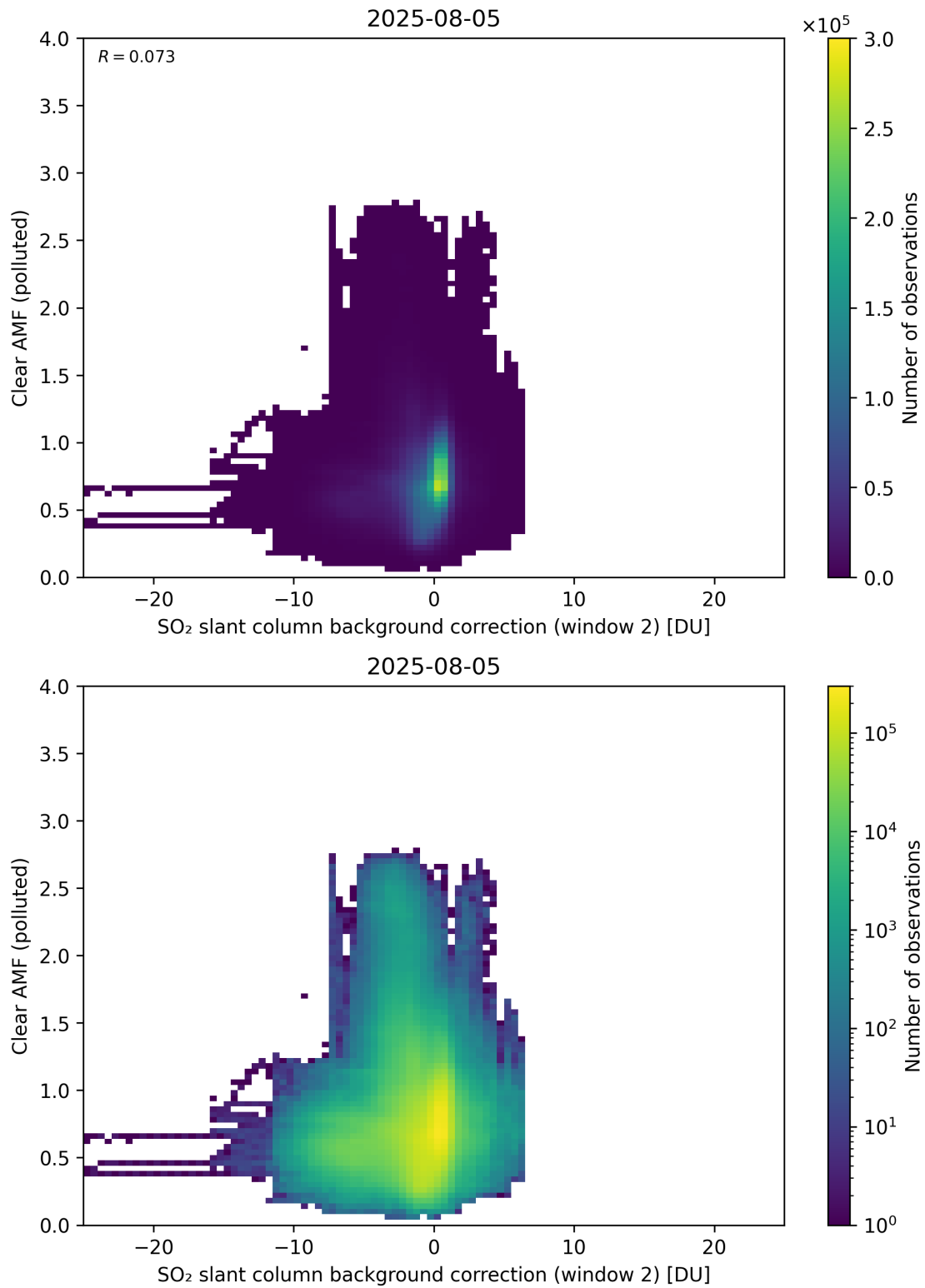
Figure 126: Scatter density plot of “SO 2 slant column background correction (window 2)” against “Clear AMF (polluted)” for 2025-08-04 to 2025-08-06.
