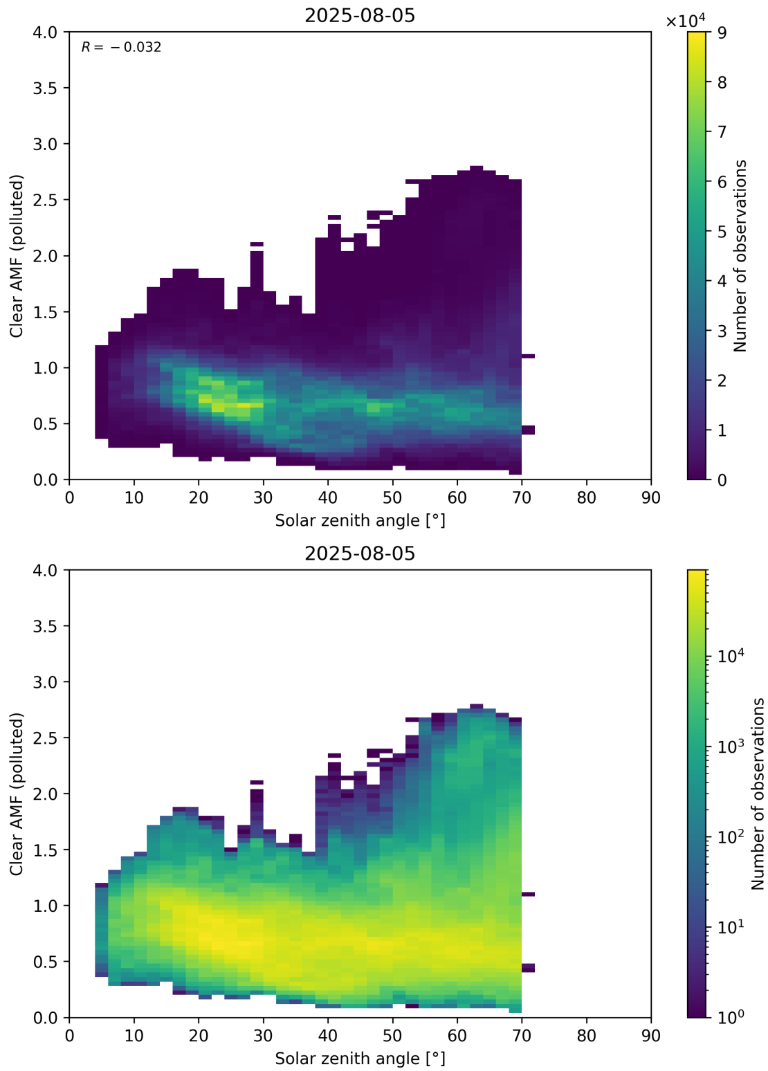
Figure 178: Scatter density plot of “Solar zenith angle” against “Clear AMF (polluted)” for 2025-08-04 to 2025-08-06.
