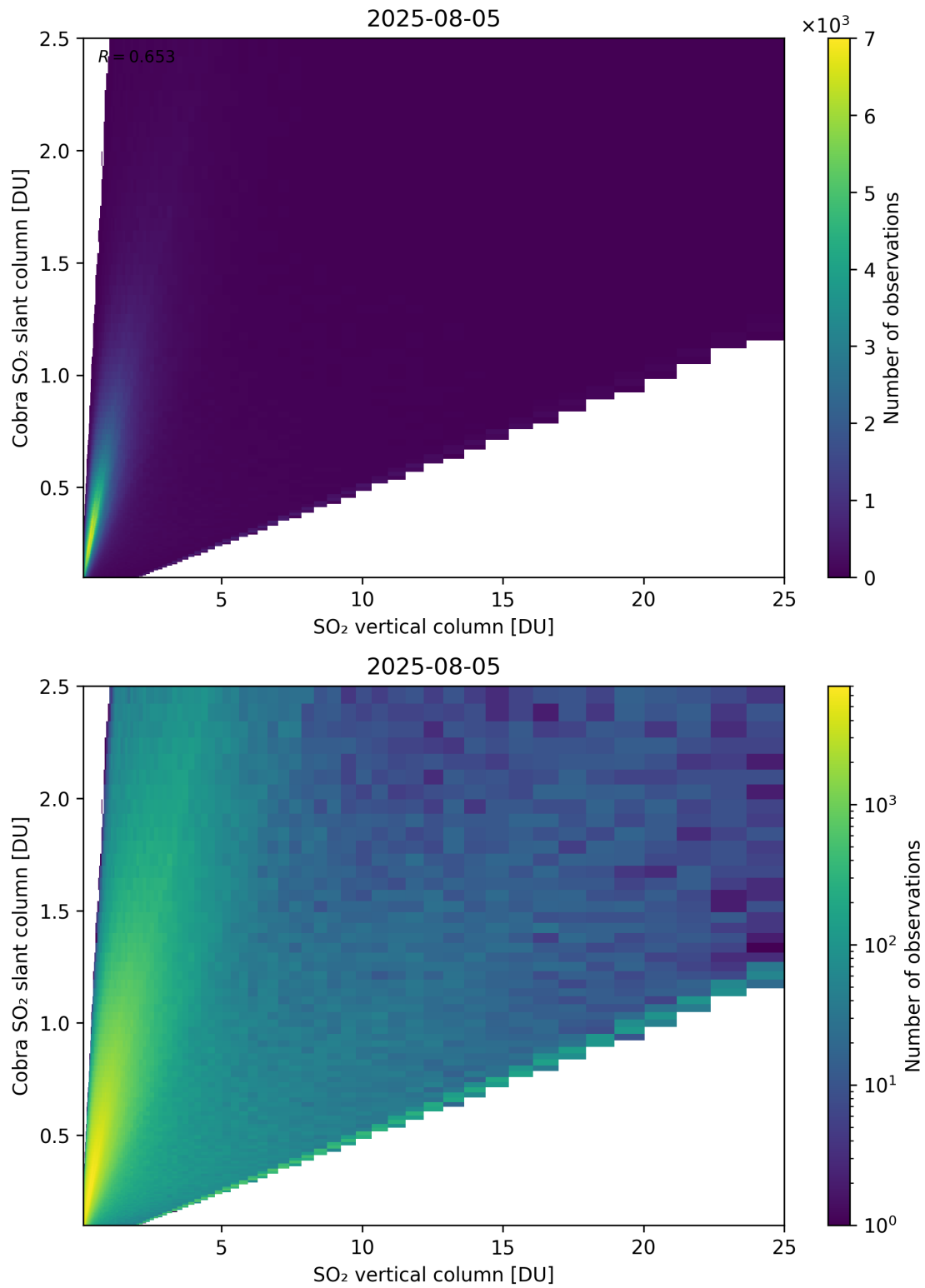
Figure 349: Scatter density plot of “SO 2 vertical column” against “Cobra SO 2 slant column” for 2025-08-04 to 2025-08-06.
