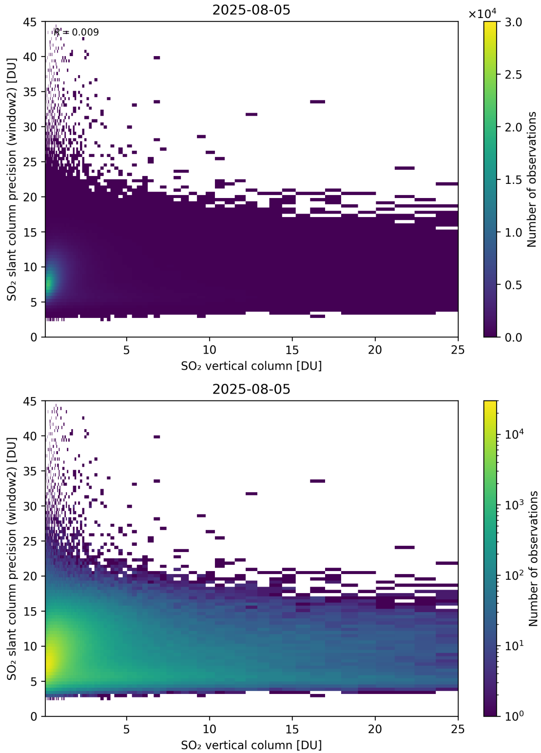
Figure 356: Scatter density plot of “SO 2 vertical column” against “SO 2 slant column precision (window2)” for 2025-08-04 to 2025-08-06.
