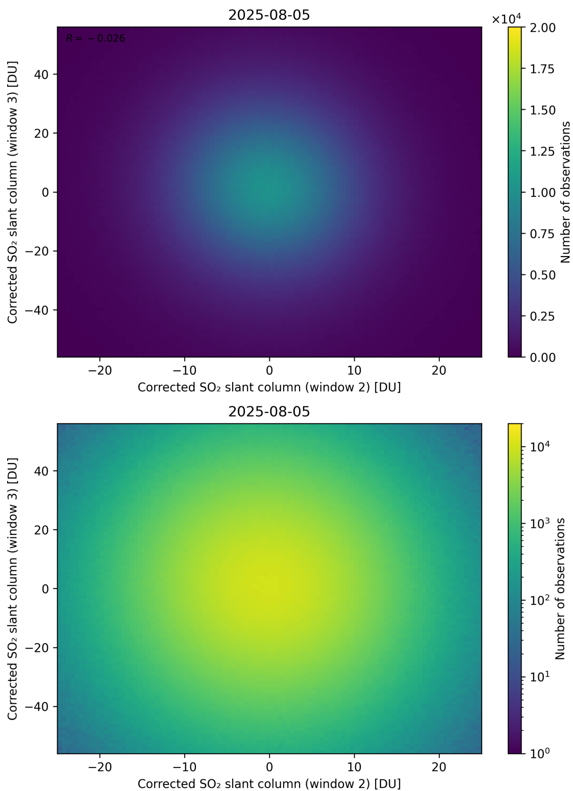
Figure 250: Scatter density plot of “Corrected SO 2 slant column (window 2)” against “Corrected SO 2 slant column (window 3)” for 2025-08-04 to 2025-08-06.
