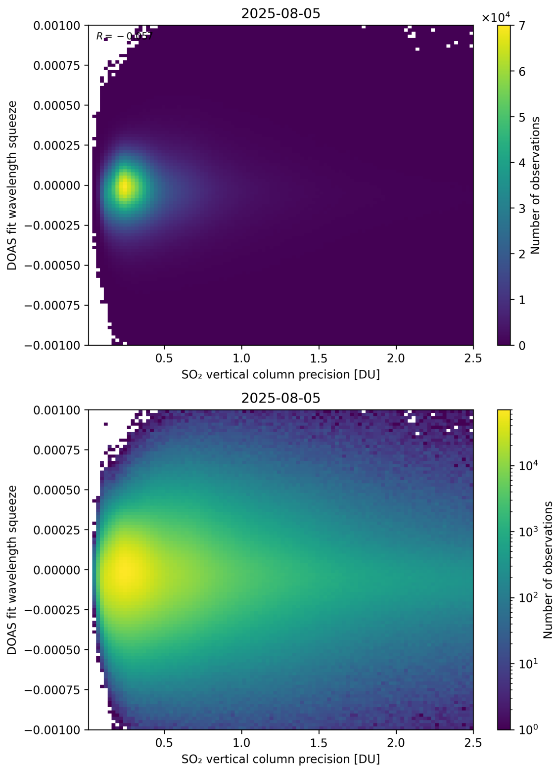
Figure 333: Scatter density plot of “SO 2 vertical column precision” against “DOAS fit wavelength squeeze” for 2025-08-04 to 2025-08-06.
