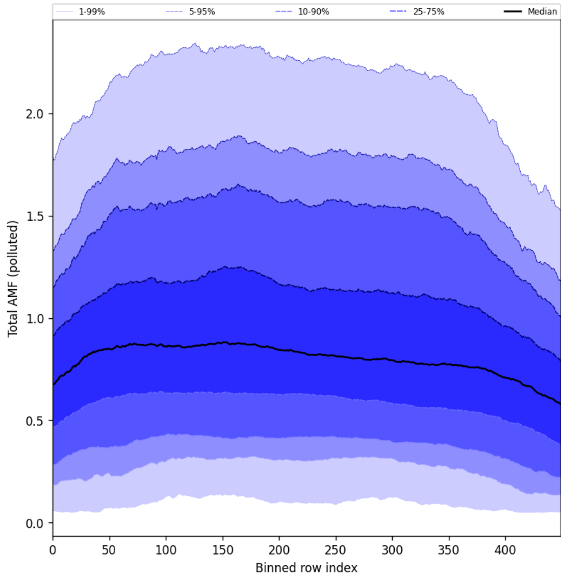
Figure 105: Along track statistics of “Total AMF (polluted)” for 2025-08-04 to 2025-08-06
