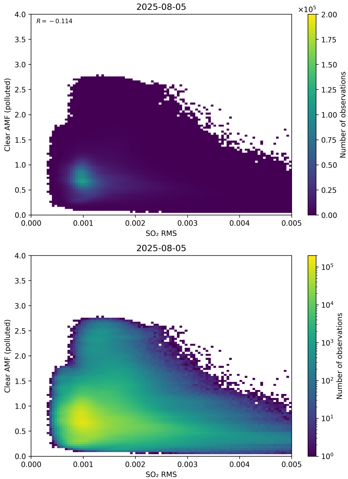
Figure 147: Scatter density plot of “SO 2 RMS” against “Clear AMF (polluted)” for 2025-08-04 to 2025-08-06.
