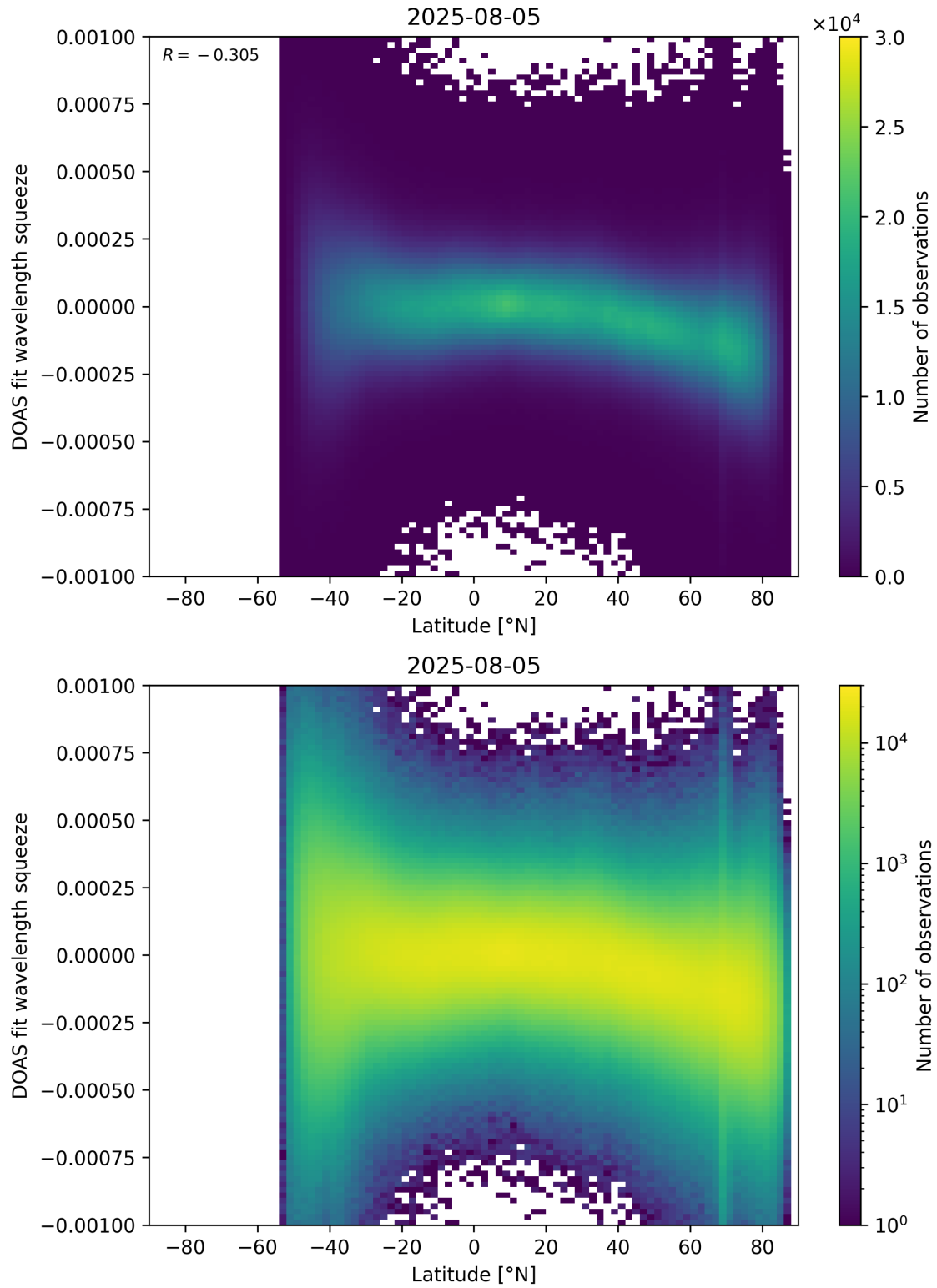
Figure 154: Scatter density plot of “Latitude” against “DOAS fit wavelength squeeze” for 2025-08-04 to 2025-08-06.
