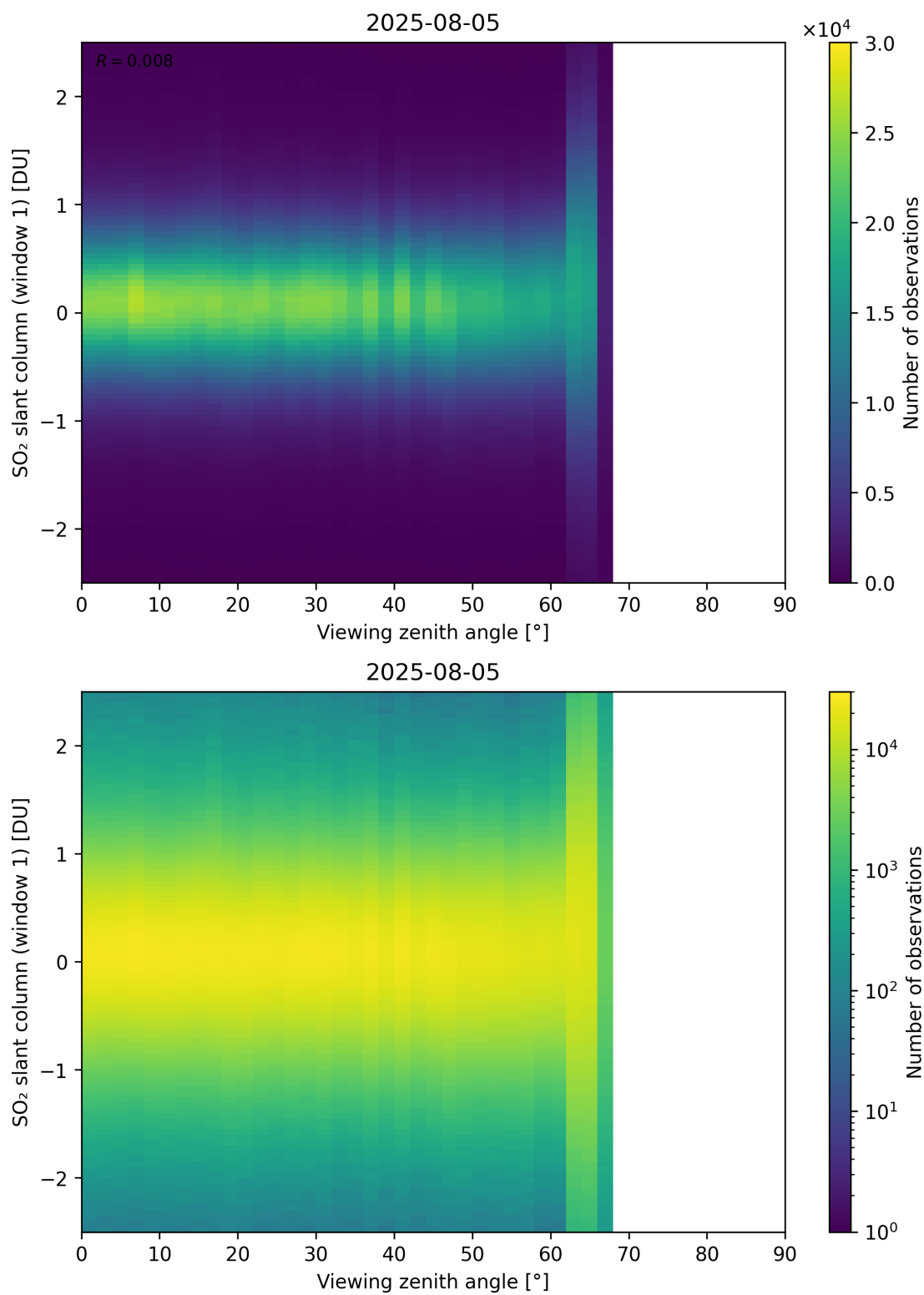
Figure 376: Scatter density plot of “Viewing zenith angle” against “SO 2 slant column (window 1)” for 2025-08-04 to 2025-08-06.
