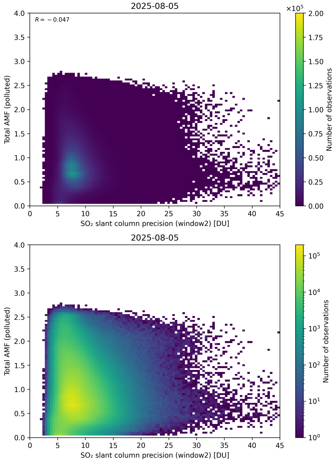
Figure 301: Scatter density plot of “SO 2 slant column precision (window2)” against “Total AMF (polluted)” for 2025-08-04 to 2025-08-06.
