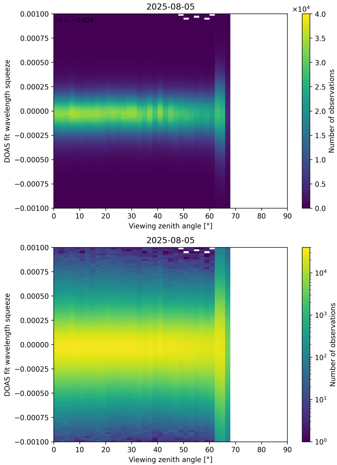
Figure 366: Scatter density plot of “Viewing zenith angle” against “DOAS fit wavelength squeeze” for 2025-08-04 to 2025-08-06.
