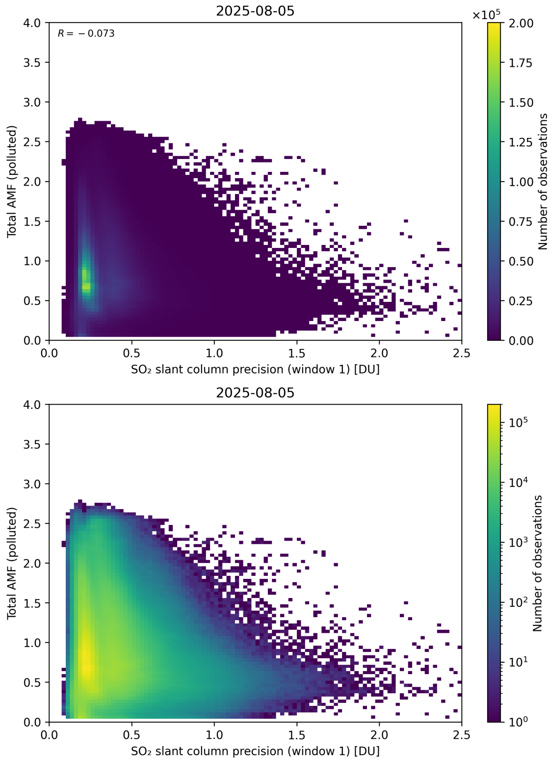
Figure 280: Scatter density plot of “SO 2 slant column precision (window 1)” against “Total AMF (polluted)” for 2025-08-04 to 2025-08-06.
