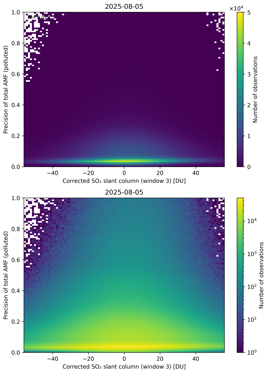
Figure 261: Scatter density plot of “Corrected SO 2 slant column (window 3)” against “Precision of total AMF (polluted)” for 2025-08-04 to 2025-08-06.
