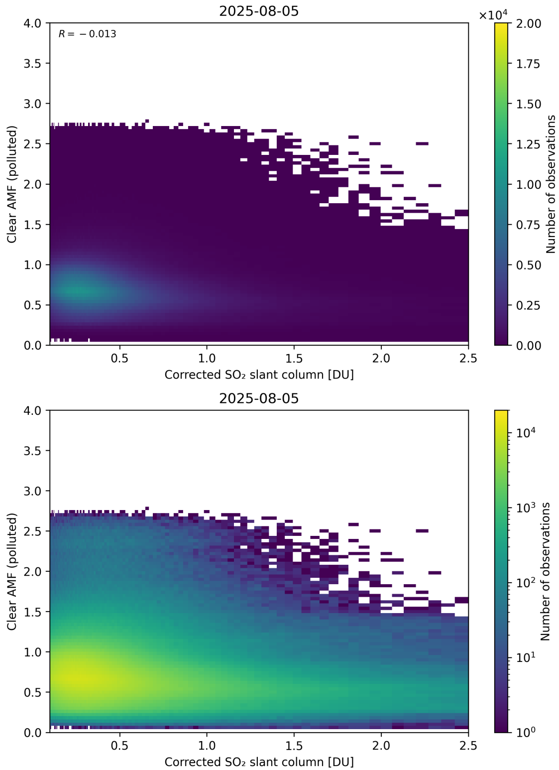
Figure 232: Scatter density plot of “Corrected SO 2 slant column” against “Clear AMF (polluted)” for 2025-08-04 to 2025-08-06.
