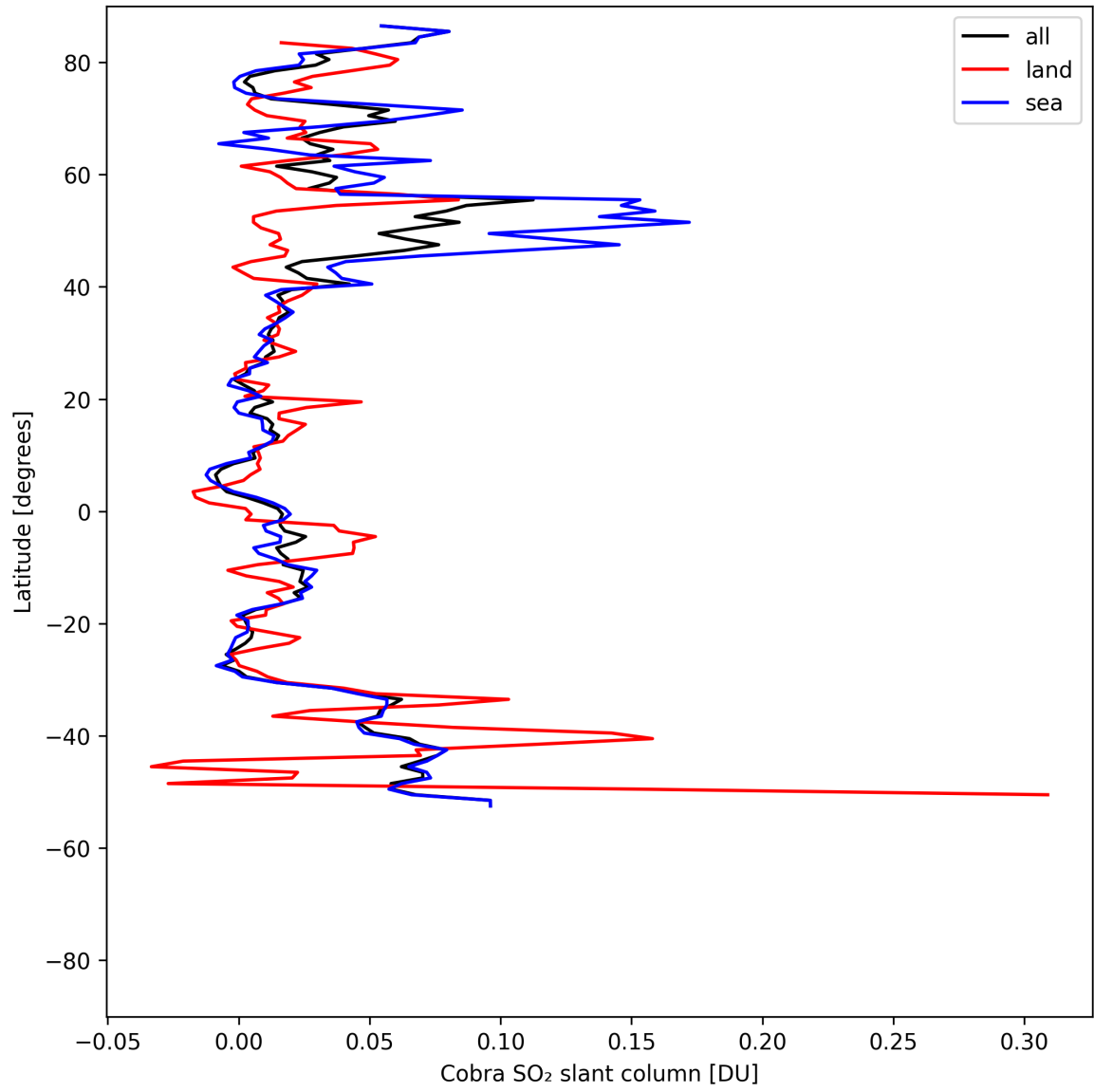
Figure 35: Zonal average of “Cobra SO 2 slant column” for 2025-08-04 to 2025-08-06.
