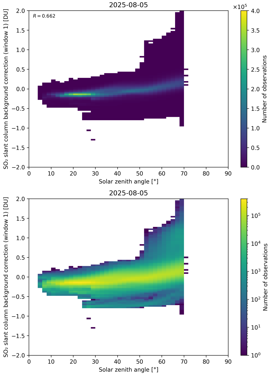
Figure 171: Scatter density plot of “Solar zenith angle” against “SO 2 slant column background correction (window 1)” for 2025-08-04 to 2025-08-06.
