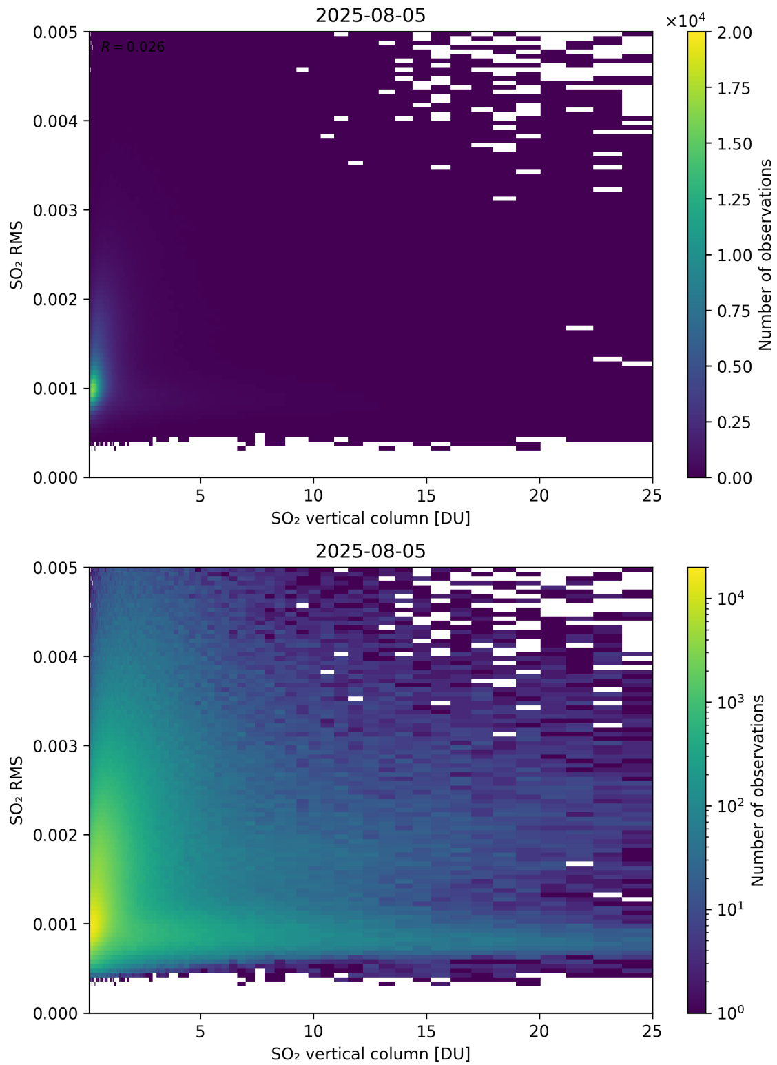
Figure 328: Scatter density plot of “SO 2 vertical column” against “SO 2 RMS” for 2025-08-04 to 2025-08-06.
