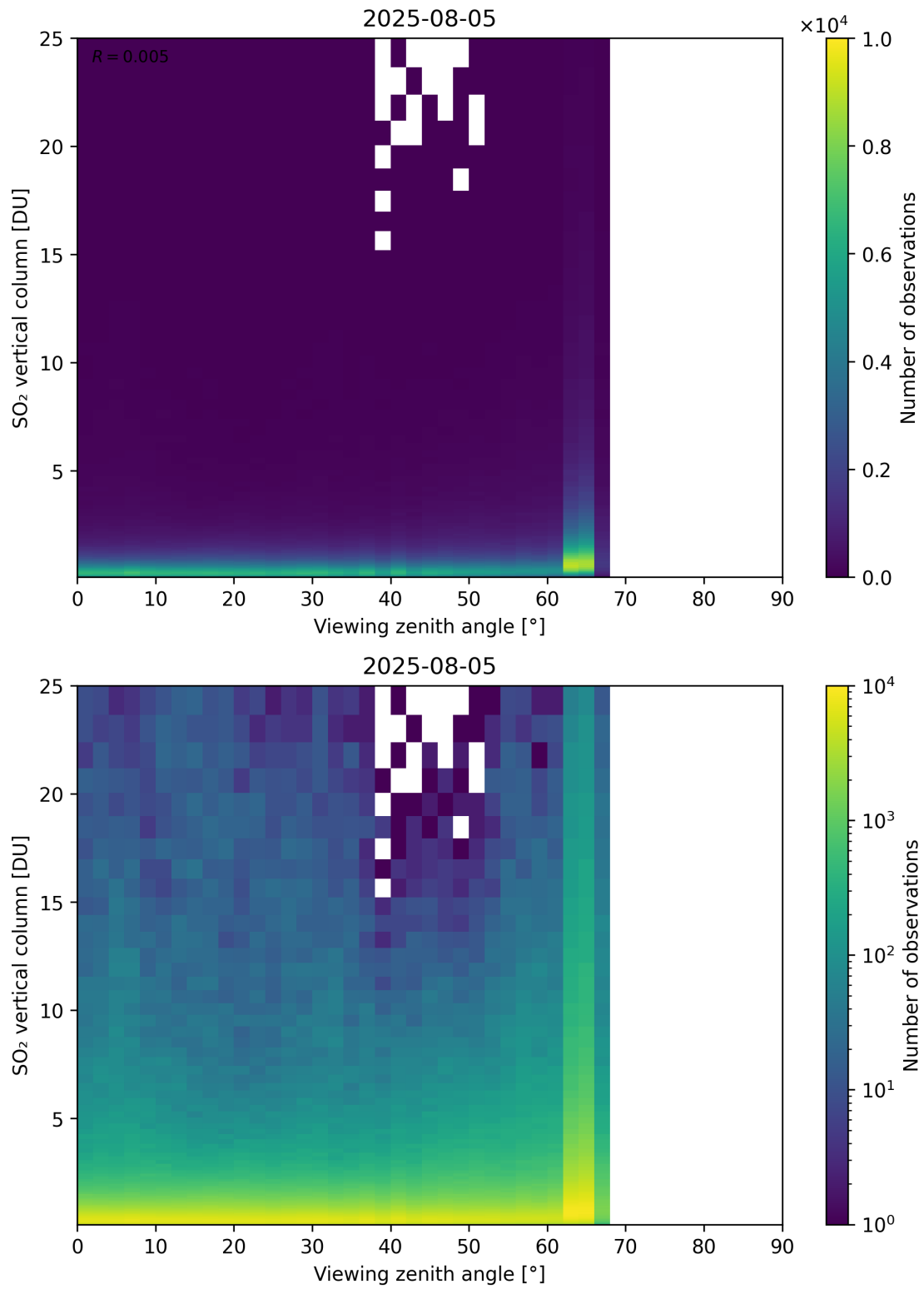
Figure 383: Scatter density plot of “Viewing zenith angle” against “SO 2 vertical column” for 2025-08-04 to 2025-08-06.
