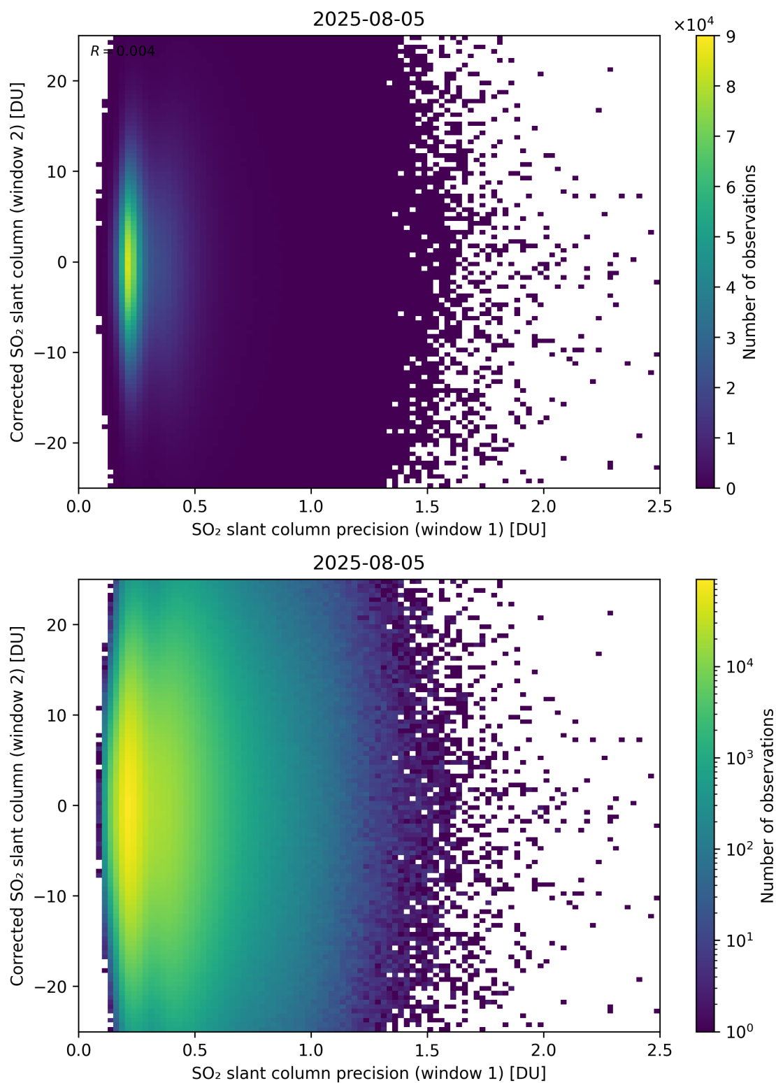
Figure 275: Scatter density plot of “SO 2 slant column precision (window 1)” against “Corrected SO 2 slant column (window 2)” for 2025-08-04 to 2025-08-06.
