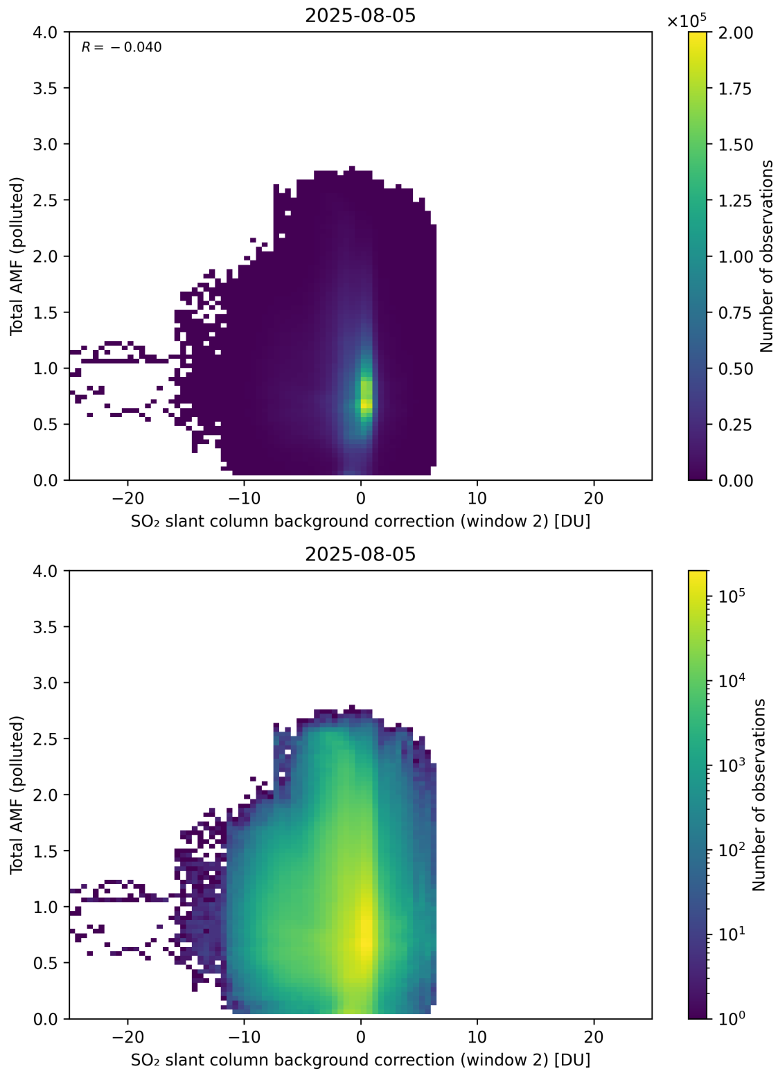
Figure 130: Scatter density plot of “SO 2 slant column background correction (window 2)” against “Total AMF (polluted)” for 2025-08-04 to 2025-08-06.
