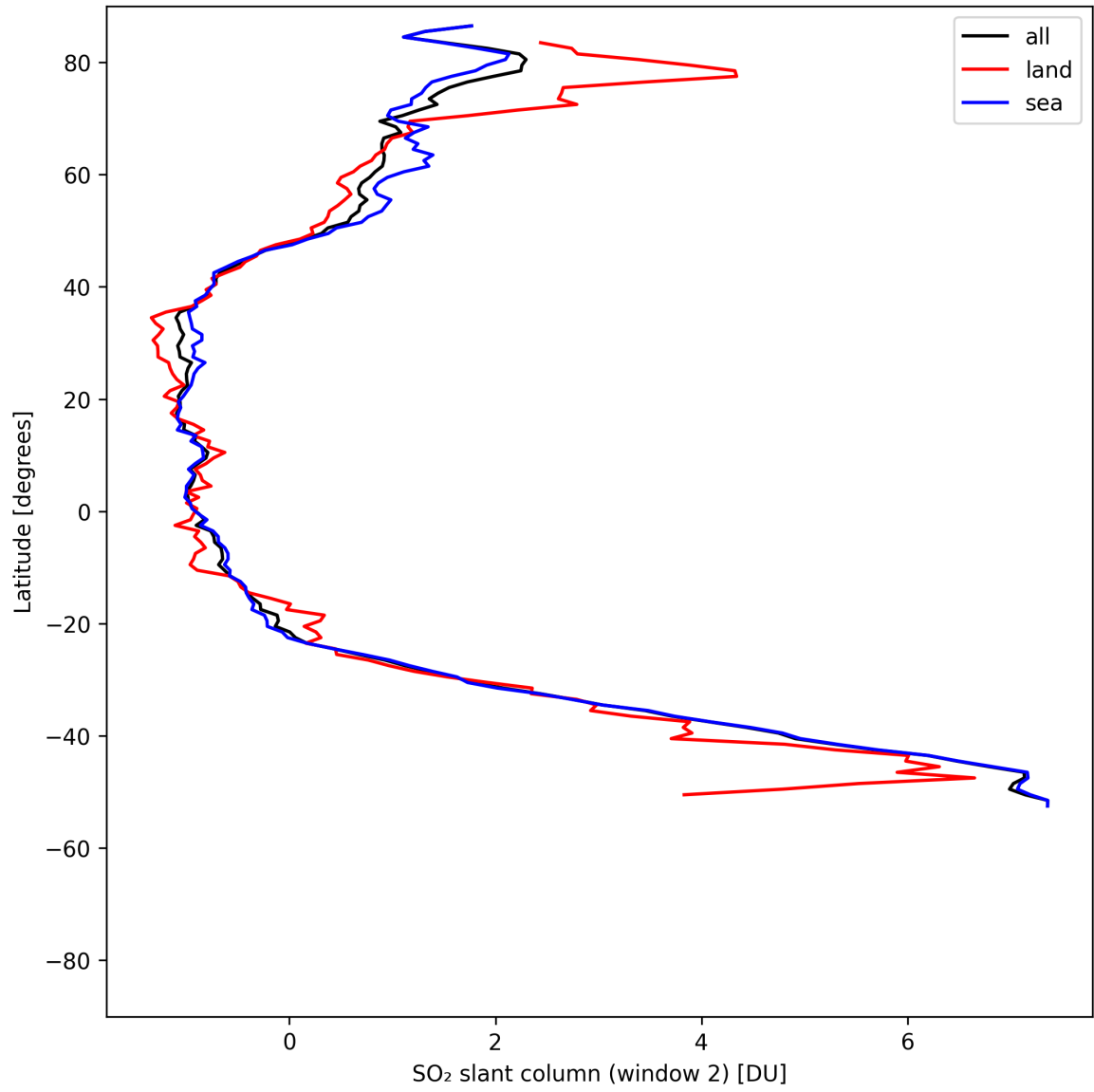
Figure 41: Zonal average of “SO 2 slant column (window 2)” for 2025-08-04 to 2025-08-06.
