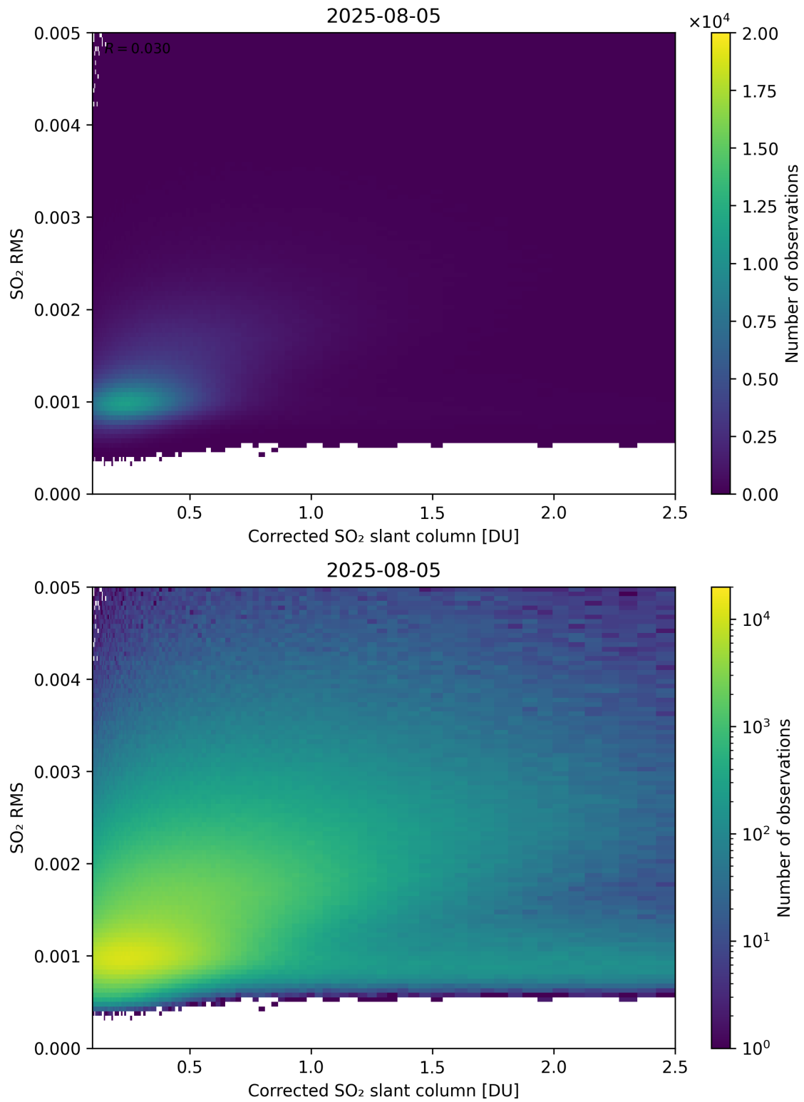
Figure 231: Scatter density plot of “Corrected SO 2 slant column” against “SO 2 RMS” for 2025-08-04 to 2025-08-06.
