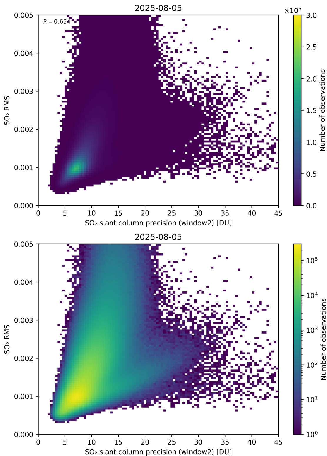
Figure 295: Scatter density plot of “SO 2 slant column precision (window2)” against “SO 2 RMS” for 2025-08-04 to 2025-08-06.
