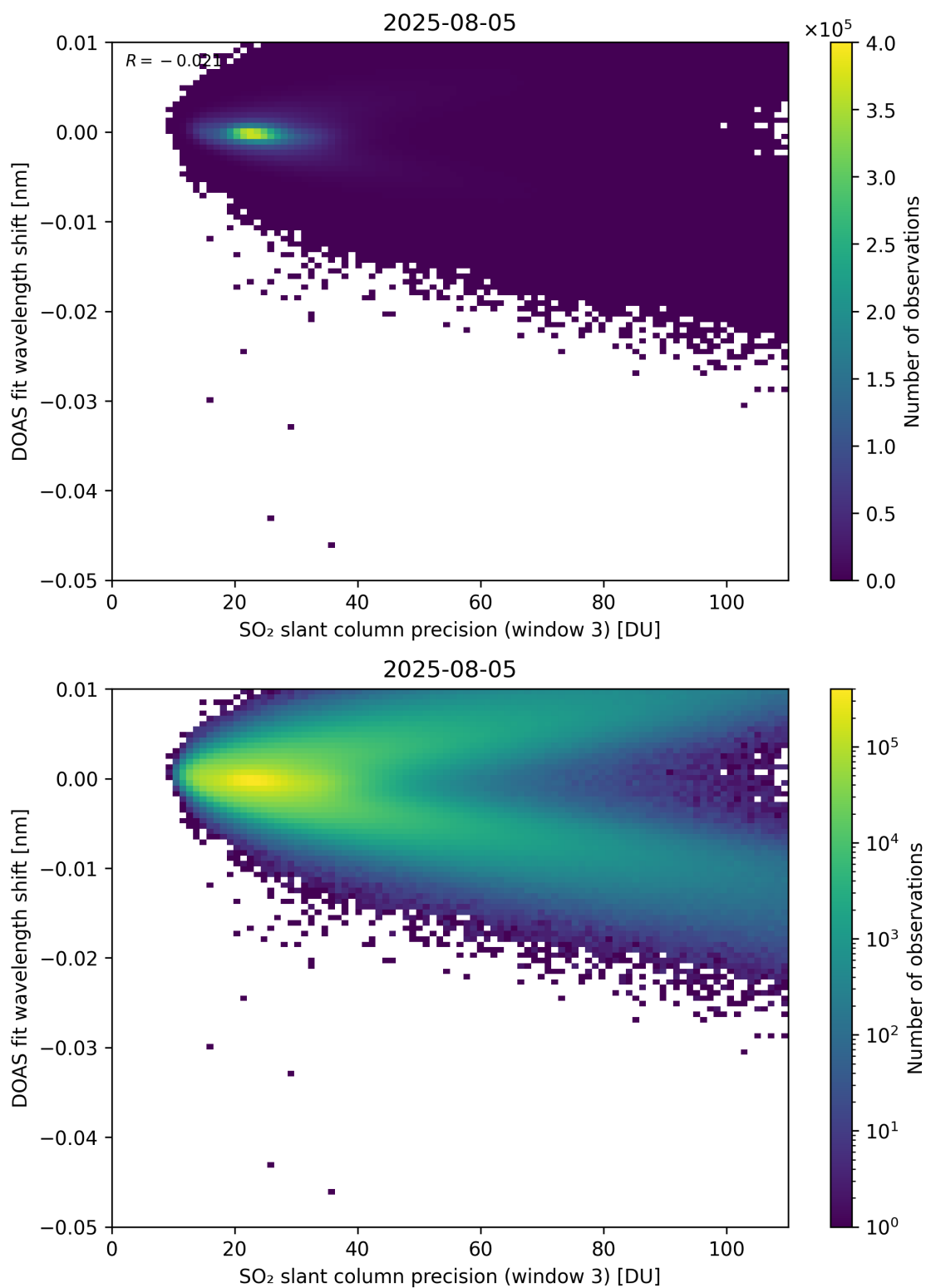
Figure 308: Scatter density plot of “SO 2 slant column precision (window 3)” against “DOAS fit wavelength shift” for 2025-08-04 to 2025-08-06.
