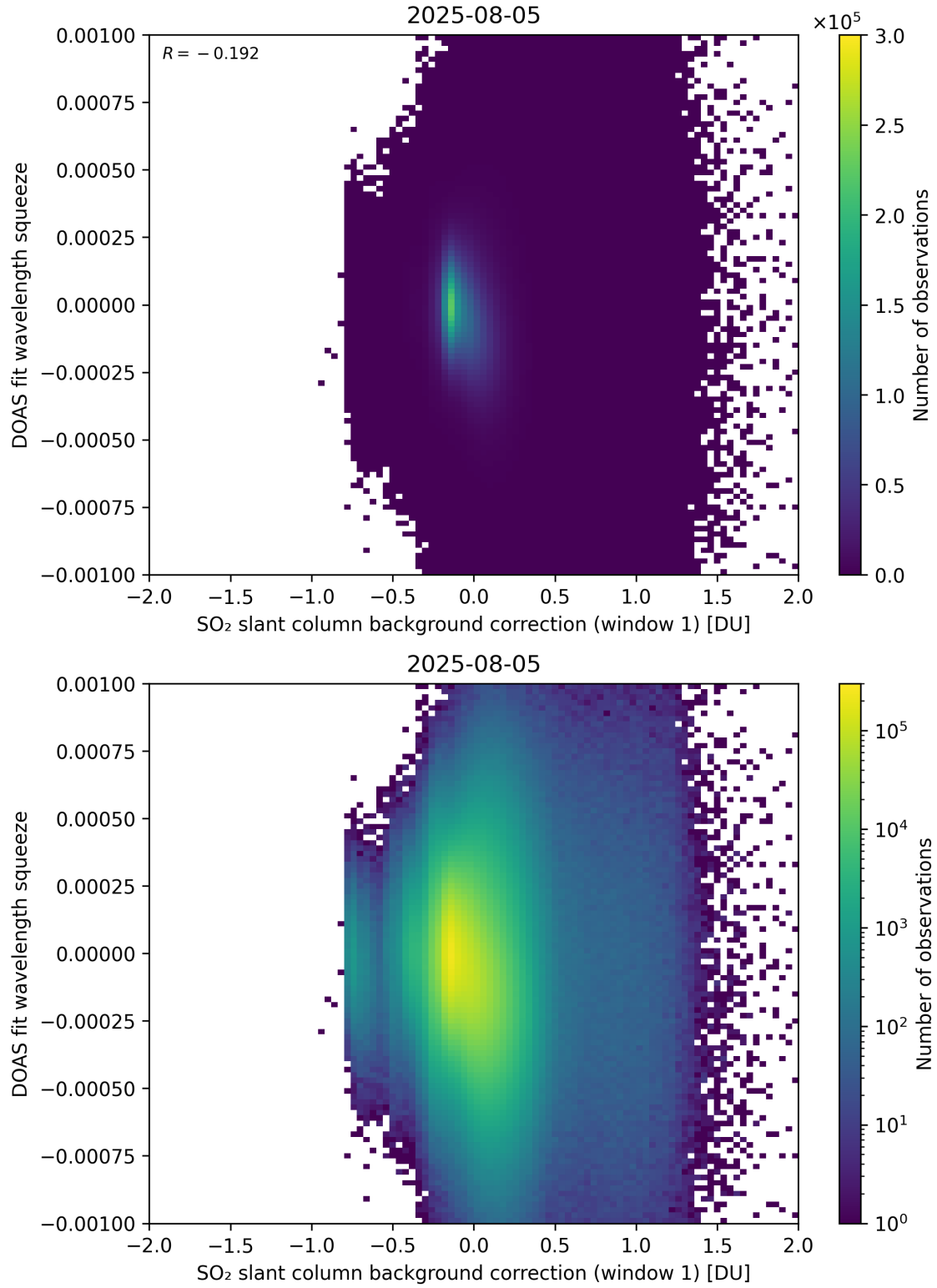
Figure 112: Scatter density plot of “SO 2 slant column background correction (window 1)” against “DOAS fit wavelength squeeze” for 2025-08-04 to 2025-08-06.
