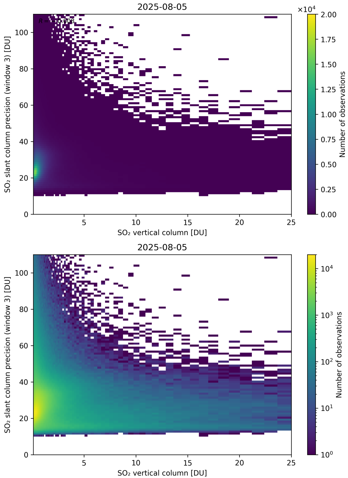
Figure 358: Scatter density plot of “SO 2 vertical column” against “SO 2 slant column precision (window 3)” for 2025-08-04 to 2025-08-06.
