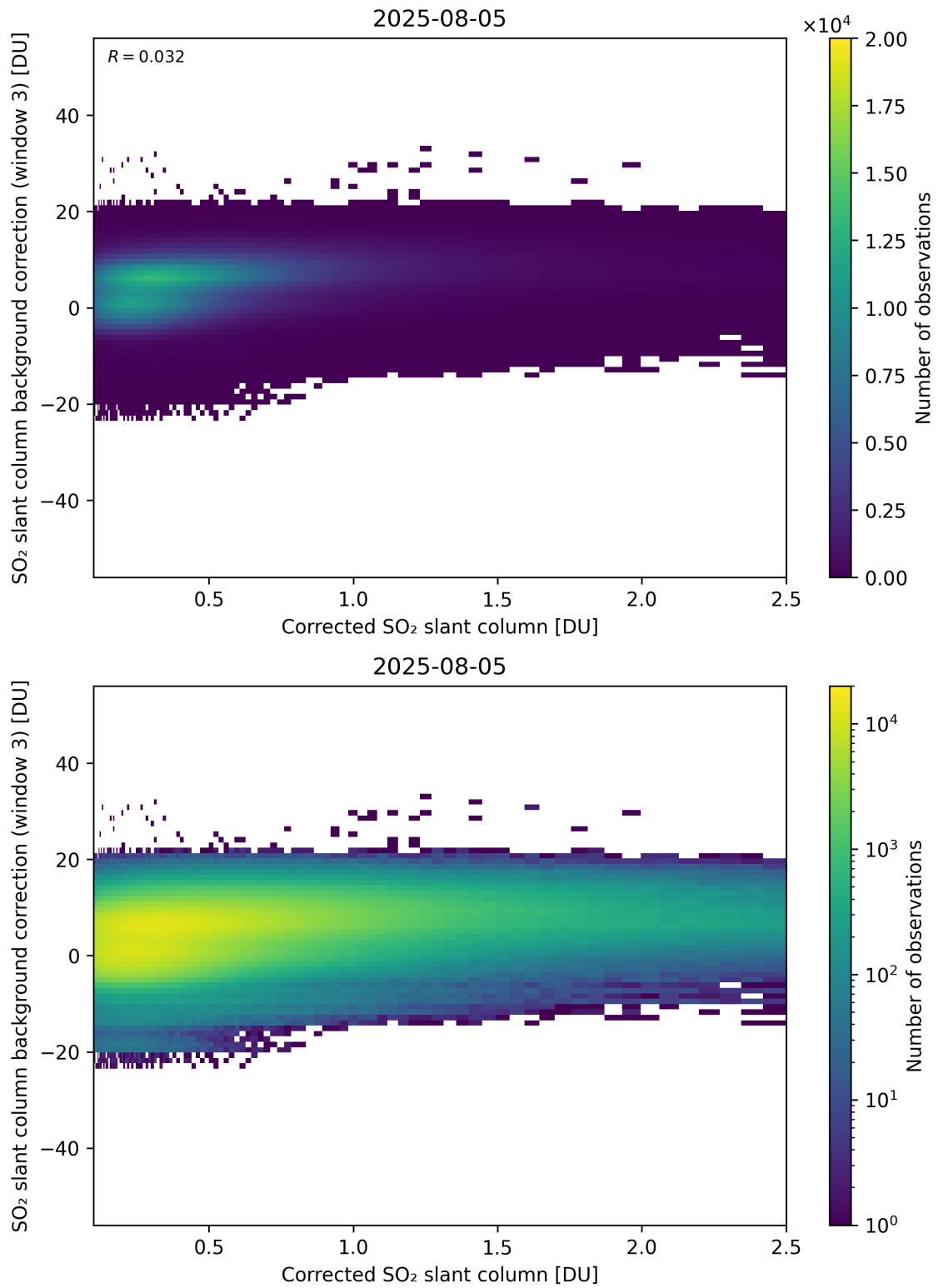
Figure 228: Scatter density plot of “Corrected SO 2 slant column” against “SO 2 slant column background correction (window 3)” for 2025-08-04 to 2025-08-06.
