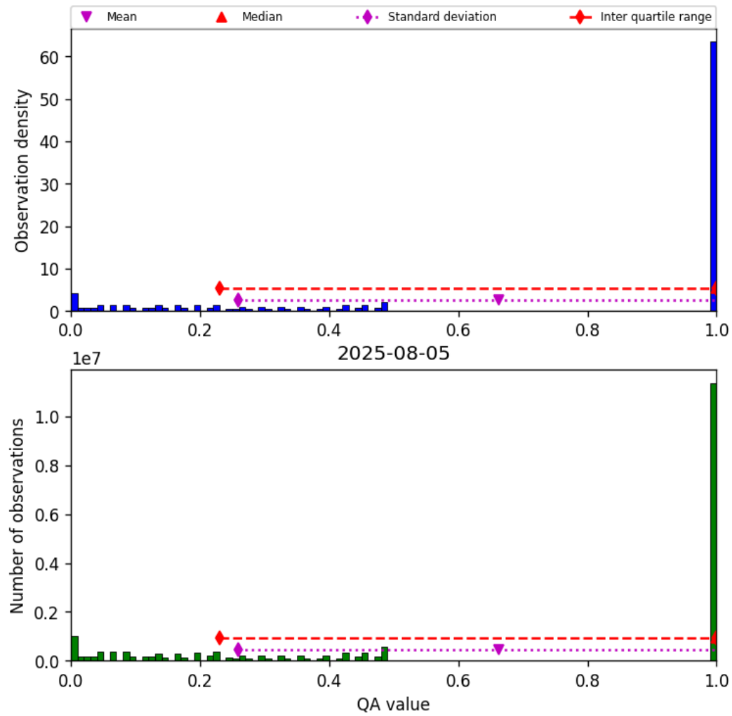
Figure 57: Histogram of “QA value” for 2025-08-04 to 2025-08-06
