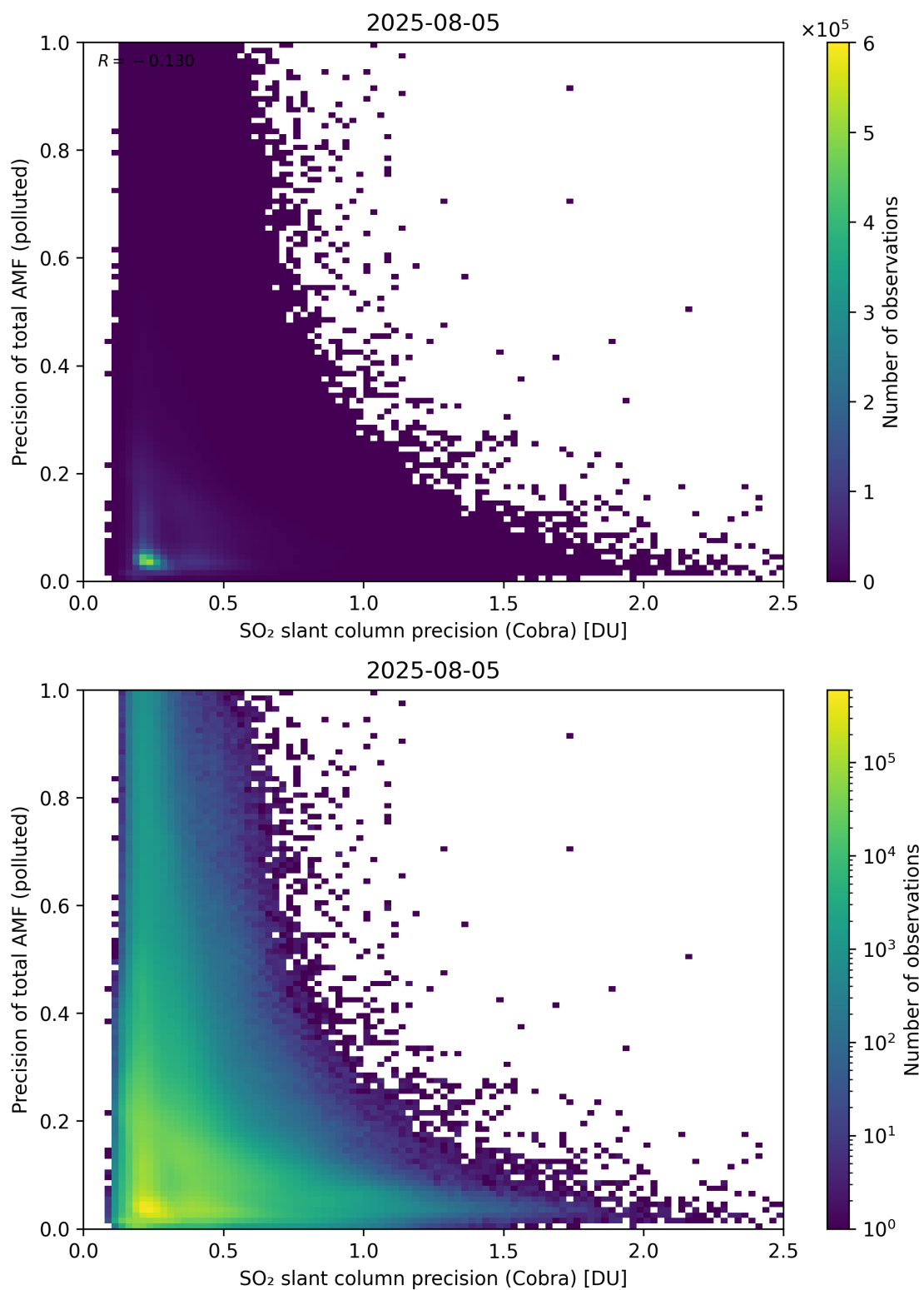
Figure 214: Scatter density plot of “SO 2 slant column precision (Cobra)” against “Precision of total AMF (polluted)” for 2025-08-04 to 2025-08-06.
