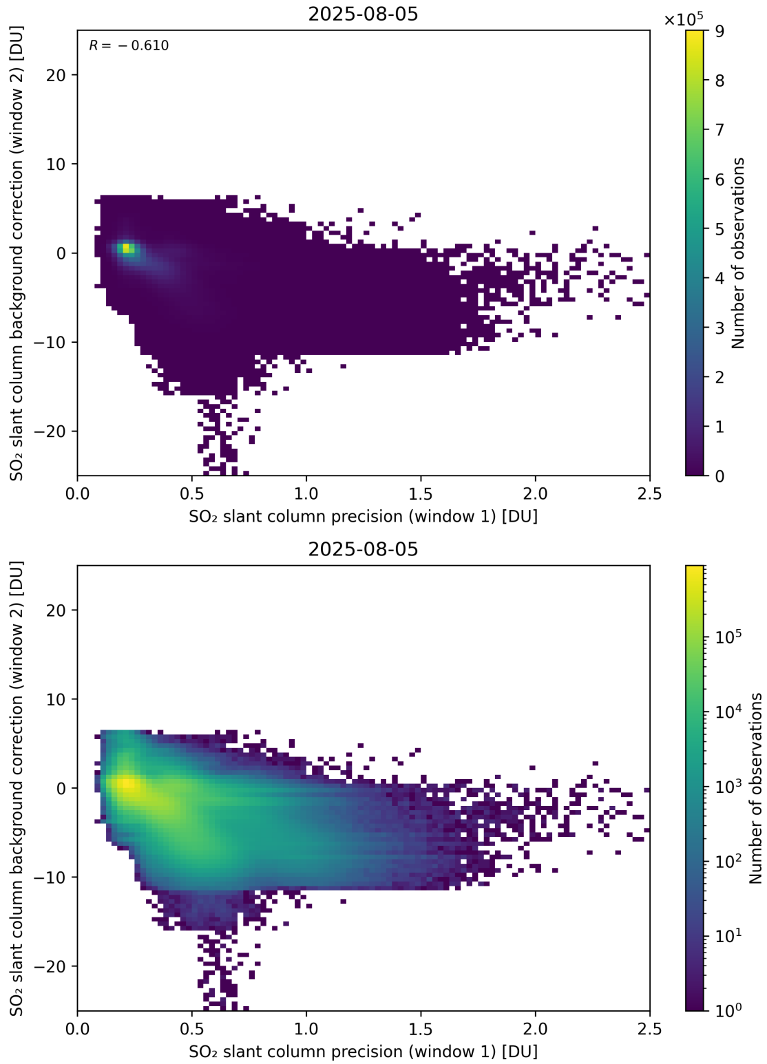
Figure 269: Scatter density plot of “SO 2 slant column precision (window 1)” against “SO 2 slant column background correction (window 2)” for 2025-08-04 to 2025-08-06.
