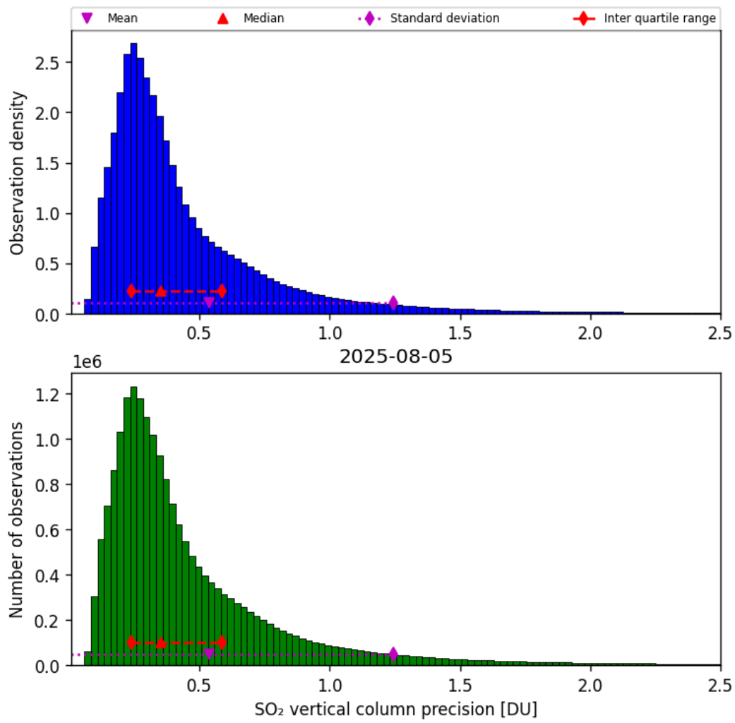
Figure 59: Histogram of “SO 2 vertical column precision” for 2025-08-04 to 2025-08-06
