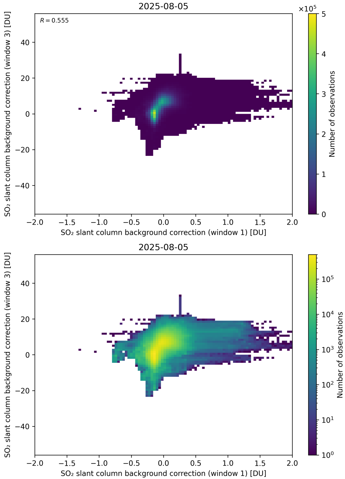
Figure 110: Scatter density plot of “SO 2 slant column background correction (window 1)” against “SO 2 slant column background correction (window 3)” for 2025-08-04 to 2025-08-06.
