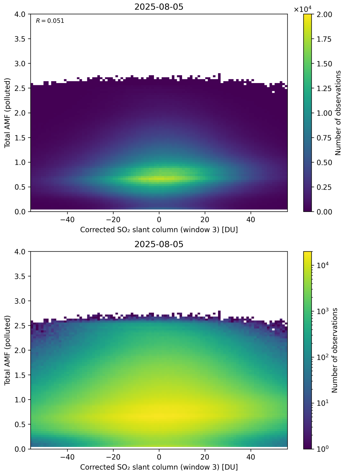
Figure 260: Scatter density plot of “Corrected SO 2 slant column (window 3)” against “Total AMF (polluted)” for 2025-08-04 to 2025-08-06.
