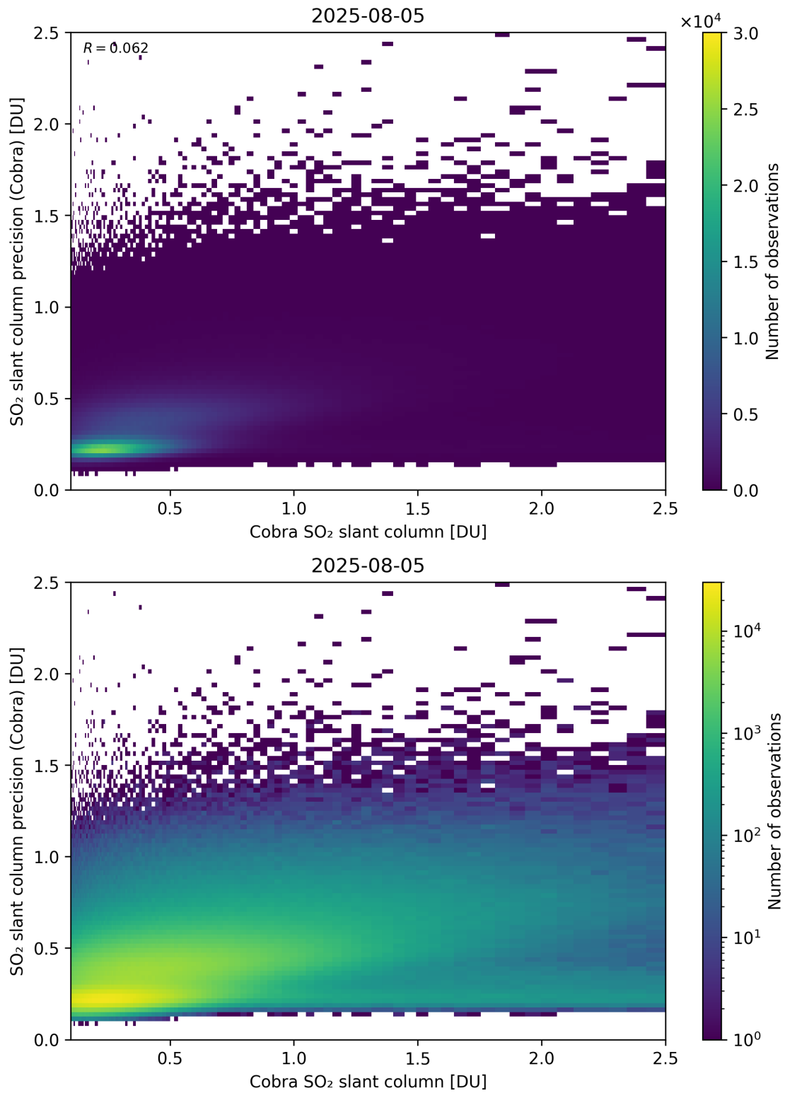
Figure 216: Scatter density plot of “Cobra SO 2 slant column” against “SO 2 slant column precision (Cobra)” for 2025-08-04 to 2025-08-06.
