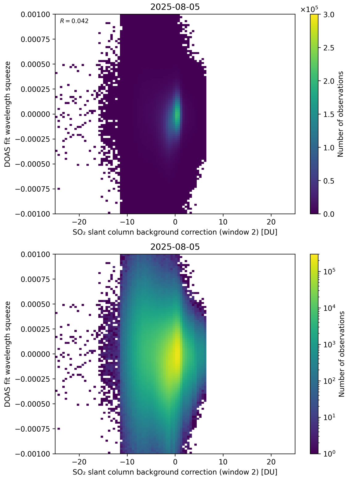
Figure 124: Scatter density plot of “SO 2 slant column background correction (window 2)” against “DOAS fit wavelength squeeze” for 2025-08-04 to 2025-08-06.
