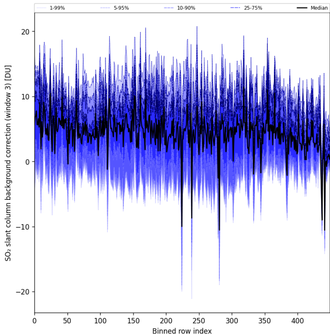
Figure 100: Along track statistics of “SO 2 slant column background correction (window 3)” for 2025-08-04 to 2025-08-06
