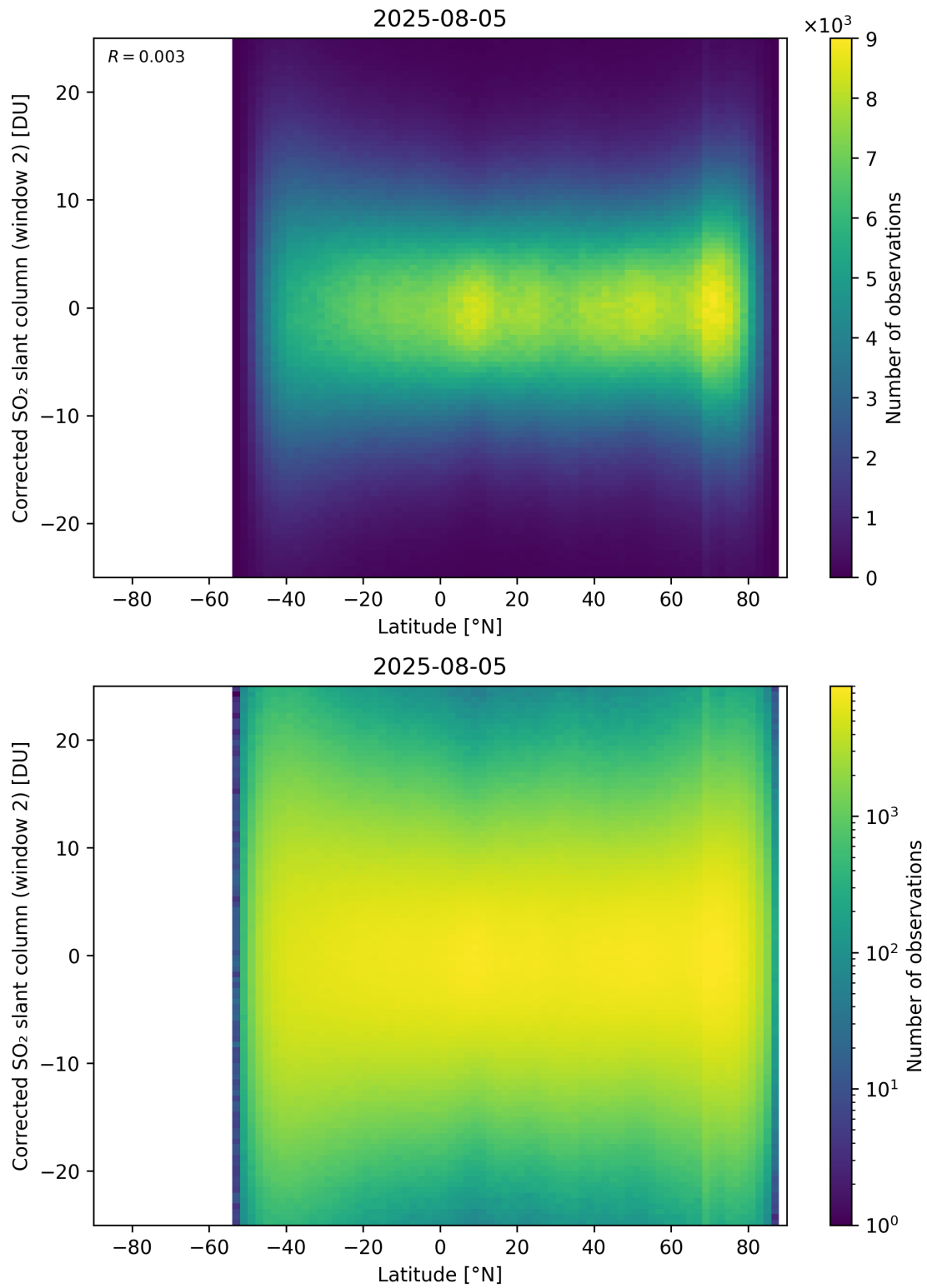
Figure 160: Scatter density plot of “Latitude” against “Corrected SO 2 slant column (window 2)” for 2025-08-04 to 2025-08-06.
