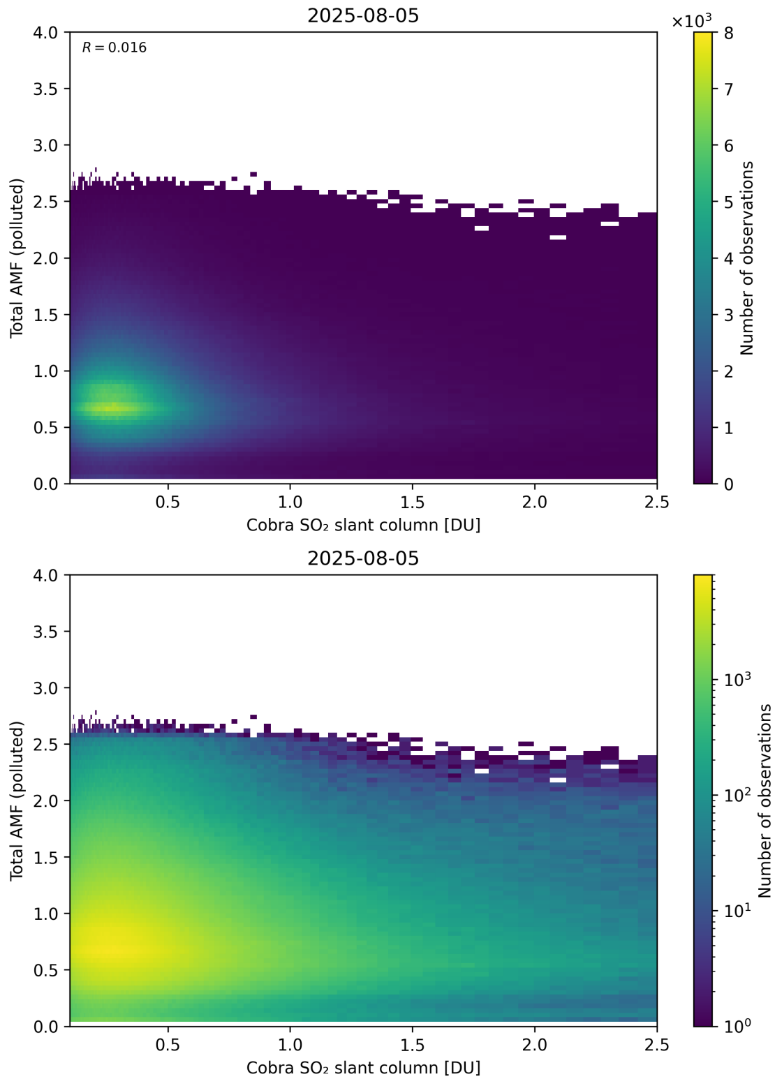
Figure 224: Scatter density plot of “Cobra SO 2 slant column” against “Total AMF (polluted)” for 2025-08-04 to 2025-08-06.
