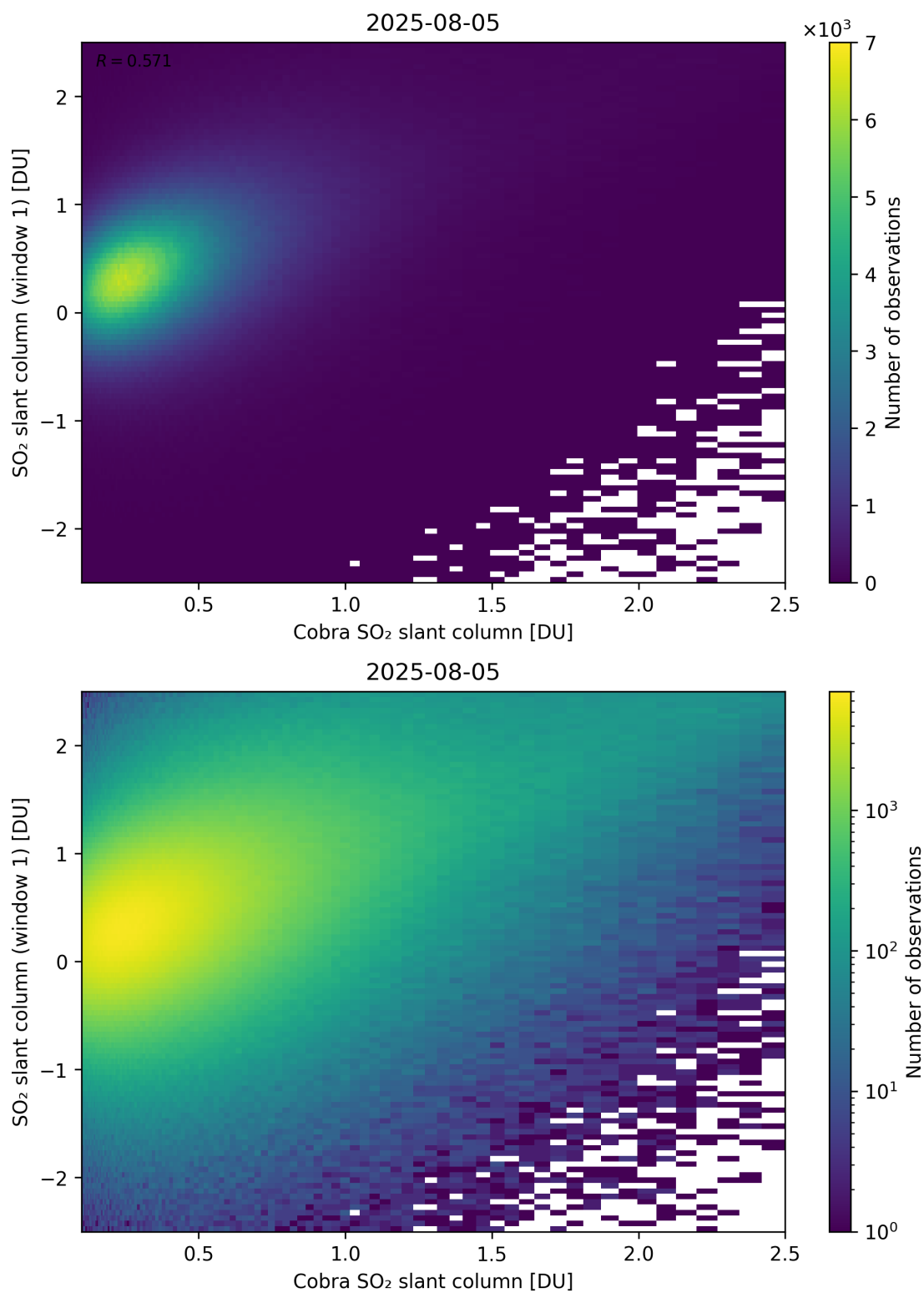
Figure 219: Scatter density plot of “Cobra SO 2 slant column” against “SO 2 slant column (window 1)” for 2025-08-04 to 2025-08-06.
