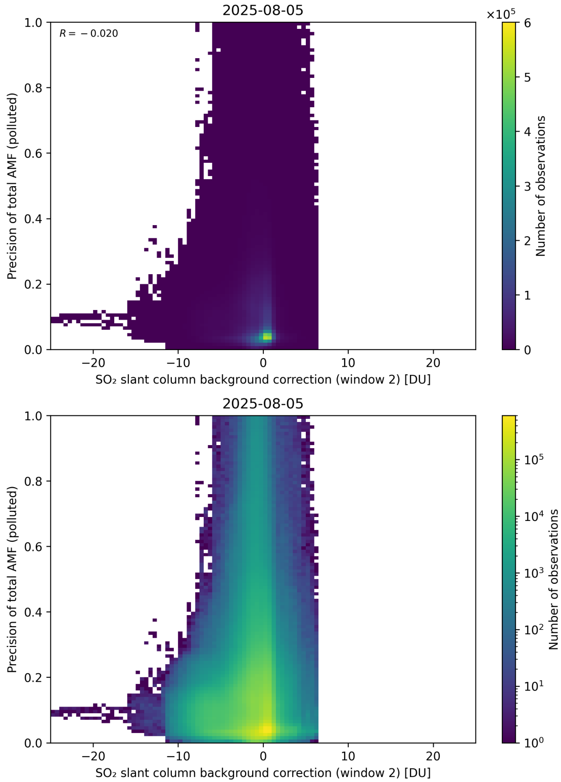
Figure 131: Scatter density plot of “SO 2 slant column background correction (window 2)” against “Precision of total AMF (polluted)” for 2025-08-04 to 2025-08-06.
