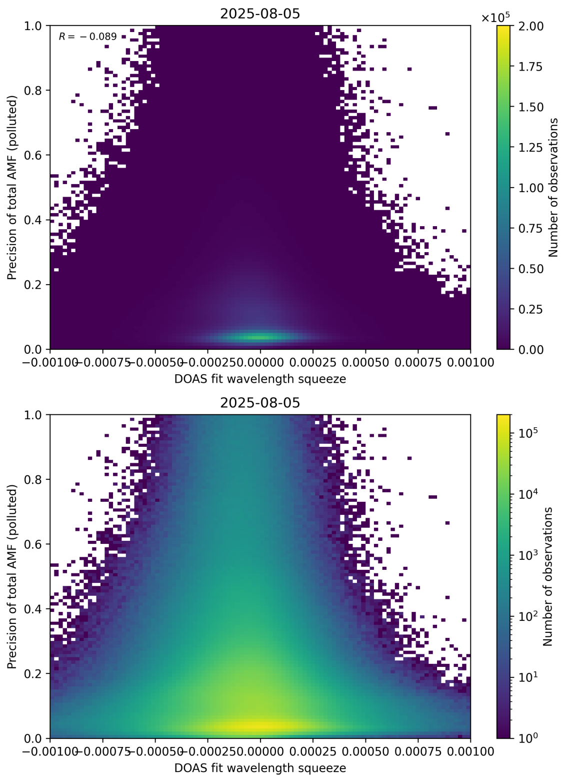
Figure 146: Scatter density plot of “DOAS fit wavelength squeeze” against “Precision of total AMF (polluted)” for 2025-08-04 to 2025-08-06.
