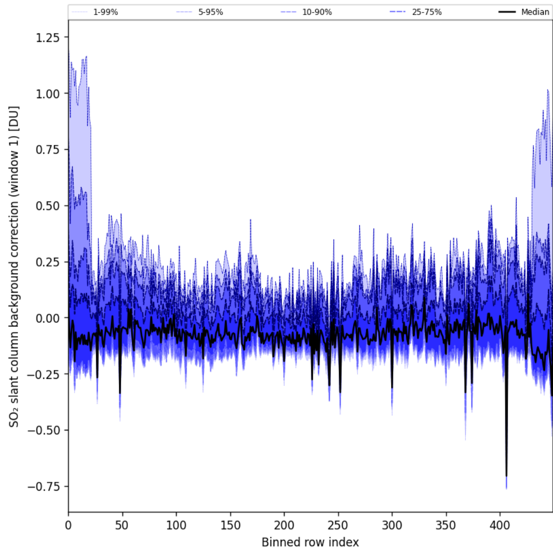
Figure 92: Along track statistics of “SO 2 slant column background correction (window 1)” for 2025-08-04 to 2025-08-06
