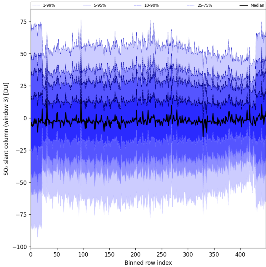
Figure 97: Along track statistics of “SO 2 slant column (window 3)” for 2025-08-04 to 2025-08-06
