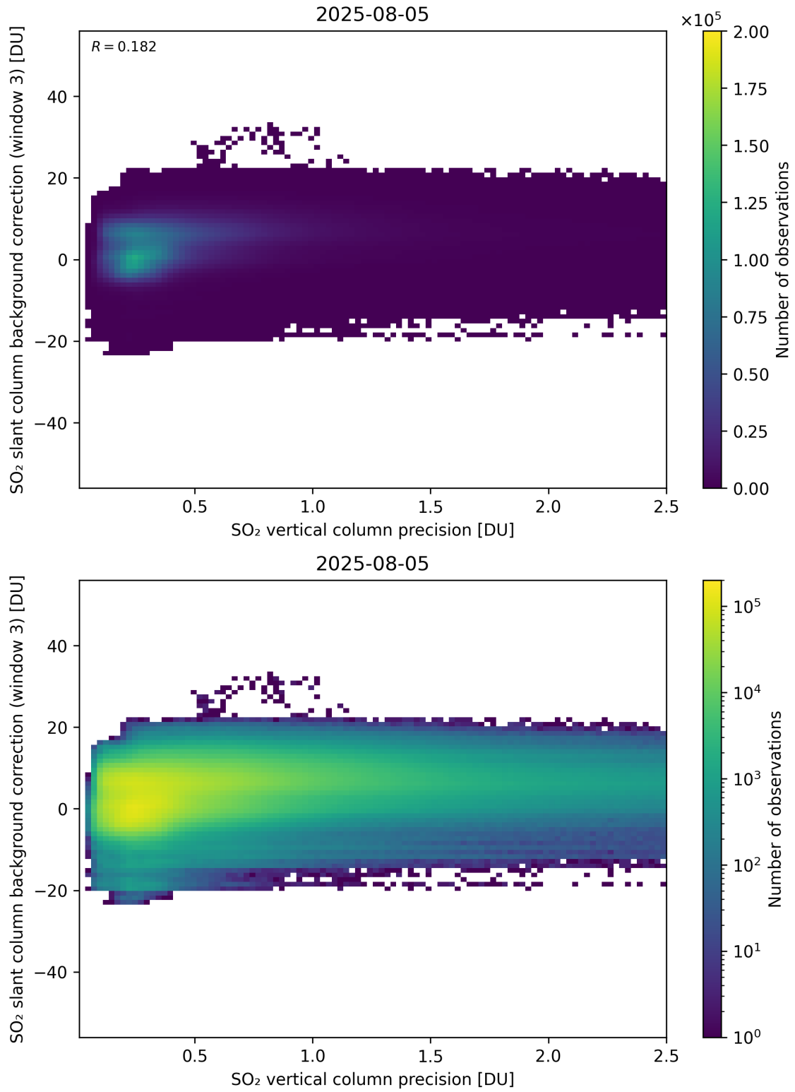
Figure 331: Scatter density plot of “SO 2 vertical column precision” against “SO 2 slant column background correction (window 3)” for 2025-08-04 to 2025-08-06.
