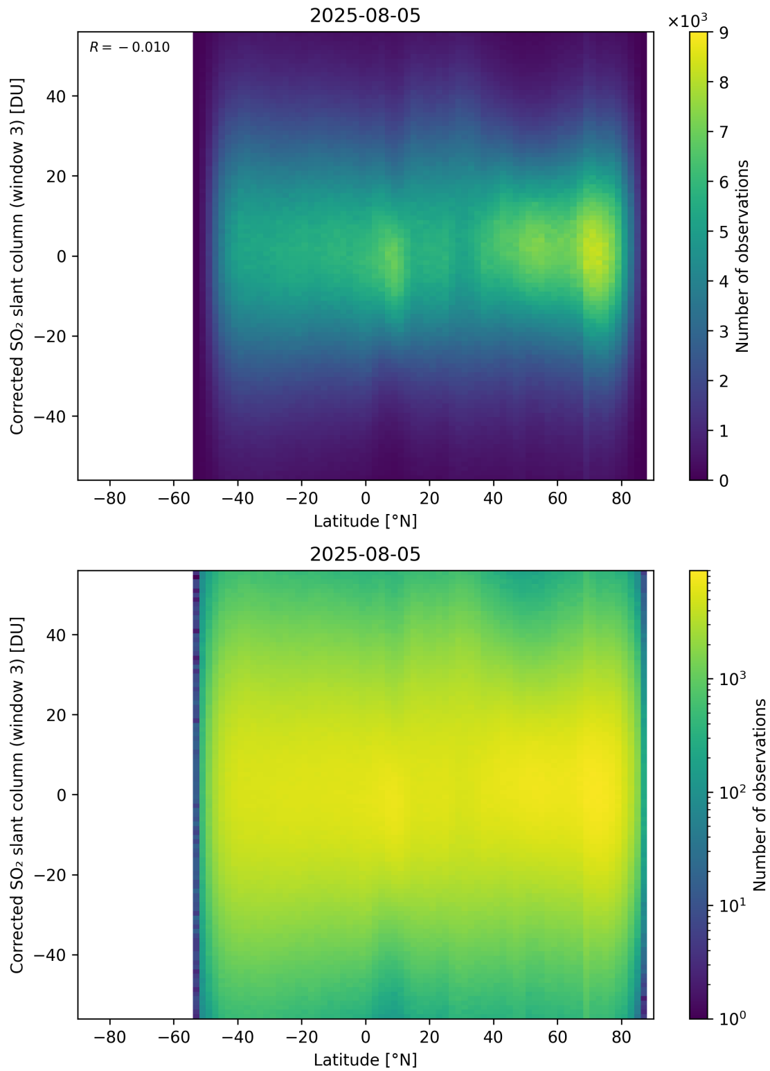
Figure 161: Scatter density plot of “Latitude” against “Corrected SO 2 slant column (window 3)” for 2025-08-04 to 2025-08-06.
