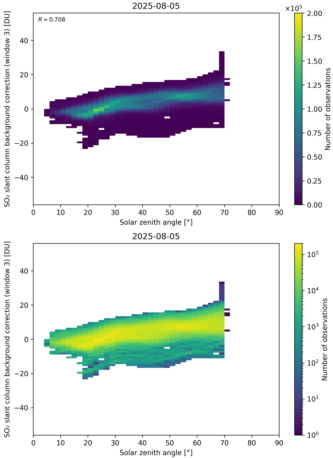
Figure 173: Scatter density plot of “Solar zenith angle” against “SO 2 slant column background correction (window 3)” for 2025-08-04 to 2025-08-06.
