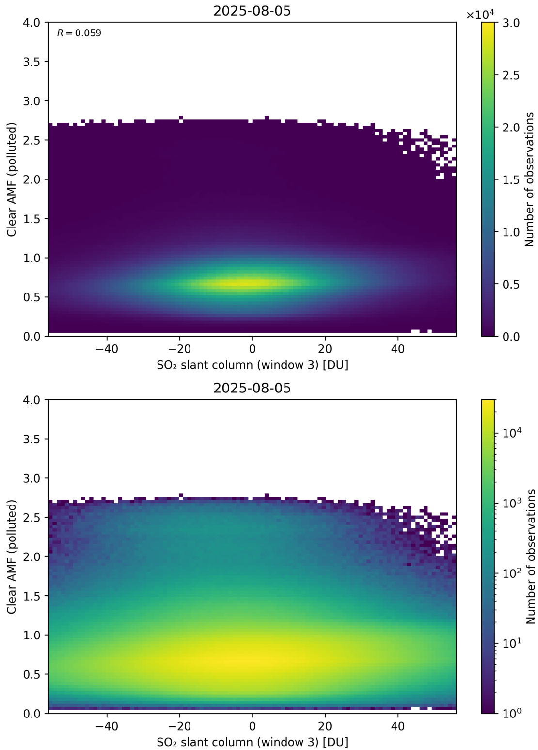
Figure 315: Scatter density plot of “SO 2 slant column (window 3)” against “Clear AMF (polluted)” for 2025-08-04 to 2025-08-06.
