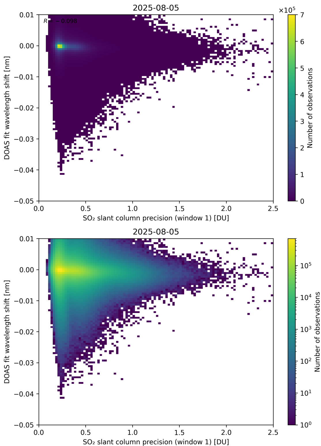
Figure 271: Scatter density plot of “SO 2 slant column precision (window 1)” against “DOAS fit wavelength shift” for 2025-08-04 to 2025-08-06.
