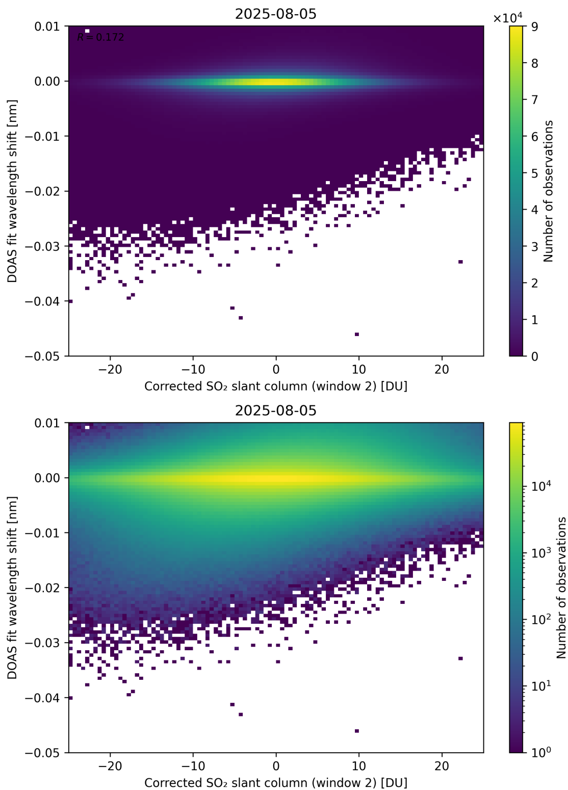
Figure 246: Scatter density plot of “Corrected SO 2 slant column (window 2)” against “DOAS fit wavelength shift” for 2025-08-04 to 2025-08-06.
