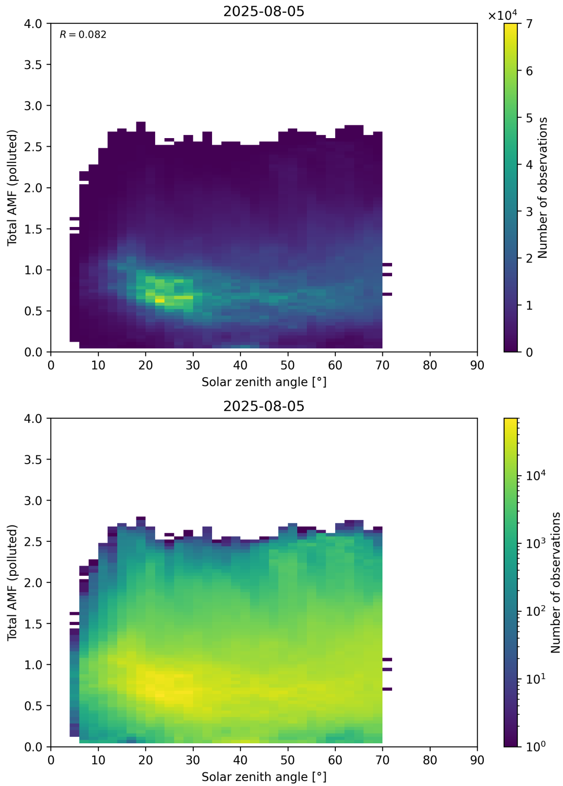
Figure 189: Scatter density plot of “Solar zenith angle” against “Total AMF (polluted)” for 2025-08-04 to 2025-08-06.
