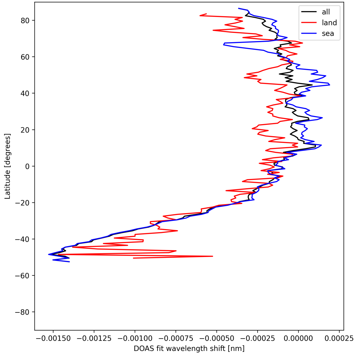
Figure 50: Zonal average of “DOAS fit wavelength shift” for 2025-08-04 to 2025-08-06.
