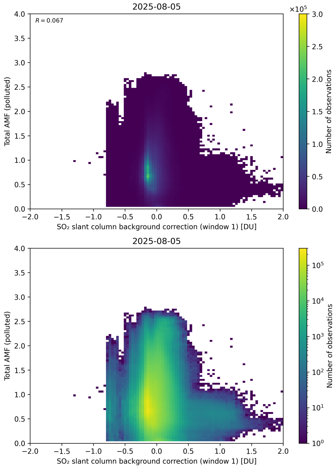
Figure 120: Scatter density plot of “SO 2 slant column background correction (window 1)” against “Total AMF (polluted)” for 2025-08-04 to 2025-08-06.
