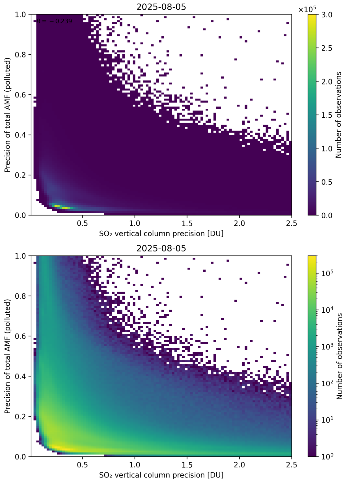
Figure 347: Scatter density plot of “SO 2 vertical column precision” against “Precision of total AMF (polluted)” for 2025-08-04 to 2025-08-06.
