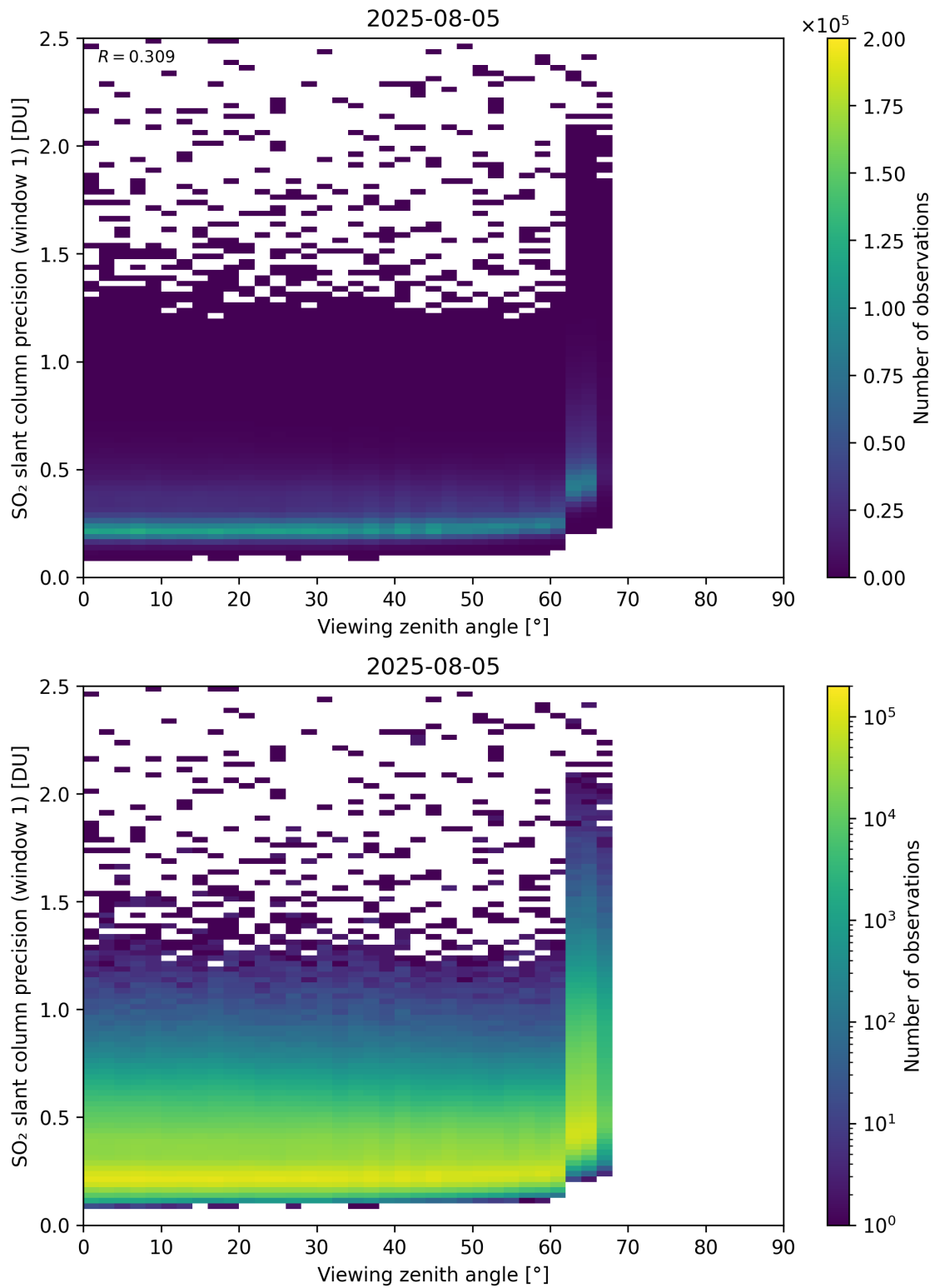
Figure 377: Scatter density plot of “Viewing zenith angle” against “SO 2 slant column precision (window 1)” for 2025-08-04 to 2025-08-06.
