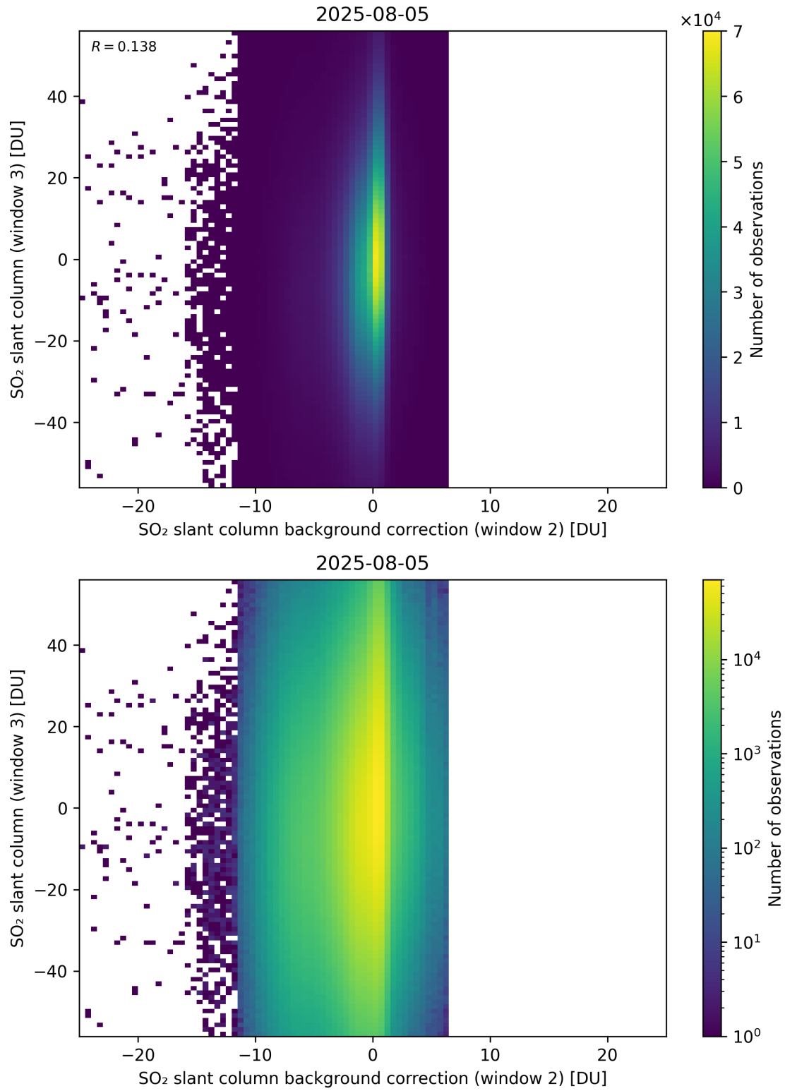
Figure 128: Scatter density plot of “SO 2 slant column background correction (window 2)” against “SO 2 slant column (window 3)” for 2025-08-04 to 2025-08-06.
