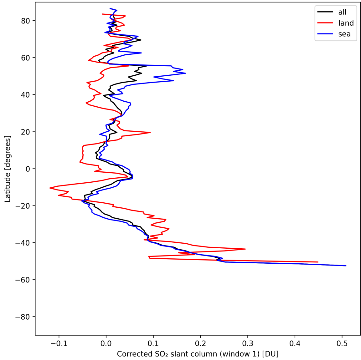
Figure 39: Zonal average of “Corrected SO 2 slant column (window 1)” for 2025-08-04 to 2025-08-06.
