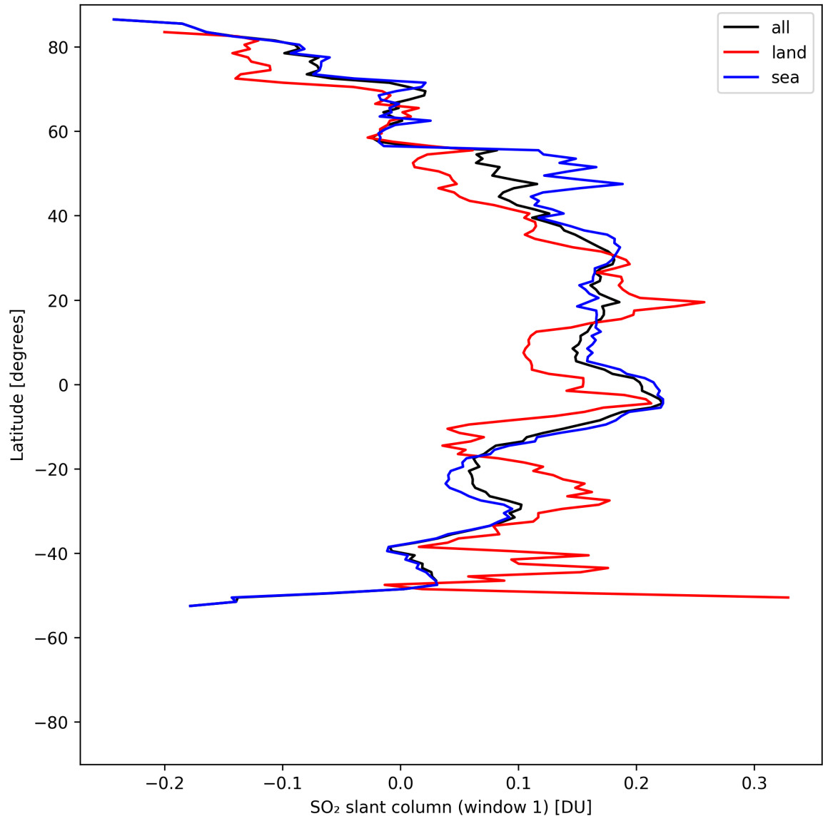
Figure 37: Zonal average of “SO 2 slant column (window 1)” for 2025-08-04 to 2025-08-06.
