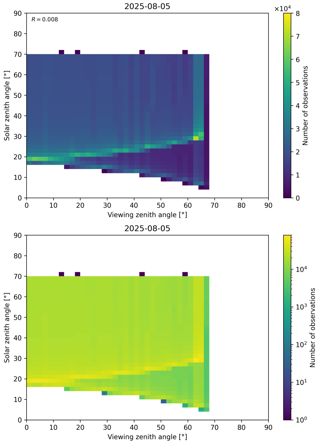
Figure 369: Scatter density plot of “Viewing zenith angle” against “Solar zenith angle” for 2025-08-04 to 2025-08-06.
