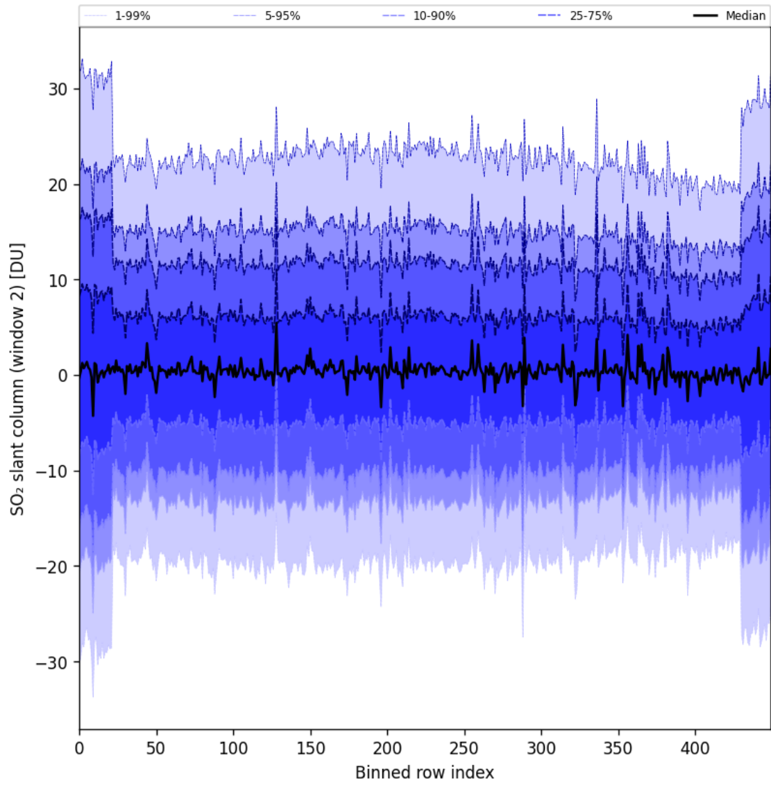
Figure 93: Along track statistics of “SO 2 slant column (window 2)” for 2025-08-04 to 2025-08-06
