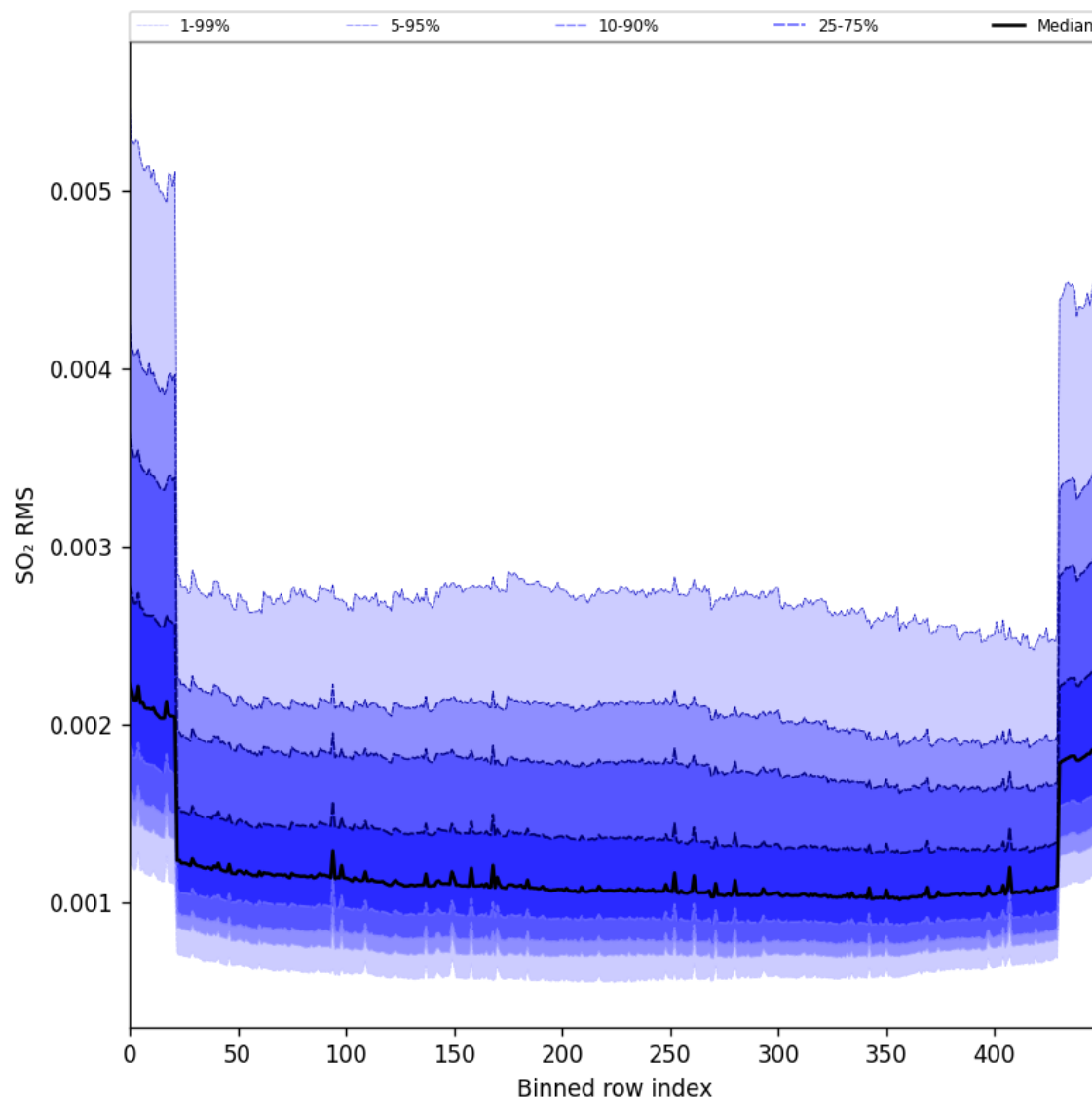
Figure 104: Along track statistics of “SO 2 RMS” for 2025-08-04 to 2025-08-06
