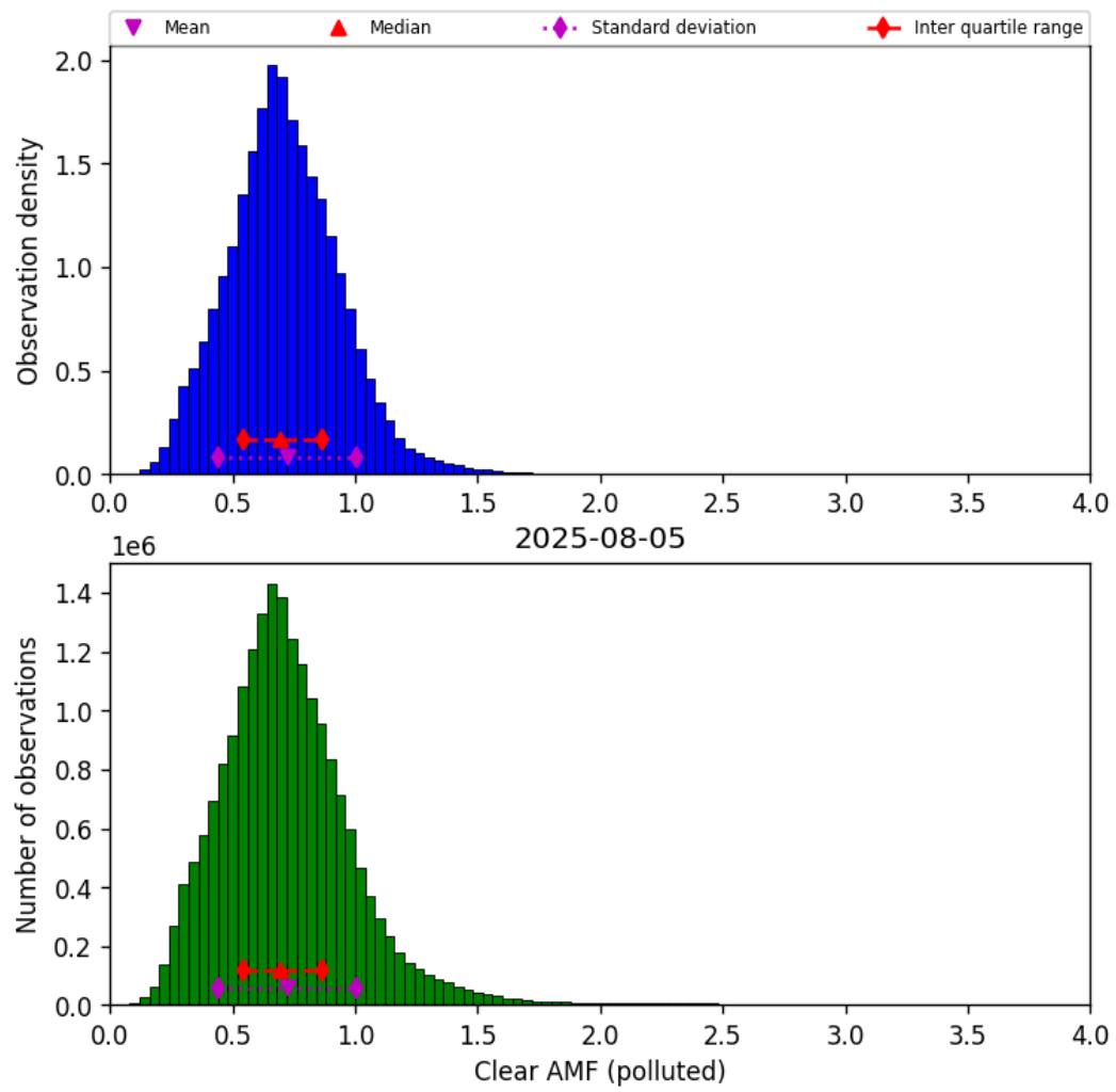
Figure 81: Histogram of “Clear AMF (polluted)” for 2025-08-04 to 2025-08-06
