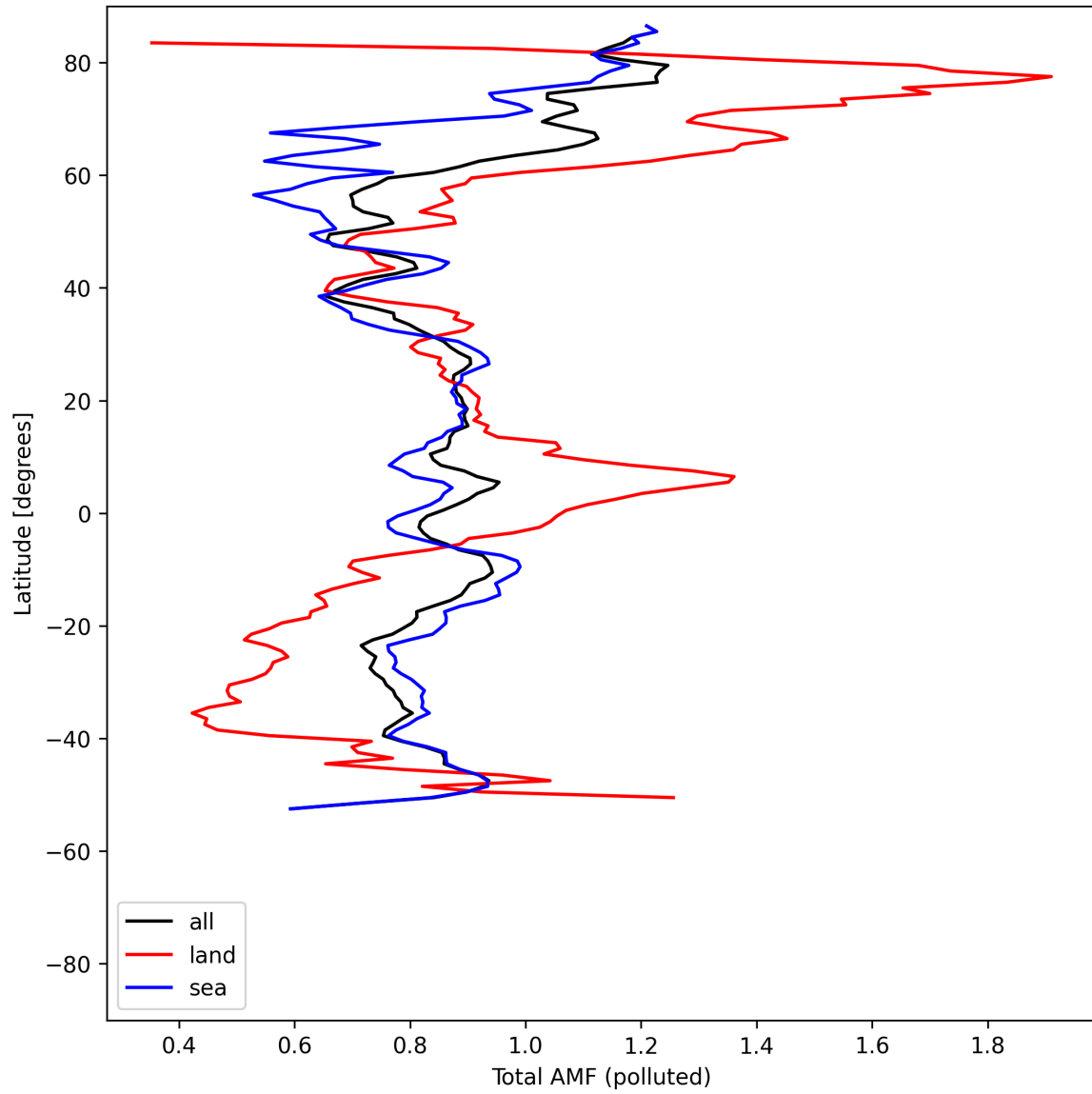
Figure 53: Zonal average of “Total AMF (polluted)” for 2025-08-04 to 2025-08-06.
