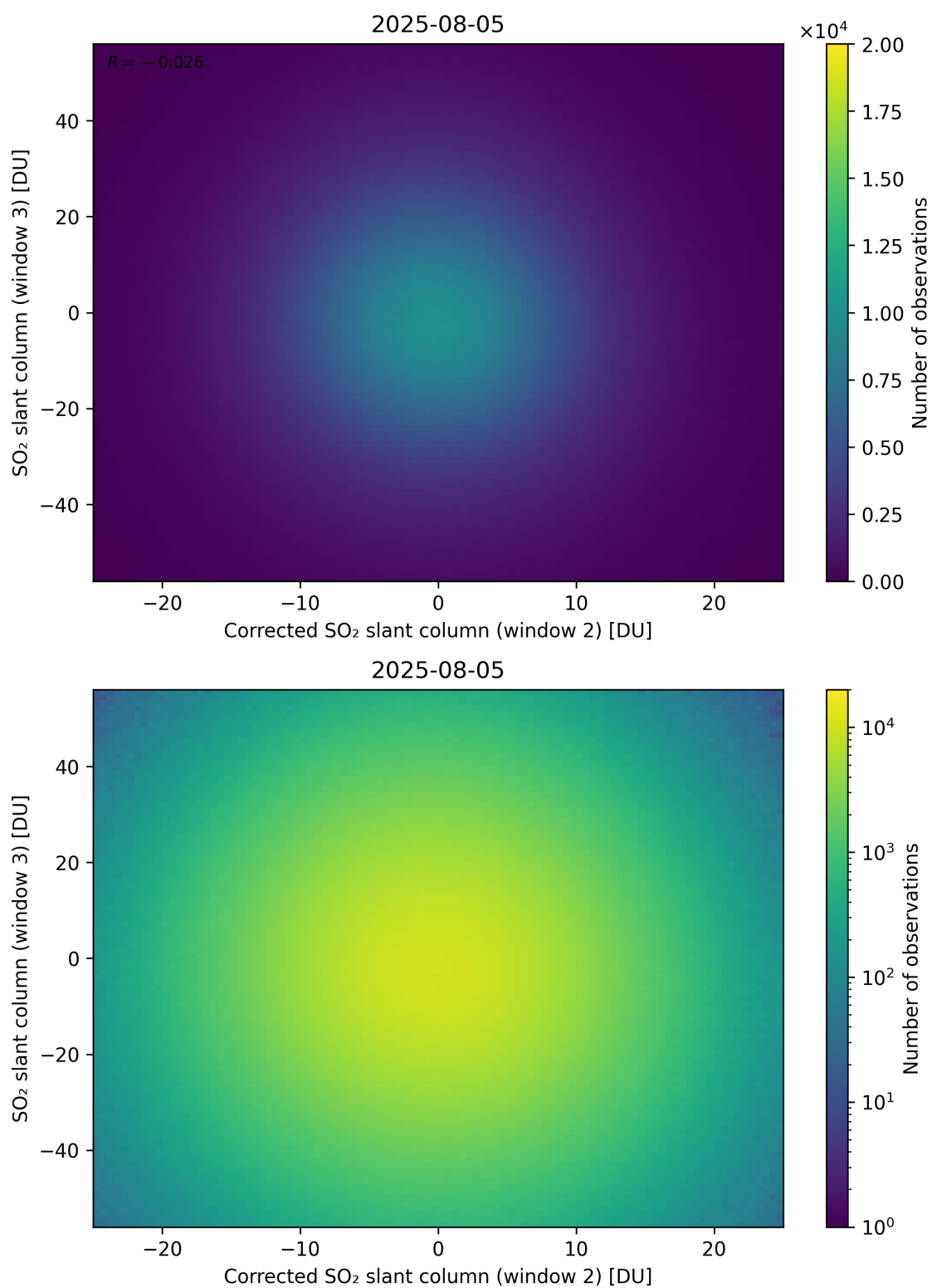
Figure 251: Scatter density plot of “Corrected SO 2 slant column (window 2)” against “SO 2 slant column (window 3)” for 2025-08-04 to 2025-08-06.
