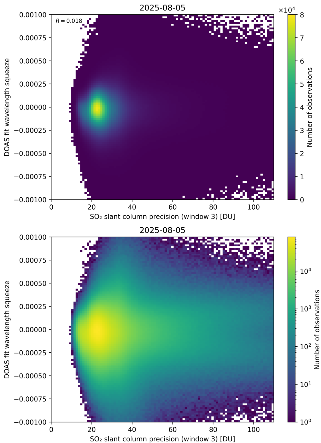
Figure 309: Scatter density plot of “SO 2 slant column precision (window 3)” against “DOAS fit wavelength squeeze” for 2025-08-04 to 2025-08-06.
