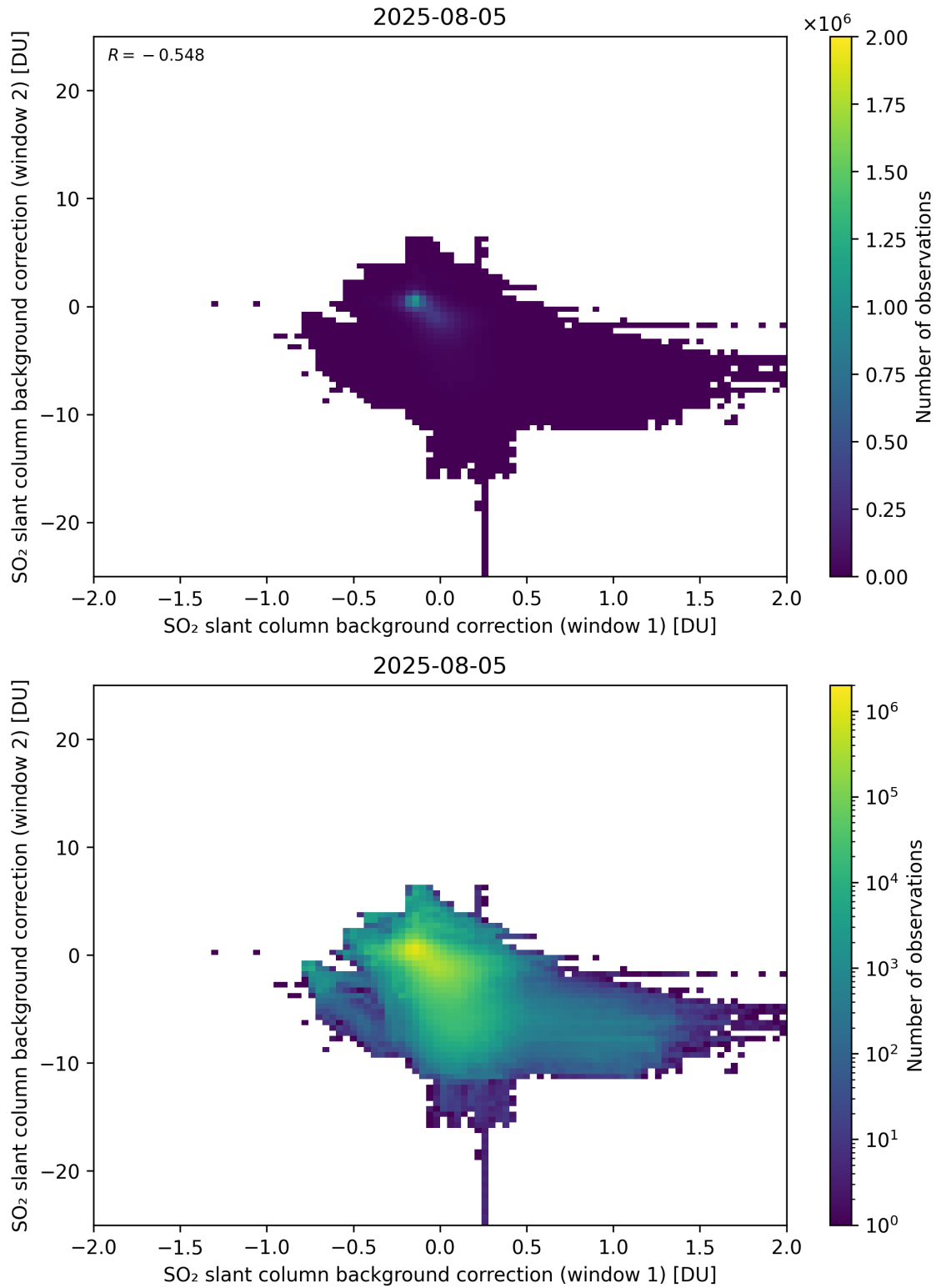
Figure 109: Scatter density plot of “SO 2 slant column background correction (window 1)” against “SO 2 slant column background correction (window 2)” for 2025-08-04 to 2025-08-06.
