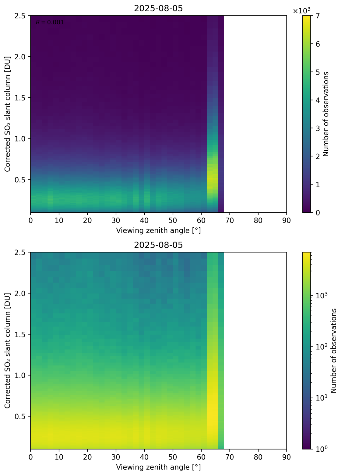
Figure 373: Scatter density plot of “Viewing zenith angle” against “Corrected SO 2 slant column” for 2025-08-04 to 2025-08-06.
