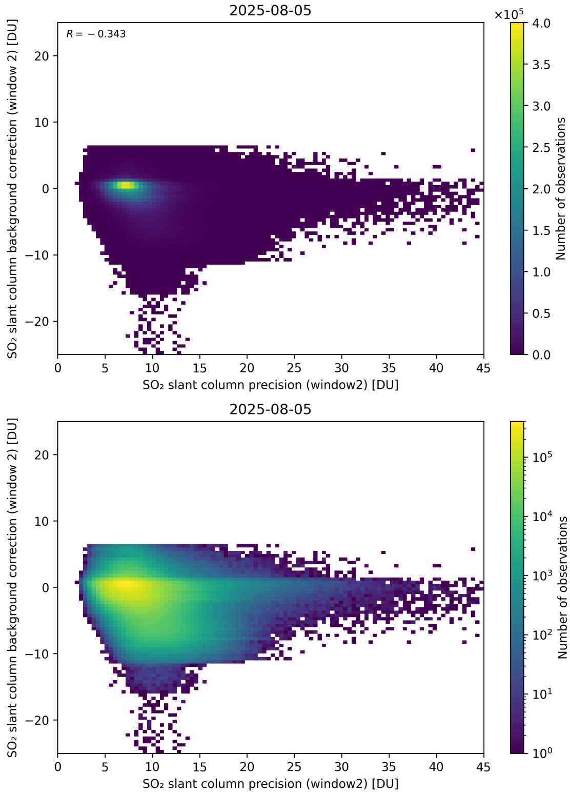
Figure 291: Scatter density plot of “SO 2 slant column precision (window2)” against “SO 2 slant column background correction (window 2)” for 2025-08-04 to 2025-08-06.
