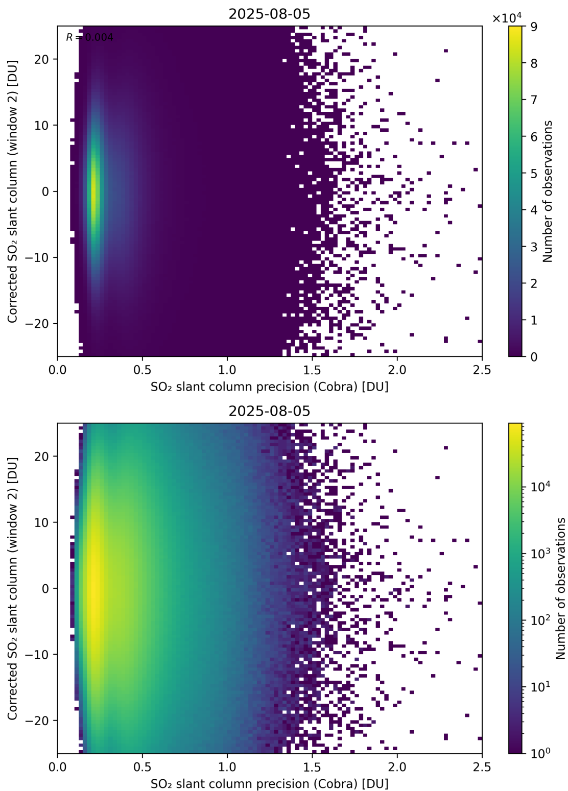
Figure 206: Scatter density plot of “SO 2 slant column precision (Cobra)” against “Corrected SO 2 slant column (window 2)” for 2025-08-04 to 2025-08-06.
