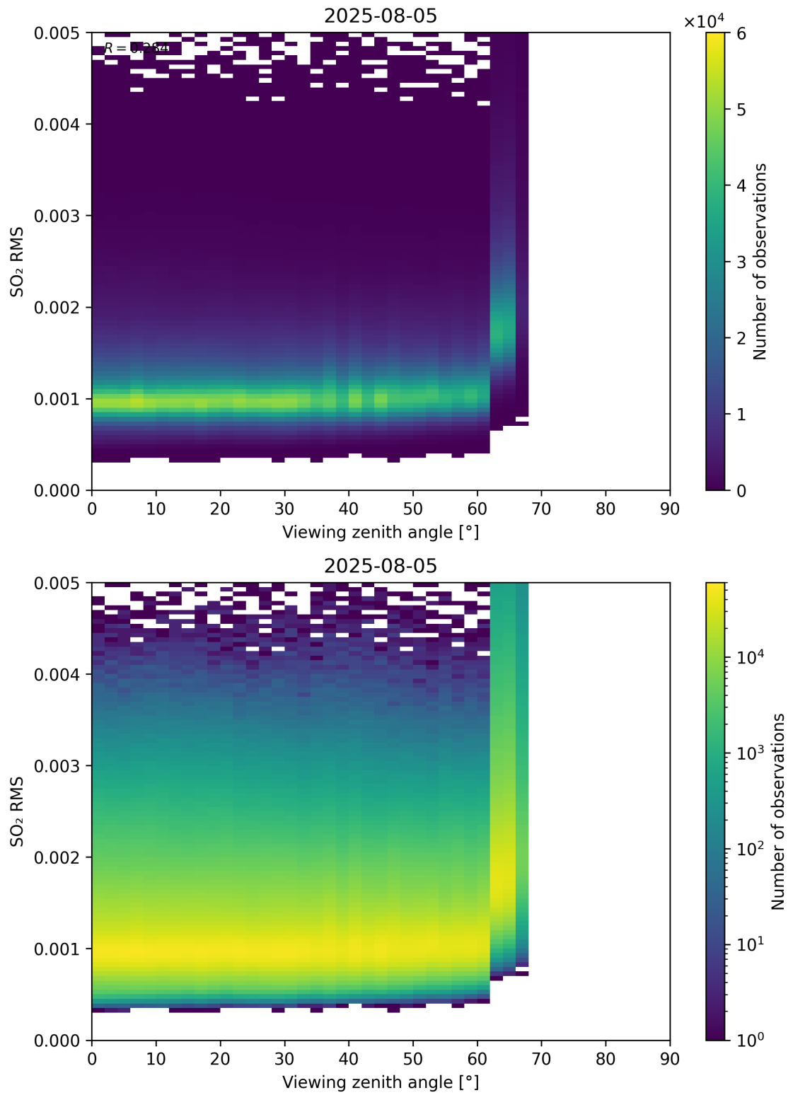
Figure 367: Scatter density plot of “Viewing zenith angle” against “SO 2 RMS” for 2025-08-04 to 2025-08-06.
