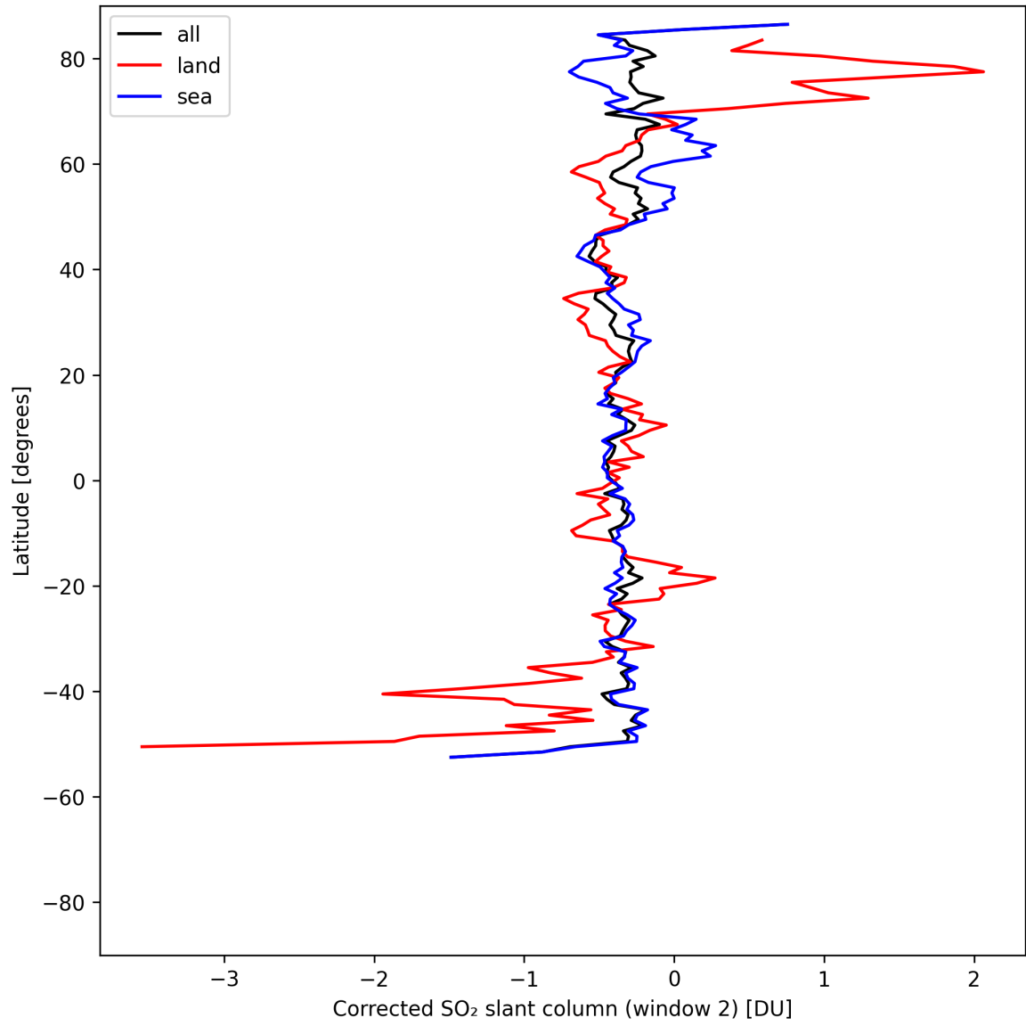
Figure 43: Zonal average of “Corrected SO 2 slant column (window 2)” for 2025-08-04 to 2025-08-06.
