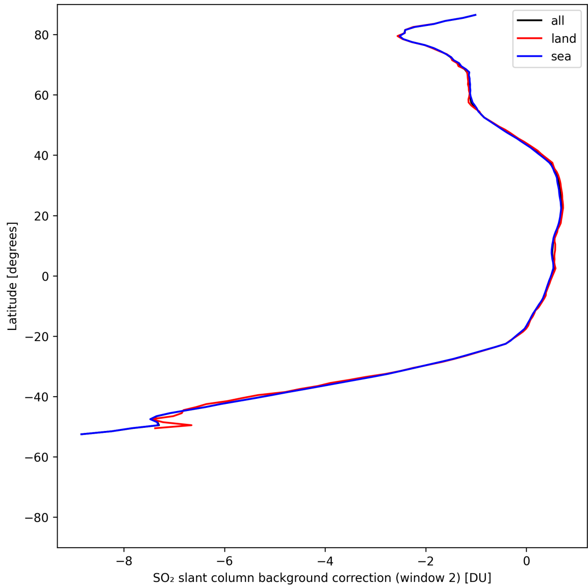
Figure 44: Zonal average of “SO 2 slant column background correction (window 2)” for 2025-08-04 to 2025-08-06.
