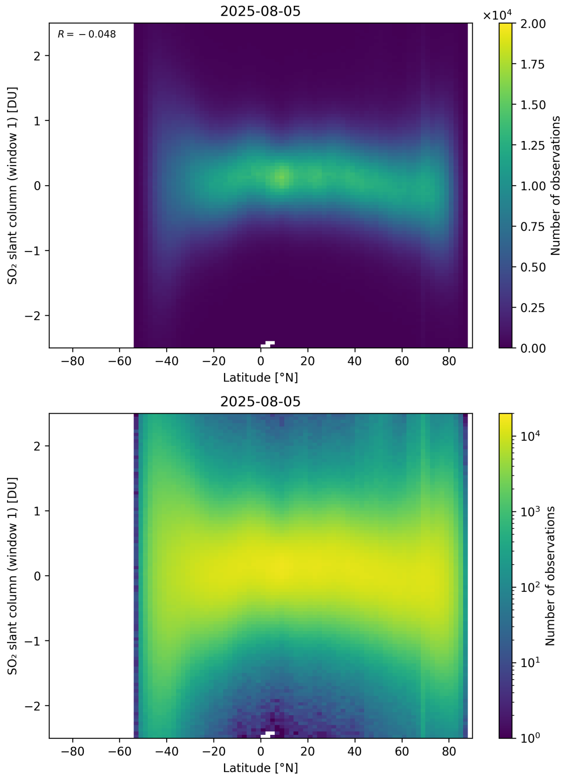
Figure 162: Scatter density plot of “Latitude” against “SO 2 slant column (window 1)” for 2025-08-04 to 2025-08-06.
