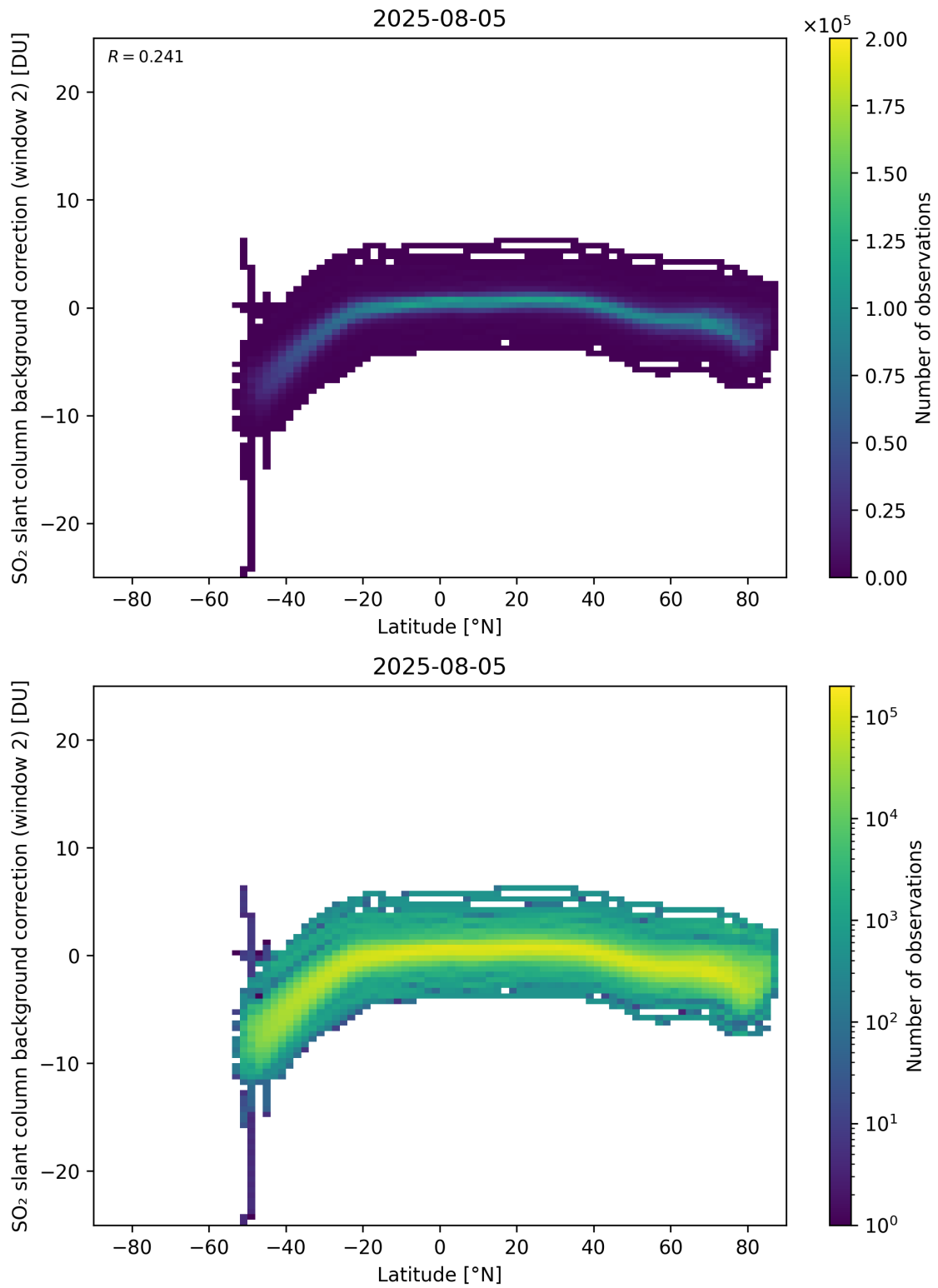
Figure 151: Scatter density plot of “Latitude” against “SO 2 slant column background correction (window 2)” for 2025-08-04 to 2025-08-06.
