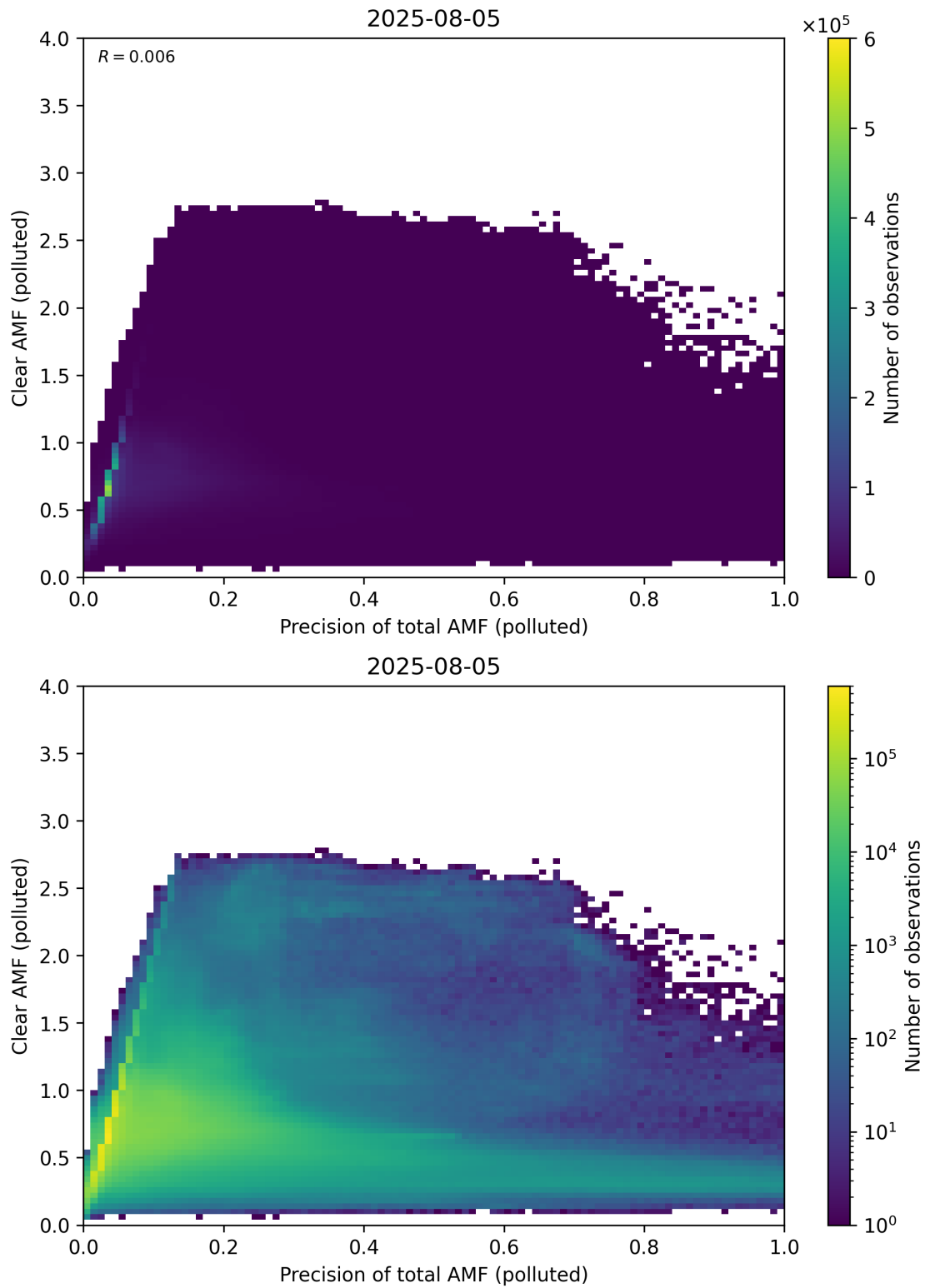
Figure 320: Scatter density plot of “Precision of total AMF (polluted)” against “Clear AMF (polluted)” for 2025-08-04 to 2025-08-06.
