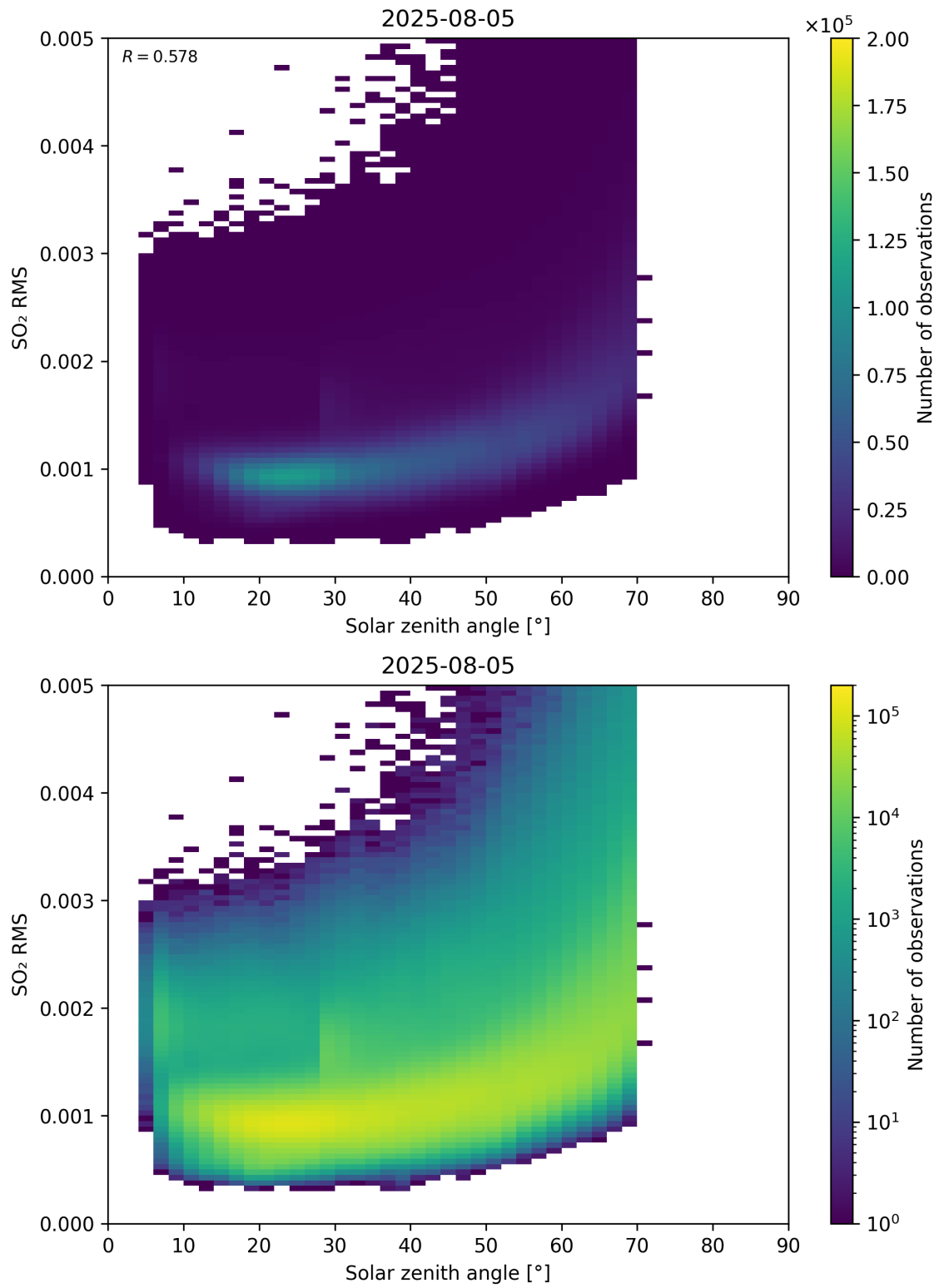
Figure 176: Scatter density plot of “Solar zenith angle” against “SO 2 RMS” for 2025-08-04 to 2025-08-06.
