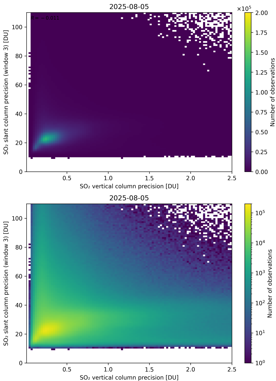
Figure 345: Scatter density plot of “SO 2 vertical column precision” against “SO 2 slant column precision (window 3)” for 2025-08-04 to 2025-08-06.
