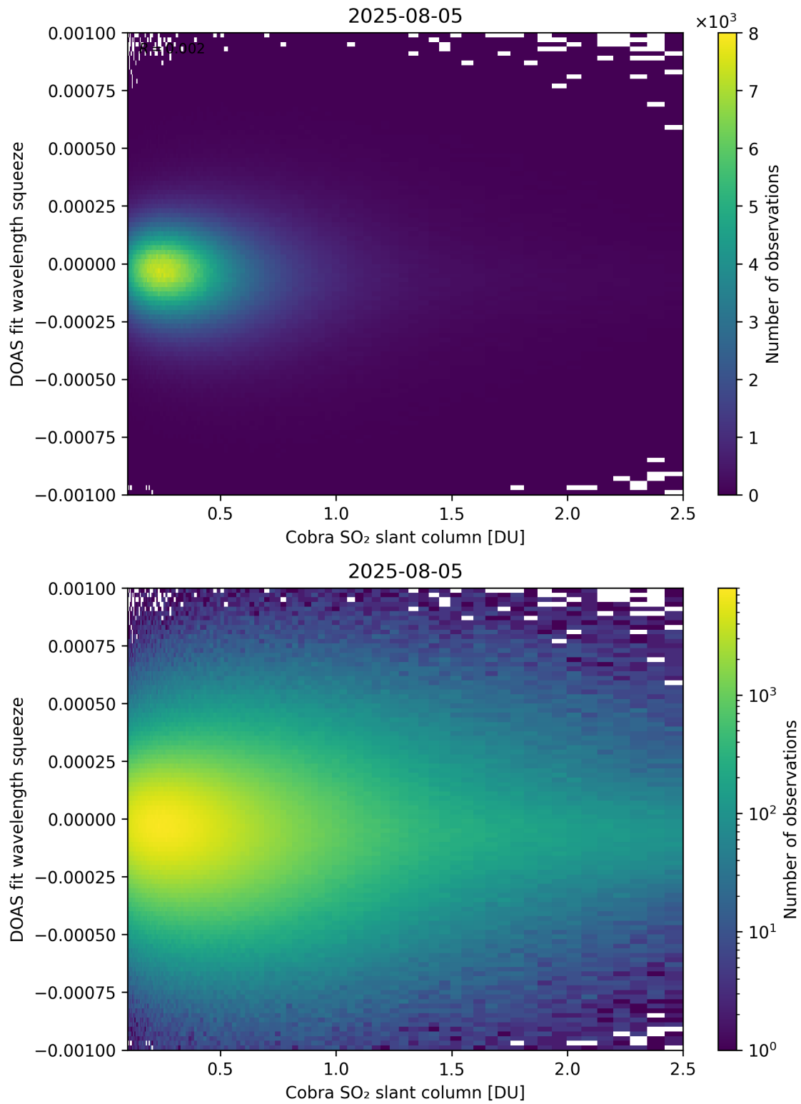
Figure 197: Scatter density plot of “Cobra SO 2 slant column” against “DOAS fit wavelength squeeze” for 2025-08-04 to 2025-08-06.
