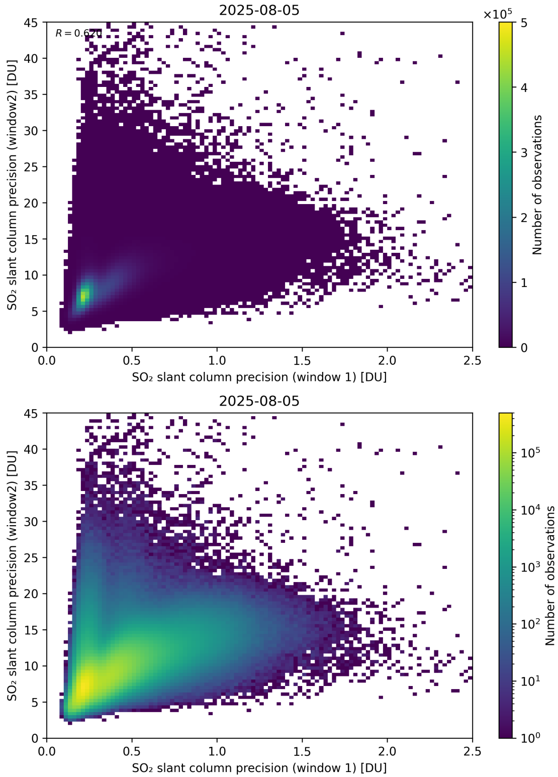
Figure 277: Scatter density plot of “SO 2 slant column precision (window 1)” against “SO 2 slant column precision (window2)” for 2025-08-04 to 2025-08-06.
