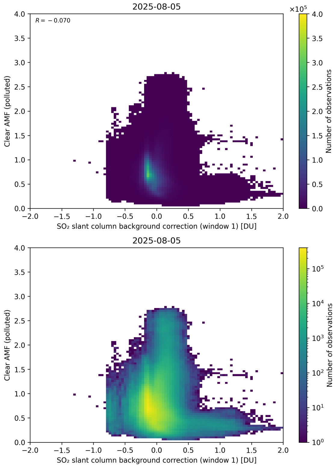
Figure 114: Scatter density plot of “SO 2 slant column background correction (window 1)” against “Clear AMF (polluted)” for 2025-08-04 to 2025-08-06.
