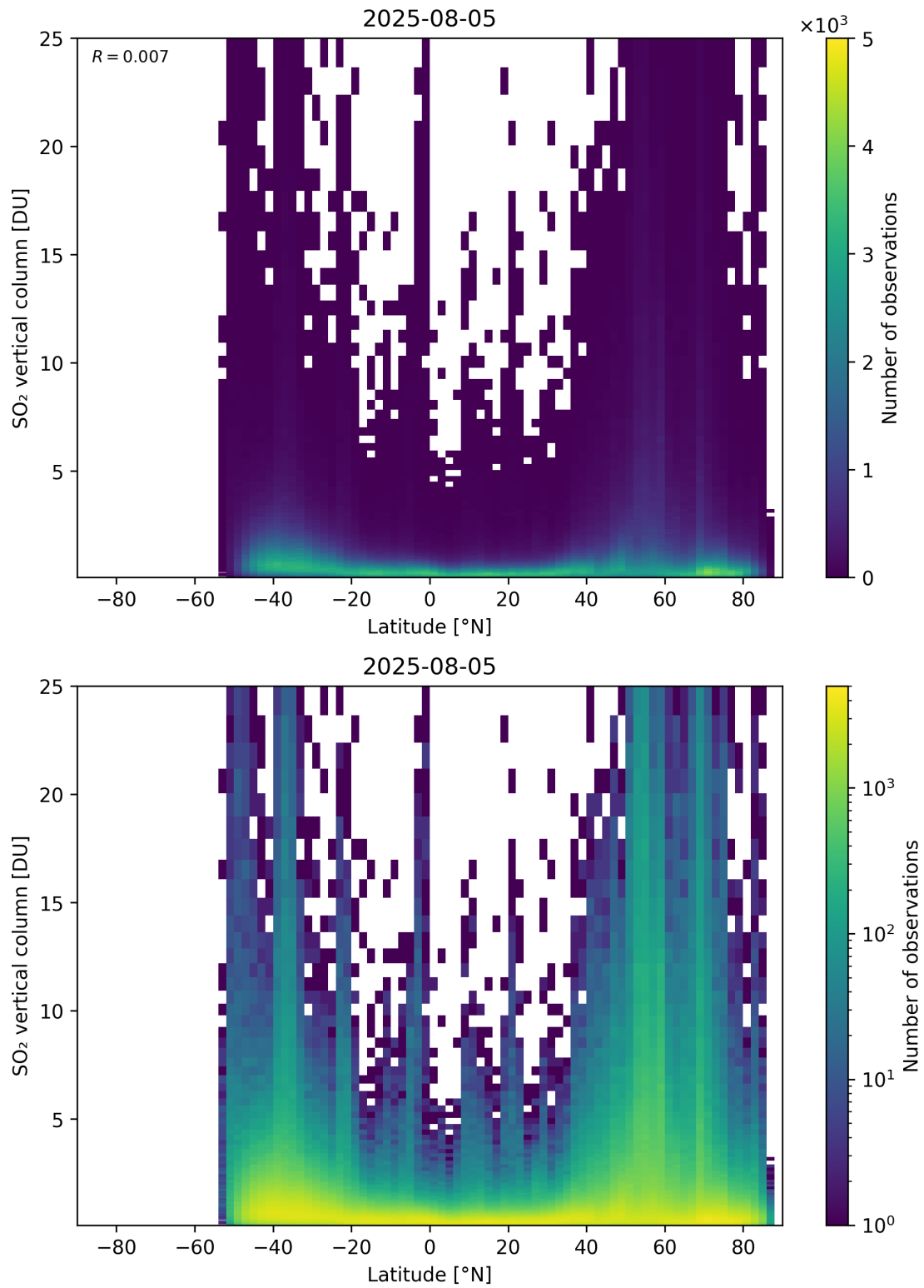
Figure 169: Scatter density plot of “Latitude” against “SO 2 vertical column” for 2025-08-04 to 2025-08-06.
