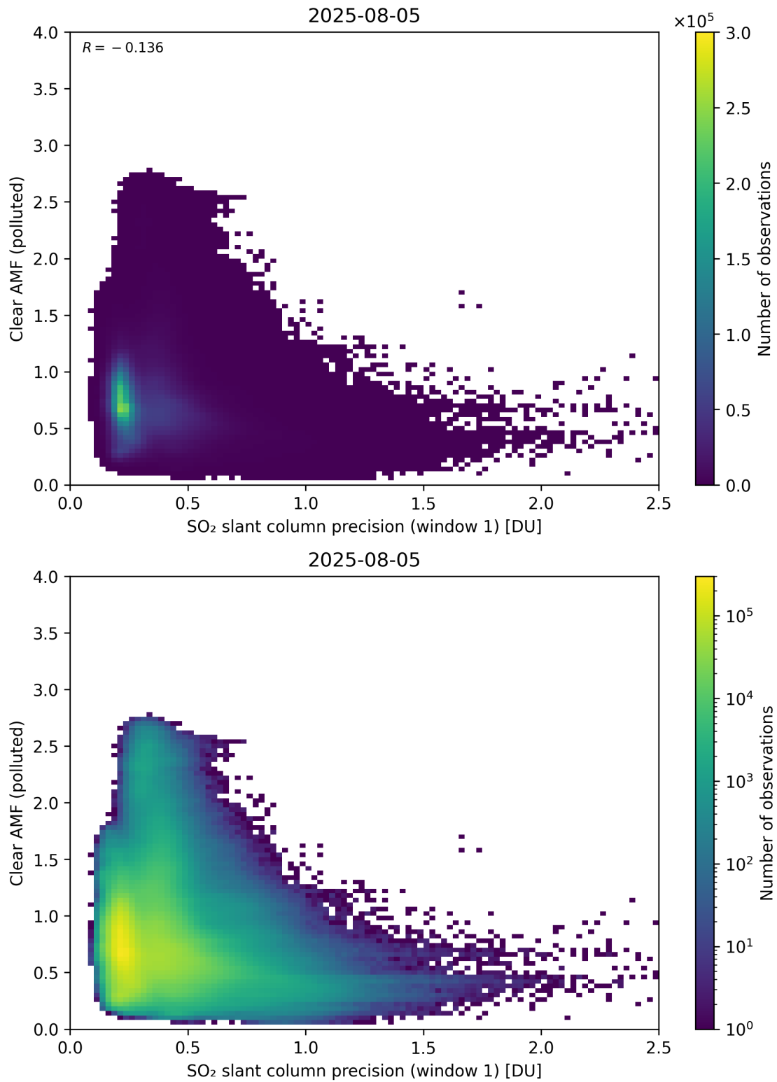
Figure 274: Scatter density plot of “SO 2 slant column precision (window 1)” against “Clear AMF (polluted)” for 2025-08-04 to 2025-08-06.
