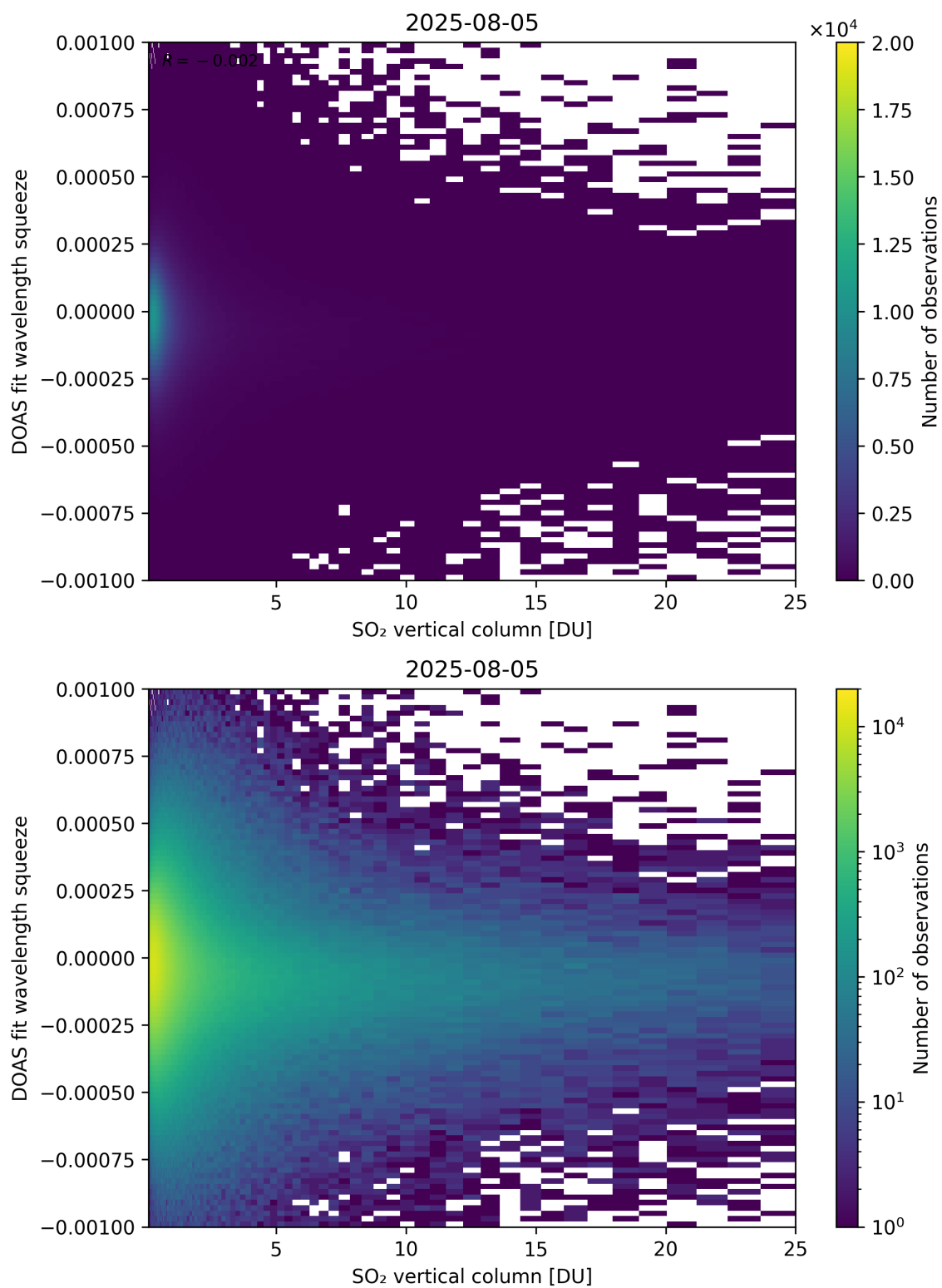
Figure 327: Scatter density plot of “SO 2 vertical column” against “DOAS fit wavelength squeeze” for 2025-08-04 to 2025-08-06.
