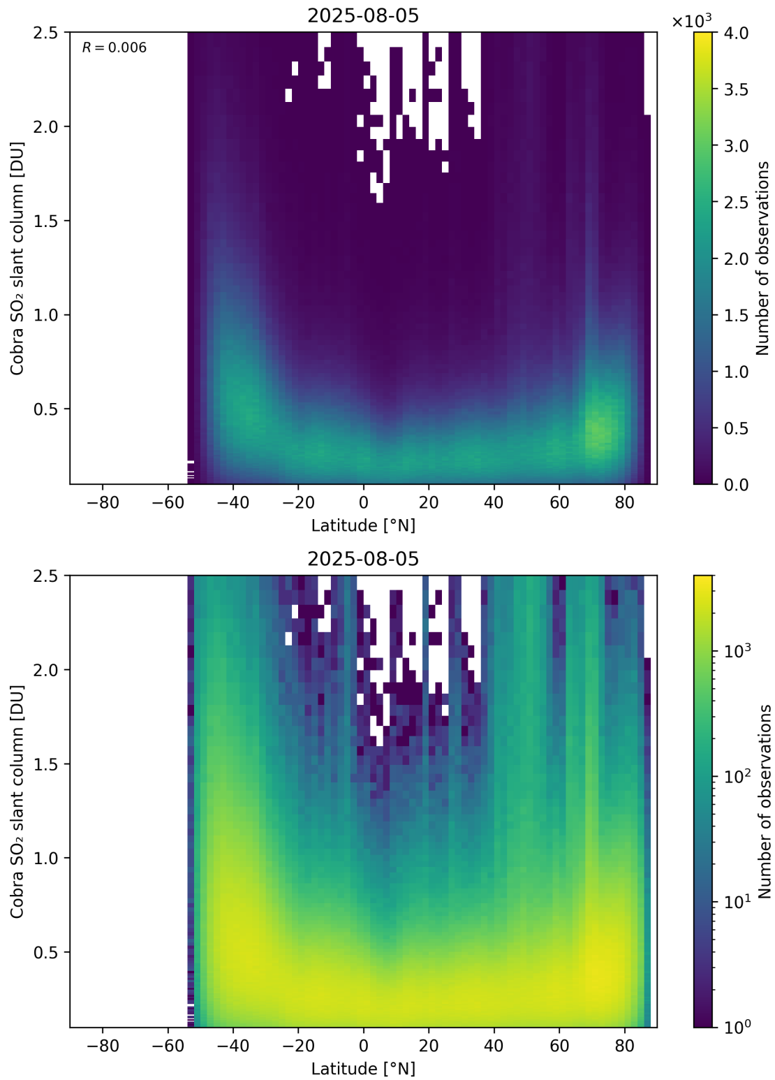
Figure 157: Scatter density plot of “Latitude” against “Cobra SO 2 slant column” for 2025-08-04 to 2025-08-06.
