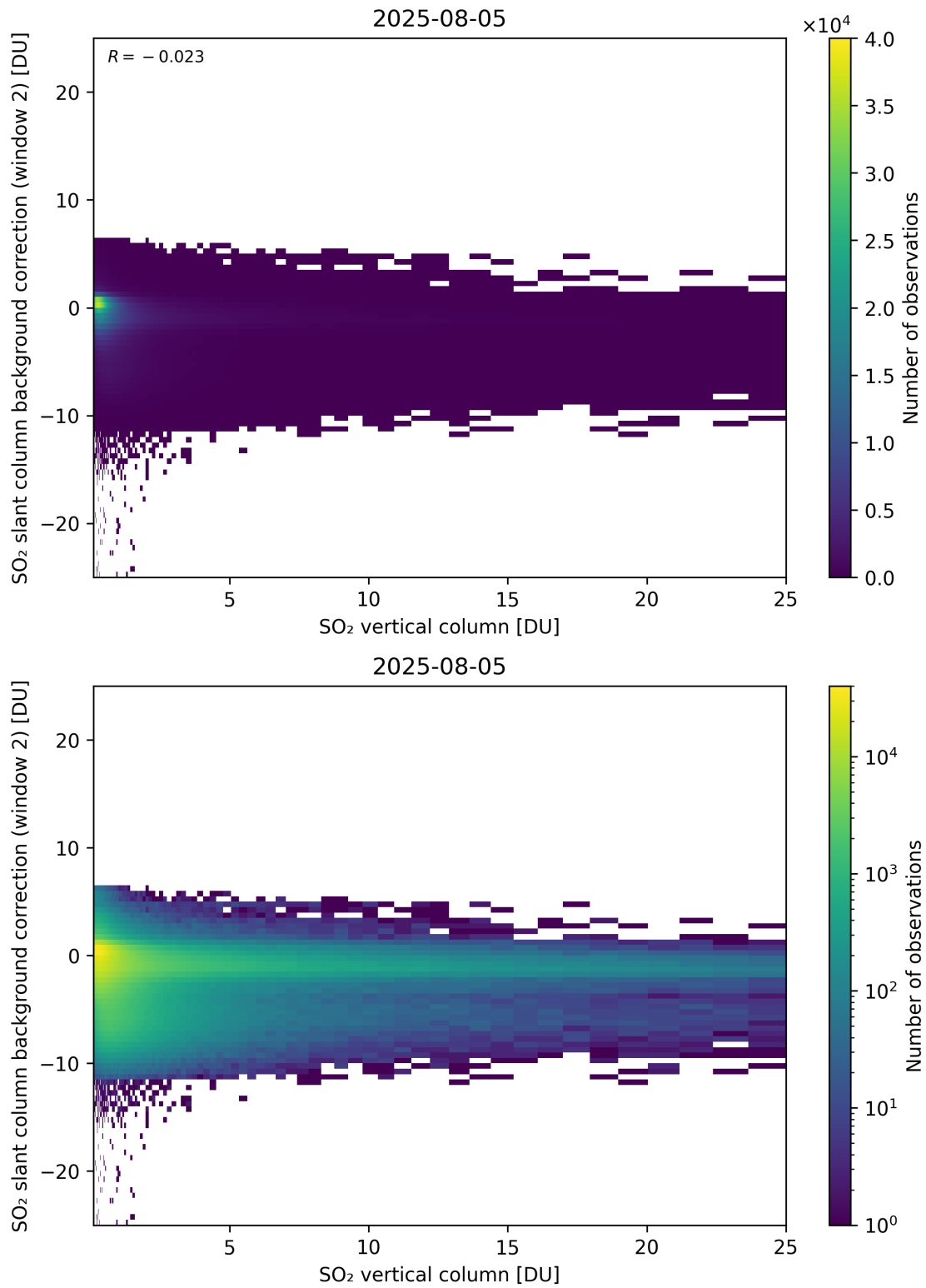
Figure 324: Scatter density plot of “SO 2 vertical column” against “SO 2 slant column background correction (window 2)” for 2025-08-04 to 2025-08-06.
