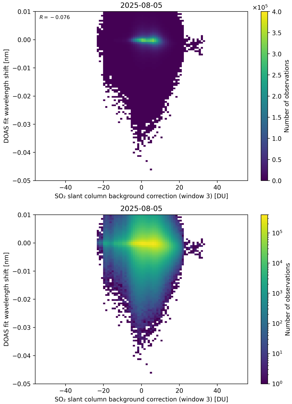
Figure 132: Scatter density plot of “SO 2 slant column background correction (window 3)” against “DOAS fit wavelength shift” for 2025-08-04 to 2025-08-06.
