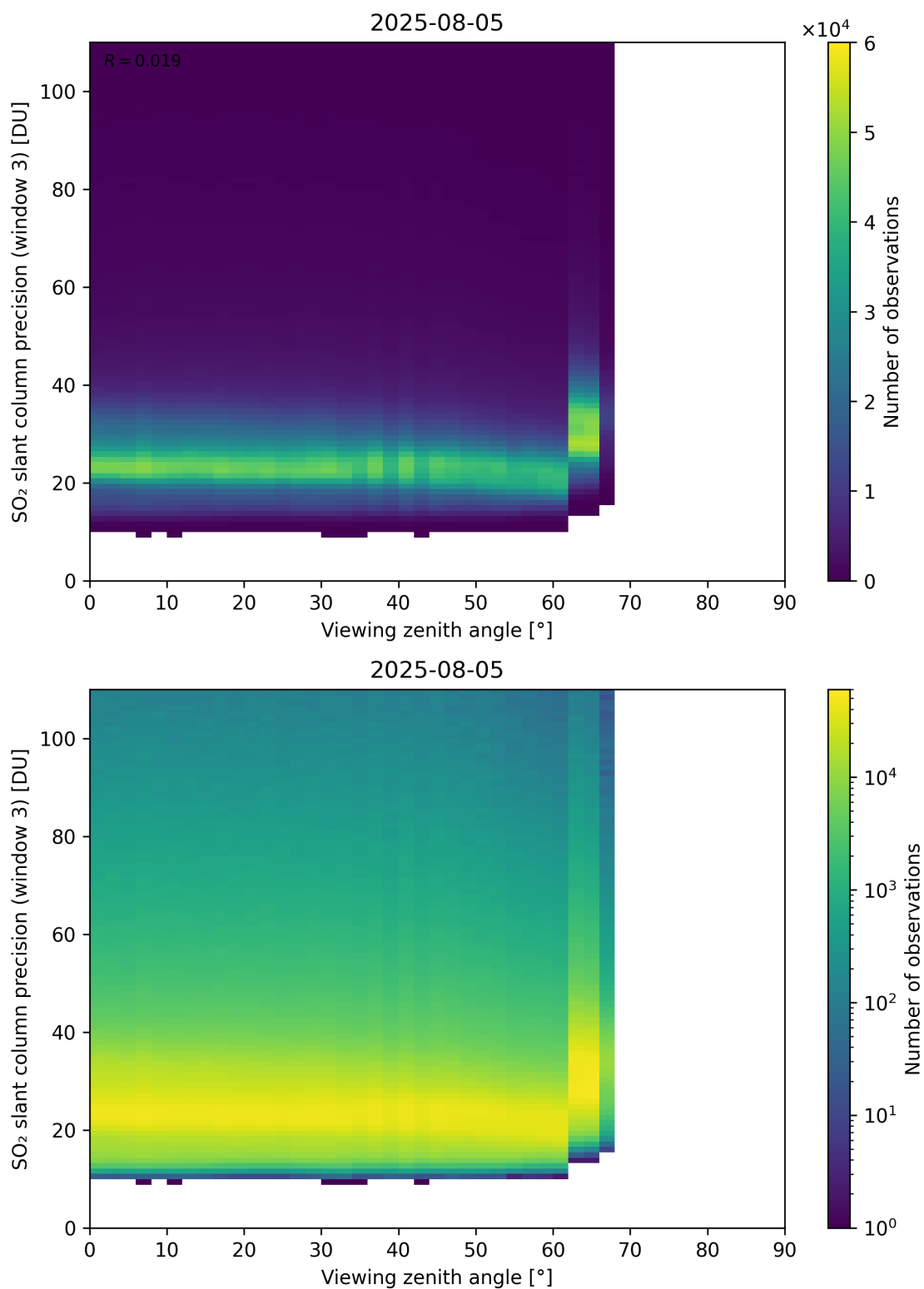
Figure 380: Scatter density plot of “Viewing zenith angle” against “SO 2 slant column precision (window 3)” for 2025-08-04 to 2025-08-06.
