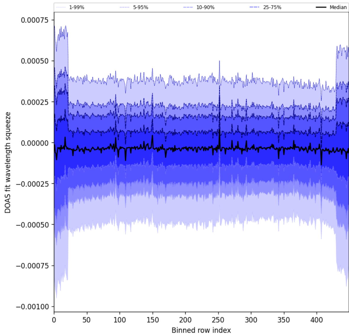
Figure 103: Along track statistics of “DOAS fit wavelength squeeze” for 2025-08-04 to 2025-08-06
