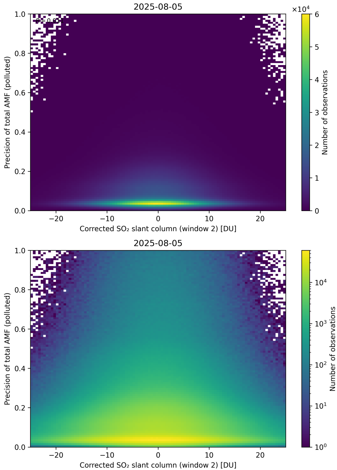
Figure 254: Scatter density plot of “Corrected SO 2 slant column (window 2)” against “Precision of total AMF (polluted)” for 2025-08-04 to 2025-08-06.
