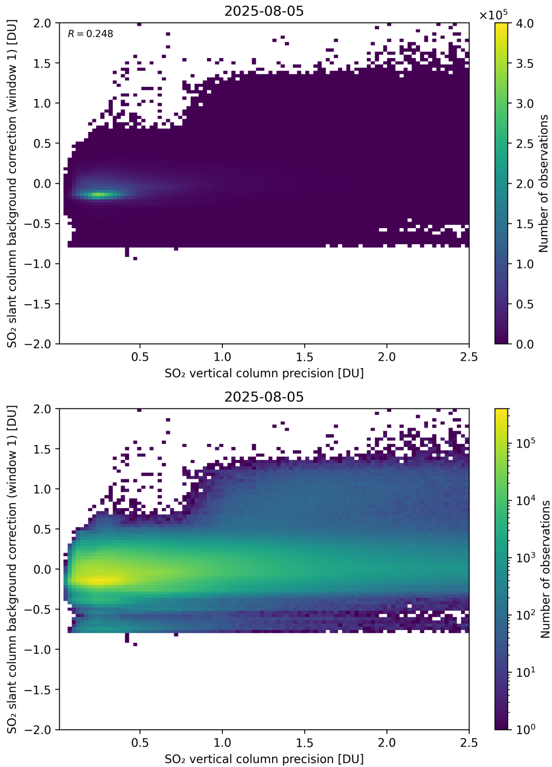
Figure 329: Scatter density plot of “SO 2 vertical column precision” against “SO 2 slant column background correction (window 1)” for 2025-08-04 to 2025-08-06.
