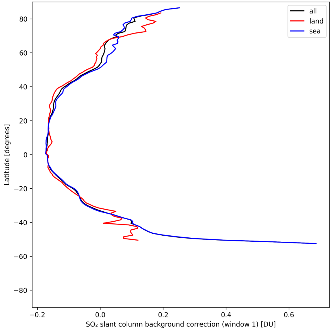
Figure 40: Zonal average of "SO 2 slant column background correction (window 1)" for 2025-08-04 to 2025-08-06.
