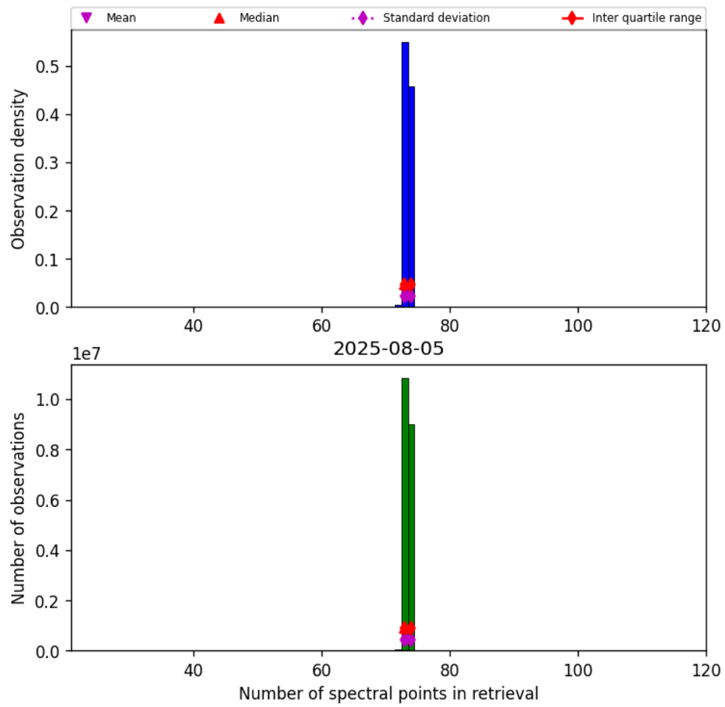
Figure 82: Histogram of “Number of spectral points in retrieval” for 2025-08-04 to 2025-08-06
