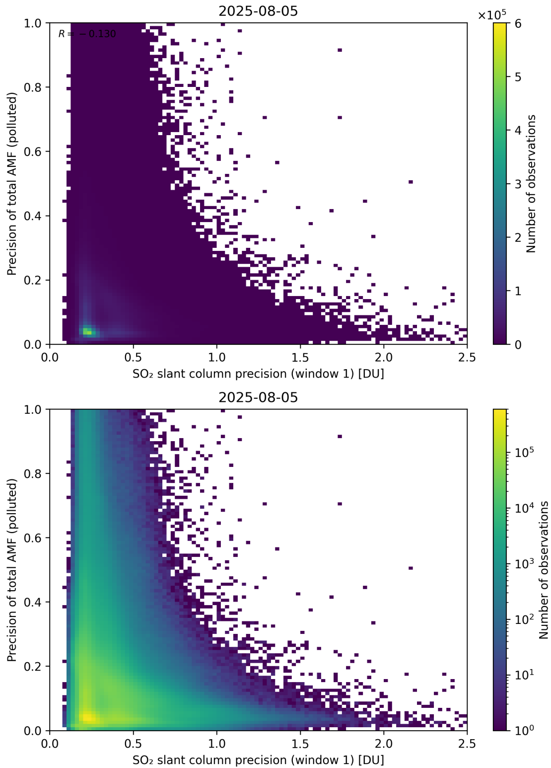
Figure 281: Scatter density plot of “SO 2 slant column precision (window 1)” against “Precision of total AMF (polluted)” for 2025-08-04 to 2025-08-06.
