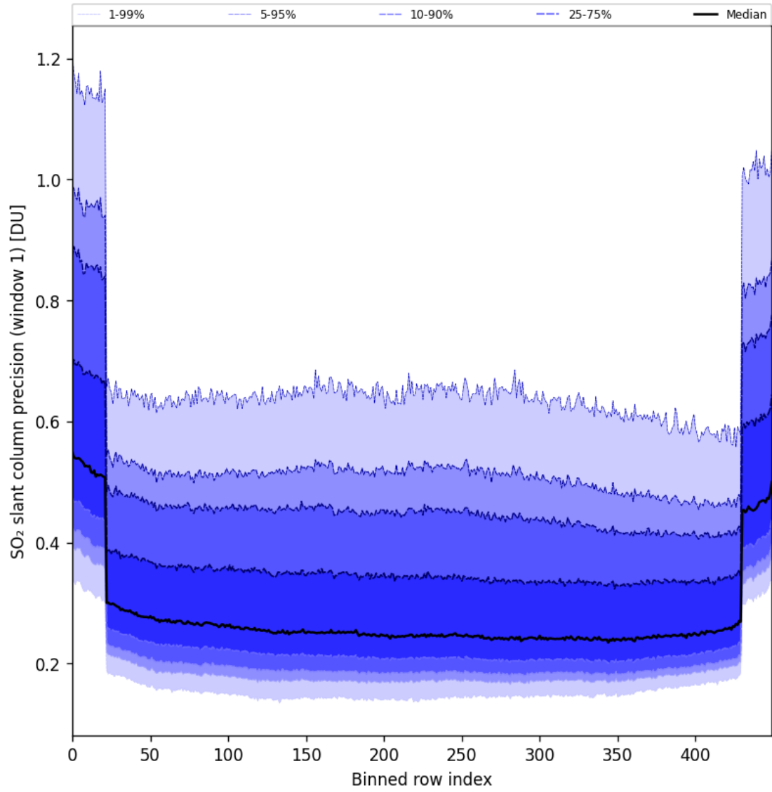
Figure 90: Along track statistics of “SO 2 slant column precision (window 1)” for 2025-08-04 to 2025-08-06
