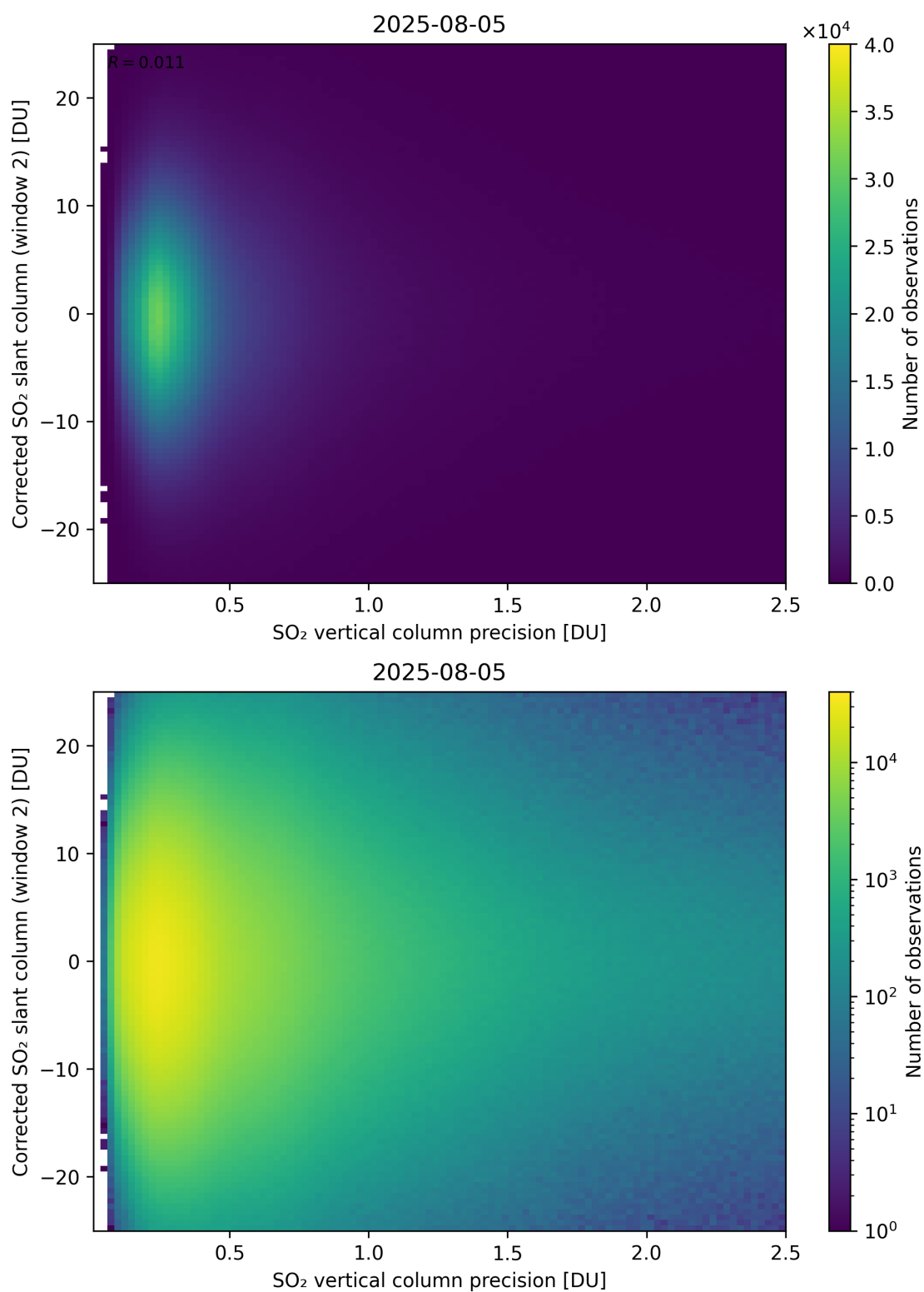
Figure 339: Scatter density plot of “SO 2 vertical column precision” against “Corrected SO 2 slant column (window 2)” for 2025-08-04 to 2025-08-06.
