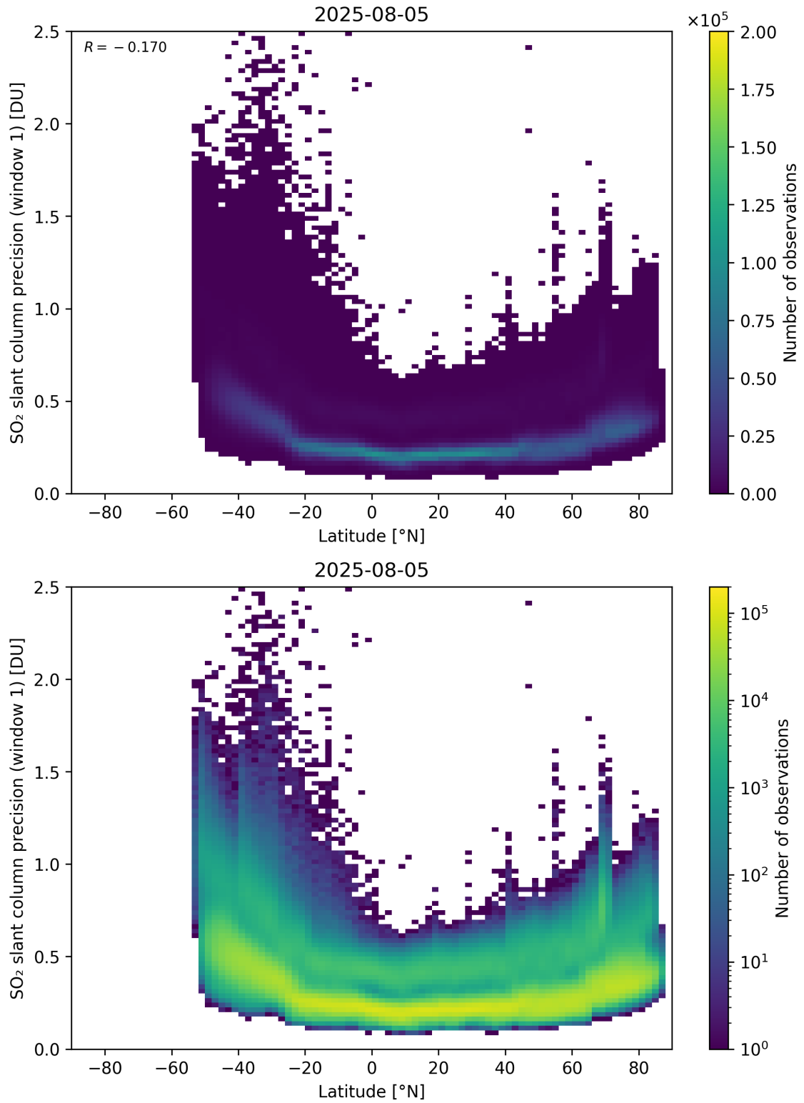
Figure 163: Scatter density plot of “Latitude” against “SO 2 slant column precision (window 1)” for 2025-08-04 to 2025-08-06.
