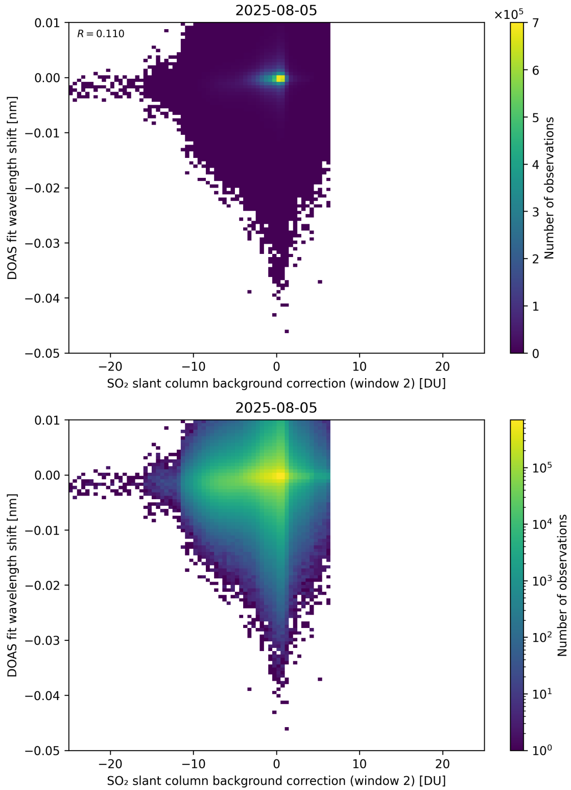
Figure 123: Scatter density plot of “SO 2 slant column background correction (window 2)” against “DOAS fit wavelength shift” for 2025-08-04 to 2025-08-06.
