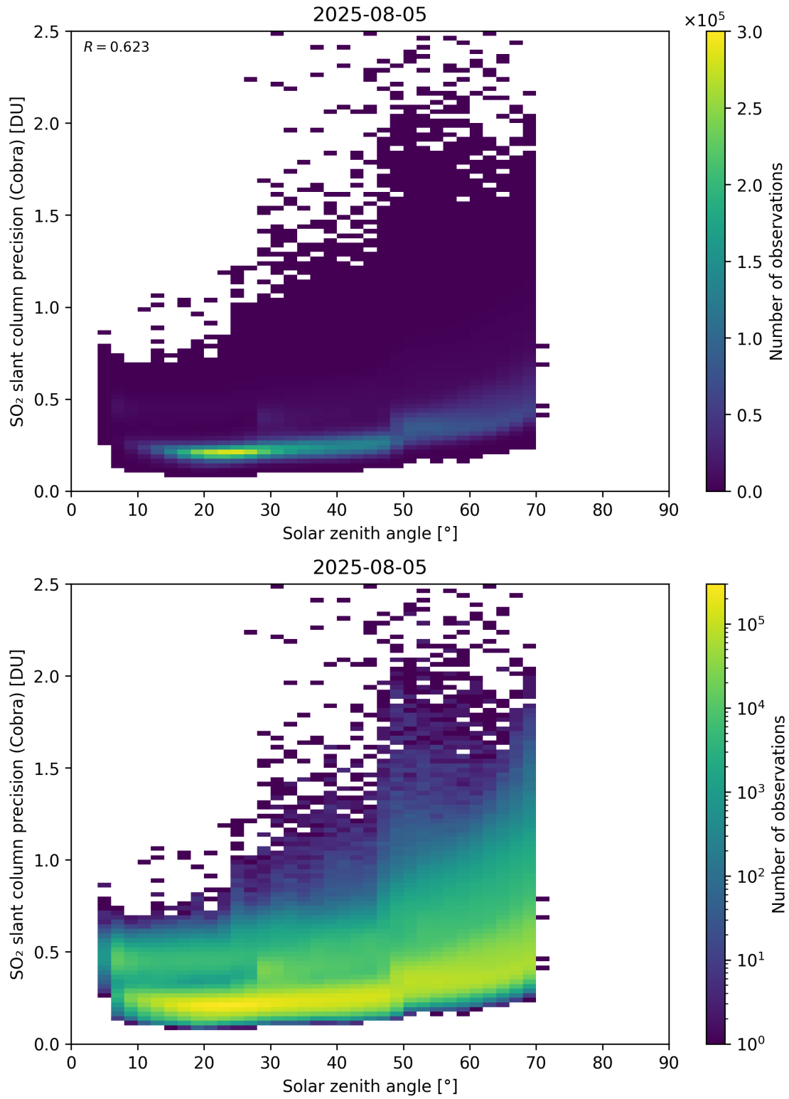
Figure 180: Scatter density plot of “Solar zenith angle” against “SO 2 slant column precision (Cobra)” for 2025-08-04 to 2025-08-06.
