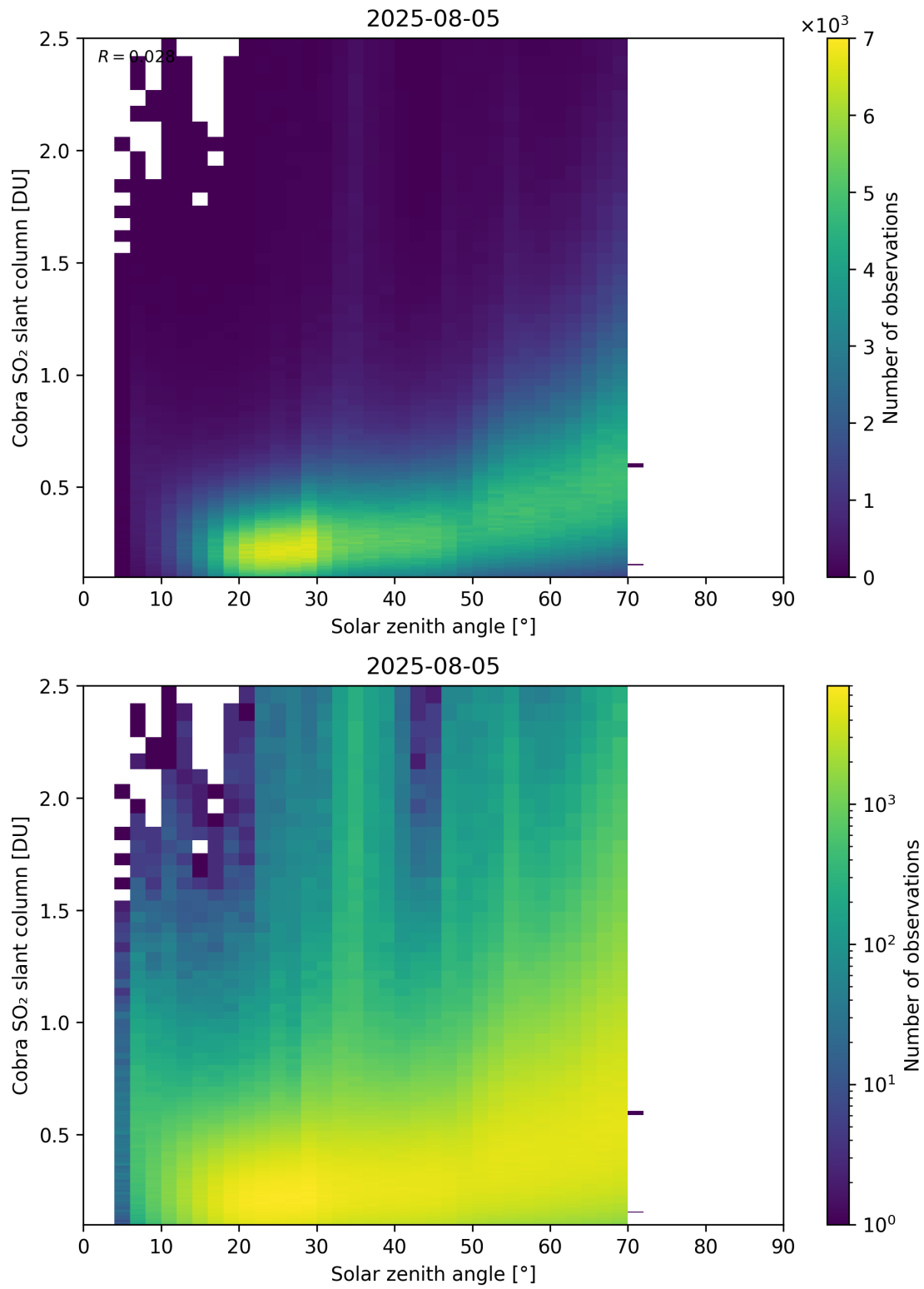
Figure 179: Scatter density plot of “Solar zenith angle” against “Cobra SO 2 slant column” for 2025-08-04 to 2025-08-06.
