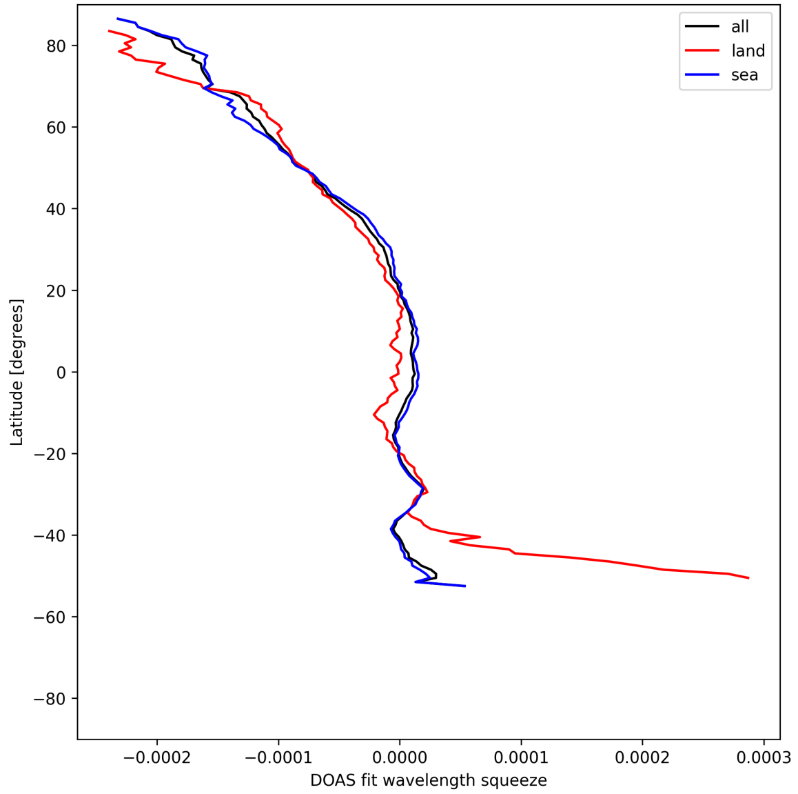
Figure 51: Zonal average of “DOAS fit wavelength squeeze” for 2025-08-04 to 2025-08-06.
