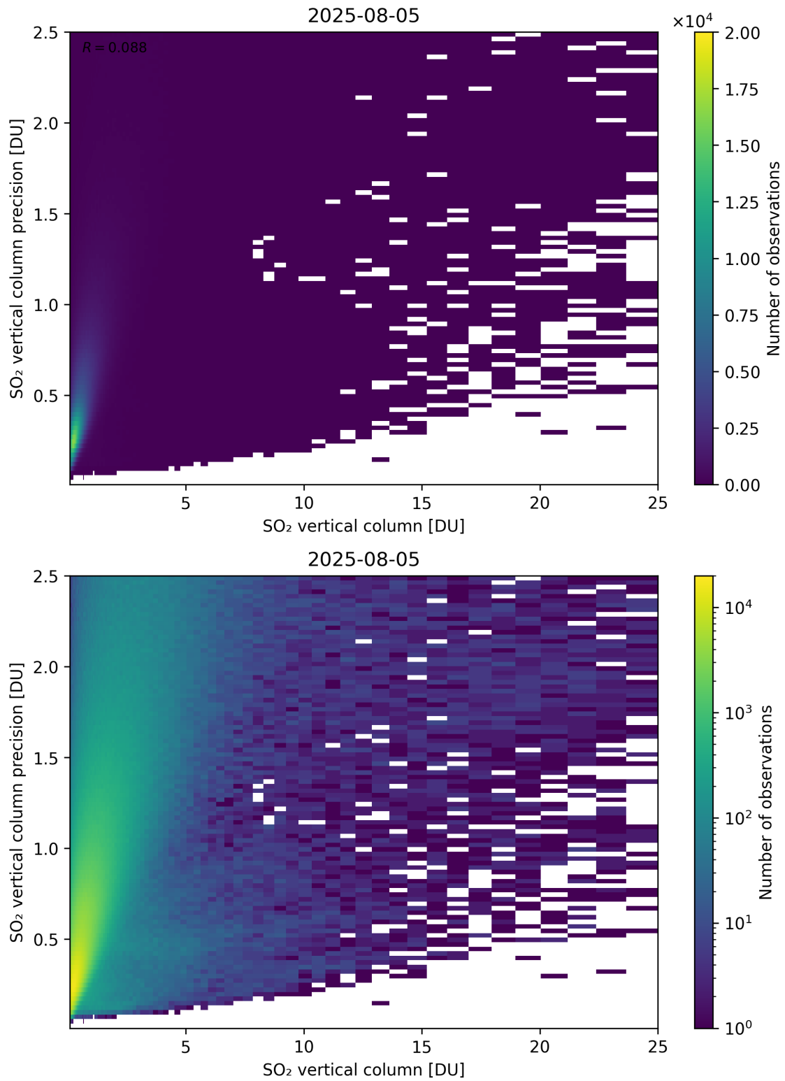
Figure 361: Scatter density plot of “SO 2 vertical column” against “SO 2 vertical column precision” for 2025-08-04 to 2025-08-06.
