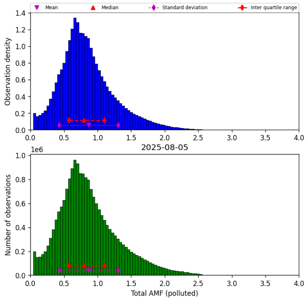
Figure 79: Histogram of “Total AMF (polluted)” for 2025-08-04 to 2025-08-06
