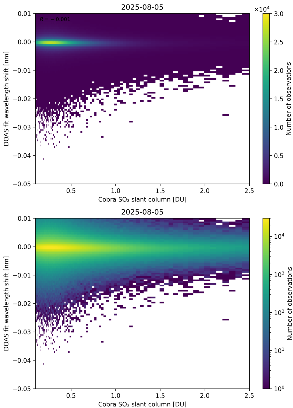
Figure 196: Scatter density plot of “Cobra SO 2 slant column” against “DOAS fit wavelength shift” for 2025-08-04 to 2025-08-06.
