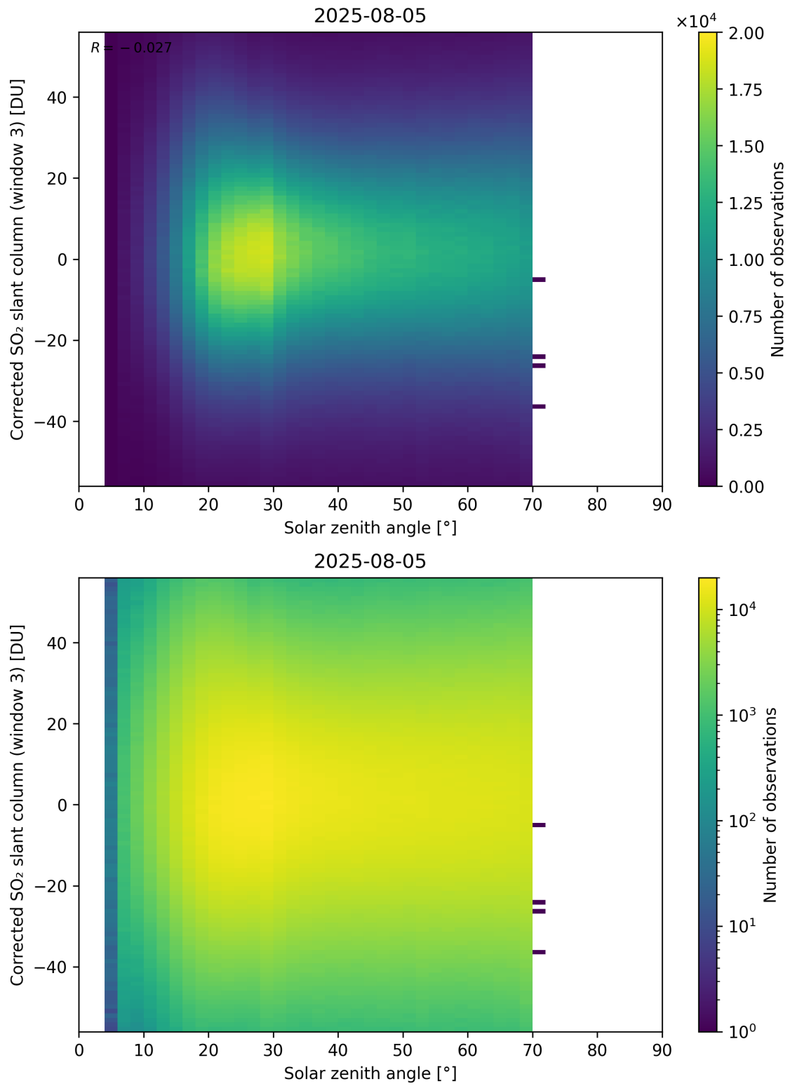
Figure 183: Scatter density plot of “Solar zenith angle” against “Corrected SO 2 slant column (window 3)” for 2025-08-04 to 2025-08-06.
