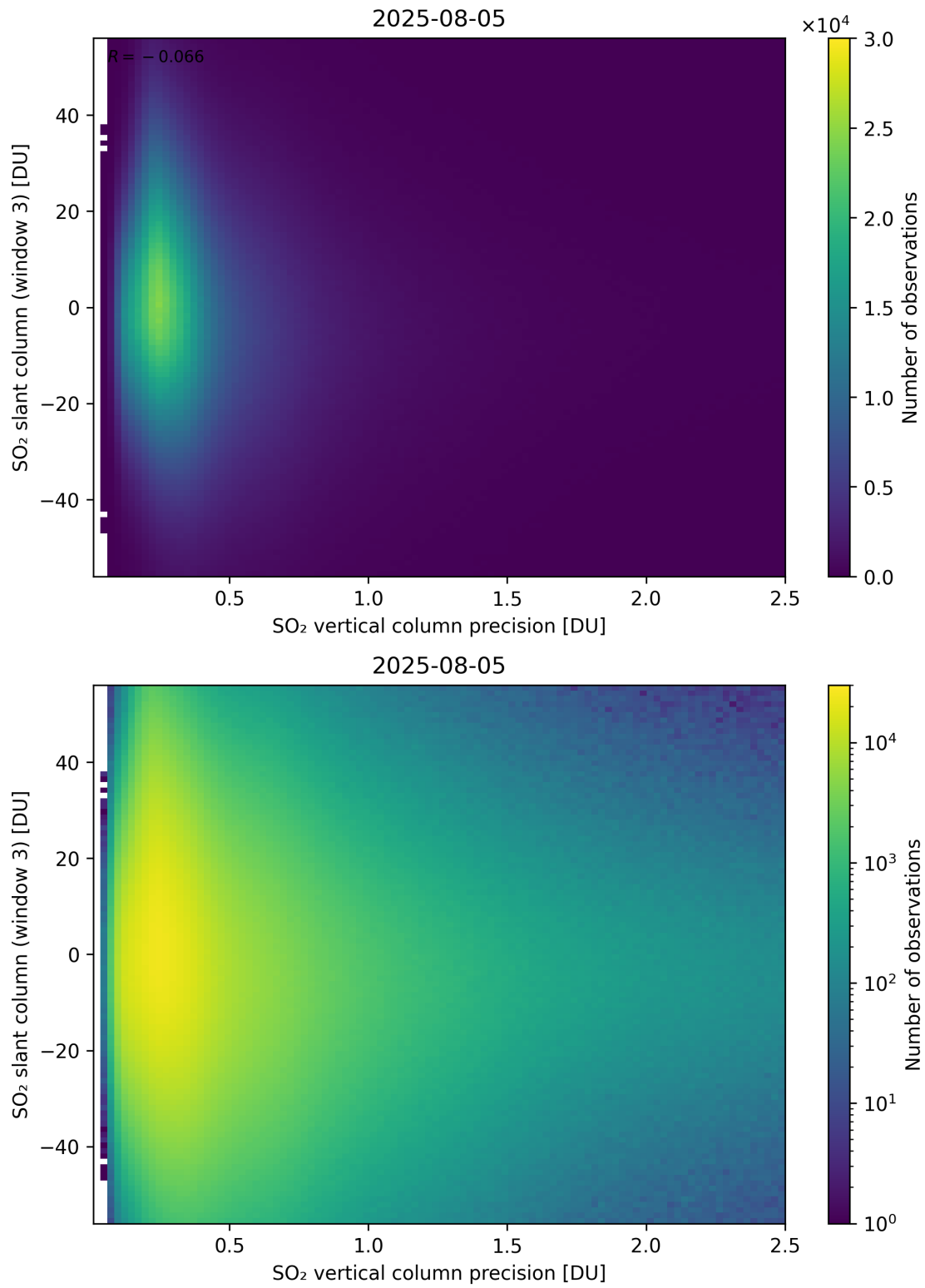
Figure 344: Scatter density plot of “SO 2 vertical column precision” against “SO 2 slant column (window 3)” for 2025-08-04 to 2025-08-06.
