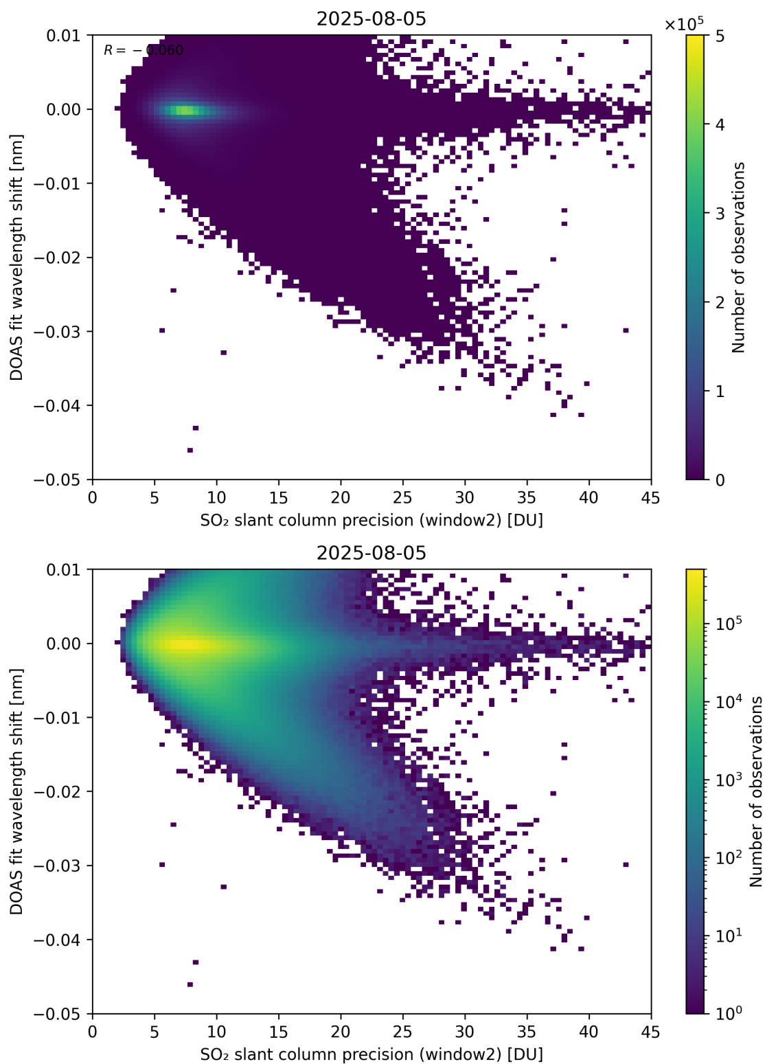
Figure 293: Scatter density plot of “SO 2 slant column precision (window2)” against “DOAS fit wavelength shift” for 2025-08-04 to 2025-08-06.
