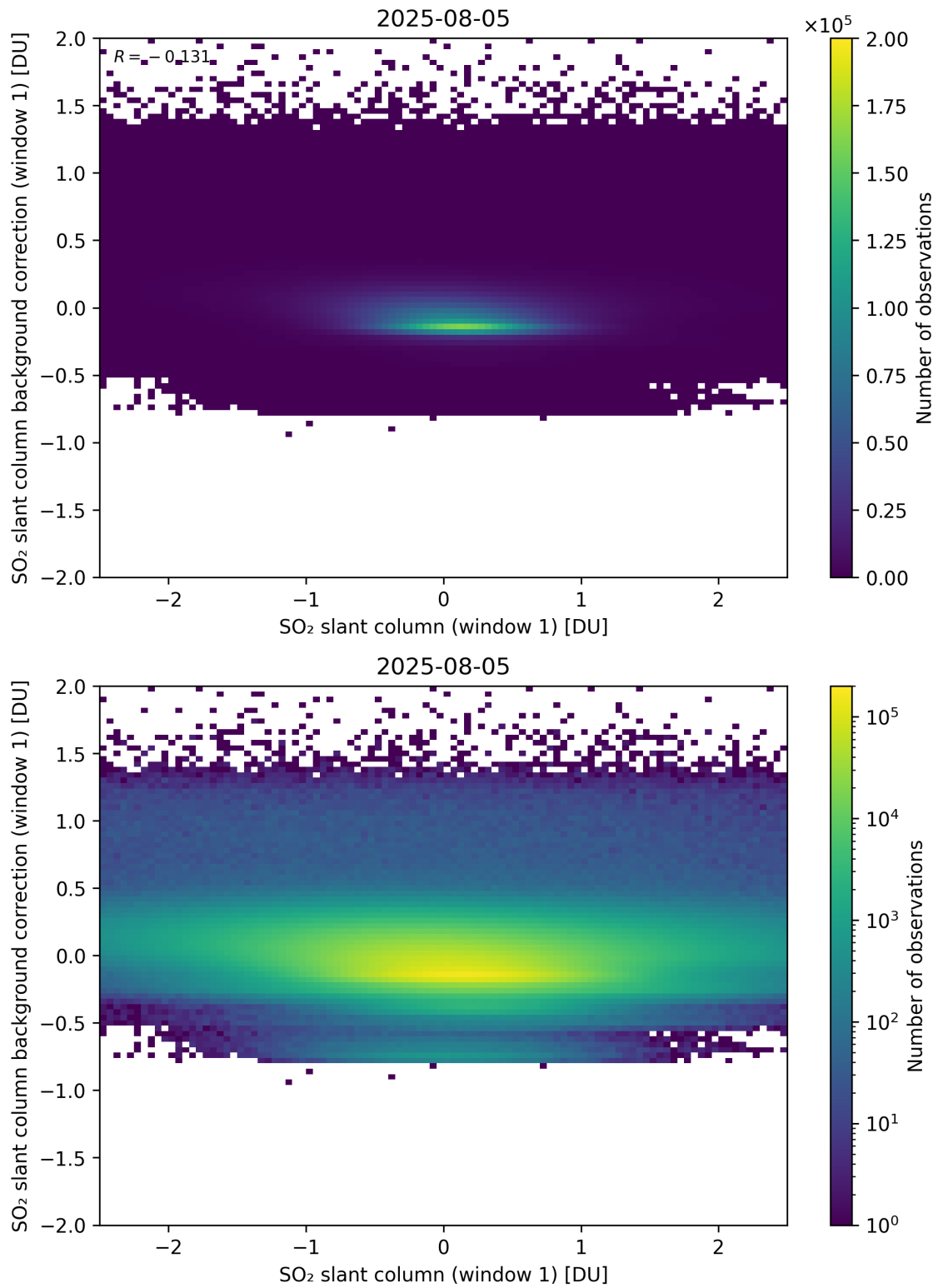
Figure 262: Scatter density plot of “SO 2 slant column (window 1)” against “SO 2 slant column background correction (window 1)” for 2025-08-04 to 2025-08-06.
