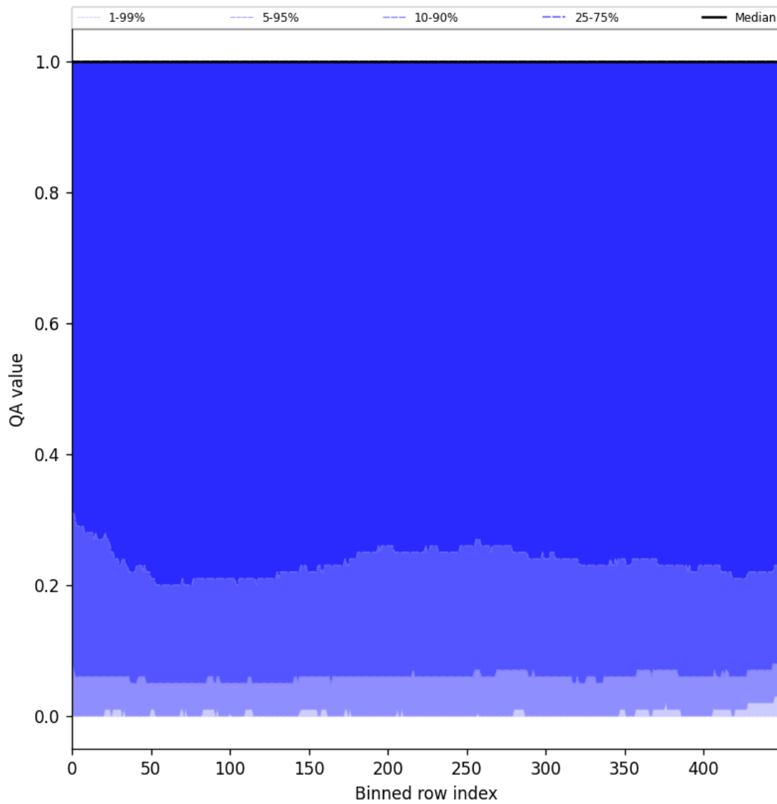
Figure 83: Along track statistics of “QA value” for 2025-08-04 to 2025-08-06
