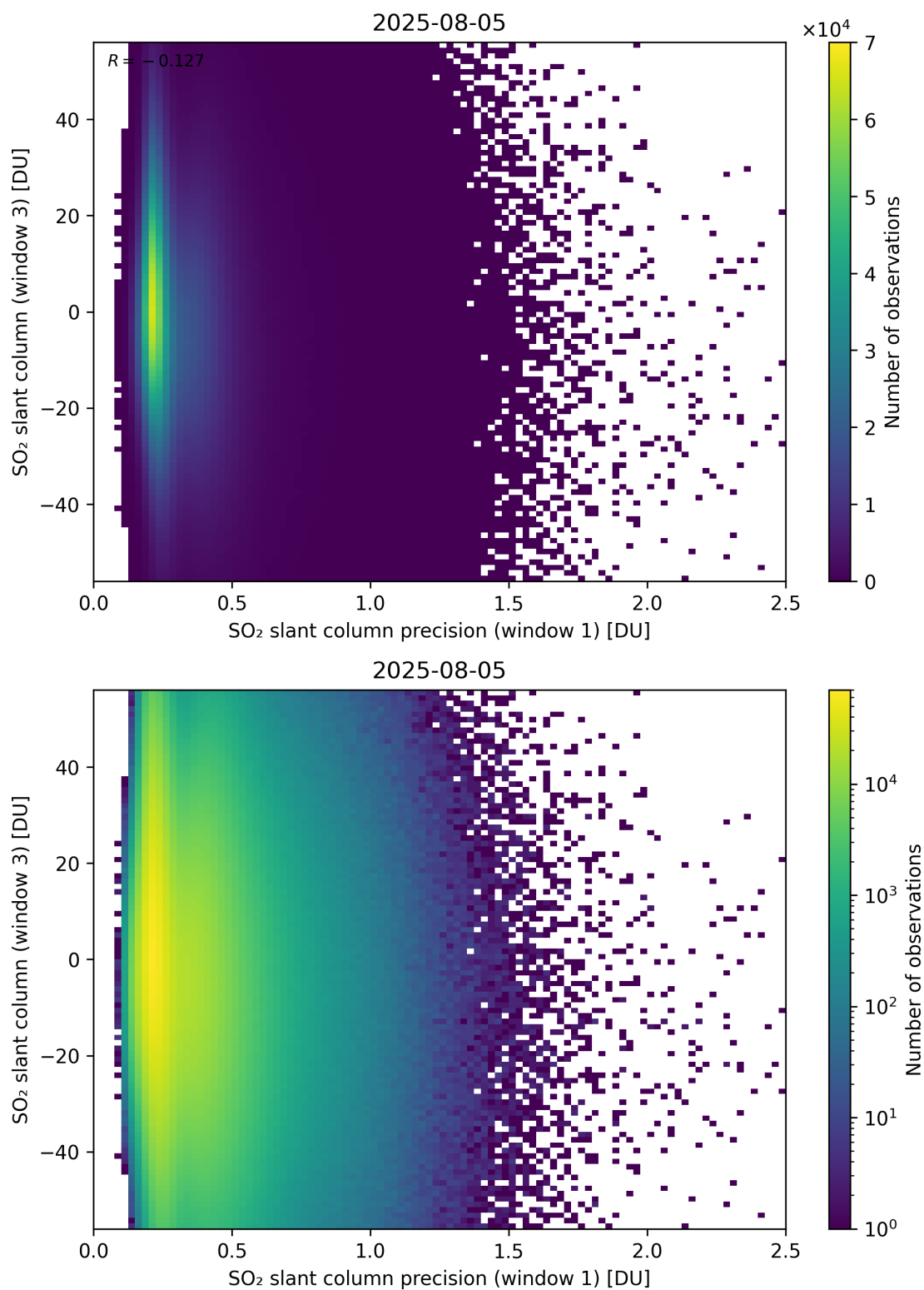
Figure 278: Scatter density plot of “SO 2 slant column precision (window 1)” against “SO 2 slant column (window 3)” for 2025-08-04 to 2025-08-06.
