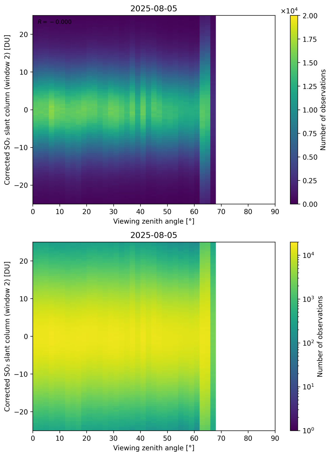
Figure 374: Scatter density plot of “Viewing zenith angle” against “Corrected SO 2 slant column (window 2)” for 2025-08-04 to 2025-08-06.
