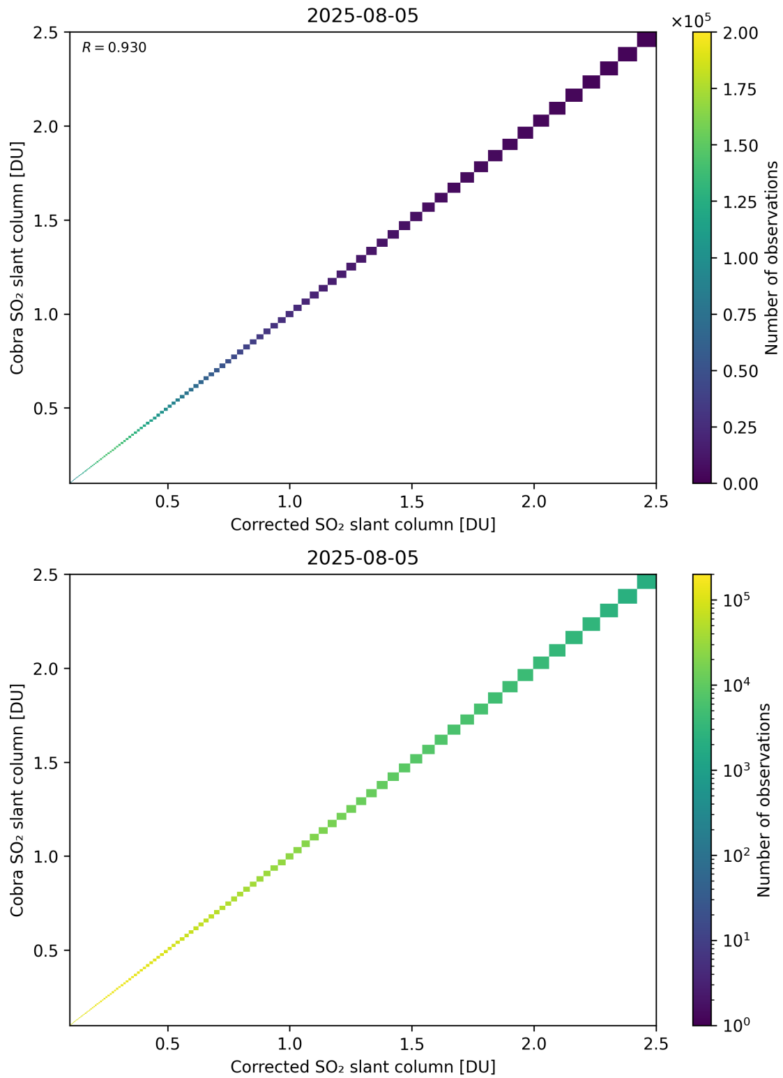
Figure 233: Scatter density plot of “Corrected SO 2 slant column” against “Cobra SO 2 slant column” for 2025-08-04 to 2025-08-06.
