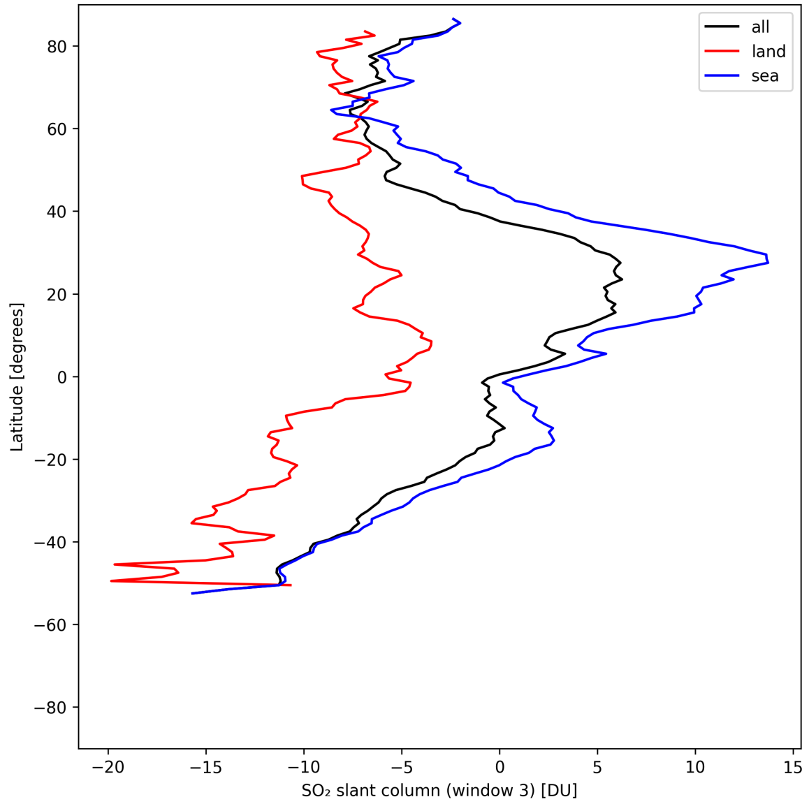
Figure 45: Zonal average of “SO 2 slant column (window 3)” for 2025-08-04 to 2025-08-06.
