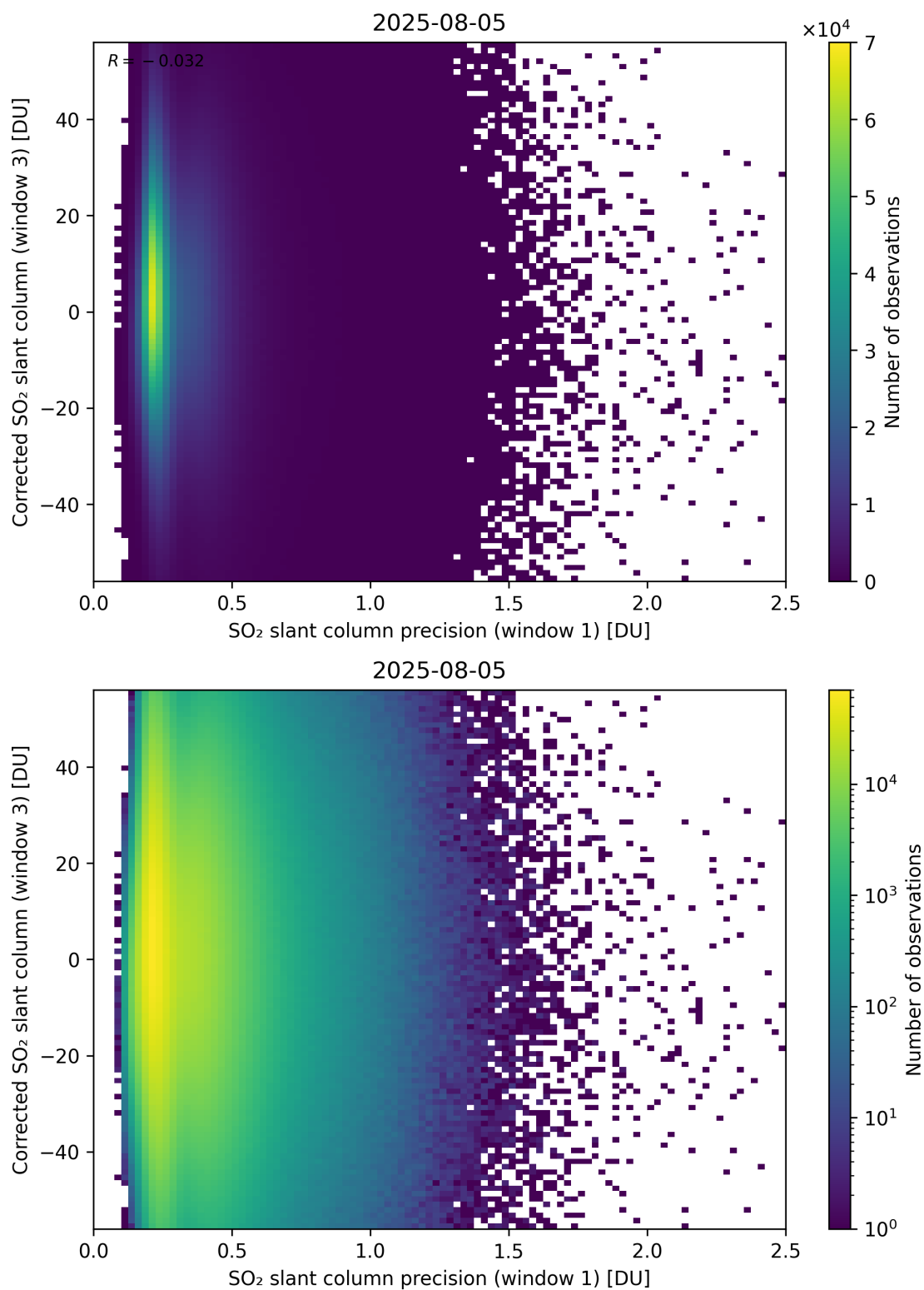
Figure 276: Scatter density plot of “SO 2 slant column precision (window 1)” against “Corrected SO 2 slant column (window 3)” for 2025-08-04 to 2025-08-06.
