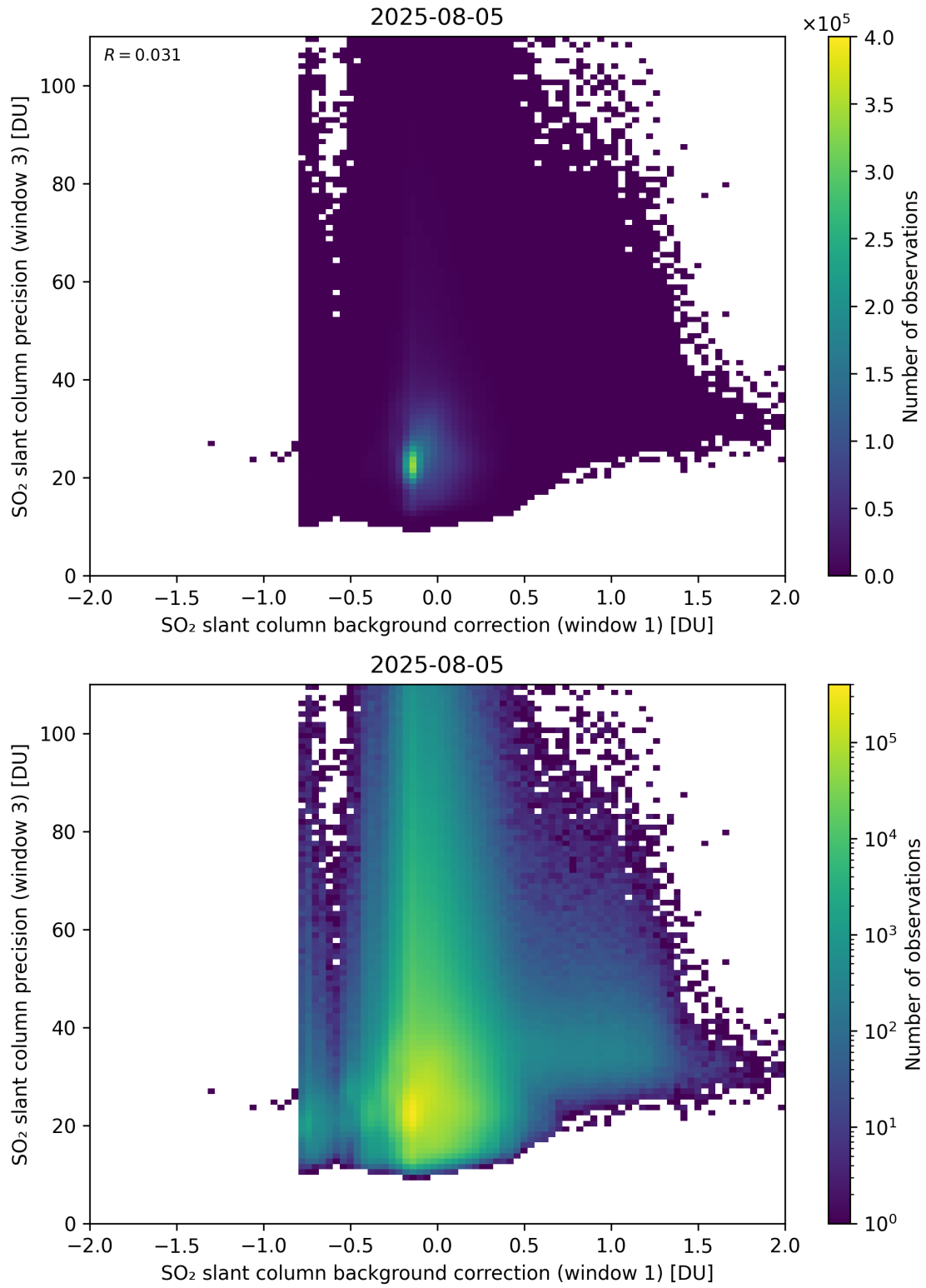
Figure 119: Scatter density plot of “SO 2 slant column background correction (window 1)” against “SO 2 slant column precision (window 3)” for 2025-08-04 to 2025-08-06.
