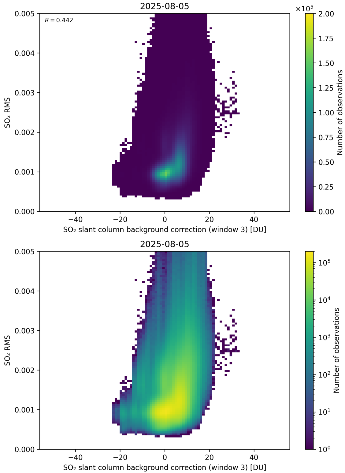
Figure 134: Scatter density plot of “SO 2 slant column background correction (window 3)” against “SO 2 RMS” for 2025-08-04 to 2025-08-06.
