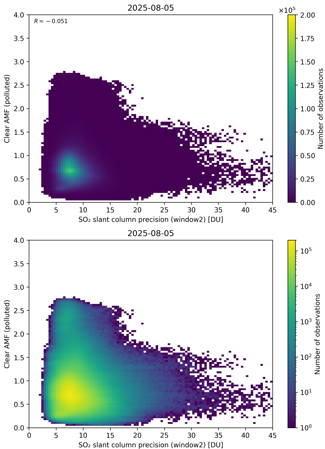
Figure 296: Scatter density plot of “SO 2 slant column precision (window2)” against “Clear AMF (polluted)” for 2025-08-04 to 2025-08-06.
