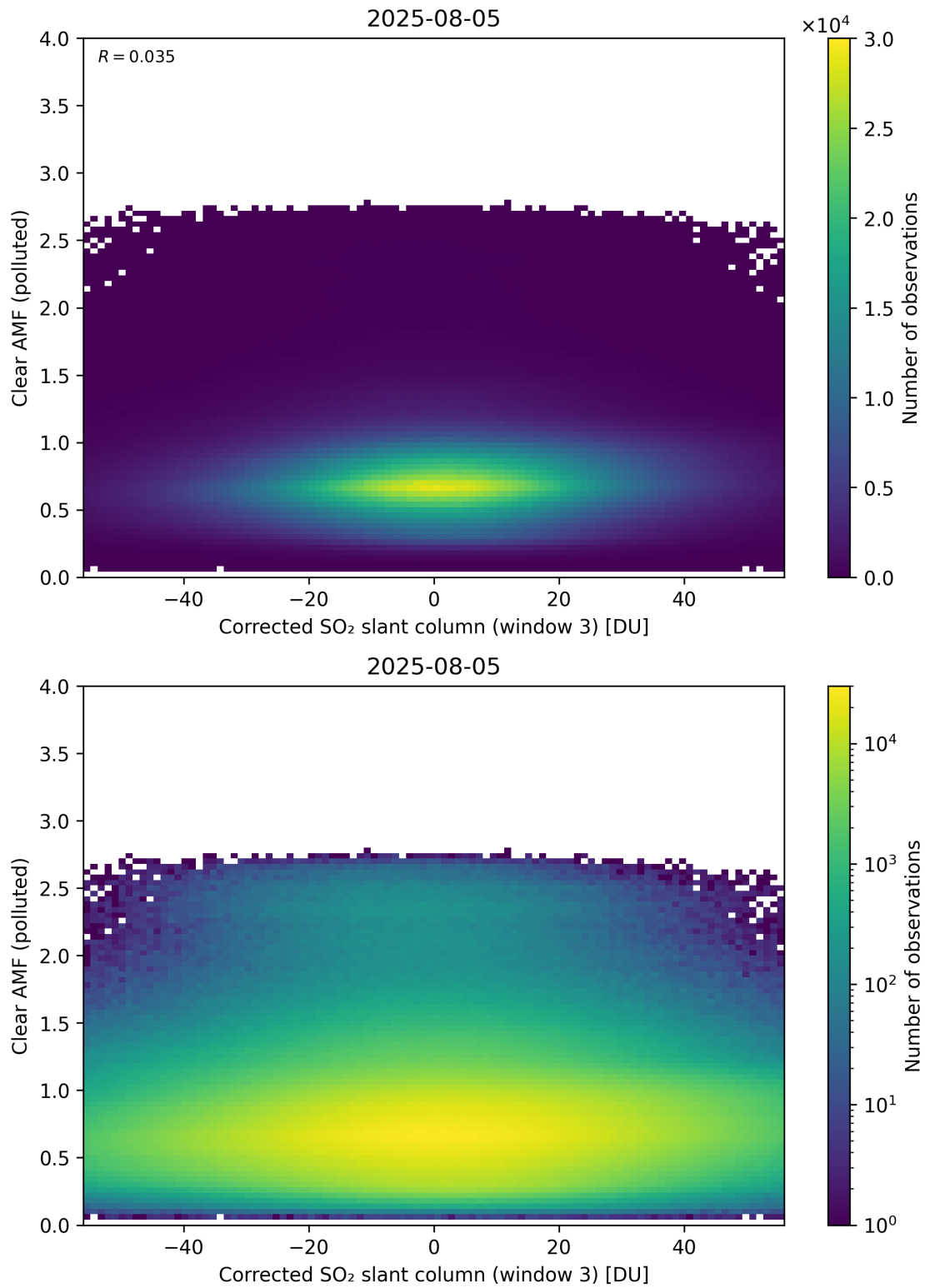
Figure 259: Scatter density plot of “Corrected SO 2 slant column (window 3)” against “Clear AMF (polluted)” for 2025-08-04 to 2025-08-06.
