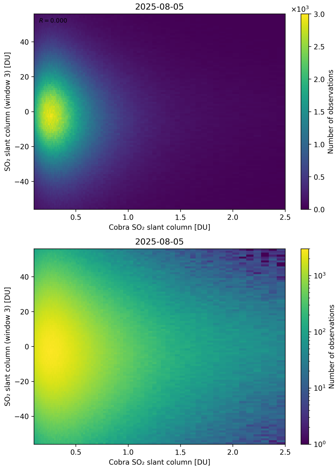
Figure 222: Scatter density plot of “Cobra SO 2 slant column” against “SO 2 slant column (window 3)” for 2025-08-04 to 2025-08-06.
