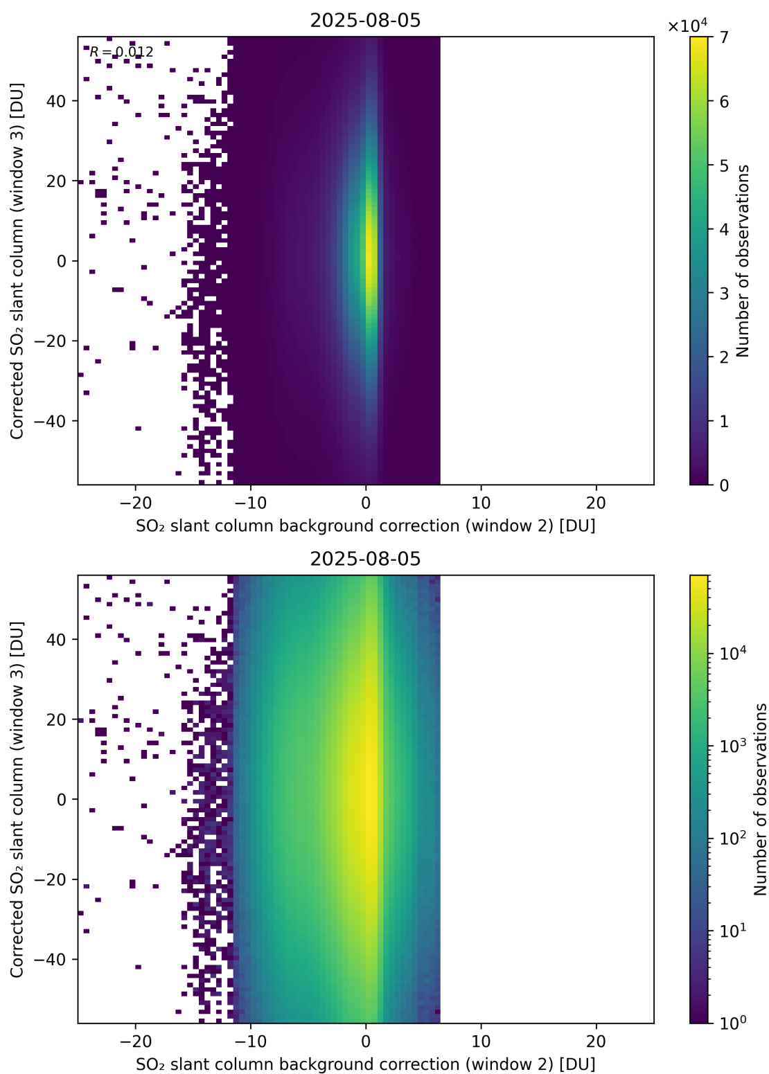
Figure 127: Scatter density plot of “SO 2 slant column background correction (window 2)” against “Corrected SO 2 slant column (window 3)” for 2025-08-04 to 2025-08-06.
