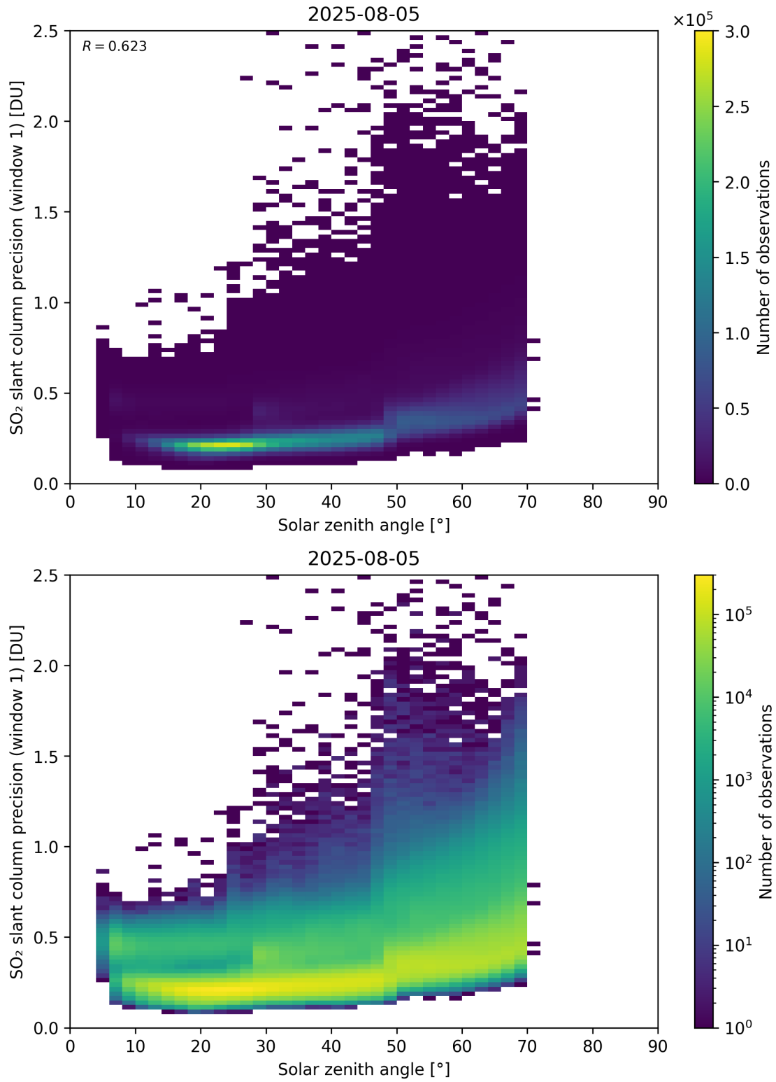
Figure 185: Scatter density plot of “Solar zenith angle” against “SO 2 slant column precision (window 1)” for 2025-08-04 to 2025-08-06.
