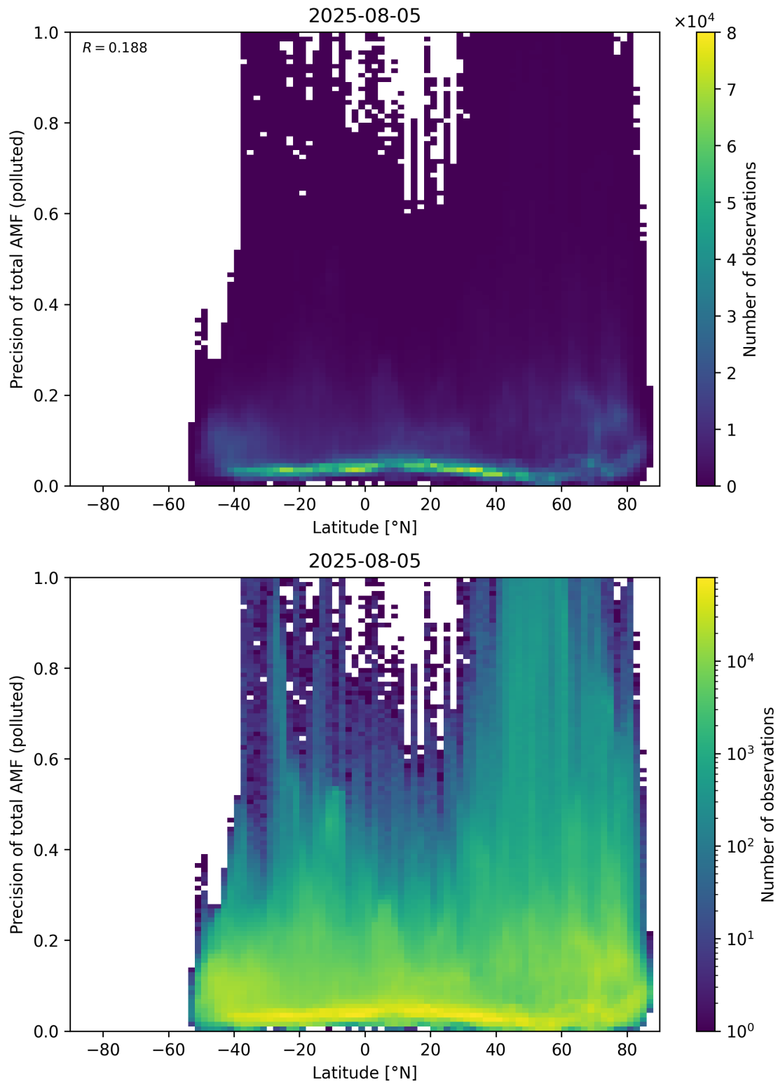
Figure 168: Scatter density plot of “Latitude” against “Precision of total AMF (polluted)” for 2025-08-04 to 2025-08-06.
