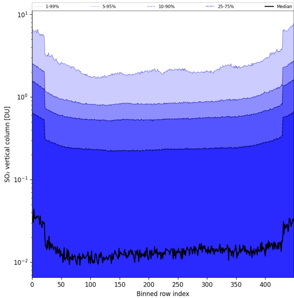
Figure 84: Along track statistics of “SO 2 vertical column” for 2025-08-04 to 2025-08-06
