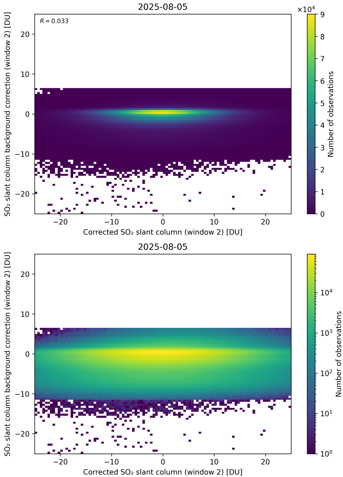
Figure 244: Scatter density plot of “Corrected SO 2 slant column (window 2)” against “SO 2 slant column background correction (window 2)” for 2025-08-04 to 2025-08-06.
