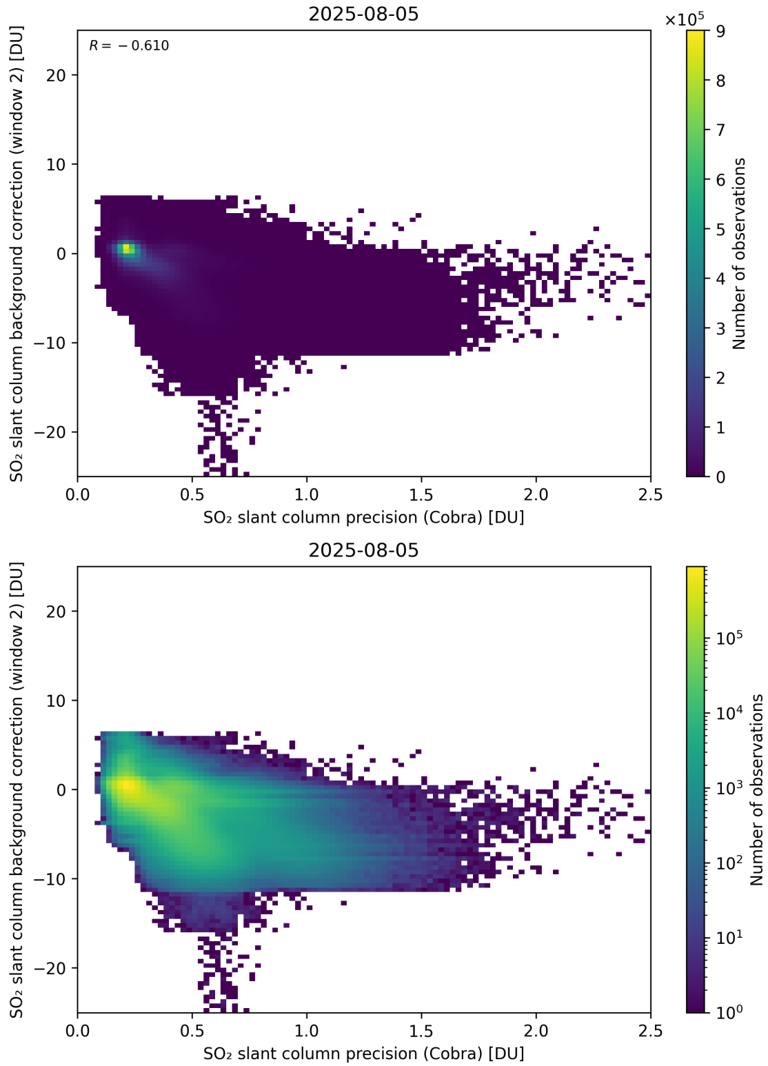
Figure 200: Scatter density plot of “SO 2 slant column precision (Cobra)” against “SO 2 slant column background correction (window 2)” for 2025-08-04 to 2025-08-06.
