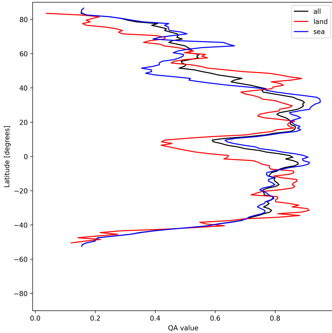
Figure 31: Zonal average of “QA value” for 2025-08-04 to 2025-08-06.
