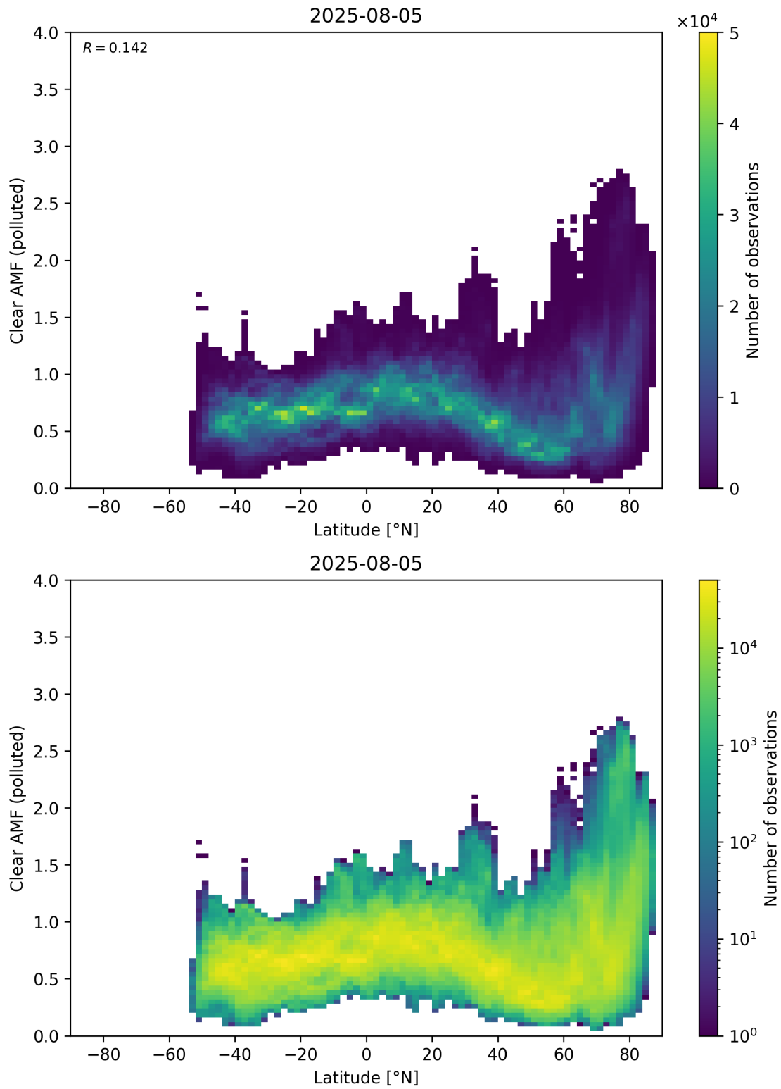
Figure 156: Scatter density plot of “Latitude” against “Clear AMF (polluted)” for 2025-08-04 to 2025-08-06.
