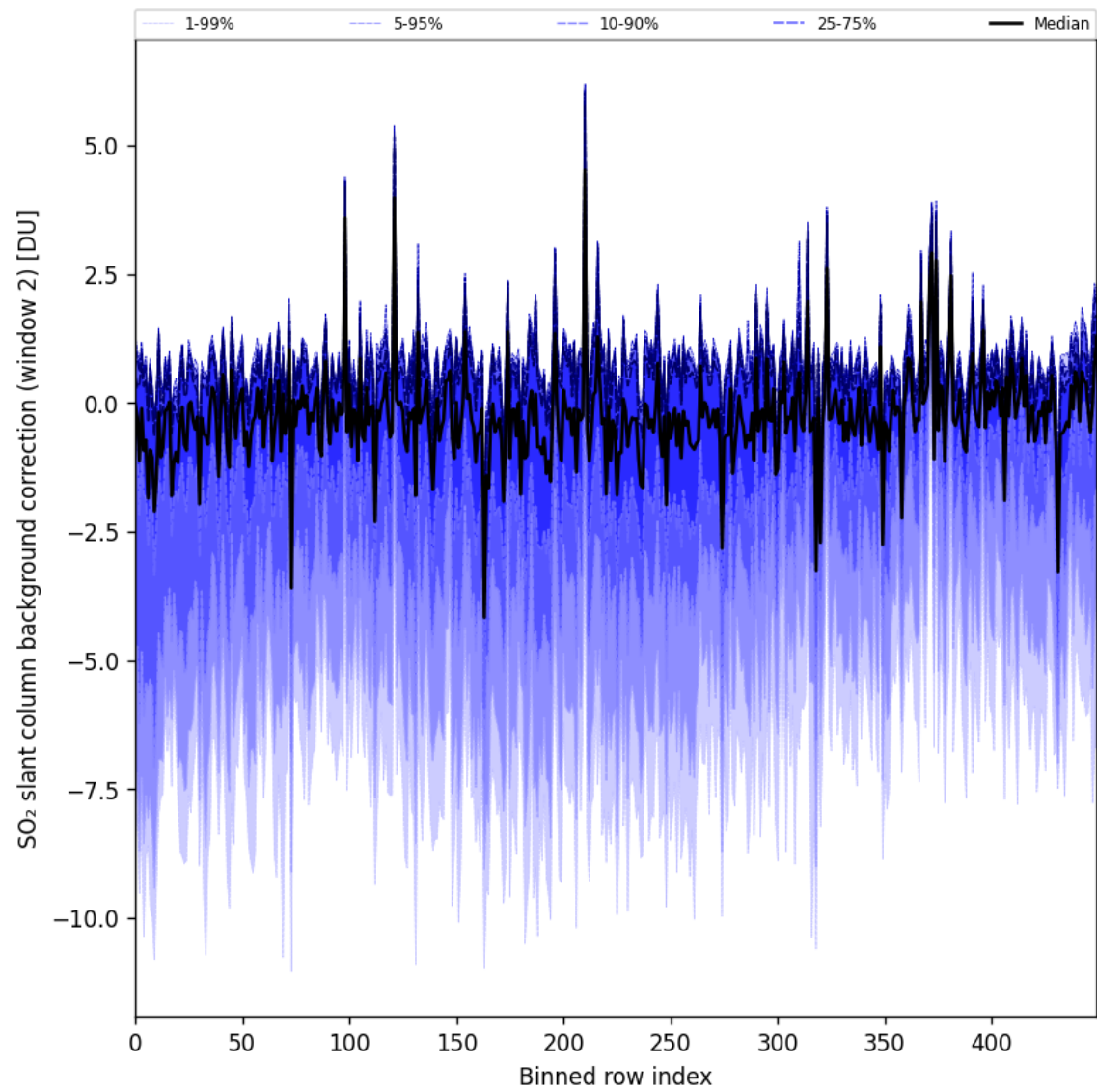
Figure 96: Along track statistics of “SO 2 slant column background correction (window 2)” for 2025-08-04 to 2025-08-06
