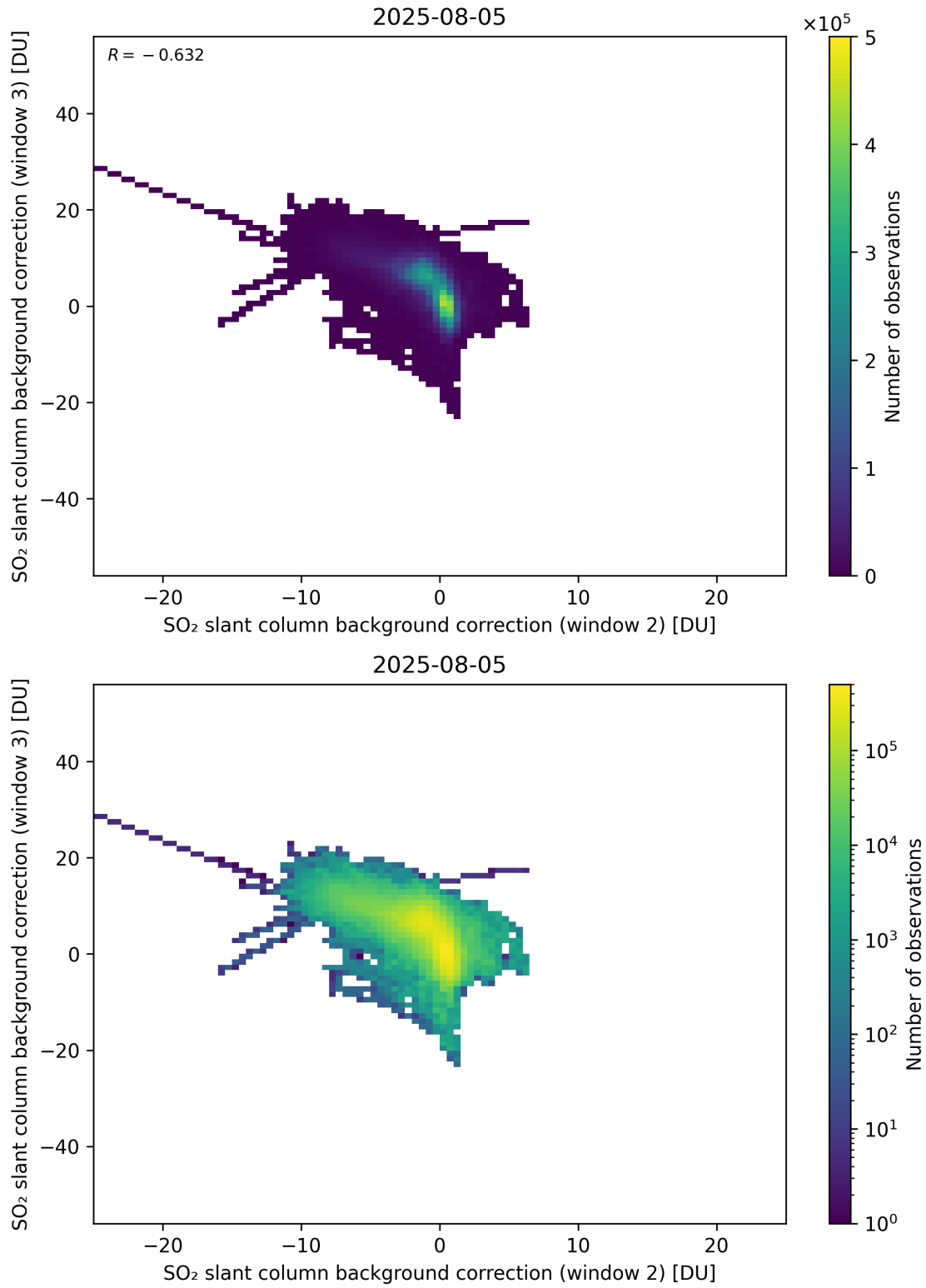
Figure 122: Scatter density plot of “SO 2 slant column background correction (window 2)” against “SO 2 slant column background correction (window 3)” for 2025-08-04 to 2025-08-06.
