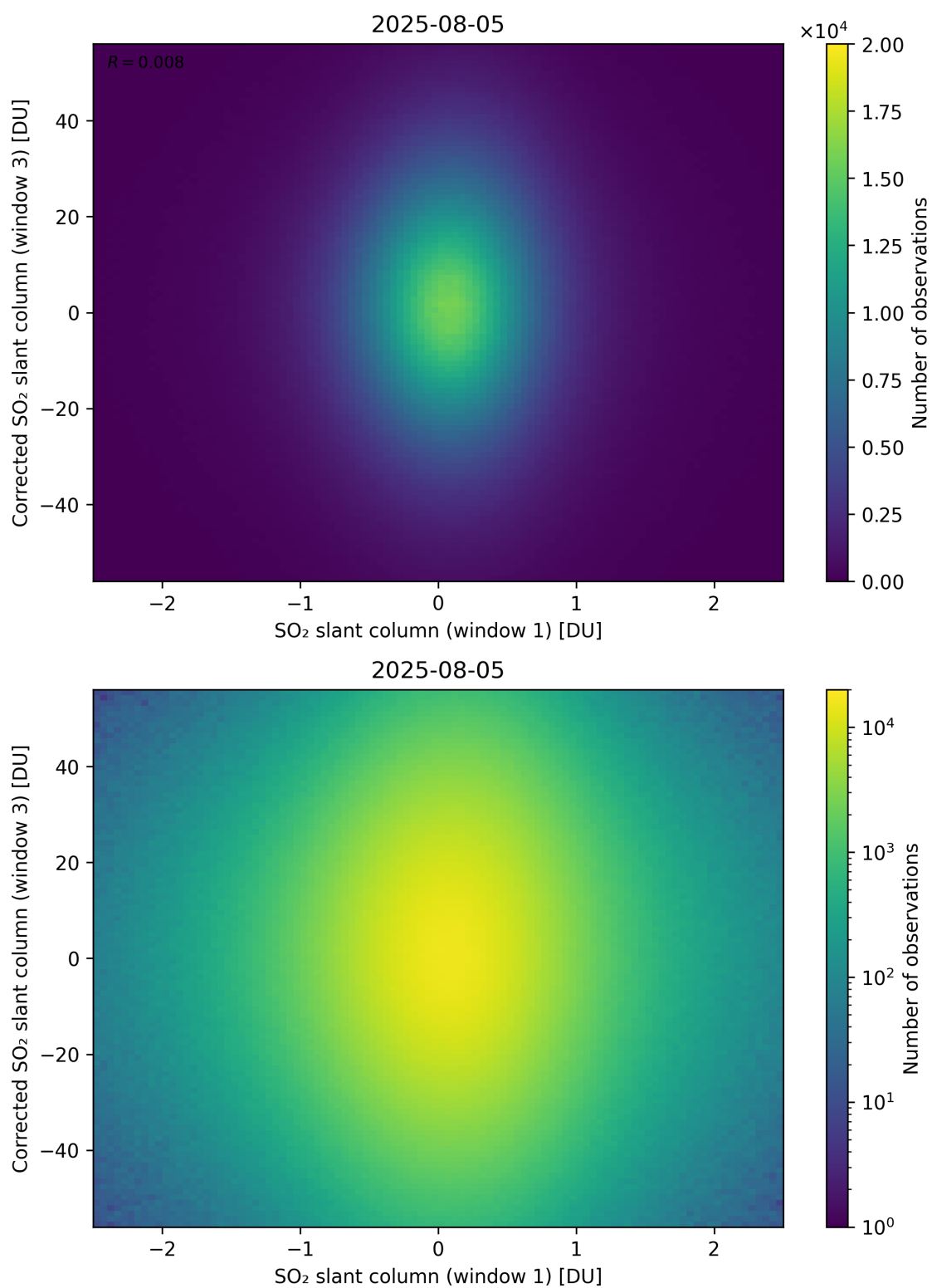
Figure 284: Scatter density plot of “SO 2 slant column (window 1)” against “Corrected SO 2 slant column (window 3)” for 2025-08-04 to 2025-08-06.
