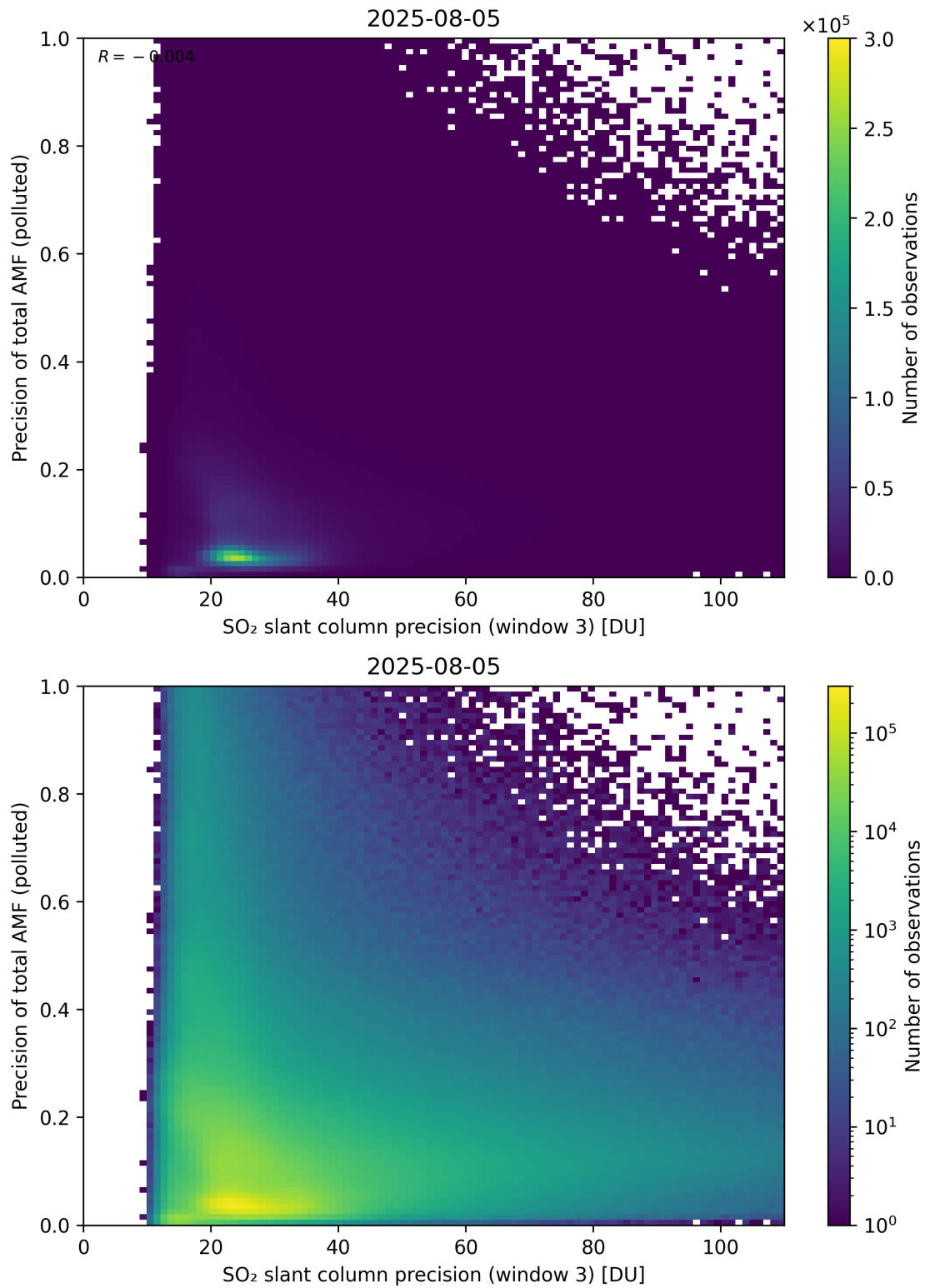
Figure 314: Scatter density plot of “SO 2 slant column precision (window 3)” against “Precision of total AMF (polluted)” for 2025-08-04 to 2025-08-06.
