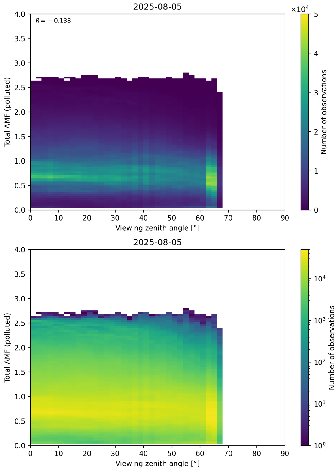
Figure 381: Scatter density plot of “Viewing zenith angle” against “Total AMF (polluted)” for 2025-08-04 to 2025-08-06.
