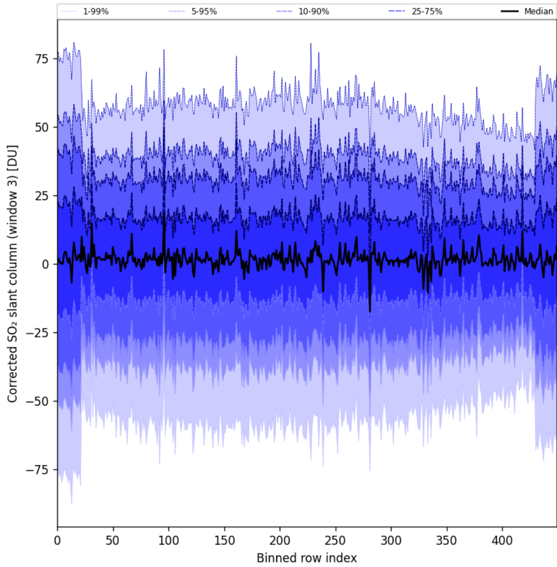
Figure 99: Along track statistics of “Corrected SO 2 slant column (window 3)” for 2025-08-04 to 2025-08-06
