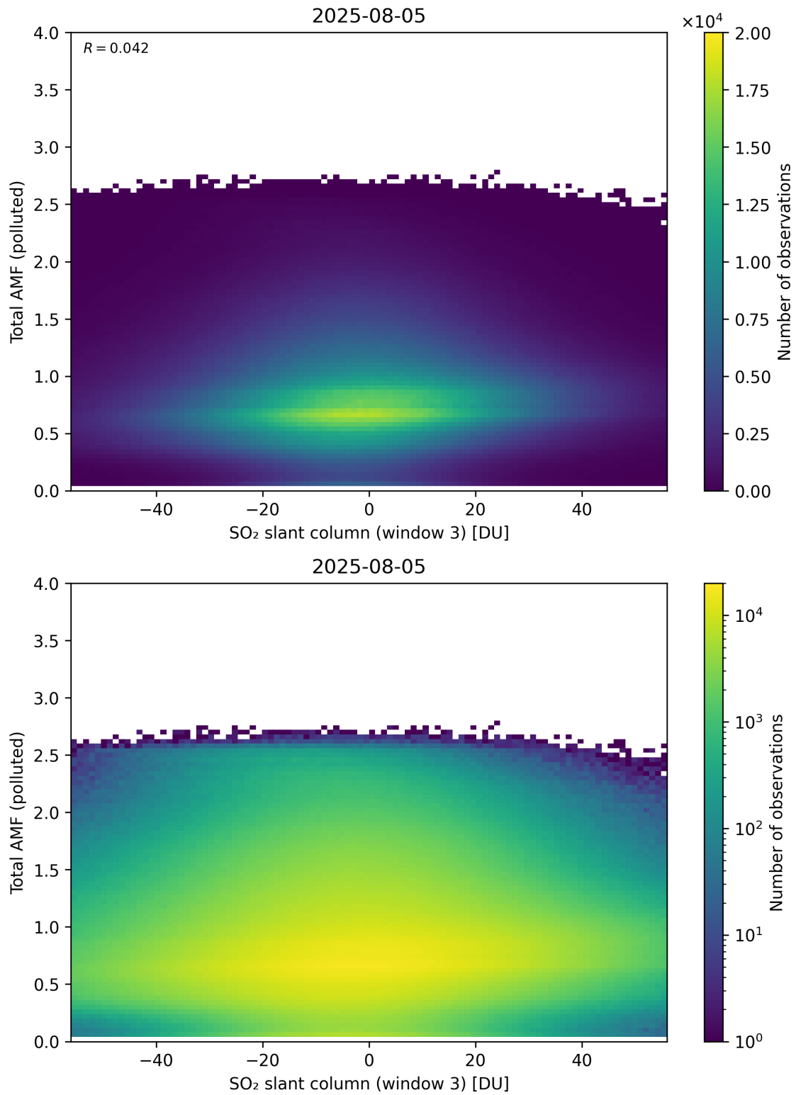
Figure 318: Scatter density plot of “SO 2 slant column (window 3)” against “Total AMF (polluted)” for 2025-08-04 to 2025-08-06.
