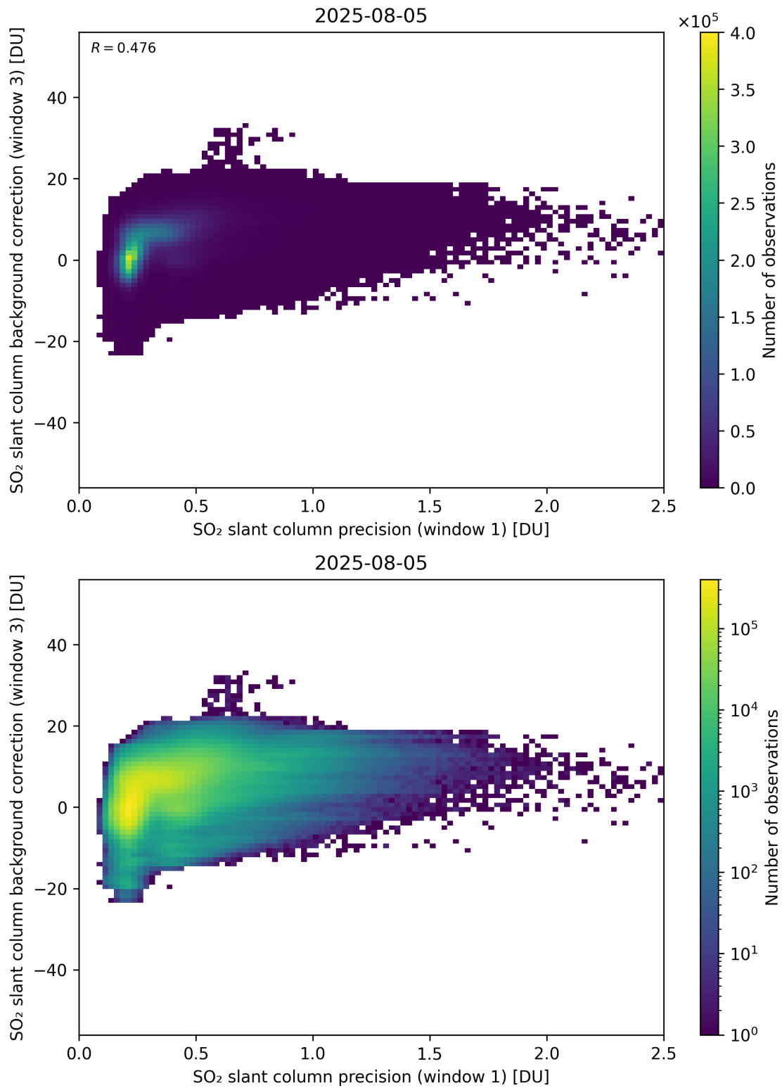
Figure 270: Scatter density plot of “SO 2 slant column precision (window 1)” against “SO 2 slant column background correction (window 3)” for 2025-08-04 to 2025-08-06.
