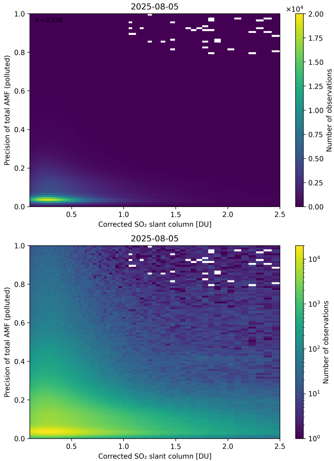
Figure 243: Scatter density plot of “Corrected SO 2 slant column” against “Precision of total AMF (polluted)” for 2025-08-04 to 2025-08-06.
