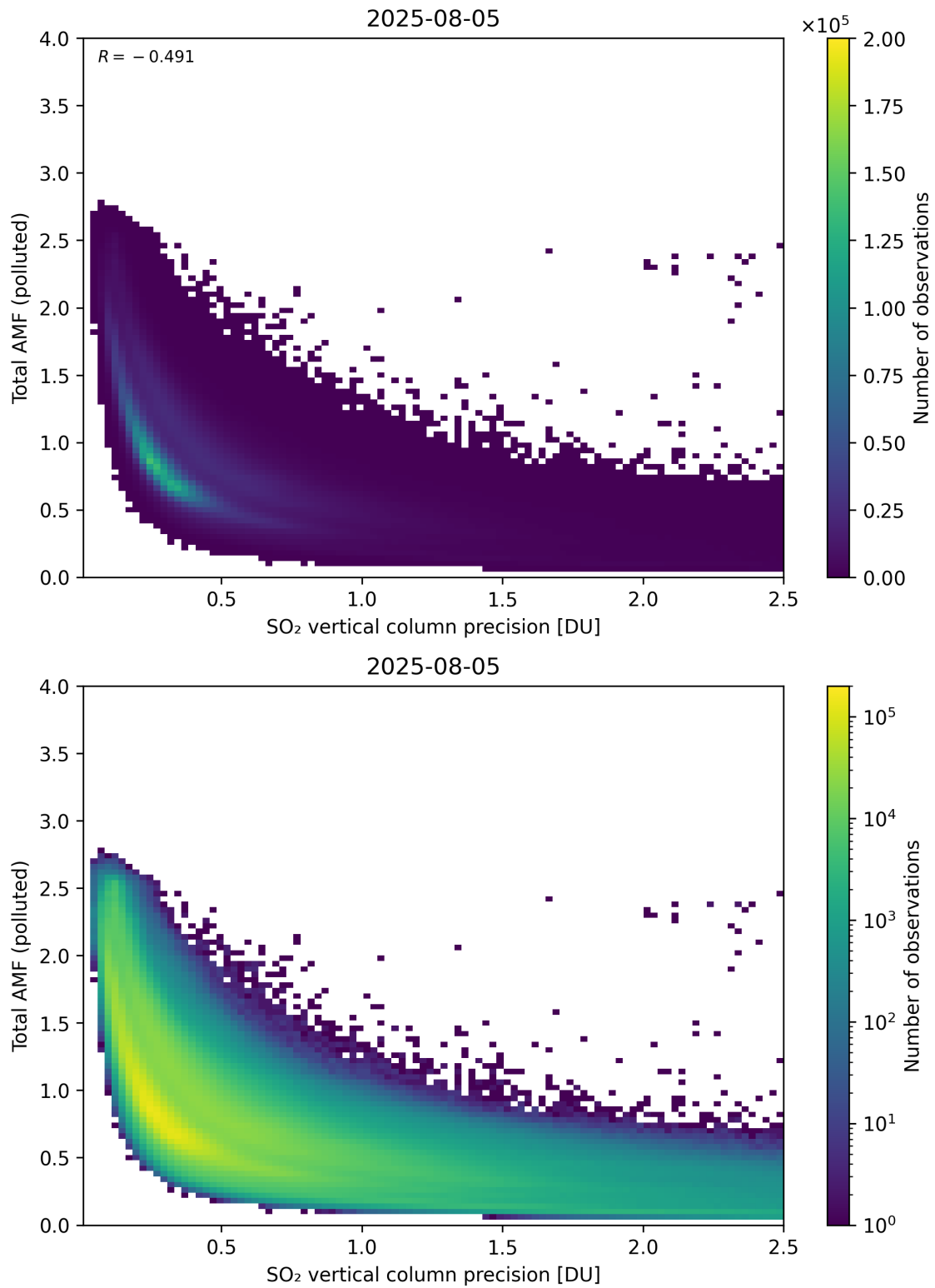
Figure 346: Scatter density plot of “SO 2 vertical column precision” against “Total AMF (polluted)” for 2025-08-04 to 2025-08-06.
