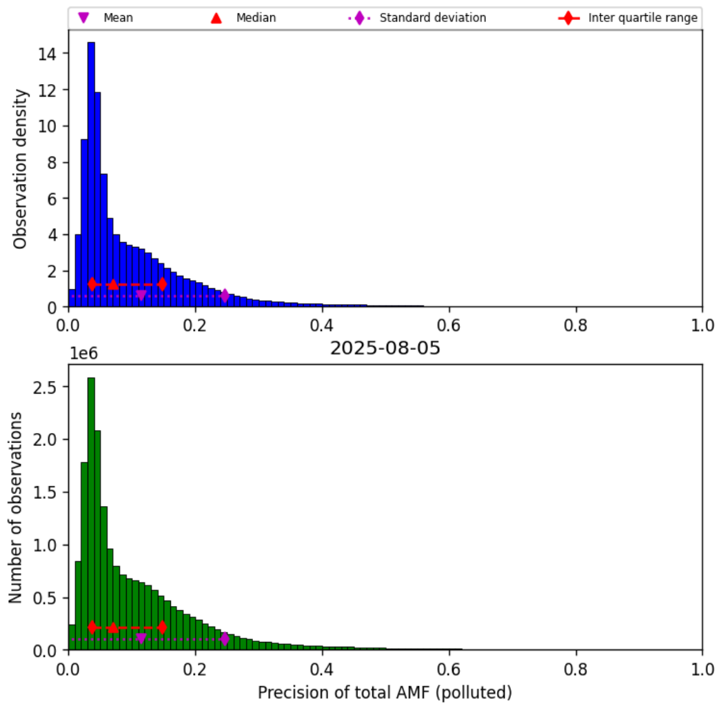
Figure 80: Histogram of “Precision of total AMF (polluted)” for 2025-08-04 to 2025-08-06
