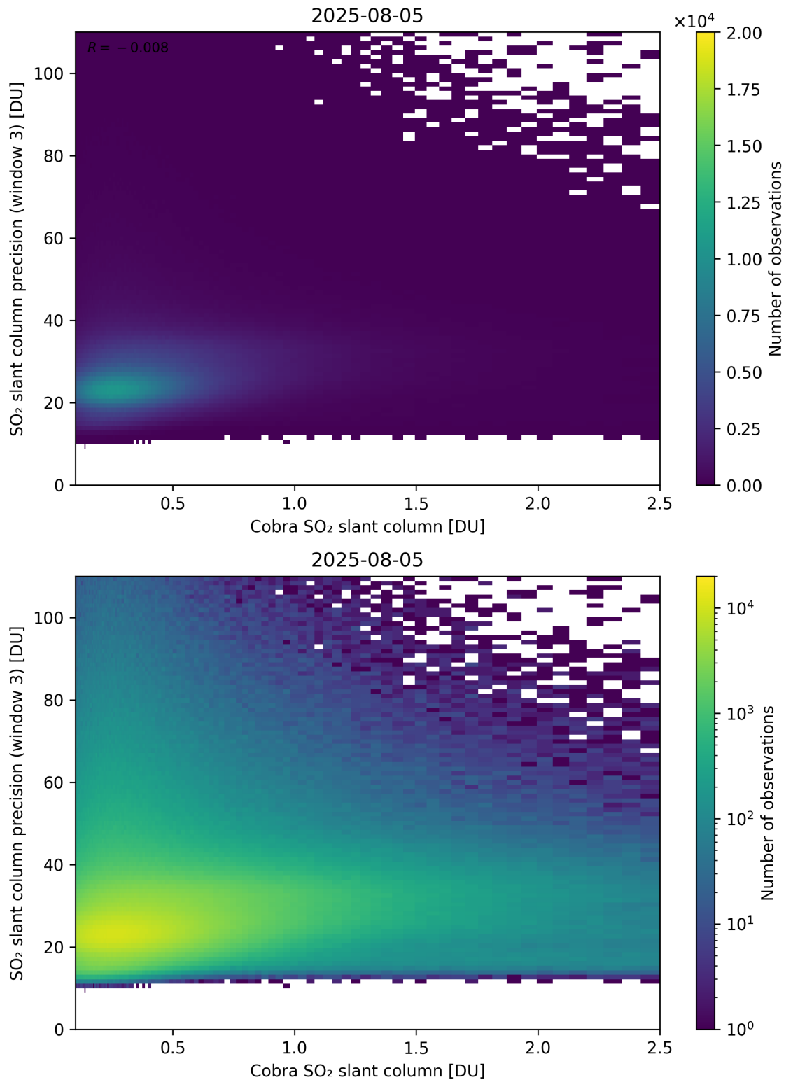
Figure 223: Scatter density plot of “Cobra SO 2 slant column” against “SO 2 slant column precision (window 3)” for 2025-08-04 to 2025-08-06.
