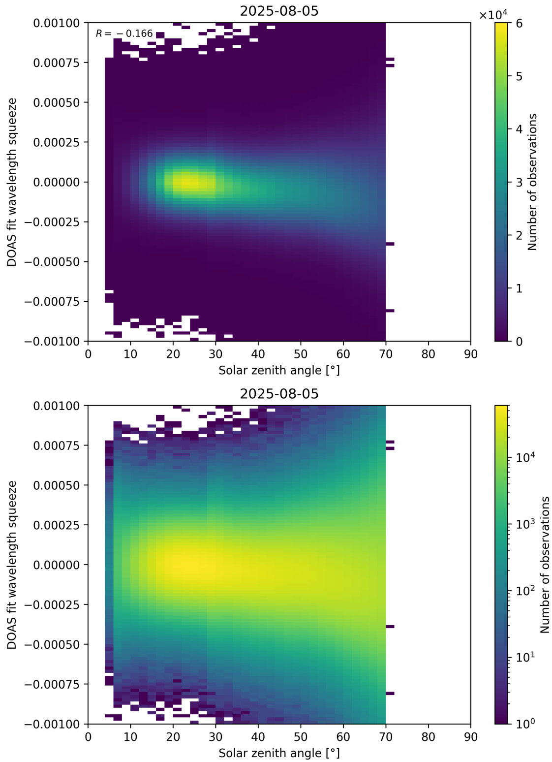
Figure 175: Scatter density plot of “Solar zenith angle” against “DOAS fit wavelength squeeze” for 2025-08-04 to 2025-08-06.
