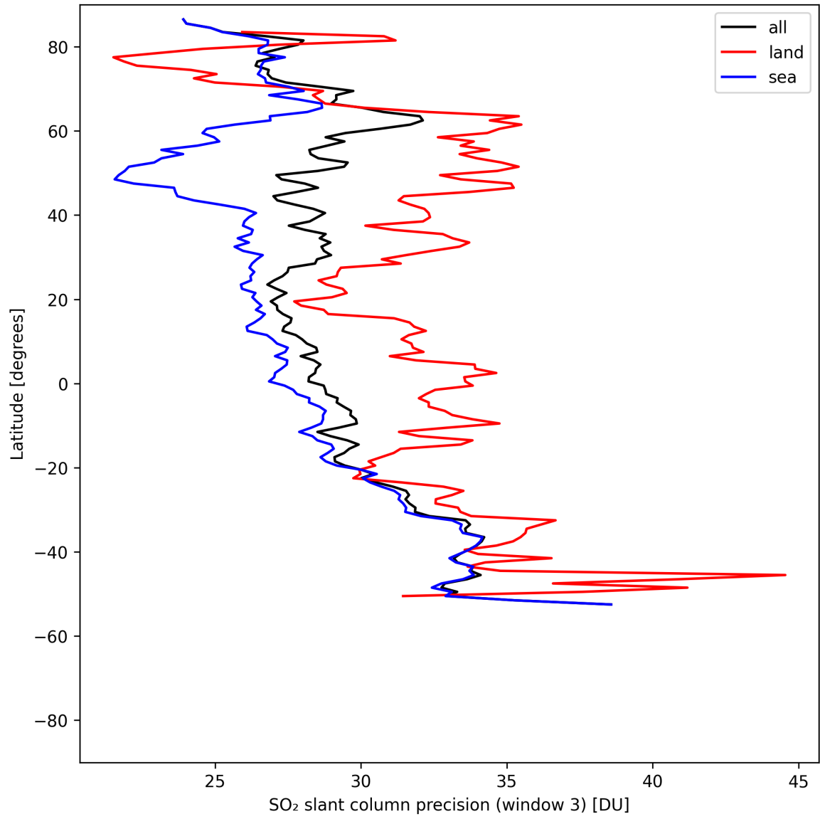
Figure 46: Zonal average of “SO 2 slant column precision (window 3)” for 2025-08-04 to 2025-08-06.
