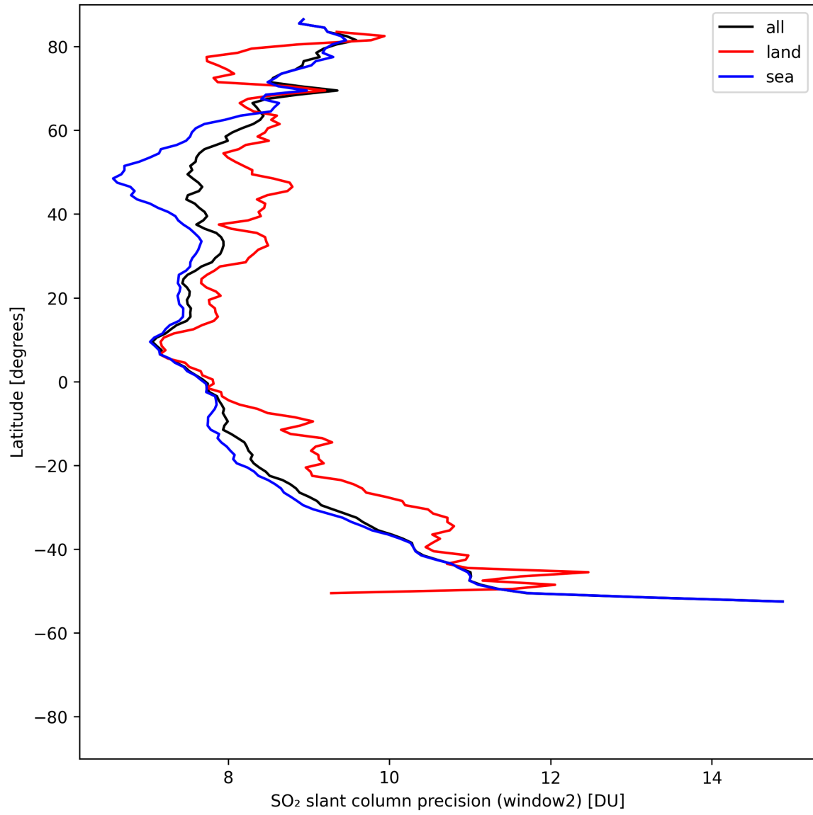
Figure 42: Zonal average of “SO 2 slant column precision (window2)” for 2025-08-04 to 2025-08-06.
