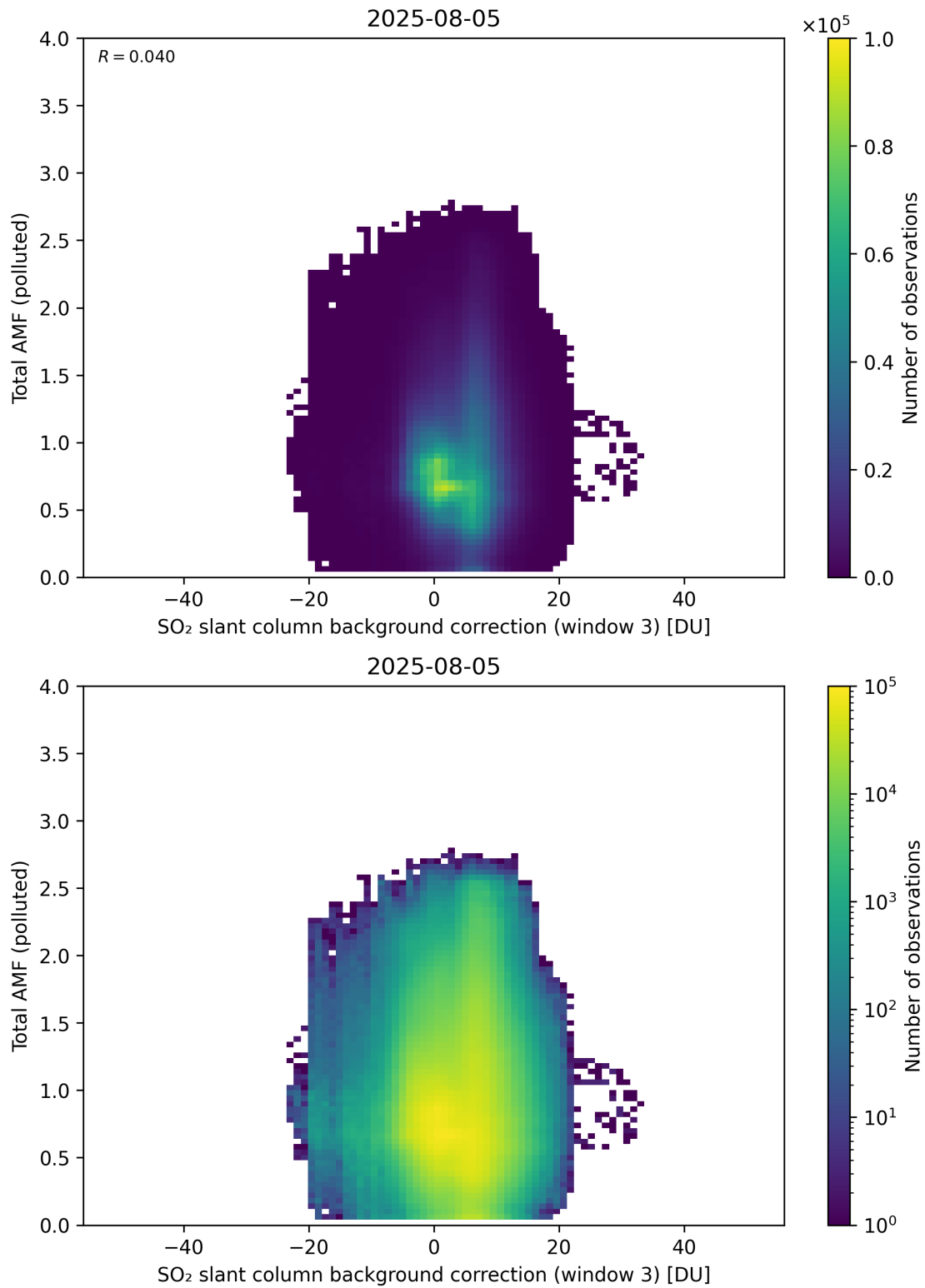
Figure 136: Scatter density plot of “SO 2 slant column background correction (window 3)” against “Total AMF (polluted)” for 2025-08-04 to 2025-08-06.
