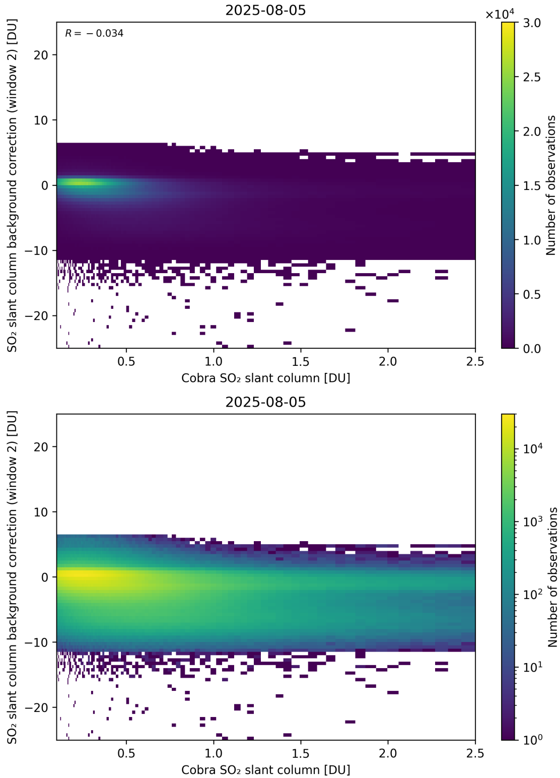
Figure 194: Scatter density plot of “Cobra SO 2 slant column” against “SO 2 slant column background correction (window 2)” for 2025-08-04 to 2025-08-06.
