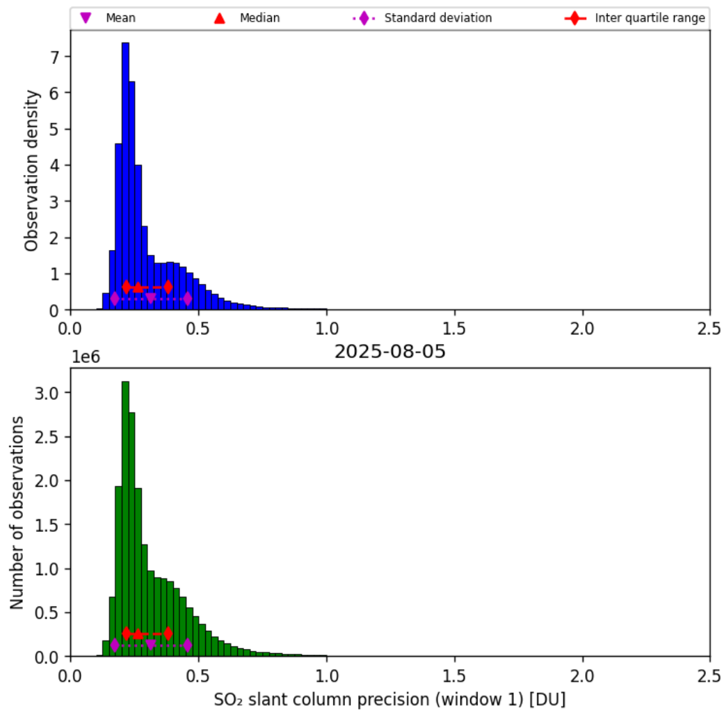
Figure 64: Histogram of “SO 2 slant column precision (window 1)” for 2025-08-04 to 2025-08-06
