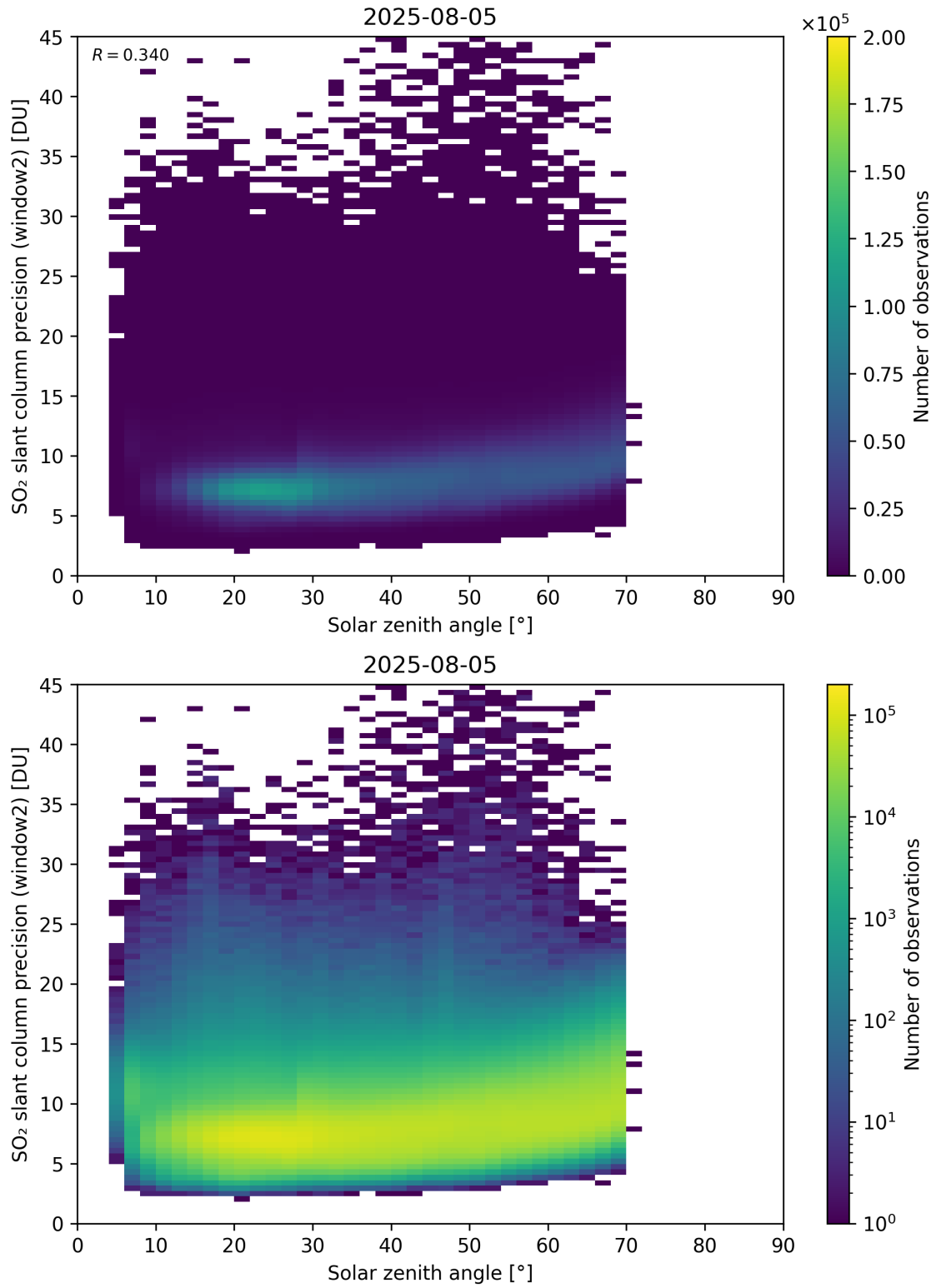
Figure 186: Scatter density plot of “Solar zenith angle” against “SO 2 slant column precision (window2)” for 2025-08-04 to 2025-08-06.
