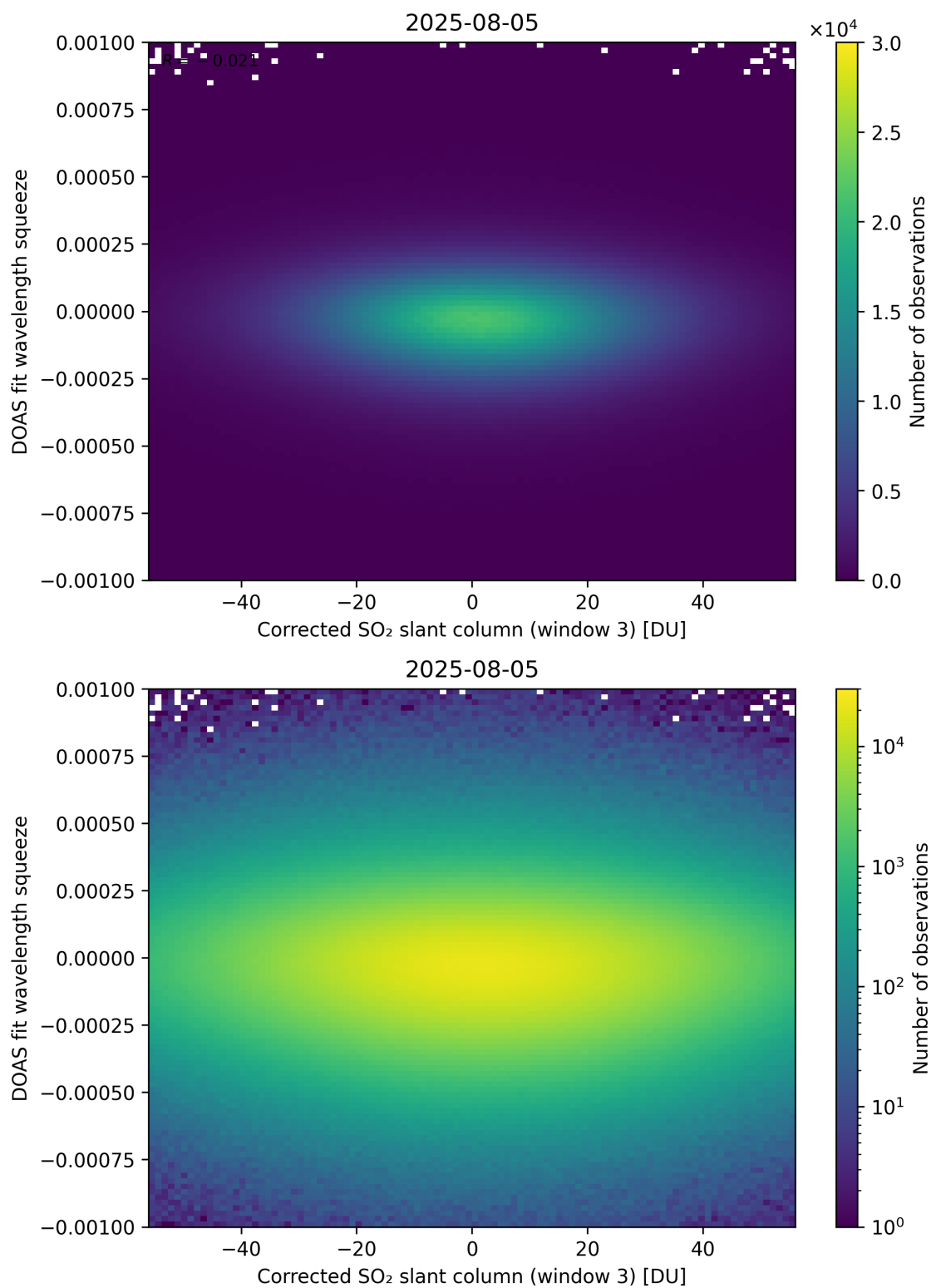
Figure 257: Scatter density plot of “Corrected SO 2 slant column (window 3)” against “DOAS fit wavelength squeeze” for 2025-08-04 to 2025-08-06.
