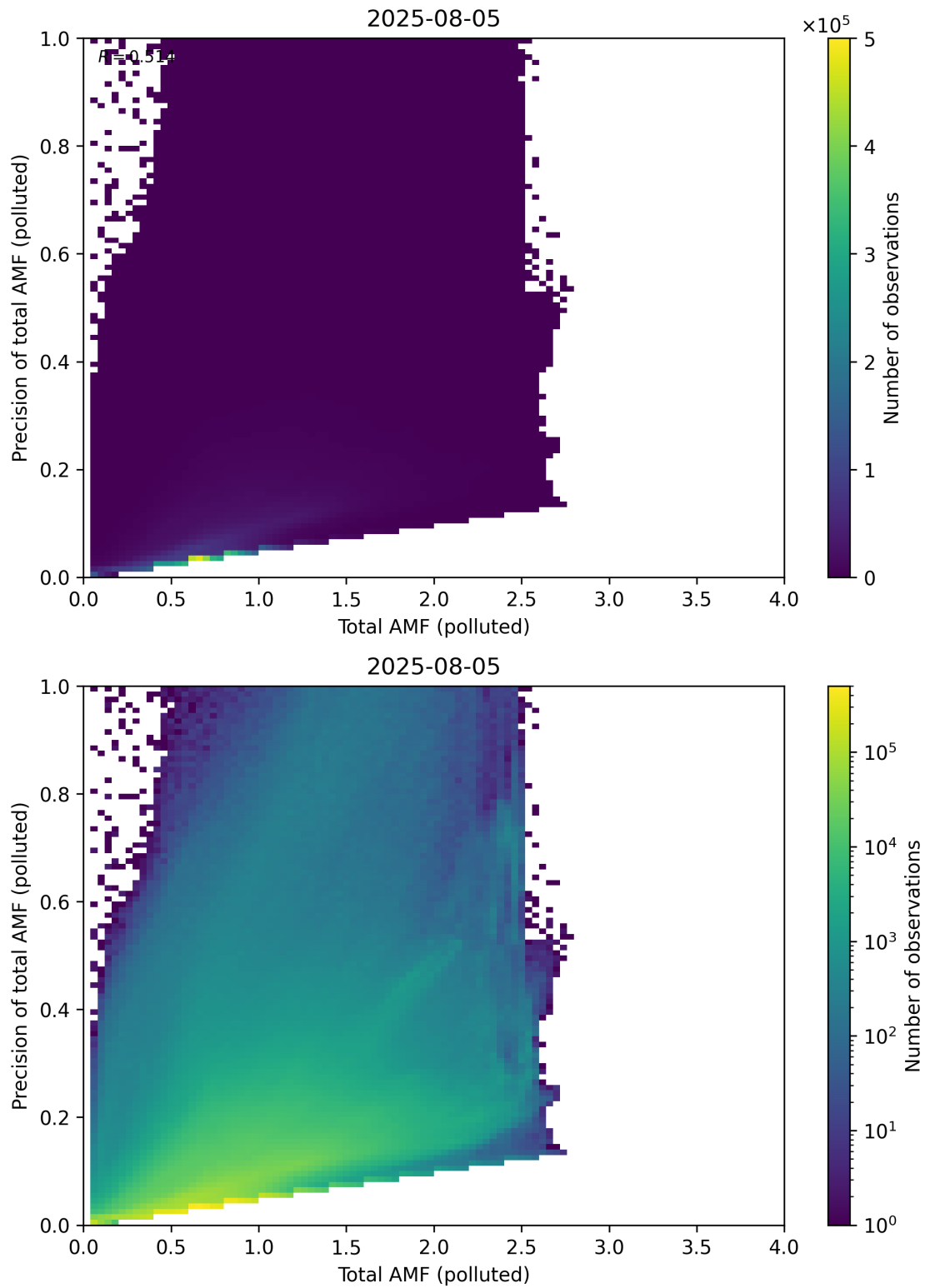
Figure 322: Scatter density plot of “Total AMF (polluted)” against “Precision of total AMF (polluted)” for 2025-08-04 to 2025-08-06.
