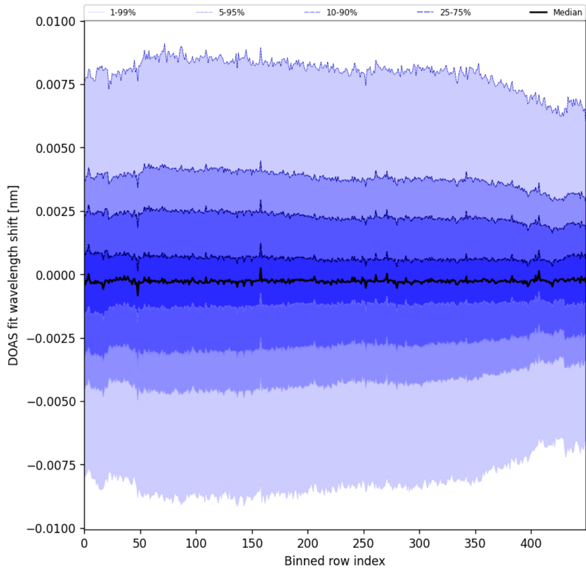
Figure 102: Along track statistics of “DOAS fit wavelength shift” for 2025-08-04 to 2025-08-06
