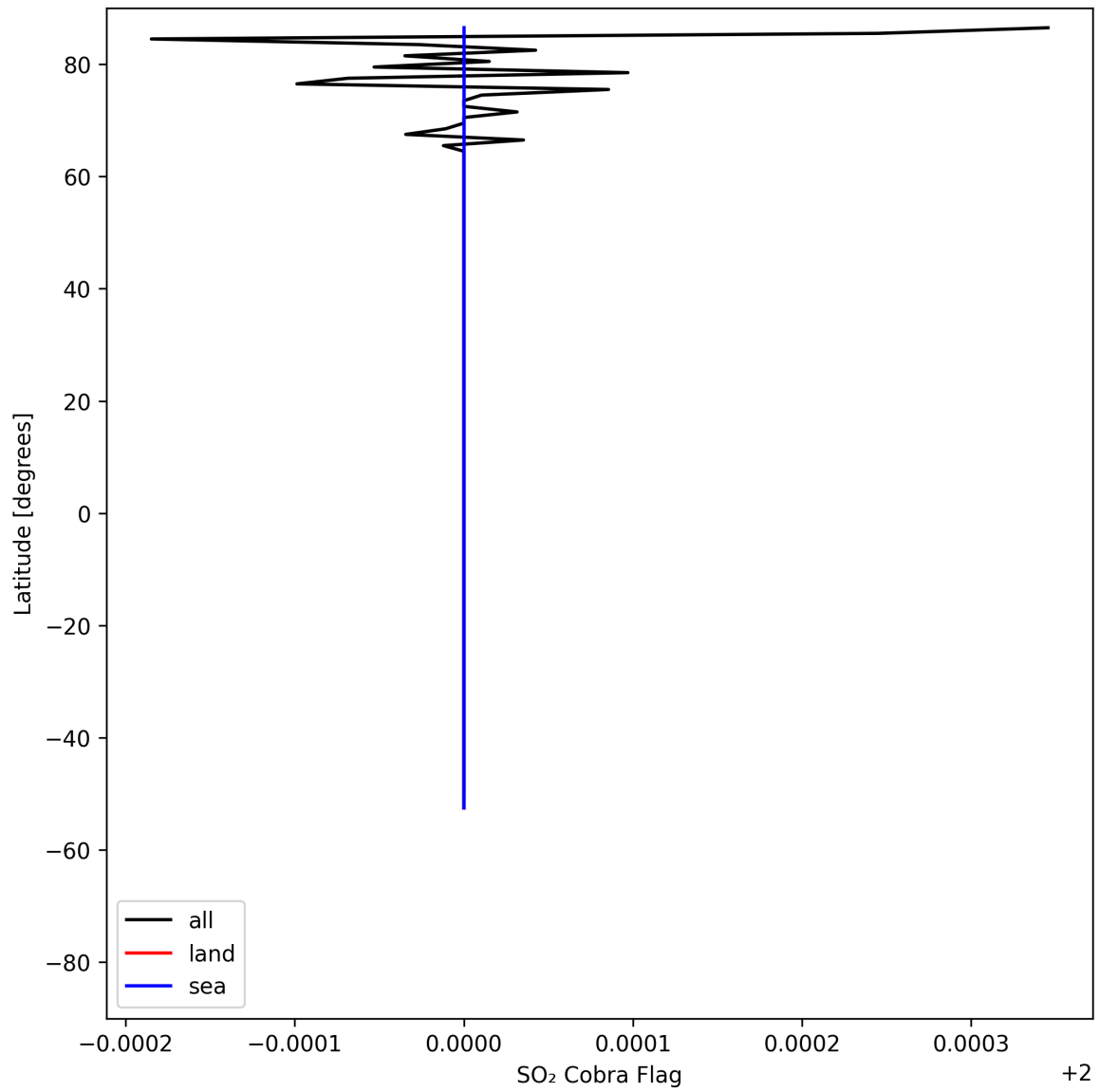
Figure 49: Zonal average of “SO 2 Cobra Flag” for 2025-08-04 to 2025-08-06.
