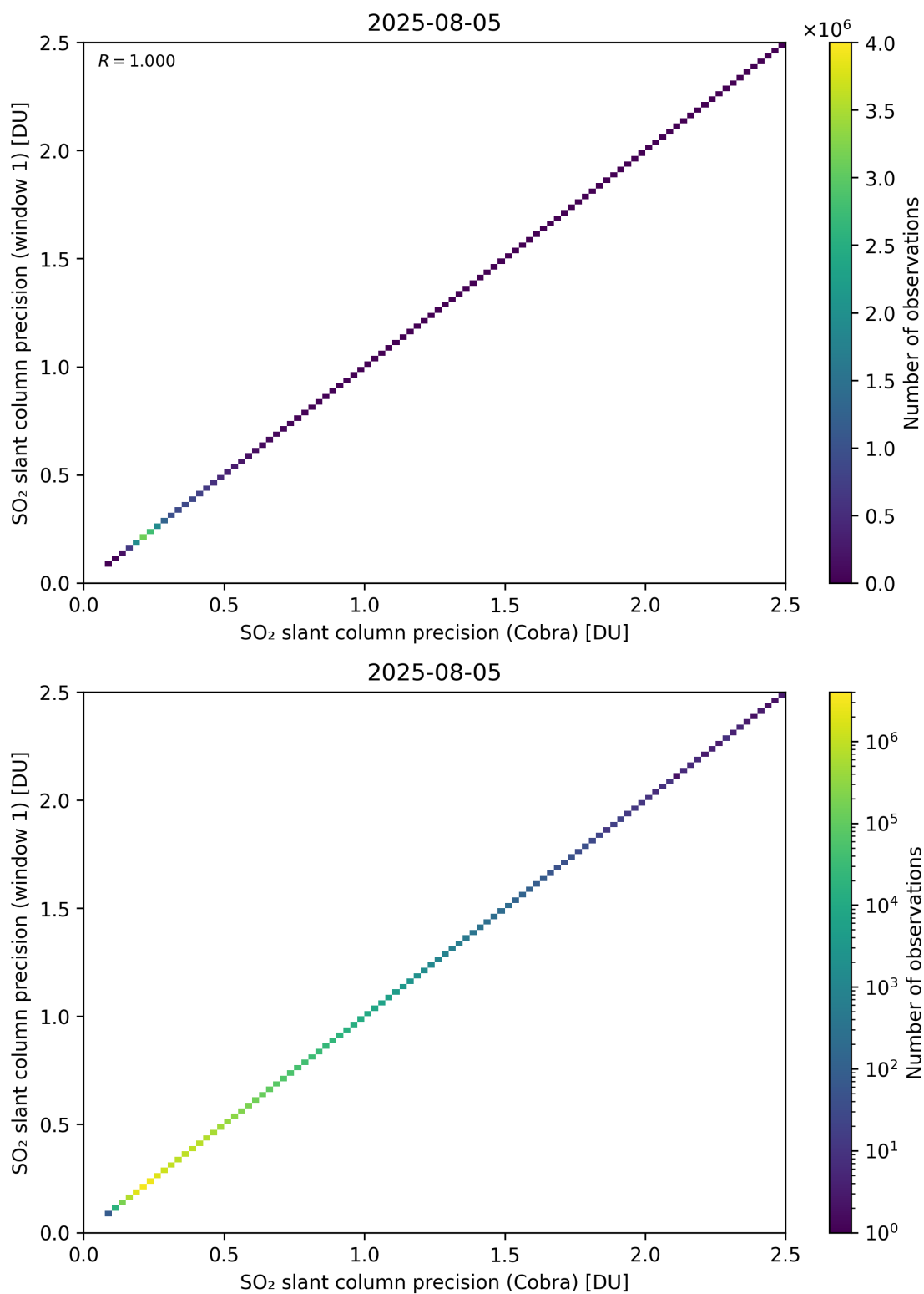
Figure 209: Scatter density plot of “SO 2 slant column precision (Cobra)” against “SO 2 slant column precision (window 1)” for 2025-08-04 to 2025-08-06.
