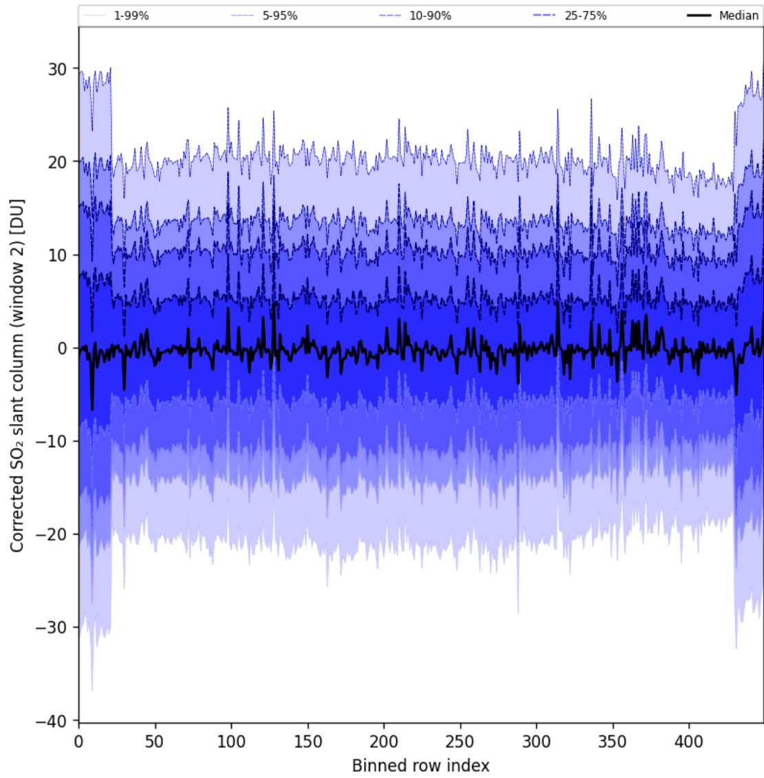
Figure 95: Along track statistics of “Corrected SO 2 slant column (window 2)” for 2025-08-04 to 2025-08-06
