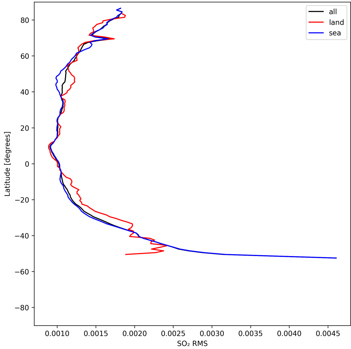
Figure 52: Zonal average of “SO 2 RMS” for 2025-08-04 to 2025-08-06.
