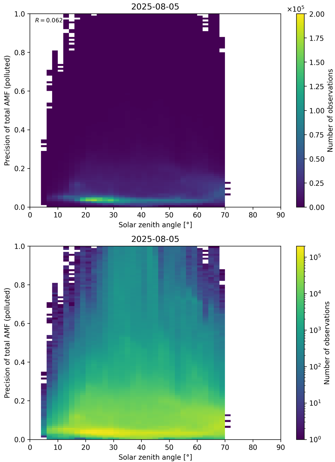
Figure 190: Scatter density plot of “Solar zenith angle” against “Precision of total AMF (polluted)” for 2025-08-04 to 2025-08-06.
