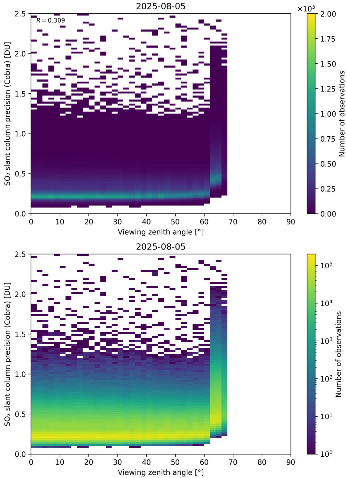
Figure 372: Scatter density plot of “Viewing zenith angle” against “SO 2 slant column precision (Cobra)” for 2025-08-04 to 2025-08-06.
