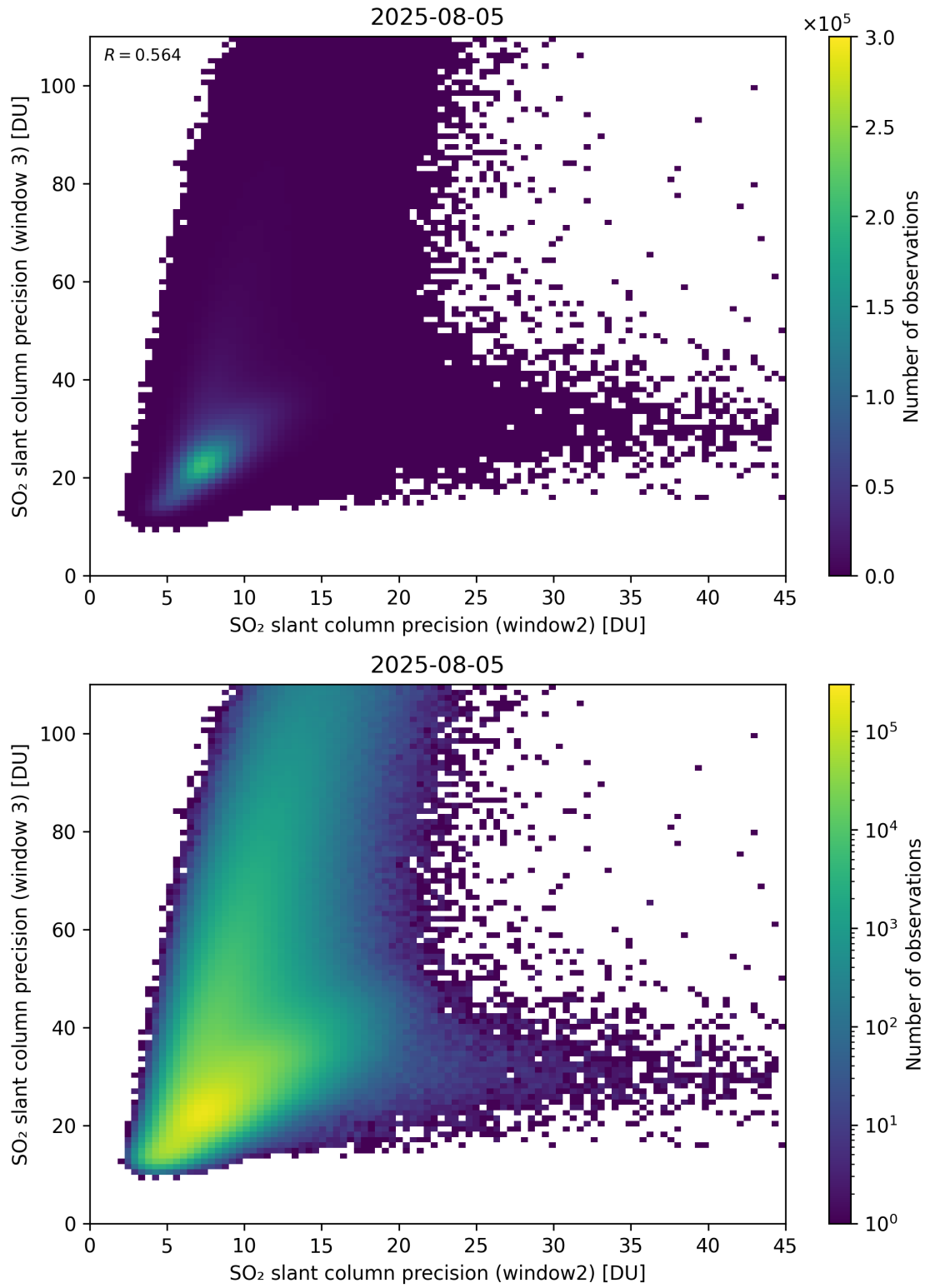
Figure 300: Scatter density plot of “SO 2 slant column precision (window2)” against “SO 2 slant column precision (window 3)” for 2025-08-04 to 2025-08-06.
