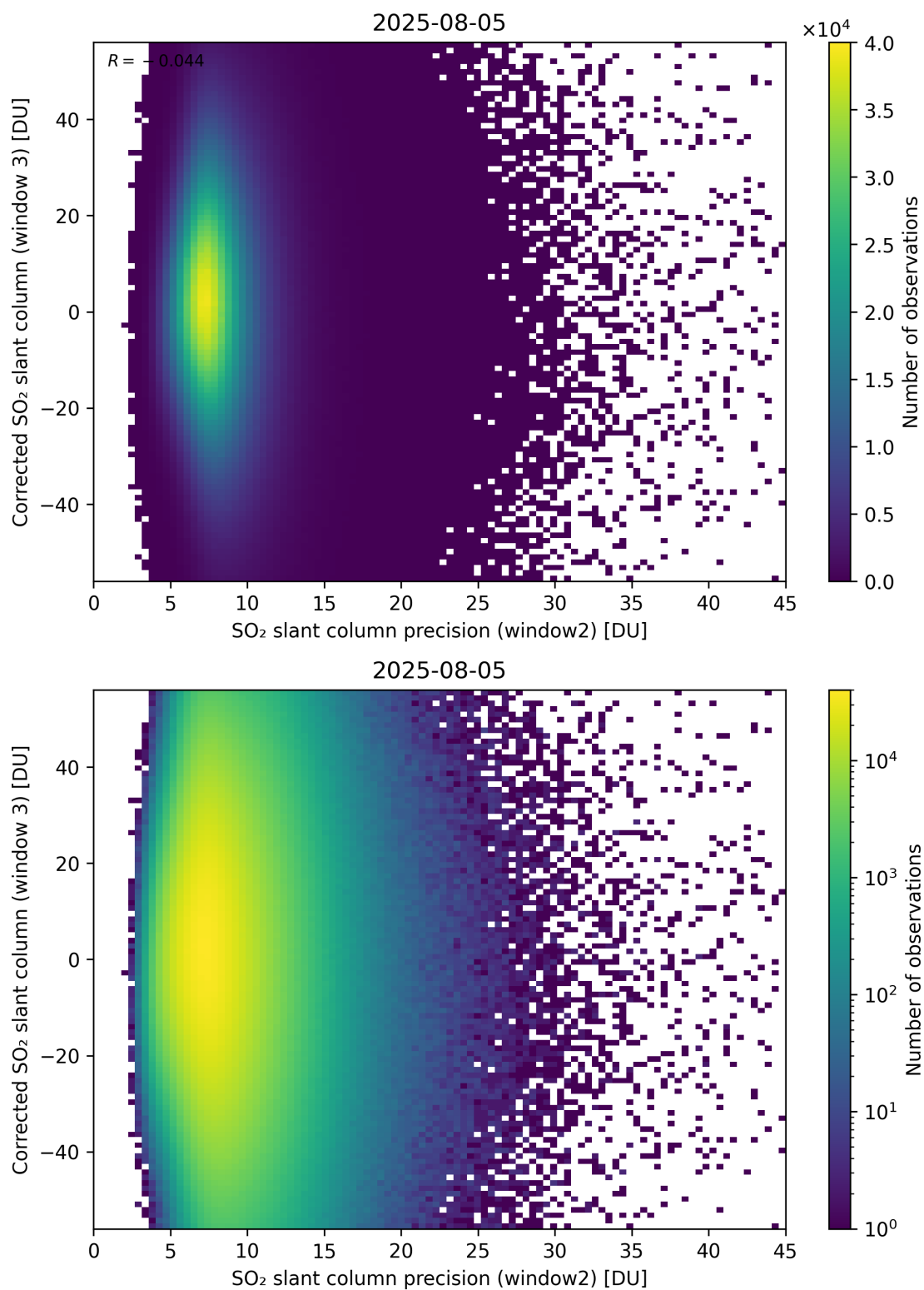
Figure 298: Scatter density plot of “SO 2 slant column precision (window2)” against “Corrected SO 2 slant column (window 3)” for 2025-08-04 to 2025-08-06.
