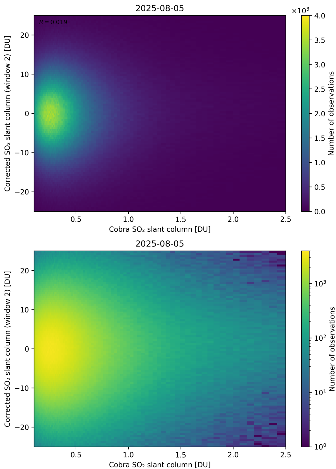
Figure 217: Scatter density plot of “Cobra SO 2 slant column” against “Corrected SO 2 slant column (window 2)” for 2025-08-04 to 2025-08-06.
