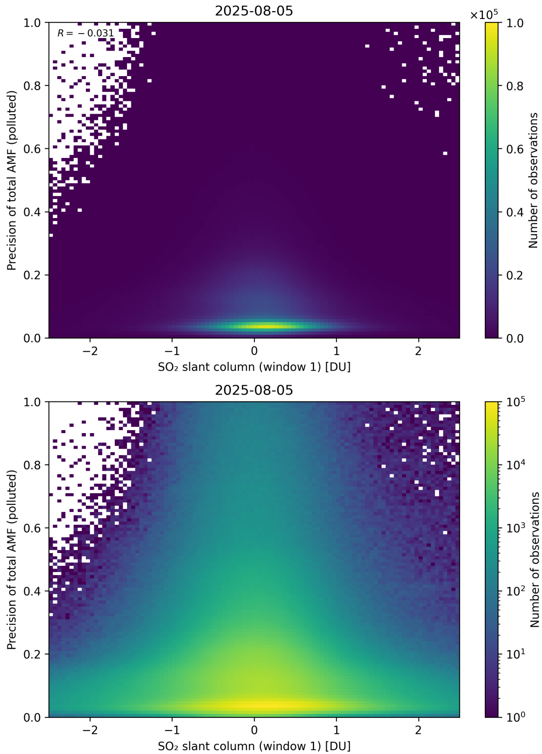
Figure 290: Scatter density plot of “SO 2 slant column (window 1)” against “Precision of total AMF (polluted)” for 2025-08-04 to 2025-08-06.
