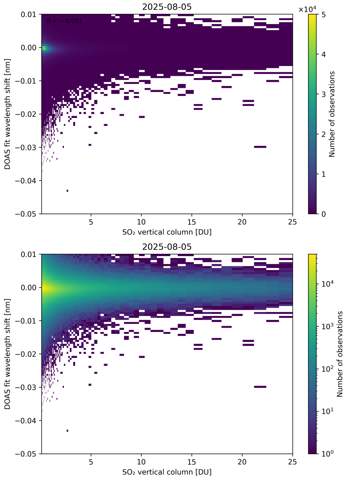
Figure 326: Scatter density plot of “SO 2 vertical column” against “DOAS fit wavelength shift” for 2025-08-04 to 2025-08-06.
