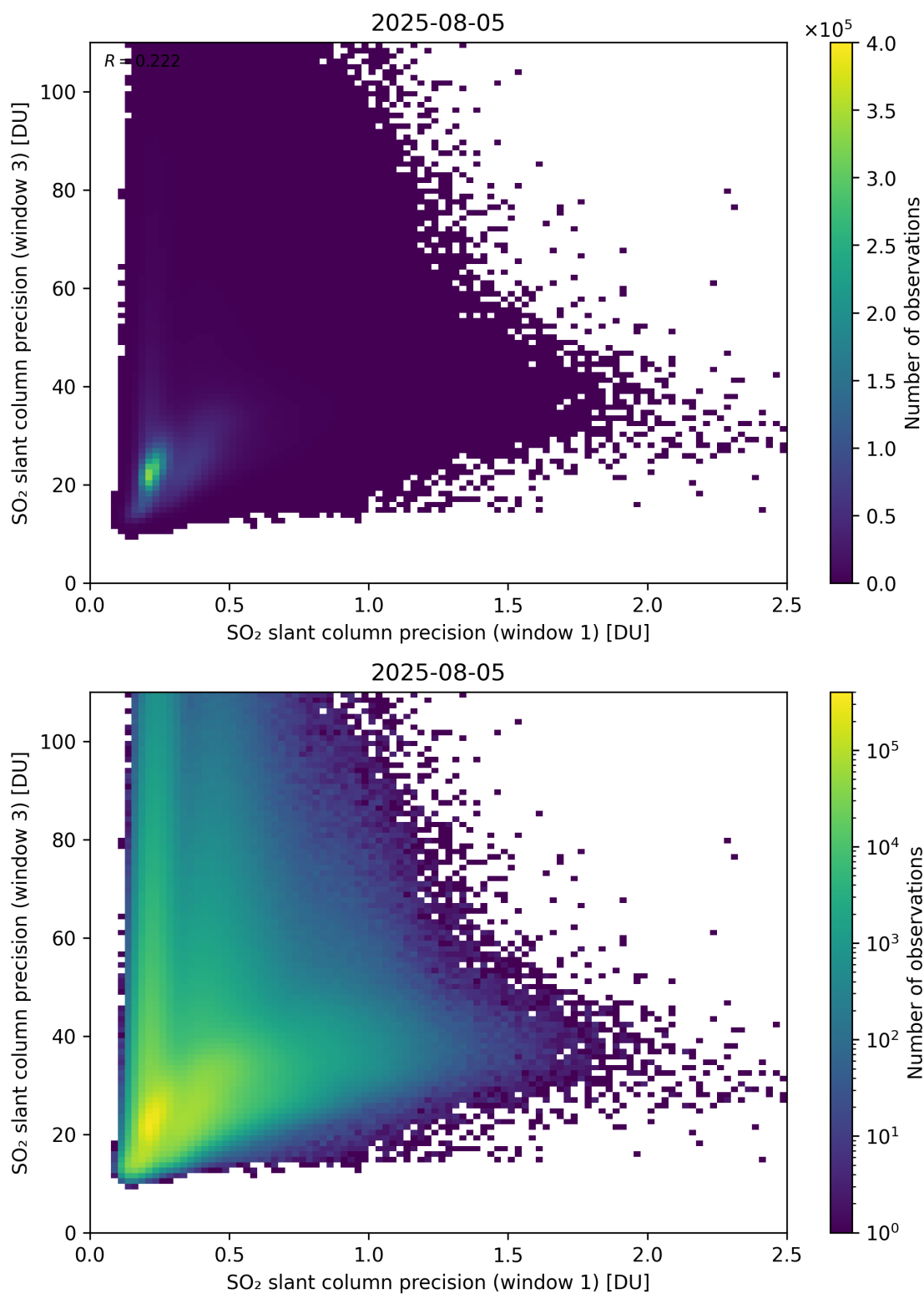
Figure 279: Scatter density plot of “SO 2 slant column precision (window 1)” against “SO 2 slant column precision (window 3)” for 2025-08-04 to 2025-08-06.
