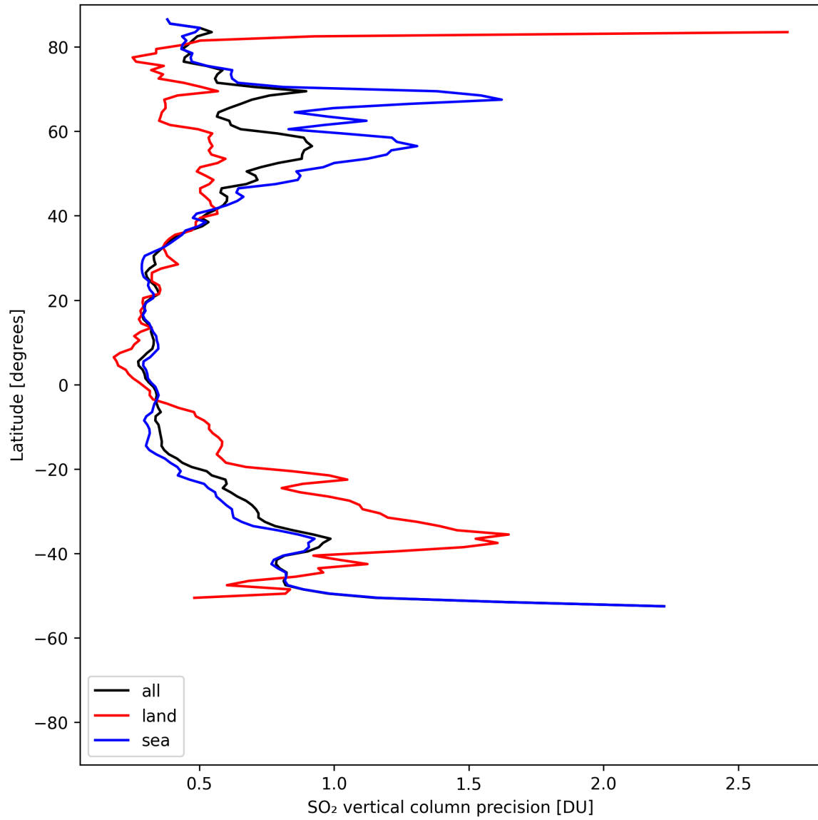
Figure 33: Zonal average of “SO 2 vertical column precision” for 2025-08-04 to 2025-08-06.
