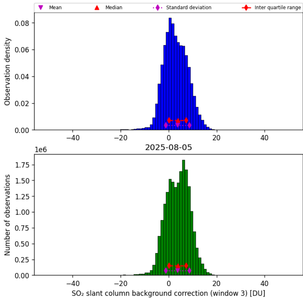
Figure 74: Histogram of “SO 2 slant column background correction (window 3)” for 2025-08-04 to 2025-08-06
