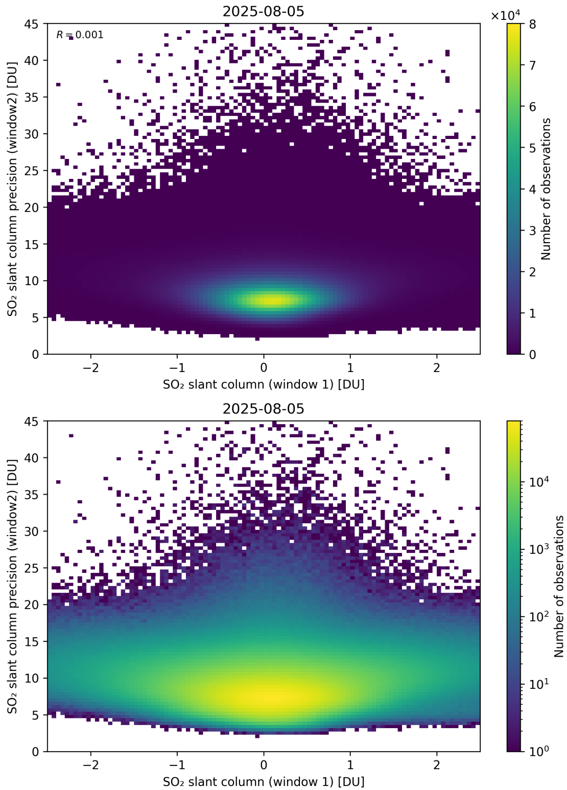
Figure 286: Scatter density plot of “SO 2 slant column (window 1)” against “SO 2 slant column precision (window2)” for 2025-08-04 to 2025-08-06.
