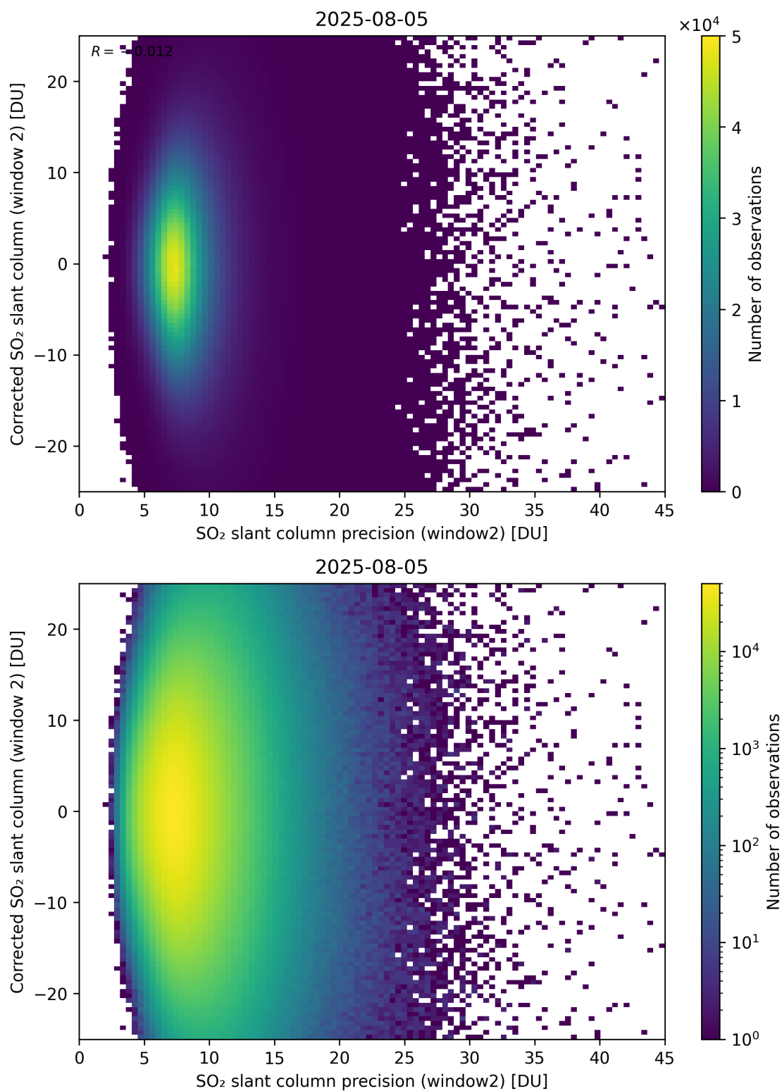
Figure 297: Scatter density plot of “SO 2 slant column precision (window2)” against “Corrected SO 2 slant column (window 2)” for 2025-08-04 to 2025-08-06.
