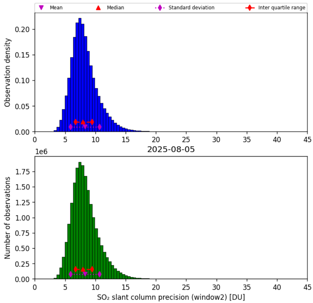
Figure 68: Histogram of “SO 2 slant column precision (window2)” for 2025-08-04 to 2025-08-06
