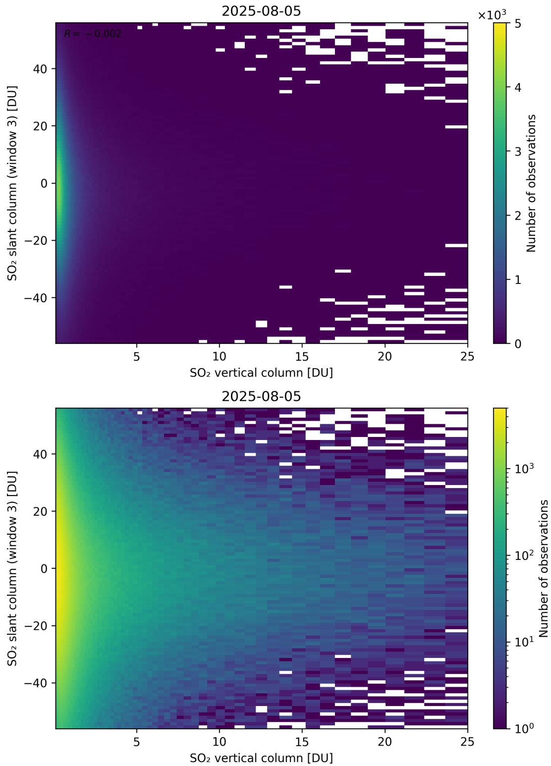
Figure 357: Scatter density plot of “SO 2 vertical column” against “SO 2 slant column (window 3)” for 2025-08-04 to 2025-08-06.
