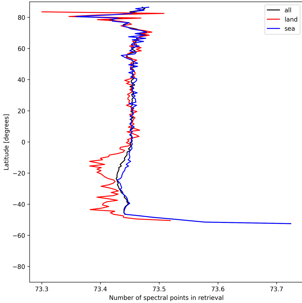
Figure 56: Zonal average of “Number of spectral points in retrieval” for 2025-08-04 to 2025-08-06.
