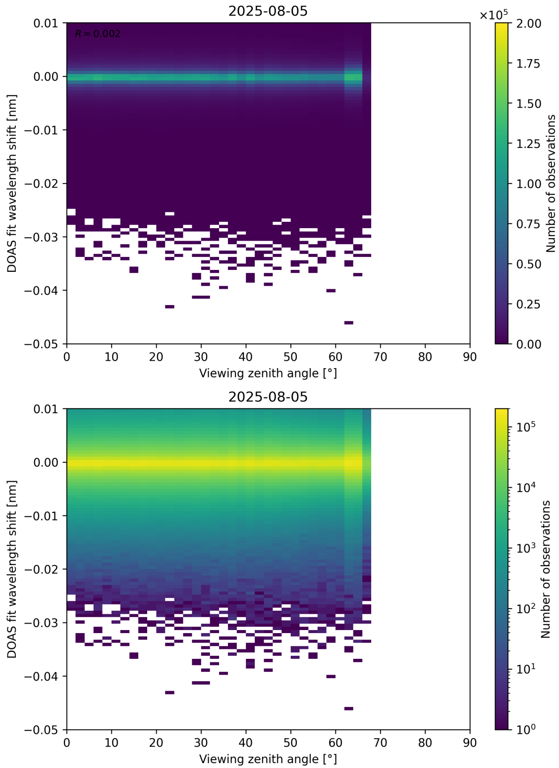
Figure 365: Scatter density plot of “Viewing zenith angle” against “DOAS fit wavelength shift” for 2025-08-04 to 2025-08-06.
