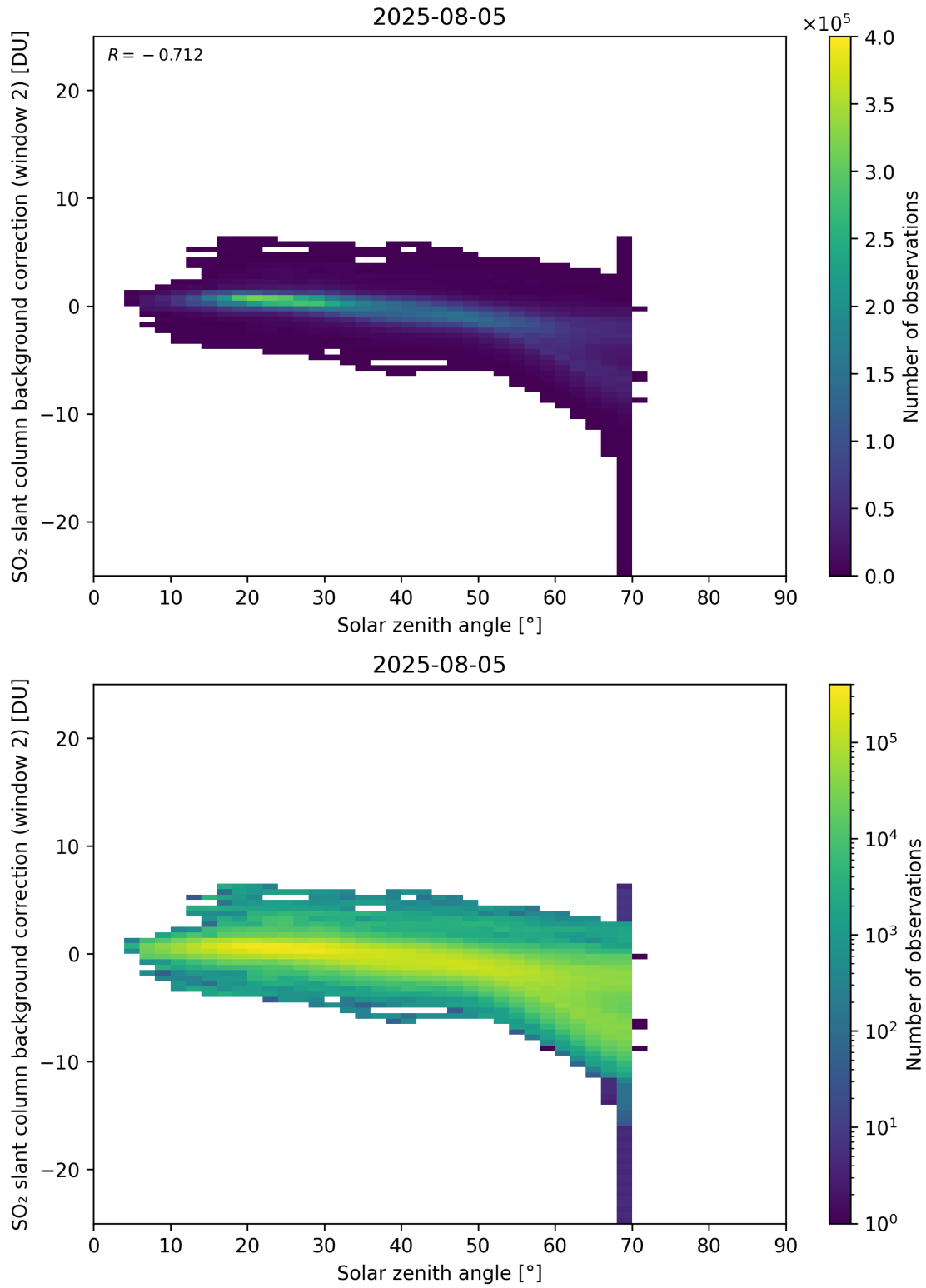
Figure 172: Scatter density plot of “Solar zenith angle” against “SO 2 slant column background correction (window 2)” for 2025-08-04 to 2025-08-06.
