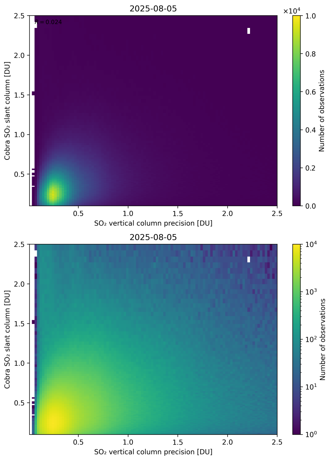
Figure 336: Scatter density plot of “SO 2 vertical column precision” against “Cobra SO 2 slant column” for 2025-08-04 to 2025-08-06.
