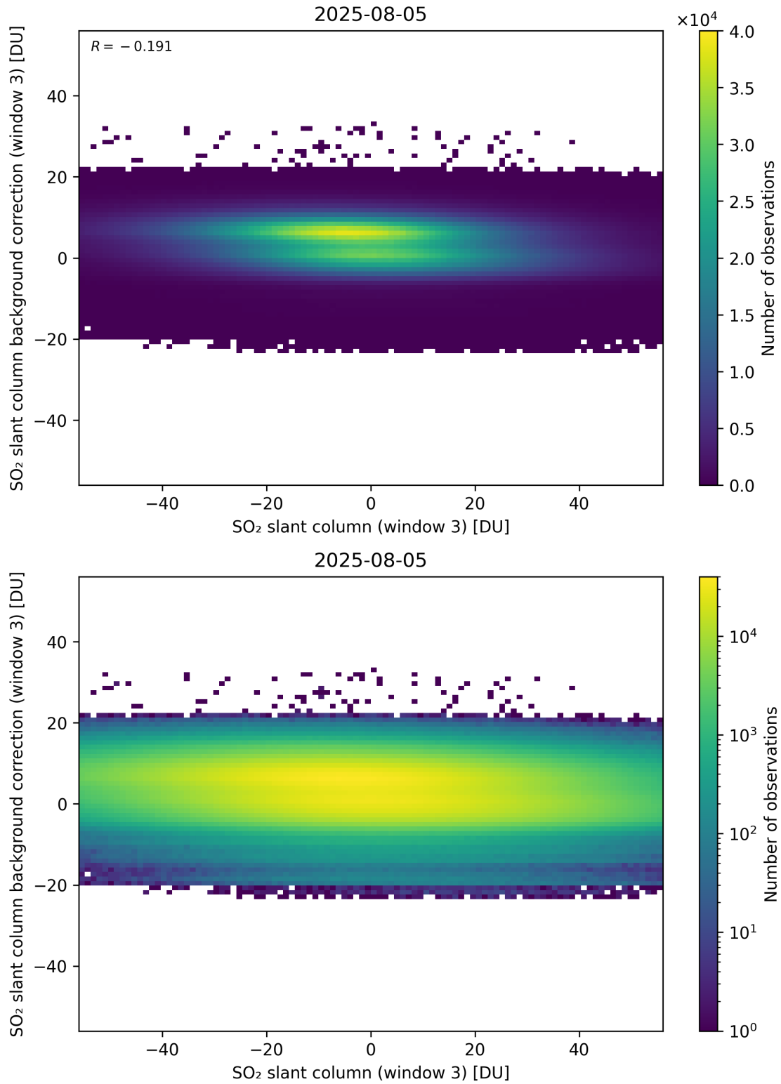
Figure 303: Scatter density plot of “SO 2 slant column (window 3)” against “SO 2 slant column background correction (window 3)” for 2025-08-04 to 2025-08-06.
