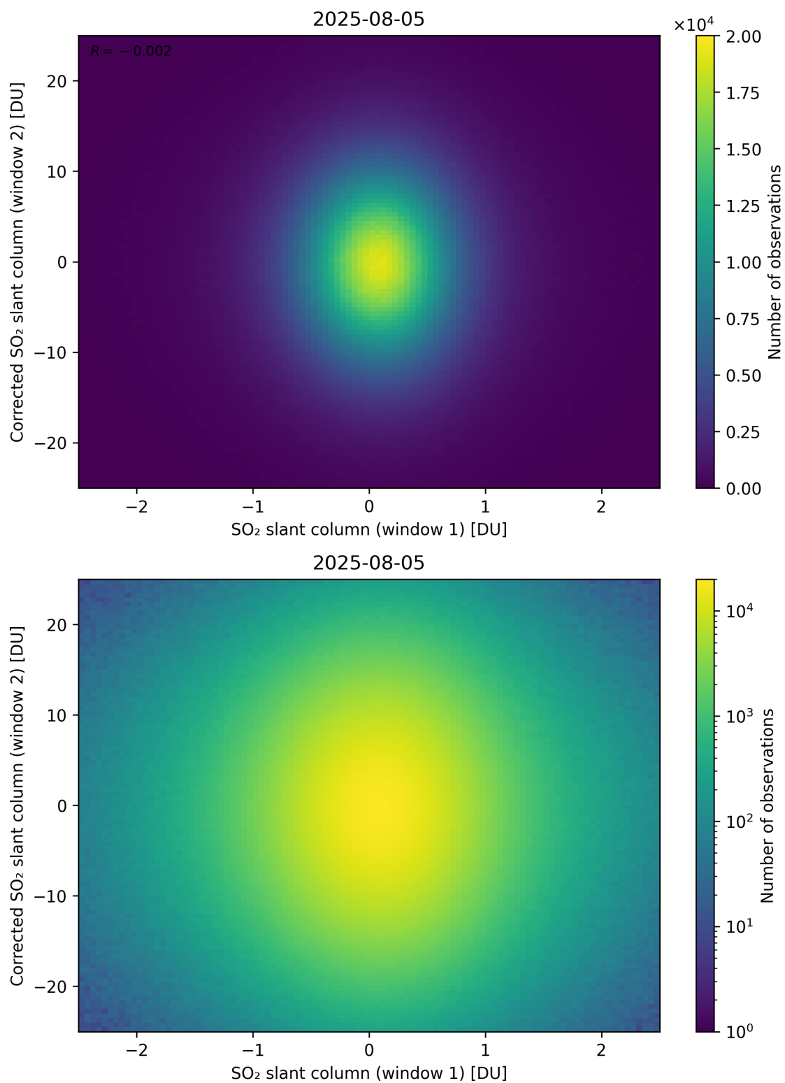
Figure 283: Scatter density plot of “SO 2 slant column (window 1)” against “Corrected SO 2 slant column (window 2)” for 2025-08-04 to 2025-08-06.
