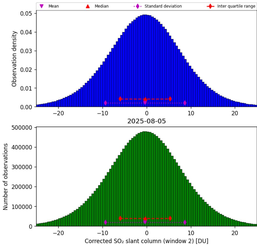
Figure 69: Histogram of “Corrected SO 2 slant column (window 2)” for 2025-08-04 to 2025-08-06
