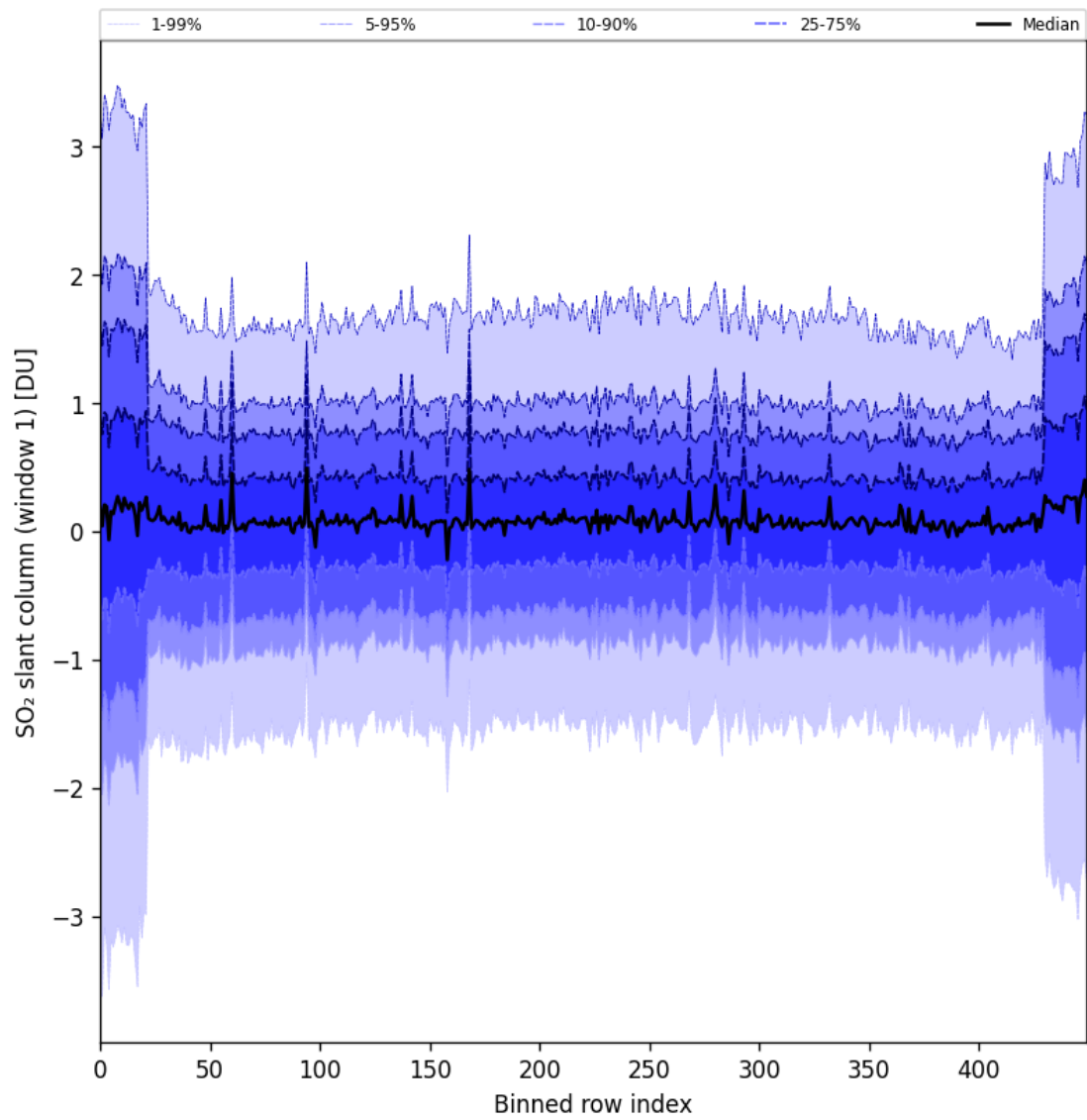
Figure 89: Along track statistics of “SO 2 slant column (window 1)” for 2025-08-04 to 2025-08-06
