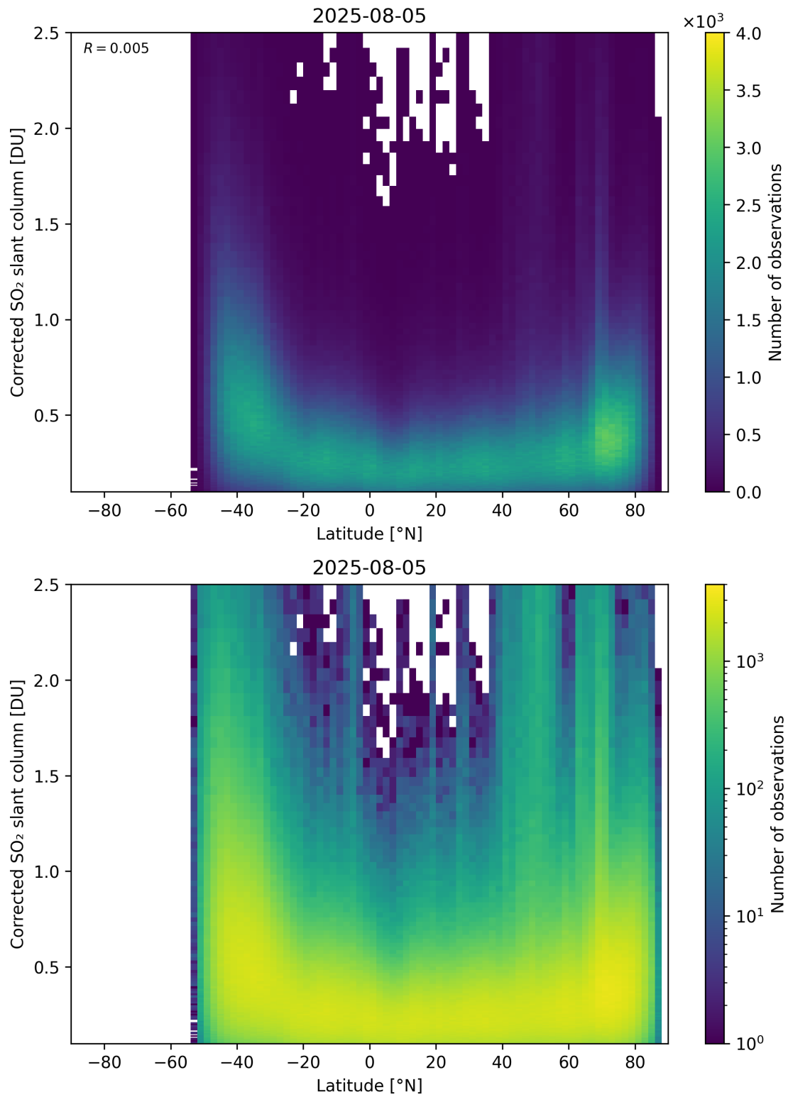
Figure 159: Scatter density plot of “Latitude” against “Corrected SO 2 slant column” for 2025-08-04 to 2025-08-06.
