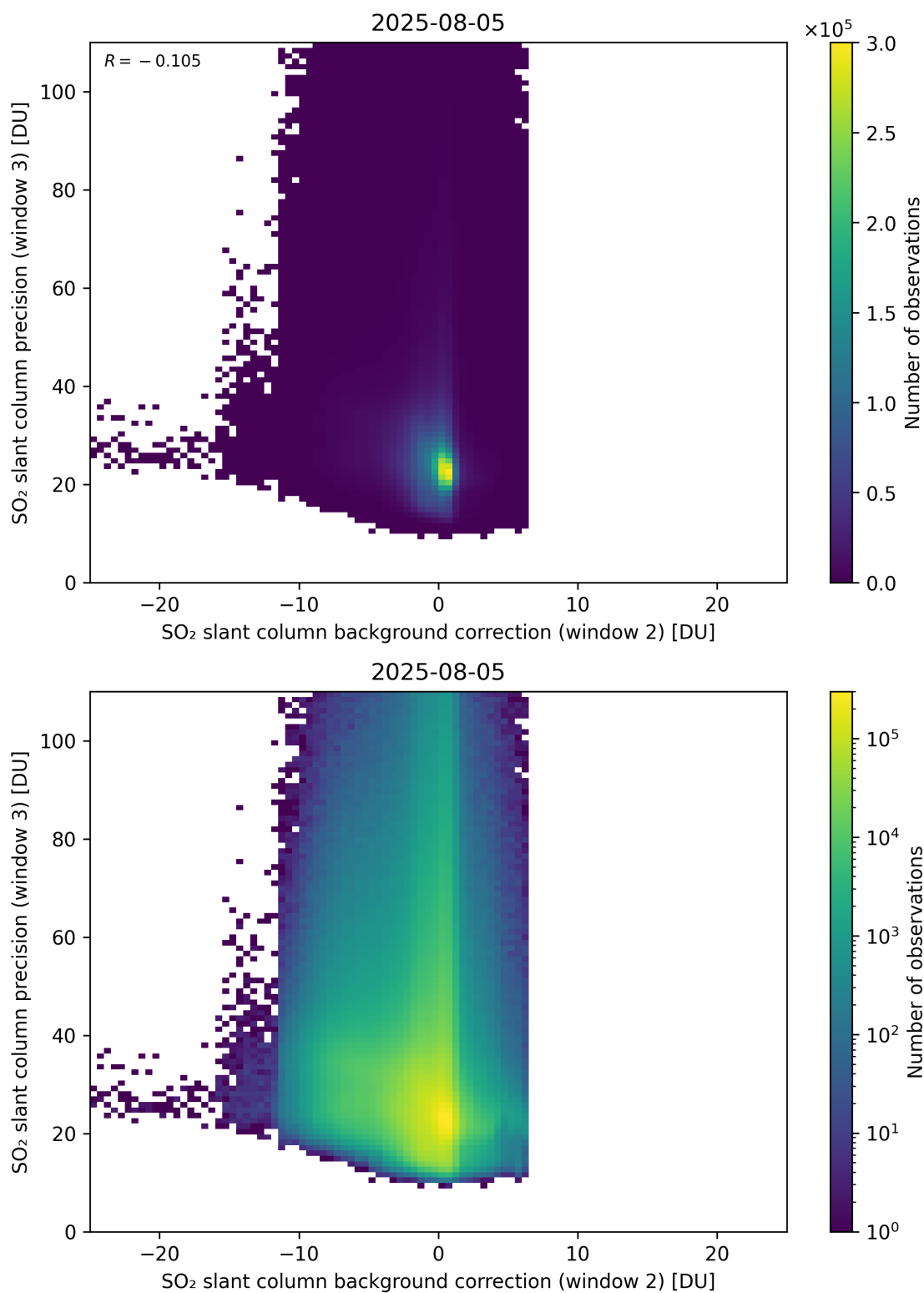
Figure 129: Scatter density plot of “SO 2 slant column background correction (window 2)” against “SO 2 slant column precision (window 3)” for 2025-08-04 to 2025-08-06.
