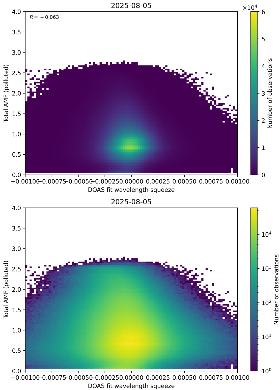
Figure 145: Scatter density plot of “DOAS fit wavelength squeeze” against “Total AMF (polluted)” for 2025-08-04 to 2025-08-06.
