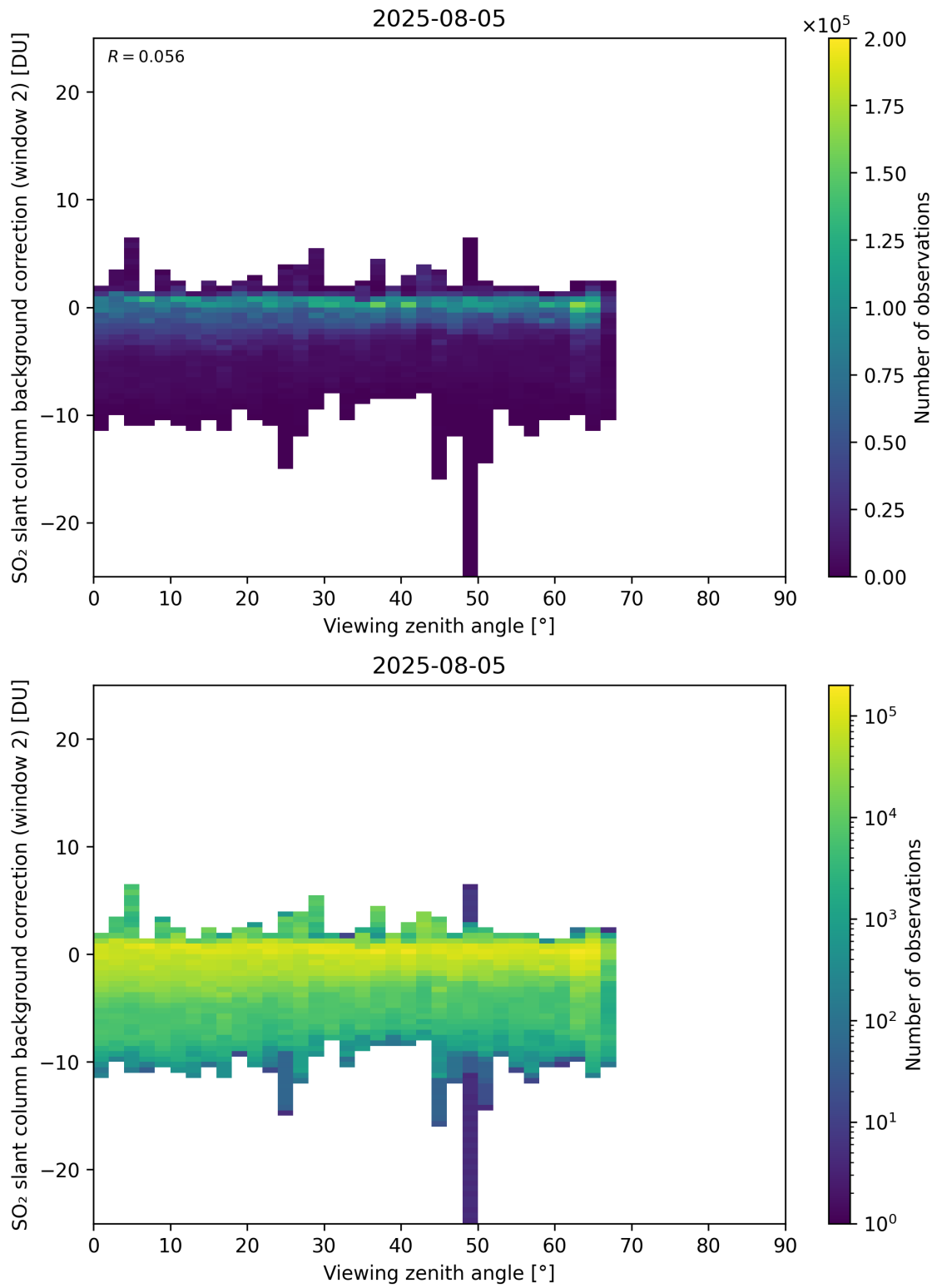
Figure 363: Scatter density plot of “Viewing zenith angle” against “SO 2 slant column background correction (window 2)” for 2025-08-04 to 2025-08-06.
