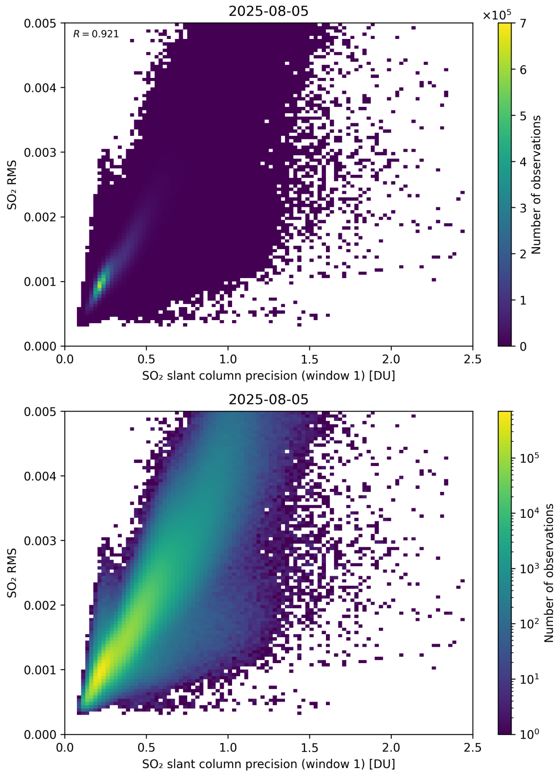
Figure 273: Scatter density plot of “SO 2 slant column precision (window 1)” against “SO 2 RMS” for 2025-08-04 to 2025-08-06.
