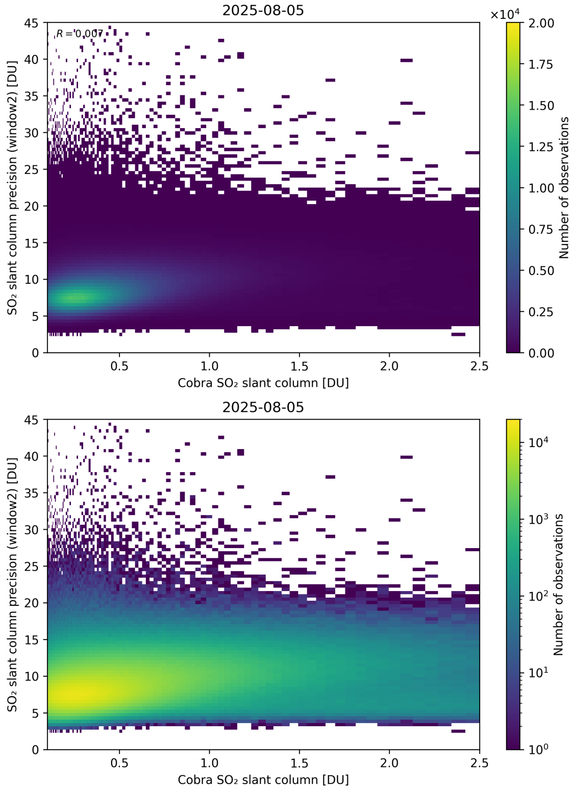
Figure 221: Scatter density plot of “Cobra SO 2 slant column” against “SO 2 slant column precision (window2)” for 2025-08-04 to 2025-08-06.
