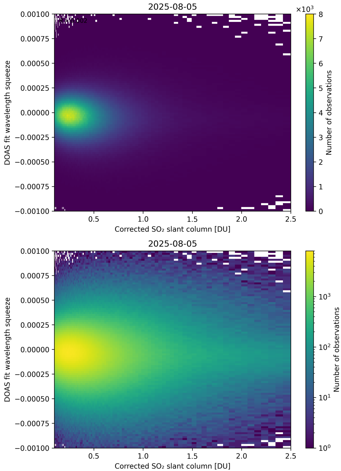
Figure 230: Scatter density plot of “Corrected SO 2 slant column” against “DOAS fit wavelength squeeze” for 2025-08-04 to 2025-08-06.
