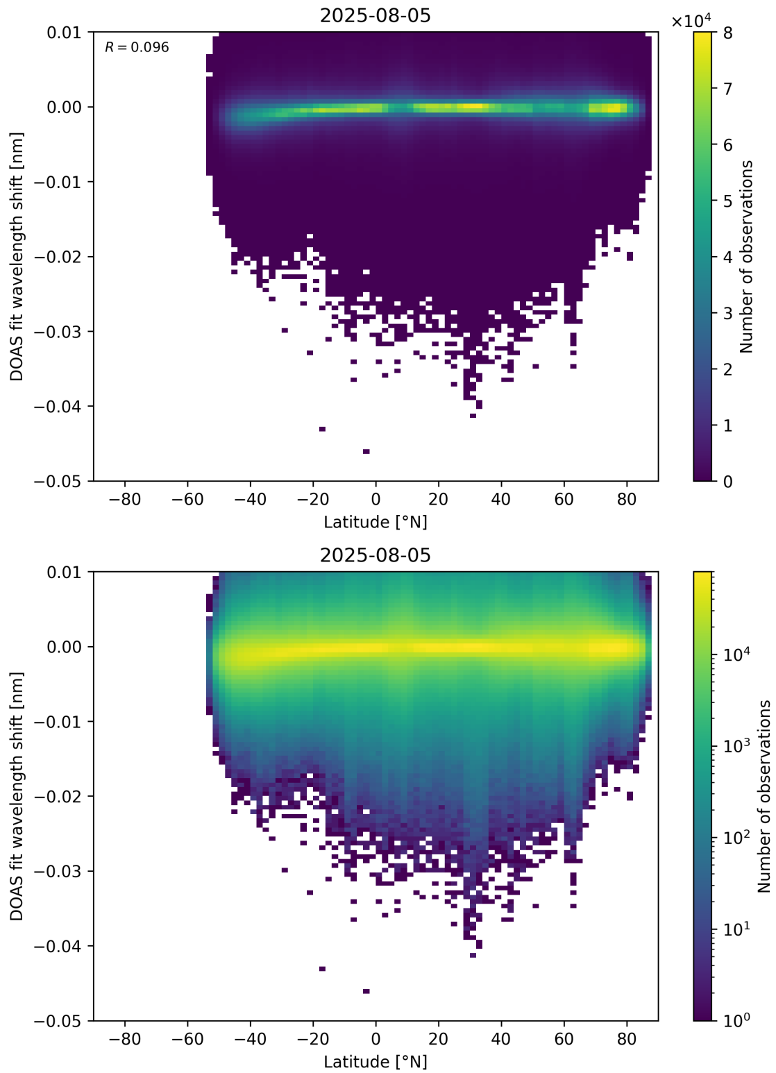
Figure 153: Scatter density plot of “Latitude” against “DOAS fit wavelength shift” for 2025-08-04 to 2025-08-06.
