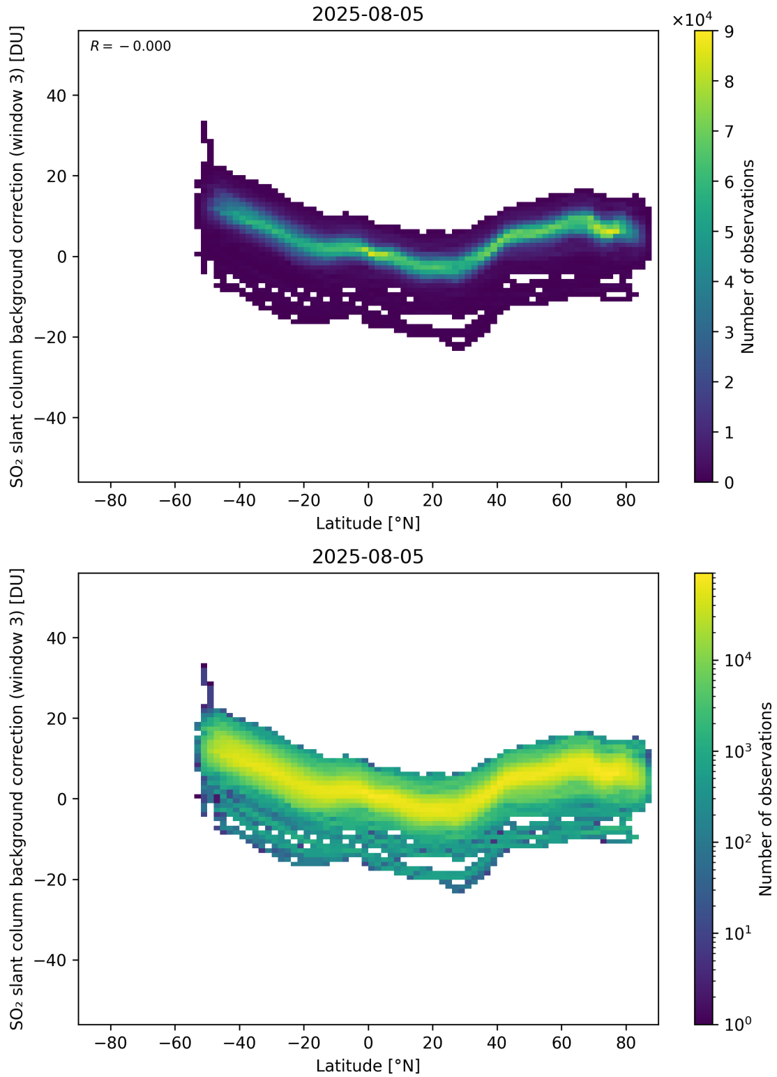
Figure 152: Scatter density plot of “Latitude” against “SO 2 slant column background correction (window 3)” for 2025-08-04 to 2025-08-06.
