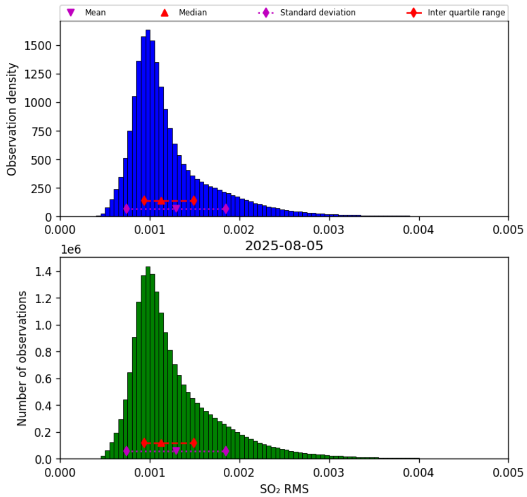
Figure 78: Histogram of “SO 2 RMS” for 2025-08-04 to 2025-08-06
