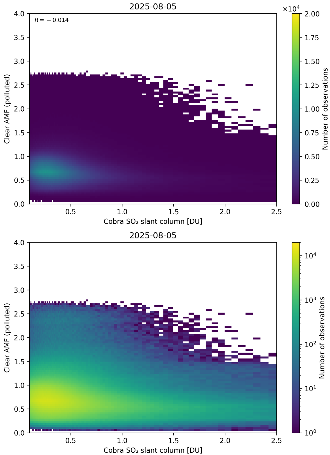
Figure 215: Scatter density plot of “Cobra SO 2 slant column” against “Clear AMF (polluted)” for 2025-08-04 to 2025-08-06.
