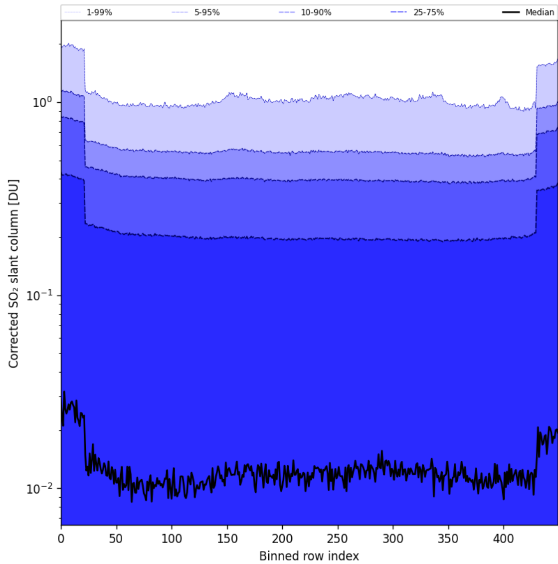
Figure 86: Along track statistics of “Corrected SO 2 slant column” for 2025-08-04 to 2025-08-06
