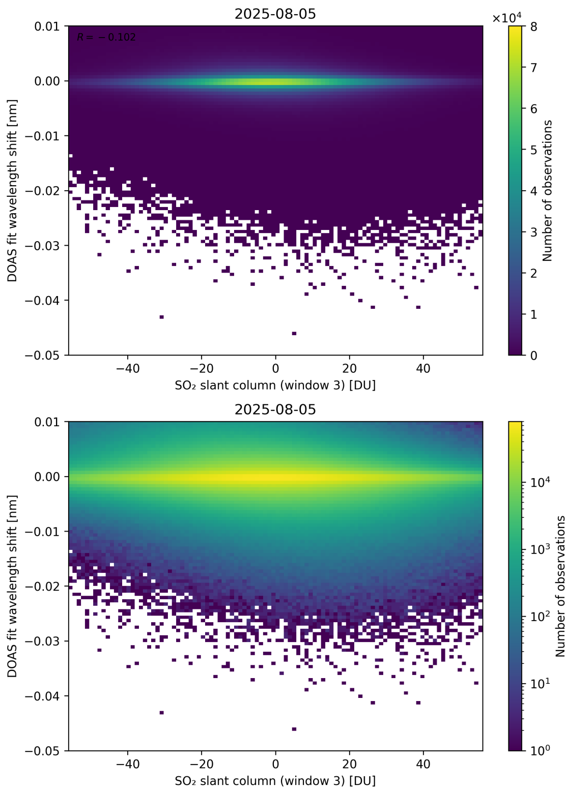
Figure 304: Scatter density plot of “SO 2 slant column (window 3)” against “DOAS fit wavelength shift” for 2025-08-04 to 2025-08-06.
