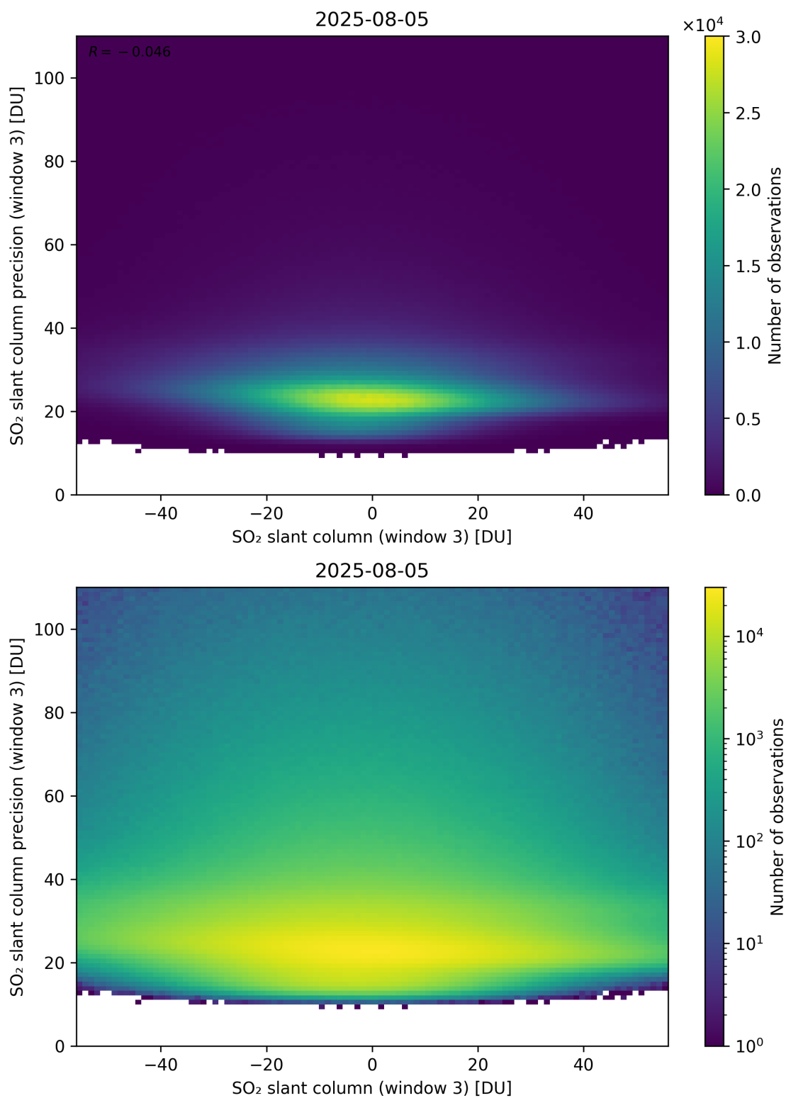
Figure 317: Scatter density plot of “SO 2 slant column (window 3)” against “SO 2 slant column precision (window 3)” for 2025-08-04 to 2025-08-06.
