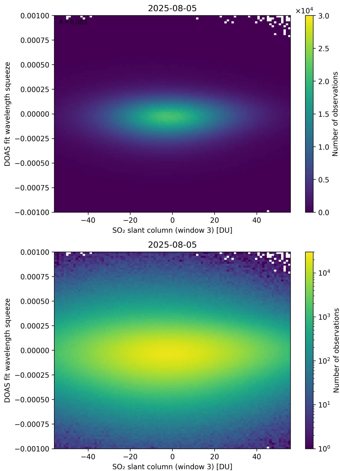
Figure 305: Scatter density plot of “SO 2 slant column (window 3)” against “DOAS fit wavelength squeeze” for 2025-08-04 to 2025-08-06.
