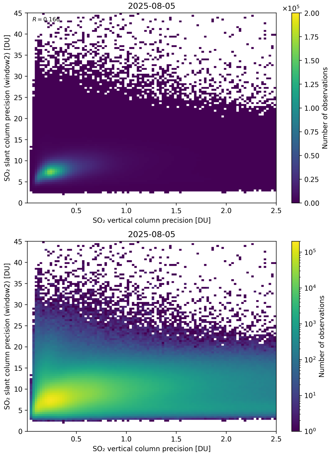
Figure 343: Scatter density plot of “SO 2 vertical column precision” against “SO 2 slant column precision (window2)” for 2025-08-04 to 2025-08-06.
