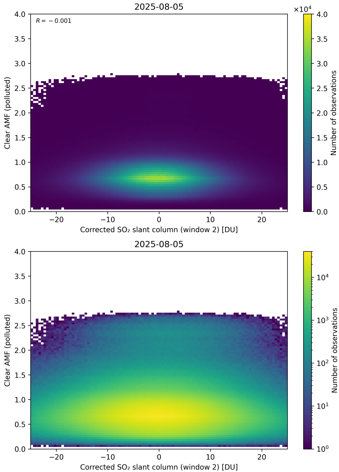
Figure 249: Scatter density plot of “Corrected SO 2 slant column (window 2)” against “Clear AMF (polluted)” for 2025-08-04 to 2025-08-06.
