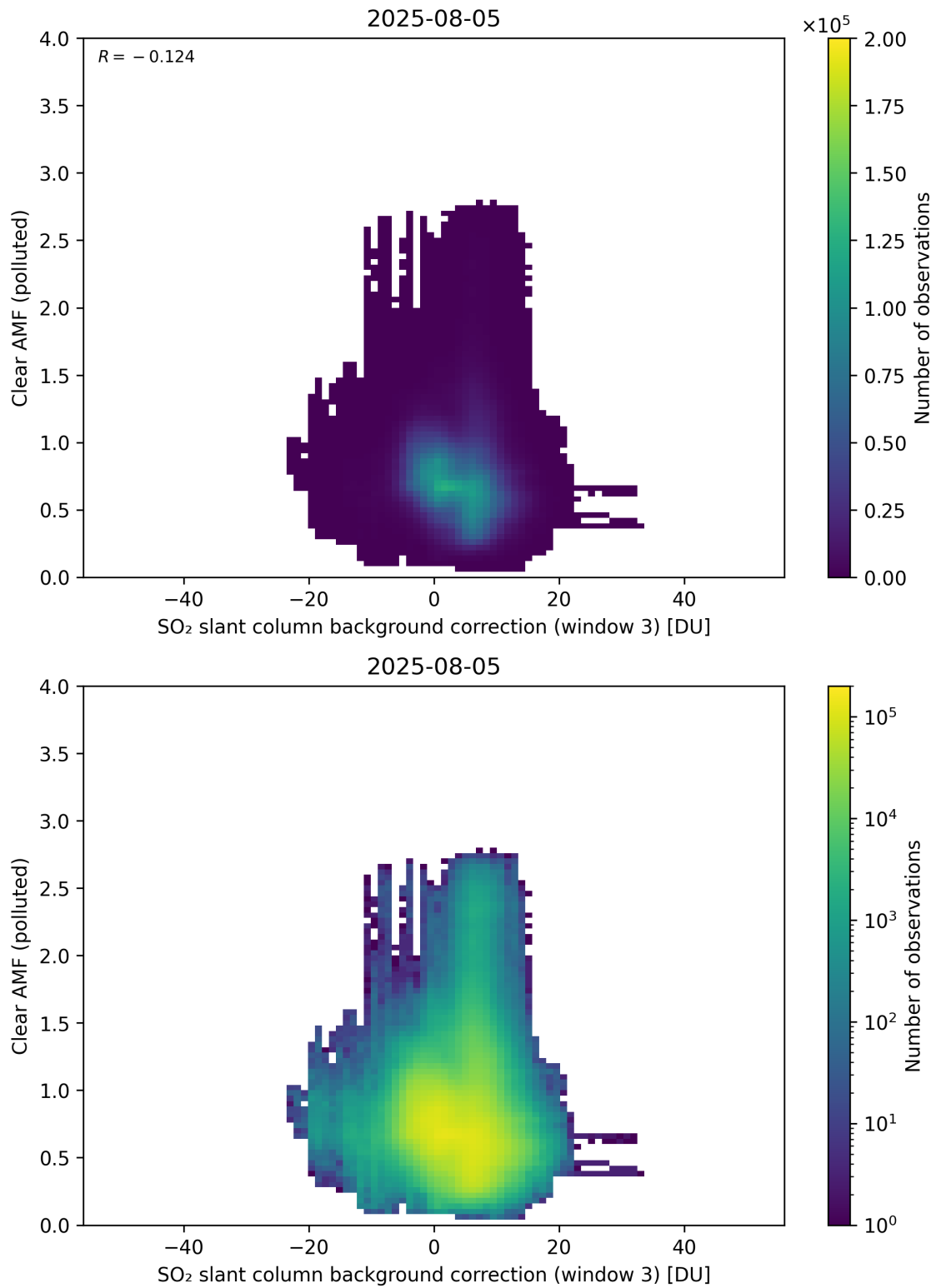
Figure 135: Scatter density plot of “SO 2 slant column background correction (window 3)” against “Clear AMF (polluted)” for 2025-08-04 to 2025-08-06.
