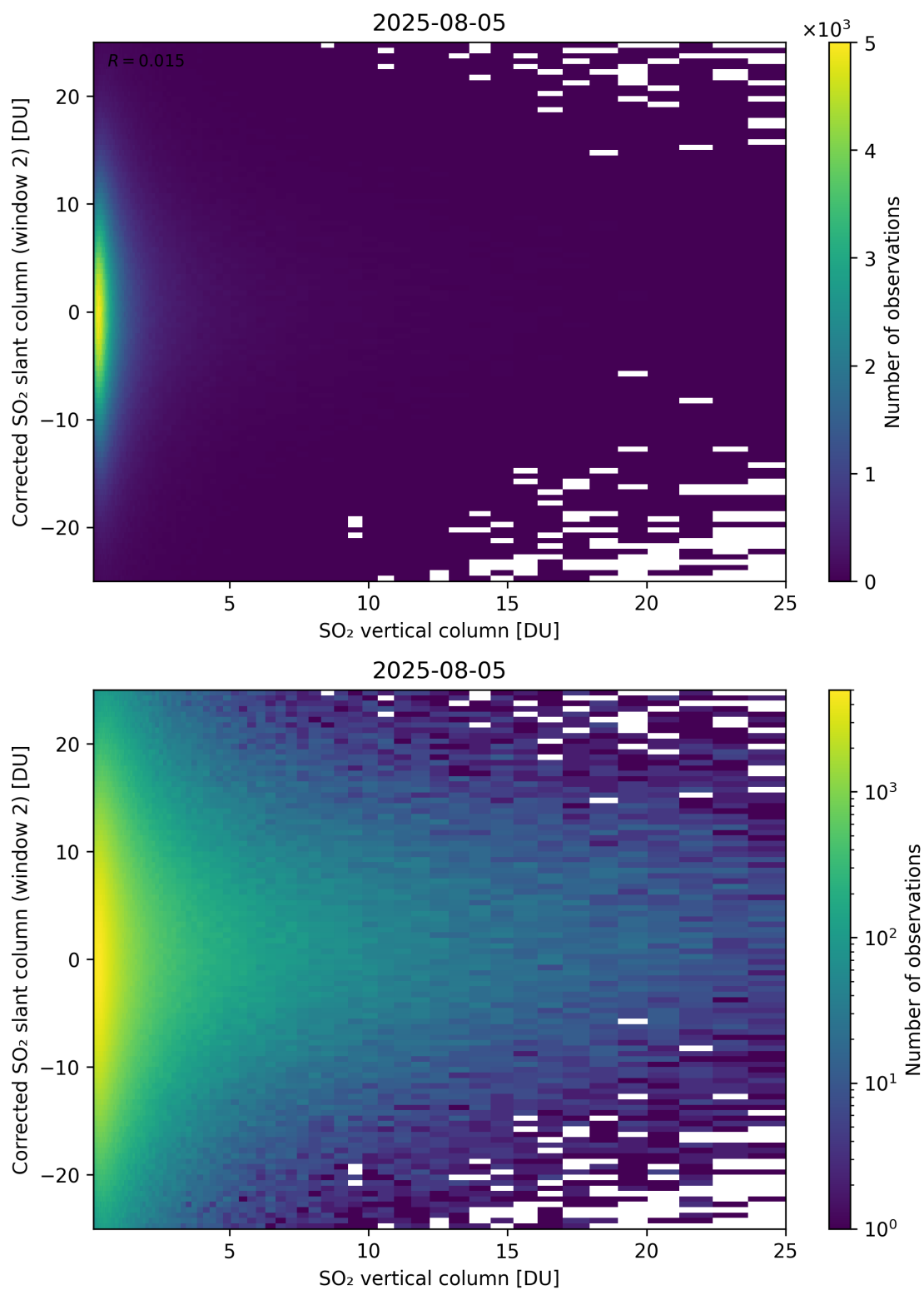
Figure 352: Scatter density plot of “SO 2 vertical column” against “Corrected SO 2 slant column (window 2)” for 2025-08-04 to 2025-08-06.
