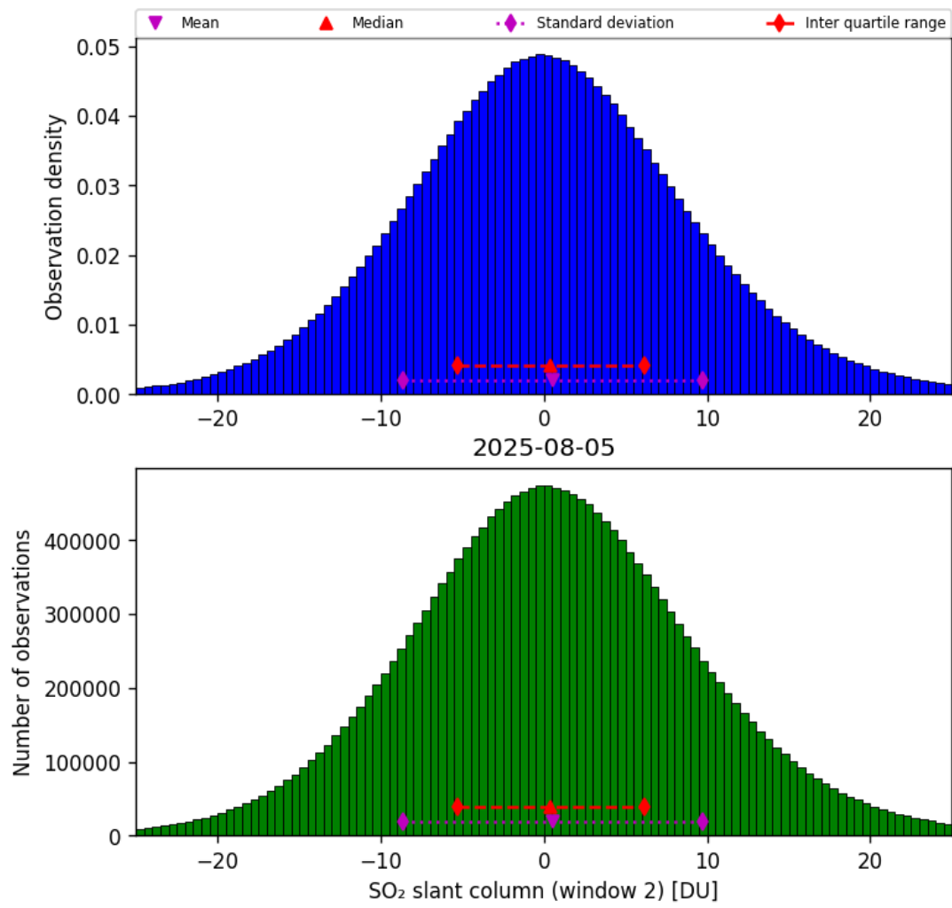
Figure 67: Histogram of “SO 2 slant column (window 2)” for 2025-08-04 to 2025-08-06
