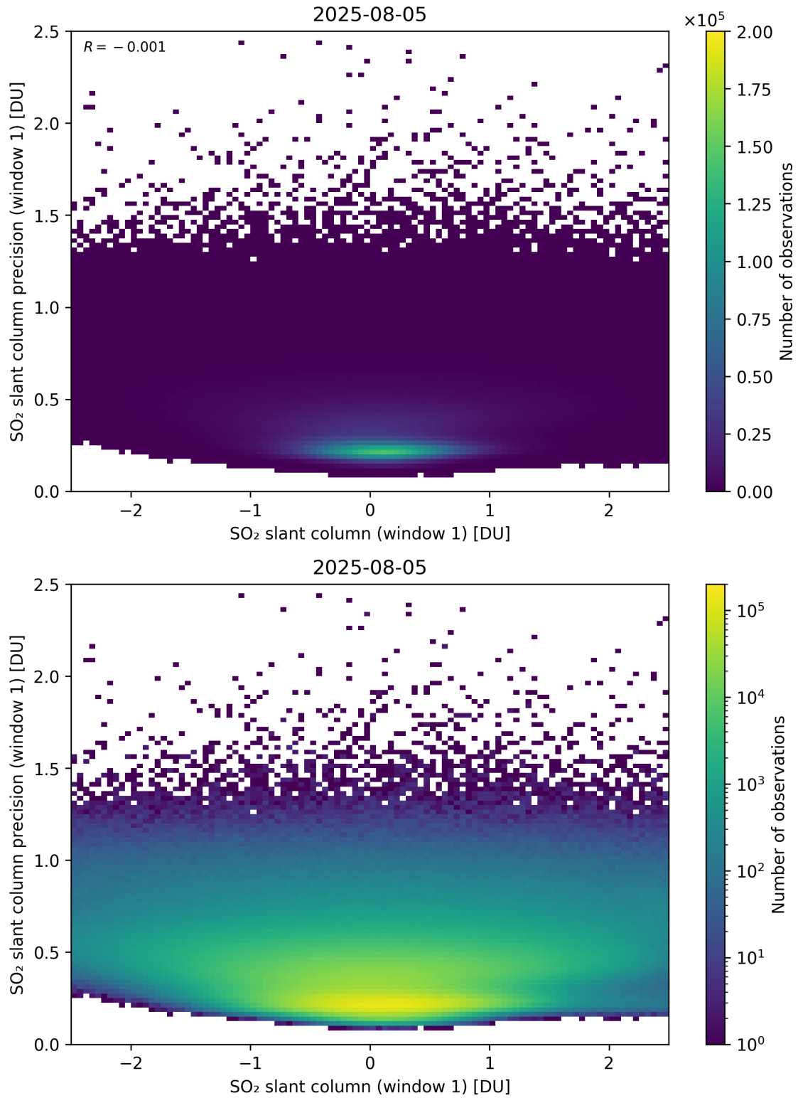
Figure 285: Scatter density plot of “SO 2 slant column (window 1)” against “SO 2 slant column precision (window 1)” for 2025-08-04 to 2025-08-06.
