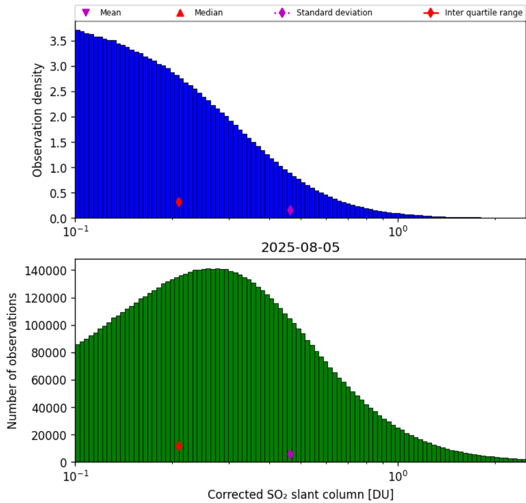
Figure 60: Histogram of "Corrected SO 2 slant column" for 2025-08-04 to 2025-08-06
