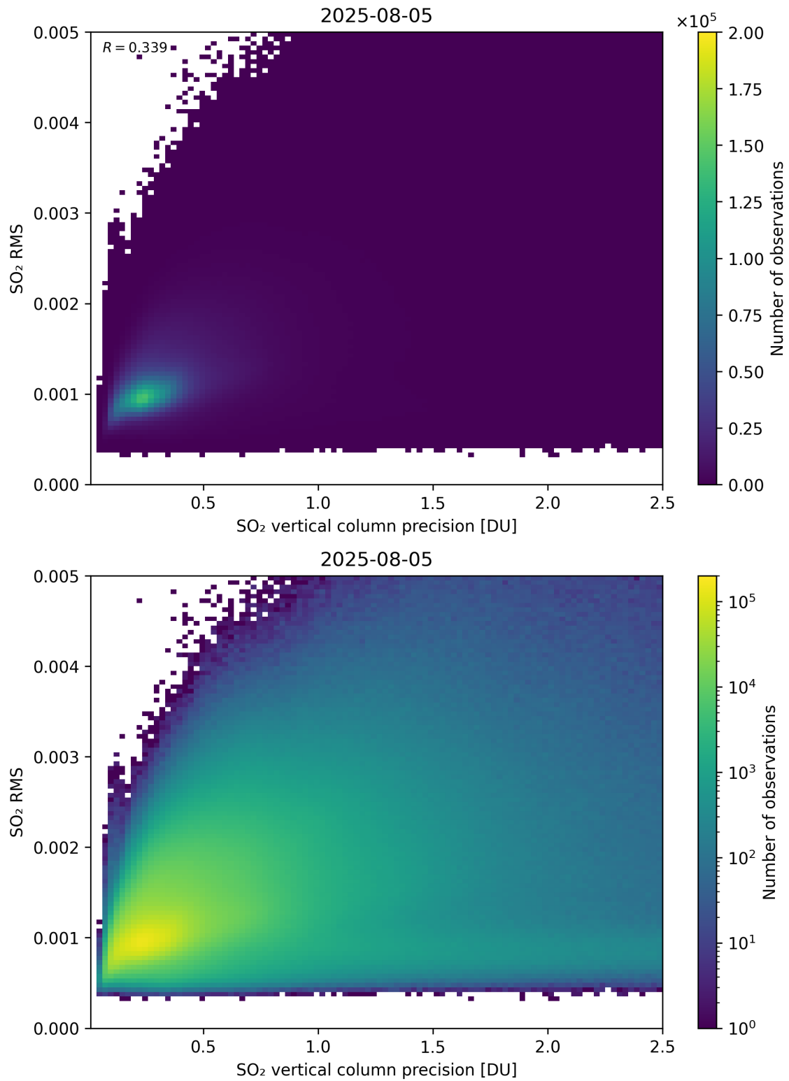
Figure 334: Scatter density plot of “SO 2 vertical column precision” against “SO 2 RMS” for 2025-08-04 to 2025-08-06.
