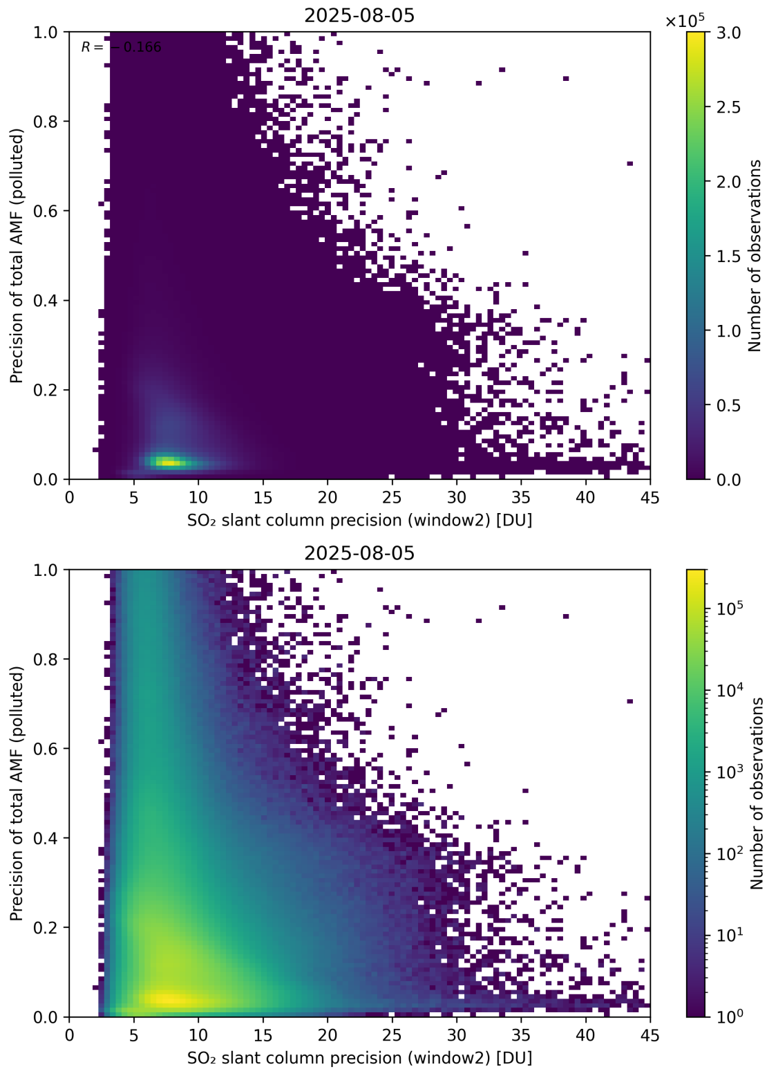
Figure 302: Scatter density plot of “SO 2 slant column precision (window2)” against “Precision of total AMF (polluted)” for 2025-08-04 to 2025-08-06.
