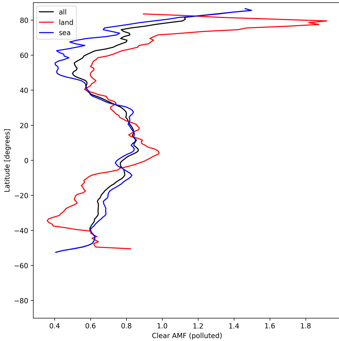
Figure 55: Zonal average of “Clear AMF (polluted)” for 2025-08-04 to 2025-08-06.
