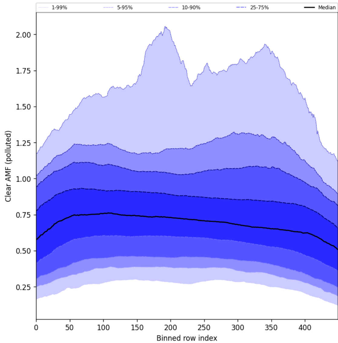
Figure 107: Along track statistics of “Clear AMF (polluted)” for 2025-08-04 to 2025-08-06
