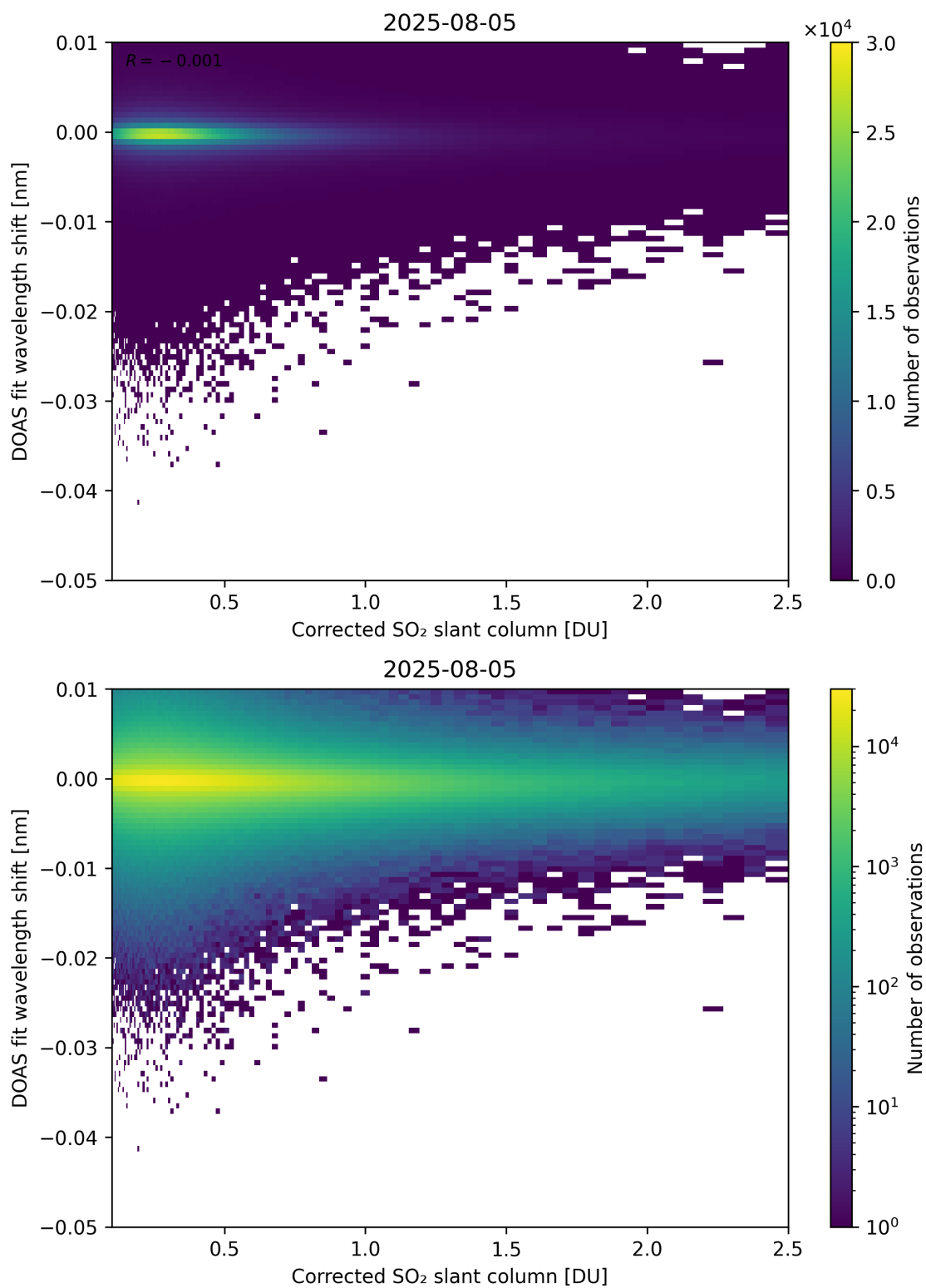
Figure 229: Scatter density plot of “Corrected SO 2 slant column” against “DOAS fit wavelength shift” for 2025-08-04 to 2025-08-06.
