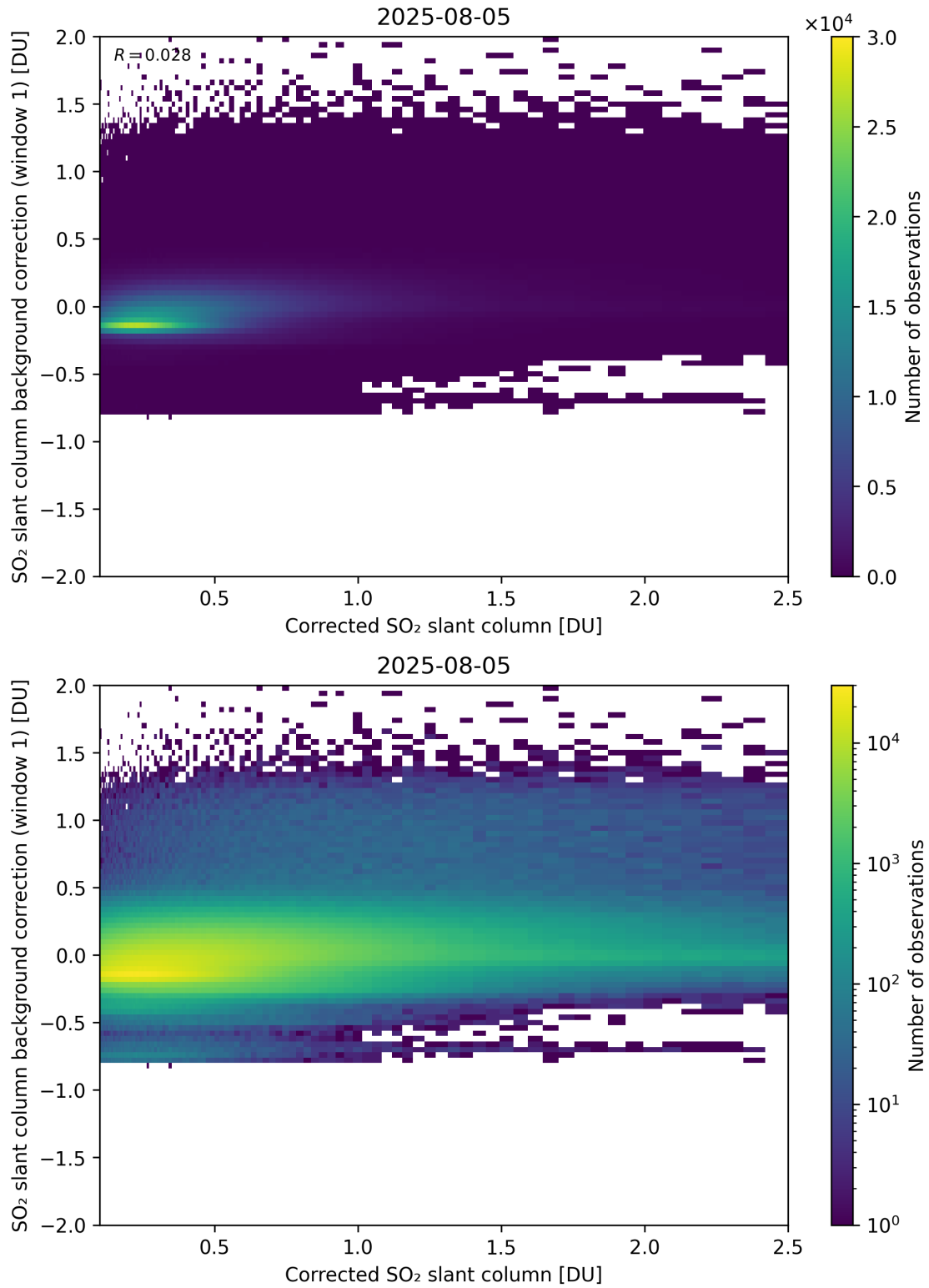
Figure 226: Scatter density plot of “Corrected SO 2 slant column” against “SO 2 slant column background correction (window 1)” for 2025-08-04 to 2025-08-06.
