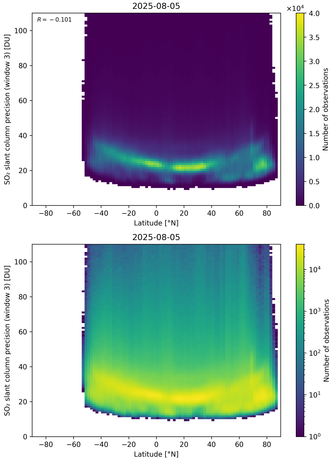
Figure 166: Scatter density plot of “Latitude” against “SO 2 slant column precision (window 3)” for 2025-08-04 to 2025-08-06.
