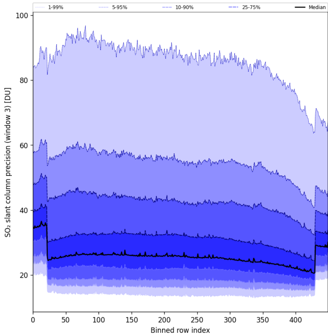
Figure 98: Along track statistics of “SO 2 slant column precision (window 3)” for 2025-08-04 to 2025-08-06
