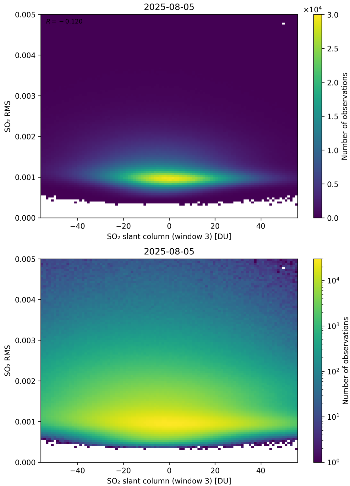
Figure 306: Scatter density plot of “SO 2 slant column (window 3)” against “SO 2 RMS” for 2025-08-04 to 2025-08-06.
