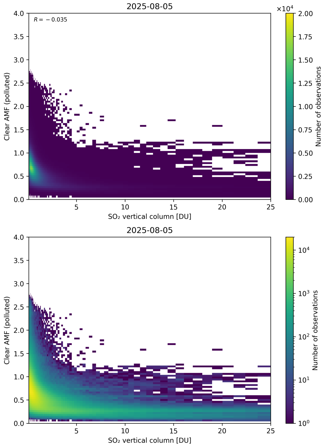
Figure 348: Scatter density plot of “SO 2 vertical column” against “Clear AMF (polluted)” for 2025-08-04 to 2025-08-06.
