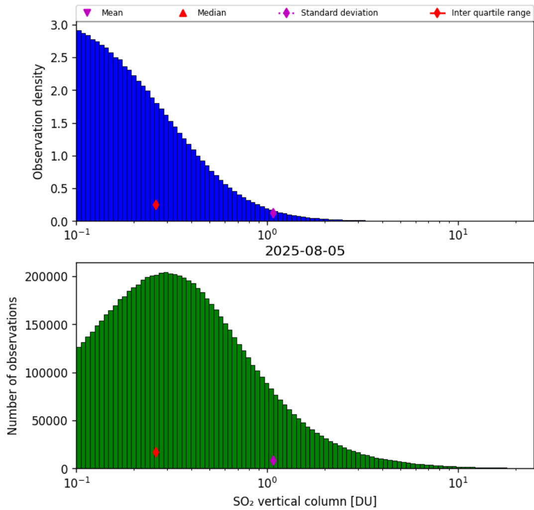
Figure 58: Histogram of “SO 2 vertical column” for 2025-08-04 to 2025-08-06
