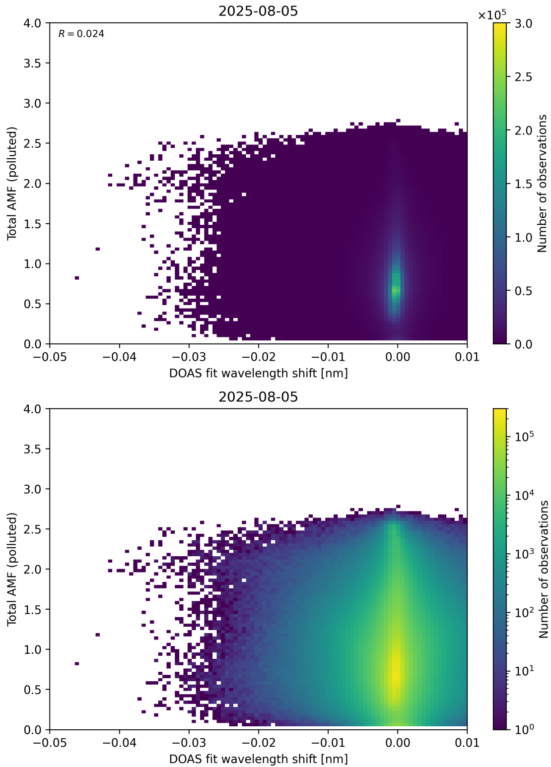
Figure 141: Scatter density plot of “DOAS fit wavelength shift” against “Total AMF (polluted)” for 2025-08-04 to 2025-08-06.
