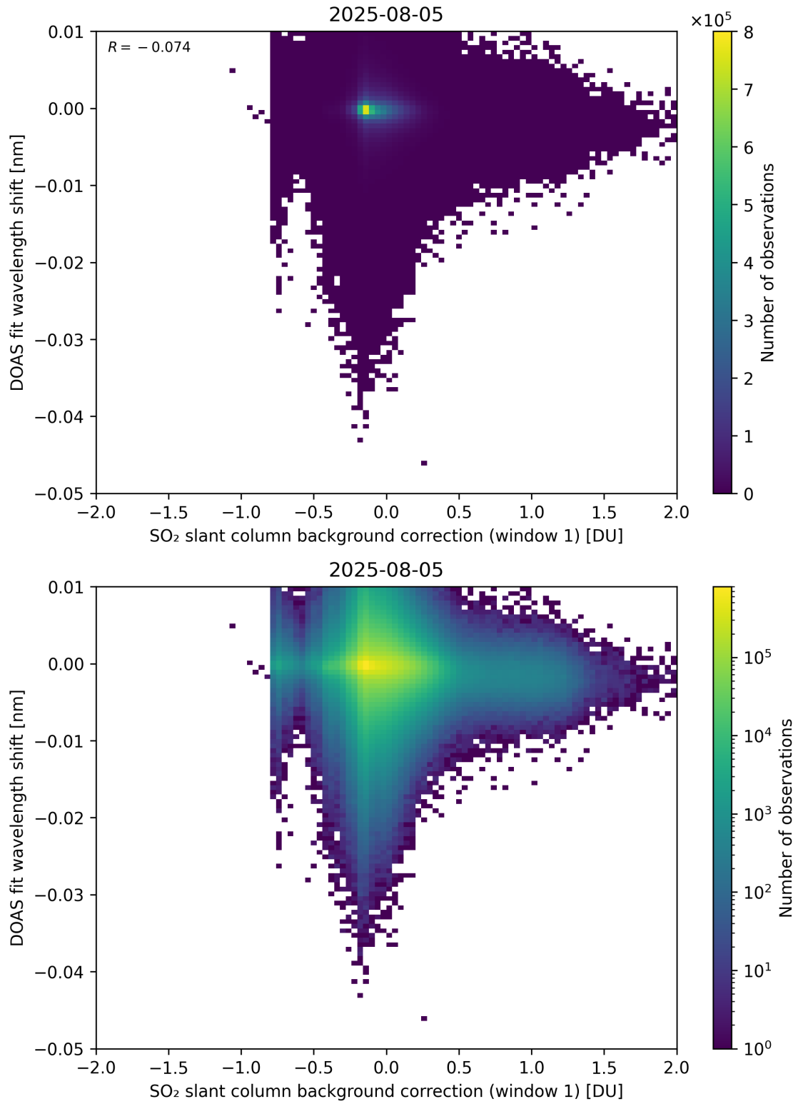
Figure 111: Scatter density plot of “SO 2 slant column background correction (window 1)” against “DOAS fit wavelength shift” for 2025-08-04 to 2025-08-06.
