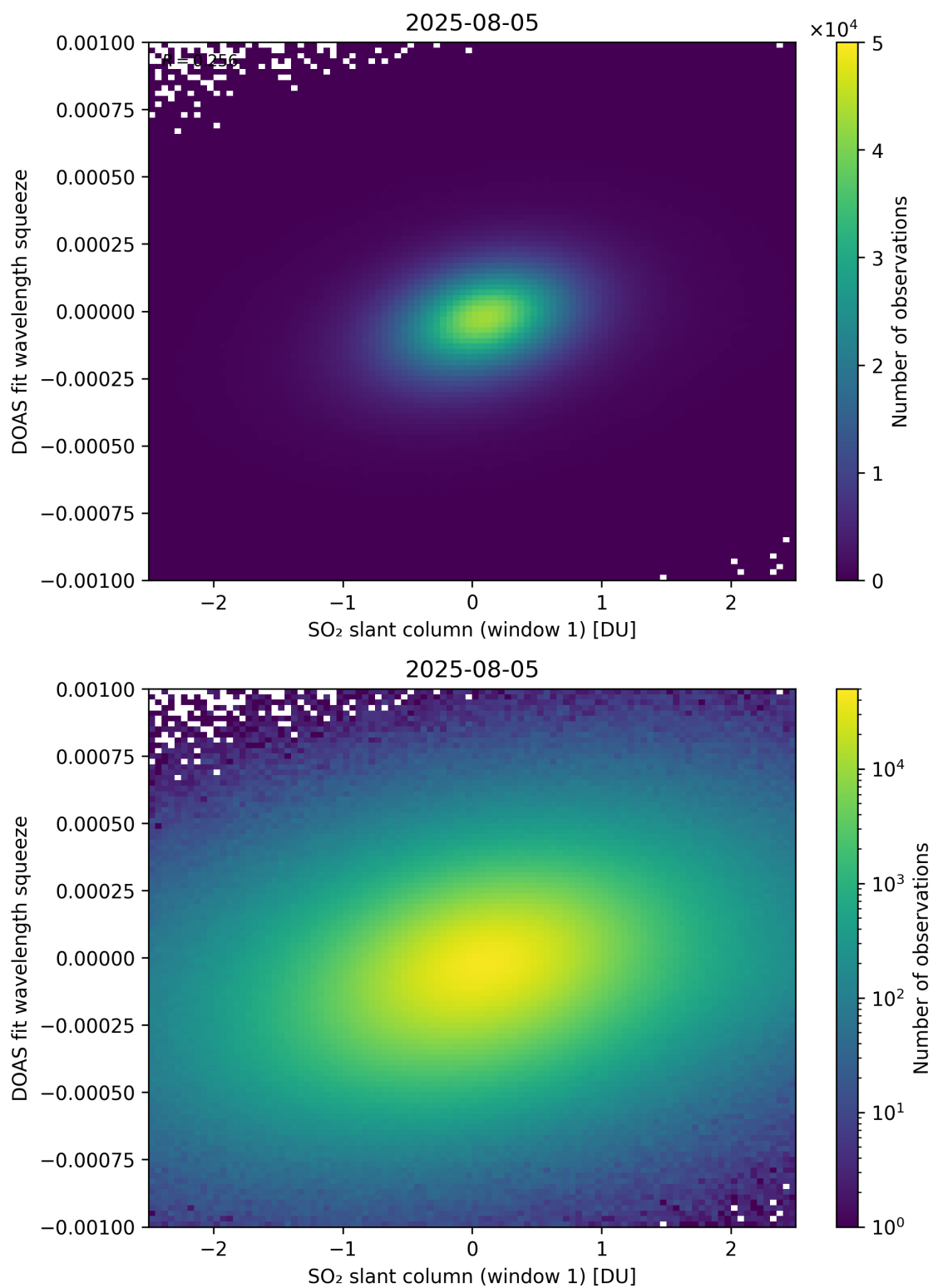
Figure 266: Scatter density plot of “SO 2 slant column (window 1)” against “DOAS fit wavelength squeeze” for 2025-08-04 to 2025-08-06.
