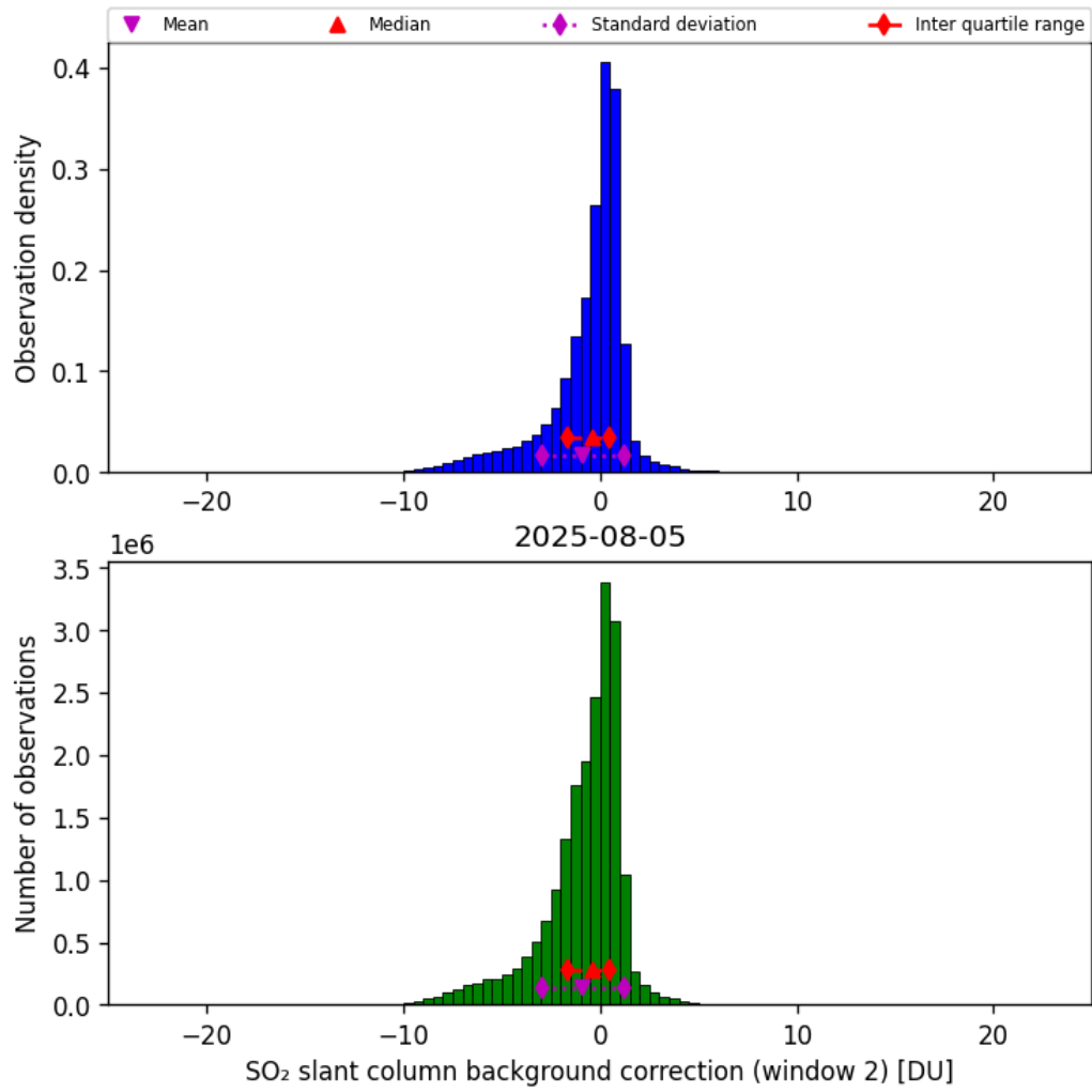
Figure 70: Histogram of “SO 2 slant column background correction (window 2)” for 2025-08-04 to 2025-08-06
