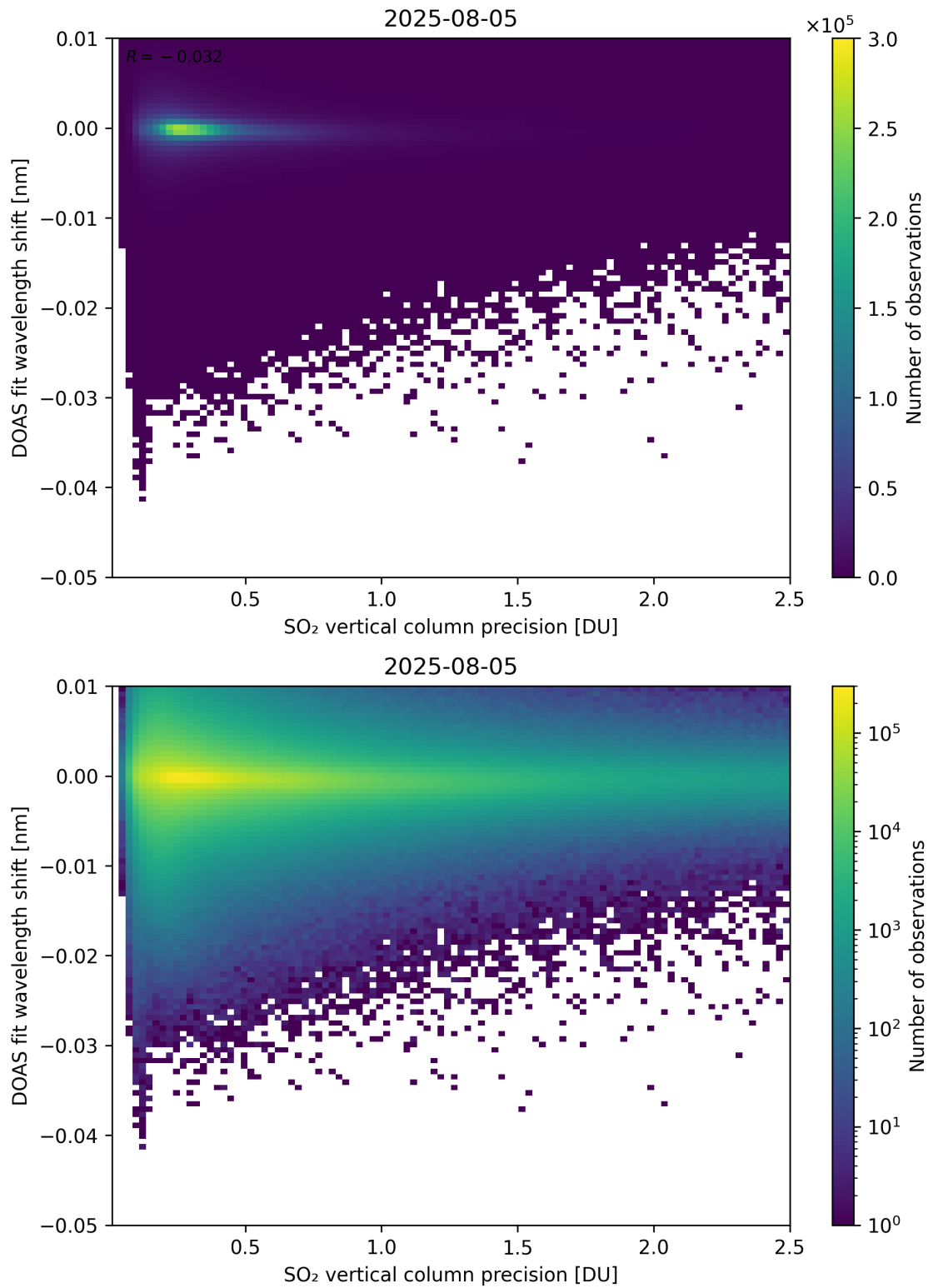
Figure 332: Scatter density plot of “SO 2 vertical column precision” against “DOAS fit wavelength shift” for 2025-08-04 to 2025-08-06.
