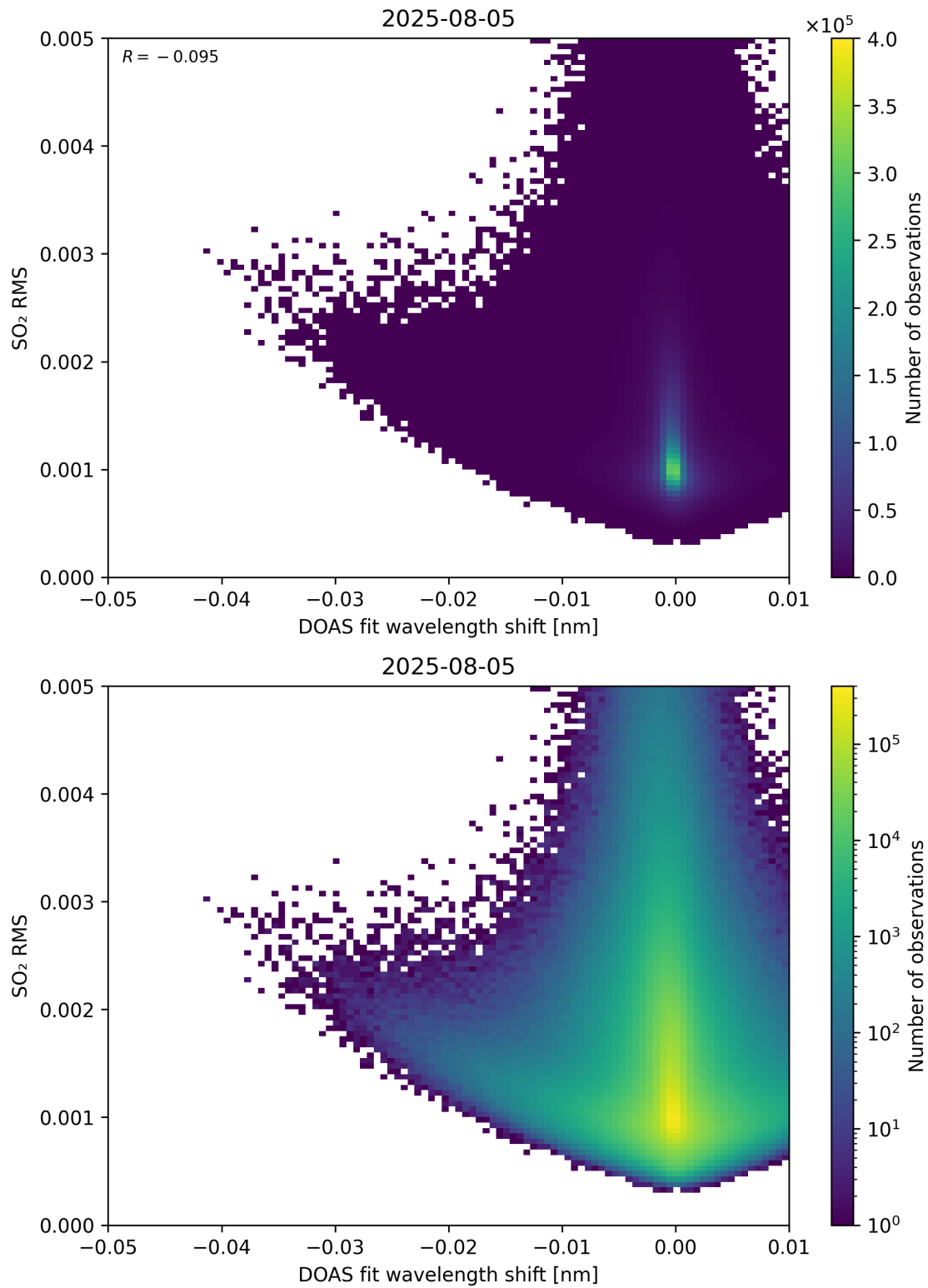
Figure 139: Scatter density plot of “DOAS fit wavelength shift” against “SO 2 RMS” for 2025-08-04 to 2025-08-06.
