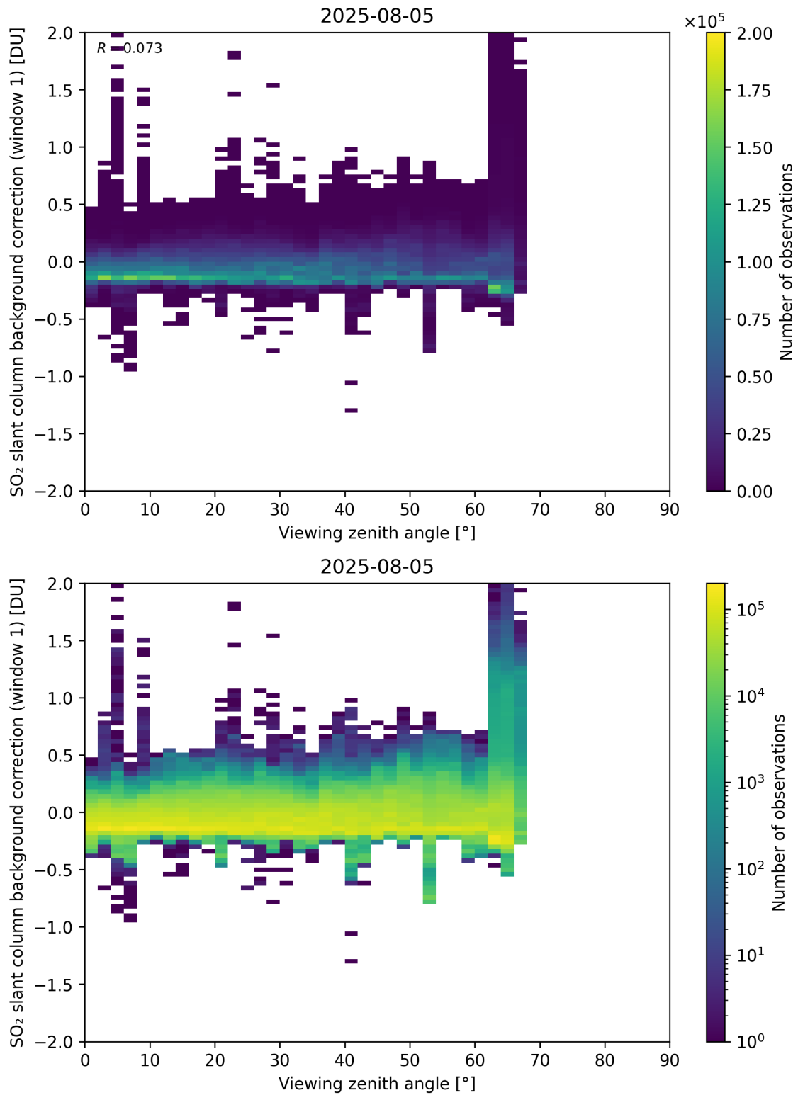
Figure 362: Scatter density plot of “Viewing zenith angle” against “SO 2 slant column background correction (window 1)” for 2025-08-04 to 2025-08-06.
