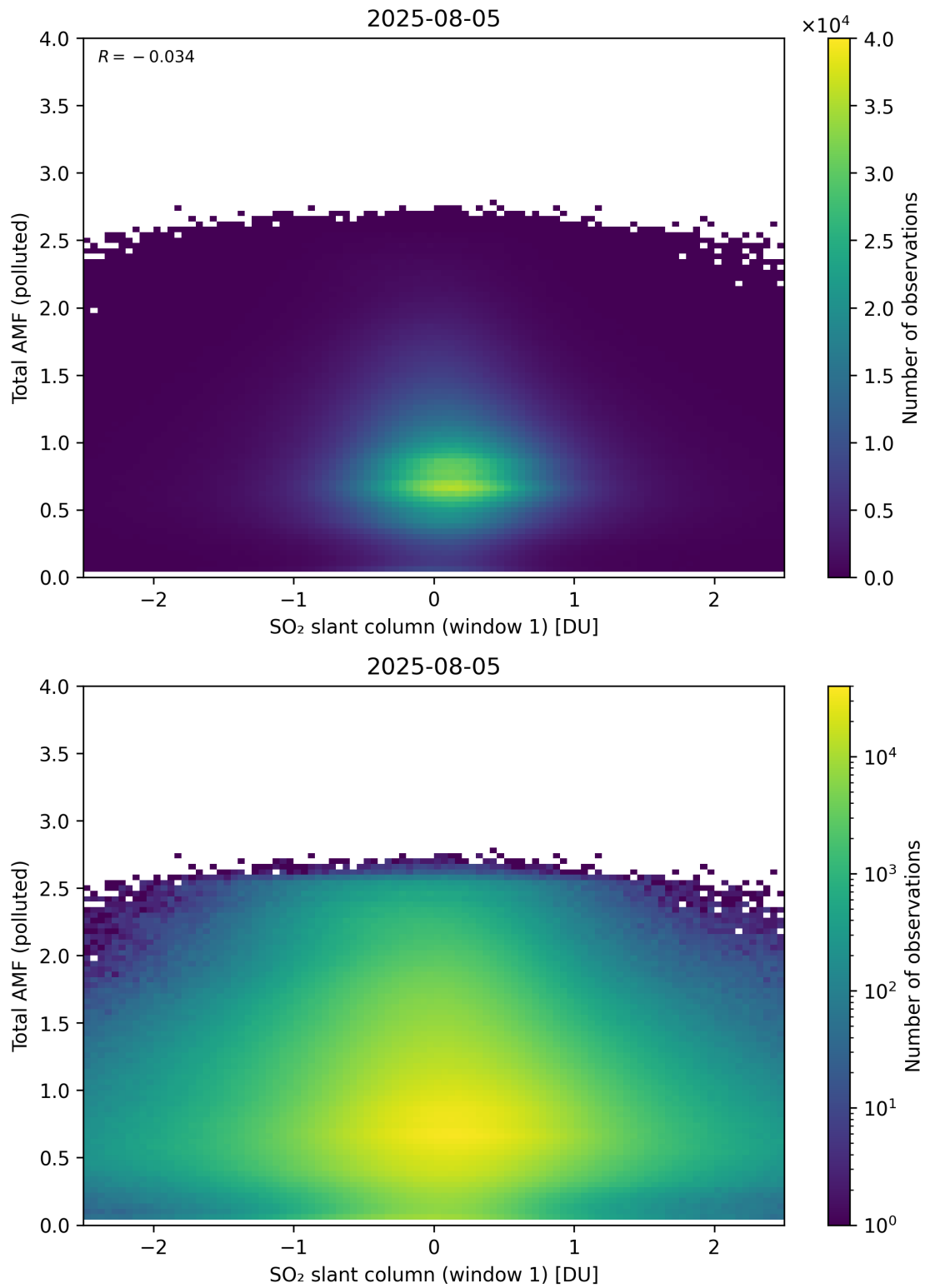
Figure 289: Scatter density plot of “SO 2 slant column (window 1)” against “Total AMF (polluted)” for 2025-08-04 to 2025-08-06.
