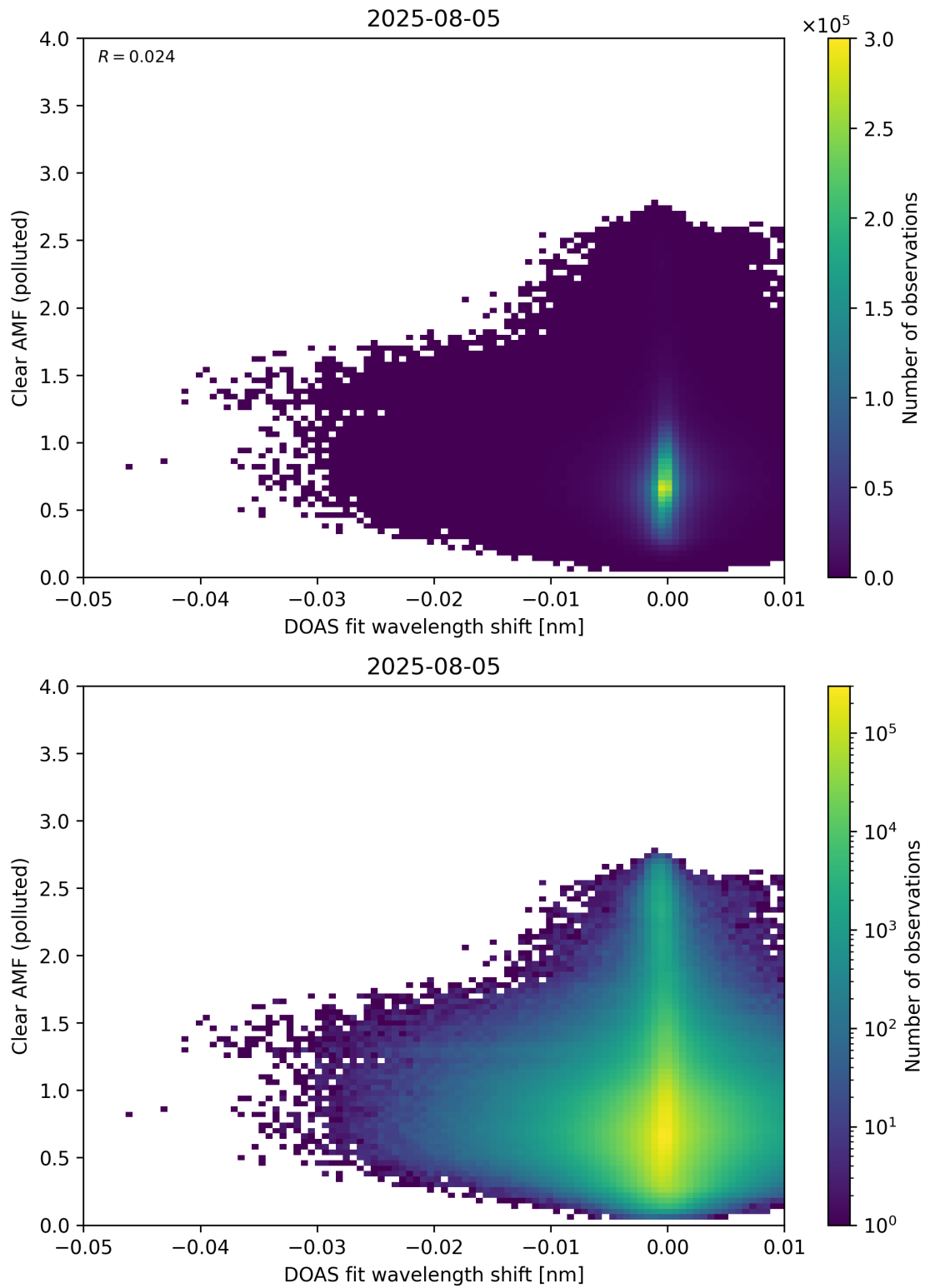
Figure 140: Scatter density plot of “DOAS fit wavelength shift” against “Clear AMF (polluted)” for 2025-08-04 to 2025-08-06.
