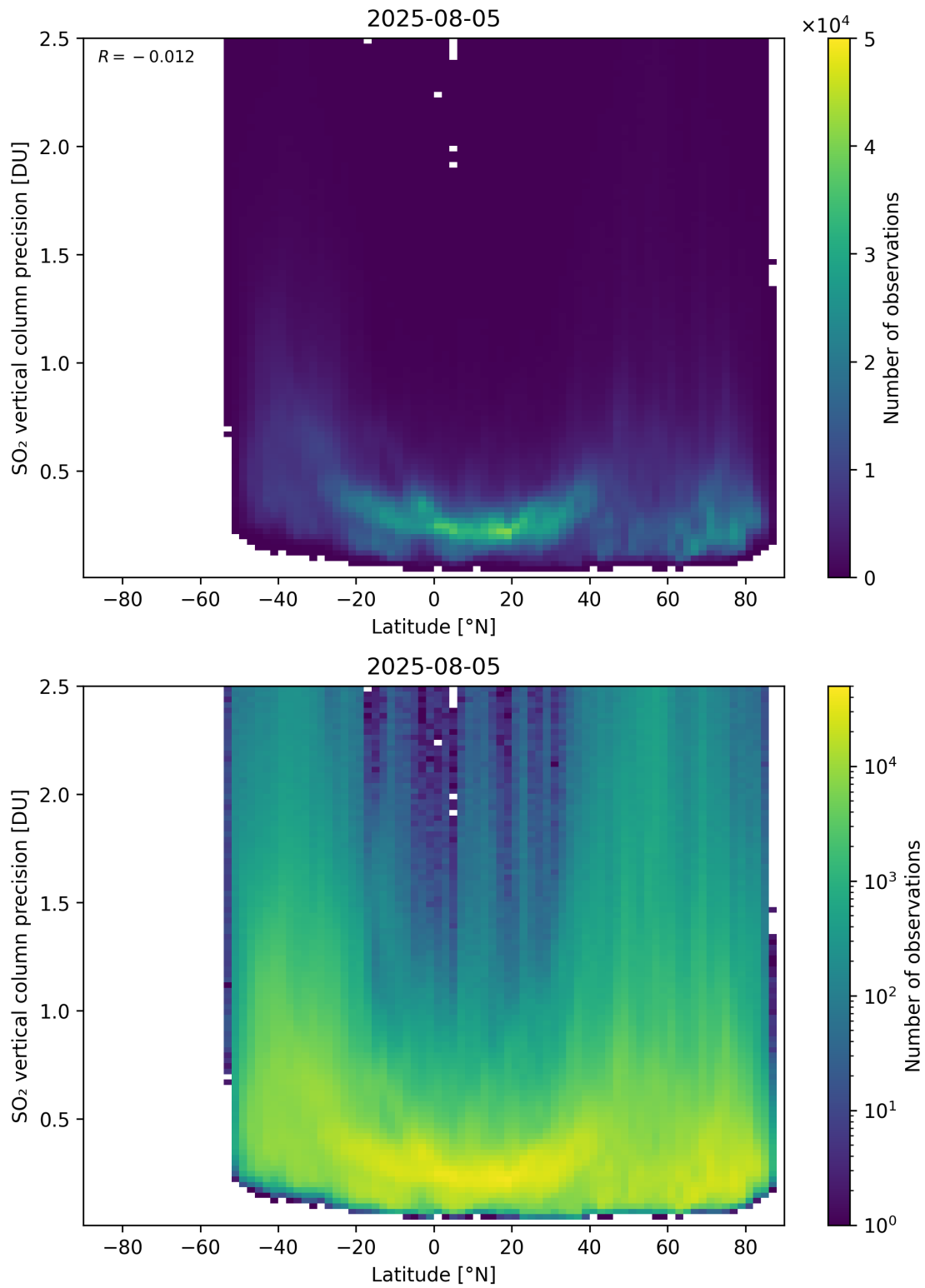
Figure 170: Scatter density plot of “Latitude” against “SO 2 vertical column precision” for 2025-08-04 to 2025-08-06.
