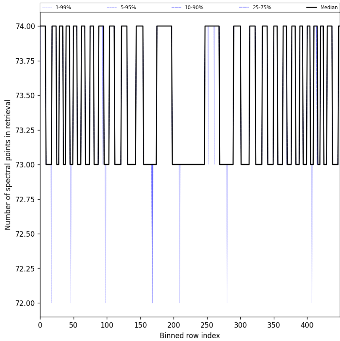
Figure 108: Along track statistics of “Number of spectral points in retrieval” for 2025-08-04 to 2025-08-06
