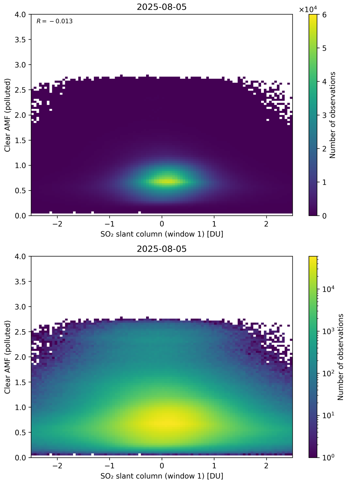
Figure 282: Scatter density plot of “SO 2 slant column (window 1)” against “Clear AMF (polluted)” for 2025-08-04 to 2025-08-06.
