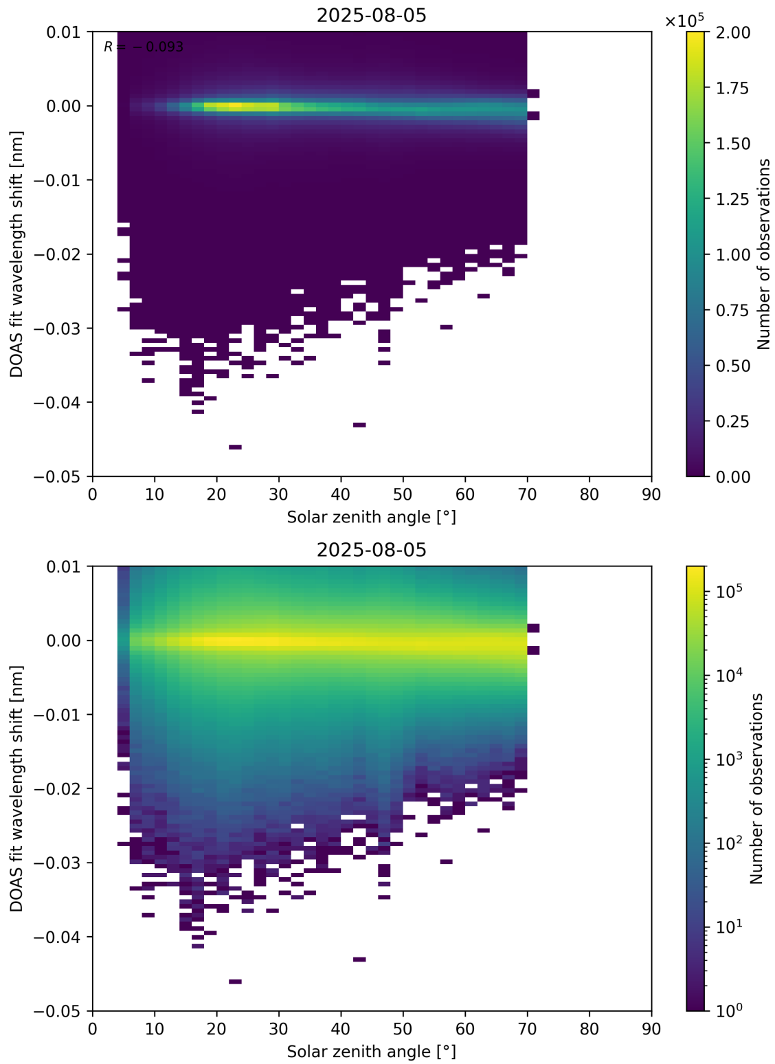
Figure 174: Scatter density plot of “Solar zenith angle” against “DOAS fit wavelength shift” for 2025-08-04 to 2025-08-06.
