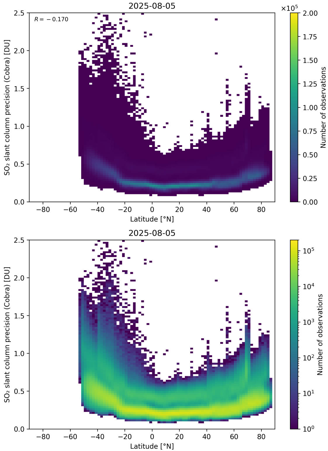
Figure 158: Scatter density plot of “Latitude” against “SO 2 slant column precision (Cobra)” for 2025-08-04 to 2025-08-06.
