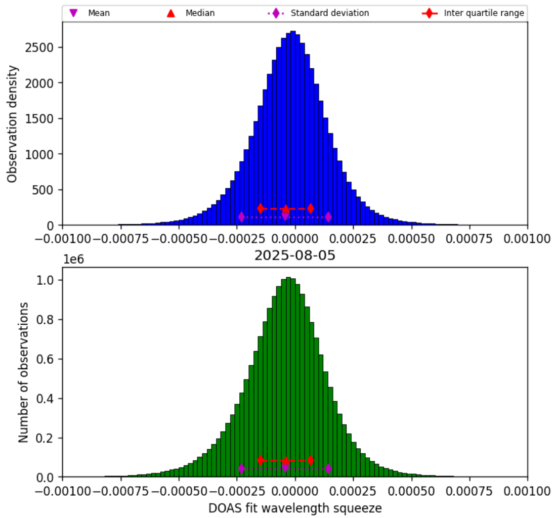
Figure 77: Histogram of “DOAS fit wavelength squeeze” for 2025-08-04 to 2025-08-06
