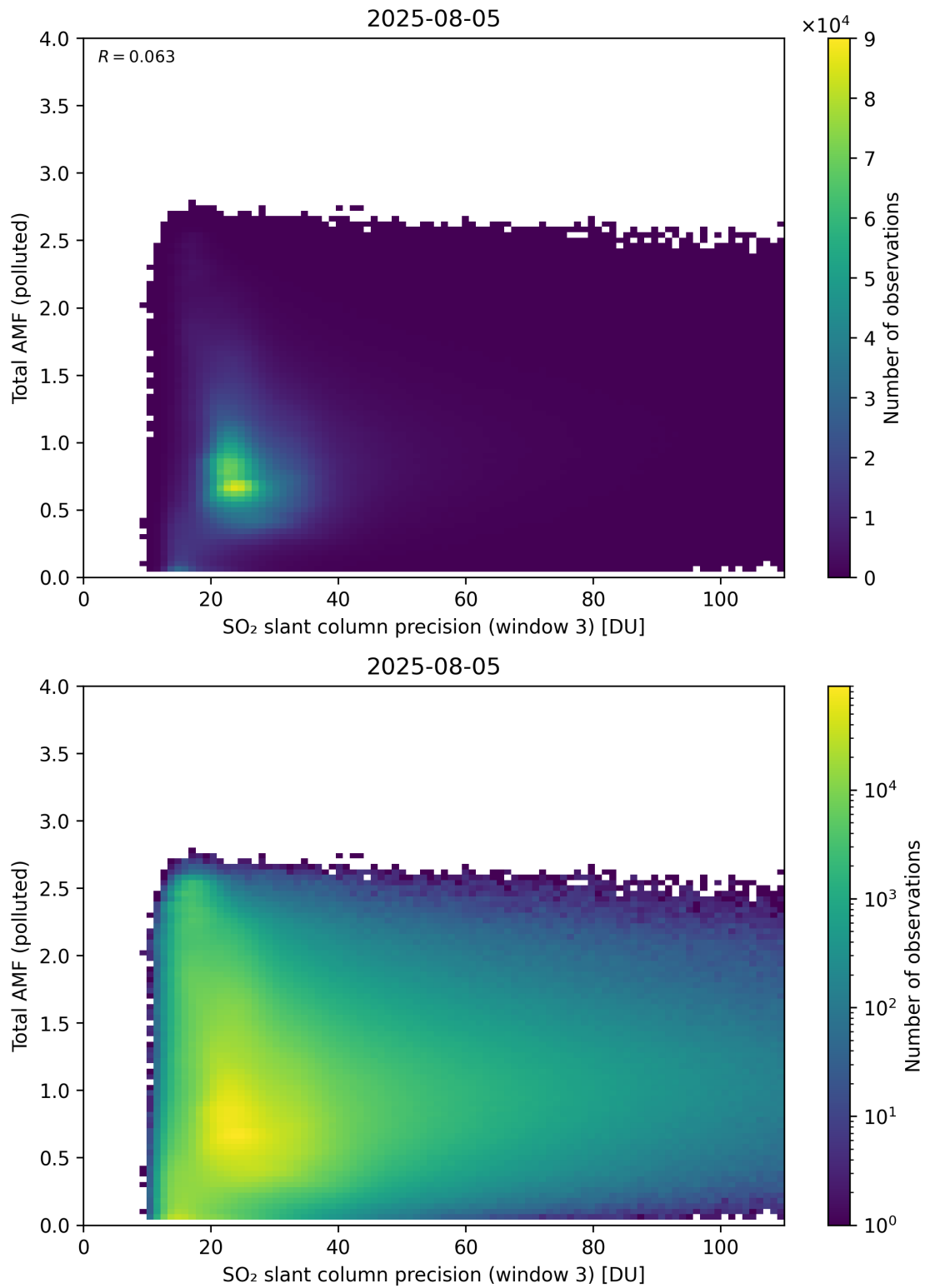
Figure 313: Scatter density plot of “SO 2 slant column precision (window 3)” against “Total AMF (polluted)” for 2025-08-04 to 2025-08-06.
