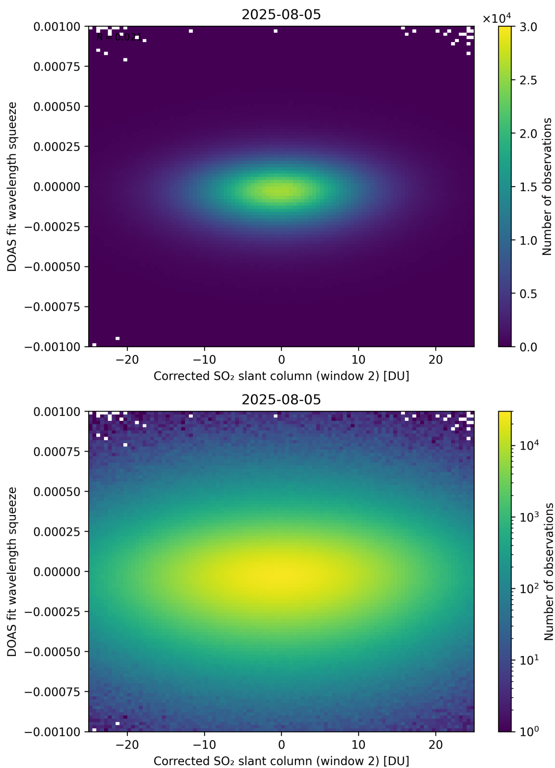
Figure 247: Scatter density plot of “Corrected SO 2 slant column (window 2)” against “DOAS fit wavelength squeeze” for 2025-08-04 to 2025-08-06.
