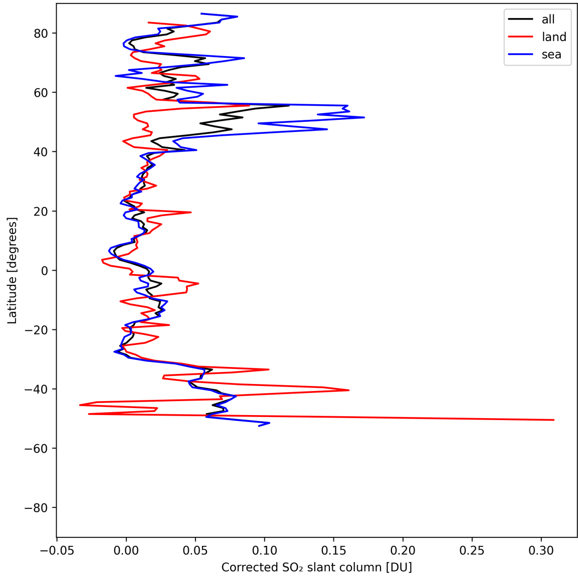
Figure 34: Zonal average of “Corrected SO 2 slant column” for 2025-08-04 to 2025-08-06.
