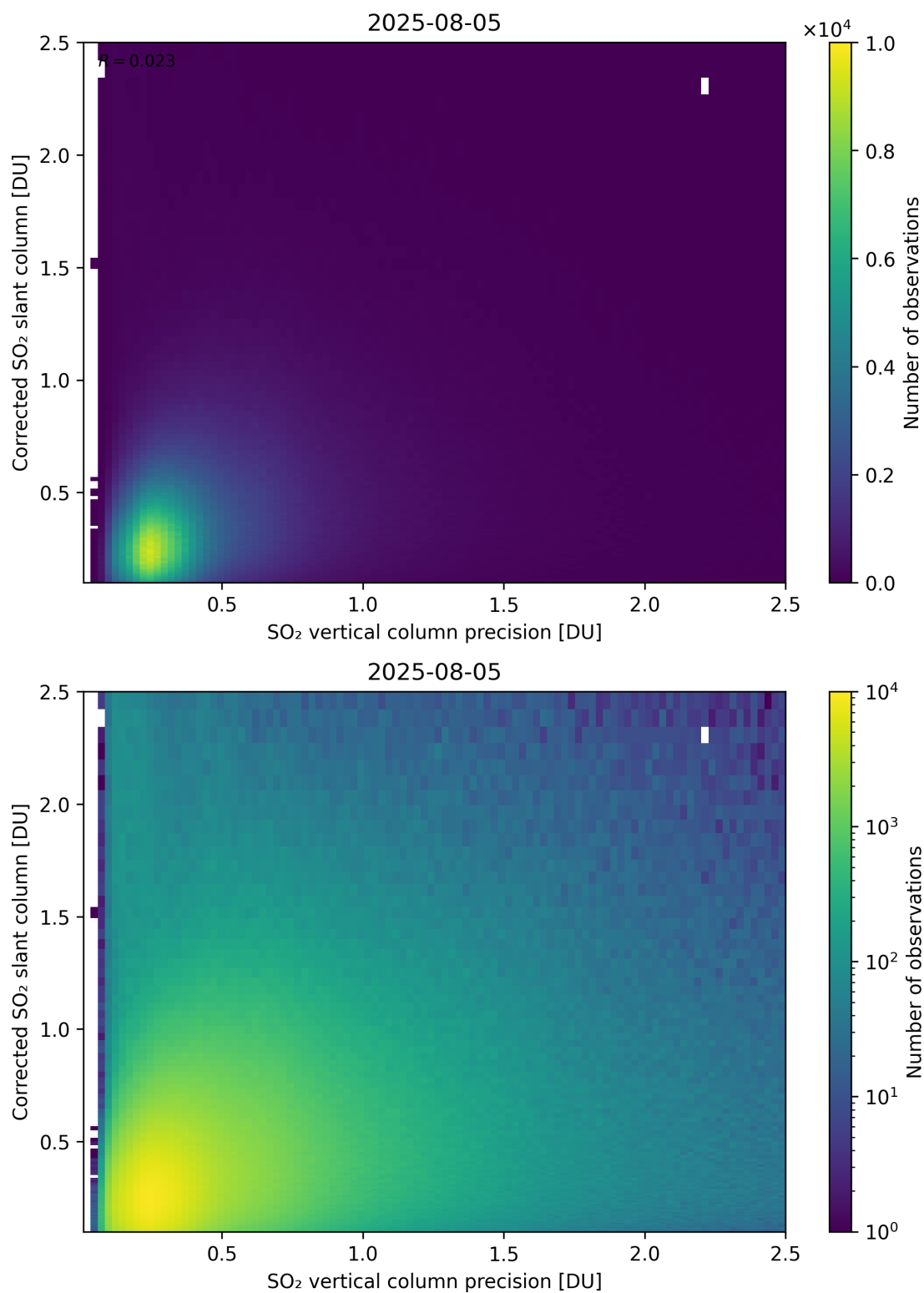
Figure 338: Scatter density plot of “SO 2 vertical column precision” against “Corrected SO 2 slant column” for 2025-08-04 to 2025-08-06.
