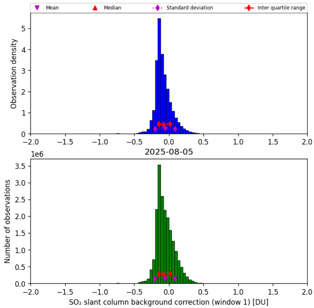
Figure 66: Histogram of “SO 2 slant column background correction (window 1)” for 2025-08-04 to 2025-08-06
