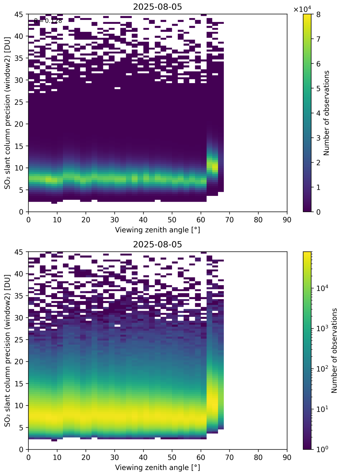
Figure 378: Scatter density plot of “Viewing zenith angle” against “SO 2 slant column precision (window2)” for 2025-08-04 to 2025-08-06.
