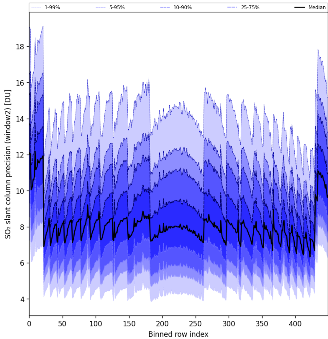
Figure 94: Along track statistics of “SO 2 slant column precision (window2)” for 2025-08-04 to 2025-08-06
