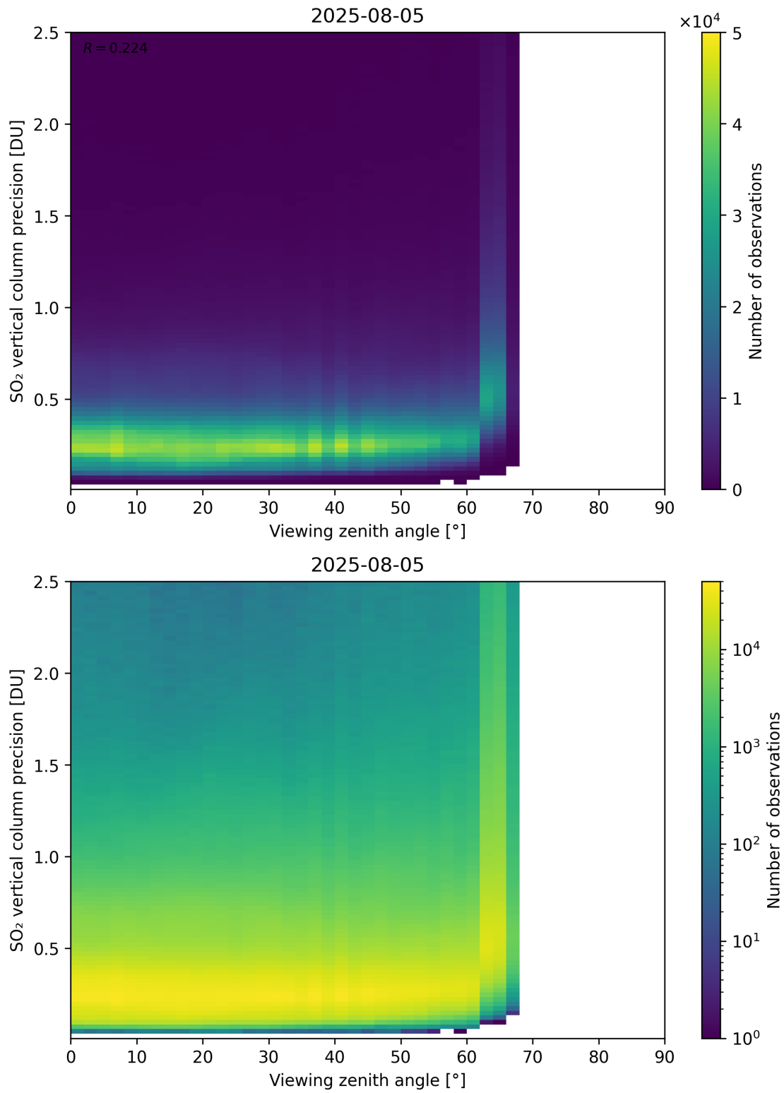
Figure 384: Scatter density plot of “Viewing zenith angle” against “SO 2 vertical column precision” for 2025-08-04 to 2025-08-06.
