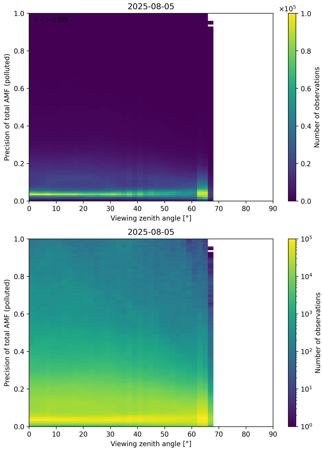
Figure 382: Scatter density plot of “Viewing zenith angle” against “Precision of total AMF (polluted)” for 2025-08-04 to 2025-08-06.
