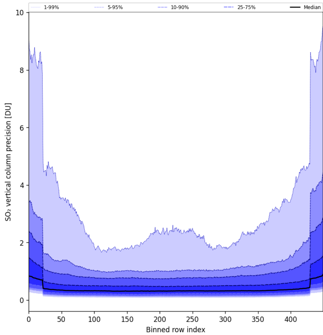
Figure 85: Along track statistics of “SO 2 vertical column precision” for 2025-08-04 to 2025-08-06
