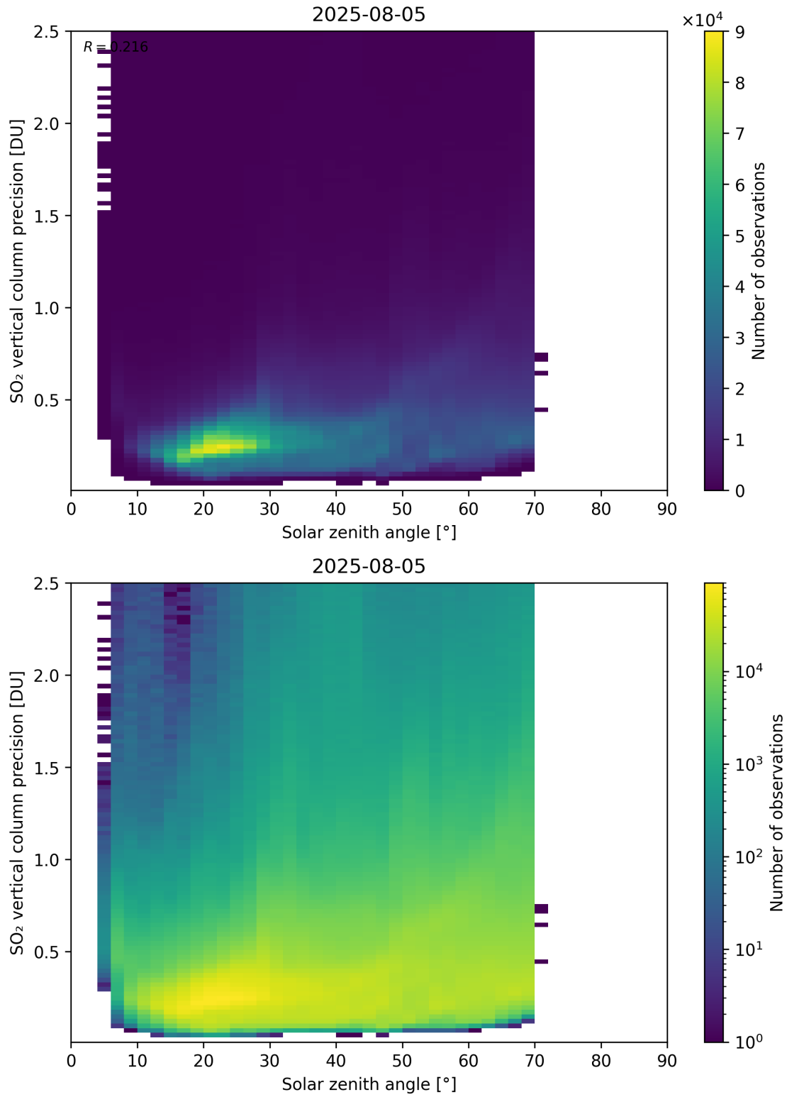
Figure 192: Scatter density plot of “Solar zenith angle” against “SO 2 vertical column precision” for 2025-08-04 to 2025-08-06.
