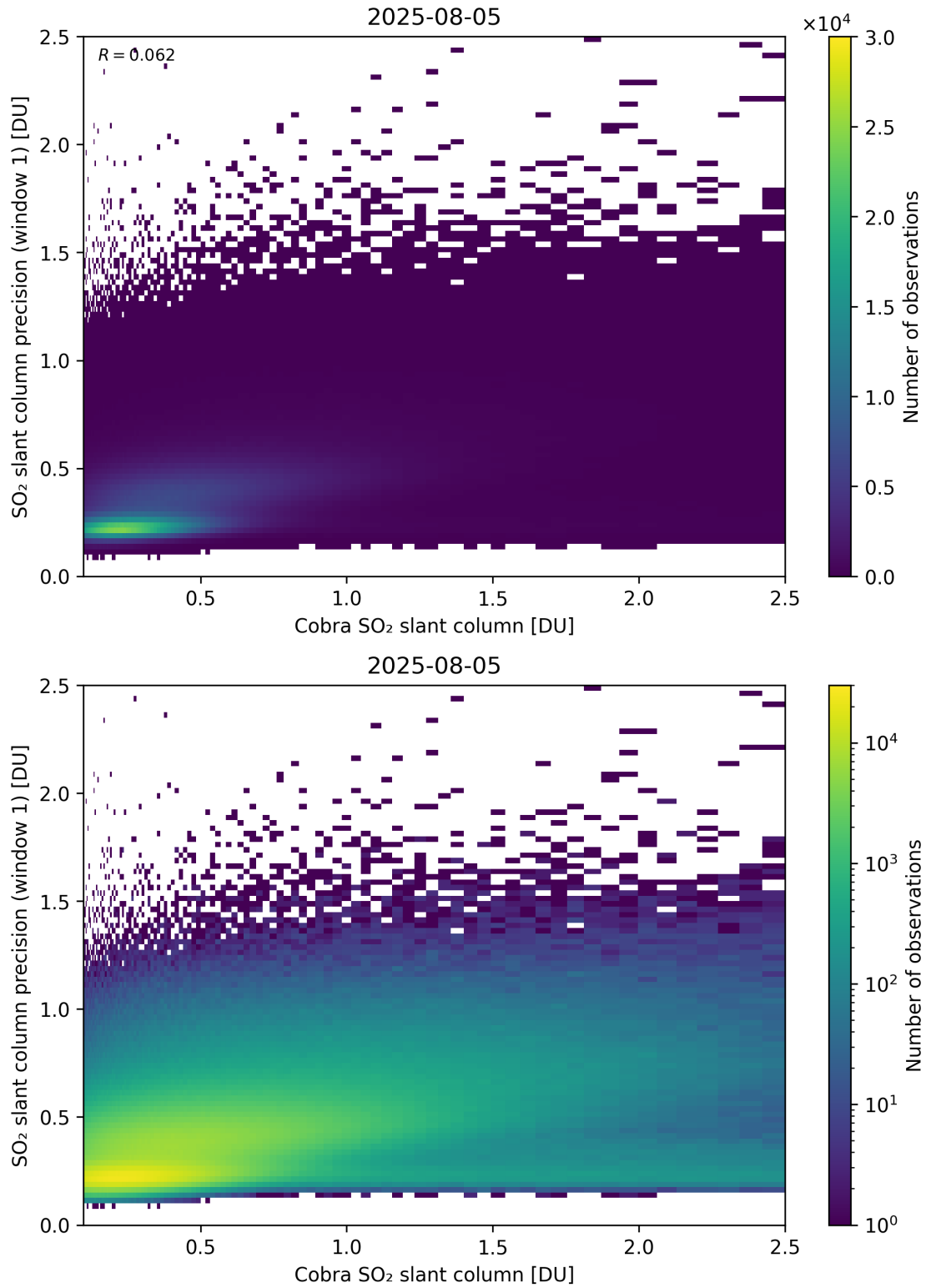
Figure 220: Scatter density plot of “Cobra SO 2 slant column” against “SO 2 slant column precision (window 1)” for 2025-08-04 to 2025-08-06.
