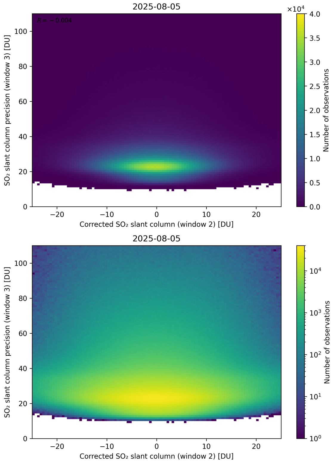
Figure 252: Scatter density plot of “Corrected SO 2 slant column (window 2)” against “SO 2 slant column precision (window 3)” for 2025-08-04 to 2025-08-06.
