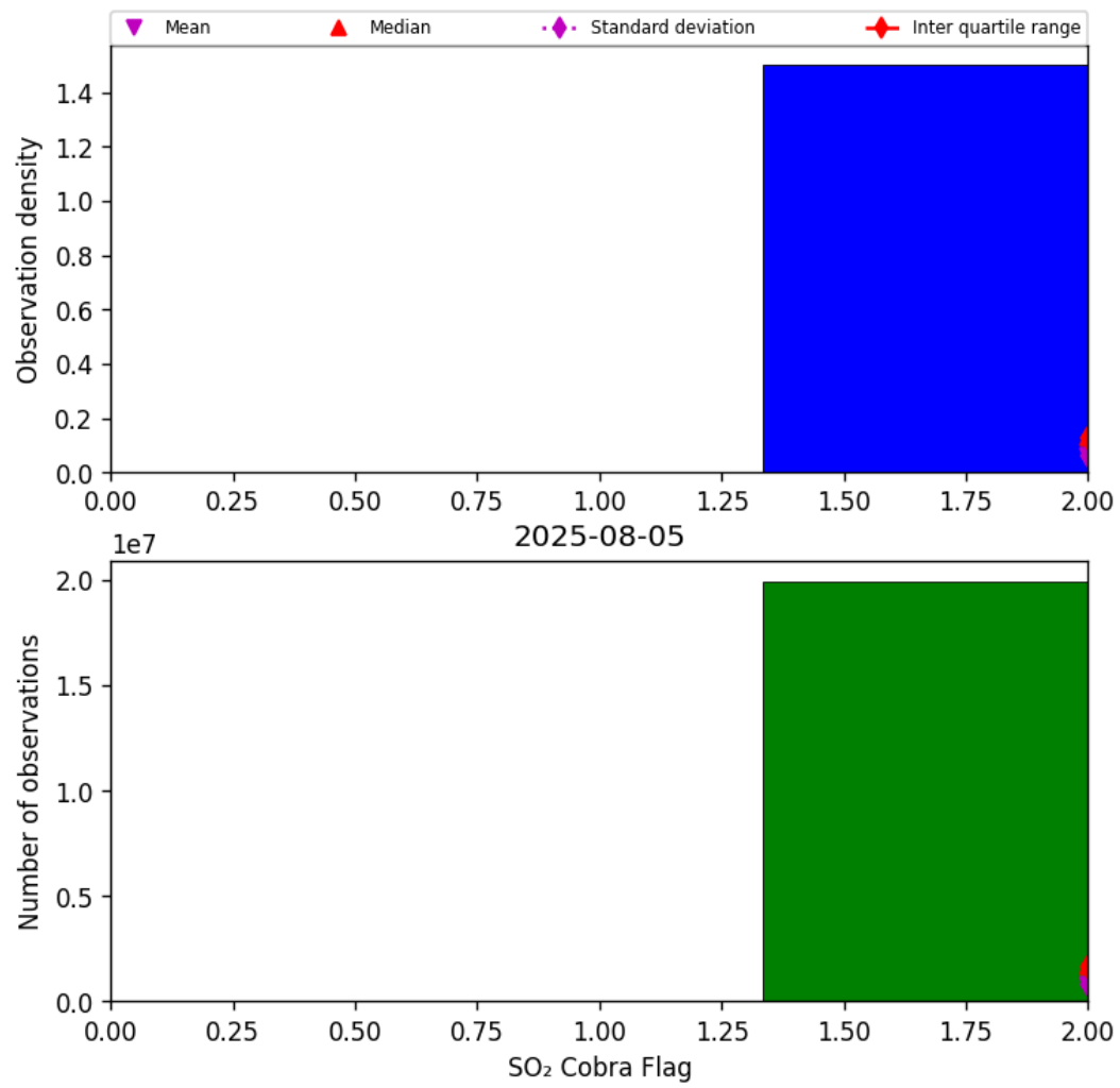
Figure 75: Histogram of “SO 2 Cobra Flag” for 2025-08-04 to 2025-08-06
