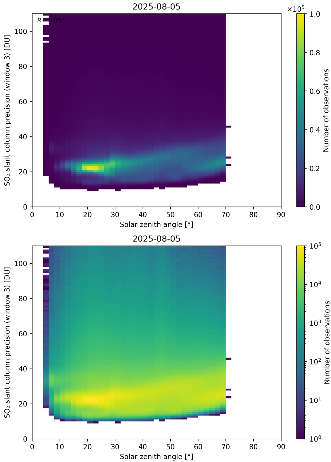
Figure 188: Scatter density plot of “Solar zenith angle” against “SO 2 slant column precision (window 3)” for 2025-08-04 to 2025-08-06.
