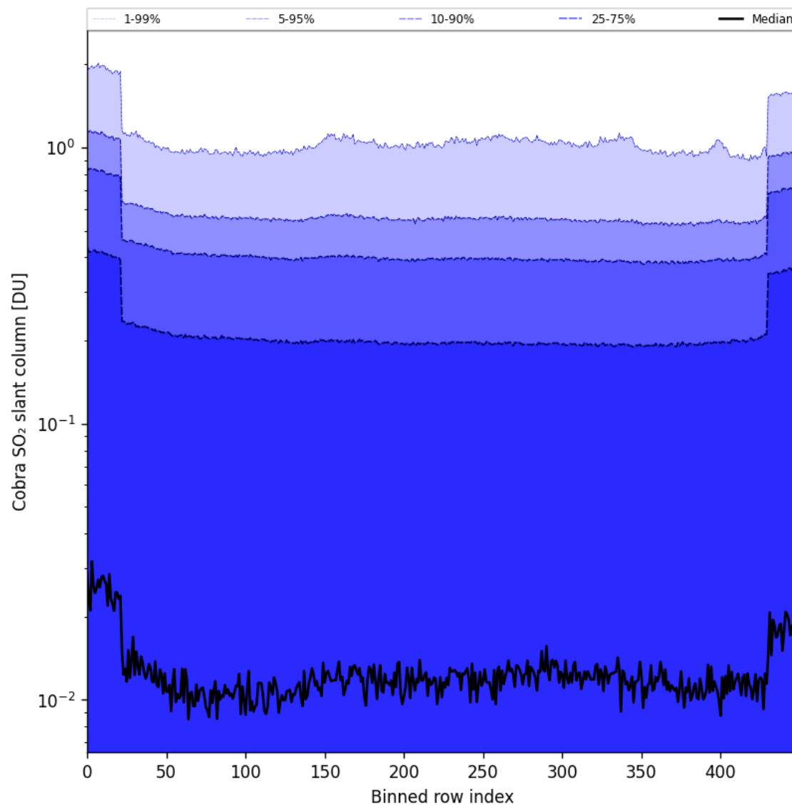
Figure 87: Along track statistics of “Cobra SO 2 slant column” for 2025-08-04 to 2025-08-06
