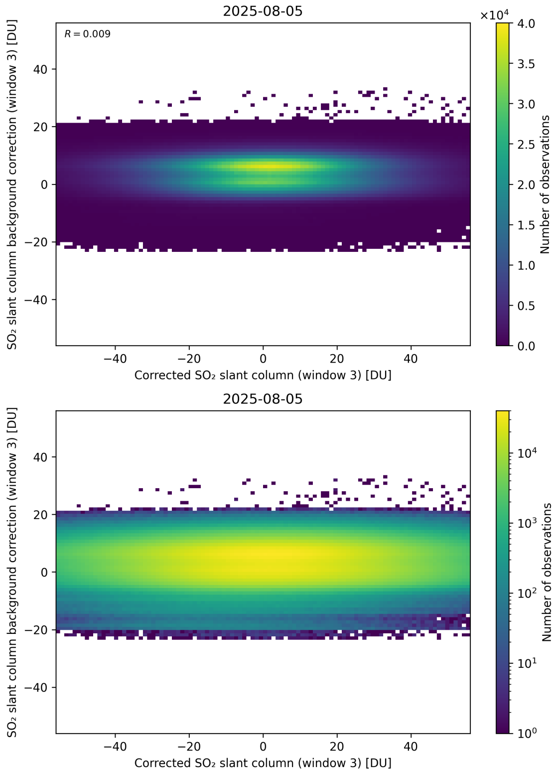
Figure 255: Scatter density plot of “Corrected SO 2 slant column (window 3)” against “SO 2 slant column background correction (window 3)” for 2025-08-04 to 2025-08-06.
