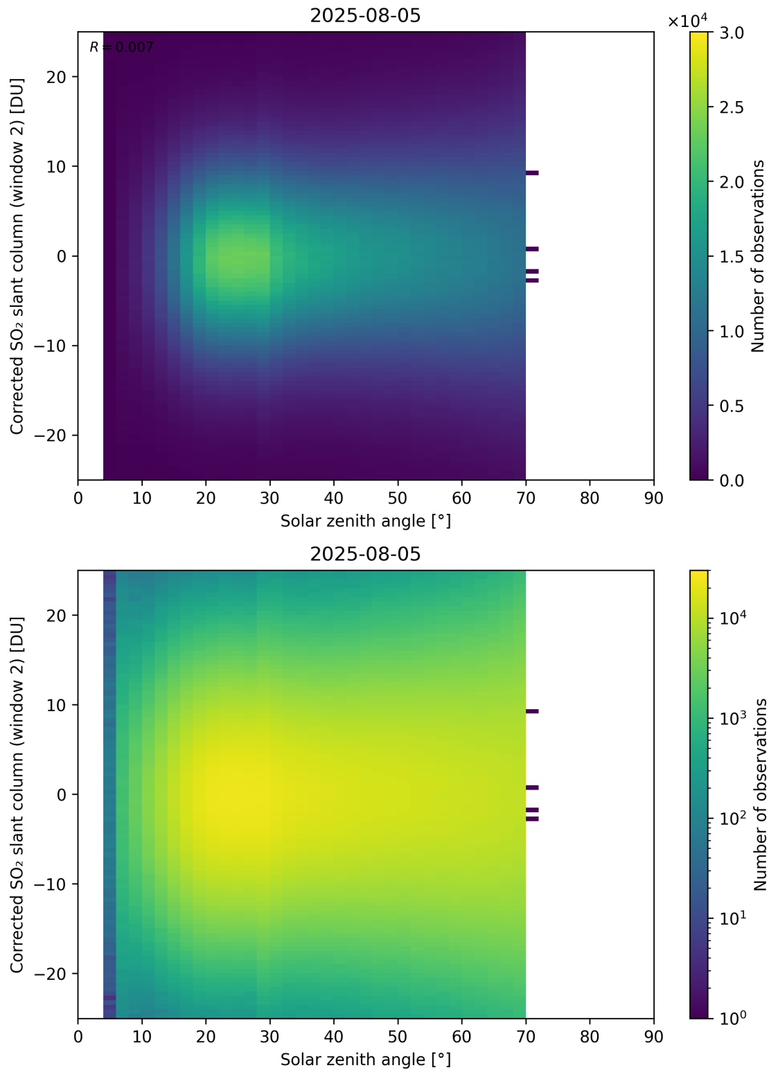
Figure 182: Scatter density plot of “Solar zenith angle” against “Corrected SO 2 slant column (window 2)” for 2025-08-04 to 2025-08-06.
