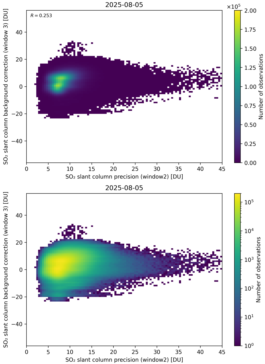
Figure 292: Scatter density plot of “SO 2 slant column precision (window2)” against “SO 2 slant column background correction (window 3)” for 2025-08-04 to 2025-08-06.
