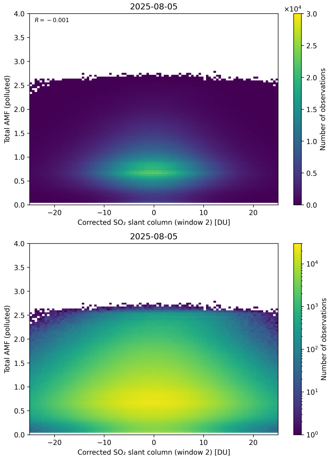
Figure 253: Scatter density plot of “Corrected SO 2 slant column (window 2)” against “Total AMF (polluted)” for 2025-08-04 to 2025-08-06.
