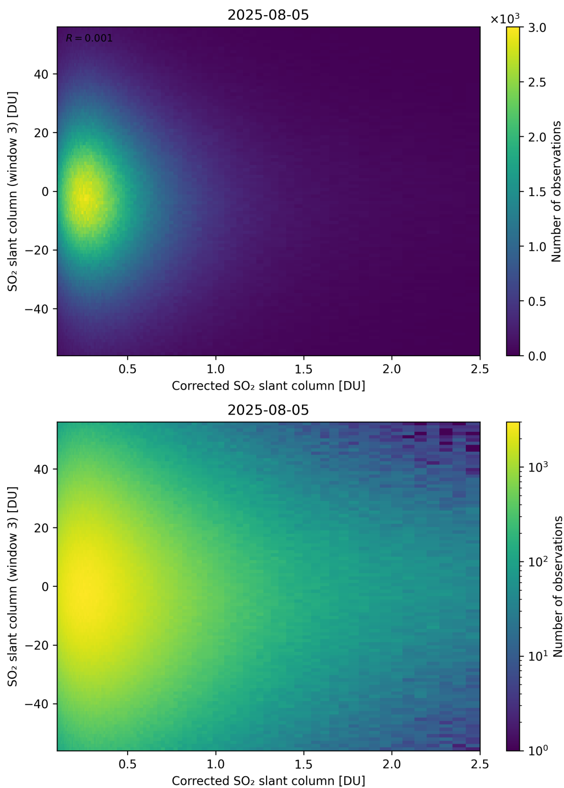
Figure 240: Scatter density plot of “Corrected SO 2 slant column” against “SO 2 slant column (window 3)” for 2025-08-04 to 2025-08-06.
