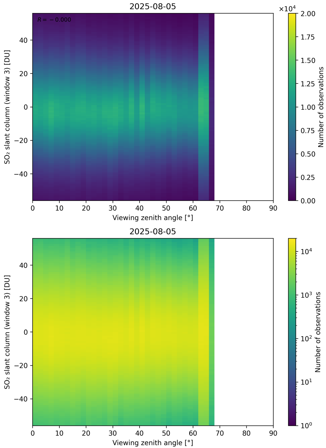
Figure 379: Scatter density plot of “Viewing zenith angle” against “SO 2 slant column (window 3)” for 2025-08-04 to 2025-08-06.
