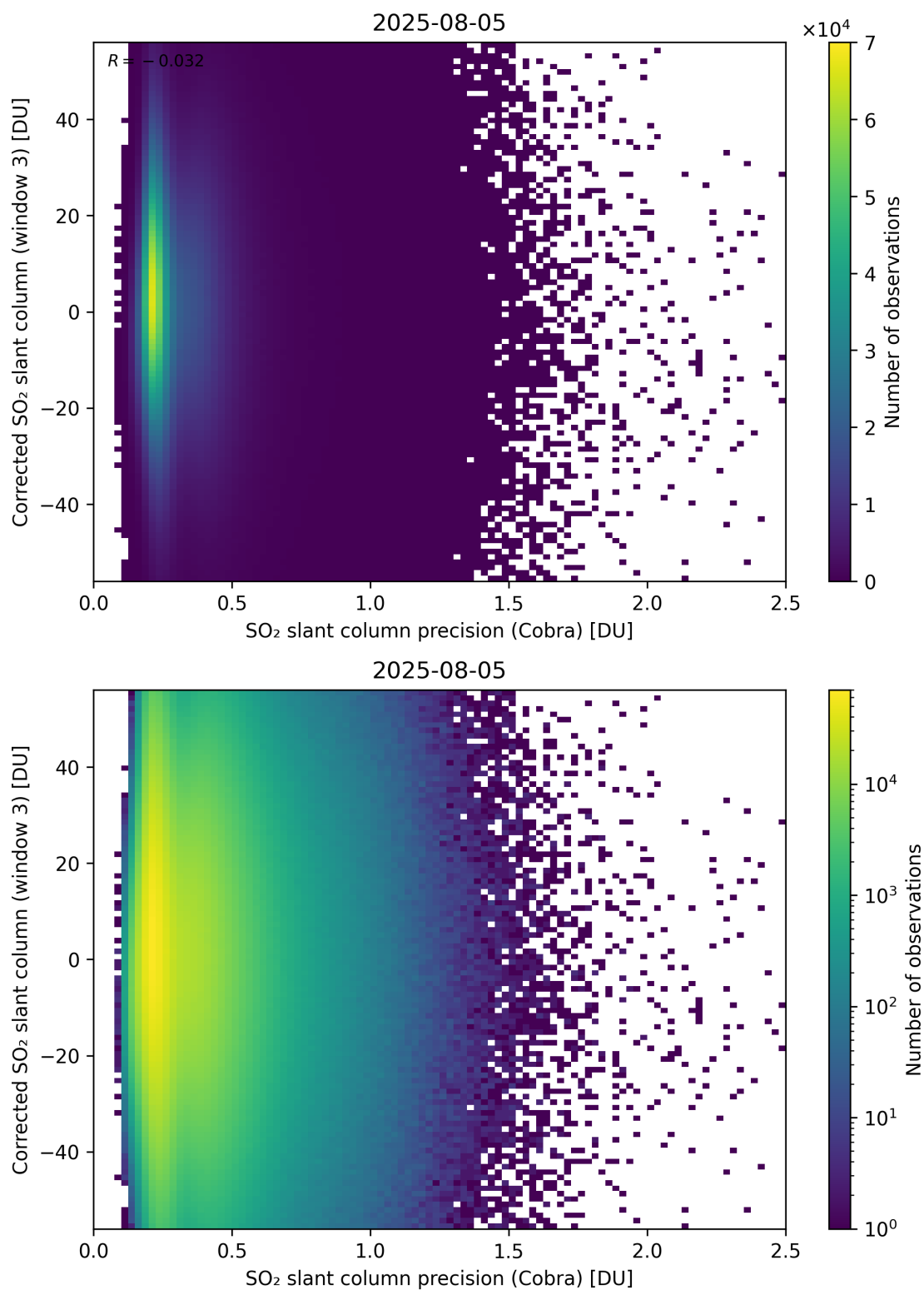
Figure 207: Scatter density plot of “SO 2 slant column precision (Cobra)” against “Corrected SO 2 slant column (window 3)” for 2025-08-04 to 2025-08-06.
