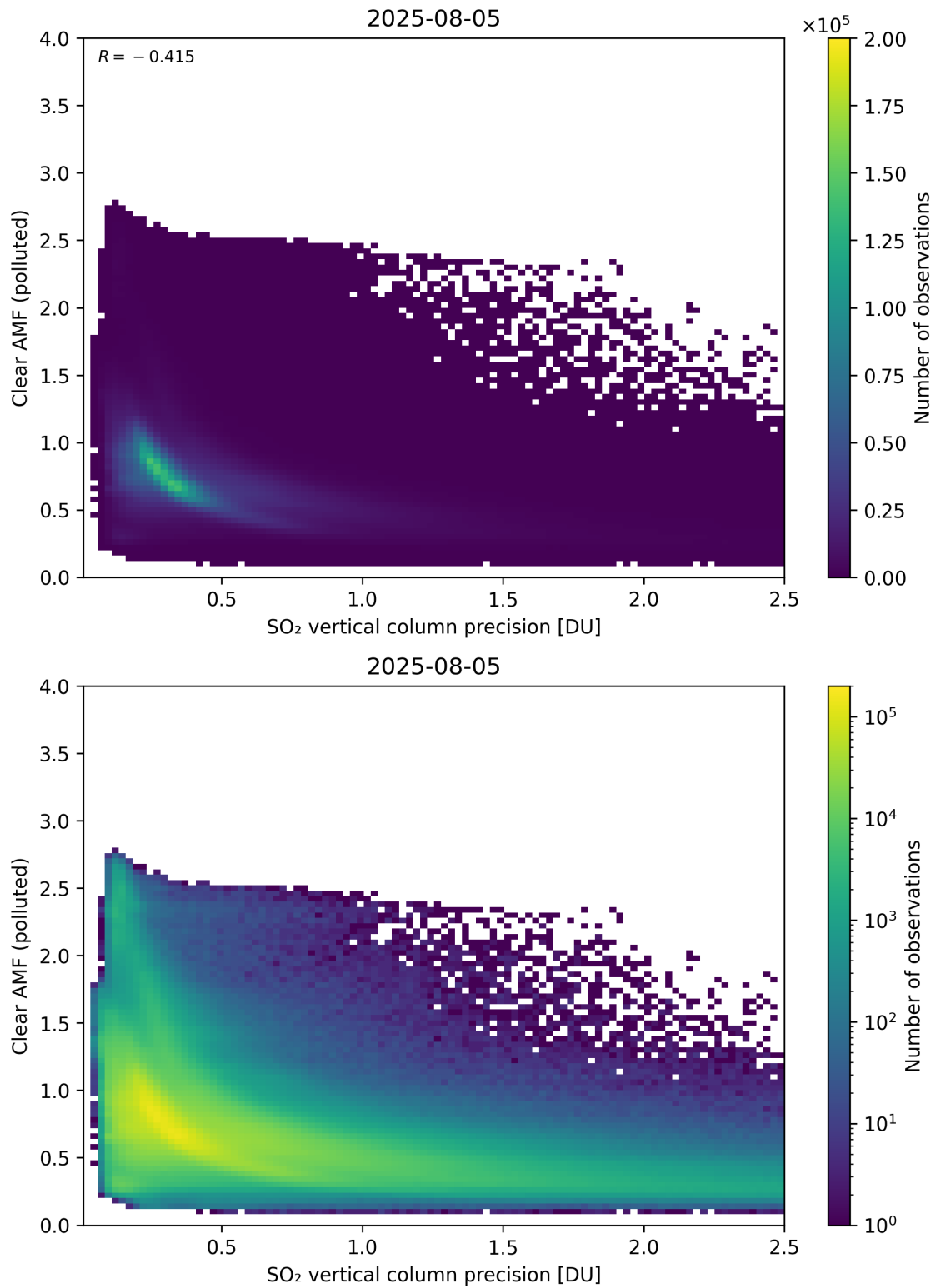
Figure 335: Scatter density plot of “SO 2 vertical column precision” against “Clear AMF (polluted)” for 2025-08-04 to 2025-08-06.
