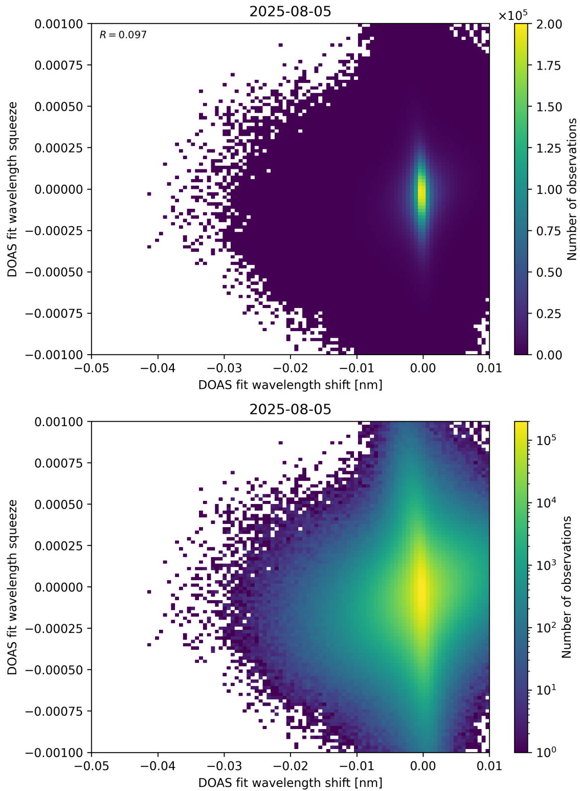
Figure 138: Scatter density plot of “DOAS fit wavelength shift” against “DOAS fit wavelength squeeze” for 2025-08-04 to 2025-08-06.
