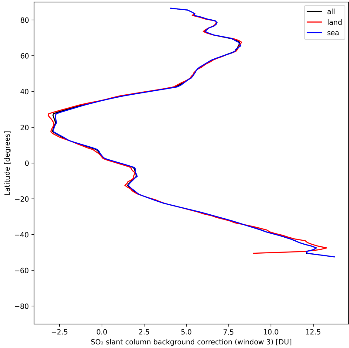
Figure 48: Zonal average of “SO 2 slant column background correction (window 3)” for 2025-08-04 to 2025-08-06.
