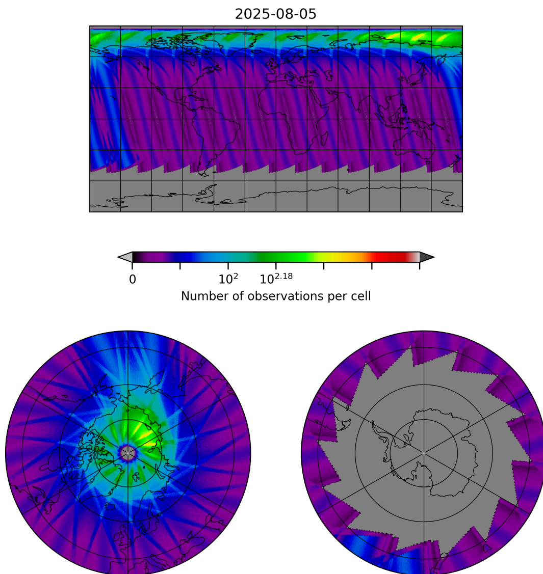
Figure 30: Map of the number of observations for 2025-08-04 to 2025-08-06
