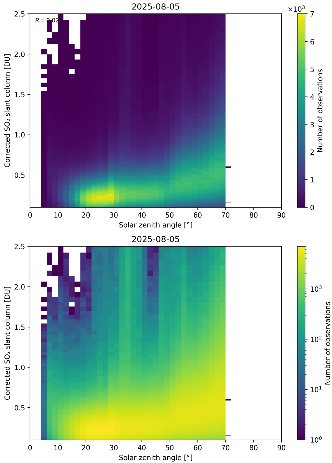
Figure 181: Scatter density plot of “Solar zenith angle” against “Corrected SO 2 slant column” for 2025-08-04 to 2025-08-06.
