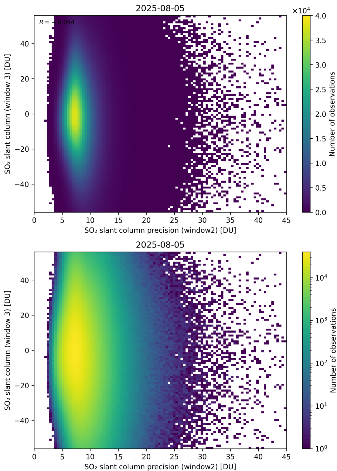
Figure 299: Scatter density plot of “SO 2 slant column precision (window2)” against “SO 2 slant column (window 3)” for 2025-08-04 to 2025-08-06.
