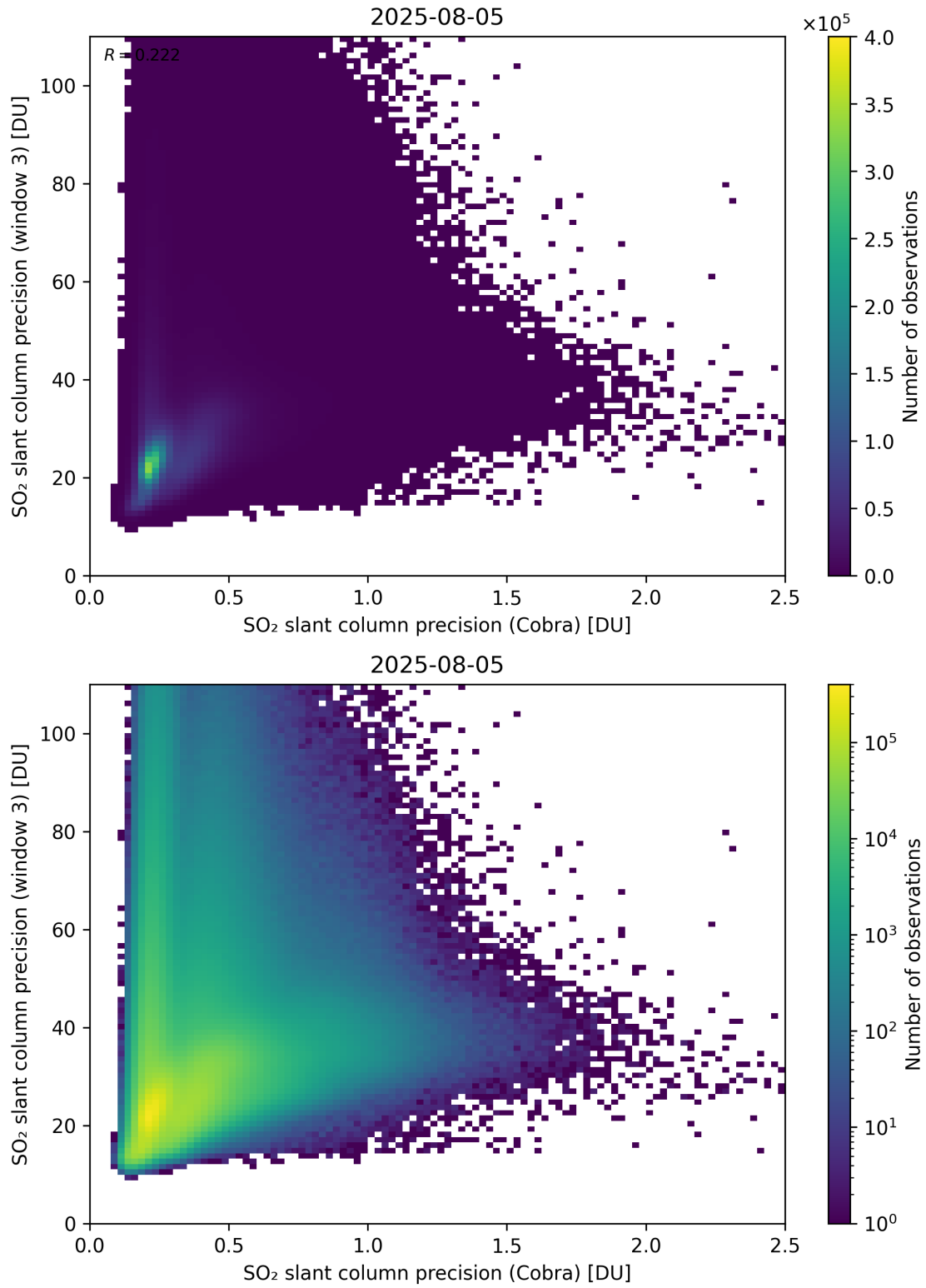
Figure 212: Scatter density plot of “SO 2 slant column precision (Cobra)” against “SO 2 slant column precision (window 3)” for 2025-08-04 to 2025-08-06.
