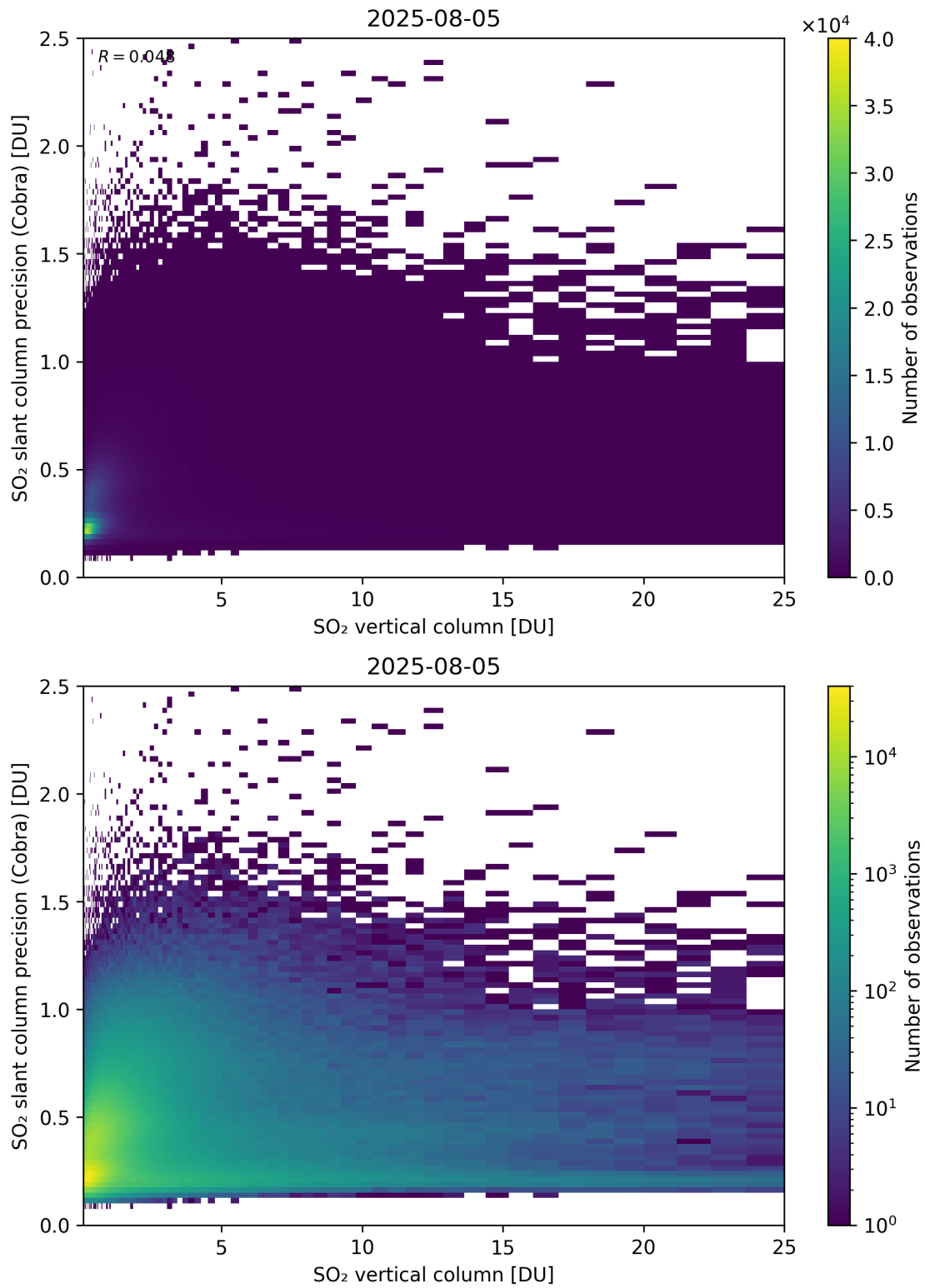
Figure 350: Scatter density plot of “SO 2 vertical column” against “SO 2 slant column precision (Cobra)” for 2025-08-04 to 2025-08-06.
