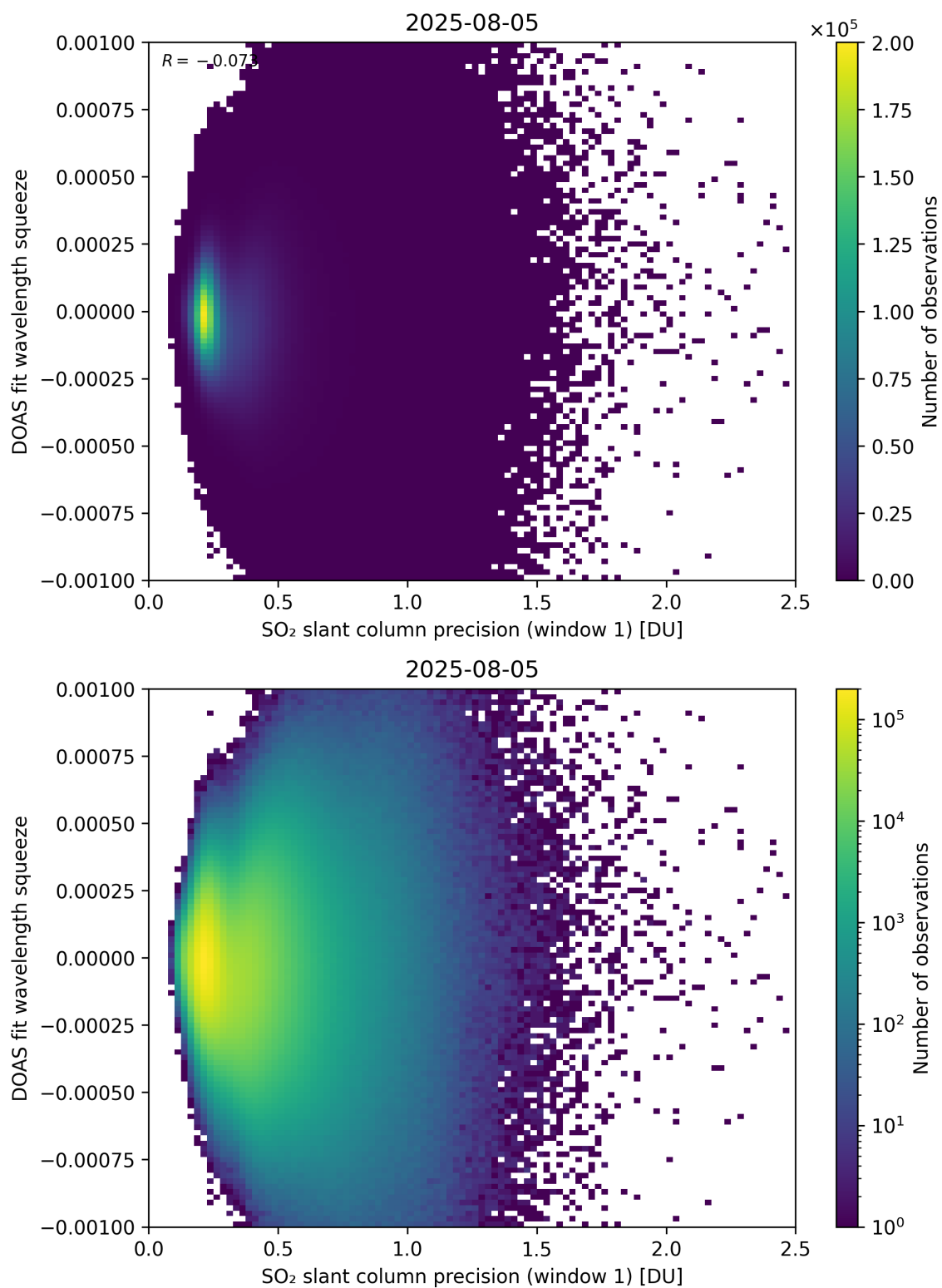
Figure 272: Scatter density plot of “SO 2 slant column precision (window 1)” against “DOAS fit wavelength squeeze” for 2025-08-04 to 2025-08-06.
