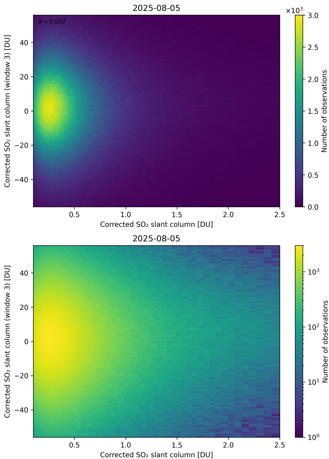
Figure 236: Scatter density plot of “Corrected SO 2 slant column” against “Corrected SO 2 slant column (window 3)” for 2025-08-04 to 2025-08-06.
