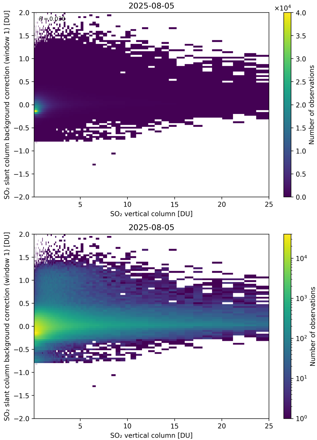
Figure 323: Scatter density plot of “SO 2 vertical column” against “SO 2 slant column background correction (window 1)” for 2025-08-04 to 2025-08-06.
