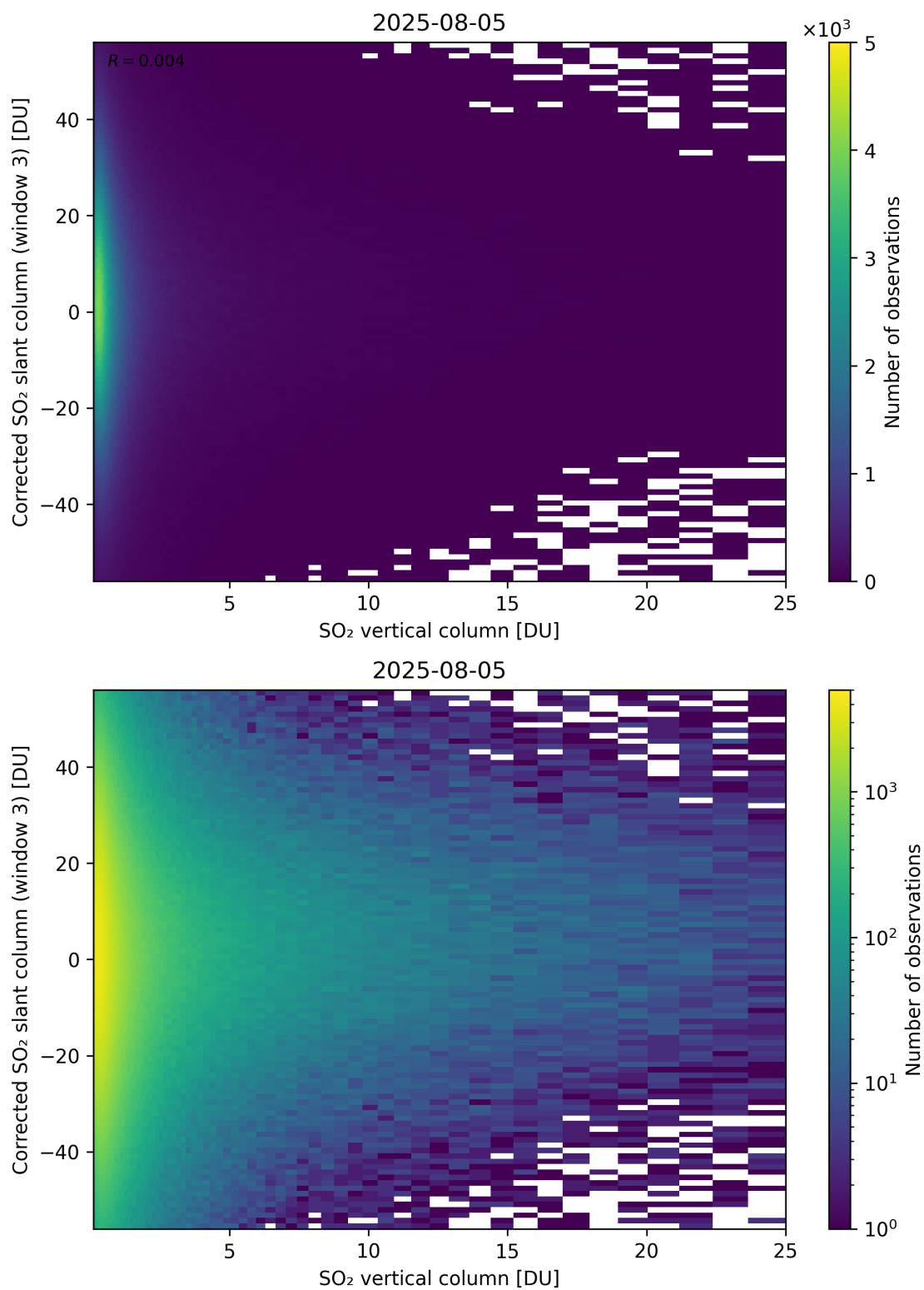
Figure 353: Scatter density plot of “SO 2 vertical column” against “Corrected SO 2 slant column (window 3)” for 2025-08-04 to 2025-08-06.
