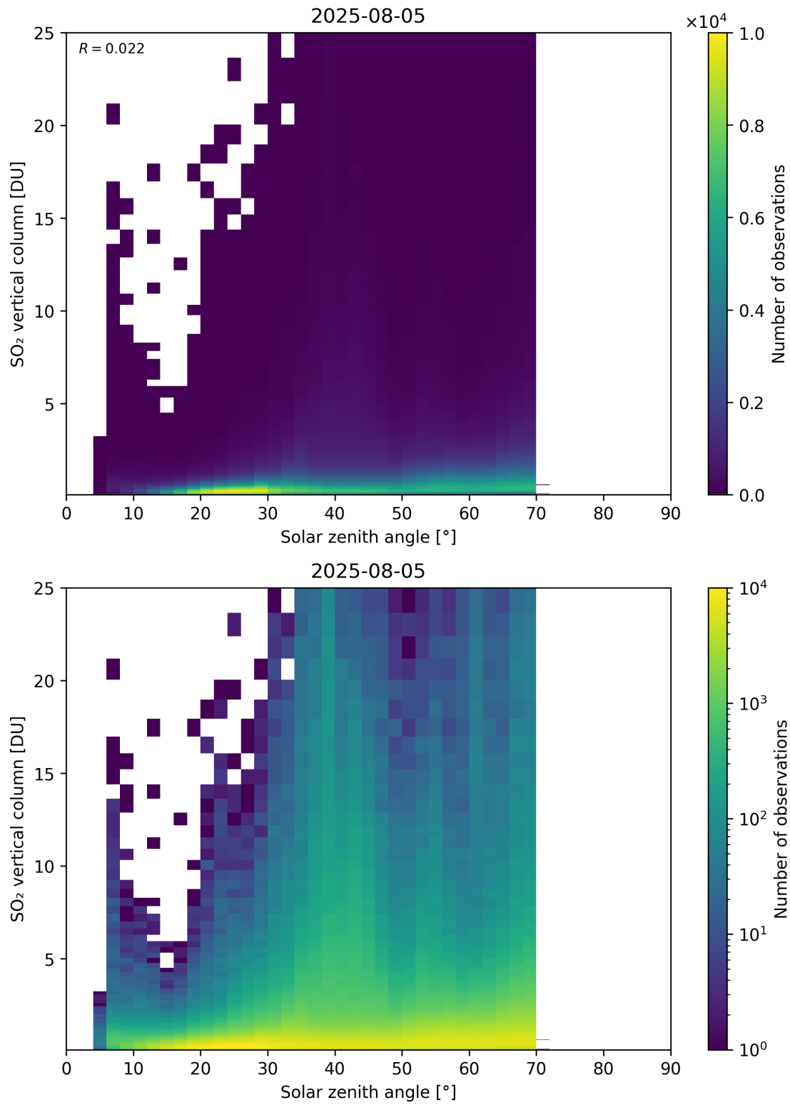
Figure 191: Scatter density plot of “Solar zenith angle” against “SO 2 vertical column” for 2025-08-04 to 2025-08-06.
