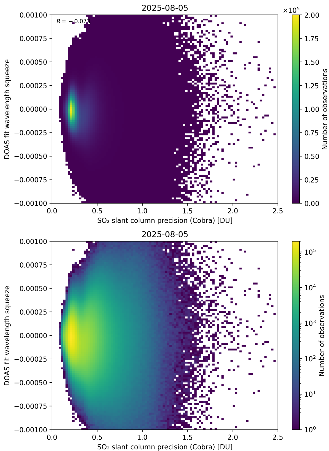
Figure 203: Scatter density plot of “SO 2 slant column precision (Cobra)” against “DOAS fit wavelength squeeze” for 2025-08-04 to 2025-08-06.
