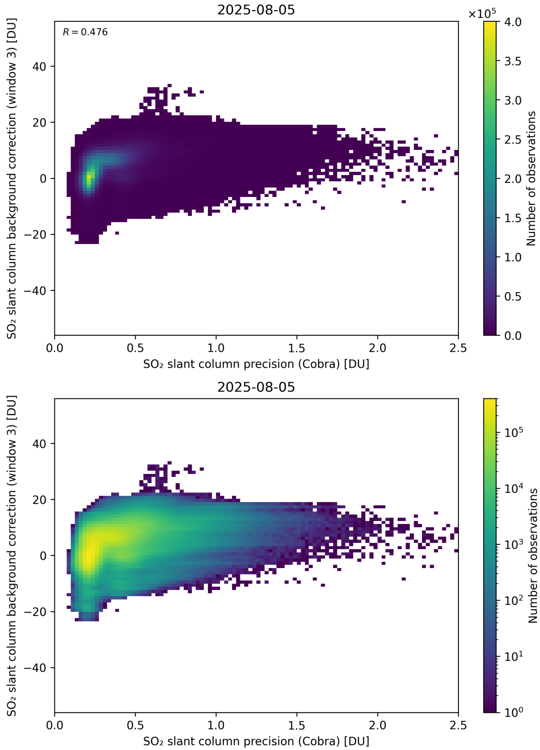
Figure 201: Scatter density plot of “SO 2 slant column precision (Cobra)” against “SO 2 slant column background correction (window 3)” for 2025-08-04 to 2025-08-06.
