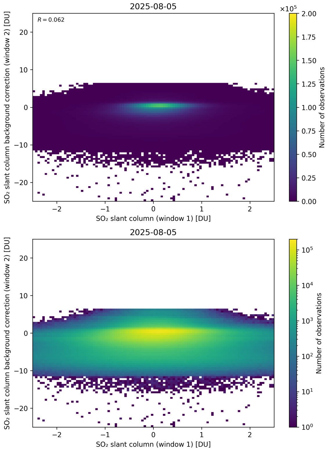
Figure 263: Scatter density plot of “SO 2 slant column (window 1)” against “SO 2 slant column background correction (window 2)” for 2025-08-04 to 2025-08-06.
