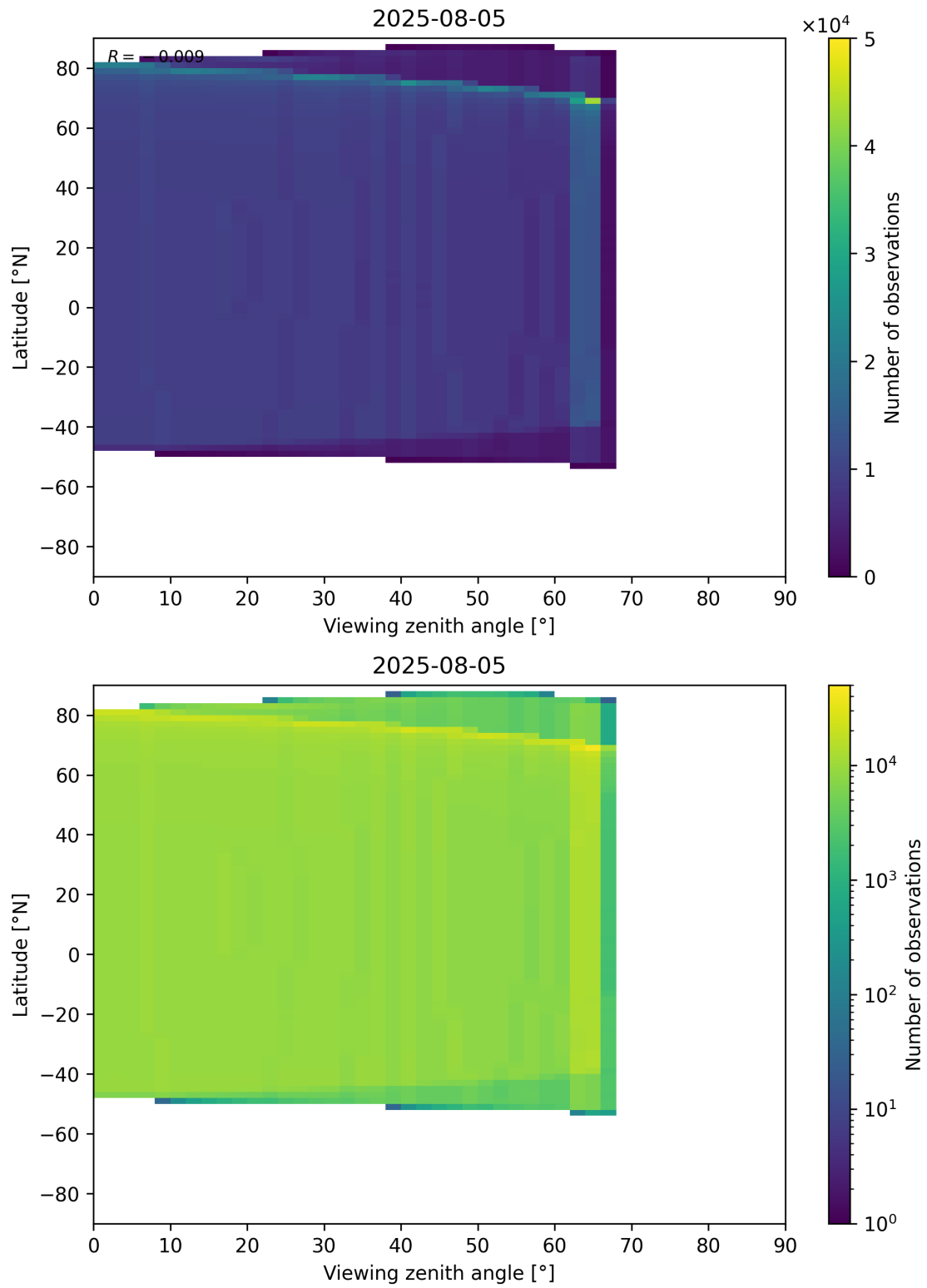
Figure 368: Scatter density plot of “Viewing zenith angle” against “Latitude” for 2025-08-04 to 2025-08-06.
