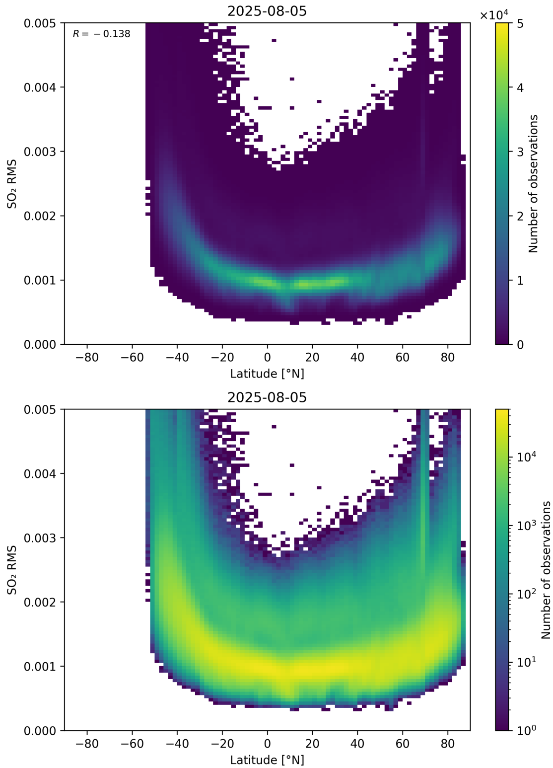
Figure 155: Scatter density plot of “Latitude” against “SO 2 RMS” for 2025-08-04 to 2025-08-06.
