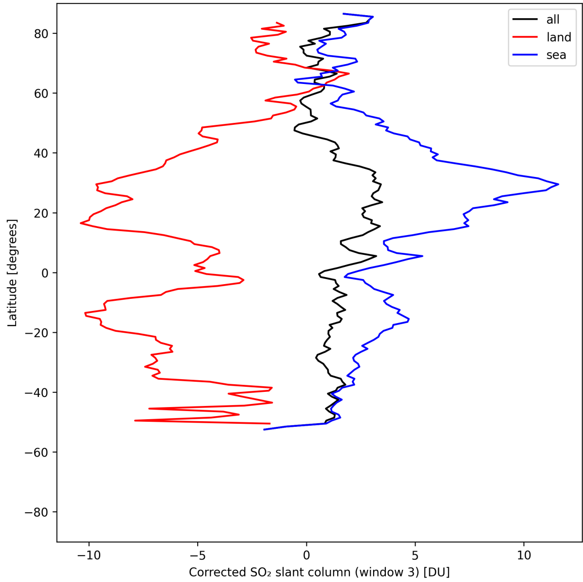
Figure 47: Zonal average of “Corrected SO 2 slant column (window 3)” for 2025-08-04 to 2025-08-06.
