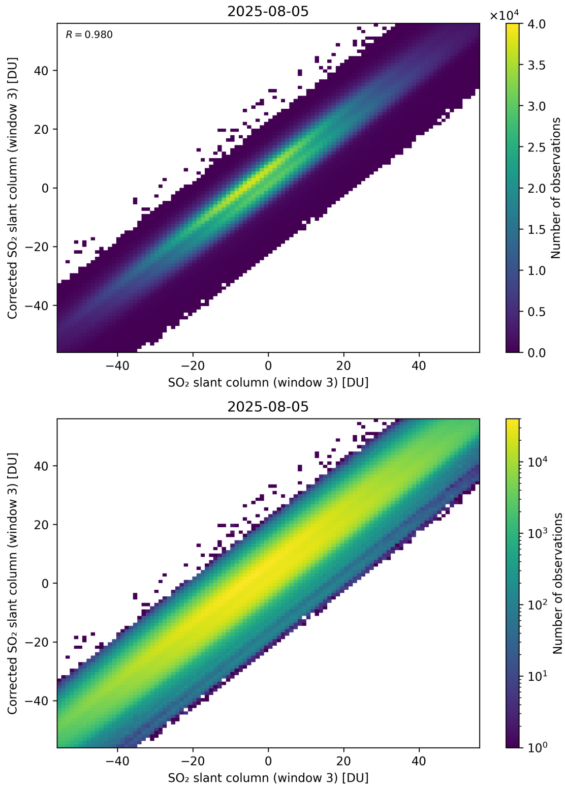
Figure 316: Scatter density plot of “SO 2 slant column (window 3)” against “Corrected SO 2 slant column (window 3)” for 2025-08-04 to 2025-08-06.
