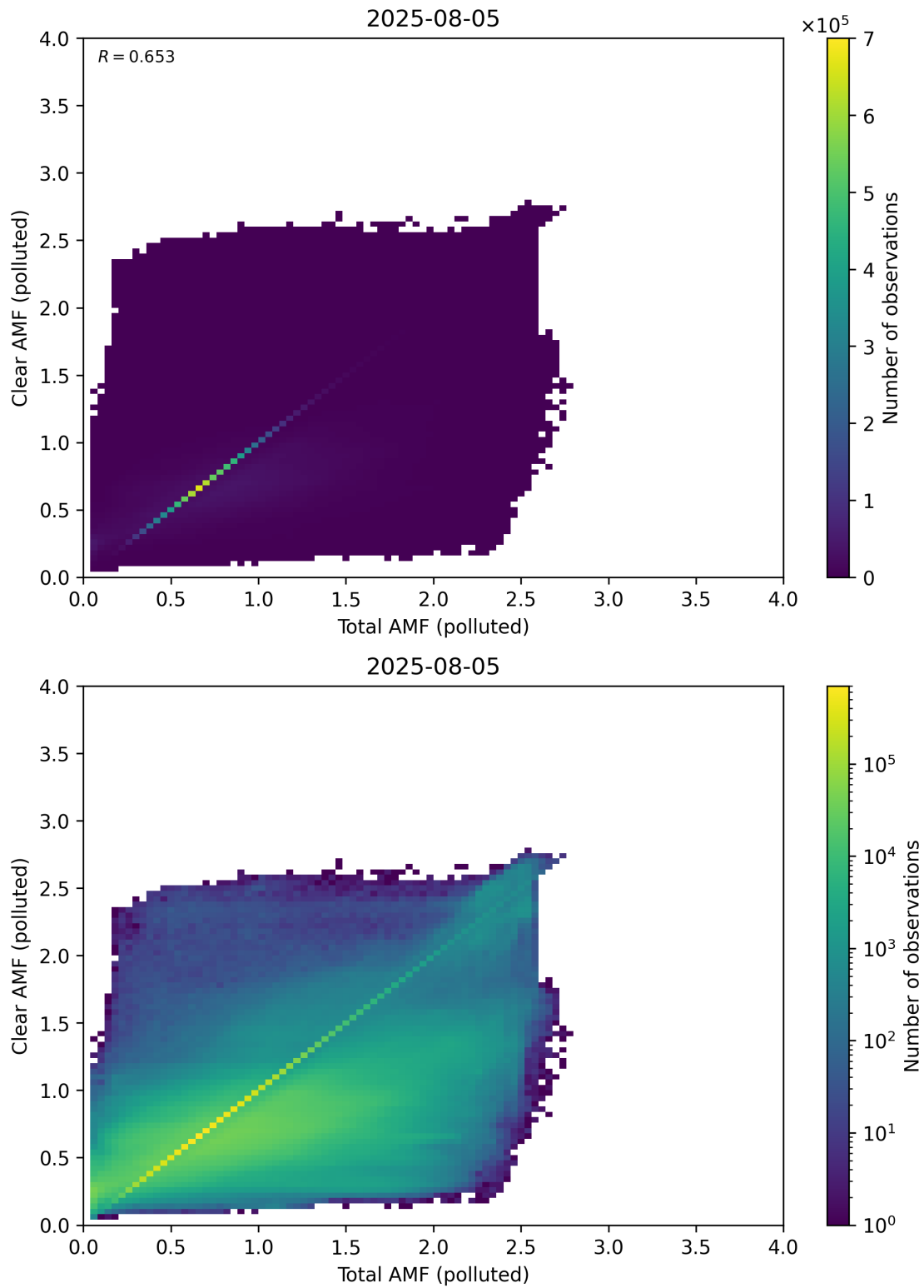
Figure 321: Scatter density plot of “Total AMF (polluted)” against “Clear AMF (polluted)” for 2025-08-04 to 2025-08-06.
