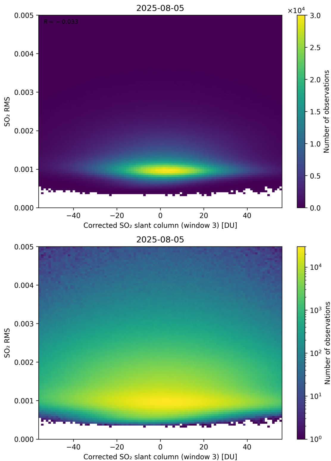
Figure 258: Scatter density plot of “Corrected SO 2 slant column (window 3)” against “SO 2 RMS” for 2025-08-04 to 2025-08-06.
