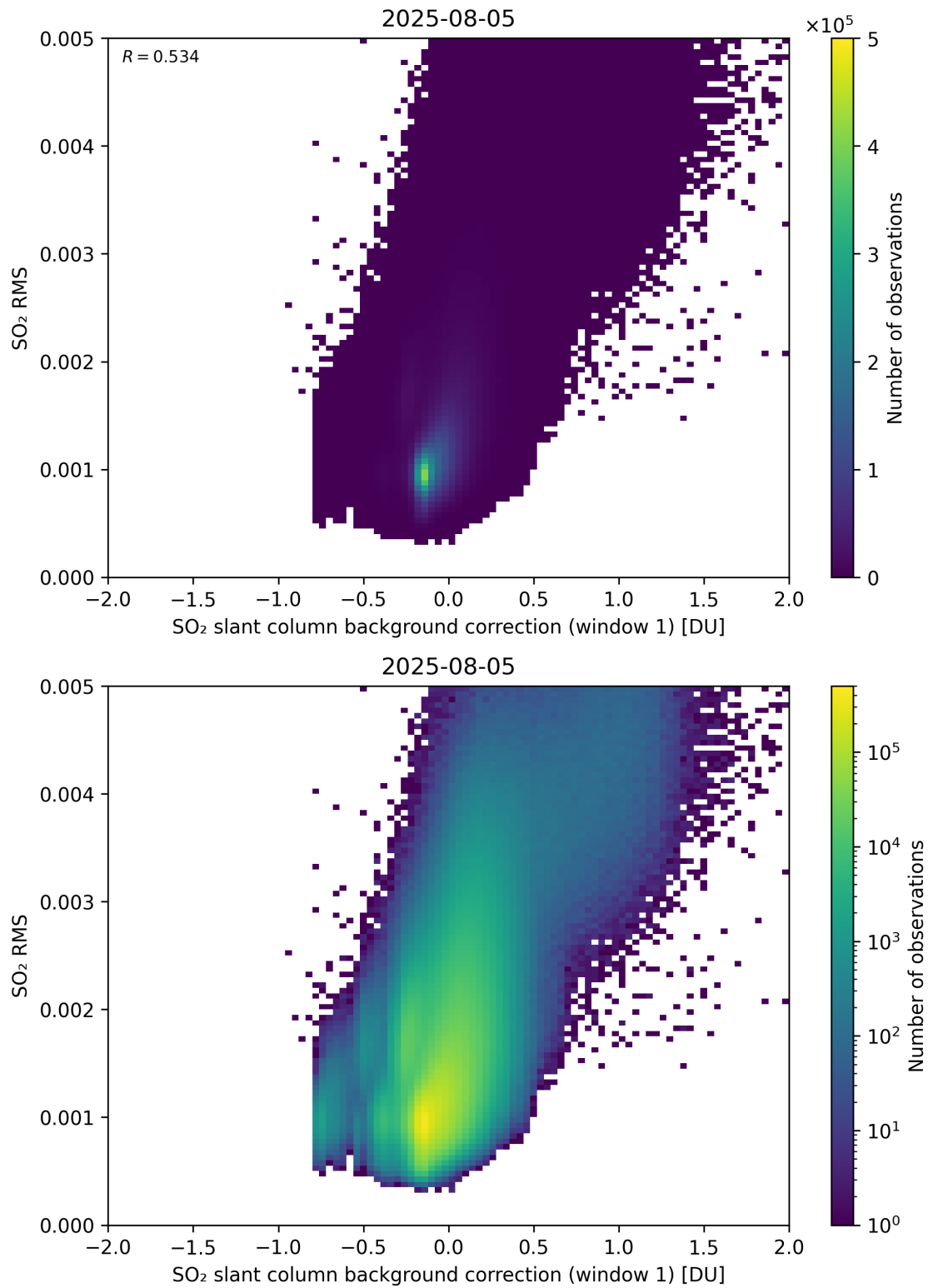
Figure 113: Scatter density plot of “SO 2 slant column background correction (window 1)” against “SO 2 RMS” for 2025-08-04 to 2025-08-06.
