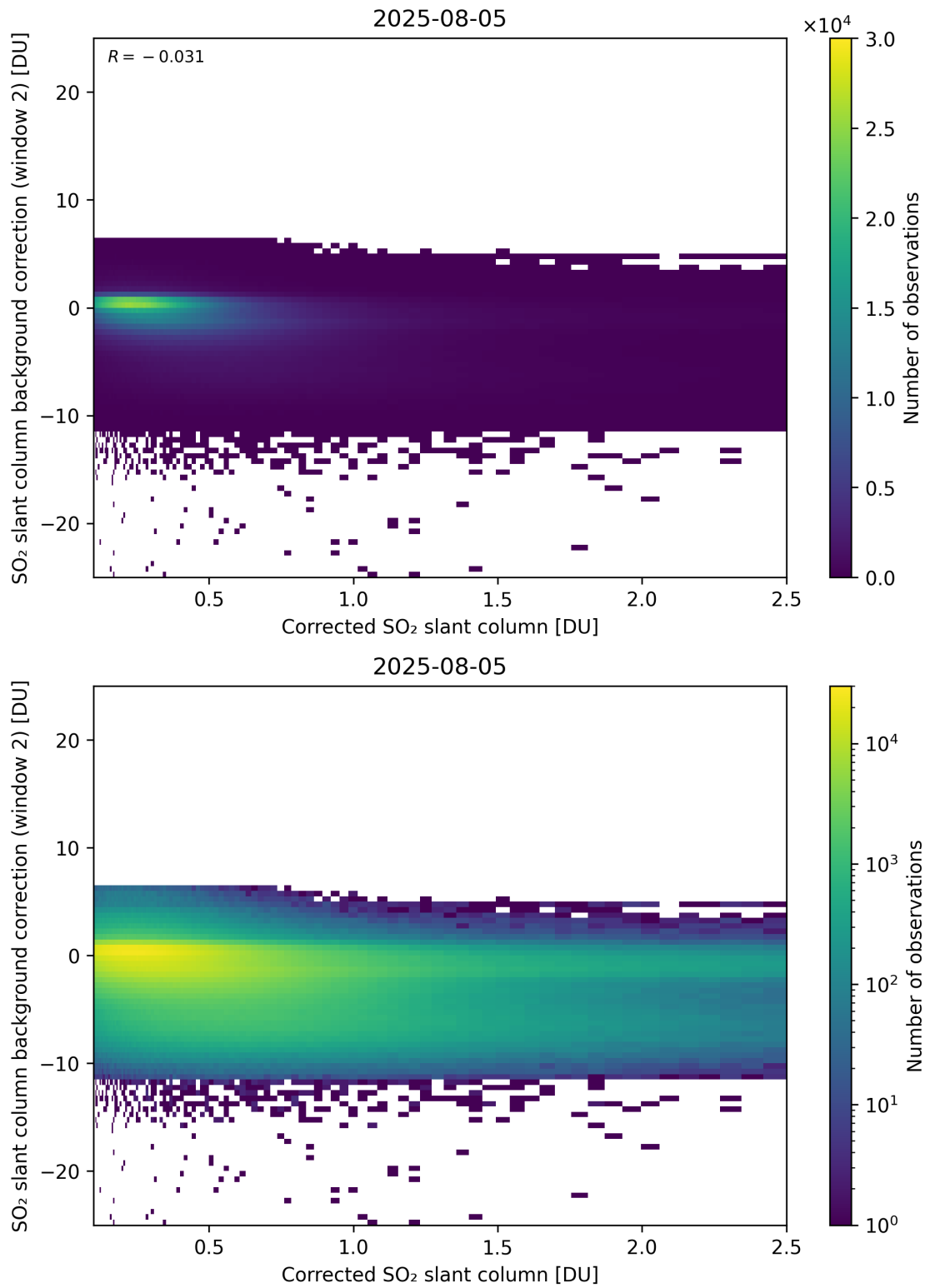
Figure 227: Scatter density plot of “Corrected SO 2 slant column” against “SO 2 slant column background correction (window 2)” for 2025-08-04 to 2025-08-06.
