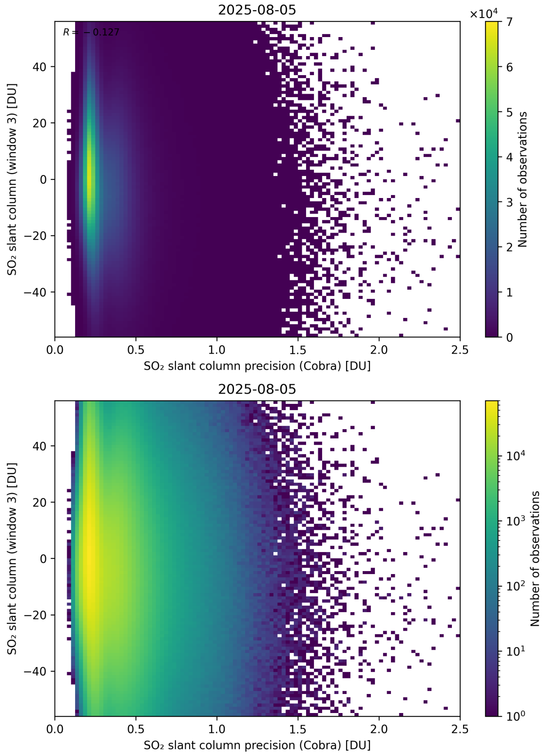
Figure 211: Scatter density plot of “SO 2 slant column precision (Cobra)” against “SO 2 slant column (window 3)” for 2025-08-04 to 2025-08-06.
