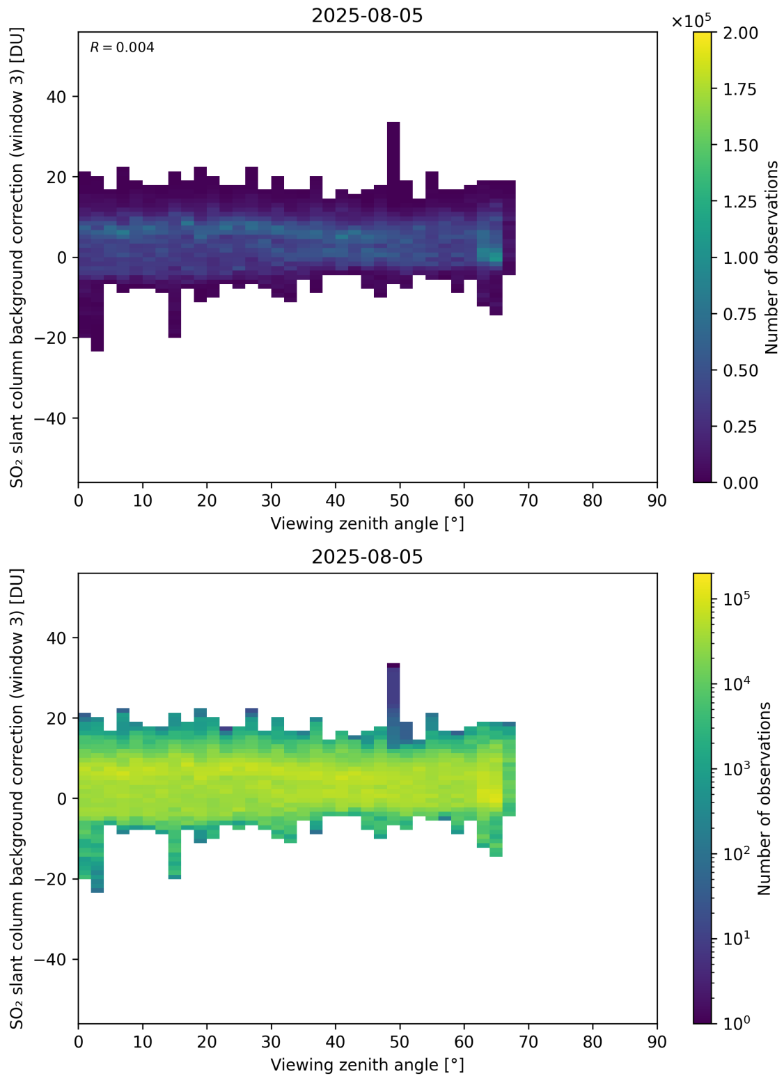
Figure 364: Scatter density plot of “Viewing zenith angle” against “SO 2 slant column background correction (window 3)” for 2025-08-04 to 2025-08-06.
