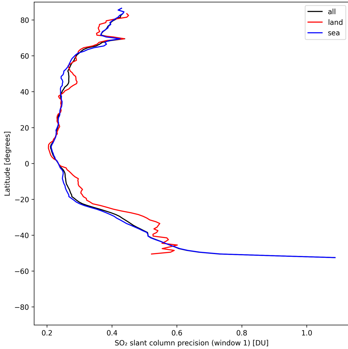
Figure 38: Zonal average of “SO 2 slant column precision (window 1)” for 2025-08-04 to 2025-08-06.
