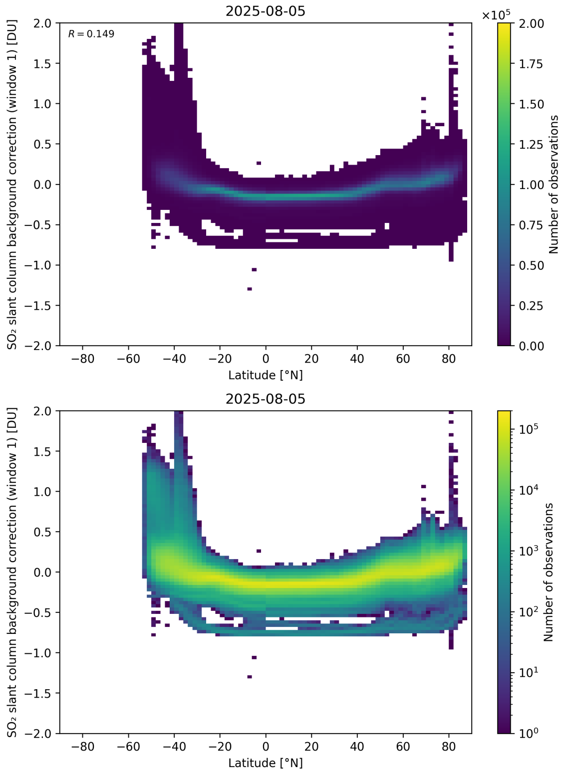
Figure 150: Scatter density plot of “Latitude” against “SO 2 slant column background correction (window 1)” for 2025-08-04 to 2025-08-06.
