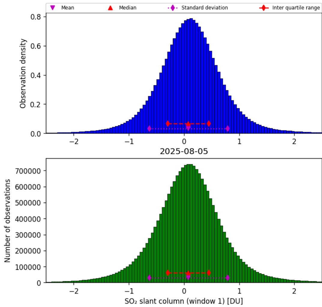
Figure 63: Histogram of “SO 2 slant column (window 1)” for 2025-08-04 to 2025-08-06
