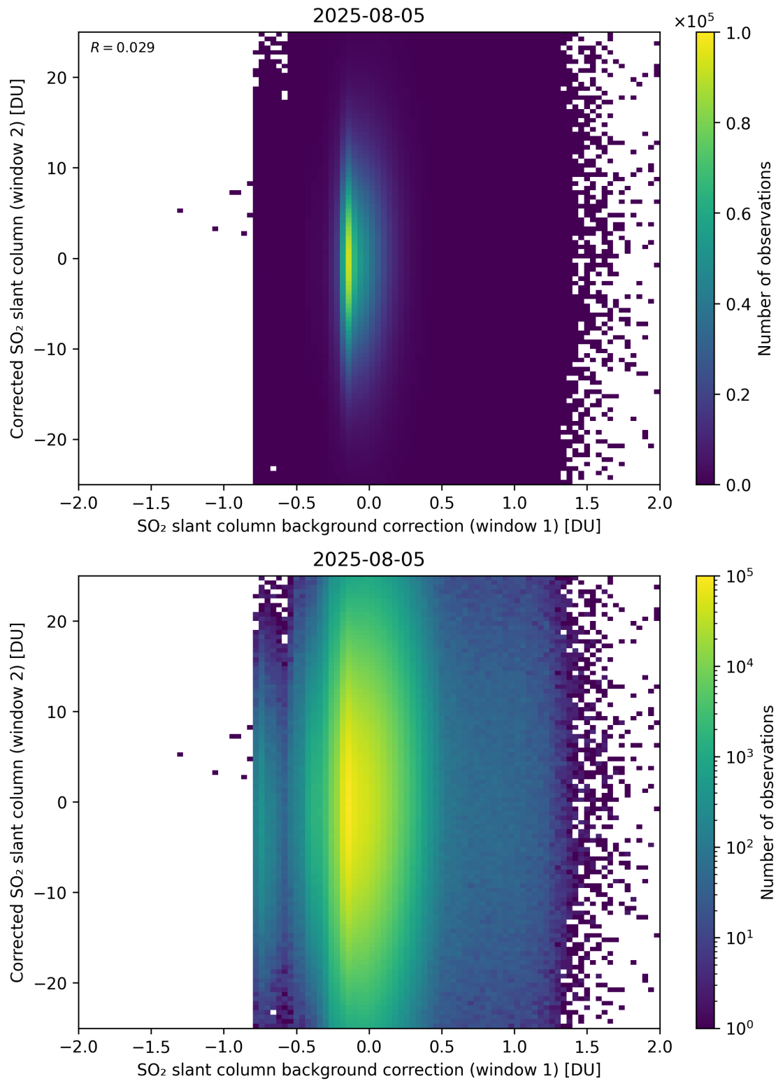
Figure 115: Scatter density plot of “SO 2 slant column background correction (window 1)” against “Corrected SO 2 slant column (window 2)” for 2025-08-04 to 2025-08-06.
