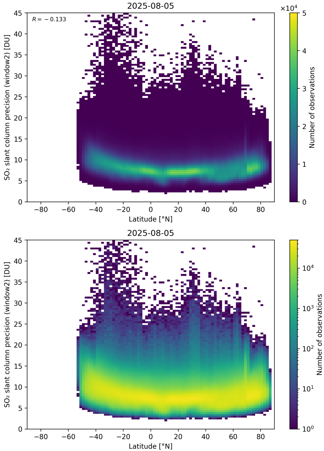
Figure 164: Scatter density plot of “Latitude” against “SO 2 slant column precision (window2)” for 2025-08-04 to 2025-08-06.
