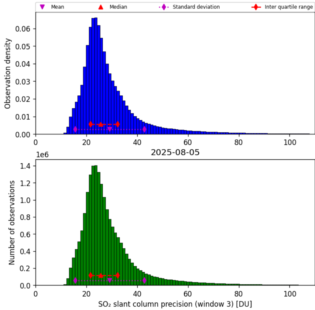
Figure 72: Histogram of “SO 2 slant column precision (window 3)” for 2025-08-04 to 2025-08-06
