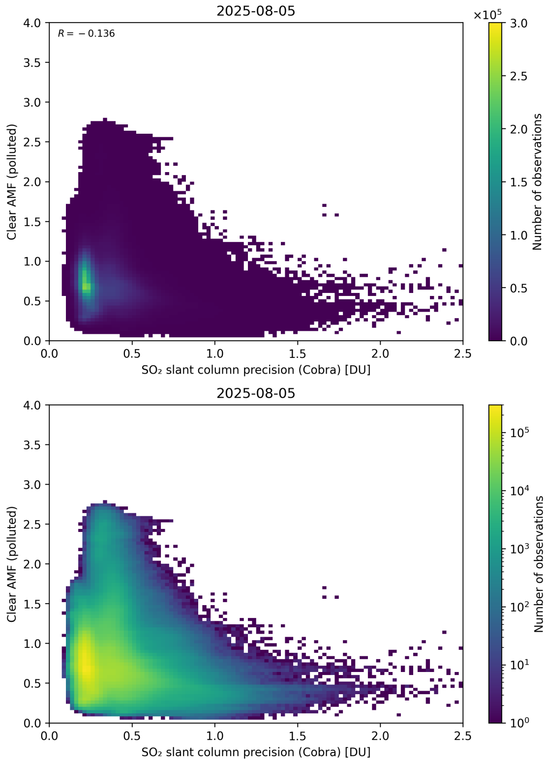
Figure 205: Scatter density plot of “SO 2 slant column precision (Cobra)” against “Clear AMF (polluted)” for 2025-08-04 to 2025-08-06.
