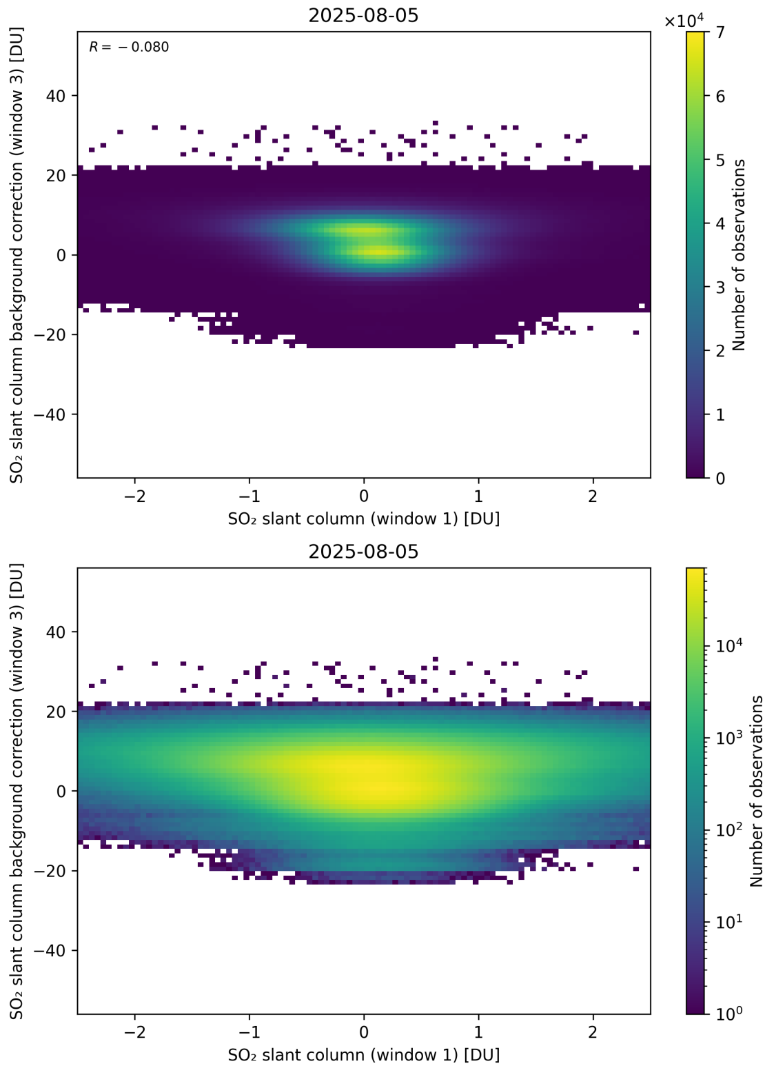
Figure 264: Scatter density plot of “SO 2 slant column (window 1)” against “SO 2 slant column background correction (window 3)” for 2025-08-04 to 2025-08-06.
