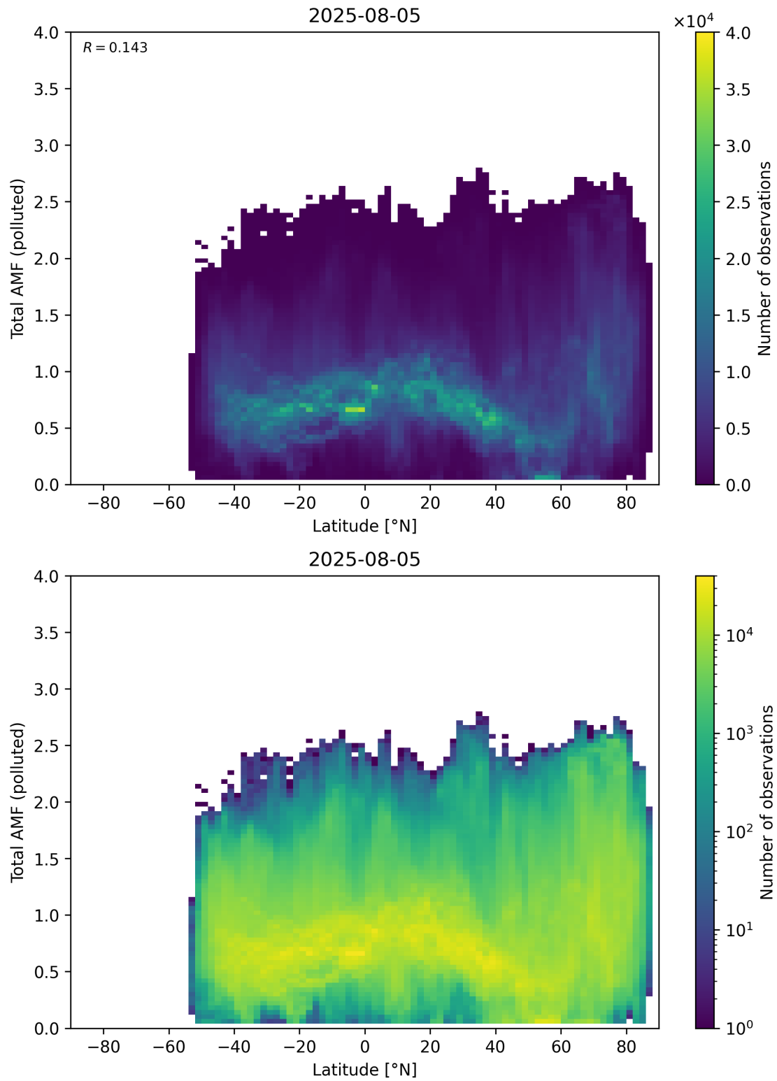
Figure 167: Scatter density plot of “Latitude” against “Total AMF (polluted)” for 2025-08-04 to 2025-08-06.
