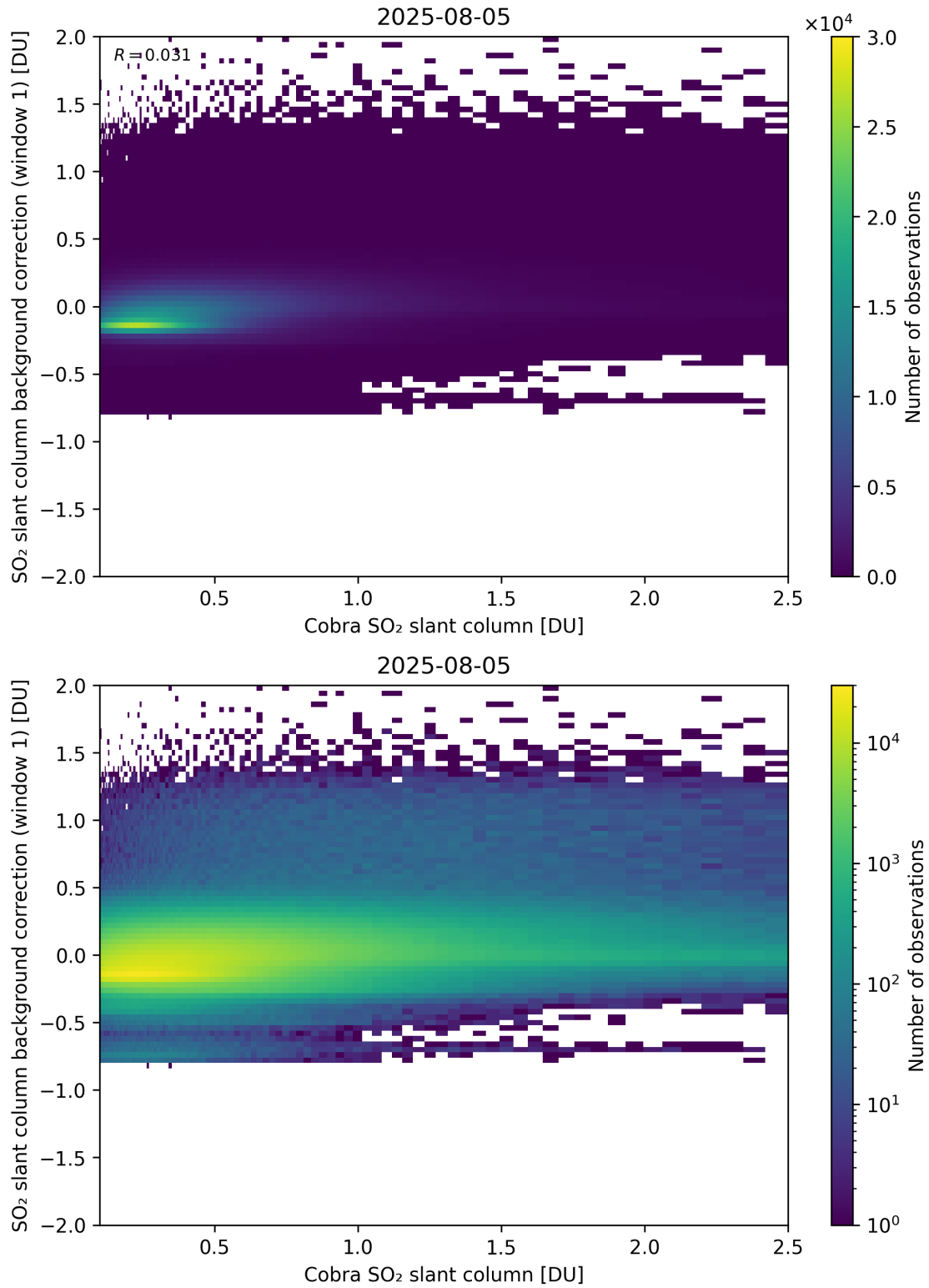
Figure 193: Scatter density plot of “Cobra SO 2 slant column” against “SO 2 slant column background correction (window 1)” for 2025-08-04 to 2025-08-06.
