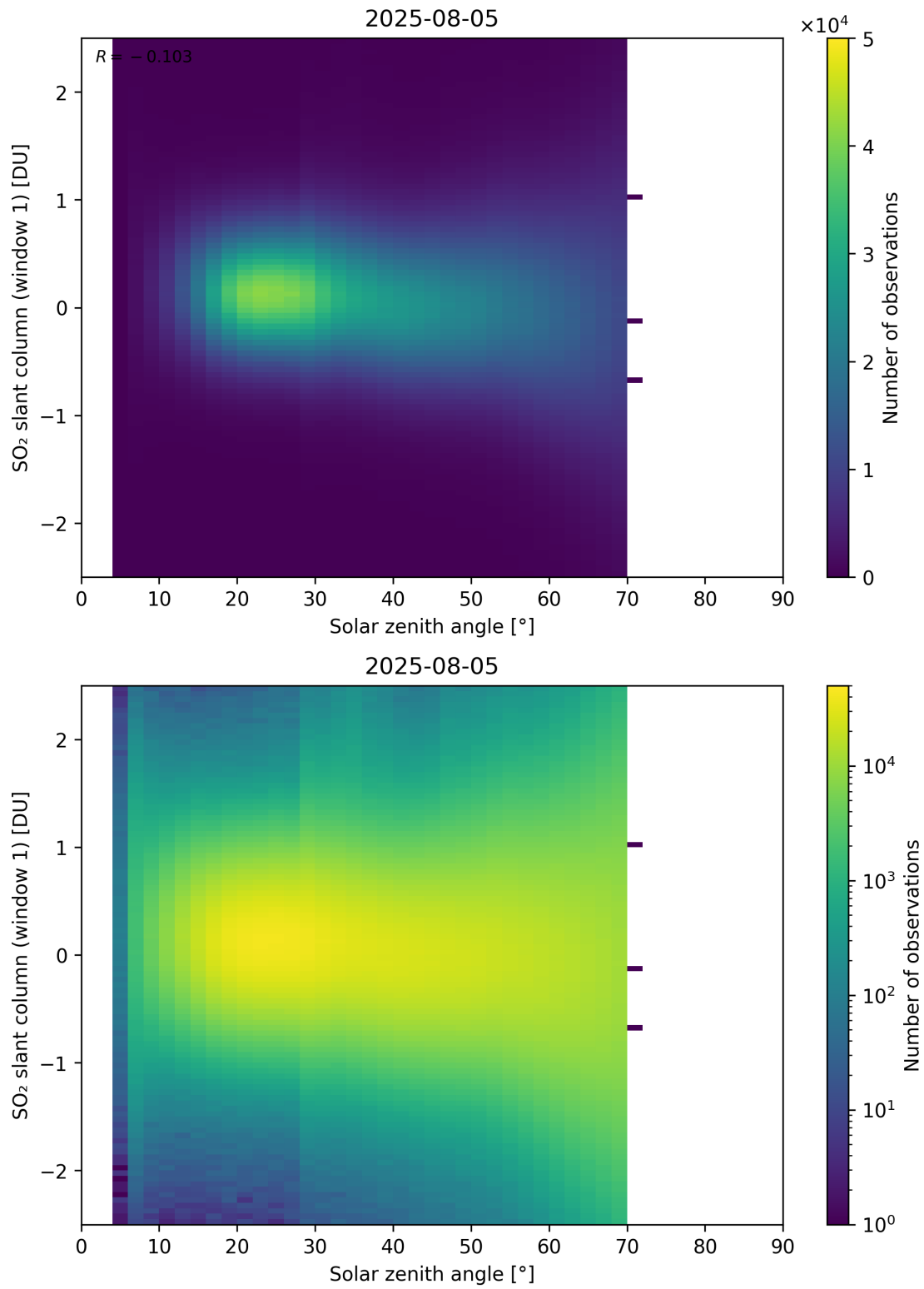
Figure 184: Scatter density plot of “Solar zenith angle” against “SO 2 slant column (window 1)” for 2025-08-04 to 2025-08-06.
