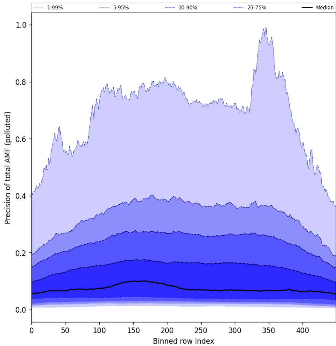
Figure 106: Along track statistics of “Precision of total AMF (polluted)” for 2025-08-04 to 2025-08-06
