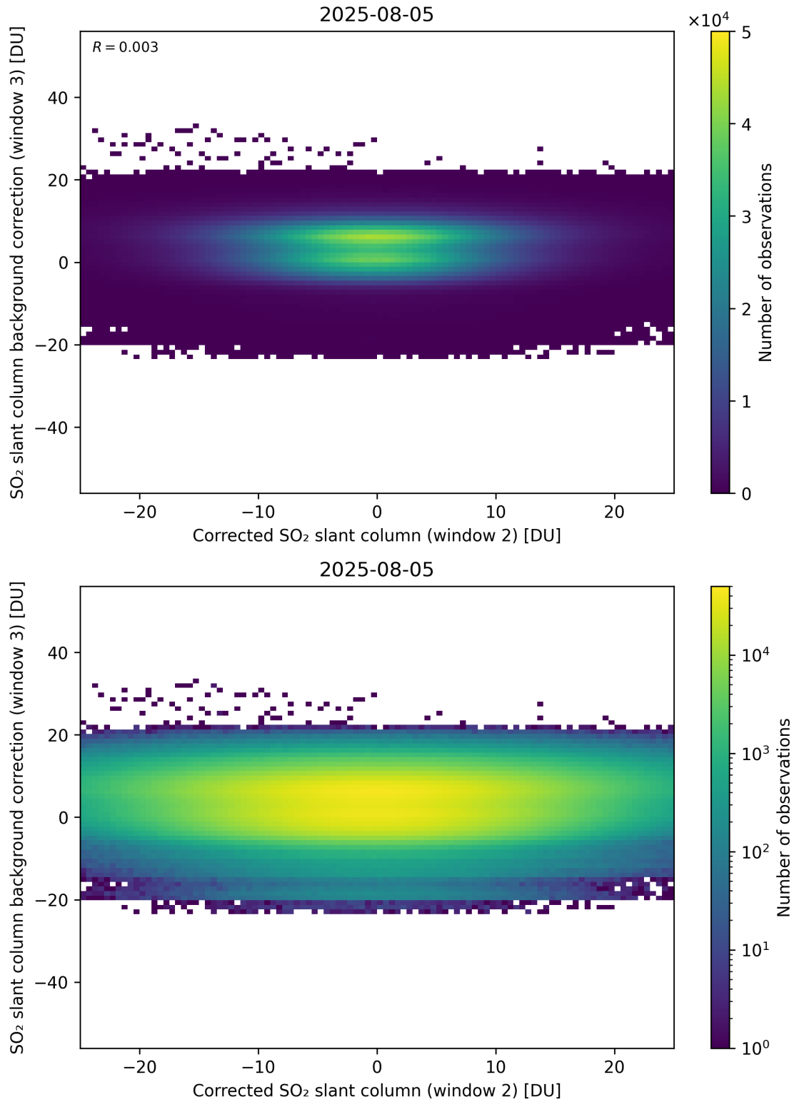
Figure 245: Scatter density plot of “Corrected SO 2 slant column (window 2)” against “SO 2 slant column background correction (window 3)” for 2025-08-04 to 2025-08-06.
