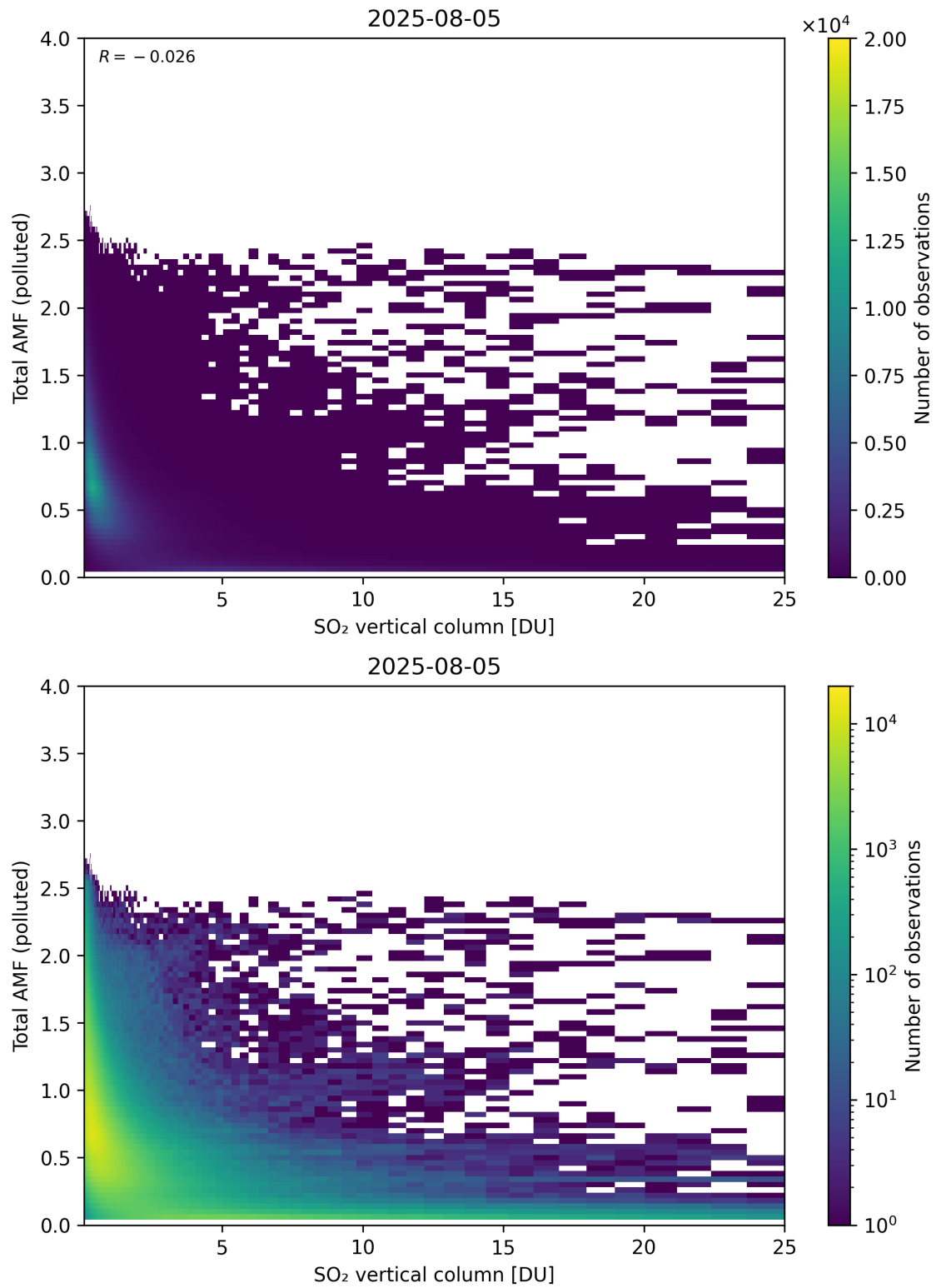
Figure 359: Scatter density plot of “SO 2 vertical column” against “Total AMF (polluted)” for 2025-08-04 to 2025-08-06.
