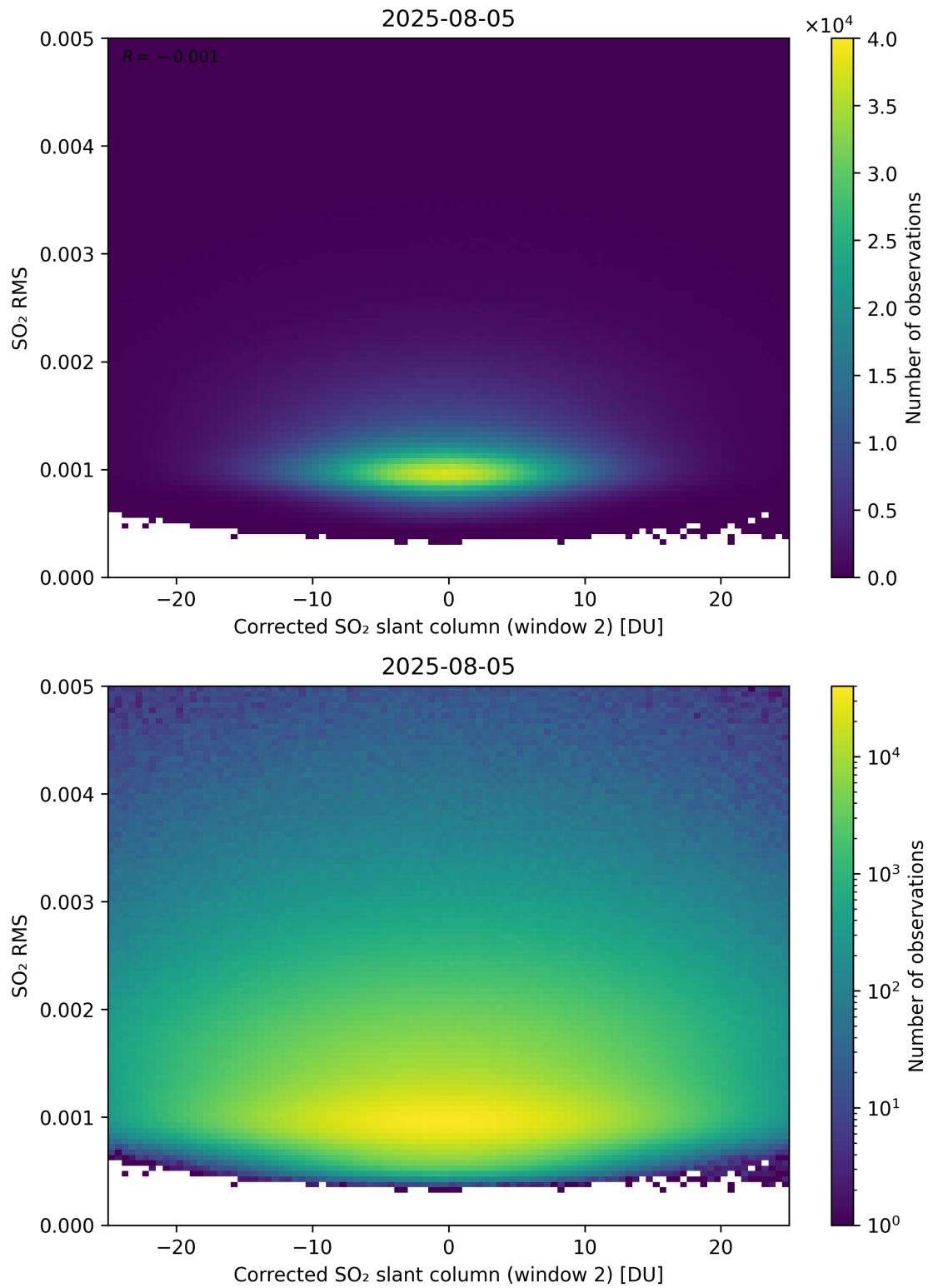
Figure 248: Scatter density plot of “Corrected SO 2 slant column (window 2)” against “SO 2 RMS” for 2025-08-04 to 2025-08-06.
