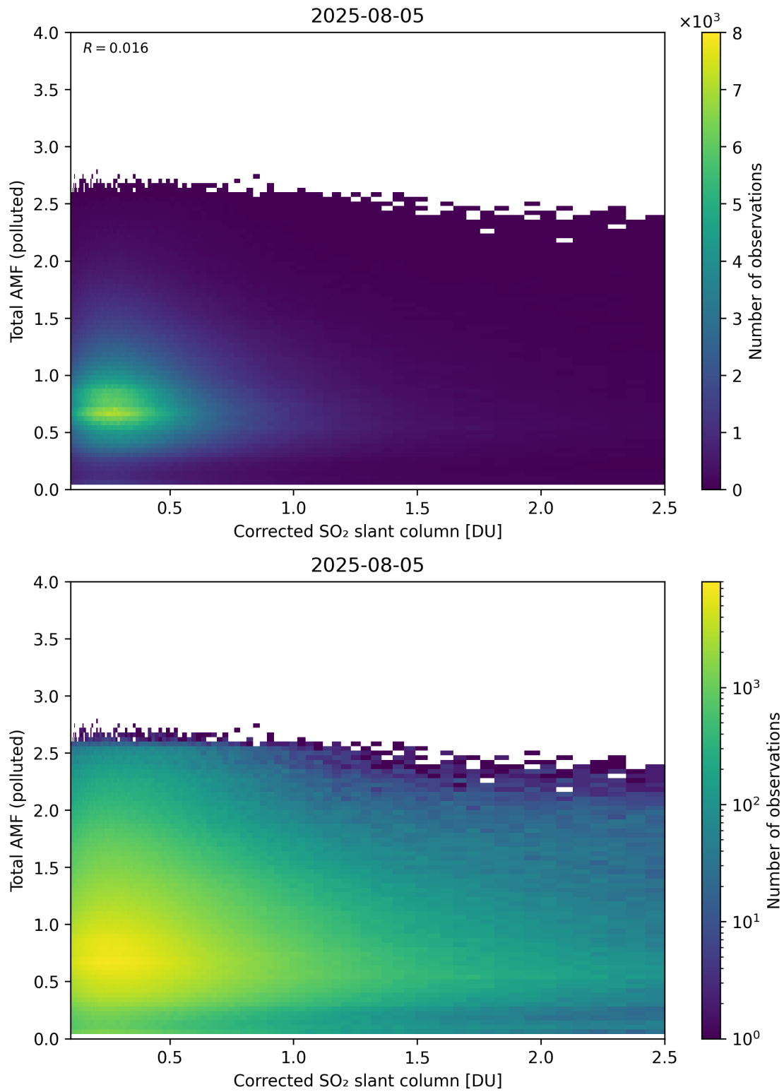
Figure 242: Scatter density plot of “Corrected SO 2 slant column” against “Total AMF (polluted)” for 2025-08-04 to 2025-08-06.
