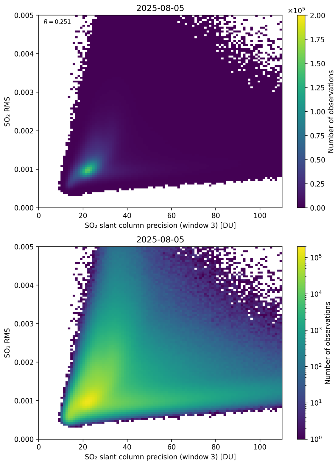
Figure 310: Scatter density plot of “SO 2 slant column precision (window 3)” against “SO 2 RMS” for 2025-08-04 to 2025-08-06.
