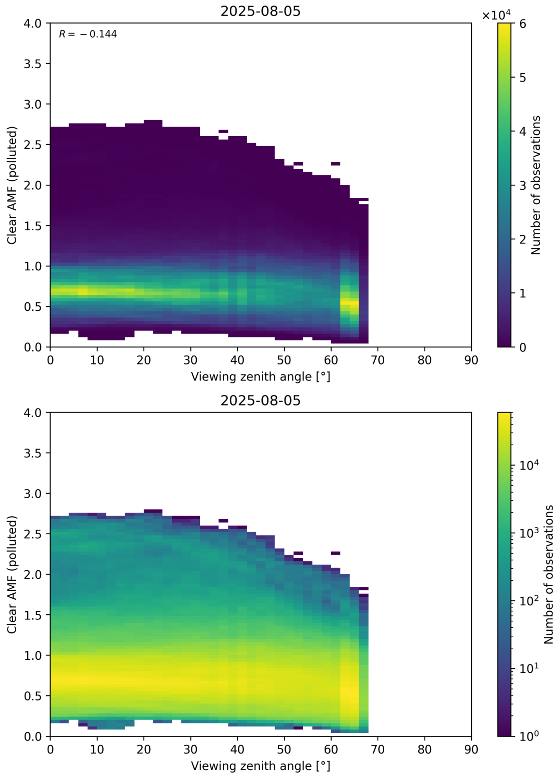
Figure 370: Scatter density plot of “Viewing zenith angle” against “Clear AMF (polluted)” for 2025-08-04 to 2025-08-06.
