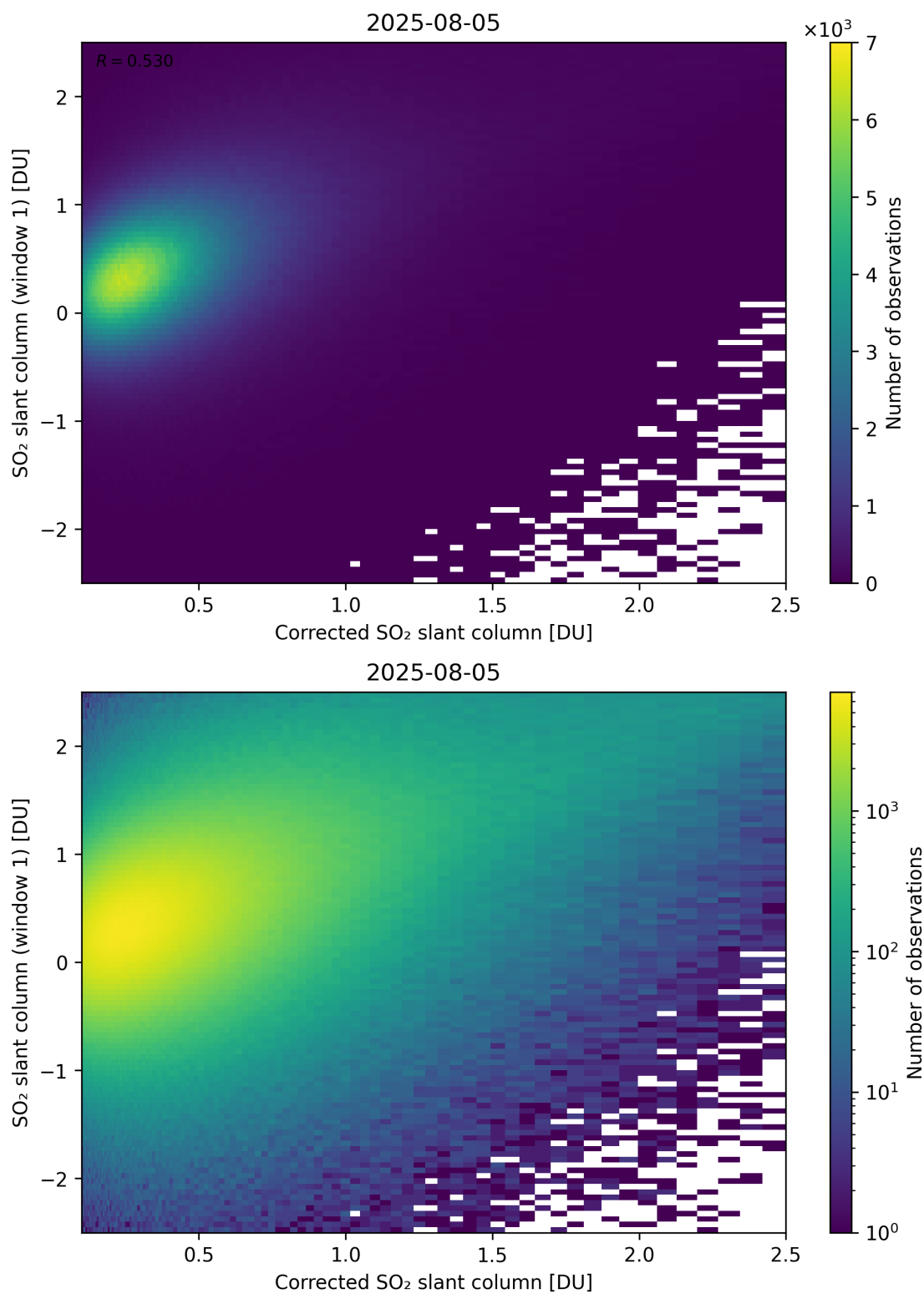
Figure 237: Scatter density plot of “Corrected SO 2 slant column” against “SO 2 slant column (window 1)” for 2025-08-04 to 2025-08-06.
