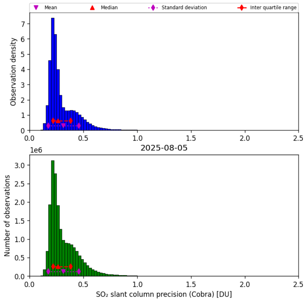
Figure 62: Histogram of “SO 2 slant column precision (Cobra)” for 2025-08-04 to 2025-08-06
