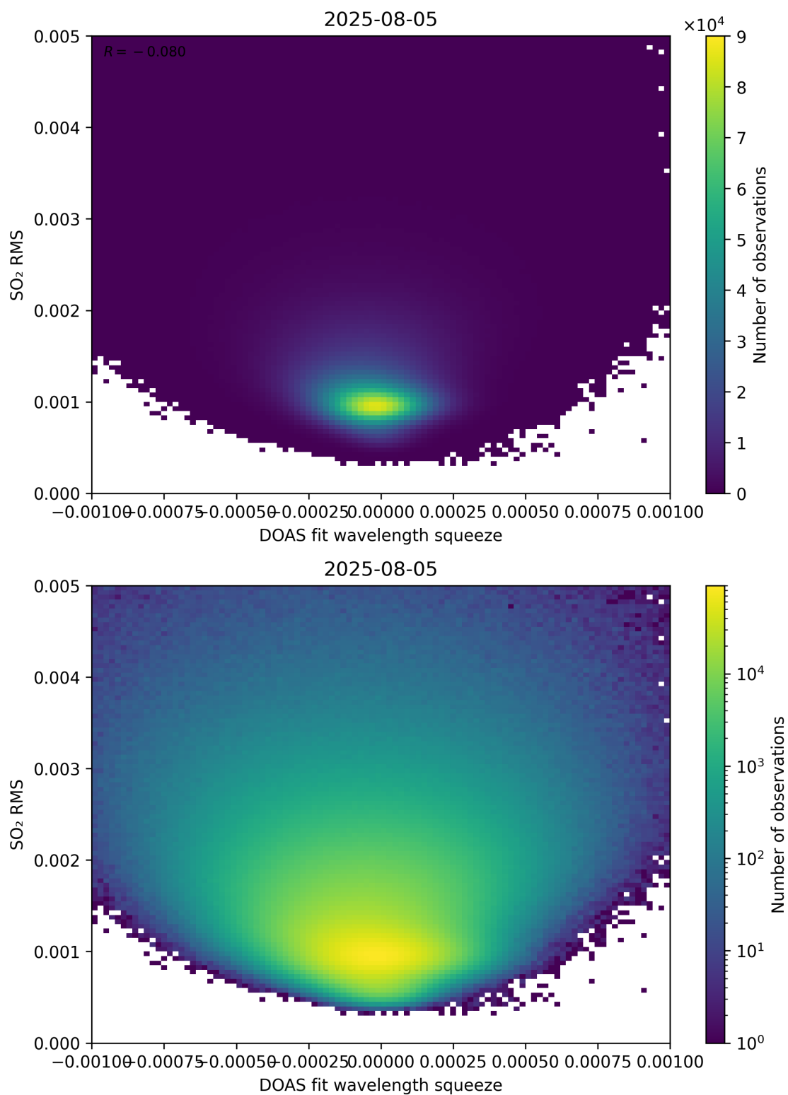
Figure 143: Scatter density plot of “DOAS fit wavelength squeeze” against “SO 2 RMS” for 2025-08-04 to 2025-08-06.
