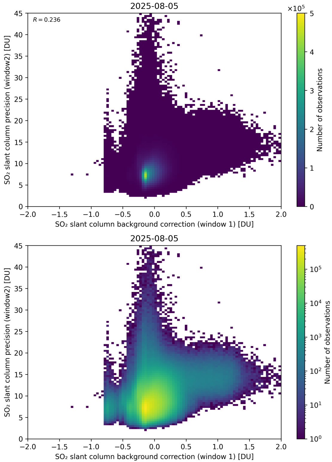
Figure 117: Scatter density plot of “SO 2 slant column background correction (window 1)” against “SO 2 slant column precision (window2)” for 2025-08-04 to 2025-08-06.
