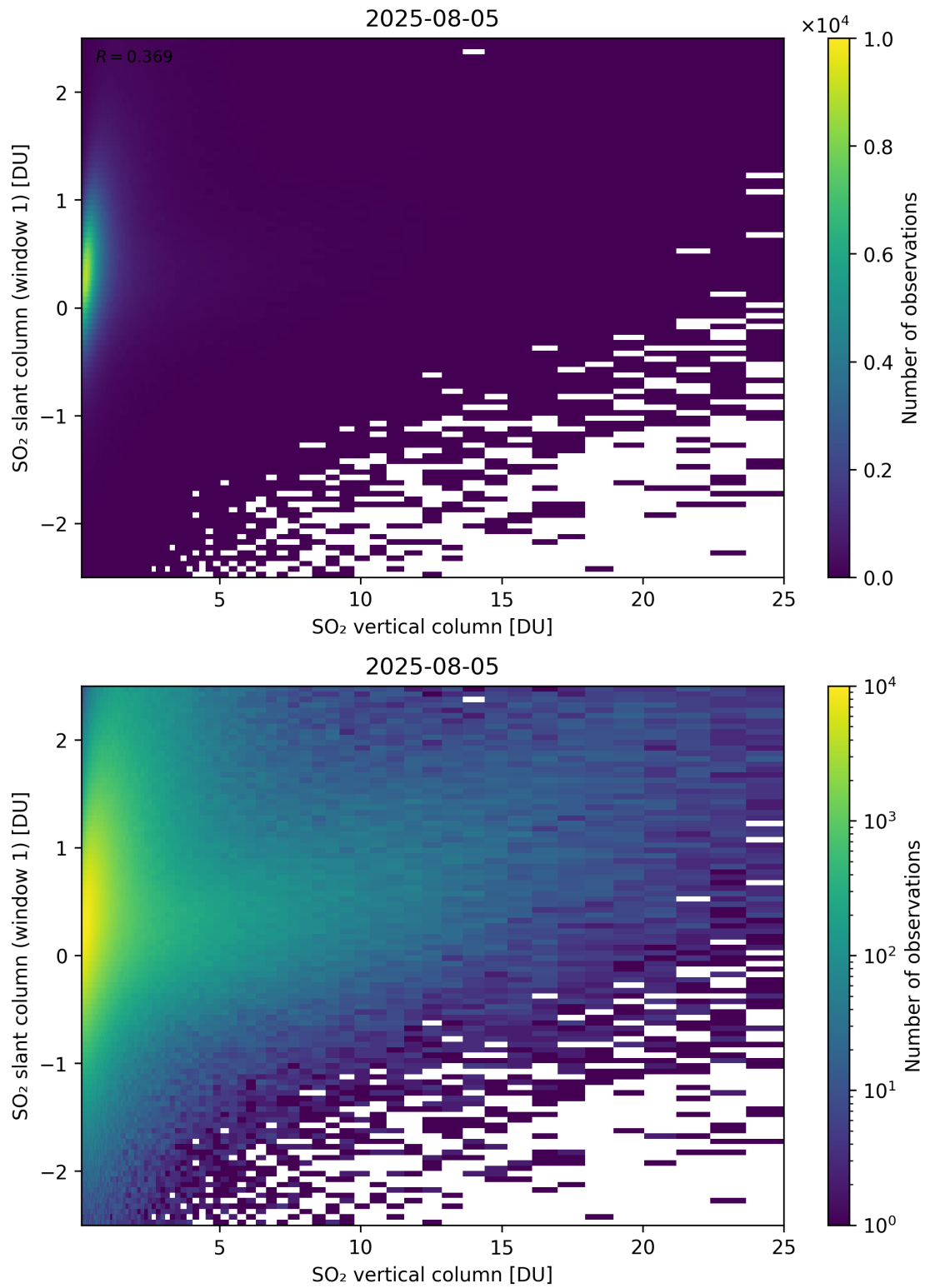
Figure 354: Scatter density plot of “SO 2 vertical column” against “SO 2 slant column (window 1)” for 2025-08-04 to 2025-08-06.
