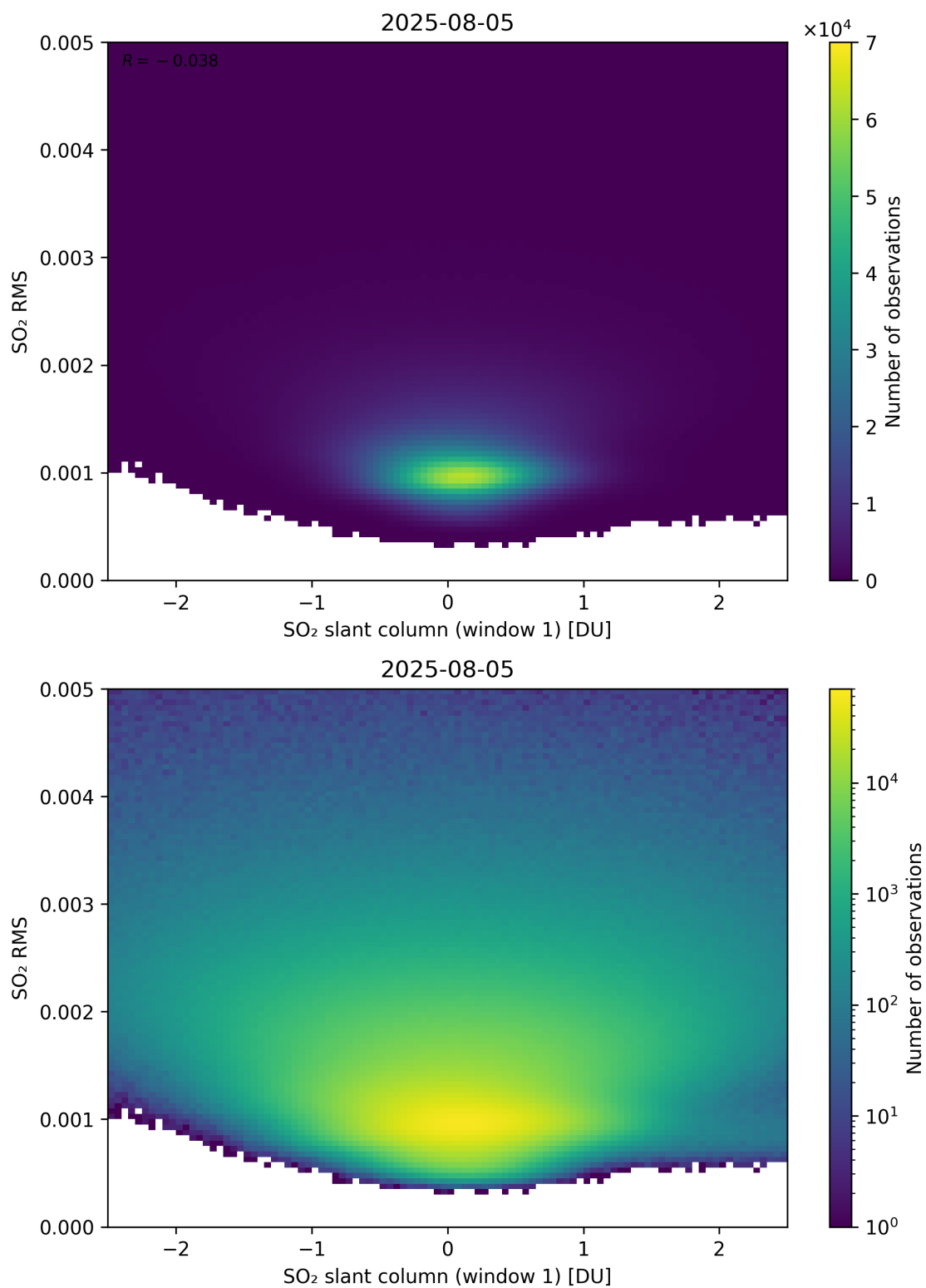
Figure 267: Scatter density plot of “SO 2 slant column (window 1)” against “SO 2 RMS” for 2025-08-04 to 2025-08-06.
