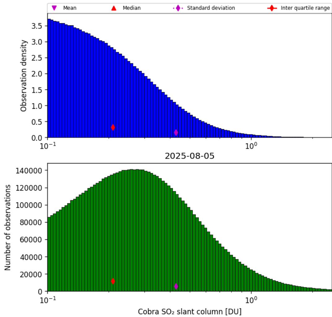
Figure 61: Histogram of “Cobra SO 2 slant column” for 2025-08-04 to 2025-08-06
