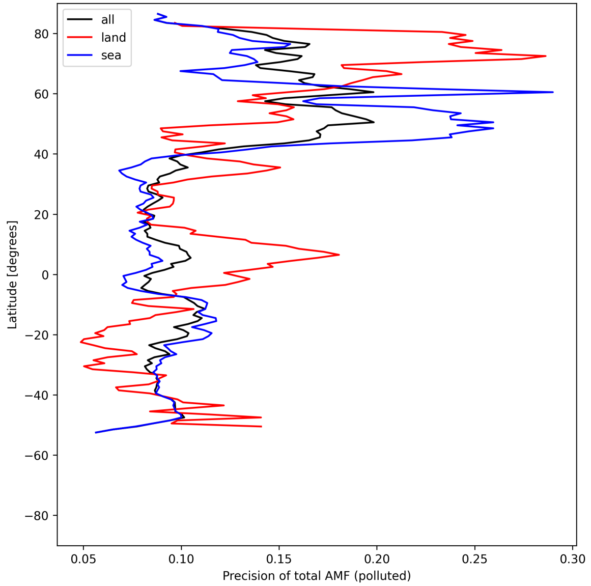
Figure 54: Zonal average of “Precision of total AMF (polluted)” for 2025-08-04 to 2025-08-06.
