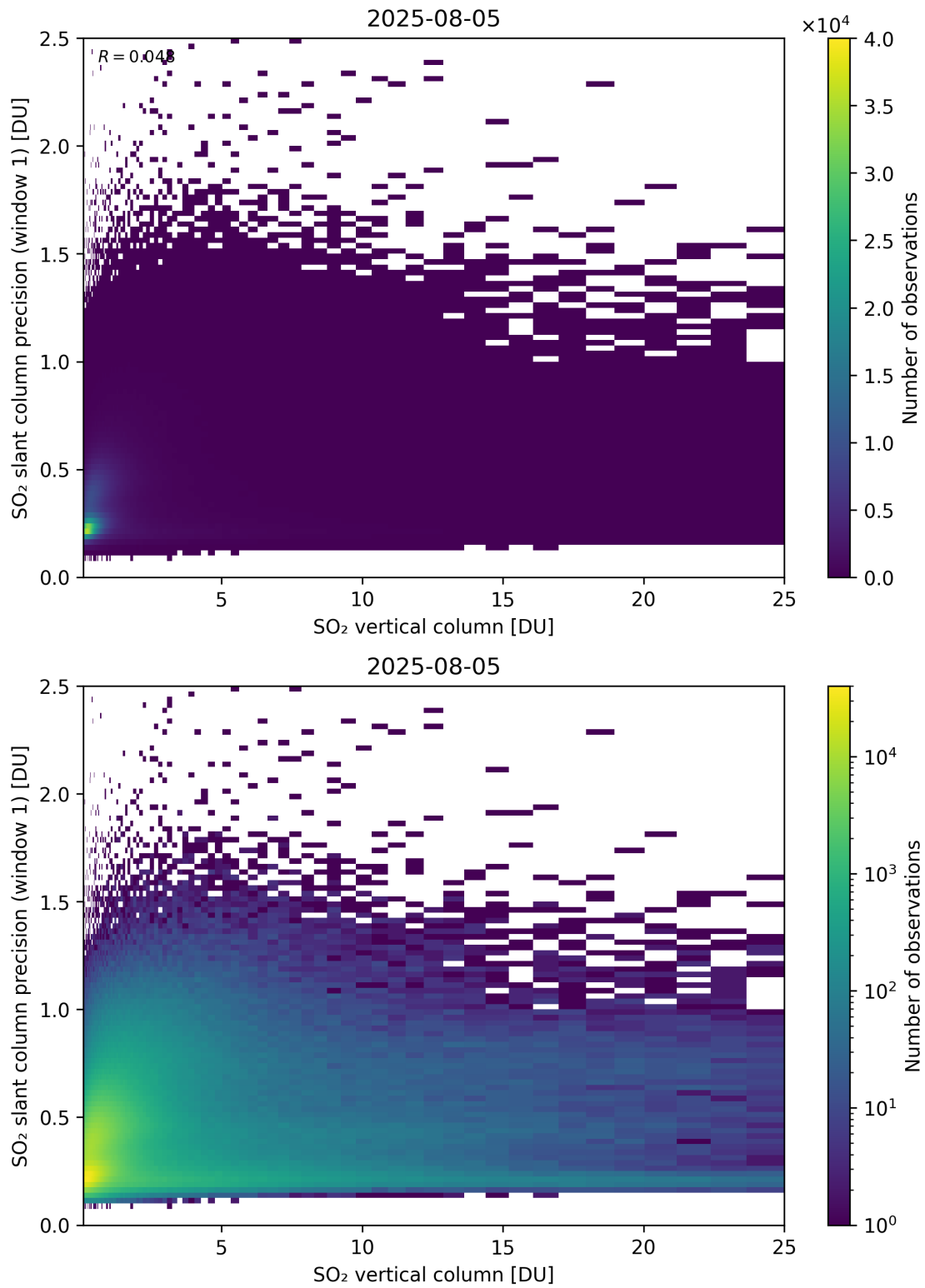
Figure 355: Scatter density plot of “SO 2 vertical column” against “SO 2 slant column precision (window 1)” for 2025-08-04 to 2025-08-06.
