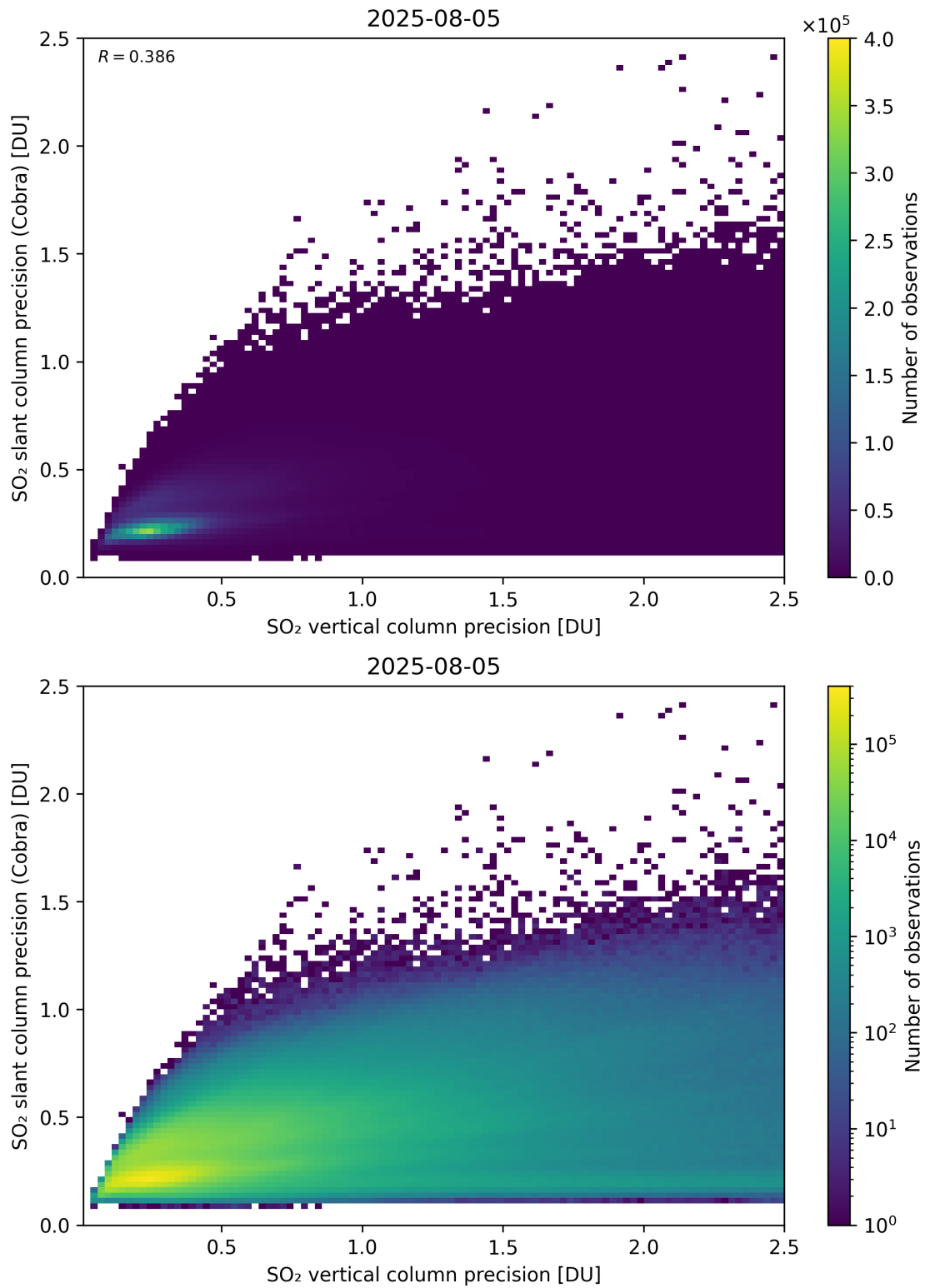
Figure 337: Scatter density plot of “SO 2 vertical column precision” against “SO 2 slant column precision (Cobra)” for 2025-08-04 to 2025-08-06.
