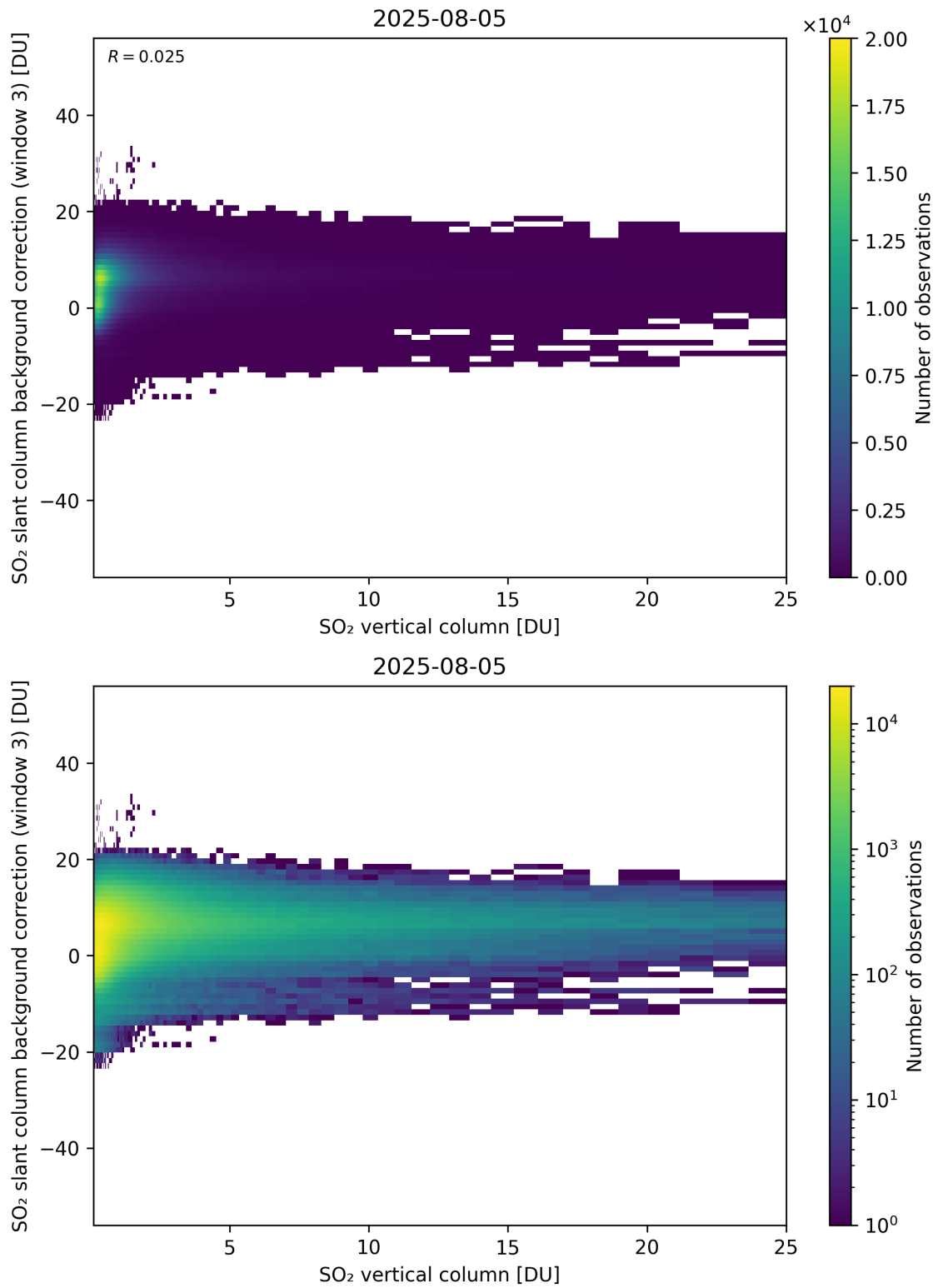
Figure 325: Scatter density plot of “SO 2 vertical column” against “SO 2 slant column background correction (window 3)” for 2025-08-04 to 2025-08-06.
