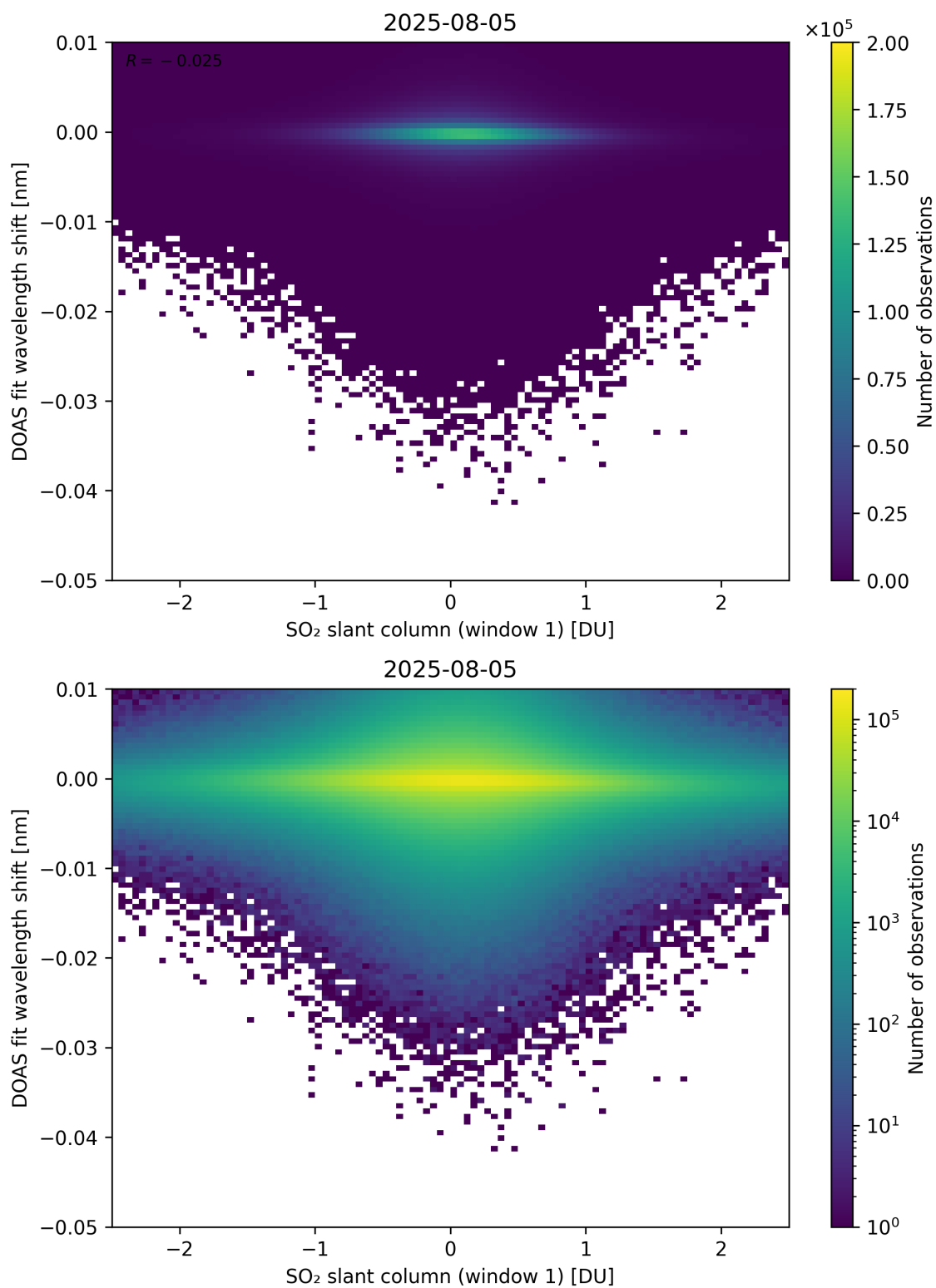
Figure 265: Scatter density plot of “SO 2 slant column (window 1)” against “DOAS fit wavelength shift” for 2025-08-04 to 2025-08-06.
