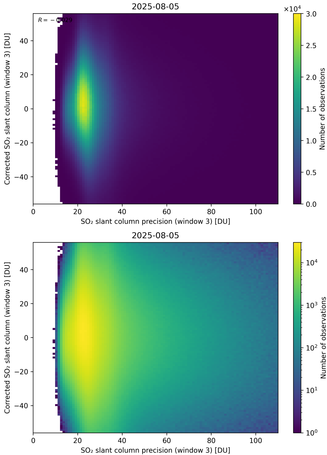
Figure 312: Scatter density plot of “SO 2 slant column precision (window 3)” against “Corrected SO 2 slant column (window 3)” for 2025-08-04 to 2025-08-06.
