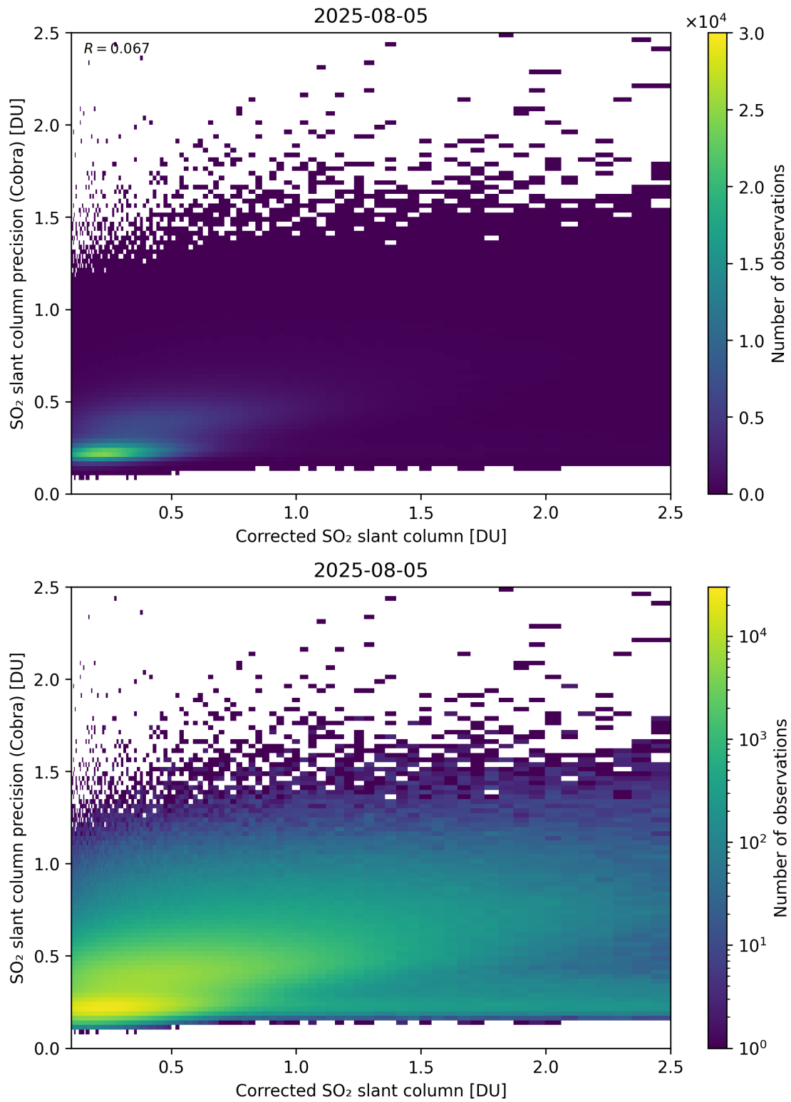
Figure 234: Scatter density plot of “Corrected SO 2 slant column” against “SO 2 slant column precision (Cobra)” for 2025-08-04 to 2025-08-06.
