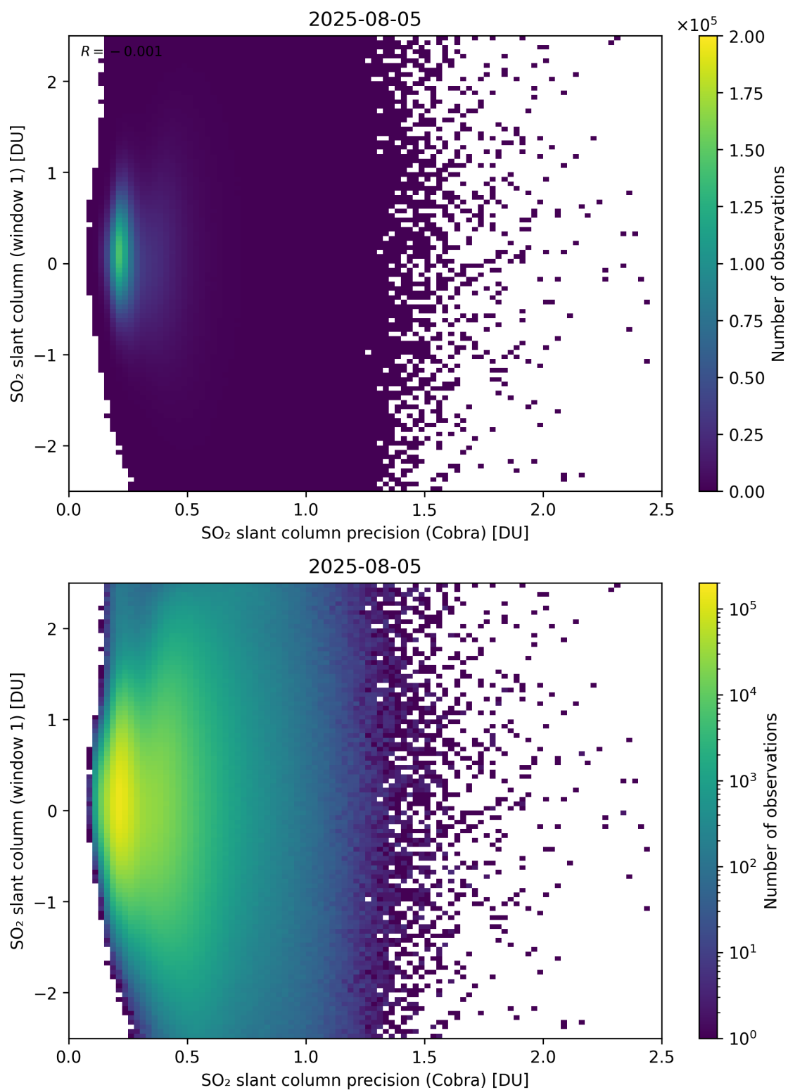
Figure 208: Scatter density plot of “SO 2 slant column precision (Cobra)” against “SO 2 slant column (window 1)” for 2025-08-04 to 2025-08-06.
