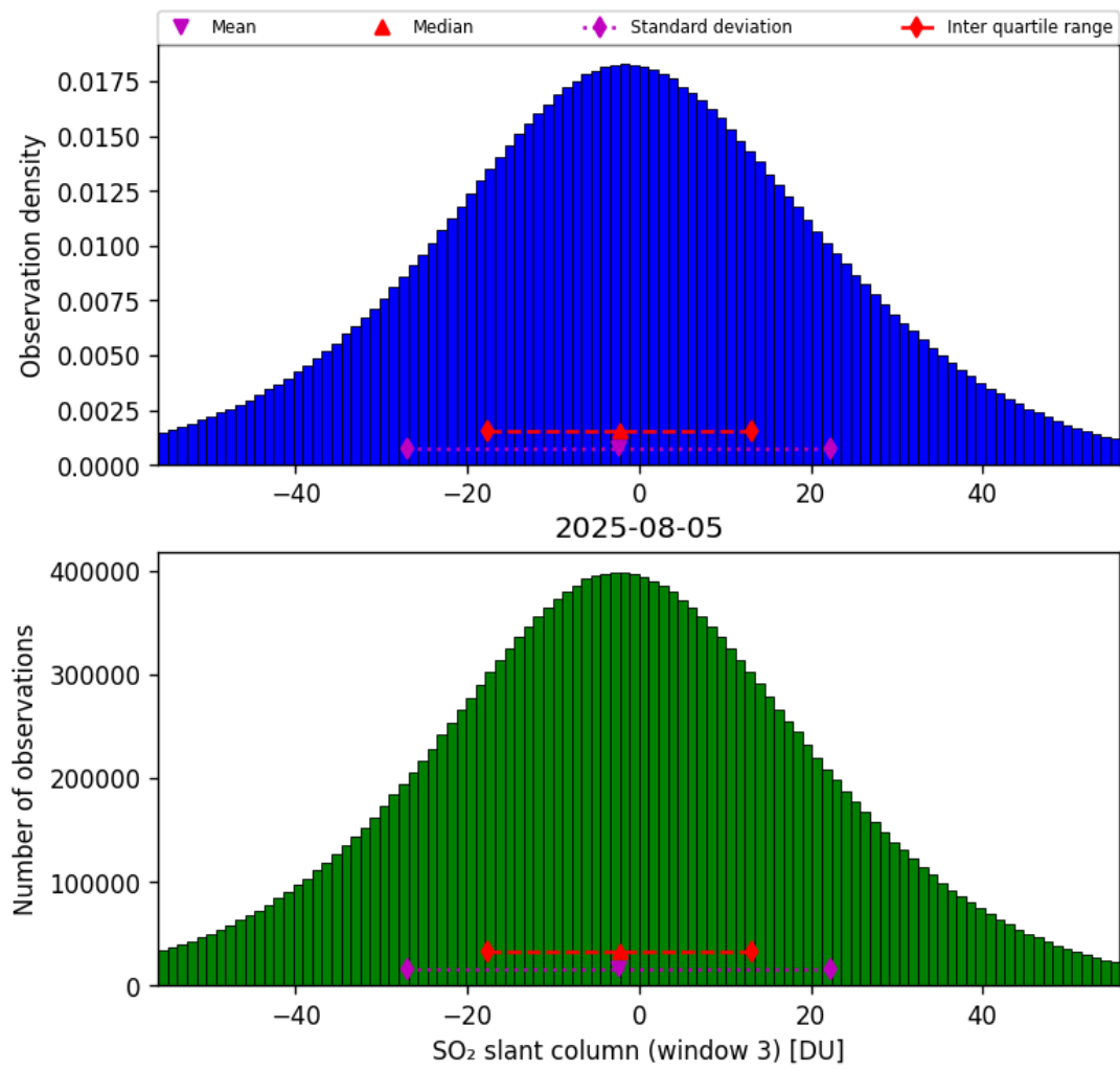
Figure 71: Histogram of “SO 2 slant column (window 3)” for 2025-08-04 to 2025-08-06
