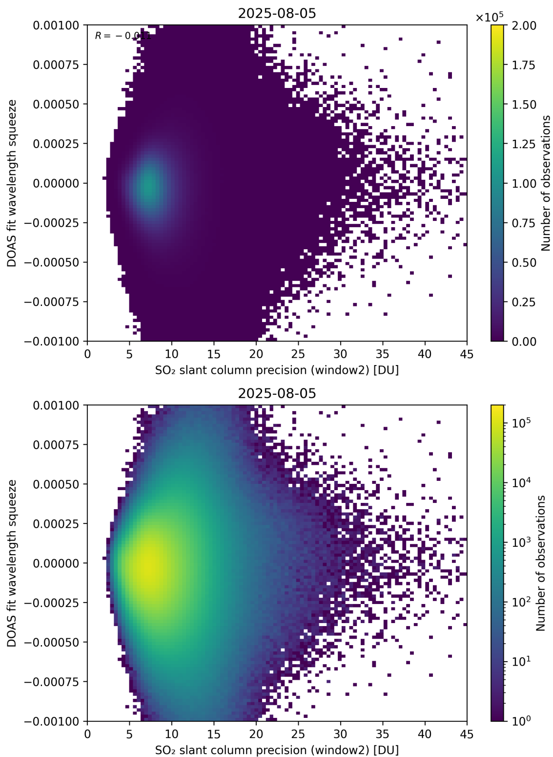
Figure 294: Scatter density plot of “SO 2 slant column precision (window2)” against “DOAS fit wavelength squeeze” for 2025-08-04 to 2025-08-06.
