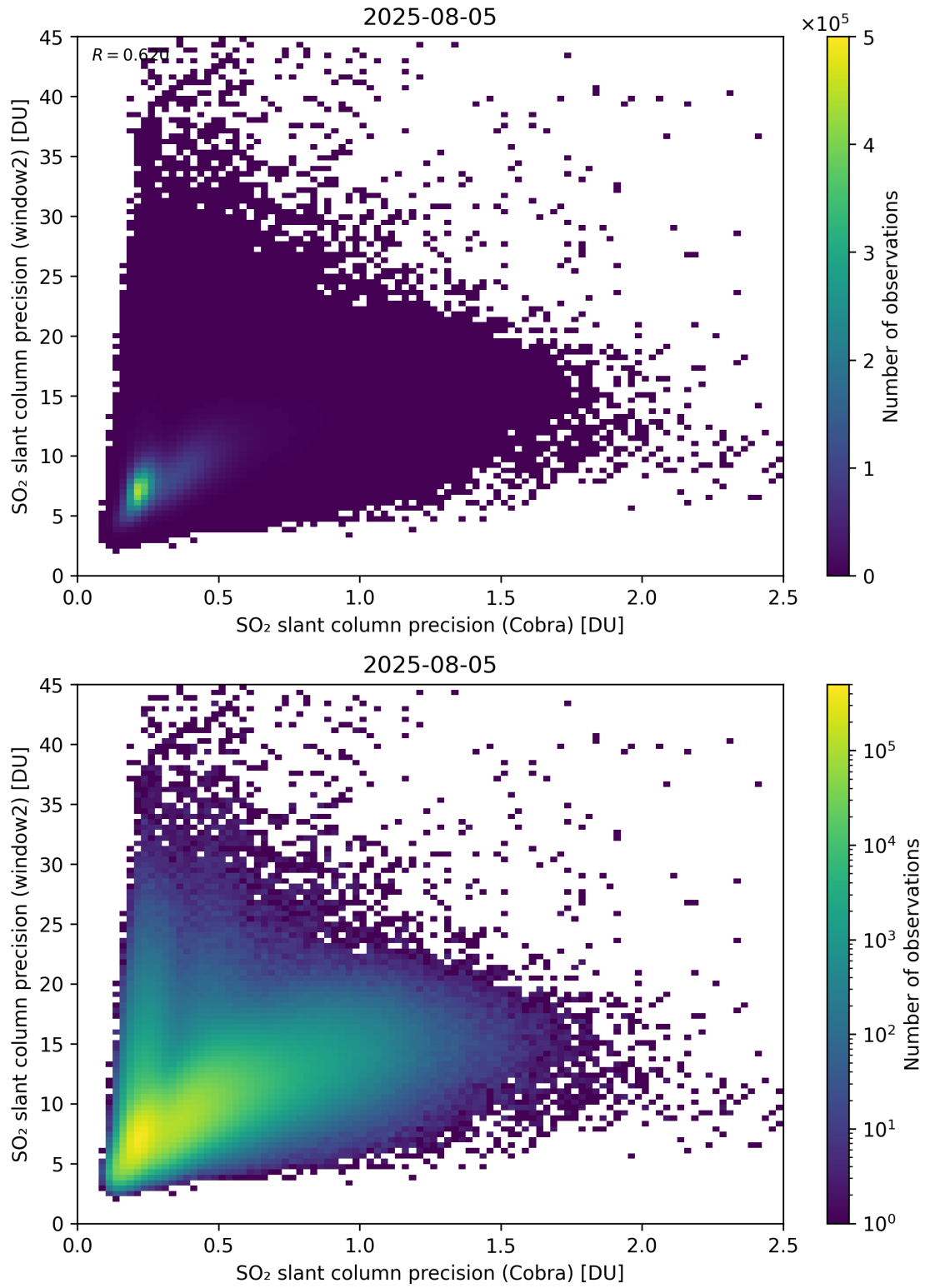
Figure 210: Scatter density plot of “SO 2 slant column precision (Cobra)” against “SO 2 slant column precision (window2)” for 2025-08-04 to 2025-08-06.
