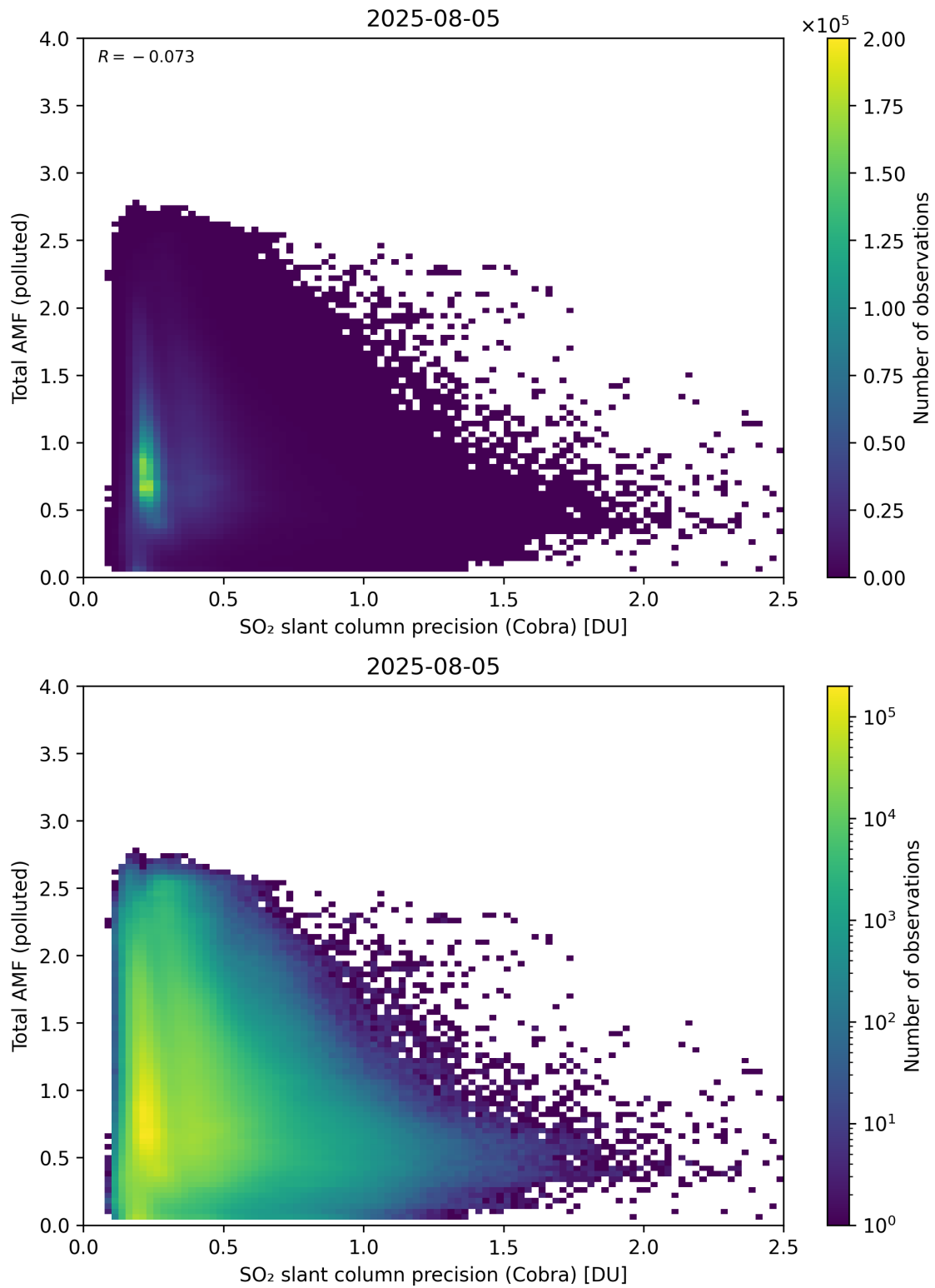
Figure 213: Scatter density plot of “SO 2 slant column precision (Cobra)” against “Total AMF (polluted)” for 2025-08-04 to 2025-08-06.
