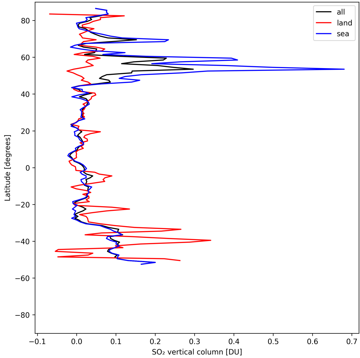
Figure 32: Zonal average of “SO 2 vertical column” for 2025-08-04 to 2025-08-06.
