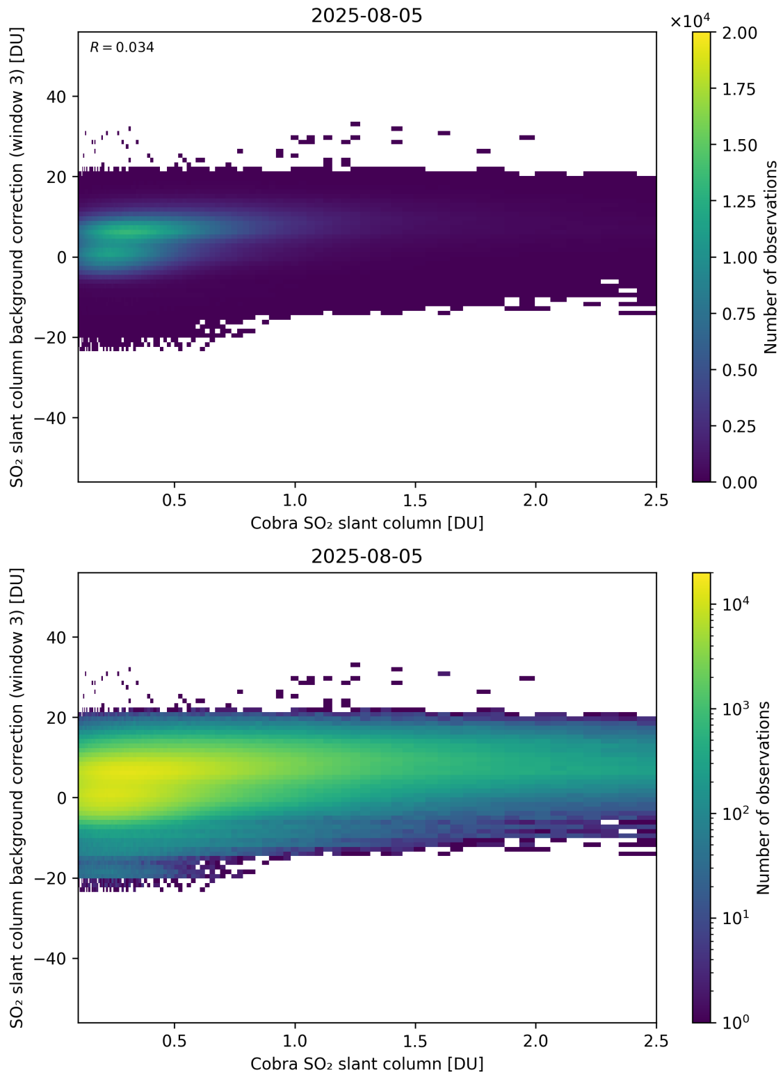
Figure 195: Scatter density plot of “Cobra SO 2 slant column” against “SO 2 slant column background correction (window 3)” for 2025-08-04 to 2025-08-06.
