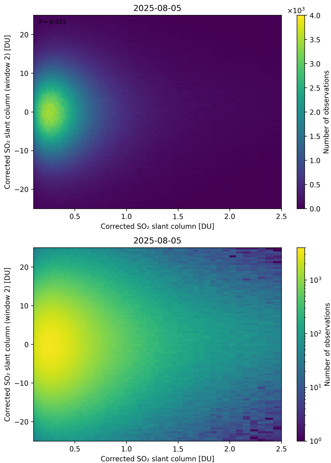
Figure 235: Scatter density plot of “Corrected SO 2 slant column” against “Corrected SO 2 slant column (window 2)” for 2025-08-04 to 2025-08-06.
