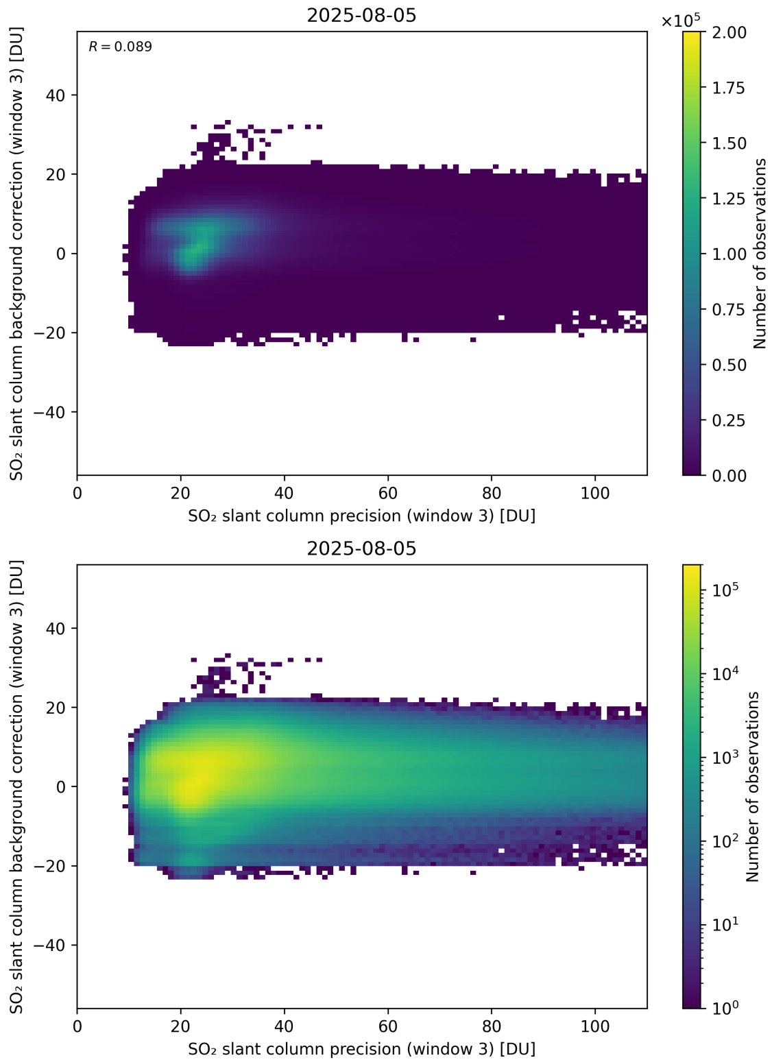
Figure 307: Scatter density plot of “SO 2 slant column precision (window 3)” against “SO 2 slant column background correction (window 3)” for 2025-08-04 to 2025-08-06.
