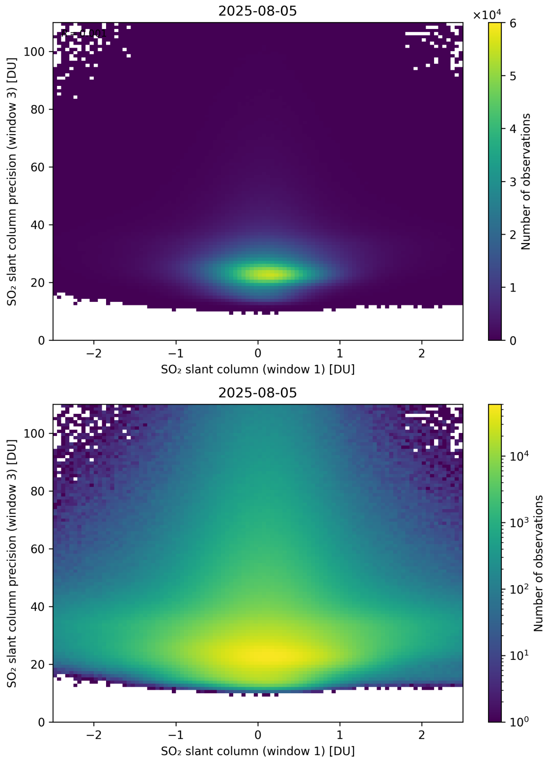
Figure 288: Scatter density plot of “SO 2 slant column (window 1)” against “SO 2 slant column precision (window 3)” for 2025-08-04 to 2025-08-06.
