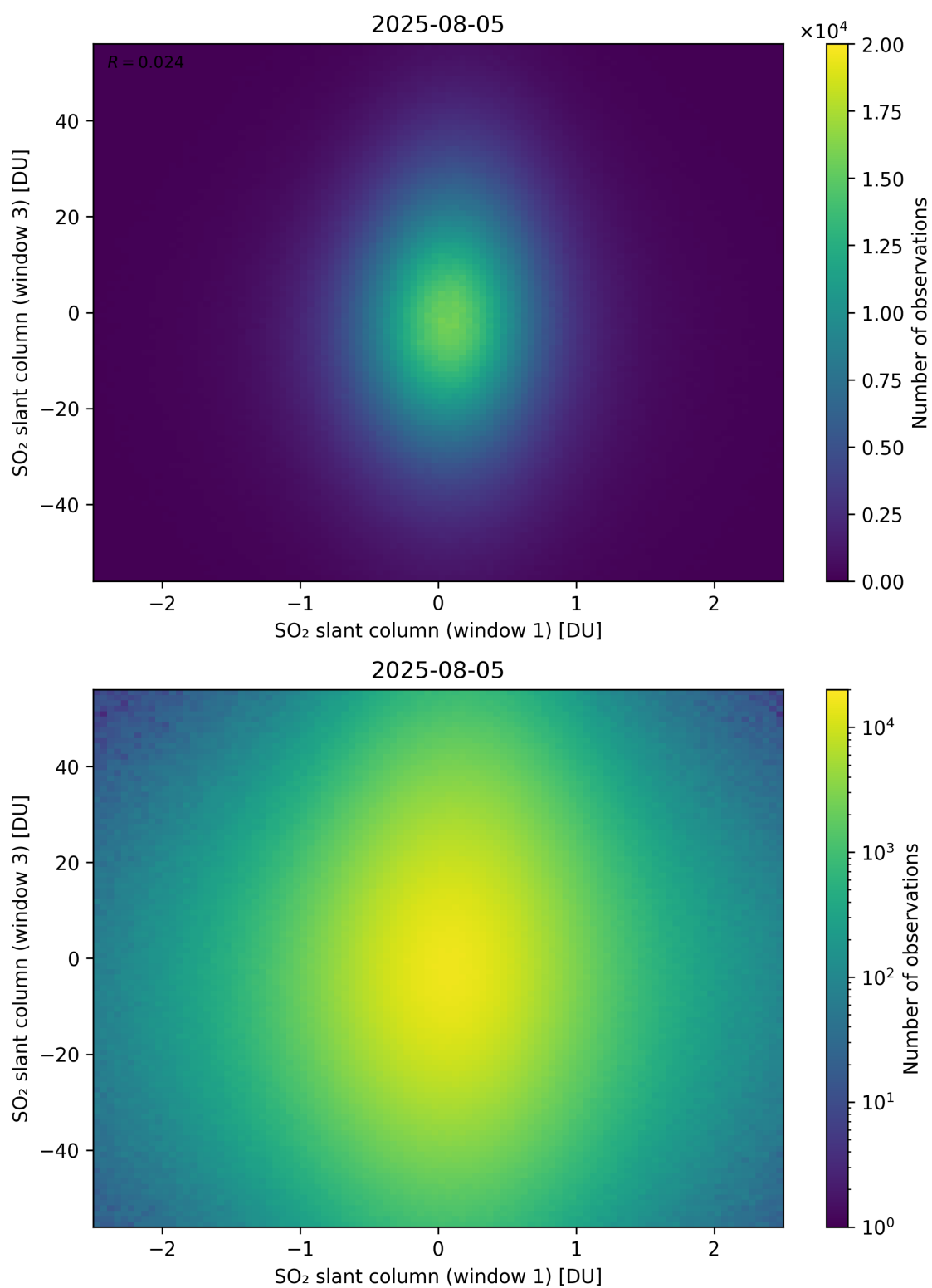
Figure 287: Scatter density plot of “SO 2 slant column (window 1)” against “SO 2 slant column (window 3)” for 2025-08-04 to 2025-08-06.
