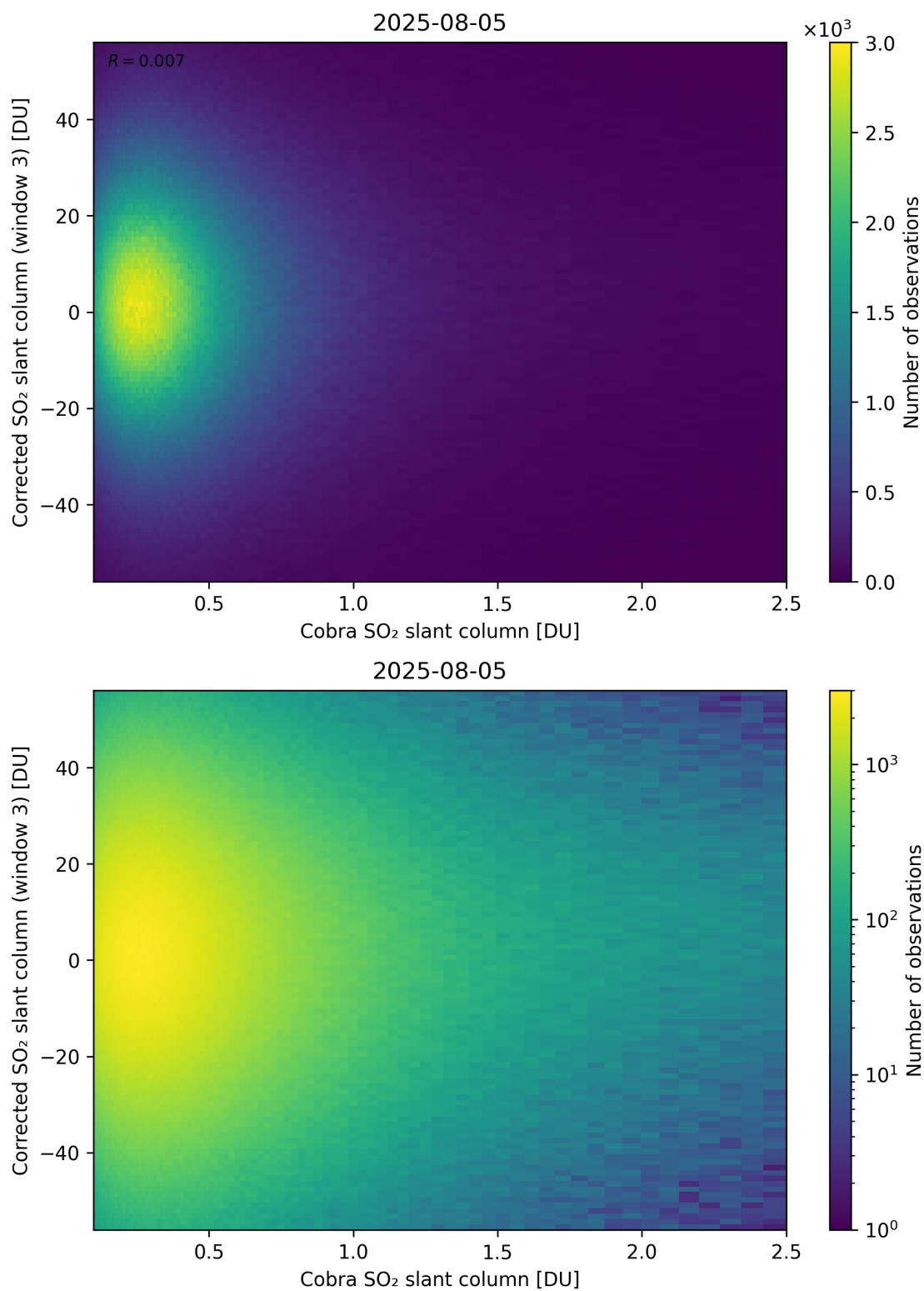
Figure 218: Scatter density plot of “Cobra SO 2 slant column” against “Corrected SO 2 slant column (window 3)” for 2025-08-04 to 2025-08-06.
