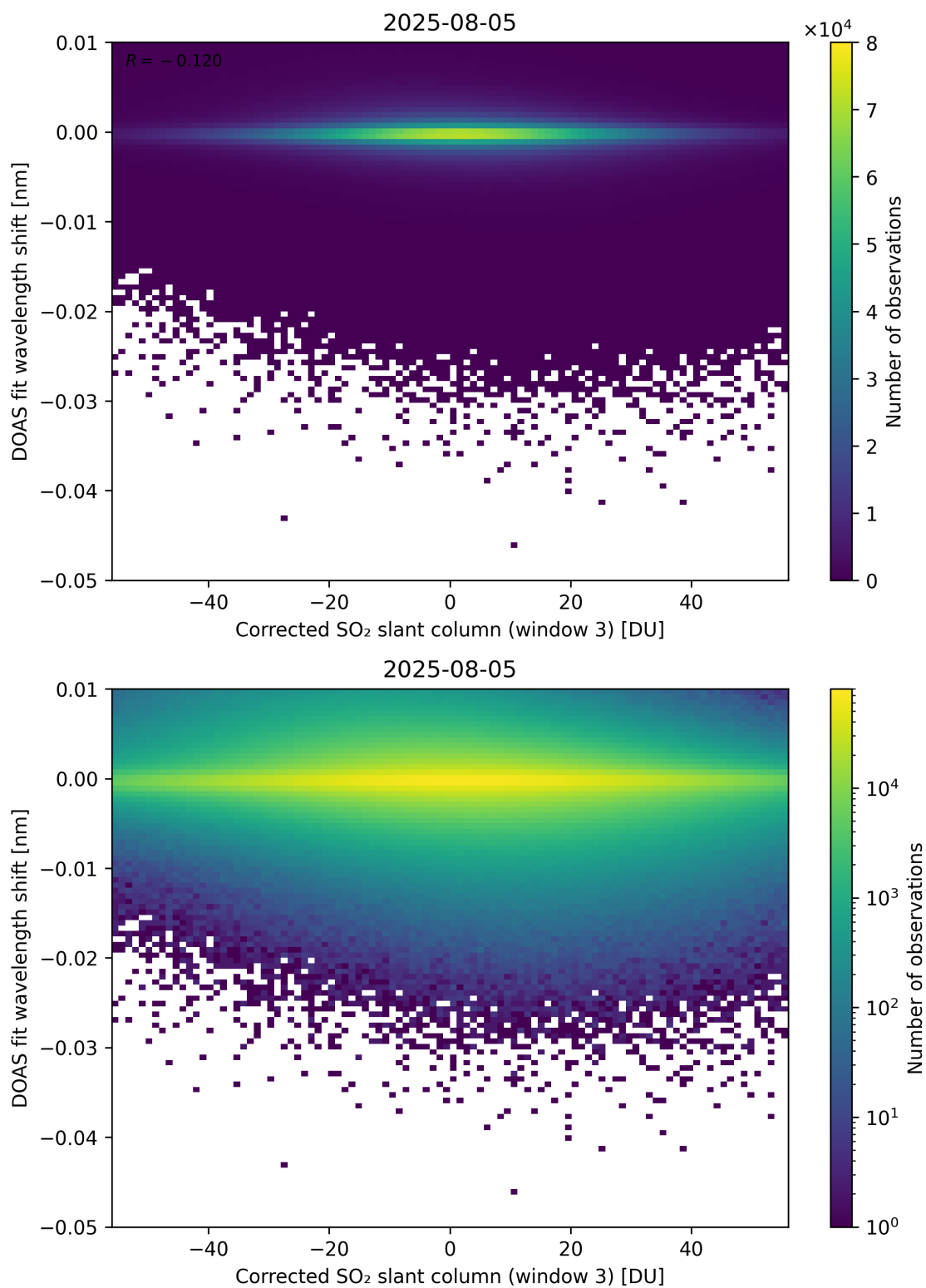
Figure 256: Scatter density plot of “Corrected SO 2 slant column (window 3)” against “DOAS fit wavelength shift” for 2025-08-04 to 2025-08-06.
