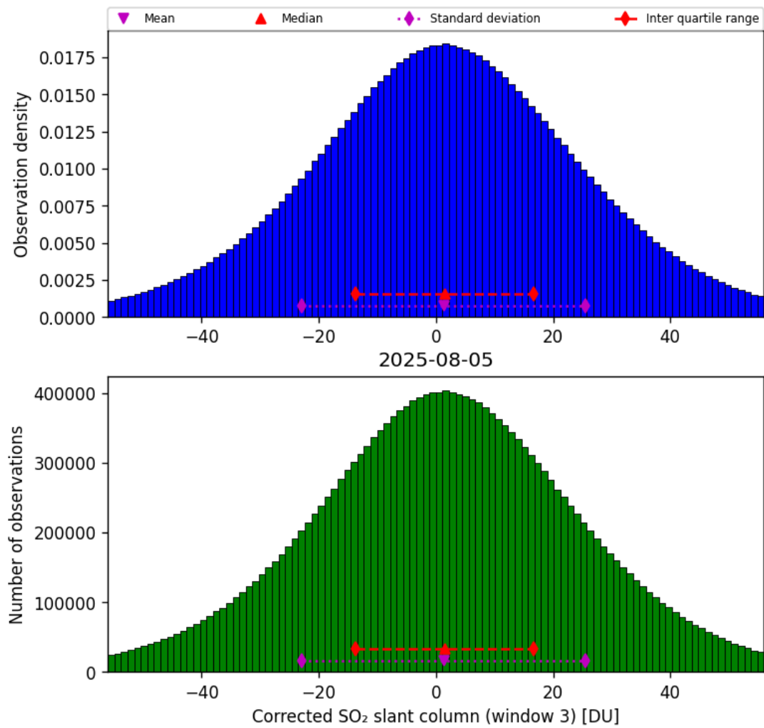
Figure 73: Histogram of “Corrected SO 2 slant column (window 3)” for 2025-08-04 to 2025-08-06
