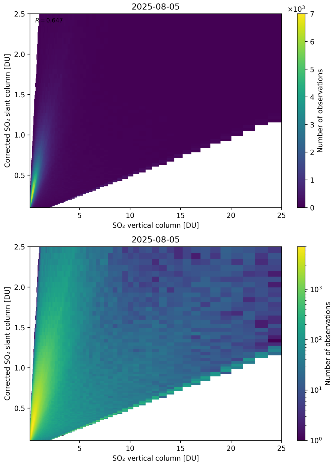
Figure 351: Scatter density plot of “SO 2 vertical column” against “Corrected SO 2 slant column” for 2025-08-04 to 2025-08-06.
