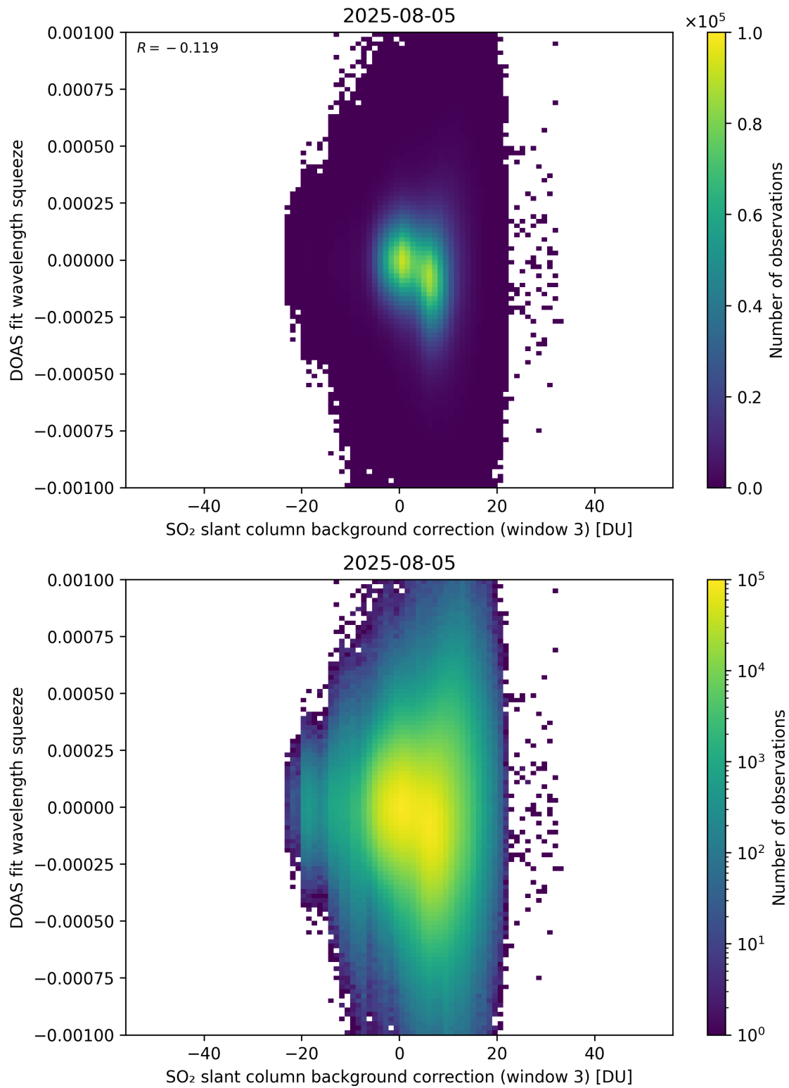
Figure 133: Scatter density plot of “SO 2 slant column background correction (window 3)” against “DOAS fit wavelength squeeze” for 2025-08-04 to 2025-08-06.
