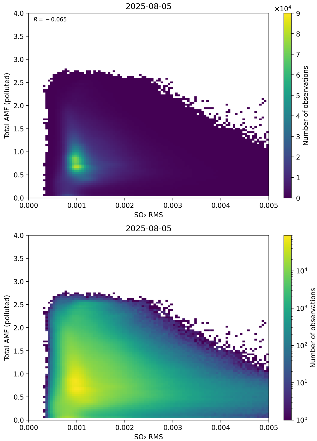
Figure 148: Scatter density plot of “SO 2 RMS” against “Total AMF (polluted)” for 2025-08-04 to 2025-08-06.
