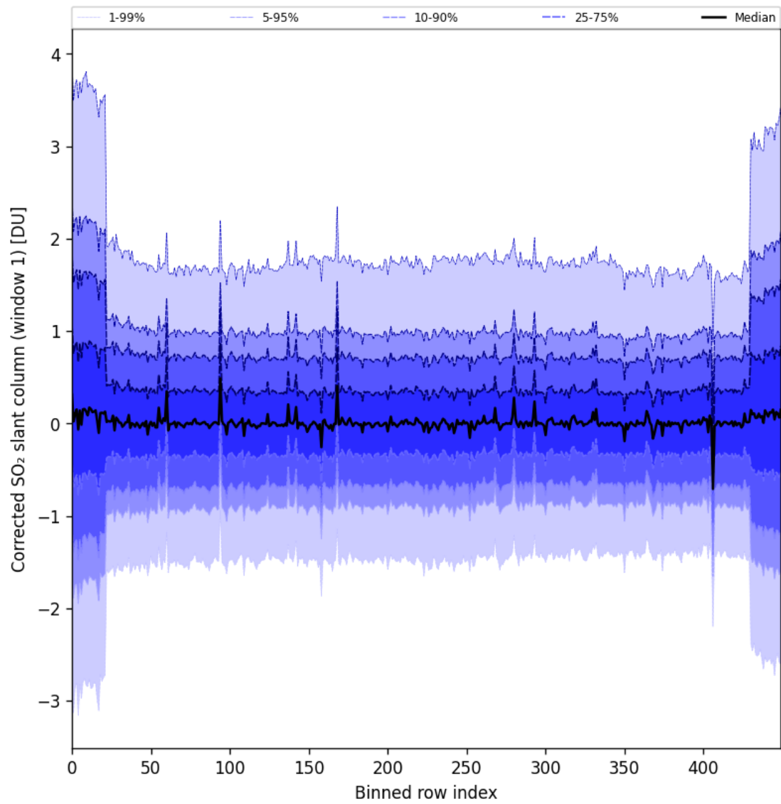
Figure 91: Along track statistics of “Corrected SO 2 slant column (window 1)” for 2025-08-04 to 2025-08-06
