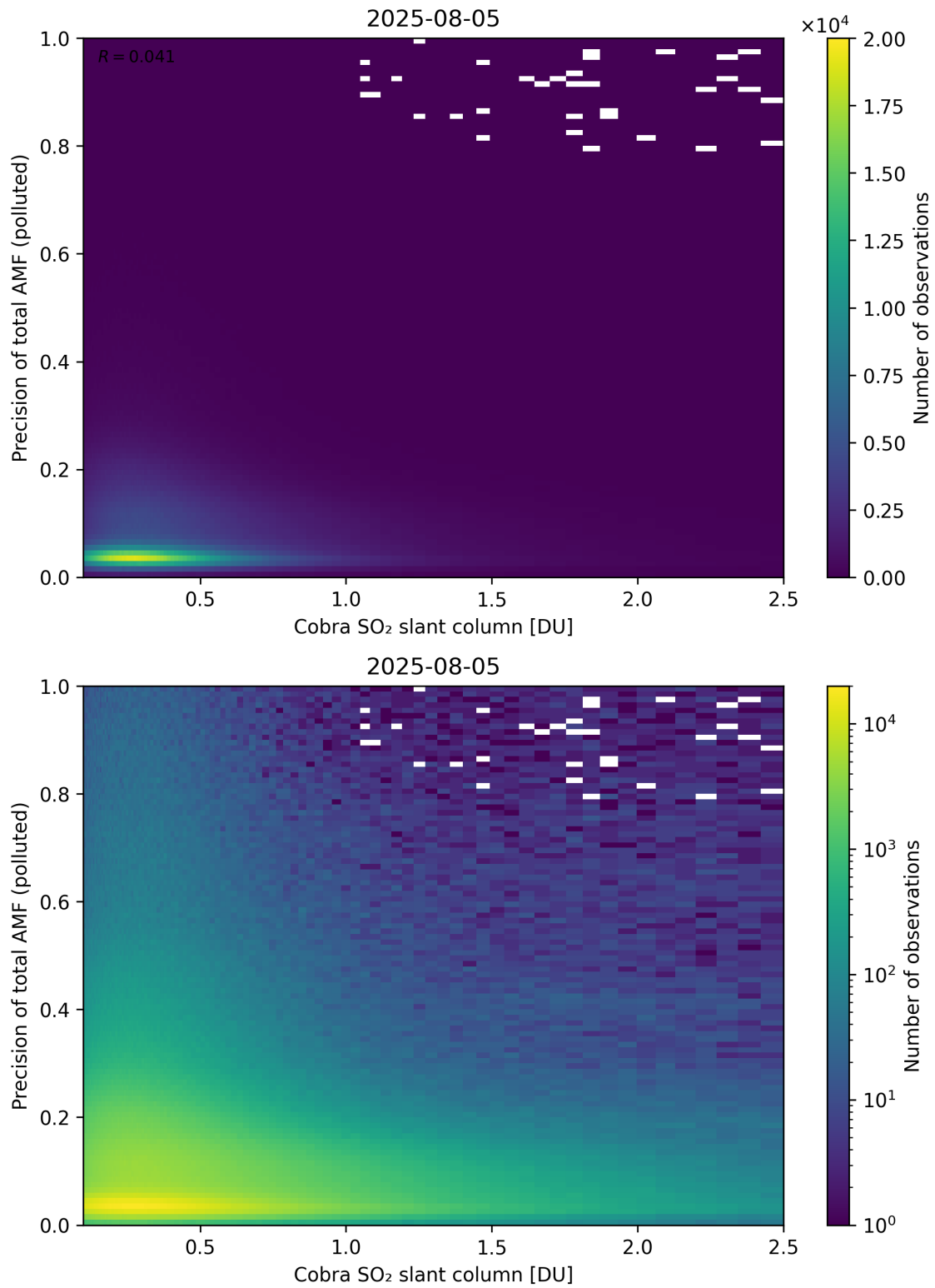
Figure 225: Scatter density plot of “Cobra SO 2 slant column” against “Precision of total AMF (polluted)” for 2025-08-04 to 2025-08-06.
