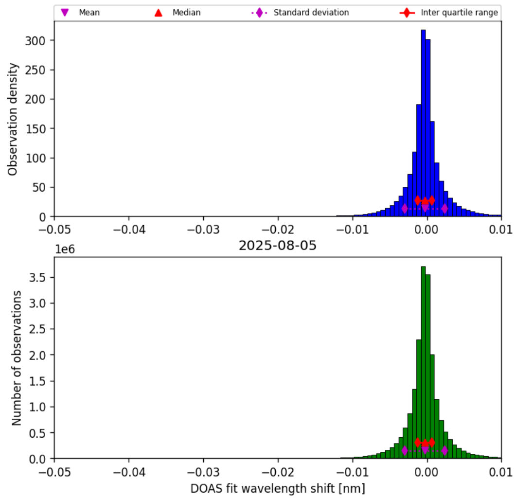
Figure 76: Histogram of “DOAS fit wavelength shift” for 2025-08-04 to 2025-08-06
