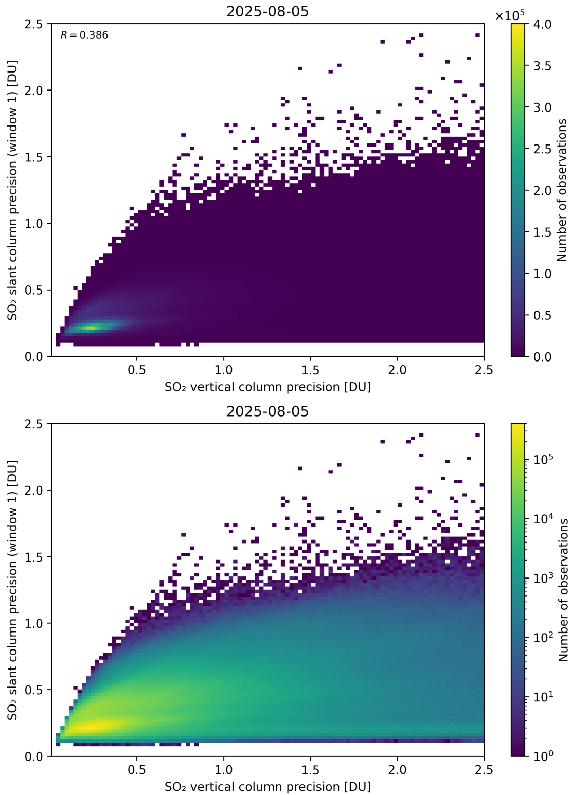
Figure 342: Scatter density plot of “SO 2 vertical column precision” against “SO 2 slant column precision (window 1)” for 2025-08-04 to 2025-08-06.
