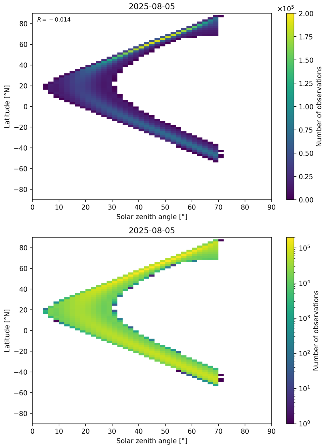
Figure 177: Scatter density plot of “Solar zenith angle” against “Latitude” for 2025-08-04 to 2025-08-06.
