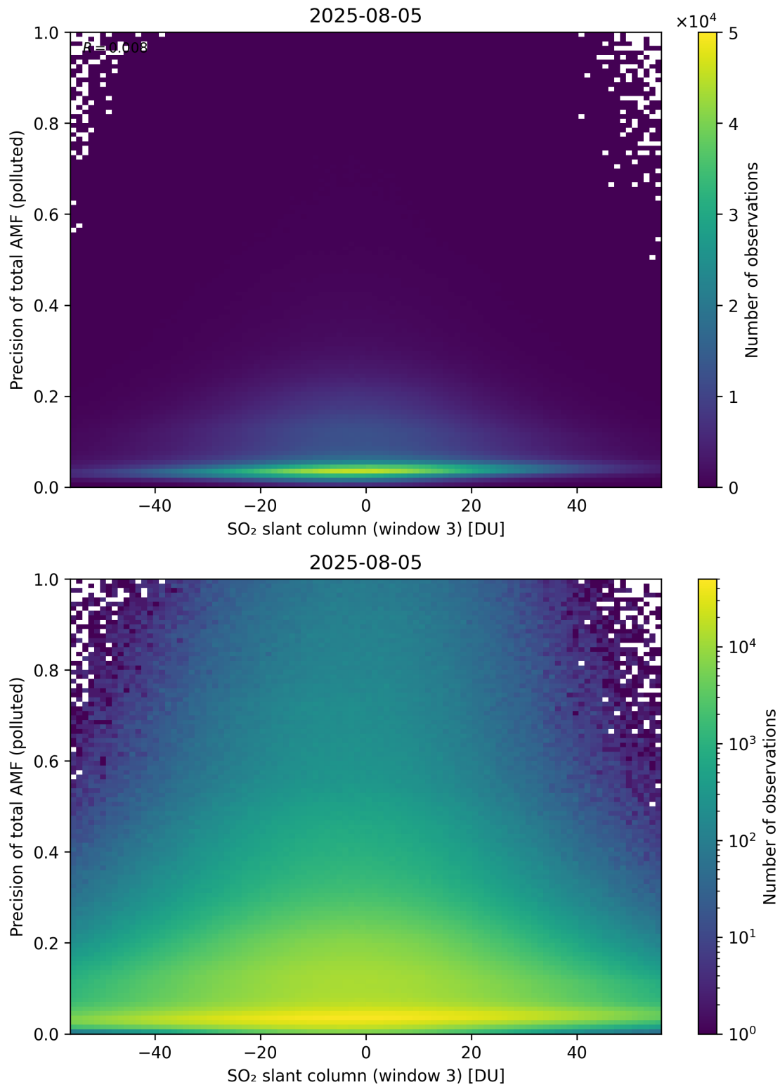
Figure 319: Scatter density plot of “SO 2 slant column (window 3)” against “Precision of total AMF (polluted)” for 2025-08-04 to 2025-08-06.
