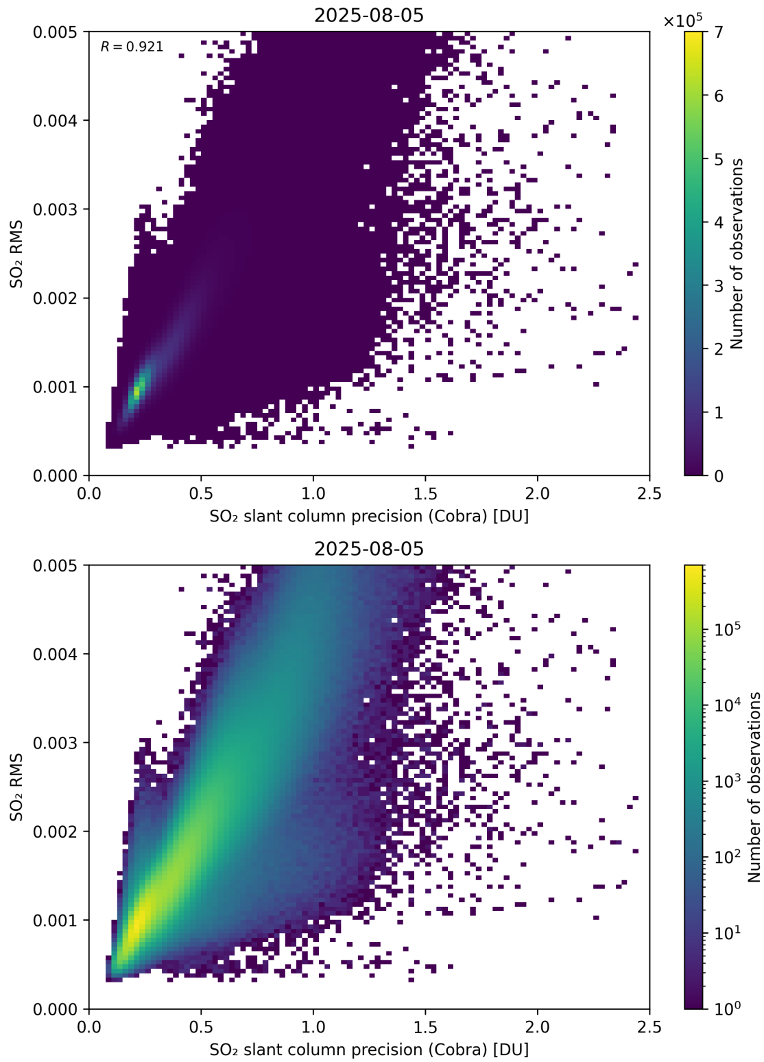
Figure 204: Scatter density plot of “SO 2 slant column precision (Cobra)” against “SO 2 RMS” for 2025-08-04 to 2025-08-06.
