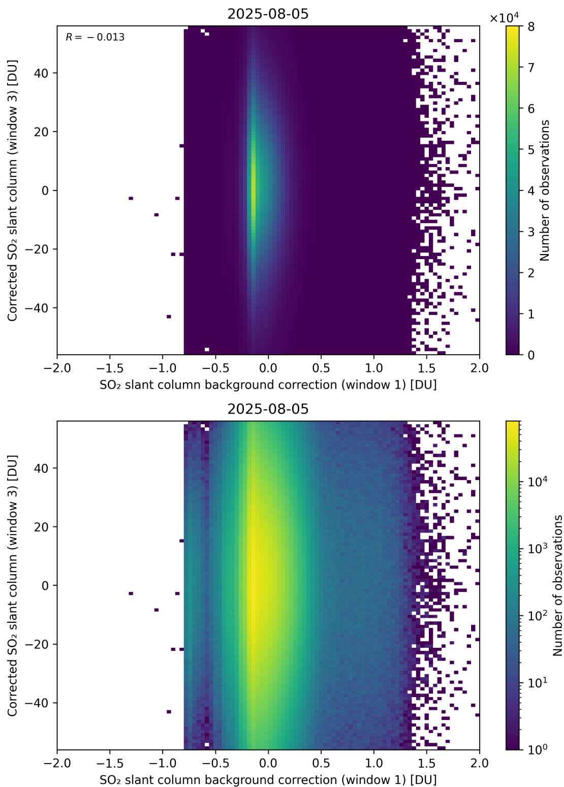
Figure 116: Scatter density plot of “SO 2 slant column background correction (window 1)” against “Corrected SO 2 slant column (window 3)” for 2025-08-04 to 2025-08-06.
