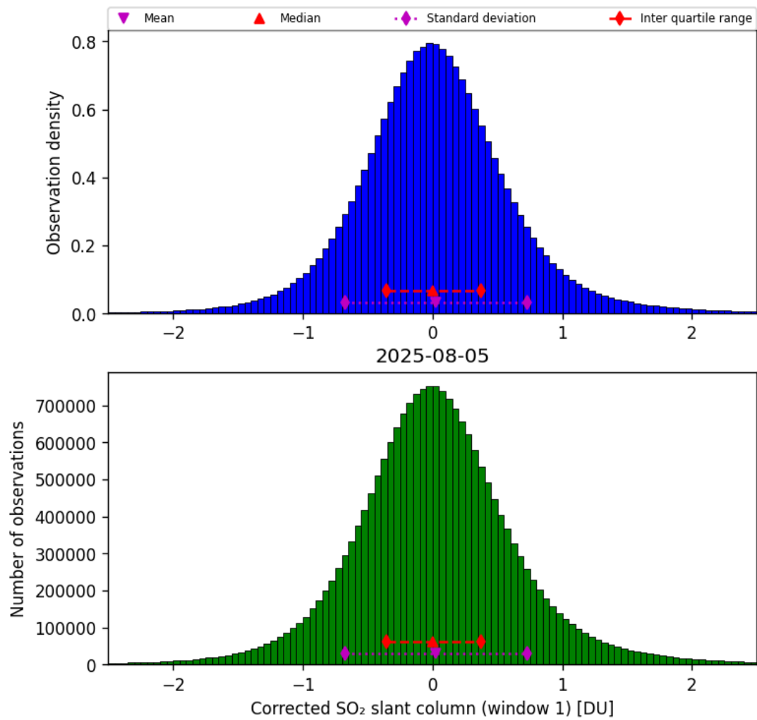
Figure 65: Histogram of “Corrected SO 2 slant column (window 1)” for 2025-08-04 to 2025-08-06
