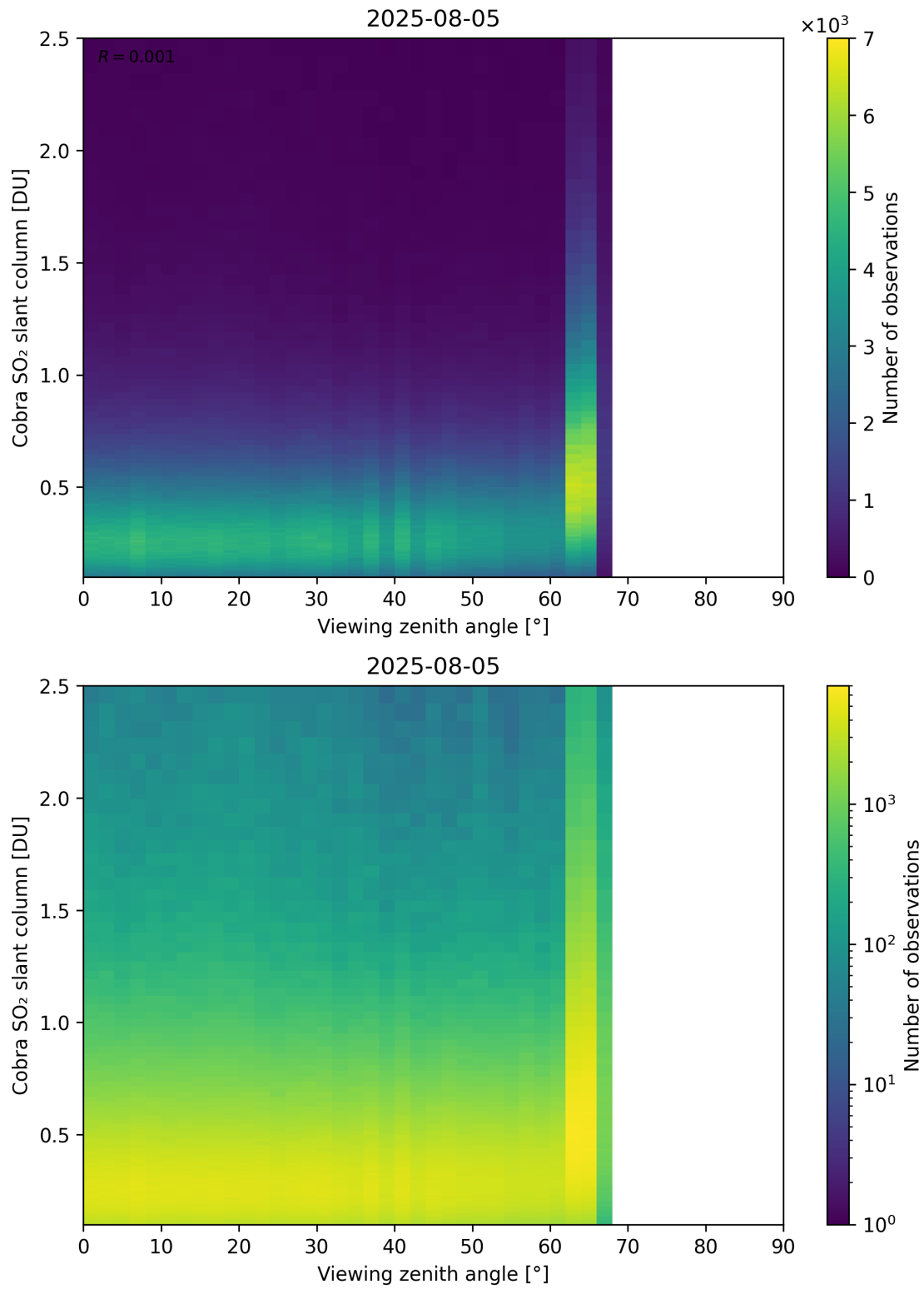
Figure 371: Scatter density plot of “Viewing zenith angle” against “Cobra SO 2 slant column” for 2025-08-04 to 2025-08-06.
