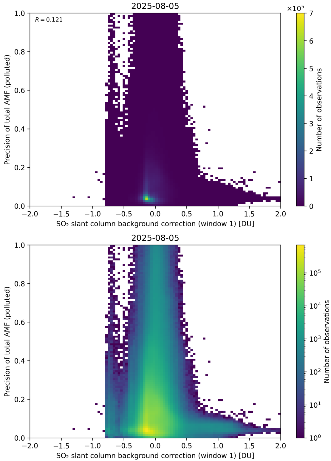
Figure 121: Scatter density plot of “SO 2 slant column background correction (window 1)” against “Precision of total AMF (polluted)” for 2025-08-04 to 2025-08-06.
