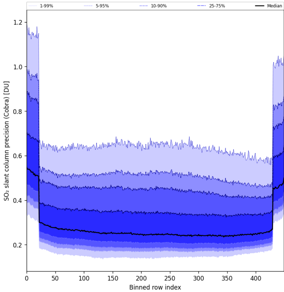
Figure 88: Along track statistics of “SO 2 slant column precision (Cobra)” for 2025-08-04 to 2025-08-06
