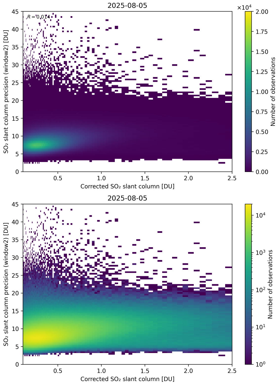
Figure 239: Scatter density plot of “Corrected SO 2 slant column” against “SO 2 slant column precision (window2)” for 2025-08-04 to 2025-08-06.
