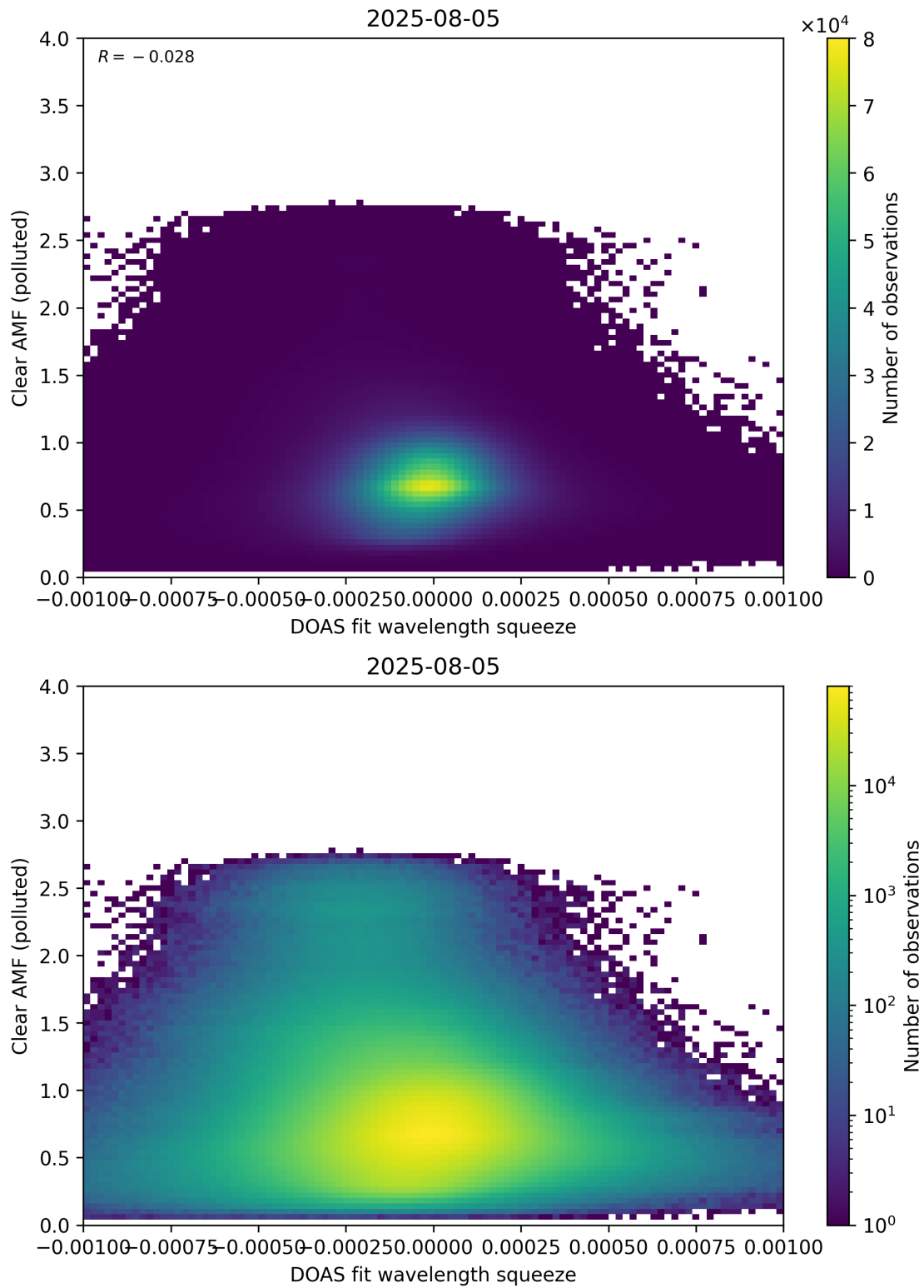
Figure 144: Scatter density plot of “DOAS fit wavelength squeeze” against “Clear AMF (polluted)” for 2025-08-04 to 2025-08-06.
