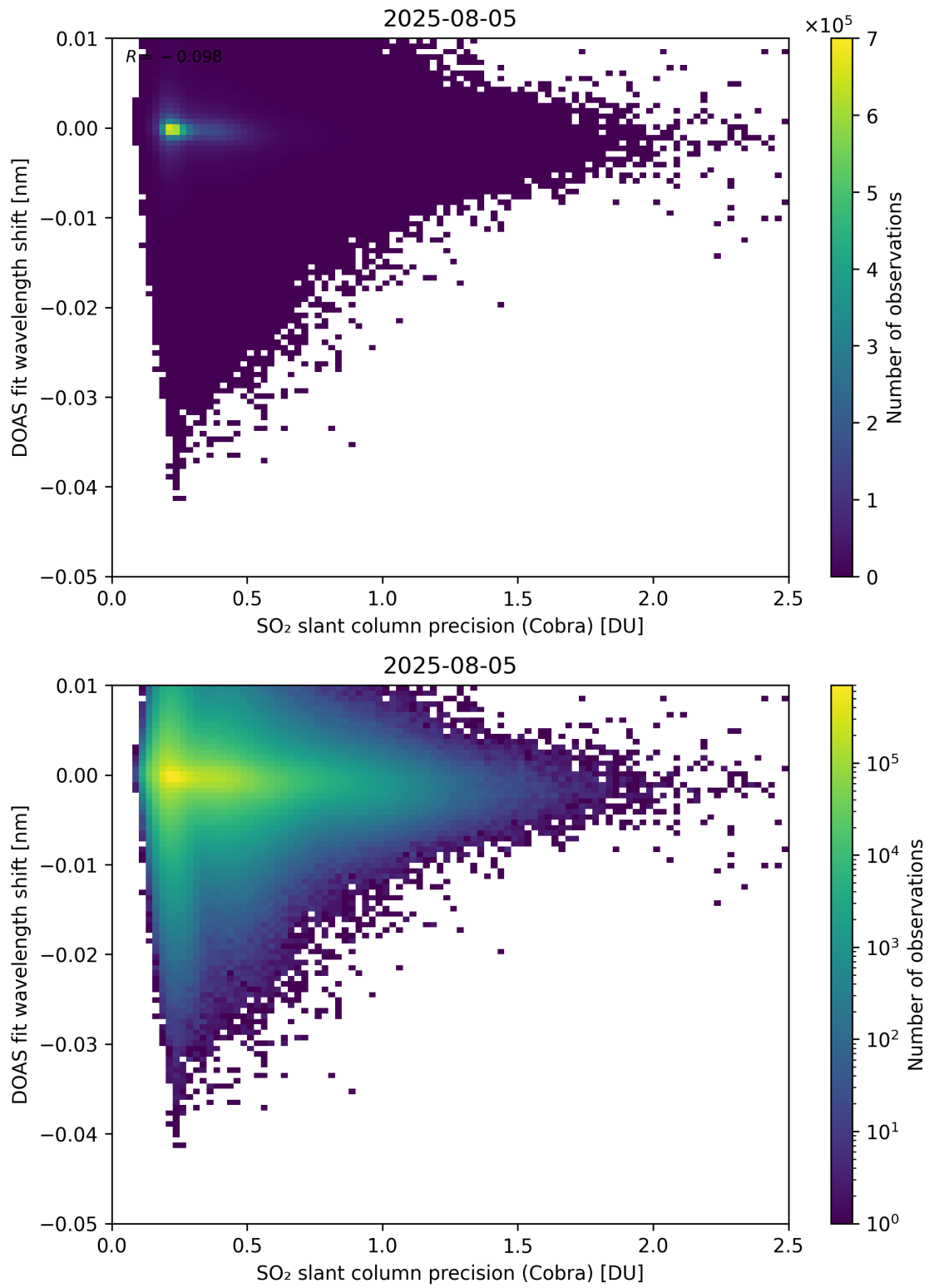
Figure 202: Scatter density plot of “SO 2 slant column precision (Cobra)” against “DOAS fit wavelength shift” for 2025-08-04 to 2025-08-06.
