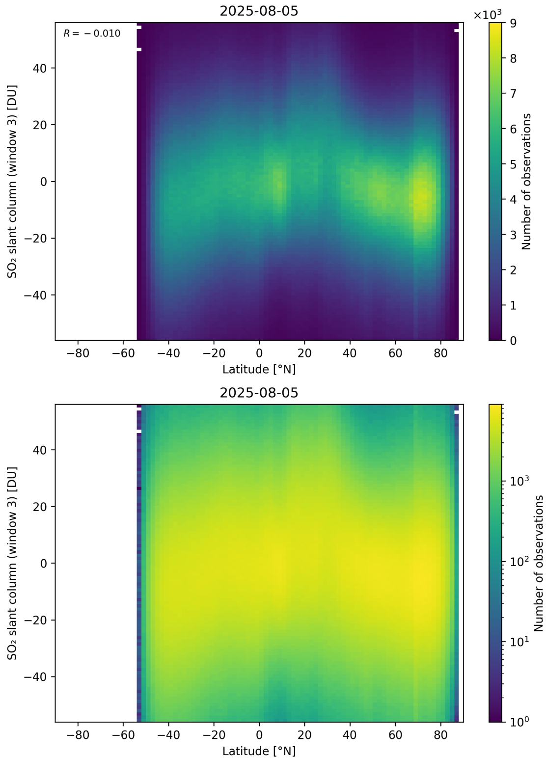
Figure 165: Scatter density plot of “Latitude” against “SO 2 slant column (window 3)” for 2025-08-04 to 2025-08-06.
