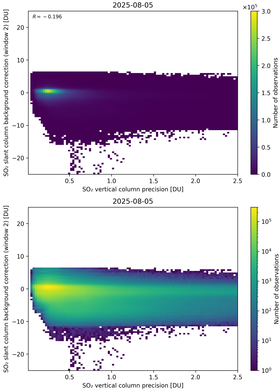
Figure 330: Scatter density plot of “SO 2 vertical column precision” against “SO 2 slant column background correction (window 2)” for 2025-08-04 to 2025-08-06.
