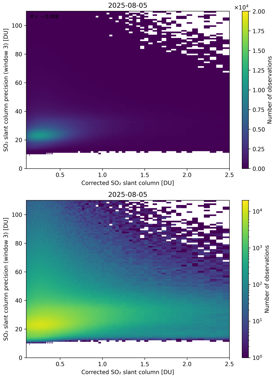
Figure 241: Scatter density plot of “Corrected SO 2 slant column” against “SO 2 slant column precision (window 3)” for 2025-08-04 to 2025-08-06.
