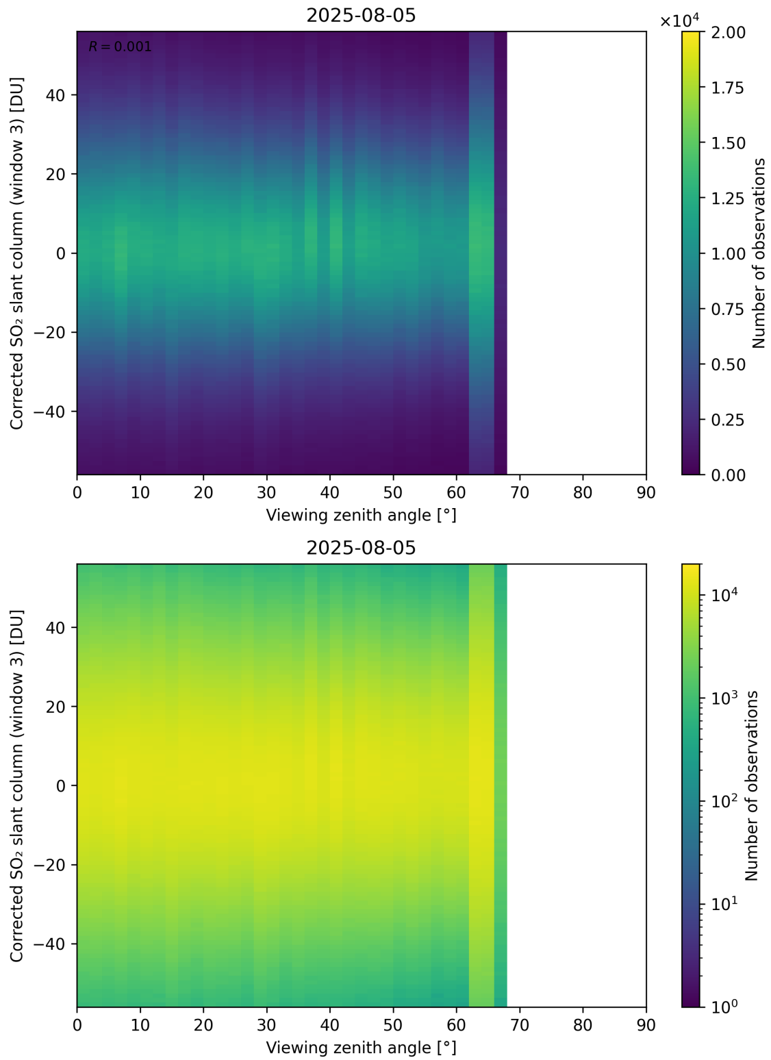
Figure 375: Scatter density plot of “Viewing zenith angle” against “Corrected SO 2 slant column (window 3)” for 2025-08-04 to 2025-08-06.
