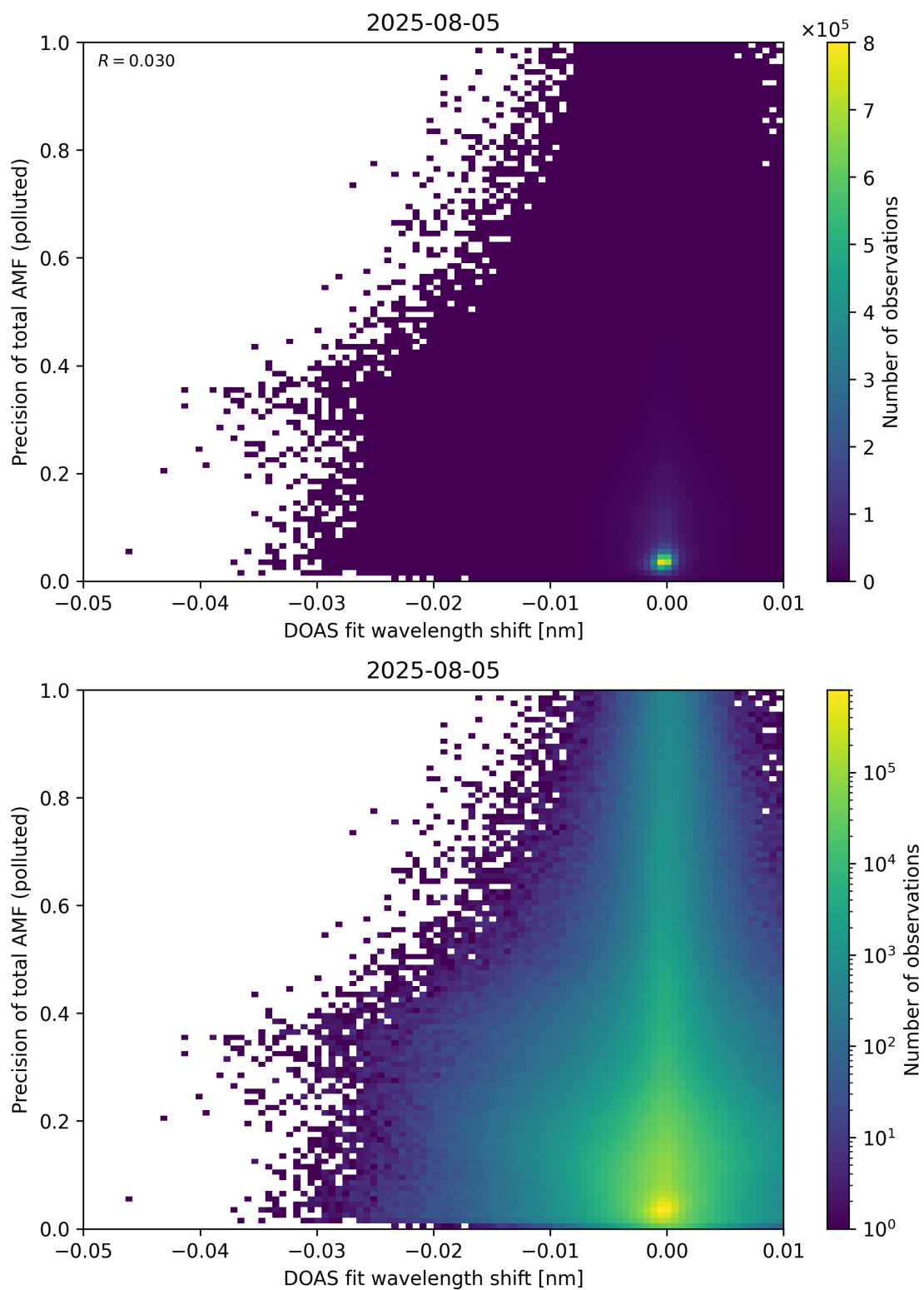
Figure 142: Scatter density plot of “DOAS fit wavelength shift” against “Precision of total AMF (polluted)” for 2025-08-04 to 2025-08-06.
