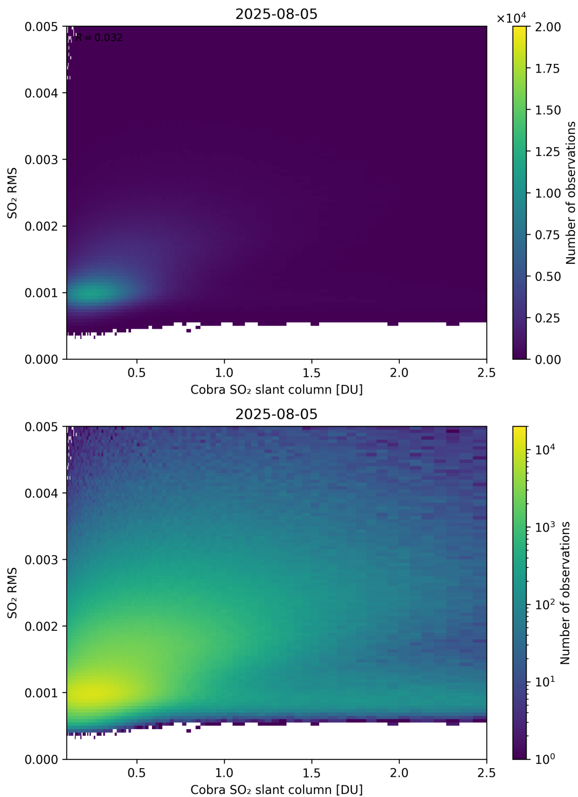
Figure 198: Scatter density plot of “Cobra SO 2 slant column” against “SO 2 RMS” for 2025-08-04 to 2025-08-06.
