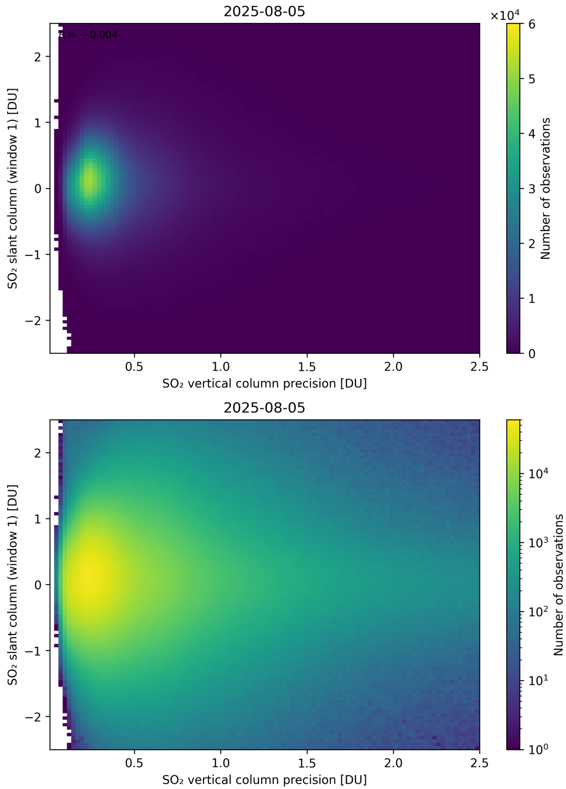
Figure 341: Scatter density plot of “SO 2 vertical column precision” against “SO 2 slant column (window 1)” for 2025-08-04 to 2025-08-06.
