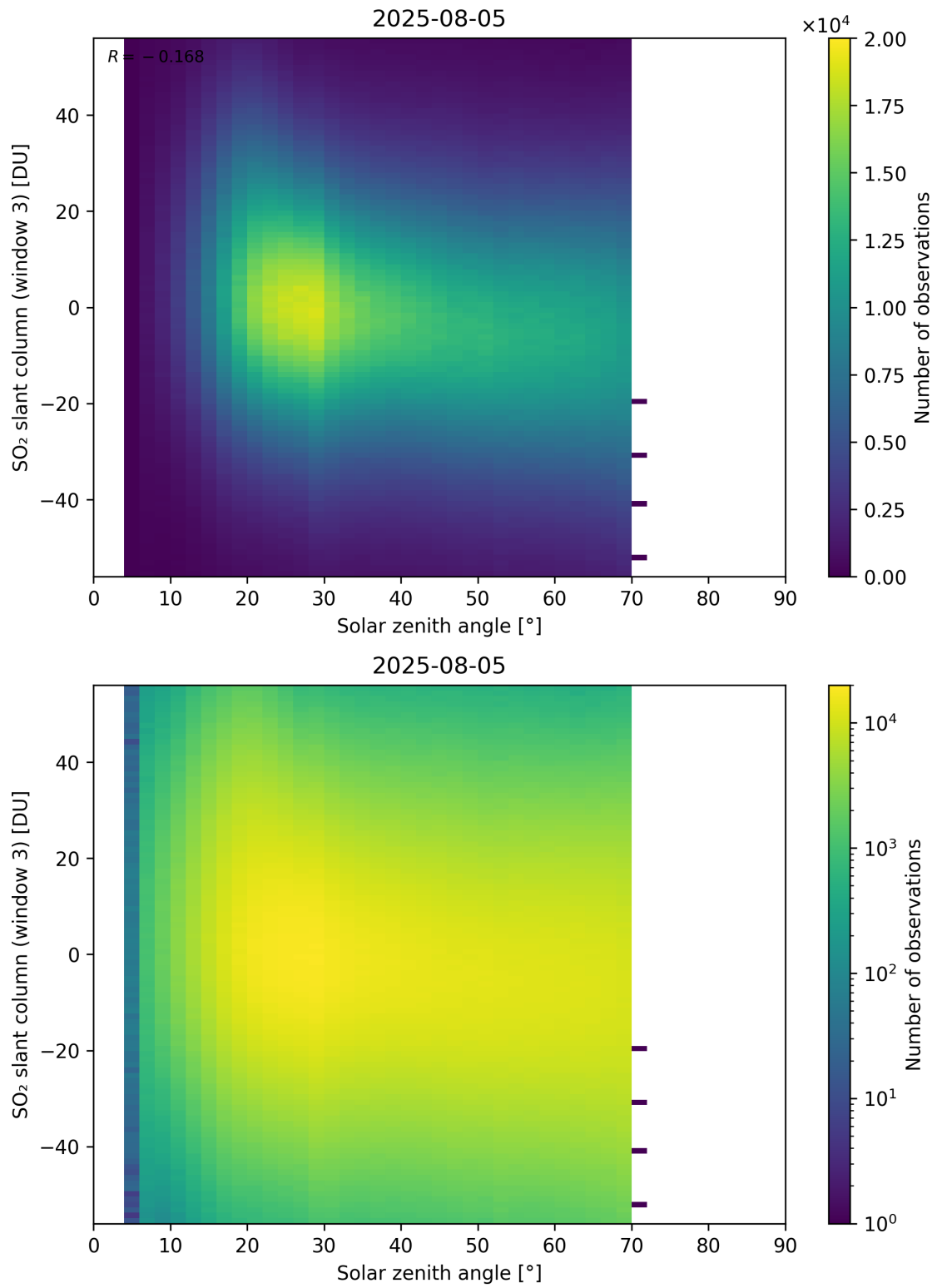
Figure 187: Scatter density plot of “Solar zenith angle” against “SO 2 slant column (window 3)” for 2025-08-04 to 2025-08-06.
