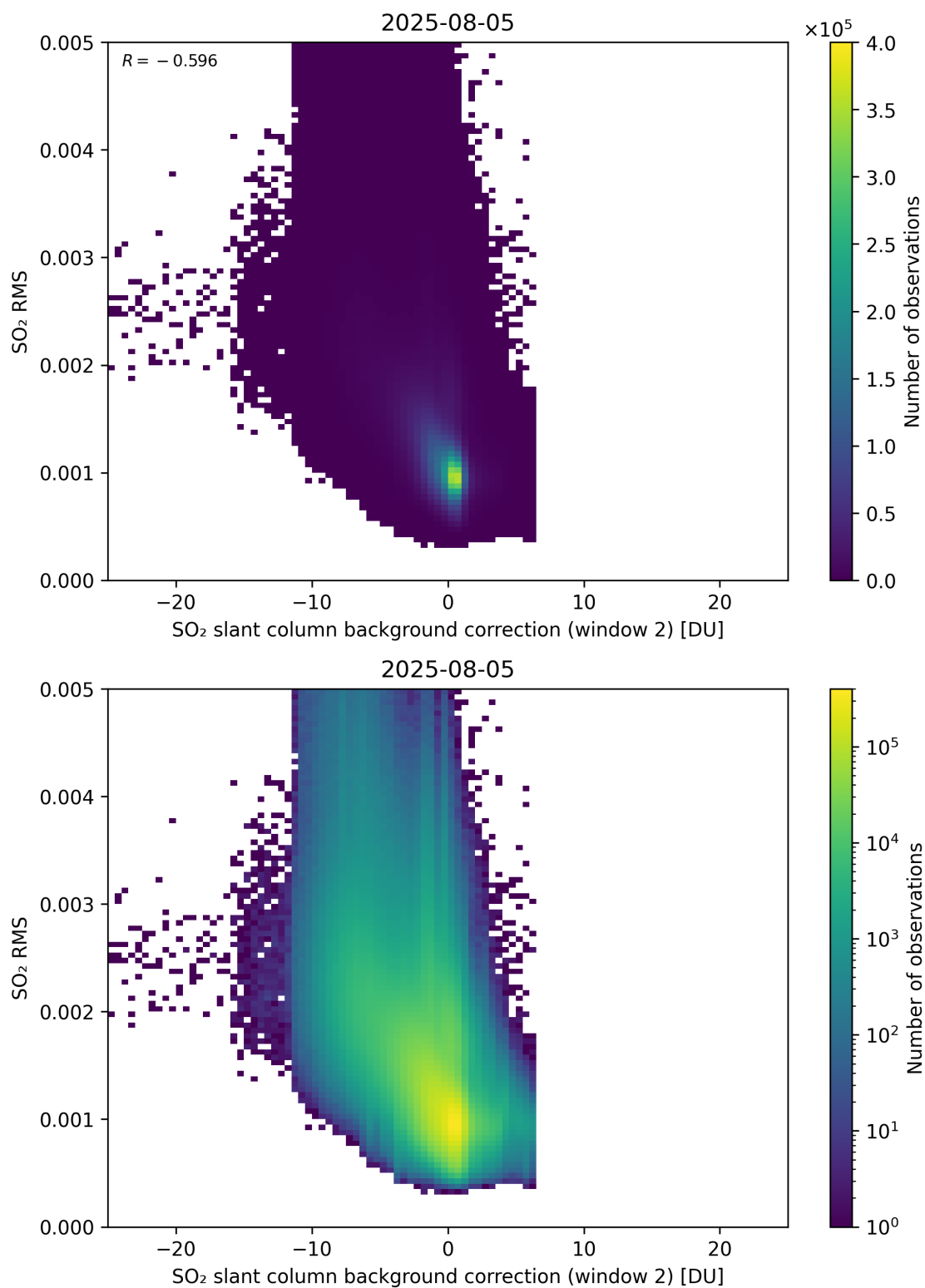
Figure 125: Scatter density plot of “SO 2 slant column background correction (window 2)” against “SO 2 RMS” for 2025-08-04 to 2025-08-06.
