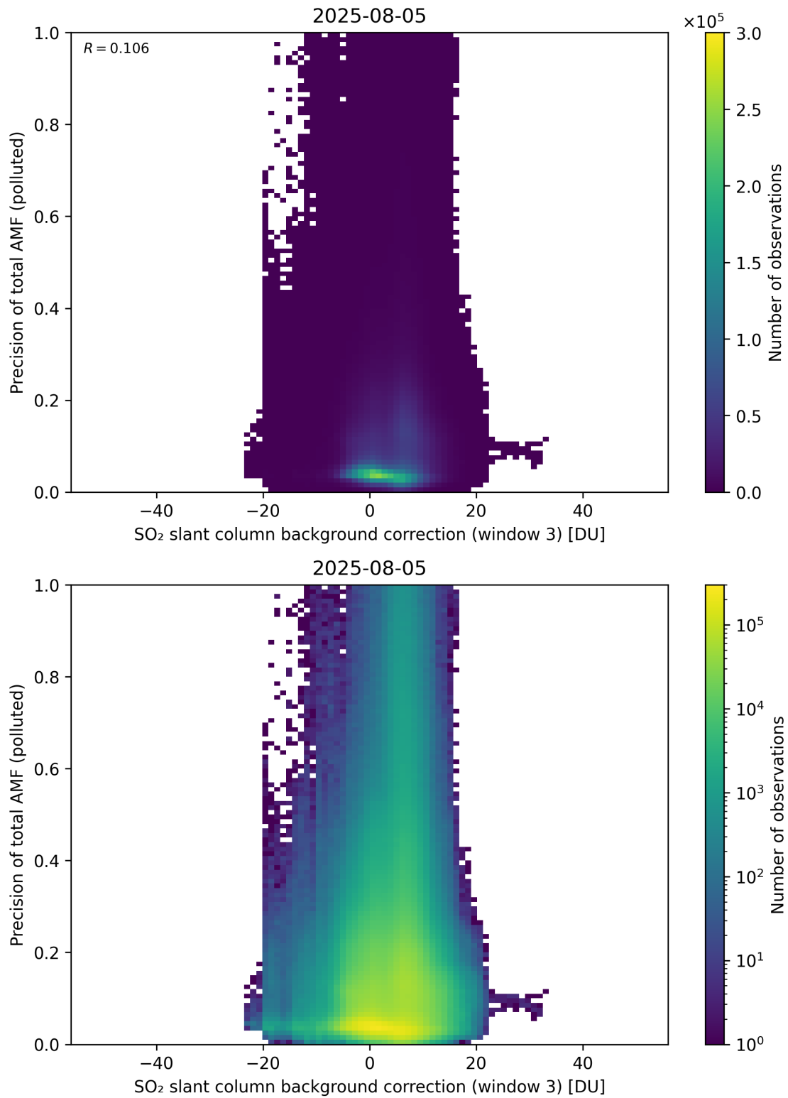
Figure 137: Scatter density plot of “SO 2 slant column background correction (window 3)” against “Precision of total AMF (polluted)” for 2025-08-04 to 2025-08-06.
