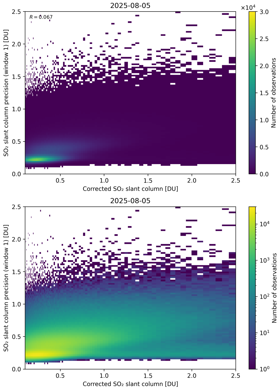
Figure 238: Scatter density plot of “Corrected SO 2 slant column” against “SO 2 slant column precision (window 1)” for 2025-08-04 to 2025-08-06.
