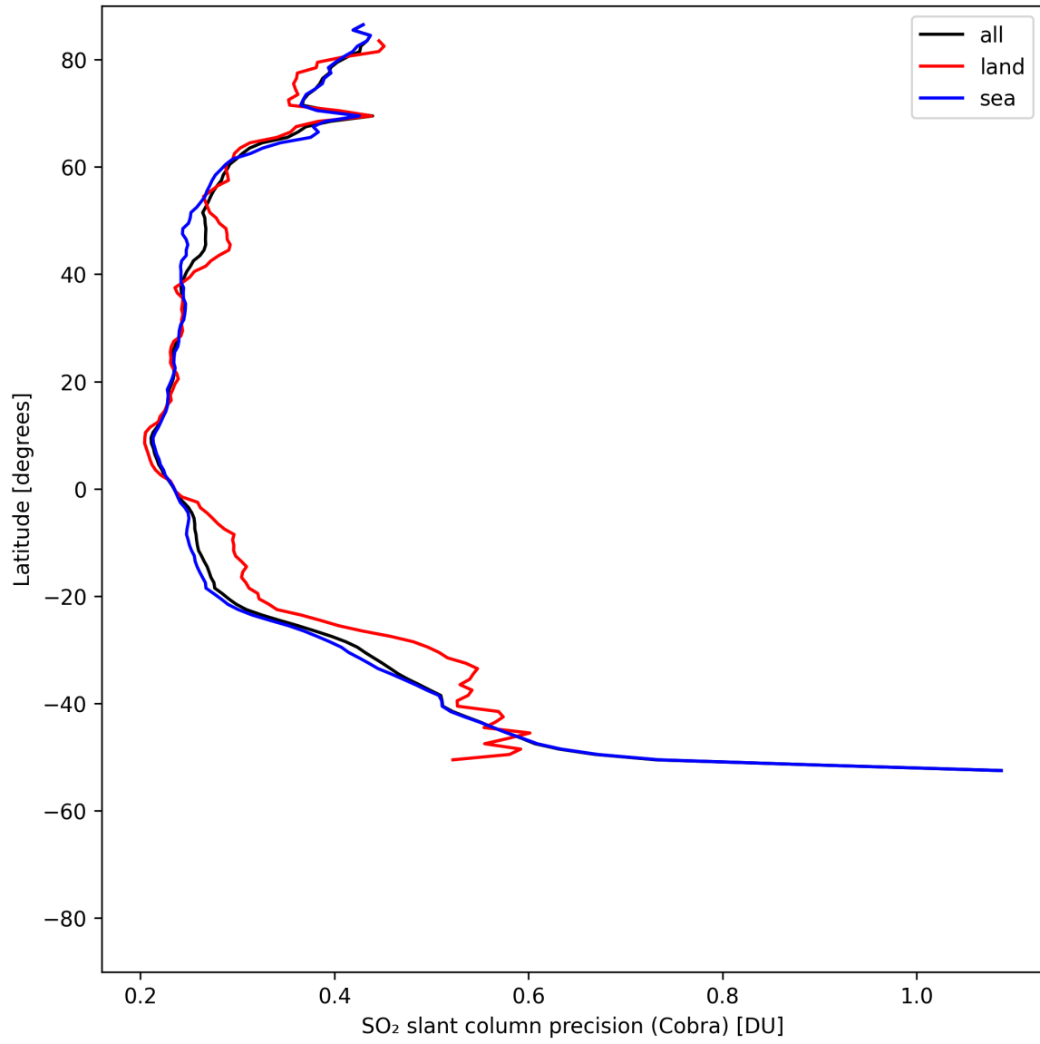
Figure 36: Zonal average of “SO 2 slant column precision (Cobra)” for 2025-08-04 to 2025-08-06.
