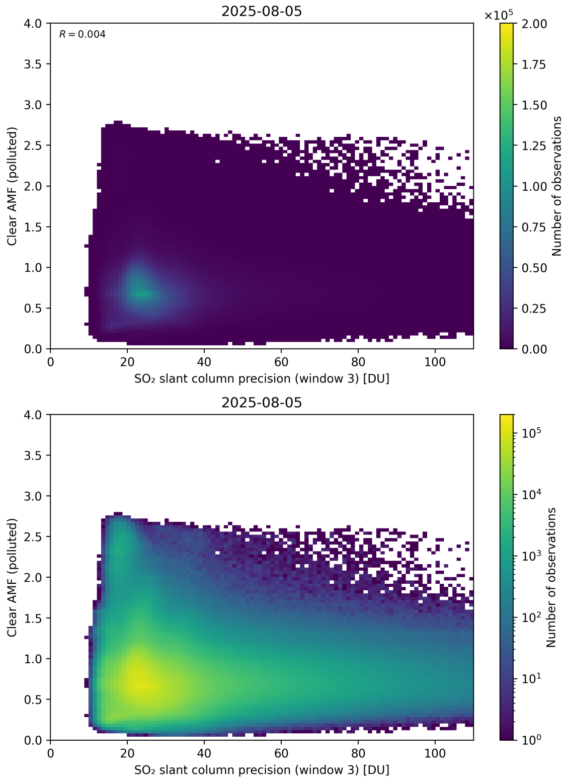
Figure 311: Scatter density plot of “SO 2 slant column precision (window 3)” against “Clear AMF (polluted)” for 2025-08-04 to 2025-08-06.
