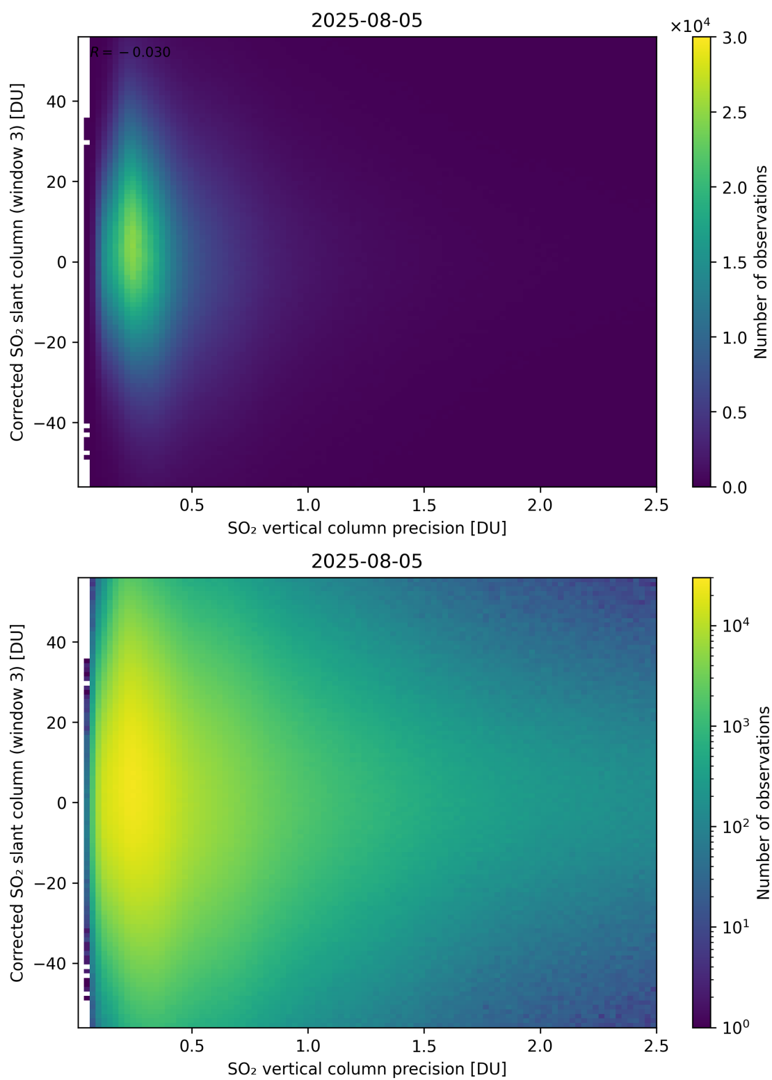
Figure 340: Scatter density plot of “SO 2 vertical column precision” against “Corrected SO 2 slant column (window 3)” for 2025-08-04 to 2025-08-06.
