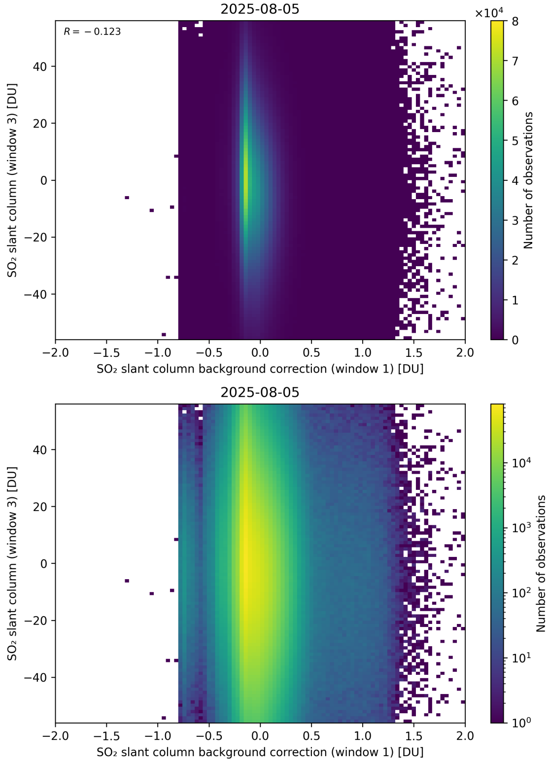
Figure 118: Scatter density plot of “SO 2 slant column background correction (window 1)” against “SO 2 slant column (window 3)” for 2025-08-04 to 2025-08-06.
