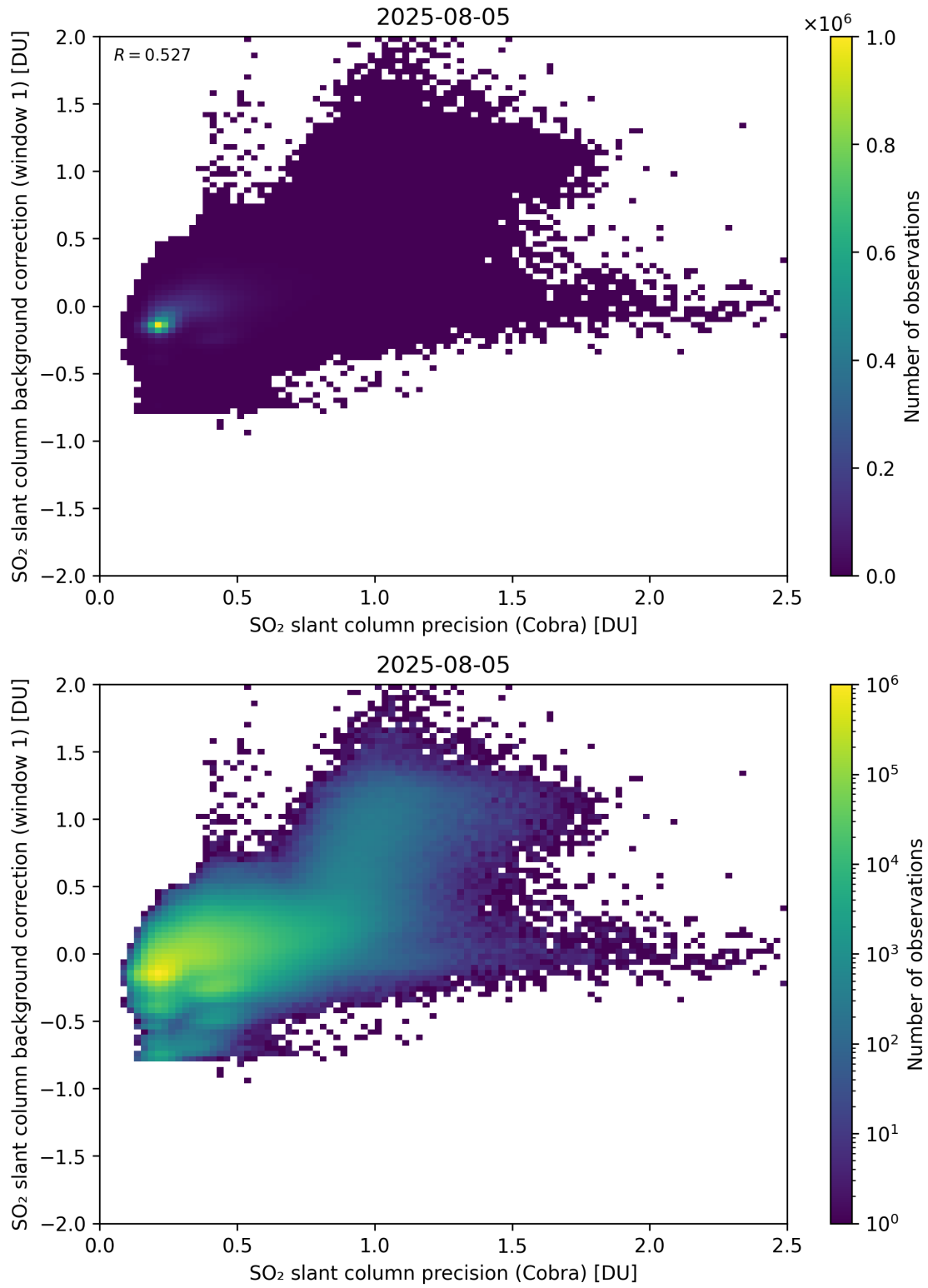
Figure 199: Scatter density plot of “SO 2 slant column precision (Cobra)” against “SO 2 slant column background correction (window 1)” for 2025-08-04 to 2025-08-06.
