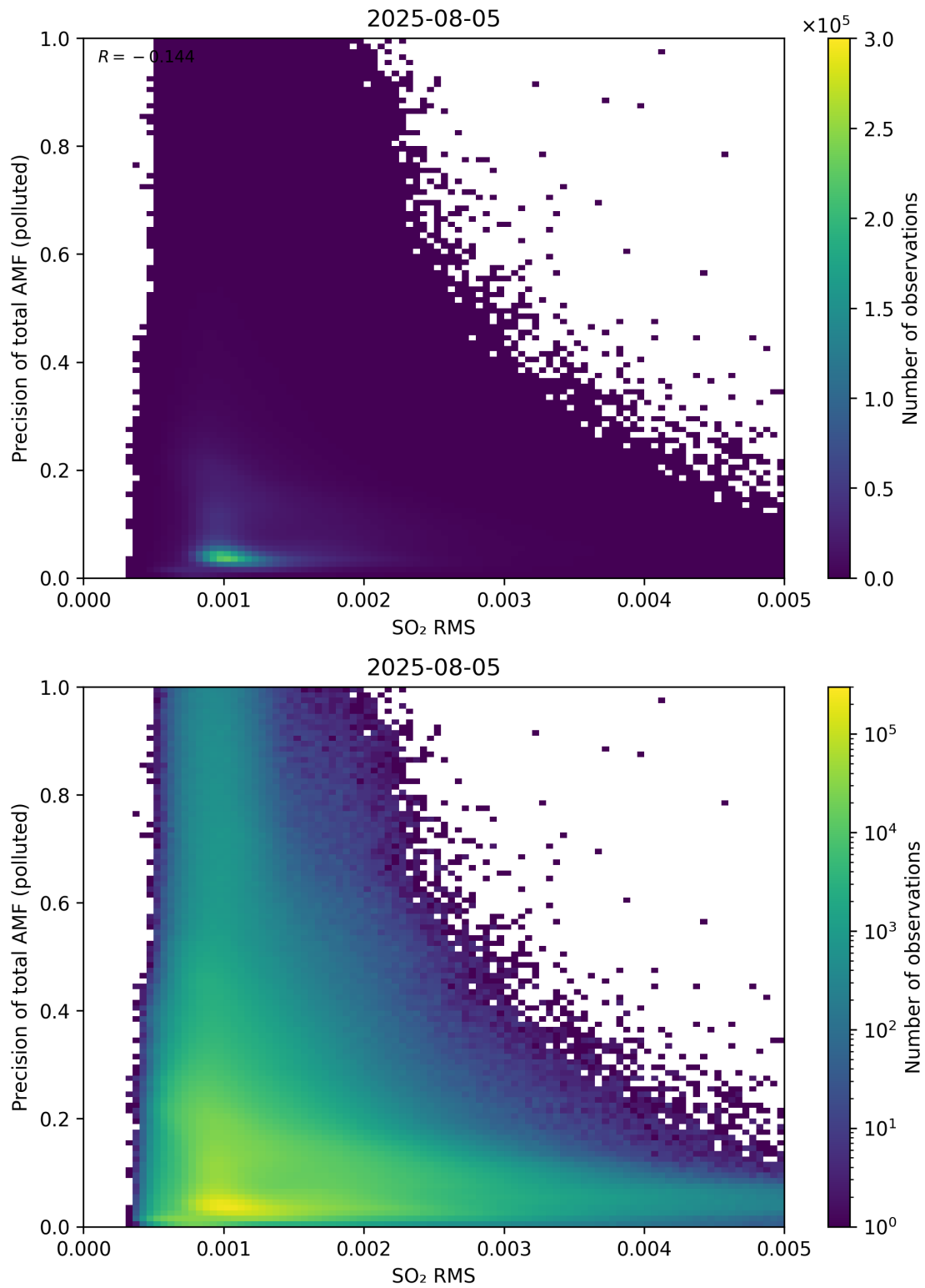
Figure 149: Scatter density plot of “SO 2 RMS” against “Precision of total AMF (polluted)” for 2025-08-04 to 2025-08-06.
