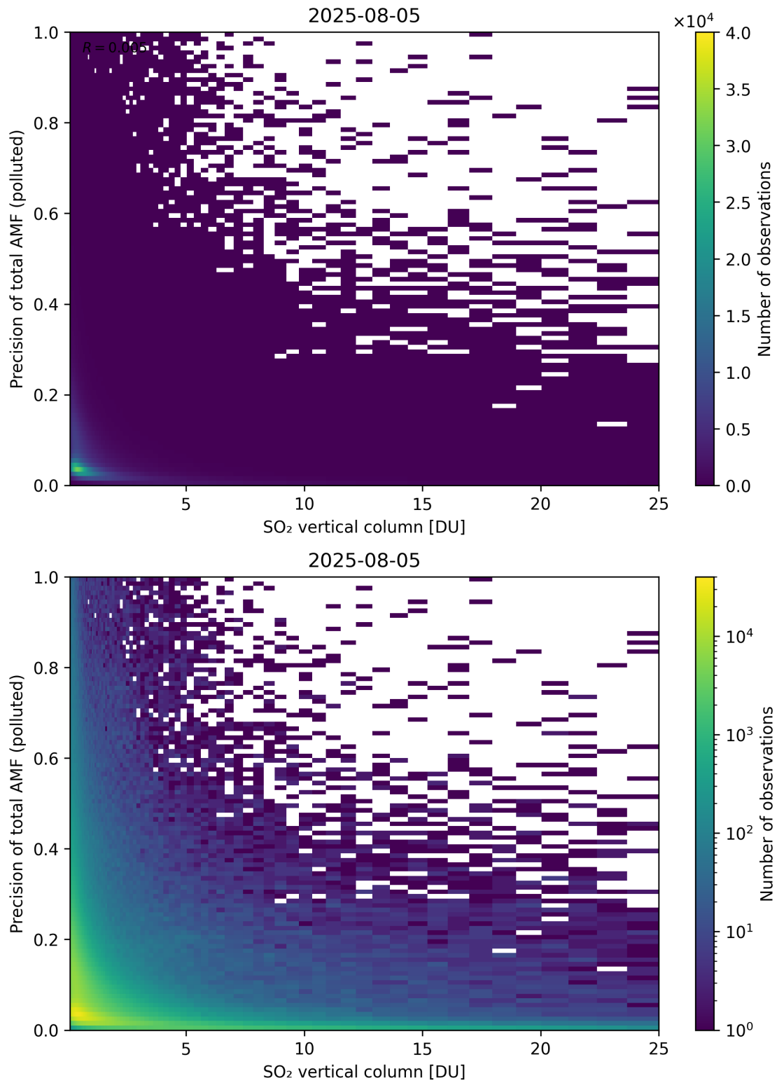
Figure 360: Scatter density plot of “SO 2 vertical column” against “Precision of total AMF (polluted)” for 2025-08-04 to 2025-08-06.
