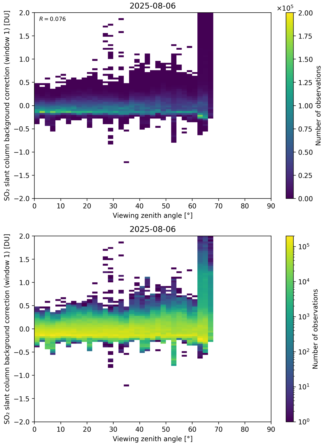
Figure 362: Scatter density plot of “Viewing zenith angle” against “SO 2 slant column background correction (window 1)” for 2025-08-05 to 2025-08-07.
