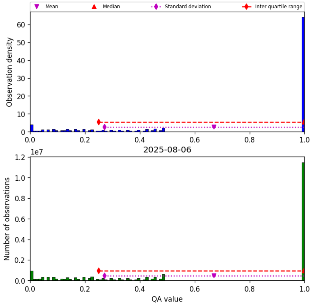
Figure 57: Histogram of “QA value” for 2025-08-05 to 2025-08-07
