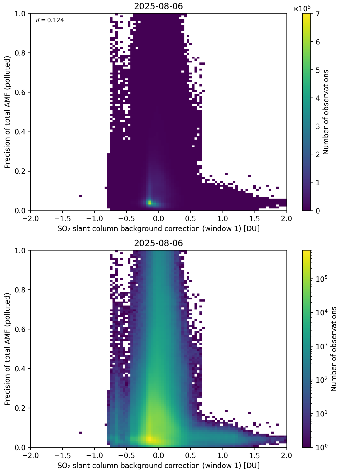
Figure 121: Scatter density plot of “SO 2 slant column background correction (window 1)” against “Precision of total AMF (polluted)” for 2025-08-05 to 2025-08-07.
