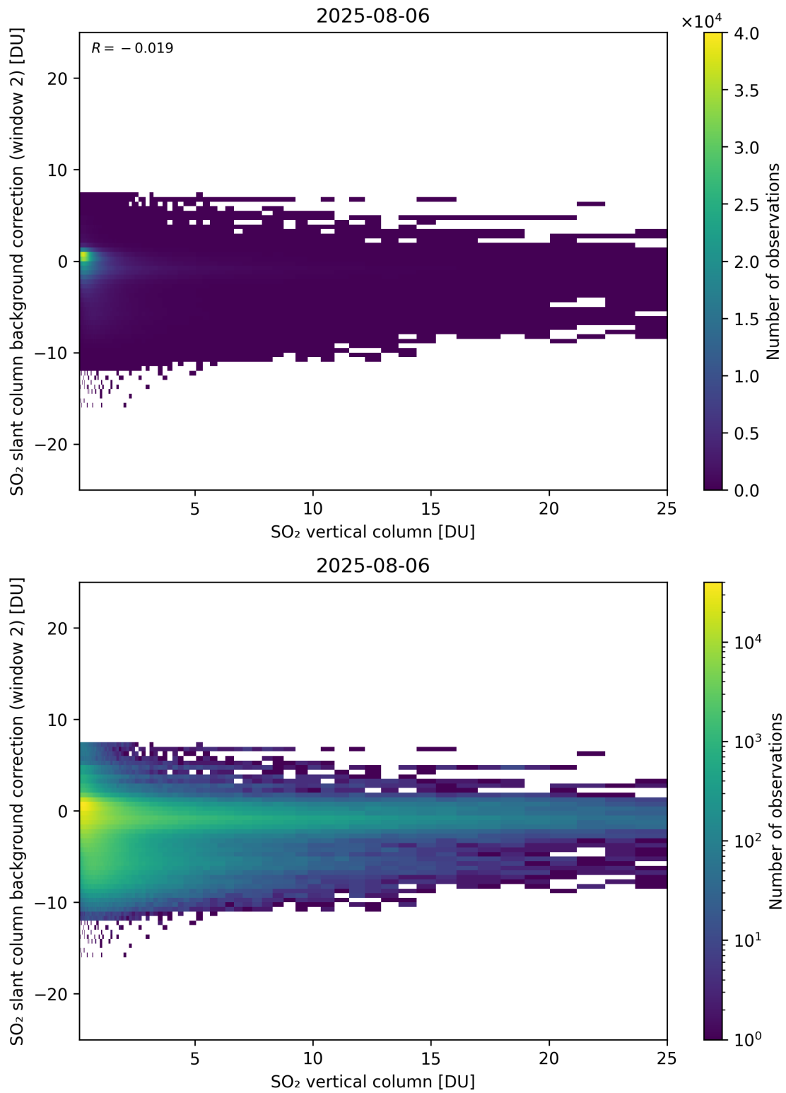
Figure 324: Scatter density plot of “SO 2 vertical column” against “SO 2 slant column background correction (window 2)” for 2025-08-05 to 2025-08-07.
