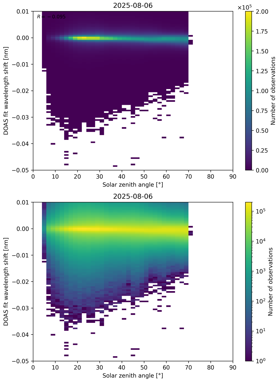
Figure 174: Scatter density plot of “Solar zenith angle” against “DOAS fit wavelength shift” for 2025-08-05 to 2025-08-07.
