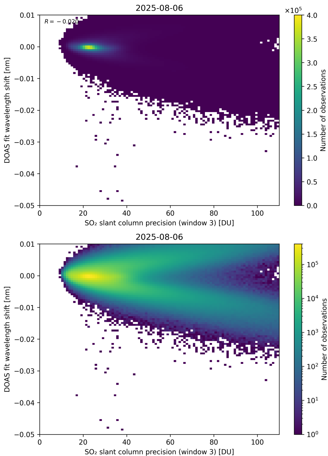
Figure 308: Scatter density plot of “SO 2 slant column precision (window 3)” against “DOAS fit wavelength shift” for 2025-08-05 to 2025-08-07.
