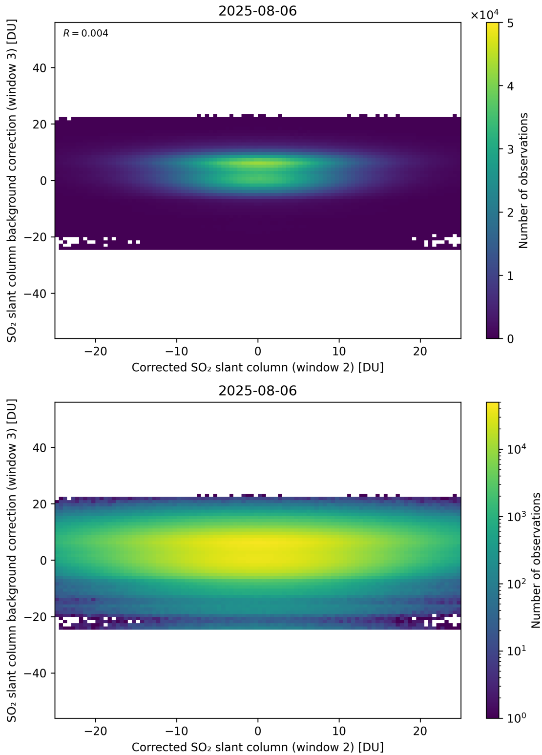
Figure 245: Scatter density plot of “Corrected SO 2 slant column (window 2)” against “SO 2 slant column background correction (window 3)” for 2025-08-05 to 2025-08-07.
