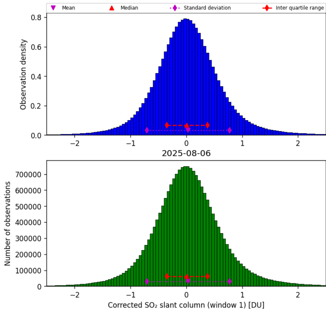
Figure 65: Histogram of “Corrected SO 2 slant column (window 1)” for 2025-08-05 to 2025-08-07
