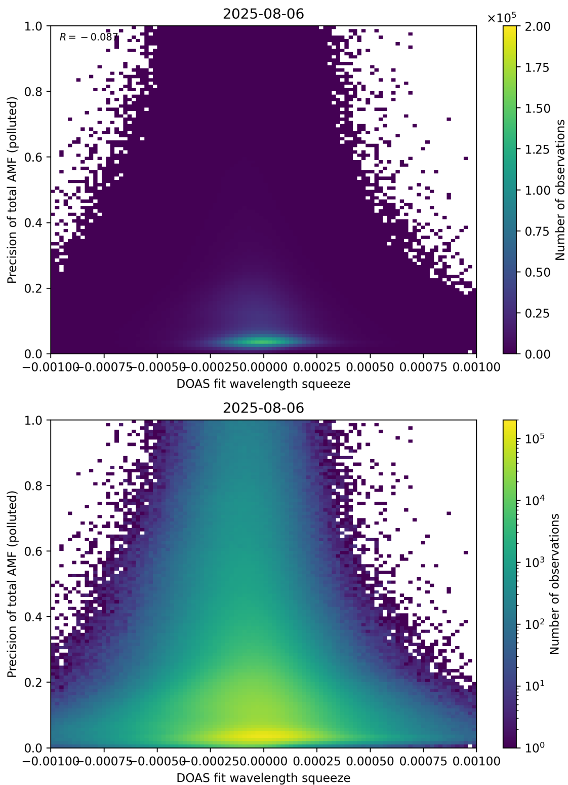
Figure 146: Scatter density plot of “DOAS fit wavelength squeeze” against “Precision of total AMF (polluted)” for 2025-08-05 to 2025-08-07.
