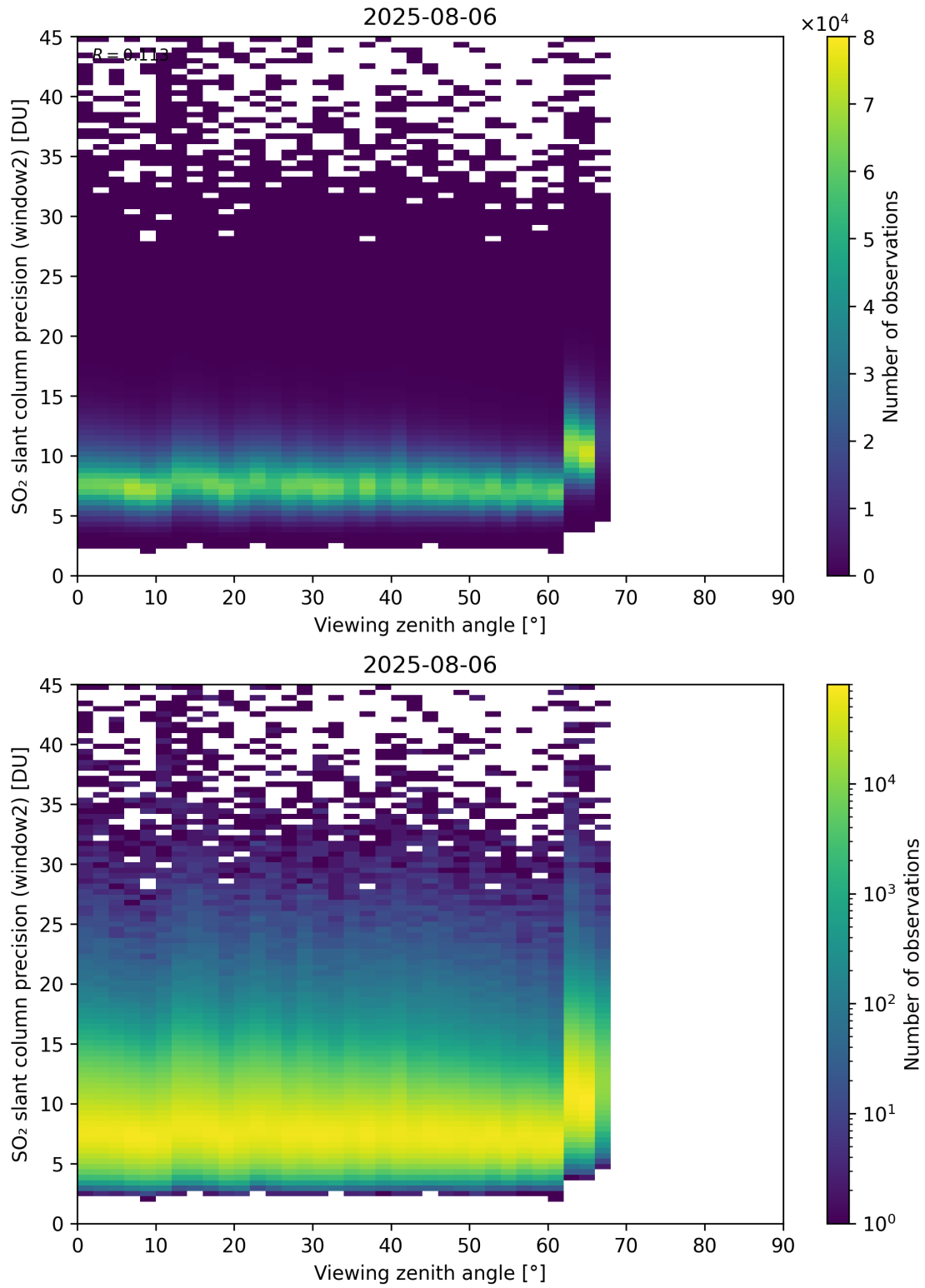
Figure 378: Scatter density plot of “Viewing zenith angle” against “SO 2 slant column precision (window2)” for 2025-08-05 to 2025-08-07.
