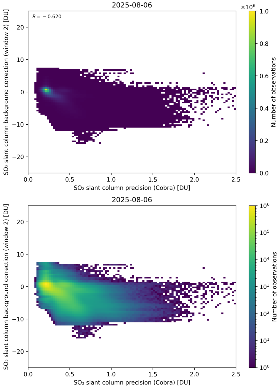
Figure 200: Scatter density plot of “SO 2 slant column precision (Cobra)” against “SO 2 slant column background correction (window 2)” for 2025-08-05 to 2025-08-07.
