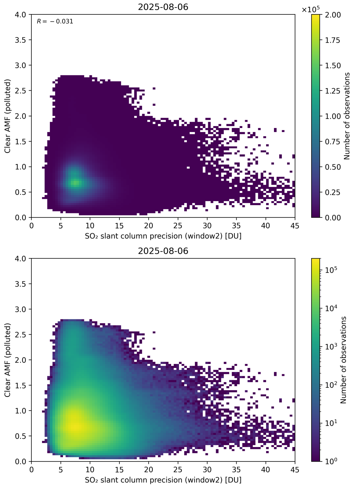
Figure 296: Scatter density plot of “SO 2 slant column precision (window2)” against “Clear AMF (polluted)” for 2025-08-05 to 2025-08-07.
