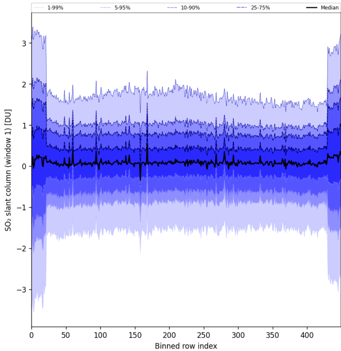
Figure 89: Along track statistics of “SO 2 slant column (window 1)” for 2025-08-05 to 2025-08-07
