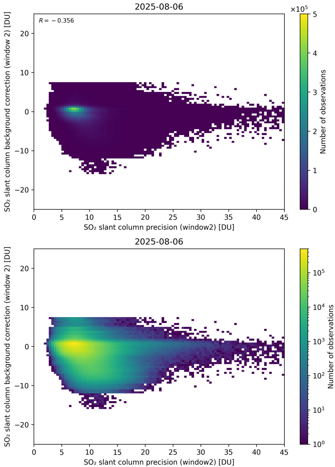
Figure 291: Scatter density plot of “SO 2 slant column precision (window2)” against “SO 2 slant column background correction (window 2)” for 2025-08-05 to 2025-08-07.
