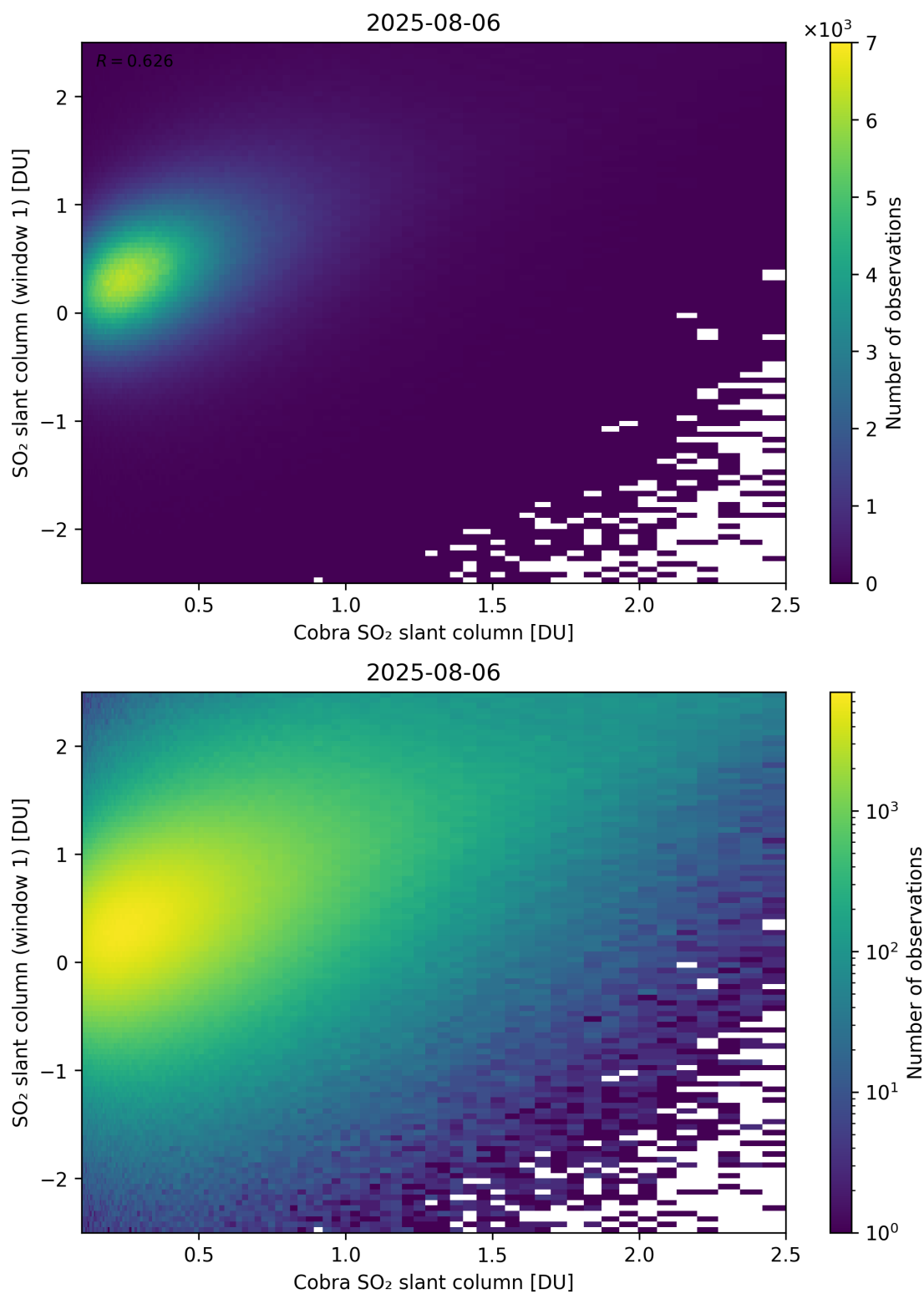
Figure 219: Scatter density plot of “Cobra SO 2 slant column” against “SO 2 slant column (window 1)” for 2025-08-05 to 2025-08-07.
