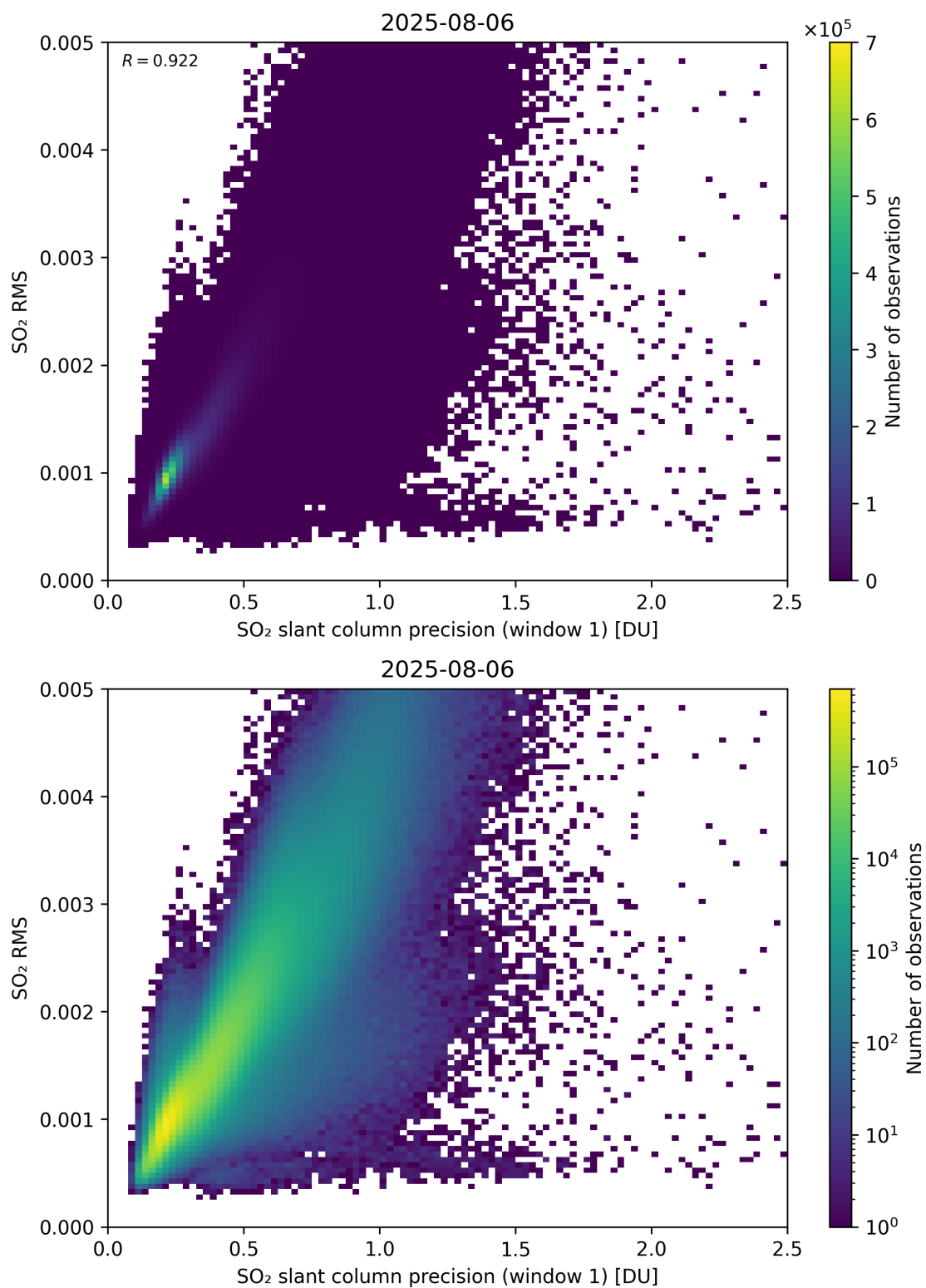
Figure 273: Scatter density plot of “SO 2 slant column precision (window 1)” against “SO 2 RMS” for 2025-08-05 to 2025-08-07.
