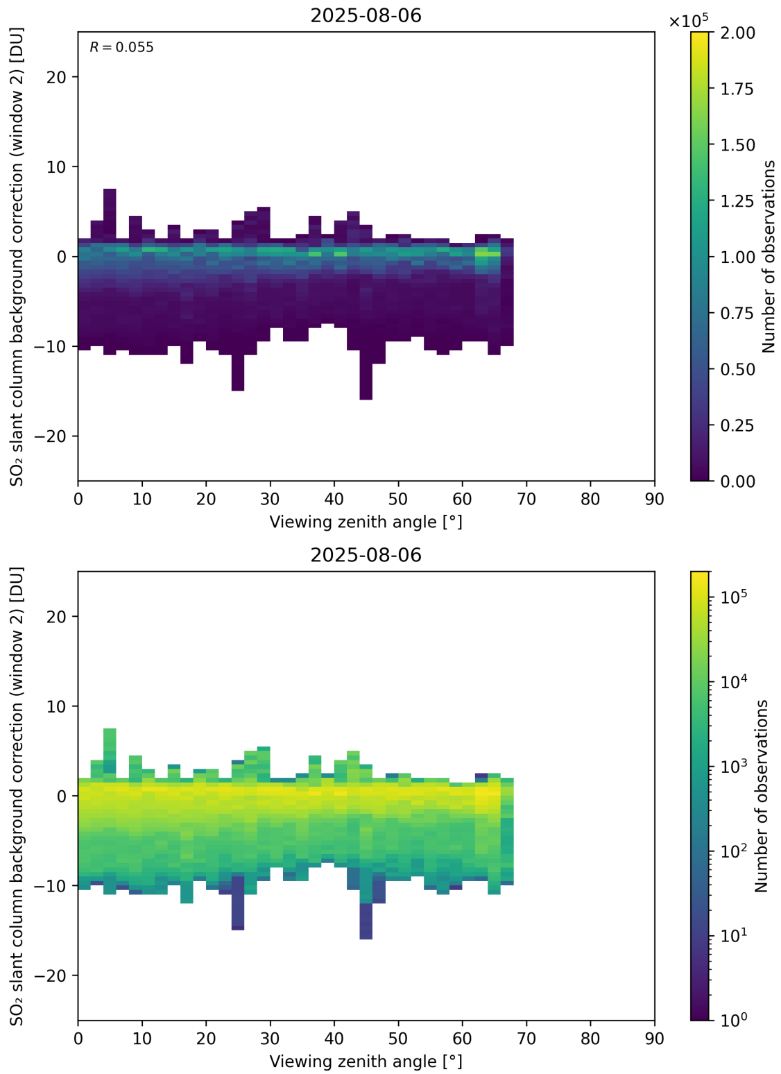
Figure 363: Scatter density plot of “Viewing zenith angle” against “SO 2 slant column background correction (window 2)” for 2025-08-05 to 2025-08-07.
