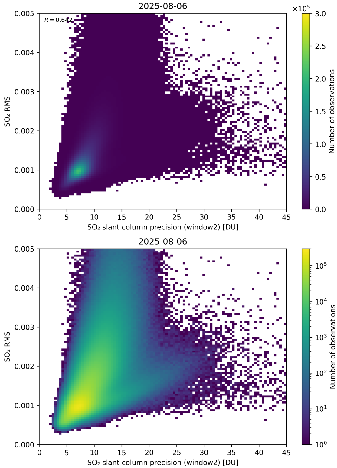
Figure 295: Scatter density plot of “SO 2 slant column precision (window2)” against “SO 2 RMS” for 2025-08-05 to 2025-08-07.
