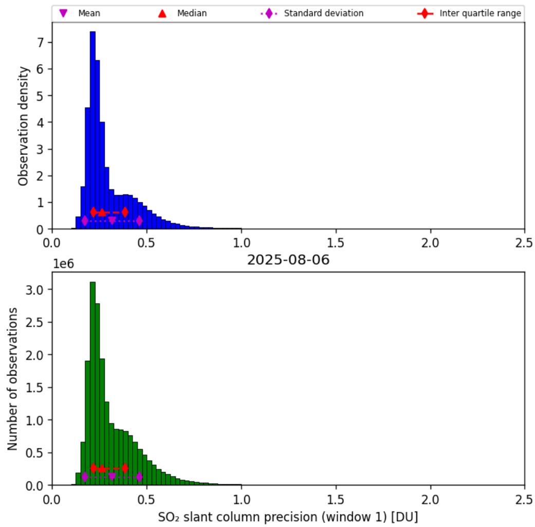
Figure 64: Histogram of “SO 2 slant column precision (window 1)” for 2025-08-05 to 2025-08-07
