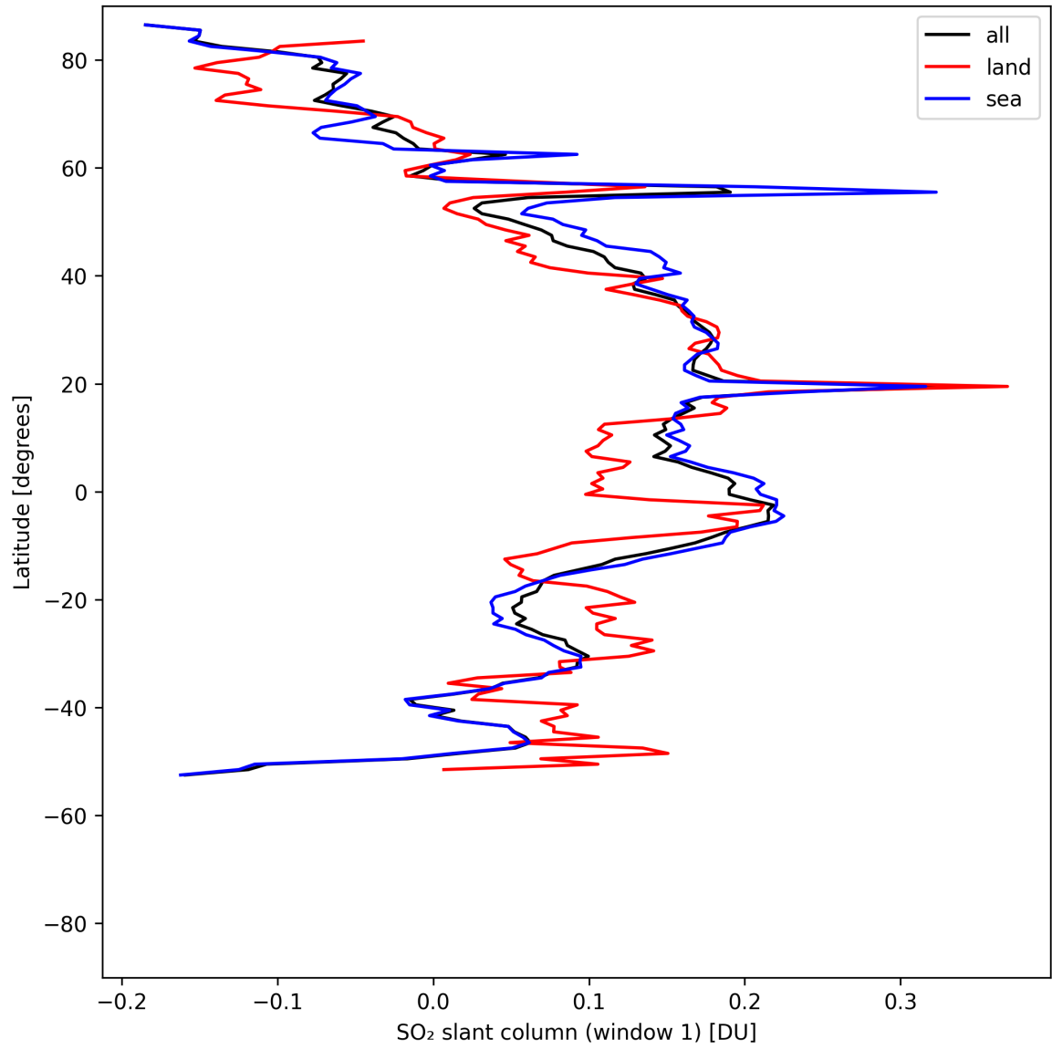
Figure 37: Zonal average of “SO 2 slant column (window 1)” for 2025-08-05 to 2025-08-07.
