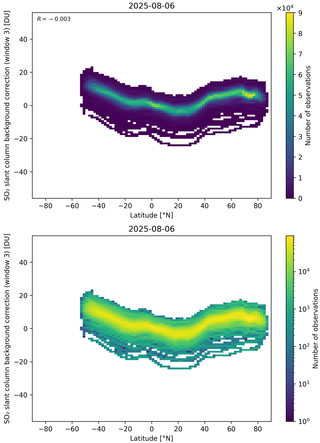
Figure 152: Scatter density plot of “Latitude” against “SO 2 slant column background correction (window 3)” for 2025-08-05 to 2025-08-07.
