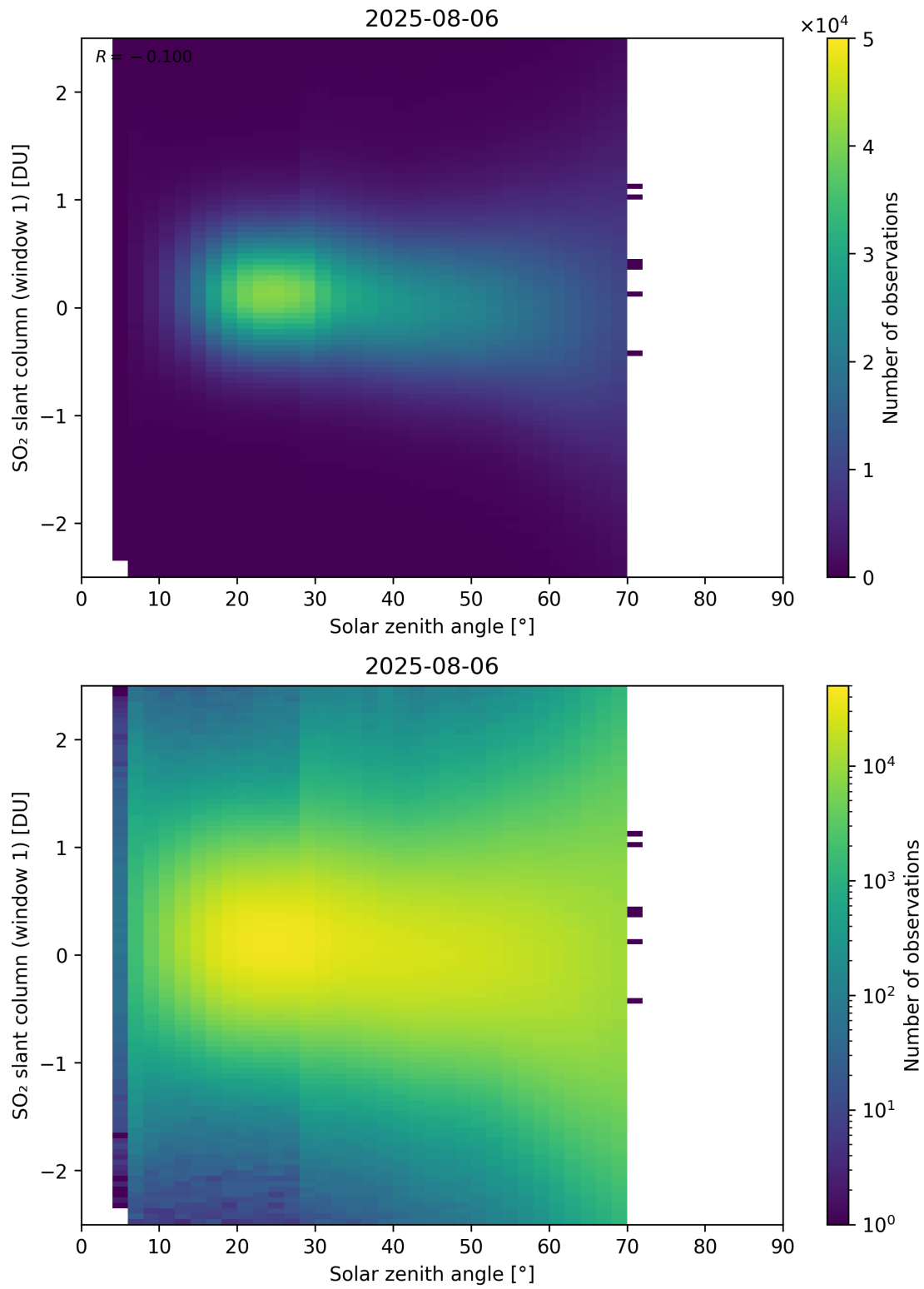
Figure 184: Scatter density plot of “Solar zenith angle” against “SO 2 slant column (window 1)” for 2025-08-05 to 2025-08-07.
