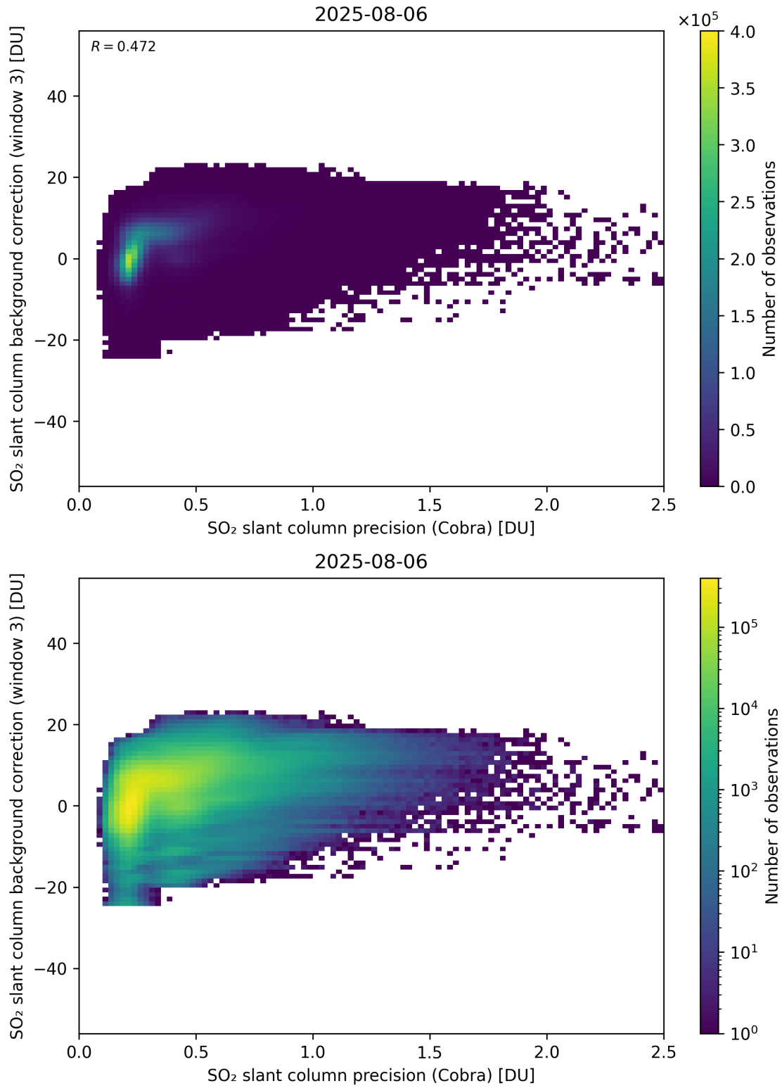
Figure 201: Scatter density plot of “SO 2 slant column precision (Cobra)” against “SO 2 slant column background correction (window 3)” for 2025-08-05 to 2025-08-07.
