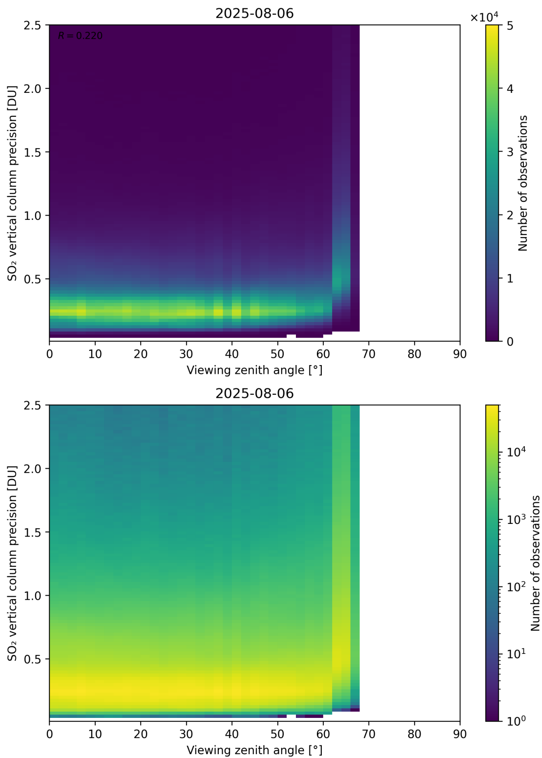
Figure 384: Scatter density plot of “Viewing zenith angle” against “SO 2 vertical column precision” for 2025-08-05 to 2025-08-07.
