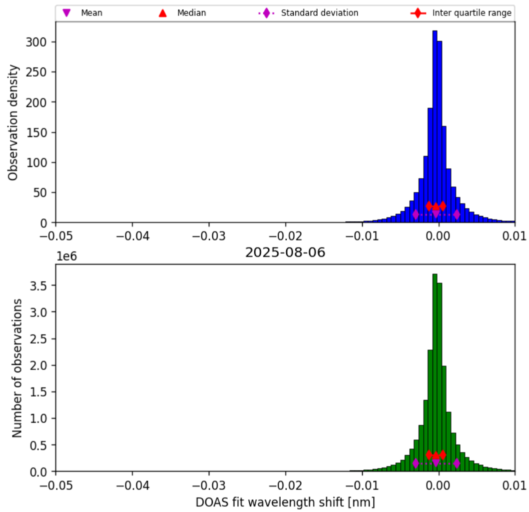
Figure 76: Histogram of “DOAS fit wavelength shift” for 2025-08-05 to 2025-08-07
