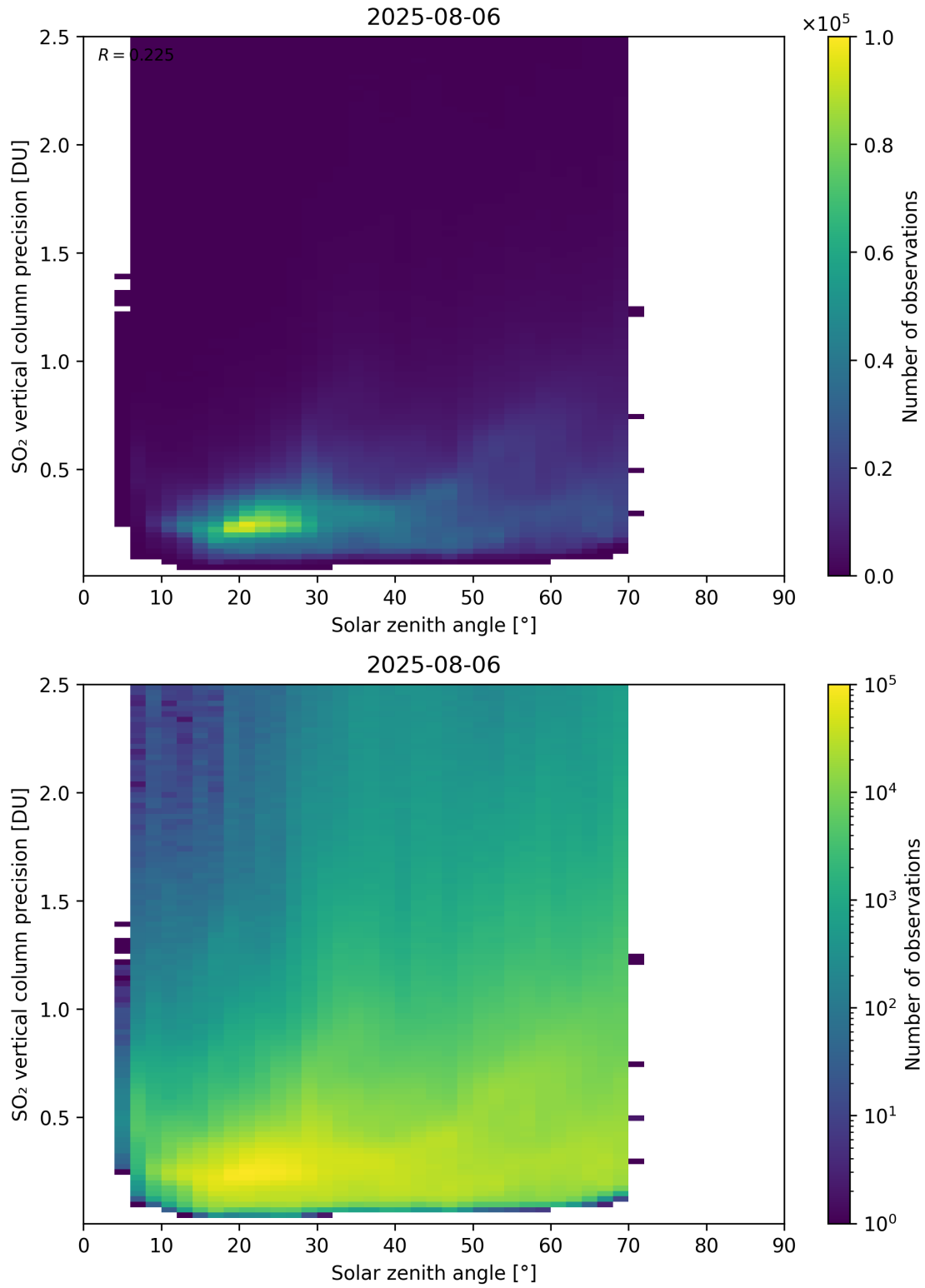
Figure 192: Scatter density plot of “Solar zenith angle” against “SO 2 vertical column precision” for 2025-08-05 to 2025-08-07.
