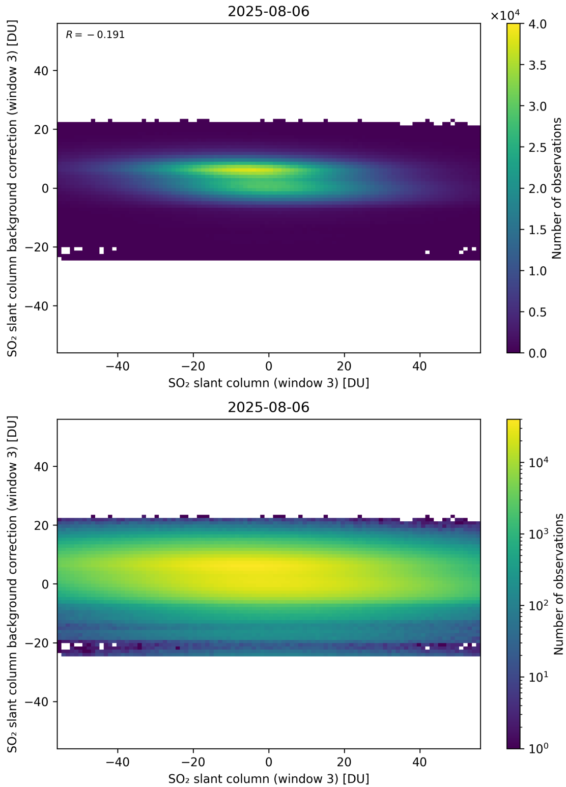
Figure 303: Scatter density plot of “SO 2 slant column (window 3)” against “SO 2 slant column background correction (window 3)” for 2025-08-05 to 2025-08-07.
