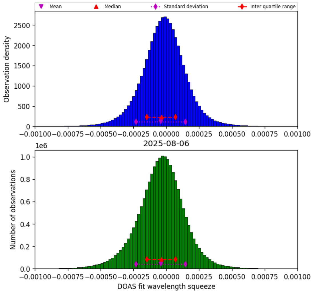
Figure 77: Histogram of “DOAS fit wavelength squeeze” for 2025-08-05 to 2025-08-07
