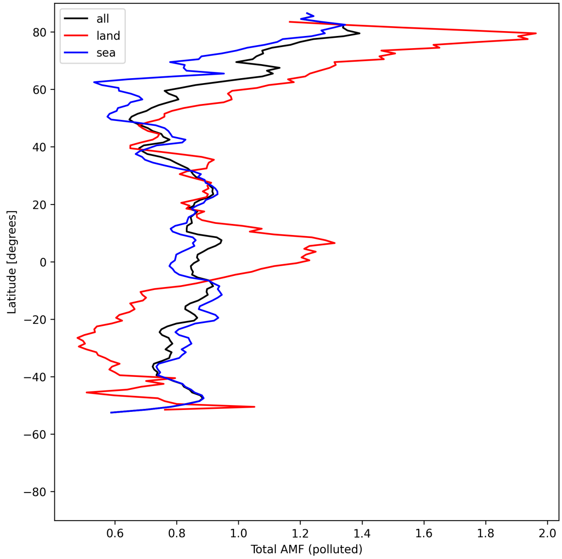
Figure 53: Zonal average of “Total AMF (polluted)” for 2025-08-05 to 2025-08-07.
