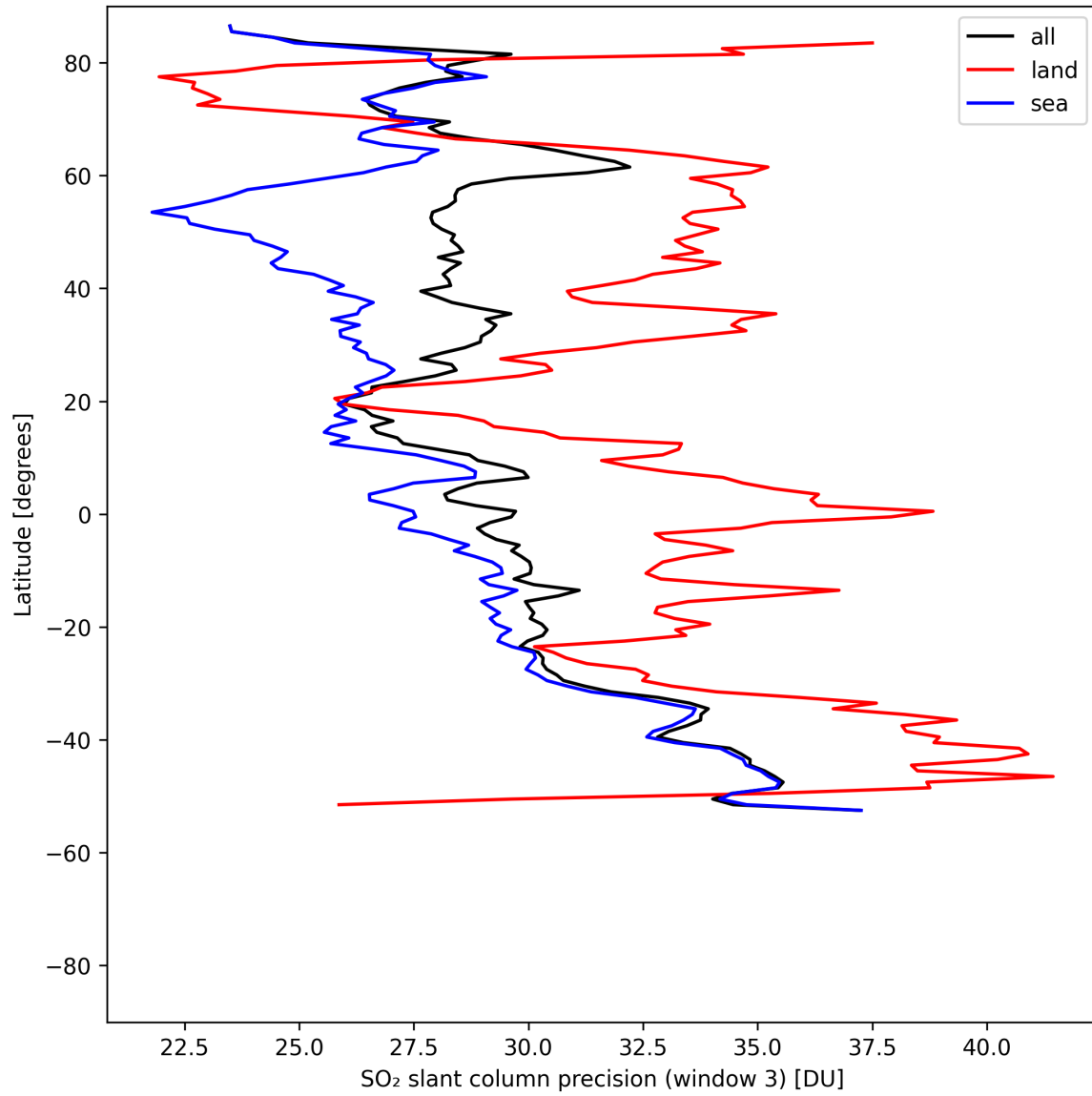
Figure 46: Zonal average of “SO 2 slant column precision (window 3)” for 2025-08-05 to 2025-08-07.
