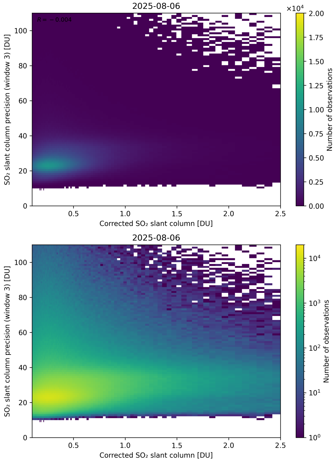
Figure 241: Scatter density plot of “Corrected SO 2 slant column” against “SO 2 slant column precision (window 3)” for 2025-08-05 to 2025-08-07.
