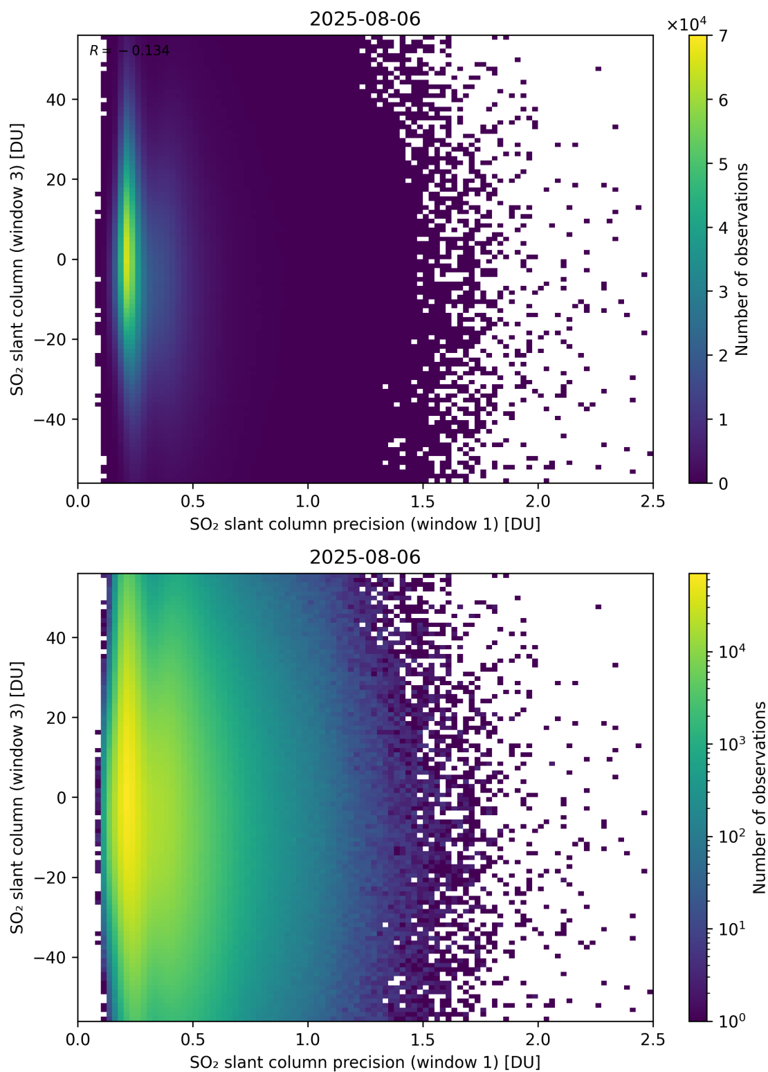
Figure 278: Scatter density plot of “SO 2 slant column precision (window 1)” against “SO 2 slant column (window 3)” for 2025-08-05 to 2025-08-07.
