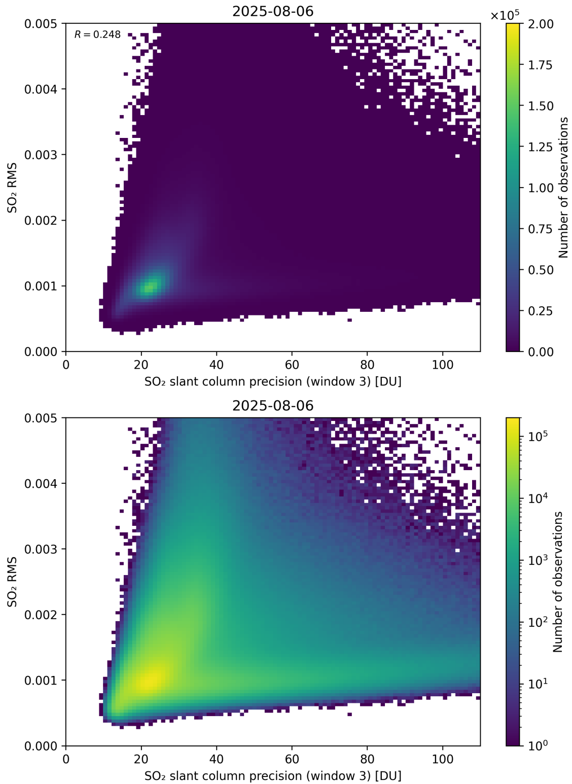
Figure 310: Scatter density plot of “SO 2 slant column precision (window 3)” against “SO 2 RMS” for 2025-08-05 to 2025-08-07.
