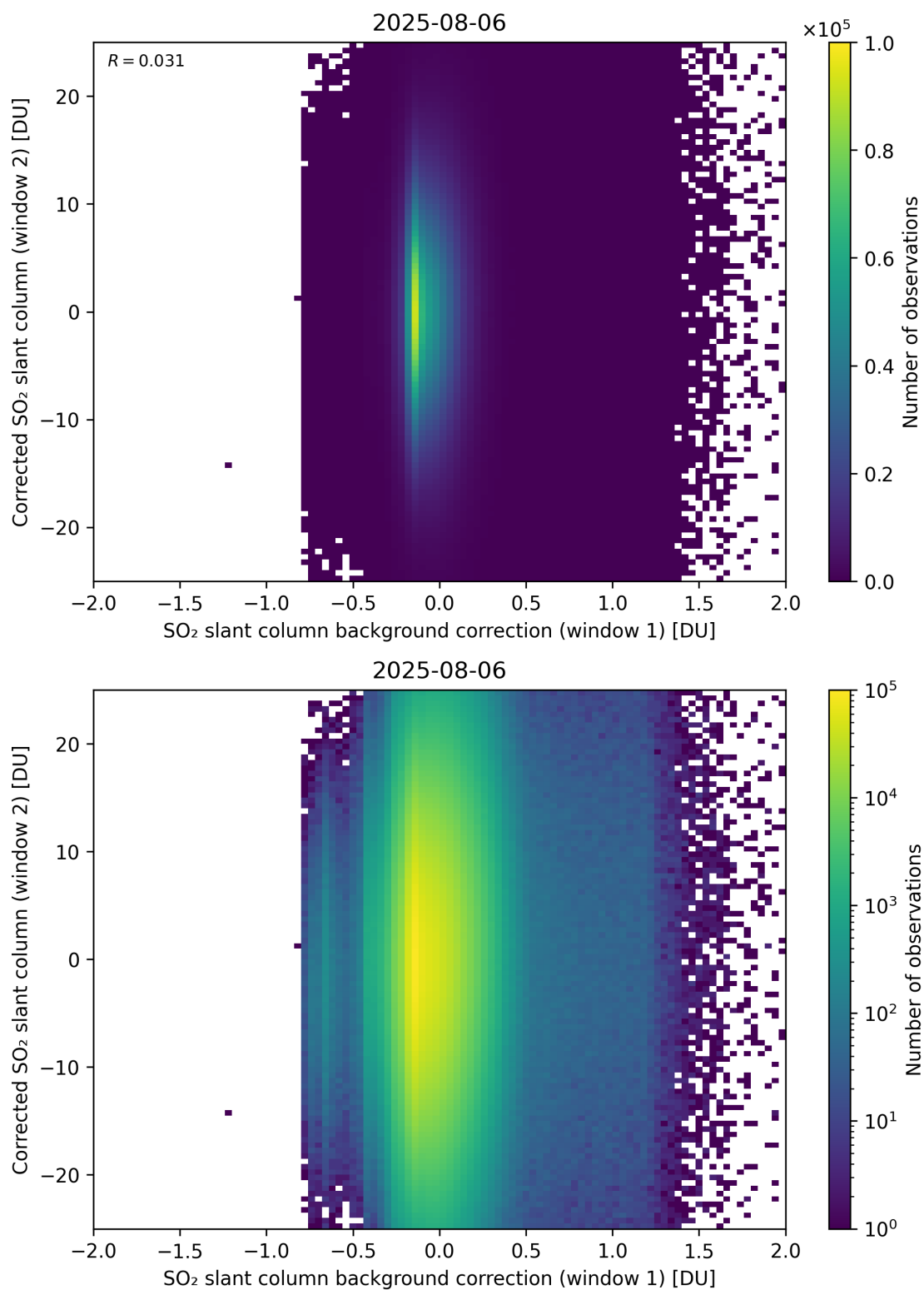
Figure 115: Scatter density plot of “SO 2 slant column background correction (window 1)” against “Corrected SO 2 slant column (window 2)” for 2025-08-05 to 2025-08-07.
