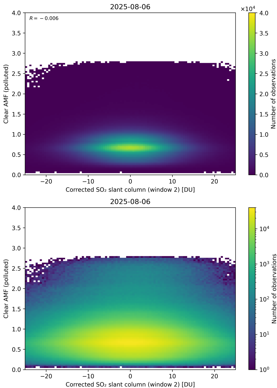
Figure 249: Scatter density plot of “Corrected SO 2 slant column (window 2)” against “Clear AMF (polluted)” for 2025-08-05 to 2025-08-07.
