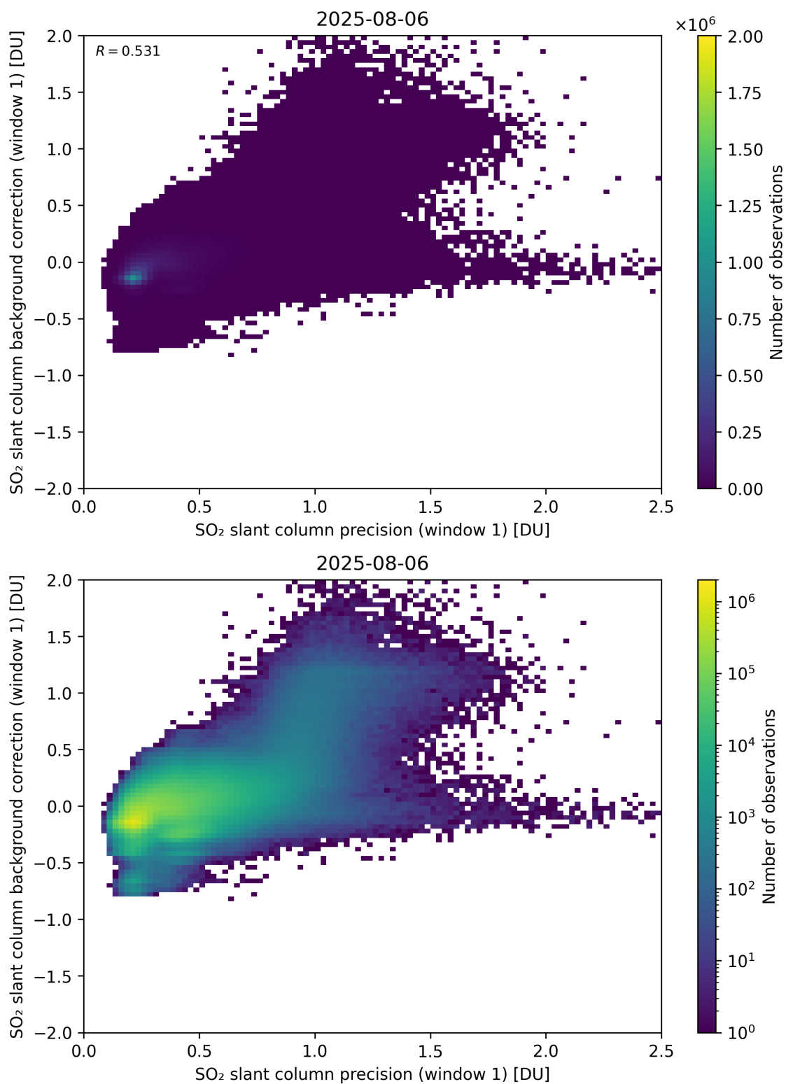
Figure 268: Scatter density plot of “SO 2 slant column precision (window 1)” against “SO 2 slant column background correction (window 1)” for 2025-08-05 to 2025-08-07.
