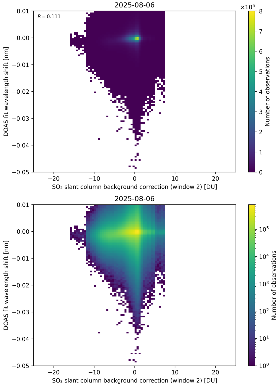
Figure 123: Scatter density plot of “SO 2 slant column background correction (window 2)” against “DOAS fit wavelength shift” for 2025-08-05 to 2025-08-07.
