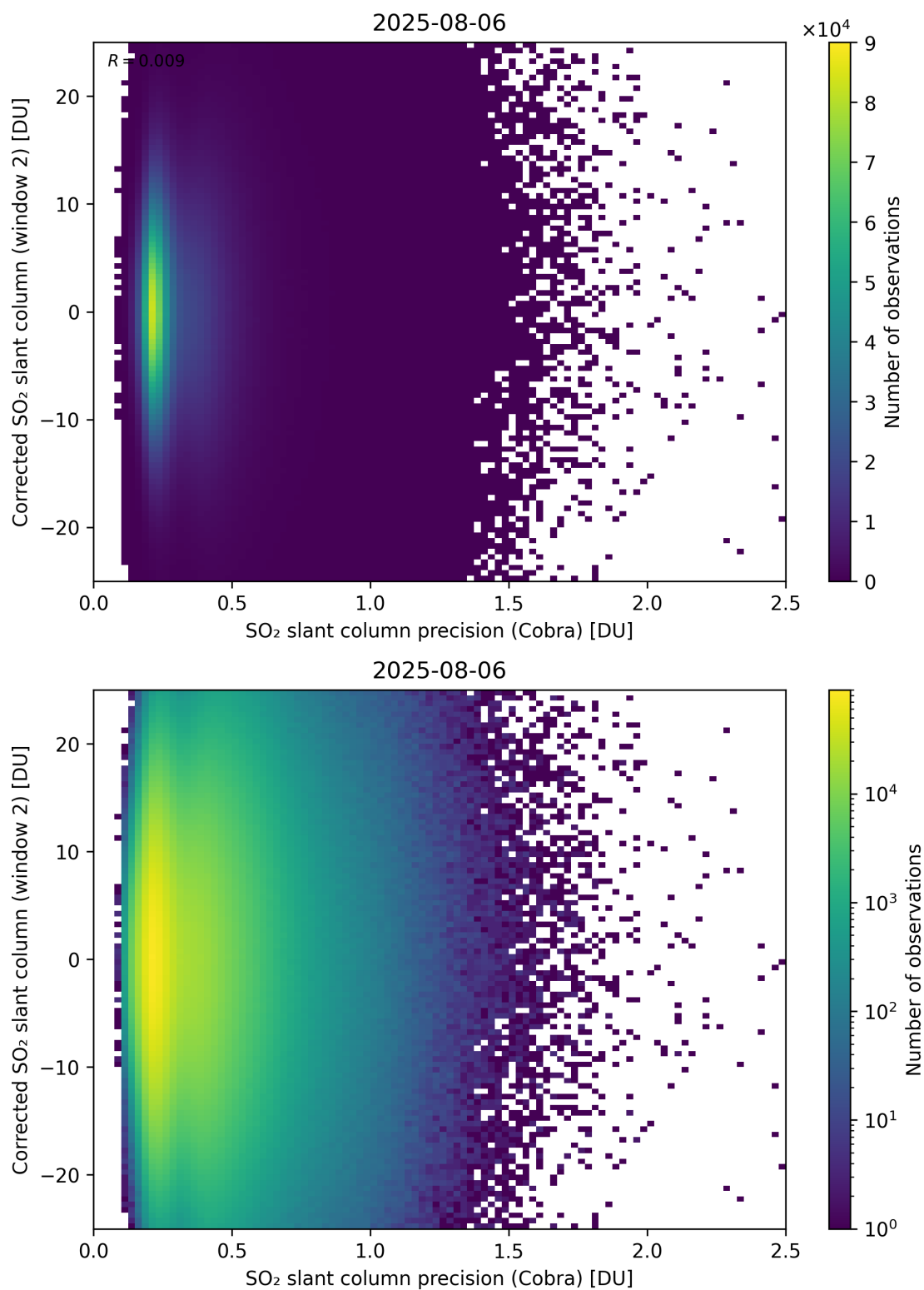
Figure 206: Scatter density plot of “SO 2 slant column precision (Cobra)” against “Corrected SO 2 slant column (window 2)” for 2025-08-05 to 2025-08-07.
