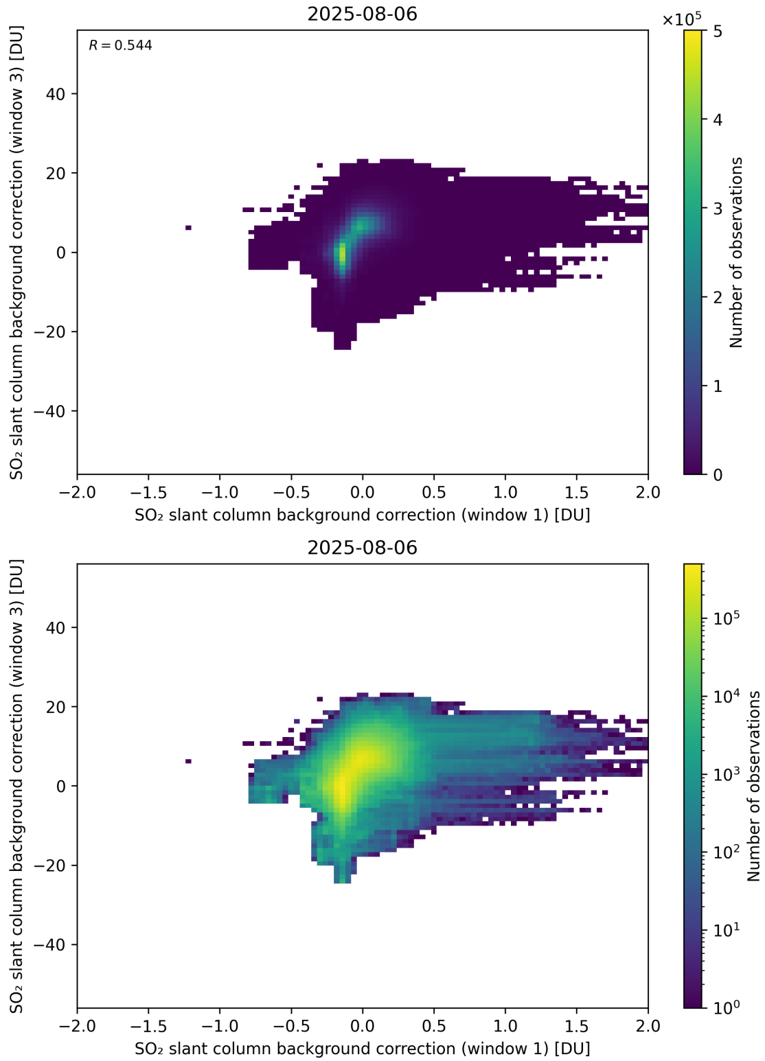
Figure 110: Scatter density plot of “SO 2 slant column background correction (window 1)” against “SO 2 slant column background correction (window 3)” for 2025-08-05 to 2025-08-07.
