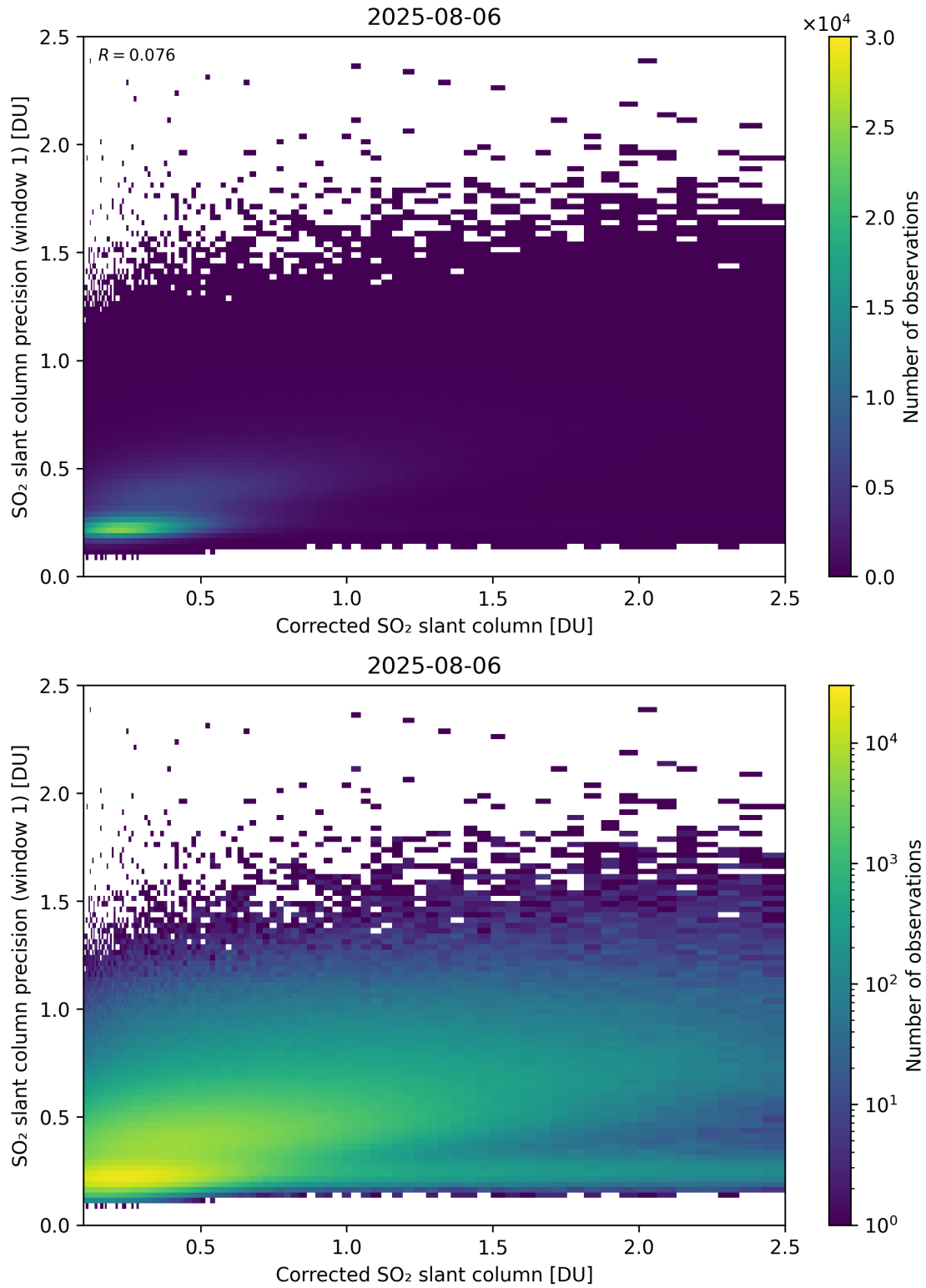
Figure 238: Scatter density plot of “Corrected SO 2 slant column” against “SO 2 slant column precision (window 1)” for 2025-08-05 to 2025-08-07.
