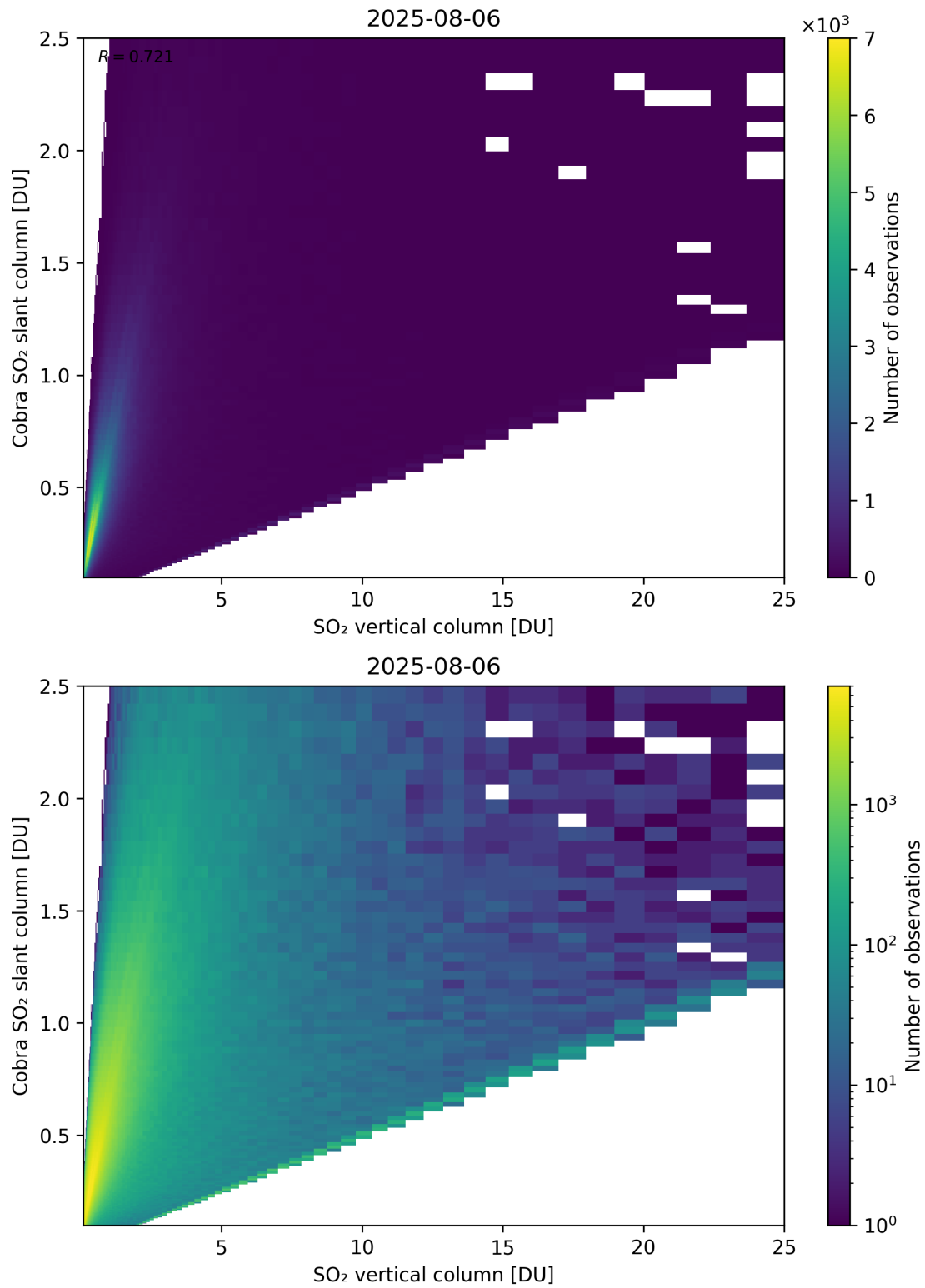
Figure 349: Scatter density plot of “SO 2 vertical column” against “Cobra SO 2 slant column” for 2025-08-05 to 2025-08-07.
