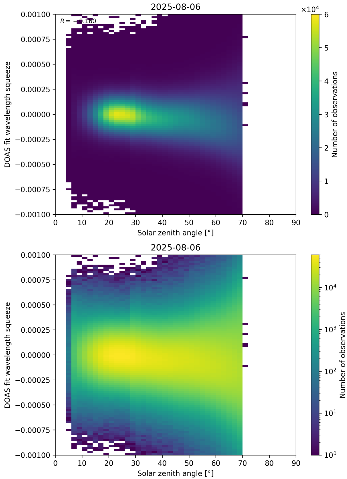
Figure 175: Scatter density plot of “Solar zenith angle” against “DOAS fit wavelength squeeze” for 2025-08-05 to 2025-08-07.
