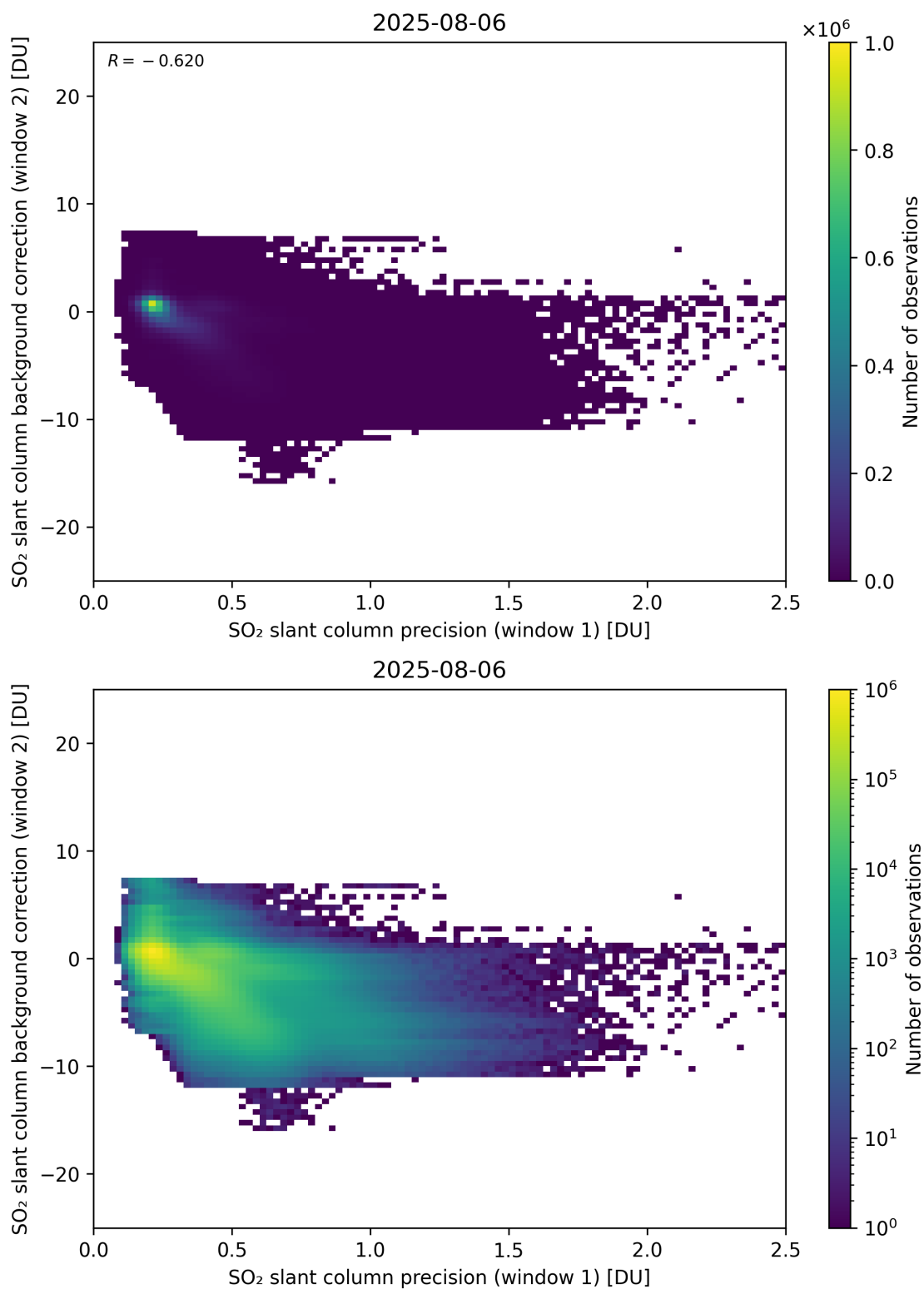
Figure 269: Scatter density plot of “SO 2 slant column precision (window 1)” against “SO 2 slant column background correction (window 2)” for 2025-08-05 to 2025-08-07.
