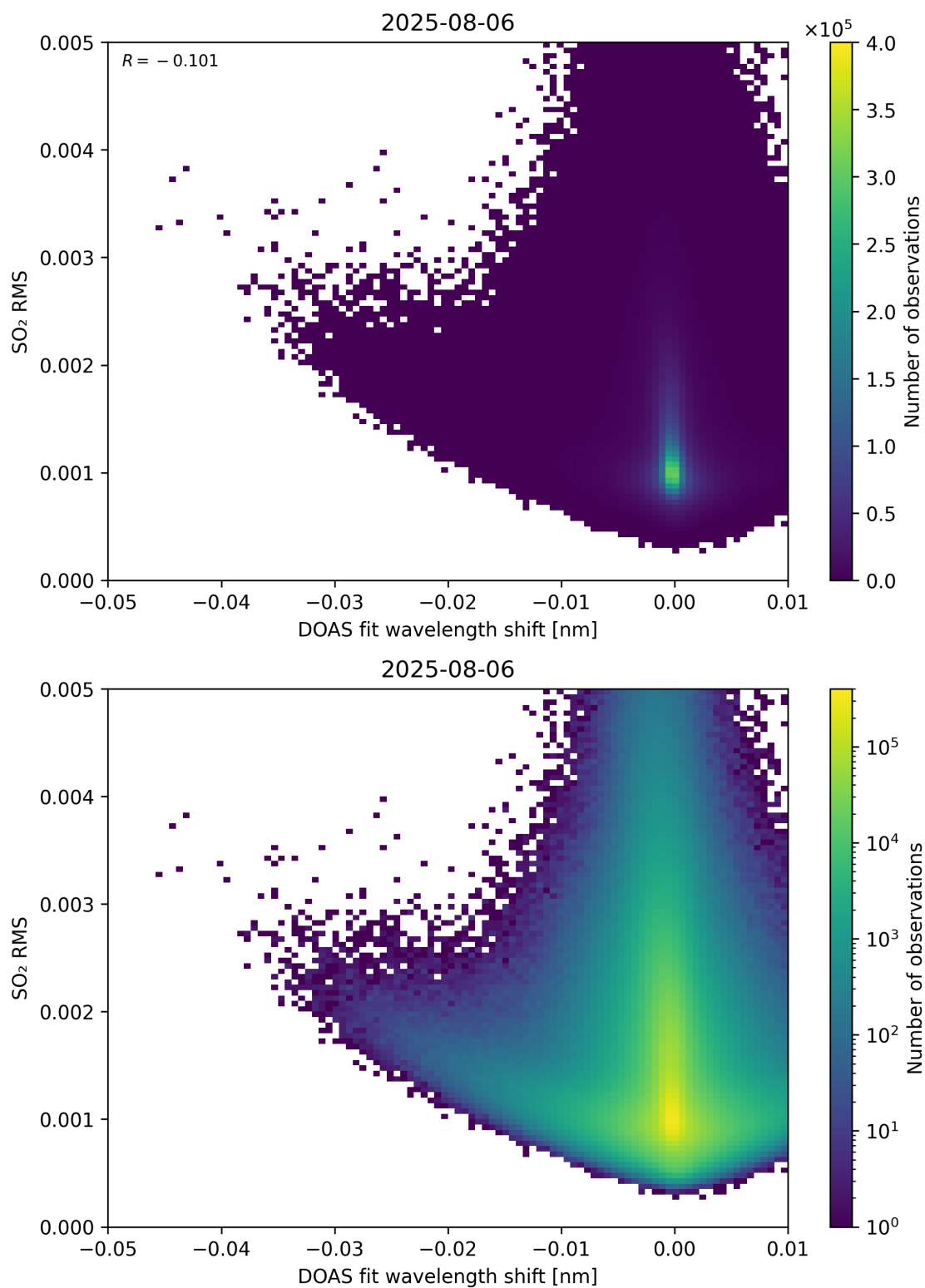
Figure 139: Scatter density plot of “DOAS fit wavelength shift” against “SO 2 RMS” for 2025-08-05 to 2025-08-07.
