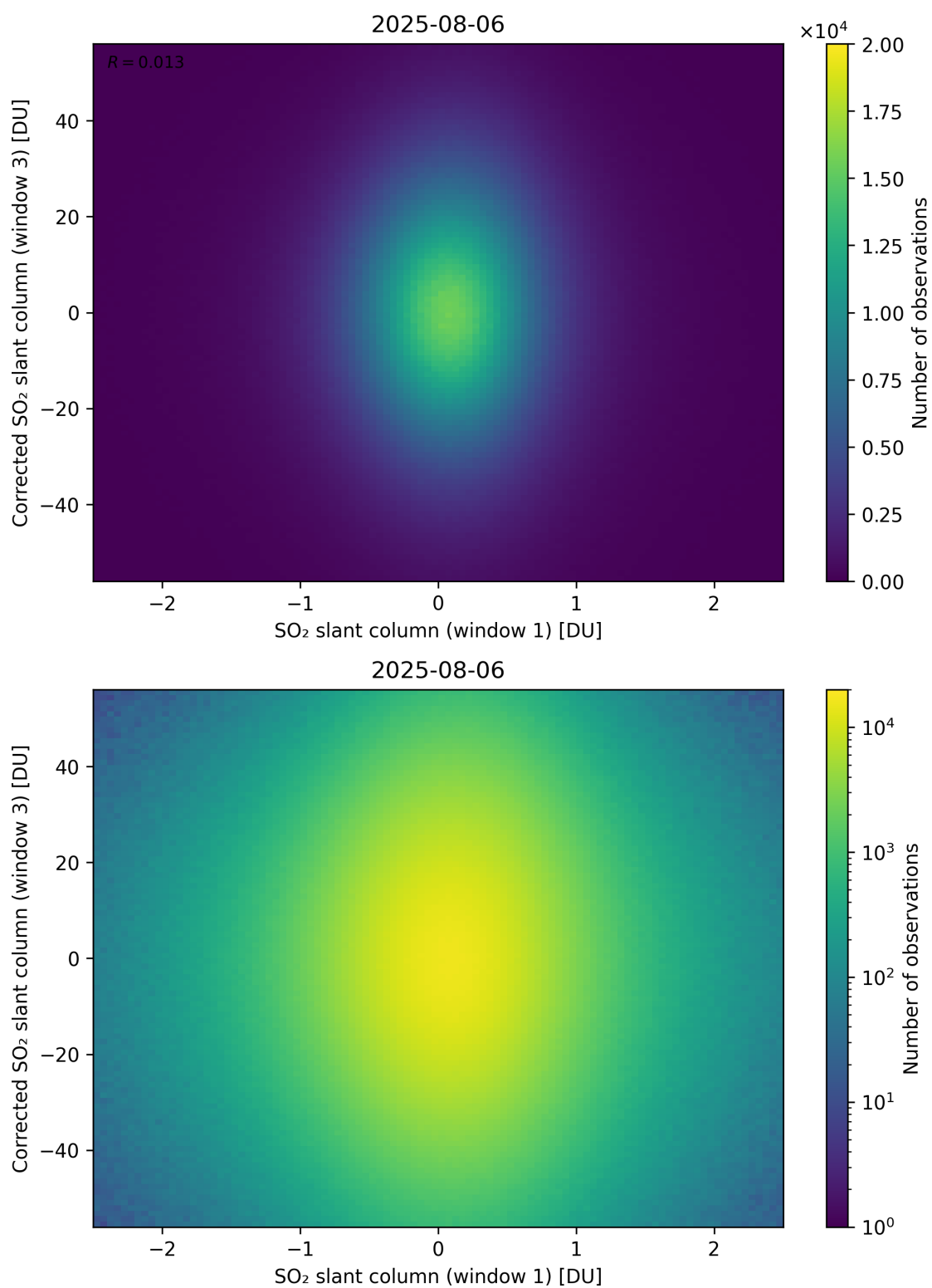
Figure 284: Scatter density plot of “SO 2 slant column (window 1)” against “Corrected SO 2 slant column (window 3)” for 2025-08-05 to 2025-08-07.
