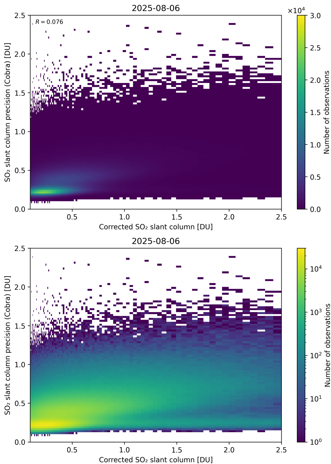
Figure 234: Scatter density plot of “Corrected SO 2 slant column” against “SO 2 slant column precision (Cobra)” for 2025-08-05 to 2025-08-07.
