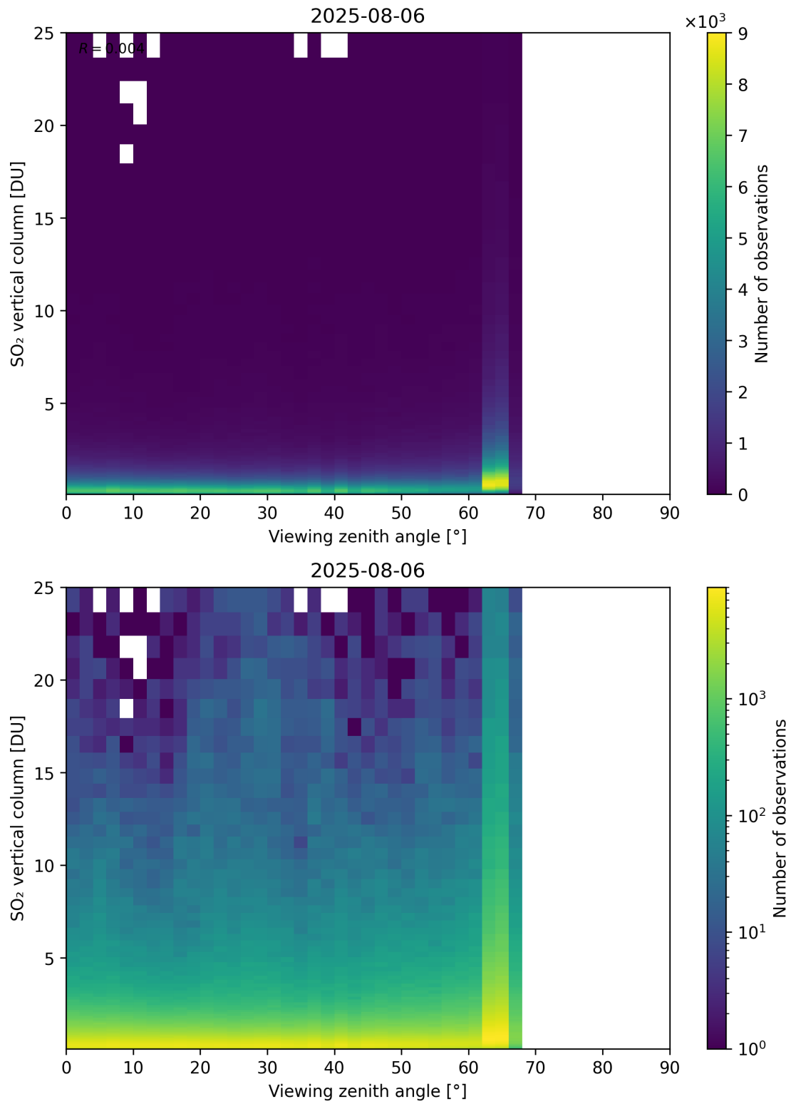
Figure 383: Scatter density plot of “Viewing zenith angle” against “SO 2 vertical column” for 2025-08-05 to 2025-08-07.
