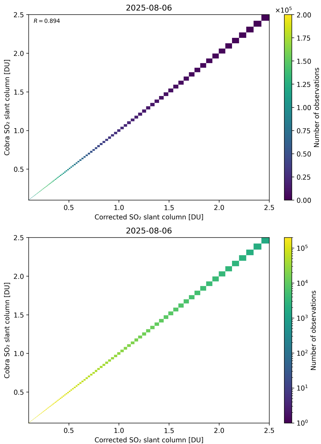
Figure 233: Scatter density plot of “Corrected SO 2 slant column” against “Cobra SO 2 slant column” for 2025-08-05 to 2025-08-07.
