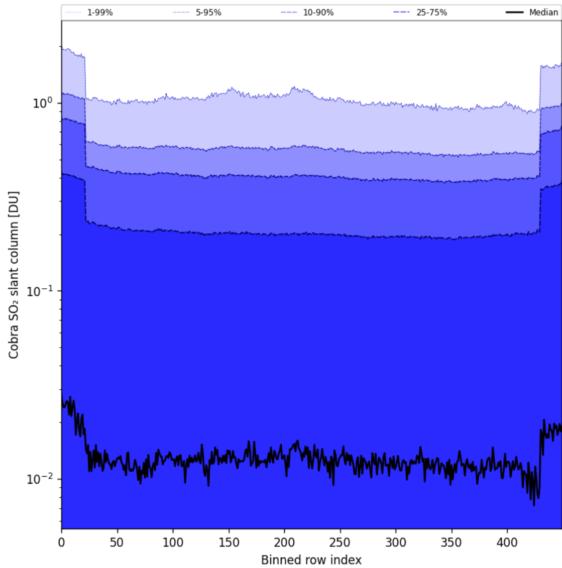
Figure 87: Along track statistics of “Cobra SO 2 slant column” for 2025-08-05 to 2025-08-07
