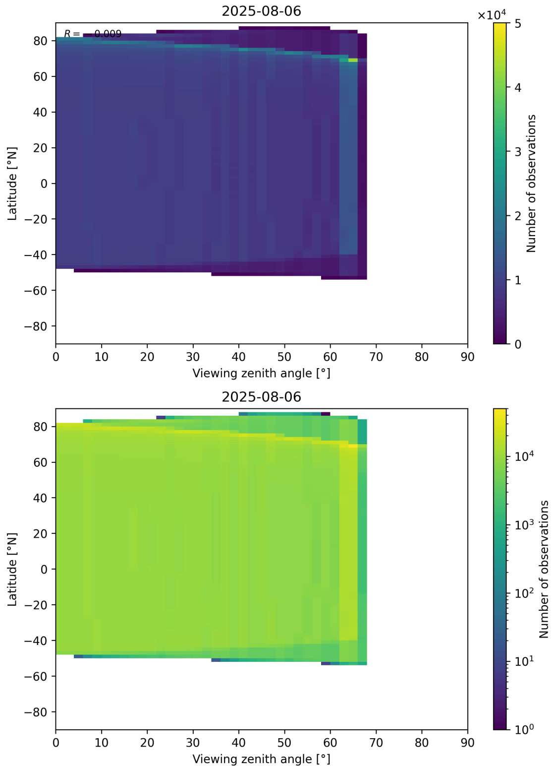
Figure 368: Scatter density plot of “Viewing zenith angle” against “Latitude” for 2025-08-05 to 2025-08-07.
