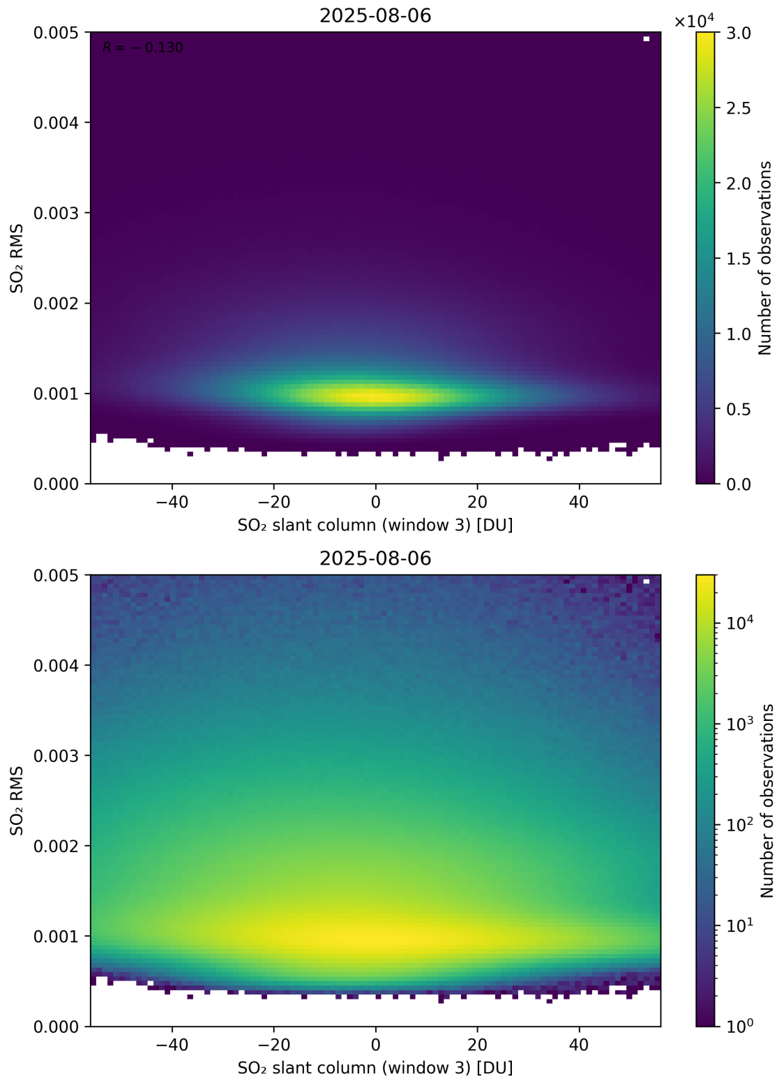
Figure 306: Scatter density plot of “SO 2 slant column (window 3)” against “SO 2 RMS” for 2025-08-05 to 2025-08-07.
