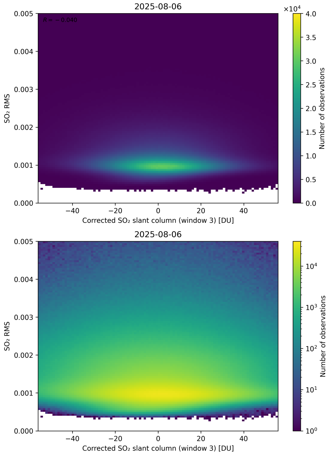
Figure 258: Scatter density plot of “Corrected SO 2 slant column (window 3)” against “SO 2 RMS” for 2025-08-05 to 2025-08-07.
