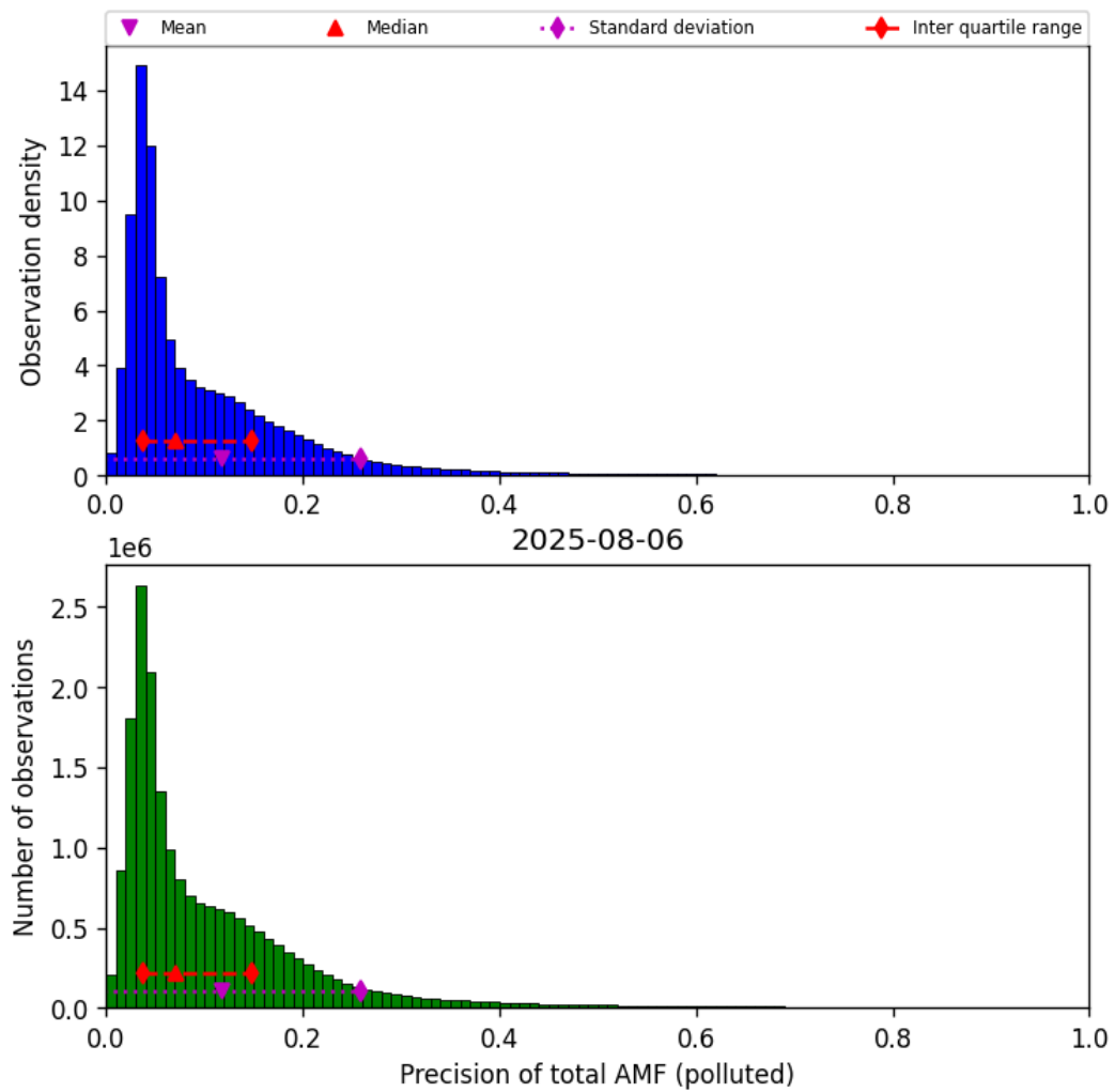
Figure 80: Histogram of “Precision of total AMF (polluted)” for 2025-08-05 to 2025-08-07
