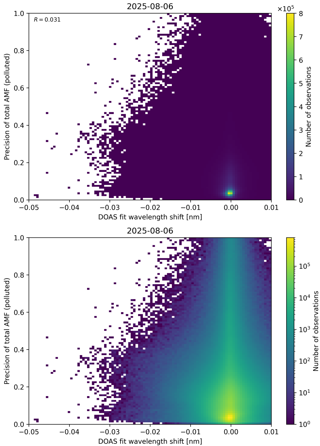
Figure 142: Scatter density plot of “DOAS fit wavelength shift” against “Precision of total AMF (polluted)” for 2025-08-05 to 2025-08-07.
