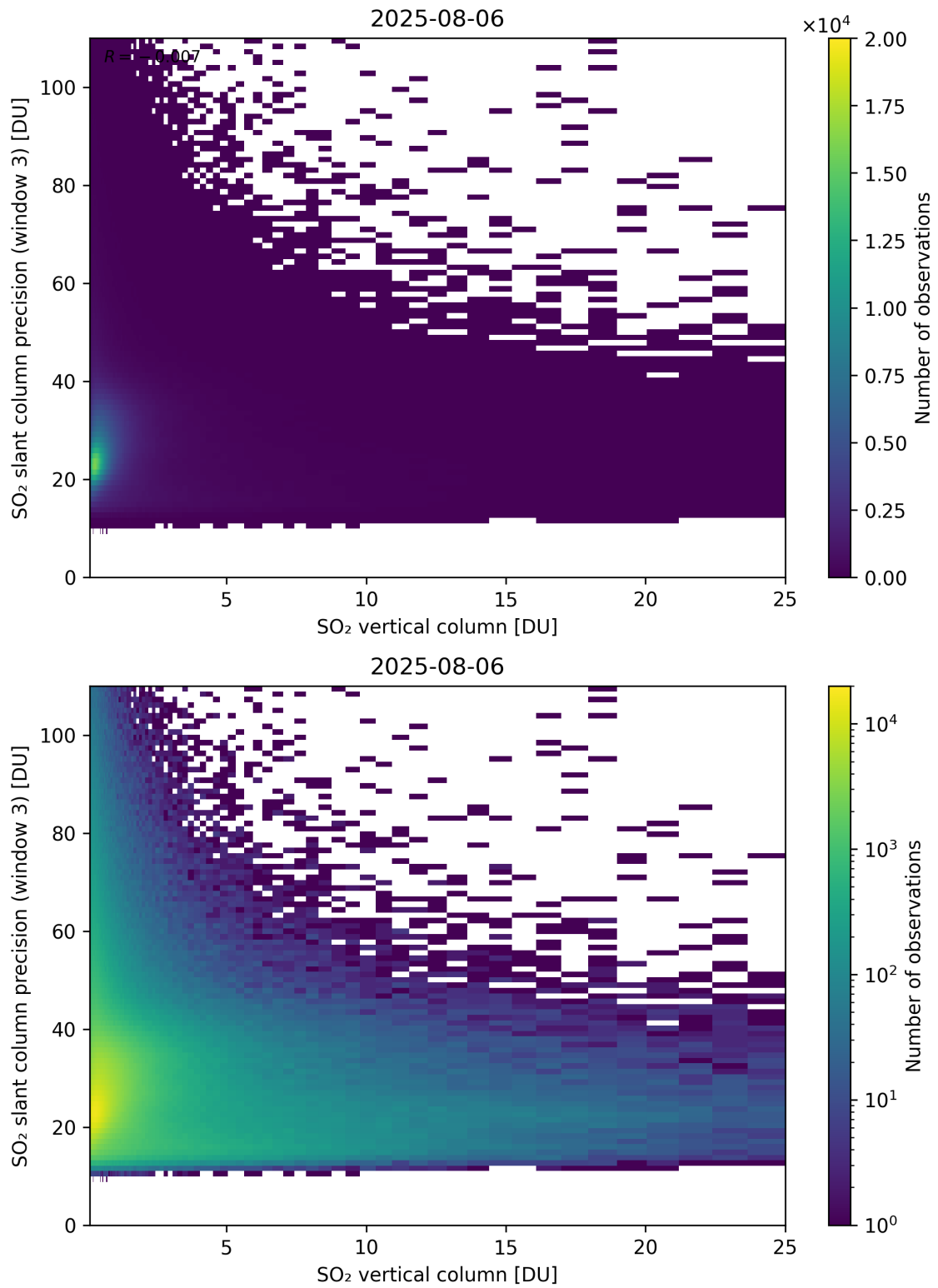
Figure 358: Scatter density plot of “SO 2 vertical column” against “SO 2 slant column precision (window 3)” for 2025-08-05 to 2025-08-07.
