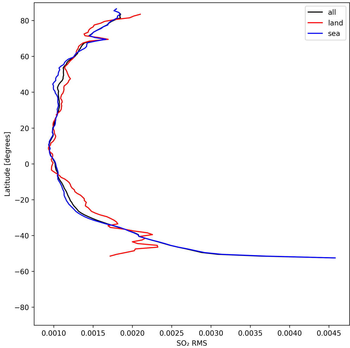
Figure 52: Zonal average of “SO 2 RMS” for 2025-08-05 to 2025-08-07.
