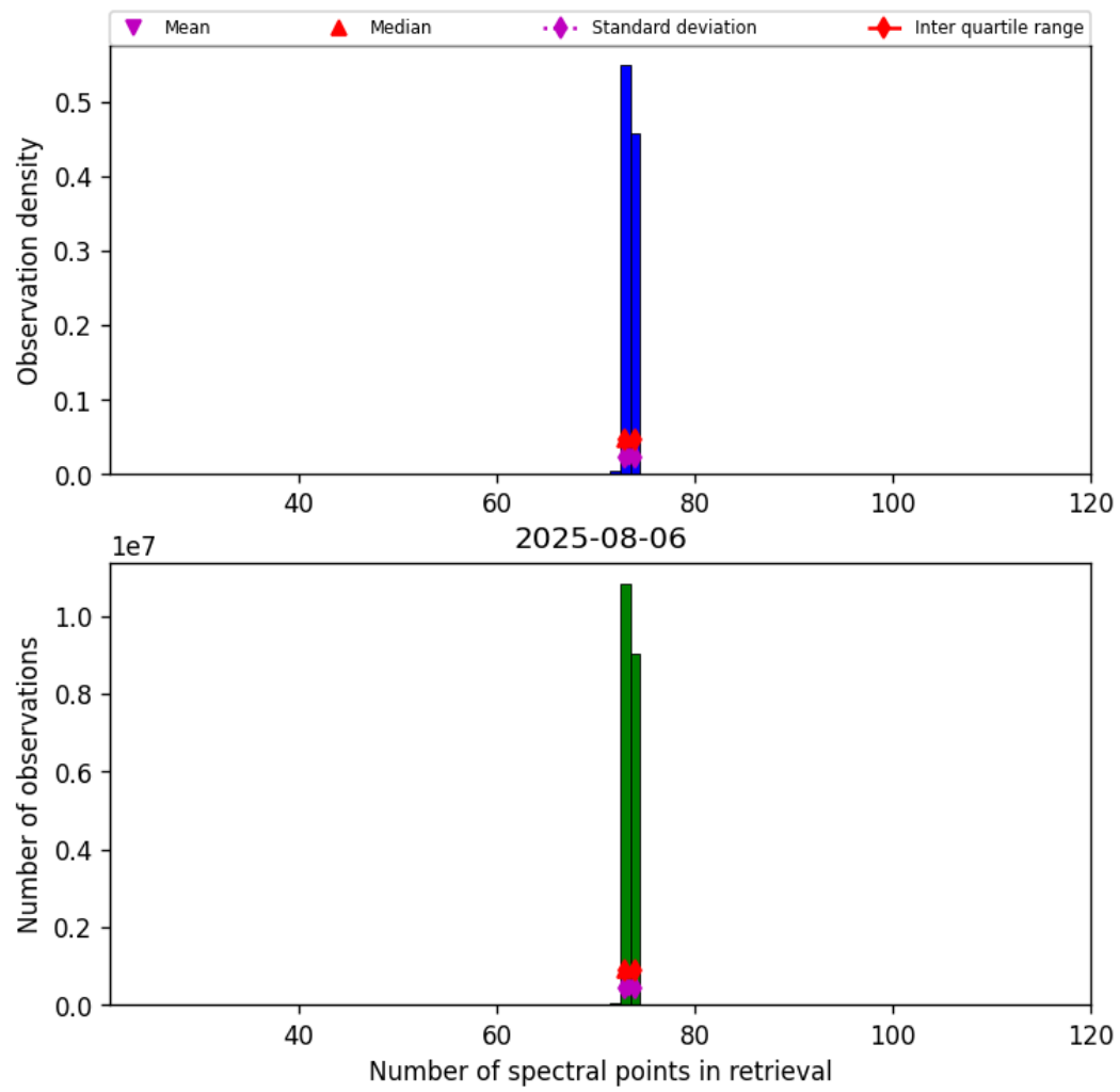
Figure 82: Histogram of “Number of spectral points in retrieval” for 2025-08-05 to 2025-08-07
