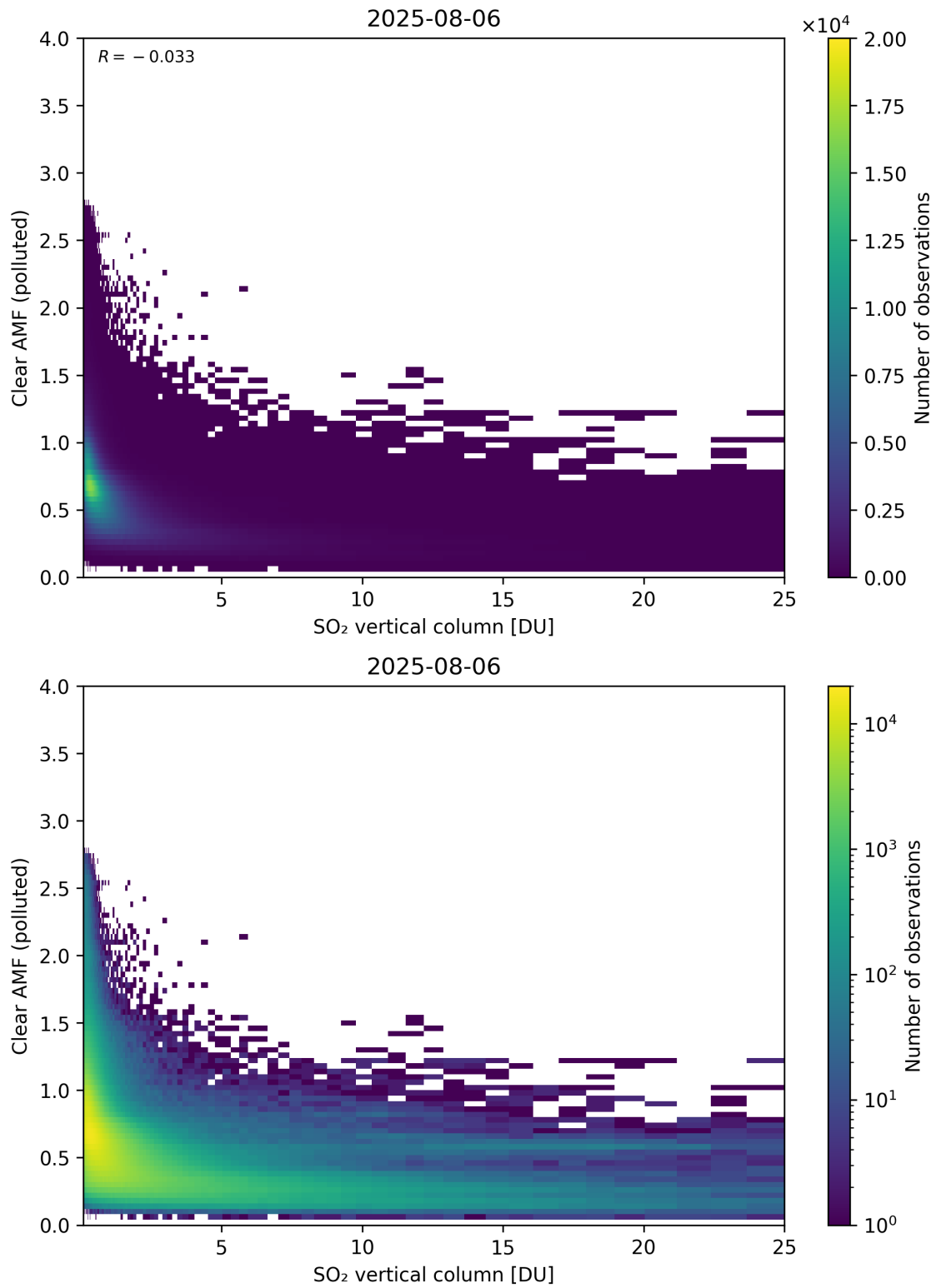
Figure 348: Scatter density plot of “SO 2 vertical column” against “Clear AMF (polluted)” for 2025-08-05 to 2025-08-07.
