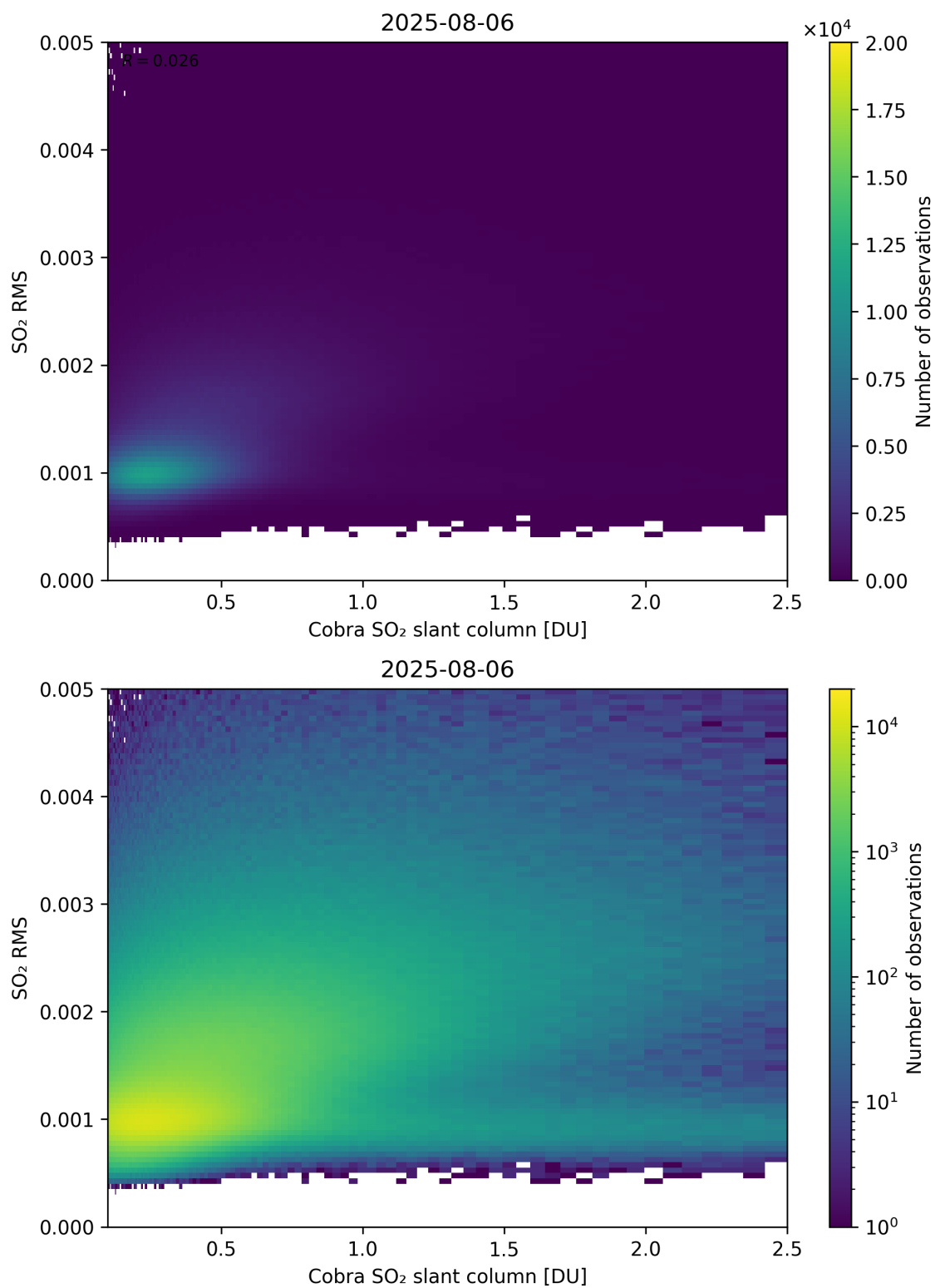
Figure 198: Scatter density plot of “Cobra SO 2 slant column” against “SO 2 RMS” for 2025-08-05 to 2025-08-07.
