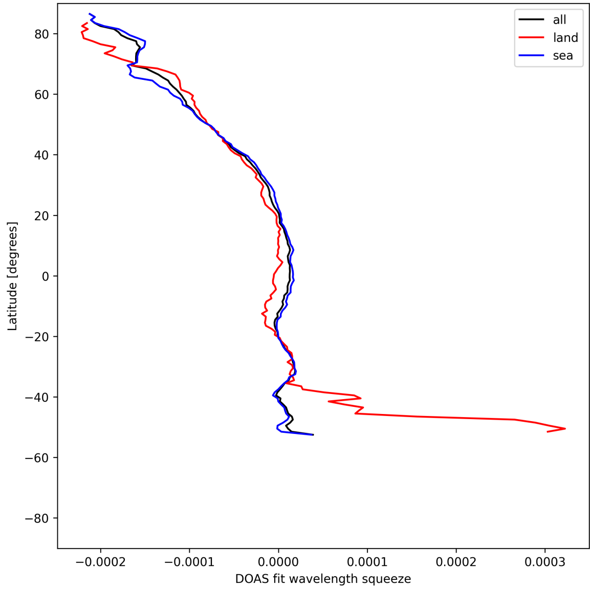
Figure 51: Zonal average of “DOAS fit wavelength squeeze” for 2025-08-05 to 2025-08-07.
