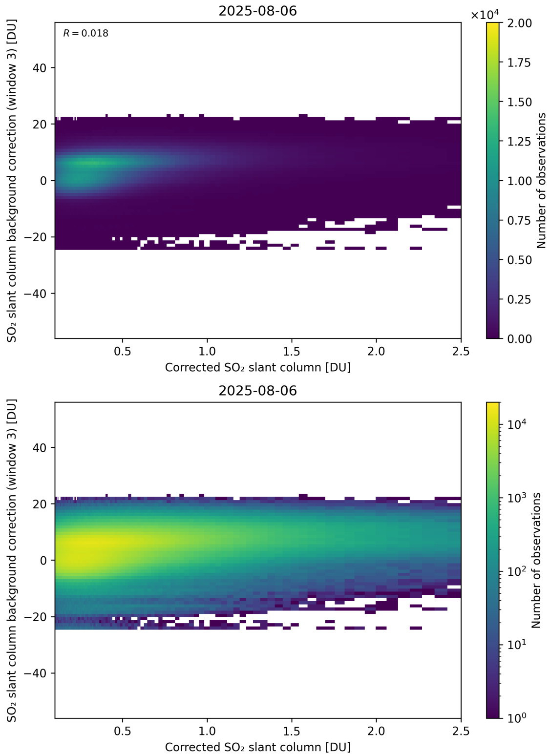
Figure 228: Scatter density plot of “Corrected SO 2 slant column” against “SO 2 slant column background correction (window 3)” for 2025-08-05 to 2025-08-07.
