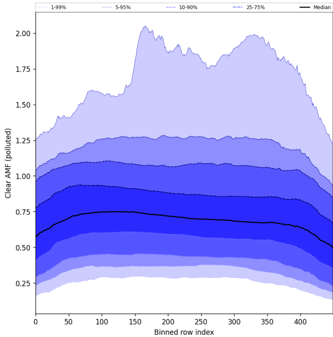
Figure 107: Along track statistics of “Clear AMF (polluted)” for 2025-08-05 to 2025-08-07
