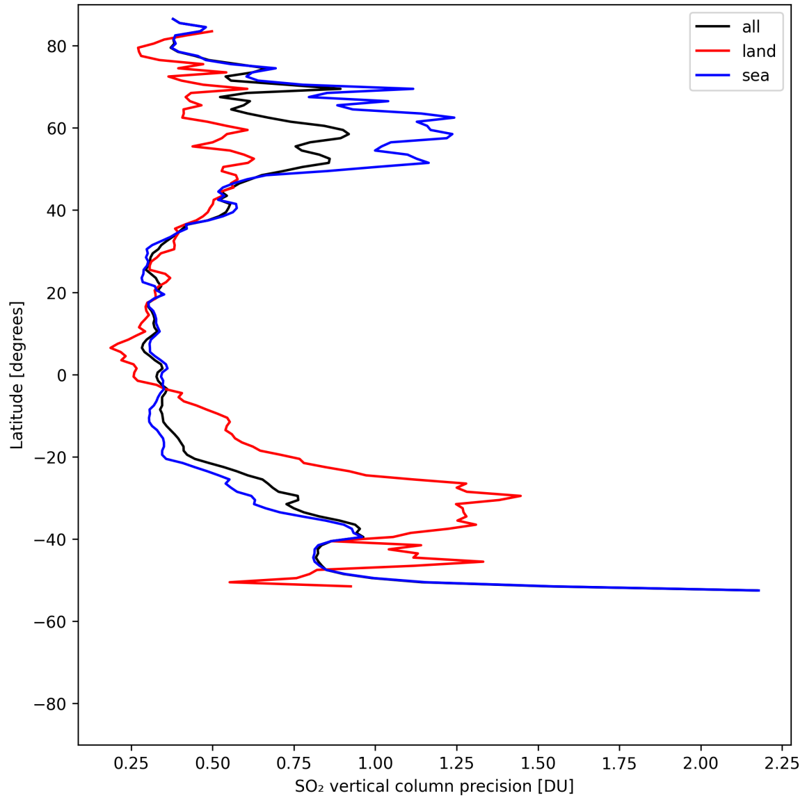
Figure 33: Zonal average of “SO 2 vertical column precision” for 2025-08-05 to 2025-08-07.
