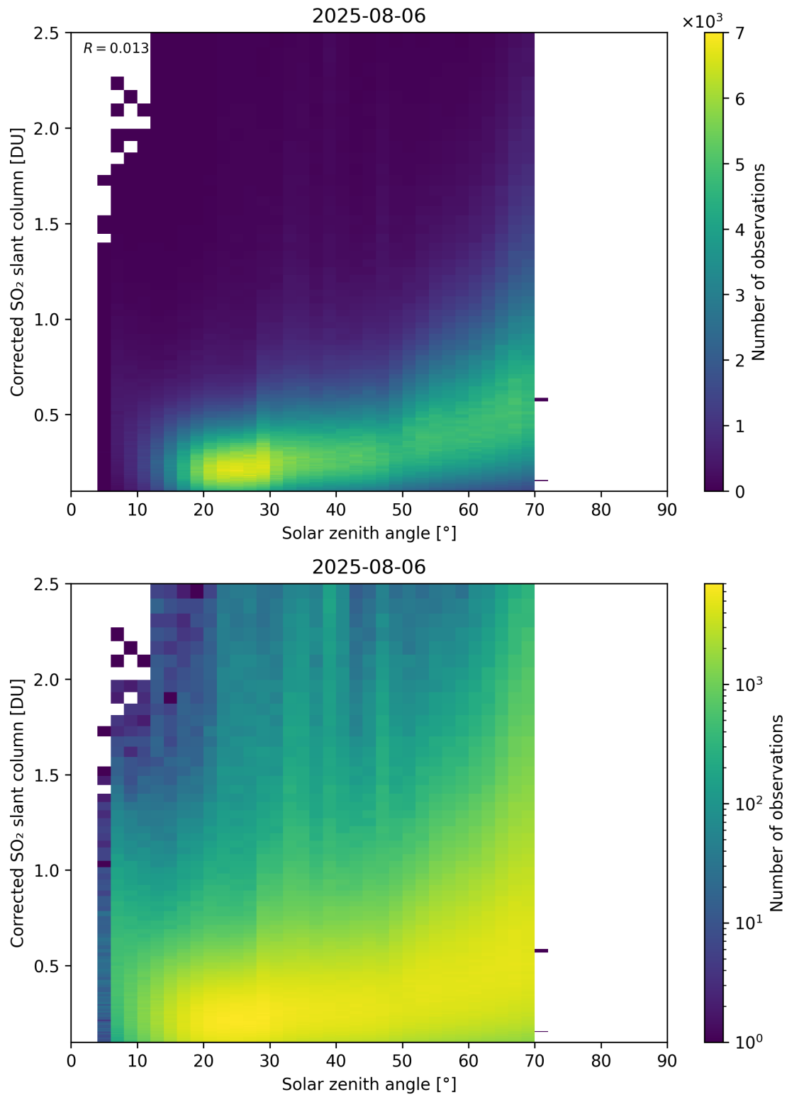
Figure 181: Scatter density plot of “Solar zenith angle” against “Corrected SO 2 slant column” for 2025-08-05 to 2025-08-07.
