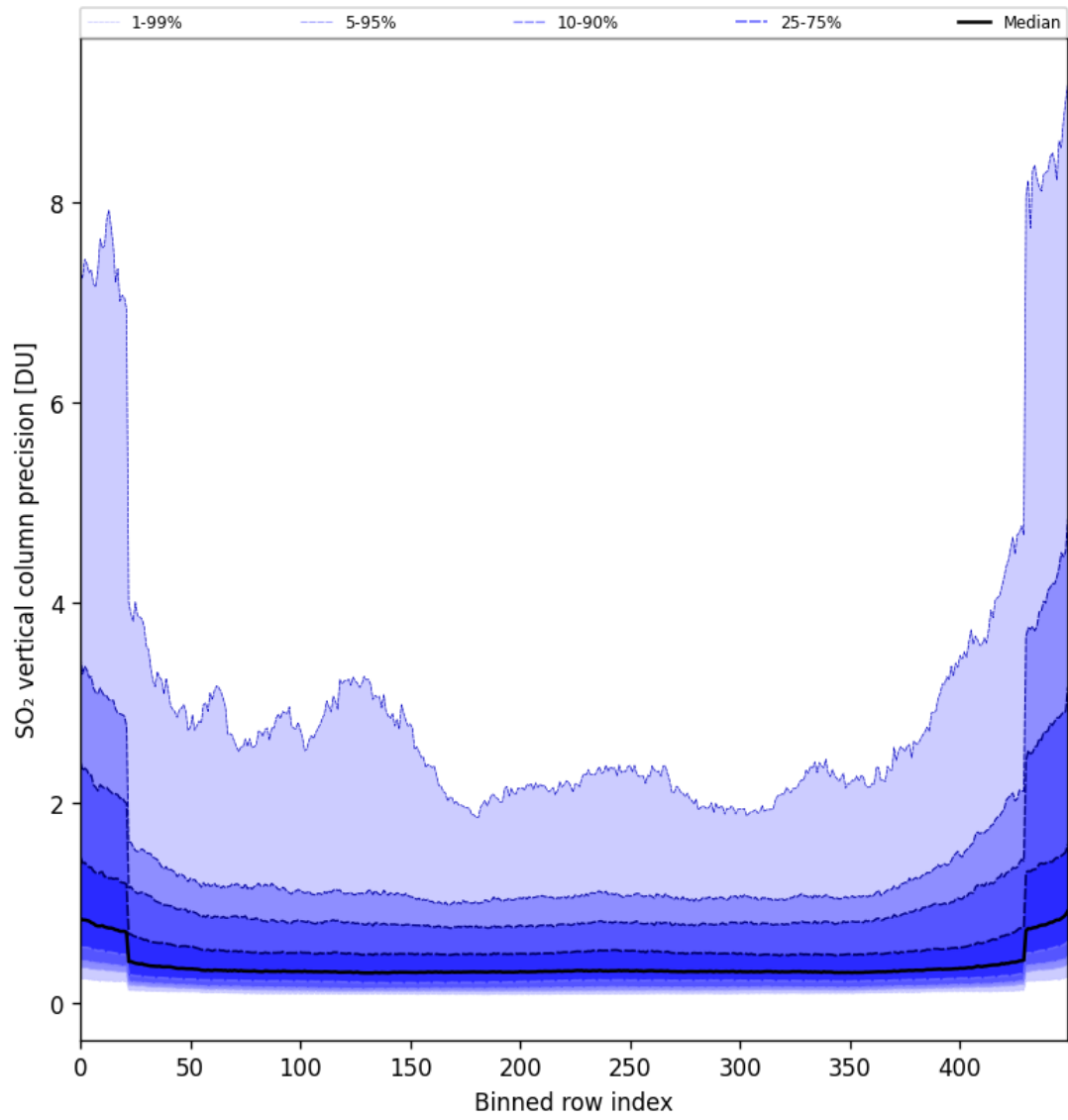
Figure 85: Along track statistics of “SO 2 vertical column precision” for 2025-08-05 to 2025-08-07
