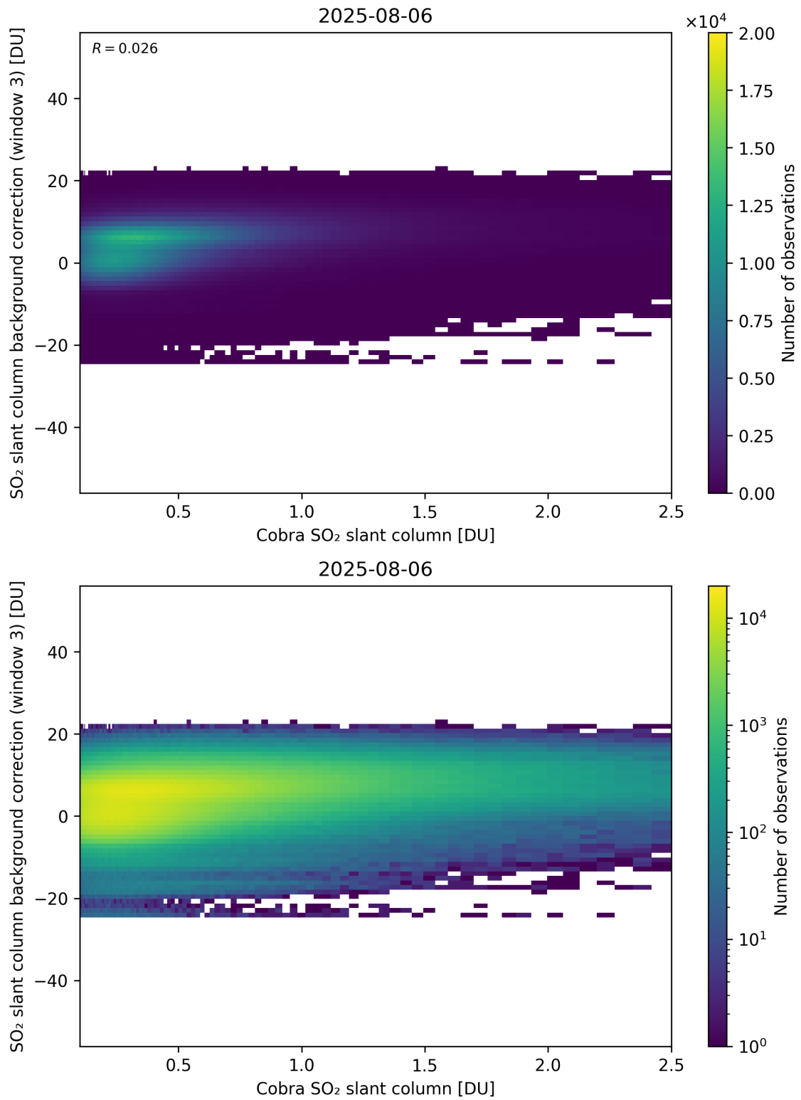
Figure 195: Scatter density plot of “Cobra SO 2 slant column” against “SO 2 slant column background correction (window 3)” for 2025-08-05 to 2025-08-07.
