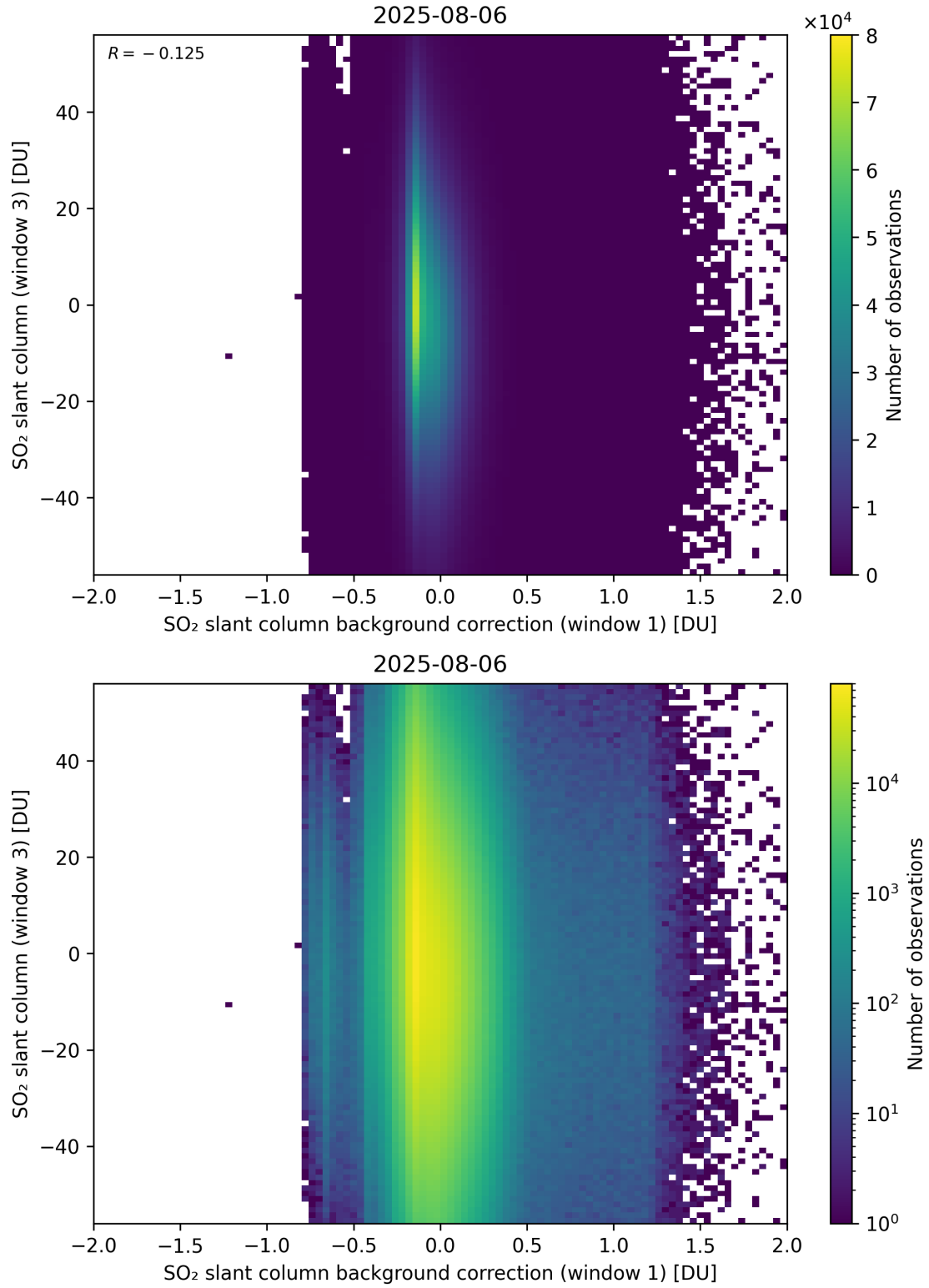
Figure 118: Scatter density plot of “SO 2 slant column background correction (window 1)” against “SO 2 slant column (window 3)” for 2025-08-05 to 2025-08-07.
