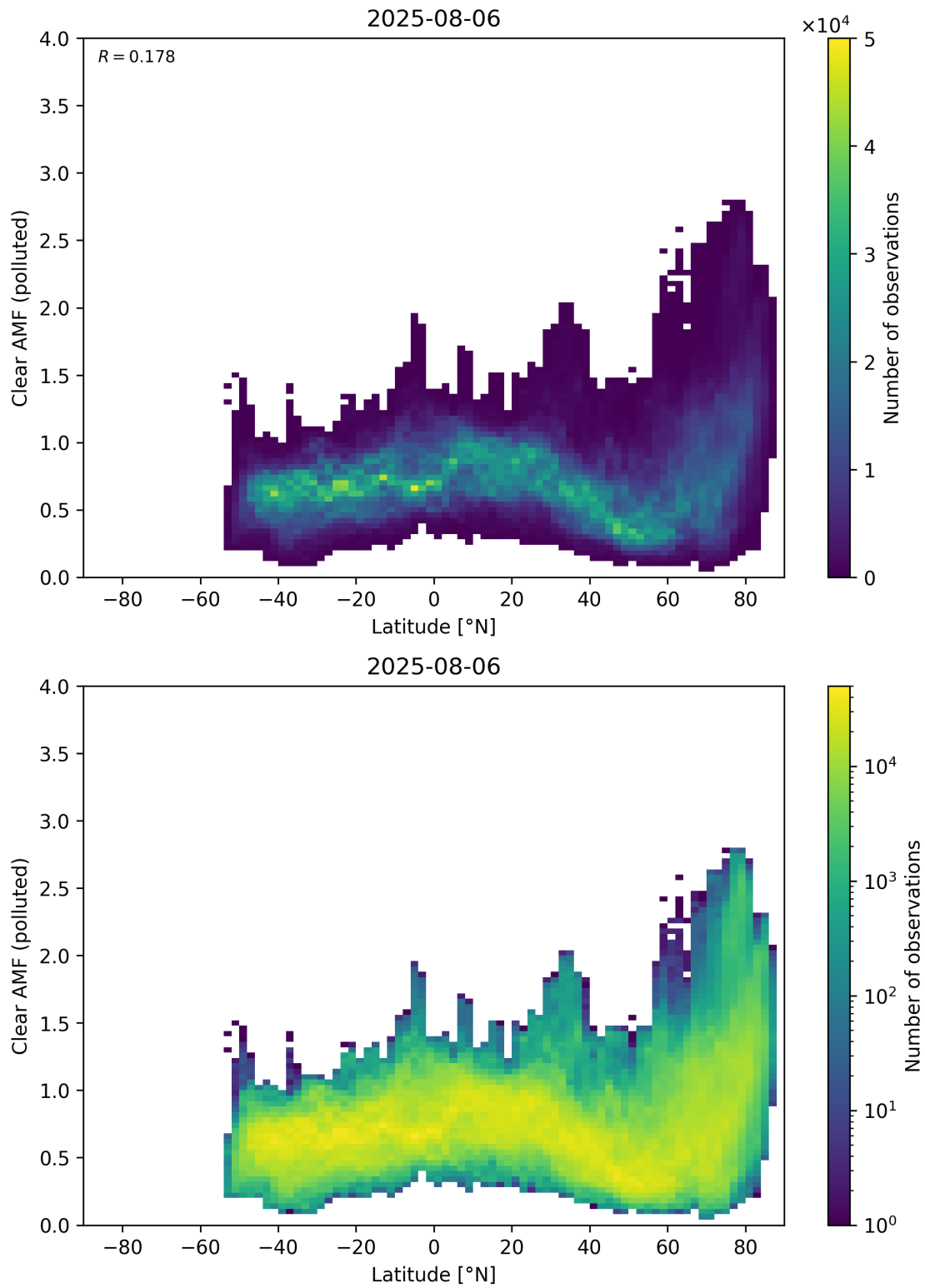
Figure 156: Scatter density plot of “Latitude” against “Clear AMF (polluted)” for 2025-08-05 to 2025-08-07.
