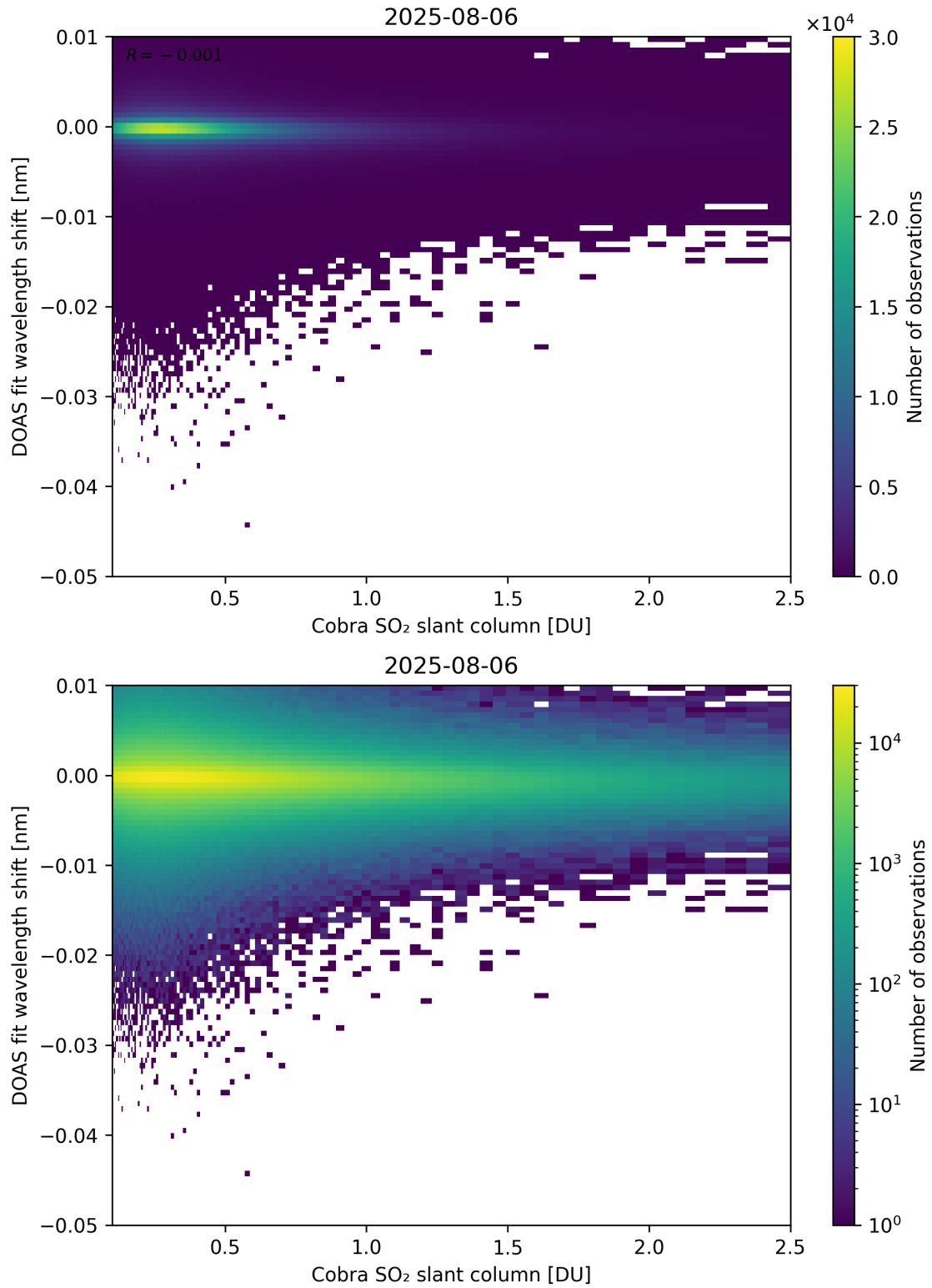
Figure 196: Scatter density plot of “Cobra SO 2 slant column” against “DOAS fit wavelength shift” for 2025-08-05 to 2025-08-07.
