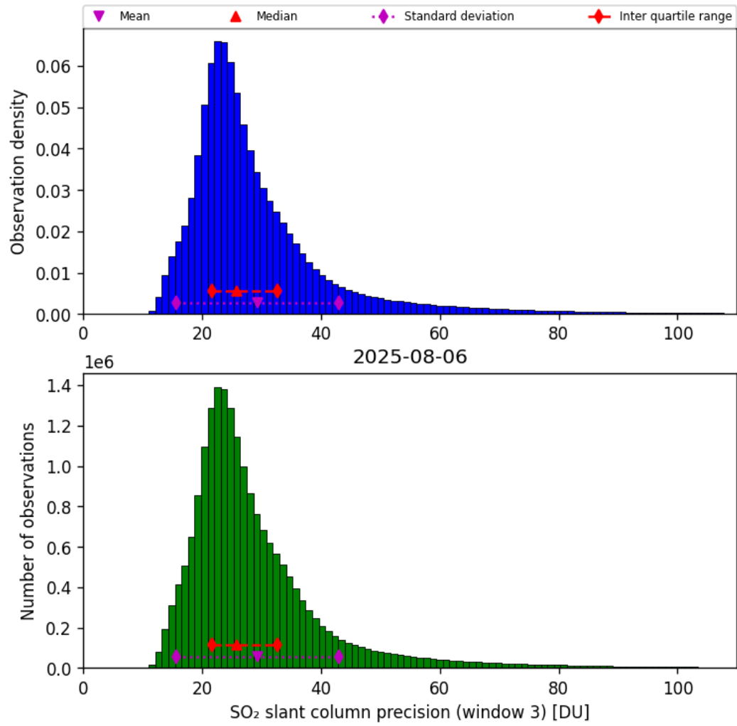
Figure 72: Histogram of “SO 2 slant column precision (window 3)” for 2025-08-05 to 2025-08-07
