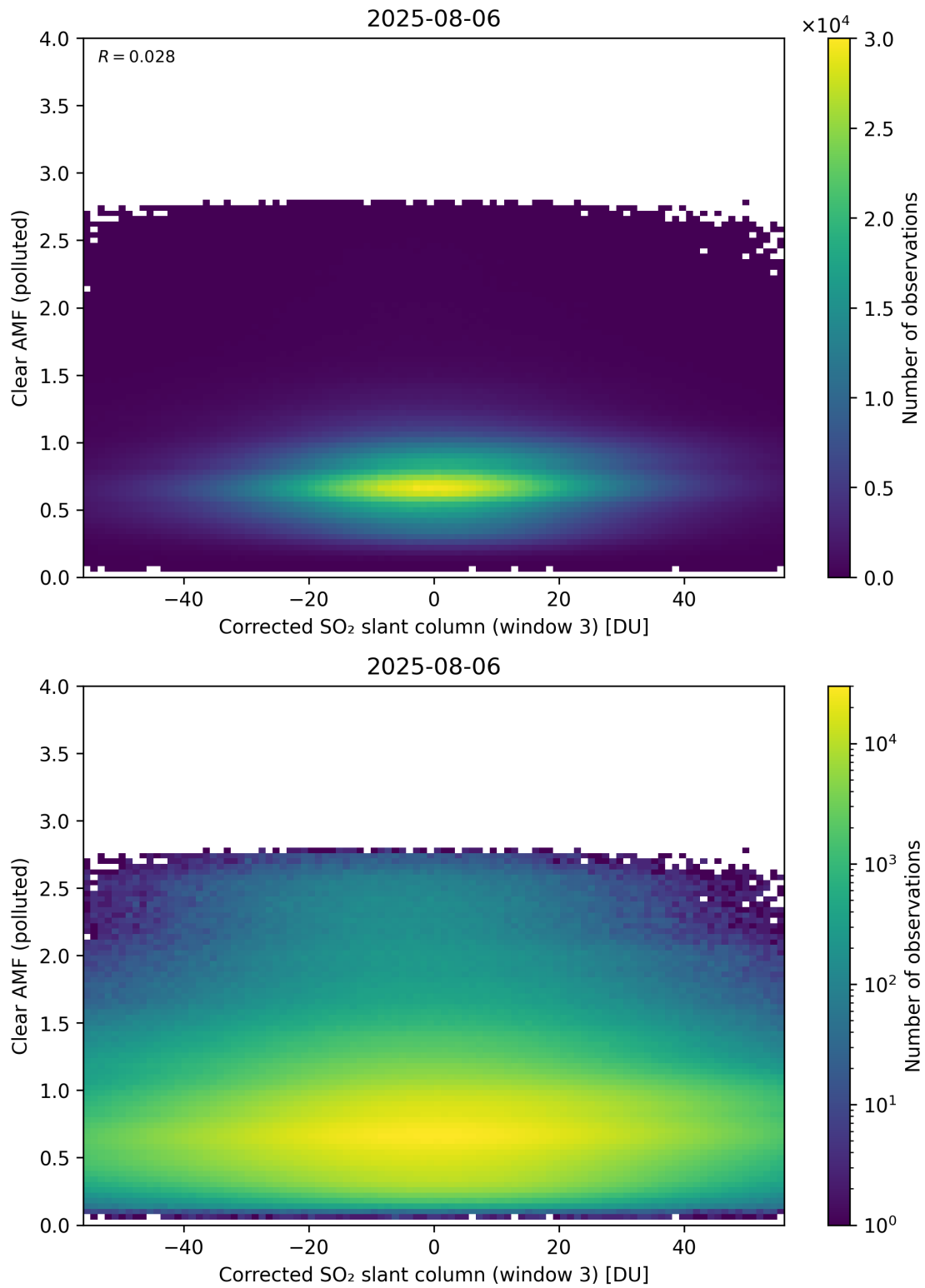
Figure 259: Scatter density plot of “Corrected SO 2 slant column (window 3)” against “Clear AMF (polluted)” for 2025-08-05 to 2025-08-07.
