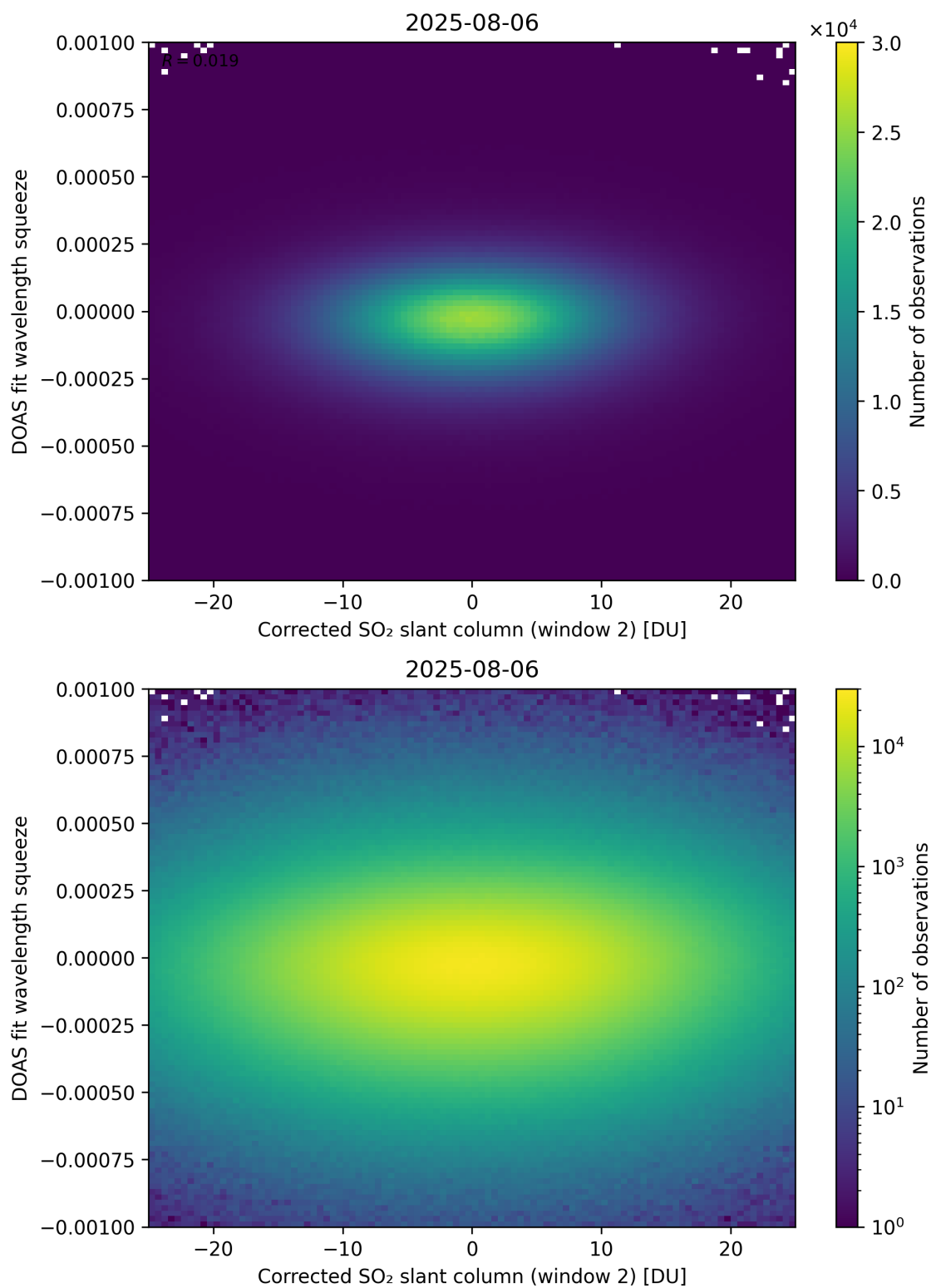
Figure 247: Scatter density plot of “Corrected SO 2 slant column (window 2)” against “DOAS fit wavelength squeeze” for 2025-08-05 to 2025-08-07.
