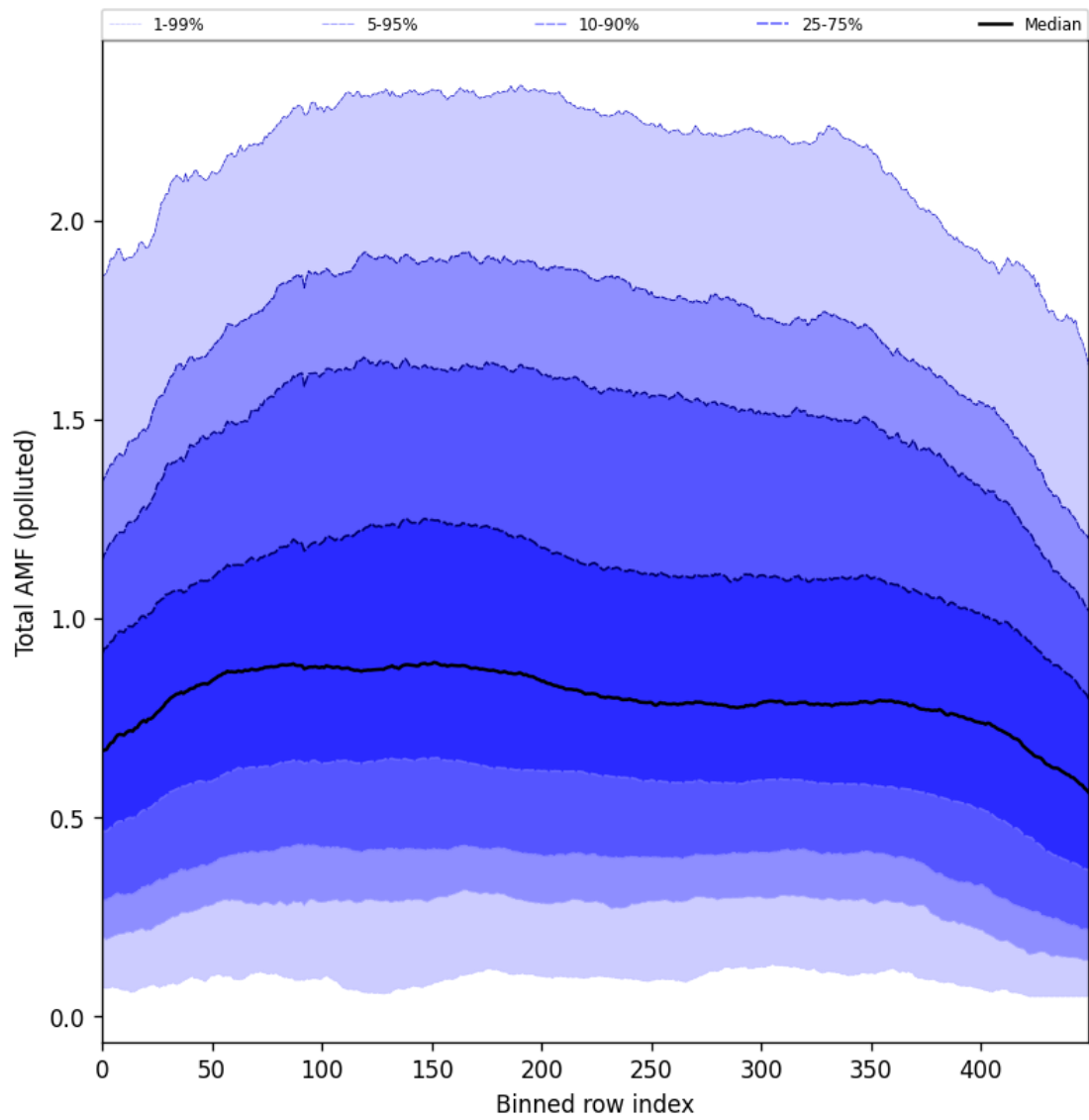
Figure 105: Along track statistics of “Total AMF (polluted)” for 2025-08-05 to 2025-08-07
