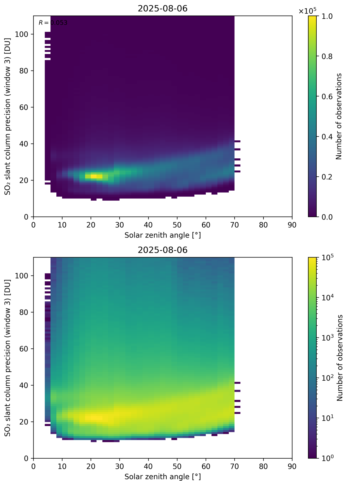
Figure 188: Scatter density plot of “Solar zenith angle” against “SO 2 slant column precision (window 3)” for 2025-08-05 to 2025-08-07.
