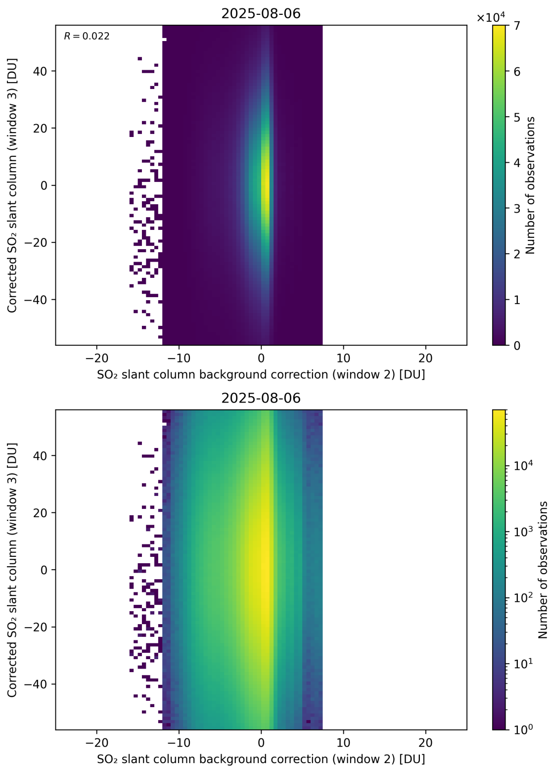
Figure 127: Scatter density plot of “SO 2 slant column background correction (window 2)” against “Corrected SO 2 slant column (window 3)” for 2025-08-05 to 2025-08-07.
