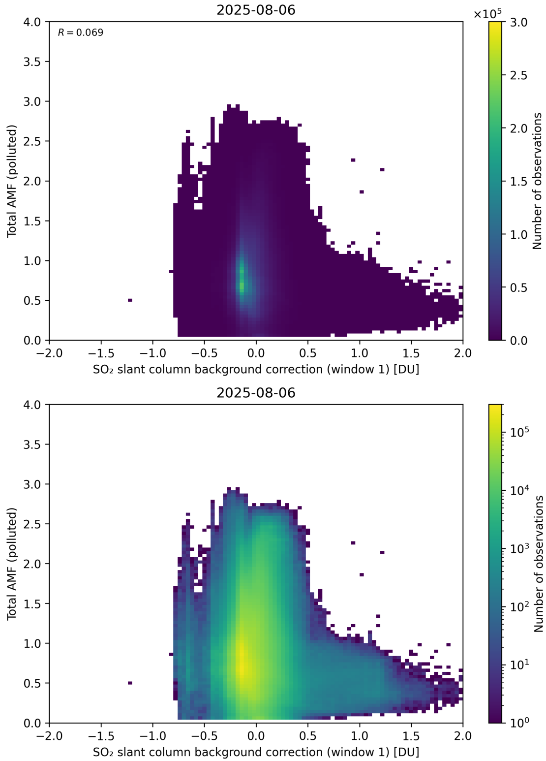
Figure 120: Scatter density plot of “SO 2 slant column background correction (window 1)” against “Total AMF (polluted)” for 2025-08-05 to 2025-08-07.
