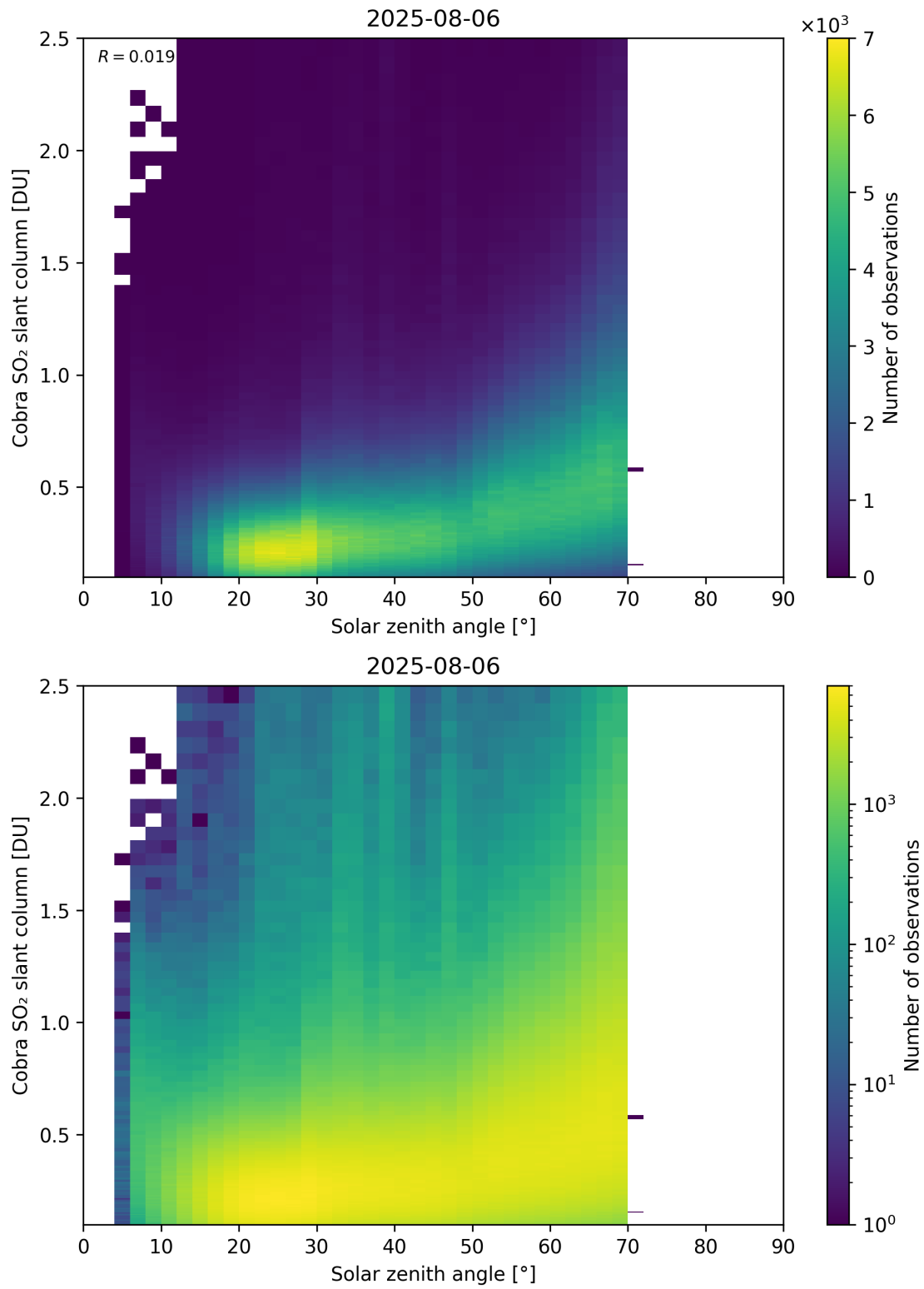
Figure 179: Scatter density plot of “Solar zenith angle” against “Cobra SO 2 slant column” for 2025-08-05 to 2025-08-07.
