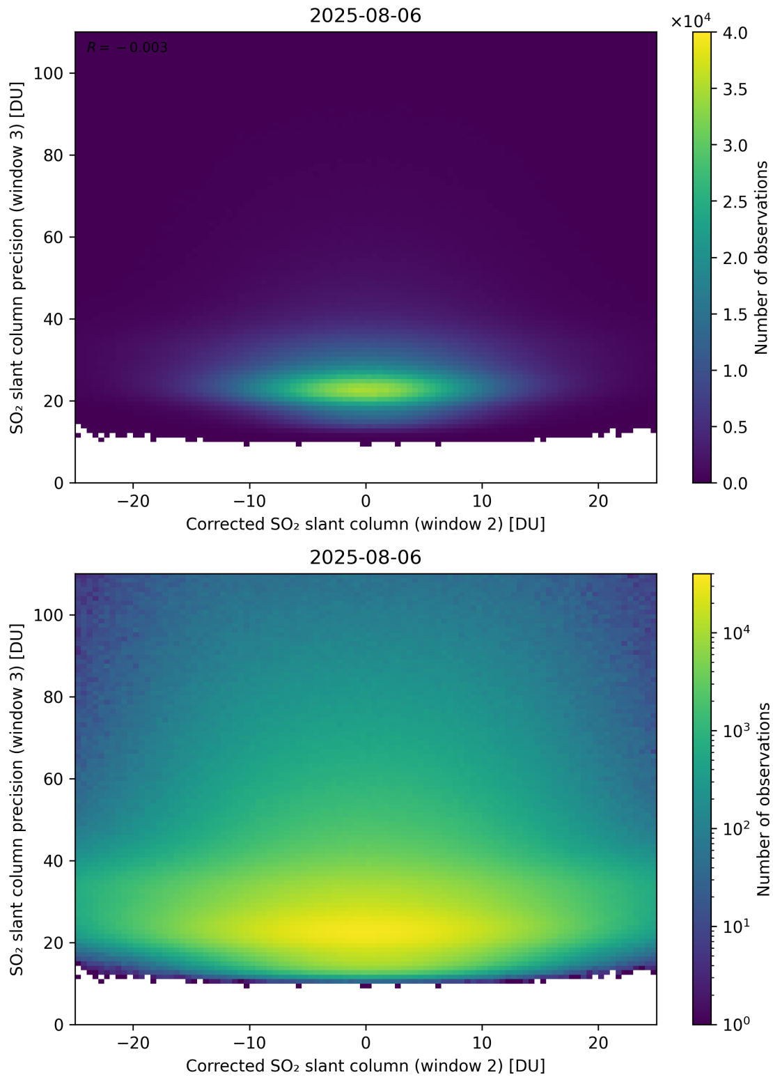
Figure 252: Scatter density plot of “Corrected SO 2 slant column (window 2)” against “SO 2 slant column precision (window 3)” for 2025-08-05 to 2025-08-07.
