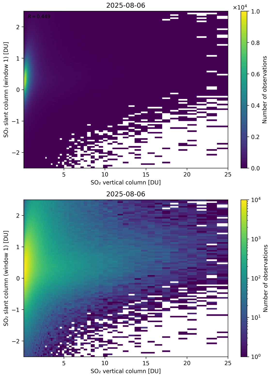
Figure 354: Scatter density plot of “SO 2 vertical column” against “SO 2 slant column (window 1)” for 2025-08-05 to 2025-08-07.
