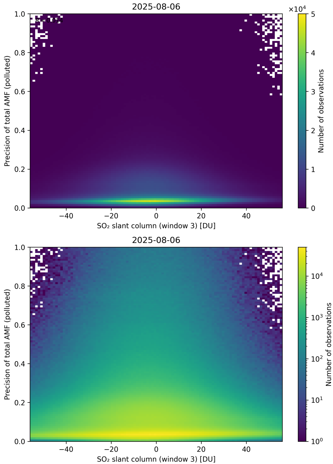
Figure 319: Scatter density plot of “SO 2 slant column (window 3)” against “Precision of total AMF (polluted)” for 2025-08-05 to 2025-08-07.
