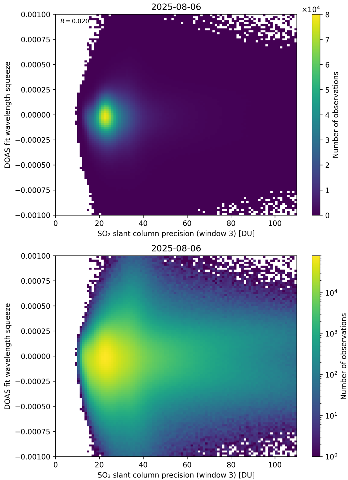
Figure 309: Scatter density plot of “SO 2 slant column precision (window 3)” against “DOAS fit wavelength squeeze” for 2025-08-05 to 2025-08-07.
