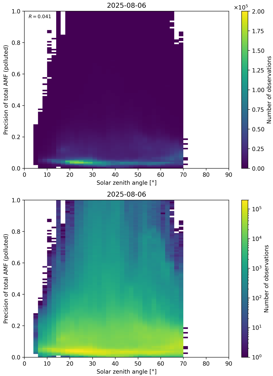
Figure 190: Scatter density plot of “Solar zenith angle” against “Precision of total AMF (polluted)” for 2025-08-05 to 2025-08-07.
