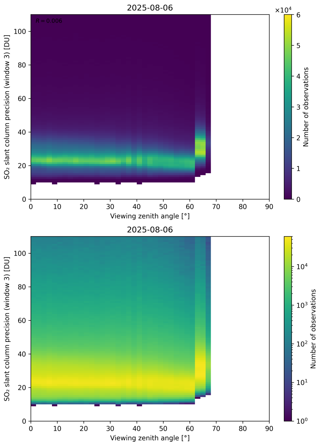
Figure 380: Scatter density plot of “Viewing zenith angle” against “SO 2 slant column precision (window 3)” for 2025-08-05 to 2025-08-07.
