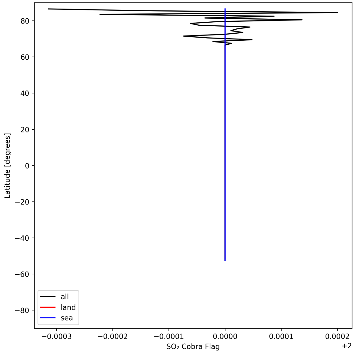
Figure 49: Zonal average of “SO 2 Cobra Flag” for 2025-08-05 to 2025-08-07.
