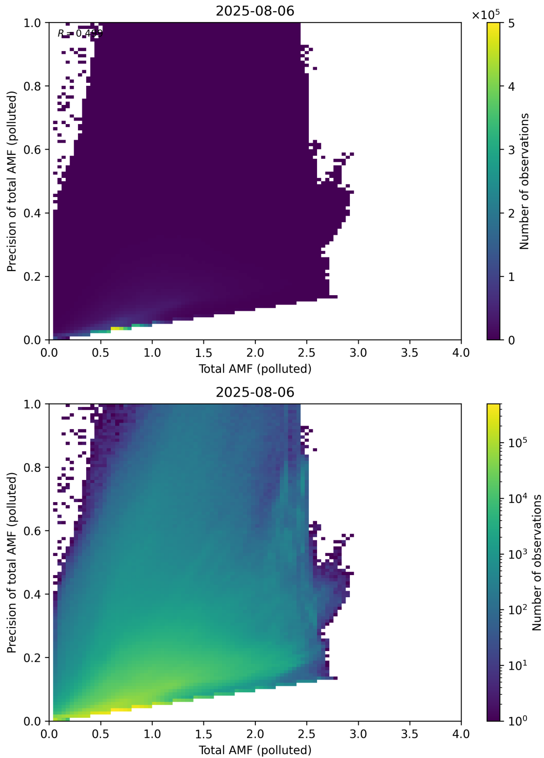
Figure 322: Scatter density plot of “Total AMF (polluted)” against “Precision of total AMF (polluted)” for 2025-08-05 to 2025-08-07.
