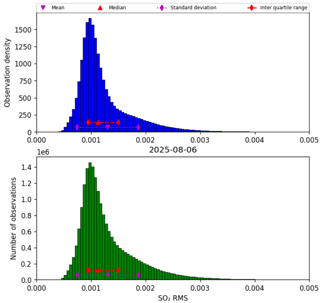
Figure 78: Histogram of “SO 2 RMS” for 2025-08-05 to 2025-08-07
