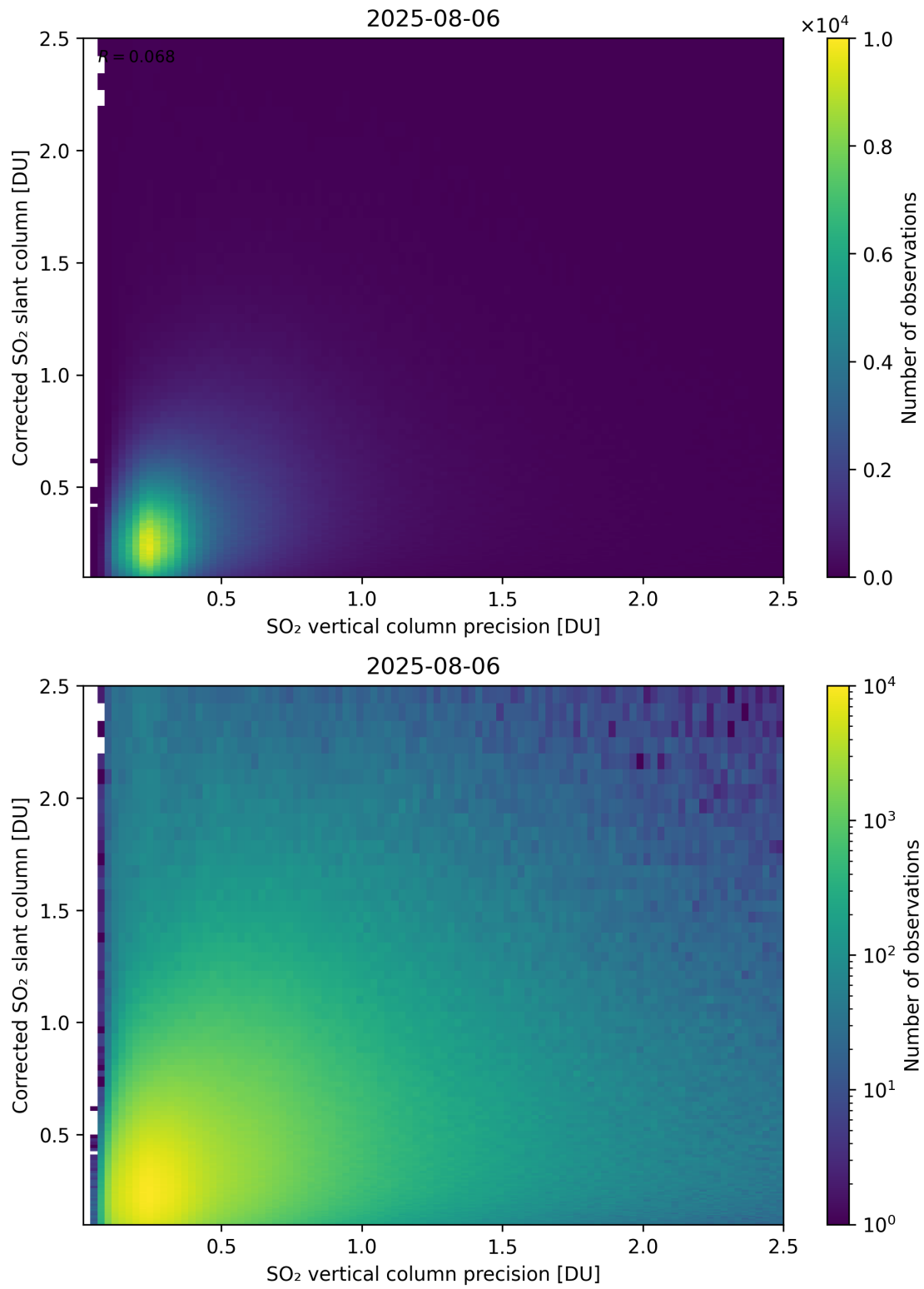
Figure 338: Scatter density plot of “SO 2 vertical column precision” against “Corrected SO 2 slant column” for 2025-08-05 to 2025-08-07.
