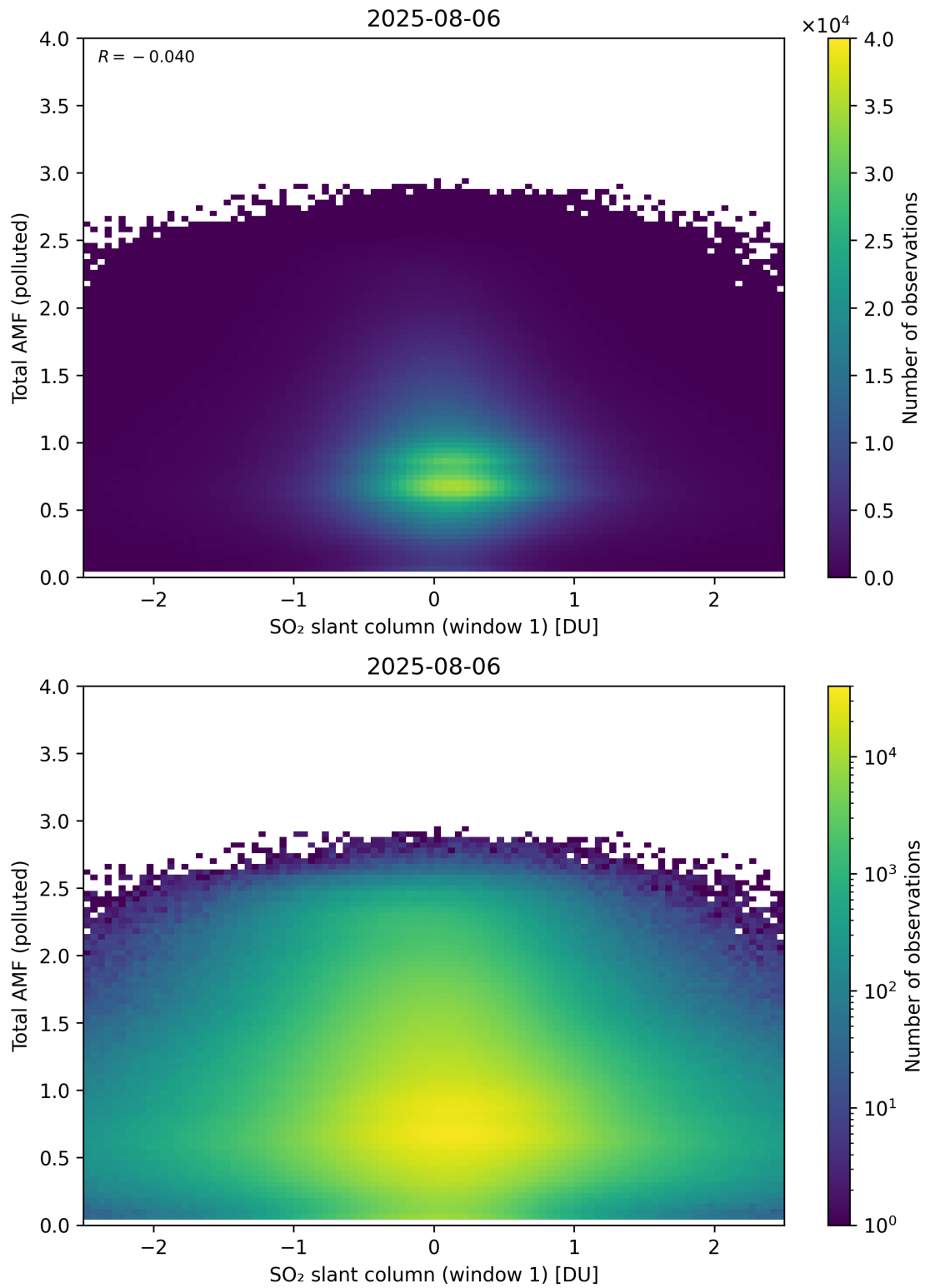
Figure 289: Scatter density plot of “SO 2 slant column (window 1)” against “Total AMF (polluted)” for 2025-08-05 to 2025-08-07.
