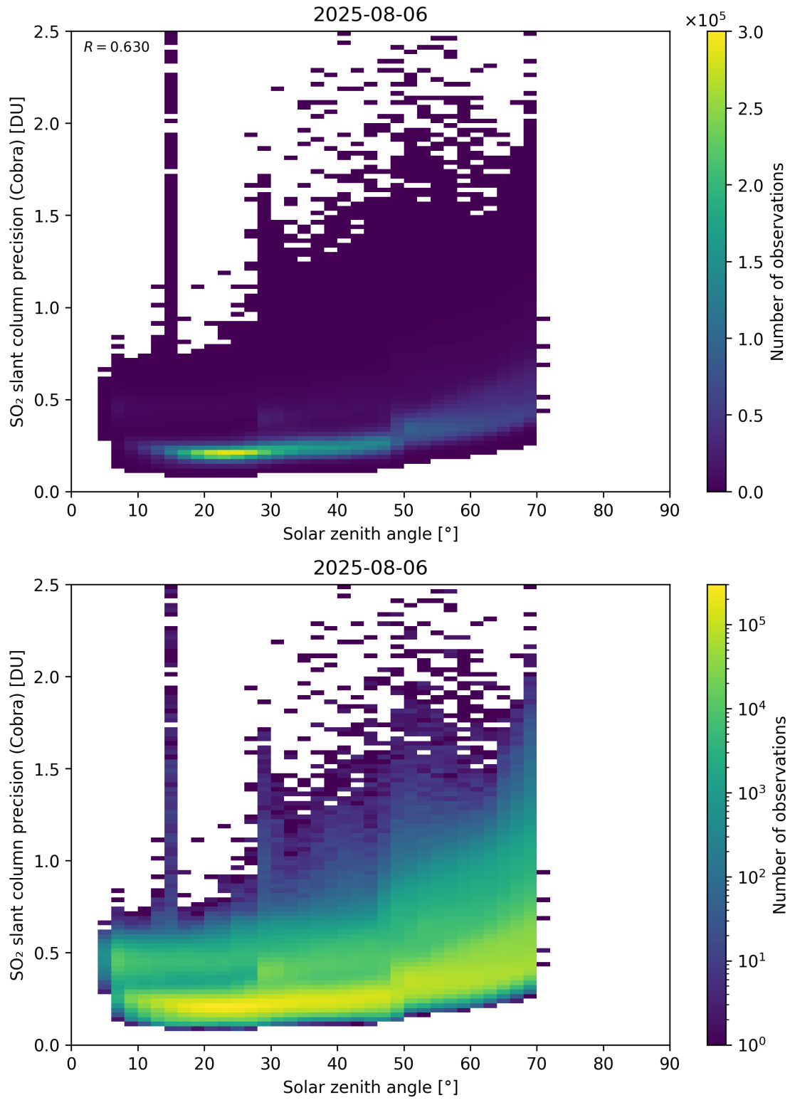
Figure 180: Scatter density plot of “Solar zenith angle” against “SO 2 slant column precision (Cobra)” for 2025-08-05 to 2025-08-07.
