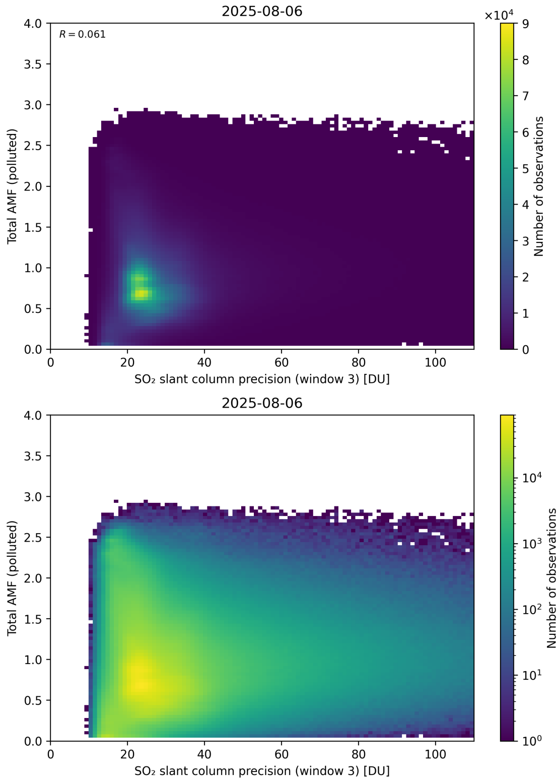
Figure 313: Scatter density plot of “SO 2 slant column precision (window 3)” against “Total AMF (polluted)” for 2025-08-05 to 2025-08-07.
