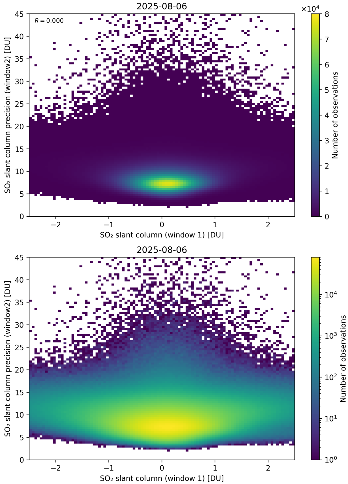
Figure 286: Scatter density plot of “SO 2 slant column (window 1)” against “SO 2 slant column precision (window2)” for 2025-08-05 to 2025-08-07.
