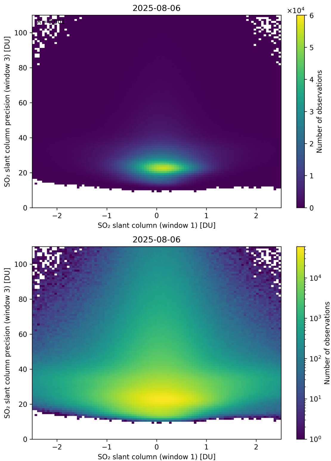
Figure 288: Scatter density plot of “SO 2 slant column (window 1)” against “SO 2 slant column precision (window 3)” for 2025-08-05 to 2025-08-07.
