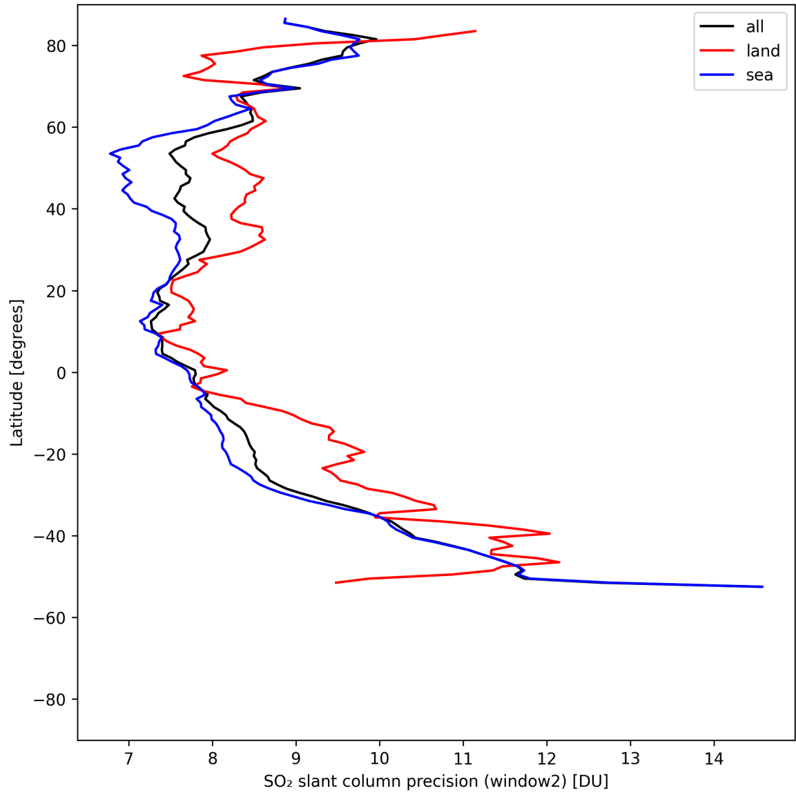
Figure 42: Zonal average of “SO 2 slant column precision (window2)” for 2025-08-05 to 2025-08-07.
