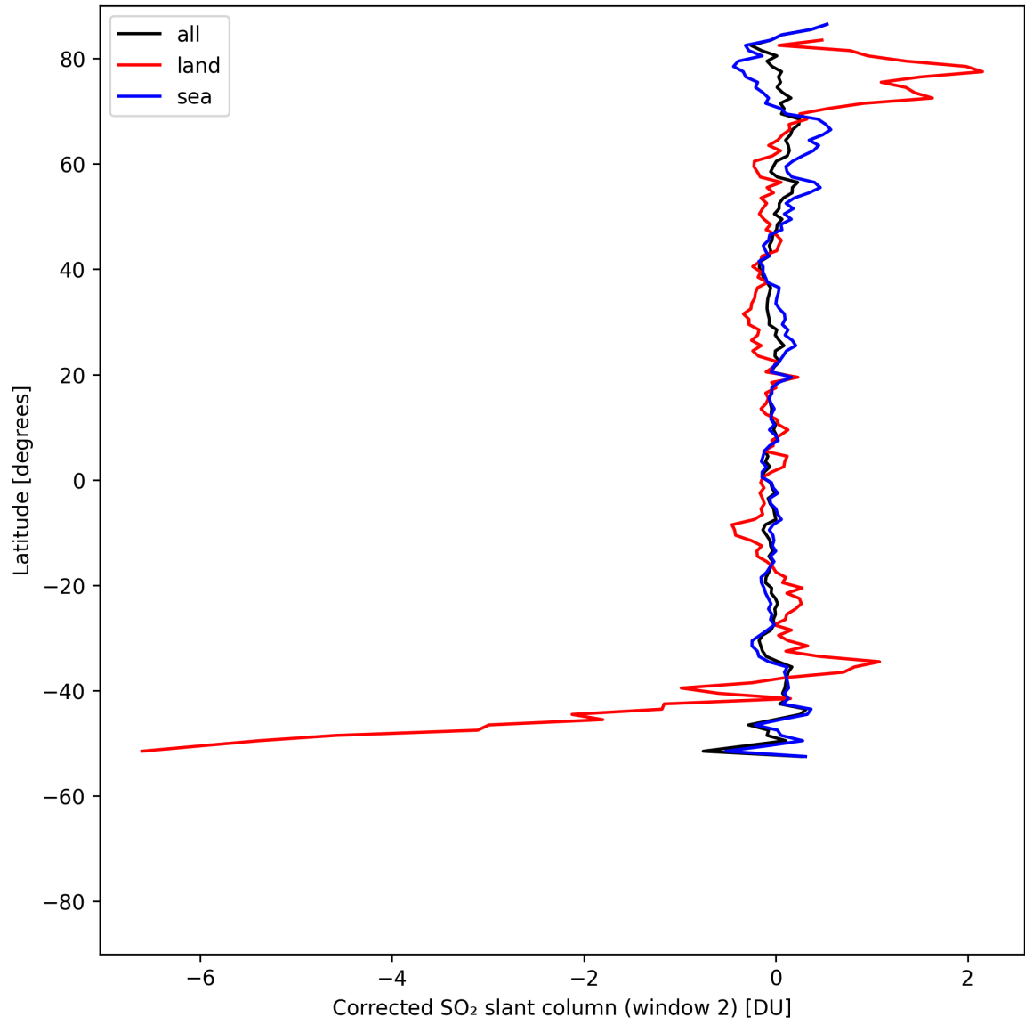
Figure 43: Zonal average of “Corrected SO 2 slant column (window 2)” for 2025-08-05 to 2025-08-07.
