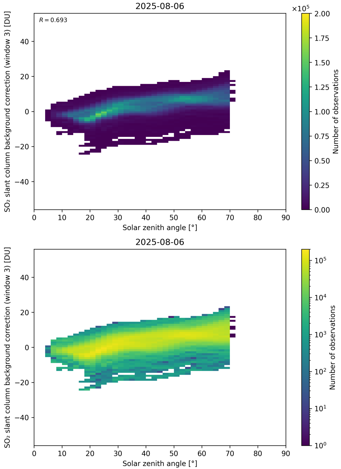
Figure 173: Scatter density plot of “Solar zenith angle” against “SO 2 slant column background correction (window 3)” for 2025-08-05 to 2025-08-07.
