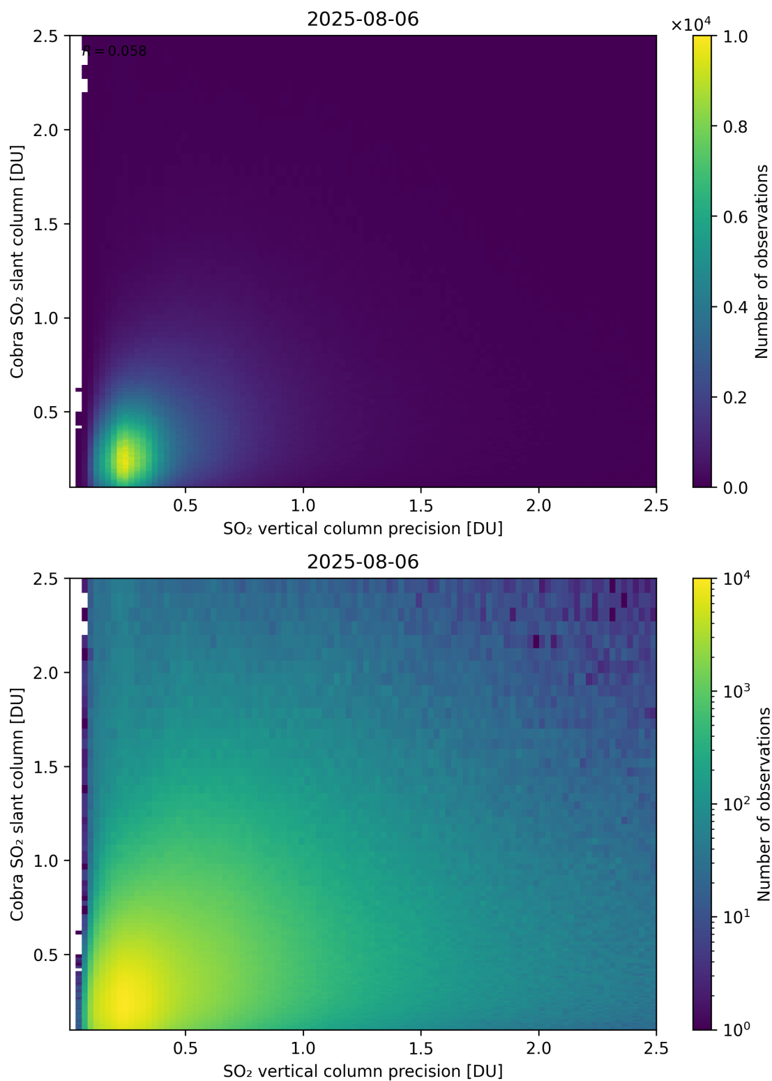
Figure 336: Scatter density plot of “SO 2 vertical column precision” against “Cobra SO 2 slant column” for 2025-08-05 to 2025-08-07.
