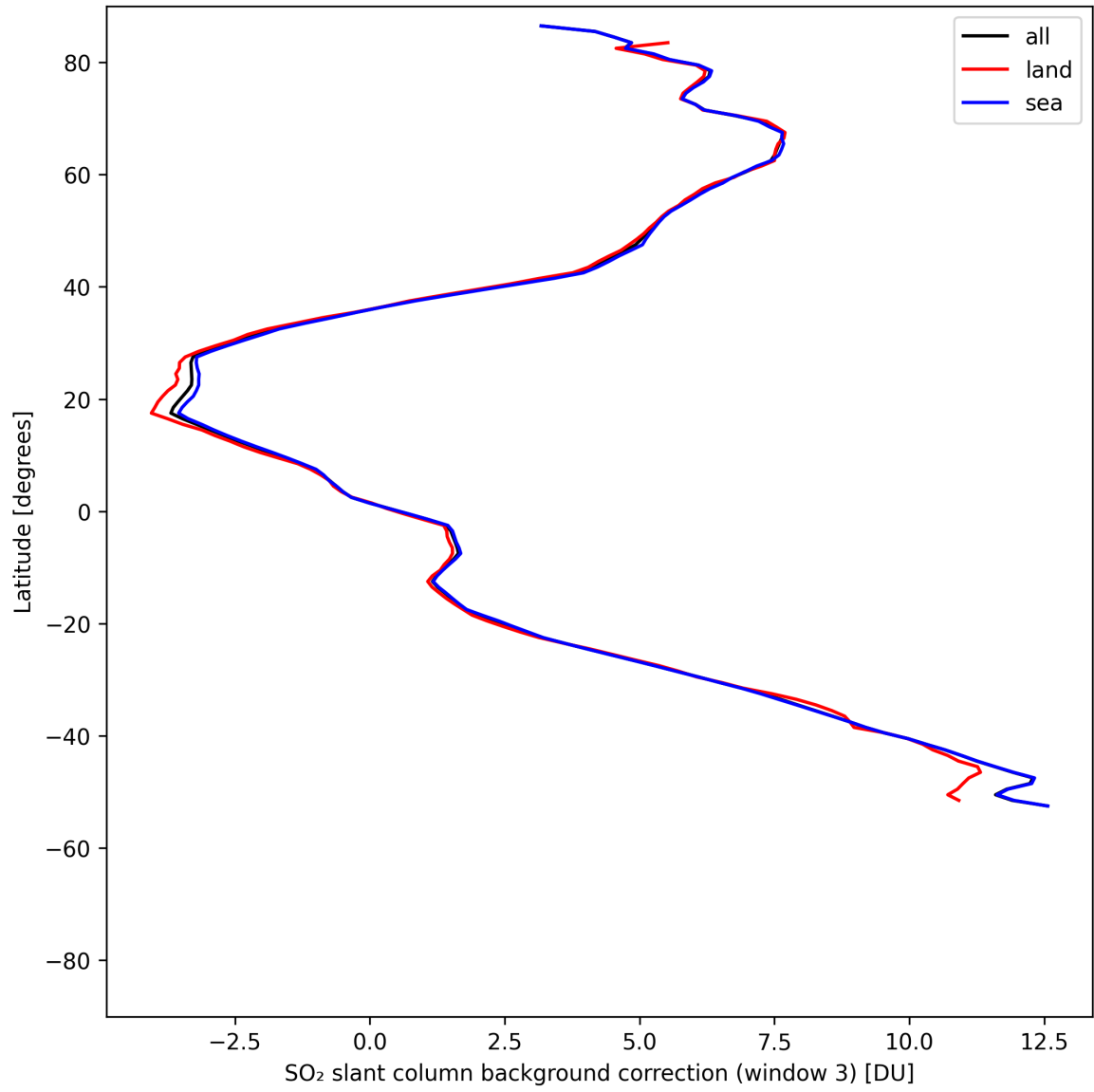
Figure 48: Zonal average of “SO 2 slant column background correction (window 3)” for 2025-08-05 to 2025-08-07.
