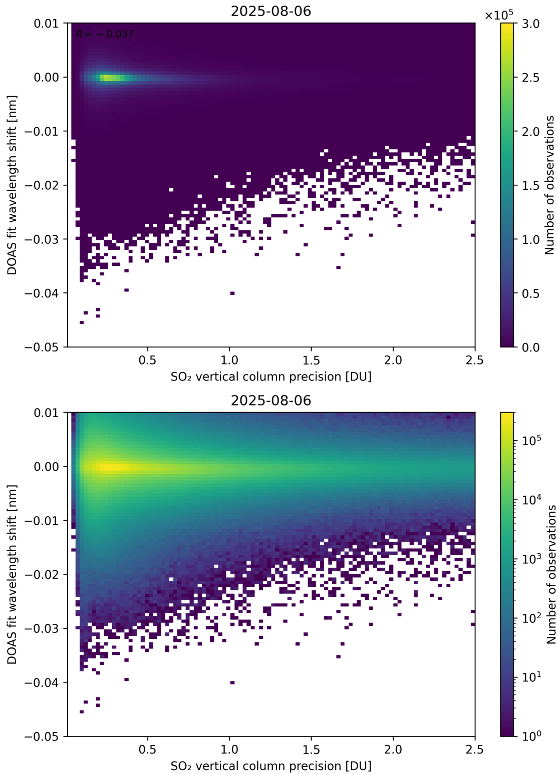
Figure 332: Scatter density plot of “SO 2 vertical column precision” against “DOAS fit wavelength shift” for 2025-08-05 to 2025-08-07.
