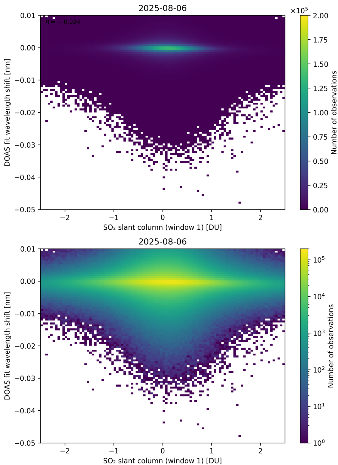
Figure 265: Scatter density plot of “SO 2 slant column (window 1)” against “DOAS fit wavelength shift” for 2025-08-05 to 2025-08-07.
