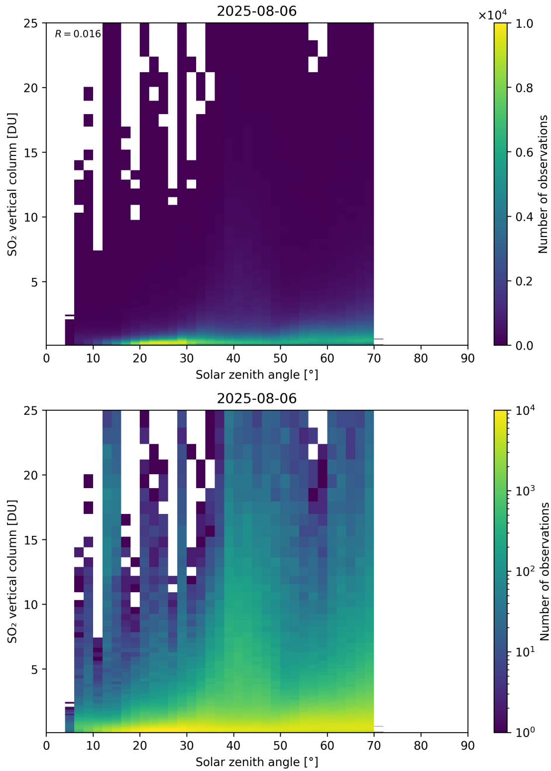
Figure 191: Scatter density plot of “Solar zenith angle” against “SO 2 vertical column” for 2025-08-05 to 2025-08-07.
