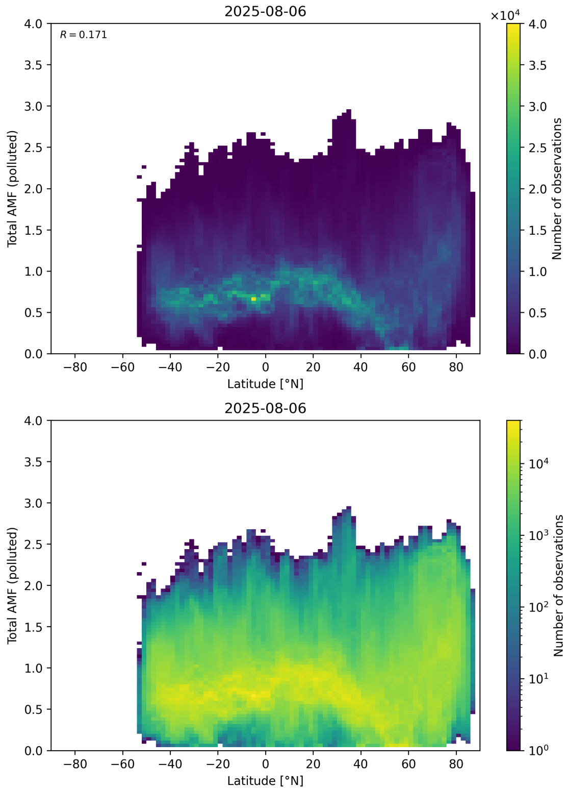
Figure 167: Scatter density plot of “Latitude” against “Total AMF (polluted)” for 2025-08-05 to 2025-08-07.
