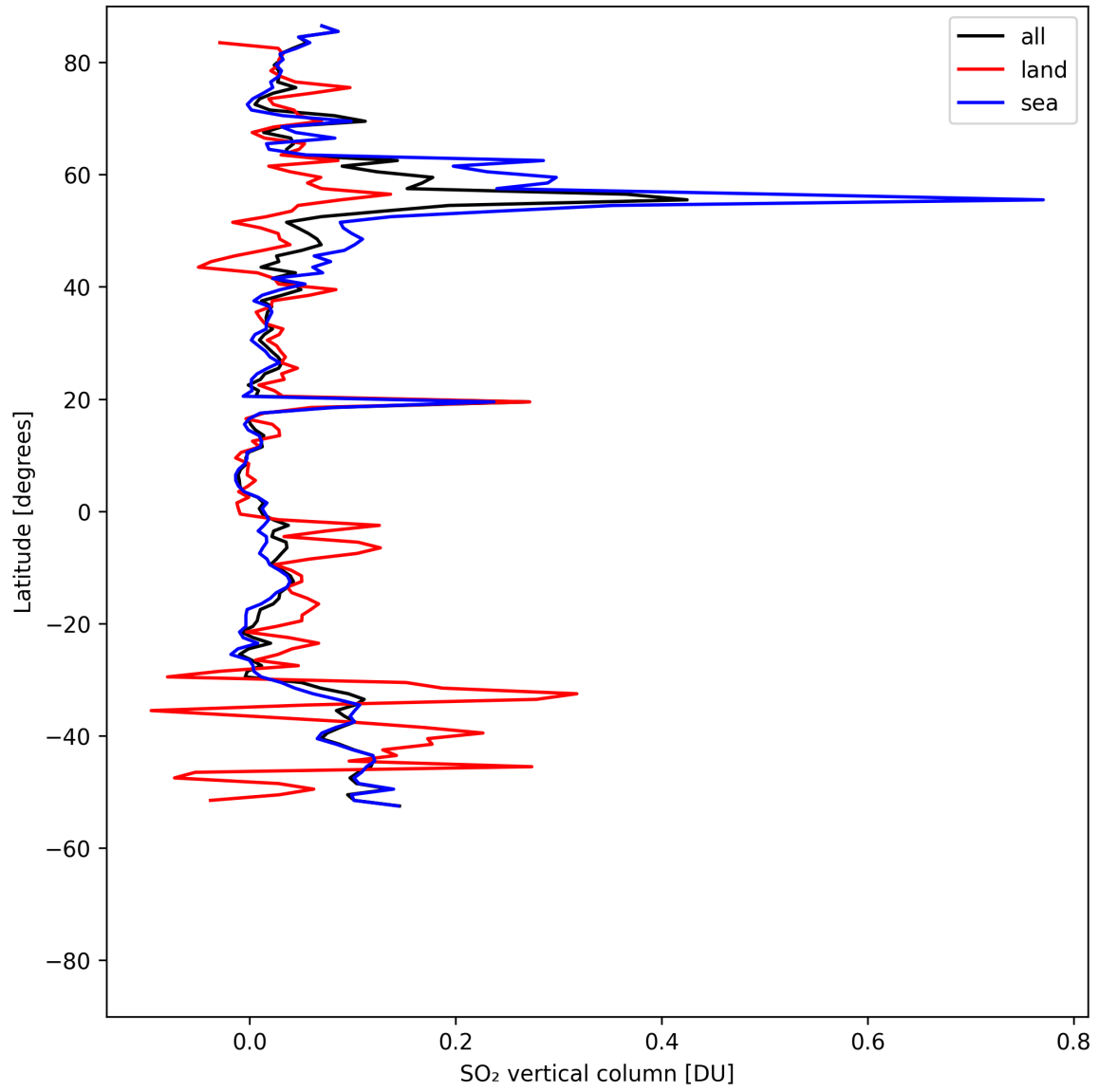
Figure 32: Zonal average of “SO 2 vertical column” for 2025-08-05 to 2025-08-07.
