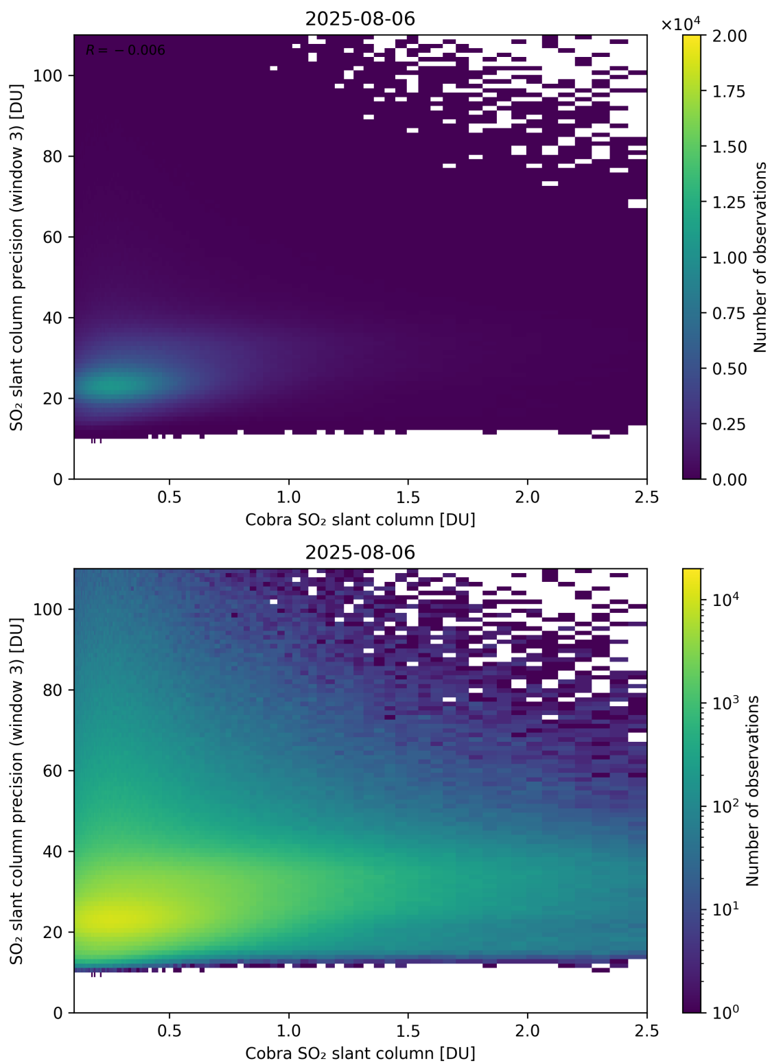
Figure 223: Scatter density plot of “Cobra SO 2 slant column” against “SO 2 slant column precision (window 3)” for 2025-08-05 to 2025-08-07.
