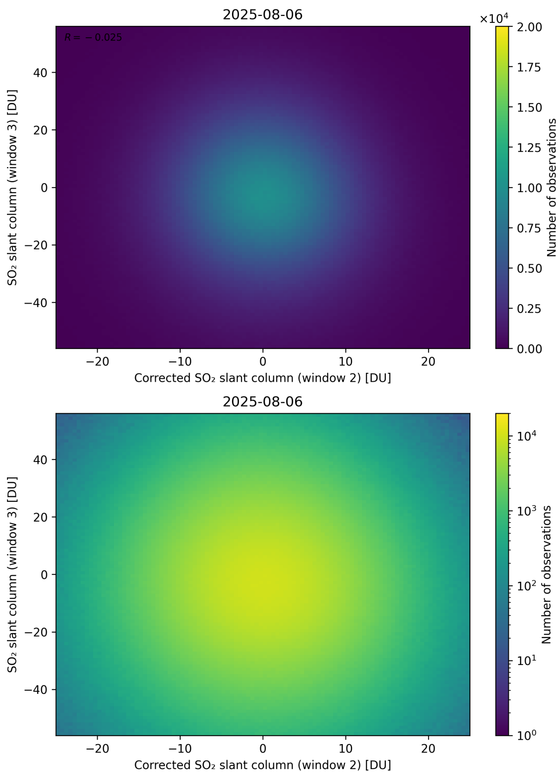
Figure 251: Scatter density plot of “Corrected SO 2 slant column (window 2)” against “SO 2 slant column (window 3)” for 2025-08-05 to 2025-08-07.
