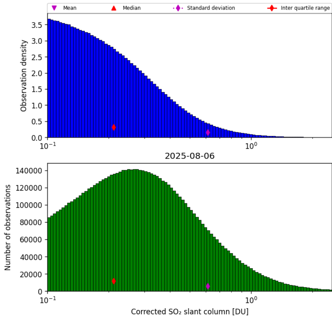
Figure 60: Histogram of "Corrected SO 2 slant column" for 2025-08-05 to 2025-08-07
