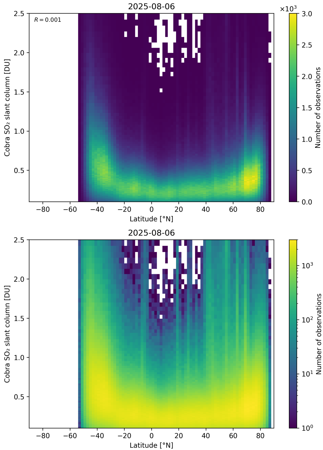
Figure 157: Scatter density plot of “Latitude” against “Cobra SO 2 slant column” for 2025-08-05 to 2025-08-07.
