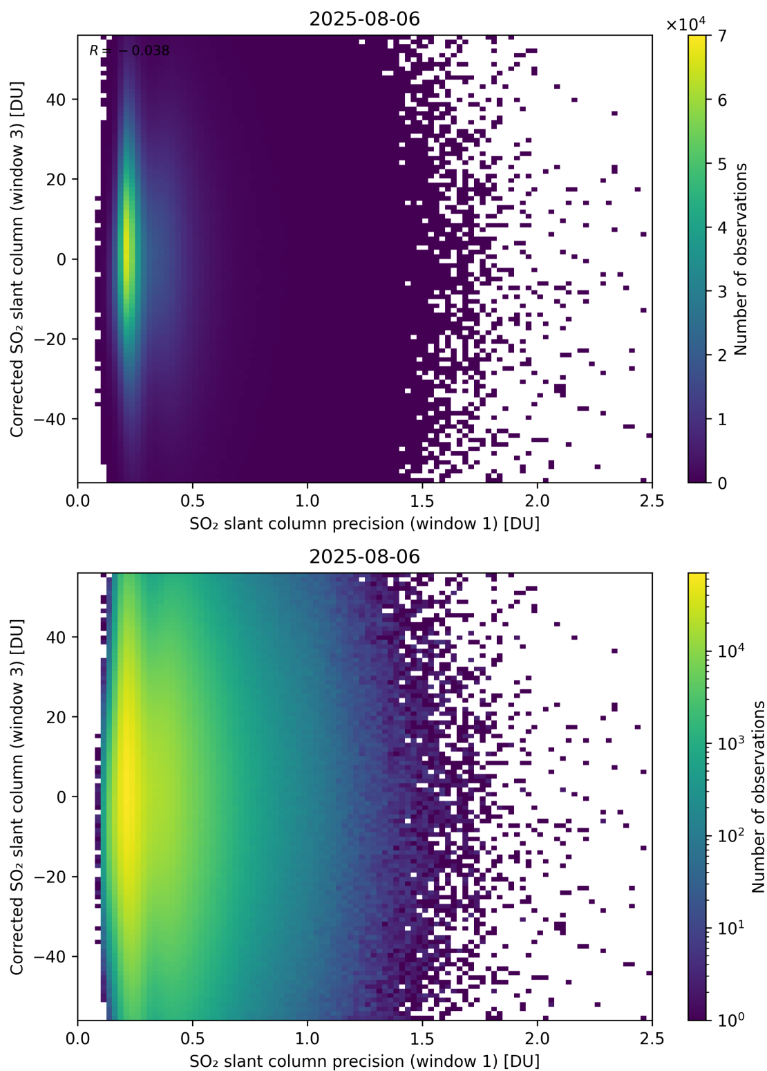
Figure 276: Scatter density plot of “SO 2 slant column precision (window 1)” against “Corrected SO 2 slant column (window 3)” for 2025-08-05 to 2025-08-07.
