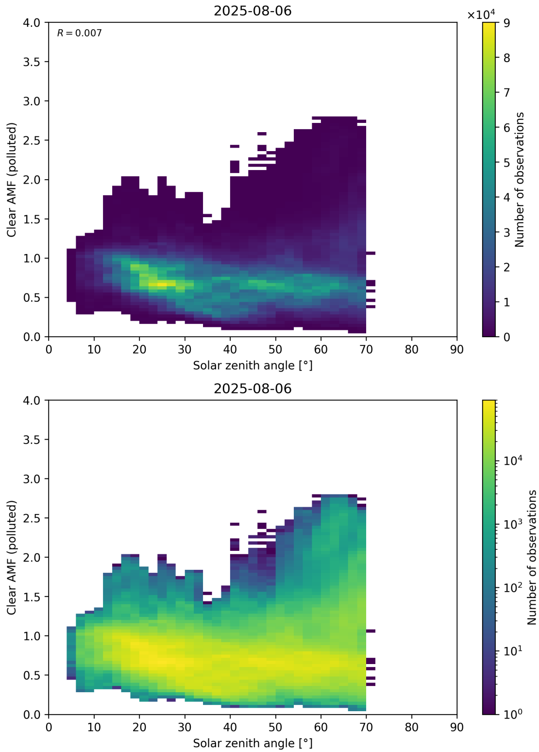
Figure 178: Scatter density plot of “Solar zenith angle” against “Clear AMF (polluted)” for 2025-08-05 to 2025-08-07.
