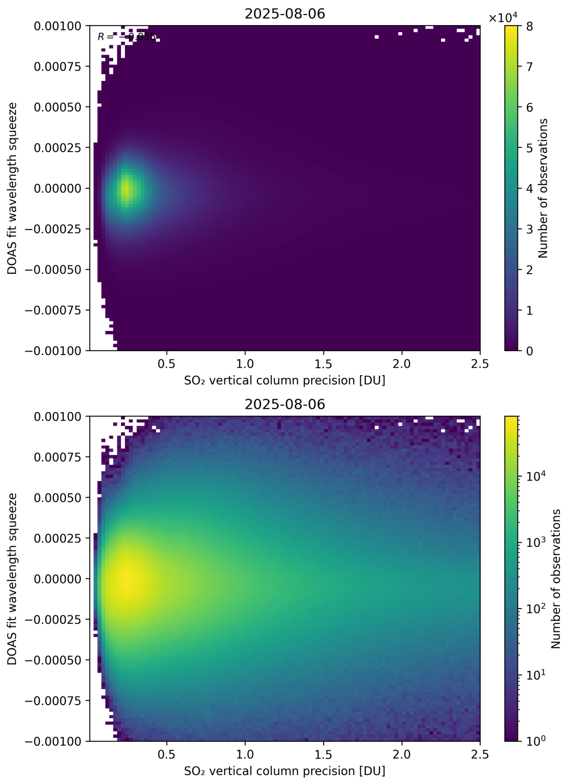
Figure 333: Scatter density plot of “SO 2 vertical column precision” against “DOAS fit wavelength squeeze” for 2025-08-05 to 2025-08-07.
