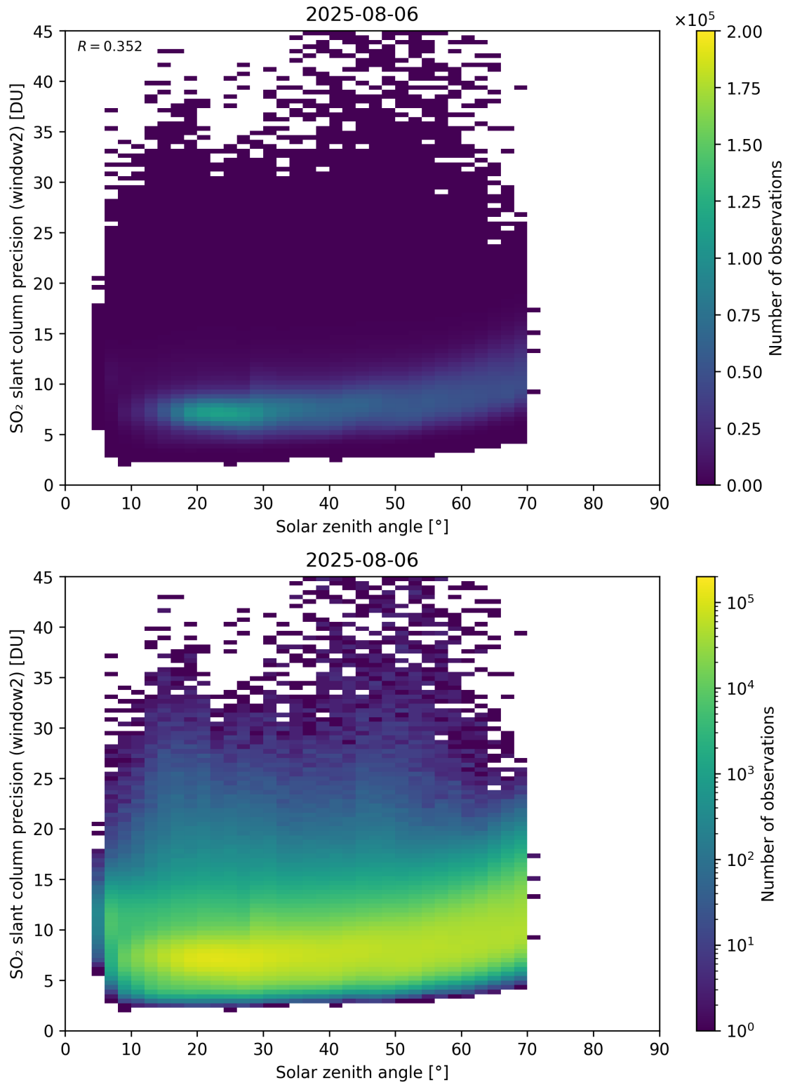
Figure 186: Scatter density plot of “Solar zenith angle” against “SO 2 slant column precision (window2)” for 2025-08-05 to 2025-08-07.
