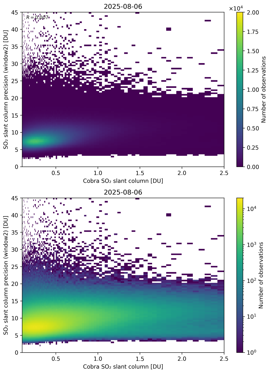
Figure 221: Scatter density plot of “Cobra SO 2 slant column” against “SO 2 slant column precision (window2)” for 2025-08-05 to 2025-08-07.
