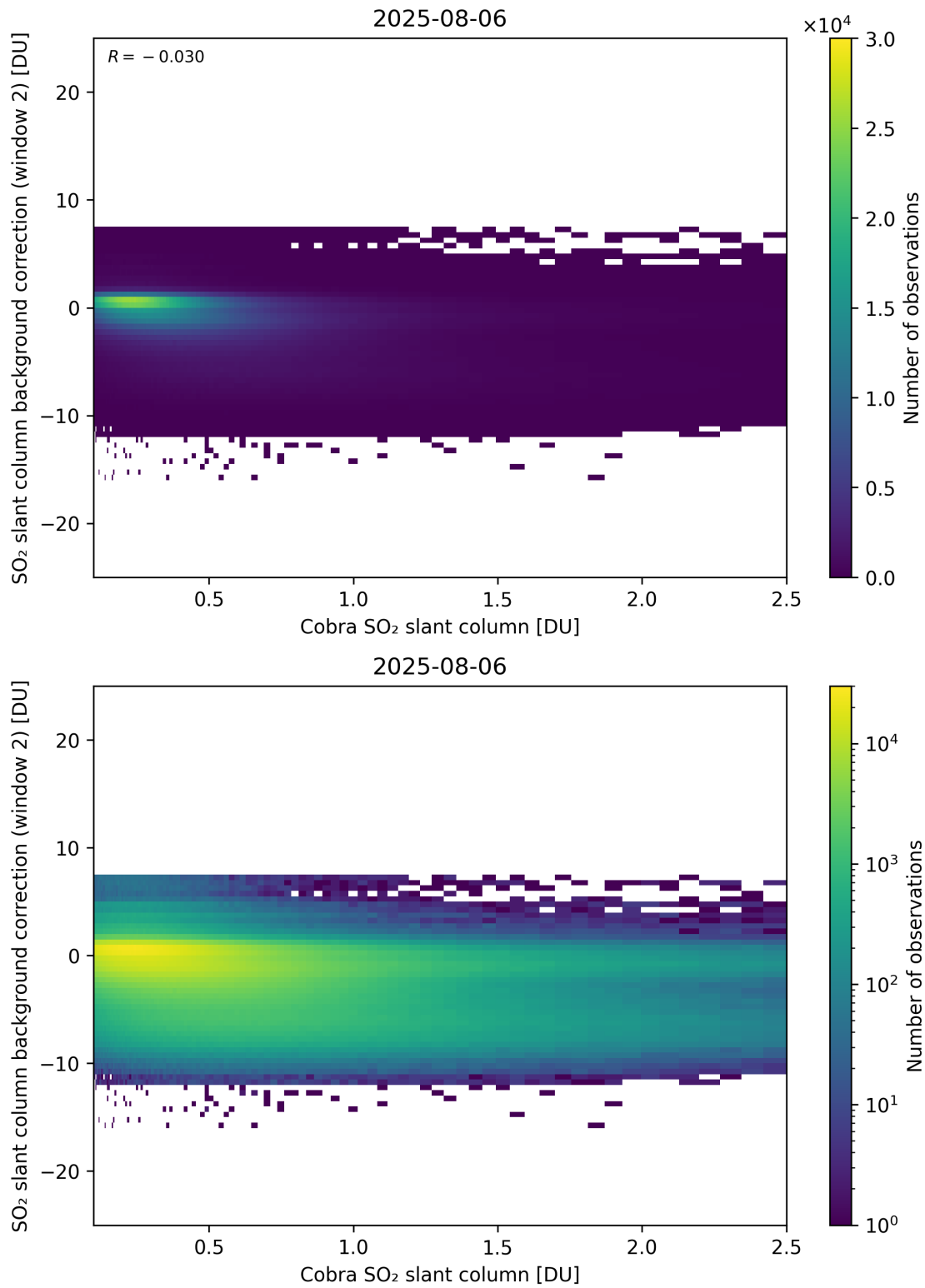
Figure 194: Scatter density plot of “Cobra SO 2 slant column” against “SO 2 slant column background correction (window 2)” for 2025-08-05 to 2025-08-07.
