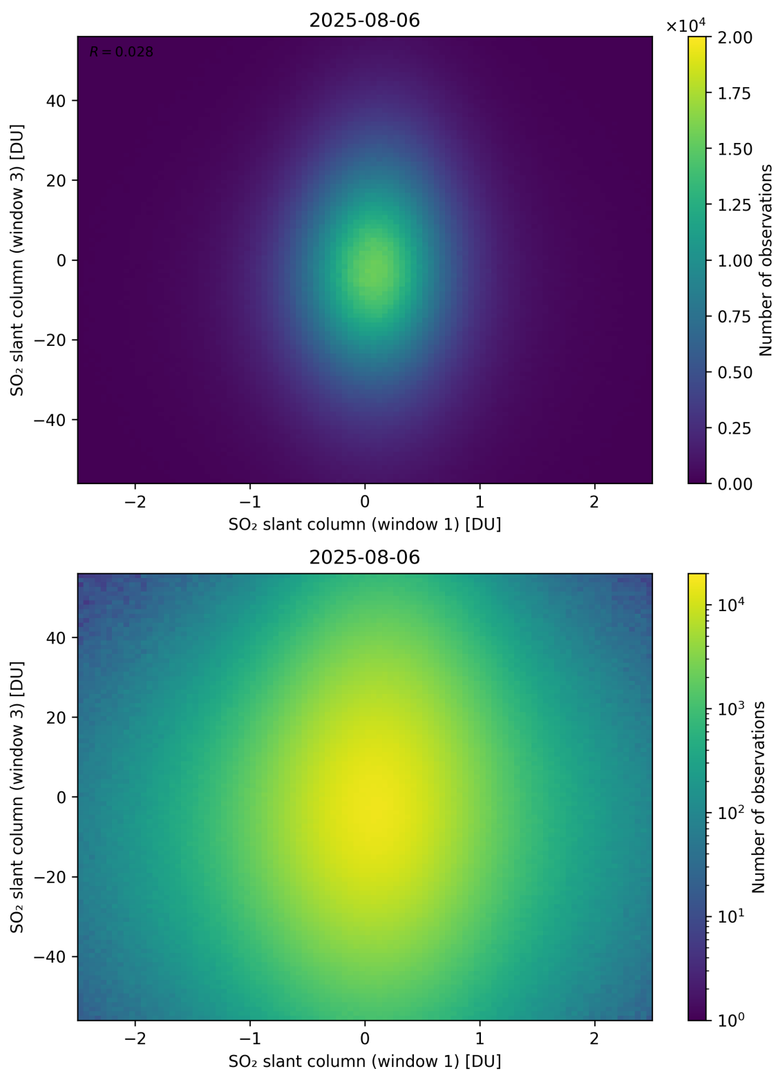
Figure 287: Scatter density plot of “SO 2 slant column (window 1)” against “SO 2 slant column (window 3)” for 2025-08-05 to 2025-08-07.
