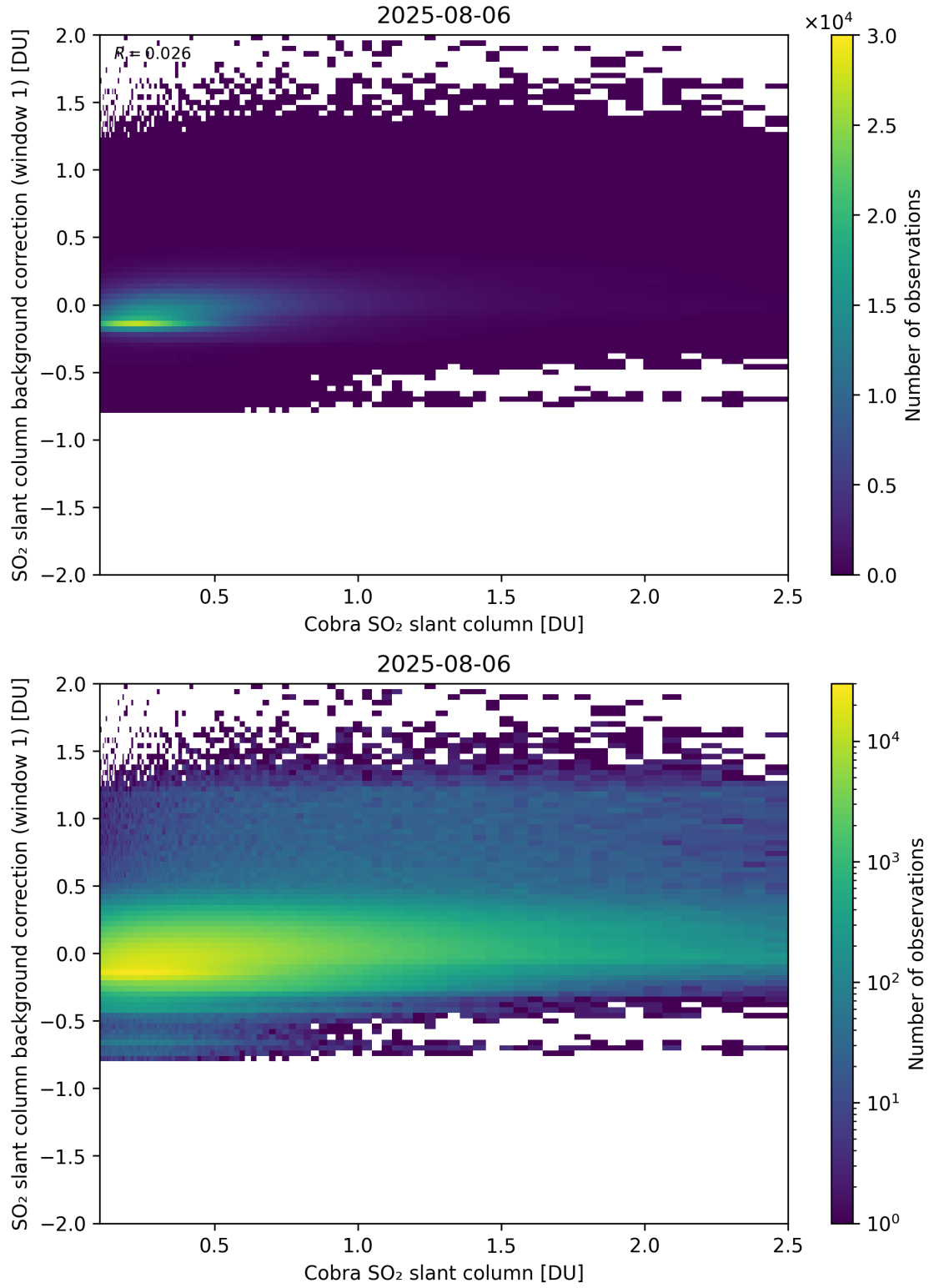
Figure 193: Scatter density plot of “Cobra SO 2 slant column” against “SO 2 slant column background correction (window 1)” for 2025-08-05 to 2025-08-07.
