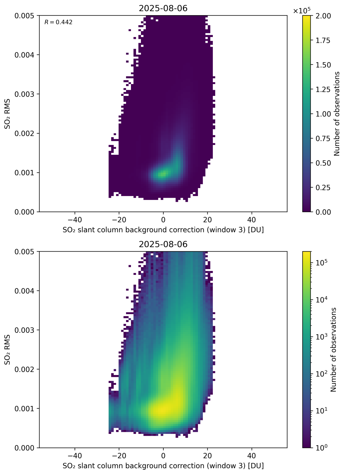
Figure 134: Scatter density plot of “SO 2 slant column background correction (window 3)” against “SO 2 RMS” for 2025-08-05 to 2025-08-07.
