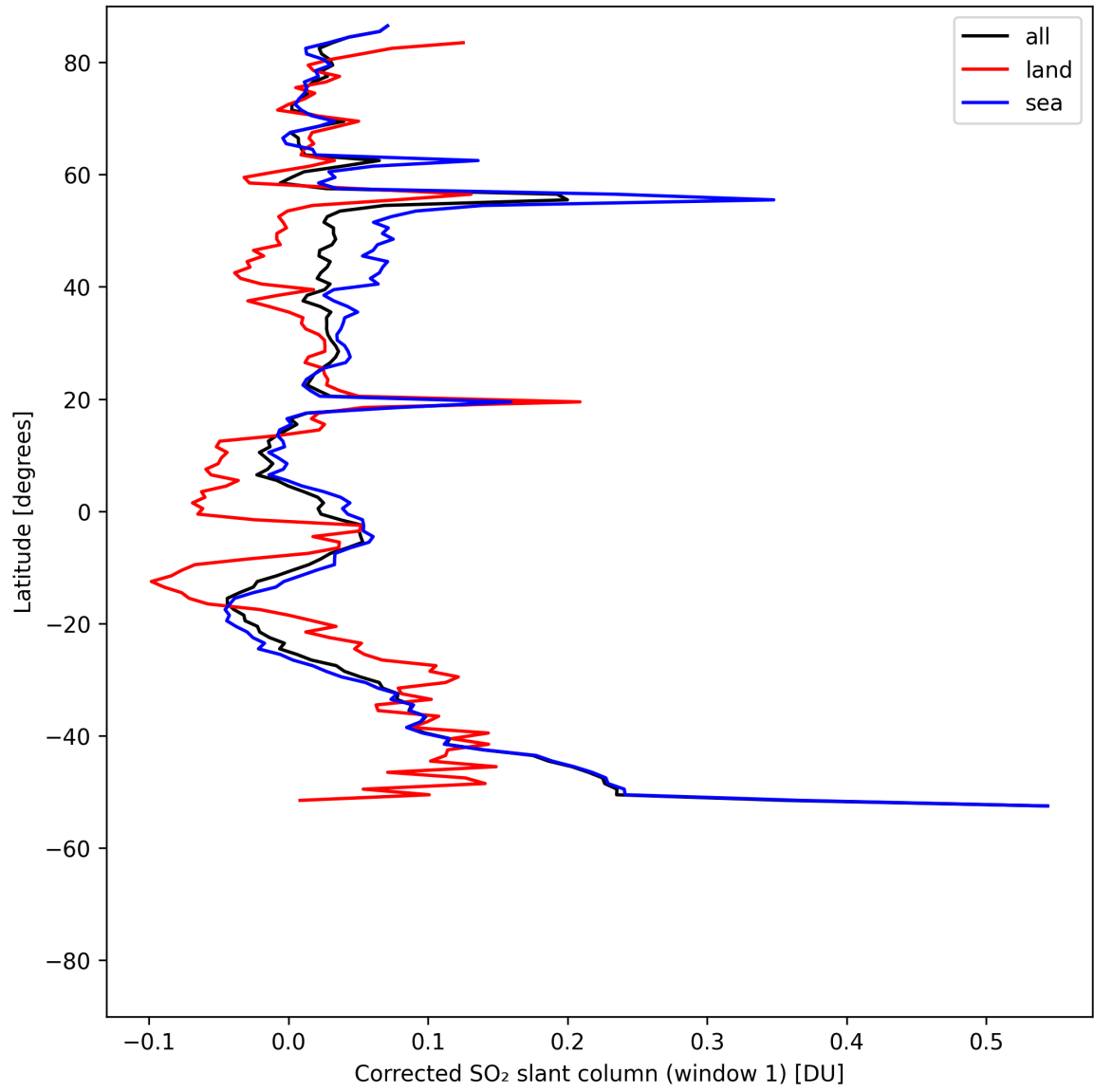
Figure 39: Zonal average of “Corrected SO 2 slant column (window 1)” for 2025-08-05 to 2025-08-07.
