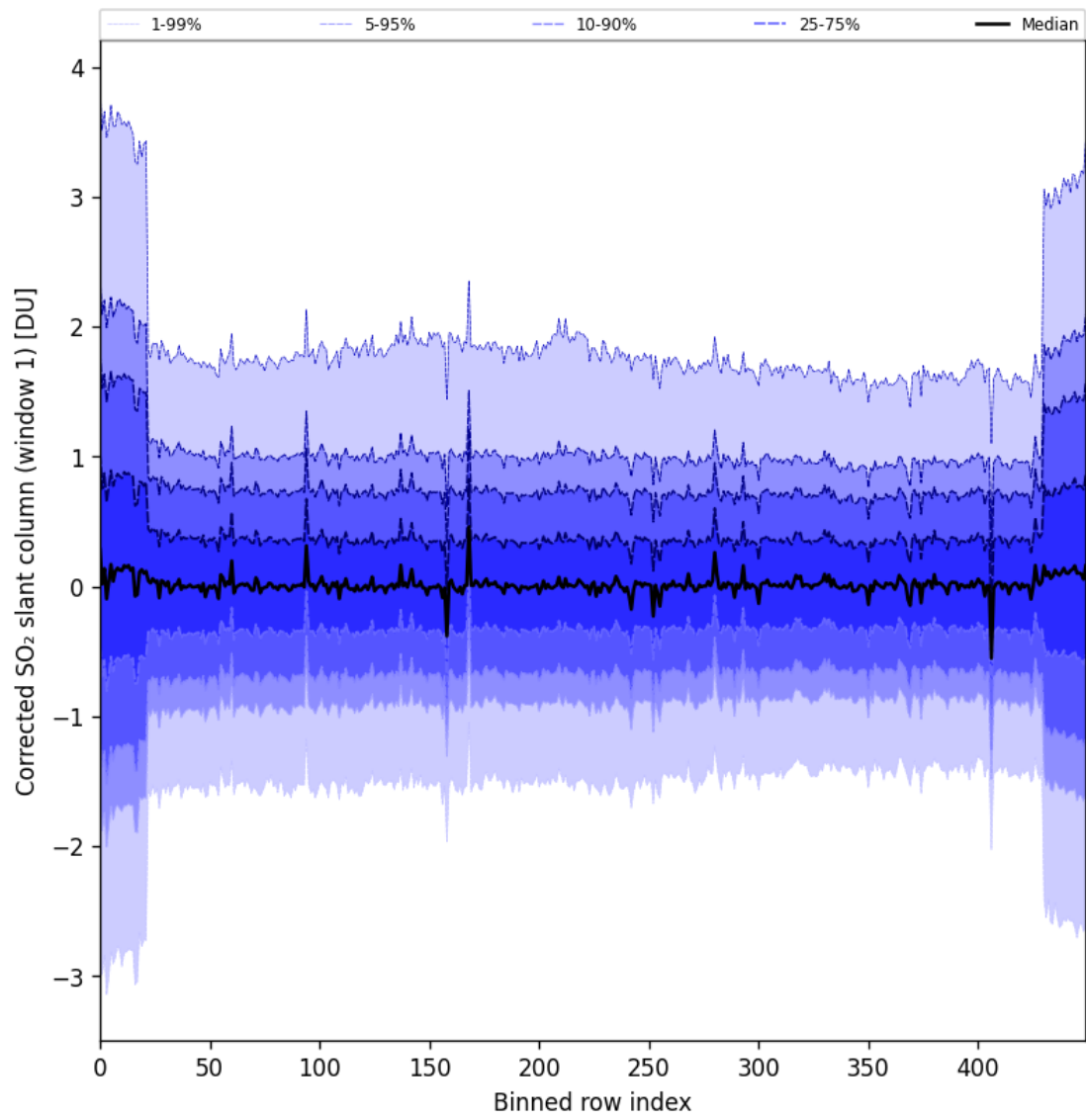
Figure 91: Along track statistics of “Corrected SO 2 slant column (window 1)” for 2025-08-05 to 2025-08-07
