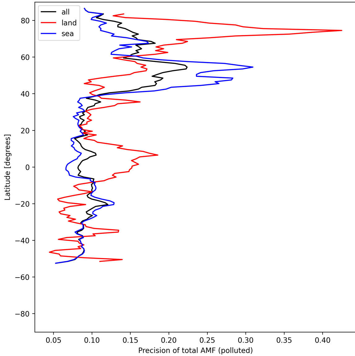
Figure 54: Zonal average of “Precision of total AMF (polluted)” for 2025-08-05 to 2025-08-07.
