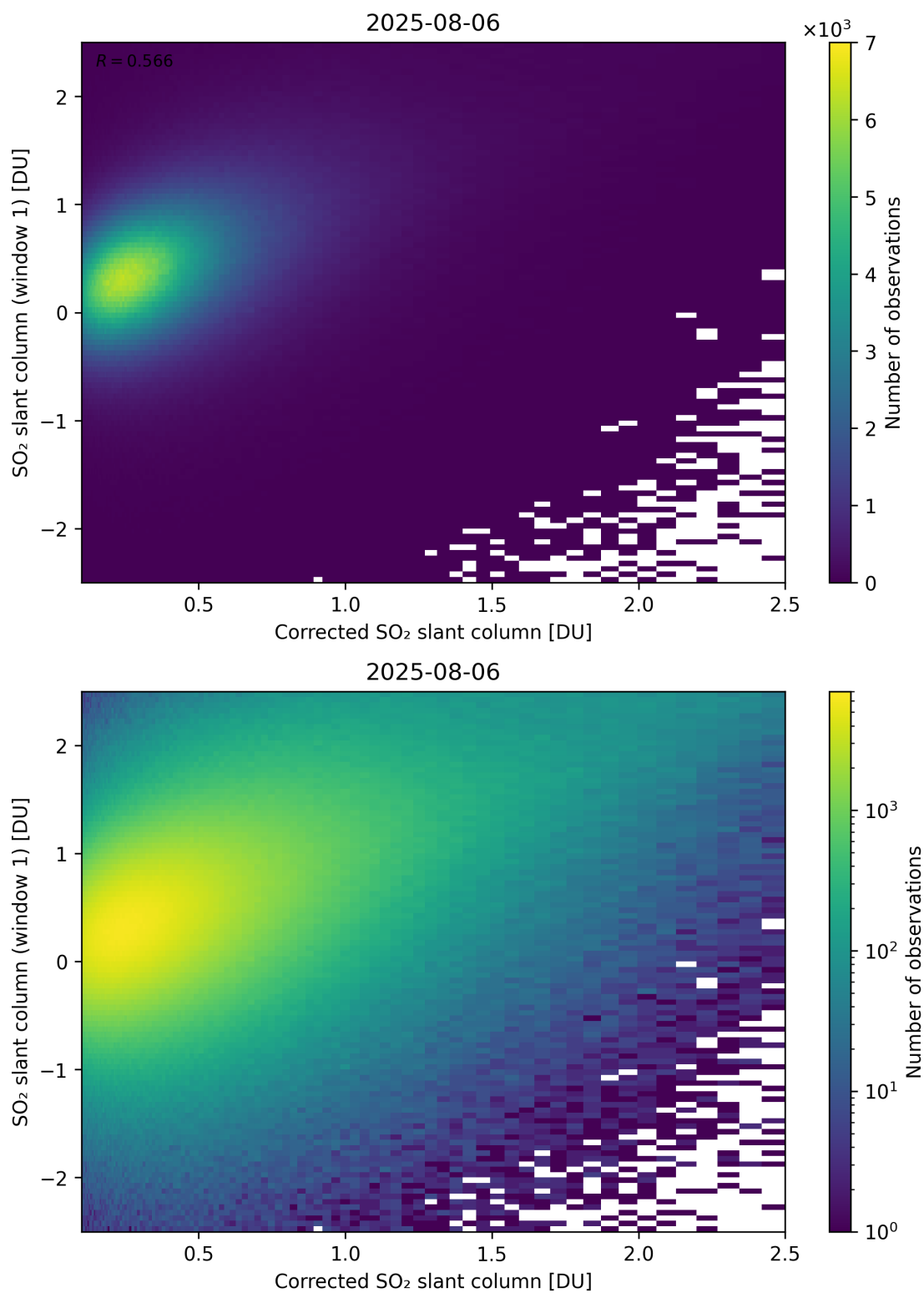
Figure 237: Scatter density plot of “Corrected SO 2 slant column” against “SO 2 slant column (window 1)” for 2025-08-05 to 2025-08-07.
