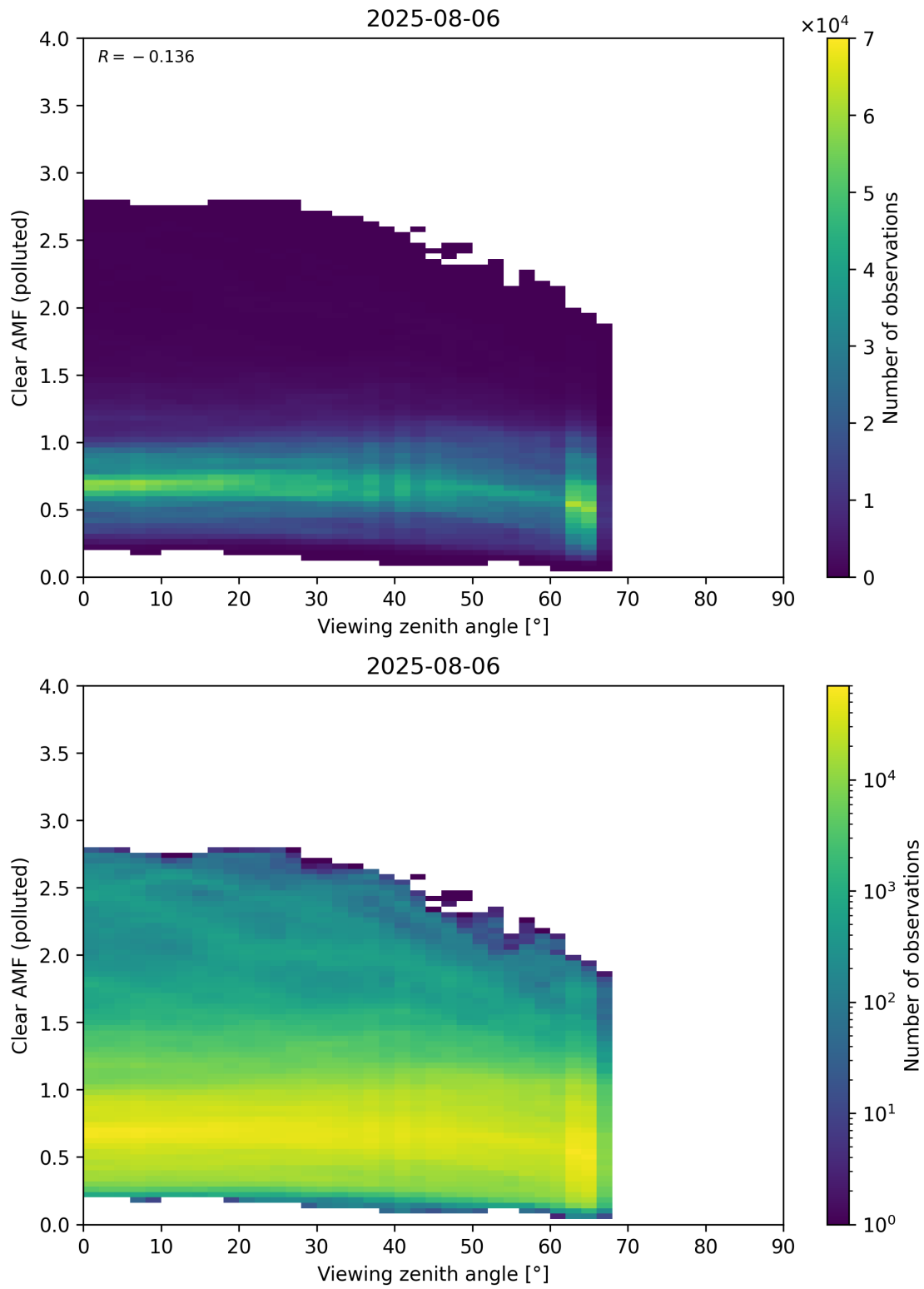
Figure 370: Scatter density plot of “Viewing zenith angle” against “Clear AMF (polluted)” for 2025-08-05 to 2025-08-07.
