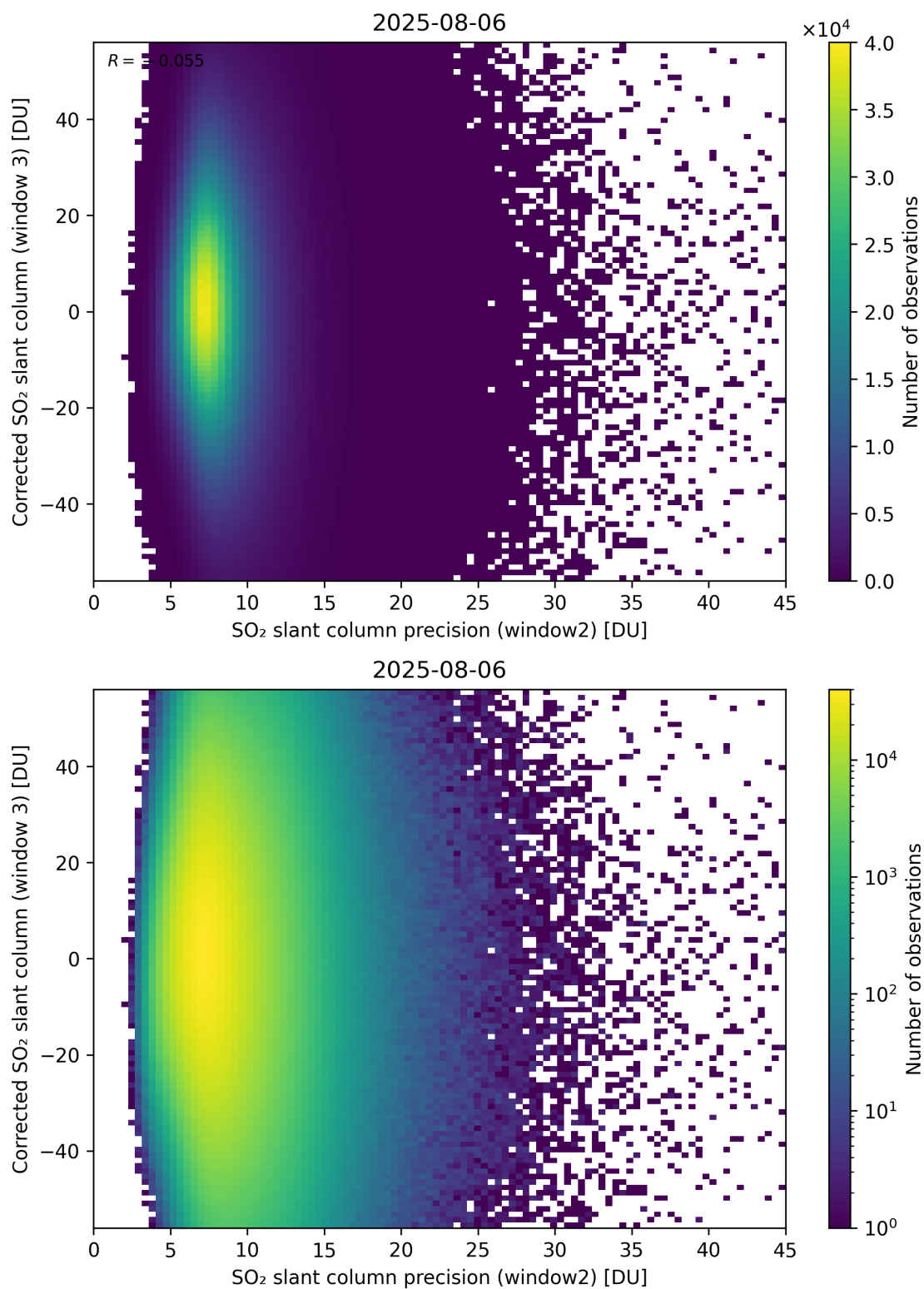
Figure 298: Scatter density plot of “SO 2 slant column precision (window2)” against “Corrected SO 2 slant column (window 3)” for 2025-08-05 to 2025-08-07.
