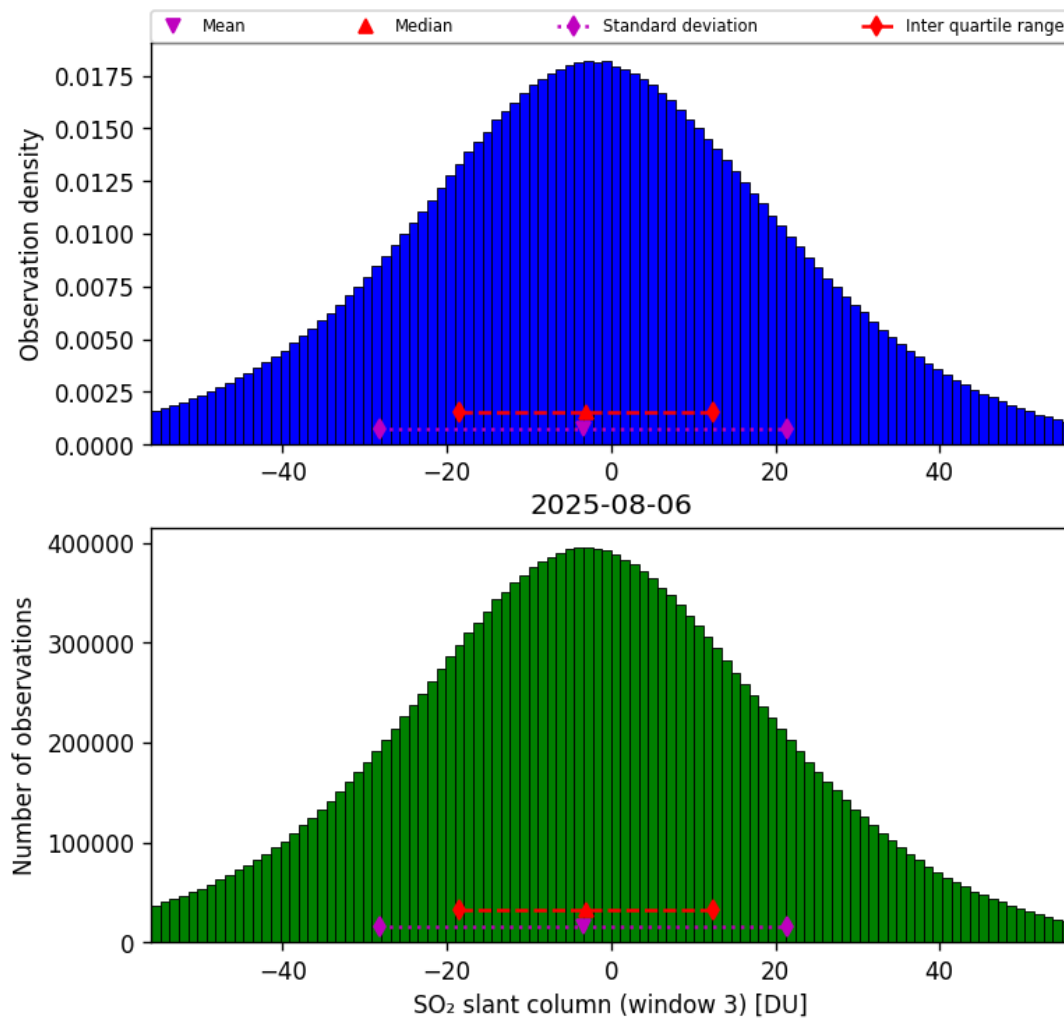
Figure 71: Histogram of “SO 2 slant column (window 3)” for 2025-08-05 to 2025-08-07
