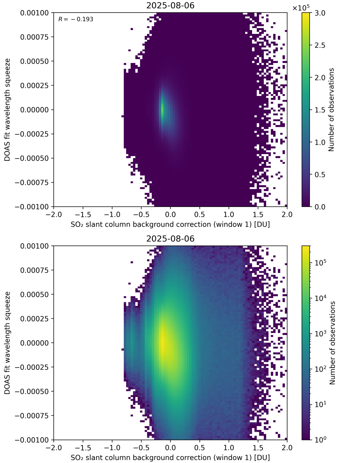
Figure 112: Scatter density plot of “SO 2 slant column background correction (window 1)” against “DOAS fit wavelength squeeze” for 2025-08-05 to 2025-08-07.
