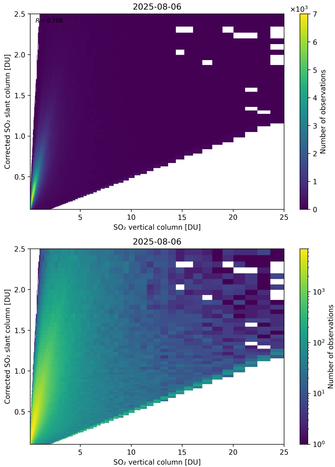
Figure 351: Scatter density plot of “SO 2 vertical column” against “Corrected SO 2 slant column” for 2025-08-05 to 2025-08-07.
