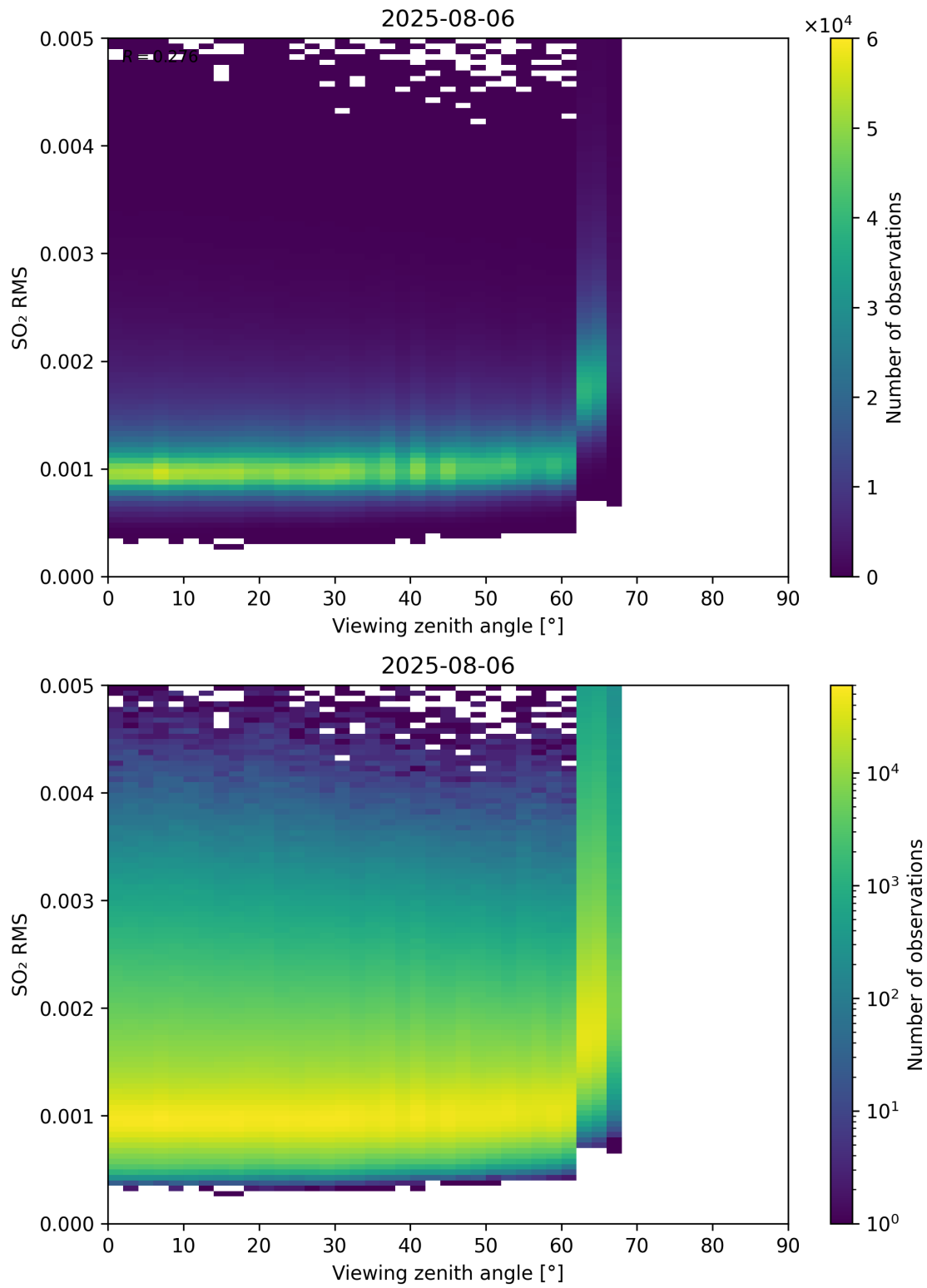
Figure 367: Scatter density plot of “Viewing zenith angle” against “SO 2 RMS” for 2025-08-05 to 2025-08-07.
