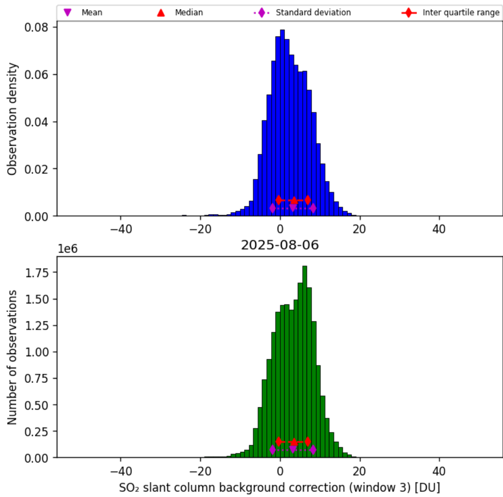
Figure 74: Histogram of “SO 2 slant column background correction (window 3)” for 2025-08-05 to 2025-08-07
