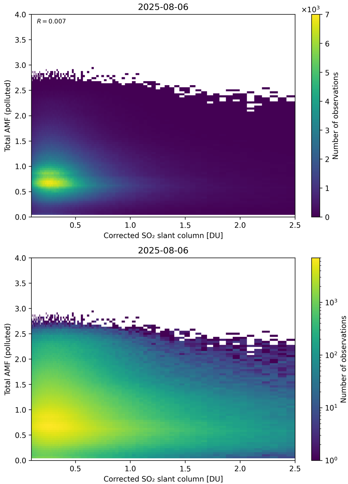
Figure 242: Scatter density plot of “Corrected SO 2 slant column” against “Total AMF (polluted)” for 2025-08-05 to 2025-08-07.
