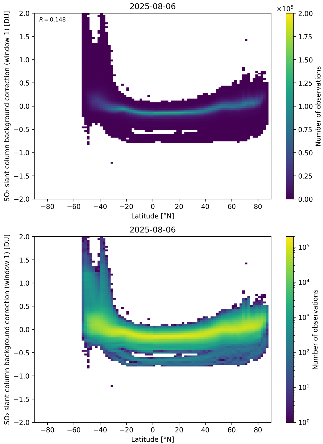
Figure 150: Scatter density plot of “Latitude” against “SO 2 slant column background correction (window 1)” for 2025-08-05 to 2025-08-07.
