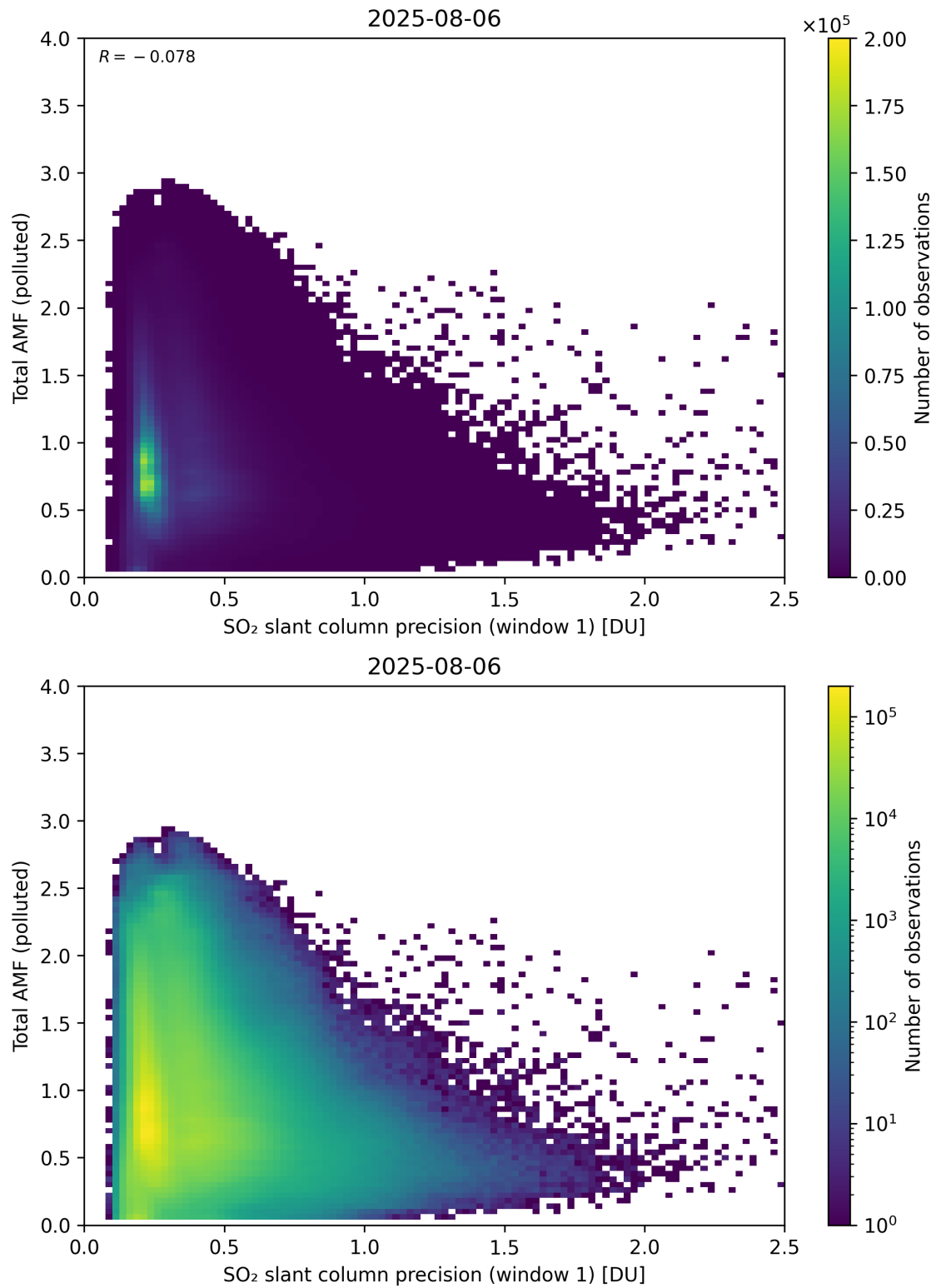
Figure 280: Scatter density plot of “SO 2 slant column precision (window 1)” against “Total AMF (polluted)” for 2025-08-05 to 2025-08-07.
