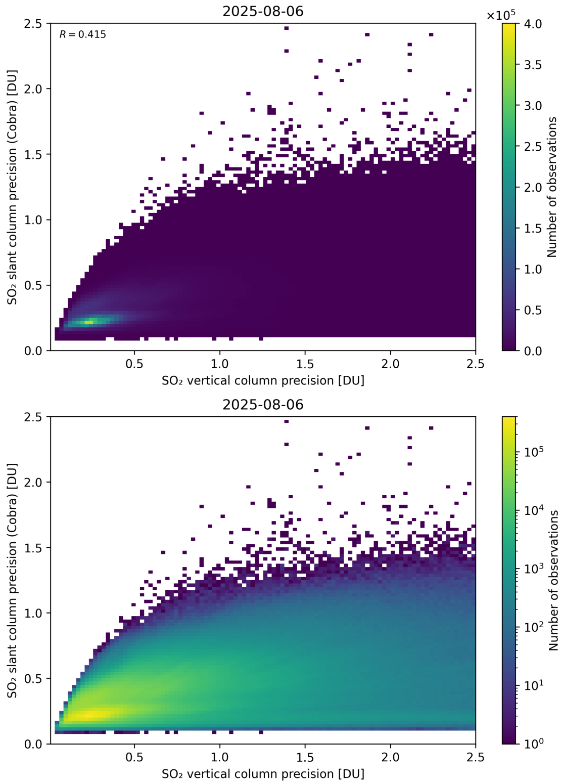
Figure 337: Scatter density plot of “SO 2 vertical column precision” against “SO 2 slant column precision (Cobra)” for 2025-08-05 to 2025-08-07.
