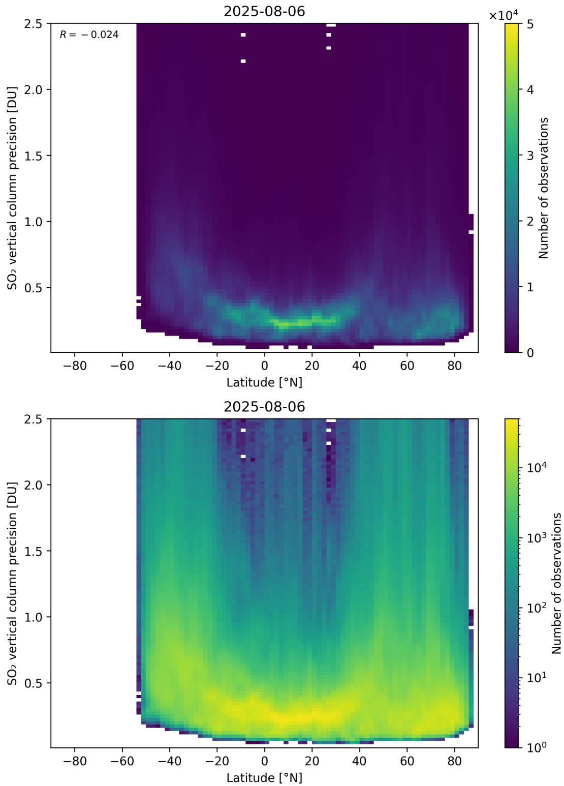
Figure 170: Scatter density plot of “Latitude” against “SO 2 vertical column precision” for 2025-08-05 to 2025-08-07.
