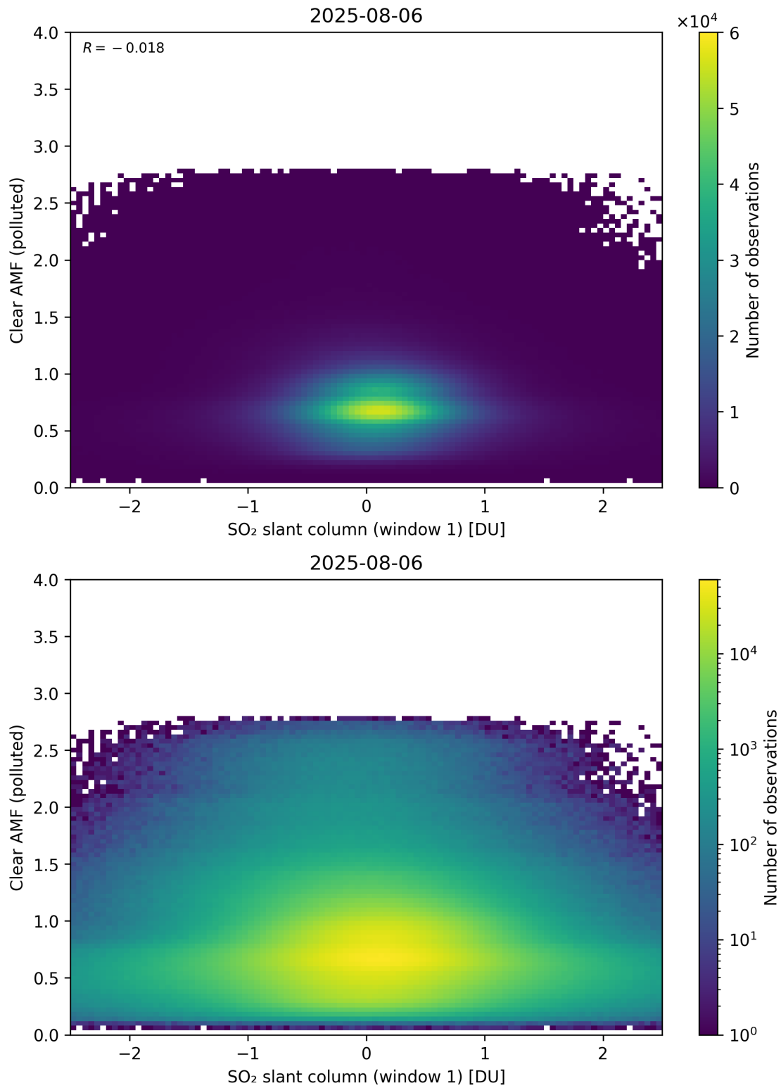
Figure 282: Scatter density plot of “SO 2 slant column (window 1)” against “Clear AMF (polluted)” for 2025-08-05 to 2025-08-07.
