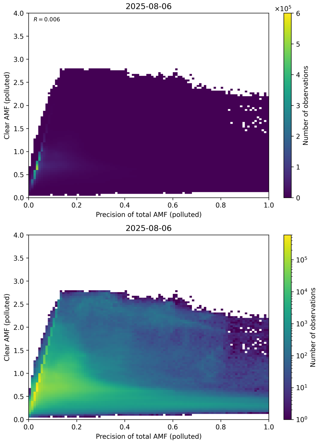
Figure 320: Scatter density plot of “Precision of total AMF (polluted)” against “Clear AMF (polluted)” for 2025-08-05 to 2025-08-07.
