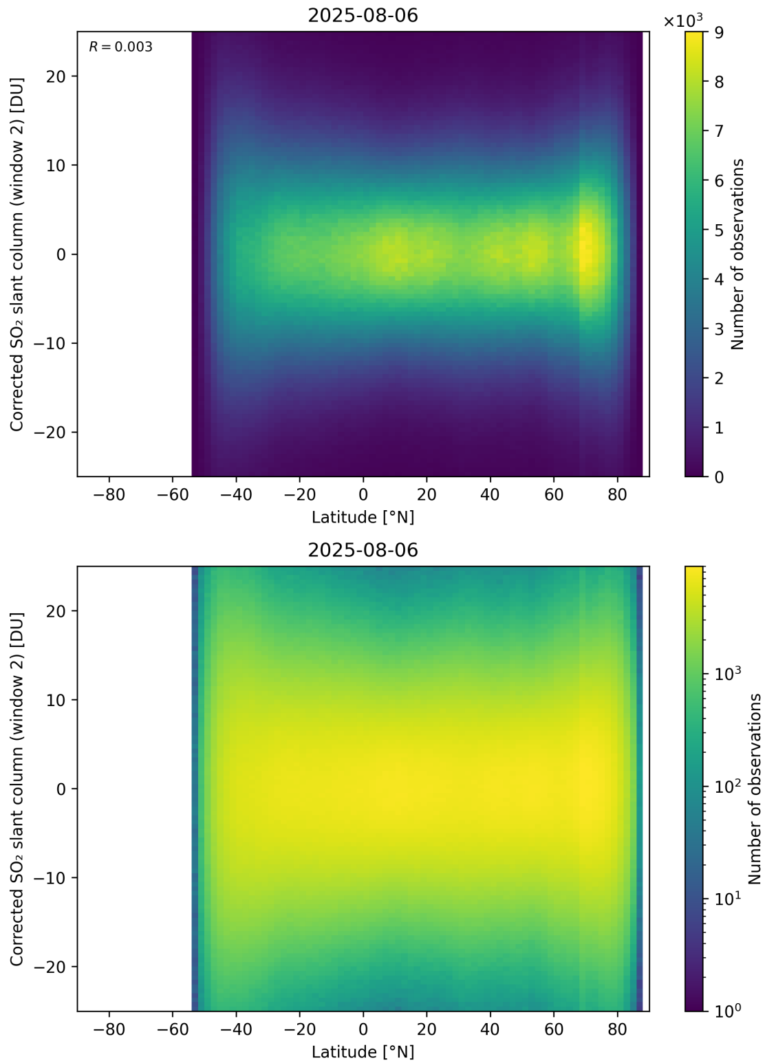
Figure 160: Scatter density plot of “Latitude” against “Corrected SO 2 slant column (window 2)” for 2025-08-05 to 2025-08-07.
