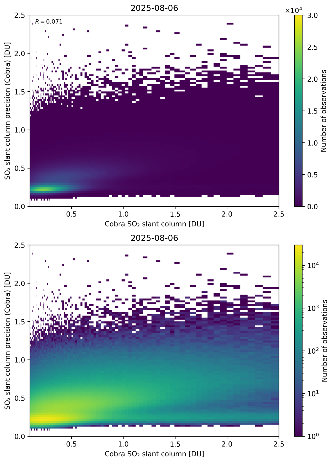
Figure 216: Scatter density plot of “Cobra SO 2 slant column” against “SO 2 slant column precision (Cobra)” for 2025-08-05 to 2025-08-07.
