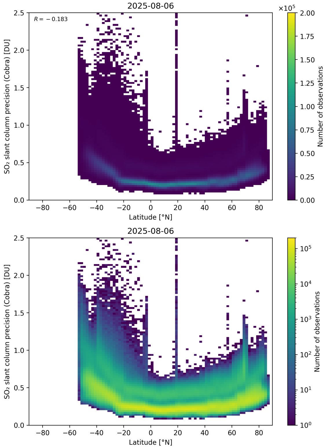
Figure 158: Scatter density plot of “Latitude” against “SO 2 slant column precision (Cobra)” for 2025-08-05 to 2025-08-07.
