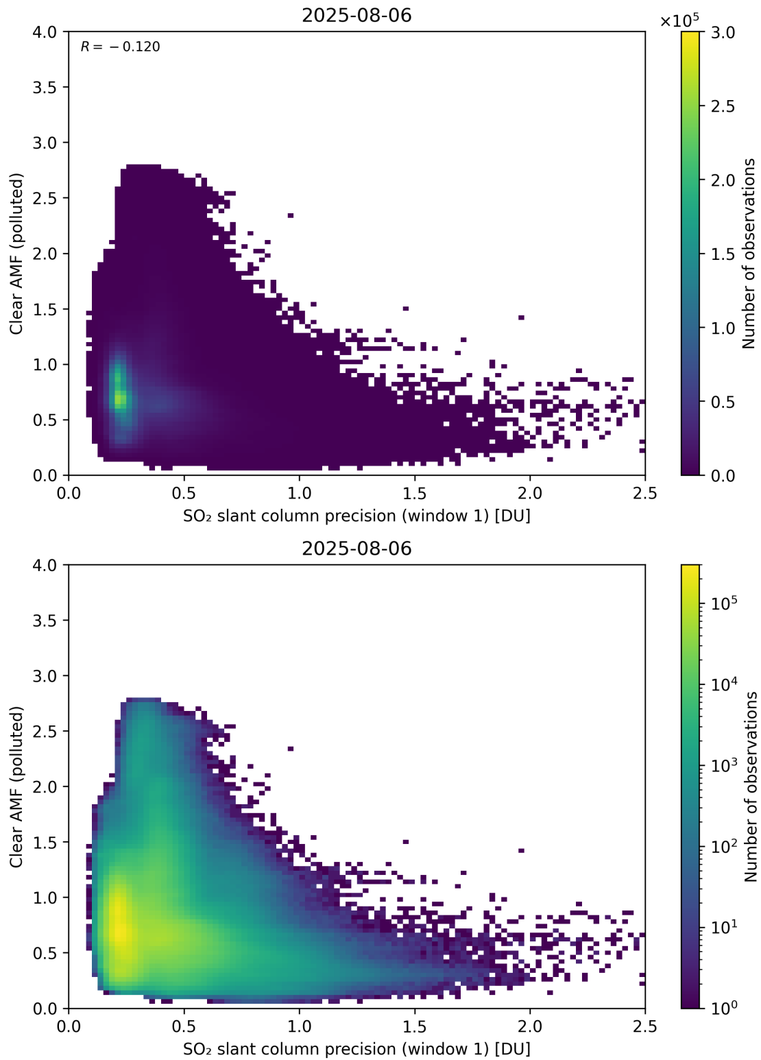
Figure 274: Scatter density plot of “SO 2 slant column precision (window 1)” against “Clear AMF (polluted)” for 2025-08-05 to 2025-08-07.
