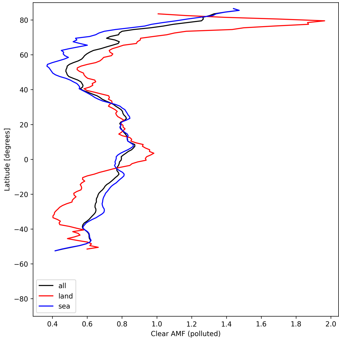
Figure 55: Zonal average of “Clear AMF (polluted)” for 2025-08-05 to 2025-08-07.
