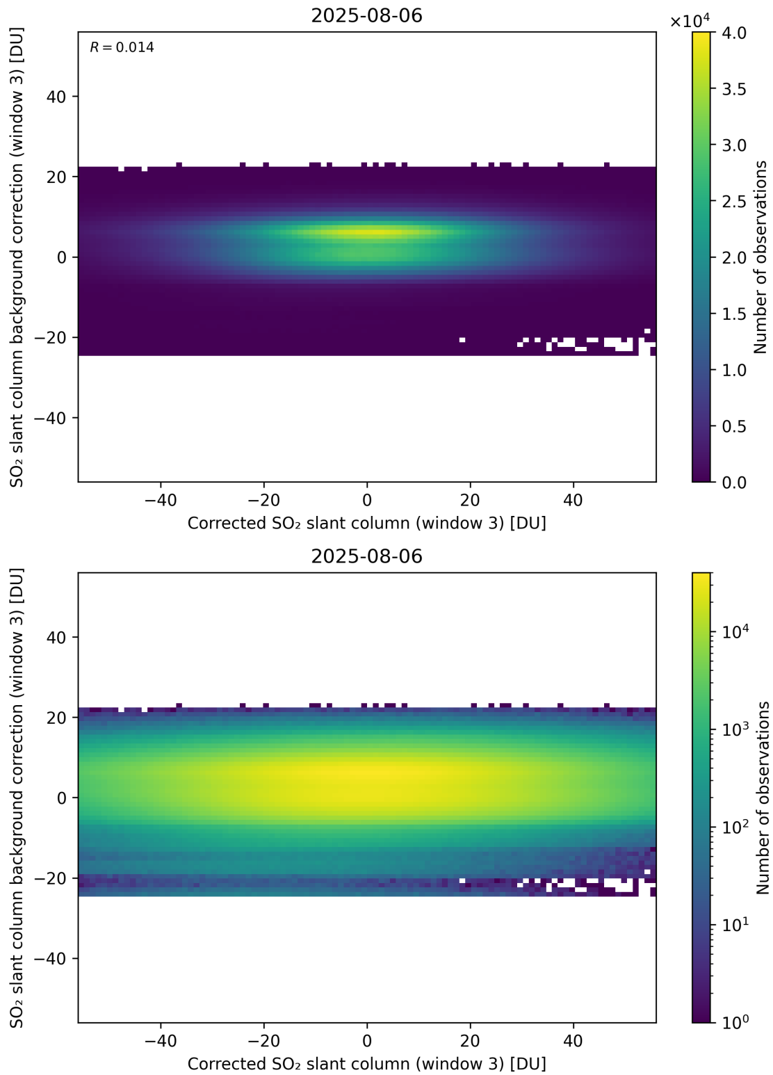
Figure 255: Scatter density plot of “Corrected SO 2 slant column (window 3)” against “SO 2 slant column background correction (window 3)” for 2025-08-05 to 2025-08-07.
