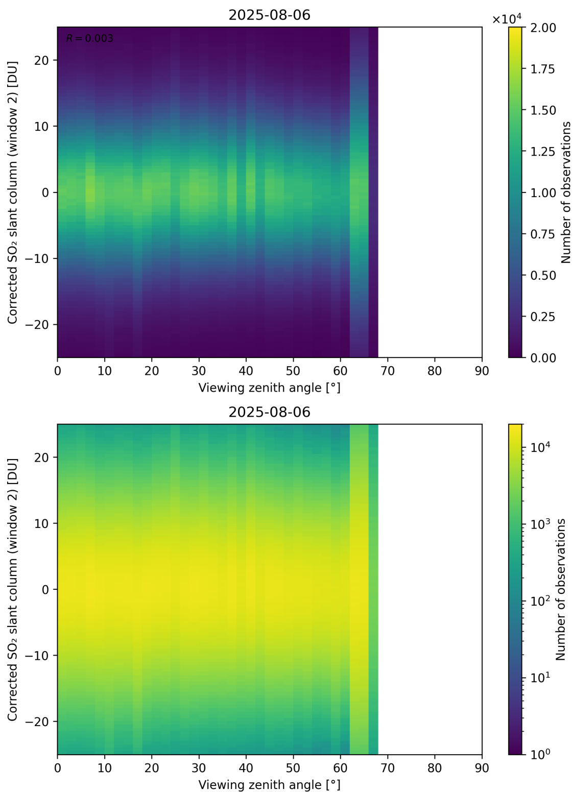
Figure 374: Scatter density plot of “Viewing zenith angle” against “Corrected SO 2 slant column (window 2)” for 2025-08-05 to 2025-08-07.
