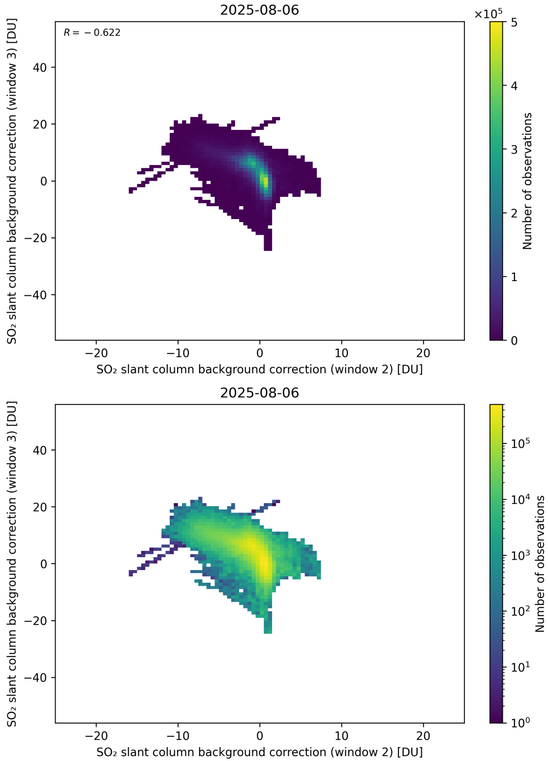
Figure 122: Scatter density plot of “SO 2 slant column background correction (window 2)” against “SO 2 slant column background correction (window 3)” for 2025-08-05 to 2025-08-07.
