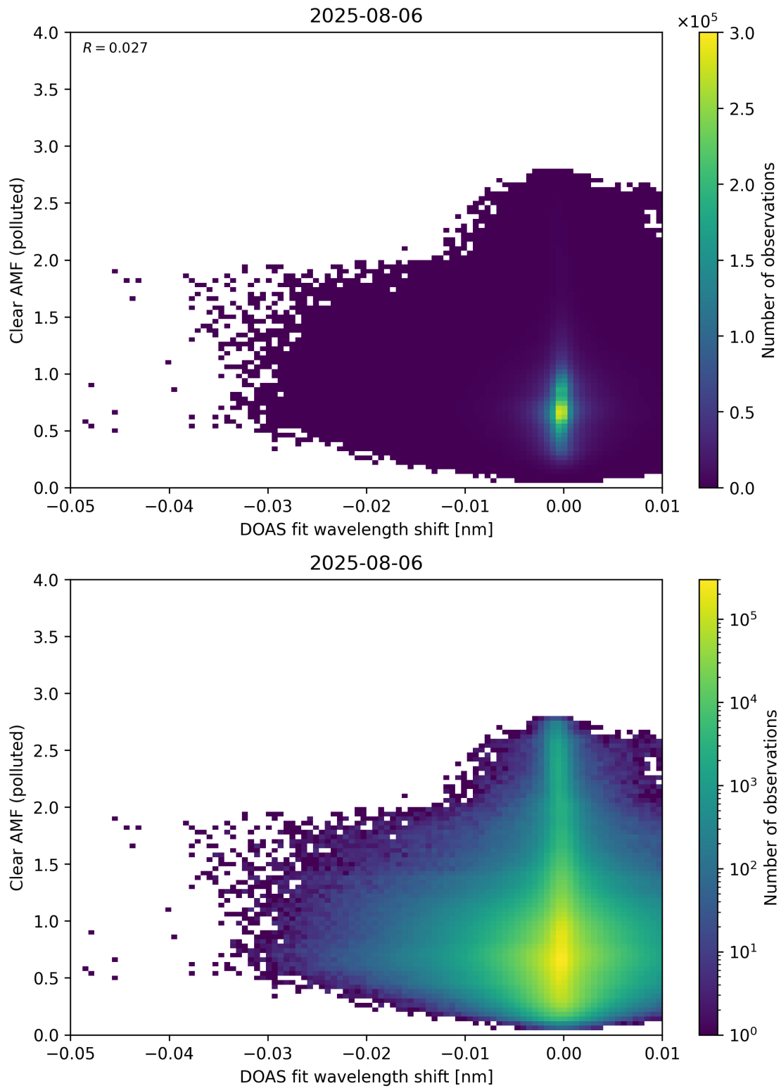
Figure 140: Scatter density plot of “DOAS fit wavelength shift” against “Clear AMF (polluted)” for 2025-08-05 to 2025-08-07.
