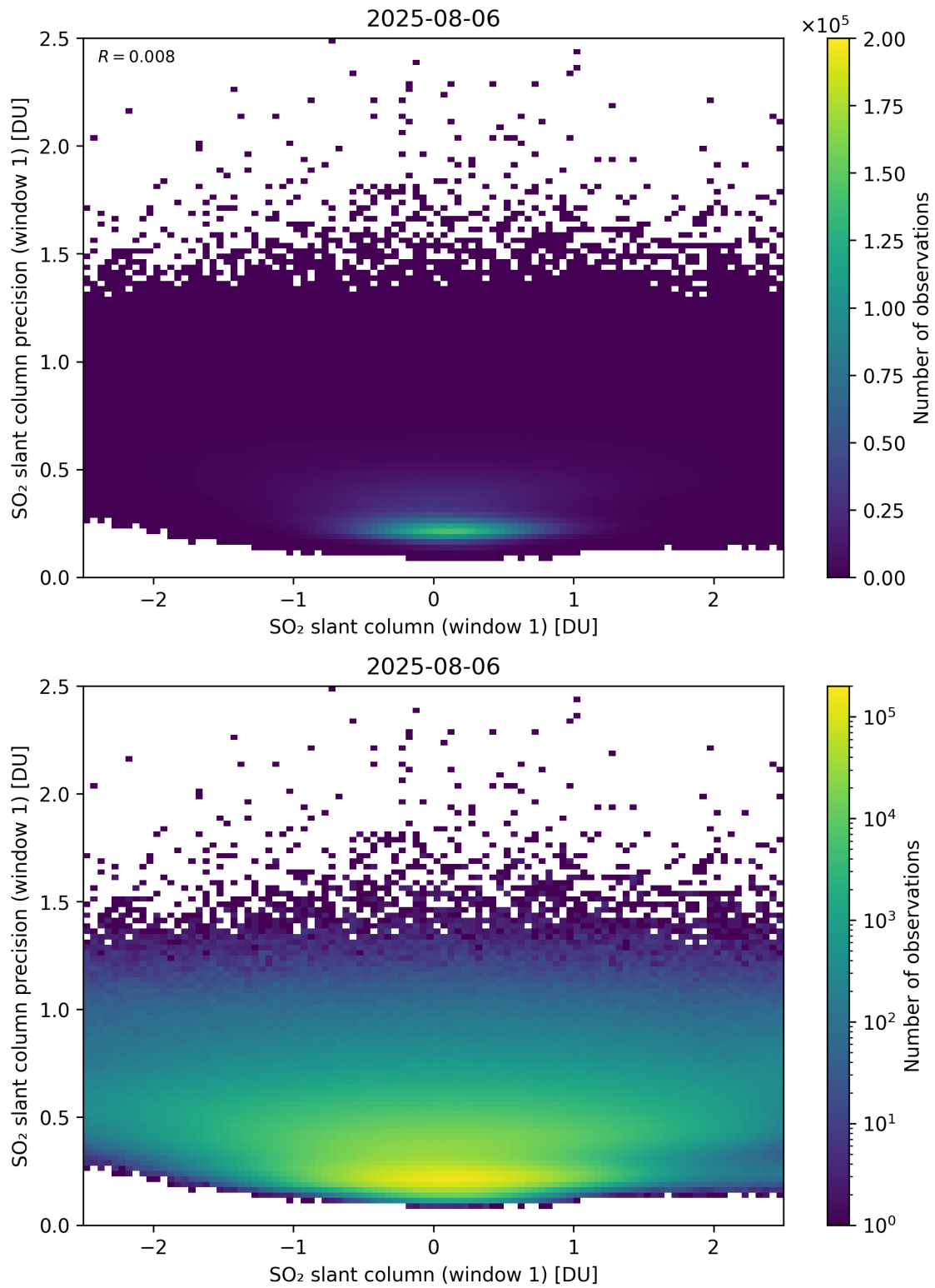
Figure 285: Scatter density plot of “SO 2 slant column (window 1)” against “SO 2 slant column precision (window 1)” for 2025-08-05 to 2025-08-07.
