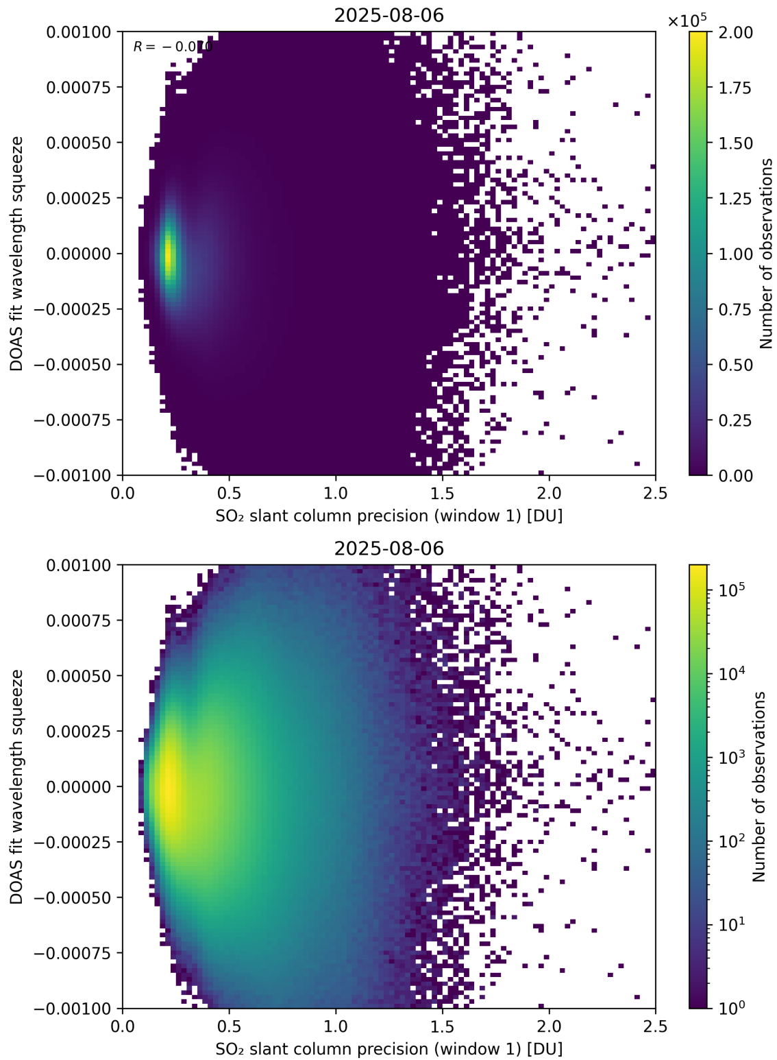
Figure 272: Scatter density plot of “SO 2 slant column precision (window 1)” against “DOAS fit wavelength squeeze” for 2025-08-05 to 2025-08-07.
