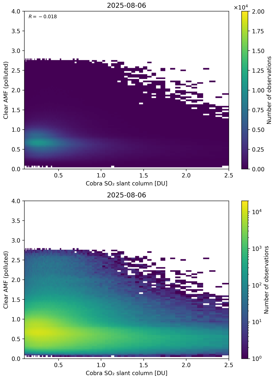
Figure 215: Scatter density plot of “Cobra SO 2 slant column” against “Clear AMF (polluted)” for 2025-08-05 to 2025-08-07.
