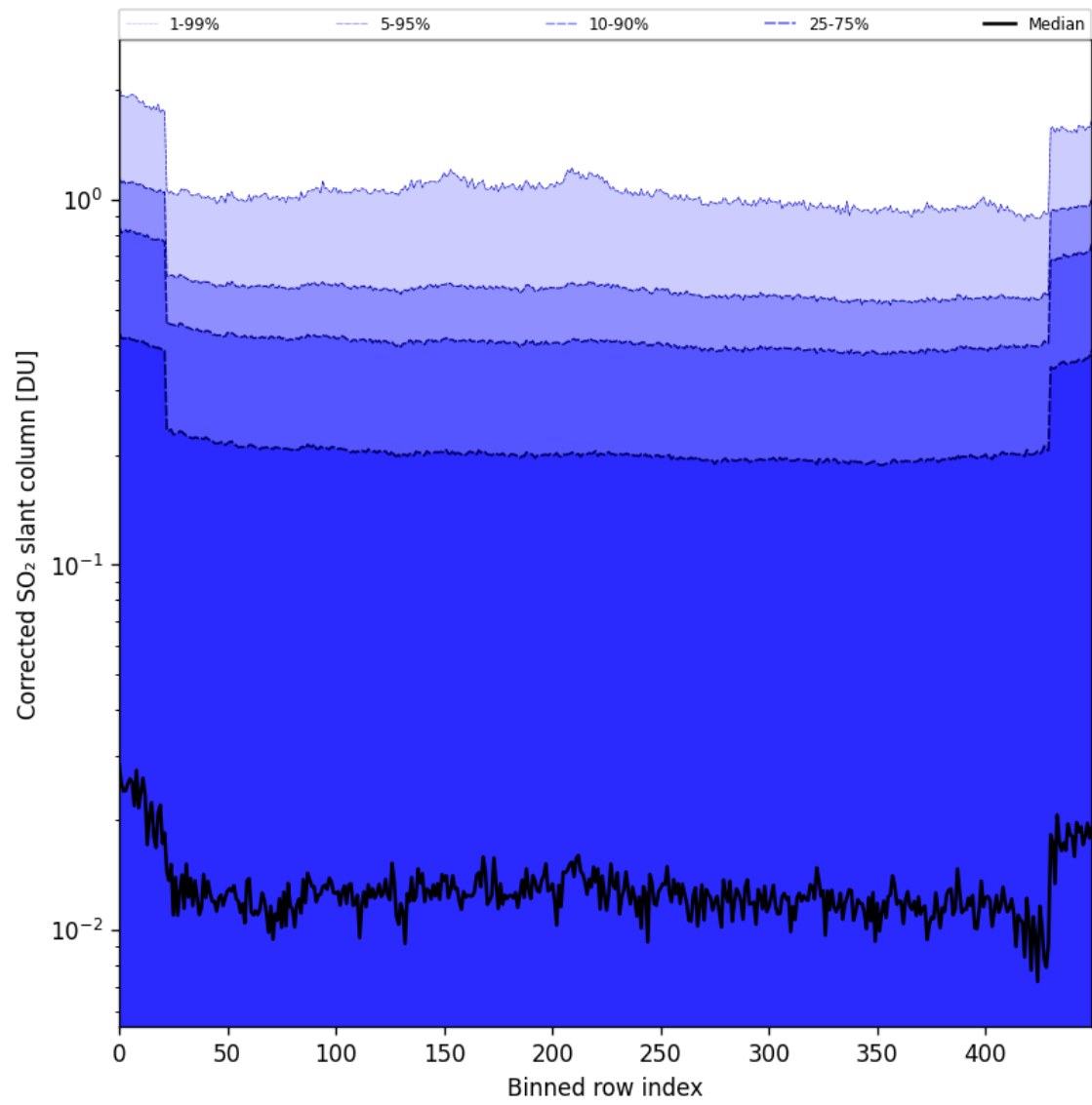
Figure 86: Along track statistics of "Corrected SO 2 slant column" for 2025-08-05 to 2025-08-07
