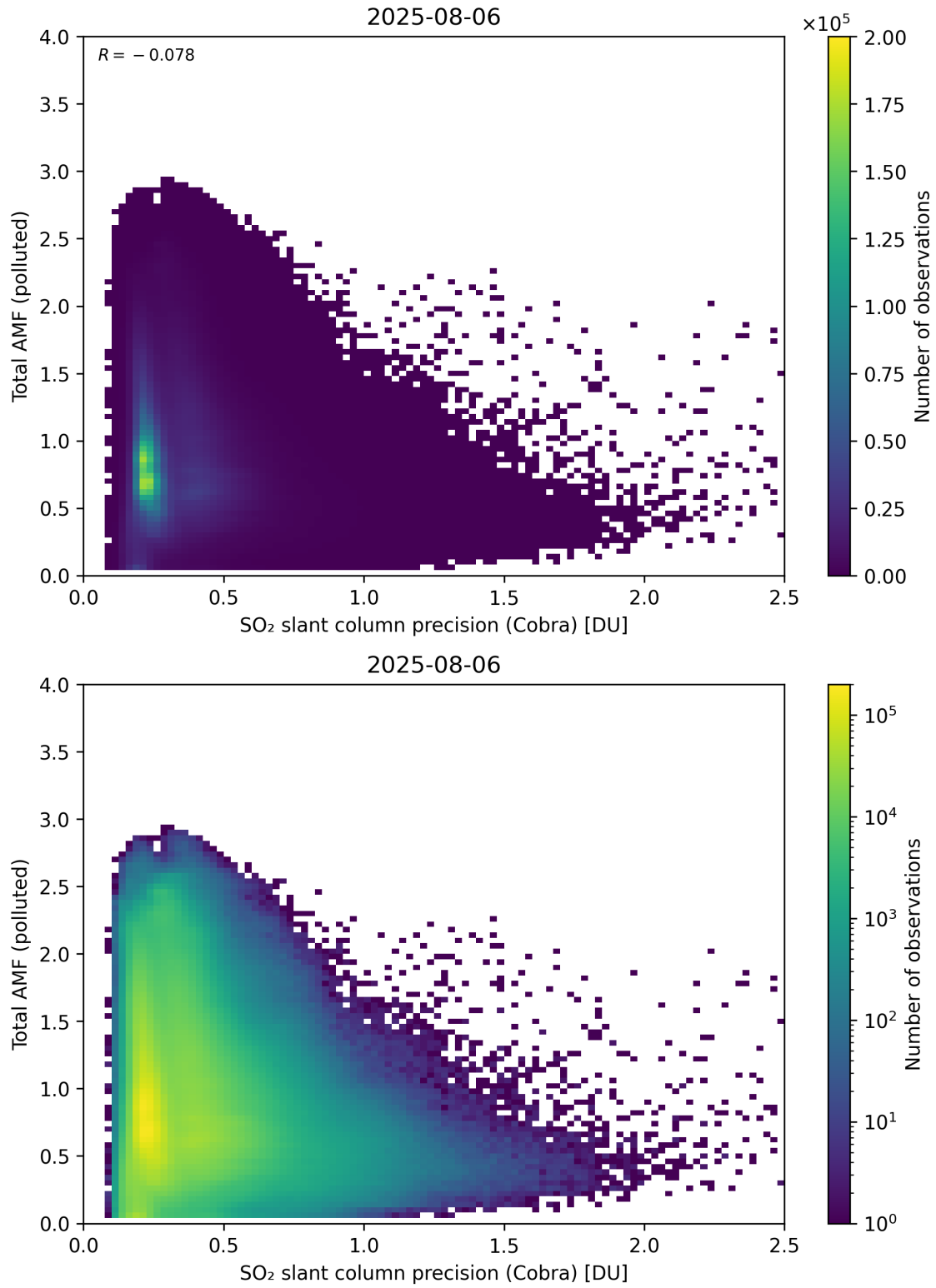
Figure 213: Scatter density plot of “SO 2 slant column precision (Cobra)” against “Total AMF (polluted)” for 2025-08-05 to 2025-08-07.
