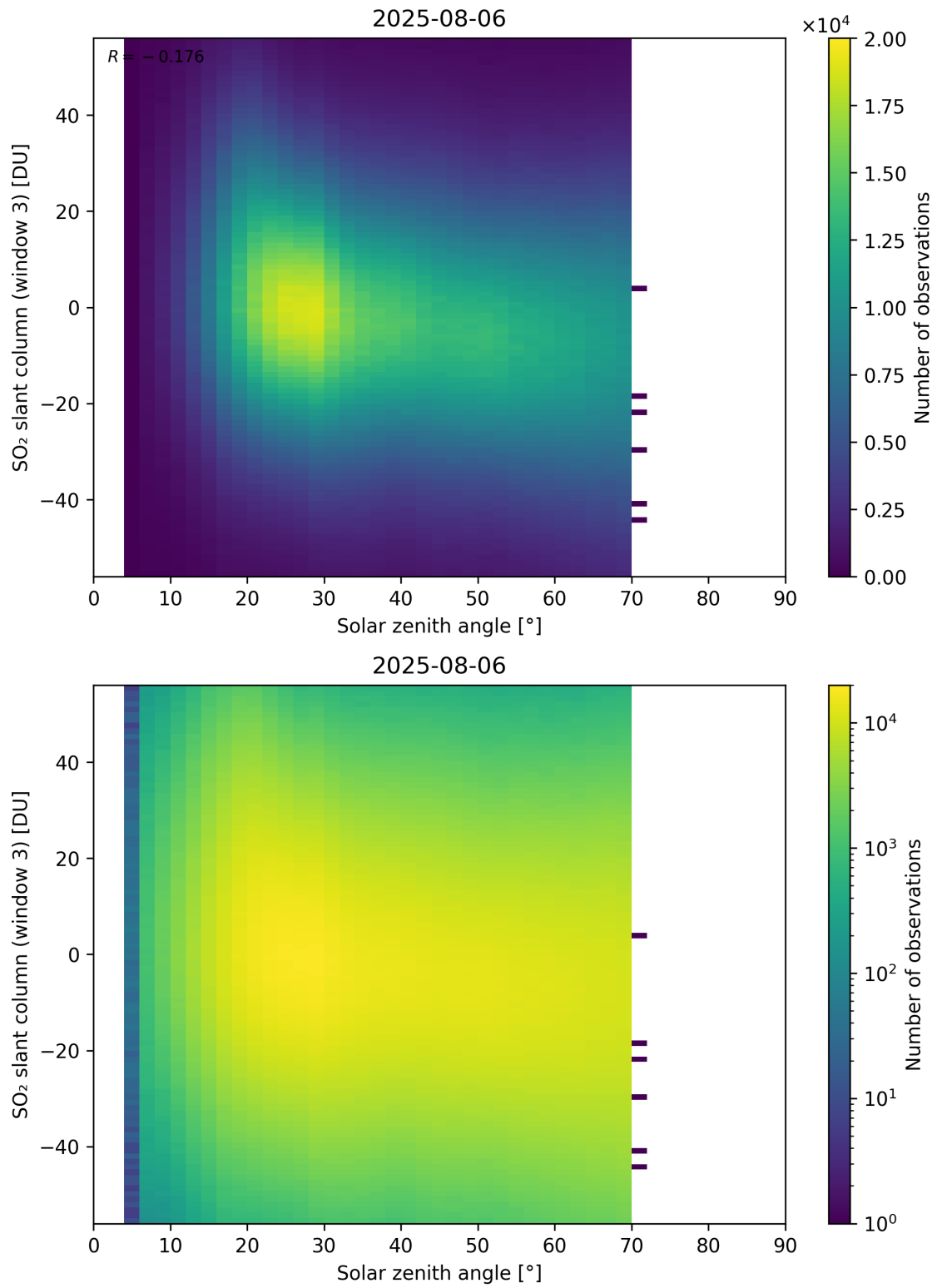
Figure 187: Scatter density plot of “Solar zenith angle” against “SO 2 slant column (window 3)” for 2025-08-05 to 2025-08-07.
