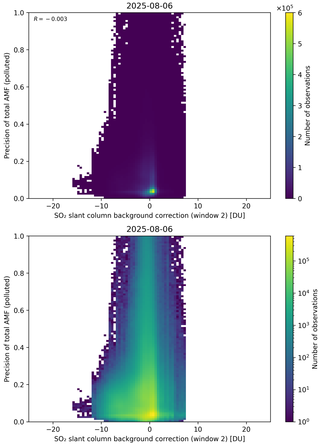
Figure 131: Scatter density plot of “SO 2 slant column background correction (window 2)” against “Precision of total AMF (polluted)” for 2025-08-05 to 2025-08-07.
