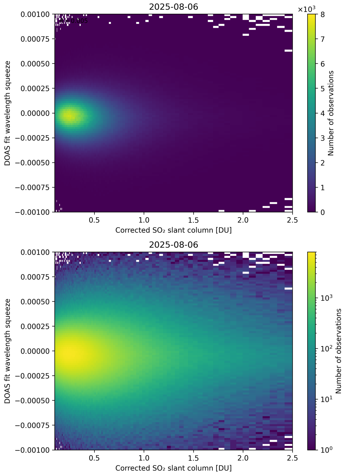
Figure 230: Scatter density plot of “Corrected SO 2 slant column” against “DOAS fit wavelength squeeze” for 2025-08-05 to 2025-08-07.
