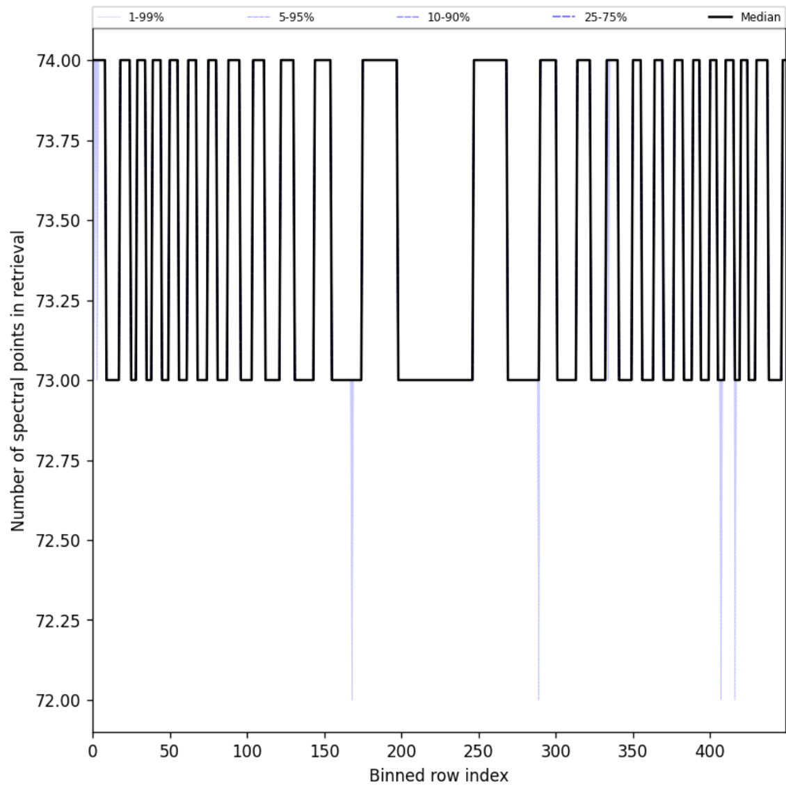
Figure 108: Along track statistics of “Number of spectral points in retrieval” for 2025-08-05 to 2025-08-07
