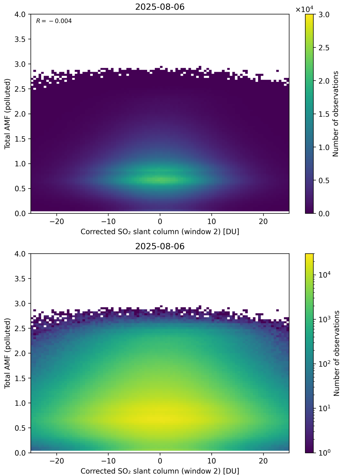
Figure 253: Scatter density plot of “Corrected SO 2 slant column (window 2)” against “Total AMF (polluted)” for 2025-08-05 to 2025-08-07.
