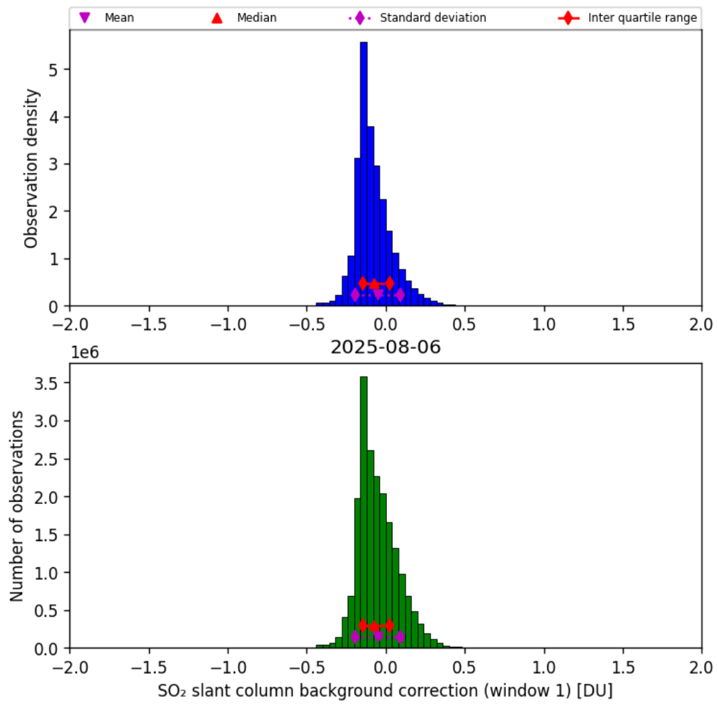
Figure 66: Histogram of “SO 2 slant column background correction (window 1)” for 2025-08-05 to 2025-08-07
