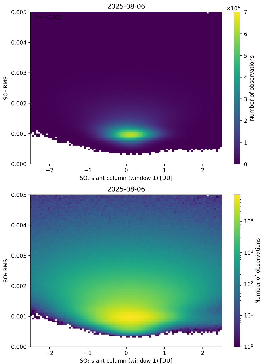
Figure 267: Scatter density plot of “SO 2 slant column (window 1)” against “SO 2 RMS” for 2025-08-05 to 2025-08-07.
