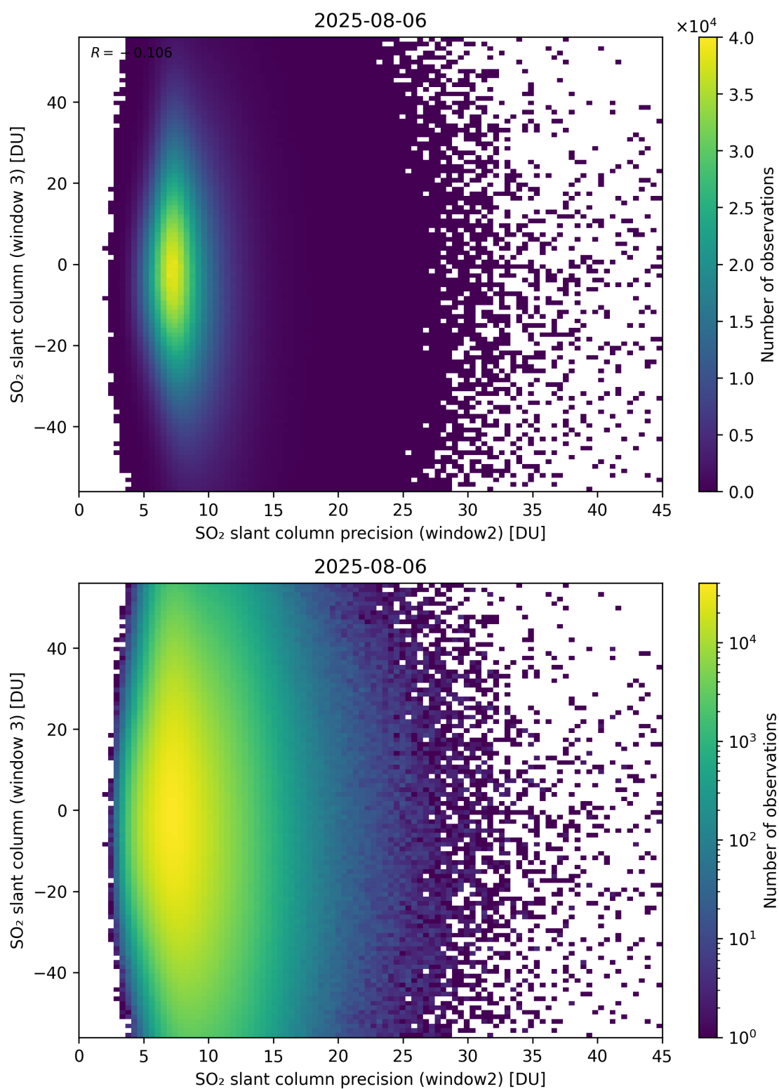
Figure 299: Scatter density plot of “SO 2 slant column precision (window2)” against “SO 2 slant column (window 3)” for 2025-08-05 to 2025-08-07.
