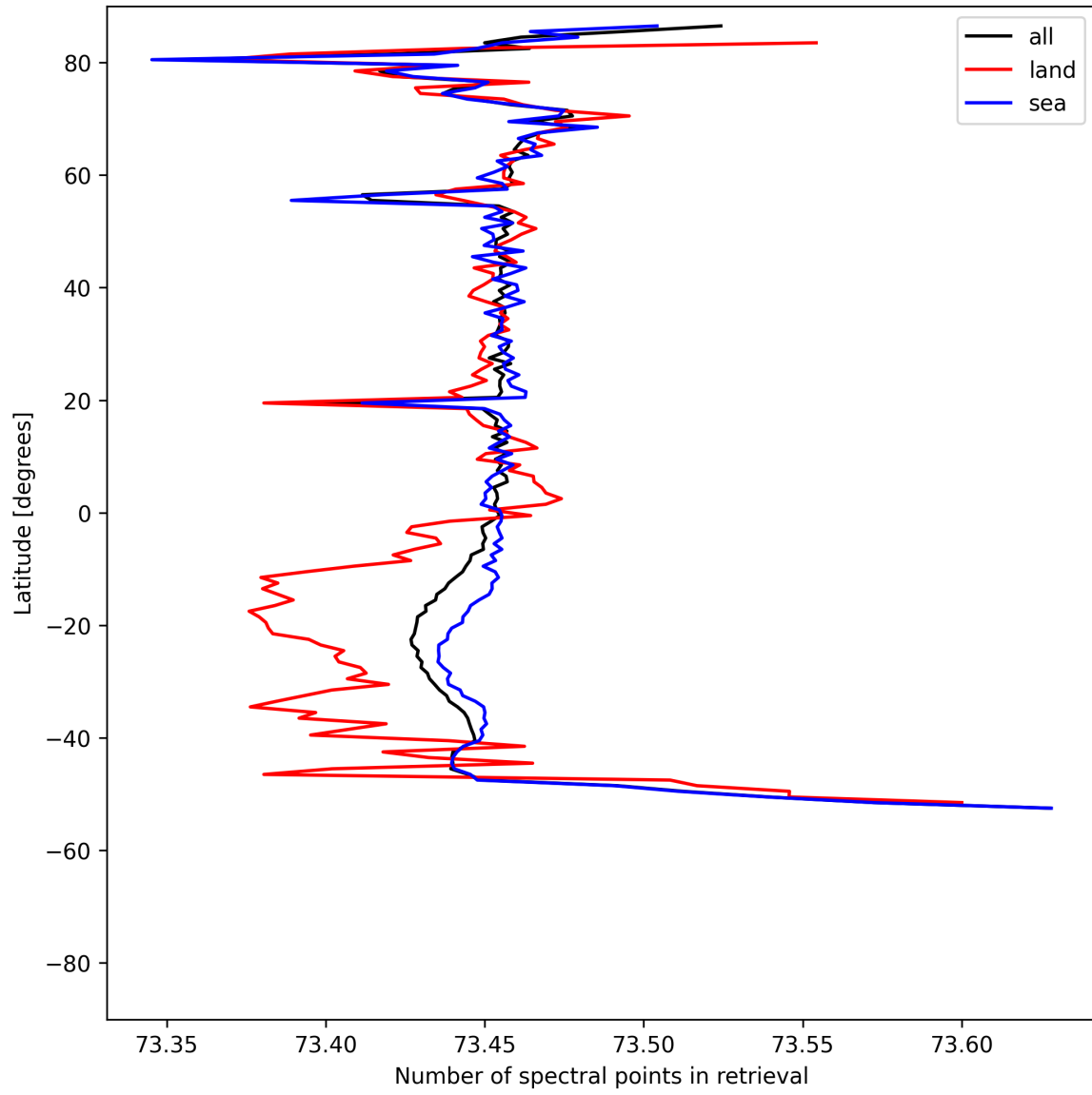
Figure 56: Zonal average of “Number of spectral points in retrieval” for 2025-08-05 to 2025-08-07.
