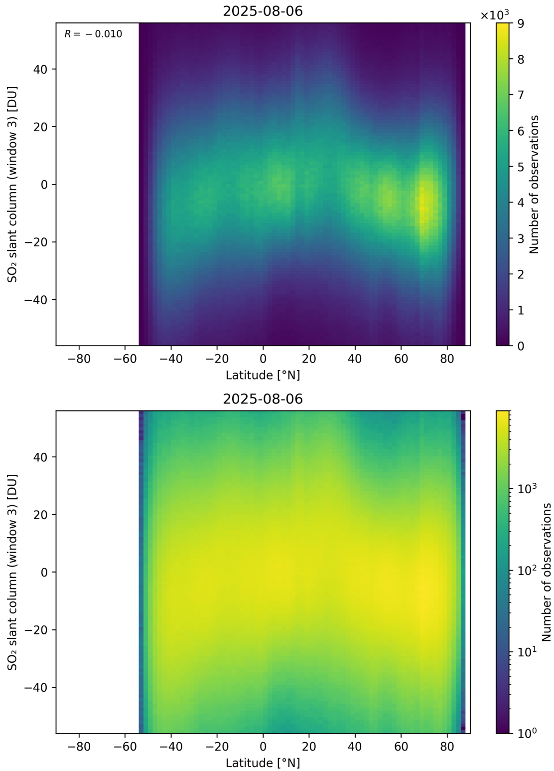
Figure 165: Scatter density plot of “Latitude” against “SO 2 slant column (window 3)” for 2025-08-05 to 2025-08-07.
