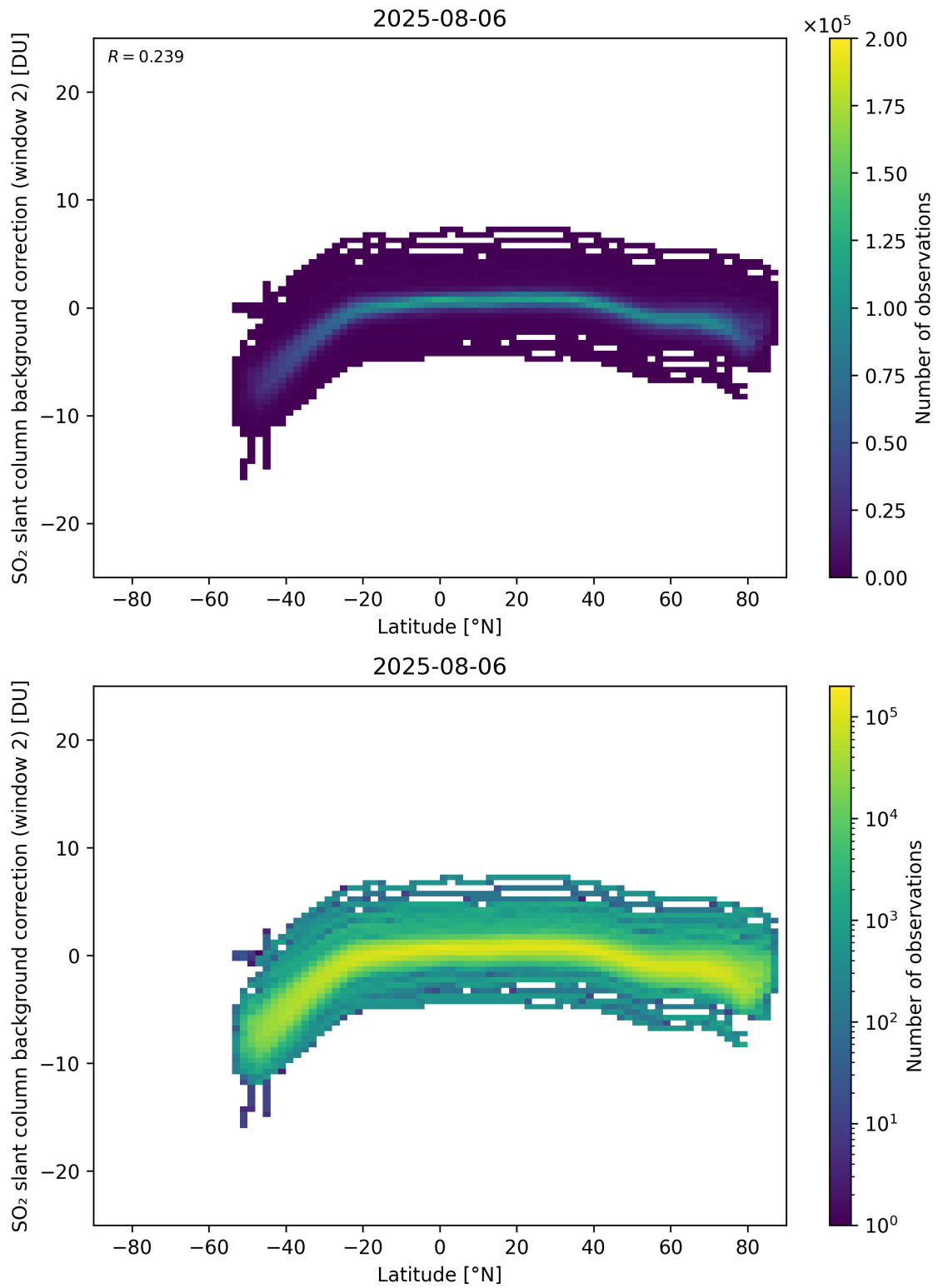
Figure 151: Scatter density plot of “Latitude” against “SO 2 slant column background correction (window 2)” for 2025-08-05 to 2025-08-07.
