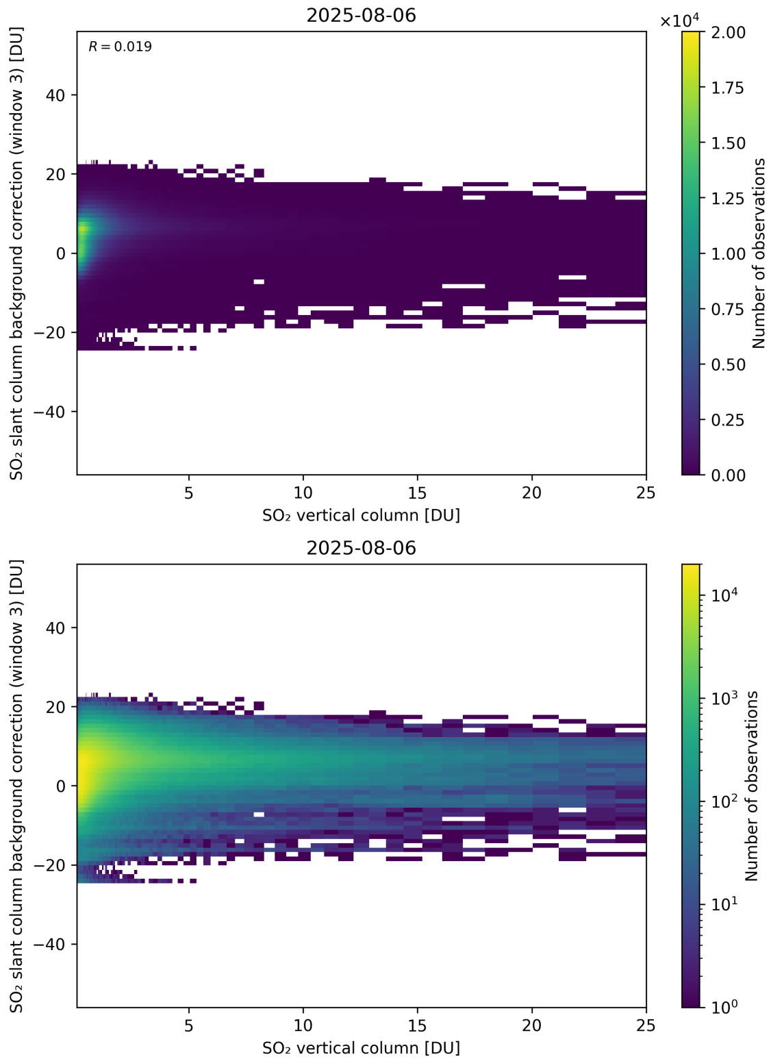
Figure 325: Scatter density plot of “SO 2 vertical column” against “SO 2 slant column background correction (window 3)” for 2025-08-05 to 2025-08-07.
