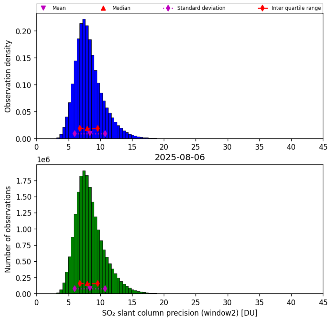
Figure 68: Histogram of “SO 2 slant column precision (window2)” for 2025-08-05 to 2025-08-07
