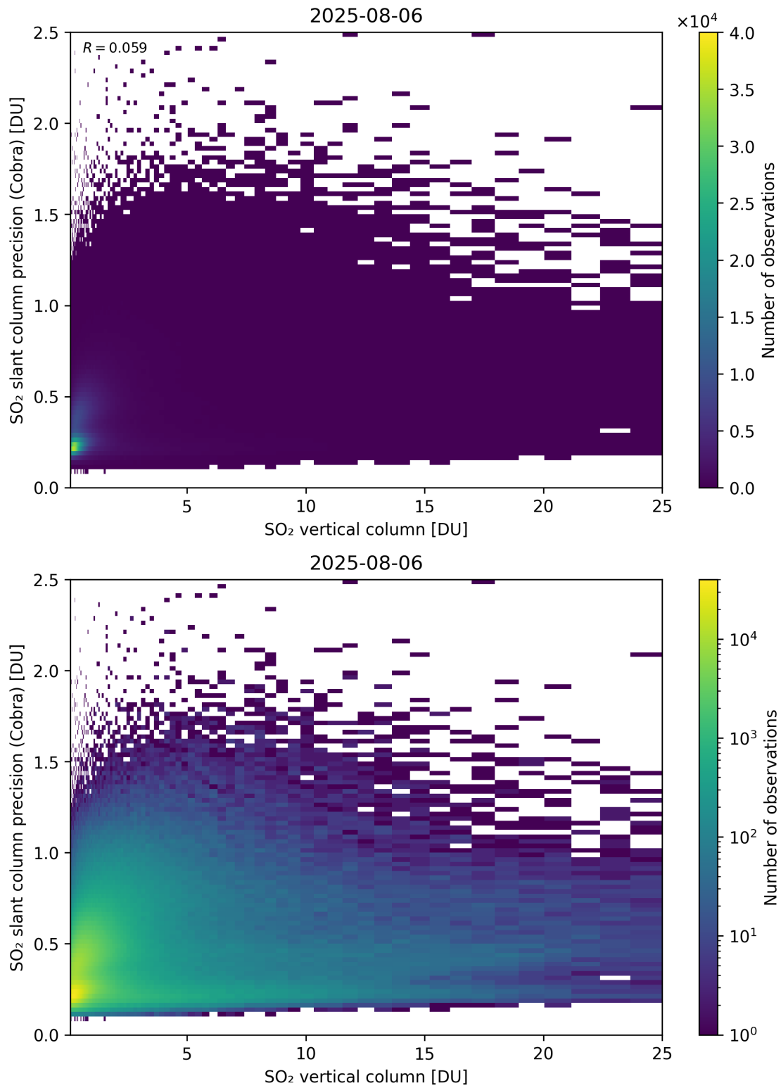
Figure 350: Scatter density plot of “SO 2 vertical column” against “SO 2 slant column precision (Cobra)” for 2025-08-05 to 2025-08-07.
