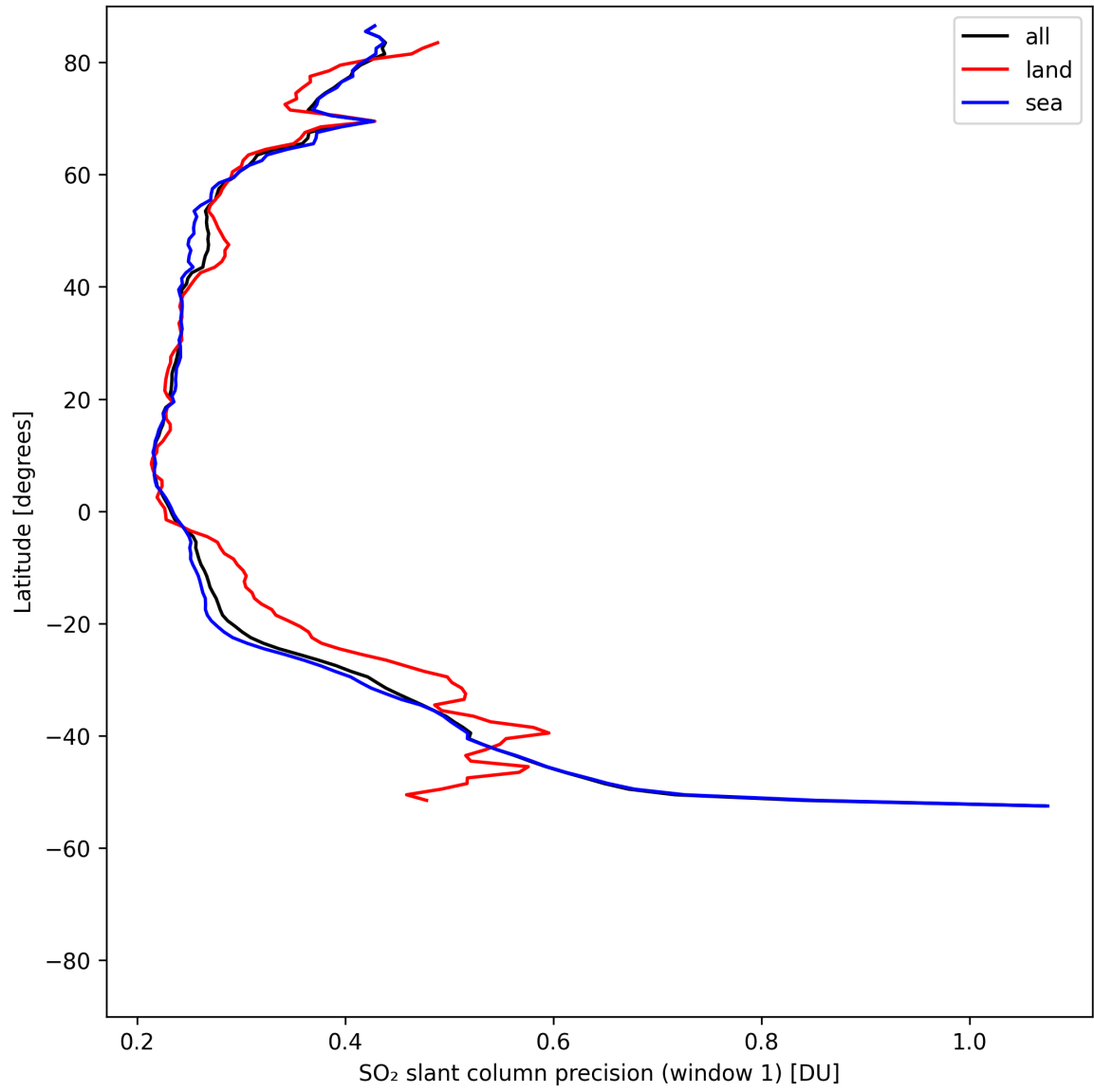
Figure 38: Zonal average of “SO 2 slant column precision (window 1)” for 2025-08-05 to 2025-08-07.
