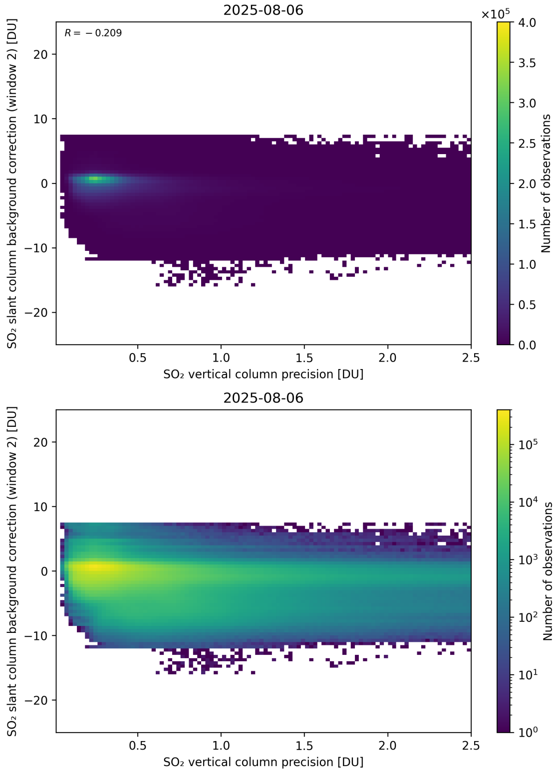
Figure 330: Scatter density plot of “SO 2 vertical column precision” against “SO 2 slant column background correction (window 2)” for 2025-08-05 to 2025-08-07.
