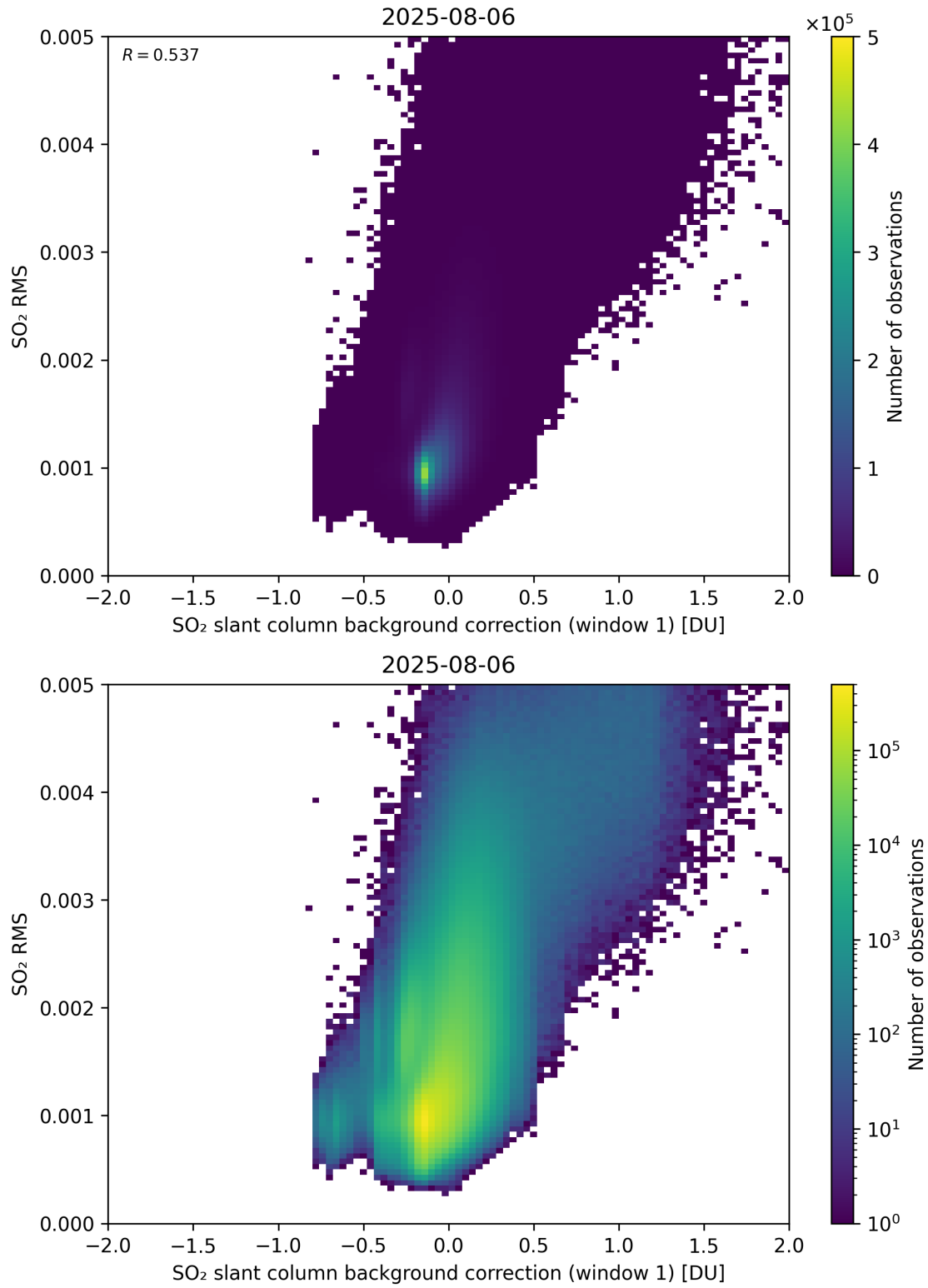
Figure 113: Scatter density plot of “SO 2 slant column background correction (window 1)” against “SO 2 RMS” for 2025-08-05 to 2025-08-07.
