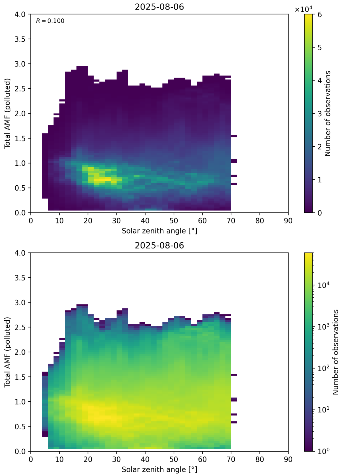
Figure 189: Scatter density plot of “Solar zenith angle” against “Total AMF (polluted)” for 2025-08-05 to 2025-08-07.
