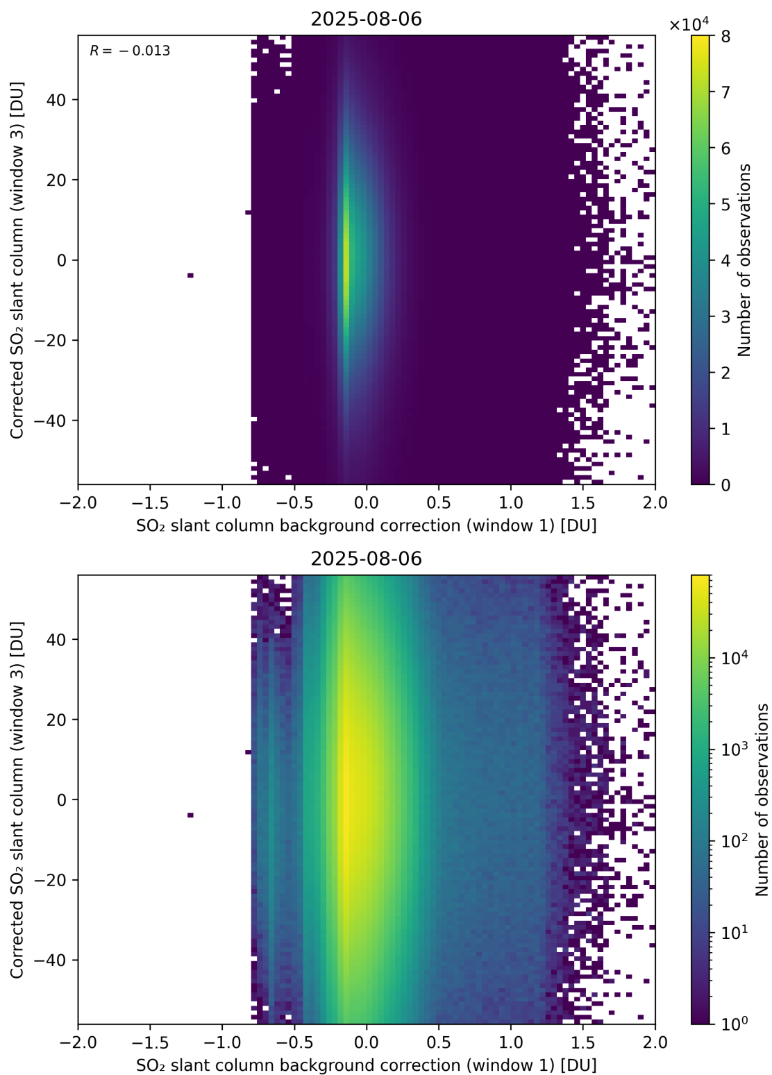
Figure 116: Scatter density plot of “SO 2 slant column background correction (window 1)” against “Corrected SO 2 slant column (window 3)” for 2025-08-05 to 2025-08-07.
