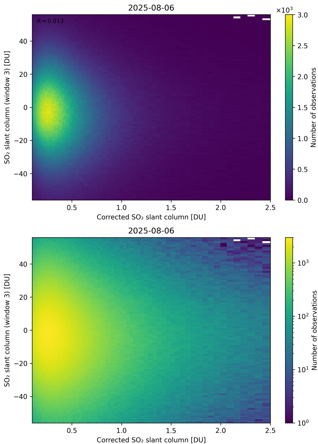
Figure 240: Scatter density plot of “Corrected SO 2 slant column” against “SO 2 slant column (window 3)” for 2025-08-05 to 2025-08-07.
