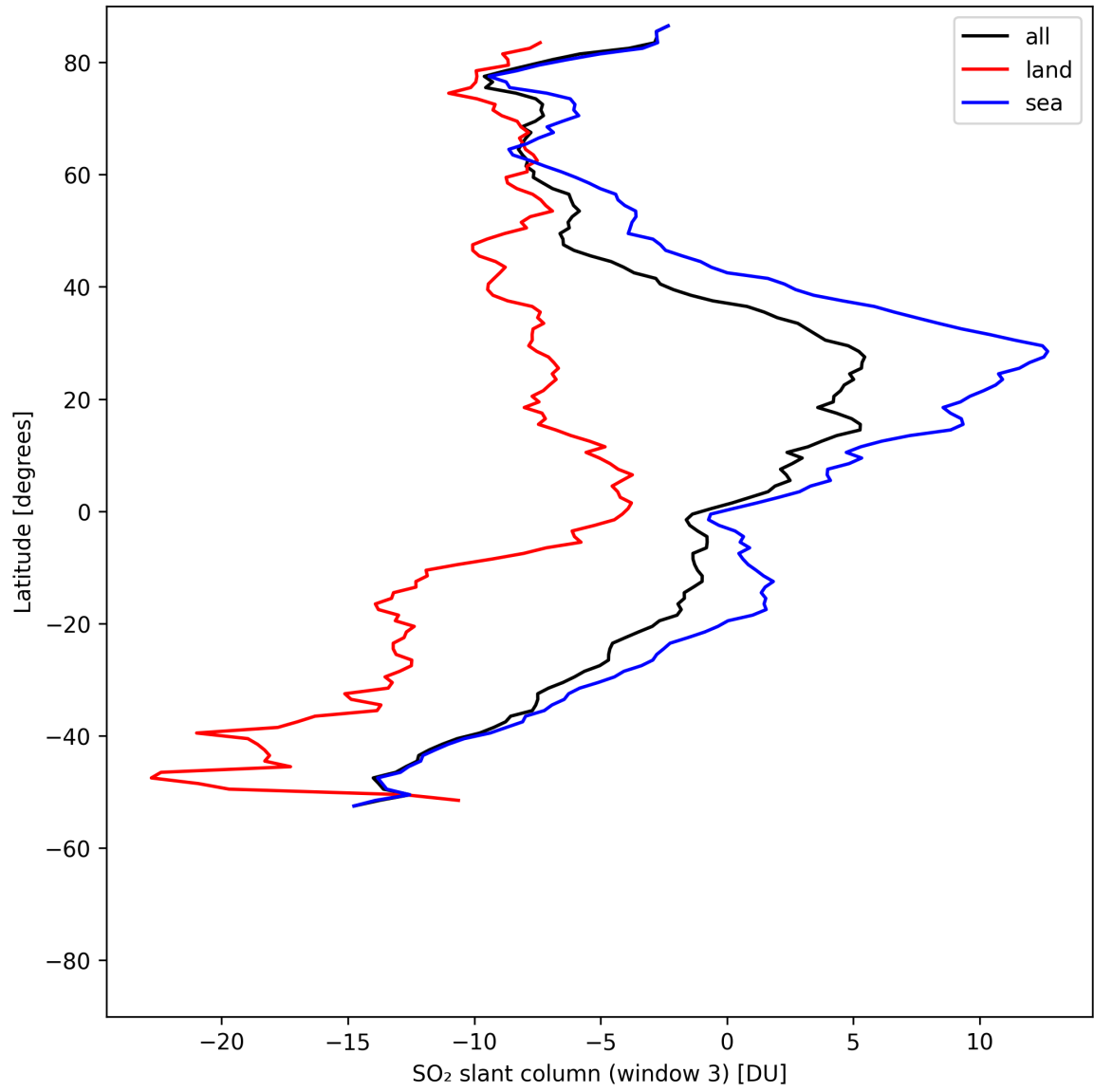
Figure 45: Zonal average of “SO 2 slant column (window 3)” for 2025-08-05 to 2025-08-07.
