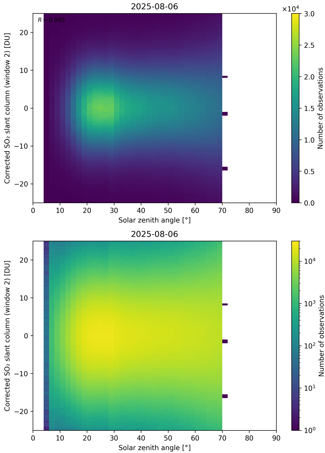
Figure 182: Scatter density plot of “Solar zenith angle” against “Corrected SO 2 slant column (window 2)” for 2025-08-05 to 2025-08-07.
