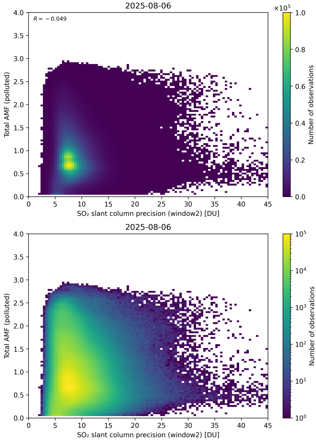
Figure 301: Scatter density plot of “SO 2 slant column precision (window2)” against “Total AMF (polluted)” for 2025-08-05 to 2025-08-07.
