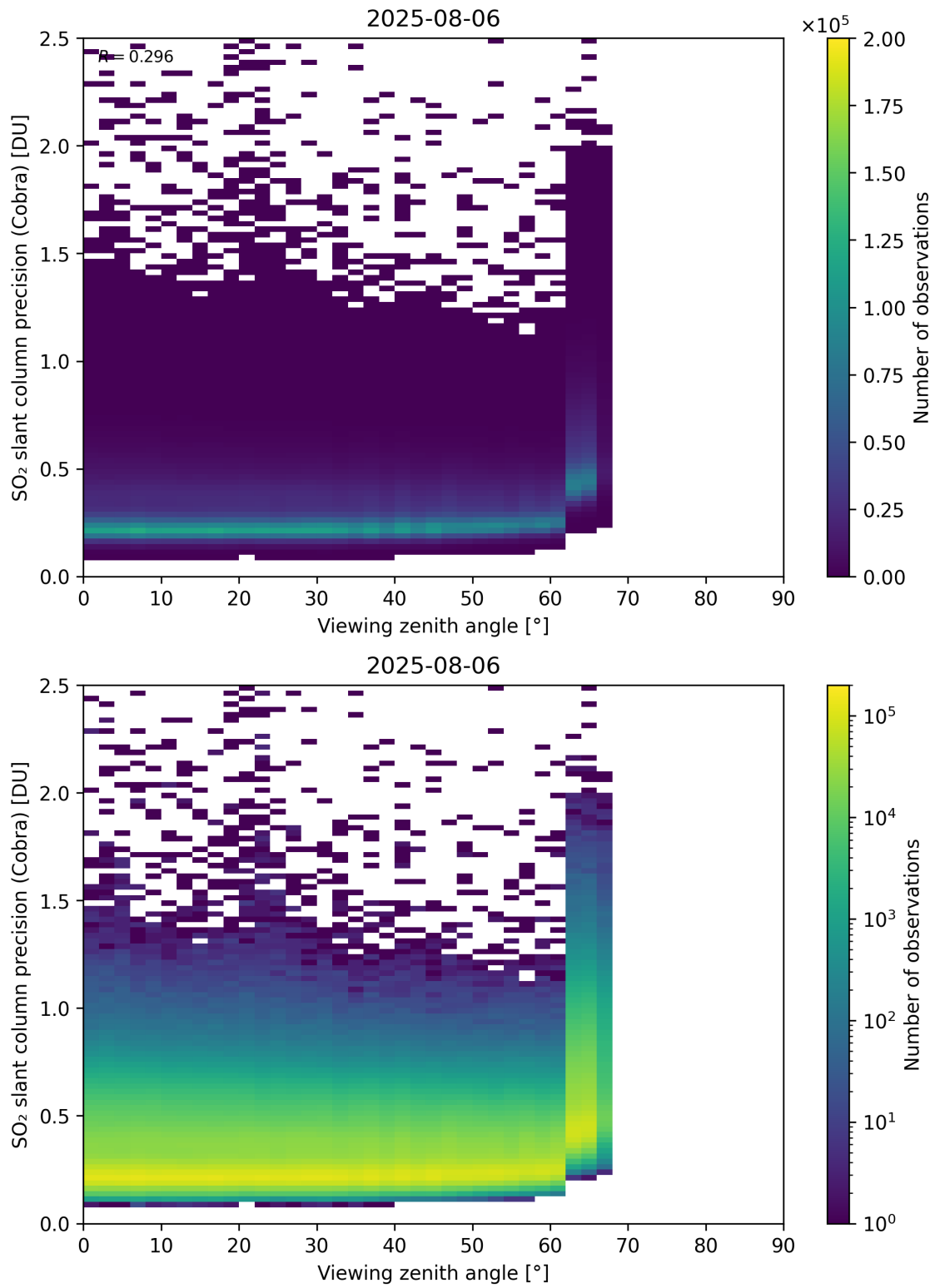
Figure 372: Scatter density plot of “Viewing zenith angle” against “SO 2 slant column precision (Cobra)” for 2025-08-05 to 2025-08-07.
