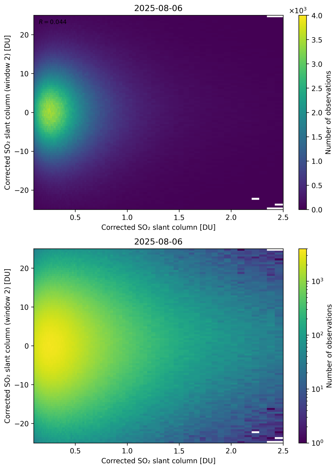
Figure 235: Scatter density plot of “Corrected SO 2 slant column” against “Corrected SO 2 slant column (window 2)” for 2025-08-05 to 2025-08-07.
