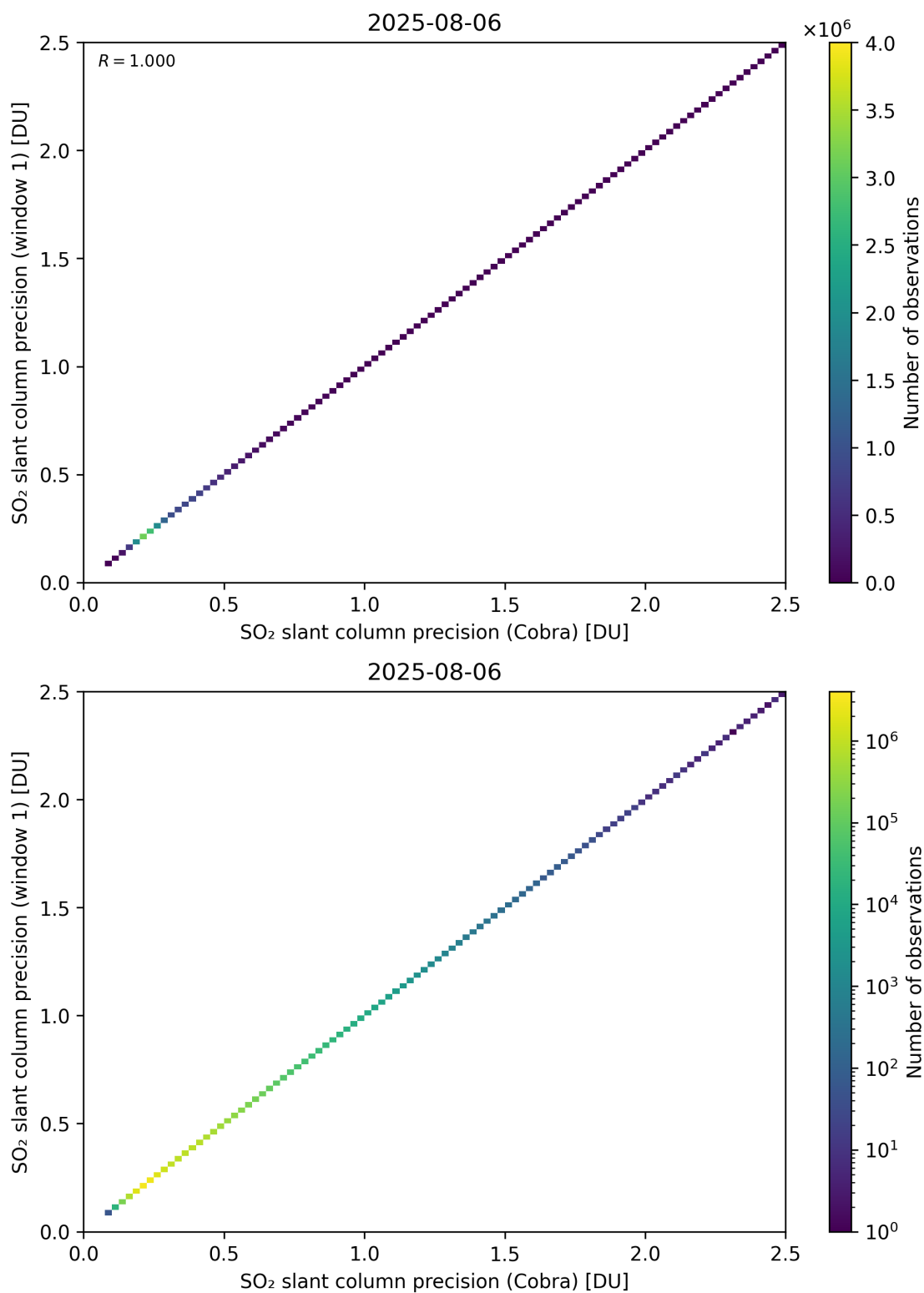
Figure 209: Scatter density plot of “SO 2 slant column precision (Cobra)” against “SO 2 slant column precision (window 1)” for 2025-08-05 to 2025-08-07.
