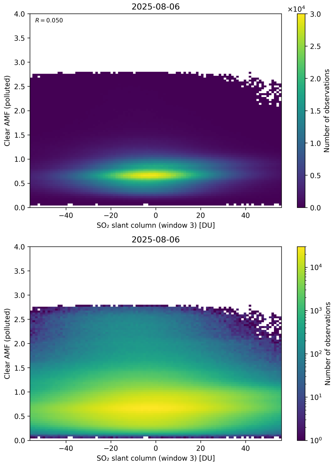
Figure 315: Scatter density plot of “SO 2 slant column (window 3)” against “Clear AMF (polluted)” for 2025-08-05 to 2025-08-07.
