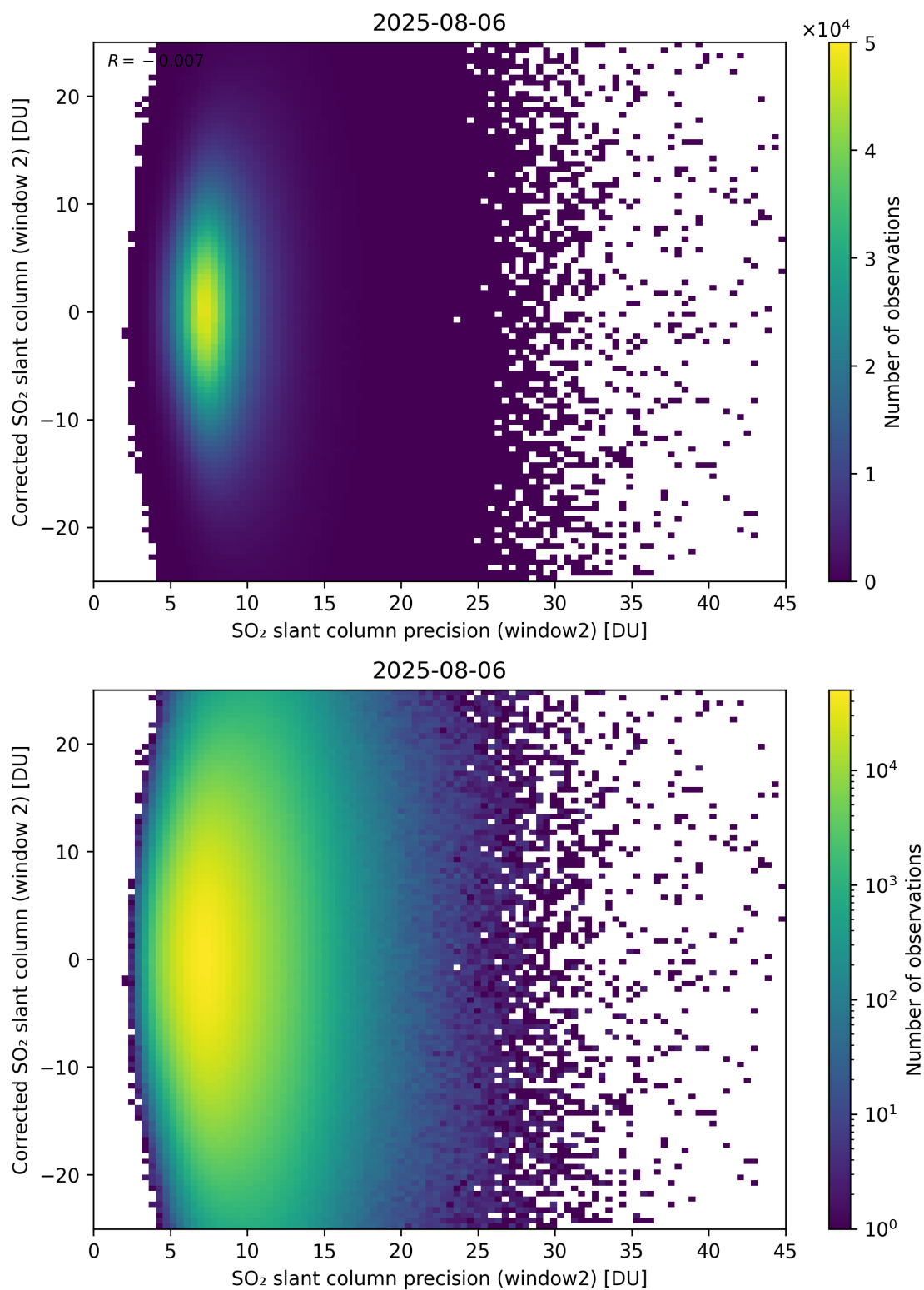
Figure 297: Scatter density plot of “SO 2 slant column precision (window2)” against “Corrected SO 2 slant column (window 2)” for 2025-08-05 to 2025-08-07.
