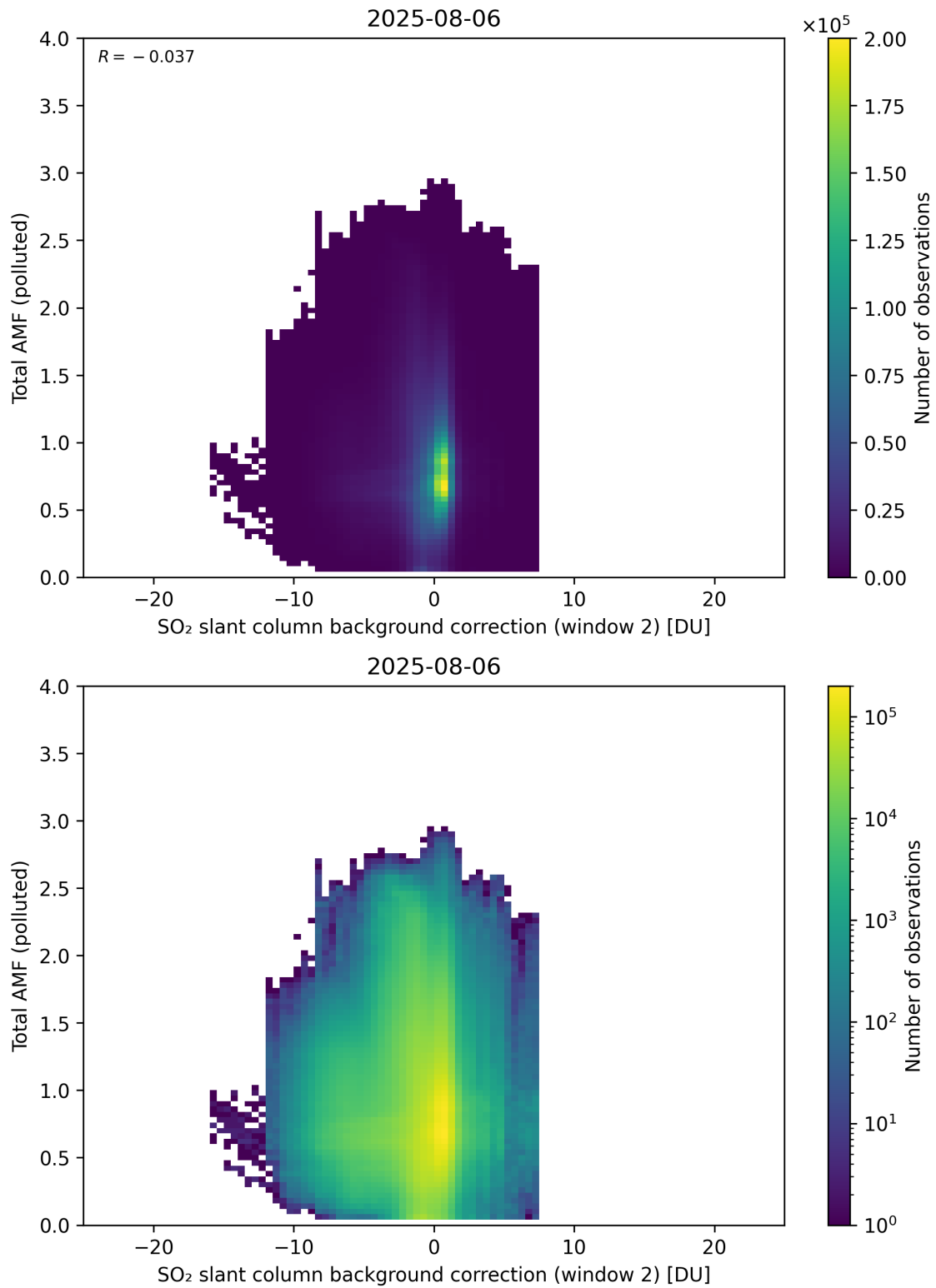
Figure 130: Scatter density plot of “SO 2 slant column background correction (window 2)” against “Total AMF (polluted)” for 2025-08-05 to 2025-08-07.
