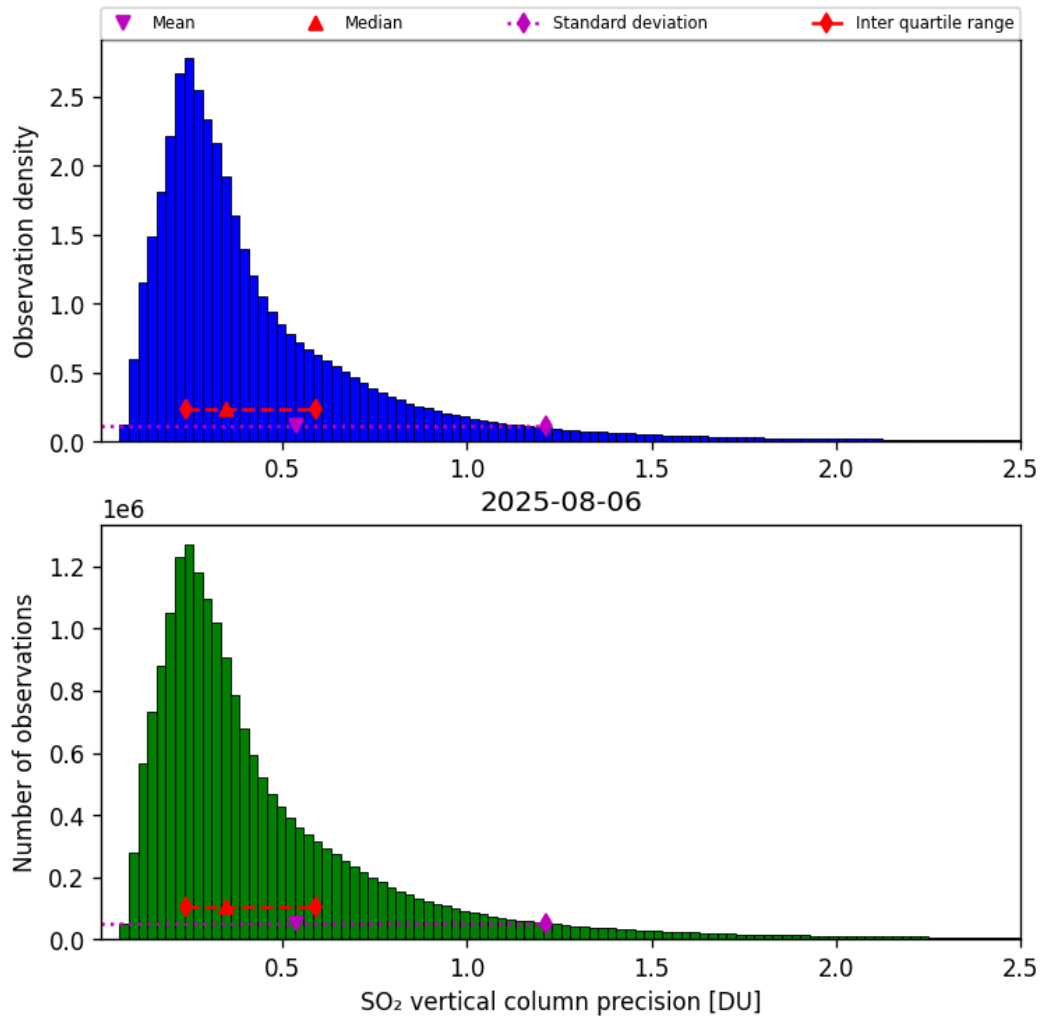
Figure 59: Histogram of “SO 2 vertical column precision” for 2025-08-05 to 2025-08-07
