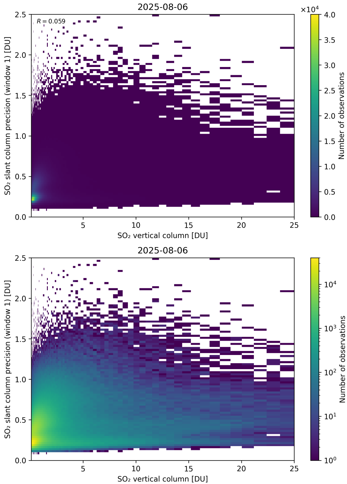
Figure 355: Scatter density plot of “SO 2 vertical column” against “SO 2 slant column precision (window 1)” for 2025-08-05 to 2025-08-07.
