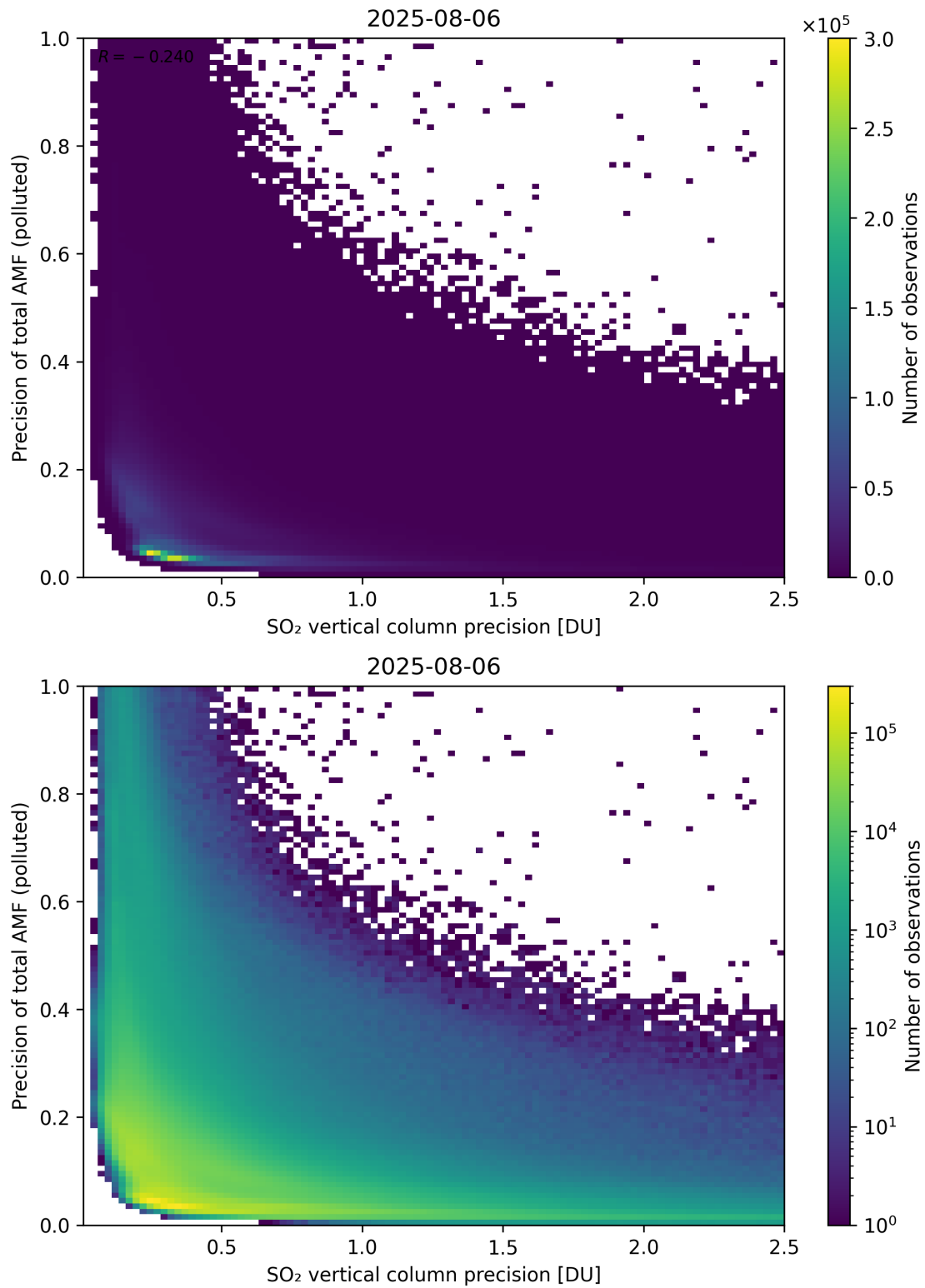
Figure 347: Scatter density plot of “SO 2 vertical column precision” against “Precision of total AMF (polluted)” for 2025-08-05 to 2025-08-07.
