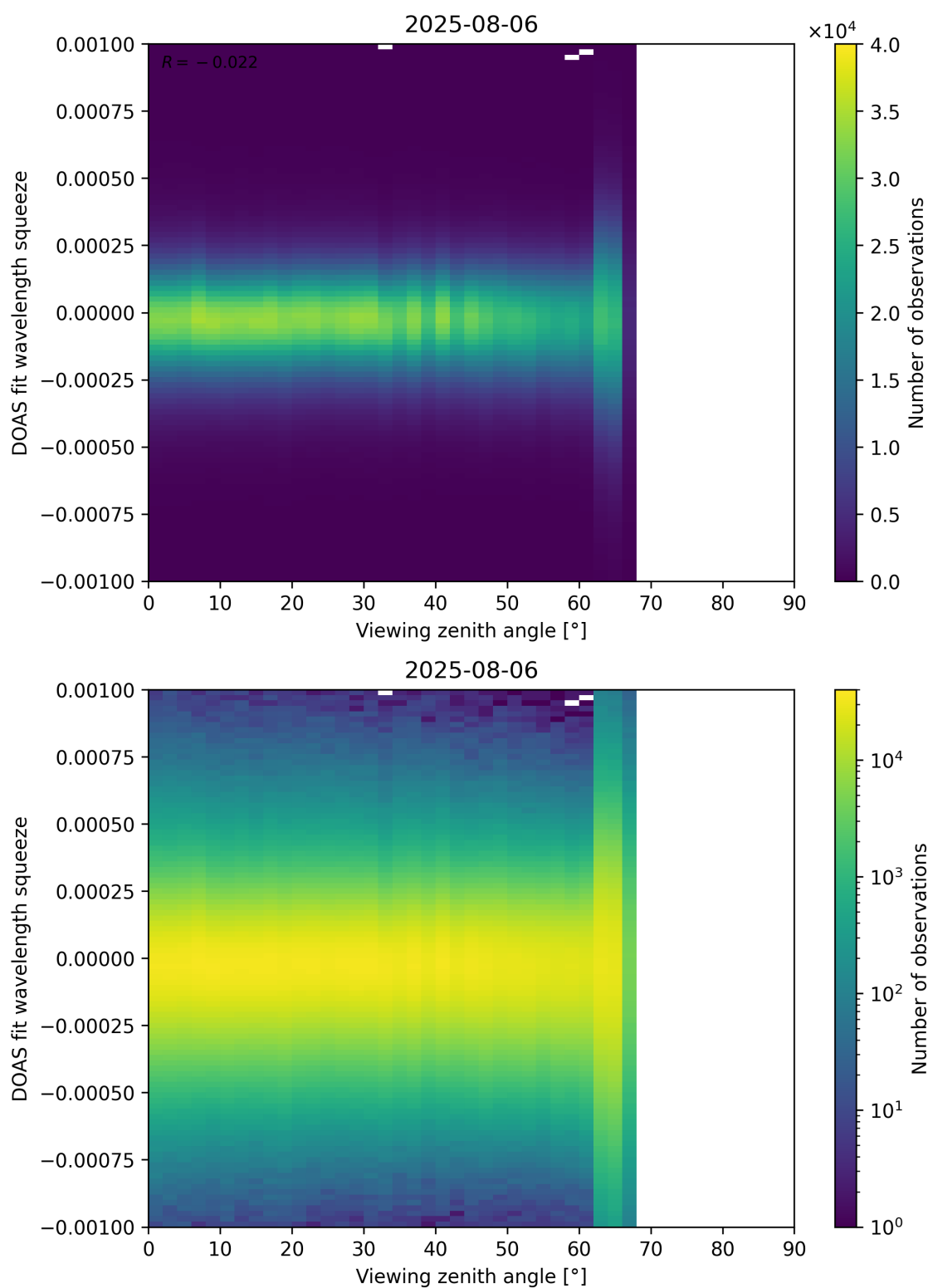
Figure 366: Scatter density plot of “Viewing zenith angle” against “DOAS fit wavelength squeeze” for 2025-08-05 to 2025-08-07.
