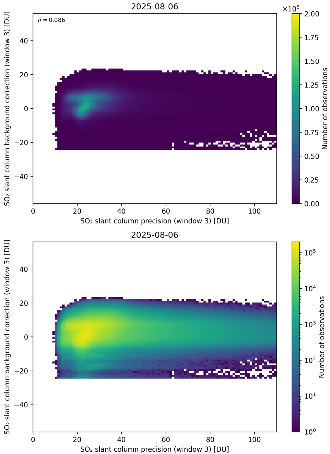
Figure 307: Scatter density plot of “SO 2 slant column precision (window 3)” against “SO 2 slant column background correction (window 3)” for 2025-08-05 to 2025-08-07.
