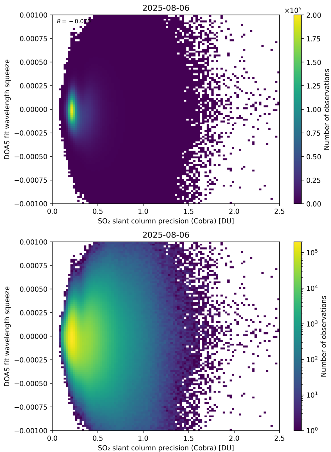
Figure 203: Scatter density plot of “SO 2 slant column precision (Cobra)” against “DOAS fit wavelength squeeze” for 2025-08-05 to 2025-08-07.
