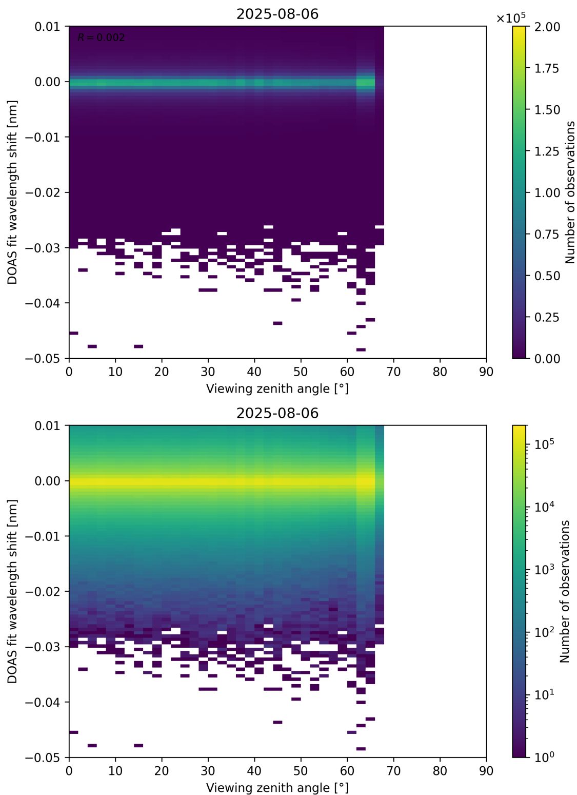
Figure 365: Scatter density plot of “Viewing zenith angle” against “DOAS fit wavelength shift” for 2025-08-05 to 2025-08-07.
