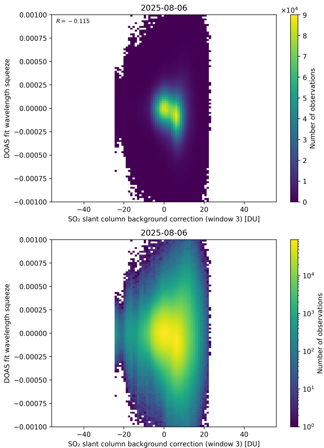
Figure 133: Scatter density plot of “SO 2 slant column background correction (window 3)” against “DOAS fit wavelength squeeze” for 2025-08-05 to 2025-08-07.
