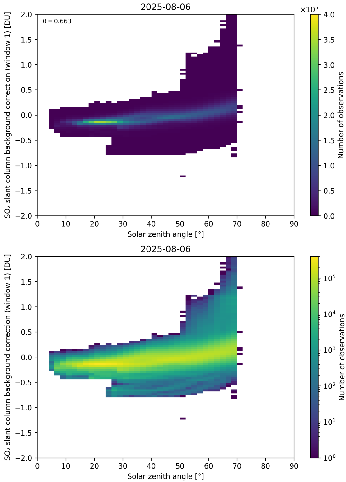
Figure 171: Scatter density plot of “Solar zenith angle” against “SO 2 slant column background correction (window 1)” for 2025-08-05 to 2025-08-07.
