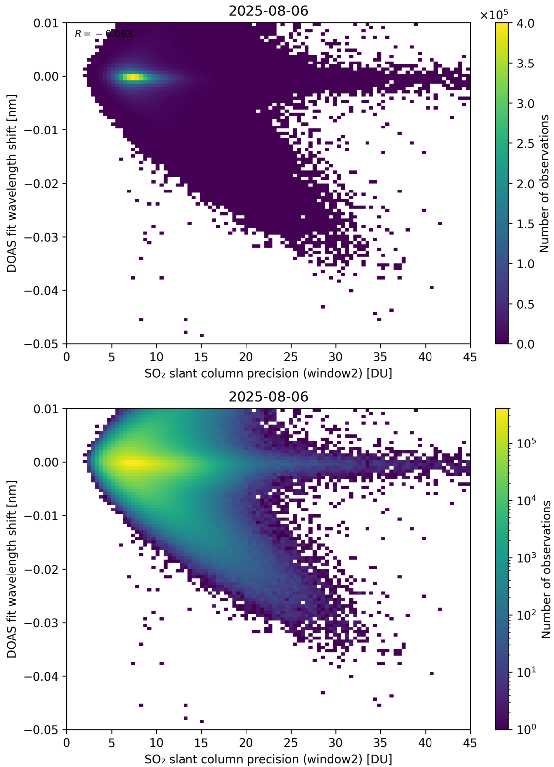
Figure 293: Scatter density plot of “SO 2 slant column precision (window2)” against “DOAS fit wavelength shift” for 2025-08-05 to 2025-08-07.
