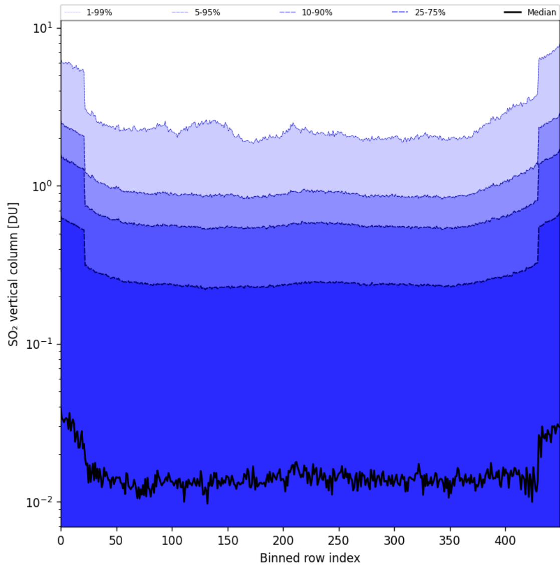
Figure 84: Along track statistics of “SO 2 vertical column” for 2025-08-05 to 2025-08-07
