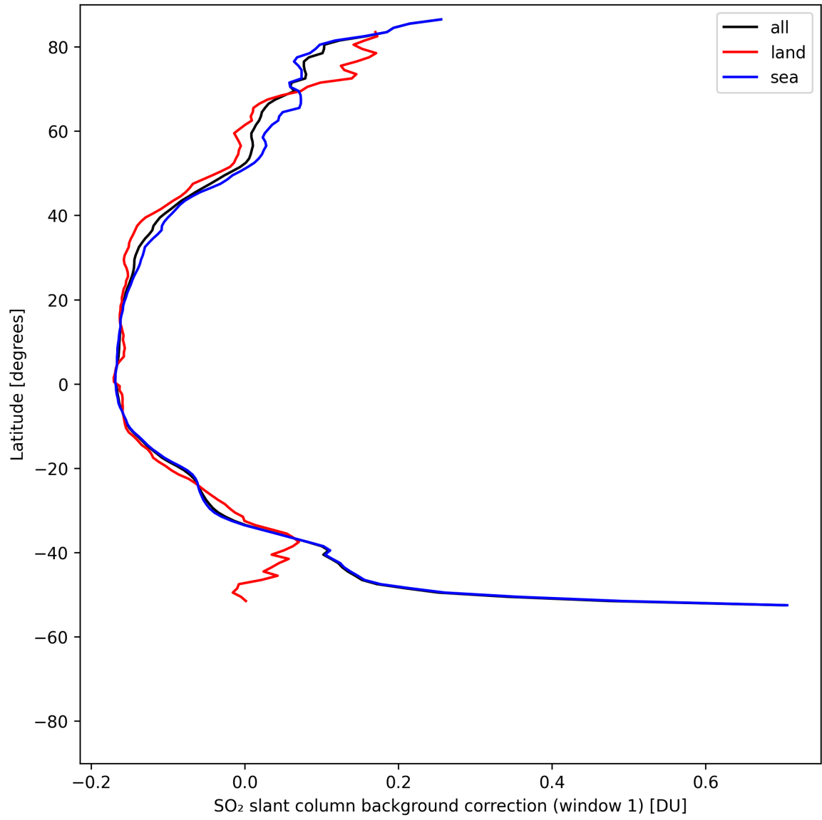
Figure 40: Zonal average of “SO 2 slant column background correction (window 1)” for 2025-08-05 to 2025-08-07.
