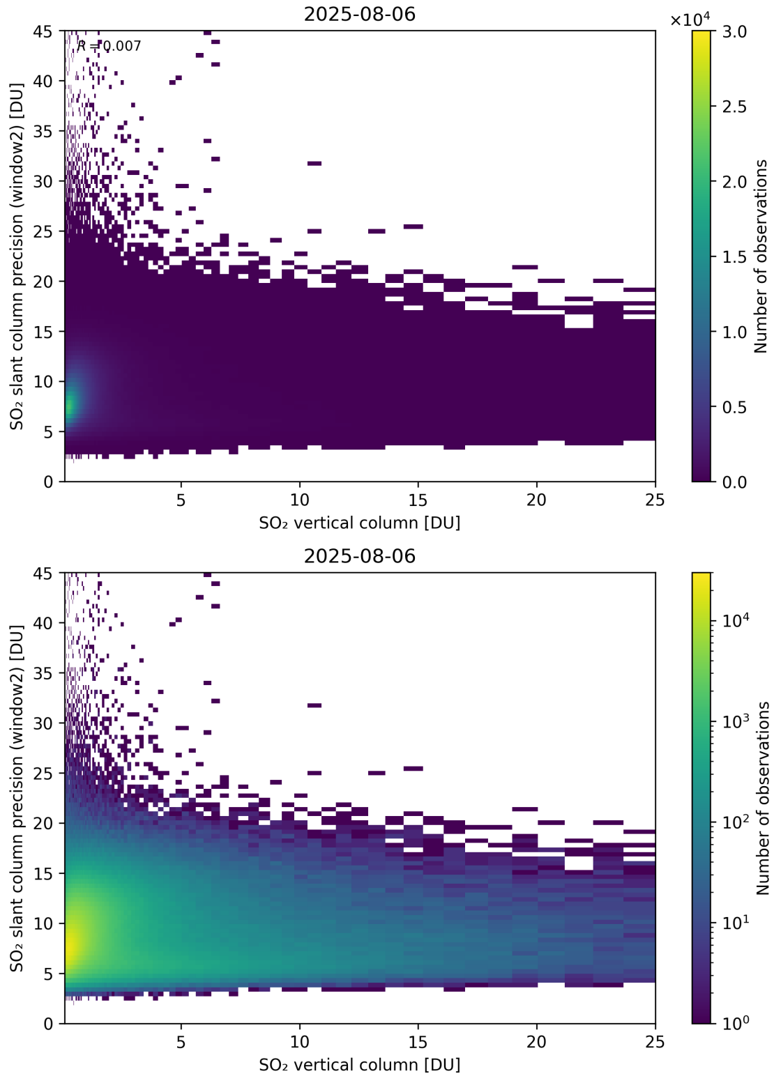
Figure 356: Scatter density plot of “SO 2 vertical column” against “SO 2 slant column precision (window2)” for 2025-08-05 to 2025-08-07.
