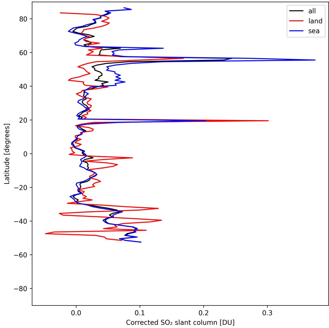
Figure 34: Zonal average of “Corrected SO 2 slant column” for 2025-08-05 to 2025-08-07.
