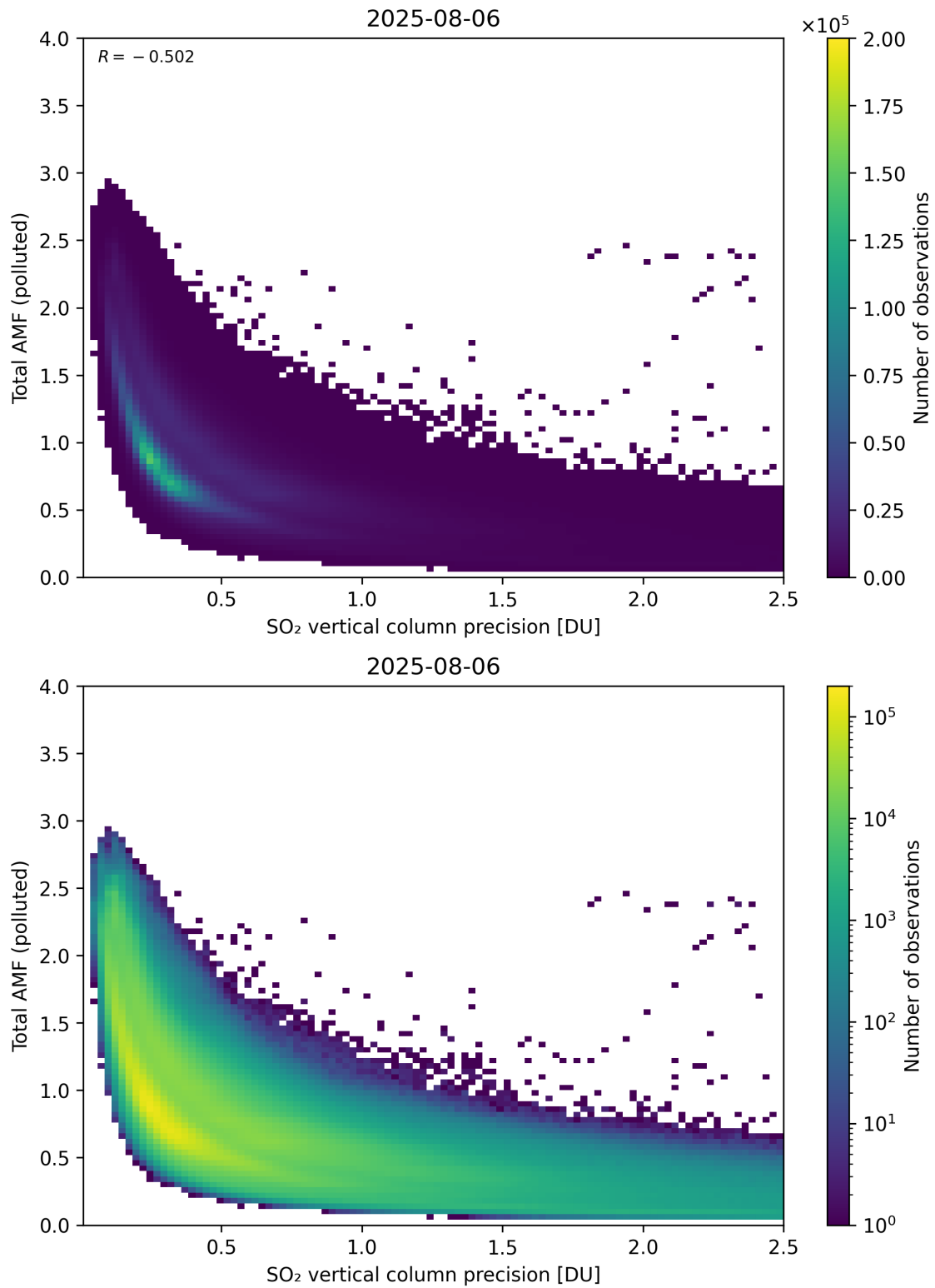
Figure 346: Scatter density plot of “SO 2 vertical column precision” against “Total AMF (polluted)” for 2025-08-05 to 2025-08-07.
