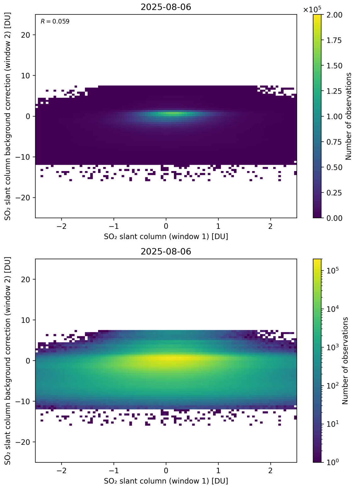
Figure 263: Scatter density plot of “SO 2 slant column (window 1)” against “SO 2 slant column background correction (window 2)” for 2025-08-05 to 2025-08-07.
