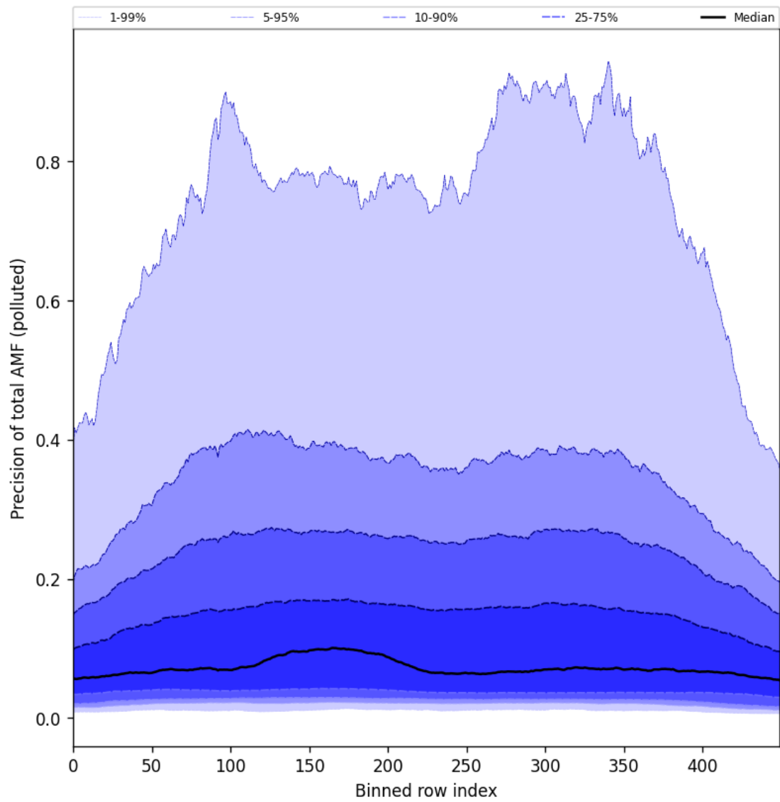
Figure 106: Along track statistics of “Precision of total AMF (polluted)” for 2025-08-05 to 2025-08-07
