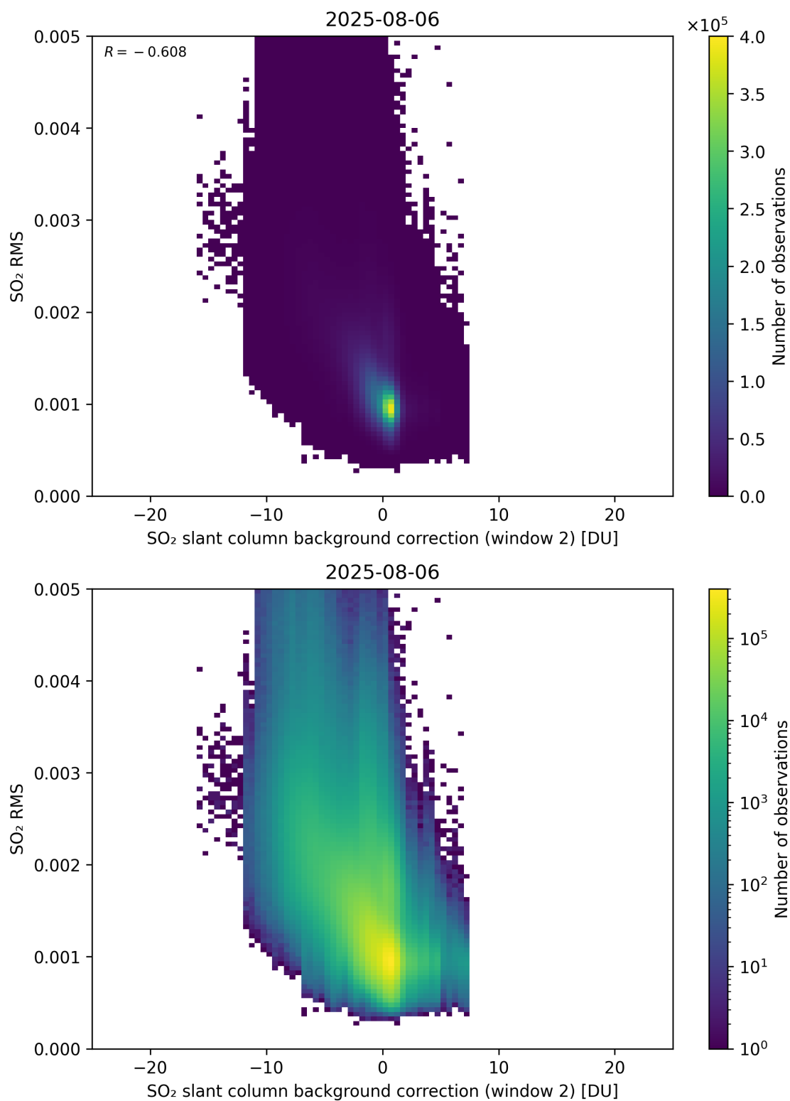
Figure 125: Scatter density plot of “SO 2 slant column background correction (window 2)” against “SO 2 RMS” for 2025-08-05 to 2025-08-07.
