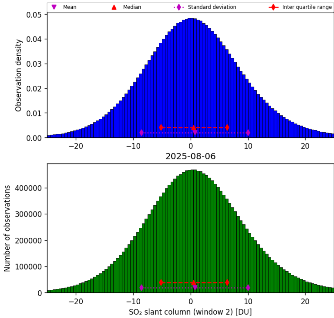
Figure 67: Histogram of “SO 2 slant column (window 2)” for 2025-08-05 to 2025-08-07
