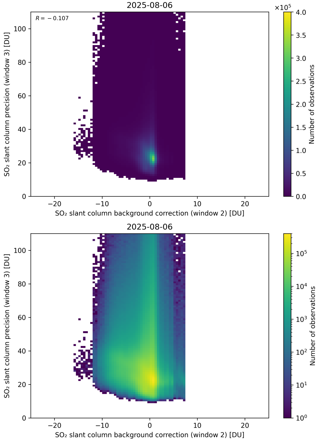
Figure 129: Scatter density plot of “SO 2 slant column background correction (window 2)” against “SO 2 slant column precision (window 3)” for 2025-08-05 to 2025-08-07.
