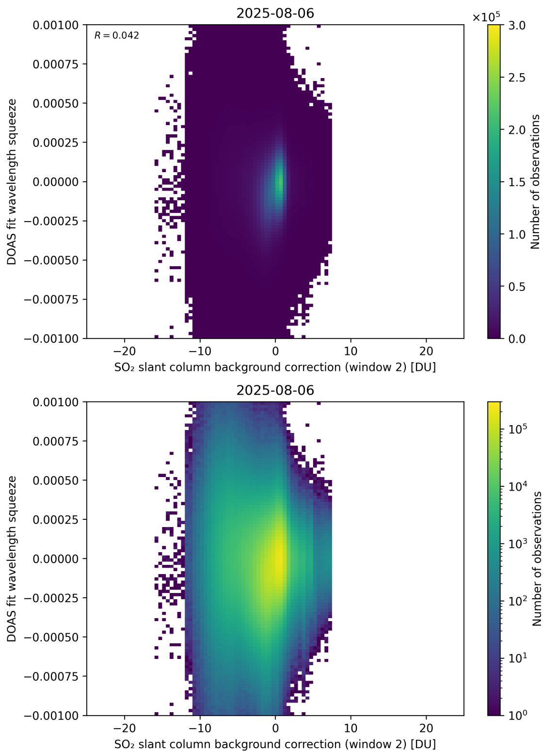
Figure 124: Scatter density plot of “SO 2 slant column background correction (window 2)” against “DOAS fit wavelength squeeze” for 2025-08-05 to 2025-08-07.
