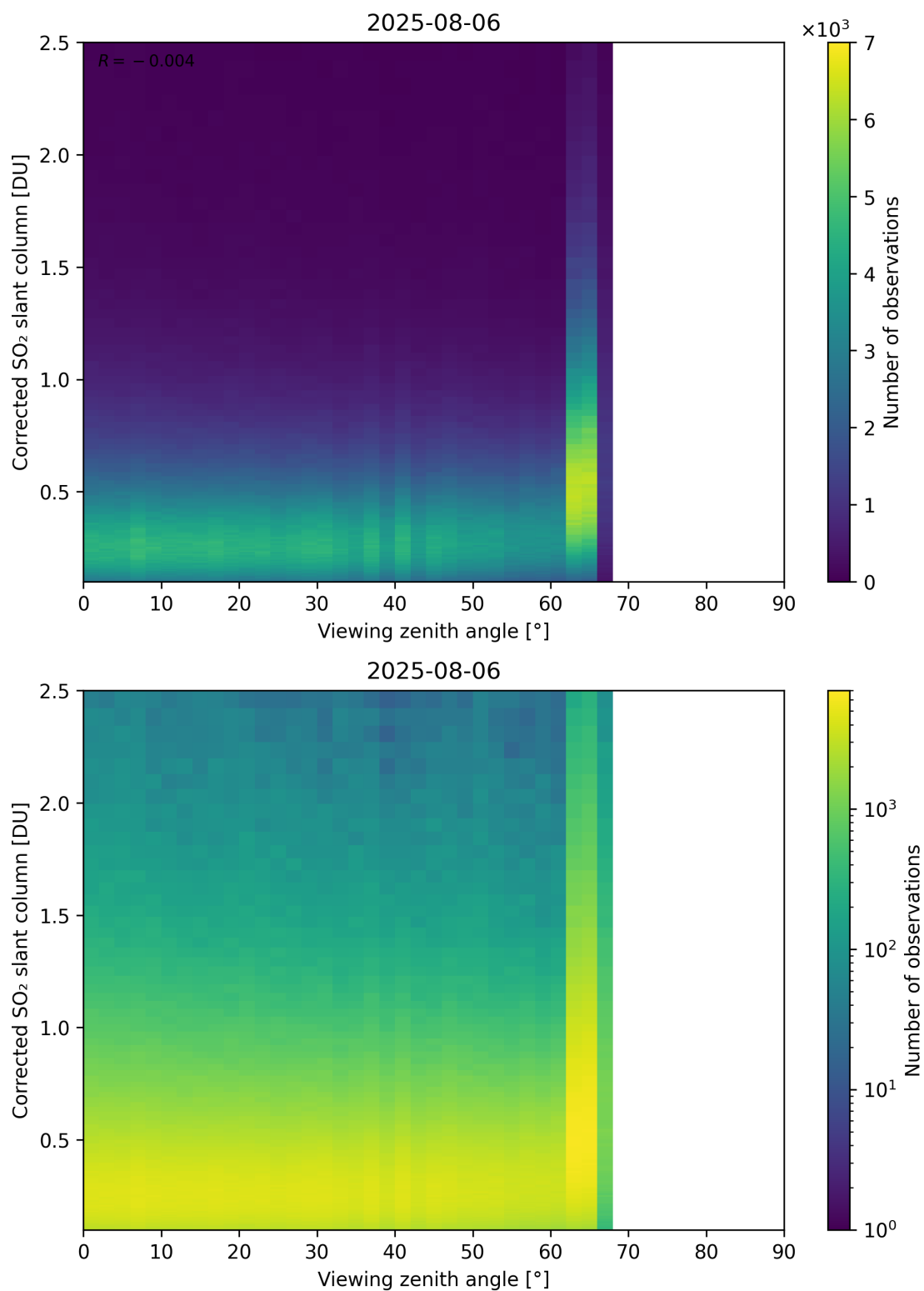
Figure 373: Scatter density plot of “Viewing zenith angle” against “Corrected SO 2 slant column” for 2025-08-05 to 2025-08-07.
