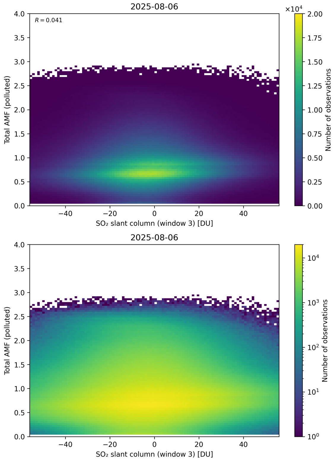
Figure 318: Scatter density plot of “SO 2 slant column (window 3)” against “Total AMF (polluted)” for 2025-08-05 to 2025-08-07.
