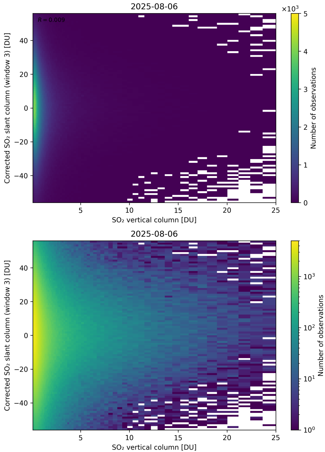
Figure 353: Scatter density plot of “SO 2 vertical column” against “Corrected SO 2 slant column (window 3)” for 2025-08-05 to 2025-08-07.
