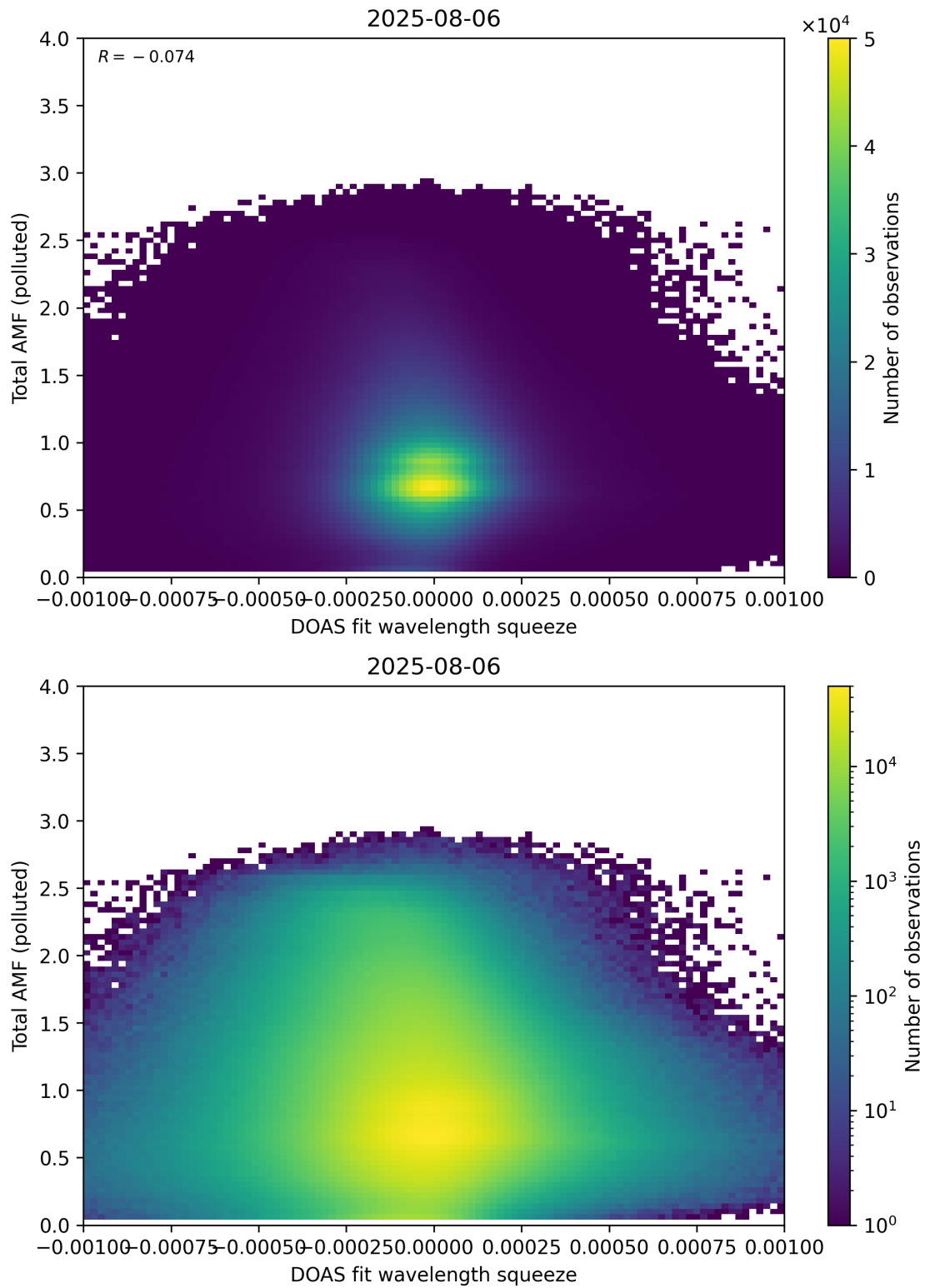
Figure 145: Scatter density plot of “DOAS fit wavelength squeeze” against “Total AMF (polluted)” for 2025-08-05 to 2025-08-07.
