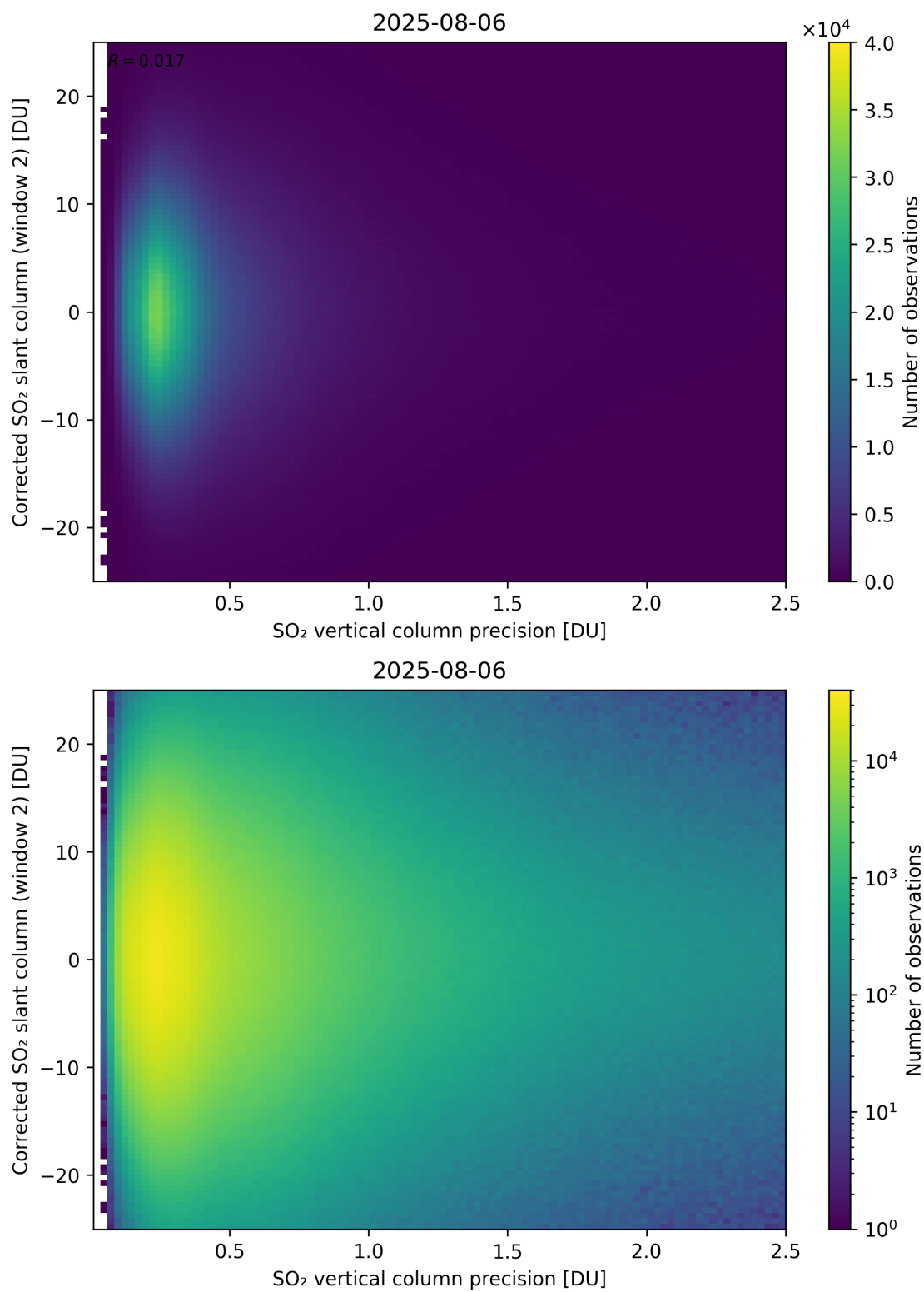
Figure 339: Scatter density plot of “SO 2 vertical column precision” against “Corrected SO 2 slant column (window 2)” for 2025-08-05 to 2025-08-07.
