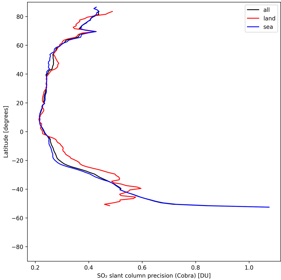
Figure 36: Zonal average of “SO 2 slant column precision (Cobra)” for 2025-08-05 to 2025-08-07.
