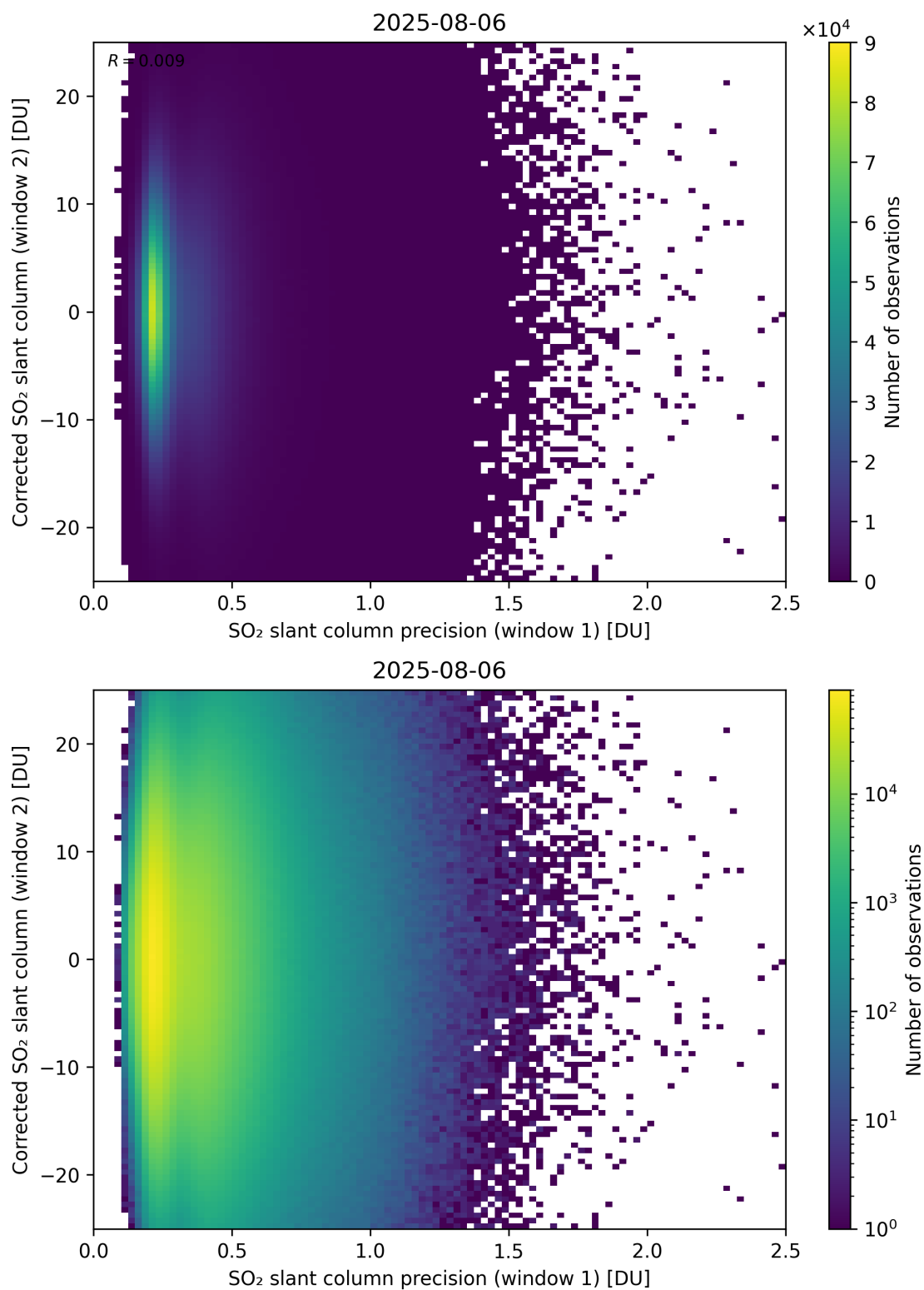
Figure 275: Scatter density plot of “SO 2 slant column precision (window 1)” against “Corrected SO 2 slant column (window 2)” for 2025-08-05 to 2025-08-07.
