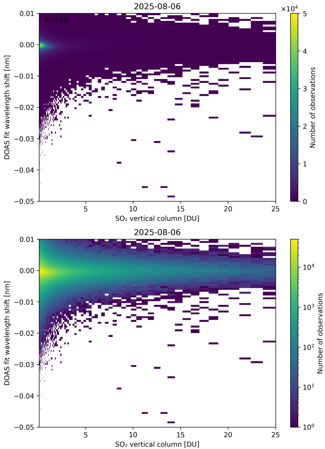
Figure 326: Scatter density plot of “SO 2 vertical column” against “DOAS fit wavelength shift” for 2025-08-05 to 2025-08-07.
