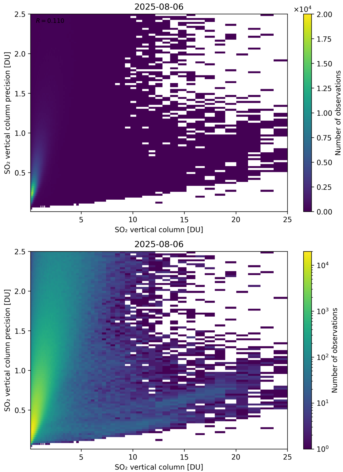
Figure 361: Scatter density plot of “SO 2 vertical column” against “SO 2 vertical column precision” for 2025-08-05 to 2025-08-07.
