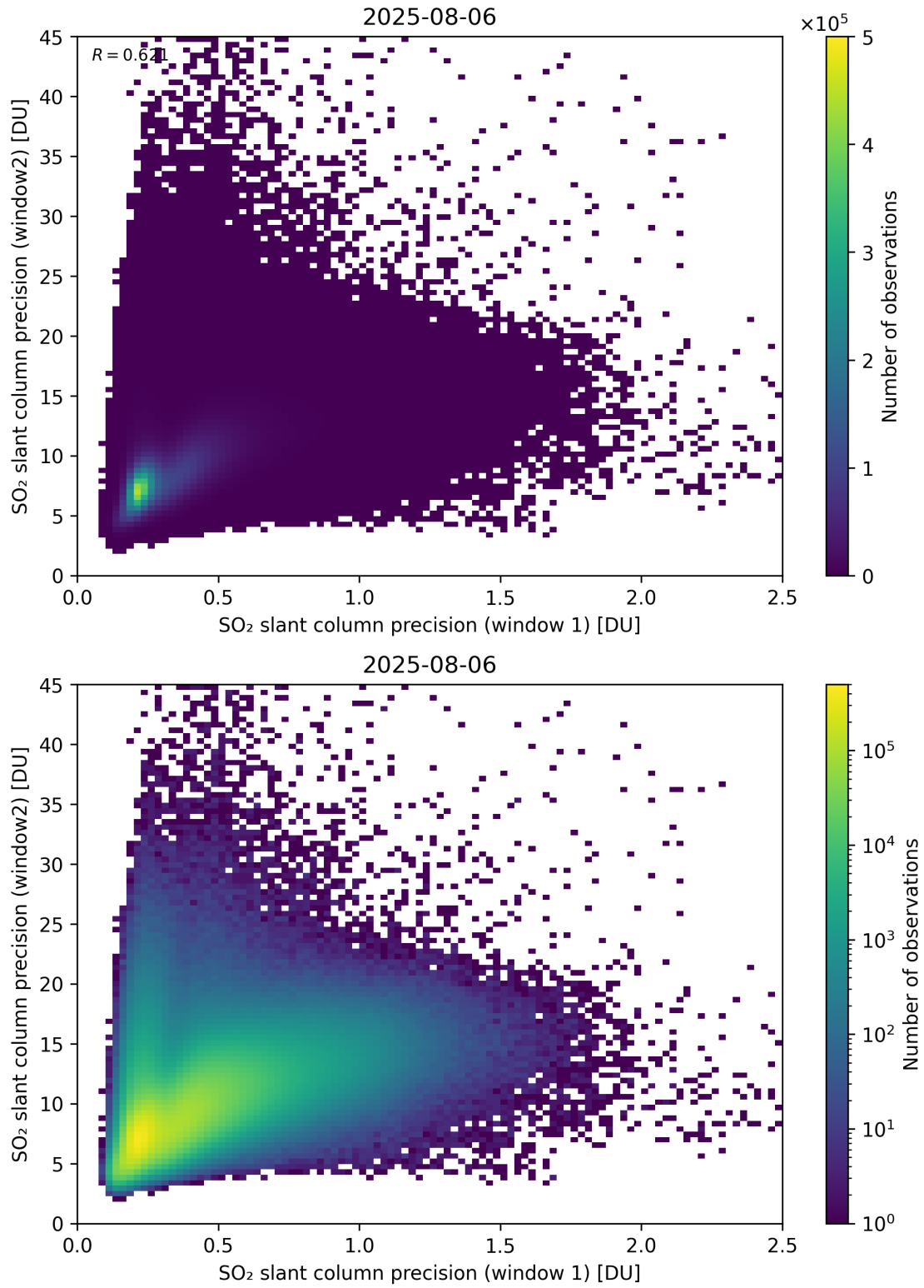
Figure 277: Scatter density plot of “SO 2 slant column precision (window 1)” against “SO 2 slant column precision (window2)” for 2025-08-05 to 2025-08-07.
