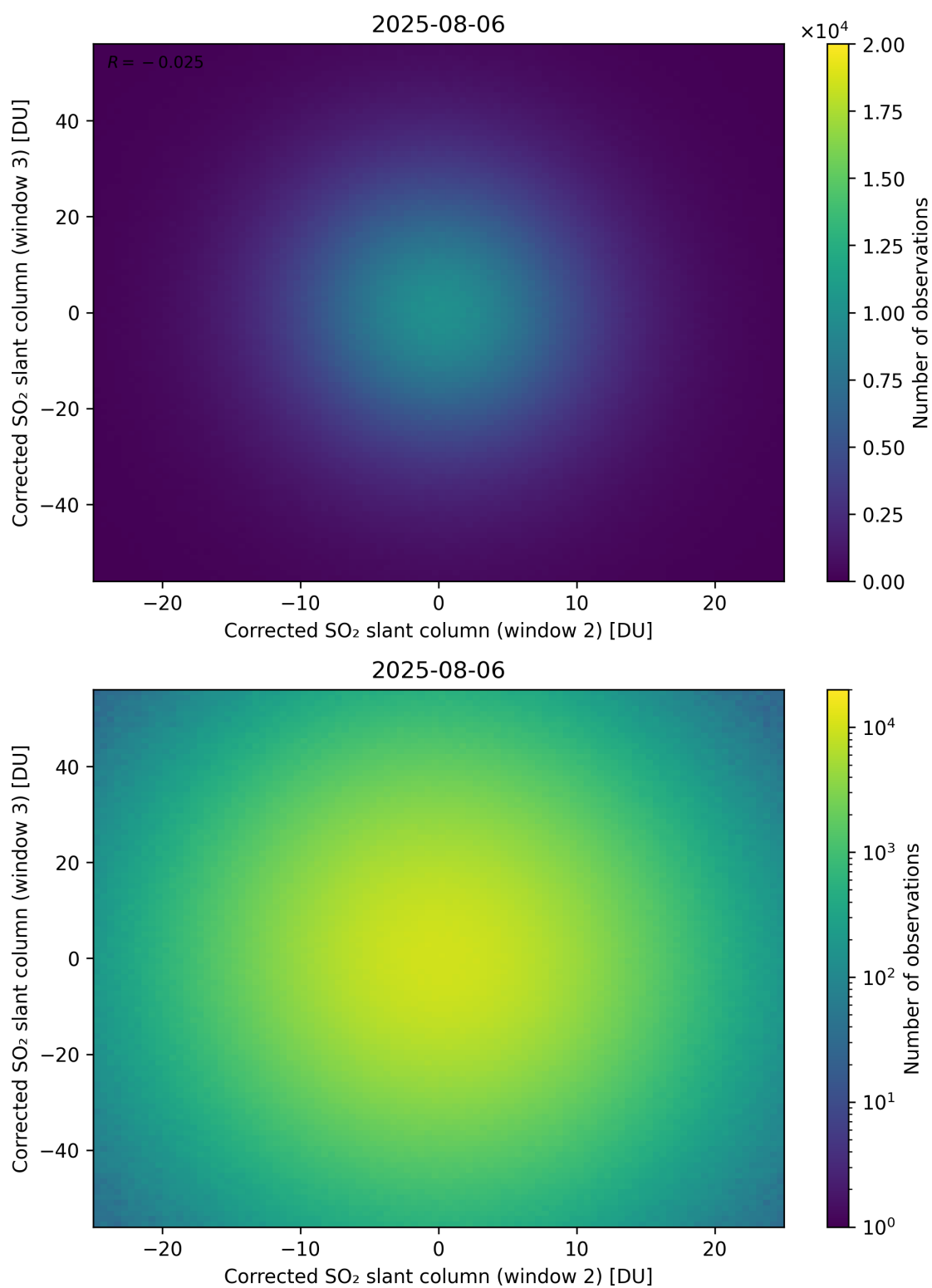
Figure 250: Scatter density plot of “Corrected SO 2 slant column (window 2)” against “Corrected SO 2 slant column (window 3)” for 2025-08-05 to 2025-08-07.
