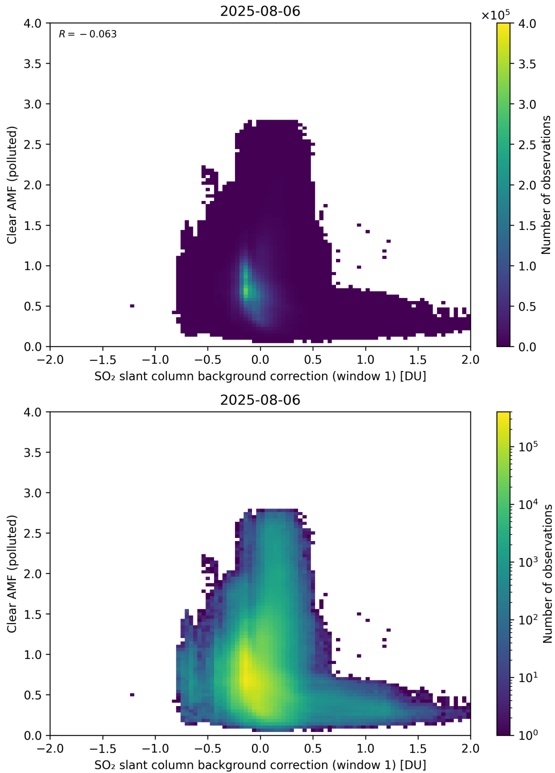
Figure 114: Scatter density plot of “SO 2 slant column background correction (window 1)” against “Clear AMF (polluted)” for 2025-08-05 to 2025-08-07.
