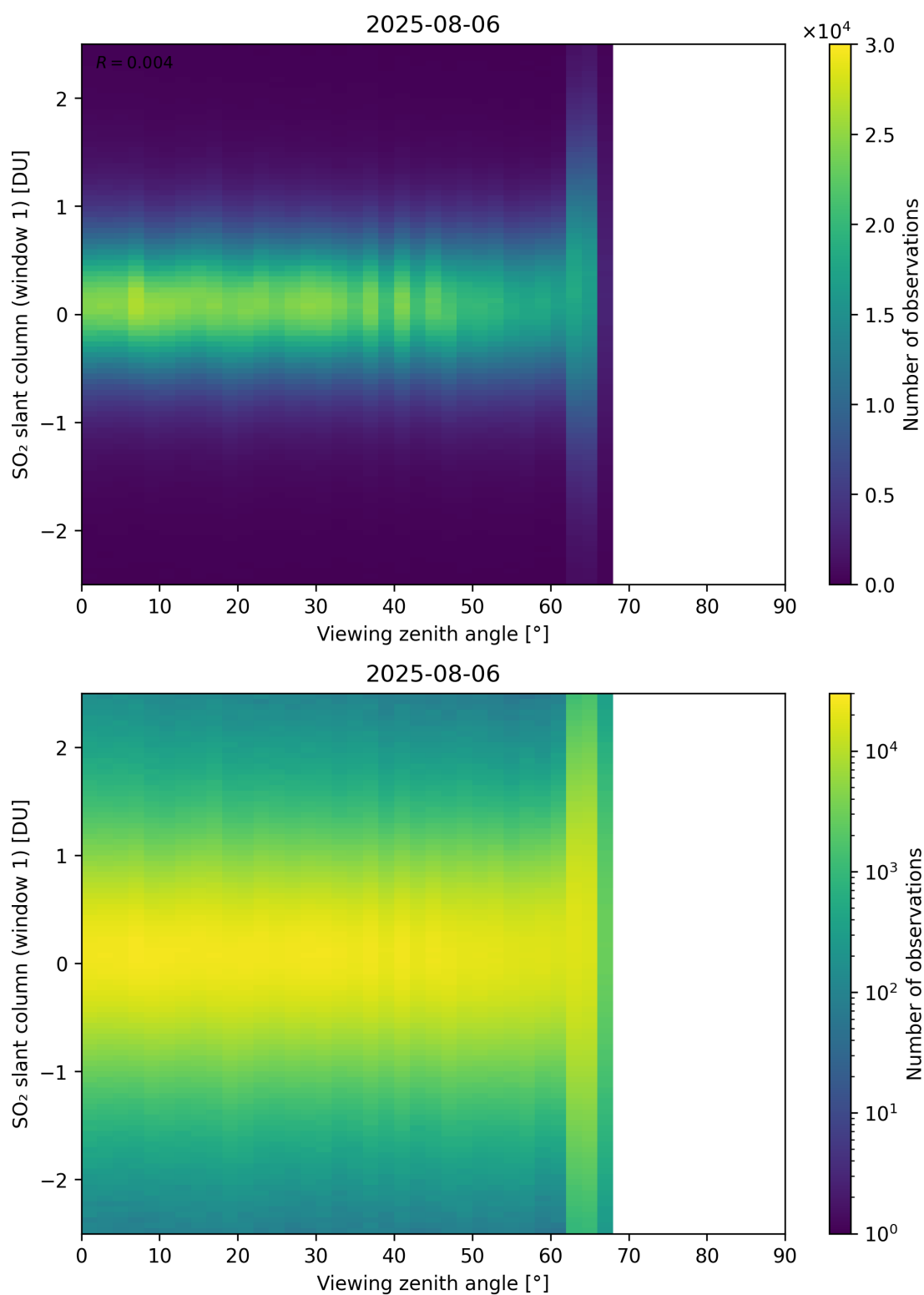
Figure 376: Scatter density plot of “Viewing zenith angle” against “SO 2 slant column (window 1)” for 2025-08-05 to 2025-08-07.
