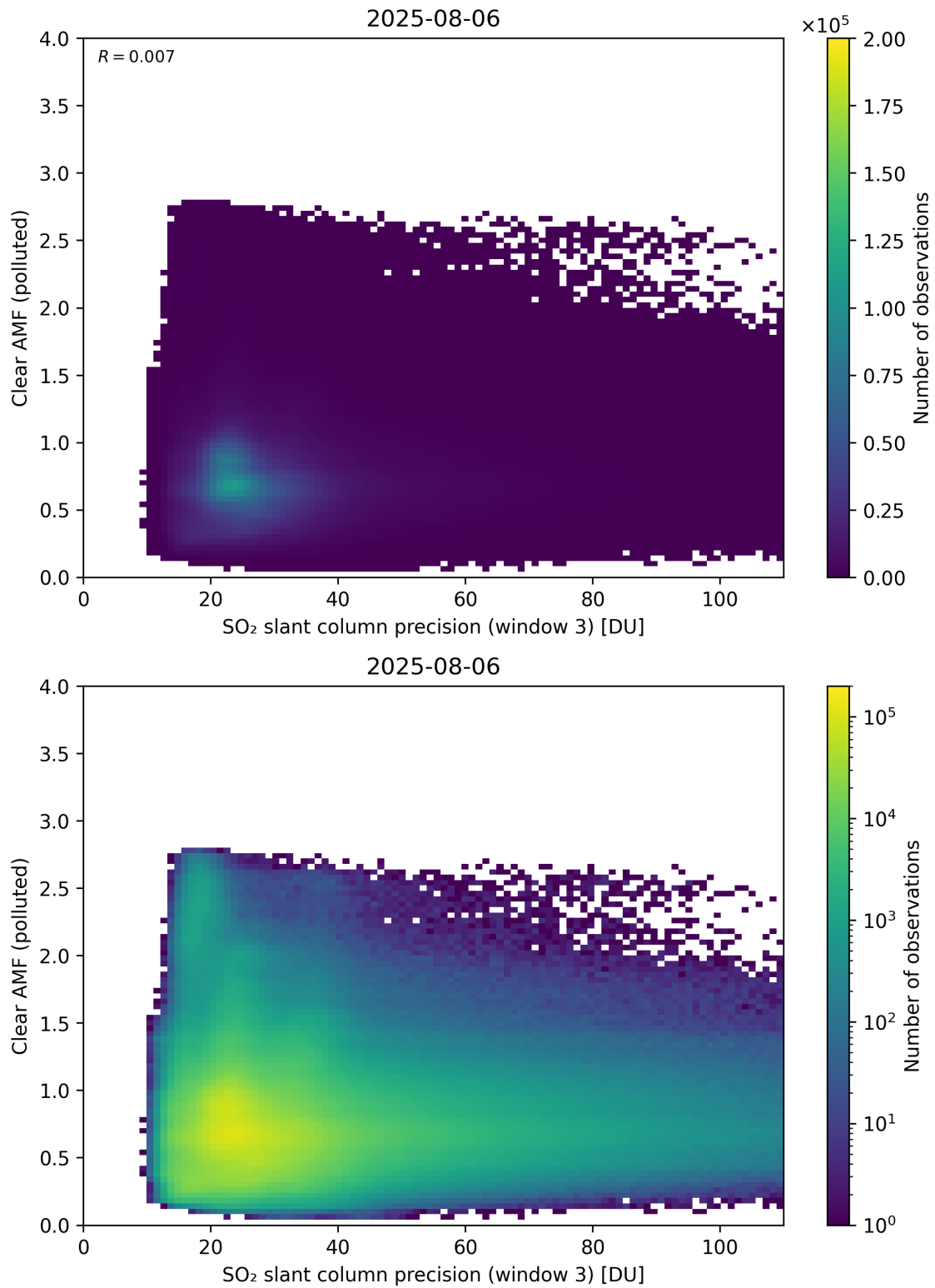
Figure 311: Scatter density plot of “SO 2 slant column precision (window 3)” against “Clear AMF (polluted)” for 2025-08-05 to 2025-08-07.
