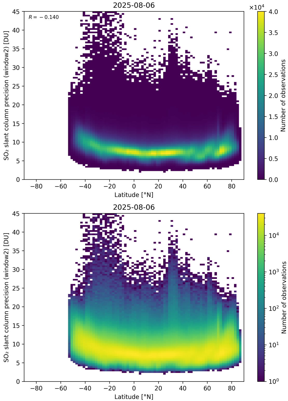
Figure 164: Scatter density plot of “Latitude” against “SO 2 slant column precision (window2)” for 2025-08-05 to 2025-08-07.
