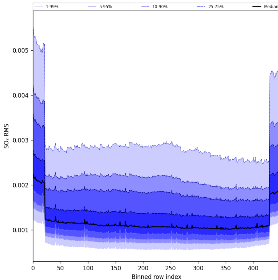
Figure 104: Along track statistics of “SO 2 RMS” for 2025-08-05 to 2025-08-07
