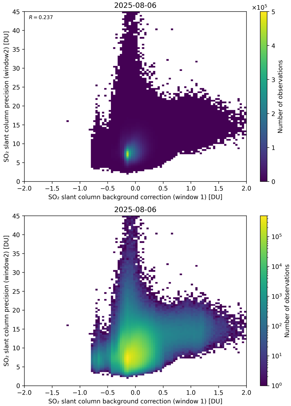
Figure 117: Scatter density plot of “SO 2 slant column background correction (window 1)” against “SO 2 slant column precision (window2)” for 2025-08-05 to 2025-08-07.
