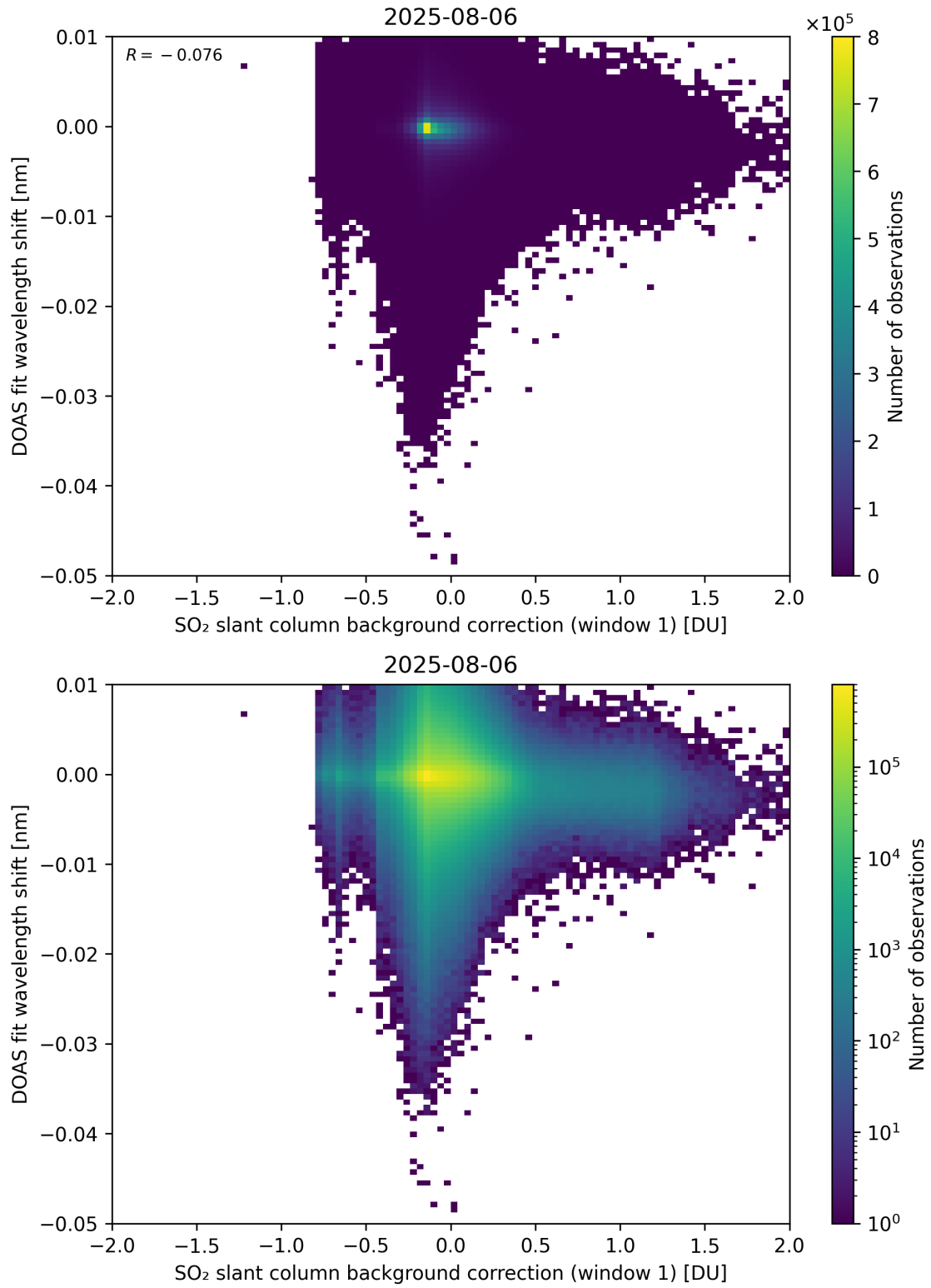
Figure 111: Scatter density plot of “SO 2 slant column background correction (window 1)” against “DOAS fit wavelength shift” for 2025-08-05 to 2025-08-07.
