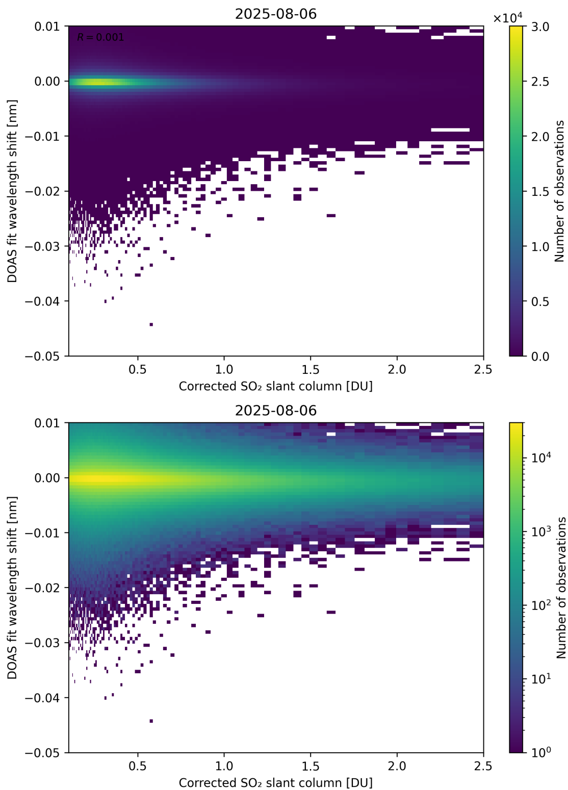
Figure 229: Scatter density plot of “Corrected SO 2 slant column” against “DOAS fit wavelength shift” for 2025-08-05 to 2025-08-07.
