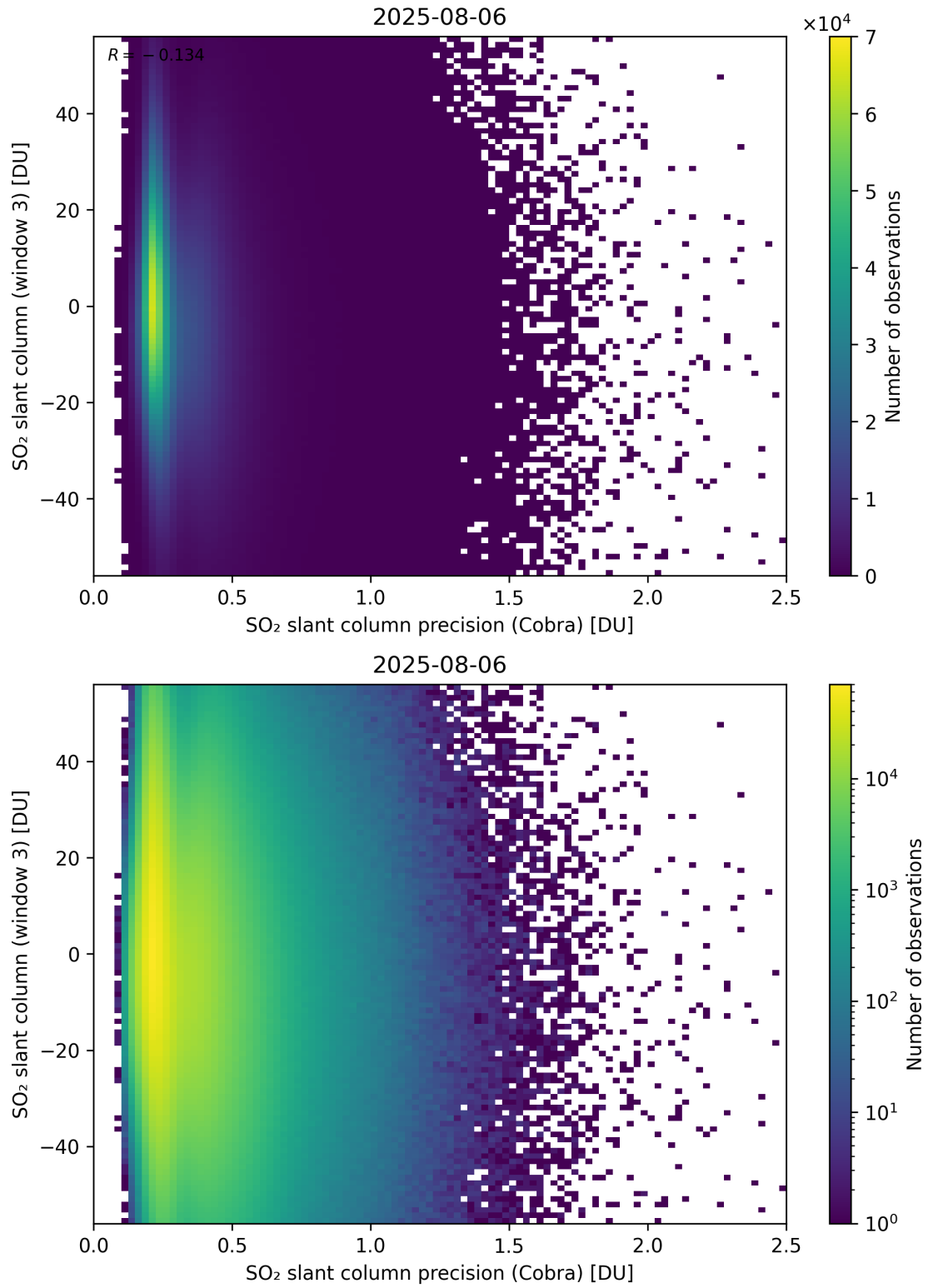
Figure 211: Scatter density plot of “SO 2 slant column precision (Cobra)” against “SO 2 slant column (window 3)” for 2025-08-05 to 2025-08-07.
