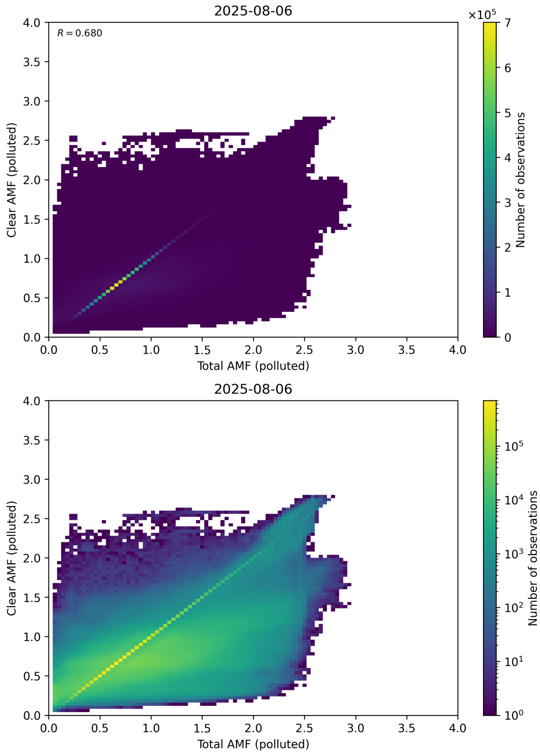
Figure 321: Scatter density plot of “Total AMF (polluted)” against “Clear AMF (polluted)” for 2025-08-05 to 2025-08-07.
