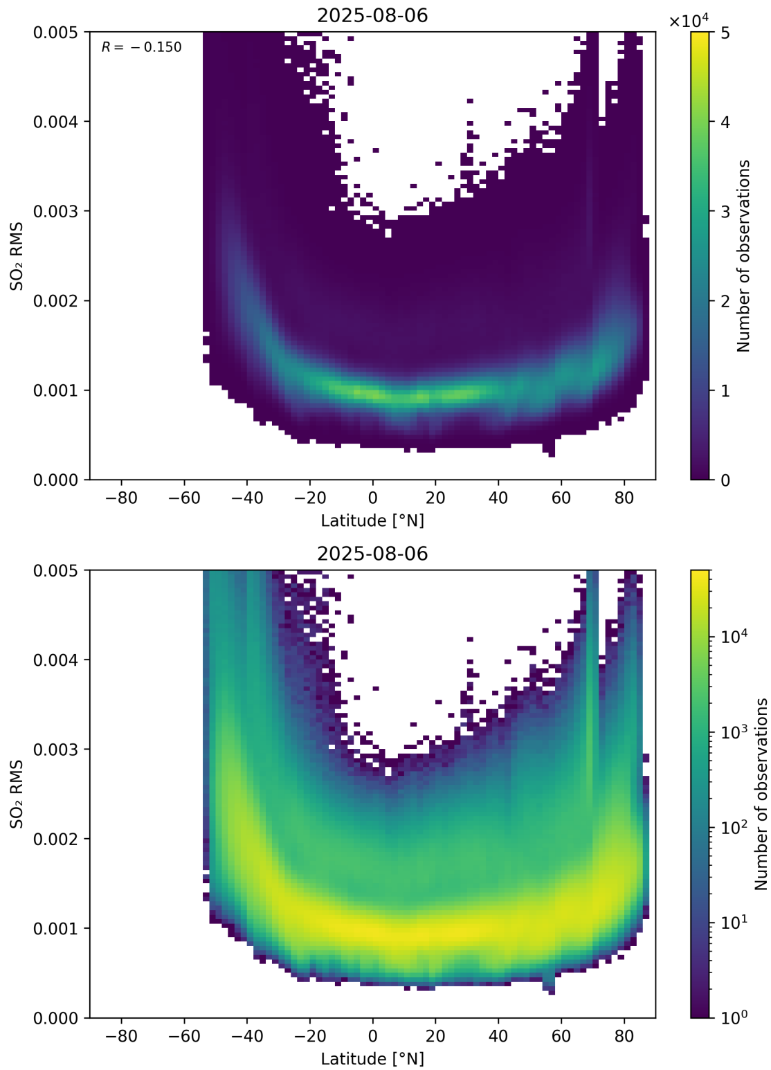
Figure 155: Scatter density plot of “Latitude” against “SO 2 RMS” for 2025-08-05 to 2025-08-07.
