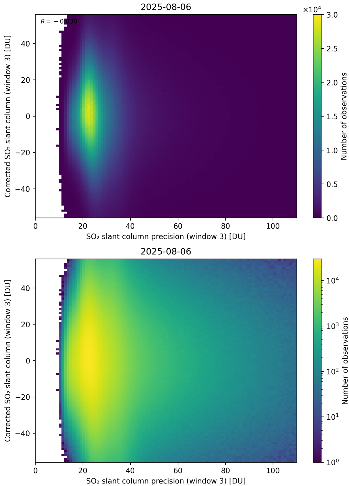
Figure 312: Scatter density plot of “SO 2 slant column precision (window 3)” against “Corrected SO 2 slant column (window 3)” for 2025-08-05 to 2025-08-07.
