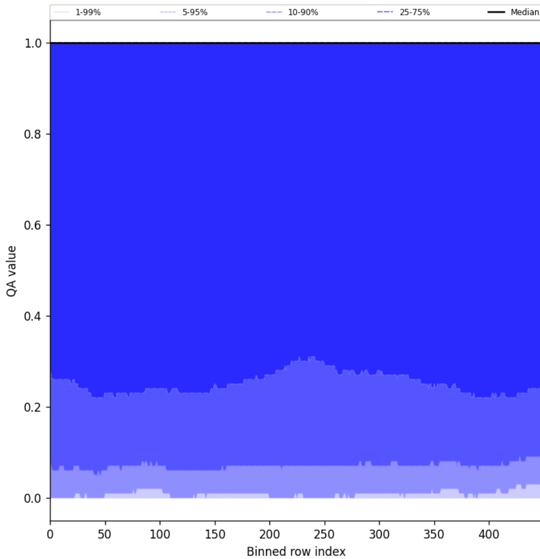
Figure 83: Along track statistics of “QA value” for 2025-08-05 to 2025-08-07
