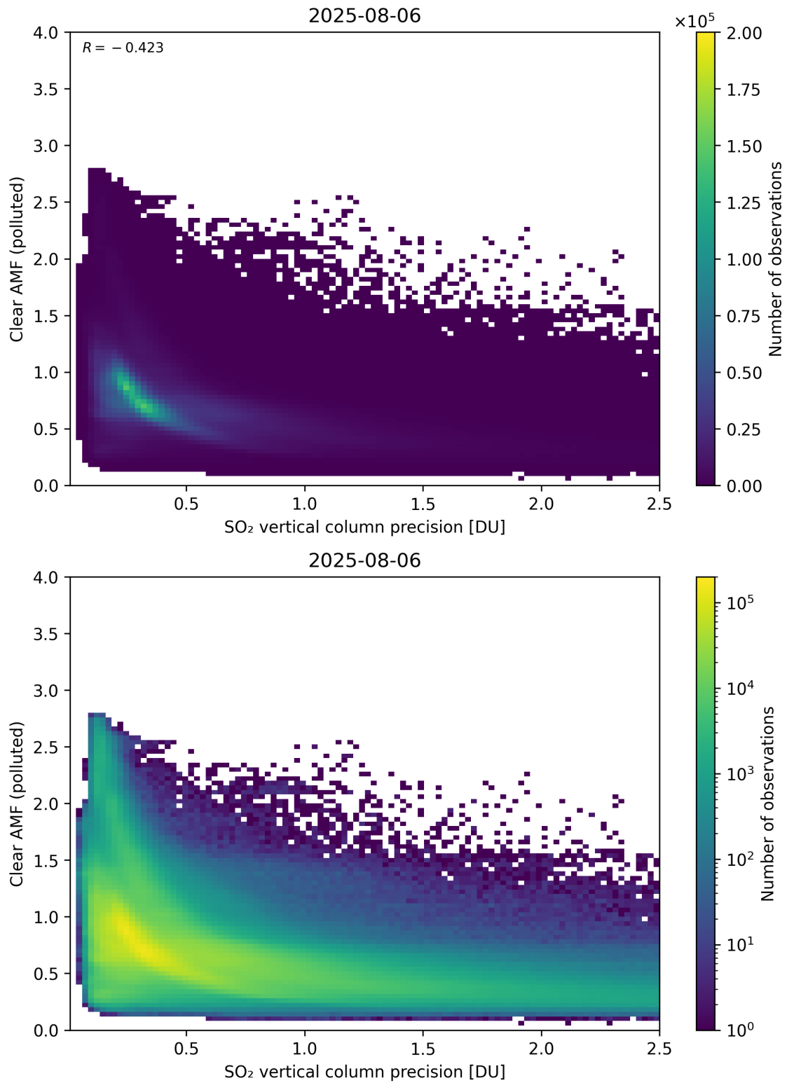
Figure 335: Scatter density plot of “SO 2 vertical column precision” against “Clear AMF (polluted)” for 2025-08-05 to 2025-08-07.
