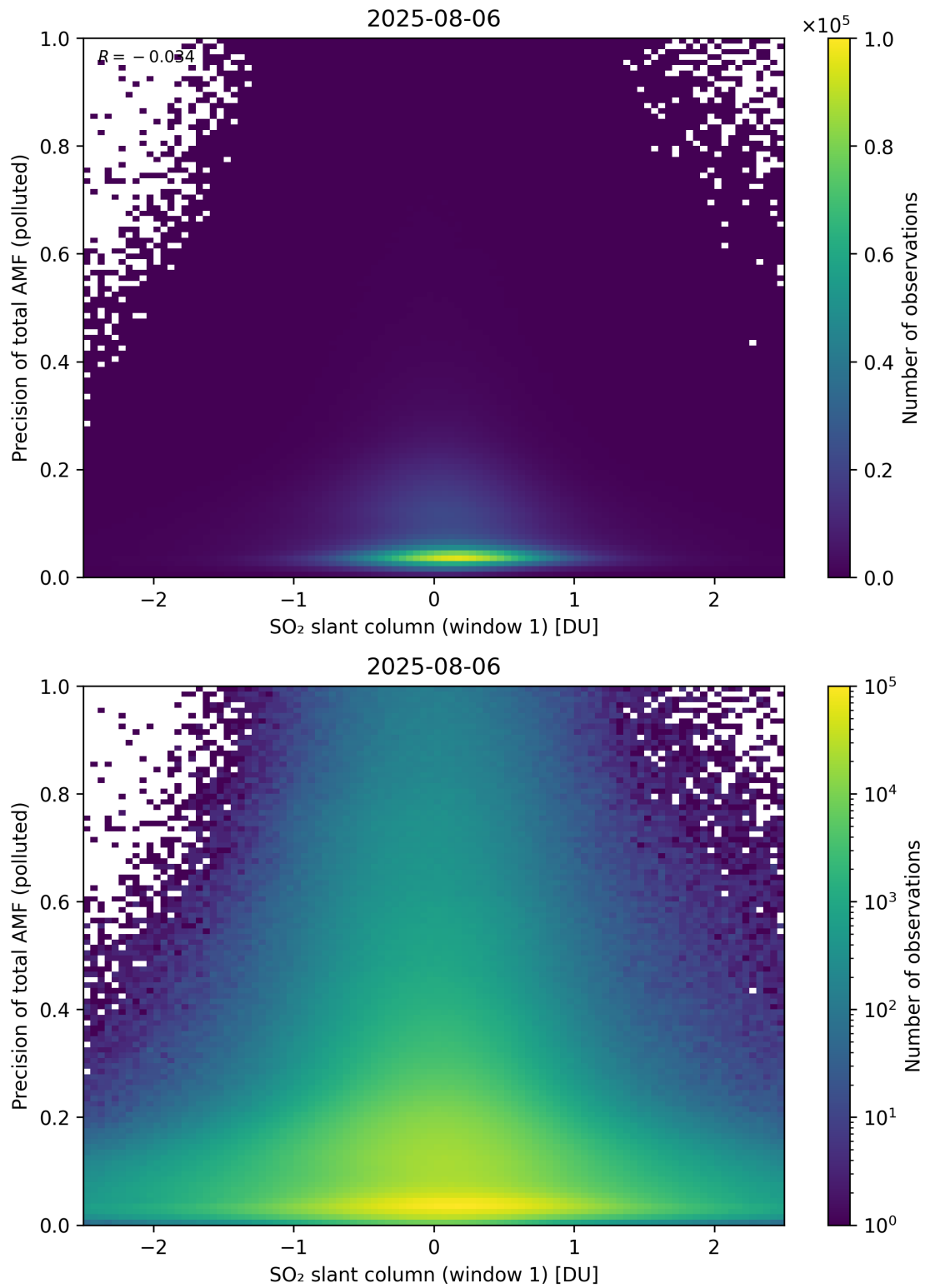
Figure 290: Scatter density plot of “SO 2 slant column (window 1)” against “Precision of total AMF (polluted)” for 2025-08-05 to 2025-08-07.
