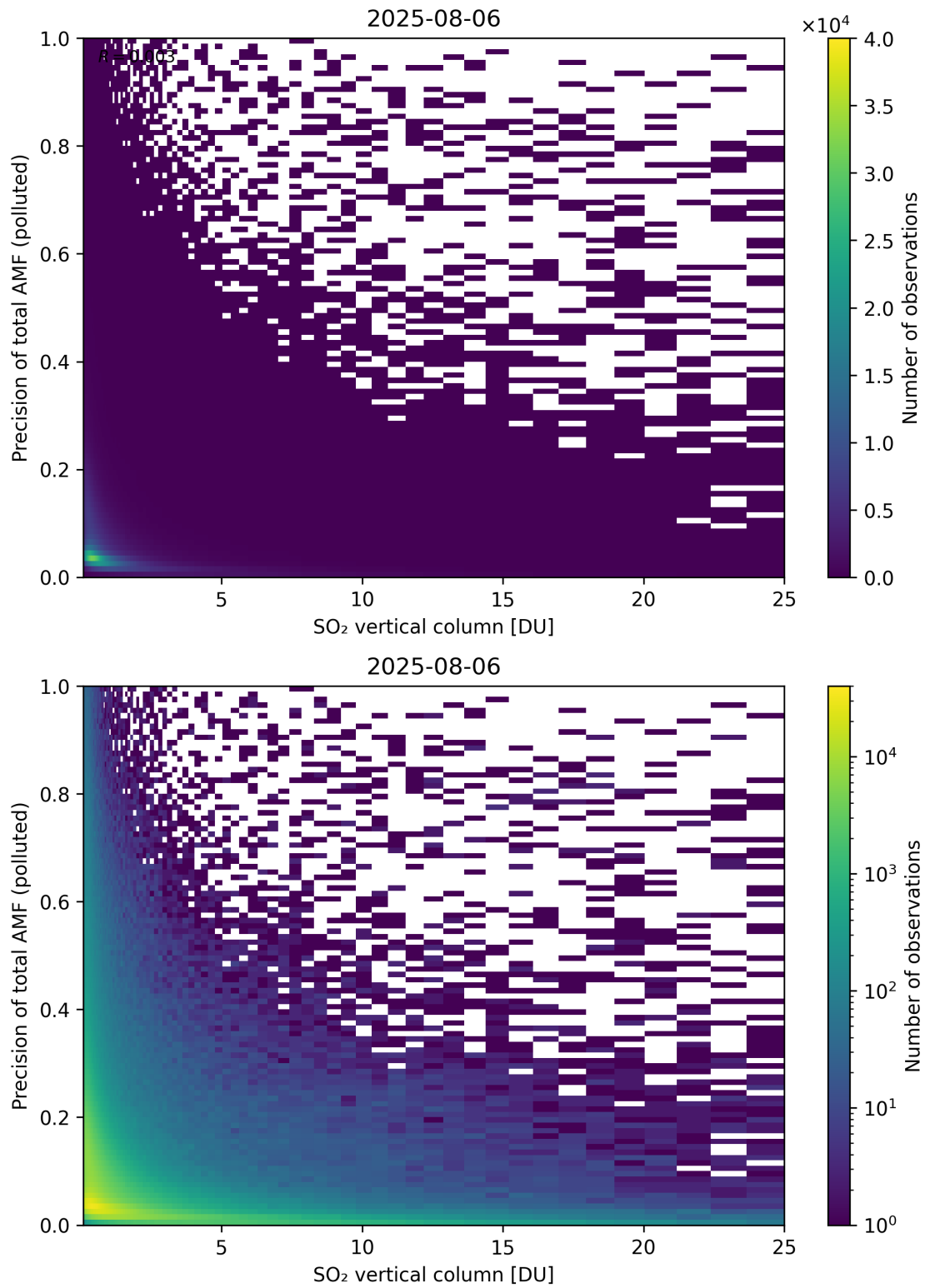
Figure 360: Scatter density plot of “SO 2 vertical column” against “Precision of total AMF (polluted)” for 2025-08-05 to 2025-08-07.
