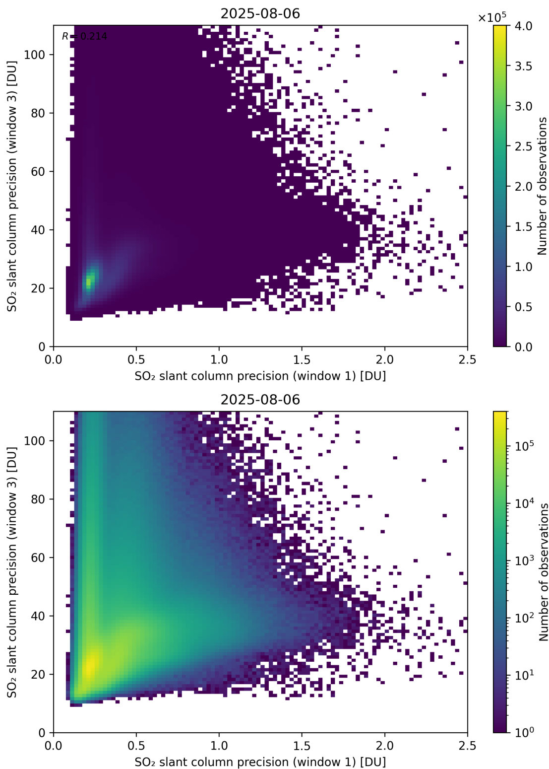
Figure 279: Scatter density plot of “SO 2 slant column precision (window 1)” against “SO 2 slant column precision (window 3)” for 2025-08-05 to 2025-08-07.
