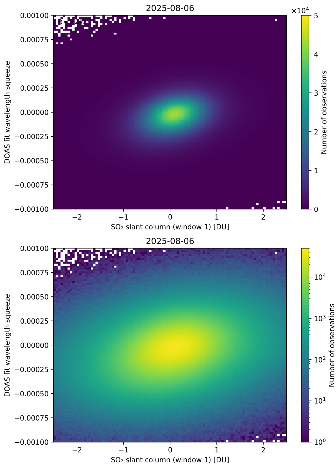
Figure 266: Scatter density plot of “SO 2 slant column (window 1)” against “DOAS fit wavelength squeeze” for 2025-08-05 to 2025-08-07.
