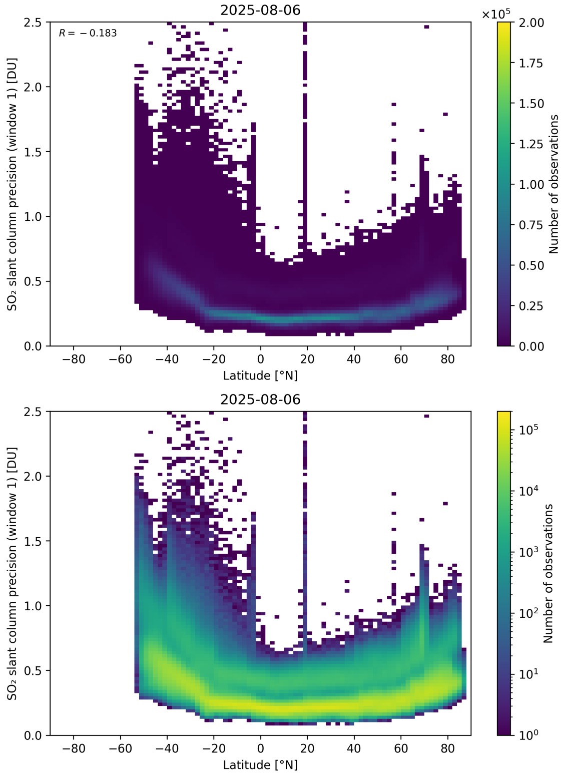
Figure 163: Scatter density plot of “Latitude” against “SO 2 slant column precision (window 1)” for 2025-08-05 to 2025-08-07.
