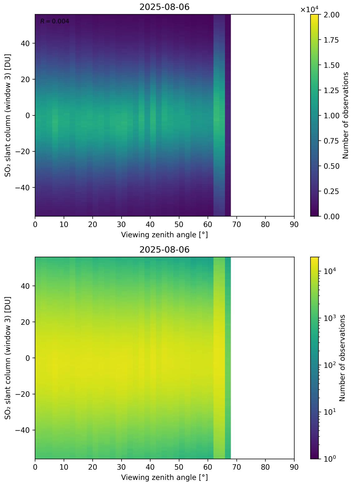
Figure 379: Scatter density plot of “Viewing zenith angle” against “SO 2 slant column (window 3)” for 2025-08-05 to 2025-08-07.
