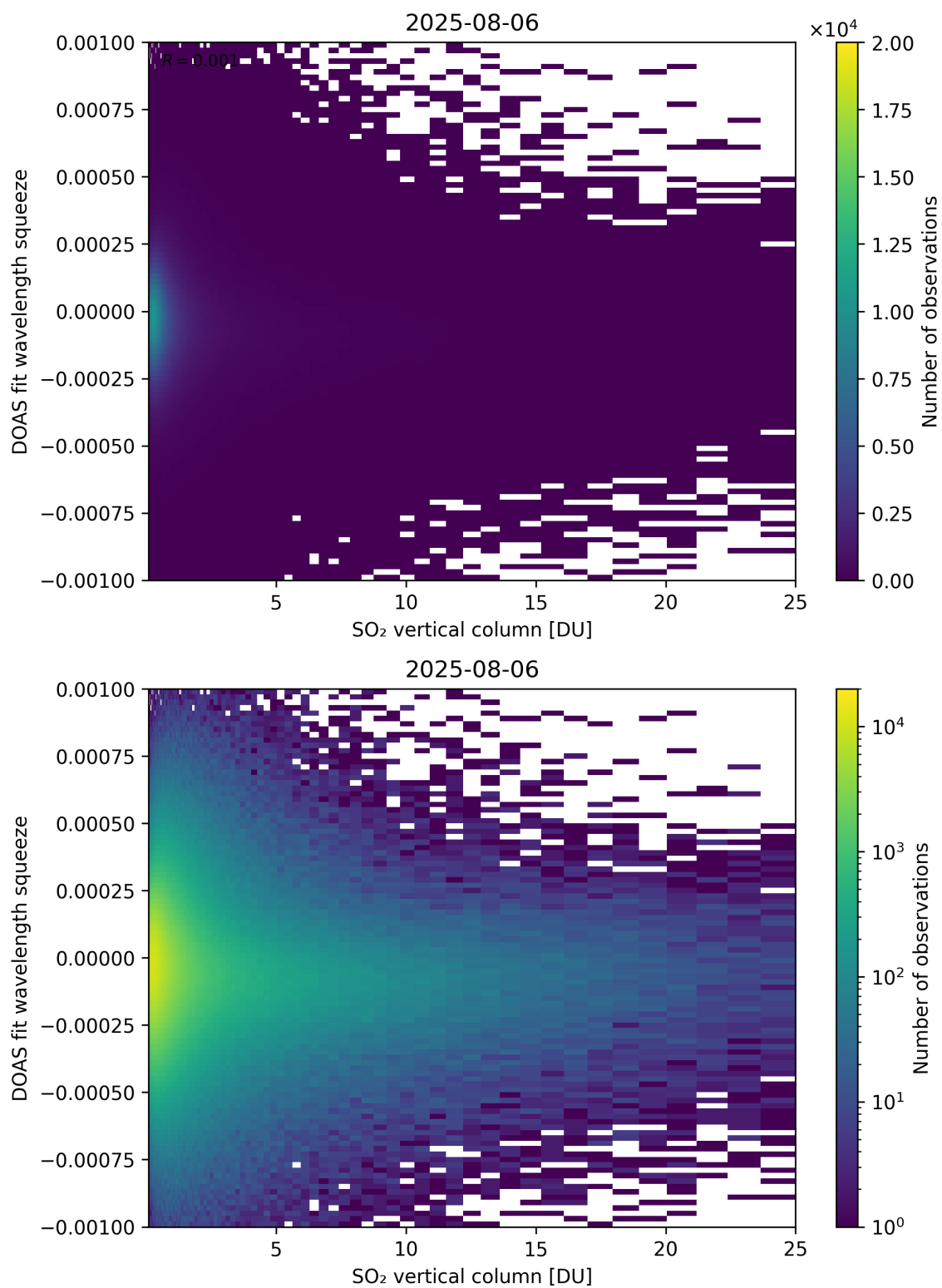
Figure 327: Scatter density plot of “SO 2 vertical column” against “DOAS fit wavelength squeeze” for 2025-08-05 to 2025-08-07.
