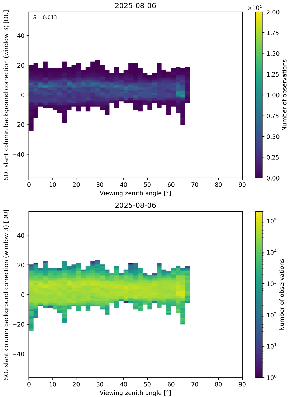
Figure 364: Scatter density plot of “Viewing zenith angle” against “SO 2 slant column background correction (window 3)” for 2025-08-05 to 2025-08-07.
