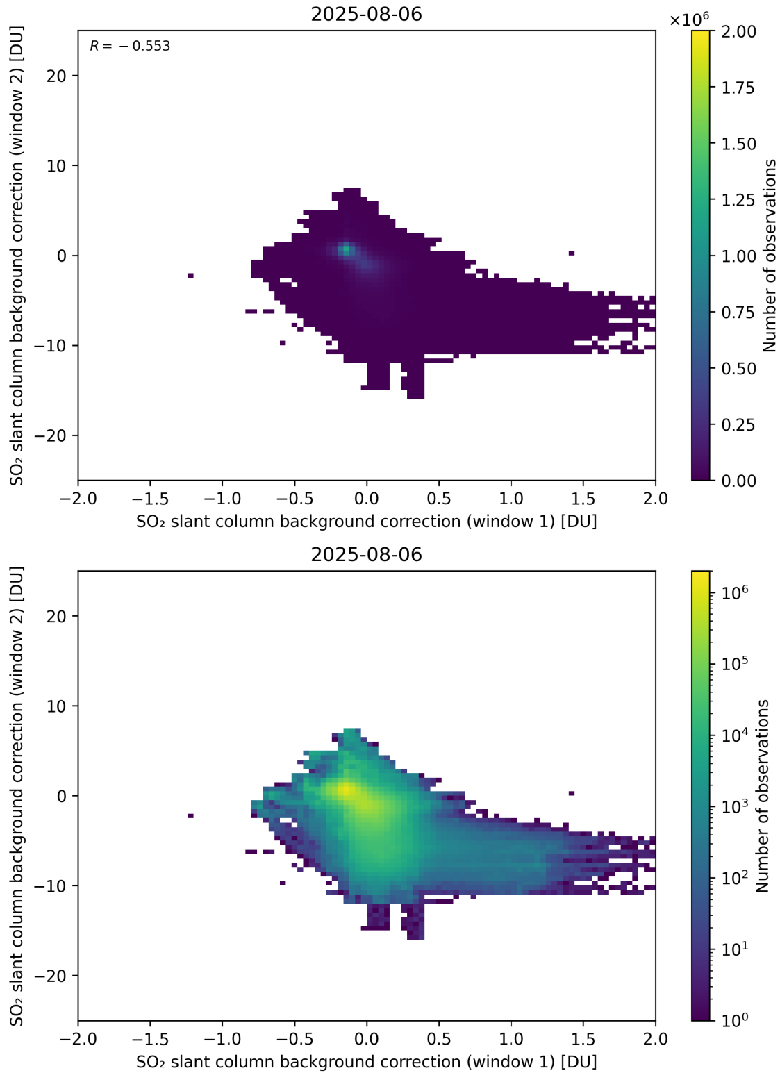
Figure 109: Scatter density plot of “SO 2 slant column background correction (window 1)” against “SO 2 slant column background correction (window 2)” for 2025-08-05 to 2025-08-07.
