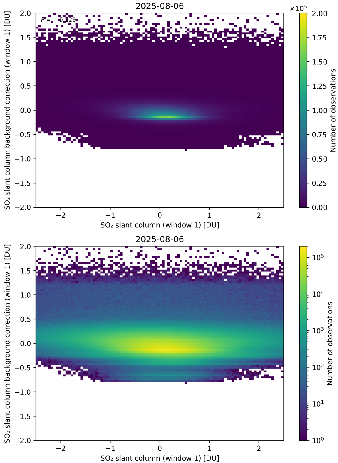
Figure 262: Scatter density plot of “SO 2 slant column (window 1)” against “SO 2 slant column background correction (window 1)” for 2025-08-05 to 2025-08-07.
