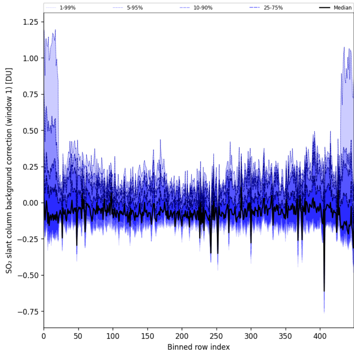
Figure 92: Along track statistics of “SO 2 slant column background correction (window 1)” for 2025-08-05 to 2025-08-07
