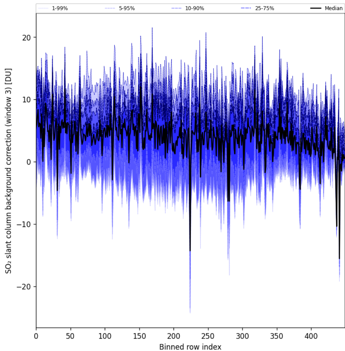
Figure 100: Along track statistics of "SO 2 slant column background correction (window 3)" for 2025-08-05 to 2025-08-07
