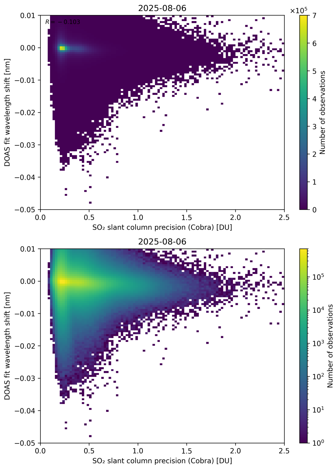
Figure 202: Scatter density plot of “SO 2 slant column precision (Cobra)” against “DOAS fit wavelength shift” for 2025-08-05 to 2025-08-07.
