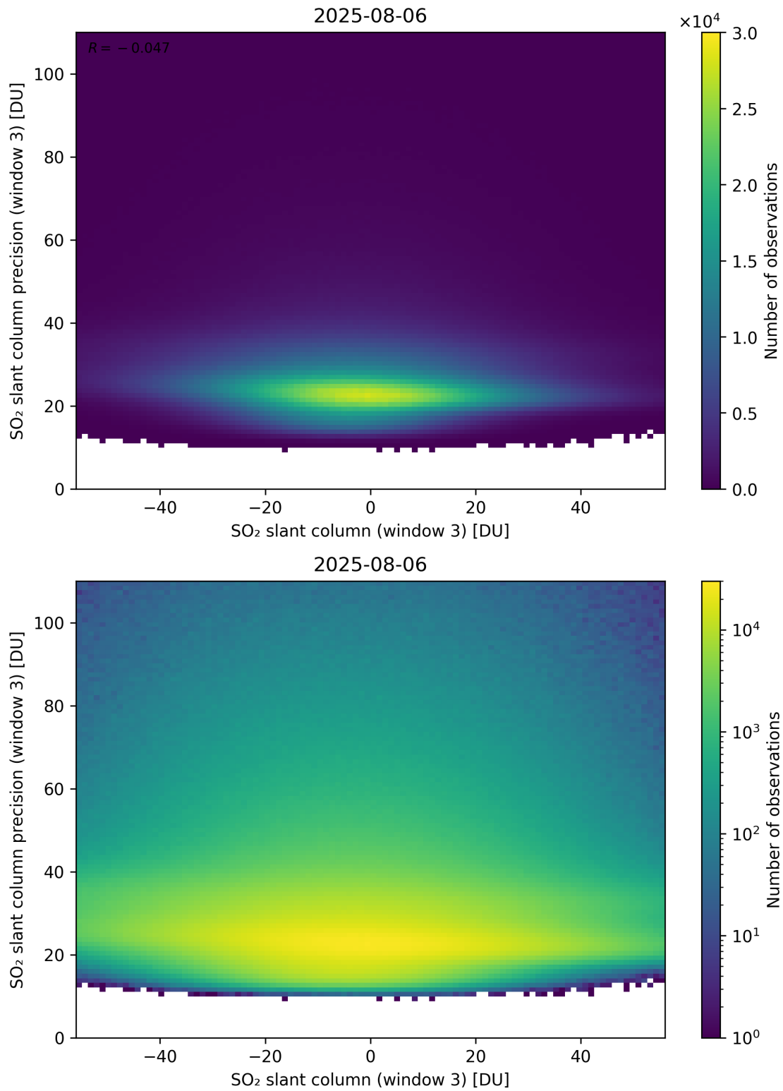
Figure 317: Scatter density plot of “SO 2 slant column (window 3)” against “SO 2 slant column precision (window 3)” for 2025-08-05 to 2025-08-07.
