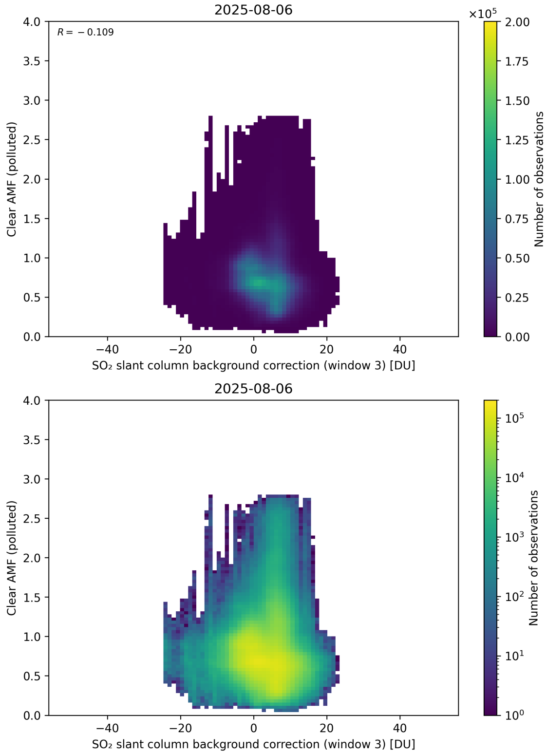
Figure 135: Scatter density plot of “SO 2 slant column background correction (window 3)” against “Clear AMF (polluted)” for 2025-08-05 to 2025-08-07.
