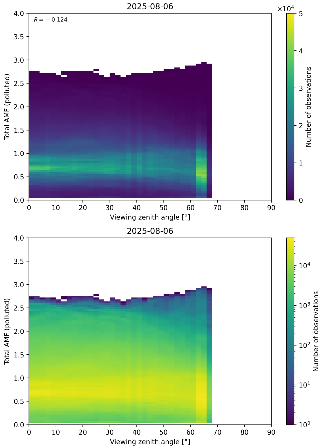
Figure 381: Scatter density plot of “Viewing zenith angle” against “Total AMF (polluted)” for 2025-08-05 to 2025-08-07.
