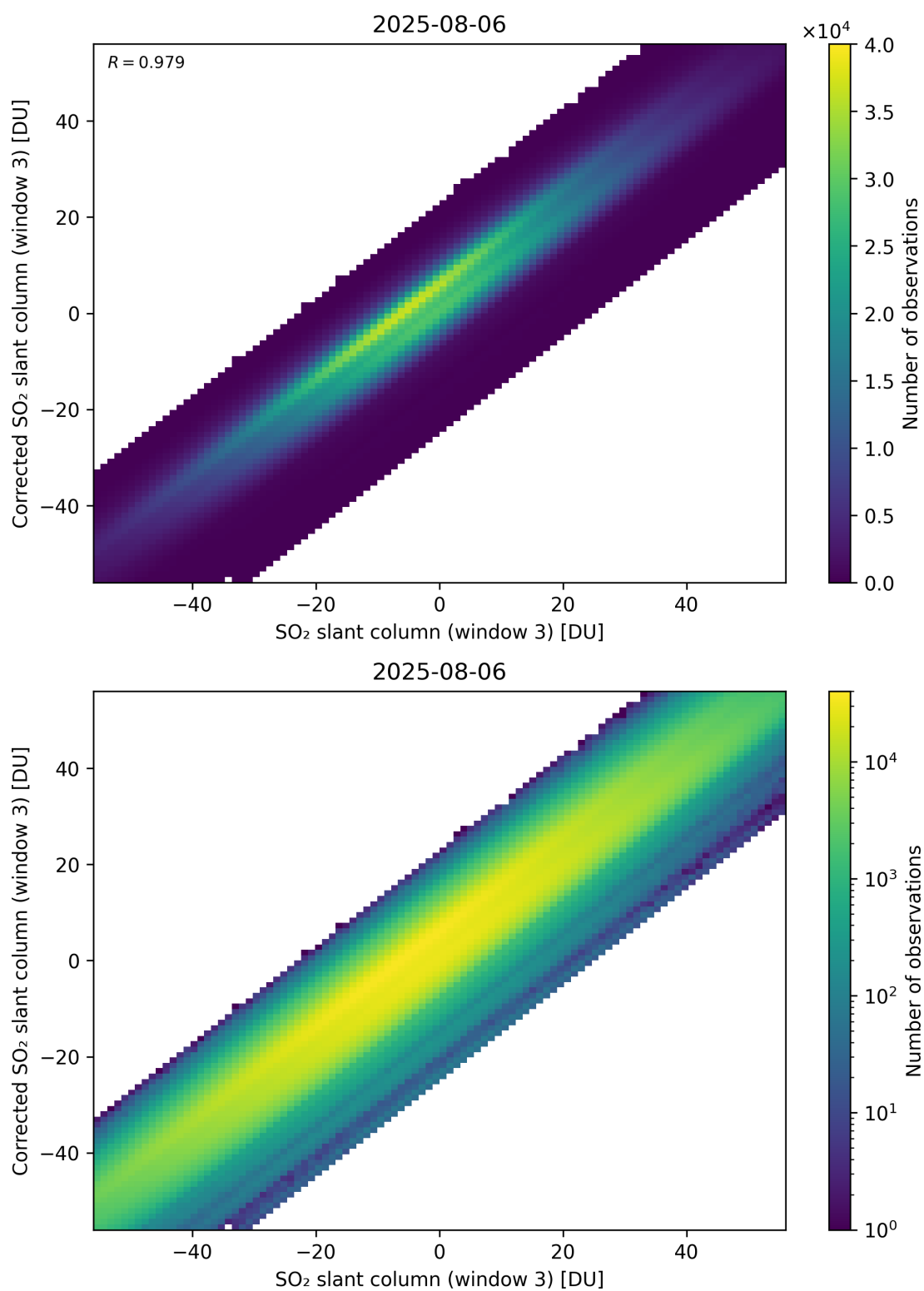
Figure 316: Scatter density plot of “SO 2 slant column (window 3)” against “Corrected SO 2 slant column (window 3)” for 2025-08-05 to 2025-08-07.
