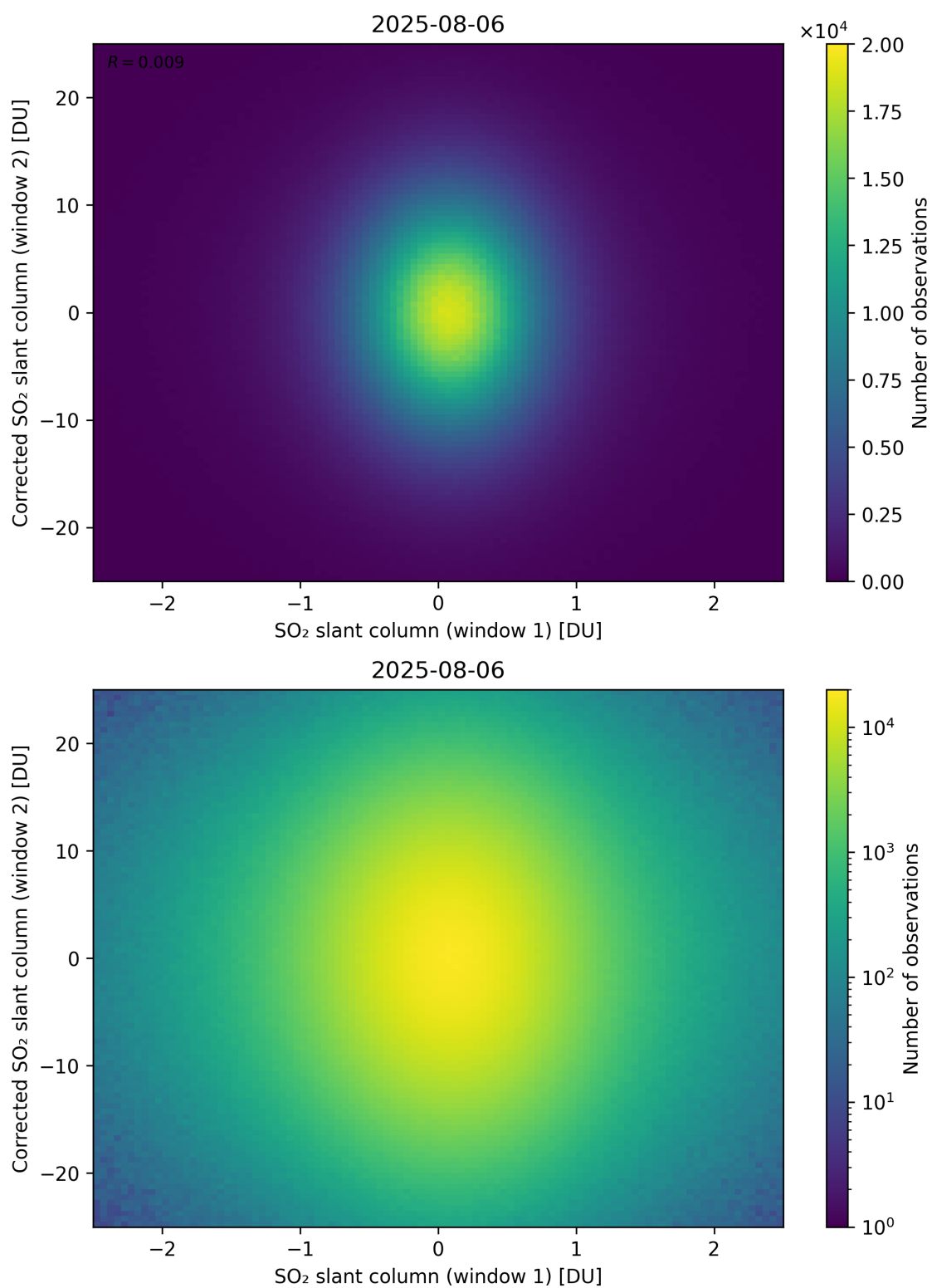
Figure 283: Scatter density plot of “SO 2 slant column (window 1)” against “Corrected SO 2 slant column (window 2)” for 2025-08-05 to 2025-08-07.
