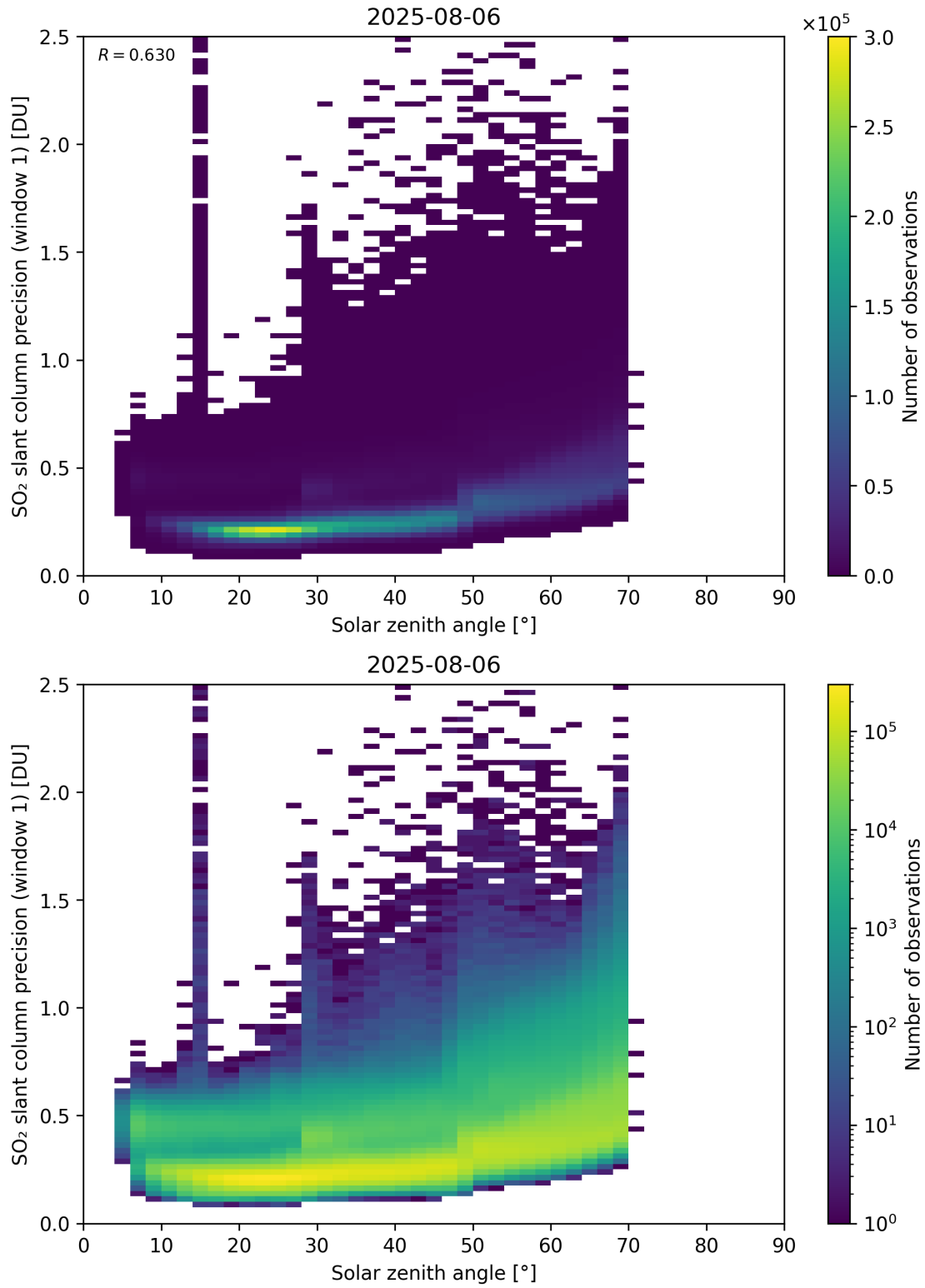
Figure 185: Scatter density plot of “Solar zenith angle” against “SO 2 slant column precision (window 1)” for 2025-08-05 to 2025-08-07.
