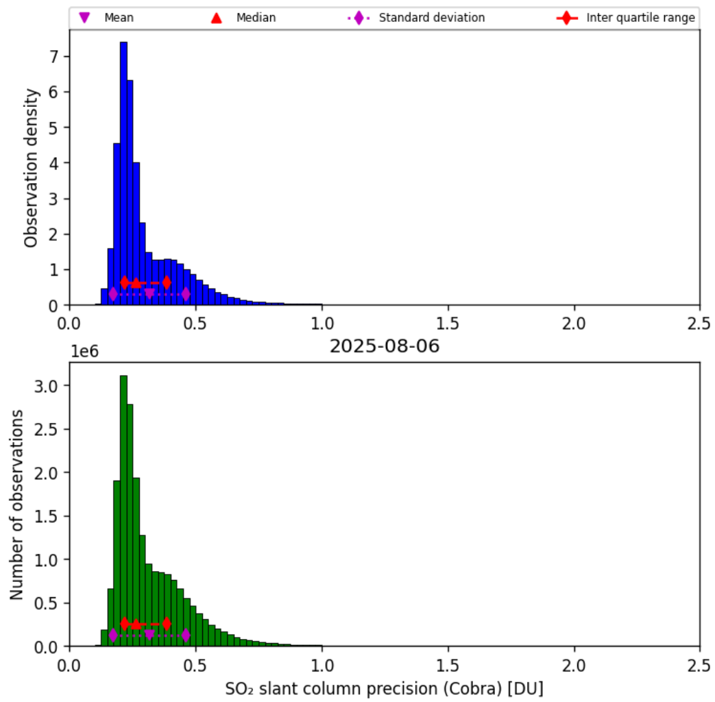
Figure 62: Histogram of “SO 2 slant column precision (Cobra)” for 2025-08-05 to 2025-08-07
