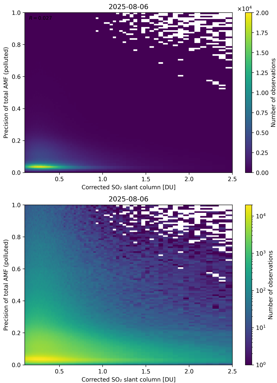
Figure 243: Scatter density plot of “Corrected SO 2 slant column” against “Precision of total AMF (polluted)” for 2025-08-05 to 2025-08-07.
