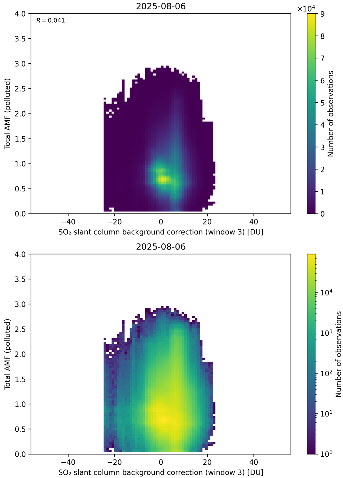
Figure 136: Scatter density plot of “SO 2 slant column background correction (window 3)” against “Total AMF (polluted)” for 2025-08-05 to 2025-08-07.
