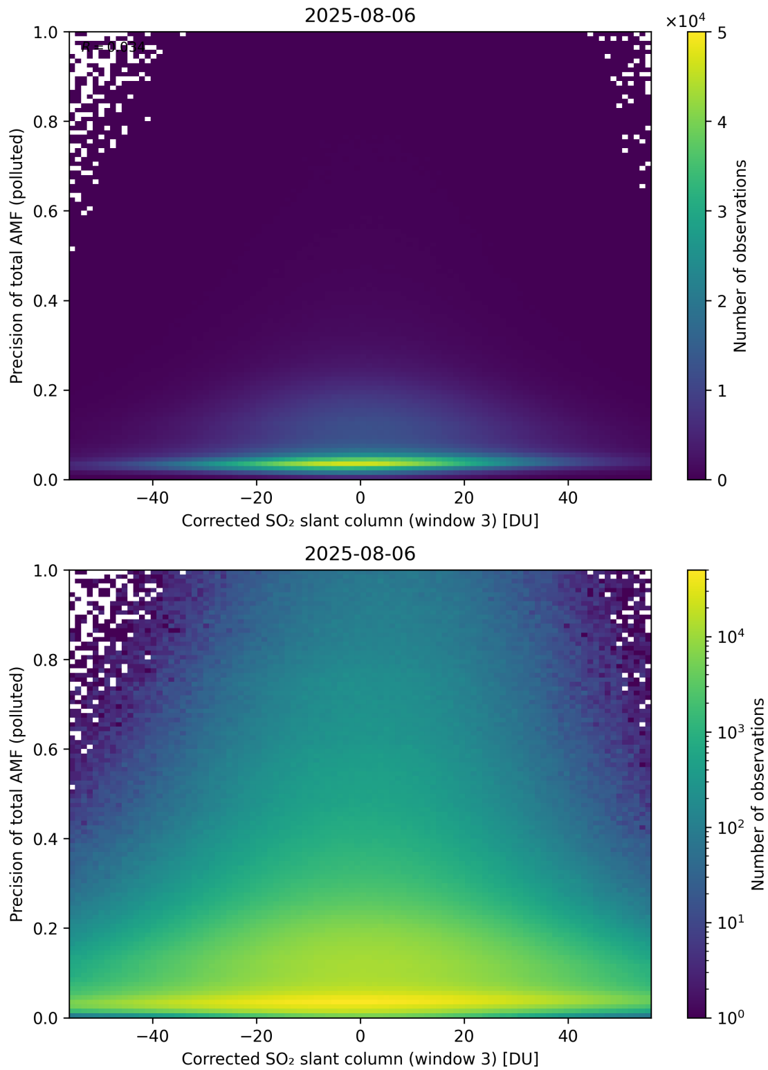
Figure 261: Scatter density plot of “Corrected SO 2 slant column (window 3)” against “Precision of total AMF (polluted)” for 2025-08-05 to 2025-08-07.
