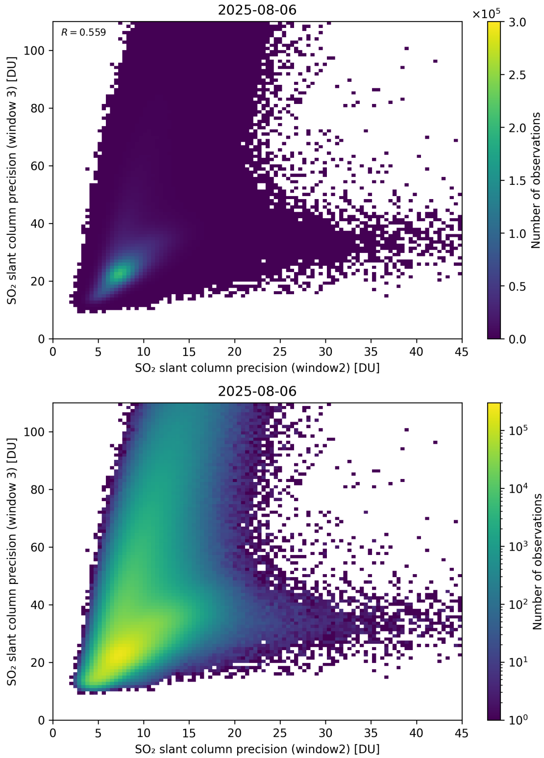
Figure 300: Scatter density plot of “SO 2 slant column precision (window2)” against “SO 2 slant column precision (window 3)” for 2025-08-05 to 2025-08-07.
