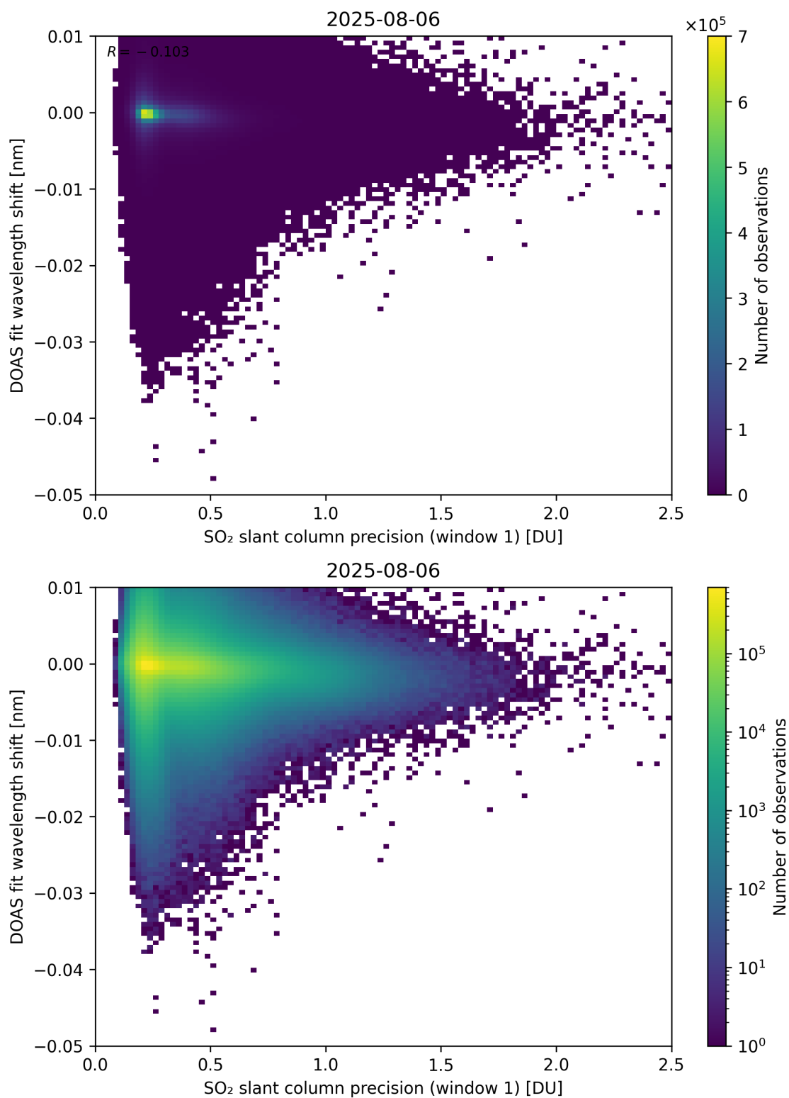
Figure 271: Scatter density plot of “SO 2 slant column precision (window 1)” against “DOAS fit wavelength shift” for 2025-08-05 to 2025-08-07.
