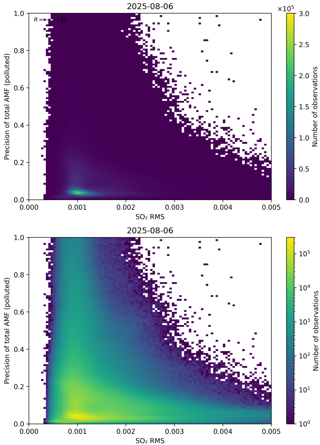
Figure 149: Scatter density plot of “SO 2 RMS” against “Precision of total AMF (polluted)” for 2025-08-05 to 2025-08-07.
