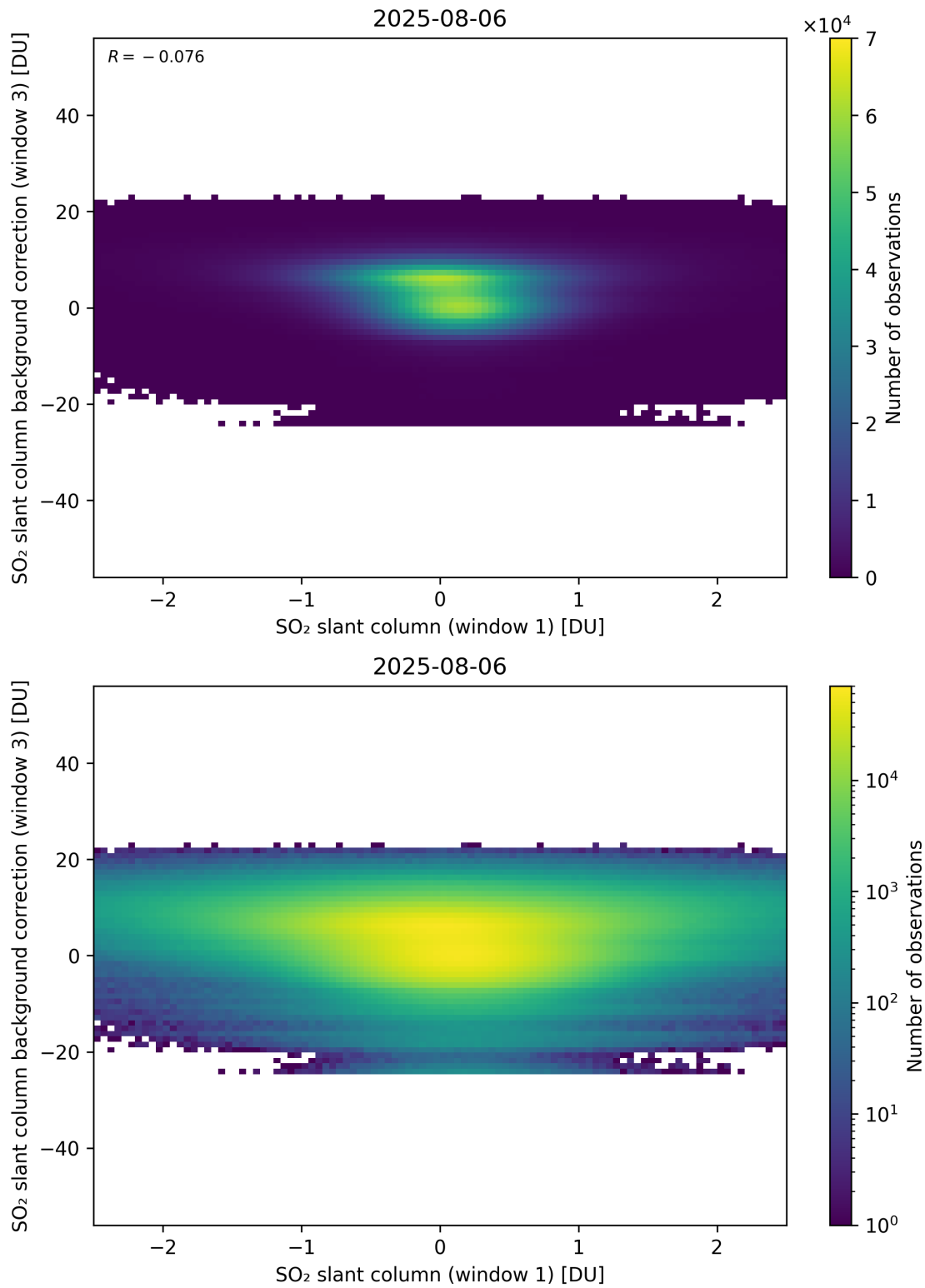
Figure 264: Scatter density plot of “SO 2 slant column (window 1)” against “SO 2 slant column background correction (window 3)” for 2025-08-05 to 2025-08-07.
