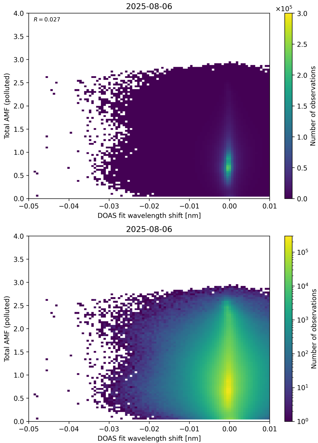
Figure 141: Scatter density plot of “DOAS fit wavelength shift” against “Total AMF (polluted)” for 2025-08-05 to 2025-08-07.
