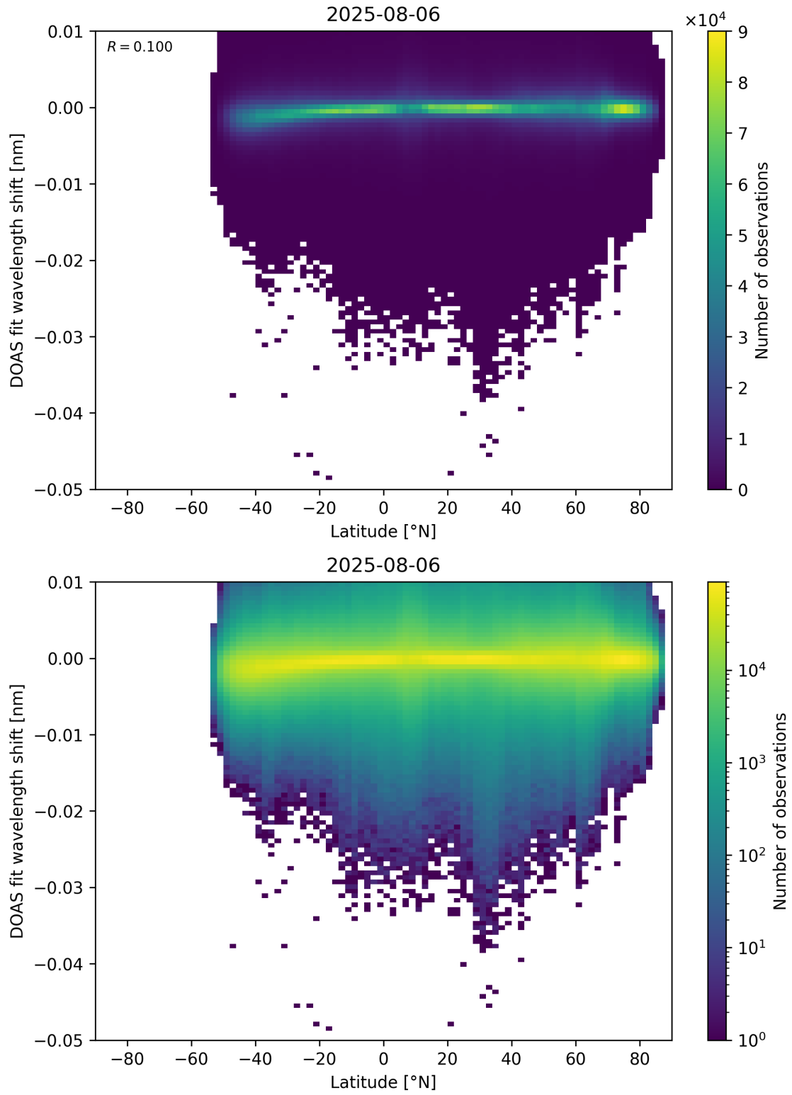
Figure 153: Scatter density plot of “Latitude” against “DOAS fit wavelength shift” for 2025-08-05 to 2025-08-07.
