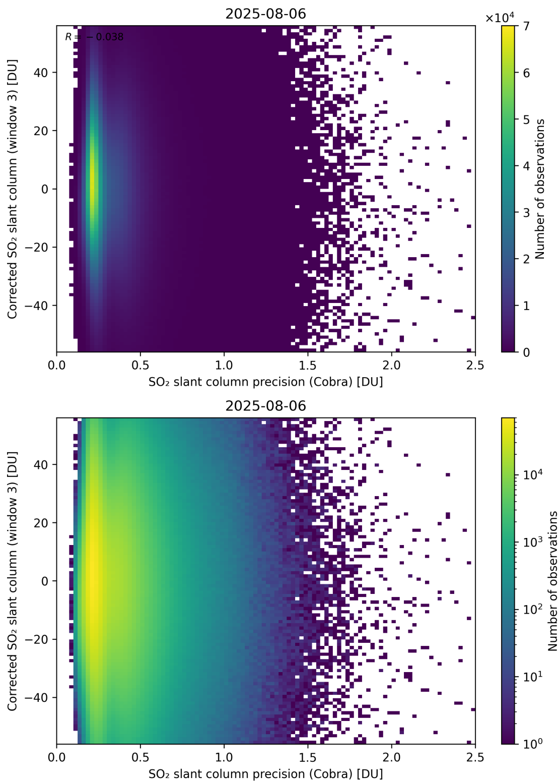
Figure 207: Scatter density plot of “SO 2 slant column precision (Cobra)” against “Corrected SO 2 slant column (window 3)” for 2025-08-05 to 2025-08-07.
