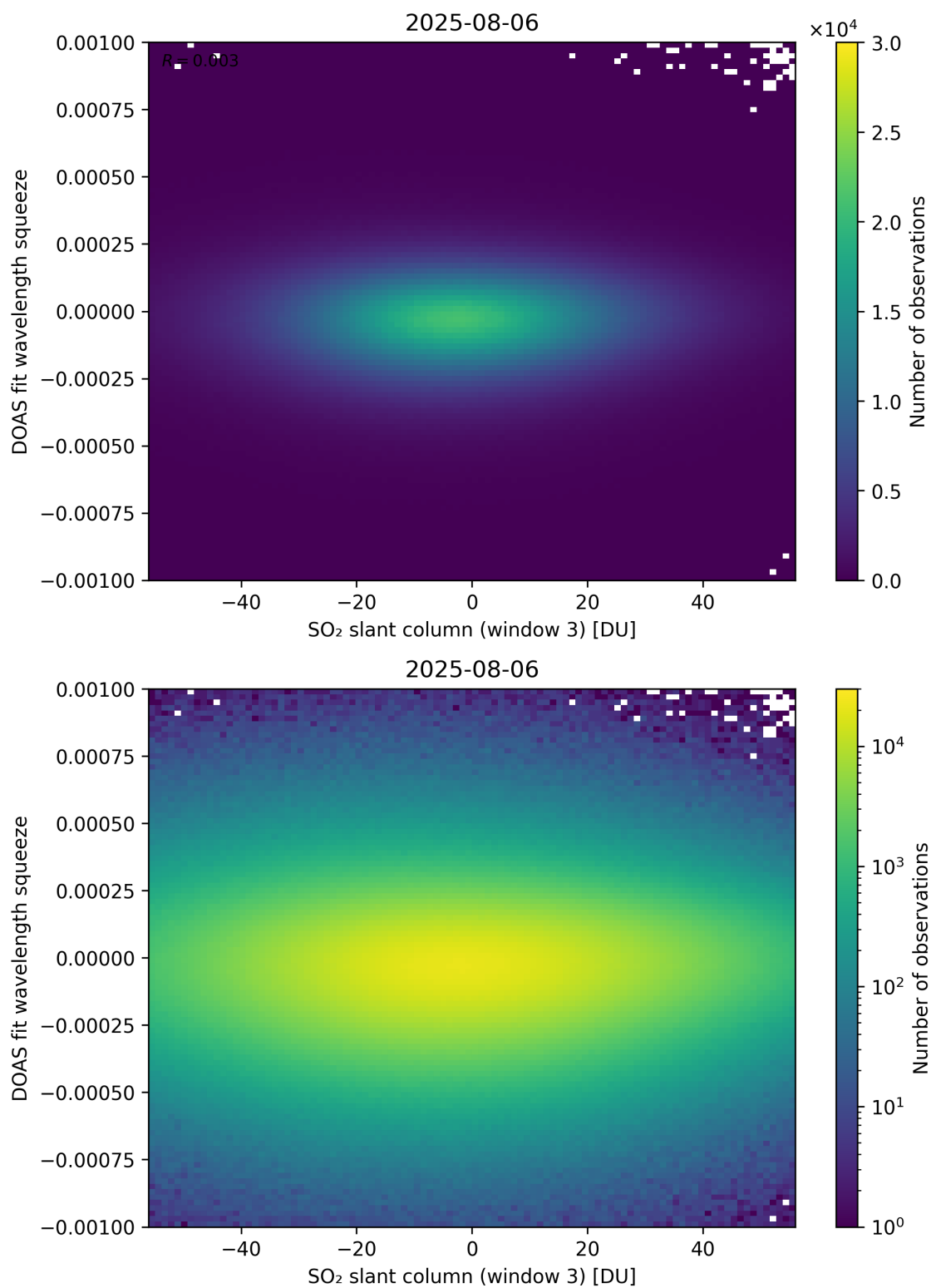
Figure 305: Scatter density plot of “SO 2 slant column (window 3)” against “DOAS fit wavelength squeeze” for 2025-08-05 to 2025-08-07.
