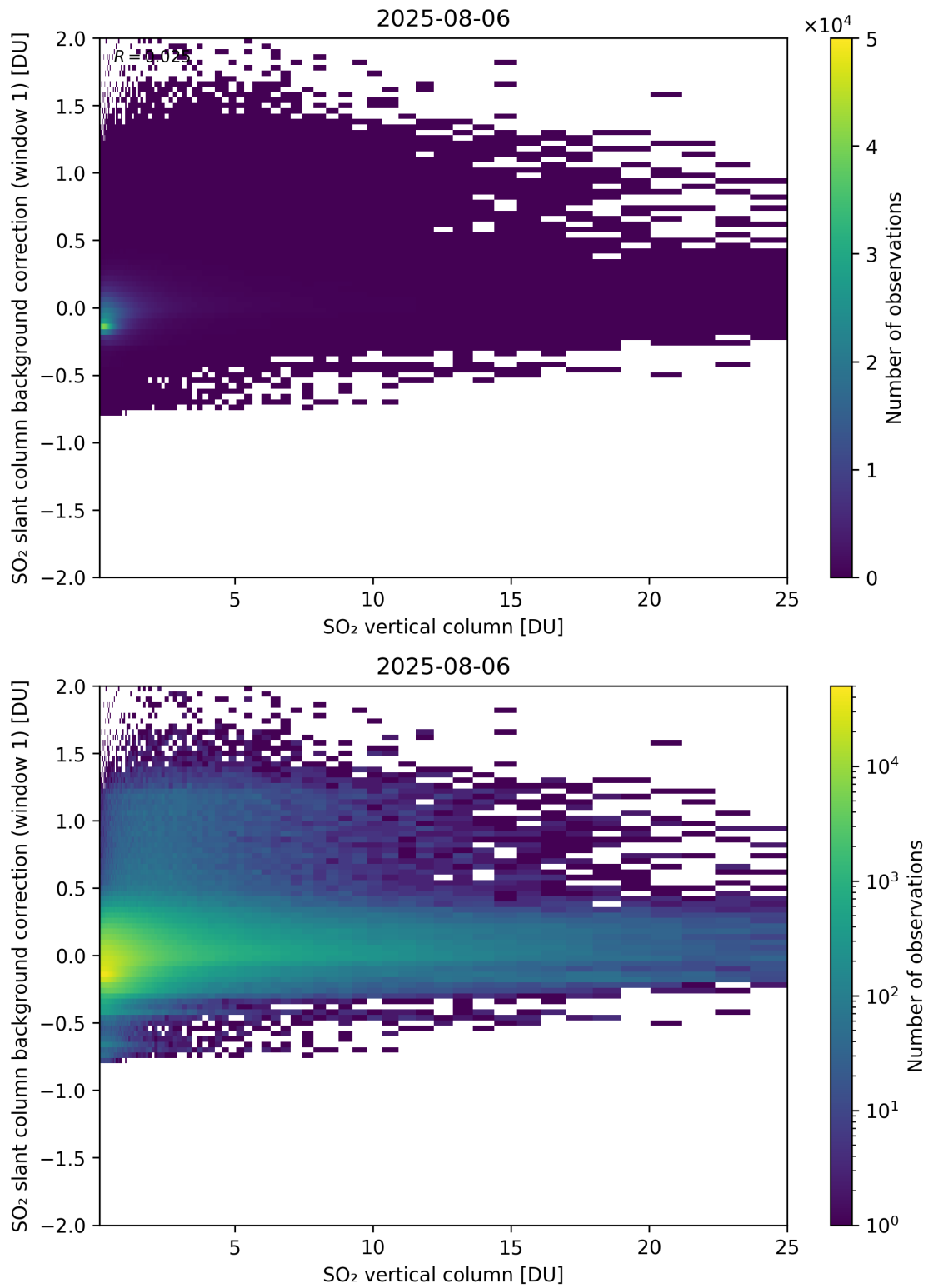
Figure 323: Scatter density plot of “SO 2 vertical column” against “SO 2 slant column background correction (window 1)” for 2025-08-05 to 2025-08-07.
