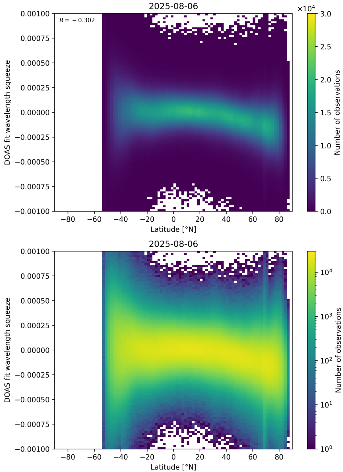
Figure 154: Scatter density plot of “Latitude” against “DOAS fit wavelength squeeze” for 2025-08-05 to 2025-08-07.
