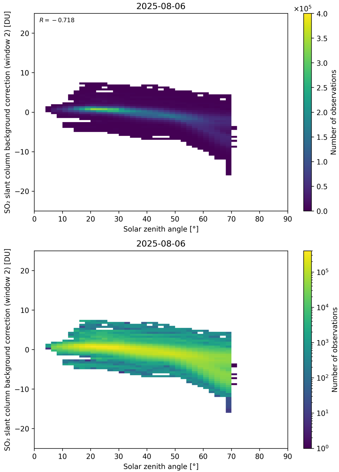
Figure 172: Scatter density plot of “Solar zenith angle” against “SO 2 slant column background correction (window 2)” for 2025-08-05 to 2025-08-07.
