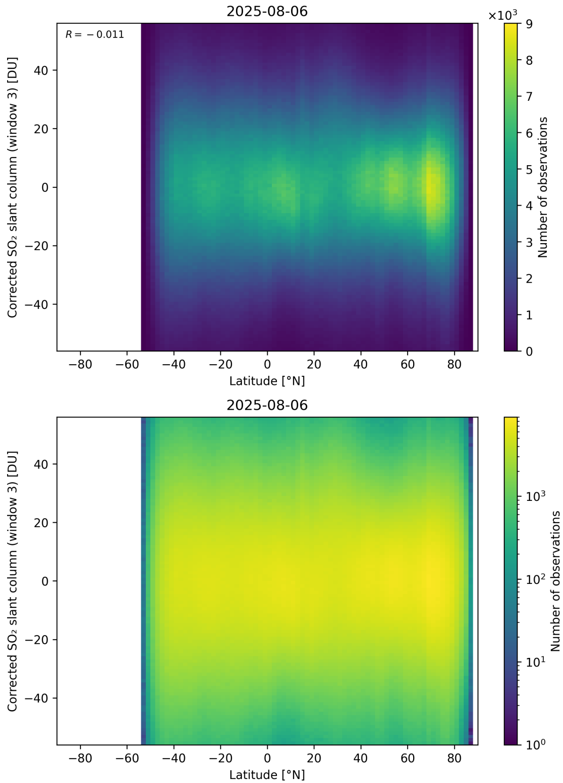
Figure 161: Scatter density plot of “Latitude” against “Corrected SO 2 slant column (window 3)” for 2025-08-05 to 2025-08-07.
