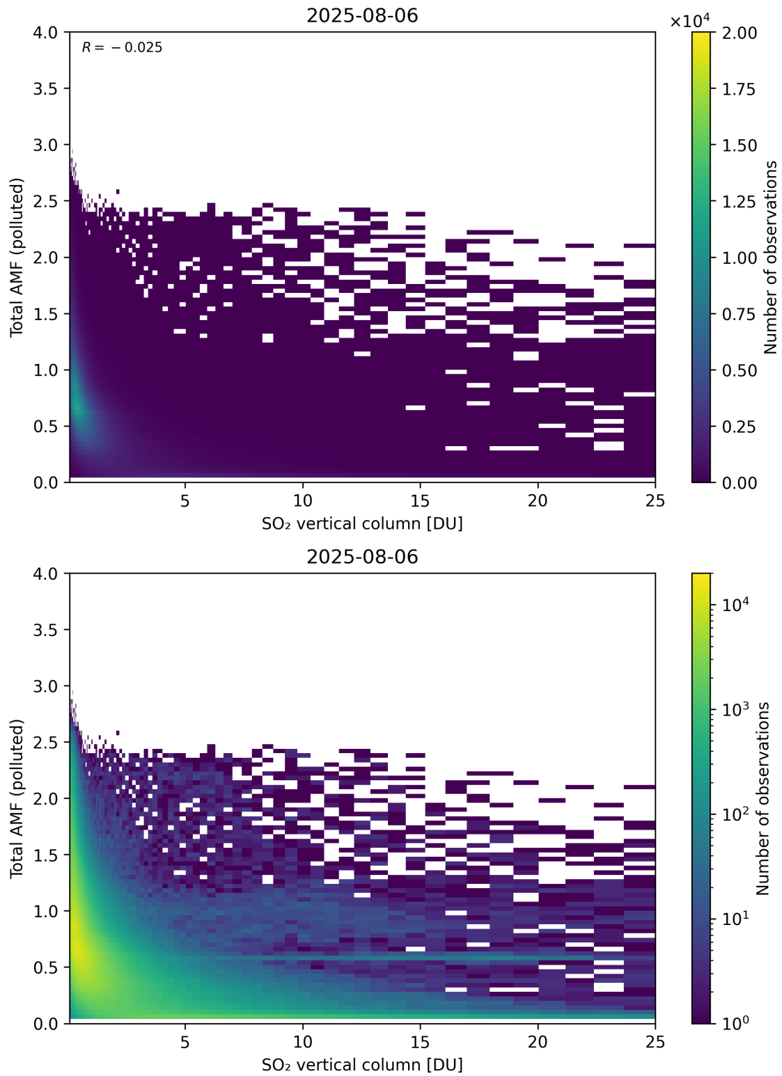
Figure 359: Scatter density plot of “SO 2 vertical column” against “Total AMF (polluted)” for 2025-08-05 to 2025-08-07.
