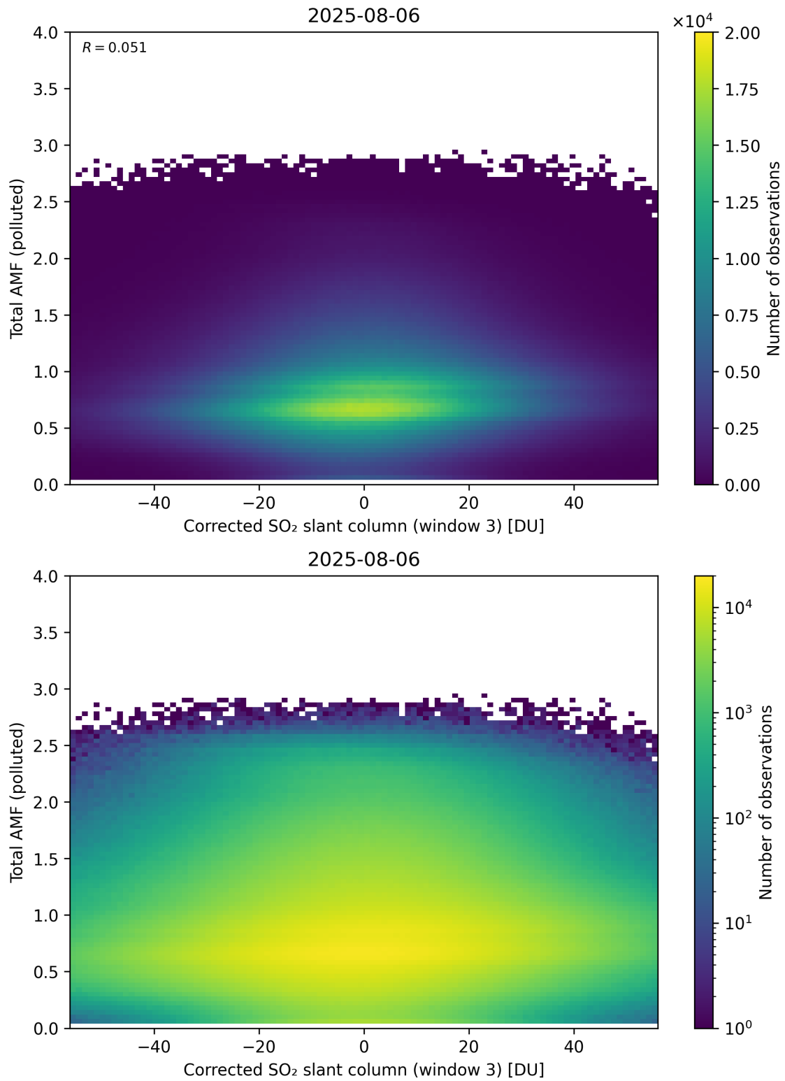
Figure 260: Scatter density plot of “Corrected SO 2 slant column (window 3)” against “Total AMF (polluted)” for 2025-08-05 to 2025-08-07.
