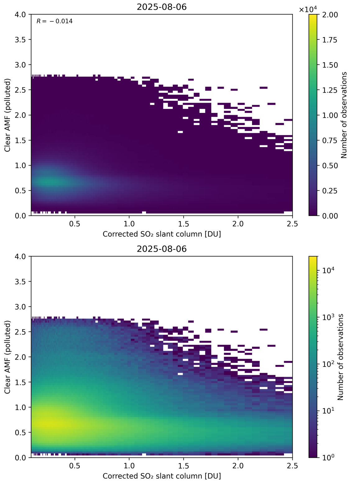
Figure 232: Scatter density plot of “Corrected SO 2 slant column” against “Clear AMF (polluted)” for 2025-08-05 to 2025-08-07.
