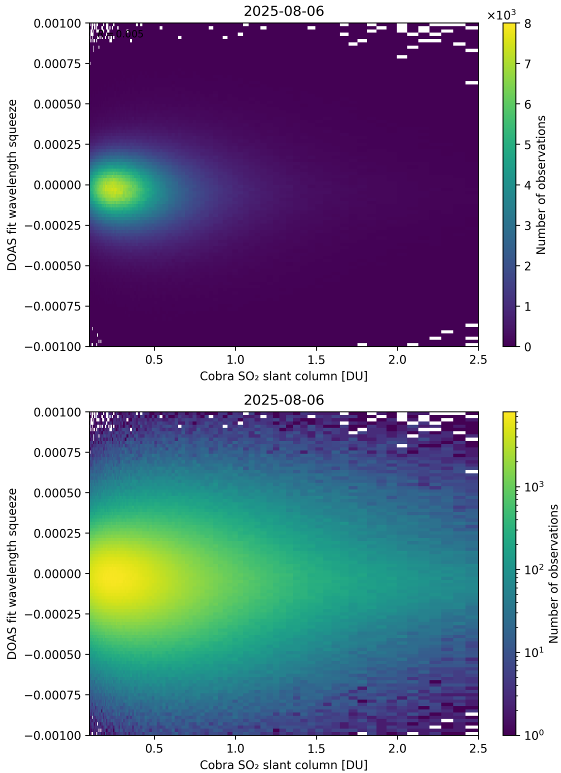
Figure 197: Scatter density plot of “Cobra SO 2 slant column” against “DOAS fit wavelength squeeze” for 2025-08-05 to 2025-08-07.
