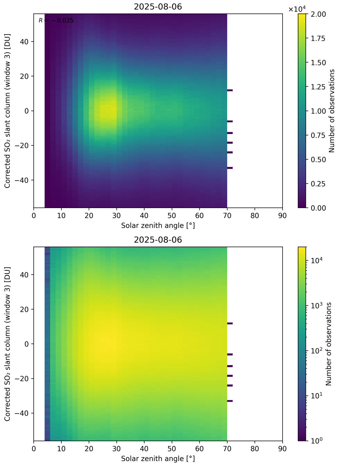
Figure 183: Scatter density plot of “Solar zenith angle” against “Corrected SO 2 slant column (window 3)” for 2025-08-05 to 2025-08-07.
