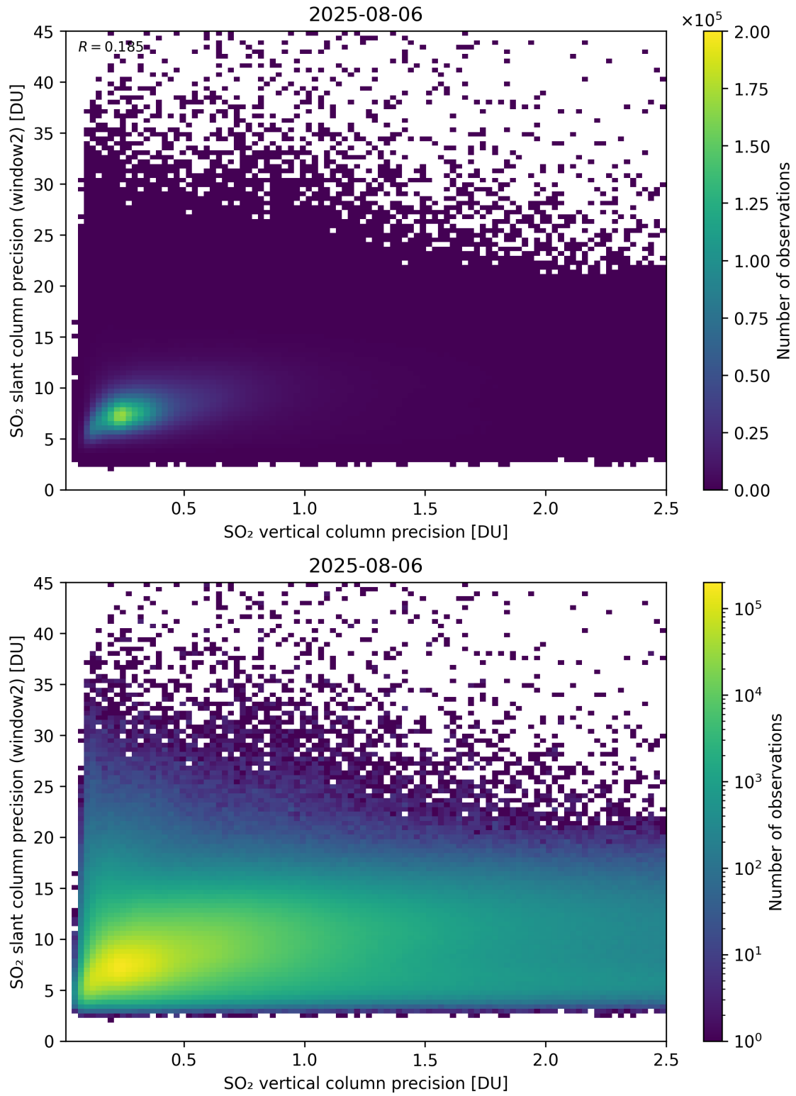
Figure 343: Scatter density plot of “SO 2 vertical column precision” against “SO 2 slant column precision (window2)” for 2025-08-05 to 2025-08-07.
