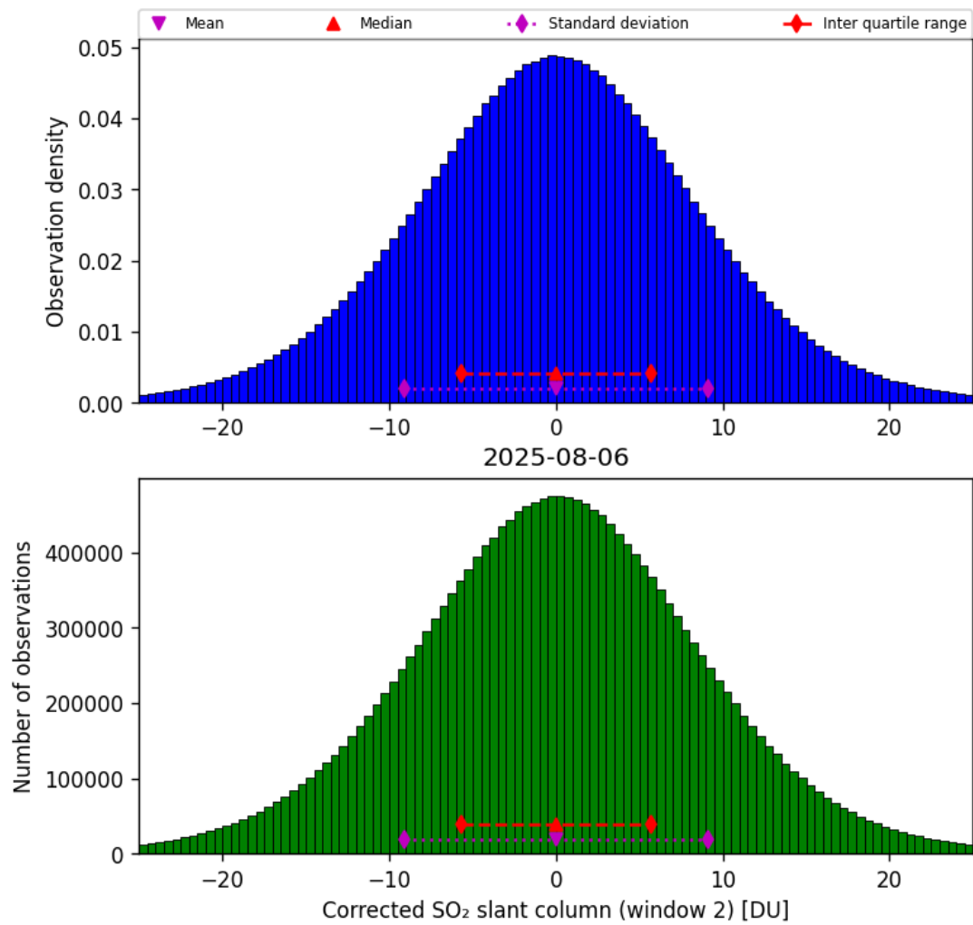
Figure 69: Histogram of “Corrected SO 2 slant column (window 2)” for 2025-08-05 to 2025-08-07
