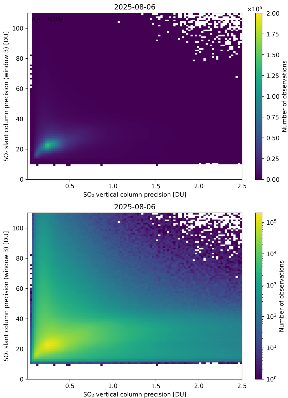
Figure 345: Scatter density plot of “SO 2 vertical column precision” against “SO 2 slant column precision (window 3)” for 2025-08-05 to 2025-08-07.
