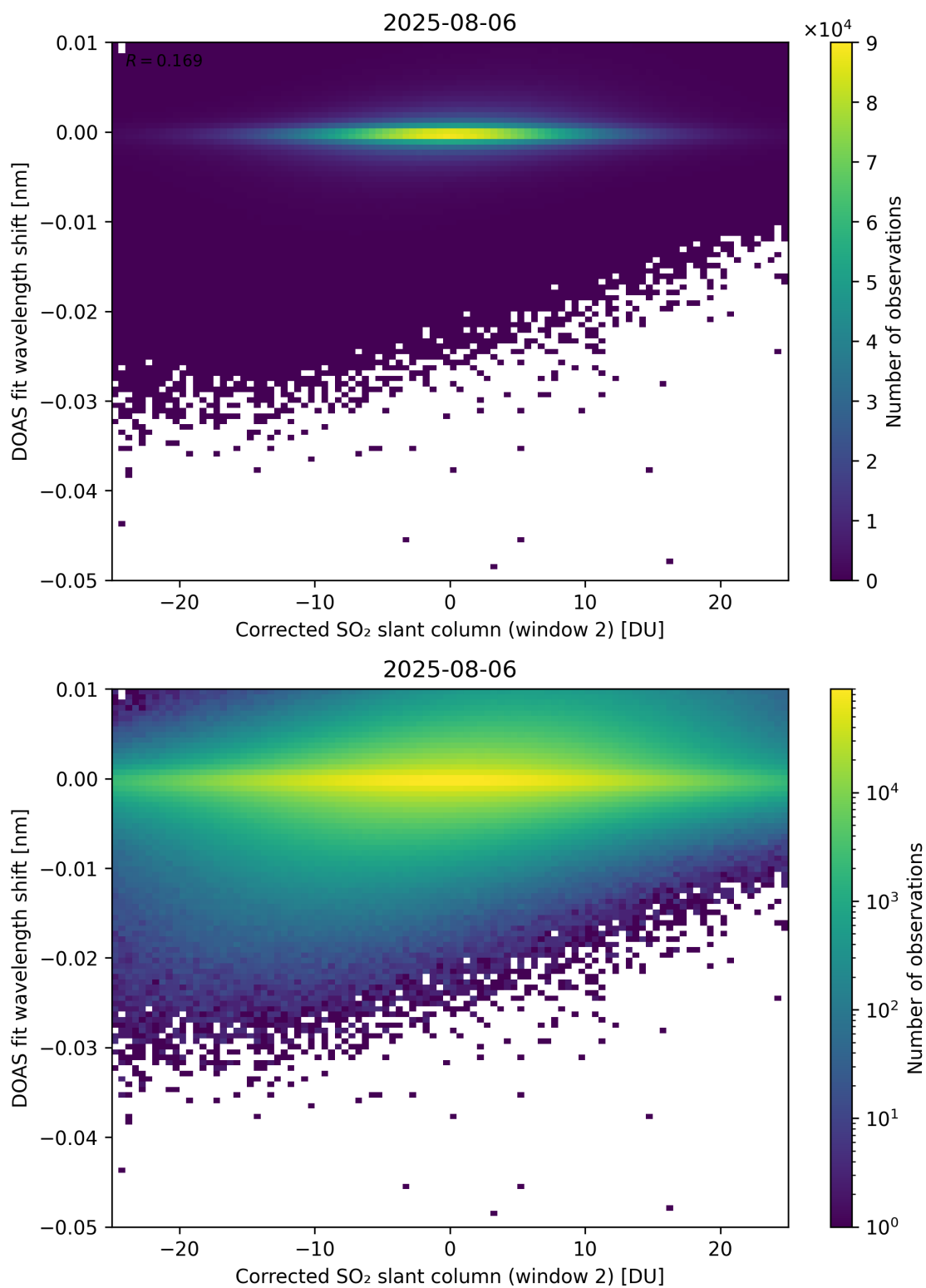
Figure 246: Scatter density plot of “Corrected SO 2 slant column (window 2)” against “DOAS fit wavelength shift” for 2025-08-05 to 2025-08-07.
