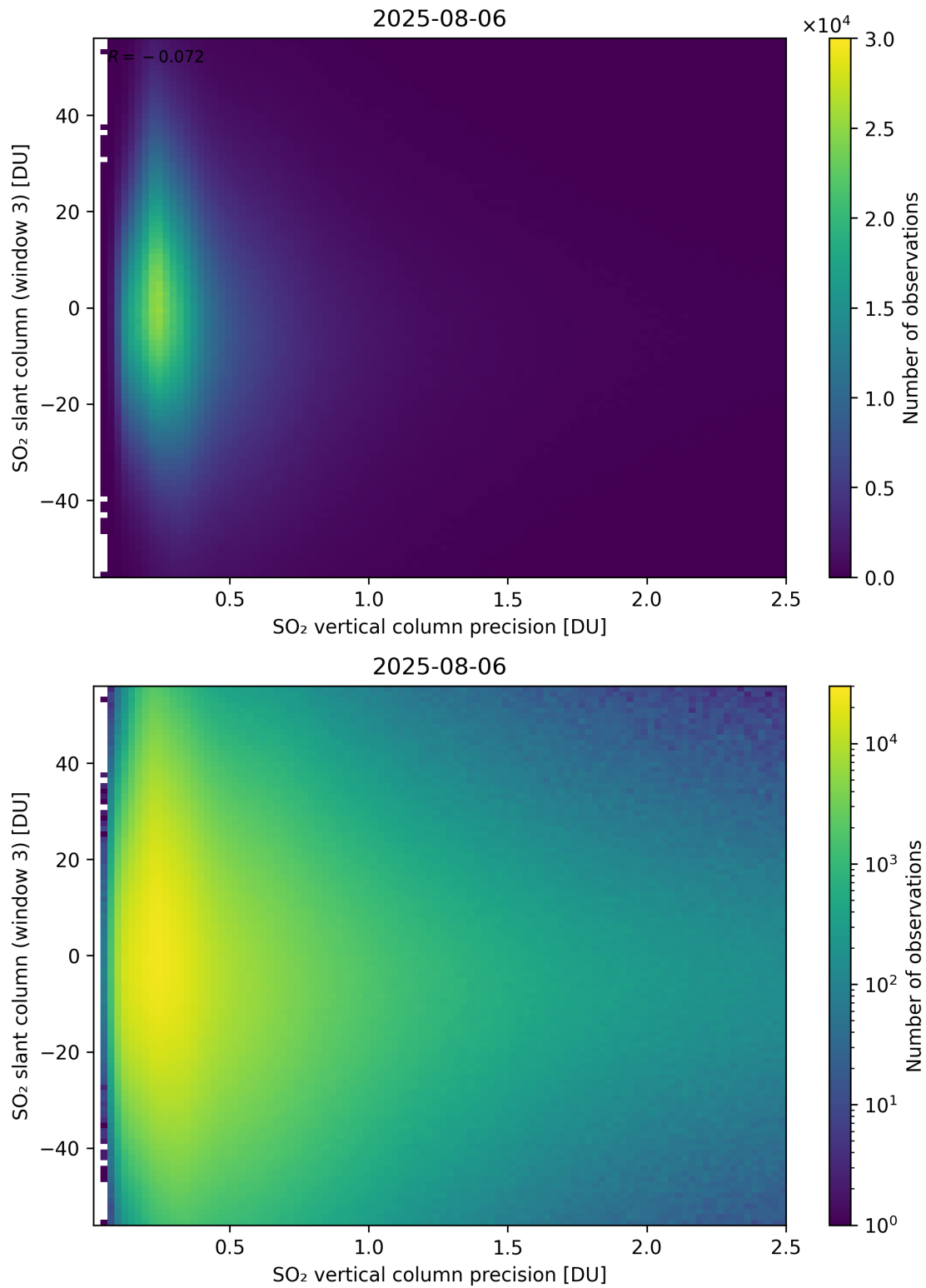
Figure 344: Scatter density plot of “SO 2 vertical column precision” against “SO 2 slant column (window 3)” for 2025-08-05 to 2025-08-07.
