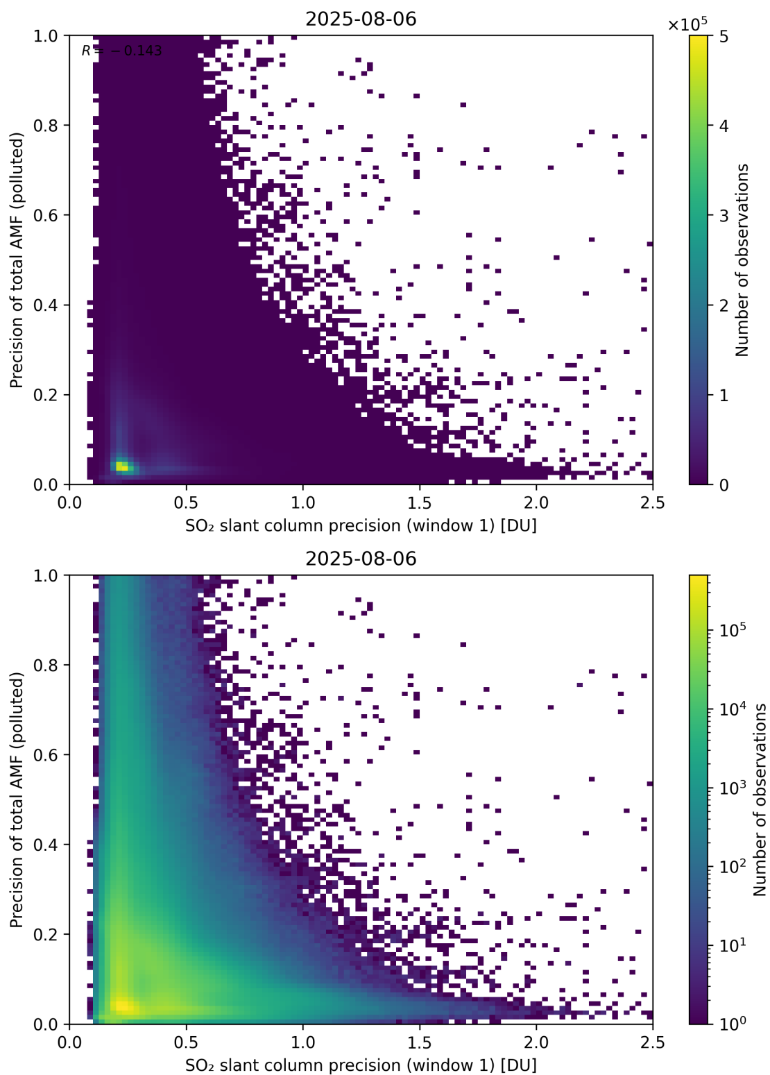
Figure 281: Scatter density plot of “SO 2 slant column precision (window 1)” against “Precision of total AMF (polluted)” for 2025-08-05 to 2025-08-07.
