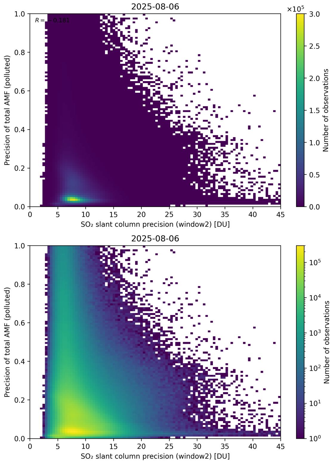
Figure 302: Scatter density plot of “SO 2 slant column precision (window2)” against “Precision of total AMF (polluted)” for 2025-08-05 to 2025-08-07.
