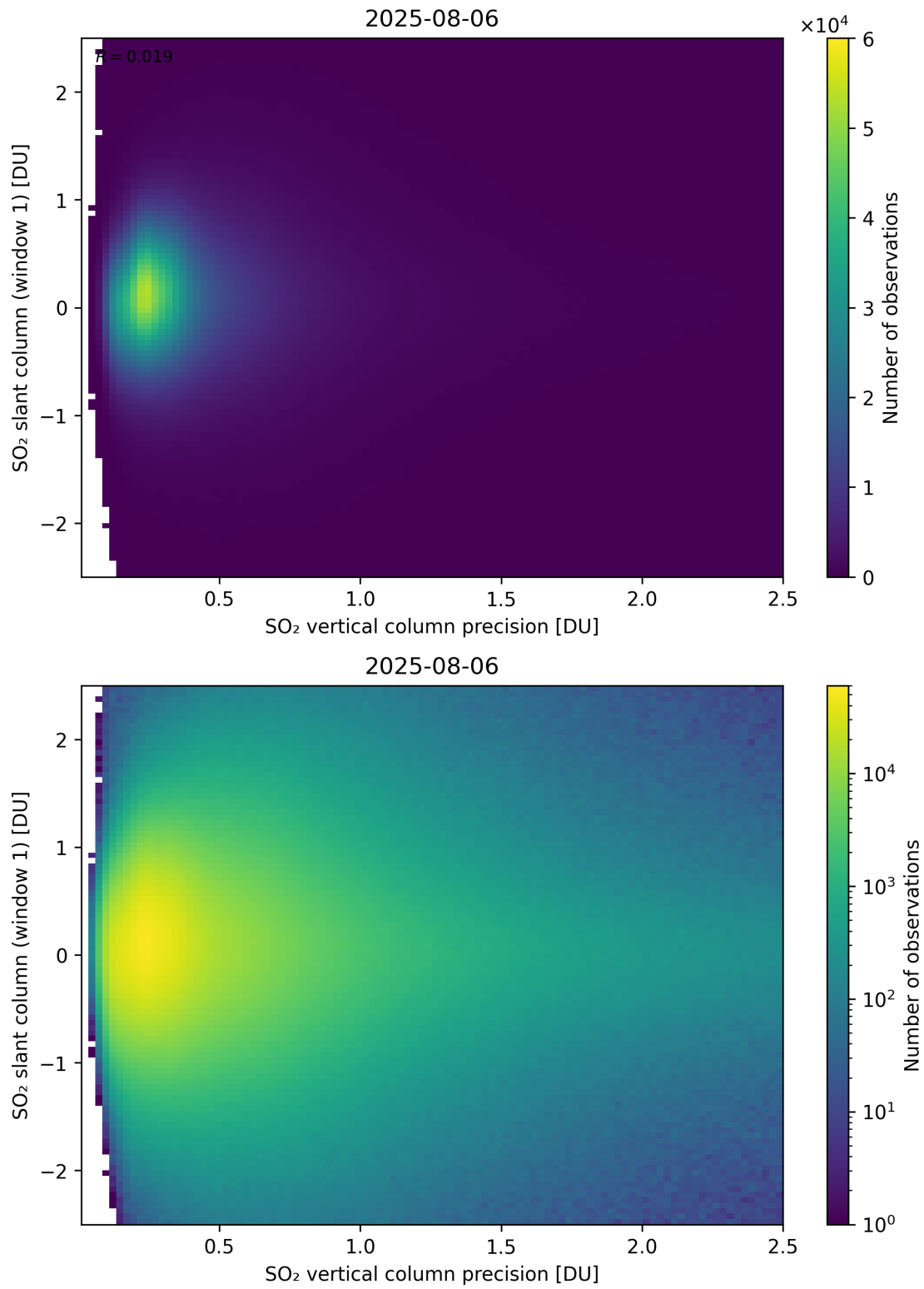
Figure 341: Scatter density plot of “SO 2 vertical column precision” against “SO 2 slant column (window 1)” for 2025-08-05 to 2025-08-07.
