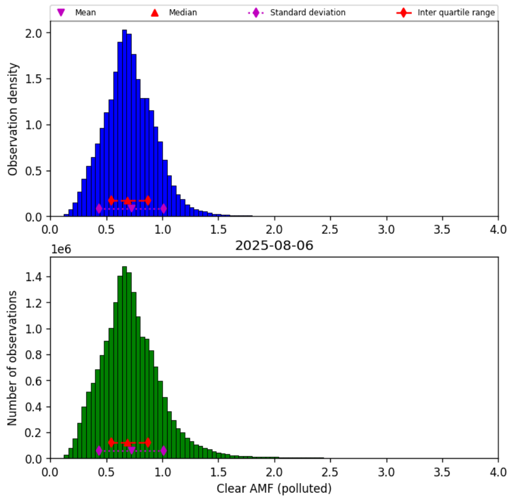
Figure 81: Histogram of “Clear AMF (polluted)” for 2025-08-05 to 2025-08-07
