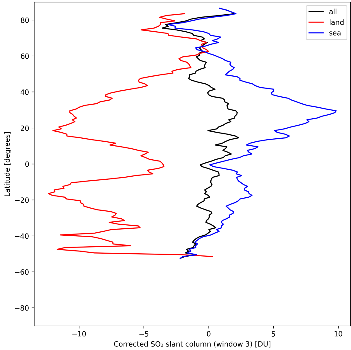
Figure 47: Zonal average of “Corrected SO 2 slant column (window 3)” for 2025-08-05 to 2025-08-07.
