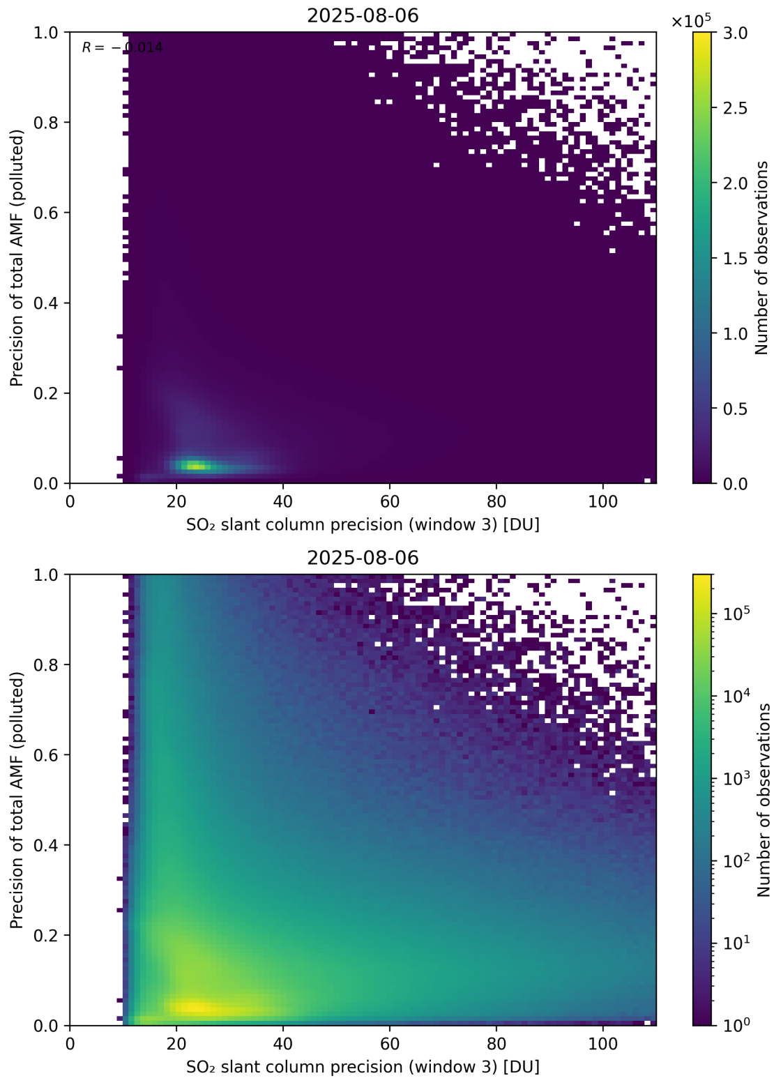
Figure 314: Scatter density plot of “SO 2 slant column precision (window 3)” against “Precision of total AMF (polluted)” for 2025-08-05 to 2025-08-07.
