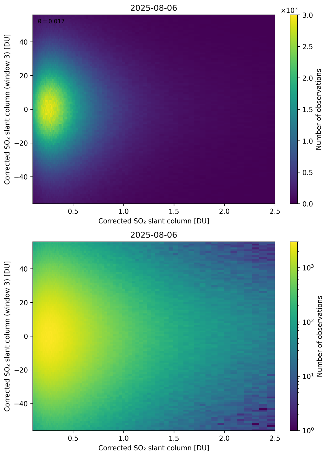
Figure 236: Scatter density plot of “Corrected SO 2 slant column” against “Corrected SO 2 slant column (window 3)” for 2025-08-05 to 2025-08-07.
