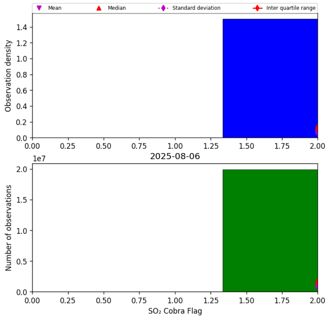
Figure 75: Histogram of “SO 2 Cobra Flag” for 2025-08-05 to 2025-08-07
