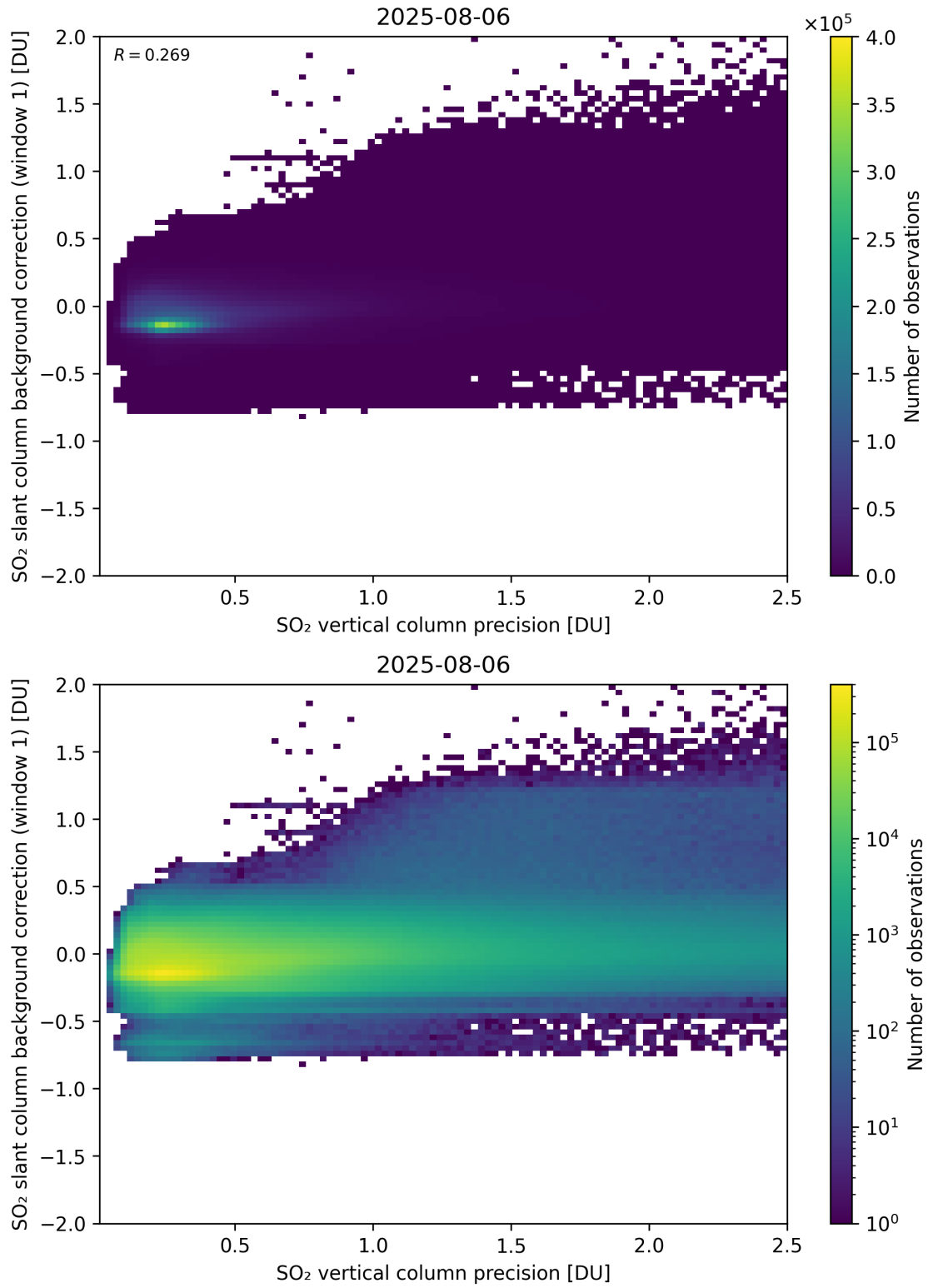
Figure 329: Scatter density plot of “SO 2 vertical column precision” against “SO 2 slant column background correction (window 1)” for 2025-08-05 to 2025-08-07.
