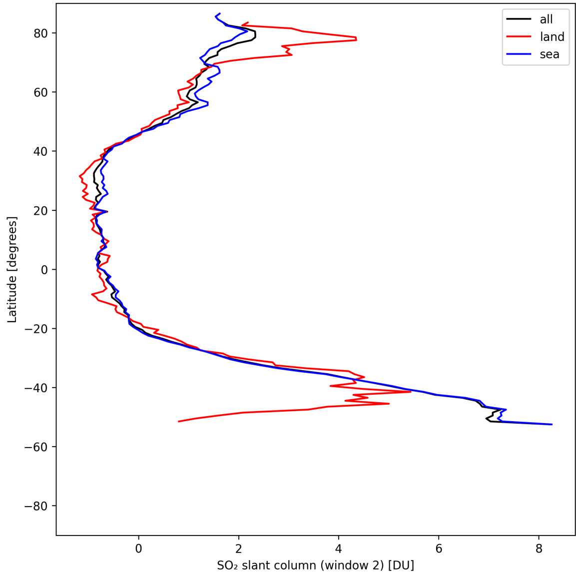
Figure 41: Zonal average of “SO 2 slant column (window 2)” for 2025-08-05 to 2025-08-07.
