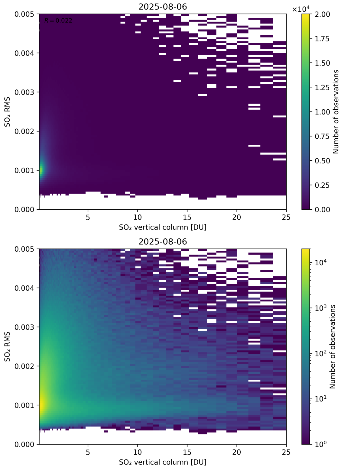
Figure 328: Scatter density plot of “SO 2 vertical column” against “SO 2 RMS” for 2025-08-05 to 2025-08-07.
