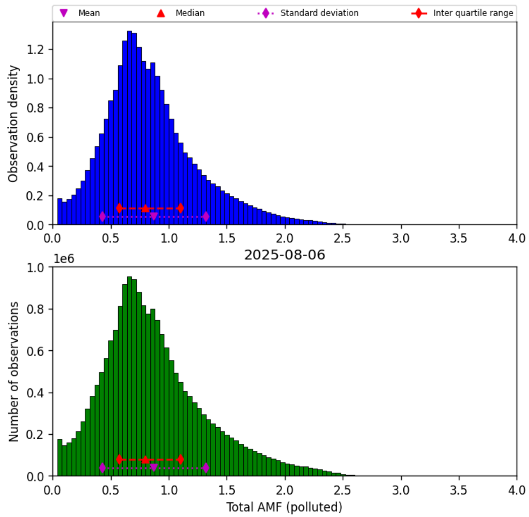
Figure 79: Histogram of “Total AMF (polluted)” for 2025-08-05 to 2025-08-07
