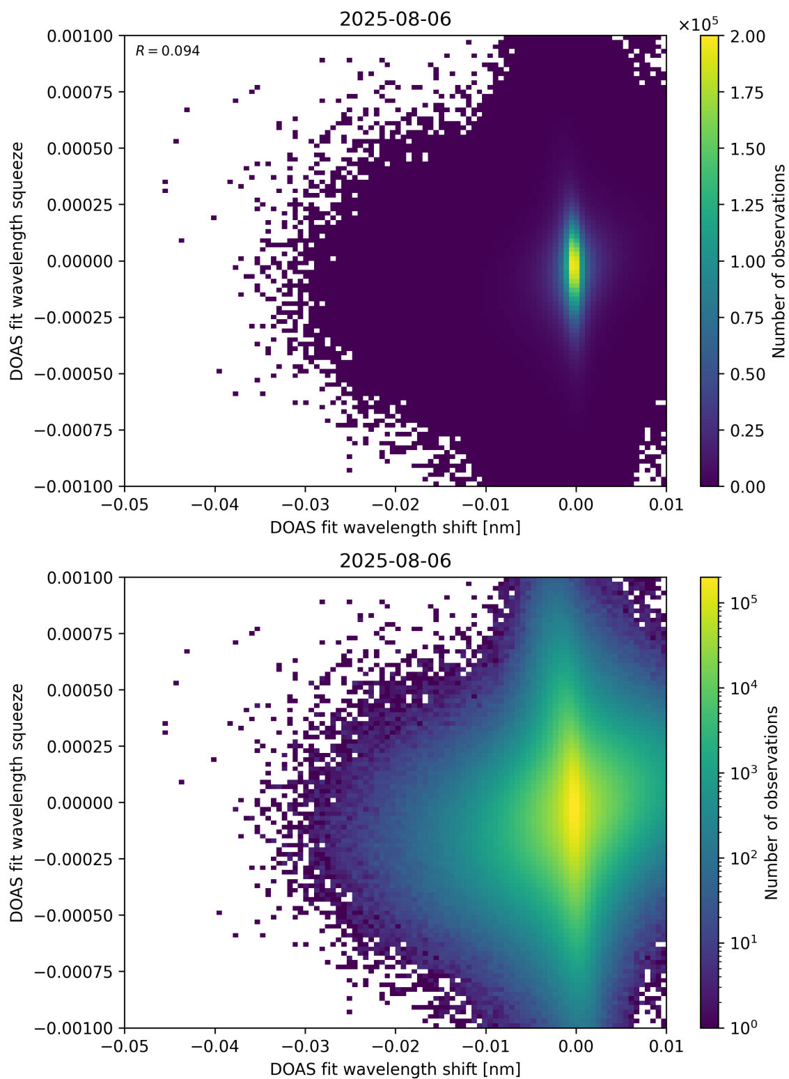
Figure 138: Scatter density plot of “DOAS fit wavelength shift” against “DOAS fit wavelength squeeze” for 2025-08-05 to 2025-08-07.
