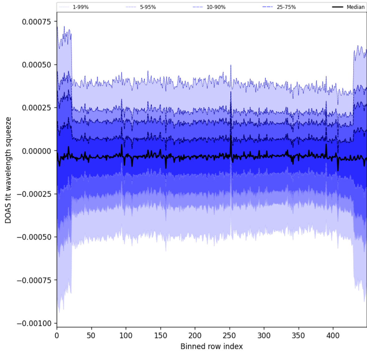
Figure 103: Along track statistics of “DOAS fit wavelength squeeze” for 2025-08-05 to 2025-08-07
