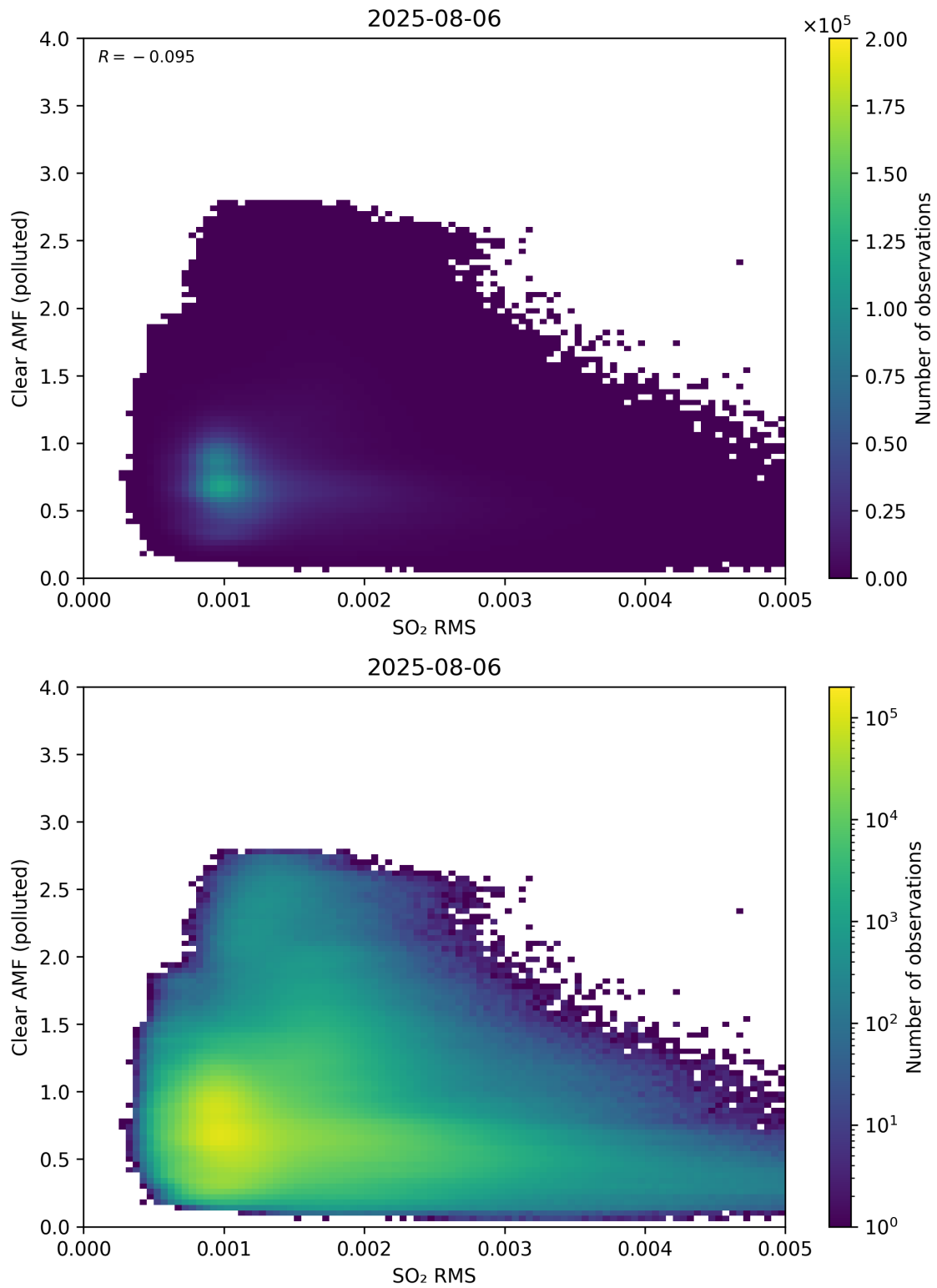
Figure 147: Scatter density plot of “SO 2 RMS” against “Clear AMF (polluted)” for 2025-08-05 to 2025-08-07.
