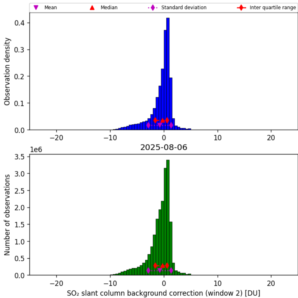
Figure 70: Histogram of “SO 2 slant column background correction (window 2)” for 2025-08-05 to 2025-08-07
