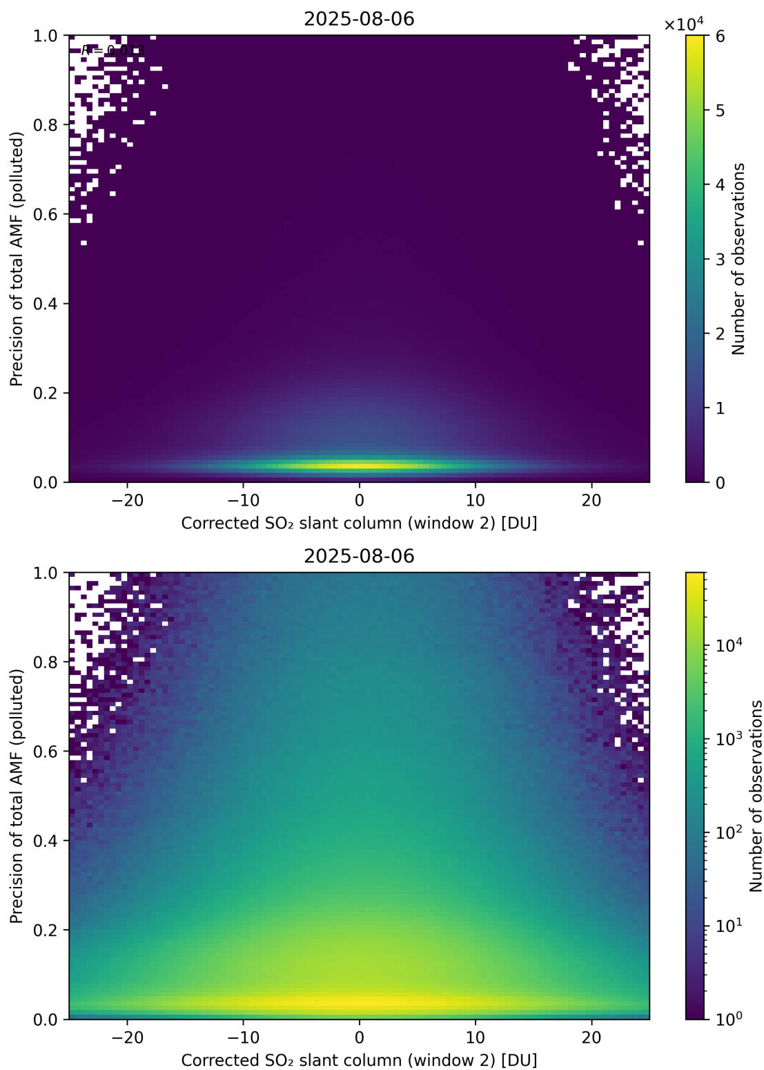
Figure 254: Scatter density plot of “Corrected SO 2 slant column (window 2)” against “Precision of total AMF (polluted)” for 2025-08-05 to 2025-08-07.
