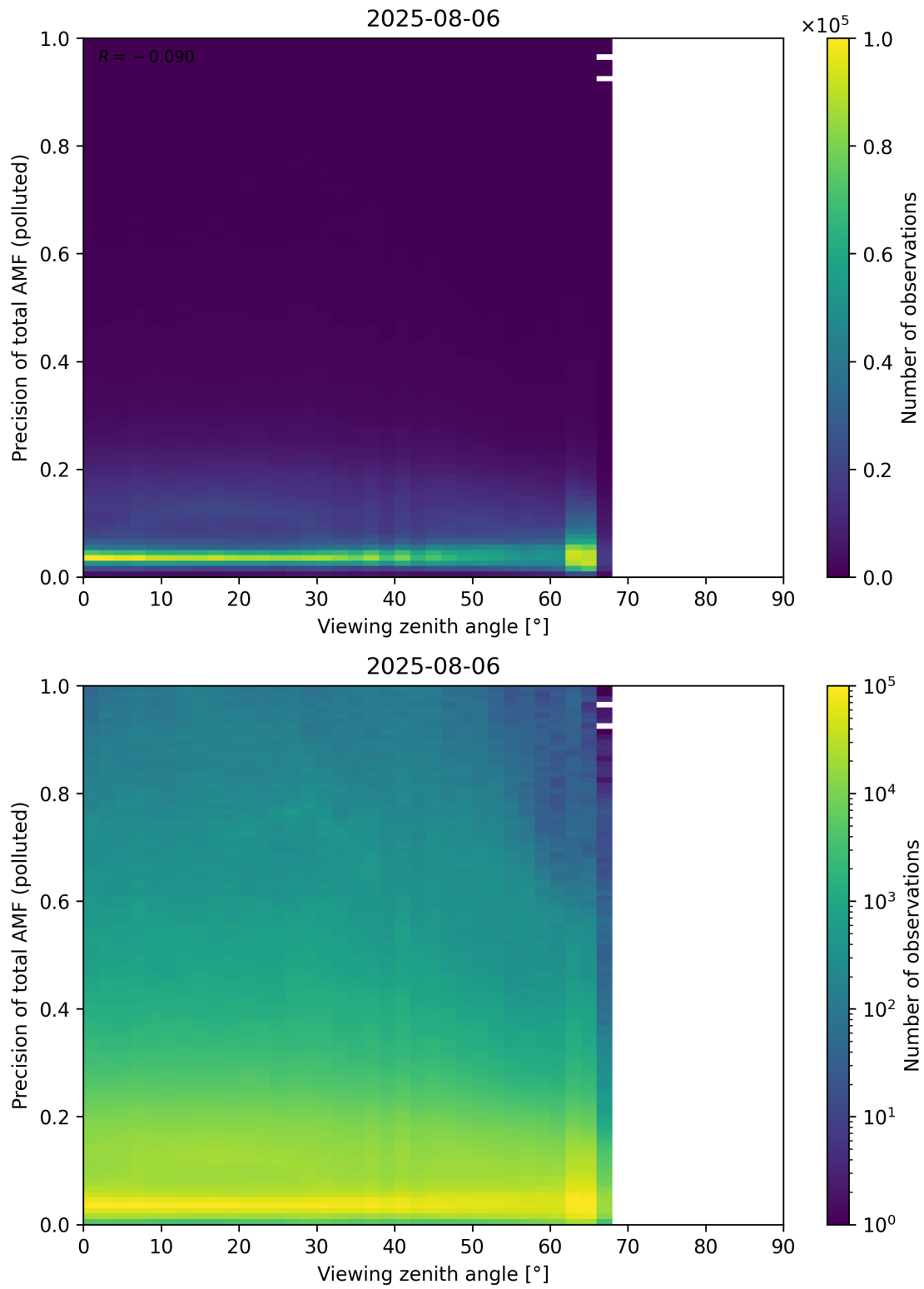
Figure 382: Scatter density plot of “Viewing zenith angle” against “Precision of total AMF (polluted)” for 2025-08-05 to 2025-08-07.
