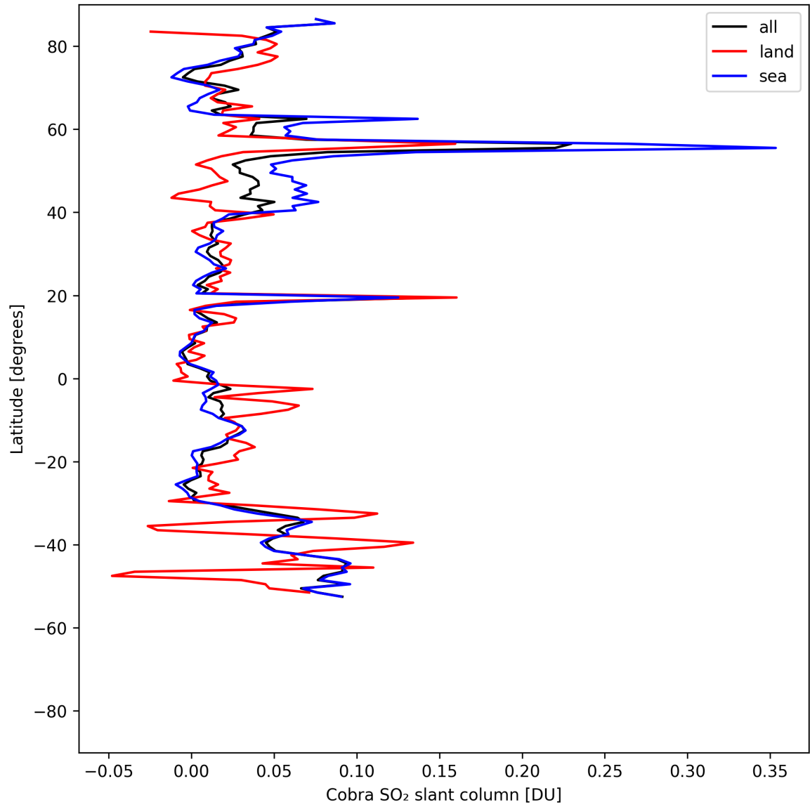
Figure 35: Zonal average of “Cobra SO 2 slant column” for 2025-08-05 to 2025-08-07.
