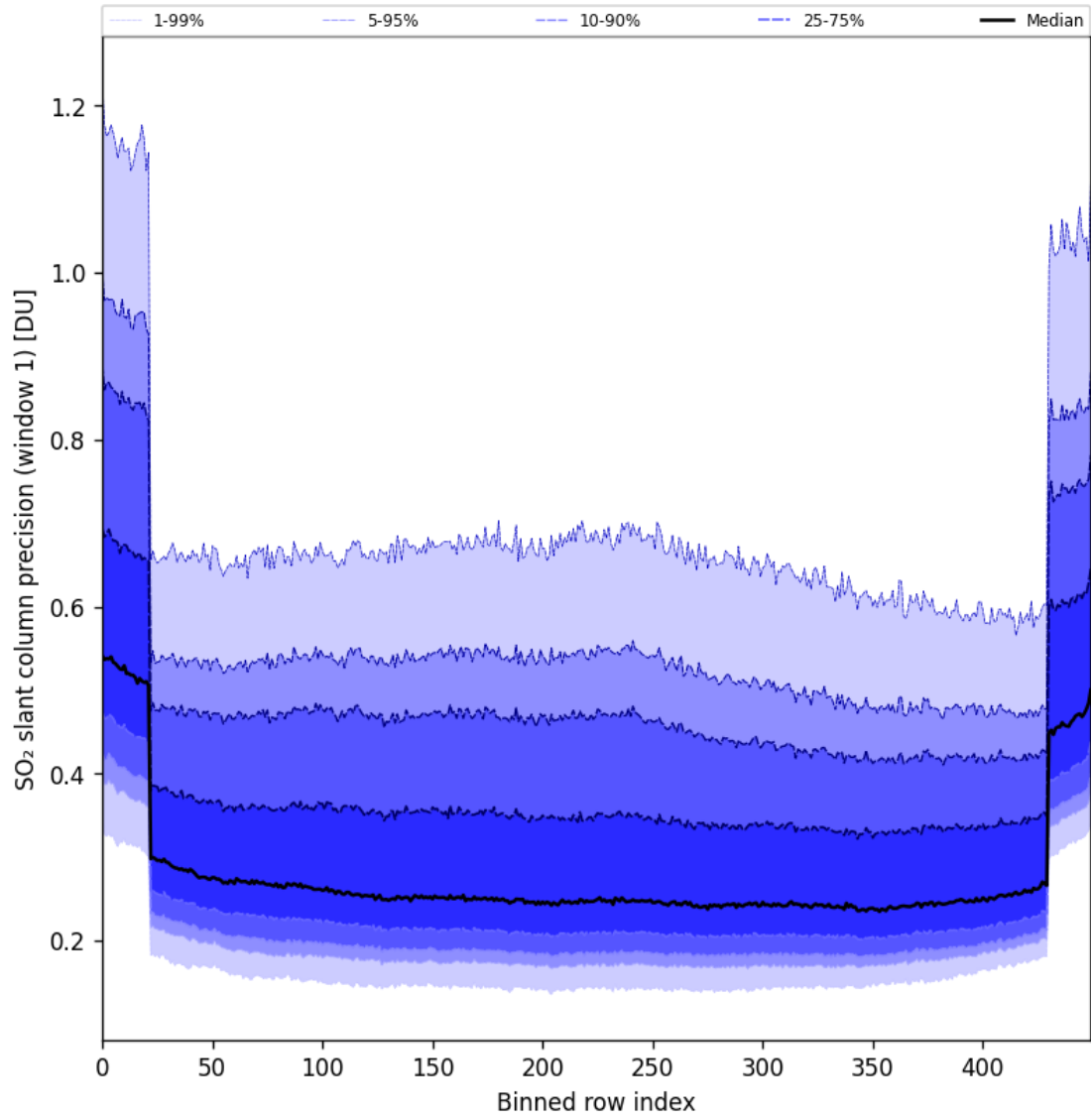
Figure 90: Along track statistics of “SO 2 slant column precision (window 1)” for 2025-08-05 to 2025-08-07
