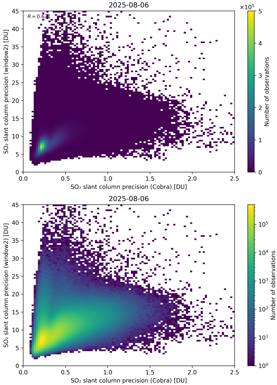
Figure 210: Scatter density plot of “SO 2 slant column precision (Cobra)” against “SO 2 slant column precision (window2)” for 2025-08-05 to 2025-08-07.
