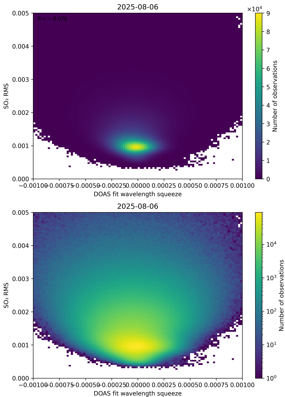
Figure 143: Scatter density plot of “DOAS fit wavelength squeeze” against “SO 2 RMS” for 2025-08-05 to 2025-08-07.
