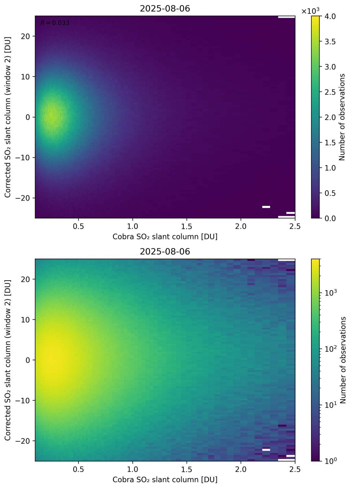
Figure 217: Scatter density plot of “Cobra SO 2 slant column” against “Corrected SO 2 slant column (window 2)” for 2025-08-05 to 2025-08-07.
