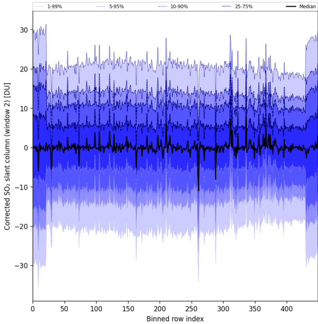
Figure 95: Along track statistics of “Corrected SO 2 slant column (window 2)” for 2025-08-05 to 2025-08-07
