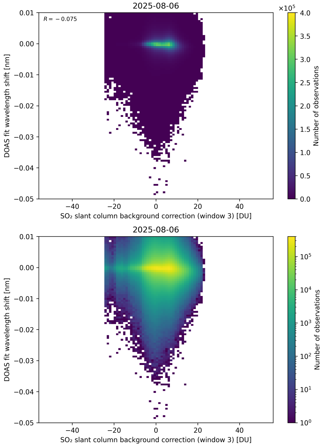
Figure 132: Scatter density plot of “SO 2 slant column background correction (window 3)” against “DOAS fit wavelength shift” for 2025-08-05 to 2025-08-07.
