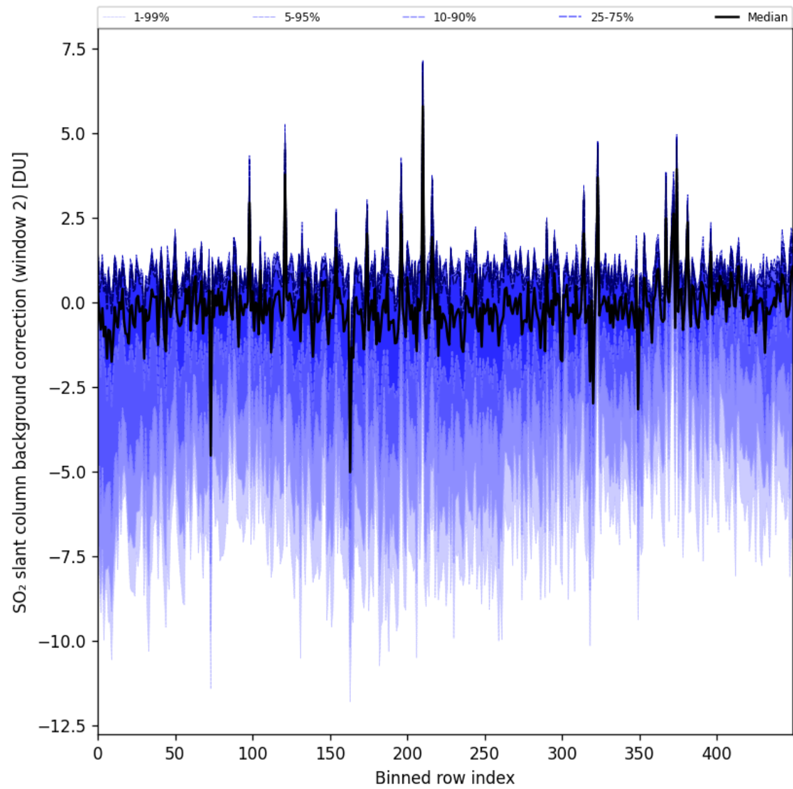
Figure 96: Along track statistics of “SO 2 slant column background correction (window 2)” for 2025-08-05 to 2025-08-07
