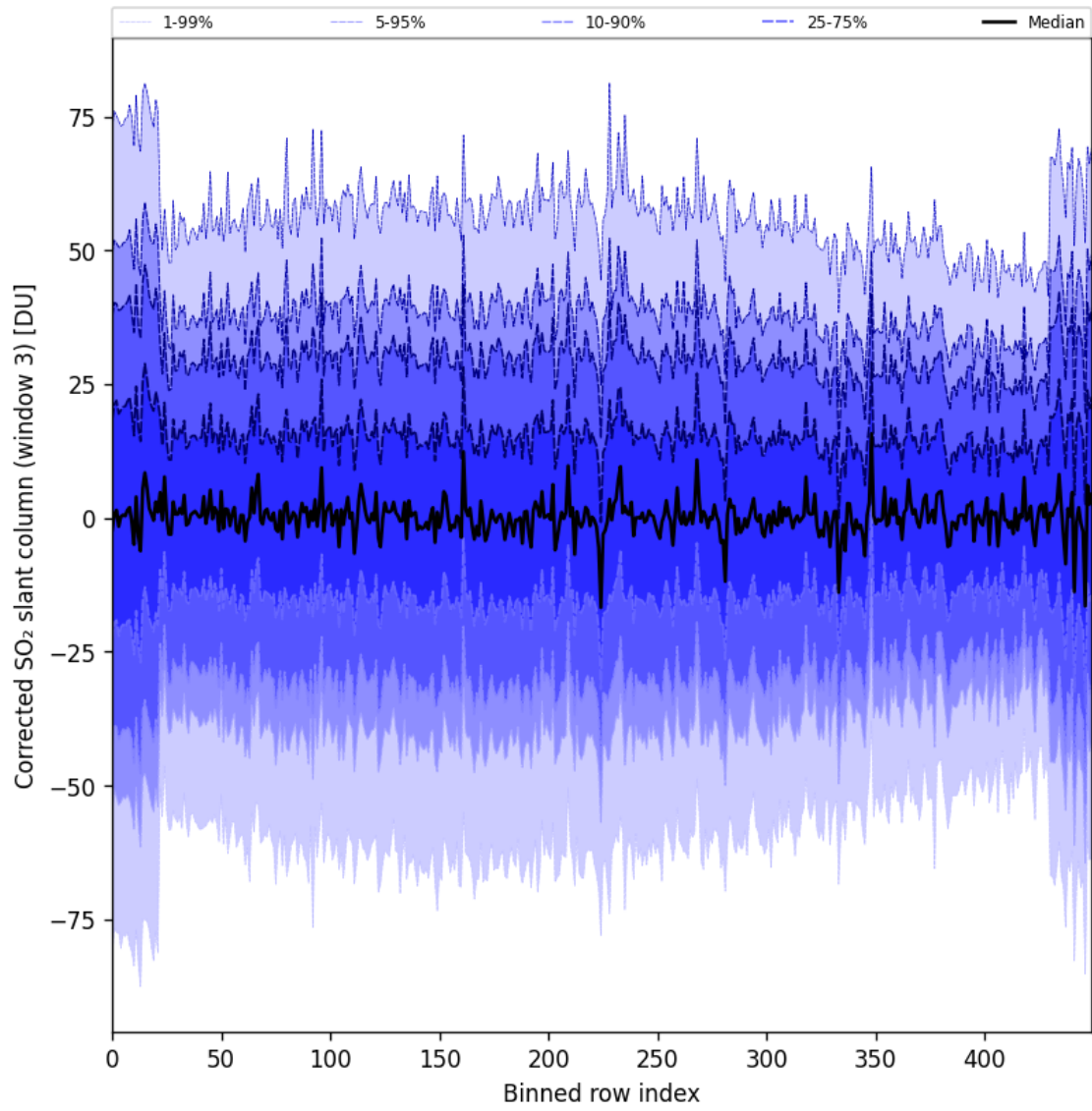
Figure 99: Along track statistics of “Corrected SO 2 slant column (window 3)” for 2025-08-05 to 2025-08-07
