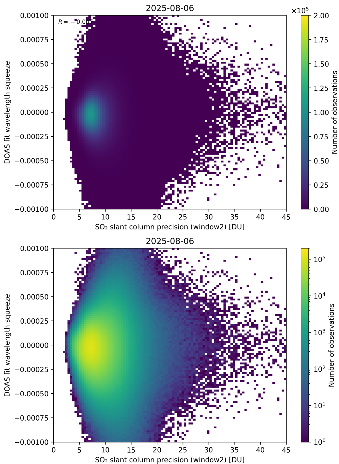
Figure 294: Scatter density plot of “SO 2 slant column precision (window2)” against “DOAS fit wavelength squeeze” for 2025-08-05 to 2025-08-07.
