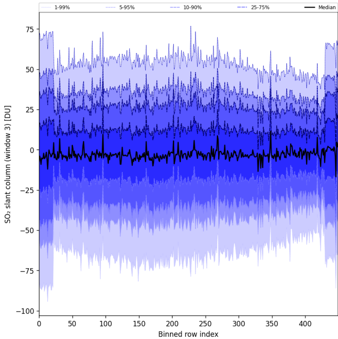
Figure 97: Along track statistics of “SO 2 slant column (window 3)” for 2025-08-05 to 2025-08-07
