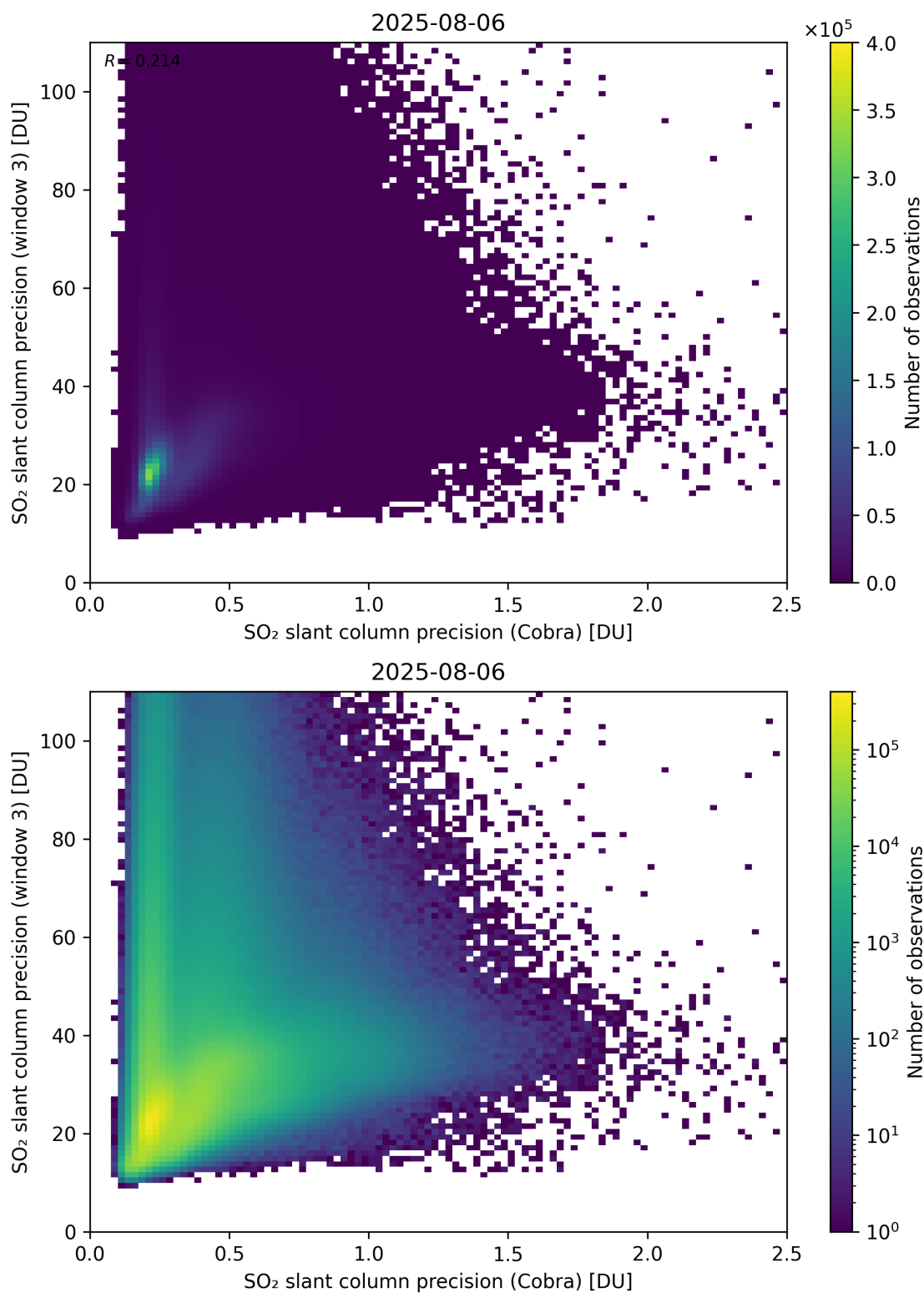
Figure 212: Scatter density plot of “SO 2 slant column precision (Cobra)” against “SO 2 slant column precision (window 3)” for 2025-08-05 to 2025-08-07.
