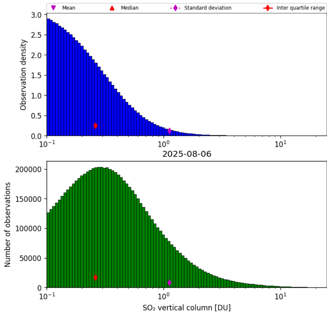
Figure 58: Histogram of “SO 2 vertical column” for 2025-08-05 to 2025-08-07
