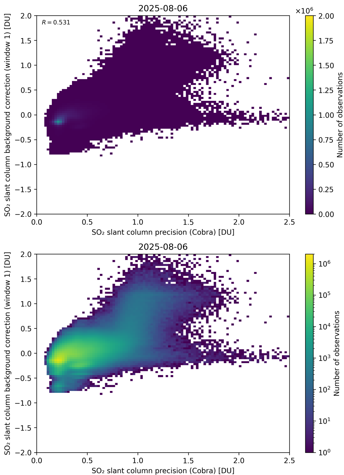
Figure 199: Scatter density plot of “SO 2 slant column precision (Cobra)” against “SO 2 slant column background correction (window 1)” for 2025-08-05 to 2025-08-07.
