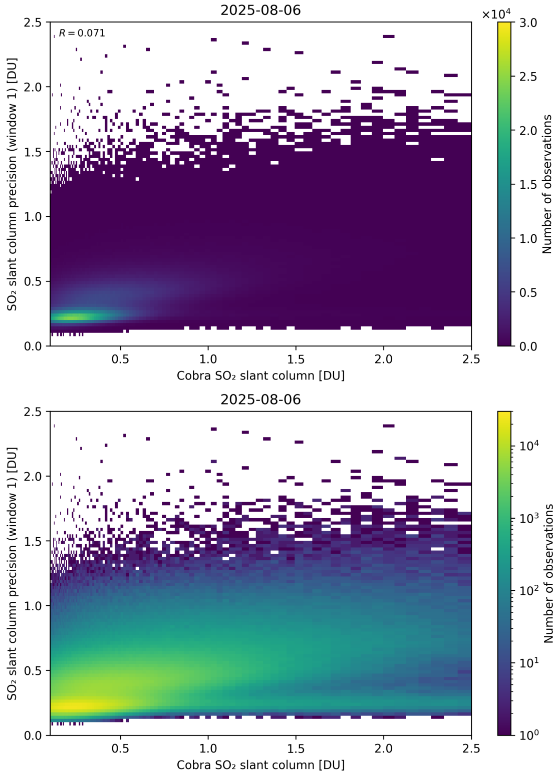
Figure 220: Scatter density plot of “Cobra SO 2 slant column” against “SO 2 slant column precision (window 1)” for 2025-08-05 to 2025-08-07.
