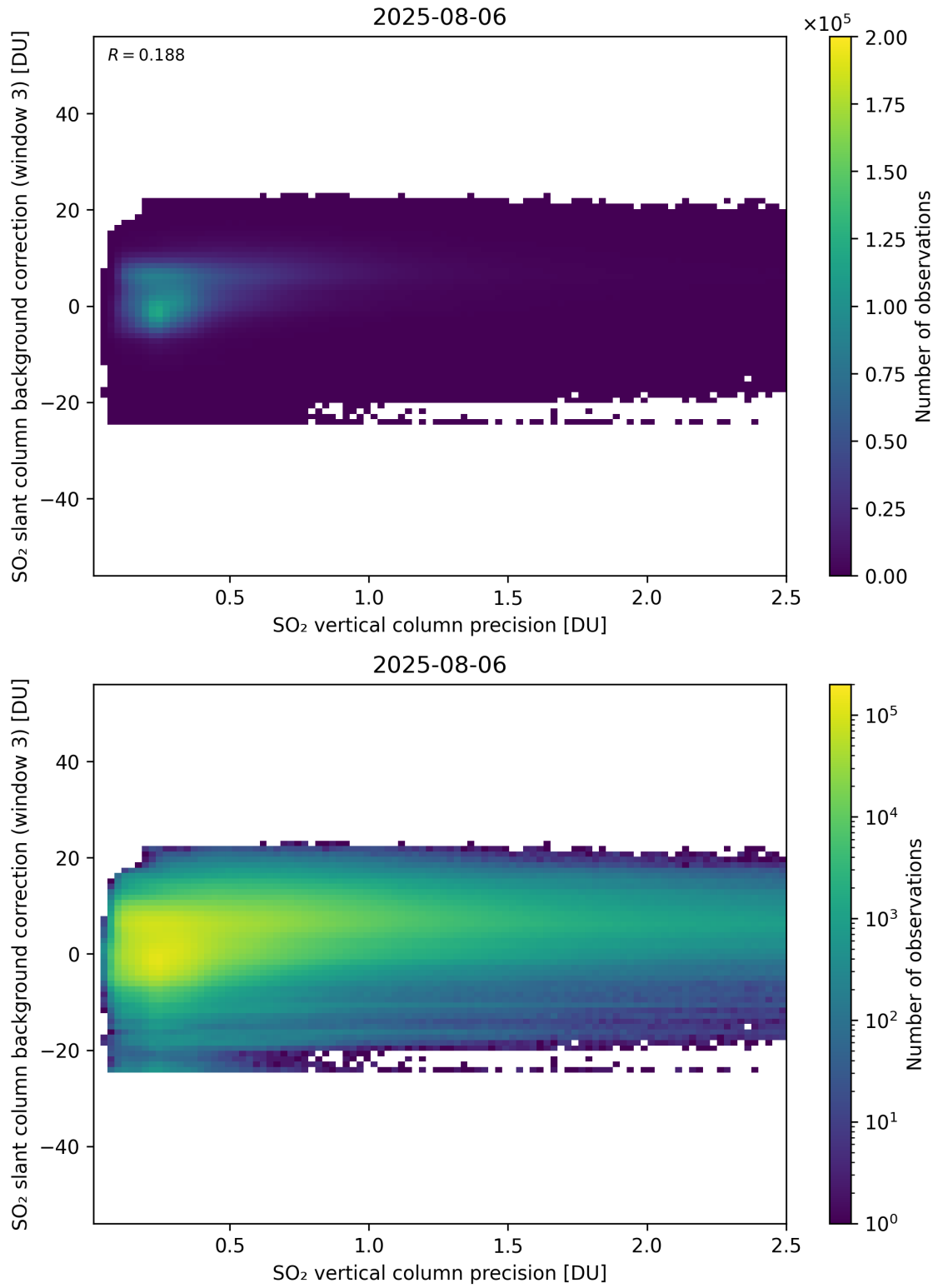
Figure 331: Scatter density plot of “SO 2 vertical column precision” against “SO 2 slant column background correction (window 3)” for 2025-08-05 to 2025-08-07.
