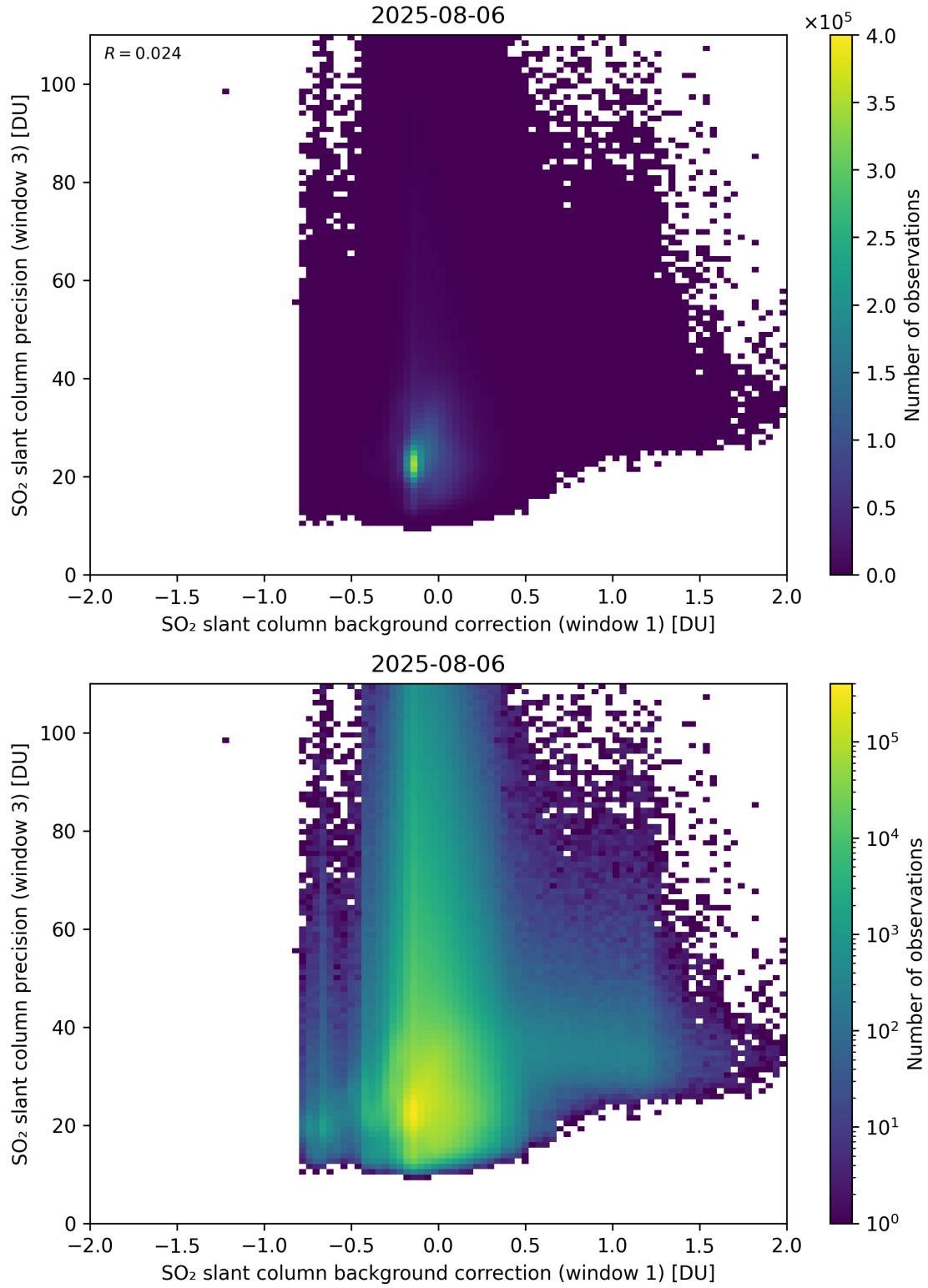
Figure 119: Scatter density plot of “SO 2 slant column background correction (window 1)” against “SO 2 slant column precision (window 3)” for 2025-08-05 to 2025-08-07.
