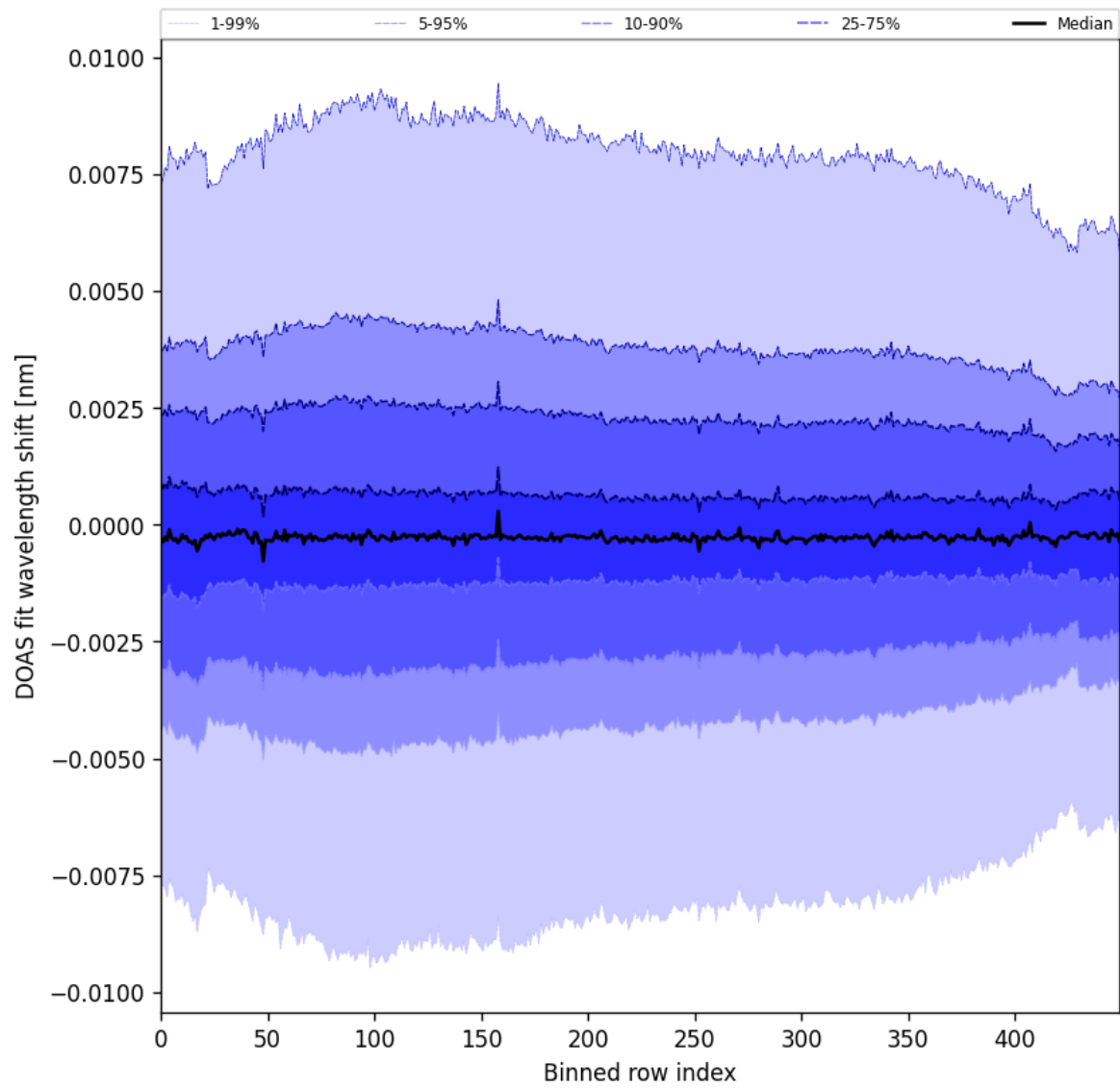
Figure 102: Along track statistics of “DOAS fit wavelength shift” for 2025-08-05 to 2025-08-07
