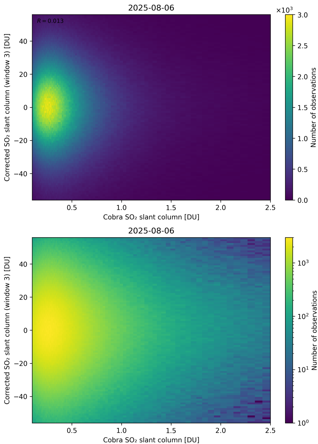
Figure 218: Scatter density plot of “Cobra SO 2 slant column” against “Corrected SO 2 slant column (window 3)” for 2025-08-05 to 2025-08-07.
