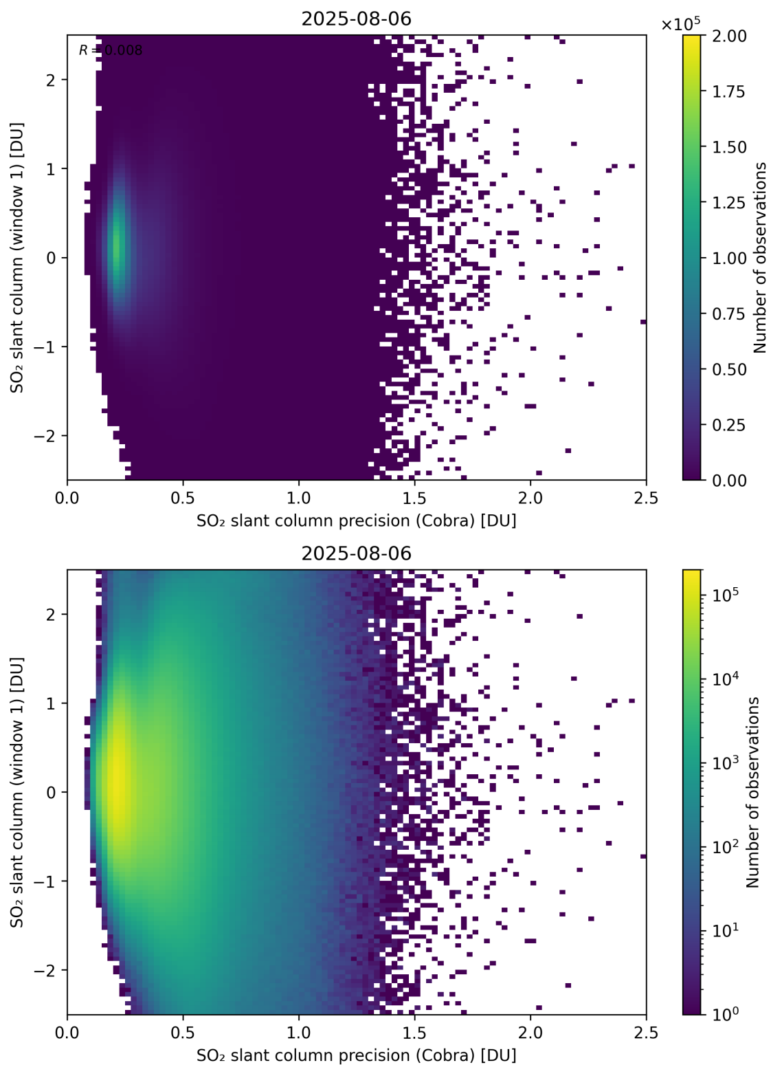
Figure 208: Scatter density plot of “SO 2 slant column precision (Cobra)” against “SO 2 slant column (window 1)” for 2025-08-05 to 2025-08-07.
