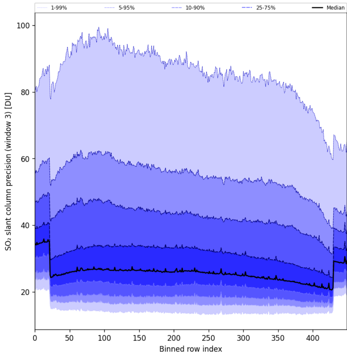
Figure 98: Along track statistics of “SO 2 slant column precision (window 3)” for 2025-08-05 to 2025-08-07
