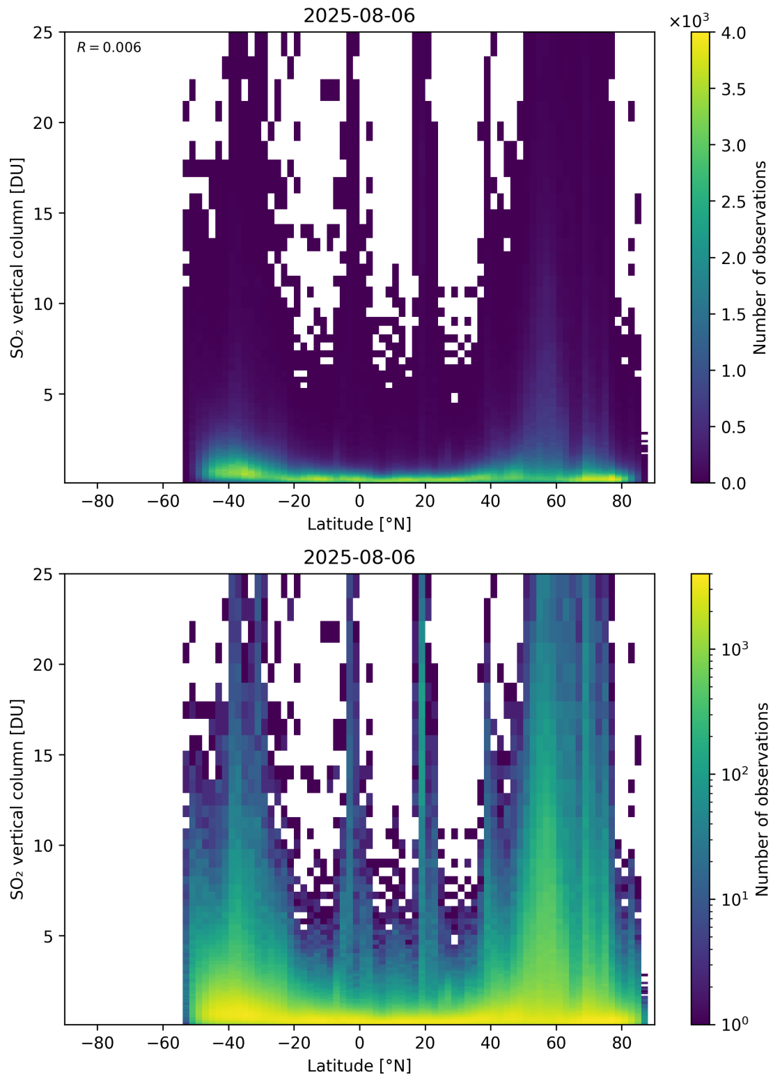
Figure 169: Scatter density plot of “Latitude” against “SO 2 vertical column” for 2025-08-05 to 2025-08-07.
