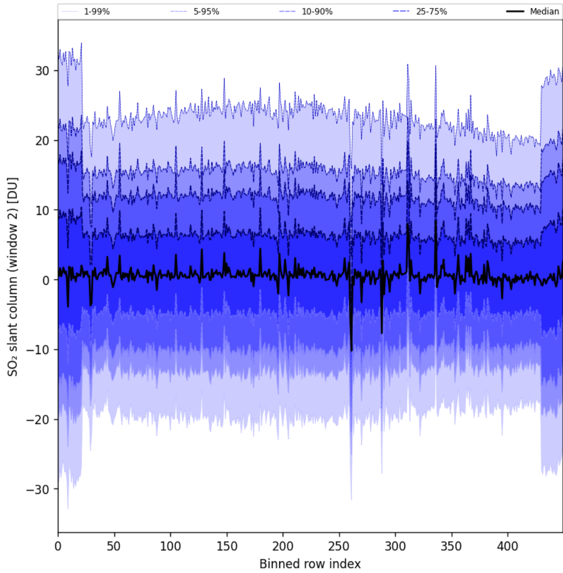
Figure 93: Along track statistics of “SO 2 slant column (window 2)” for 2025-08-05 to 2025-08-07
