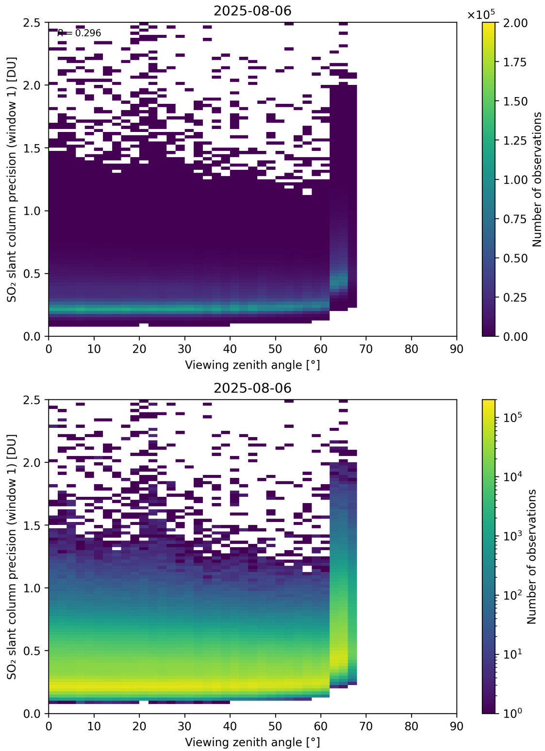
Figure 377: Scatter density plot of “Viewing zenith angle” against “SO 2 slant column precision (window 1)” for 2025-08-05 to 2025-08-07.
