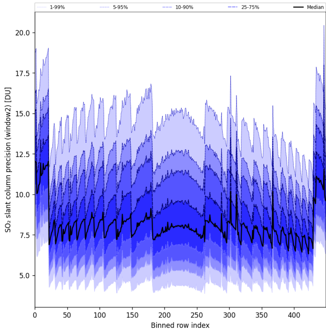
Figure 94: Along track statistics of “SO 2 slant column precision (window2)” for 2025-08-05 to 2025-08-07
