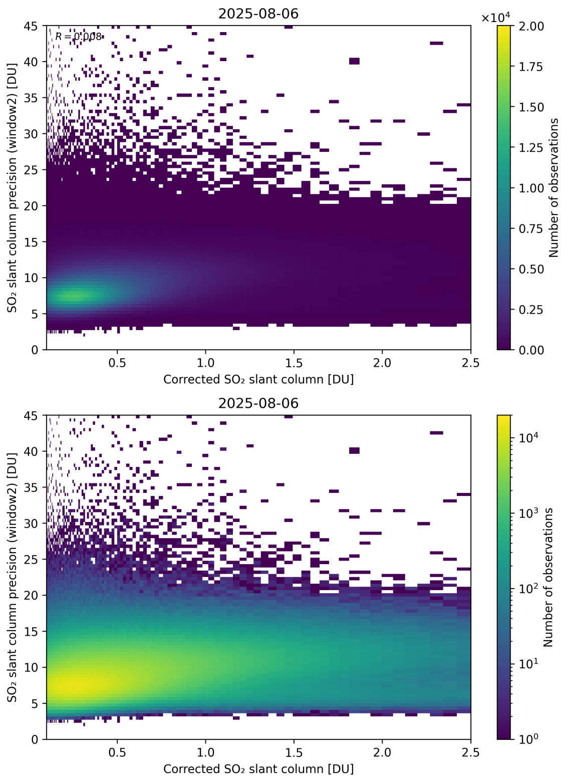
Figure 239: Scatter density plot of “Corrected SO 2 slant column” against “SO 2 slant column precision (window2)” for 2025-08-05 to 2025-08-07.
