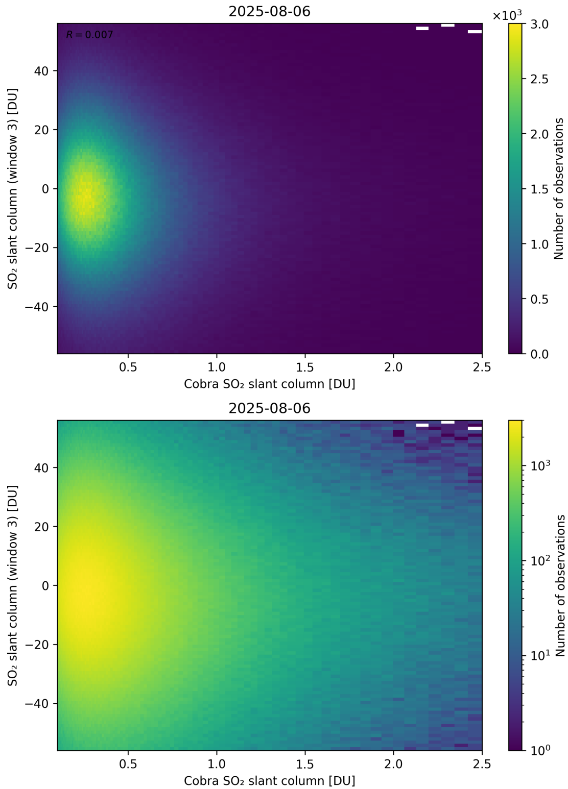
Figure 222: Scatter density plot of “Cobra SO 2 slant column” against “SO 2 slant column (window 3)” for 2025-08-05 to 2025-08-07.
