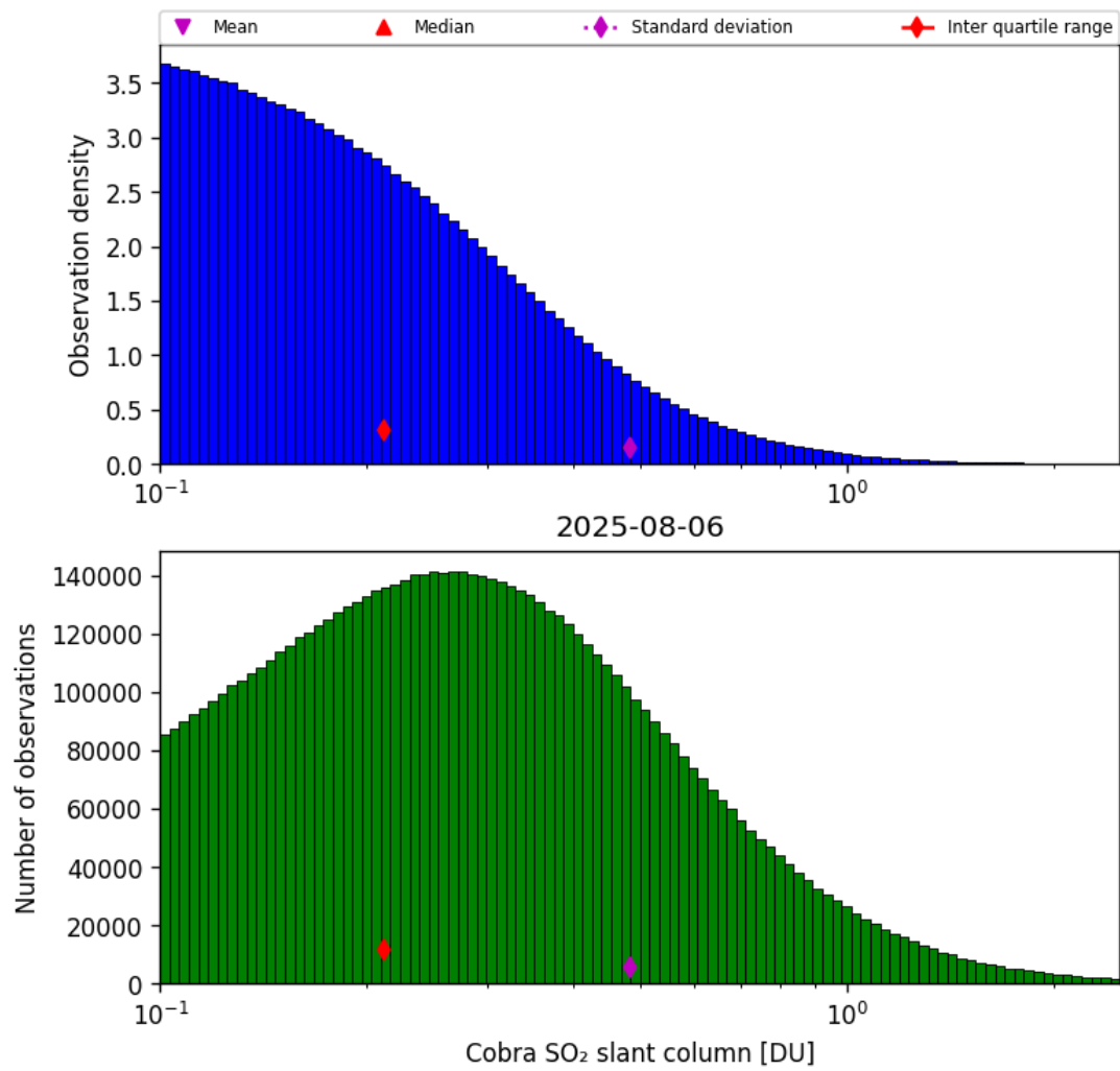
Figure 61: Histogram of “Cobra SO 2 slant column” for 2025-08-05 to 2025-08-07
