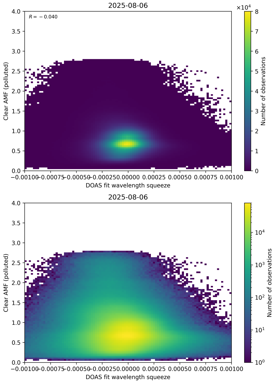
Figure 144: Scatter density plot of “DOAS fit wavelength squeeze” against “Clear AMF (polluted)” for 2025-08-05 to 2025-08-07.
