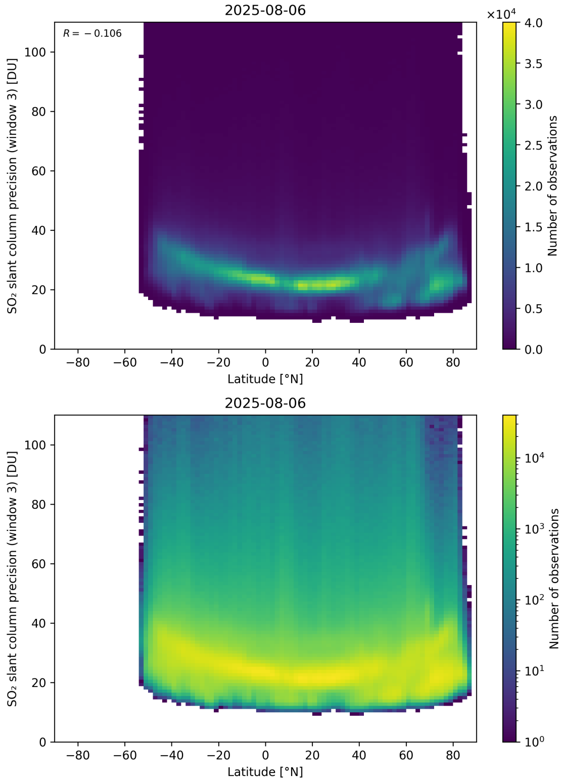
Figure 166: Scatter density plot of “Latitude” against “SO 2 slant column precision (window 3)” for 2025-08-05 to 2025-08-07.
