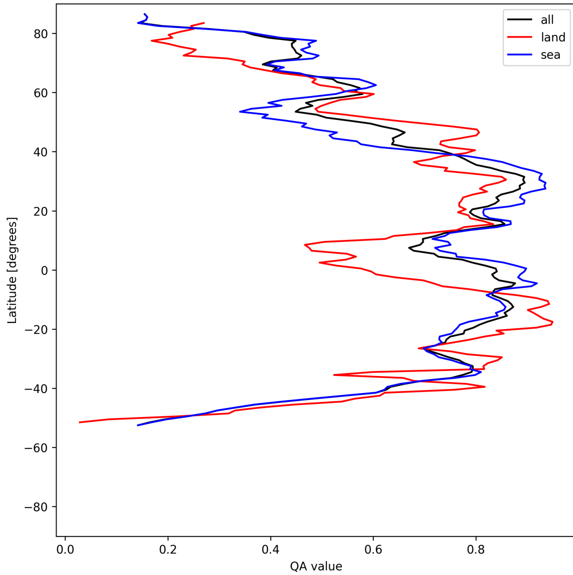
Figure 31: Zonal average of “QA value” for 2025-08-05 to 2025-08-07.
