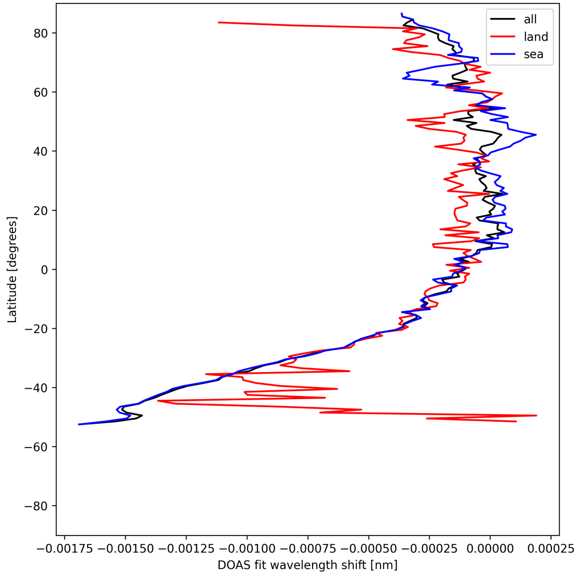
Figure 50: Zonal average of “DOAS fit wavelength shift” for 2025-08-05 to 2025-08-07.
