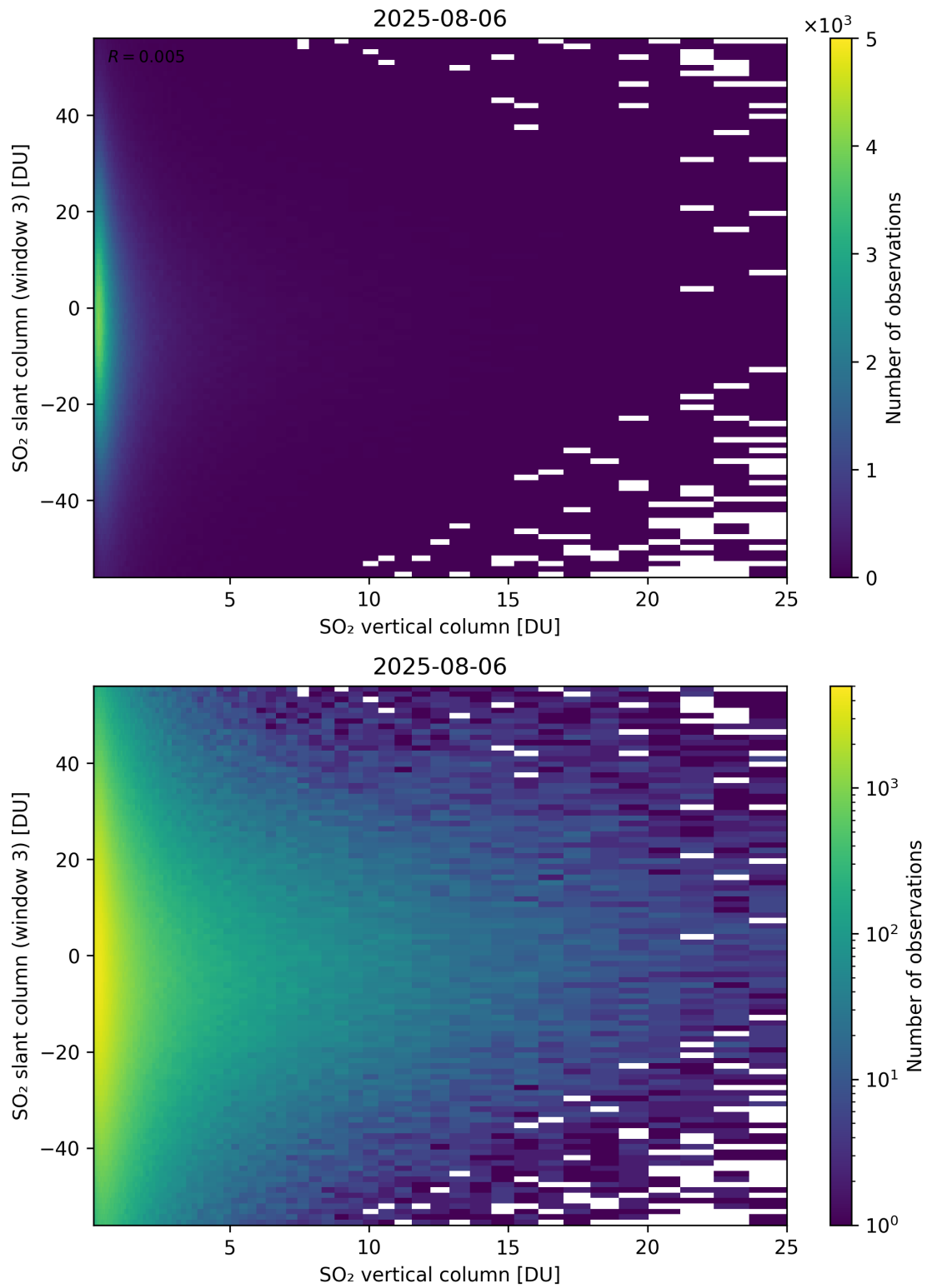
Figure 357: Scatter density plot of “SO 2 vertical column” against “SO 2 slant column (window 3)” for 2025-08-05 to 2025-08-07.
