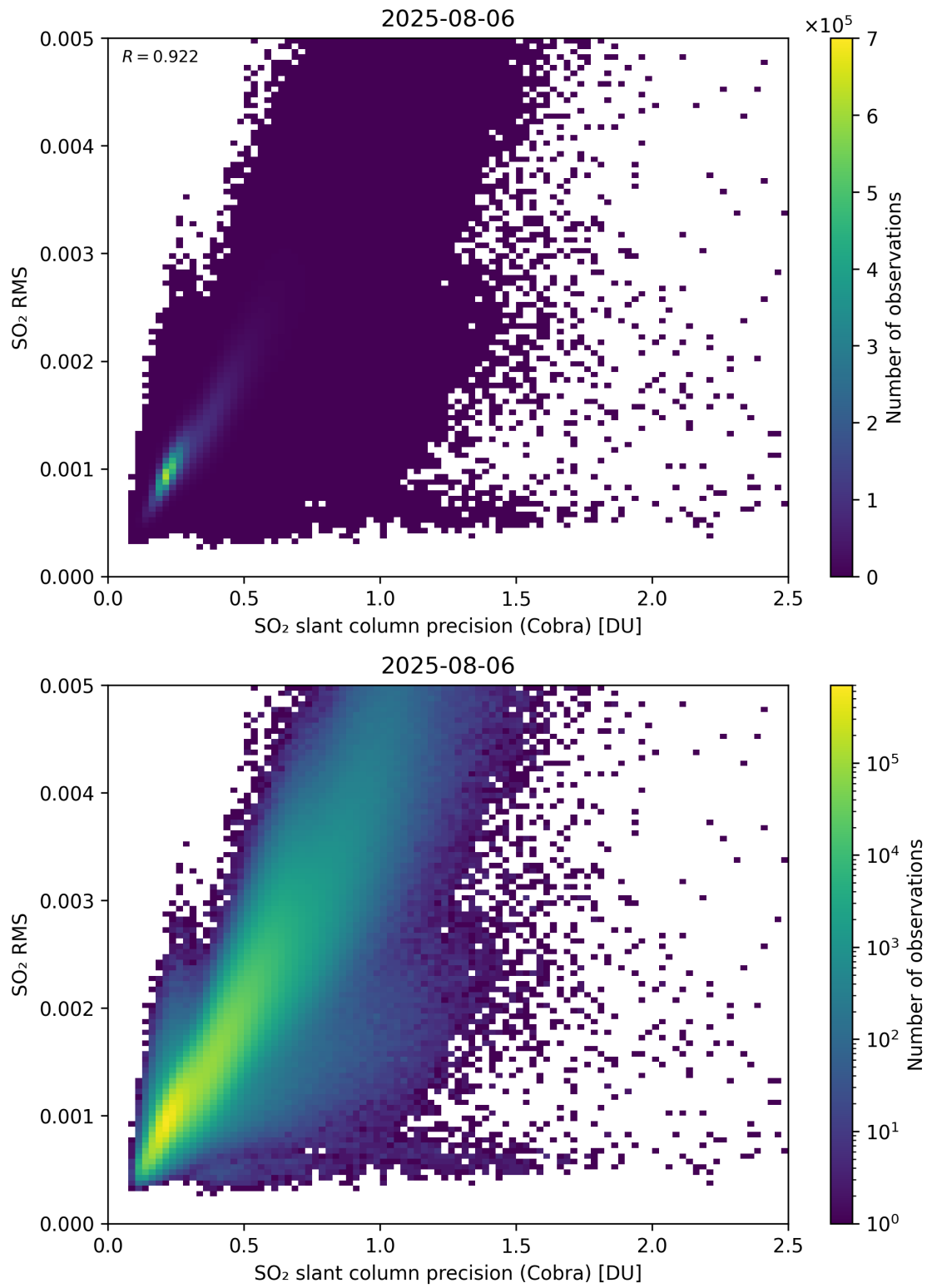
Figure 204: Scatter density plot of “SO 2 slant column precision (Cobra)” against “SO 2 RMS” for 2025-08-05 to 2025-08-07.
