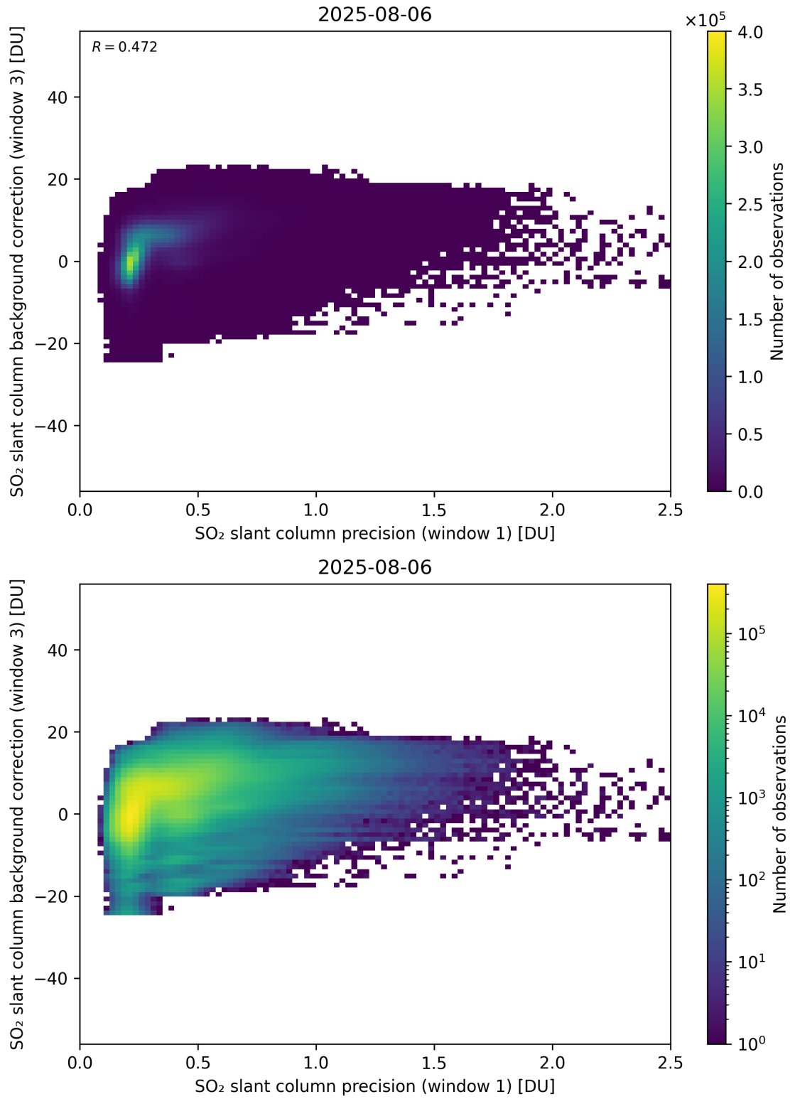
Figure 270: Scatter density plot of “SO 2 slant column precision (window 1)” against “SO 2 slant column background correction (window 3)” for 2025-08-05 to 2025-08-07.
