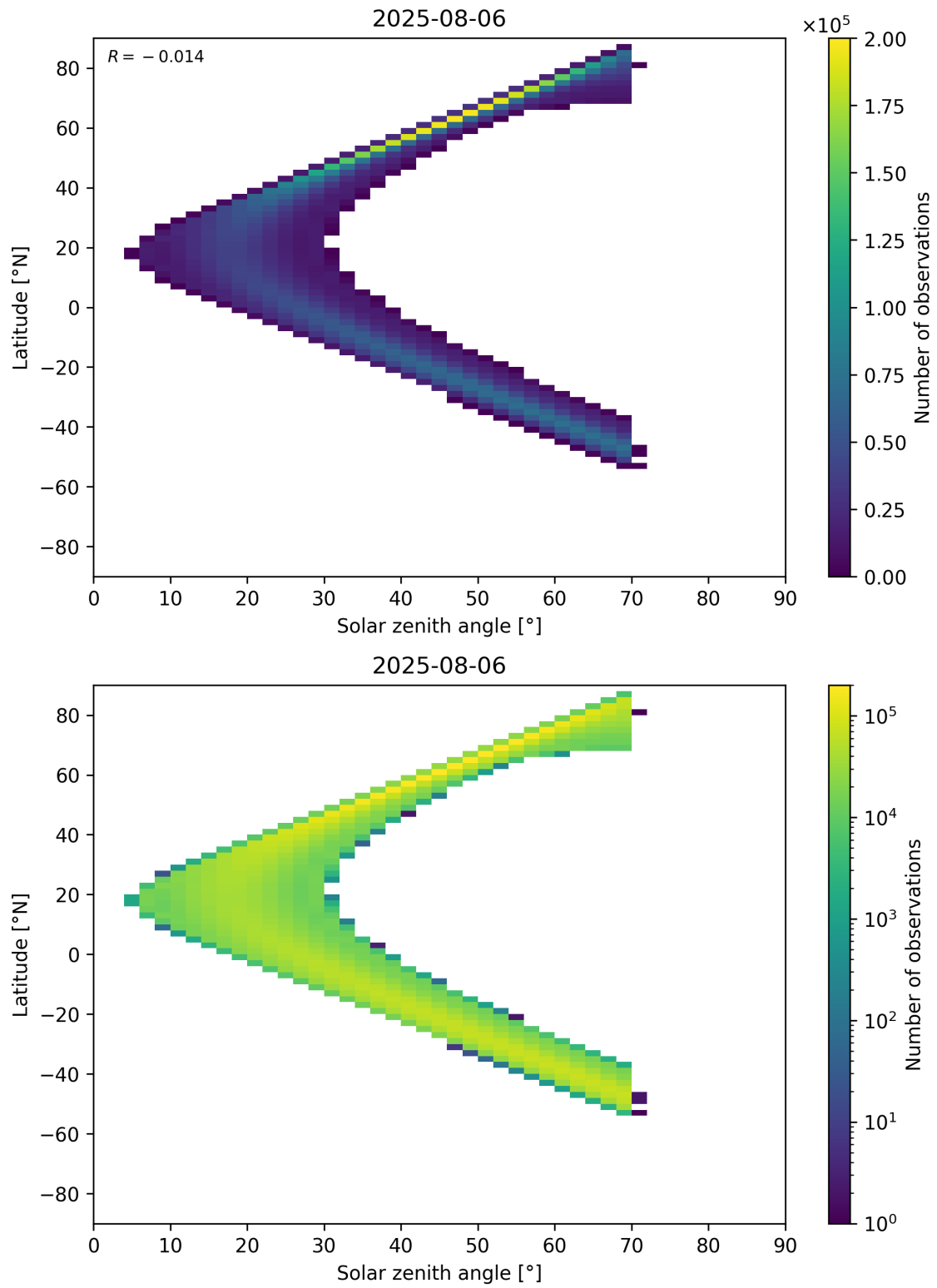
Figure 177: Scatter density plot of “Solar zenith angle” against “Latitude” for 2025-08-05 to 2025-08-07.
