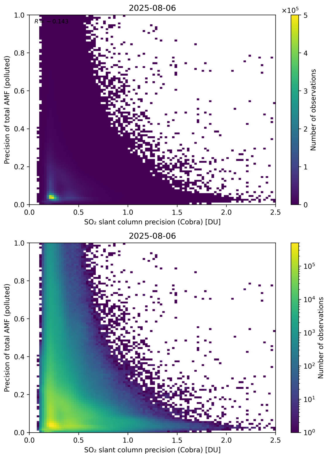
Figure 214: Scatter density plot of “SO 2 slant column precision (Cobra)” against “Precision of total AMF (polluted)” for 2025-08-05 to 2025-08-07.
