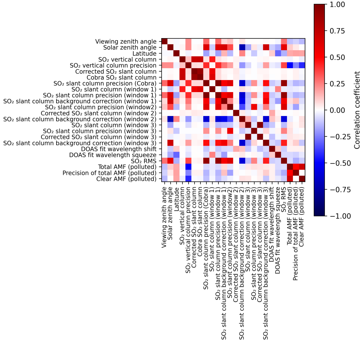
Figure 2: Map of correlation matrix for 2025-08-05 to 2025-08-07.
