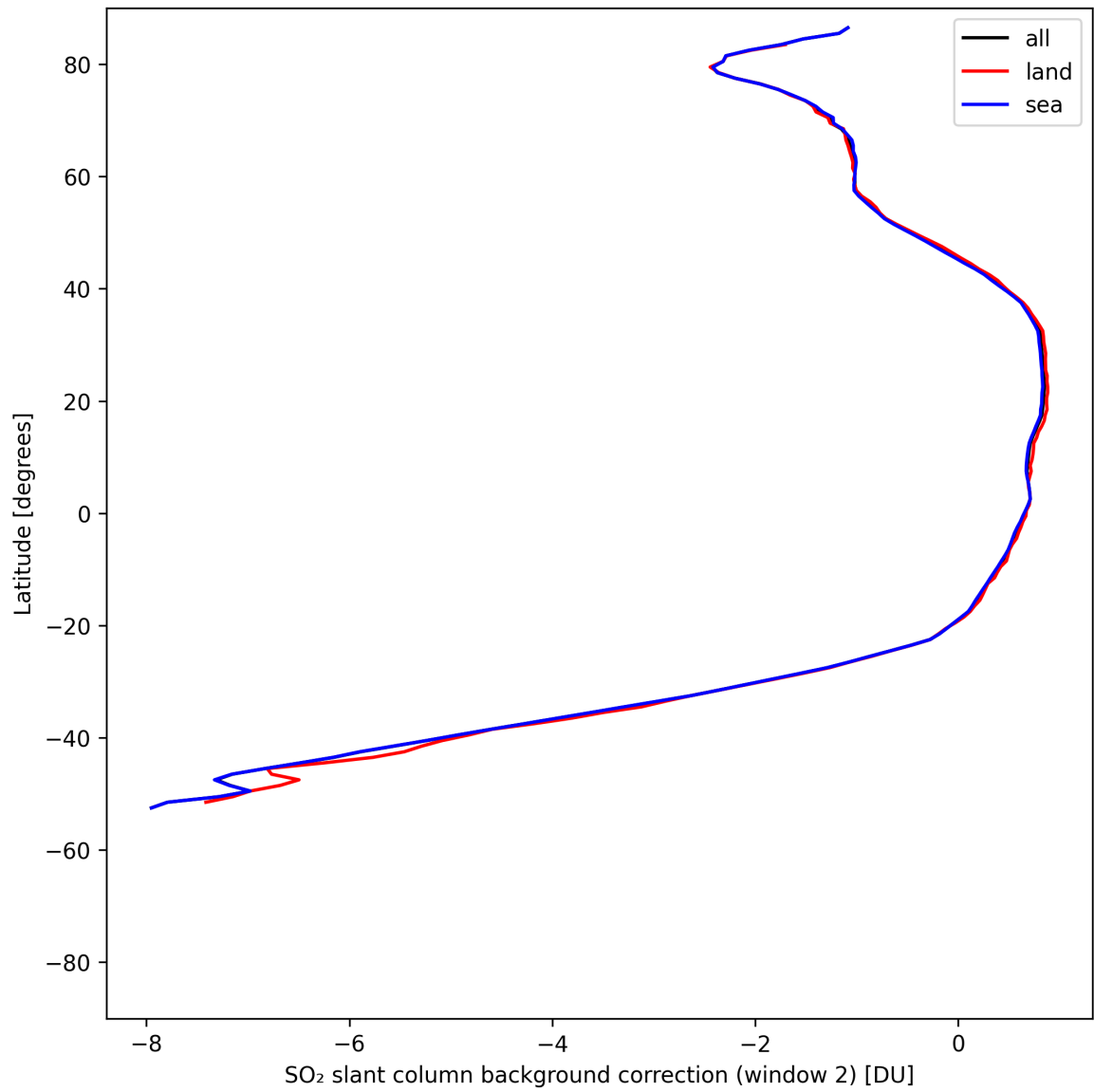
Figure 44: Zonal average of “SO 2 slant column background correction (window 2)” for 2025-08-05 to 2025-08-07.
