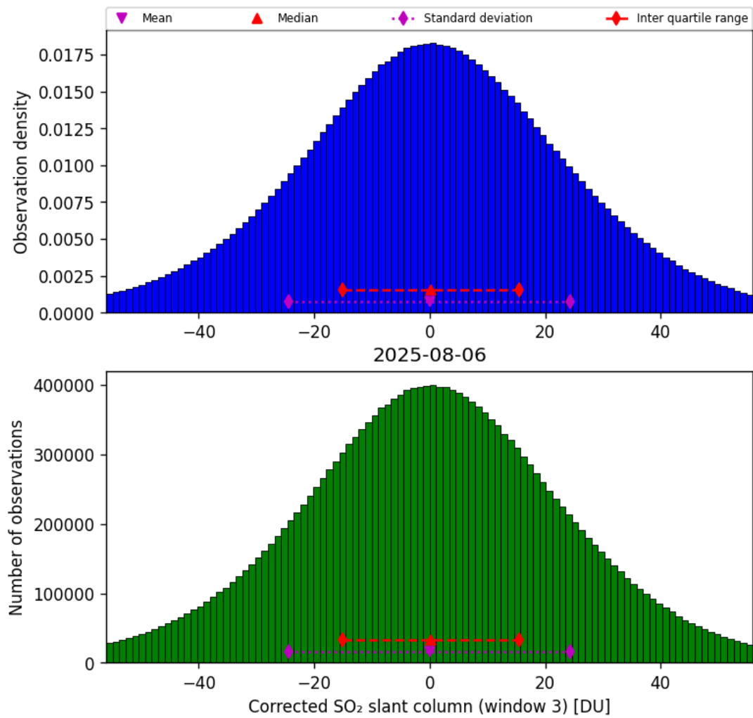
Figure 73: Histogram of “Corrected SO 2 slant column (window 3)” for 2025-08-05 to 2025-08-07
