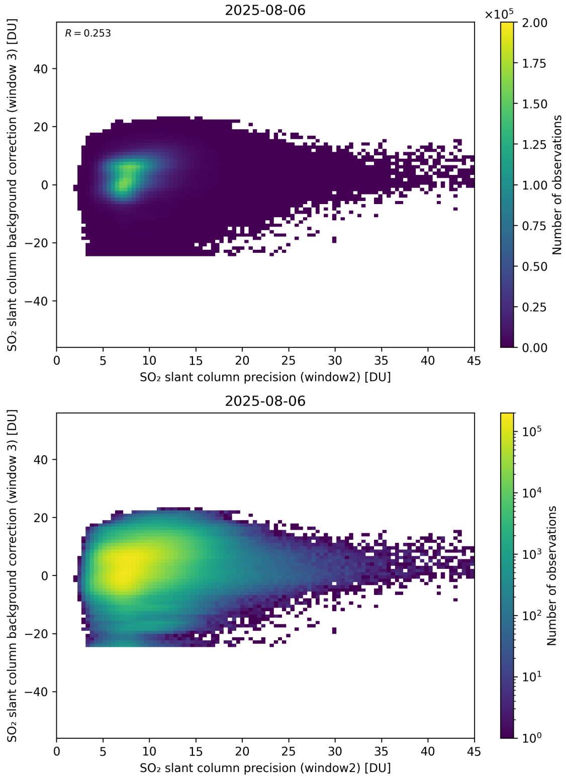
Figure 292: Scatter density plot of “SO 2 slant column precision (window2)” against “SO 2 slant column background correction (window 3)” for 2025-08-05 to 2025-08-07.
