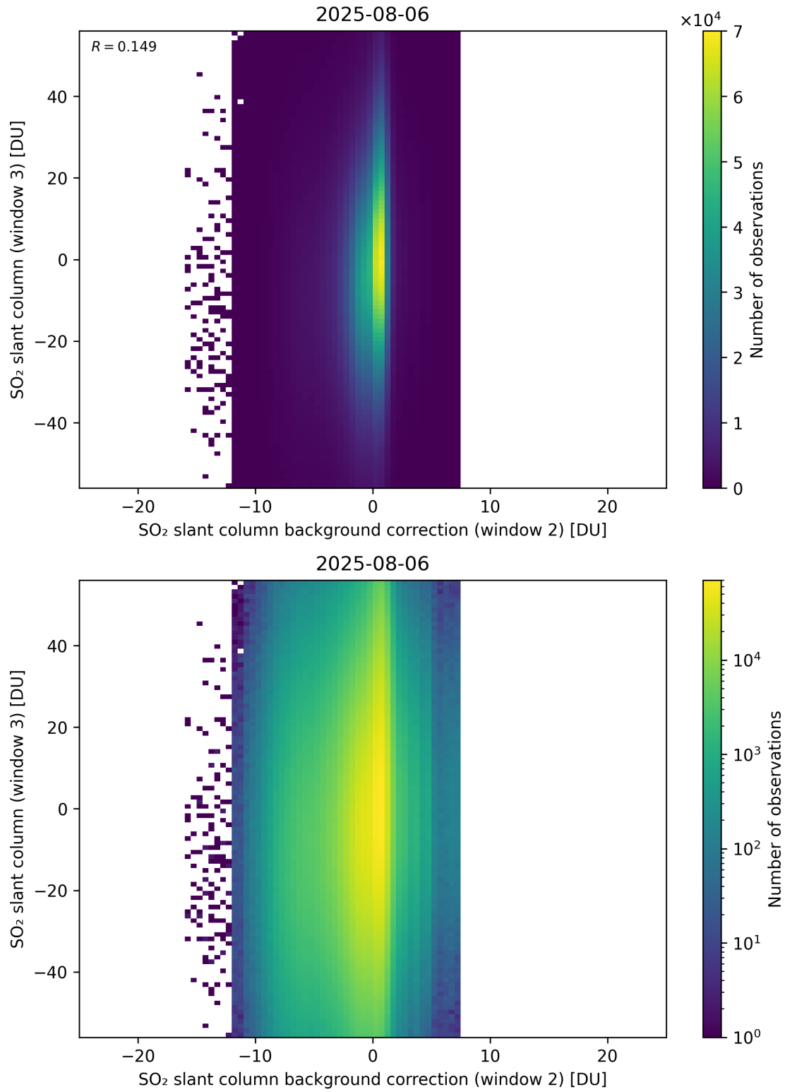
Figure 128: Scatter density plot of “SO 2 slant column background correction (window 2)” against “SO 2 slant column (window 3)” for 2025-08-05 to 2025-08-07.
