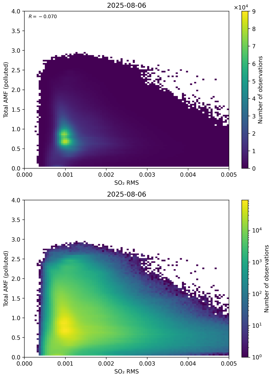
Figure 148: Scatter density plot of “SO 2 RMS” against “Total AMF (polluted)” for 2025-08-05 to 2025-08-07.
