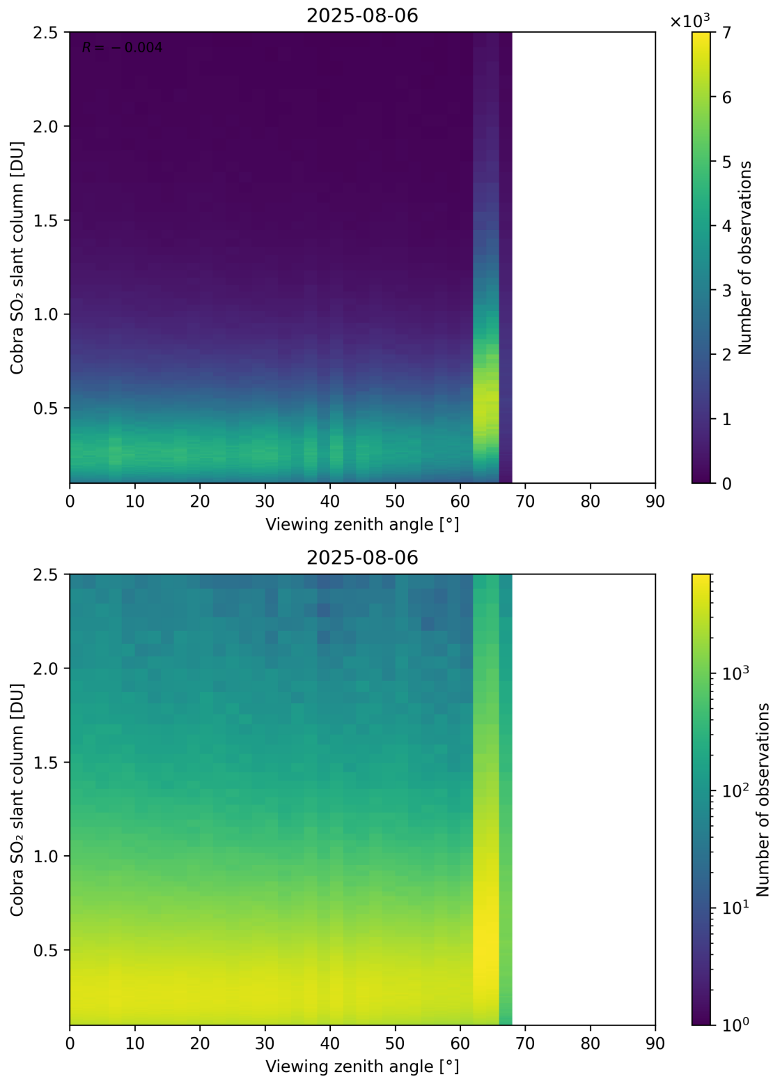
Figure 371: Scatter density plot of “Viewing zenith angle” against “Cobra SO 2 slant column” for 2025-08-05 to 2025-08-07.
