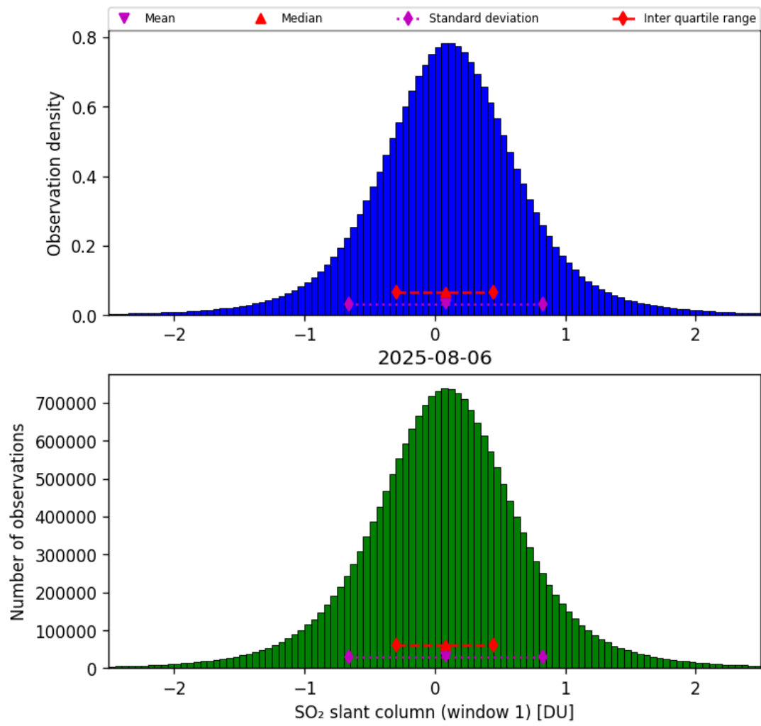
Figure 63: Histogram of “SO 2 slant column (window 1)” for 2025-08-05 to 2025-08-07
