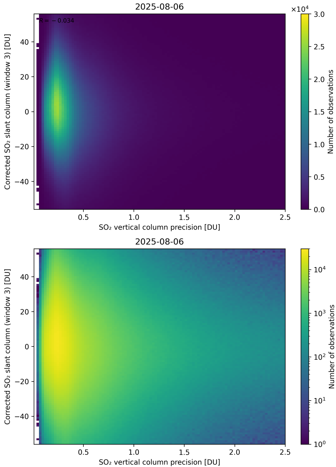
Figure 340: Scatter density plot of “SO 2 vertical column precision” against “Corrected SO 2 slant column (window 3)” for 2025-08-05 to 2025-08-07.
