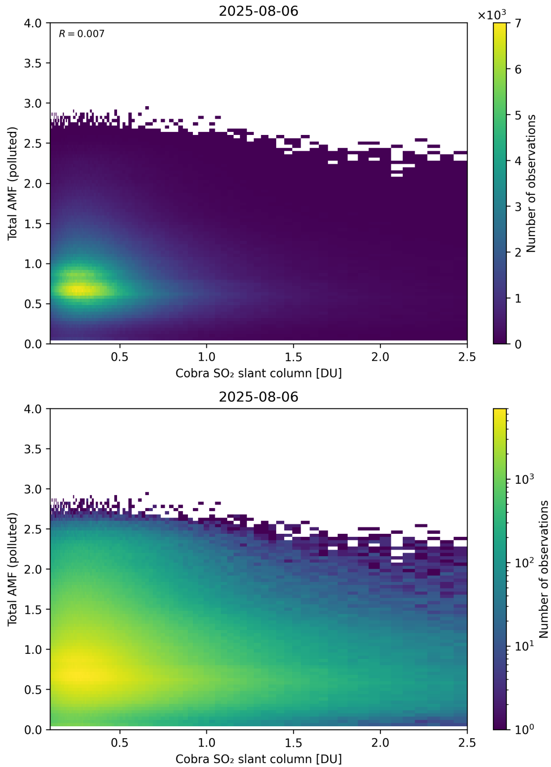
Figure 224: Scatter density plot of “Cobra SO 2 slant column” against “Total AMF (polluted)” for 2025-08-05 to 2025-08-07.
