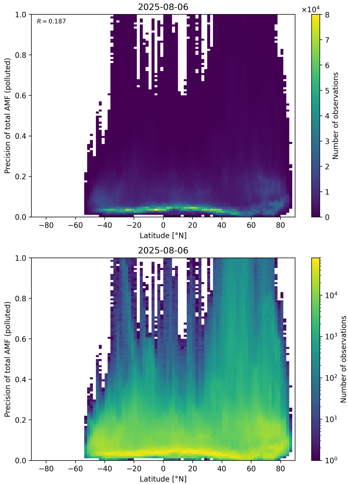
Figure 168: Scatter density plot of “Latitude” against “Precision of total AMF (polluted)” for 2025-08-05 to 2025-08-07.
