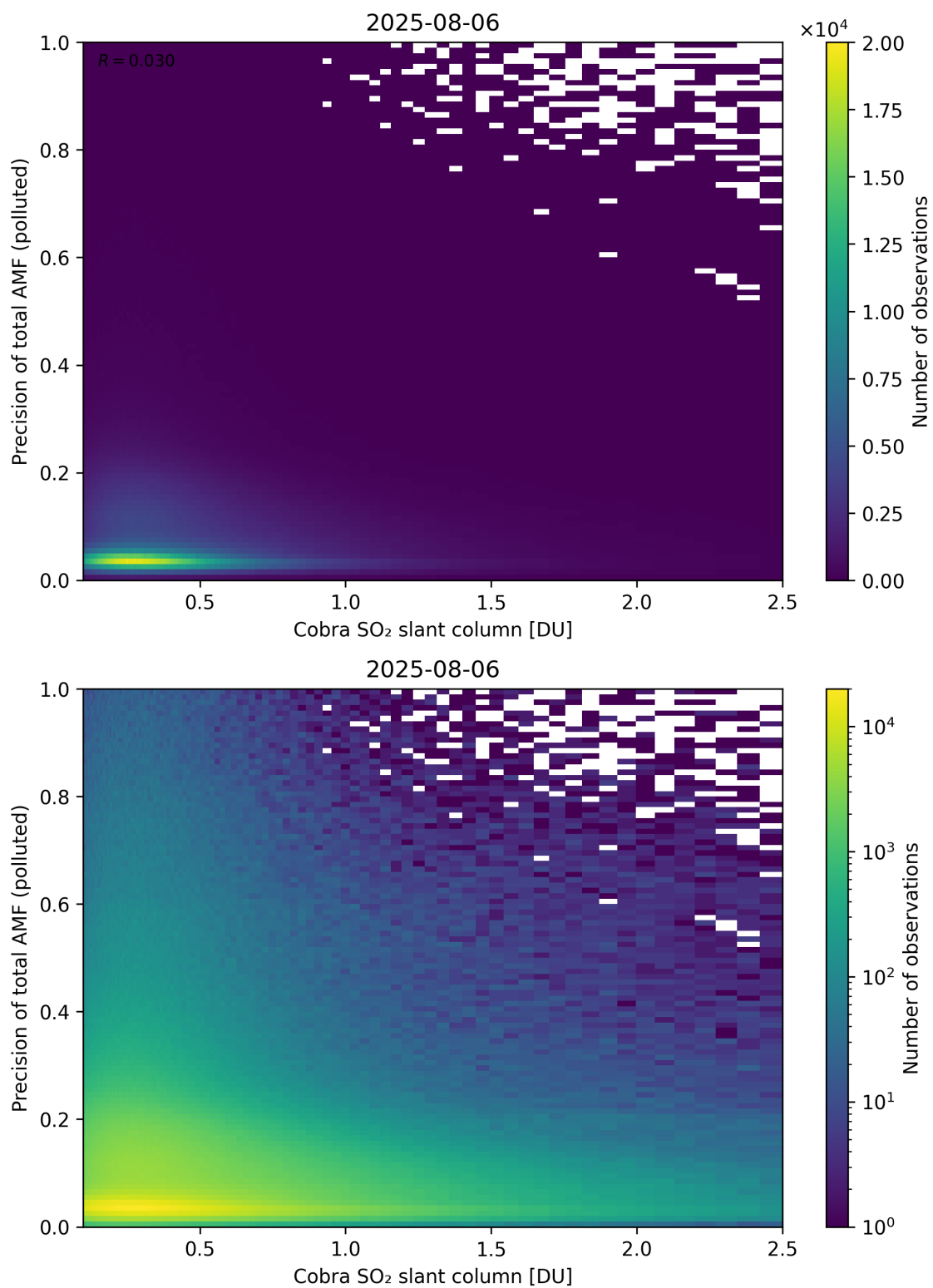
Figure 225: Scatter density plot of “Cobra SO 2 slant column” against “Precision of total AMF (polluted)” for 2025-08-05 to 2025-08-07.
