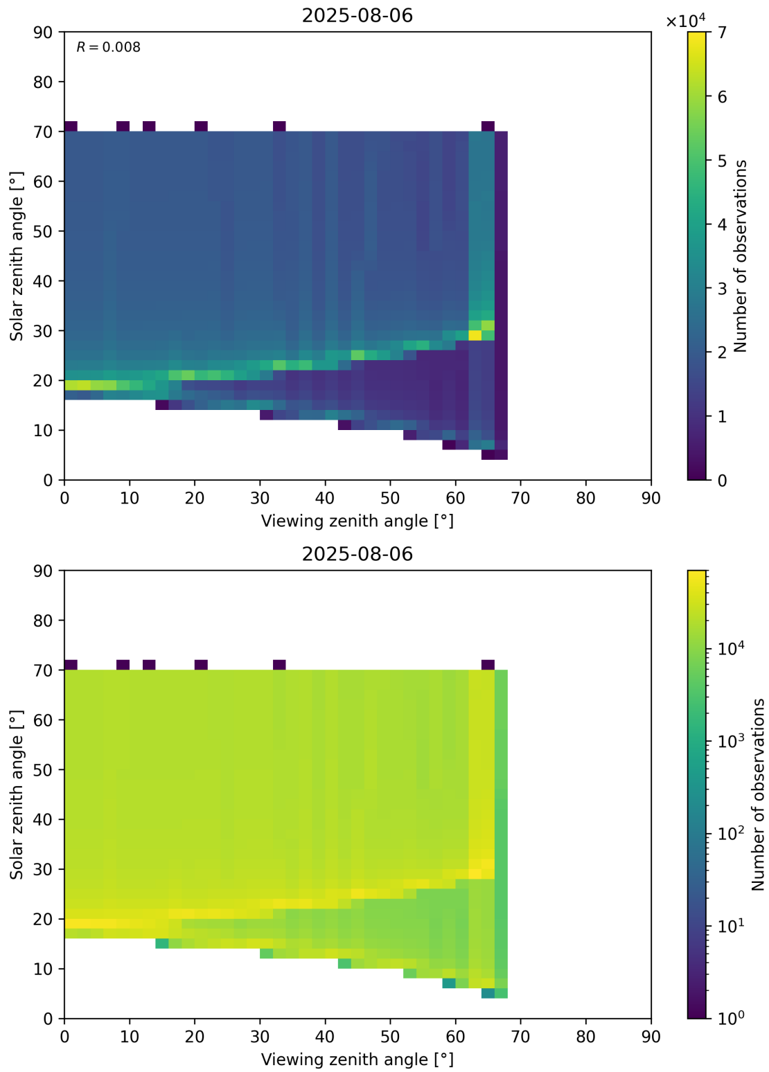
Figure 369: Scatter density plot of “Viewing zenith angle” against “Solar zenith angle” for 2025-08-05 to 2025-08-07.
