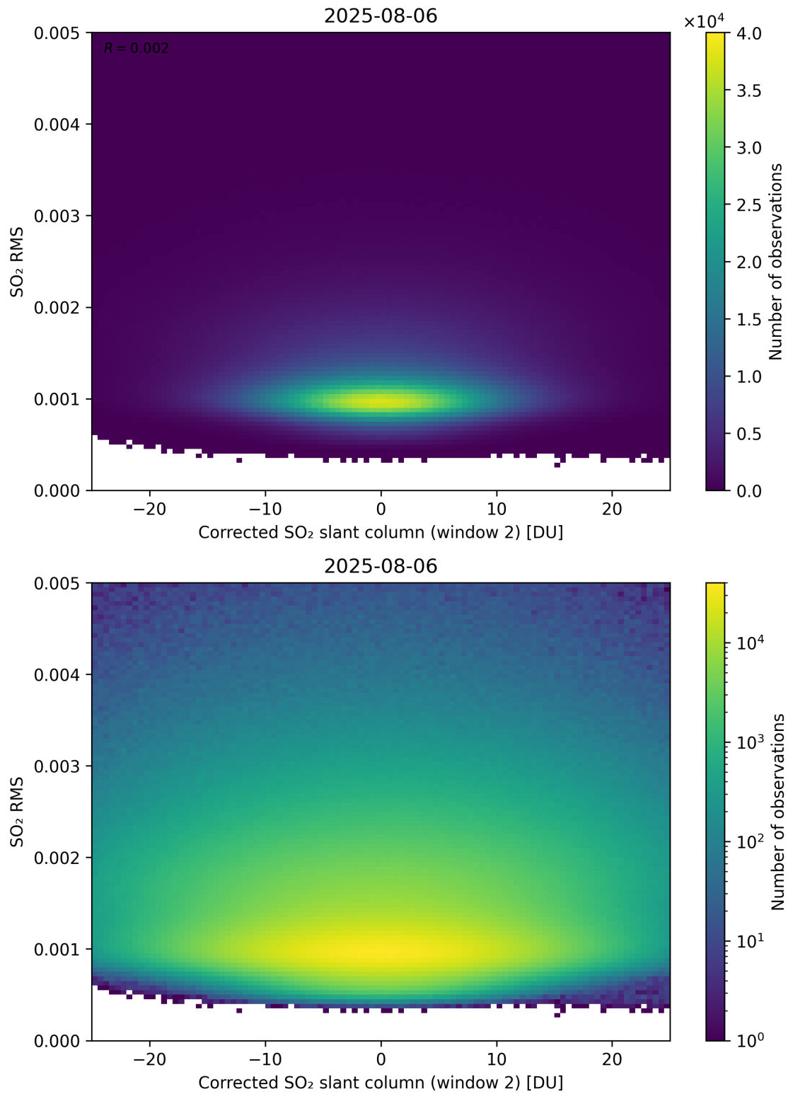
Figure 248: Scatter density plot of “Corrected SO 2 slant column (window 2)” against “SO 2 RMS” for 2025-08-05 to 2025-08-07.
