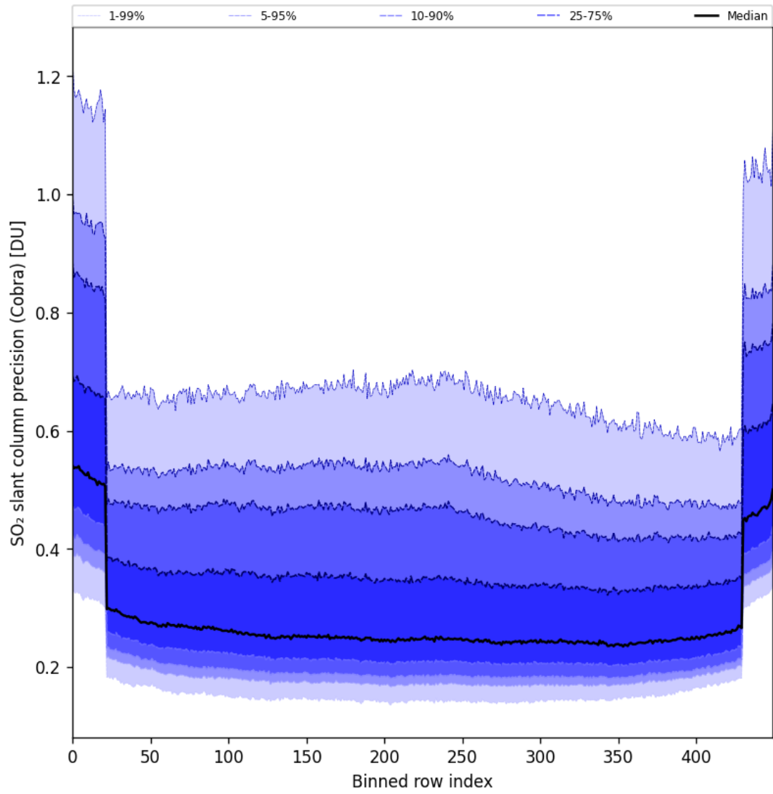
Figure 88: Along track statistics of “SO 2 slant column precision (Cobra)” for 2025-08-05 to 2025-08-07
