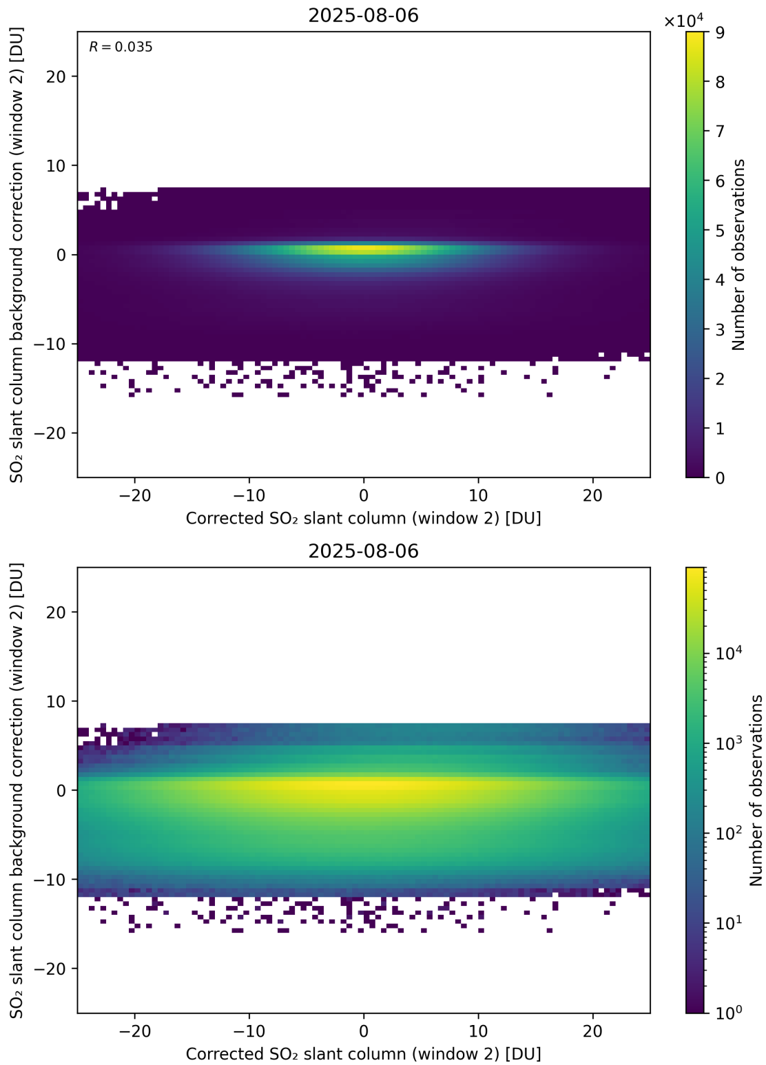
Figure 244: Scatter density plot of “Corrected SO 2 slant column (window 2)” against “SO 2 slant column background correction (window 2)” for 2025-08-05 to 2025-08-07.
