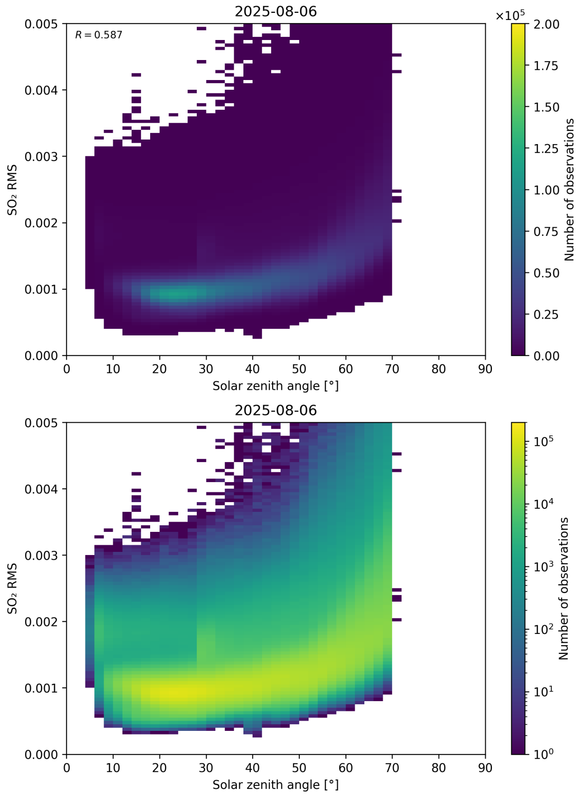
Figure 176: Scatter density plot of “Solar zenith angle” against “SO 2 RMS” for 2025-08-05 to 2025-08-07.
