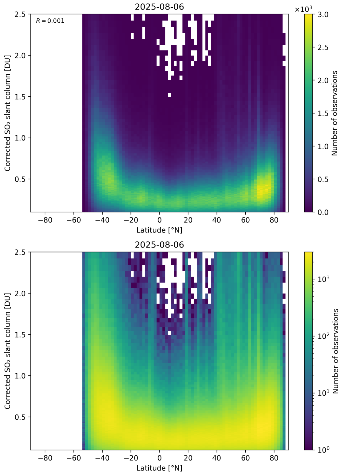
Figure 159: Scatter density plot of “Latitude” against “Corrected SO 2 slant column” for 2025-08-05 to 2025-08-07.
