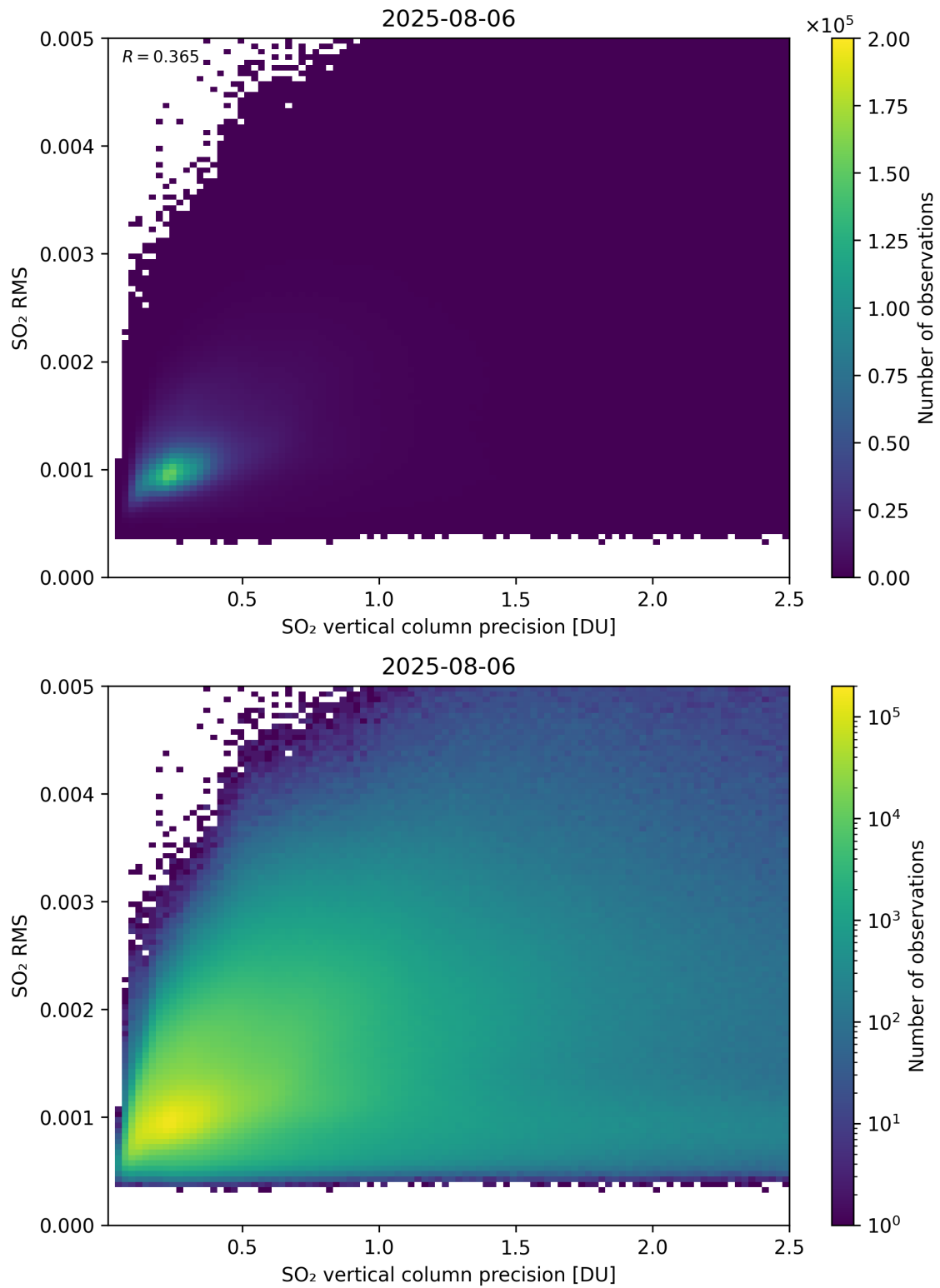
Figure 334: Scatter density plot of “SO 2 vertical column precision” against “SO 2 RMS” for 2025-08-05 to 2025-08-07.
