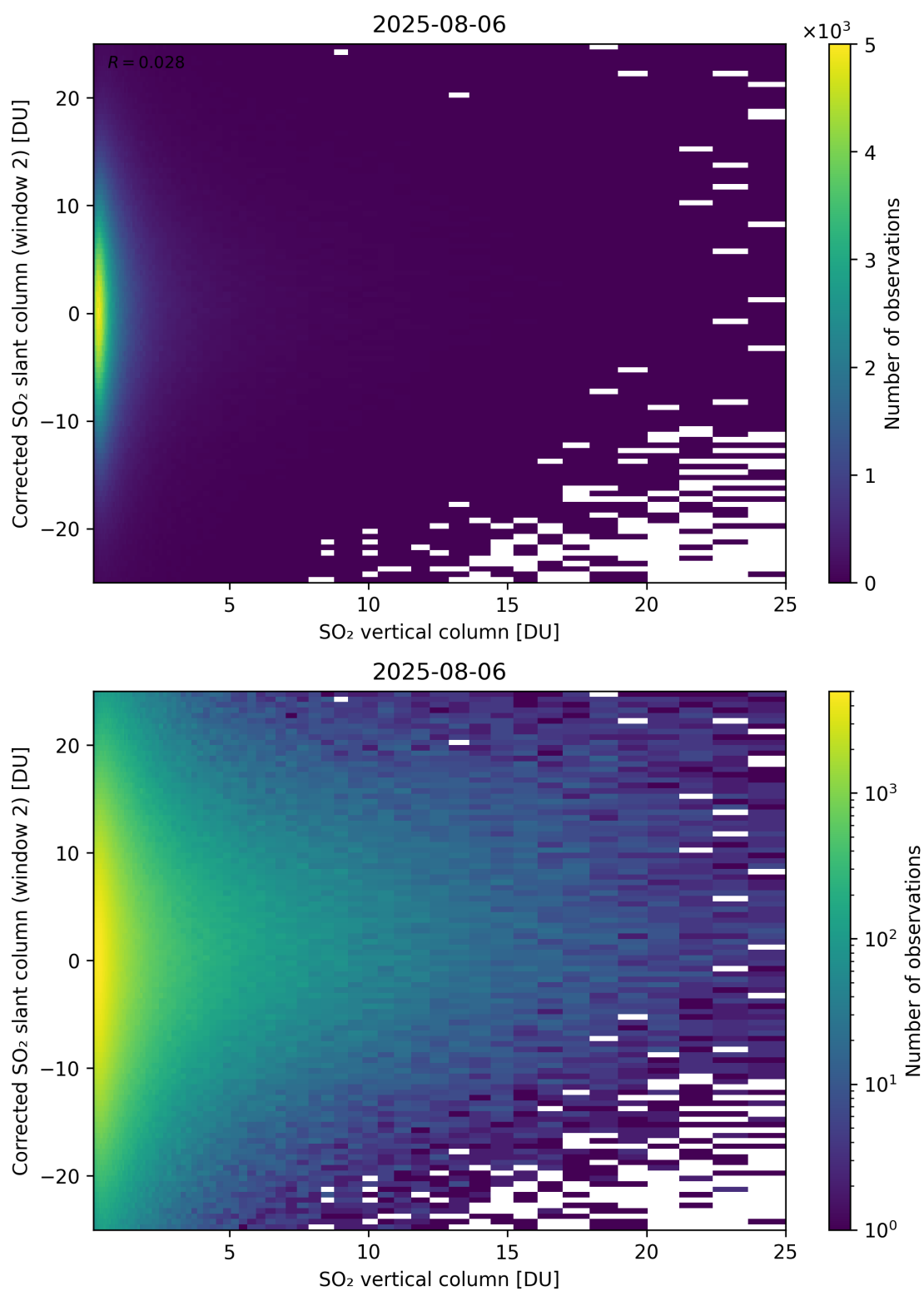
Figure 352: Scatter density plot of “SO 2 vertical column” against “Corrected SO 2 slant column (window 2)” for 2025-08-05 to 2025-08-07.
