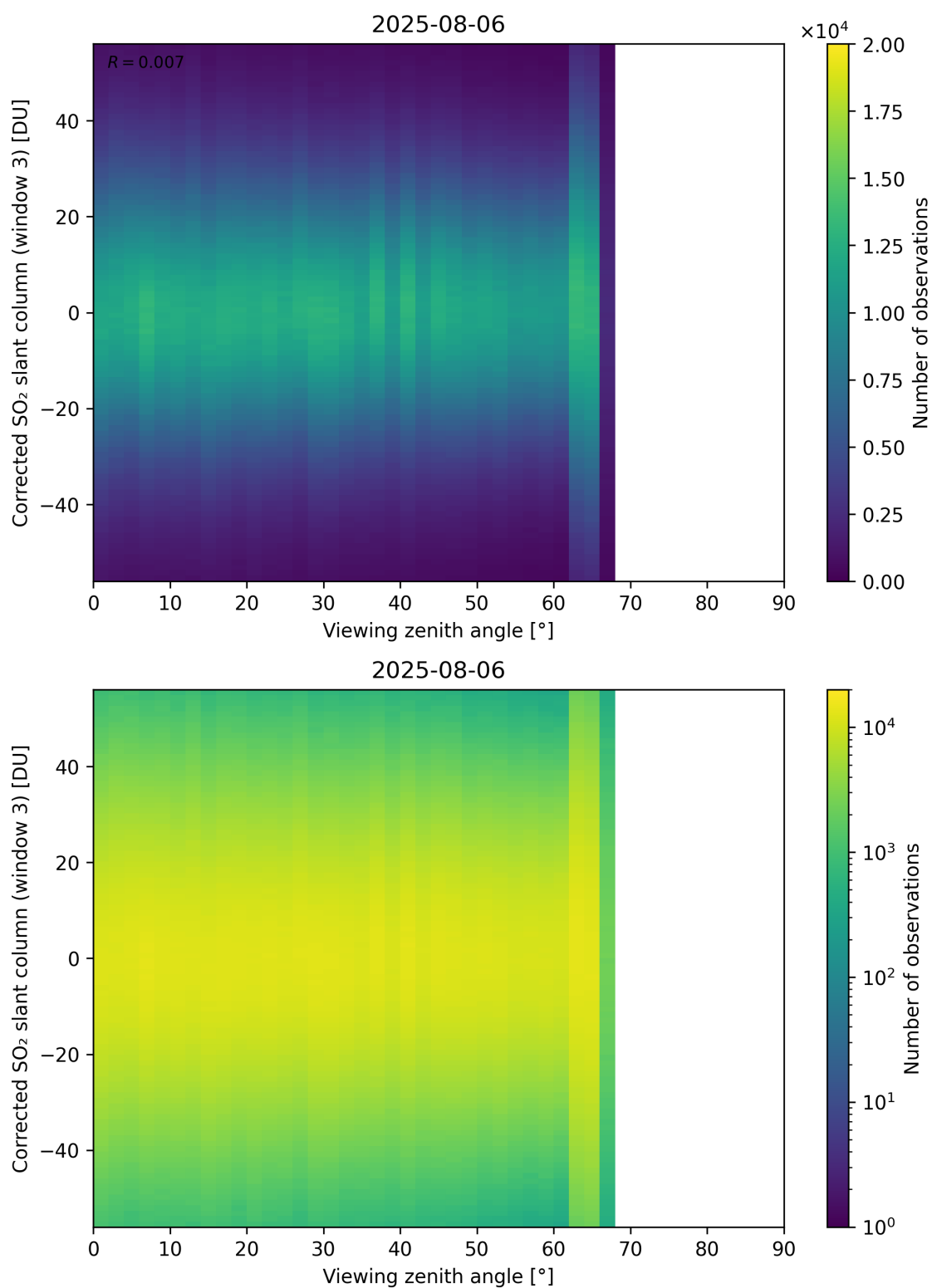
Figure 375: Scatter density plot of “Viewing zenith angle” against “Corrected SO 2 slant column (window 3)” for 2025-08-05 to 2025-08-07.
