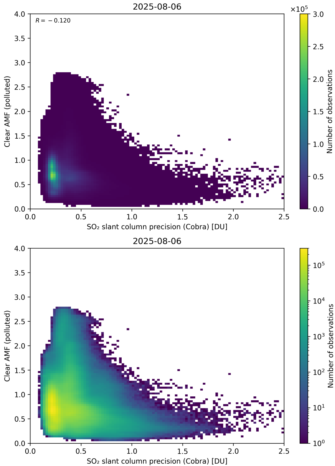
Figure 205: Scatter density plot of “SO 2 slant column precision (Cobra)” against “Clear AMF (polluted)” for 2025-08-05 to 2025-08-07.
