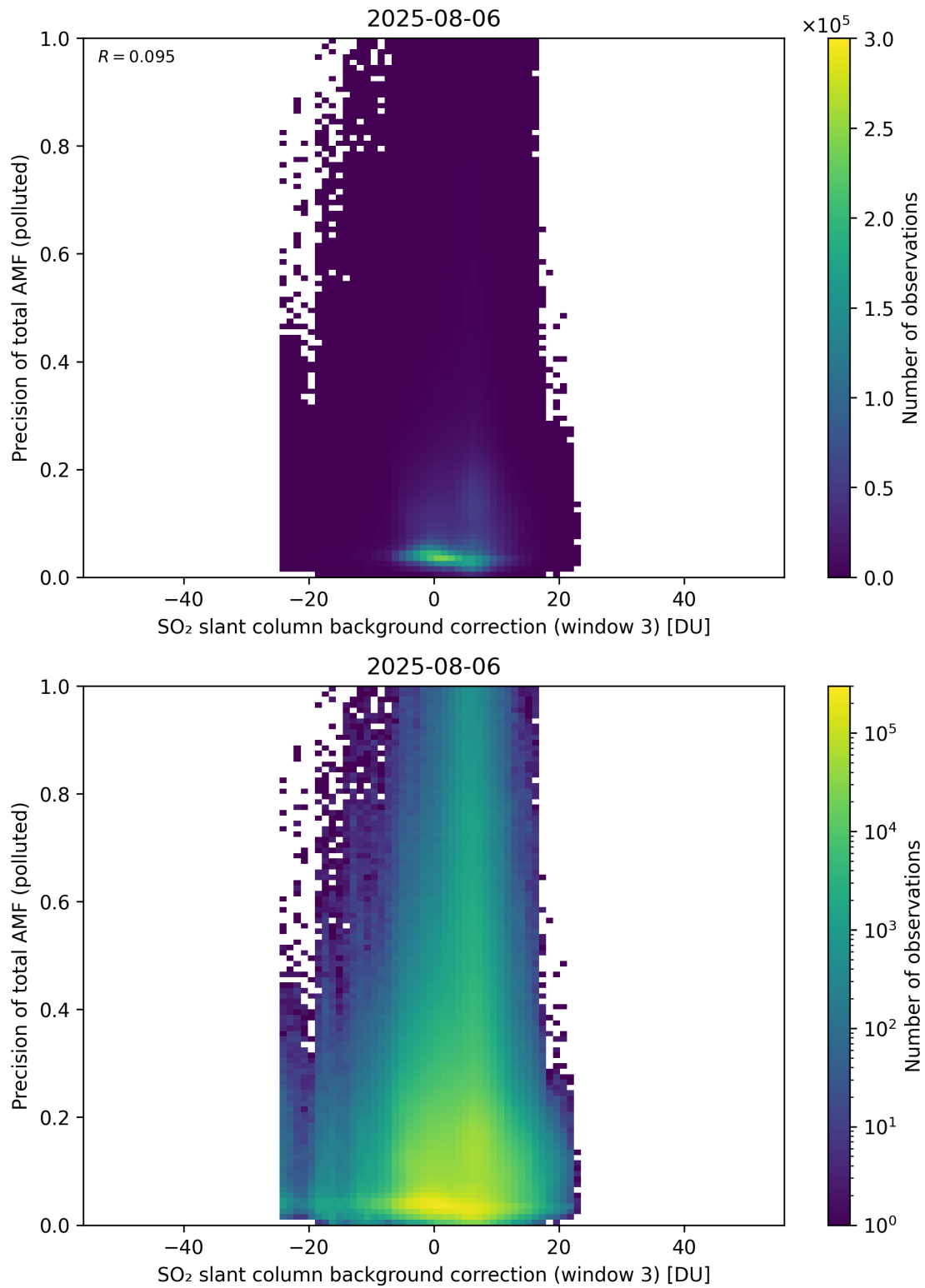
Figure 137: Scatter density plot of “SO 2 slant column background correction (window 3)” against “Precision of total AMF (polluted)” for 2025-08-05 to 2025-08-07.
