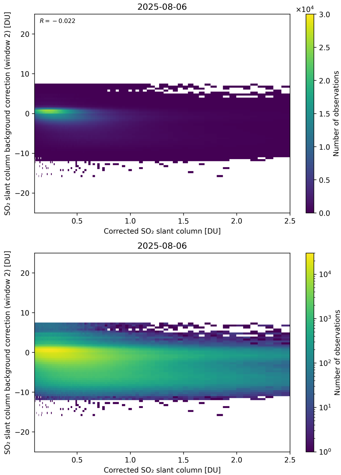
Figure 227: Scatter density plot of “Corrected SO 2 slant column” against “SO 2 slant column background correction (window 2)” for 2025-08-05 to 2025-08-07.
