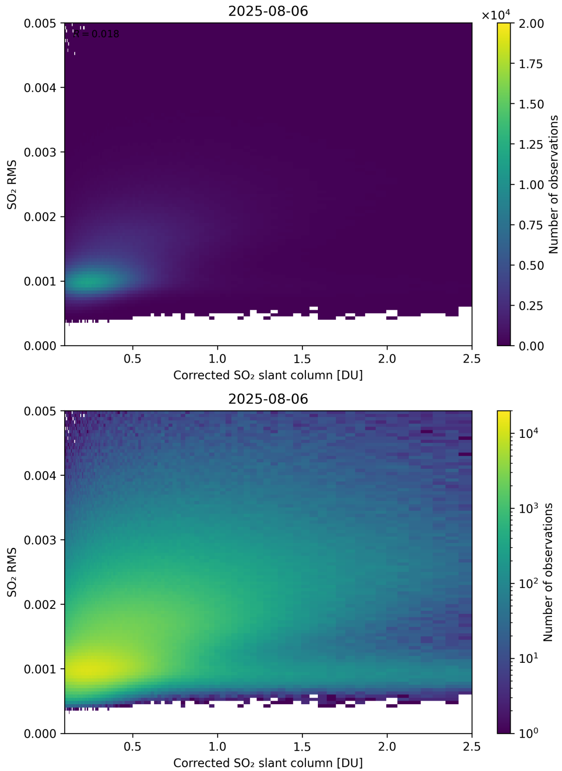
Figure 231: Scatter density plot of “Corrected SO 2 slant column” against “SO 2 RMS” for 2025-08-05 to 2025-08-07.
