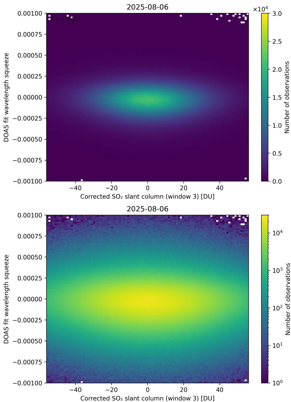
Figure 257: Scatter density plot of “Corrected SO 2 slant column (window 3)” against “DOAS fit wavelength squeeze” for 2025-08-05 to 2025-08-07.
