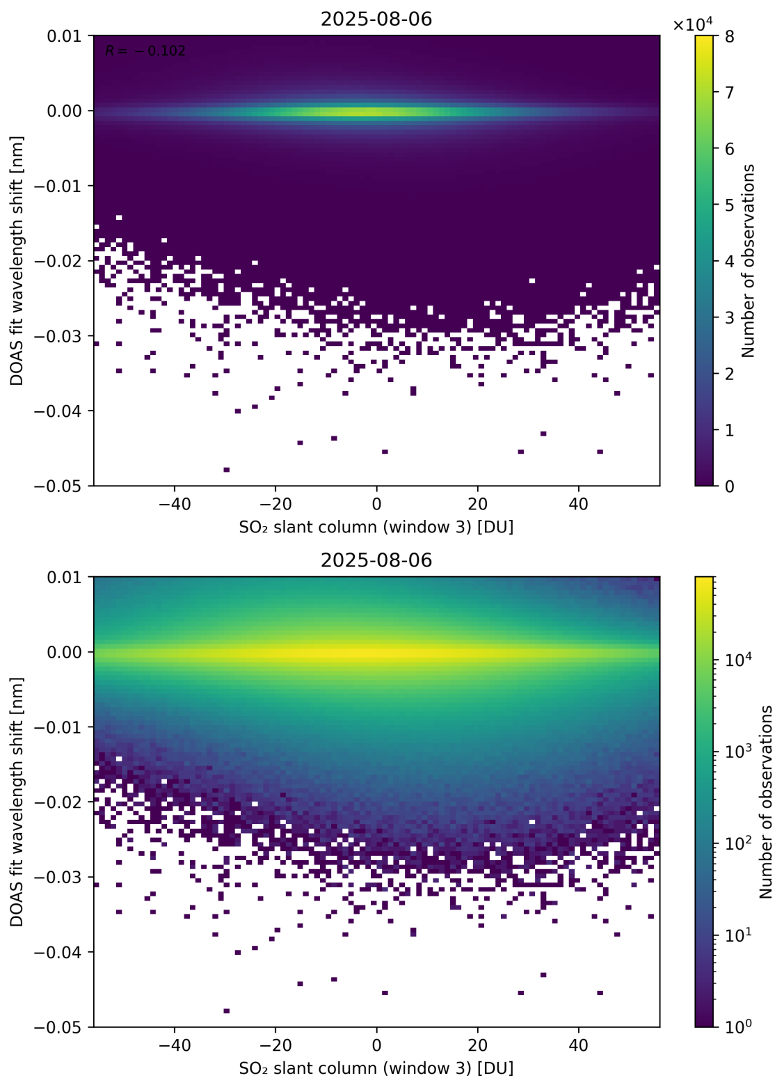
Figure 304: Scatter density plot of “SO 2 slant column (window 3)” against “DOAS fit wavelength shift” for 2025-08-05 to 2025-08-07.
