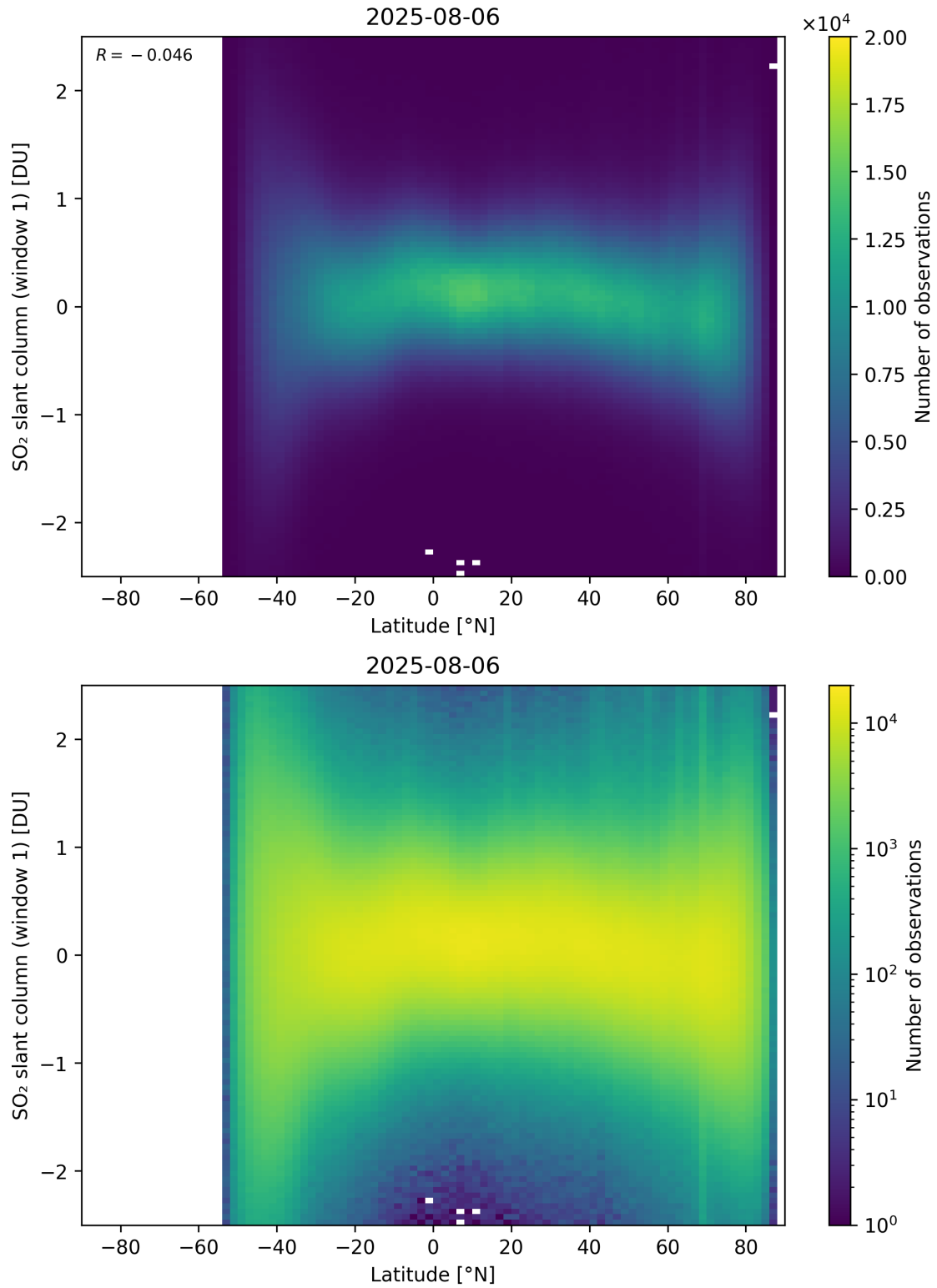
Figure 162: Scatter density plot of “Latitude” against “SO 2 slant column (window 1)” for 2025-08-05 to 2025-08-07.
