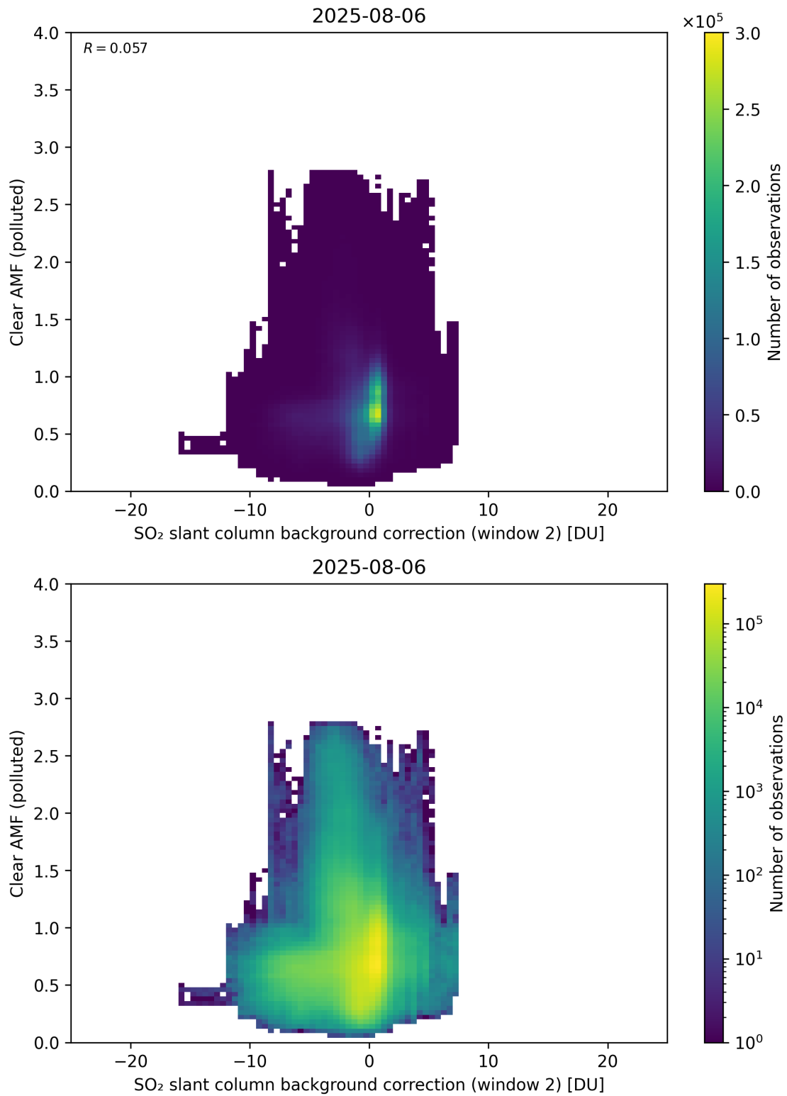
Figure 126: Scatter density plot of “SO 2 slant column background correction (window 2)” against “Clear AMF (polluted)” for 2025-08-05 to 2025-08-07.
