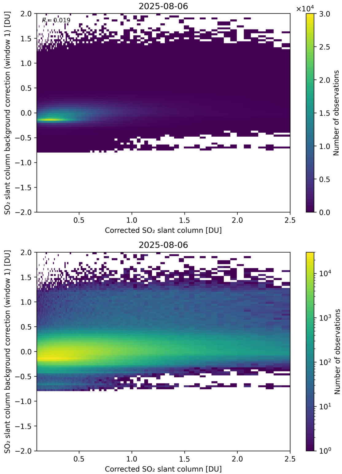
Figure 226: Scatter density plot of “Corrected SO 2 slant column” against “SO 2 slant column background correction (window 1)” for 2025-08-05 to 2025-08-07.
