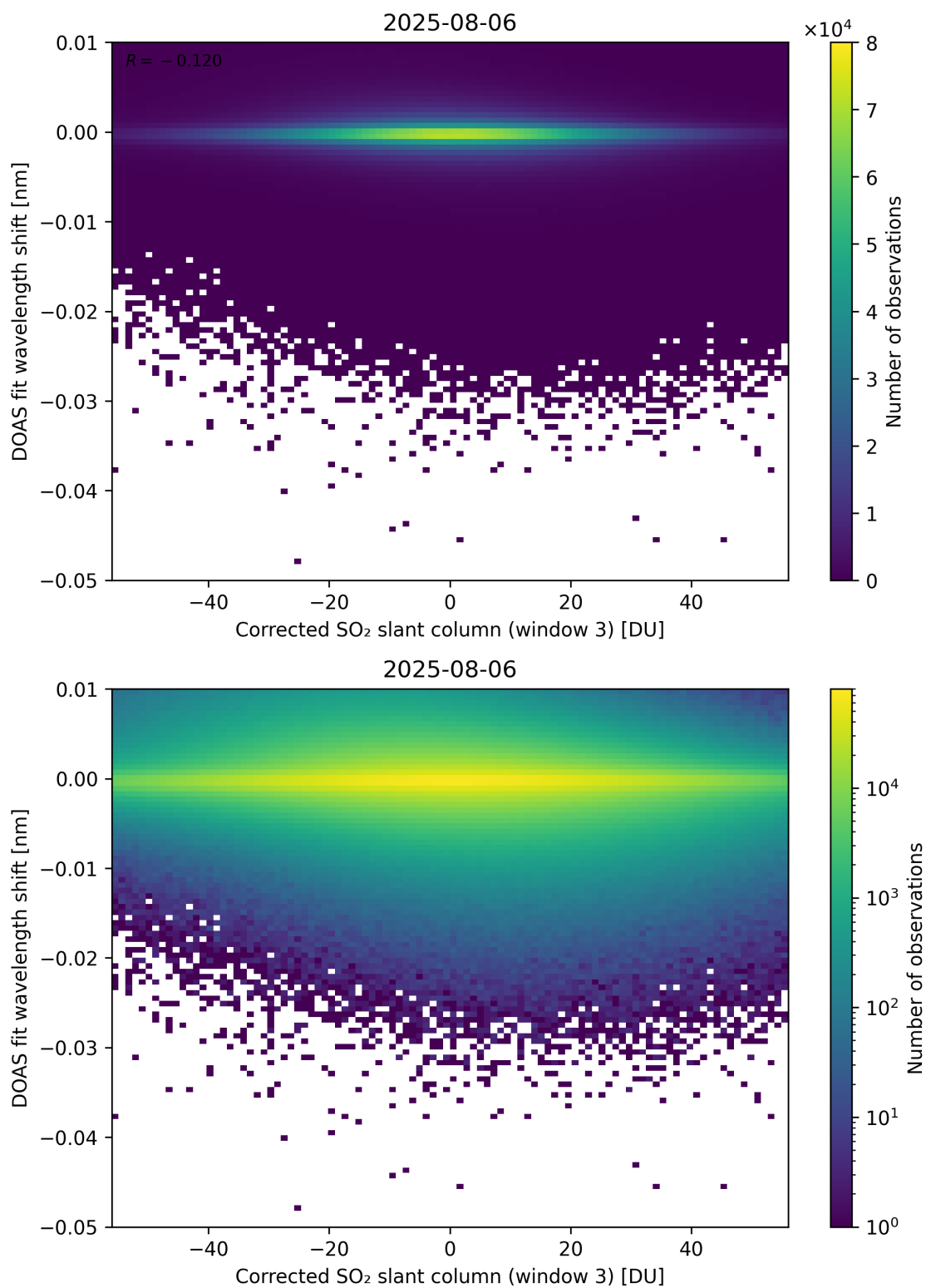
Figure 256: Scatter density plot of “Corrected SO 2 slant column (window 3)” against “DOAS fit wavelength shift” for 2025-08-05 to 2025-08-07.
