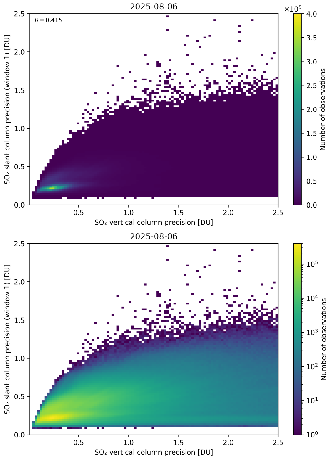
Figure 342: Scatter density plot of “SO 2 vertical column precision” against “SO 2 slant column precision (window 1)” for 2025-08-05 to 2025-08-07.
