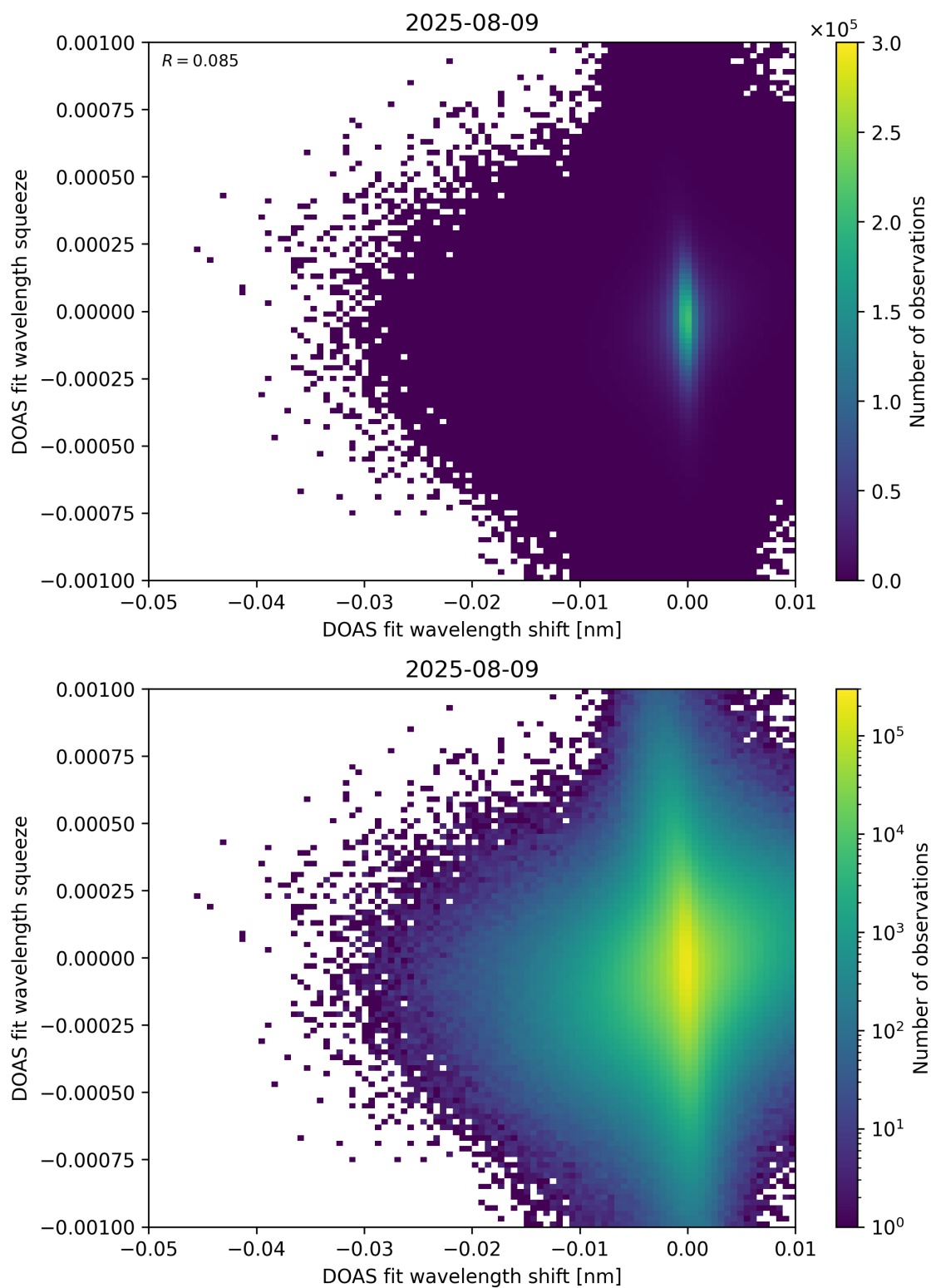
Figure 138: Scatter density plot of “DOAS fit wavelength shift” against “DOAS fit wavelength squeeze” for 2025-08-09 to 2025-08-10.
