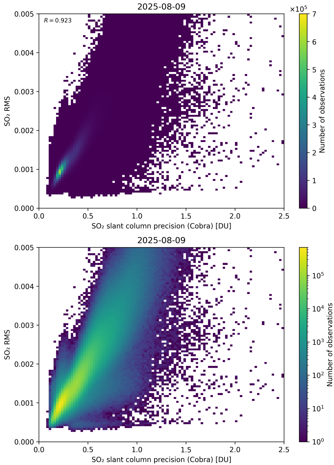
Figure 204: Scatter density plot of “SO 2 slant column precision (Cobra)” against “SO 2 RMS” for 2025-08-09 to 2025-08-10.
