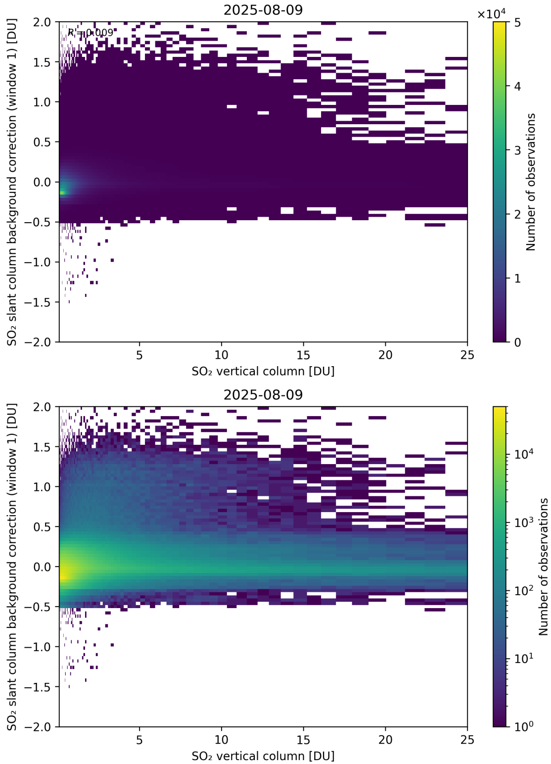
Figure 323: Scatter density plot of “SO 2 vertical column” against “SO 2 slant column background correction (window 1)” for 2025-08-09 to 2025-08-10.
