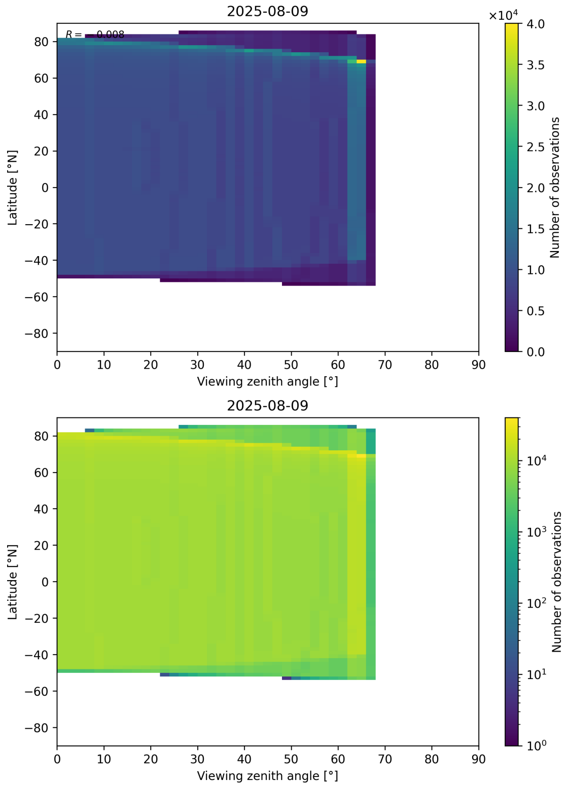
Figure 368: Scatter density plot of “Viewing zenith angle” against “Latitude” for 2025-08-09 to 2025-08-10.
