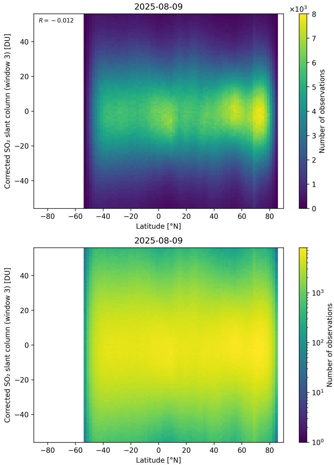
Figure 161: Scatter density plot of “Latitude” against “Corrected SO 2 slant column (window 3)” for 2025-08-09 to 2025-08-10.
