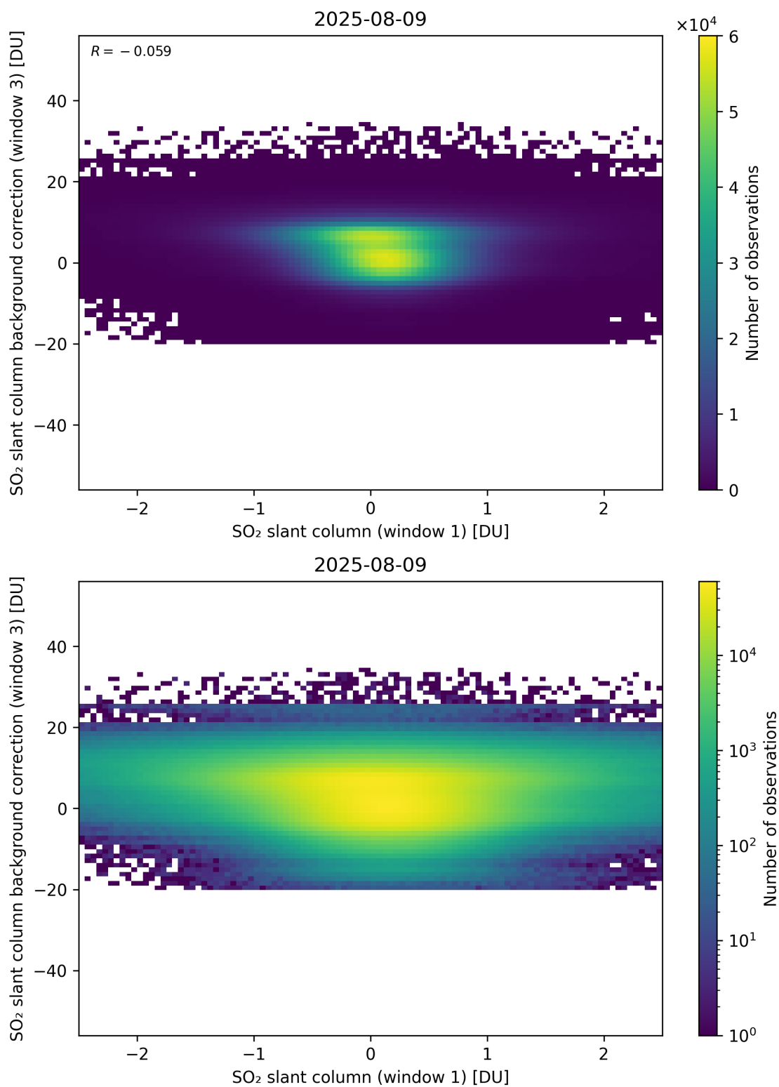
Figure 264: Scatter density plot of “SO 2 slant column (window 1)” against “SO 2 slant column background correction (window 3)” for 2025-08-09 to 2025-08-10.
