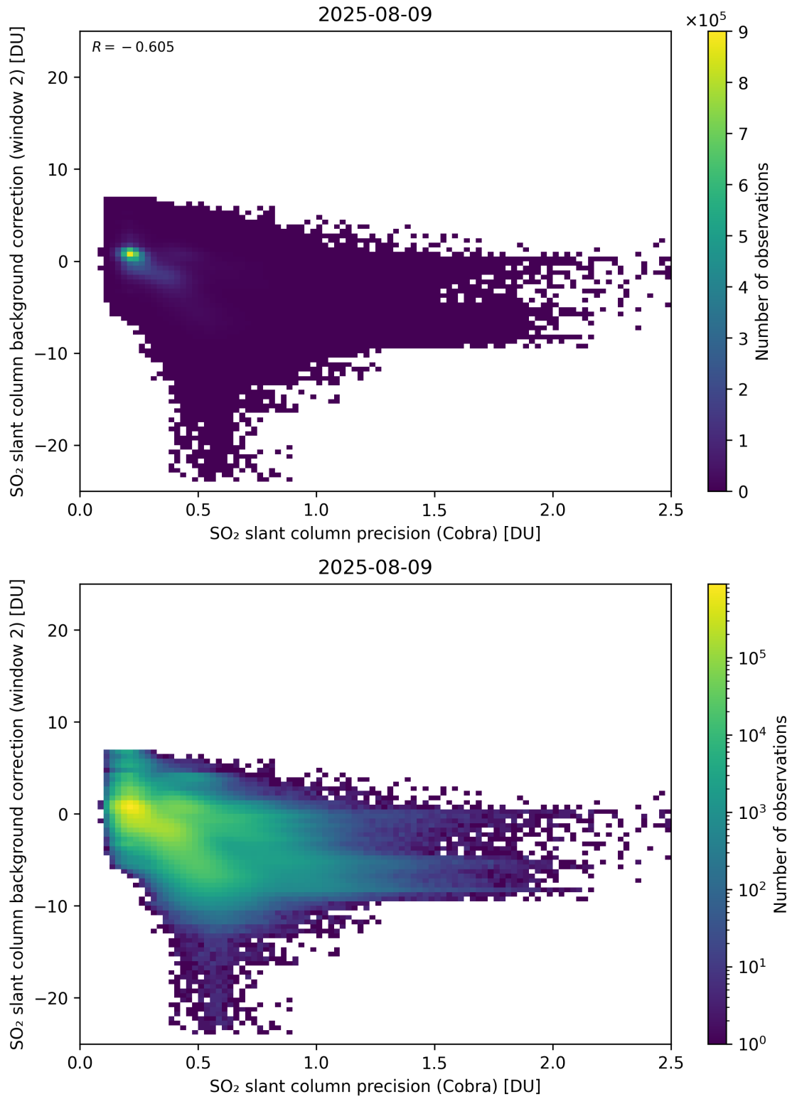
Figure 200: Scatter density plot of “SO 2 slant column precision (Cobra)” against “SO 2 slant column background correction (window 2)” for 2025-08-09 to 2025-08-10.
