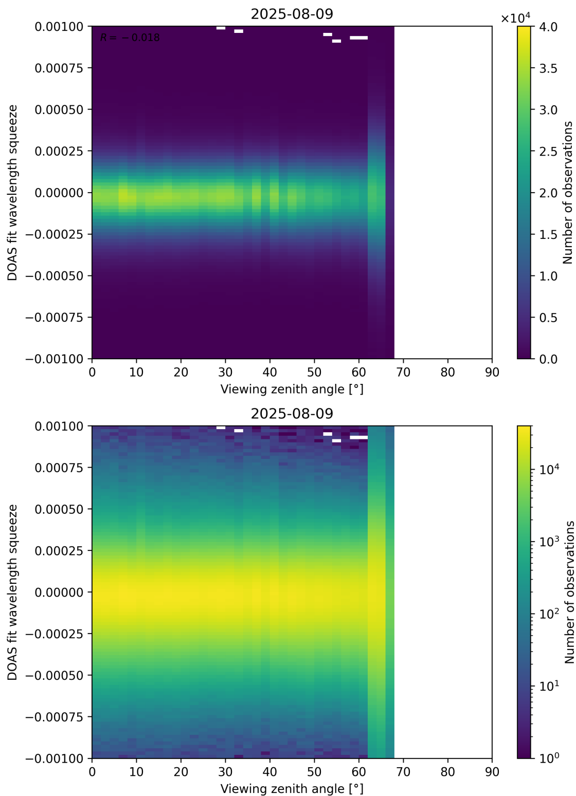
Figure 366: Scatter density plot of “Viewing zenith angle” against “DOAS fit wavelength squeeze” for 2025-08-09 to 2025-08-10.
