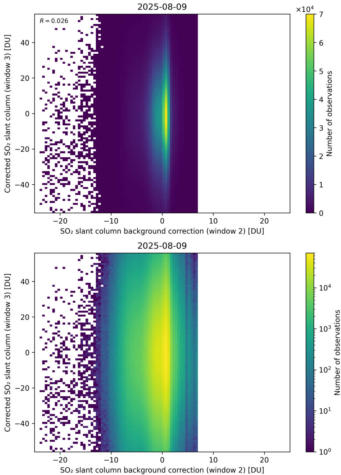
Figure 127: Scatter density plot of “SO 2 slant column background correction (window 2)” against “Corrected SO 2 slant column (window 3)” for 2025-08-09 to 2025-08-10.
