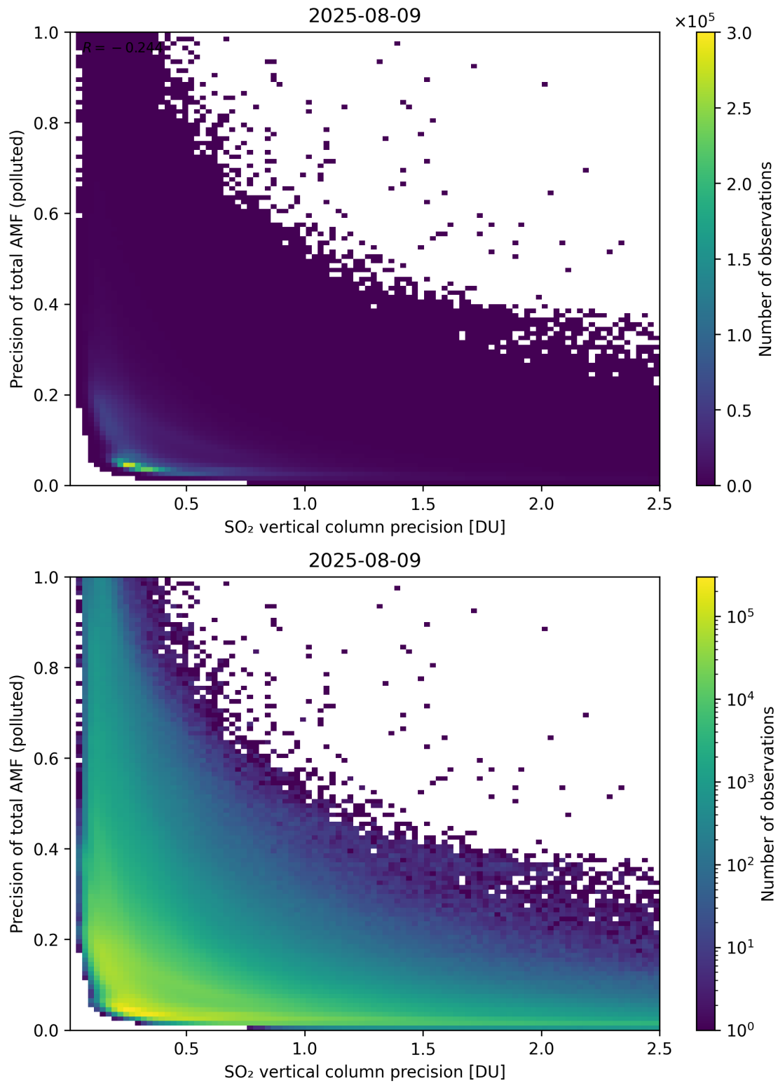
Figure 347: Scatter density plot of “SO 2 vertical column precision” against “Precision of total AMF (polluted)” for 2025-08-09 to 2025-08-10.
