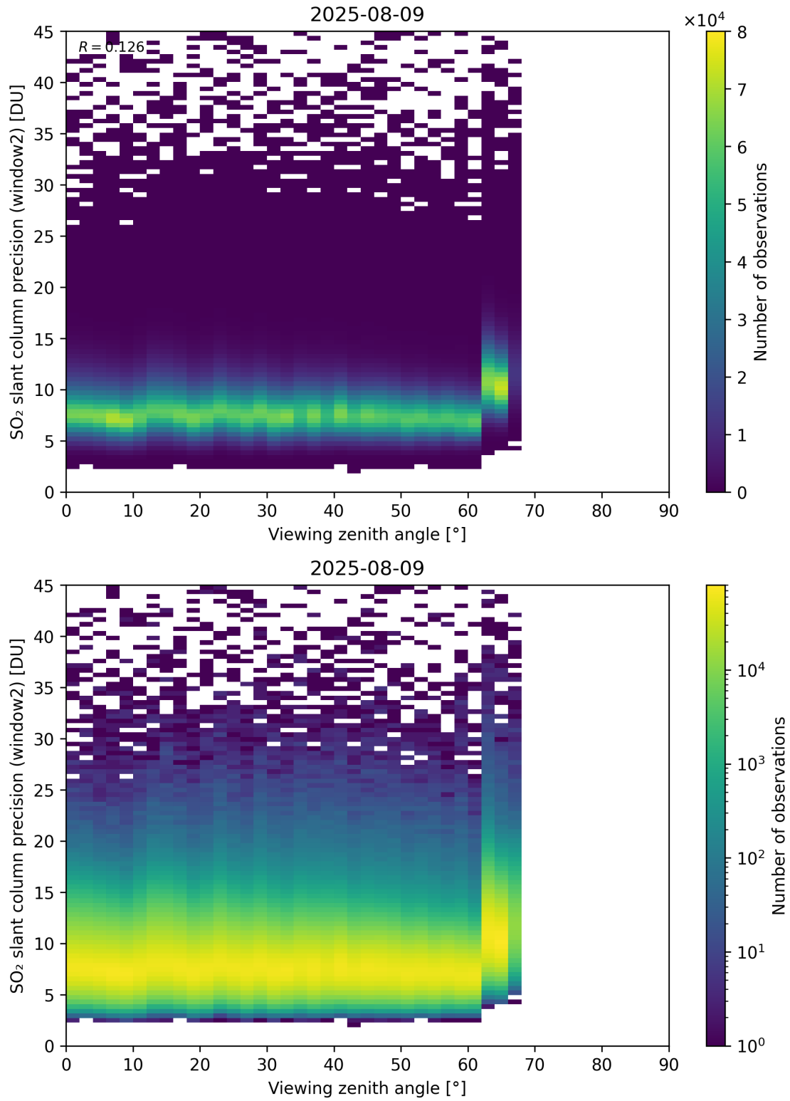
Figure 378: Scatter density plot of “Viewing zenith angle” against “SO 2 slant column precision (window2)” for 2025-08-09 to 2025-08-10.
