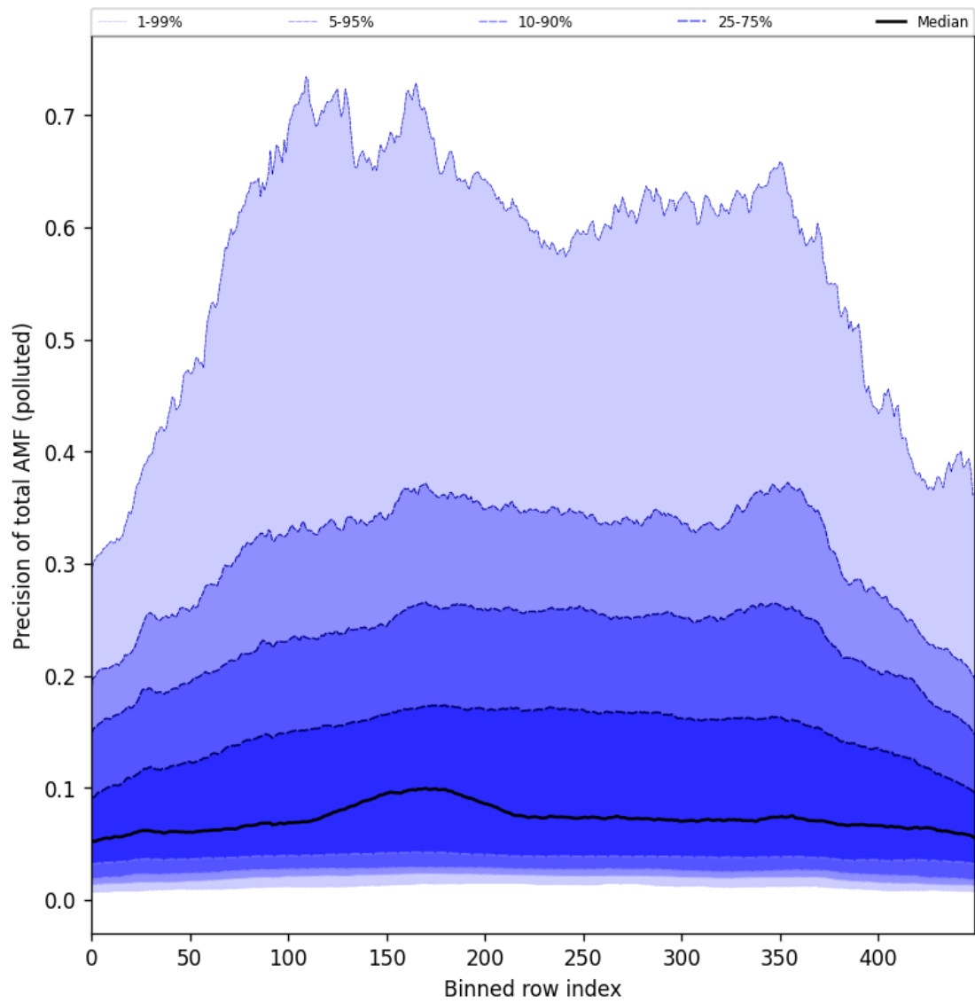
Figure 106: Along track statistics of “Precision of total AMF (polluted)” for 2025-08-09 to 2025-08-10
