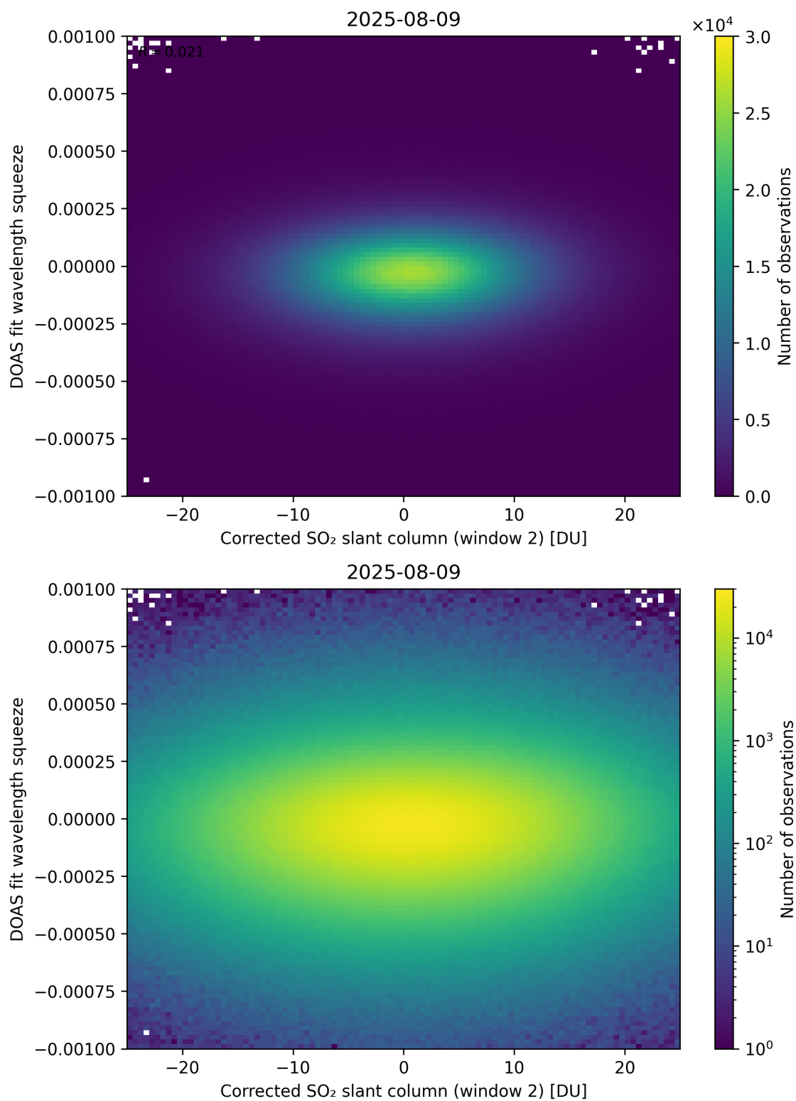
Figure 247: Scatter density plot of “Corrected SO 2 slant column (window 2)” against “DOAS fit wavelength squeeze” for 2025-08-09 to 2025-08-10.
