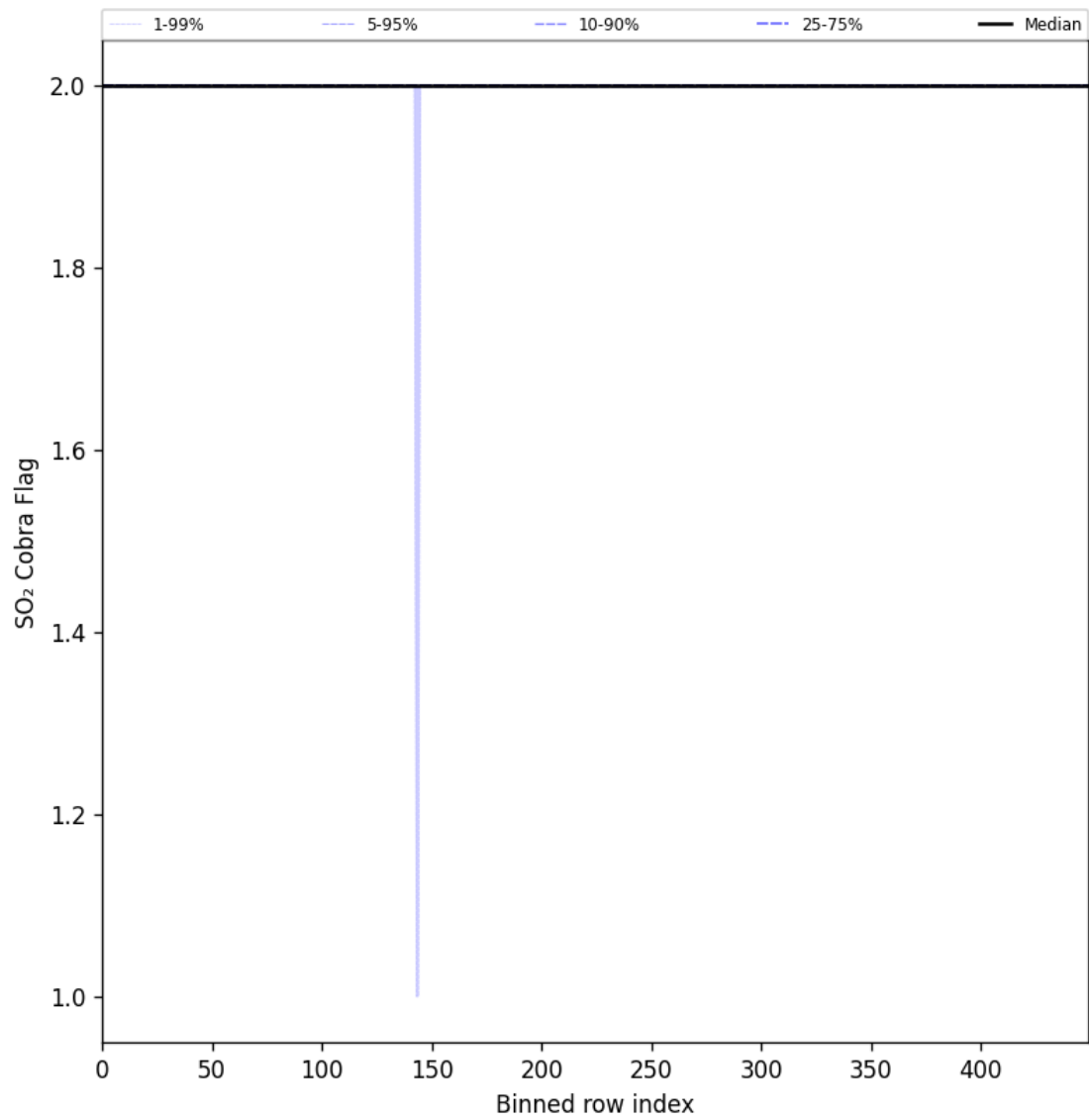
Figure 101: Along track statistics of “SO 2 Cobra Flag” for 2025-08-09 to 2025-08-10
