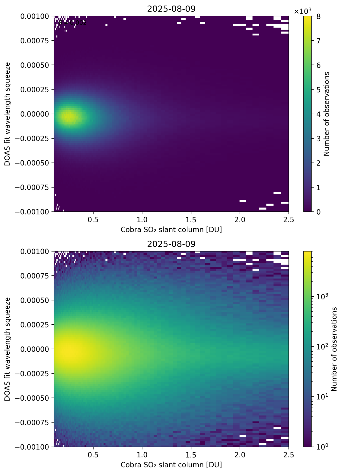
Figure 197: Scatter density plot of “Cobra SO 2 slant column” against “DOAS fit wavelength squeeze” for 2025-08-09 to 2025-08-10.
