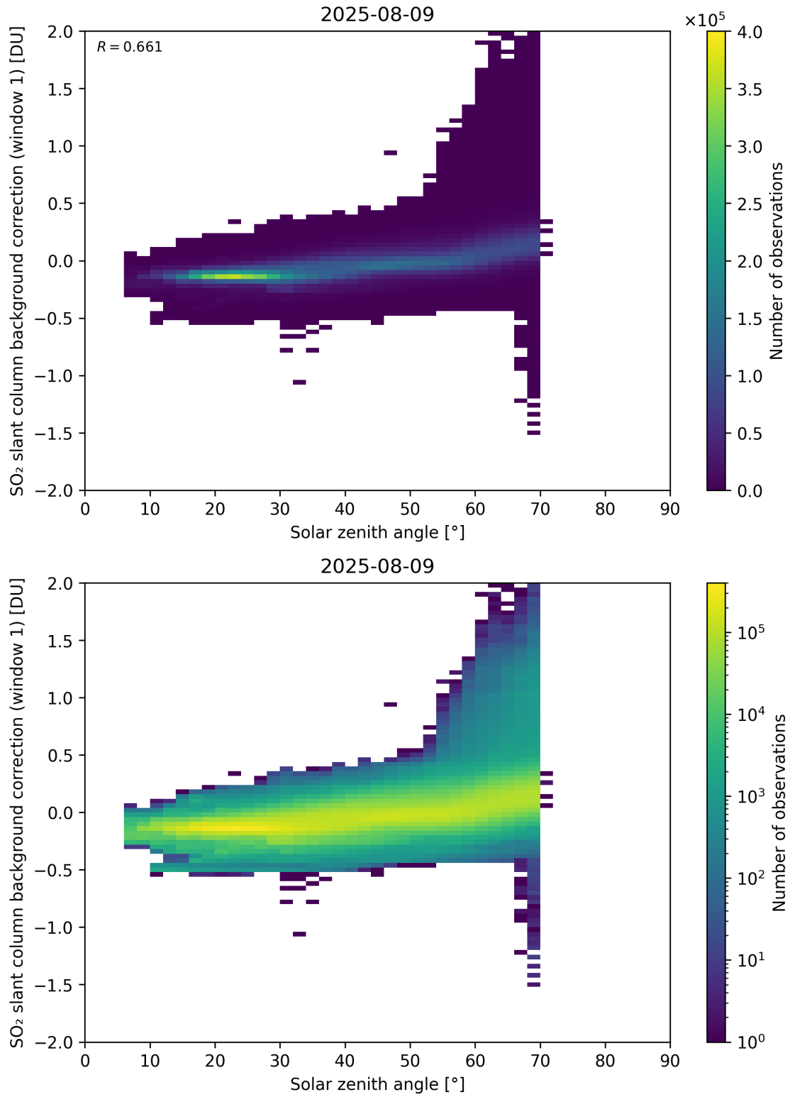
Figure 171: Scatter density plot of “Solar zenith angle” against “SO 2 slant column background correction (window 1)” for 2025-08-09 to 2025-08-10.
