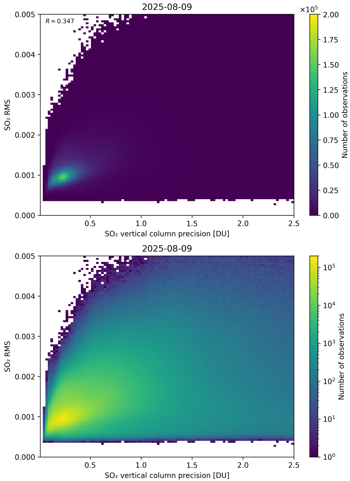
Figure 334: Scatter density plot of “SO 2 vertical column precision” against “SO 2 RMS” for 2025-08-09 to 2025-08-10.
