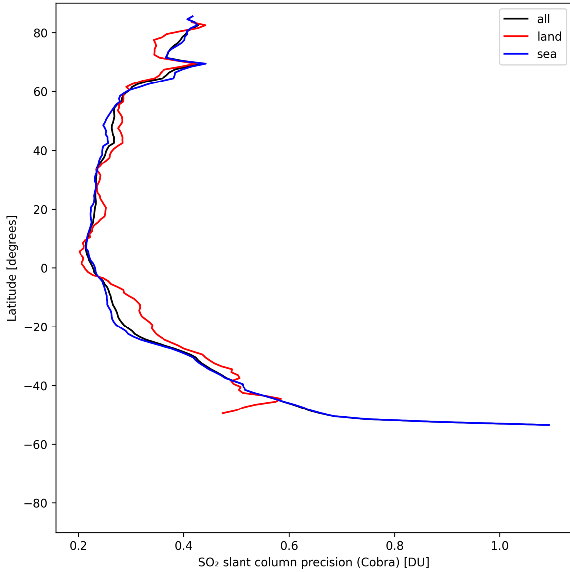
Figure 36: Zonal average of “SO 2 slant column precision (Cobra)” for 2025-08-09 to 2025-08-10.
