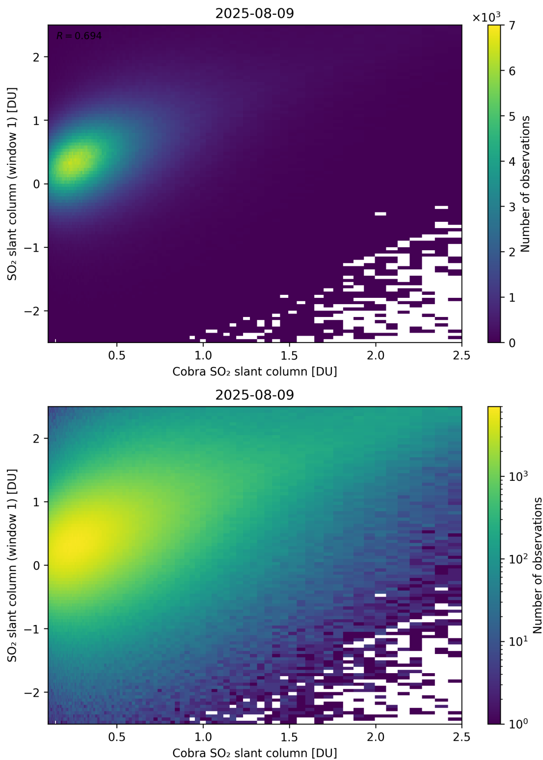
Figure 219: Scatter density plot of “Cobra SO 2 slant column” against “SO 2 slant column (window 1)” for 2025-08-09 to 2025-08-10.
