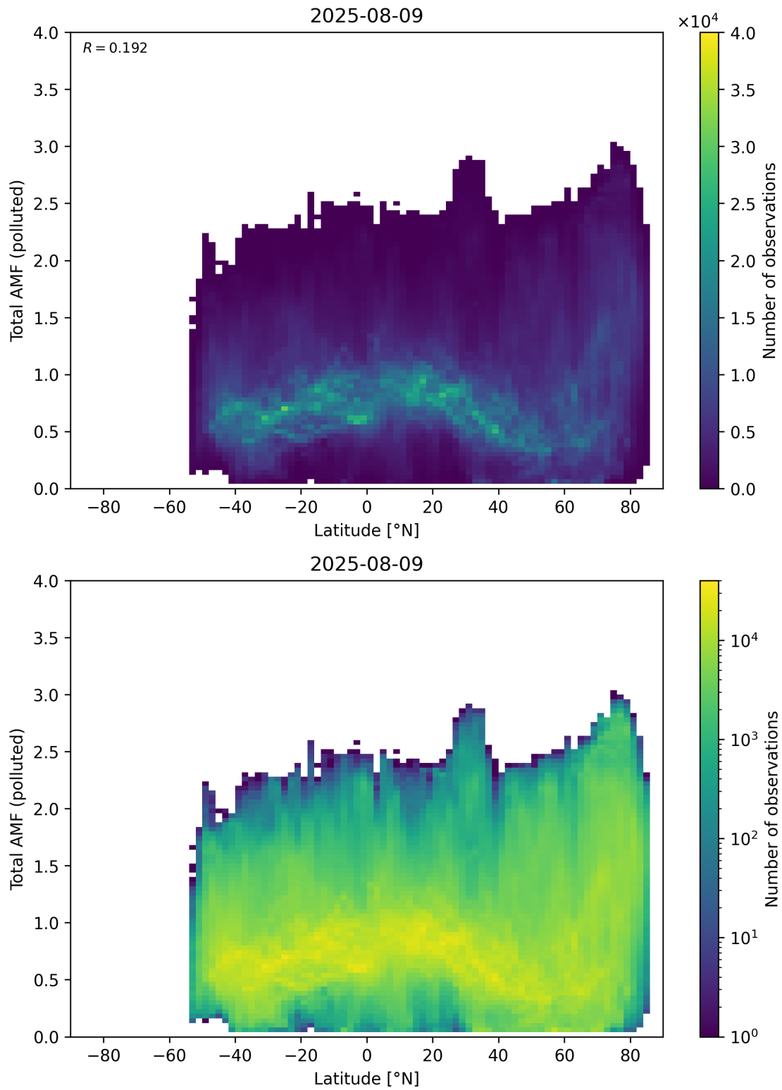
Figure 167: Scatter density plot of “Latitude” against “Total AMF (polluted)” for 2025-08-09 to 2025-08-10.
