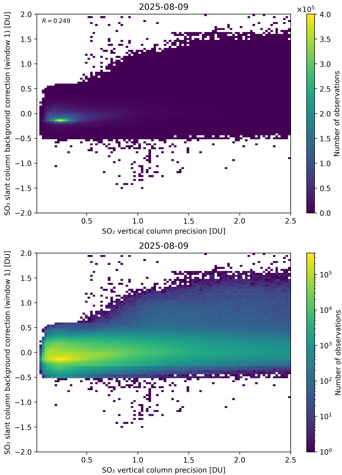
Figure 329: Scatter density plot of “SO 2 vertical column precision” against “SO 2 slant column background correction (window 1)” for 2025-08-09 to 2025-08-10.
