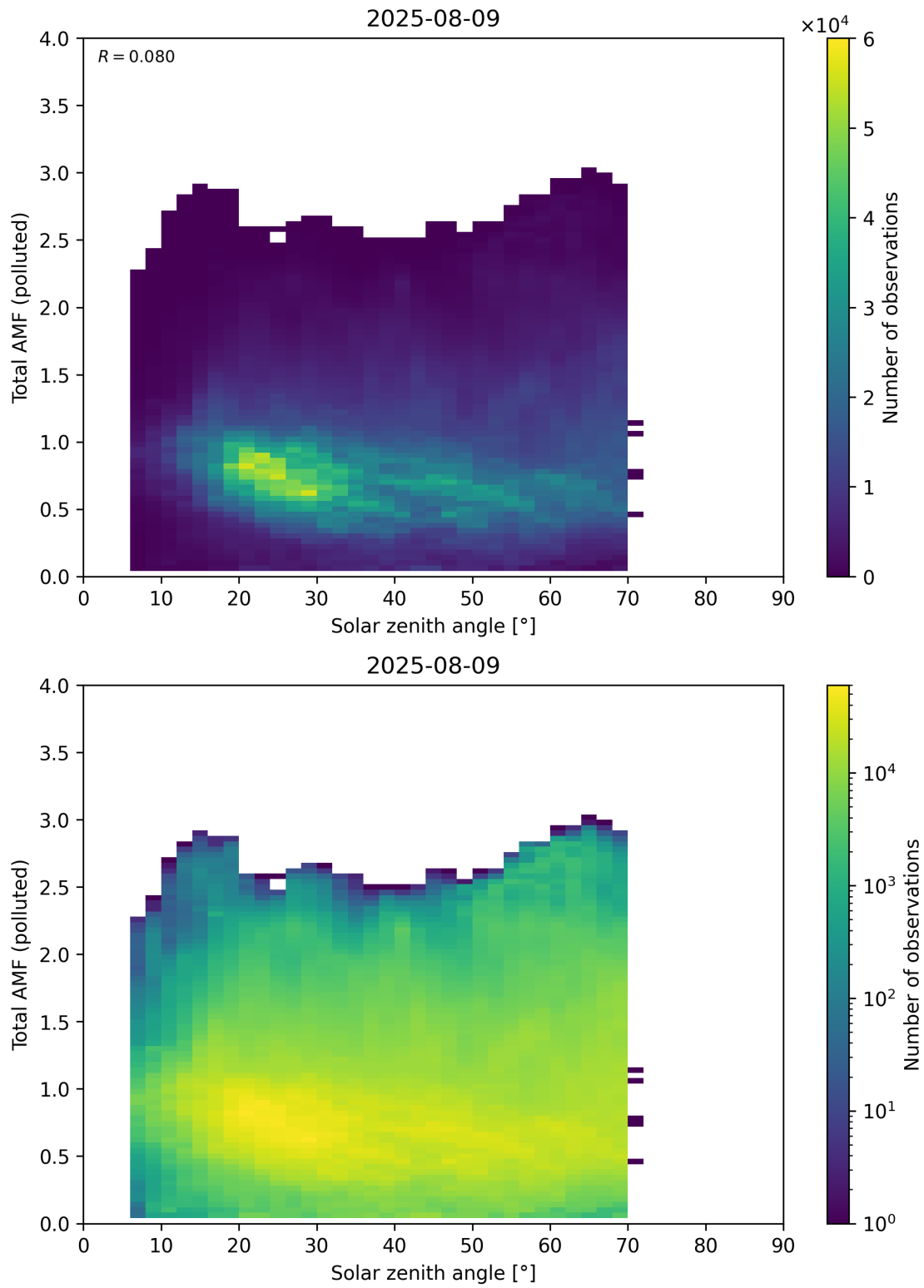
Figure 189: Scatter density plot of “Solar zenith angle” against “Total AMF (polluted)” for 2025-08-09 to 2025-08-10.
