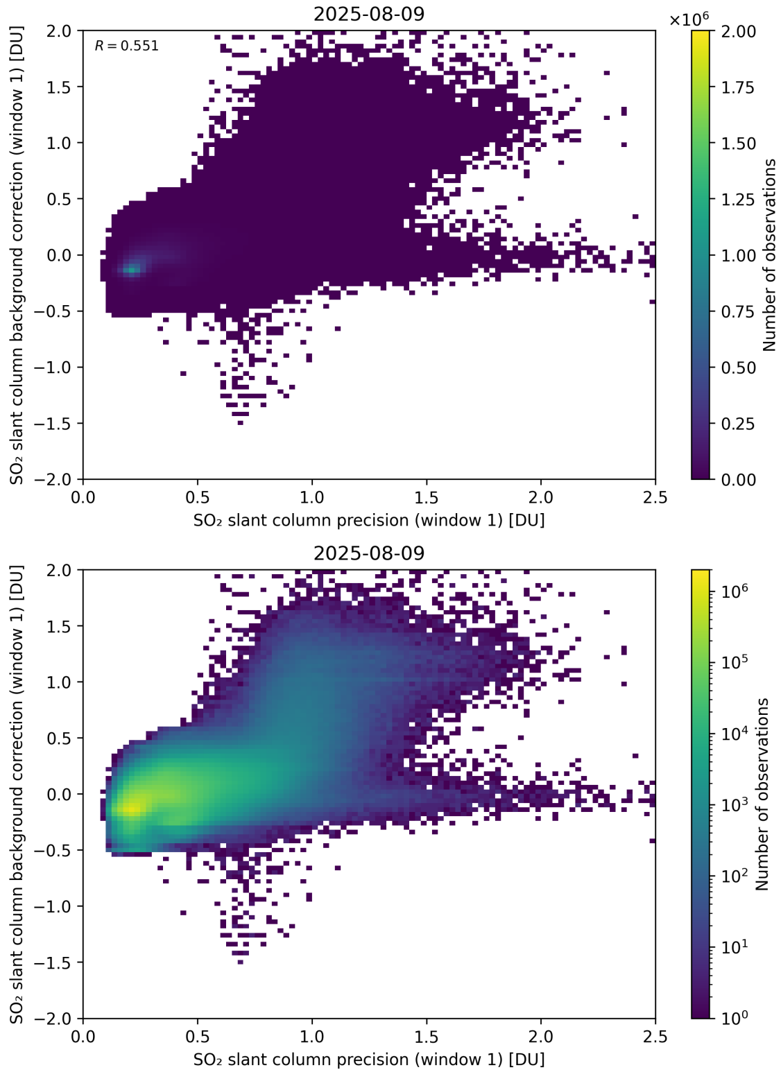
Figure 268: Scatter density plot of “SO 2 slant column precision (window 1)” against “SO 2 slant column background correction (window 1)” for 2025-08-09 to 2025-08-10.
