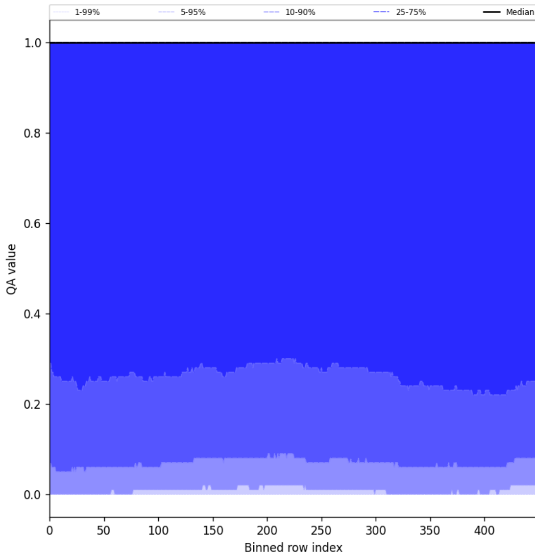
Figure 83: Along track statistics of “QA value” for 2025-08-09 to 2025-08-10
