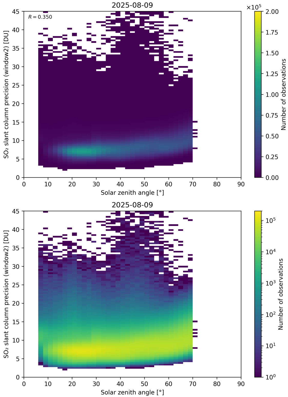
Figure 186: Scatter density plot of “Solar zenith angle” against “SO 2 slant column precision (window2)” for 2025-08-09 to 2025-08-10.
