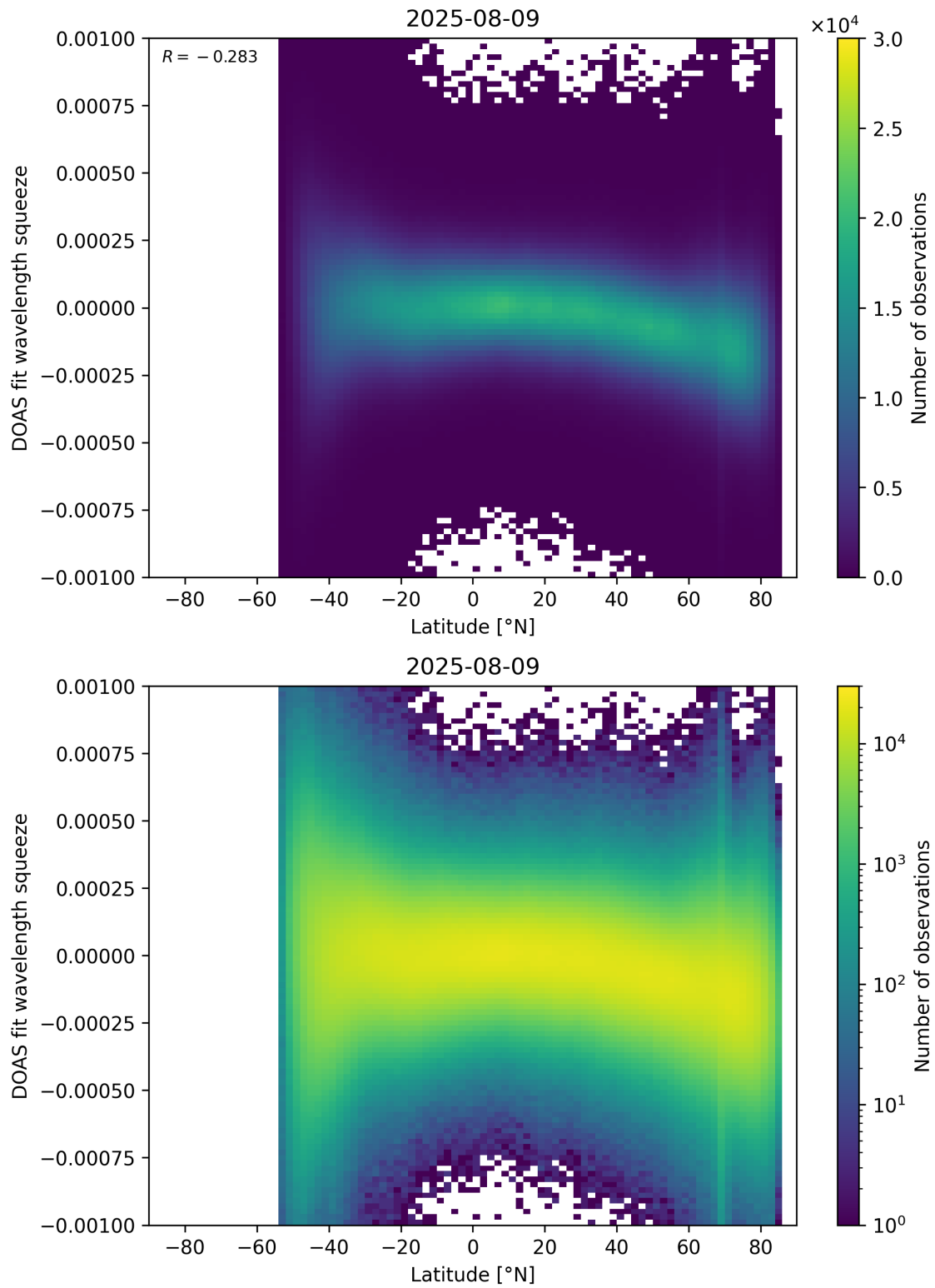
Figure 154: Scatter density plot of “Latitude” against “DOAS fit wavelength squeeze” for 2025-08-09 to 2025-08-10.
