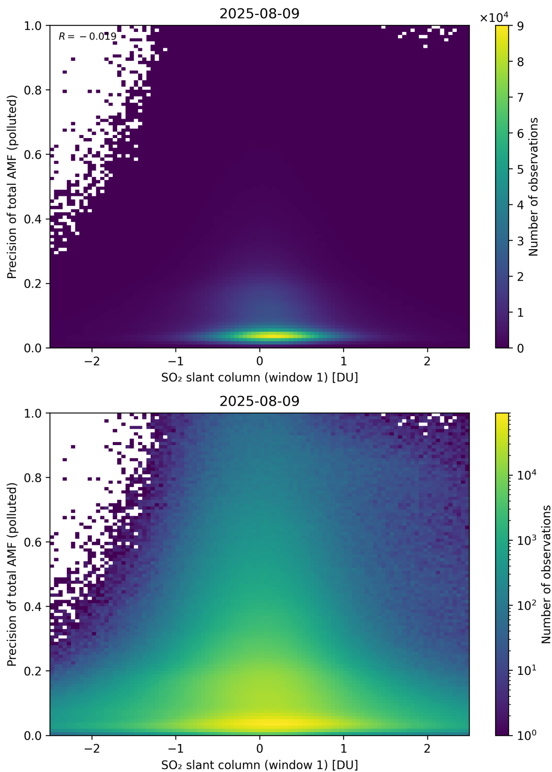
Figure 290: Scatter density plot of “SO 2 slant column (window 1)” against “Precision of total AMF (polluted)” for 2025-08-09 to 2025-08-10.
