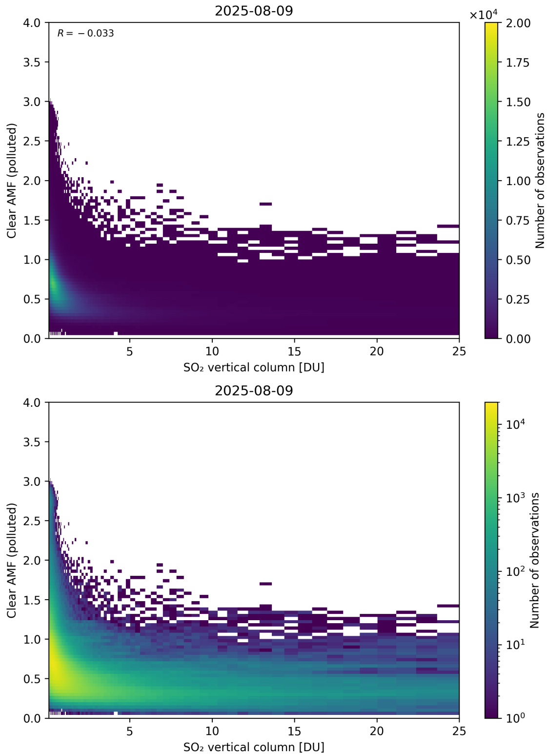
Figure 348: Scatter density plot of “SO 2 vertical column” against “Clear AMF (polluted)” for 2025-08-09 to 2025-08-10.
