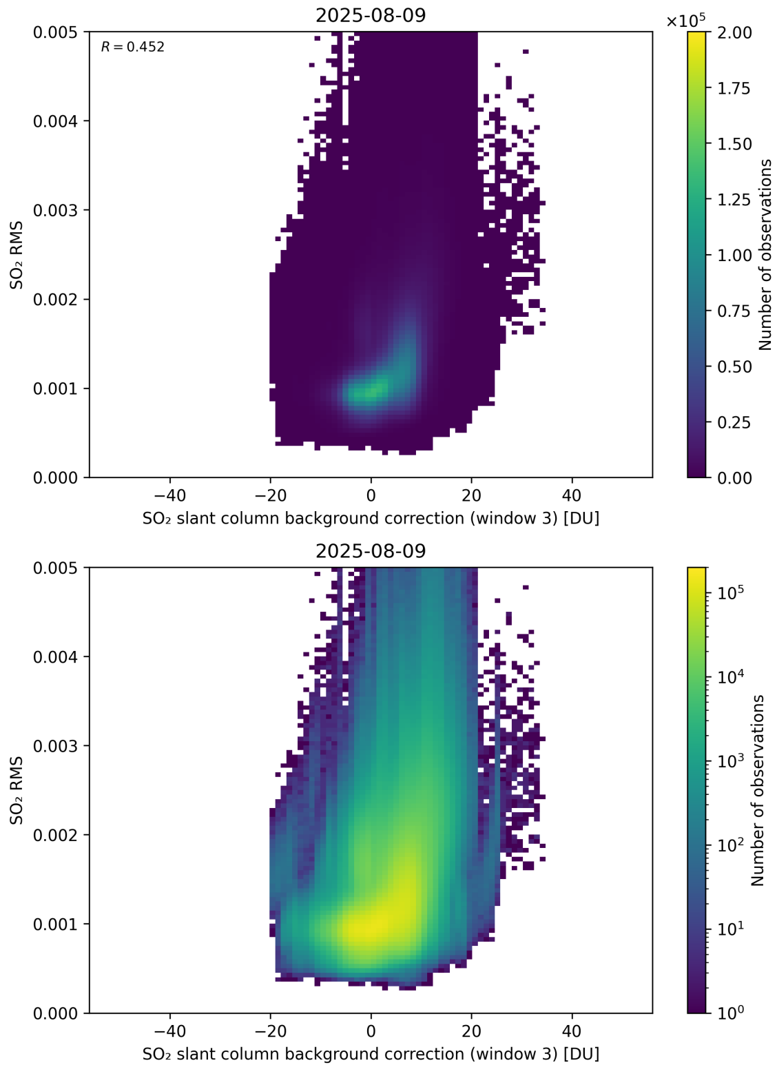
Figure 134: Scatter density plot of “SO 2 slant column background correction (window 3)” against “SO 2 RMS” for 2025-08-09 to 2025-08-10.
