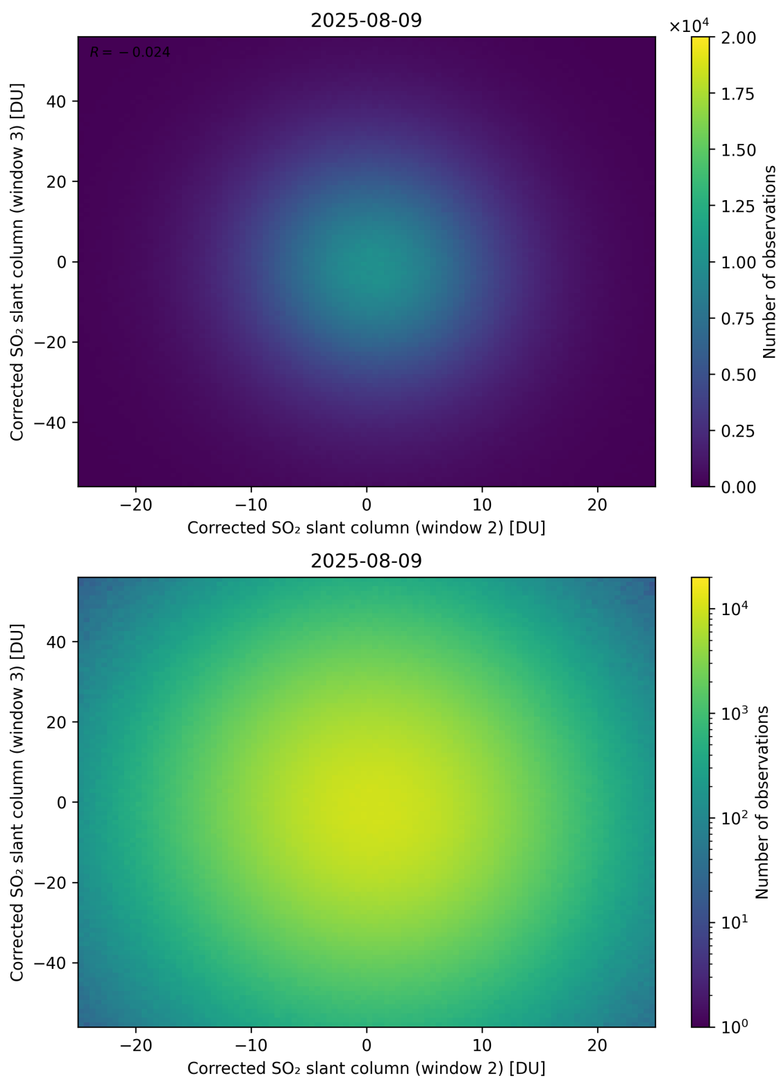
Figure 250: Scatter density plot of “Corrected SO 2 slant column (window 2)” against “Corrected SO 2 slant column (window 3)” for 2025-08-09 to 2025-08-10.
