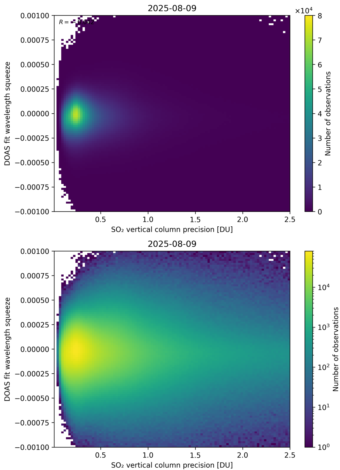
Figure 333: Scatter density plot of “SO 2 vertical column precision” against “DOAS fit wavelength squeeze” for 2025-08-09 to 2025-08-10.
