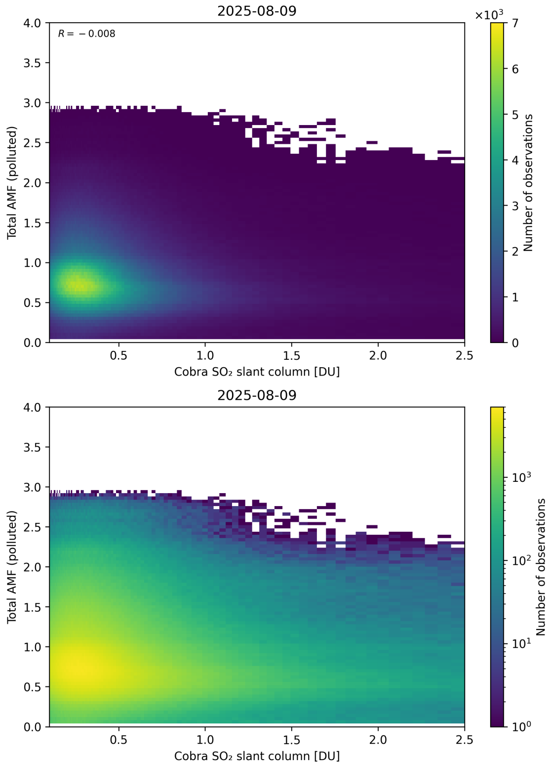
Figure 224: Scatter density plot of “Cobra SO 2 slant column” against “Total AMF (polluted)” for 2025-08-09 to 2025-08-10.
