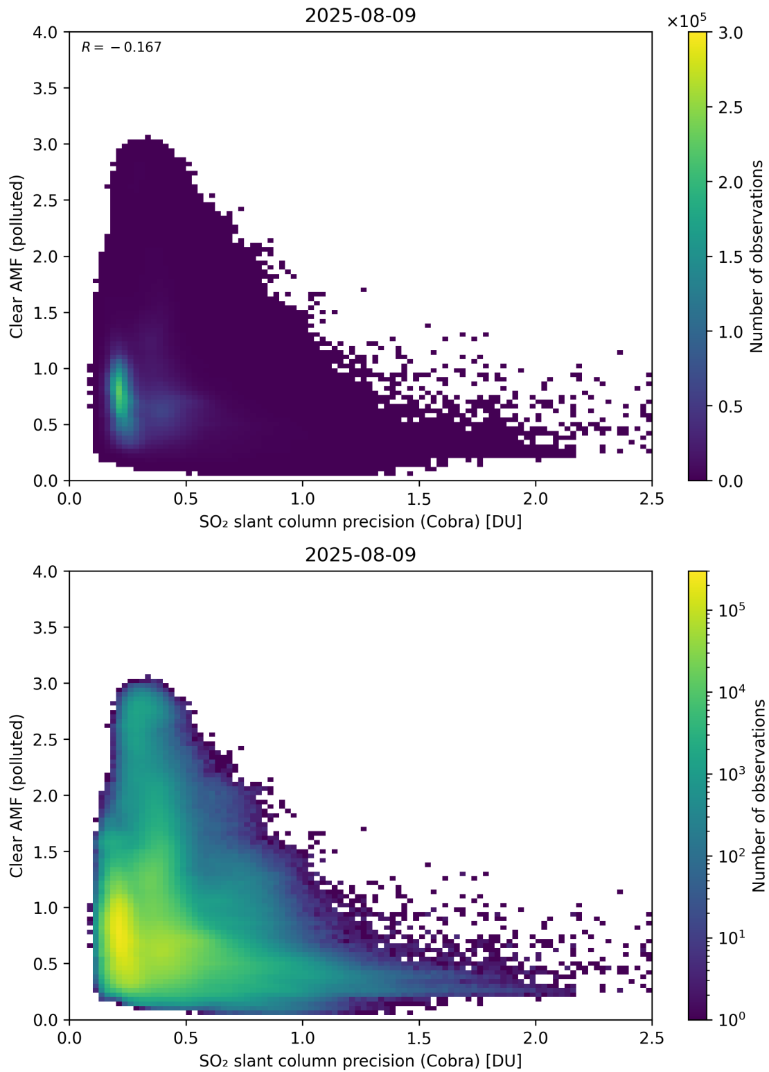
Figure 205: Scatter density plot of “SO 2 slant column precision (Cobra)” against “Clear AMF (polluted)” for 2025-08-09 to 2025-08-10.
