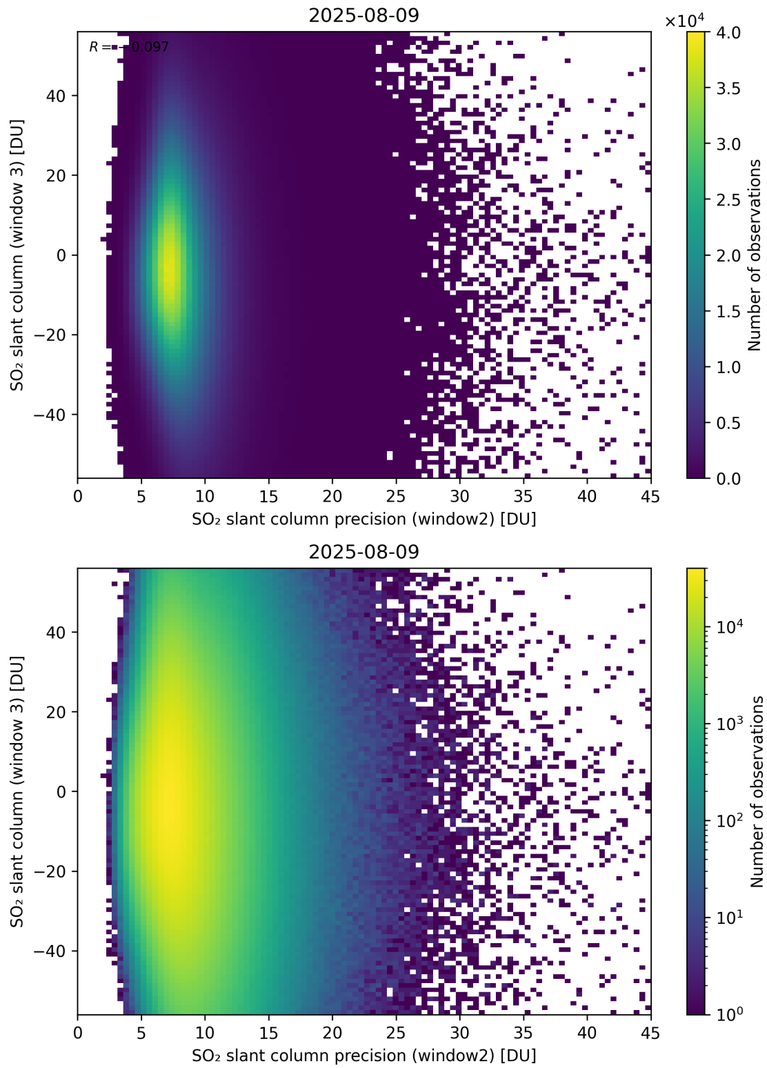
Figure 299: Scatter density plot of “SO 2 slant column precision (window2)” against “SO 2 slant column (window 3)” for 2025-08-09 to 2025-08-10.
