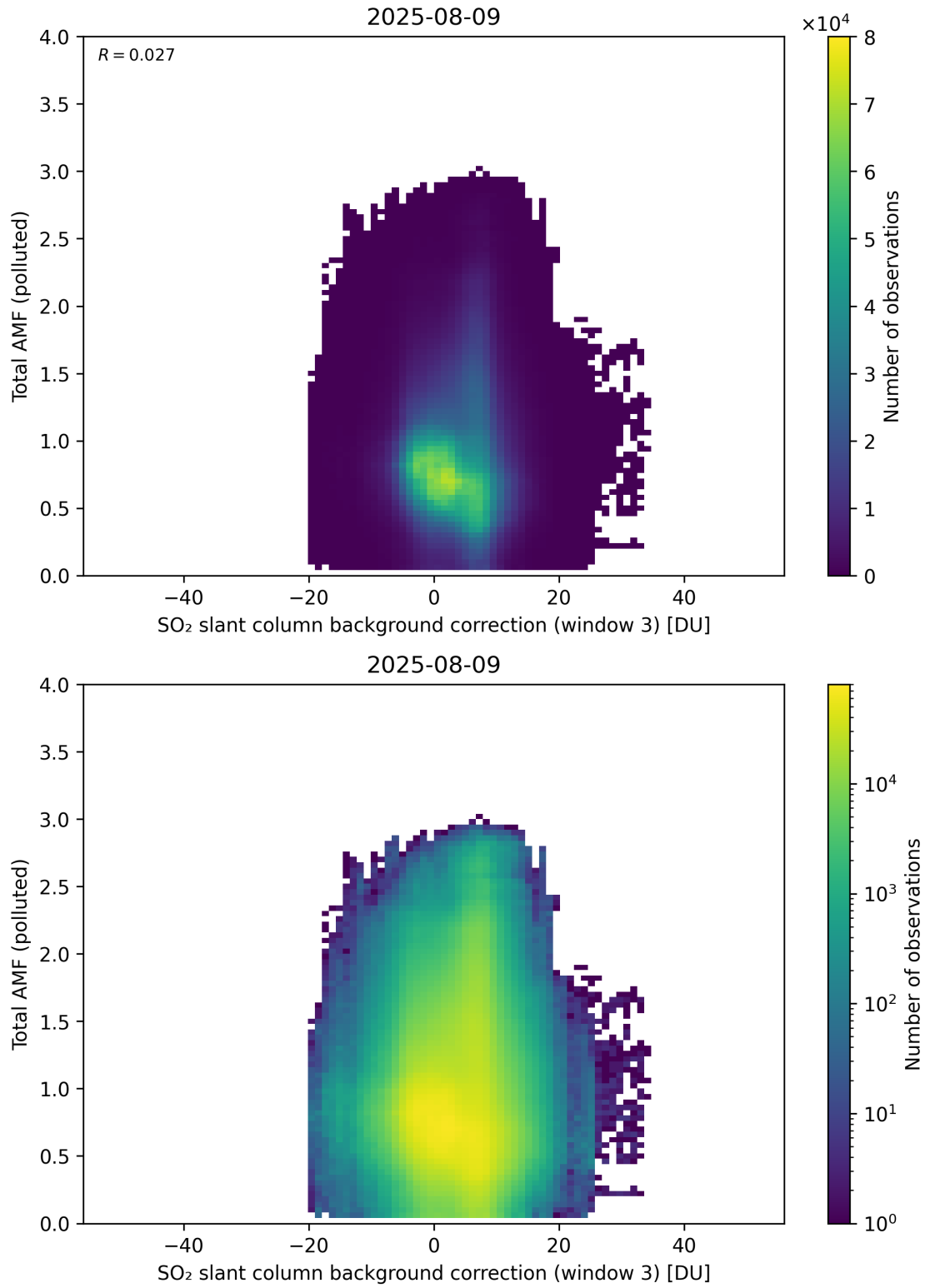
Figure 136: Scatter density plot of “SO 2 slant column background correction (window 3)” against “Total AMF (polluted)” for 2025-08-09 to 2025-08-10.
