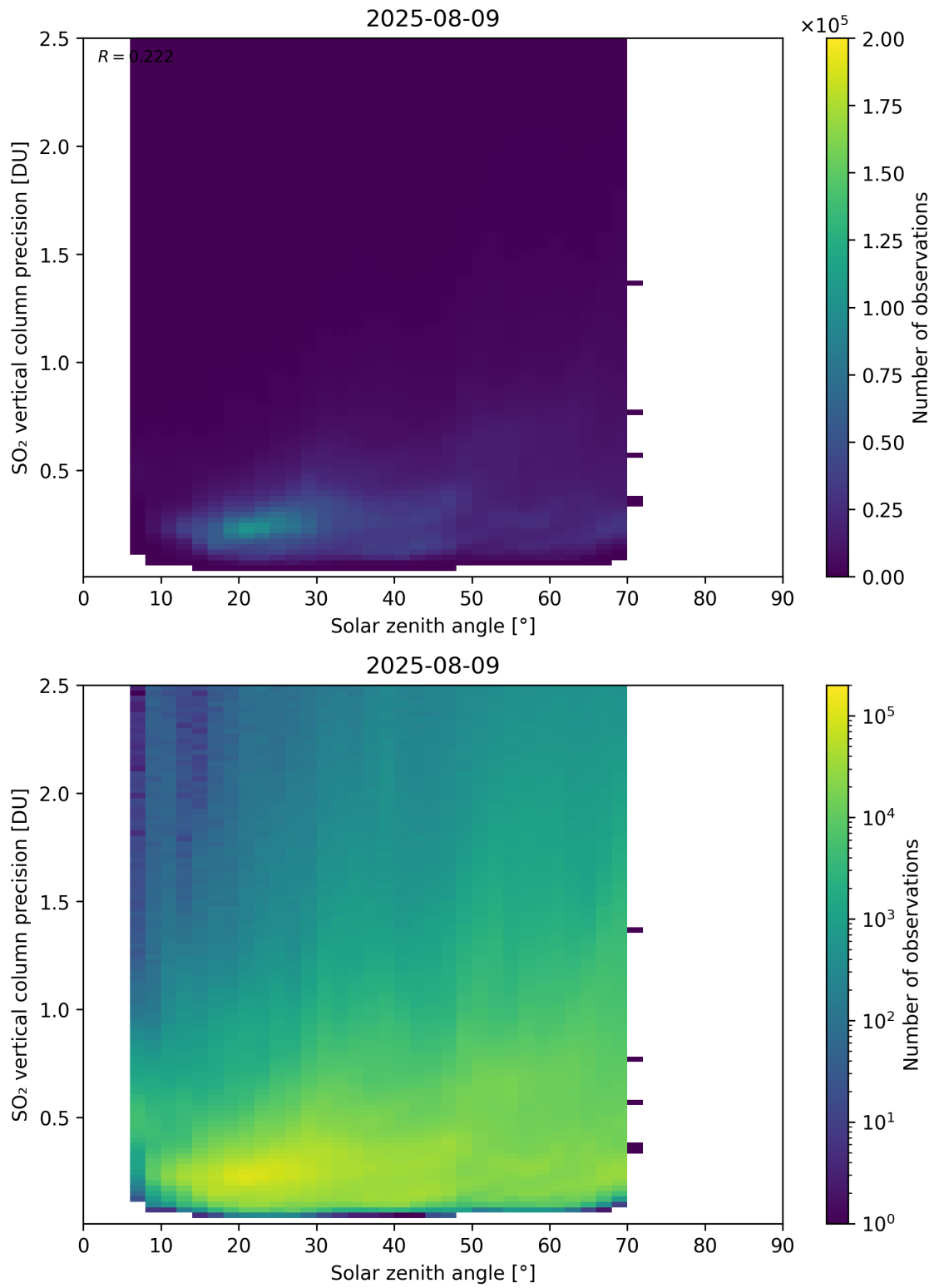
Figure 192: Scatter density plot of “Solar zenith angle” against “SO 2 vertical column precision” for 2025-08-09 to 2025-08-10.
