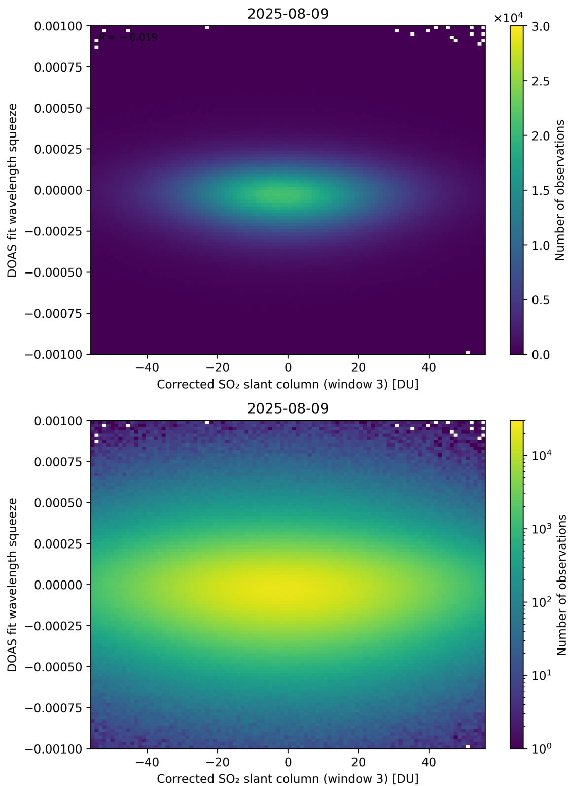
Figure 257: Scatter density plot of “Corrected SO 2 slant column (window 3)” against “DOAS fit wavelength squeeze” for 2025-08-09 to 2025-08-10.
