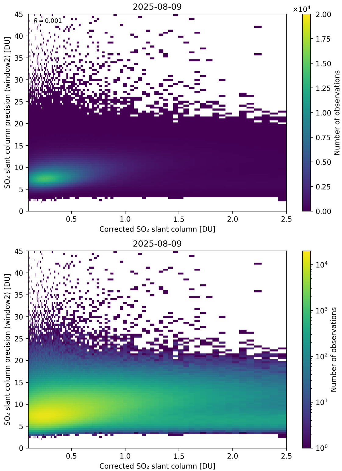
Figure 239: Scatter density plot of “Corrected SO 2 slant column” against “SO 2 slant column precision (window2)” for 2025-08-09 to 2025-08-10.
