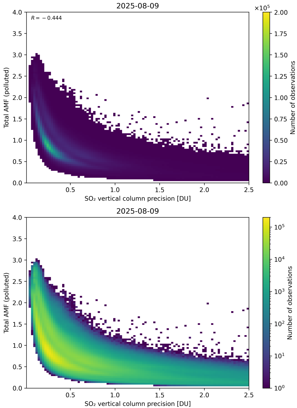
Figure 346: Scatter density plot of “SO 2 vertical column precision” against “Total AMF (polluted)” for 2025-08-09 to 2025-08-10.
