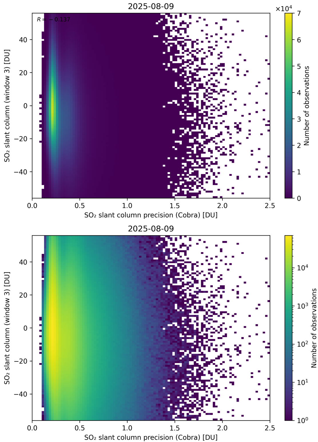
Figure 211: Scatter density plot of “SO 2 slant column precision (Cobra)” against “SO 2 slant column (window 3)” for 2025-08-09 to 2025-08-10.
