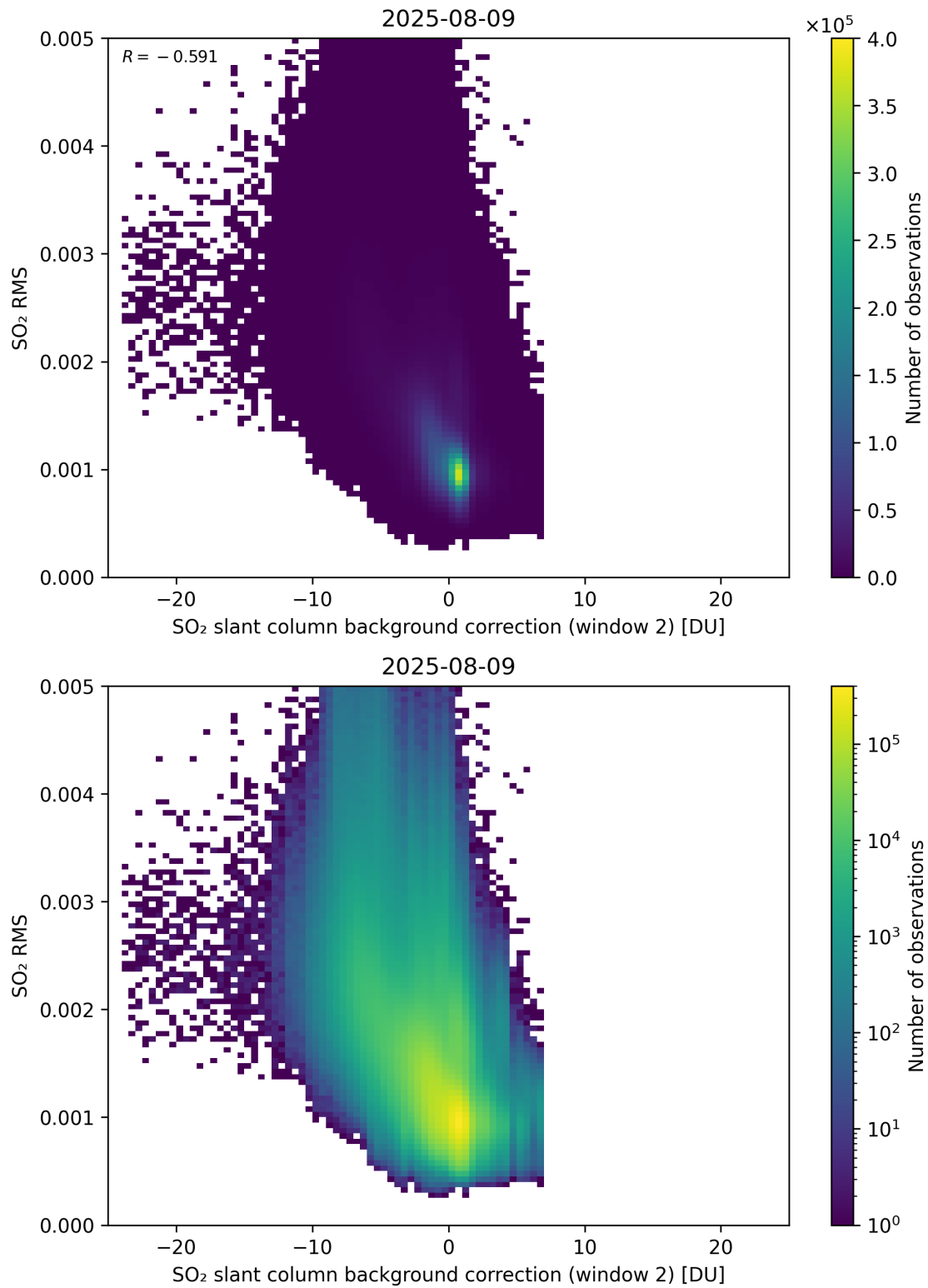
Figure 125: Scatter density plot of “SO 2 slant column background correction (window 2)” against “SO 2 RMS” for 2025-08-09 to 2025-08-10.
