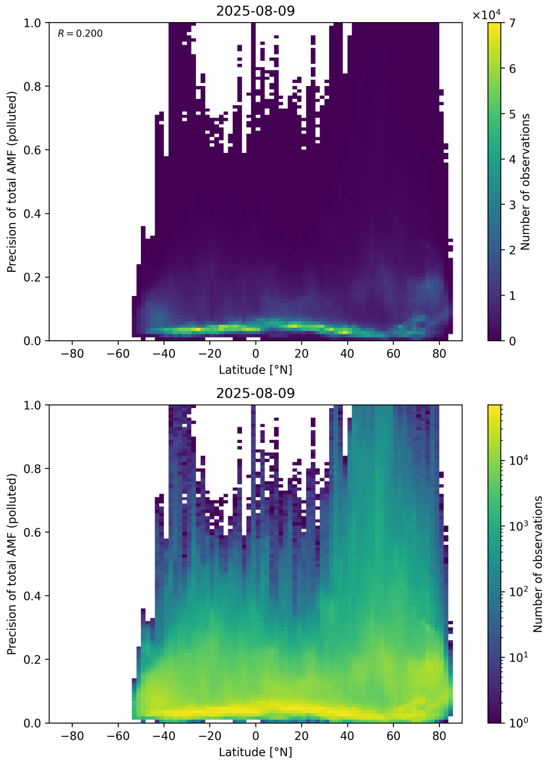
Figure 168: Scatter density plot of “Latitude” against “Precision of total AMF (polluted)” for 2025-08-09 to 2025-08-10.
