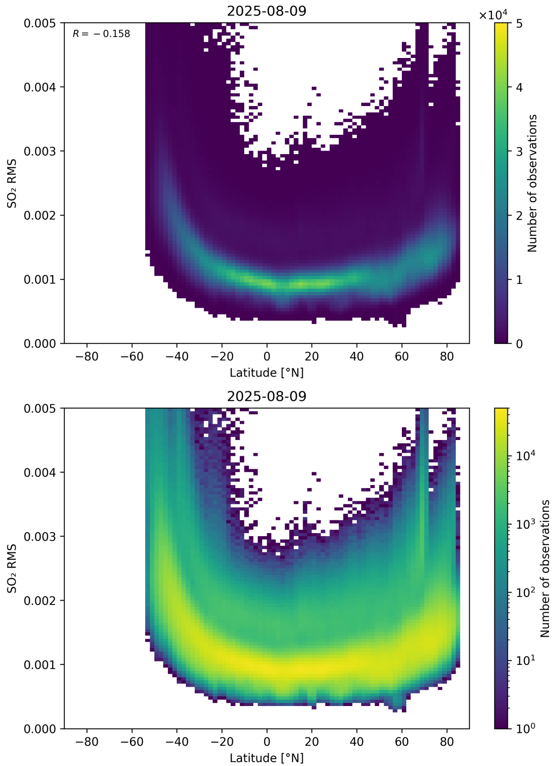
Figure 155: Scatter density plot of “Latitude” against “SO 2 RMS” for 2025-08-09 to 2025-08-10.
