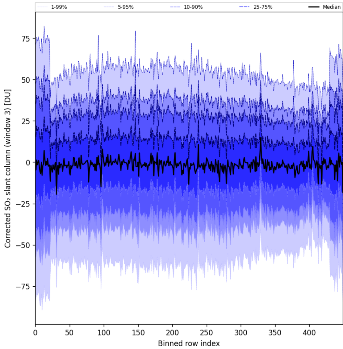
Figure 99: Along track statistics of “Corrected SO 2 slant column (window 3)” for 2025-08-09 to 2025-08-10
