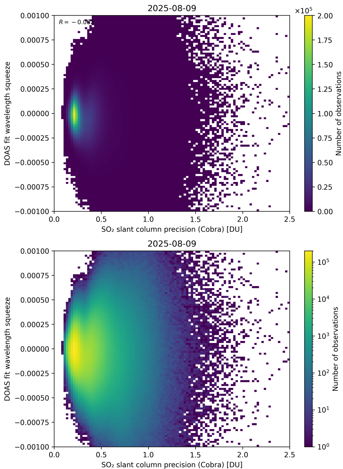
Figure 203: Scatter density plot of “SO 2 slant column precision (Cobra)” against “DOAS fit wavelength squeeze” for 2025-08-09 to 2025-08-10.
