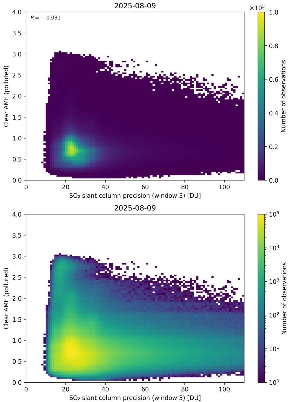
Figure 311: Scatter density plot of “SO 2 slant column precision (window 3)” against “Clear AMF (polluted)” for 2025-08-09 to 2025-08-10.
