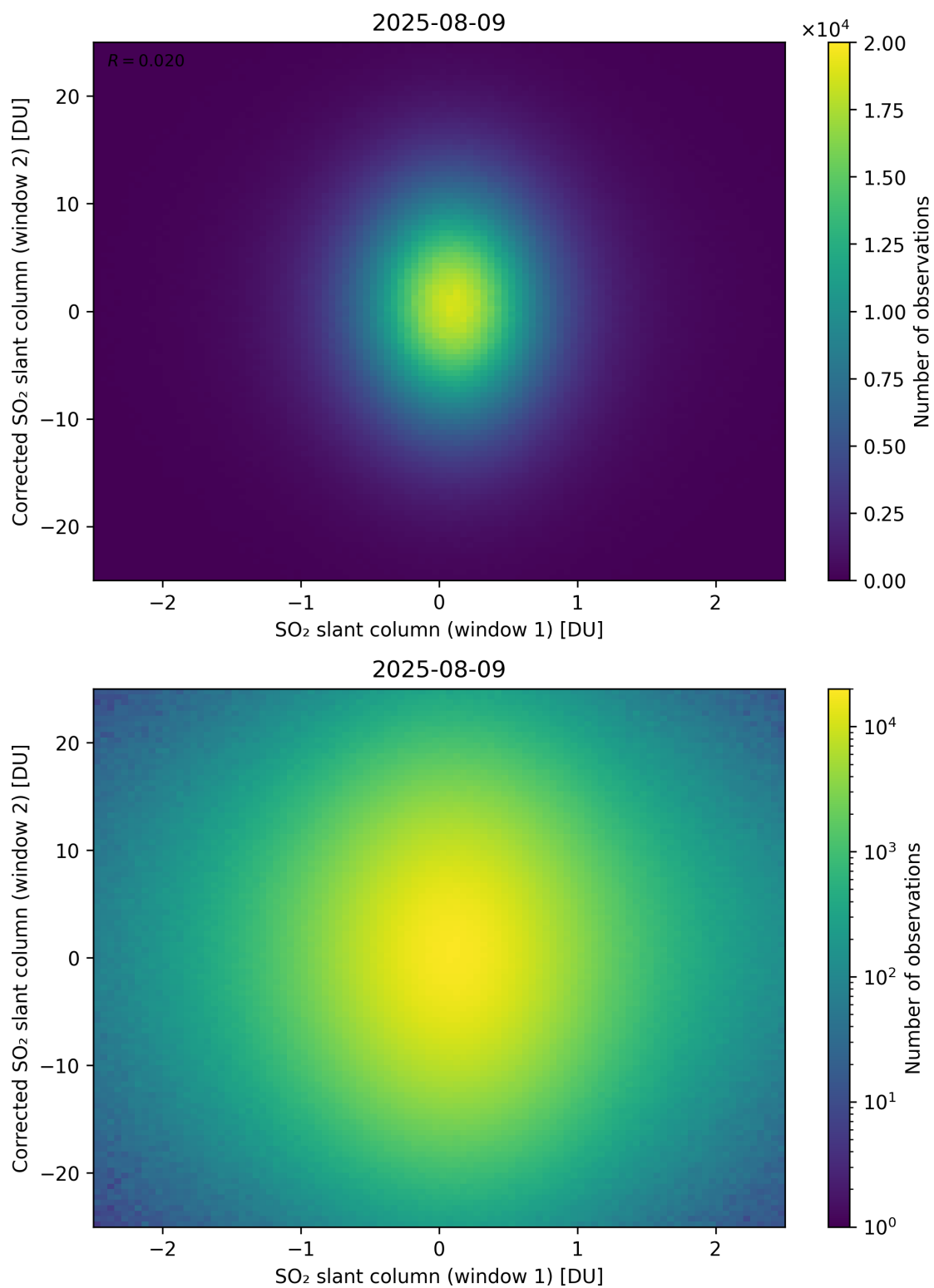
Figure 283: Scatter density plot of “SO 2 slant column (window 1)” against “Corrected SO 2 slant column (window 2)” for 2025-08-09 to 2025-08-10.
