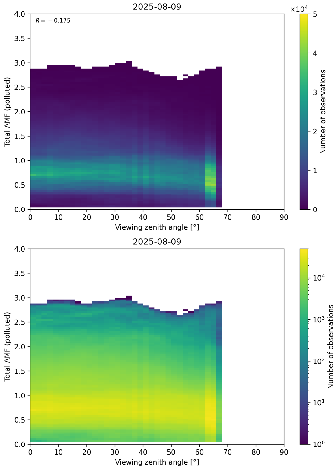
Figure 381: Scatter density plot of “Viewing zenith angle” against “Total AMF (polluted)” for 2025-08-09 to 2025-08-10.
