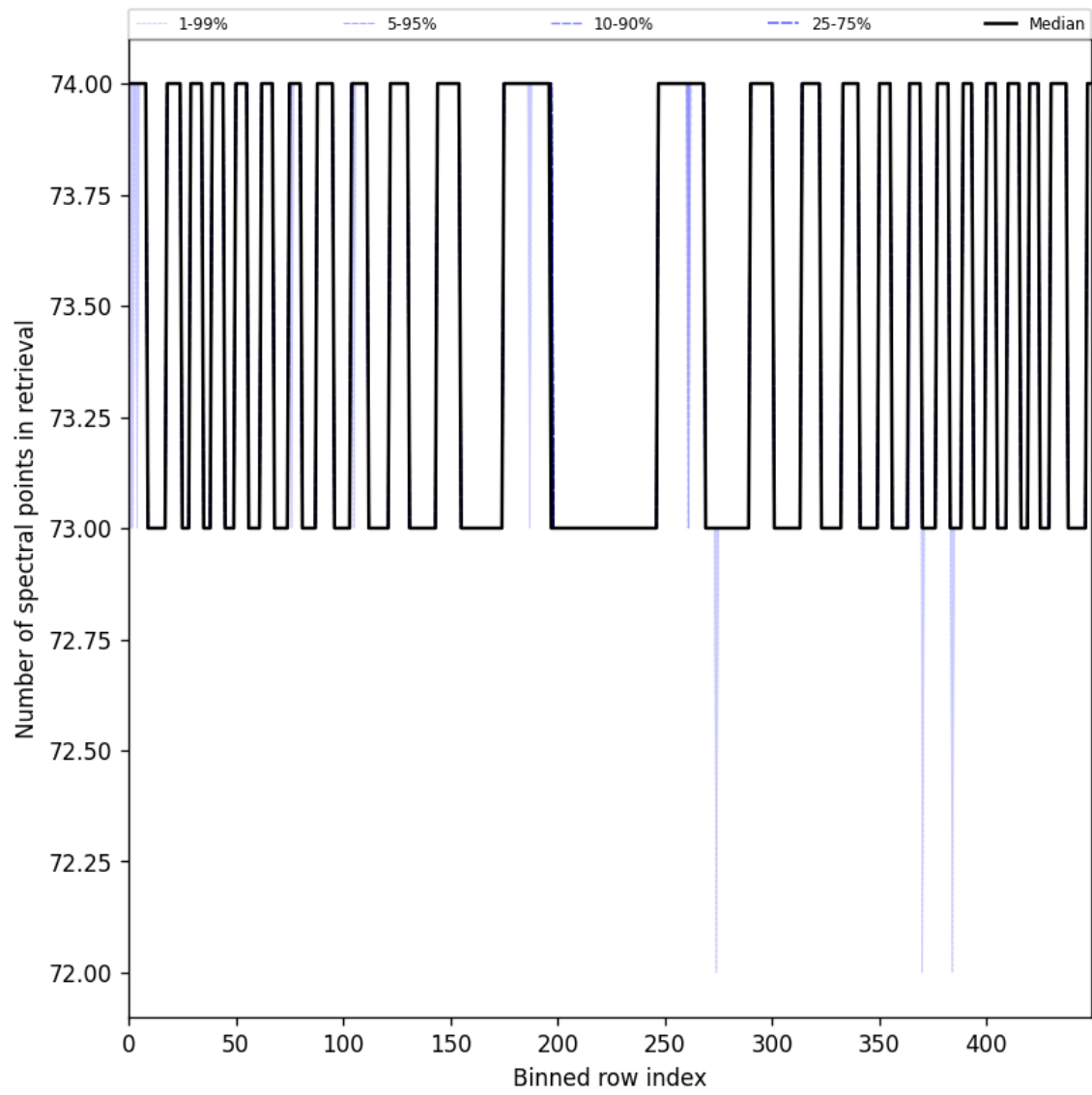
Figure 108: Along track statistics of “Number of spectral points in retrieval” for 2025-08-09 to 2025-08-10
