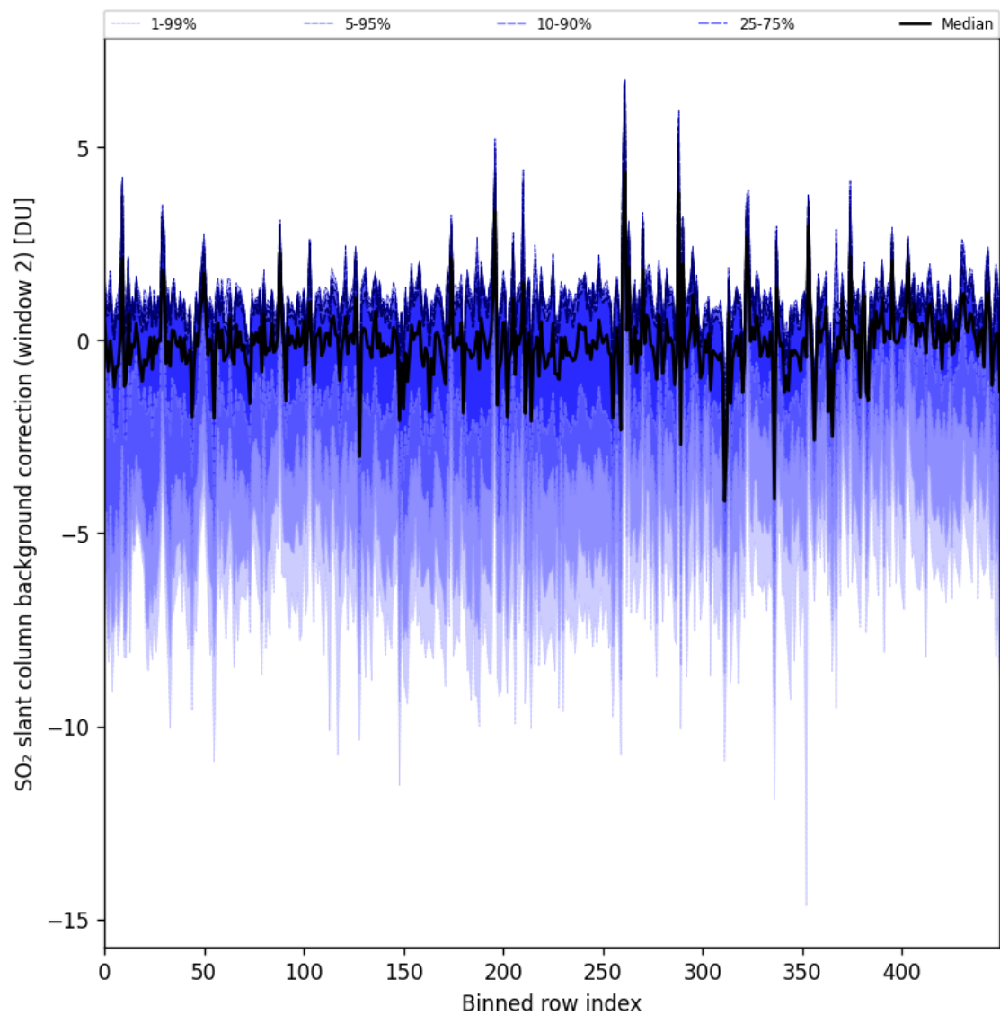
Figure 96: Along track statistics of “SO 2 slant column background correction (window 2)” for 2025-08-09 to 2025-08-10
