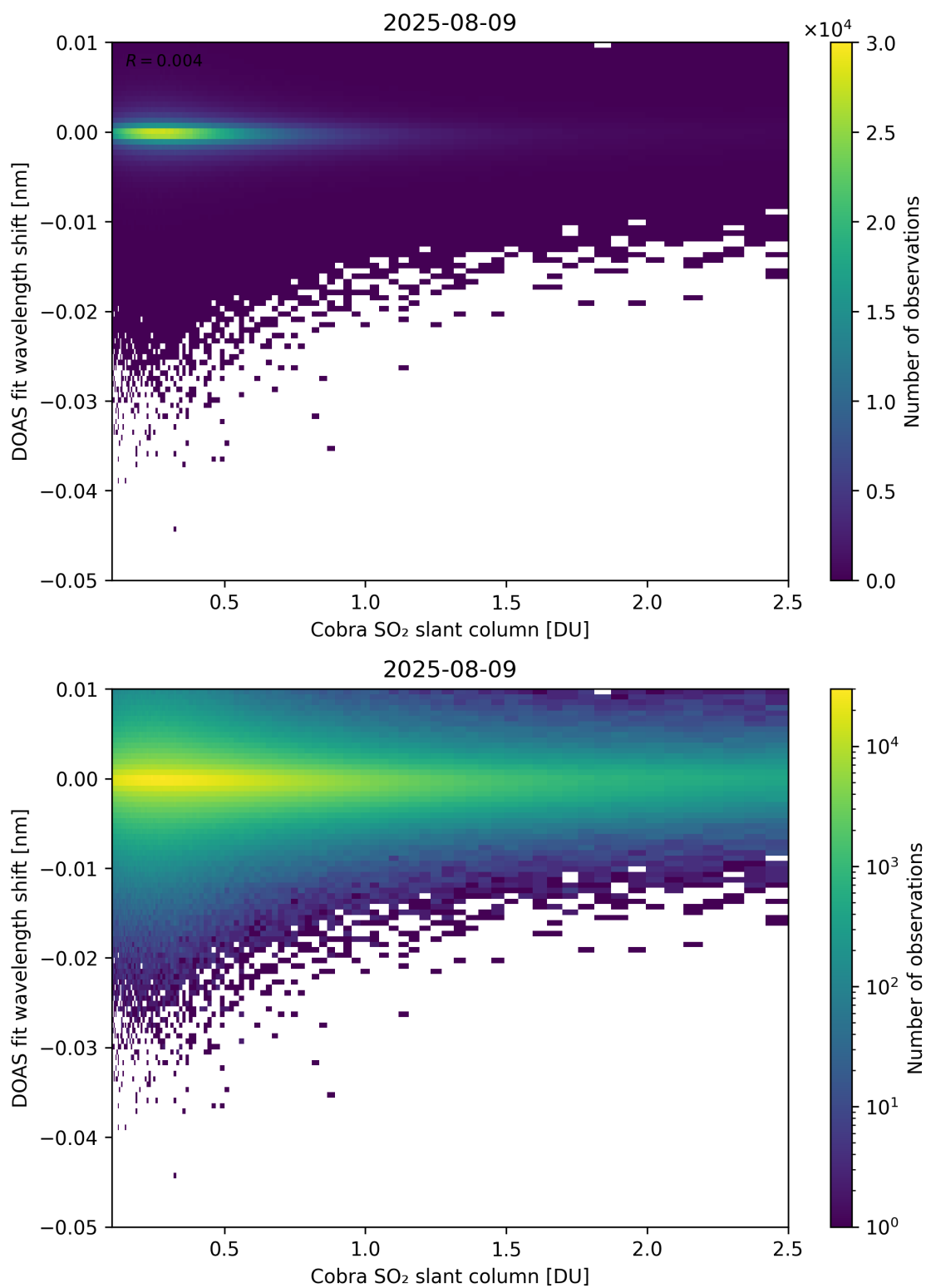
Figure 196: Scatter density plot of “Cobra SO 2 slant column” against “DOAS fit wavelength shift” for 2025-08-09 to 2025-08-10.
