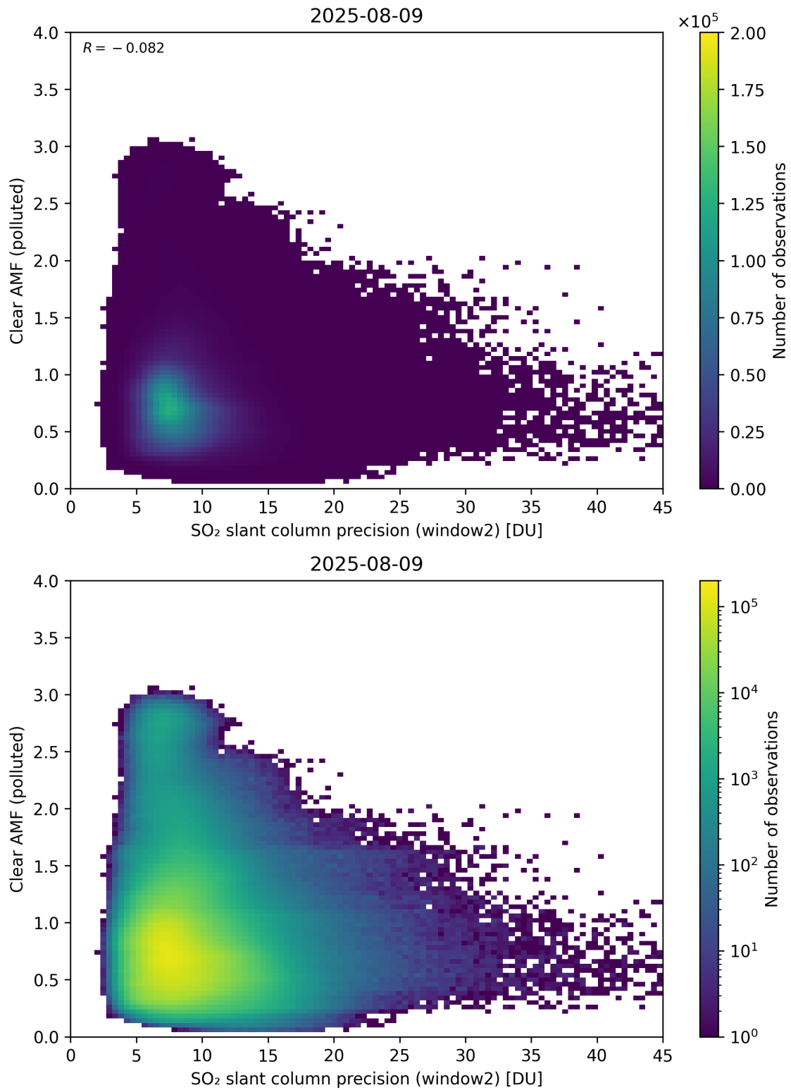
Figure 296: Scatter density plot of “SO 2 slant column precision (window2)” against “Clear AMF (polluted)” for 2025-08-09 to 2025-08-10.
