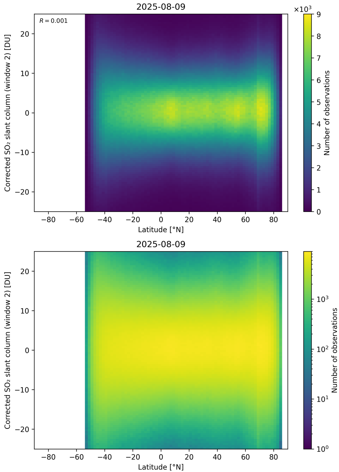
Figure 160: Scatter density plot of “Latitude” against “Corrected SO 2 slant column (window 2)” for 2025-08-09 to 2025-08-10.
