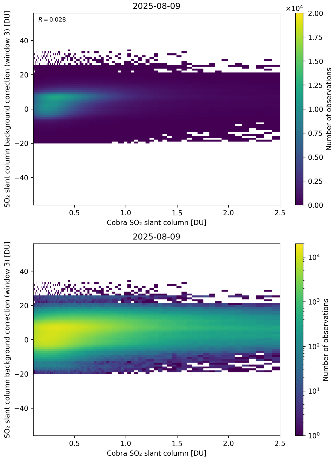
Figure 195: Scatter density plot of “Cobra SO 2 slant column” against “SO 2 slant column background correction (window 3)” for 2025-08-09 to 2025-08-10.
