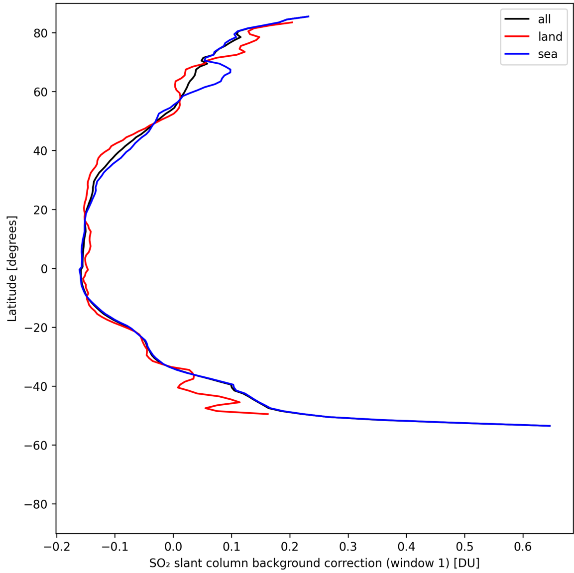
Figure 40: Zonal average of “SO 2 slant column background correction (window 1)” for 2025-08-09 to 2025-08-10.
