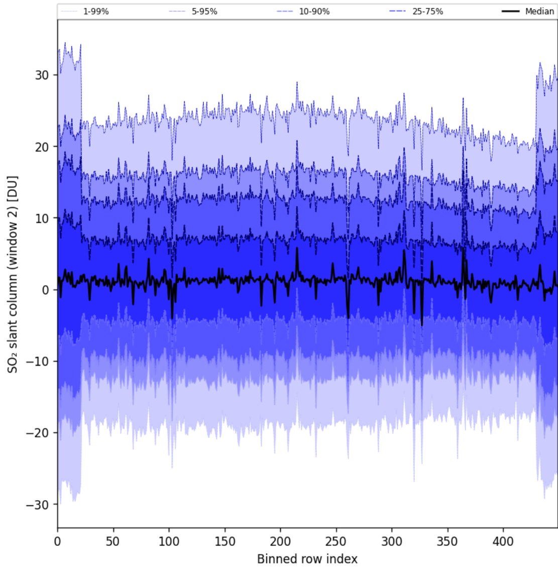
Figure 93: Along track statistics of “SO 2 slant column (window 2)” for 2025-08-09 to 2025-08-10
