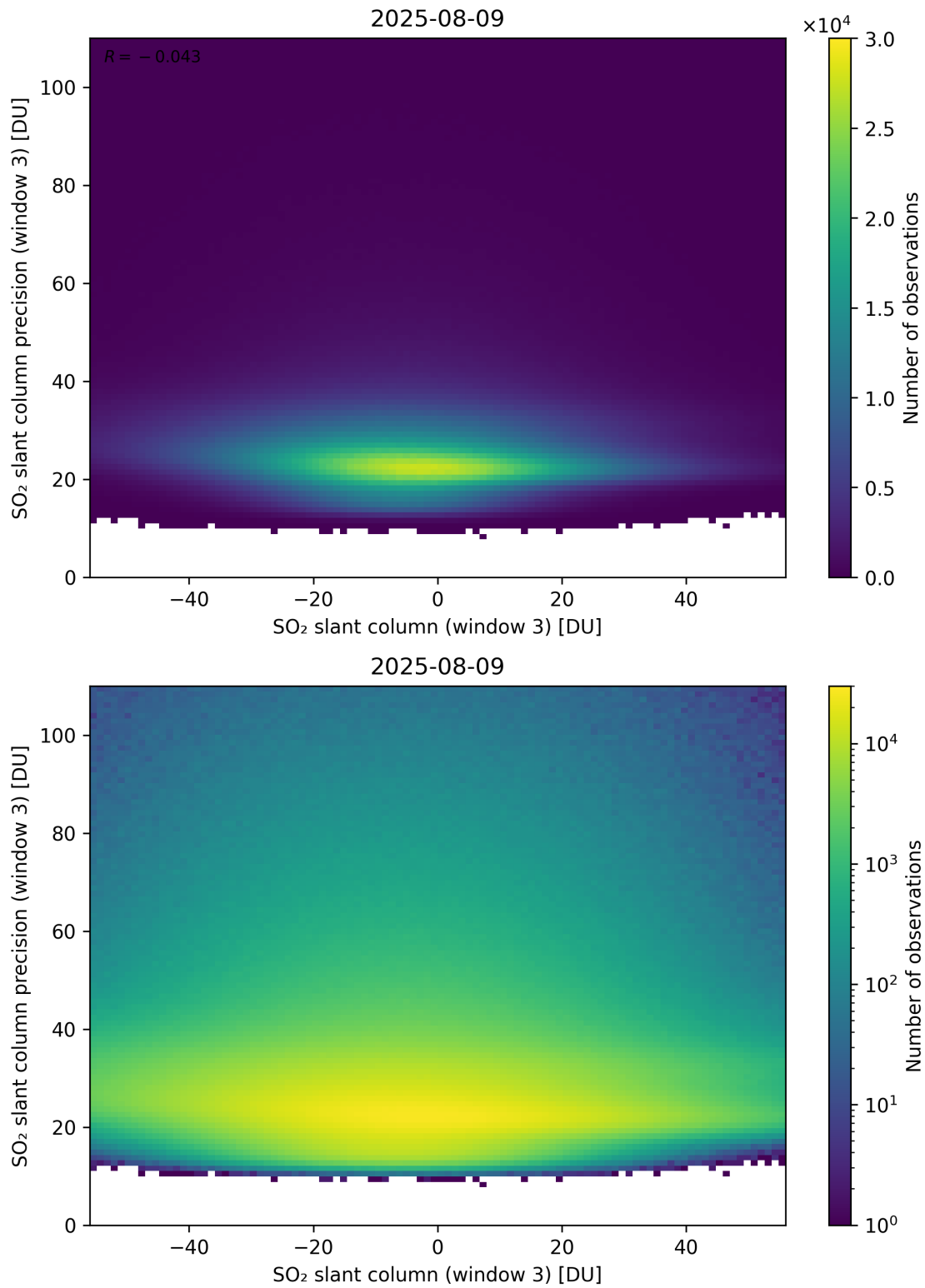
Figure 317: Scatter density plot of “SO 2 slant column (window 3)” against “SO 2 slant column precision (window 3)” for 2025-08-09 to 2025-08-10.
