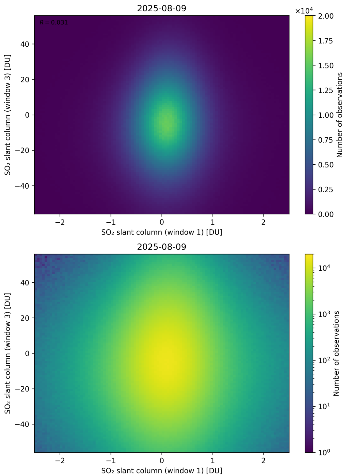
Figure 287: Scatter density plot of “SO 2 slant column (window 1)” against “SO 2 slant column (window 3)” for 2025-08-09 to 2025-08-10.
