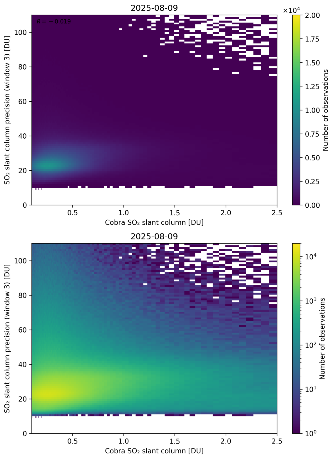
Figure 223: Scatter density plot of “Cobra SO 2 slant column” against “SO 2 slant column precision (window 3)” for 2025-08-09 to 2025-08-10.
