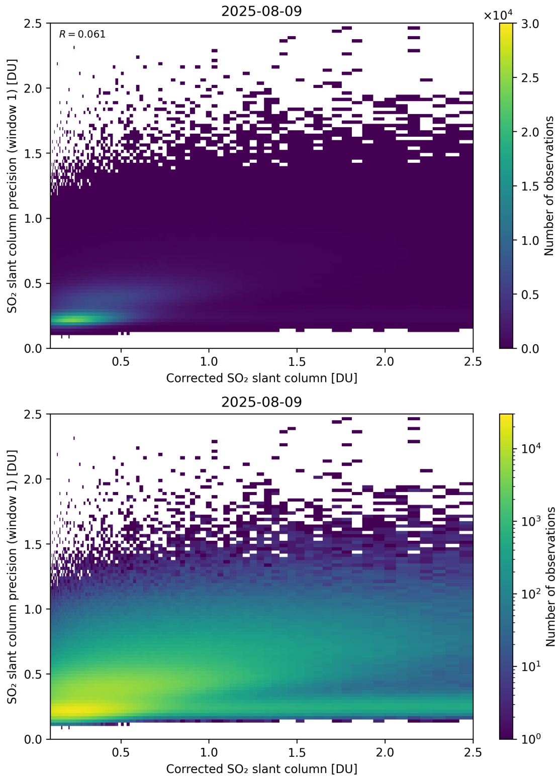
Figure 238: Scatter density plot of “Corrected SO 2 slant column” against “SO 2 slant column precision (window 1)” for 2025-08-09 to 2025-08-10.
