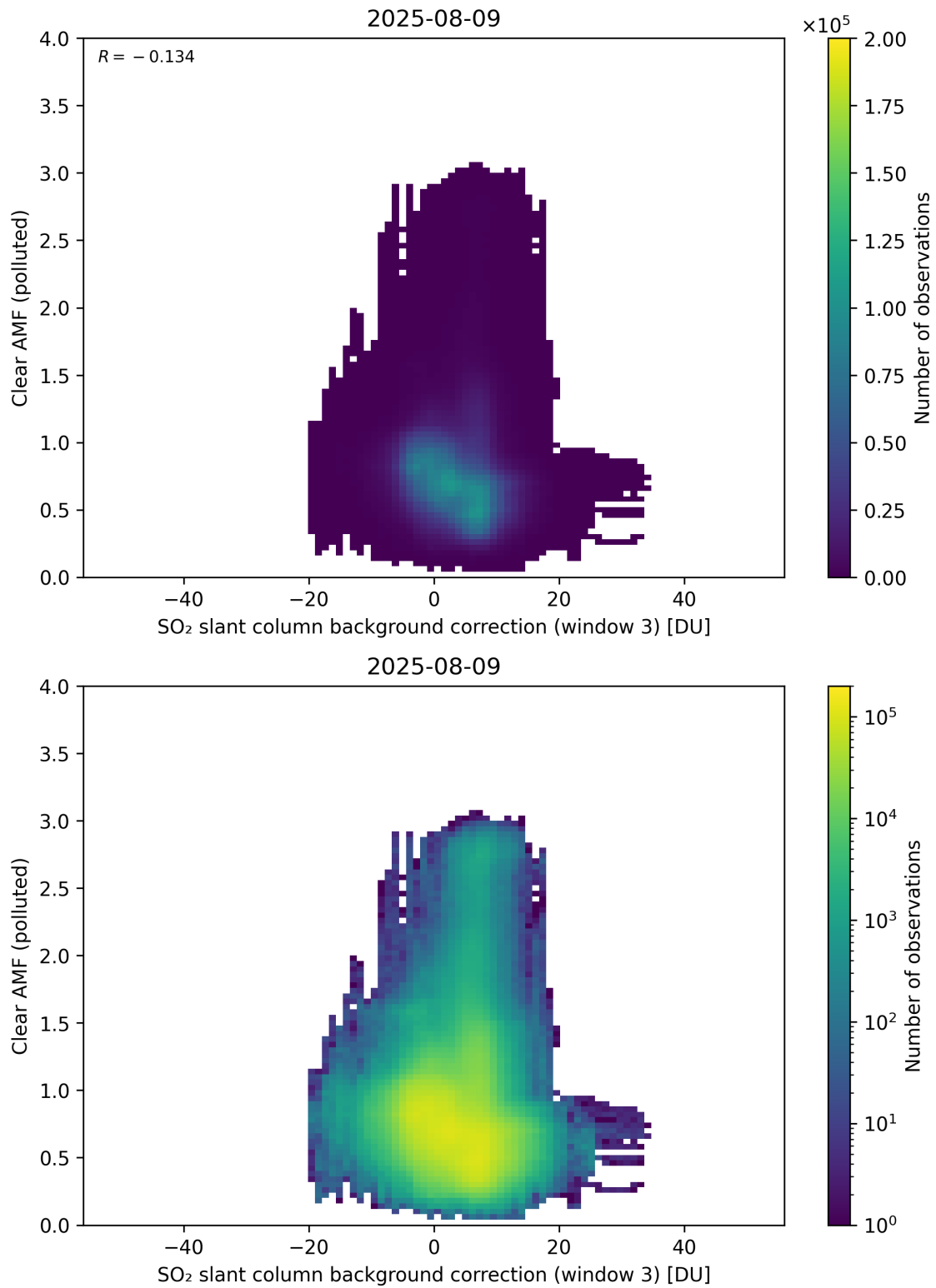
Figure 135: Scatter density plot of “SO 2 slant column background correction (window 3)” against “Clear AMF (polluted)” for 2025-08-09 to 2025-08-10.
