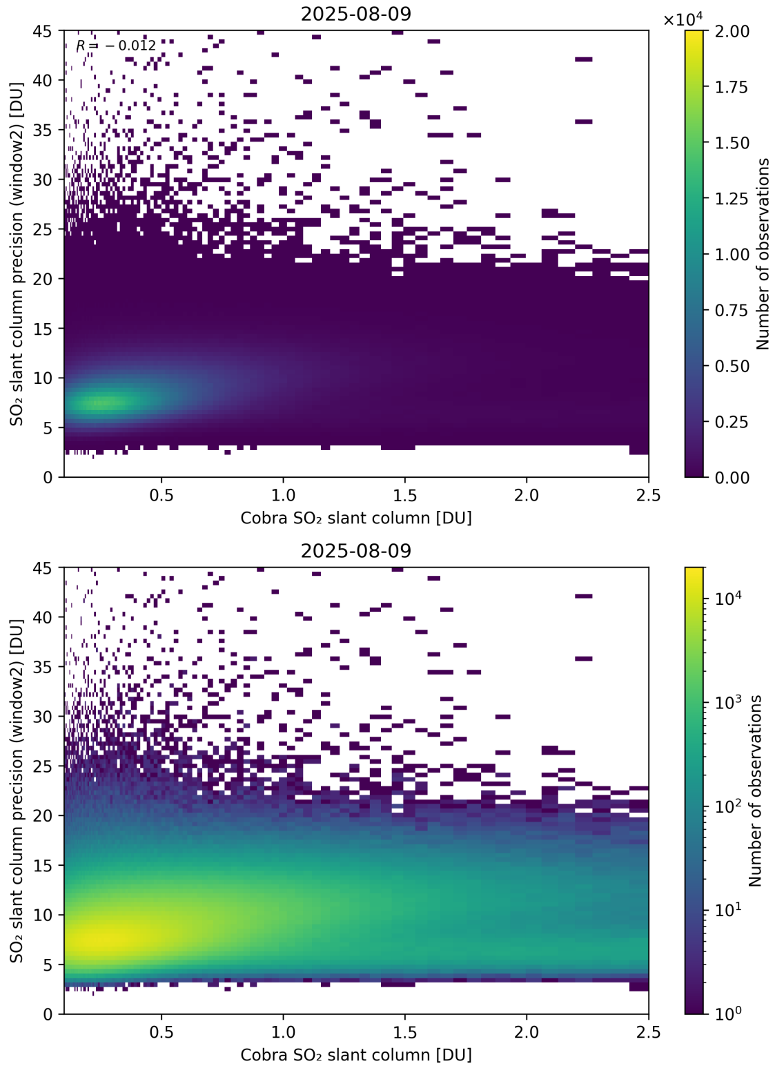
Figure 221: Scatter density plot of “Cobra SO 2 slant column” against “SO 2 slant column precision (window2)” for 2025-08-09 to 2025-08-10.
