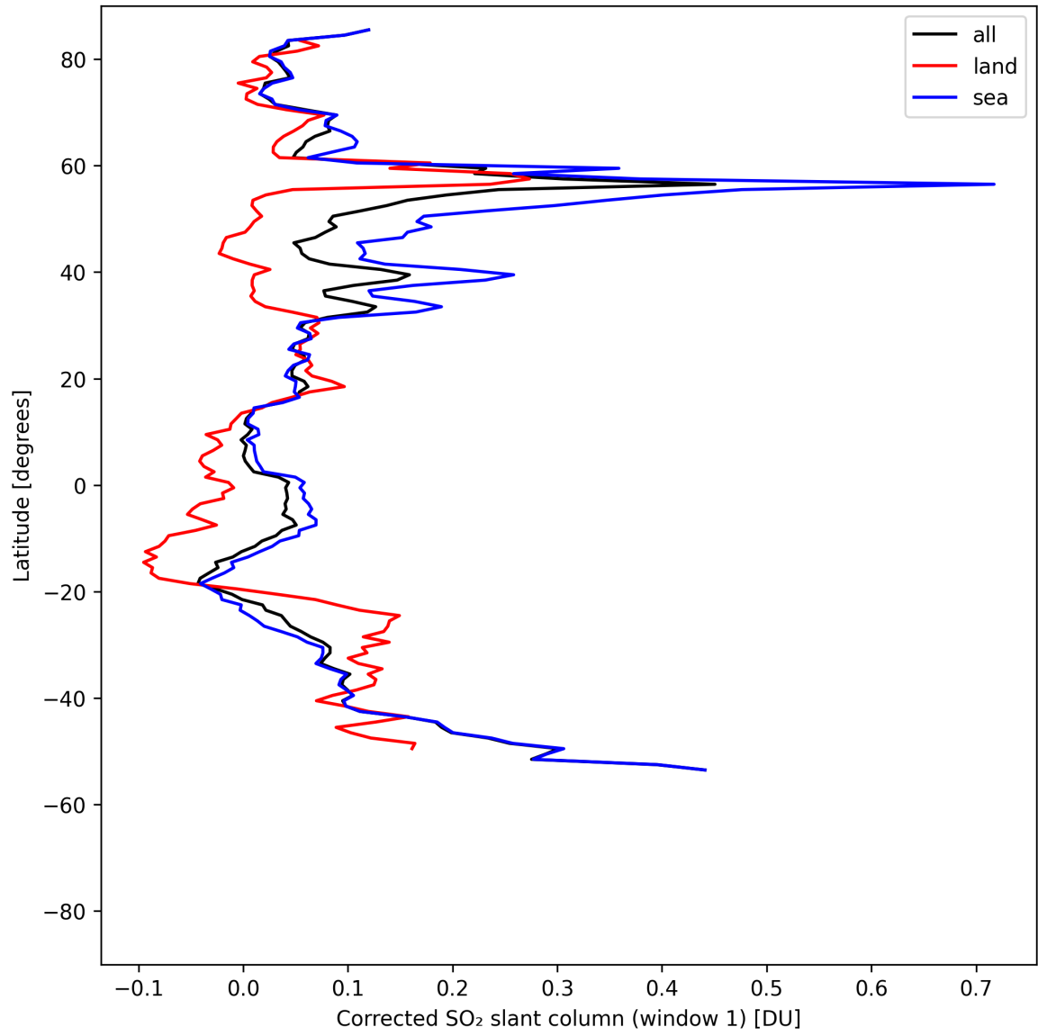
Figure 39: Zonal average of “Corrected SO 2 slant column (window 1)” for 2025-08-09 to 2025-08-10.
