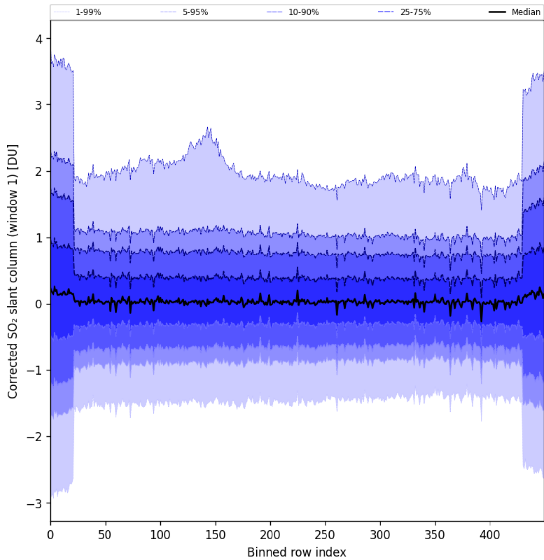
Figure 91: Along track statistics of “Corrected SO 2 slant column (window 1)” for 2025-08-09 to 2025-08-10
