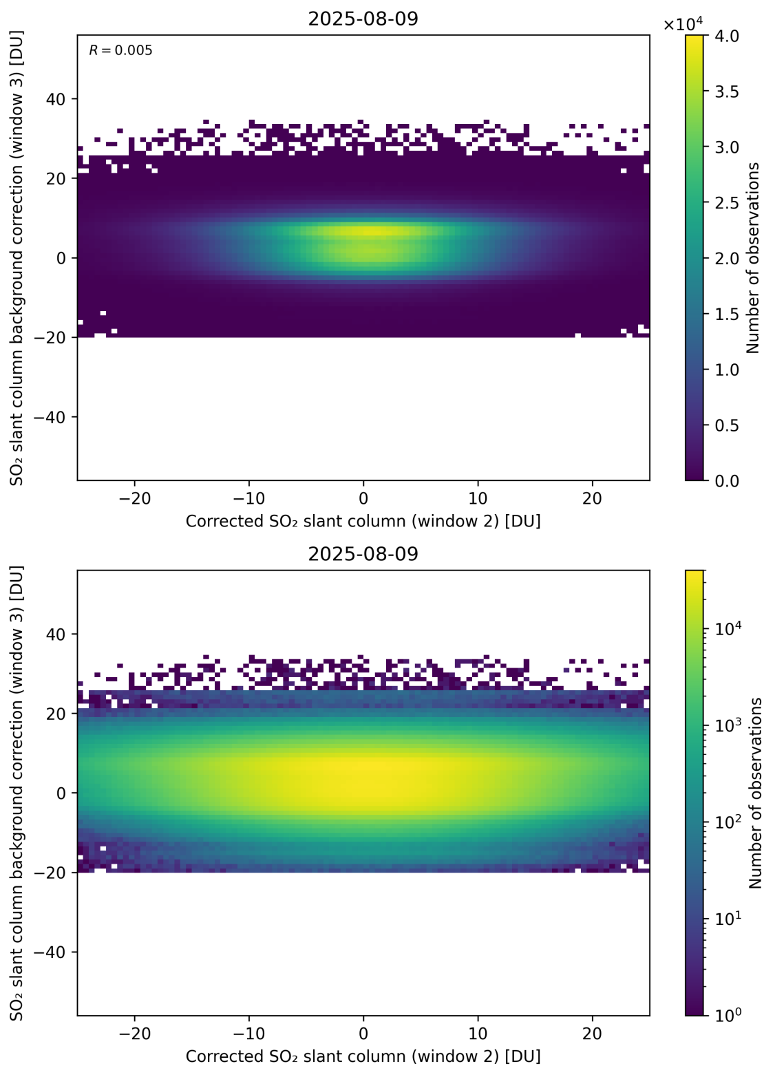
Figure 245: Scatter density plot of “Corrected SO 2 slant column (window 2)” against “SO 2 slant column background correction (window 3)” for 2025-08-09 to 2025-08-10.
