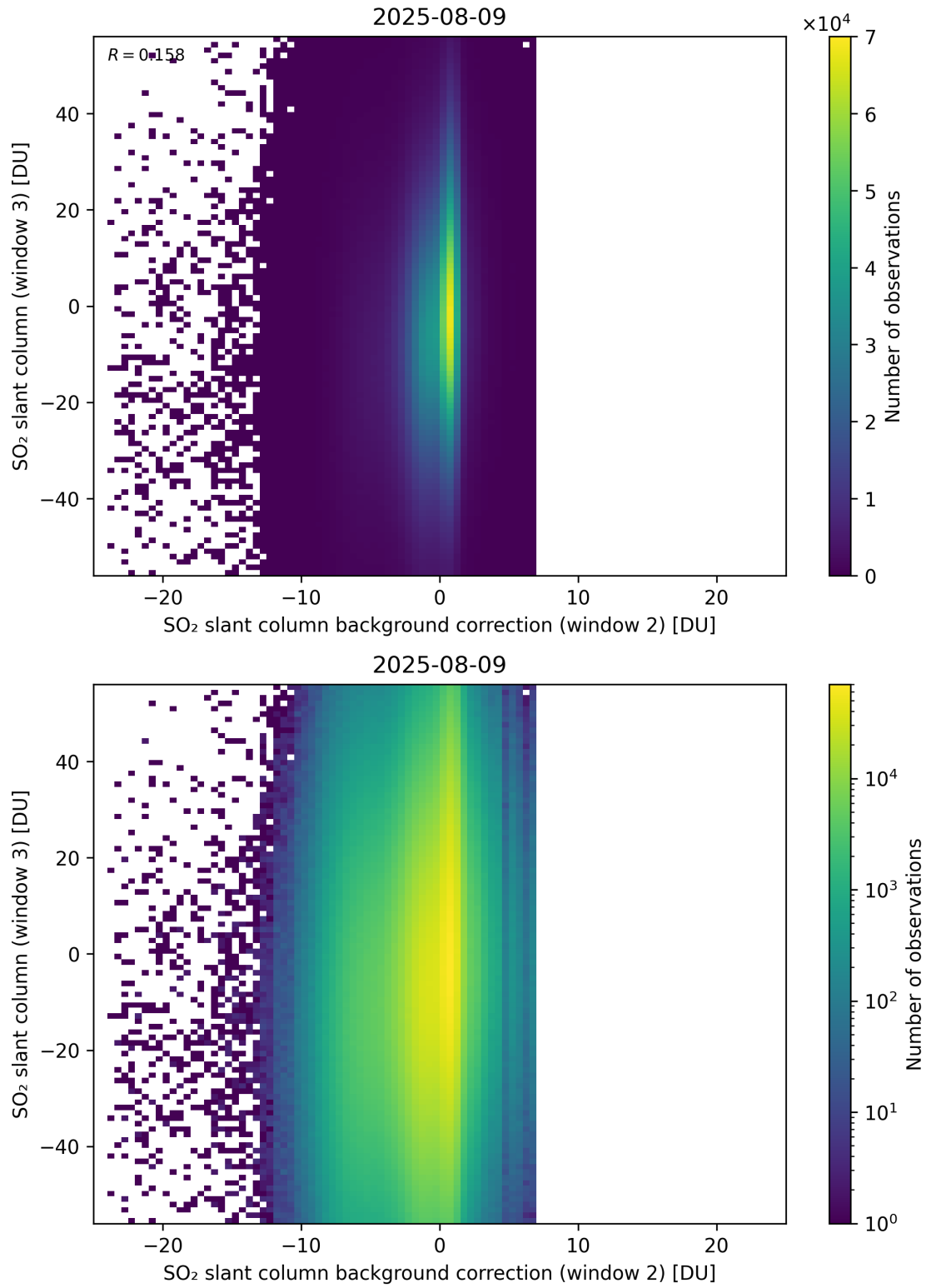
Figure 128: Scatter density plot of “SO 2 slant column background correction (window 2)” against “SO 2 slant column (window 3)” for 2025-08-09 to 2025-08-10.
