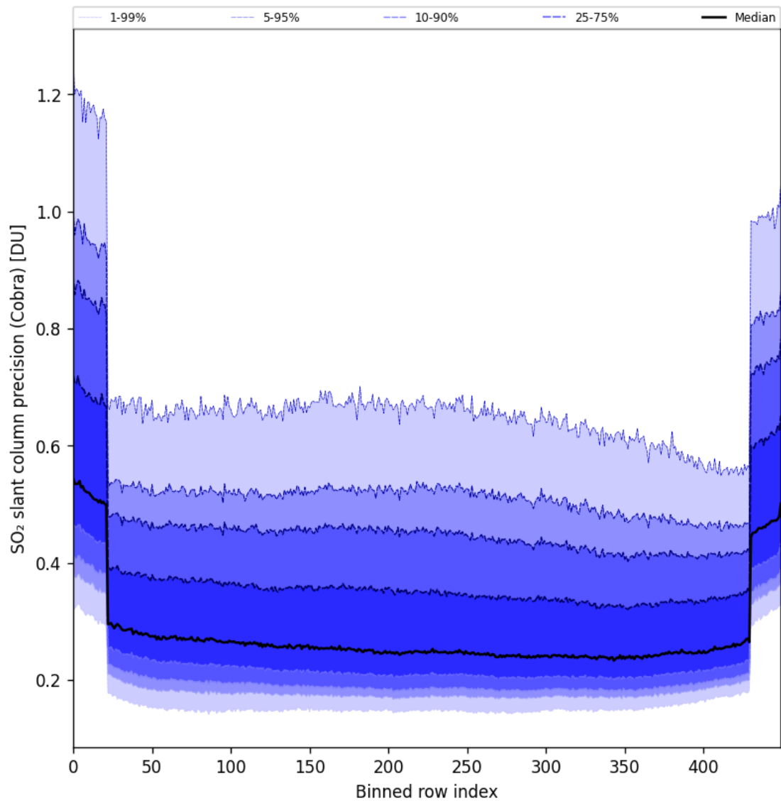
Figure 88: Along track statistics of “SO 2 slant column precision (Cobra)” for 2025-08-09 to 2025-08-10
