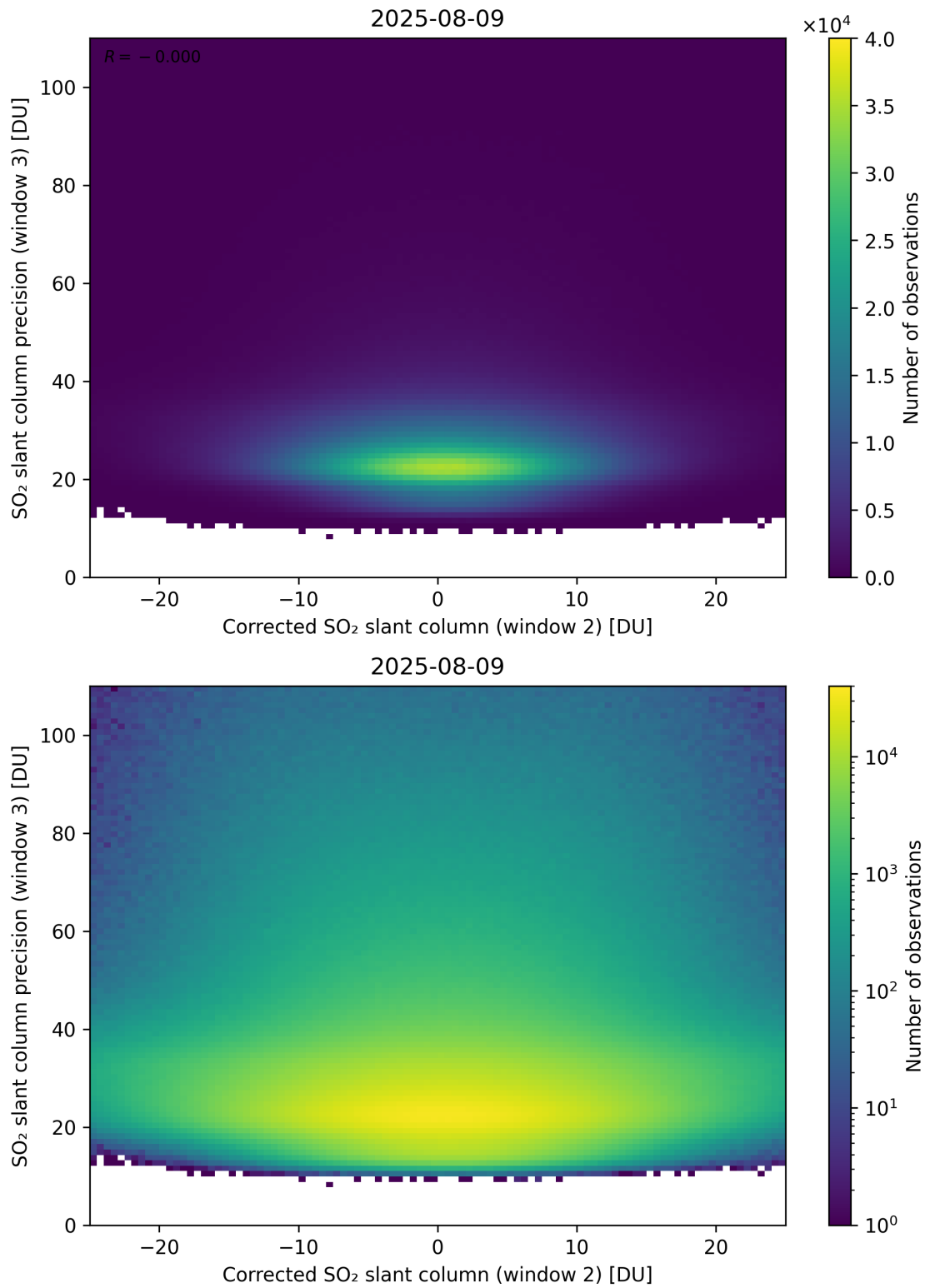
Figure 252: Scatter density plot of “Corrected SO 2 slant column (window 2)” against “SO 2 slant column precision (window 3)” for 2025-08-09 to 2025-08-10.
