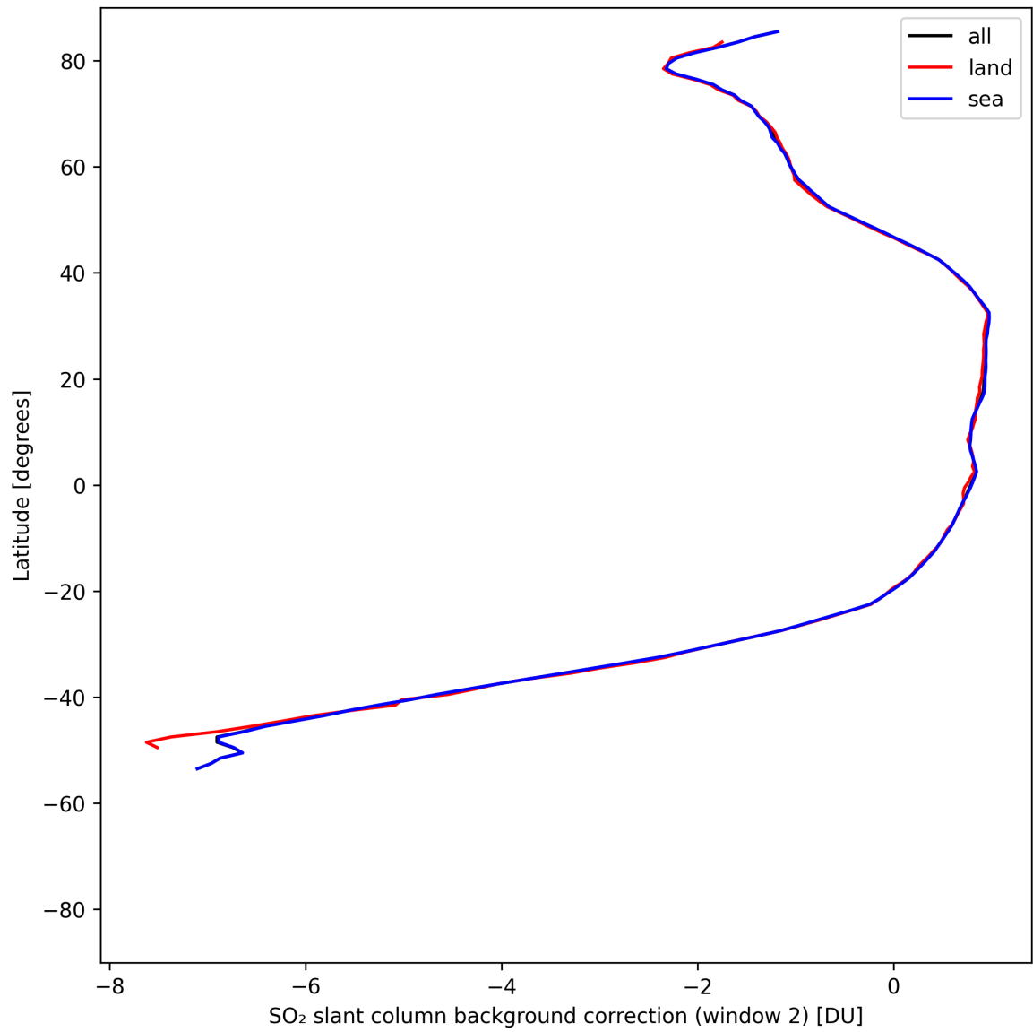
Figure 44: Zonal average of “SO 2 slant column background correction (window 2)” for 2025-08-09 to 2025-08-10.
