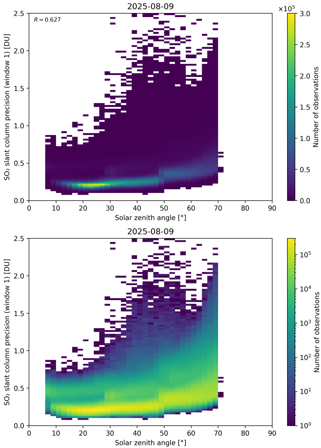
Figure 185: Scatter density plot of “Solar zenith angle” against “SO 2 slant column precision (window 1)” for 2025-08-09 to 2025-08-10.
