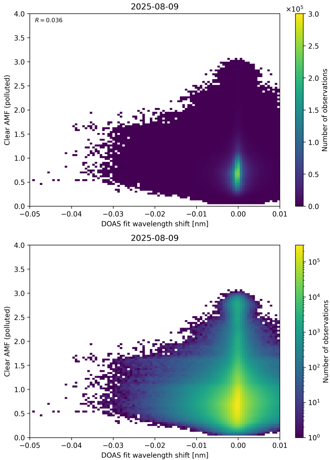
Figure 140: Scatter density plot of “DOAS fit wavelength shift” against “Clear AMF (polluted)” for 2025-08-09 to 2025-08-10.
