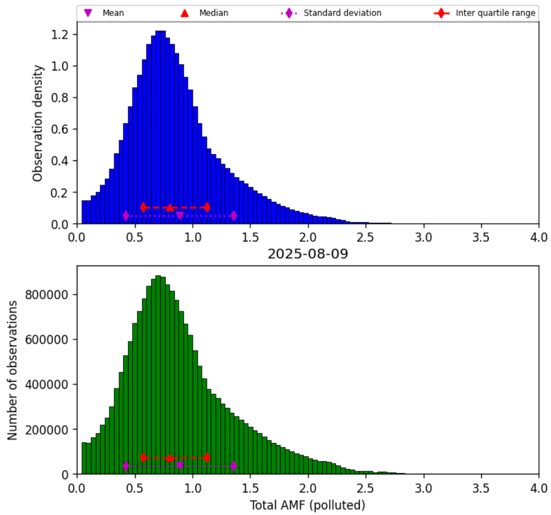
Figure 79: Histogram of “Total AMF (polluted)” for 2025-08-09 to 2025-08-10
