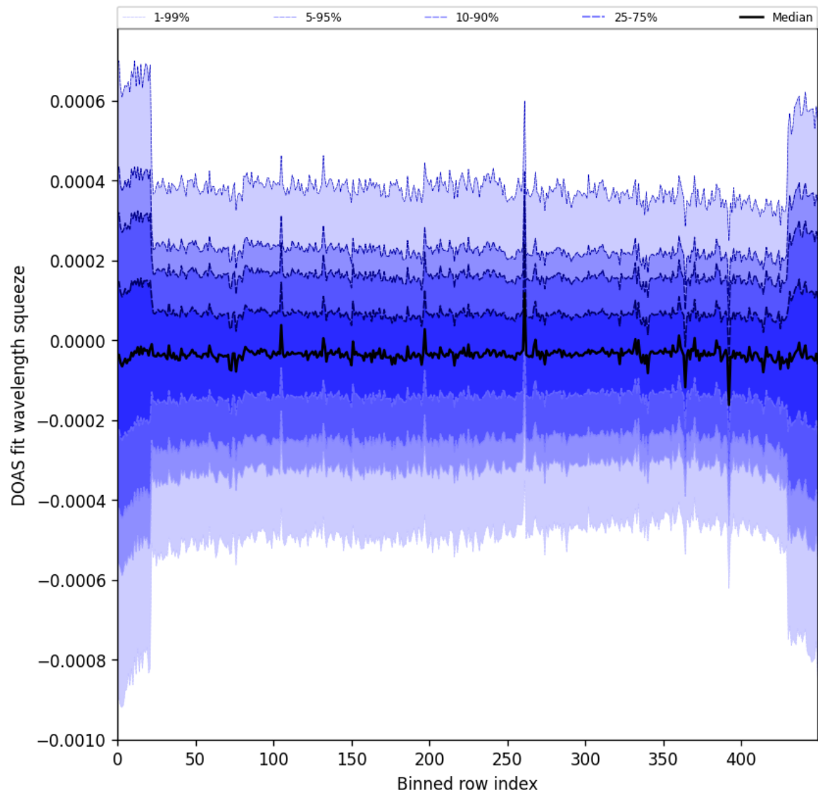
Figure 103: Along track statistics of “DOAS fit wavelength squeeze” for 2025-08-09 to 2025-08-10
