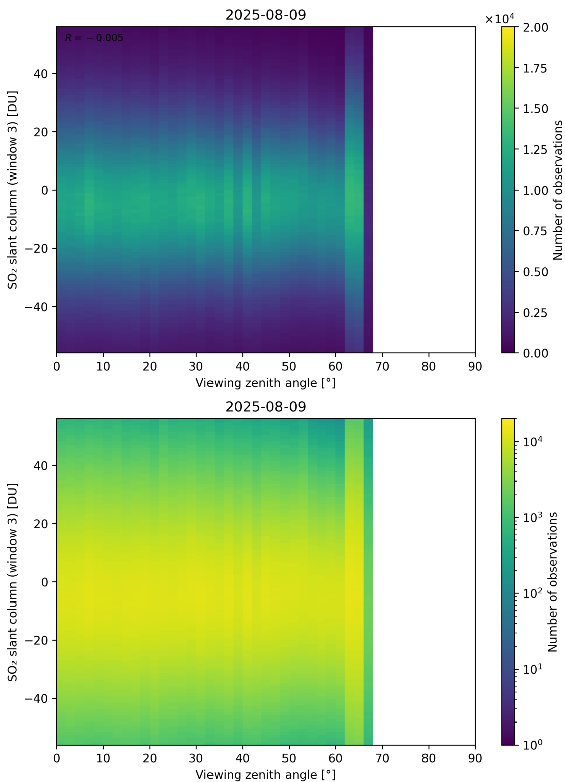
Figure 379: Scatter density plot of “Viewing zenith angle” against “SO 2 slant column (window 3)” for 2025-08-09 to 2025-08-10.
