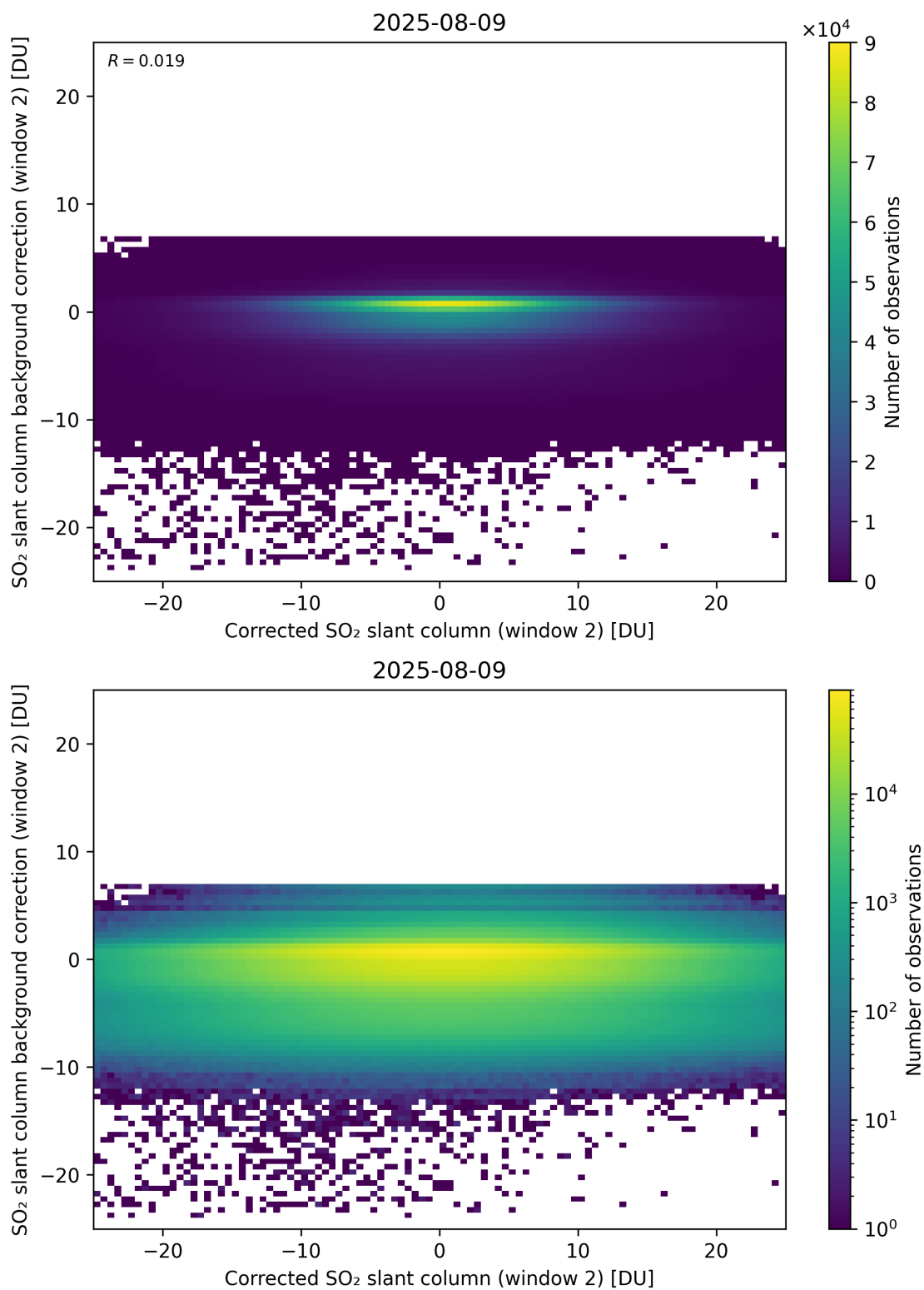
Figure 244: Scatter density plot of “Corrected SO 2 slant column (window 2)” against “SO 2 slant column background correction (window 2)” for 2025-08-09 to 2025-08-10.
