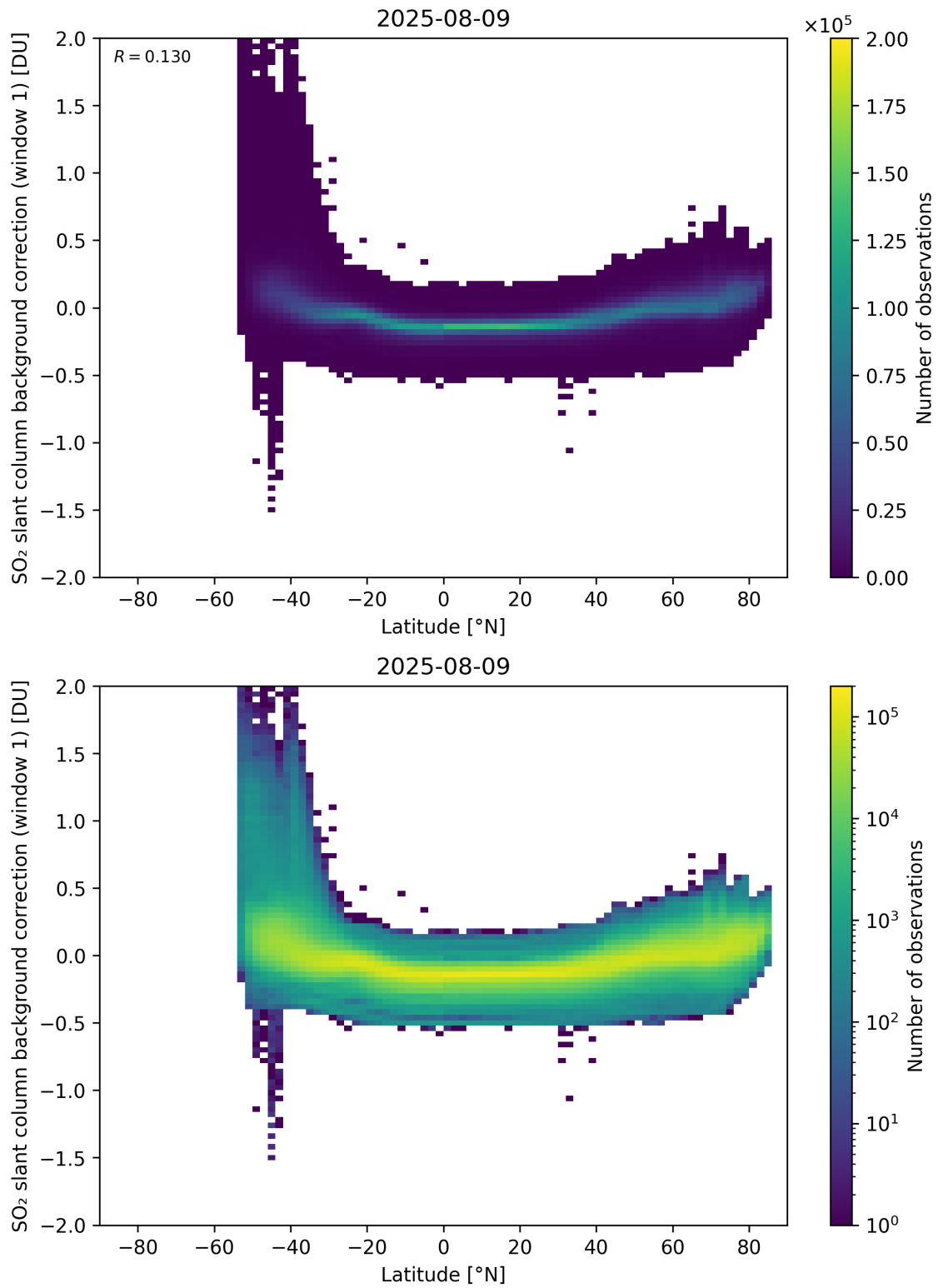
Figure 150: Scatter density plot of “Latitude” against “SO 2 slant column background correction (window 1)” for 2025-08-09 to 2025-08-10.
