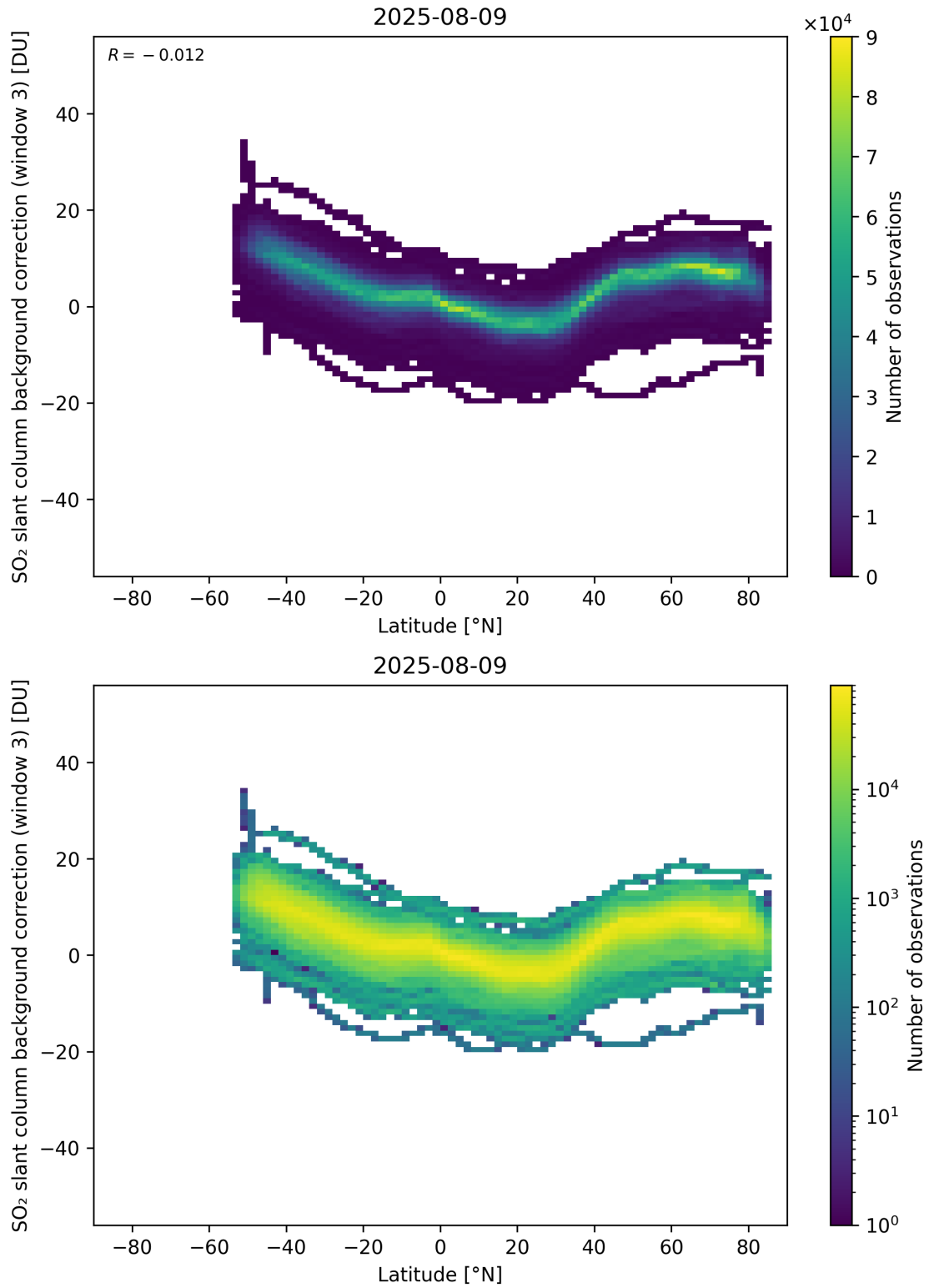
Figure 152: Scatter density plot of “Latitude” against “SO 2 slant column background correction (window 3)” for 2025-08-09 to 2025-08-10.
