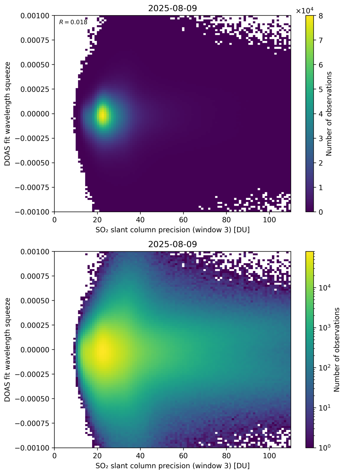
Figure 309: Scatter density plot of “SO 2 slant column precision (window 3)” against “DOAS fit wavelength squeeze” for 2025-08-09 to 2025-08-10.
