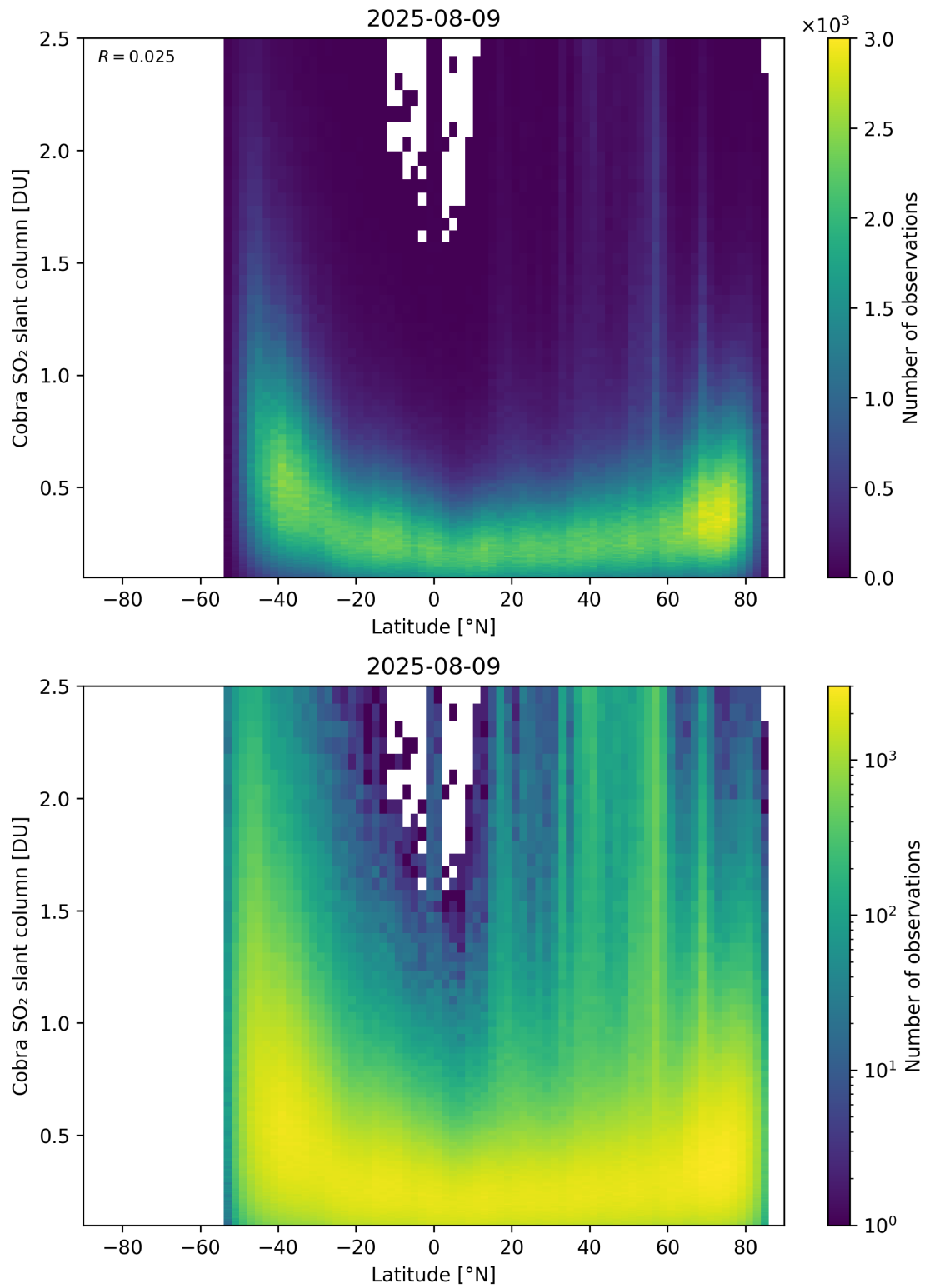
Figure 157: Scatter density plot of “Latitude” against “Cobra SO 2 slant column” for 2025-08-09 to 2025-08-10.
