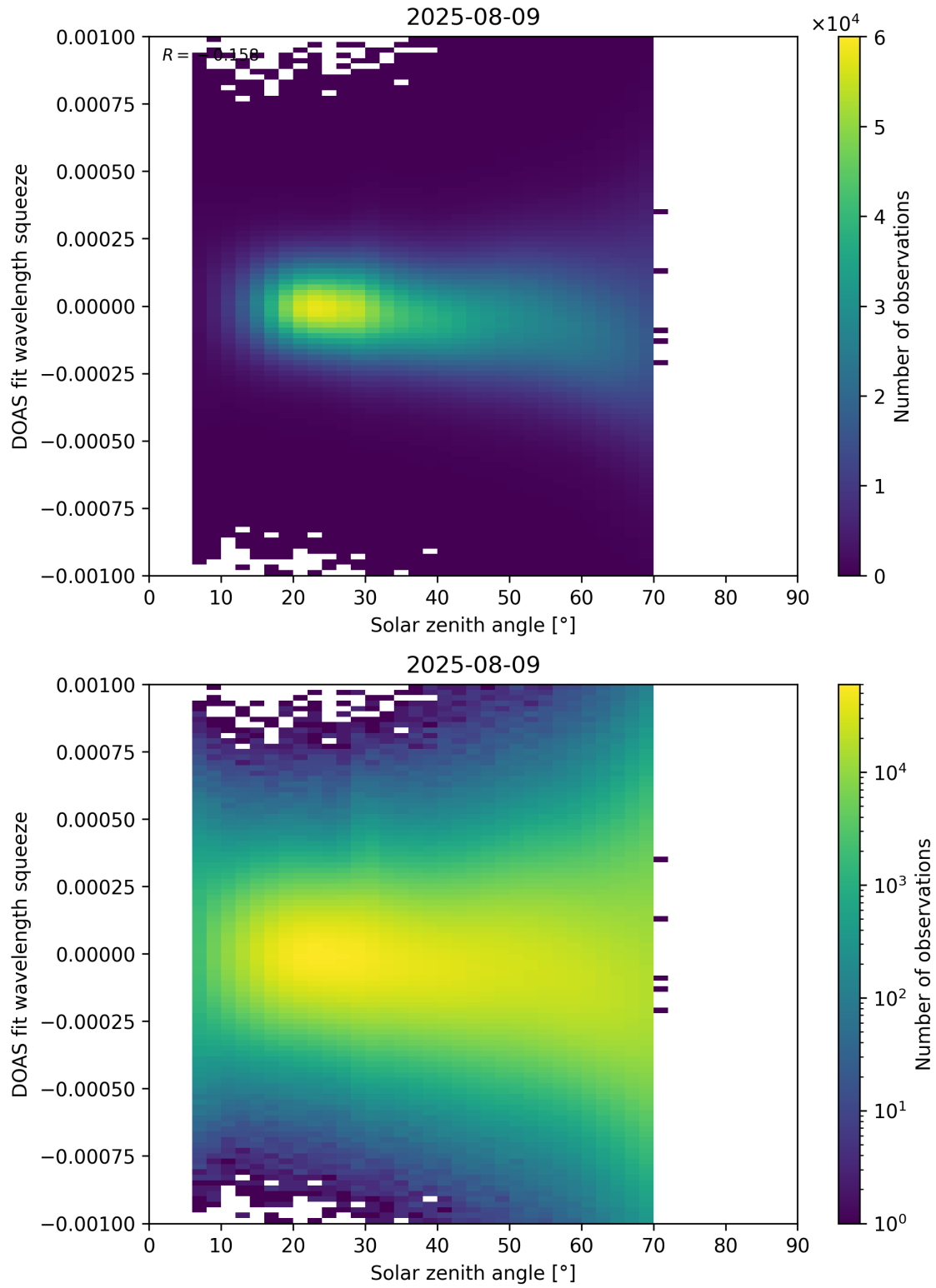
Figure 175: Scatter density plot of “Solar zenith angle” against “DOAS fit wavelength squeeze” for 2025-08-09 to 2025-08-10.
