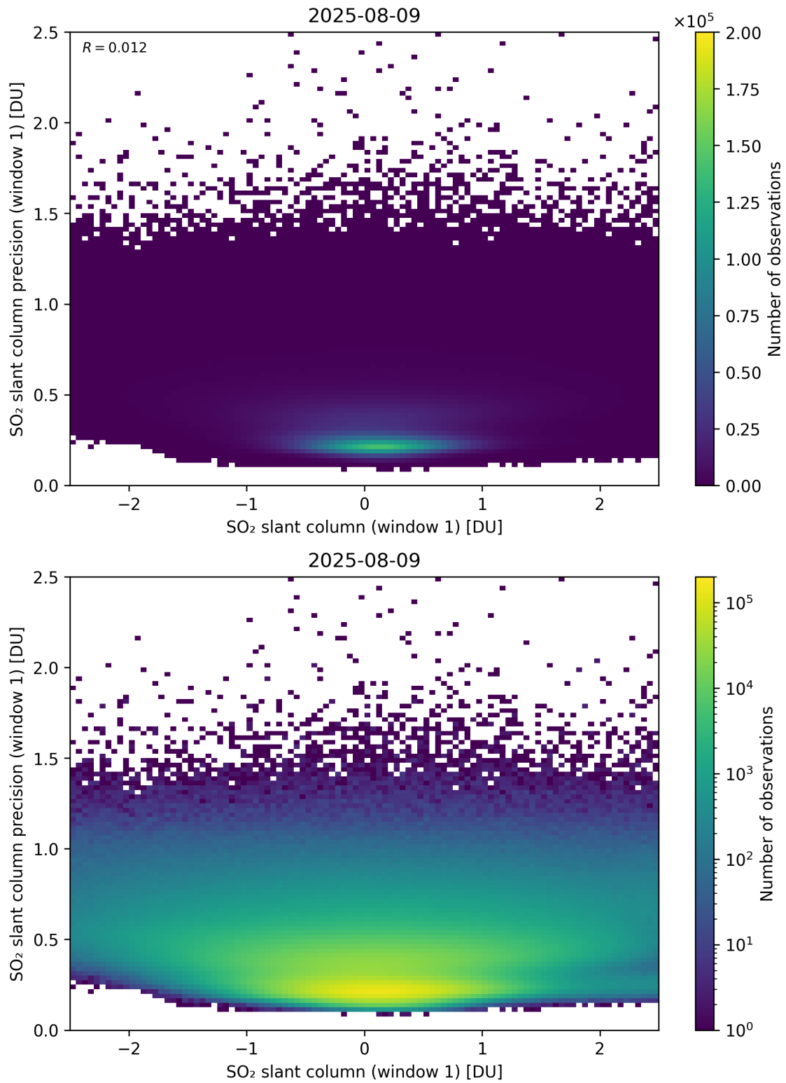
Figure 285: Scatter density plot of “SO 2 slant column (window 1)” against “SO 2 slant column precision (window 1)” for 2025-08-09 to 2025-08-10.
