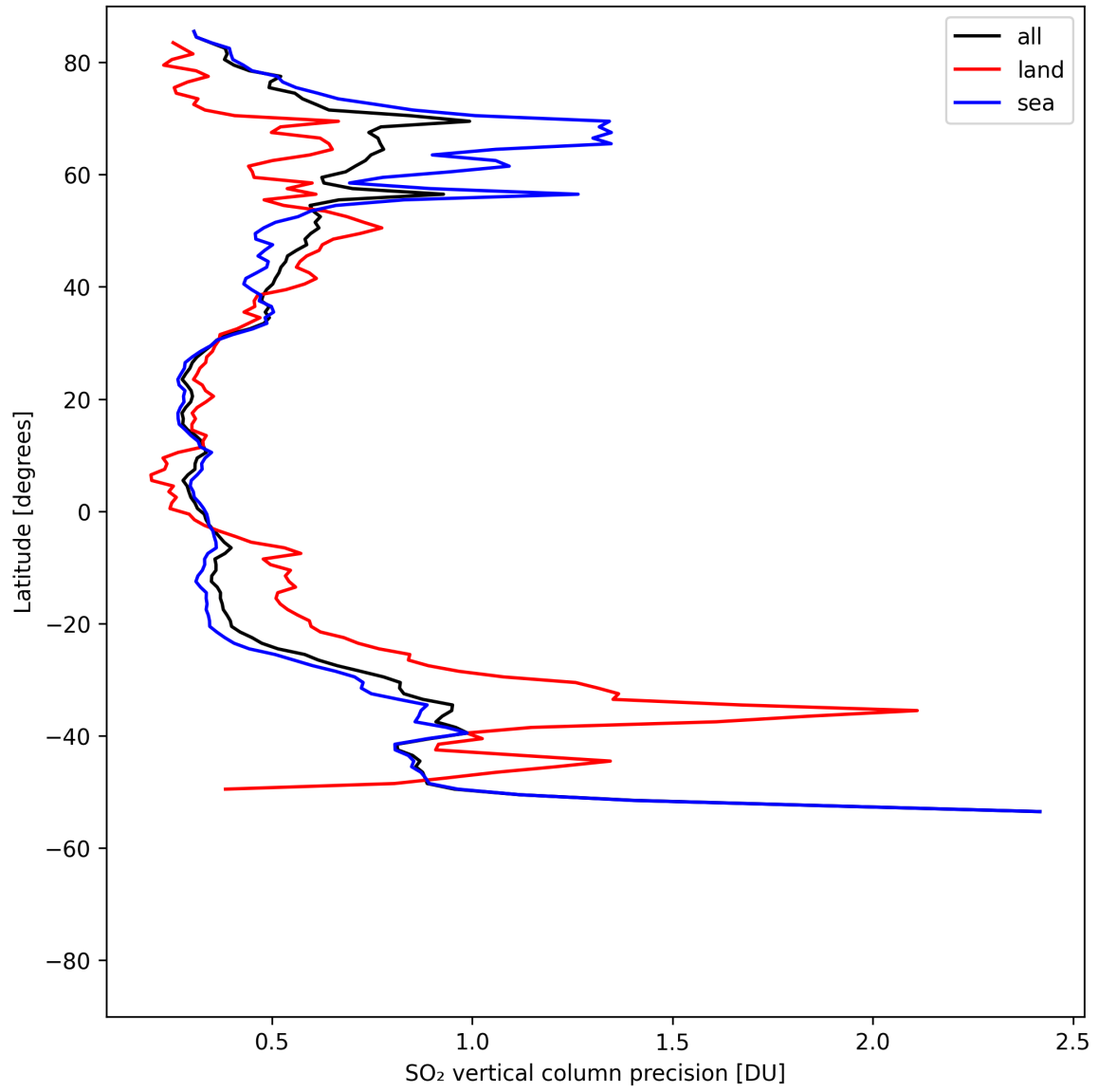
Figure 33: Zonal average of “SO 2 vertical column precision” for 2025-08-09 to 2025-08-10.
