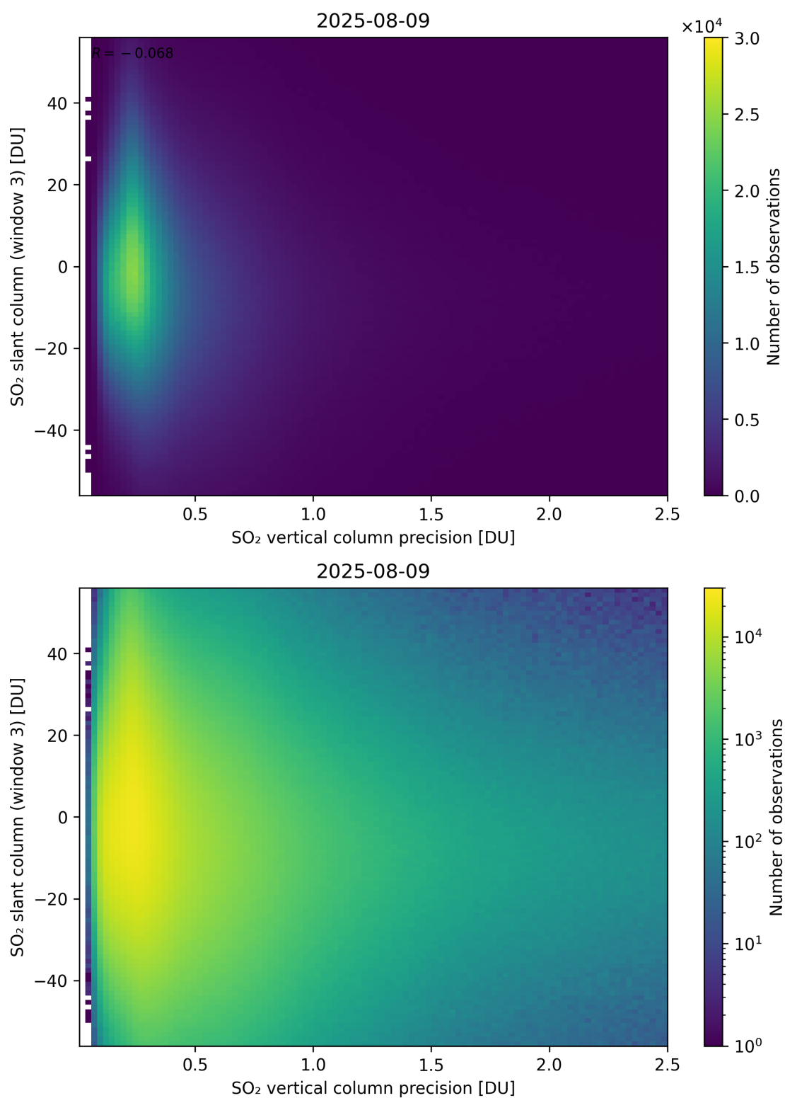
Figure 344: Scatter density plot of “SO 2 vertical column precision” against “SO 2 slant column (window 3)” for 2025-08-09 to 2025-08-10.
