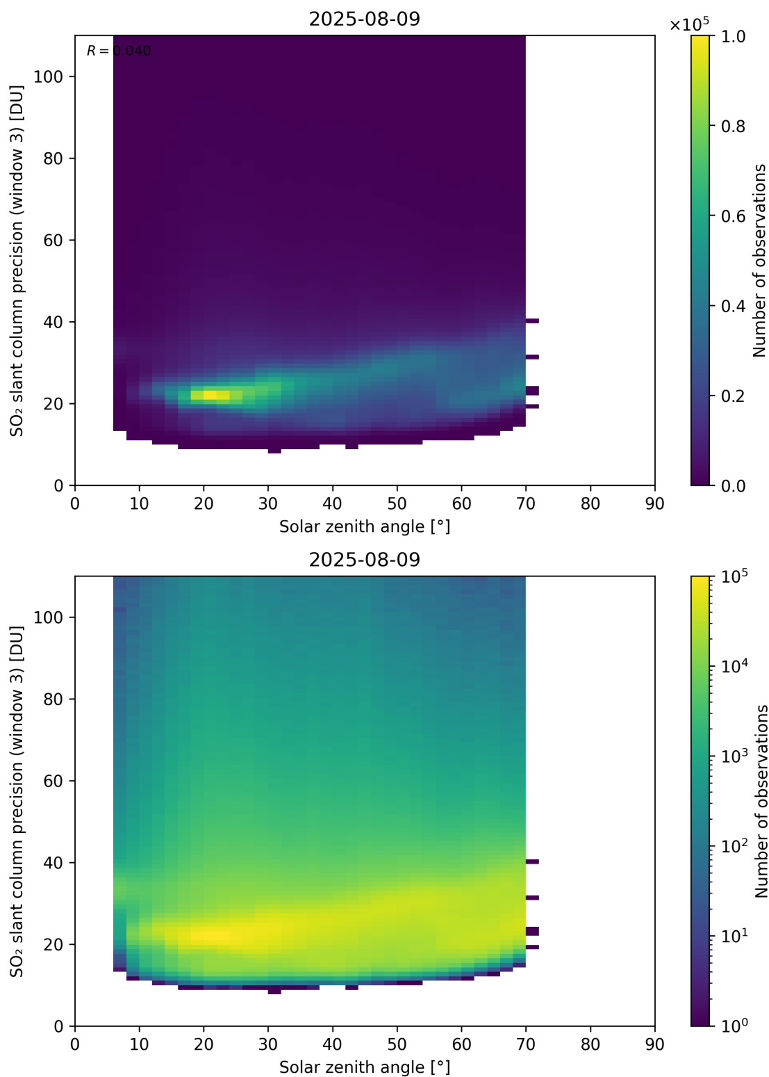
Figure 188: Scatter density plot of “Solar zenith angle” against “SO 2 slant column precision (window 3)” for 2025-08-09 to 2025-08-10.
