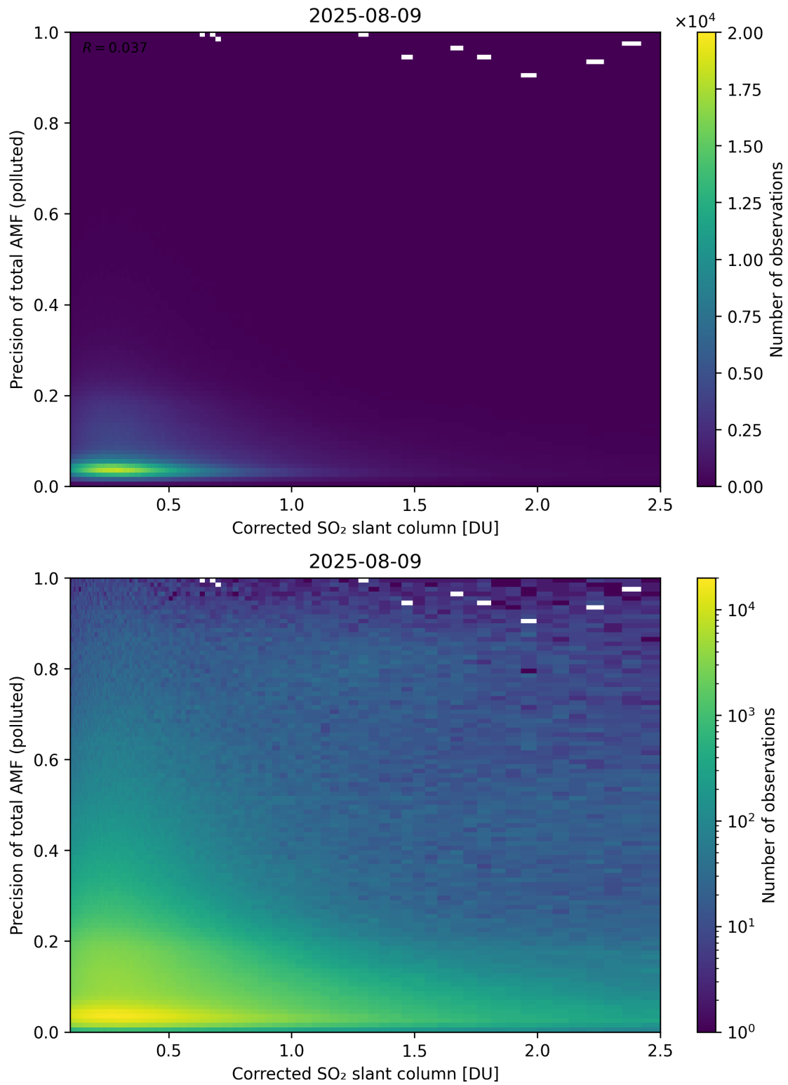
Figure 243: Scatter density plot of “Corrected SO 2 slant column” against “Precision of total AMF (polluted)” for 2025-08-09 to 2025-08-10.
