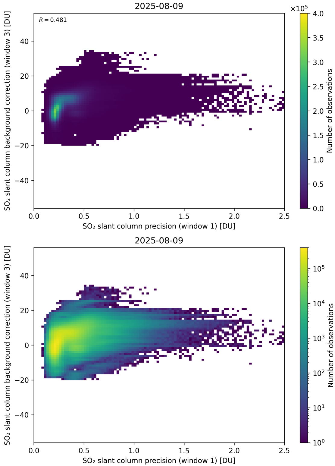
Figure 270: Scatter density plot of “SO 2 slant column precision (window 1)” against “SO 2 slant column background correction (window 3)” for 2025-08-09 to 2025-08-10.
