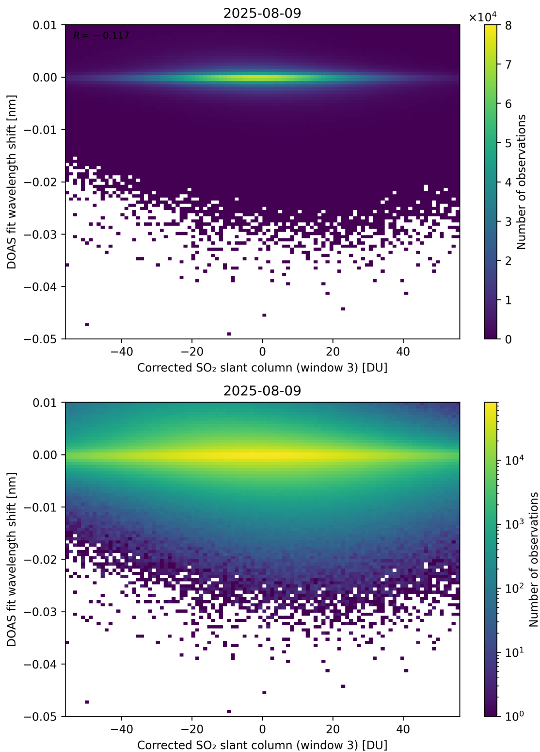
Figure 256: Scatter density plot of “Corrected SO 2 slant column (window 3)” against “DOAS fit wavelength shift” for 2025-08-09 to 2025-08-10.
