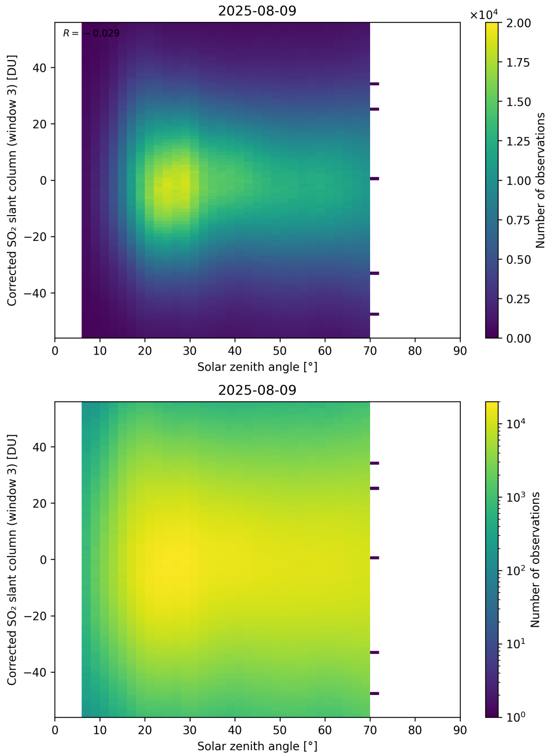
Figure 183: Scatter density plot of “Solar zenith angle” against “Corrected SO 2 slant column (window 3)” for 2025-08-09 to 2025-08-10.
