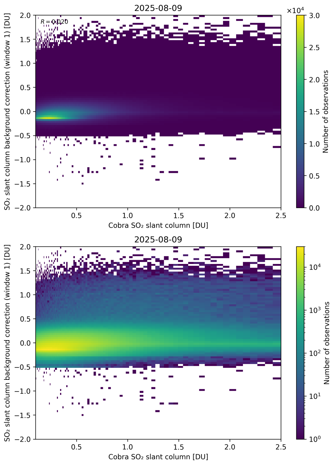
Figure 193: Scatter density plot of “Cobra SO 2 slant column” against “SO 2 slant column background correction (window 1)” for 2025-08-09 to 2025-08-10.
