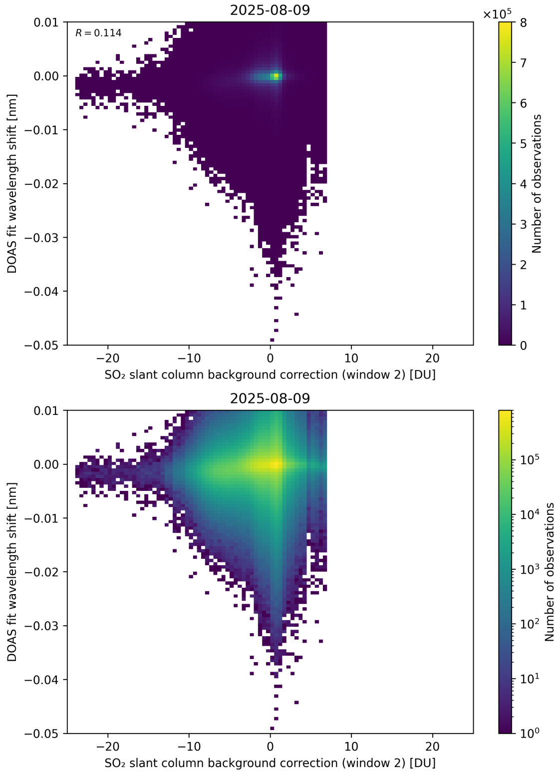
Figure 123: Scatter density plot of “SO 2 slant column background correction (window 2)” against “DOAS fit wavelength shift” for 2025-08-09 to 2025-08-10.
