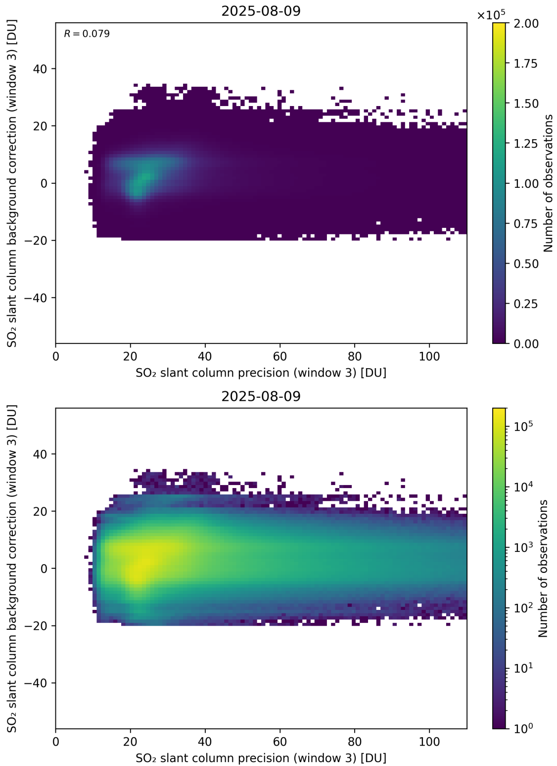
Figure 307: Scatter density plot of “SO 2 slant column precision (window 3)” against “SO 2 slant column background correction (window 3)” for 2025-08-09 to 2025-08-10.
