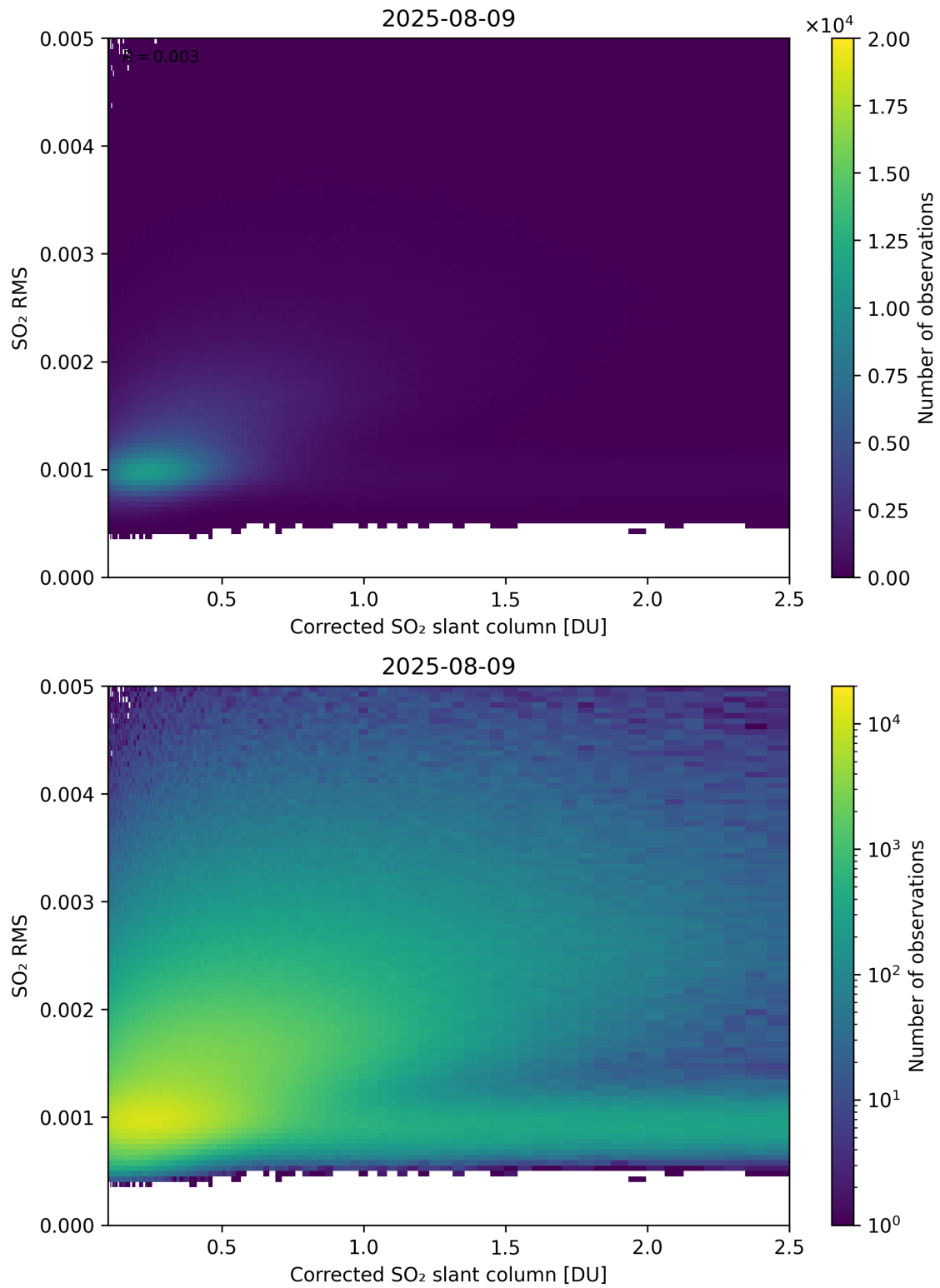
Figure 231: Scatter density plot of “Corrected SO 2 slant column” against “SO 2 RMS” for 2025-08-09 to 2025-08-10.
