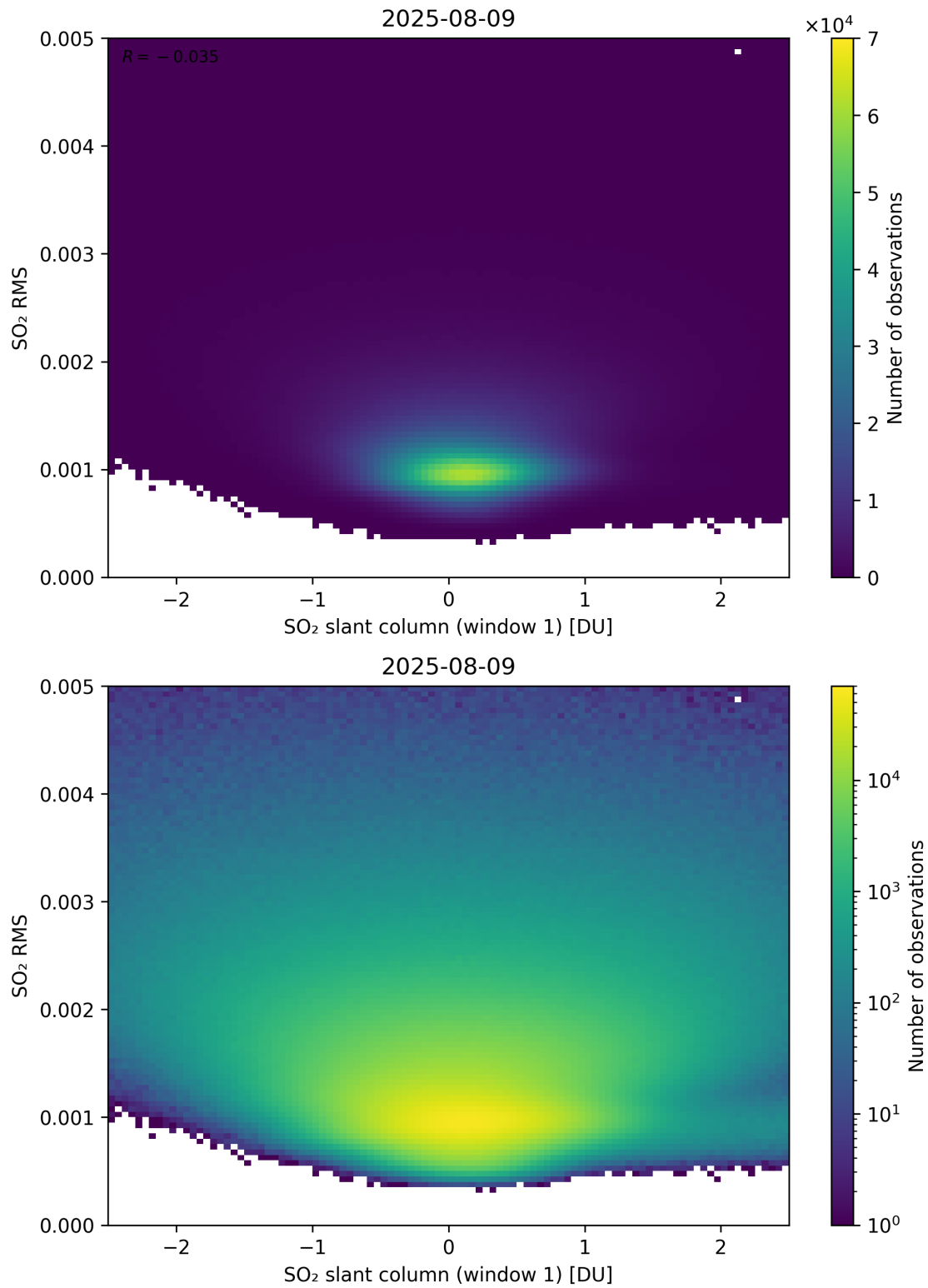
Figure 267: Scatter density plot of “SO 2 slant column (window 1)” against “SO 2 RMS” for 2025-08-09 to 2025-08-10.
