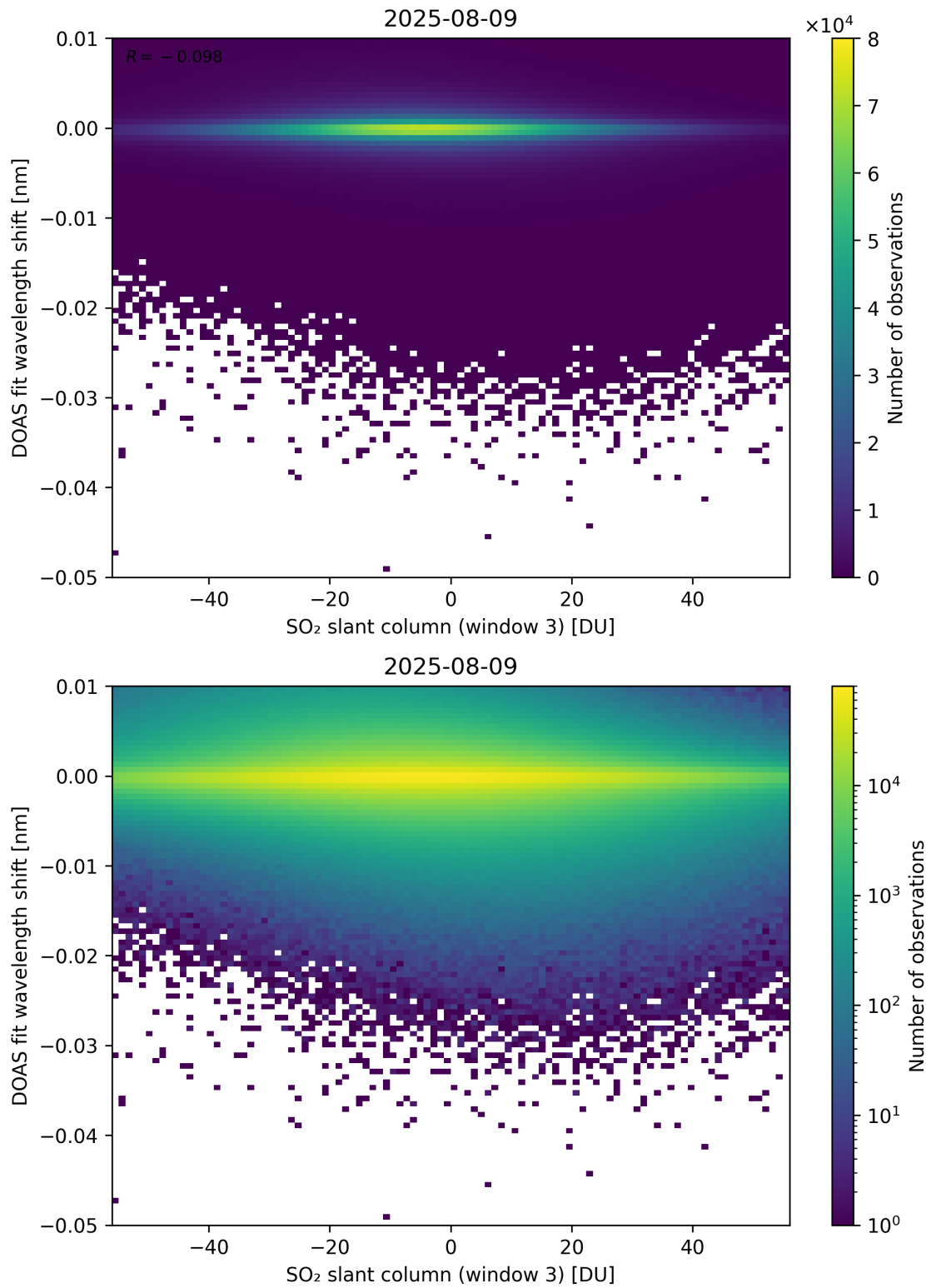
Figure 304: Scatter density plot of “SO 2 slant column (window 3)” against “DOAS fit wavelength shift” for 2025-08-09 to 2025-08-10.
