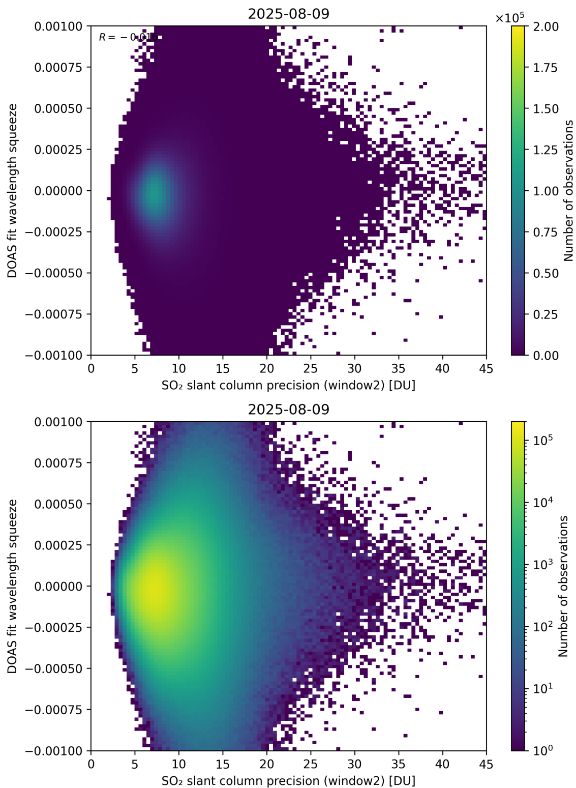
Figure 294: Scatter density plot of “SO 2 slant column precision (window2)” against “DOAS fit wavelength squeeze” for 2025-08-09 to 2025-08-10.
