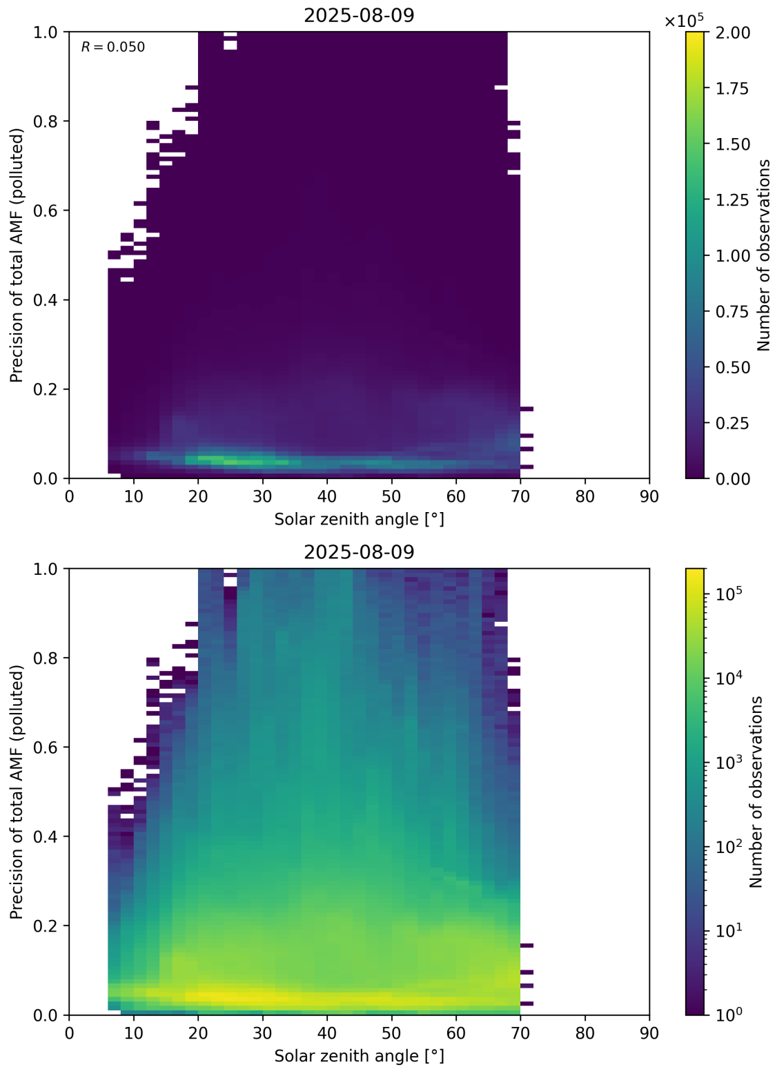
Figure 190: Scatter density plot of “Solar zenith angle” against “Precision of total AMF (polluted)” for 2025-08-09 to 2025-08-10.
