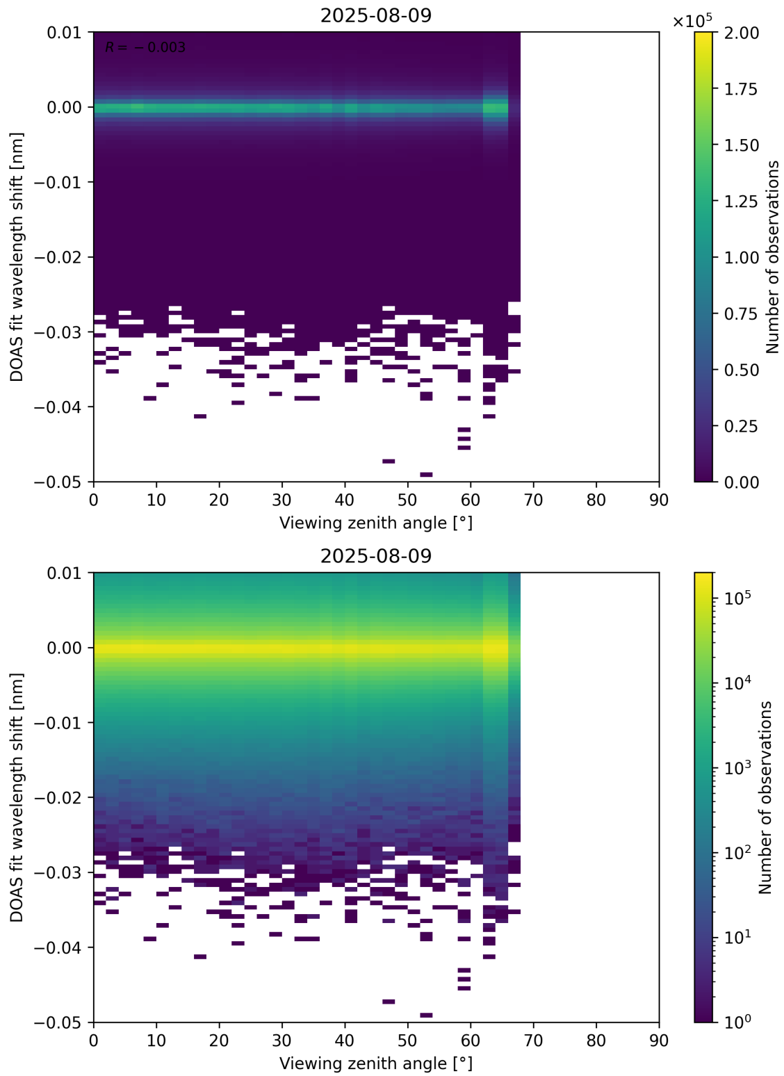
Figure 365: Scatter density plot of “Viewing zenith angle” against “DOAS fit wavelength shift” for 2025-08-09 to 2025-08-10.
