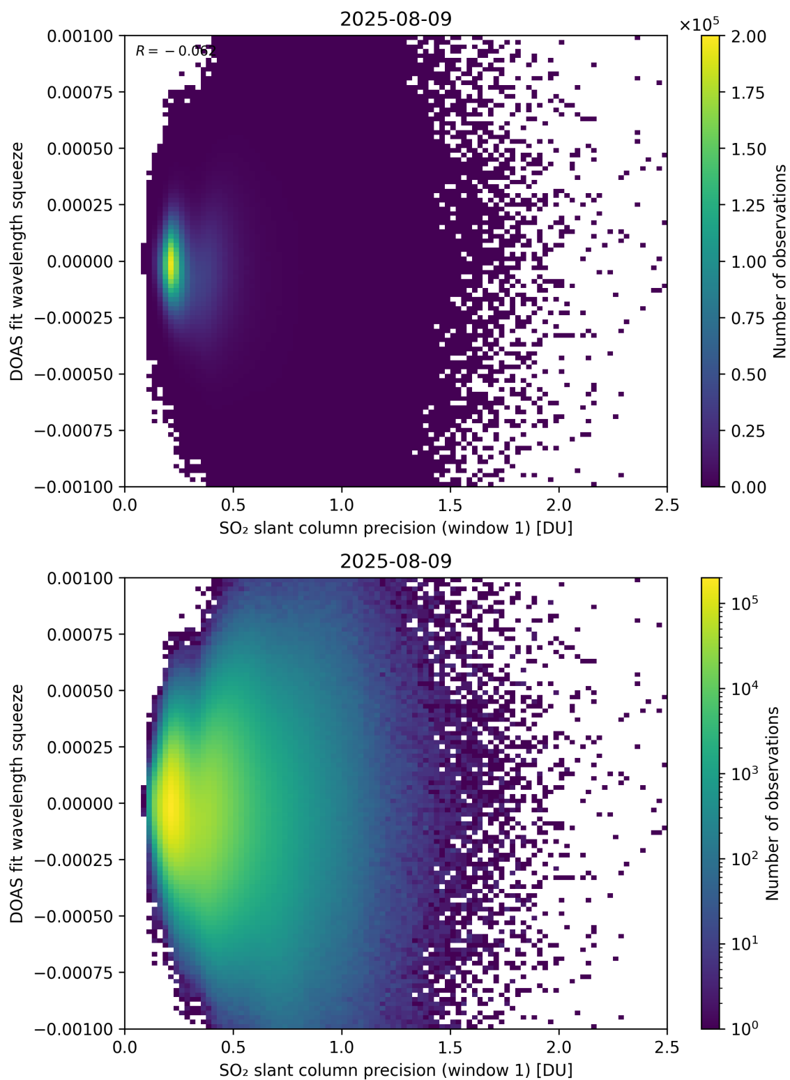
Figure 272: Scatter density plot of “SO 2 slant column precision (window 1)” against “DOAS fit wavelength squeeze” for 2025-08-09 to 2025-08-10.
