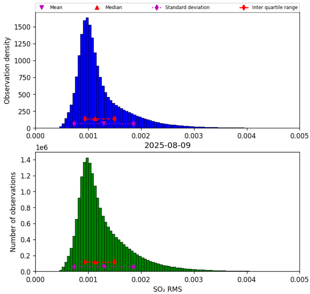
Figure 78: Histogram of “SO 2 RMS” for 2025-08-09 to 2025-08-10
