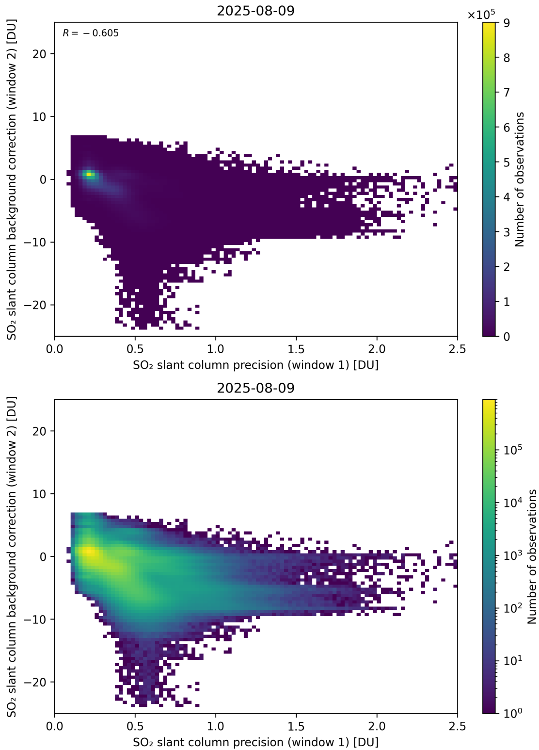
Figure 269: Scatter density plot of “SO 2 slant column precision (window 1)” against “SO 2 slant column background correction (window 2)” for 2025-08-09 to 2025-08-10.
