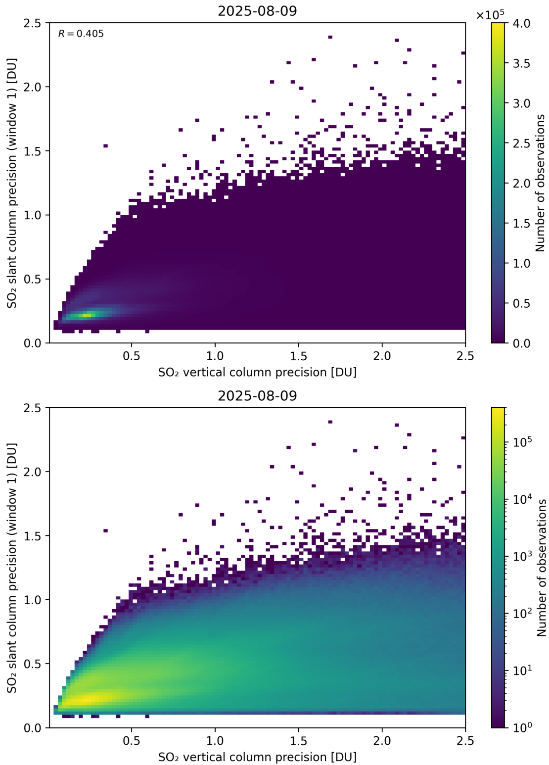
Figure 342: Scatter density plot of “SO 2 vertical column precision” against “SO 2 slant column precision (window 1)” for 2025-08-09 to 2025-08-10.
