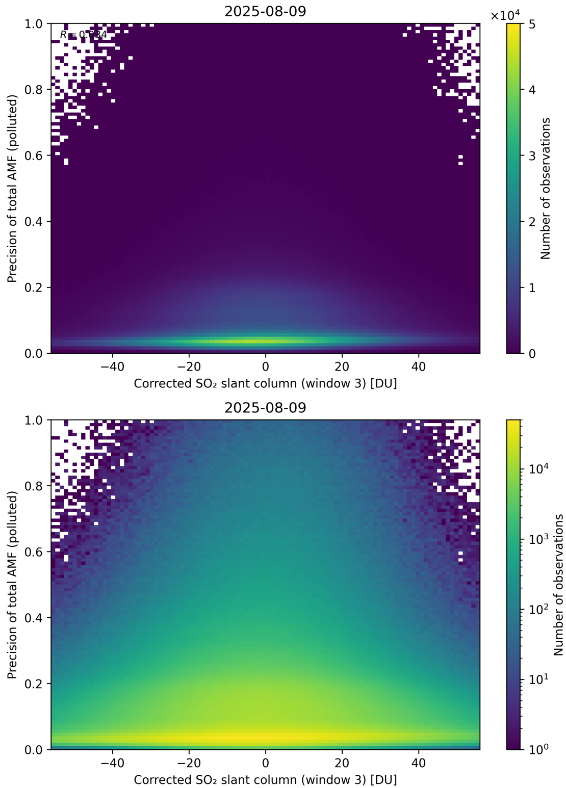
Figure 261: Scatter density plot of “Corrected SO 2 slant column (window 3)” against “Precision of total AMF (polluted)” for 2025-08-09 to 2025-08-10.
