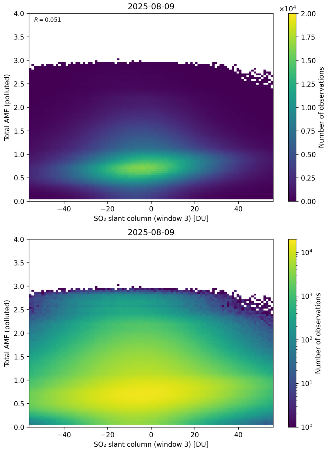
Figure 318: Scatter density plot of “SO 2 slant column (window 3)” against “Total AMF (polluted)” for 2025-08-09 to 2025-08-10.
