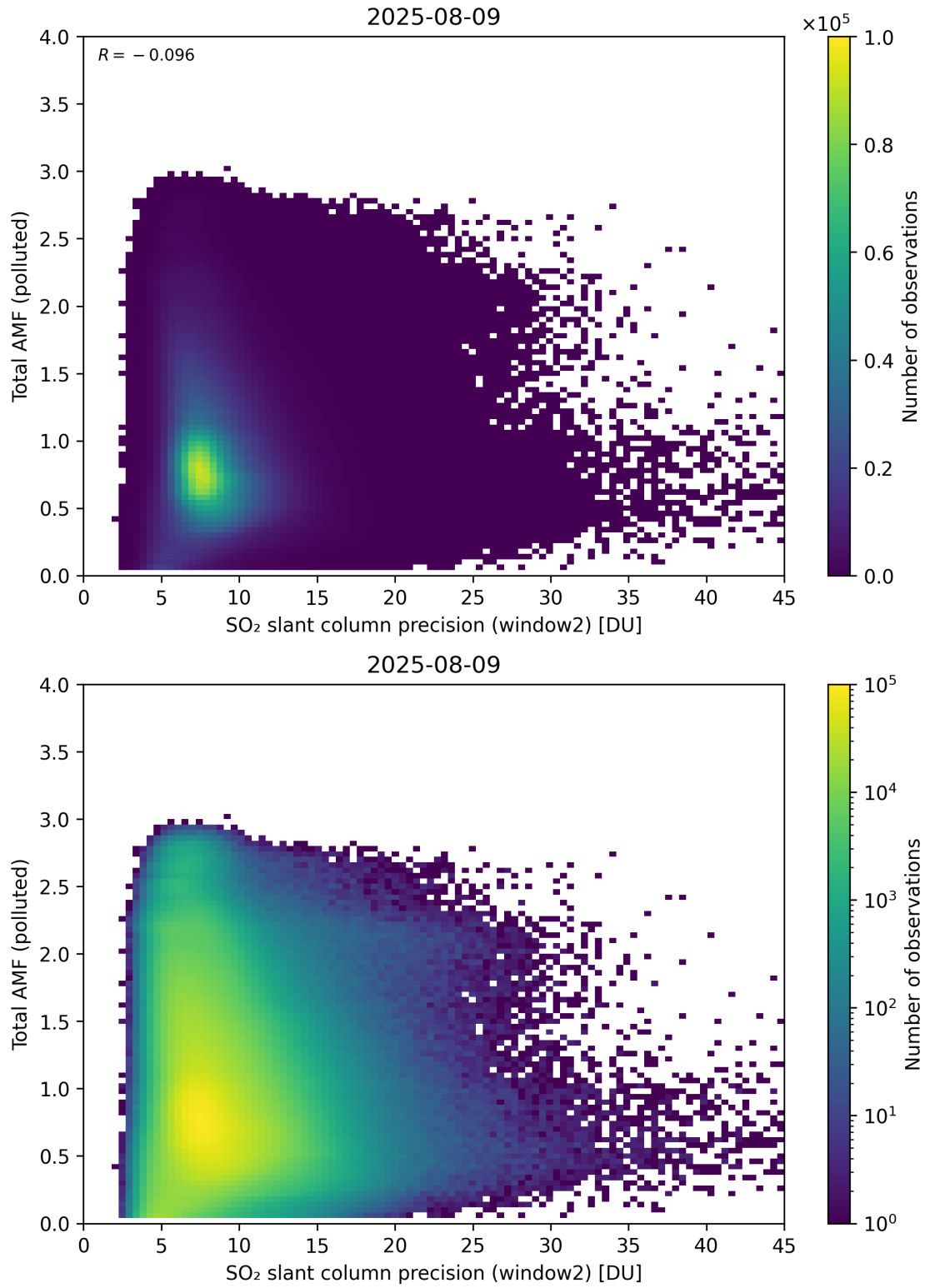
Figure 301: Scatter density plot of “SO 2 slant column precision (window2)” against “Total AMF (polluted)” for 2025-08-09 to 2025-08-10.
