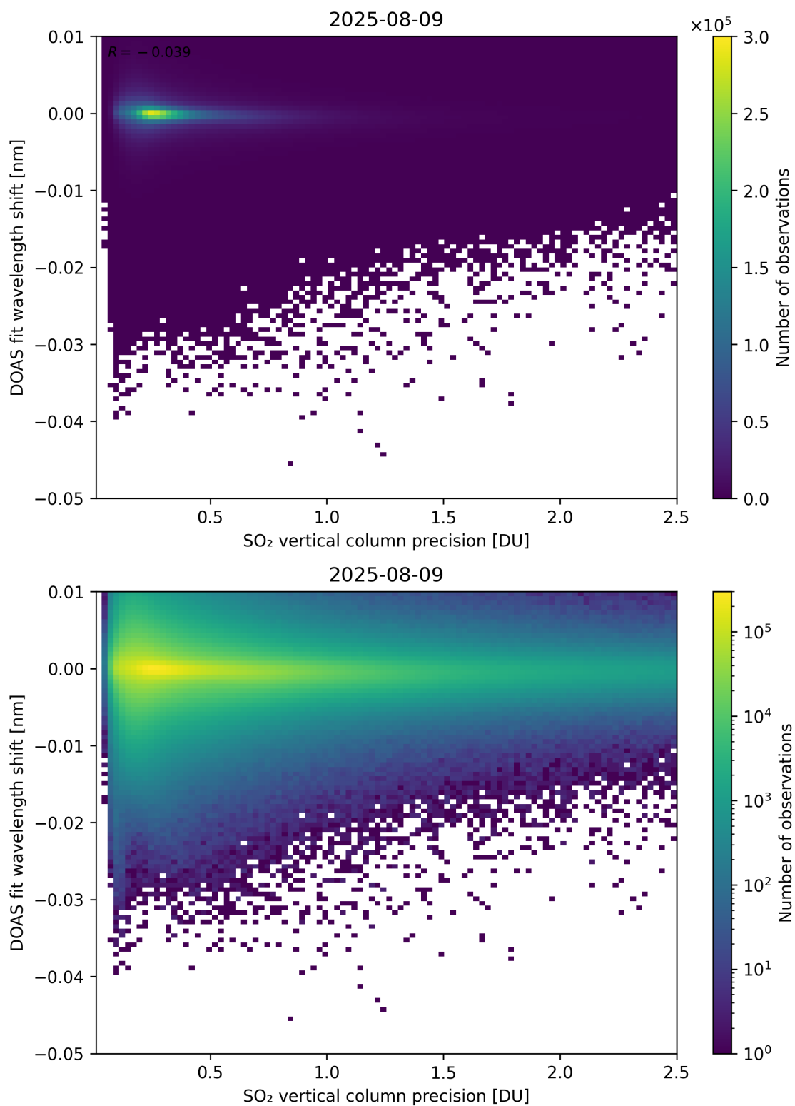
Figure 332: Scatter density plot of “SO 2 vertical column precision” against “DOAS fit wavelength shift” for 2025-08-09 to 2025-08-10.
