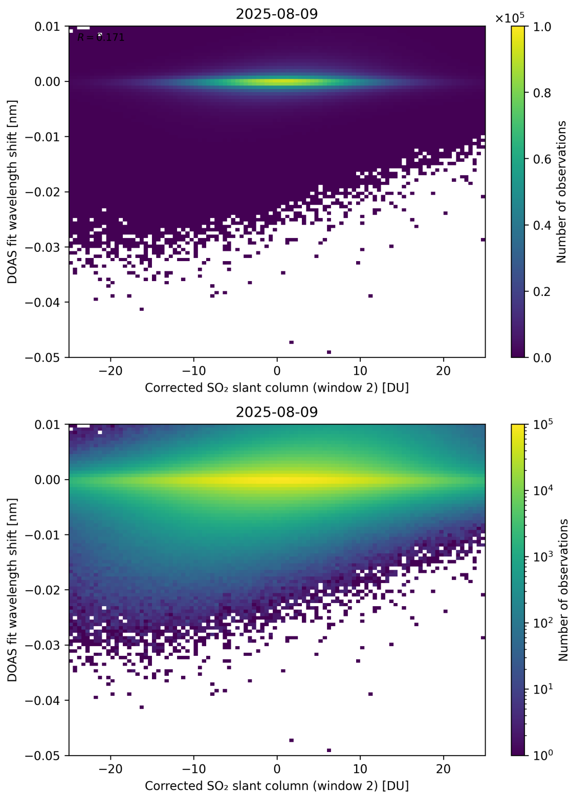
Figure 246: Scatter density plot of “Corrected SO 2 slant column (window 2)” against “DOAS fit wavelength shift” for 2025-08-09 to 2025-08-10.
