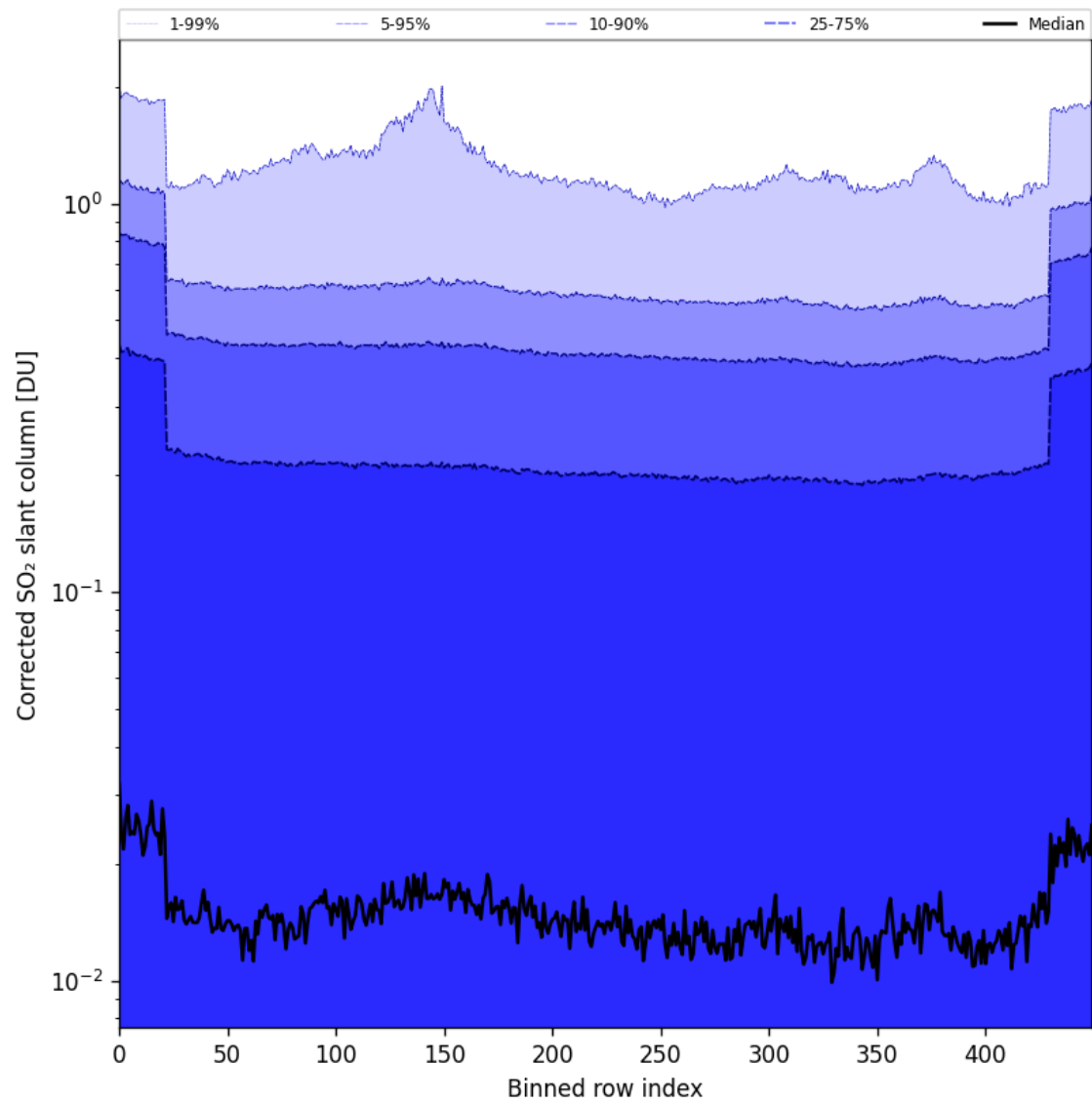
Figure 86: Along track statistics of “Corrected SO 2 slant column” for 2025-08-09 to 2025-08-10
