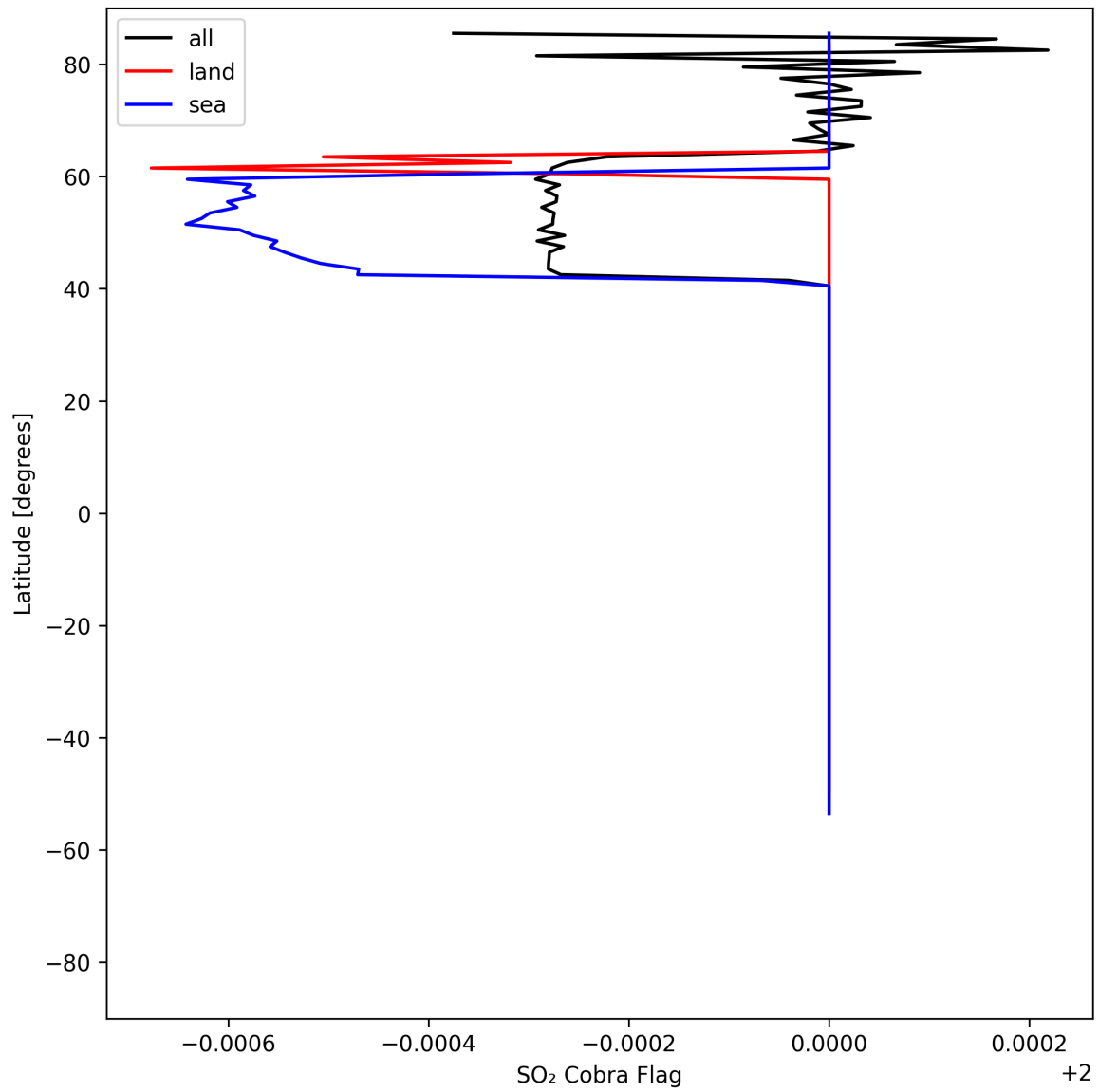
Figure 49: Zonal average of "SO 2 Cobra Flag" for 2025-08-09 to 2025-08-10.
