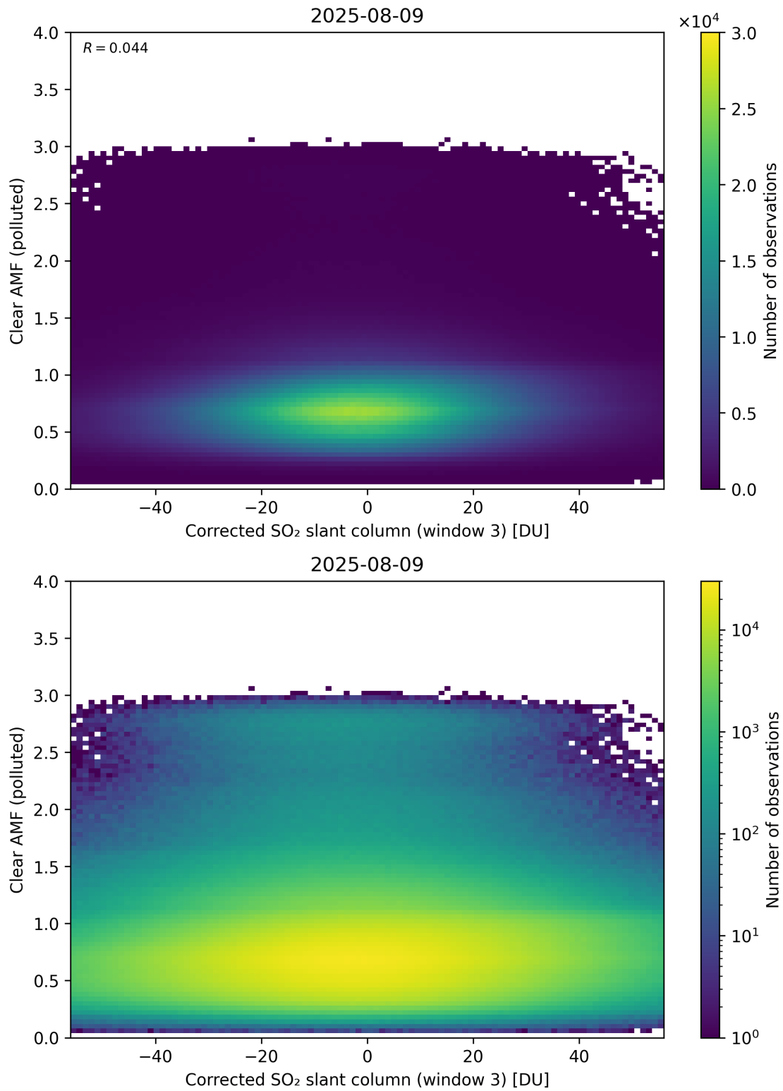
Figure 259: Scatter density plot of “Corrected SO 2 slant column (window 3)” against “Clear AMF (polluted)” for 2025-08-09 to 2025-08-10.
