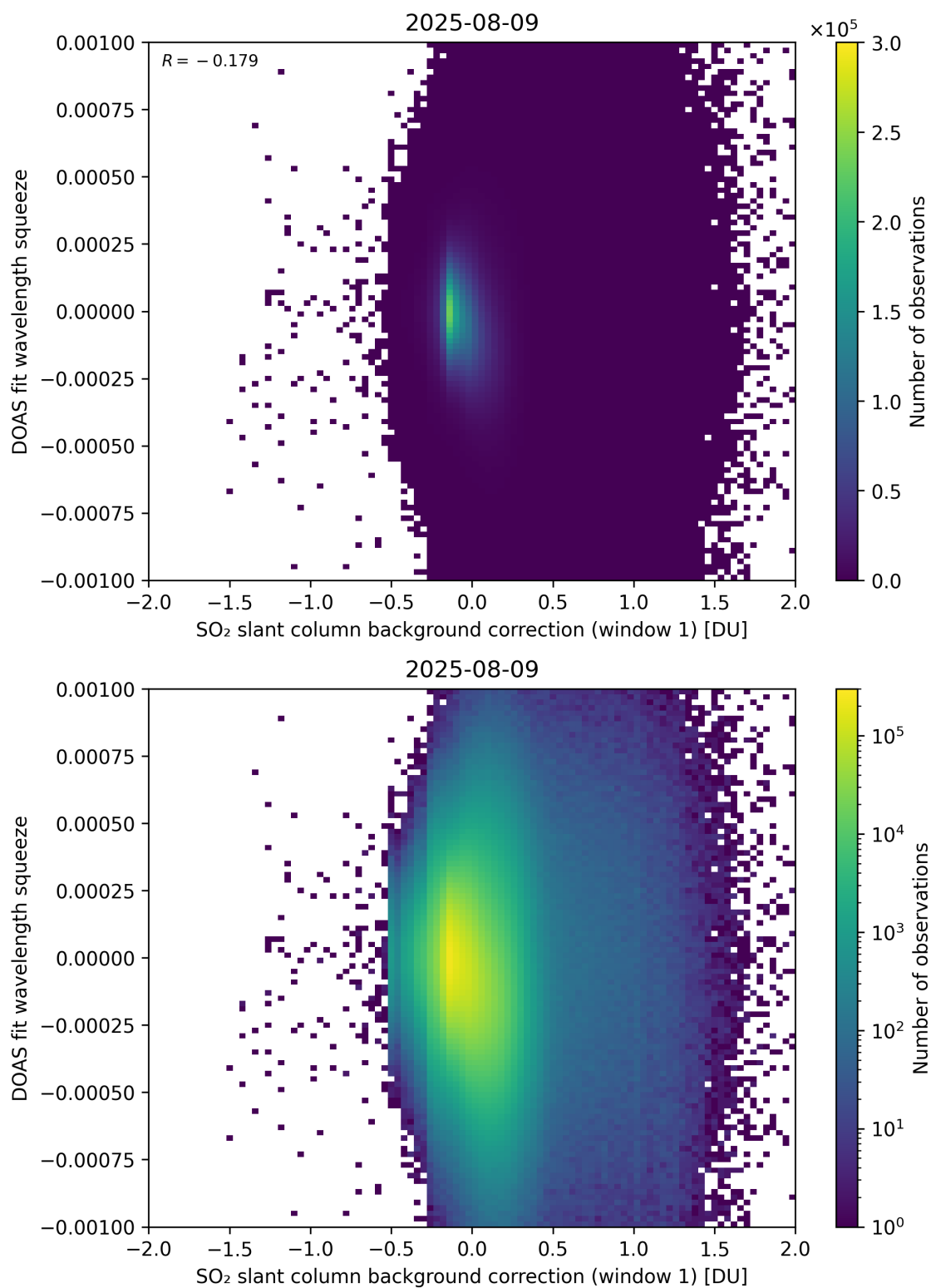
Figure 112: Scatter density plot of “SO 2 slant column background correction (window 1)” against “DOAS fit wavelength squeeze” for 2025-08-09 to 2025-08-10.
