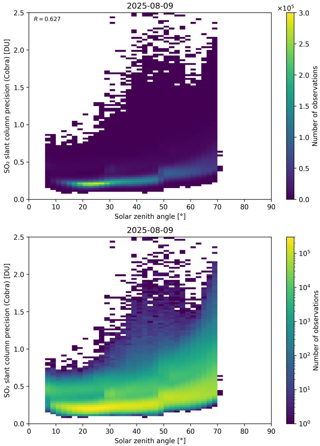
Figure 180: Scatter density plot of “Solar zenith angle” against “SO 2 slant column precision (Cobra)” for 2025-08-09 to 2025-08-10.
