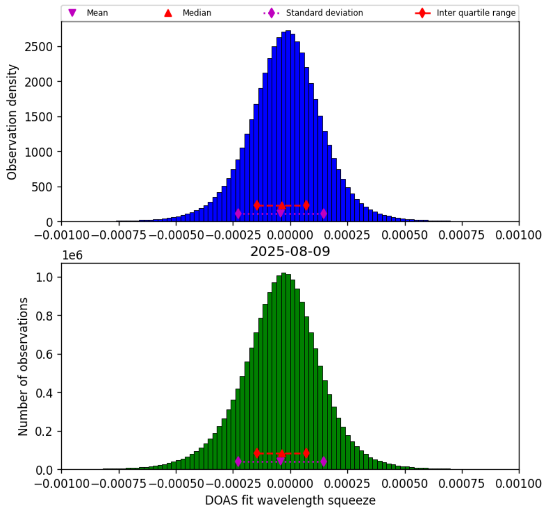
Figure 77: Histogram of “DOAS fit wavelength squeeze” for 2025-08-09 to 2025-08-10
