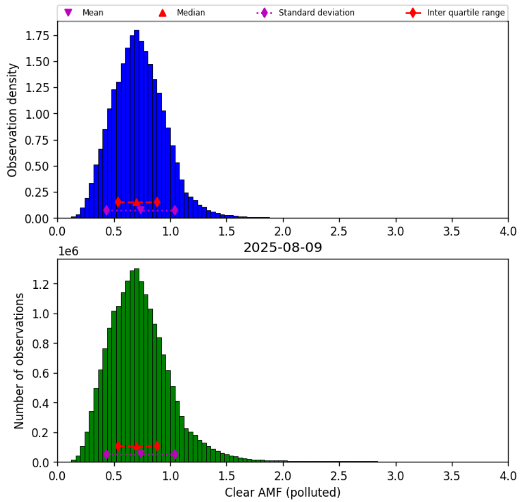
Figure 81: Histogram of “Clear AMF (polluted)” for 2025-08-09 to 2025-08-10
