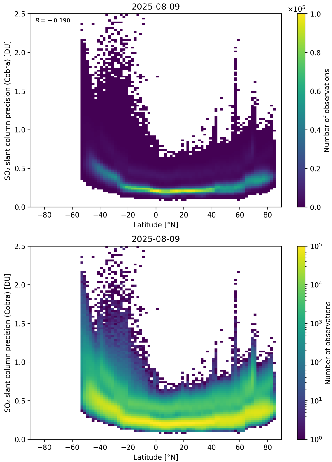
Figure 158: Scatter density plot of “Latitude” against “SO 2 slant column precision (Cobra)” for 2025-08-09 to 2025-08-10.
