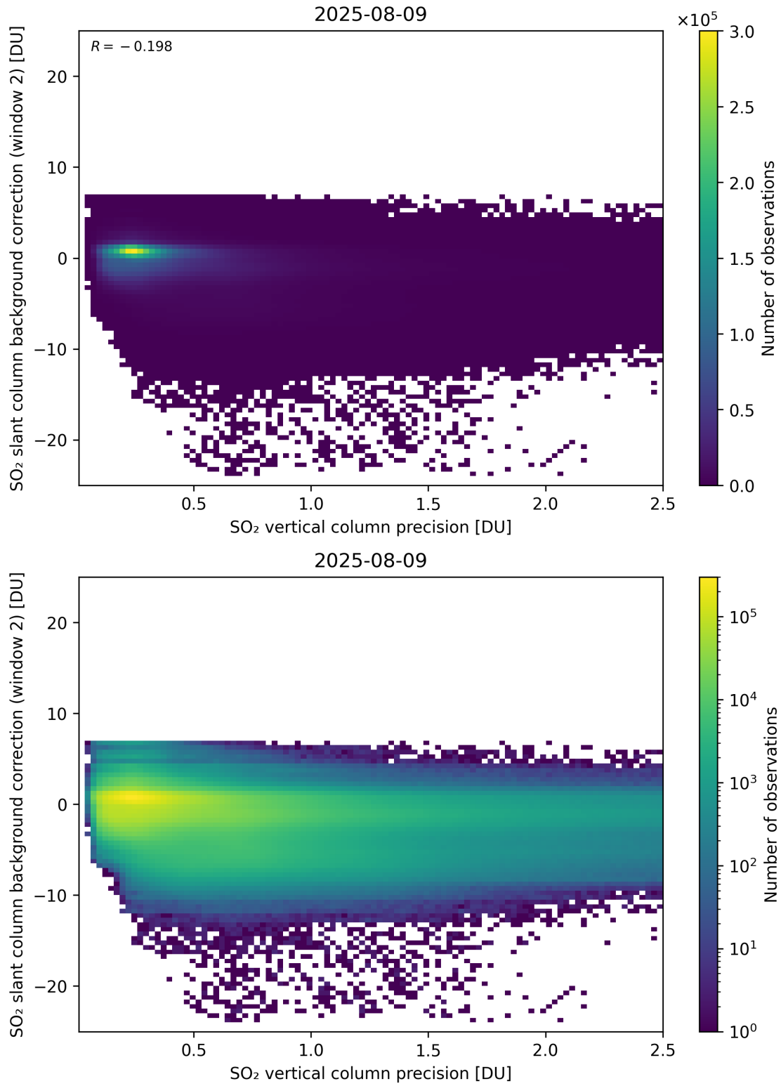
Figure 330: Scatter density plot of “SO 2 vertical column precision” against “SO 2 slant column background correction (window 2)” for 2025-08-09 to 2025-08-10.
