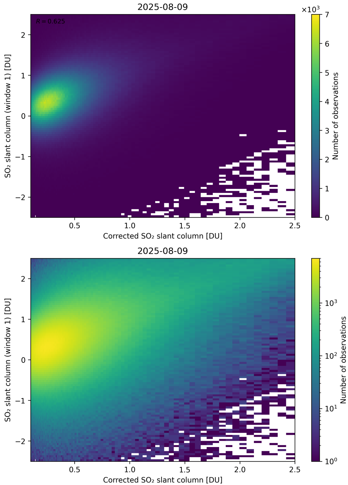
Figure 237: Scatter density plot of “Corrected SO 2 slant column” against “SO 2 slant column (window 1)” for 2025-08-09 to 2025-08-10.
