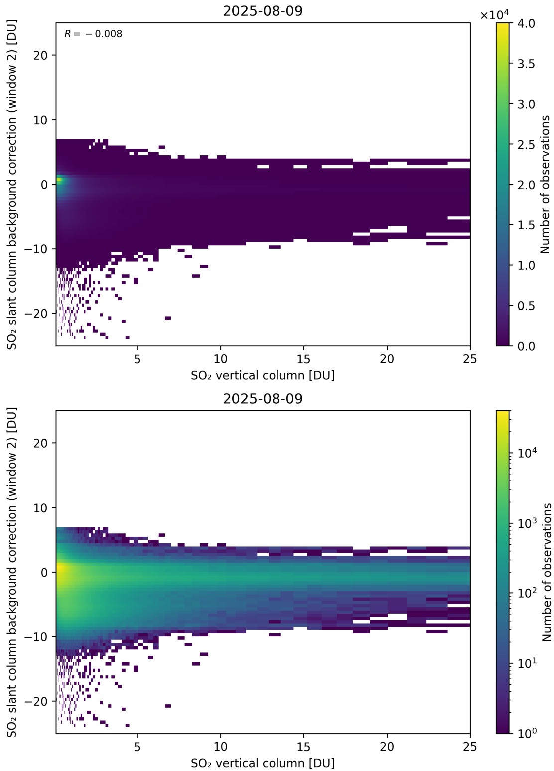
Figure 324: Scatter density plot of “SO 2 vertical column” against “SO 2 slant column background correction (window 2)” for 2025-08-09 to 2025-08-10.
