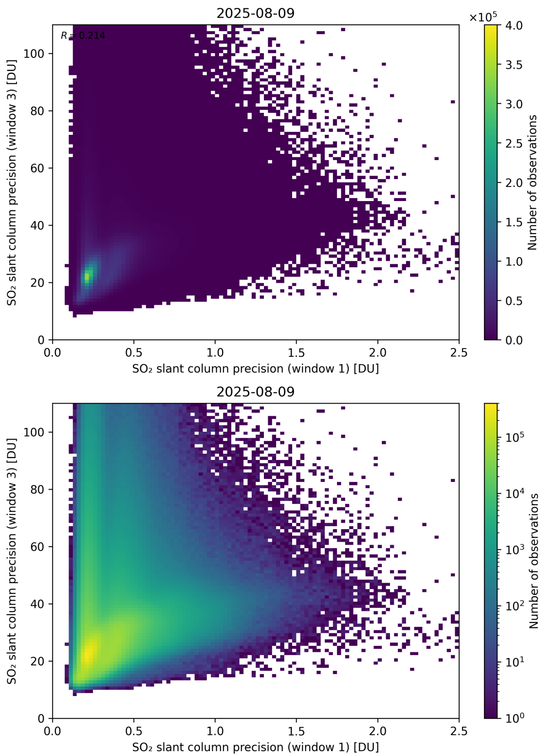
Figure 279: Scatter density plot of “SO 2 slant column precision (window 1)” against “SO 2 slant column precision (window 3)” for 2025-08-09 to 2025-08-10.
