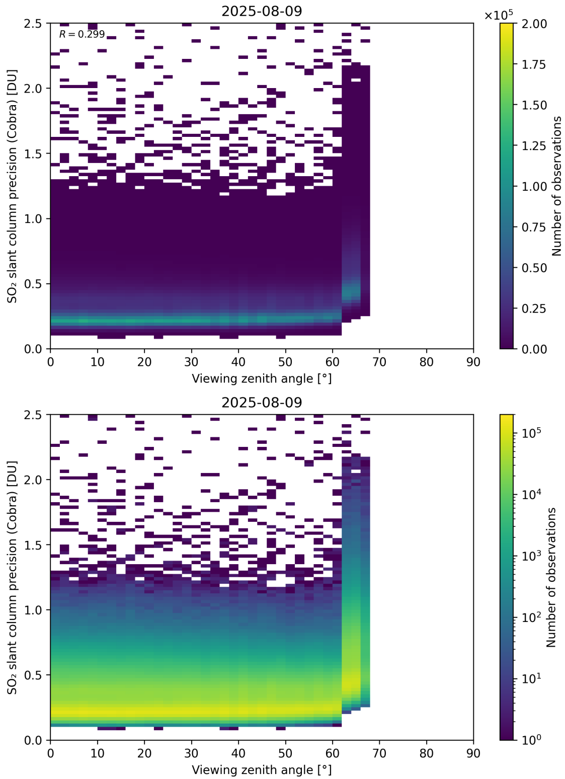
Figure 372: Scatter density plot of “Viewing zenith angle” against “SO 2 slant column precision (Cobra)” for 2025-08-09 to 2025-08-10.
