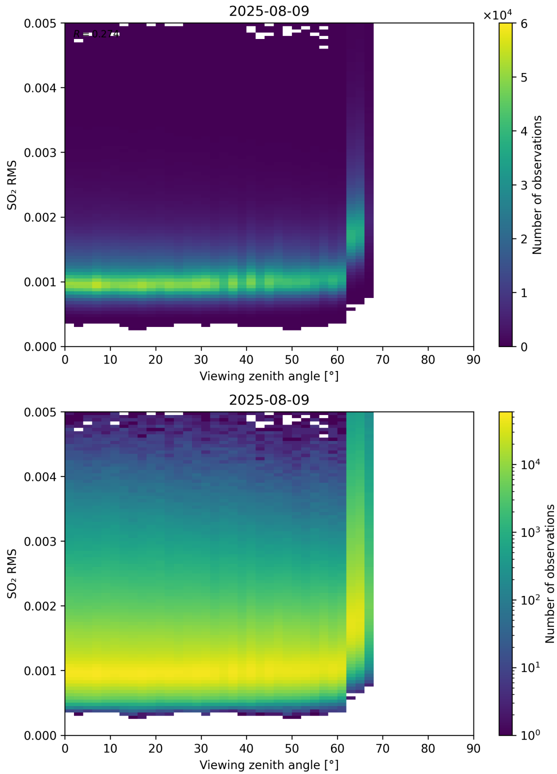
Figure 367: Scatter density plot of “Viewing zenith angle” against “SO 2 RMS” for 2025-08-09 to 2025-08-10.
