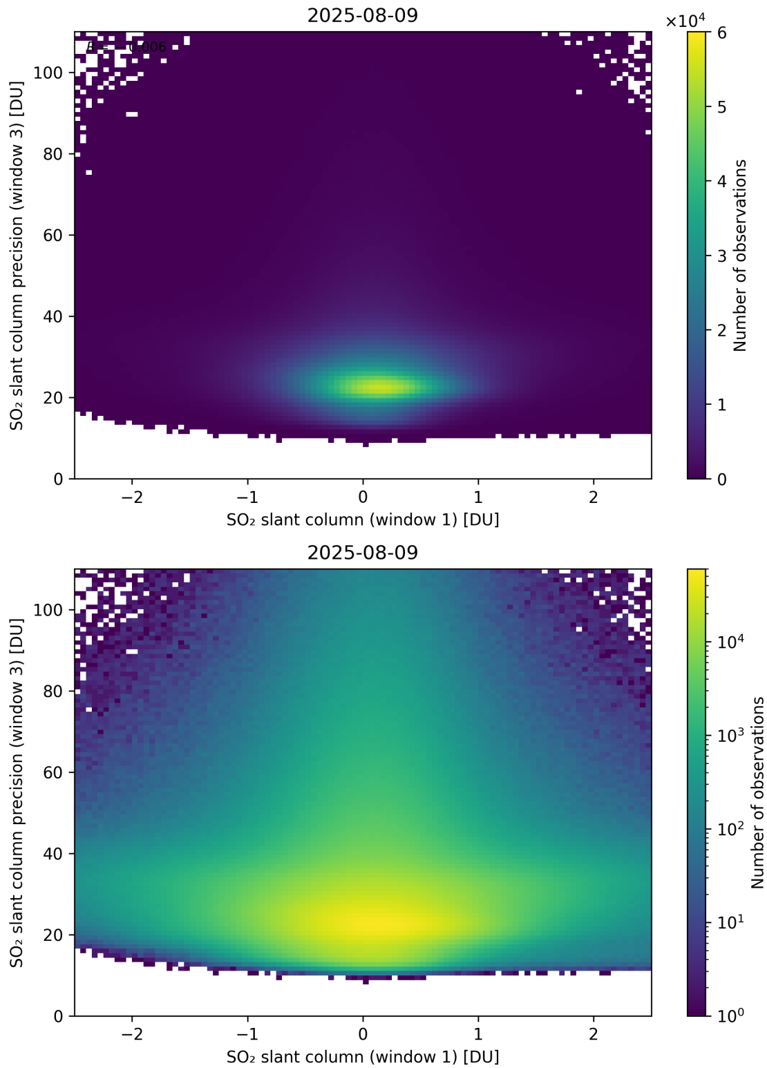
Figure 288: Scatter density plot of “SO 2 slant column (window 1)” against “SO 2 slant column precision (window 3)” for 2025-08-09 to 2025-08-10.
