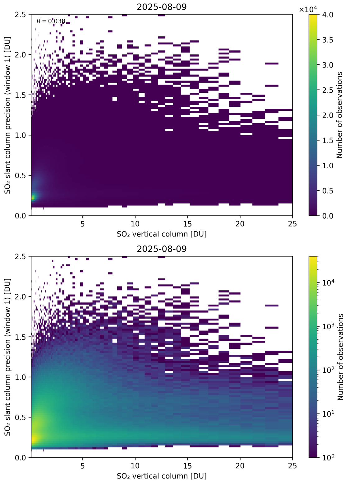
Figure 355: Scatter density plot of “SO 2 vertical column” against “SO 2 slant column precision (window 1)” for 2025-08-09 to 2025-08-10.
