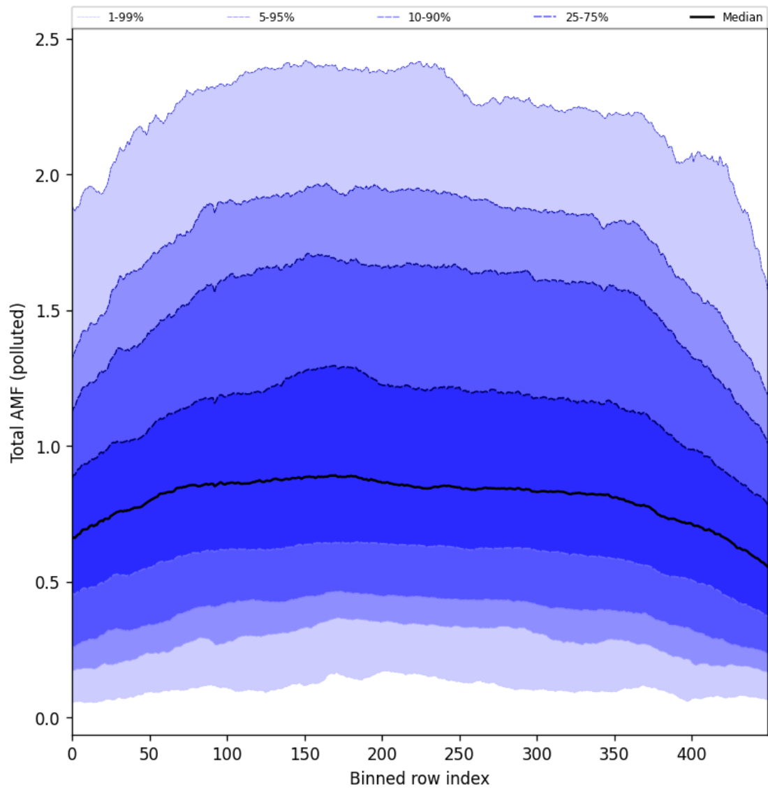
Figure 105: Along track statistics of “Total AMF (polluted)” for 2025-08-09 to 2025-08-10
