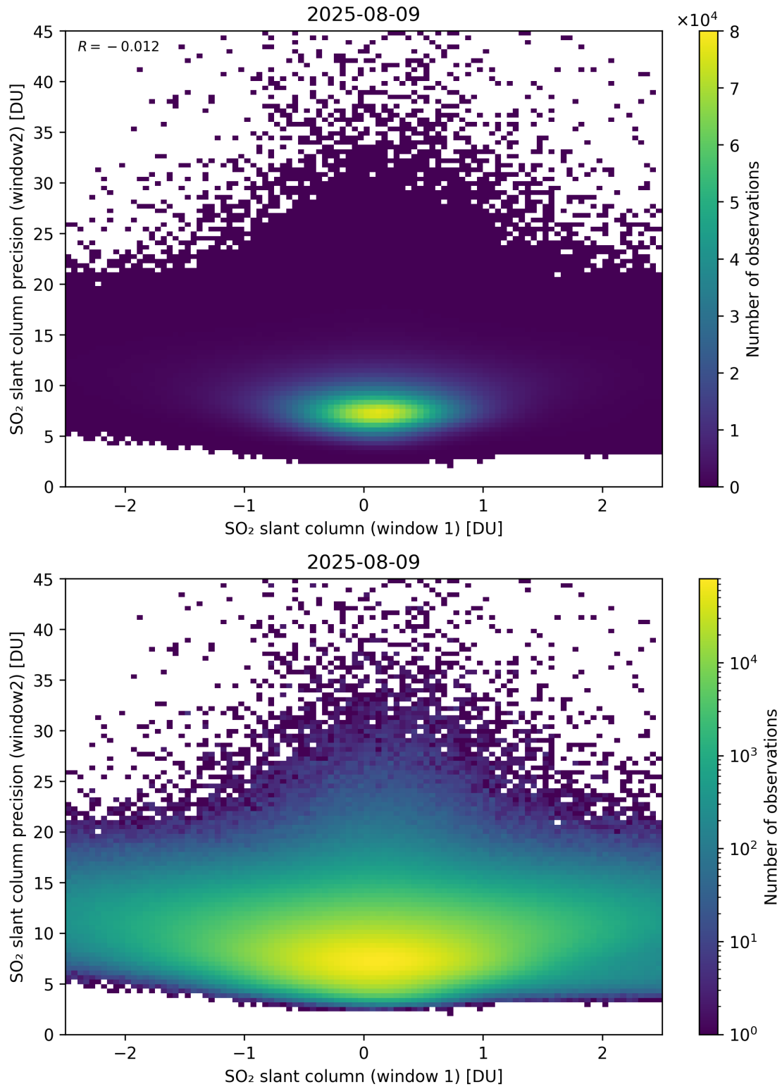
Figure 286: Scatter density plot of “SO 2 slant column (window 1)” against “SO 2 slant column precision (window2)” for 2025-08-09 to 2025-08-10.
