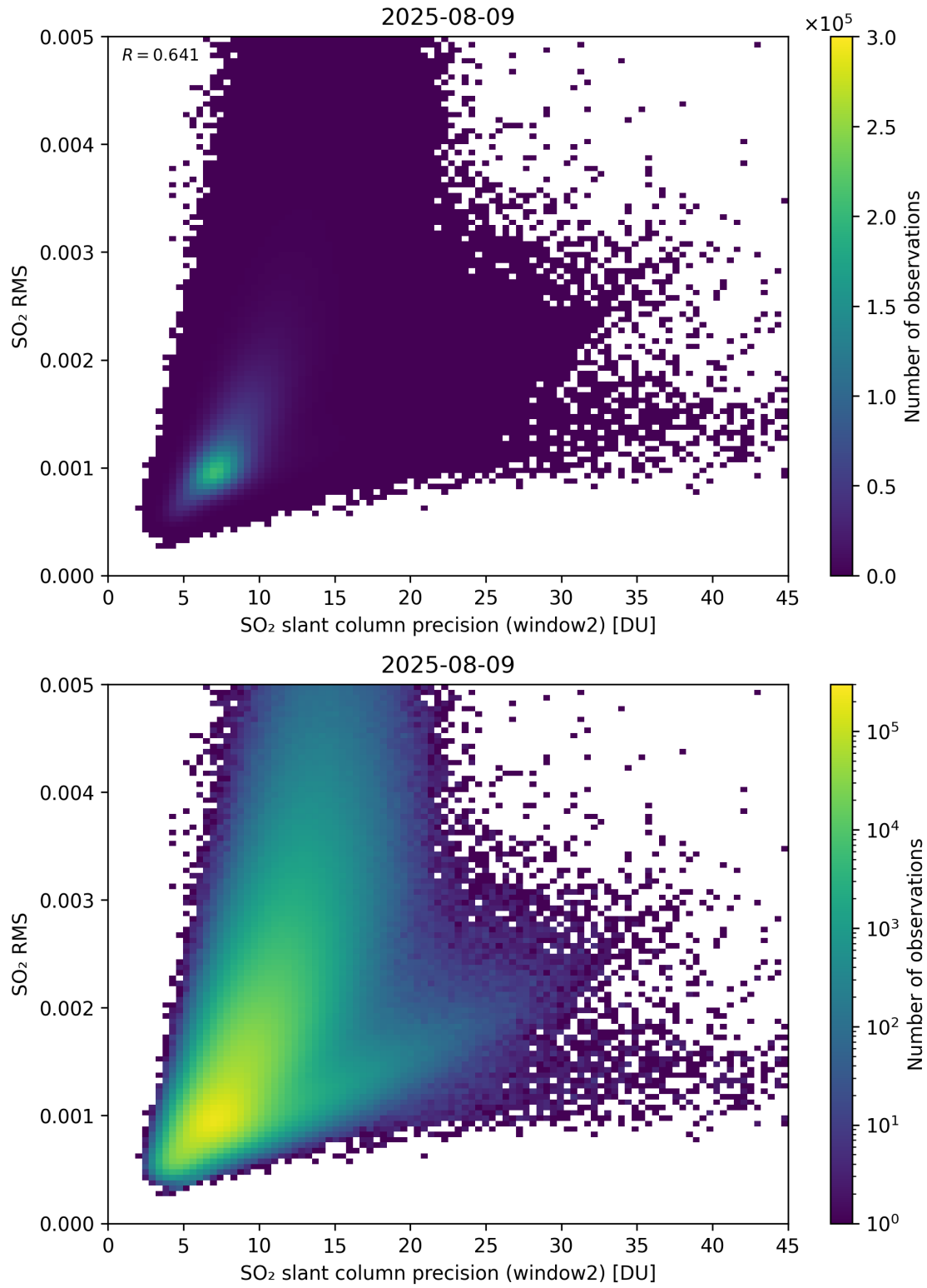
Figure 295: Scatter density plot of “SO 2 slant column precision (window2)” against “SO 2 RMS” for 2025-08-09 to 2025-08-10.
