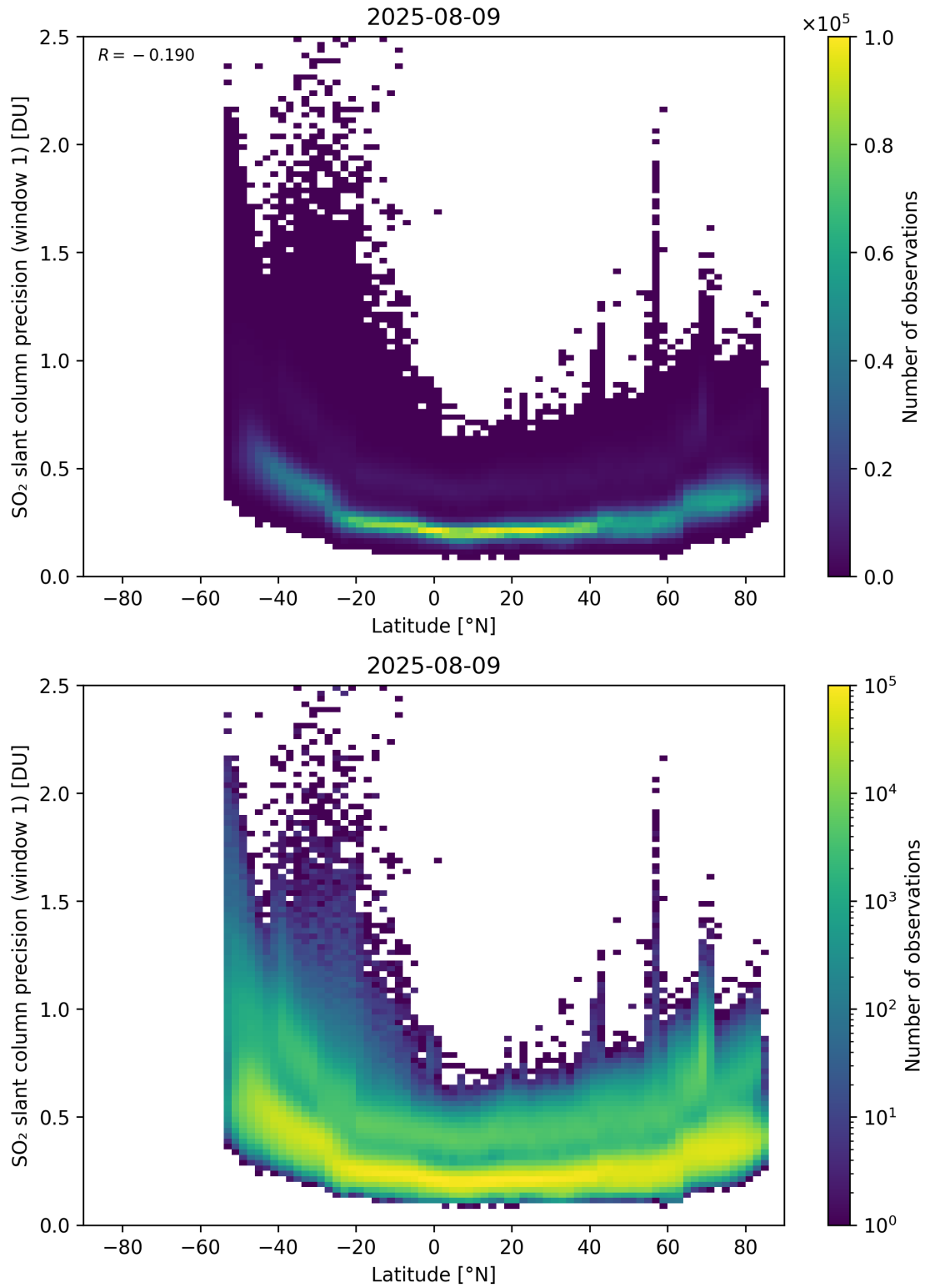
Figure 163: Scatter density plot of “Latitude” against “SO 2 slant column precision (window 1)” for 2025-08-09 to 2025-08-10.
