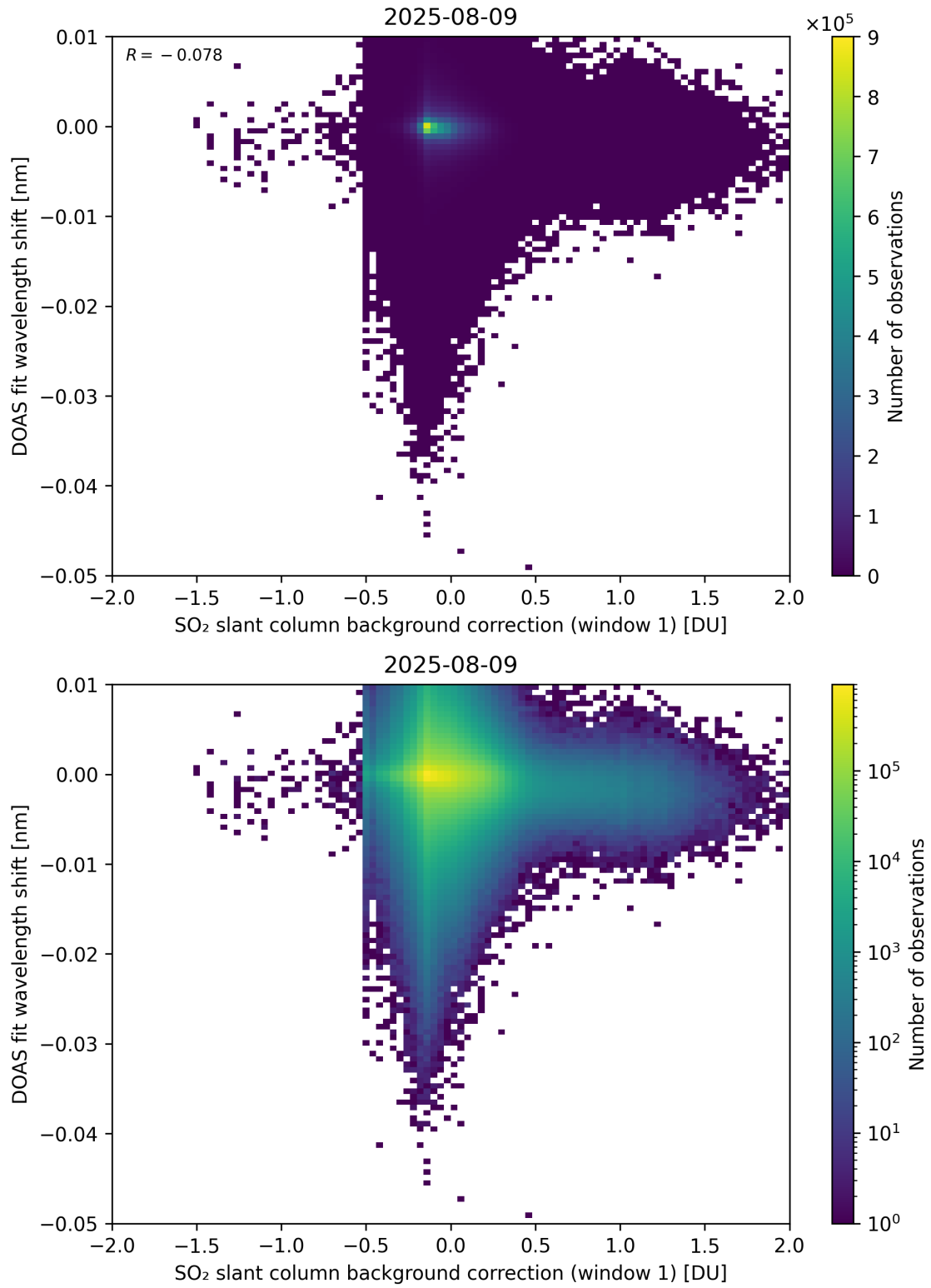
Figure 111: Scatter density plot of “SO 2 slant column background correction (window 1)” against “DOAS fit wavelength shift” for 2025-08-09 to 2025-08-10.
