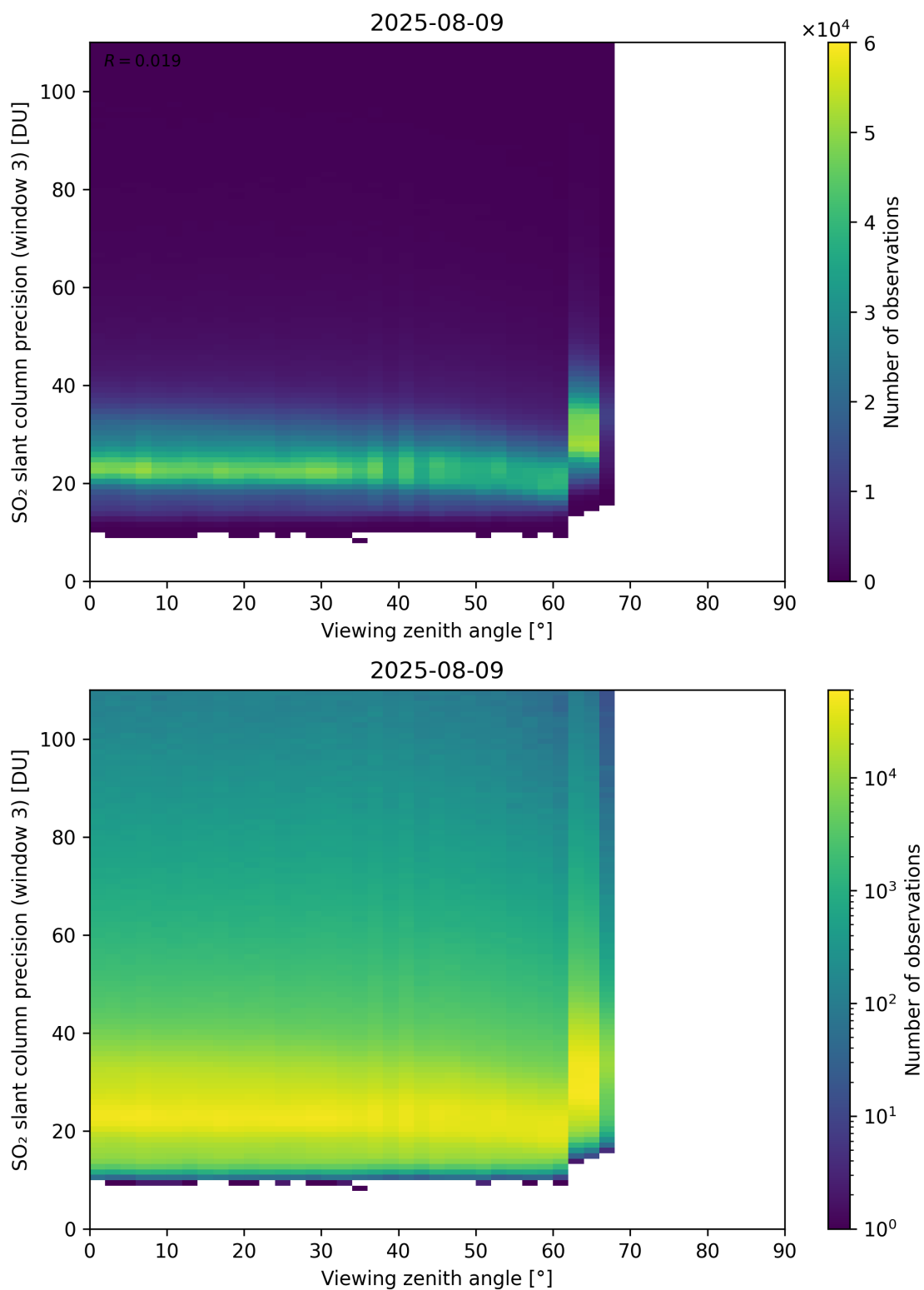
Figure 380: Scatter density plot of “Viewing zenith angle” against “SO 2 slant column precision (window 3)” for 2025-08-09 to 2025-08-10.
