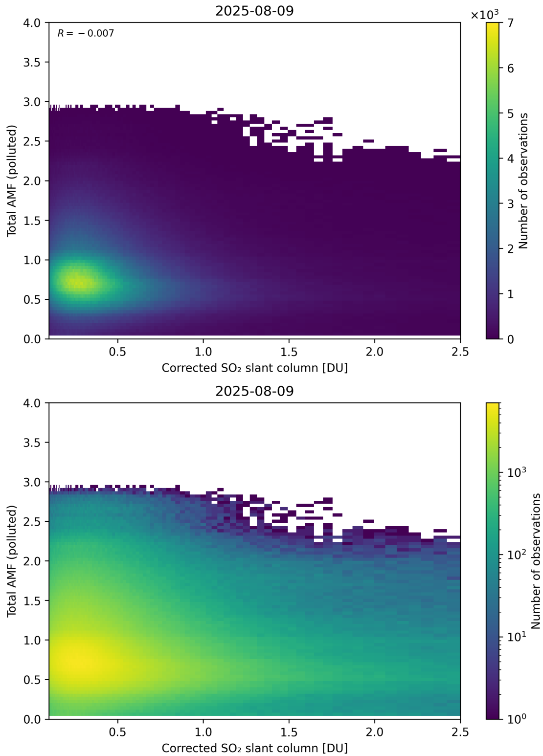
Figure 242: Scatter density plot of “Corrected SO 2 slant column” against “Total AMF (polluted)” for 2025-08-09 to 2025-08-10.
