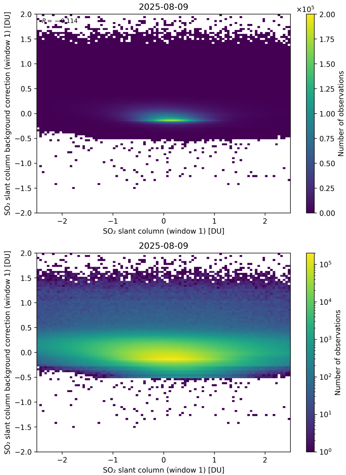
Figure 262: Scatter density plot of “SO 2 slant column (window 1)” against “SO 2 slant column background correction (window 1)” for 2025-08-09 to 2025-08-10.
