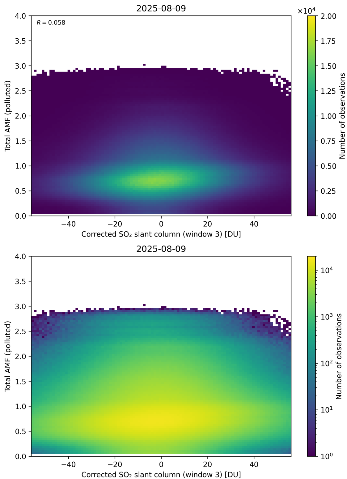
Figure 260: Scatter density plot of “Corrected SO 2 slant column (window 3)” against “Total AMF (polluted)” for 2025-08-09 to 2025-08-10.
