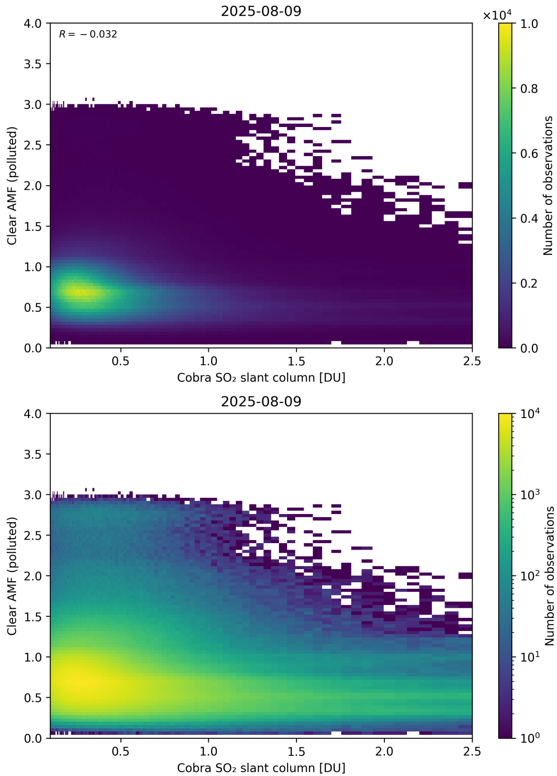
Figure 215: Scatter density plot of “Cobra SO 2 slant column” against “Clear AMF (polluted)” for 2025-08-09 to 2025-08-10.
