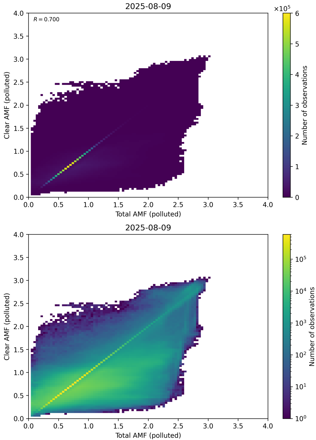
Figure 321: Scatter density plot of “Total AMF (polluted)” against “Clear AMF (polluted)” for 2025-08-09 to 2025-08-10.
