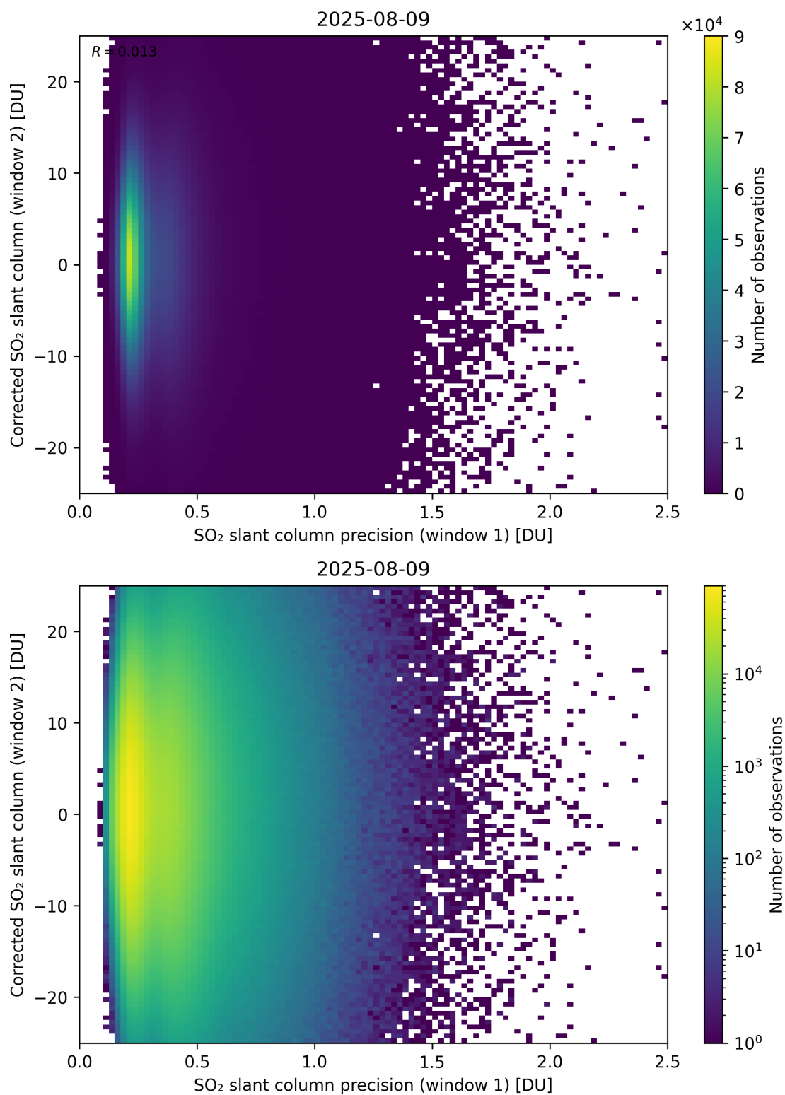
Figure 275: Scatter density plot of “SO 2 slant column precision (window 1)” against “Corrected SO 2 slant column (window 2)” for 2025-08-09 to 2025-08-10.
