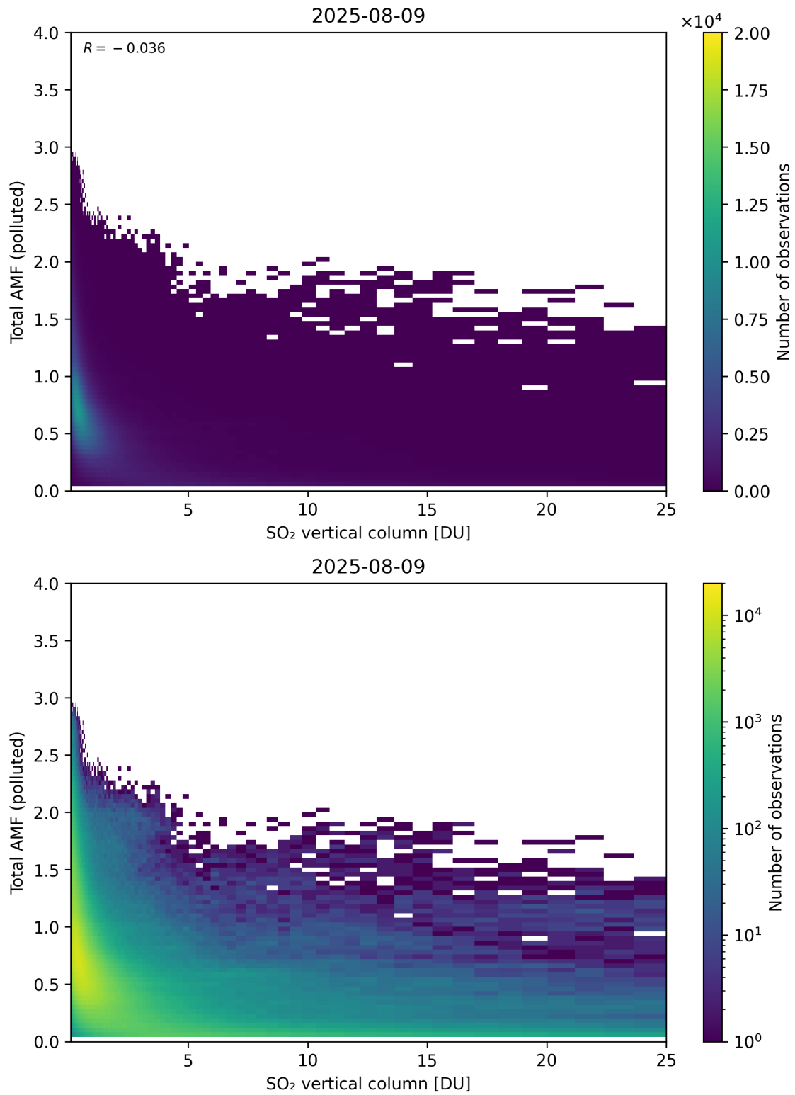
Figure 359: Scatter density plot of “SO 2 vertical column” against “Total AMF (polluted)” for 2025-08-09 to 2025-08-10.
