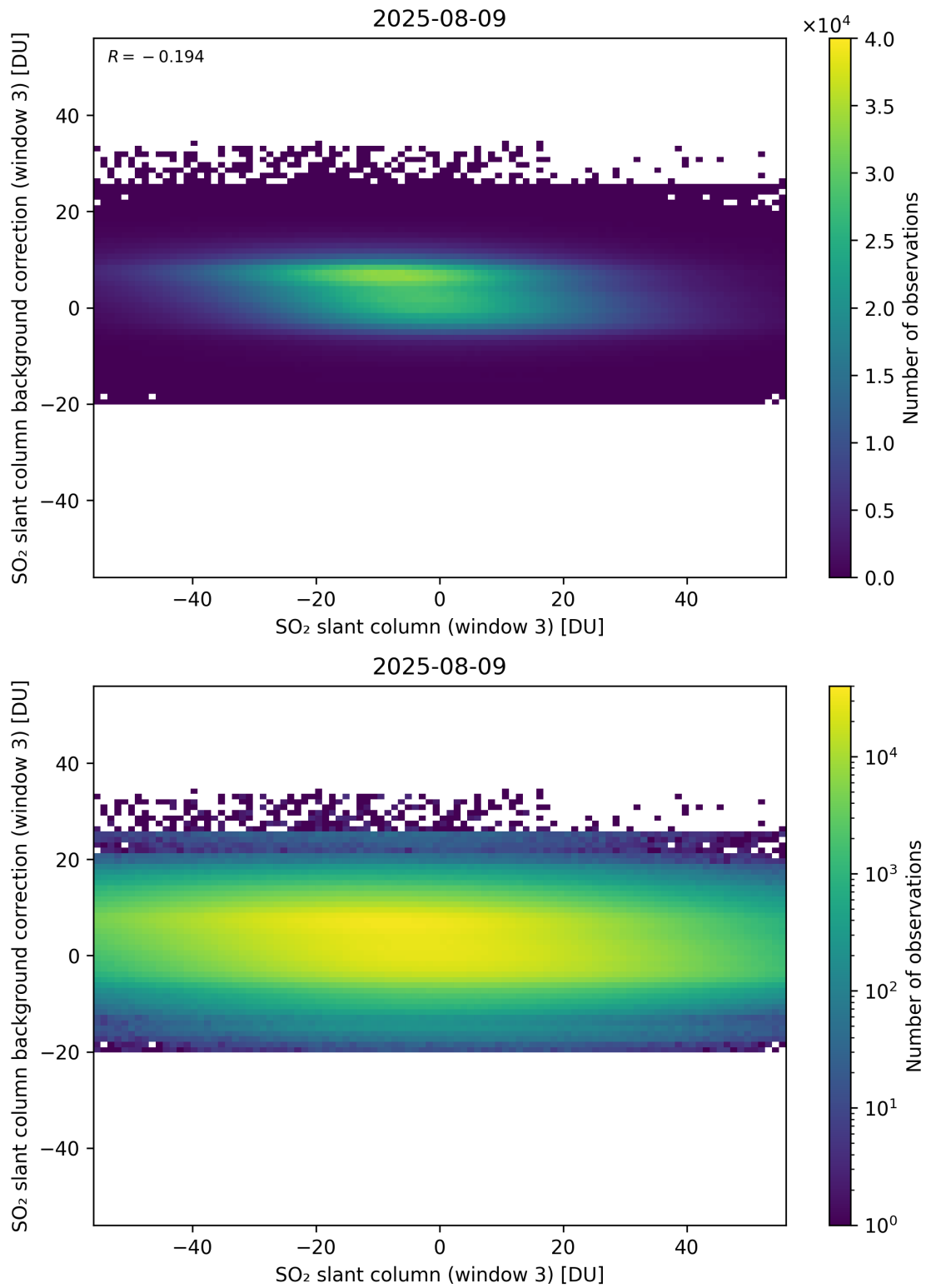
Figure 303: Scatter density plot of “SO 2 slant column (window 3)” against “SO 2 slant column background correction (window 3)” for 2025-08-09 to 2025-08-10.
