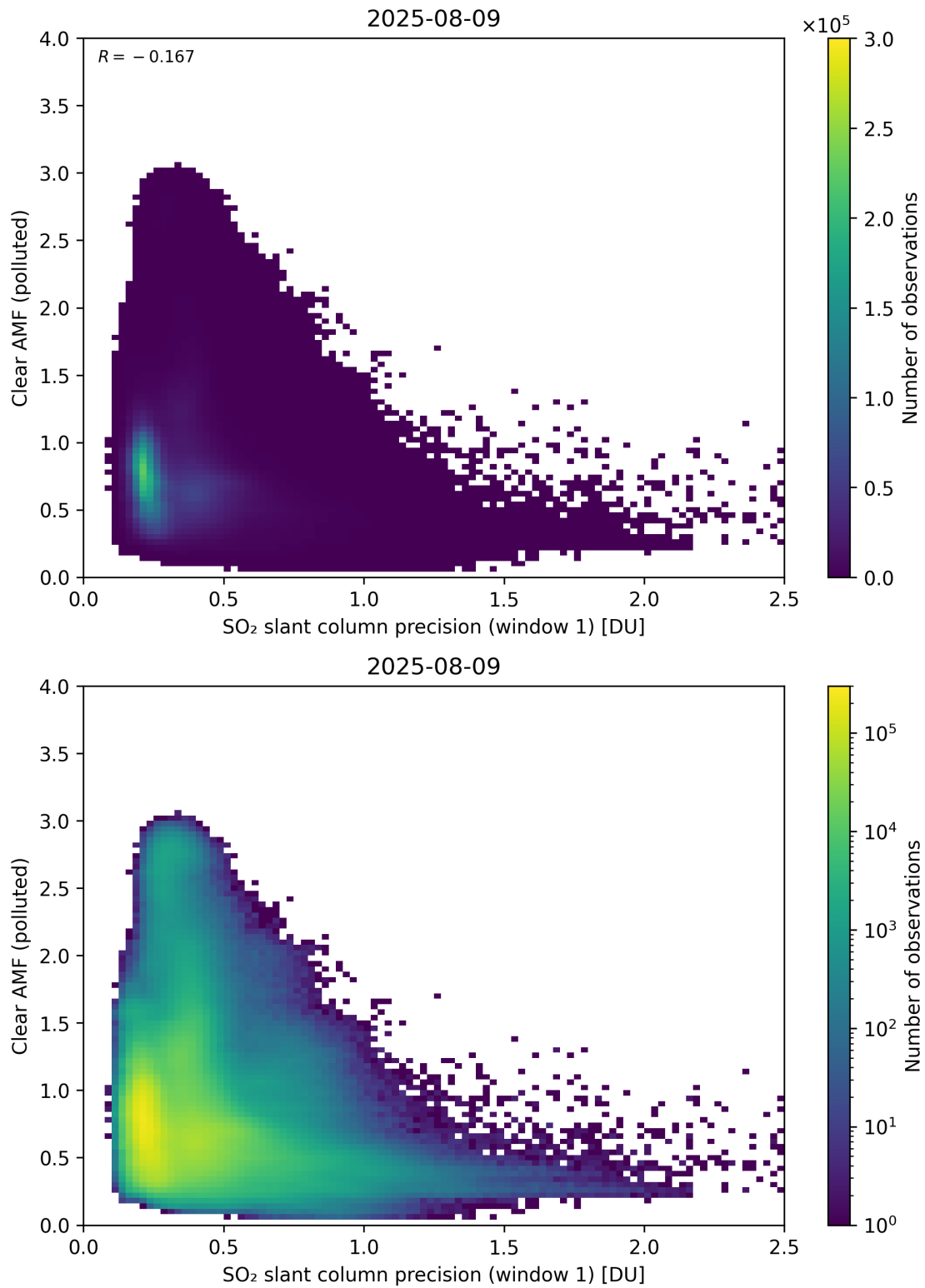
Figure 274: Scatter density plot of “SO 2 slant column precision (window 1)” against “Clear AMF (polluted)” for 2025-08-09 to 2025-08-10.
