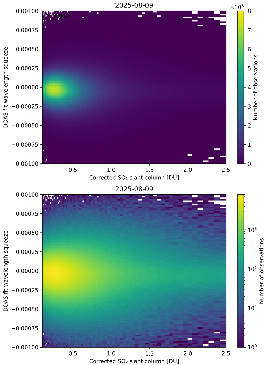
Figure 230: Scatter density plot of “Corrected SO 2 slant column” against “DOAS fit wavelength squeeze” for 2025-08-09 to 2025-08-10.
