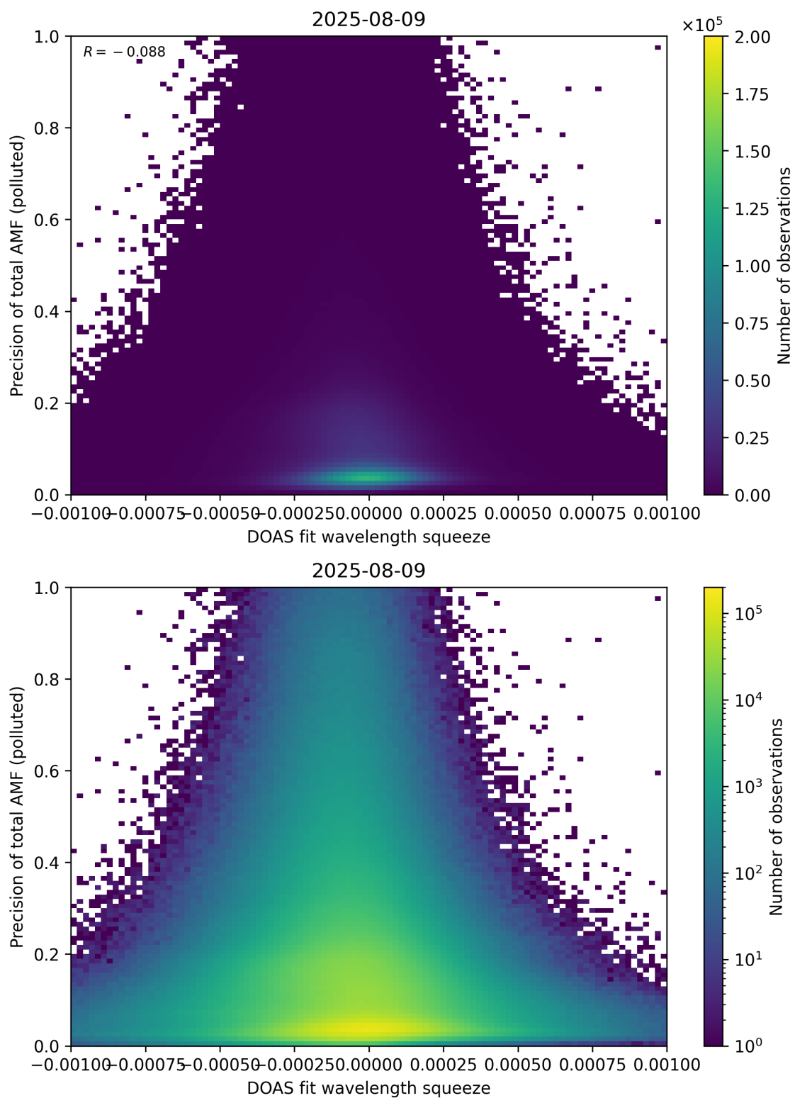
Figure 146: Scatter density plot of “DOAS fit wavelength squeeze” against “Precision of total AMF (polluted)” for 2025-08-09 to 2025-08-10.
