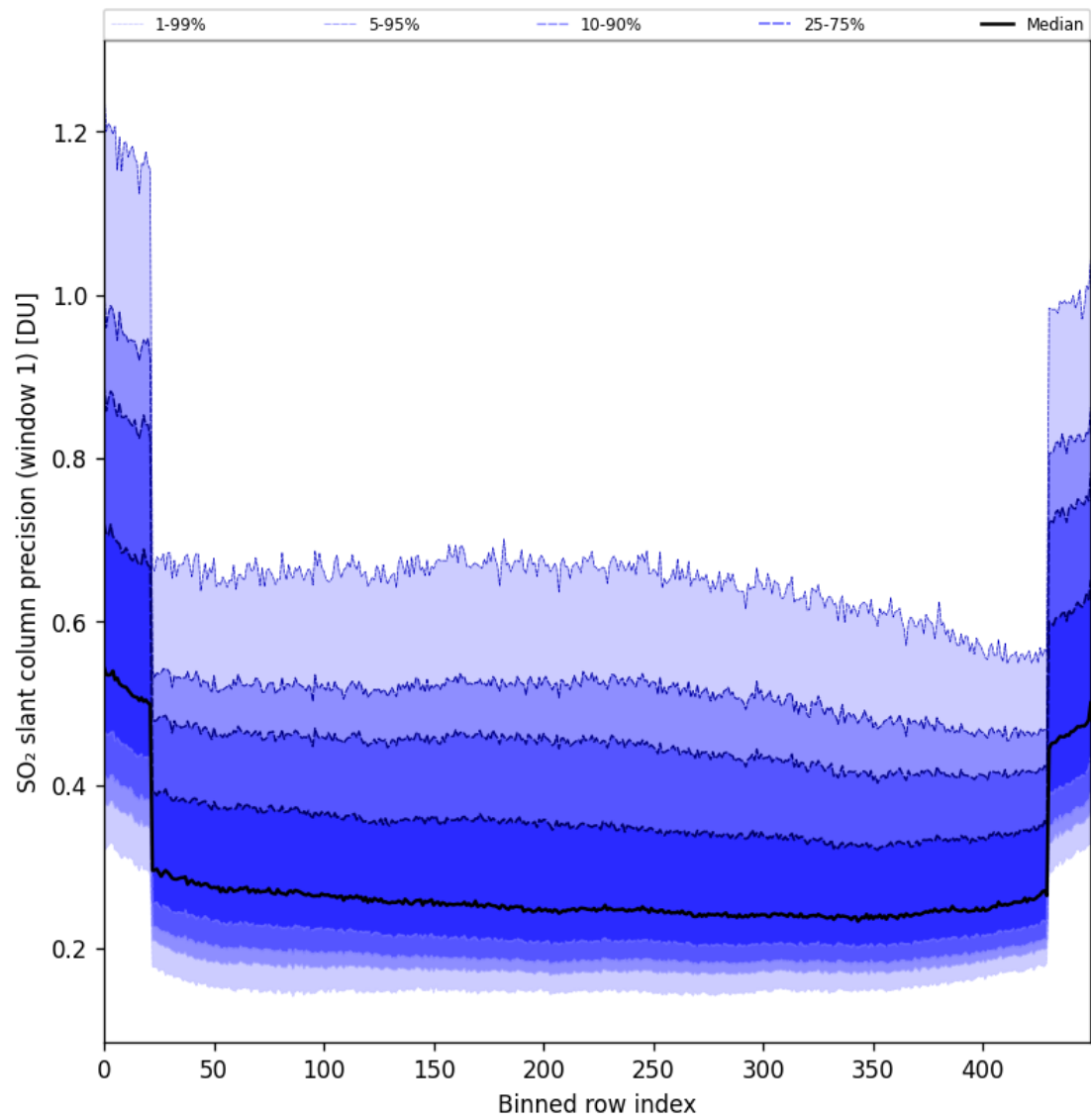
Figure 90: Along track statistics of “SO 2 slant column precision (window 1)” for 2025-08-09 to 2025-08-10
