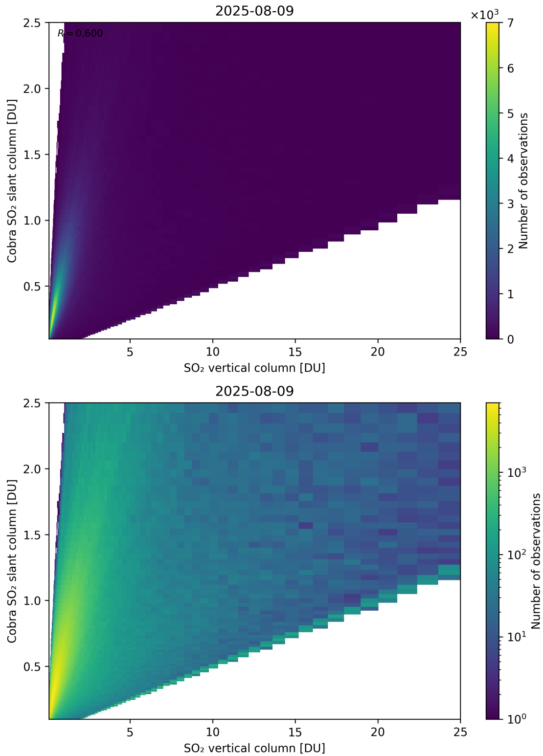
Figure 349: Scatter density plot of “SO 2 vertical column” against “Cobra SO 2 slant column” for 2025-08-09 to 2025-08-10.
