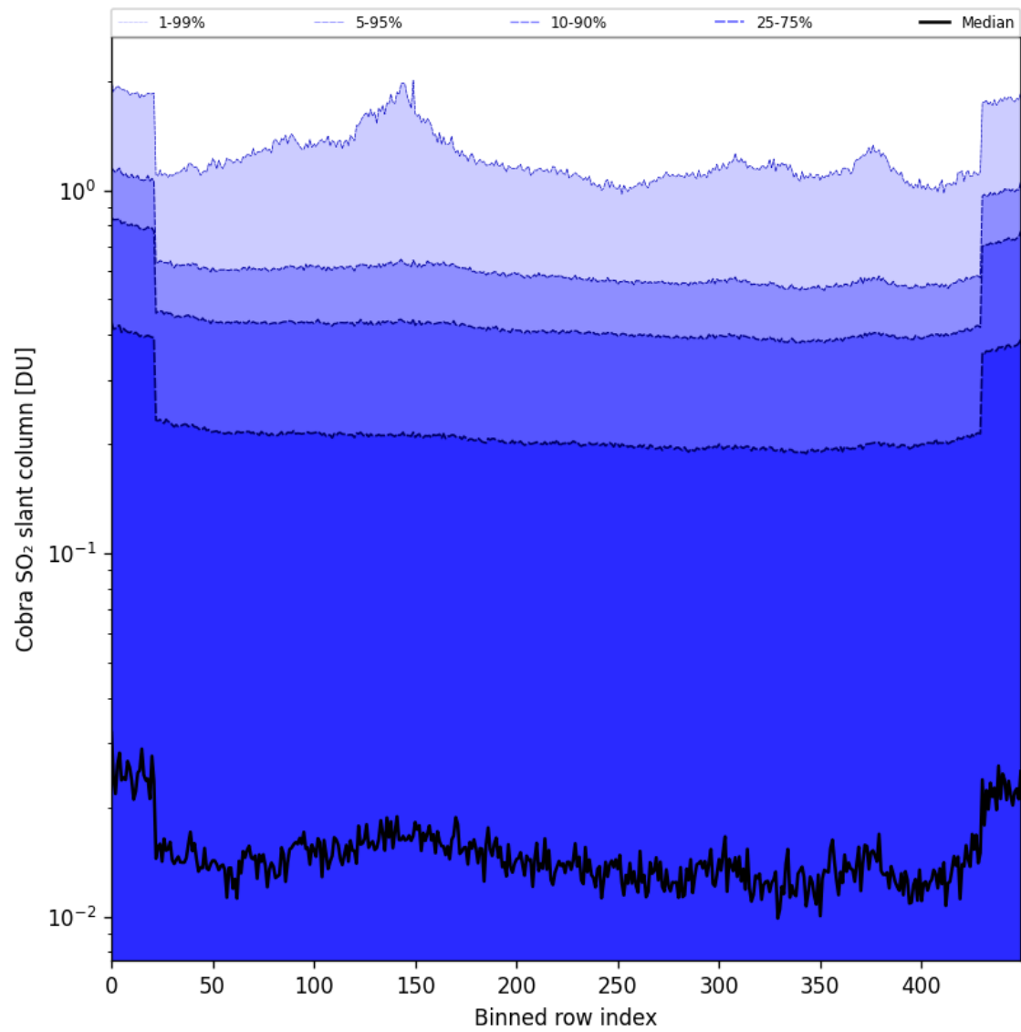
Figure 87: Along track statistics of “Cobra SO 2 slant column” for 2025-08-09 to 2025-08-10
