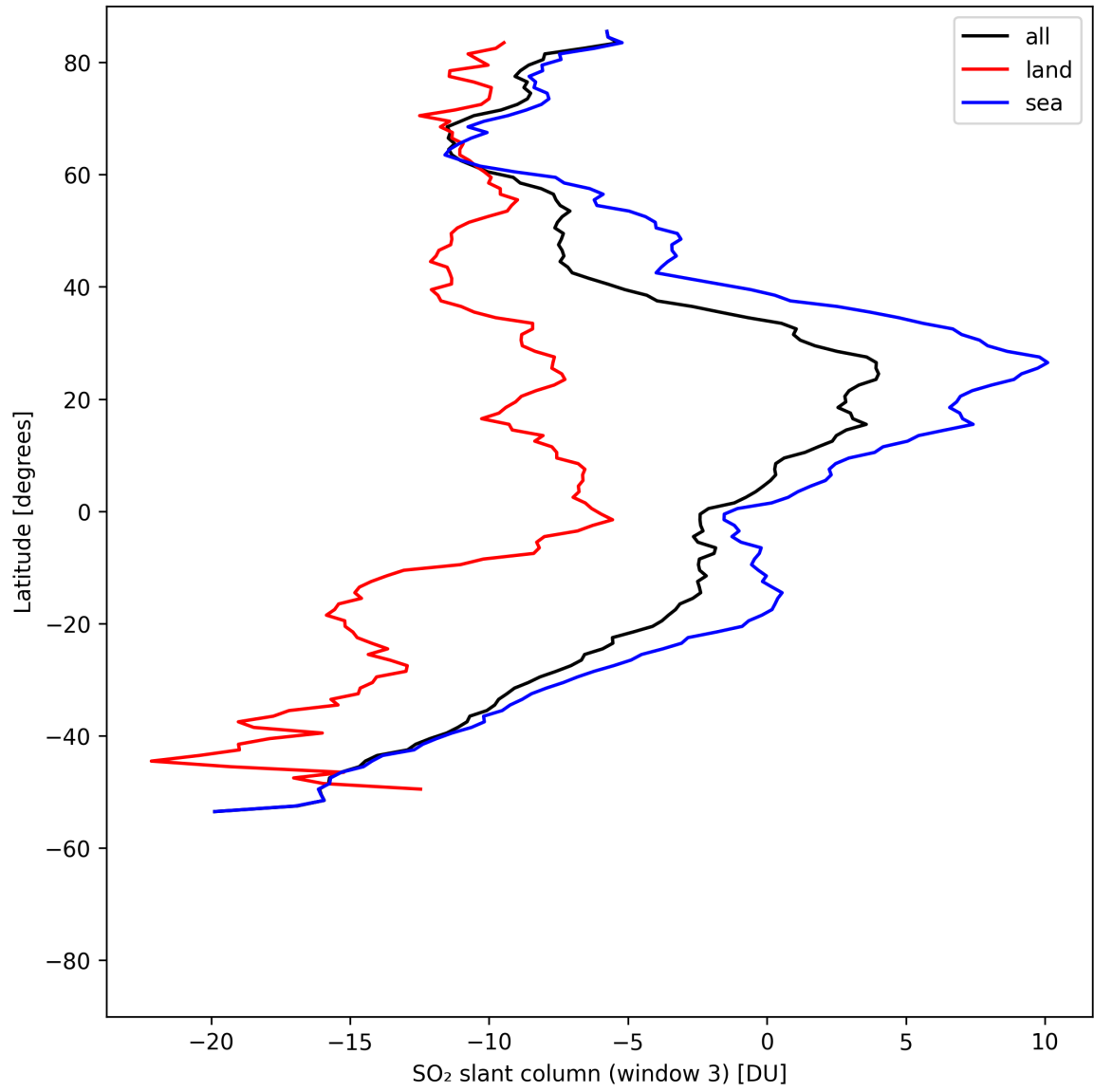
Figure 45: Zonal average of “SO 2 slant column (window 3)” for 2025-08-09 to 2025-08-10.
