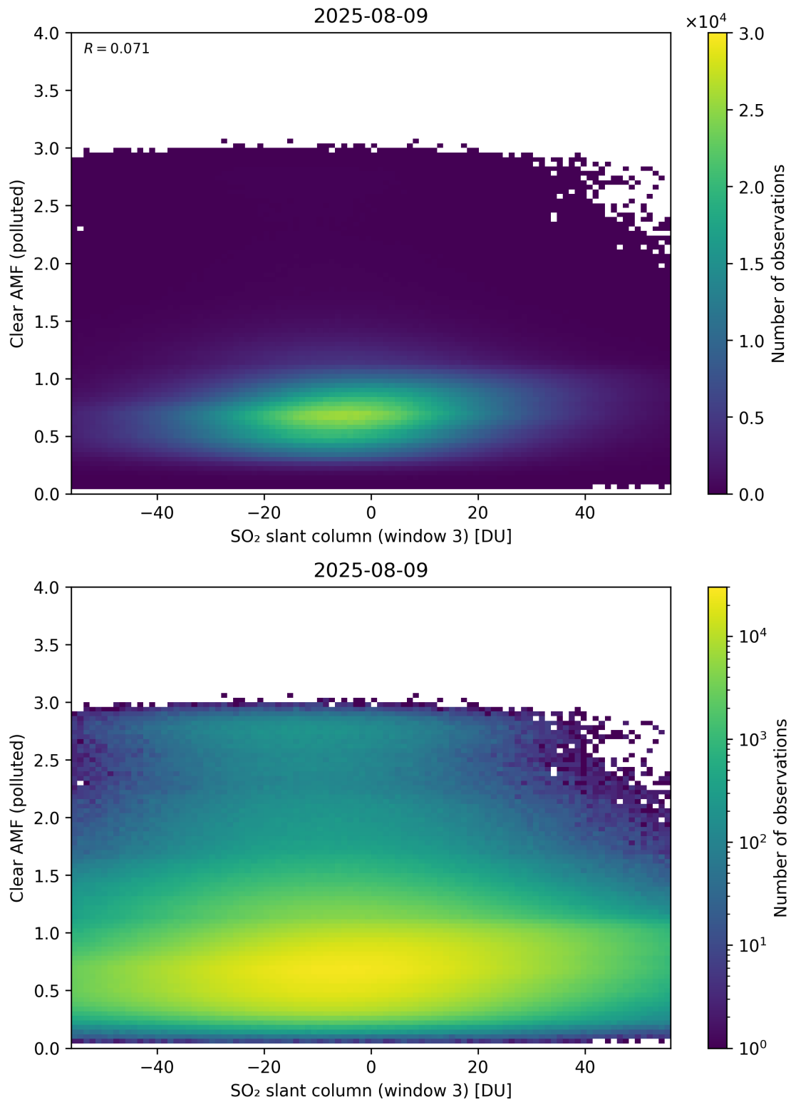
Figure 315: Scatter density plot of “SO 2 slant column (window 3)” against “Clear AMF (polluted)” for 2025-08-09 to 2025-08-10.
