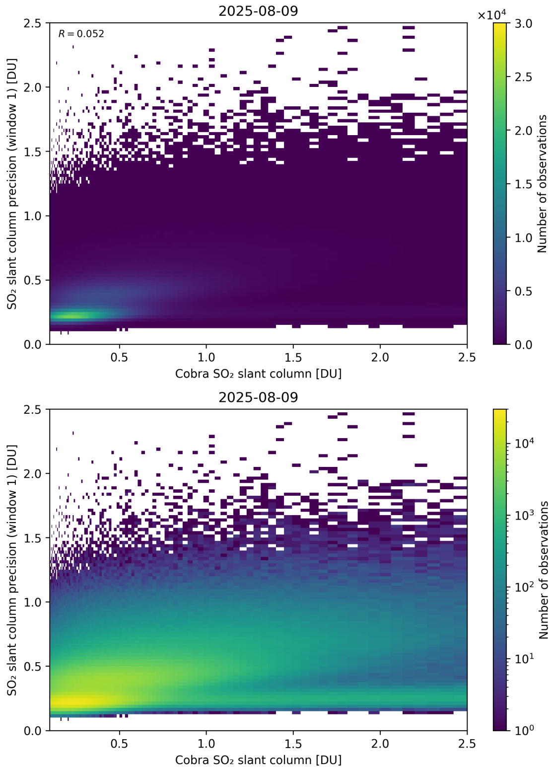
Figure 220: Scatter density plot of “Cobra SO 2 slant column” against “SO 2 slant column precision (window 1)” for 2025-08-09 to 2025-08-10.
