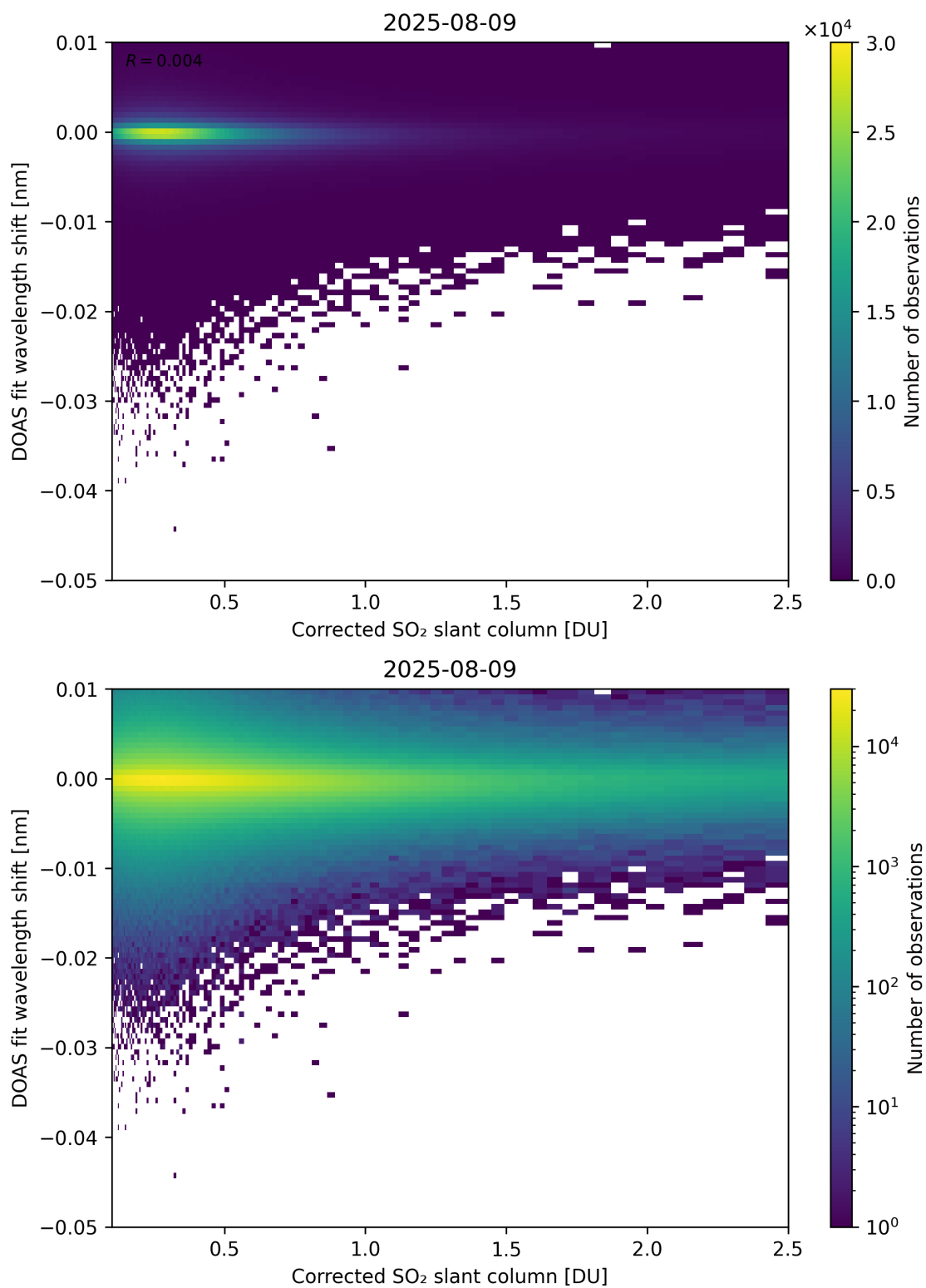
Figure 229: Scatter density plot of “Corrected SO 2 slant column” against “DOAS fit wavelength shift” for 2025-08-09 to 2025-08-10.
