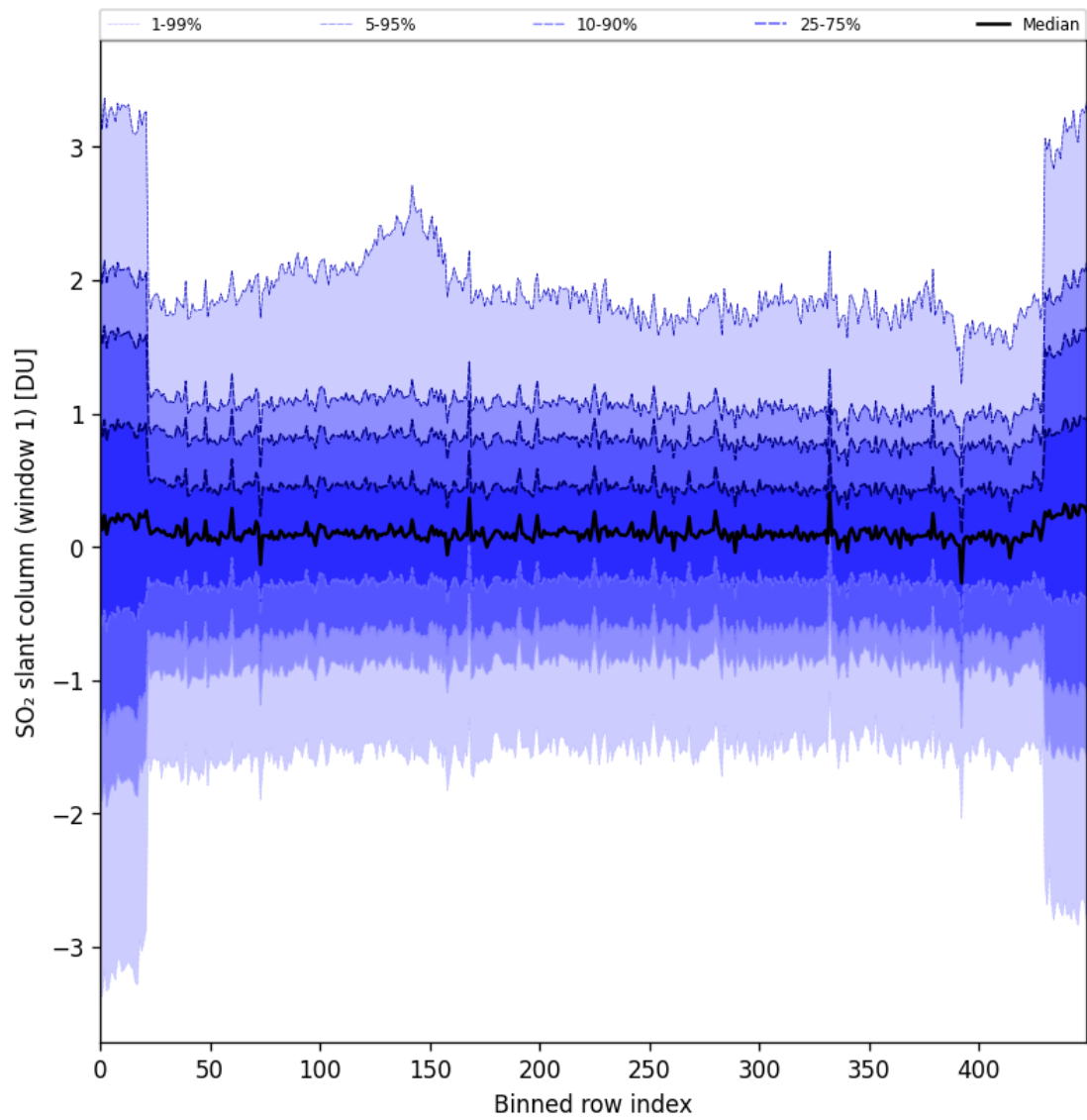
Figure 89: Along track statistics of “SO 2 slant column (window 1)” for 2025-08-09 to 2025-08-10
