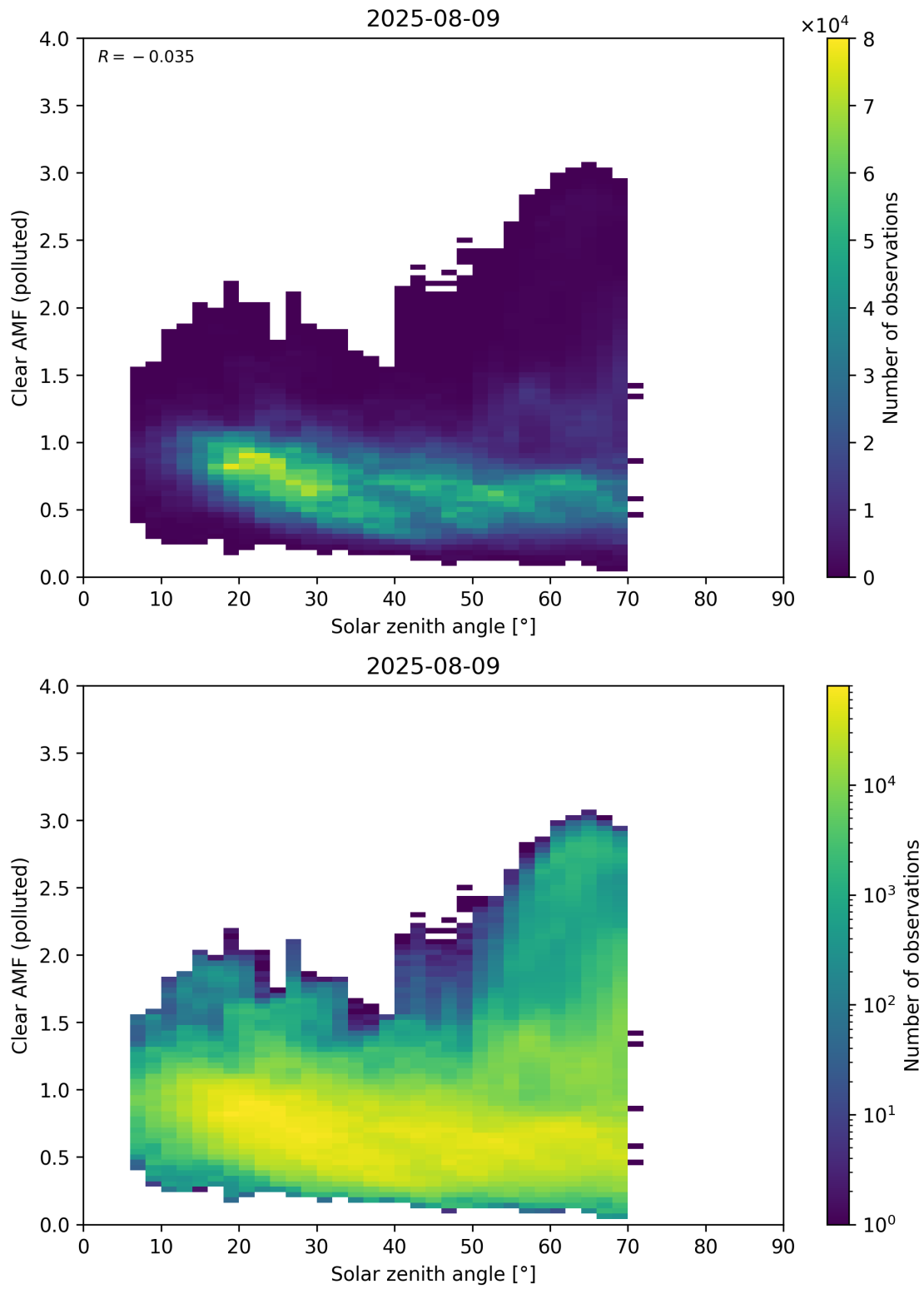
Figure 178: Scatter density plot of “Solar zenith angle” against “Clear AMF (polluted)” for 2025-08-09 to 2025-08-10.
