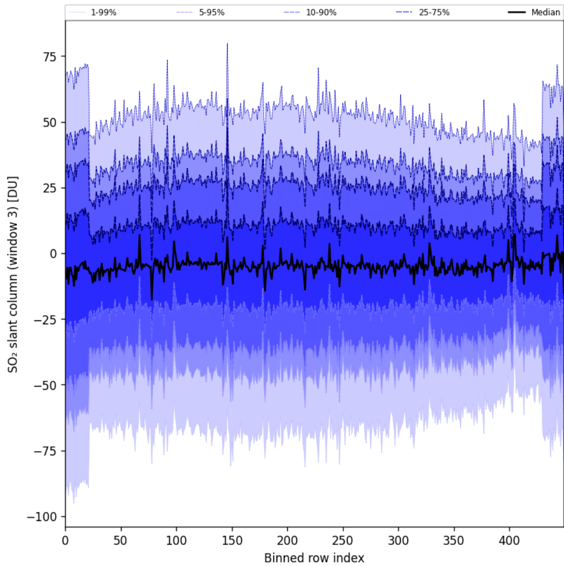
Figure 97: Along track statistics of “SO 2 slant column (window 3)” for 2025-08-09 to 2025-08-10
