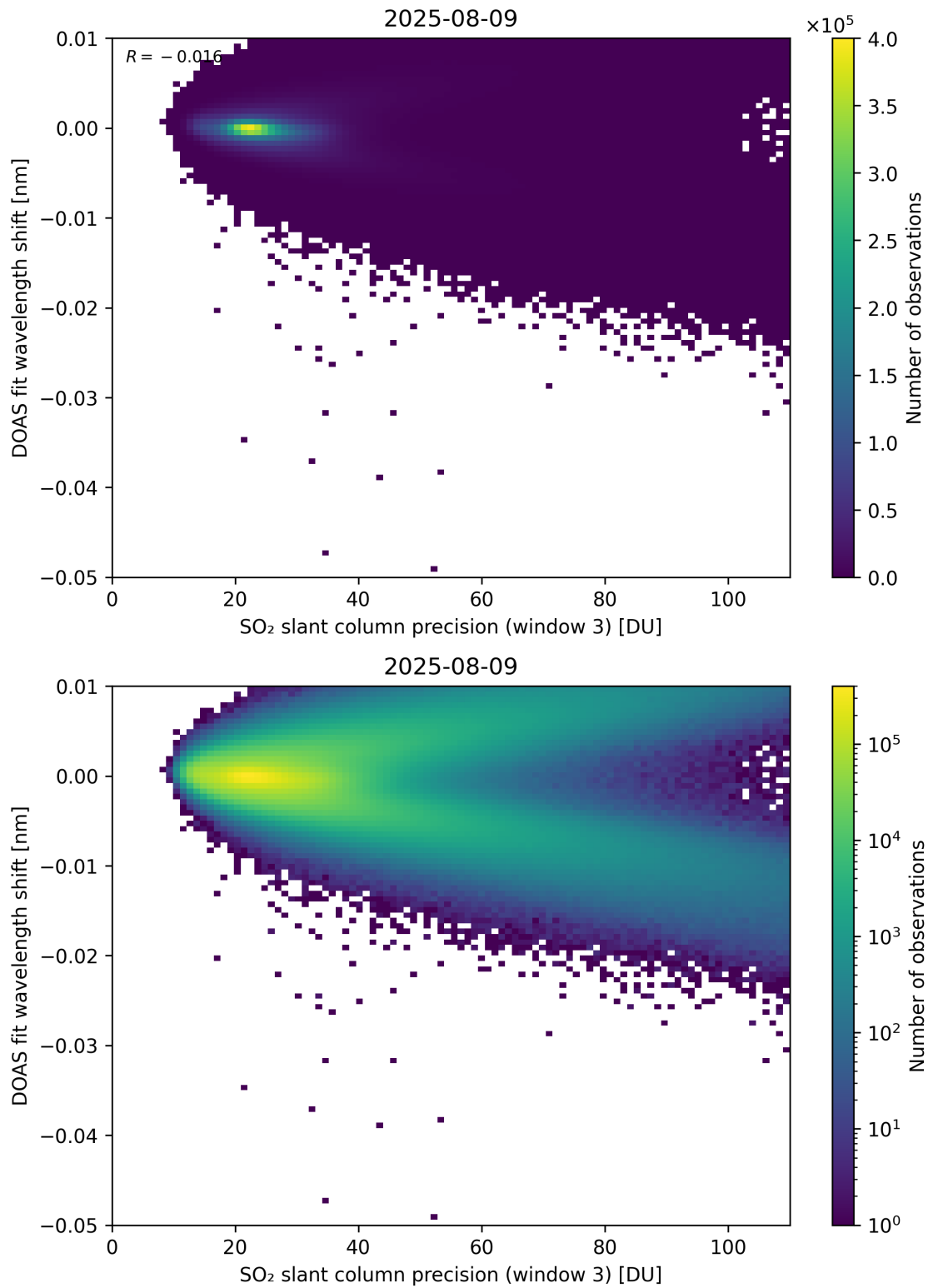
Figure 308: Scatter density plot of “SO 2 slant column precision (window 3)” against “DOAS fit wavelength shift” for 2025-08-09 to 2025-08-10.
