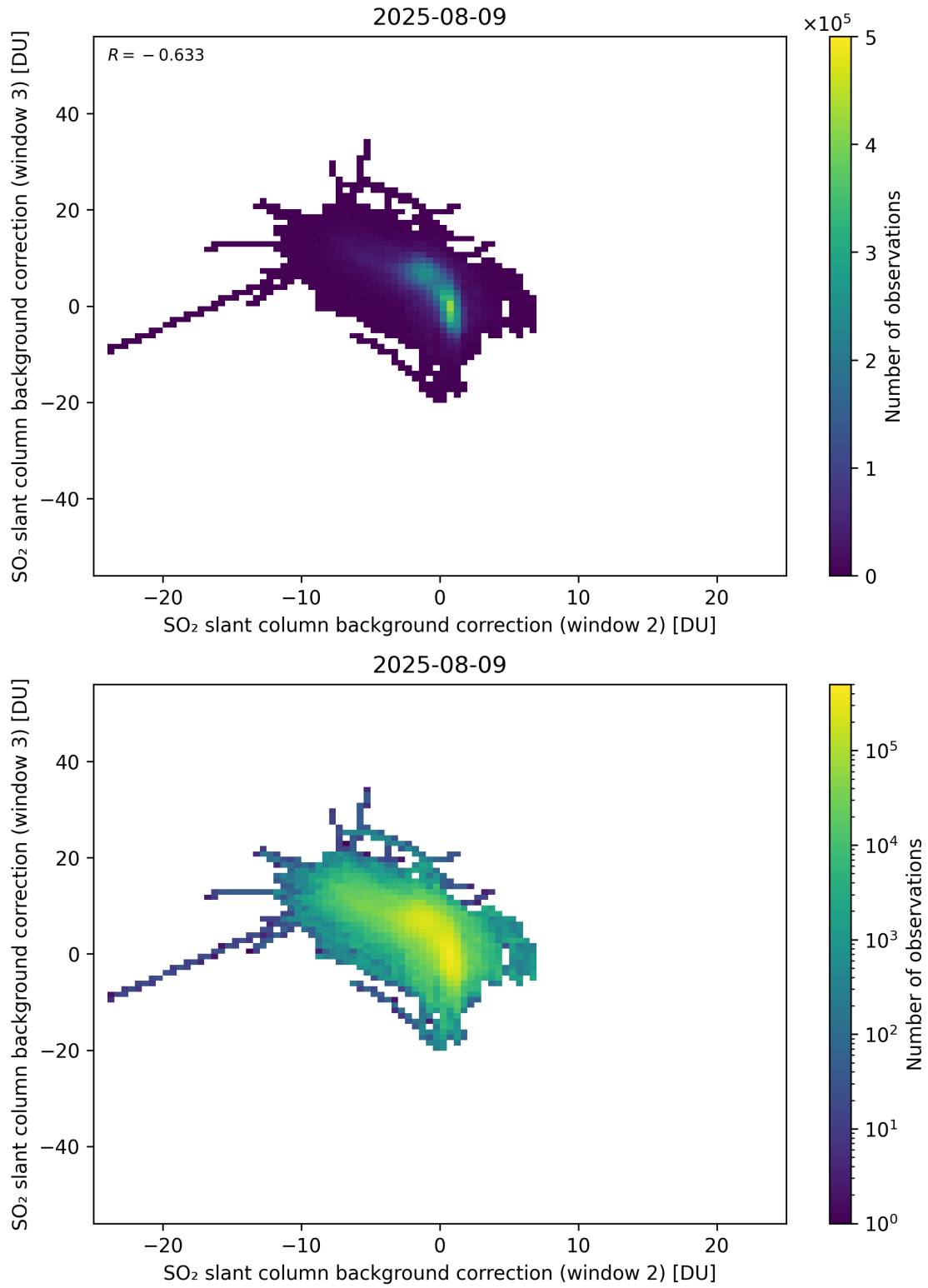
Figure 122: Scatter density plot of “SO 2 slant column background correction (window 2)” against “SO 2 slant column background correction (window 3)” for 2025-08-09 to 2025-08-10.
