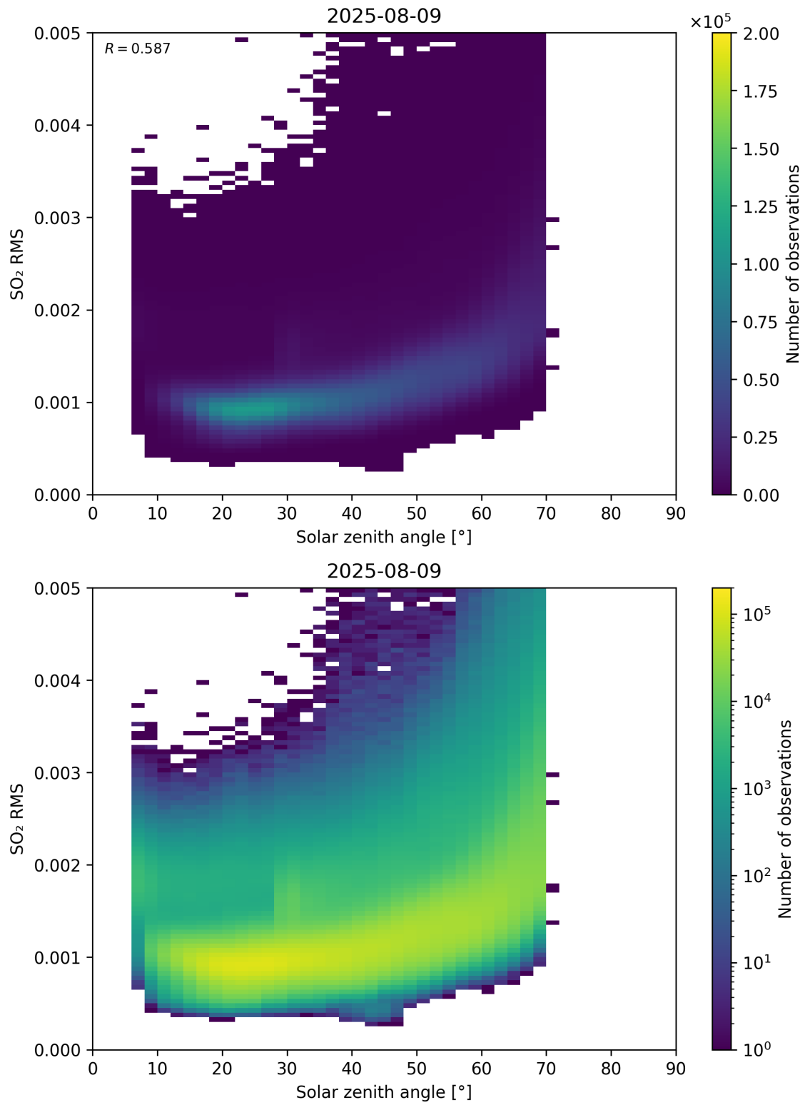
Figure 176: Scatter density plot of “Solar zenith angle” against “SO 2 RMS” for 2025-08-09 to 2025-08-10.
