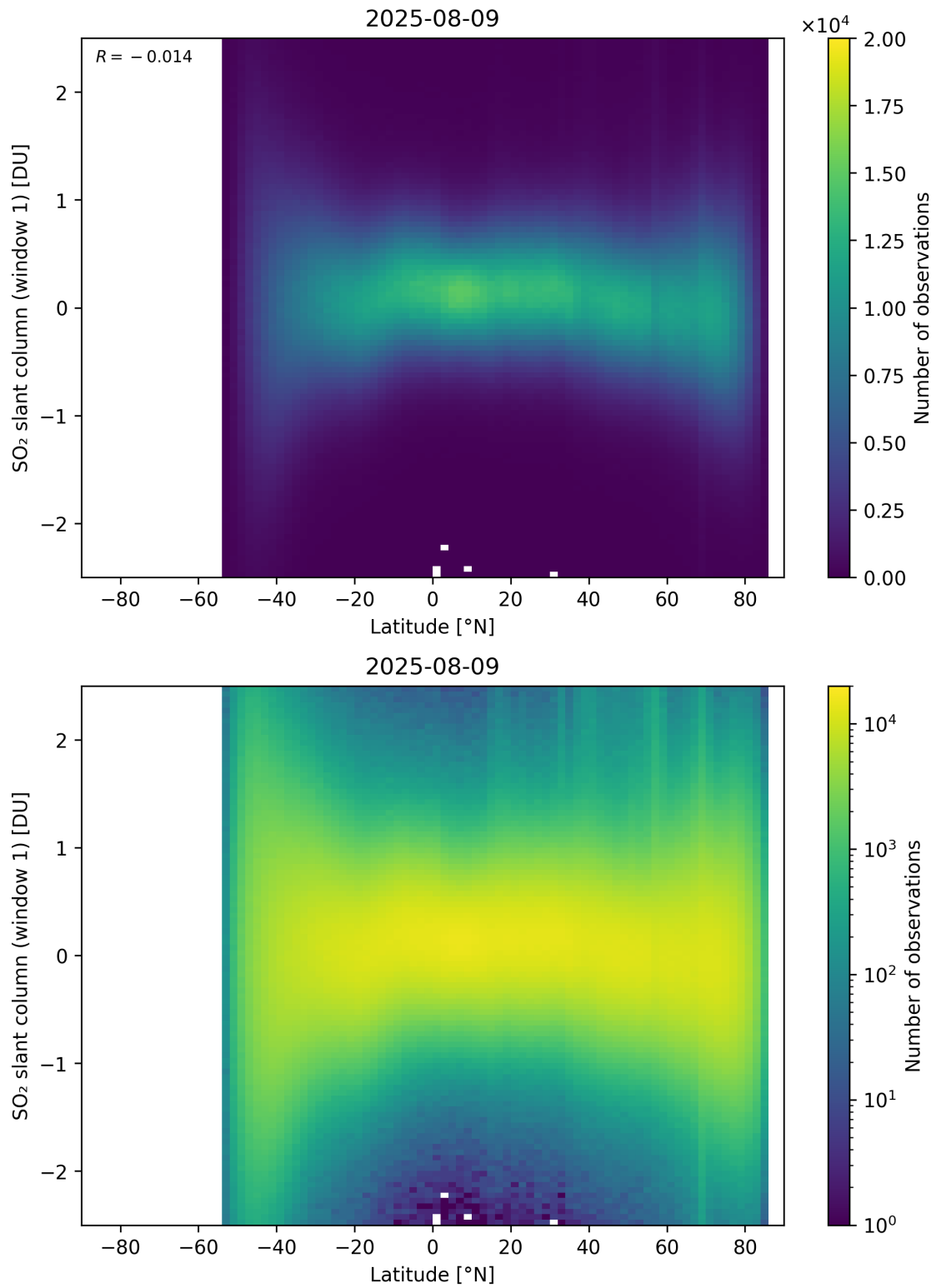
Figure 162: Scatter density plot of “Latitude” against “SO 2 slant column (window 1)” for 2025-08-09 to 2025-08-10.
