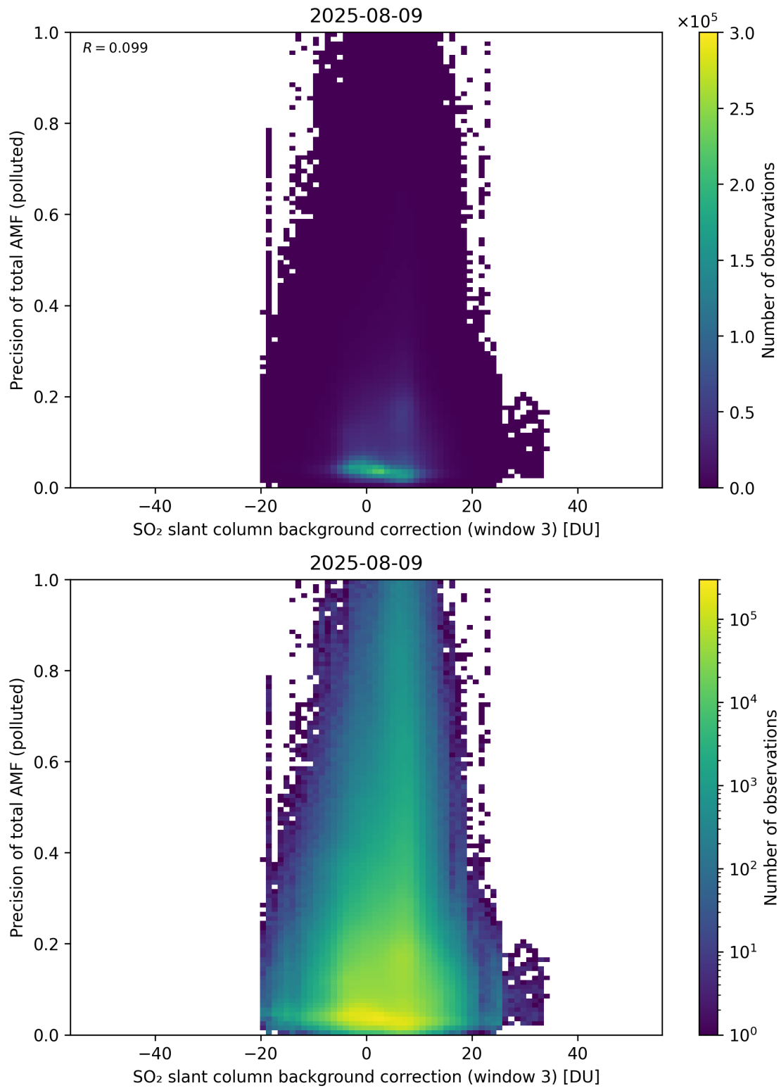
Figure 137: Scatter density plot of “SO 2 slant column background correction (window 3)” against “Precision of total AMF (polluted)” for 2025-08-09 to 2025-08-10.
