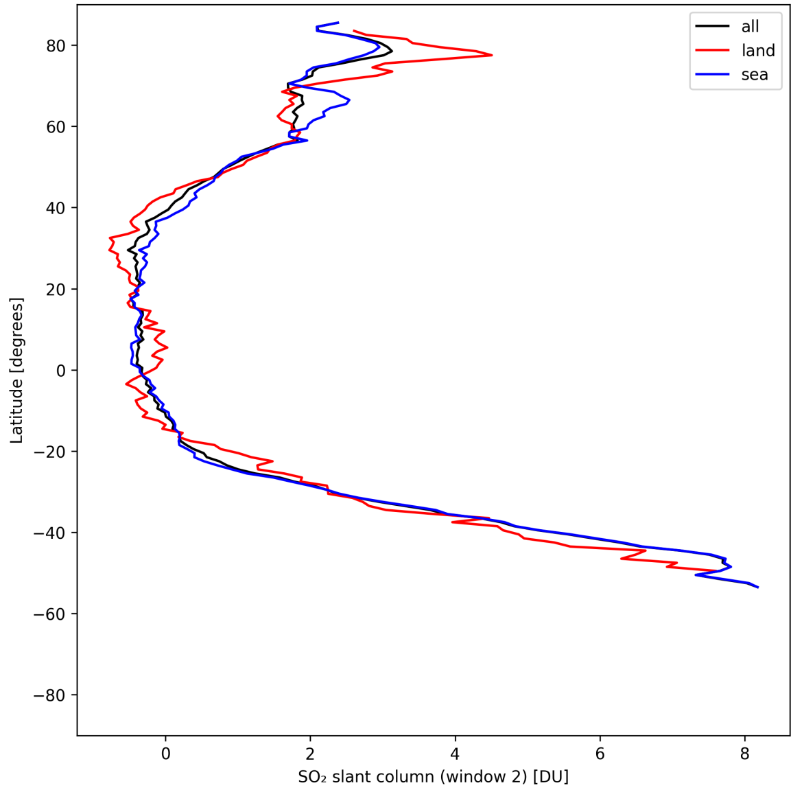
Figure 41: Zonal average of “SO 2 slant column (window 2)” for 2025-08-09 to 2025-08-10.
