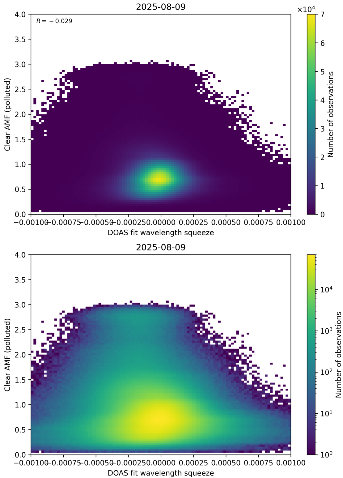
Figure 144: Scatter density plot of “DOAS fit wavelength squeeze” against “Clear AMF (polluted)” for 2025-08-09 to 2025-08-10.
