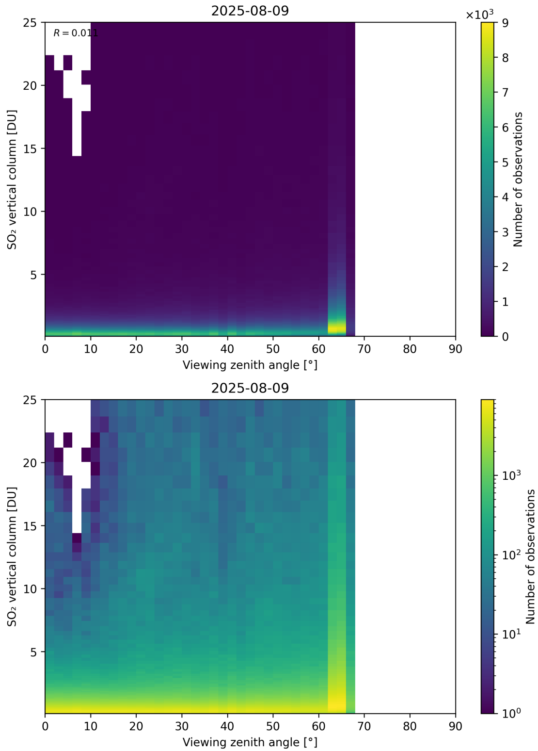
Figure 383: Scatter density plot of “Viewing zenith angle” against “SO 2 vertical column” for 2025-08-09 to 2025-08-10.
