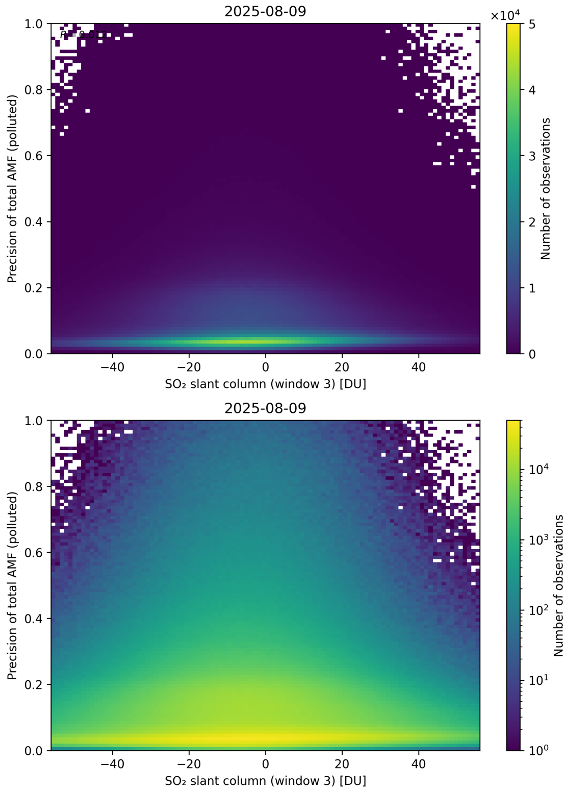
Figure 319: Scatter density plot of “SO 2 slant column (window 3)” against “Precision of total AMF (polluted)” for 2025-08-09 to 2025-08-10.
