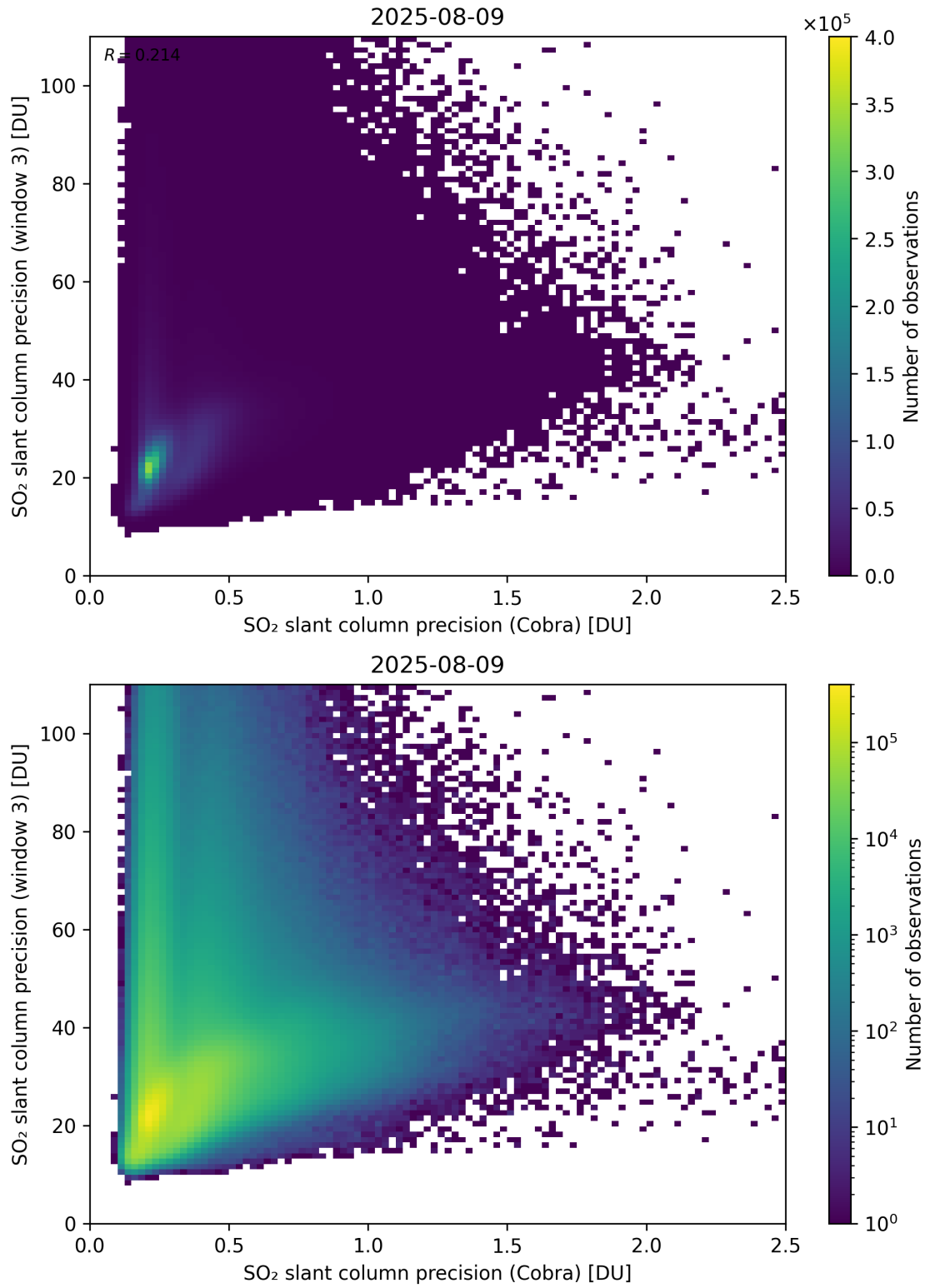
Figure 212: Scatter density plot of “SO 2 slant column precision (Cobra)” against “SO 2 slant column precision (window 3)” for 2025-08-09 to 2025-08-10.
