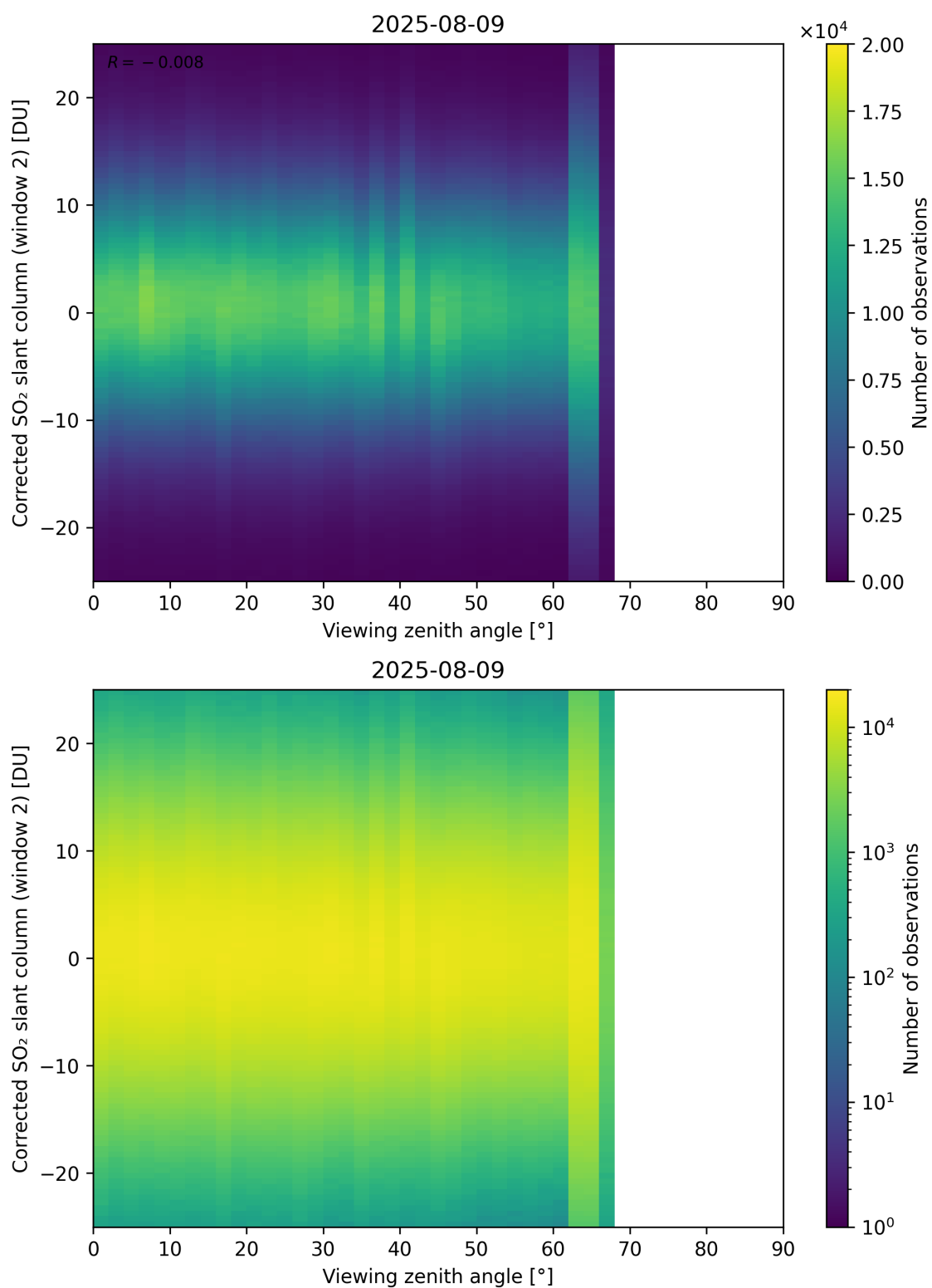
Figure 374: Scatter density plot of “Viewing zenith angle” against “Corrected SO 2 slant column (window 2)” for 2025-08-09 to 2025-08-10.
