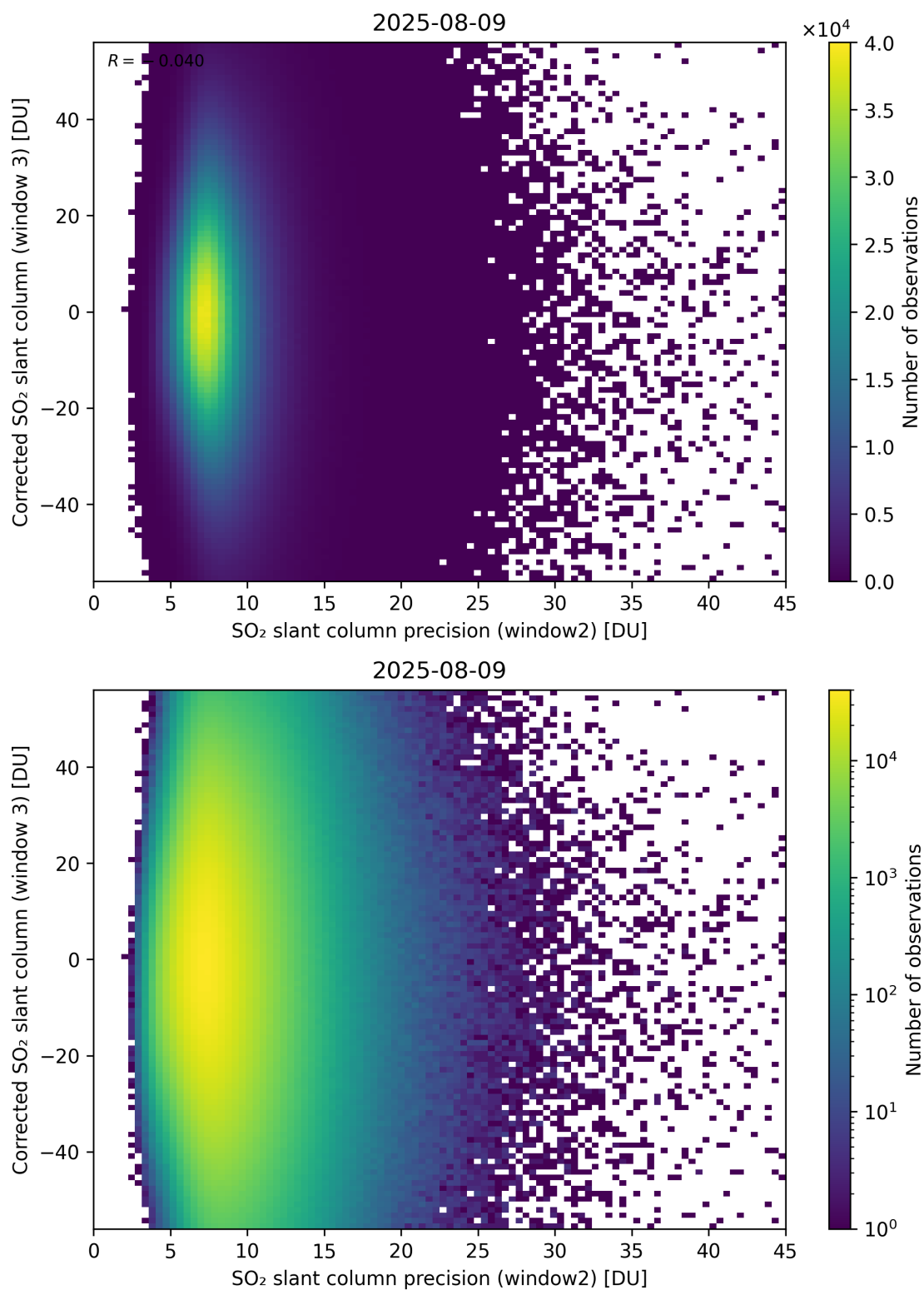
Figure 298: Scatter density plot of “SO 2 slant column precision (window2)” against “Corrected SO 2 slant column (window 3)” for 2025-08-09 to 2025-08-10.
