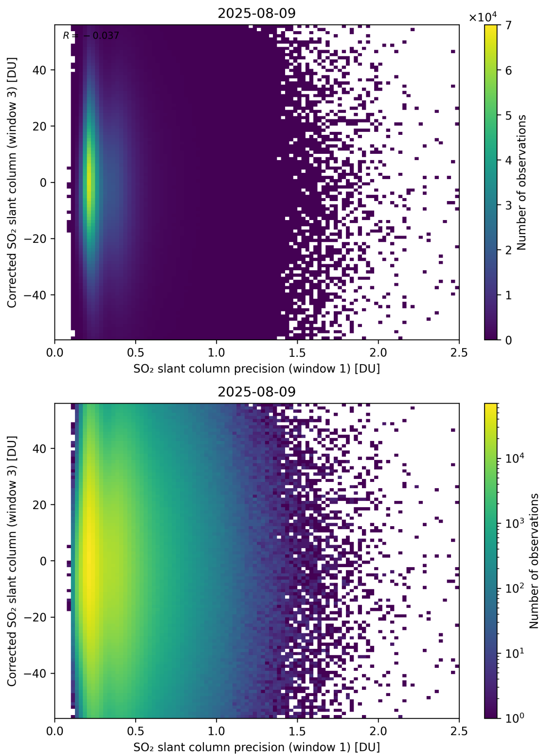
Figure 276: Scatter density plot of “SO 2 slant column precision (window 1)” against “Corrected SO 2 slant column (window 3)” for 2025-08-09 to 2025-08-10.
