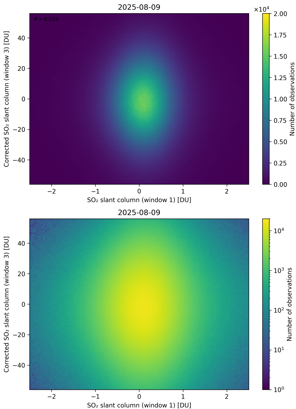
Figure 284: Scatter density plot of “SO 2 slant column (window 1)” against “Corrected SO 2 slant column (window 3)” for 2025-08-09 to 2025-08-10.
