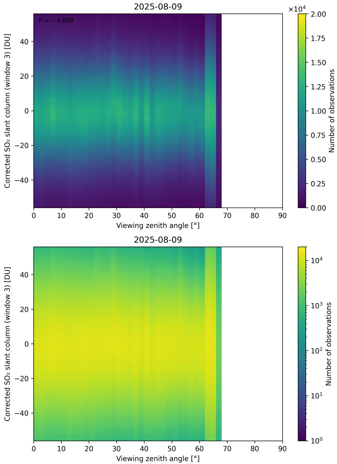
Figure 375: Scatter density plot of “Viewing zenith angle” against “Corrected SO 2 slant column (window 3)” for 2025-08-09 to 2025-08-10.
