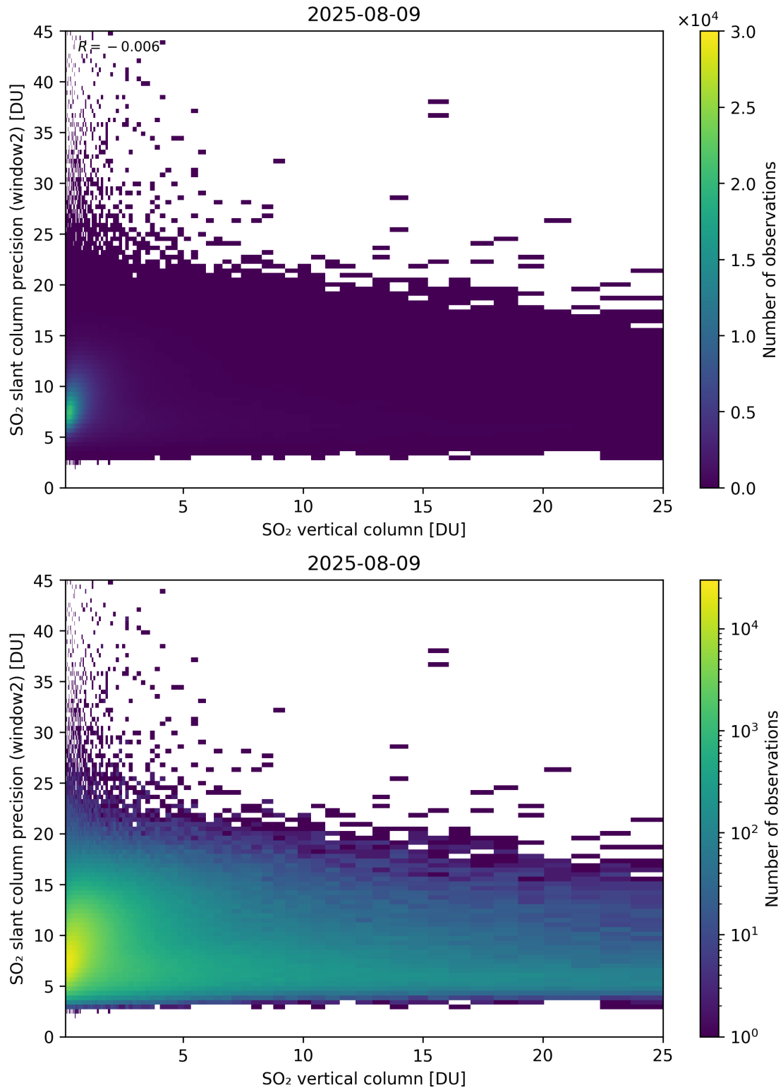
Figure 356: Scatter density plot of “SO 2 vertical column” against “SO 2 slant column precision (window2)” for 2025-08-09 to 2025-08-10.
