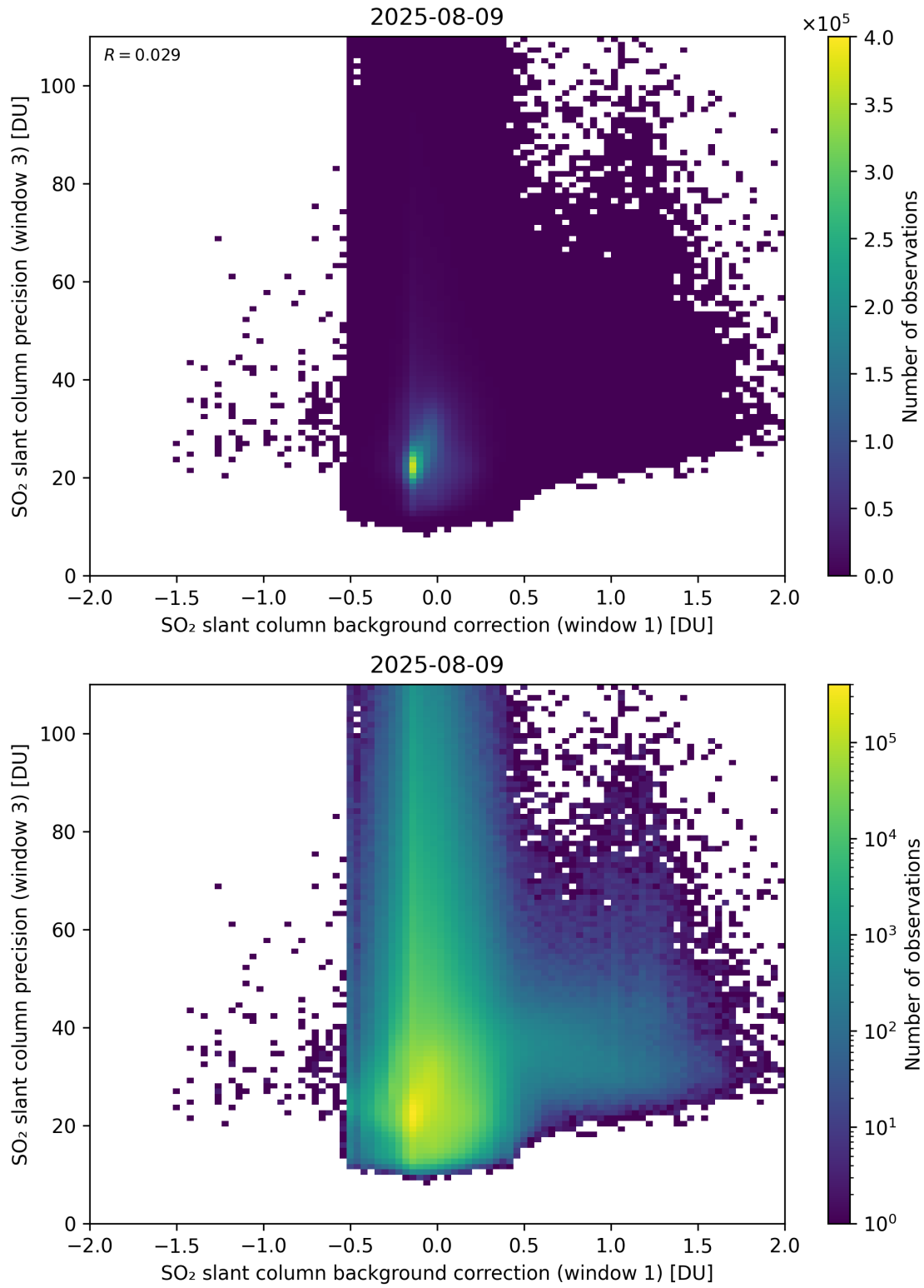
Figure 119: Scatter density plot of “SO 2 slant column background correction (window 1)” against “SO 2 slant column precision (window 3)” for 2025-08-09 to 2025-08-10.
