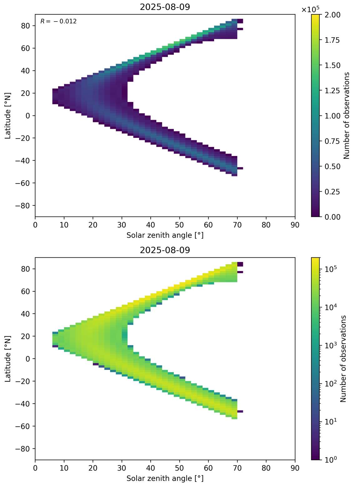
Figure 177: Scatter density plot of “Solar zenith angle” against “Latitude” for 2025-08-09 to 2025-08-10.
