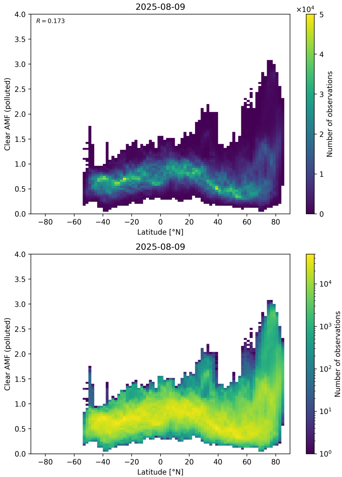
Figure 156: Scatter density plot of “Latitude” against “Clear AMF (polluted)” for 2025-08-09 to 2025-08-10.
