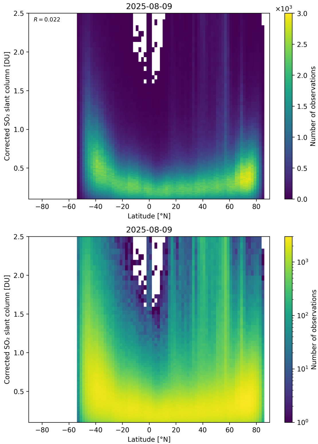
Figure 159: Scatter density plot of “Latitude” against “Corrected SO 2 slant column” for 2025-08-09 to 2025-08-10.
