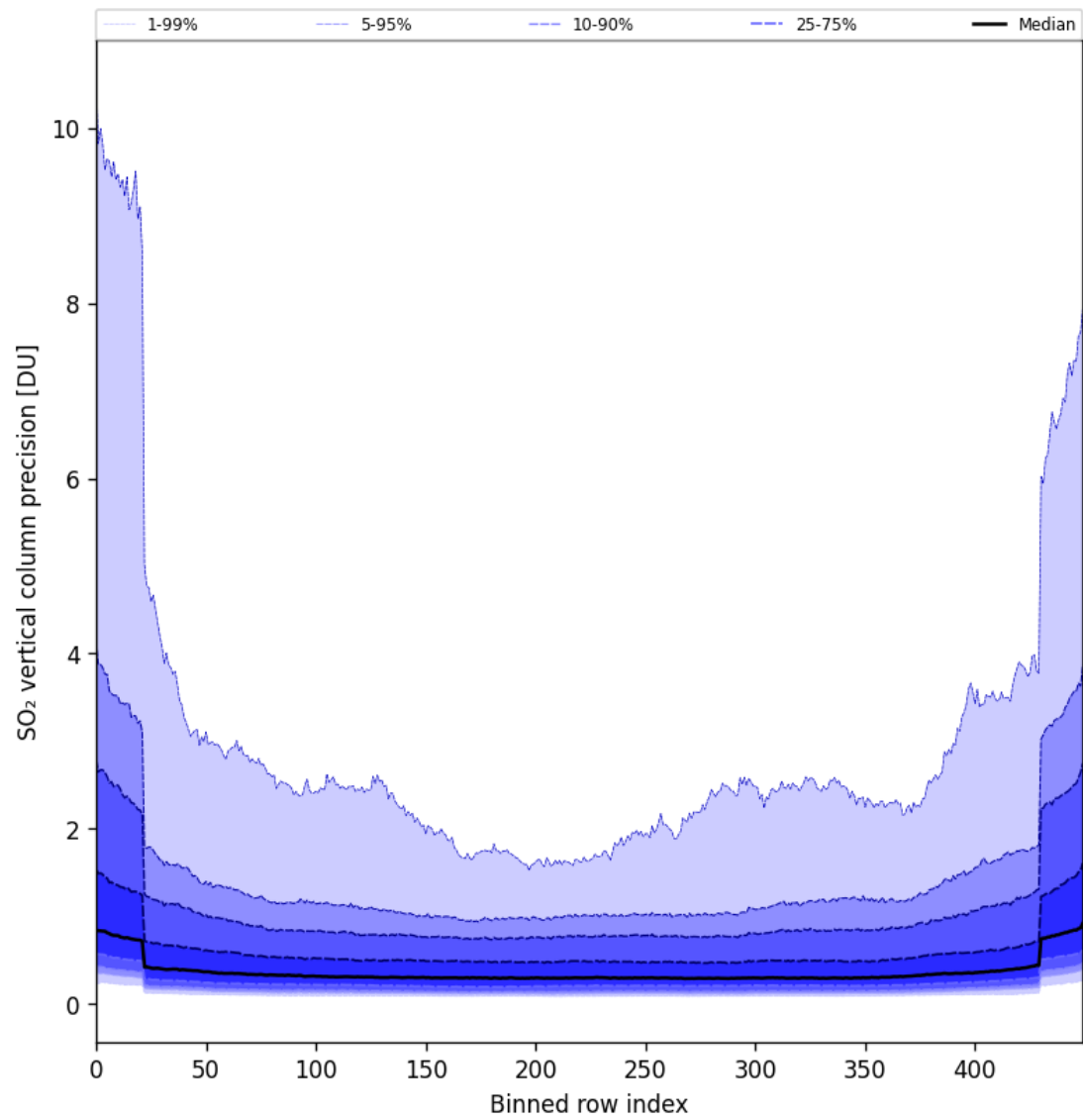
Figure 85: Along track statistics of “SO 2 vertical column precision” for 2025-08-09 to 2025-08-10
