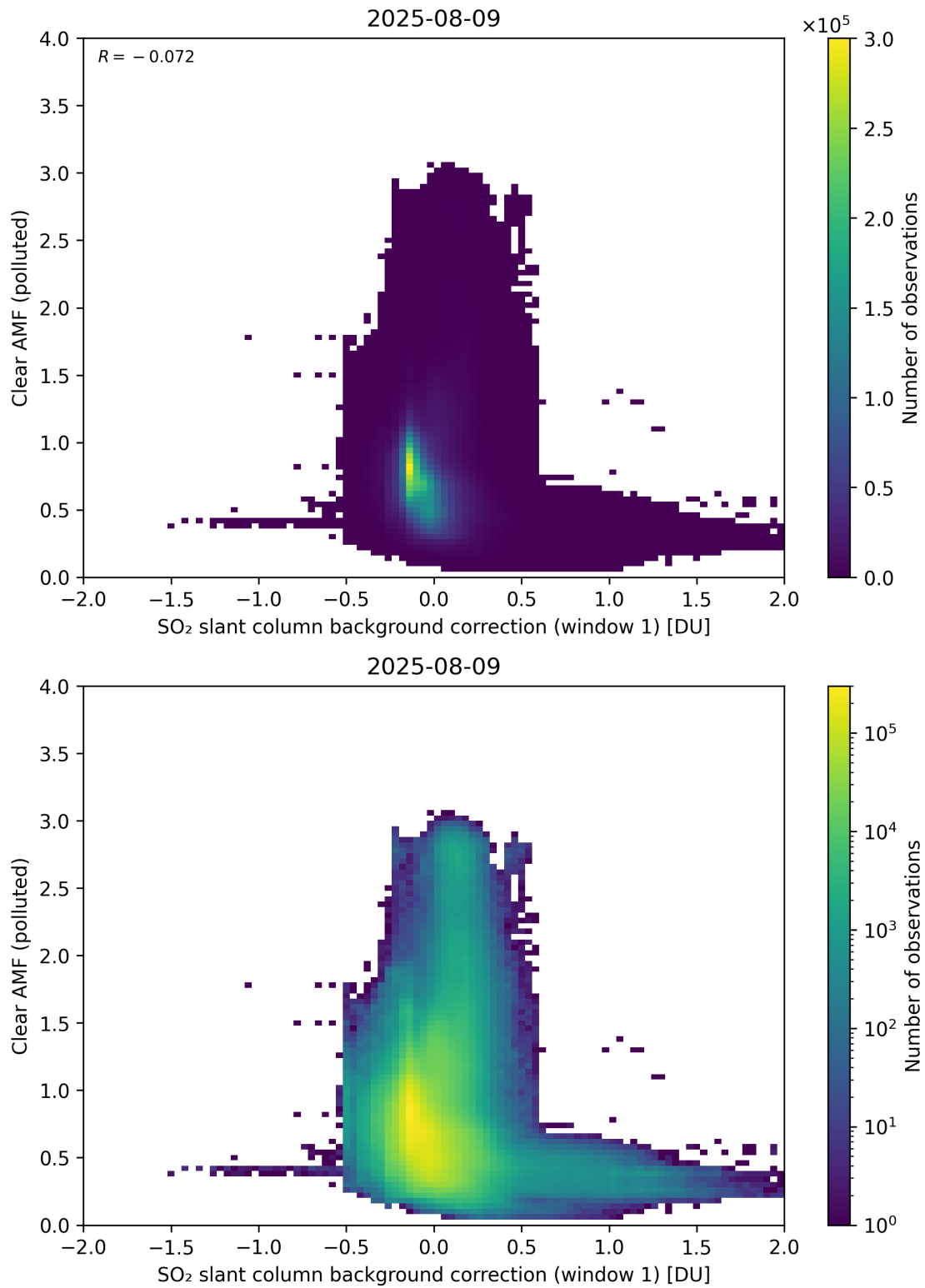
Figure 114: Scatter density plot of “SO 2 slant column background correction (window 1)” against “Clear AMF (polluted)” for 2025-08-09 to 2025-08-10.
