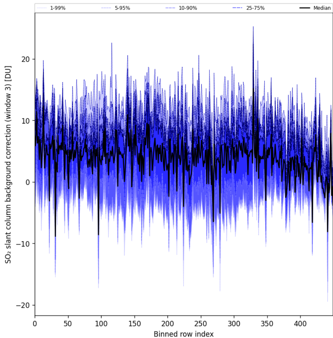
Figure 100: Along track statistics of “SO 2 slant column background correction (window 3)” for 2025-08-09 to 2025-08-10
