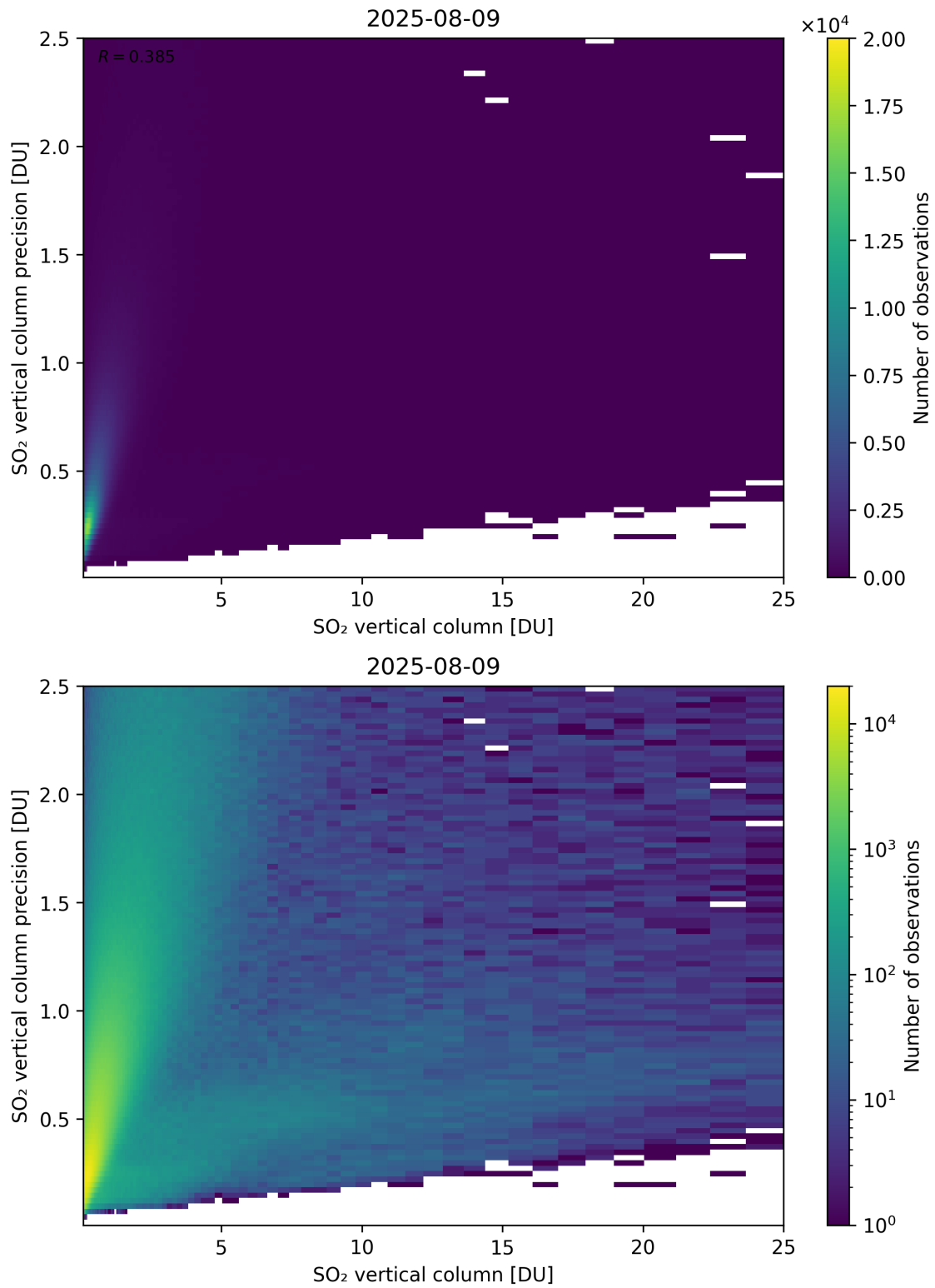
Figure 361: Scatter density plot of “SO 2 vertical column” against “SO 2 vertical column precision” for 2025-08-09 to 2025-08-10.
