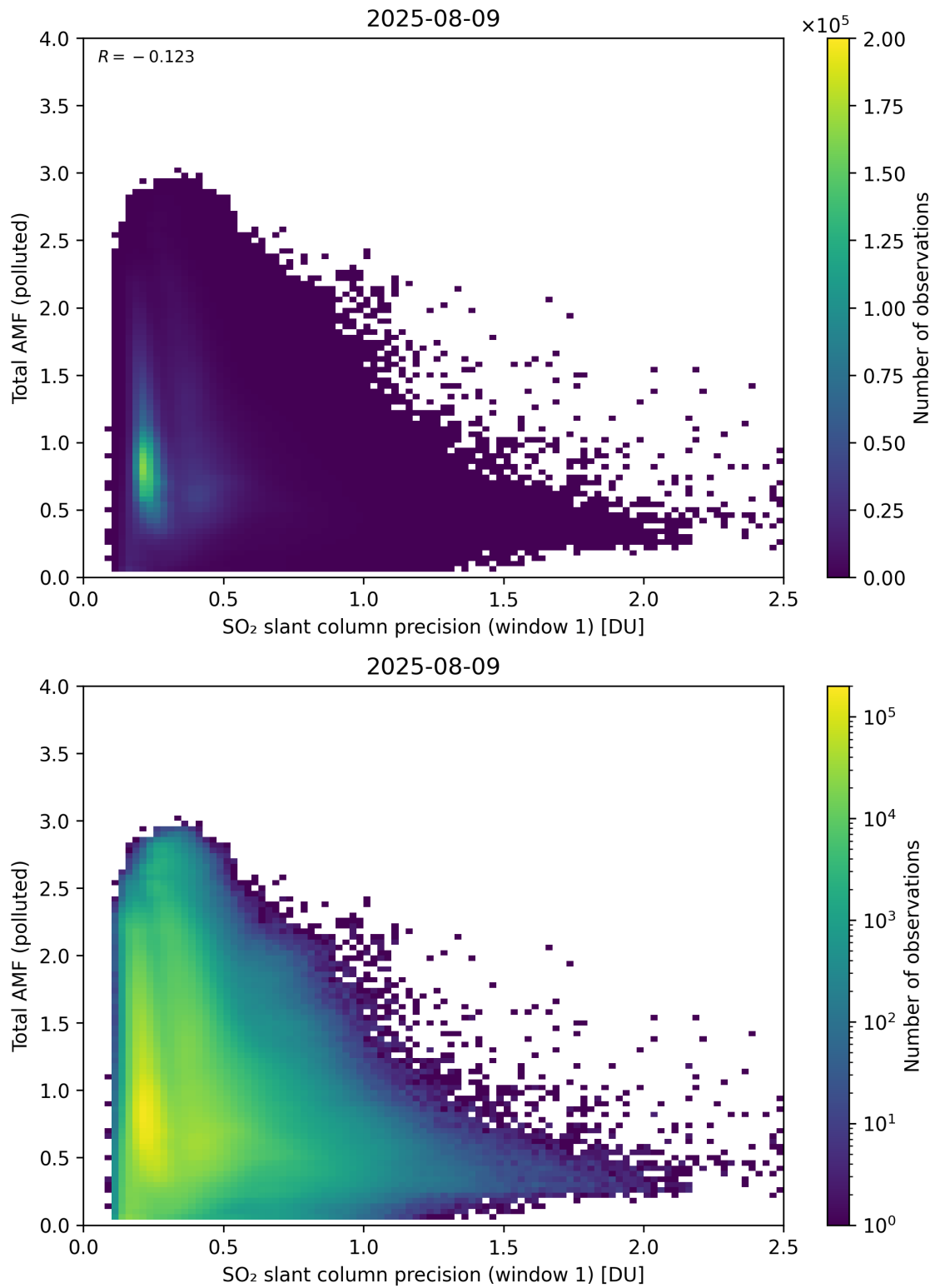
Figure 280: Scatter density plot of “SO 2 slant column precision (window 1)” against “Total AMF (polluted)” for 2025-08-09 to 2025-08-10.
