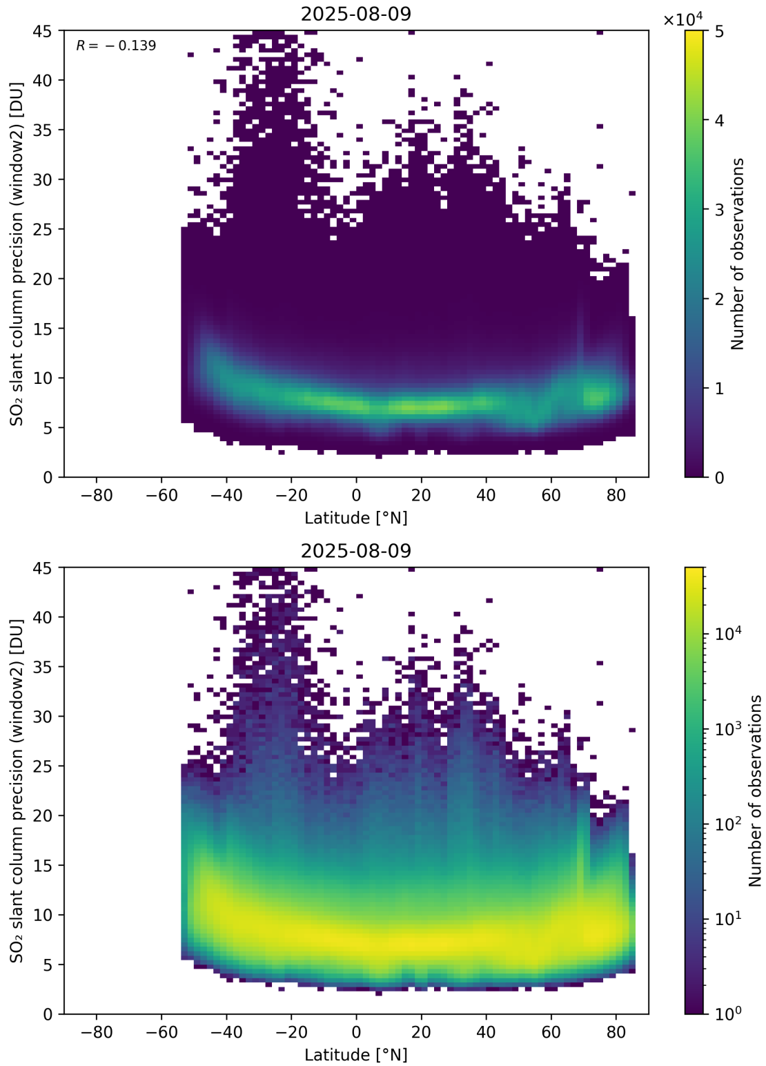
Figure 164: Scatter density plot of “Latitude” against “SO 2 slant column precision (window2)” for 2025-08-09 to 2025-08-10.
