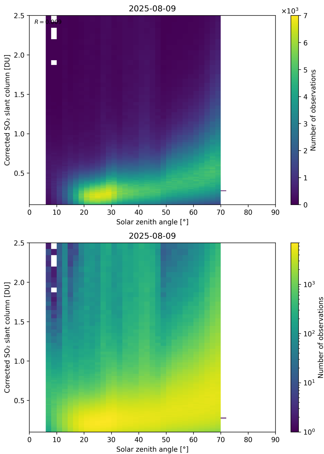
Figure 181: Scatter density plot of “Solar zenith angle” against “Corrected SO 2 slant column” for 2025-08-09 to 2025-08-10.
