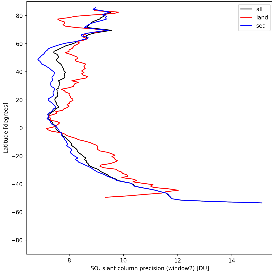
Figure 42: Zonal average of “SO 2 slant column precision (window2)” for 2025-08-09 to 2025-08-10.
