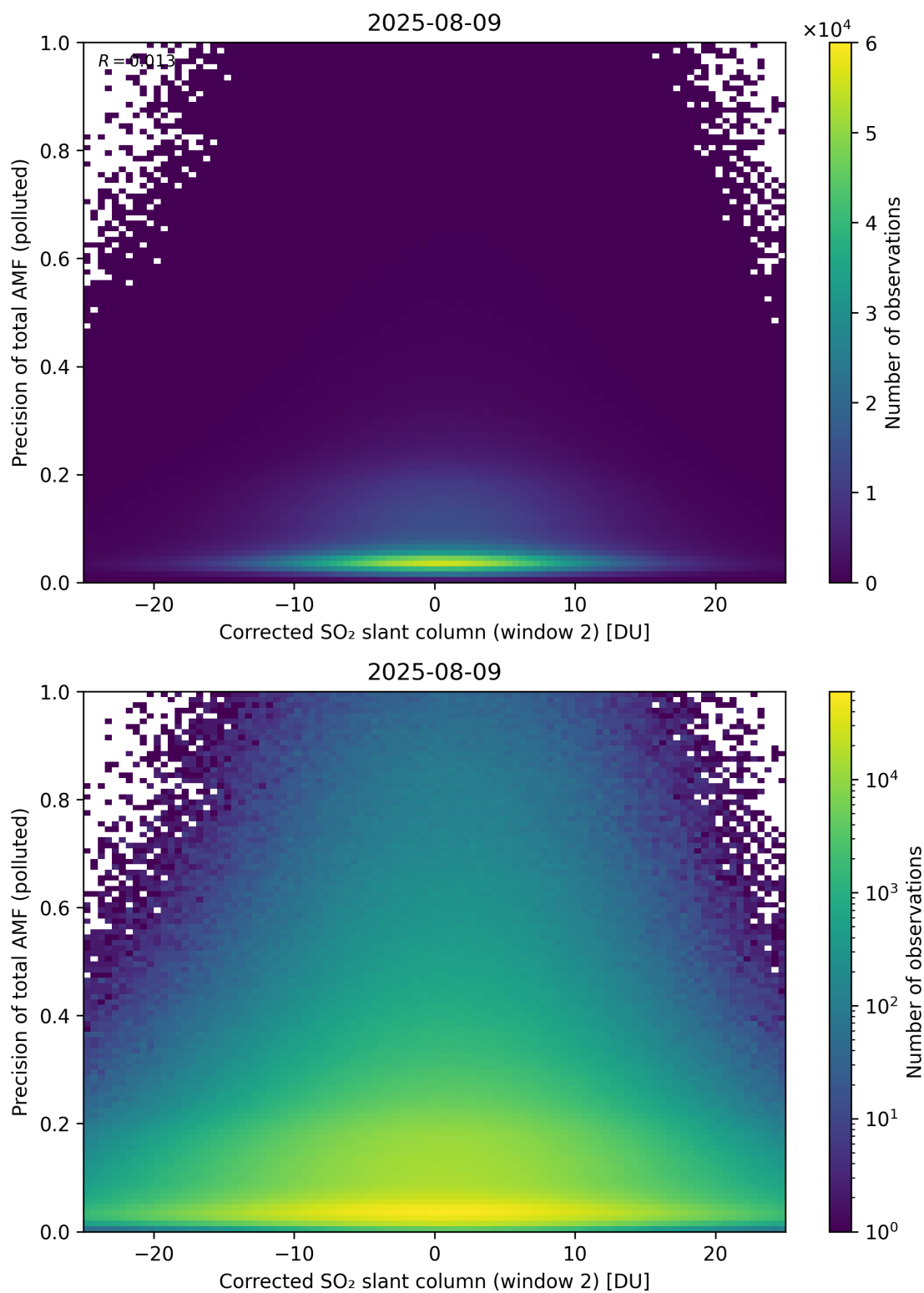
Figure 254: Scatter density plot of “Corrected SO 2 slant column (window 2)” against “Precision of total AMF (polluted)” for 2025-08-09 to 2025-08-10.
