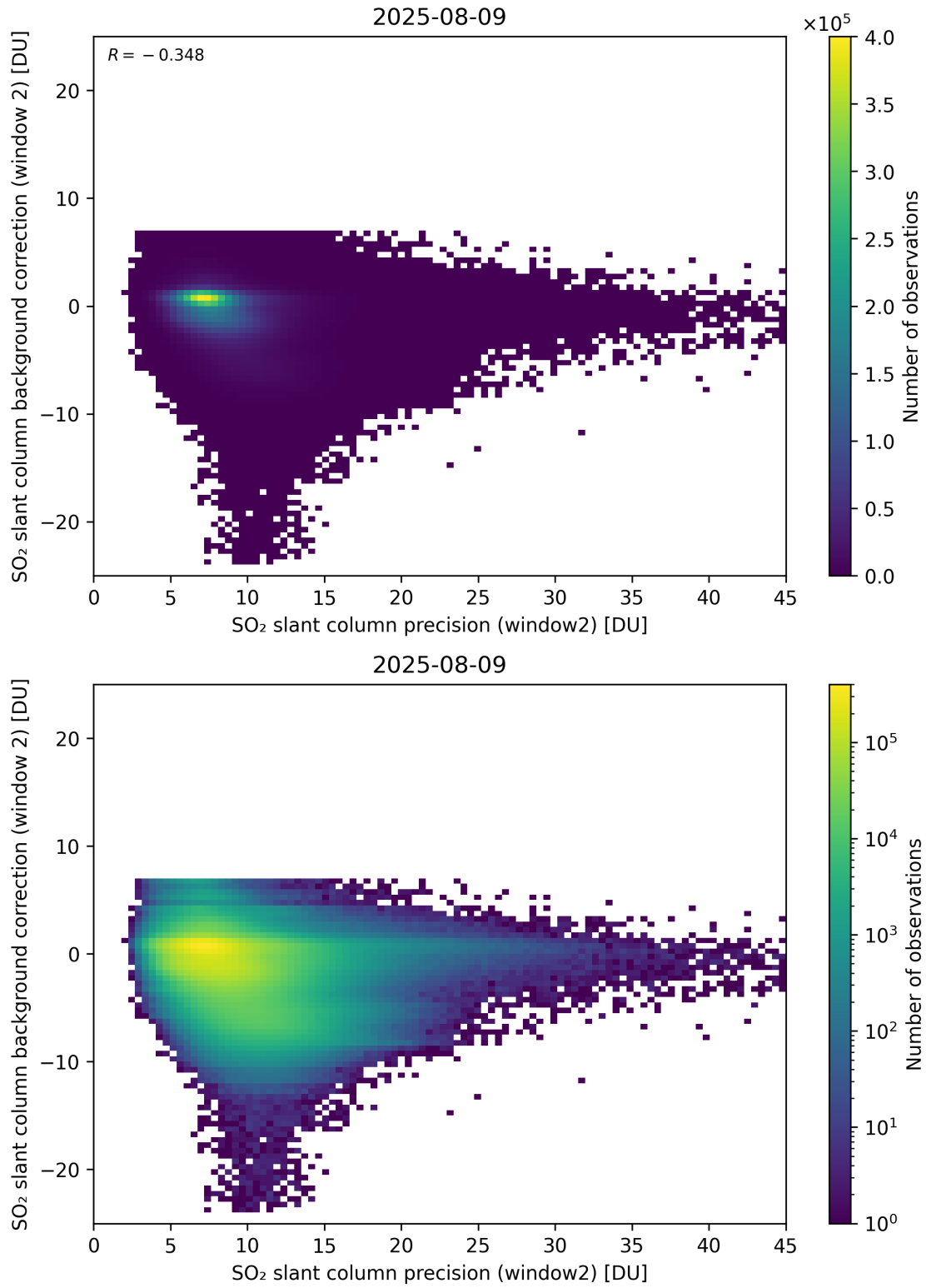
Figure 291: Scatter density plot of “SO 2 slant column precision (window2)” against “SO 2 slant column background correction (window 2)” for 2025-08-09 to 2025-08-10.
