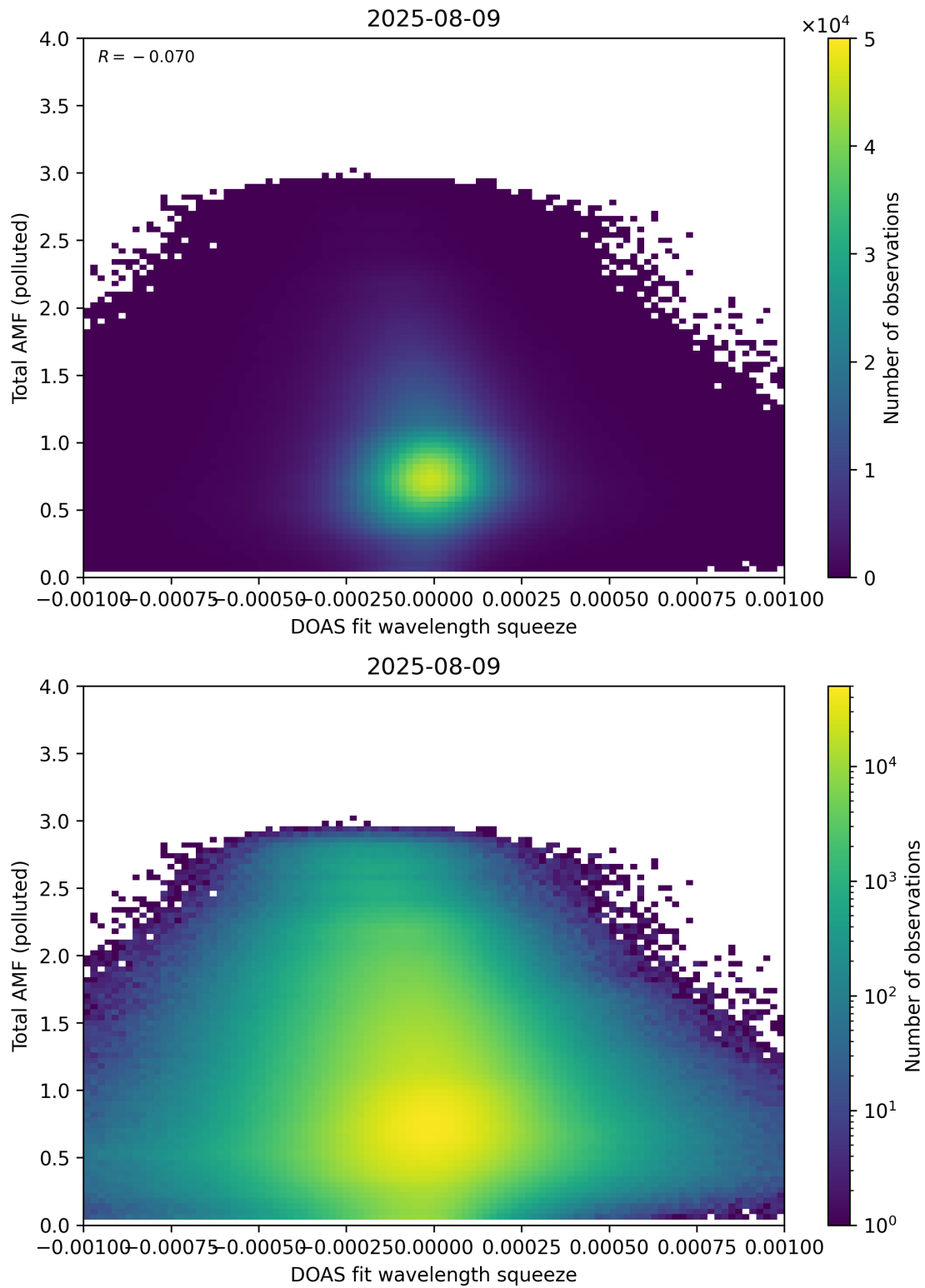
Figure 145: Scatter density plot of “DOAS fit wavelength squeeze” against “Total AMF (polluted)” for 2025-08-09 to 2025-08-10.
