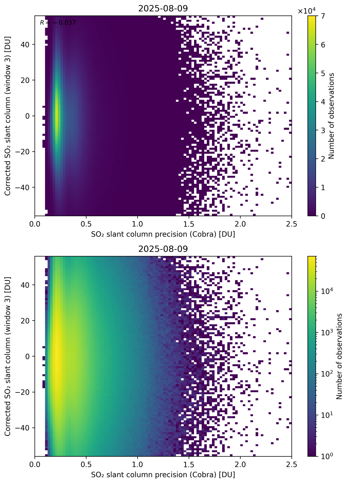
Figure 207: Scatter density plot of “SO 2 slant column precision (Cobra)” against “Corrected SO 2 slant column (window 3)” for 2025-08-09 to 2025-08-10.
