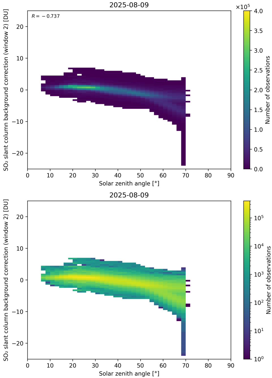
Figure 172: Scatter density plot of “Solar zenith angle” against “SO 2 slant column background correction (window 2)” for 2025-08-09 to 2025-08-10.
