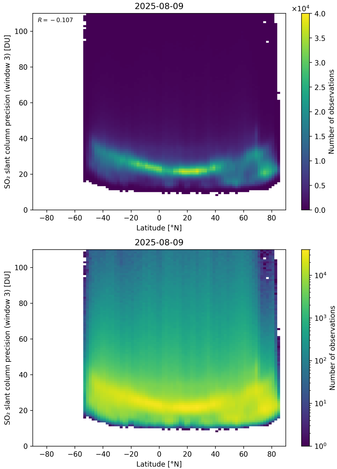
Figure 166: Scatter density plot of “Latitude” against “SO 2 slant column precision (window 3)” for 2025-08-09 to 2025-08-10.
