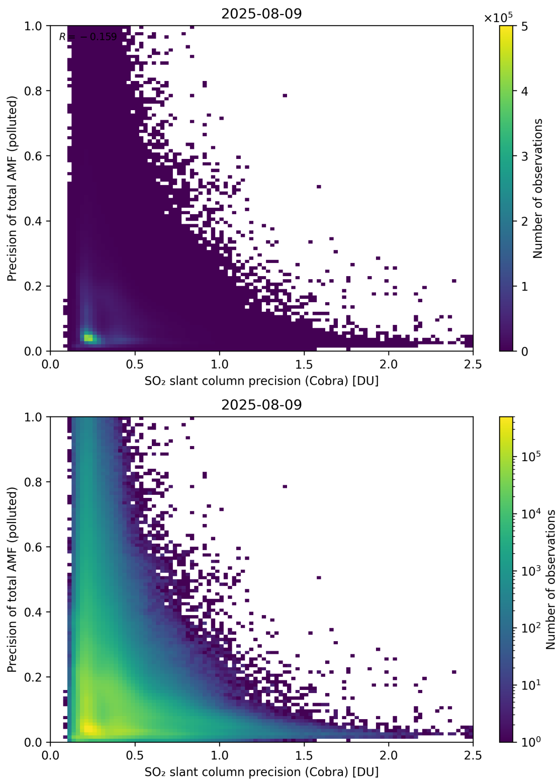
Figure 214: Scatter density plot of “SO 2 slant column precision (Cobra)” against “Precision of total AMF (polluted)” for 2025-08-09 to 2025-08-10.
