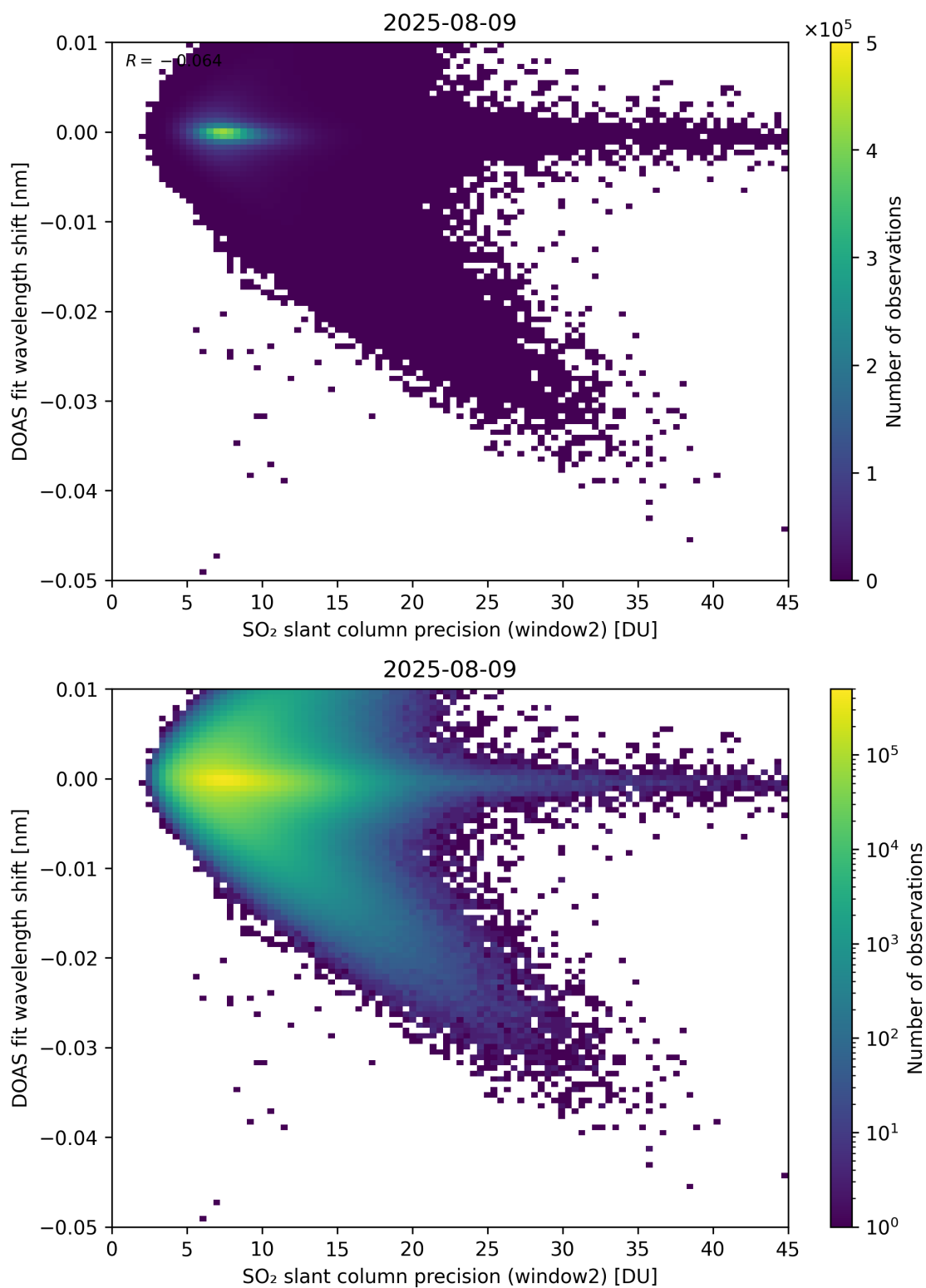
Figure 293: Scatter density plot of “SO 2 slant column precision (window2)” against “DOAS fit wavelength shift” for 2025-08-09 to 2025-08-10.
