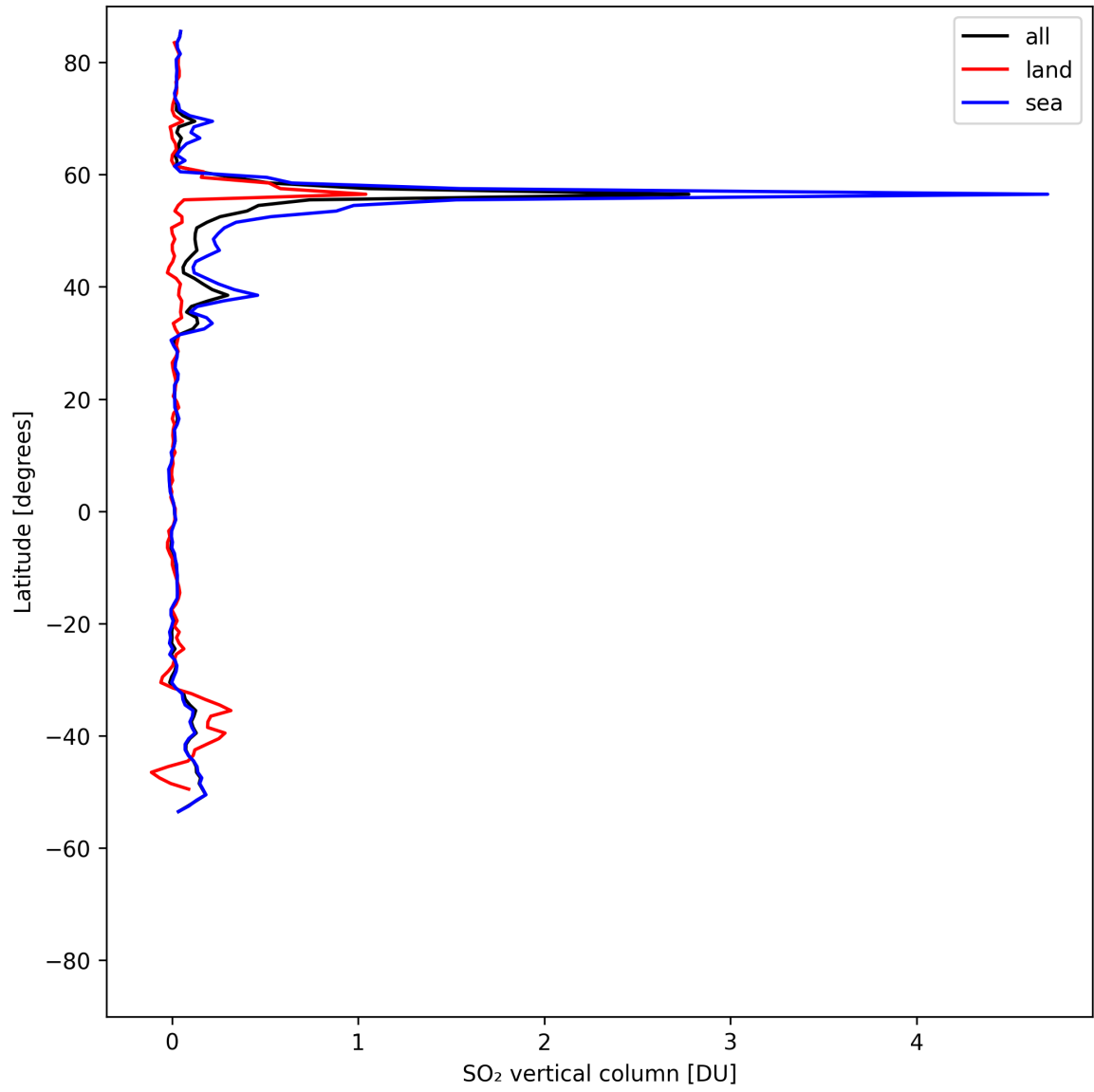
Figure 32: Zonal average of “SO 2 vertical column” for 2025-08-09 to 2025-08-10.
