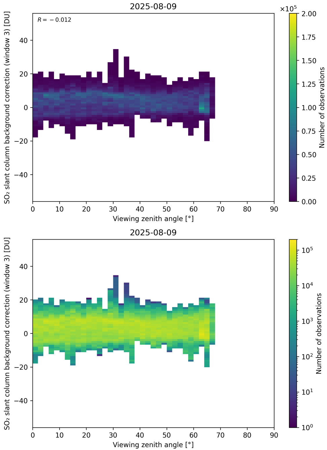
Figure 364: Scatter density plot of “Viewing zenith angle” against “SO 2 slant column background correction (window 3)” for 2025-08-09 to 2025-08-10.
