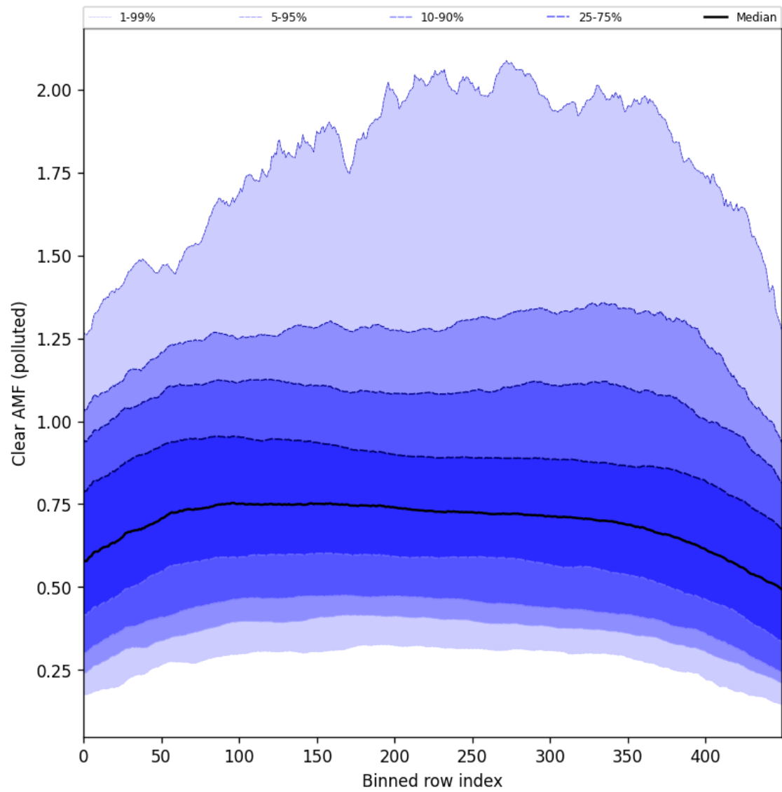
Figure 107: Along track statistics of “Clear AMF (polluted)” for 2025-08-09 to 2025-08-10
