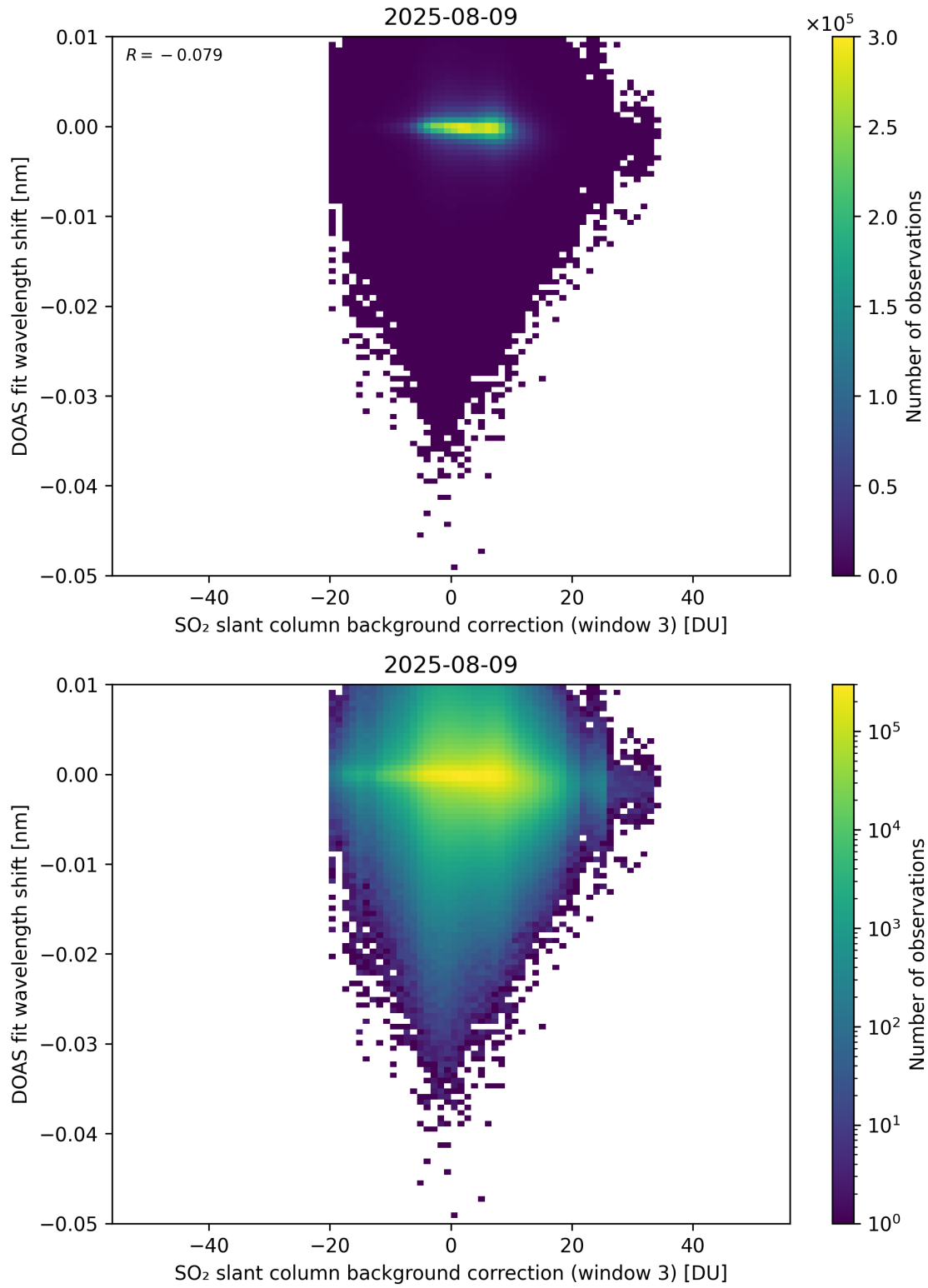
Figure 132: Scatter density plot of “SO 2 slant column background correction (window 3)” against “DOAS fit wavelength shift” for 2025-08-09 to 2025-08-10.
