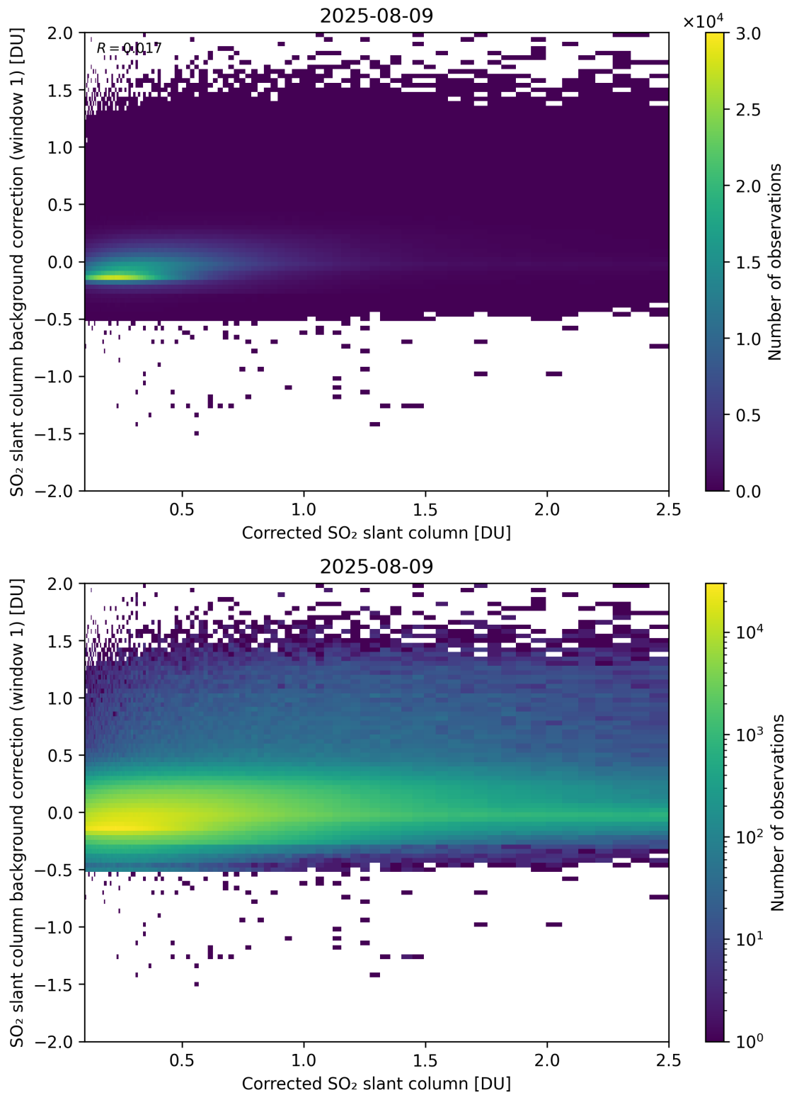
Figure 226: Scatter density plot of “Corrected SO 2 slant column” against “SO 2 slant column background correction (window 1)” for 2025-08-09 to 2025-08-10.
