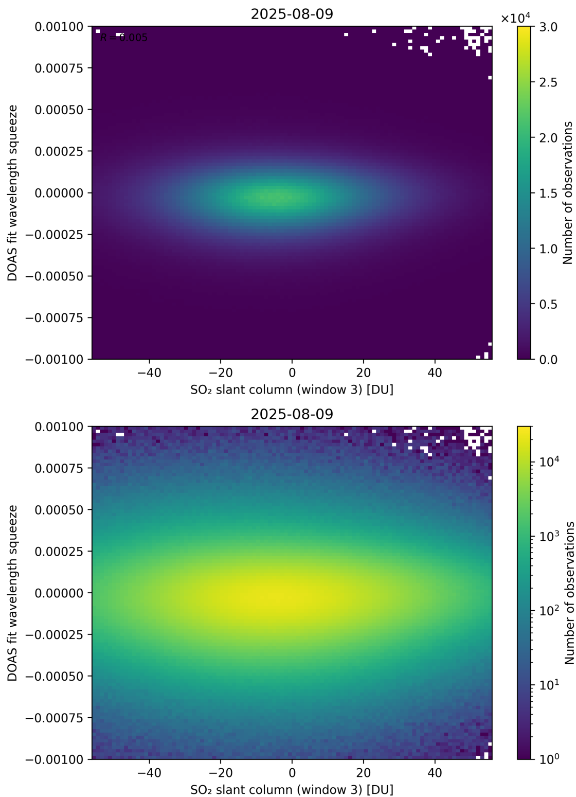
Figure 305: Scatter density plot of “SO 2 slant column (window 3)” against “DOAS fit wavelength squeeze” for 2025-08-09 to 2025-08-10.
