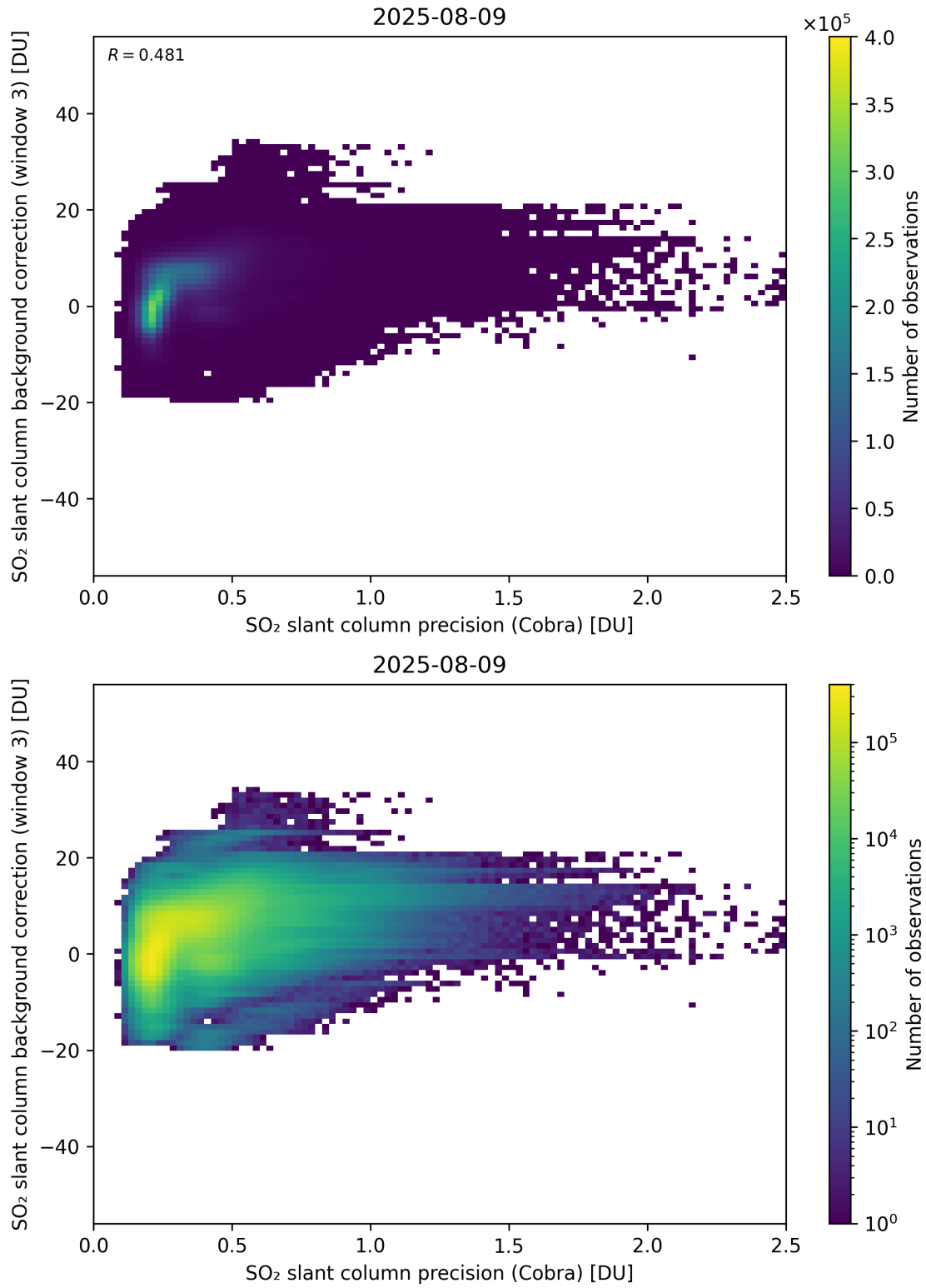
Figure 201: Scatter density plot of “SO 2 slant column precision (Cobra)” against “SO 2 slant column background correction (window 3)” for 2025-08-09 to 2025-08-10.
