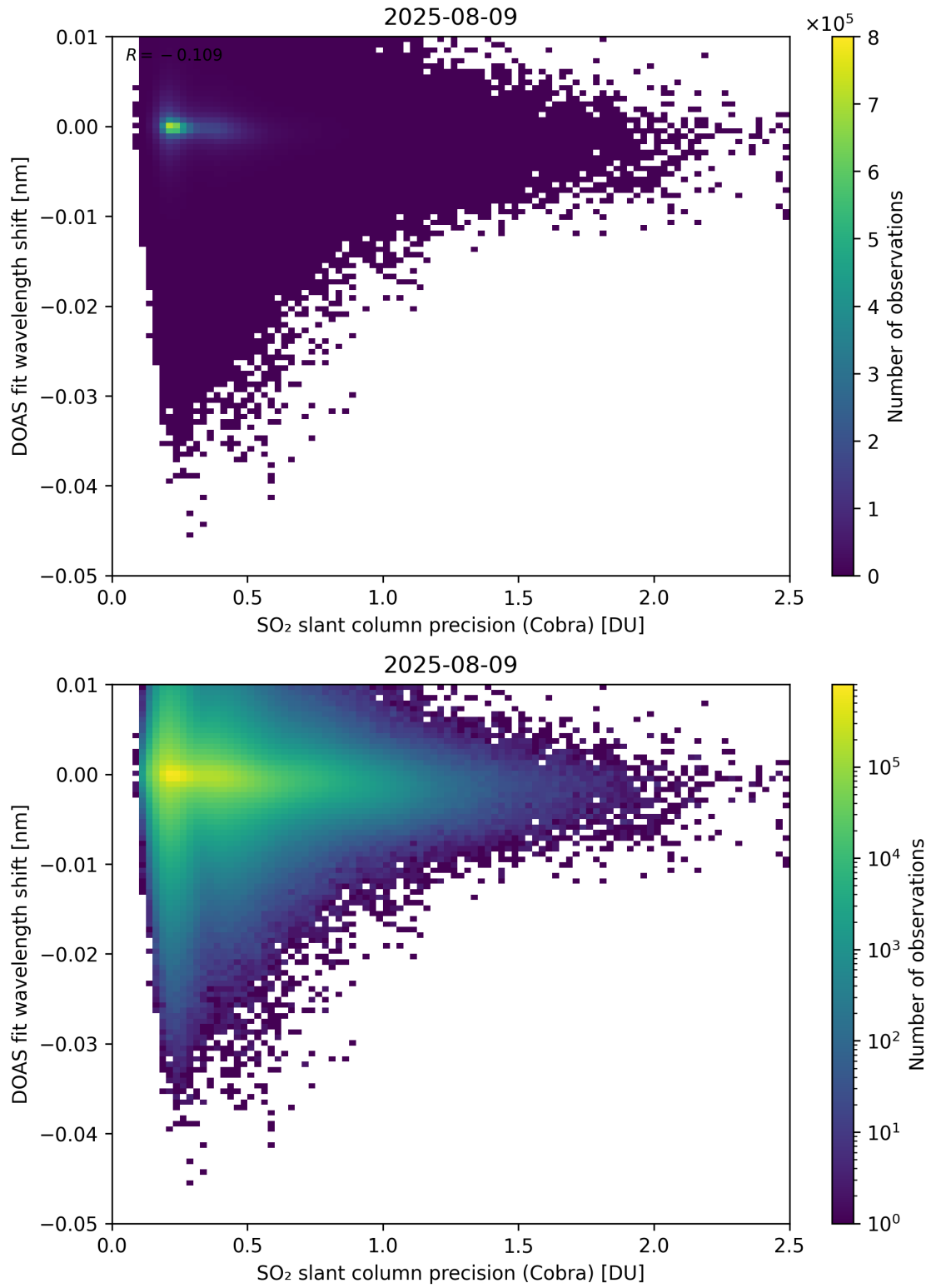
Figure 202: Scatter density plot of “SO 2 slant column precision (Cobra)” against “DOAS fit wavelength shift” for 2025-08-09 to 2025-08-10.
