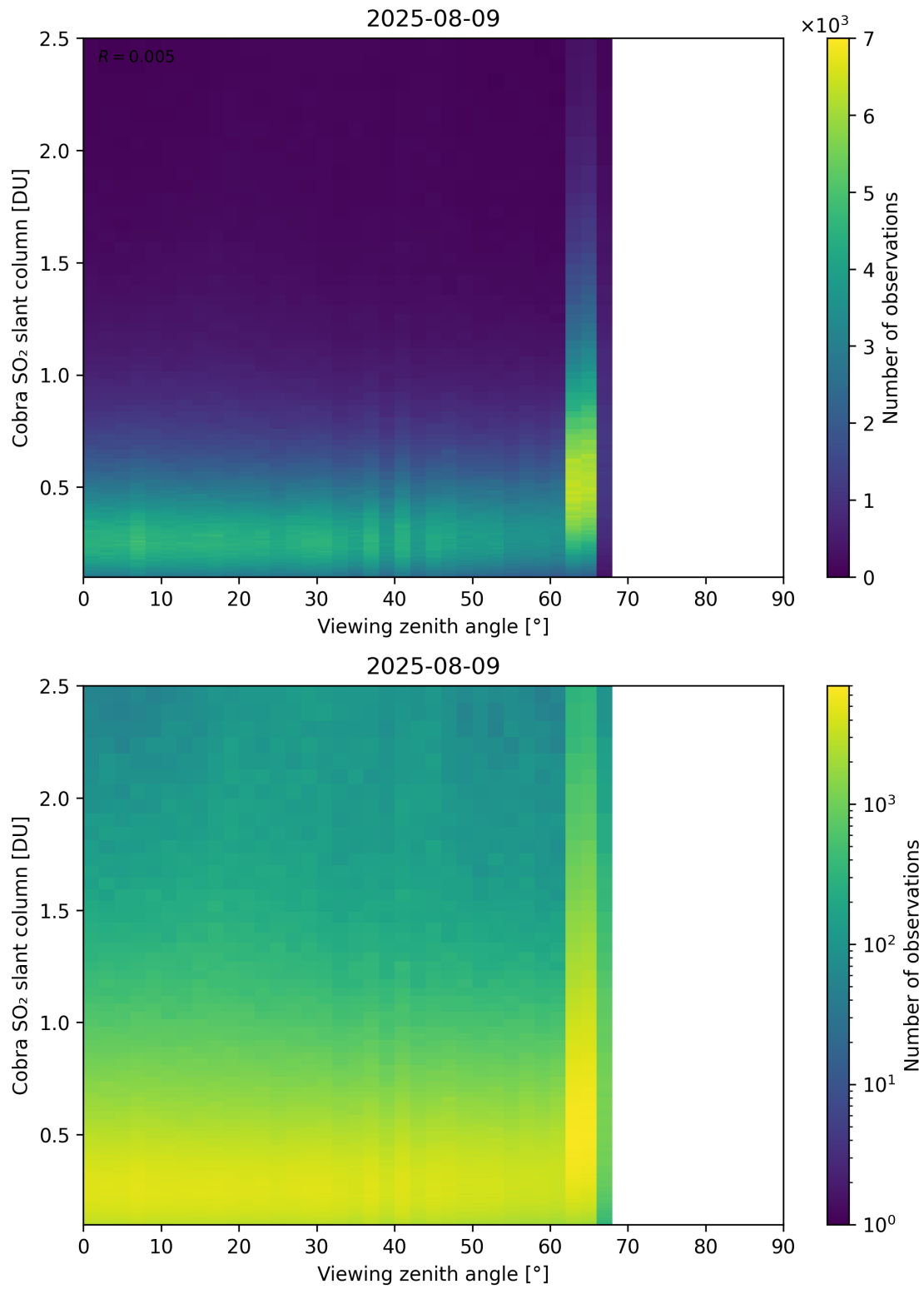
Figure 371: Scatter density plot of “Viewing zenith angle” against “Cobra SO 2 slant column” for 2025-08-09 to 2025-08-10.
