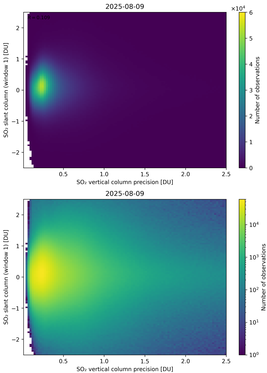
Figure 341: Scatter density plot of “SO 2 vertical column precision” against “SO 2 slant column (window 1)” for 2025-08-09 to 2025-08-10.
