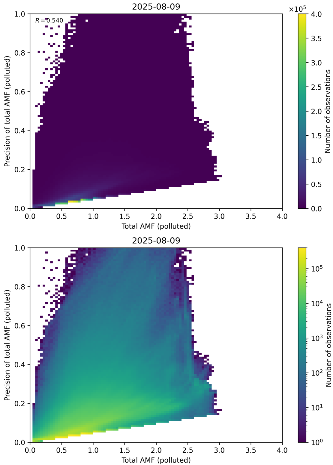
Figure 322: Scatter density plot of “Total AMF (polluted)” against “Precision of total AMF (polluted)” for 2025-08-09 to 2025-08-10.
