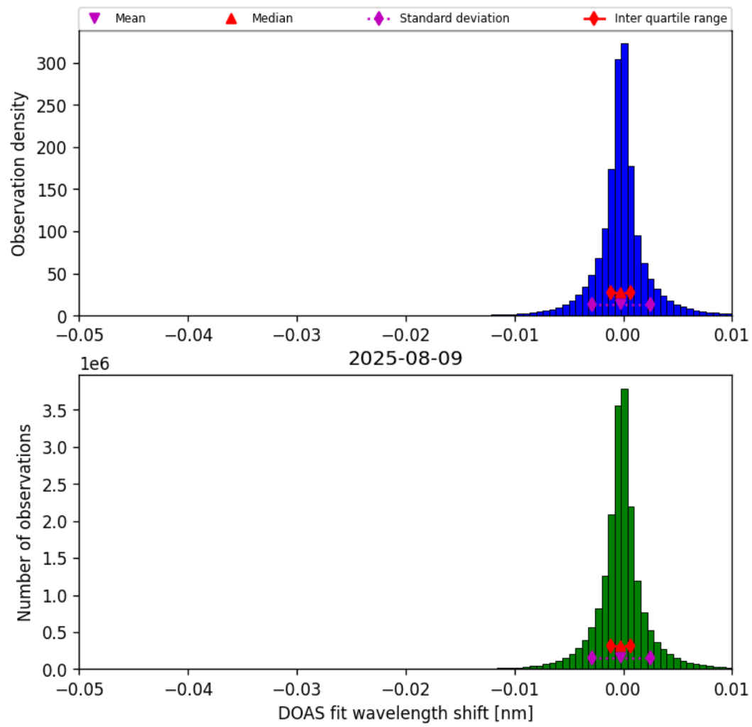
Figure 76: Histogram of “DOAS fit wavelength shift” for 2025-08-09 to 2025-08-10
