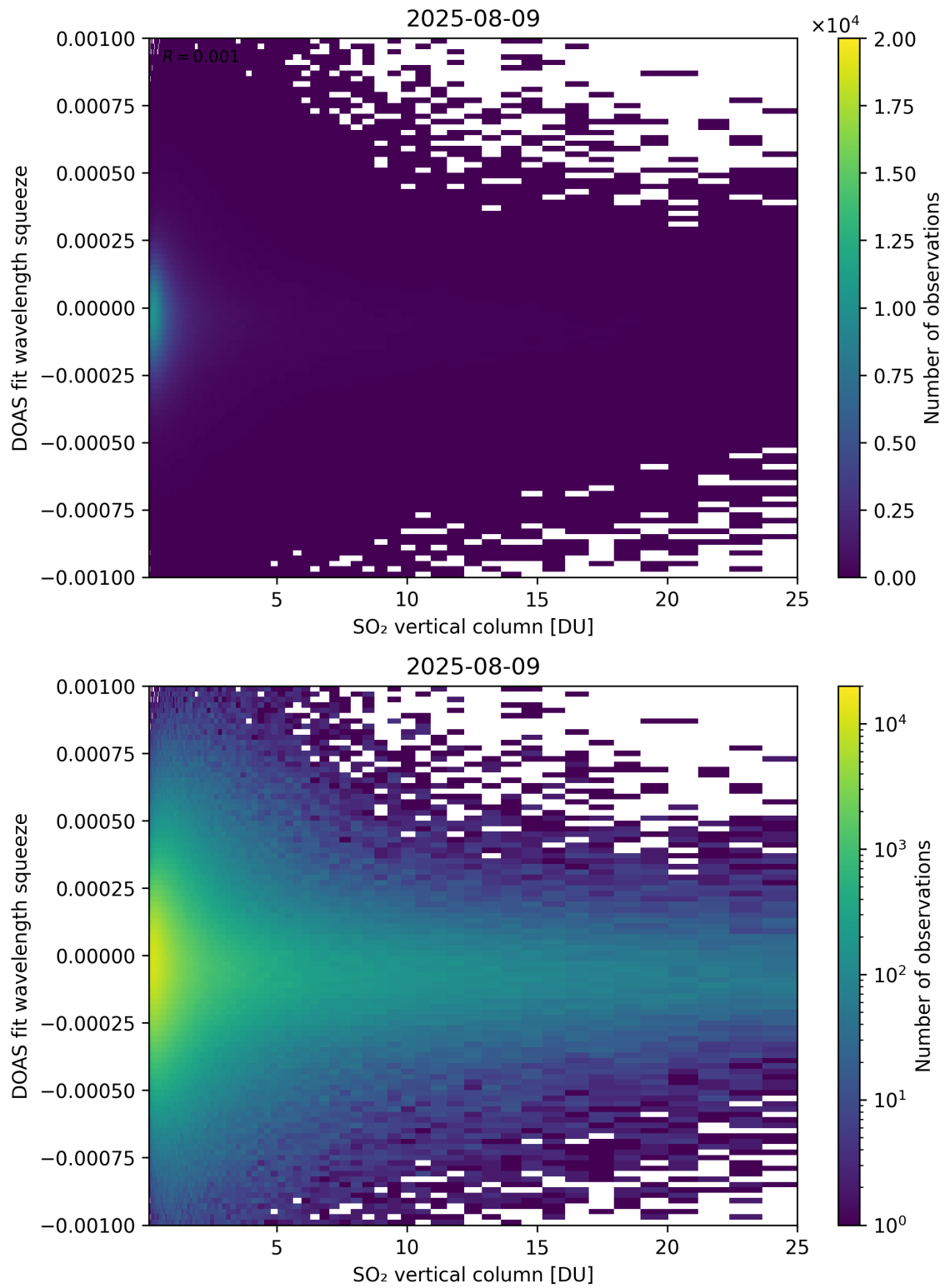
Figure 327: Scatter density plot of “SO 2 vertical column” against “DOAS fit wavelength squeeze” for 2025-08-09 to 2025-08-10.
