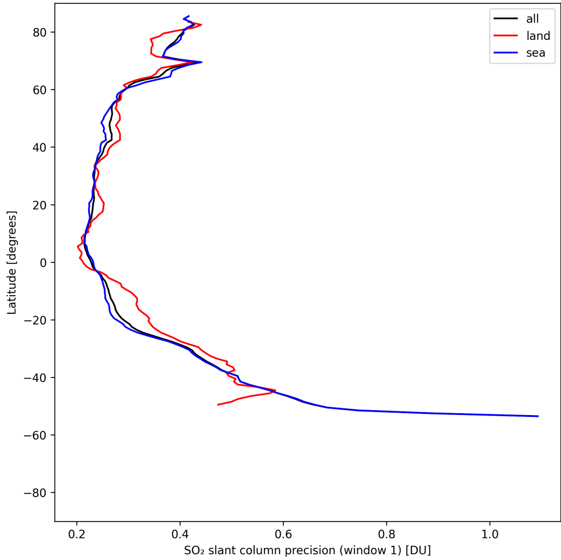
Figure 38: Zonal average of “SO 2 slant column precision (window 1)” for 2025-08-09 to 2025-08-10.
