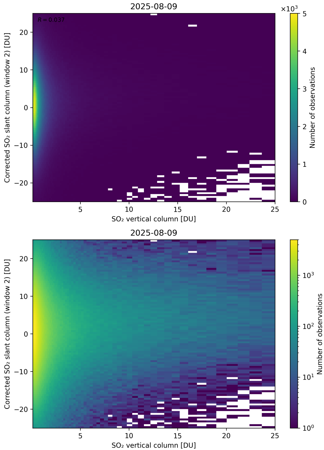
Figure 352: Scatter density plot of “SO 2 vertical column” against “Corrected SO 2 slant column (window 2)” for 2025-08-09 to 2025-08-10.
