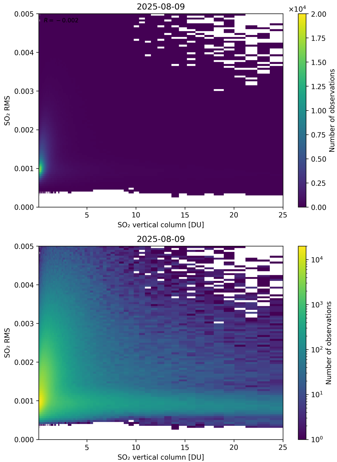
Figure 328: Scatter density plot of “SO 2 vertical column” against “SO 2 RMS” for 2025-08-09 to 2025-08-10.
