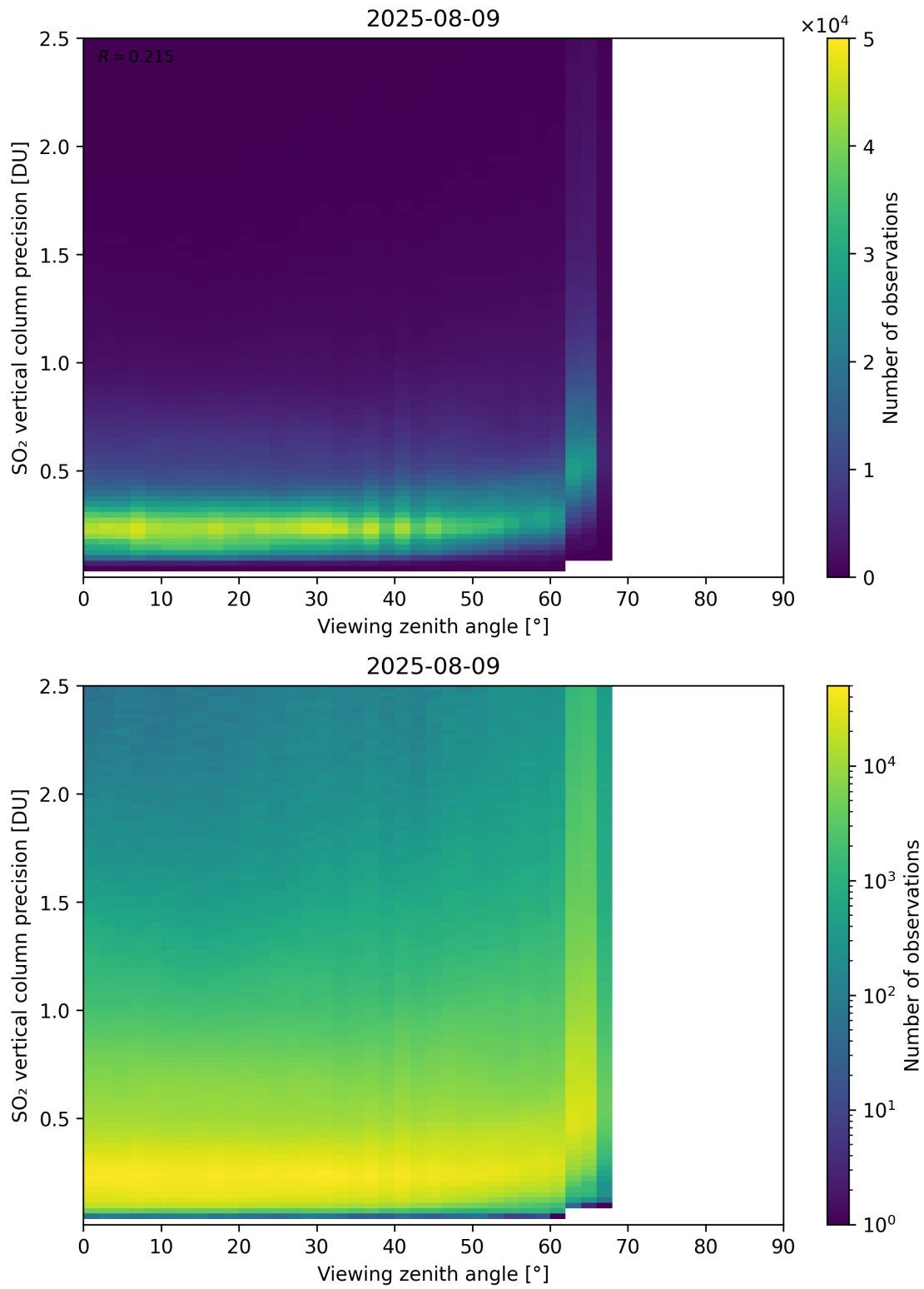
Figure 384: Scatter density plot of “Viewing zenith angle” against “SO 2 vertical column precision” for 2025-08-09 to 2025-08-10.
