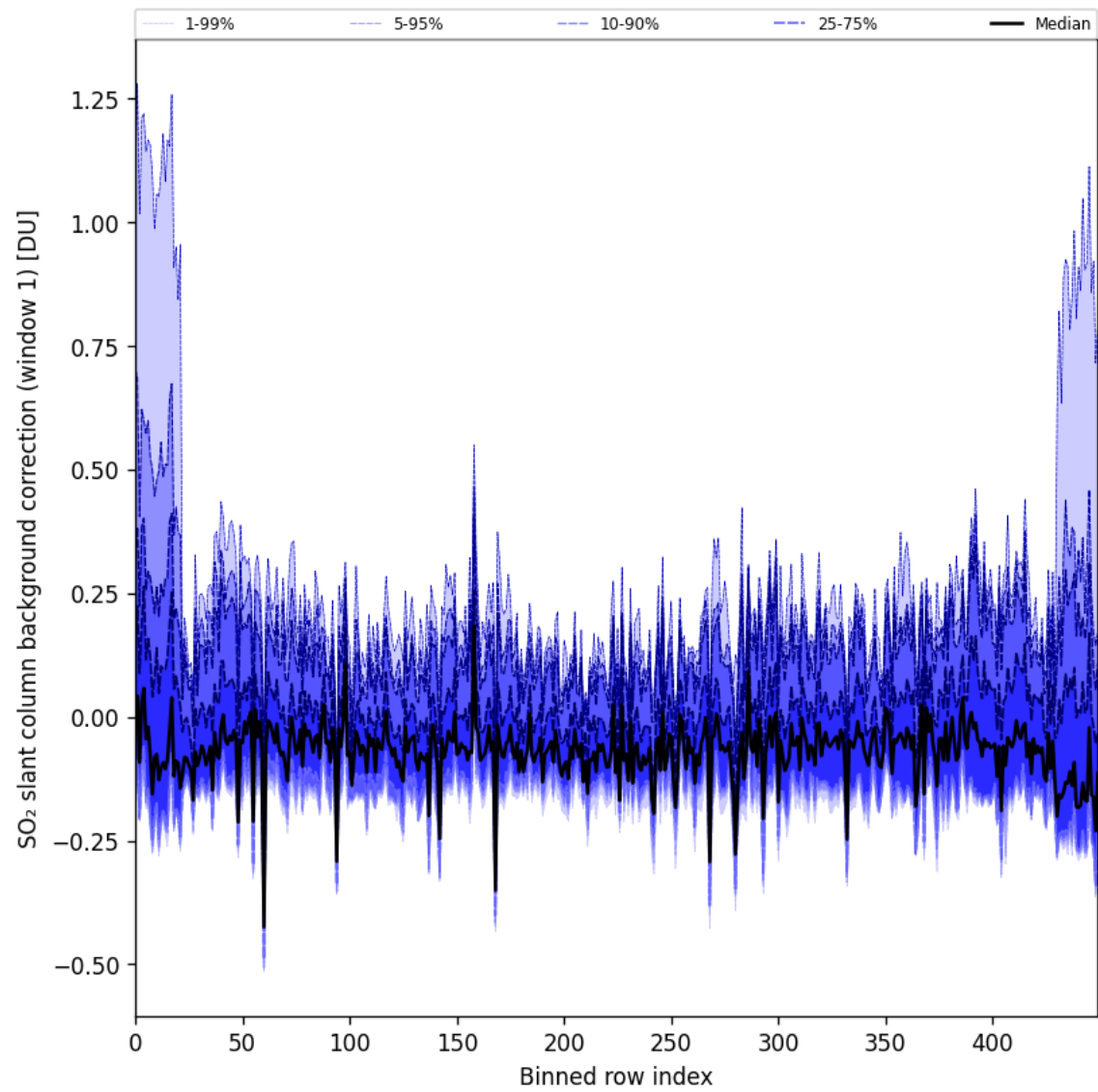
Figure 92: Along track statistics of “SO 2 slant column background correction (window 1)” for 2025-08-09 to 2025-08-10
