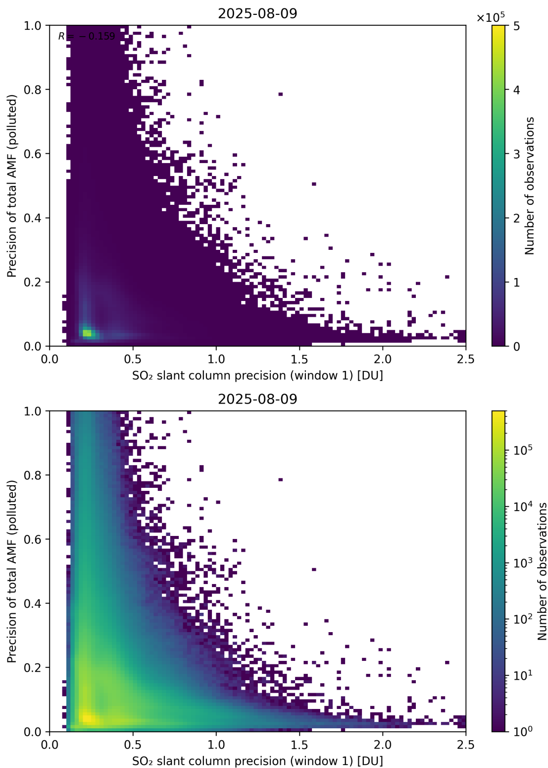
Figure 281: Scatter density plot of “SO 2 slant column precision (window 1)” against “Precision of total AMF (polluted)” for 2025-08-09 to 2025-08-10.
