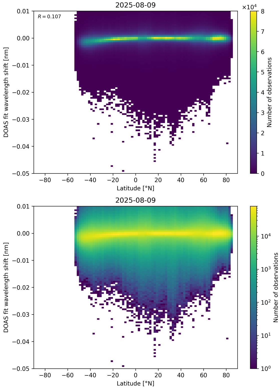
Figure 153: Scatter density plot of “Latitude” against “DOAS fit wavelength shift” for 2025-08-09 to 2025-08-10.
