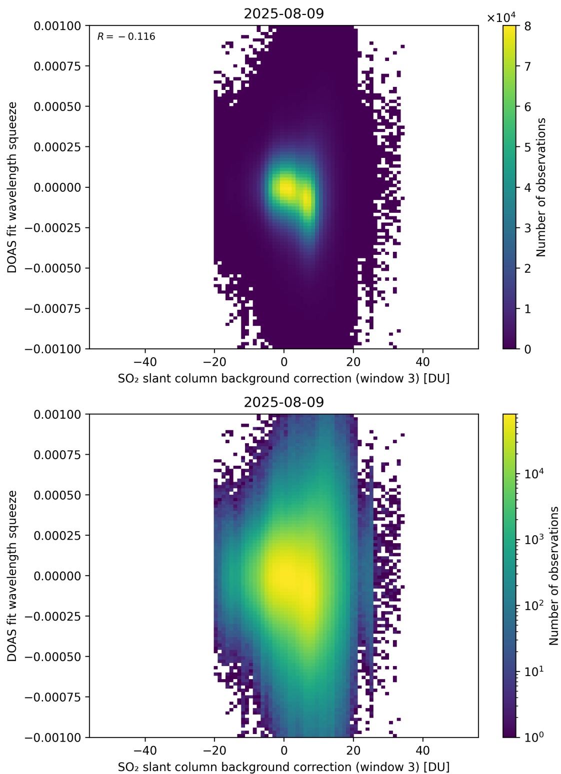
Figure 133: Scatter density plot of “SO 2 slant column background correction (window 3)” against “DOAS fit wavelength squeeze” for 2025-08-09 to 2025-08-10.
