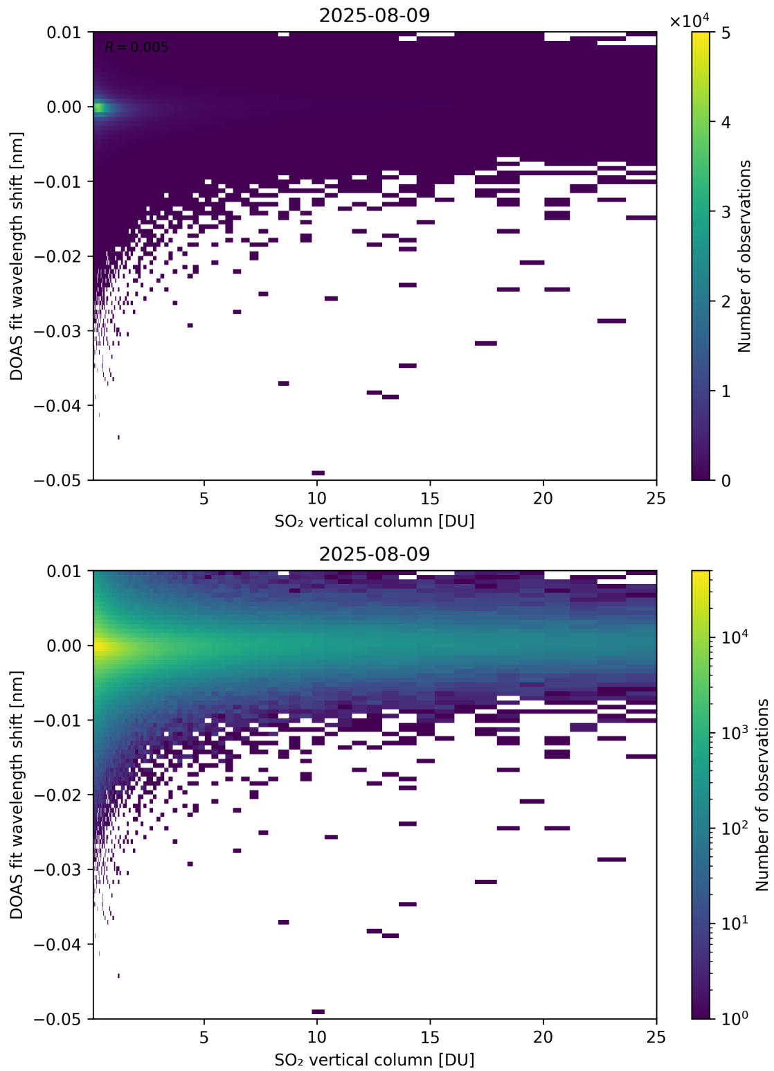
Figure 326: Scatter density plot of “SO 2 vertical column” against “DOAS fit wavelength shift” for 2025-08-09 to 2025-08-10.
