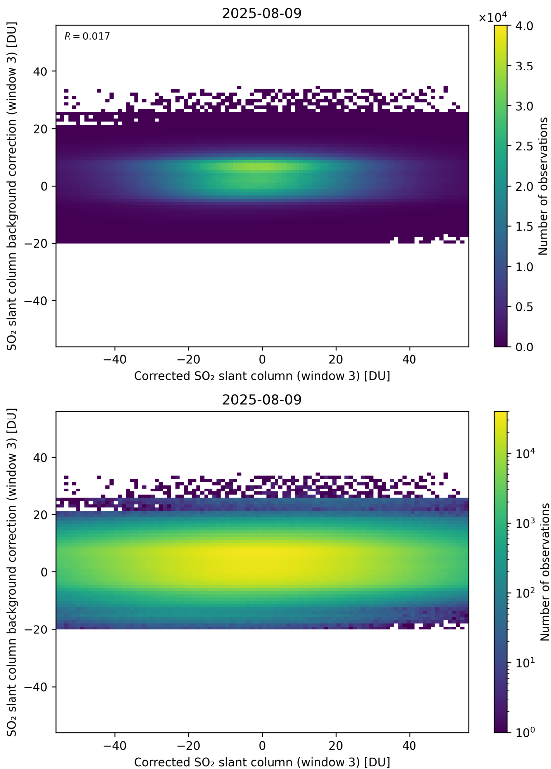
Figure 255: Scatter density plot of “Corrected SO 2 slant column (window 3)” against “SO 2 slant column background correction (window 3)” for 2025-08-09 to 2025-08-10.
