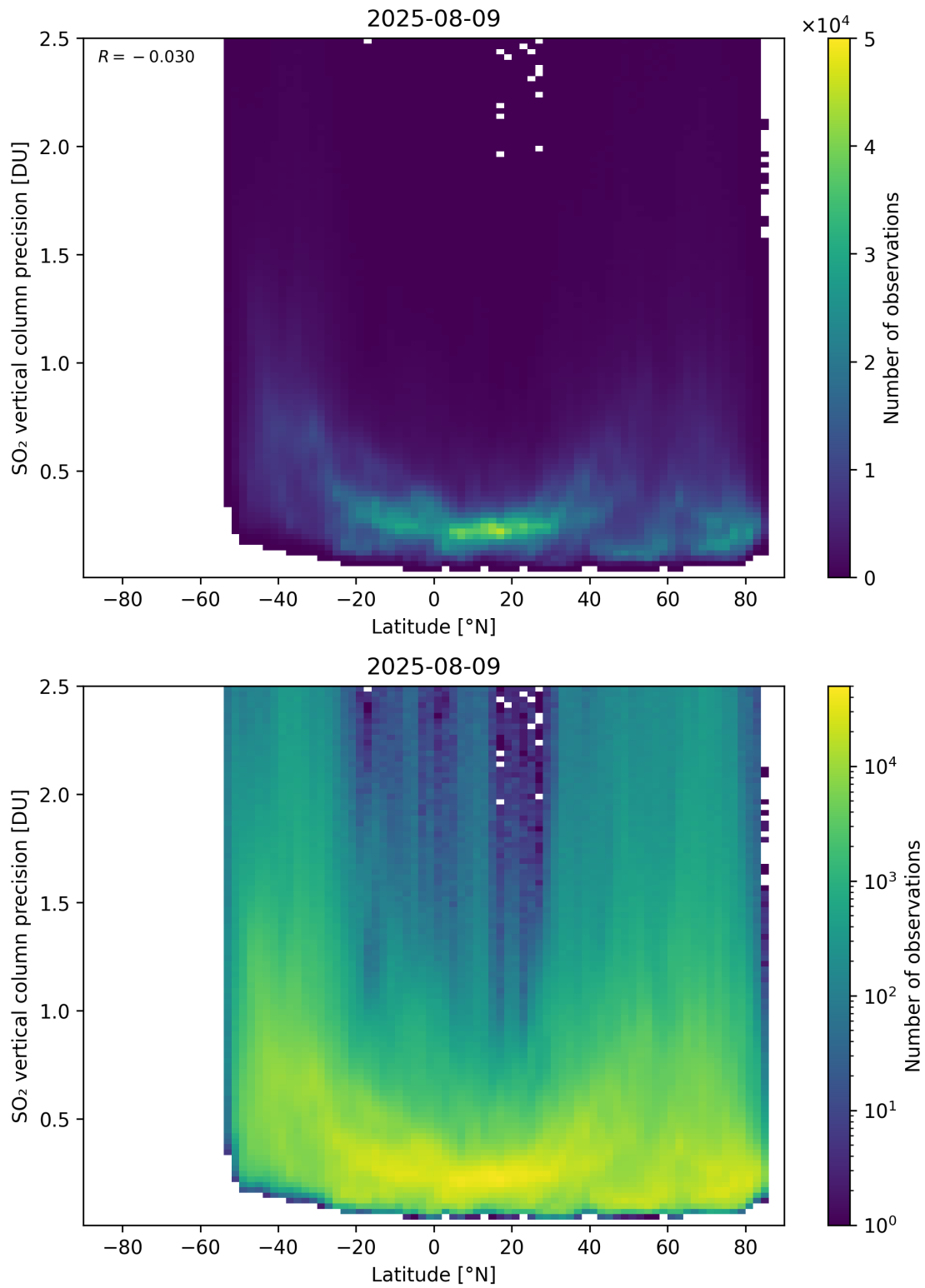
Figure 170: Scatter density plot of “Latitude” against “SO 2 vertical column precision” for 2025-08-09 to 2025-08-10.
