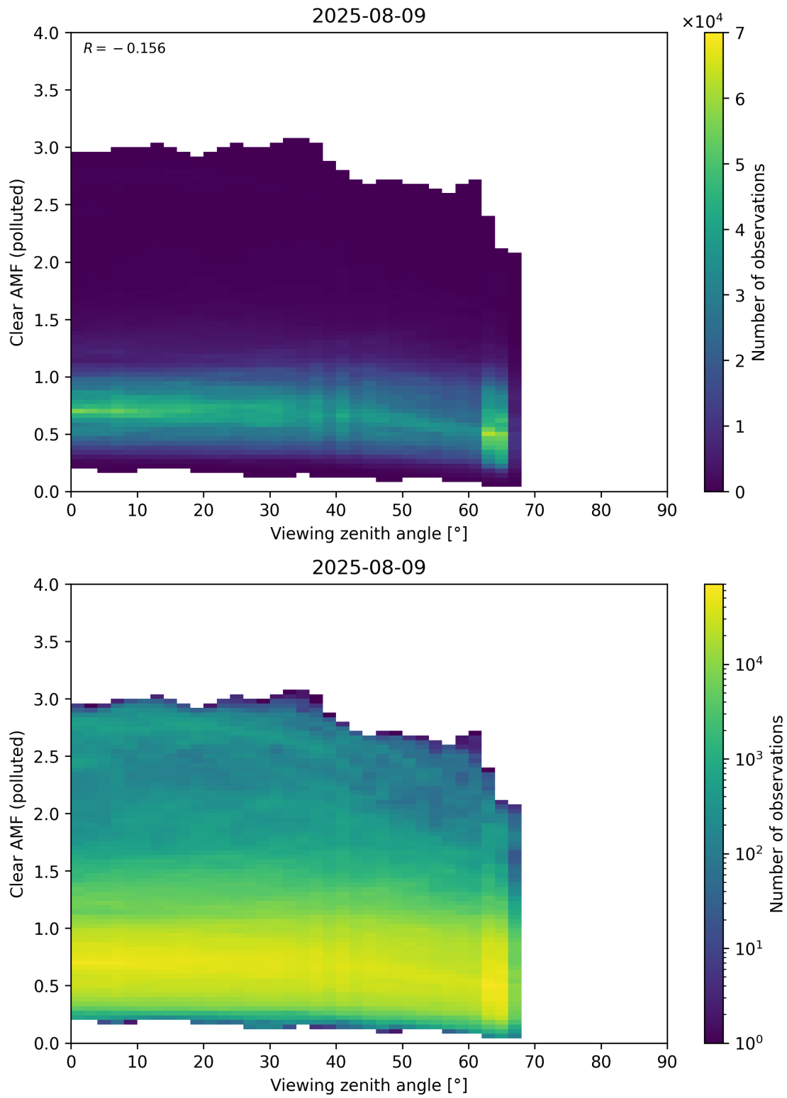
Figure 370: Scatter density plot of “Viewing zenith angle” against “Clear AMF (polluted)” for 2025-08-09 to 2025-08-10.
