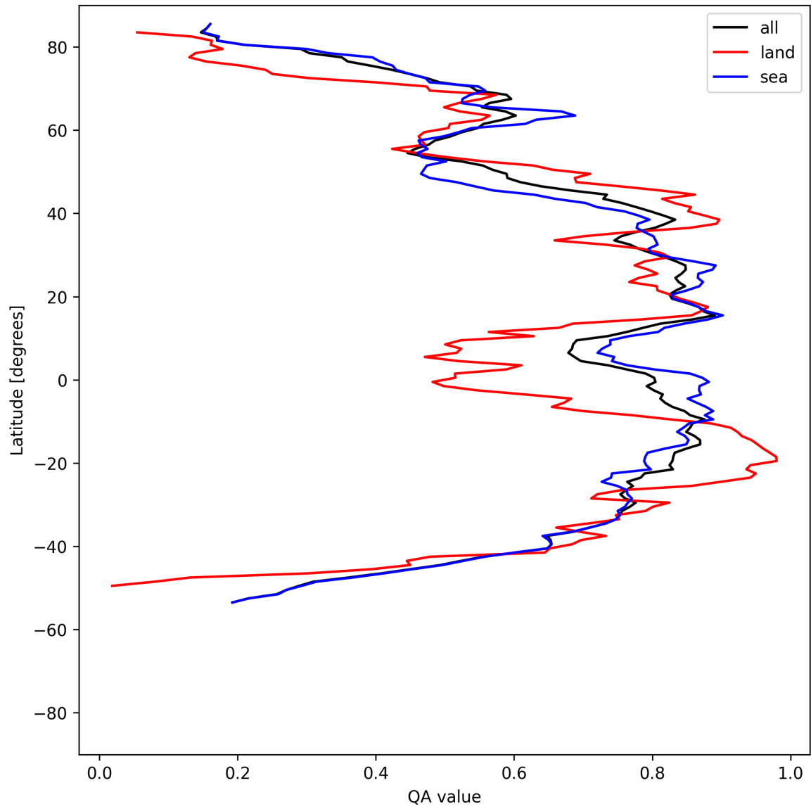
Figure 31: Zonal average of “QA value” for 2025-08-09 to 2025-08-10.
