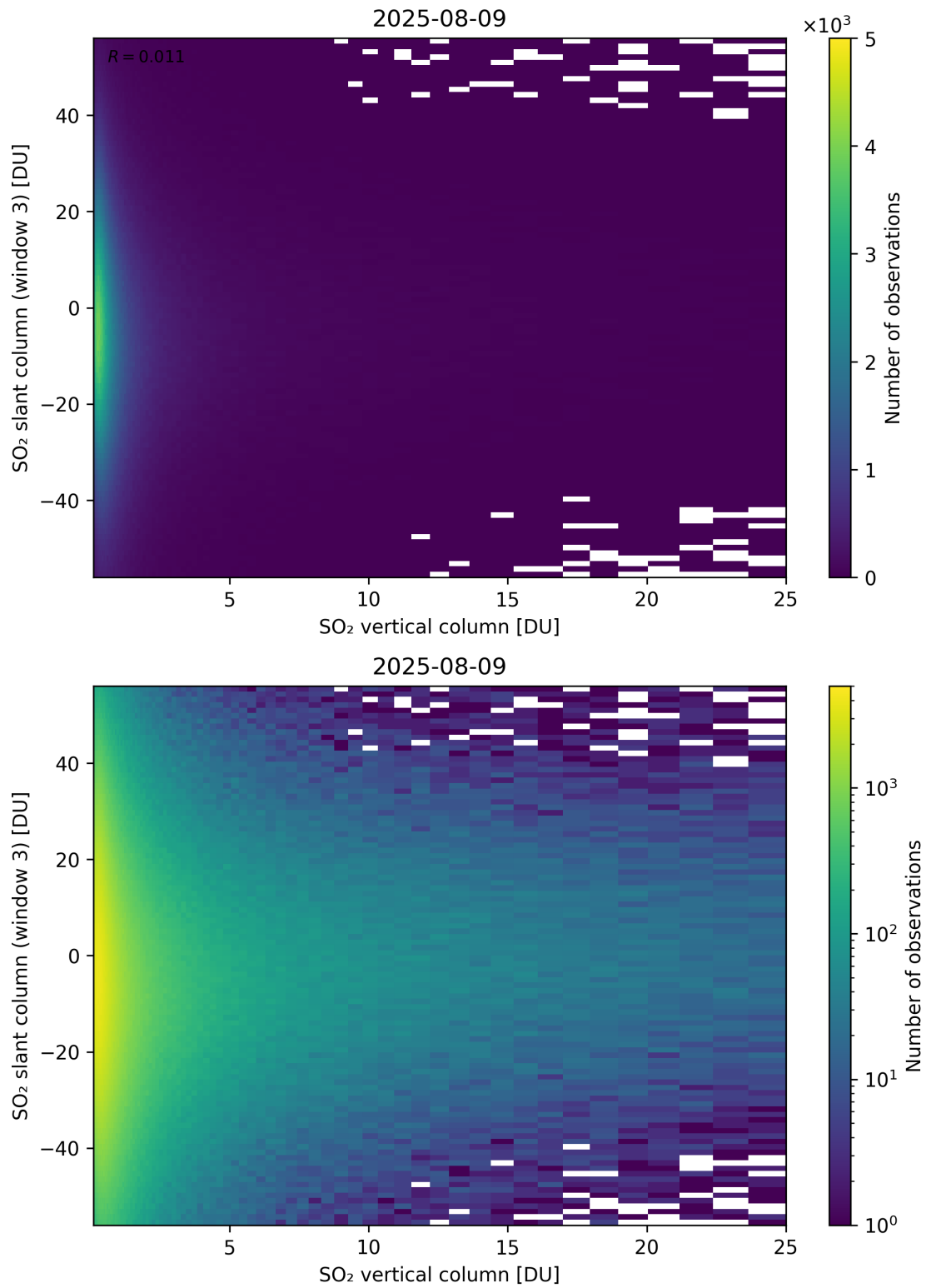
Figure 357: Scatter density plot of “SO 2 vertical column” against “SO 2 slant column (window 3)” for 2025-08-09 to 2025-08-10.
