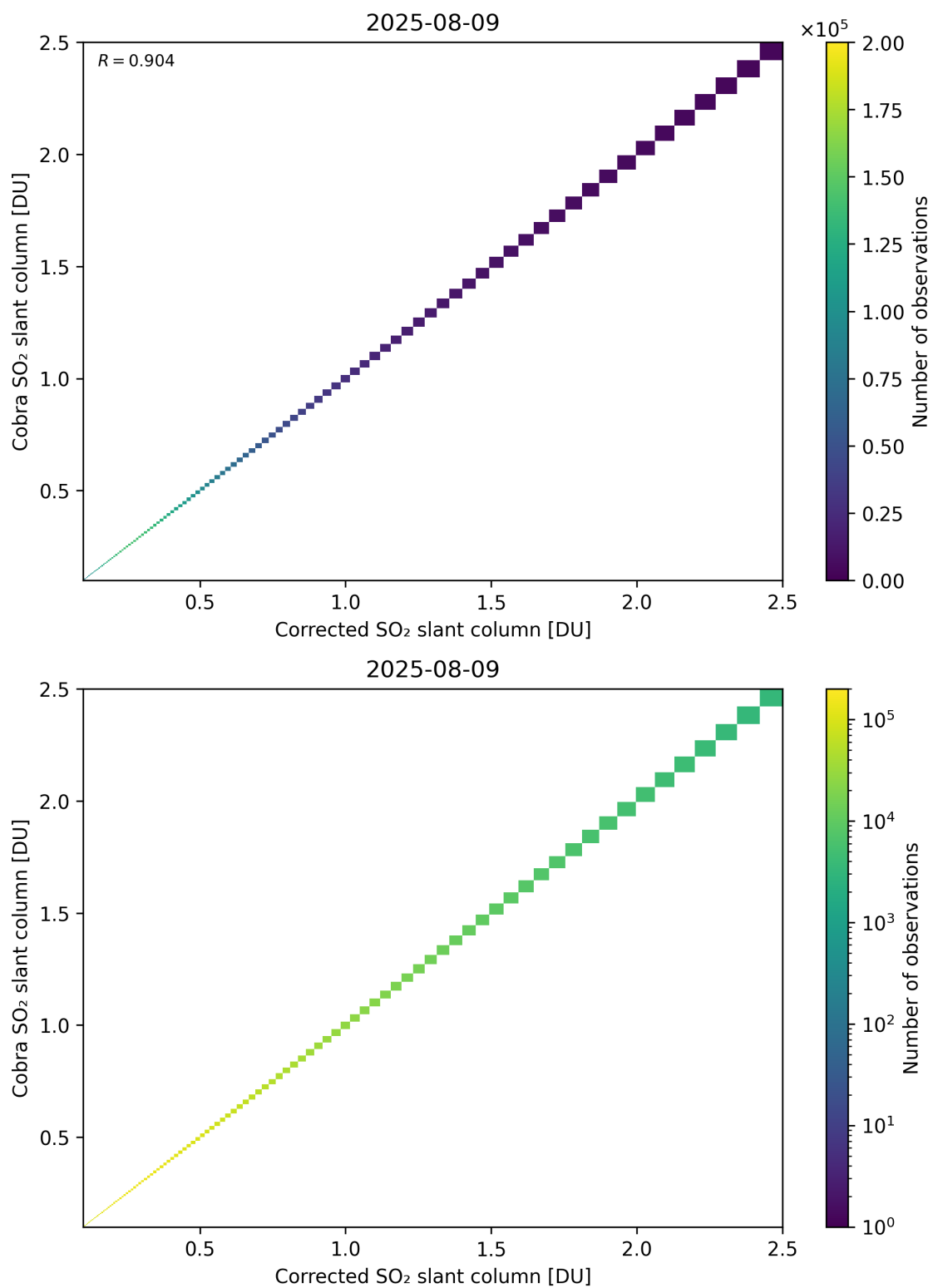
Figure 233: Scatter density plot of “Corrected SO 2 slant column” against “Cobra SO 2 slant column” for 2025-08-09 to 2025-08-10.
