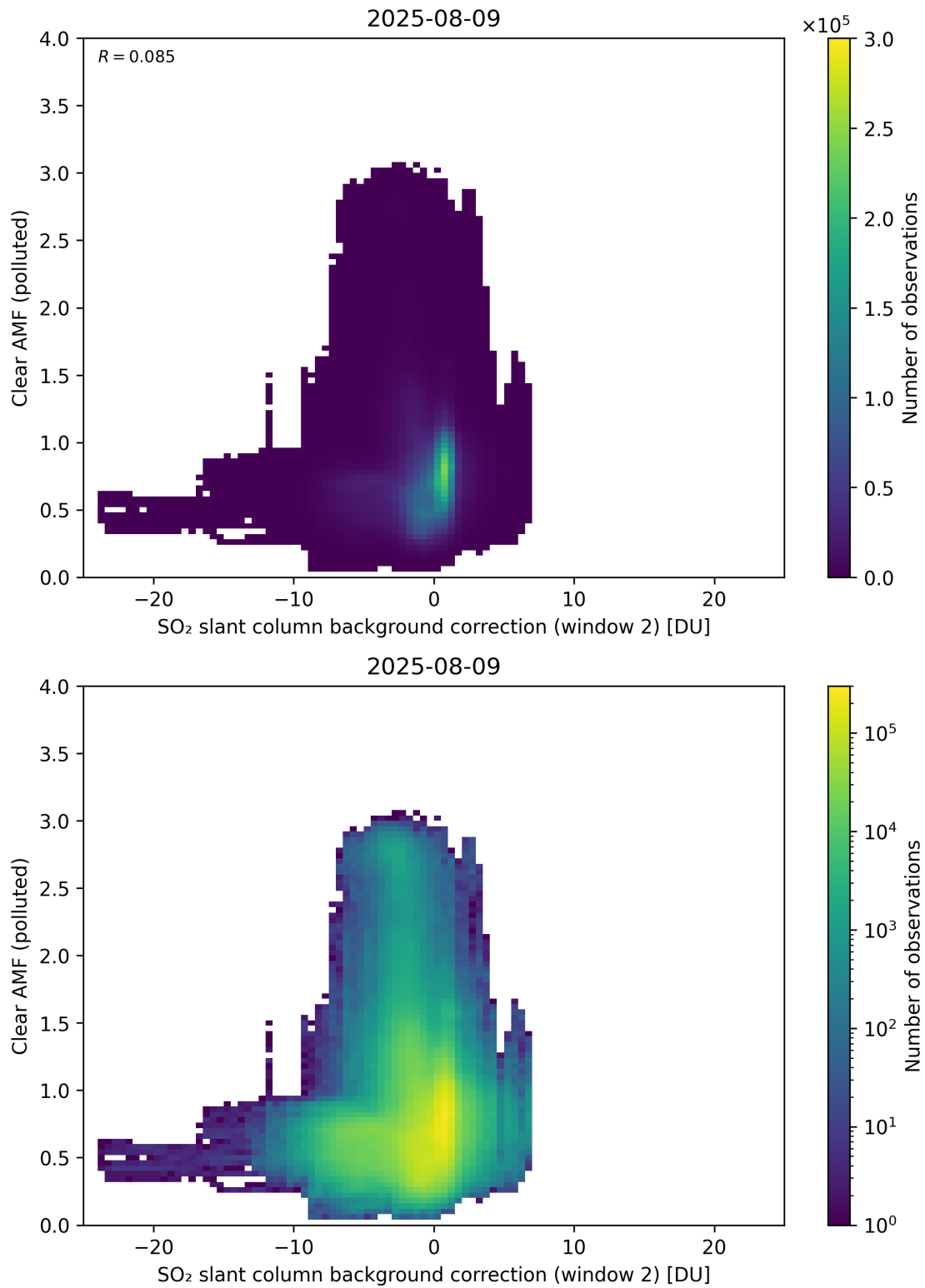
Figure 126: Scatter density plot of “SO 2 slant column background correction (window 2)” against “Clear AMF (polluted)” for 2025-08-09 to 2025-08-10.
