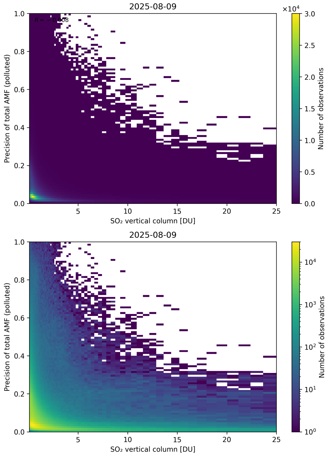
Figure 360: Scatter density plot of “SO 2 vertical column” against “Precision of total AMF (polluted)” for 2025-08-09 to 2025-08-10.
