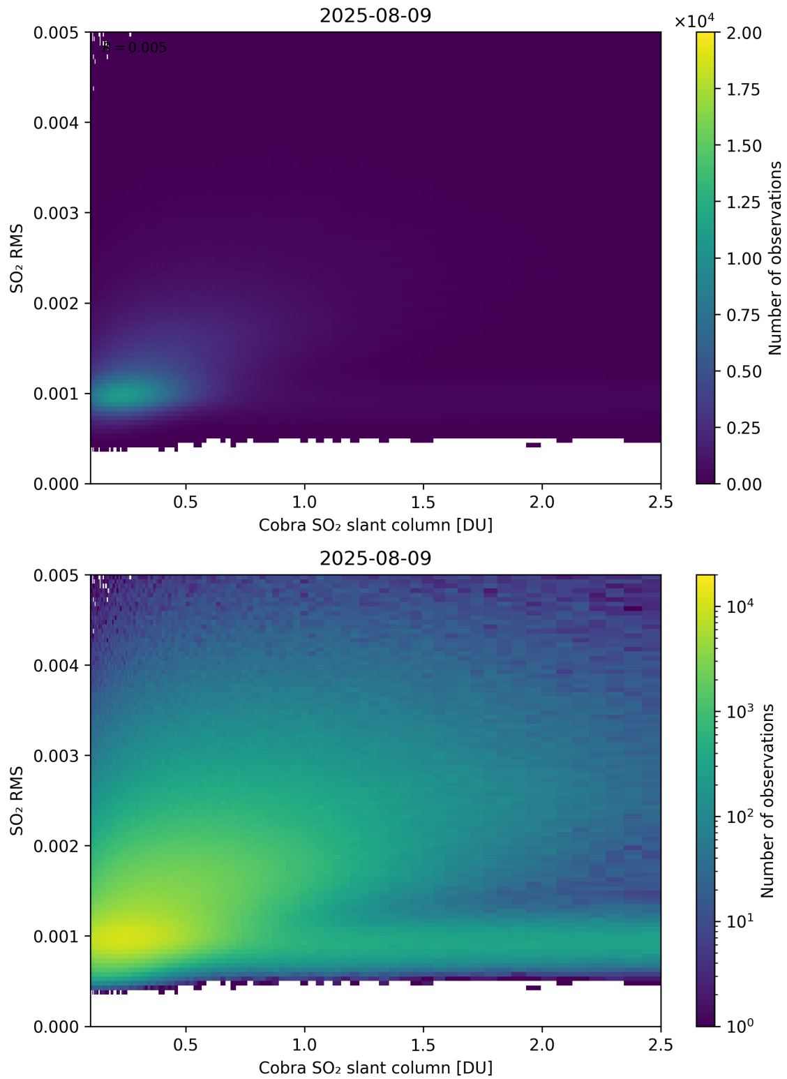
Figure 198: Scatter density plot of “Cobra SO 2 slant column” against “SO 2 RMS” for 2025-08-09 to 2025-08-10.
