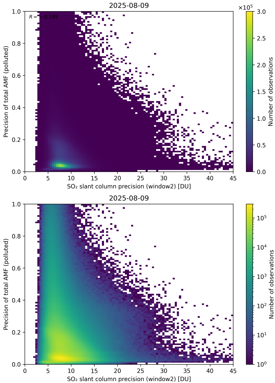
Figure 302: Scatter density plot of “SO 2 slant column precision (window2)” against “Precision of total AMF (polluted)” for 2025-08-09 to 2025-08-10.
