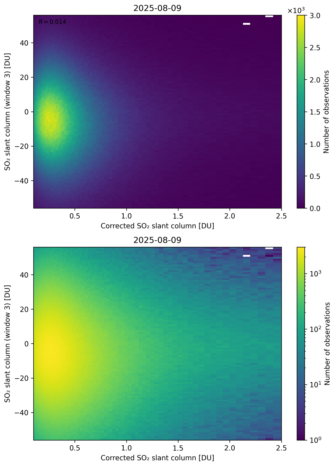
Figure 240: Scatter density plot of “Corrected SO 2 slant column” against “SO 2 slant column (window 3)” for 2025-08-09 to 2025-08-10.
