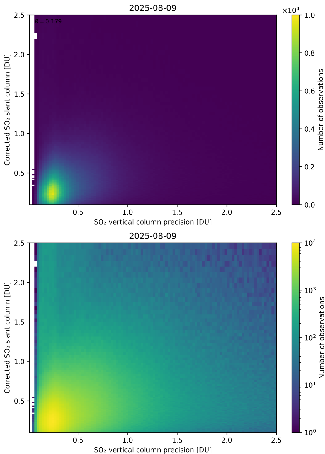
Figure 338: Scatter density plot of “SO 2 vertical column precision” against “Corrected SO 2 slant column” for 2025-08-09 to 2025-08-10.
