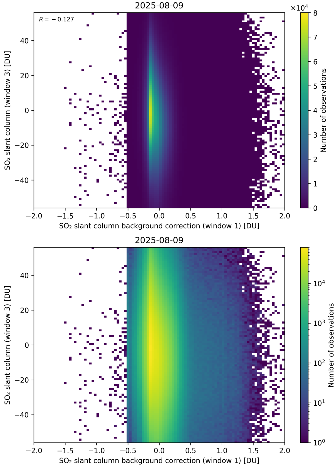
Figure 118: Scatter density plot of “SO 2 slant column background correction (window 1)” against “SO 2 slant column (window 3)” for 2025-08-09 to 2025-08-10.
