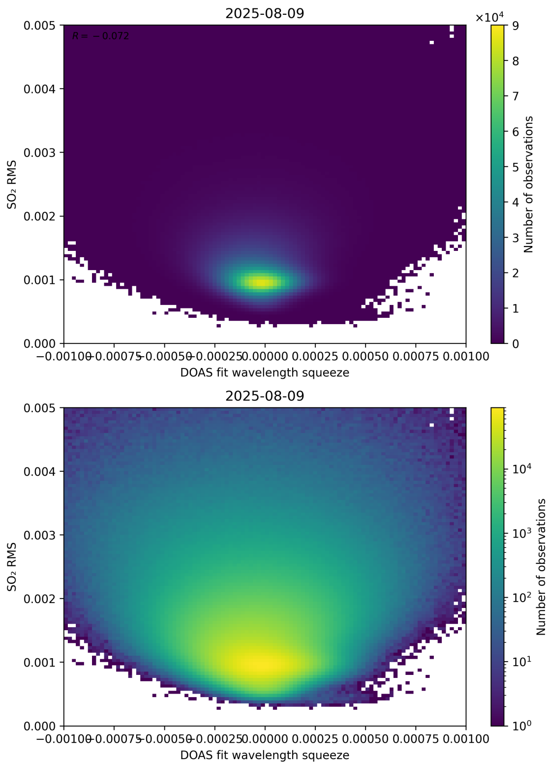
Figure 143: Scatter density plot of “DOAS fit wavelength squeeze” against “SO 2 RMS” for 2025-08-09 to 2025-08-10.
