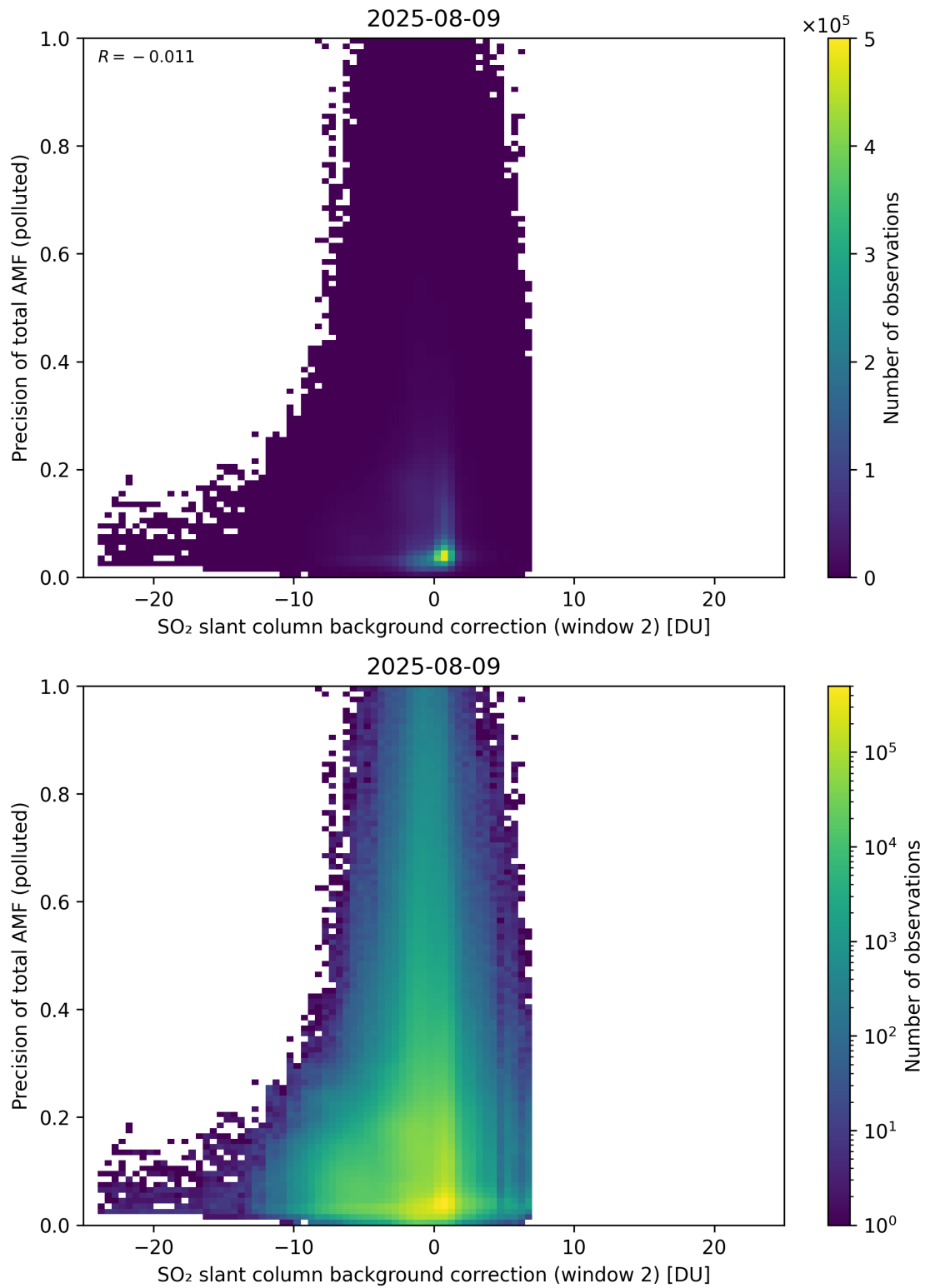
Figure 131: Scatter density plot of “SO 2 slant column background correction (window 2)” against “Precision of total AMF (polluted)” for 2025-08-09 to 2025-08-10.
