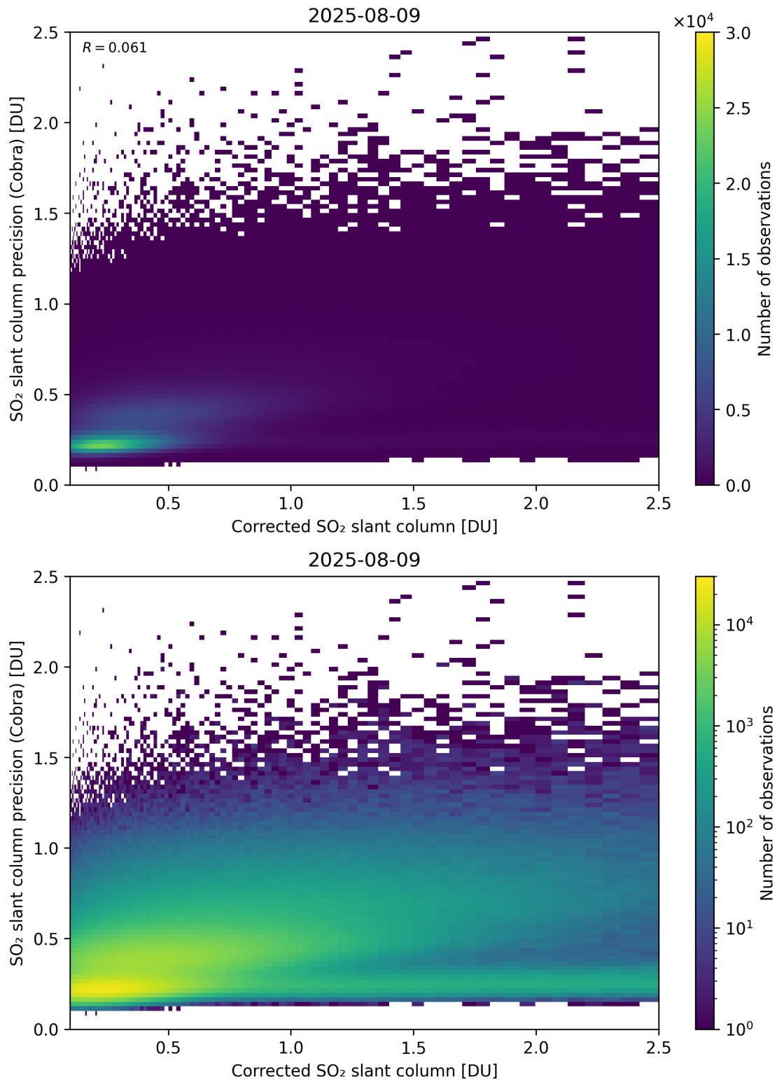
Figure 234: Scatter density plot of “Corrected SO 2 slant column” against “SO 2 slant column precision (Cobra)” for 2025-08-09 to 2025-08-10.
