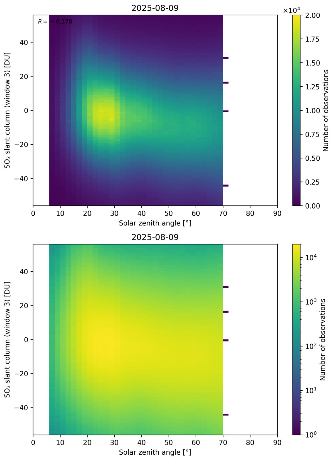
Figure 187: Scatter density plot of “Solar zenith angle” against “SO 2 slant column (window 3)” for 2025-08-09 to 2025-08-10.
