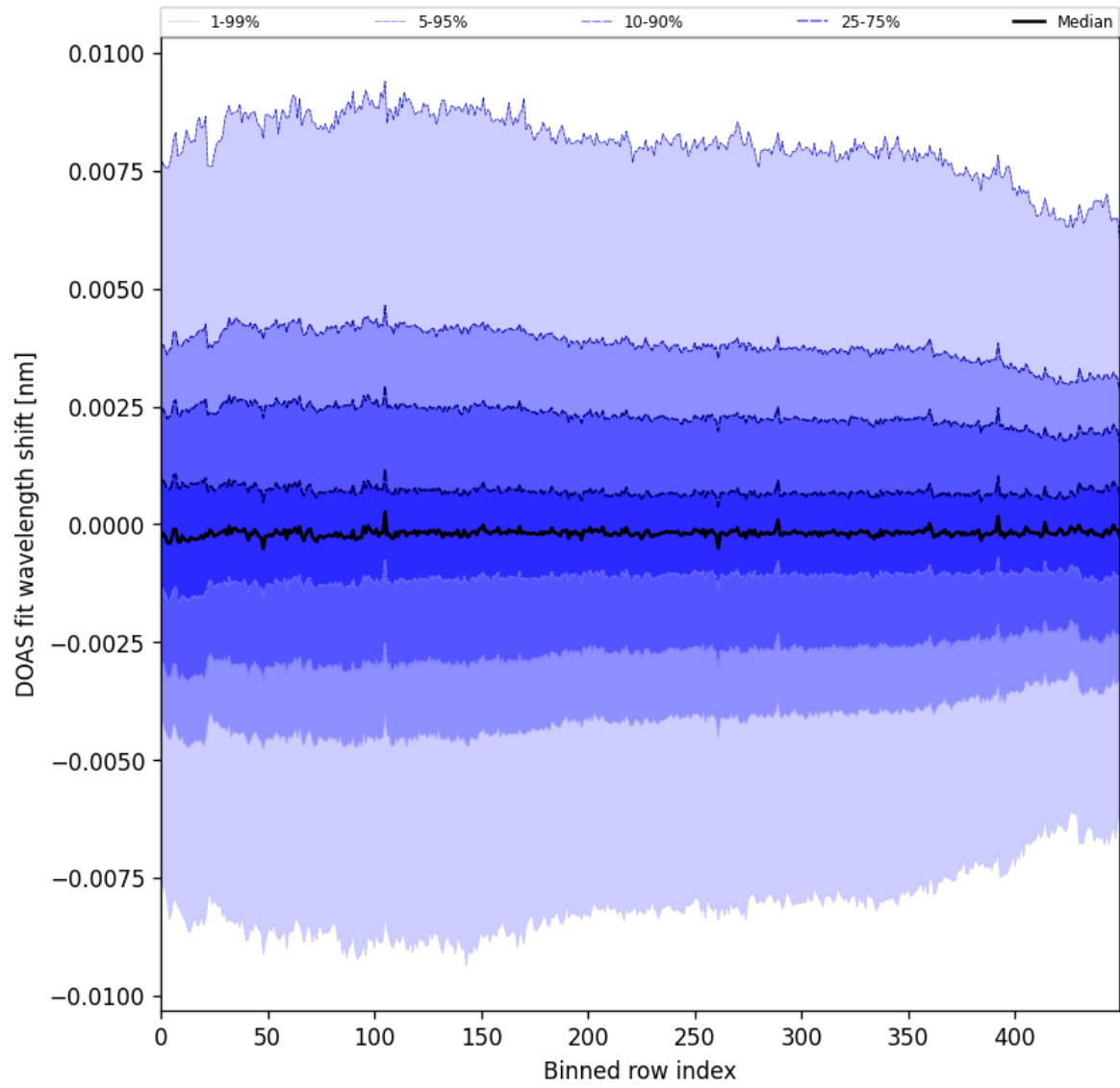
Figure 102: Along track statistics of “DOAS fit wavelength shift” for 2025-08-09 to 2025-08-10
