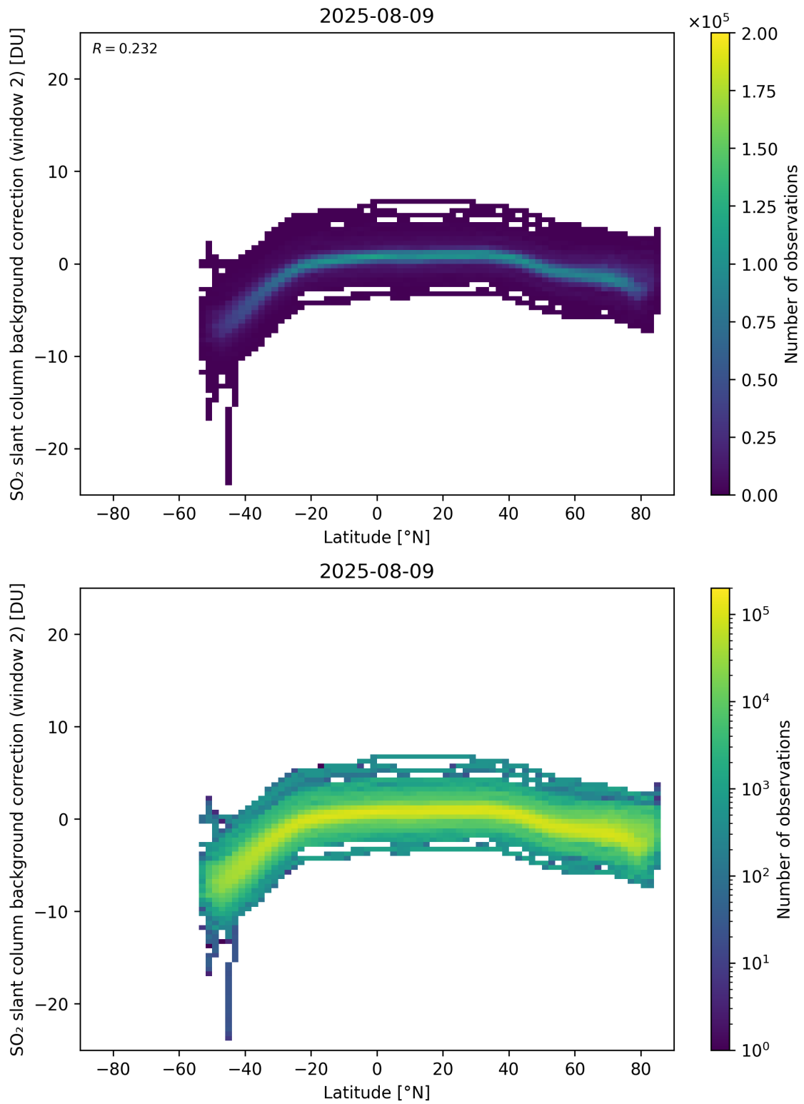
Figure 151: Scatter density plot of “Latitude” against “SO 2 slant column background correction (window 2)” for 2025-08-09 to 2025-08-10.
