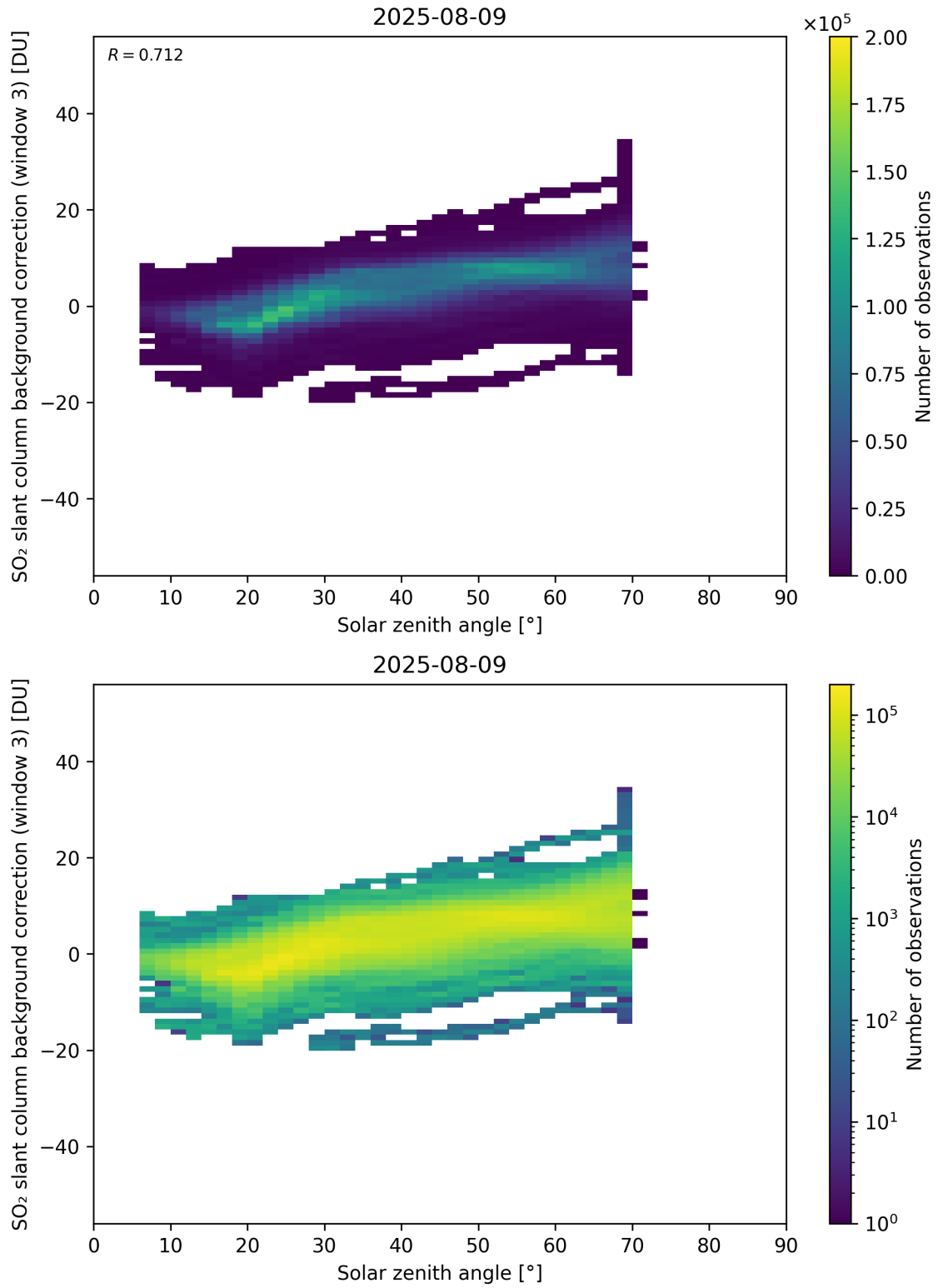
Figure 173: Scatter density plot of “Solar zenith angle” against “SO 2 slant column background correction (window 3)” for 2025-08-09 to 2025-08-10.
