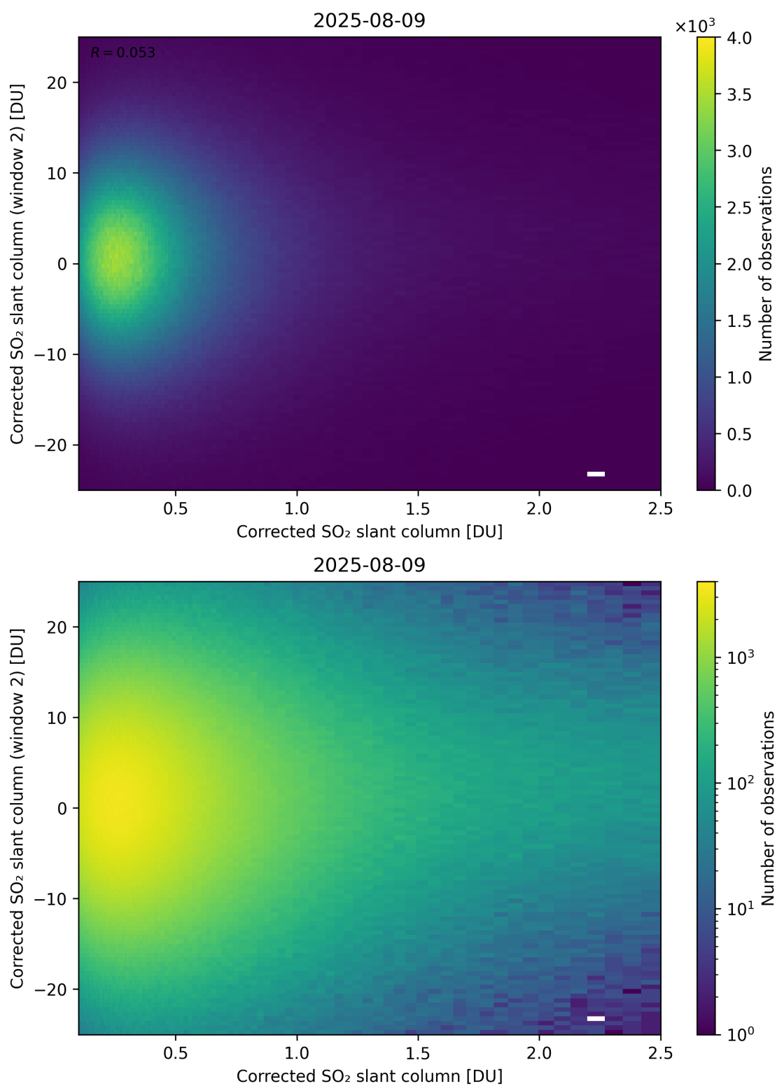
Figure 235: Scatter density plot of “Corrected SO 2 slant column” against “Corrected SO 2 slant column (window 2)” for 2025-08-09 to 2025-08-10.
