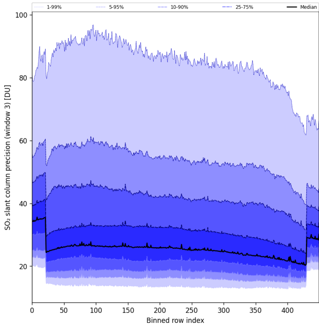
Figure 98: Along track statistics of “SO 2 slant column precision (window 3)” for 2025-08-09 to 2025-08-10
