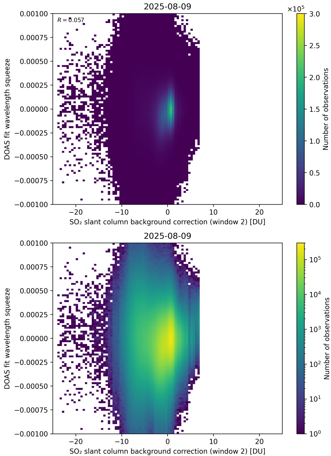
Figure 124: Scatter density plot of “SO 2 slant column background correction (window 2)” against “DOAS fit wavelength squeeze” for 2025-08-09 to 2025-08-10.
