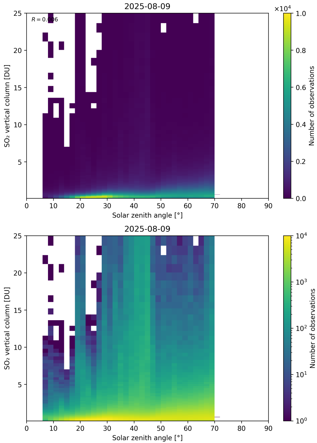
Figure 191: Scatter density plot of “Solar zenith angle” against “SO 2 vertical column” for 2025-08-09 to 2025-08-10.
