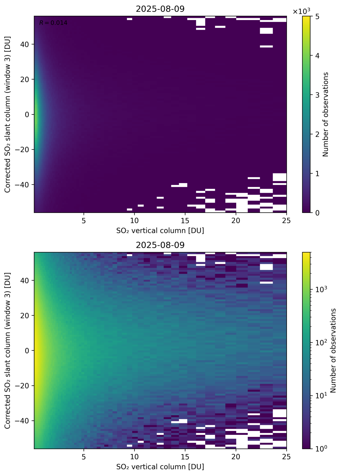
Figure 353: Scatter density plot of “SO 2 vertical column” against “Corrected SO 2 slant column (window 3)” for 2025-08-09 to 2025-08-10.
