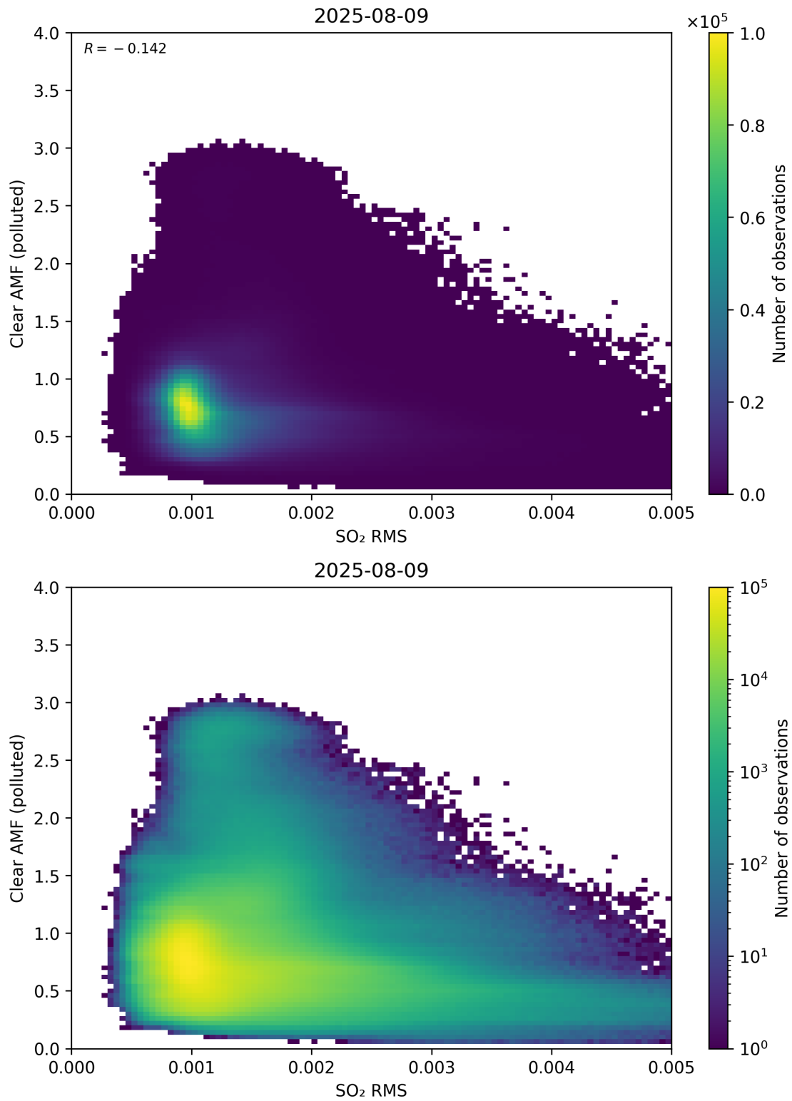
Figure 147: Scatter density plot of “SO 2 RMS” against “Clear AMF (polluted)” for 2025-08-09 to 2025-08-10.
