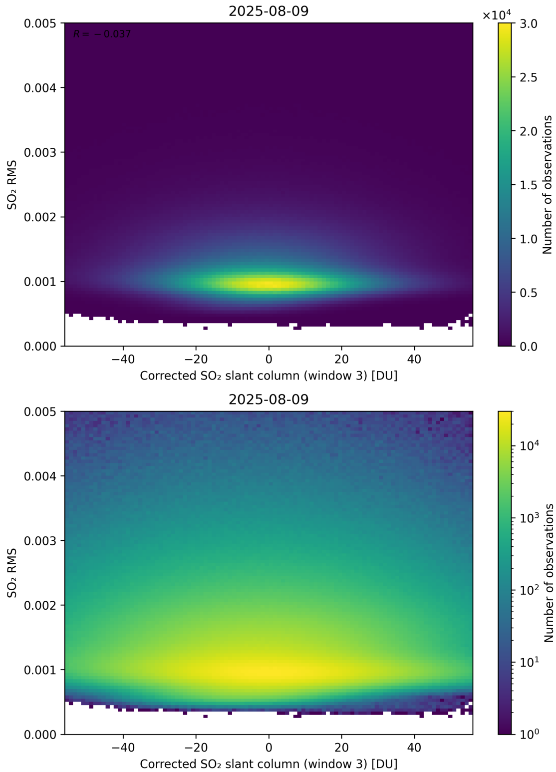
Figure 258: Scatter density plot of “Corrected SO 2 slant column (window 3)” against “SO 2 RMS” for 2025-08-09 to 2025-08-10.
