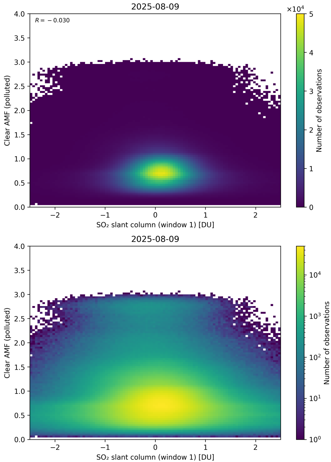
Figure 282: Scatter density plot of “SO 2 slant column (window 1)” against “Clear AMF (polluted)” for 2025-08-09 to 2025-08-10.
