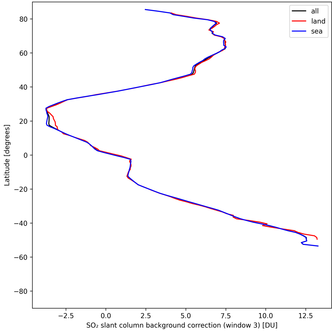
Figure 48: Zonal average of “SO 2 slant column background correction (window 3)” for 2025-08-09 to 2025-08-10.
