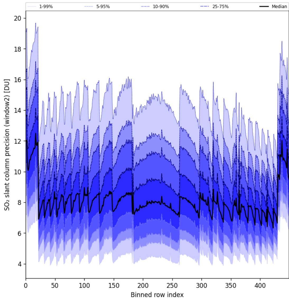
Figure 94: Along track statistics of “SO 2 slant column precision (window2)” for 2025-08-09 to 2025-08-10
