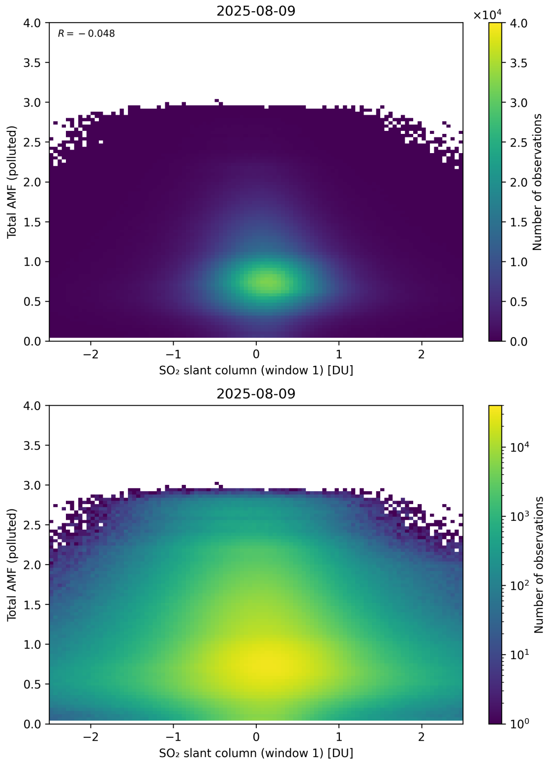
Figure 289: Scatter density plot of “SO 2 slant column (window 1)” against “Total AMF (polluted)” for 2025-08-09 to 2025-08-10.
