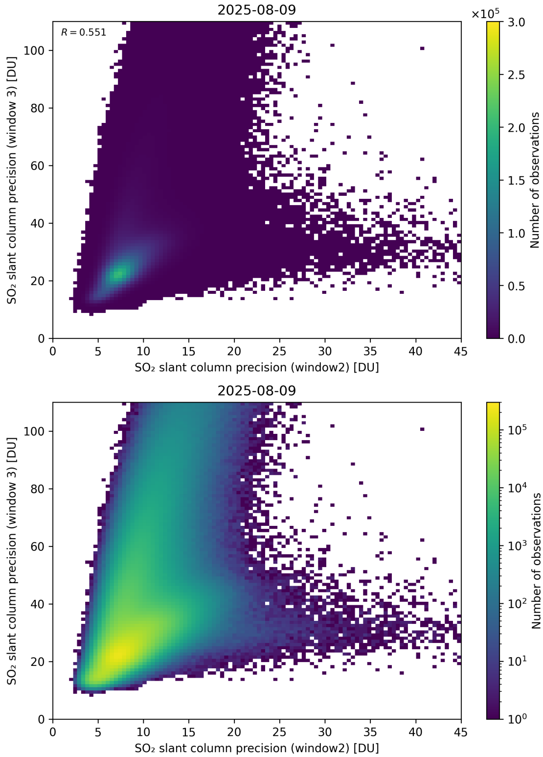
Figure 300: Scatter density plot of “SO 2 slant column precision (window2)” against “SO 2 slant column precision (window 3)” for 2025-08-09 to 2025-08-10.
