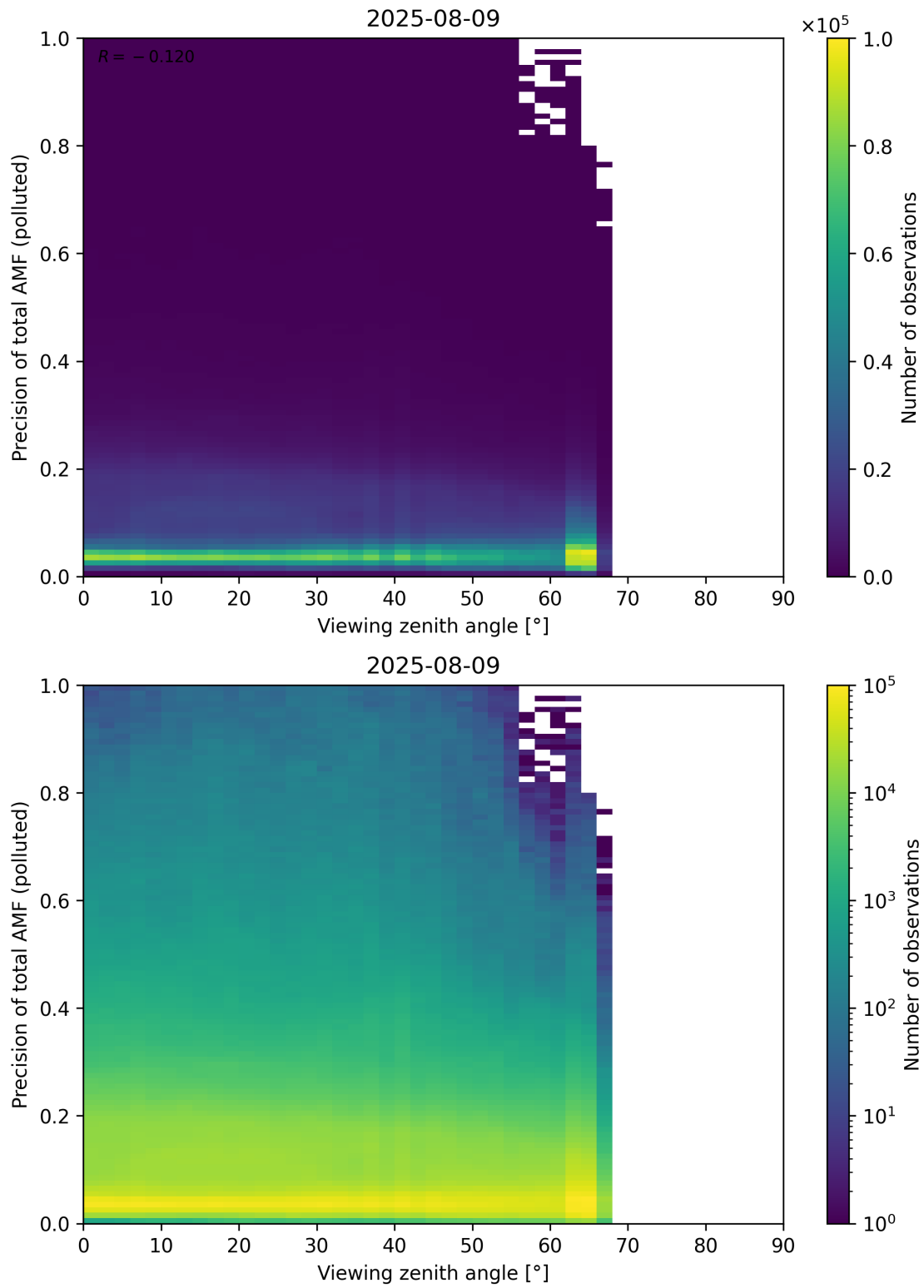
Figure 382: Scatter density plot of “Viewing zenith angle” against “Precision of total AMF (polluted)” for 2025-08-09 to 2025-08-10.
