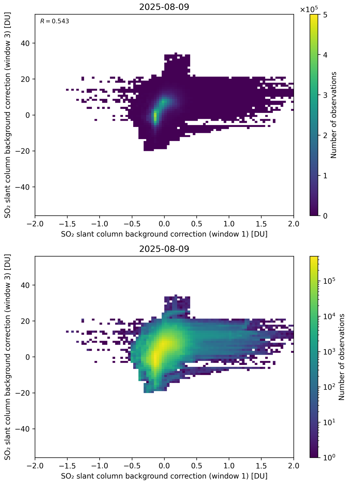
Figure 110: Scatter density plot of “SO 2 slant column background correction (window 1)” against “SO 2 slant column background correction (window 3)” for 2025-08-09 to 2025-08-10.
