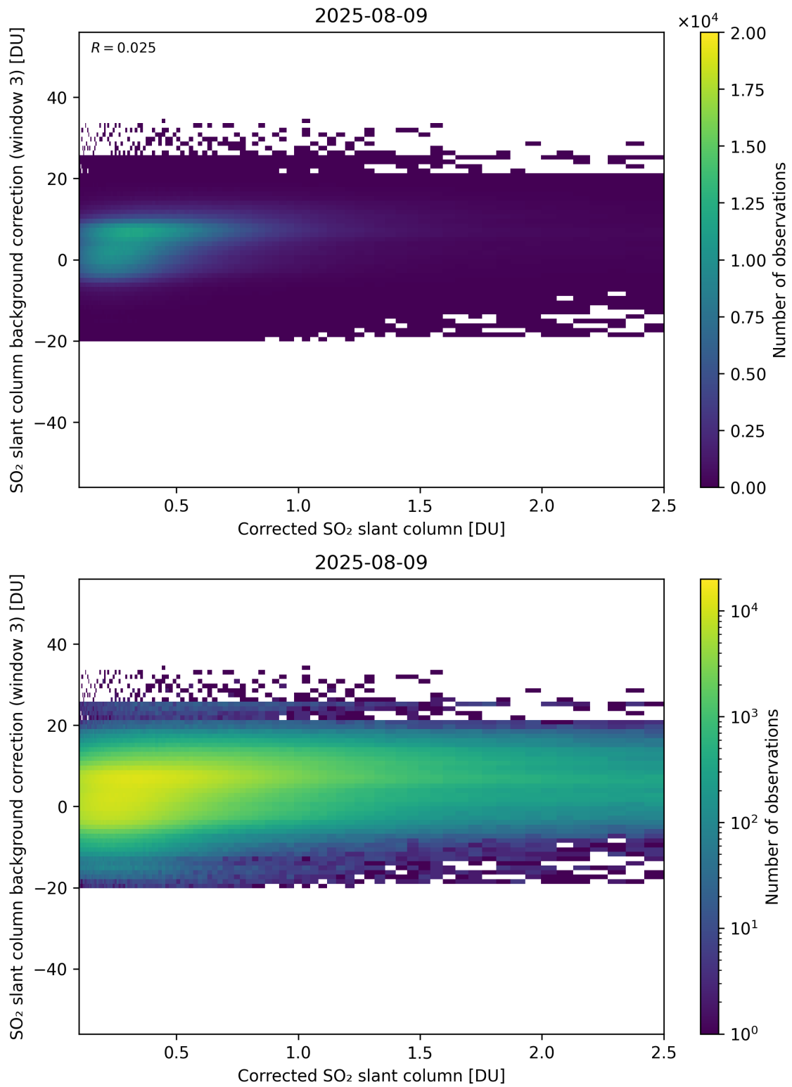
Figure 228: Scatter density plot of “Corrected SO 2 slant column” against “SO 2 slant column background correction (window 3)” for 2025-08-09 to 2025-08-10.
