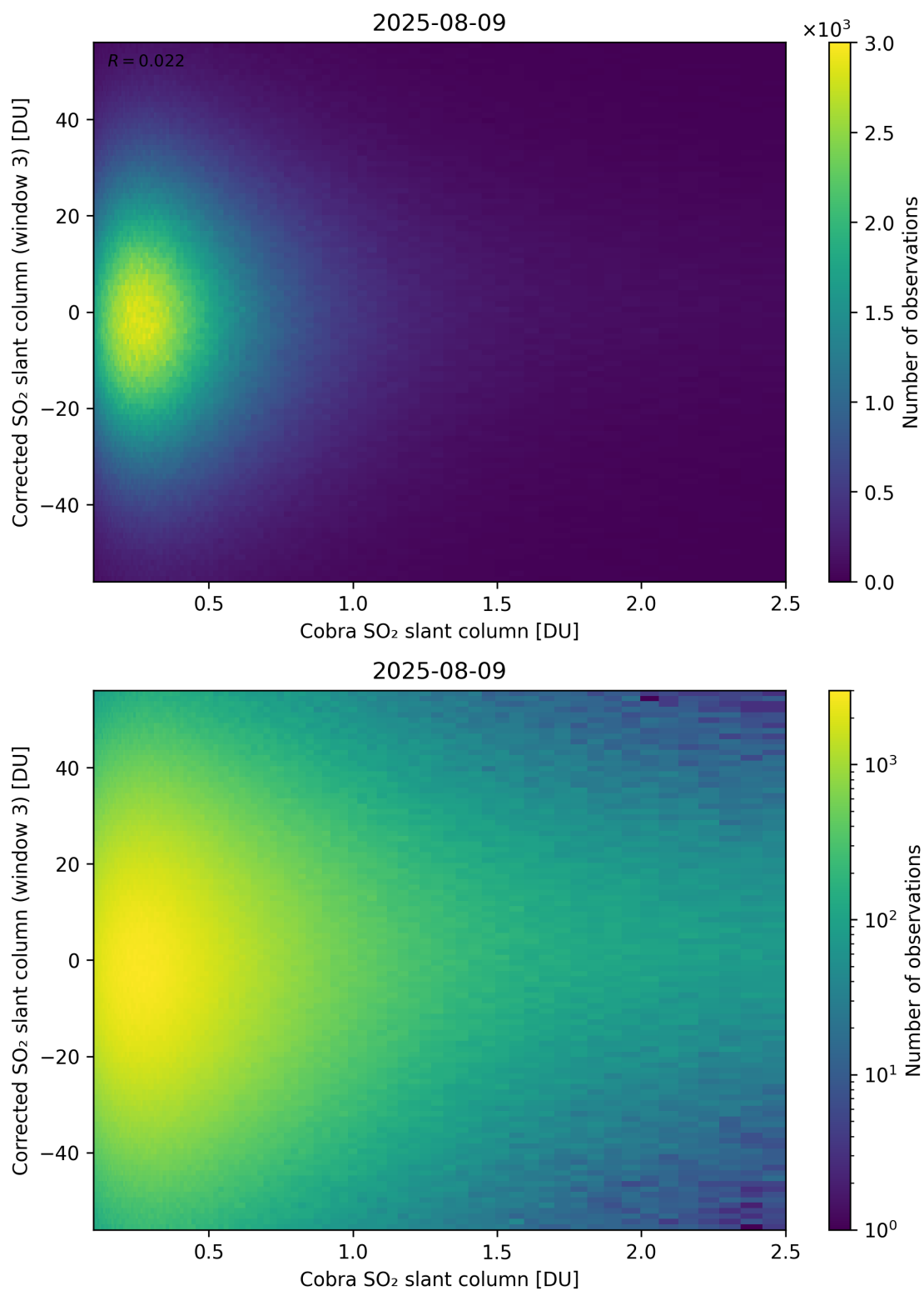
Figure 218: Scatter density plot of “Cobra SO 2 slant column” against “Corrected SO 2 slant column (window 3)” for 2025-08-09 to 2025-08-10.
