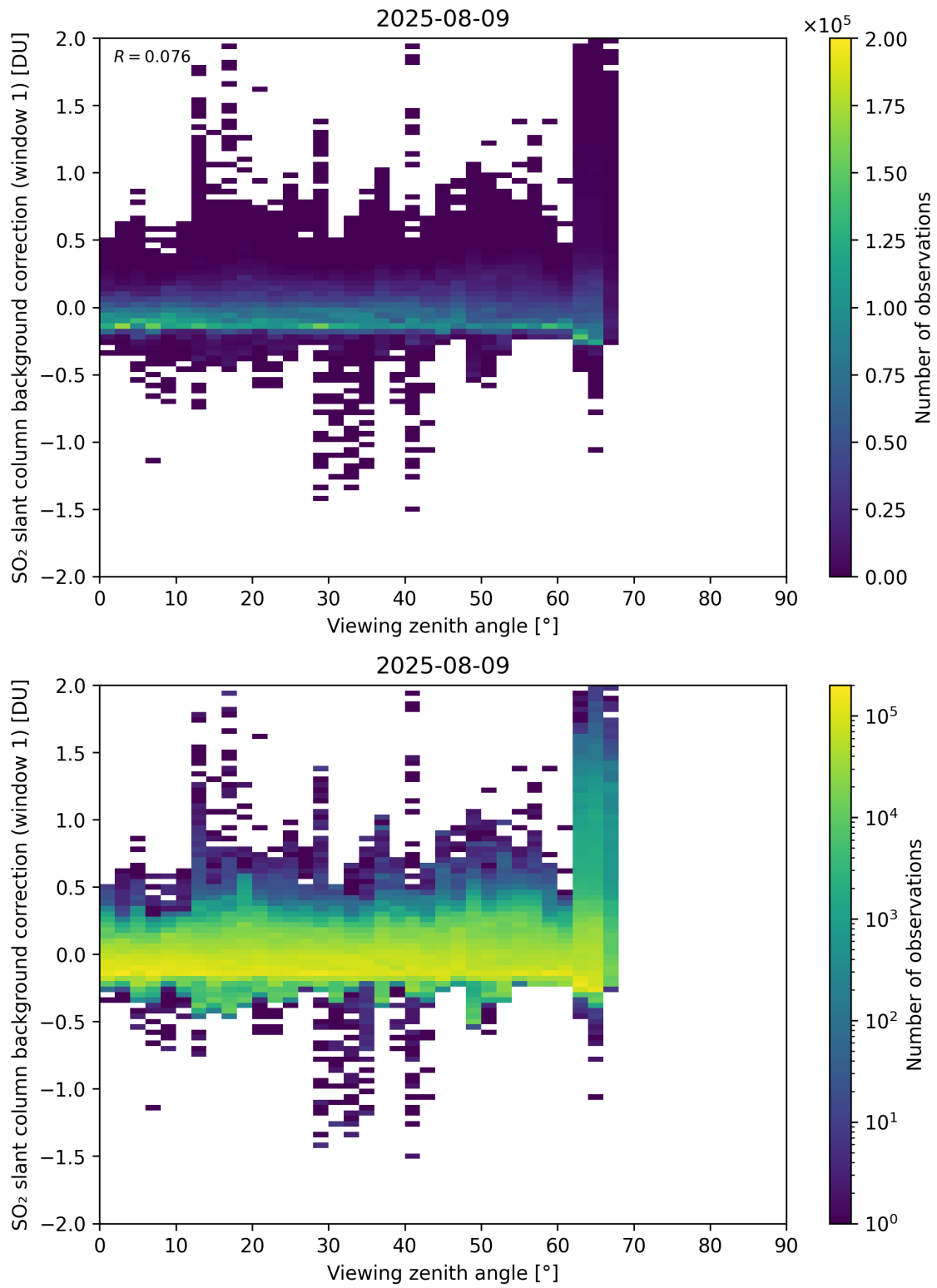
Figure 362: Scatter density plot of “Viewing zenith angle” against “SO 2 slant column background correction (window 1)” for 2025-08-09 to 2025-08-10.
