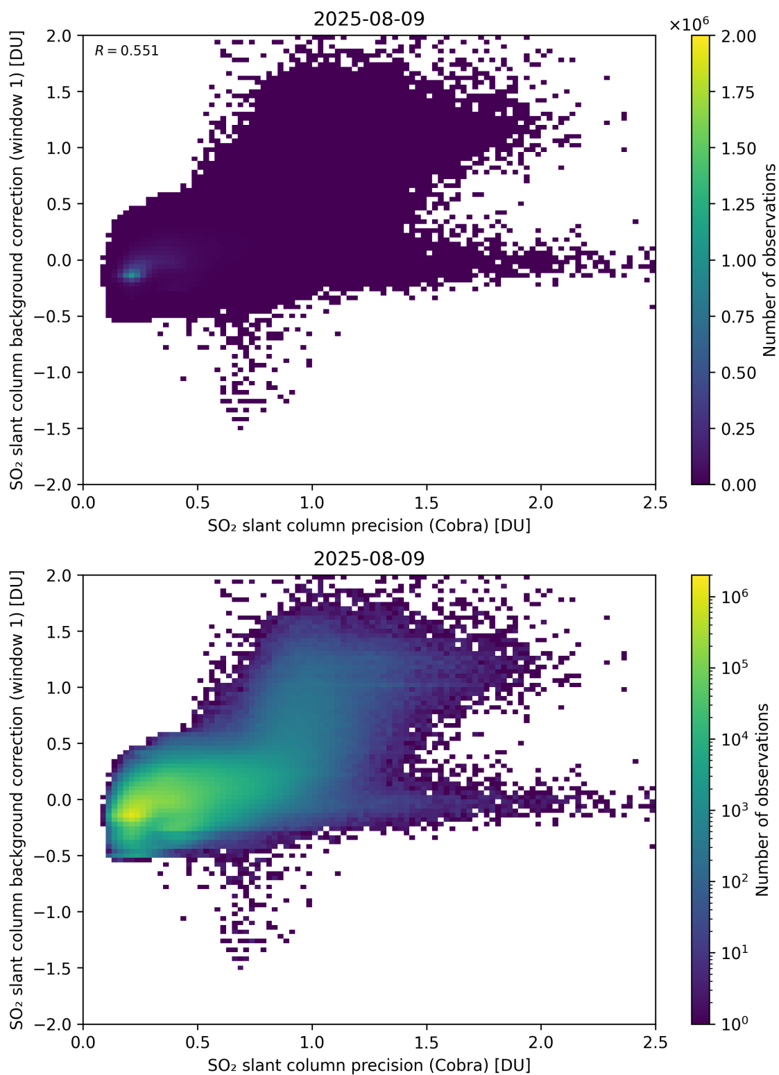
Figure 199: Scatter density plot of “SO 2 slant column precision (Cobra)” against “SO 2 slant column background correction (window 1)” for 2025-08-09 to 2025-08-10.
