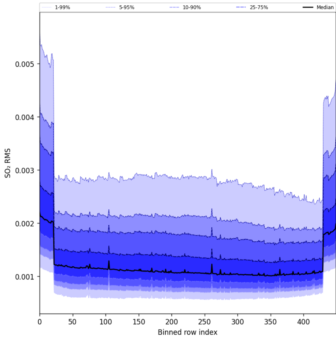
Figure 104: Along track statistics of “SO 2 RMS” for 2025-08-09 to 2025-08-10
