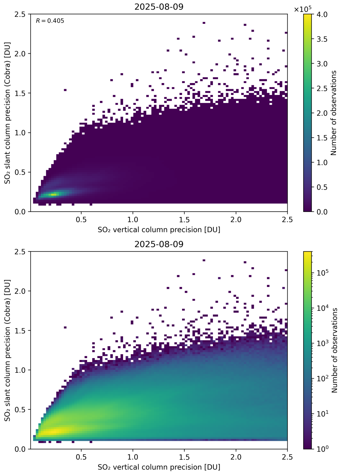
Figure 337: Scatter density plot of “SO 2 vertical column precision” against “SO 2 slant column precision (Cobra)” for 2025-08-09 to 2025-08-10.
