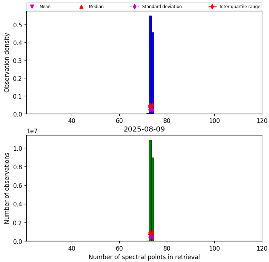
Figure 82: Histogram of “Number of spectral points in retrieval” for 2025-08-09 to 2025-08-10
