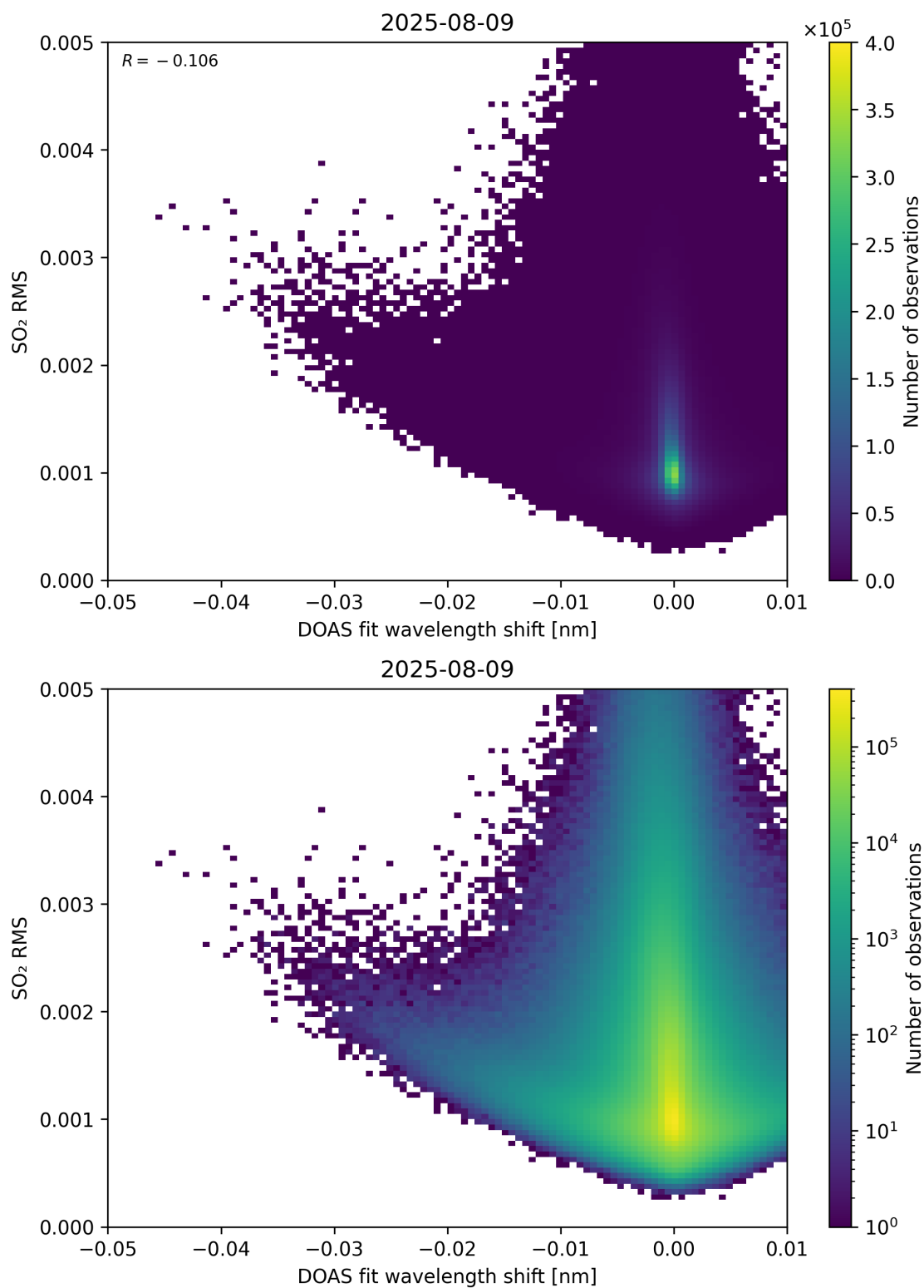
Figure 139: Scatter density plot of “DOAS fit wavelength shift” against “SO 2 RMS” for 2025-08-09 to 2025-08-10.
