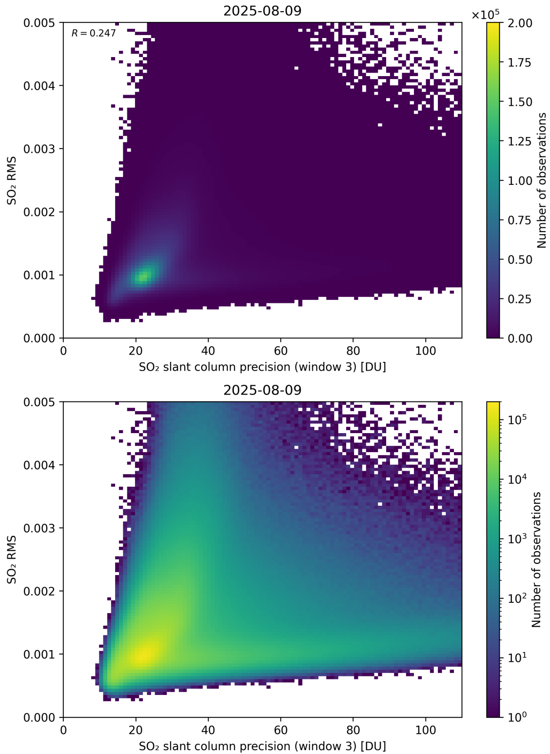
Figure 310: Scatter density plot of “SO 2 slant column precision (window 3)” against “SO 2 RMS” for 2025-08-09 to 2025-08-10.
