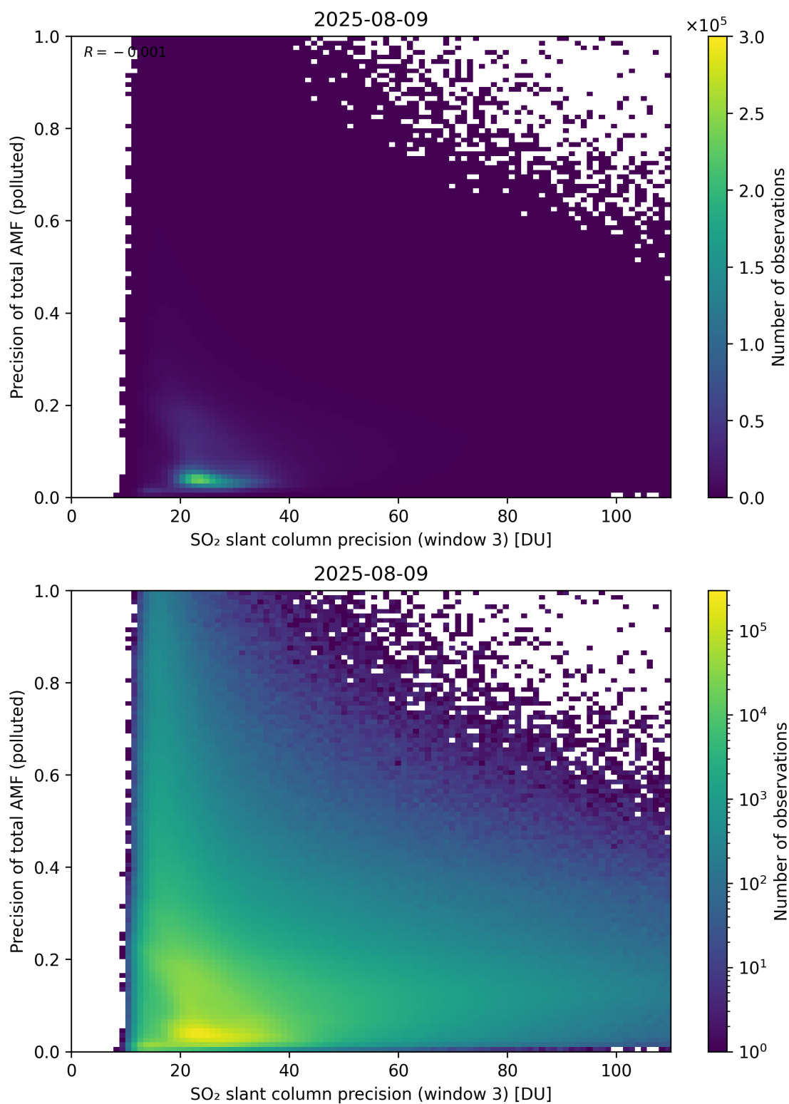
Figure 314: Scatter density plot of “SO 2 slant column precision (window 3)” against “Precision of total AMF (polluted)” for 2025-08-09 to 2025-08-10.
