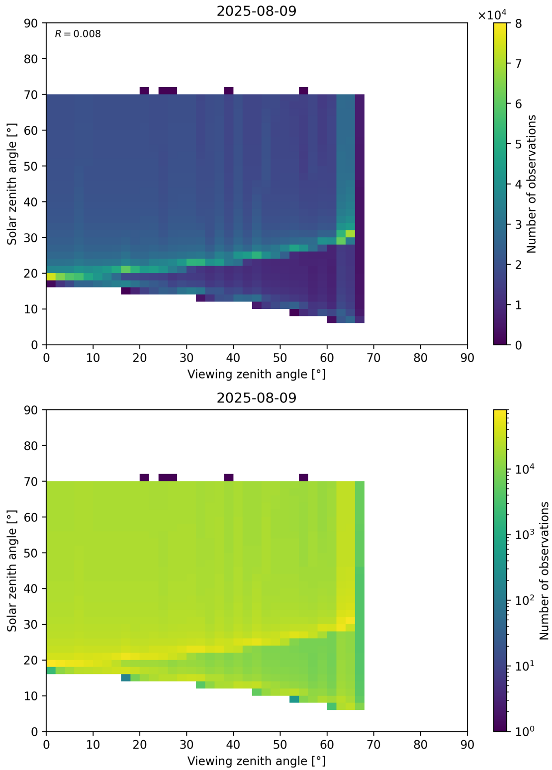
Figure 369: Scatter density plot of “Viewing zenith angle” against “Solar zenith angle” for 2025-08-09 to 2025-08-10.
