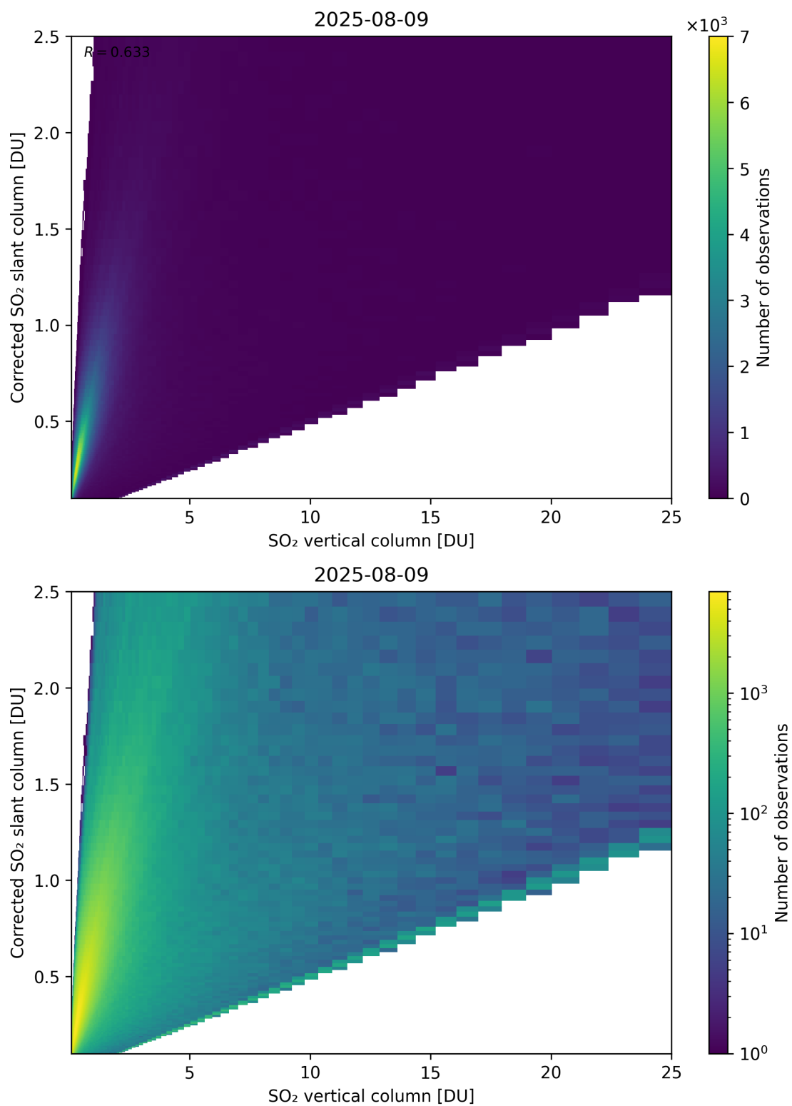
Figure 351: Scatter density plot of “SO 2 vertical column” against “Corrected SO 2 slant column” for 2025-08-09 to 2025-08-10.
