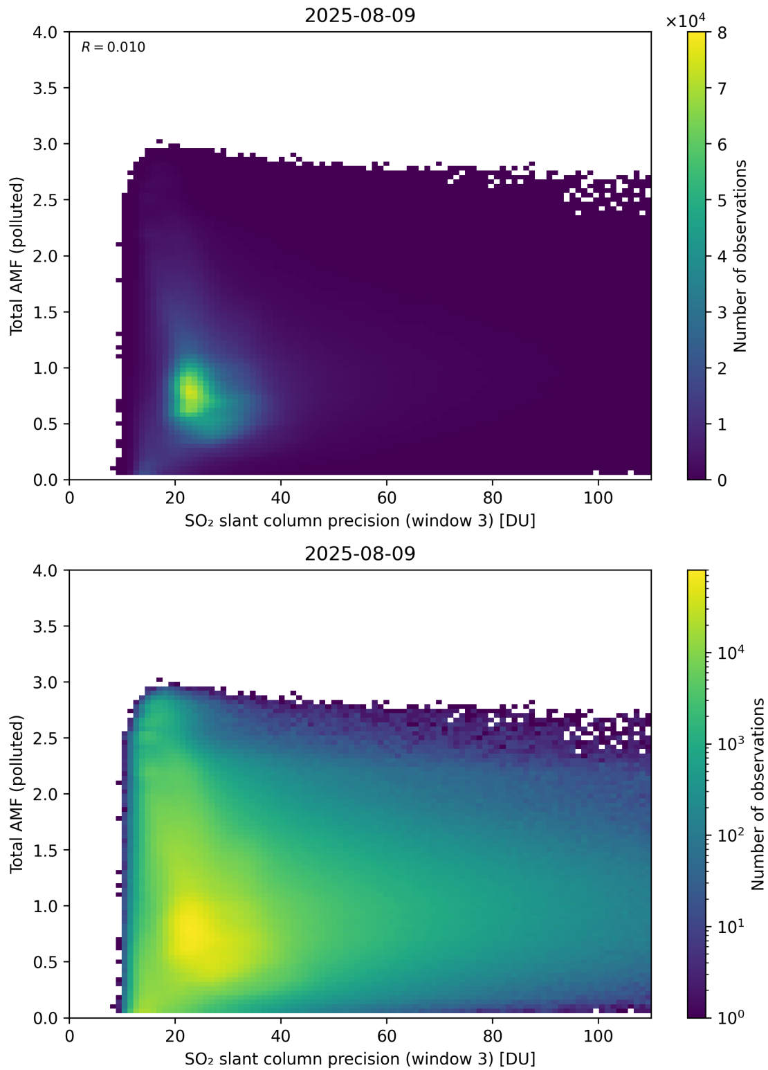
Figure 313: Scatter density plot of “SO 2 slant column precision (window 3)” against “Total AMF (polluted)” for 2025-08-09 to 2025-08-10.
