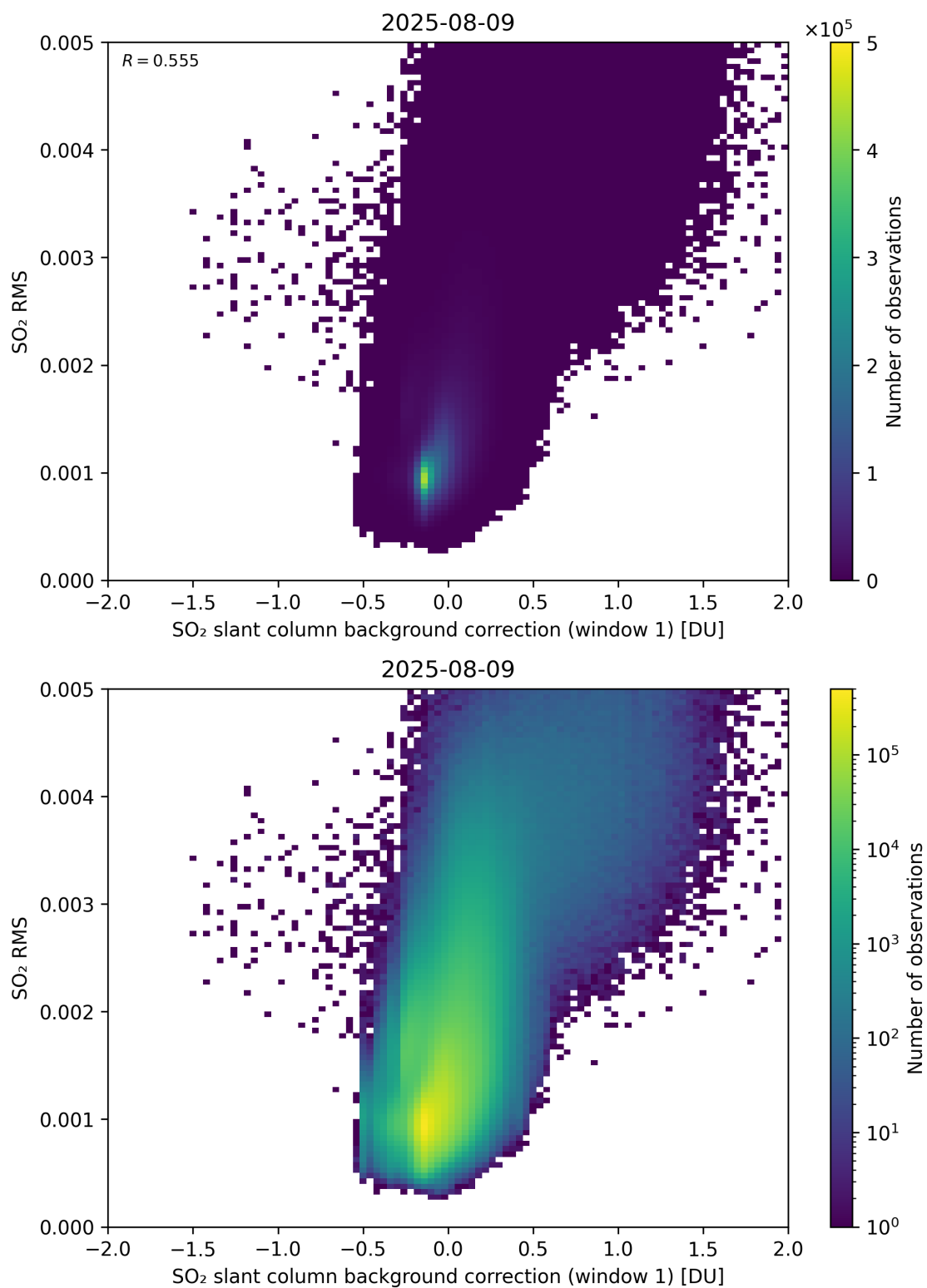
Figure 113: Scatter density plot of “SO 2 slant column background correction (window 1)” against “SO 2 RMS” for 2025-08-09 to 2025-08-10.
