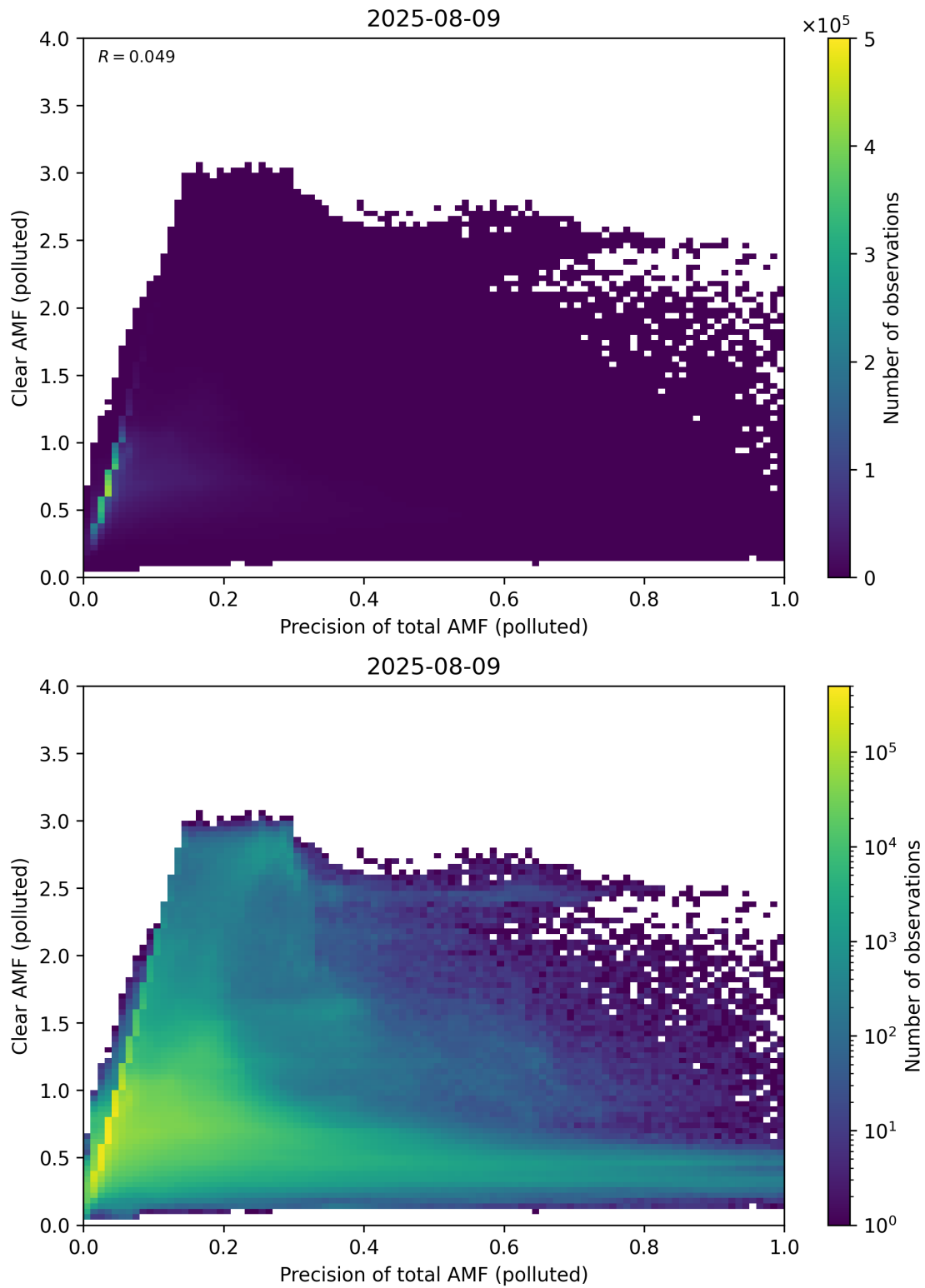
Figure 320: Scatter density plot of “Precision of total AMF (polluted)” against “Clear AMF (polluted)” for 2025-08-09 to 2025-08-10.
