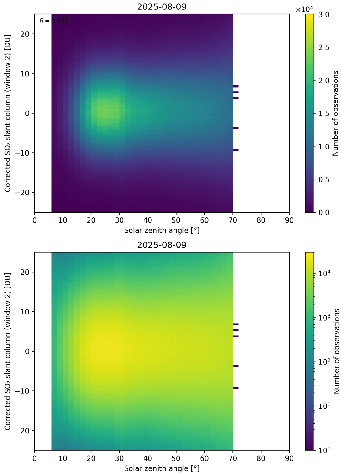
Figure 182: Scatter density plot of “Solar zenith angle” against “Corrected SO 2 slant column (window 2)” for 2025-08-09 to 2025-08-10.
