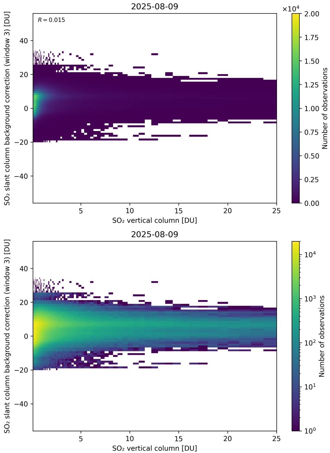
Figure 325: Scatter density plot of “SO 2 vertical column” against “SO 2 slant column background correction (window 3)” for 2025-08-09 to 2025-08-10.
