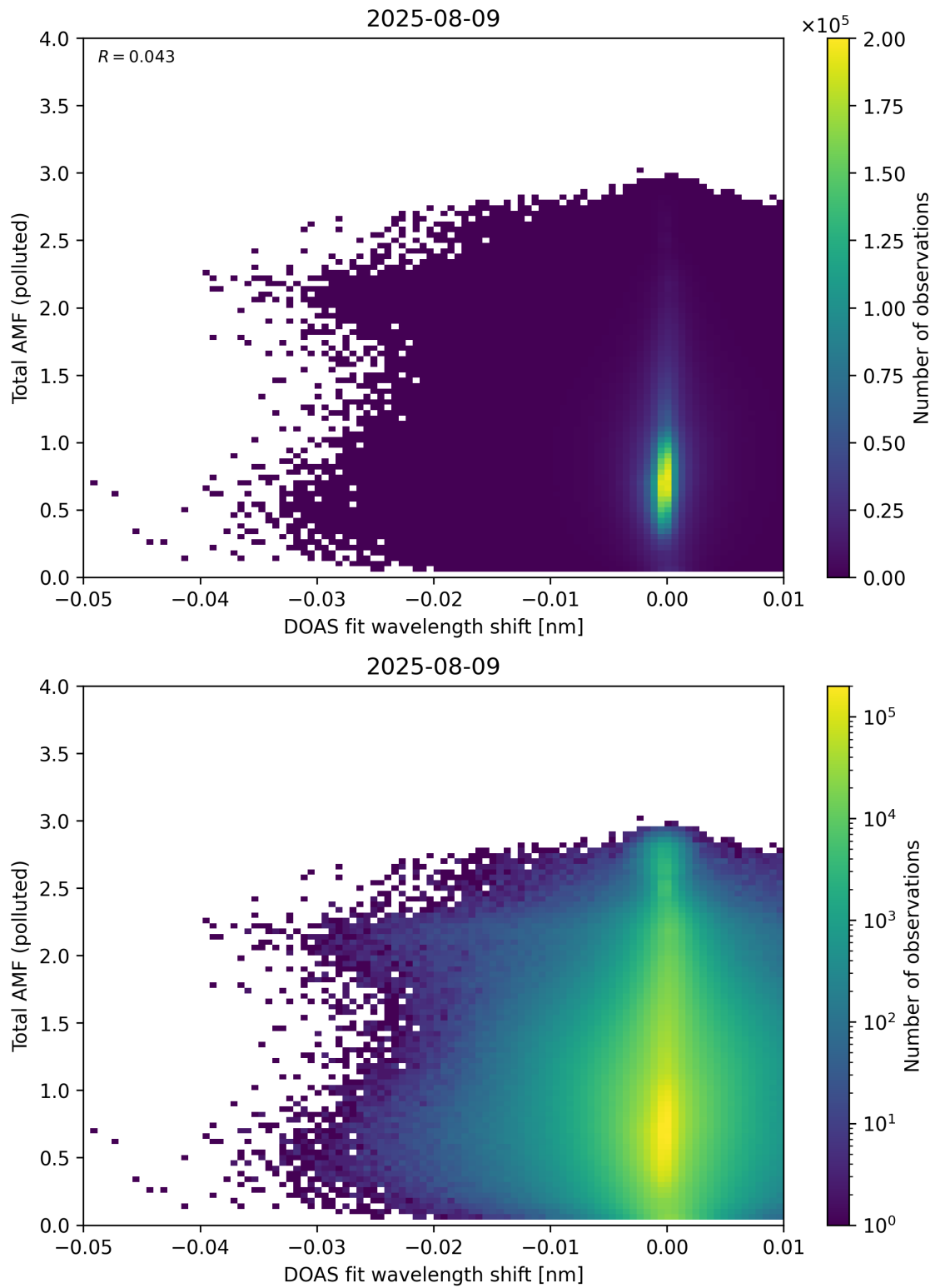
Figure 141: Scatter density plot of “DOAS fit wavelength shift” against “Total AMF (polluted)” for 2025-08-09 to 2025-08-10.
