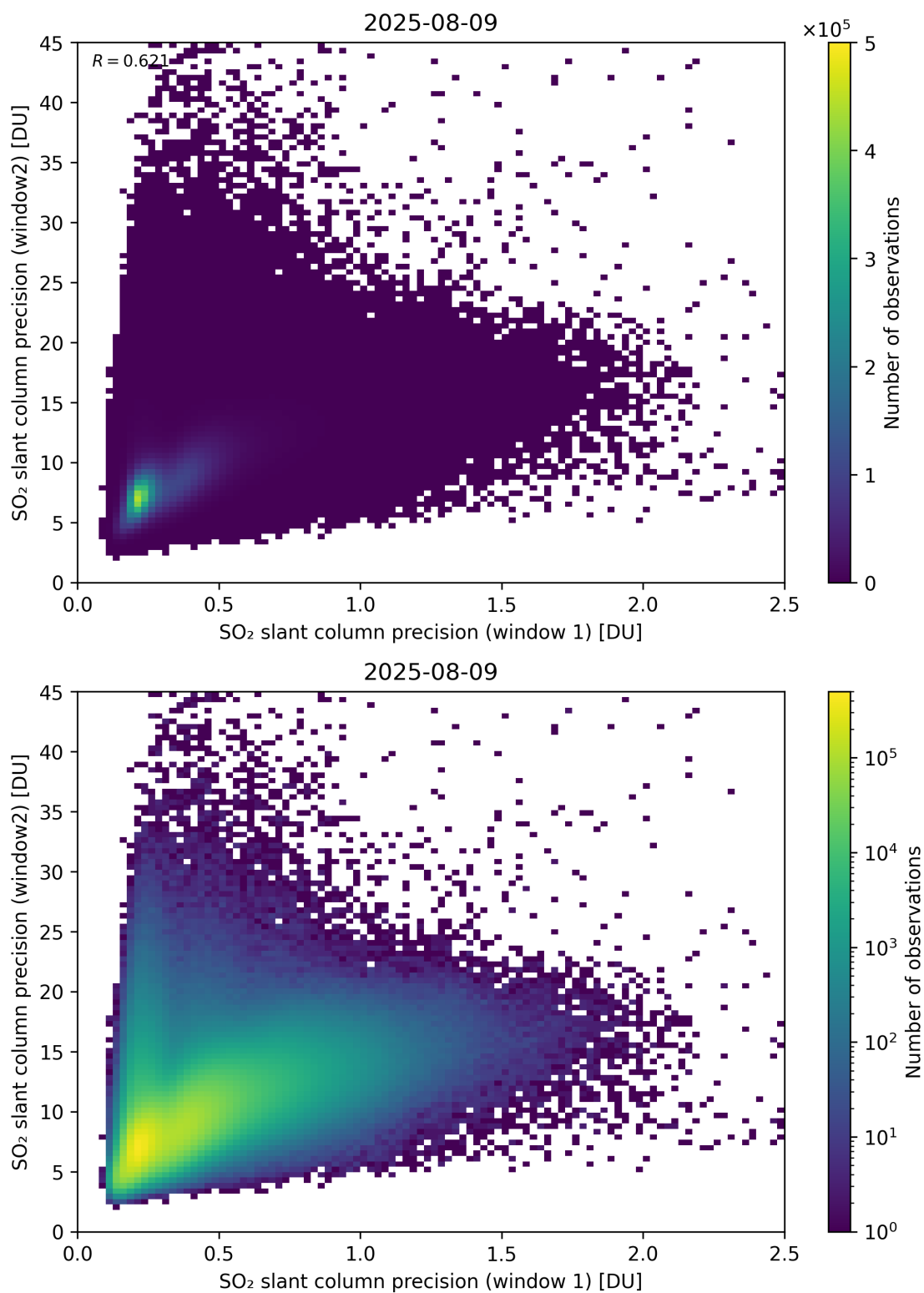
Figure 277: Scatter density plot of “SO 2 slant column precision (window 1)” against “SO 2 slant column precision (window2)” for 2025-08-09 to 2025-08-10.
