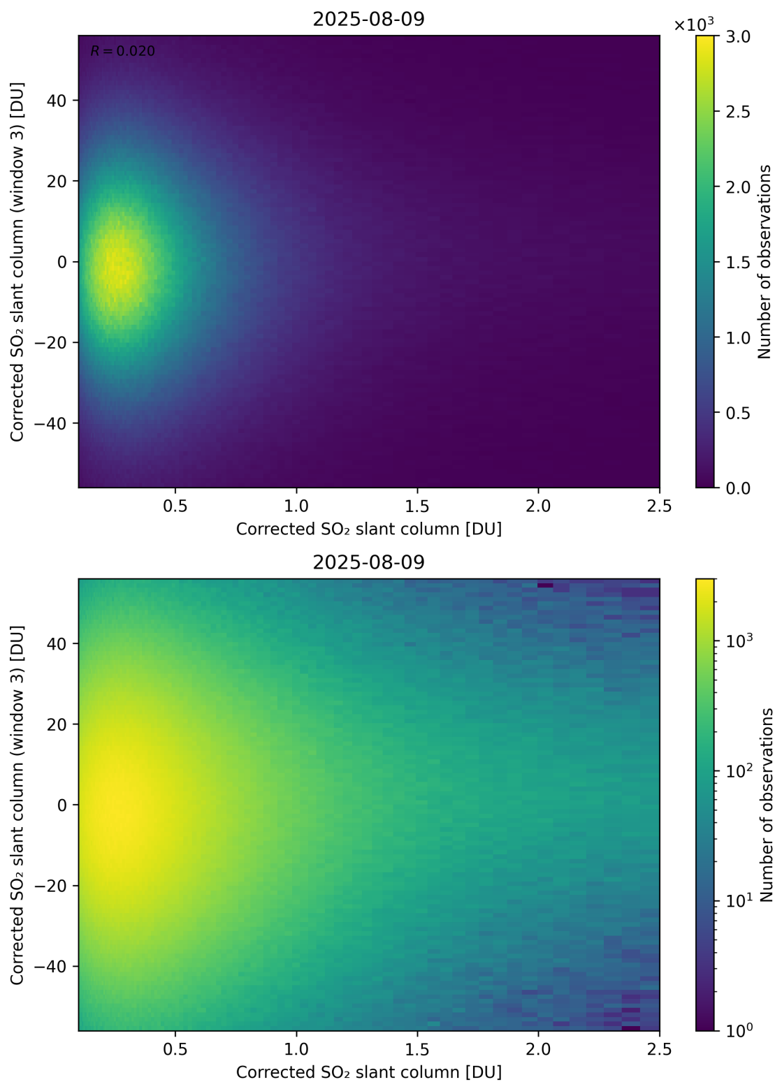
Figure 236: Scatter density plot of “Corrected SO 2 slant column” against “Corrected SO 2 slant column (window 3)” for 2025-08-09 to 2025-08-10.
