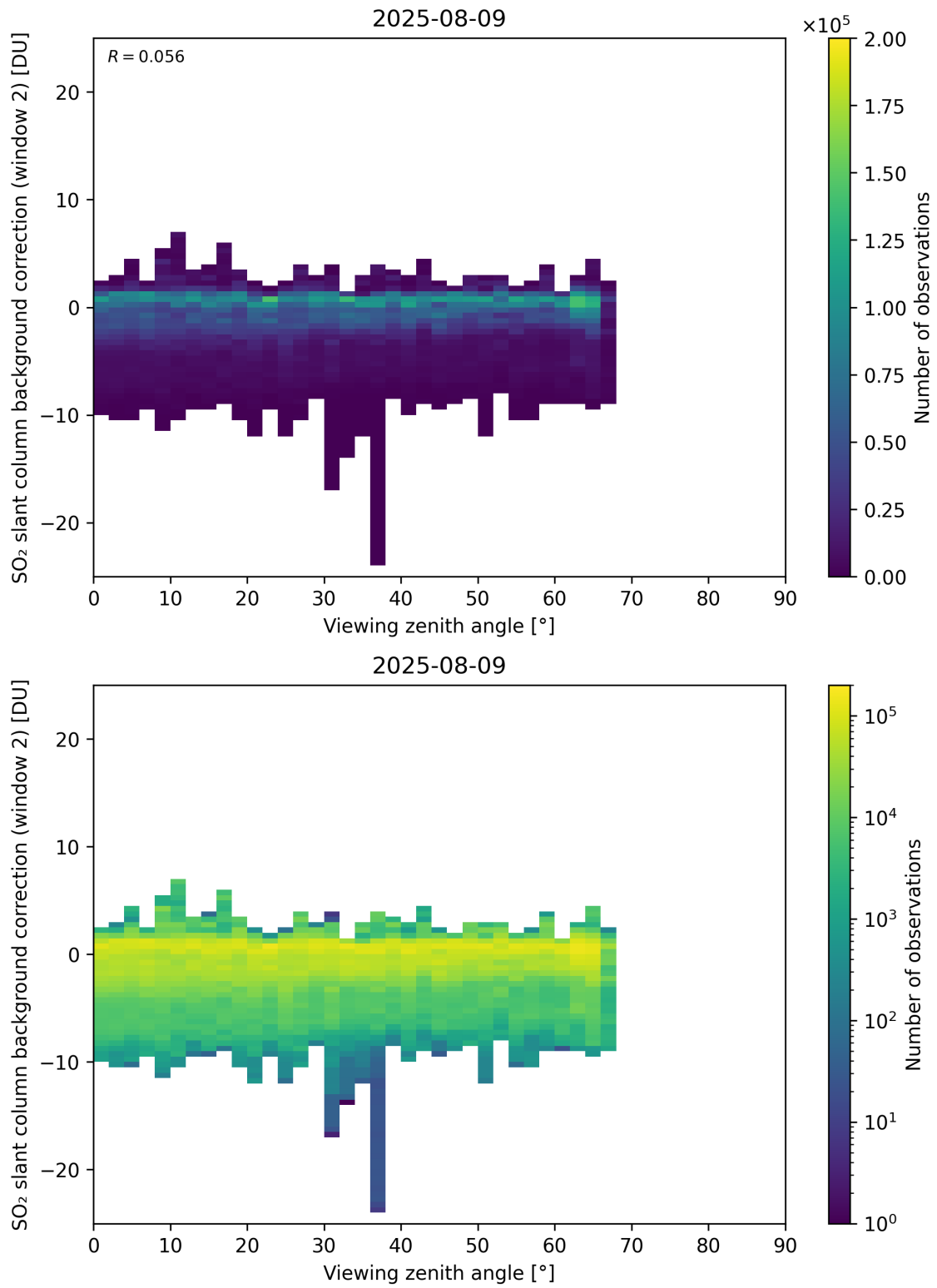
Figure 363: Scatter density plot of “Viewing zenith angle” against “SO 2 slant column background correction (window 2)” for 2025-08-09 to 2025-08-10.
