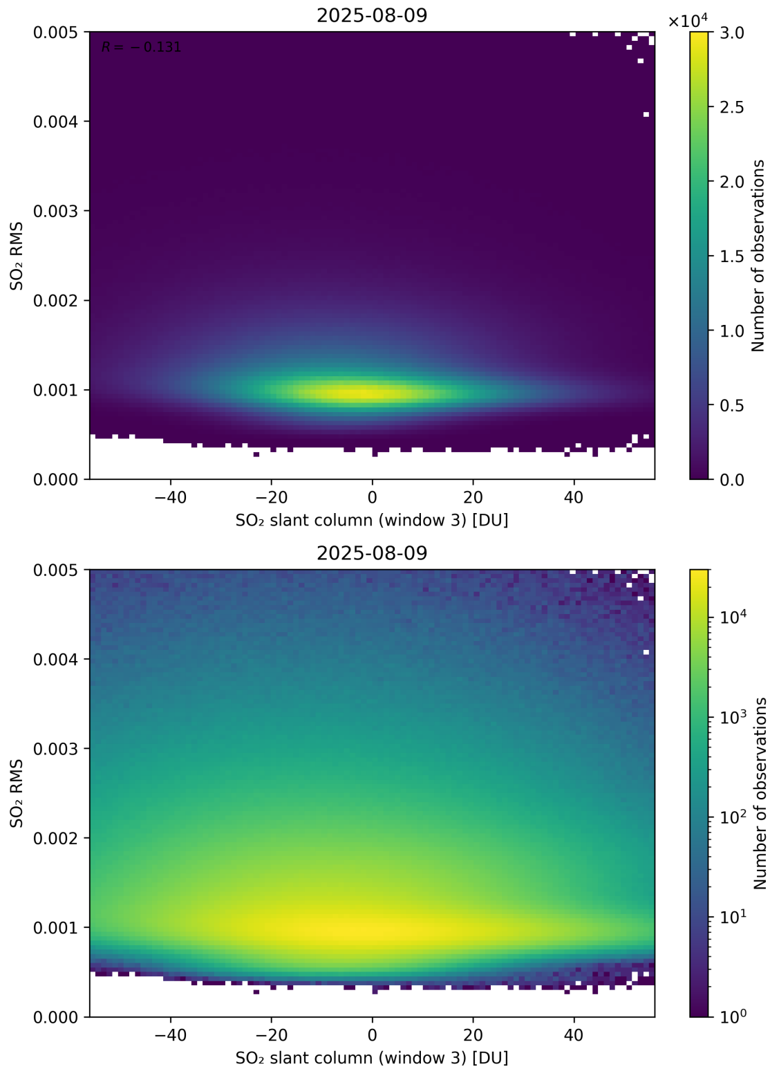
Figure 306: Scatter density plot of “SO 2 slant column (window 3)” against “SO 2 RMS” for 2025-08-09 to 2025-08-10.
