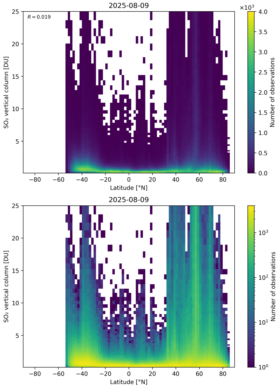
Figure 169: Scatter density plot of “Latitude” against “SO 2 vertical column” for 2025-08-09 to 2025-08-10.
