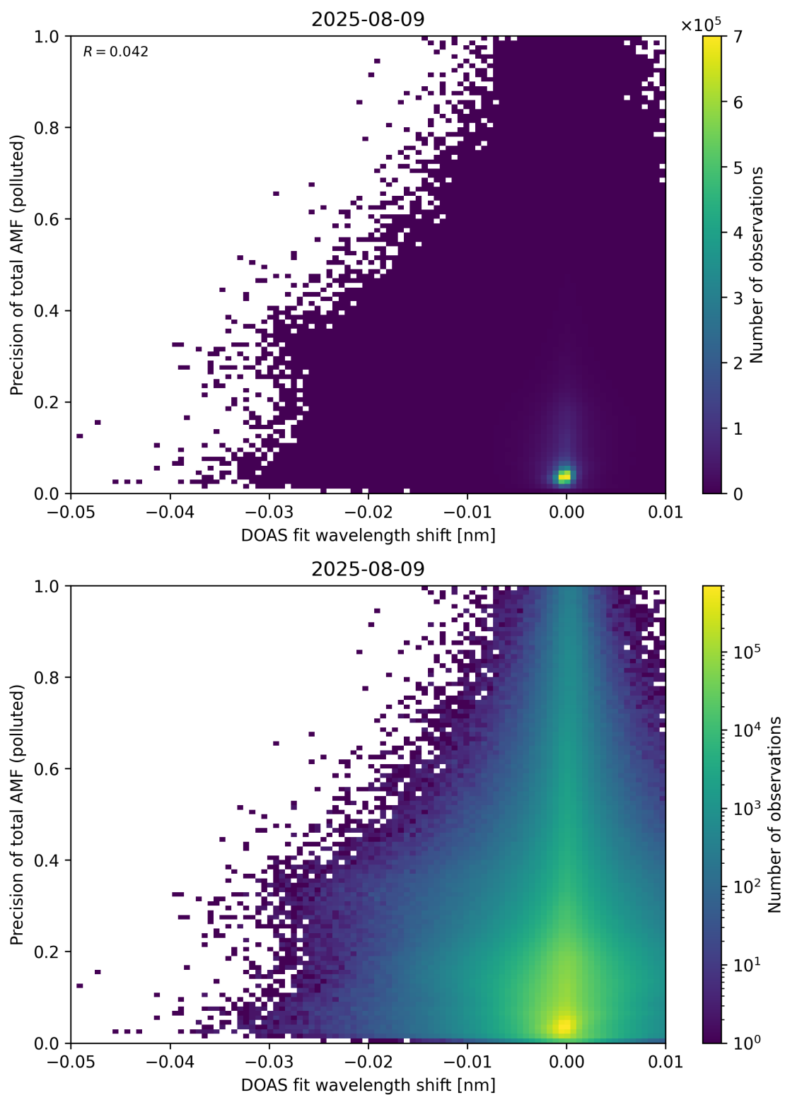
Figure 142: Scatter density plot of “DOAS fit wavelength shift” against “Precision of total AMF (polluted)” for 2025-08-09 to 2025-08-10.
