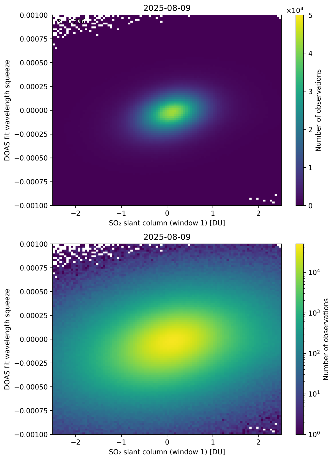
Figure 266: Scatter density plot of “SO 2 slant column (window 1)” against “DOAS fit wavelength squeeze” for 2025-08-09 to 2025-08-10.
