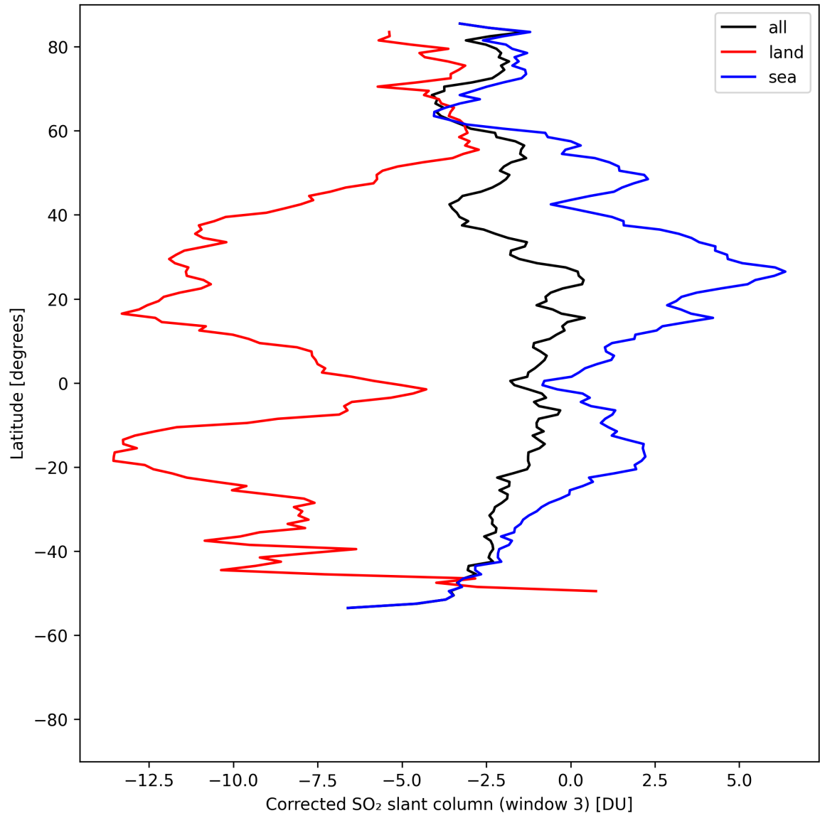
Figure 47: Zonal average of “Corrected SO 2 slant column (window 3)” for 2025-08-09 to 2025-08-10.
