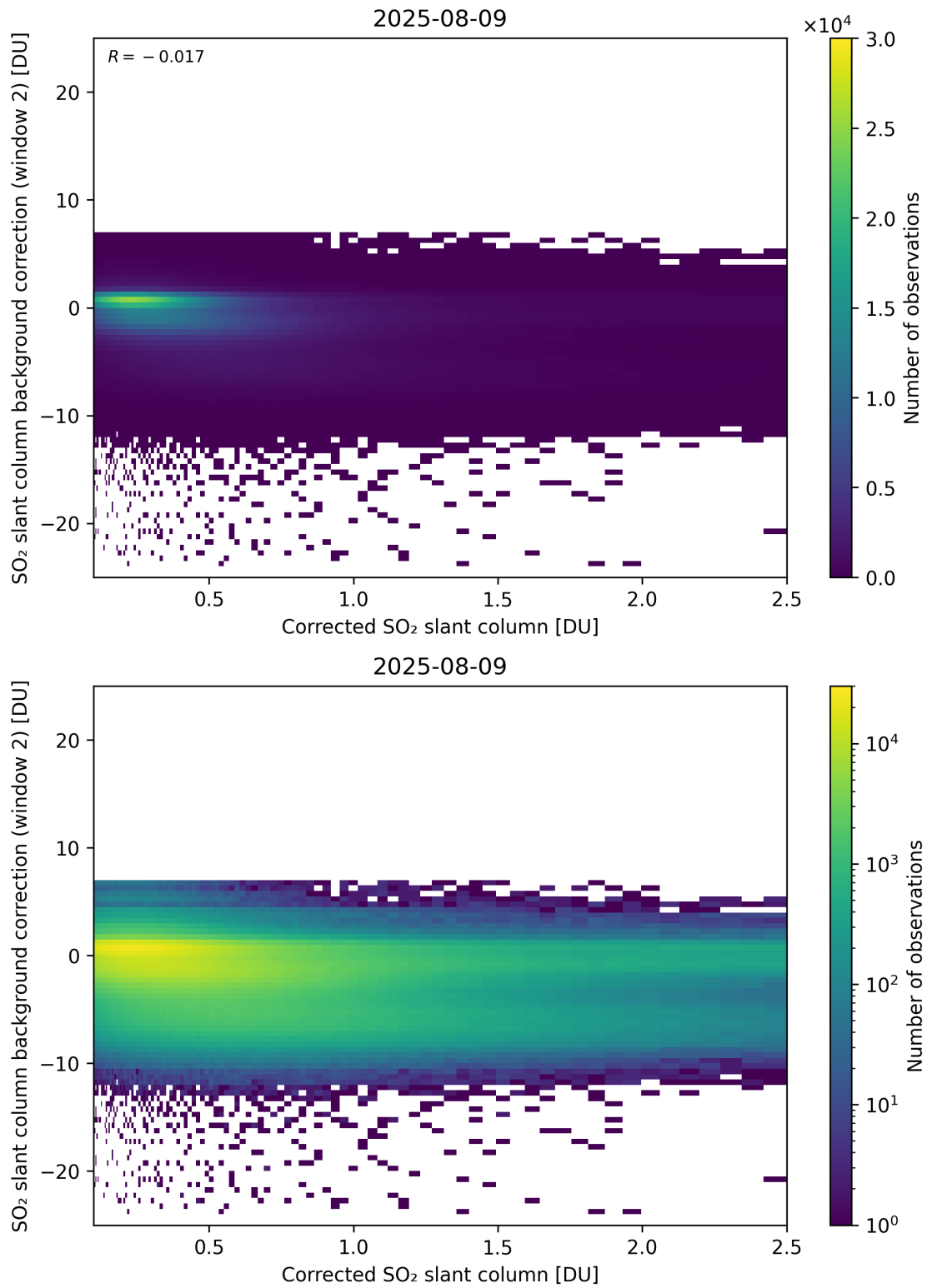
Figure 227: Scatter density plot of “Corrected SO 2 slant column” against “SO 2 slant column background correction (window 2)” for 2025-08-09 to 2025-08-10.
