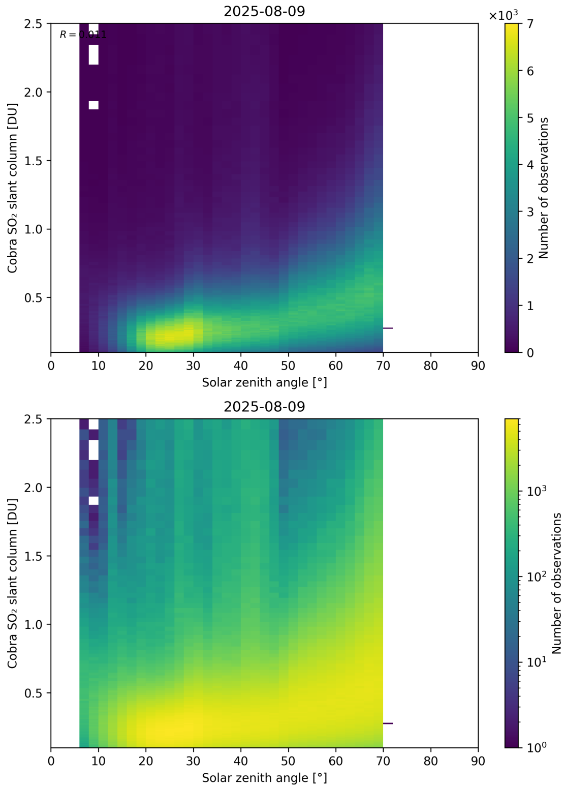
Figure 179: Scatter density plot of “Solar zenith angle” against “Cobra SO 2 slant column” for 2025-08-09 to 2025-08-10.
