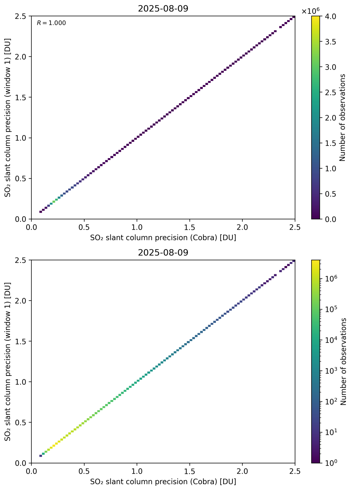
Figure 209: Scatter density plot of “SO 2 slant column precision (Cobra)” against “SO 2 slant column precision (window 1)” for 2025-08-09 to 2025-08-10.
