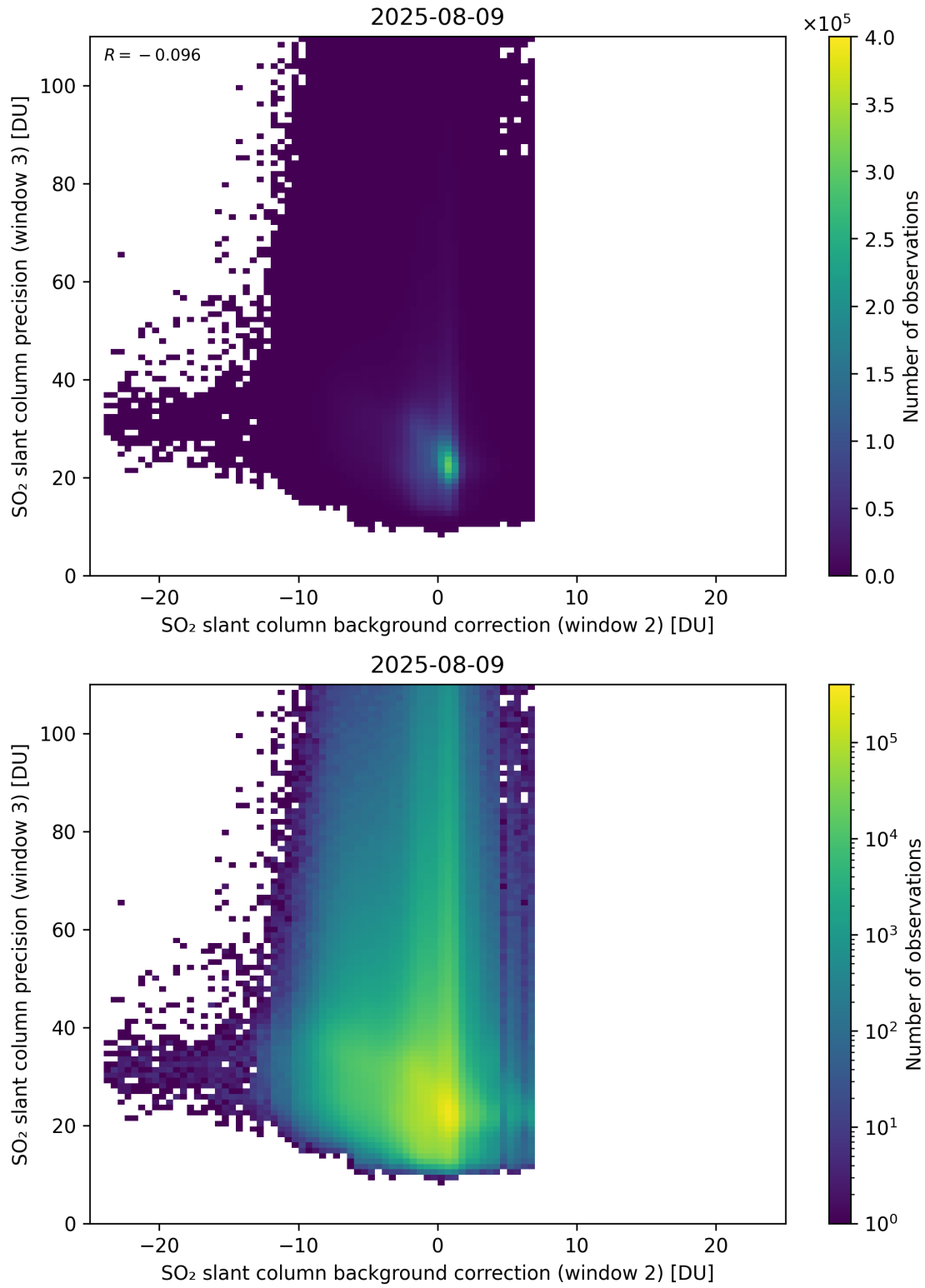
Figure 129: Scatter density plot of “SO 2 slant column background correction (window 2)” against “SO 2 slant column precision (window 3)” for 2025-08-09 to 2025-08-10.
