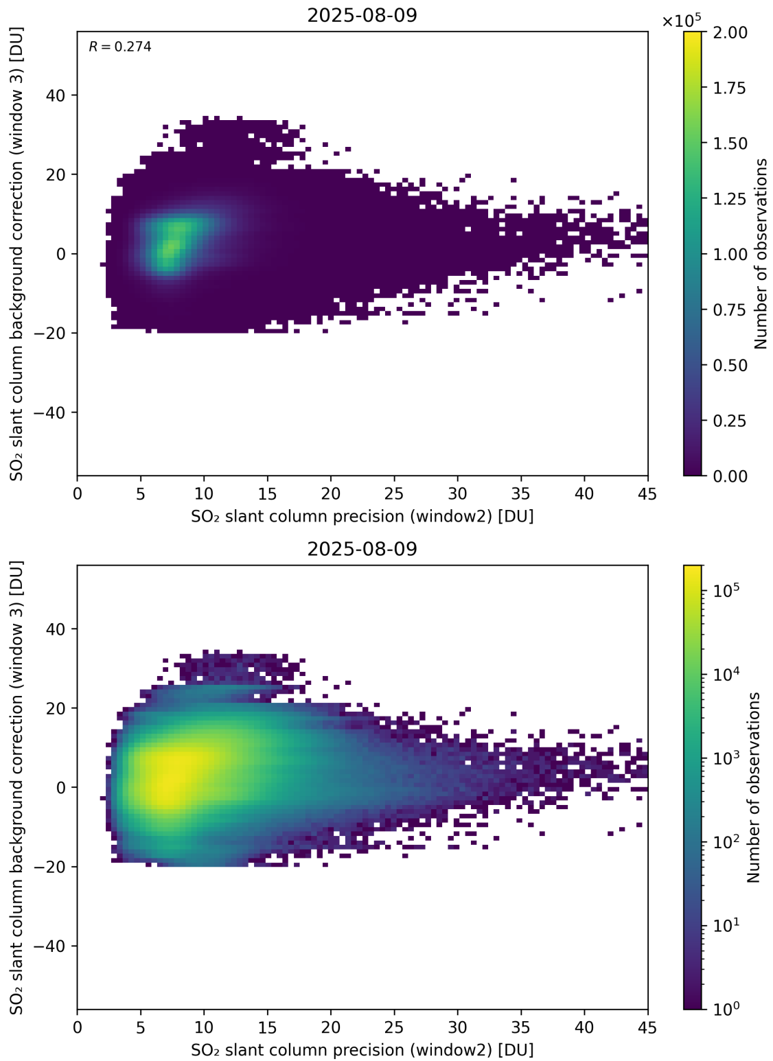
Figure 292: Scatter density plot of “SO 2 slant column precision (window2)” against “SO 2 slant column background correction (window 3)” for 2025-08-09 to 2025-08-10.
