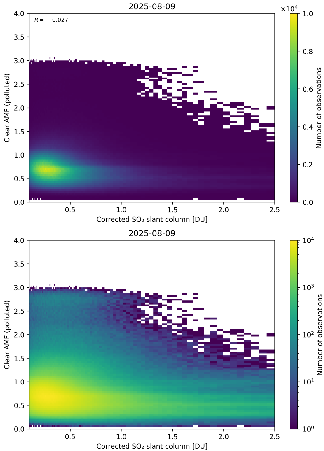
Figure 232: Scatter density plot of “Corrected SO 2 slant column” against “Clear AMF (polluted)” for 2025-08-09 to 2025-08-10.
