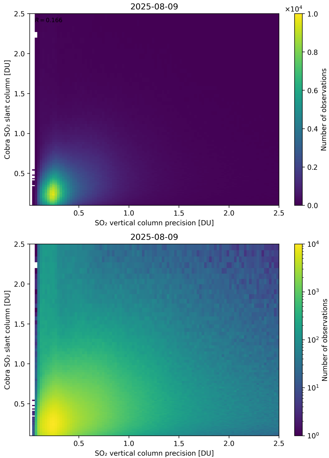
Figure 336: Scatter density plot of “SO 2 vertical column precision” against “Cobra SO 2 slant column” for 2025-08-09 to 2025-08-10.
