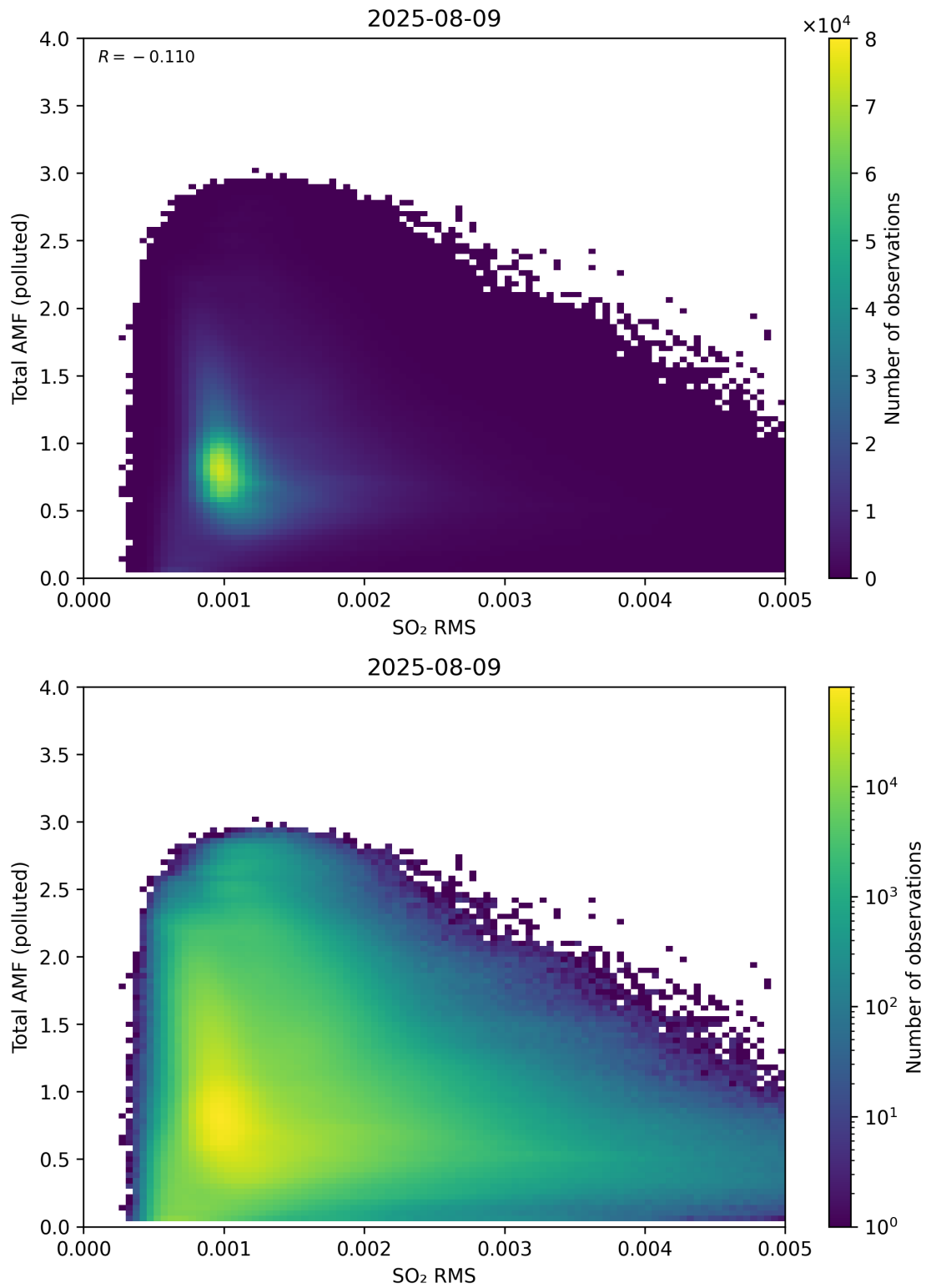
Figure 148: Scatter density plot of “SO 2 RMS” against “Total AMF (polluted)” for 2025-08-09 to 2025-08-10.
