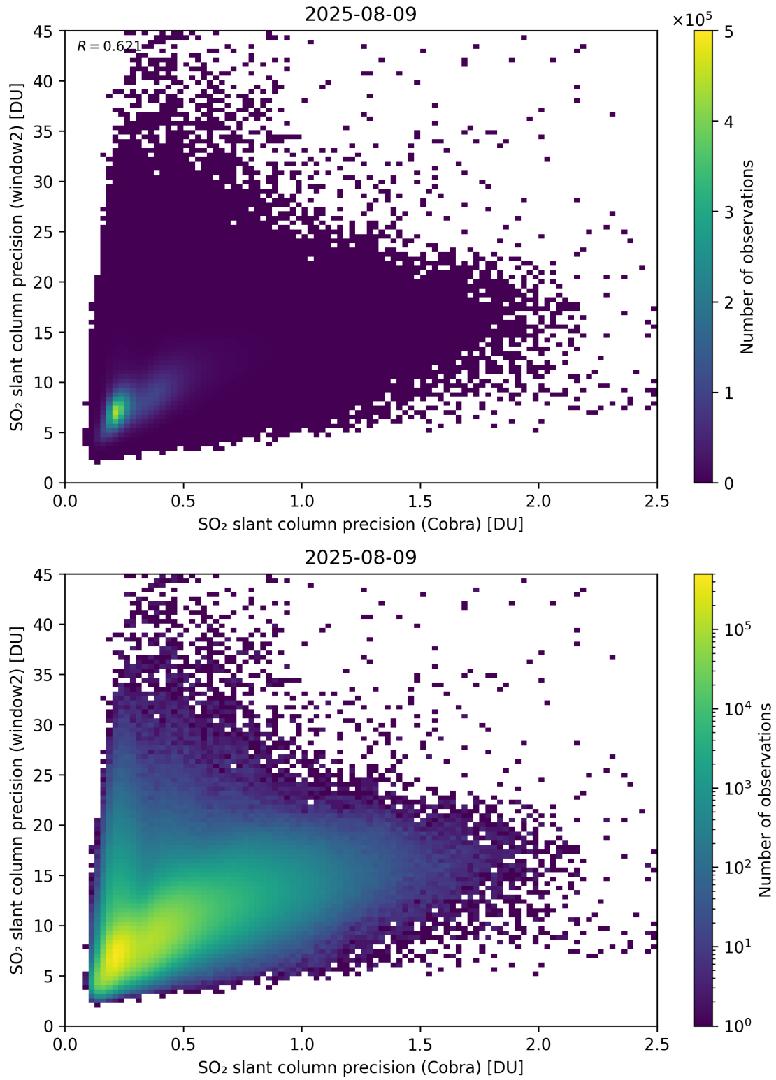
Figure 210: Scatter density plot of “SO 2 slant column precision (Cobra)” against “SO 2 slant column precision (window2)” for 2025-08-09 to 2025-08-10.
