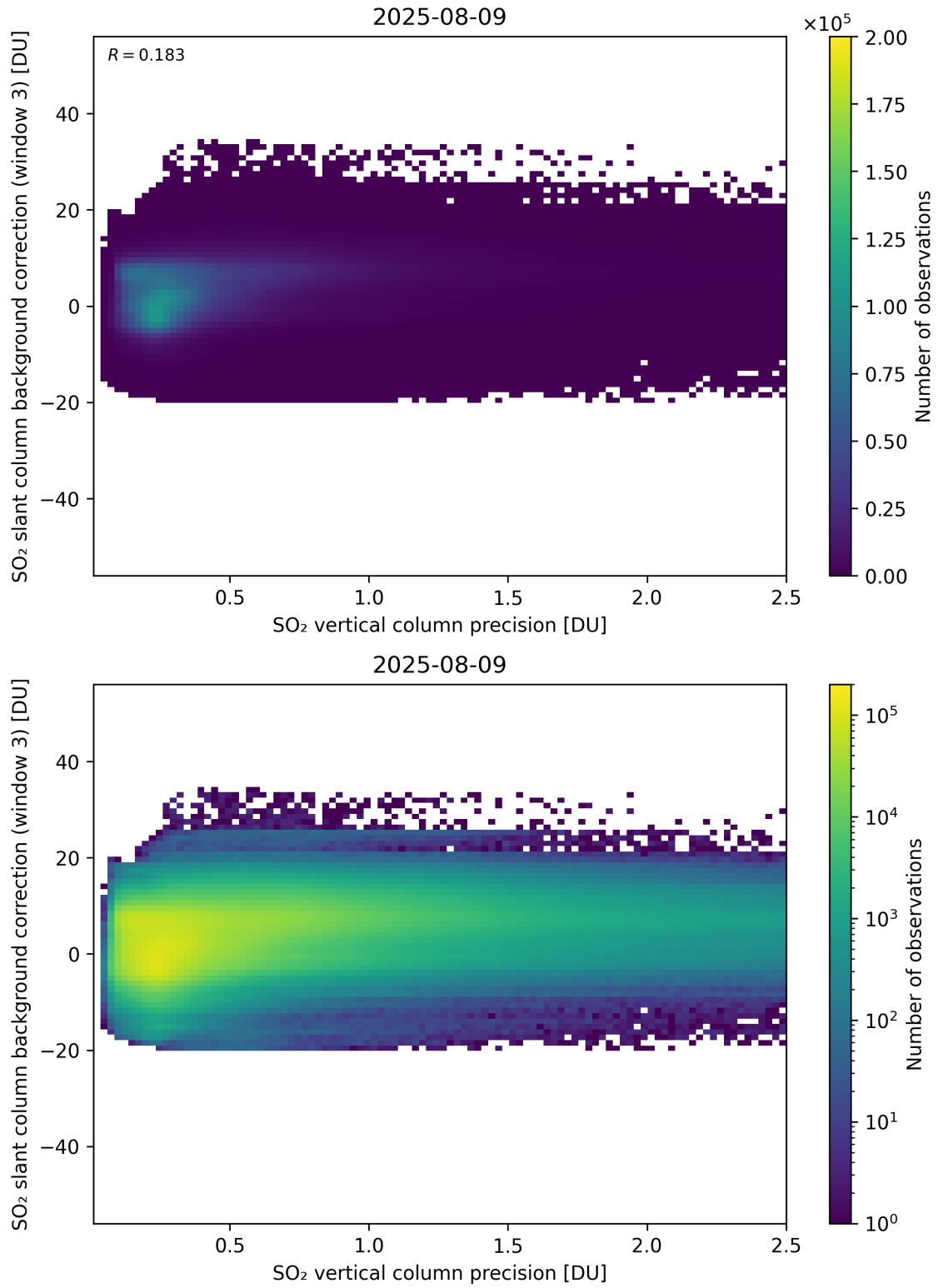
Figure 331: Scatter density plot of “SO 2 vertical column precision” against “SO 2 slant column background correction (window 3)” for 2025-08-09 to 2025-08-10.
