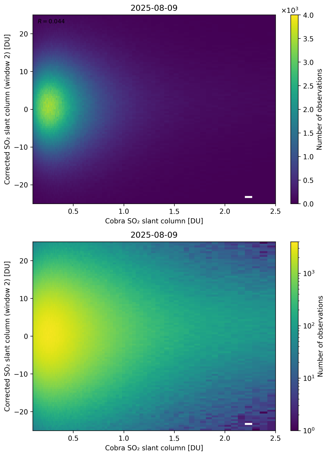
Figure 217: Scatter density plot of “Cobra SO 2 slant column” against “Corrected SO 2 slant column (window 2)” for 2025-08-09 to 2025-08-10.
