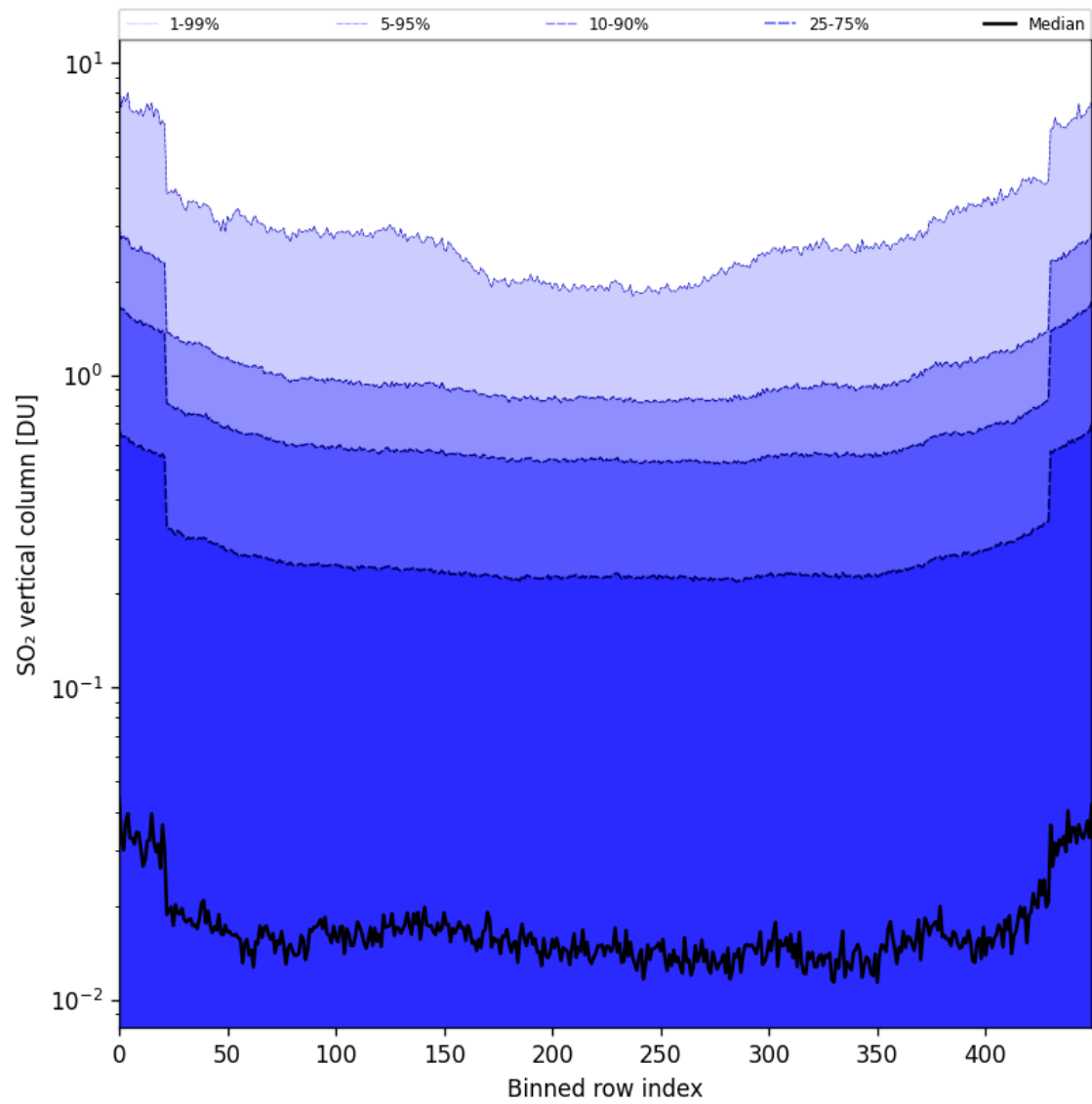
Figure 84: Along track statistics of “SO 2 vertical column” for 2025-08-09 to 2025-08-10
