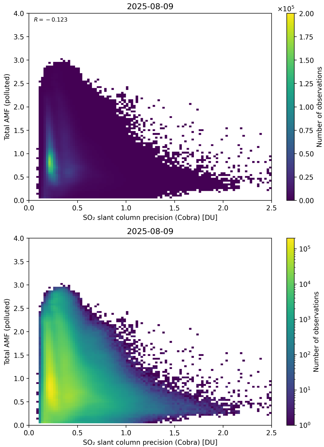
Figure 213: Scatter density plot of “SO 2 slant column precision (Cobra)” against “Total AMF (polluted)” for 2025-08-09 to 2025-08-10.
