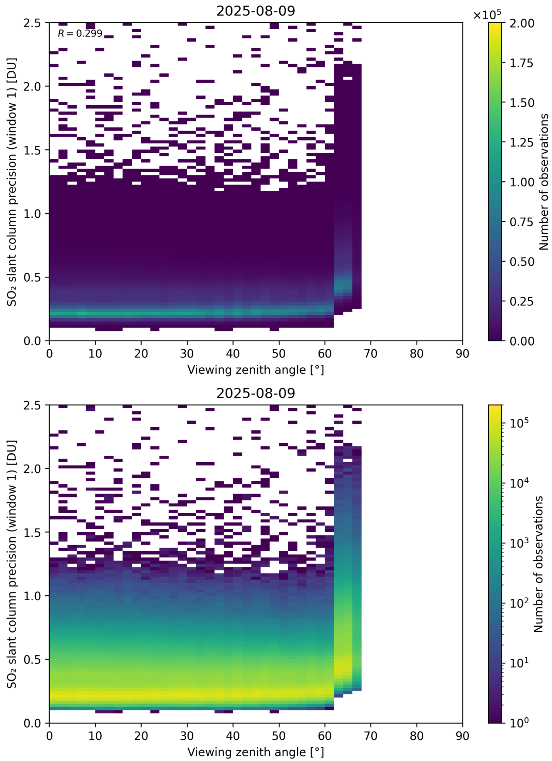
Figure 377: Scatter density plot of “Viewing zenith angle” against “SO 2 slant column precision (window 1)” for 2025-08-09 to 2025-08-10.
