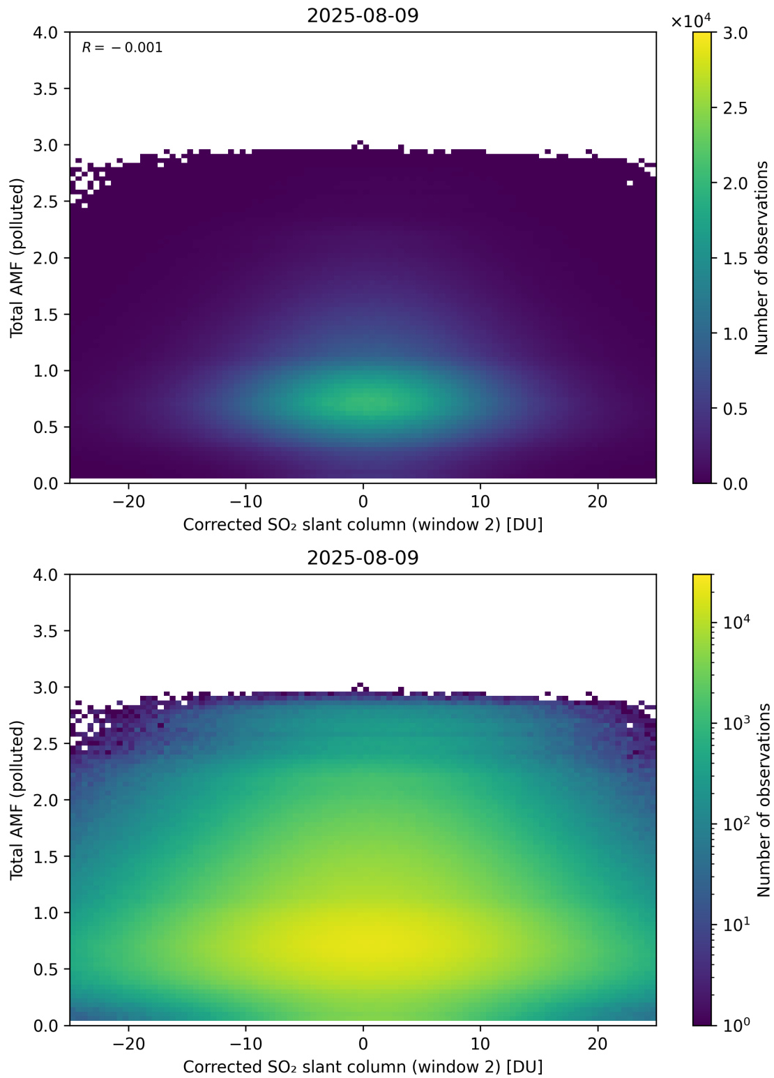
Figure 253: Scatter density plot of “Corrected SO 2 slant column (window 2)” against “Total AMF (polluted)” for 2025-08-09 to 2025-08-10.
