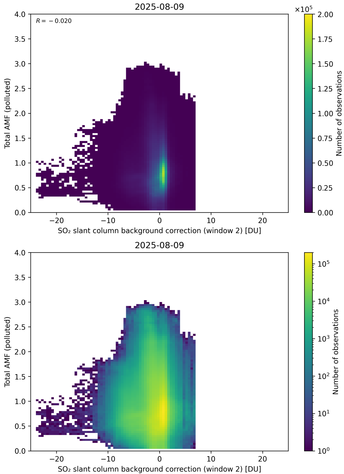
Figure 130: Scatter density plot of “SO 2 slant column background correction (window 2)” against “Total AMF (polluted)” for 2025-08-09 to 2025-08-10.
