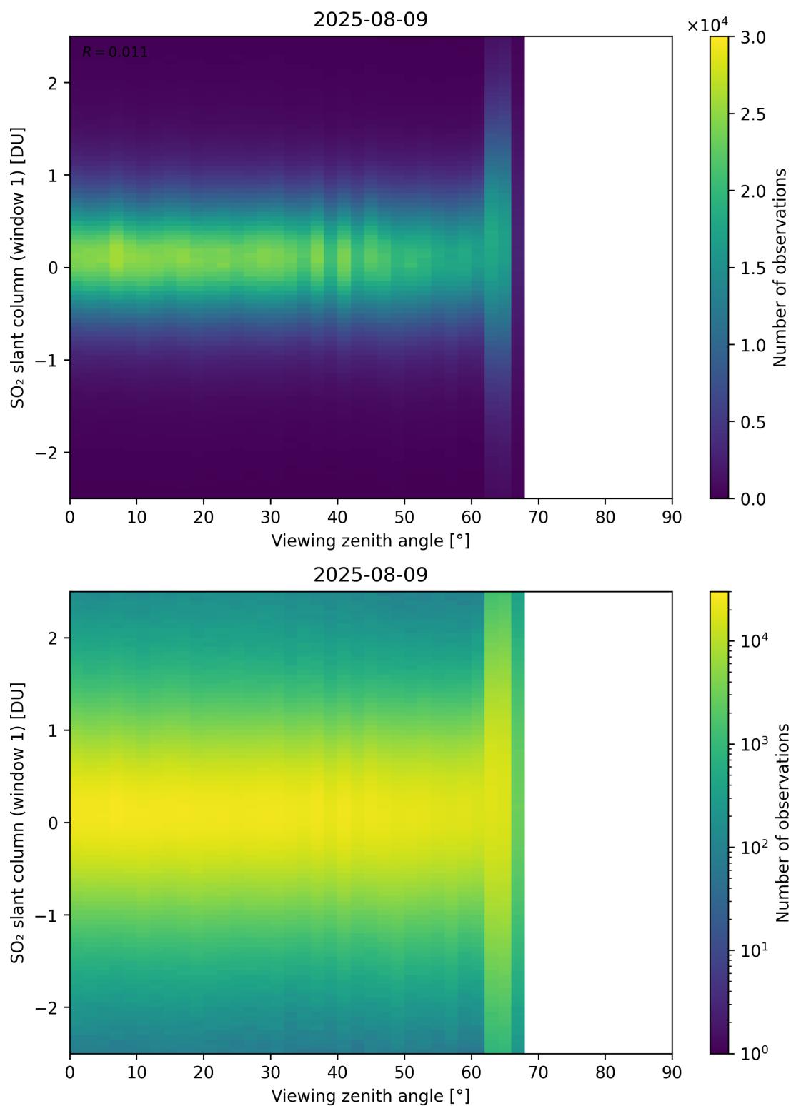
Figure 376: Scatter density plot of “Viewing zenith angle” against “SO 2 slant column (window 1)” for 2025-08-09 to 2025-08-10.
