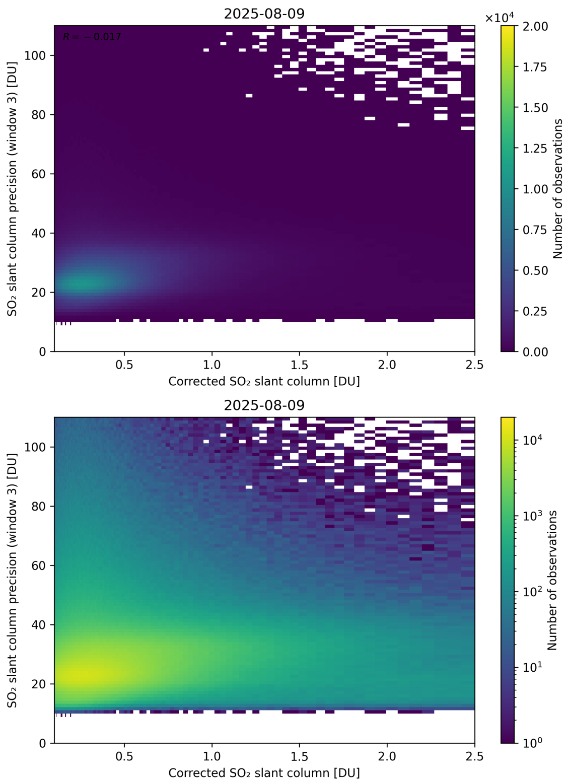
Figure 241: Scatter density plot of “Corrected SO 2 slant column” against “SO 2 slant column precision (window 3)” for 2025-08-09 to 2025-08-10.
