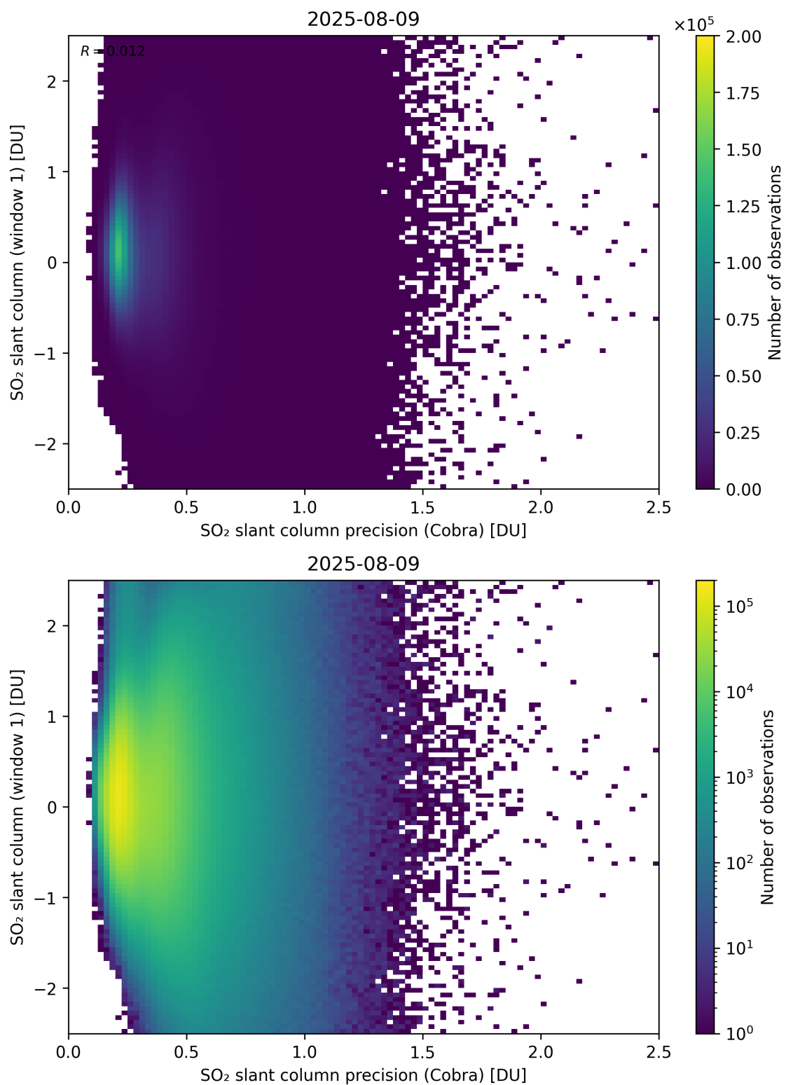
Figure 208: Scatter density plot of “SO 2 slant column precision (Cobra)” against “SO 2 slant column (window 1)” for 2025-08-09 to 2025-08-10.
