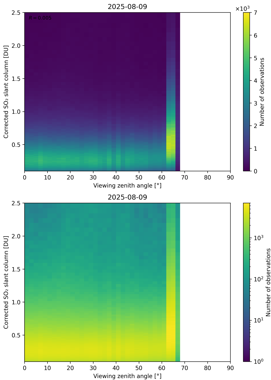
Figure 373: Scatter density plot of “Viewing zenith angle” against “Corrected SO 2 slant column” for 2025-08-09 to 2025-08-10.
