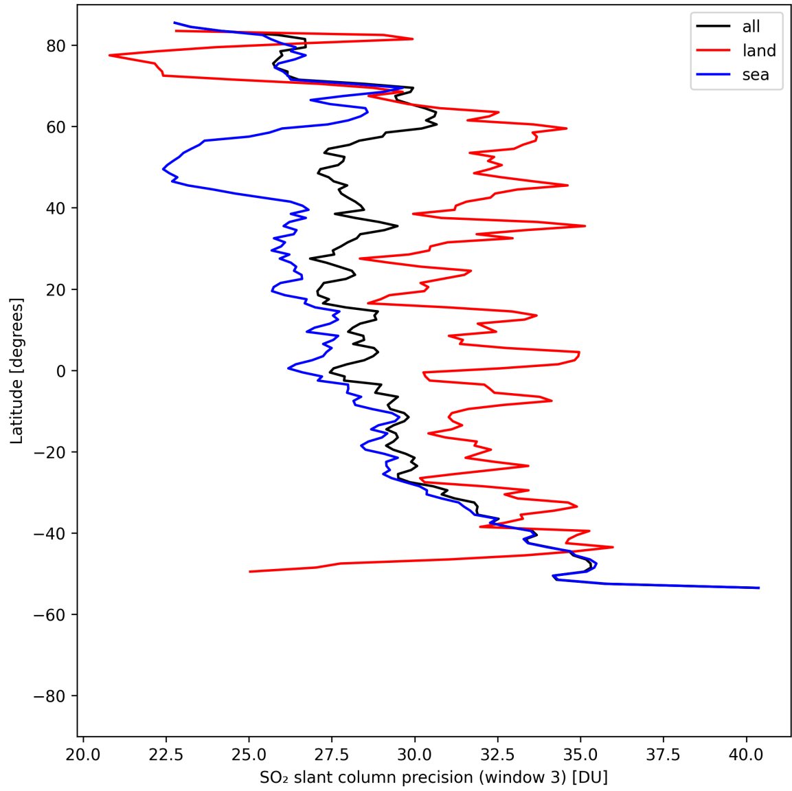
Figure 46: Zonal average of “SO 2 slant column precision (window 3)” for 2025-08-09 to 2025-08-10.
