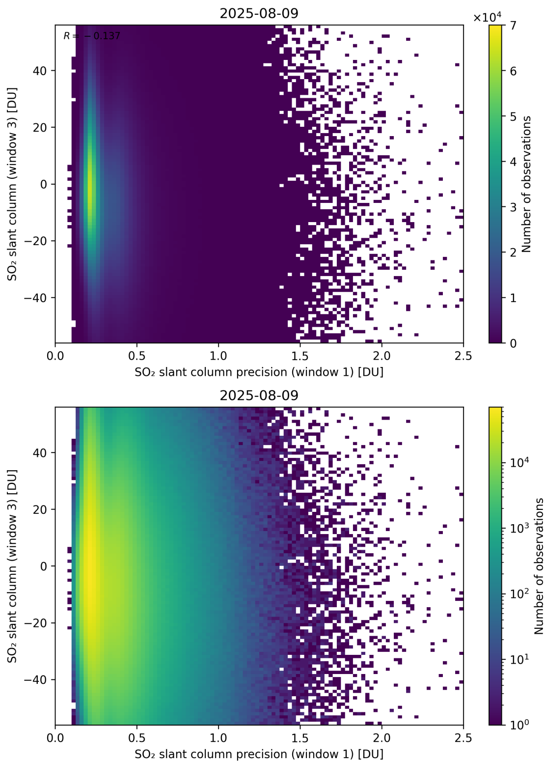
Figure 278: Scatter density plot of “SO 2 slant column precision (window 1)” against “SO 2 slant column (window 3)” for 2025-08-09 to 2025-08-10.
