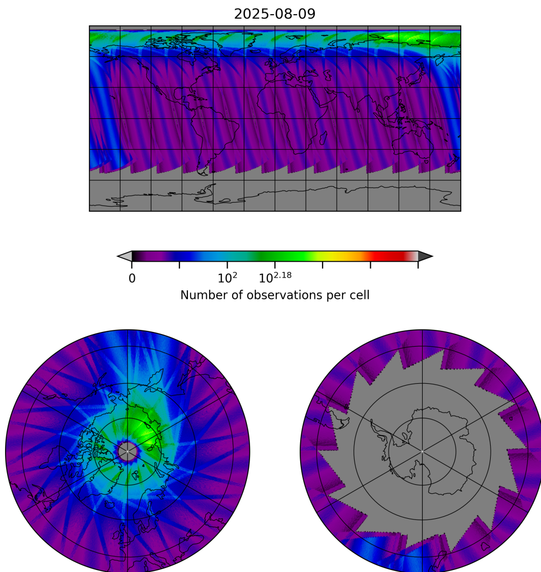
Figure 30: Map of the number of observations for 2025-08-09 to 2025-08-10
