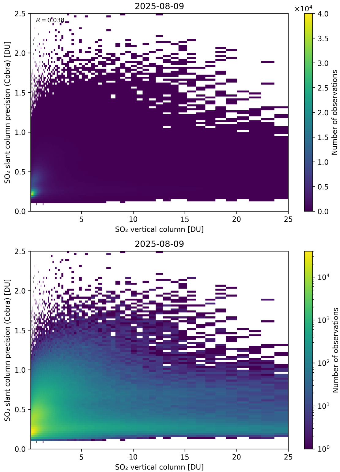
Figure 350: Scatter density plot of “SO 2 vertical column” against “SO 2 slant column precision (Cobra)” for 2025-08-09 to 2025-08-10.
