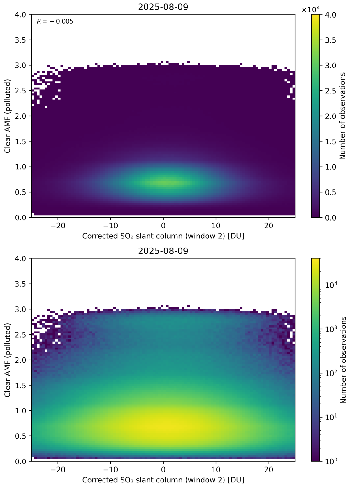
Figure 249: Scatter density plot of “Corrected SO 2 slant column (window 2)” against “Clear AMF (polluted)” for 2025-08-09 to 2025-08-10.
