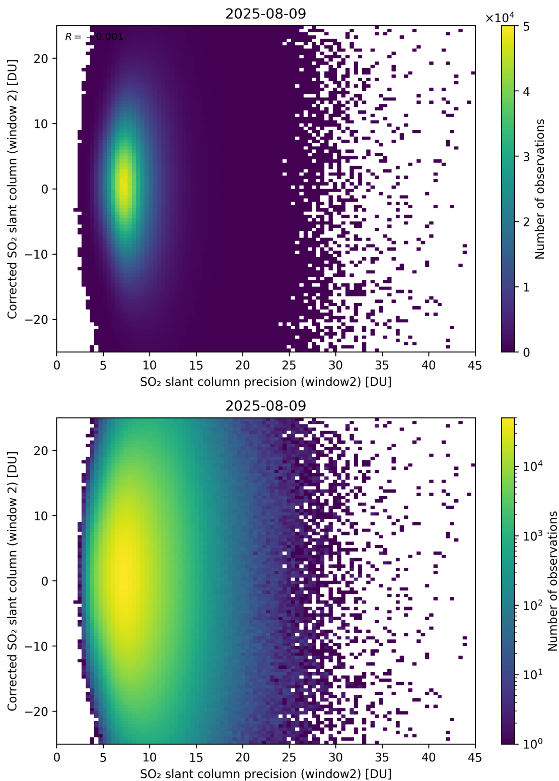
Figure 297: Scatter density plot of “SO 2 slant column precision (window2)” against “Corrected SO 2 slant column (window 2)” for 2025-08-09 to 2025-08-10.
