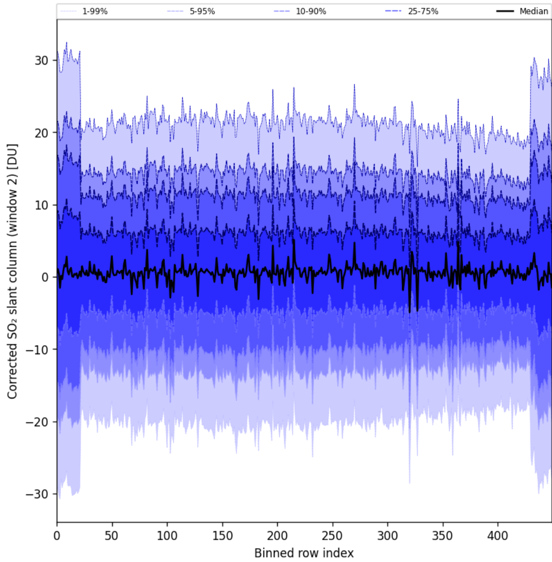
Figure 95: Along track statistics of “Corrected SO 2 slant column (window 2)” for 2025-08-09 to 2025-08-10
