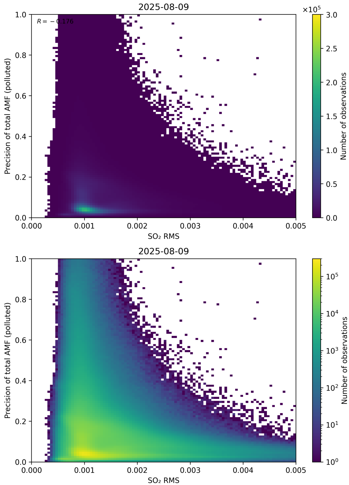
Figure 149: Scatter density plot of “SO 2 RMS” against “Precision of total AMF (polluted)” for 2025-08-09 to 2025-08-10.
