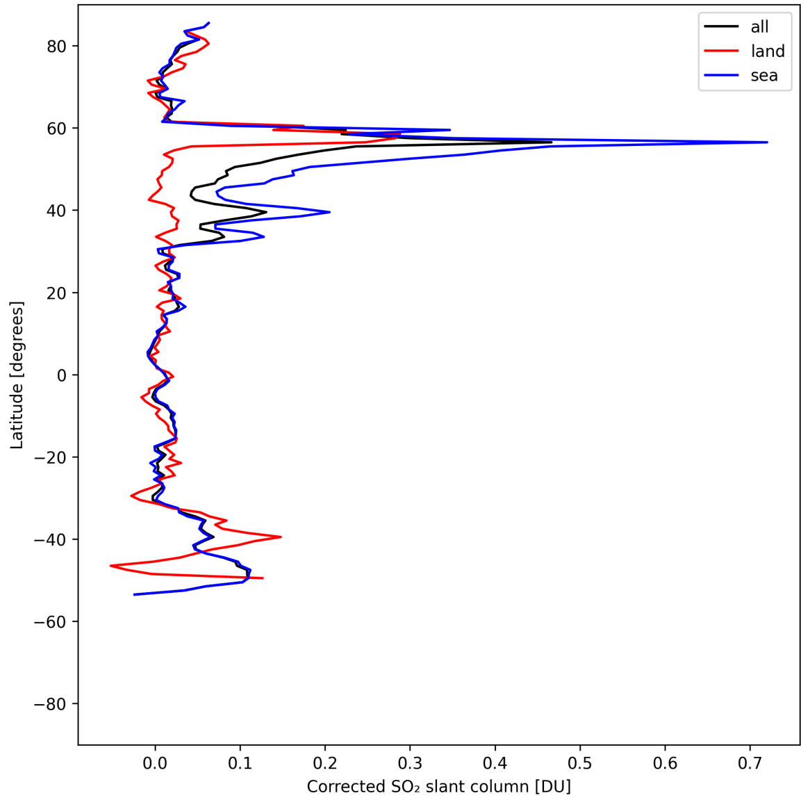
Figure 34: Zonal average of “Corrected SO 2 slant column” for 2025-08-09 to 2025-08-10.
