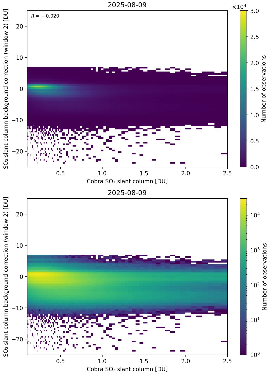
Figure 194: Scatter density plot of “Cobra SO 2 slant column” against “SO 2 slant column background correction (window 2)” for 2025-08-09 to 2025-08-10.
