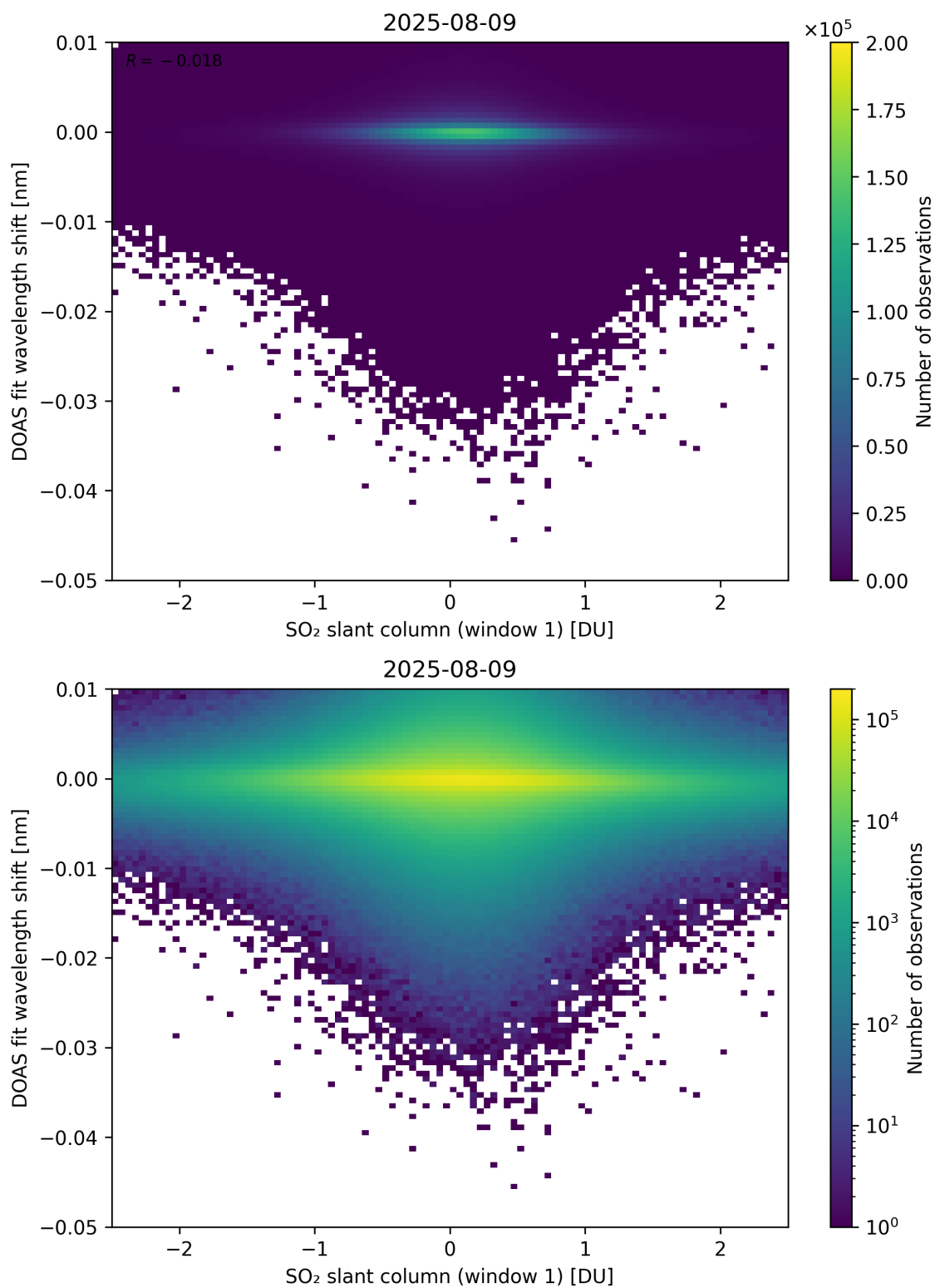
Figure 265: Scatter density plot of “SO 2 slant column (window 1)” against “DOAS fit wavelength shift” for 2025-08-09 to 2025-08-10.
