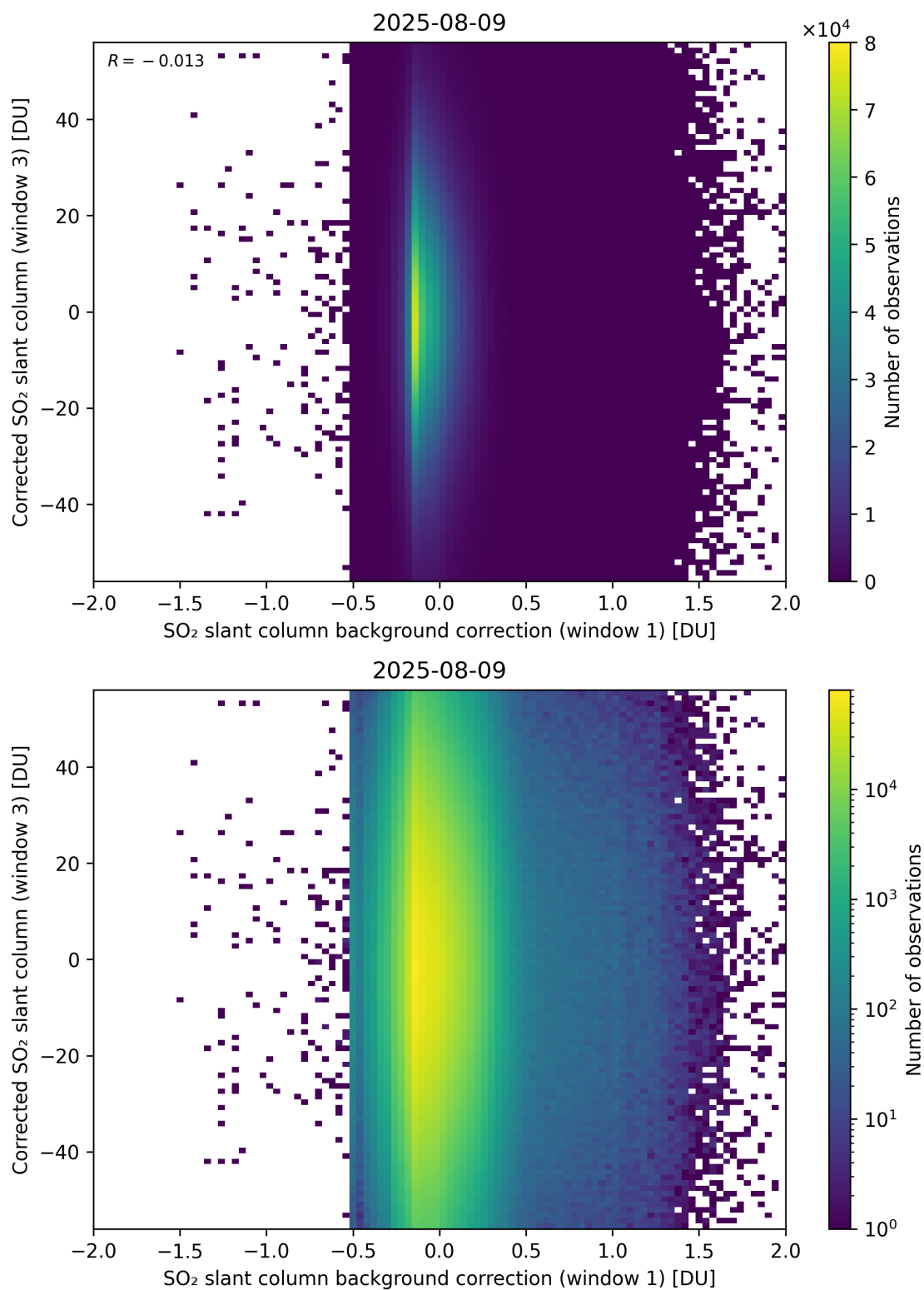
Figure 116: Scatter density plot of “SO 2 slant column background correction (window 1)” against “Corrected SO 2 slant column (window 3)” for 2025-08-09 to 2025-08-10.
