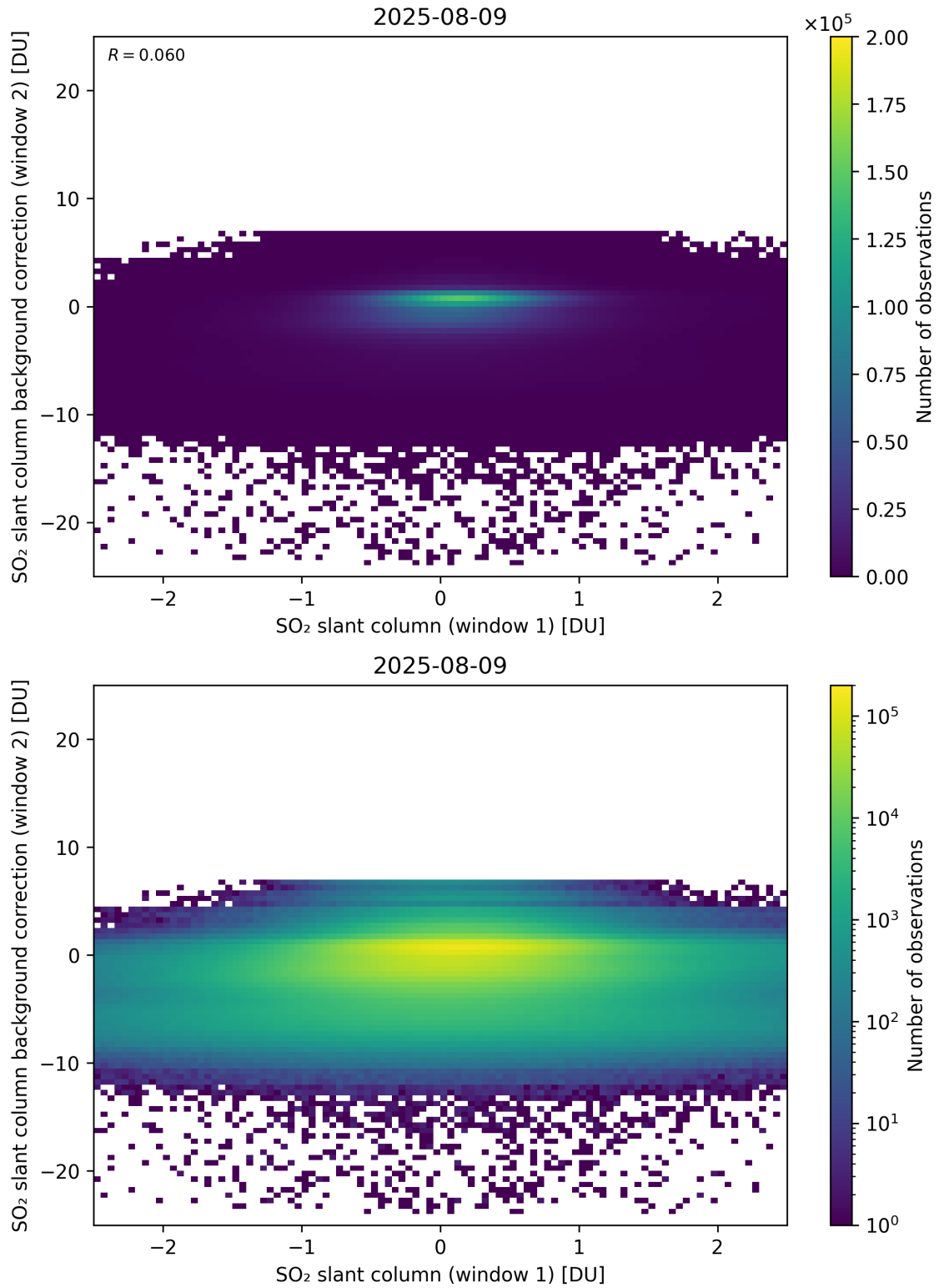
Figure 263: Scatter density plot of “SO 2 slant column (window 1)” against “SO 2 slant column background correction (window 2)” for 2025-08-09 to 2025-08-10.
