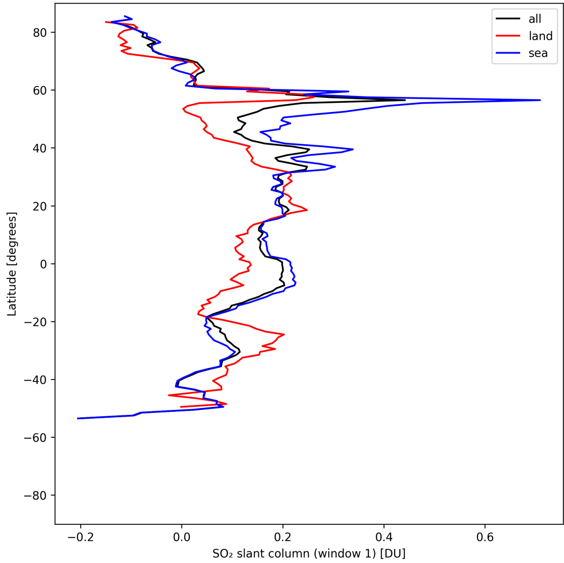
Figure 37: Zonal average of “SO 2 slant column (window 1)” for 2025-08-09 to 2025-08-10.
