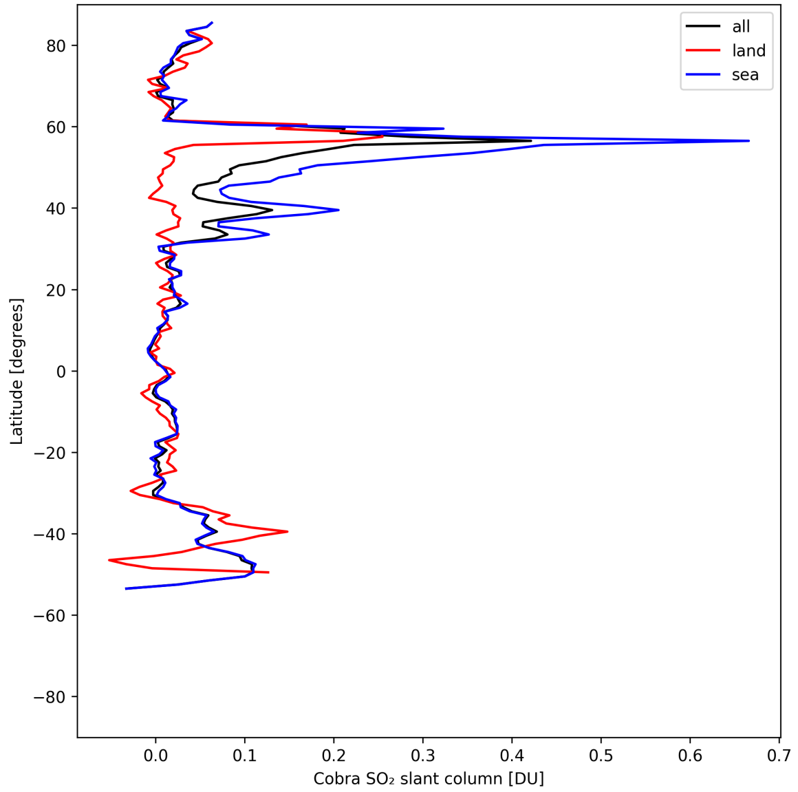
Figure 35: Zonal average of “Cobra SO 2 slant column” for 2025-08-09 to 2025-08-10.
