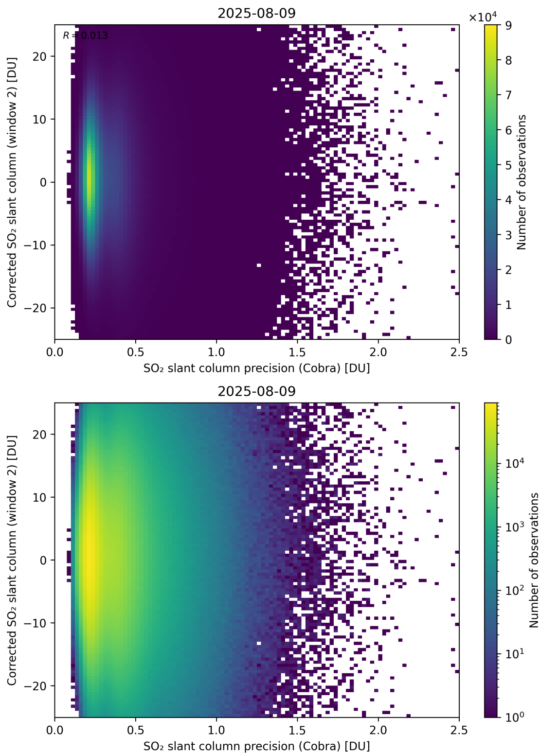
Figure 206: Scatter density plot of “SO 2 slant column precision (Cobra)” against “Corrected SO 2 slant column (window 2)” for 2025-08-09 to 2025-08-10.
