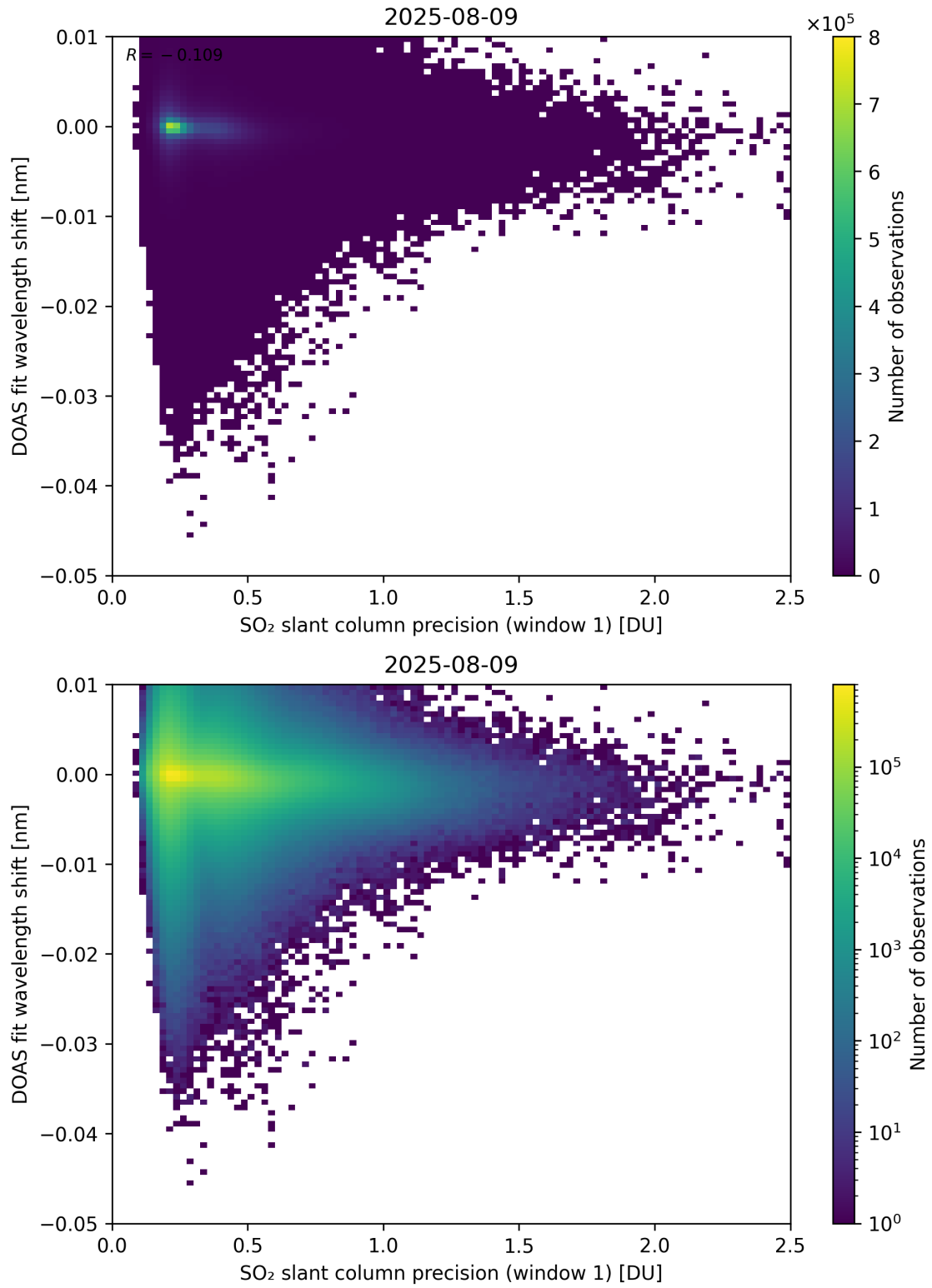
Figure 271: Scatter density plot of “SO 2 slant column precision (window 1)” against “DOAS fit wavelength shift” for 2025-08-09 to 2025-08-10.
