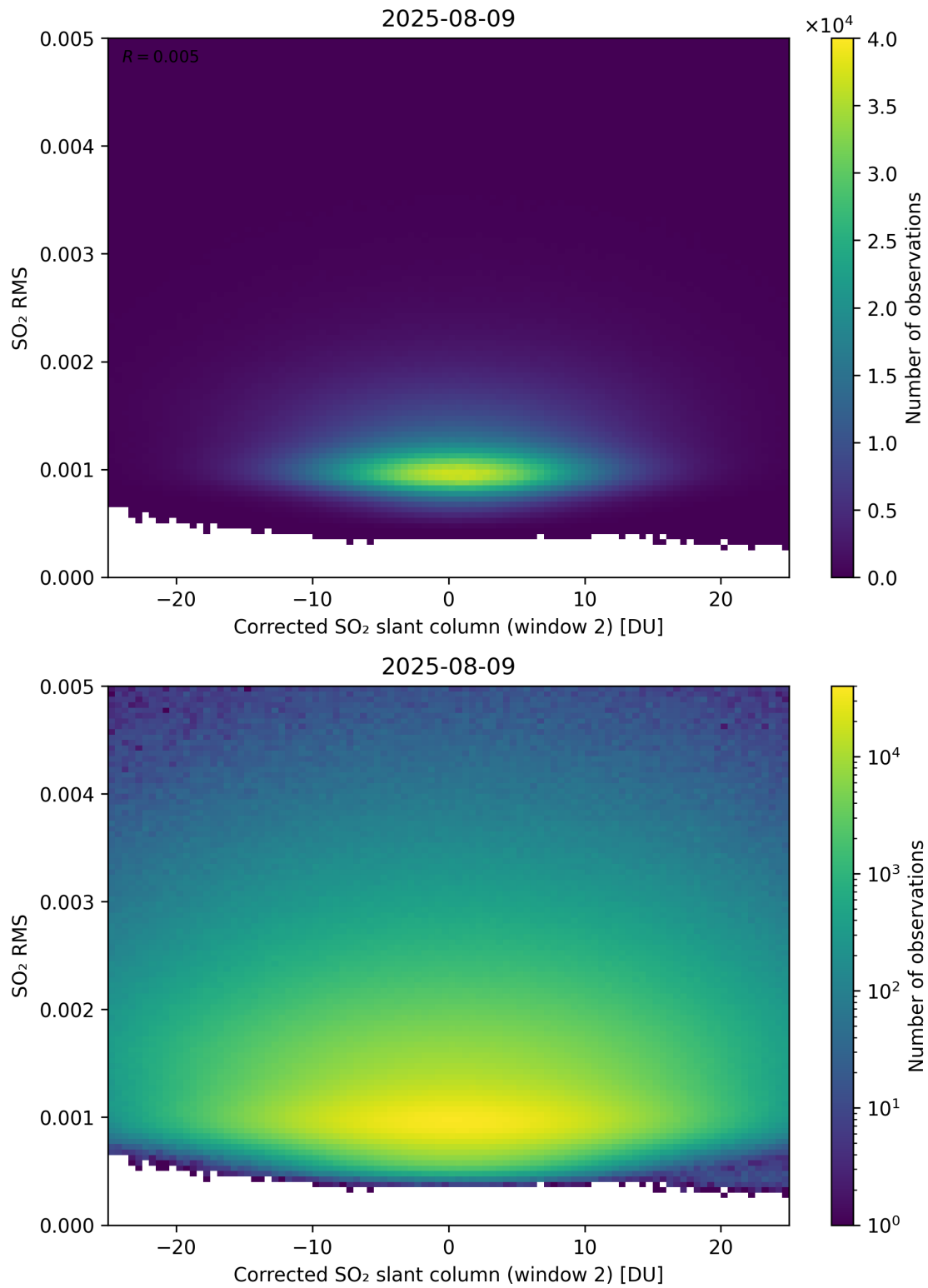
Figure 248: Scatter density plot of “Corrected SO 2 slant column (window 2)” against “SO 2 RMS” for 2025-08-09 to 2025-08-10.
