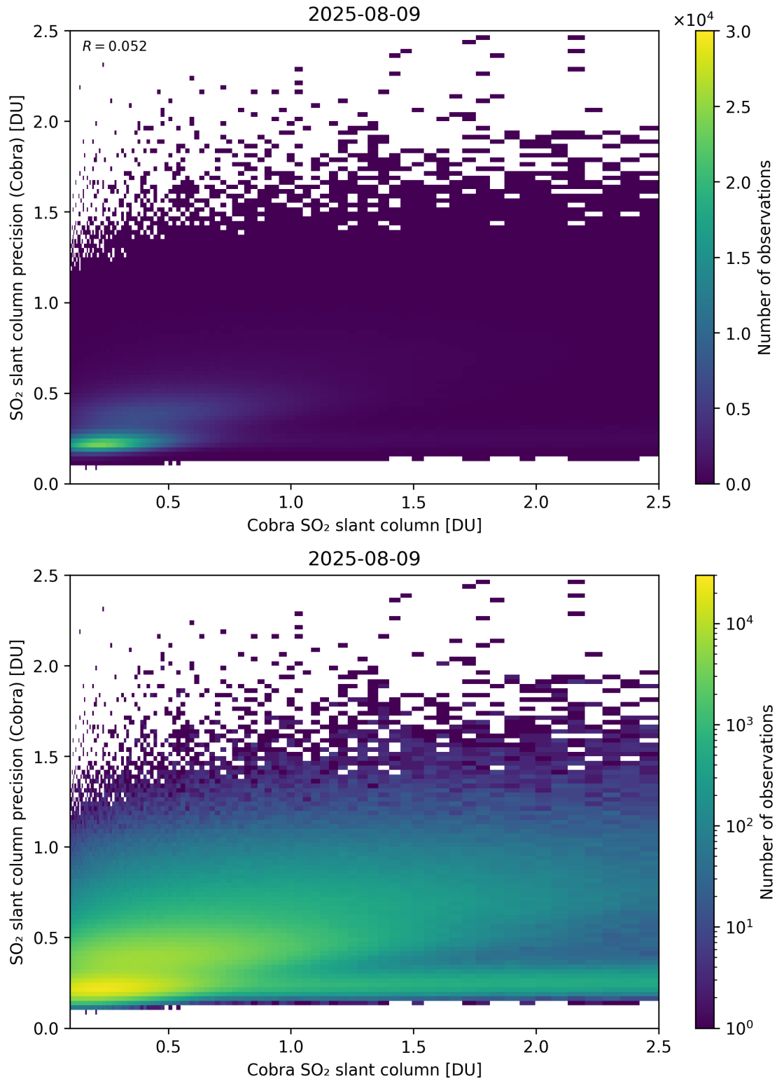
Figure 216: Scatter density plot of “Cobra SO 2 slant column” against “SO 2 slant column precision (Cobra)” for 2025-08-09 to 2025-08-10.
