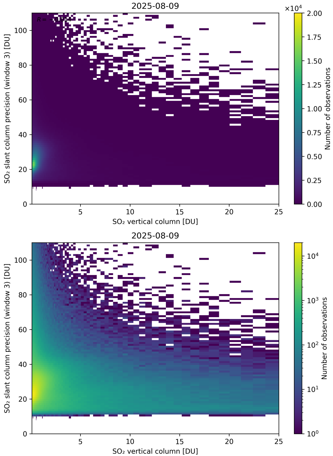
Figure 358: Scatter density plot of “SO 2 vertical column” against “SO 2 slant column precision (window 3)” for 2025-08-09 to 2025-08-10.
