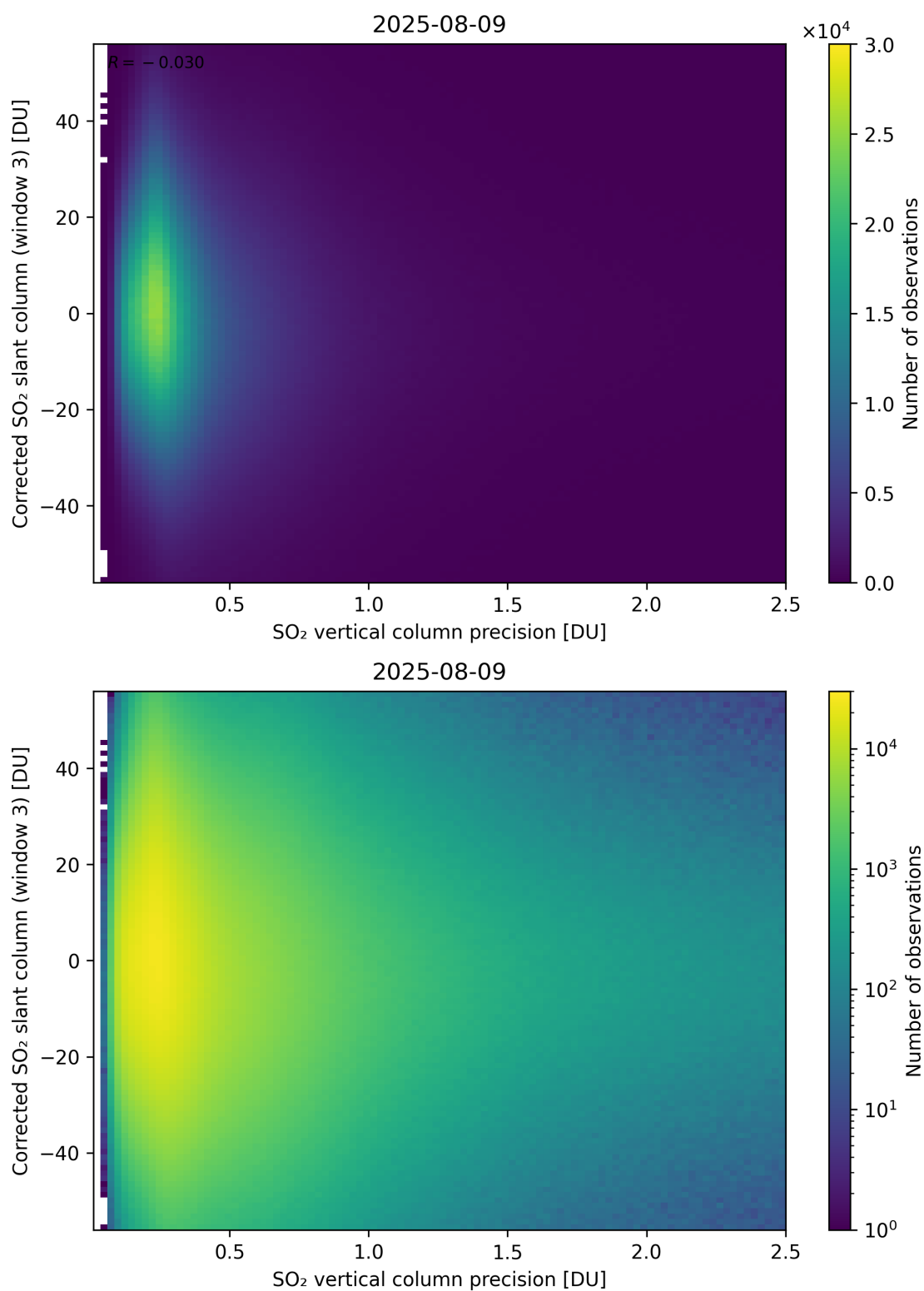
Figure 340: Scatter density plot of “SO 2 vertical column precision” against “Corrected SO 2 slant column (window 3)” for 2025-08-09 to 2025-08-10.
