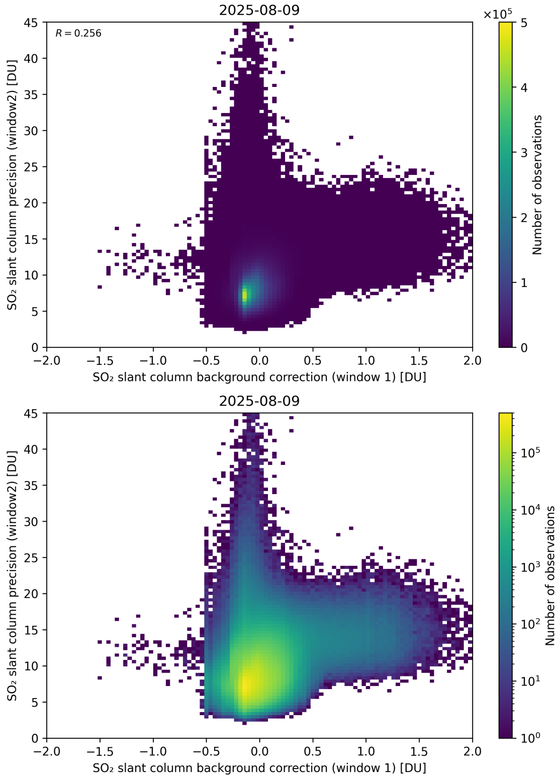
Figure 117: Scatter density plot of “SO 2 slant column background correction (window 1)” against “SO 2 slant column precision (window2)” for 2025-08-09 to 2025-08-10.
