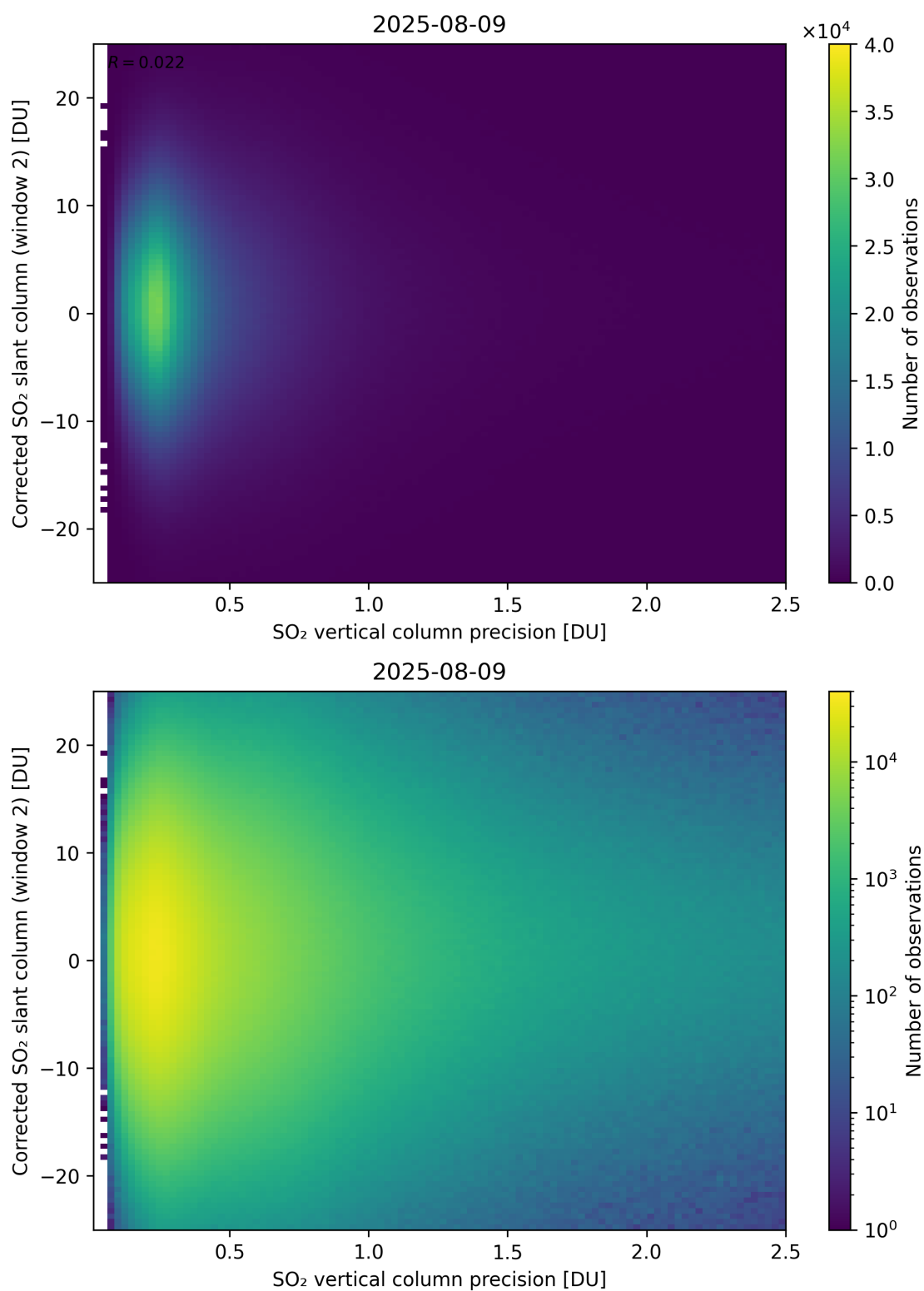
Figure 339: Scatter density plot of “SO 2 vertical column precision” against “Corrected SO 2 slant column (window 2)” for 2025-08-09 to 2025-08-10.
