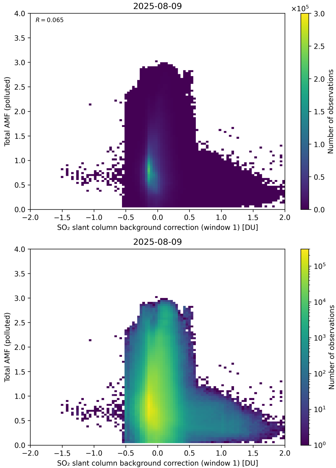
Figure 120: Scatter density plot of “SO 2 slant column background correction (window 1)” against “Total AMF (polluted)” for 2025-08-09 to 2025-08-10.
