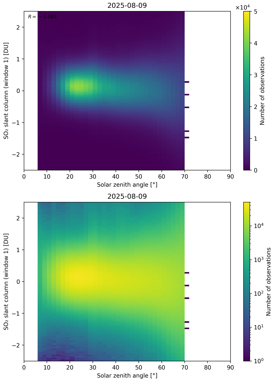
Figure 184: Scatter density plot of “Solar zenith angle” against “SO 2 slant column (window 1)” for 2025-08-09 to 2025-08-10.
