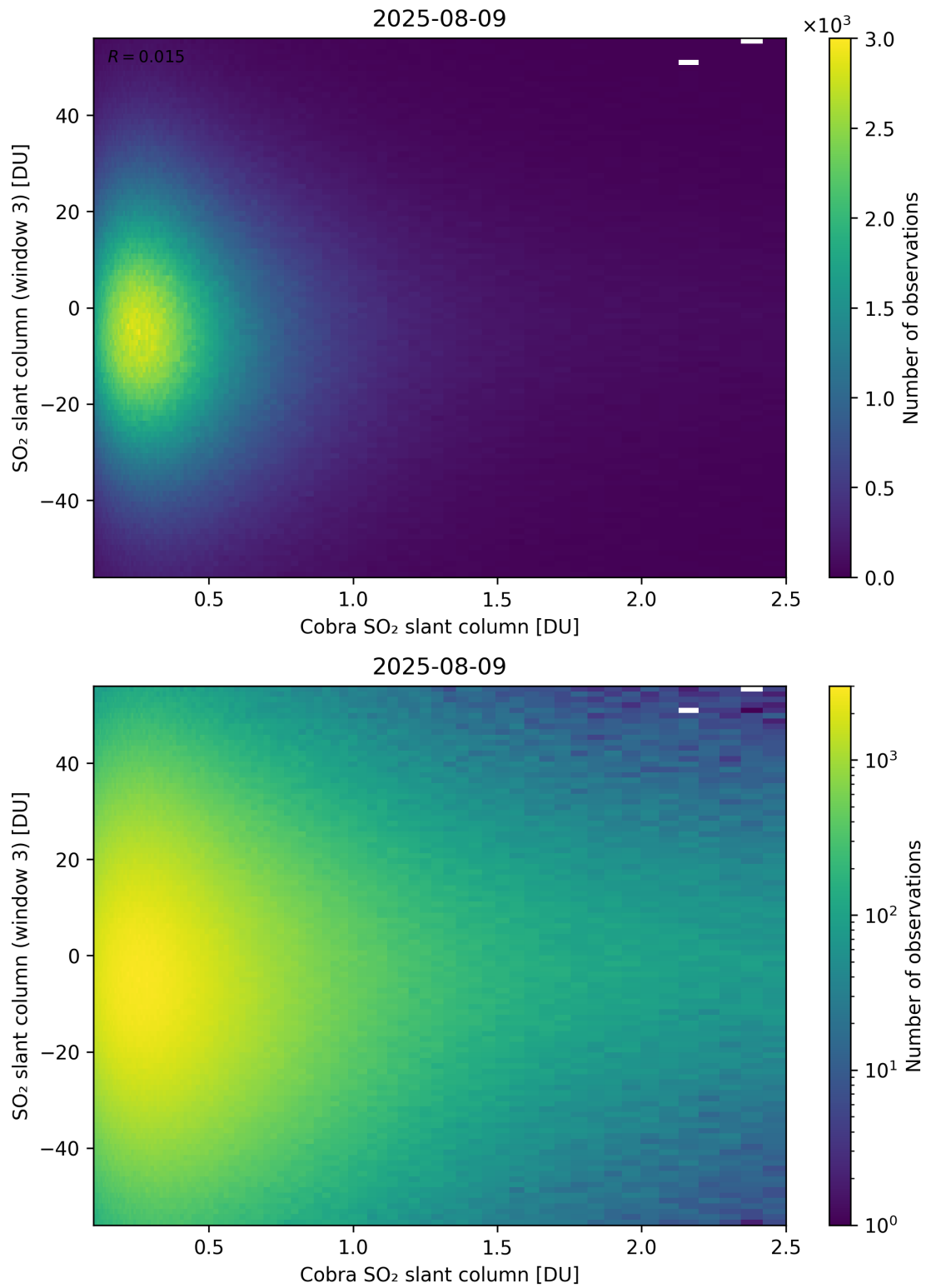
Figure 222: Scatter density plot of “Cobra SO 2 slant column” against “SO 2 slant column (window 3)” for 2025-08-09 to 2025-08-10.
