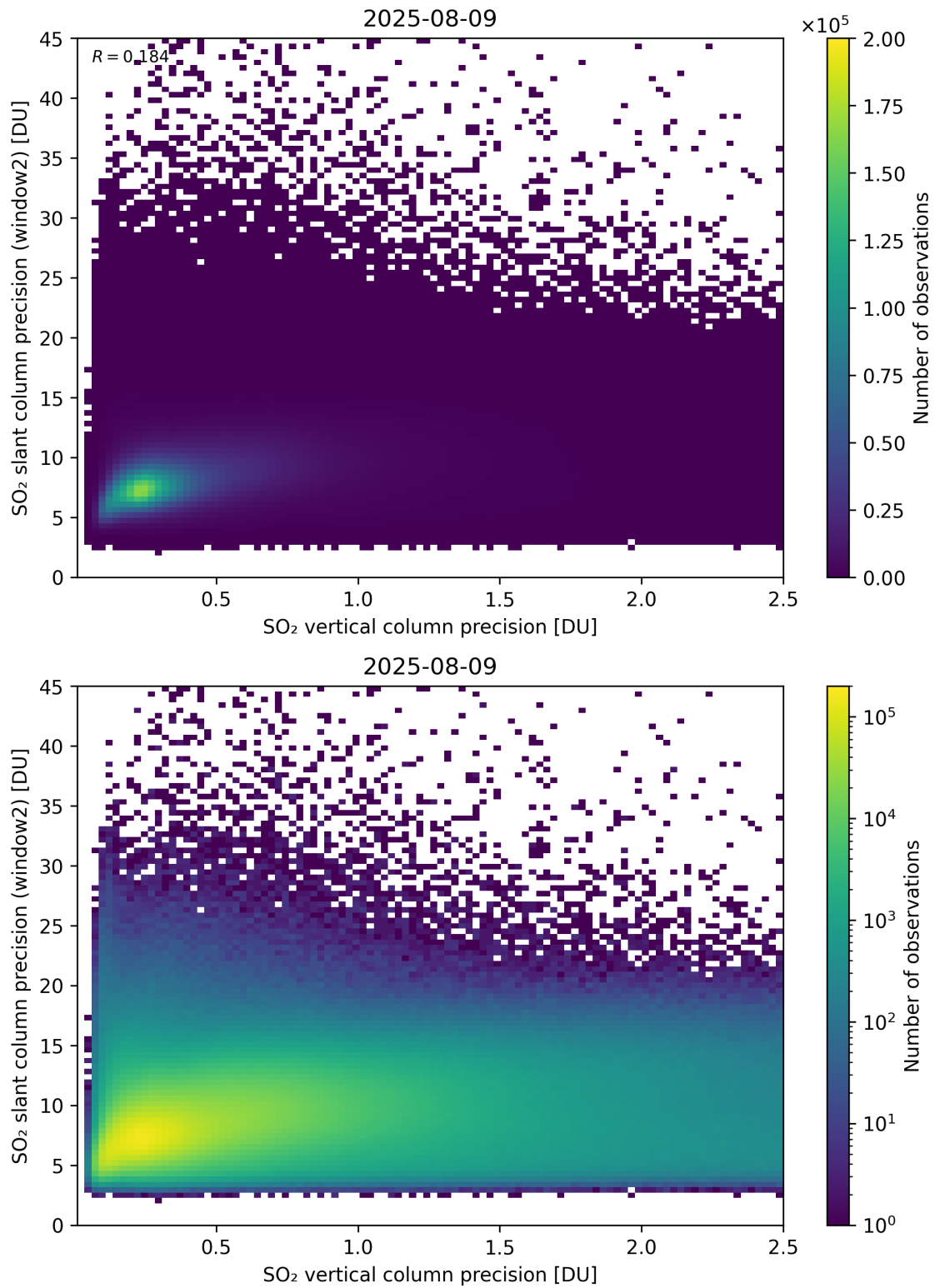
Figure 343: Scatter density plot of “SO 2 vertical column precision” against “SO 2 slant column precision (window2)” for 2025-08-09 to 2025-08-10.
