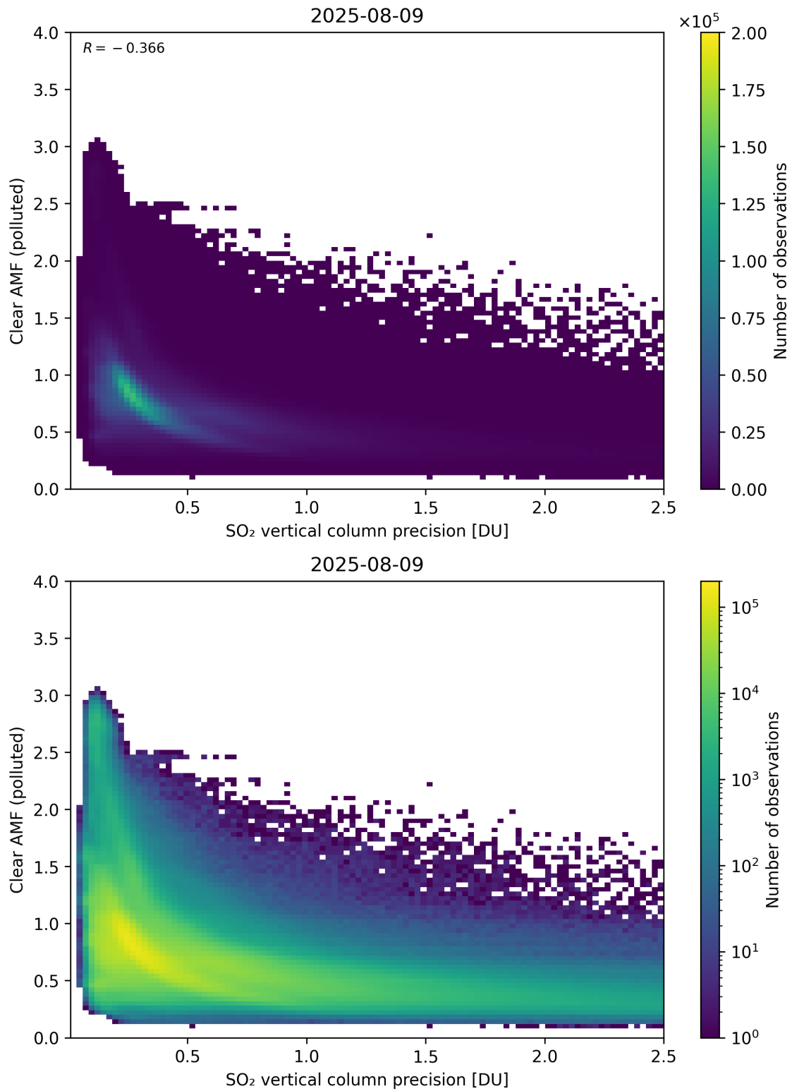
Figure 335: Scatter density plot of “SO 2 vertical column precision” against “Clear AMF (polluted)” for 2025-08-09 to 2025-08-10.
