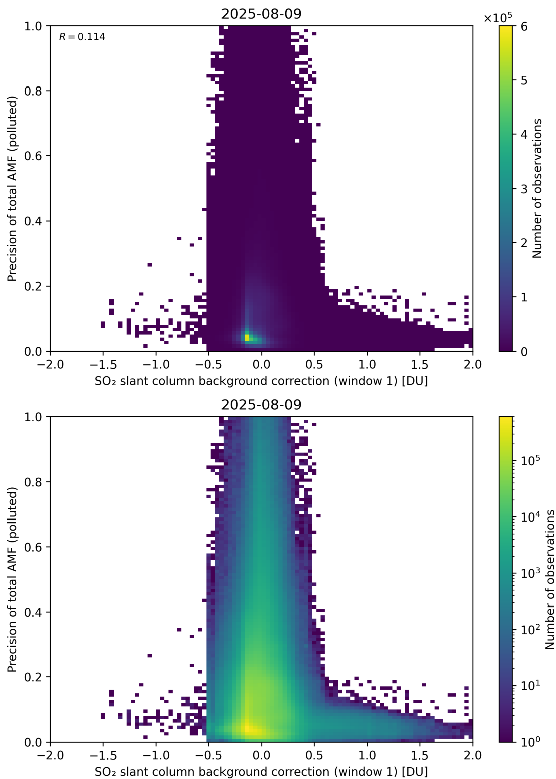
Figure 121: Scatter density plot of “SO 2 slant column background correction (window 1)” against “Precision of total AMF (polluted)” for 2025-08-09 to 2025-08-10.
