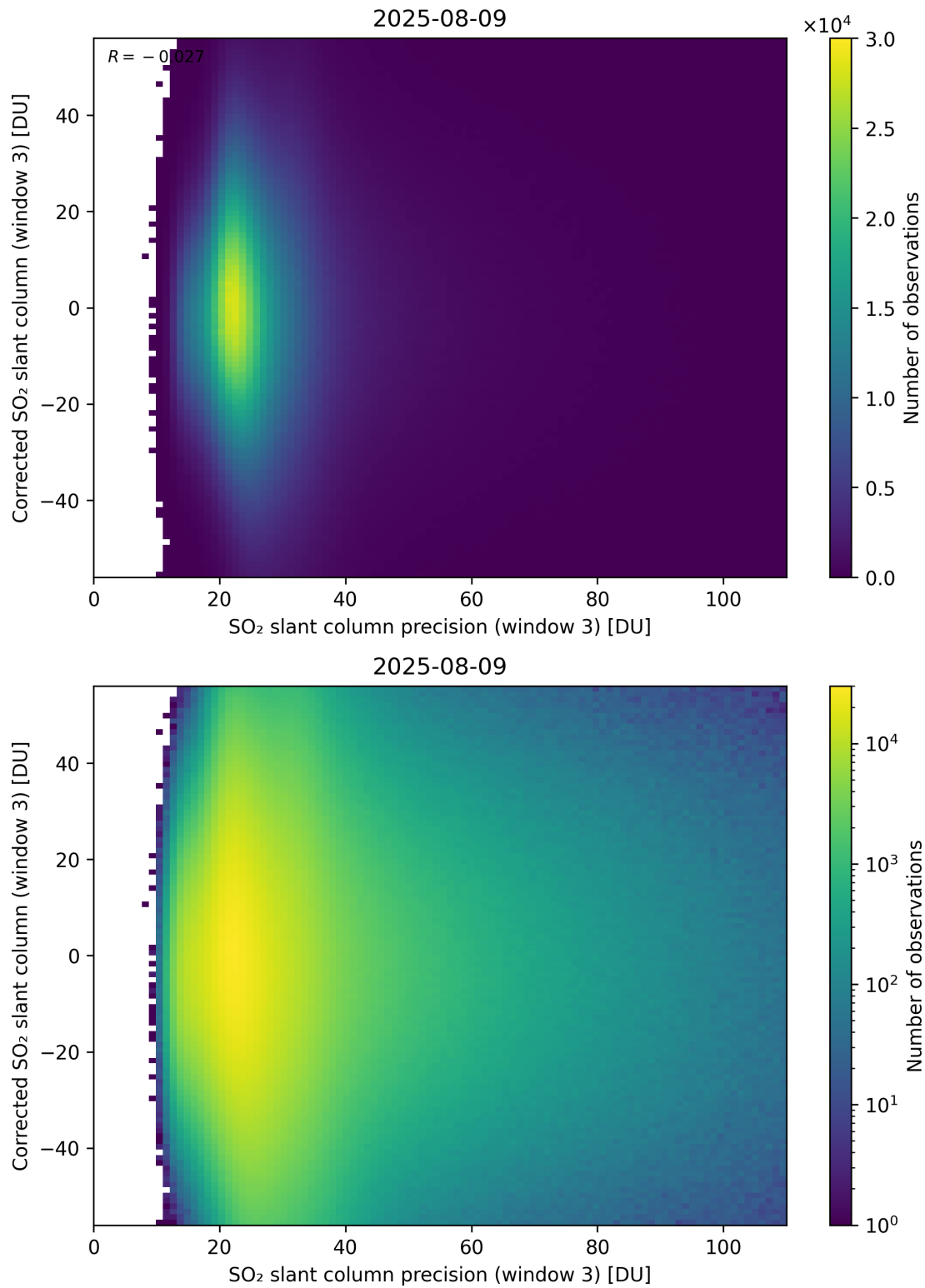
Figure 312: Scatter density plot of “SO 2 slant column precision (window 3)” against “Corrected SO 2 slant column (window 3)” for 2025-08-09 to 2025-08-10.
