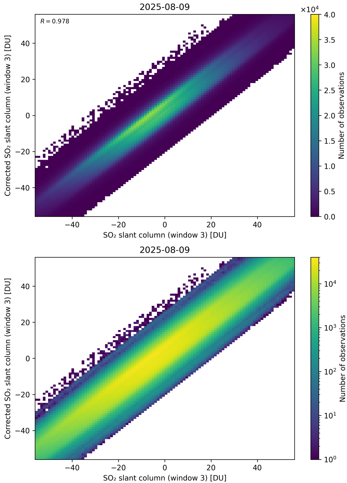
Figure 316: Scatter density plot of “SO 2 slant column (window 3)” against “Corrected SO 2 slant column (window 3)” for 2025-08-09 to 2025-08-10.
