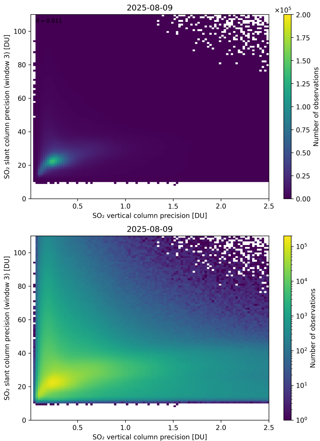
Figure 345: Scatter density plot of “SO 2 vertical column precision” against “SO 2 slant column precision (window 3)” for 2025-08-09 to 2025-08-10.
