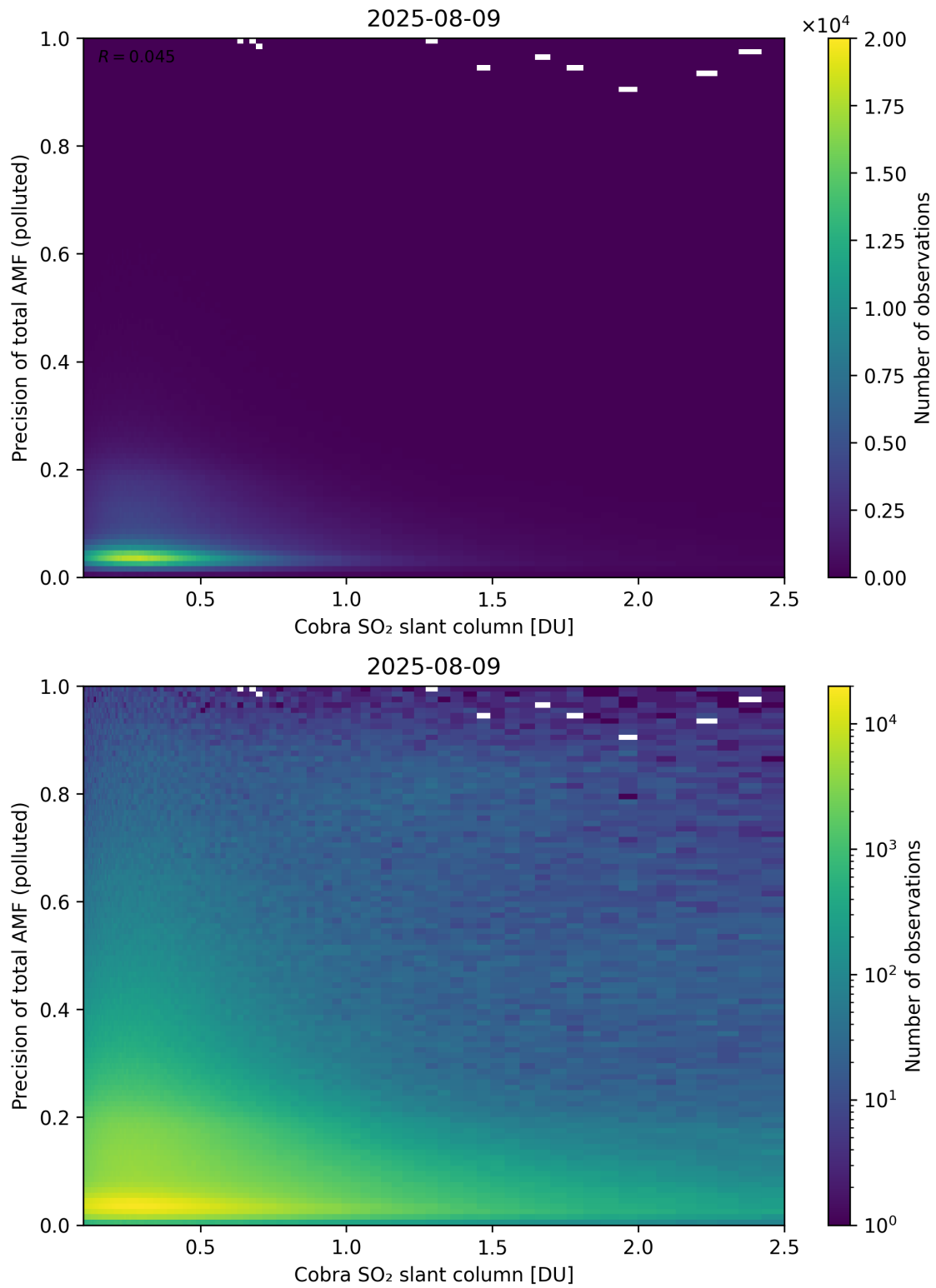
Figure 225: Scatter density plot of “Cobra SO 2 slant column” against “Precision of total AMF (polluted)” for 2025-08-09 to 2025-08-10.
