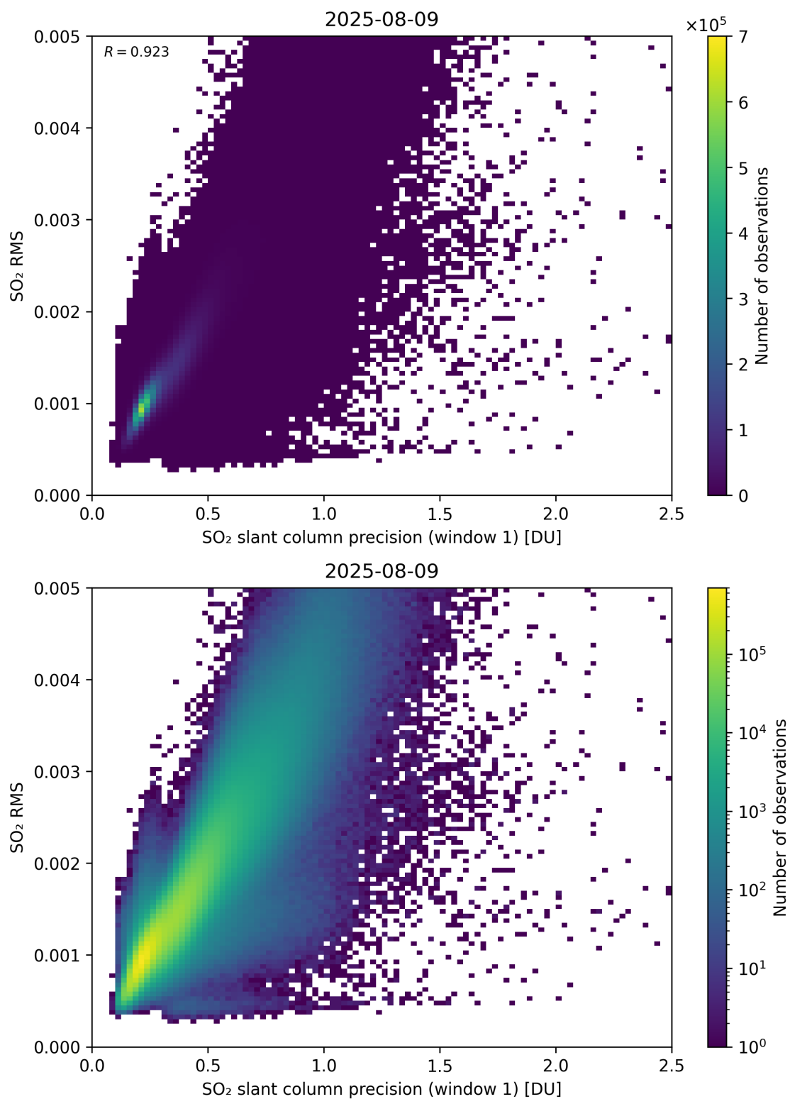
Figure 273: Scatter density plot of “SO 2 slant column precision (window 1)” against “SO 2 RMS” for 2025-08-09 to 2025-08-10.
