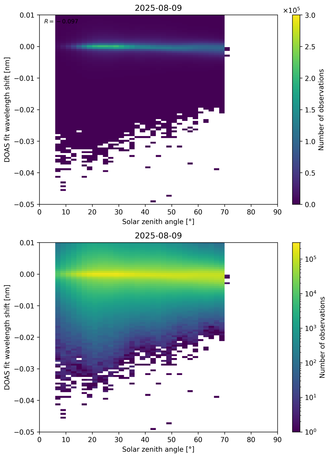
Figure 174: Scatter density plot of “Solar zenith angle” against “DOAS fit wavelength shift” for 2025-08-09 to 2025-08-10.
