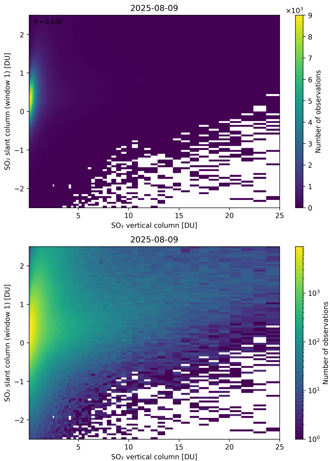
Figure 354: Scatter density plot of “SO 2 vertical column” against “SO 2 slant column (window 1)” for 2025-08-09 to 2025-08-10.
