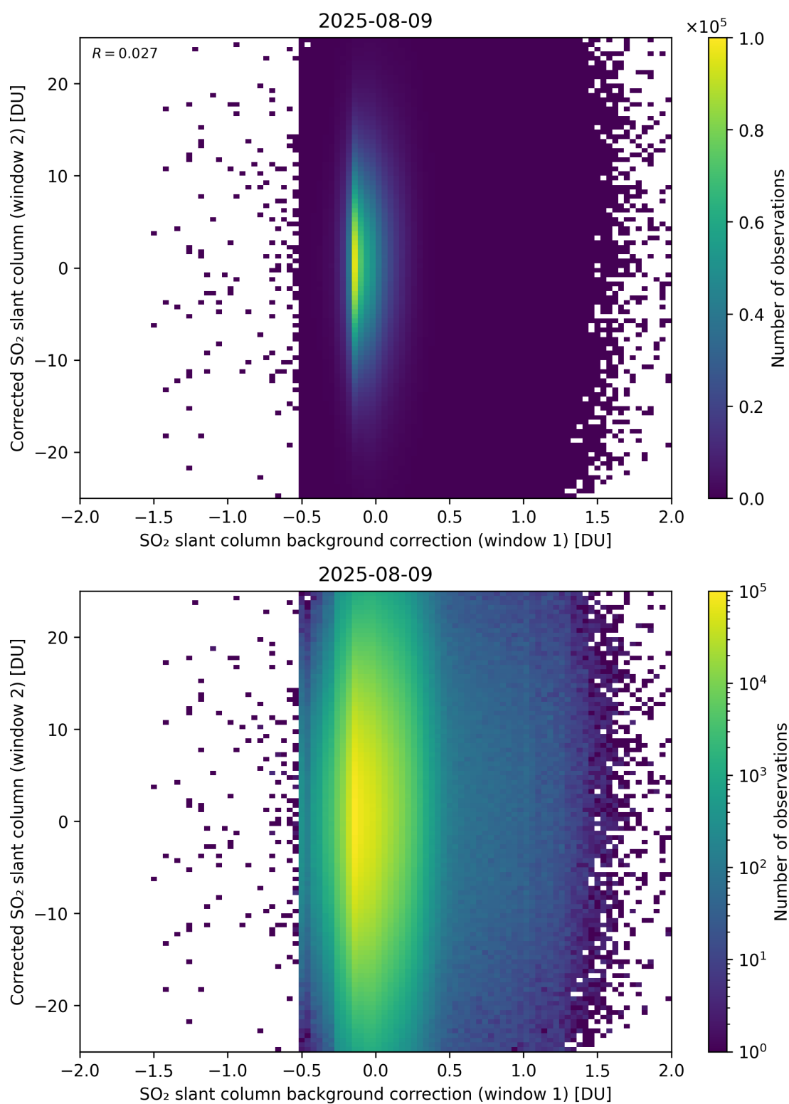
Figure 115: Scatter density plot of “SO 2 slant column background correction (window 1)” against “Corrected SO 2 slant column (window 2)” for 2025-08-09 to 2025-08-10.
