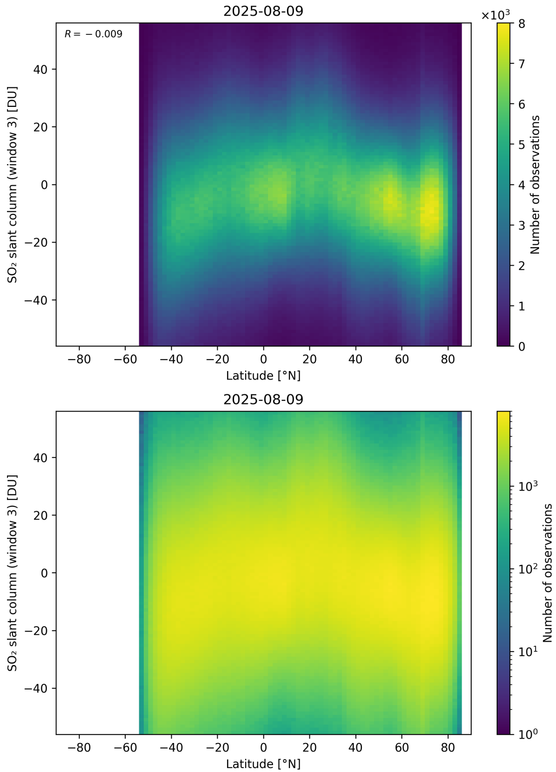
Figure 165: Scatter density plot of “Latitude” against “SO 2 slant column (window 3)” for 2025-08-09 to 2025-08-10.
