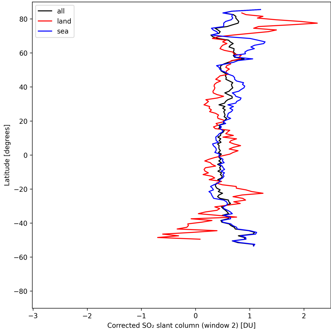
Figure 43: Zonal average of “Corrected SO 2 slant column (window 2)” for 2025-08-09 to 2025-08-10.
