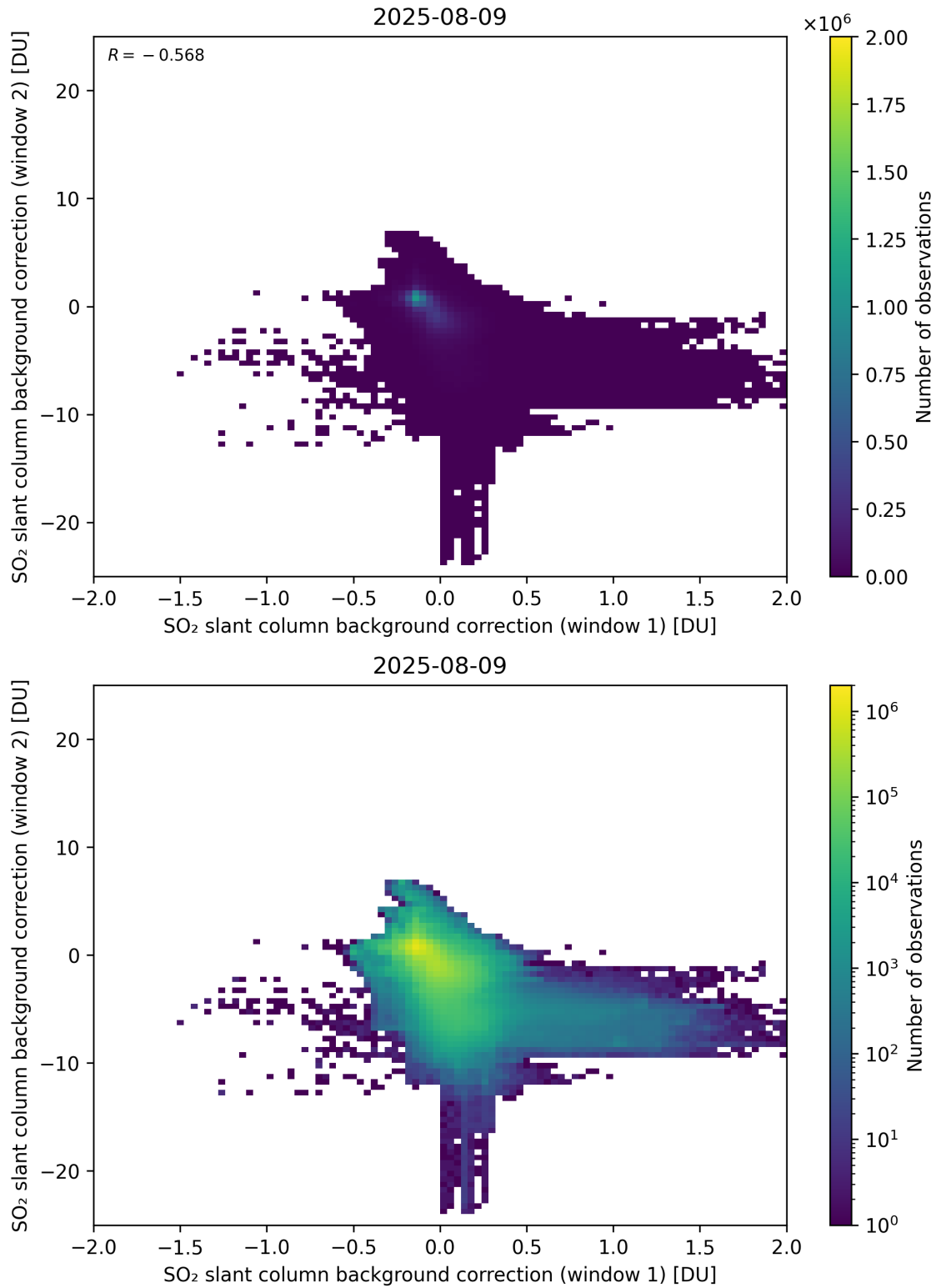
Figure 109: Scatter density plot of “SO 2 slant column background correction (window 1)” against “SO 2 slant column background correction (window 2)” for 2025-08-09 to 2025-08-10.
