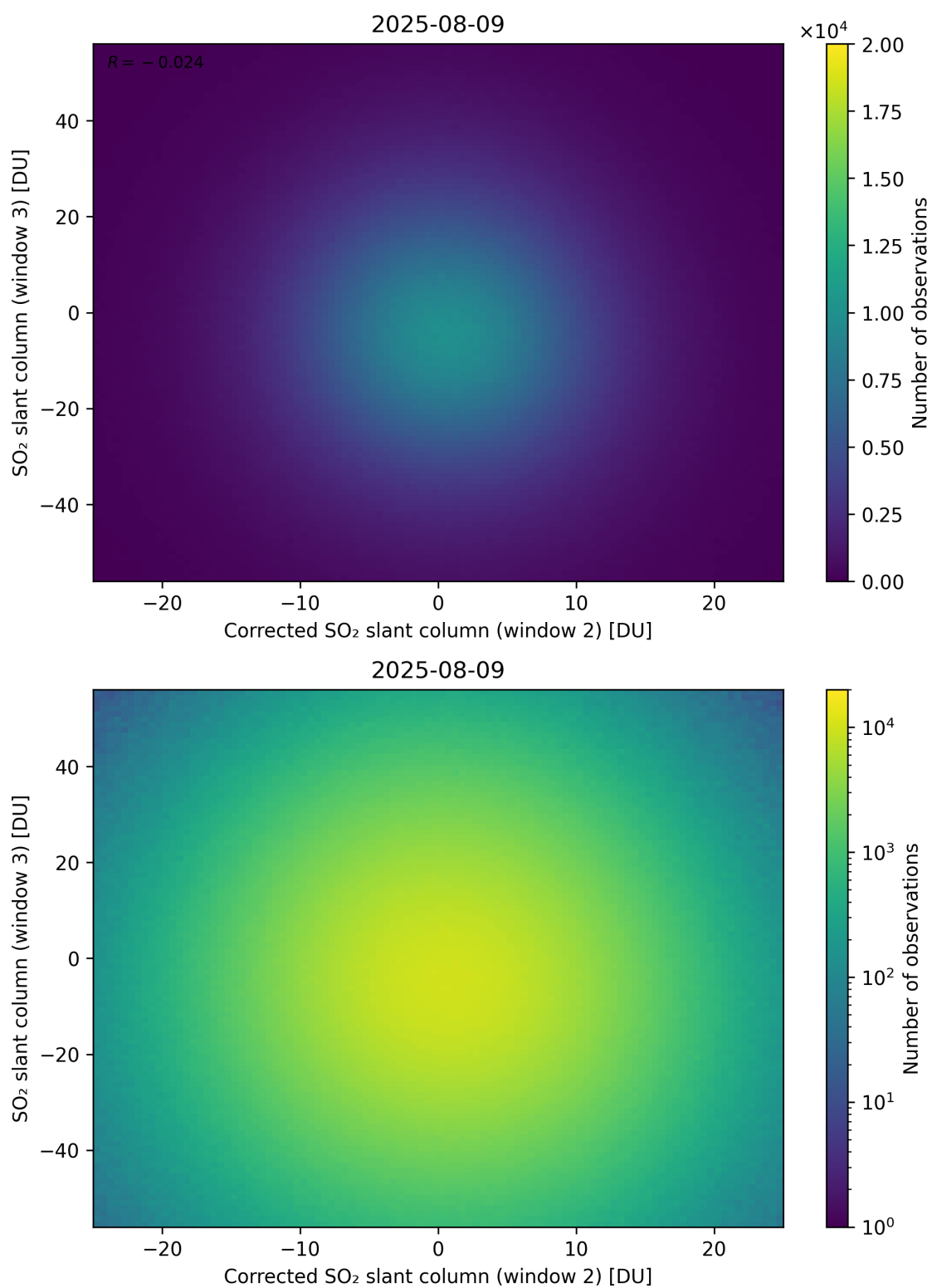
Figure 251: Scatter density plot of “Corrected SO 2 slant column (window 2)” against “SO 2 slant column (window 3)” for 2025-08-09 to 2025-08-10.
