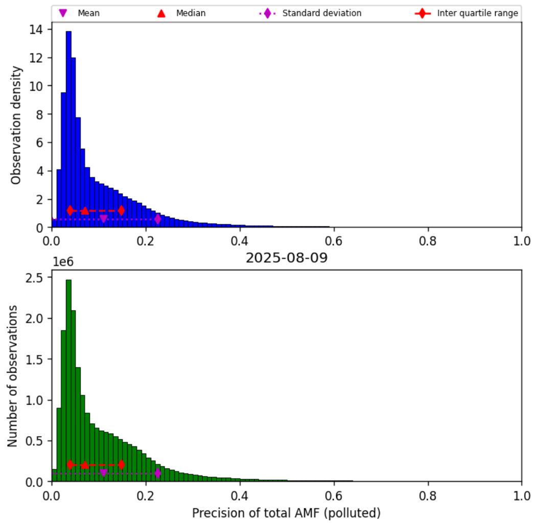
Figure 80: Histogram of “Precision of total AMF (polluted)” for 2025-08-09 to 2025-08-10
