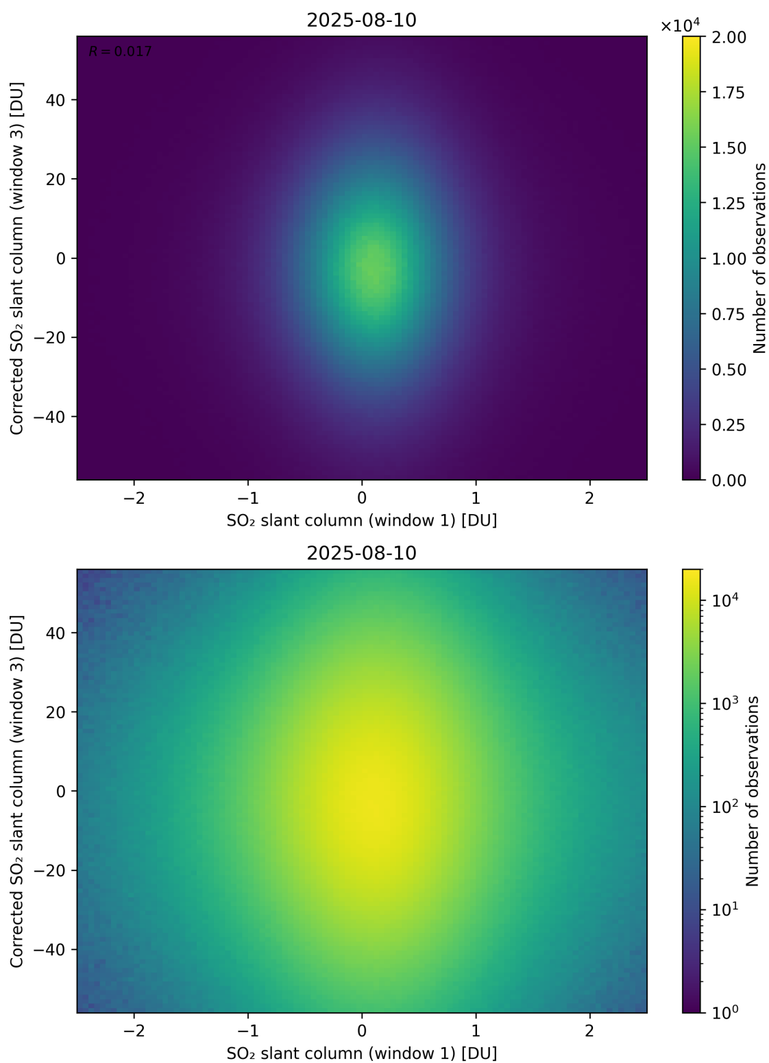
Figure 284: Scatter density plot of “SO 2 slant column (window 1)” against “Corrected SO 2 slant column (window 3)” for 2025-08-09 to 2025-08-11.
