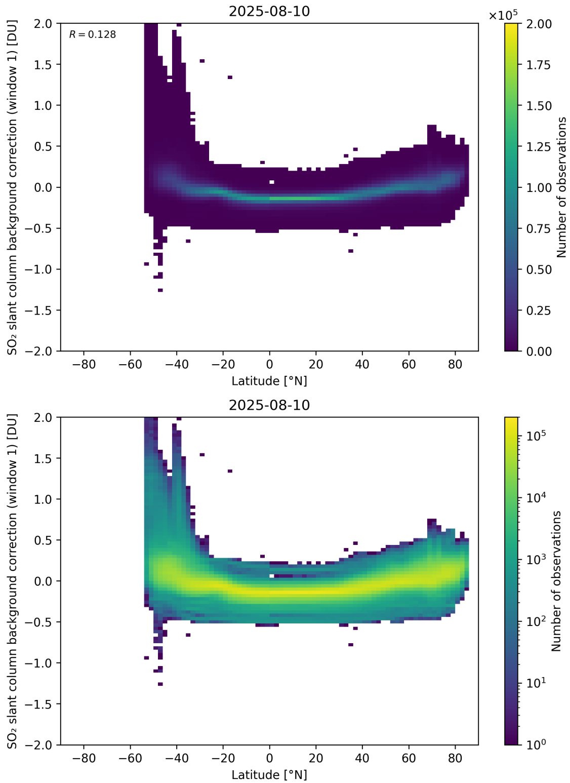
Figure 150: Scatter density plot of “Latitude” against “SO 2 slant column background correction (window 1)” for 2025-08-09 to 2025-08-11.
