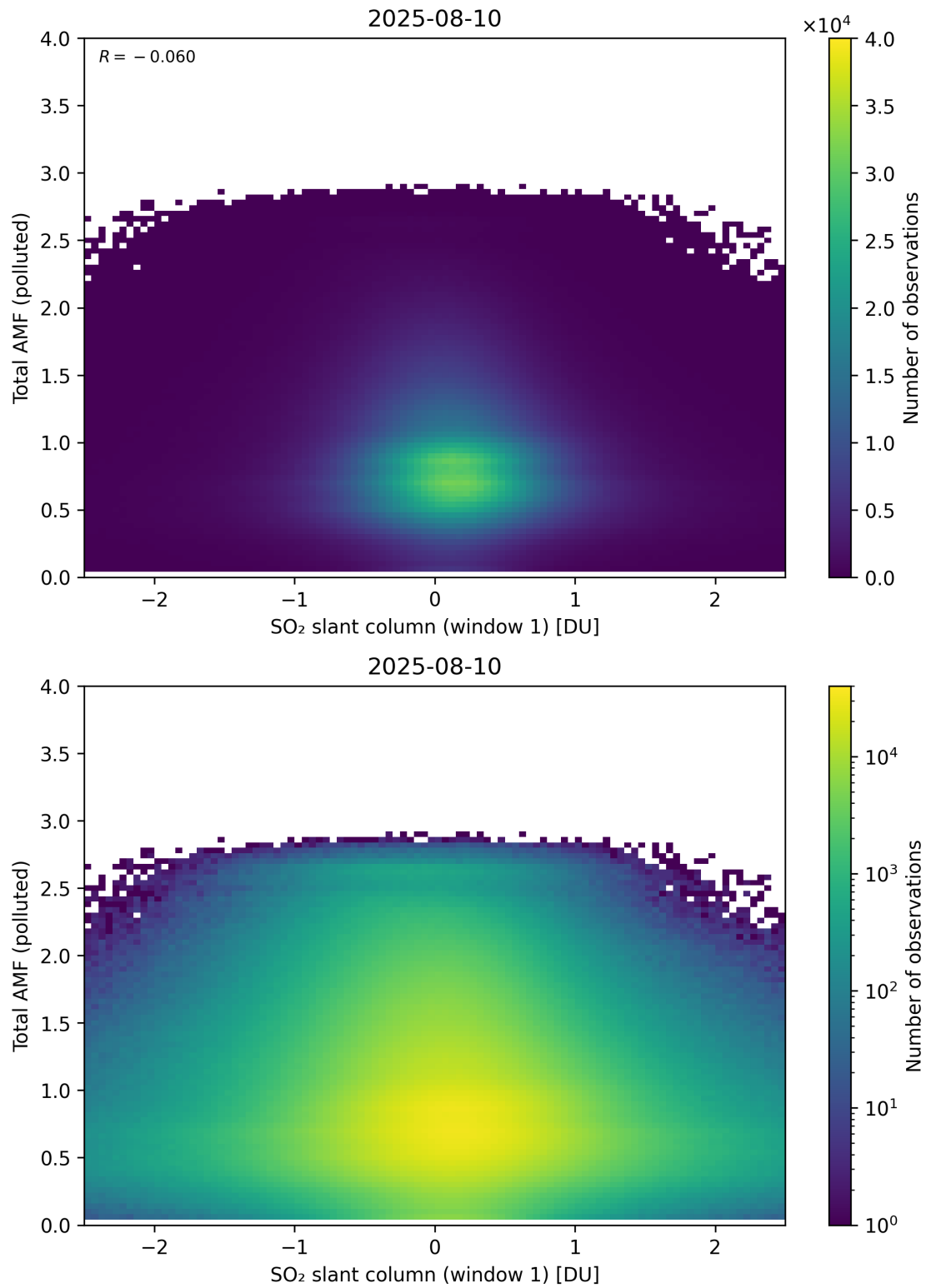
Figure 289: Scatter density plot of “SO 2 slant column (window 1)” against “Total AMF (polluted)” for 2025-08-09 to 2025-08-11.
