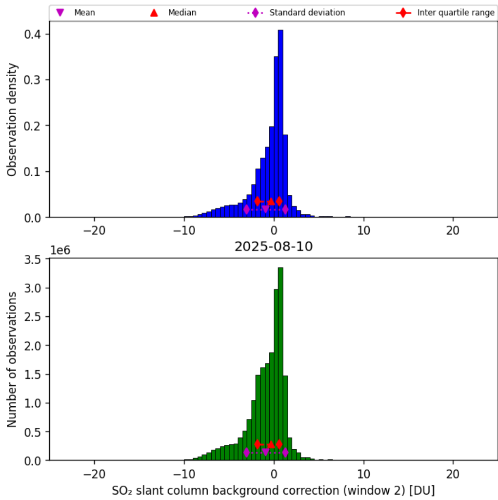
Figure 70: Histogram of “SO 2 slant column background correction (window 2)” for 2025-08-09 to 2025-08-11
