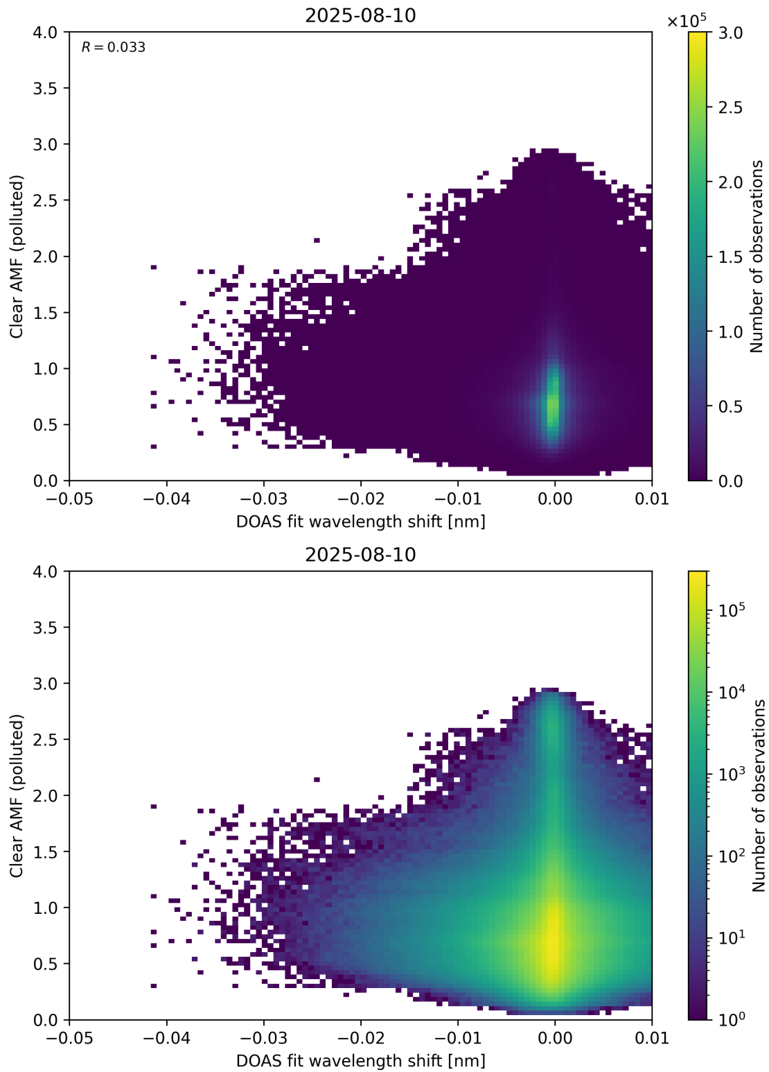
Figure 140: Scatter density plot of “DOAS fit wavelength shift” against “Clear AMF (polluted)” for 2025-08-09 to 2025-08-11.
