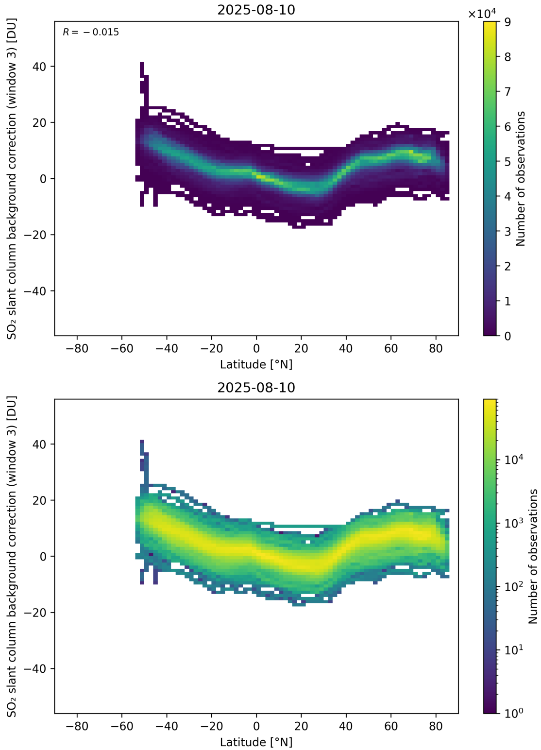
Figure 152: Scatter density plot of “Latitude” against “SO 2 slant column background correction (window 3)” for 2025-08-09 to 2025-08-11.
