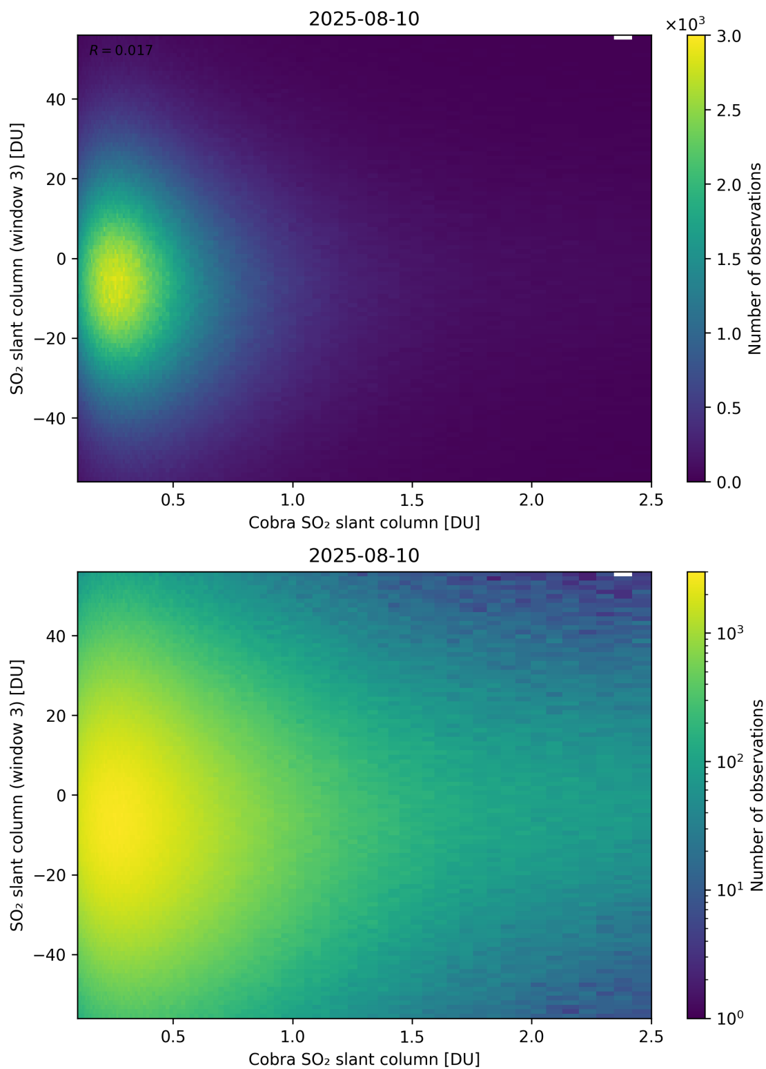
Figure 222: Scatter density plot of “Cobra SO 2 slant column” against “SO 2 slant column (window 3)” for 2025-08-09 to 2025-08-11.
