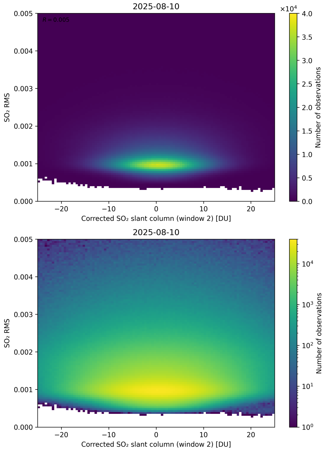
Figure 248: Scatter density plot of “Corrected SO 2 slant column (window 2)” against “SO 2 RMS” for 2025-08-09 to 2025-08-11.
