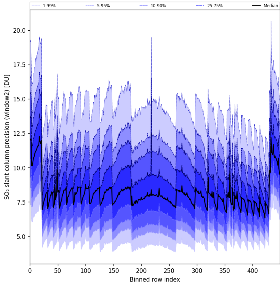
Figure 94: Along track statistics of “SO 2 slant column precision (window2)” for 2025-08-09 to 2025-08-11
