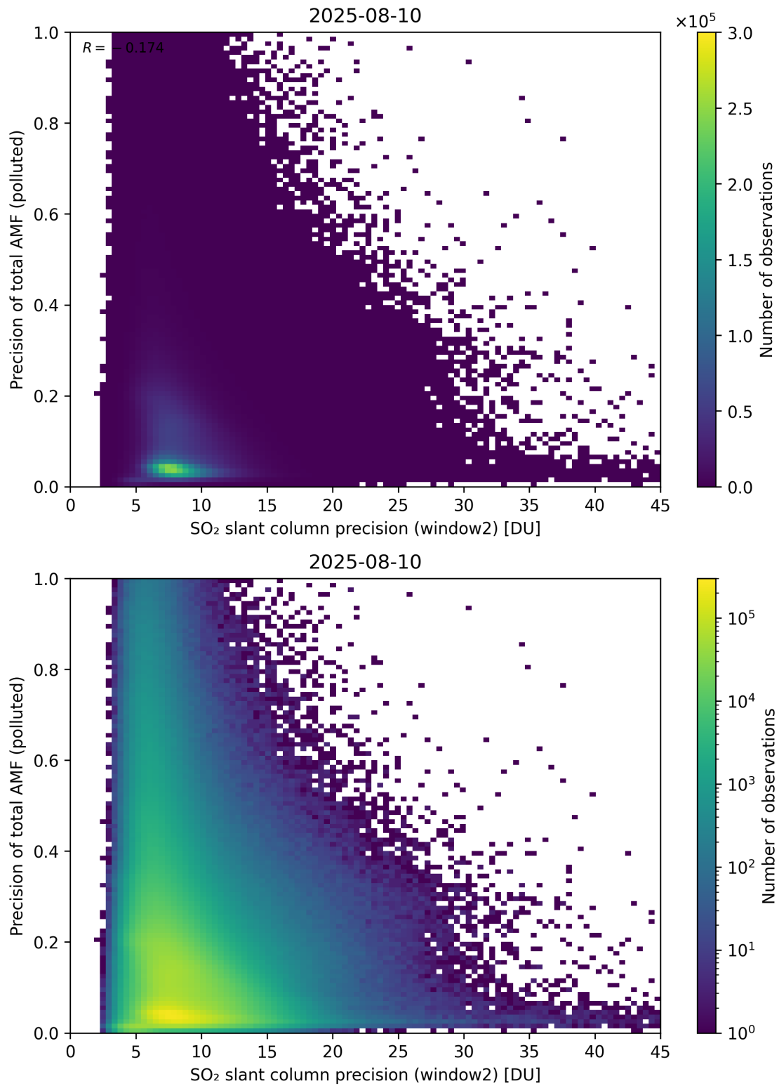
Figure 302: Scatter density plot of “SO 2 slant column precision (window2)” against “Precision of total AMF (polluted)” for 2025-08-09 to 2025-08-11.
