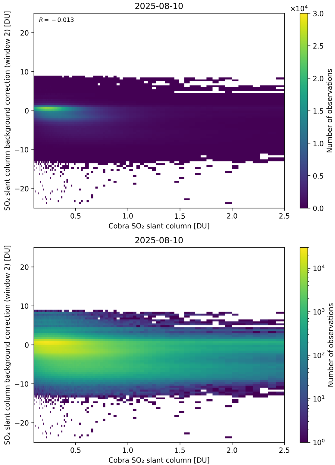
Figure 194: Scatter density plot of “Cobra SO 2 slant column” against “SO 2 slant column background correction (window 2)” for 2025-08-09 to 2025-08-11.
