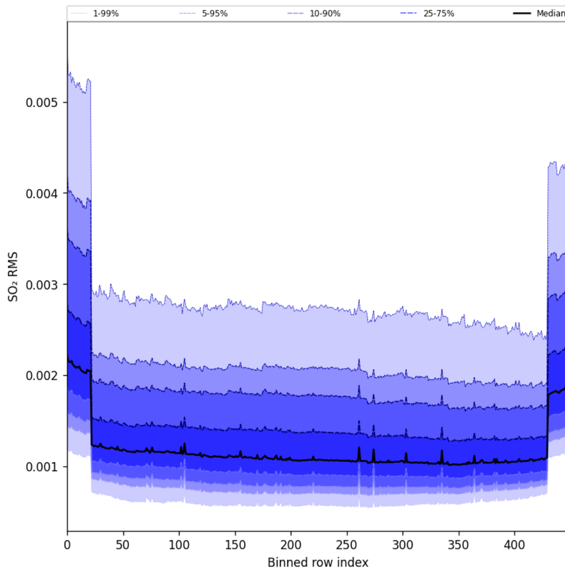
Figure 104: Along track statistics of “SO 2 RMS” for 2025-08-09 to 2025-08-11
