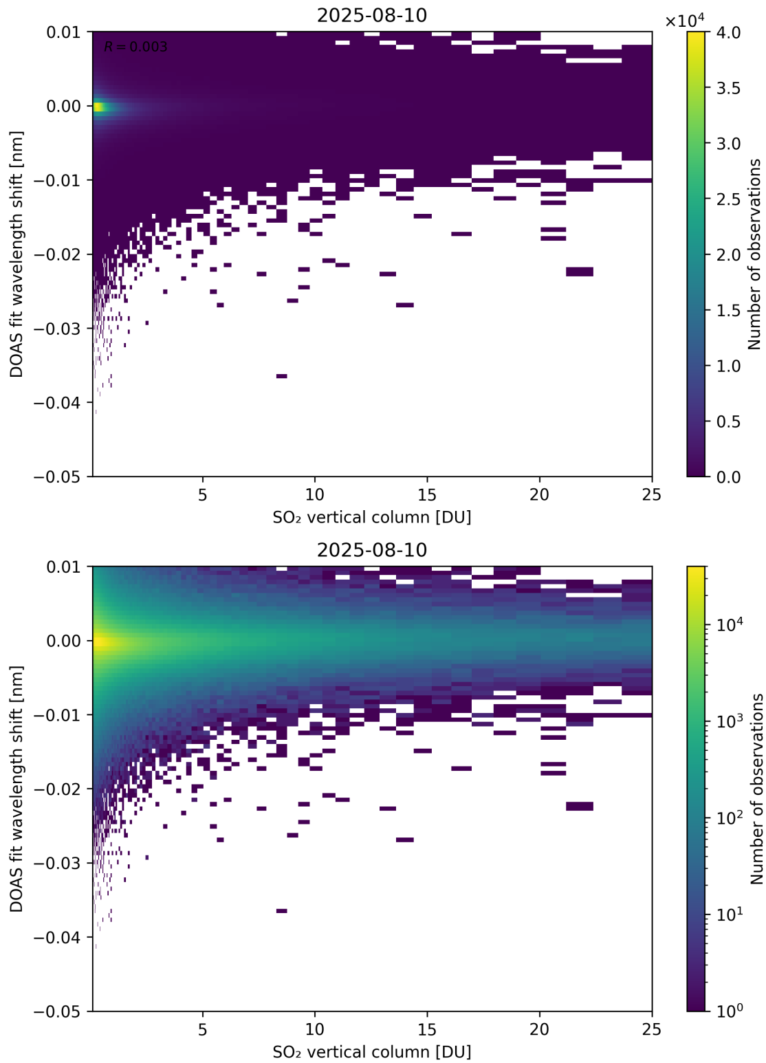
Figure 326: Scatter density plot of “SO 2 vertical column” against “DOAS fit wavelength shift” for 2025-08-09 to 2025-08-11.
