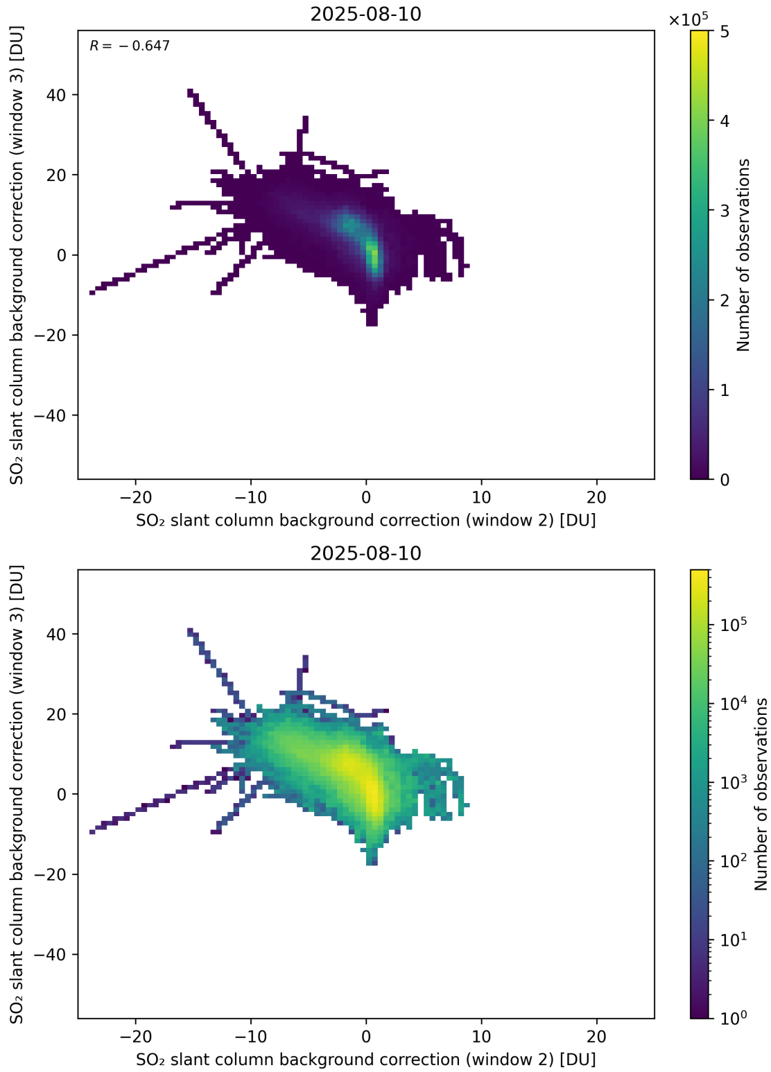
Figure 122: Scatter density plot of “SO 2 slant column background correction (window 2)” against “SO 2 slant column background correction (window 3)” for 2025-08-09 to 2025-08-11.
