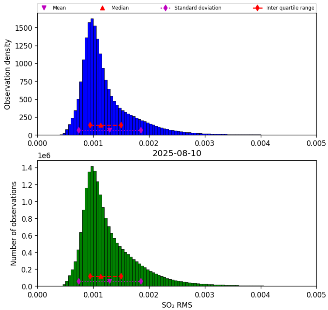
Figure 78: Histogram of “SO 2 RMS” for 2025-08-09 to 2025-08-11
