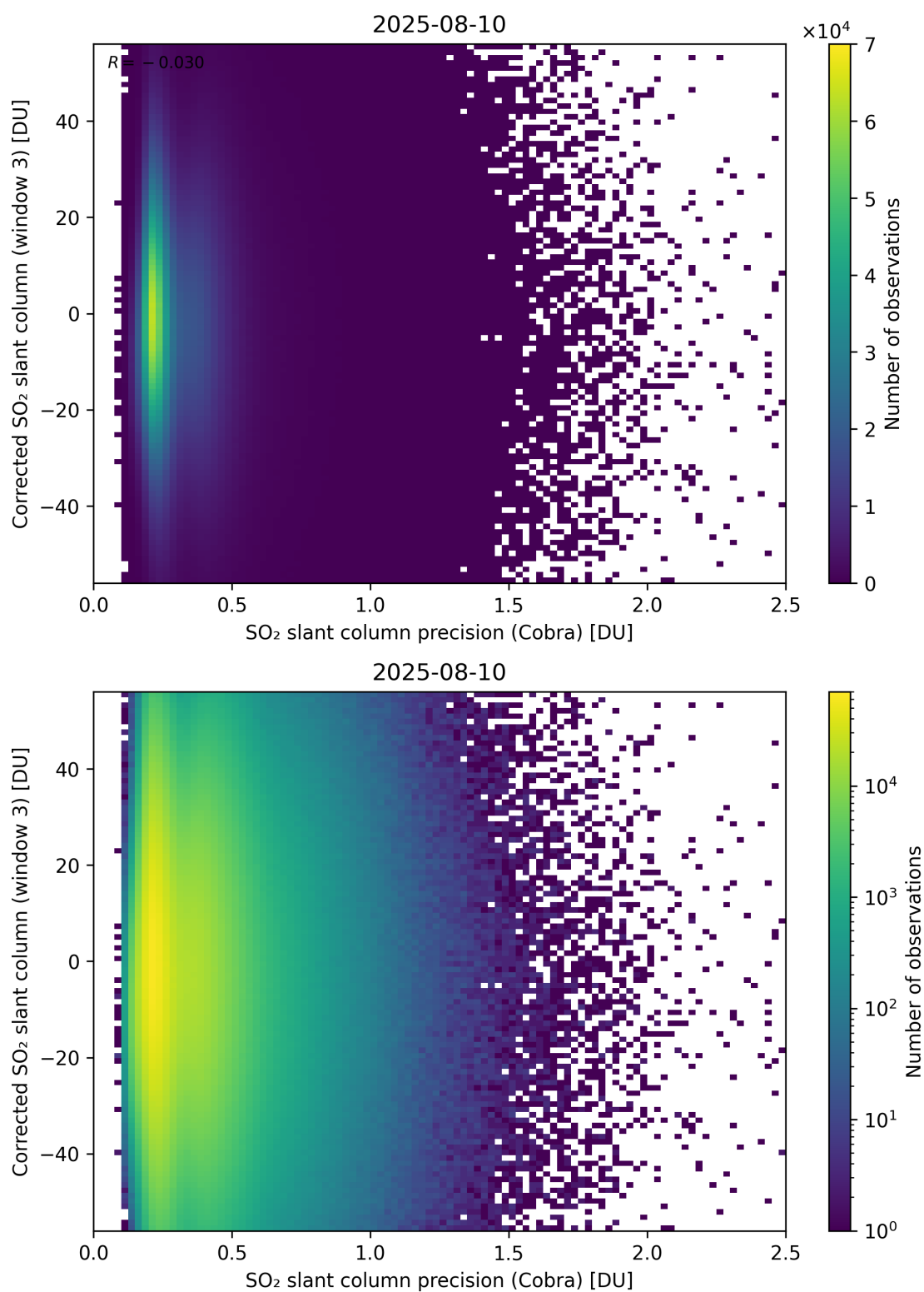
Figure 207: Scatter density plot of “SO 2 slant column precision (Cobra)” against “Corrected SO 2 slant column (window 3)” for 2025-08-09 to 2025-08-11.
