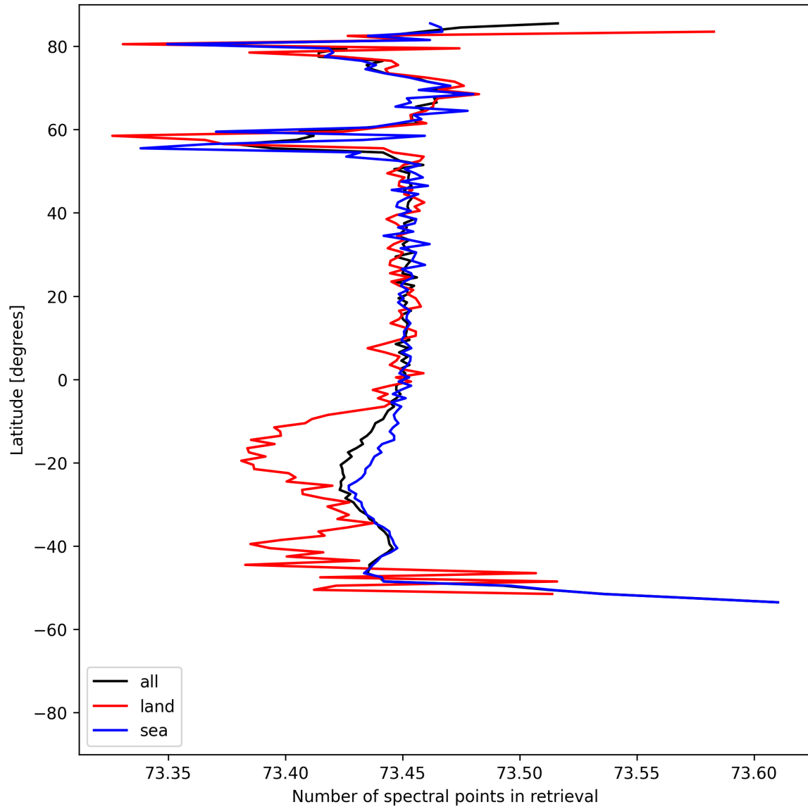
Figure 56: Zonal average of “Number of spectral points in retrieval” for 2025-08-09 to 2025-08-11.
