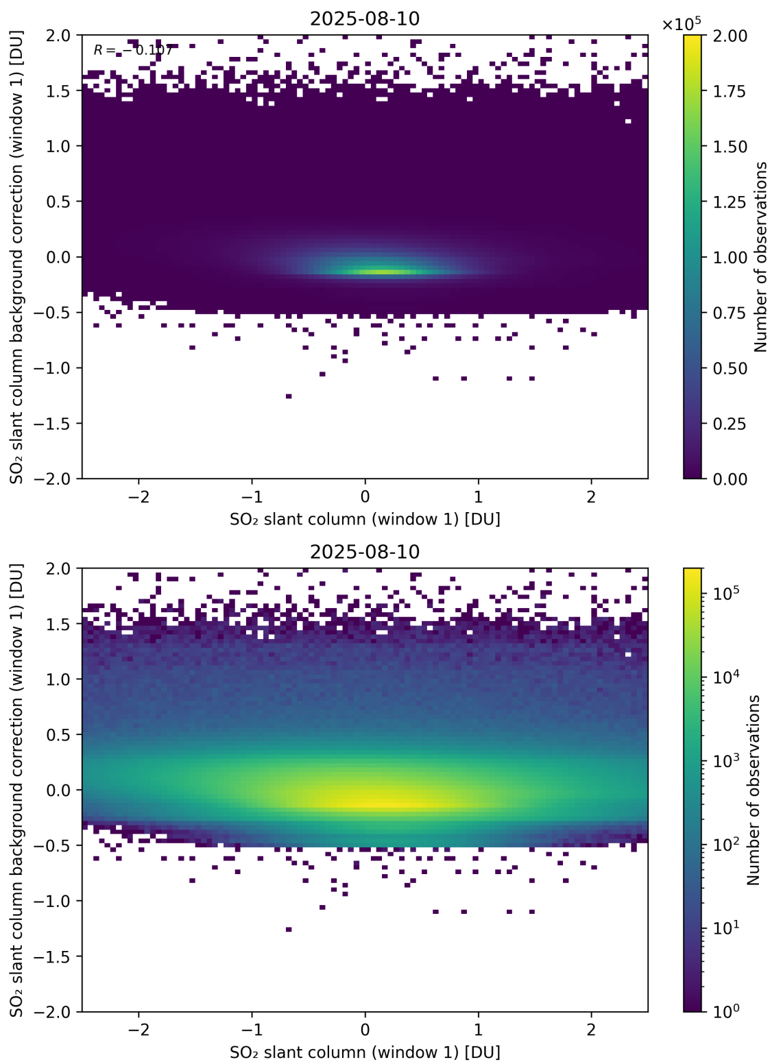
Figure 262: Scatter density plot of “SO 2 slant column (window 1)” against “SO 2 slant column background correction (window 1)” for 2025-08-09 to 2025-08-11.
