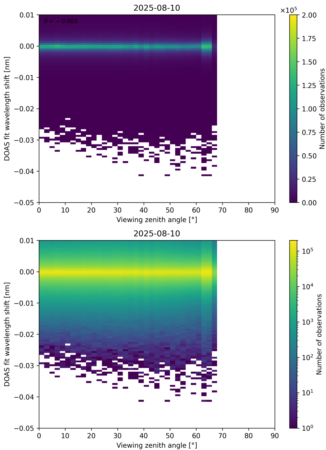
Figure 365: Scatter density plot of “Viewing zenith angle” against “DOAS fit wavelength shift” for 2025-08-09 to 2025-08-11.
