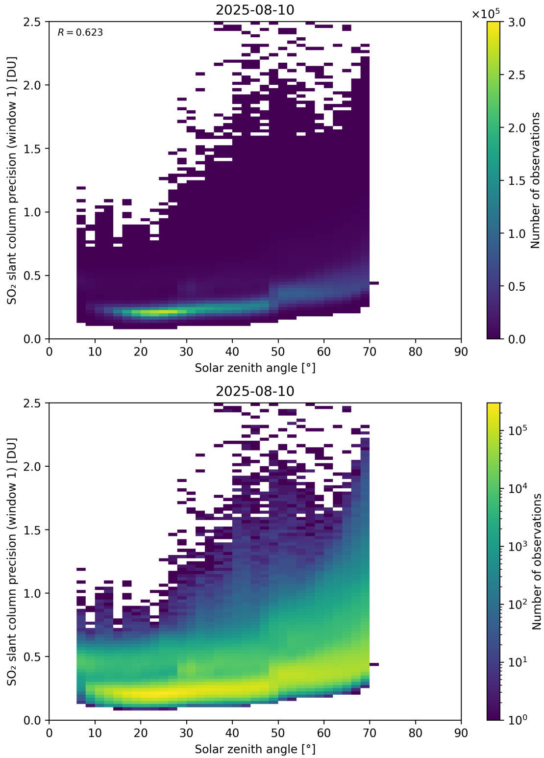
Figure 185: Scatter density plot of “Solar zenith angle” against “SO 2 slant column precision (window 1)” for 2025-08-09 to 2025-08-11.
