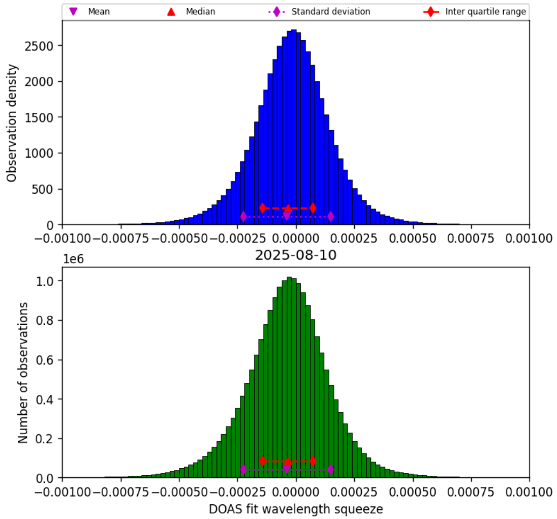
Figure 77: Histogram of “DOAS fit wavelength squeeze” for 2025-08-09 to 2025-08-11
