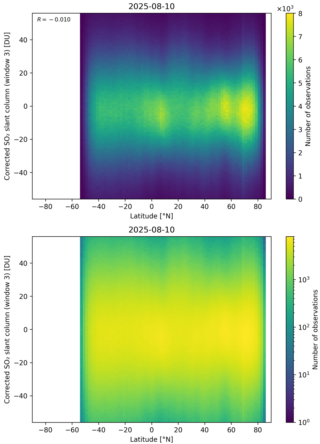
Figure 161: Scatter density plot of “Latitude” against “Corrected SO 2 slant column (window 3)” for 2025-08-09 to 2025-08-11.
