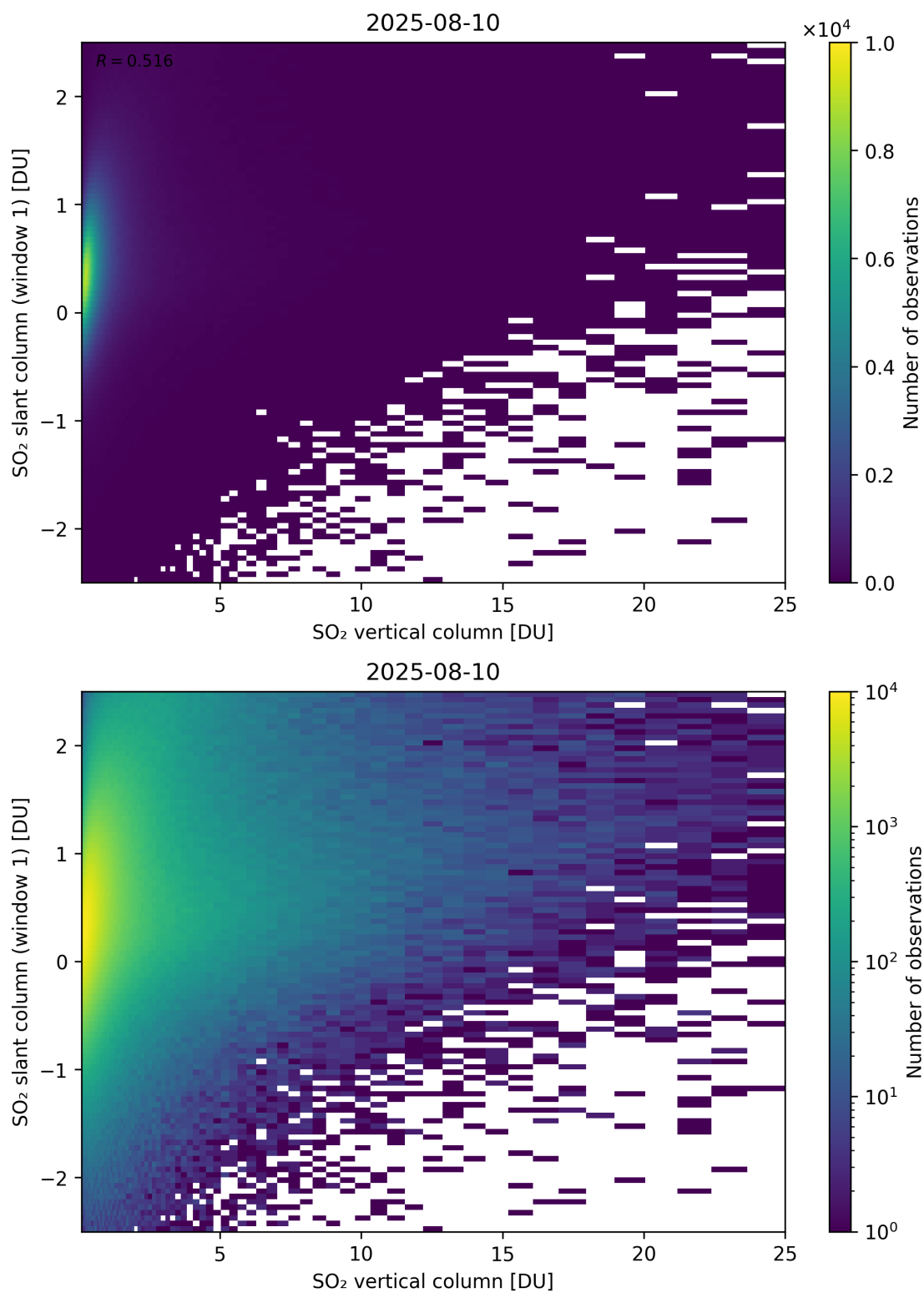
Figure 354: Scatter density plot of “SO 2 vertical column” against “SO 2 slant column (window 1)” for 2025-08-09 to 2025-08-11.
