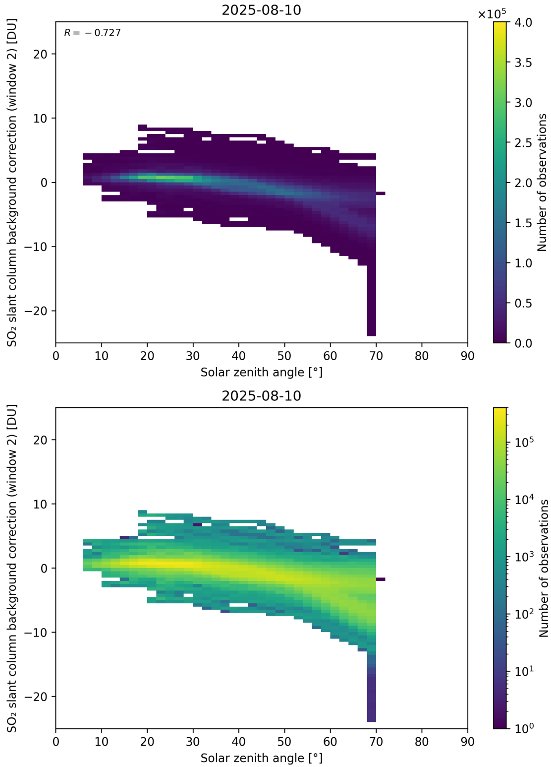
Figure 172: Scatter density plot of “Solar zenith angle” against “SO 2 slant column background correction (window 2)” for 2025-08-09 to 2025-08-11.
