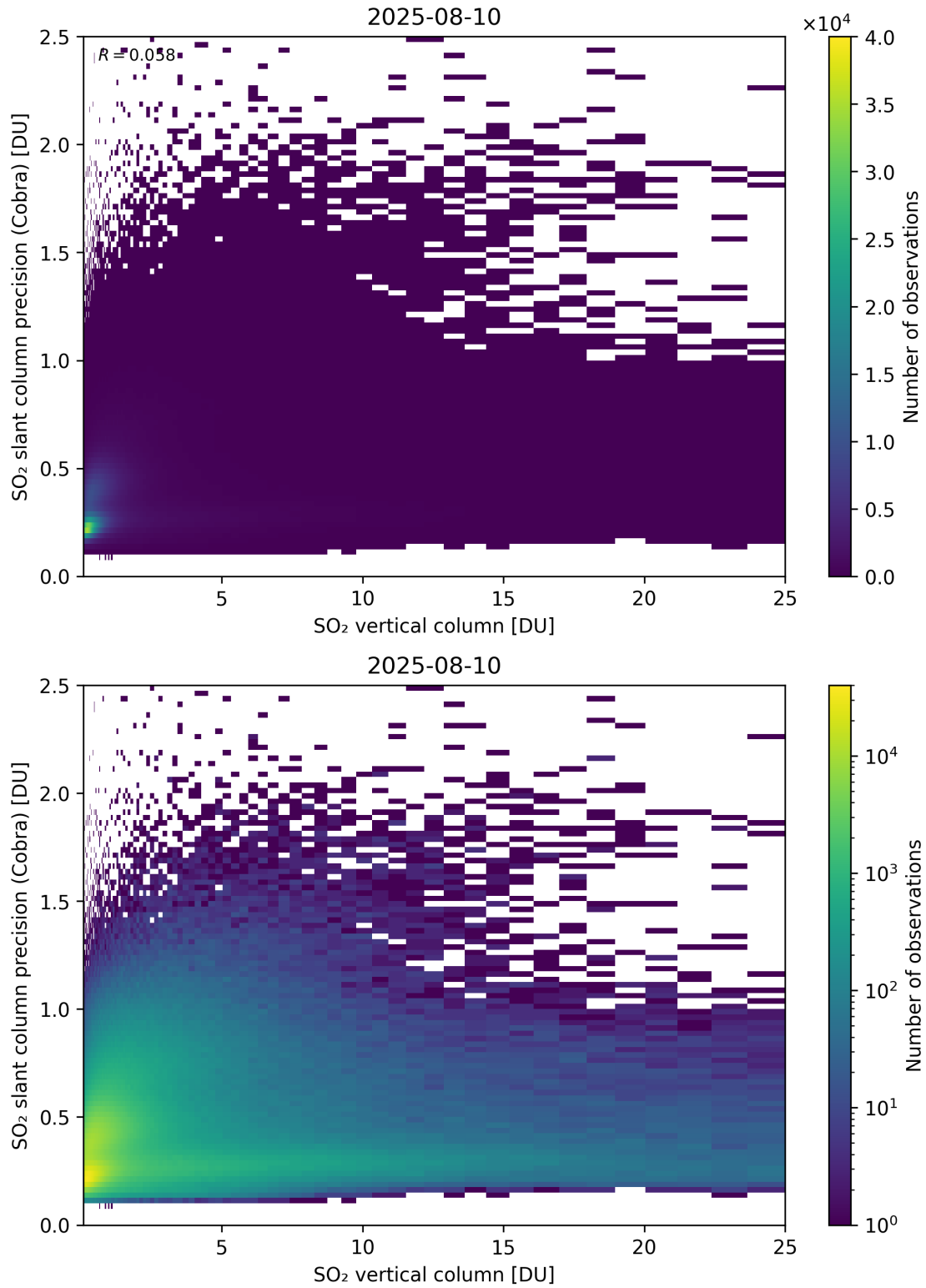
Figure 350: Scatter density plot of “SO 2 vertical column” against “SO 2 slant column precision (Cobra)” for 2025-08-09 to 2025-08-11.
