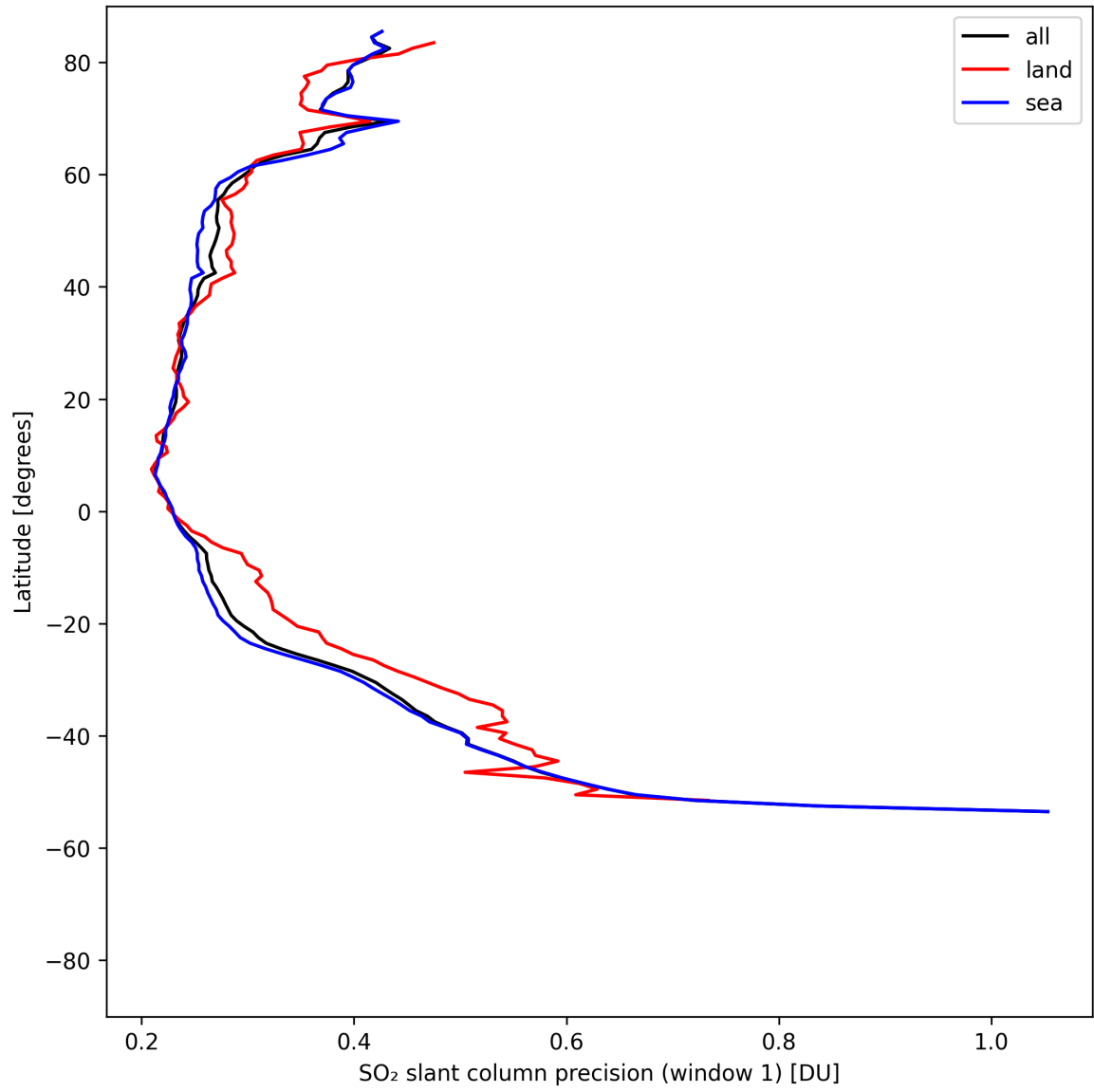
Figure 38: Zonal average of “SO 2 slant column precision (window 1)” for 2025-08-09 to 2025-08-11.
