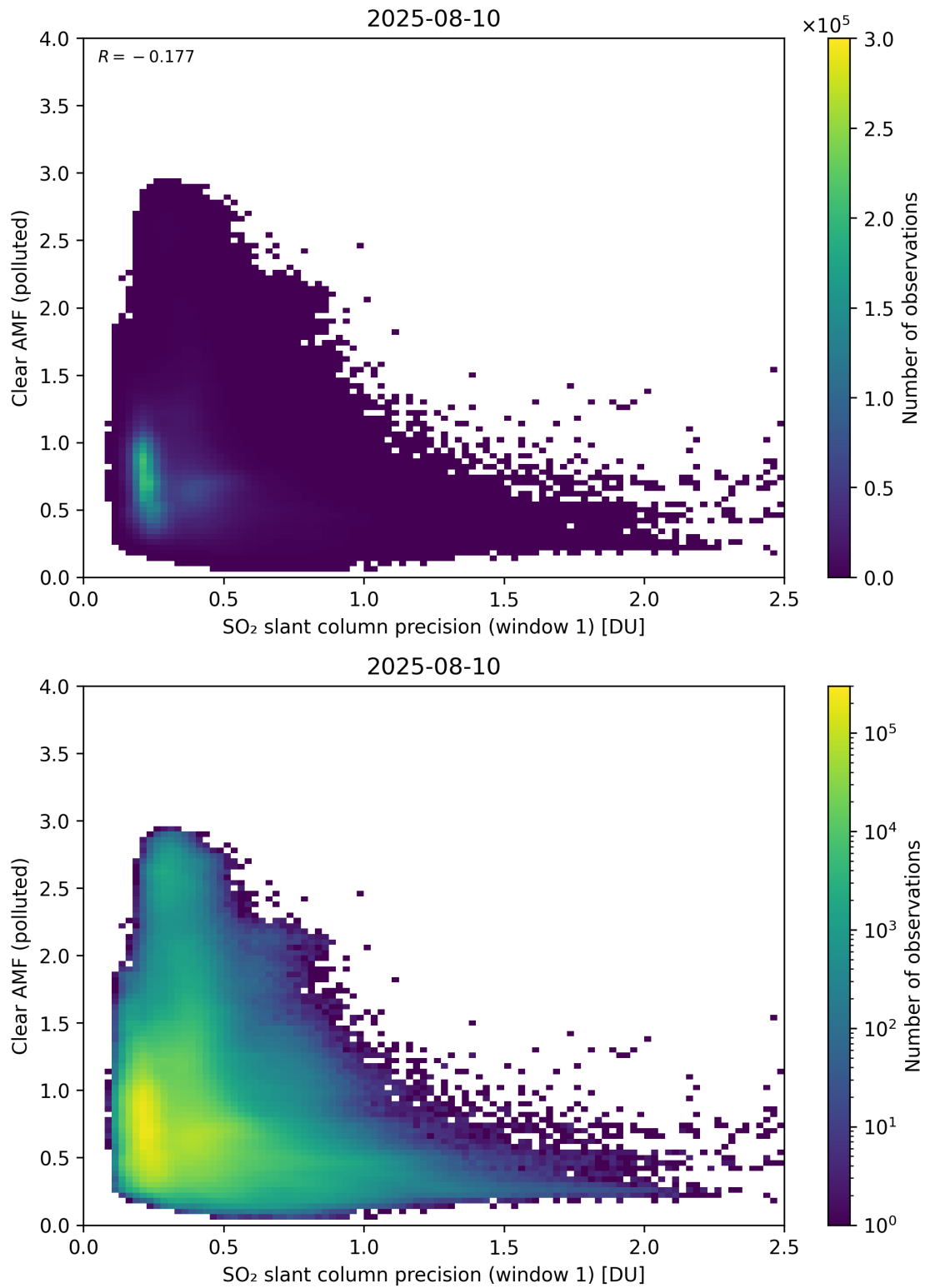
Figure 274: Scatter density plot of “SO 2 slant column precision (window 1)” against “Clear AMF (polluted)” for 2025-08-09 to 2025-08-11.
