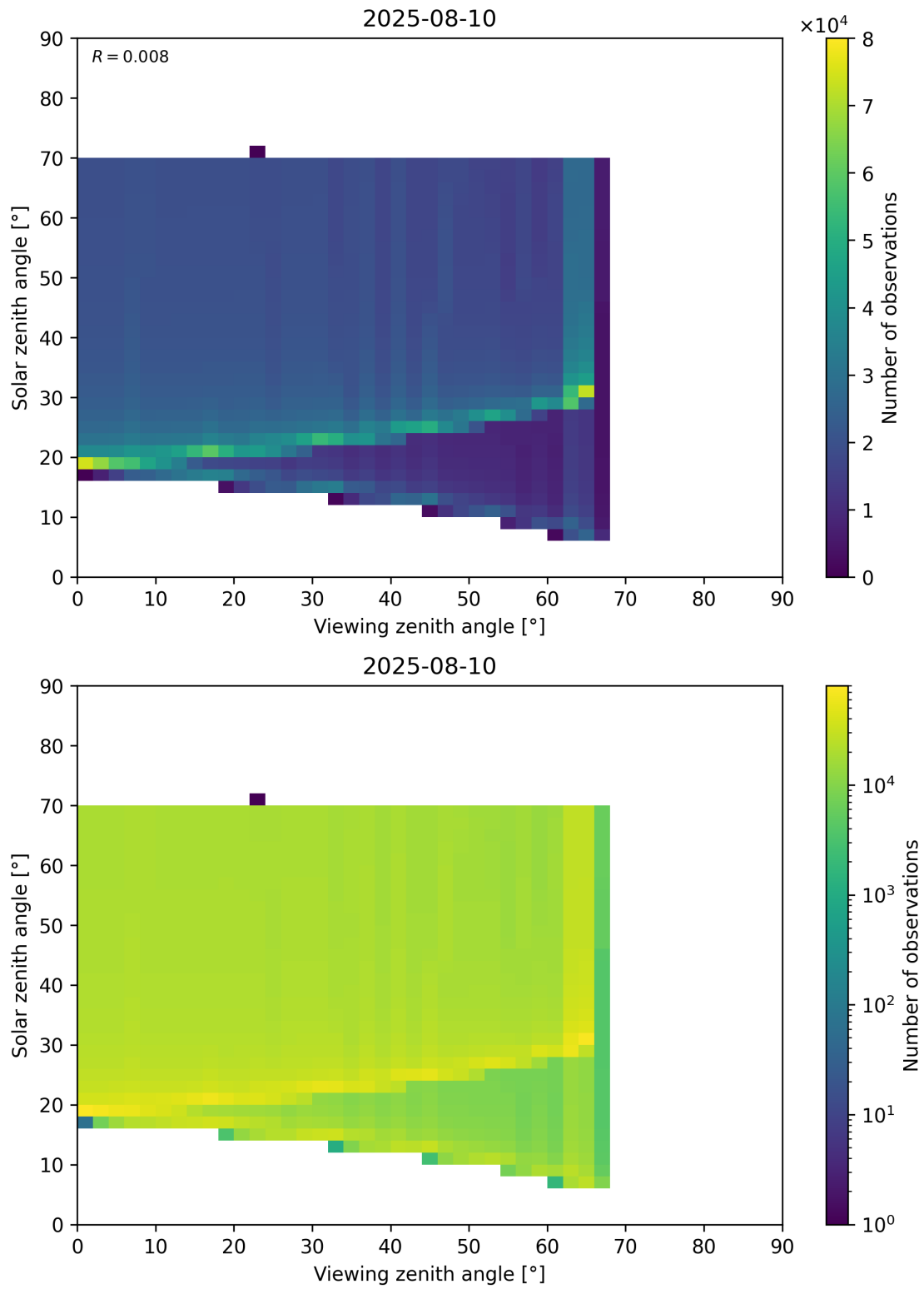
Figure 369: Scatter density plot of “Viewing zenith angle” against “Solar zenith angle” for 2025-08-09 to 2025-08-11.
