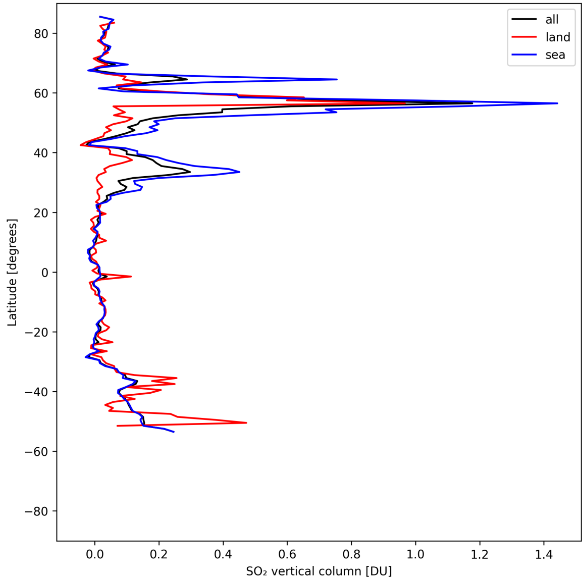
Figure 32: Zonal average of “SO 2 vertical column” for 2025-08-09 to 2025-08-11.
