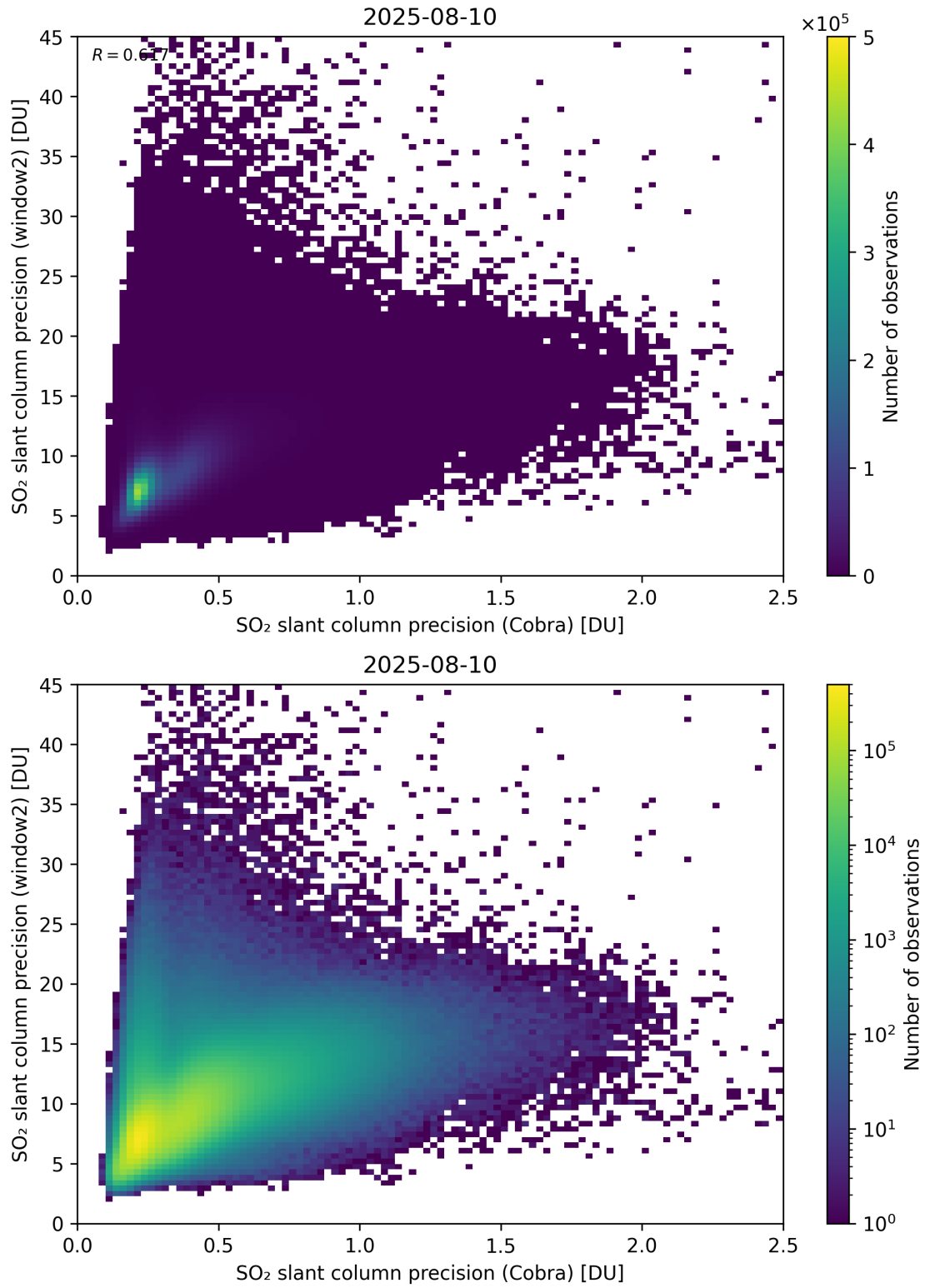
Figure 210: Scatter density plot of “SO 2 slant column precision (Cobra)” against “SO 2 slant column precision (window2)” for 2025-08-09 to 2025-08-11.
