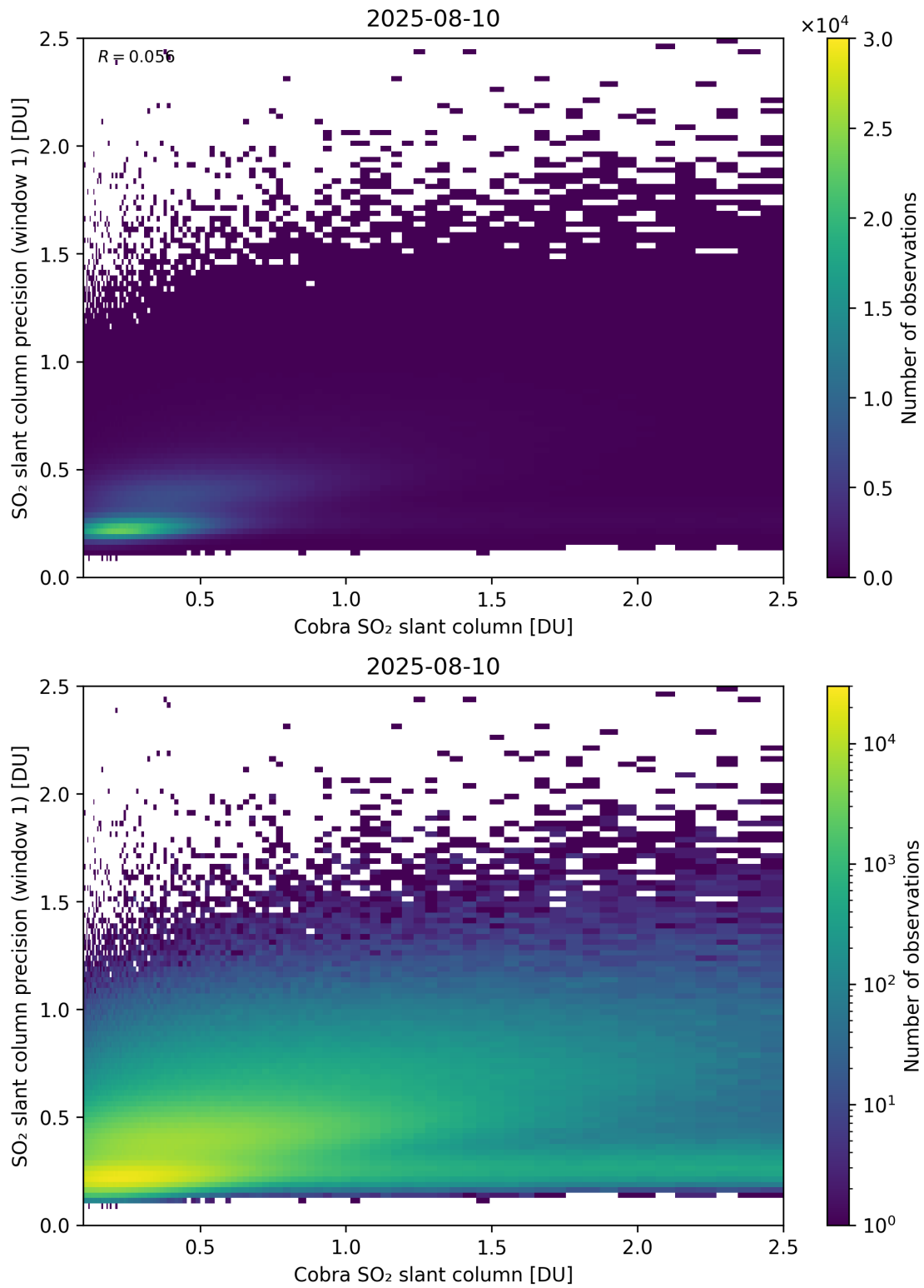
Figure 220: Scatter density plot of “Cobra SO 2 slant column” against “SO 2 slant column precision (window 1)” for 2025-08-09 to 2025-08-11.
