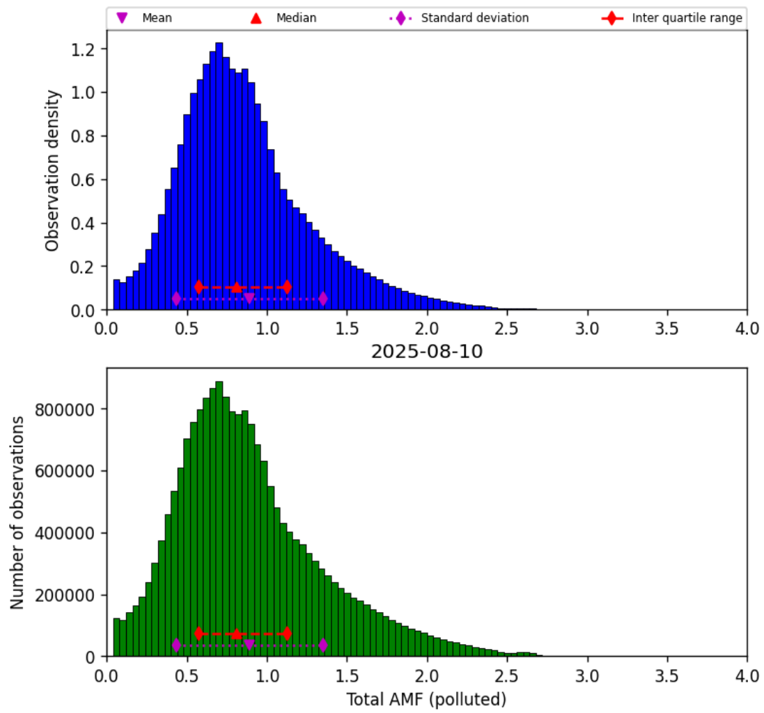
Figure 79: Histogram of “Total AMF (polluted)” for 2025-08-09 to 2025-08-11
