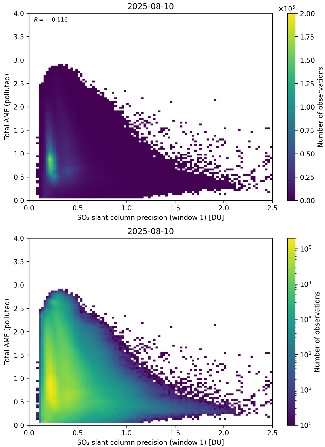
Figure 280: Scatter density plot of “SO 2 slant column precision (window 1)” against “Total AMF (polluted)” for 2025-08-09 to 2025-08-11.
