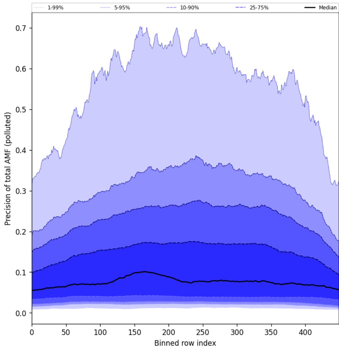
Figure 106: Along track statistics of “Precision of total AMF (polluted)” for 2025-08-09 to 2025-08-11
