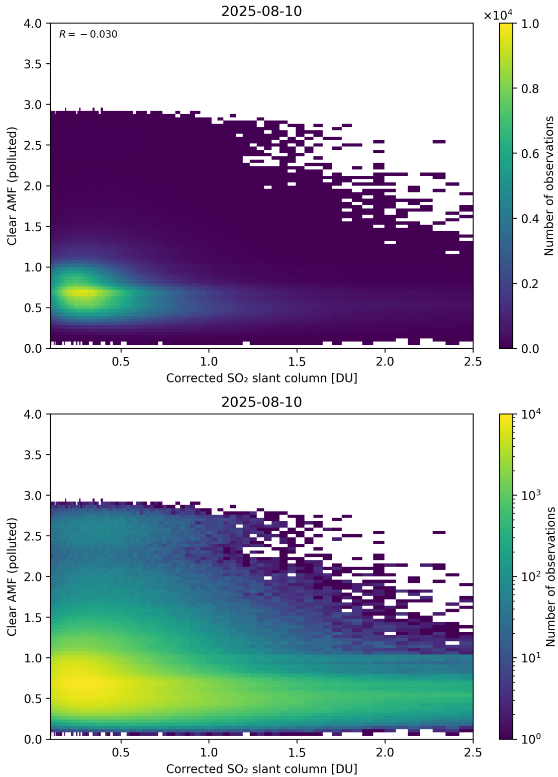
Figure 232: Scatter density plot of “Corrected SO 2 slant column” against “Clear AMF (polluted)” for 2025-08-09 to 2025-08-11.
