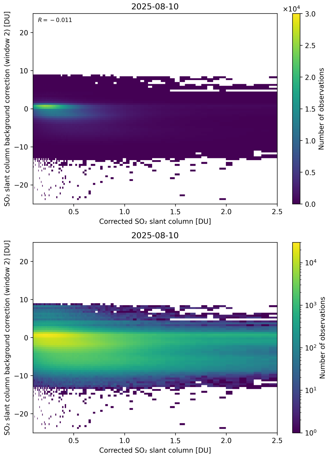
Figure 227: Scatter density plot of “Corrected SO 2 slant column” against “SO 2 slant column background correction (window 2)” for 2025-08-09 to 2025-08-11.
