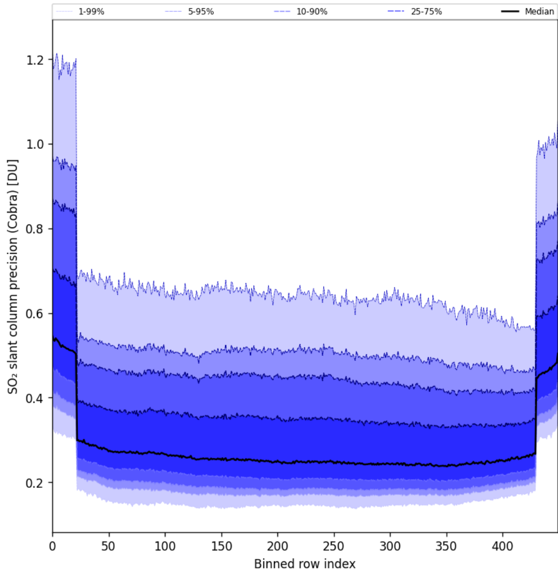
Figure 88: Along track statistics of “SO 2 slant column precision (Cobra)” for 2025-08-09 to 2025-08-11
