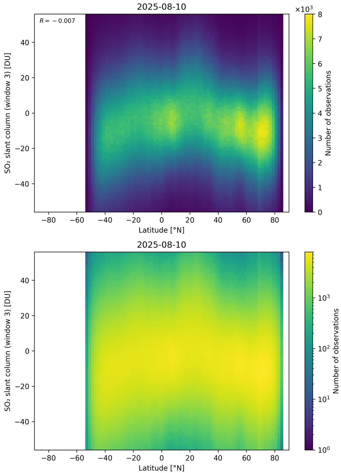
Figure 165: Scatter density plot of “Latitude” against “SO 2 slant column (window 3)” for 2025-08-09 to 2025-08-11.
