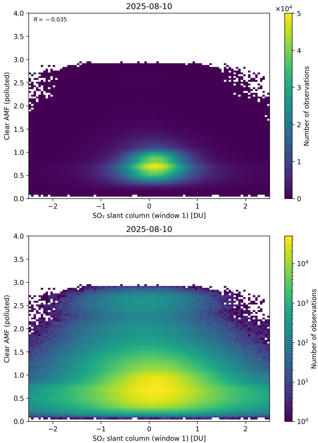
Figure 282: Scatter density plot of “SO 2 slant column (window 1)” against “Clear AMF (polluted)” for 2025-08-09 to 2025-08-11.
