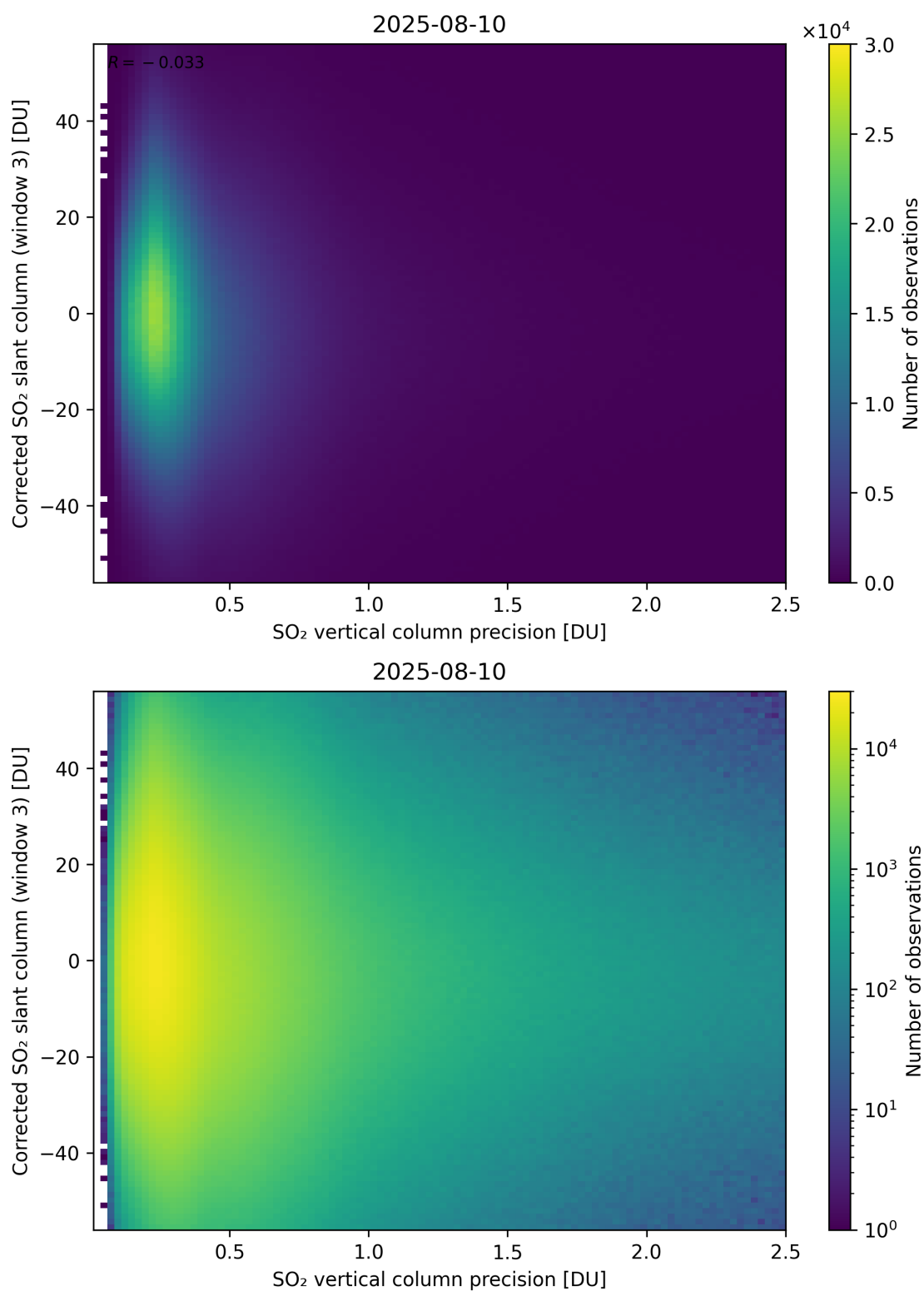
Figure 340: Scatter density plot of “SO 2 vertical column precision” against “Corrected SO 2 slant column (window 3)” for 2025-08-09 to 2025-08-11.
