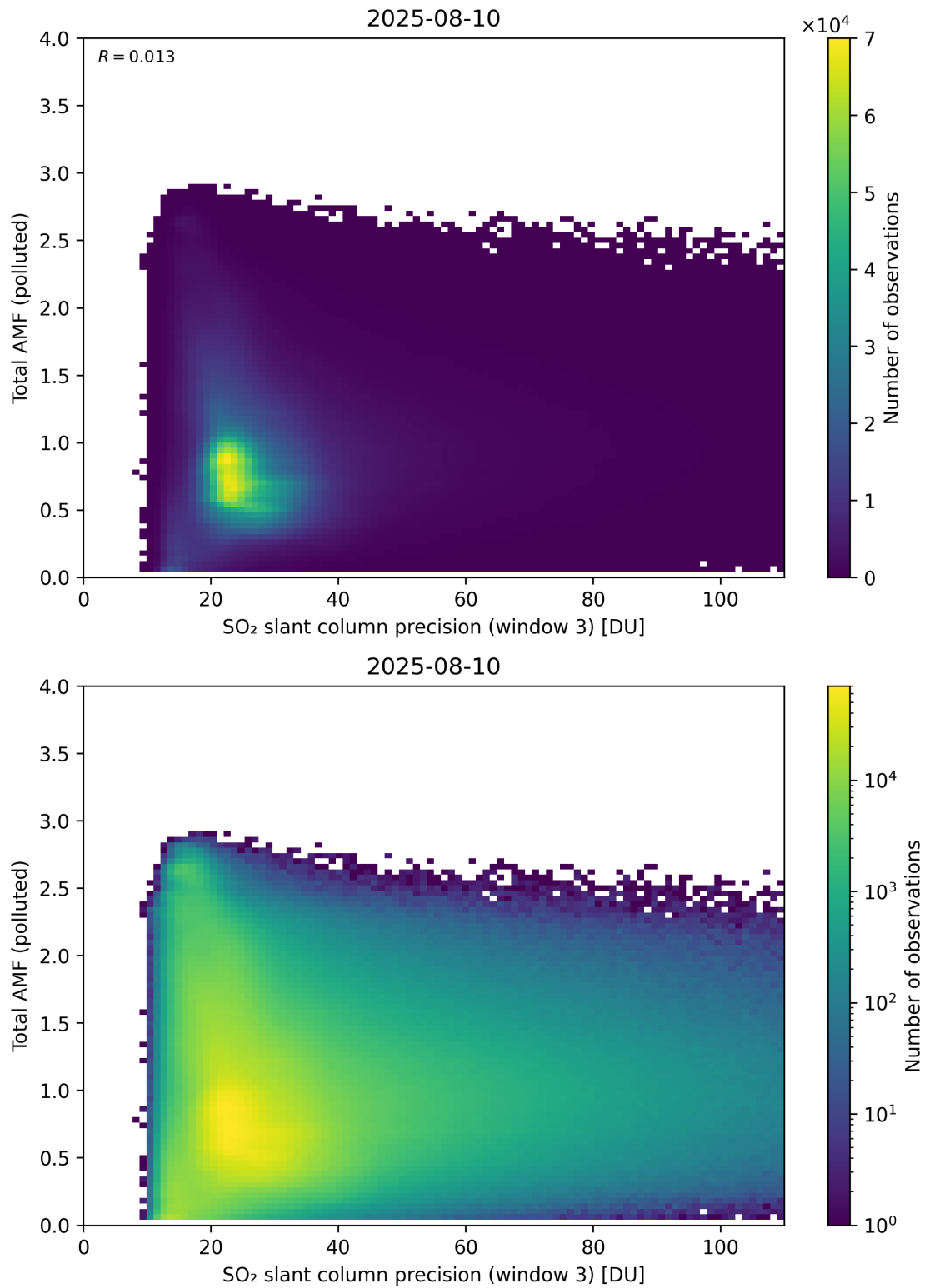
Figure 313: Scatter density plot of “SO 2 slant column precision (window 3)” against “Total AMF (polluted)” for 2025-08-09 to 2025-08-11.
