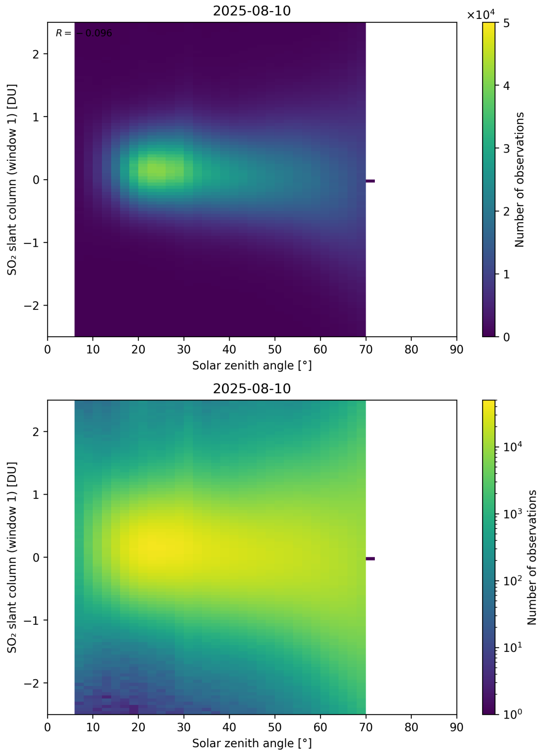
Figure 184: Scatter density plot of “Solar zenith angle” against “SO 2 slant column (window 1)” for 2025-08-09 to 2025-08-11.
