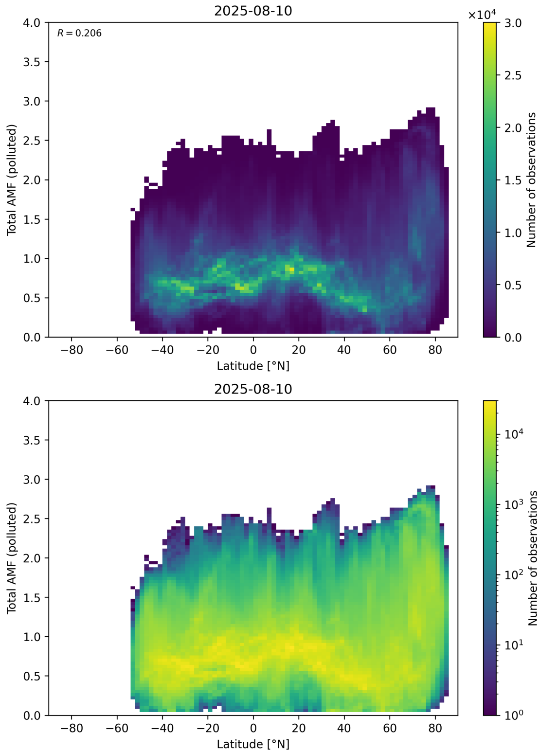
Figure 167: Scatter density plot of “Latitude” against “Total AMF (polluted)” for 2025-08-09 to 2025-08-11.
