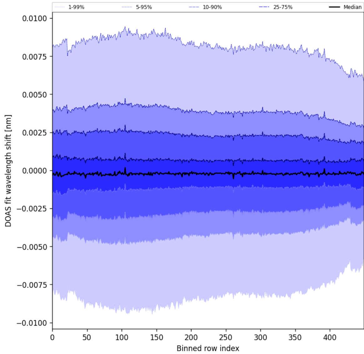
Figure 102: Along track statistics of “DOAS fit wavelength shift” for 2025-08-09 to 2025-08-11
