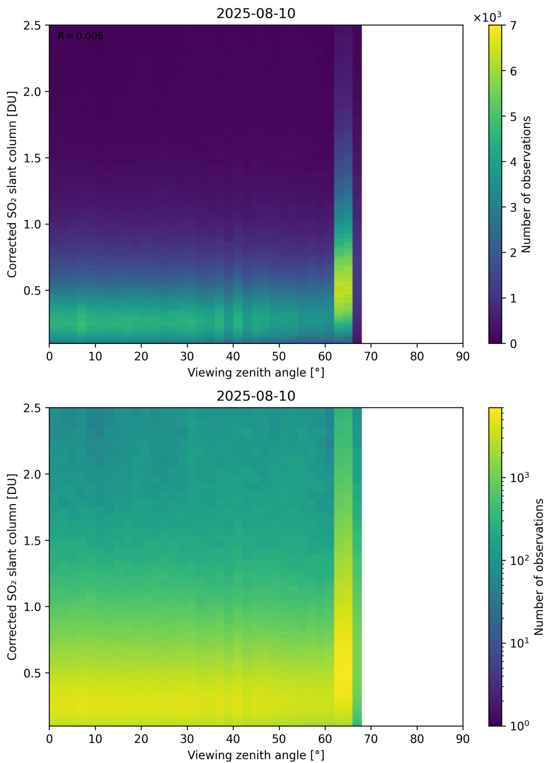
Figure 373: Scatter density plot of “Viewing zenith angle” against “Corrected SO 2 slant column” for 2025-08-09 to 2025-08-11.
