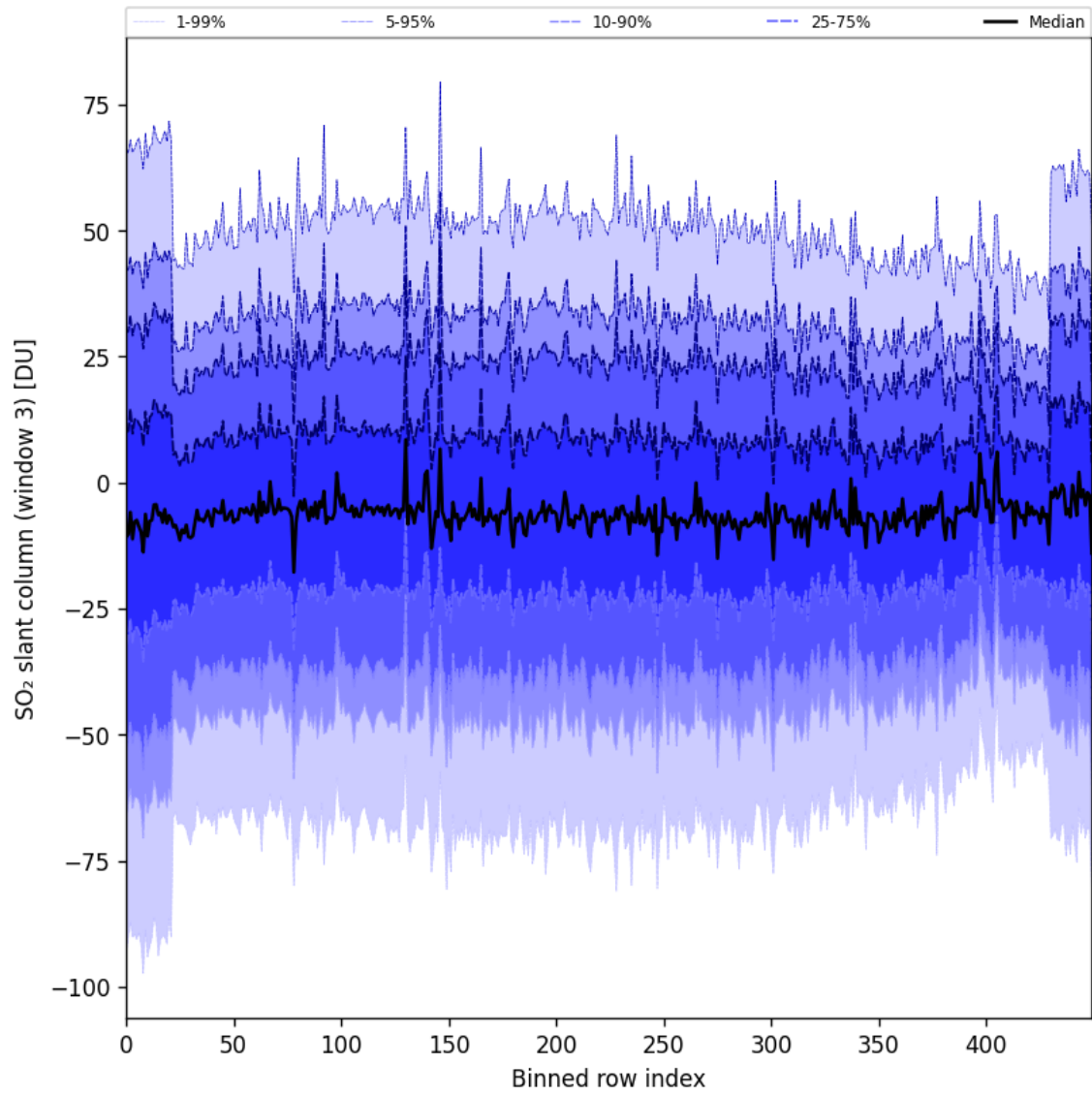
Figure 97: Along track statistics of “SO 2 slant column (window 3)” for 2025-08-09 to 2025-08-11
