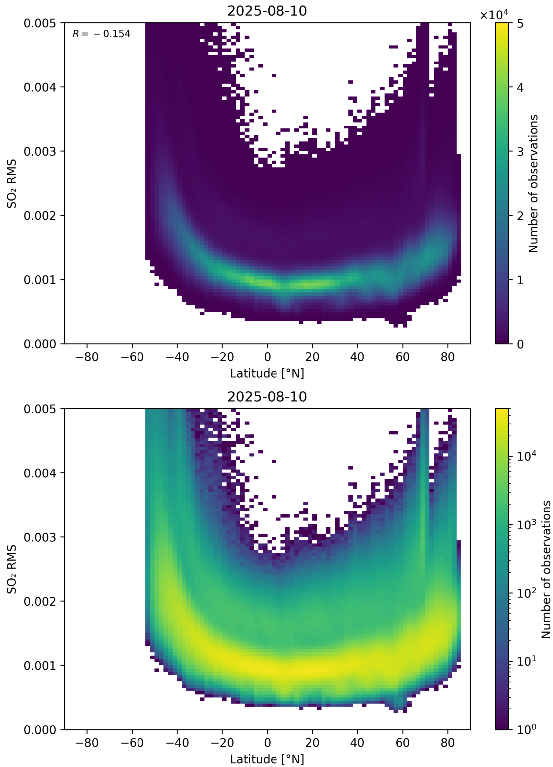
Figure 155: Scatter density plot of “Latitude” against “SO 2 RMS” for 2025-08-09 to 2025-08-11.
