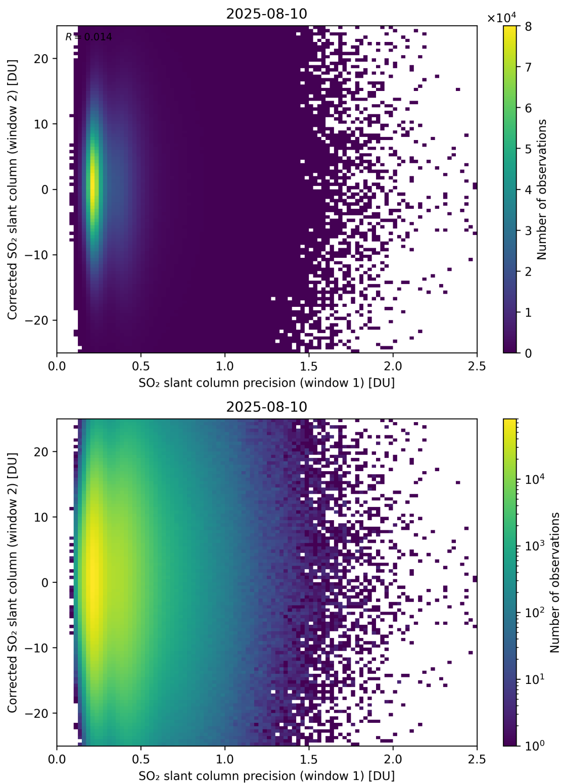
Figure 275: Scatter density plot of “SO 2 slant column precision (window 1)” against “Corrected SO 2 slant column (window 2)” for 2025-08-09 to 2025-08-11.
