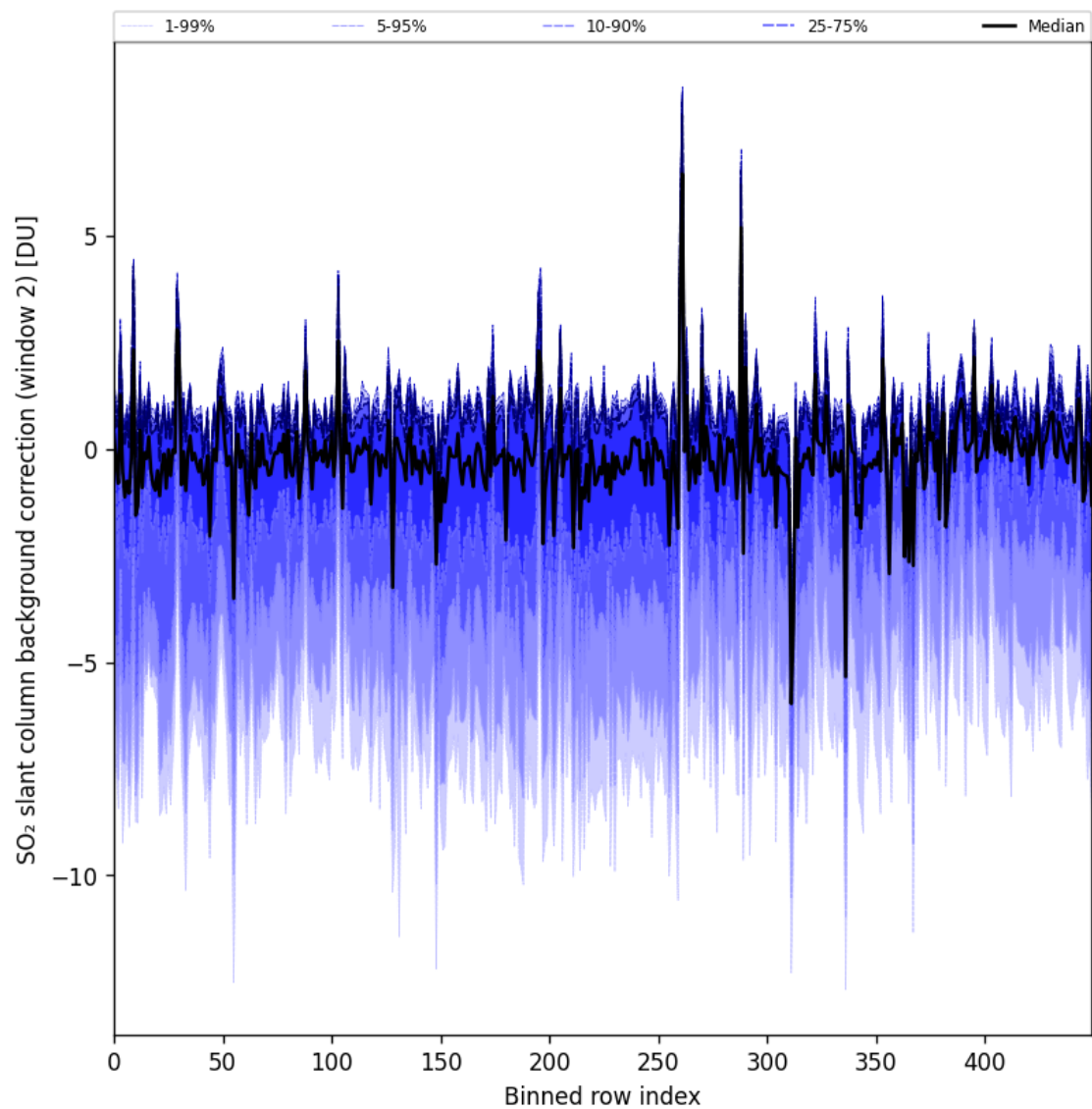
Figure 96: Along track statistics of “SO 2 slant column background correction (window 2)” for 2025-08-09 to 2025-08-11
