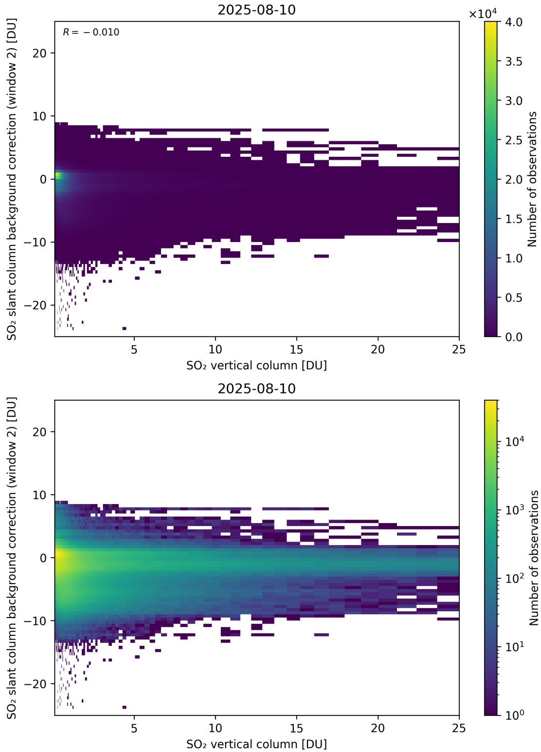
Figure 324: Scatter density plot of “SO 2 vertical column” against “SO 2 slant column background correction (window 2)” for 2025-08-09 to 2025-08-11.
