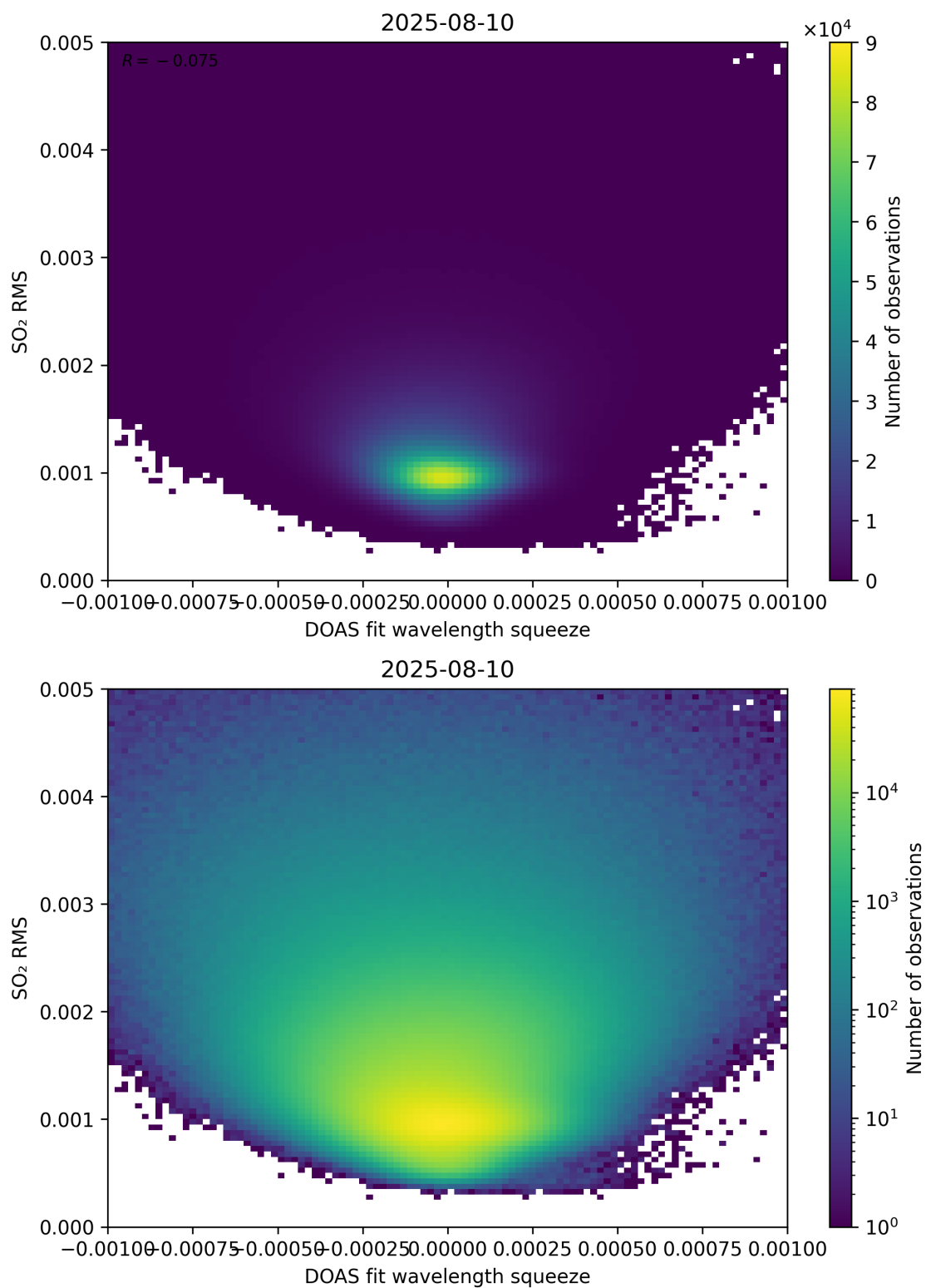
Figure 143: Scatter density plot of “DOAS fit wavelength squeeze” against “SO 2 RMS” for 2025-08-09 to 2025-08-11.
