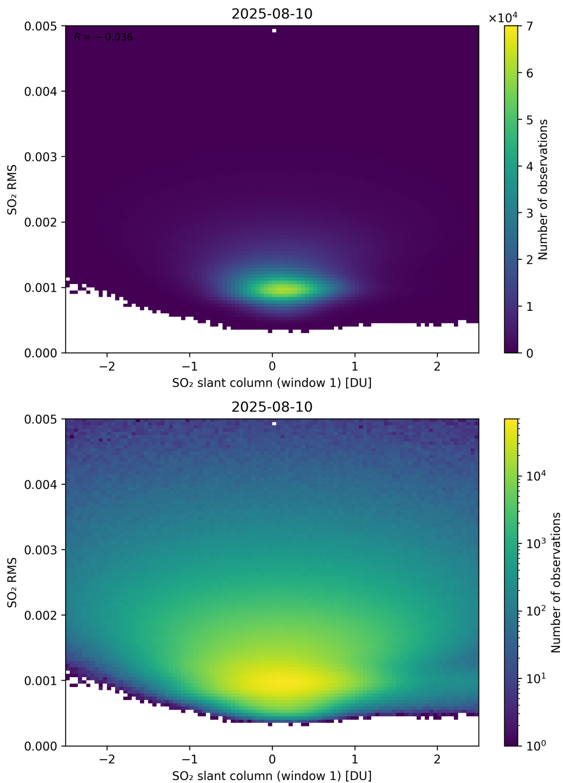
Figure 267: Scatter density plot of “SO 2 slant column (window 1)” against “SO 2 RMS” for 2025-08-09 to 2025-08-11.
