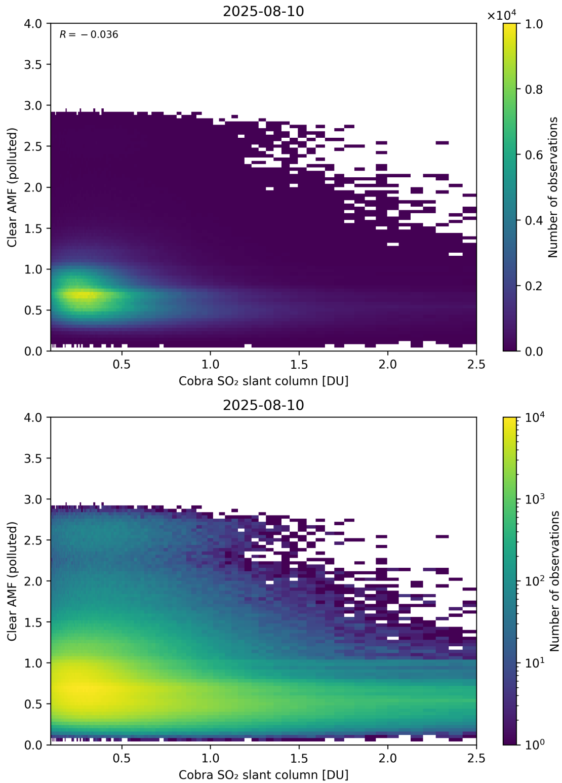
Figure 215: Scatter density plot of “Cobra SO 2 slant column” against “Clear AMF (polluted)” for 2025-08-09 to 2025-08-11.
