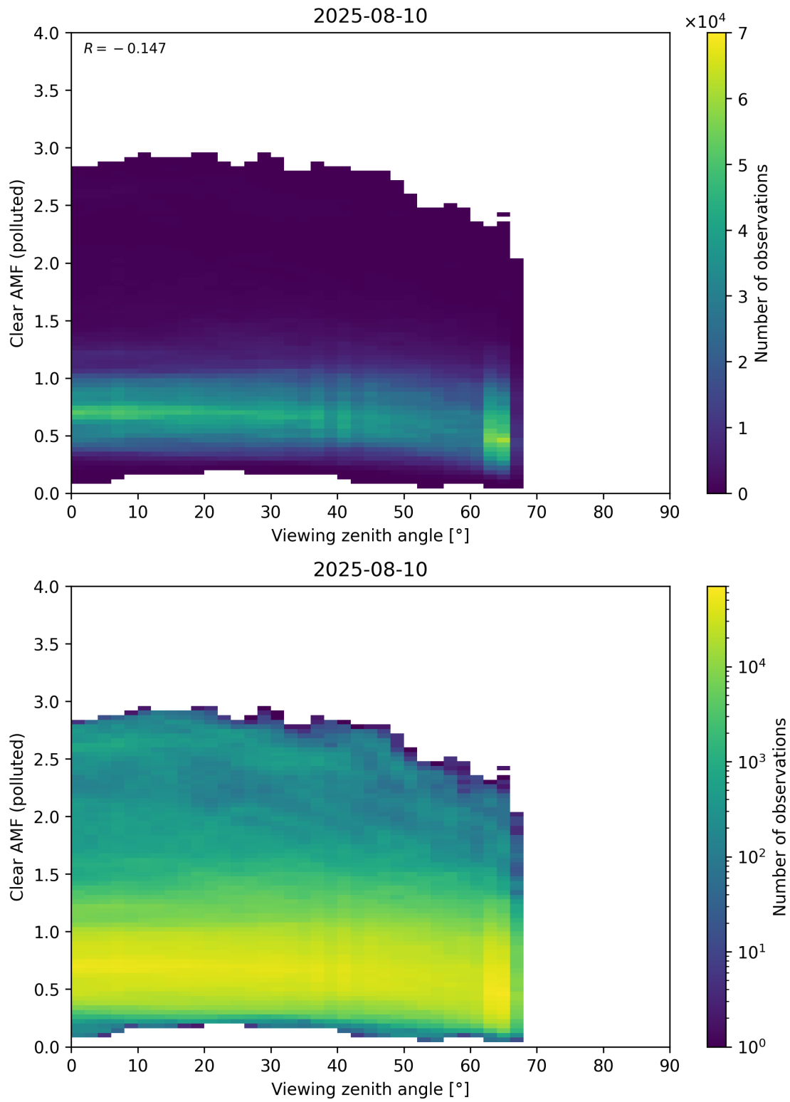
Figure 370: Scatter density plot of “Viewing zenith angle” against “Clear AMF (polluted)” for 2025-08-09 to 2025-08-11.
