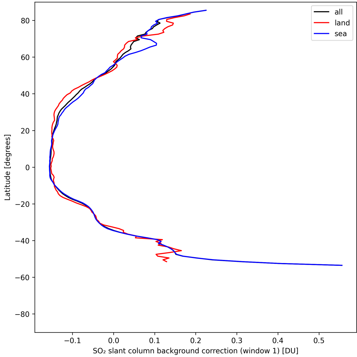
Figure 40: Zonal average of “SO 2 slant column background correction (window 1)” for 2025-08-09 to 2025-08-11.
