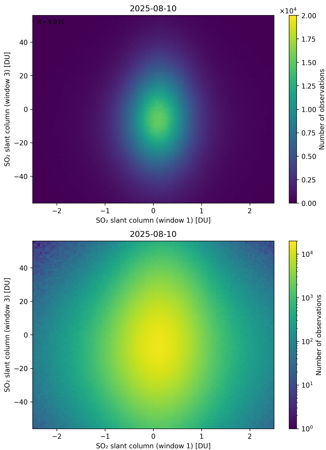
Figure 287: Scatter density plot of “SO 2 slant column (window 1)” against “SO 2 slant column (window 3)” for 2025-08-09 to 2025-08-11.
