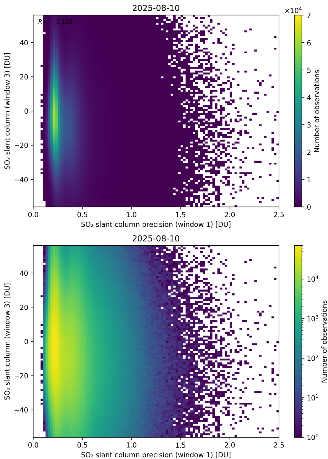
Figure 278: Scatter density plot of “SO 2 slant column precision (window 1)” against “SO 2 slant column (window 3)” for 2025-08-09 to 2025-08-11.
