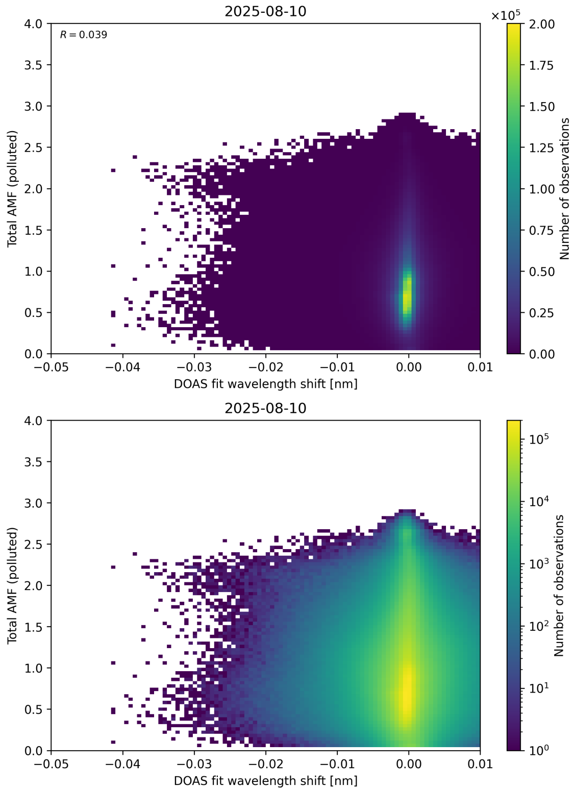
Figure 141: Scatter density plot of “DOAS fit wavelength shift” against “Total AMF (polluted)” for 2025-08-09 to 2025-08-11.
