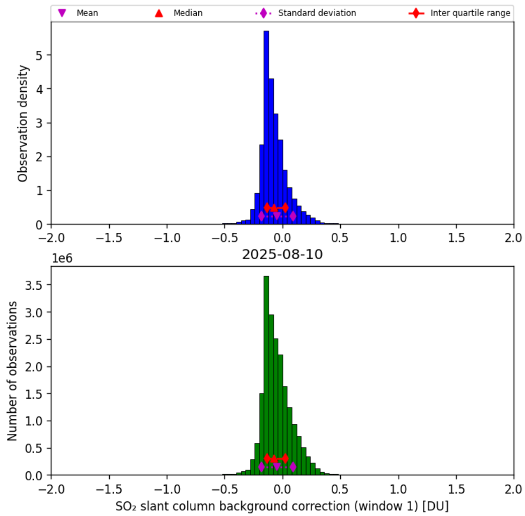
Figure 66: Histogram of “SO 2 slant column background correction (window 1)” for 2025-08-09 to 2025-08-11
