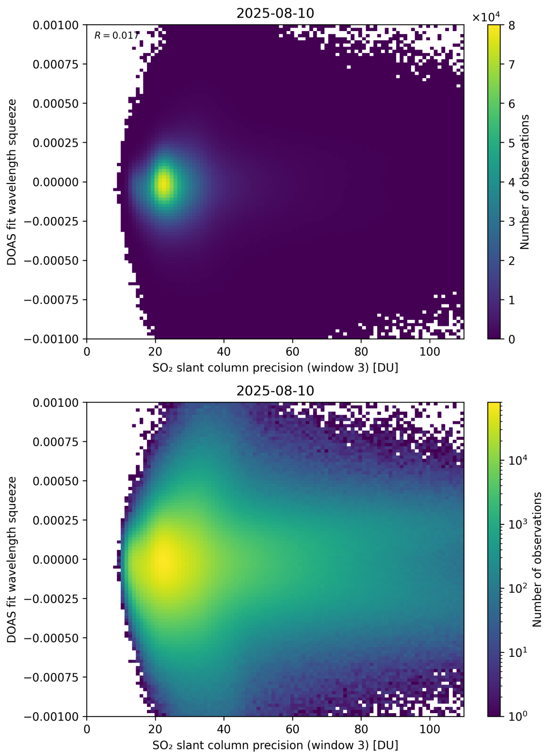
Figure 309: Scatter density plot of “SO 2 slant column precision (window 3)” against “DOAS fit wavelength squeeze” for 2025-08-09 to 2025-08-11.
