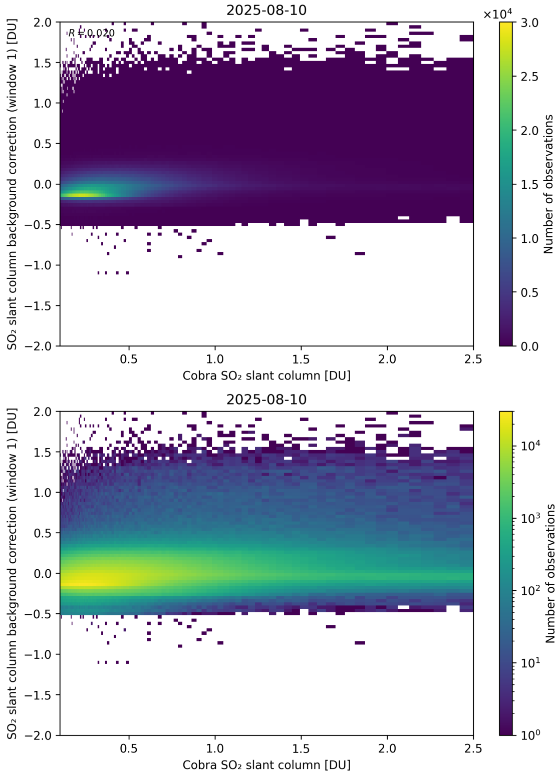
Figure 193: Scatter density plot of “Cobra SO 2 slant column” against “SO 2 slant column background correction (window 1)” for 2025-08-09 to 2025-08-11.
