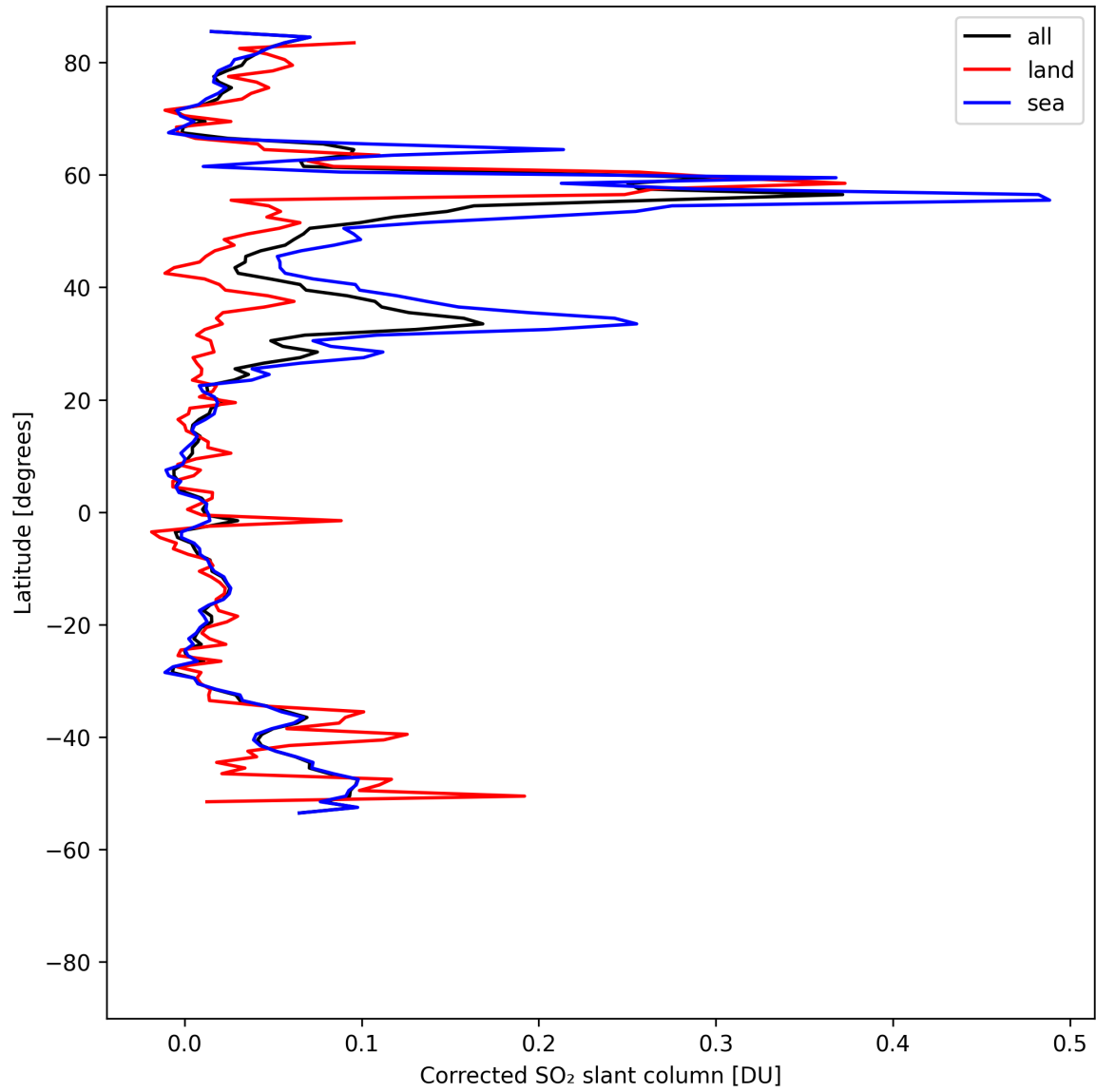
Figure 34: Zonal average of “Corrected SO 2 slant column” for 2025-08-09 to 2025-08-11.
