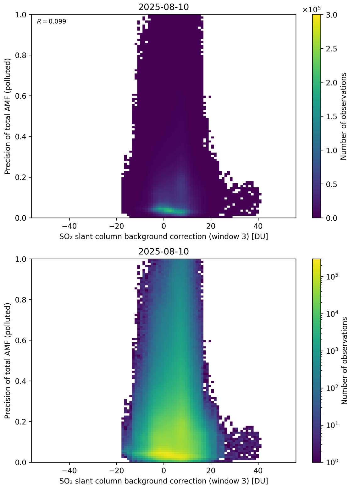
Figure 137: Scatter density plot of “SO 2 slant column background correction (window 3)” against “Precision of total AMF (polluted)” for 2025-08-09 to 2025-08-11.
