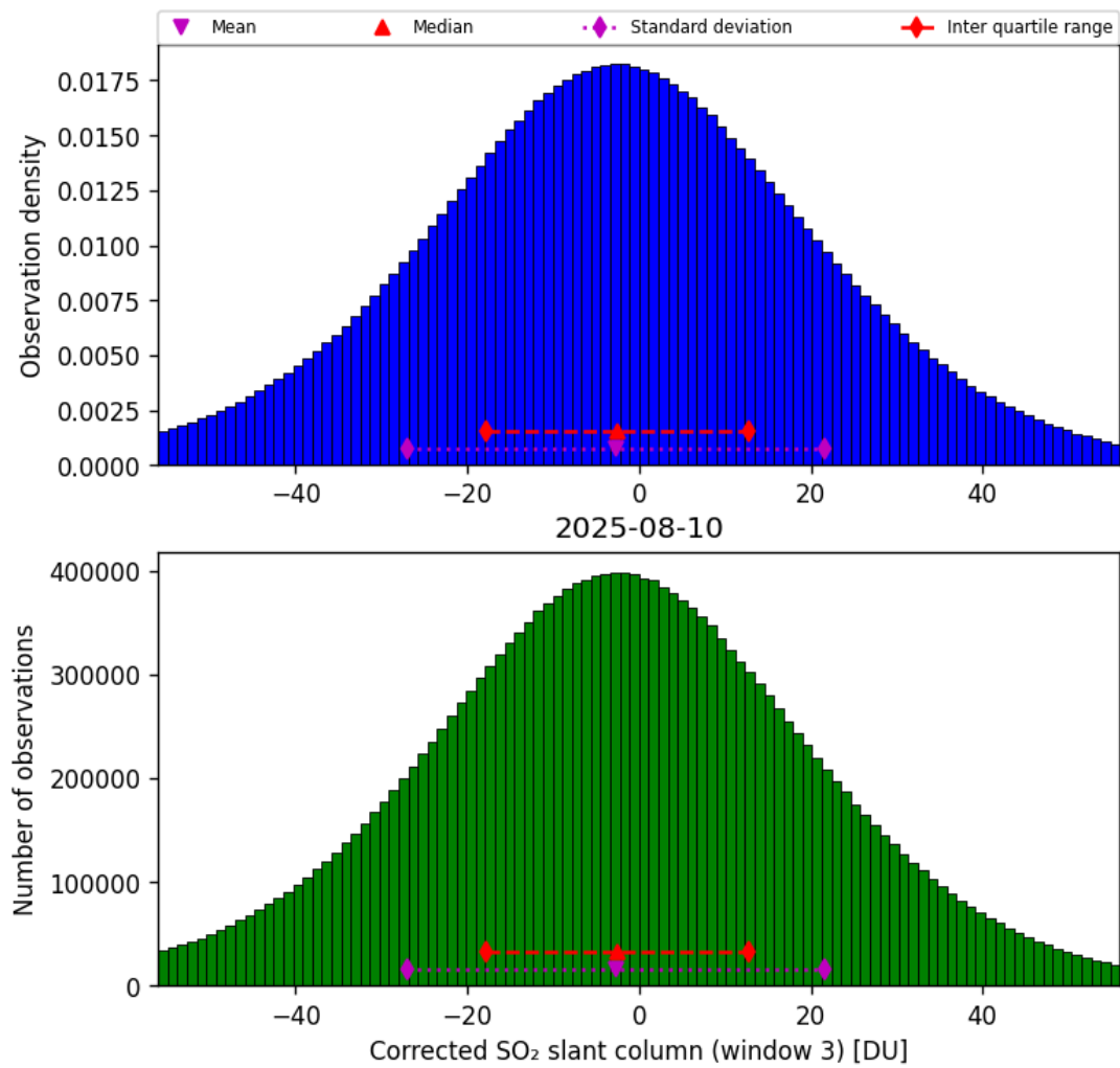
Figure 73: Histogram of “Corrected SO 2 slant column (window 3)” for 2025-08-09 to 2025-08-11
