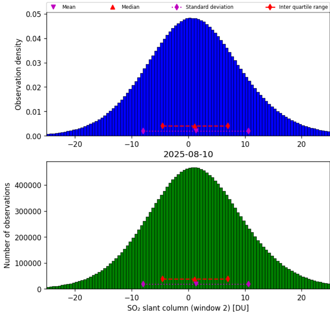
Figure 67: Histogram of “SO 2 slant column (window 2)” for 2025-08-09 to 2025-08-11
