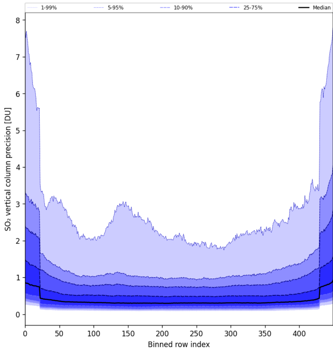
Figure 85: Along track statistics of “SO 2 vertical column precision” for 2025-08-09 to 2025-08-11
