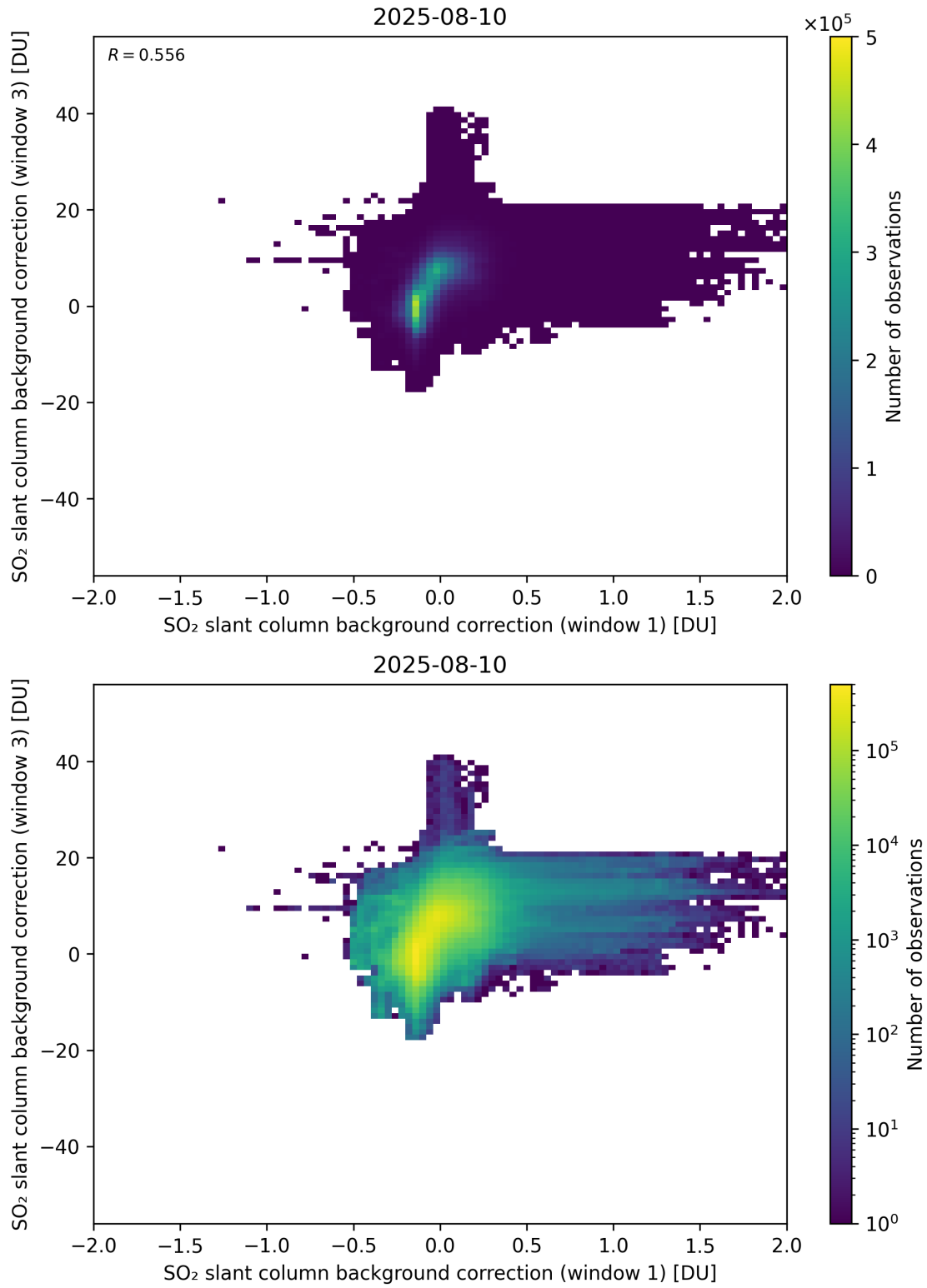
Figure 110: Scatter density plot of “SO 2 slant column background correction (window 1)” against “SO 2 slant column background correction (window 3)” for 2025-08-09 to 2025-08-11.
