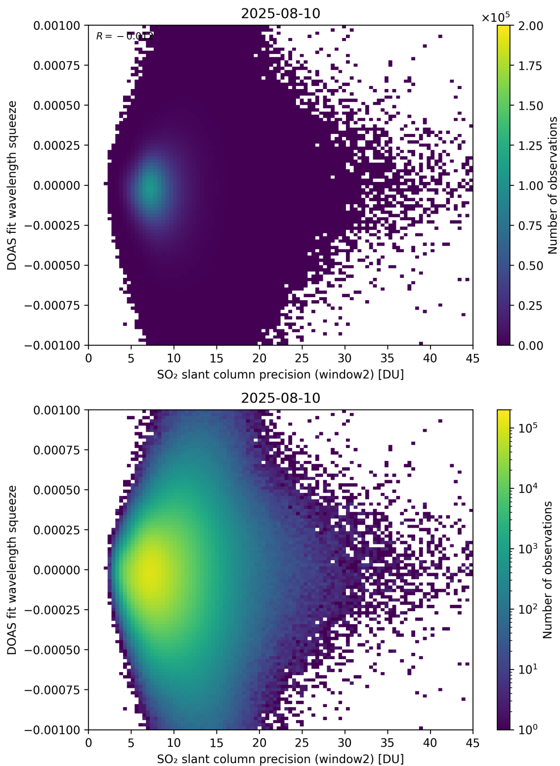
Figure 294: Scatter density plot of “SO 2 slant column precision (window2)” against “DOAS fit wavelength squeeze” for 2025-08-09 to 2025-08-11.
