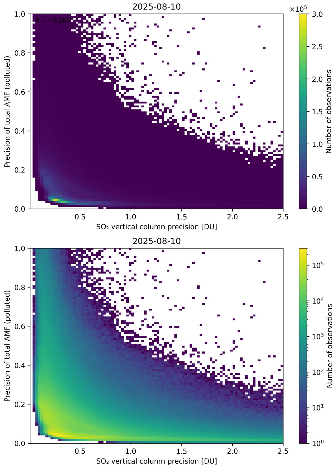
Figure 347: Scatter density plot of “SO 2 vertical column precision” against “Precision of total AMF (polluted)” for 2025-08-09 to 2025-08-11.
