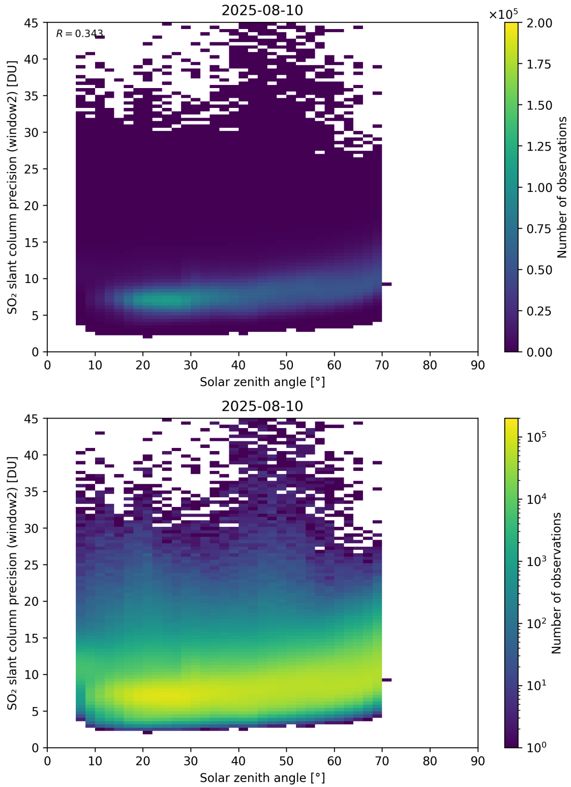
Figure 186: Scatter density plot of “Solar zenith angle” against “SO 2 slant column precision (window2)” for 2025-08-09 to 2025-08-11.
