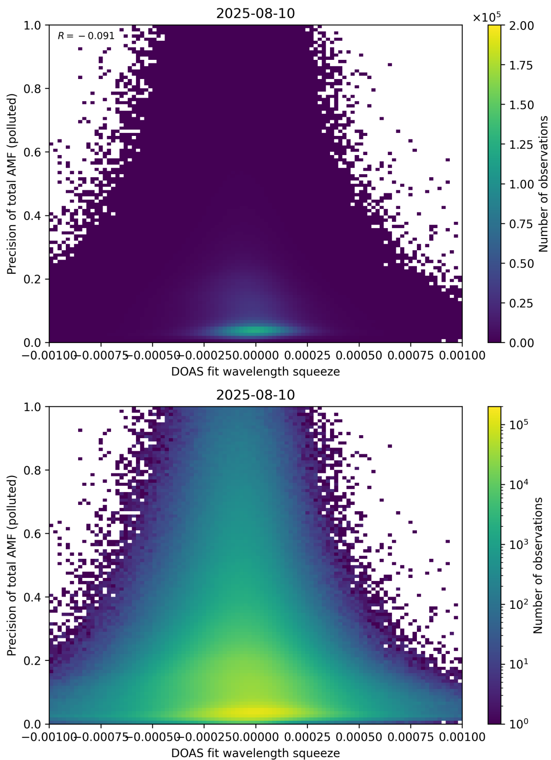
Figure 146: Scatter density plot of “DOAS fit wavelength squeeze” against “Precision of total AMF (polluted)” for 2025-08-09 to 2025-08-11.
