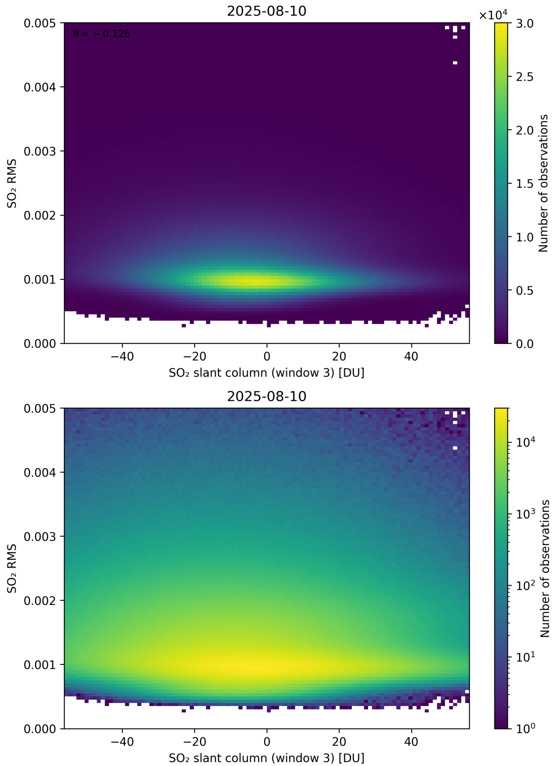
Figure 306: Scatter density plot of “SO 2 slant column (window 3)” against “SO 2 RMS” for 2025-08-09 to 2025-08-11.
