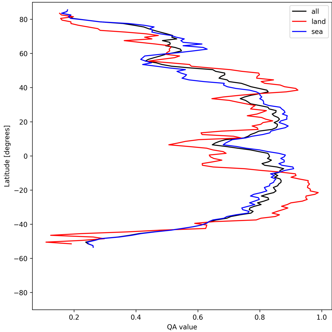
Figure 31: Zonal average of “QA value” for 2025-08-09 to 2025-08-11.
