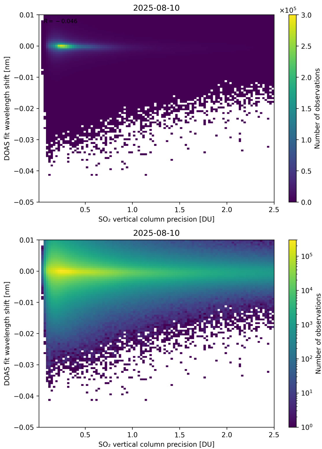
Figure 332: Scatter density plot of “SO 2 vertical column precision” against “DOAS fit wavelength shift” for 2025-08-09 to 2025-08-11.
