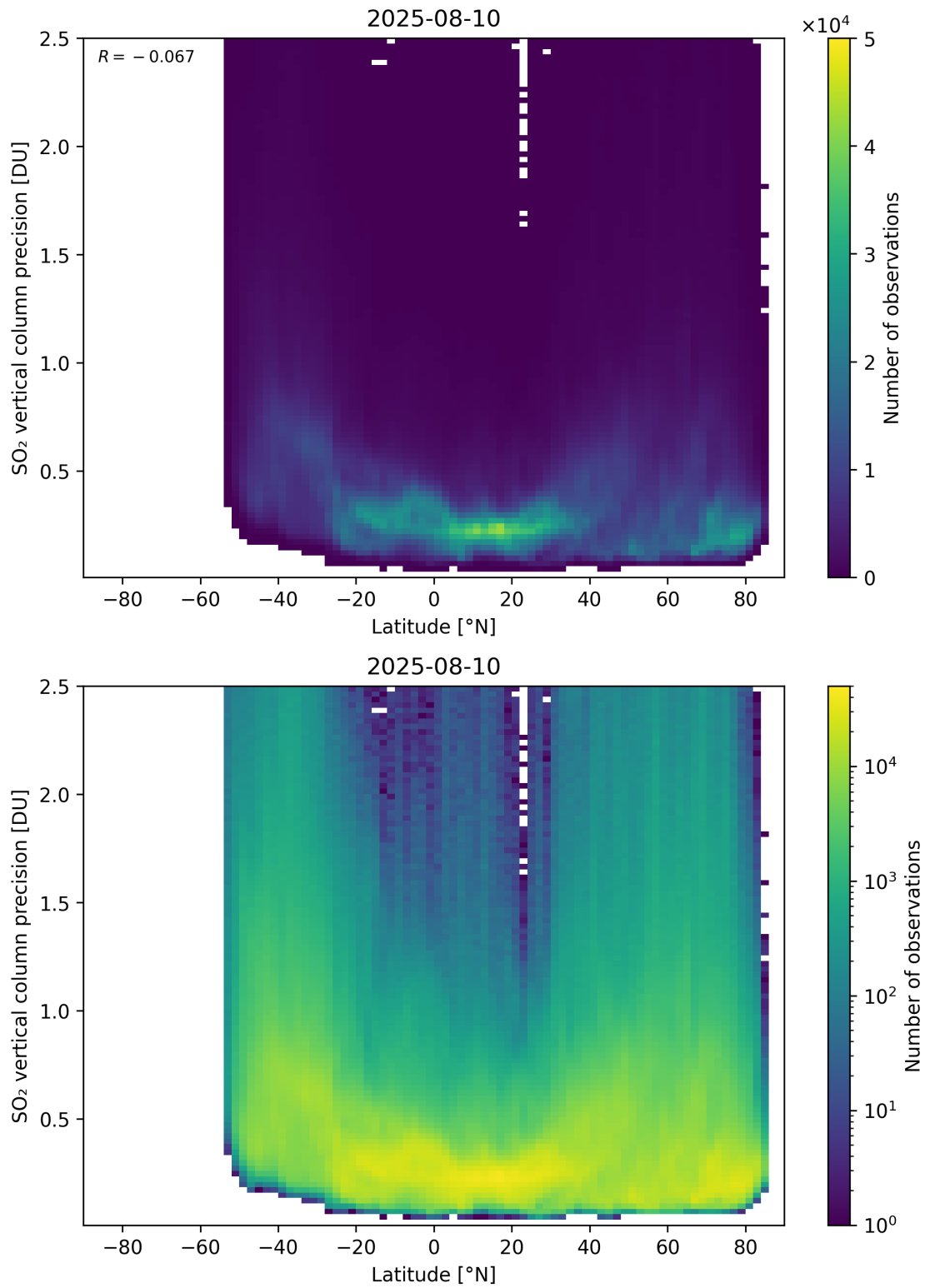
Figure 170: Scatter density plot of “Latitude” against “SO 2 vertical column precision” for 2025-08-09 to 2025-08-11.
