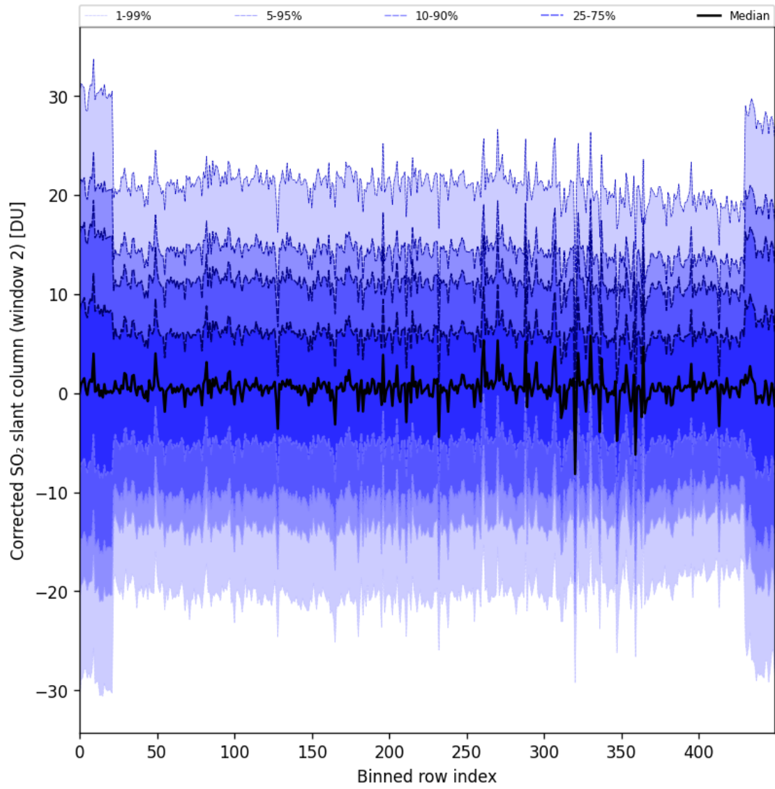
Figure 95: Along track statistics of “Corrected SO 2 slant column (window 2)” for 2025-08-09 to 2025-08-11
