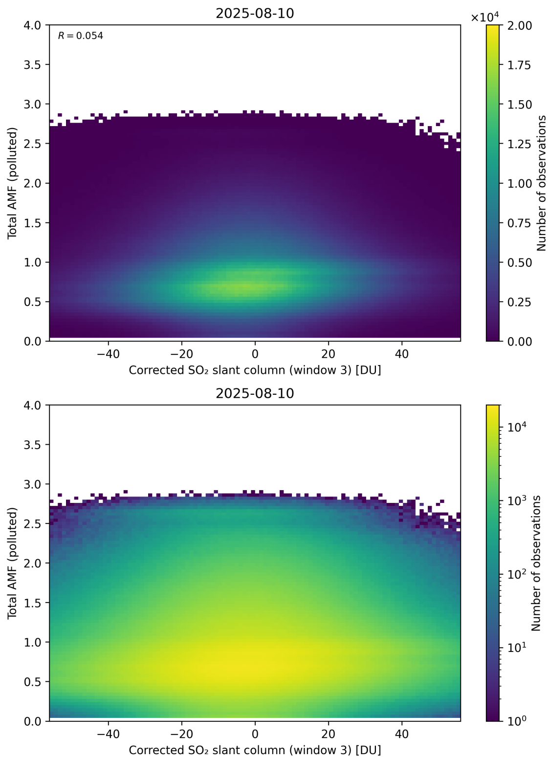
Figure 260: Scatter density plot of “Corrected SO 2 slant column (window 3)” against “Total AMF (polluted)” for 2025-08-09 to 2025-08-11.
