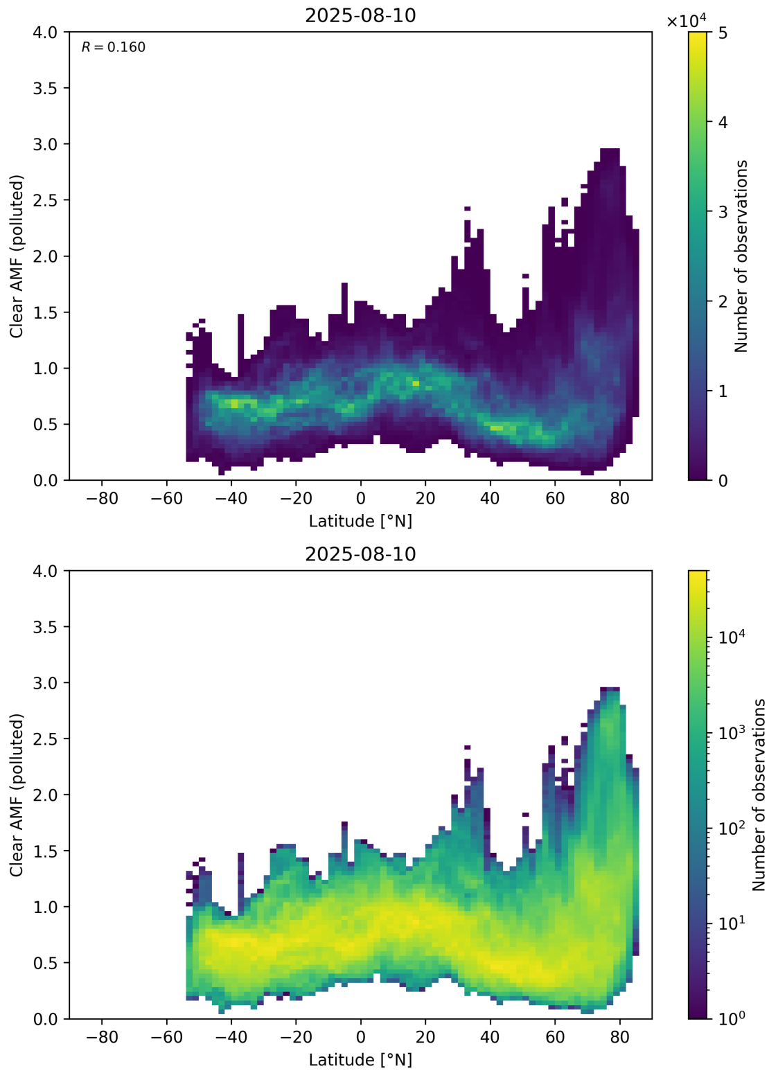
Figure 156: Scatter density plot of “Latitude” against “Clear AMF (polluted)” for 2025-08-09 to 2025-08-11.
