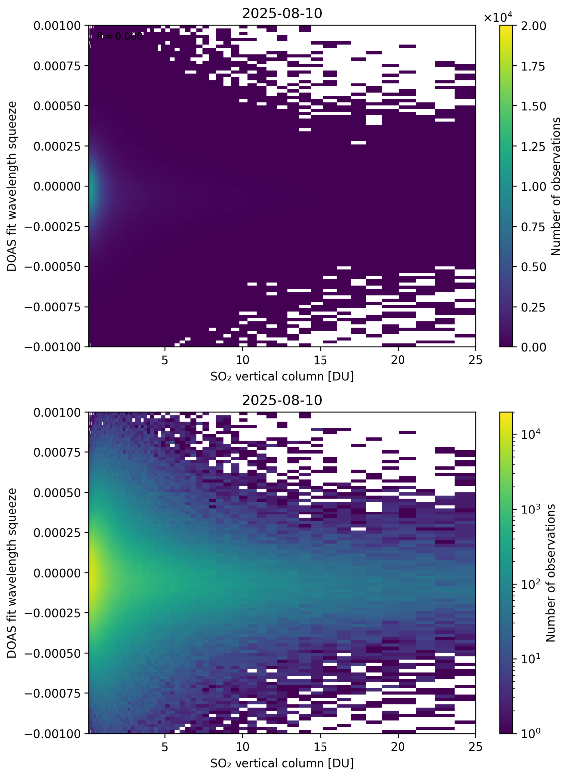
Figure 327: Scatter density plot of “SO 2 vertical column” against “DOAS fit wavelength squeeze” for 2025-08-09 to 2025-08-11.
