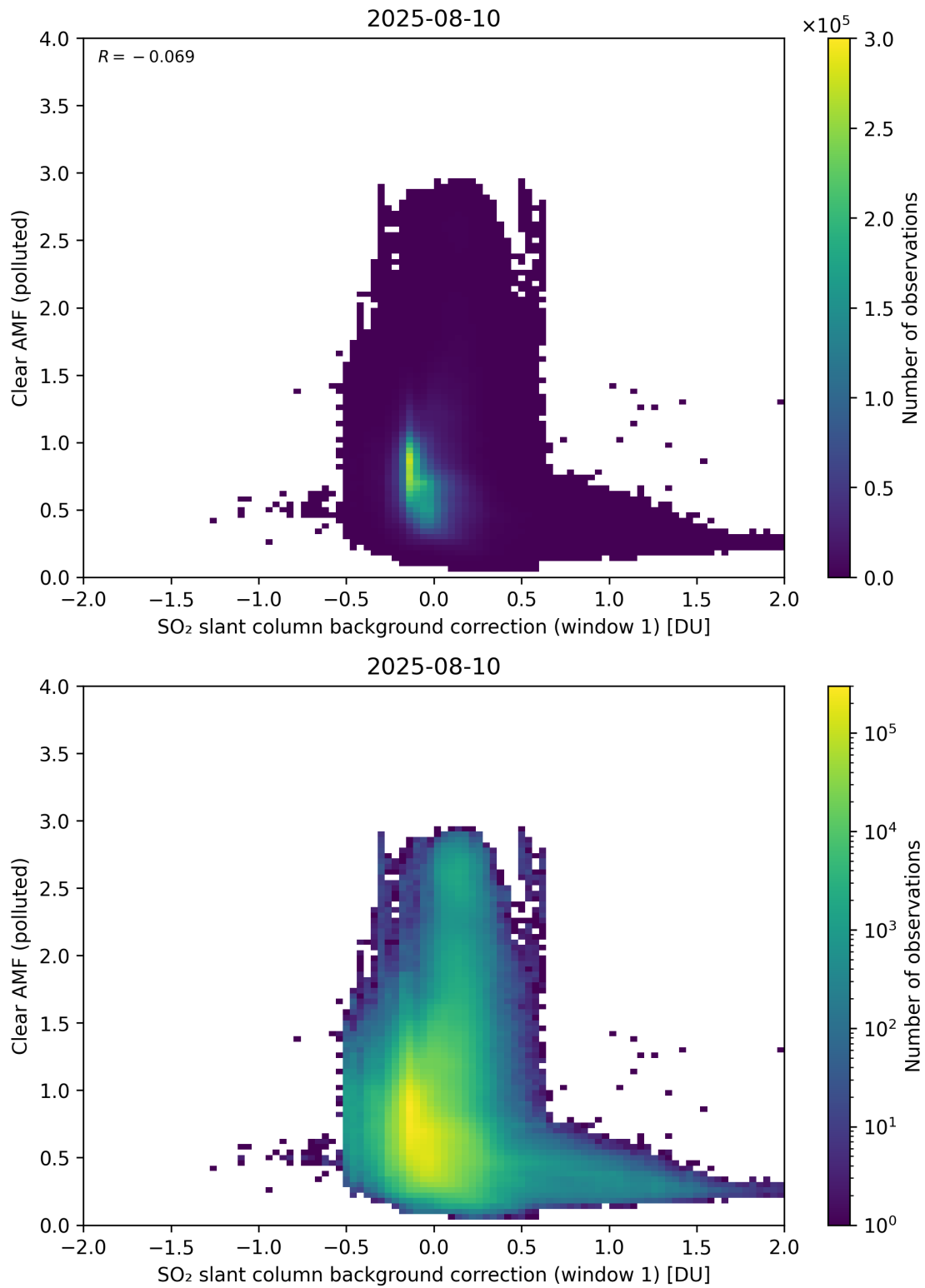
Figure 114: Scatter density plot of “SO 2 slant column background correction (window 1)” against “Clear AMF (polluted)” for 2025-08-09 to 2025-08-11.
