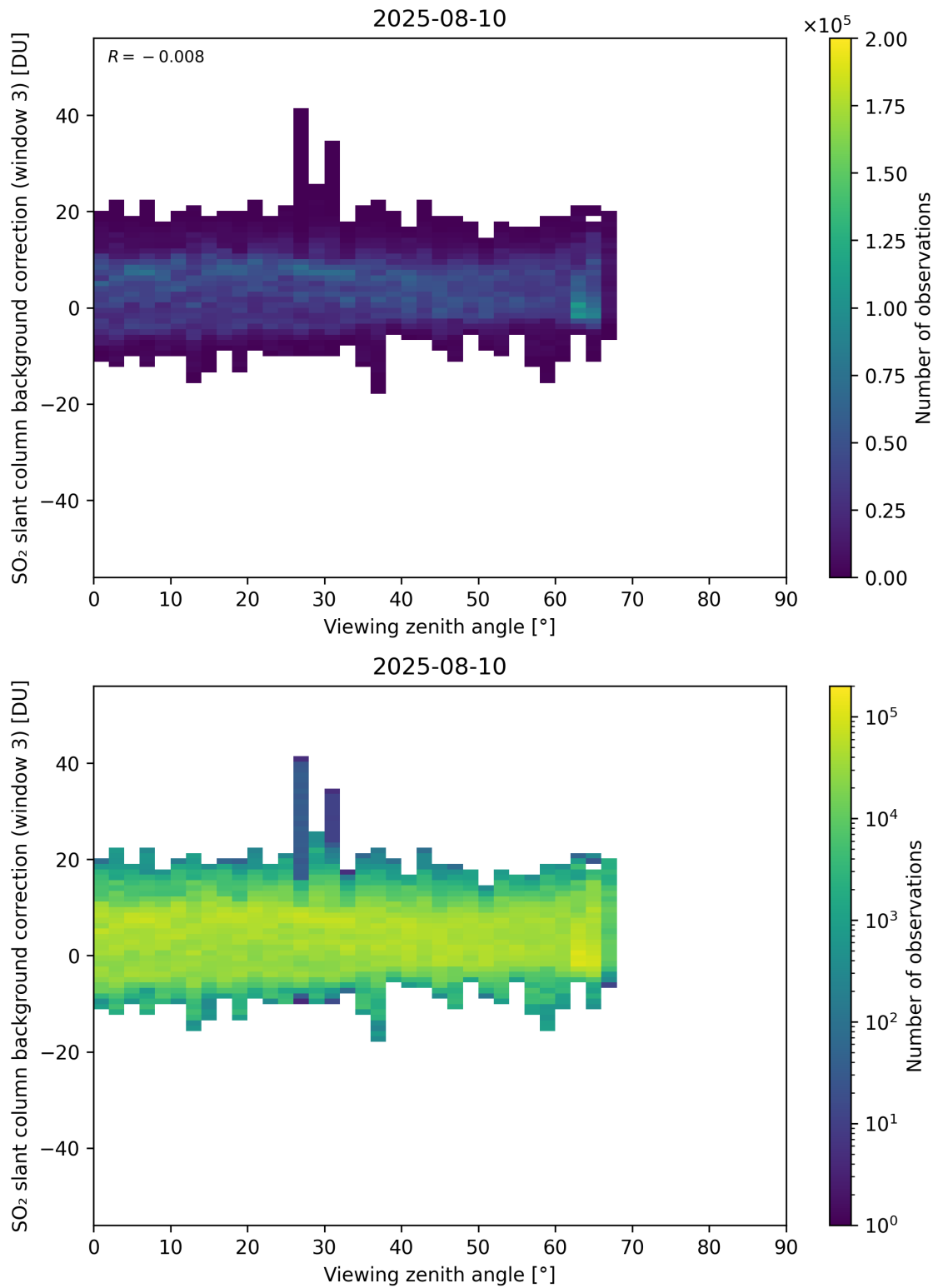
Figure 364: Scatter density plot of “Viewing zenith angle” against “SO 2 slant column background correction (window 3)” for 2025-08-09 to 2025-08-11.
