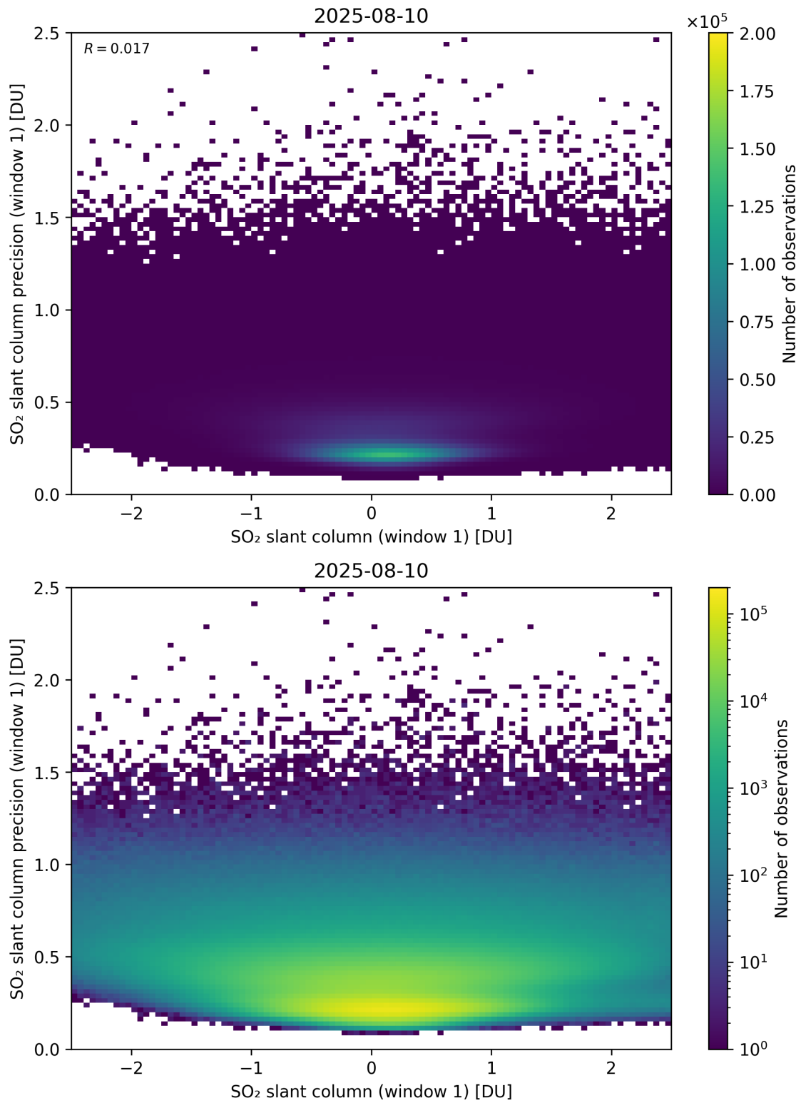
Figure 285: Scatter density plot of “SO 2 slant column (window 1)” against “SO 2 slant column precision (window 1)” for 2025-08-09 to 2025-08-11.
