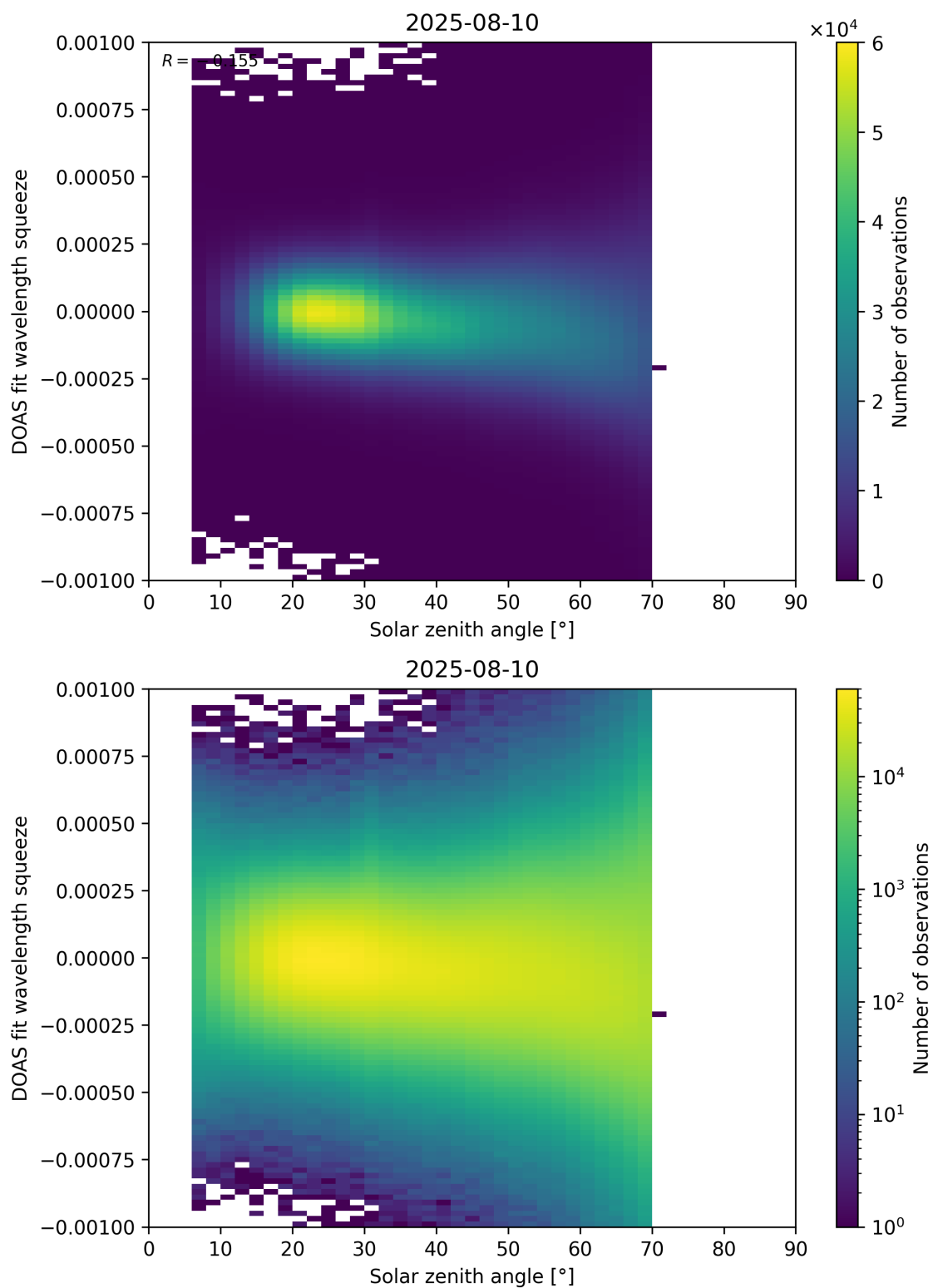
Figure 175: Scatter density plot of “Solar zenith angle” against “DOAS fit wavelength squeeze” for 2025-08-09 to 2025-08-11.
