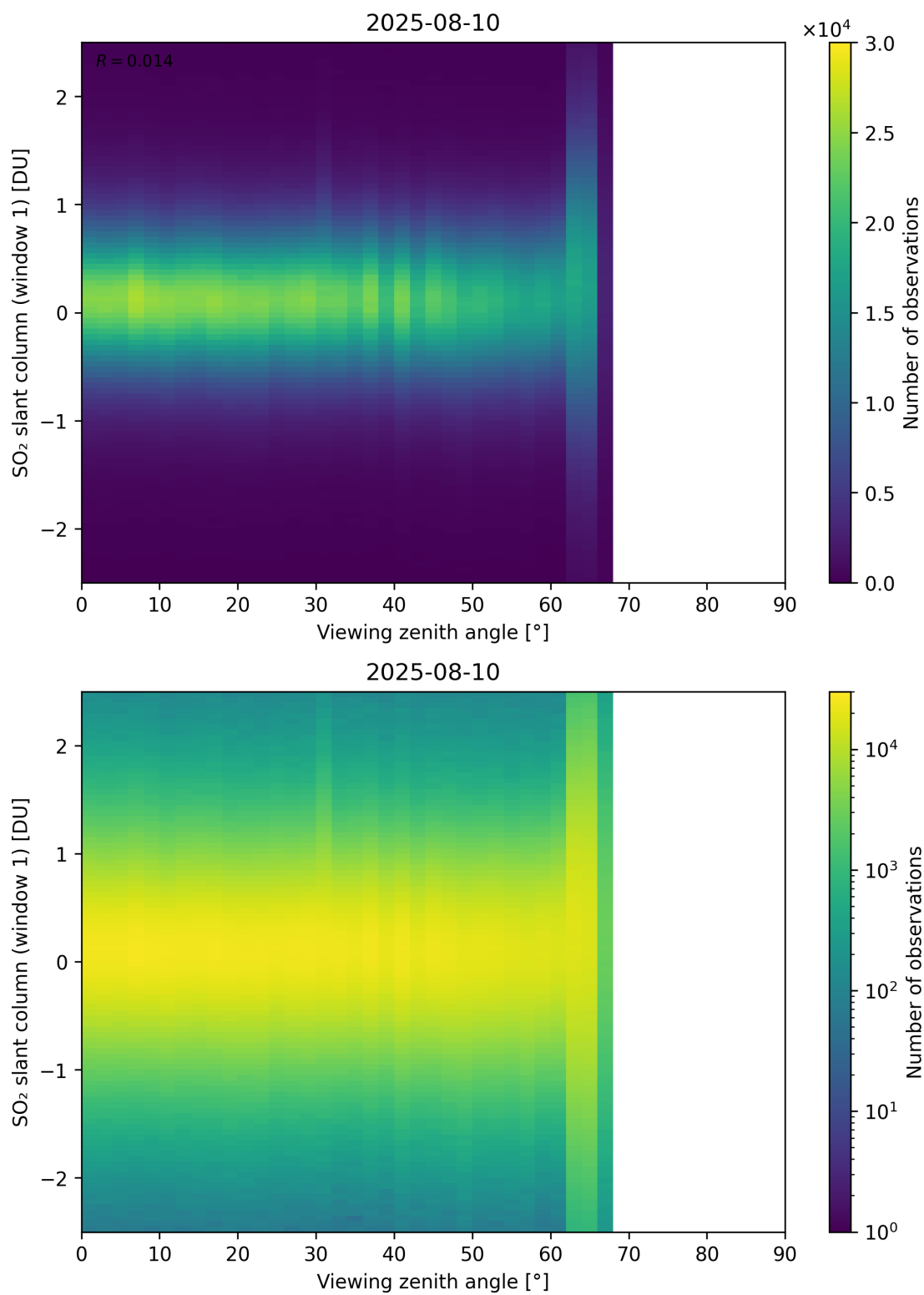
Figure 376: Scatter density plot of “Viewing zenith angle” against “SO 2 slant column (window 1)” for 2025-08-09 to 2025-08-11.
