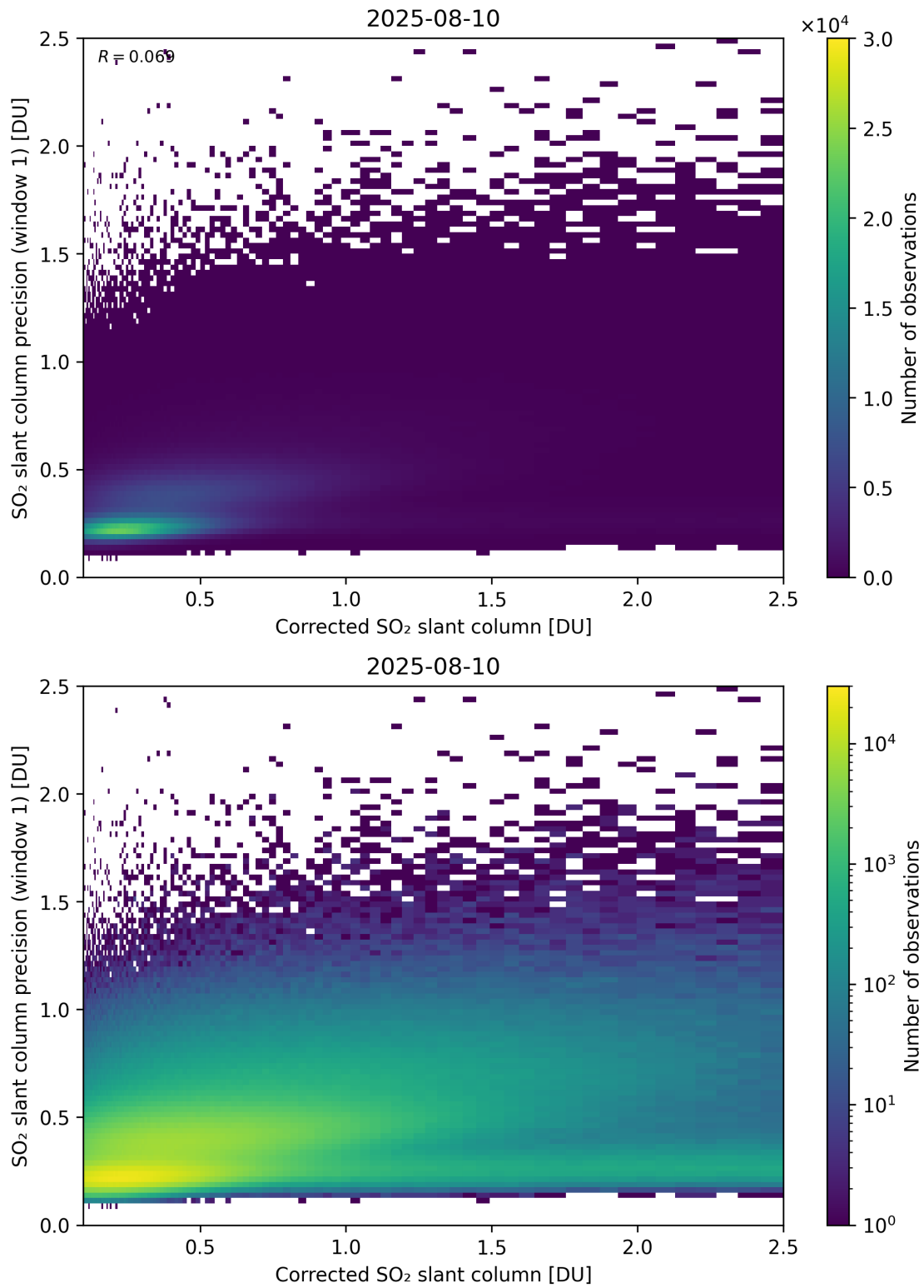
Figure 238: Scatter density plot of “Corrected SO 2 slant column” against “SO 2 slant column precision (window 1)” for 2025-08-09 to 2025-08-11.
