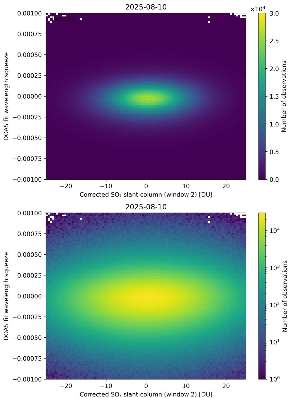
Figure 247: Scatter density plot of “Corrected SO 2 slant column (window 2)” against “DOAS fit wavelength squeeze” for 2025-08-09 to 2025-08-11.
