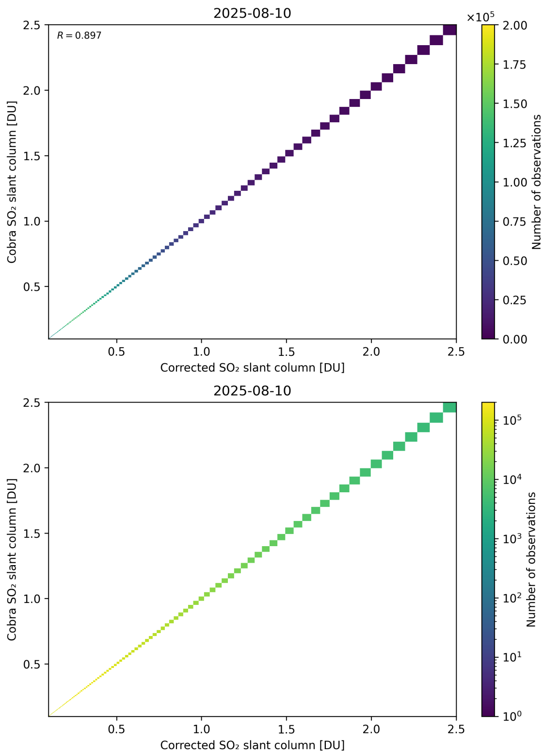
Figure 233: Scatter density plot of “Corrected SO 2 slant column” against “Cobra SO 2 slant column” for 2025-08-09 to 2025-08-11.
