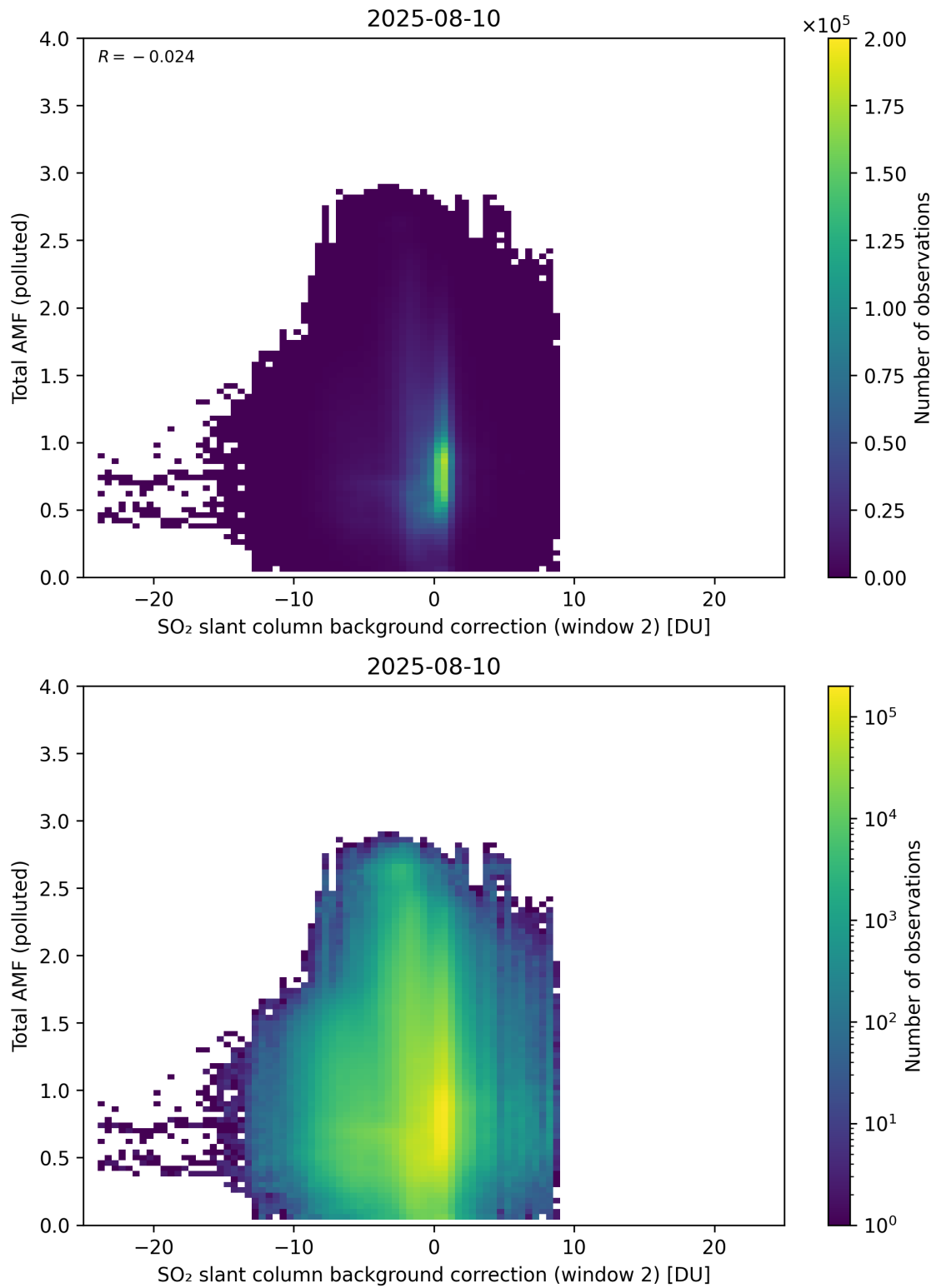
Figure 130: Scatter density plot of “SO 2 slant column background correction (window 2)” against “Total AMF (polluted)” for 2025-08-09 to 2025-08-11.
