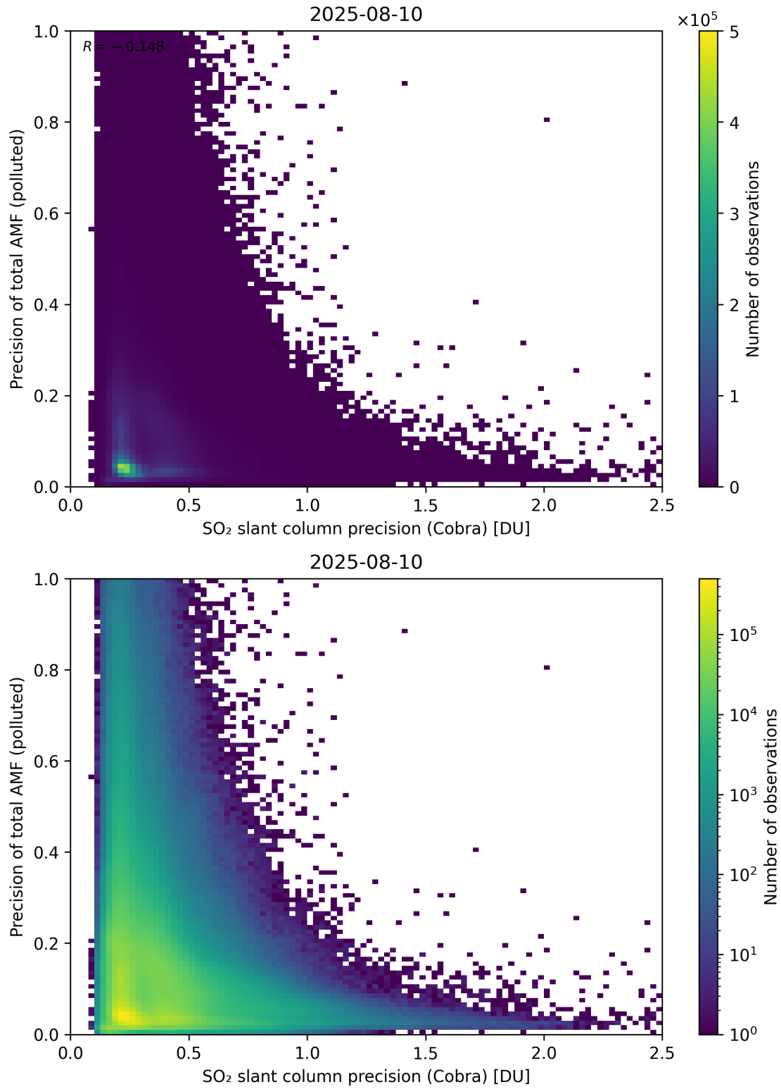
Figure 214: Scatter density plot of “SO 2 slant column precision (Cobra)” against “Precision of total AMF (polluted)” for 2025-08-09 to 2025-08-11.
