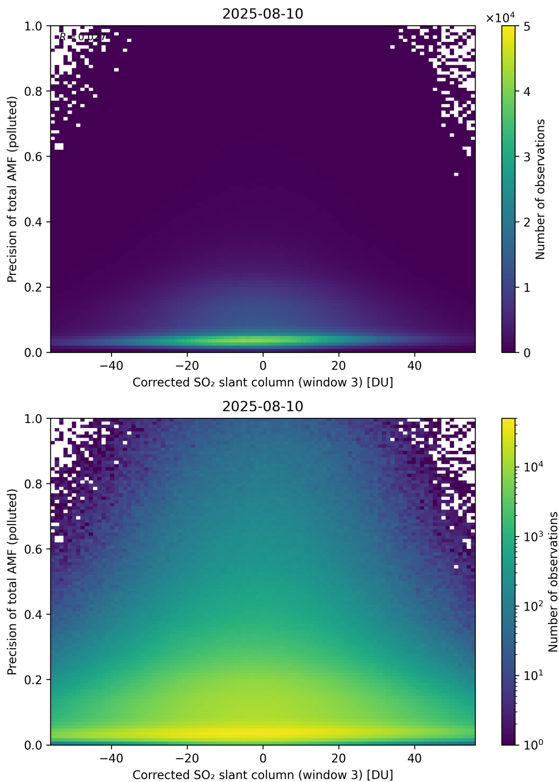
Figure 261: Scatter density plot of “Corrected SO 2 slant column (window 3)” against “Precision of total AMF (polluted)” for 2025-08-09 to 2025-08-11.
