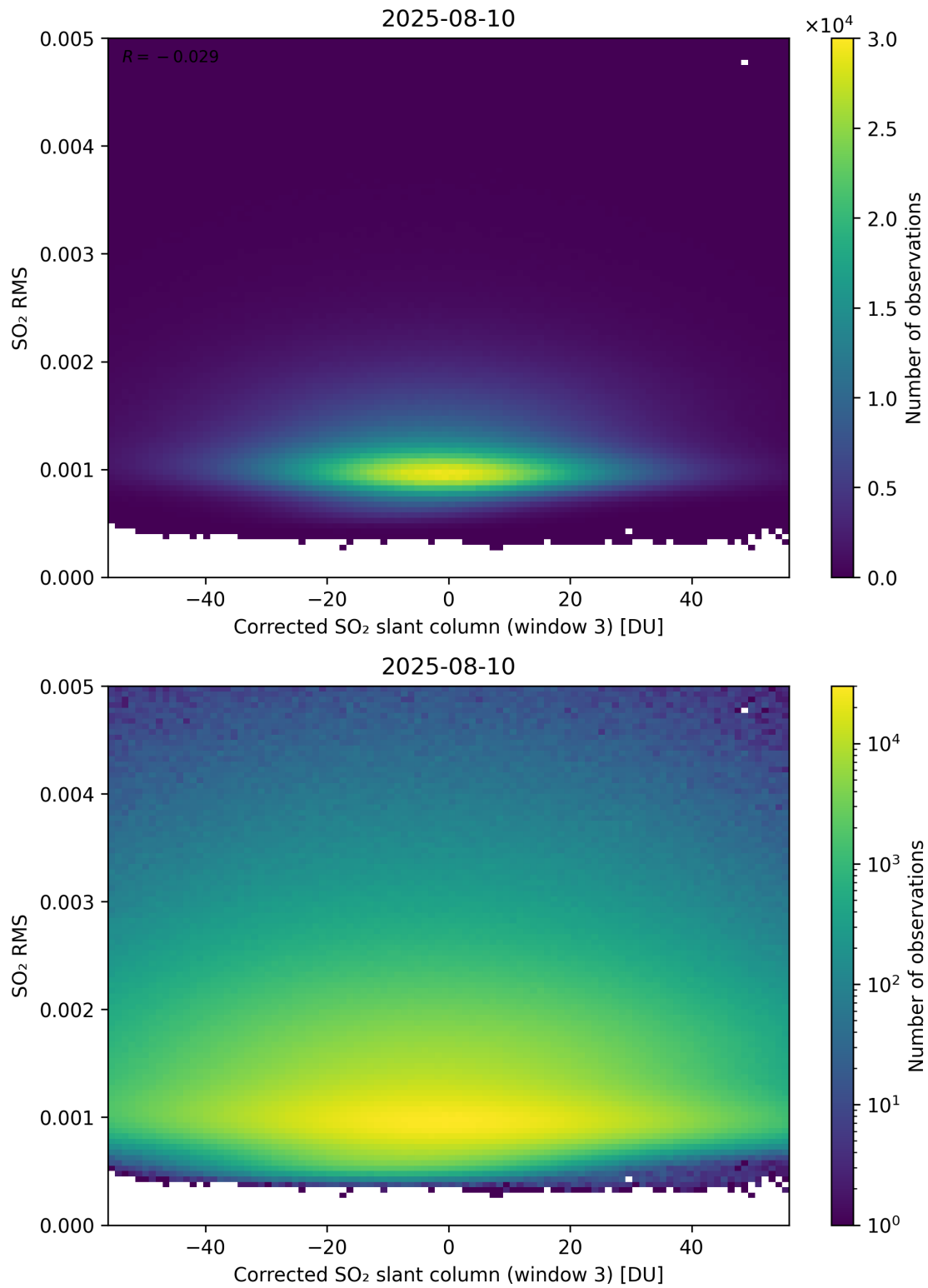
Figure 258: Scatter density plot of “Corrected SO 2 slant column (window 3)” against “SO 2 RMS” for 2025-08-09 to 2025-08-11.
