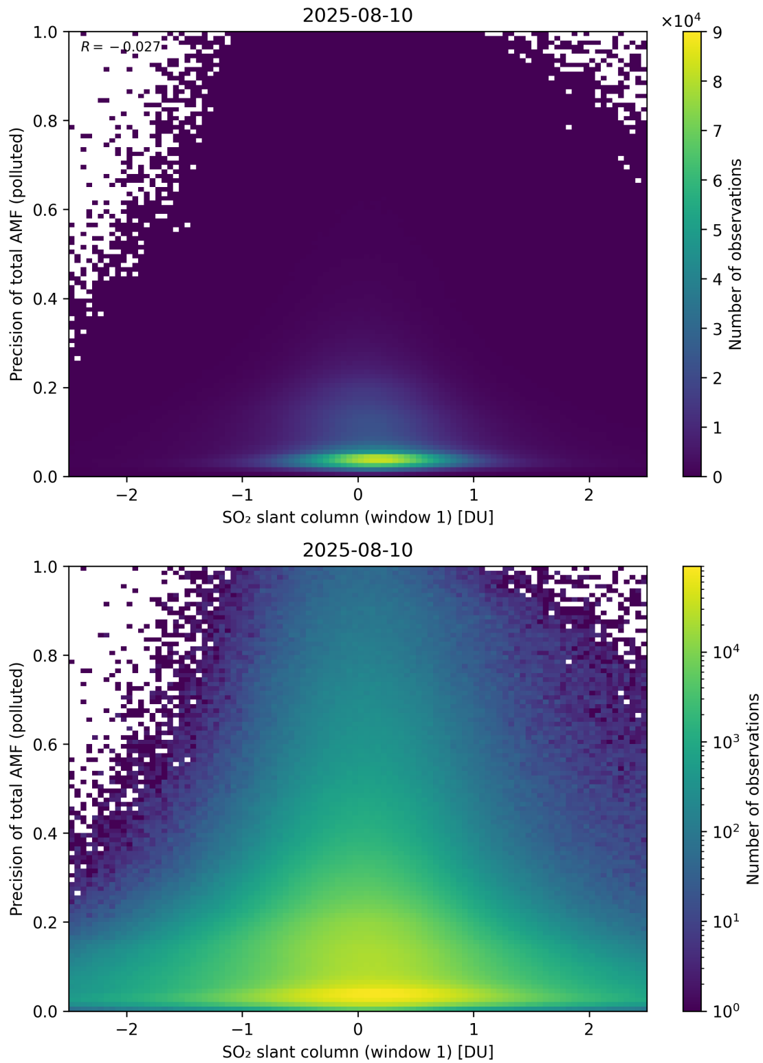
Figure 290: Scatter density plot of “SO 2 slant column (window 1)” against “Precision of total AMF (polluted)” for 2025-08-09 to 2025-08-11.
