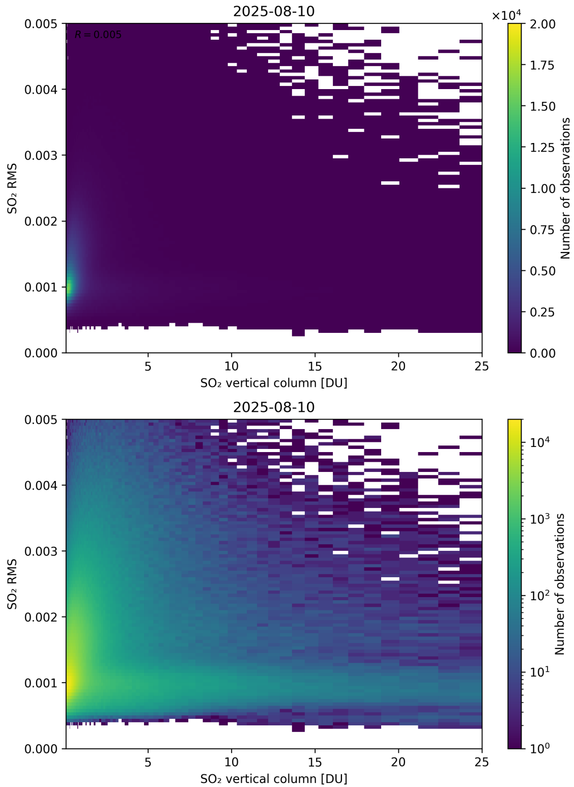
Figure 328: Scatter density plot of “SO 2 vertical column” against “SO 2 RMS” for 2025-08-09 to 2025-08-11.
