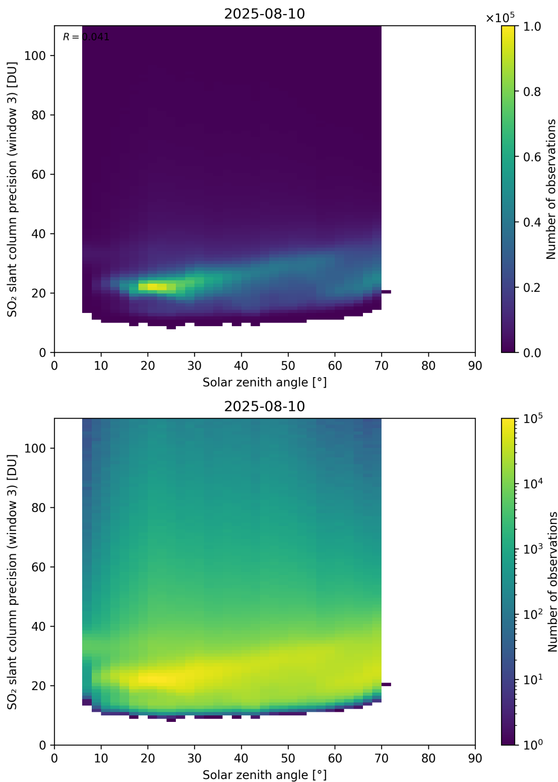
Figure 188: Scatter density plot of “Solar zenith angle” against “SO 2 slant column precision (window 3)” for 2025-08-09 to 2025-08-11.
