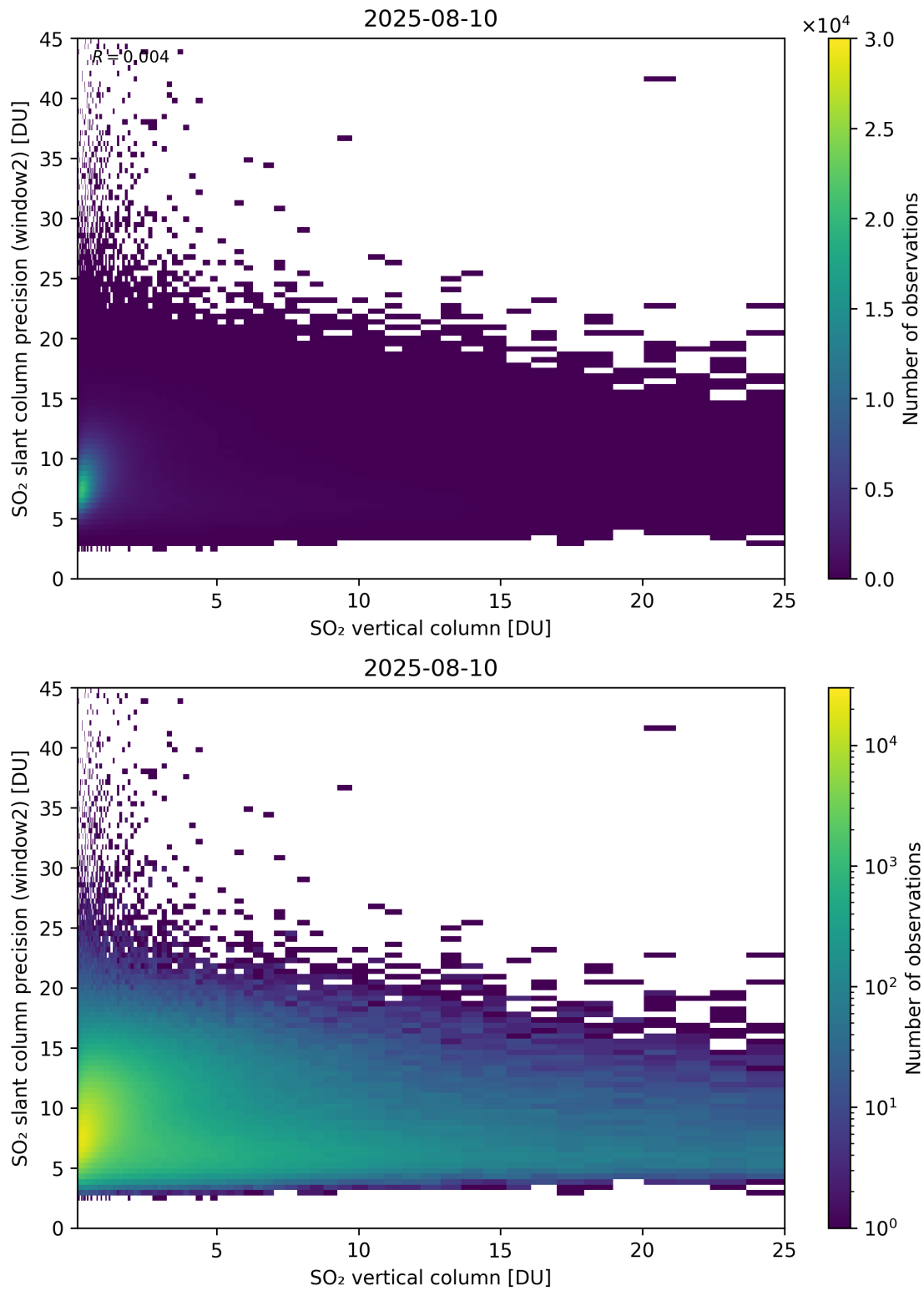
Figure 356: Scatter density plot of “SO 2 vertical column” against “SO 2 slant column precision (window2)” for 2025-08-09 to 2025-08-11.
