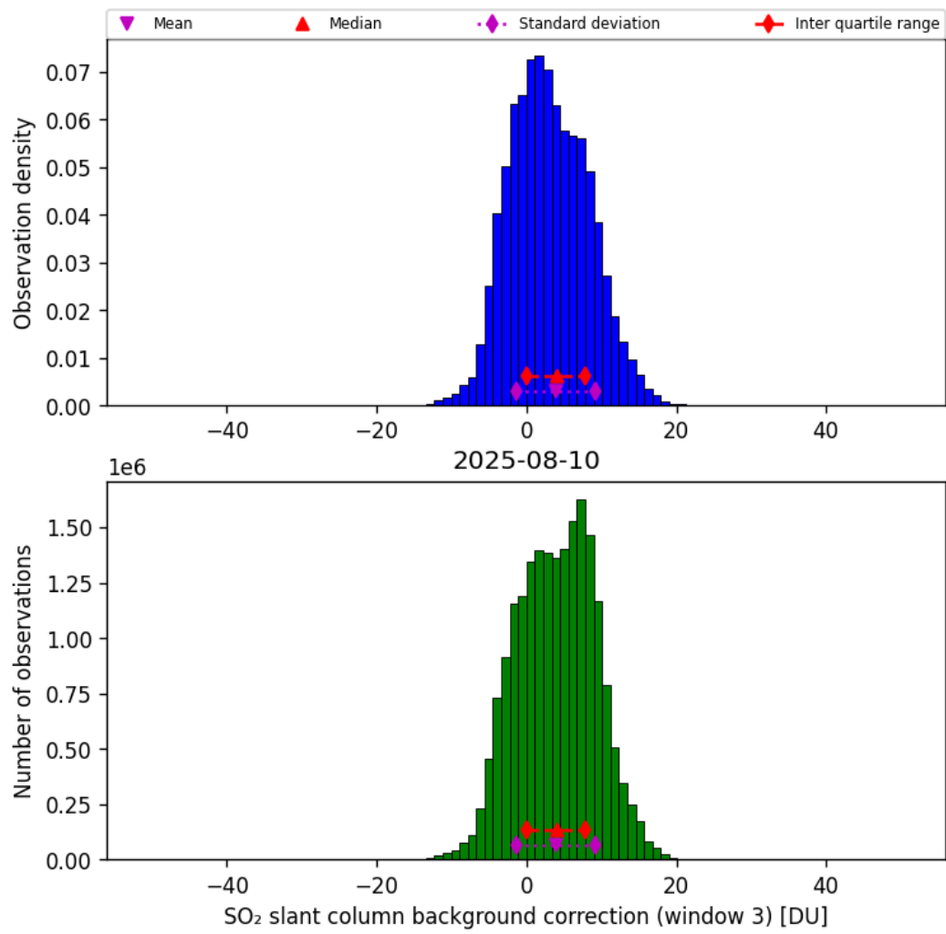
Figure 74: Histogram of “SO 2 slant column background correction (window 3)” for 2025-08-09 to 2025-08-11
