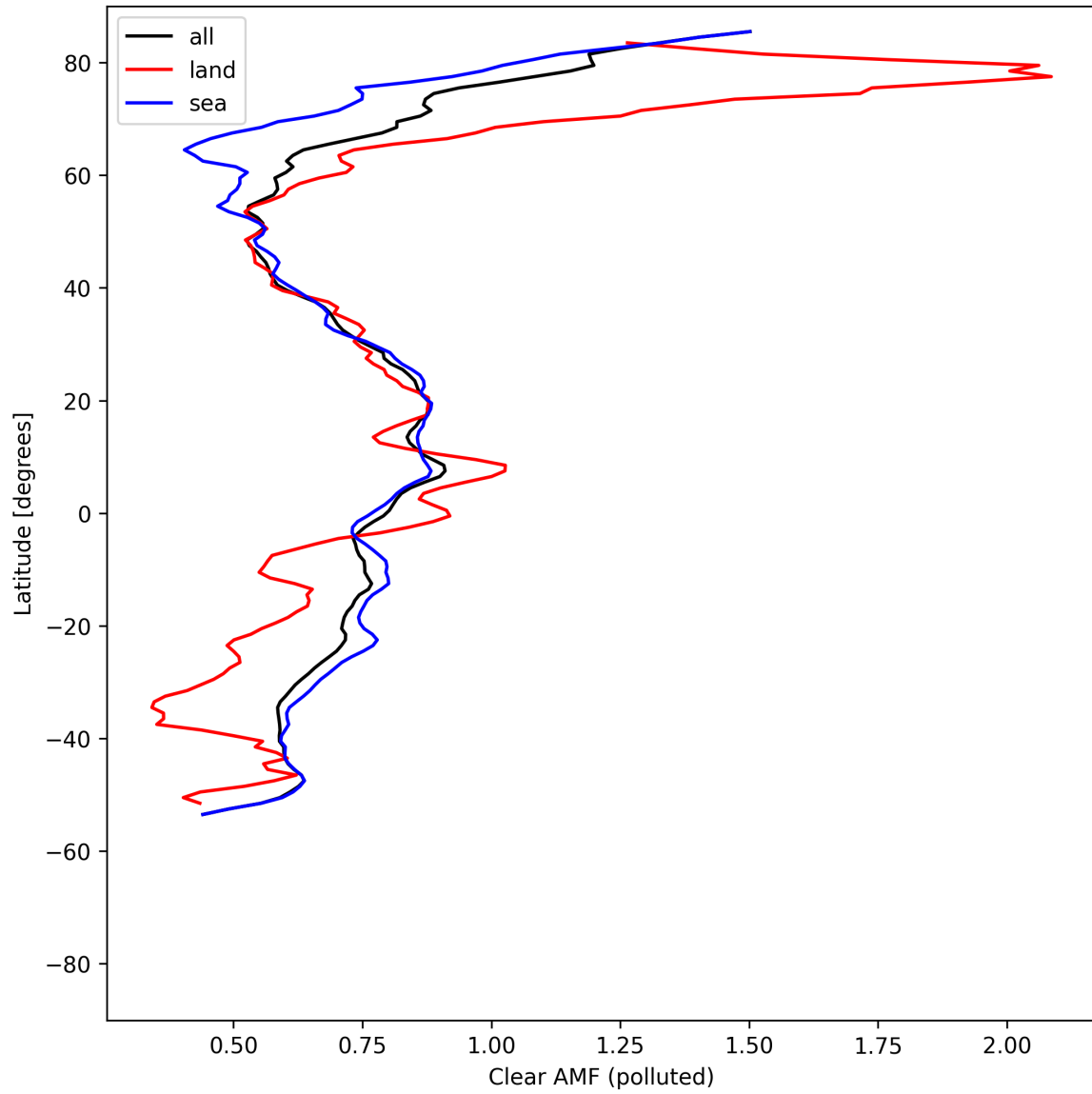
Figure 55: Zonal average of “Clear AMF (polluted)” for 2025-08-09 to 2025-08-11.
