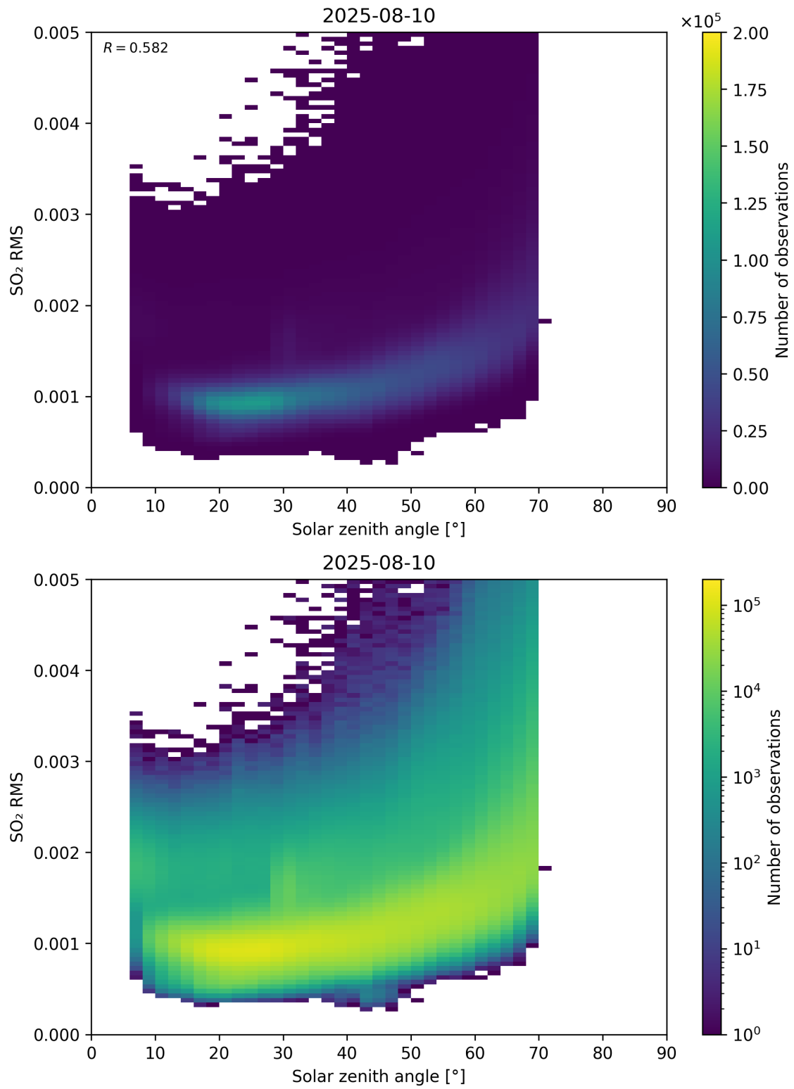
Figure 176: Scatter density plot of “Solar zenith angle” against “SO 2 RMS” for 2025-08-09 to 2025-08-11.
