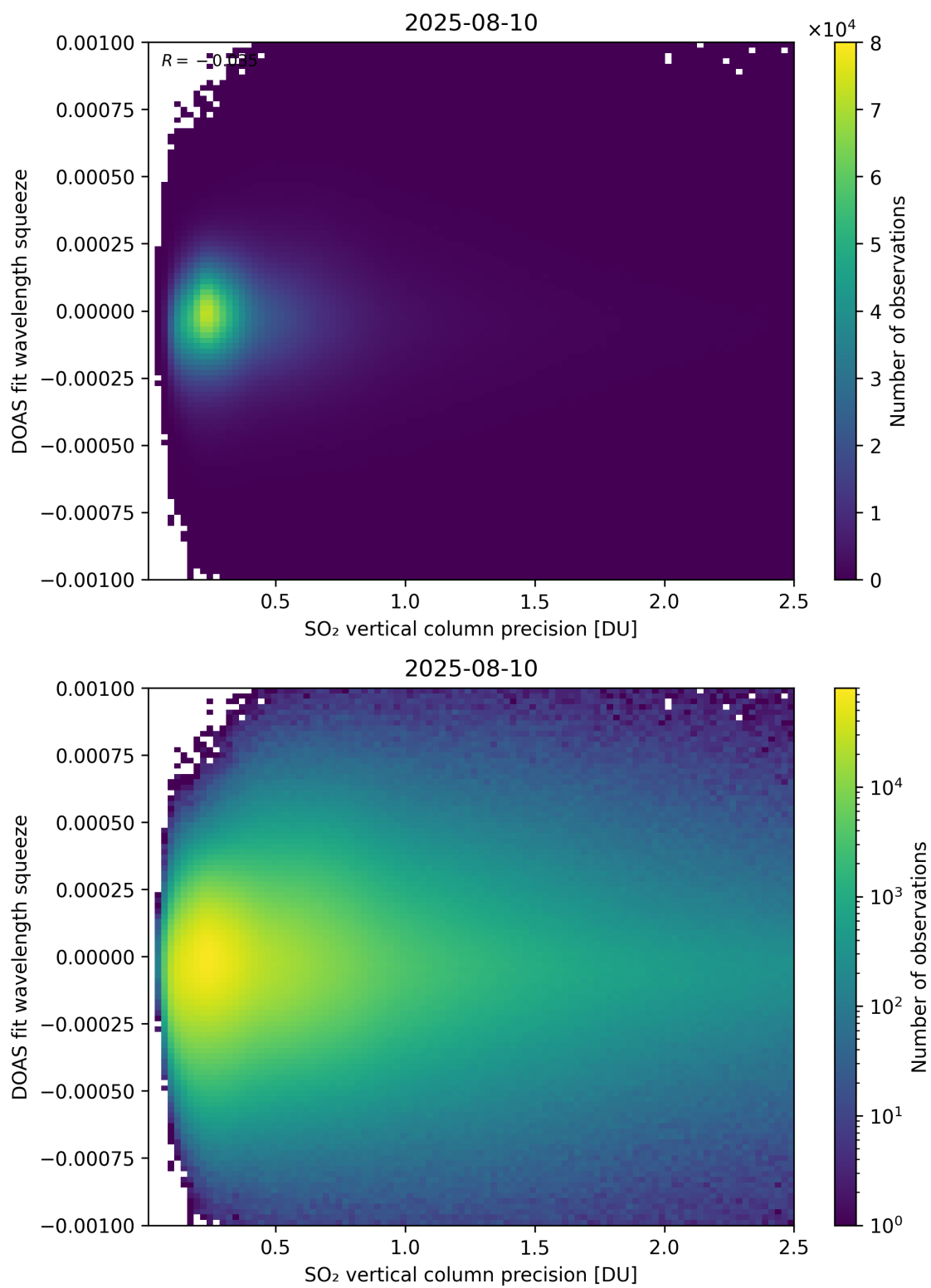
Figure 333: Scatter density plot of “SO 2 vertical column precision” against “DOAS fit wavelength squeeze” for 2025-08-09 to 2025-08-11.
