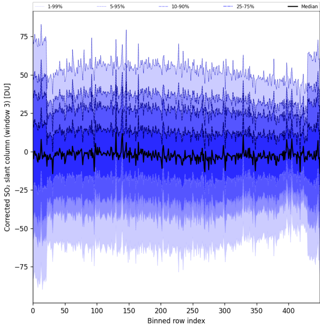
Figure 99: Along track statistics of “Corrected SO 2 slant column (window 3)” for 2025-08-09 to 2025-08-11
