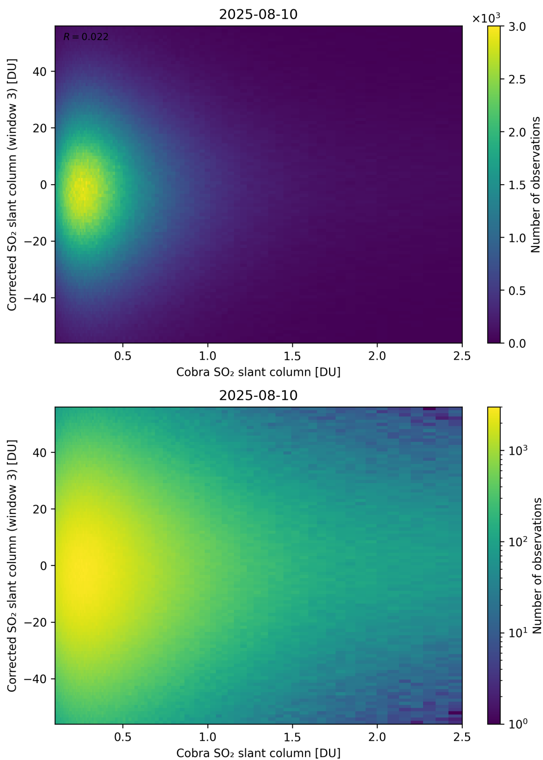
Figure 218: Scatter density plot of “Cobra SO 2 slant column” against “Corrected SO 2 slant column (window 3)” for 2025-08-09 to 2025-08-11.
