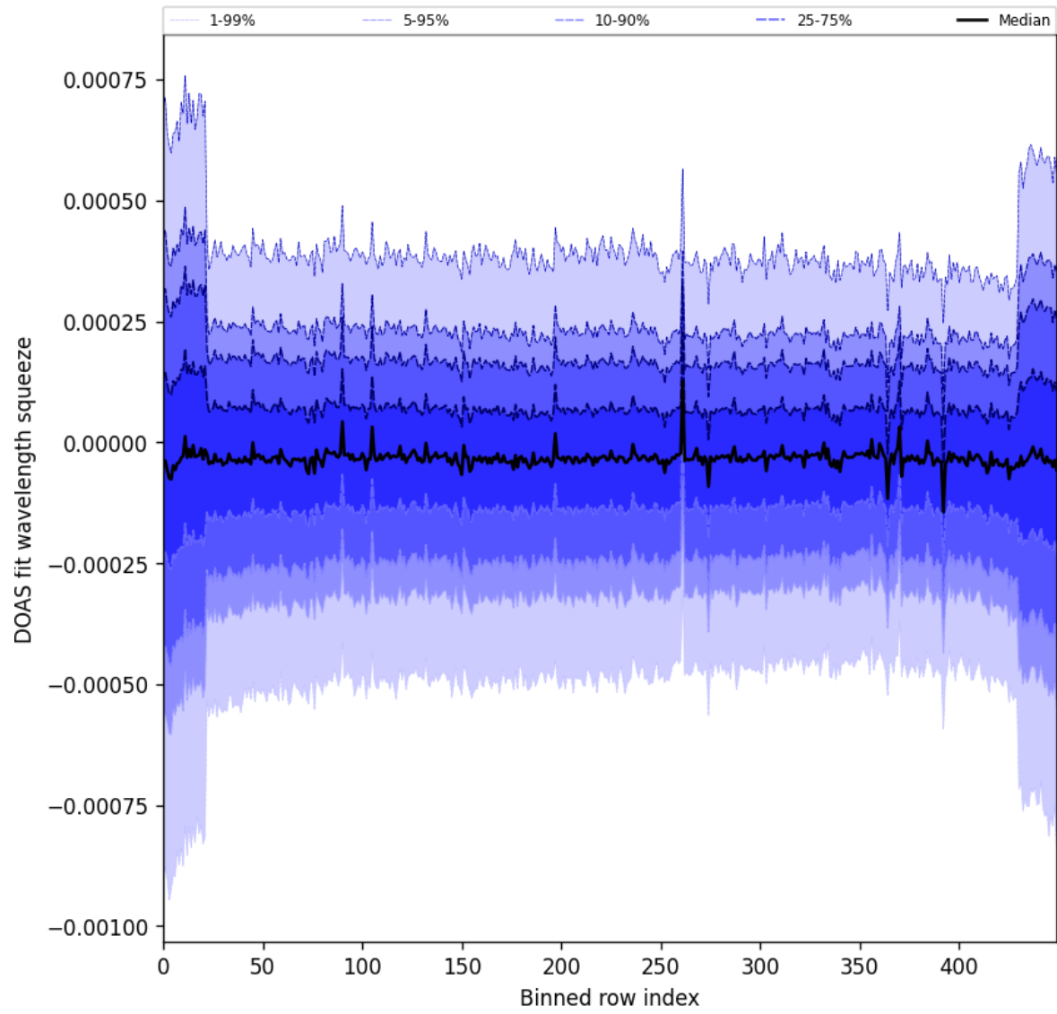
Figure 103: Along track statistics of “DOAS fit wavelength squeeze” for 2025-08-09 to 2025-08-11
