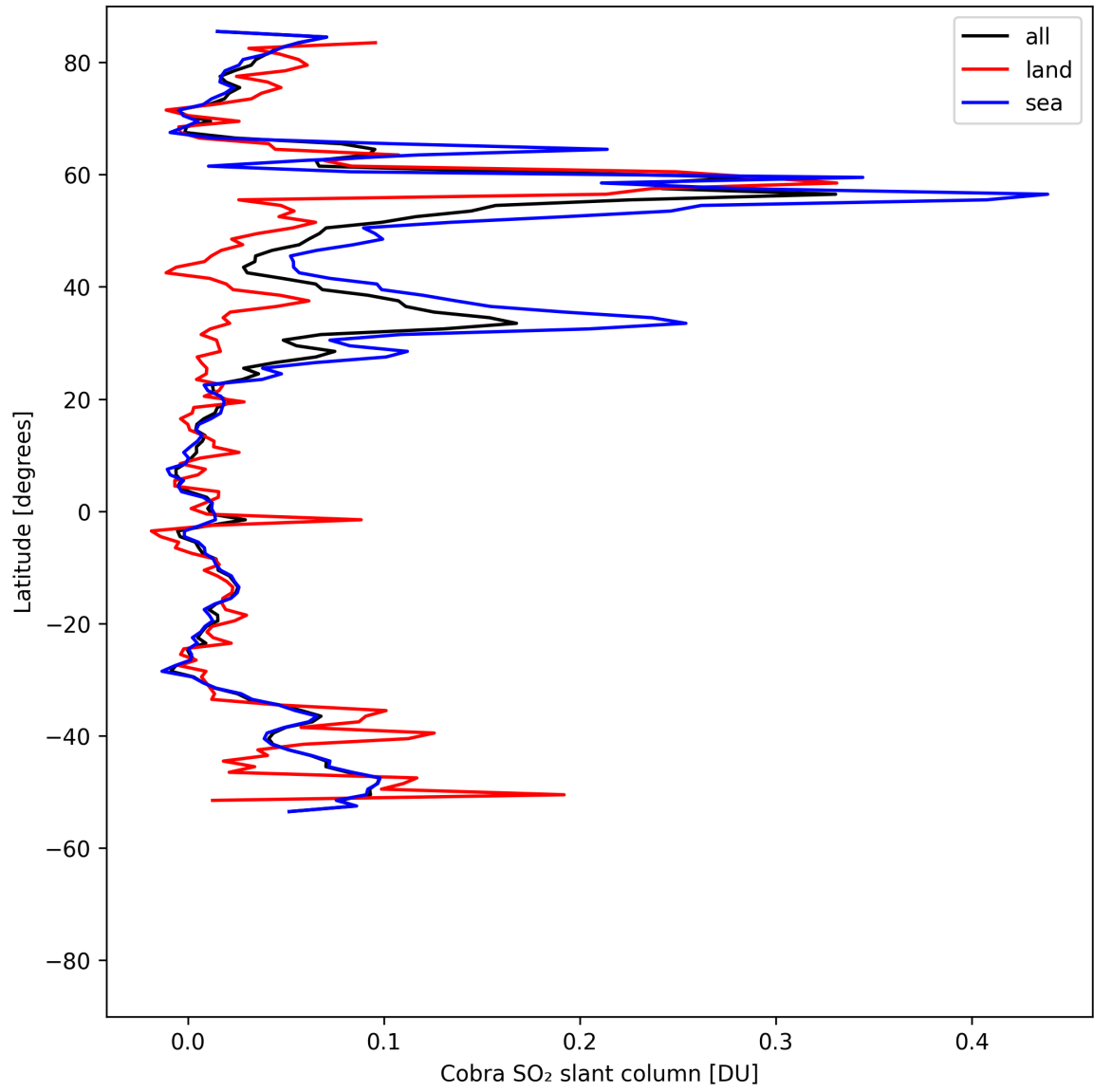
Figure 35: Zonal average of “Cobra SO 2 slant column” for 2025-08-09 to 2025-08-11.
