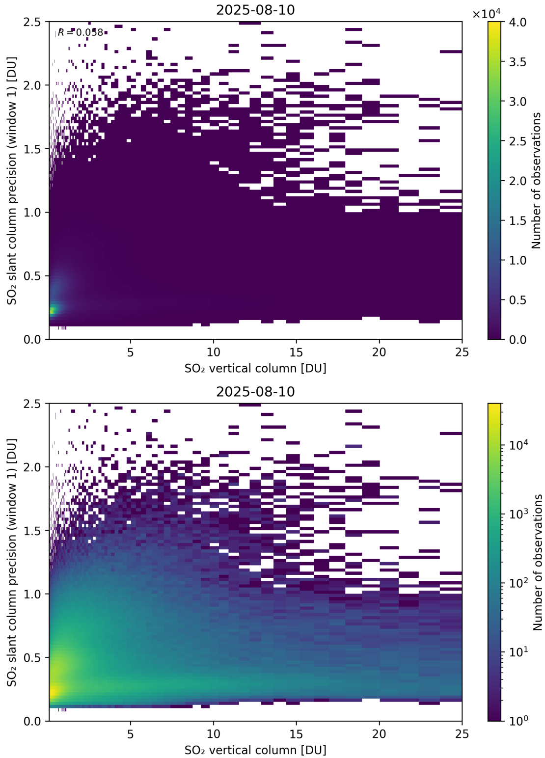
Figure 355: Scatter density plot of “SO 2 vertical column” against “SO 2 slant column precision (window 1)” for 2025-08-09 to 2025-08-11.
