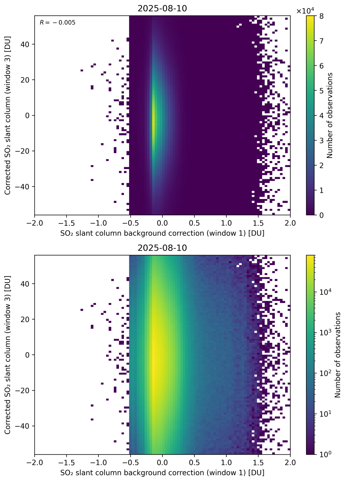
Figure 116: Scatter density plot of “SO 2 slant column background correction (window 1)” against “Corrected SO 2 slant column (window 3)” for 2025-08-09 to 2025-08-11.
