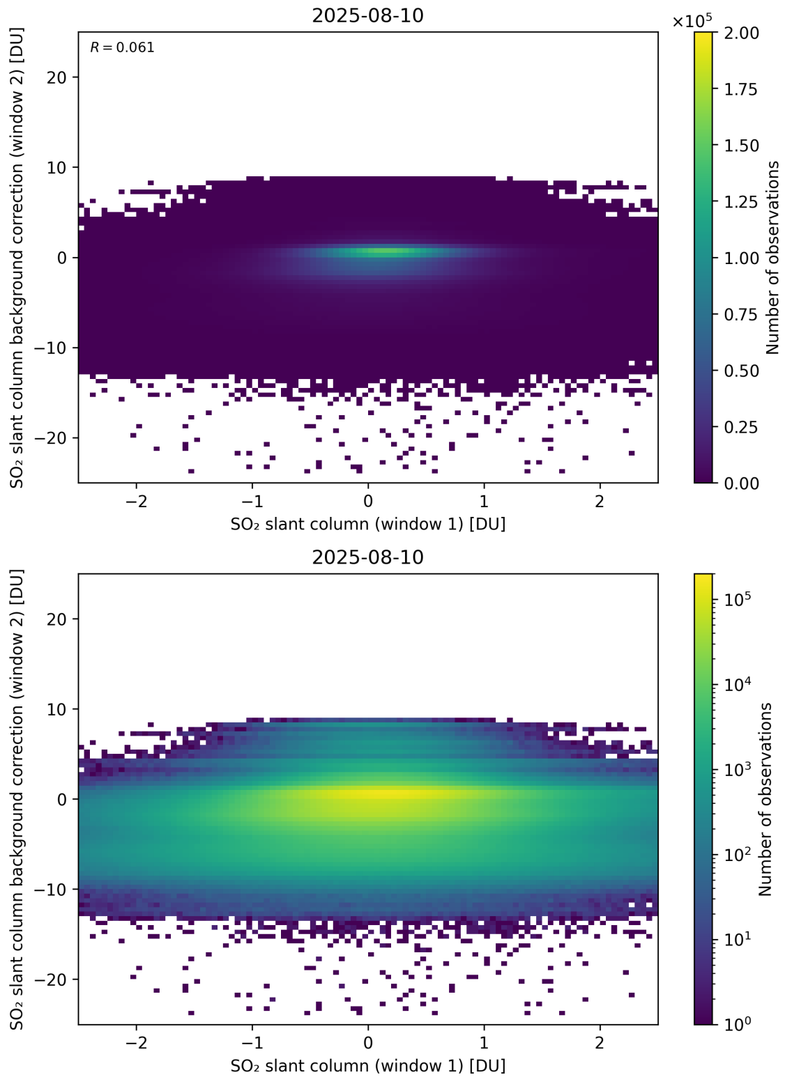
Figure 263: Scatter density plot of “SO 2 slant column (window 1)” against “SO 2 slant column background correction (window 2)” for 2025-08-09 to 2025-08-11.
