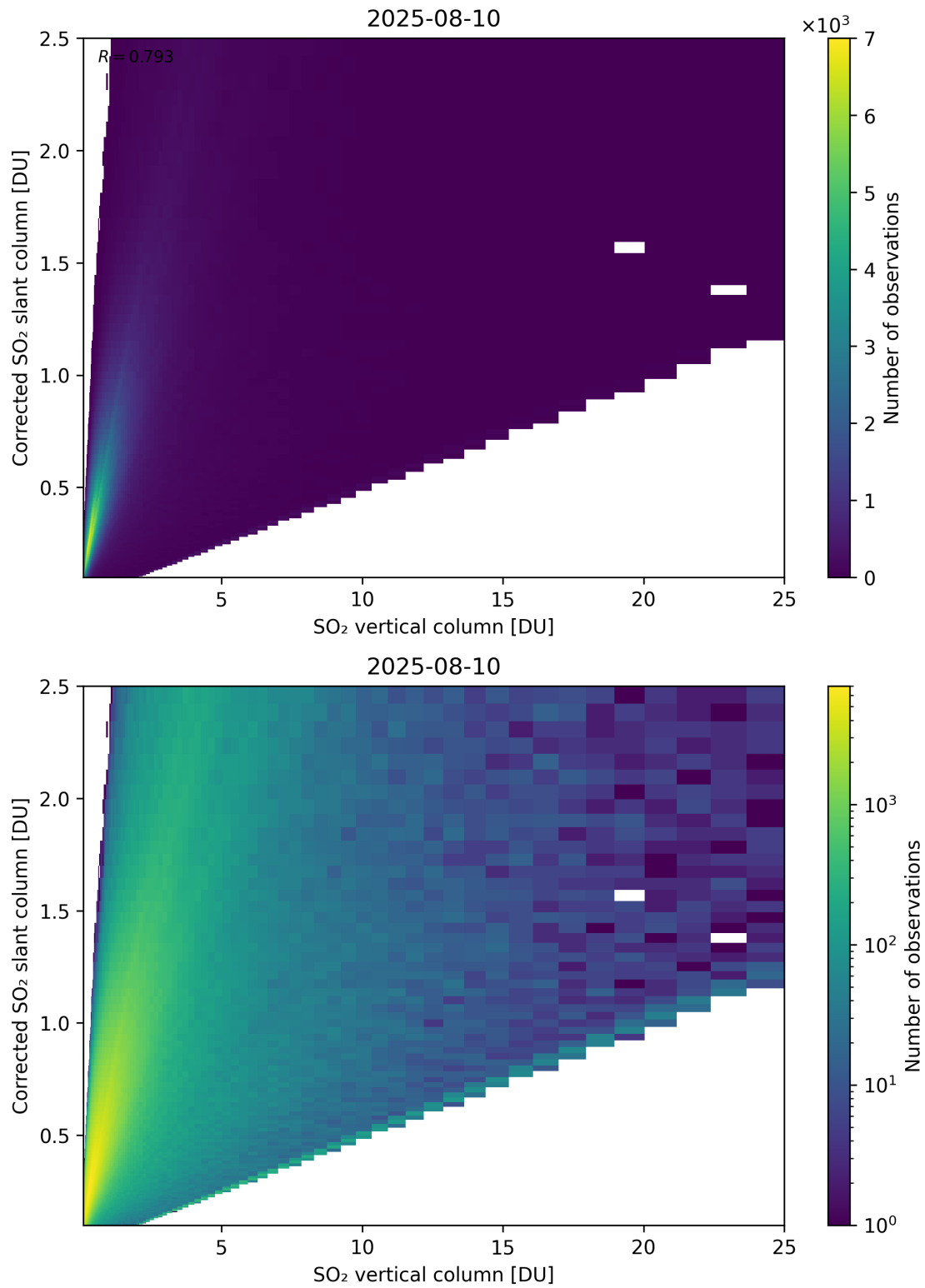
Figure 351: Scatter density plot of “SO 2 vertical column” against “Corrected SO 2 slant column” for 2025-08-09 to 2025-08-11.
