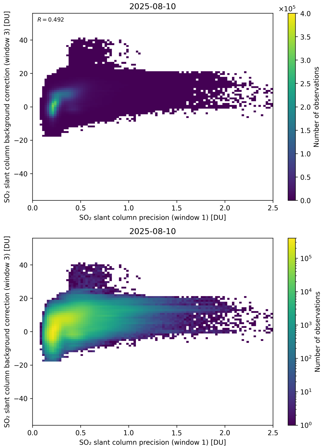
Figure 270: Scatter density plot of “SO 2 slant column precision (window 1)” against “SO 2 slant column background correction (window 3)” for 2025-08-09 to 2025-08-11.
