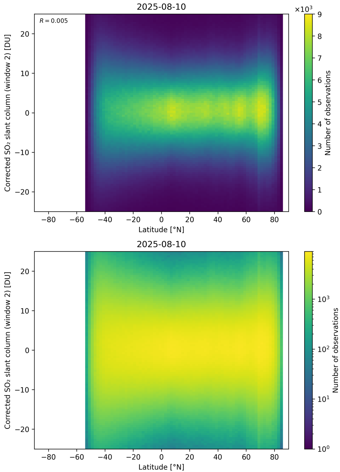
Figure 160: Scatter density plot of “Latitude” against “Corrected SO 2 slant column (window 2)” for 2025-08-09 to 2025-08-11.
