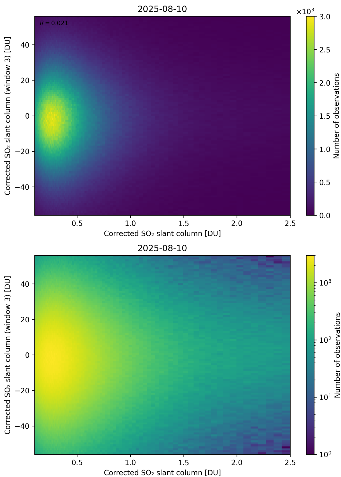
Figure 236: Scatter density plot of “Corrected SO 2 slant column” against “Corrected SO 2 slant column (window 3)” for 2025-08-09 to 2025-08-11.
