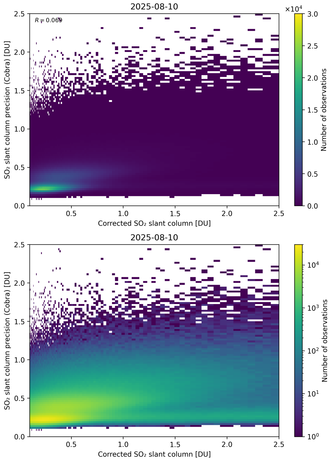
Figure 234: Scatter density plot of “Corrected SO 2 slant column” against “SO 2 slant column precision (Cobra)” for 2025-08-09 to 2025-08-11.
