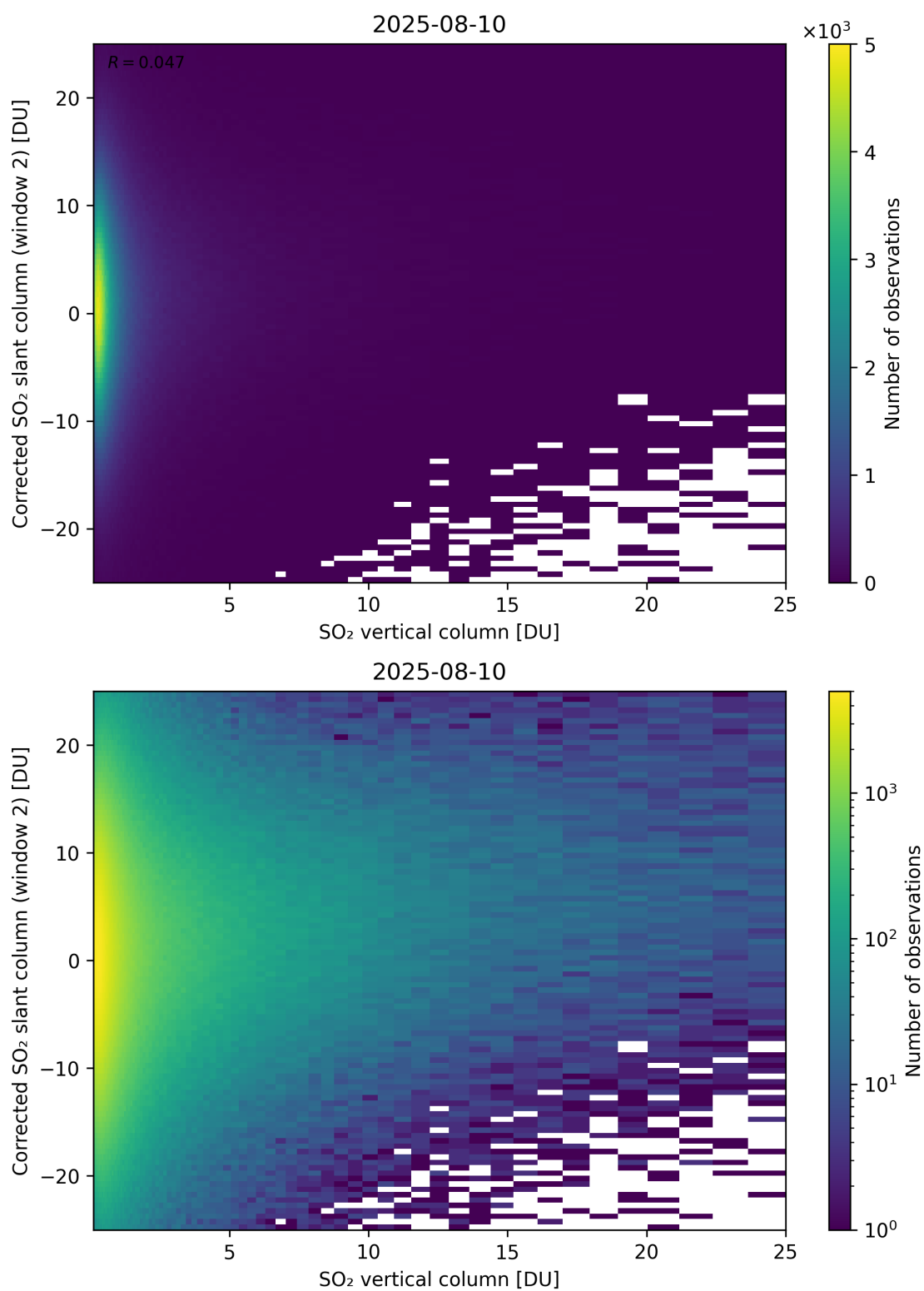
Figure 352: Scatter density plot of “SO 2 vertical column” against “Corrected SO 2 slant column (window 2)” for 2025-08-09 to 2025-08-11.
