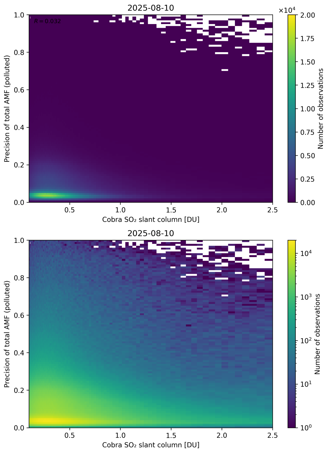
Figure 225: Scatter density plot of “Cobra SO 2 slant column” against “Precision of total AMF (polluted)” for 2025-08-09 to 2025-08-11.
