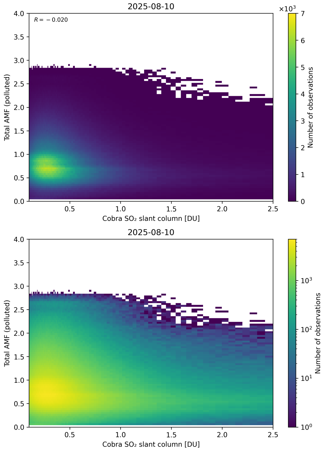
Figure 224: Scatter density plot of “Cobra SO 2 slant column” against “Total AMF (polluted)” for 2025-08-09 to 2025-08-11.
