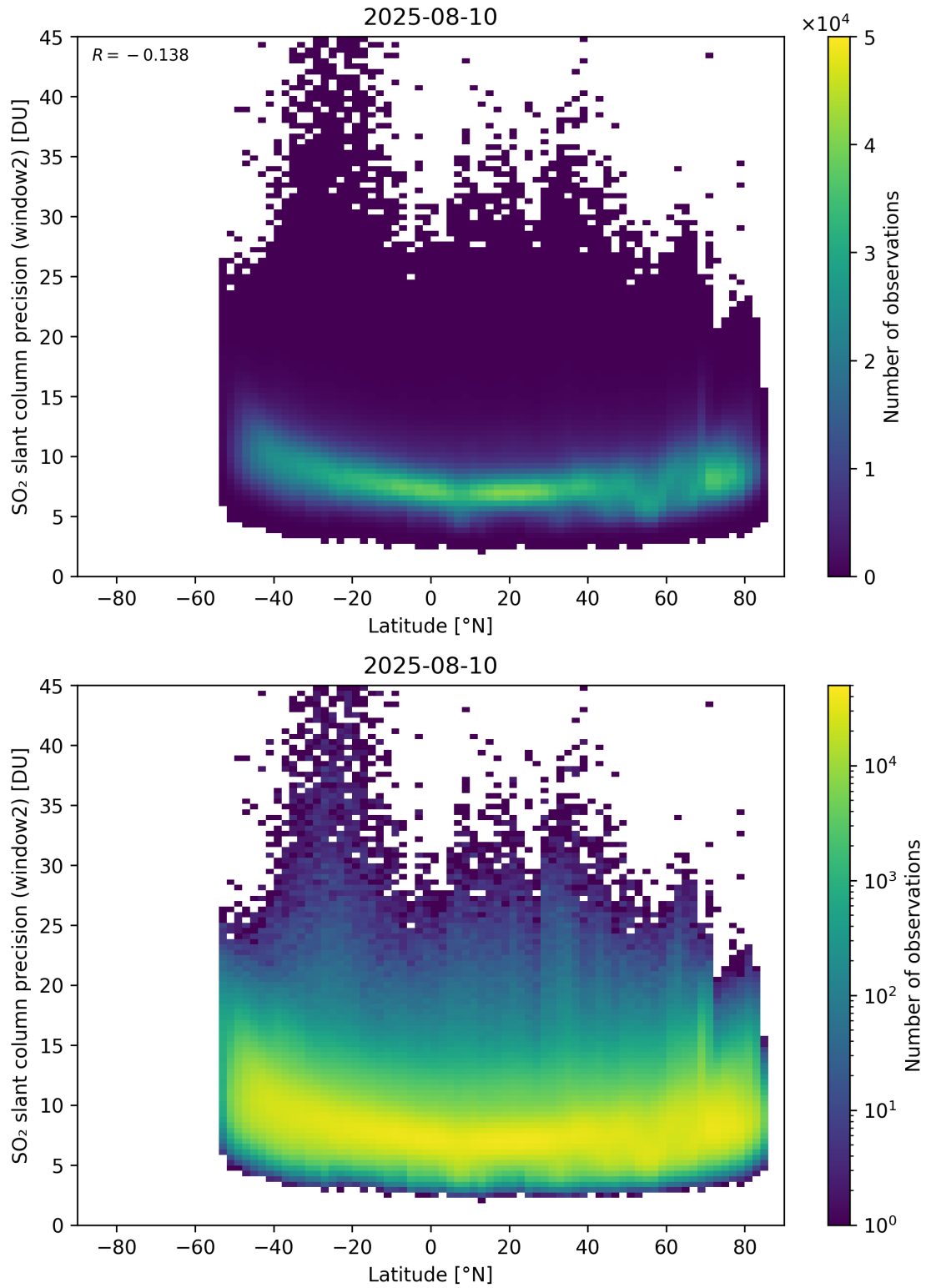
Figure 164: Scatter density plot of “Latitude” against “SO 2 slant column precision (window2)” for 2025-08-09 to 2025-08-11.
