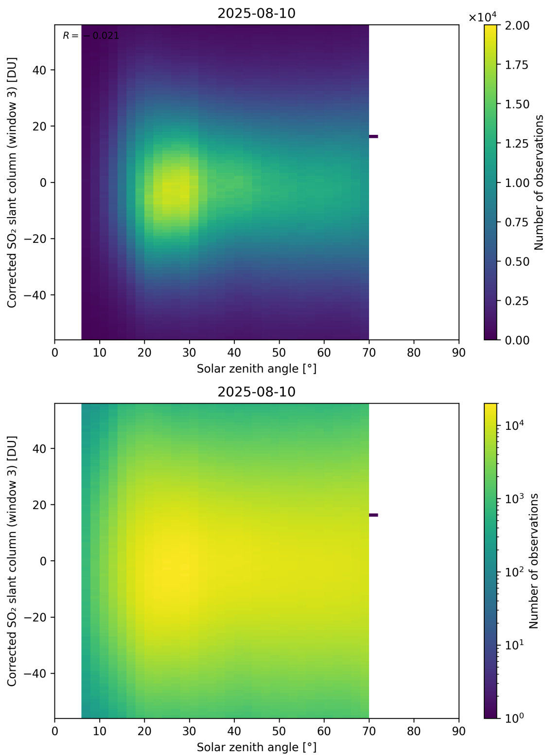
Figure 183: Scatter density plot of “Solar zenith angle” against “Corrected SO 2 slant column (window 3)” for 2025-08-09 to 2025-08-11.
