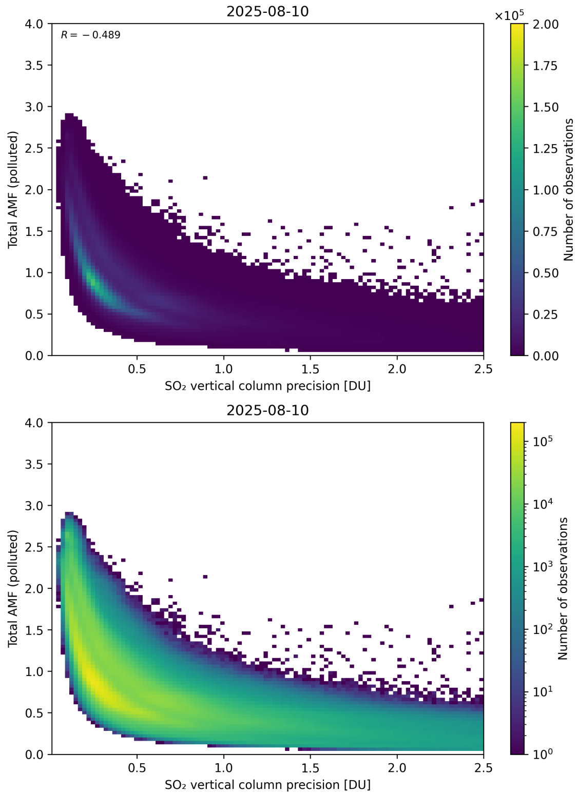
Figure 346: Scatter density plot of “SO 2 vertical column precision” against “Total AMF (polluted)” for 2025-08-09 to 2025-08-11.
