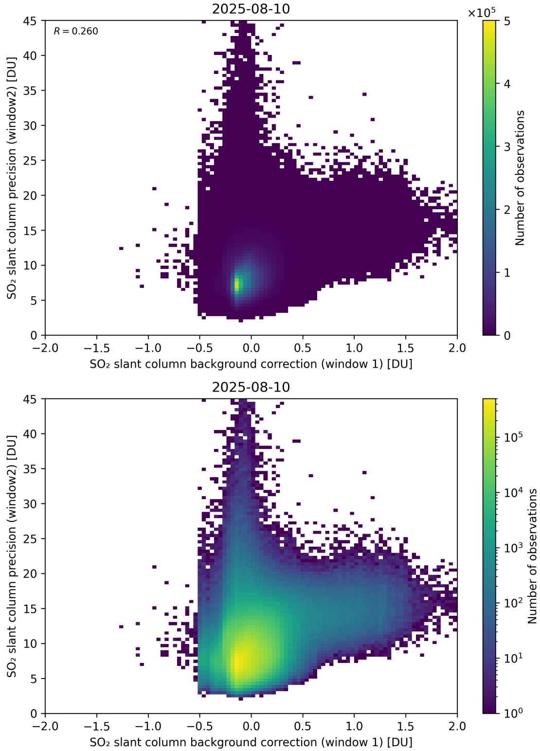
Figure 117: Scatter density plot of “SO 2 slant column background correction (window 1)” against “SO 2 slant column precision (window2)” for 2025-08-09 to 2025-08-11.
