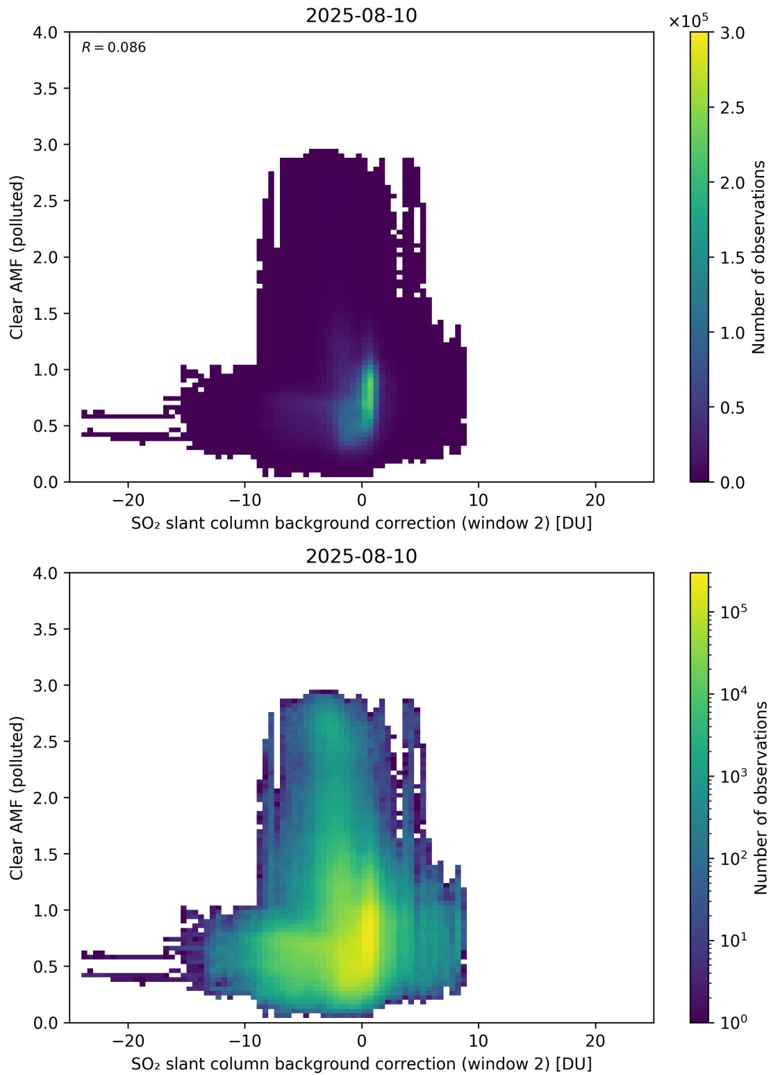
Figure 126: Scatter density plot of “SO 2 slant column background correction (window 2)” against “Clear AMF (polluted)” for 2025-08-09 to 2025-08-11.
