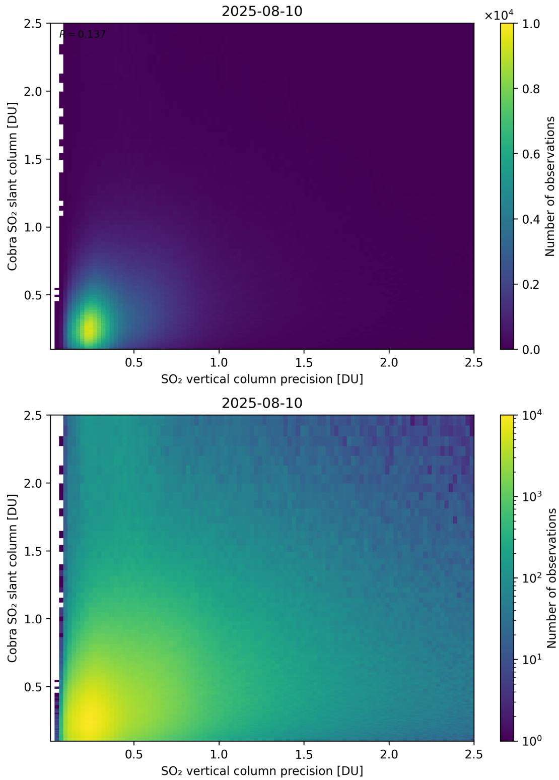
Figure 336: Scatter density plot of “SO 2 vertical column precision” against “Cobra SO 2 slant column” for 2025-08-09 to 2025-08-11.
