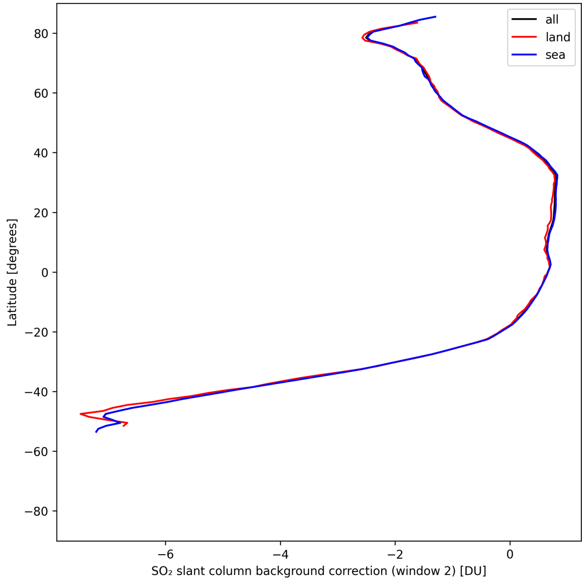
Figure 44: Zonal average of “SO 2 slant column background correction (window 2)” for 2025-08-09 to 2025-08-11.
