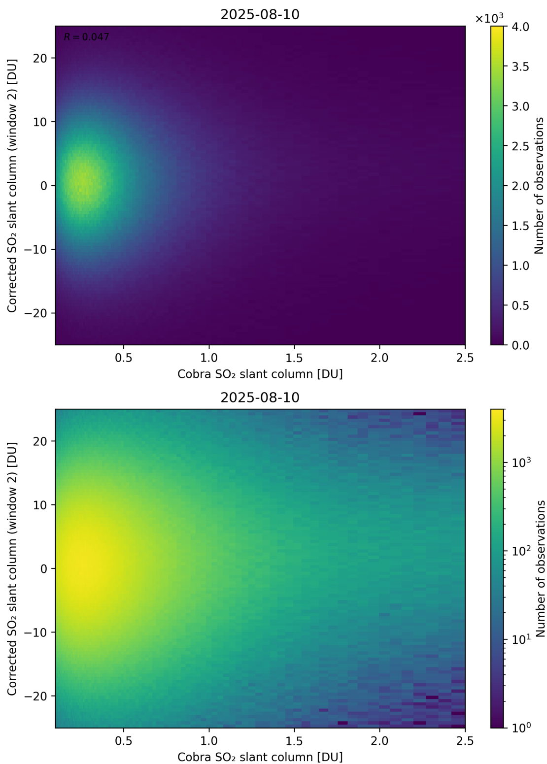
Figure 217: Scatter density plot of “Cobra SO 2 slant column” against “Corrected SO 2 slant column (window 2)” for 2025-08-09 to 2025-08-11.
