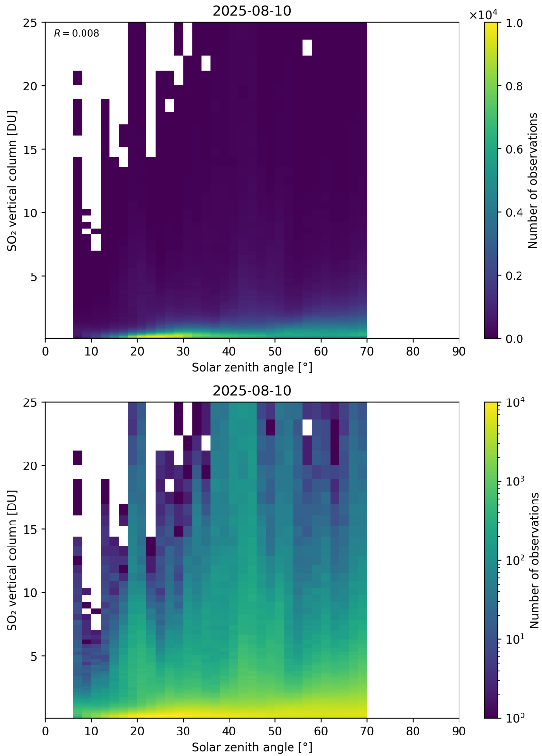
Figure 191: Scatter density plot of “Solar zenith angle” against “SO 2 vertical column” for 2025-08-09 to 2025-08-11.
