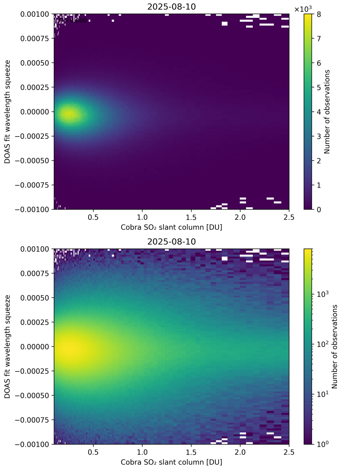
Figure 197: Scatter density plot of “Cobra SO 2 slant column” against “DOAS fit wavelength squeeze” for 2025-08-09 to 2025-08-11.
