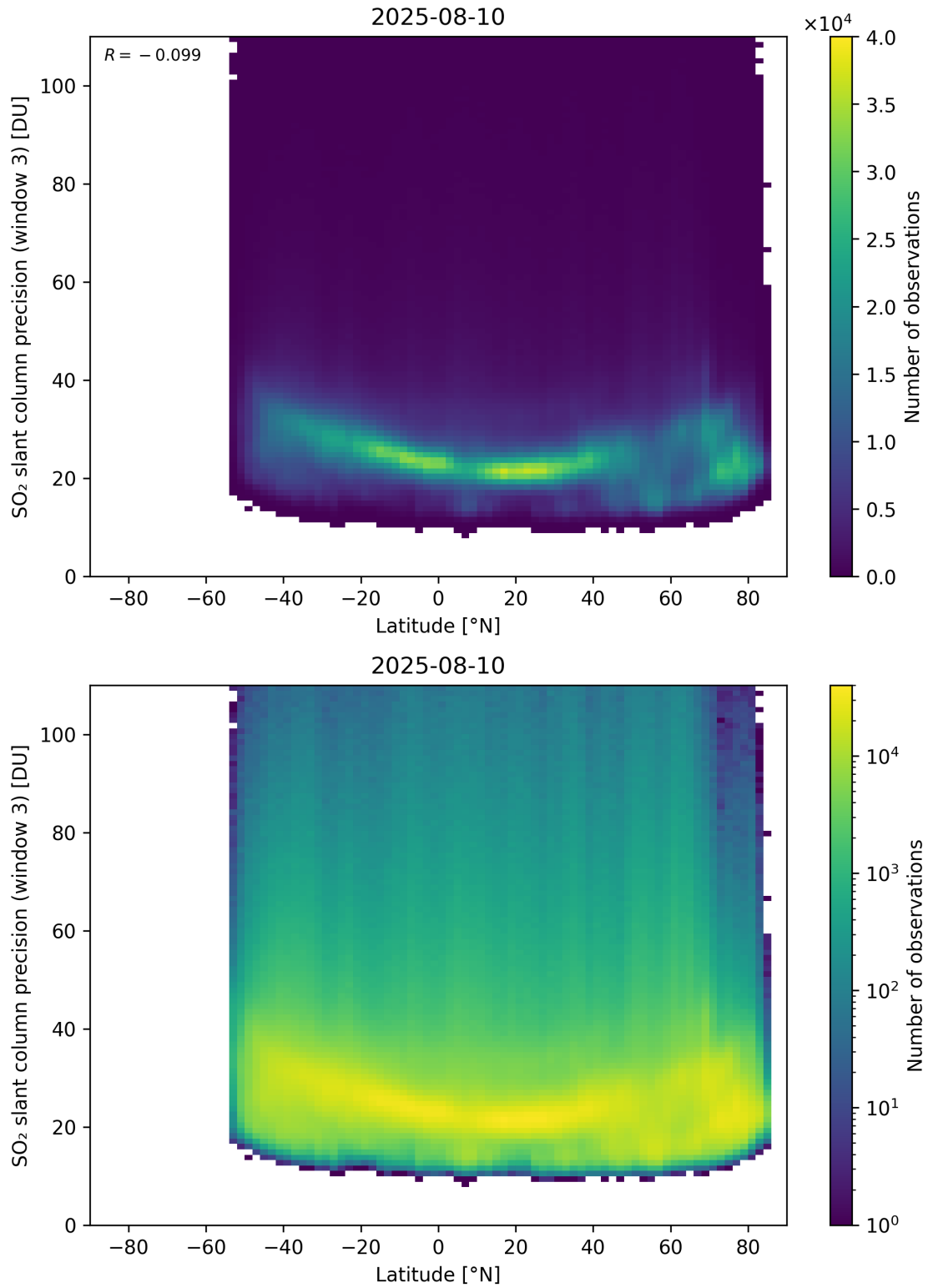
Figure 166: Scatter density plot of “Latitude” against “SO 2 slant column precision (window 3)” for 2025-08-09 to 2025-08-11.
