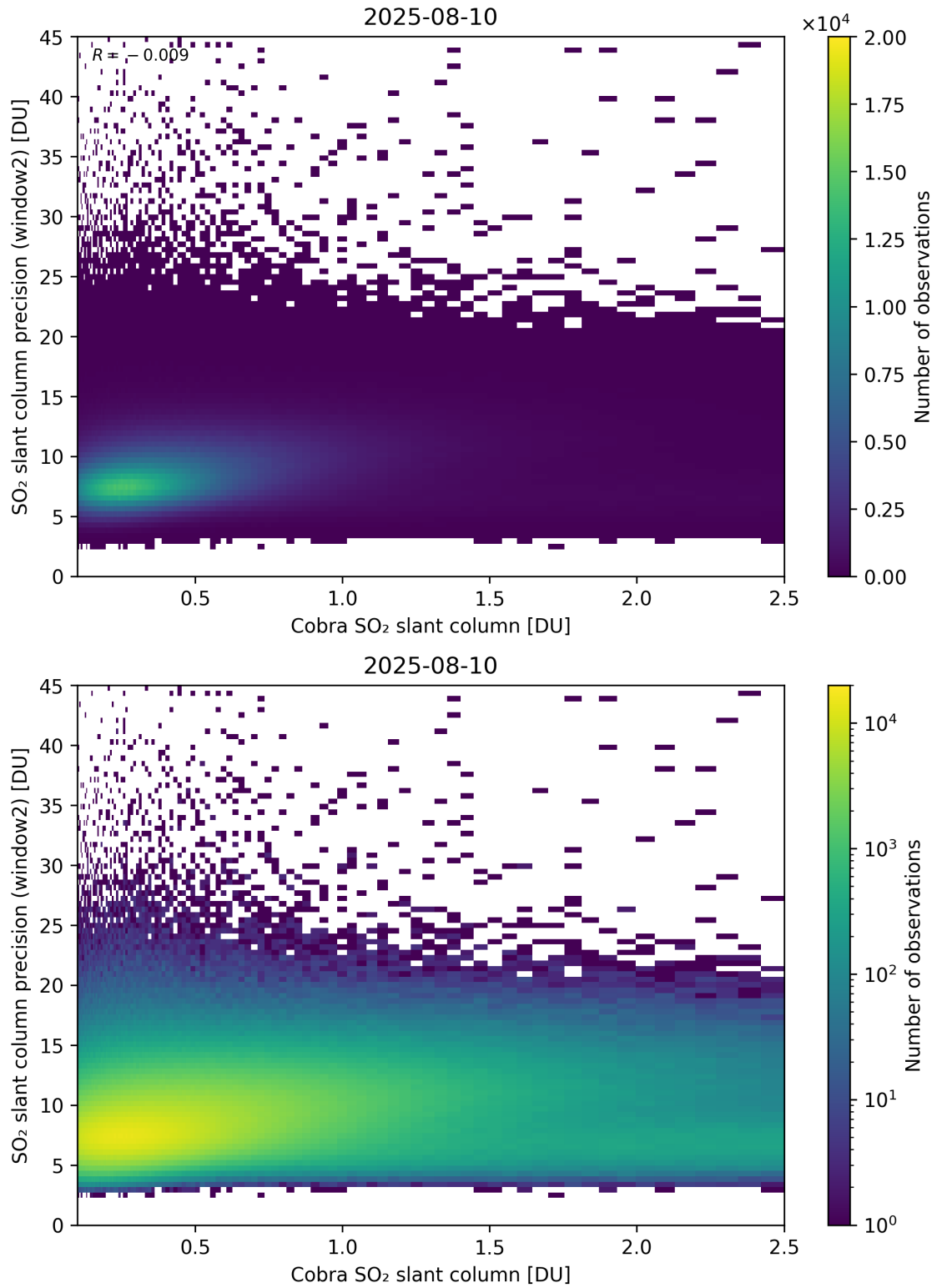
Figure 221: Scatter density plot of “Cobra SO 2 slant column” against “SO 2 slant column precision (window2)” for 2025-08-09 to 2025-08-11.
