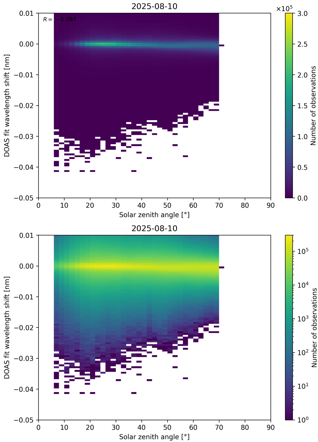
Figure 174: Scatter density plot of “Solar zenith angle” against “DOAS fit wavelength shift” for 2025-08-09 to 2025-08-11.
