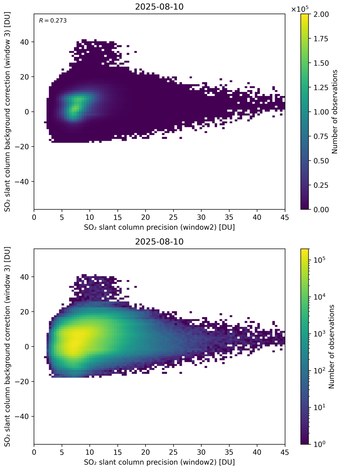
Figure 292: Scatter density plot of “SO 2 slant column precision (window2)” against “SO 2 slant column background correction (window 3)” for 2025-08-09 to 2025-08-11.
