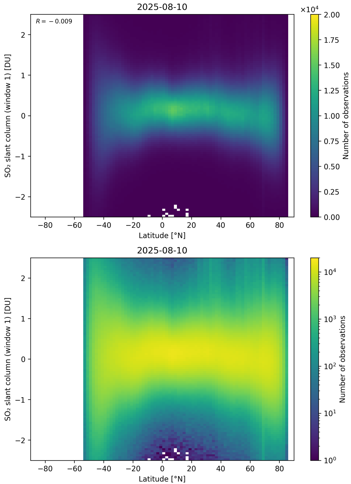
Figure 162: Scatter density plot of “Latitude” against “SO 2 slant column (window 1)” for 2025-08-09 to 2025-08-11.
