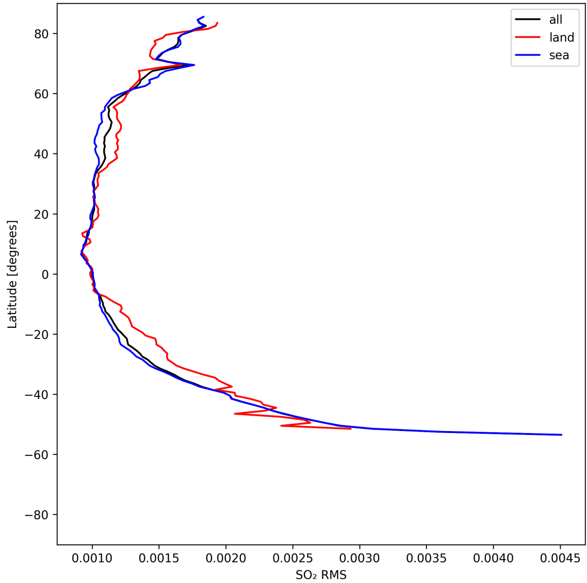
Figure 52: Zonal average of “SO 2 RMS” for 2025-08-09 to 2025-08-11.
