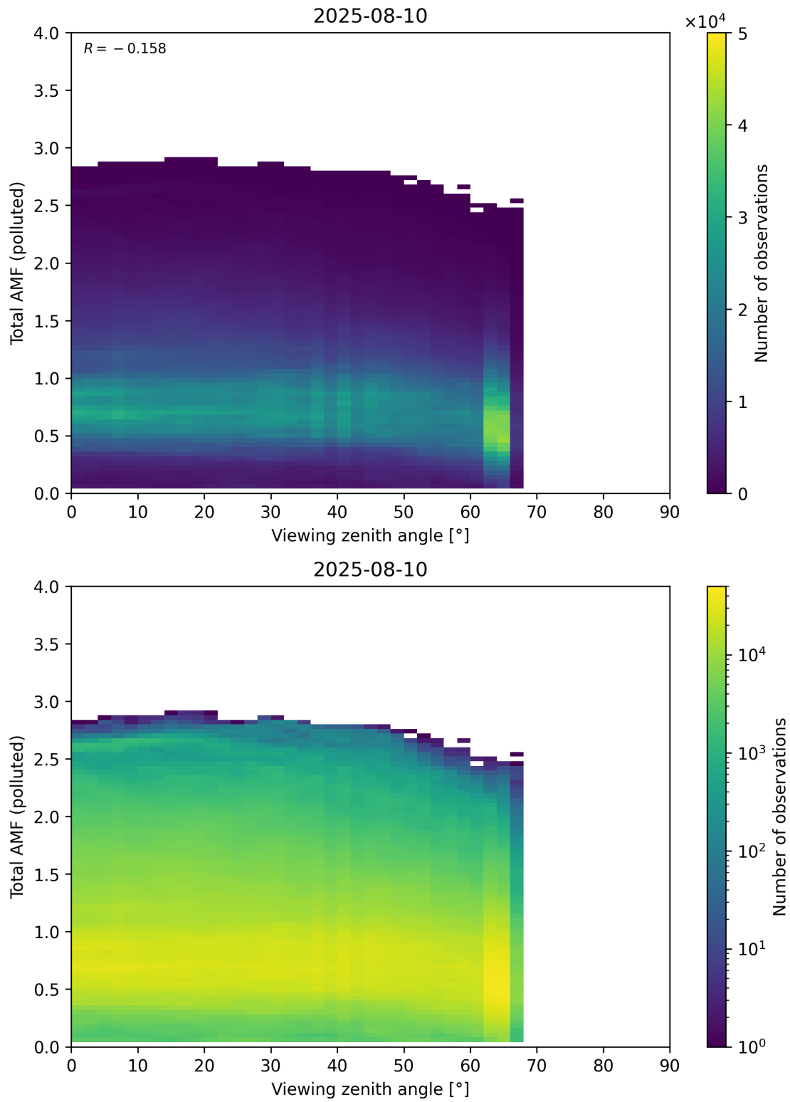
Figure 381: Scatter density plot of “Viewing zenith angle” against “Total AMF (polluted)” for 2025-08-09 to 2025-08-11.
