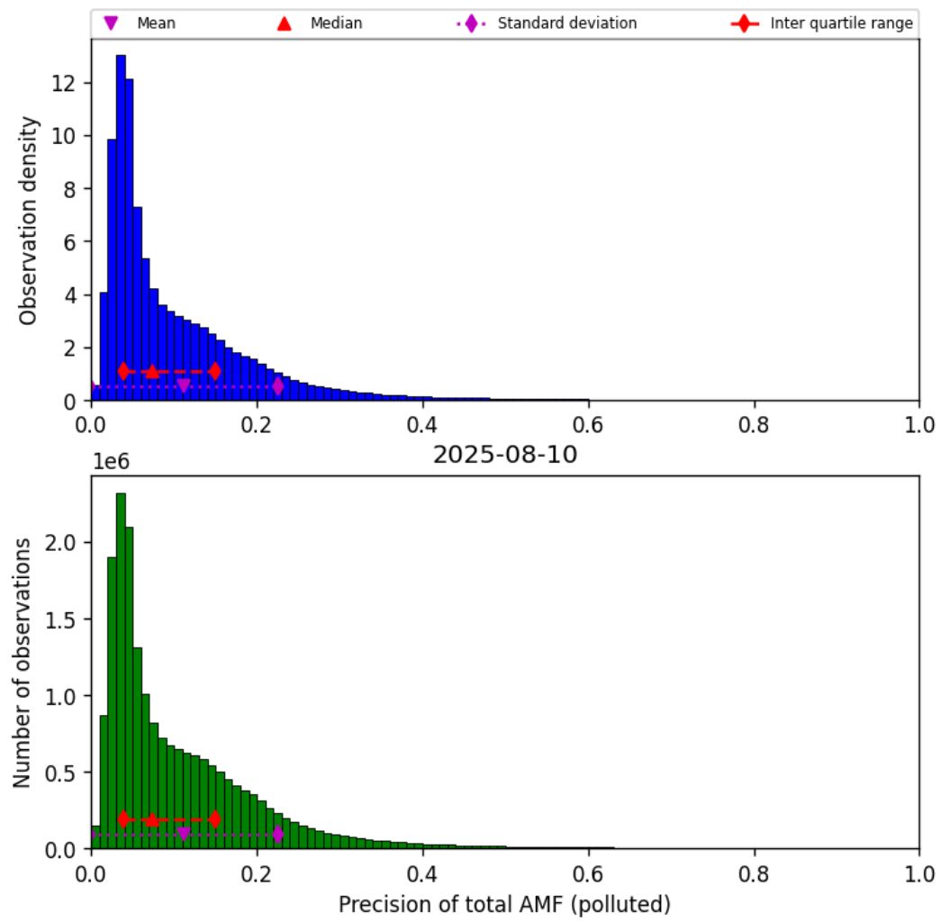
Figure 80: Histogram of “Precision of total AMF (polluted)” for 2025-08-09 to 2025-08-11
