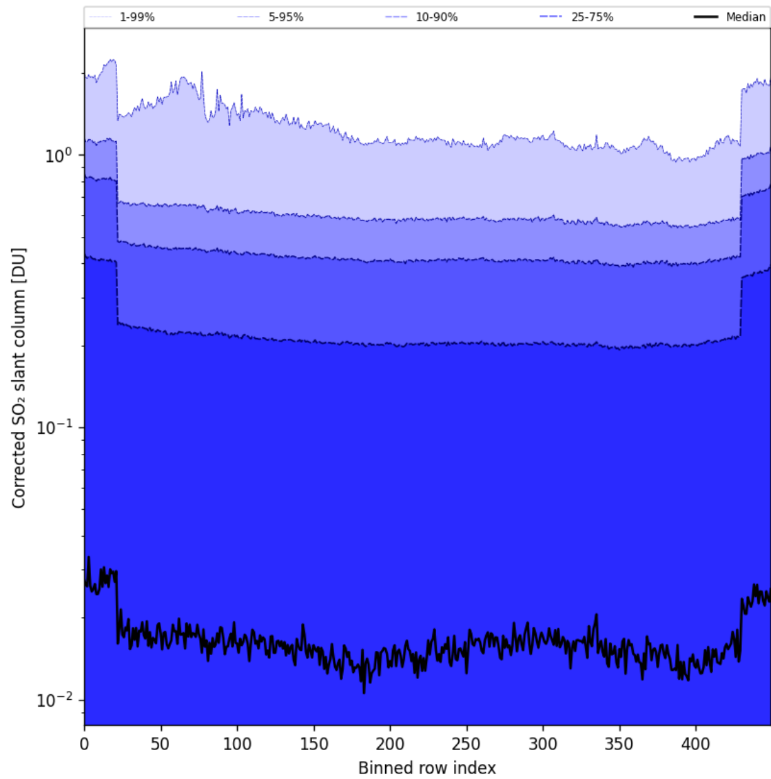
Figure 86: Along track statistics of “Corrected SO 2 slant column” for 2025-08-09 to 2025-08-11
