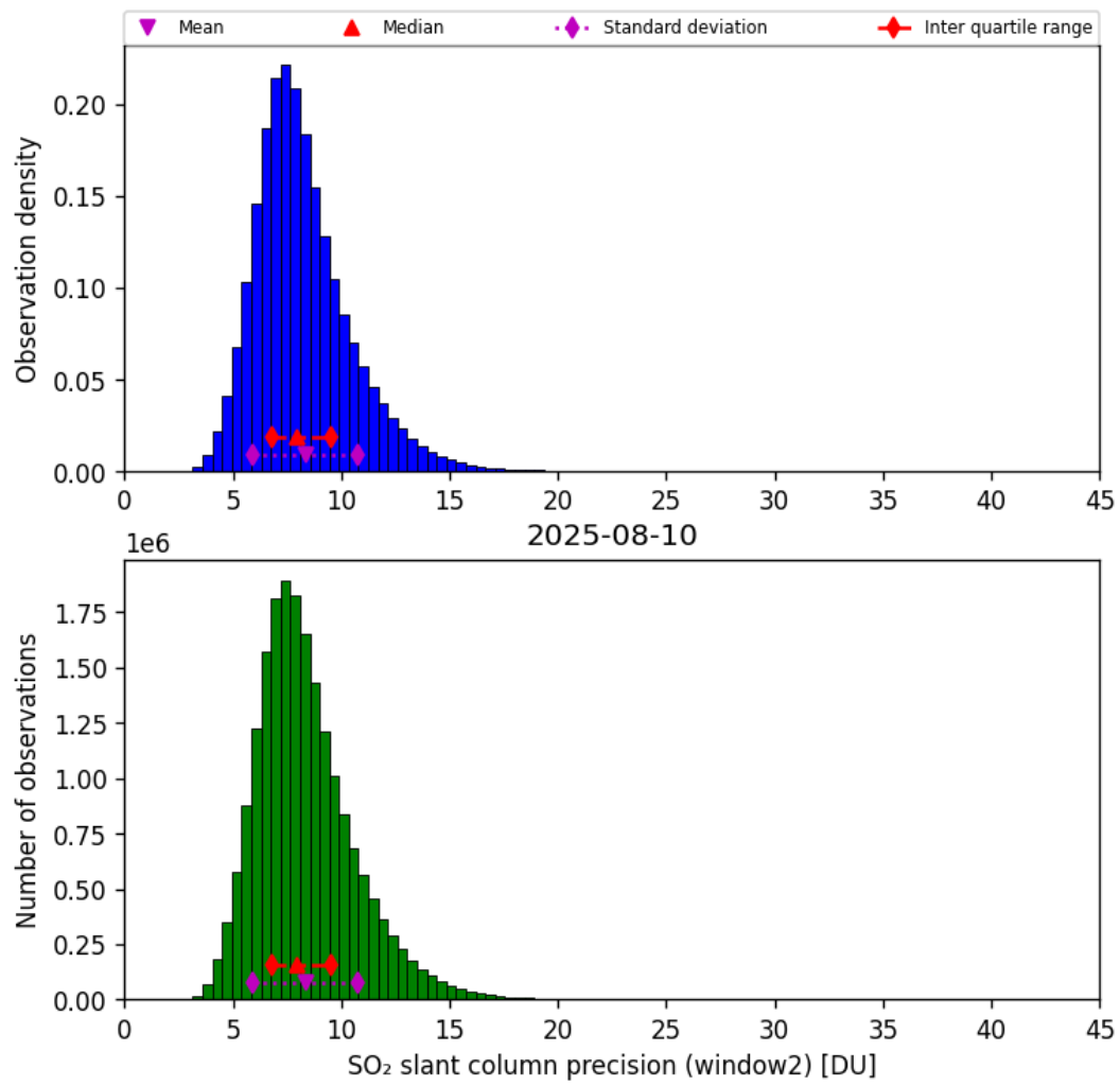
Figure 68: Histogram of “SO 2 slant column precision (window2)” for 2025-08-09 to 2025-08-11
