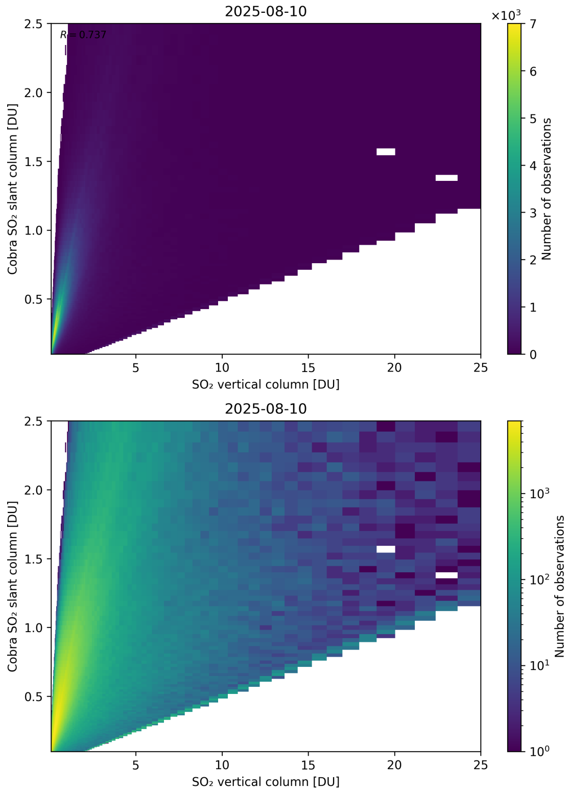
Figure 349: Scatter density plot of “SO 2 vertical column” against “Cobra SO 2 slant column” for 2025-08-09 to 2025-08-11.
