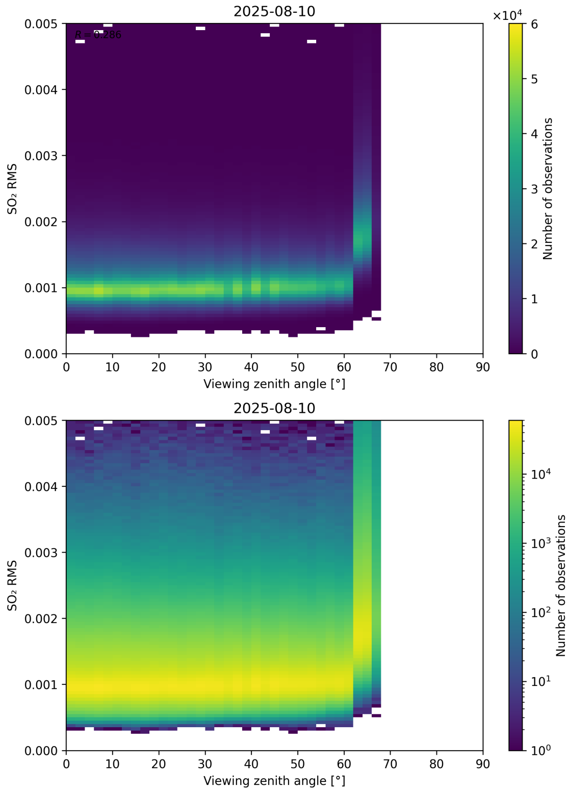
Figure 367: Scatter density plot of “Viewing zenith angle” against “SO 2 RMS” for 2025-08-09 to 2025-08-11.
