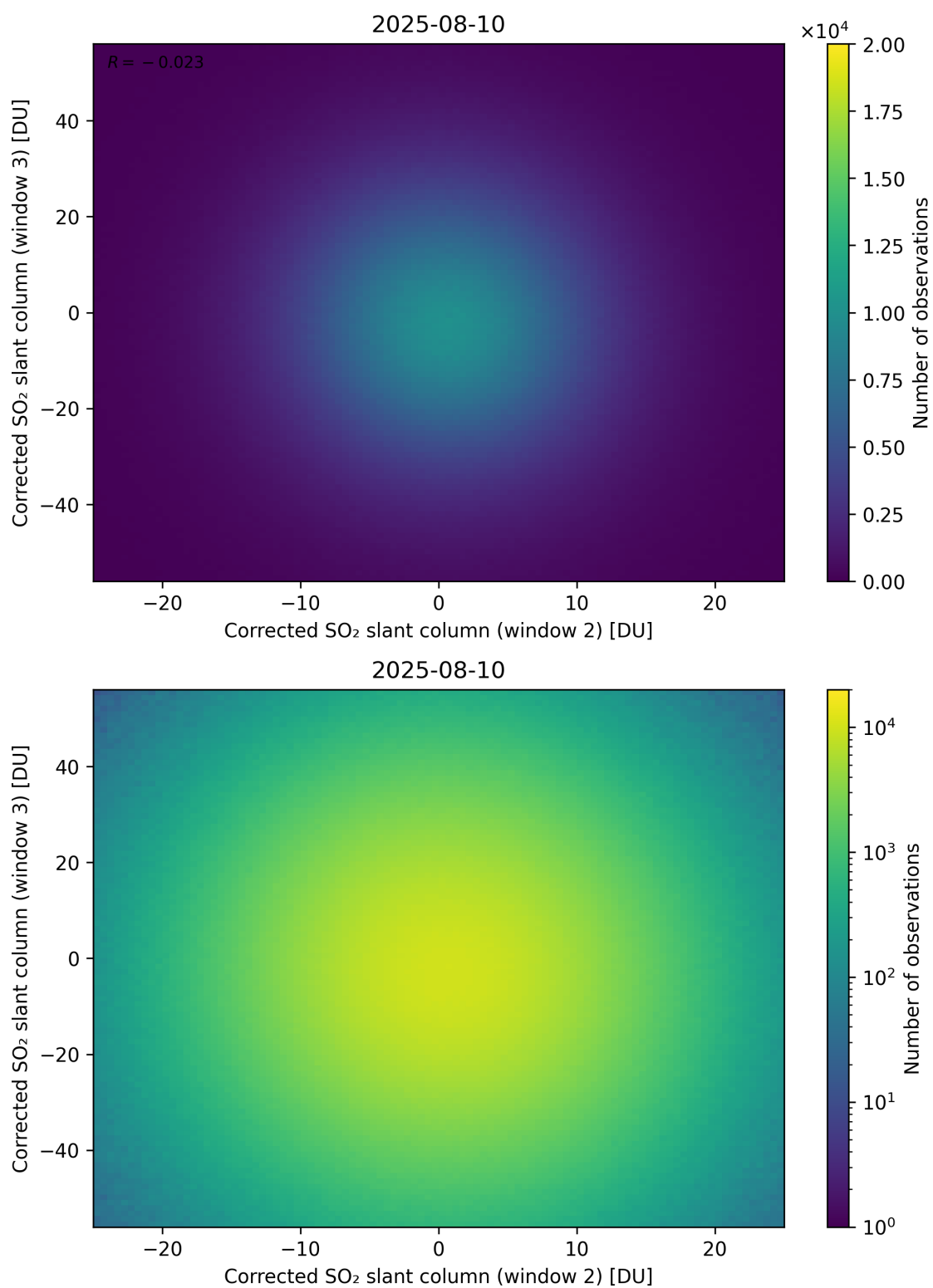
Figure 250: Scatter density plot of “Corrected SO 2 slant column (window 2)” against “Corrected SO 2 slant column (window 3)” for 2025-08-09 to 2025-08-11.
