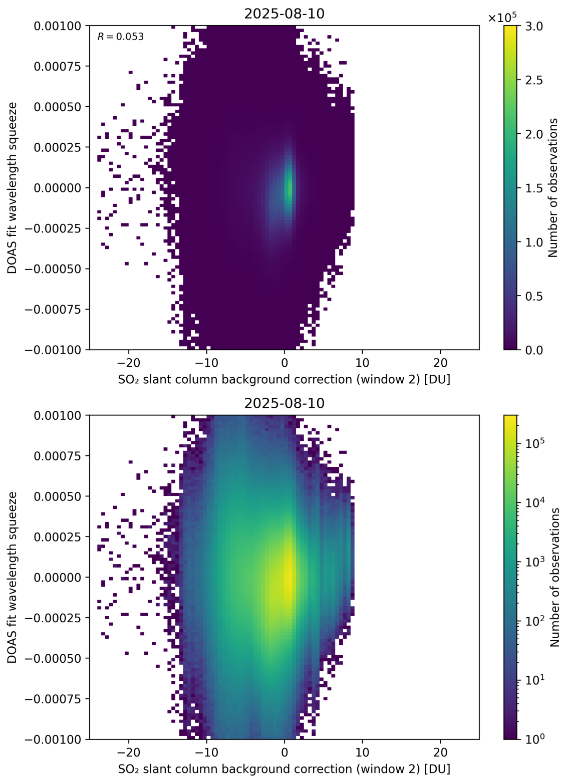
Figure 124: Scatter density plot of “SO 2 slant column background correction (window 2)” against “DOAS fit wavelength squeeze” for 2025-08-09 to 2025-08-11.
