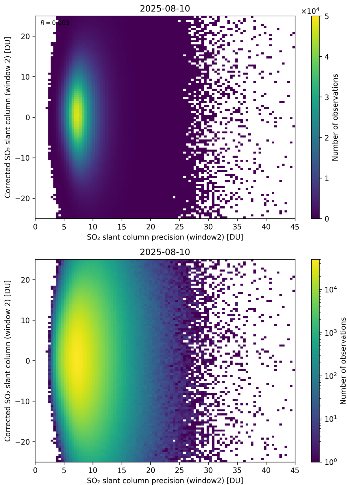
Figure 297: Scatter density plot of “SO 2 slant column precision (window2)” against “Corrected SO 2 slant column (window 2)” for 2025-08-09 to 2025-08-11.
