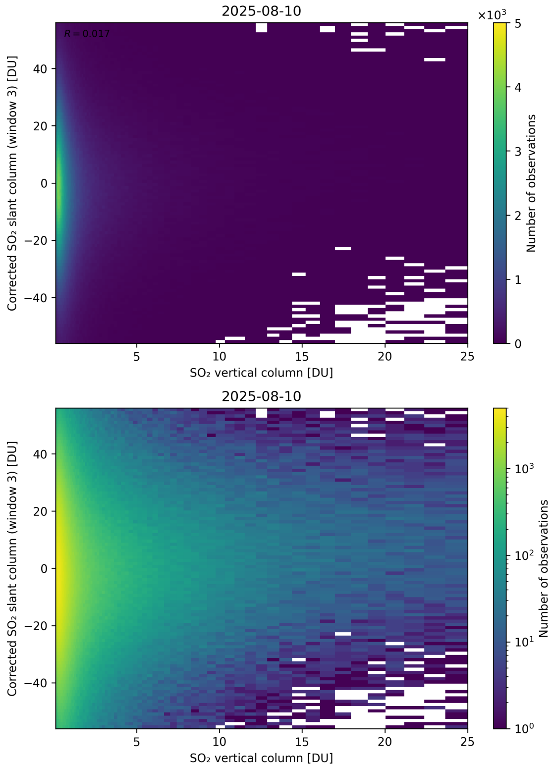
Figure 353: Scatter density plot of “SO 2 vertical column” against “Corrected SO 2 slant column (window 3)” for 2025-08-09 to 2025-08-11.
