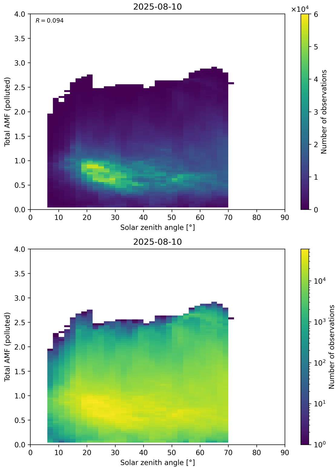
Figure 189: Scatter density plot of “Solar zenith angle” against “Total AMF (polluted)” for 2025-08-09 to 2025-08-11.
