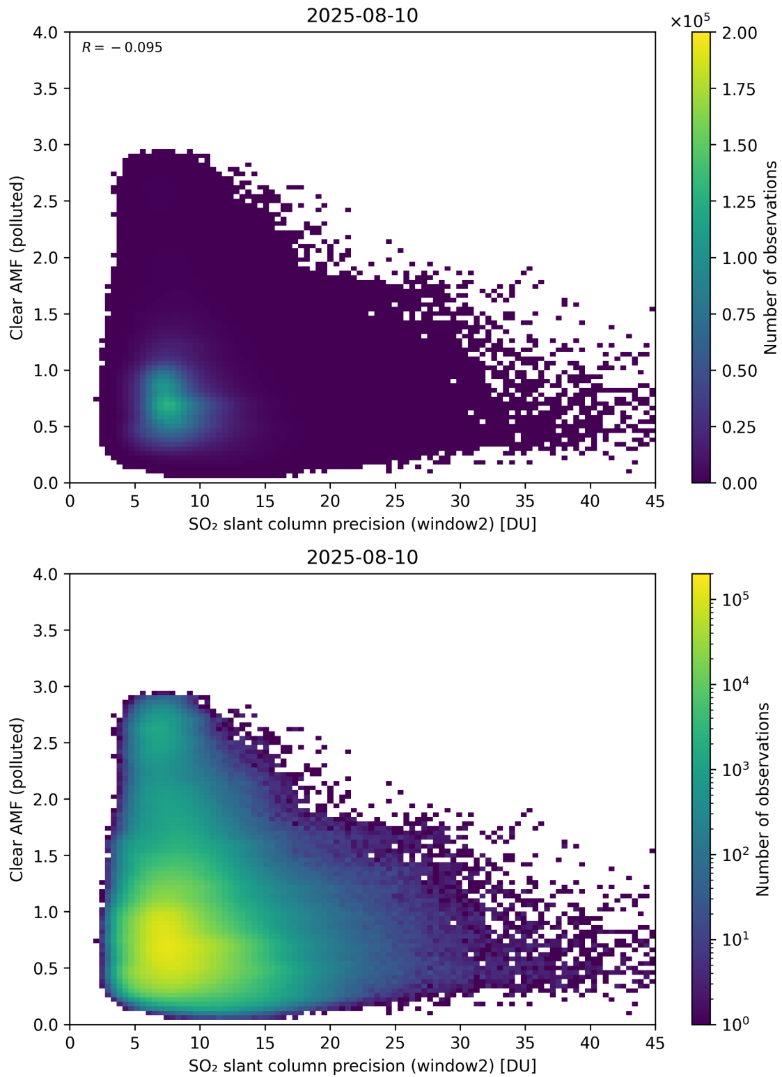
Figure 296: Scatter density plot of “SO 2 slant column precision (window2)” against “Clear AMF (polluted)” for 2025-08-09 to 2025-08-11.
