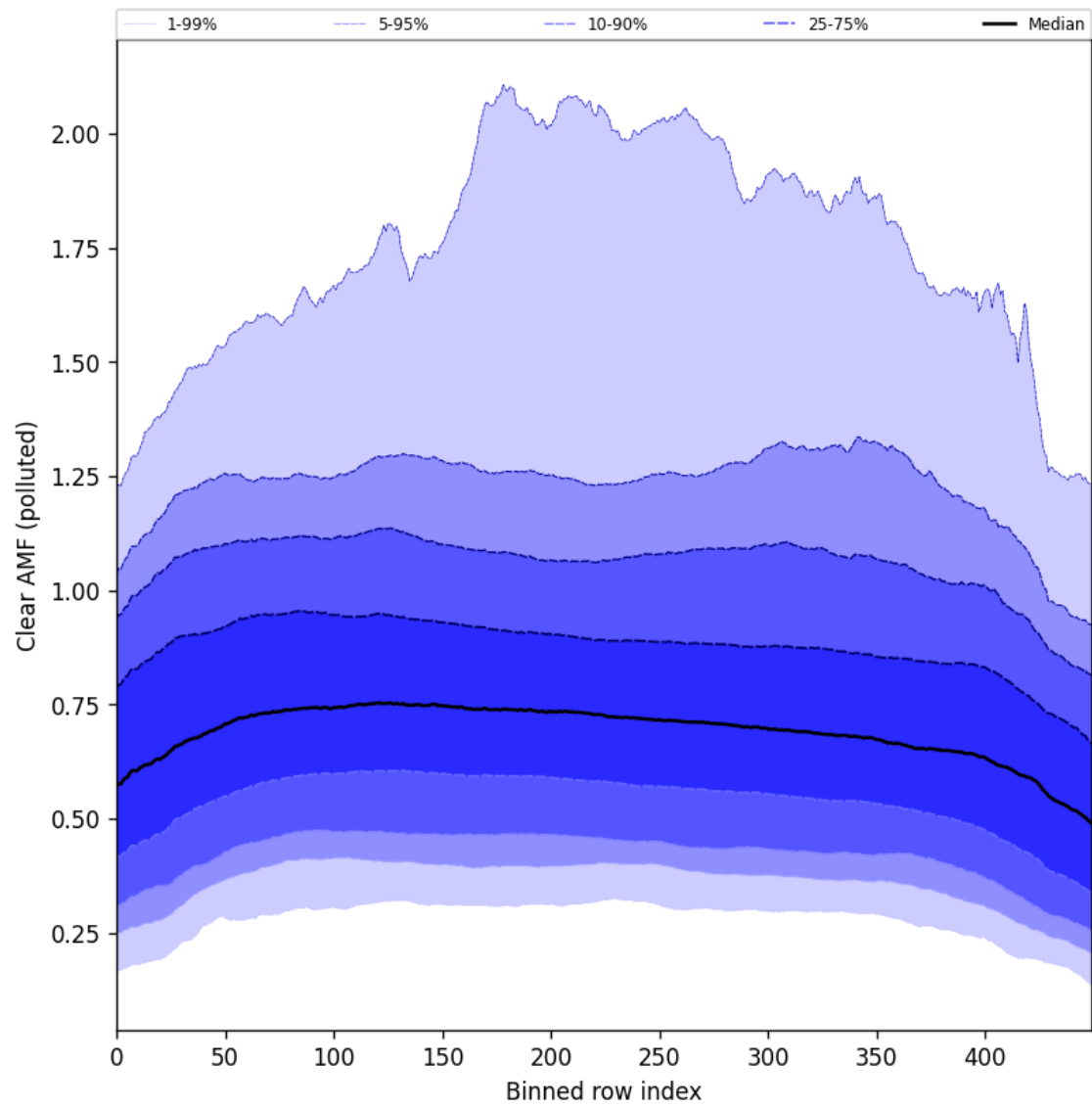
Figure 107: Along track statistics of “Clear AMF (polluted)” for 2025-08-09 to 2025-08-11
