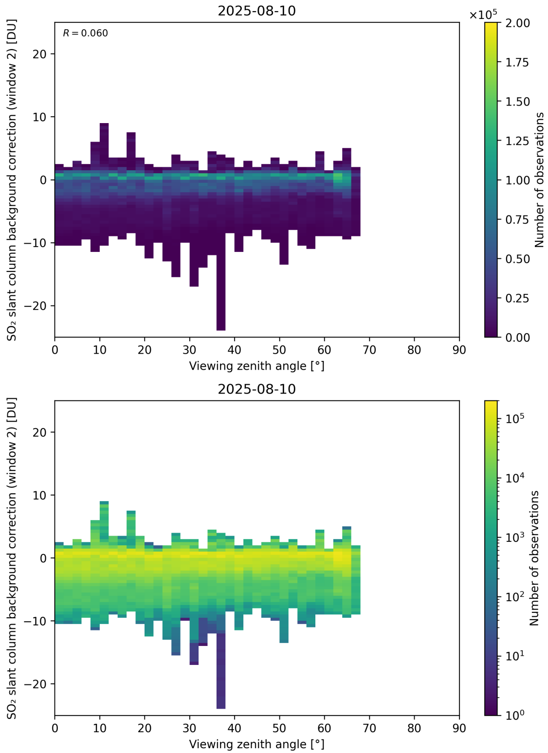
Figure 363: Scatter density plot of “Viewing zenith angle” against “SO 2 slant column background correction (window 2)” for 2025-08-09 to 2025-08-11.
