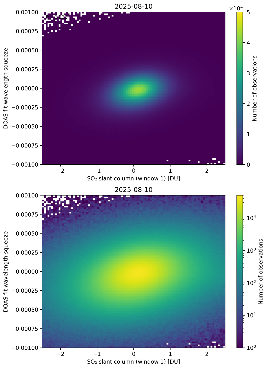
Figure 266: Scatter density plot of “SO 2 slant column (window 1)” against “DOAS fit wavelength squeeze” for 2025-08-09 to 2025-08-11.
