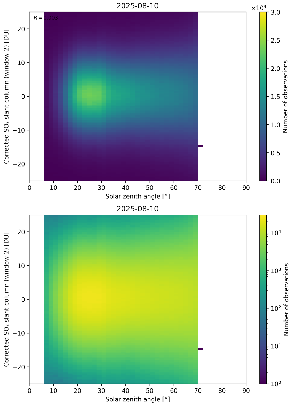
Figure 182: Scatter density plot of “Solar zenith angle” against “Corrected SO 2 slant column (window 2)” for 2025-08-09 to 2025-08-11.
