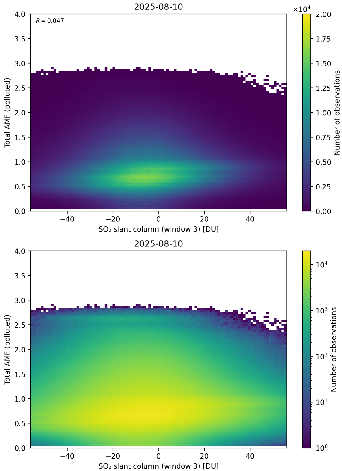
Figure 318: Scatter density plot of “SO 2 slant column (window 3)” against “Total AMF (polluted)” for 2025-08-09 to 2025-08-11.
