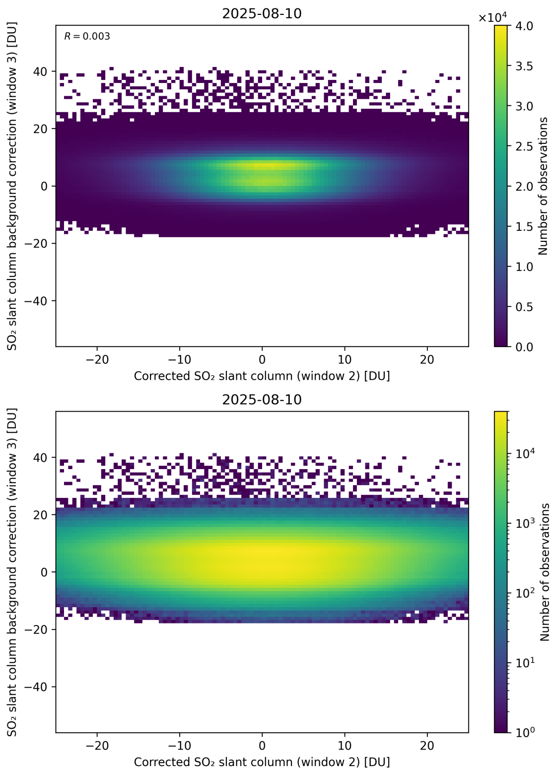
Figure 245: Scatter density plot of “Corrected SO 2 slant column (window 2)” against “SO 2 slant column background correction (window 3)” for 2025-08-09 to 2025-08-11.
