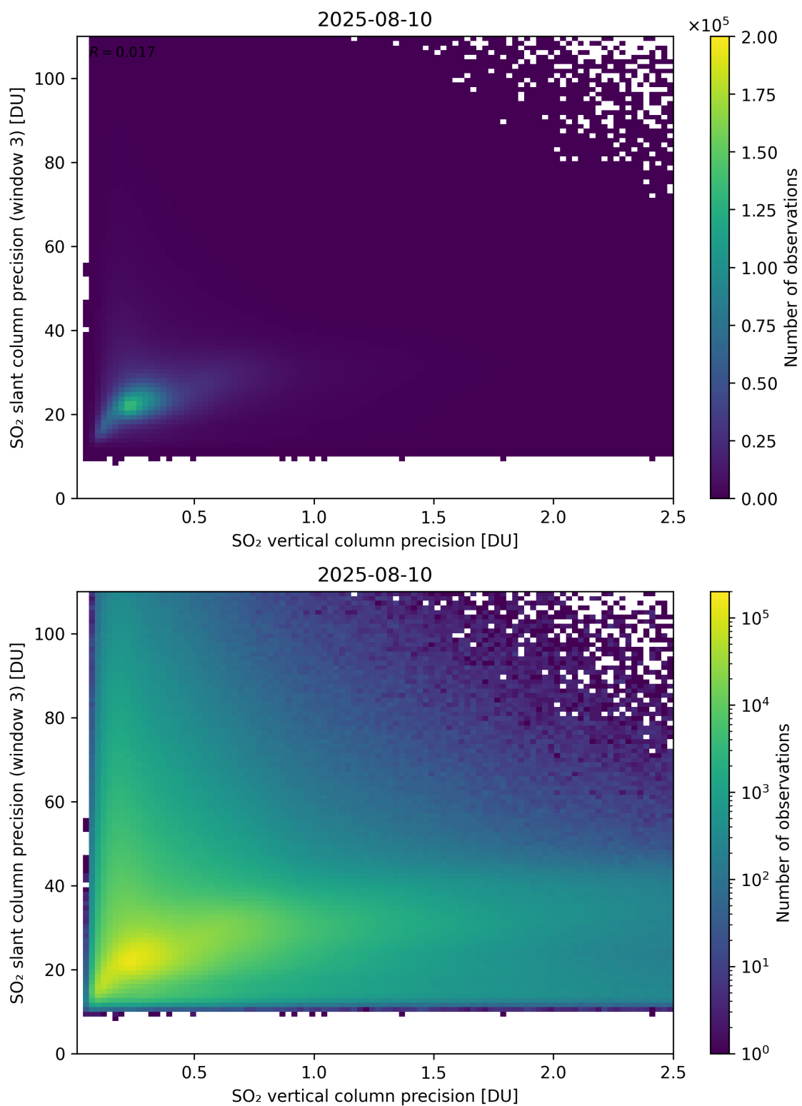
Figure 345: Scatter density plot of “SO 2 vertical column precision” against “SO 2 slant column precision (window 3)” for 2025-08-09 to 2025-08-11.
