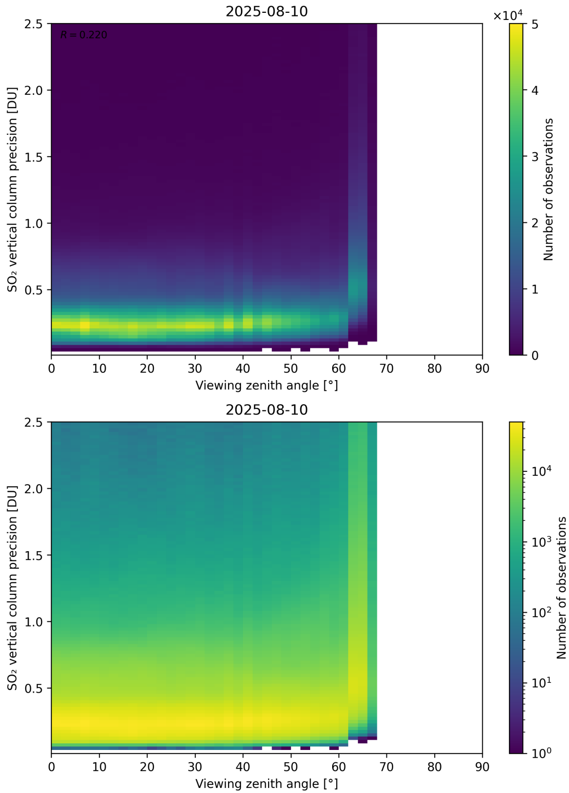
Figure 384: Scatter density plot of “Viewing zenith angle” against “SO 2 vertical column precision” for 2025-08-09 to 2025-08-11.
