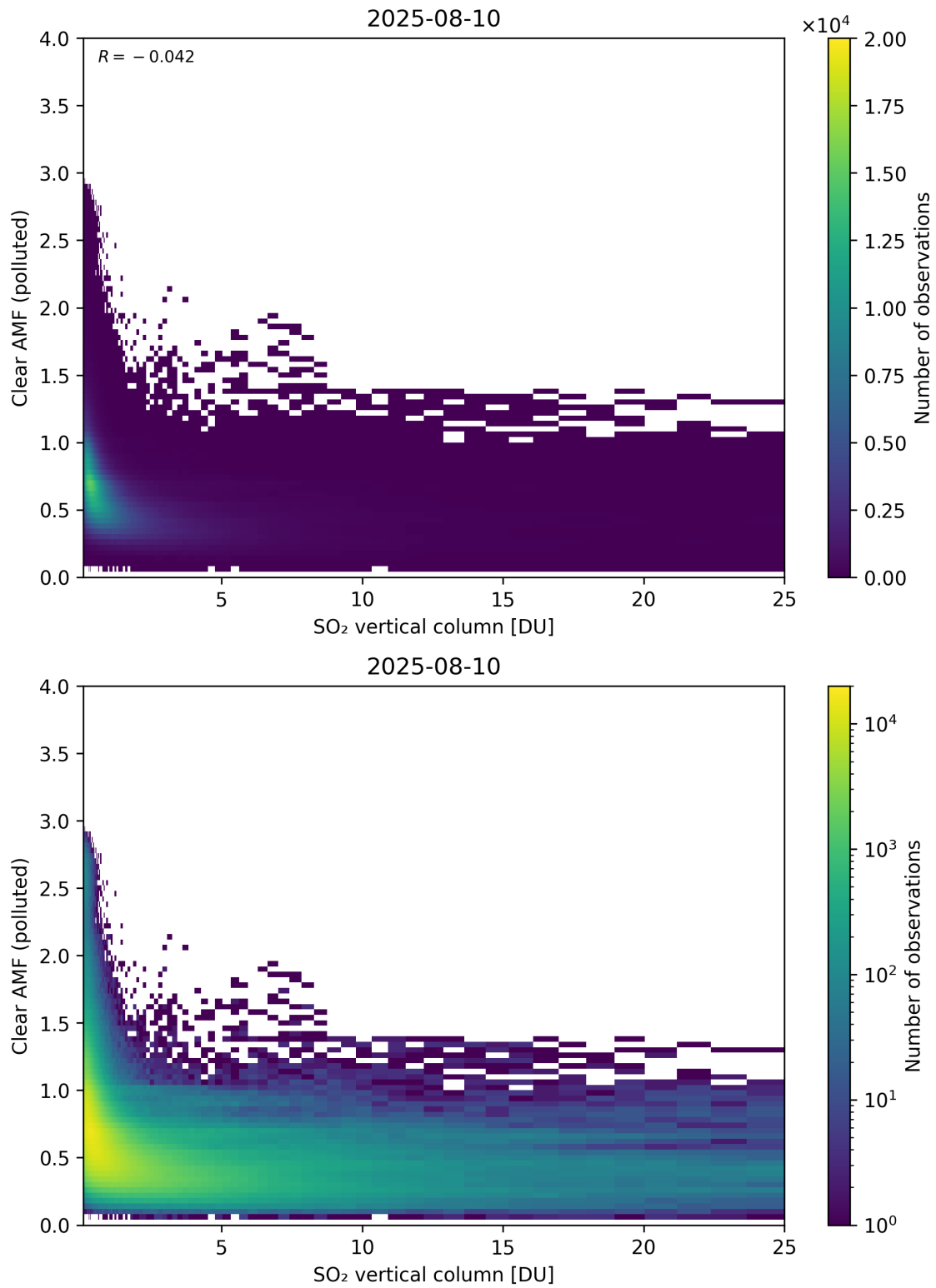
Figure 348: Scatter density plot of “SO 2 vertical column” against “Clear AMF (polluted)” for 2025-08-09 to 2025-08-11.
