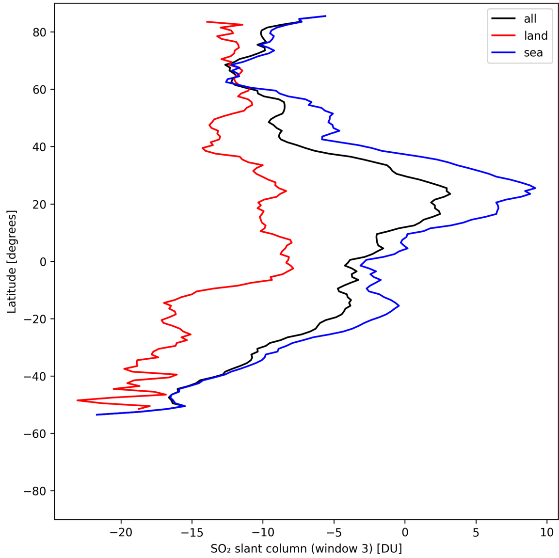
Figure 45: Zonal average of “SO 2 slant column (window 3)” for 2025-08-09 to 2025-08-11.
