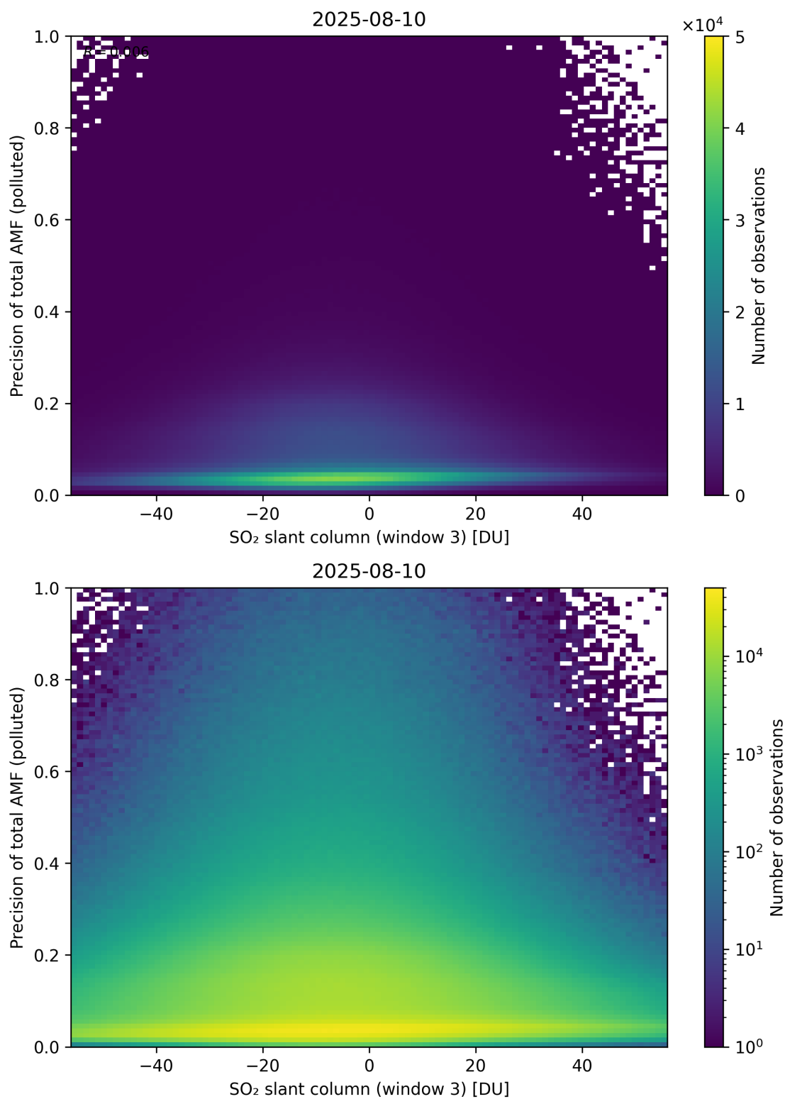
Figure 319: Scatter density plot of “SO 2 slant column (window 3)” against “Precision of total AMF (polluted)” for 2025-08-09 to 2025-08-11.
