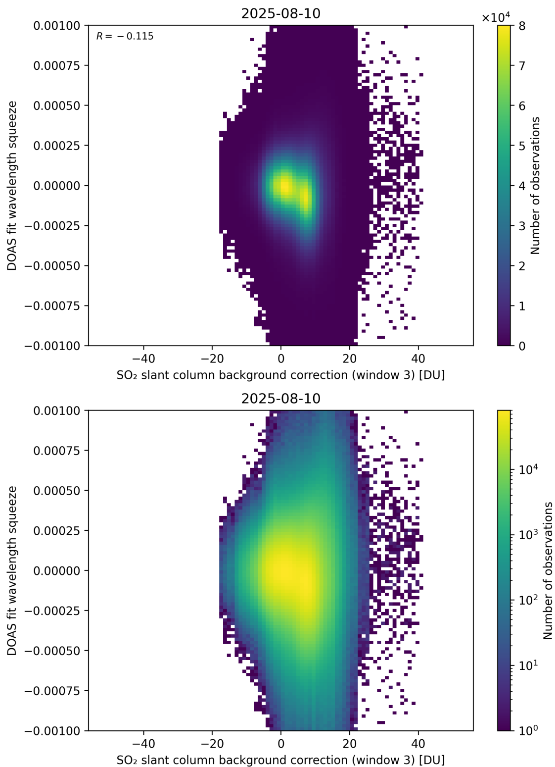
Figure 133: Scatter density plot of “SO 2 slant column background correction (window 3)” against “DOAS fit wavelength squeeze” for 2025-08-09 to 2025-08-11.
