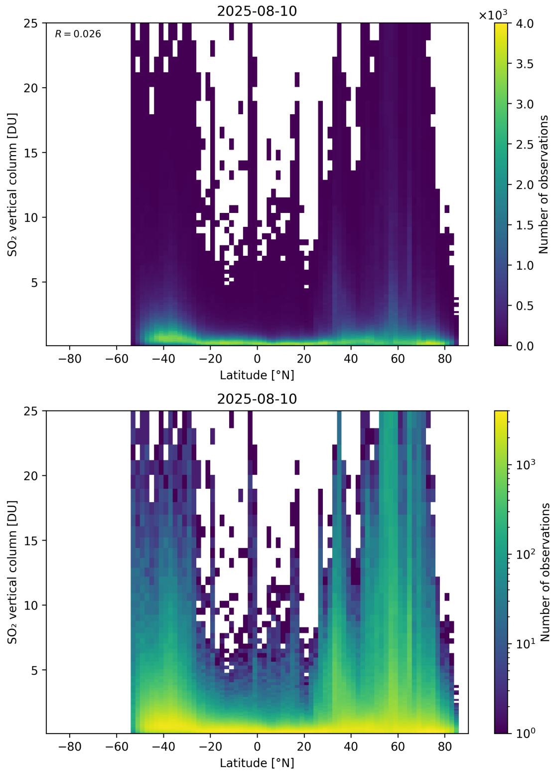
Figure 169: Scatter density plot of “Latitude” against “SO 2 vertical column” for 2025-08-09 to 2025-08-11.
