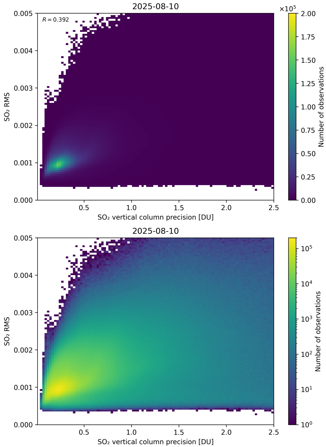
Figure 334: Scatter density plot of “SO 2 vertical column precision” against “SO 2 RMS” for 2025-08-09 to 2025-08-11.
