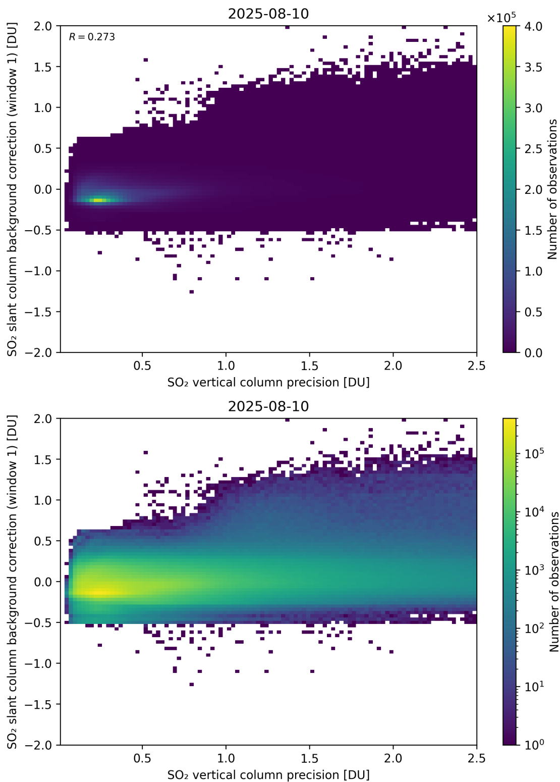
Figure 329: Scatter density plot of “SO 2 vertical column precision” against “SO 2 slant column background correction (window 1)” for 2025-08-09 to 2025-08-11.
