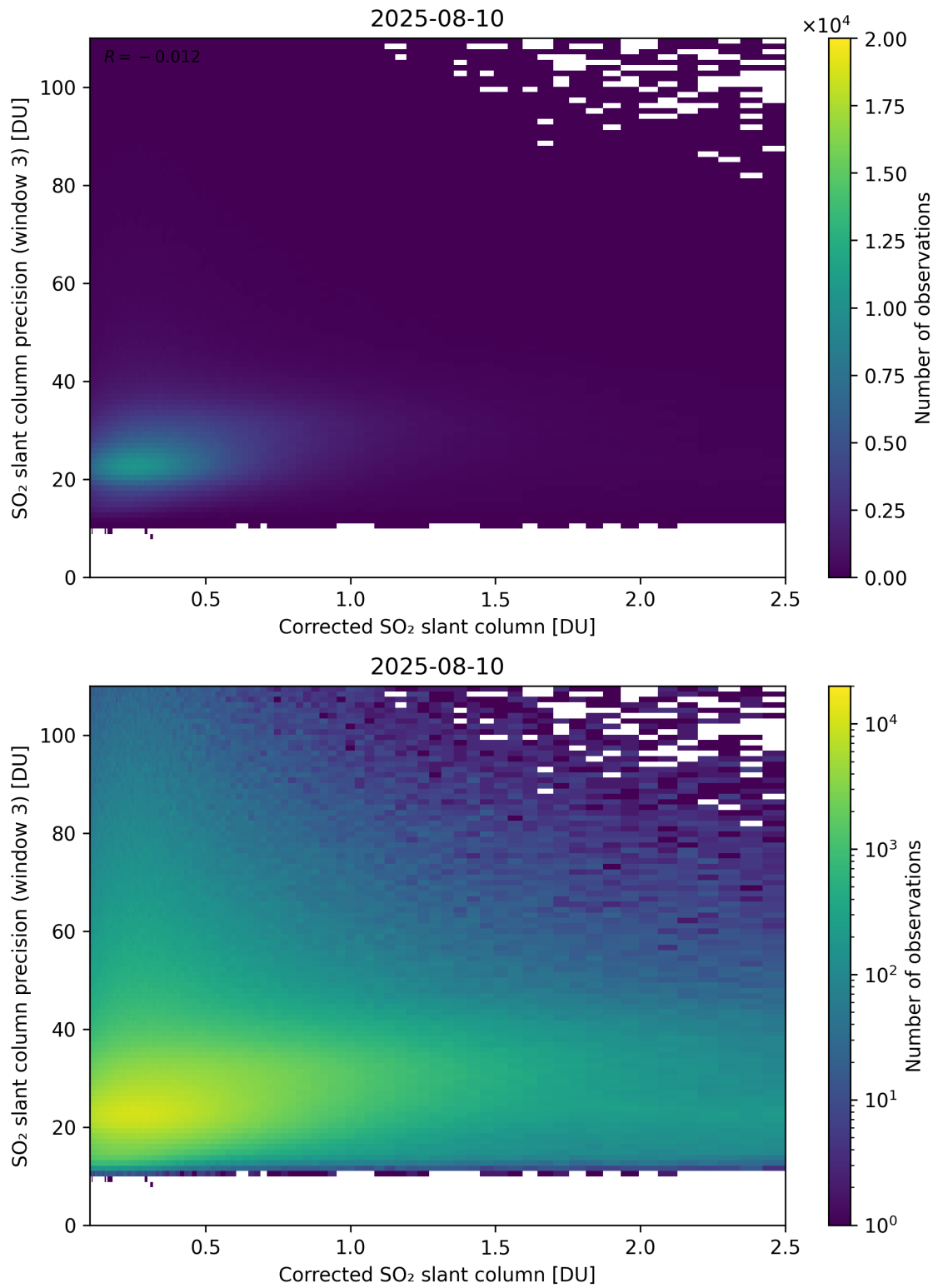
Figure 241: Scatter density plot of “Corrected SO 2 slant column” against “SO 2 slant column precision (window 3)” for 2025-08-09 to 2025-08-11.
