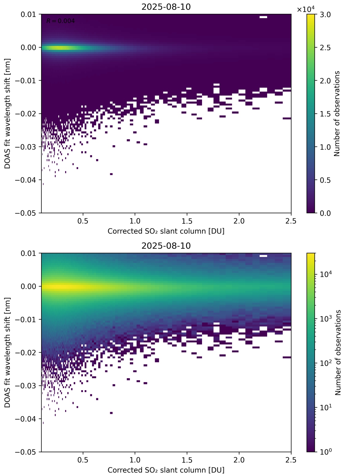
Figure 229: Scatter density plot of “Corrected SO 2 slant column” against “DOAS fit wavelength shift” for 2025-08-09 to 2025-08-11.
