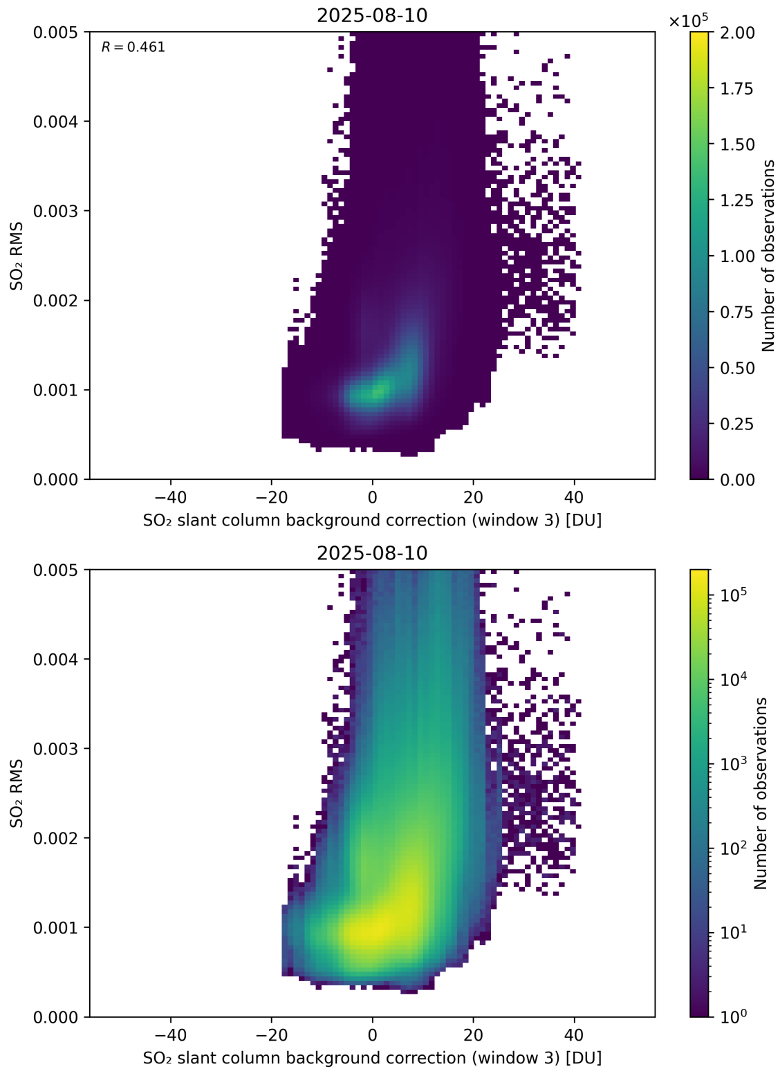
Figure 134: Scatter density plot of “SO 2 slant column background correction (window 3)” against “SO 2 RMS” for 2025-08-09 to 2025-08-11.
