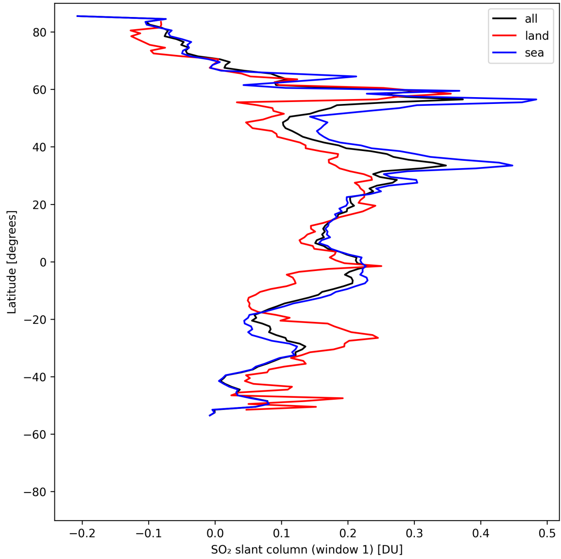
Figure 37: Zonal average of “SO 2 slant column (window 1)” for 2025-08-09 to 2025-08-11.
