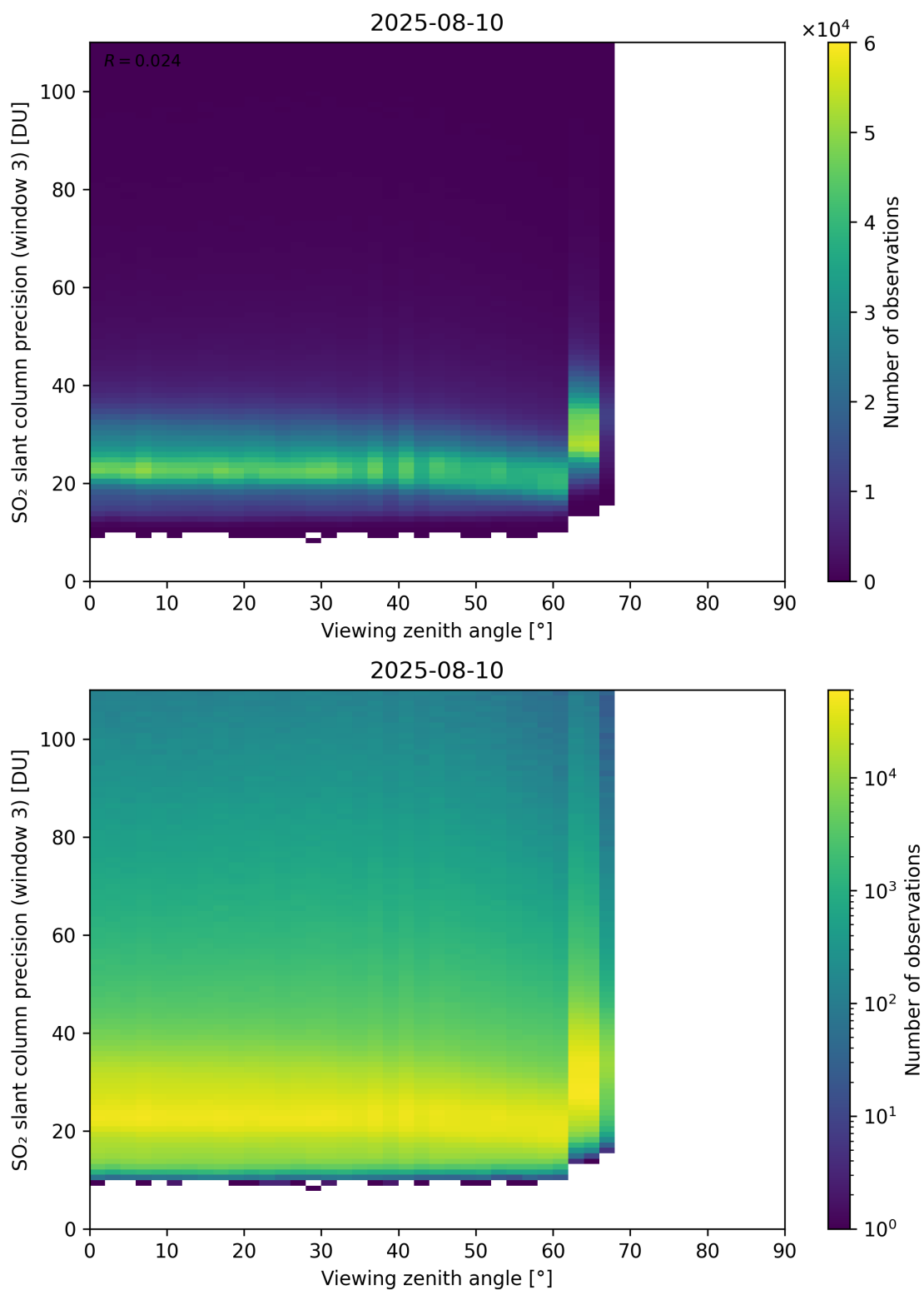
Figure 380: Scatter density plot of “Viewing zenith angle” against “SO 2 slant column precision (window 3)” for 2025-08-09 to 2025-08-11.
