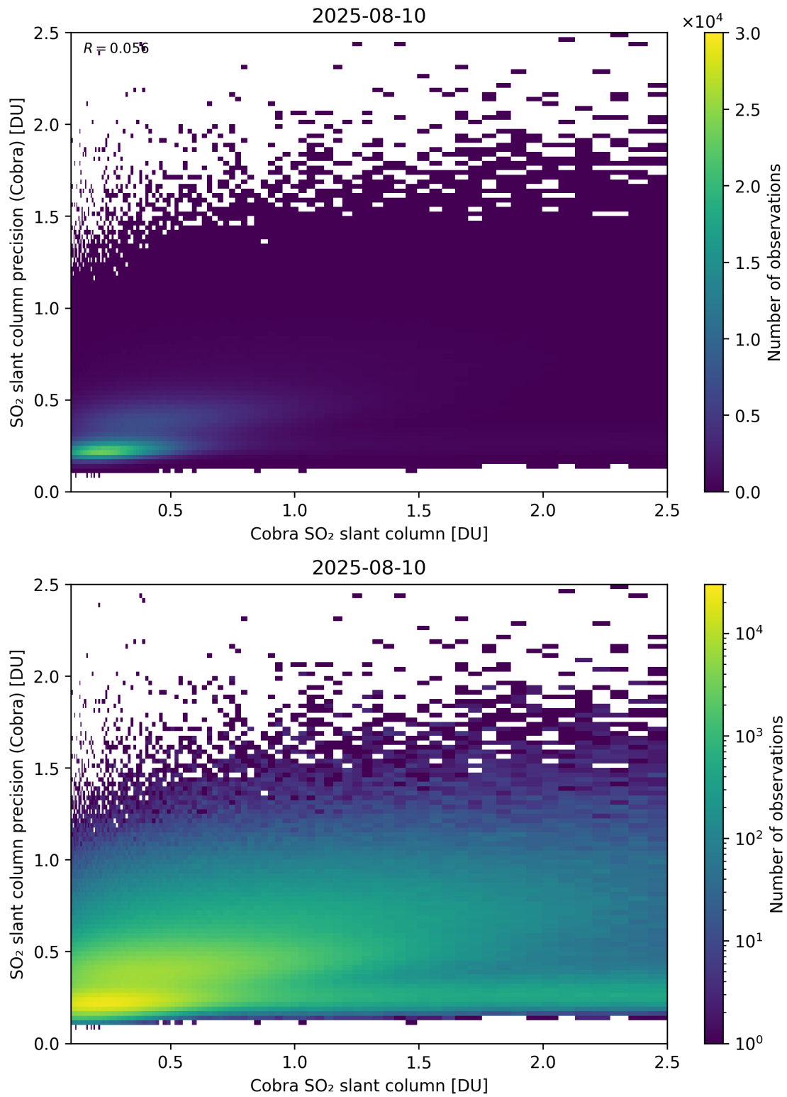
Figure 216: Scatter density plot of “Cobra SO 2 slant column” against “SO 2 slant column precision (Cobra)” for 2025-08-09 to 2025-08-11.
