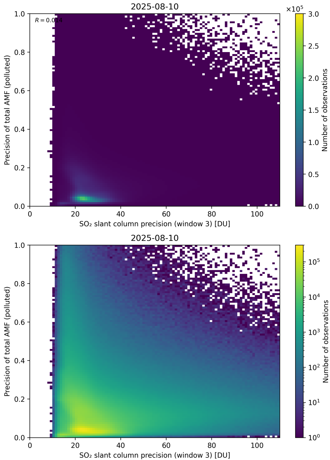
Figure 314: Scatter density plot of “SO 2 slant column precision (window 3)” against “Precision of total AMF (polluted)” for 2025-08-09 to 2025-08-11.
