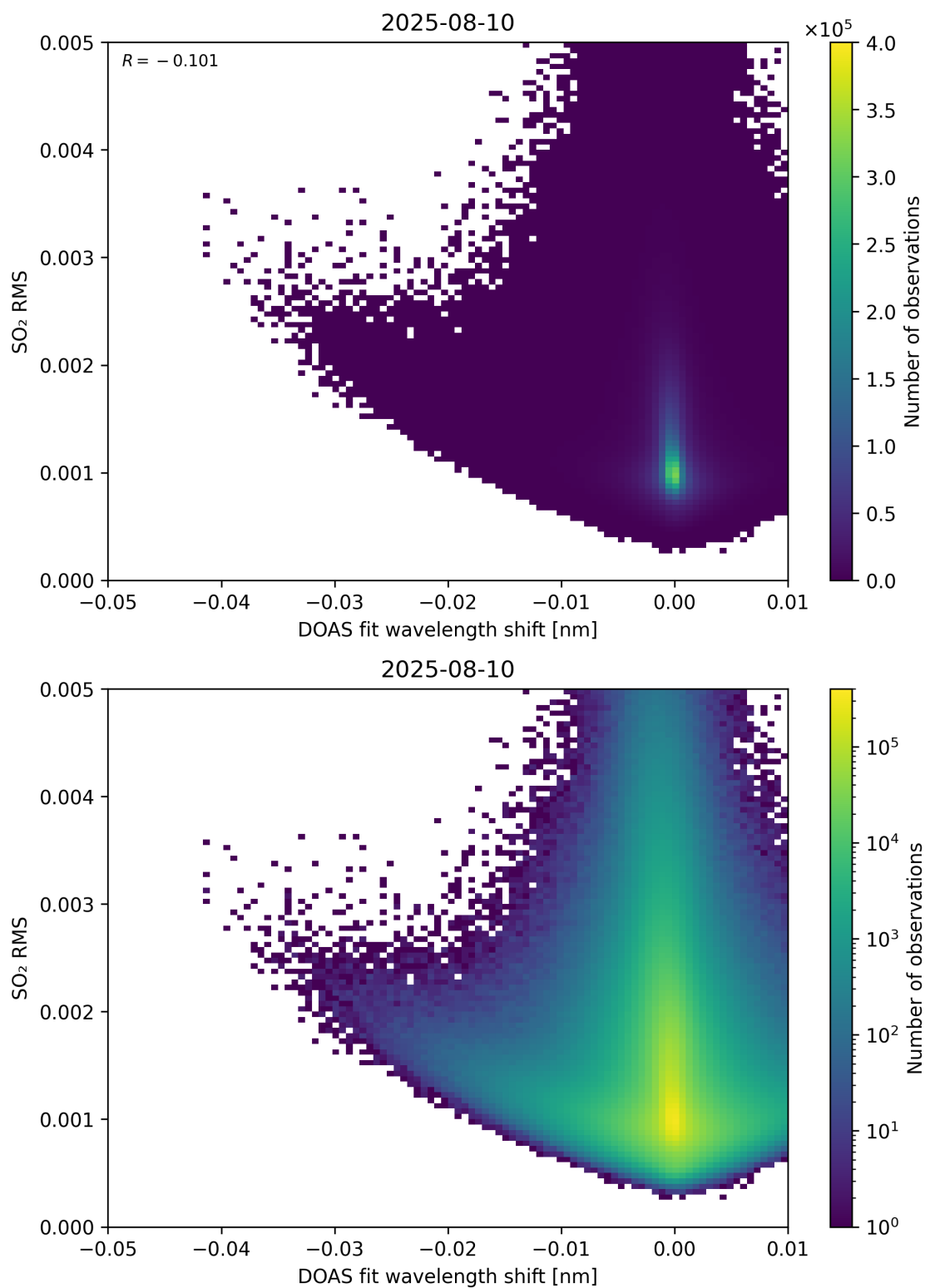
Figure 139: Scatter density plot of “DOAS fit wavelength shift” against “SO 2 RMS” for 2025-08-09 to 2025-08-11.
