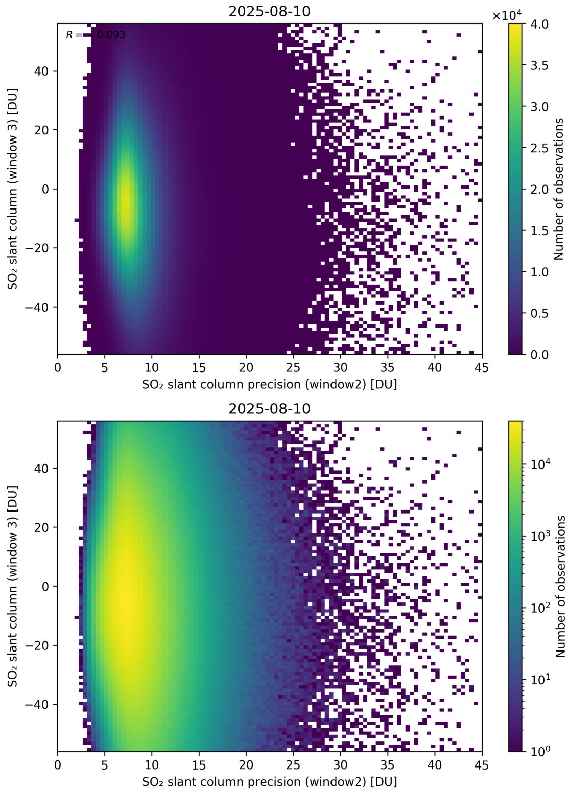
Figure 299: Scatter density plot of “SO 2 slant column precision (window2)” against “SO 2 slant column (window 3)” for 2025-08-09 to 2025-08-11.
