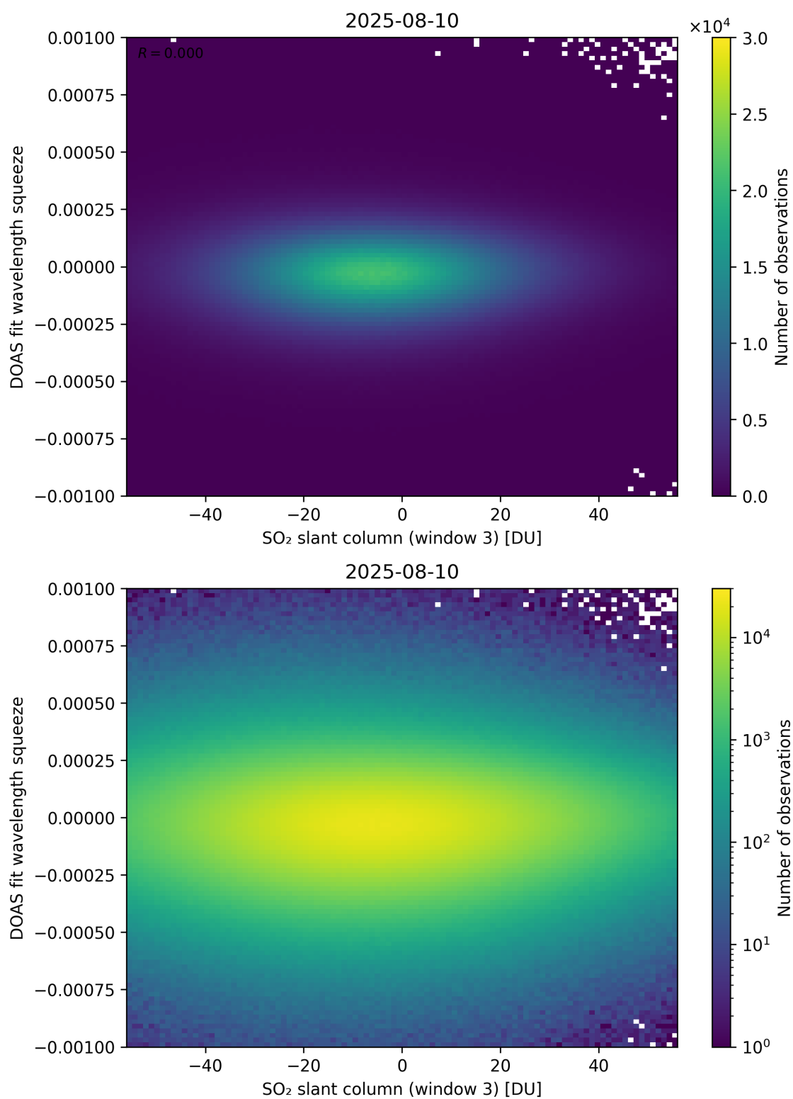
Figure 305: Scatter density plot of “SO 2 slant column (window 3)” against “DOAS fit wavelength squeeze” for 2025-08-09 to 2025-08-11.
