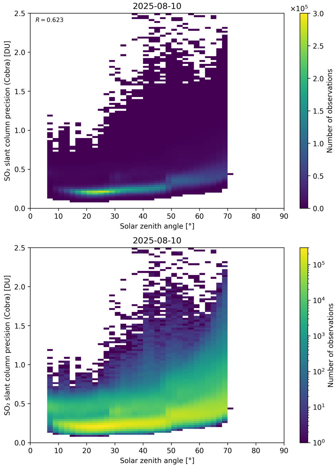
Figure 180: Scatter density plot of “Solar zenith angle” against “SO 2 slant column precision (Cobra)” for 2025-08-09 to 2025-08-11.
