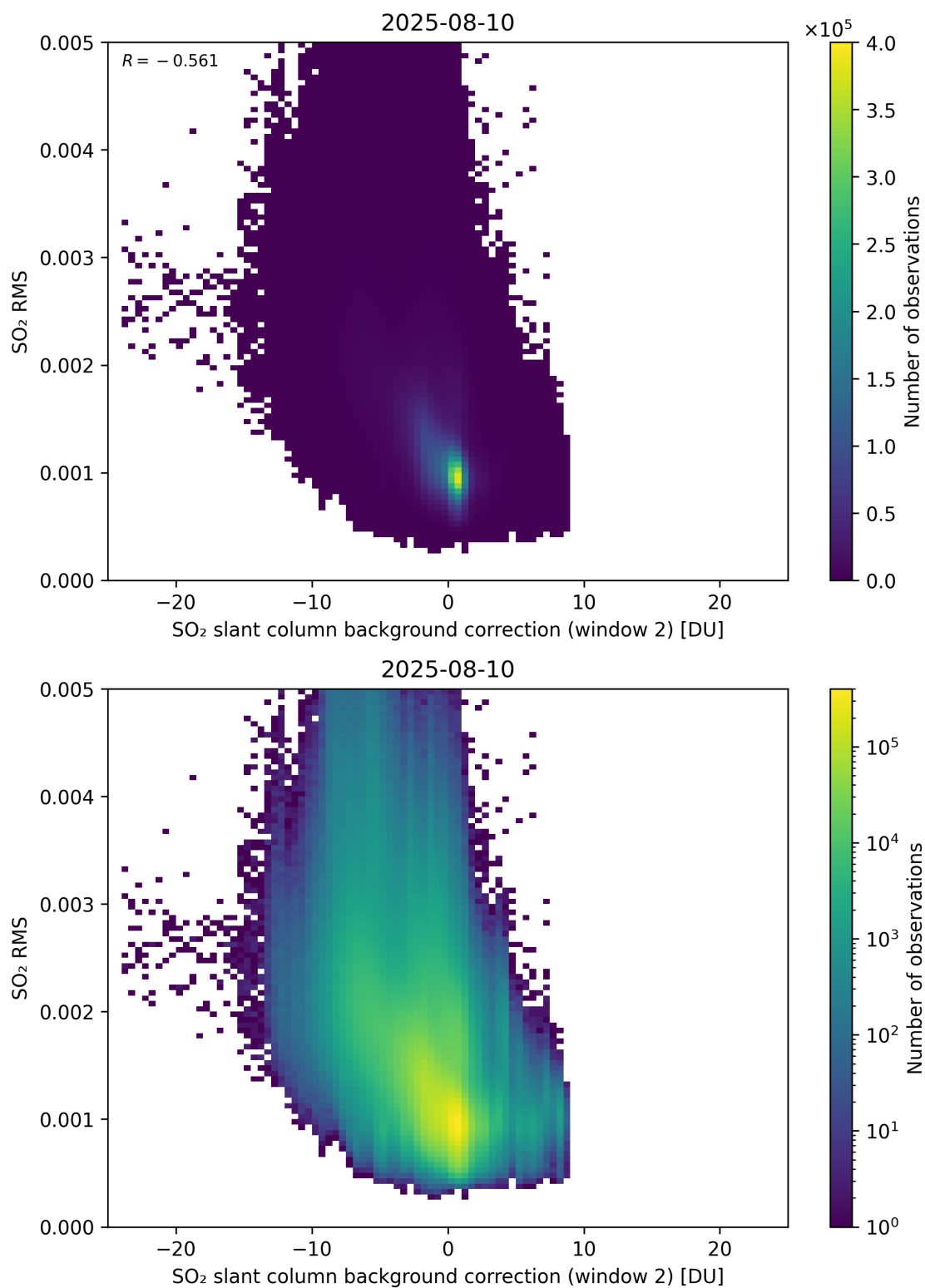
Figure 125: Scatter density plot of “SO 2 slant column background correction (window 2)” against “SO 2 RMS” for 2025-08-09 to 2025-08-11.
