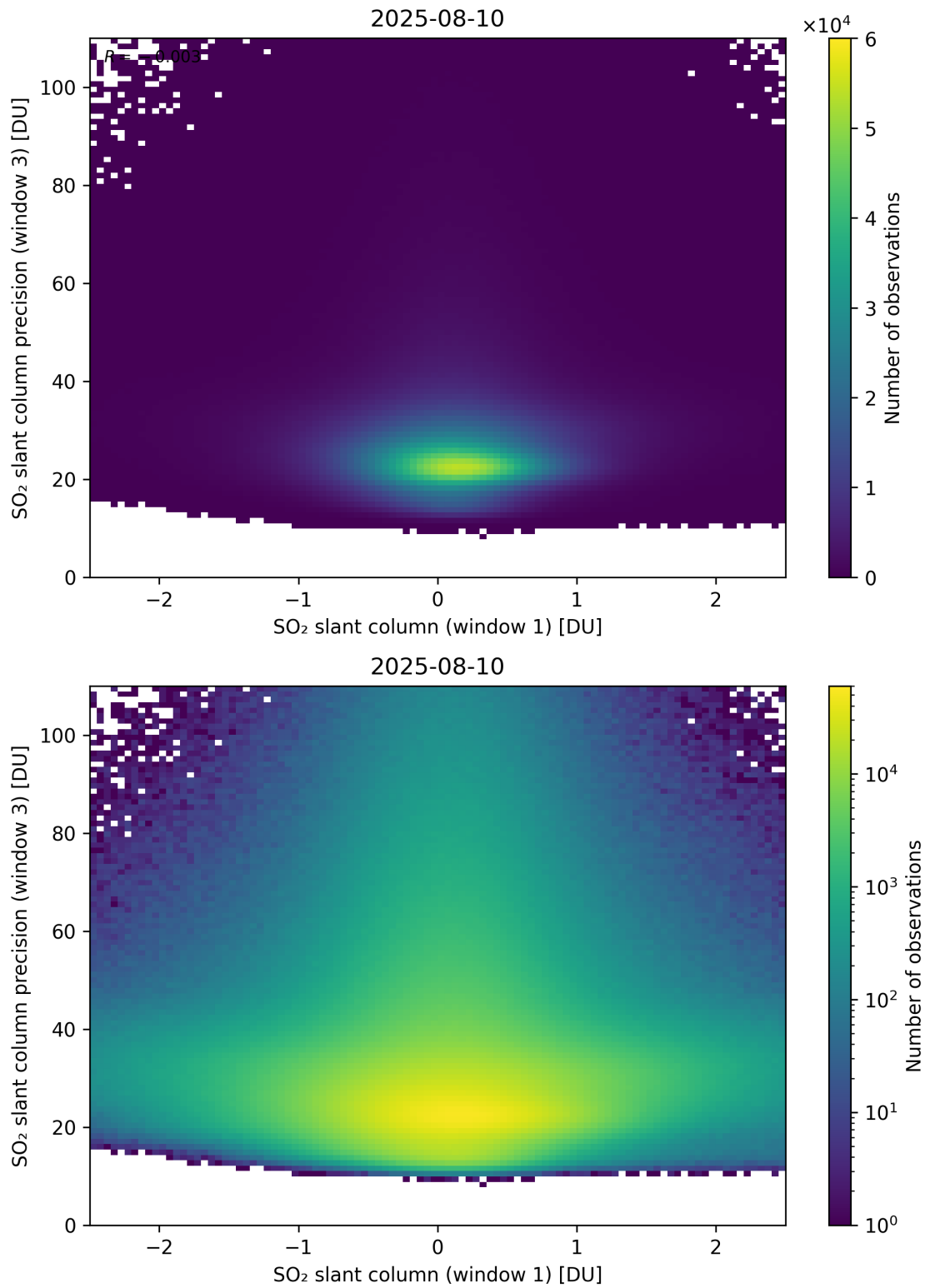
Figure 288: Scatter density plot of “SO 2 slant column (window 1)” against “SO 2 slant column precision (window 3)” for 2025-08-09 to 2025-08-11.
