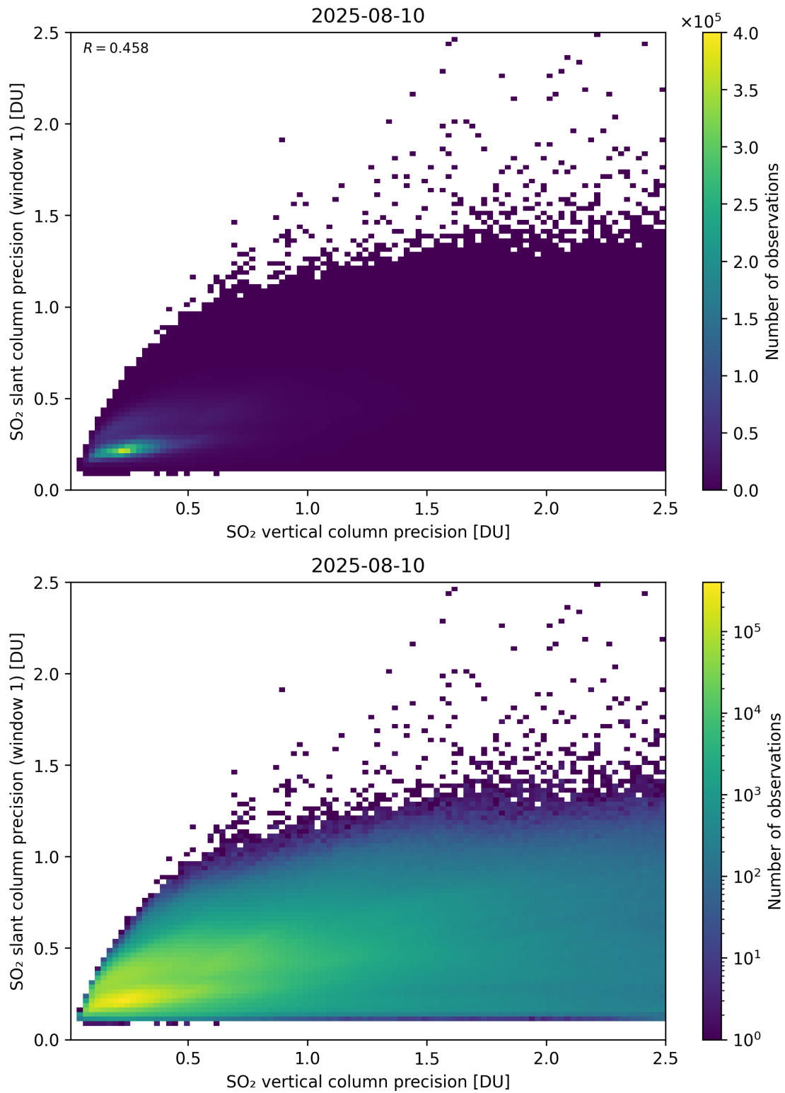
Figure 342: Scatter density plot of “SO 2 vertical column precision” against “SO 2 slant column precision (window 1)” for 2025-08-09 to 2025-08-11.
