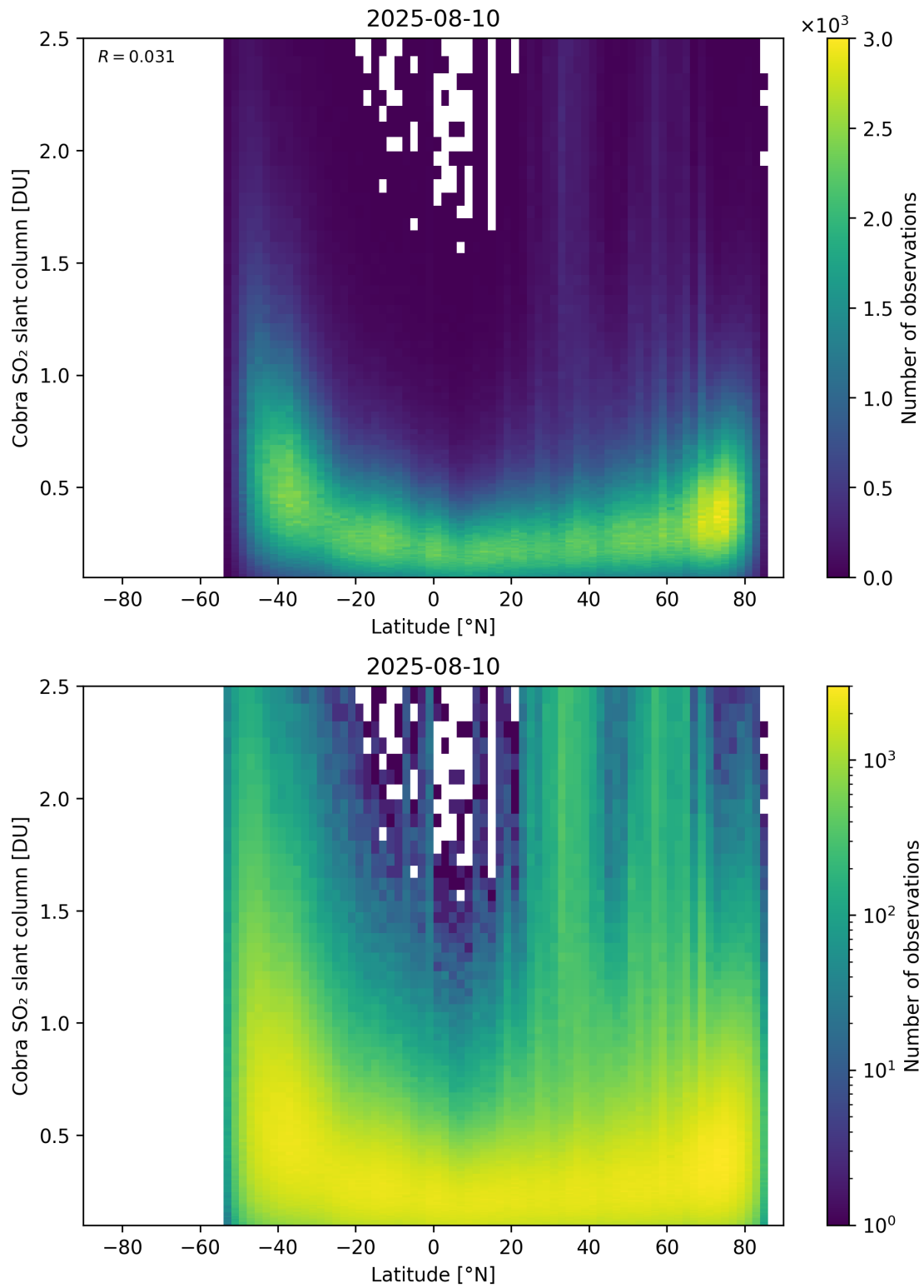
Figure 157: Scatter density plot of “Latitude” against “Cobra SO 2 slant column” for 2025-08-09 to 2025-08-11.
