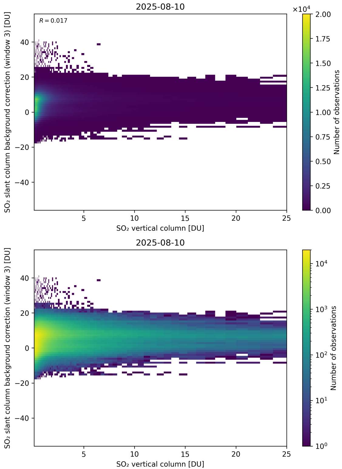
Figure 325: Scatter density plot of “SO 2 vertical column” against “SO 2 slant column background correction (window 3)” for 2025-08-09 to 2025-08-11.
