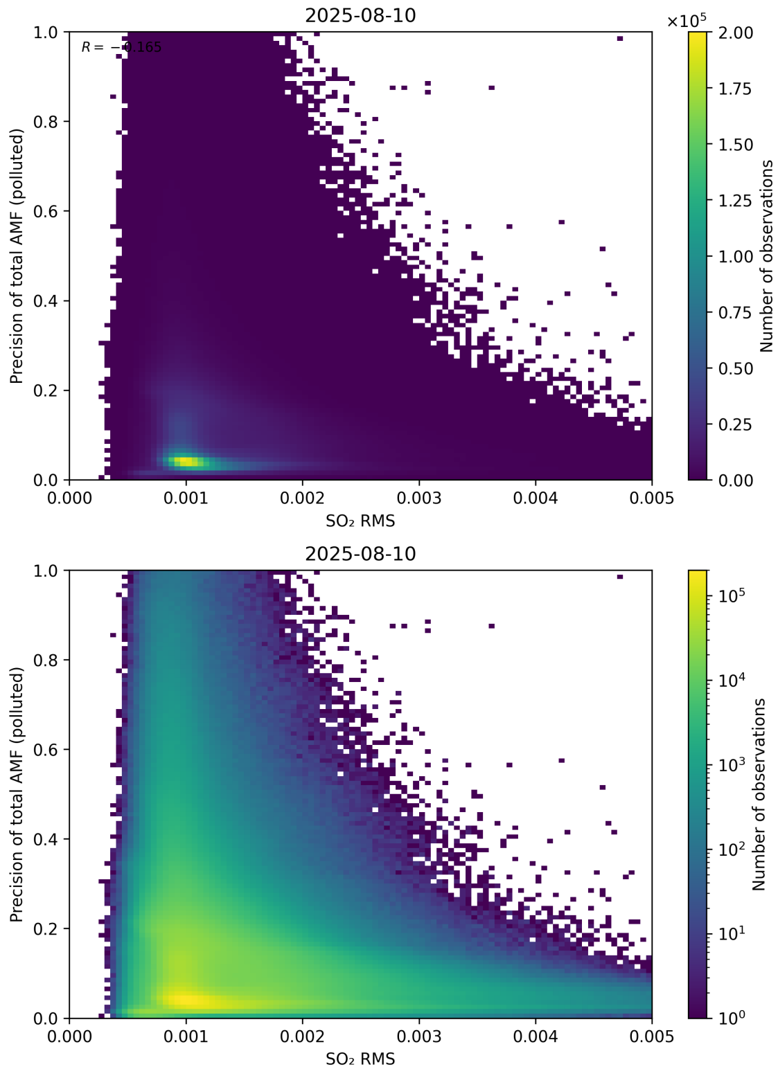
Figure 149: Scatter density plot of “SO 2 RMS” against “Precision of total AMF (polluted)” for 2025-08-09 to 2025-08-11.
