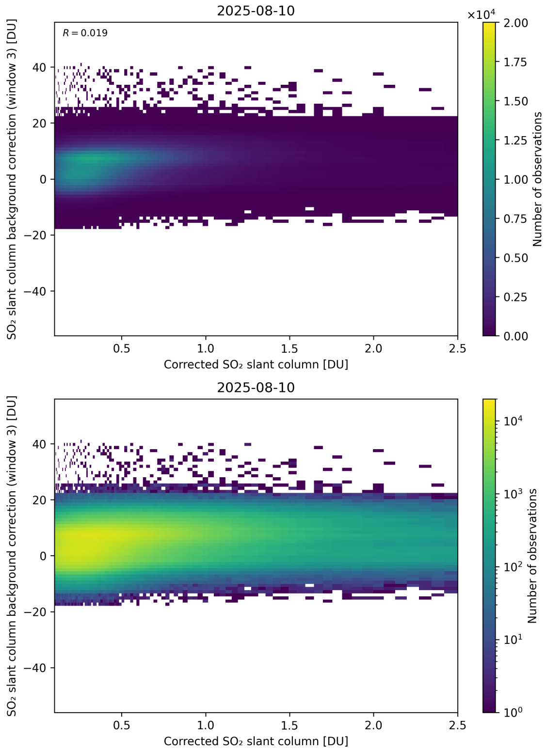
Figure 228: Scatter density plot of “Corrected SO 2 slant column” against “SO 2 slant column background correction (window 3)” for 2025-08-09 to 2025-08-11.
