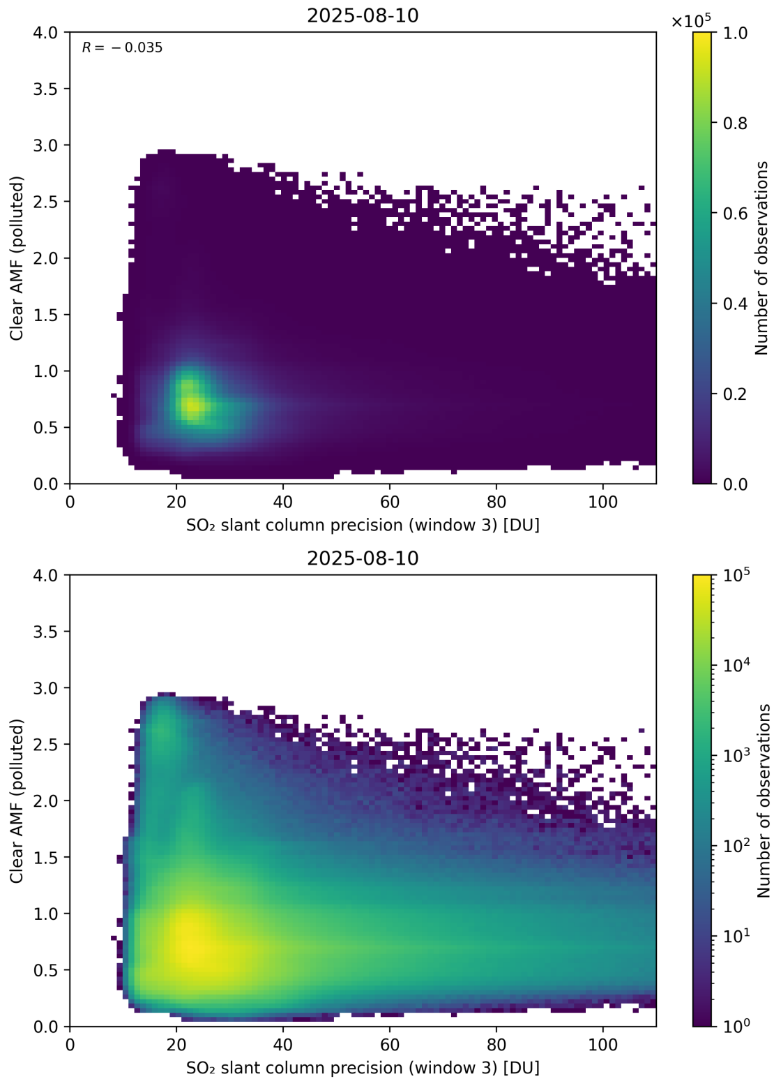
Figure 311: Scatter density plot of “SO 2 slant column precision (window 3)” against “Clear AMF (polluted)” for 2025-08-09 to 2025-08-11.
