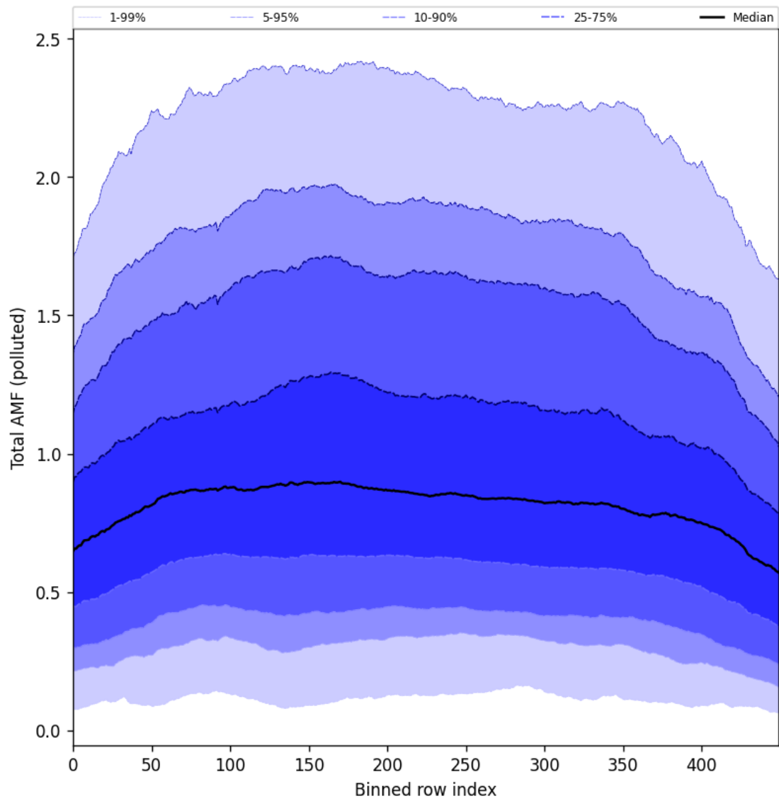
Figure 105: Along track statistics of “Total AMF (polluted)” for 2025-08-09 to 2025-08-11
