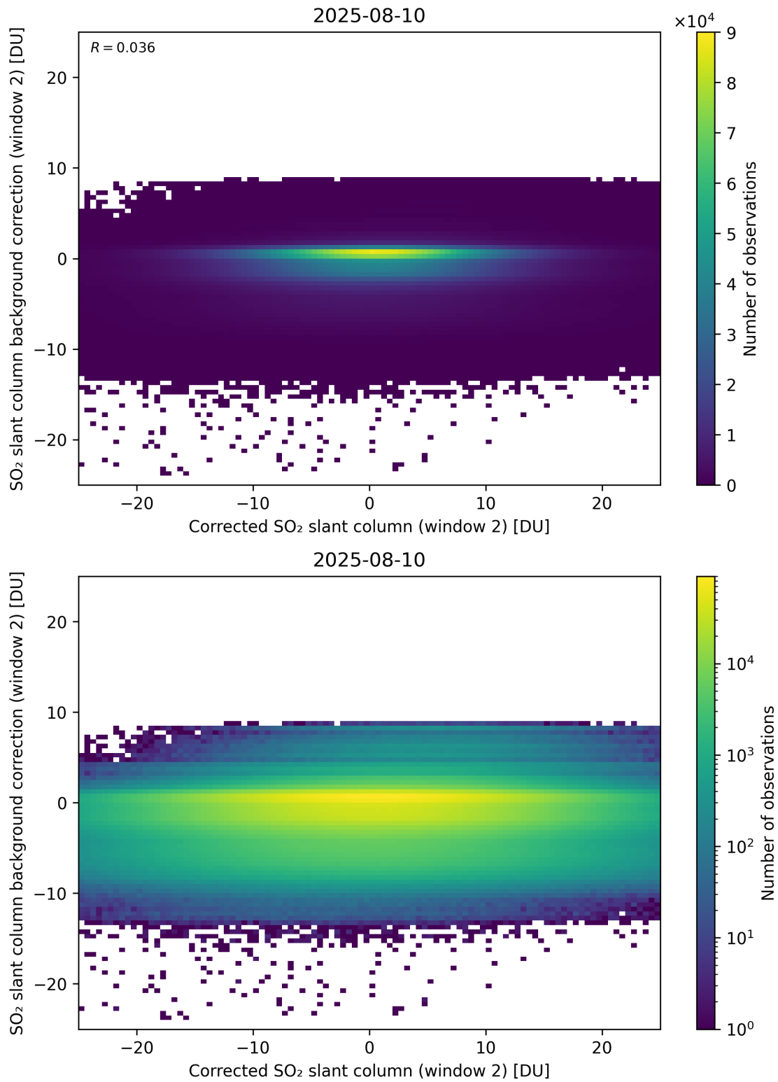
Figure 244: Scatter density plot of “Corrected SO 2 slant column (window 2)” against “SO 2 slant column background correction (window 2)” for 2025-08-09 to 2025-08-11.
