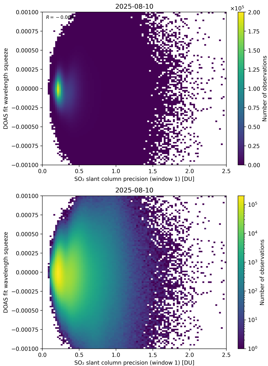
Figure 272: Scatter density plot of “SO 2 slant column precision (window 1)” against “DOAS fit wavelength squeeze” for 2025-08-09 to 2025-08-11.
