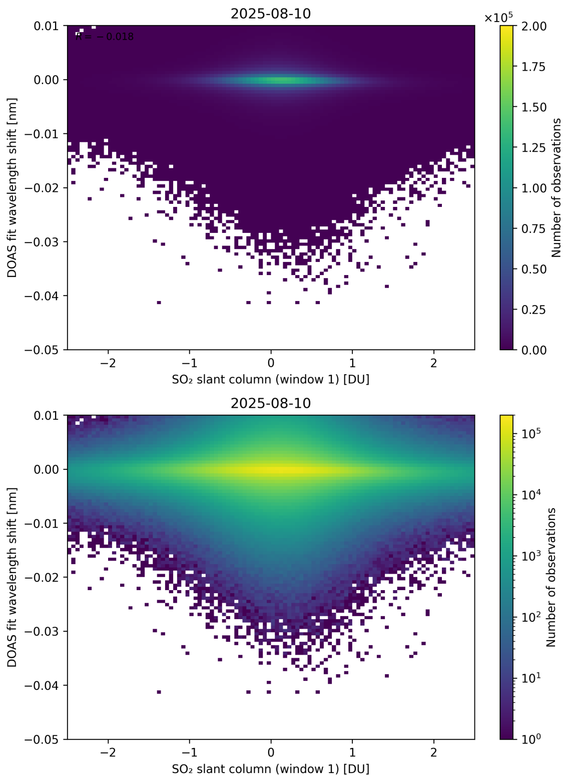
Figure 265: Scatter density plot of “SO 2 slant column (window 1)” against “DOAS fit wavelength shift” for 2025-08-09 to 2025-08-11.
