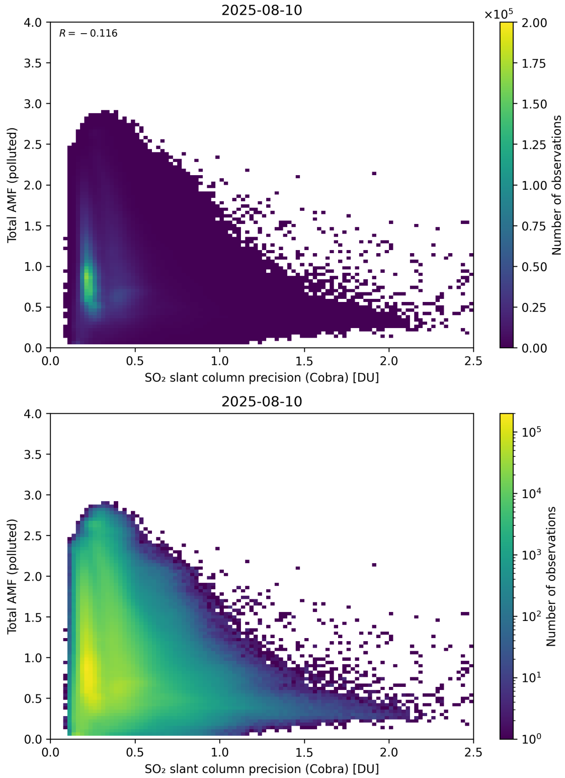
Figure 213: Scatter density plot of “SO 2 slant column precision (Cobra)” against “Total AMF (polluted)” for 2025-08-09 to 2025-08-11.
