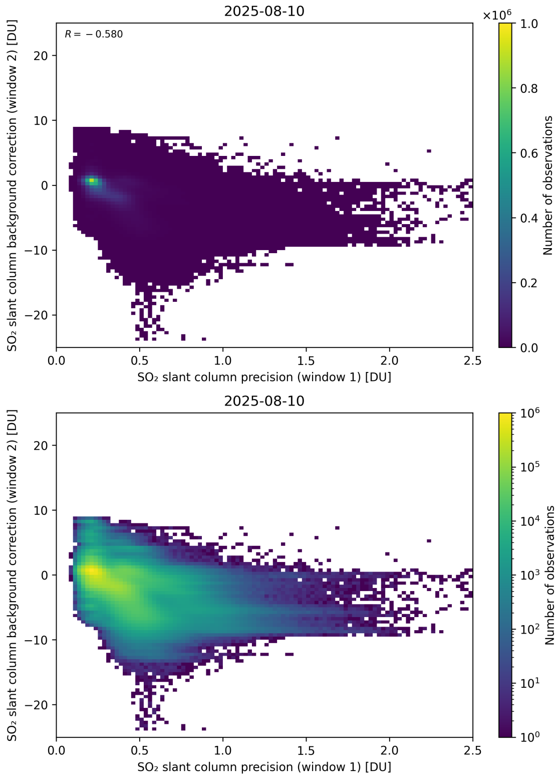
Figure 269: Scatter density plot of “SO 2 slant column precision (window 1)” against “SO 2 slant column background correction (window 2)” for 2025-08-09 to 2025-08-11.
