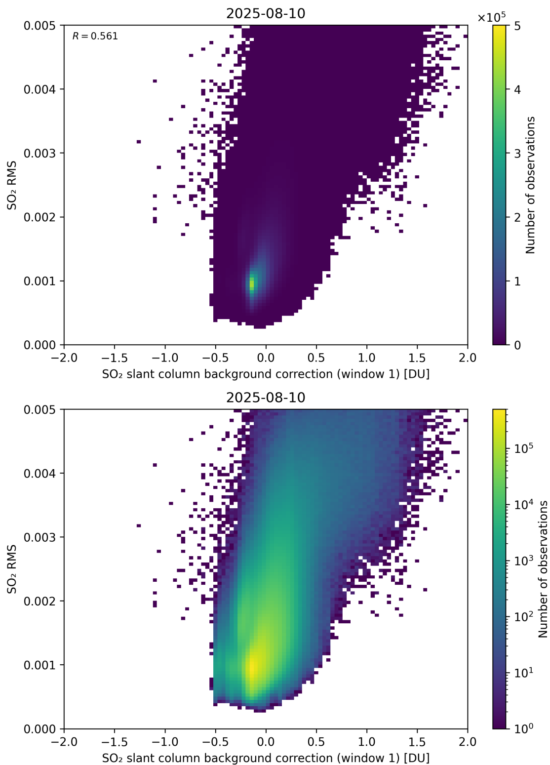
Figure 113: Scatter density plot of “SO 2 slant column background correction (window 1)” against “SO 2 RMS” for 2025-08-09 to 2025-08-11.
