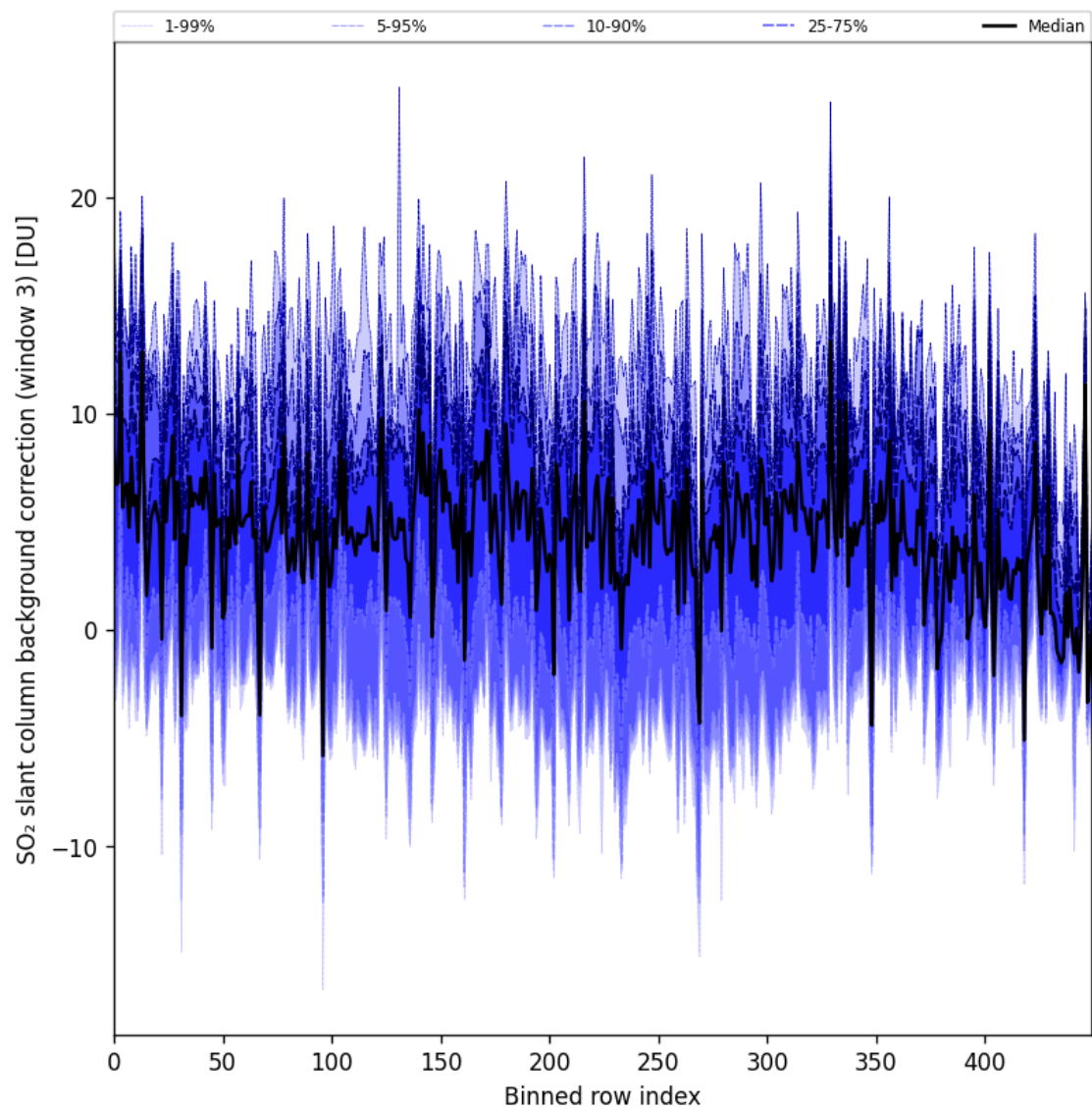
Figure 100: Along track statistics of "SO 2 slant column background correction (window 3)" for 2025-08-09 to 2025-08-11
