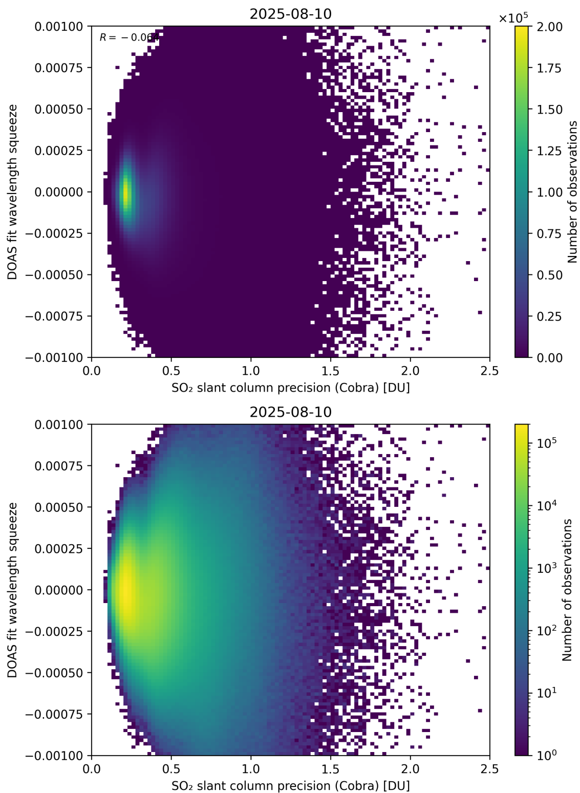
Figure 203: Scatter density plot of “SO 2 slant column precision (Cobra)” against “DOAS fit wavelength squeeze” for 2025-08-09 to 2025-08-11.
