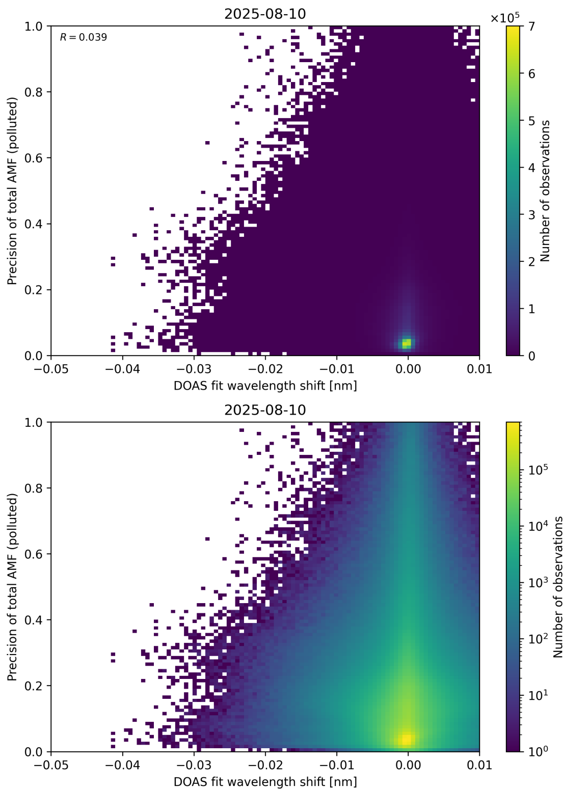
Figure 142: Scatter density plot of “DOAS fit wavelength shift” against “Precision of total AMF (polluted)” for 2025-08-09 to 2025-08-11.
