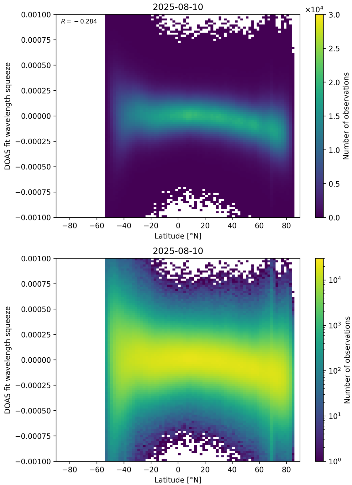
Figure 154: Scatter density plot of “Latitude” against “DOAS fit wavelength squeeze” for 2025-08-09 to 2025-08-11.
