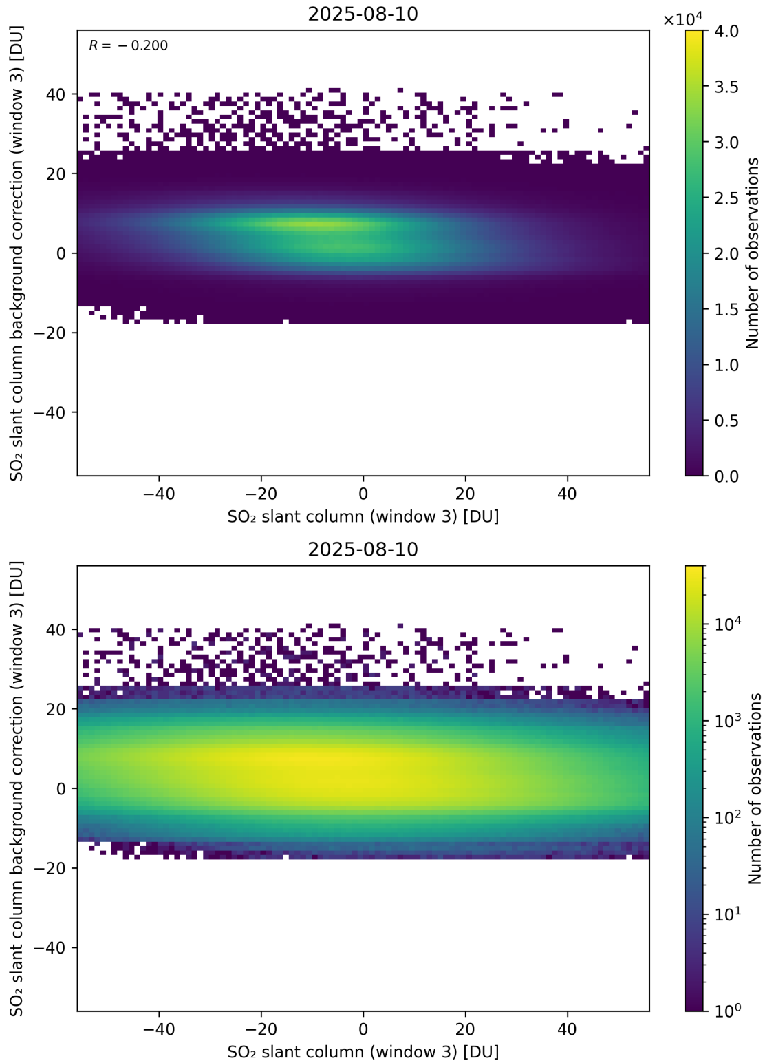
Figure 303: Scatter density plot of “SO 2 slant column (window 3)” against “SO 2 slant column background correction (window 3)” for 2025-08-09 to 2025-08-11.
