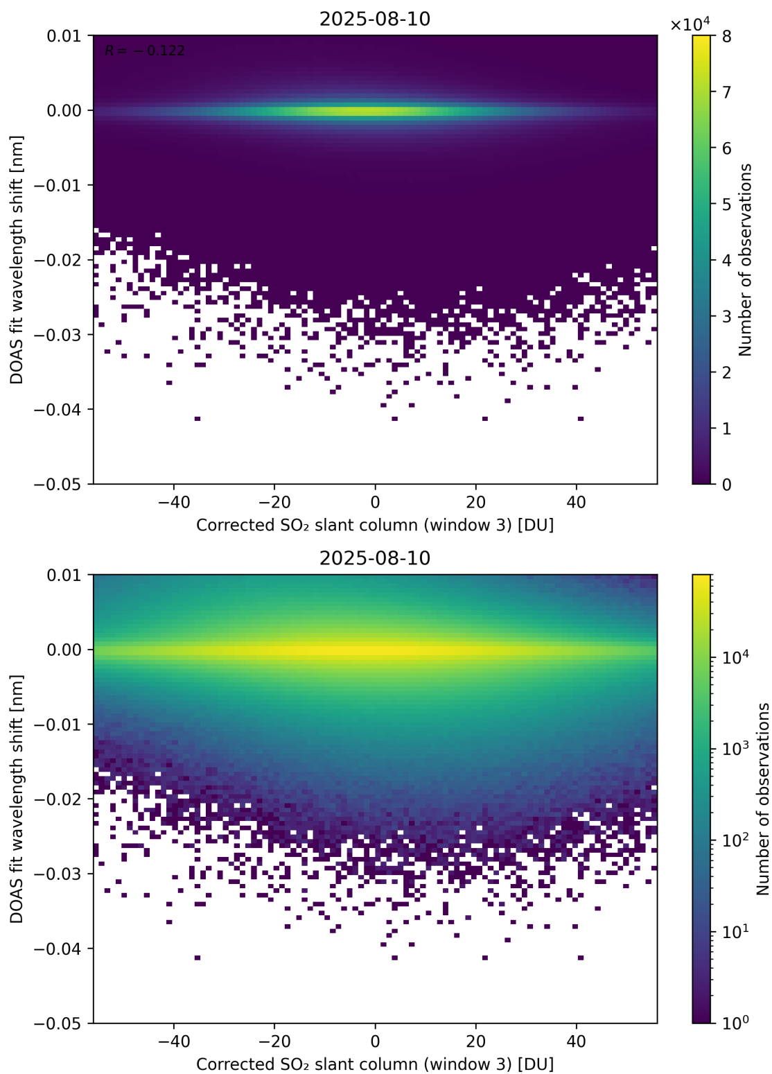
Figure 256: Scatter density plot of “Corrected SO 2 slant column (window 3)” against “DOAS fit wavelength shift” for 2025-08-09 to 2025-08-11.
