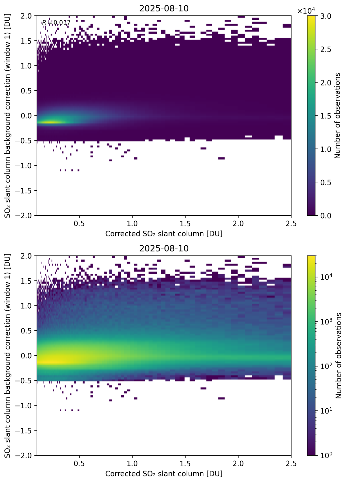
Figure 226: Scatter density plot of “Corrected SO 2 slant column” against “SO 2 slant column background correction (window 1)” for 2025-08-09 to 2025-08-11.
