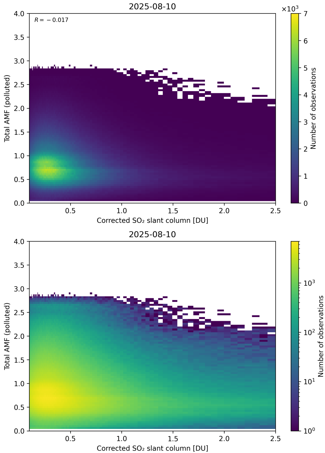
Figure 242: Scatter density plot of “Corrected SO 2 slant column” against “Total AMF (polluted)” for 2025-08-09 to 2025-08-11.
