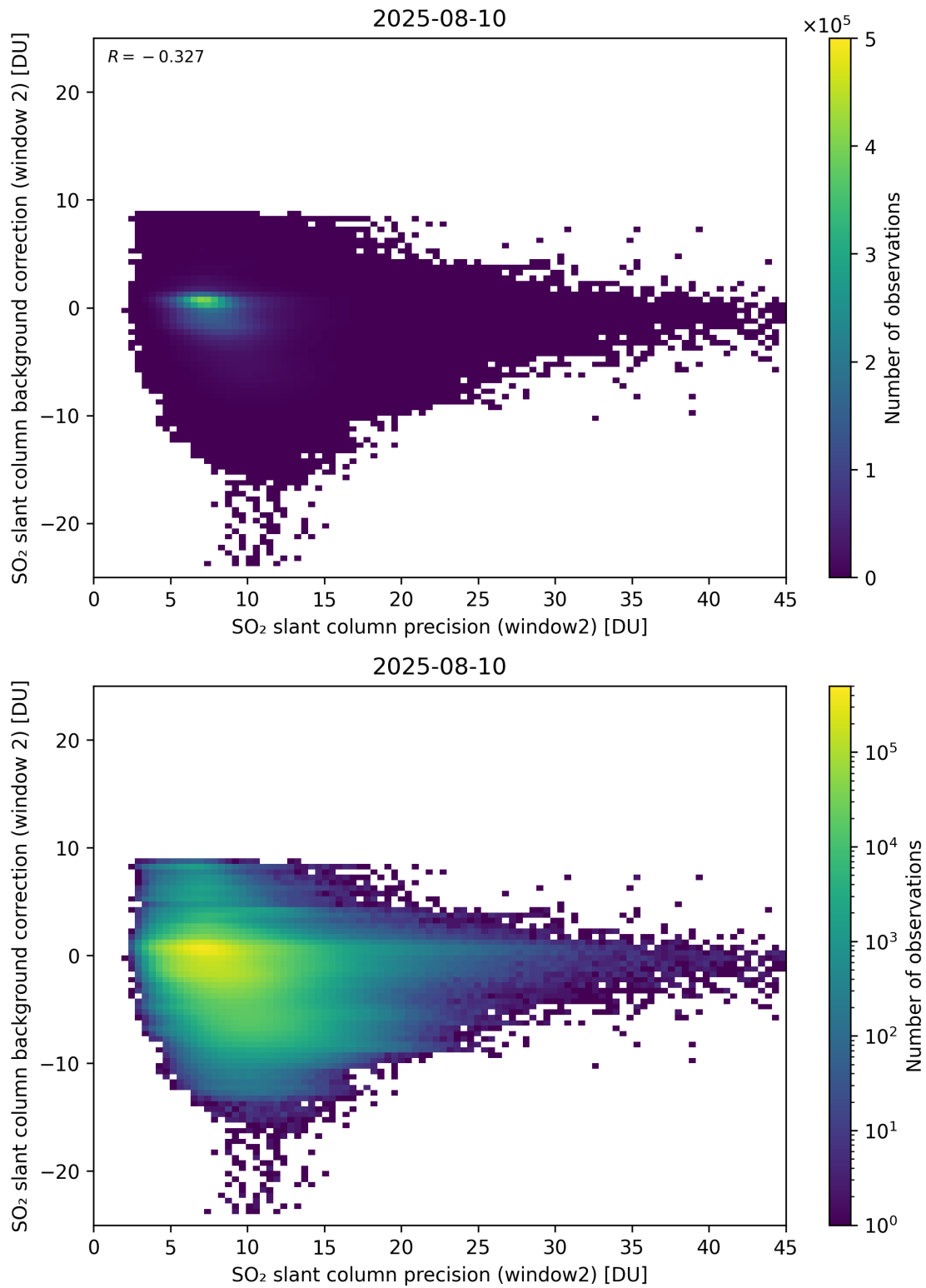
Figure 291: Scatter density plot of “SO 2 slant column precision (window2)” against “SO 2 slant column background correction (window 2)” for 2025-08-09 to 2025-08-11.
