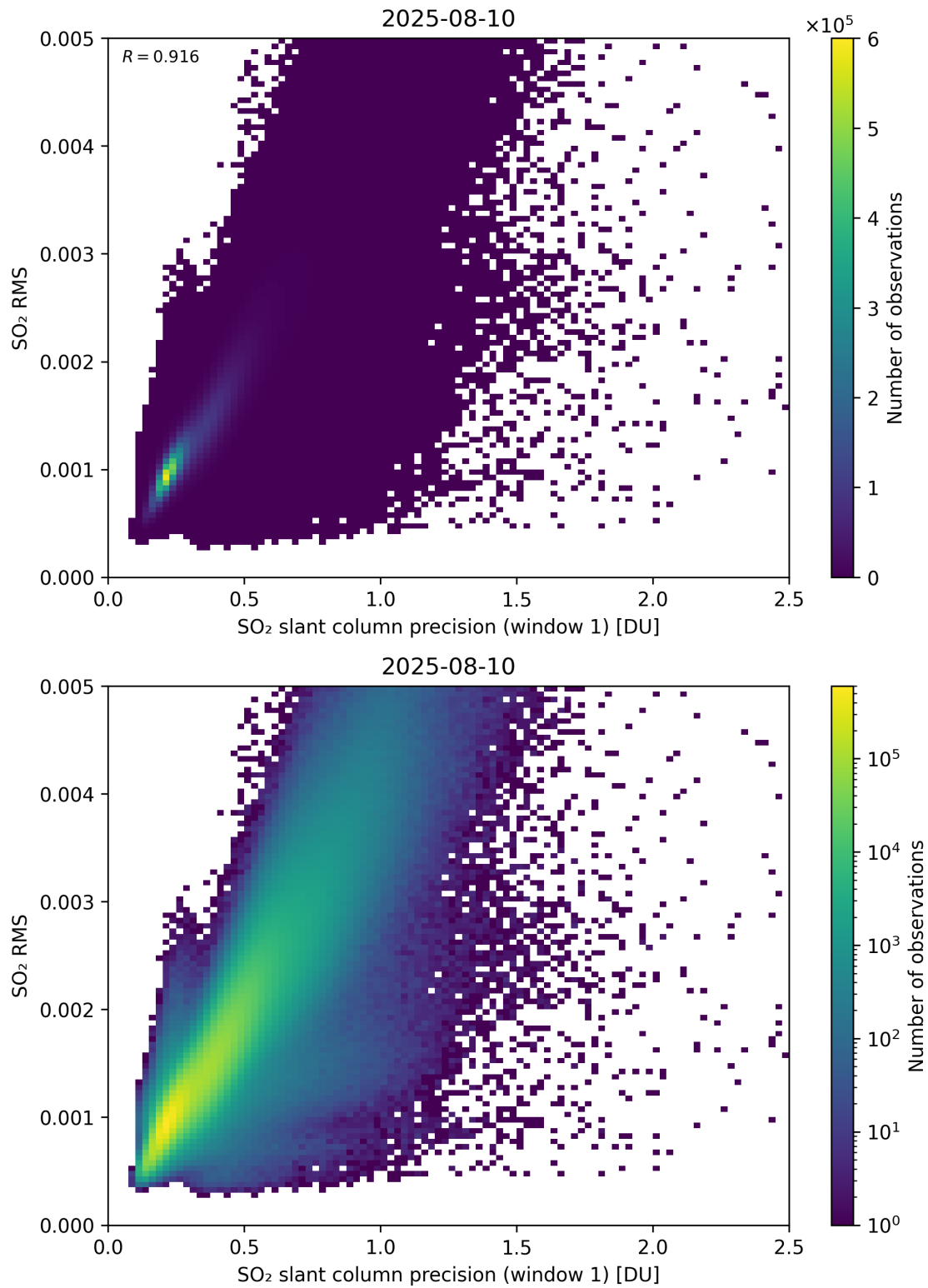
Figure 273: Scatter density plot of “SO 2 slant column precision (window 1)” against “SO 2 RMS” for 2025-08-09 to 2025-08-11.
