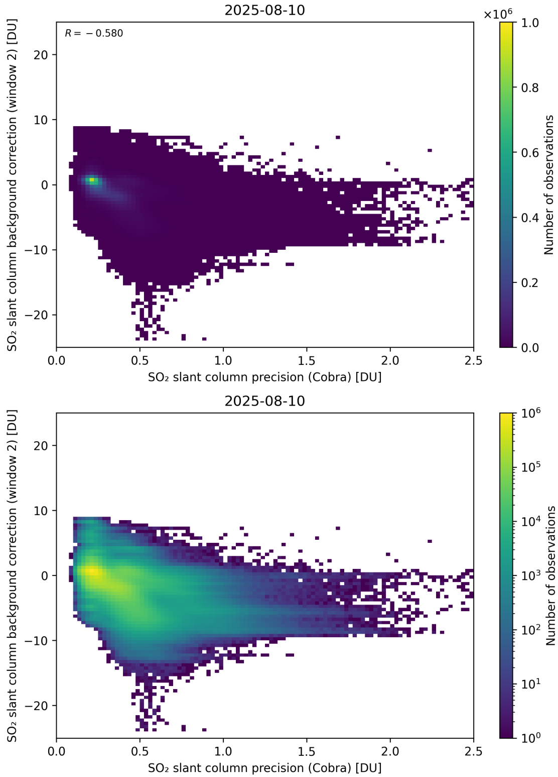
Figure 200: Scatter density plot of “SO 2 slant column precision (Cobra)” against “SO 2 slant column background correction (window 2)” for 2025-08-09 to 2025-08-11.
