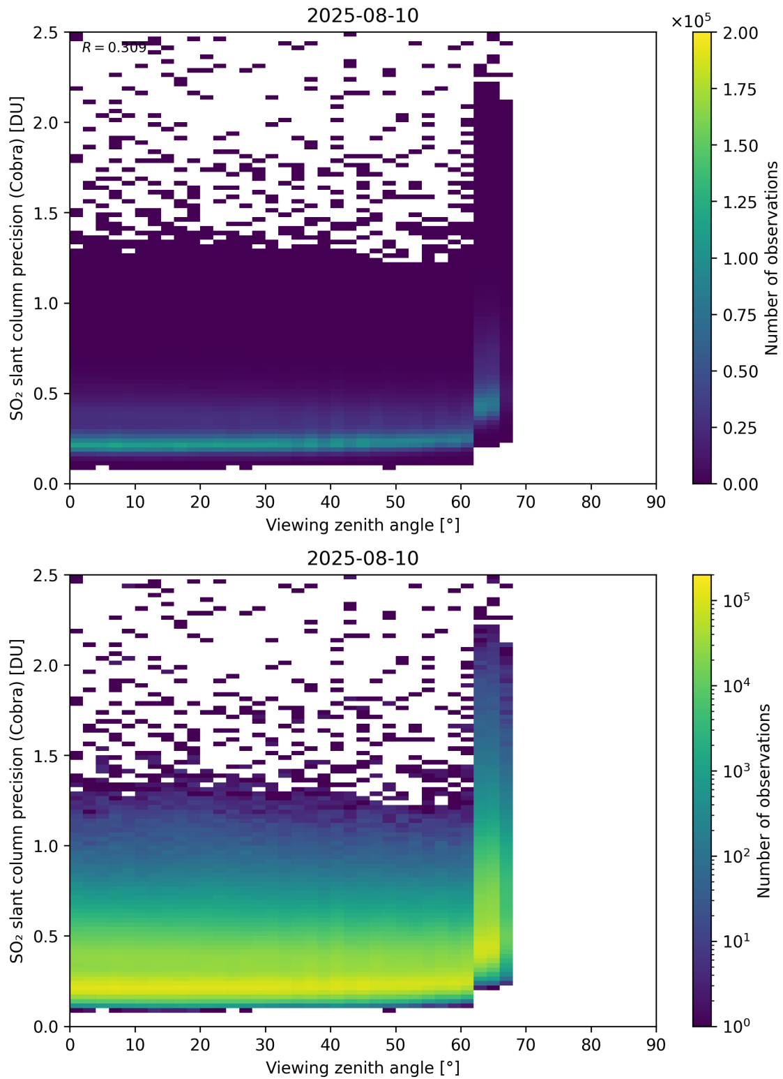
Figure 372: Scatter density plot of “Viewing zenith angle” against “SO 2 slant column precision (Cobra)” for 2025-08-09 to 2025-08-11.
