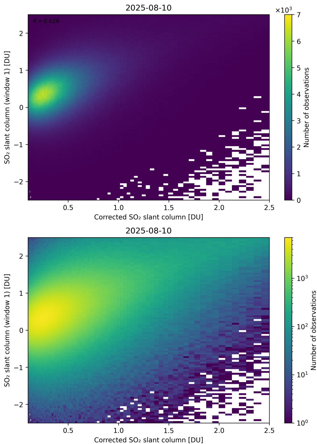
Figure 237: Scatter density plot of “Corrected SO 2 slant column” against “SO 2 slant column (window 1)” for 2025-08-09 to 2025-08-11.
