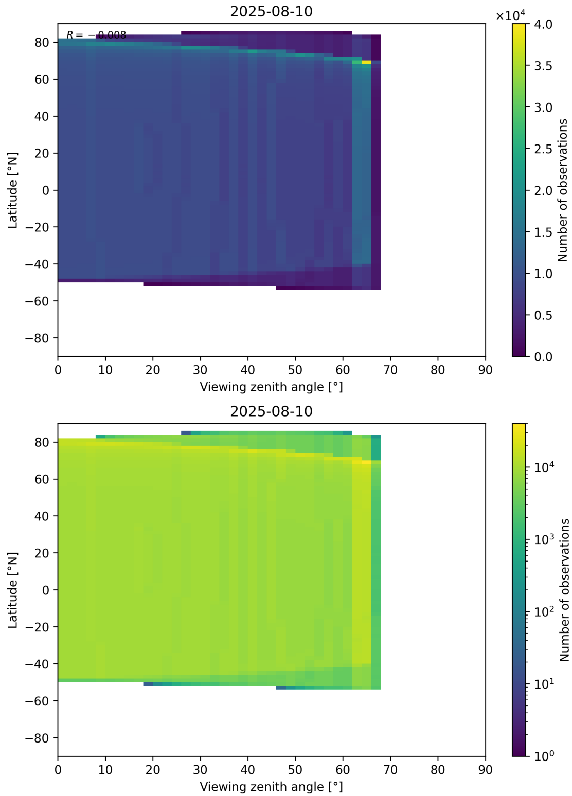
Figure 368: Scatter density plot of “Viewing zenith angle” against “Latitude” for 2025-08-09 to 2025-08-11.
