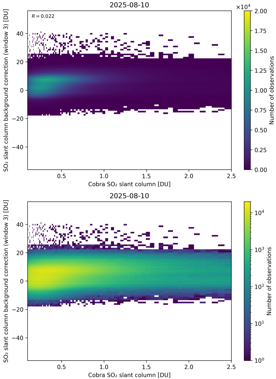
Figure 195: Scatter density plot of “Cobra SO 2 slant column” against “SO 2 slant column background correction (window 3)” for 2025-08-09 to 2025-08-11.
