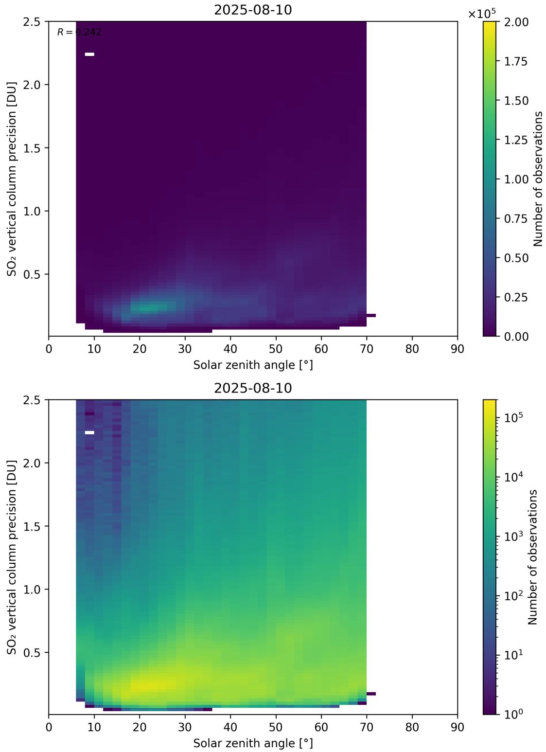
Figure 192: Scatter density plot of “Solar zenith angle” against “SO 2 vertical column precision” for 2025-08-09 to 2025-08-11.
