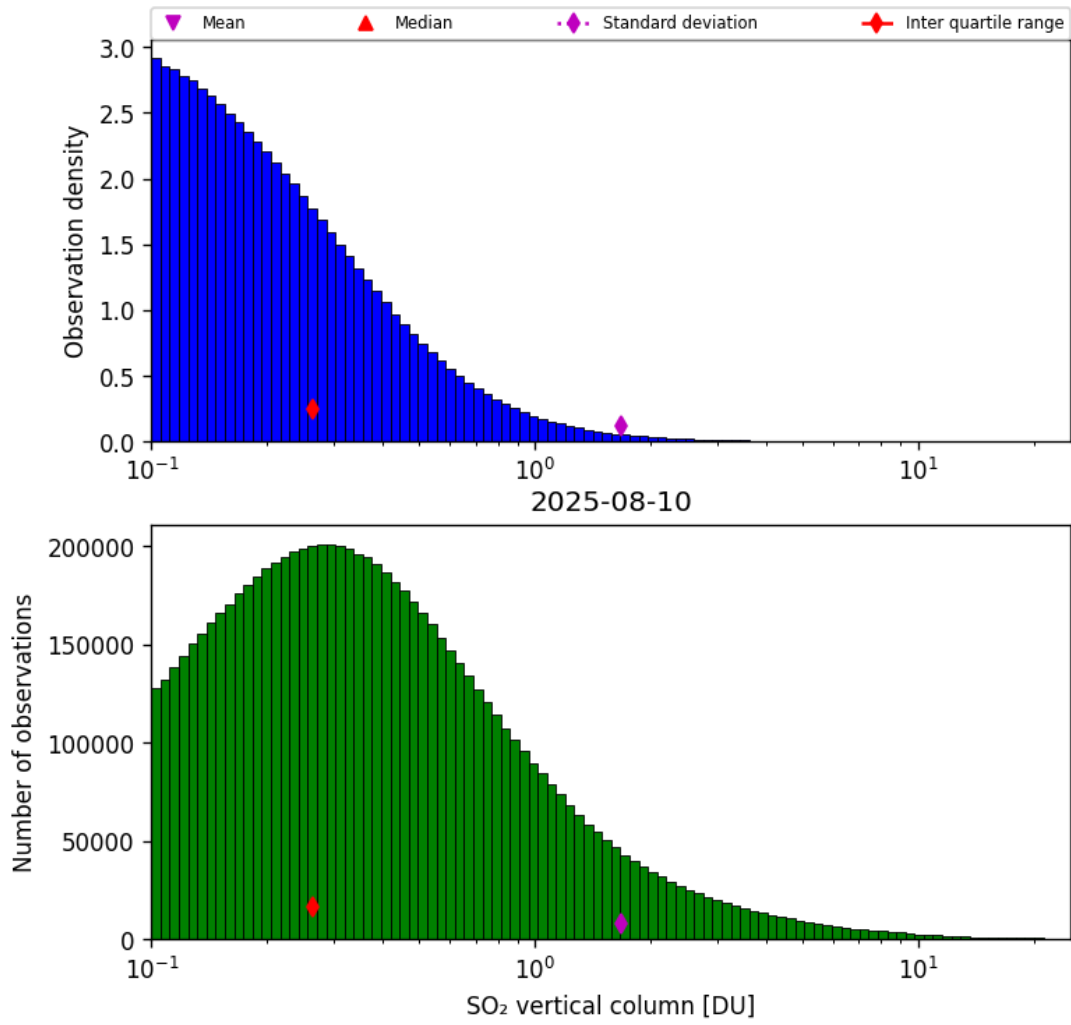
Figure 58: Histogram of “SO 2 vertical column” for 2025-08-09 to 2025-08-11
