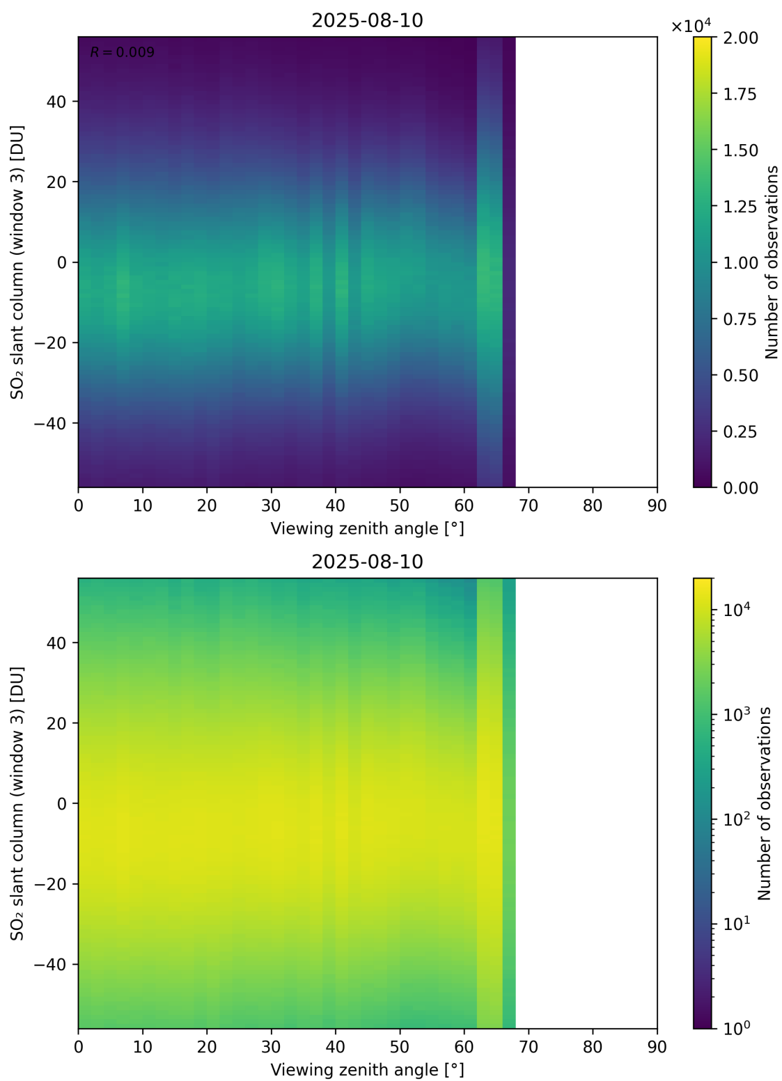
Figure 379: Scatter density plot of “Viewing zenith angle” against “SO 2 slant column (window 3)” for 2025-08-09 to 2025-08-11.
