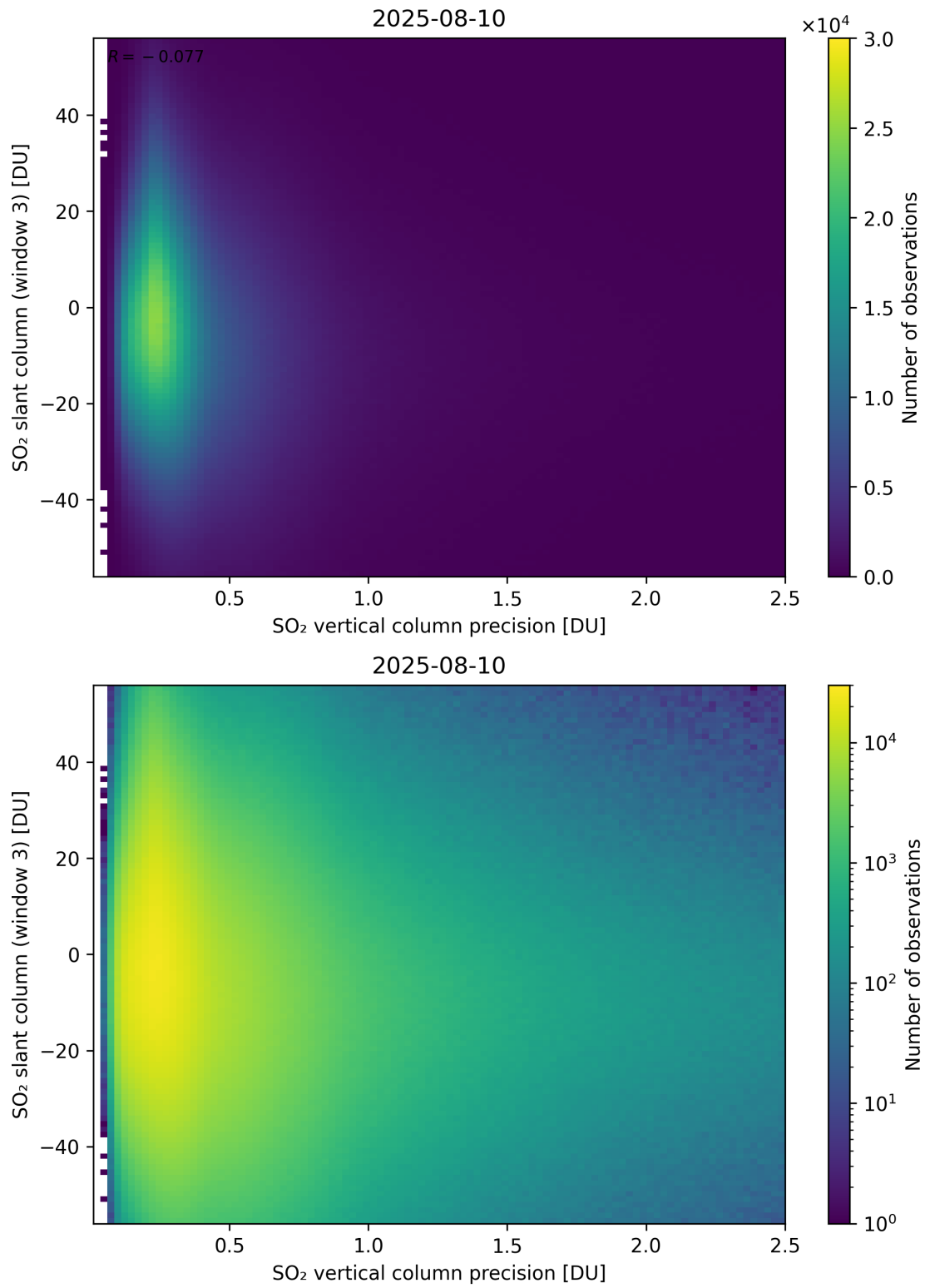
Figure 344: Scatter density plot of “SO 2 vertical column precision” against “SO 2 slant column (window 3)” for 2025-08-09 to 2025-08-11.
