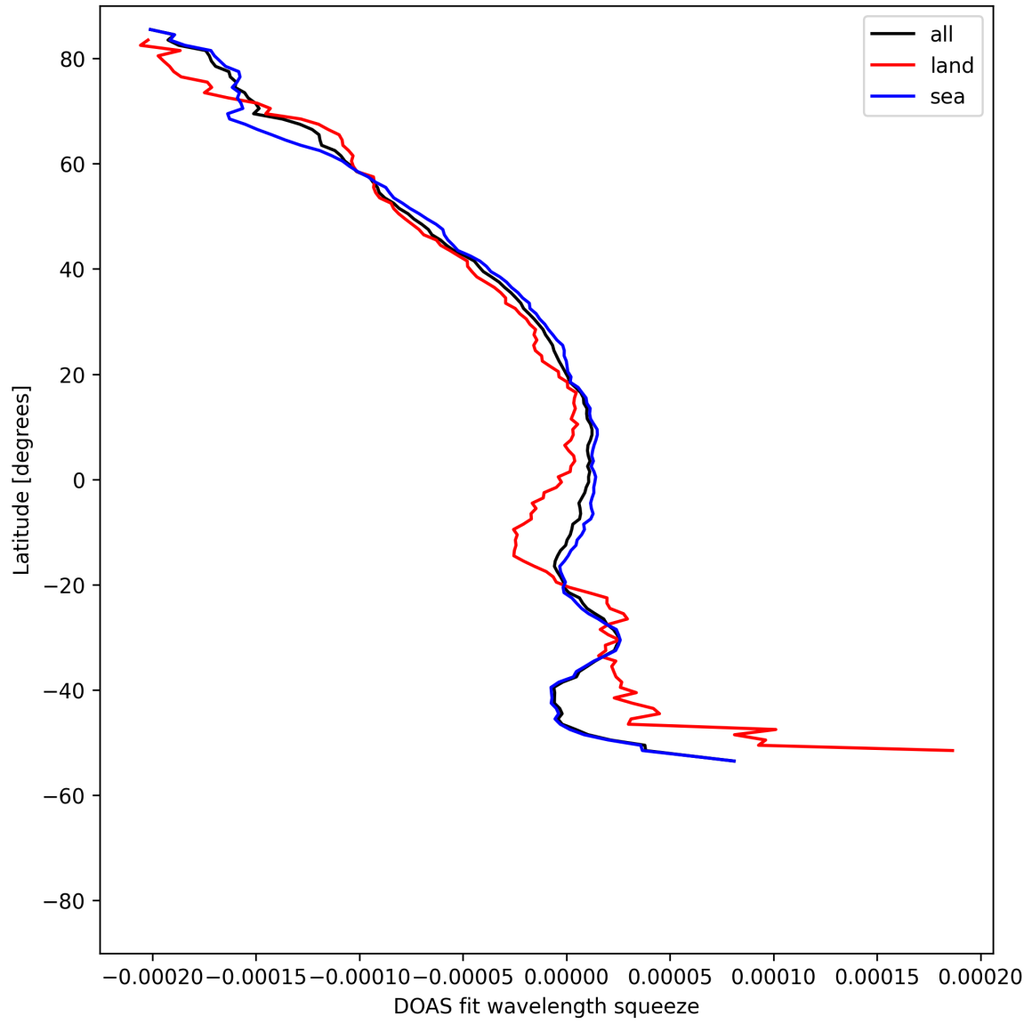
Figure 51: Zonal average of “DOAS fit wavelength squeeze” for 2025-08-09 to 2025-08-11.
