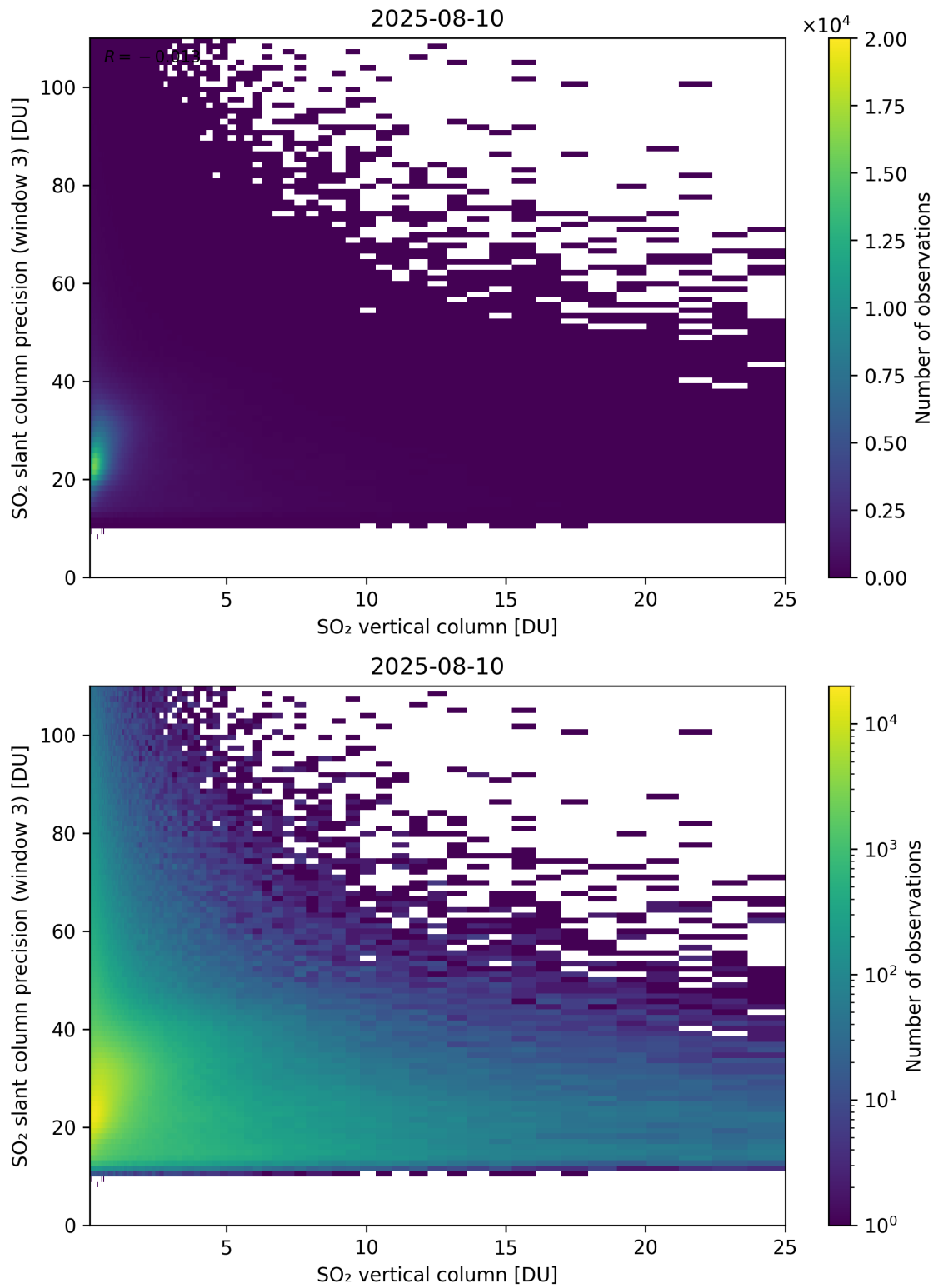
Figure 358: Scatter density plot of “SO 2 vertical column” against “SO 2 slant column precision (window 3)” for 2025-08-09 to 2025-08-11.
