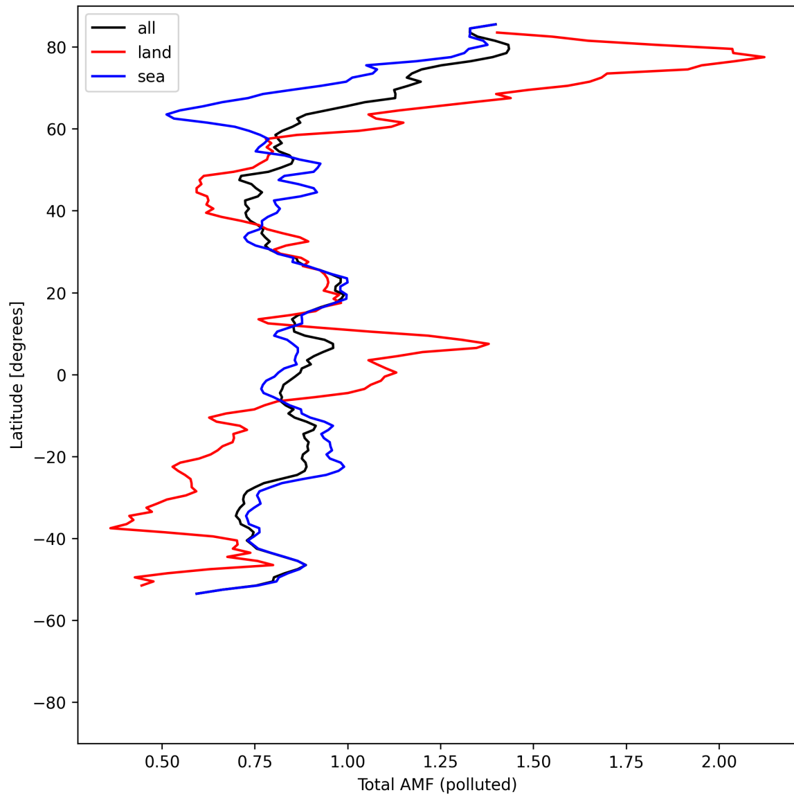
Figure 53: Zonal average of “Total AMF (polluted)” for 2025-08-09 to 2025-08-11.
