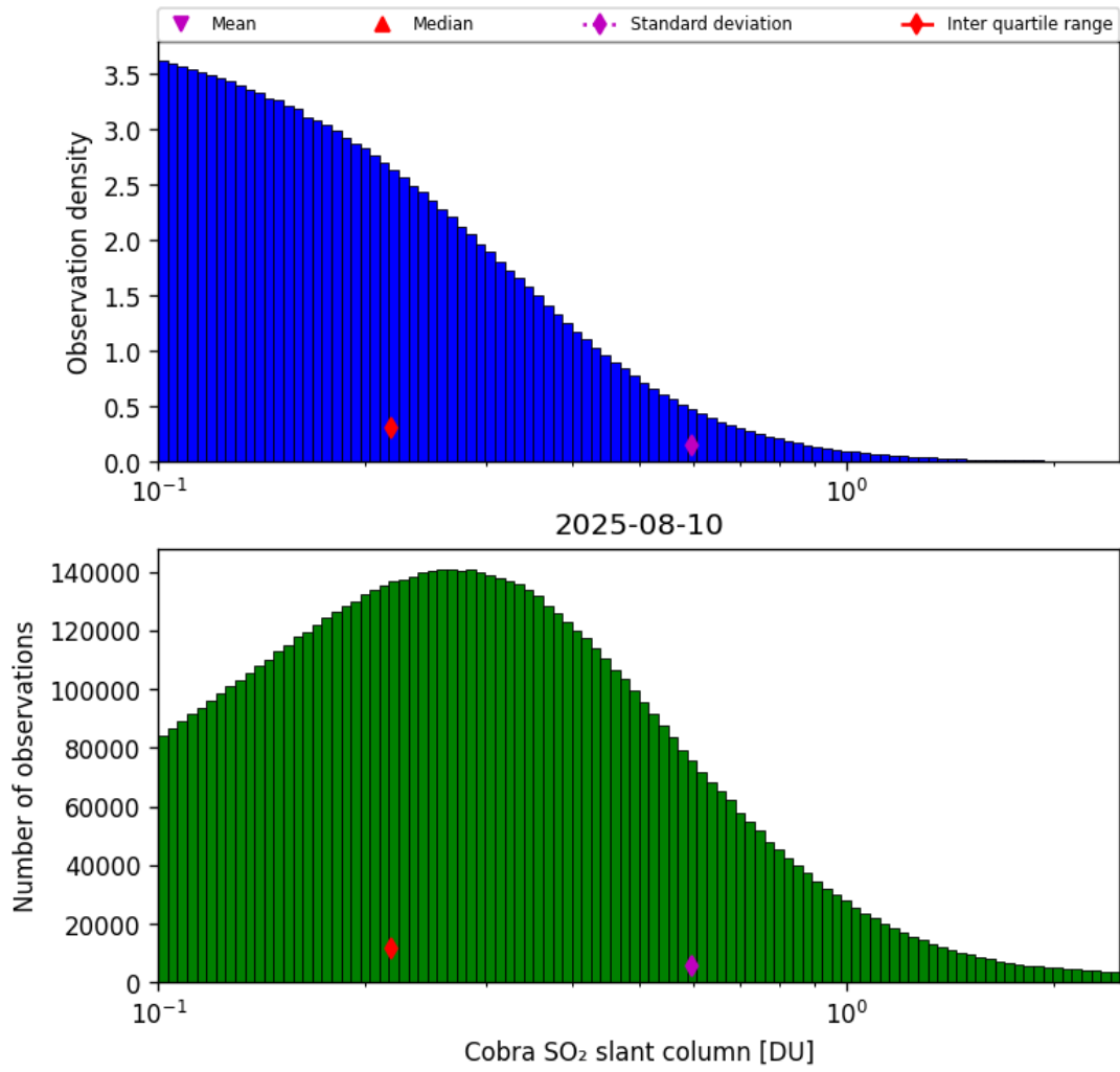
Figure 61: Histogram of “Cobra SO 2 slant column” for 2025-08-09 to 2025-08-11
