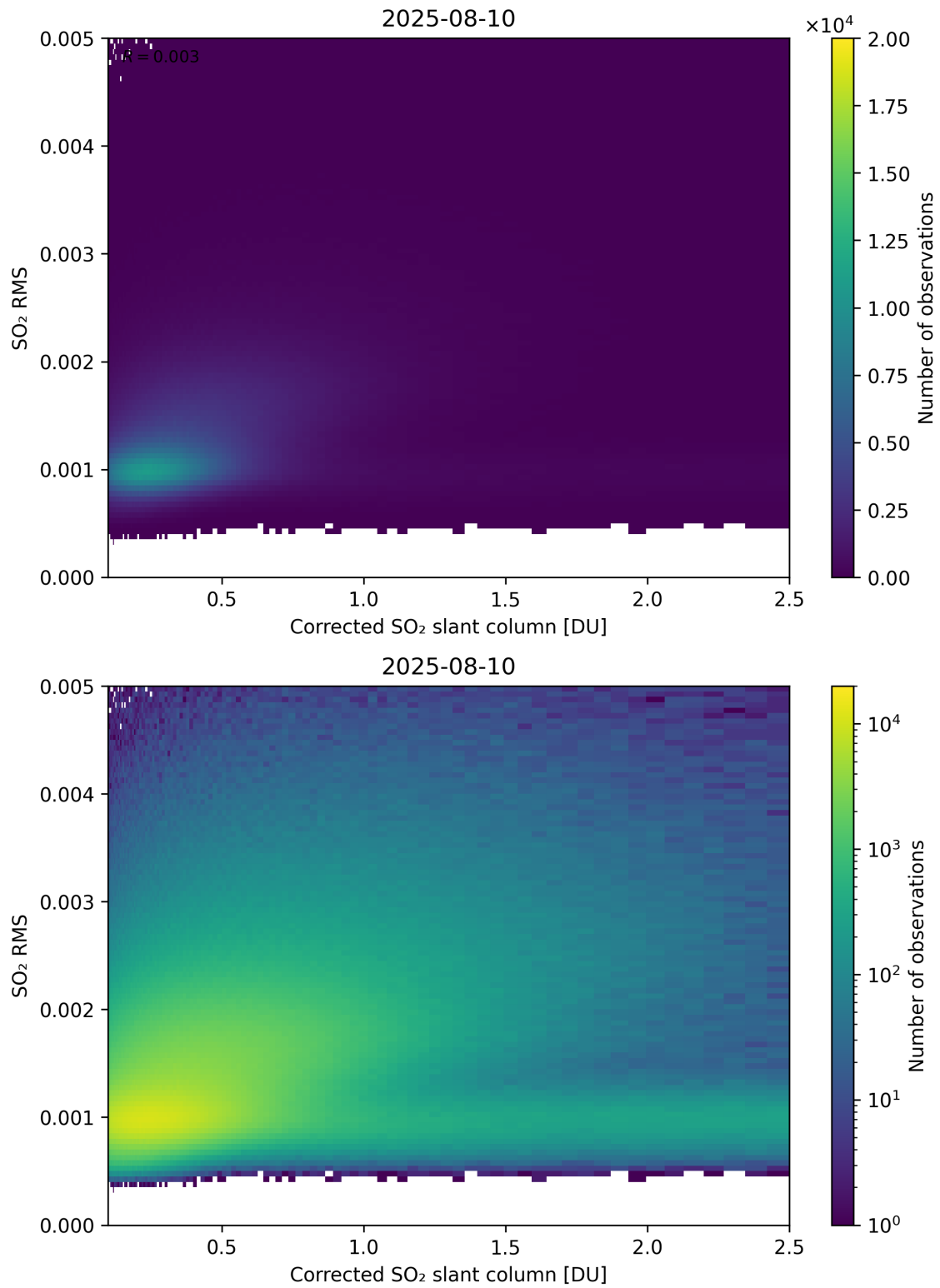
Figure 231: Scatter density plot of “Corrected SO 2 slant column” against “SO 2 RMS” for 2025-08-09 to 2025-08-11.
