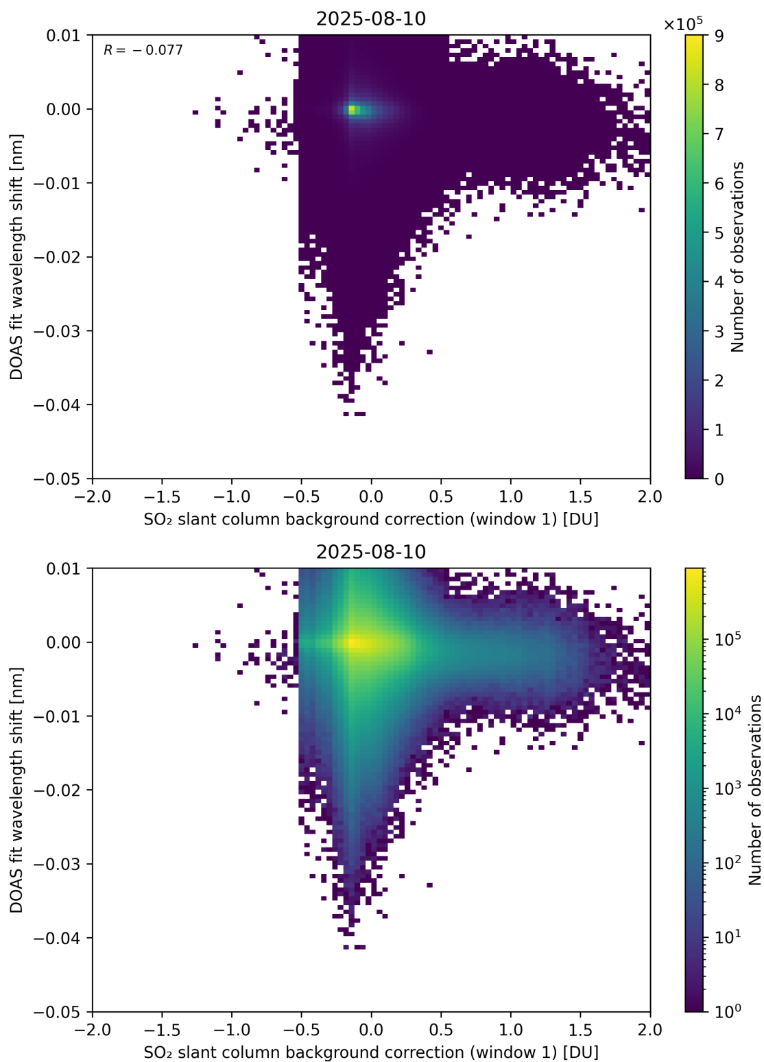
Figure 111: Scatter density plot of “SO 2 slant column background correction (window 1)” against “DOAS fit wavelength shift” for 2025-08-09 to 2025-08-11.
