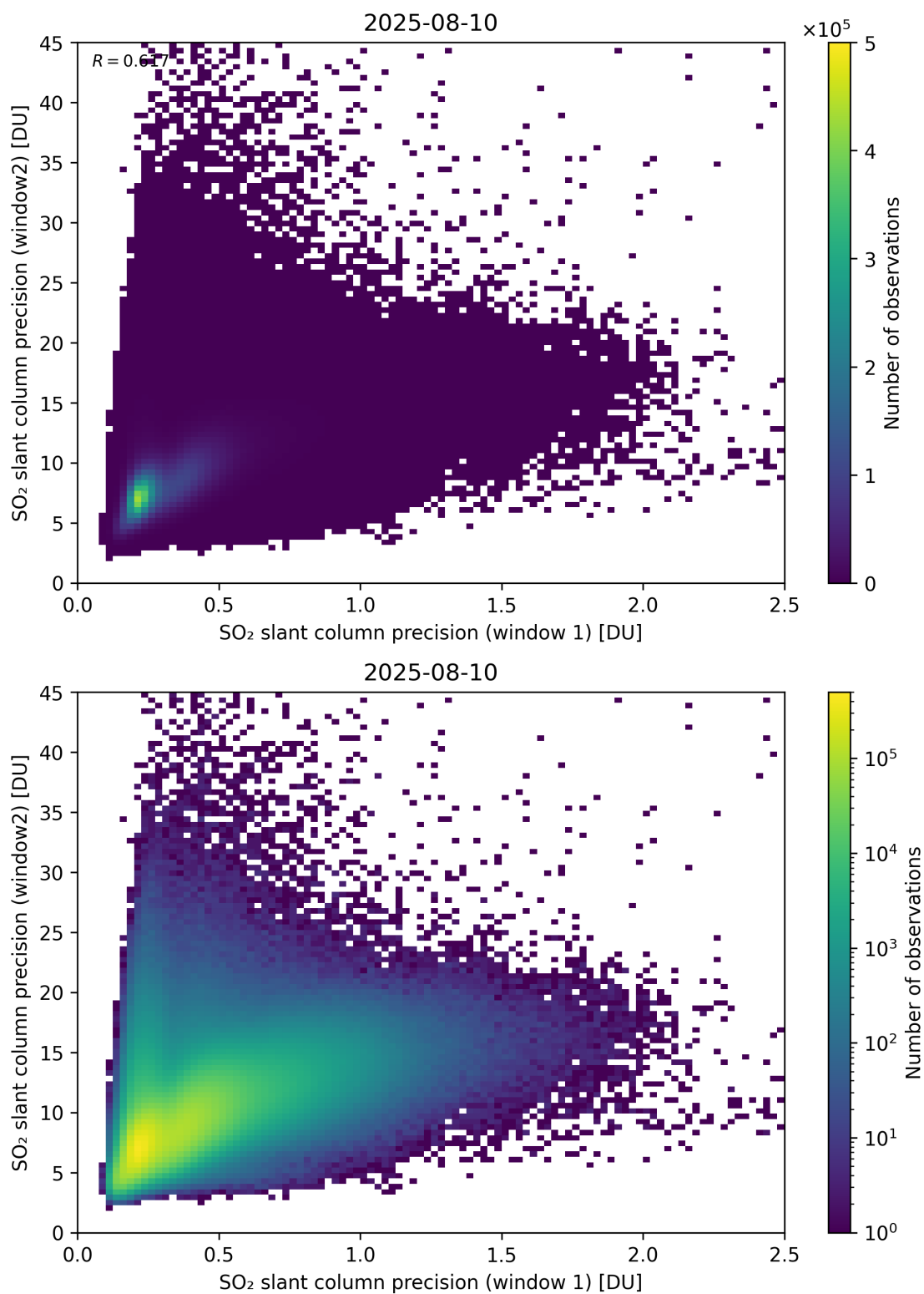
Figure 277: Scatter density plot of “SO 2 slant column precision (window 1)” against “SO 2 slant column precision (window2)” for 2025-08-09 to 2025-08-11.
