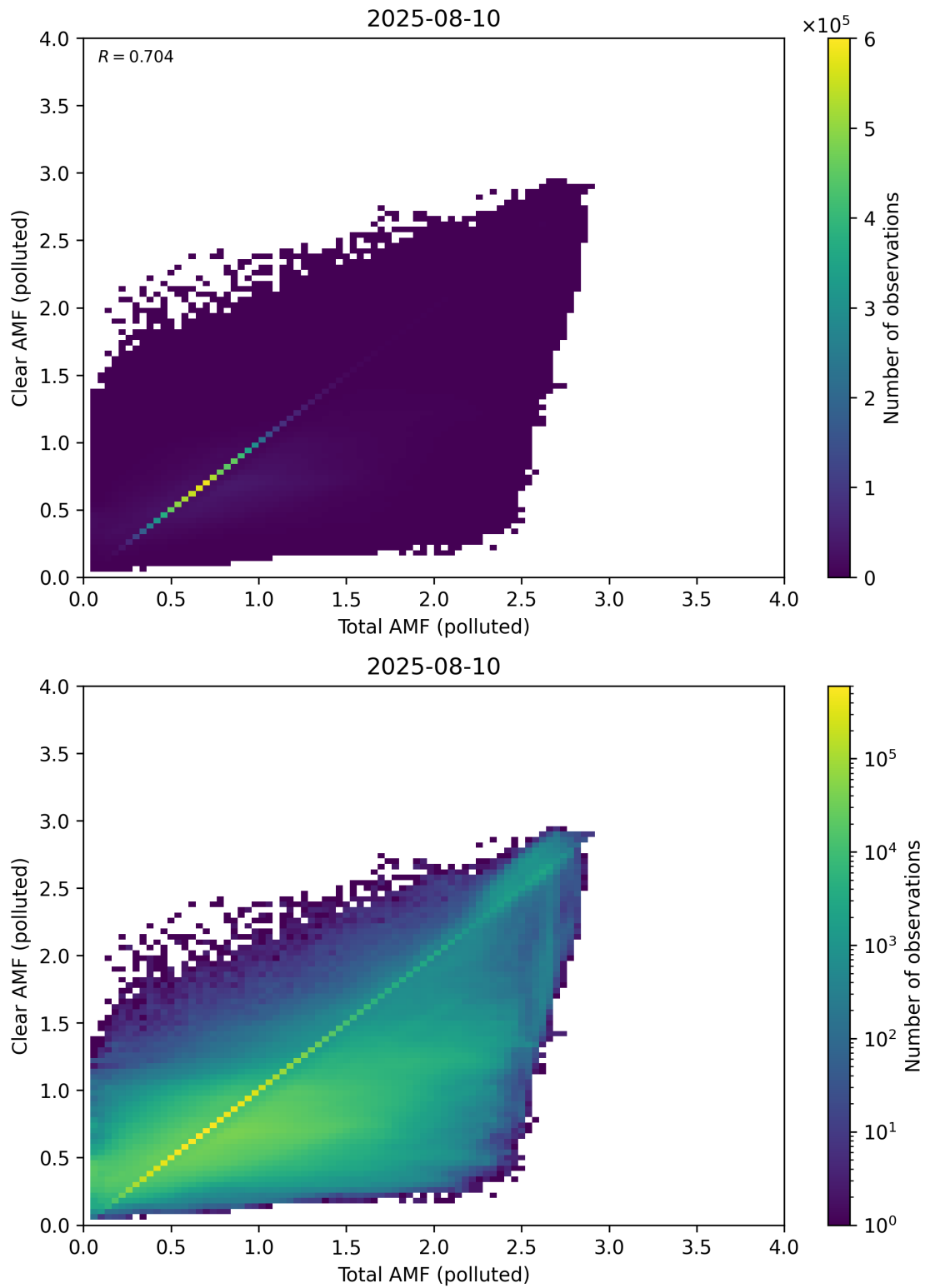
Figure 321: Scatter density plot of “Total AMF (polluted)” against “Clear AMF (polluted)” for 2025-08-09 to 2025-08-11.
