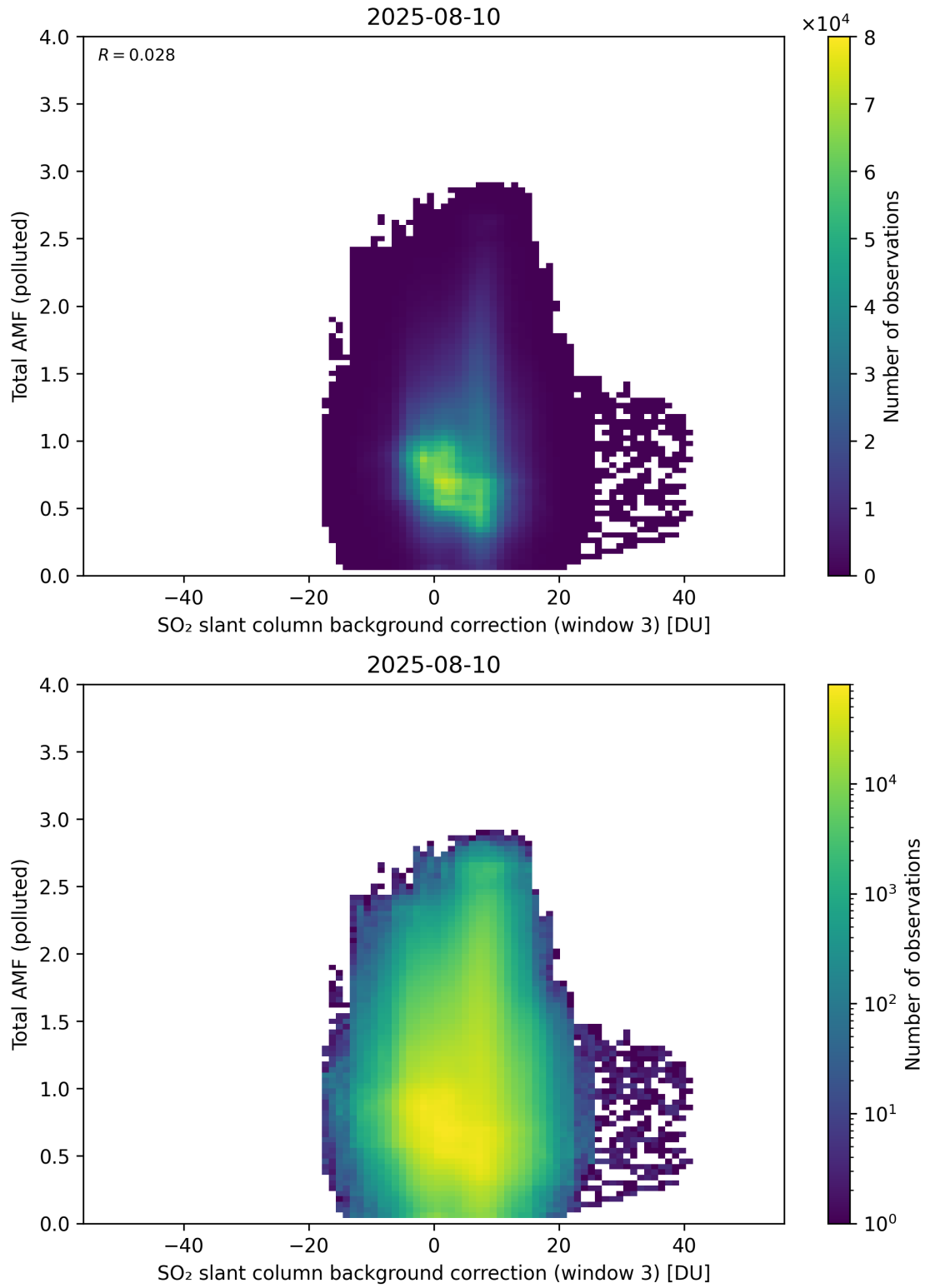
Figure 136: Scatter density plot of “SO 2 slant column background correction (window 3)” against “Total AMF (polluted)” for 2025-08-09 to 2025-08-11.
