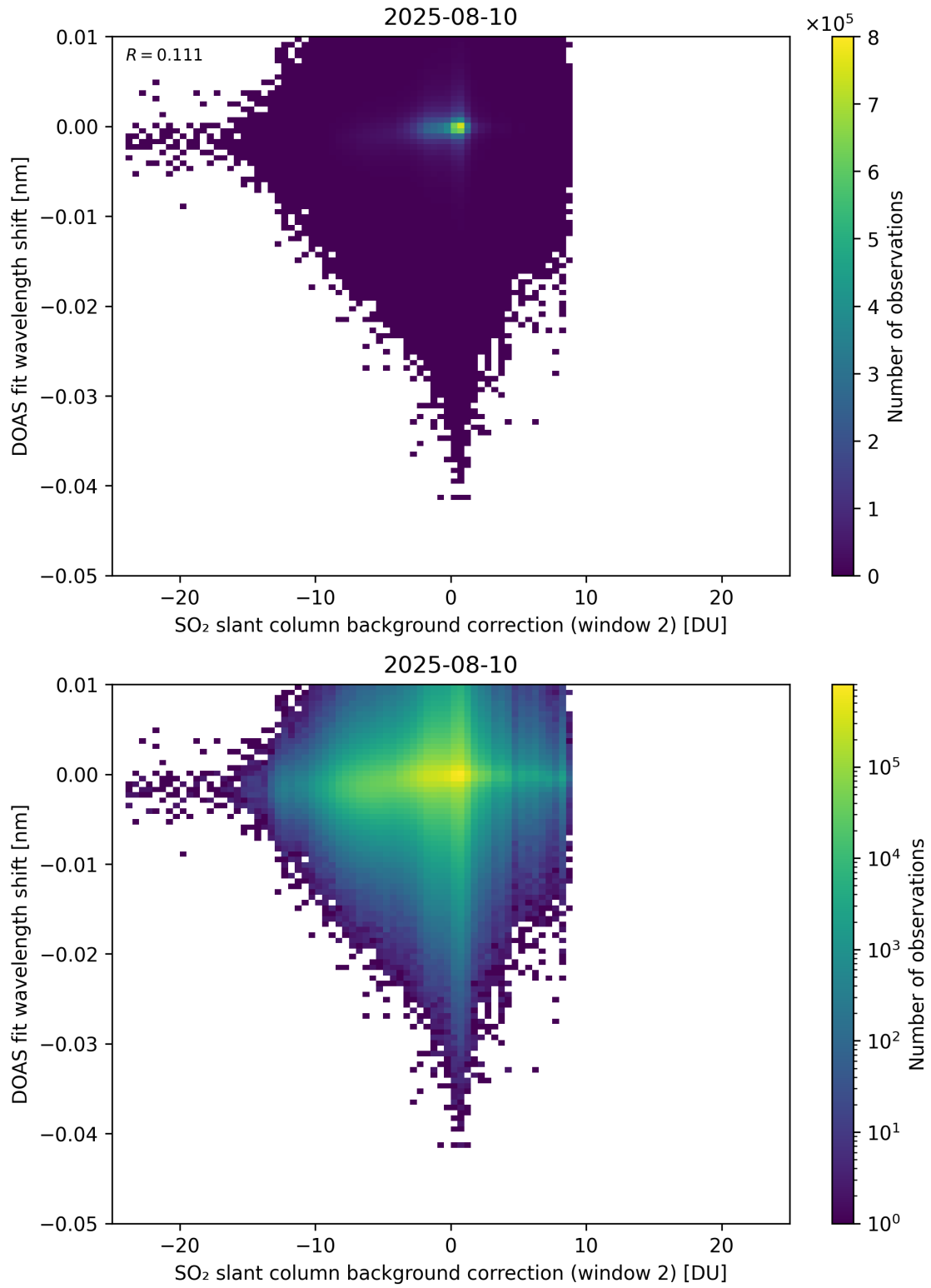
Figure 123: Scatter density plot of “SO 2 slant column background correction (window 2)” against “DOAS fit wavelength shift” for 2025-08-09 to 2025-08-11.
