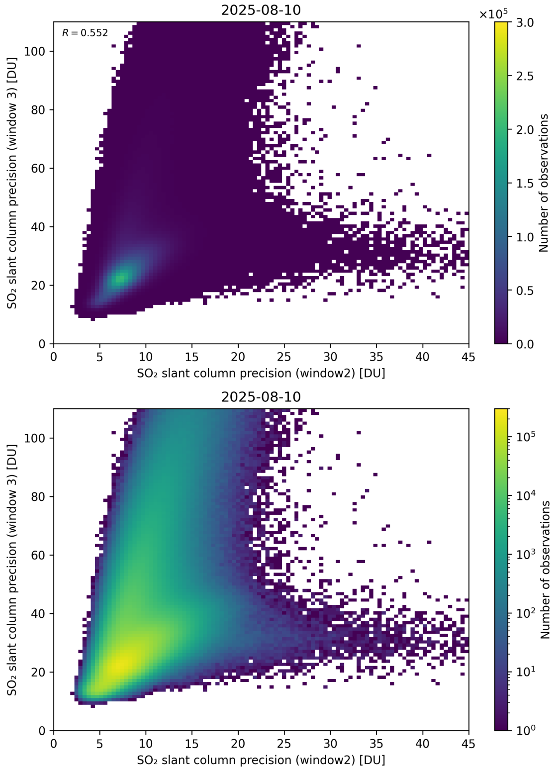
Figure 300: Scatter density plot of “SO 2 slant column precision (window2)” against “SO 2 slant column precision (window 3)” for 2025-08-09 to 2025-08-11.
