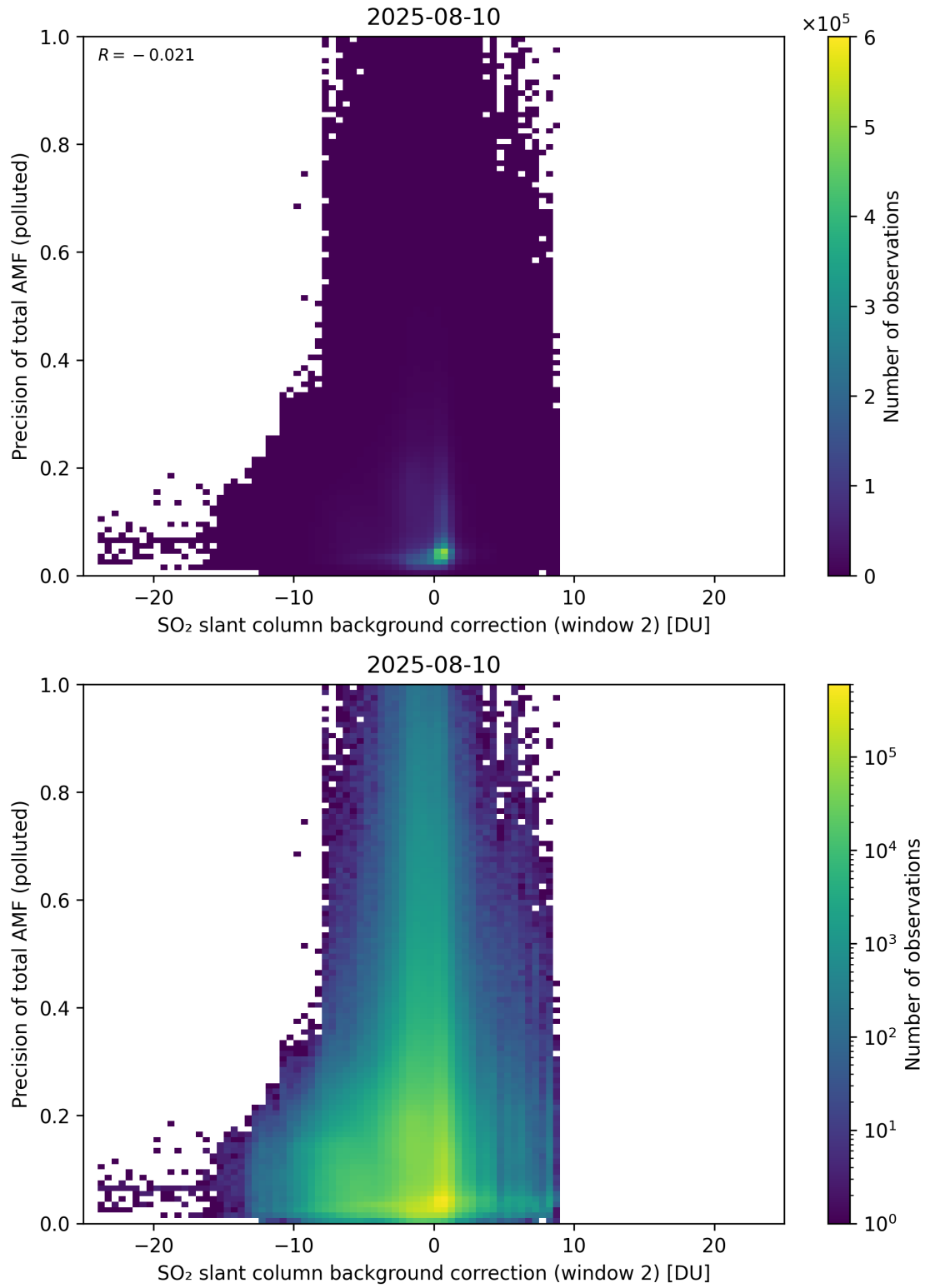
Figure 131: Scatter density plot of “SO 2 slant column background correction (window 2)” against “Precision of total AMF (polluted)” for 2025-08-09 to 2025-08-11.
