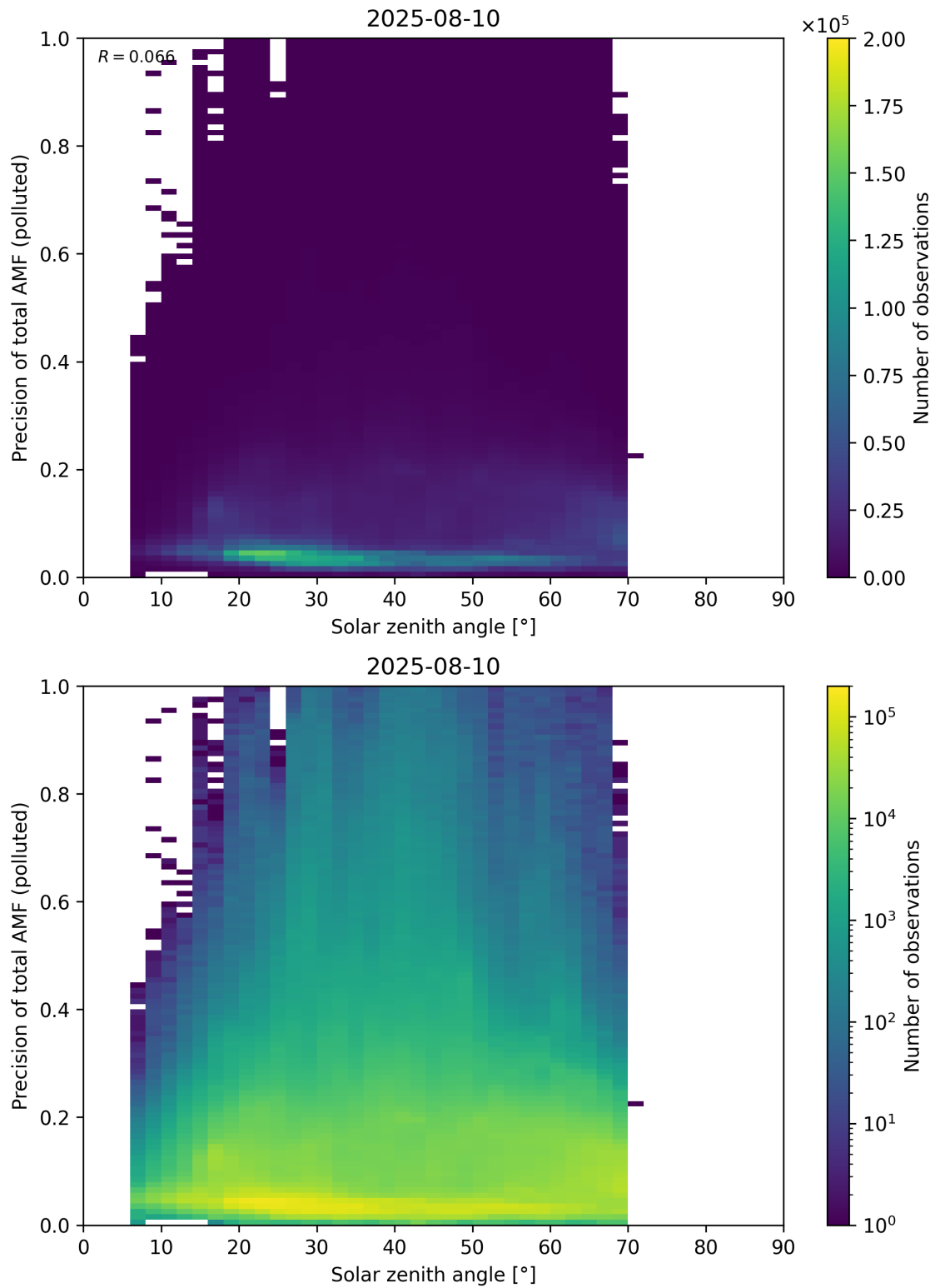
Figure 190: Scatter density plot of “Solar zenith angle” against “Precision of total AMF (polluted)” for 2025-08-09 to 2025-08-11.
