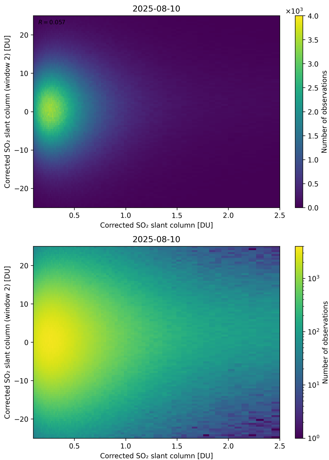
Figure 235: Scatter density plot of “Corrected SO 2 slant column” against “Corrected SO 2 slant column (window 2)” for 2025-08-09 to 2025-08-11.
