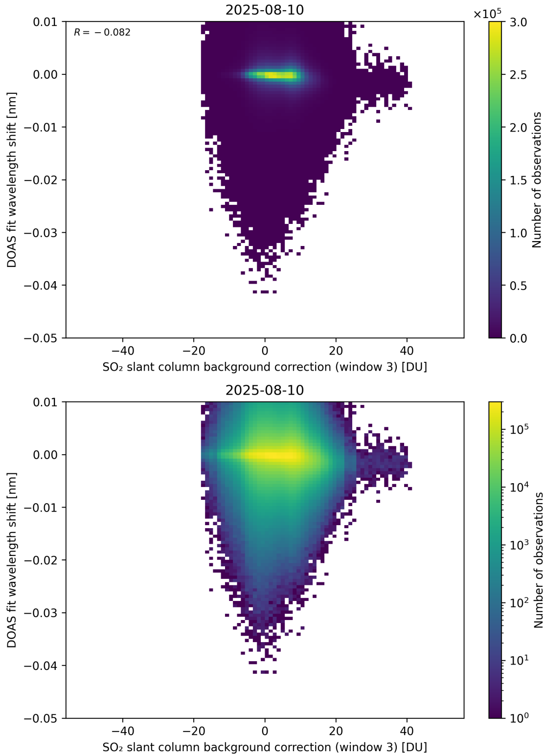
Figure 132: Scatter density plot of “SO 2 slant column background correction (window 3)” against “DOAS fit wavelength shift” for 2025-08-09 to 2025-08-11.
