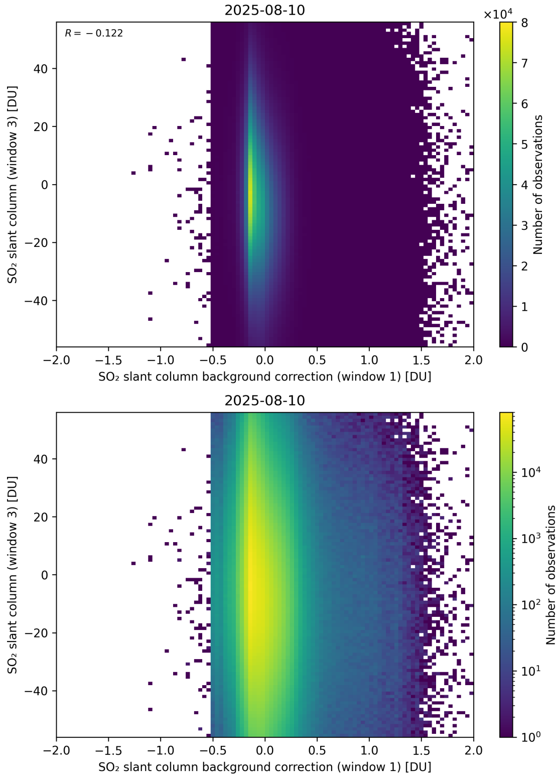
Figure 118: Scatter density plot of “SO 2 slant column background correction (window 1)” against “SO 2 slant column (window 3)” for 2025-08-09 to 2025-08-11.
