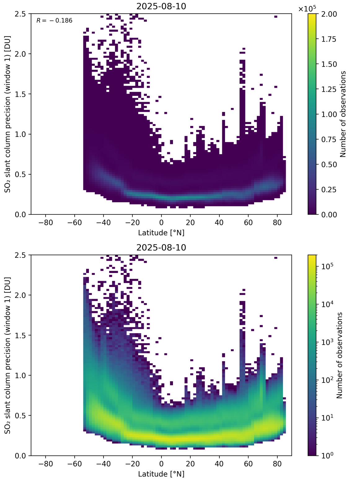
Figure 163: Scatter density plot of “Latitude” against “SO 2 slant column precision (window 1)” for 2025-08-09 to 2025-08-11.
