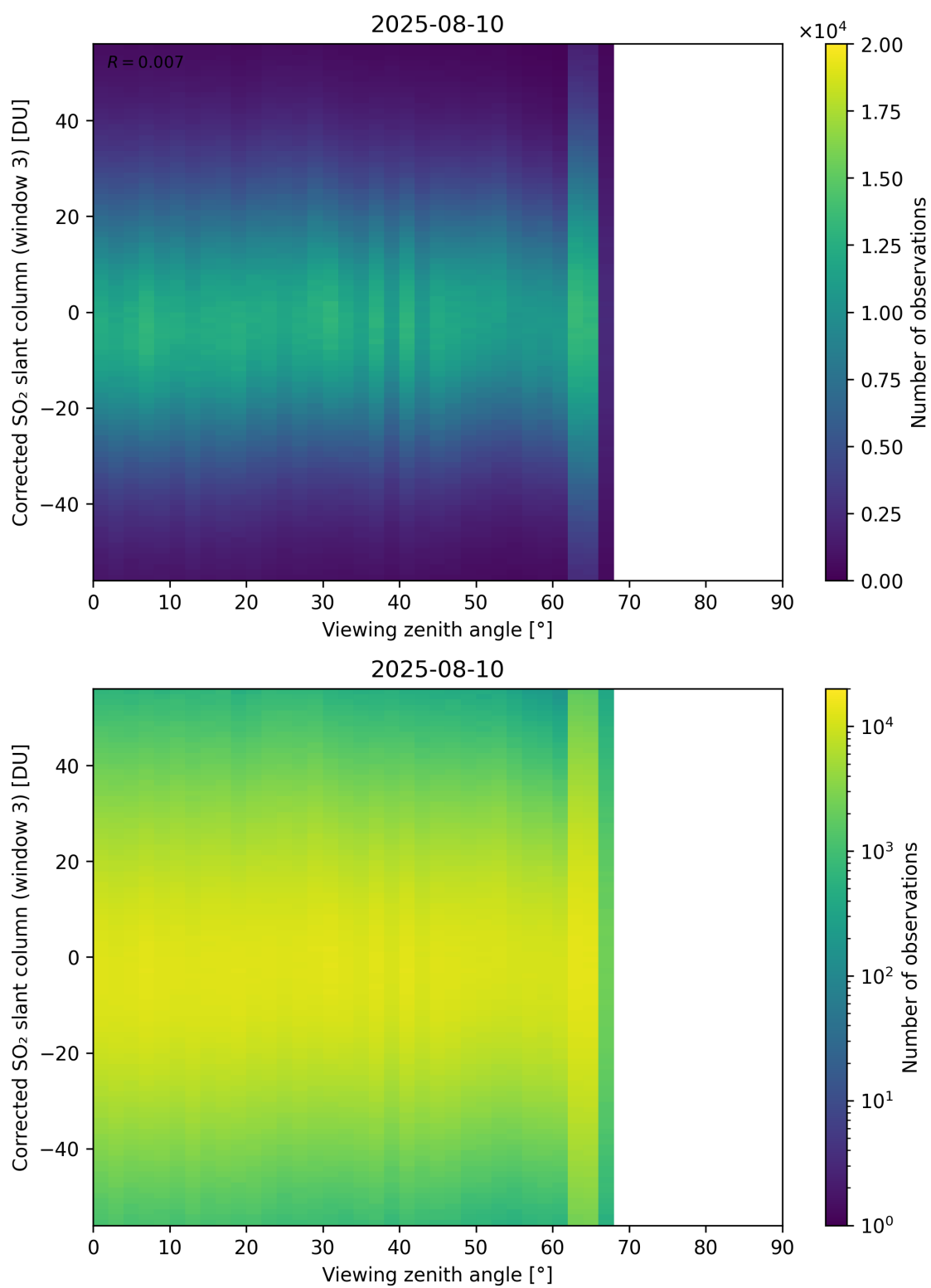
Figure 375: Scatter density plot of “Viewing zenith angle” against “Corrected SO 2 slant column (window 3)” for 2025-08-09 to 2025-08-11.
