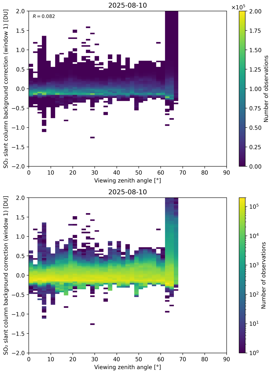
Figure 362: Scatter density plot of “Viewing zenith angle” against “SO 2 slant column background correction (window 1)” for 2025-08-09 to 2025-08-11.
