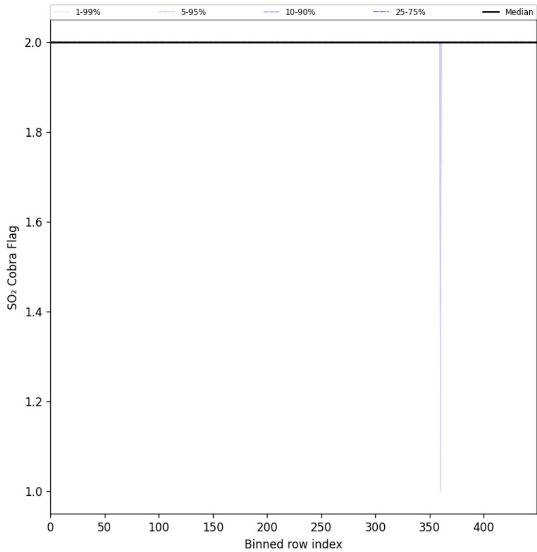
Figure 101: Along track statistics of “SO 2 Cobra Flag” for 2025-08-09 to 2025-08-11
