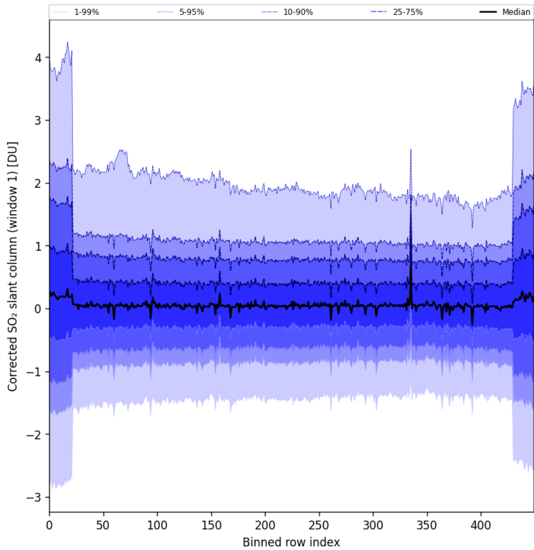
Figure 91: Along track statistics of “Corrected SO 2 slant column (window 1)” for 2025-08-09 to 2025-08-11
