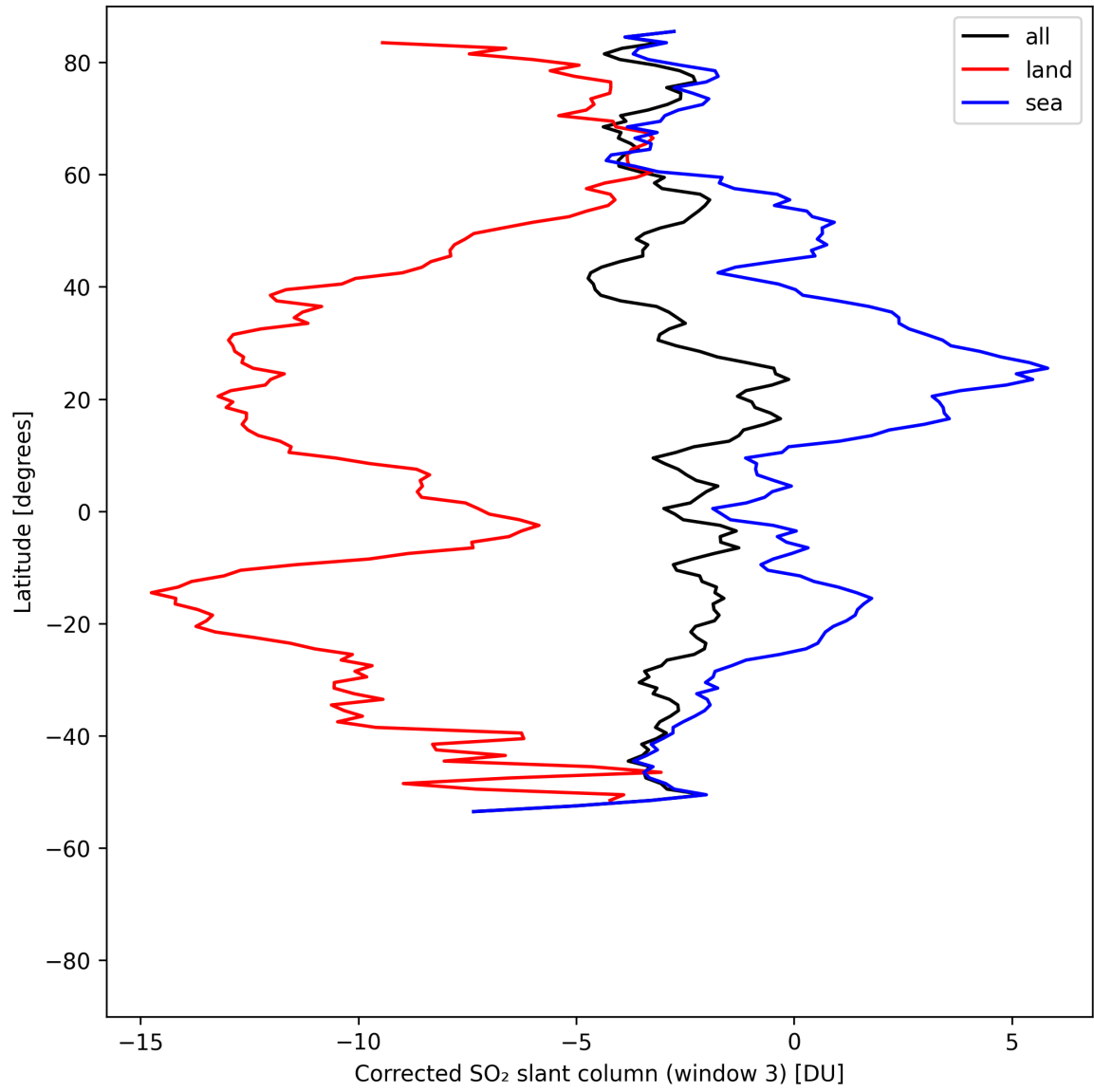
Figure 47: Zonal average of “Corrected SO 2 slant column (window 3)” for 2025-08-09 to 2025-08-11.
