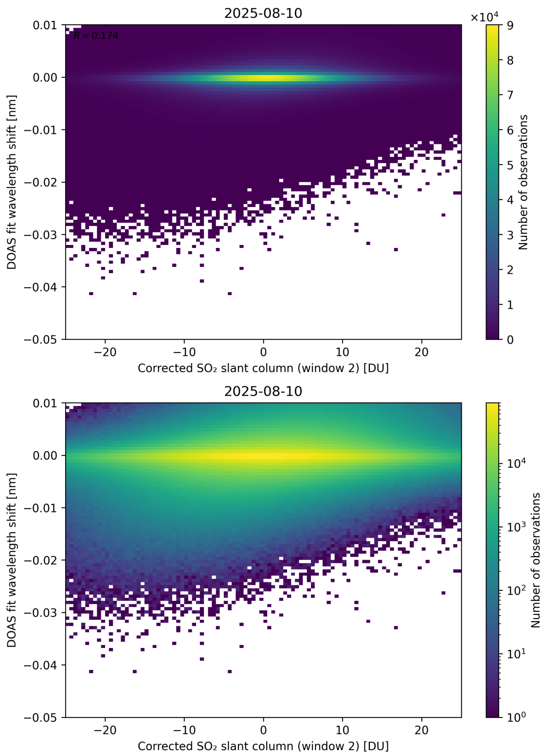
Figure 246: Scatter density plot of “Corrected SO 2 slant column (window 2)” against “DOAS fit wavelength shift” for 2025-08-09 to 2025-08-11.
