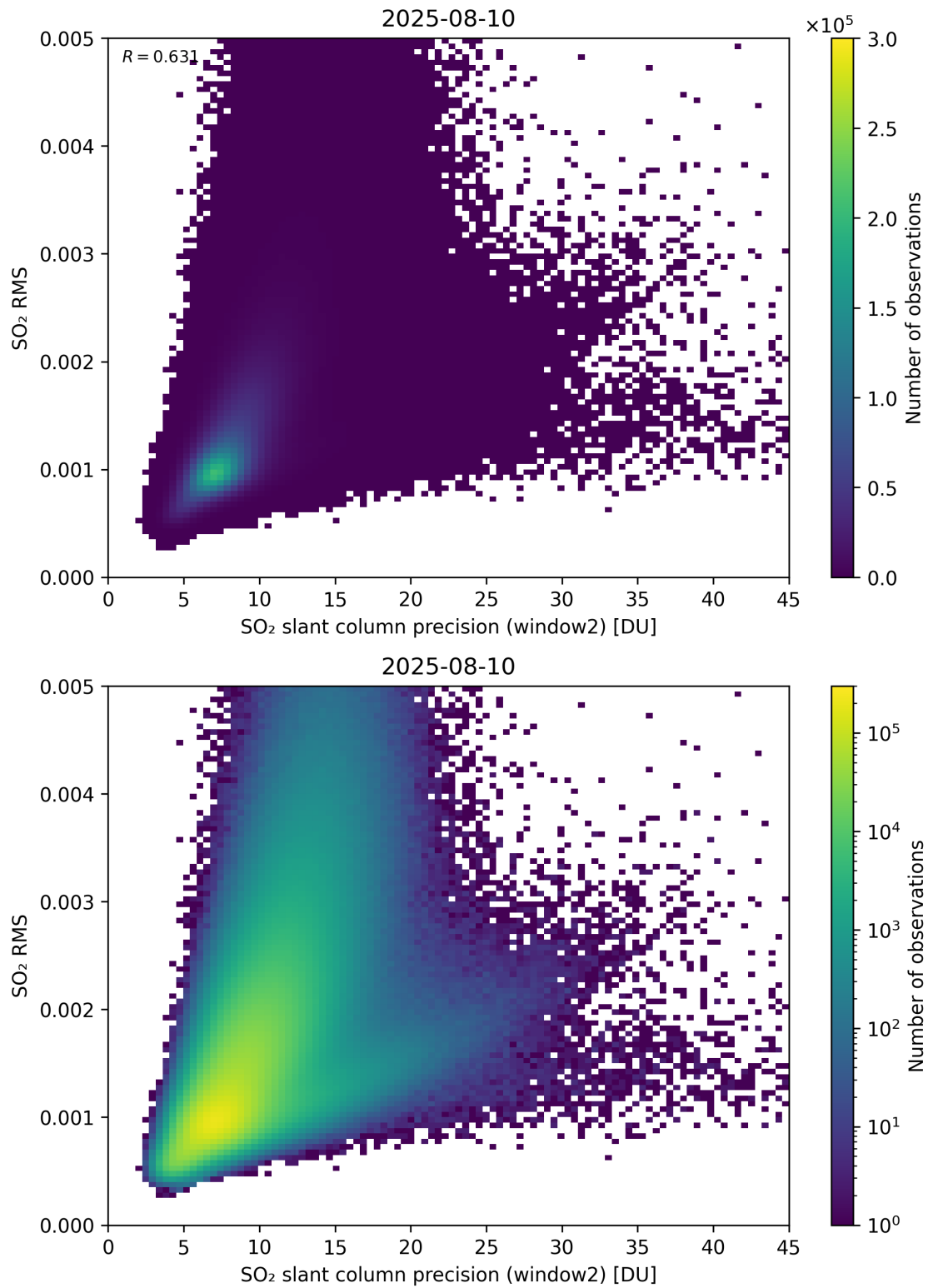
Figure 295: Scatter density plot of “SO 2 slant column precision (window2)” against “SO 2 RMS” for 2025-08-09 to 2025-08-11.
