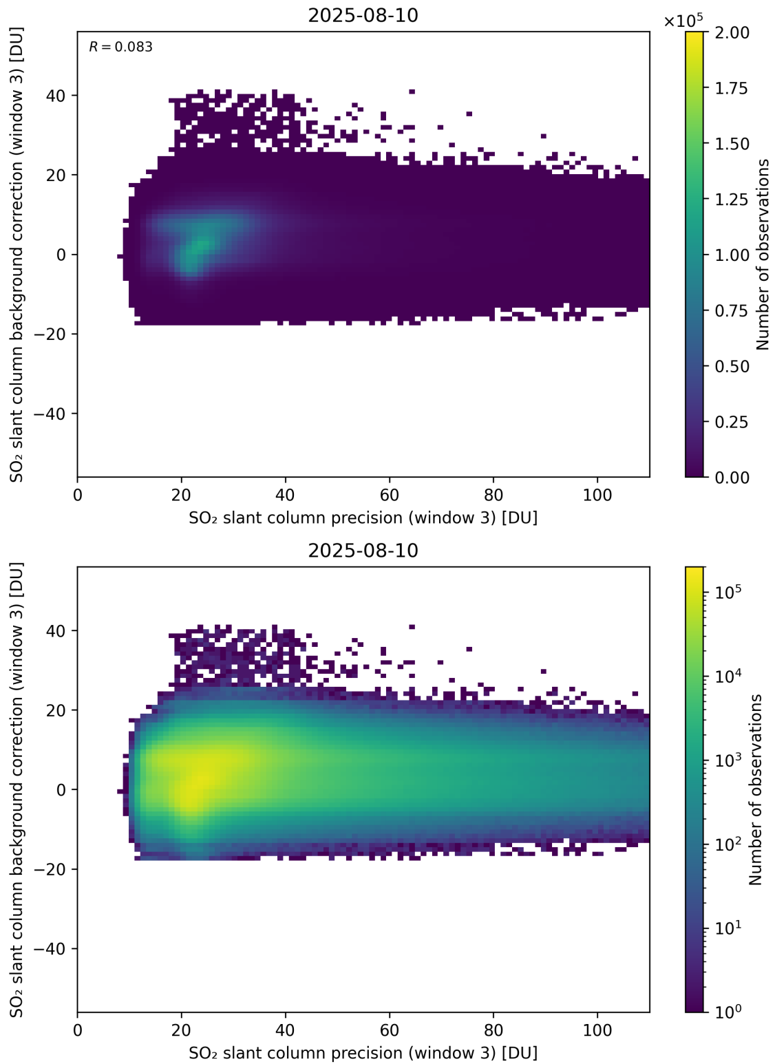
Figure 307: Scatter density plot of “SO 2 slant column precision (window 3)” against “SO 2 slant column background correction (window 3)” for 2025-08-09 to 2025-08-11.
