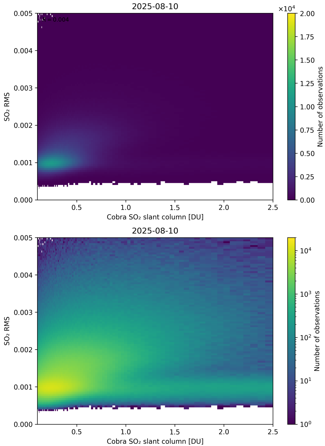
Figure 198: Scatter density plot of “Cobra SO 2 slant column” against “SO 2 RMS” for 2025-08-09 to 2025-08-11.
