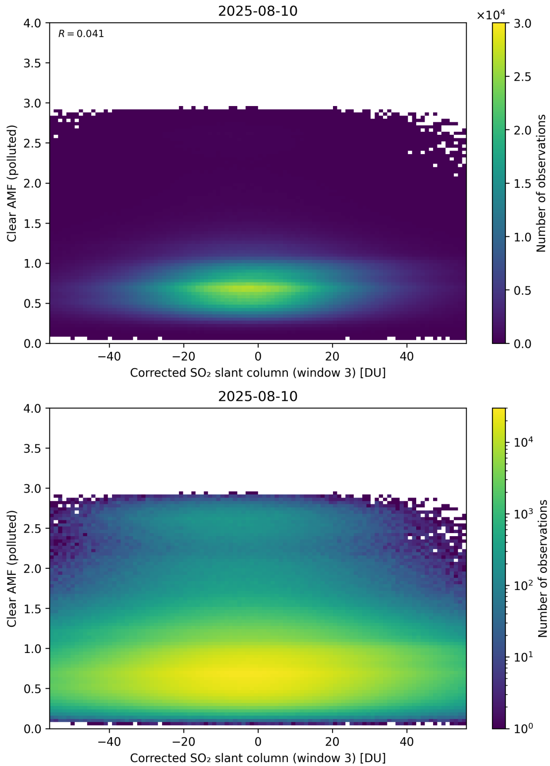
Figure 259: Scatter density plot of “Corrected SO 2 slant column (window 3)” against “Clear AMF (polluted)” for 2025-08-09 to 2025-08-11.
