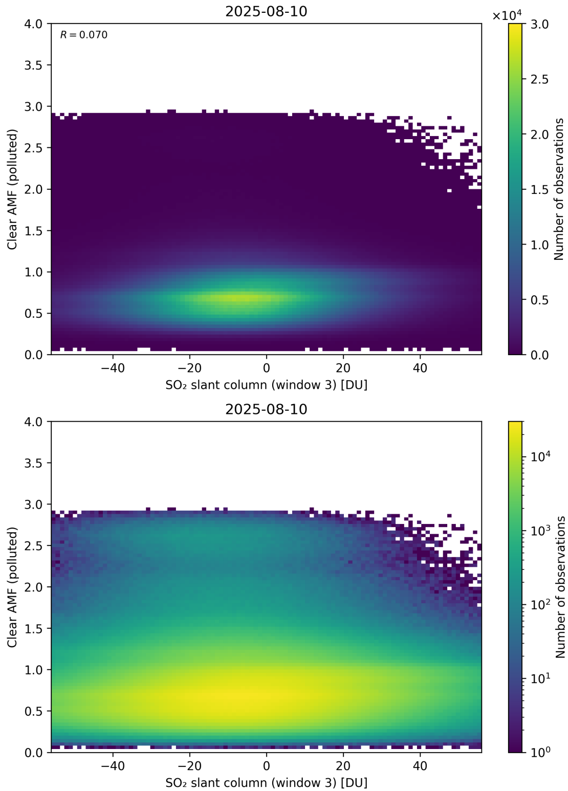
Figure 315: Scatter density plot of “SO 2 slant column (window 3)” against “Clear AMF (polluted)” for 2025-08-09 to 2025-08-11.
