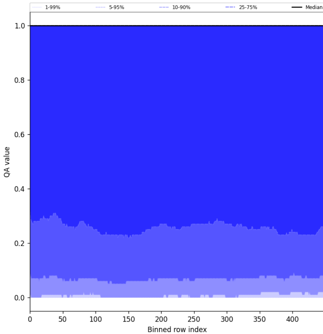
Figure 83: Along track statistics of “QA value” for 2025-08-09 to 2025-08-11
