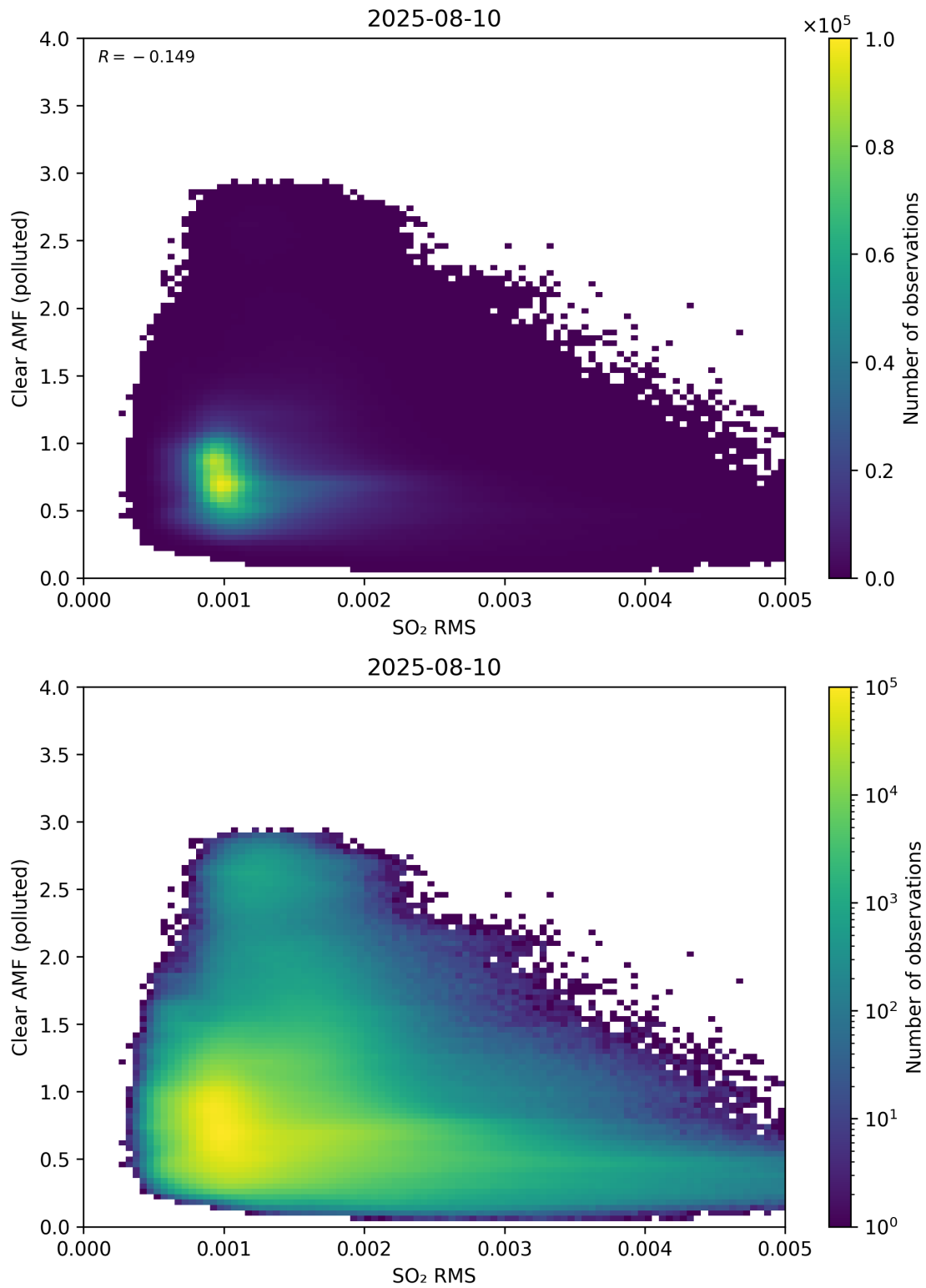
Figure 147: Scatter density plot of “SO 2 RMS” against “Clear AMF (polluted)” for 2025-08-09 to 2025-08-11.
