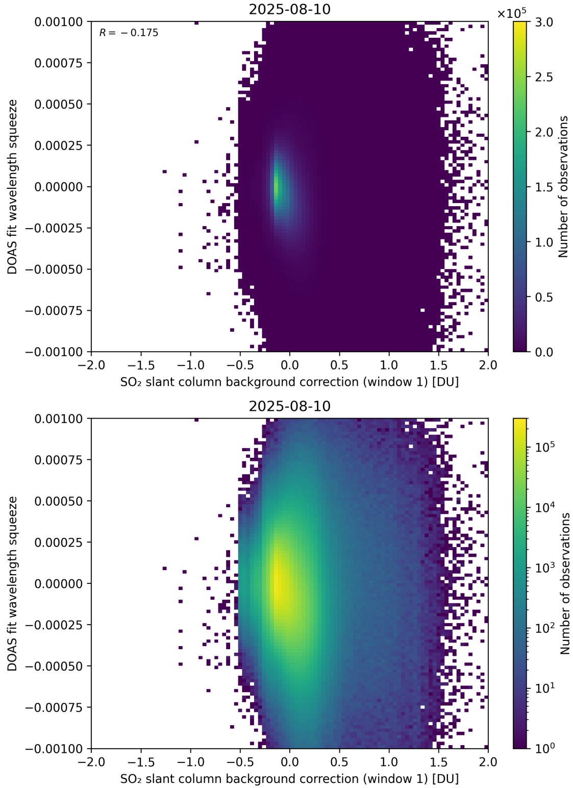
Figure 112: Scatter density plot of “SO 2 slant column background correction (window 1)” against “DOAS fit wavelength squeeze” for 2025-08-09 to 2025-08-11.
