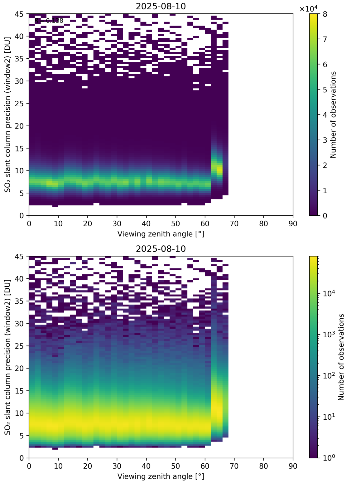
Figure 378: Scatter density plot of “Viewing zenith angle” against “SO 2 slant column precision (window2)” for 2025-08-09 to 2025-08-11.
