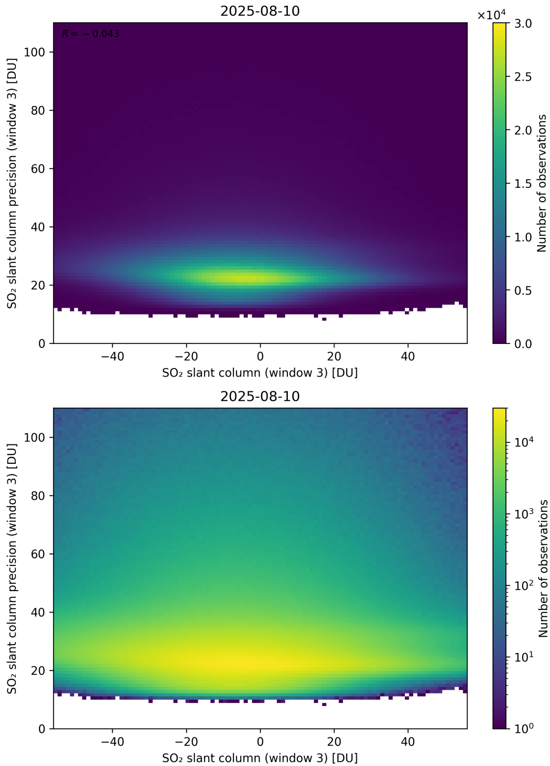
Figure 317: Scatter density plot of “SO 2 slant column (window 3)” against “SO 2 slant column precision (window 3)” for 2025-08-09 to 2025-08-11.
