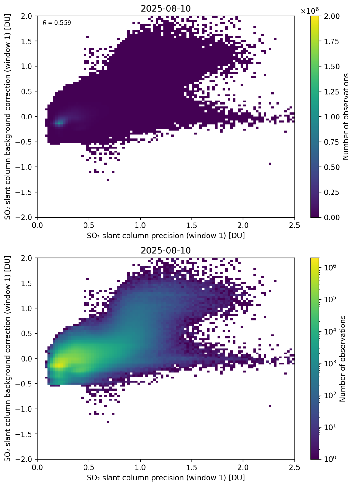
Figure 268: Scatter density plot of “SO 2 slant column precision (window 1)” against “SO 2 slant column background correction (window 1)” for 2025-08-09 to 2025-08-11.
