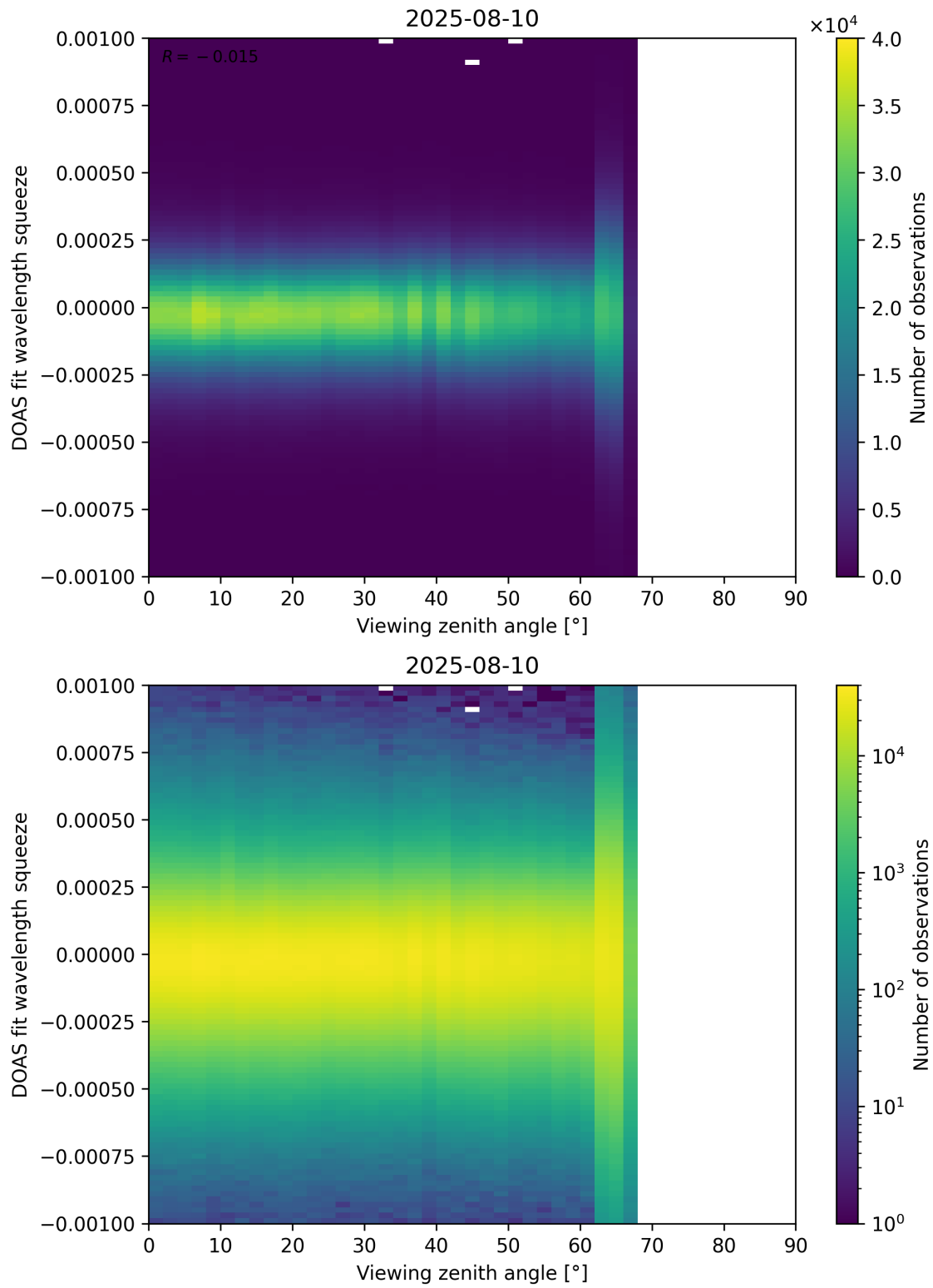
Figure 366: Scatter density plot of “Viewing zenith angle” against “DOAS fit wavelength squeeze” for 2025-08-09 to 2025-08-11.
