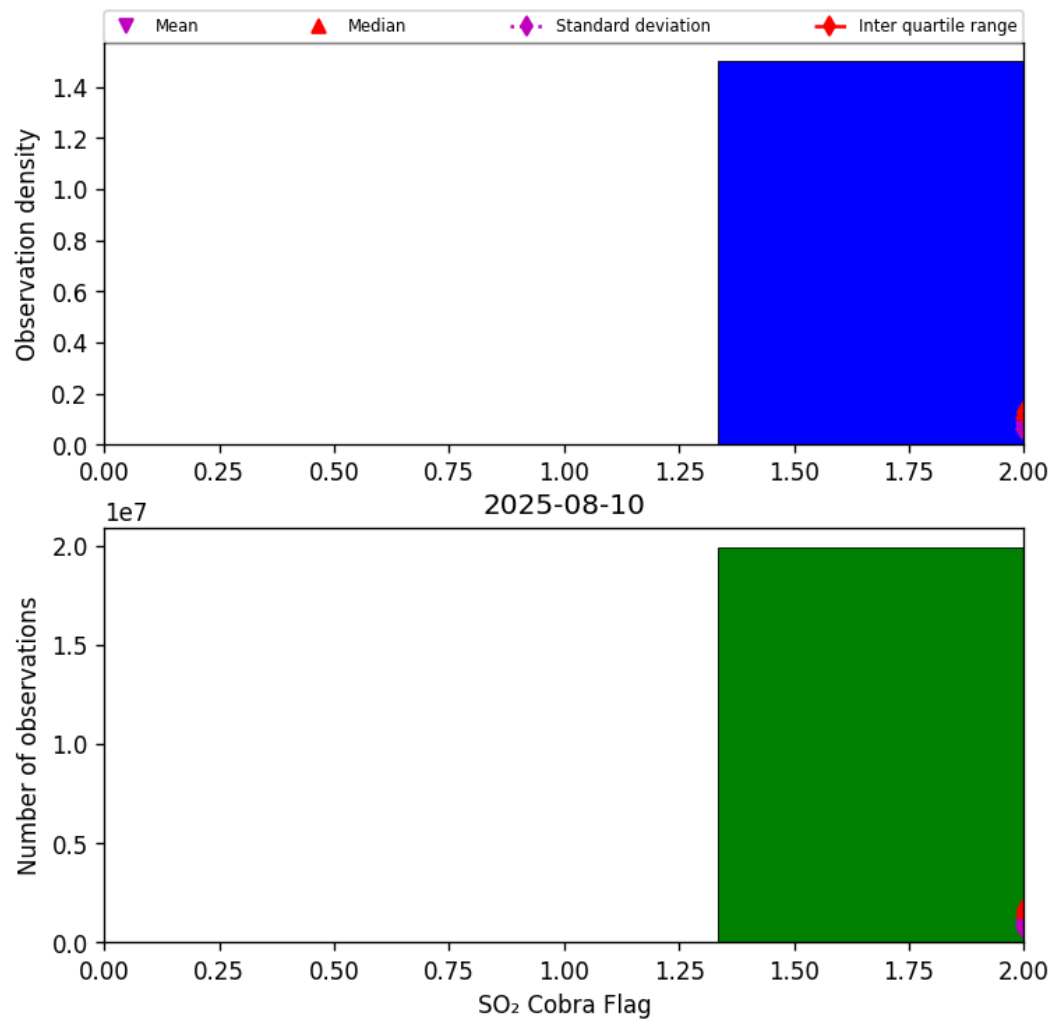
Figure 75: Histogram of “SO 2 Cobra Flag” for 2025-08-09 to 2025-08-11
