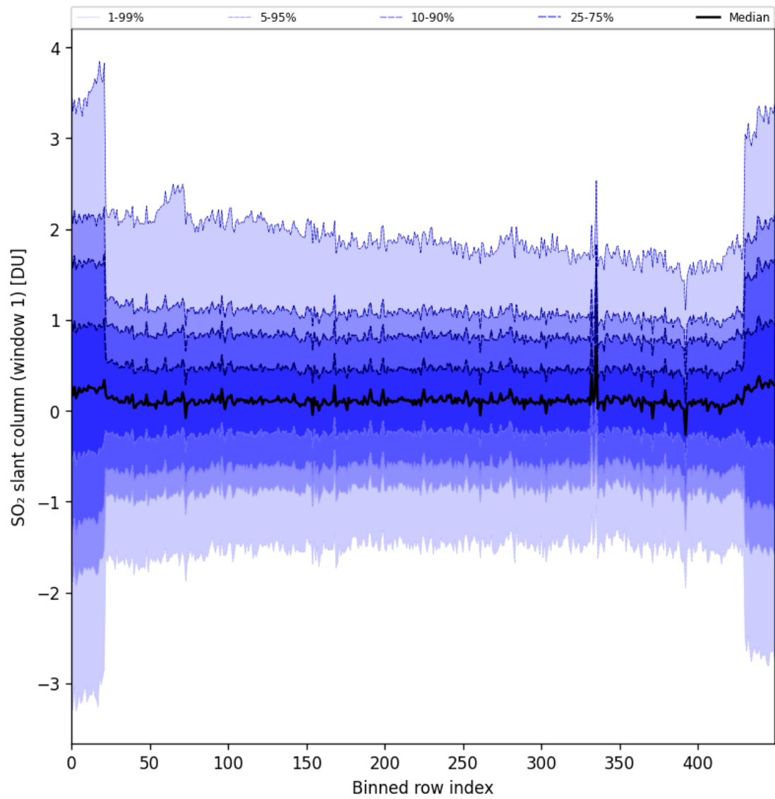
Figure 89: Along track statistics of “SO 2 slant column (window 1)” for 2025-08-09 to 2025-08-11
