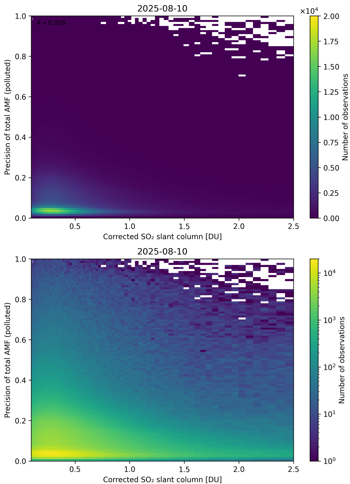
Figure 243: Scatter density plot of “Corrected SO 2 slant column” against “Precision of total AMF (polluted)” for 2025-08-09 to 2025-08-11.
