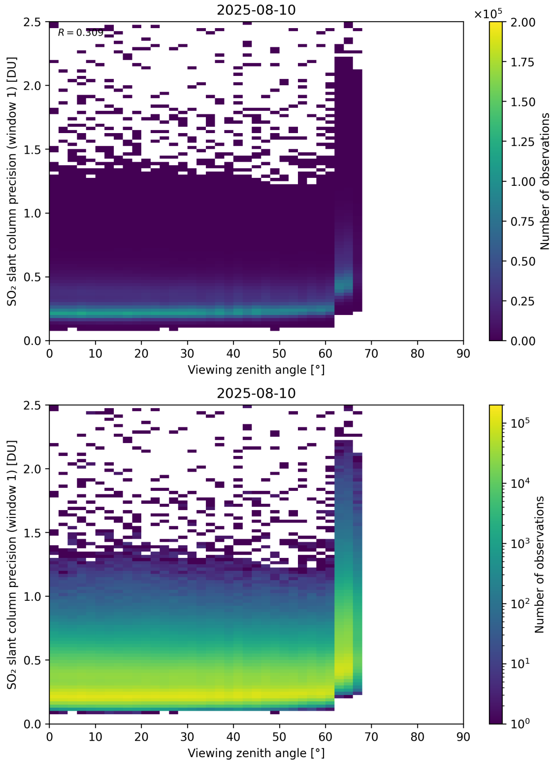
Figure 377: Scatter density plot of “Viewing zenith angle” against “SO 2 slant column precision (window 1)” for 2025-08-09 to 2025-08-11.
