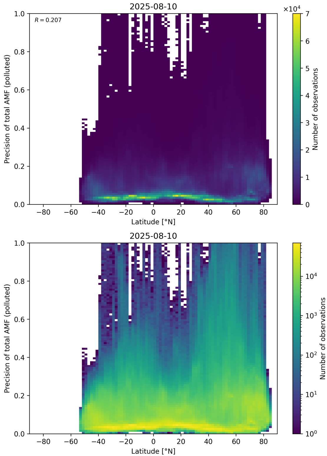
Figure 168: Scatter density plot of “Latitude” against “Precision of total AMF (polluted)” for 2025-08-09 to 2025-08-11.
