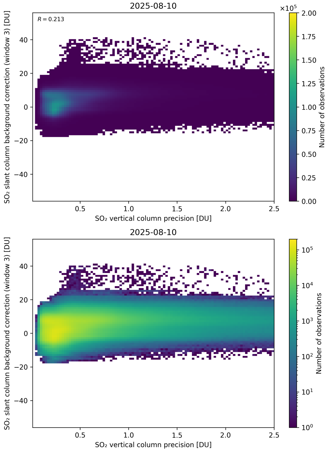
Figure 331: Scatter density plot of “SO 2 vertical column precision” against “SO 2 slant column background correction (window 3)” for 2025-08-09 to 2025-08-11.
