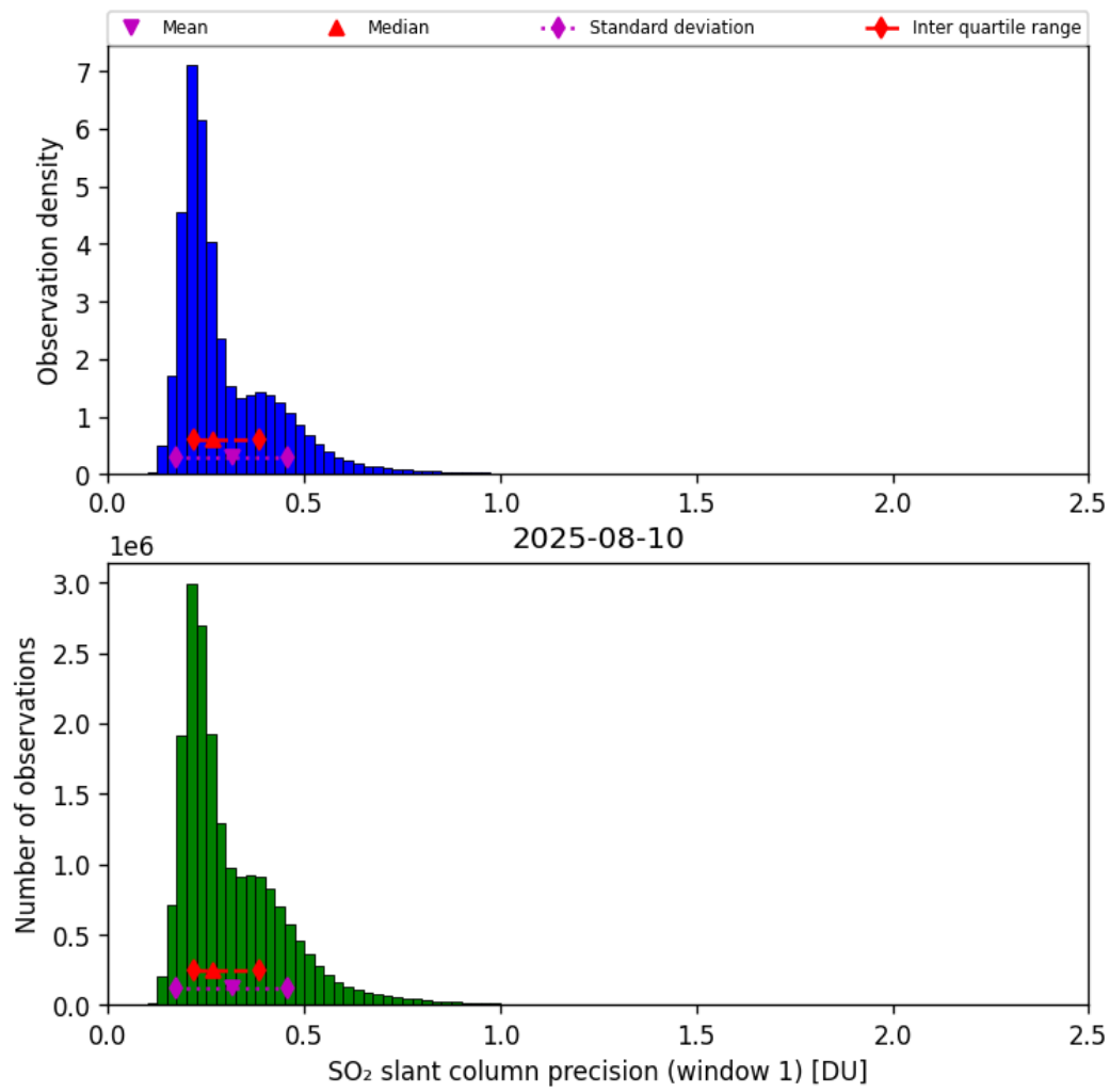
Figure 64: Histogram of “SO 2 slant column precision (window 1)” for 2025-08-09 to 2025-08-11
