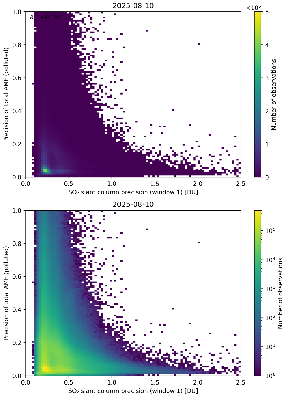
Figure 281: Scatter density plot of “SO 2 slant column precision (window 1)” against “Precision of total AMF (polluted)” for 2025-08-09 to 2025-08-11.
