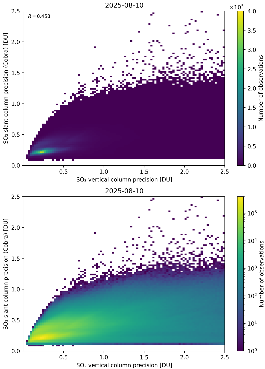
Figure 337: Scatter density plot of “SO 2 vertical column precision” against “SO 2 slant column precision (Cobra)” for 2025-08-09 to 2025-08-11.
