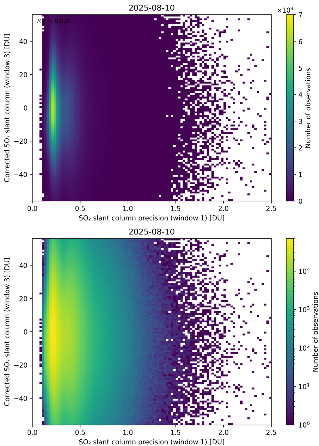
Figure 276: Scatter density plot of “SO 2 slant column precision (window 1)” against “Corrected SO 2 slant column (window 3)” for 2025-08-09 to 2025-08-11.
