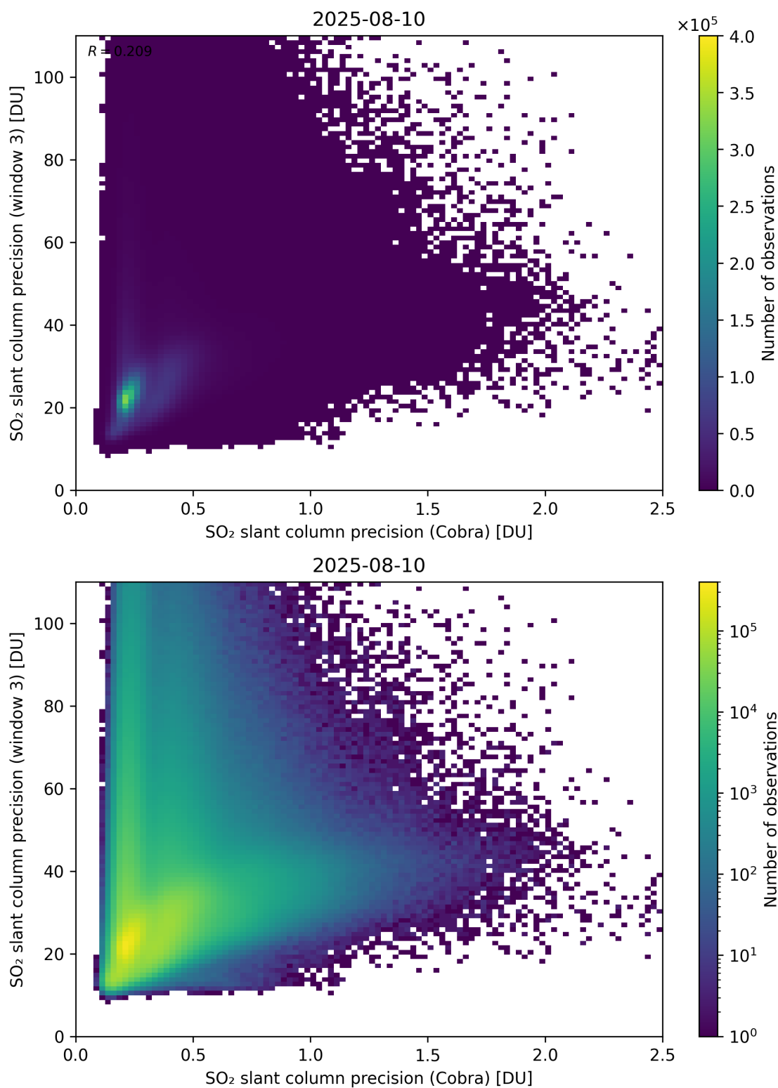
Figure 212: Scatter density plot of “SO 2 slant column precision (Cobra)” against “SO 2 slant column precision (window 3)” for 2025-08-09 to 2025-08-11.
