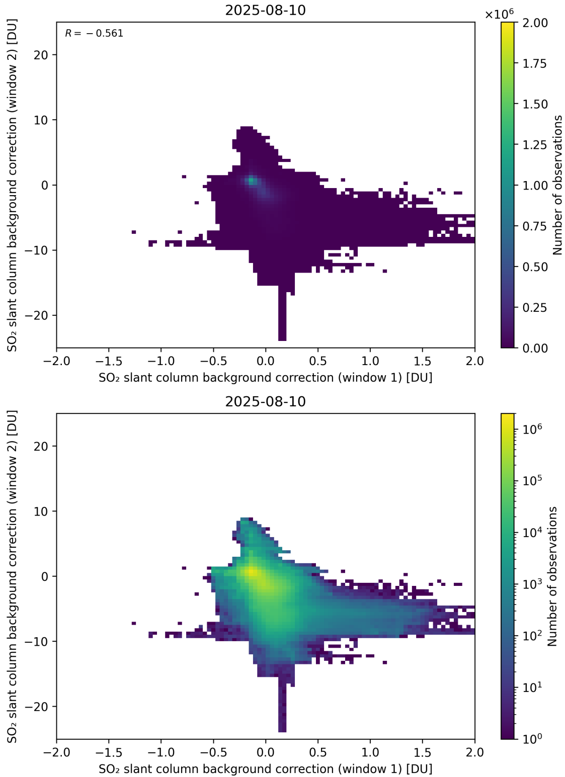
Figure 109: Scatter density plot of “SO 2 slant column background correction (window 1)” against “SO 2 slant column background correction (window 2)” for 2025-08-09 to 2025-08-11.
