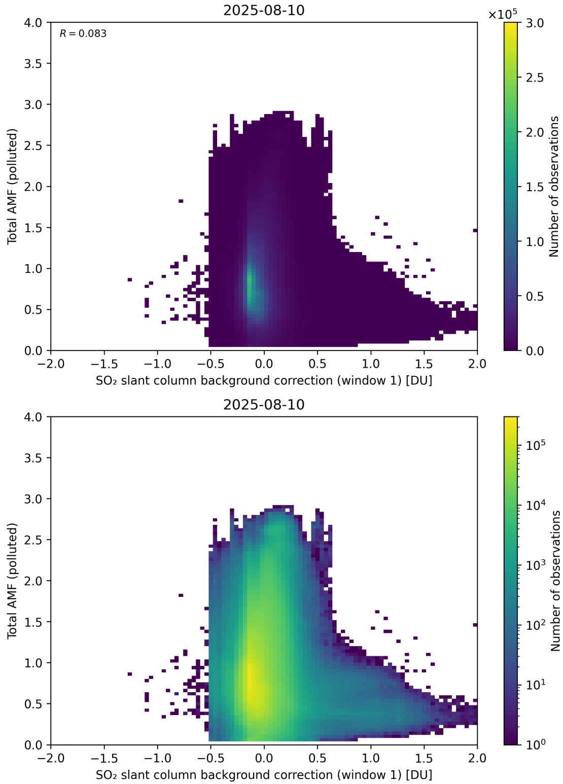
Figure 120: Scatter density plot of “SO 2 slant column background correction (window 1)” against “Total AMF (polluted)” for 2025-08-09 to 2025-08-11.
