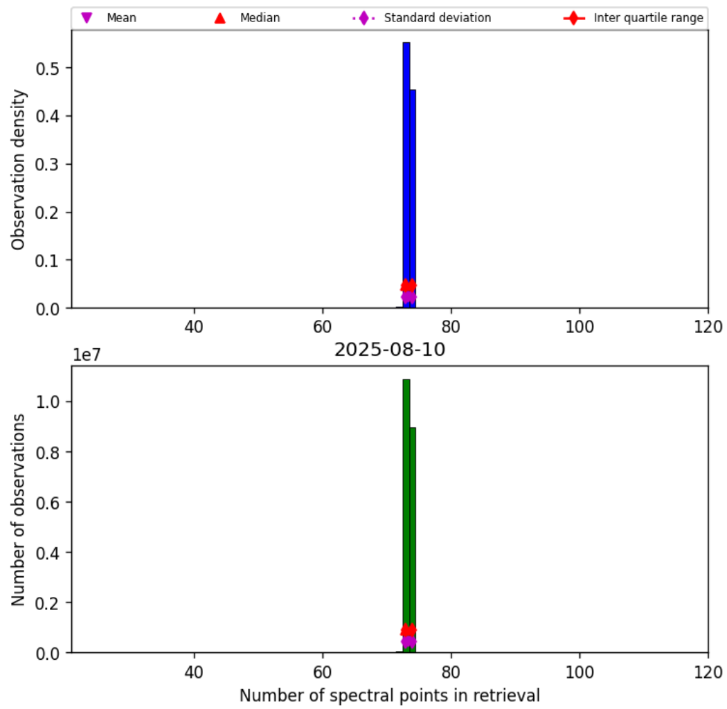
Figure 82: Histogram of “Number of spectral points in retrieval” for 2025-08-09 to 2025-08-11
