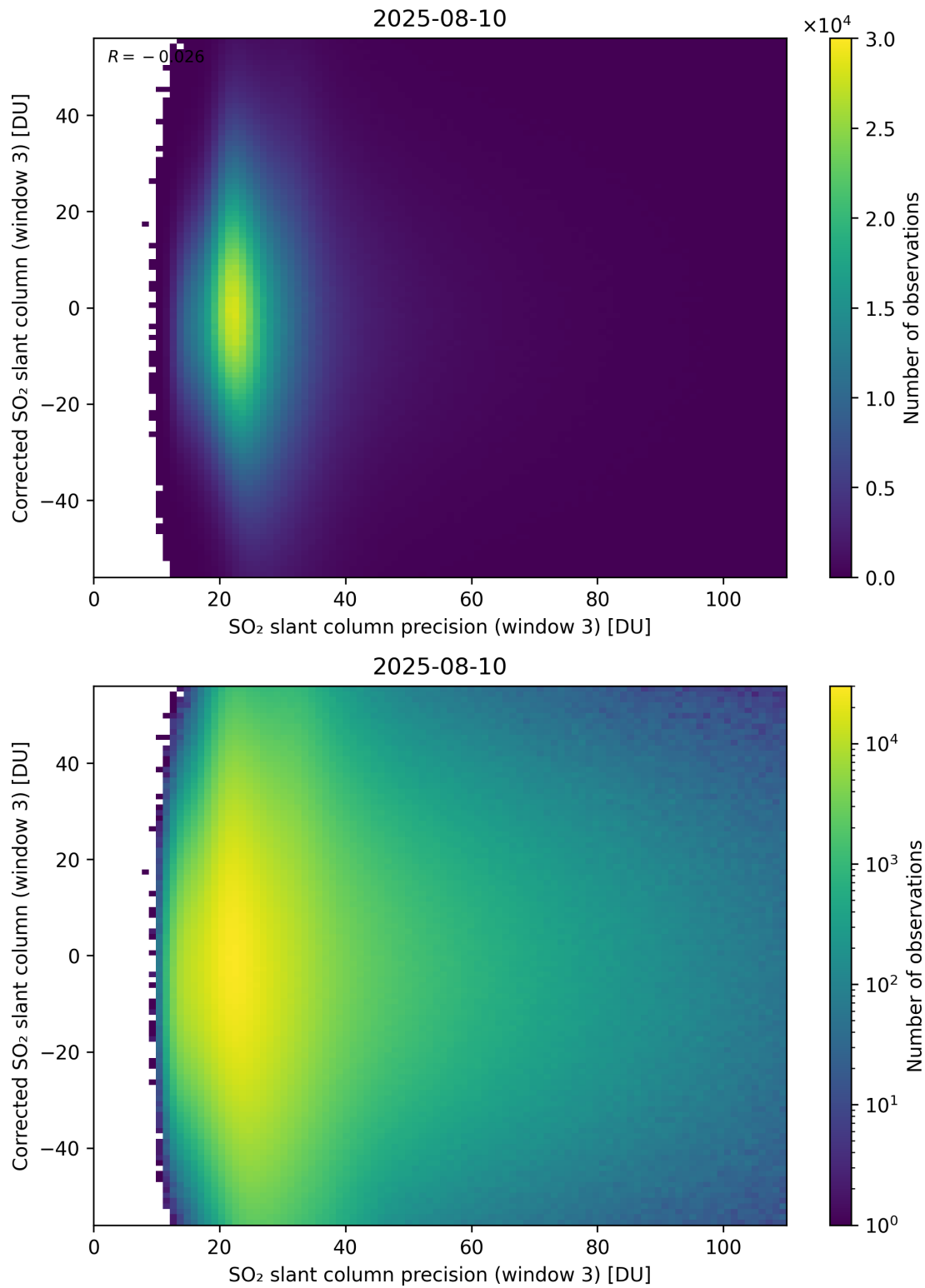
Figure 312: Scatter density plot of “SO 2 slant column precision (window 3)” against “Corrected SO 2 slant column (window 3)” for 2025-08-09 to 2025-08-11.
