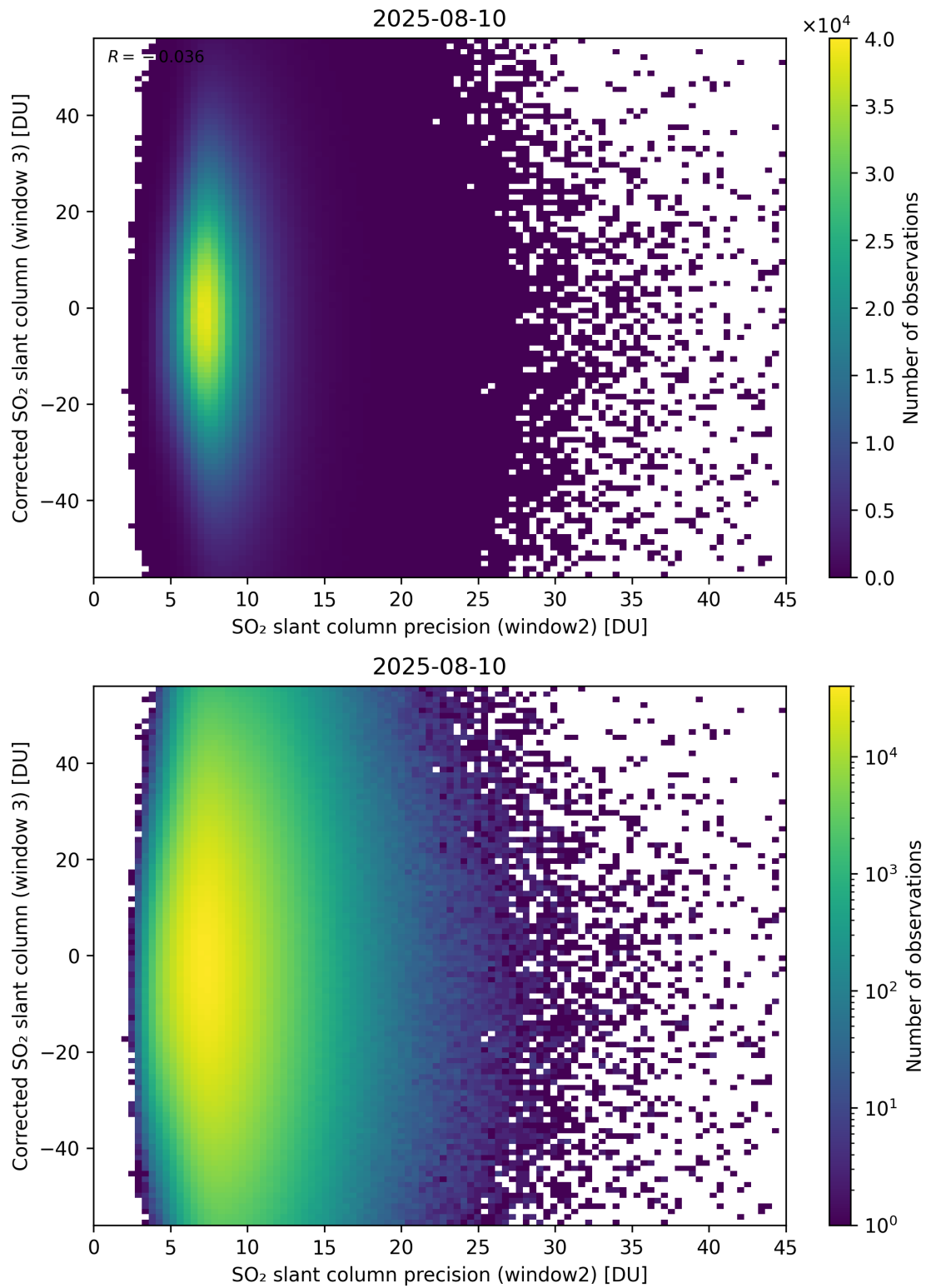
Figure 298: Scatter density plot of “SO 2 slant column precision (window2)” against “Corrected SO 2 slant column (window 3)” for 2025-08-09 to 2025-08-11.
