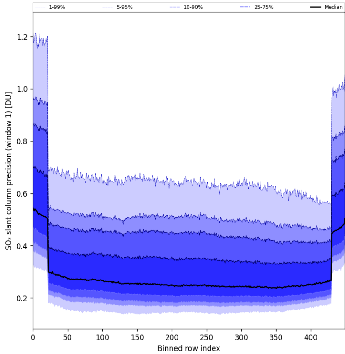
Figure 90: Along track statistics of “SO 2 slant column precision (window 1)” for 2025-08-09 to 2025-08-11
