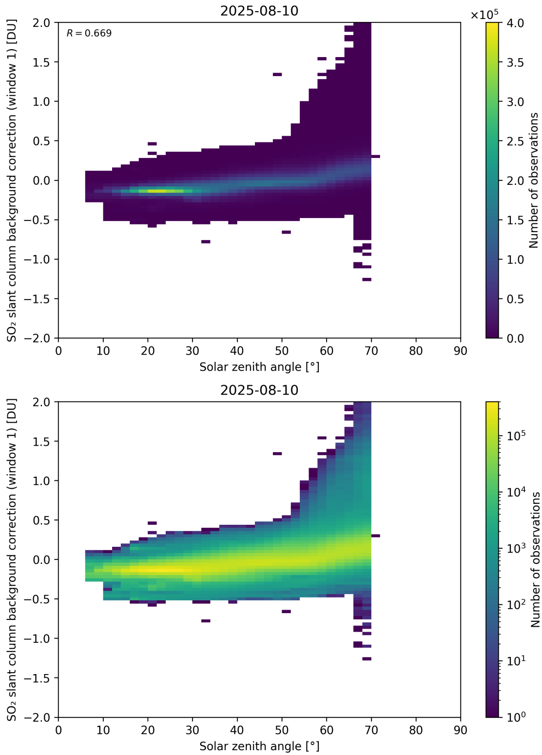
Figure 171: Scatter density plot of “Solar zenith angle” against “SO 2 slant column background correction (window 1)” for 2025-08-09 to 2025-08-11.
