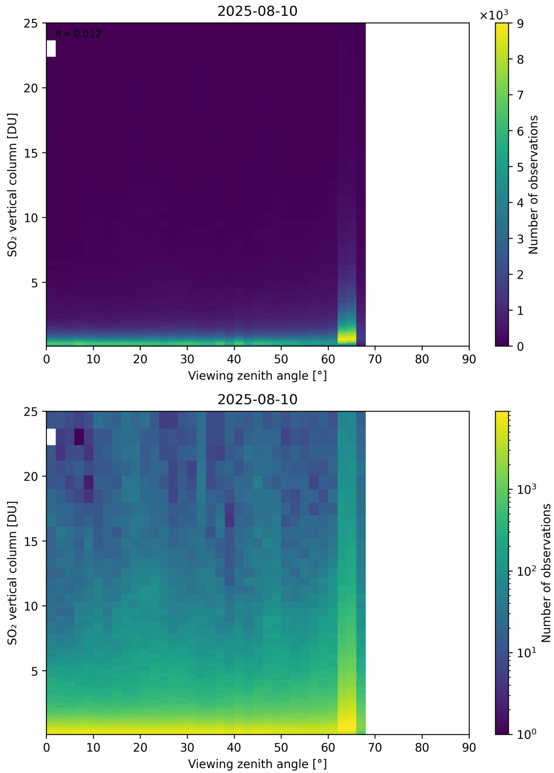
Figure 383: Scatter density plot of “Viewing zenith angle” against “SO 2 vertical column” for 2025-08-09 to 2025-08-11.
