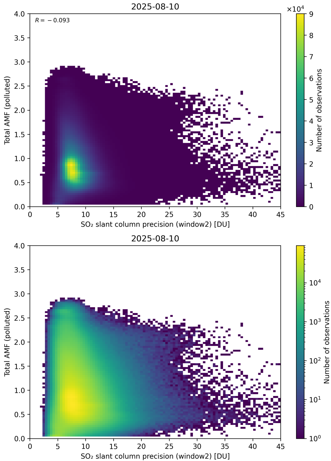
Figure 301: Scatter density plot of “SO 2 slant column precision (window2)” against “Total AMF (polluted)” for 2025-08-09 to 2025-08-11.
