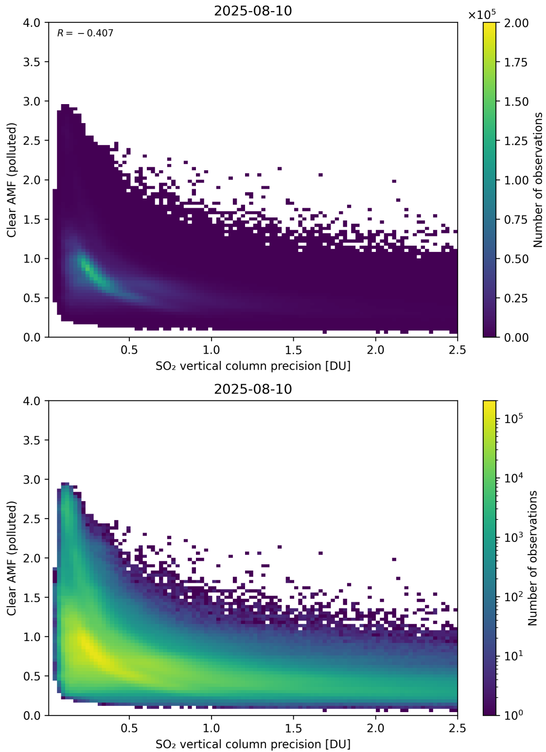
Figure 335: Scatter density plot of “SO 2 vertical column precision” against “Clear AMF (polluted)” for 2025-08-09 to 2025-08-11.
