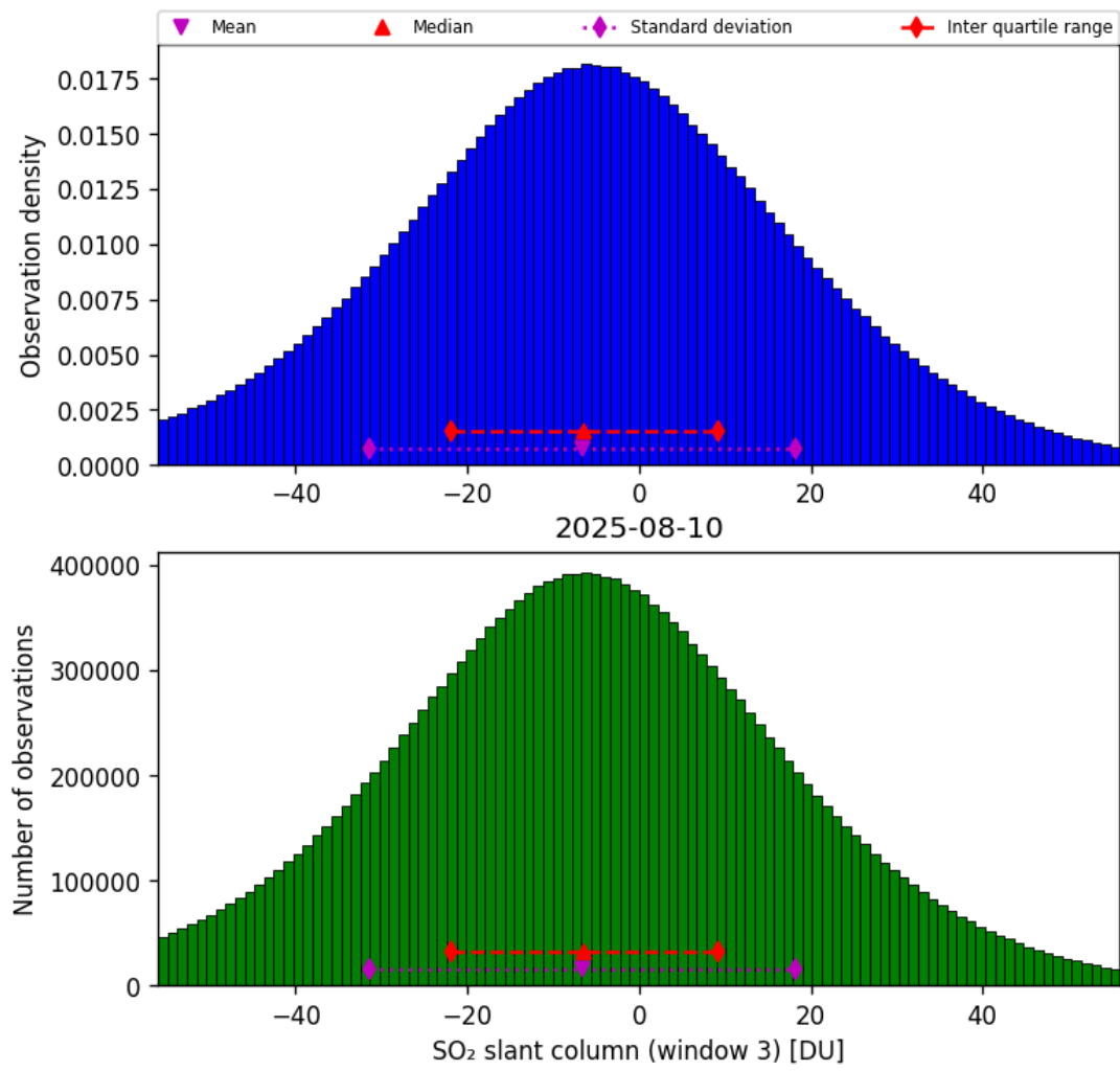
Figure 71: Histogram of “SO 2 slant column (window 3)” for 2025-08-09 to 2025-08-11
