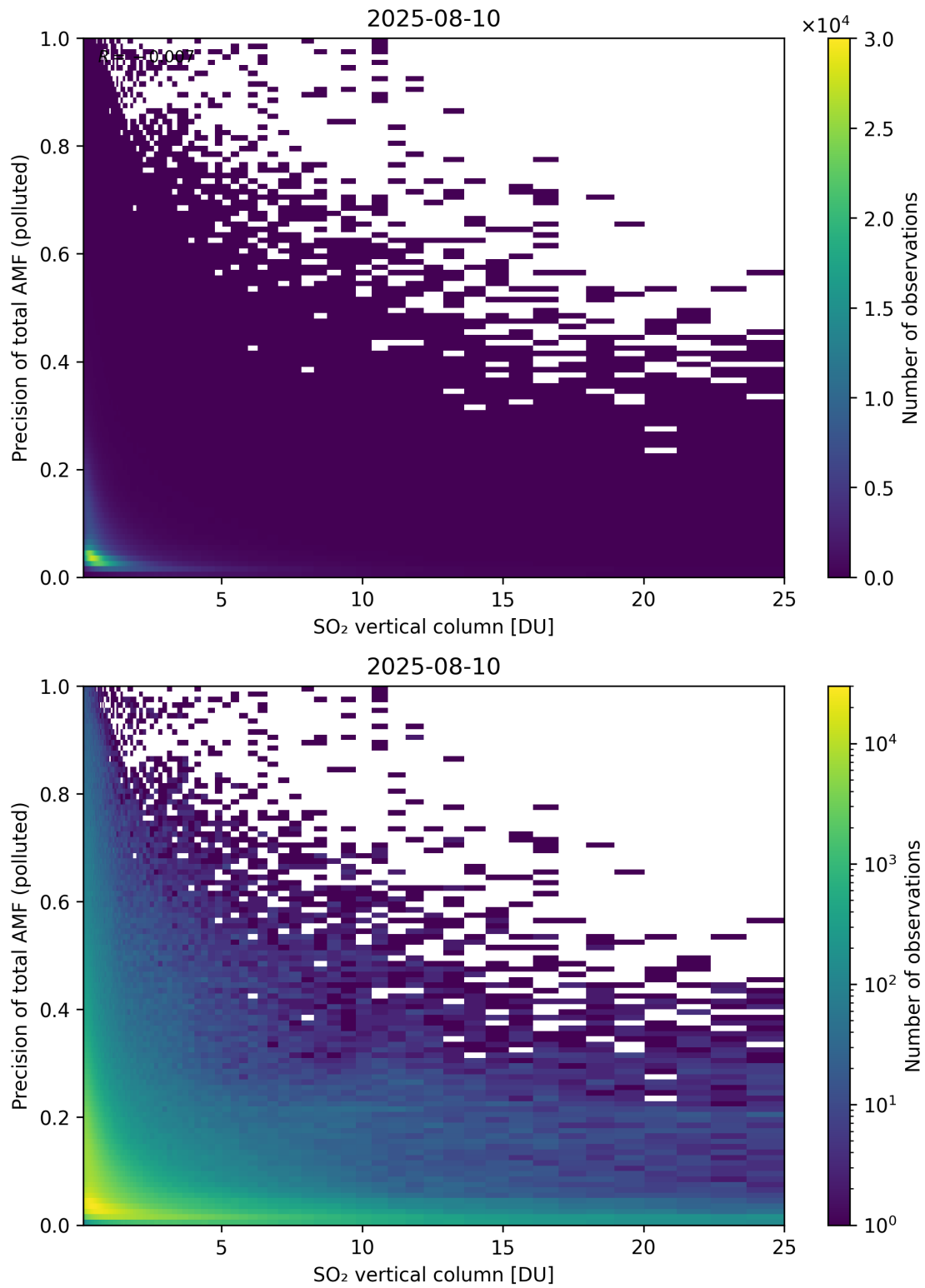
Figure 360: Scatter density plot of “SO 2 vertical column” against “Precision of total AMF (polluted)” for 2025-08-09 to 2025-08-11.
