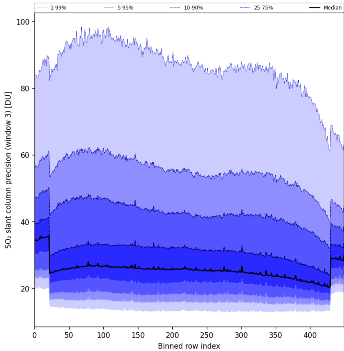
Figure 98: Along track statistics of “SO 2 slant column precision (window 3)” for 2025-08-09 to 2025-08-11
