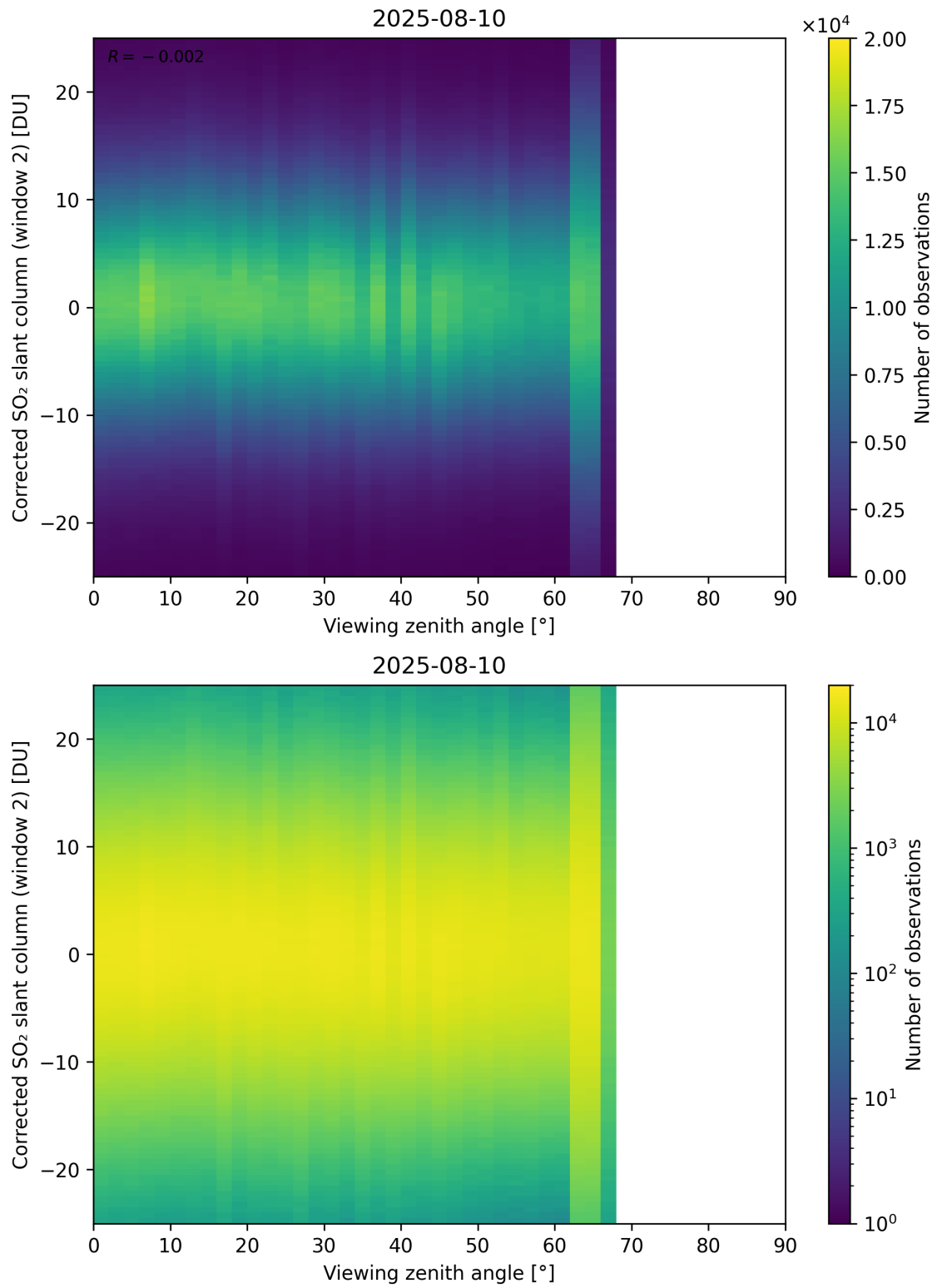
Figure 374: Scatter density plot of “Viewing zenith angle” against “Corrected SO 2 slant column (window 2)” for 2025-08-09 to 2025-08-11.
