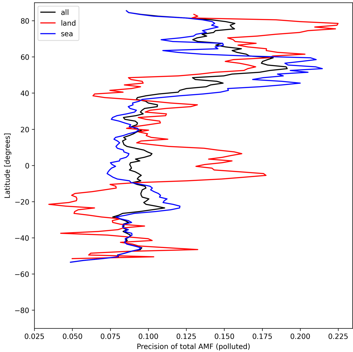
Figure 54: Zonal average of “Precision of total AMF (polluted)” for 2025-08-09 to 2025-08-11.
