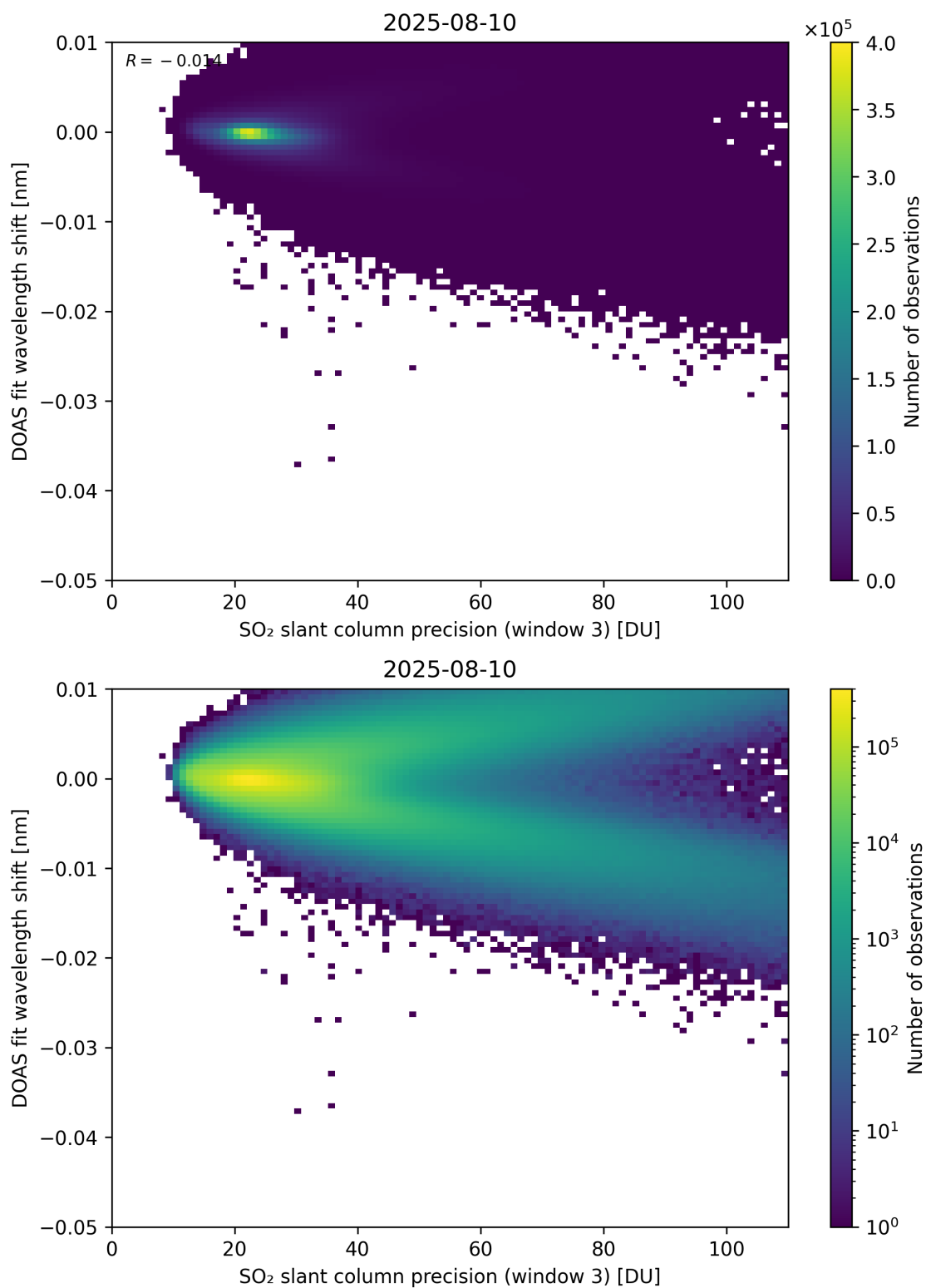
Figure 308: Scatter density plot of “SO 2 slant column precision (window 3)” against “DOAS fit wavelength shift” for 2025-08-09 to 2025-08-11.
