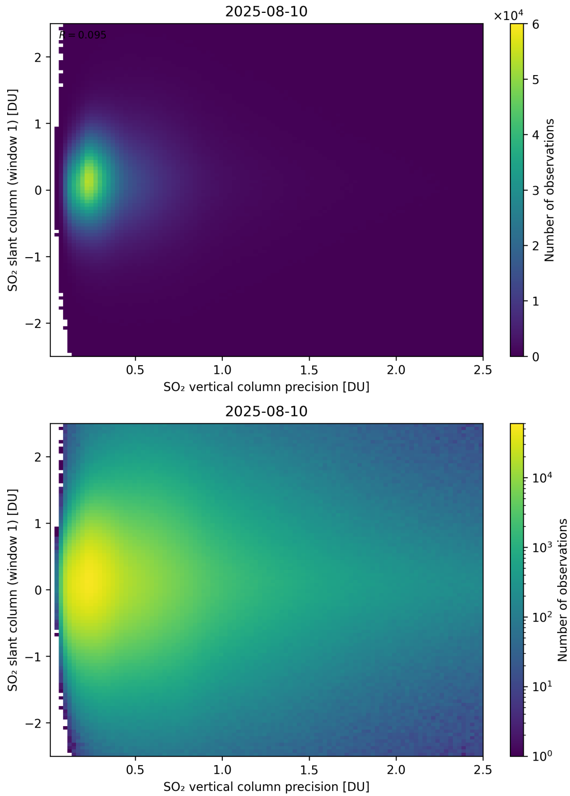
Figure 341: Scatter density plot of “SO 2 vertical column precision” against “SO 2 slant column (window 1)” for 2025-08-09 to 2025-08-11.
