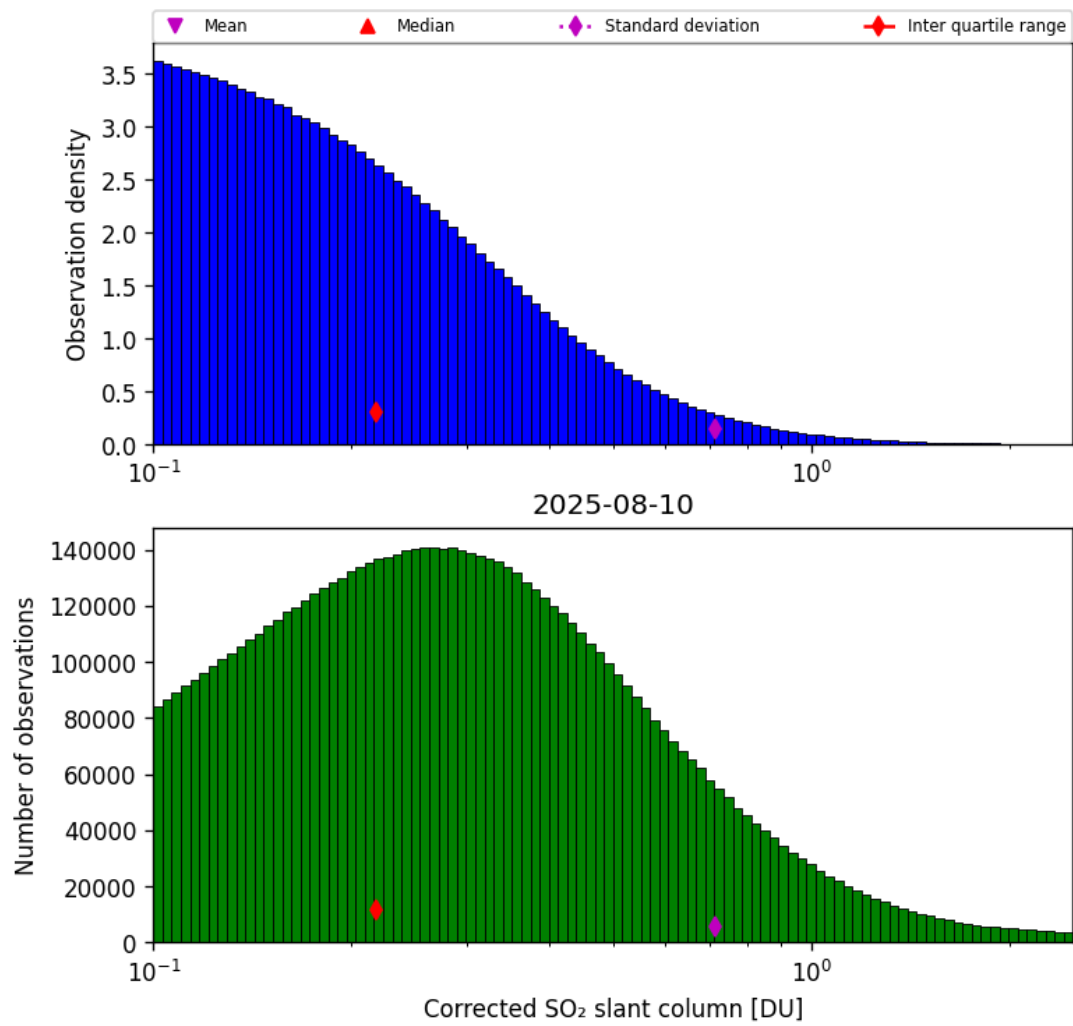
Figure 60: Histogram of “Corrected SO 2 slant column” for 2025-08-09 to 2025-08-11
