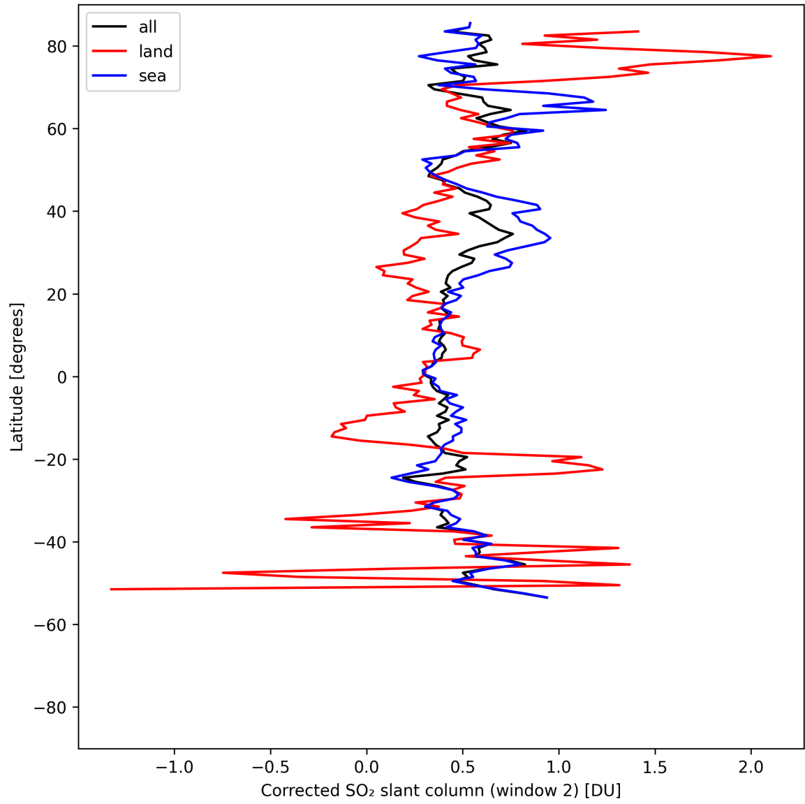
Figure 43: Zonal average of "Corrected SO 2 slant column (window 2)" for 2025-08-09 to 2025-08-11.
