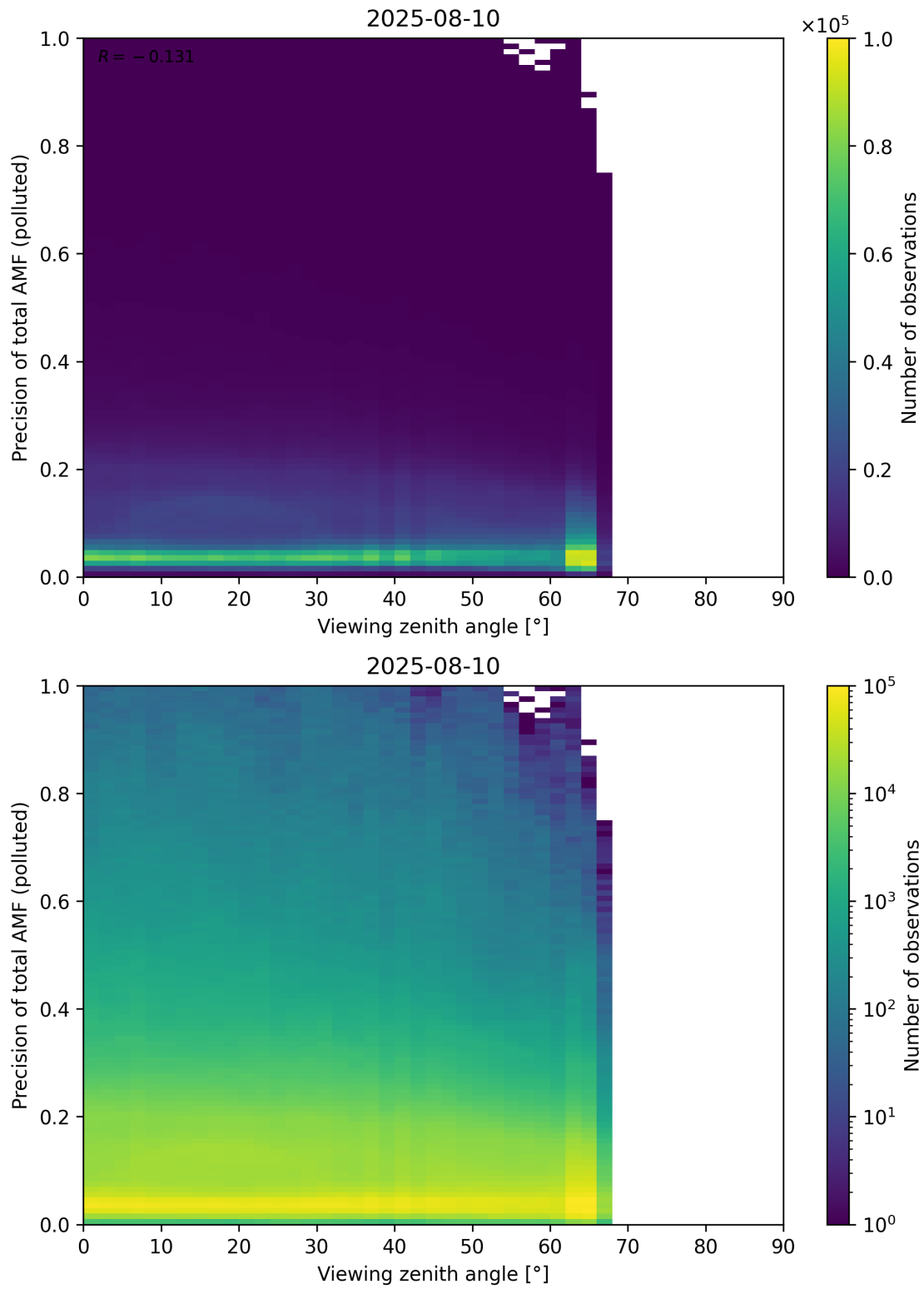
Figure 382: Scatter density plot of “Viewing zenith angle” against “Precision of total AMF (polluted)” for 2025-08-09 to 2025-08-11.
