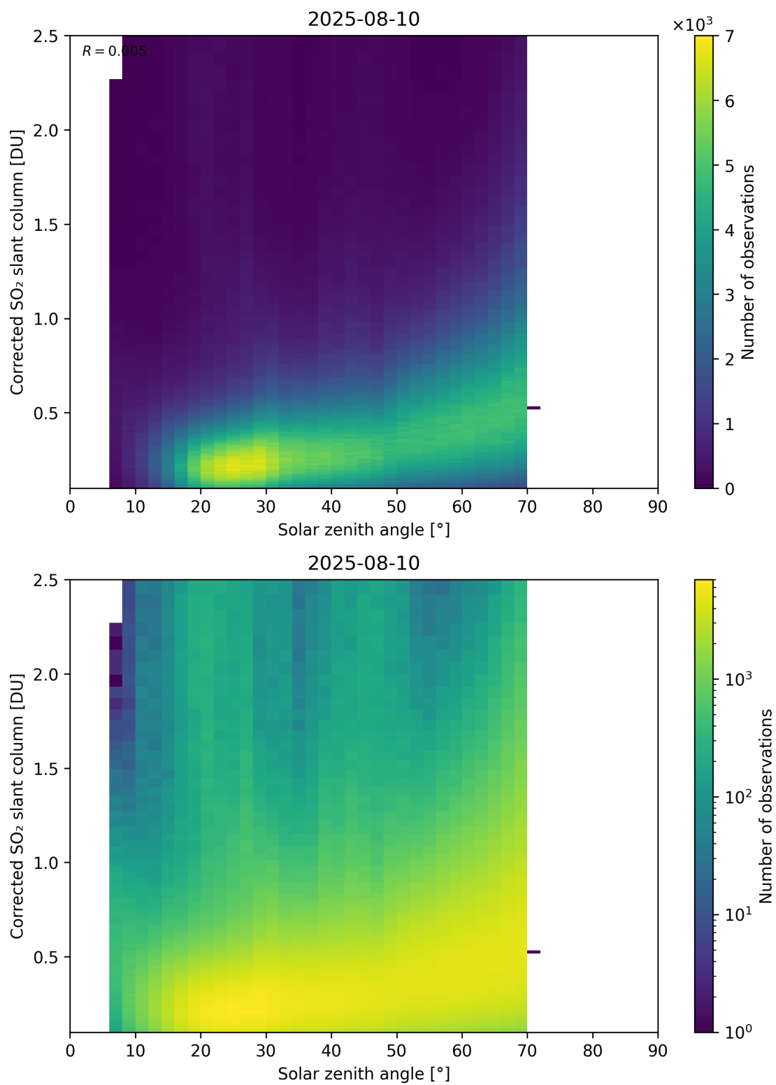
Figure 181: Scatter density plot of “Solar zenith angle” against “Corrected SO 2 slant column” for 2025-08-09 to 2025-08-11.
