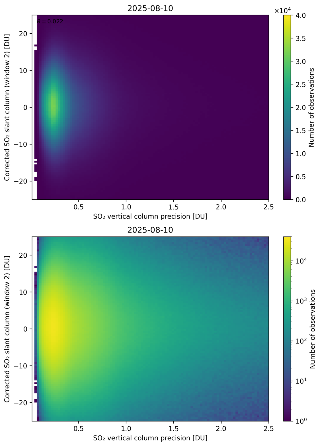
Figure 339: Scatter density plot of “SO 2 vertical column precision” against “Corrected SO 2 slant column (window 2)” for 2025-08-09 to 2025-08-11.
