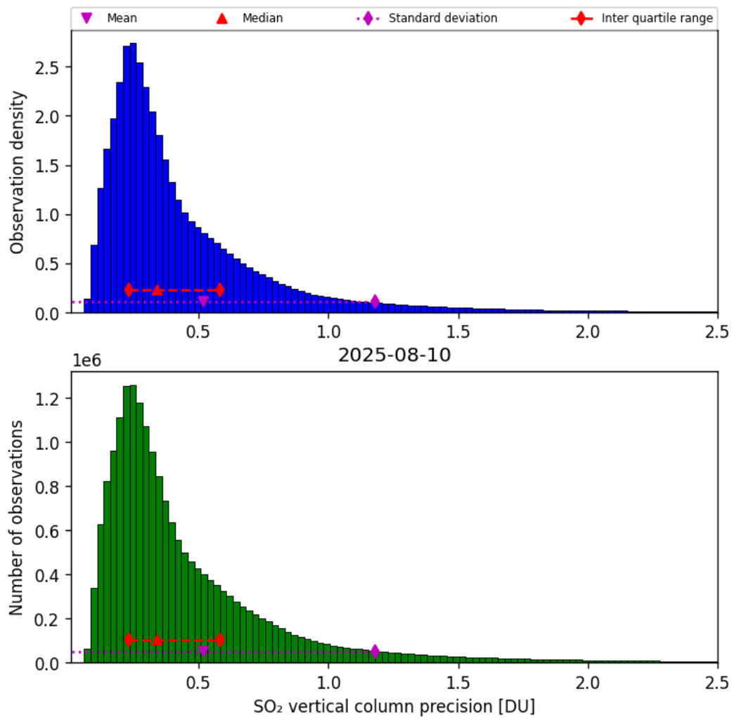
Figure 59: Histogram of “SO 2 vertical column precision” for 2025-08-09 to 2025-08-11
