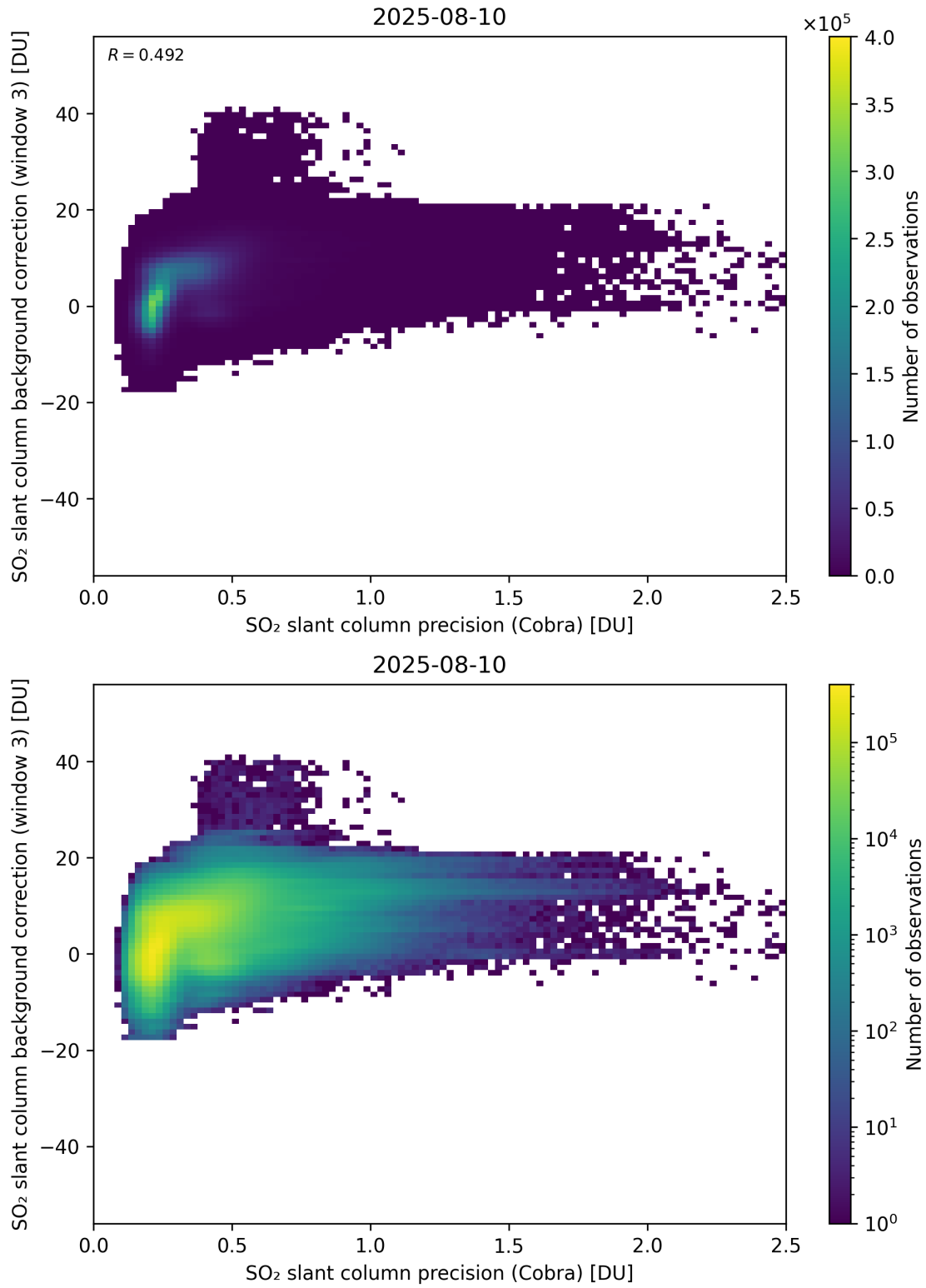
Figure 201: Scatter density plot of “SO 2 slant column precision (Cobra)” against “SO 2 slant column background correction (window 3)” for 2025-08-09 to 2025-08-11.
