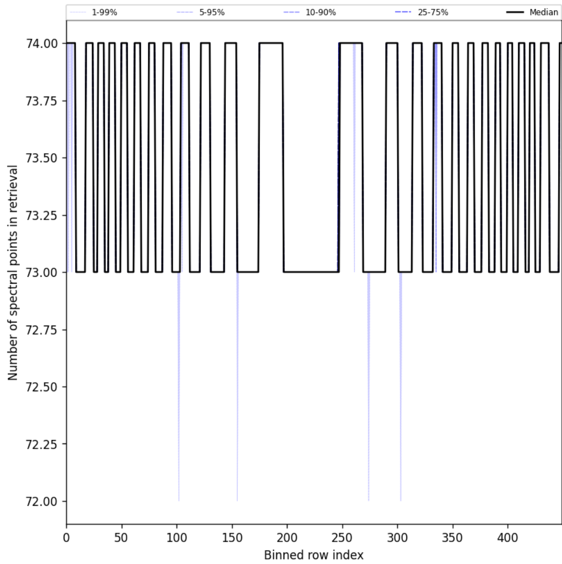
Figure 108: Along track statistics of “Number of spectral points in retrieval” for 2025-08-09 to 2025-08-11
