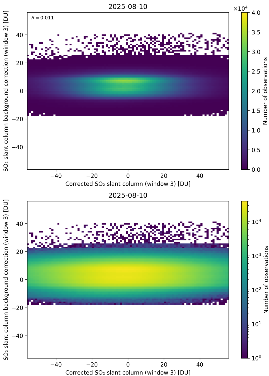
Figure 255: Scatter density plot of “Corrected SO 2 slant column (window 3)” against “SO 2 slant column background correction (window 3)” for 2025-08-09 to 2025-08-11.
