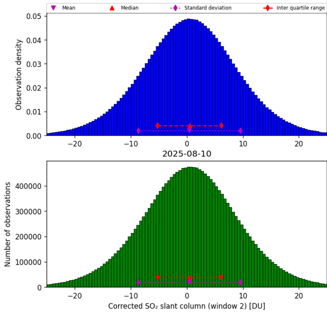
Figure 69: Histogram of “Corrected SO 2 slant column (window 2)” for 2025-08-09 to 2025-08-11
