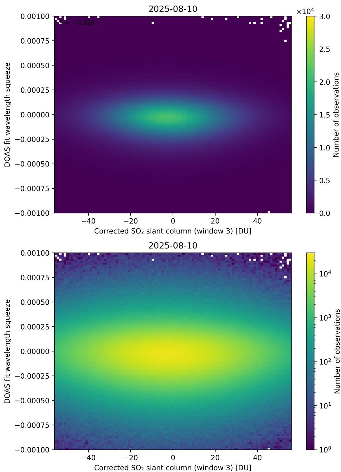
Figure 257: Scatter density plot of “Corrected SO 2 slant column (window 3)” against “DOAS fit wavelength squeeze” for 2025-08-09 to 2025-08-11.
