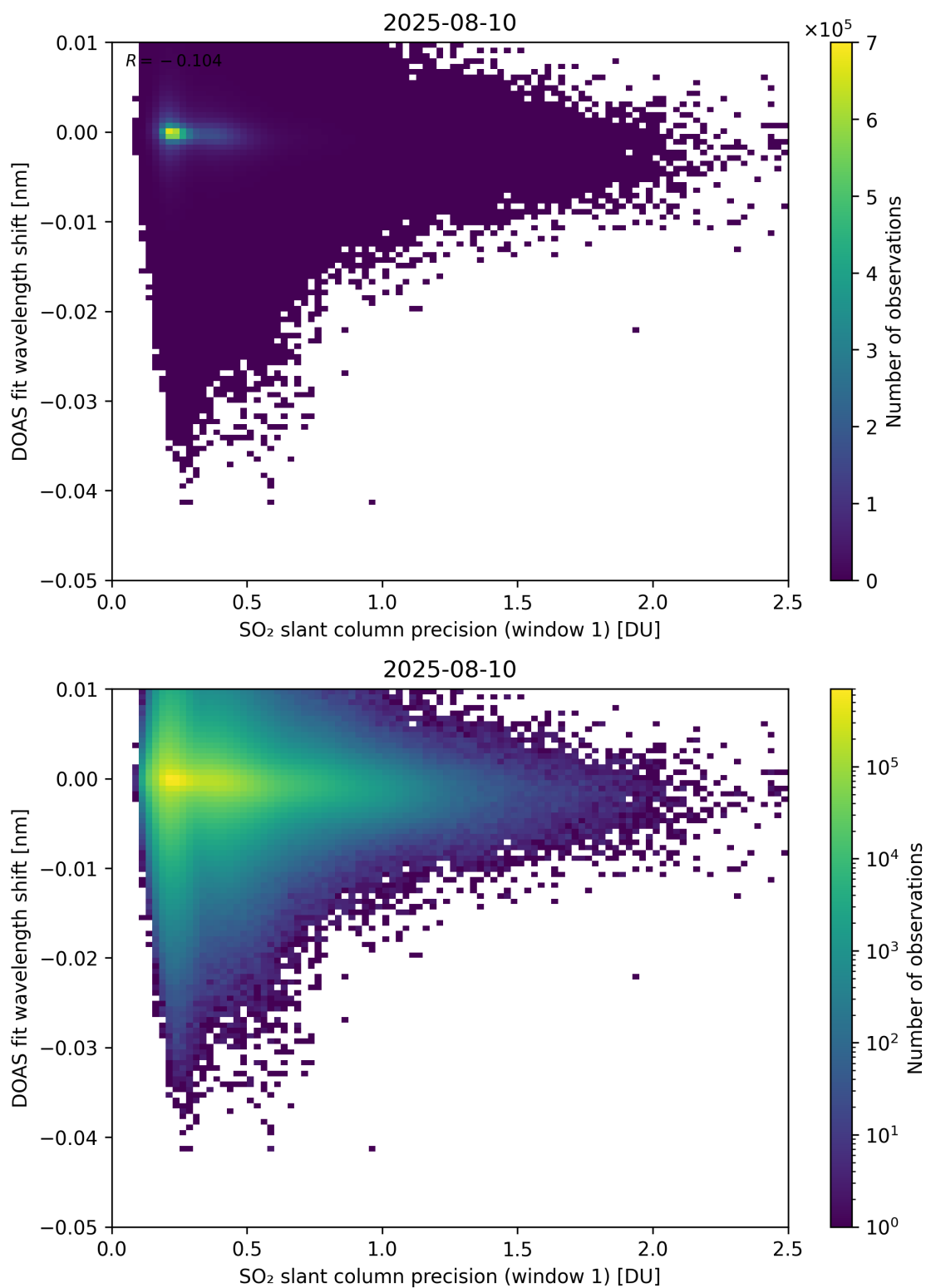
Figure 271: Scatter density plot of “SO 2 slant column precision (window 1)” against “DOAS fit wavelength shift” for 2025-08-09 to 2025-08-11.
