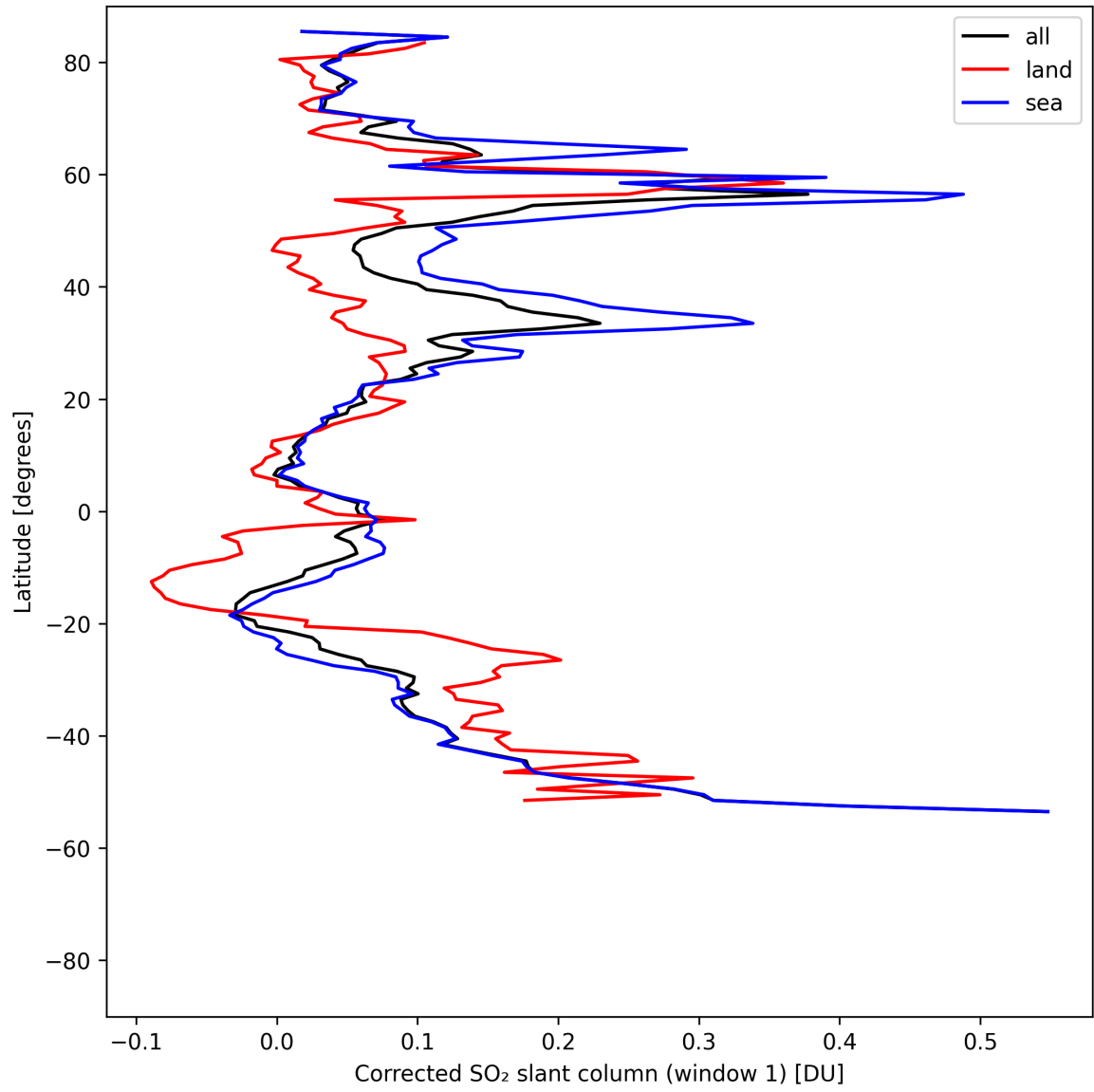
Figure 39: Zonal average of “Corrected SO 2 slant column (window 1)” for 2025-08-09 to 2025-08-11.
