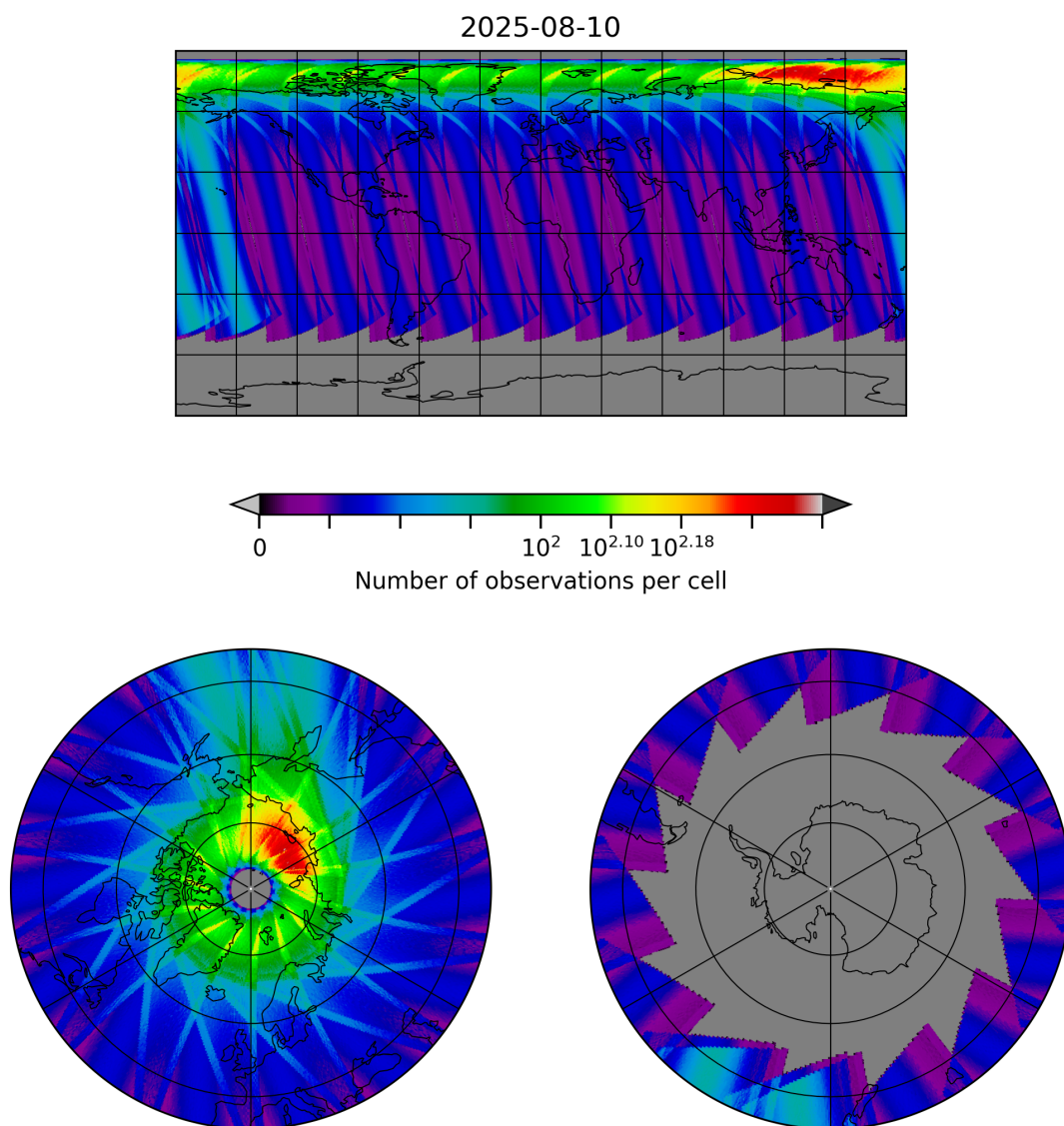
Figure 30: Map of the number of observations for 2025-08-09 to 2025-08-11
