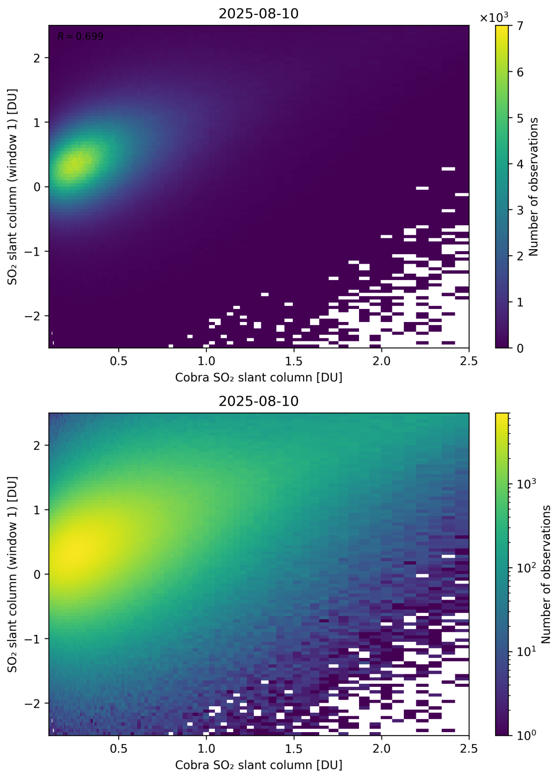
Figure 219: Scatter density plot of “Cobra SO 2 slant column” against “SO 2 slant column (window 1)” for 2025-08-09 to 2025-08-11.
