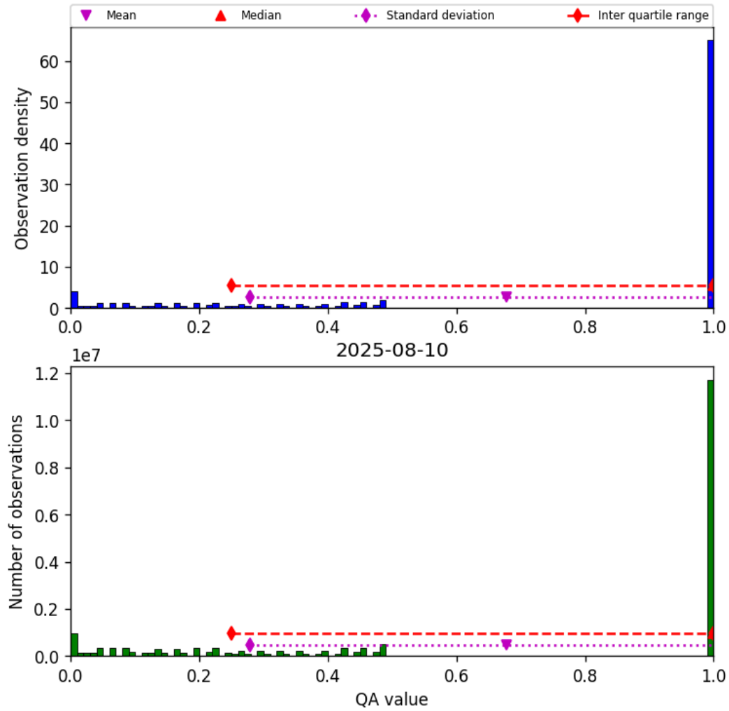
Figure 57: Histogram of “QA value” for 2025-08-09 to 2025-08-11
