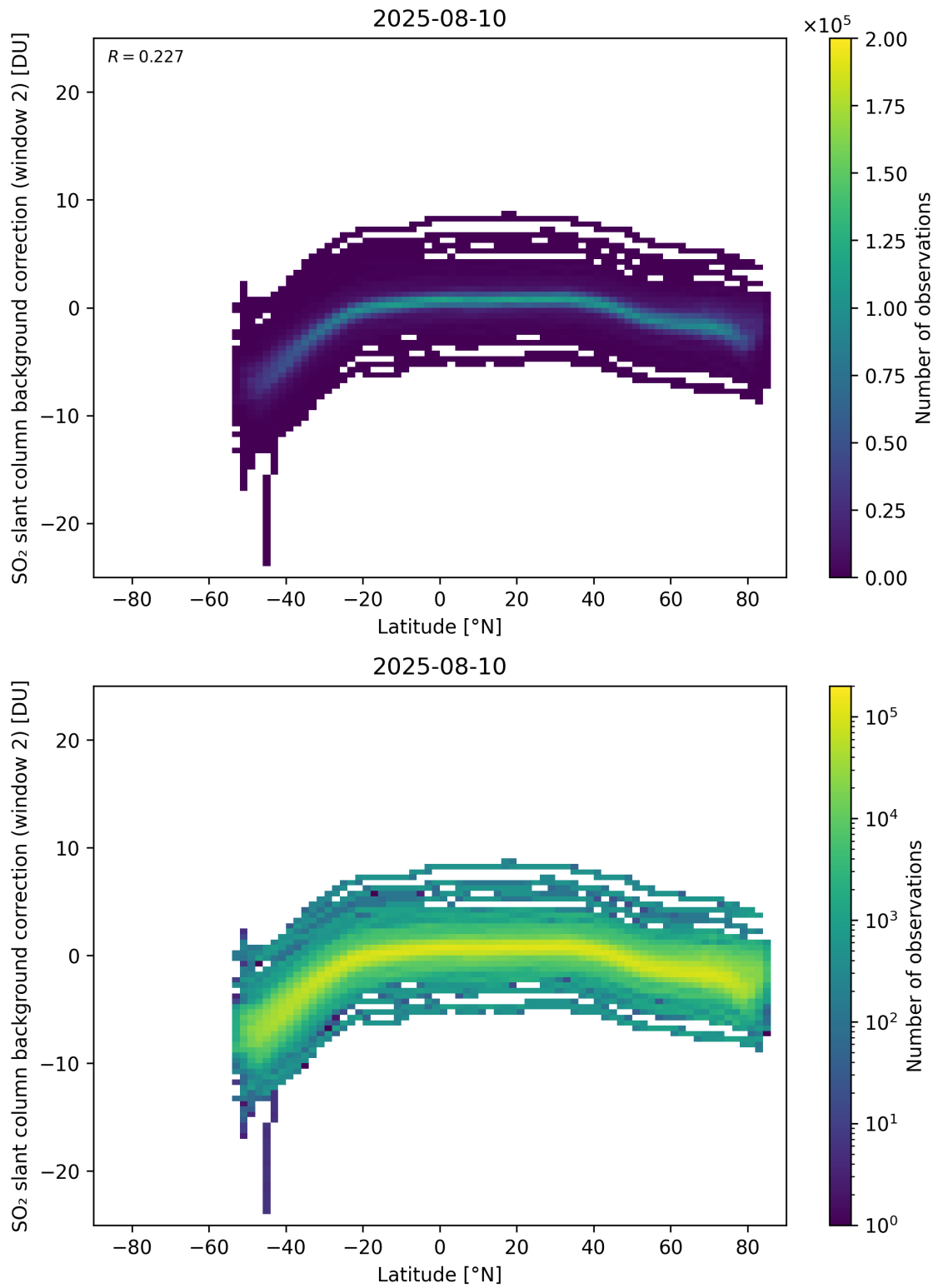
Figure 151: Scatter density plot of “Latitude” against “SO 2 slant column background correction (window 2)” for 2025-08-09 to 2025-08-11.
