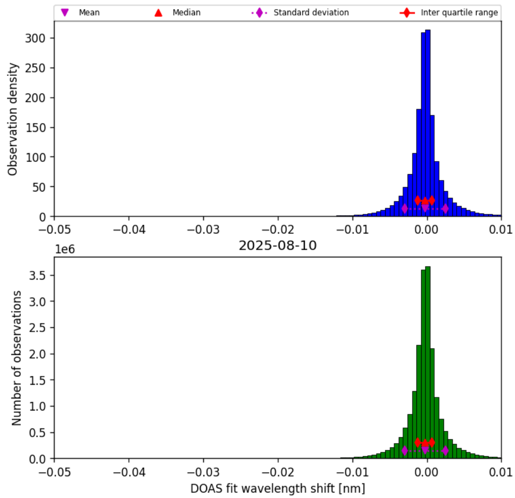
Figure 76: Histogram of “DOAS fit wavelength shift” for 2025-08-09 to 2025-08-11
