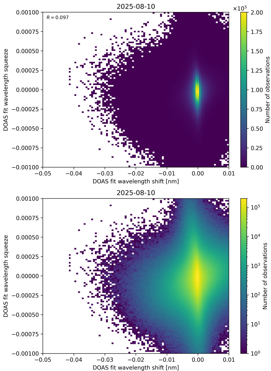
Figure 138: Scatter density plot of “DOAS fit wavelength shift” against “DOAS fit wavelength squeeze” for 2025-08-09 to 2025-08-11.
