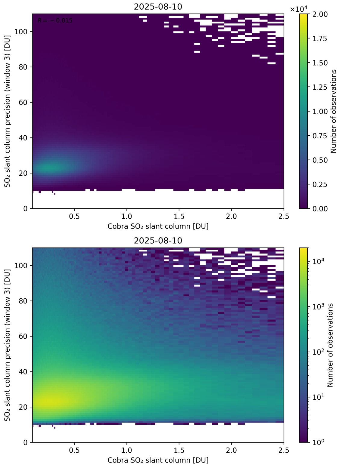
Figure 223: Scatter density plot of “Cobra SO 2 slant column” against “SO 2 slant column precision (window 3)” for 2025-08-09 to 2025-08-11.
