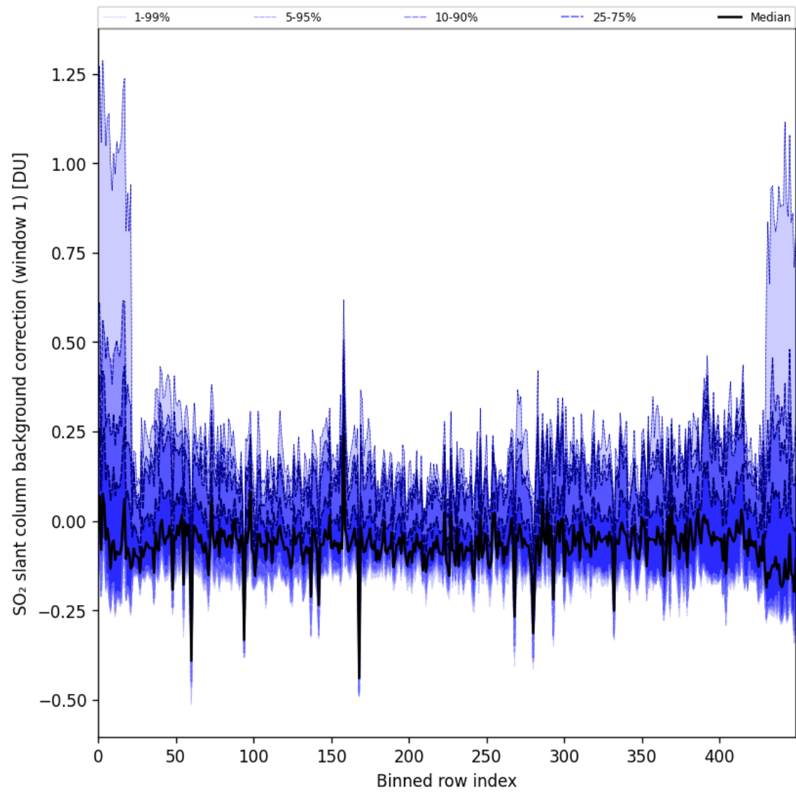
Figure 92: Along track statistics of “SO 2 slant column background correction (window 1)” for 2025-08-09 to 2025-08-11
