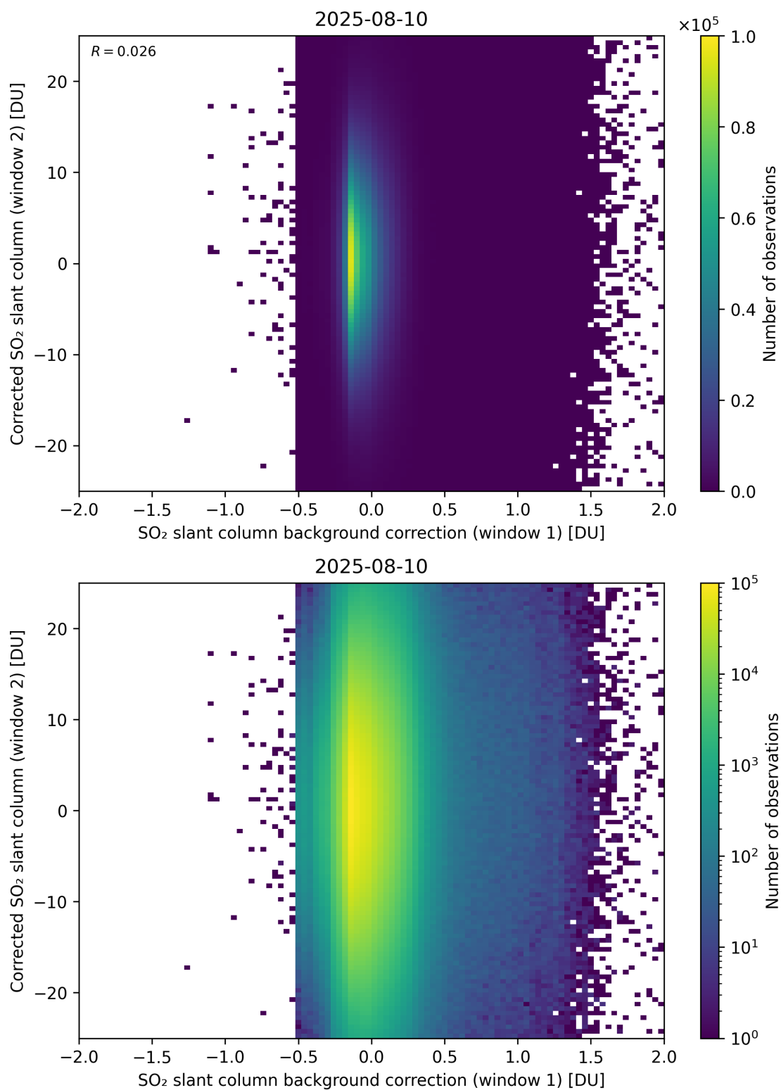
Figure 115: Scatter density plot of “SO 2 slant column background correction (window 1)” against “Corrected SO 2 slant column (window 2)” for 2025-08-09 to 2025-08-11.
