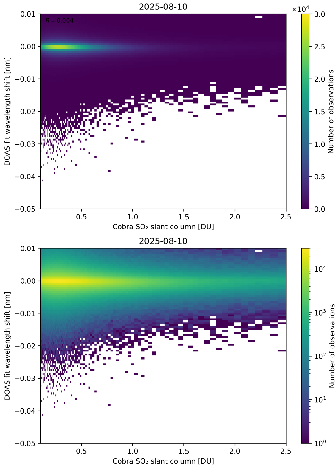
Figure 196: Scatter density plot of “Cobra SO 2 slant column” against “DOAS fit wavelength shift” for 2025-08-09 to 2025-08-11.
