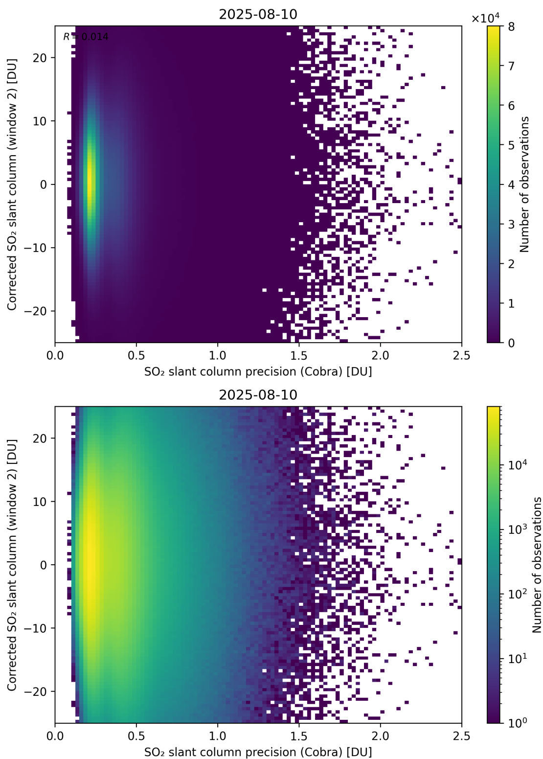
Figure 206: Scatter density plot of “SO 2 slant column precision (Cobra)” against “Corrected SO 2 slant column (window 2)” for 2025-08-09 to 2025-08-11.
