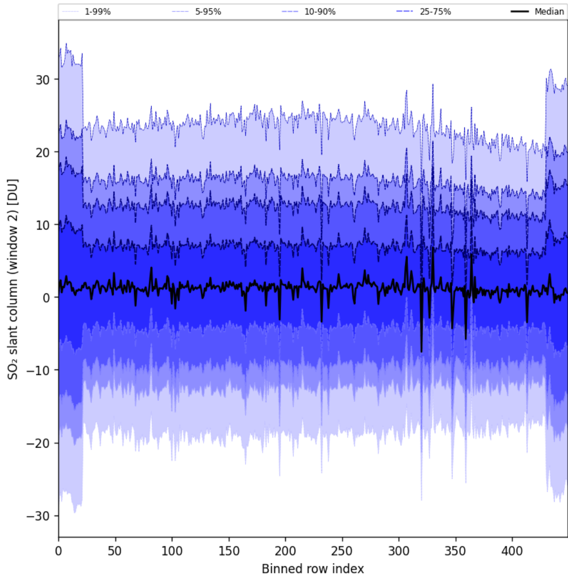
Figure 93: Along track statistics of “SO 2 slant column (window 2)” for 2025-08-09 to 2025-08-11
