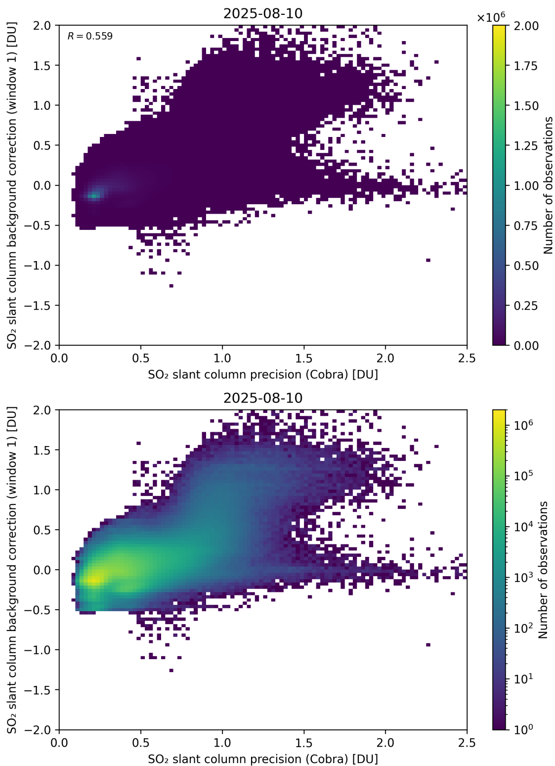
Figure 199: Scatter density plot of “SO 2 slant column precision (Cobra)” against “SO 2 slant column background correction (window 1)” for 2025-08-09 to 2025-08-11.
