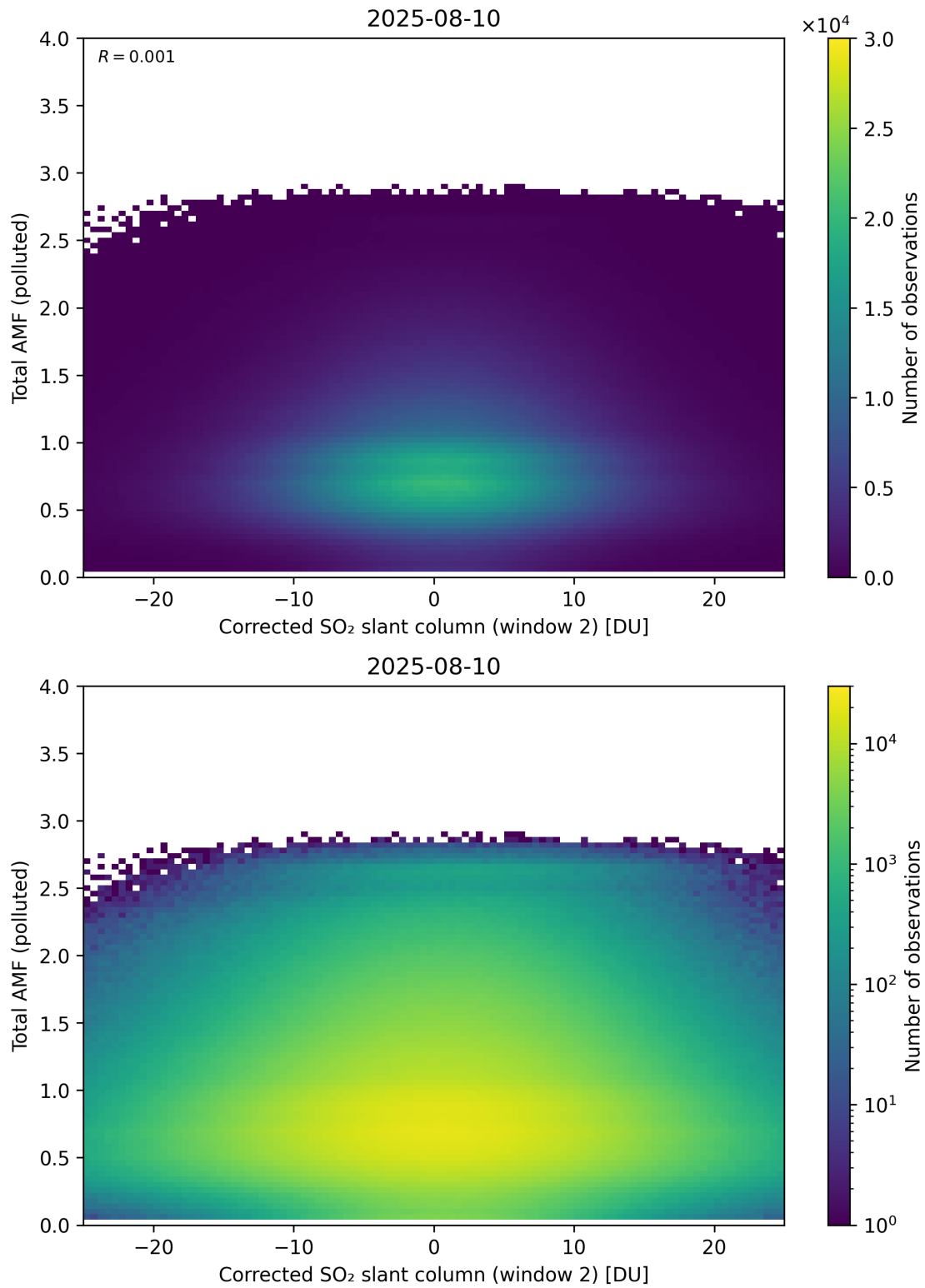
Figure 253: Scatter density plot of “Corrected SO 2 slant column (window 2)” against “Total AMF (polluted)” for 2025-08-09 to 2025-08-11.
