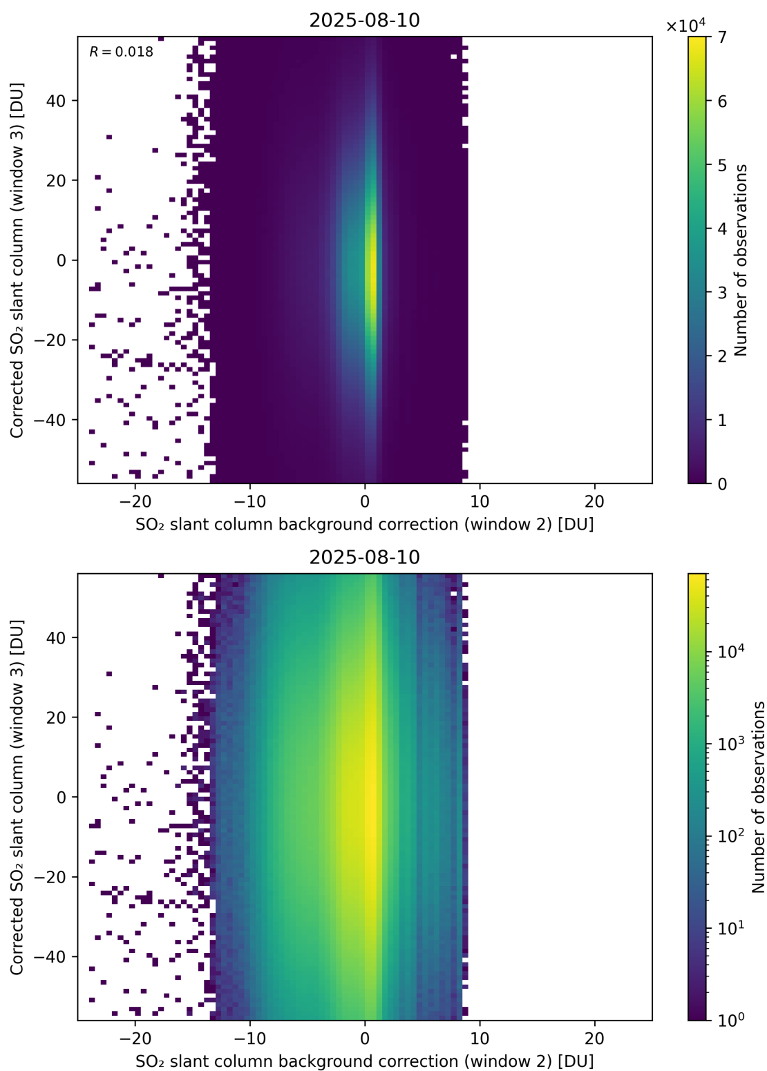
Figure 127: Scatter density plot of “SO 2 slant column background correction (window 2)” against “Corrected SO 2 slant column (window 3)” for 2025-08-09 to 2025-08-11.
