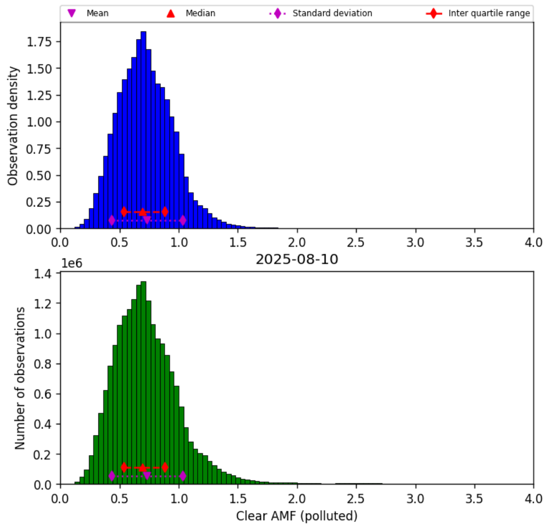
Figure 81: Histogram of “Clear AMF (polluted)” for 2025-08-09 to 2025-08-11
