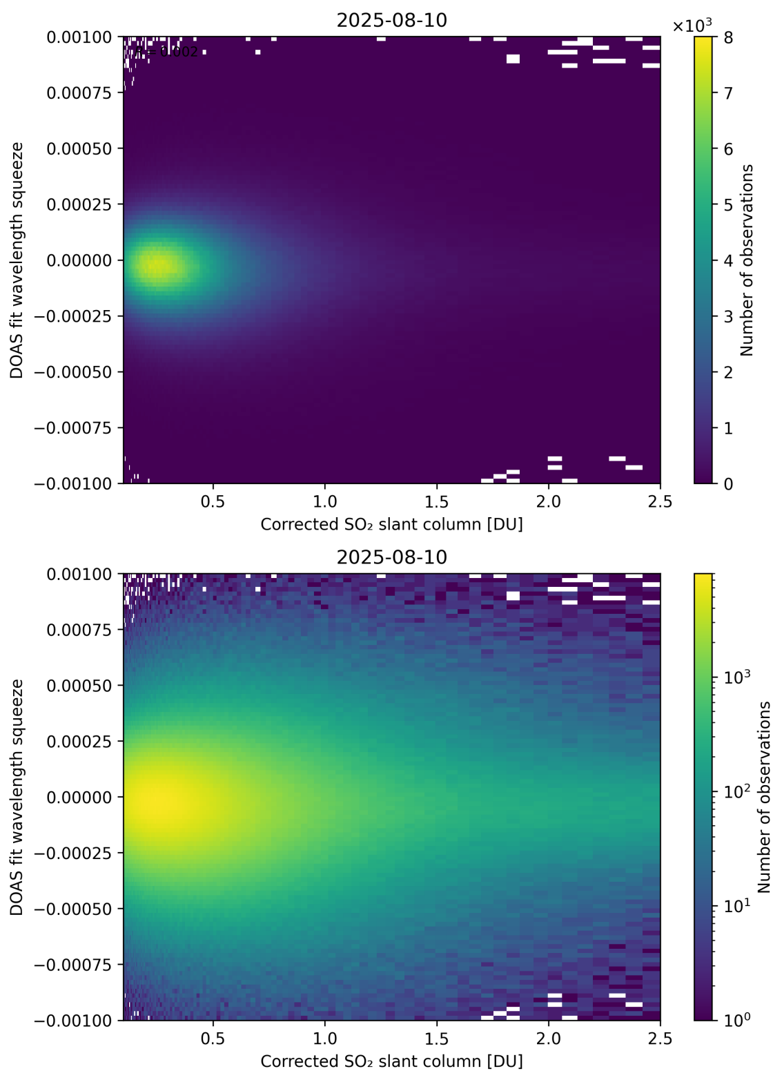
Figure 230: Scatter density plot of "Corrected SO 2 slant column" against "DOAS fit wavelength squeeze" for 2025-08-09 to 2025-08-11.
