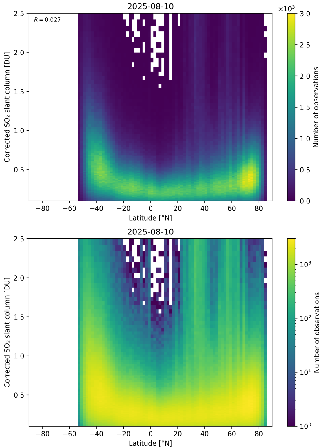
Figure 159: Scatter density plot of “Latitude” against “Corrected SO 2 slant column” for 2025-08-09 to 2025-08-11.
