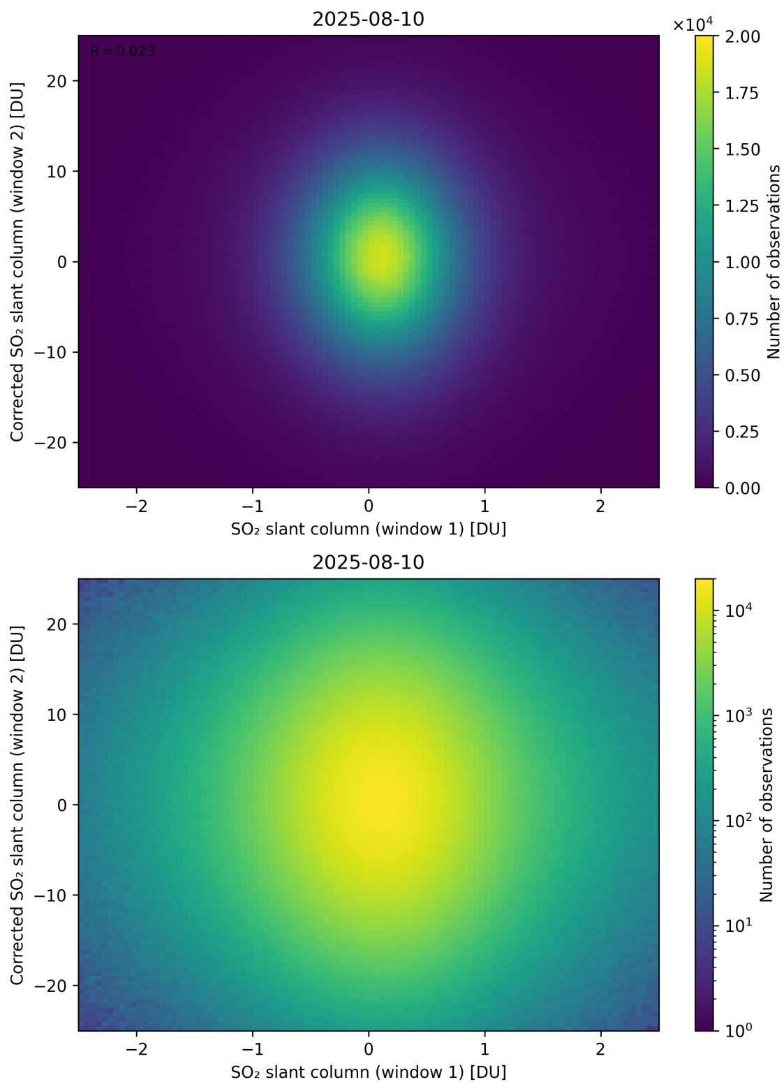
Figure 283: Scatter density plot of “SO 2 slant column (window 1)” against “Corrected SO 2 slant column (window 2)” for 2025-08-09 to 2025-08-11.
