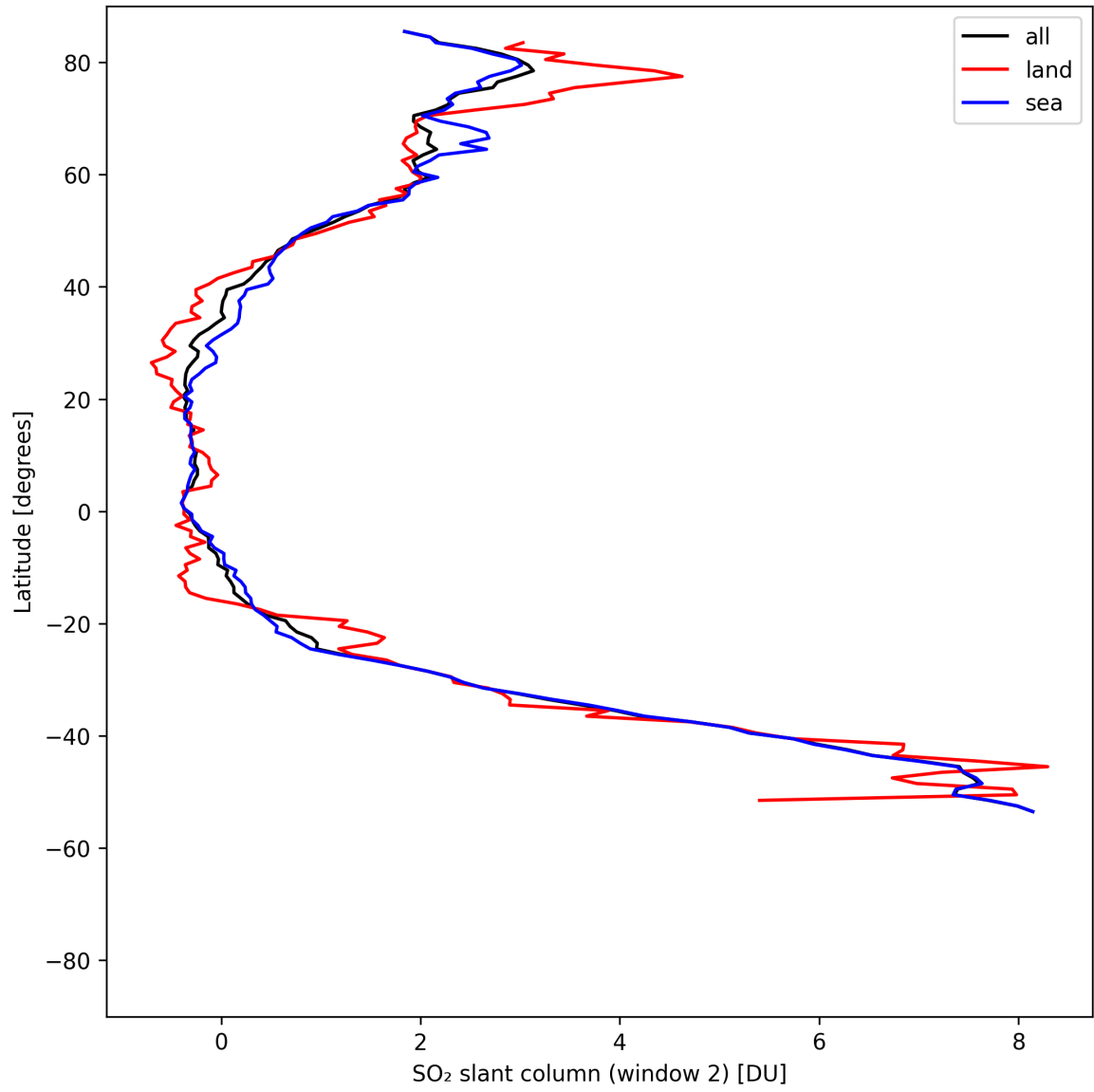
Figure 41: Zonal average of “SO 2 slant column (window 2)” for 2025-08-09 to 2025-08-11.
