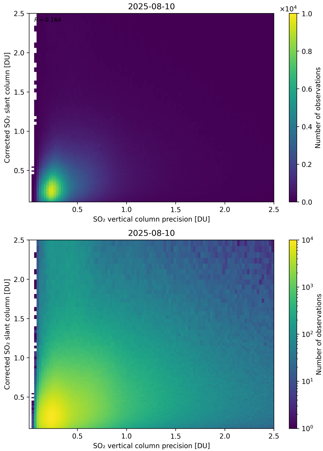
Figure 338: Scatter density plot of “SO 2 vertical column precision” against “Corrected SO 2 slant column” for 2025-08-09 to 2025-08-11.
