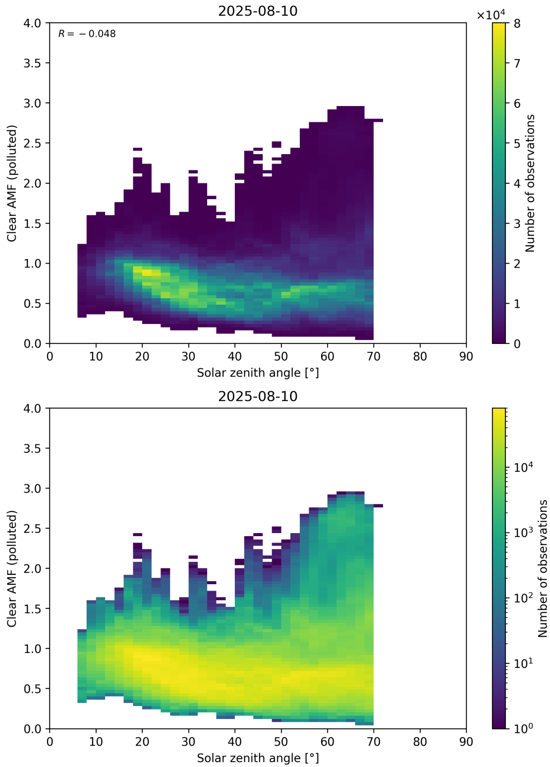
Figure 178: Scatter density plot of “Solar zenith angle” against “Clear AMF (polluted)” for 2025-08-09 to 2025-08-11.
