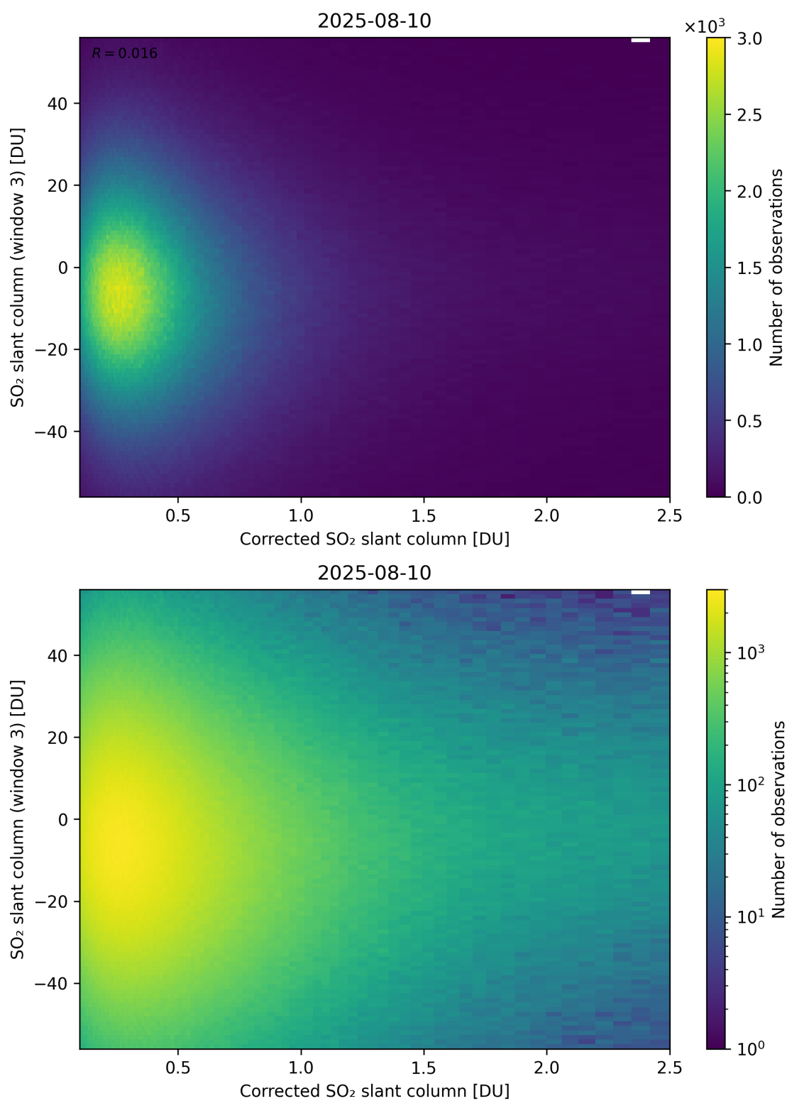
Figure 240: Scatter density plot of “Corrected SO 2 slant column” against “SO 2 slant column (window 3)” for 2025-08-09 to 2025-08-11.
