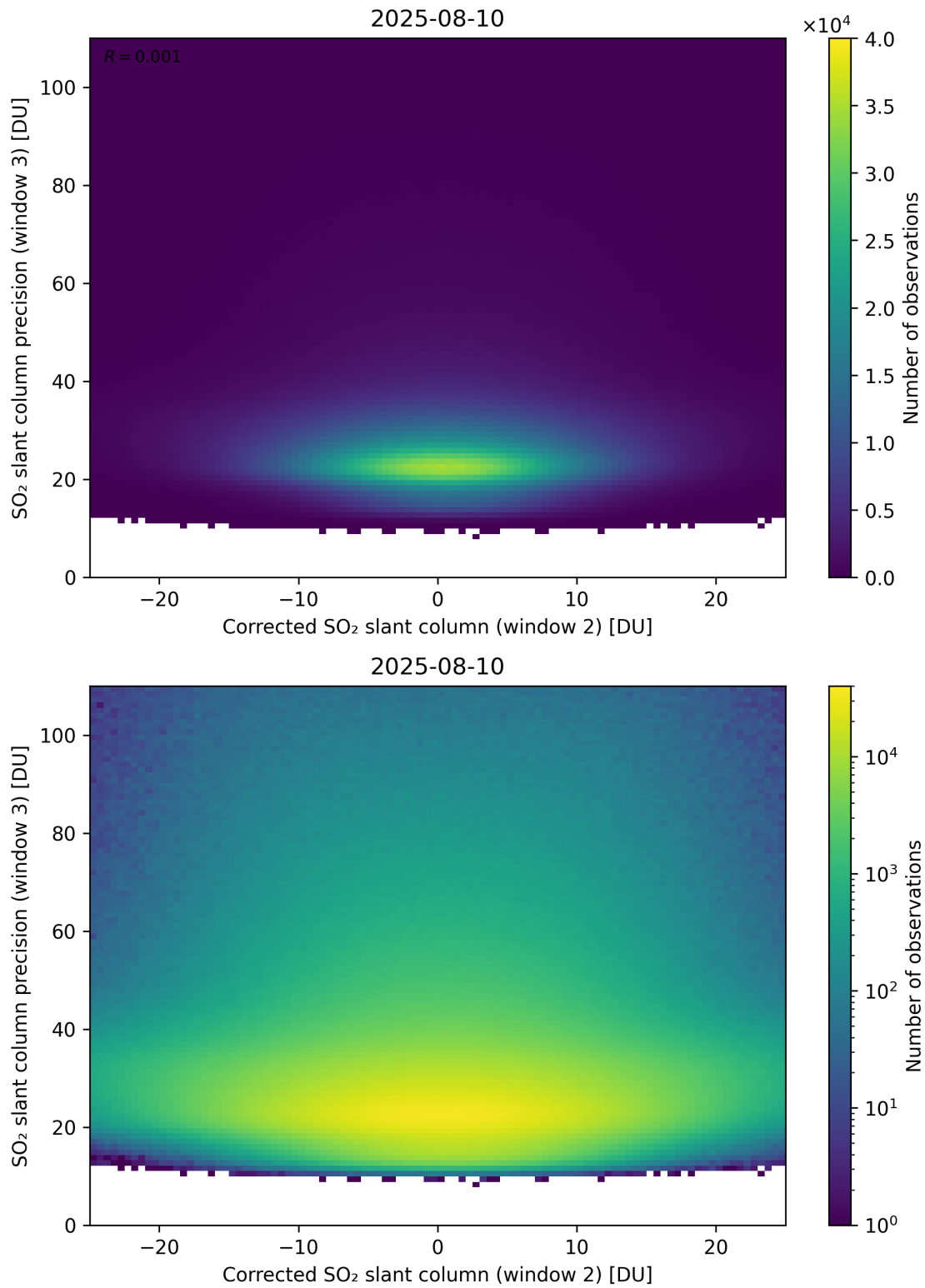
Figure 252: Scatter density plot of “Corrected SO 2 slant column (window 2)” against “SO 2 slant column precision (window 3)” for 2025-08-09 to 2025-08-11.
