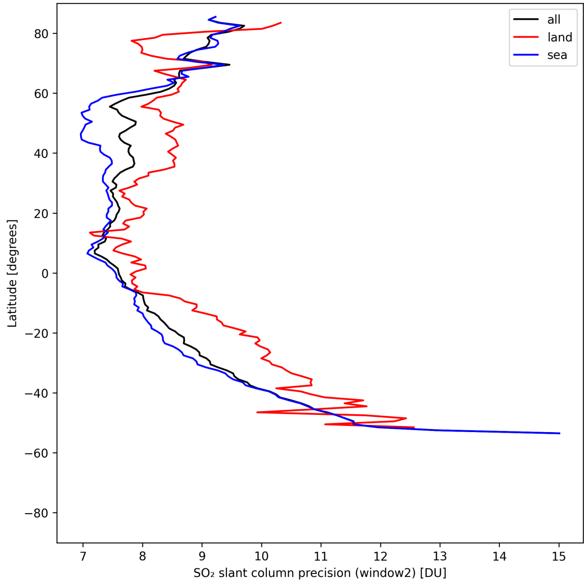
Figure 42: Zonal average of “SO 2 slant column precision (window2)” for 2025-08-09 to 2025-08-11.
