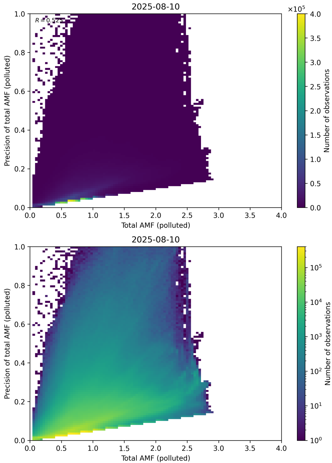
Figure 322: Scatter density plot of “Total AMF (polluted)” against “Precision of total AMF (polluted)” for 2025-08-09 to 2025-08-11.
