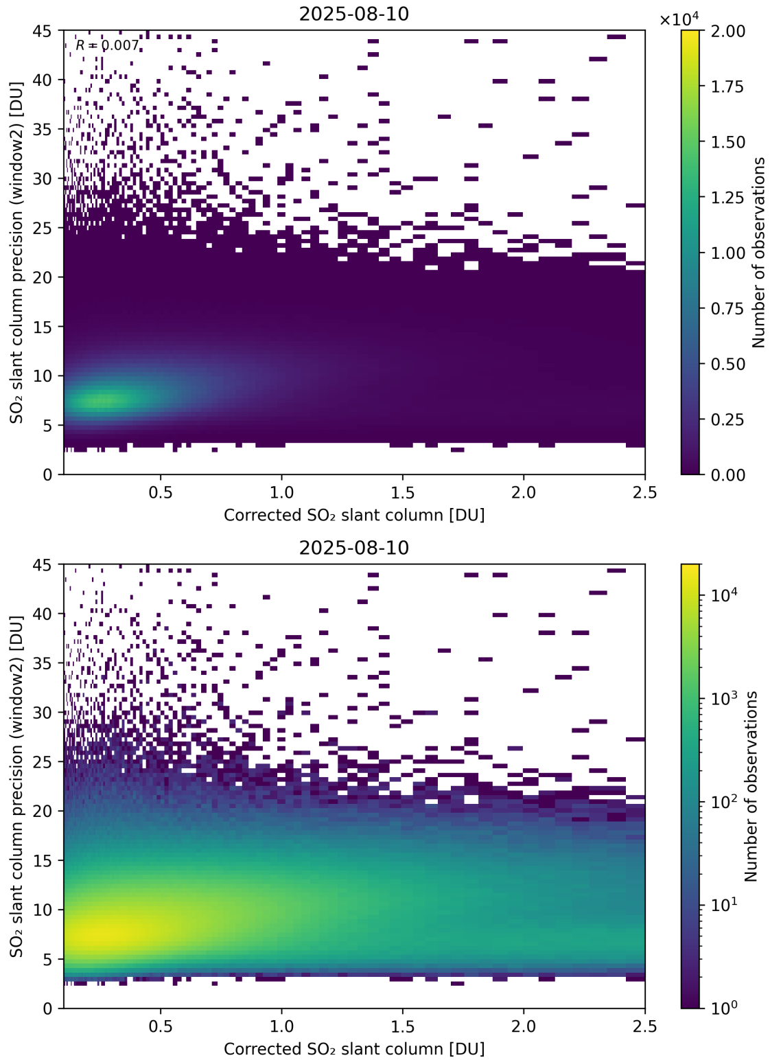
Figure 239: Scatter density plot of “Corrected SO 2 slant column” against “SO 2 slant column precision (window2)” for 2025-08-09 to 2025-08-11.
