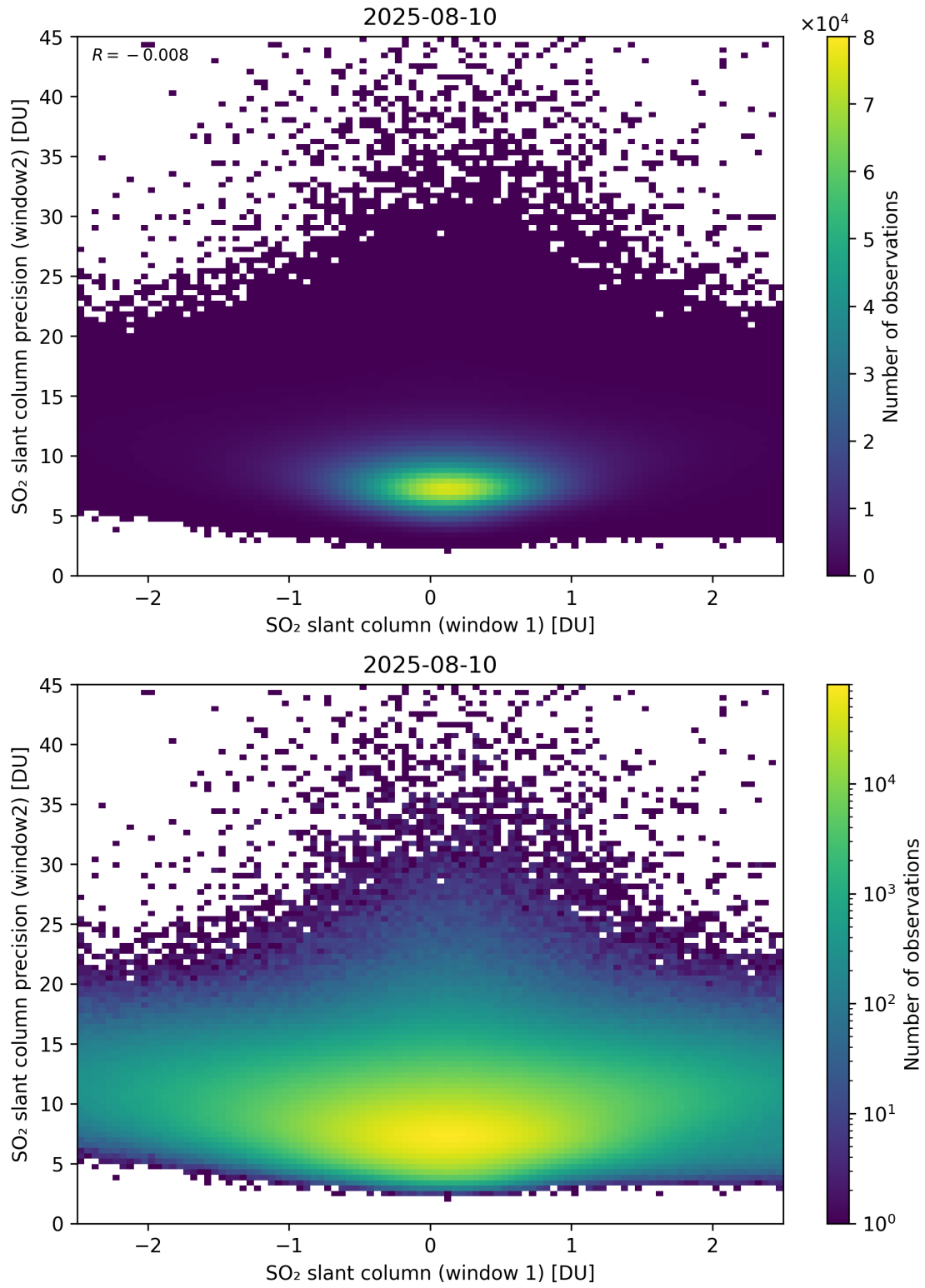
Figure 286: Scatter density plot of “SO 2 slant column (window 1)” against “SO 2 slant column precision (window2)” for 2025-08-09 to 2025-08-11.
