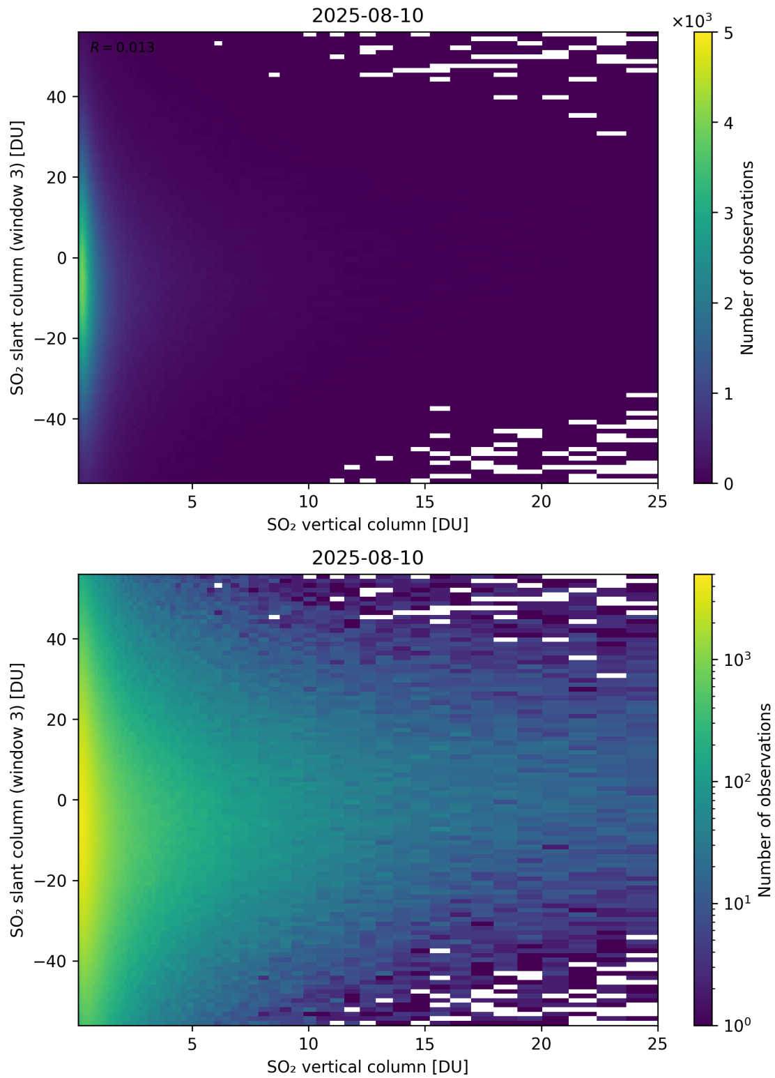
Figure 357: Scatter density plot of “SO 2 vertical column” against “SO 2 slant column (window 3)” for 2025-08-09 to 2025-08-11.
