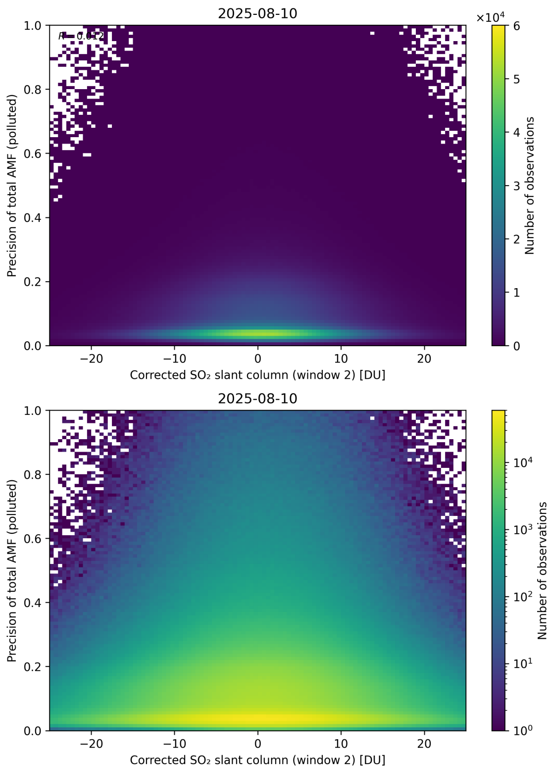
Figure 254: Scatter density plot of “Corrected SO 2 slant column (window 2)” against “Precision of total AMF (polluted)” for 2025-08-09 to 2025-08-11.
