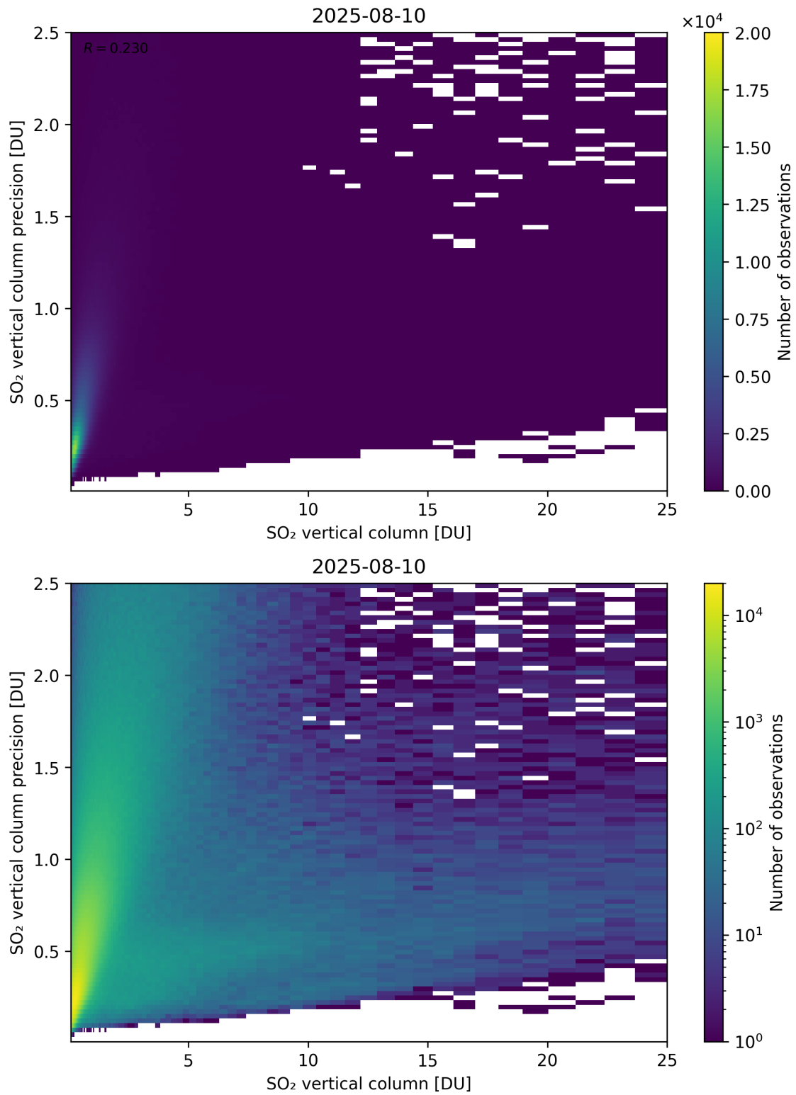
Figure 361: Scatter density plot of “SO 2 vertical column” against “SO 2 vertical column precision” for 2025-08-09 to 2025-08-11.
