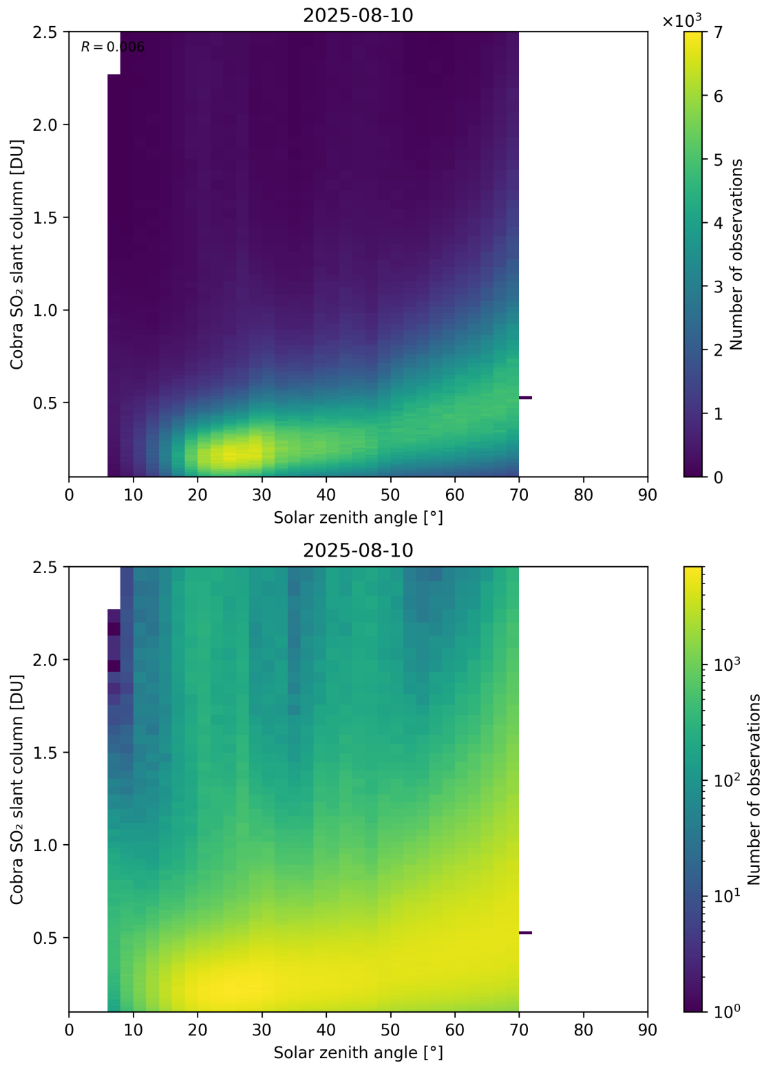
Figure 179: Scatter density plot of “Solar zenith angle” against “Cobra SO 2 slant column” for 2025-08-09 to 2025-08-11.
