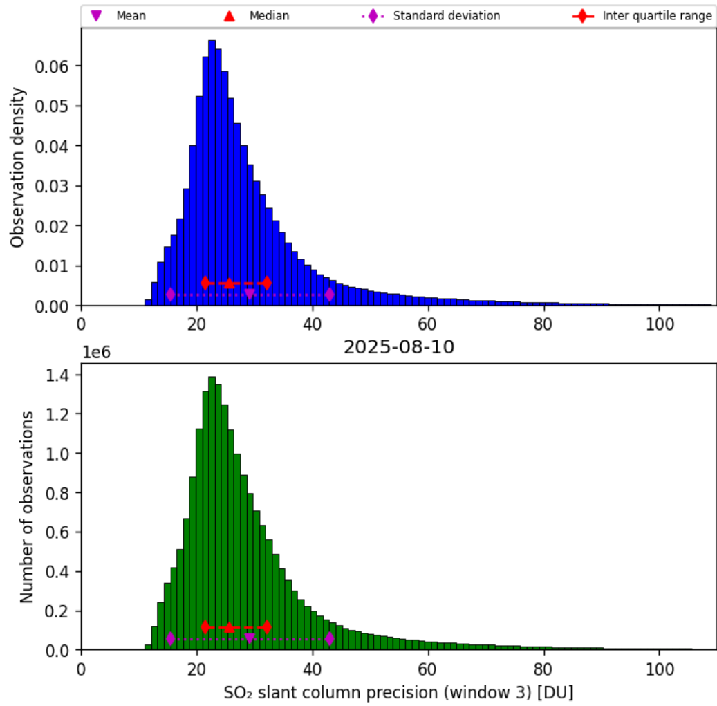
Figure 72: Histogram of “SO 2 slant column precision (window 3)” for 2025-08-09 to 2025-08-11
