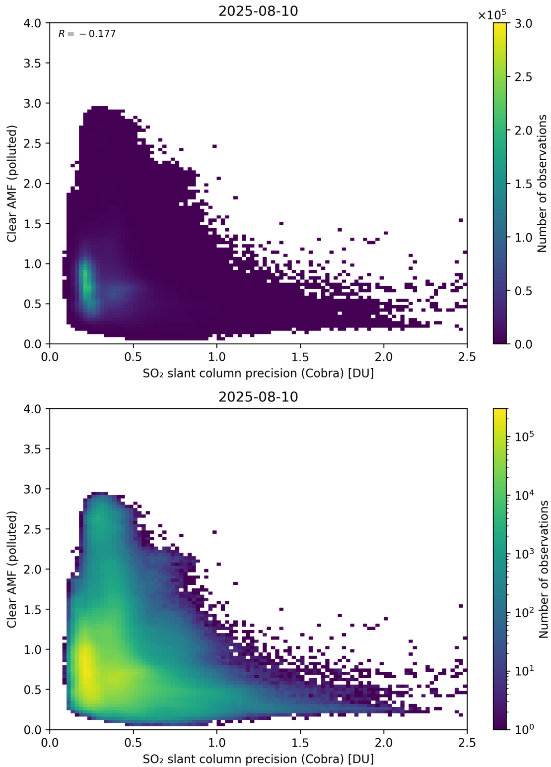
Figure 205: Scatter density plot of “SO 2 slant column precision (Cobra)” against “Clear AMF (polluted)” for 2025-08-09 to 2025-08-11.
