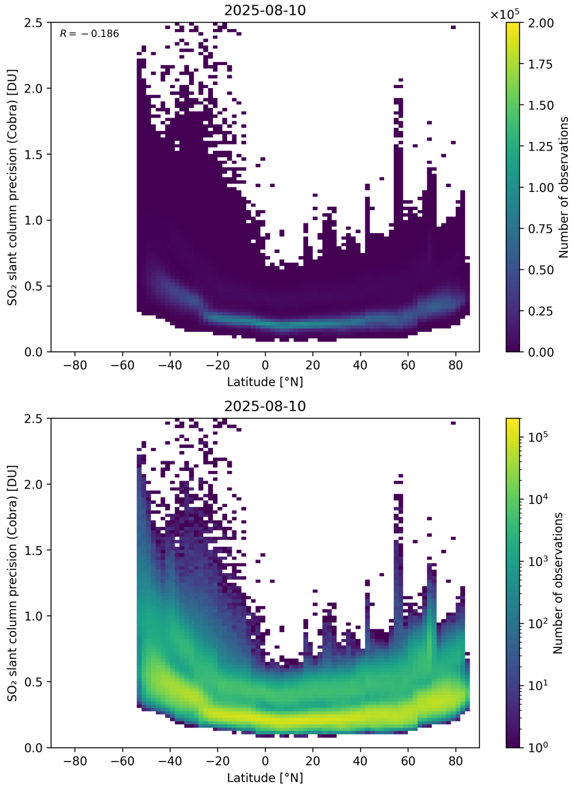
Figure 158: Scatter density plot of “Latitude” against “SO 2 slant column precision (Cobra)” for 2025-08-09 to 2025-08-11.
