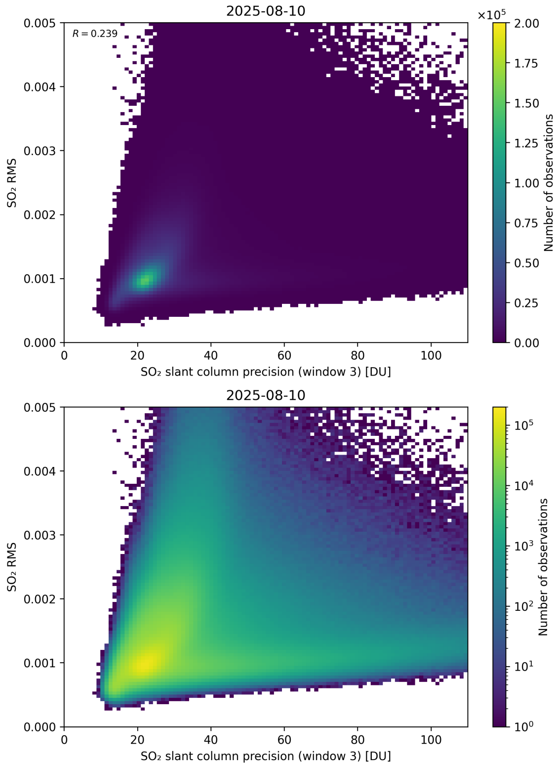
Figure 310: Scatter density plot of “SO 2 slant column precision (window 3)” against “SO 2 RMS” for 2025-08-09 to 2025-08-11.
