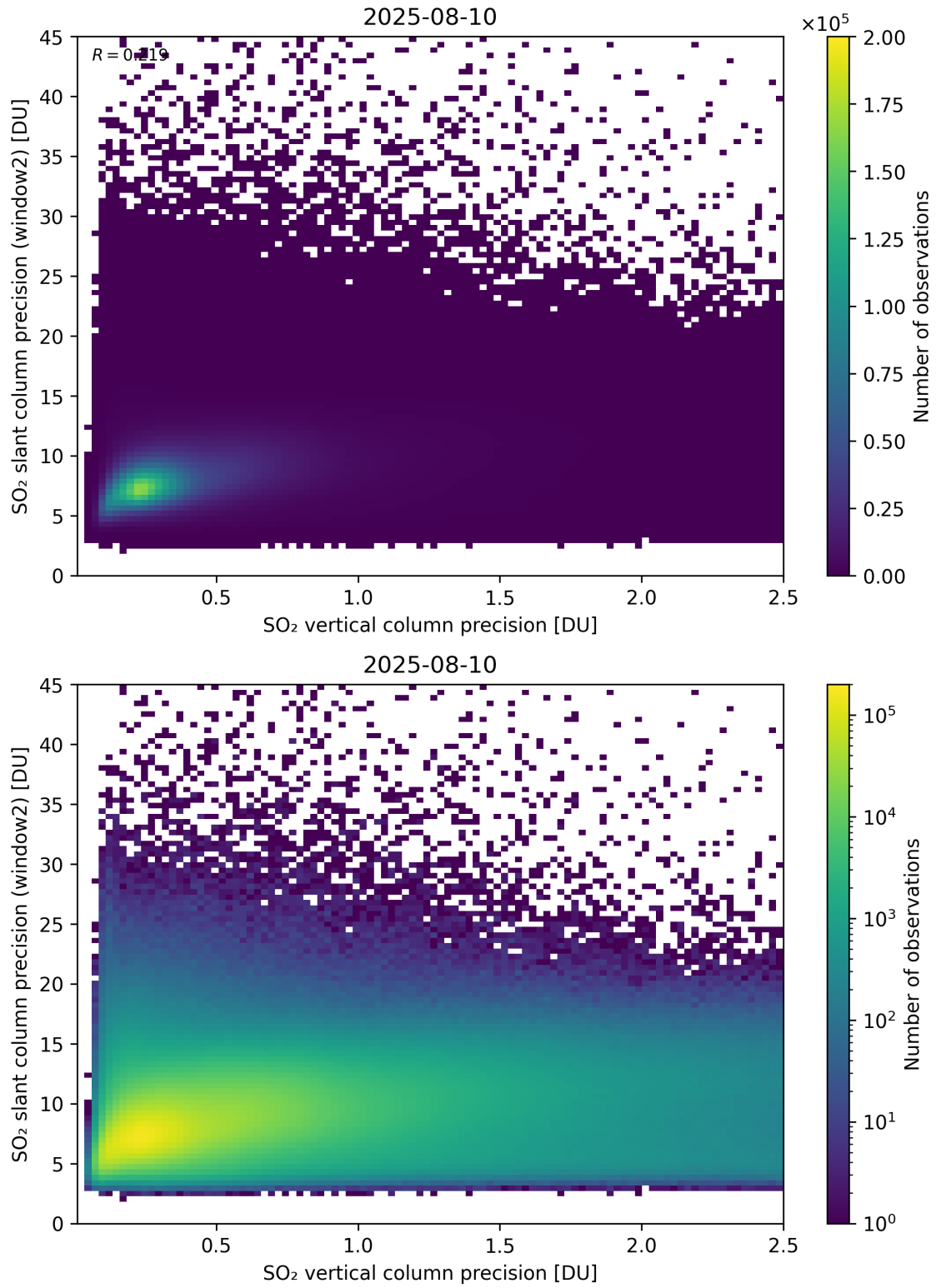
Figure 343: Scatter density plot of “SO 2 vertical column precision” against “SO 2 slant column precision (window2)” for 2025-08-09 to 2025-08-11.
