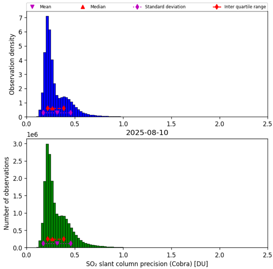
Figure 62: Histogram of “SO 2 slant column precision (Cobra)” for 2025-08-09 to 2025-08-11
