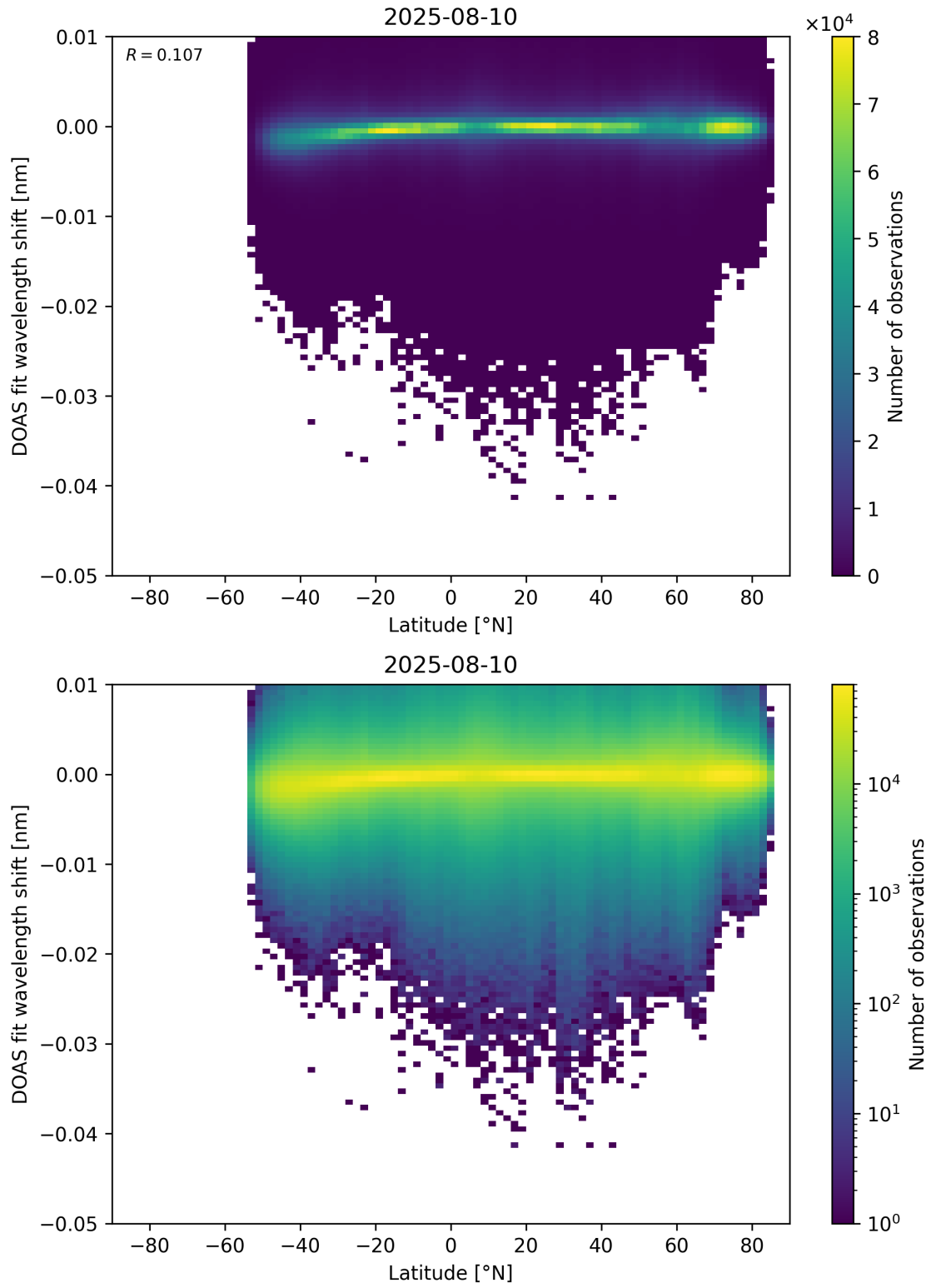
Figure 153: Scatter density plot of “Latitude” against “DOAS fit wavelength shift” for 2025-08-09 to 2025-08-11.
