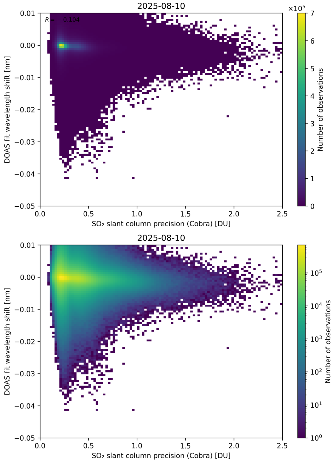
Figure 202: Scatter density plot of “SO 2 slant column precision (Cobra)” against “DOAS fit wavelength shift” for 2025-08-09 to 2025-08-11.
