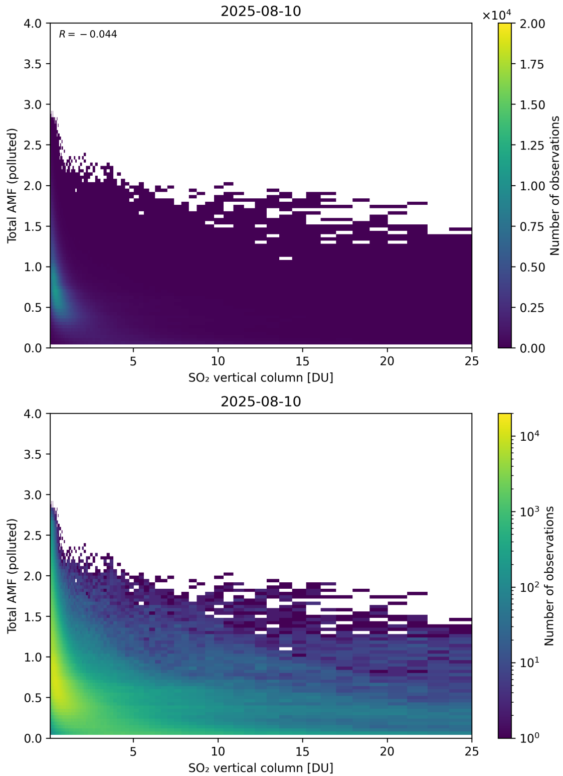
Figure 359: Scatter density plot of “SO 2 vertical column” against “Total AMF (polluted)” for 2025-08-09 to 2025-08-11.
