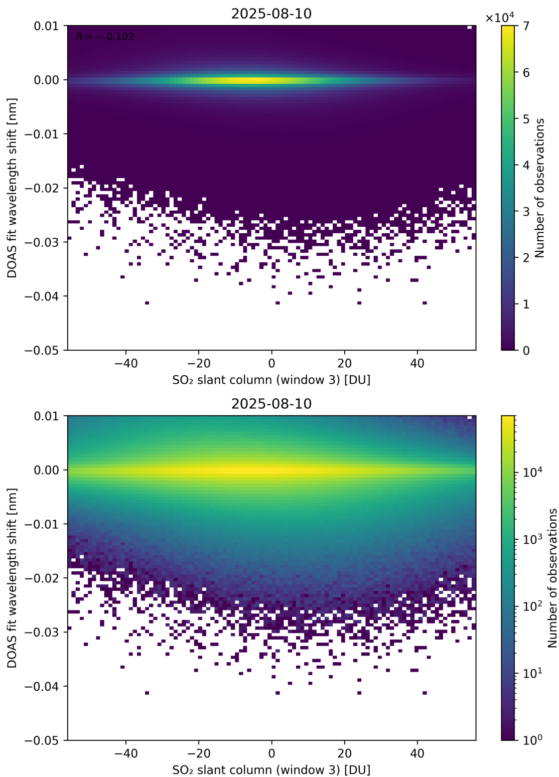
Figure 304: Scatter density plot of “SO 2 slant column (window 3)” against “DOAS fit wavelength shift” for 2025-08-09 to 2025-08-11.
