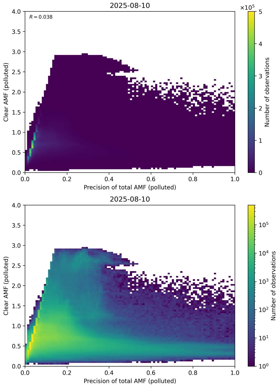
Figure 320: Scatter density plot of “Precision of total AMF (polluted)” against “Clear AMF (polluted)” for 2025-08-09 to 2025-08-11.
