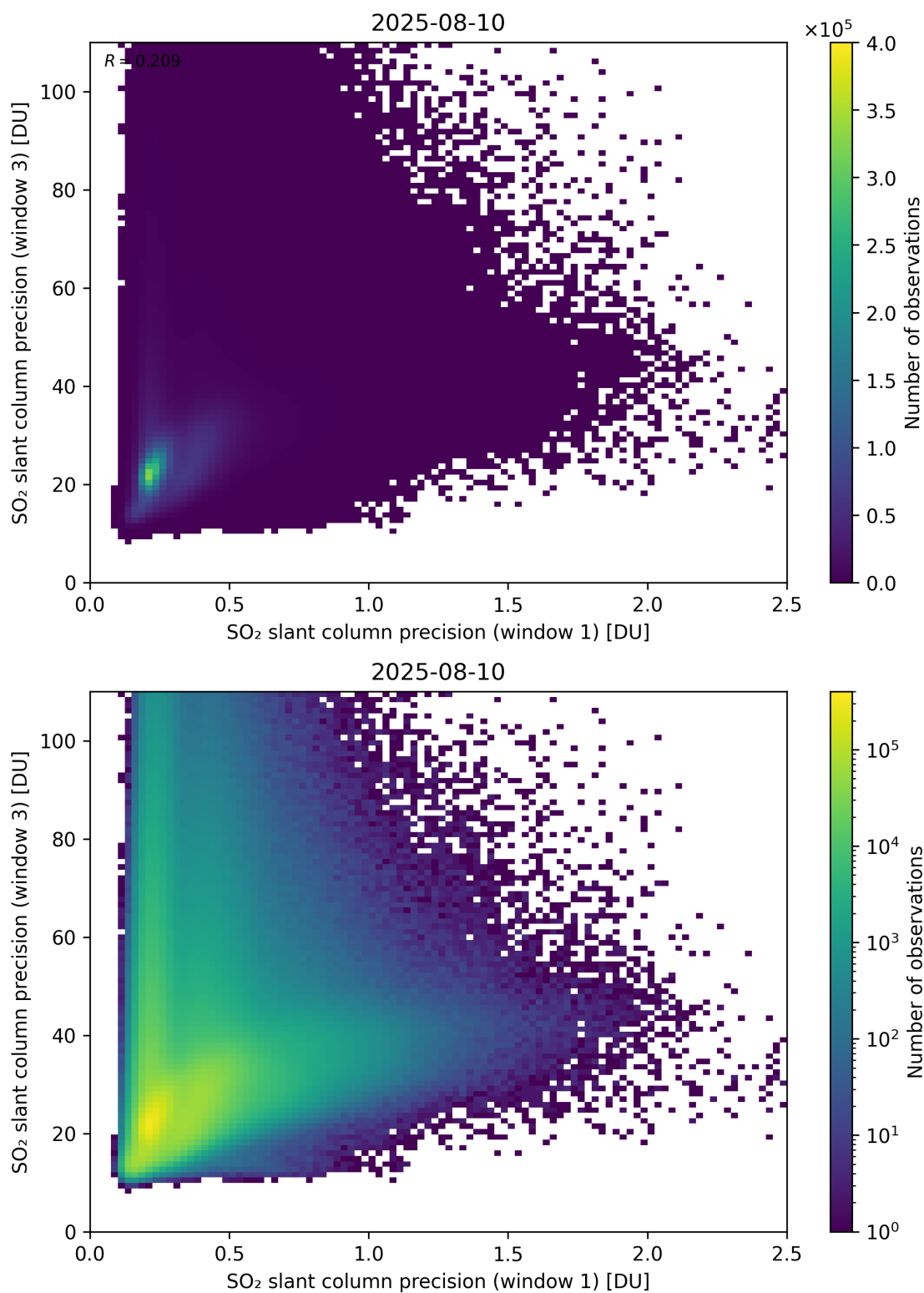
Figure 279: Scatter density plot of “SO 2 slant column precision (window 1)” against “SO 2 slant column precision (window 3)” for 2025-08-09 to 2025-08-11.
