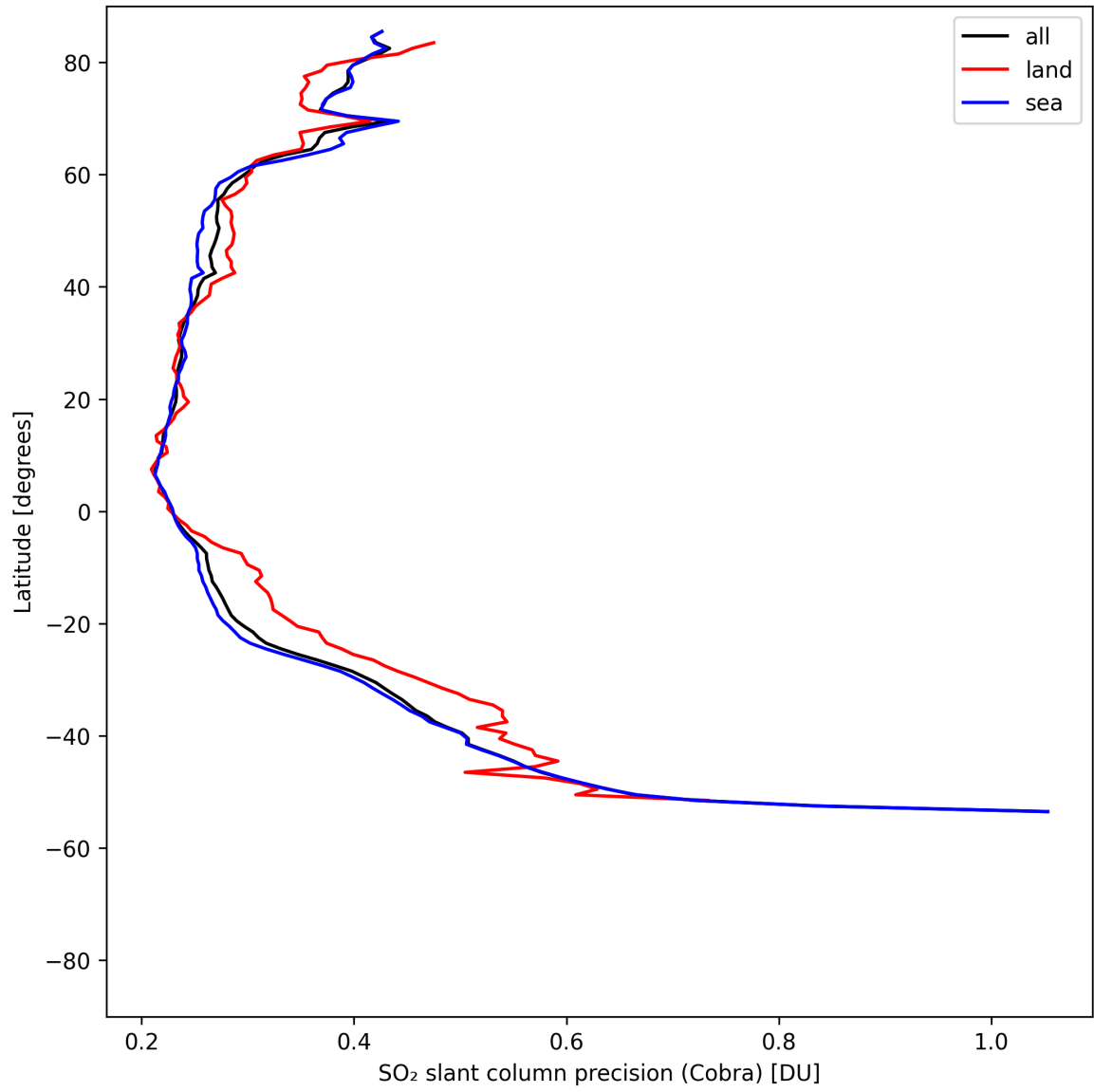
Figure 36: Zonal average of “SO 2 slant column precision (Cobra)” for 2025-08-09 to 2025-08-11.
