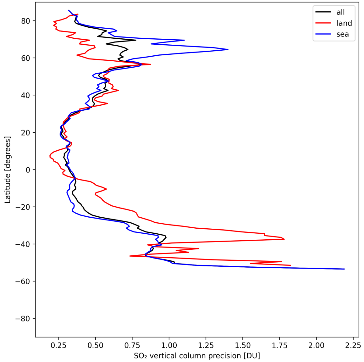
Figure 33: Zonal average of “SO 2 vertical column precision” for 2025-08-09 to 2025-08-11.
