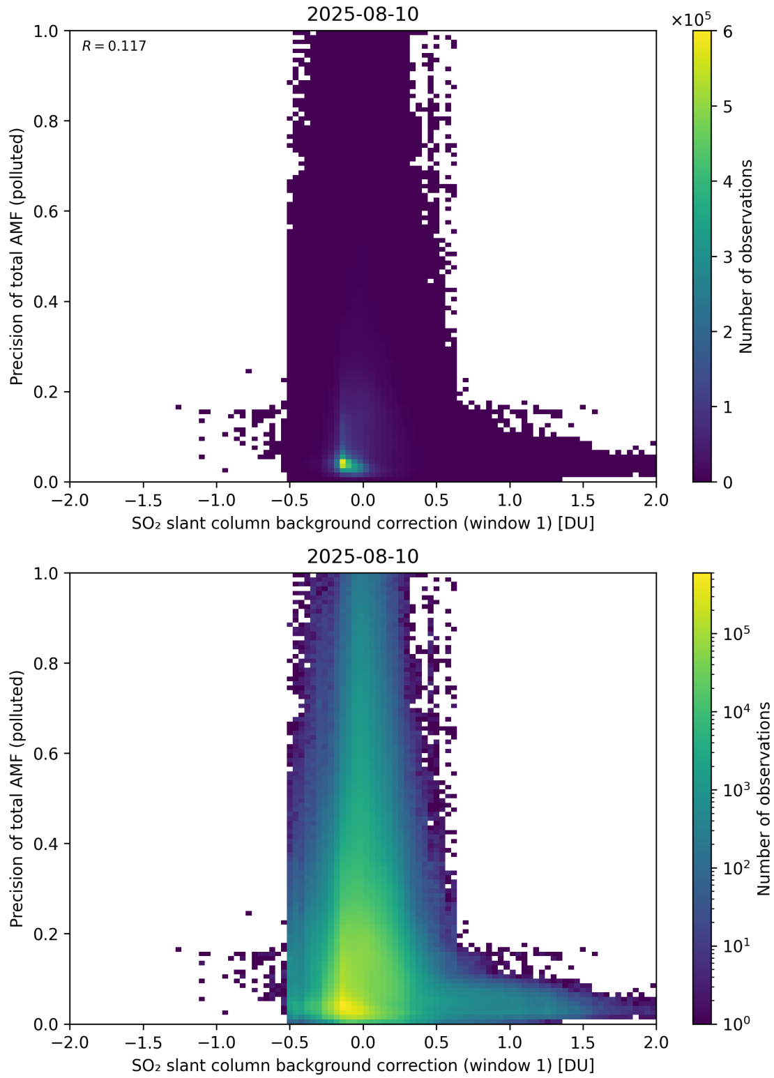
Figure 121: Scatter density plot of “SO 2 slant column background correction (window 1)” against “Precision of total AMF (polluted)” for 2025-08-09 to 2025-08-11.
