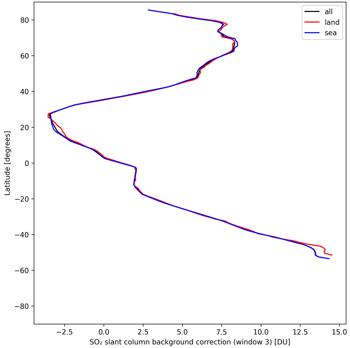
Figure 48: Zonal average of “SO 2 slant column background correction (window 3)” for 2025-08-09 to 2025-08-11.
