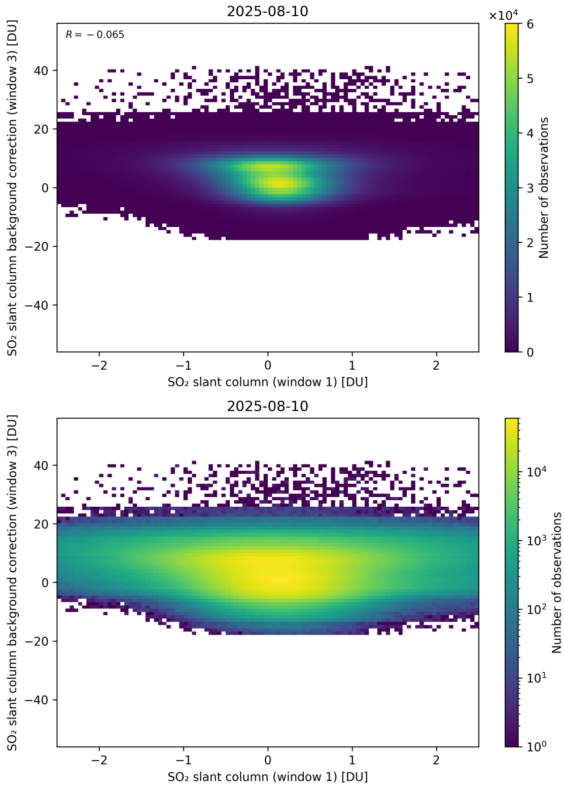
Figure 264: Scatter density plot of “SO 2 slant column (window 1)” against “SO 2 slant column background correction (window 3)” for 2025-08-09 to 2025-08-11.
