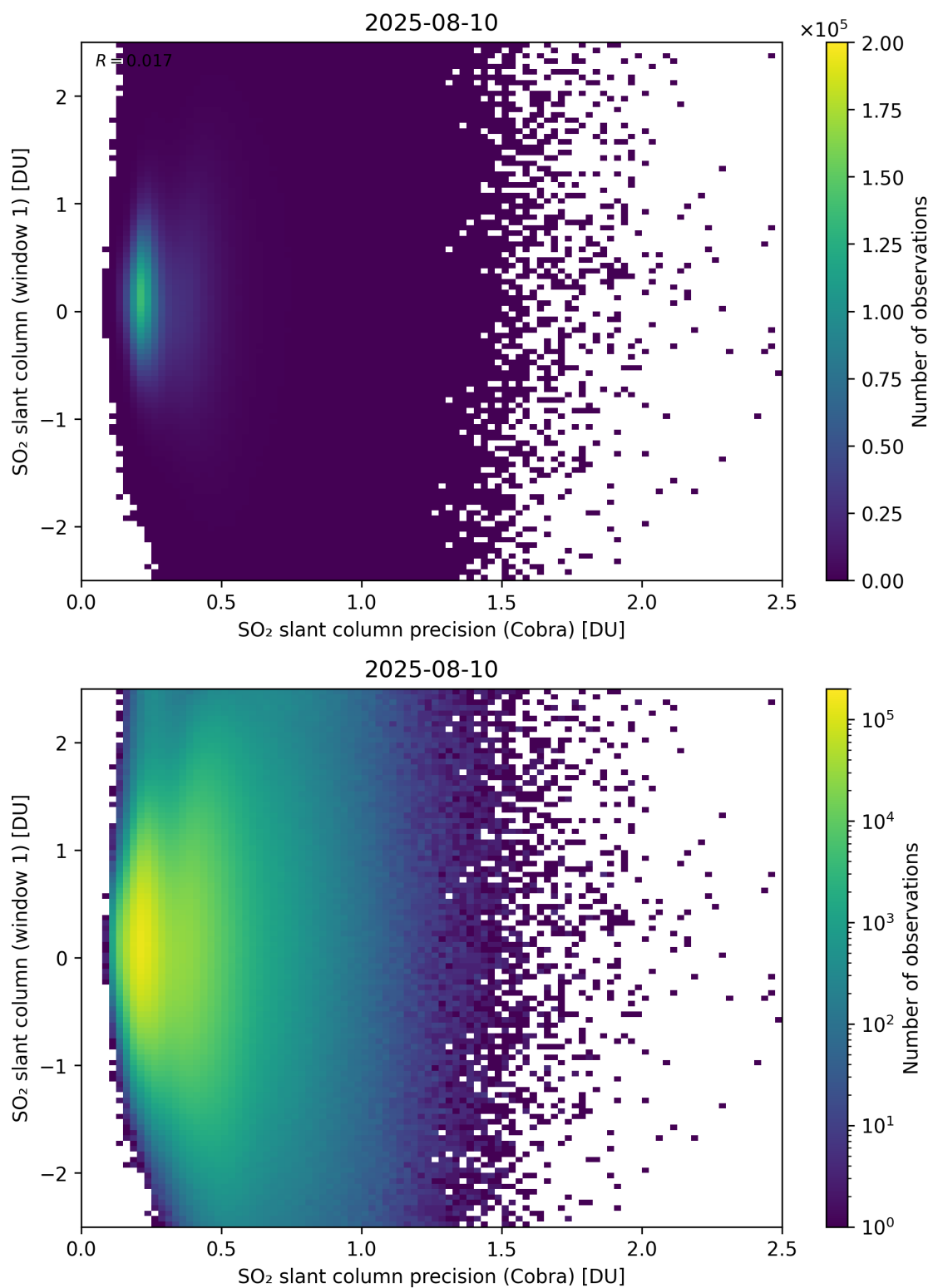
Figure 208: Scatter density plot of “SO 2 slant column precision (Cobra)” against “SO 2 slant column (window 1)” for 2025-08-09 to 2025-08-11.
