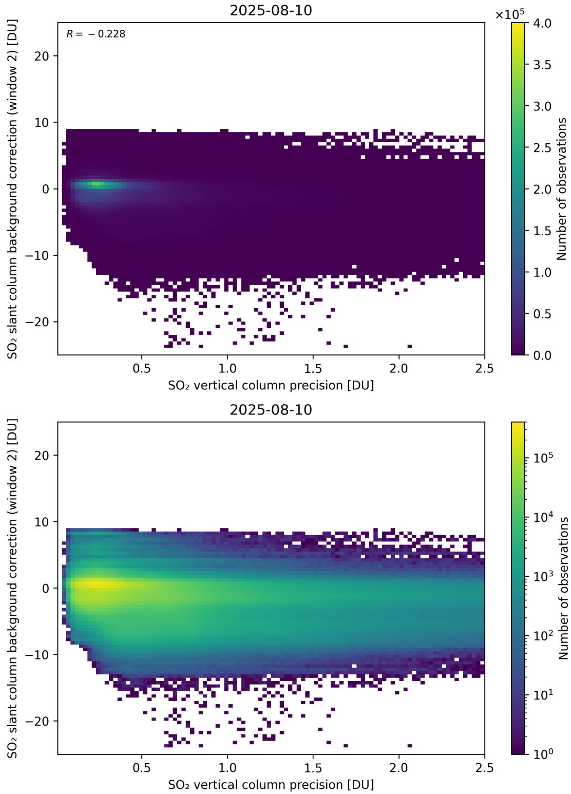
Figure 330: Scatter density plot of “SO 2 vertical column precision” against “SO 2 slant column background correction (window 2)” for 2025-08-09 to 2025-08-11.
