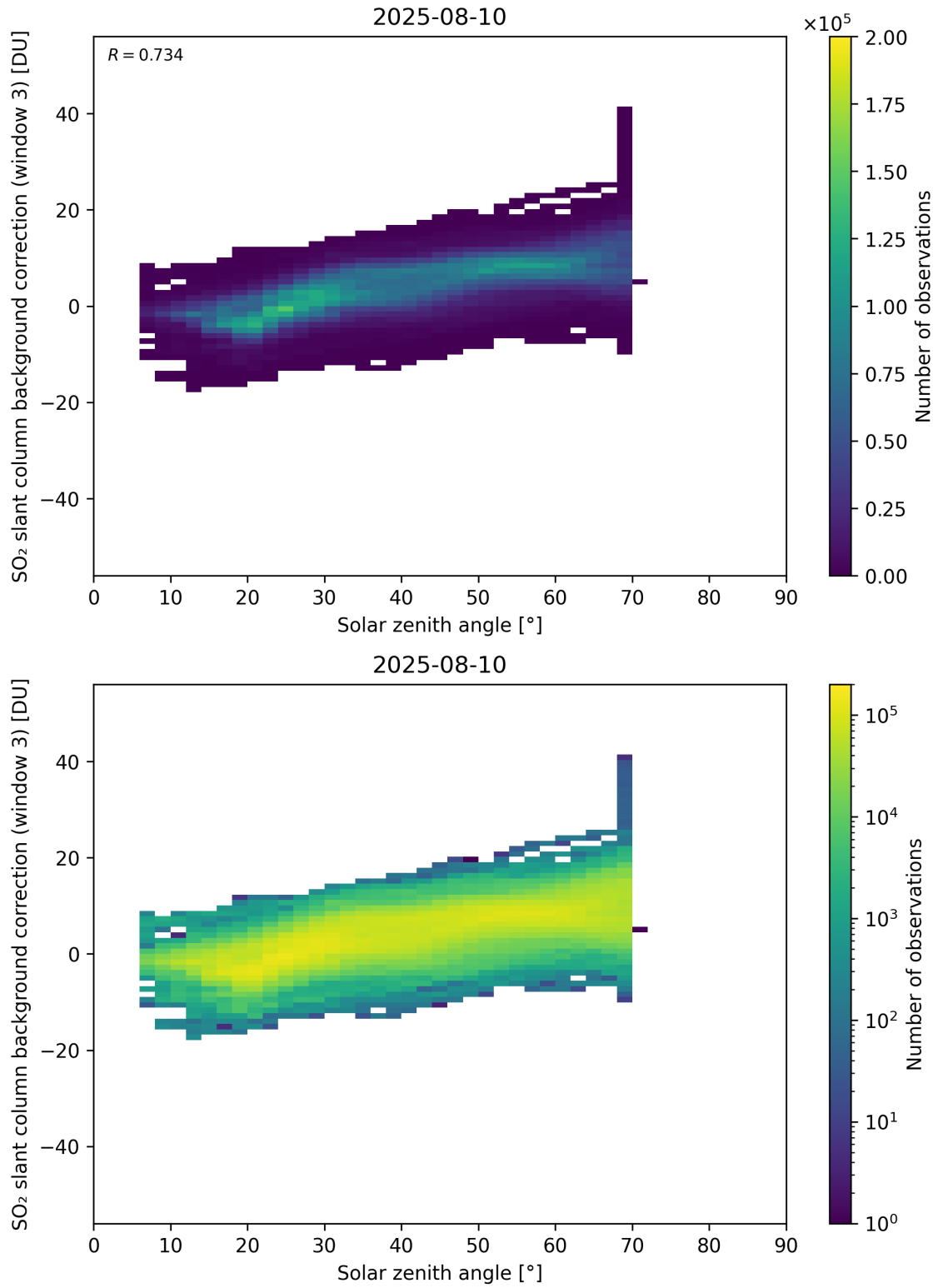
Figure 173: Scatter density plot of “Solar zenith angle” against “SO 2 slant column background correction (window 3)” for 2025-08-09 to 2025-08-11.
