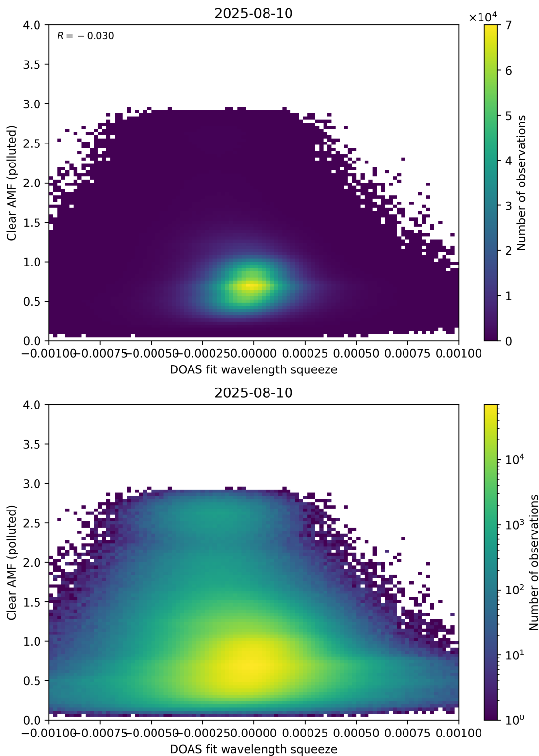
Figure 144: Scatter density plot of “DOAS fit wavelength squeeze” against “Clear AMF (polluted)” for 2025-08-09 to 2025-08-11.
