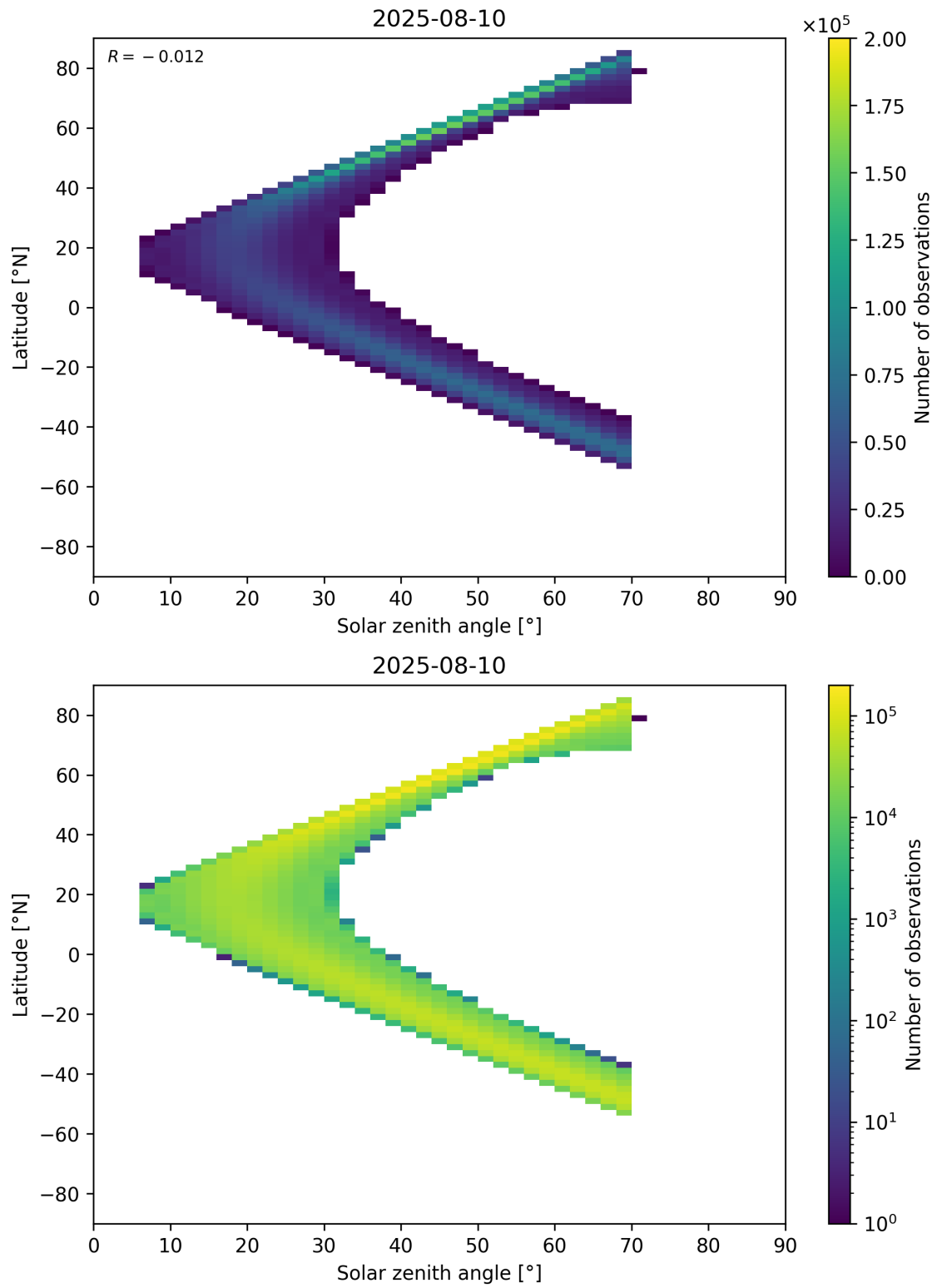
Figure 177: Scatter density plot of “Solar zenith angle” against “Latitude” for 2025-08-09 to 2025-08-11.
