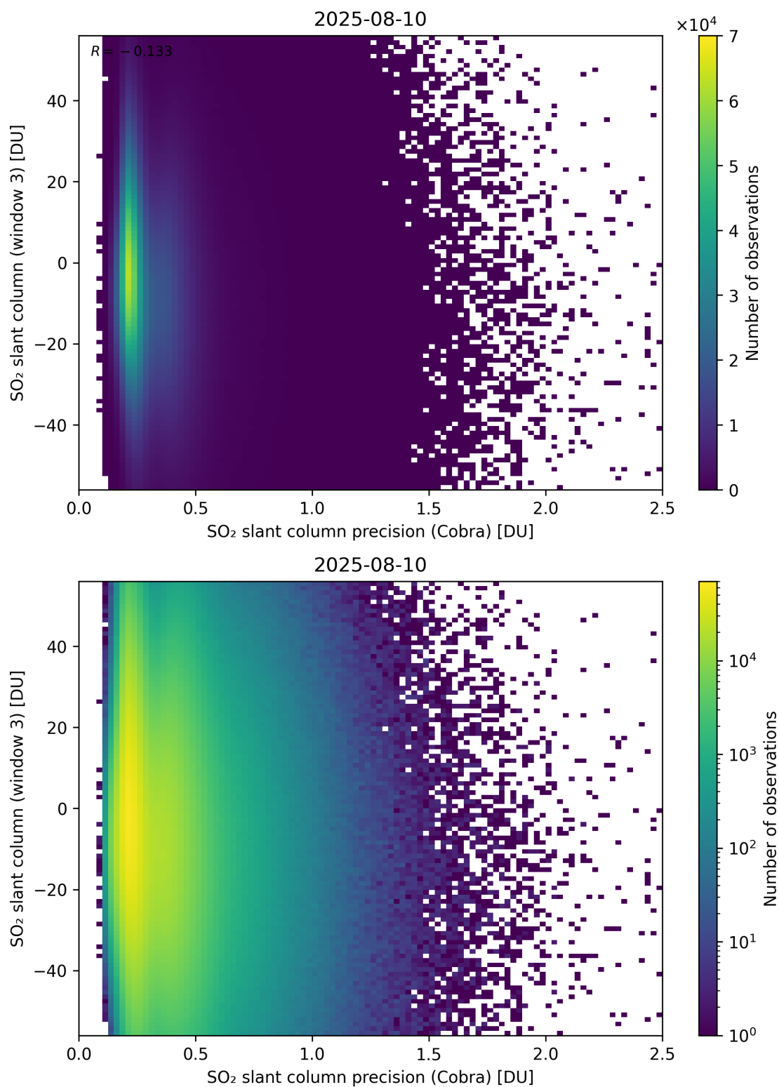
Figure 211: Scatter density plot of “SO 2 slant column precision (Cobra)” against “SO 2 slant column (window 3)” for 2025-08-09 to 2025-08-11.
