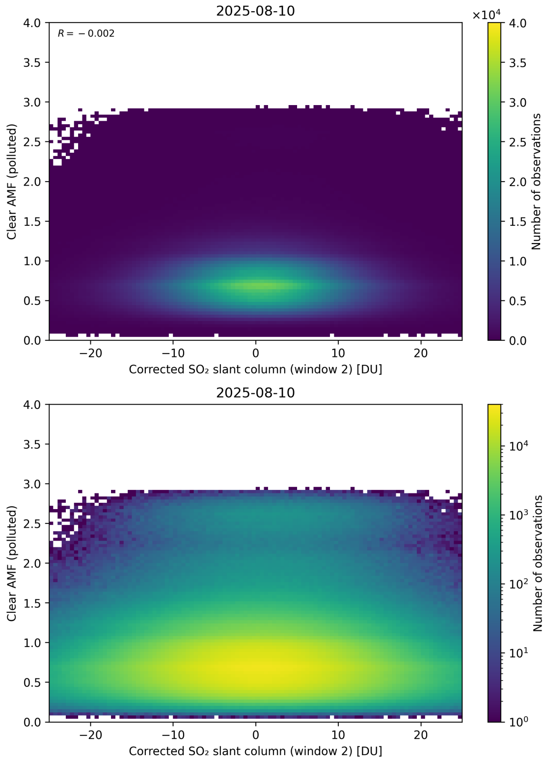
Figure 249: Scatter density plot of “Corrected SO 2 slant column (window 2)” against “Clear AMF (polluted)” for 2025-08-09 to 2025-08-11.
