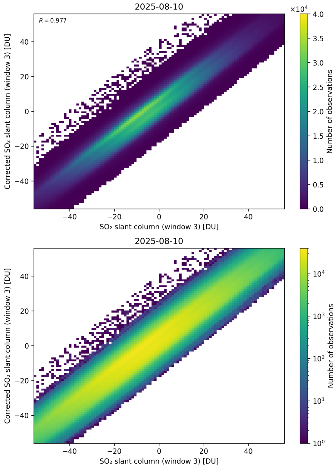
Figure 316: Scatter density plot of “SO 2 slant column (window 3)” against “Corrected SO 2 slant column (window 3)” for 2025-08-09 to 2025-08-11.
