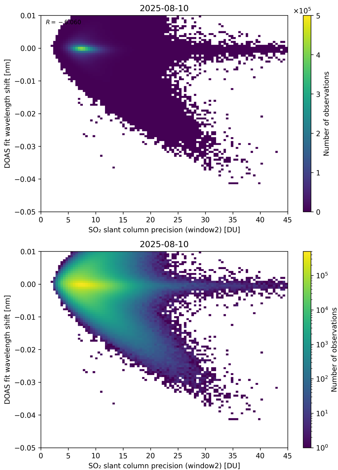
Figure 293: Scatter density plot of “SO 2 slant column precision (window2)” against “DOAS fit wavelength shift” for 2025-08-09 to 2025-08-11.
