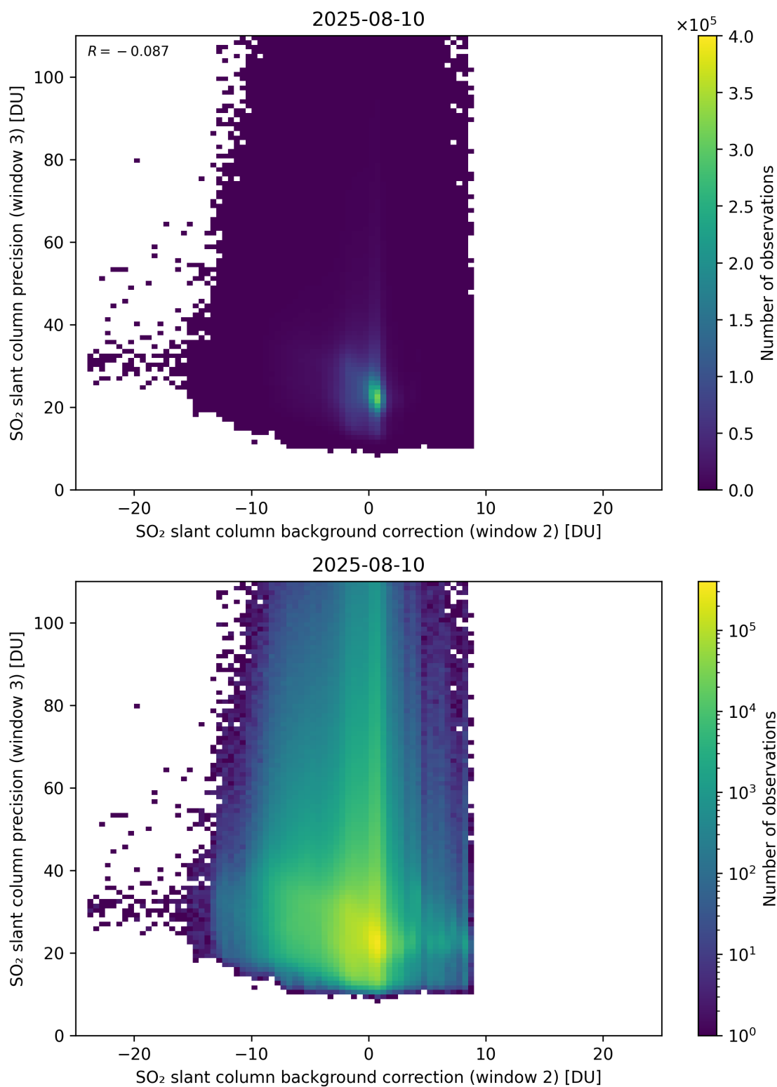
Figure 129: Scatter density plot of “SO 2 slant column background correction (window 2)” against “SO 2 slant column precision (window 3)” for 2025-08-09 to 2025-08-11.
