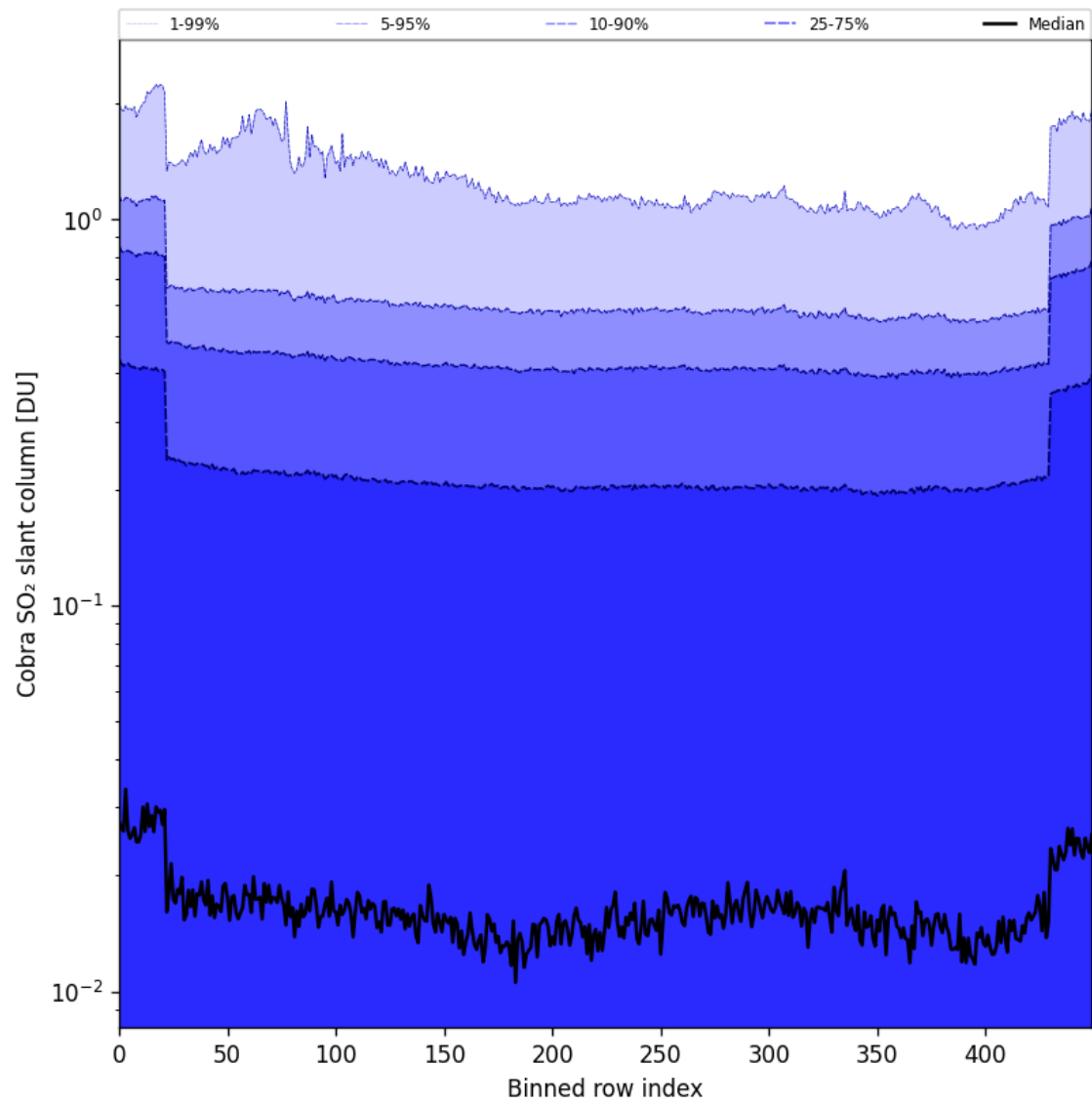
Figure 87: Along track statistics of “Cobra SO 2 slant column” for 2025-08-09 to 2025-08-11
