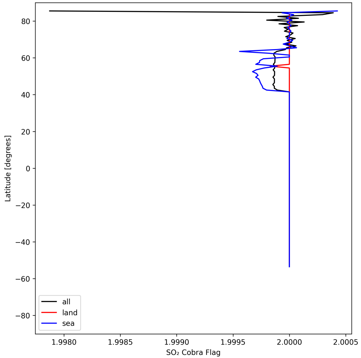
Figure 49: Zonal average of "SO 2 Cobra Flag" for 2025-08-09 to 2025-08-11.
