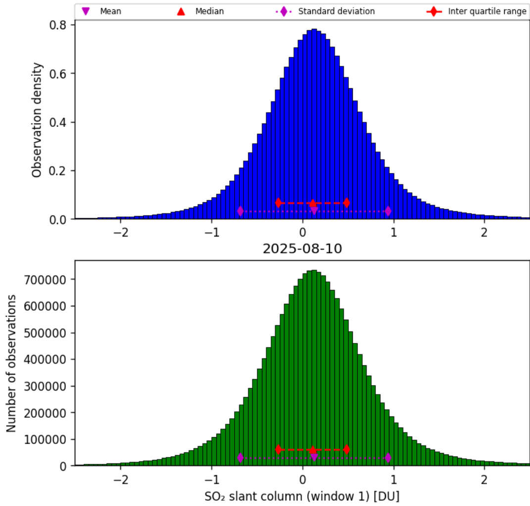
Figure 63: Histogram of “SO 2 slant column (window 1)” for 2025-08-09 to 2025-08-11
