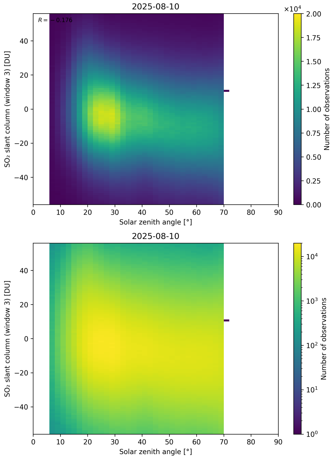
Figure 187: Scatter density plot of “Solar zenith angle” against “SO 2 slant column (window 3)” for 2025-08-09 to 2025-08-11.
