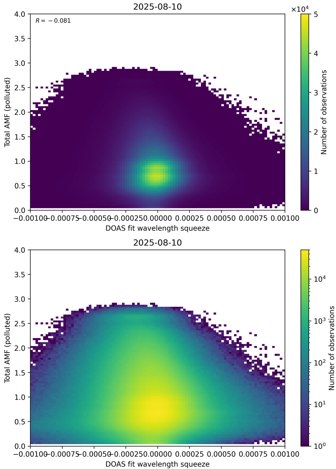
Figure 145: Scatter density plot of “DOAS fit wavelength squeeze” against “Total AMF (polluted)” for 2025-08-09 to 2025-08-11.
