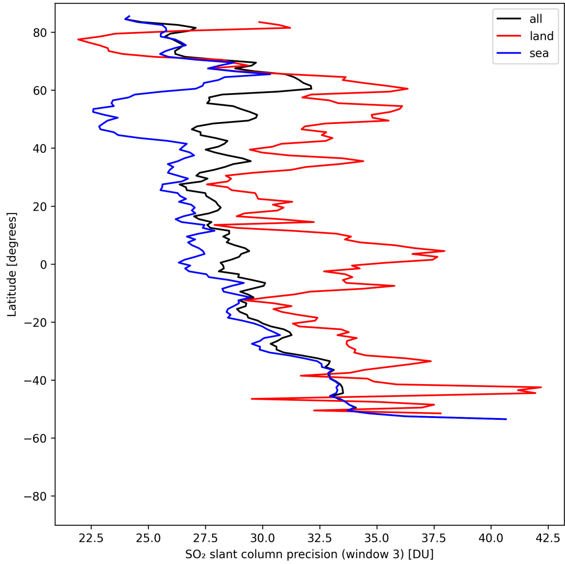
Figure 46: Zonal average of “SO 2 slant column precision (window 3)” for 2025-08-09 to 2025-08-11.
