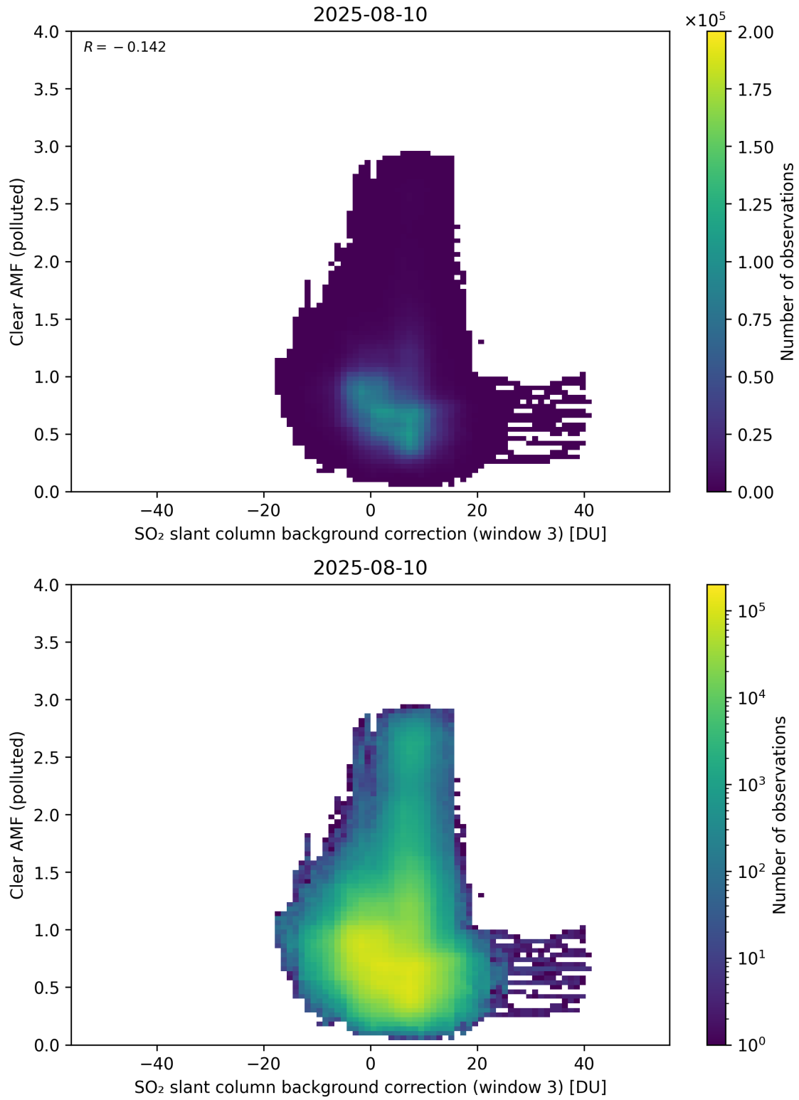
Figure 135: Scatter density plot of “SO 2 slant column background correction (window 3)” against “Clear AMF (polluted)” for 2025-08-09 to 2025-08-11.
