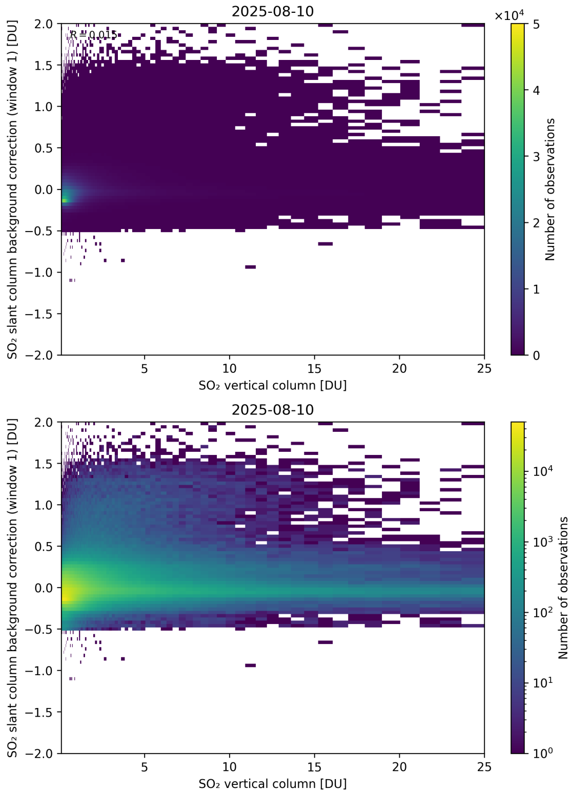
Figure 323: Scatter density plot of “SO 2 vertical column” against “SO 2 slant column background correction (window 1)” for 2025-08-09 to 2025-08-11.
