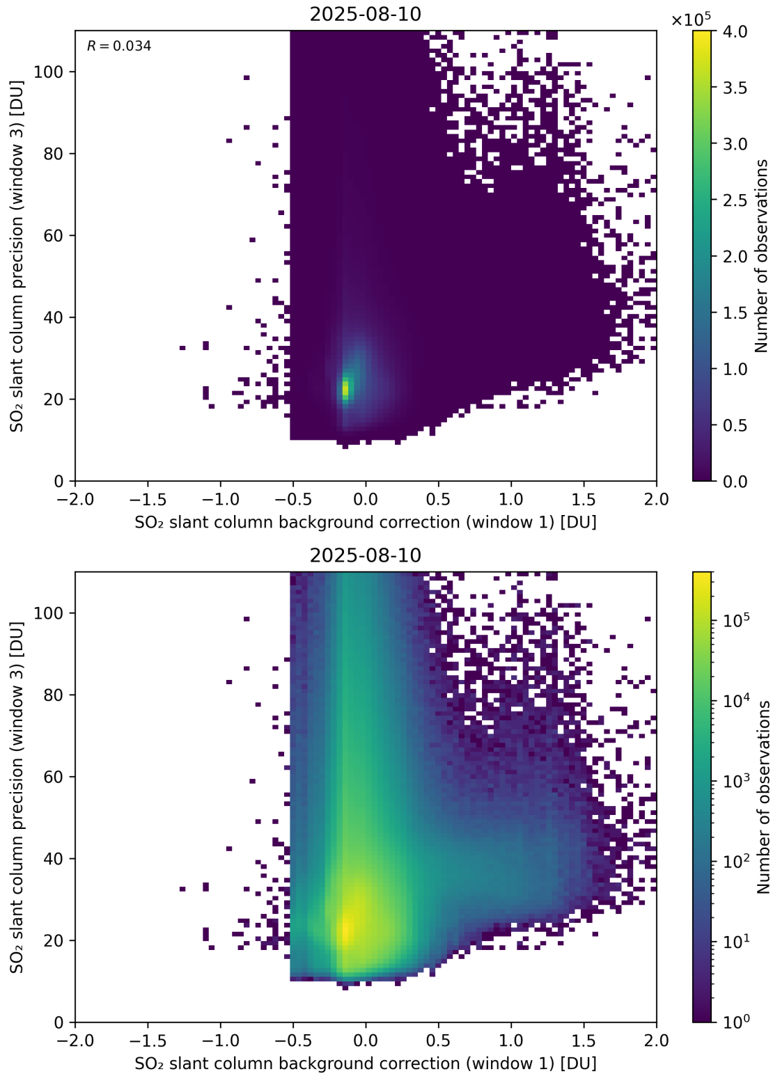
Figure 119: Scatter density plot of “SO 2 slant column background correction (window 1)” against “SO 2 slant column precision (window 3)” for 2025-08-09 to 2025-08-11.
