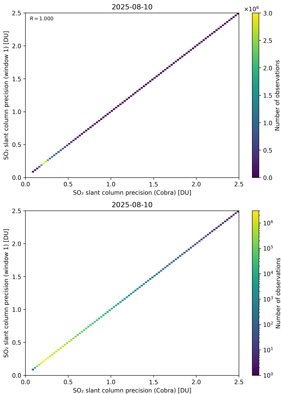
Figure 209: Scatter density plot of “SO 2 slant column precision (Cobra)” against “SO 2 slant column precision (window 1)” for 2025-08-09 to 2025-08-11.
