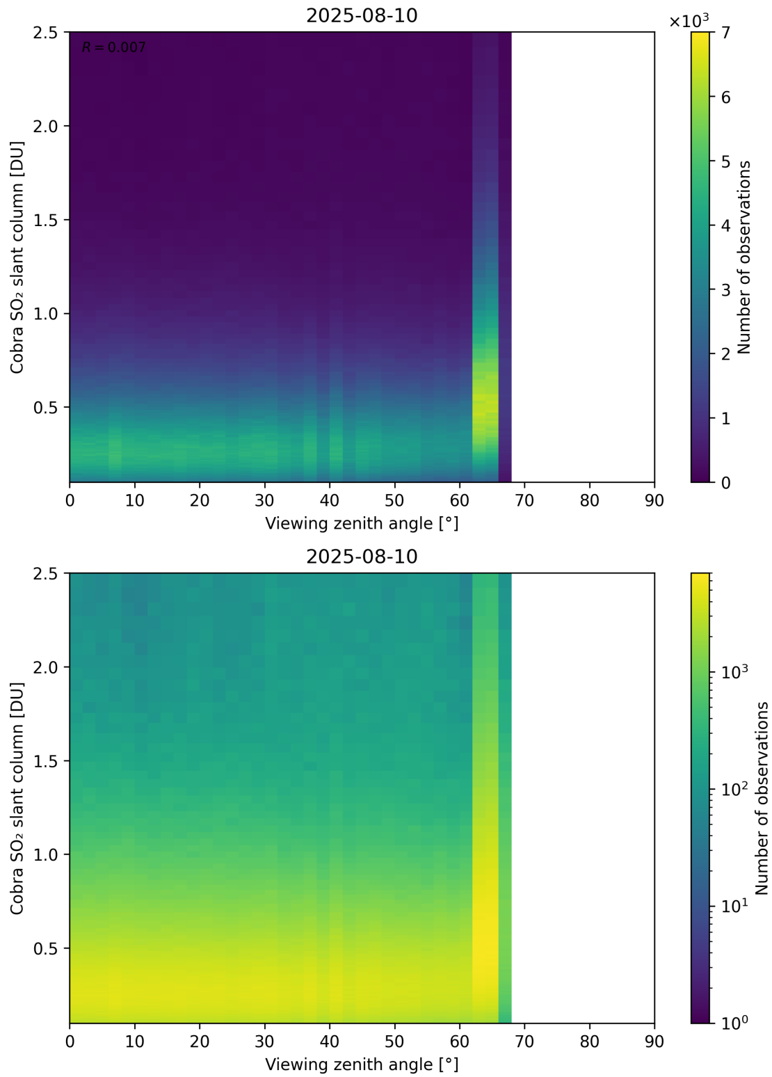
Figure 371: Scatter density plot of “Viewing zenith angle” against “Cobra SO 2 slant column” for 2025-08-09 to 2025-08-11.
