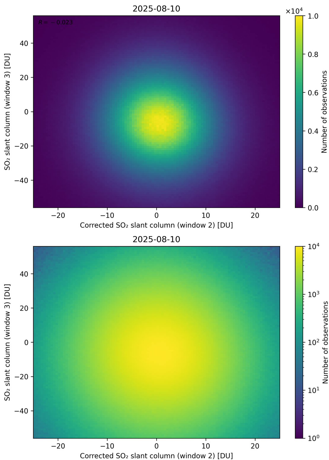
Figure 251: Scatter density plot of “Corrected SO 2 slant column (window 2)” against “SO 2 slant column (window 3)” for 2025-08-09 to 2025-08-11.
