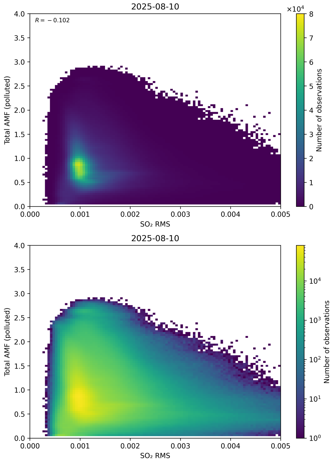
Figure 148: Scatter density plot of “SO 2 RMS” against “Total AMF (polluted)” for 2025-08-09 to 2025-08-11.
