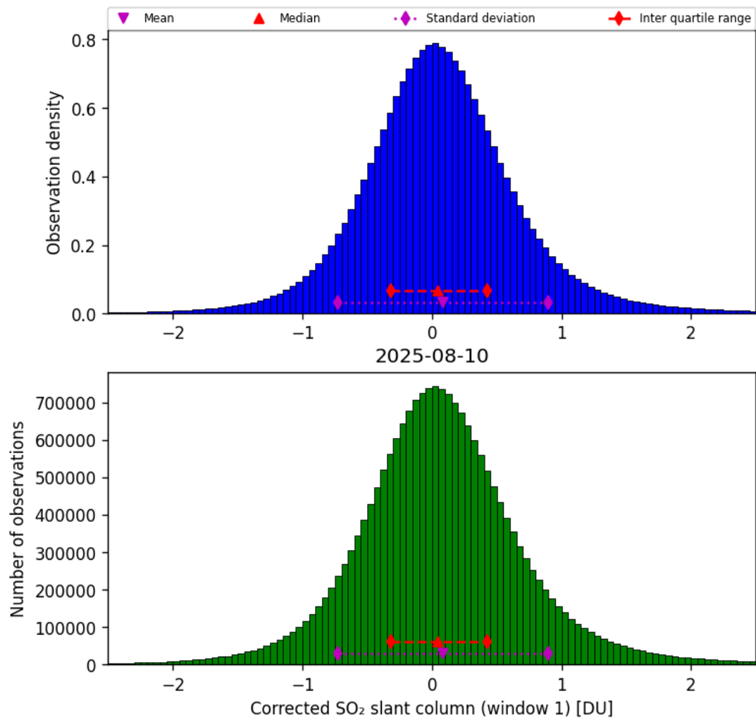
Figure 65: Histogram of “Corrected SO 2 slant column (window 1)” for 2025-08-09 to 2025-08-11
