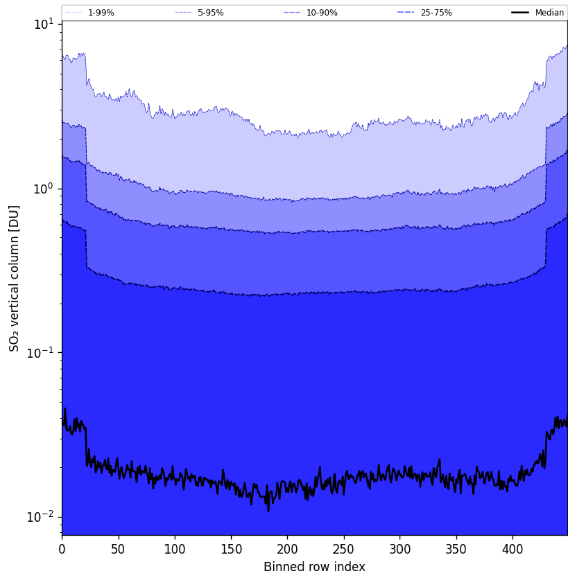
Figure 84: Along track statistics of “SO 2 vertical column” for 2025-08-09 to 2025-08-11
