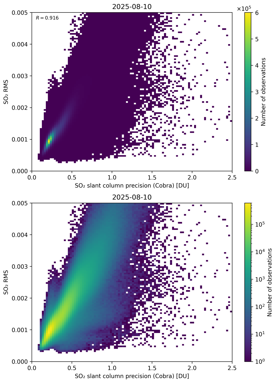
Figure 204: Scatter density plot of “SO 2 slant column precision (Cobra)” against “SO 2 RMS” for 2025-08-09 to 2025-08-11.
