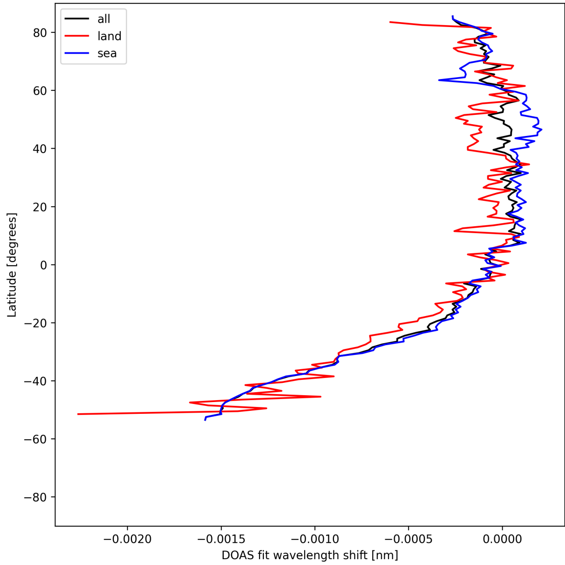
Figure 50: Zonal average of “DOAS fit wavelength shift” for 2025-08-09 to 2025-08-11.
