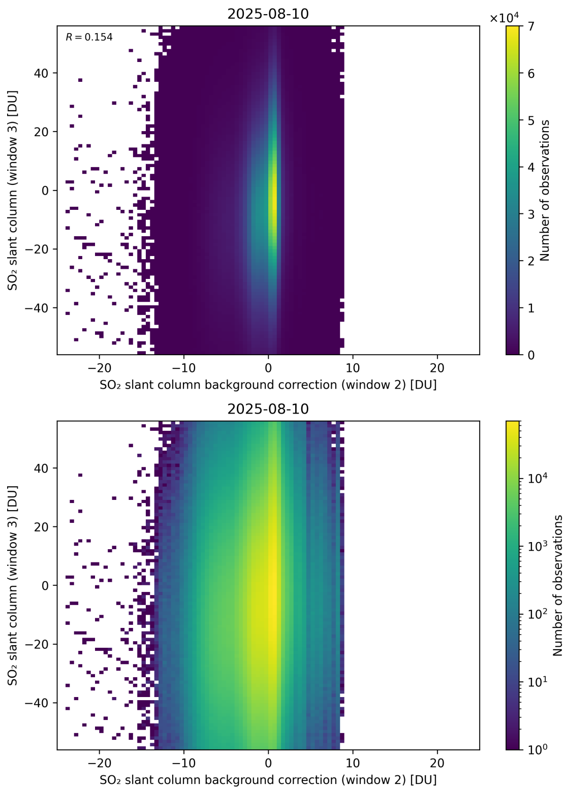
Figure 128: Scatter density plot of “SO 2 slant column background correction (window 2)” against “SO 2 slant column (window 3)” for 2025-08-09 to 2025-08-11.
