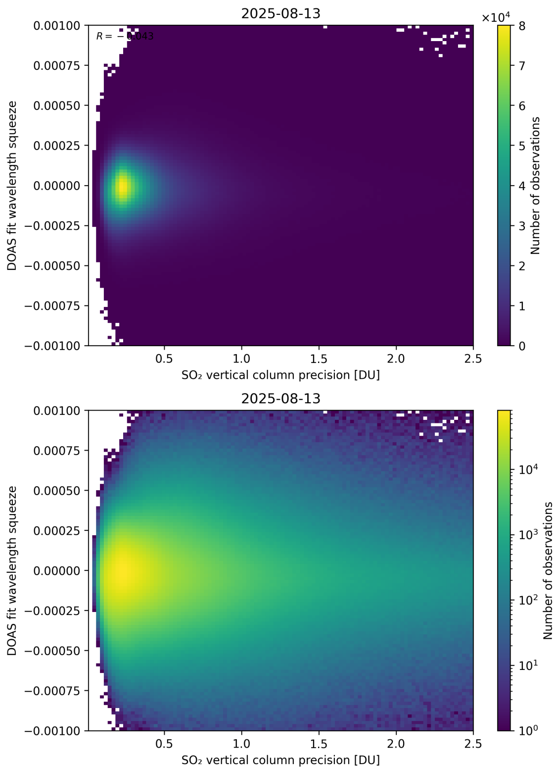
Figure 333: Scatter density plot of “SO 2 vertical column precision” against “DOAS fit wavelength squeeze” for 2025-08-12 to 2025-08-14.
