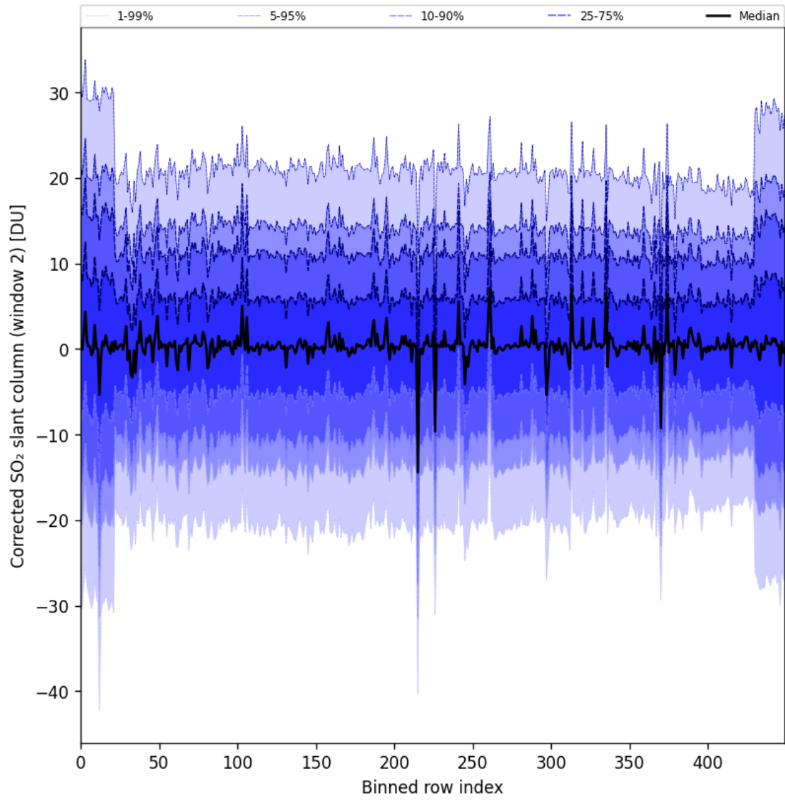
Figure 95: Along track statistics of “Corrected SO 2 slant column (window 2)” for 2025-08-12 to 2025-08-14
