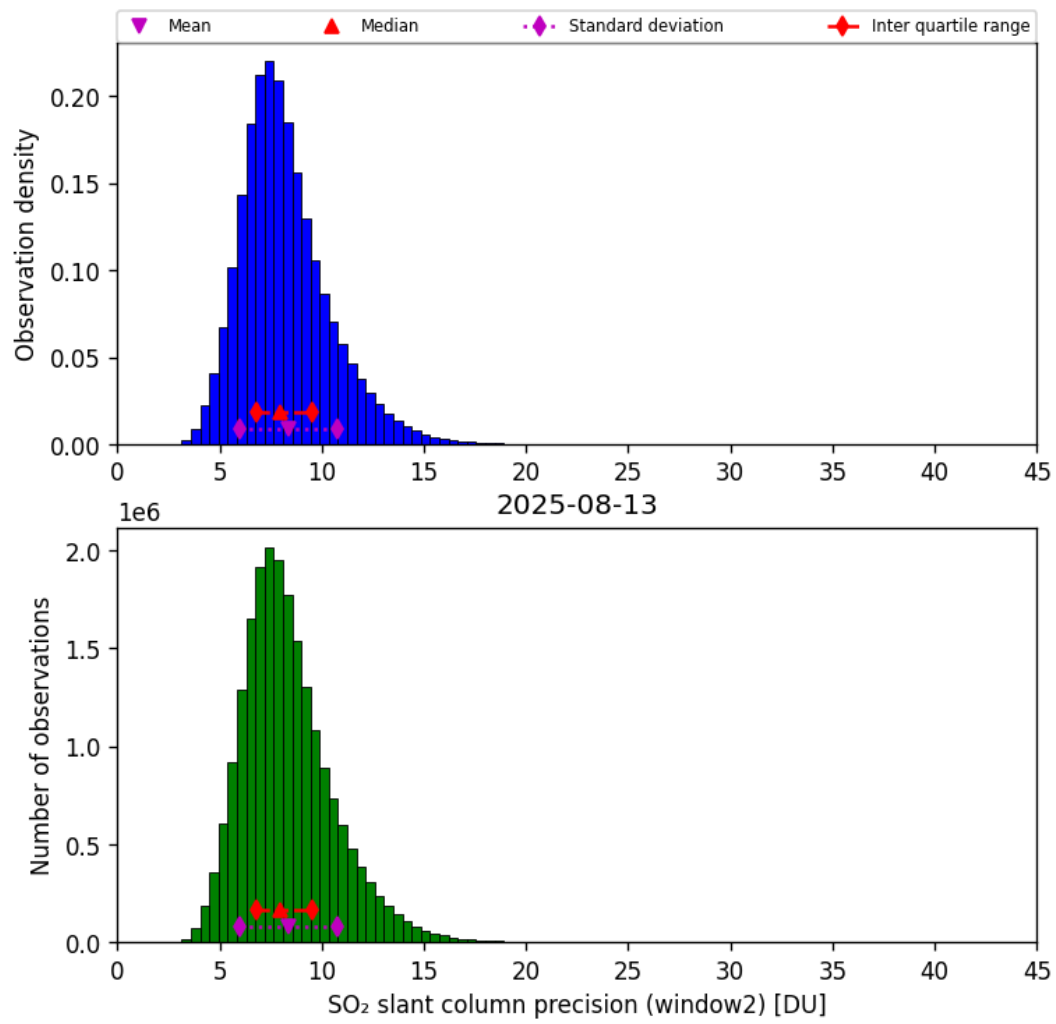
Figure 68: Histogram of “SO 2 slant column precision (window2)” for 2025-08-12 to 2025-08-14
