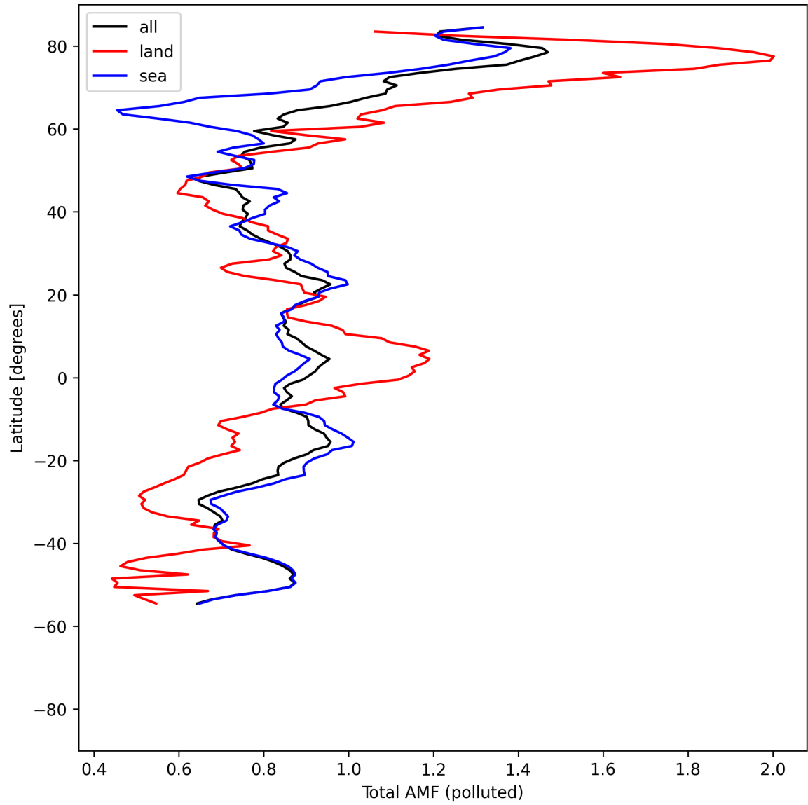
Figure 53: Zonal average of “Total AMF (polluted)” for 2025-08-12 to 2025-08-14.
