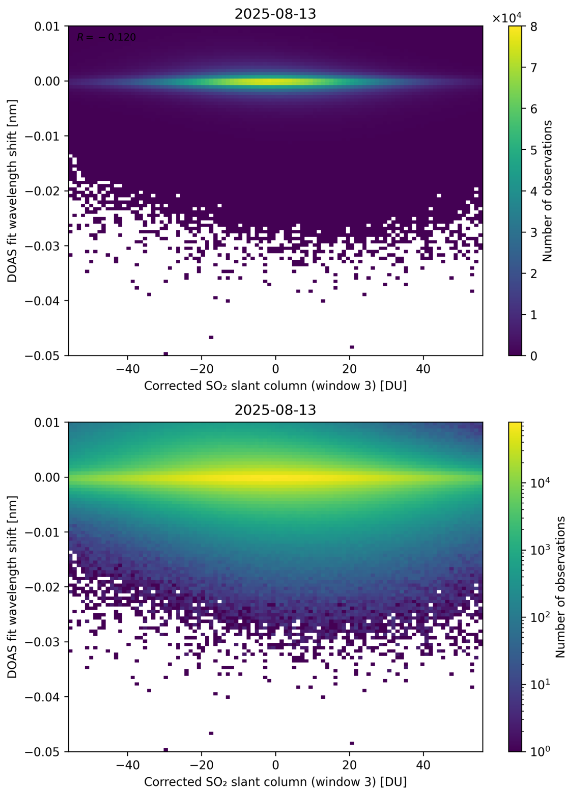
Figure 256: Scatter density plot of “Corrected SO 2 slant column (window 3)” against “DOAS fit wavelength shift” for 2025-08-12 to 2025-08-14.
