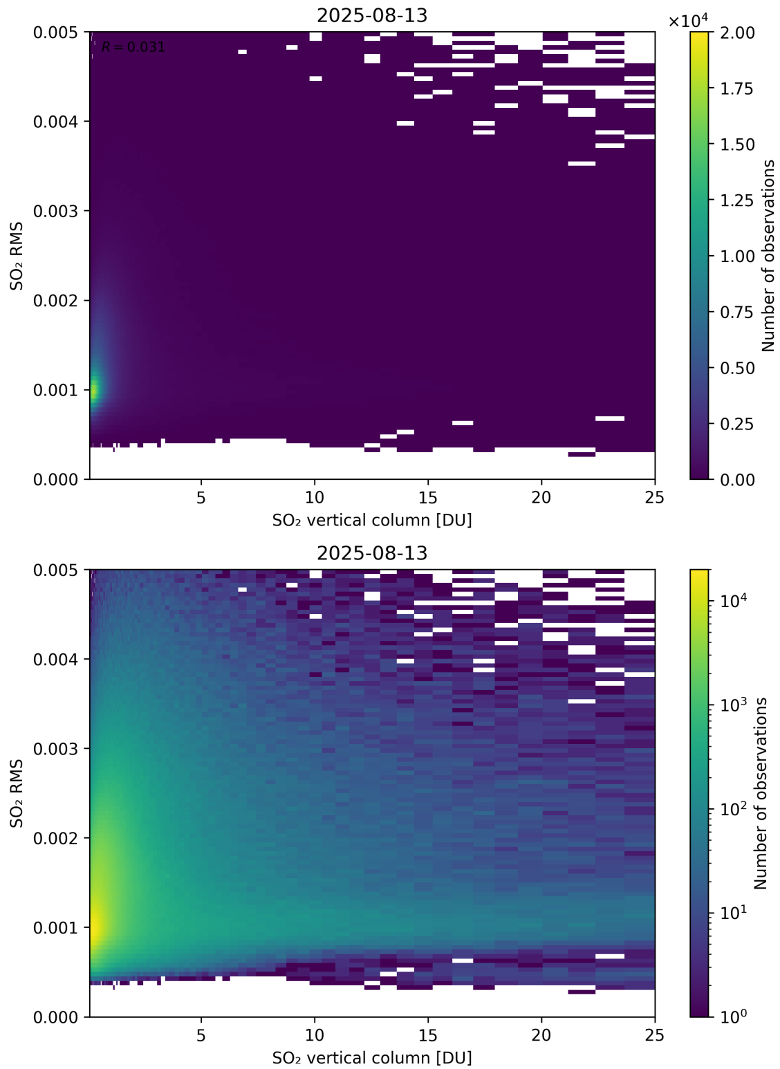
Figure 328: Scatter density plot of “SO 2 vertical column” against “SO 2 RMS” for 2025-08-12 to 2025-08-14.
