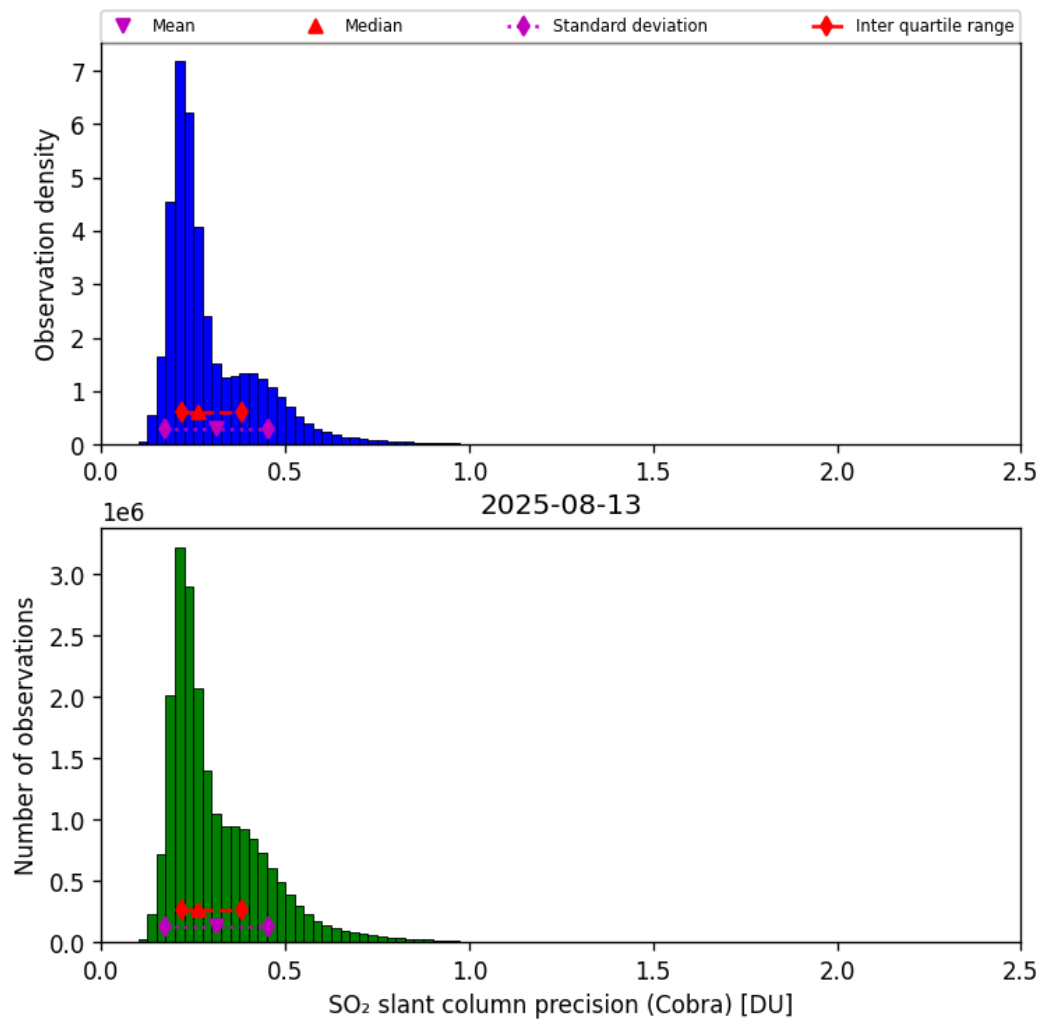
Figure 62: Histogram of “SO 2 slant column precision (Cobra)” for 2025-08-12 to 2025-08-14
