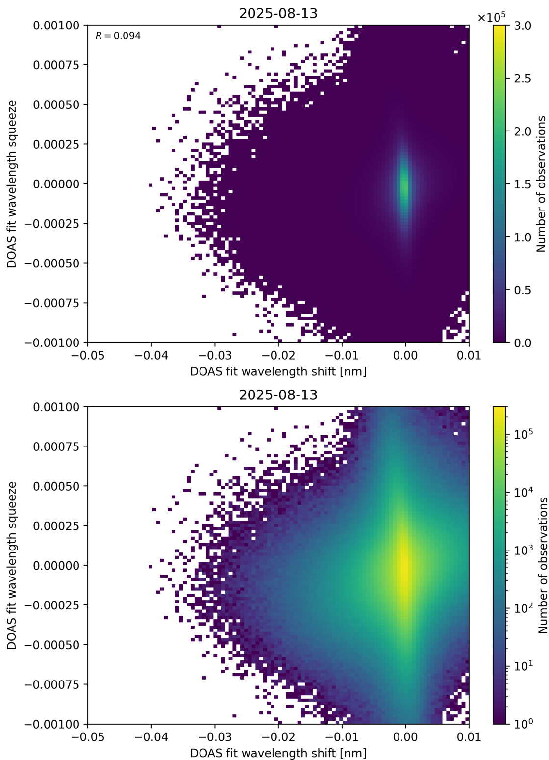
Figure 138: Scatter density plot of “DOAS fit wavelength shift” against “DOAS fit wavelength squeeze” for 2025-08-12 to 2025-08-14.
