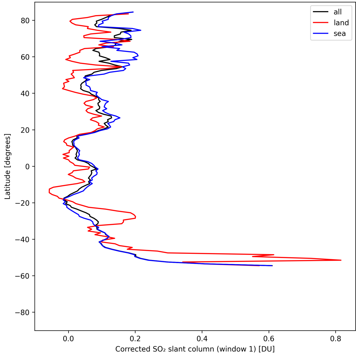
Figure 39: Zonal average of “Corrected SO 2 slant column (window 1)” for 2025-08-12 to 2025-08-14.
