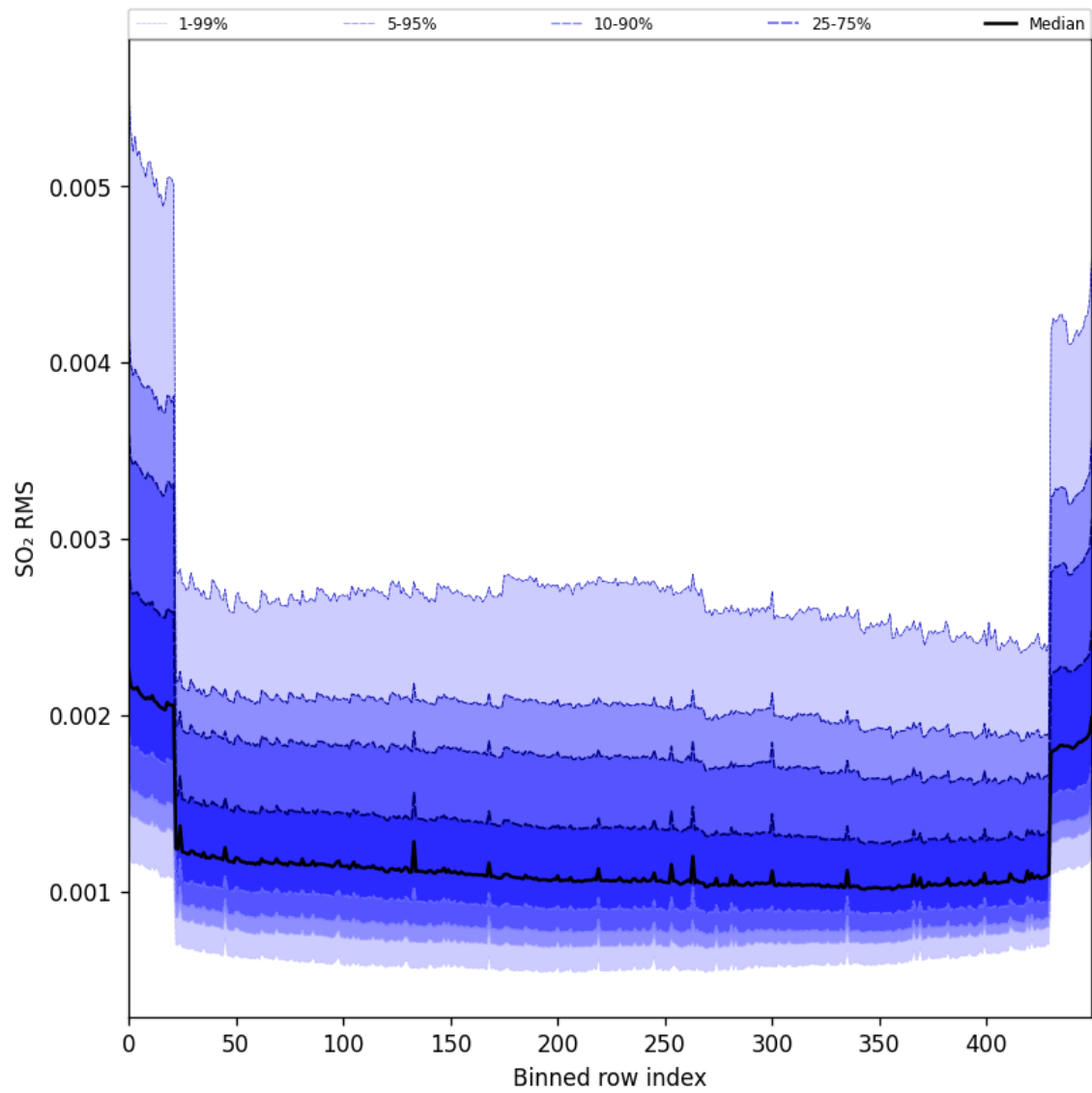
Figure 104: Along track statistics of “SO 2 RMS” for 2025-08-12 to 2025-08-14
