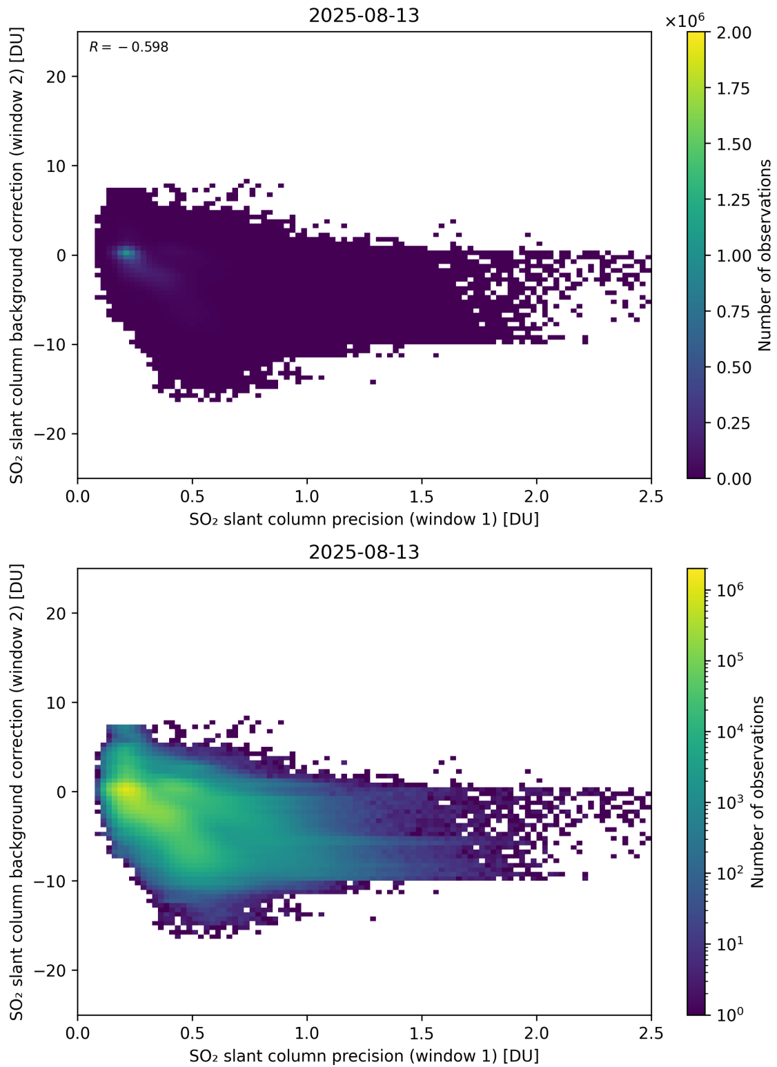
Figure 269: Scatter density plot of “SO 2 slant column precision (window 1)” against “SO 2 slant column background correction (window 2)” for 2025-08-12 to 2025-08-14.
