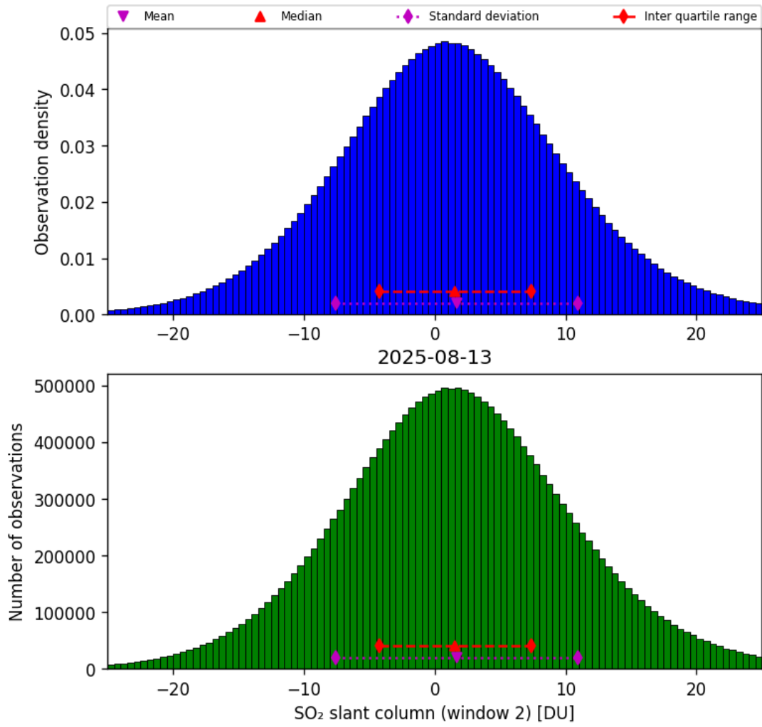
Figure 67: Histogram of “SO 2 slant column (window 2)” for 2025-08-12 to 2025-08-14
