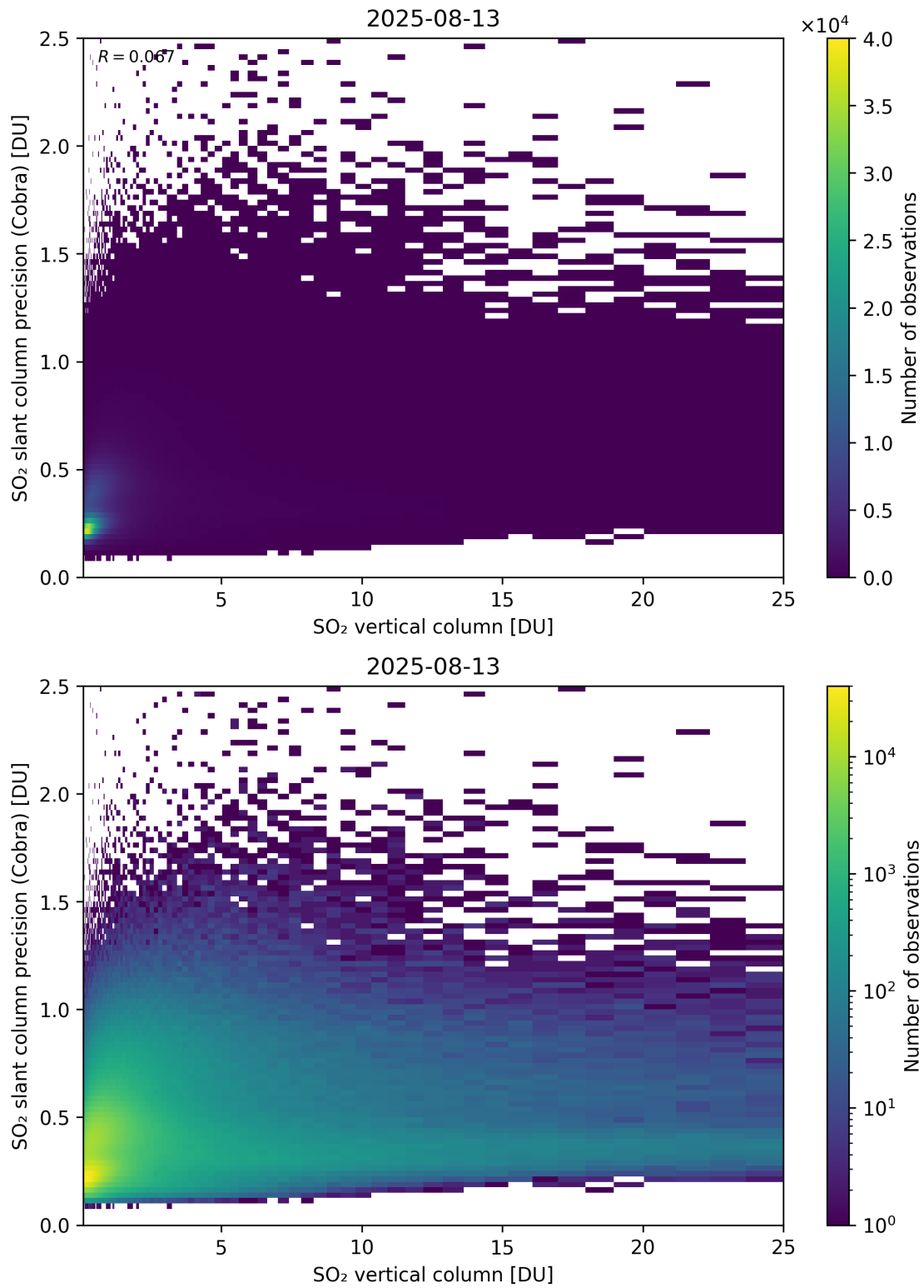
Figure 350: Scatter density plot of “SO 2 vertical column” against “SO 2 slant column precision (Cobra)” for 2025-08-12 to 2025-08-14.
