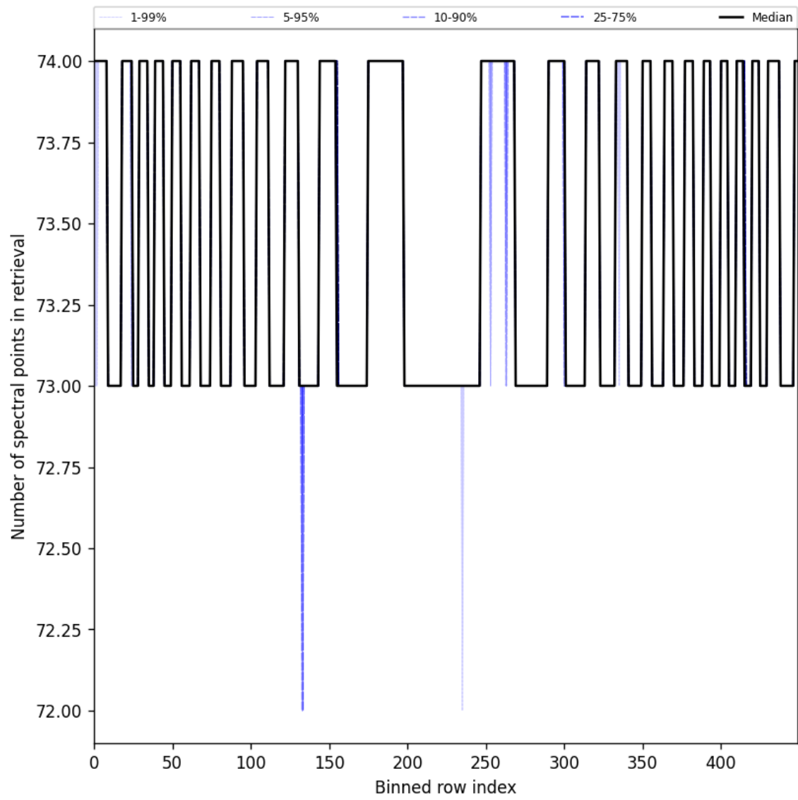
Figure 108: Along track statistics of “Number of spectral points in retrieval” for 2025-08-12 to 2025-08-14
