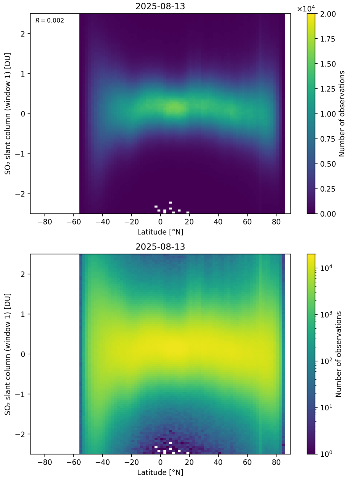
Figure 162: Scatter density plot of “Latitude” against “SO 2 slant column (window 1)” for 2025-08-12 to 2025-08-14.
