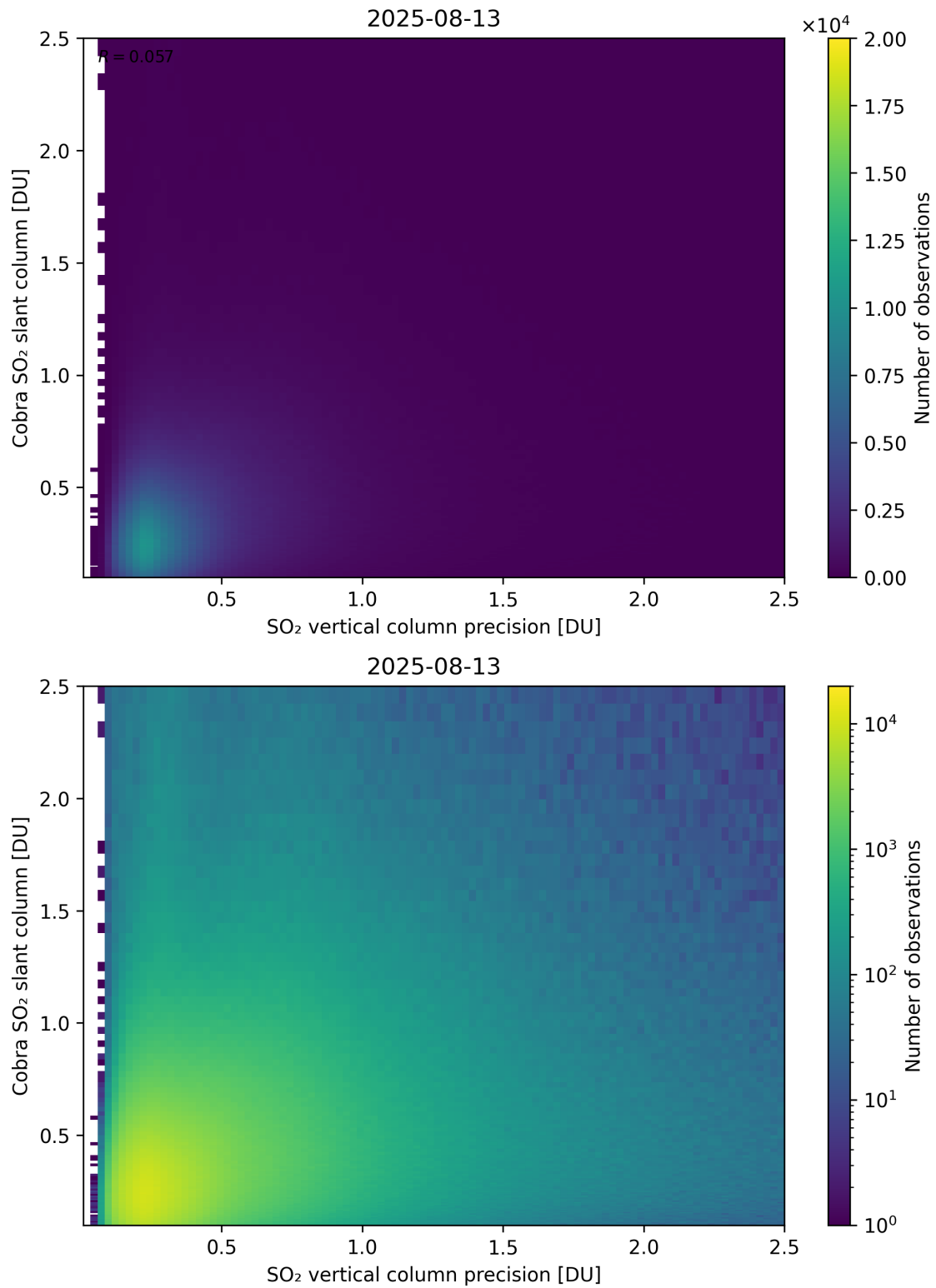
Figure 336: Scatter density plot of “SO 2 vertical column precision” against “Cobra SO 2 slant column” for 2025-08-12 to 2025-08-14.
