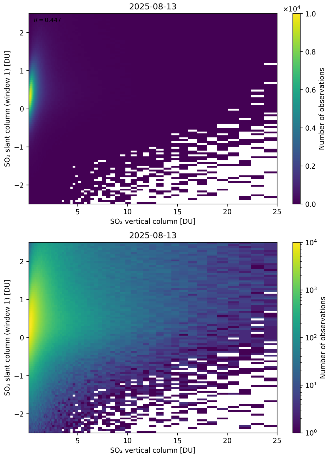
Figure 354: Scatter density plot of “SO 2 vertical column” against “SO 2 slant column (window 1)” for 2025-08-12 to 2025-08-14.
