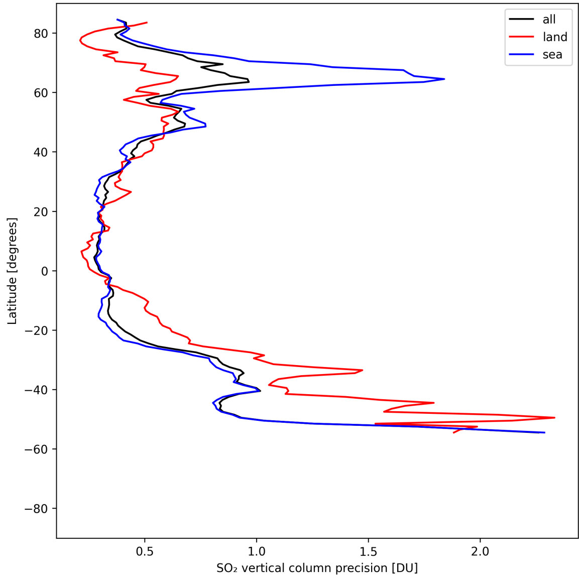
Figure 33: Zonal average of “SO 2 vertical column precision” for 2025-08-12 to 2025-08-14.
