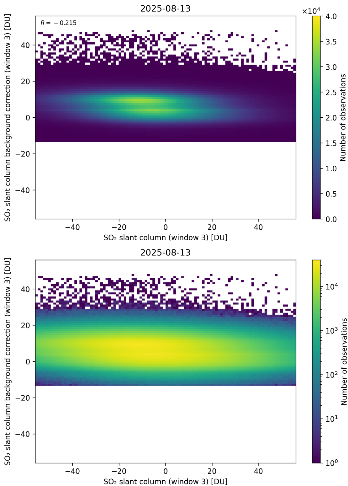
Figure 303: Scatter density plot of “SO 2 slant column (window 3)” against “SO 2 slant column background correction (window 3)” for 2025-08-12 to 2025-08-14.
