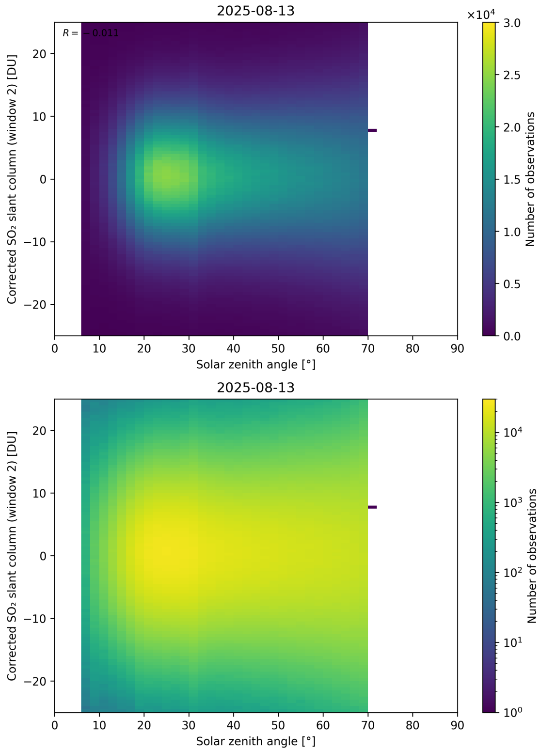
Figure 182: Scatter density plot of “Solar zenith angle” against “Corrected SO 2 slant column (window 2)” for 2025-08-12 to 2025-08-14.
