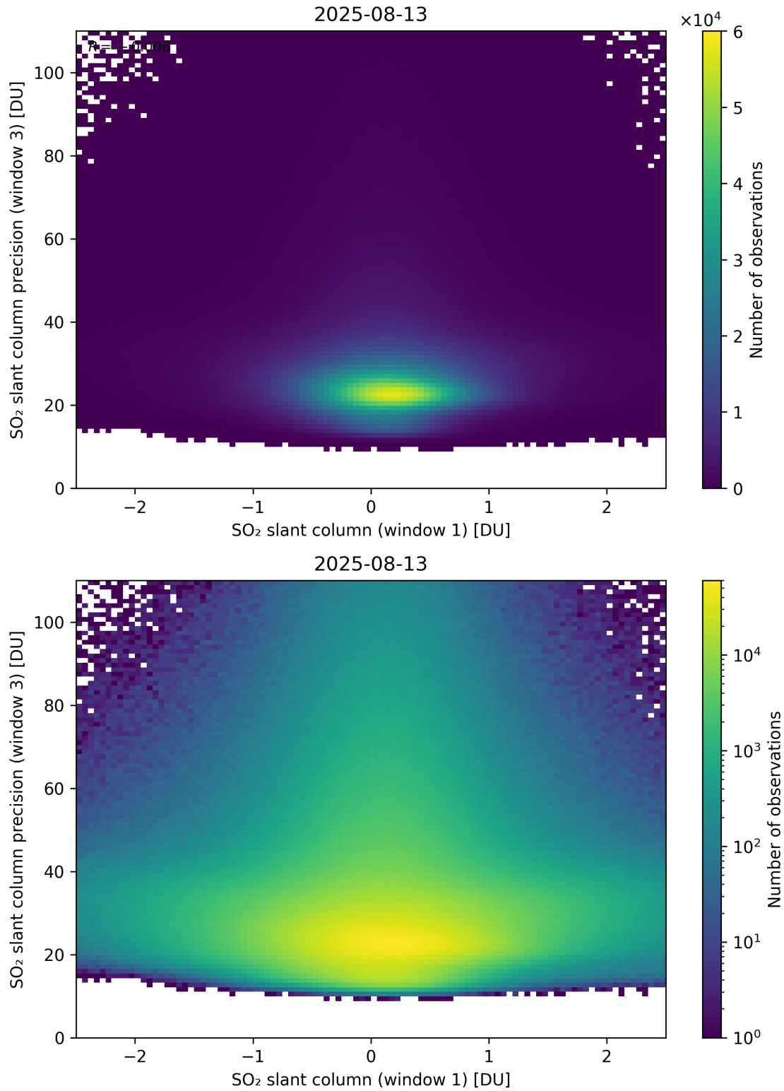
Figure 288: Scatter density plot of “SO 2 slant column (window 1)” against “SO 2 slant column precision (window 3)” for 2025-08-12 to 2025-08-14.
