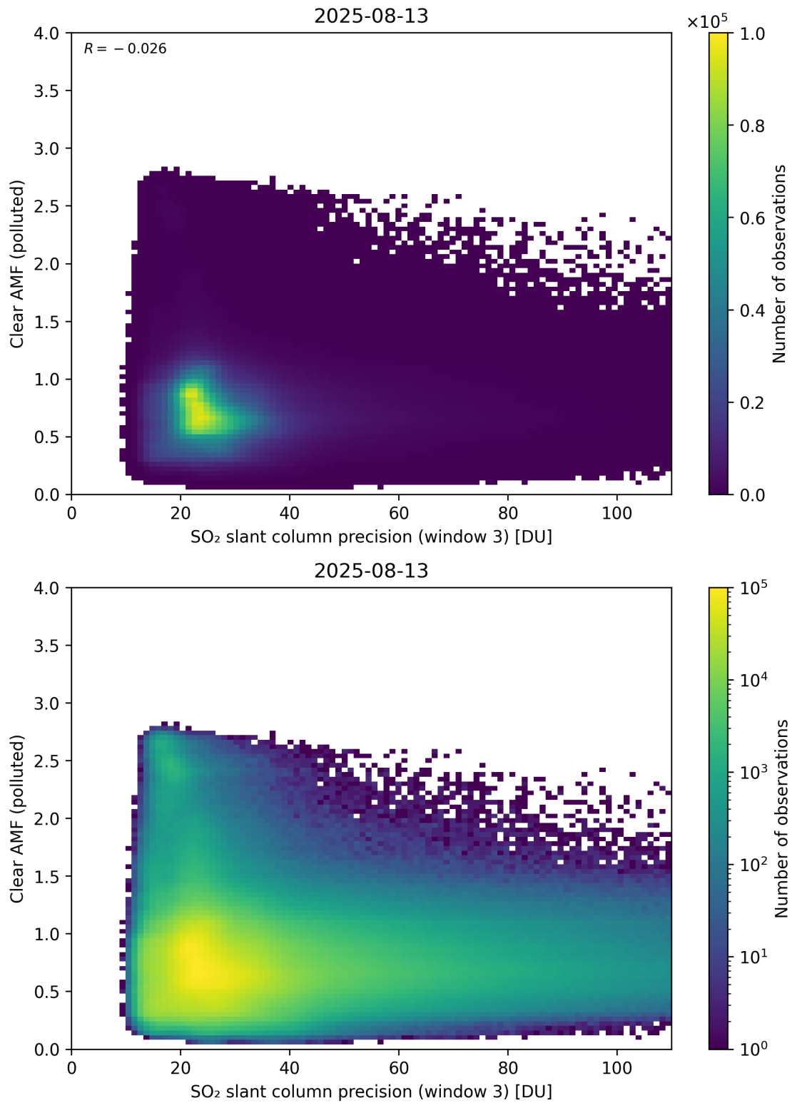
Figure 311: Scatter density plot of “SO 2 slant column precision (window 3)” against “Clear AMF (polluted)” for 2025-08-12 to 2025-08-14.
