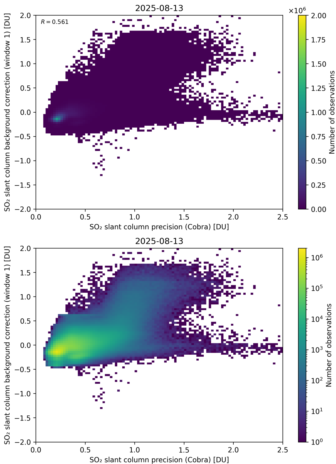
Figure 199: Scatter density plot of “SO 2 slant column precision (Cobra)” against “SO 2 slant column background correction (window 1)” for 2025-08-12 to 2025-08-14.
