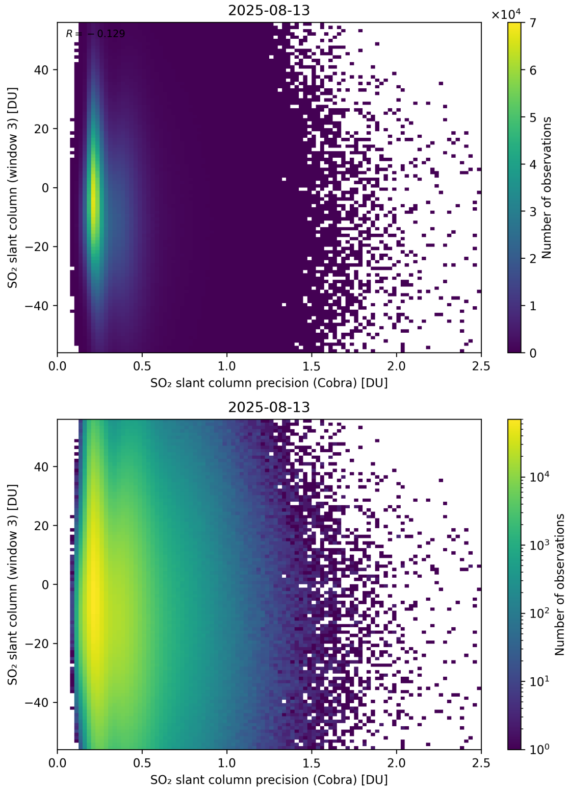
Figure 211: Scatter density plot of “SO 2 slant column precision (Cobra)” against “SO 2 slant column (window 3)” for 2025-08-12 to 2025-08-14.
