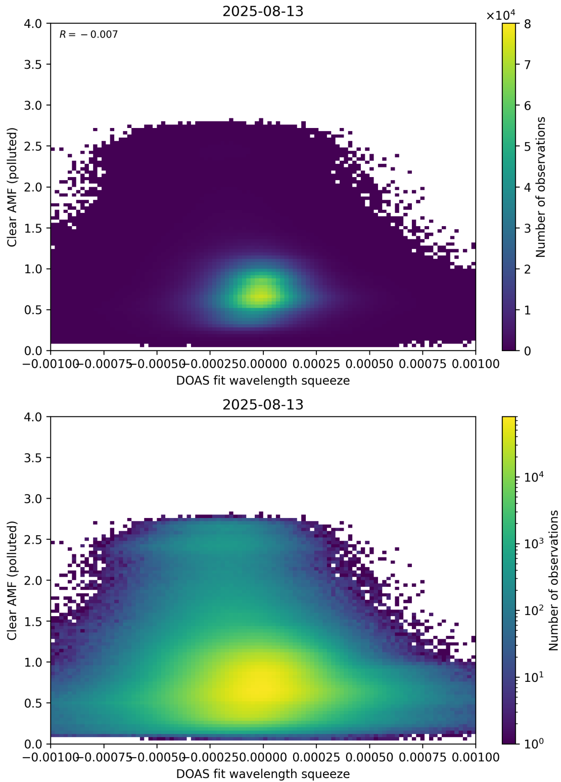
Figure 144: Scatter density plot of “DOAS fit wavelength squeeze” against “Clear AMF (polluted)” for 2025-08-12 to 2025-08-14.
