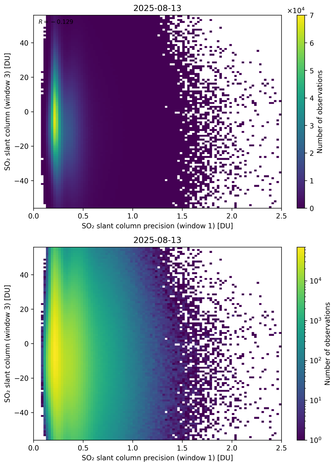
Figure 278: Scatter density plot of “SO 2 slant column precision (window 1)” against “SO 2 slant column (window 3)” for 2025-08-12 to 2025-08-14.
