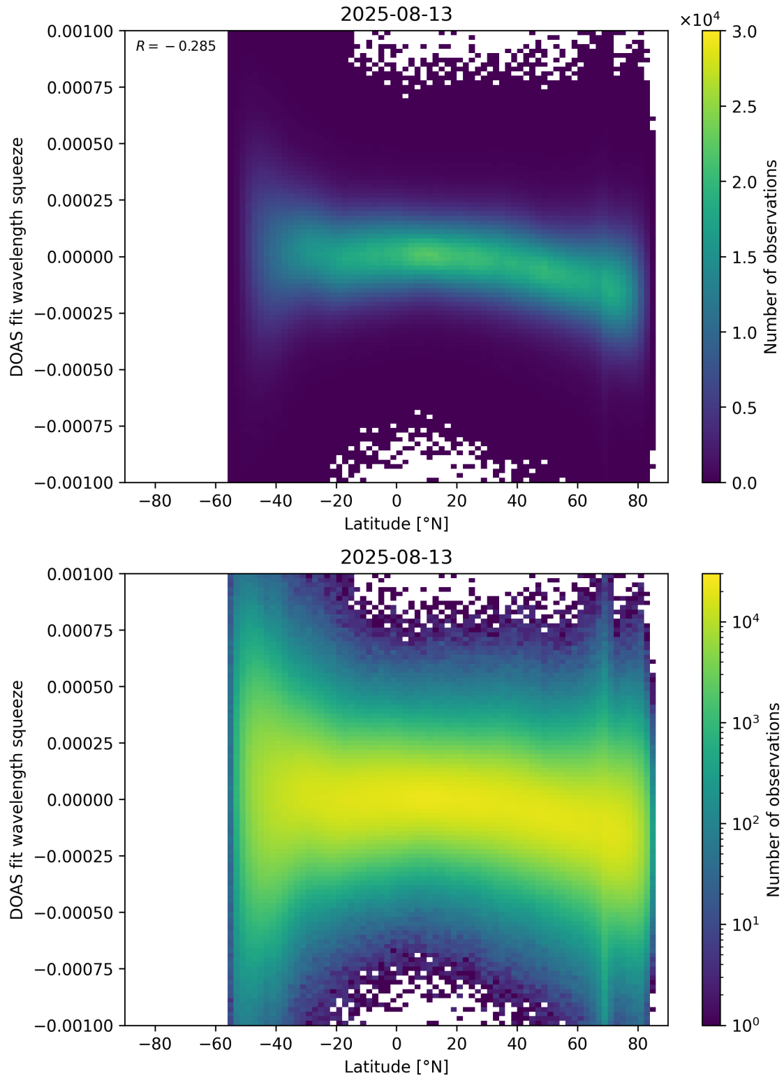
Figure 154: Scatter density plot of “Latitude” against “DOAS fit wavelength squeeze” for 2025-08-12 to 2025-08-14.
