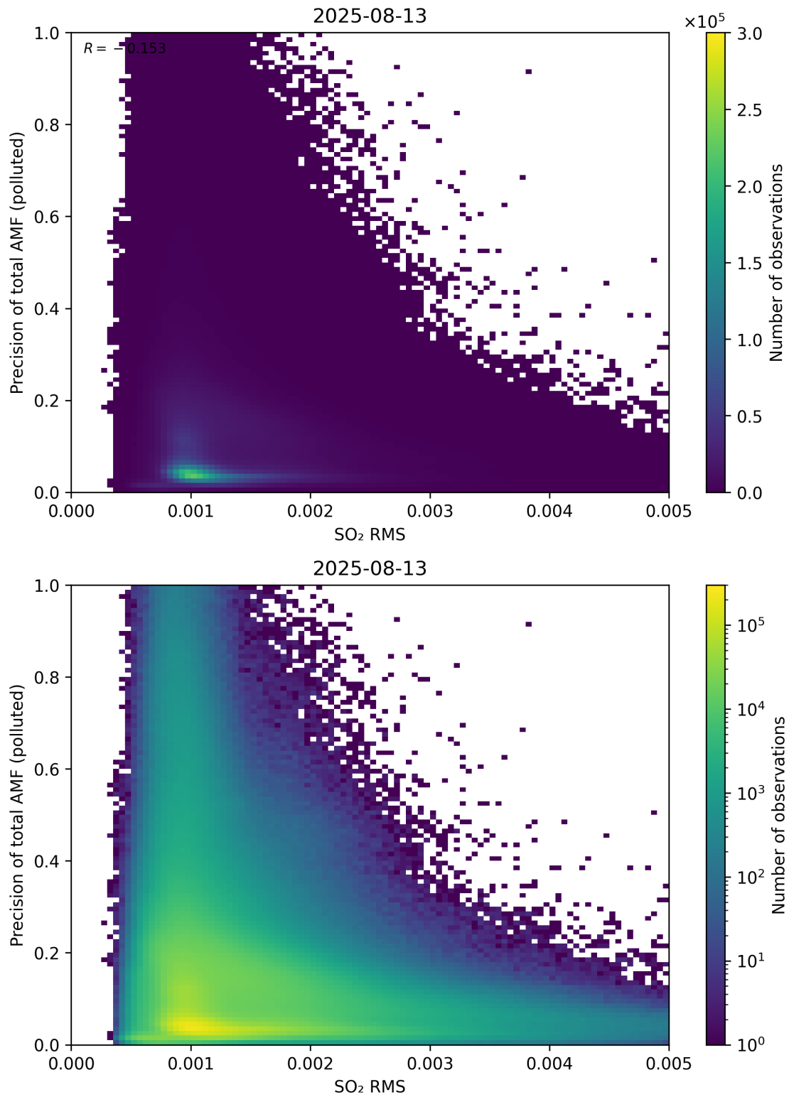
Figure 149: Scatter density plot of “SO 2 RMS” against “Precision of total AMF (polluted)” for 2025-08-12 to 2025-08-14.
