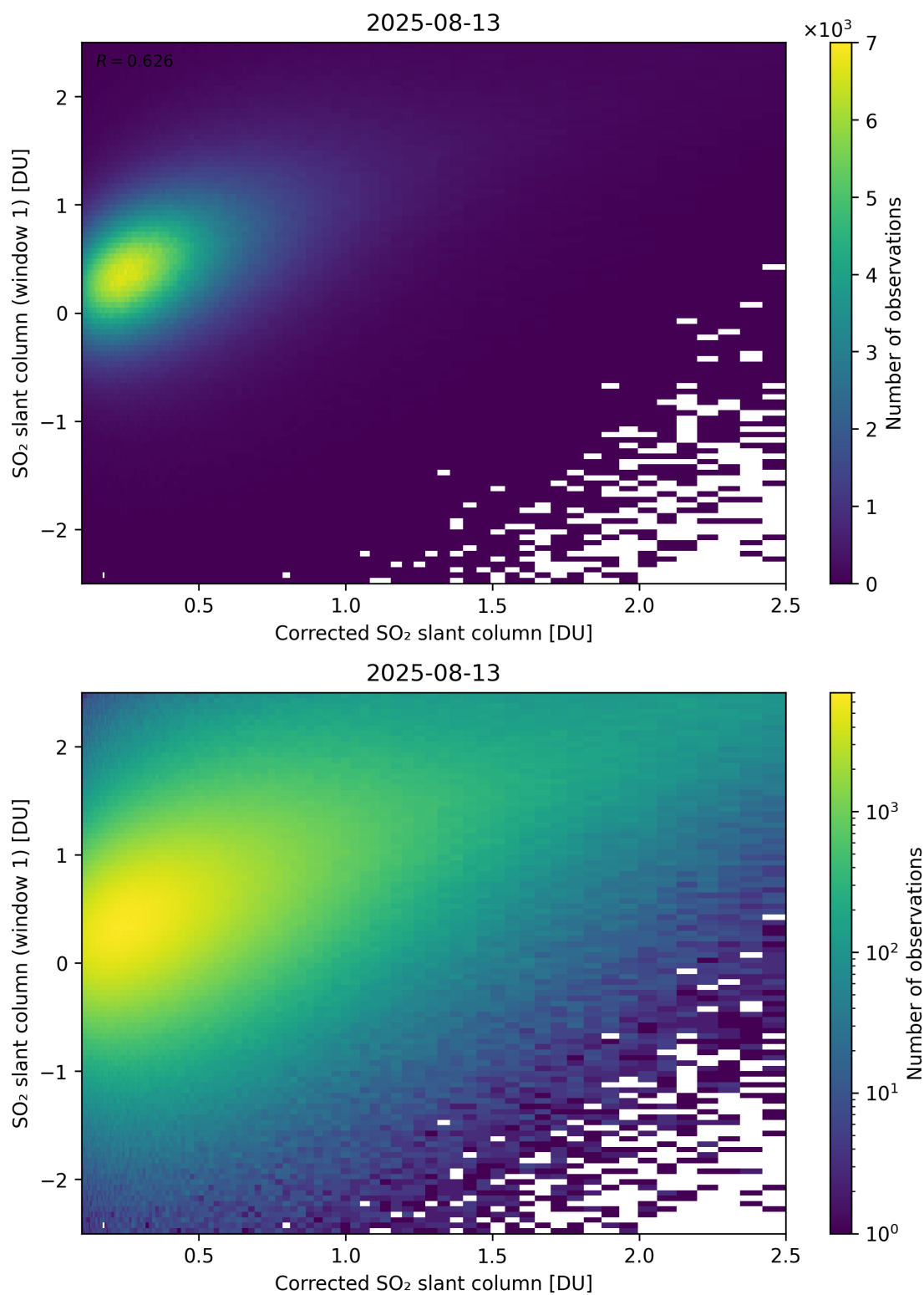
Figure 237: Scatter density plot of “Corrected SO 2 slant column” against “SO 2 slant column (window 1)” for 2025-08-12 to 2025-08-14.
