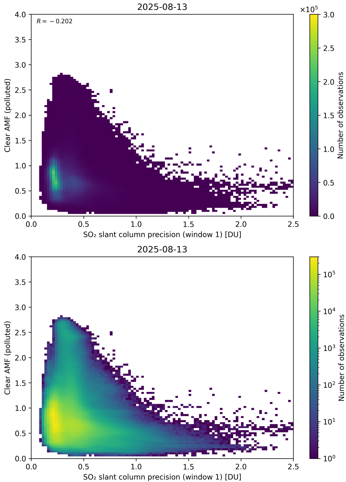
Figure 274: Scatter density plot of “SO 2 slant column precision (window 1)” against “Clear AMF (polluted)” for 2025-08-12 to 2025-08-14.
