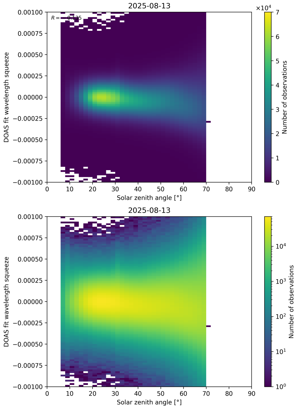
Figure 175: Scatter density plot of “Solar zenith angle” against “DOAS fit wavelength squeeze” for 2025-08-12 to 2025-08-14.
