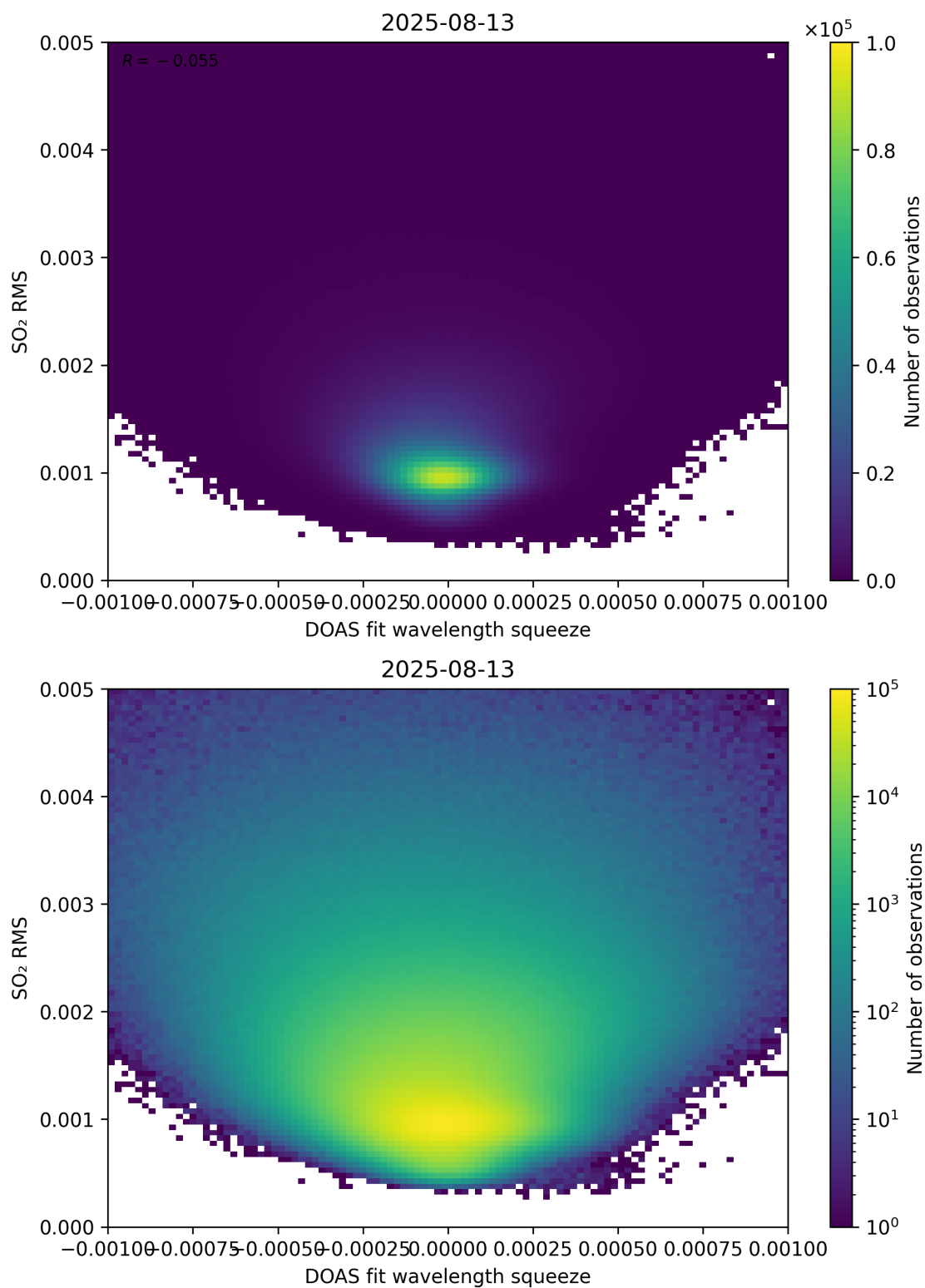
Figure 143: Scatter density plot of “DOAS fit wavelength squeeze” against “SO 2 RMS” for 2025-08-12 to 2025-08-14.
