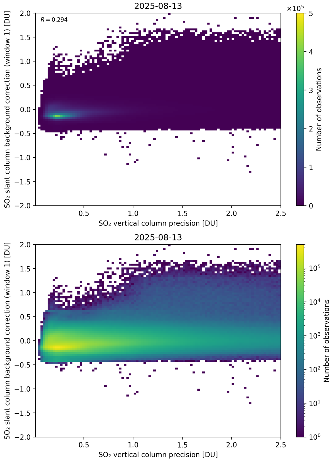
Figure 329: Scatter density plot of “SO 2 vertical column precision” against “SO 2 slant column background correction (window 1)” for 2025-08-12 to 2025-08-14.
