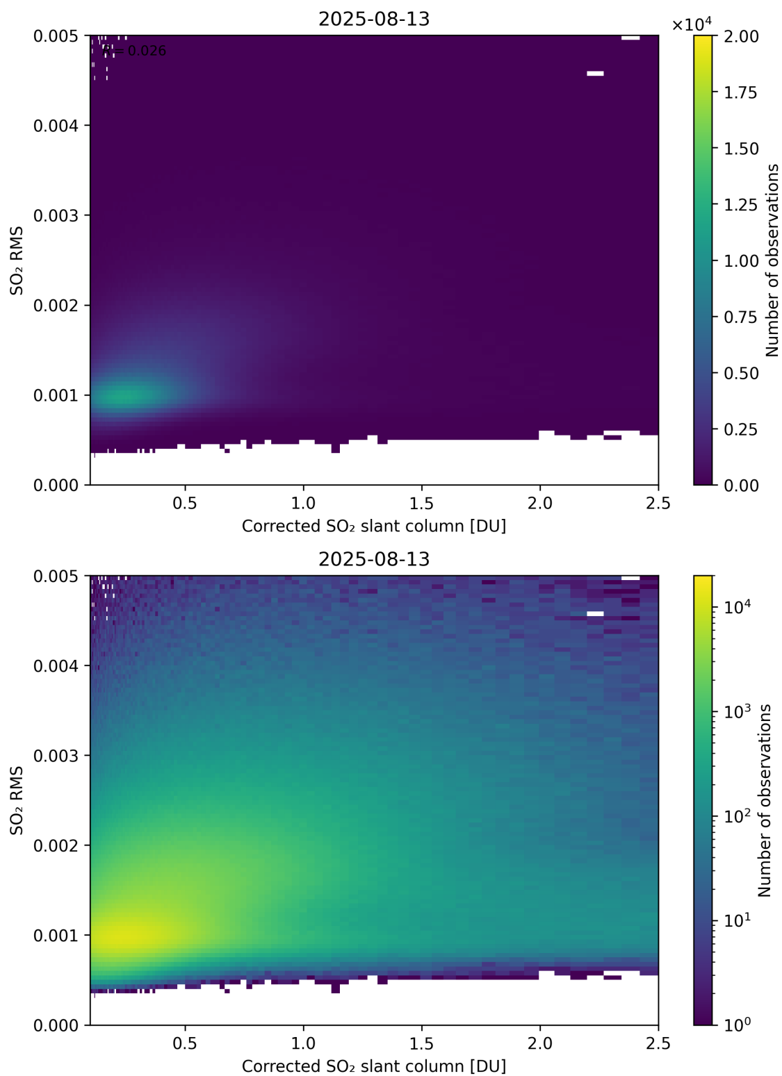
Figure 231: Scatter density plot of “Corrected SO 2 slant column” against “SO 2 RMS” for 2025-08-12 to 2025-08-14.
