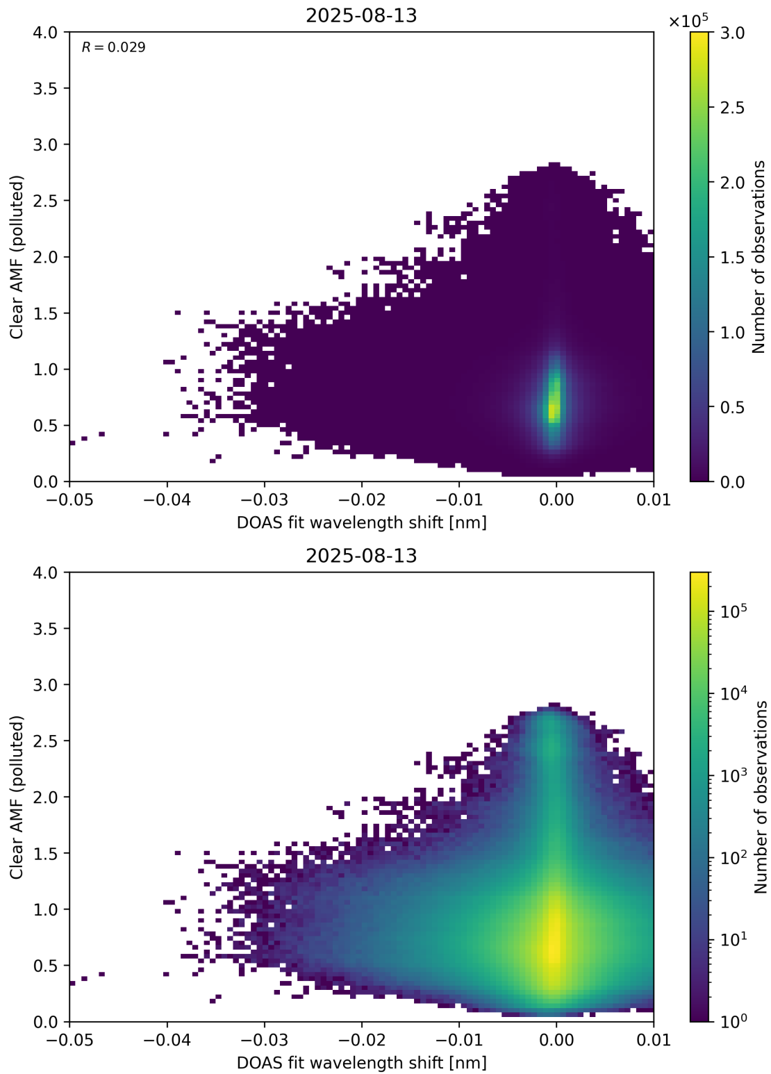
Figure 140: Scatter density plot of “DOAS fit wavelength shift” against “Clear AMF (polluted)” for 2025-08-12 to 2025-08-14.
