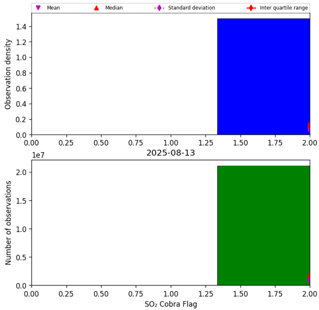
Figure 75: Histogram of “SO 2 Cobra Flag” for 2025-08-12 to 2025-08-14
