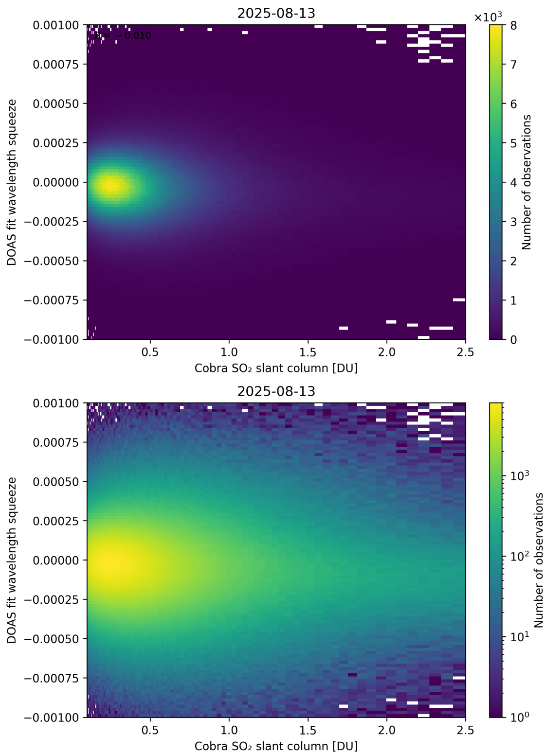
Figure 197: Scatter density plot of “Cobra SO 2 slant column” against “DOAS fit wavelength squeeze” for 2025-08-12 to 2025-08-14.
