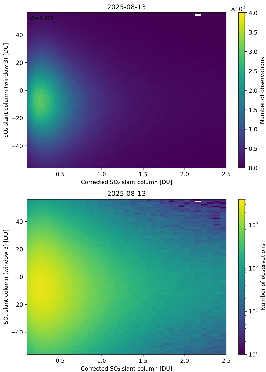
Figure 240: Scatter density plot of “Corrected SO 2 slant column” against “SO 2 slant column (window 3)” for 2025-08-12 to 2025-08-14.
