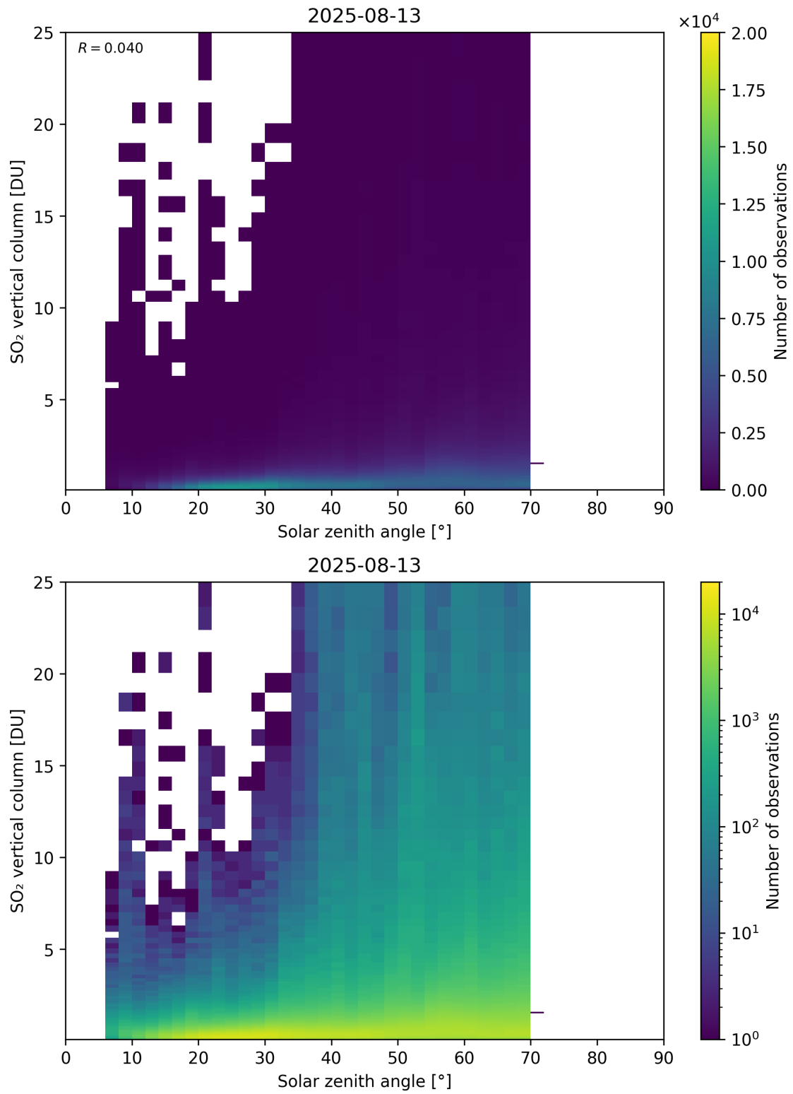
Figure 191: Scatter density plot of “Solar zenith angle” against “SO 2 vertical column” for 2025-08-12 to 2025-08-14.
