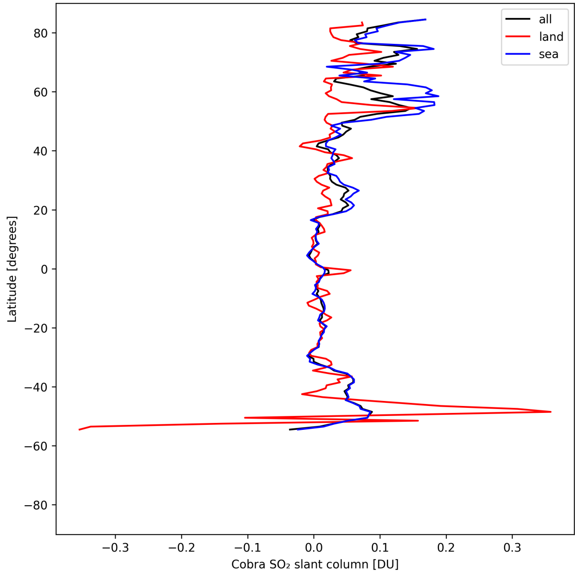
Figure 35: Zonal average of “Cobra SO 2 slant column” for 2025-08-12 to 2025-08-14.
