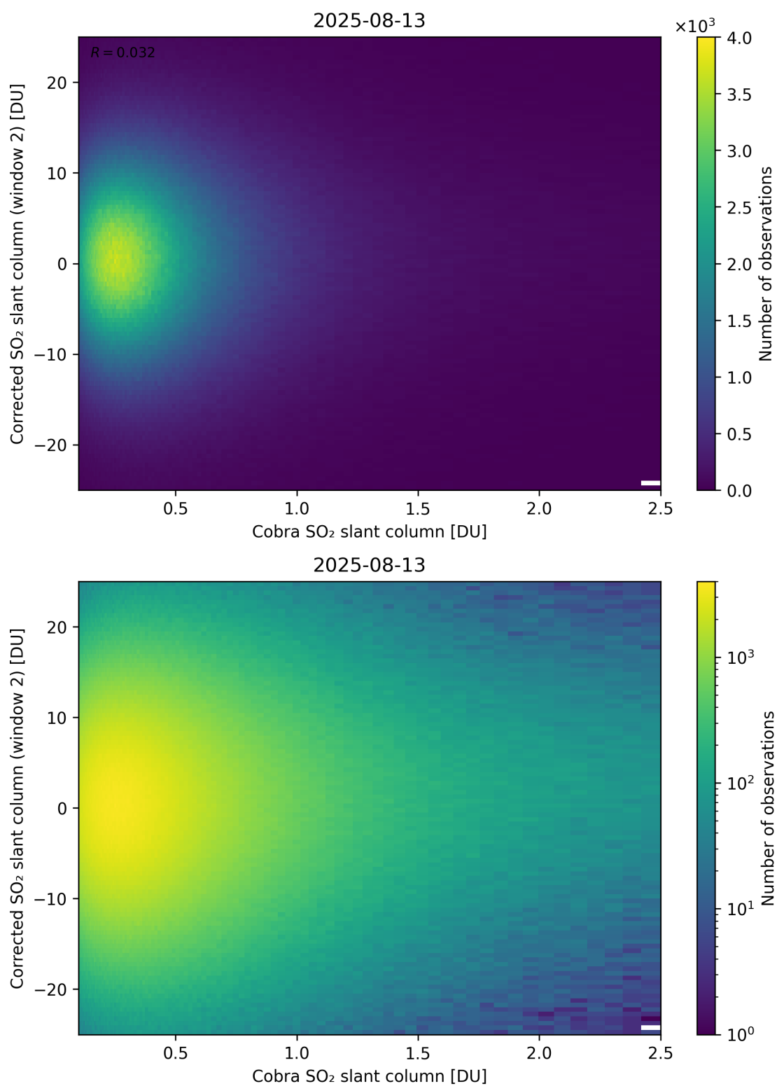
Figure 217: Scatter density plot of “Cobra SO 2 slant column” against “Corrected SO 2 slant column (window 2)” for 2025-08-12 to 2025-08-14.
