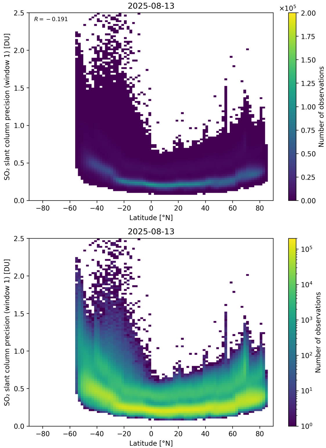
Figure 163: Scatter density plot of “Latitude” against “SO 2 slant column precision (window 1)” for 2025-08-12 to 2025-08-14.
