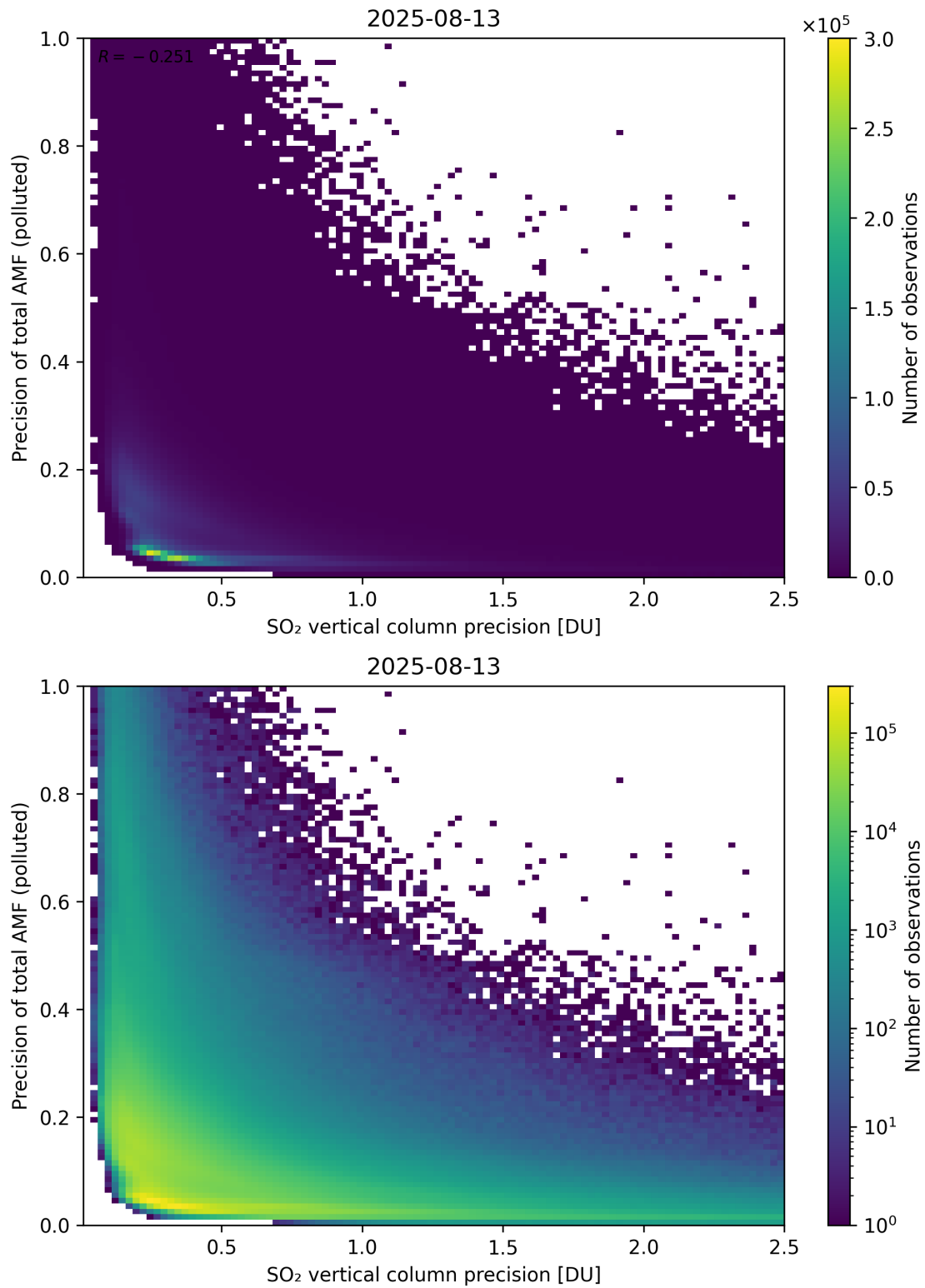
Figure 347: Scatter density plot of “SO 2 vertical column precision” against “Precision of total AMF (polluted)” for 2025-08-12 to 2025-08-14.
