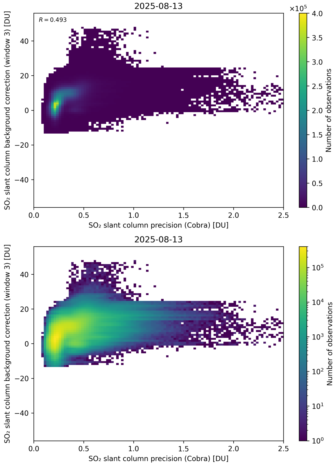
Figure 201: Scatter density plot of “SO 2 slant column precision (Cobra)” against “SO 2 slant column background correction (window 3)” for 2025-08-12 to 2025-08-14.
