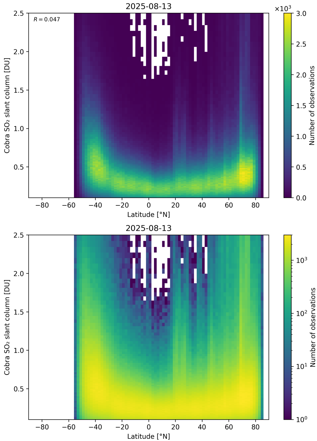
Figure 157: Scatter density plot of “Latitude” against “Cobra SO 2 slant column” for 2025-08-12 to 2025-08-14.
