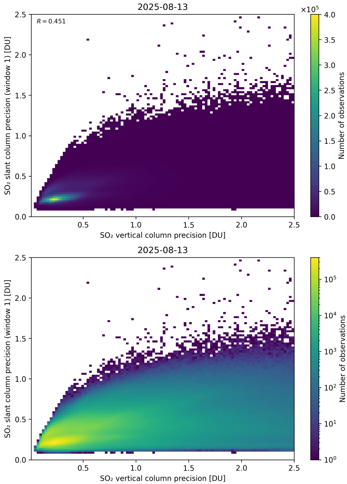
Figure 342: Scatter density plot of “SO 2 vertical column precision” against “SO 2 slant column precision (window 1)” for 2025-08-12 to 2025-08-14.
