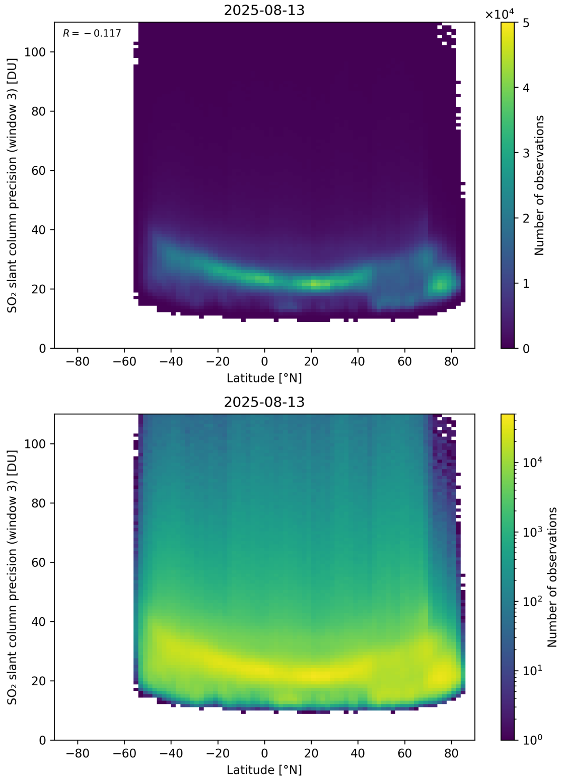
Figure 166: Scatter density plot of “Latitude” against “SO 2 slant column precision (window 3)” for 2025-08-12 to 2025-08-14.
