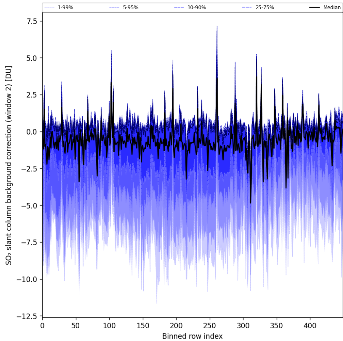
Figure 96: Along track statistics of “SO 2 slant column background correction (window 2)” for 2025-08-12 to 2025-08-14
