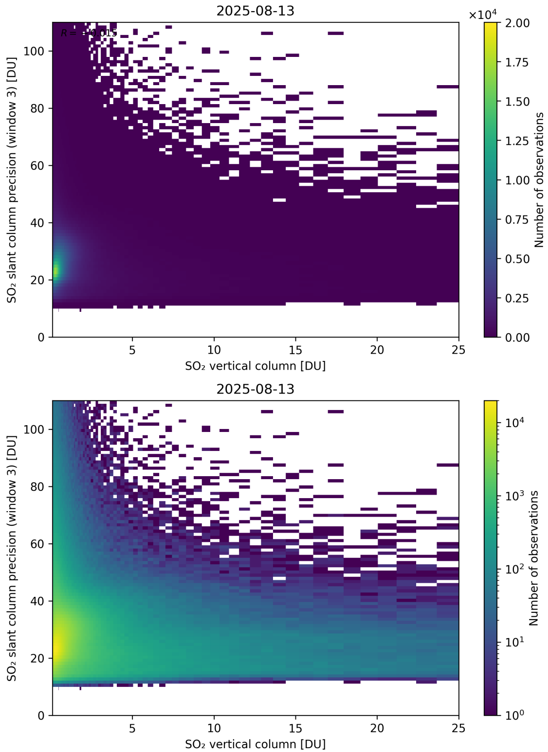
Figure 358: Scatter density plot of “SO 2 vertical column” against “SO 2 slant column precision (window 3)” for 2025-08-12 to 2025-08-14.
