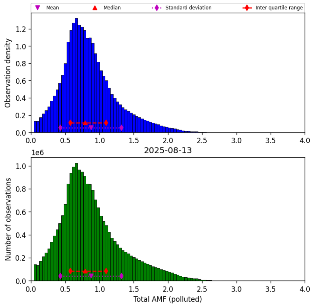
Figure 79: Histogram of “Total AMF (polluted)” for 2025-08-12 to 2025-08-14
