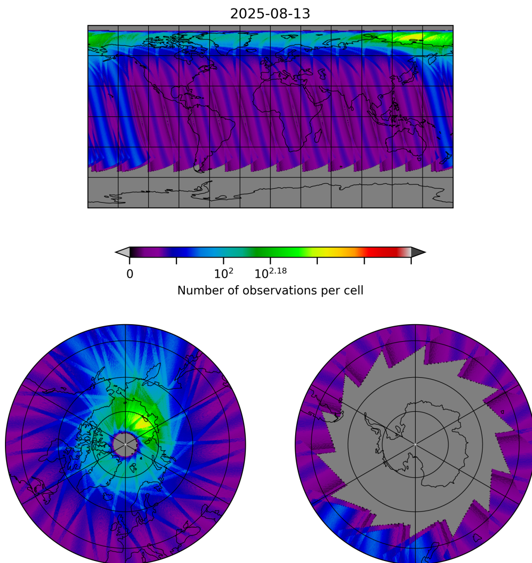
Figure 30: Map of the number of observations for 2025-08-12 to 2025-08-14
