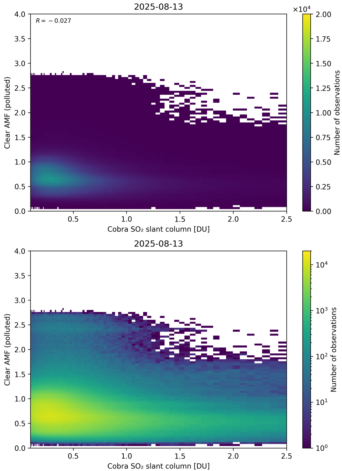
Figure 215: Scatter density plot of “Cobra SO 2 slant column” against “Clear AMF (polluted)” for 2025-08-12 to 2025-08-14.
