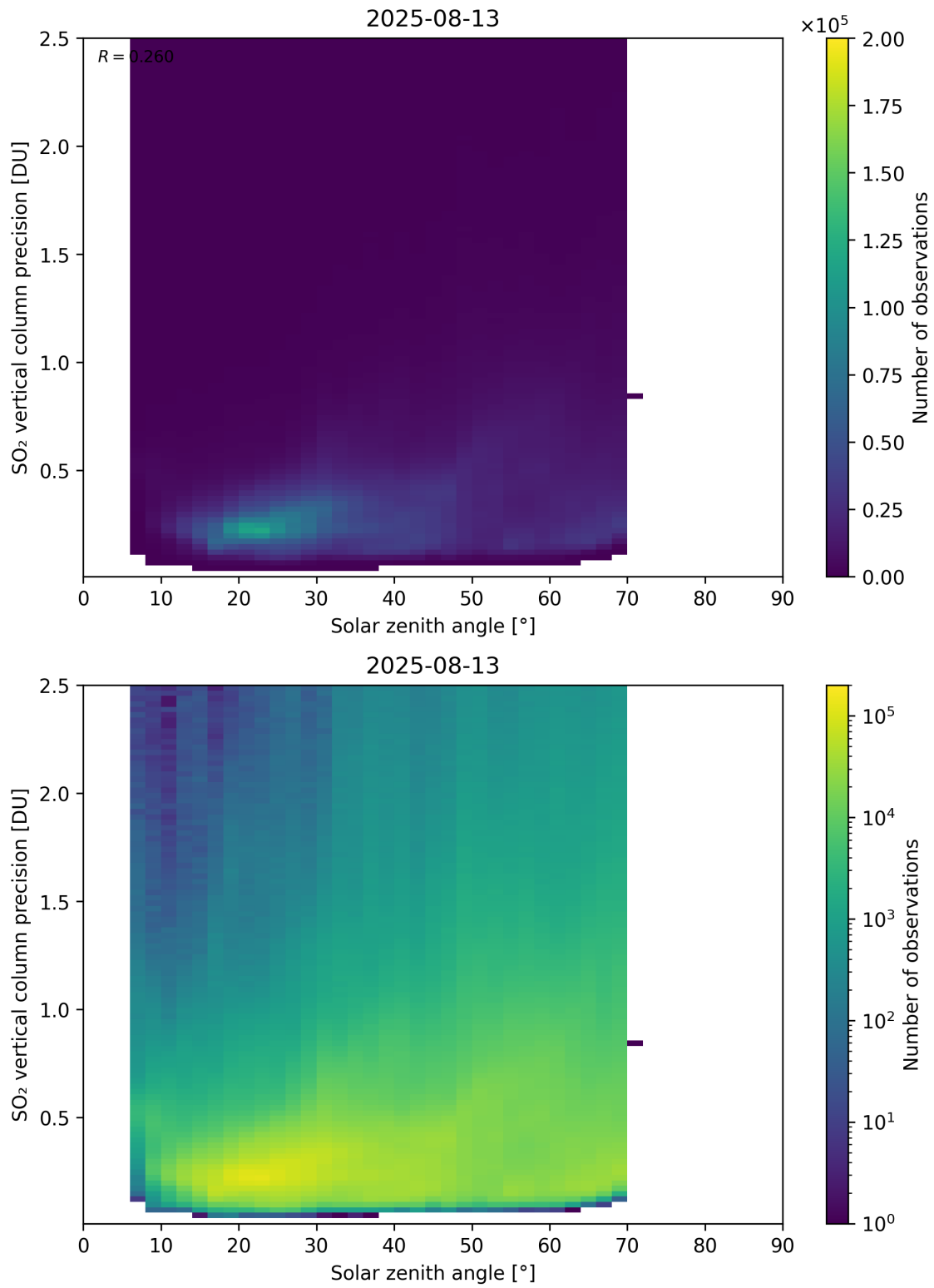
Figure 192: Scatter density plot of “Solar zenith angle” against “SO 2 vertical column precision” for 2025-08-12 to 2025-08-14.
