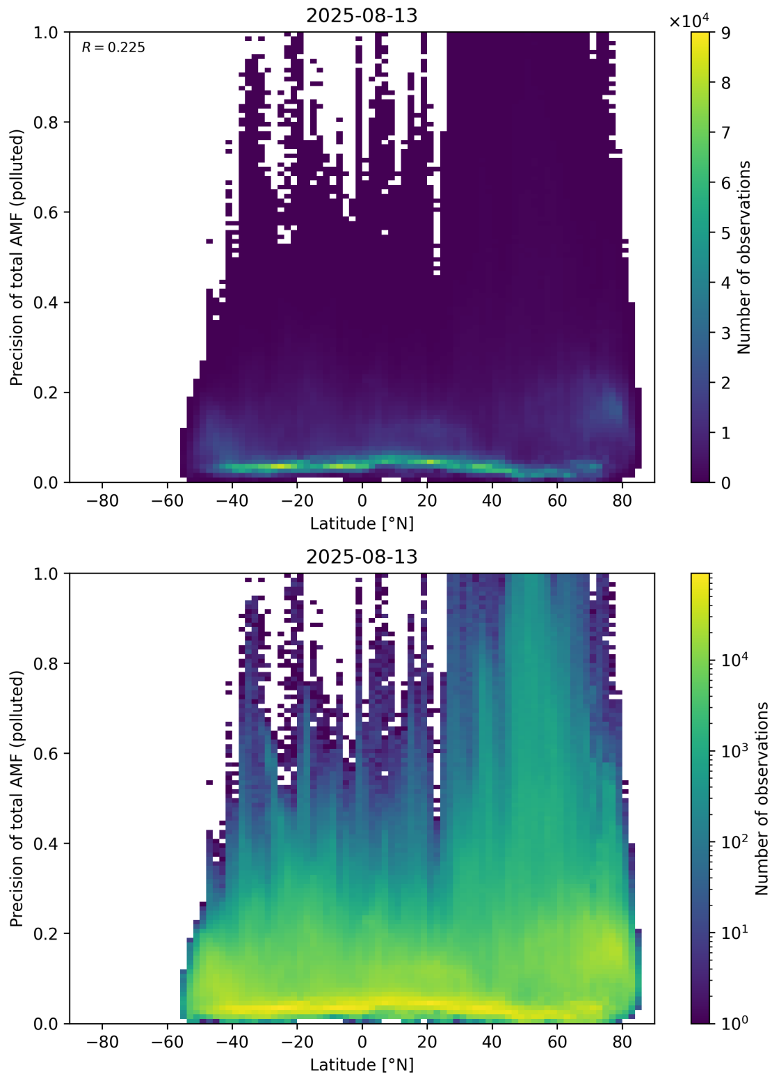
Figure 168: Scatter density plot of “Latitude” against “Precision of total AMF (polluted)” for 2025-08-12 to 2025-08-14.
