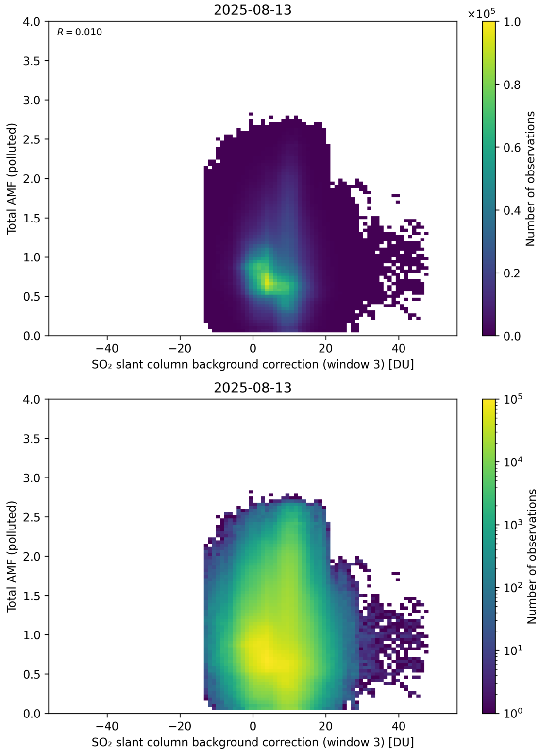
Figure 136: Scatter density plot of “SO 2 slant column background correction (window 3)” against “Total AMF (polluted)” for 2025-08-12 to 2025-08-14.
