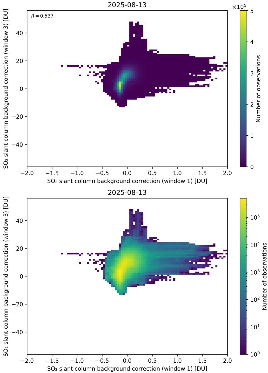
Figure 110: Scatter density plot of “SO 2 slant column background correction (window 1)” against “SO 2 slant column background correction (window 3)” for 2025-08-12 to 2025-08-14.
