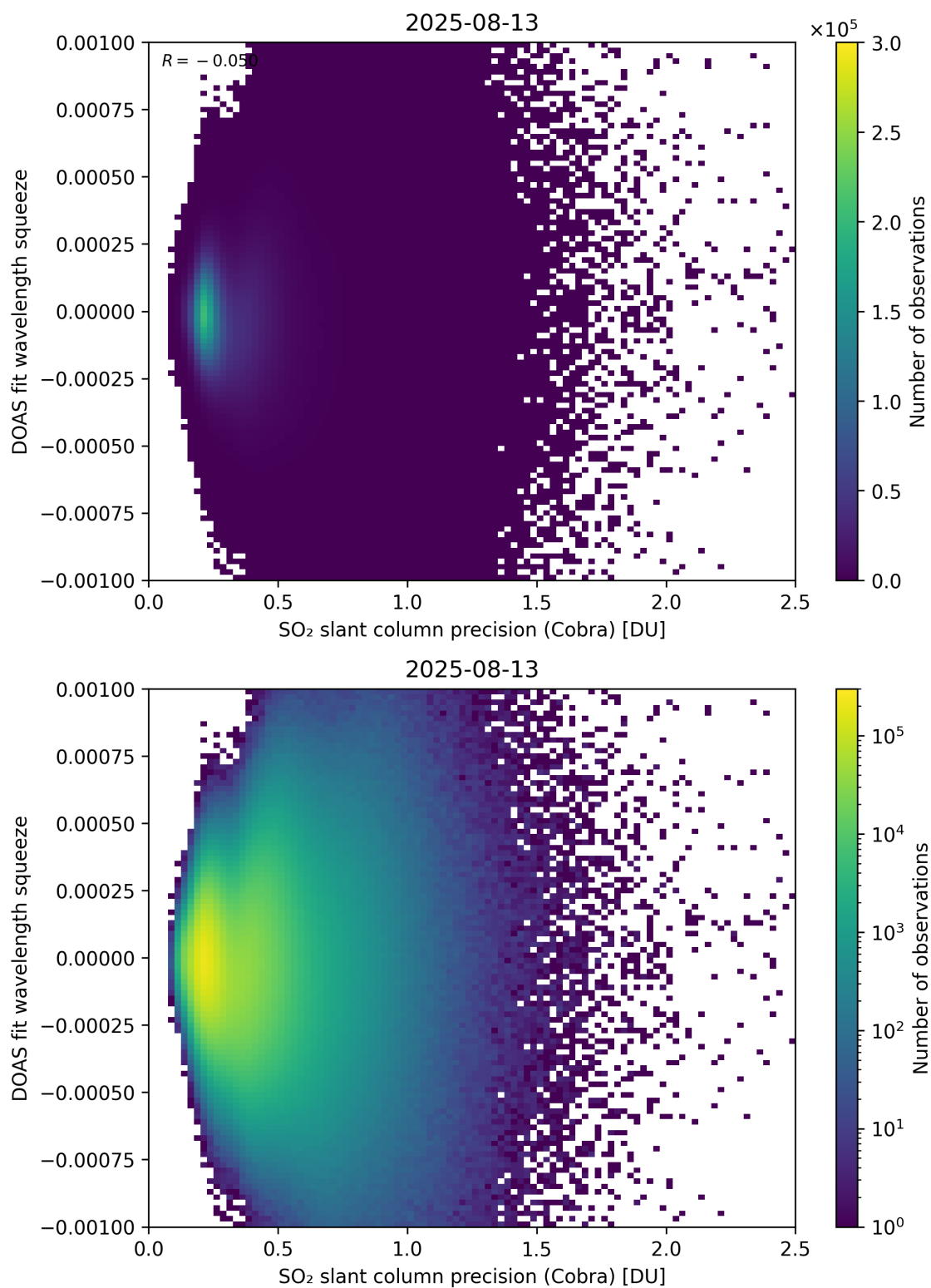
Figure 203: Scatter density plot of “SO 2 slant column precision (Cobra)” against “DOAS fit wavelength squeeze” for 2025-08-12 to 2025-08-14.
