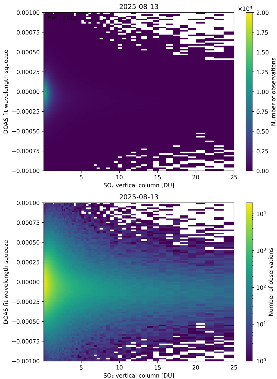
Figure 327: Scatter density plot of “SO 2 vertical column” against “DOAS fit wavelength squeeze” for 2025-08-12 to 2025-08-14.
