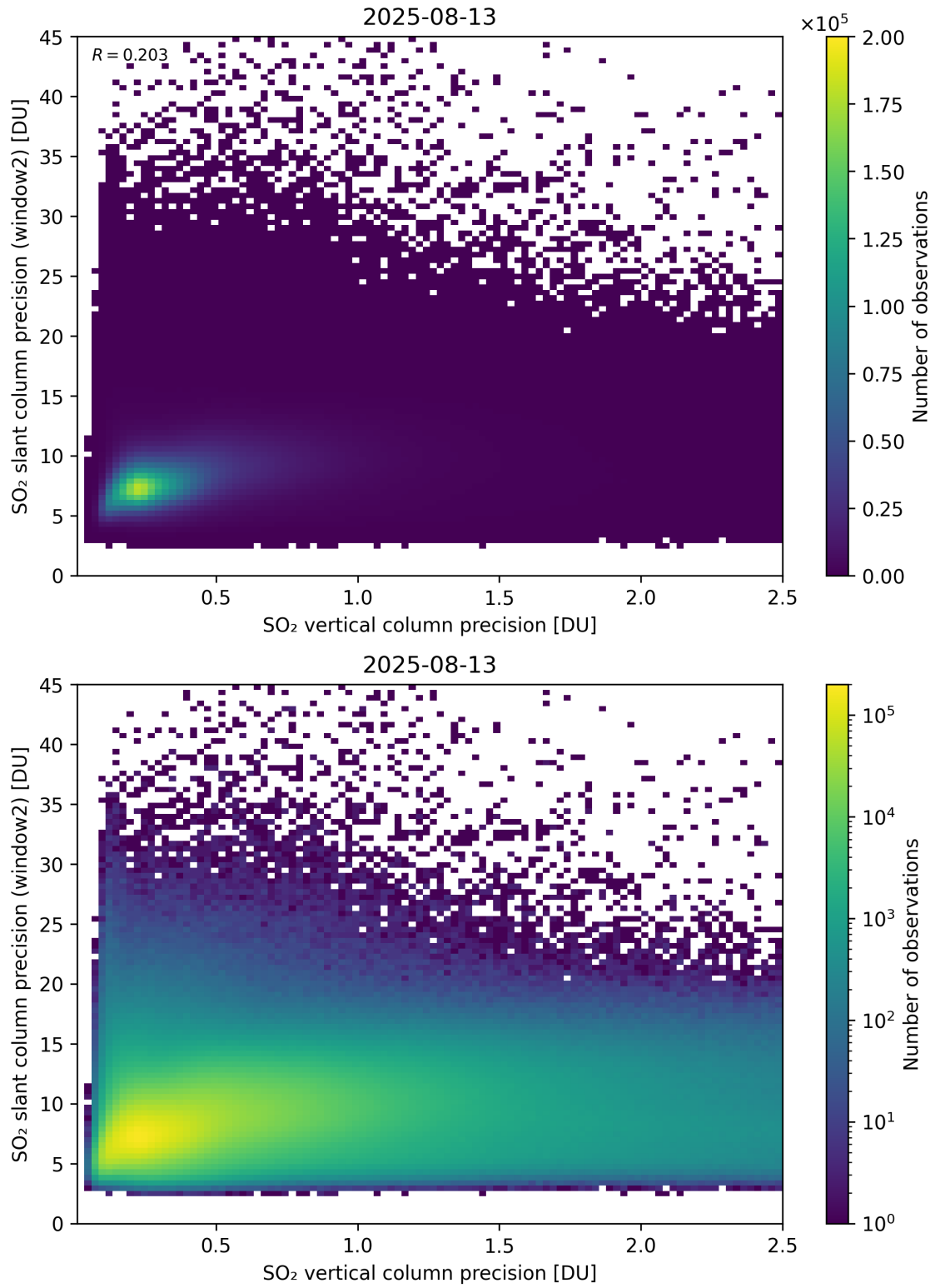
Figure 343: Scatter density plot of “SO 2 vertical column precision” against “SO 2 slant column precision (window2)” for 2025-08-12 to 2025-08-14.
