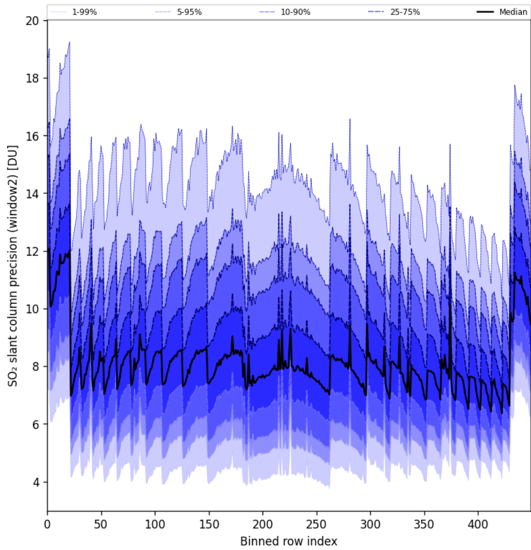
Figure 94: Along track statistics of “SO 2 slant column precision (window2)” for 2025-08-12 to 2025-08-14
