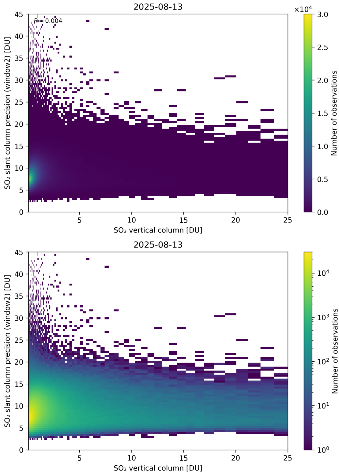
Figure 356: Scatter density plot of “SO 2 vertical column” against “SO 2 slant column precision (window2)” for 2025-08-12 to 2025-08-14.
