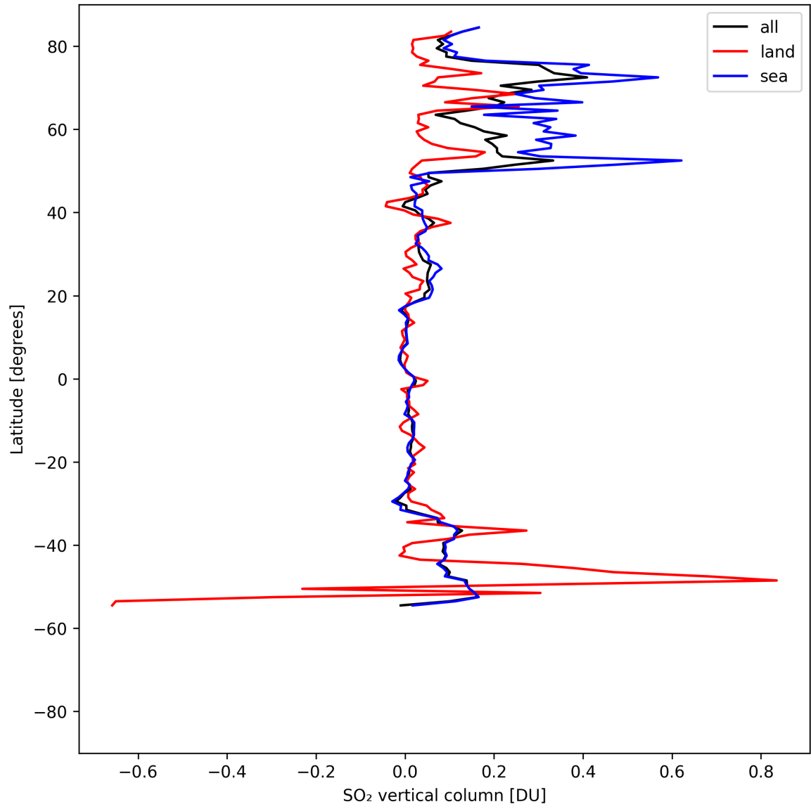
Figure 32: Zonal average of “SO 2 vertical column” for 2025-08-12 to 2025-08-14.
