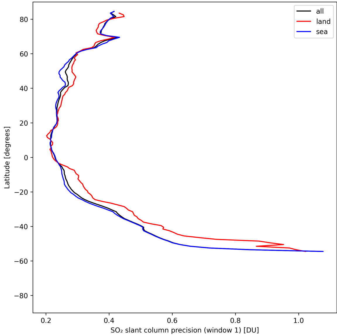
Figure 38: Zonal average of “SO 2 slant column precision (window 1)” for 2025-08-12 to 2025-08-14.
