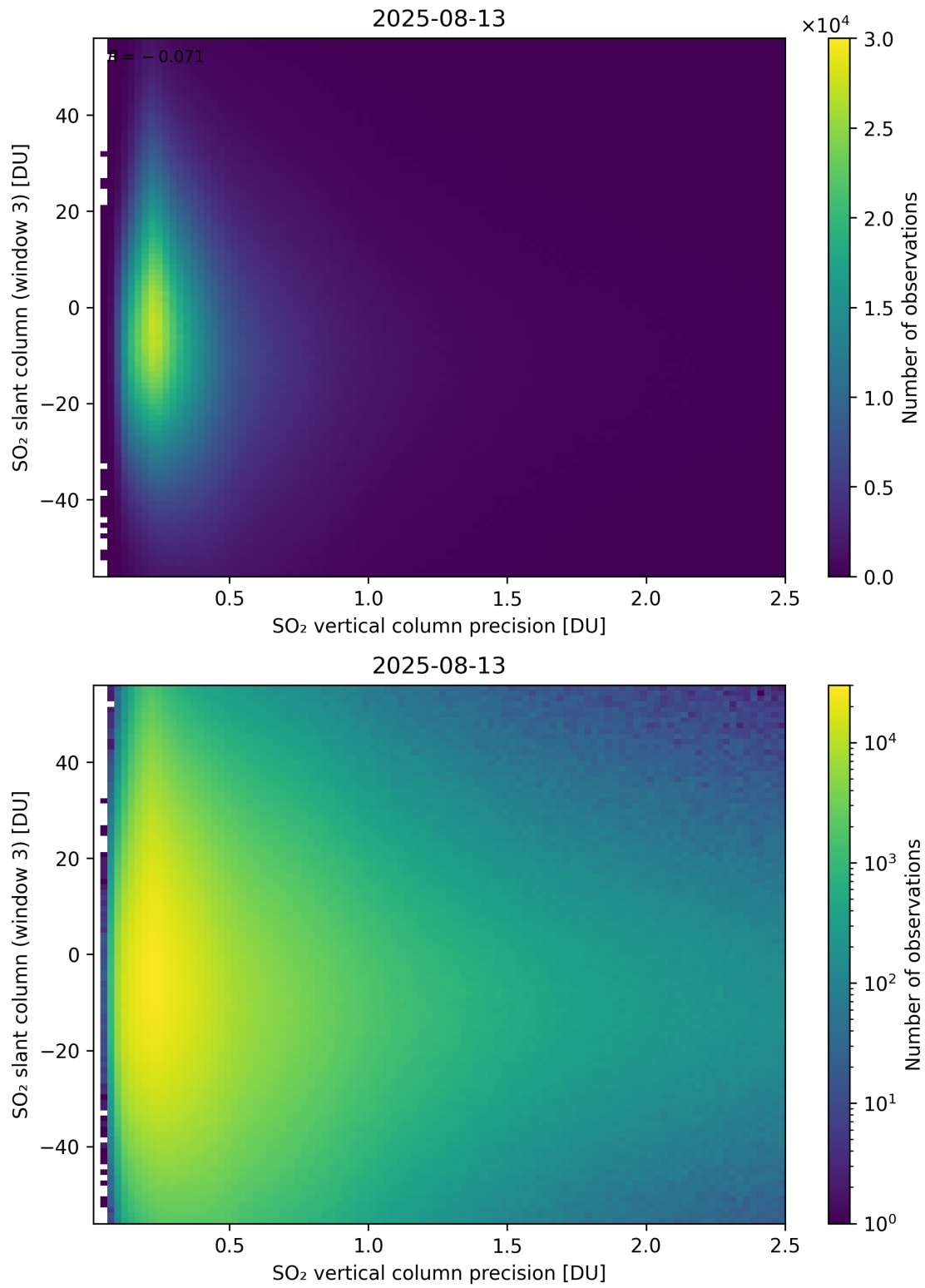
Figure 344: Scatter density plot of “SO 2 vertical column precision” against “SO 2 slant column (window 3)” for 2025-08-12 to 2025-08-14.
