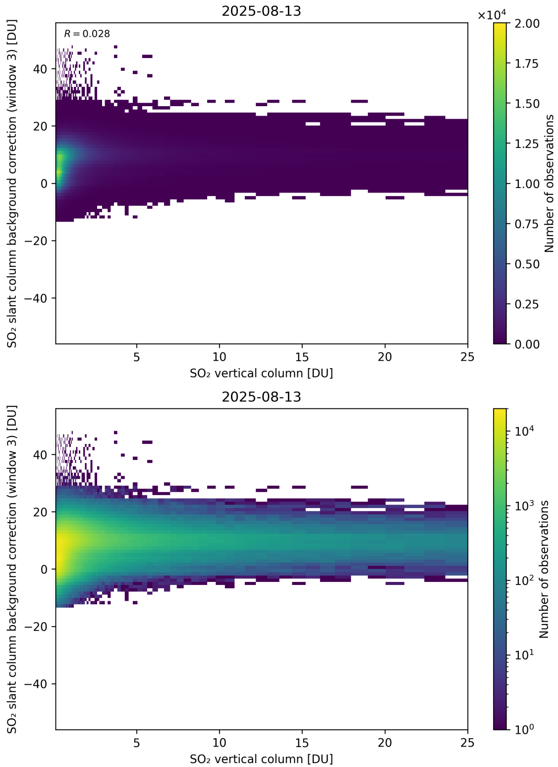
Figure 325: Scatter density plot of “SO 2 vertical column” against “SO 2 slant column background correction (window 3)” for 2025-08-12 to 2025-08-14.
