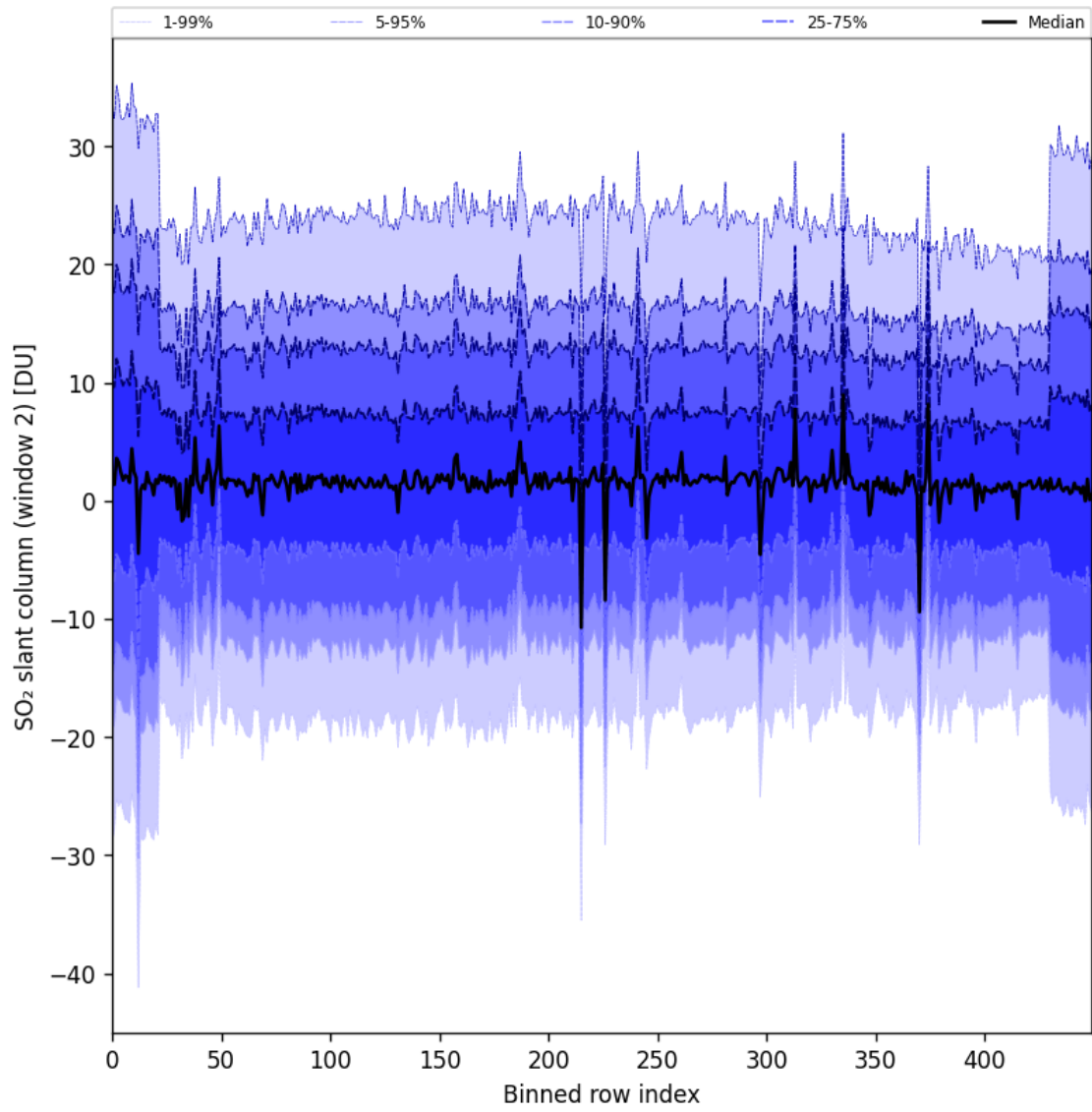
Figure 93: Along track statistics of “SO 2 slant column (window 2)” for 2025-08-12 to 2025-08-14
