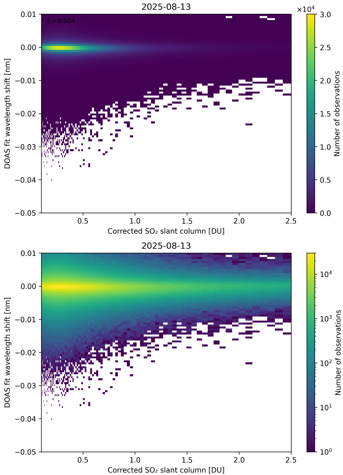
Figure 229: Scatter density plot of “Corrected SO 2 slant column” against “DOAS fit wavelength shift” for 2025-08-12 to 2025-08-14.
