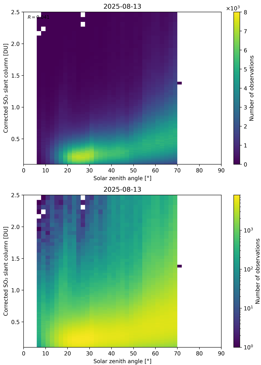
Figure 181: Scatter density plot of “Solar zenith angle” against “Corrected SO 2 slant column” for 2025-08-12 to 2025-08-14.
