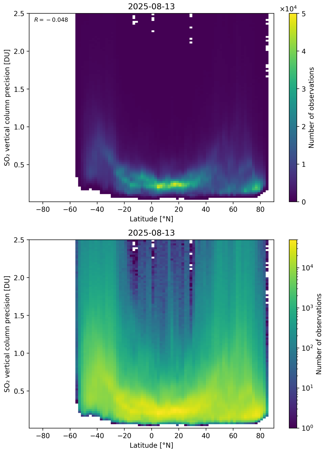
Figure 170: Scatter density plot of “Latitude” against “SO 2 vertical column precision” for 2025-08-12 to 2025-08-14.
