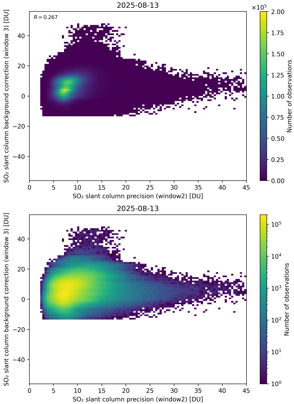
Figure 292: Scatter density plot of “SO 2 slant column precision (window2)” against “SO 2 slant column background correction (window 3)” for 2025-08-12 to 2025-08-14.
