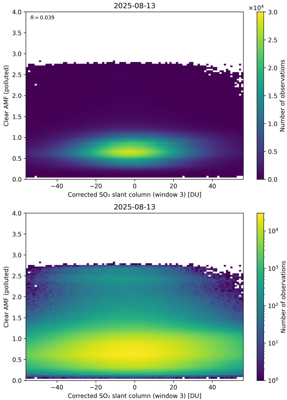
Figure 259: Scatter density plot of “Corrected SO 2 slant column (window 3)” against “Clear AMF (polluted)” for 2025-08-12 to 2025-08-14.
