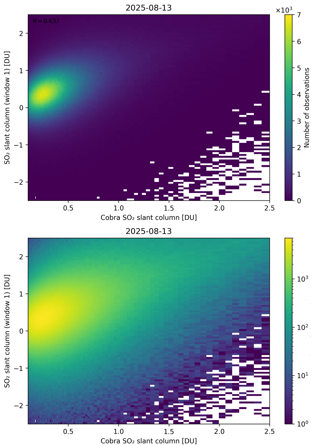
Figure 219: Scatter density plot of “Cobra SO 2 slant column” against “SO 2 slant column (window 1)” for 2025-08-12 to 2025-08-14.
