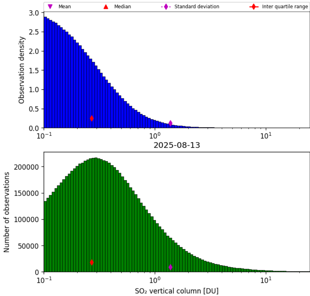
Figure 58: Histogram of “SO 2 vertical column” for 2025-08-12 to 2025-08-14
