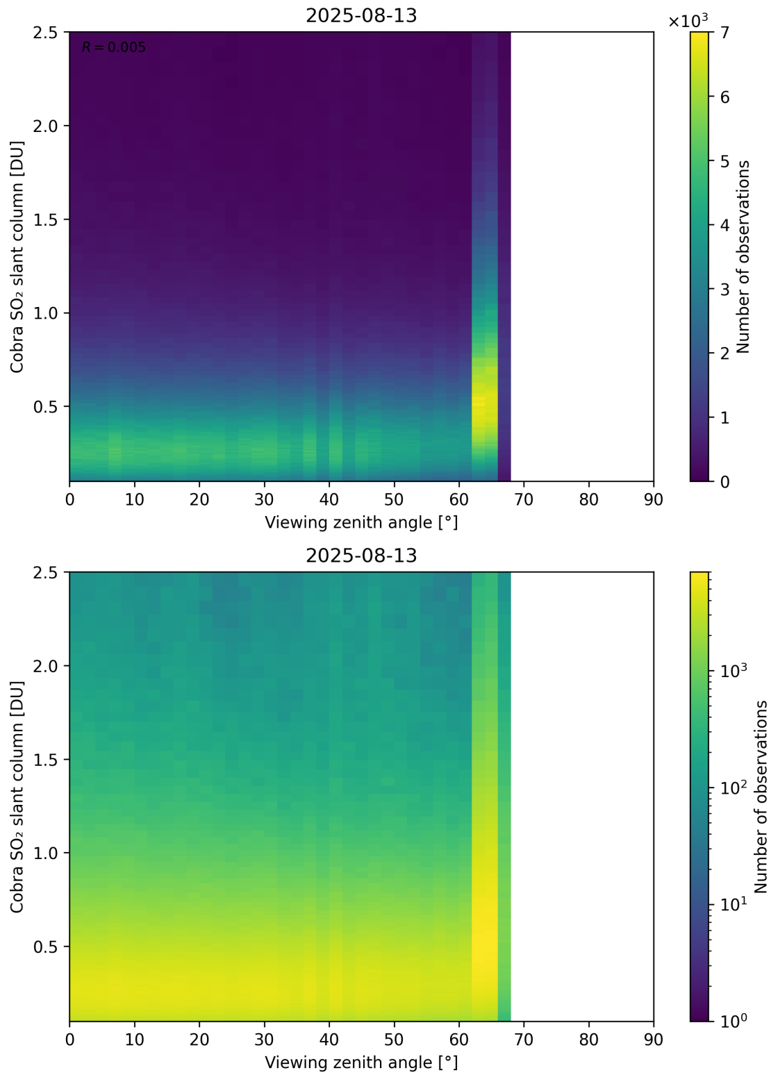
Figure 371: Scatter density plot of “Viewing zenith angle” against “Cobra SO 2 slant column” for 2025-08-12 to 2025-08-14.
