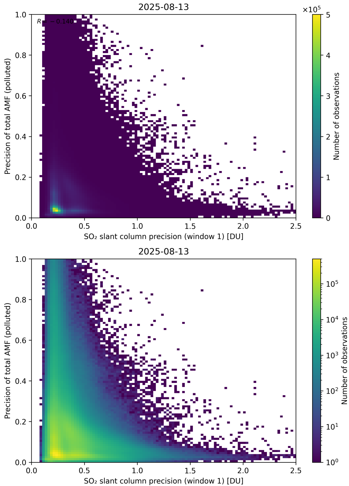
Figure 281: Scatter density plot of “SO 2 slant column precision (window 1)” against “Precision of total AMF (polluted)” for 2025-08-12 to 2025-08-14.
