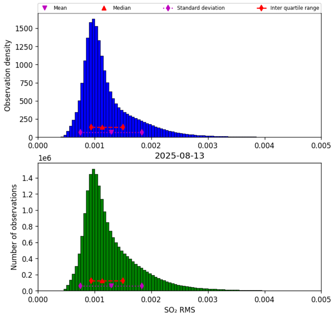
Figure 78: Histogram of “SO 2 RMS” for 2025-08-12 to 2025-08-14
