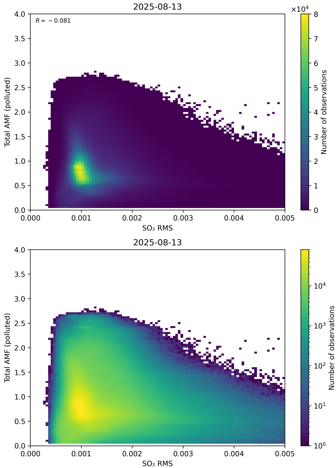
Figure 148: Scatter density plot of “SO 2 RMS” against “Total AMF (polluted)” for 2025-08-12 to 2025-08-14.
