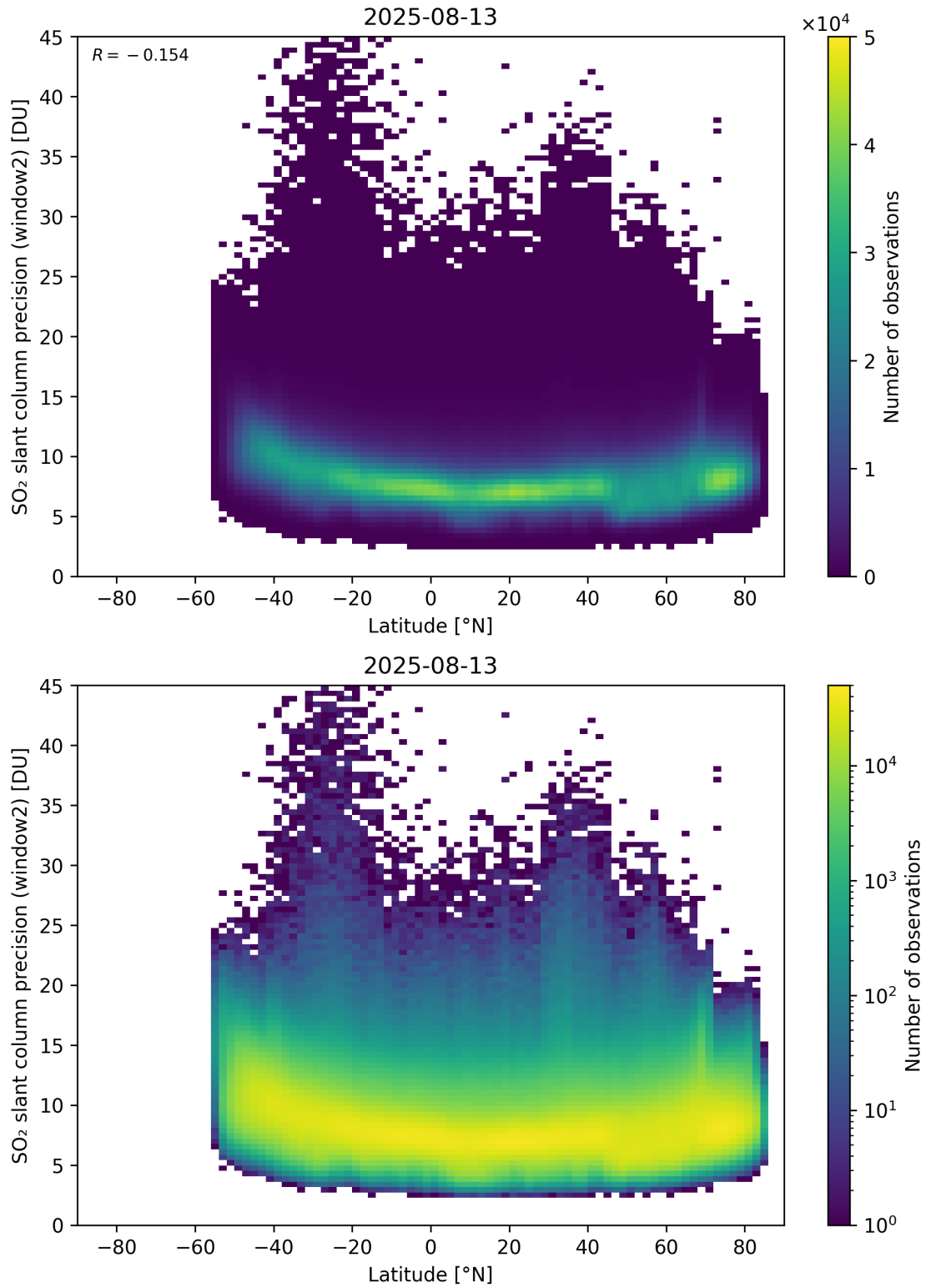
Figure 164: Scatter density plot of “Latitude” against “SO 2 slant column precision (window2)” for 2025-08-12 to 2025-08-14.
