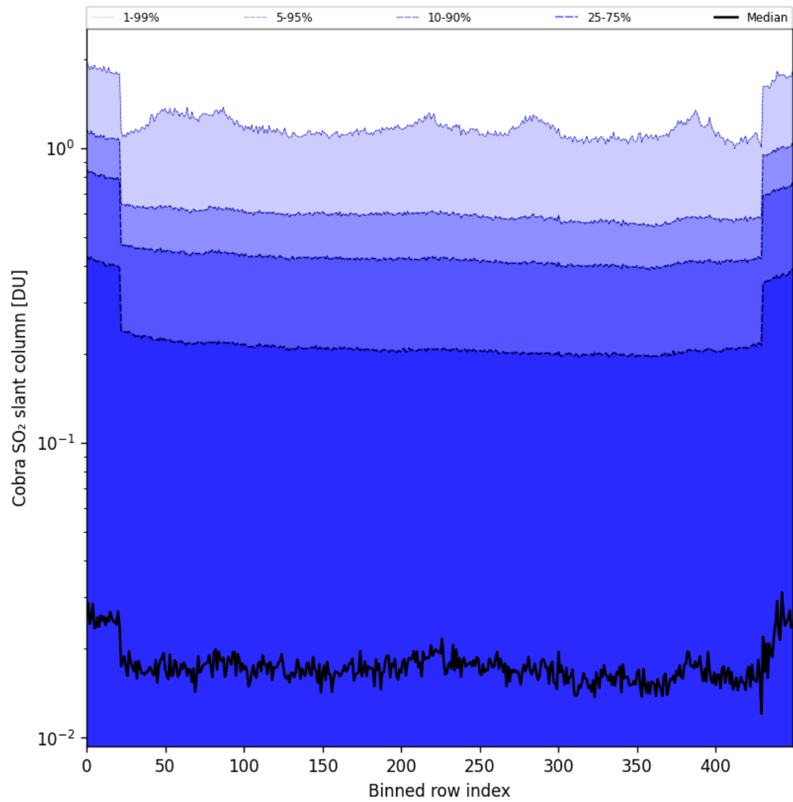
Figure 87: Along track statistics of “Cobra SO 2 slant column” for 2025-08-12 to 2025-08-14
