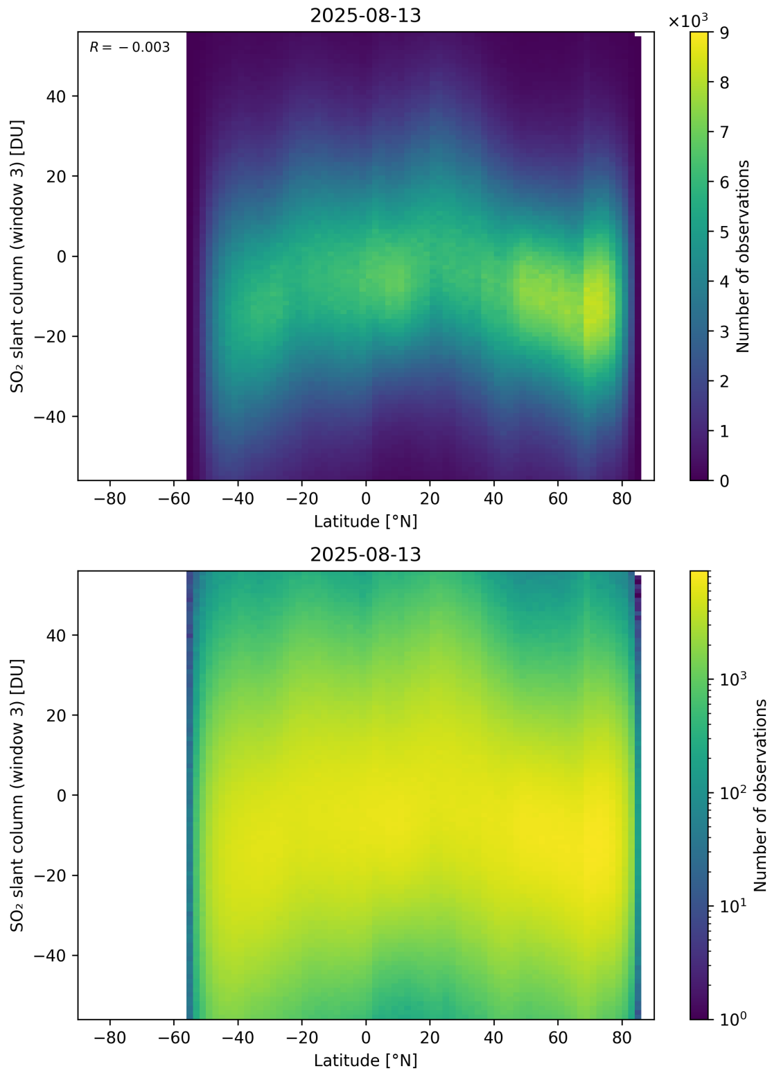
Figure 165: Scatter density plot of “Latitude” against “SO 2 slant column (window 3)” for 2025-08-12 to 2025-08-14.
