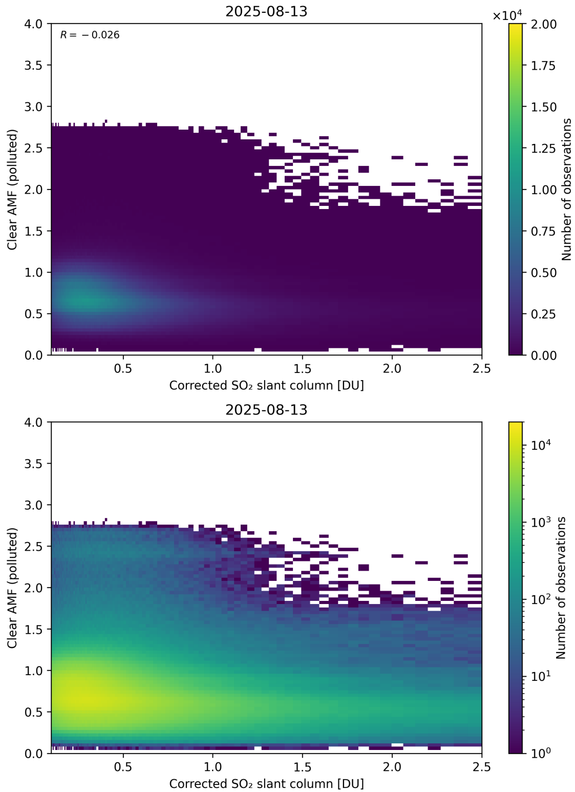
Figure 232: Scatter density plot of “Corrected SO 2 slant column” against “Clear AMF (polluted)” for 2025-08-12 to 2025-08-14.
