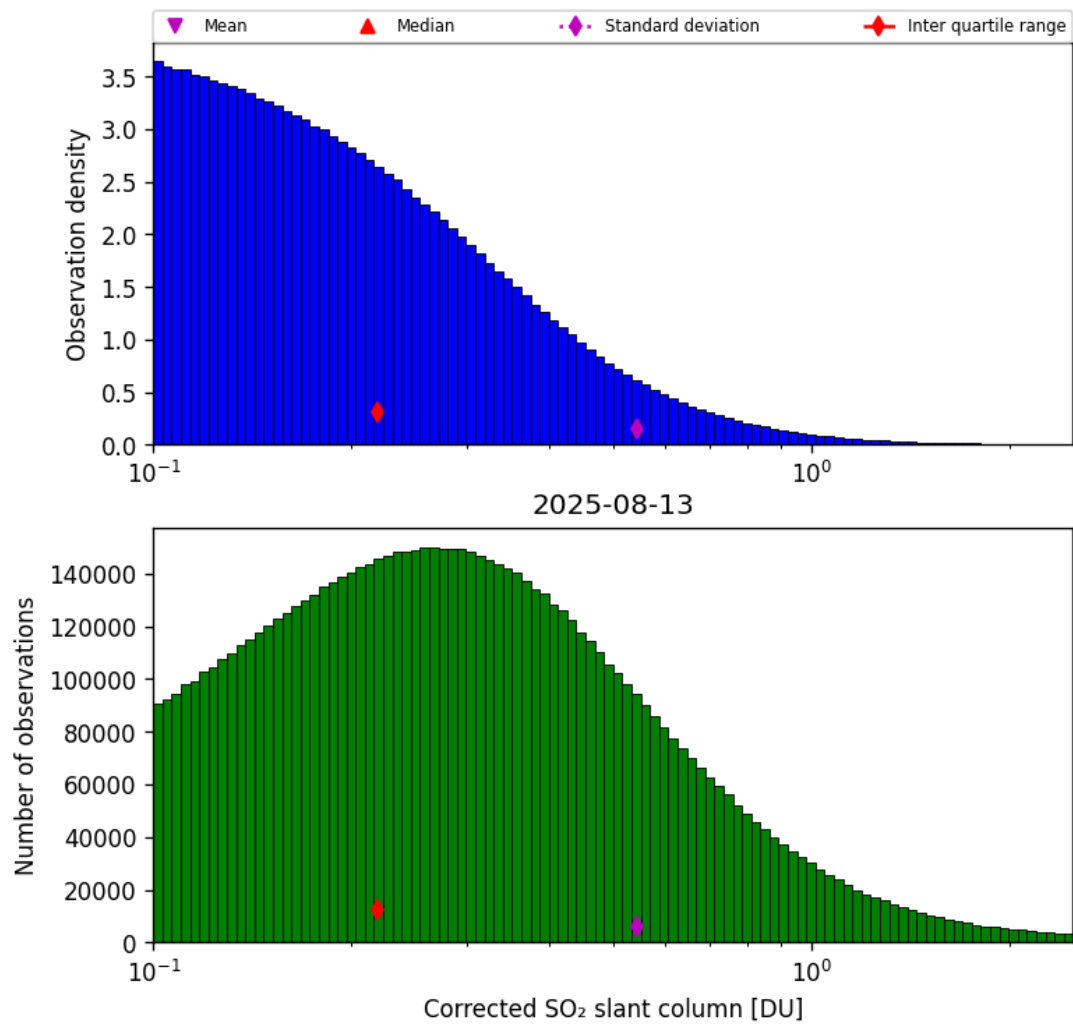
Figure 60: Histogram of "Corrected SO 2 slant column" for 2025-08-12 to 2025-08-14
