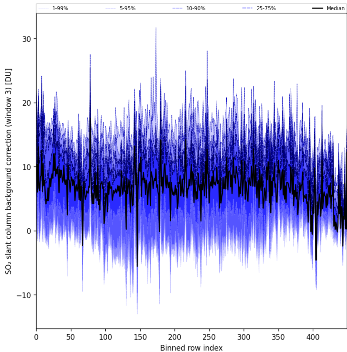
Figure 100: Along track statistics of “SO 2 slant column background correction (window 3)” for 2025-08-12 to 2025-08-14
