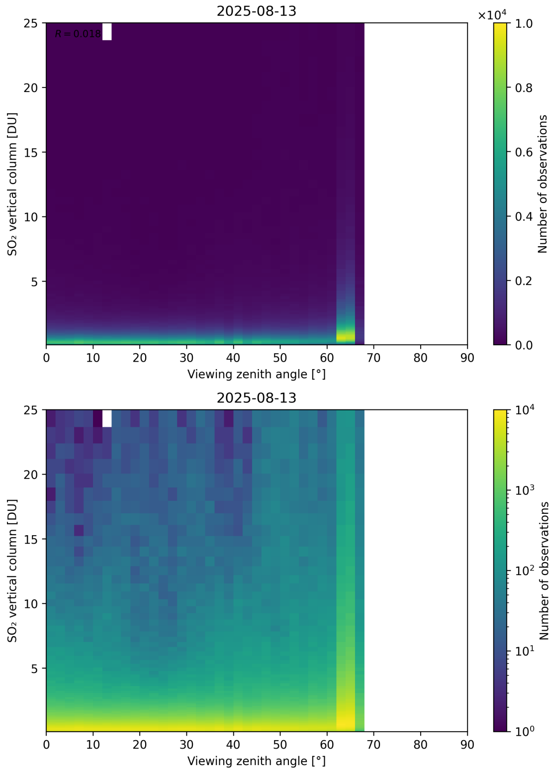
Figure 383: Scatter density plot of “Viewing zenith angle” against “SO 2 vertical column” for 2025-08-12 to 2025-08-14.
