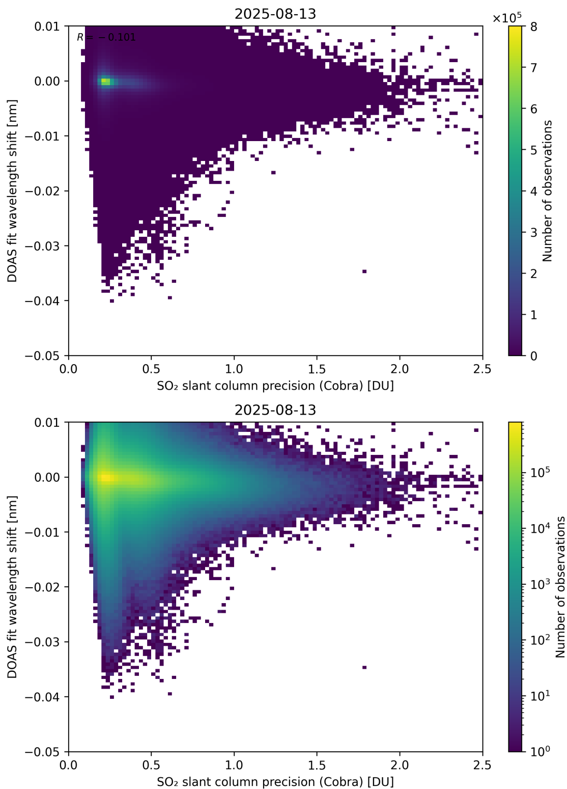
Figure 202: Scatter density plot of “SO 2 slant column precision (Cobra)” against “DOAS fit wavelength shift” for 2025-08-12 to 2025-08-14.
