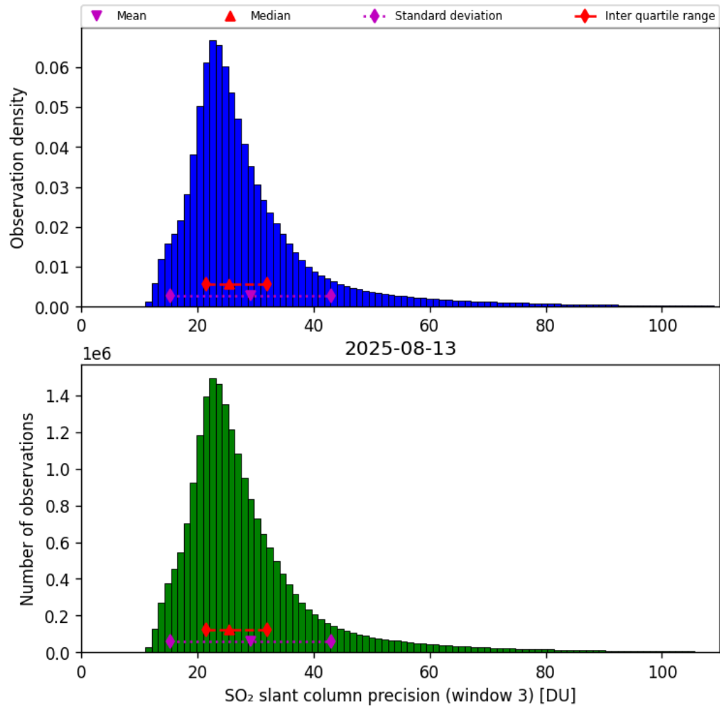
Figure 72: Histogram of “SO 2 slant column precision (window 3)” for 2025-08-12 to 2025-08-14
