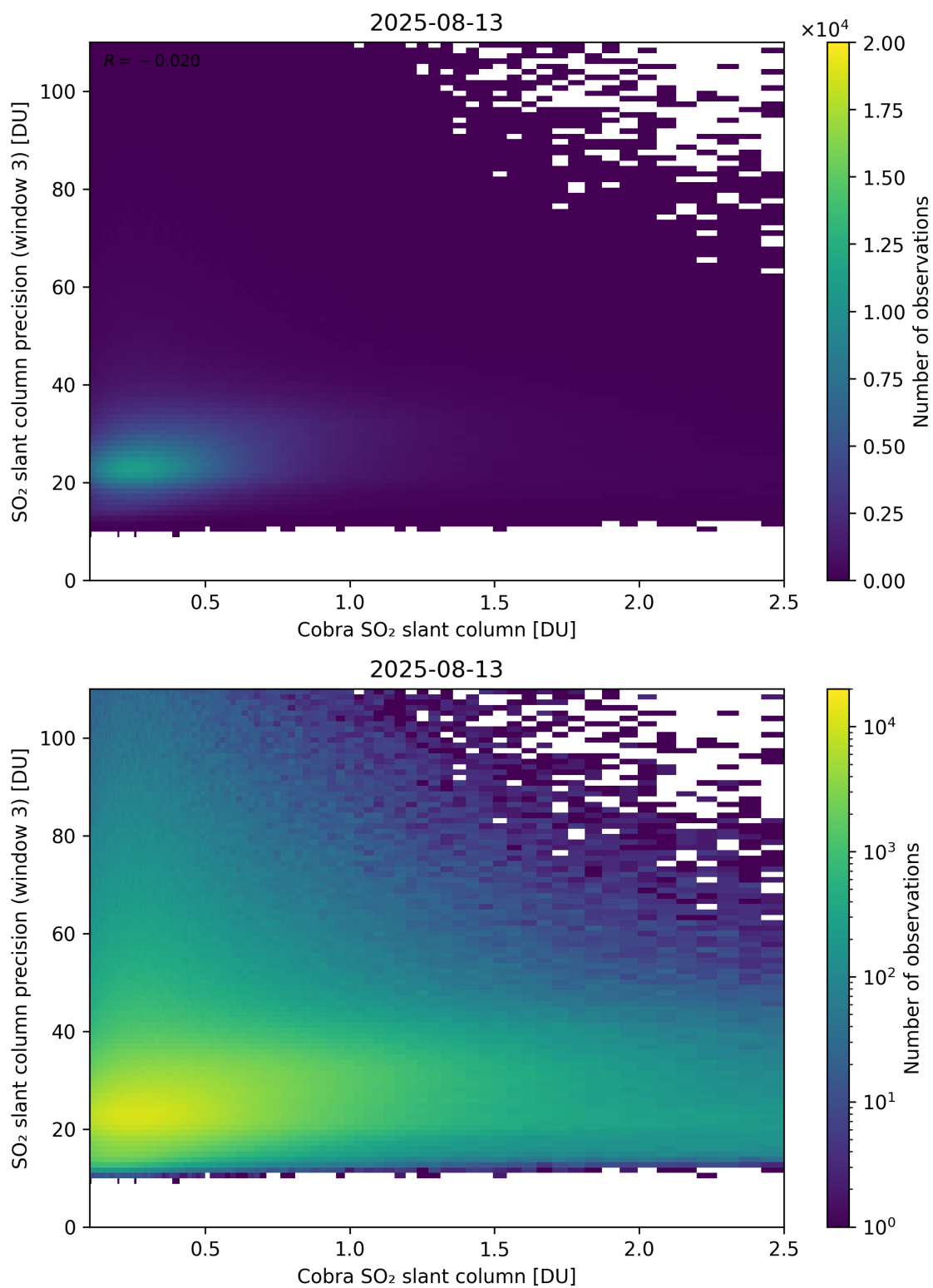
Figure 223: Scatter density plot of “Cobra SO 2 slant column” against “SO 2 slant column precision (window 3)” for 2025-08-12 to 2025-08-14.
