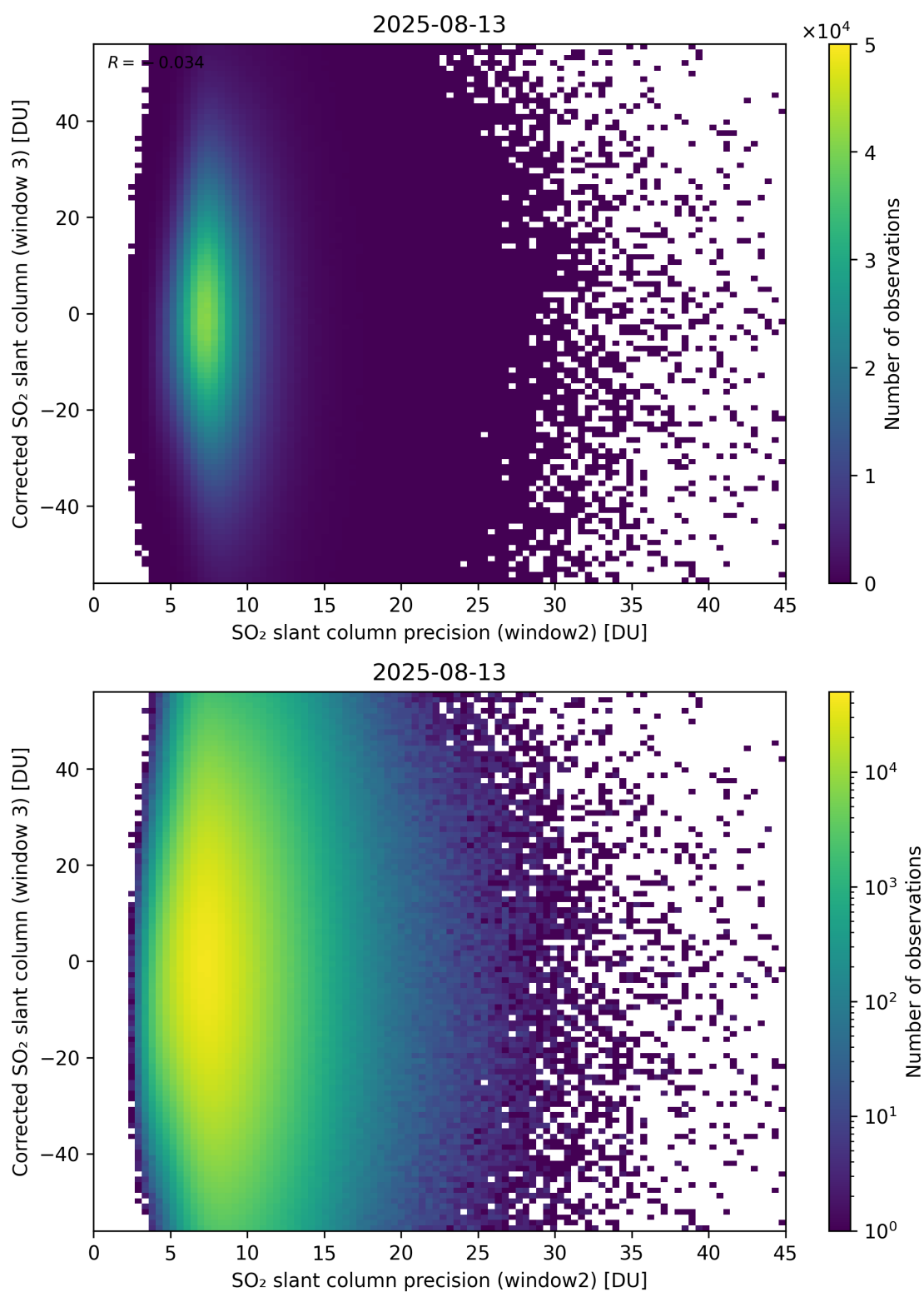
Figure 298: Scatter density plot of “SO 2 slant column precision (window2)” against “Corrected SO 2 slant column (window 3)” for 2025-08-12 to 2025-08-14.
