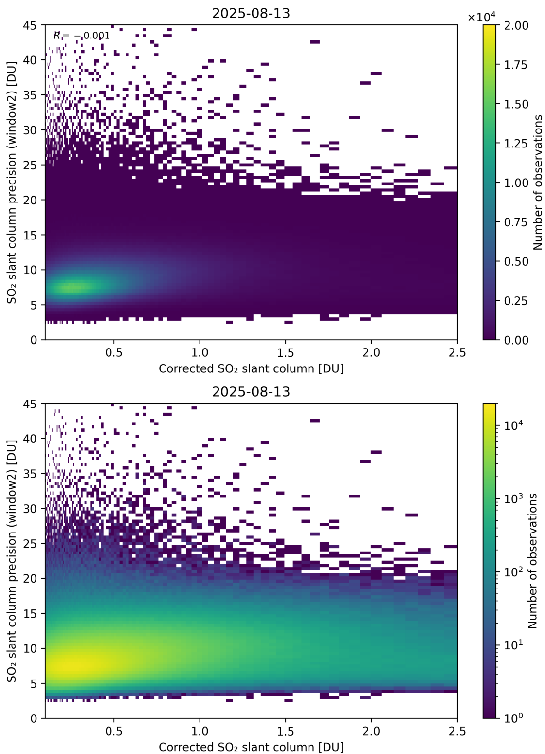
Figure 239: Scatter density plot of “Corrected SO 2 slant column” against “SO 2 slant column precision (window2)” for 2025-08-12 to 2025-08-14.
