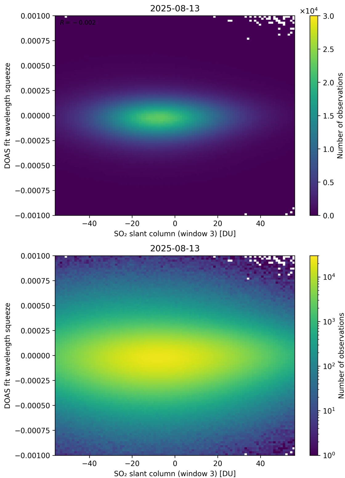
Figure 305: Scatter density plot of “SO 2 slant column (window 3)” against “DOAS fit wavelength squeeze” for 2025-08-12 to 2025-08-14.
