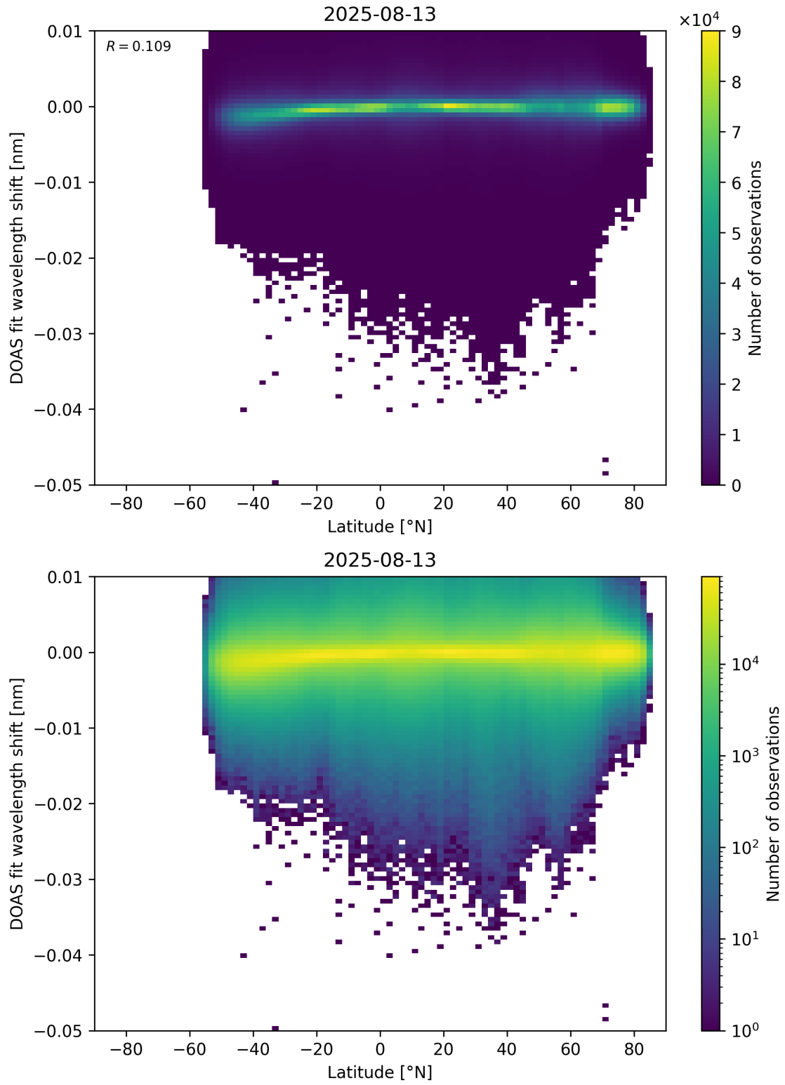
Figure 153: Scatter density plot of “Latitude” against “DOAS fit wavelength shift” for 2025-08-12 to 2025-08-14.
