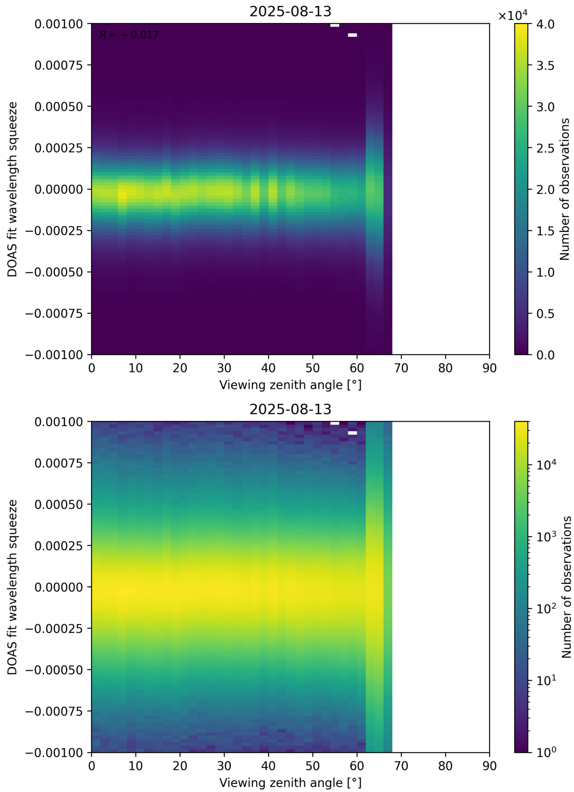
Figure 366: Scatter density plot of “Viewing zenith angle” against “DOAS fit wavelength squeeze” for 2025-08-12 to 2025-08-14.
