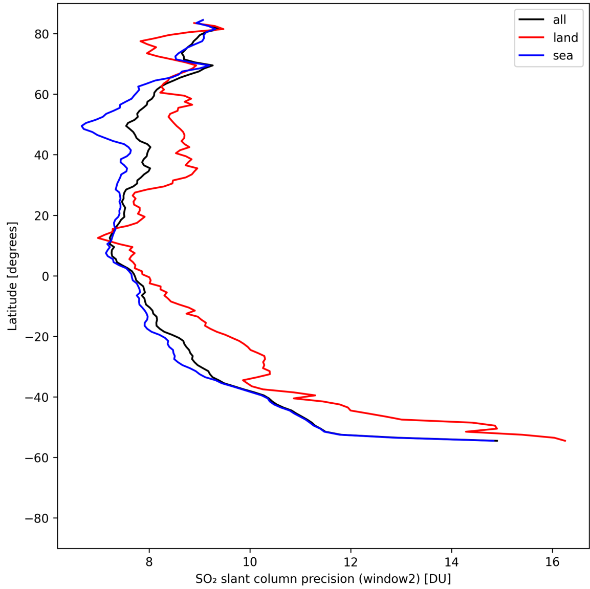
Figure 42: Zonal average of “SO 2 slant column precision (window2)” for 2025-08-12 to 2025-08-14.
