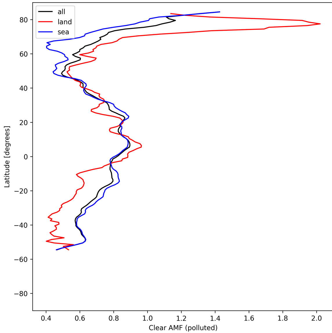
Figure 55: Zonal average of “Clear AMF (polluted)” for 2025-08-12 to 2025-08-14.
