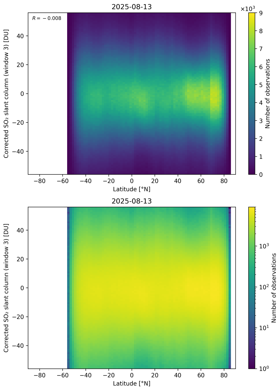
Figure 161: Scatter density plot of “Latitude” against “Corrected SO 2 slant column (window 3)” for 2025-08-12 to 2025-08-14.
