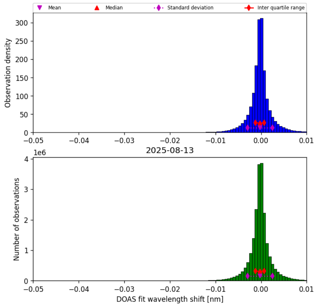
Figure 76: Histogram of “DOAS fit wavelength shift” for 2025-08-12 to 2025-08-14
