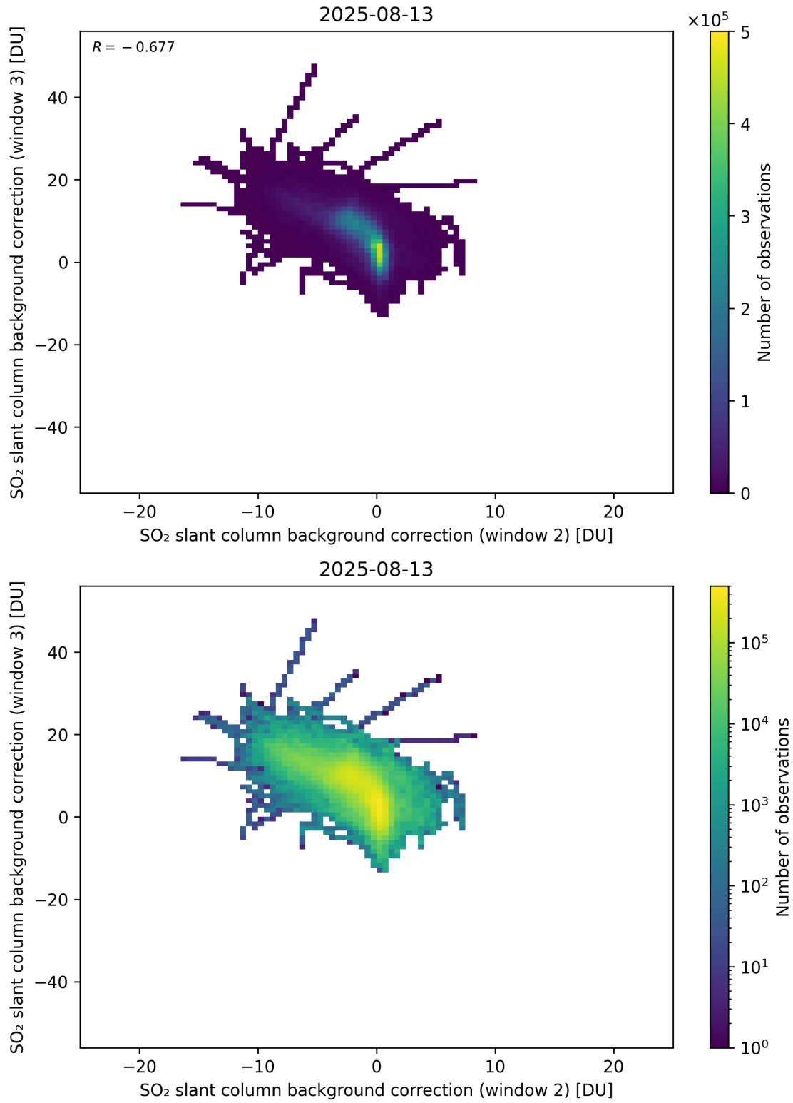
Figure 122: Scatter density plot of “SO 2 slant column background correction (window 2)” against “SO 2 slant column background correction (window 3)” for 2025-08-12 to 2025-08-14.
