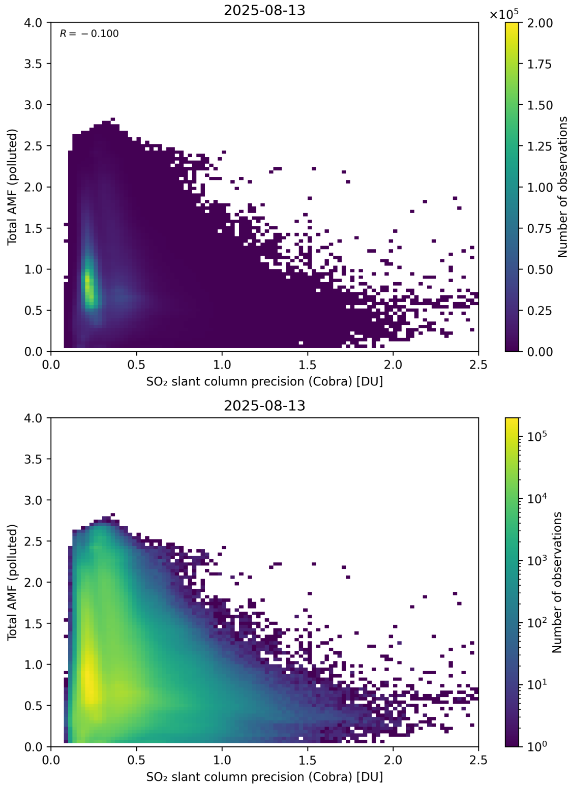
Figure 213: Scatter density plot of “SO 2 slant column precision (Cobra)” against “Total AMF (polluted)” for 2025-08-12 to 2025-08-14.
