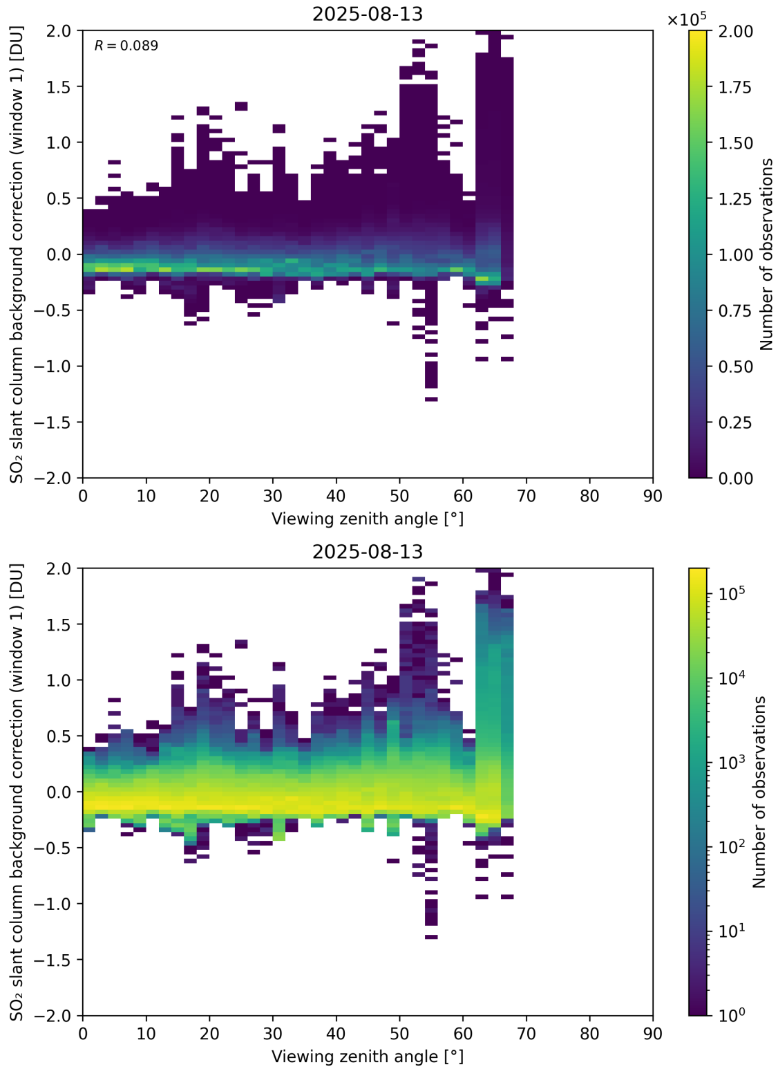
Figure 362: Scatter density plot of “Viewing zenith angle” against “SO 2 slant column background correction (window 1)” for 2025-08-12 to 2025-08-14.
