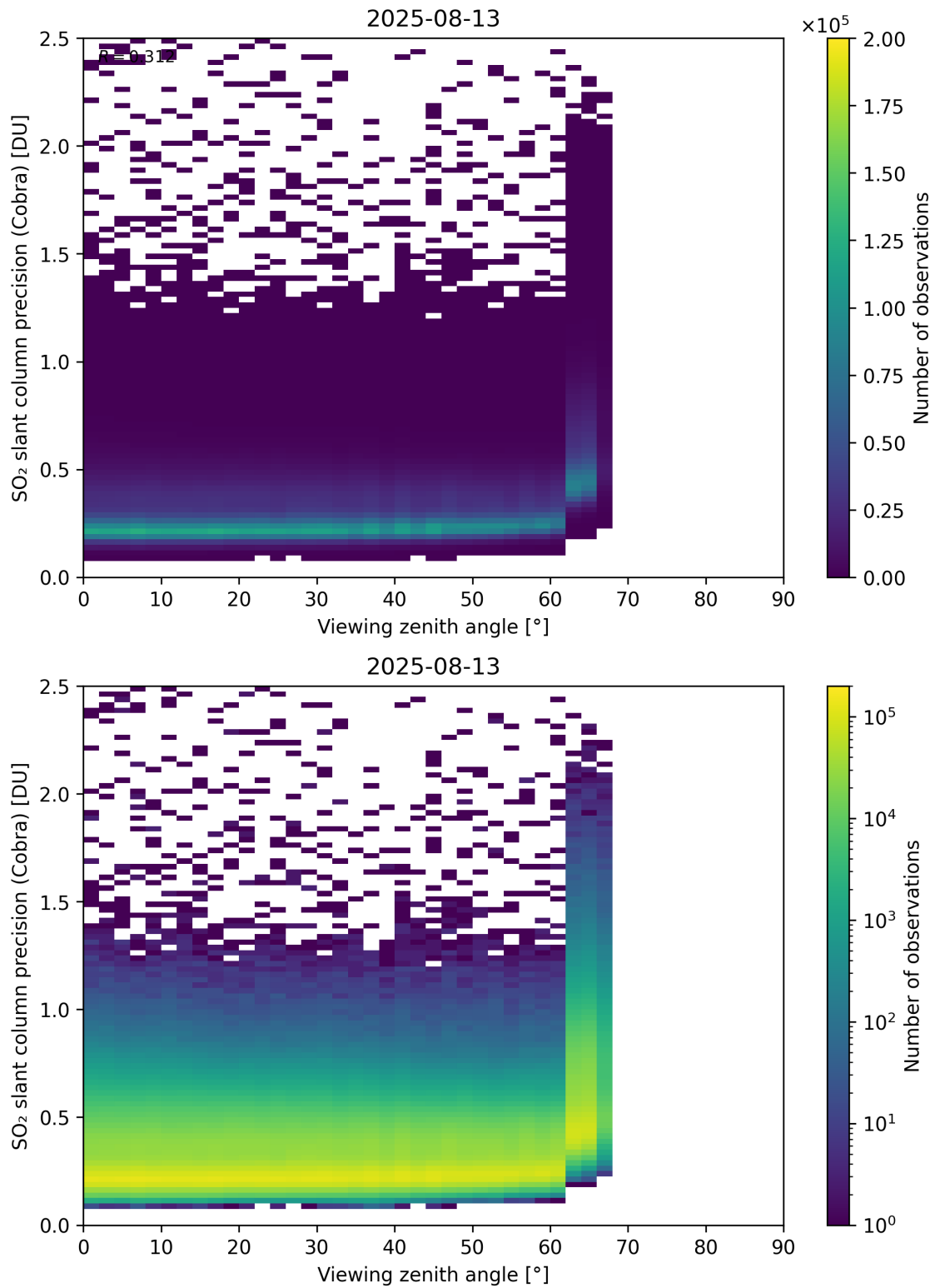
Figure 372: Scatter density plot of “Viewing zenith angle” against “SO 2 slant column precision (Cobra)” for 2025-08-12 to 2025-08-14.
