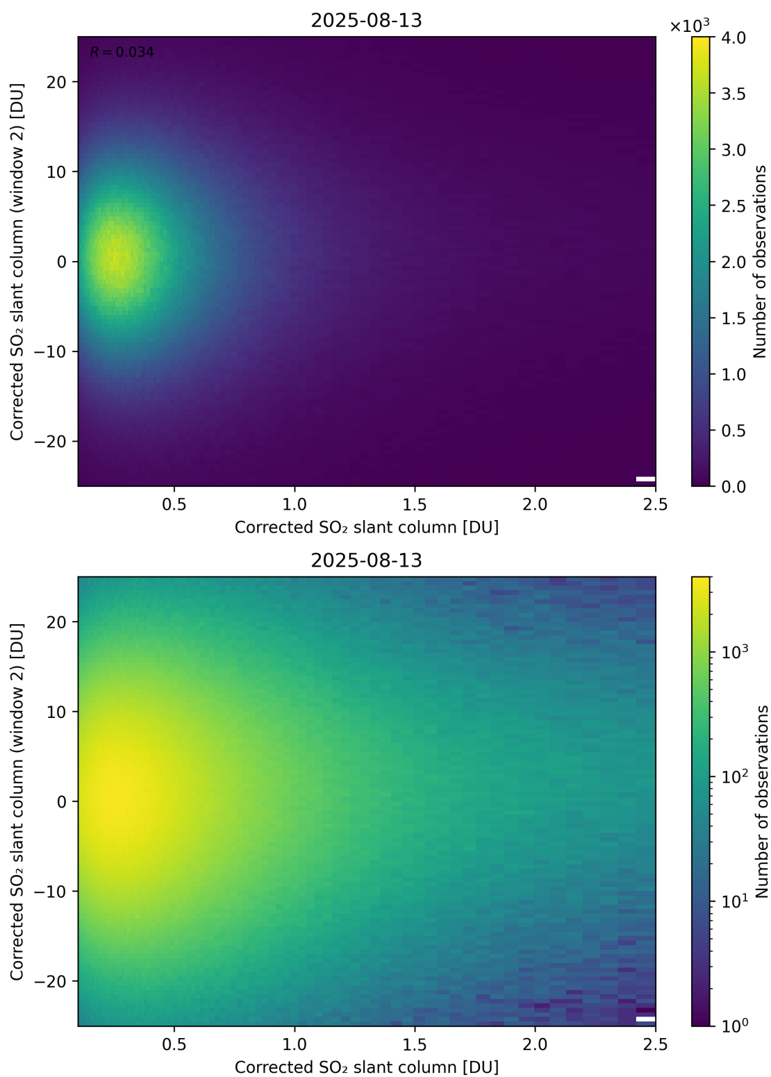
Figure 235: Scatter density plot of “Corrected SO 2 slant column” against “Corrected SO 2 slant column (window 2)” for 2025-08-12 to 2025-08-14.
