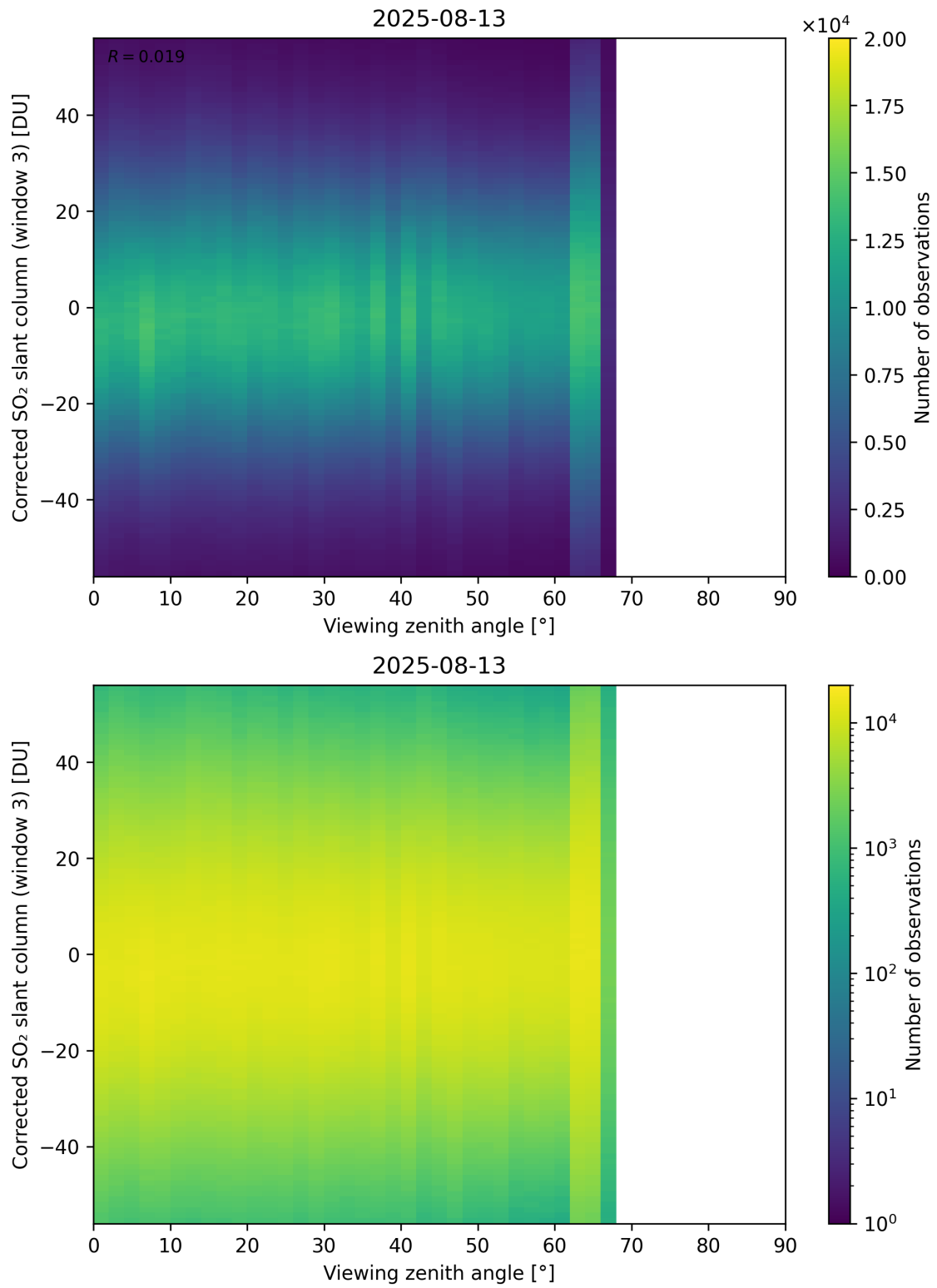
Figure 375: Scatter density plot of “Viewing zenith angle” against “Corrected SO 2 slant column (window 3)” for 2025-08-12 to 2025-08-14.
