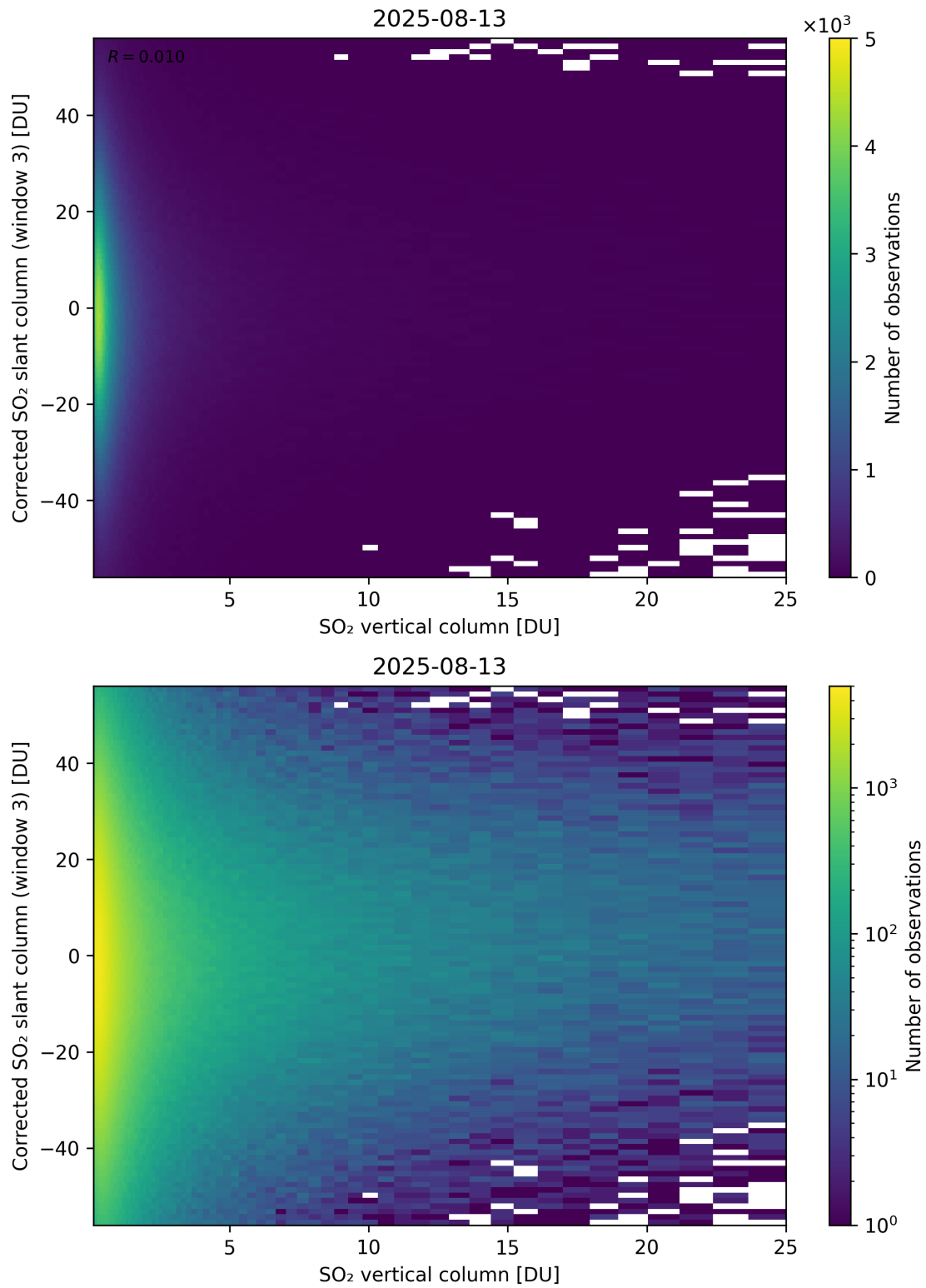
Figure 353: Scatter density plot of “SO 2 vertical column” against “Corrected SO 2 slant column (window 3)” for 2025-08-12 to 2025-08-14.
