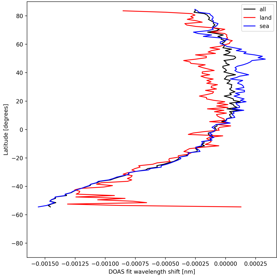
Figure 50: Zonal average of "DOAS fit wavelength shift" for 2025-08-12 to 2025-08-14.
