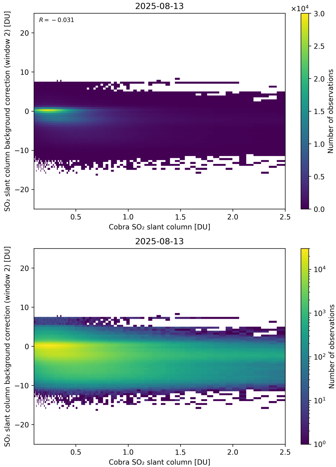
Figure 194: Scatter density plot of “Cobra SO 2 slant column” against “SO 2 slant column background correction (window 2)” for 2025-08-12 to 2025-08-14.
