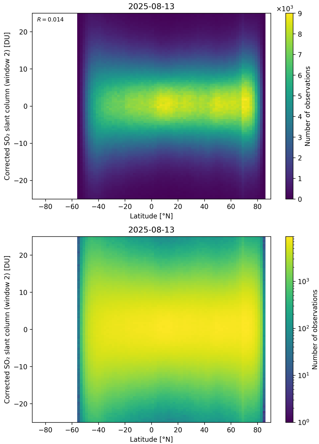
Figure 160: Scatter density plot of “Latitude” against “Corrected SO 2 slant column (window 2)” for 2025-08-12 to 2025-08-14.
