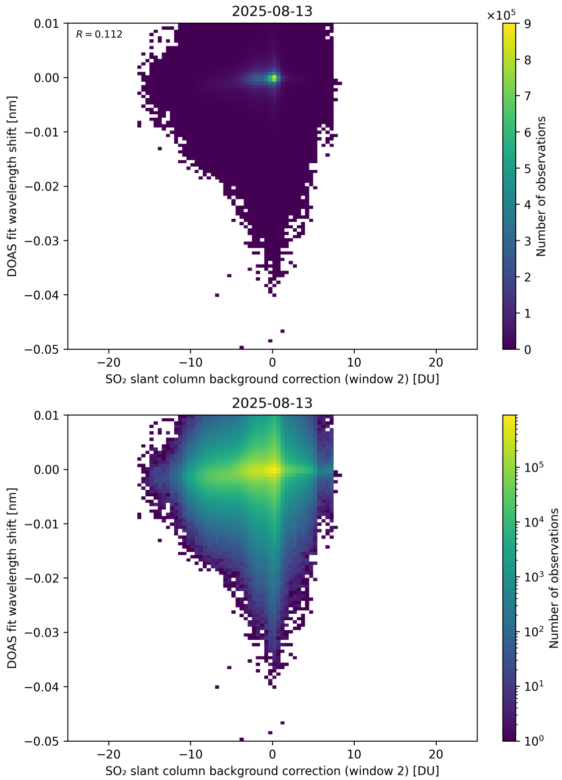
Figure 123: Scatter density plot of “SO 2 slant column background correction (window 2)” against “DOAS fit wavelength shift” for 2025-08-12 to 2025-08-14.
