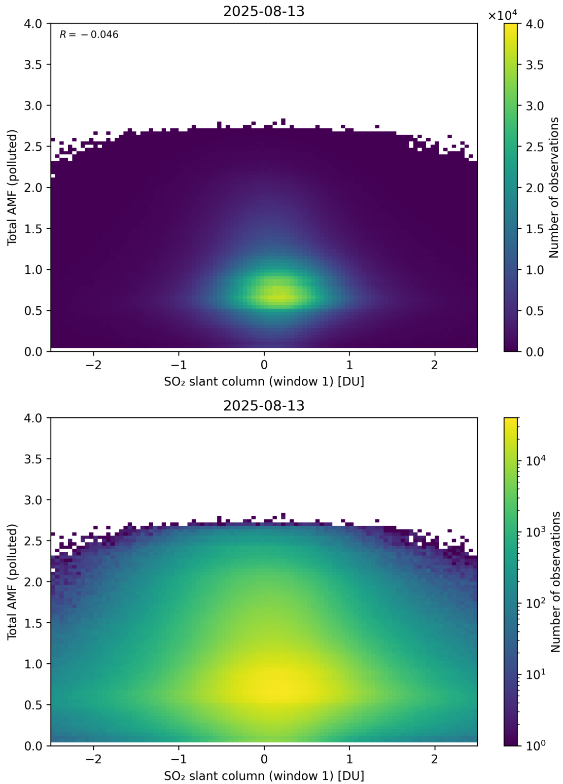
Figure 289: Scatter density plot of “SO 2 slant column (window 1)” against “Total AMF (polluted)” for 2025-08-12 to 2025-08-14.
