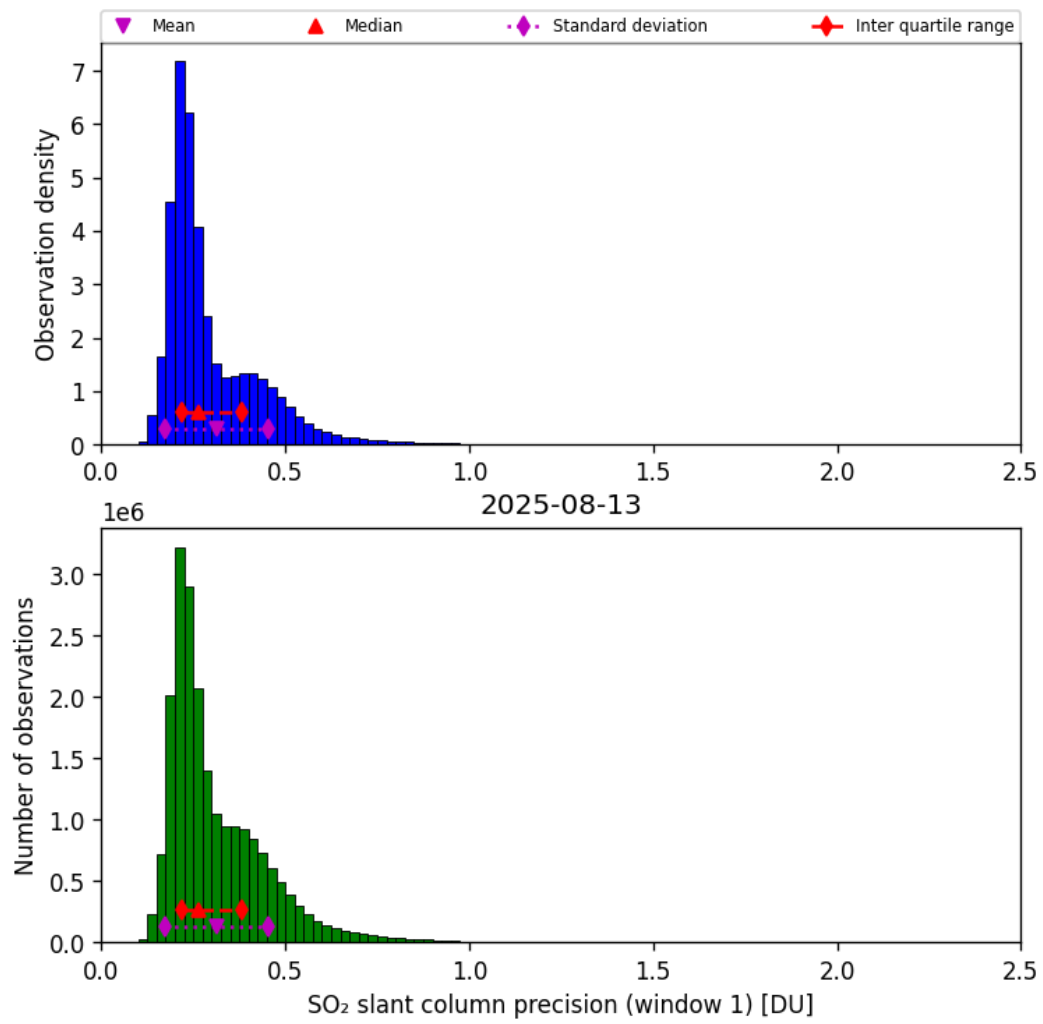
Figure 64: Histogram of “SO 2 slant column precision (window 1)” for 2025-08-12 to 2025-08-14
