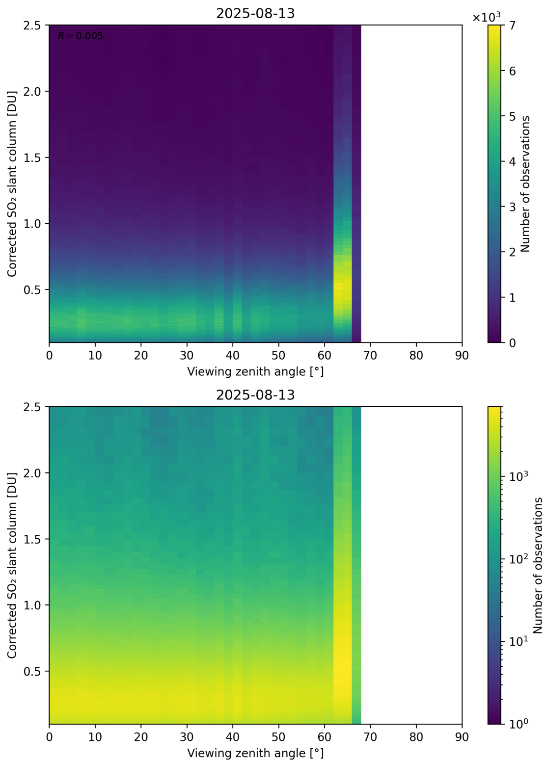
Figure 373: Scatter density plot of “Viewing zenith angle” against “Corrected SO 2 slant column” for 2025-08-12 to 2025-08-14.
