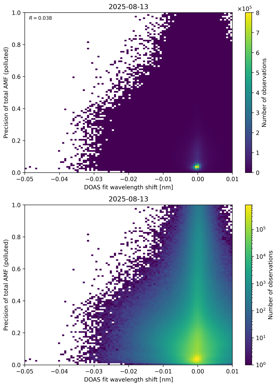
Figure 142: Scatter density plot of “DOAS fit wavelength shift” against “Precision of total AMF (polluted)” for 2025-08-12 to 2025-08-14.
