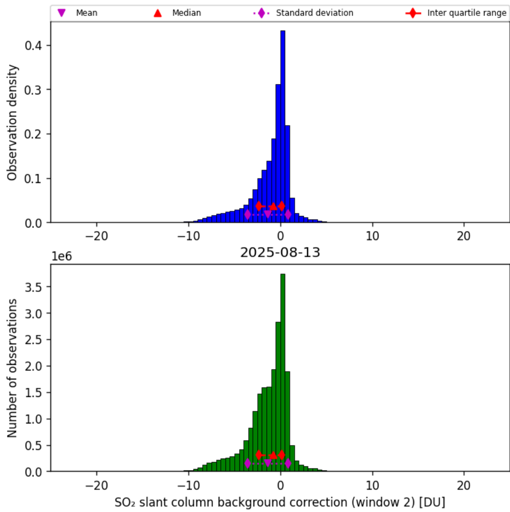
Figure 70: Histogram of “SO 2 slant column background correction (window 2)” for 2025-08-12 to 2025-08-14
