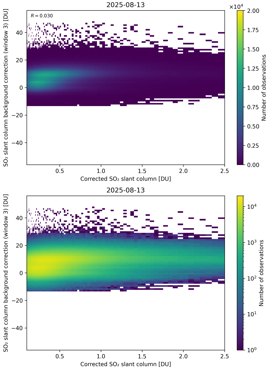
Figure 228: Scatter density plot of “Corrected SO 2 slant column” against “SO 2 slant column background correction (window 3)” for 2025-08-12 to 2025-08-14.
