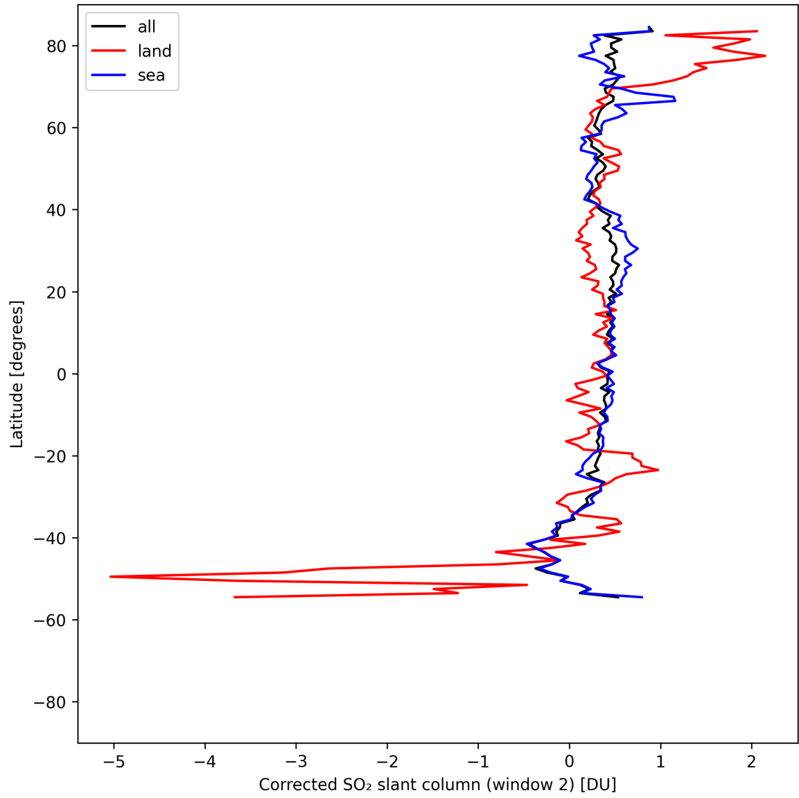
Figure 43: Zonal average of “Corrected SO 2 slant column (window 2)” for 2025-08-12 to 2025-08-14.
