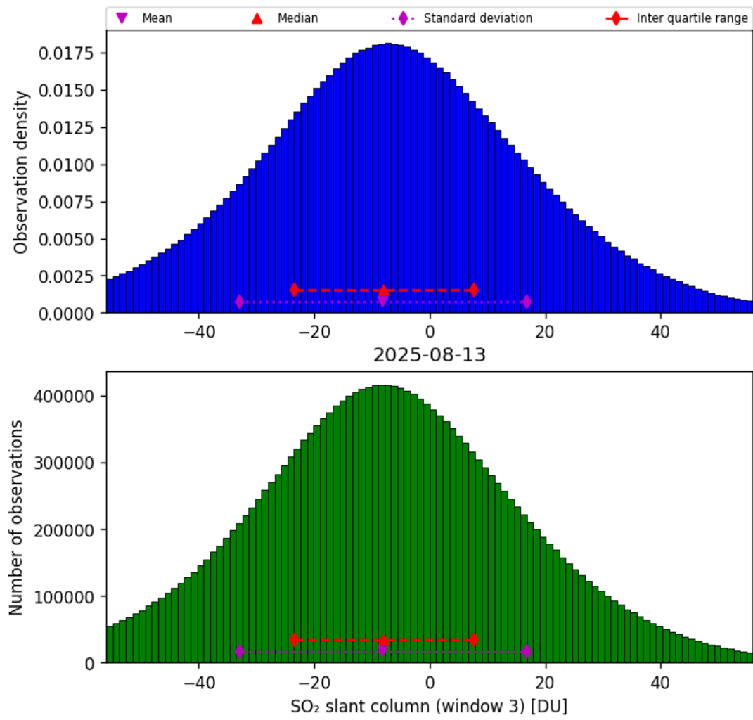
Figure 71: Histogram of “SO 2 slant column (window 3)” for 2025-08-12 to 2025-08-14
