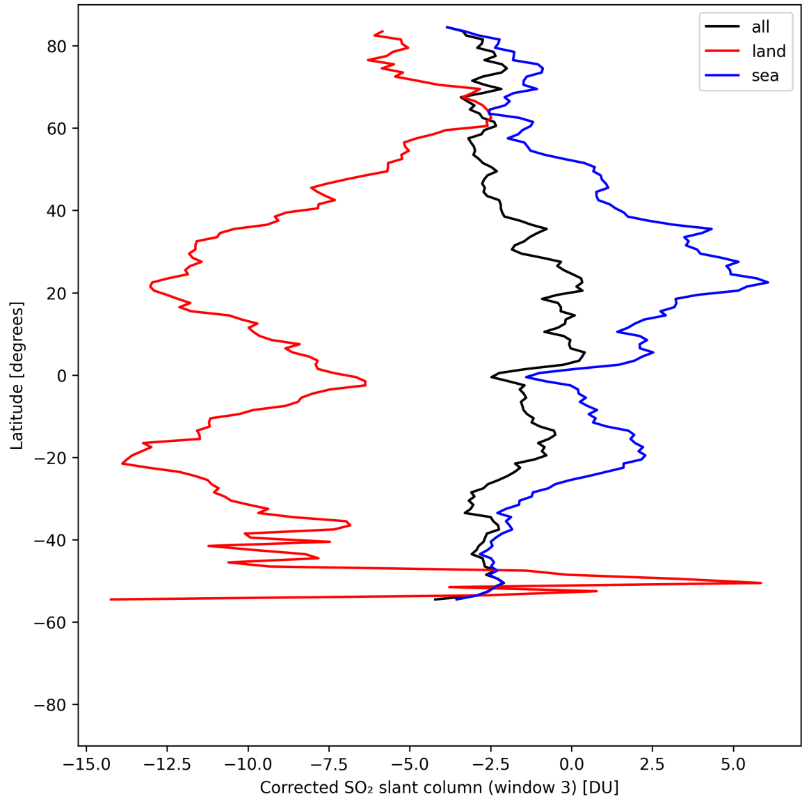
Figure 47: Zonal average of “Corrected SO 2 slant column (window 3)” for 2025-08-12 to 2025-08-14.
