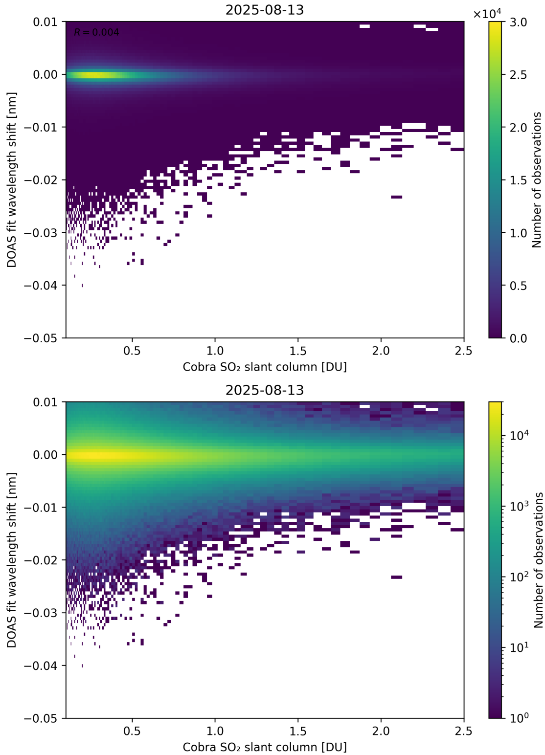
Figure 196: Scatter density plot of “Cobra SO 2 slant column” against “DOAS fit wavelength shift” for 2025-08-12 to 2025-08-14.
