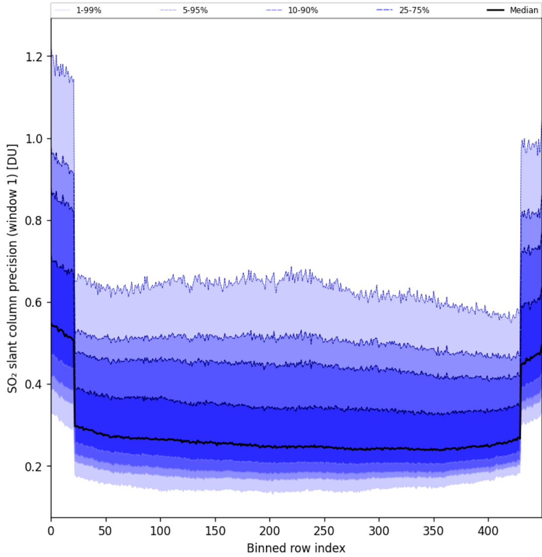
Figure 90: Along track statistics of “SO 2 slant column precision (window 1)” for 2025-08-12 to 2025-08-14
