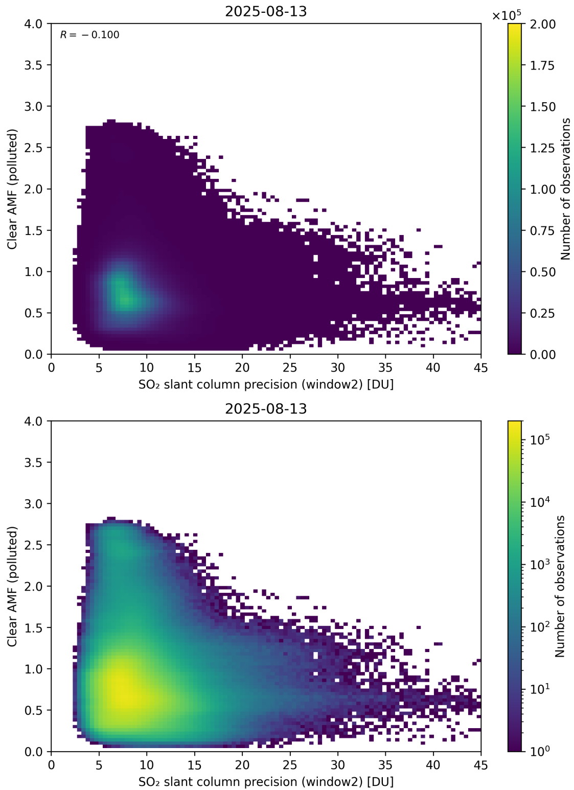
Figure 296: Scatter density plot of “SO 2 slant column precision (window2)” against “Clear AMF (polluted)” for 2025-08-12 to 2025-08-14.
