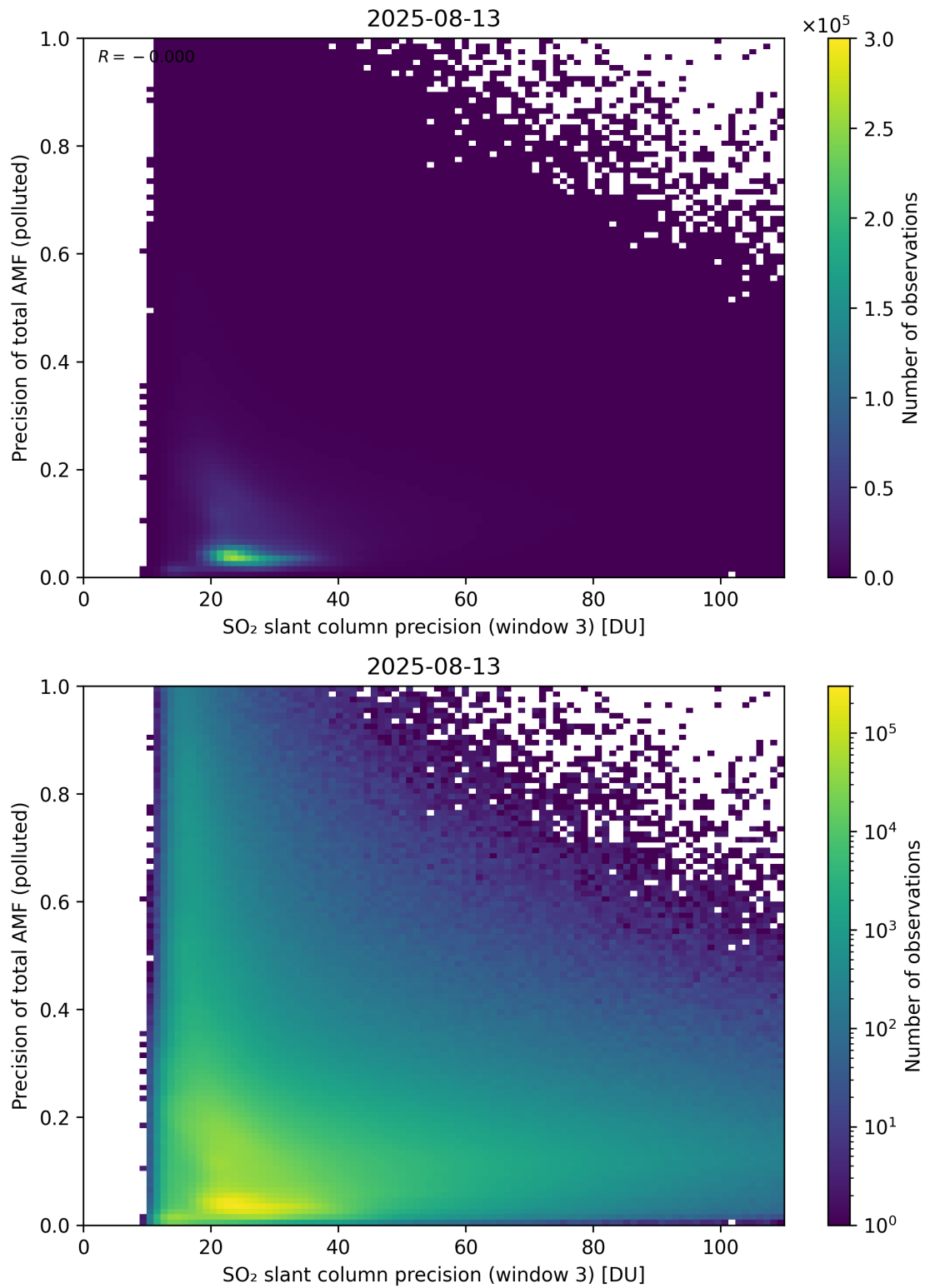
Figure 314: Scatter density plot of “SO 2 slant column precision (window 3)” against “Precision of total AMF (polluted)” for 2025-08-12 to 2025-08-14.
