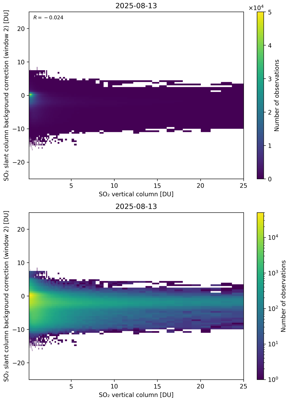
Figure 324: Scatter density plot of “SO 2 vertical column” against “SO 2 slant column background correction (window 2)” for 2025-08-12 to 2025-08-14.
