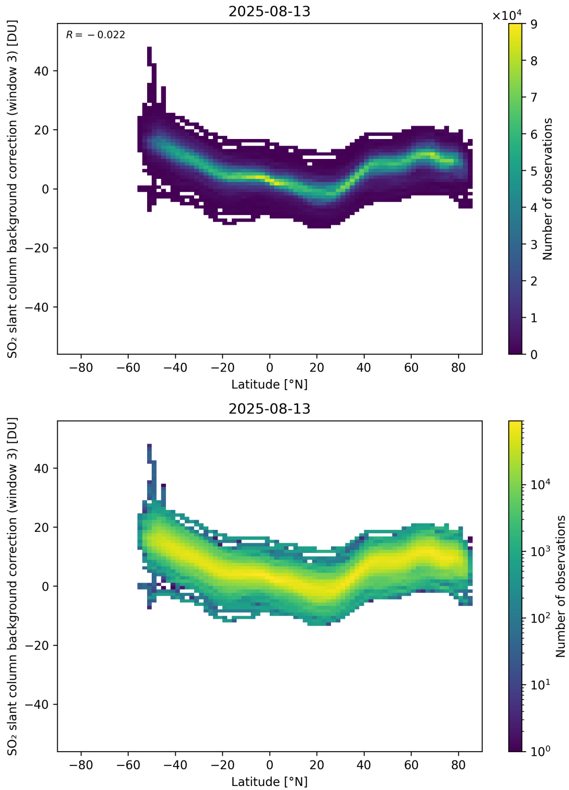
Figure 152: Scatter density plot of “Latitude” against “SO 2 slant column background correction (window 3)” for 2025-08-12 to 2025-08-14.
