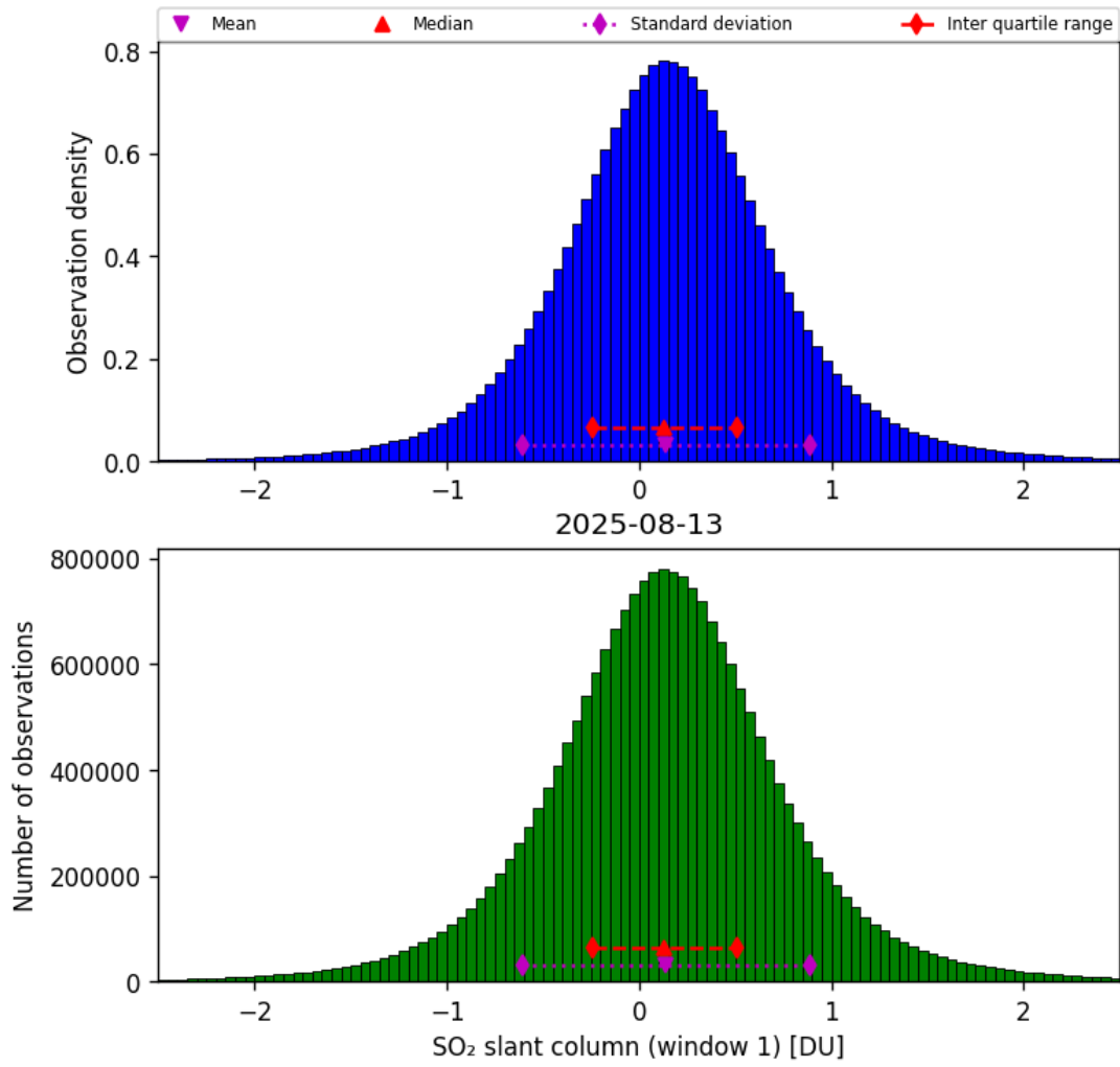
Figure 63: Histogram of “SO 2 slant column (window 1)” for 2025-08-12 to 2025-08-14
