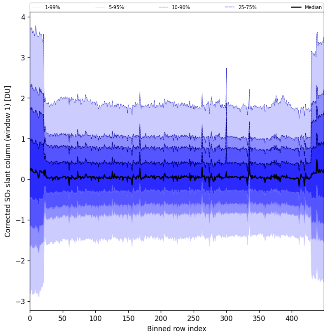
Figure 91: Along track statistics of “Corrected SO 2 slant column (window 1)” for 2025-08-12 to 2025-08-14
