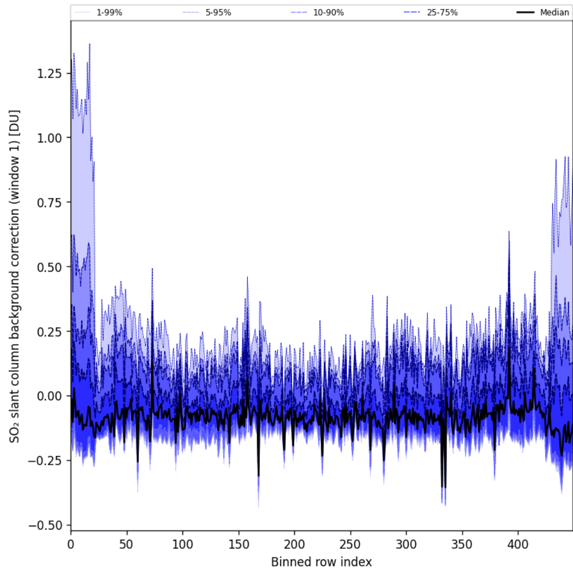
Figure 92: Along track statistics of “SO 2 slant column background correction (window 1)” for 2025-08-12 to 2025-08-14
