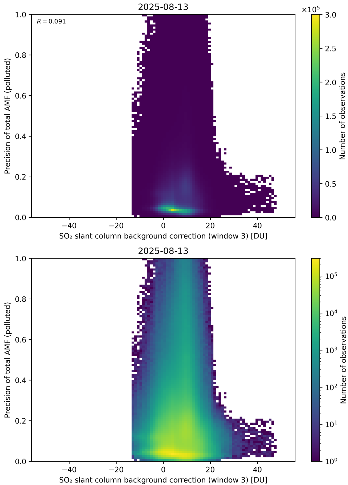
Figure 137: Scatter density plot of “SO 2 slant column background correction (window 3)” against “Precision of total AMF (polluted)” for 2025-08-12 to 2025-08-14.
