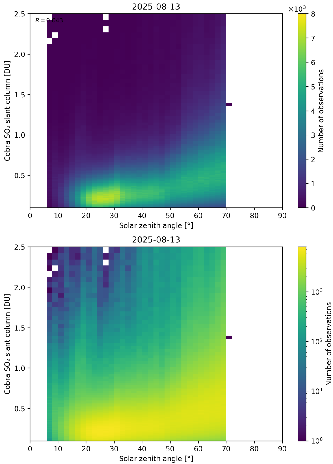
Figure 179: Scatter density plot of “Solar zenith angle” against “Cobra SO 2 slant column” for 2025-08-12 to 2025-08-14.
