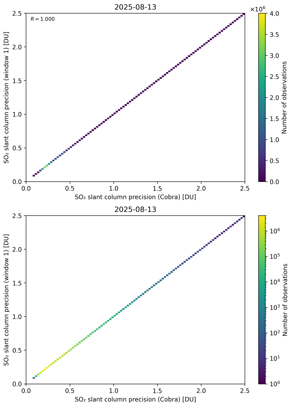
Figure 209: Scatter density plot of “SO 2 slant column precision (Cobra)” against “SO 2 slant column precision (window 1)” for 2025-08-12 to 2025-08-14.
