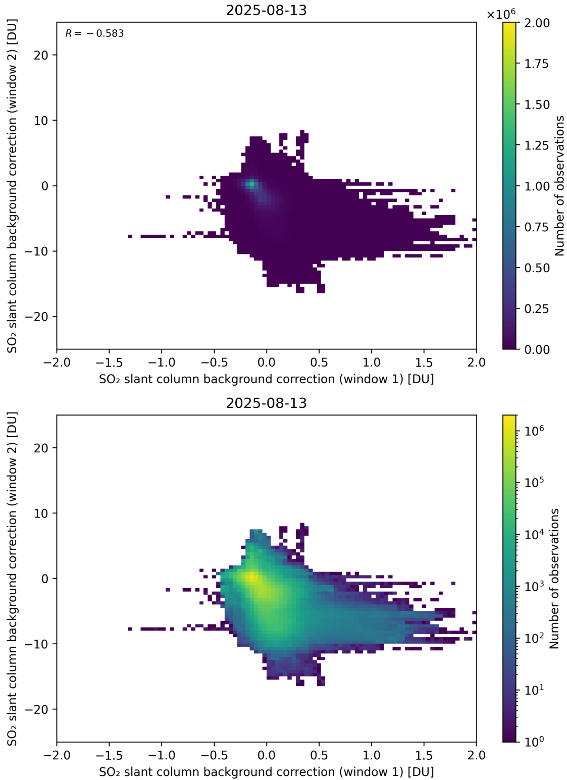
Figure 109: Scatter density plot of “SO 2 slant column background correction (window 1)” against “SO 2 slant column background correction (window 2)” for 2025-08-12 to 2025-08-14.
