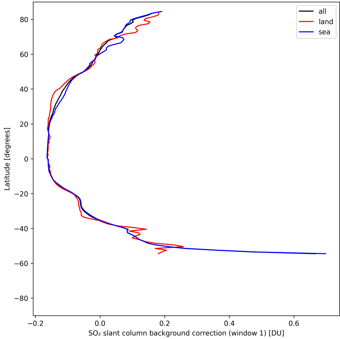
Figure 40: Zonal average of “SO 2 slant column background correction (window 1)” for 2025-08-12 to 2025-08-14.
