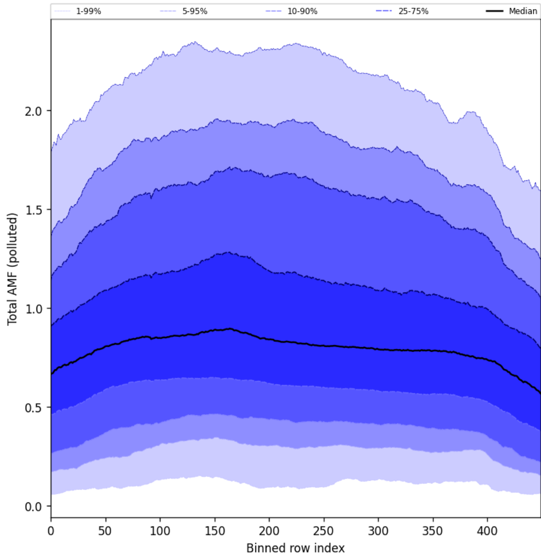
Figure 105: Along track statistics of “Total AMF (polluted)” for 2025-08-12 to 2025-08-14
