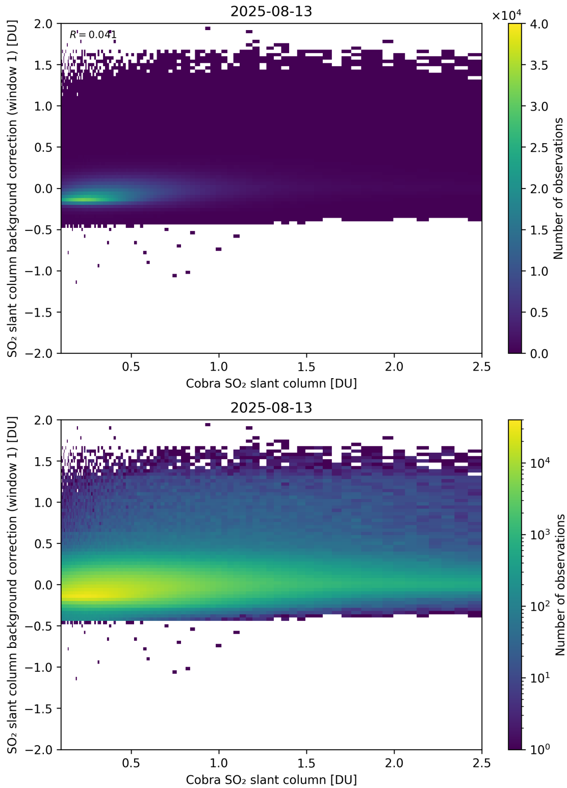
Figure 193: Scatter density plot of “Cobra SO 2 slant column” against “SO 2 slant column background correction (window 1)” for 2025-08-12 to 2025-08-14.
