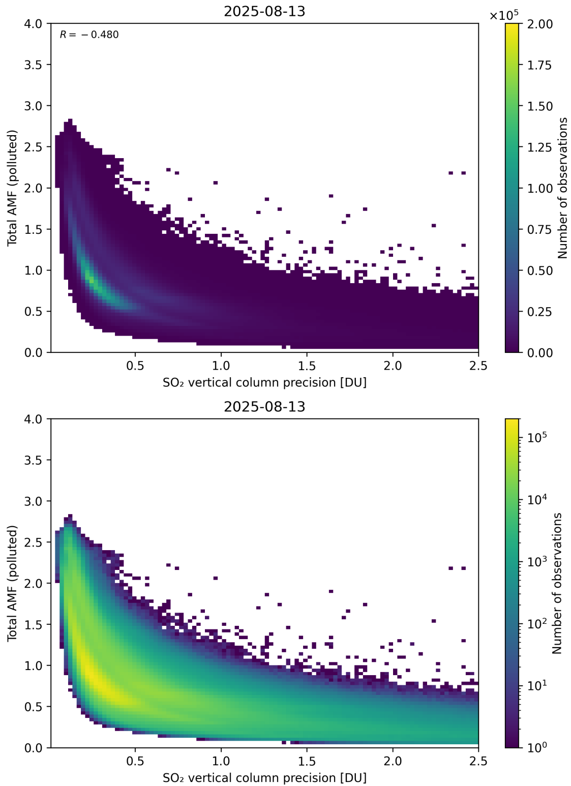
Figure 346: Scatter density plot of “SO 2 vertical column precision” against “Total AMF (polluted)” for 2025-08-12 to 2025-08-14.
