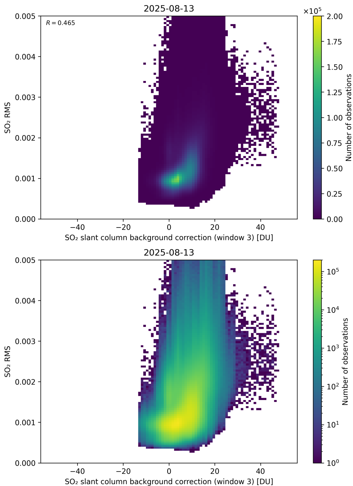
Figure 134: Scatter density plot of “SO 2 slant column background correction (window 3)” against “SO 2 RMS” for 2025-08-12 to 2025-08-14.
