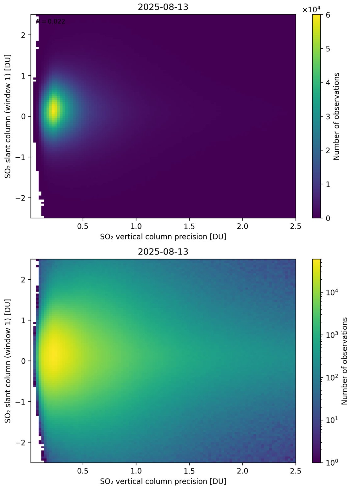
Figure 341: Scatter density plot of “SO 2 vertical column precision” against “SO 2 slant column (window 1)” for 2025-08-12 to 2025-08-14.
