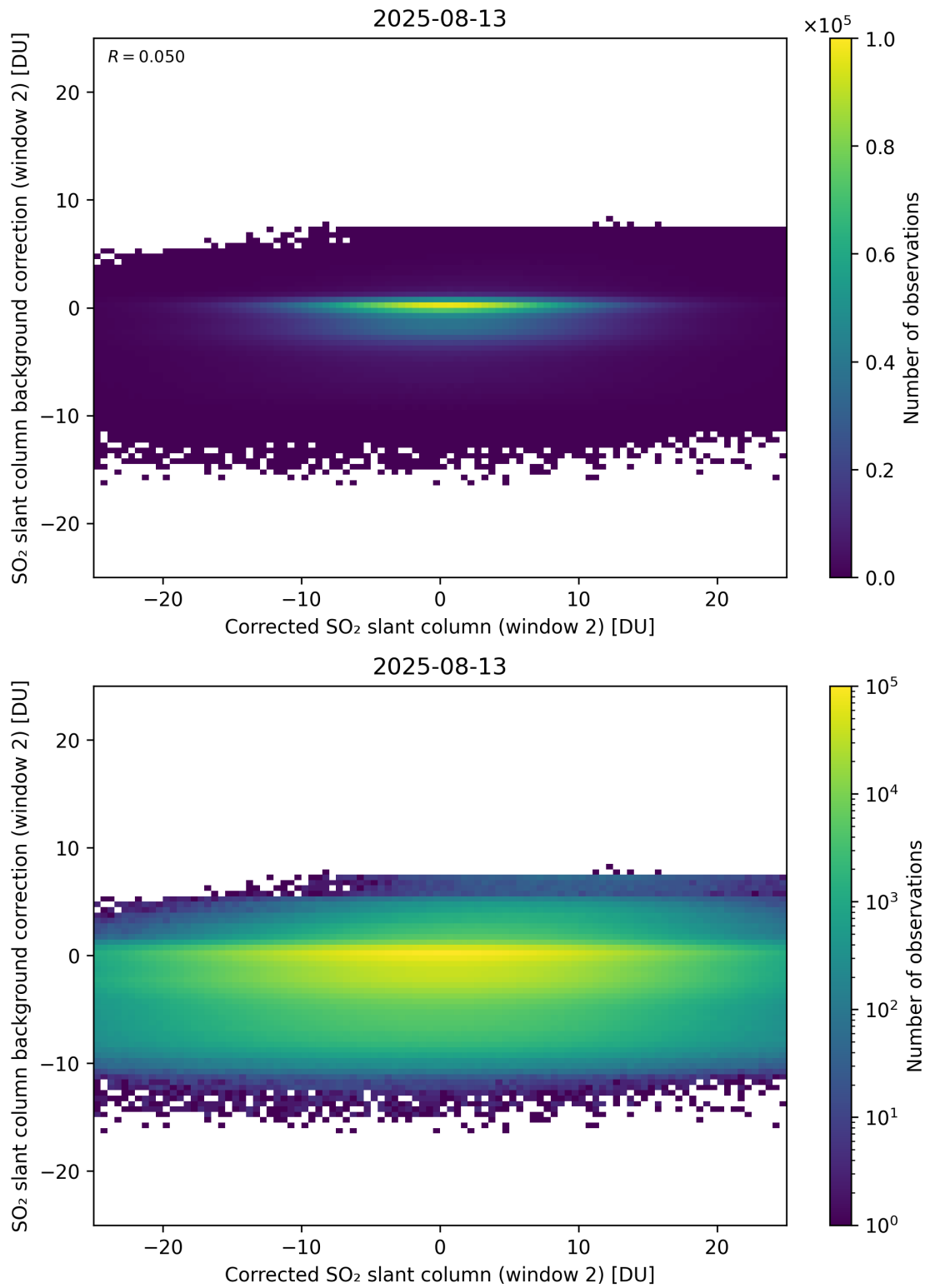
Figure 244: Scatter density plot of “Corrected SO 2 slant column (window 2)” against “SO 2 slant column background correction (window 2)” for 2025-08-12 to 2025-08-14.
