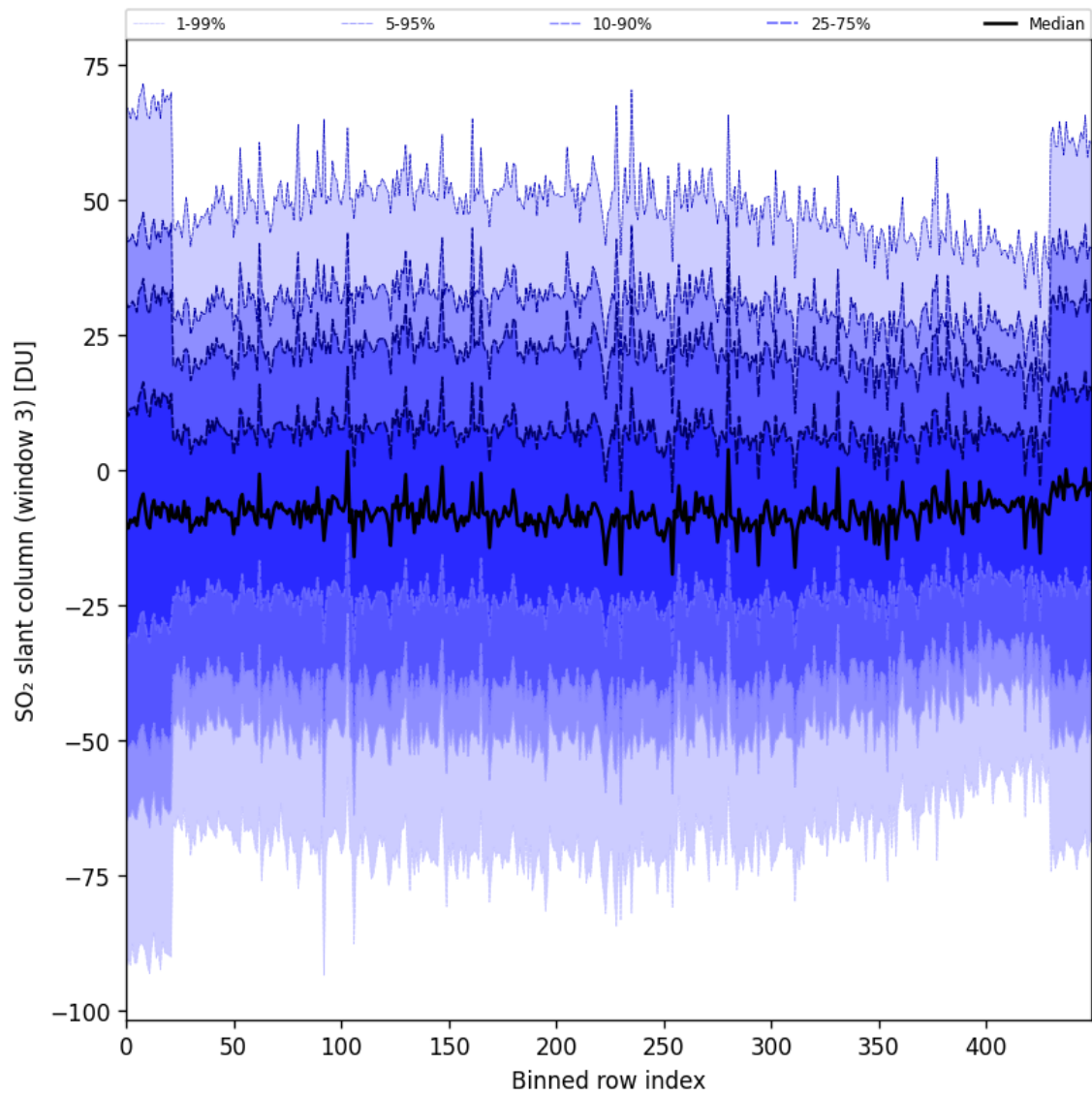
Figure 97: Along track statistics of “SO 2 slant column (window 3)” for 2025-08-12 to 2025-08-14
