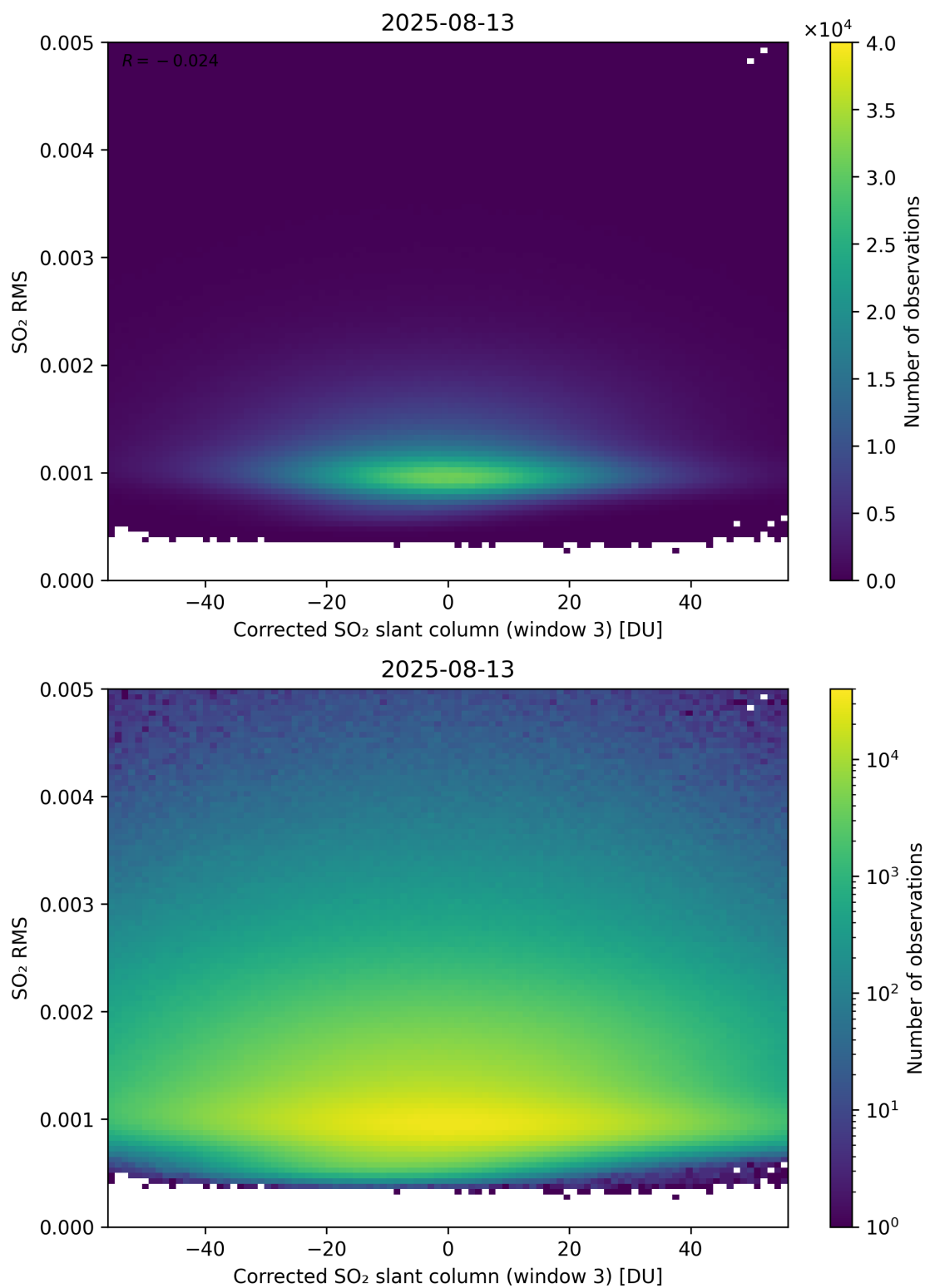
Figure 258: Scatter density plot of “Corrected SO 2 slant column (window 3)” against “SO 2 RMS” for 2025-08-12 to 2025-08-14.
