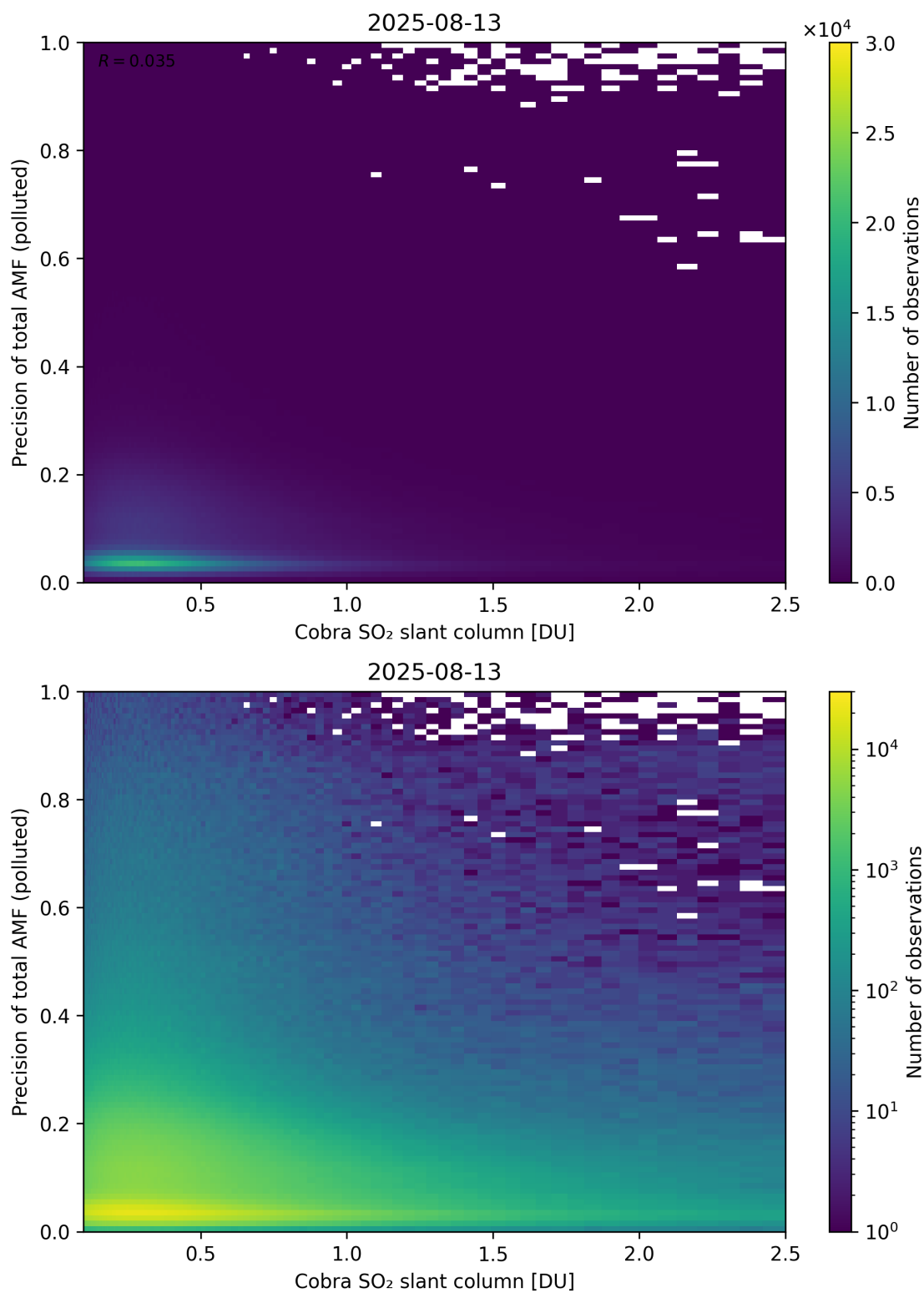
Figure 225: Scatter density plot of “Cobra SO 2 slant column” against “Precision of total AMF (polluted)” for 2025-08-12 to 2025-08-14.
