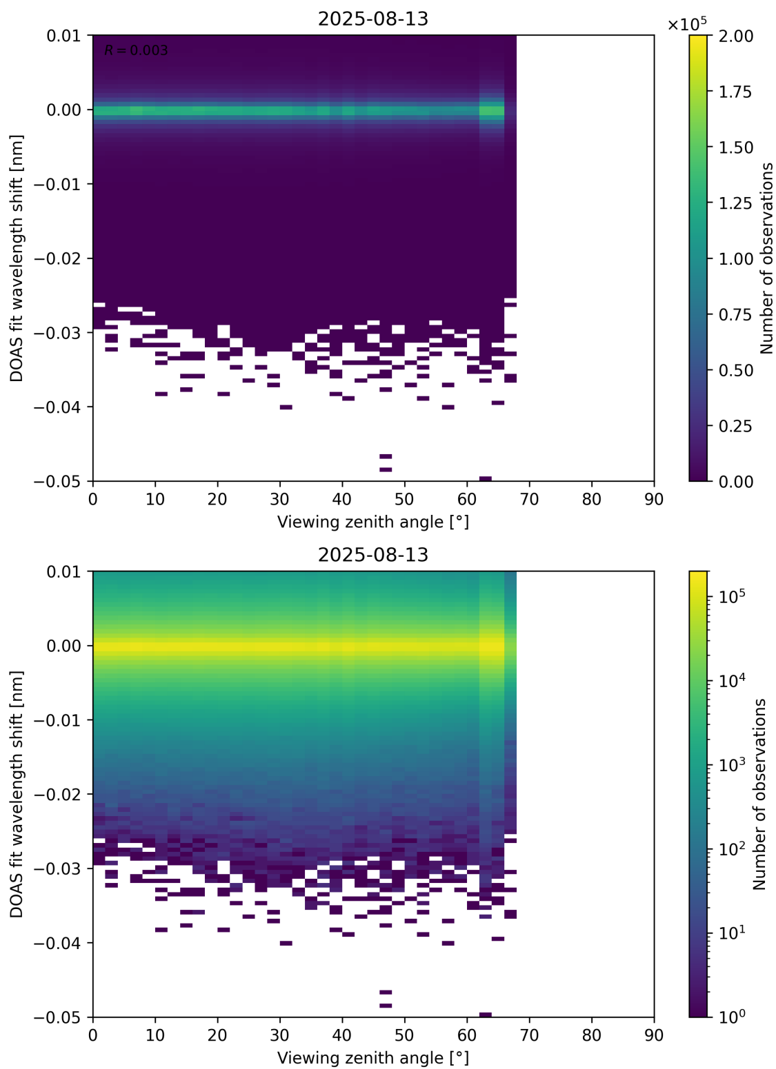
Figure 365: Scatter density plot of “Viewing zenith angle” against “DOAS fit wavelength shift” for 2025-08-12 to 2025-08-14.
