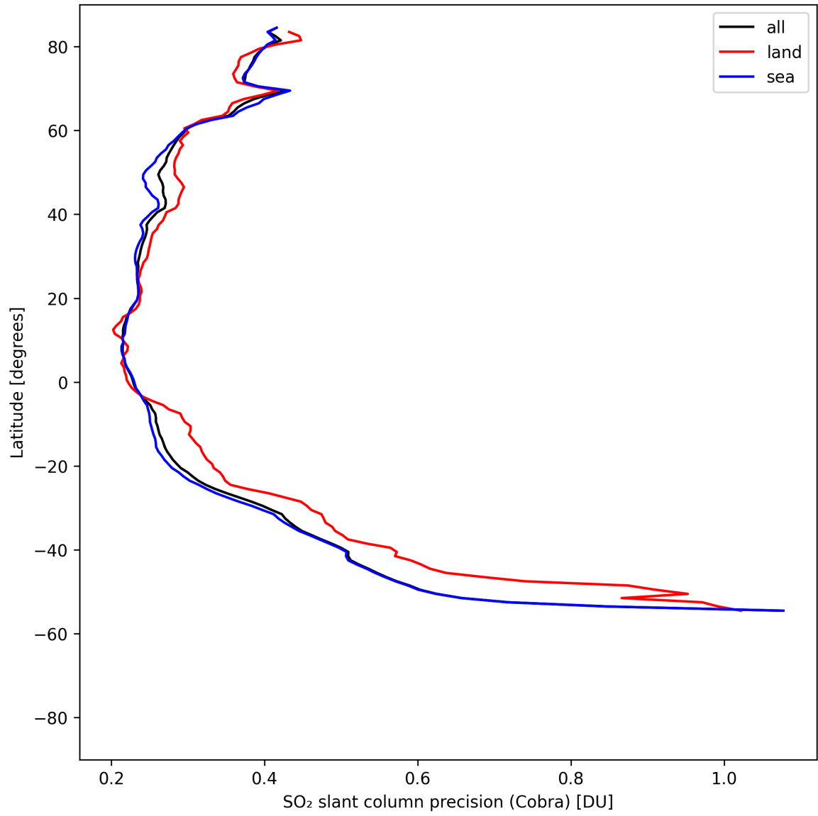
Figure 36: Zonal average of “SO 2 slant column precision (Cobra)” for 2025-08-12 to 2025-08-14.
