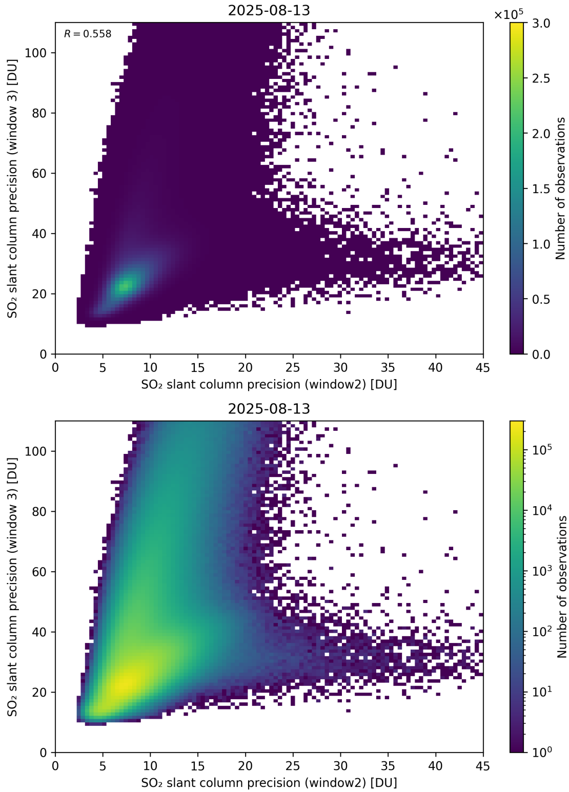
Figure 300: Scatter density plot of “SO 2 slant column precision (window2)” against “SO 2 slant column precision (window 3)” for 2025-08-12 to 2025-08-14.
