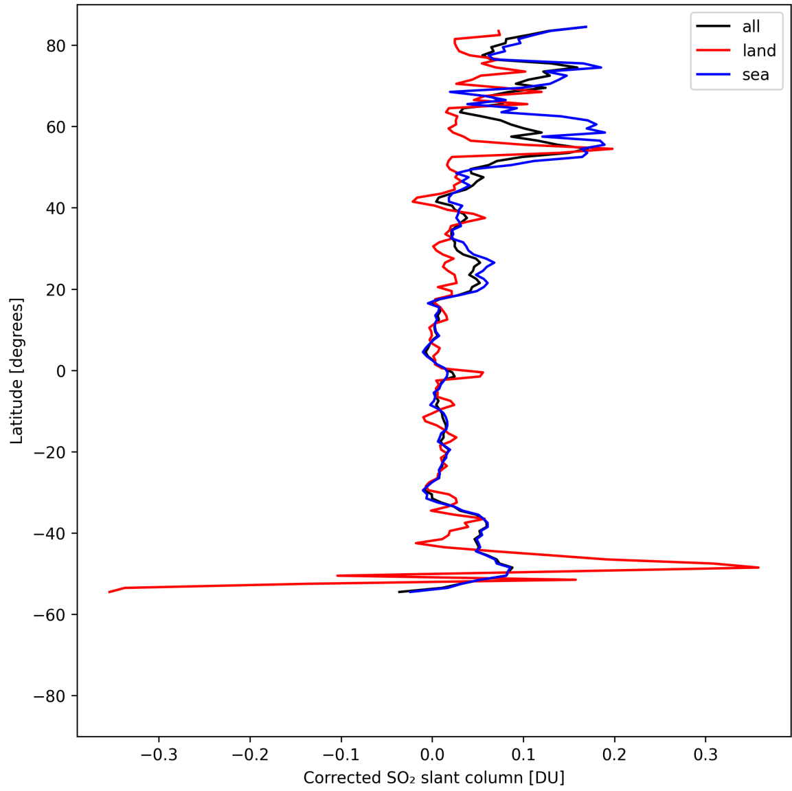
Figure 34: Zonal average of “Corrected SO 2 slant column” for 2025-08-12 to 2025-08-14.
