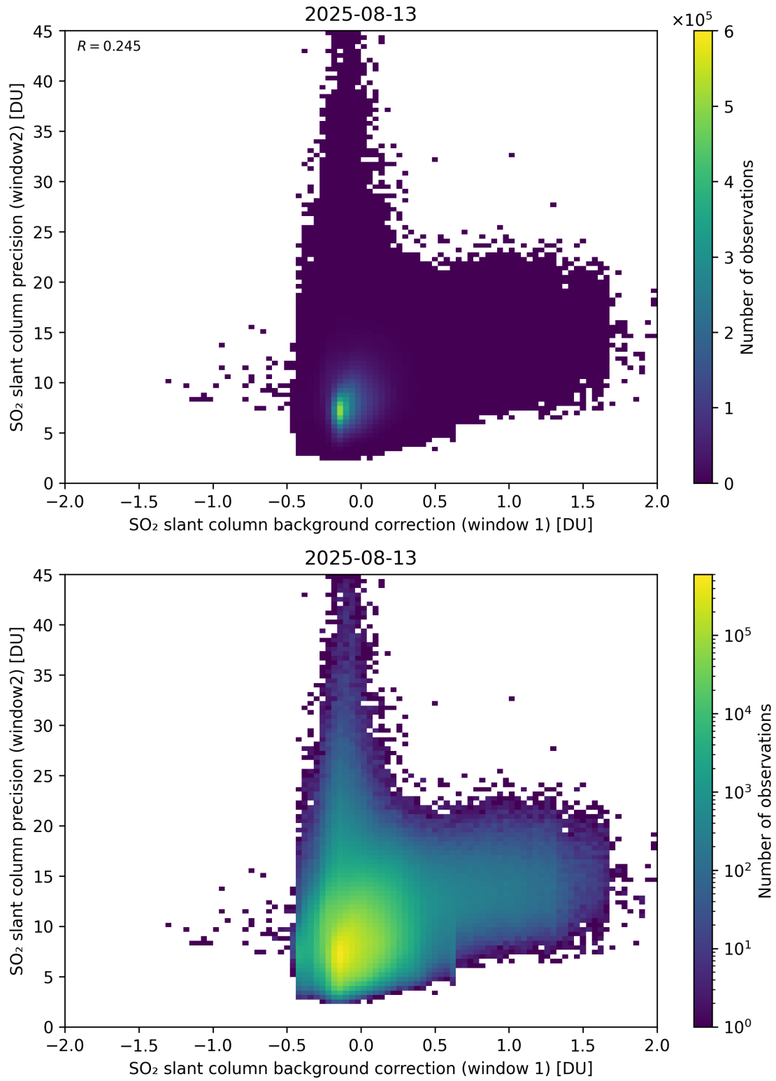
Figure 117: Scatter density plot of “SO 2 slant column background correction (window 1)” against “SO 2 slant column precision (window2)” for 2025-08-12 to 2025-08-14.
