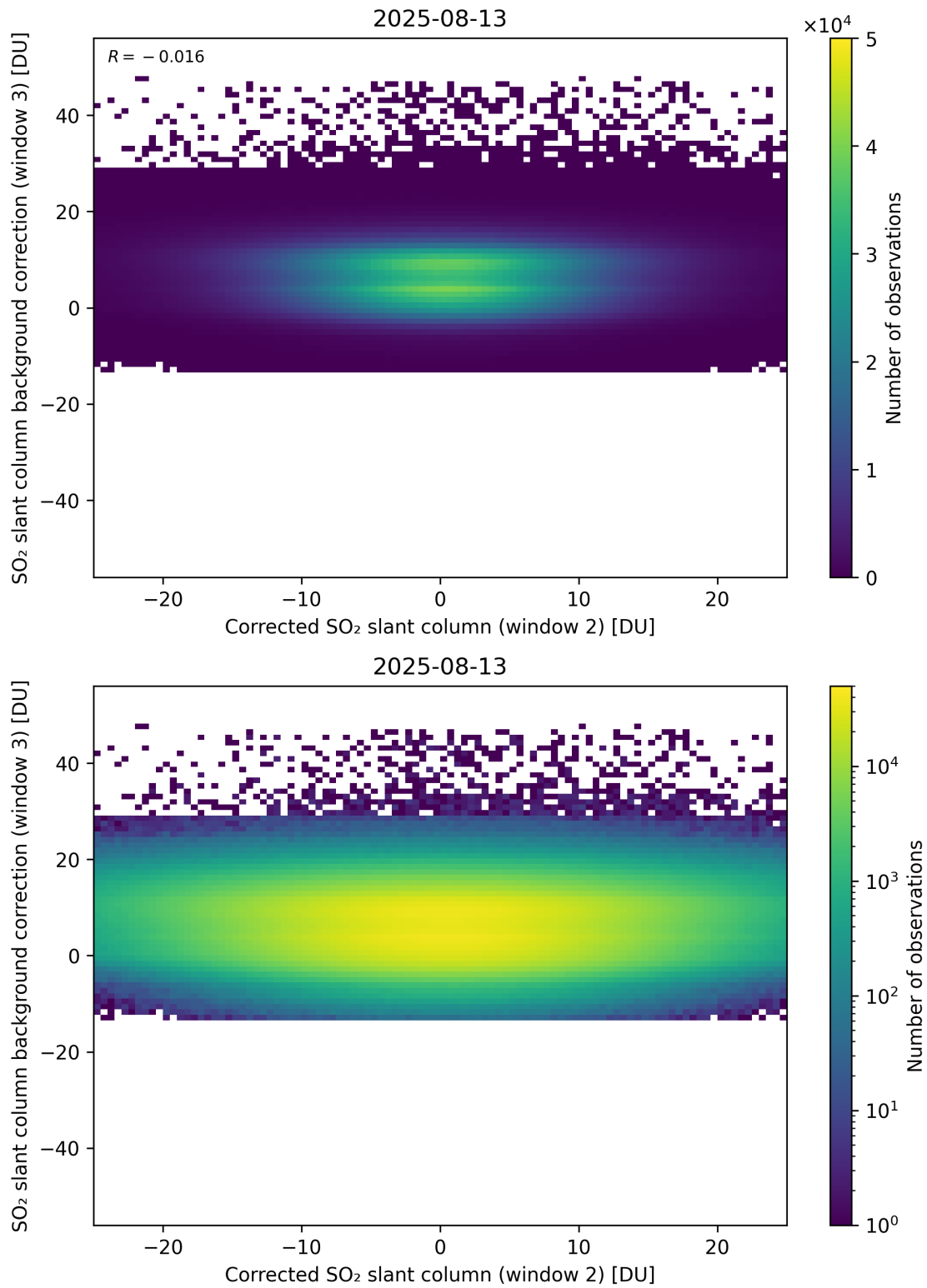
Figure 245: Scatter density plot of “Corrected SO 2 slant column (window 2)” against “SO 2 slant column background correction (window 3)” for 2025-08-12 to 2025-08-14.
