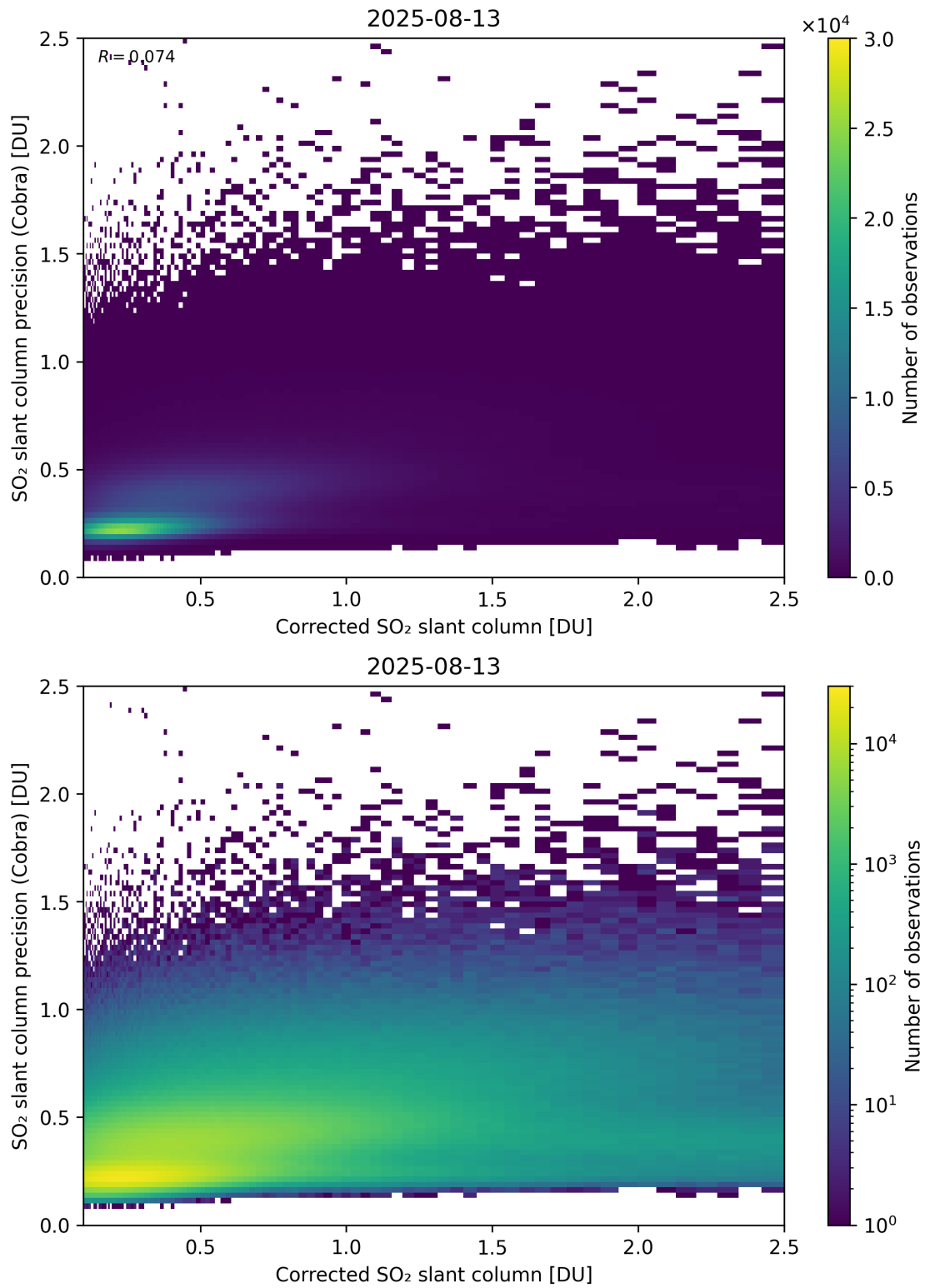
Figure 234: Scatter density plot of “Corrected SO 2 slant column” against “SO 2 slant column precision (Cobra)” for 2025-08-12 to 2025-08-14.
