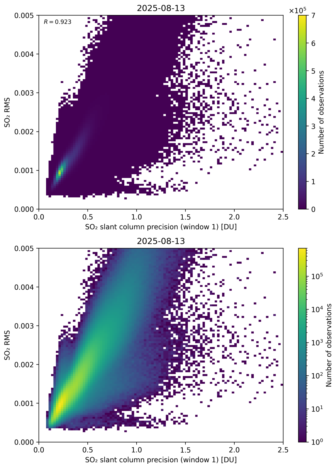
Figure 273: Scatter density plot of “SO 2 slant column precision (window 1)” against “SO 2 RMS” for 2025-08-12 to 2025-08-14.
