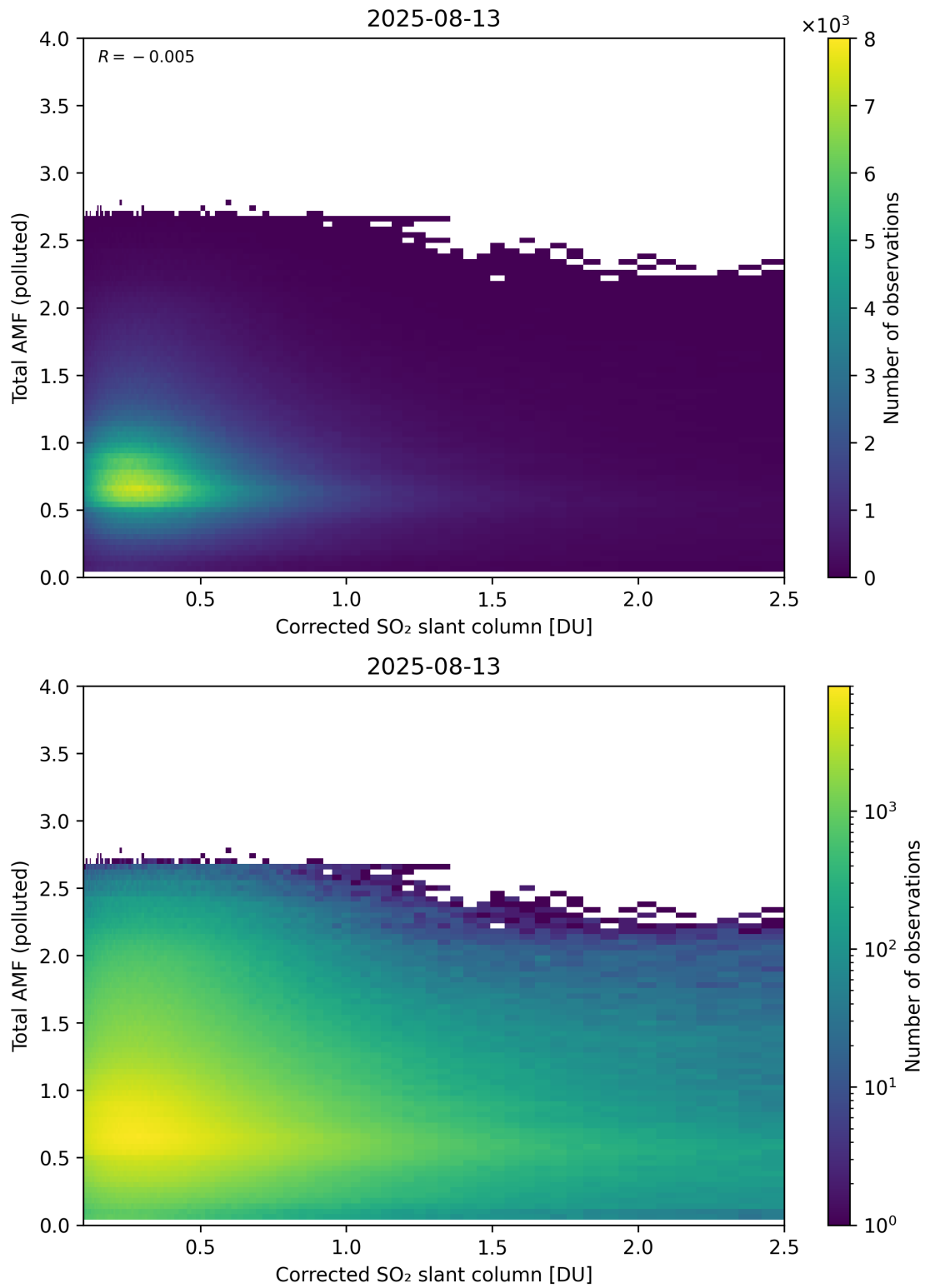
Figure 242: Scatter density plot of “Corrected SO 2 slant column” against “Total AMF (polluted)” for 2025-08-12 to 2025-08-14.
