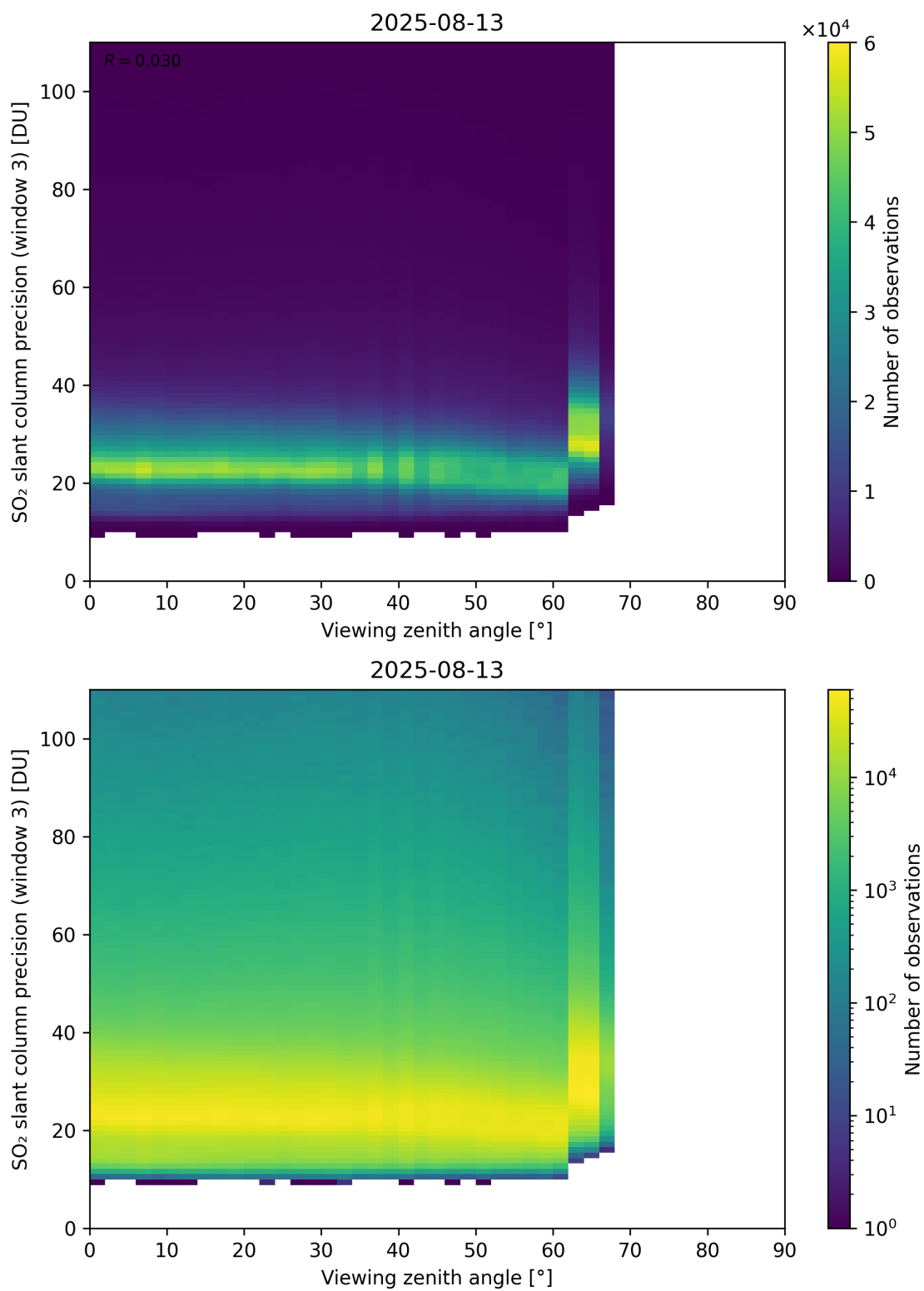
Figure 380: Scatter density plot of “Viewing zenith angle” against “SO 2 slant column precision (window 3)” for 2025-08-12 to 2025-08-14.
