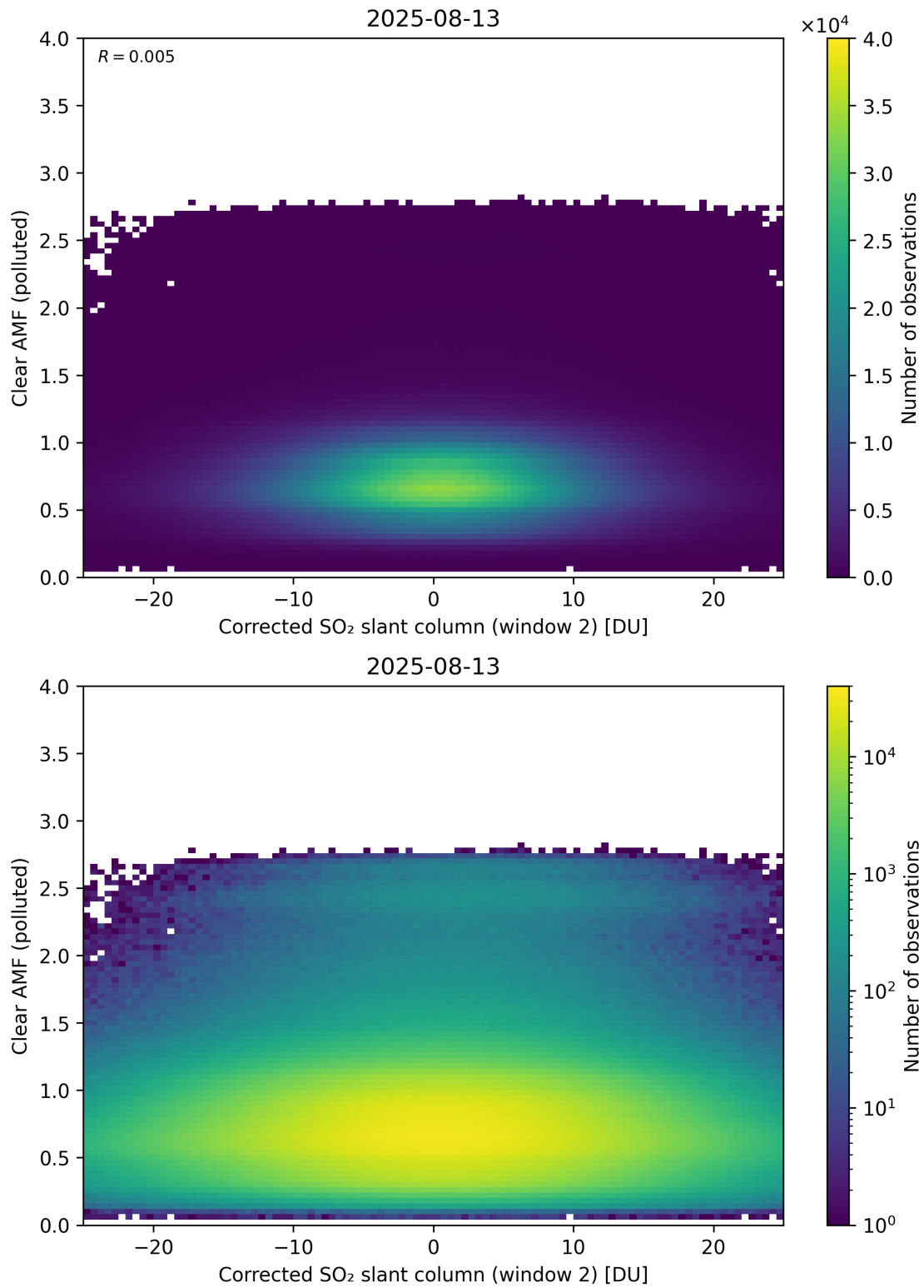
Figure 249: Scatter density plot of “Corrected SO 2 slant column (window 2)” against “Clear AMF (polluted)” for 2025-08-12 to 2025-08-14.
