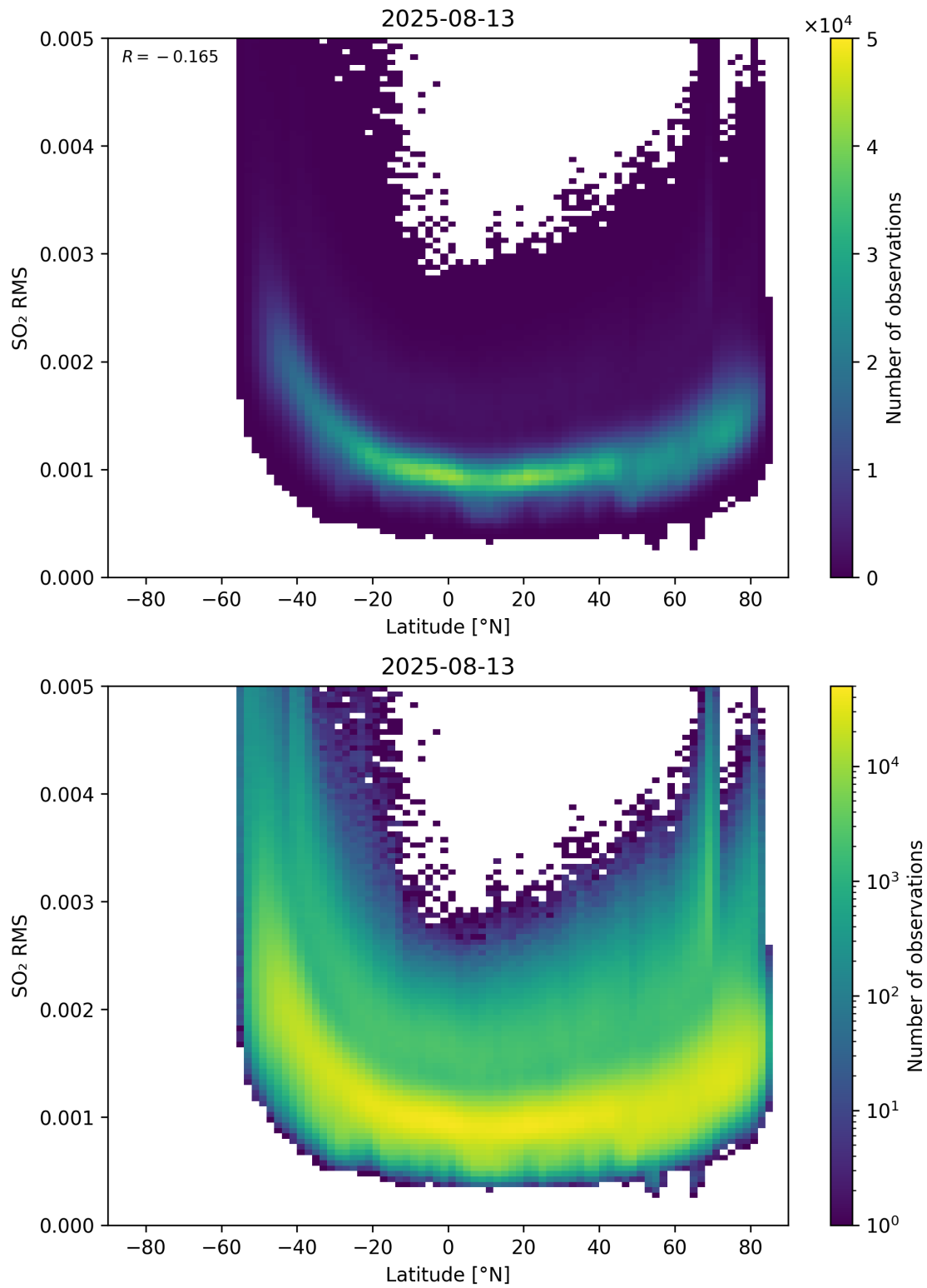
Figure 155: Scatter density plot of “Latitude” against “SO 2 RMS” for 2025-08-12 to 2025-08-14.
