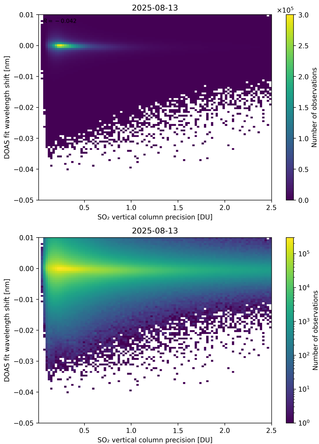
Figure 332: Scatter density plot of “SO 2 vertical column precision” against “DOAS fit wavelength shift” for 2025-08-12 to 2025-08-14.
