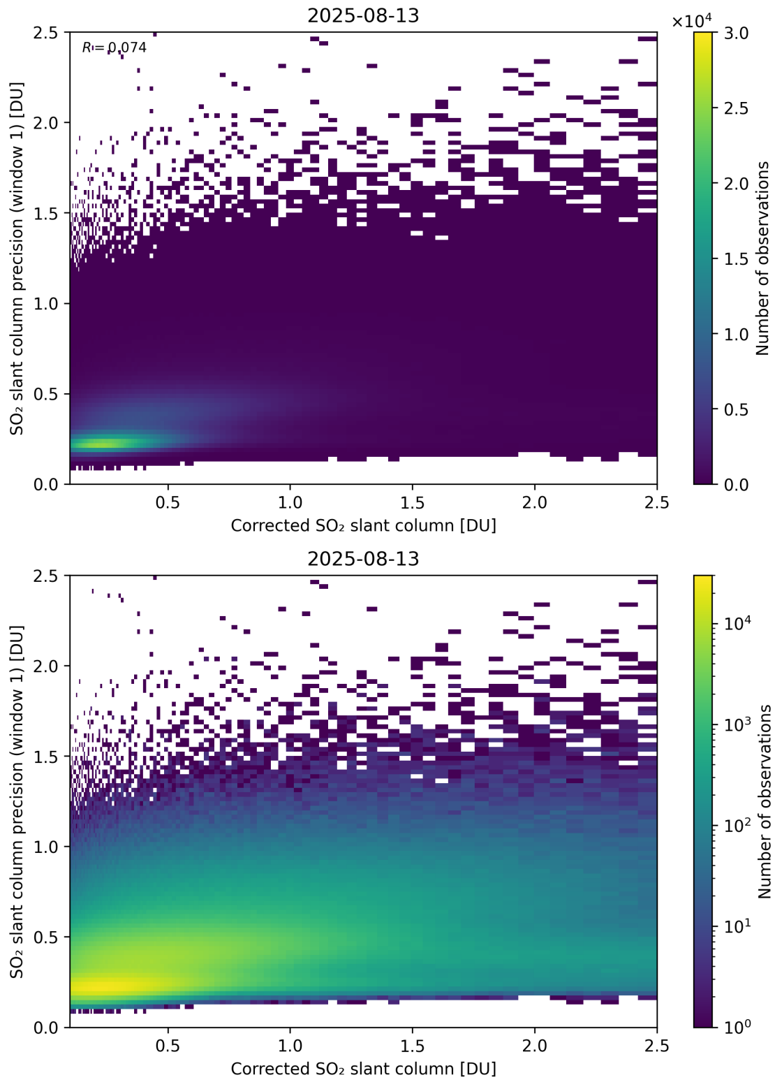
Figure 238: Scatter density plot of “Corrected SO 2 slant column” against “SO 2 slant column precision (window 1)” for 2025-08-12 to 2025-08-14.
