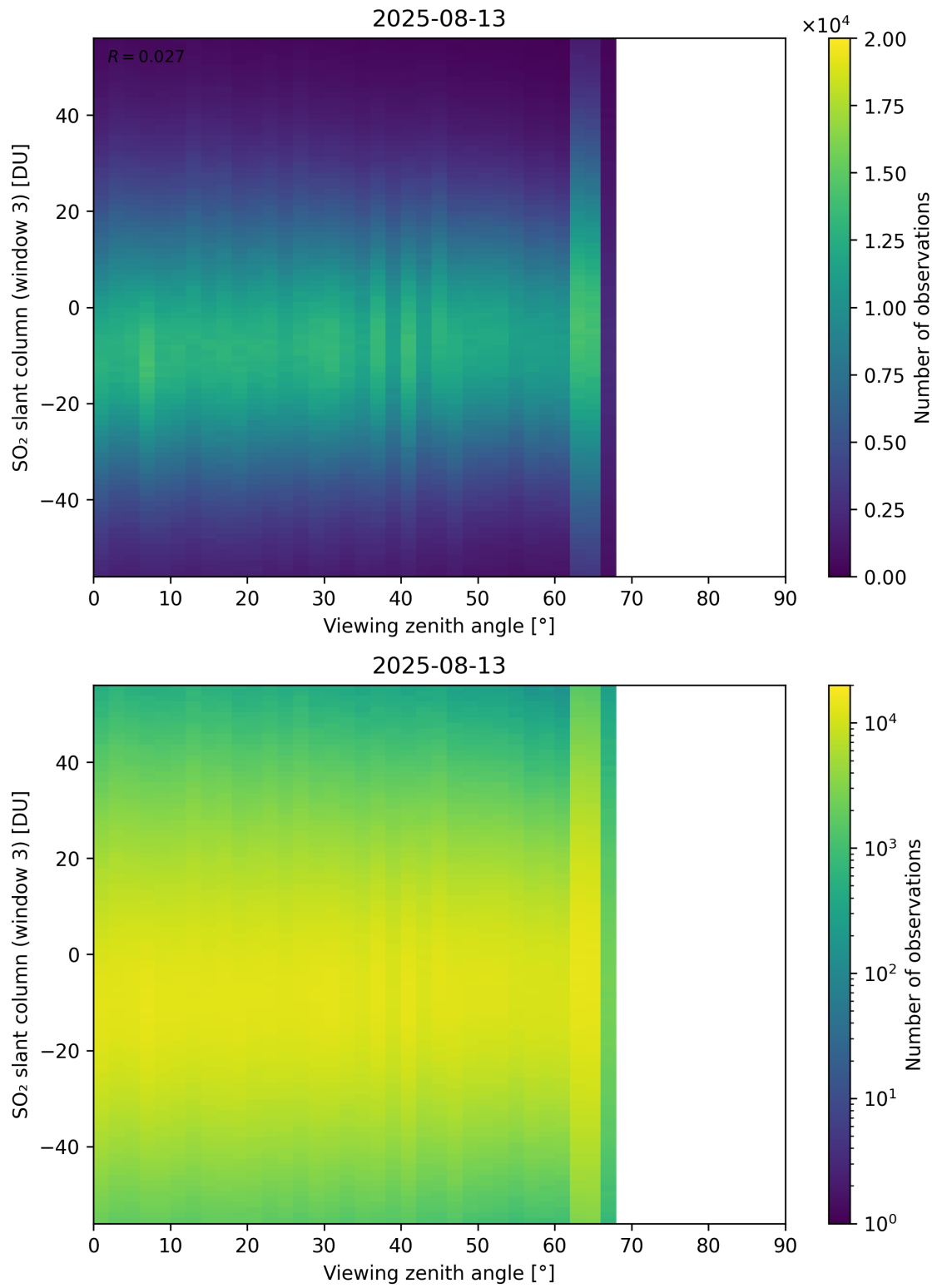
Figure 379: Scatter density plot of “Viewing zenith angle” against “SO 2 slant column (window 3)” for 2025-08-12 to 2025-08-14.
