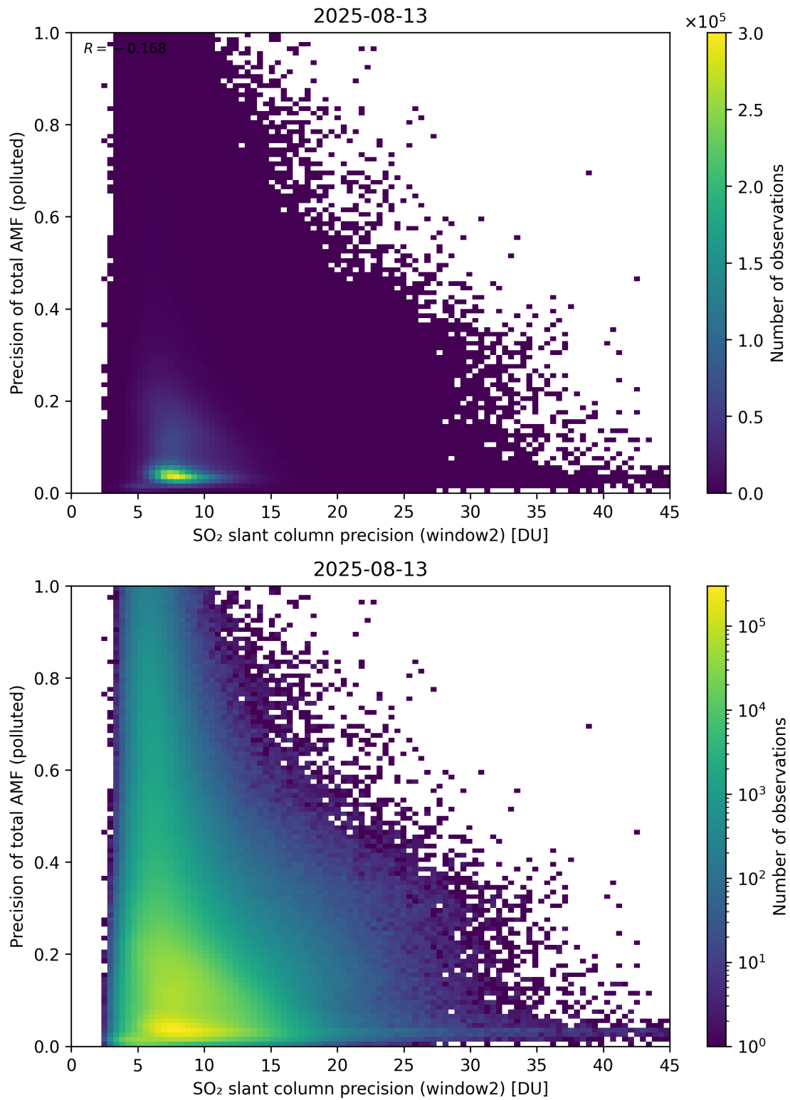
Figure 302: Scatter density plot of “SO 2 slant column precision (window2)” against “Precision of total AMF (polluted)” for 2025-08-12 to 2025-08-14.
