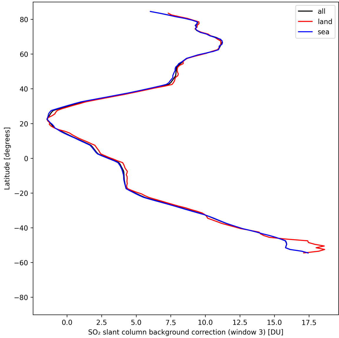
Figure 48: Zonal average of “SO 2 slant column background correction (window 3)” for 2025-08-12 to 2025-08-14.
