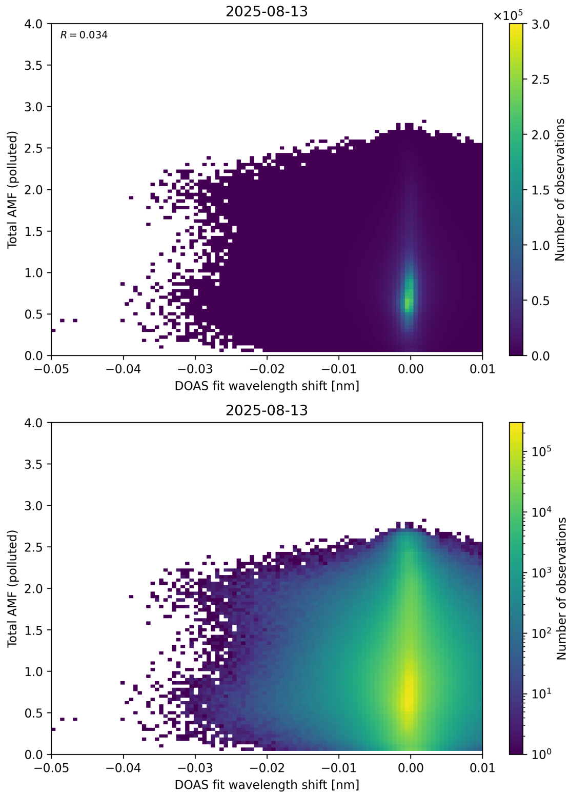
Figure 141: Scatter density plot of “DOAS fit wavelength shift” against “Total AMF (polluted)” for 2025-08-12 to 2025-08-14.
