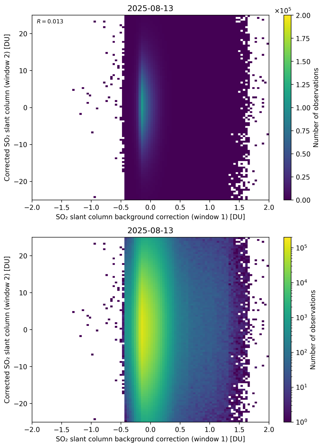
Figure 115: Scatter density plot of “SO 2 slant column background correction (window 1)” against “Corrected SO 2 slant column (window 2)” for 2025-08-12 to 2025-08-14.
