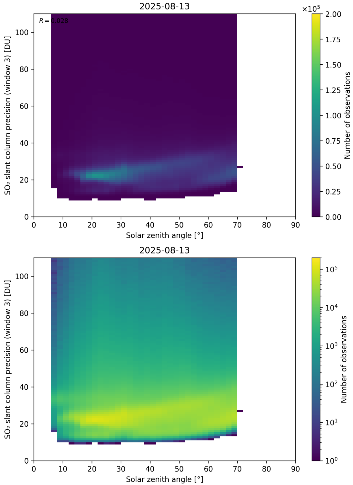
Figure 188: Scatter density plot of “Solar zenith angle” against “SO 2 slant column precision (window 3)” for 2025-08-12 to 2025-08-14.
