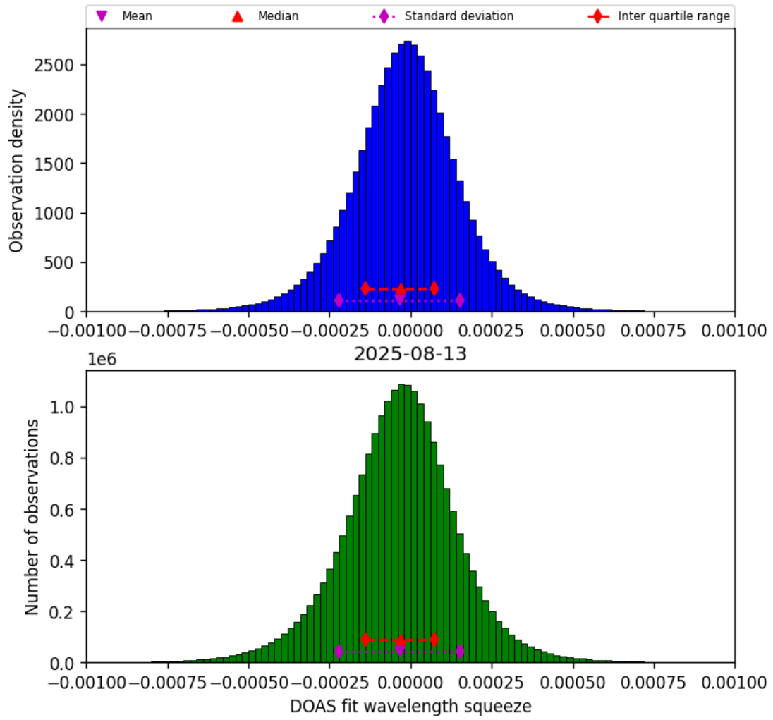
Figure 77: Histogram of “DOAS fit wavelength squeeze” for 2025-08-12 to 2025-08-14
