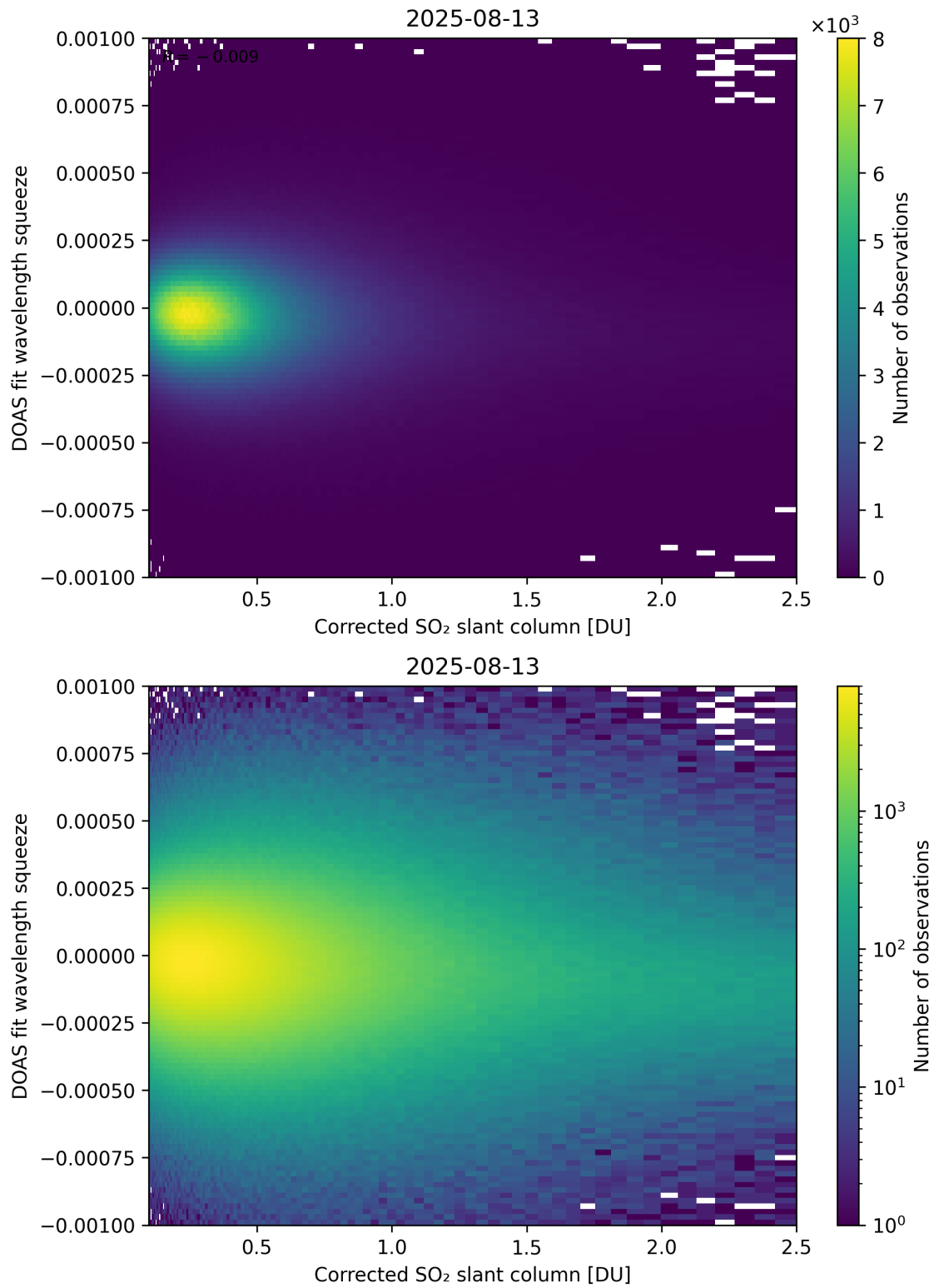
Figure 230: Scatter density plot of “Corrected SO 2 slant column” against “DOAS fit wavelength squeeze” for 2025-08-12 to 2025-08-14.
