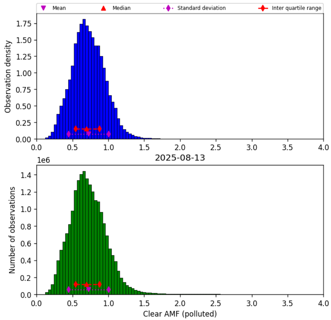
Figure 81: Histogram of “Clear AMF (polluted)” for 2025-08-12 to 2025-08-14
