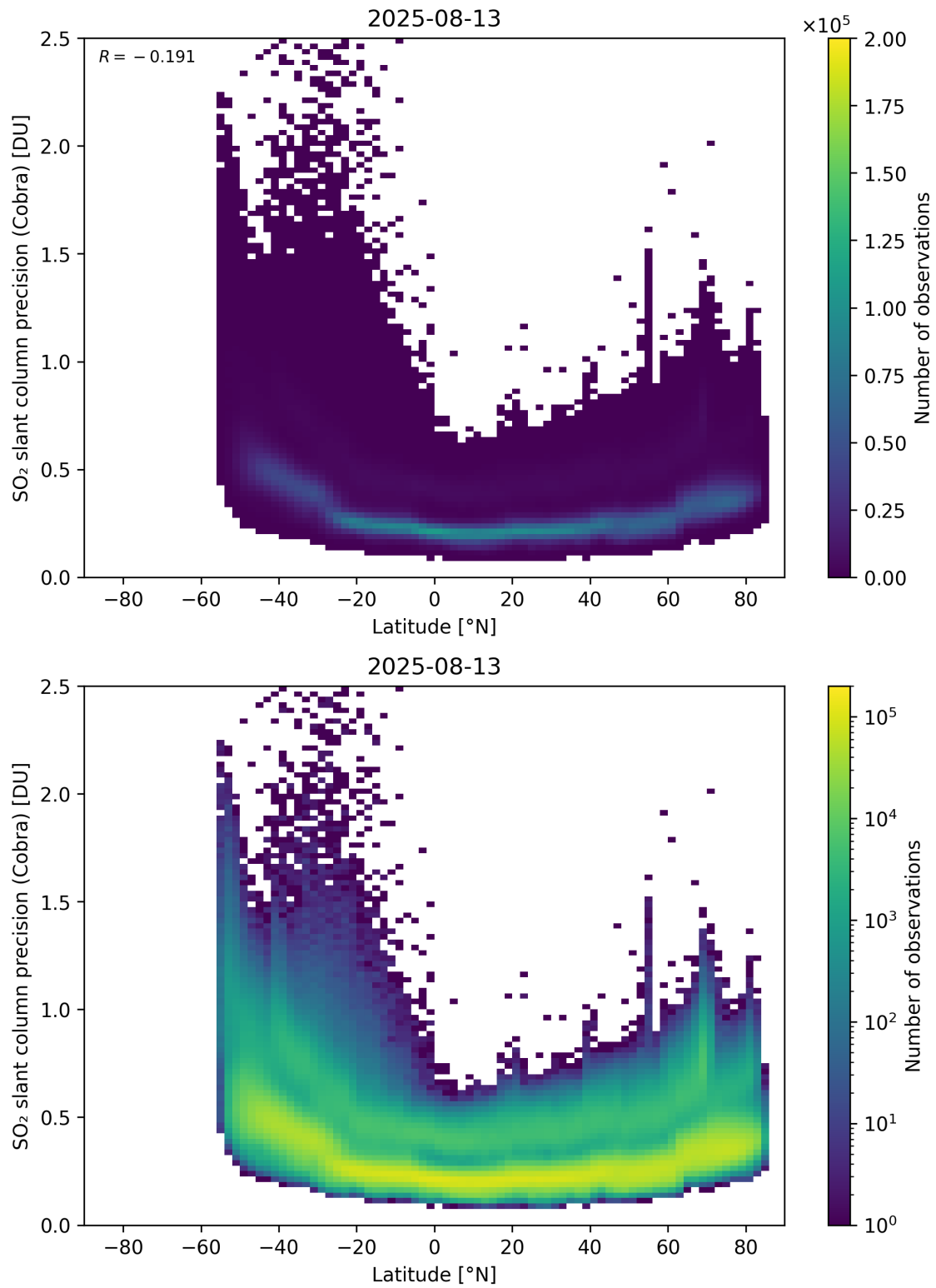
Figure 158: Scatter density plot of “Latitude” against “SO 2 slant column precision (Cobra)” for 2025-08-12 to 2025-08-14.
