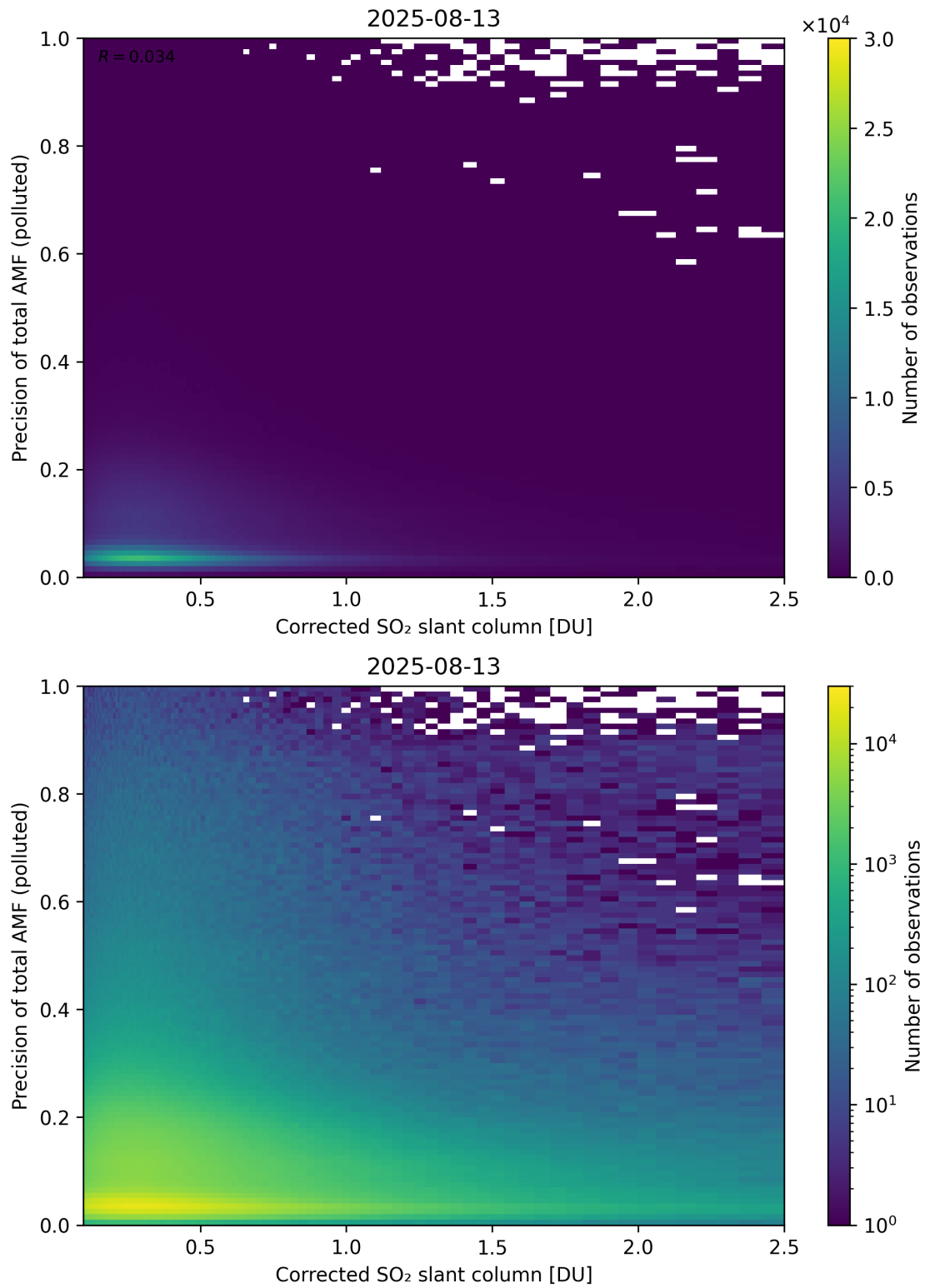
Figure 243: Scatter density plot of “Corrected SO 2 slant column” against “Precision of total AMF (polluted)” for 2025-08-12 to 2025-08-14.
