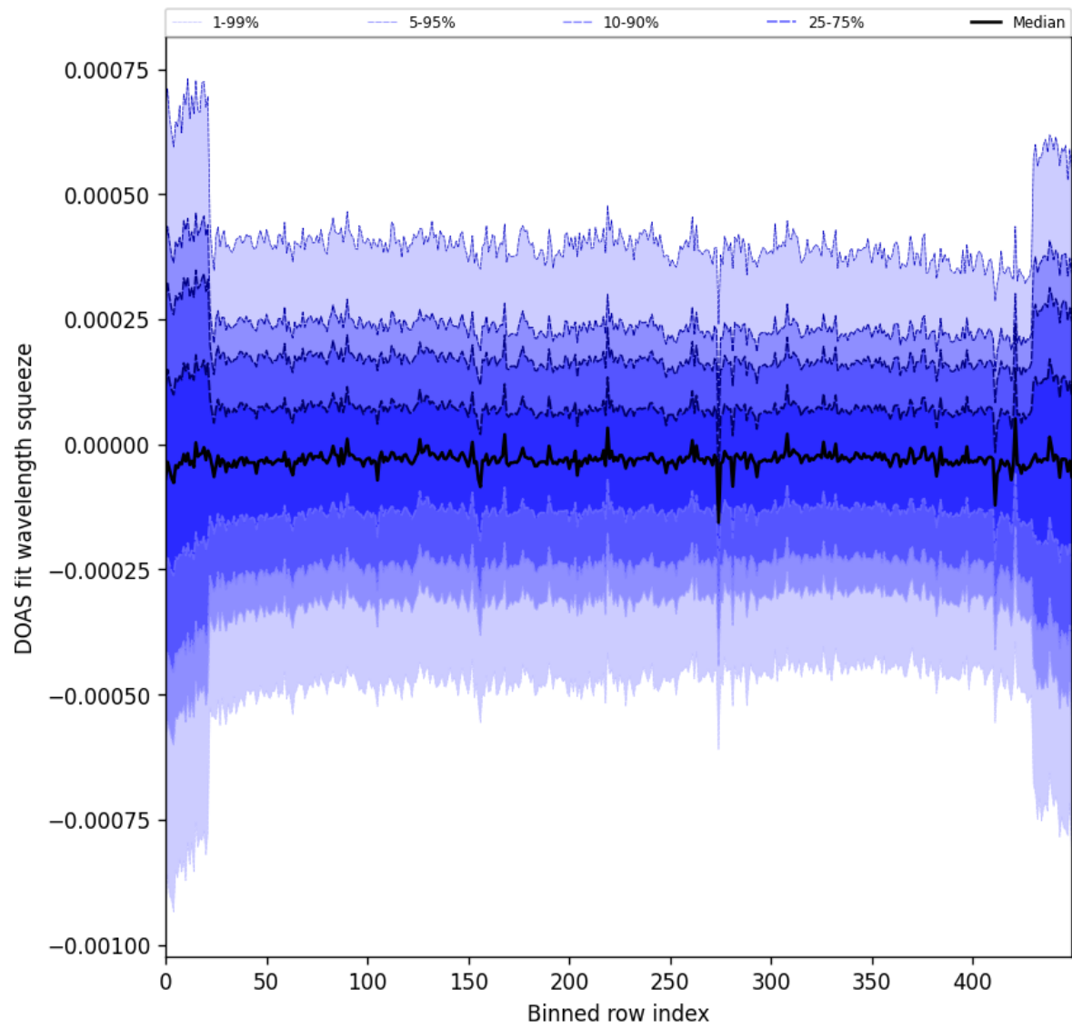
Figure 103: Along track statistics of “DOAS fit wavelength squeeze” for 2025-08-12 to 2025-08-14
