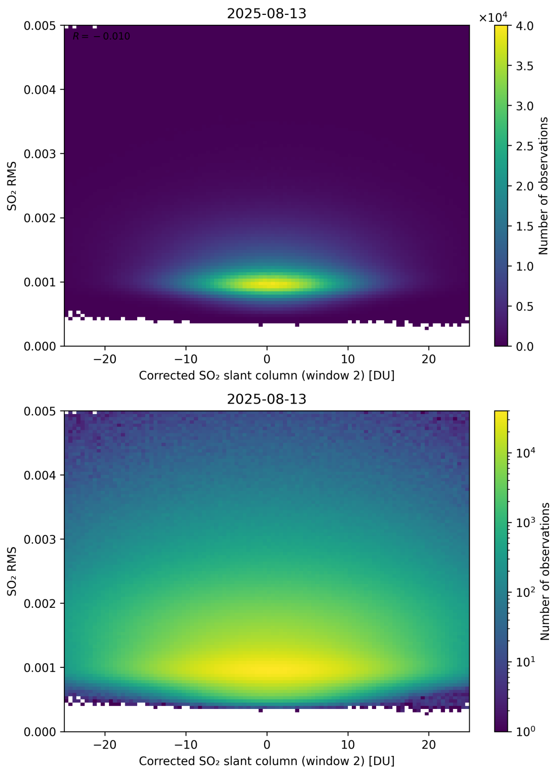
Figure 248: Scatter density plot of “Corrected SO 2 slant column (window 2)” against “SO 2 RMS” for 2025-08-12 to 2025-08-14.
