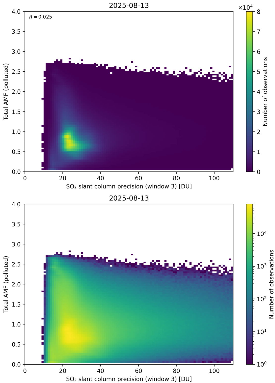
Figure 313: Scatter density plot of “SO 2 slant column precision (window 3)” against “Total AMF (polluted)” for 2025-08-12 to 2025-08-14.
