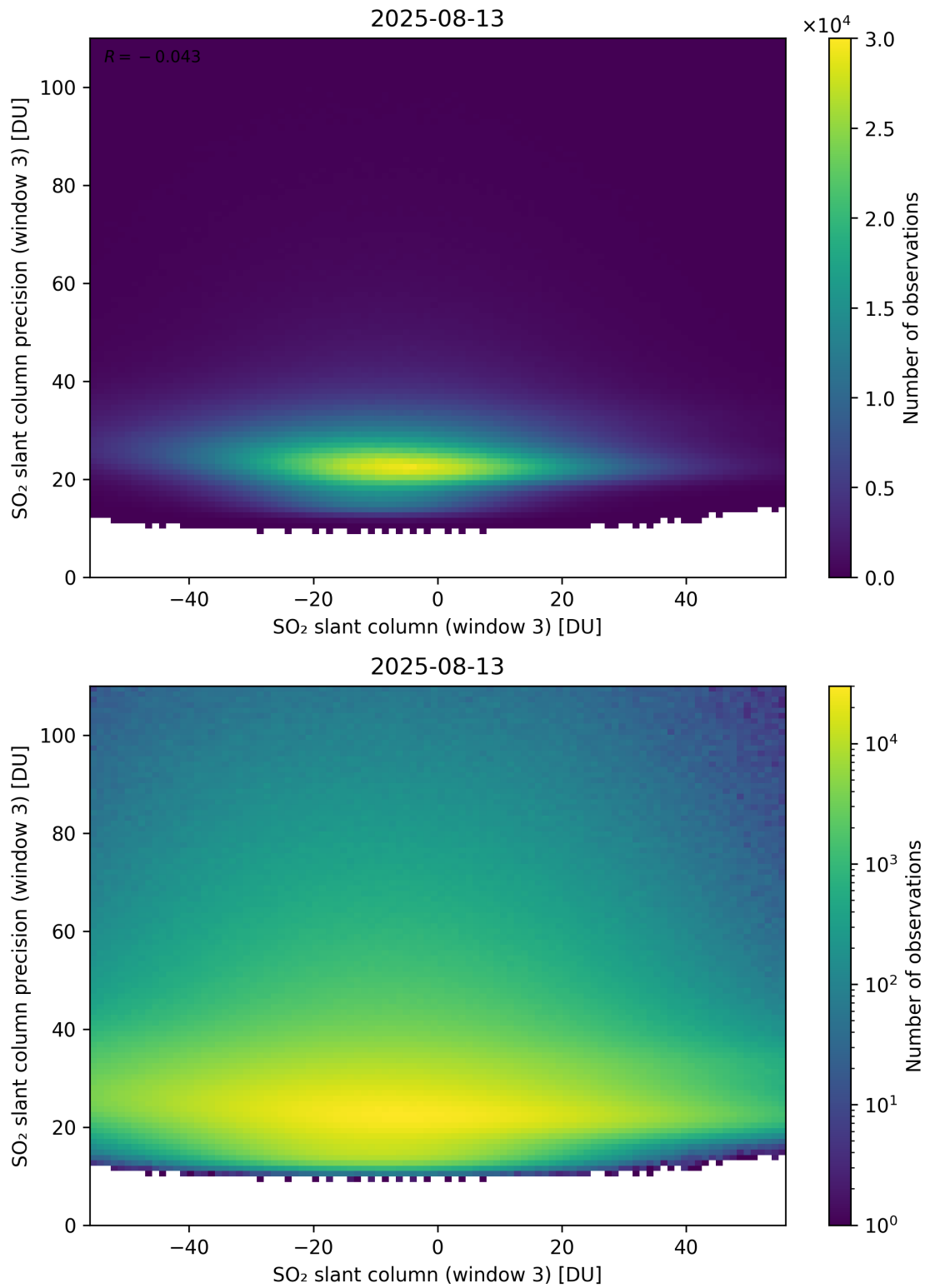
Figure 317: Scatter density plot of “SO 2 slant column (window 3)” against “SO 2 slant column precision (window 3)” for 2025-08-12 to 2025-08-14.
