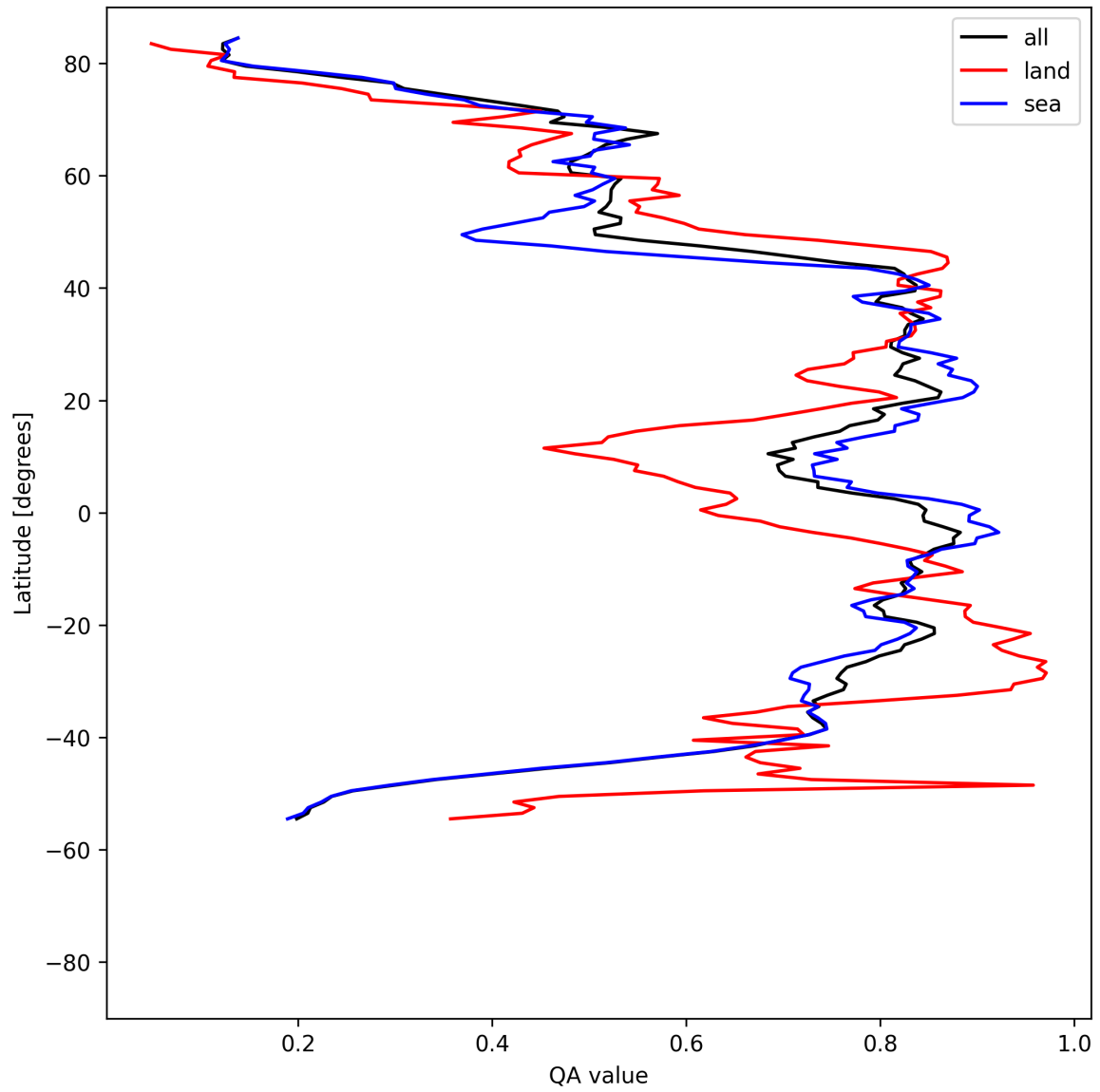
Figure 31: Zonal average of “QA value” for 2025-08-12 to 2025-08-14.
