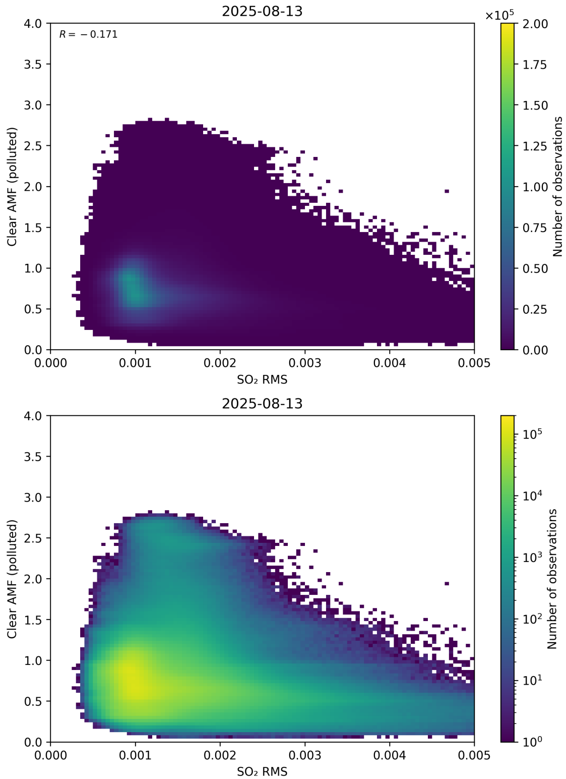
Figure 147: Scatter density plot of “SO 2 RMS” against “Clear AMF (polluted)” for 2025-08-12 to 2025-08-14.
