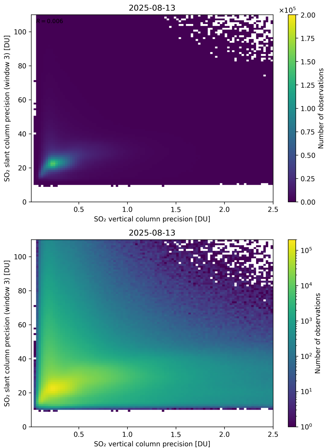
Figure 345: Scatter density plot of “SO 2 vertical column precision” against “SO 2 slant column precision (window 3)” for 2025-08-12 to 2025-08-14.
