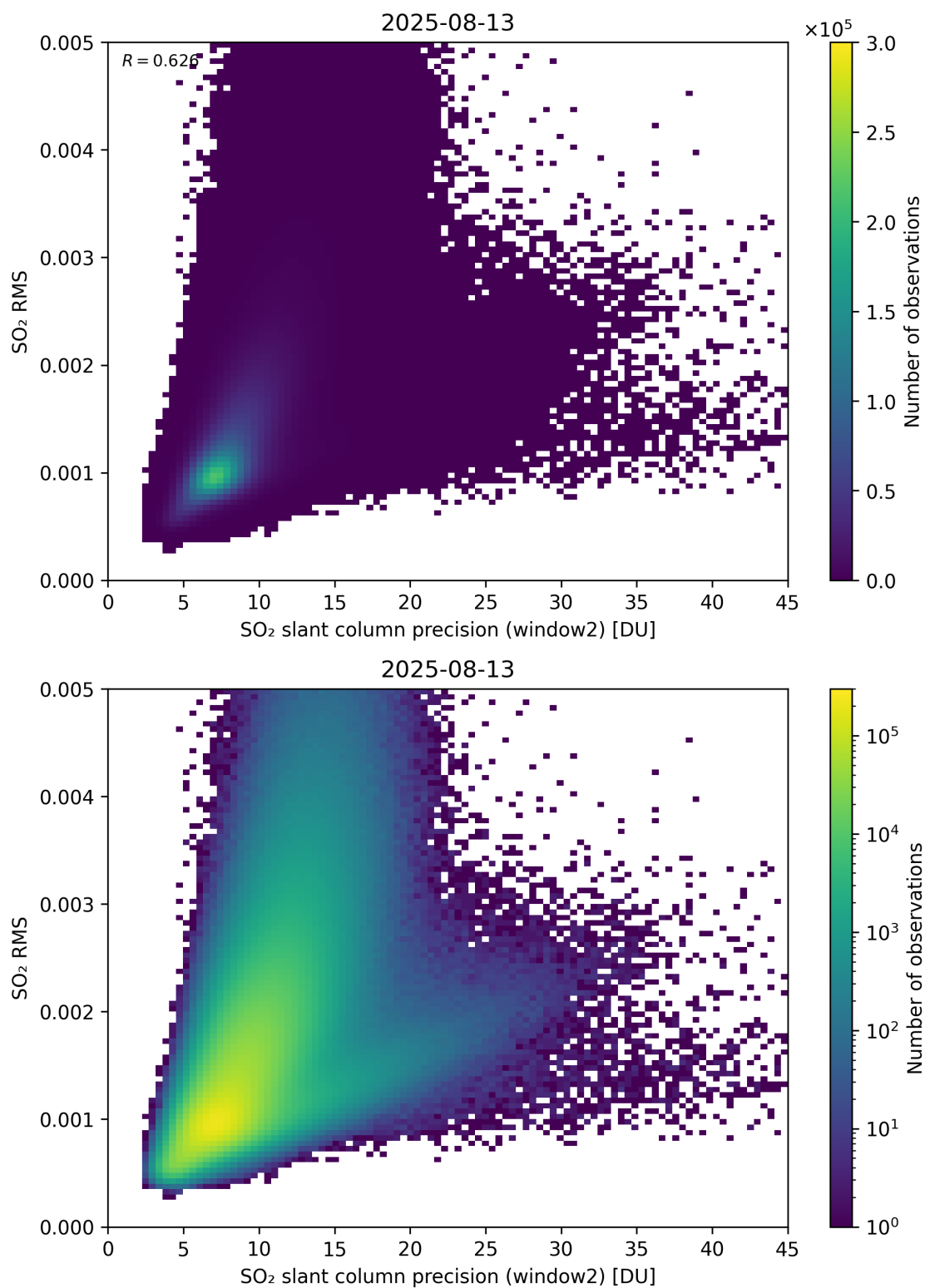
Figure 295: Scatter density plot of “SO 2 slant column precision (window2)” against “SO 2 RMS” for 2025-08-12 to 2025-08-14.
