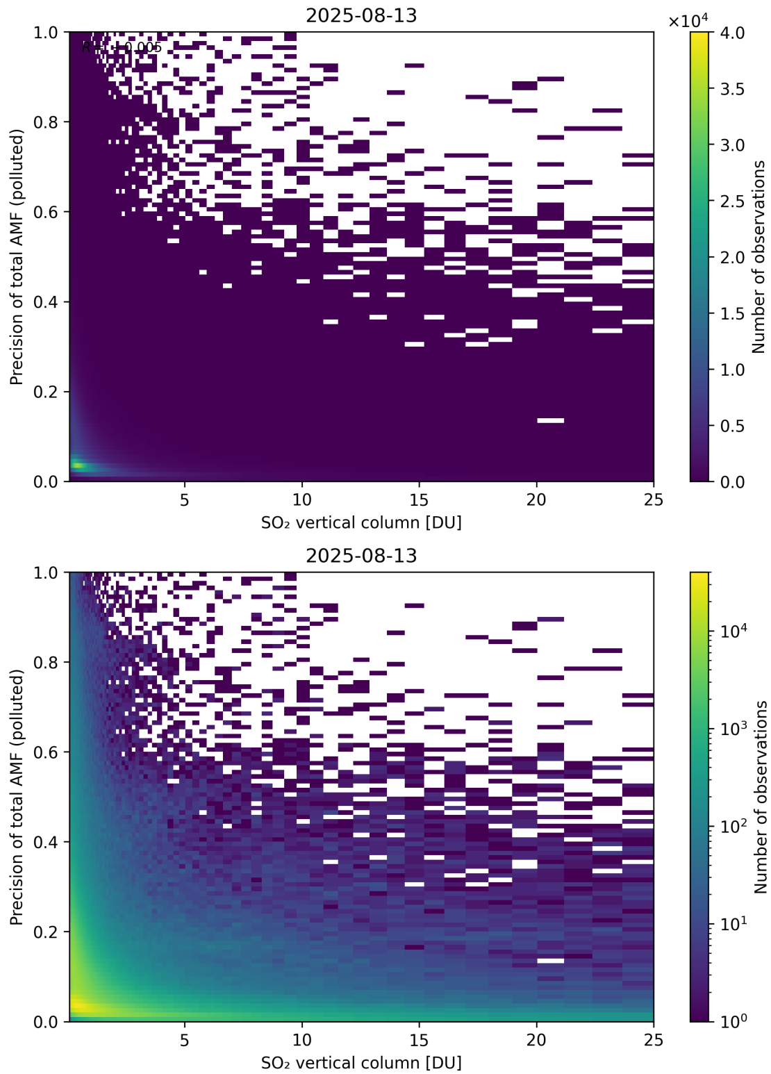
Figure 360: Scatter density plot of “SO 2 vertical column” against “Precision of total AMF (polluted)” for 2025-08-12 to 2025-08-14.
