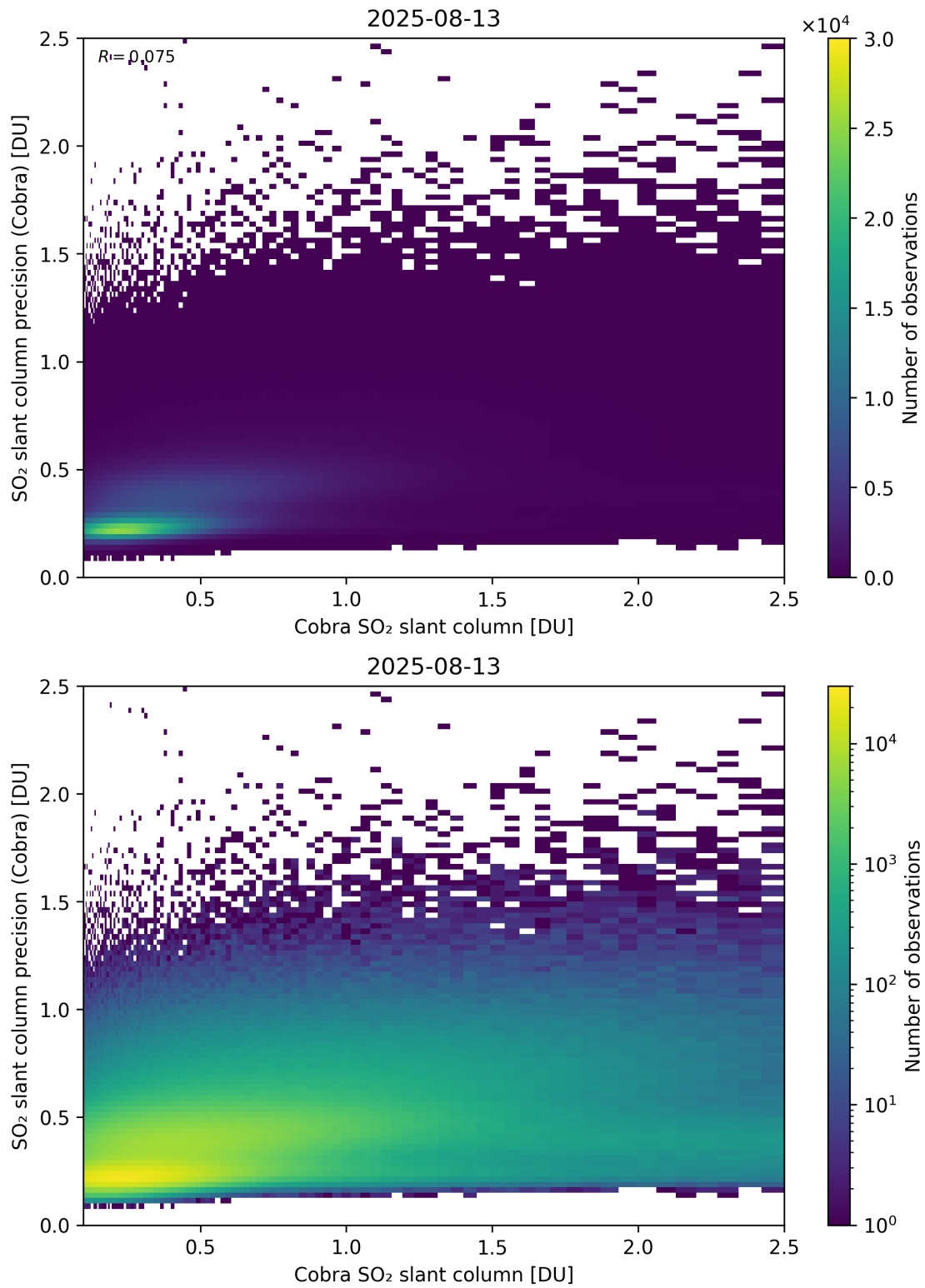
Figure 216: Scatter density plot of “Cobra SO 2 slant column” against “SO 2 slant column precision (Cobra)” for 2025-08-12 to 2025-08-14.
