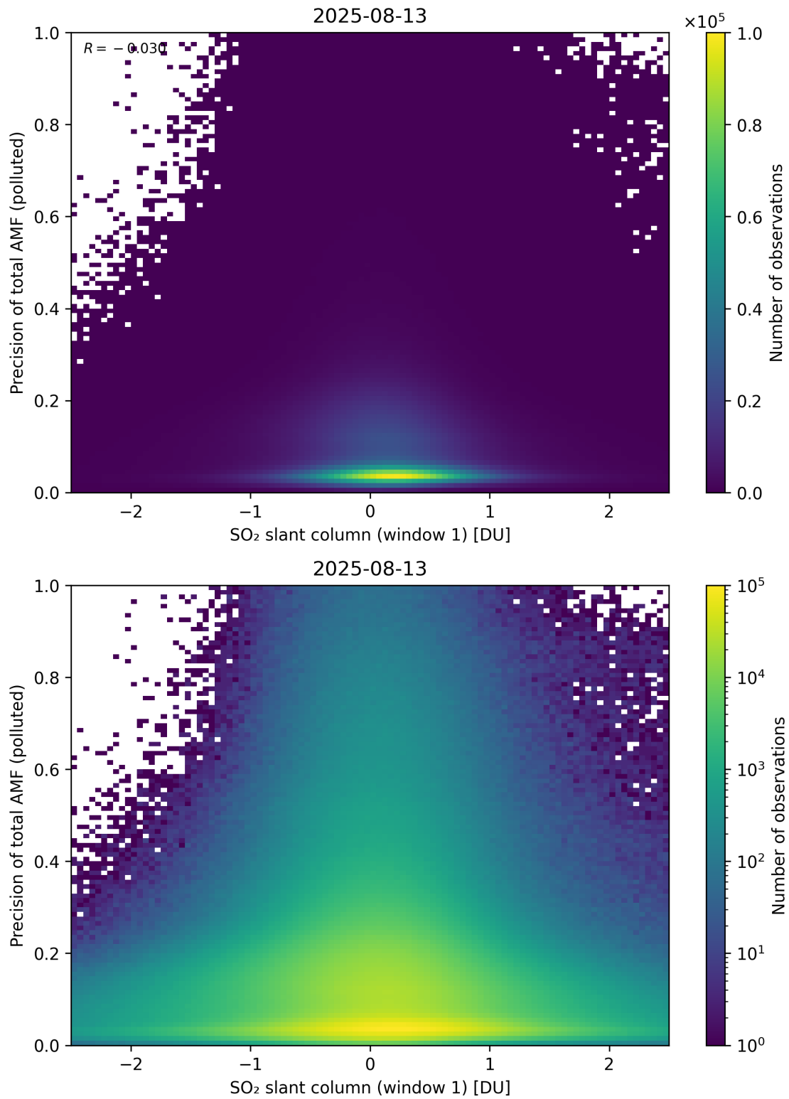
Figure 290: Scatter density plot of “SO 2 slant column (window 1)” against “Precision of total AMF (polluted)” for 2025-08-12 to 2025-08-14.
