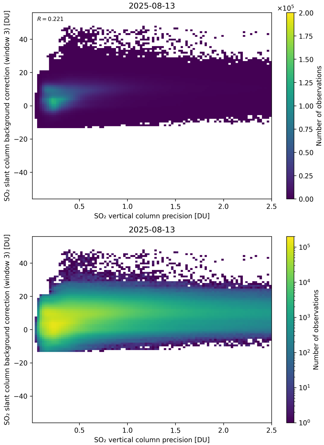
Figure 331: Scatter density plot of “SO 2 vertical column precision” against “SO 2 slant column background correction (window 3)” for 2025-08-12 to 2025-08-14.
