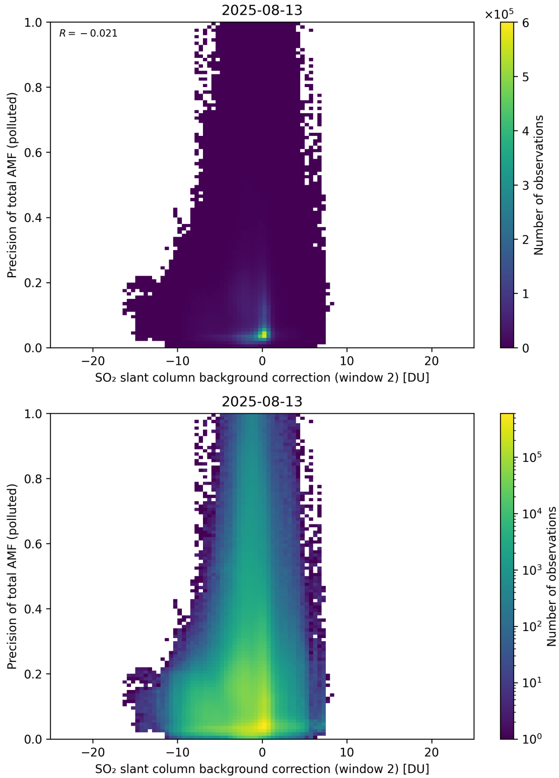
Figure 131: Scatter density plot of “SO 2 slant column background correction (window 2)” against “Precision of total AMF (polluted)” for 2025-08-12 to 2025-08-14.
