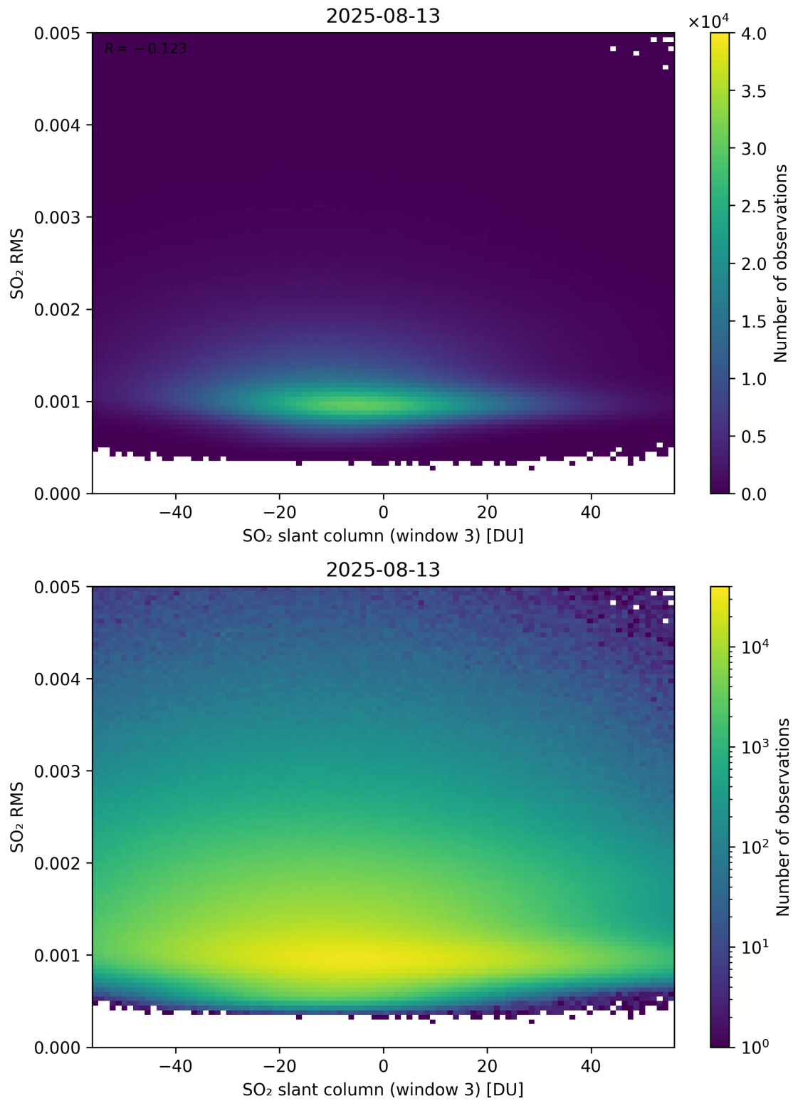
Figure 306: Scatter density plot of “SO 2 slant column (window 3)” against “SO 2 RMS” for 2025-08-12 to 2025-08-14.
