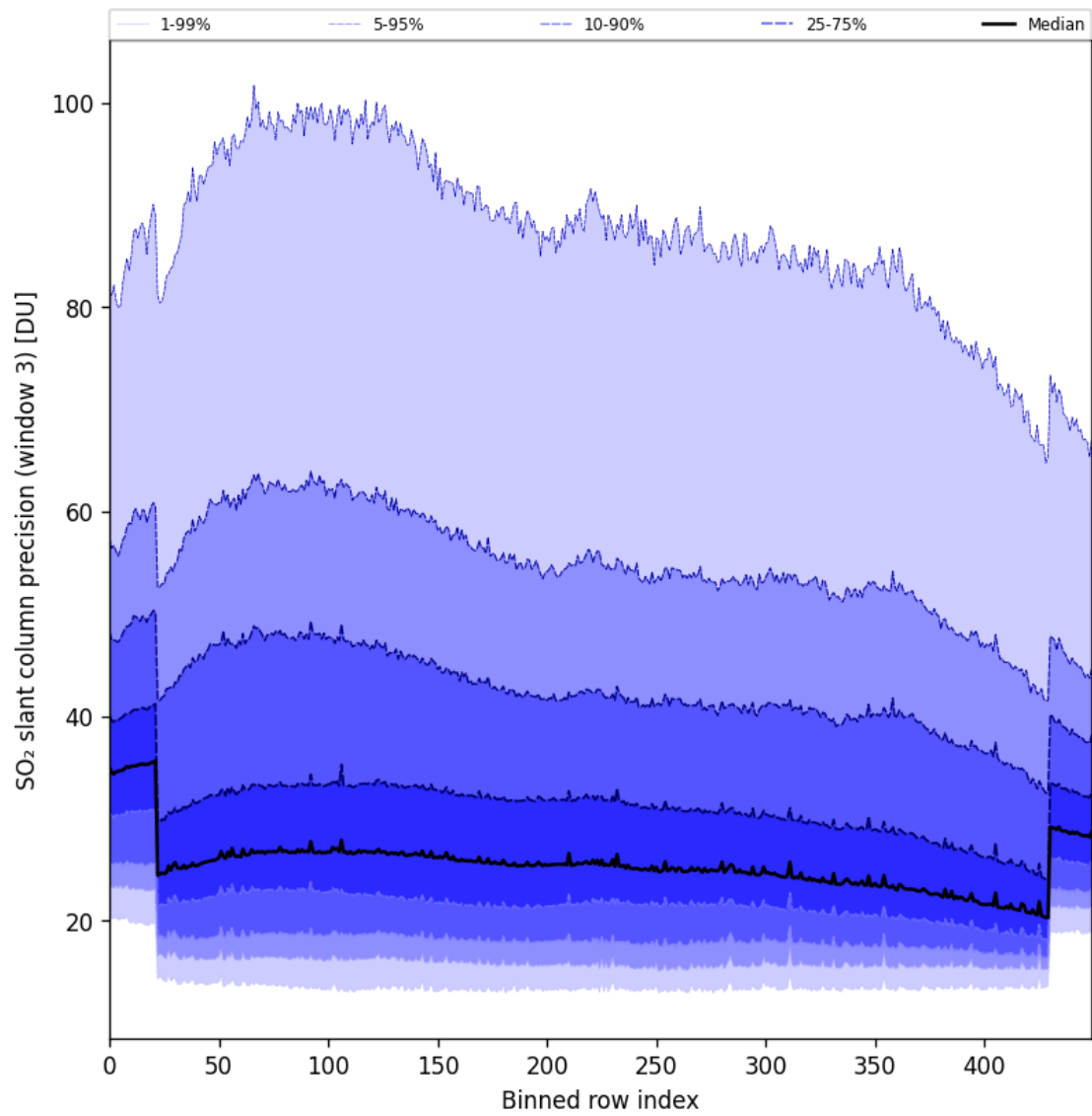
Figure 98: Along track statistics of “SO 2 slant column precision (window 3)” for 2025-08-12 to 2025-08-14
