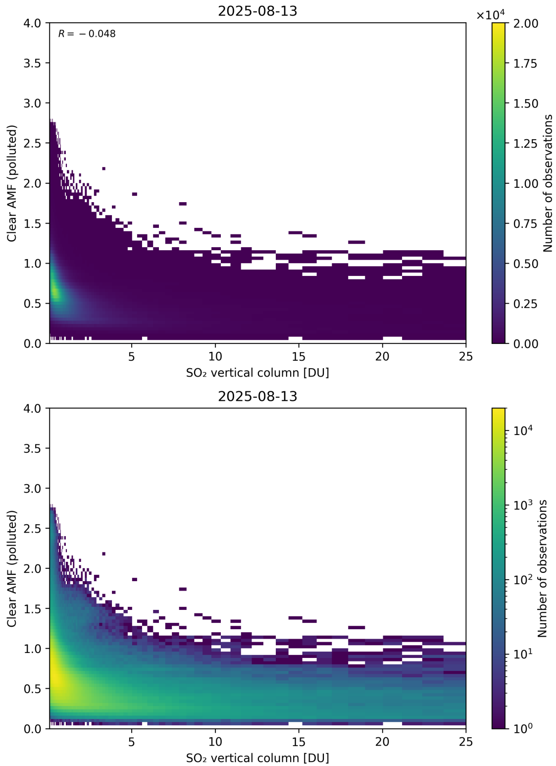
Figure 348: Scatter density plot of “SO 2 vertical column” against “Clear AMF (polluted)” for 2025-08-12 to 2025-08-14.
