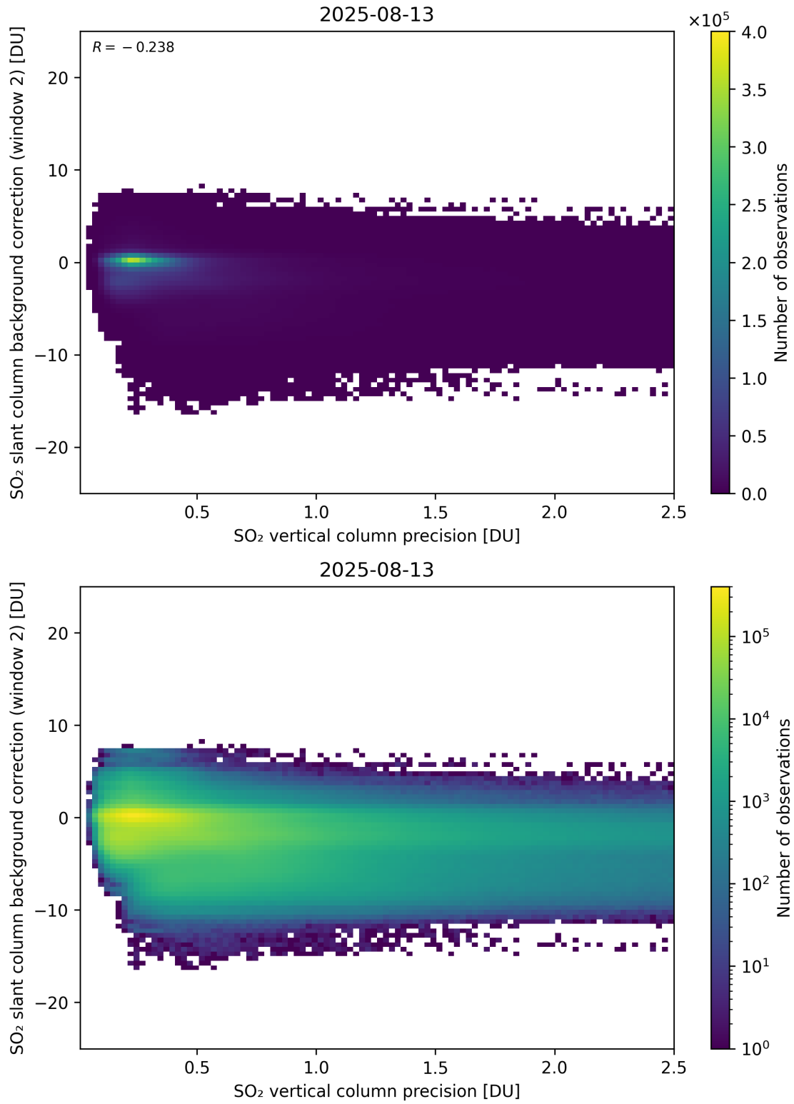
Figure 330: Scatter density plot of “SO 2 vertical column precision” against “SO 2 slant column background correction (window 2)” for 2025-08-12 to 2025-08-14.
