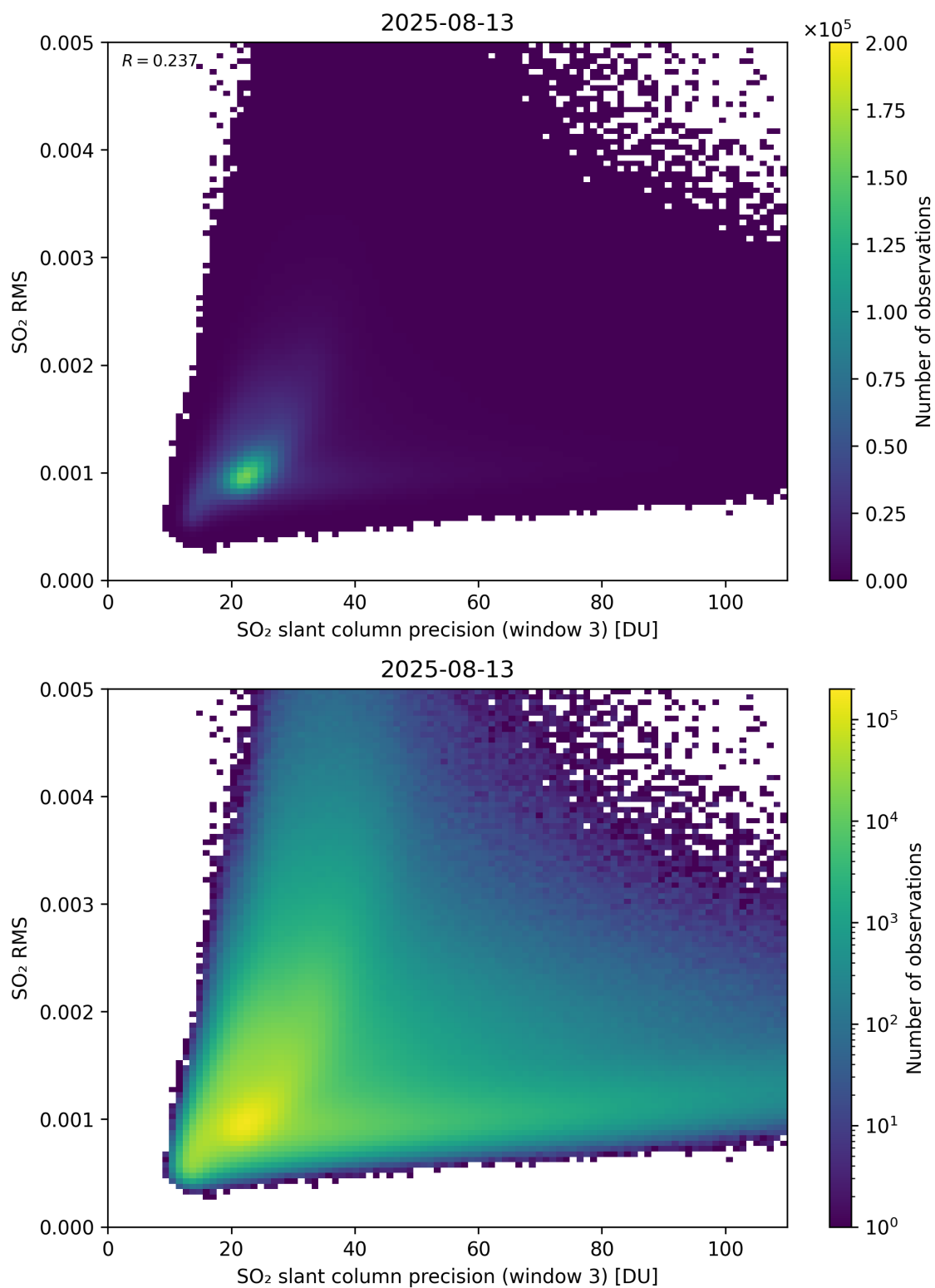
Figure 310: Scatter density plot of “SO 2 slant column precision (window 3)” against “SO 2 RMS” for 2025-08-12 to 2025-08-14.
