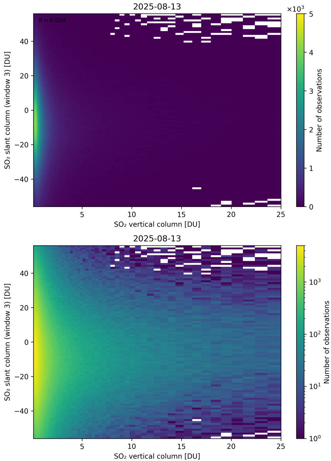
Figure 357: Scatter density plot of “SO 2 vertical column” against “SO 2 slant column (window 3)” for 2025-08-12 to 2025-08-14.
