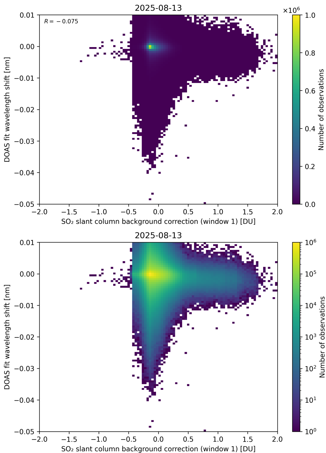
Figure 111: Scatter density plot of “SO 2 slant column background correction (window 1)” against “DOAS fit wavelength shift” for 2025-08-12 to 2025-08-14.
