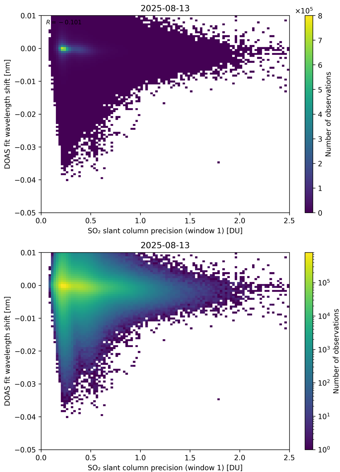
Figure 271: Scatter density plot of “SO 2 slant column precision (window 1)” against “DOAS fit wavelength shift” for 2025-08-12 to 2025-08-14.
