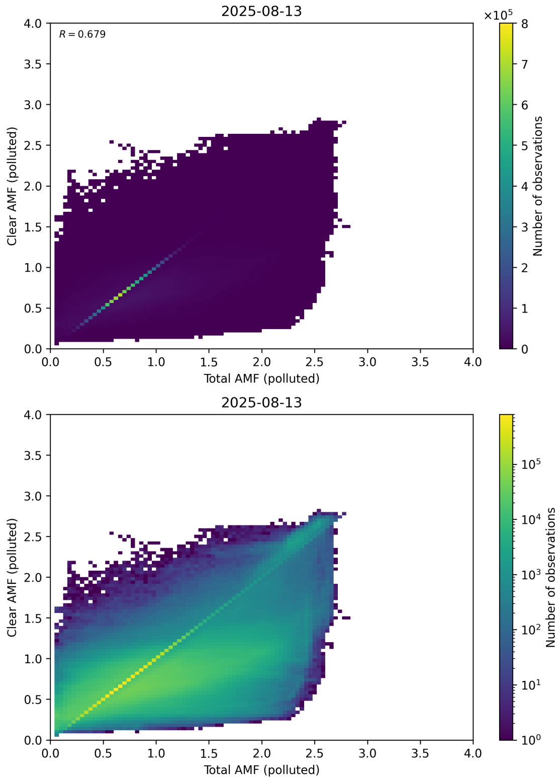
Figure 321: Scatter density plot of “Total AMF (polluted)” against “Clear AMF (polluted)” for 2025-08-12 to 2025-08-14.
