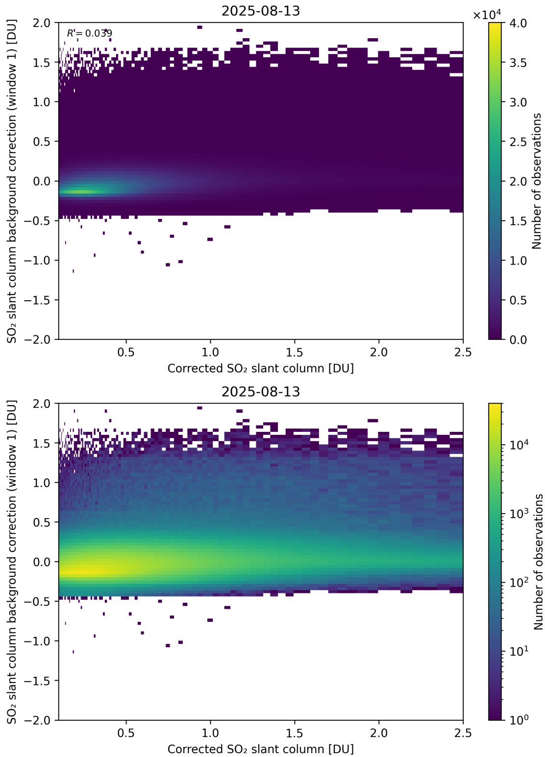
Figure 226: Scatter density plot of “Corrected SO 2 slant column” against “SO 2 slant column background correction (window 1)” for 2025-08-12 to 2025-08-14.
