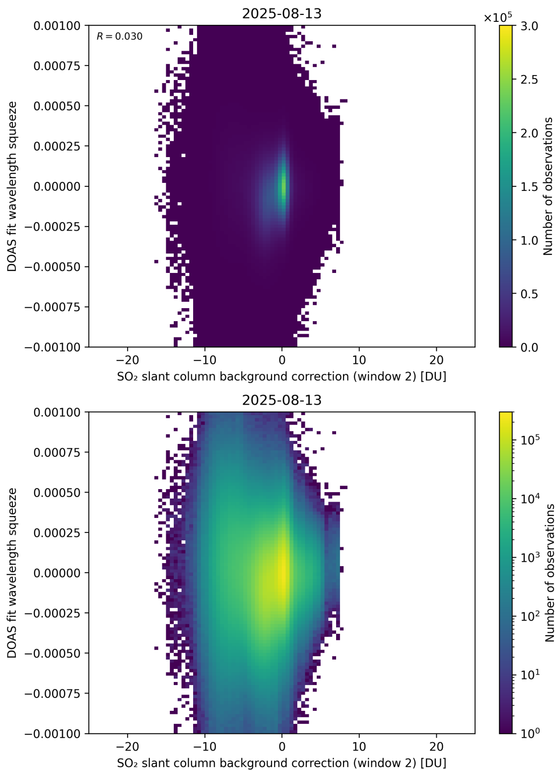
Figure 124: Scatter density plot of “SO 2 slant column background correction (window 2)” against “DOAS fit wavelength squeeze” for 2025-08-12 to 2025-08-14.
