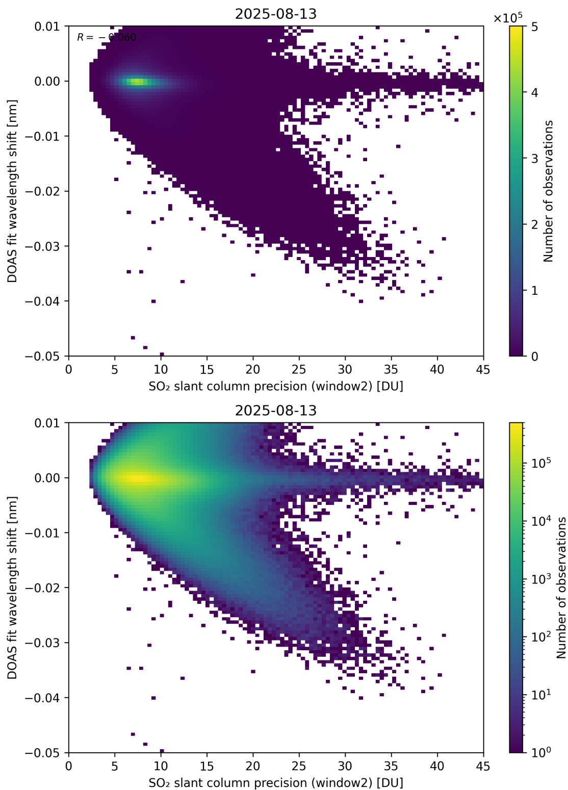
Figure 293: Scatter density plot of “SO 2 slant column precision (window2)” against “DOAS fit wavelength shift” for 2025-08-12 to 2025-08-14.
