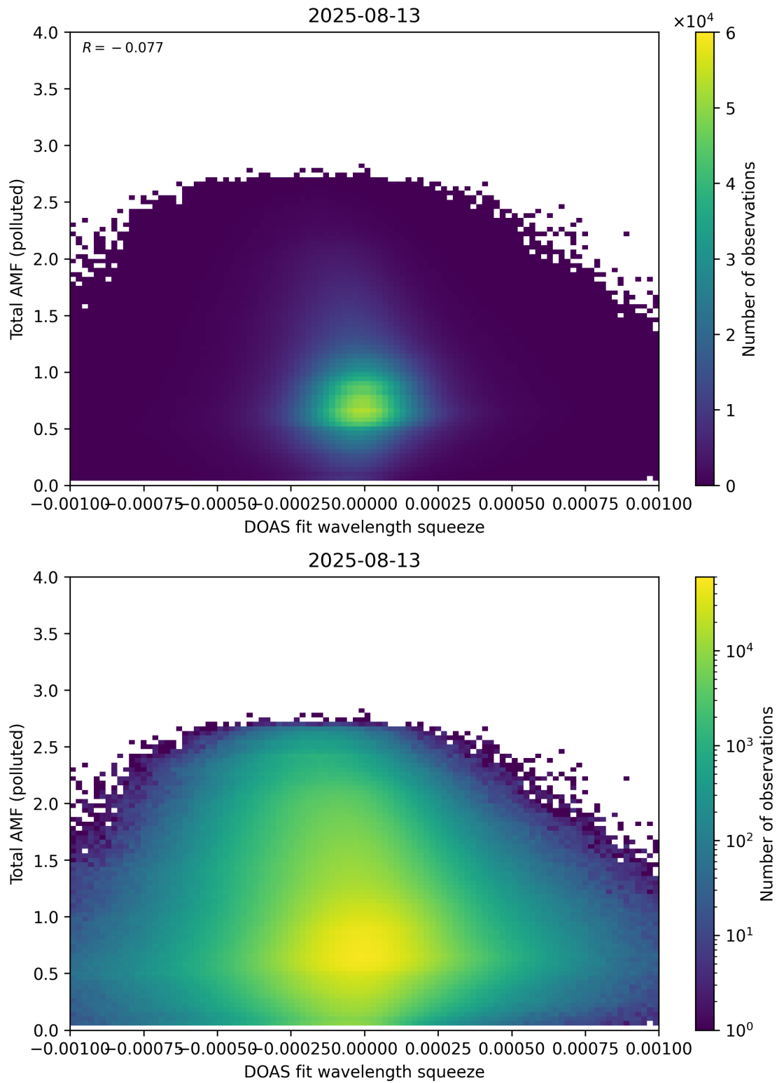
Figure 145: Scatter density plot of “DOAS fit wavelength squeeze” against “Total AMF (polluted)” for 2025-08-12 to 2025-08-14.
