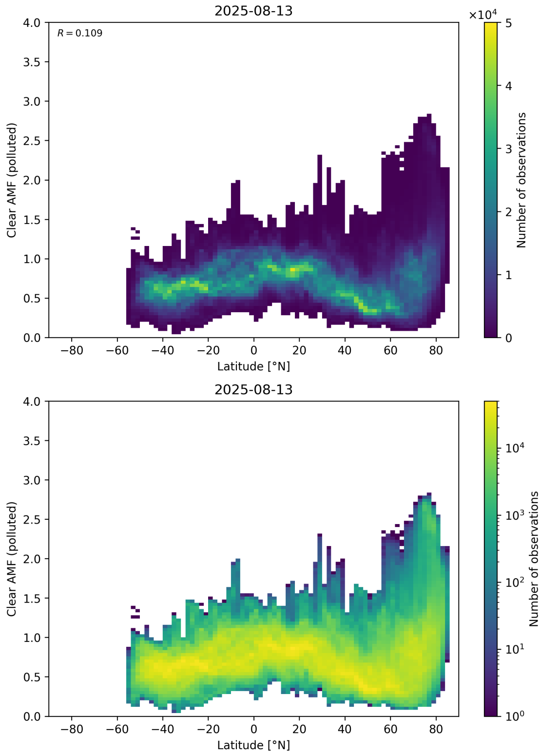
Figure 156: Scatter density plot of “Latitude” against “Clear AMF (polluted)” for 2025-08-12 to 2025-08-14.
