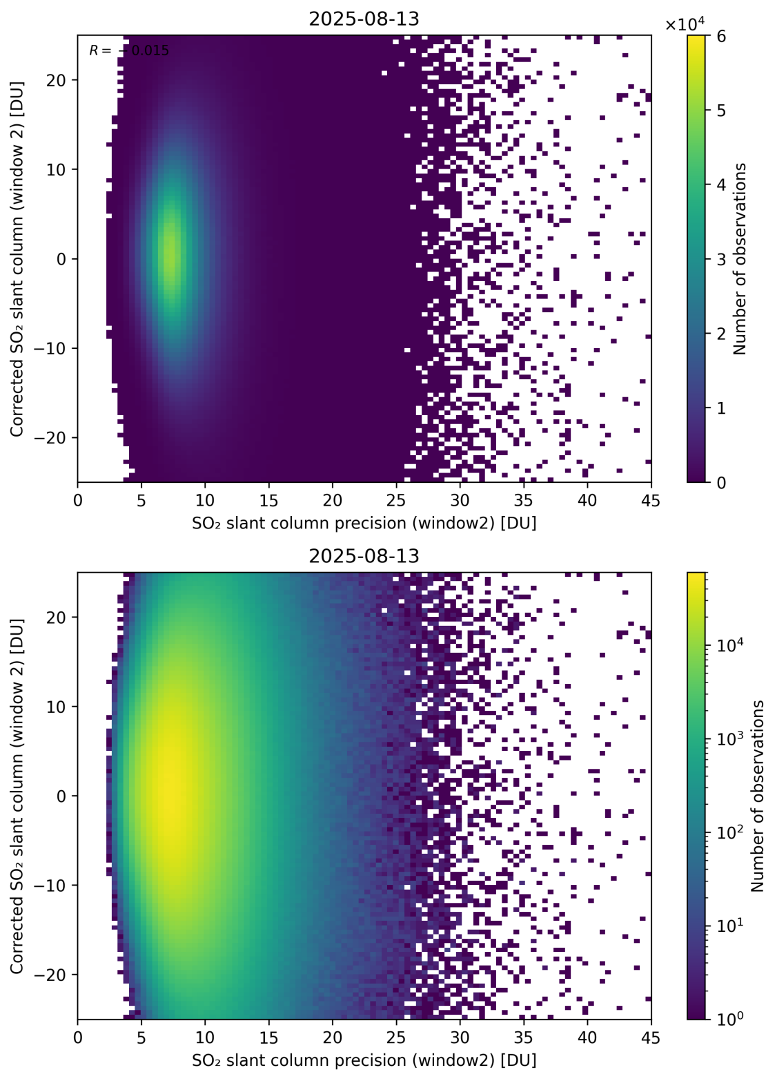
Figure 297: Scatter density plot of “SO 2 slant column precision (window2)” against “Corrected SO 2 slant column (window 2)” for 2025-08-12 to 2025-08-14.
