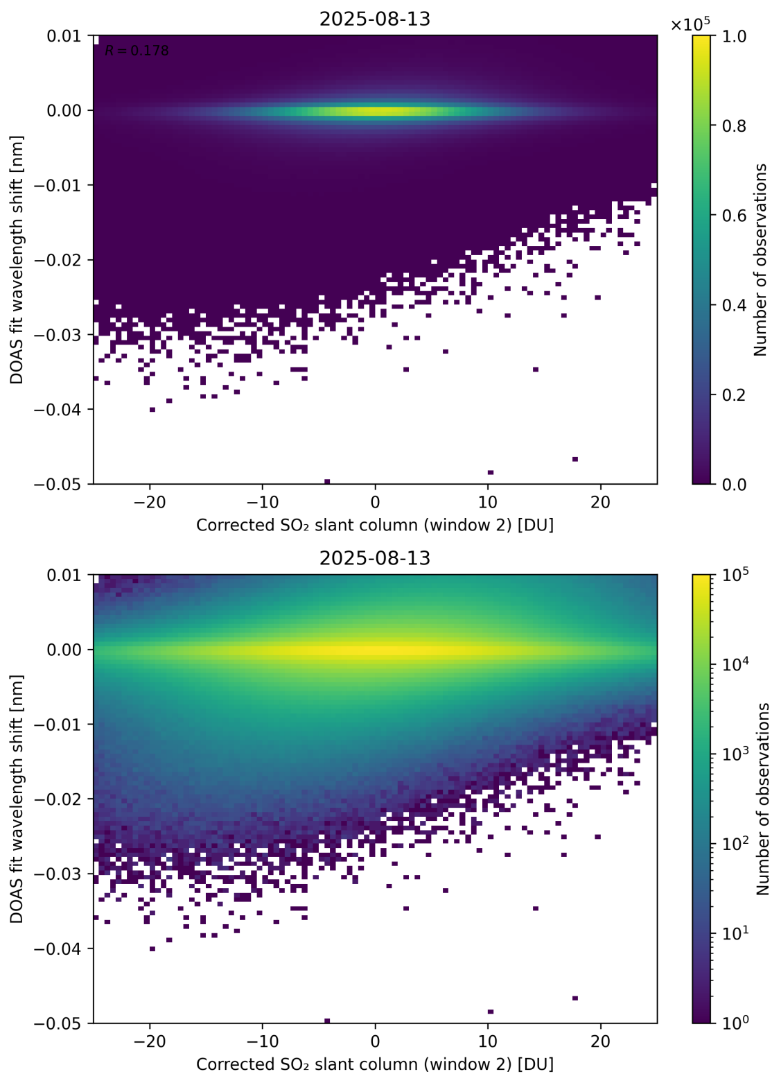
Figure 246: Scatter density plot of “Corrected SO 2 slant column (window 2)” against “DOAS fit wavelength shift” for 2025-08-12 to 2025-08-14.
