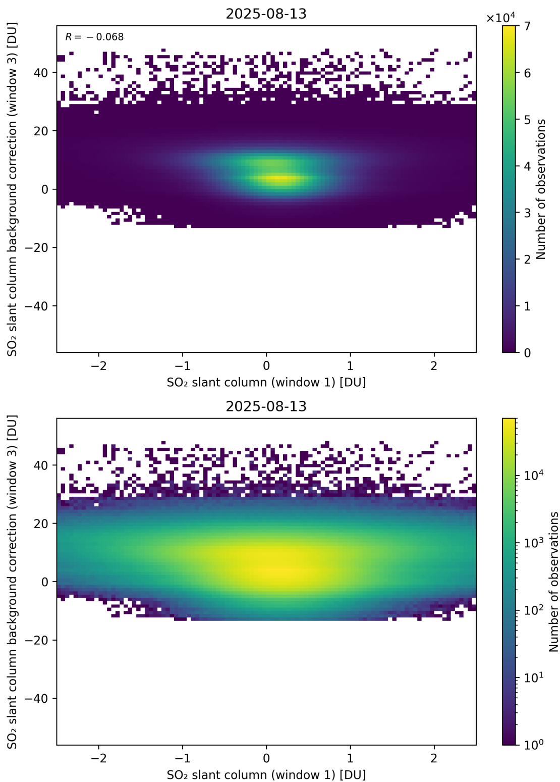
Figure 264: Scatter density plot of “SO 2 slant column (window 1)” against “SO 2 slant column background correction (window 3)” for 2025-08-12 to 2025-08-14.
