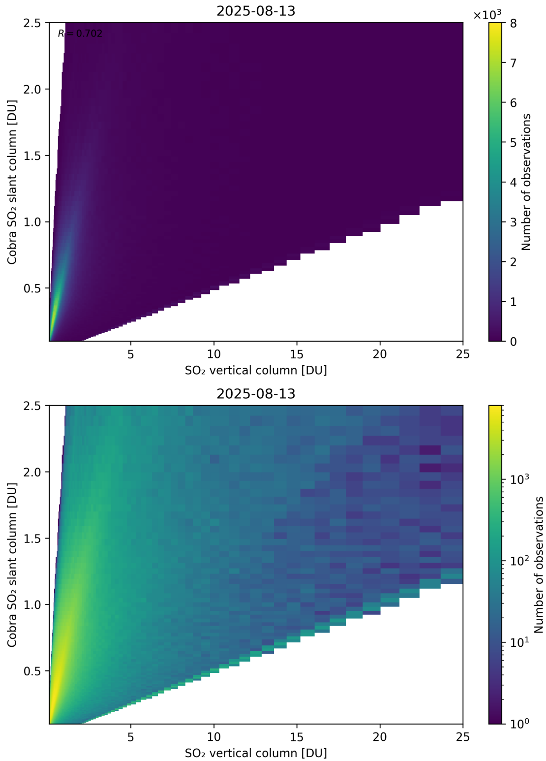
Figure 349: Scatter density plot of “SO 2 vertical column” against “Cobra SO 2 slant column” for 2025-08-12 to 2025-08-14.
