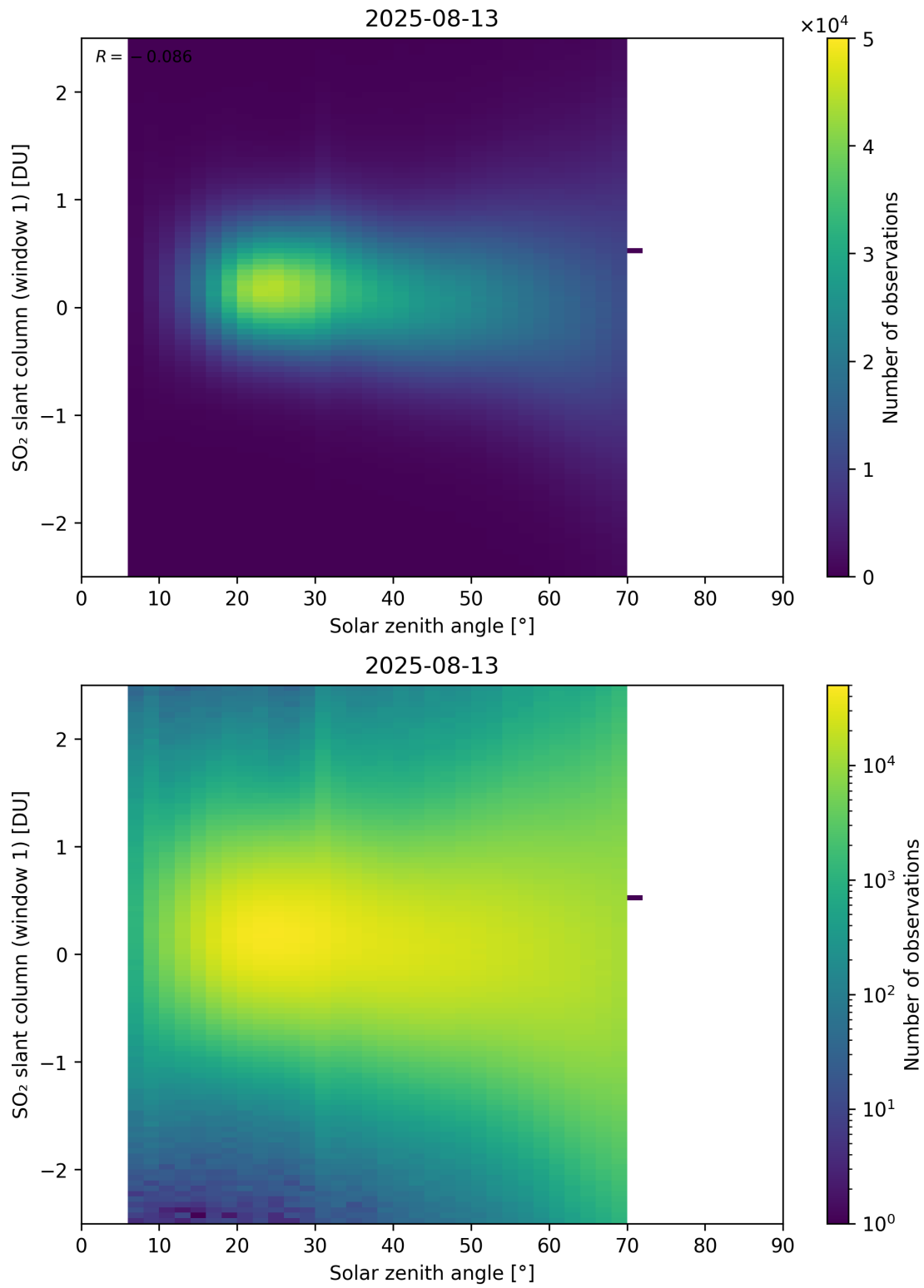
Figure 184: Scatter density plot of “Solar zenith angle” against “SO 2 slant column (window 1)” for 2025-08-12 to 2025-08-14.
