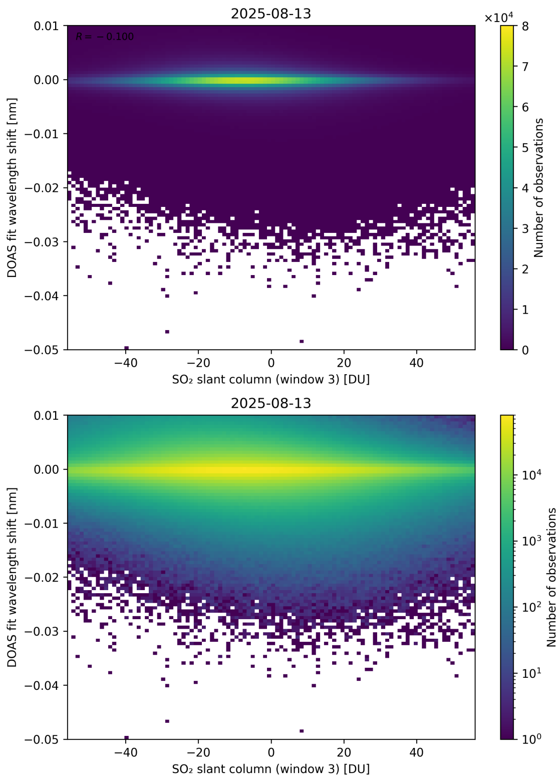
Figure 304: Scatter density plot of “SO 2 slant column (window 3)” against “DOAS fit wavelength shift” for 2025-08-12 to 2025-08-14.
