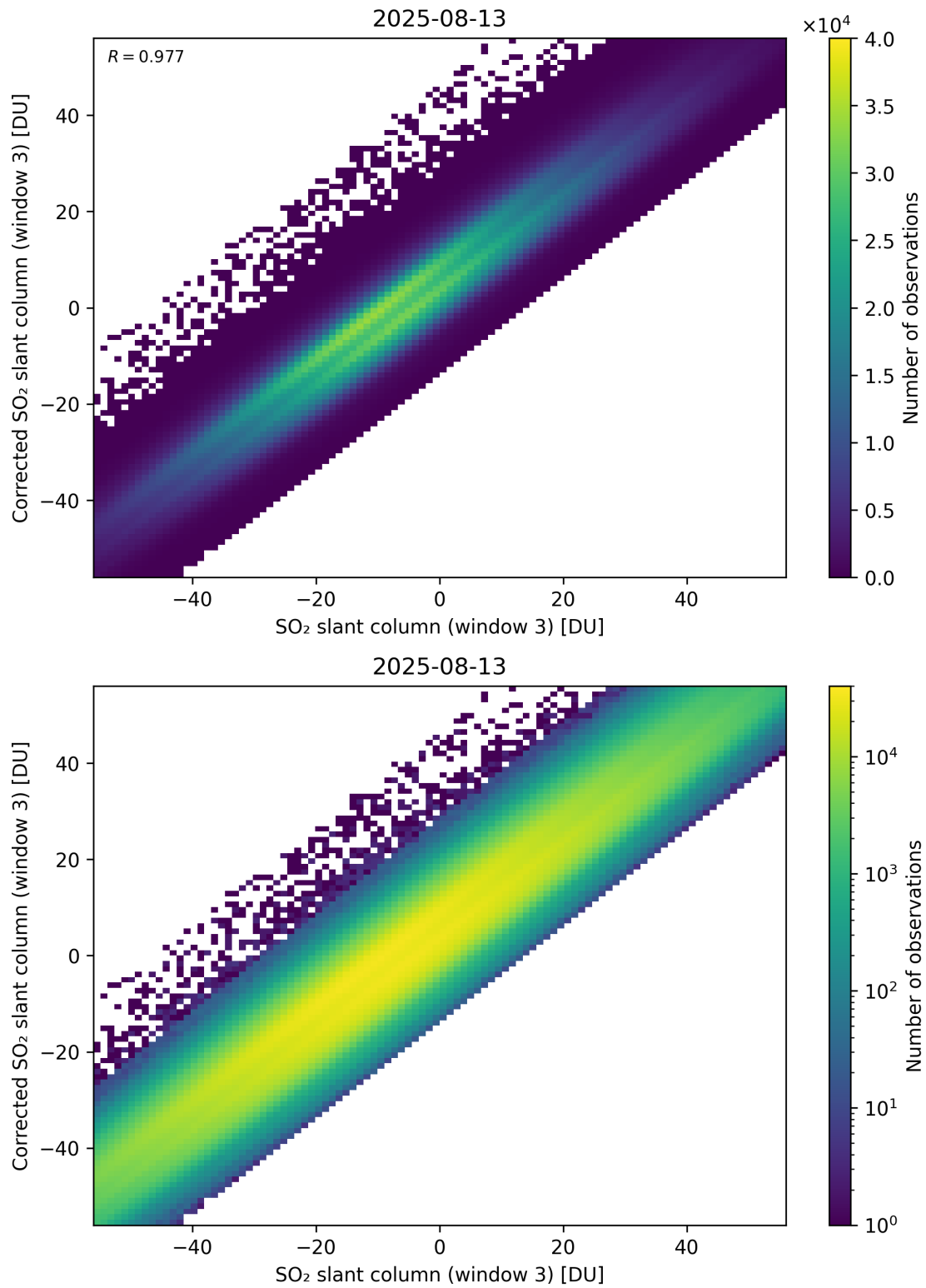
Figure 316: Scatter density plot of “SO 2 slant column (window 3)” against “Corrected SO 2 slant column (window 3)” for 2025-08-12 to 2025-08-14.
