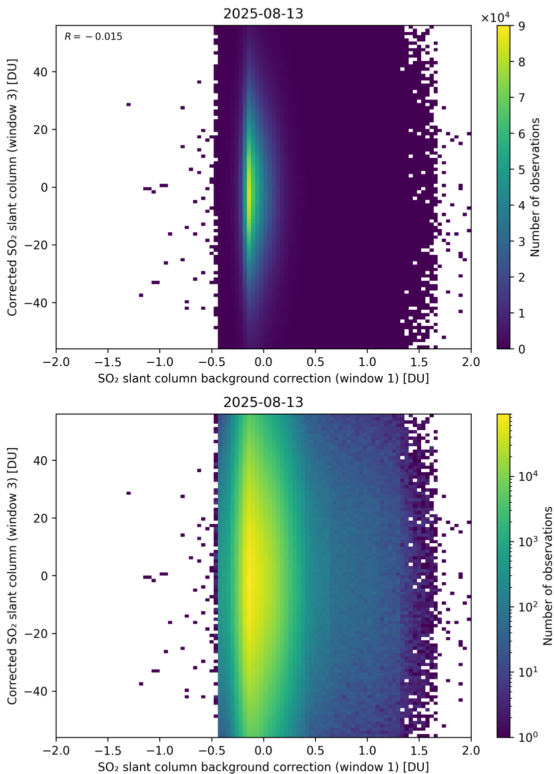
Figure 116: Scatter density plot of “SO 2 slant column background correction (window 1)” against “Corrected SO 2 slant column (window 3)” for 2025-08-12 to 2025-08-14.
