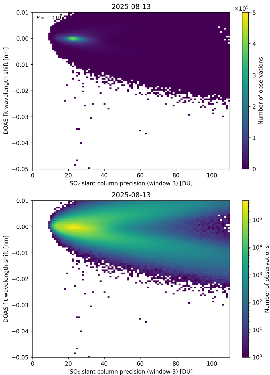
Figure 308: Scatter density plot of “SO 2 slant column precision (window 3)” against “DOAS fit wavelength shift” for 2025-08-12 to 2025-08-14.
