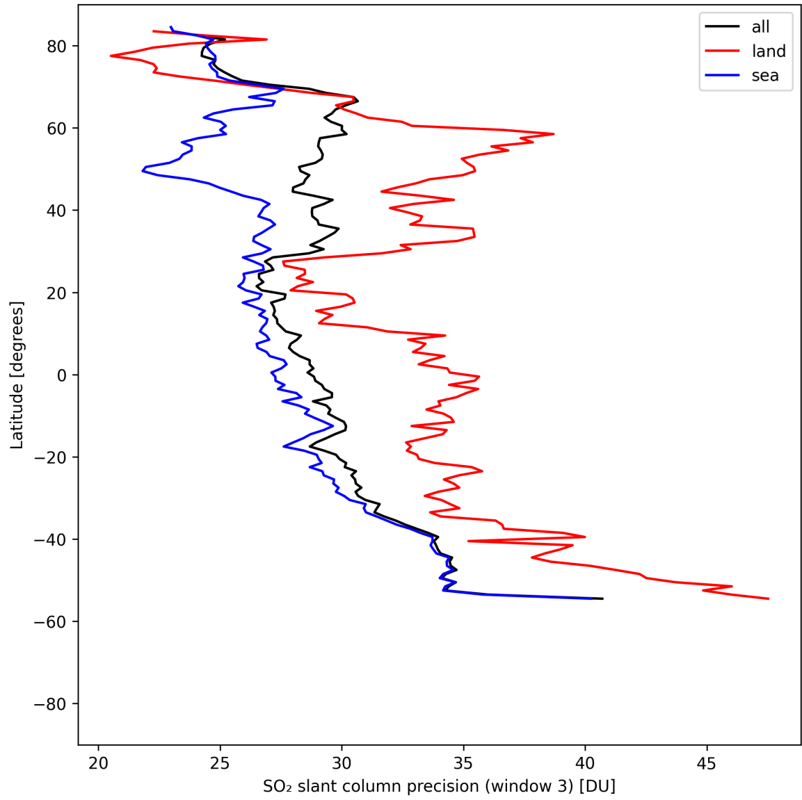
Figure 46: Zonal average of “SO 2 slant column precision (window 3)” for 2025-08-12 to 2025-08-14.
