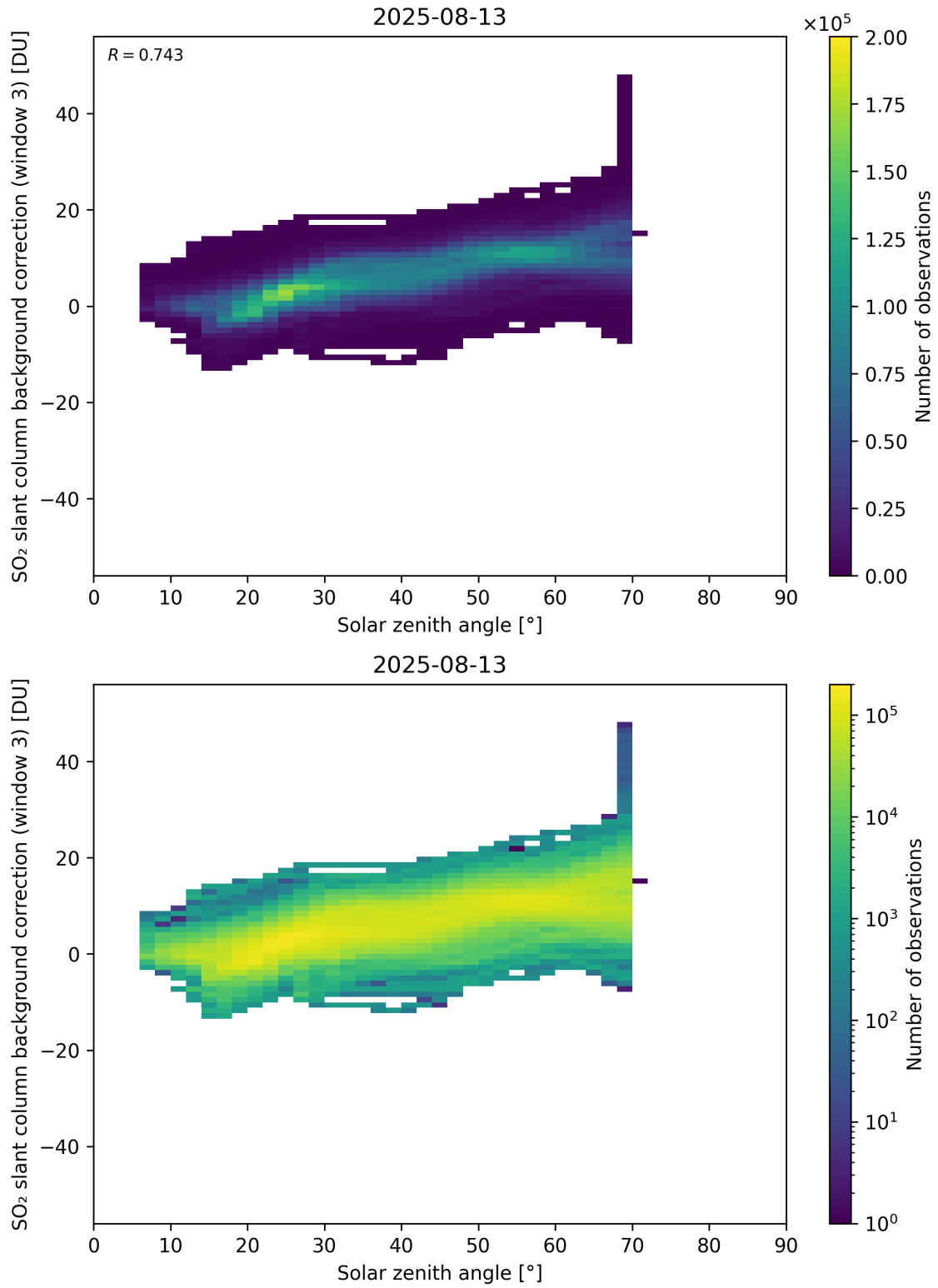
Figure 173: Scatter density plot of “Solar zenith angle” against “SO 2 slant column background correction (window 3)” for 2025-08-12 to 2025-08-14.
