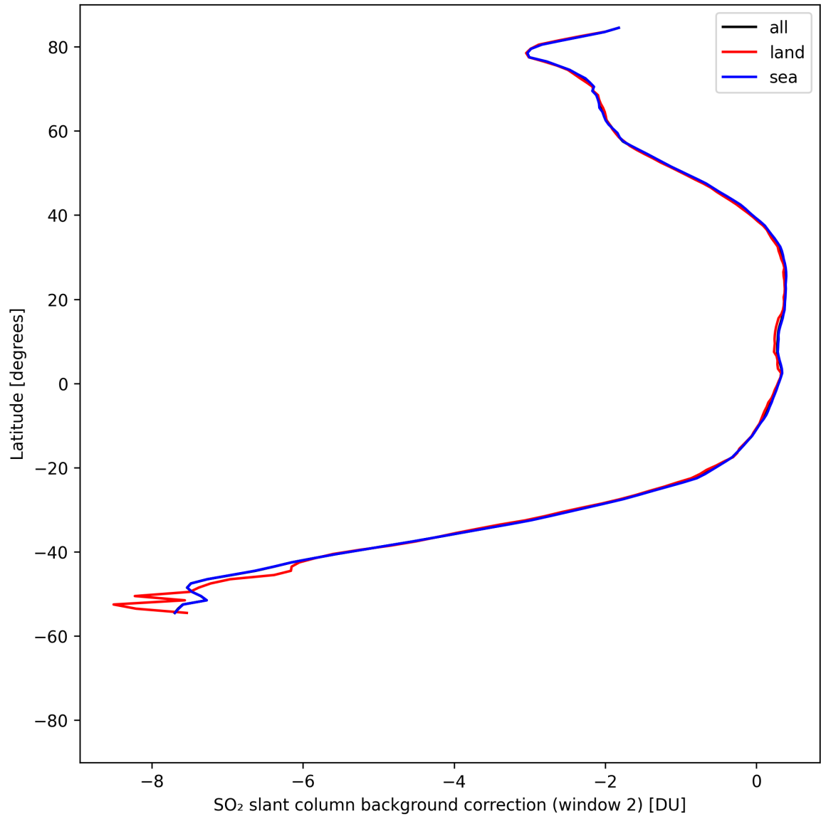
Figure 44: Zonal average of “SO 2 slant column background correction (window 2)” for 2025-08-12 to 2025-08-14.
