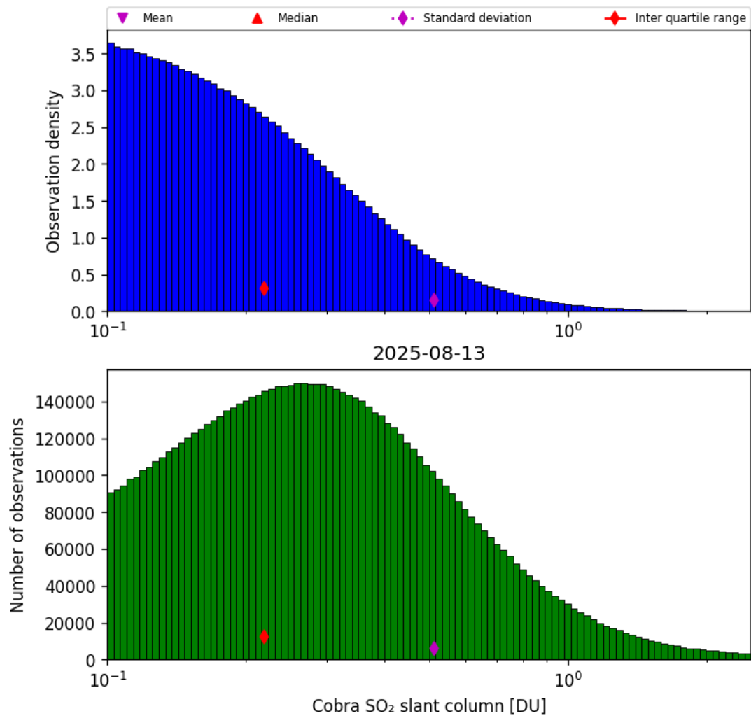
Figure 61: Histogram of “Cobra SO 2 slant column” for 2025-08-12 to 2025-08-14
