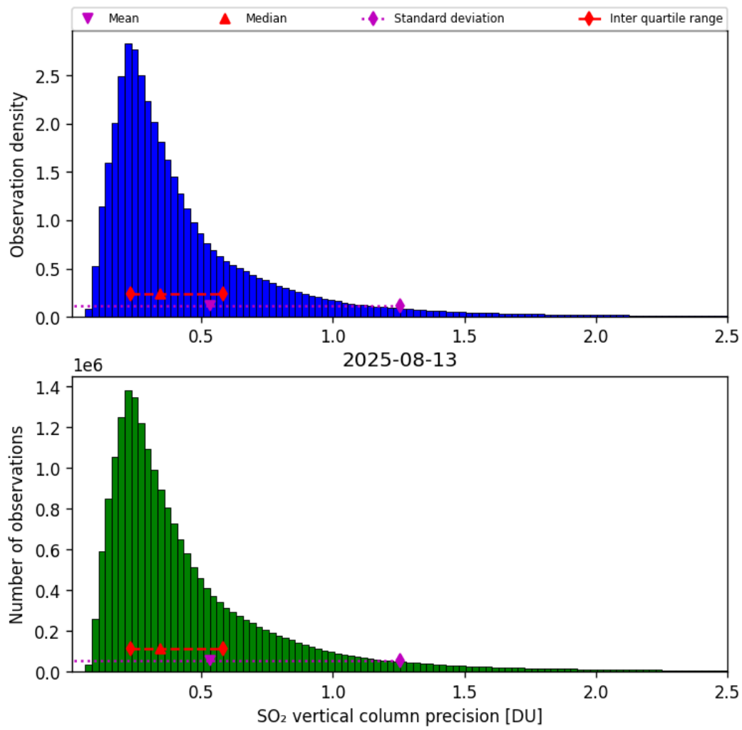
Figure 59: Histogram of “SO 2 vertical column precision” for 2025-08-12 to 2025-08-14
