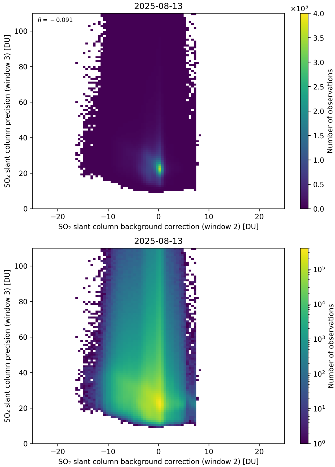
Figure 129: Scatter density plot of “SO 2 slant column background correction (window 2)” against “SO 2 slant column precision (window 3)” for 2025-08-12 to 2025-08-14.
