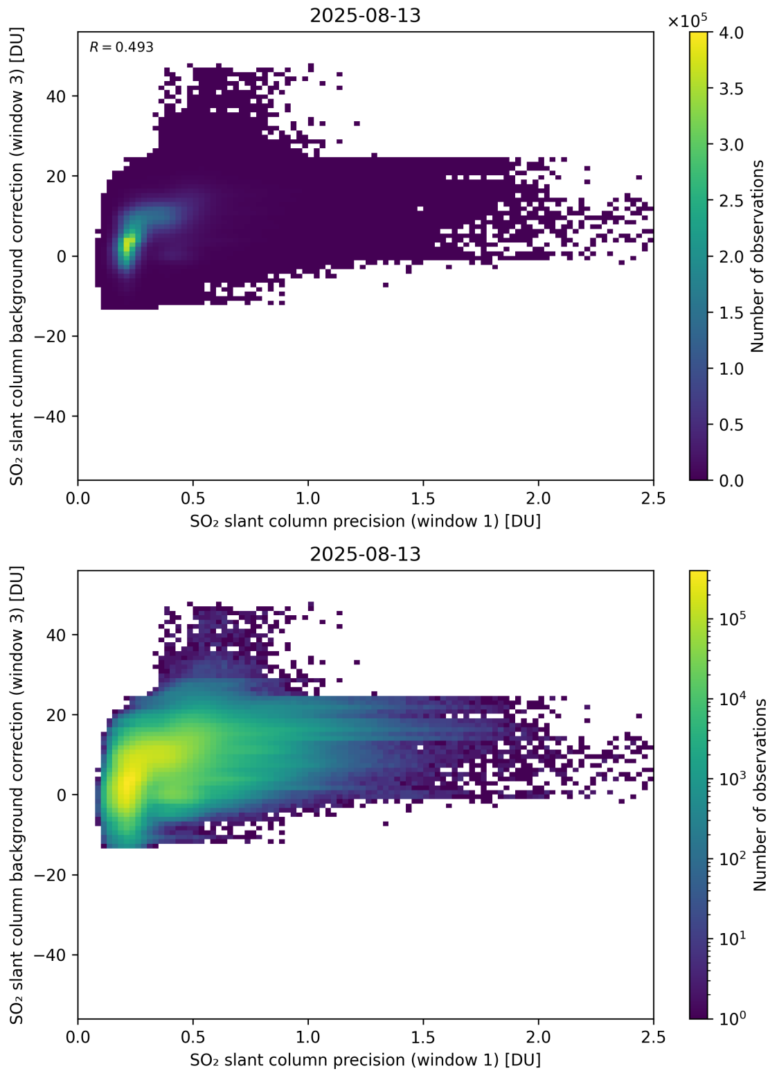
Figure 270: Scatter density plot of “SO 2 slant column precision (window 1)” against “SO 2 slant column background correction (window 3)” for 2025-08-12 to 2025-08-14.
