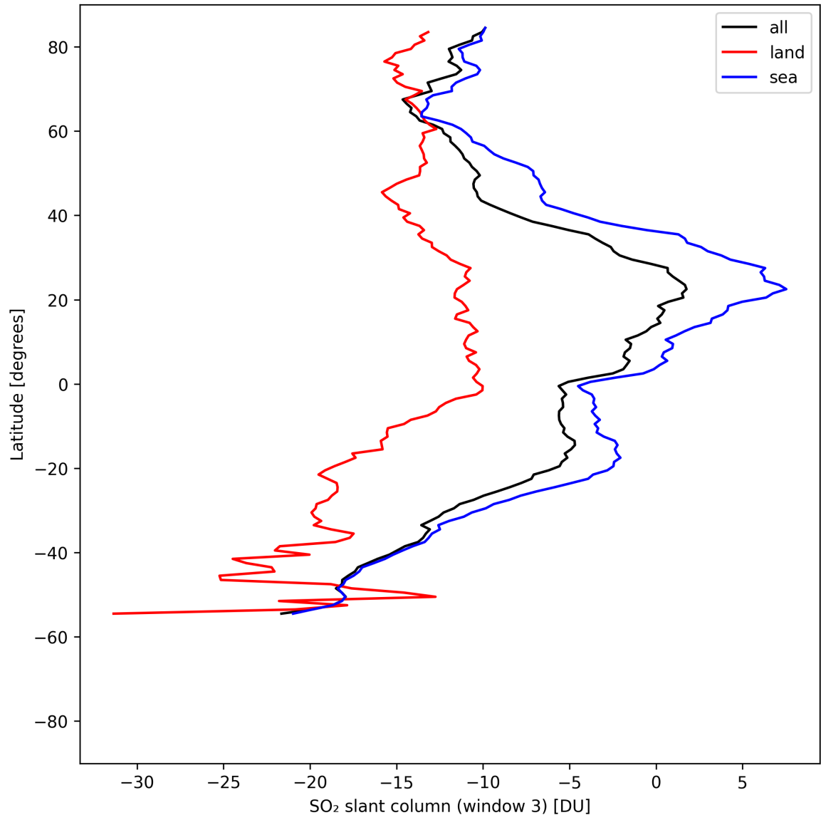
Figure 45: Zonal average of “SO 2 slant column (window 3)” for 2025-08-12 to 2025-08-14.
