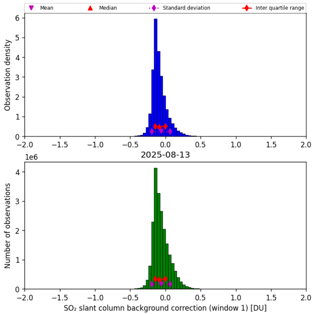
Figure 66: Histogram of “SO 2 slant column background correction (window 1)” for 2025-08-12 to 2025-08-14
