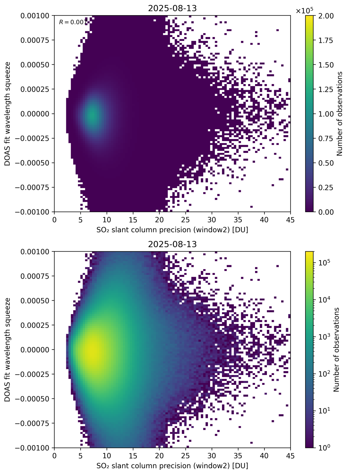
Figure 294: Scatter density plot of “SO 2 slant column precision (window2)” against “DOAS fit wavelength squeeze” for 2025-08-12 to 2025-08-14.
