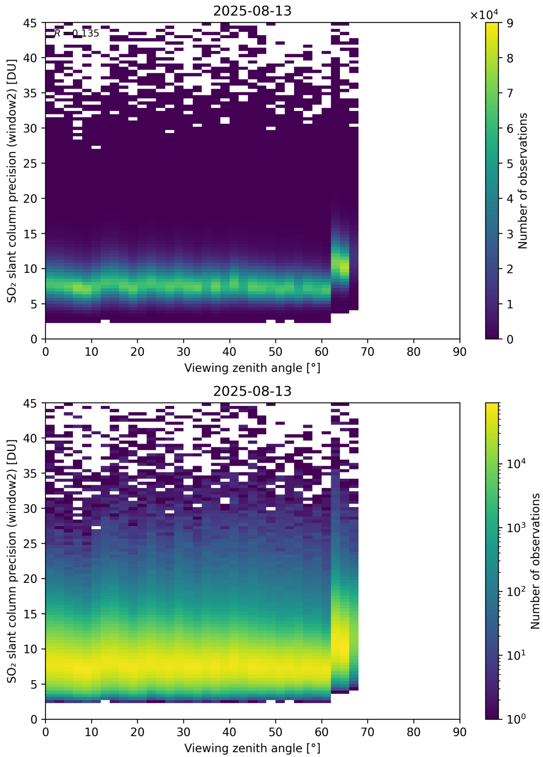
Figure 378: Scatter density plot of “Viewing zenith angle” against “SO 2 slant column precision (window2)” for 2025-08-12 to 2025-08-14.
