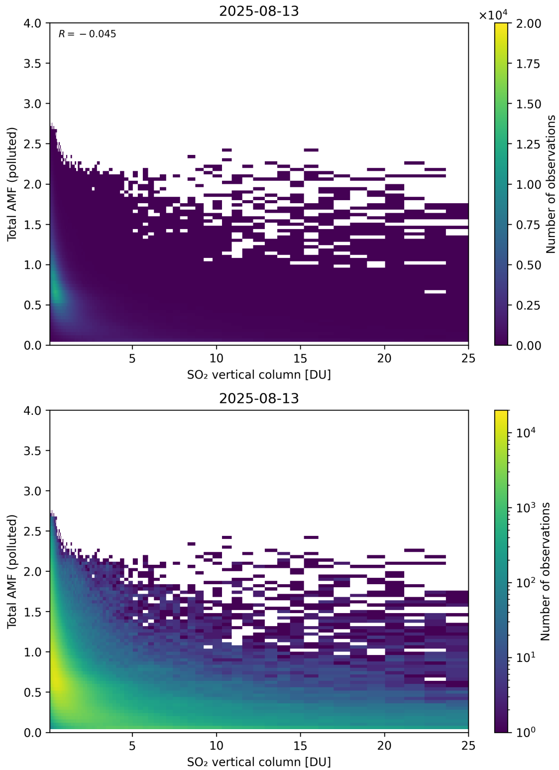
Figure 359: Scatter density plot of “SO 2 vertical column” against “Total AMF (polluted)” for 2025-08-12 to 2025-08-14.
