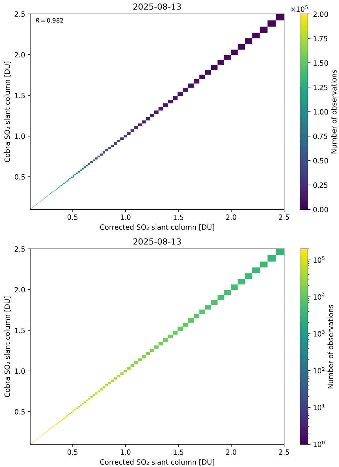
Figure 233: Scatter density plot of “Corrected SO 2 slant column” against “Cobra SO 2 slant column” for 2025-08-12 to 2025-08-14.
