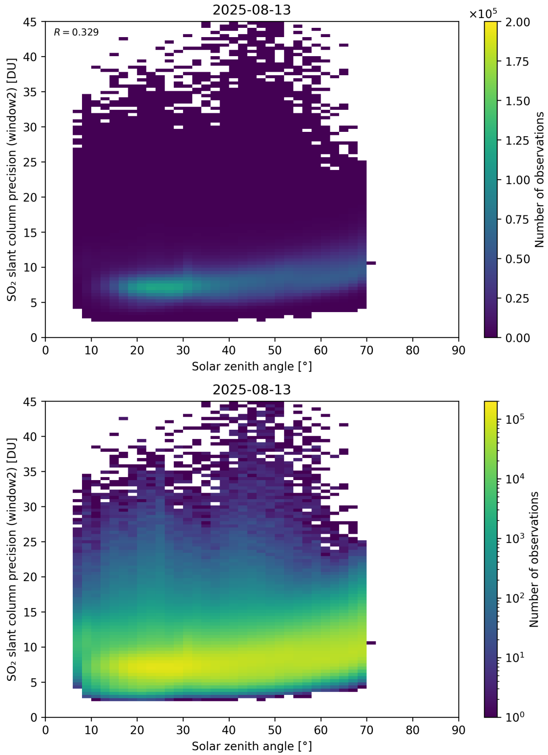
Figure 186: Scatter density plot of “Solar zenith angle” against “SO 2 slant column precision (window2)” for 2025-08-12 to 2025-08-14.
