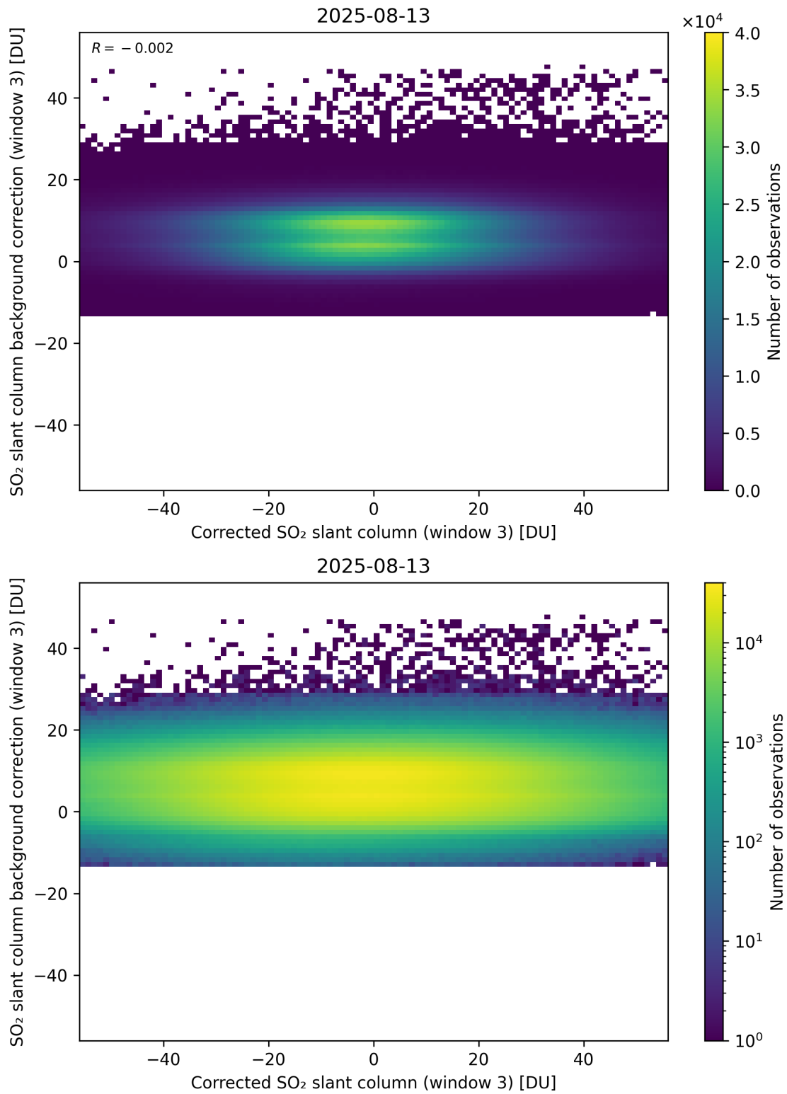
Figure 255: Scatter density plot of “Corrected SO 2 slant column (window 3)” against “SO 2 slant column background correction (window 3)” for 2025-08-12 to 2025-08-14.
