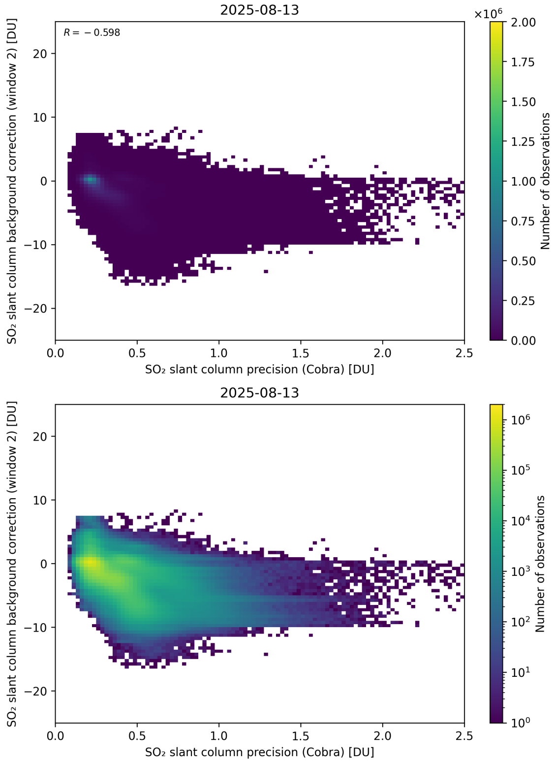
Figure 200: Scatter density plot of “SO 2 slant column precision (Cobra)” against “SO 2 slant column background correction (window 2)” for 2025-08-12 to 2025-08-14.
