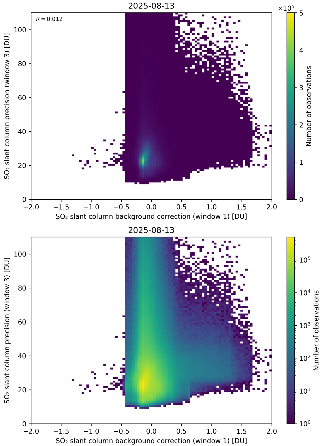
Figure 119: Scatter density plot of “SO 2 slant column background correction (window 1)” against “SO 2 slant column precision (window 3)” for 2025-08-12 to 2025-08-14.
