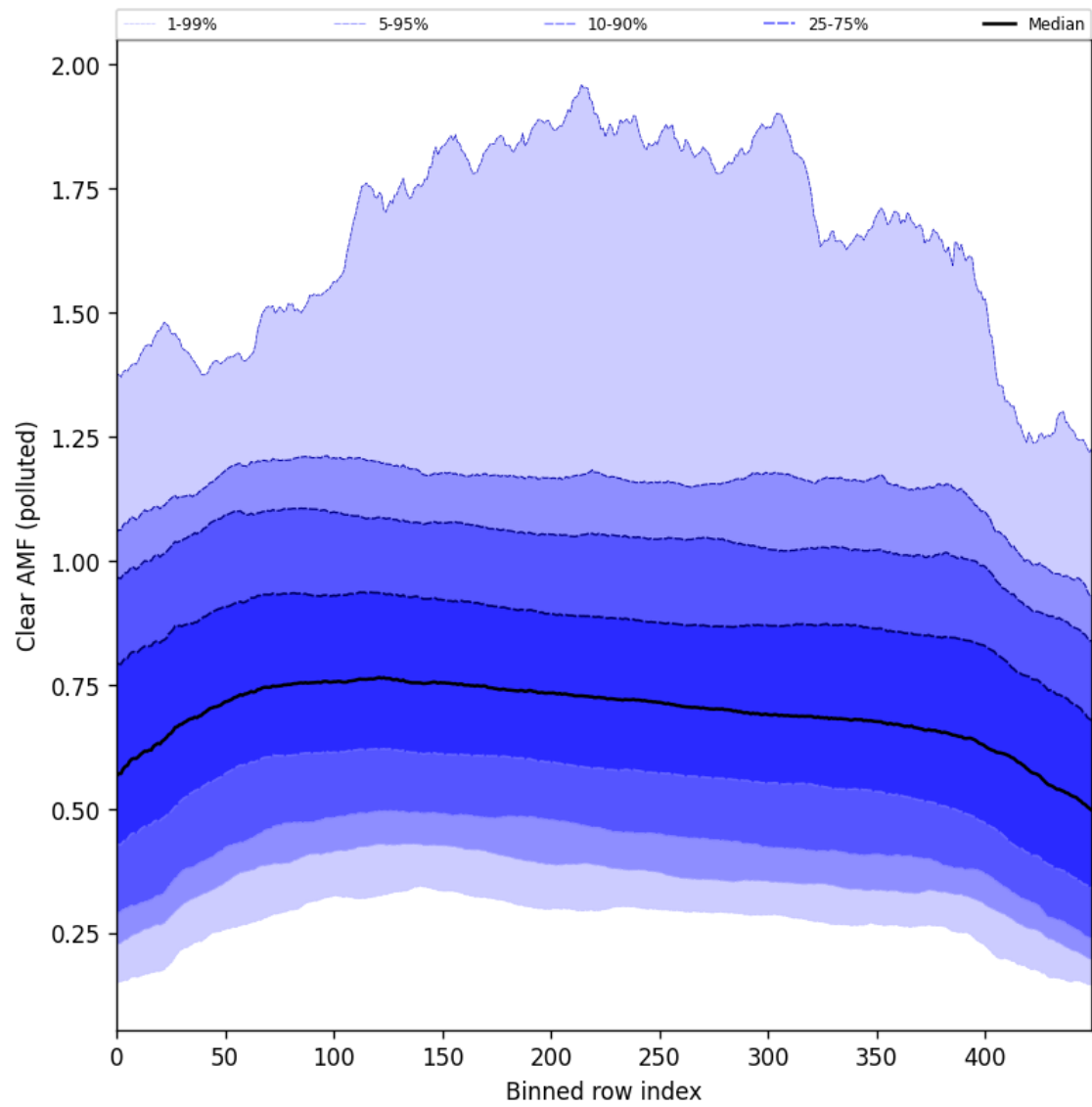
Figure 107: Along track statistics of “Clear AMF (polluted)” for 2025-08-12 to 2025-08-14
