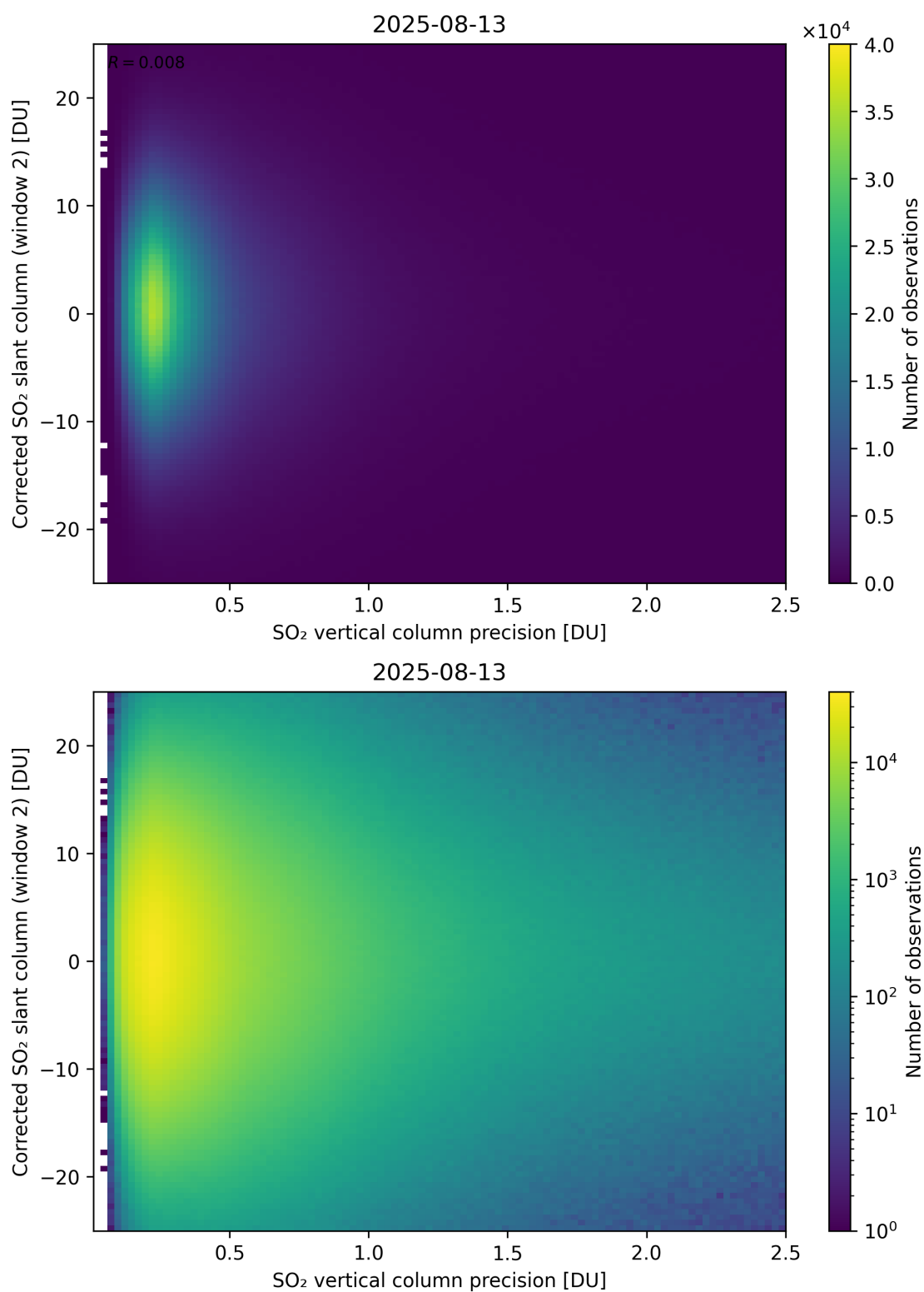
Figure 339: Scatter density plot of “SO 2 vertical column precision” against “Corrected SO 2 slant column (window 2)” for 2025-08-12 to 2025-08-14.
