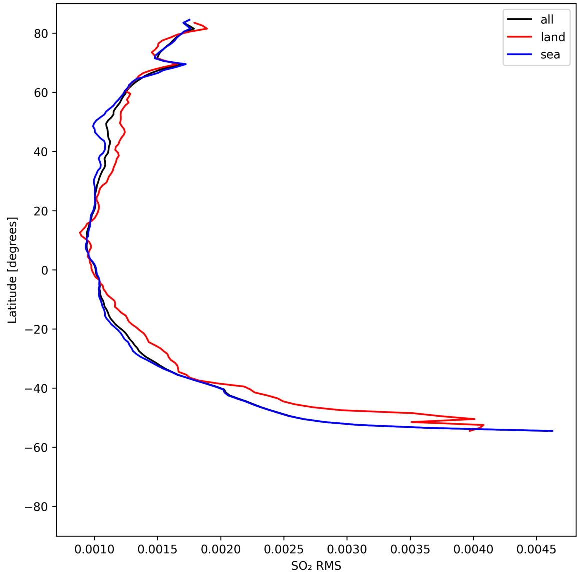
Figure 52: Zonal average of “SO 2 RMS” for 2025-08-12 to 2025-08-14.
