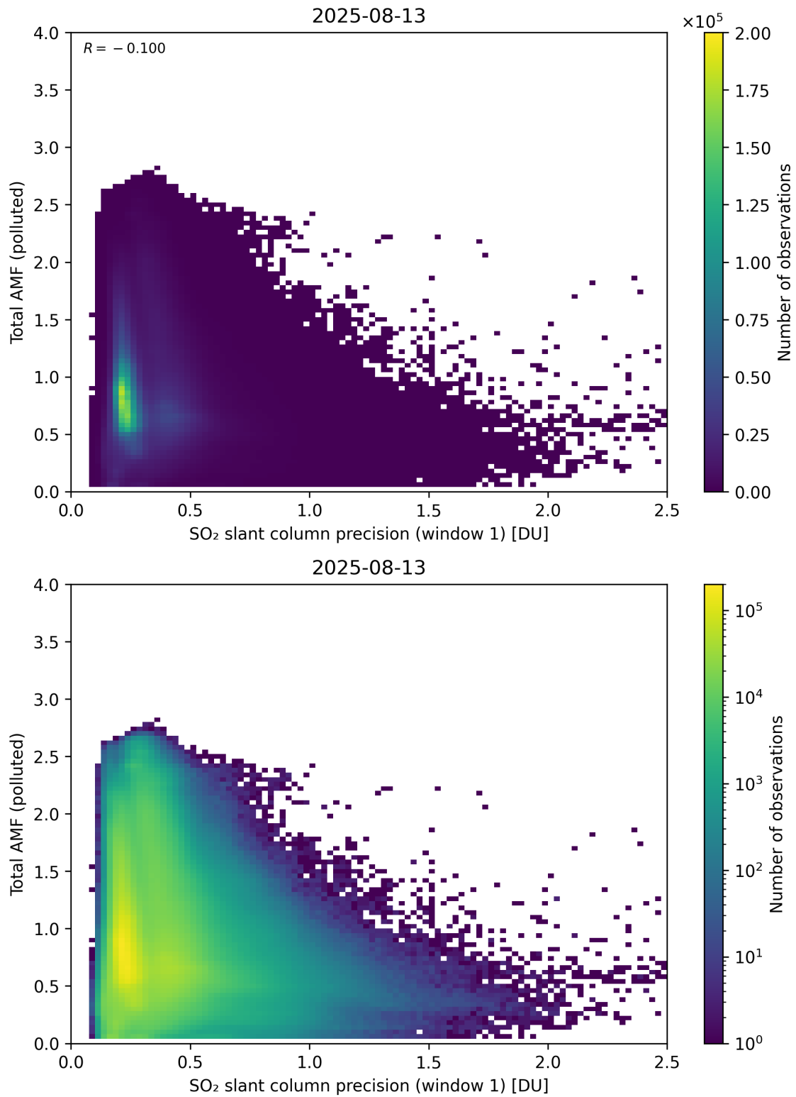
Figure 280: Scatter density plot of “SO 2 slant column precision (window 1)” against “Total AMF (polluted)” for 2025-08-12 to 2025-08-14.
