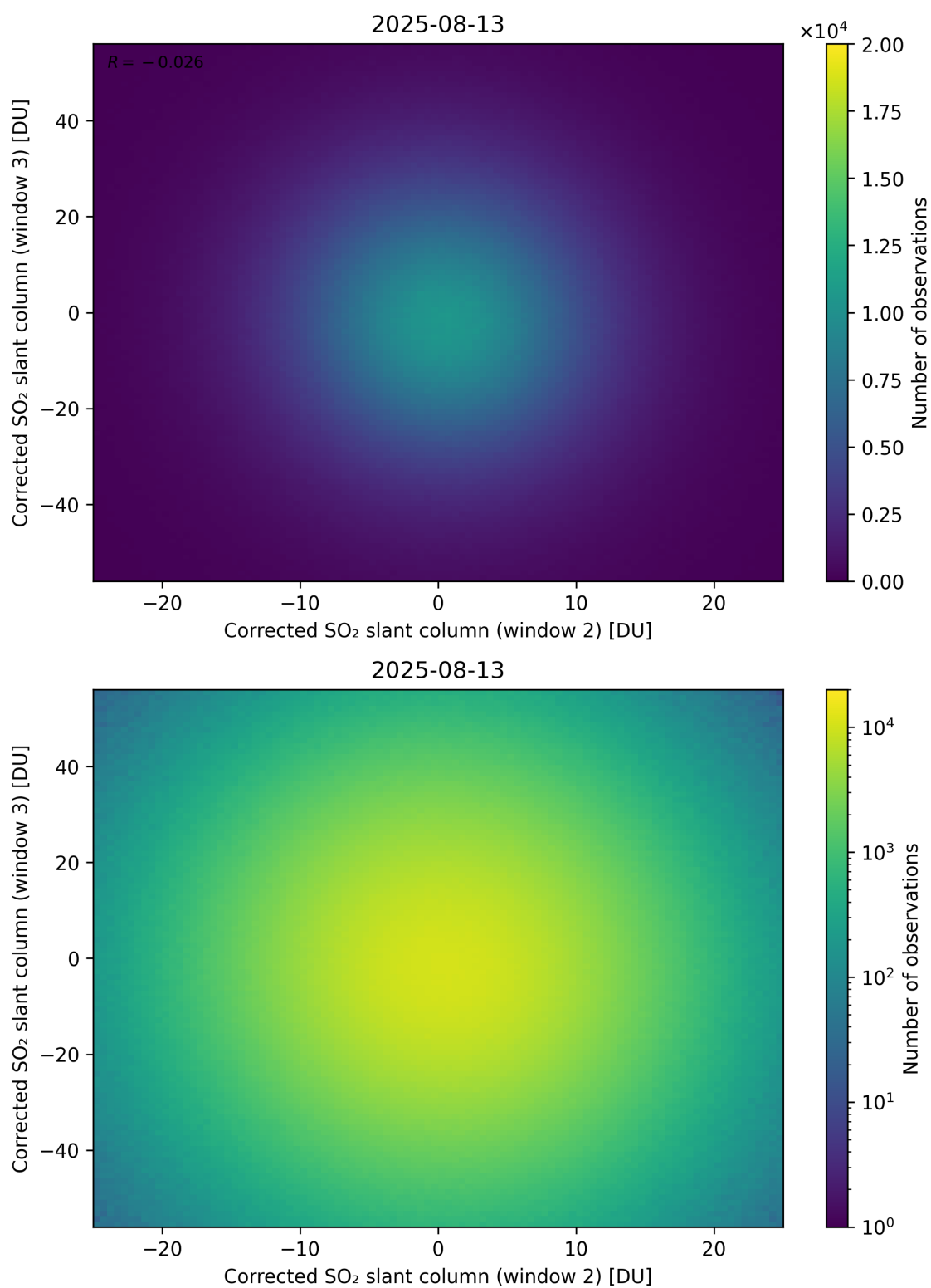
Figure 250: Scatter density plot of “Corrected SO 2 slant column (window 2)” against “Corrected SO 2 slant column (window 3)” for 2025-08-12 to 2025-08-14.
