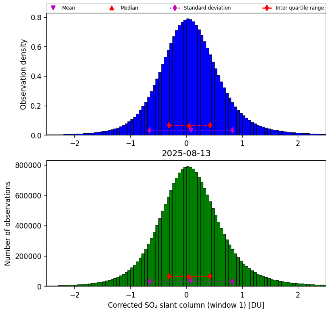
Figure 65: Histogram of “Corrected SO 2 slant column (window 1)” for 2025-08-12 to 2025-08-14
