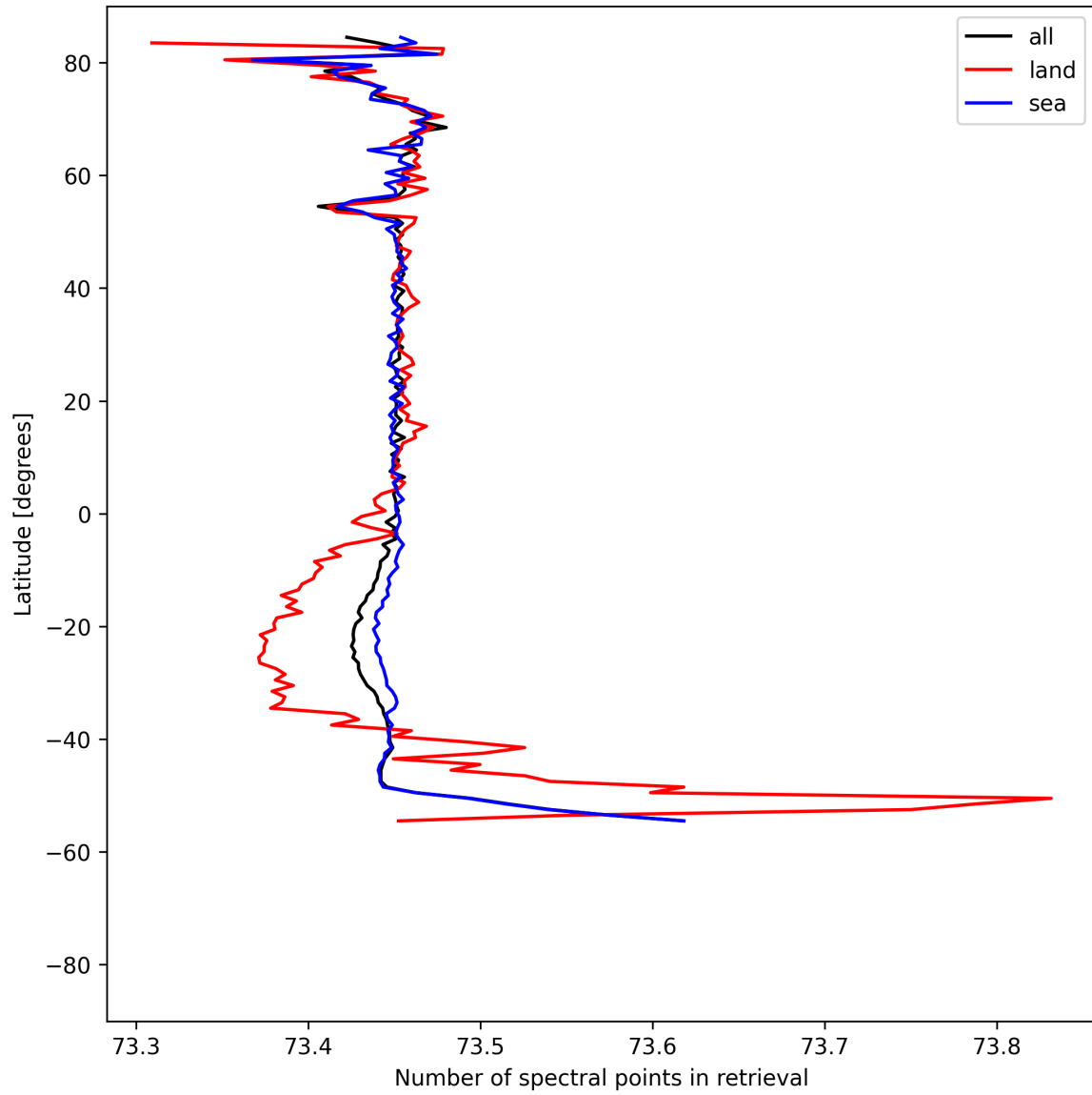
Figure 56: Zonal average of “Number of spectral points in retrieval” for 2025-08-12 to 2025-08-14.
