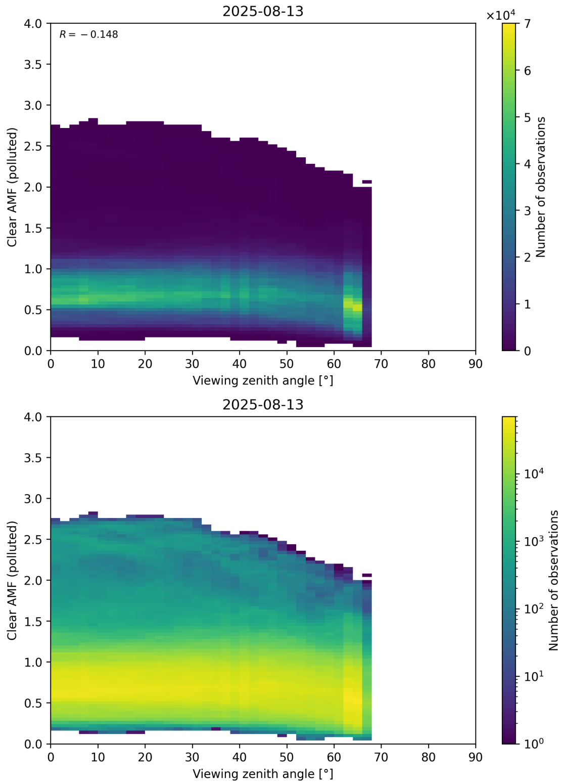
Figure 370: Scatter density plot of “Viewing zenith angle” against “Clear AMF (polluted)” for 2025-08-12 to 2025-08-14.
