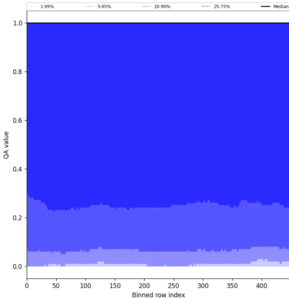
Figure 83: Along track statistics of “QA value” for 2025-08-12 to 2025-08-14
