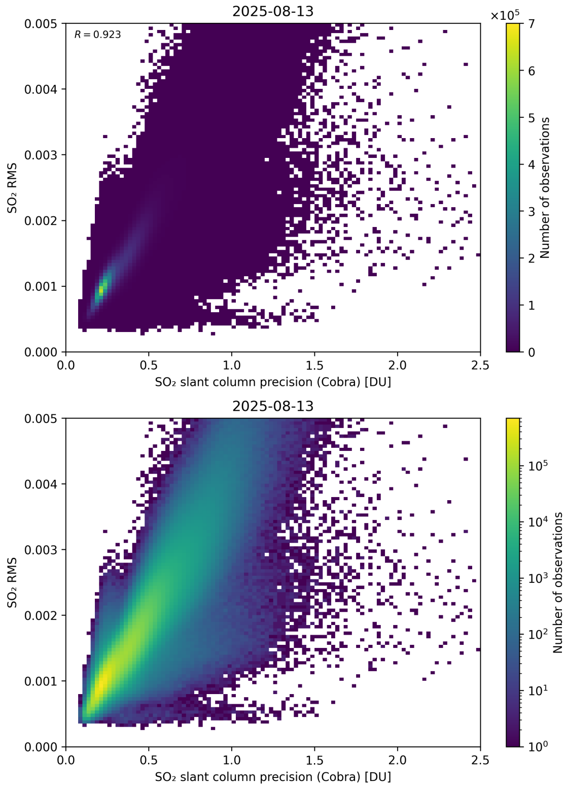
Figure 204: Scatter density plot of “SO 2 slant column precision (Cobra)” against “SO 2 RMS” for 2025-08-12 to 2025-08-14.
