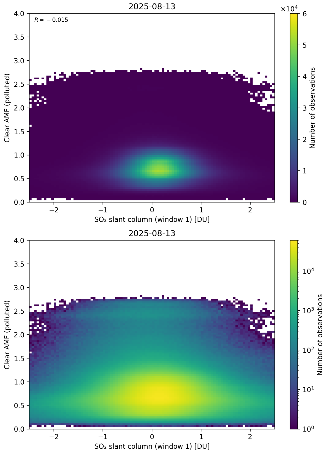
Figure 282: Scatter density plot of “SO 2 slant column (window 1)” against “Clear AMF (polluted)” for 2025-08-12 to 2025-08-14.
