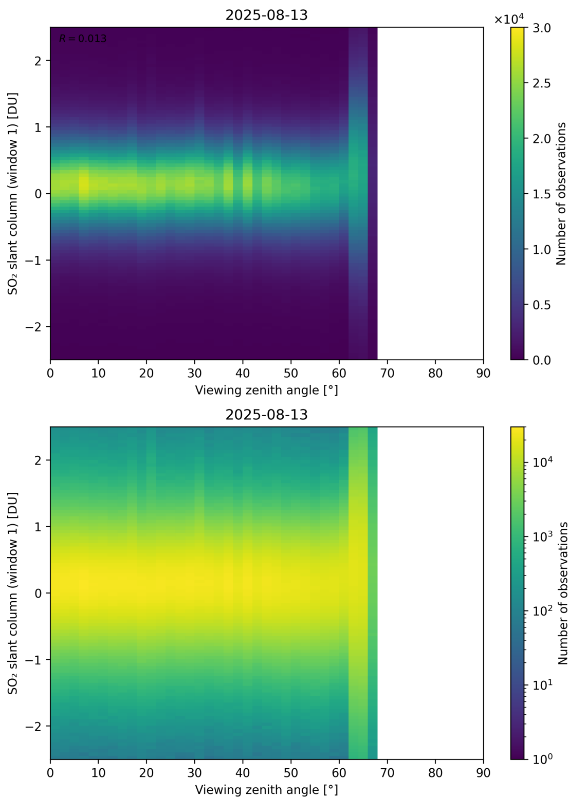
Figure 376: Scatter density plot of “Viewing zenith angle” against “SO 2 slant column (window 1)” for 2025-08-12 to 2025-08-14.
