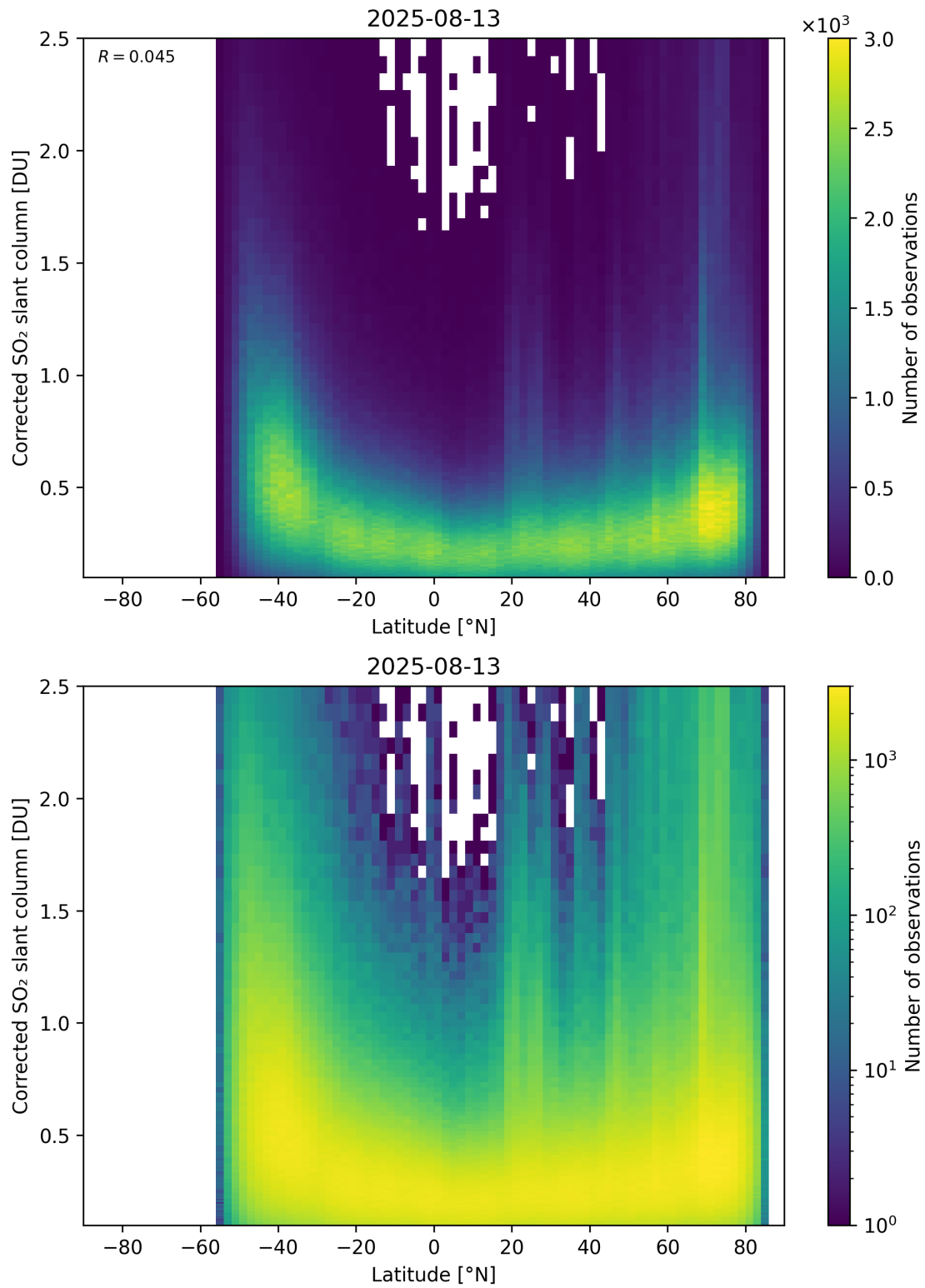
Figure 159: Scatter density plot of “Latitude” against “Corrected SO 2 slant column” for 2025-08-12 to 2025-08-14.
