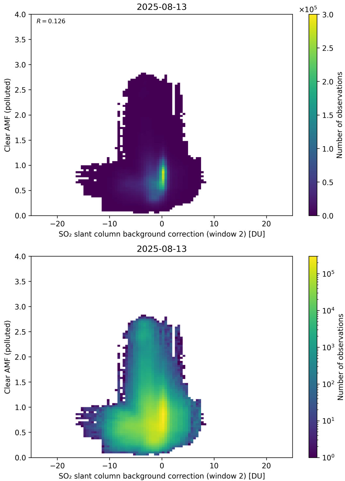
Figure 126: Scatter density plot of “SO 2 slant column background correction (window 2)” against “Clear AMF (polluted)” for 2025-08-12 to 2025-08-14.
