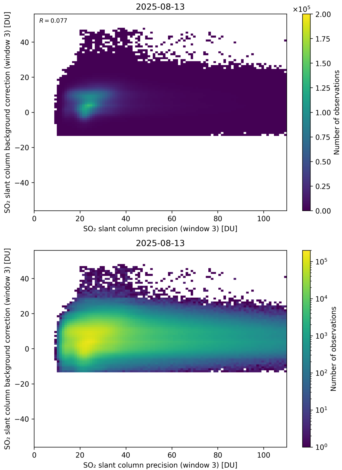
Figure 307: Scatter density plot of “SO 2 slant column precision (window 3)” against “SO 2 slant column background correction (window 3)” for 2025-08-12 to 2025-08-14.
