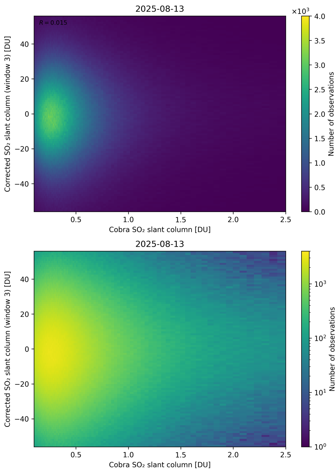
Figure 218: Scatter density plot of “Cobra SO 2 slant column” against “Corrected SO 2 slant column (window 3)” for 2025-08-12 to 2025-08-14.
