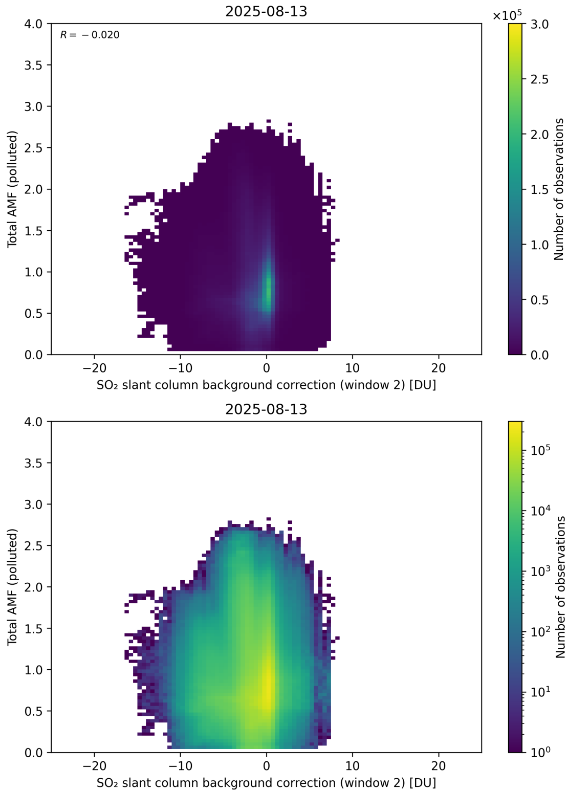
Figure 130: Scatter density plot of “SO 2 slant column background correction (window 2)” against “Total AMF (polluted)” for 2025-08-12 to 2025-08-14.
