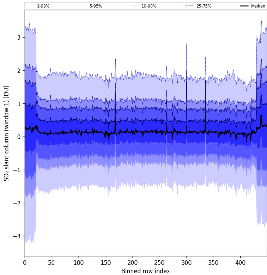
Figure 89: Along track statistics of “SO 2 slant column (window 1)” for 2025-08-12 to 2025-08-14
