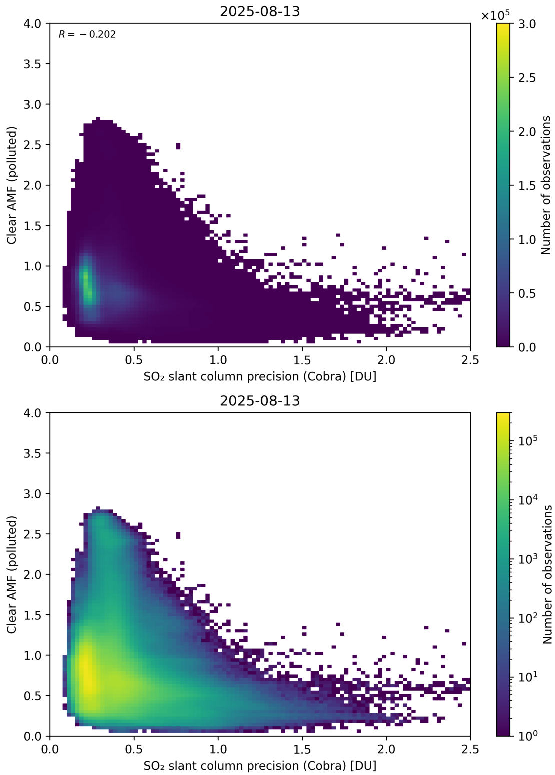
Figure 205: Scatter density plot of “SO 2 slant column precision (Cobra)” against “Clear AMF (polluted)” for 2025-08-12 to 2025-08-14.
