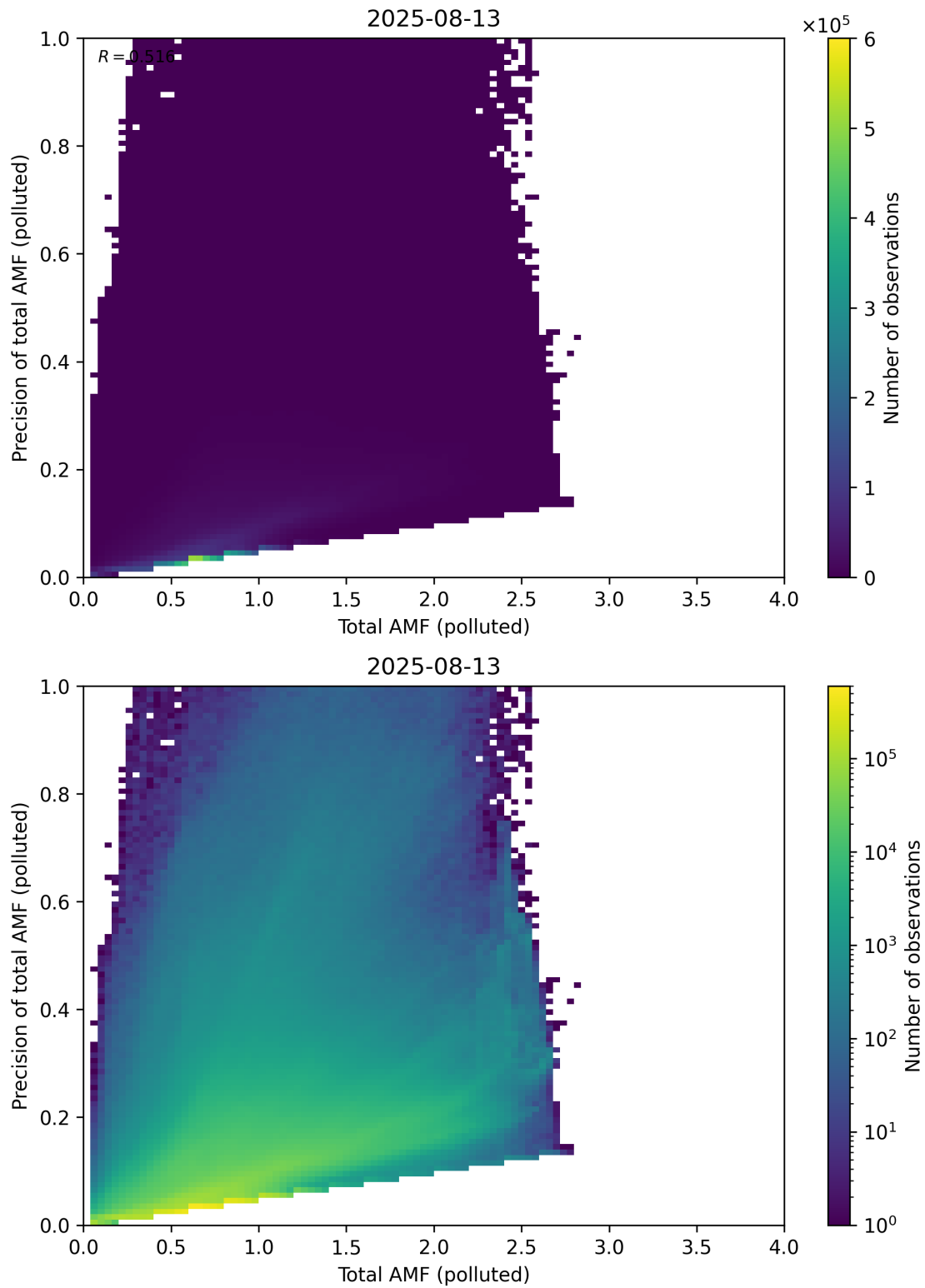
Figure 322: Scatter density plot of “Total AMF (polluted)” against “Precision of total AMF (polluted)” for 2025-08-12 to 2025-08-14.
