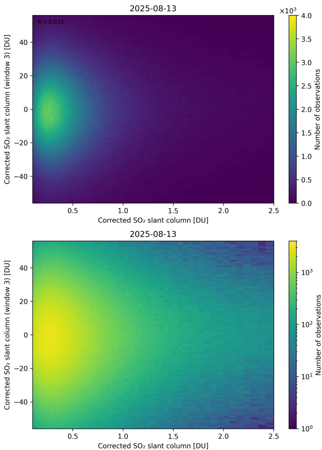
Figure 236: Scatter density plot of “Corrected SO 2 slant column” against “Corrected SO 2 slant column (window 3)” for 2025-08-12 to 2025-08-14.
