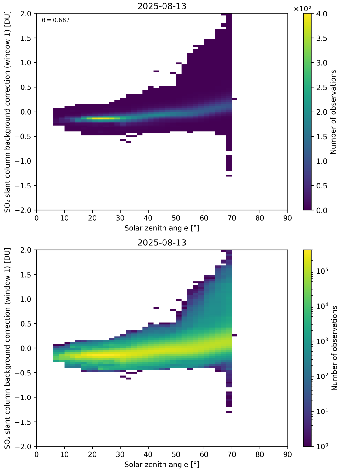
Figure 171: Scatter density plot of “Solar zenith angle” against “SO 2 slant column background correction (window 1)” for 2025-08-12 to 2025-08-14.
