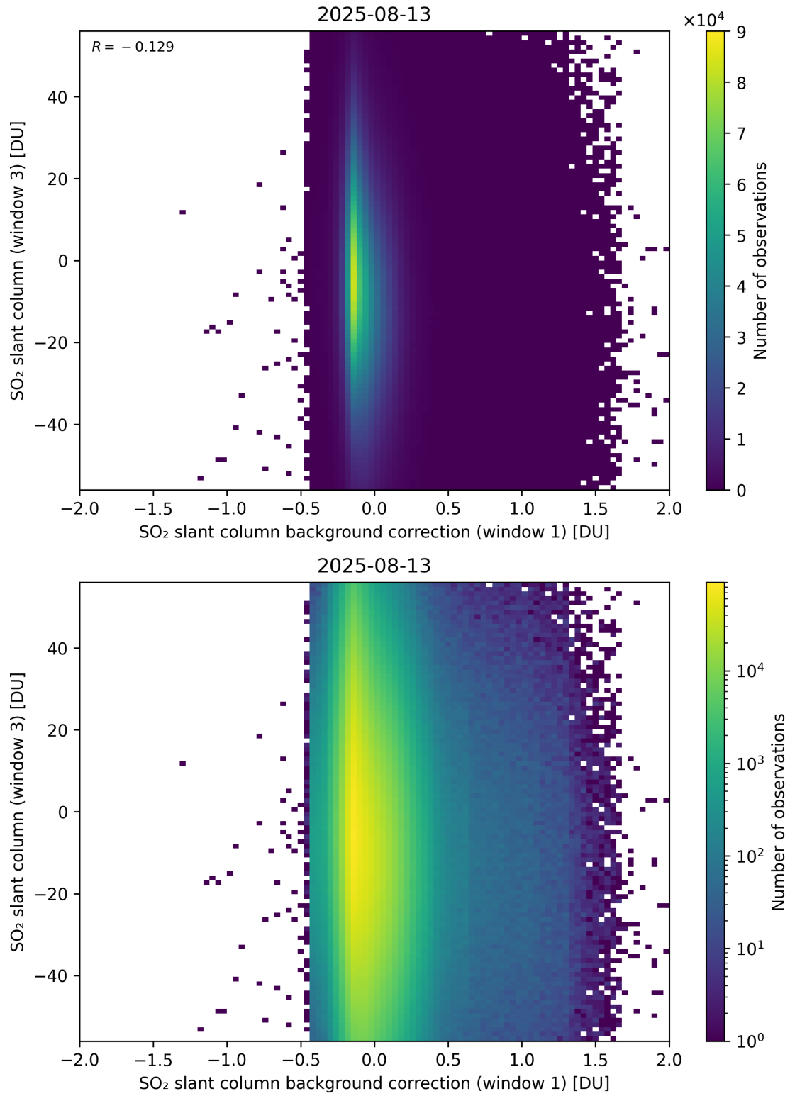
Figure 118: Scatter density plot of “SO 2 slant column background correction (window 1)” against “SO 2 slant column (window 3)” for 2025-08-12 to 2025-08-14.
