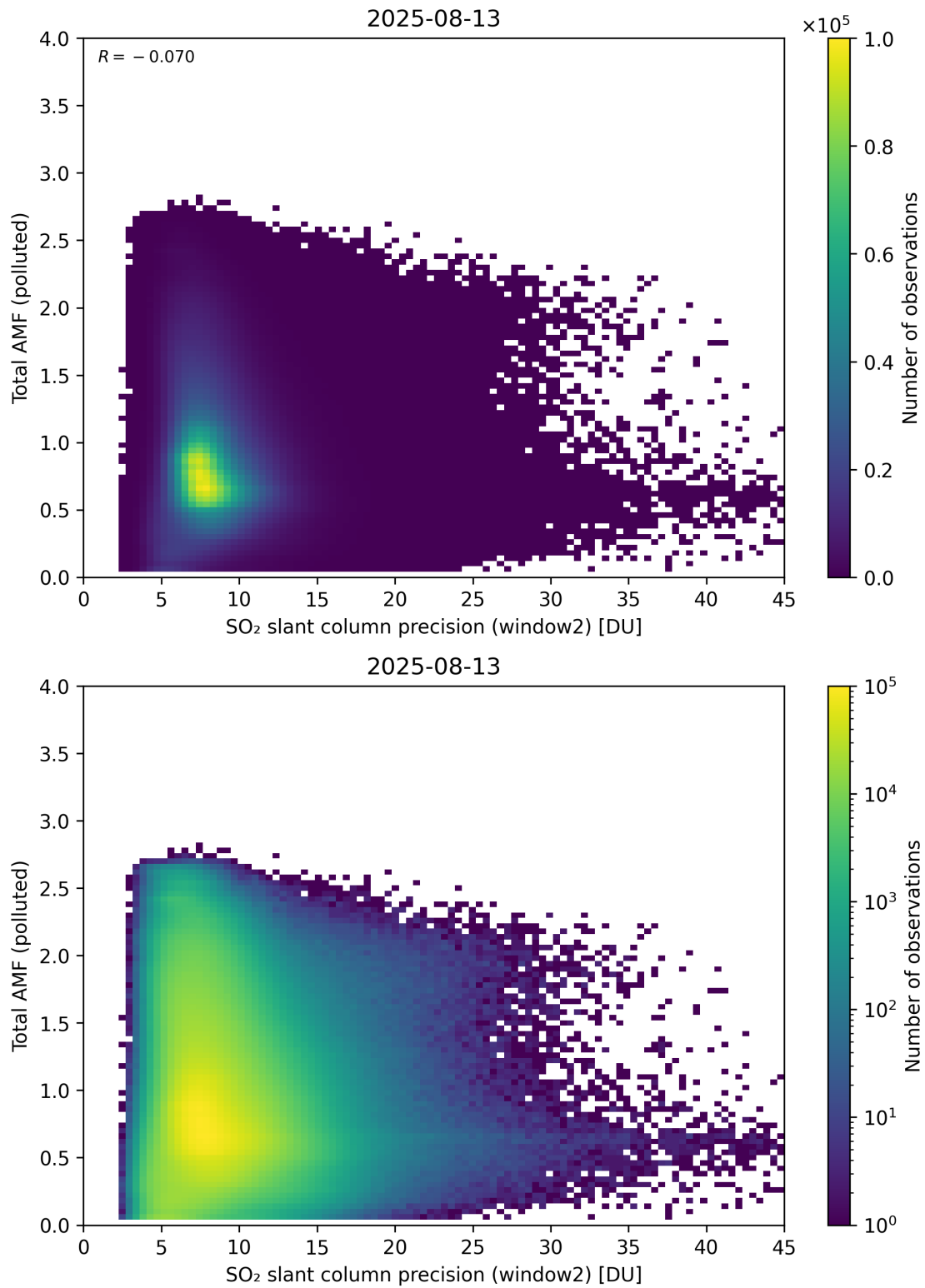
Figure 301: Scatter density plot of “SO 2 slant column precision (window2)” against “Total AMF (polluted)” for 2025-08-12 to 2025-08-14.
