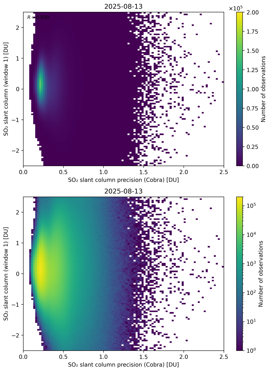
Figure 208: Scatter density plot of “SO 2 slant column precision (Cobra)” against “SO 2 slant column (window 1)” for 2025-08-12 to 2025-08-14.
