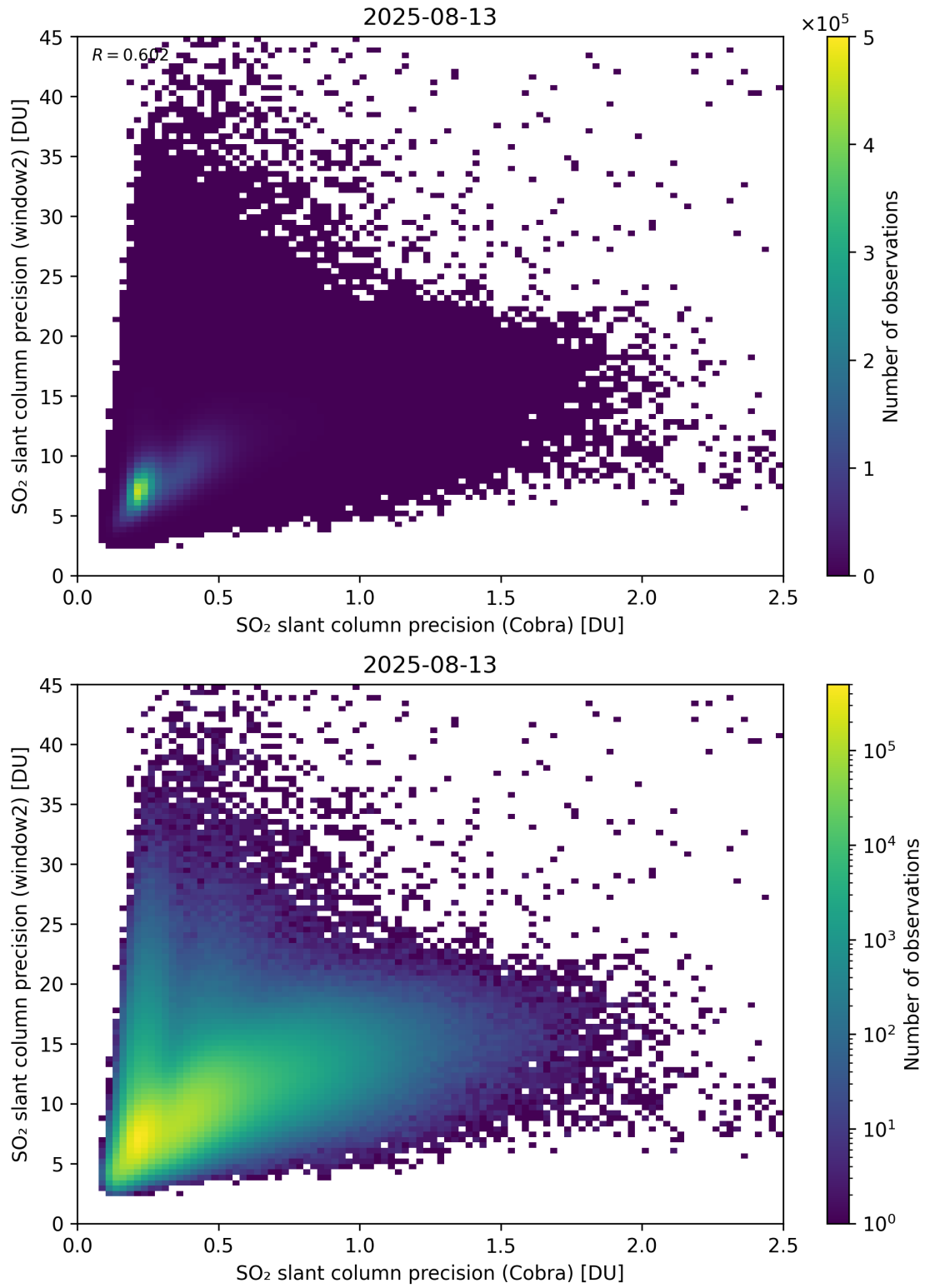
Figure 210: Scatter density plot of “SO 2 slant column precision (Cobra)” against “SO 2 slant column precision (window2)” for 2025-08-12 to 2025-08-14.
