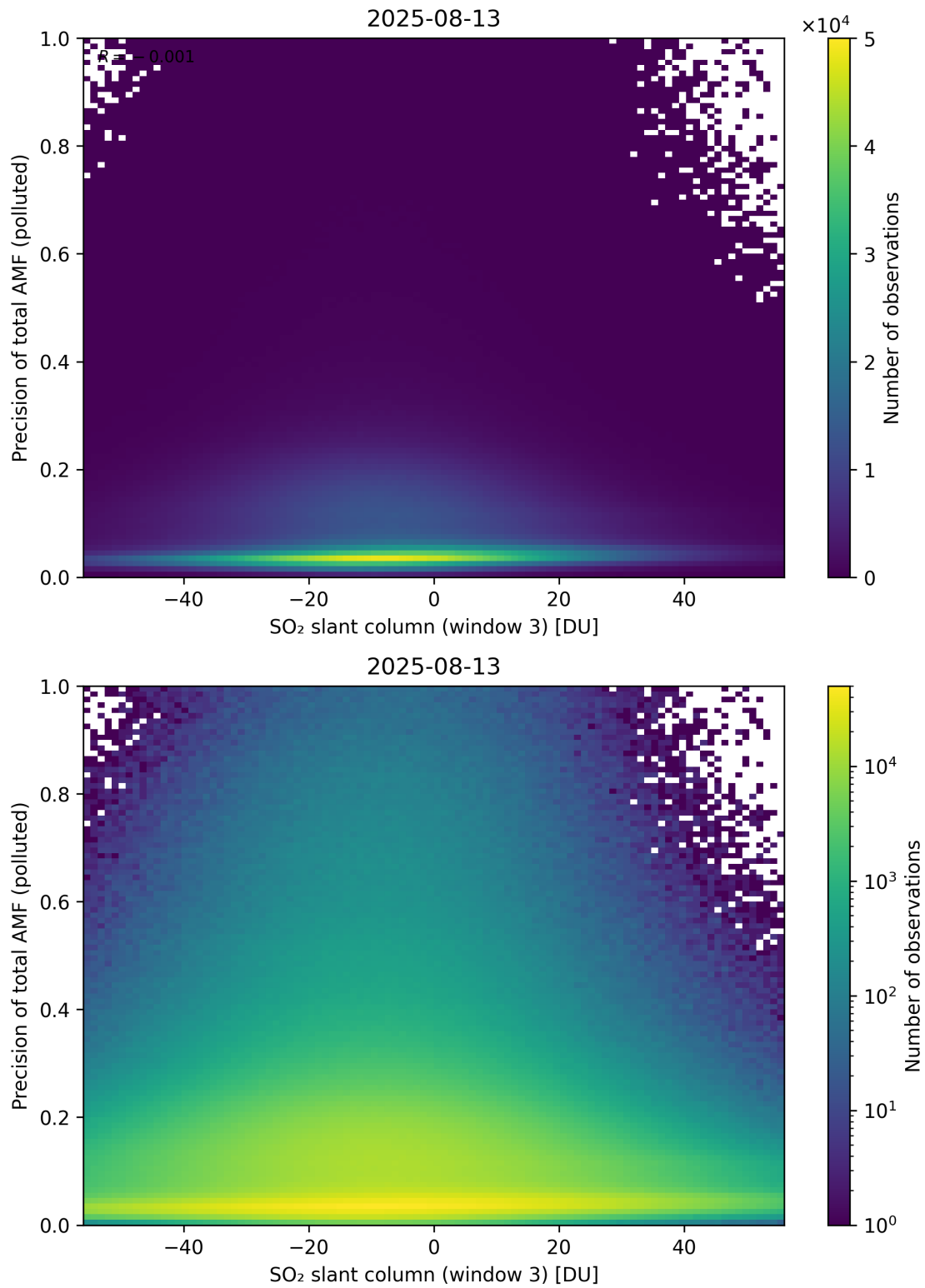
Figure 319: Scatter density plot of “SO 2 slant column (window 3)” against “Precision of total AMF (polluted)” for 2025-08-12 to 2025-08-14.
