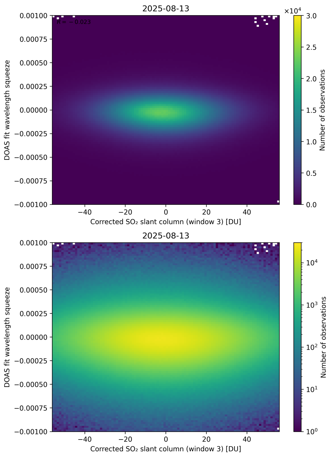
Figure 257: Scatter density plot of “Corrected SO 2 slant column (window 3)” against “DOAS fit wavelength squeeze” for 2025-08-12 to 2025-08-14.
