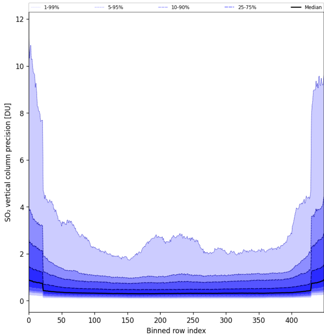
Figure 85: Along track statistics of “SO 2 vertical column precision” for 2025-08-12 to 2025-08-14
