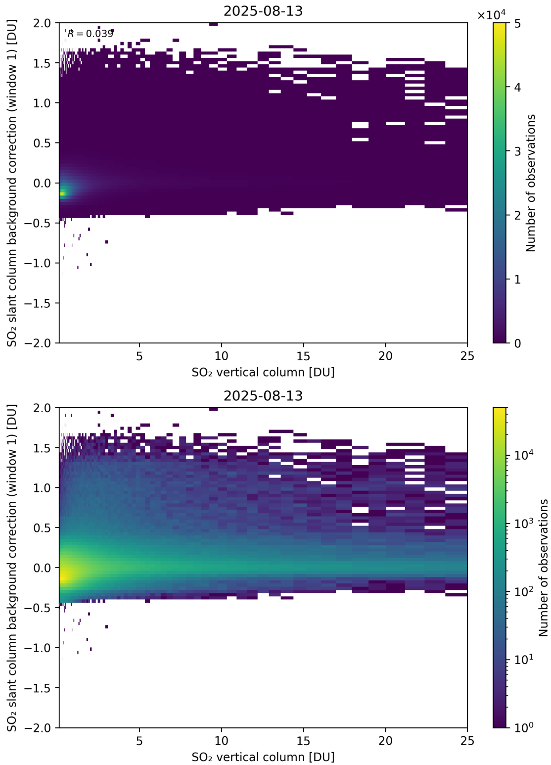
Figure 323: Scatter density plot of “SO 2 vertical column” against “SO 2 slant column background correction (window 1)” for 2025-08-12 to 2025-08-14.
