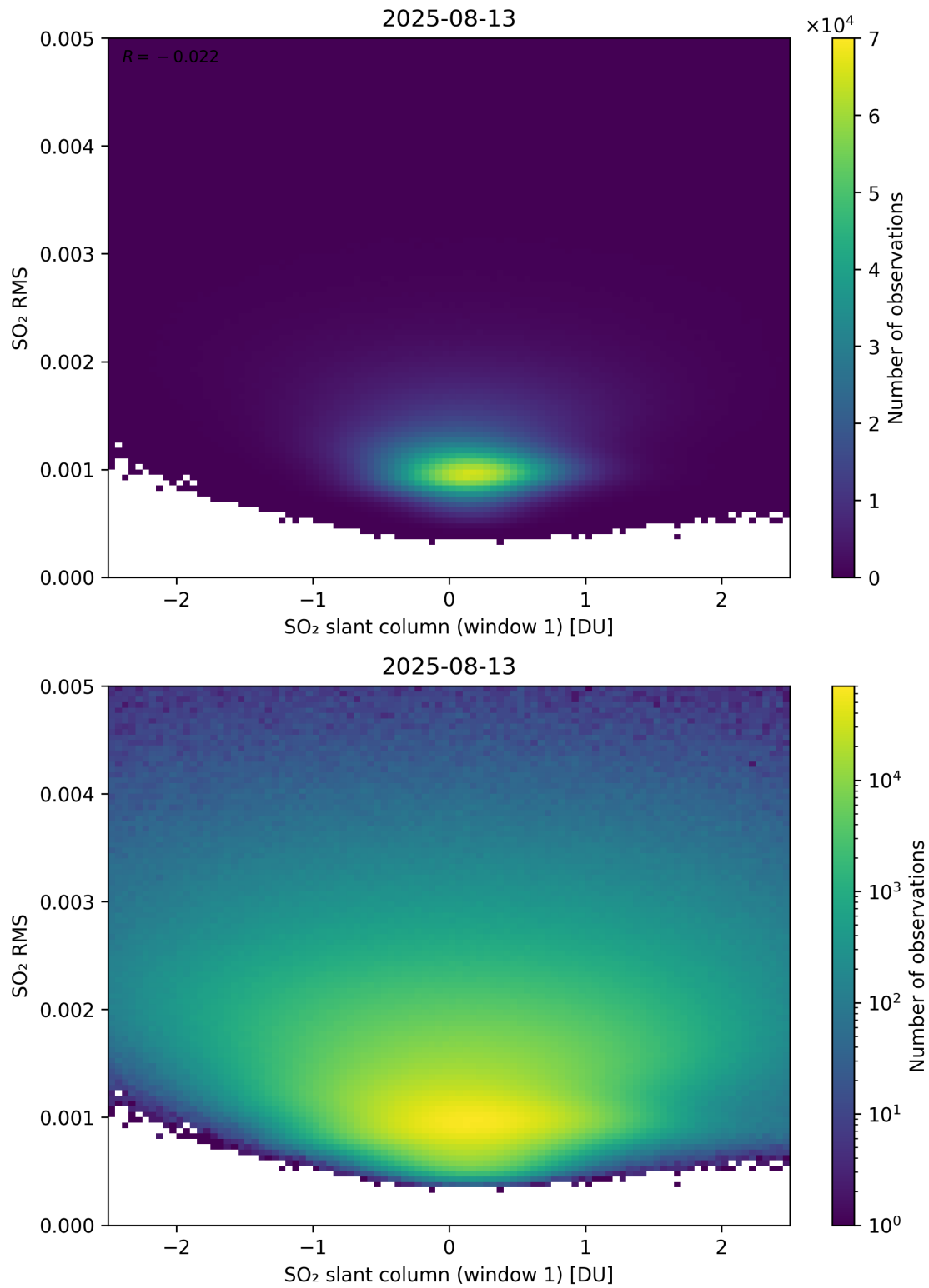
Figure 267: Scatter density plot of “SO 2 slant column (window 1)” against “SO 2 RMS” for 2025-08-12 to 2025-08-14.
