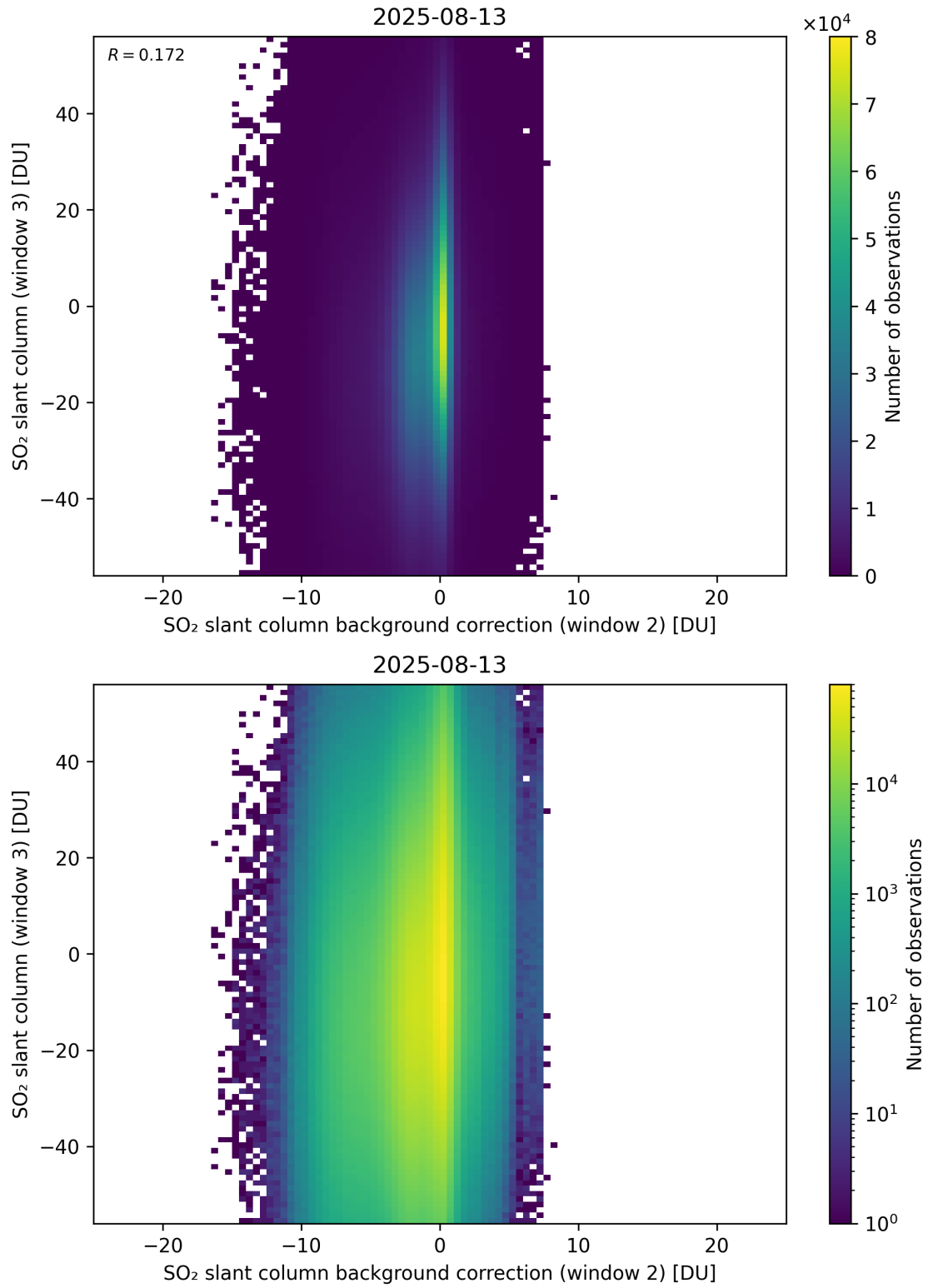
Figure 128: Scatter density plot of “SO 2 slant column background correction (window 2)” against “SO 2 slant column (window 3)” for 2025-08-12 to 2025-08-14.
