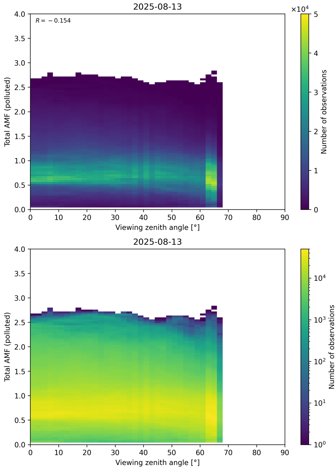
Figure 381: Scatter density plot of “Viewing zenith angle” against “Total AMF (polluted)” for 2025-08-12 to 2025-08-14.
