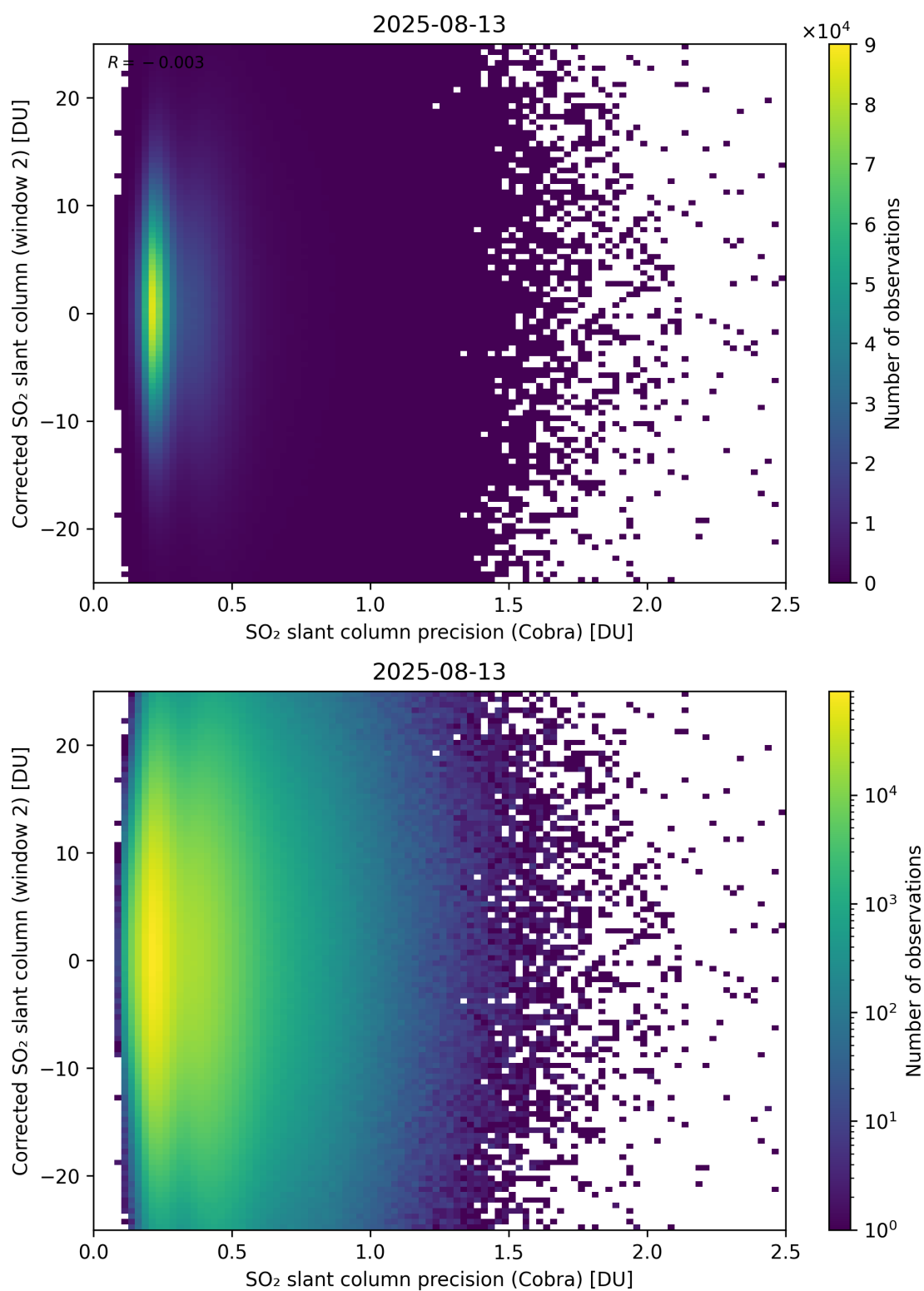
Figure 206: Scatter density plot of “SO 2 slant column precision (Cobra)” against “Corrected SO 2 slant column (window 2)” for 2025-08-12 to 2025-08-14.
