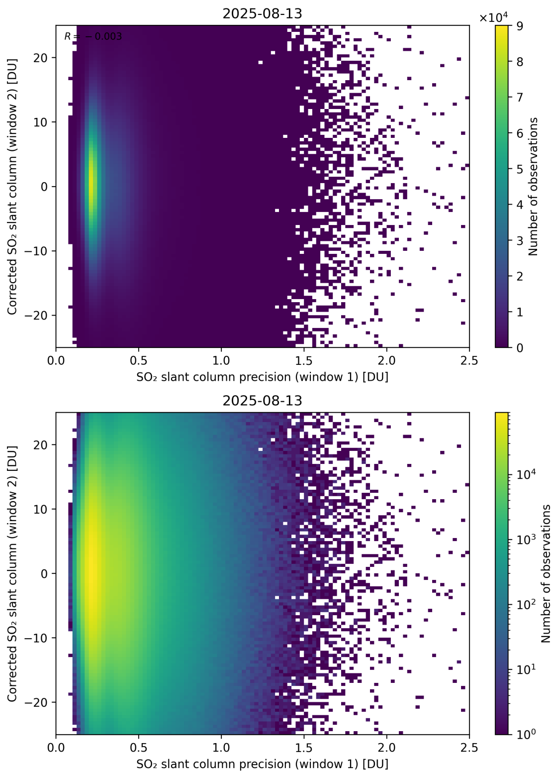
Figure 275: Scatter density plot of “SO 2 slant column precision (window 1)” against “Corrected SO 2 slant column (window 2)” for 2025-08-12 to 2025-08-14.
