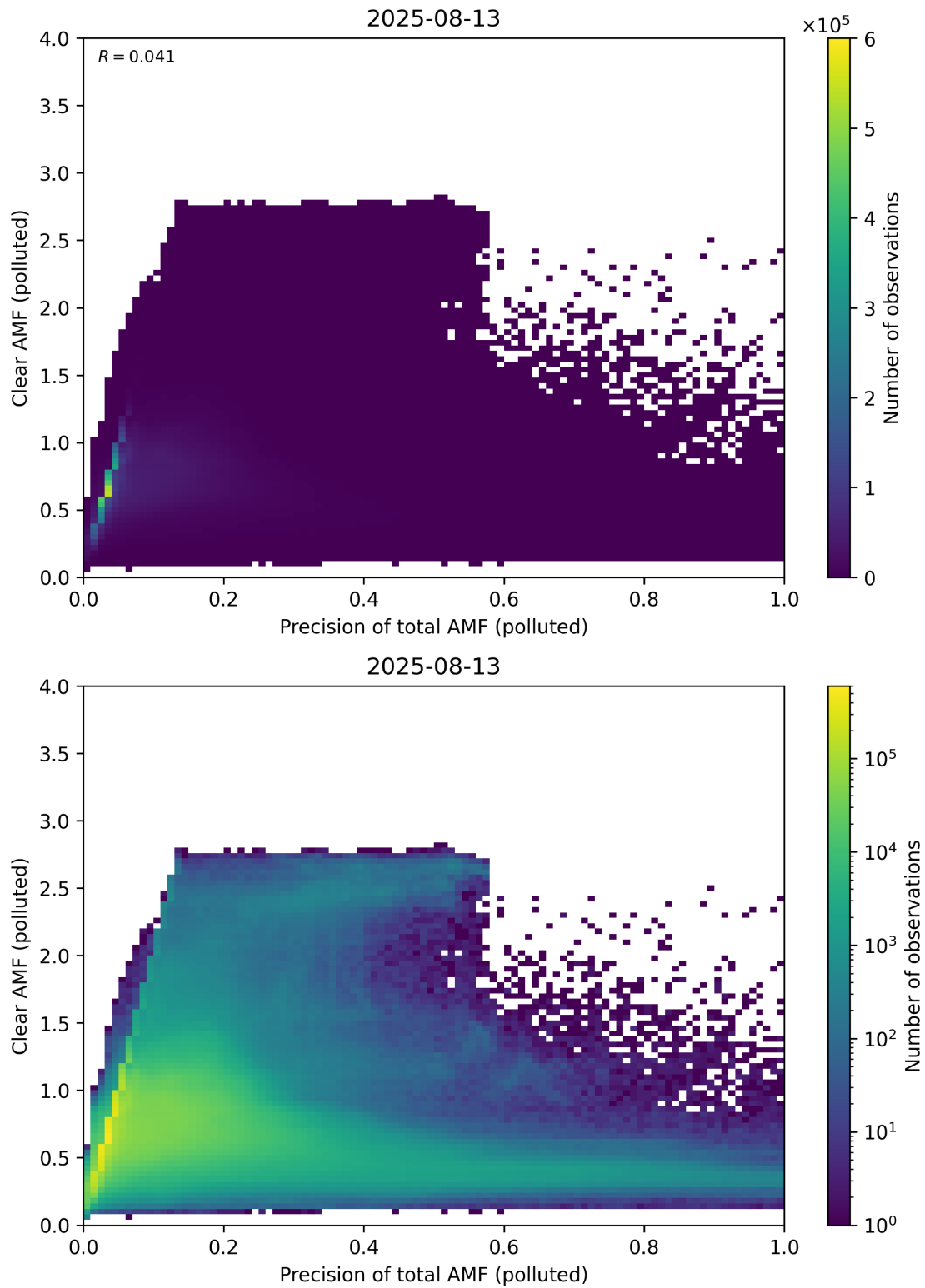
Figure 320: Scatter density plot of “Precision of total AMF (polluted)” against “Clear AMF (polluted)” for 2025-08-12 to 2025-08-14.
