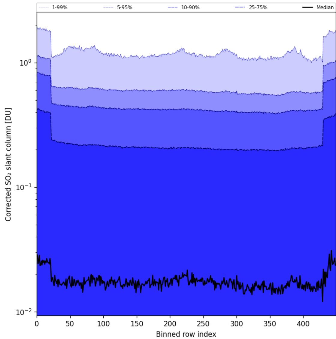
Figure 86: Along track statistics of “Corrected SO 2 slant column” for 2025-08-12 to 2025-08-14
