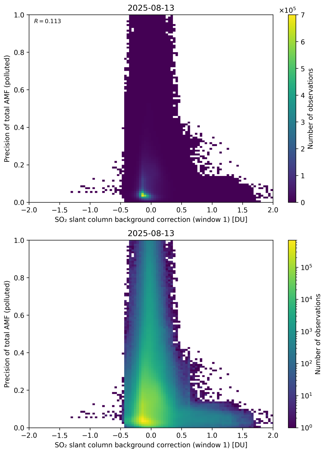
Figure 121: Scatter density plot of “SO 2 slant column background correction (window 1)” against “Precision of total AMF (polluted)” for 2025-08-12 to 2025-08-14.
