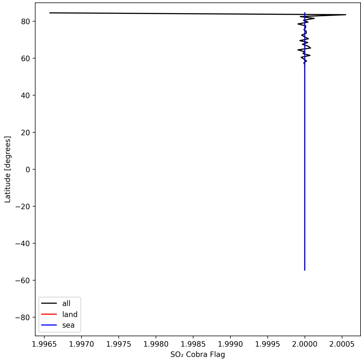
Figure 49: Zonal average of “SO 2 Cobra Flag” for 2025-08-12 to 2025-08-14.
