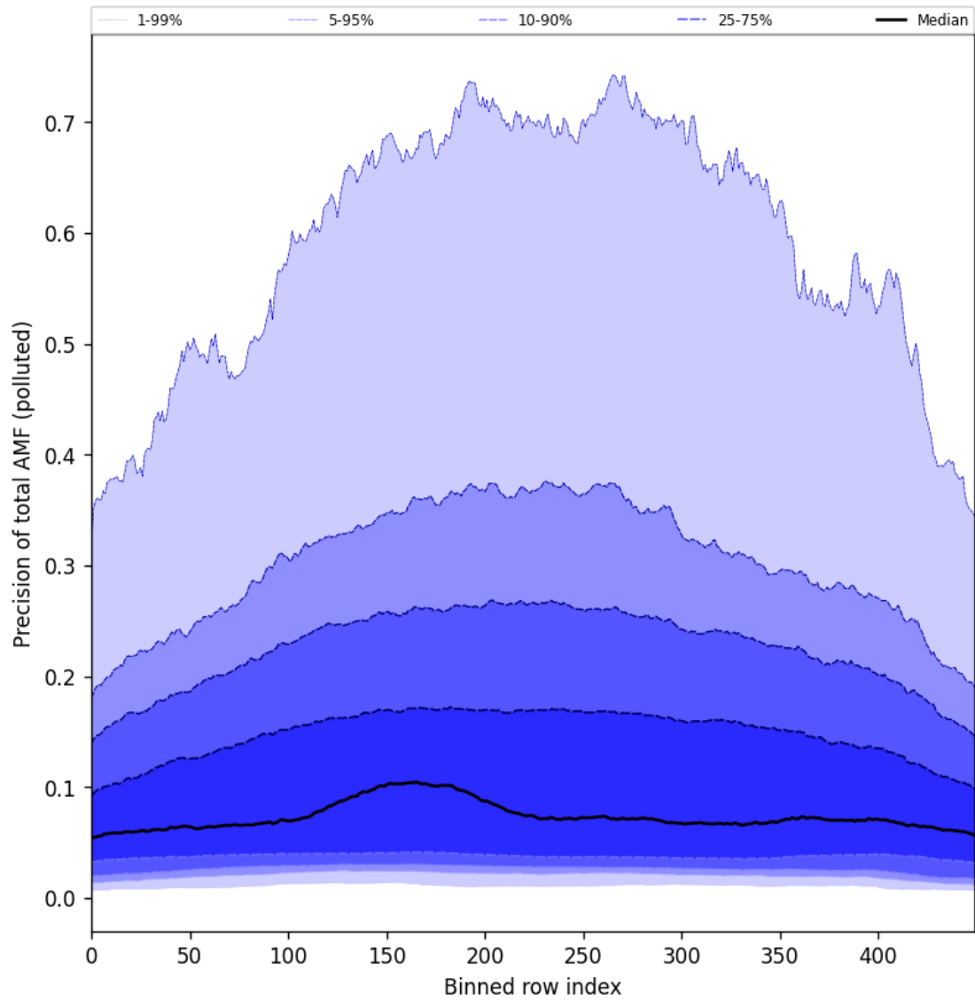
Figure 106: Along track statistics of “Precision of total AMF (polluted)” for 2025-08-12 to 2025-08-14
