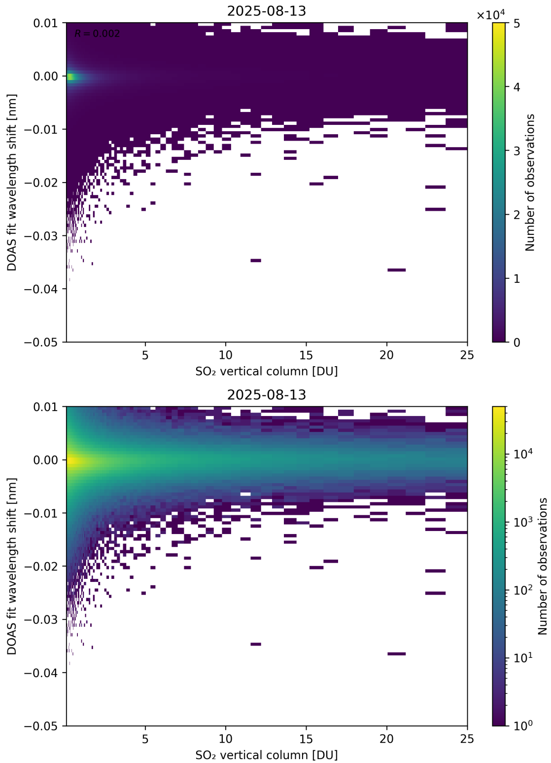
Figure 326: Scatter density plot of “SO 2 vertical column” against “DOAS fit wavelength shift” for 2025-08-12 to 2025-08-14.
