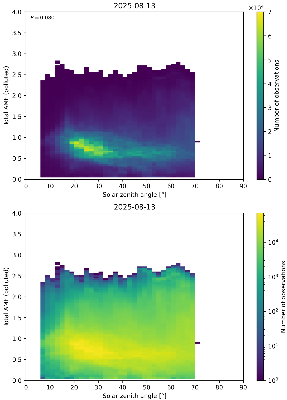
Figure 189: Scatter density plot of “Solar zenith angle” against “Total AMF (polluted)” for 2025-08-12 to 2025-08-14.
