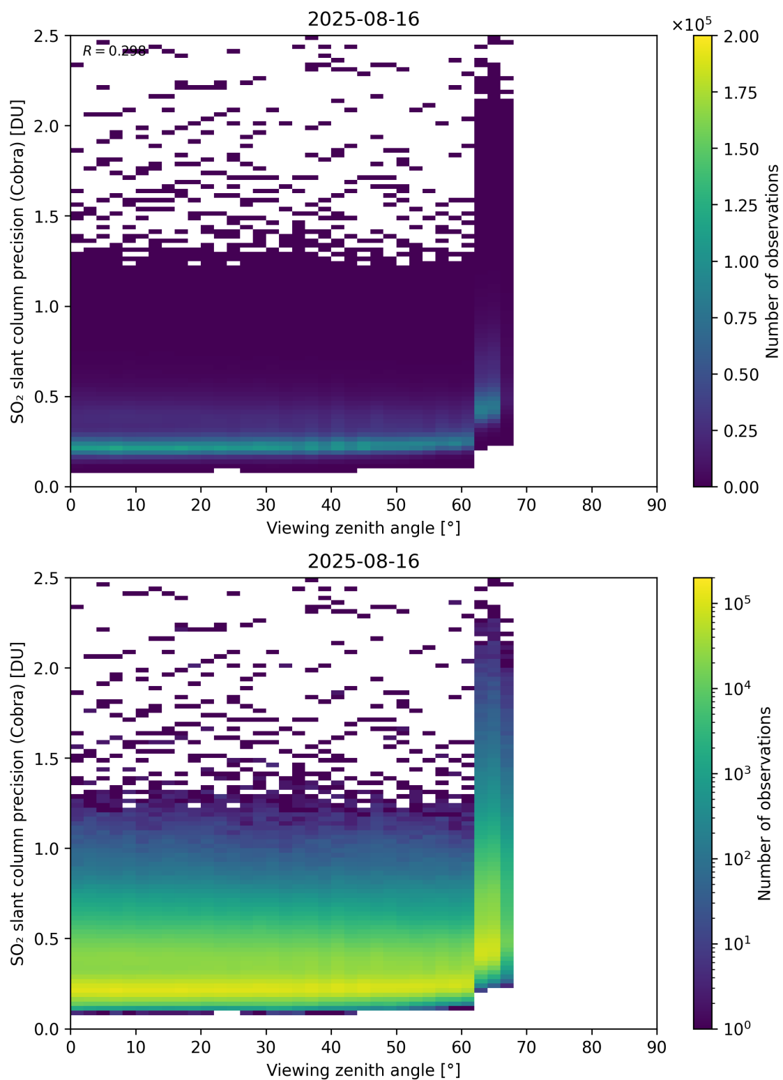
Figure 372: Scatter density plot of “Viewing zenith angle” against “SO 2 slant column precision (Cobra)” for 2025-08-15 to 2025-08-17.
