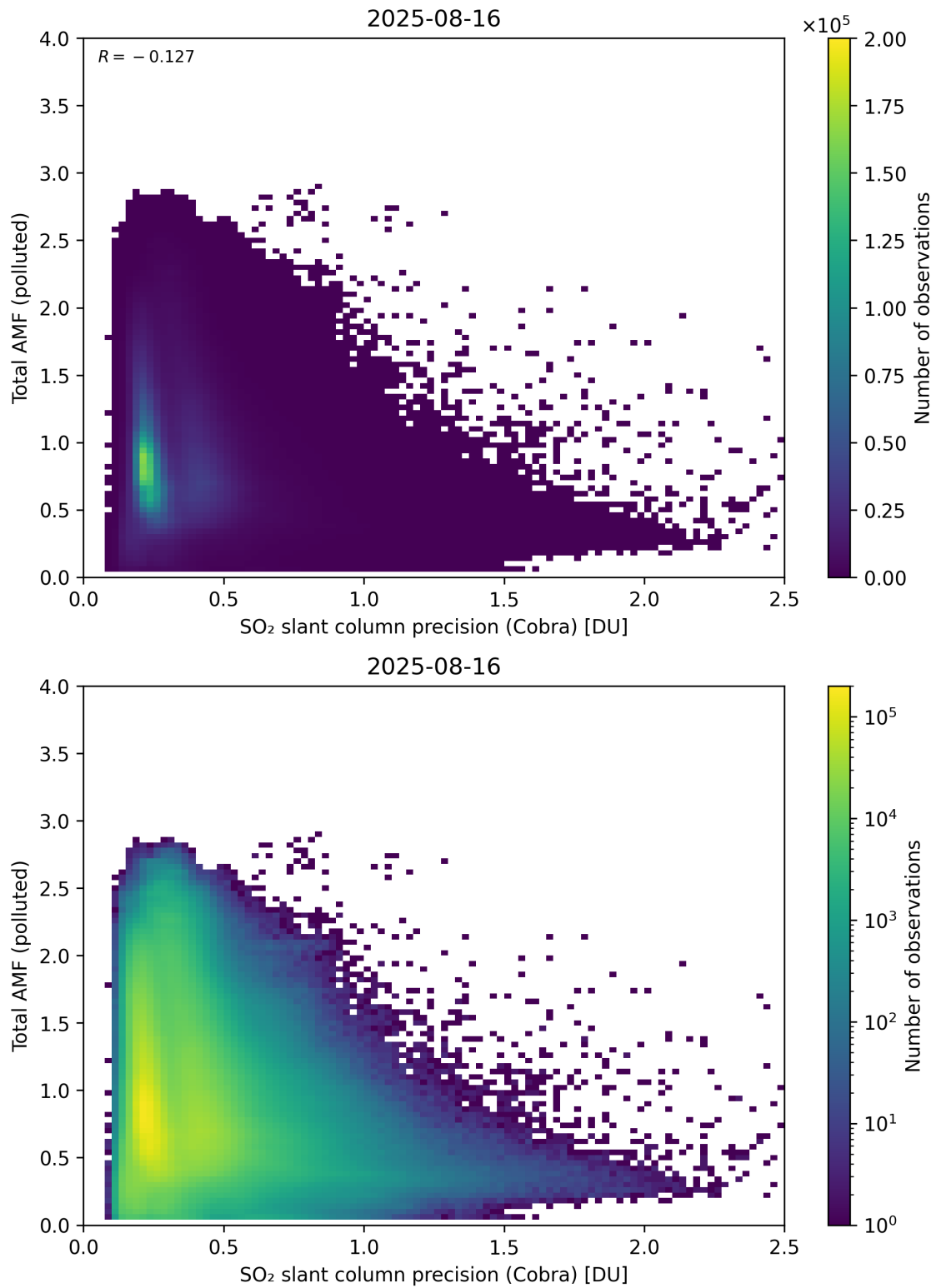
Figure 213: Scatter density plot of “SO 2 slant column precision (Cobra)” against “Total AMF (polluted)” for 2025-08-15 to 2025-08-17.
