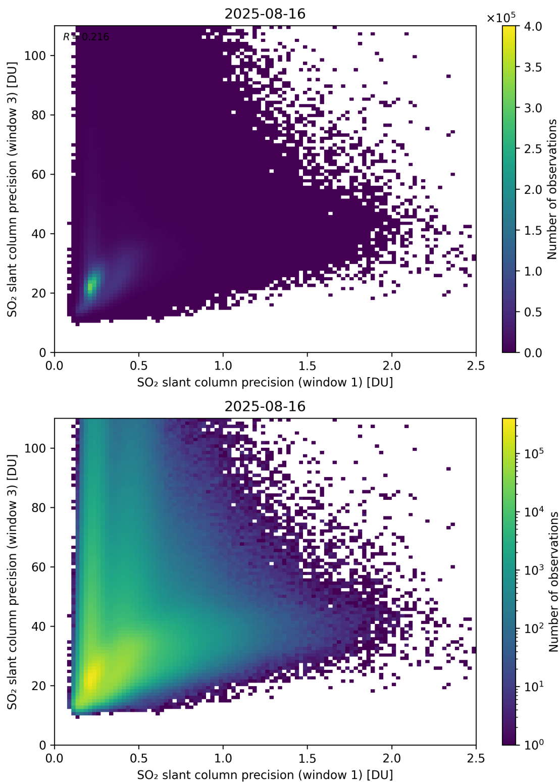
Figure 279: Scatter density plot of “SO 2 slant column precision (window 1)” against “SO 2 slant column precision (window 3)” for 2025-08-15 to 2025-08-17.
