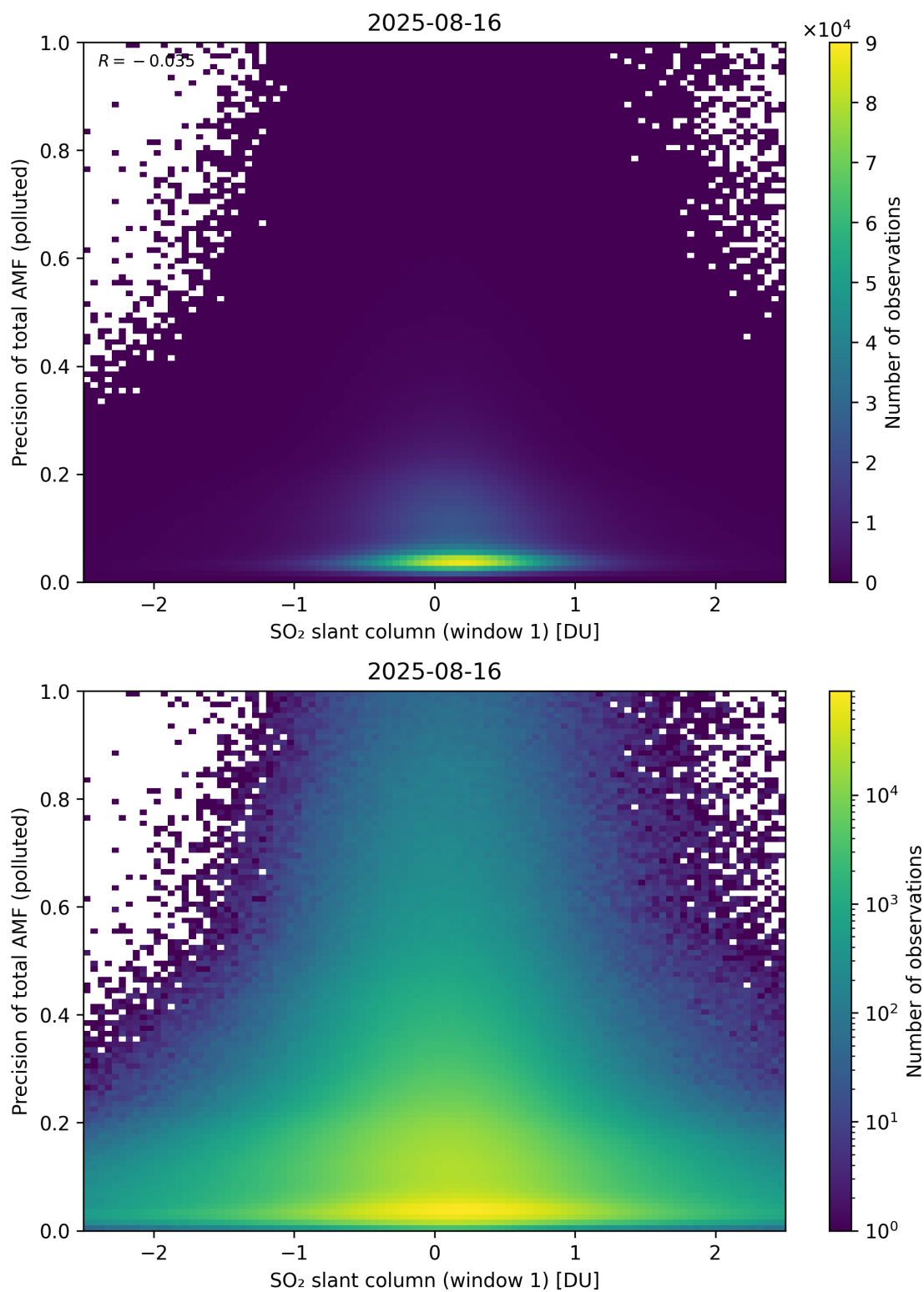
Figure 290: Scatter density plot of “SO 2 slant column (window 1)” against “Precision of total AMF (polluted)” for 2025-08-15 to 2025-08-17.
