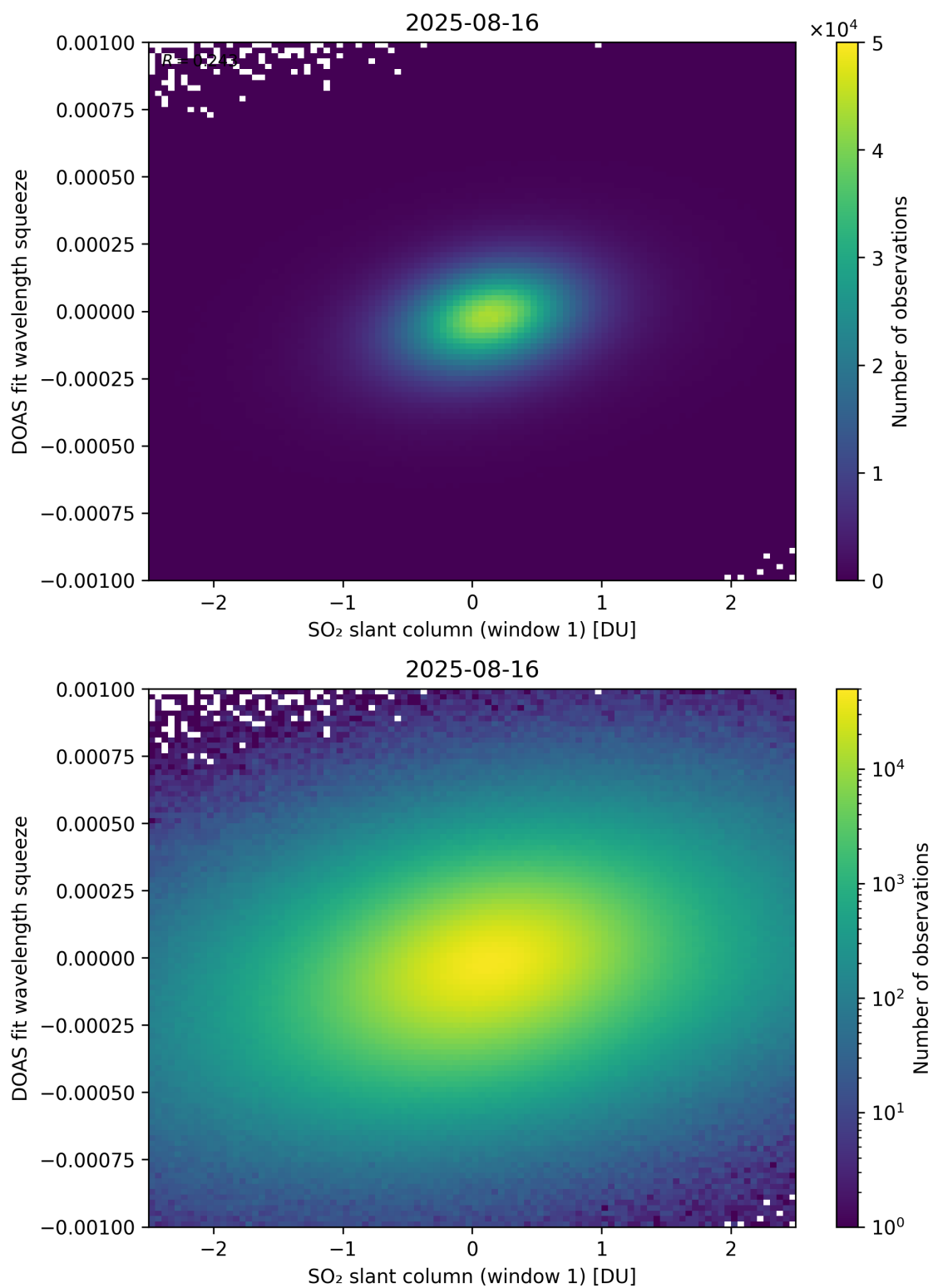
Figure 266: Scatter density plot of “SO 2 slant column (window 1)” against “DOAS fit wavelength squeeze” for 2025-08-15 to 2025-08-17.
