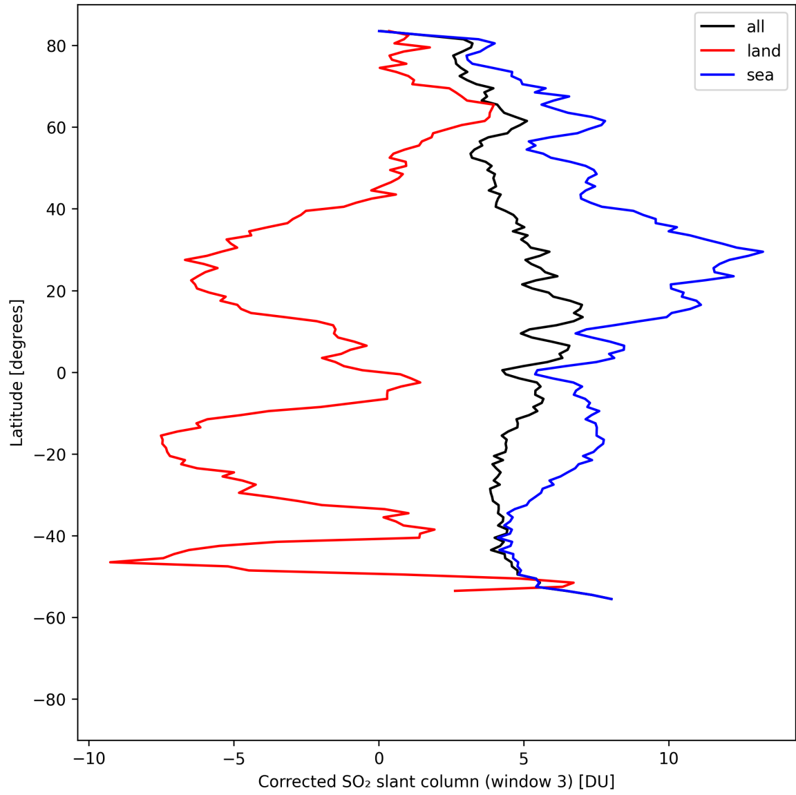
Figure 47: Zonal average of “Corrected SO 2 slant column (window 3)” for 2025-08-15 to 2025-08-17.
