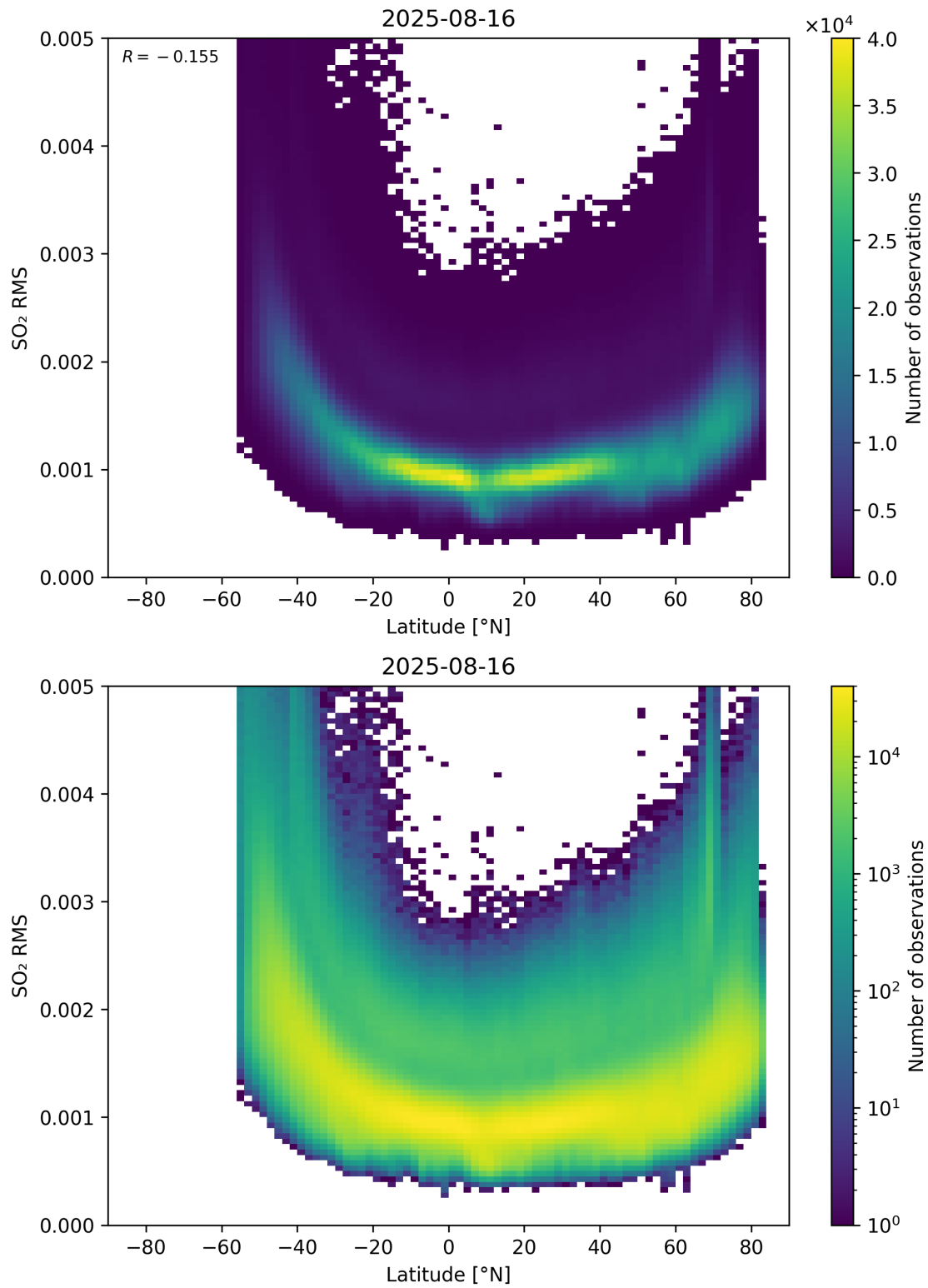
Figure 155: Scatter density plot of “Latitude” against “SO 2 RMS” for 2025-08-15 to 2025-08-17.
