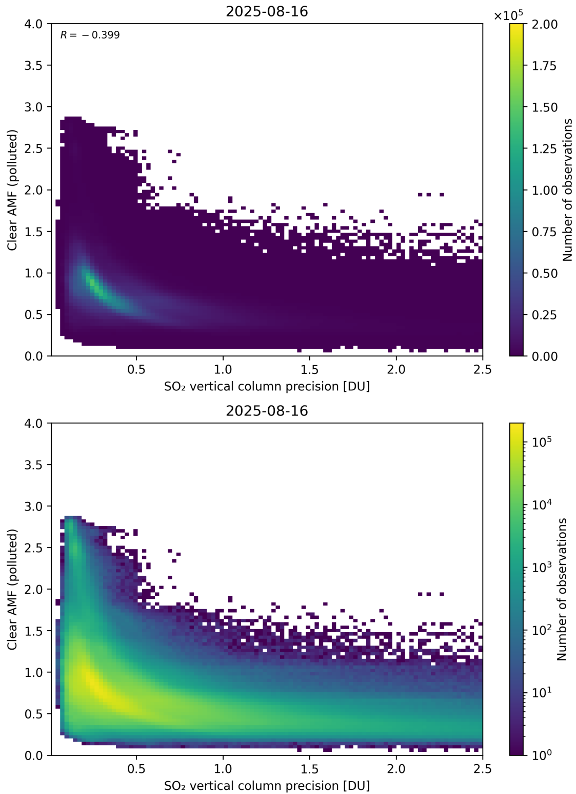
Figure 335: Scatter density plot of “SO 2 vertical column precision” against “Clear AMF (polluted)” for 2025-08-15 to 2025-08-17.
