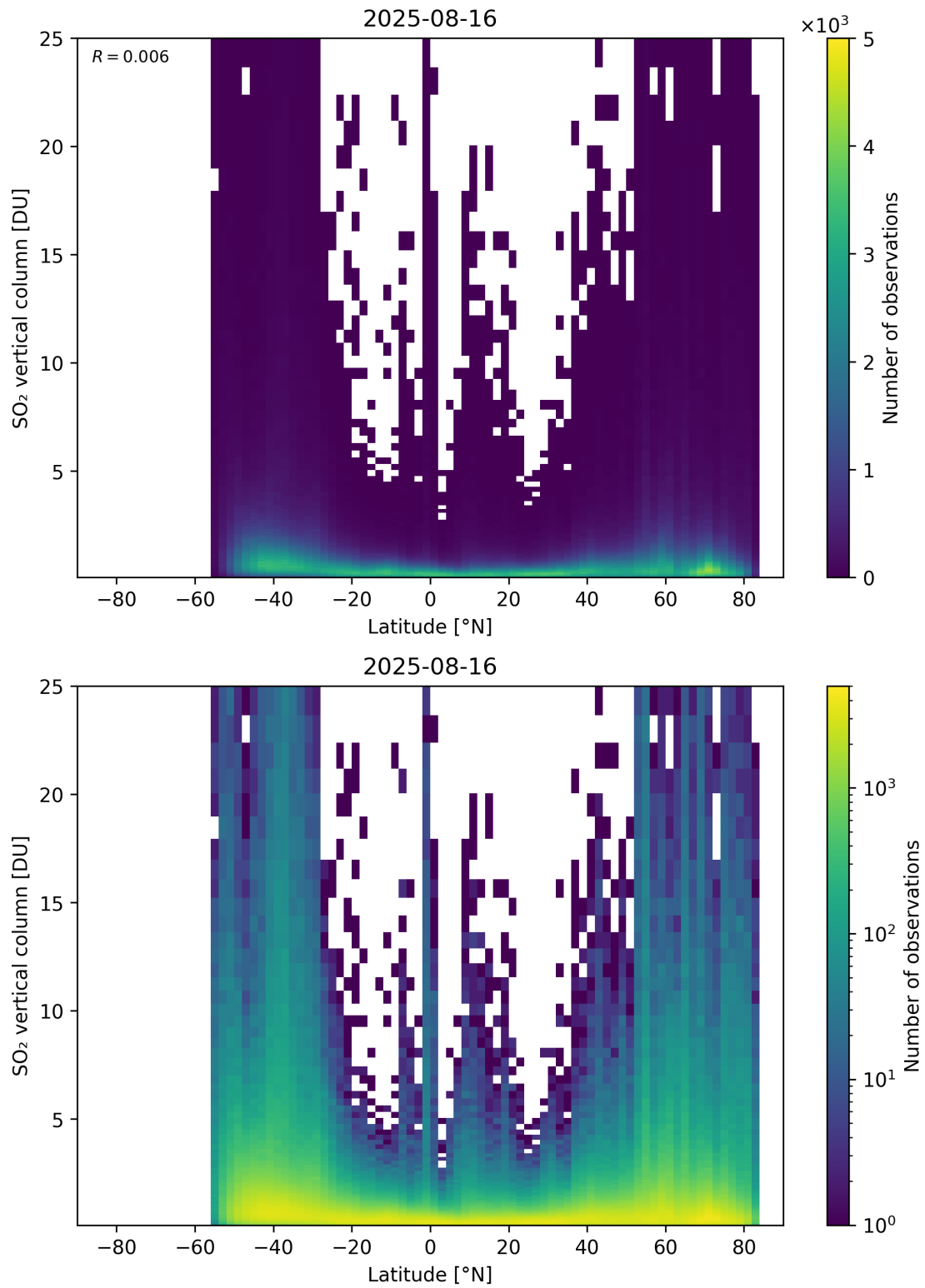
Figure 169: Scatter density plot of “Latitude” against “SO 2 vertical column” for 2025-08-15 to 2025-08-17.
