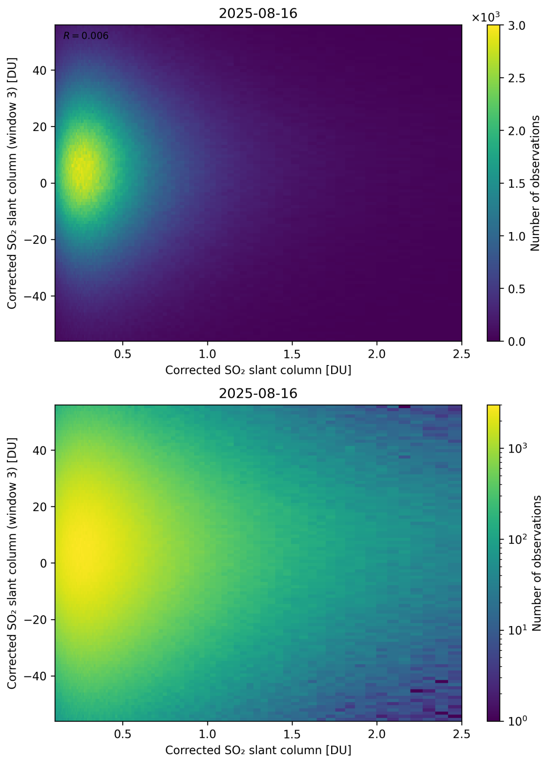
Figure 236: Scatter density plot of “Corrected SO 2 slant column” against “Corrected SO 2 slant column (window 3)” for 2025-08-15 to 2025-08-17.
