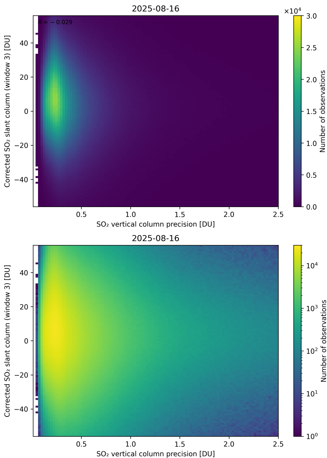
Figure 340: Scatter density plot of “SO 2 vertical column precision” against “Corrected SO 2 slant column (window 3)” for 2025-08-15 to 2025-08-17.
