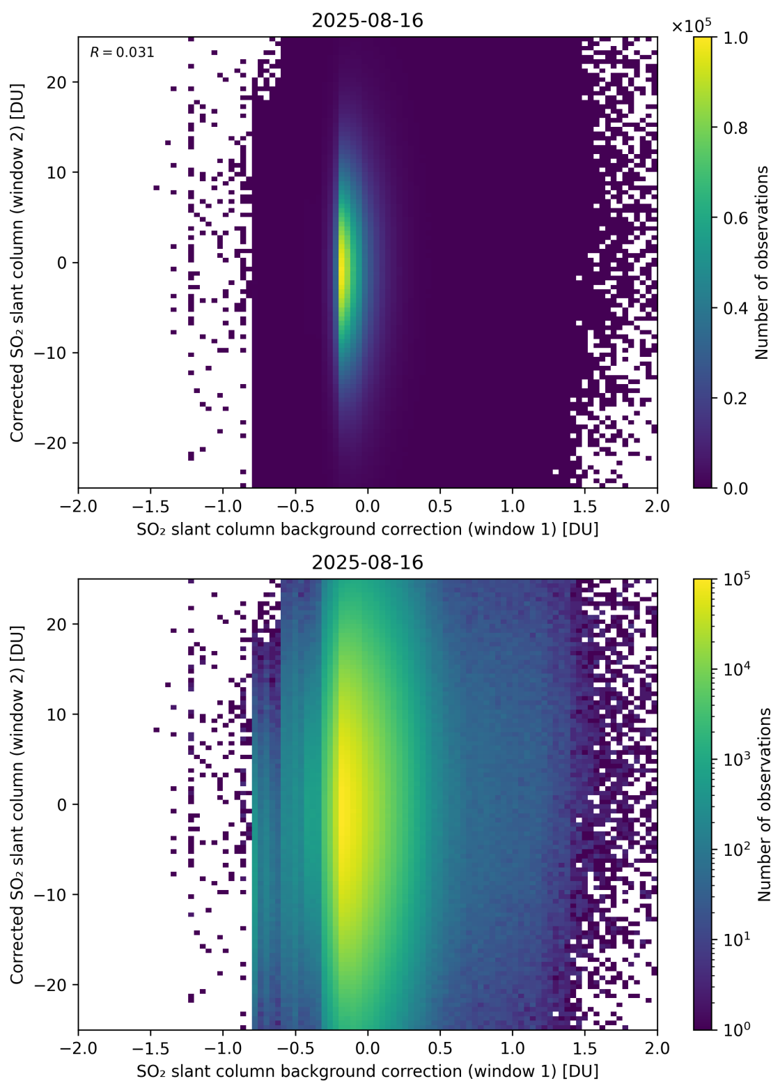
Figure 115: Scatter density plot of “SO 2 slant column background correction (window 1)” against “Corrected SO 2 slant column (window 2)” for 2025-08-15 to 2025-08-17.
