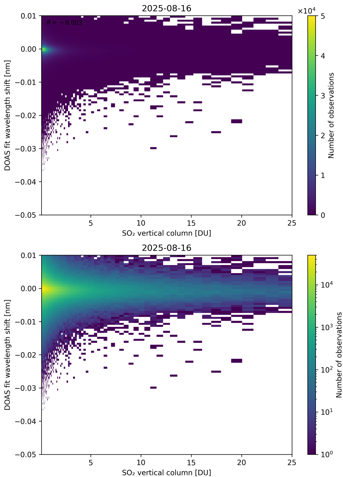
Figure 326: Scatter density plot of “SO 2 vertical column” against “DOAS fit wavelength shift” for 2025-08-15 to 2025-08-17.
