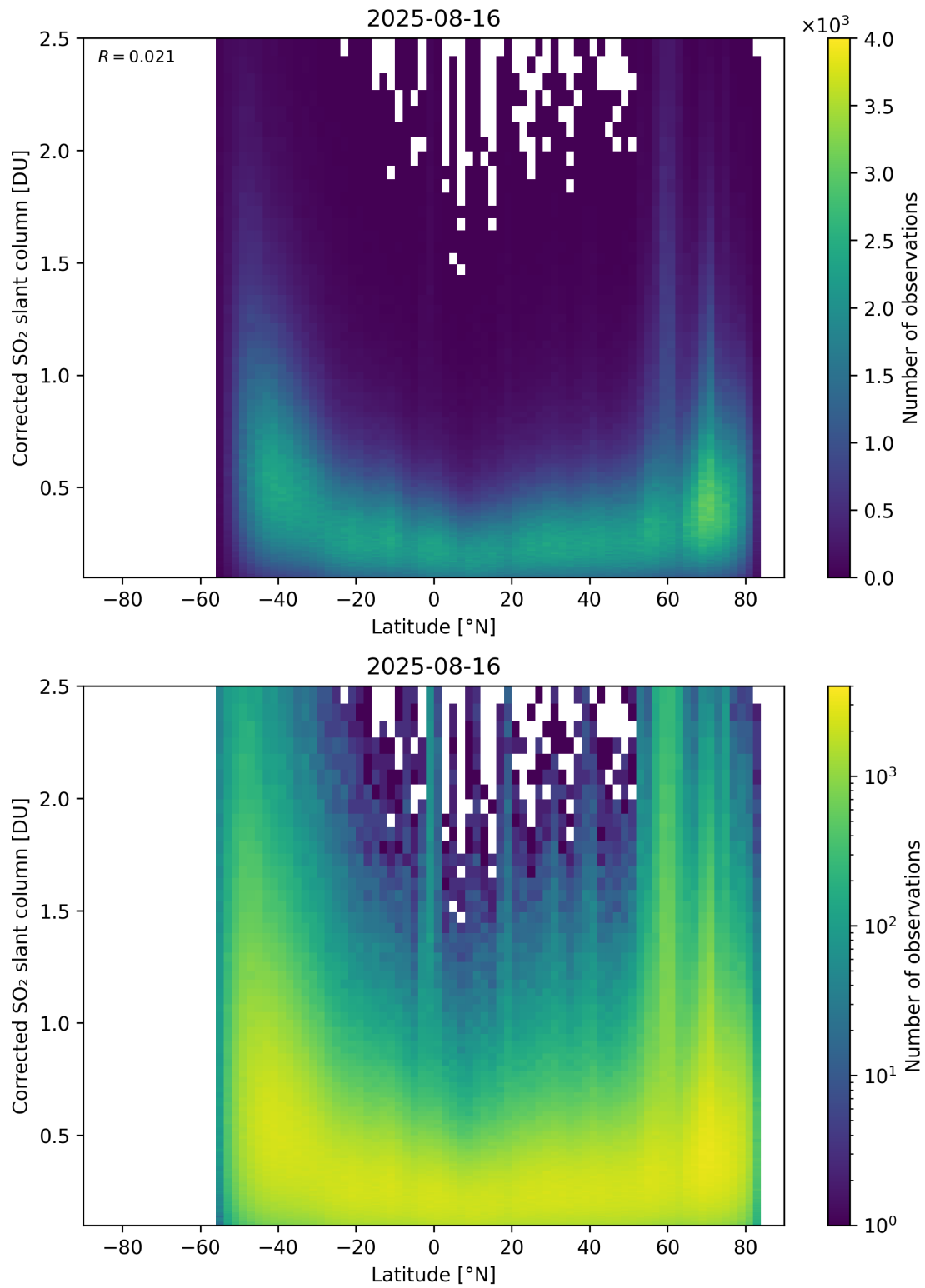
Figure 159: Scatter density plot of “Latitude” against “Corrected SO 2 slant column” for 2025-08-15 to 2025-08-17.
