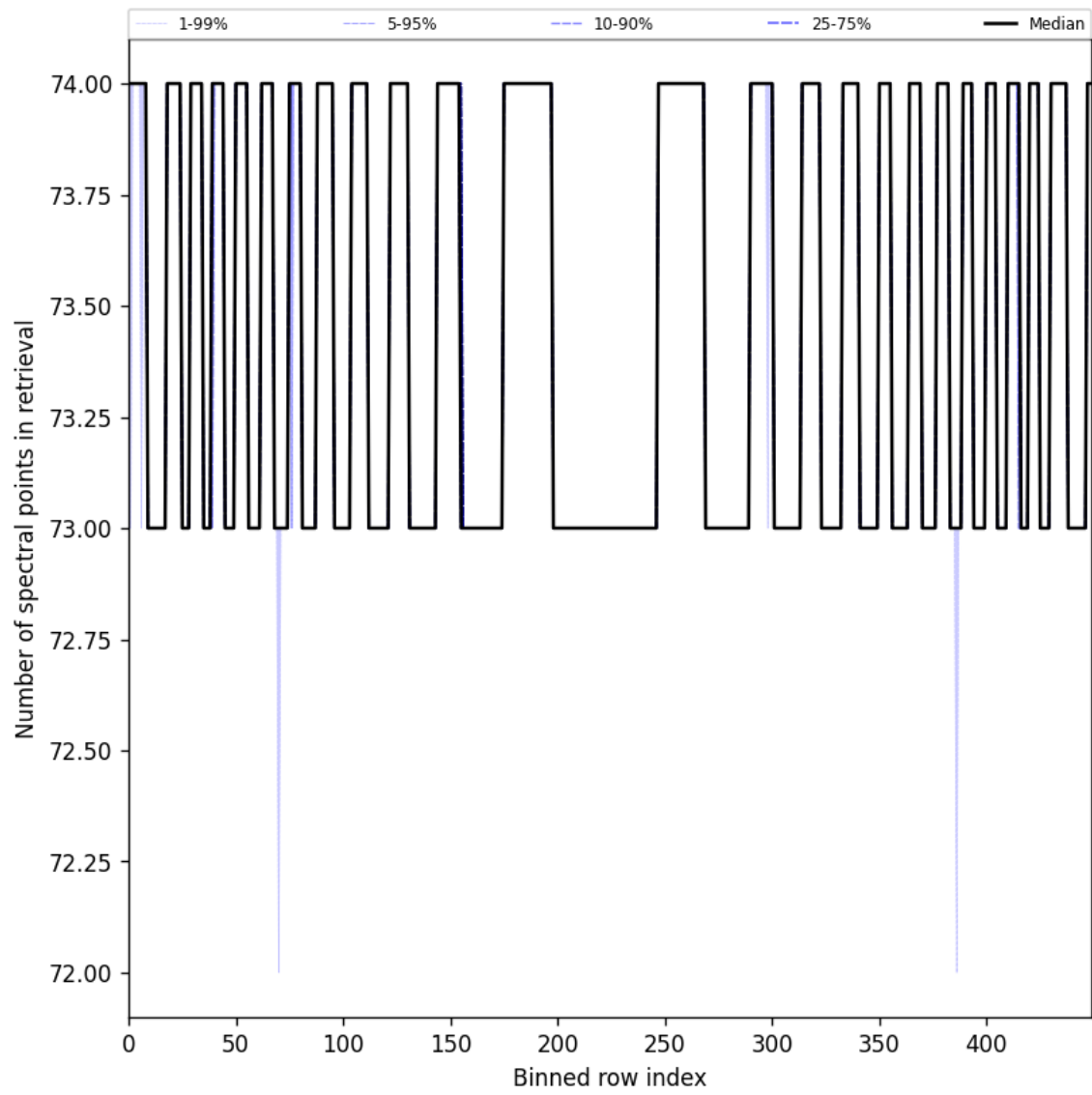
Figure 108: Along track statistics of “Number of spectral points in retrieval” for 2025-08-15 to 2025-08-17
