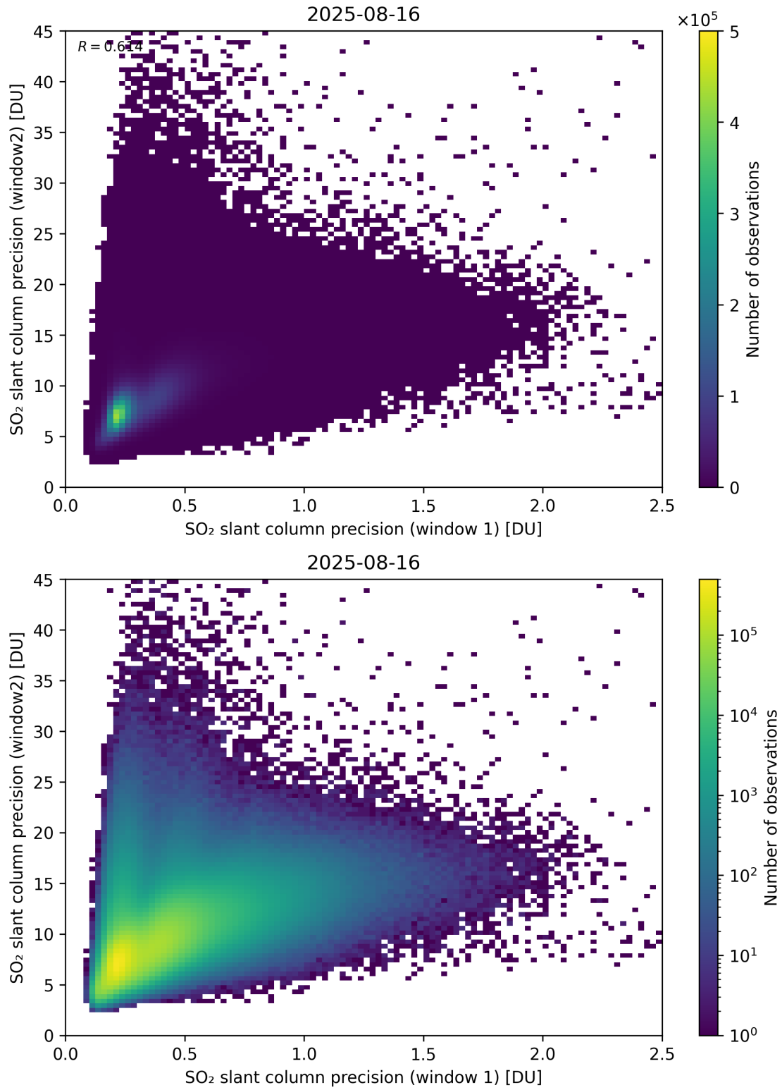
Figure 277: Scatter density plot of “SO 2 slant column precision (window 1)” against “SO 2 slant column precision (window2)” for 2025-08-15 to 2025-08-17.
