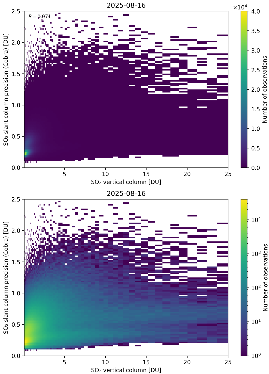
Figure 350: Scatter density plot of “SO 2 vertical column” against “SO 2 slant column precision (Cobra)” for 2025-08-15 to 2025-08-17.
