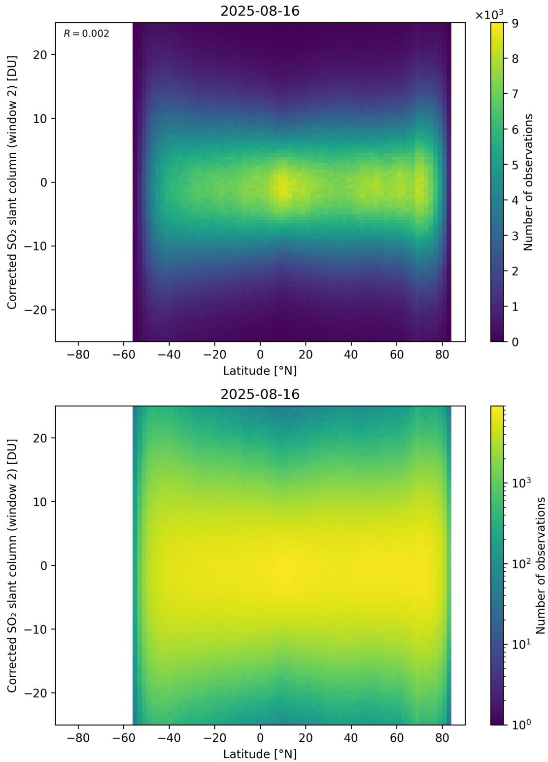
Figure 160: Scatter density plot of “Latitude” against “Corrected SO 2 slant column (window 2)” for 2025-08-15 to 2025-08-17.
