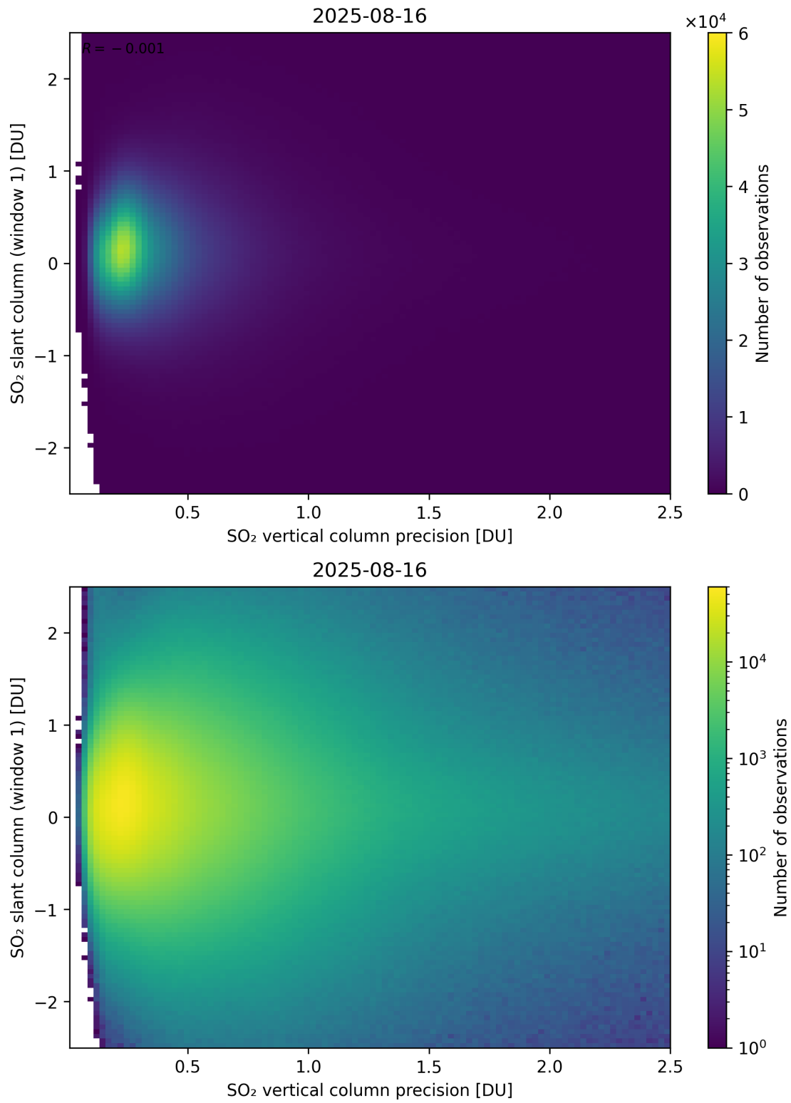
Figure 341: Scatter density plot of “SO 2 vertical column precision” against “SO 2 slant column (window 1)” for 2025-08-15 to 2025-08-17.
