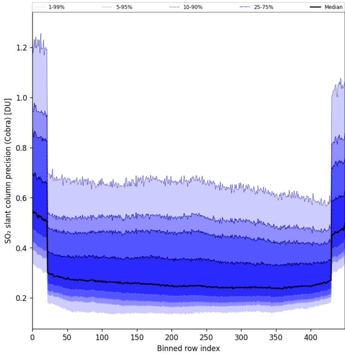
Figure 88: Along track statistics of “SO 2 slant column precision (Cobra)” for 2025-08-15 to 2025-08-17
