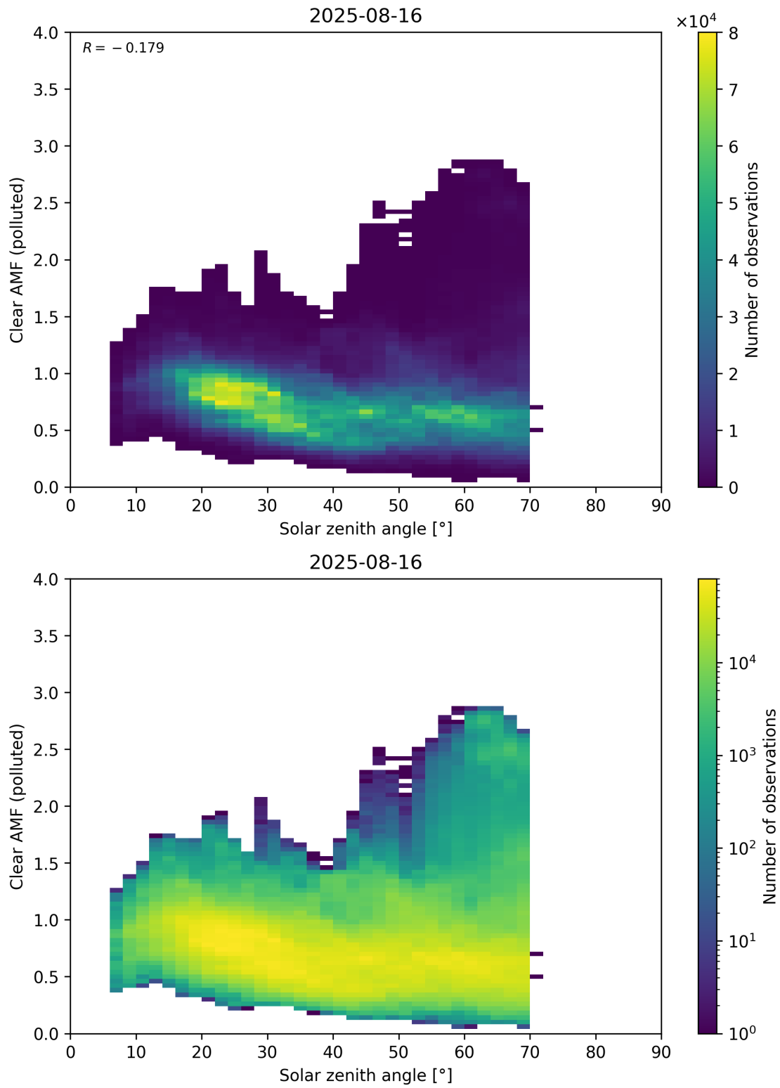
Figure 178: Scatter density plot of “Solar zenith angle” against “Clear AMF (polluted)” for 2025-08-15 to 2025-08-17.
