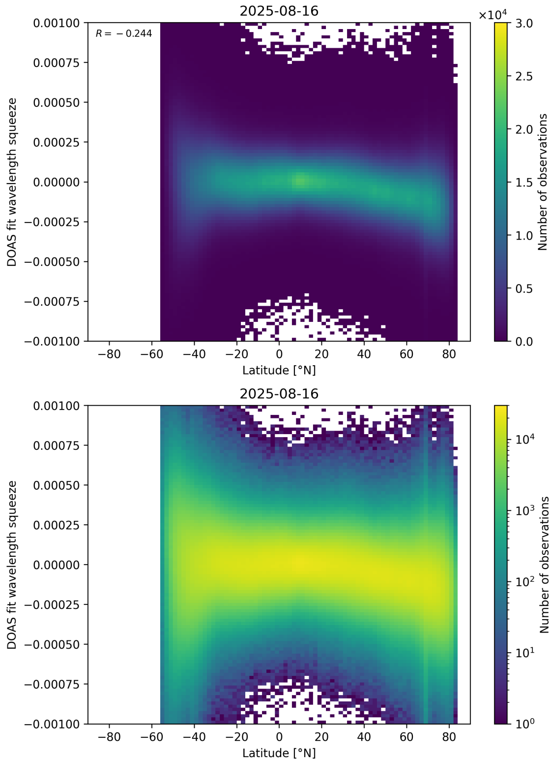
Figure 154: Scatter density plot of “Latitude” against “DOAS fit wavelength squeeze” for 2025-08-15 to 2025-08-17.
