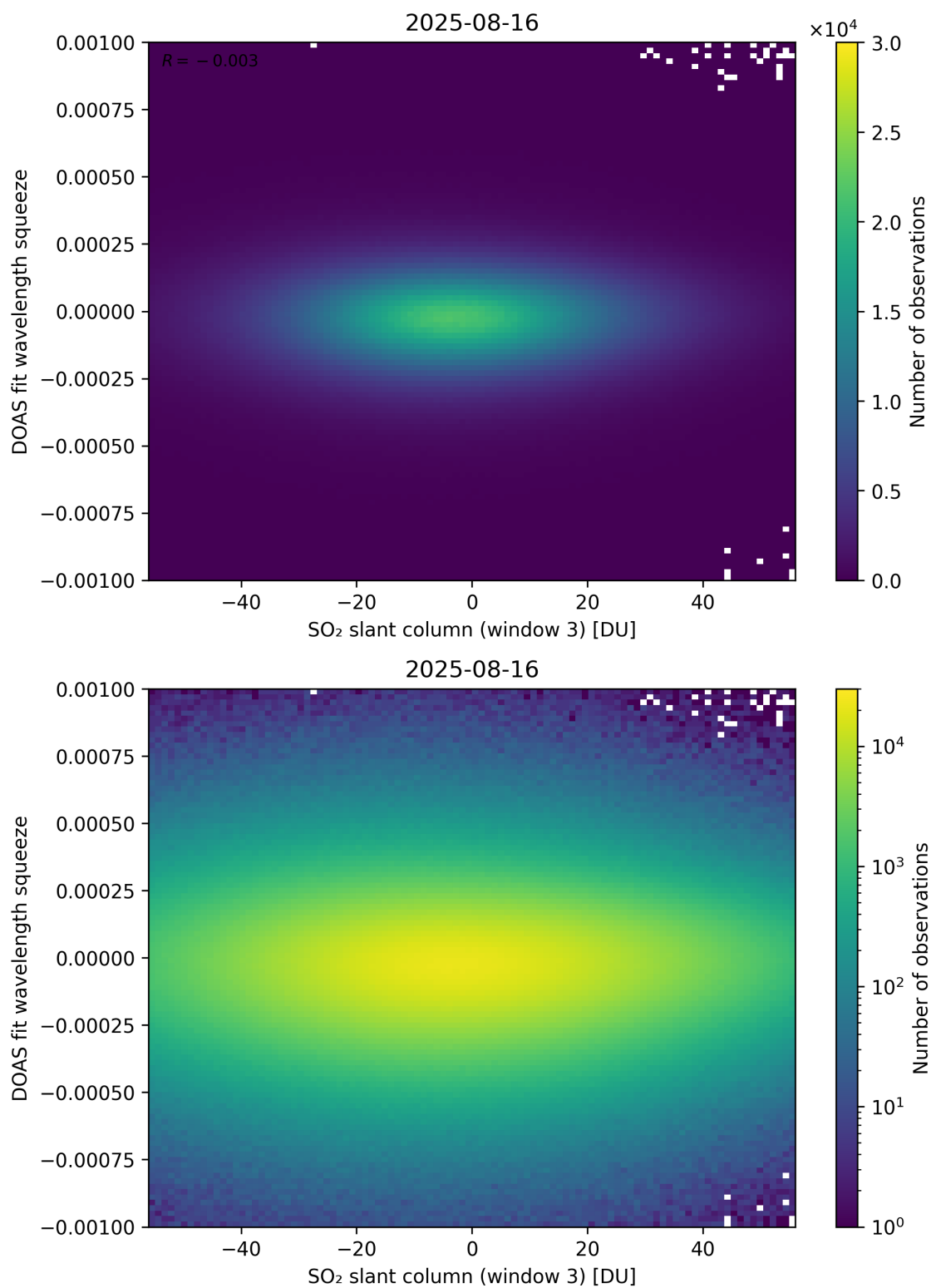
Figure 305: Scatter density plot of “SO 2 slant column (window 3)” against “DOAS fit wavelength squeeze” for 2025-08-15 to 2025-08-17.
