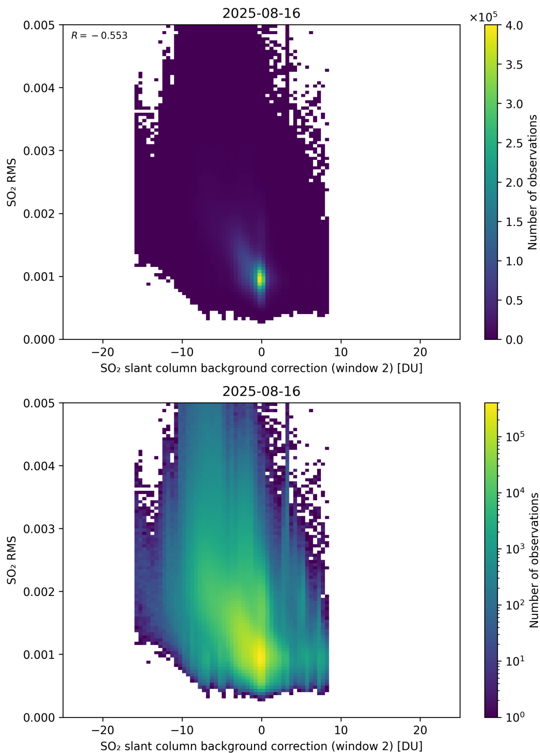
Figure 125: Scatter density plot of “SO 2 slant column background correction (window 2)” against “SO 2 RMS” for 2025-08-15 to 2025-08-17.
