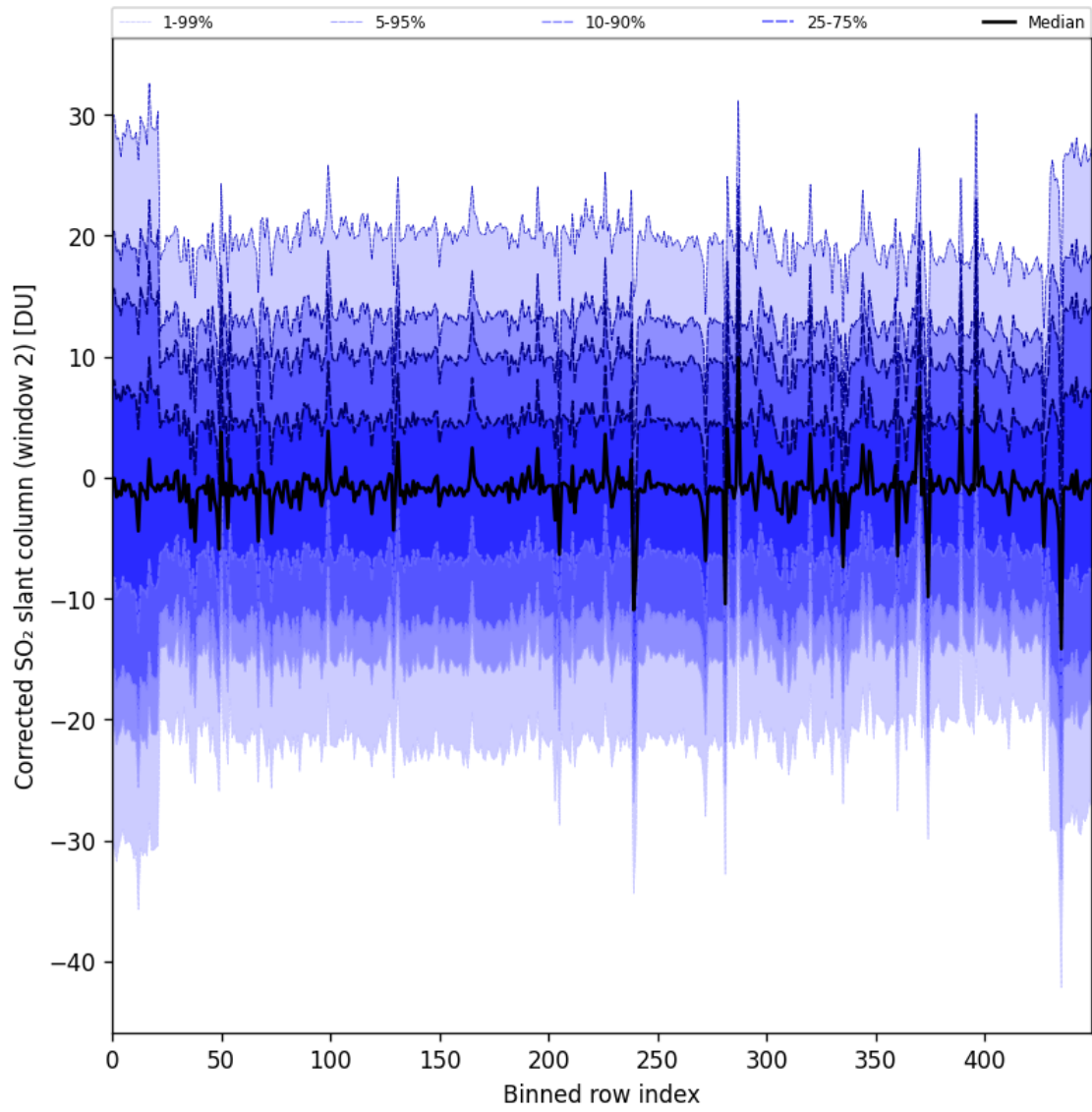
Figure 95: Along track statistics of “Corrected SO 2 slant column (window 2)” for 2025-08-15 to 2025-08-17
