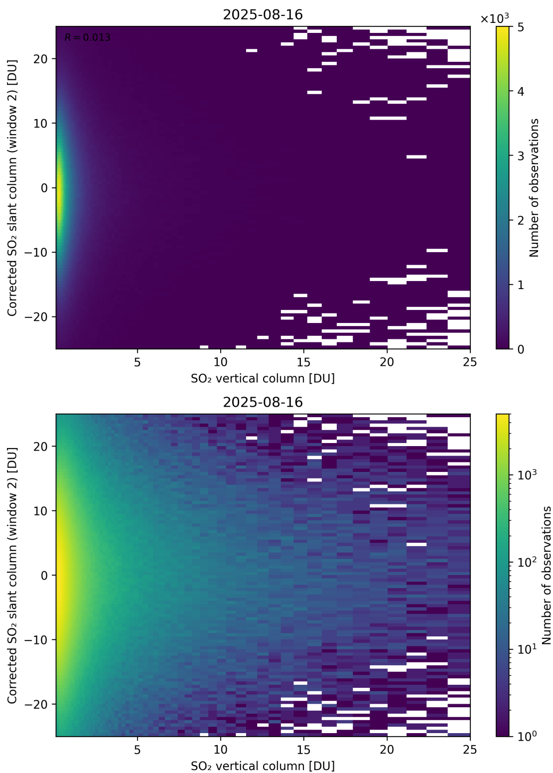
Figure 352: Scatter density plot of “SO 2 vertical column” against “Corrected SO 2 slant column (window 2)” for 2025-08-15 to 2025-08-17.
