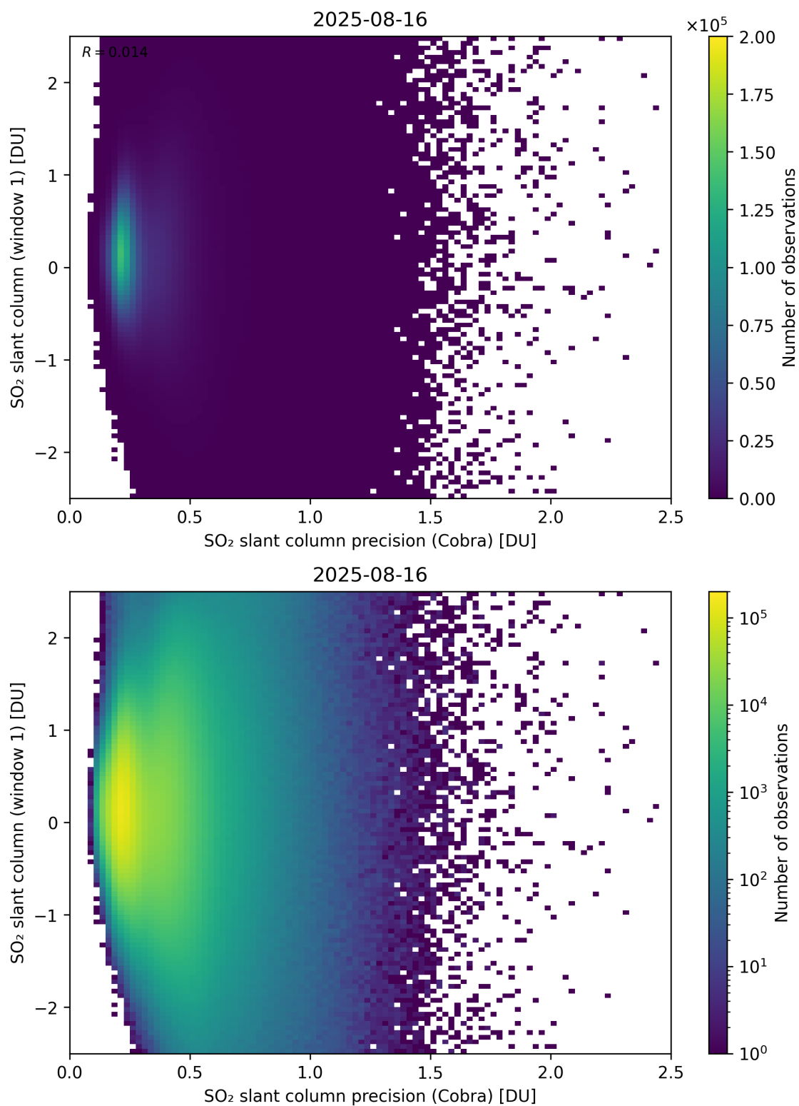
Figure 208: Scatter density plot of “SO 2 slant column precision (Cobra)” against “SO 2 slant column (window 1)” for 2025-08-15 to 2025-08-17.
