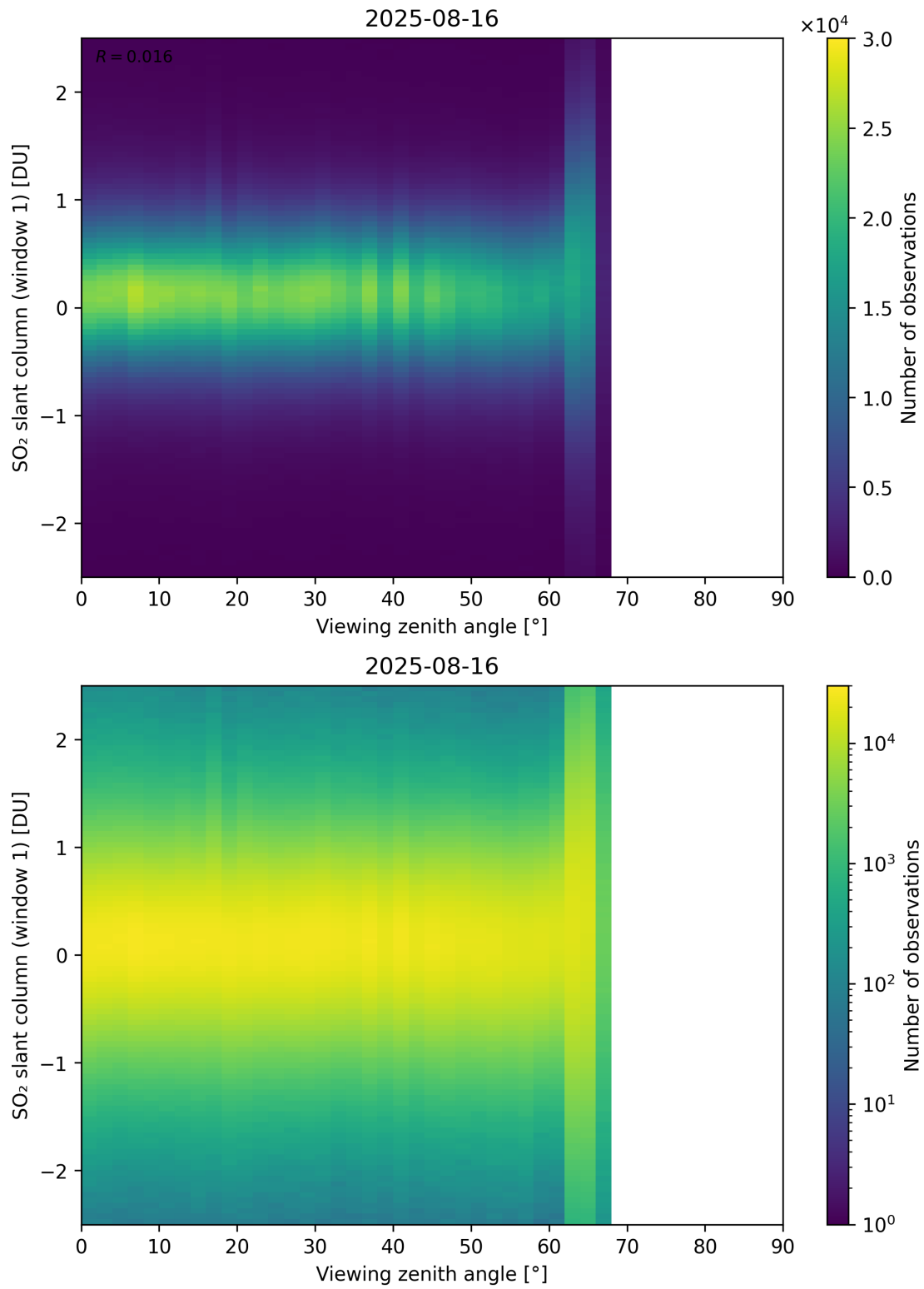
Figure 376: Scatter density plot of “Viewing zenith angle” against “SO 2 slant column (window 1)” for 2025-08-15 to 2025-08-17.
