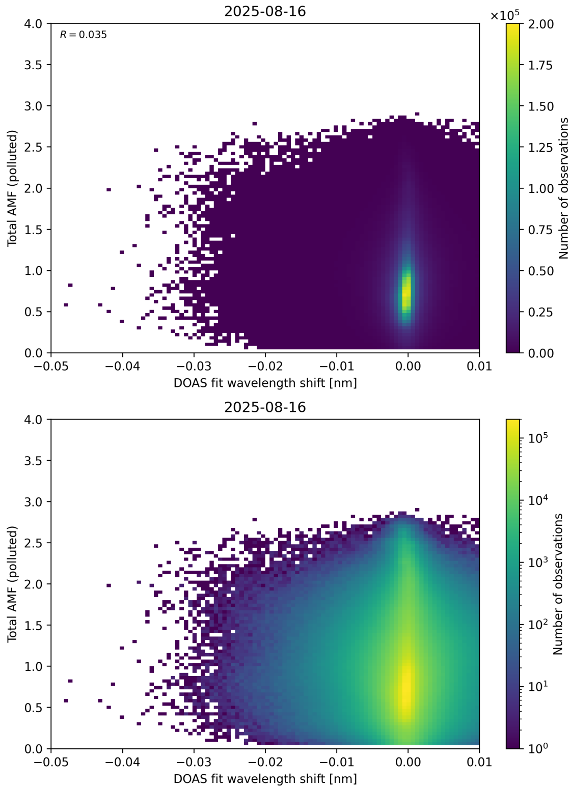
Figure 141: Scatter density plot of “DOAS fit wavelength shift” against “Total AMF (polluted)” for 2025-08-15 to 2025-08-17.
