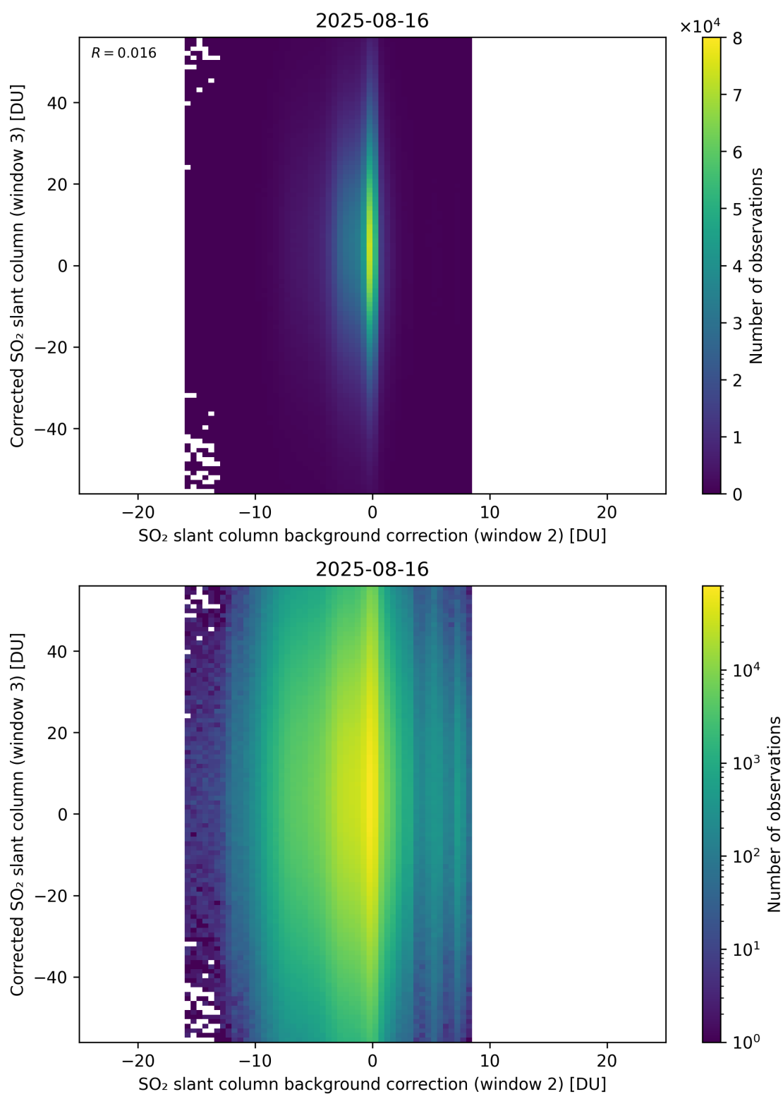
Figure 127: Scatter density plot of “SO 2 slant column background correction (window 2)” against “Corrected SO 2 slant column (window 3)” for 2025-08-15 to 2025-08-17.
