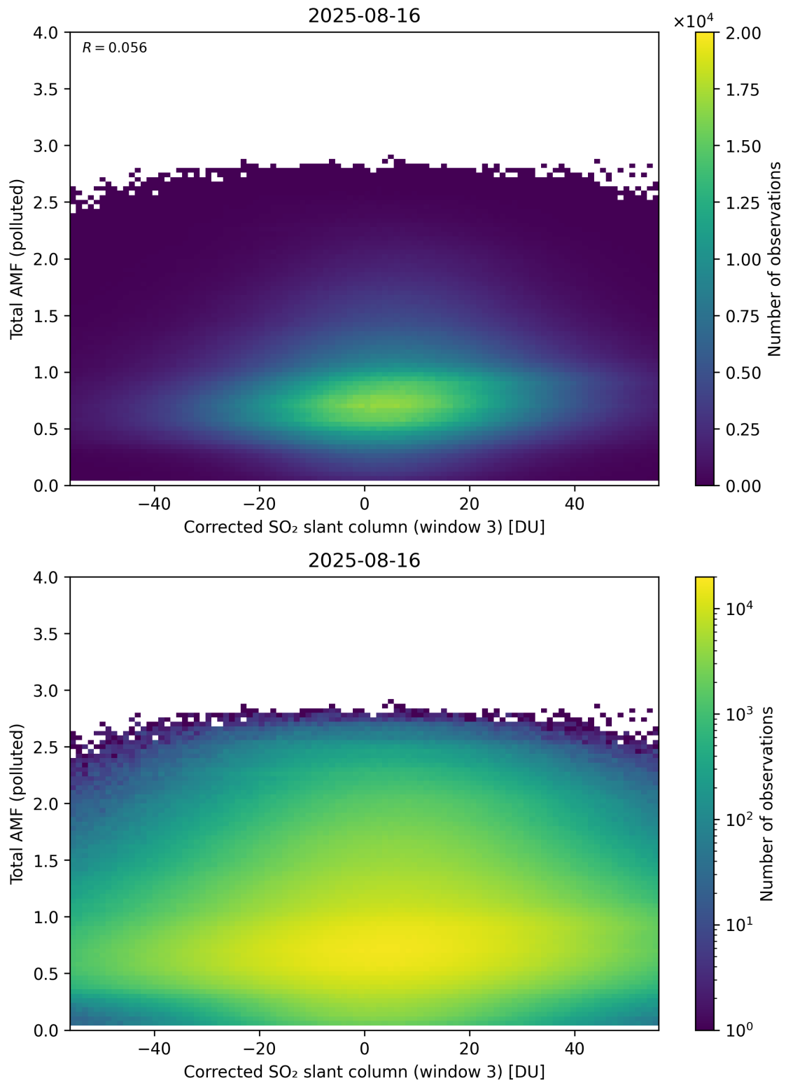
Figure 260: Scatter density plot of “Corrected SO 2 slant column (window 3)” against “Total AMF (polluted)” for 2025-08-15 to 2025-08-17.
