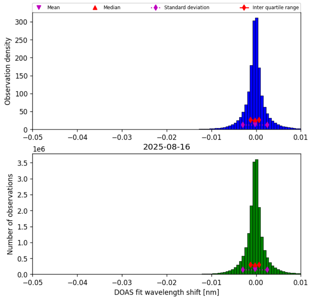
Figure 76: Histogram of “DOAS fit wavelength shift” for 2025-08-15 to 2025-08-17
