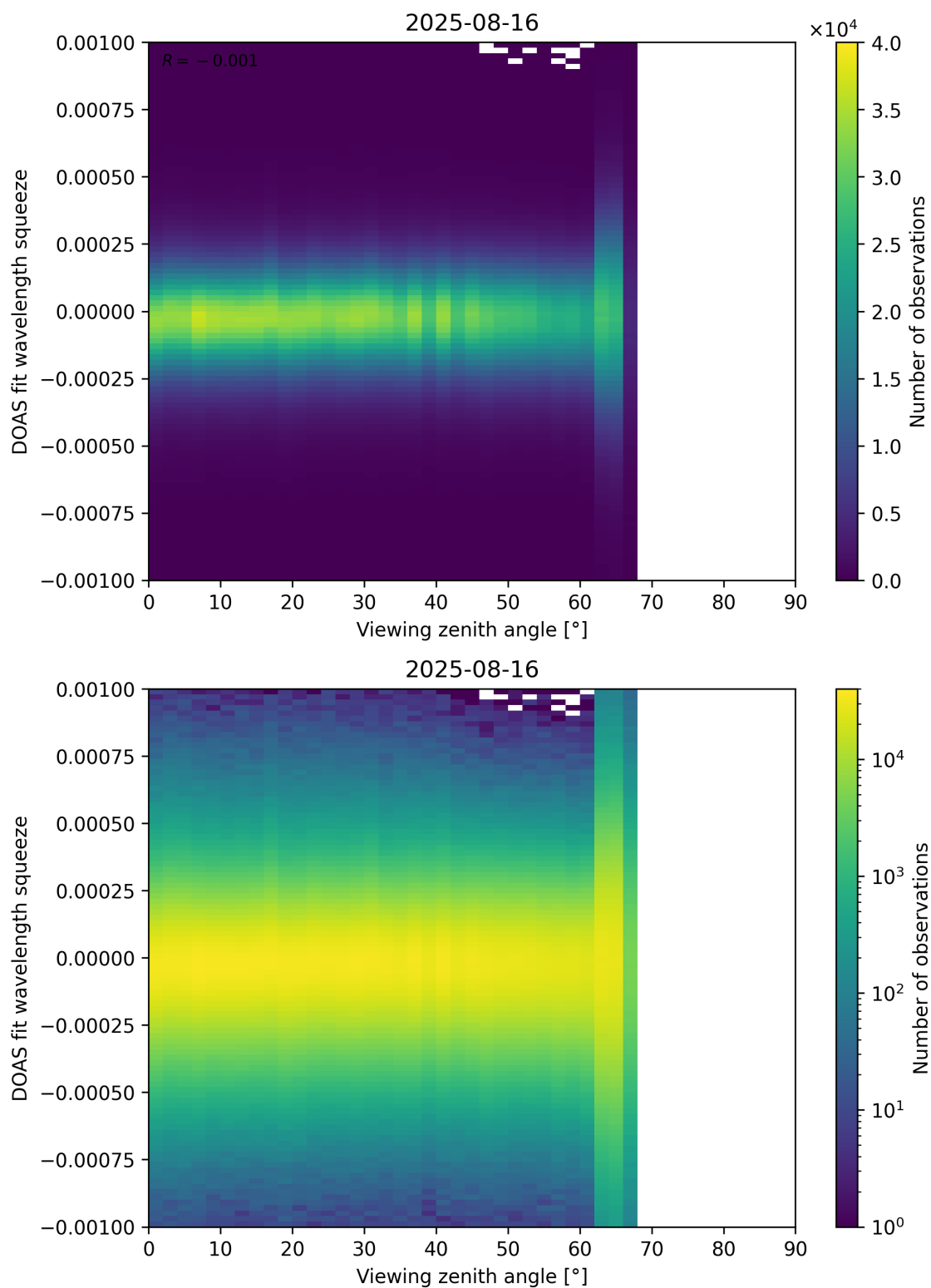
Figure 366: Scatter density plot of “Viewing zenith angle” against “DOAS fit wavelength squeeze” for 2025-08-15 to 2025-08-17.
