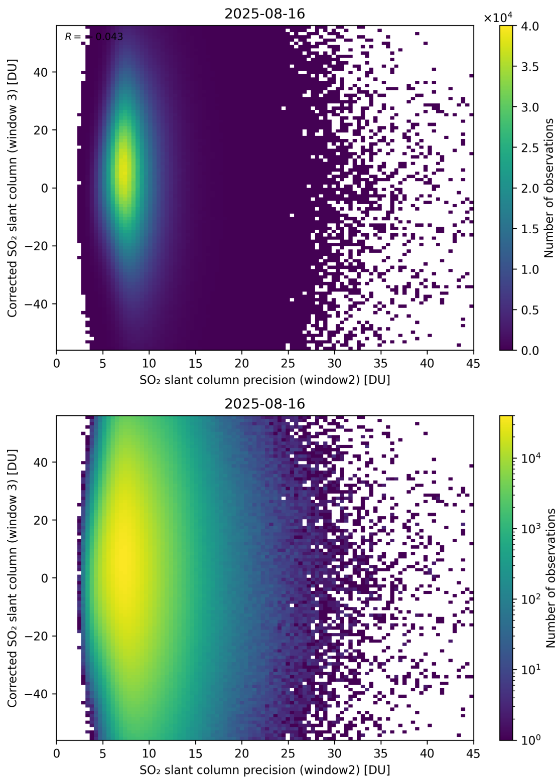
Figure 298: Scatter density plot of “SO 2 slant column precision (window2)” against “Corrected SO 2 slant column (window 3)” for 2025-08-15 to 2025-08-17.
