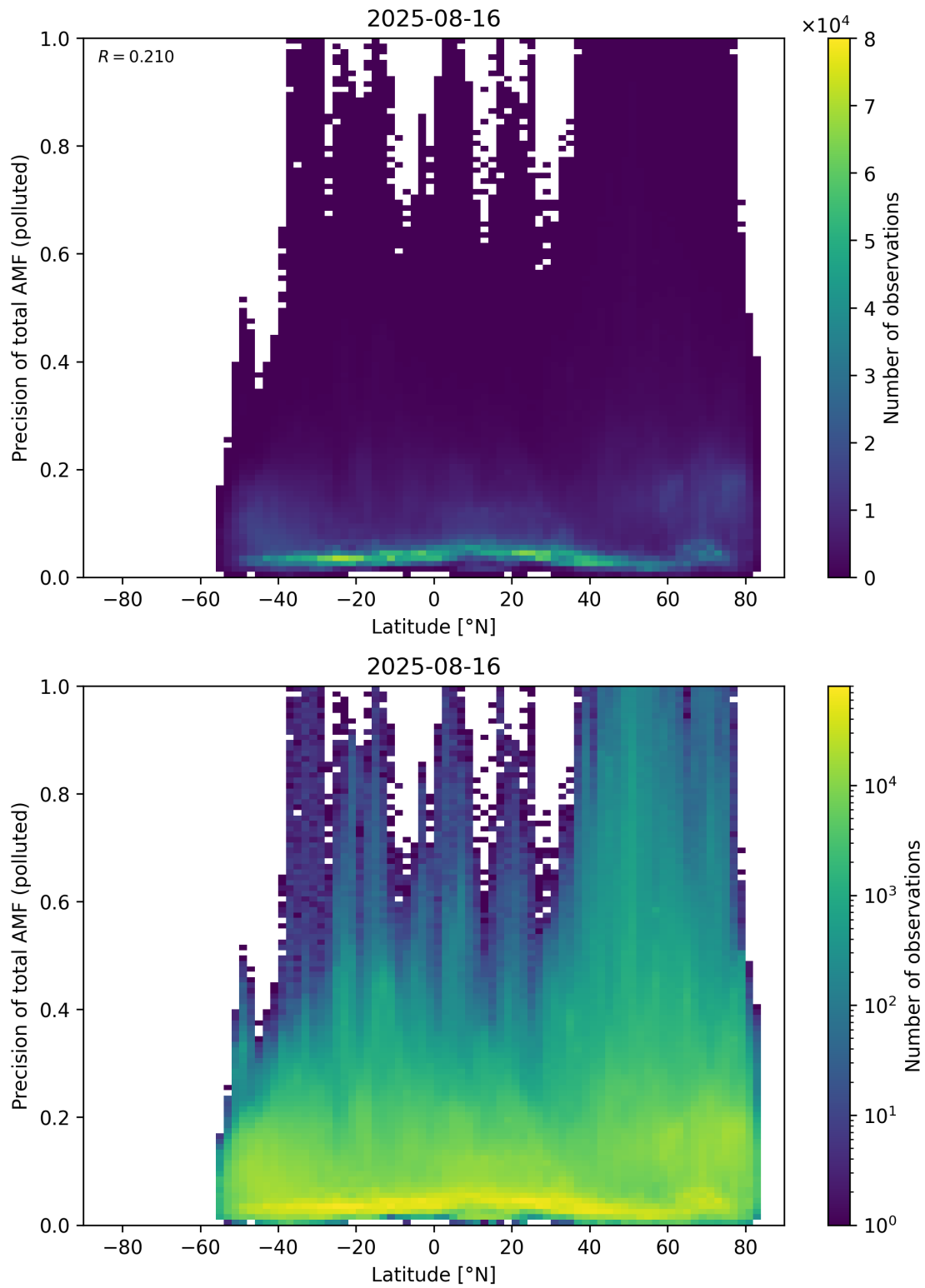
Figure 168: Scatter density plot of “Latitude” against “Precision of total AMF (polluted)” for 2025-08-15 to 2025-08-17.
