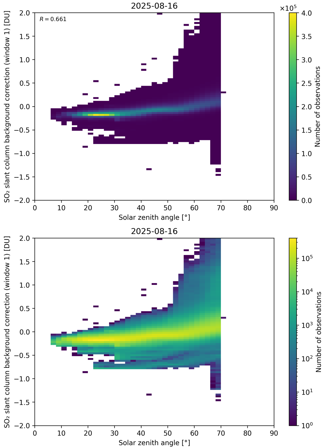
Figure 171: Scatter density plot of “Solar zenith angle” against “SO 2 slant column background correction (window 1)” for 2025-08-15 to 2025-08-17.
