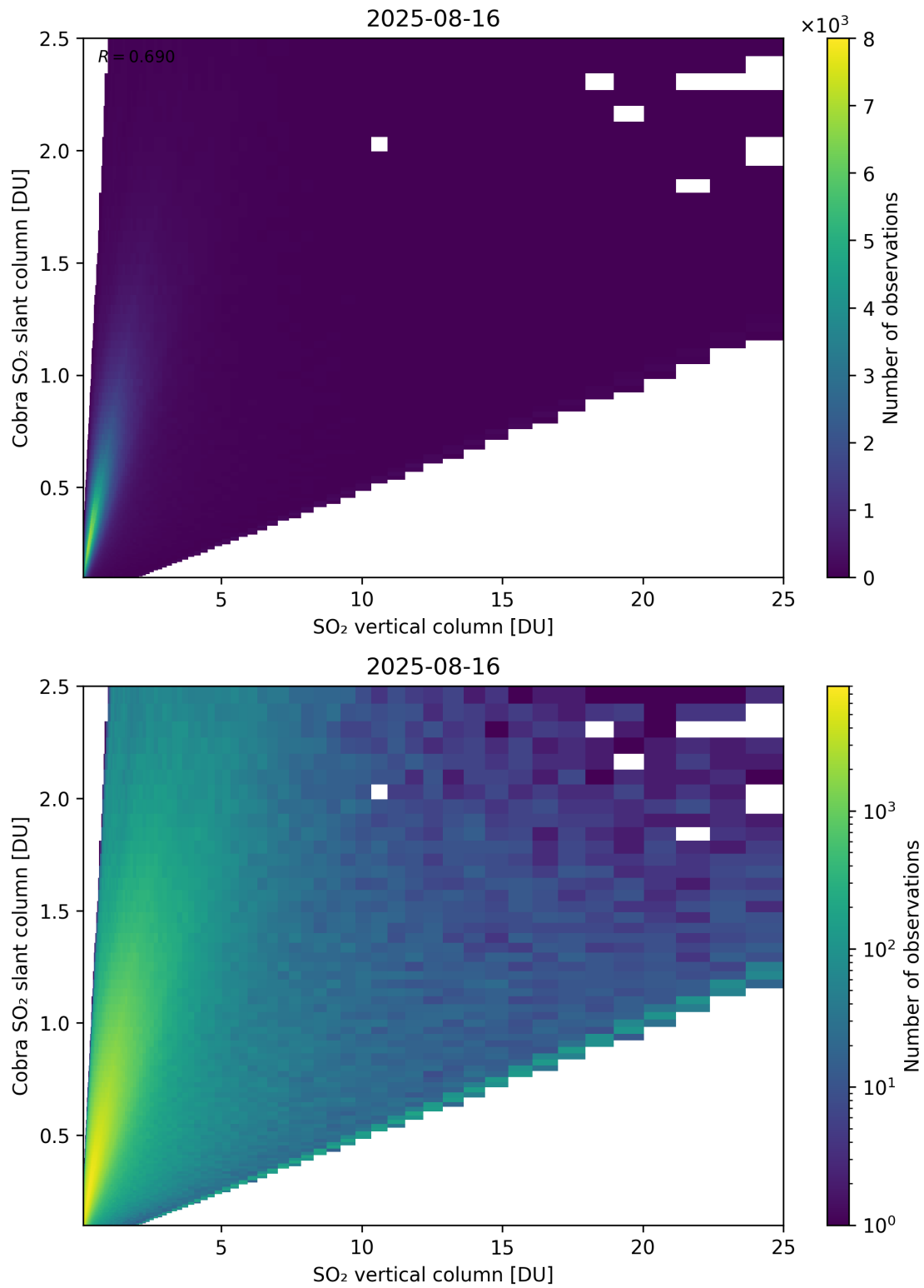
Figure 349: Scatter density plot of “SO 2 vertical column” against “Cobra SO 2 slant column” for 2025-08-15 to 2025-08-17.
