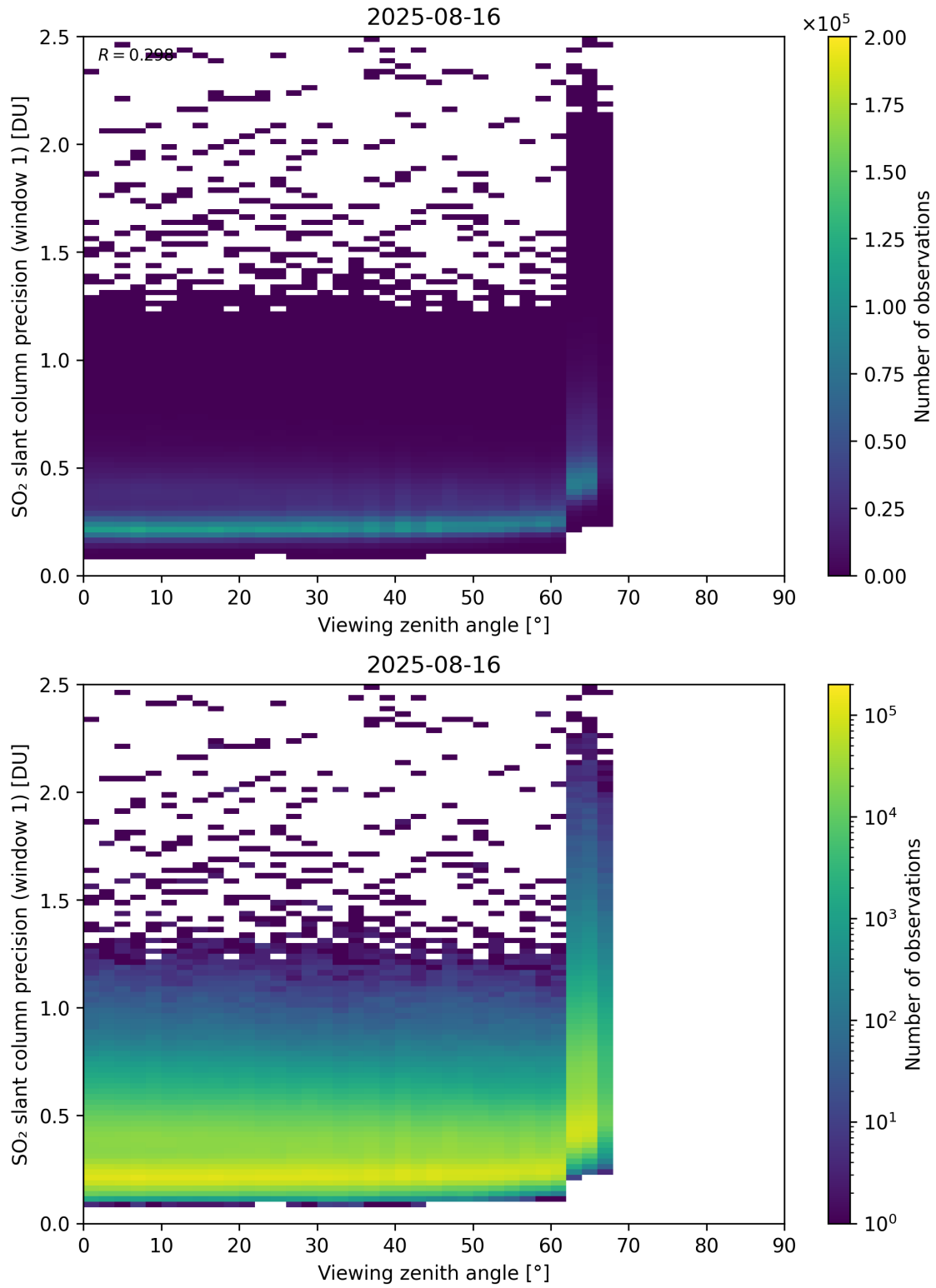
Figure 377: Scatter density plot of “Viewing zenith angle” against “SO 2 slant column precision (window 1)” for 2025-08-15 to 2025-08-17.
