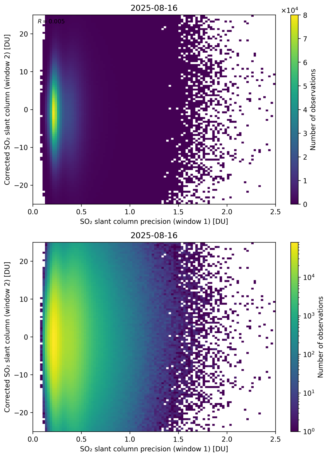
Figure 275: Scatter density plot of “SO 2 slant column precision (window 1)” against “Corrected SO 2 slant column (window 2)” for 2025-08-15 to 2025-08-17.
