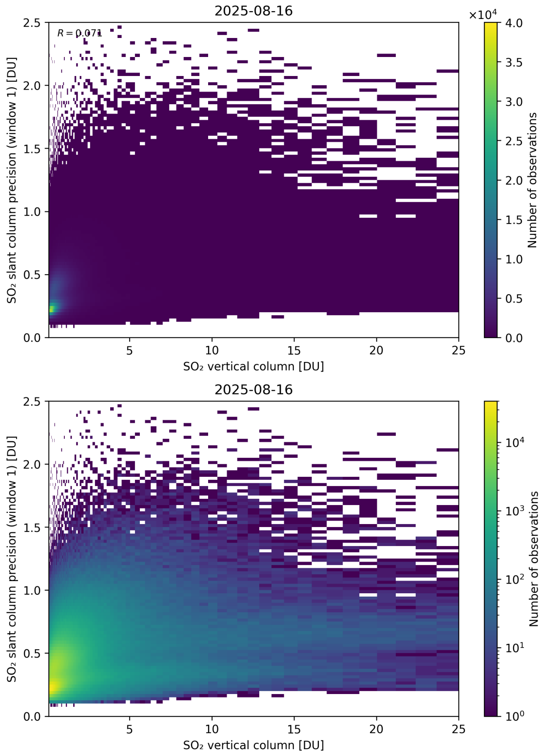
Figure 355: Scatter density plot of “SO 2 vertical column” against “SO 2 slant column precision (window 1)” for 2025-08-15 to 2025-08-17.
