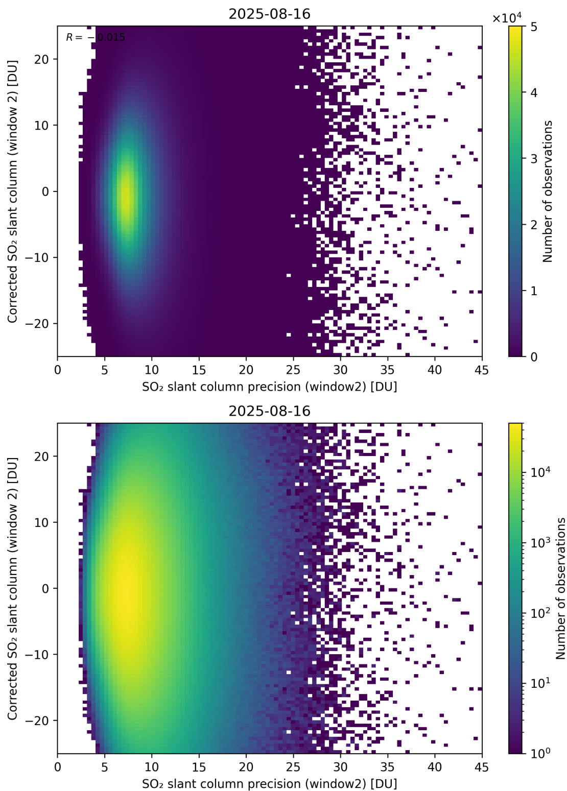
Figure 297: Scatter density plot of “SO 2 slant column precision (window2)” against “Corrected SO 2 slant column (window 2)” for 2025-08-15 to 2025-08-17.
