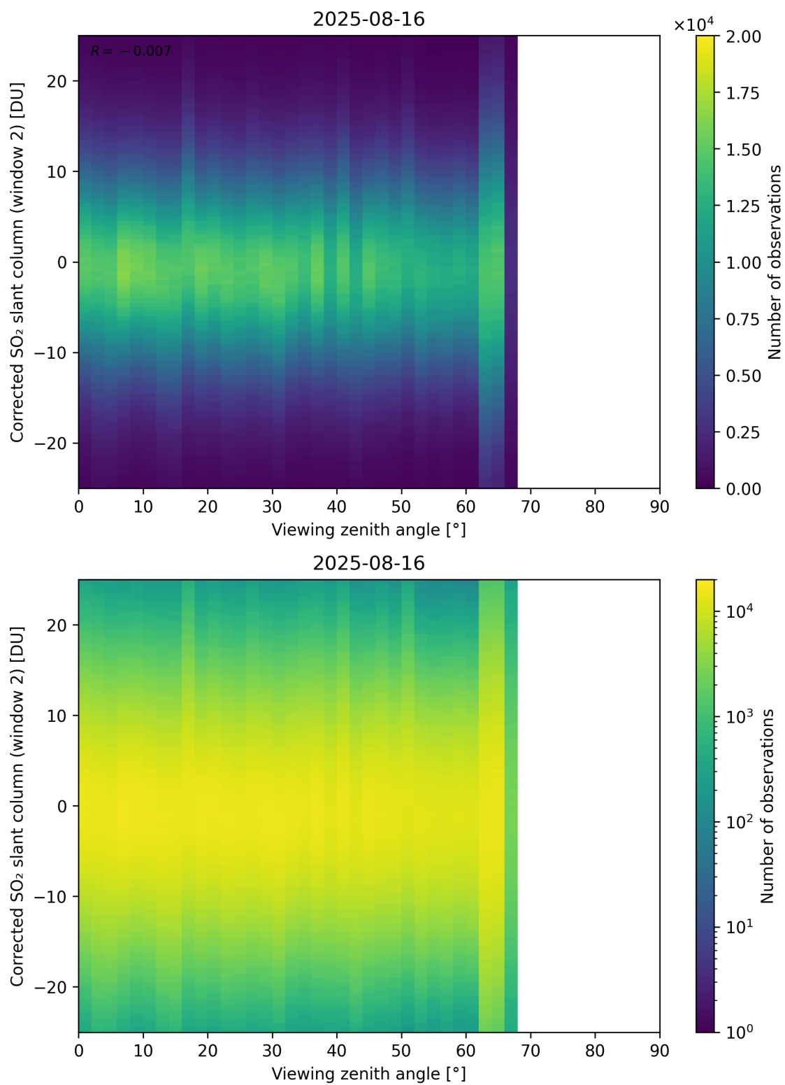
Figure 374: Scatter density plot of “Viewing zenith angle” against “Corrected SO 2 slant column (window 2)” for 2025-08-15 to 2025-08-17.
