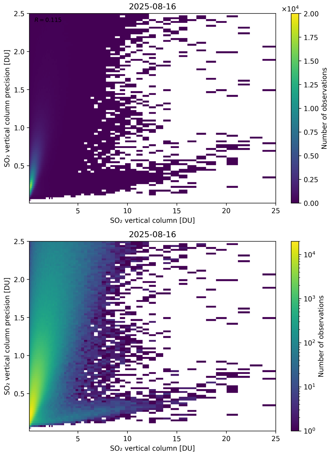
Figure 361: Scatter density plot of “SO 2 vertical column” against “SO 2 vertical column precision” for 2025-08-15 to 2025-08-17.
