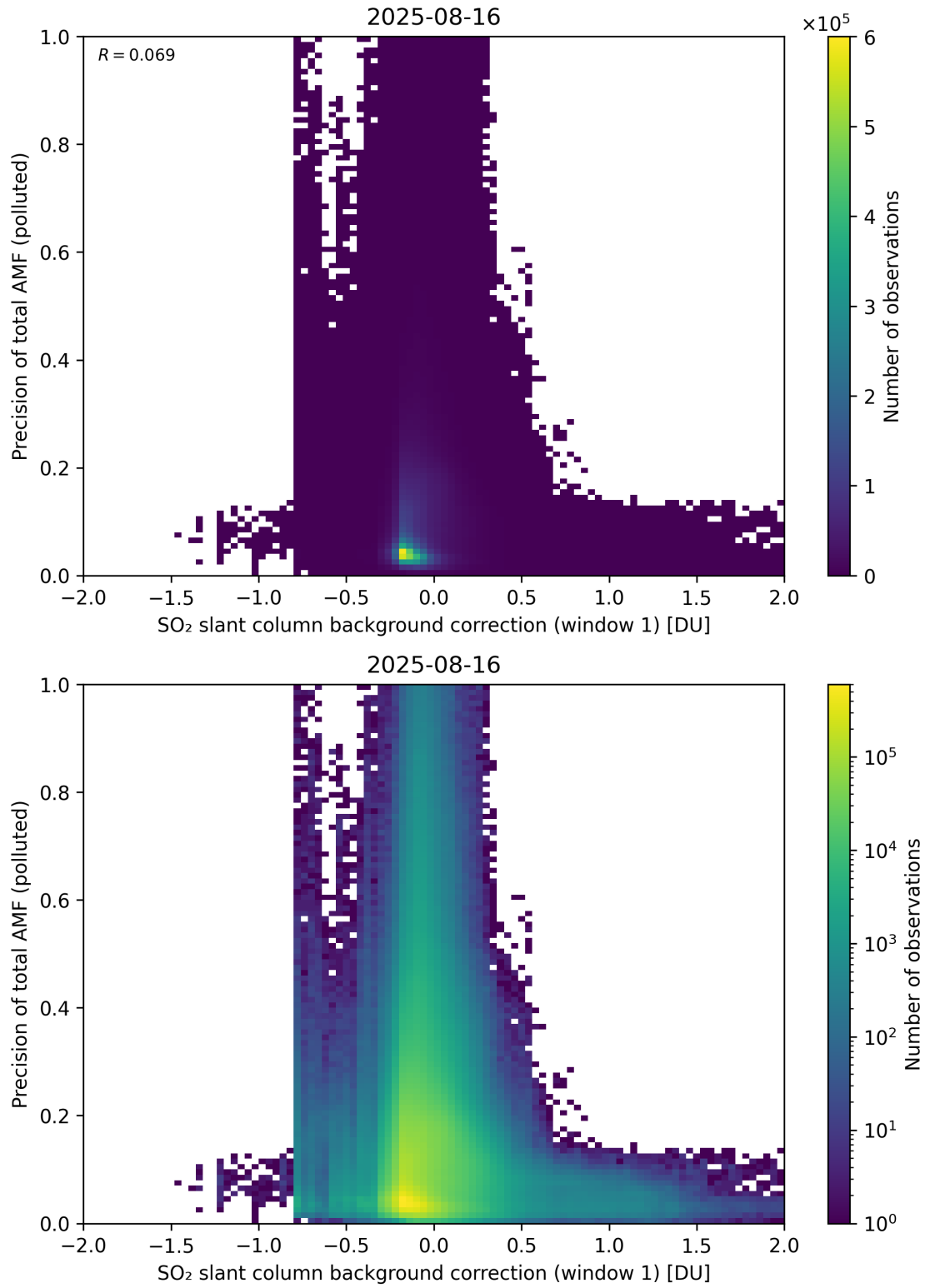
Figure 121: Scatter density plot of “SO 2 slant column background correction (window 1)” against “Precision of total AMF (polluted)” for 2025-08-15 to 2025-08-17.
