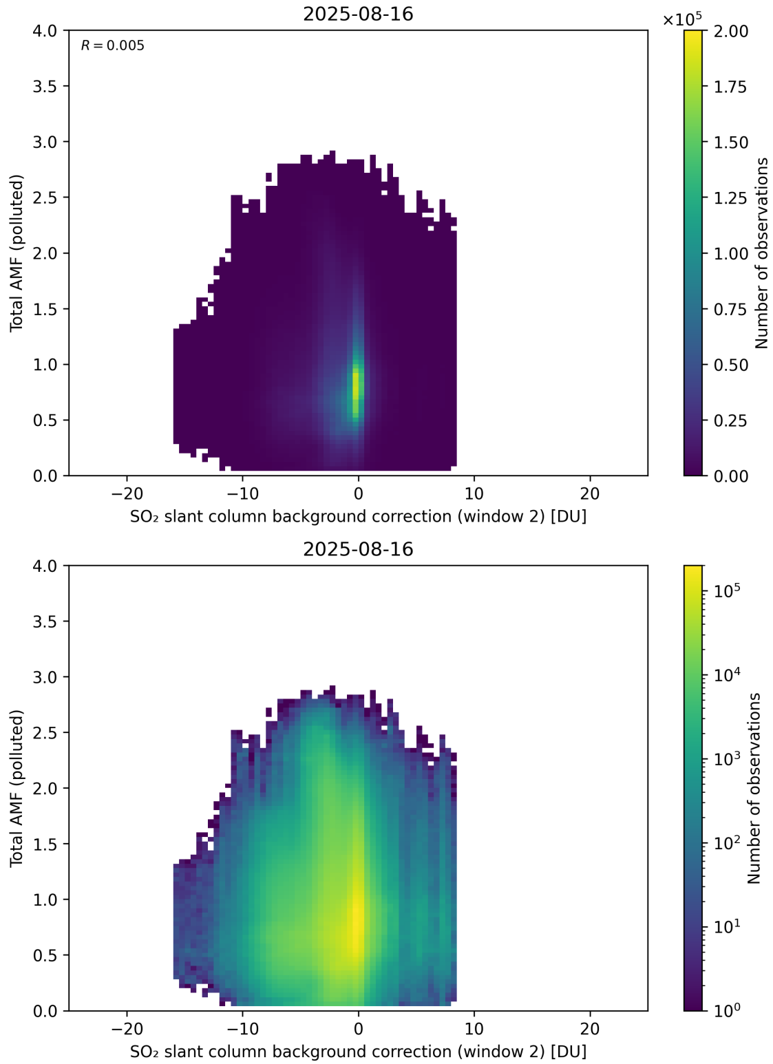
Figure 130: Scatter density plot of “SO 2 slant column background correction (window 2)” against “Total AMF (polluted)” for 2025-08-15 to 2025-08-17.
