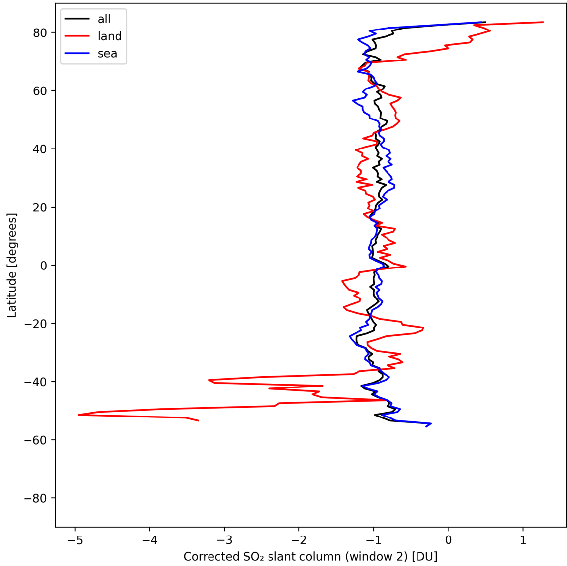
Figure 43: Zonal average of “Corrected SO 2 slant column (window 2)” for 2025-08-15 to 2025-08-17.
