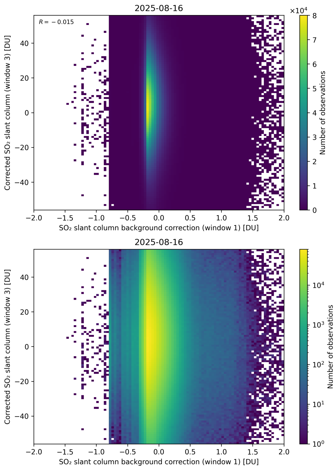
Figure 116: Scatter density plot of “SO 2 slant column background correction (window 1)” against “Corrected SO 2 slant column (window 3)” for 2025-08-15 to 2025-08-17.
