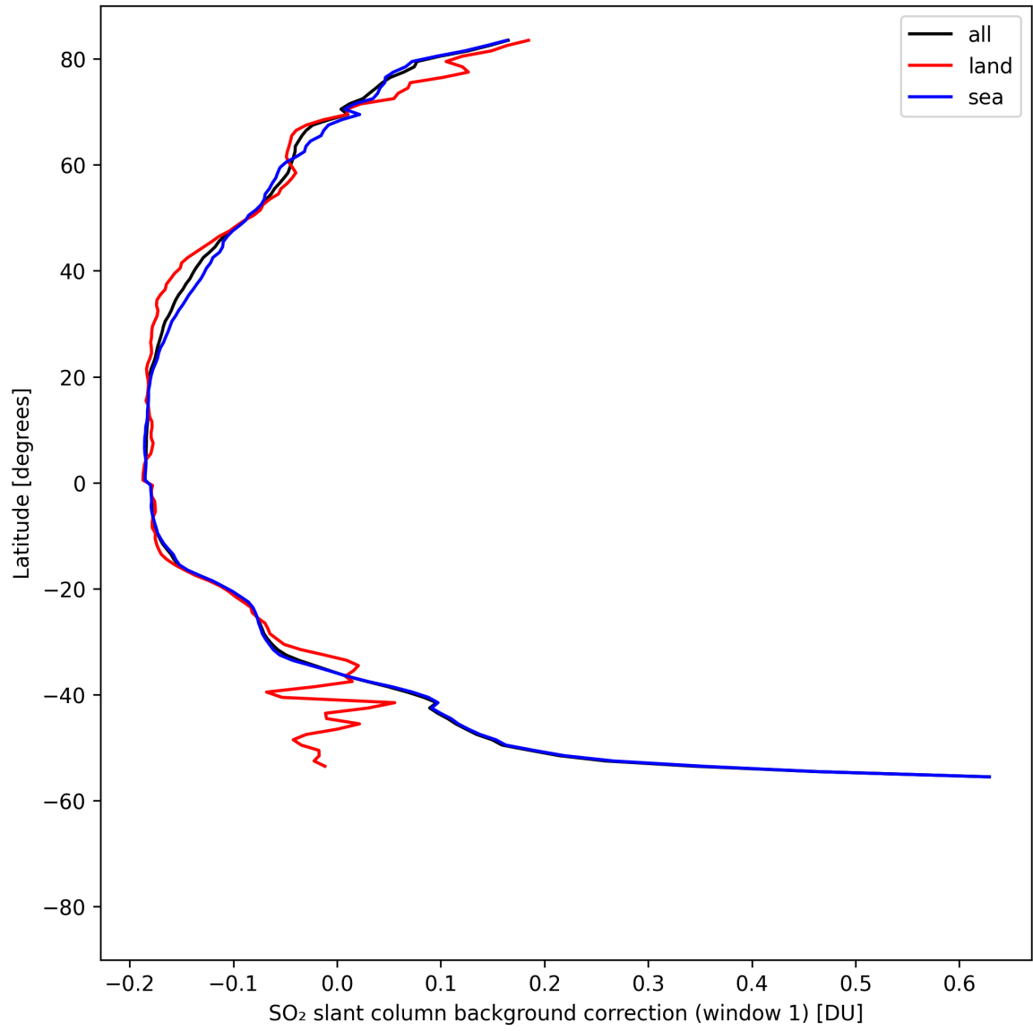
Figure 40: Zonal average of “SO 2 slant column background correction (window 1)” for 2025-08-15 to 2025-08-17.
