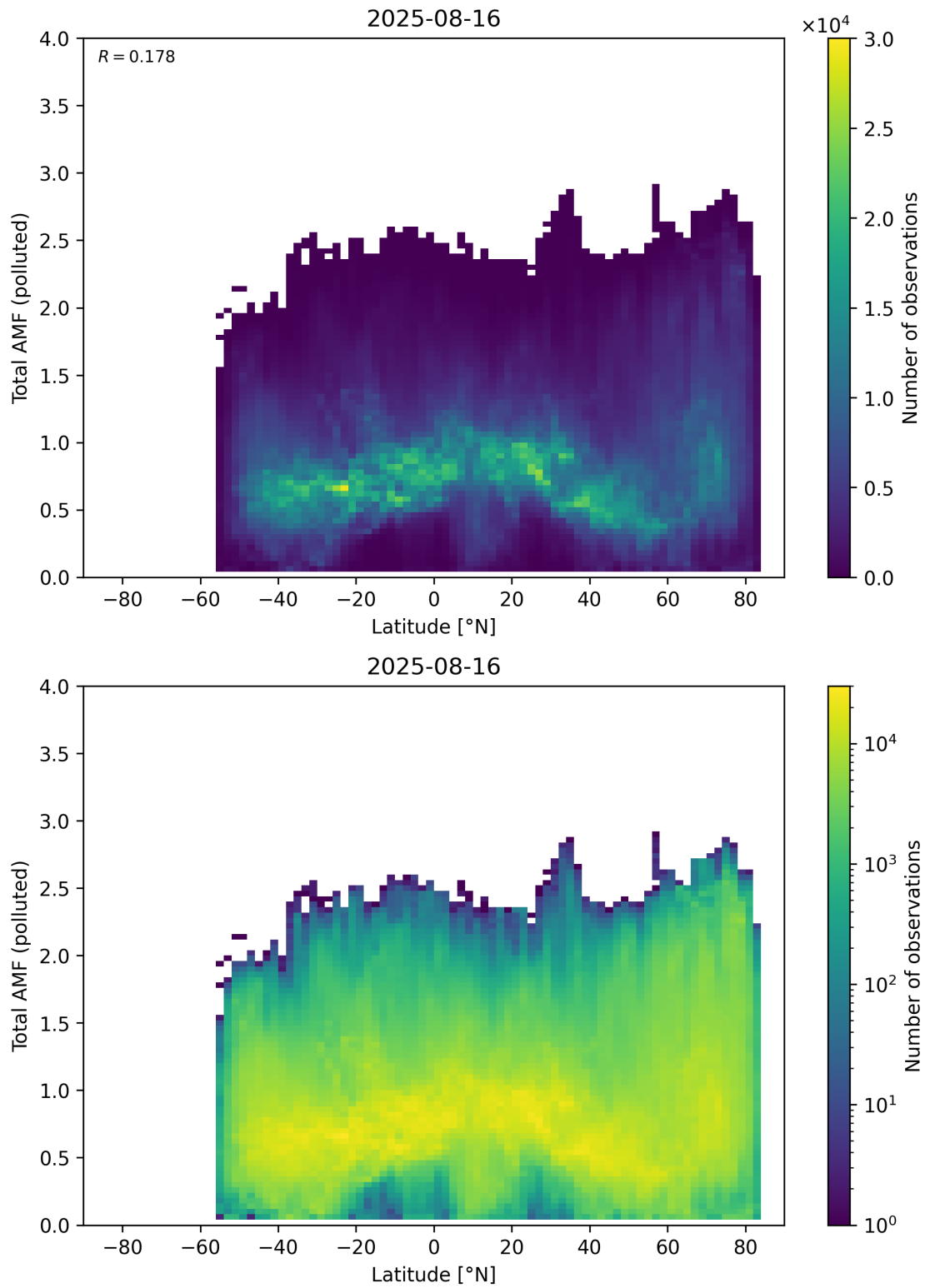
Figure 167: Scatter density plot of “Latitude” against “Total AMF (polluted)” for 2025-08-15 to 2025-08-17.
