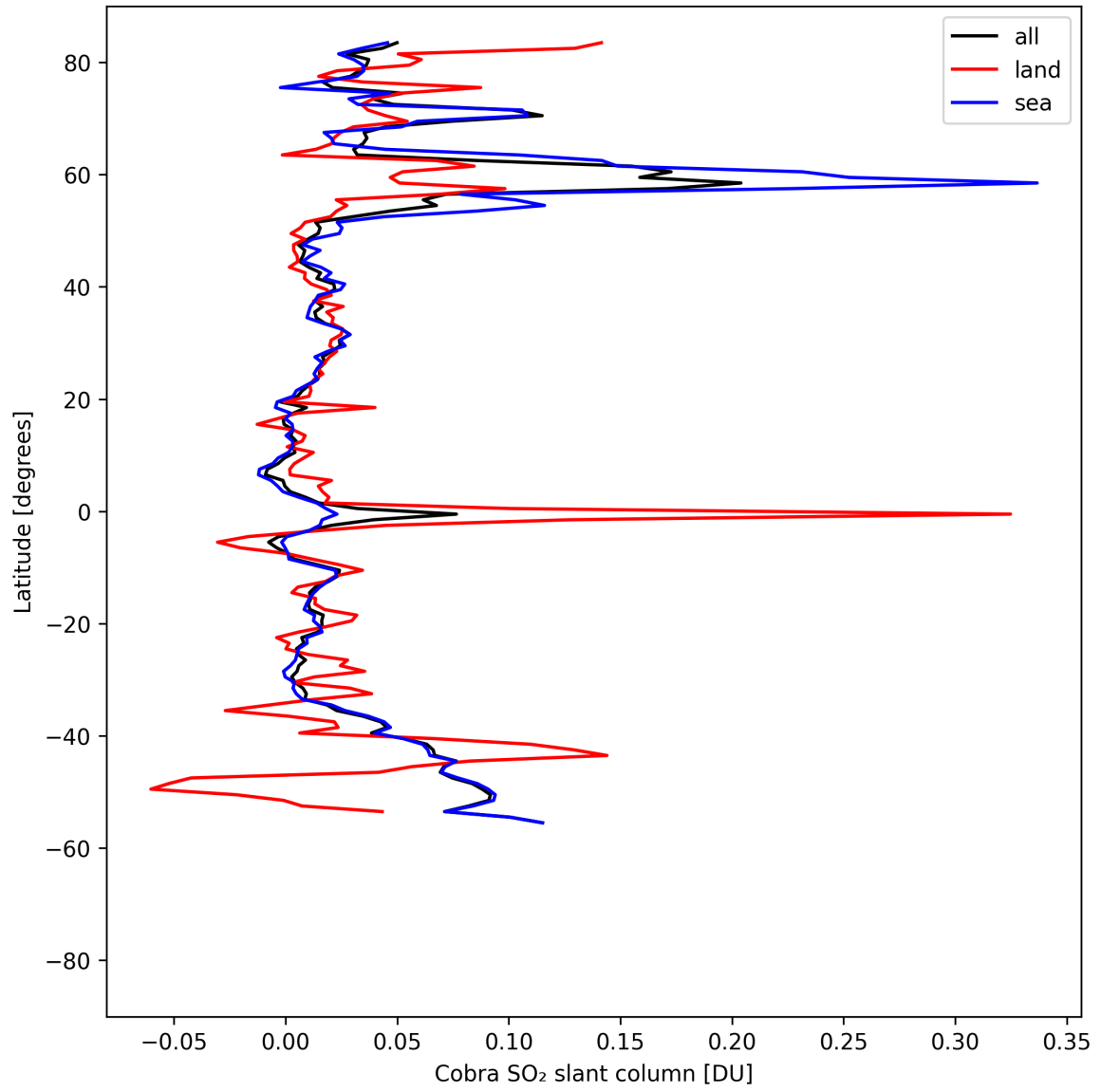
Figure 35: Zonal average of “Cobra SO 2 slant column” for 2025-08-15 to 2025-08-17.
