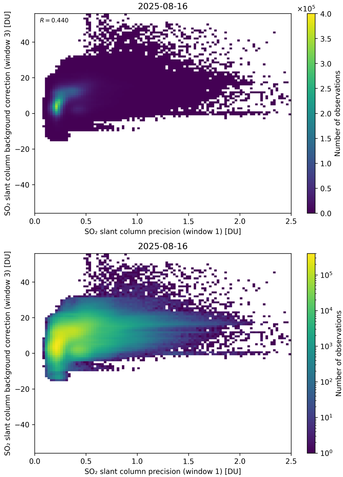
Figure 270: Scatter density plot of “SO 2 slant column precision (window 1)” against “SO 2 slant column background correction (window 3)” for 2025-08-15 to 2025-08-17.
