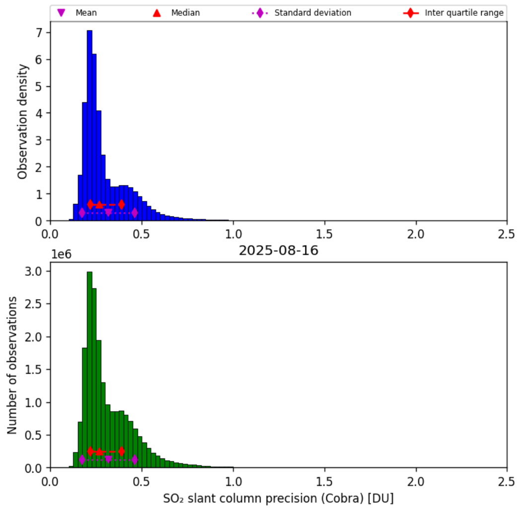
Figure 62: Histogram of “SO 2 slant column precision (Cobra)” for 2025-08-15 to 2025-08-17
