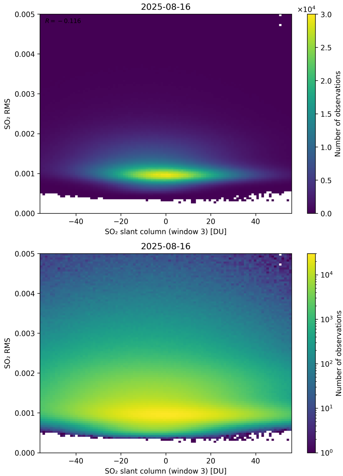
Figure 306: Scatter density plot of “SO 2 slant column (window 3)” against “SO 2 RMS” for 2025-08-15 to 2025-08-17.
