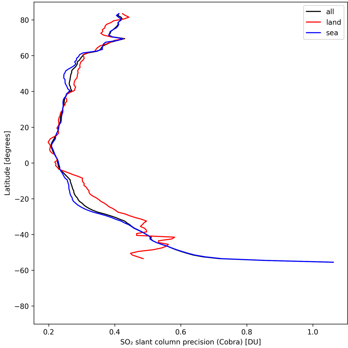
Figure 36: Zonal average of “SO 2 slant column precision (Cobra)” for 2025-08-15 to 2025-08-17.
