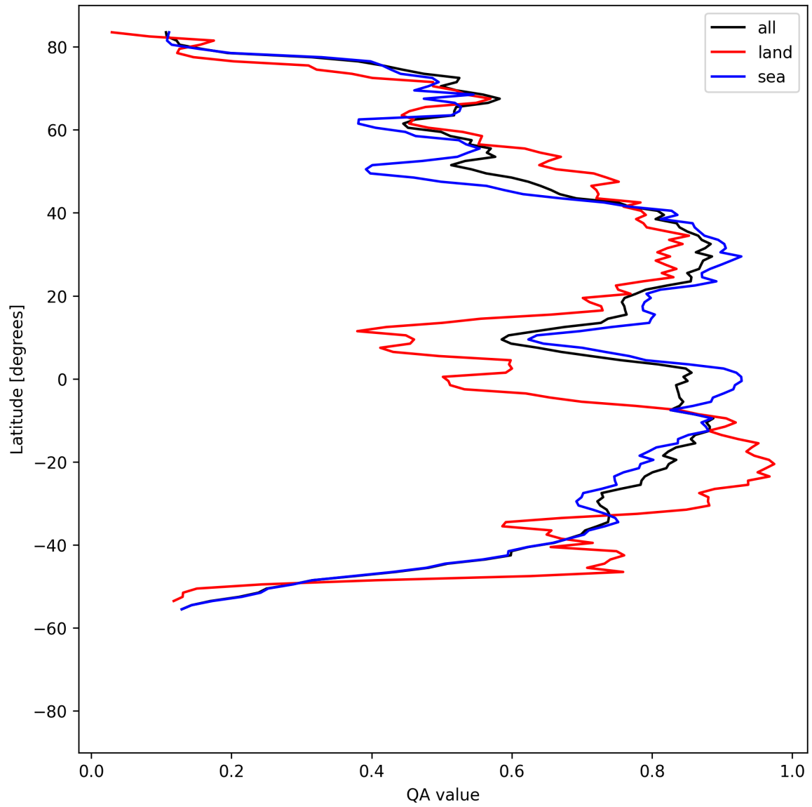
Figure 31: Zonal average of “QA value” for 2025-08-15 to 2025-08-17.
