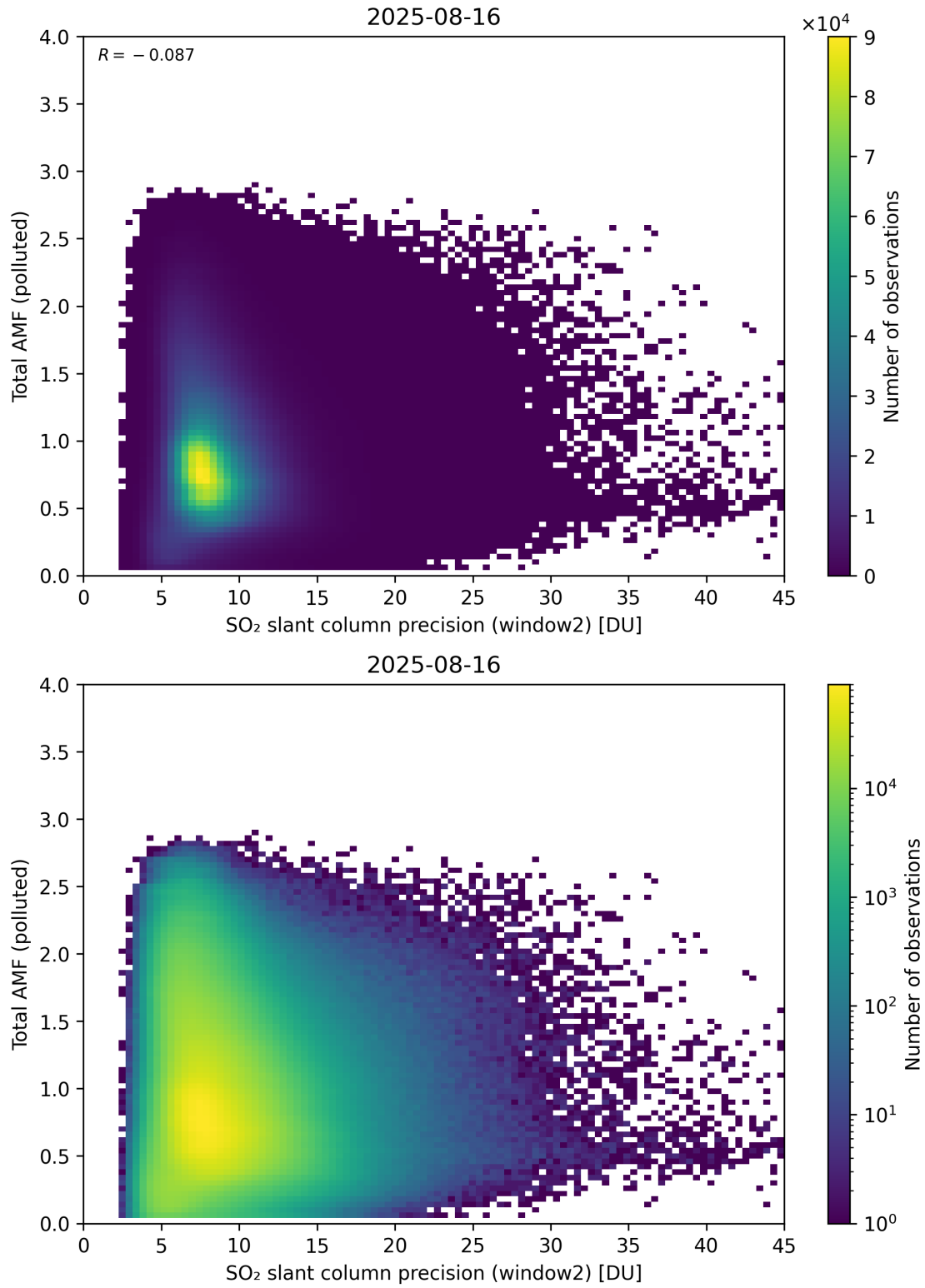
Figure 301: Scatter density plot of “SO 2 slant column precision (window2)” against “Total AMF (polluted)” for 2025-08-15 to 2025-08-17.
