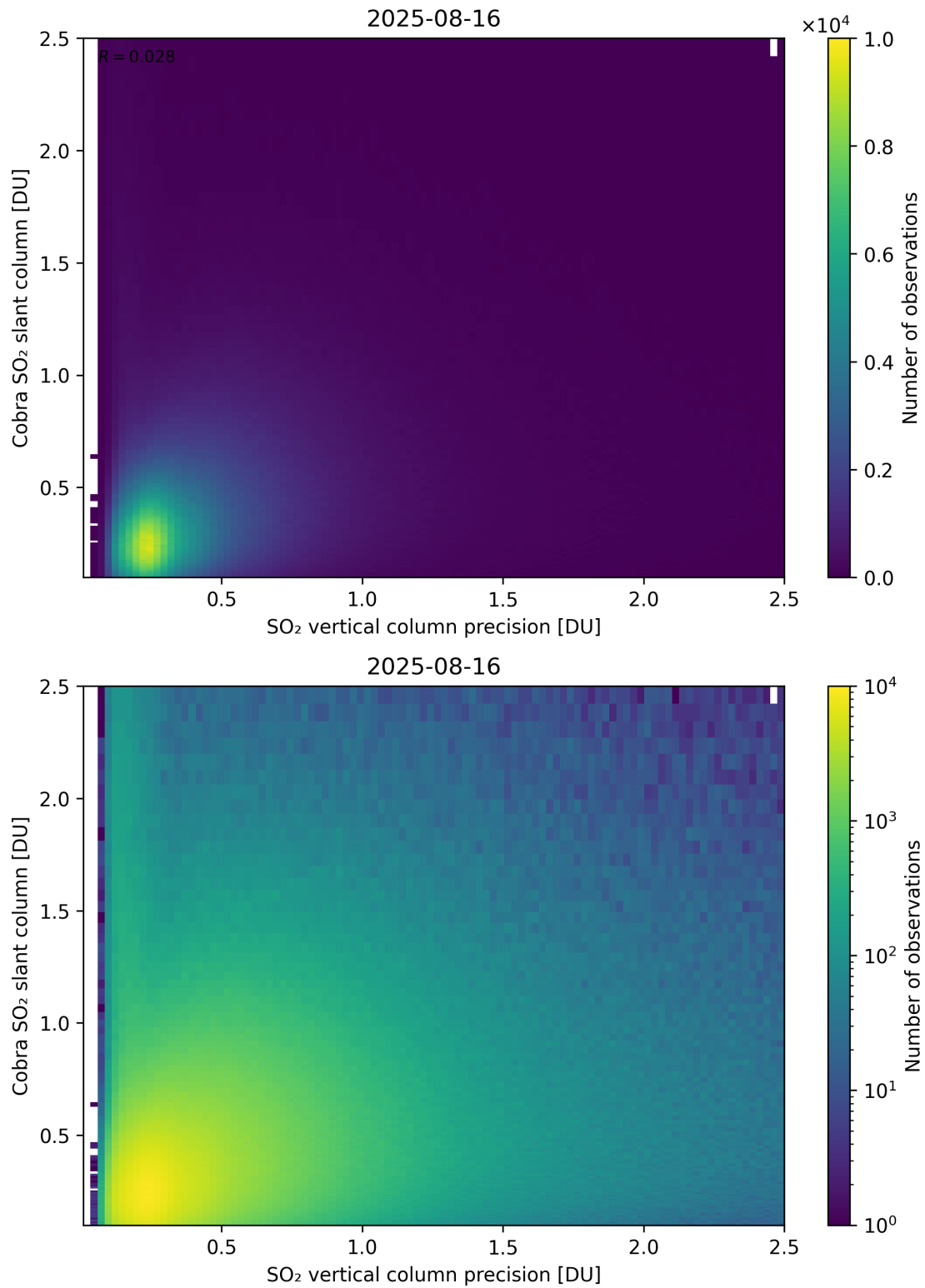
Figure 336: Scatter density plot of “SO 2 vertical column precision” against “Cobra SO 2 slant column” for 2025-08-15 to 2025-08-17.
