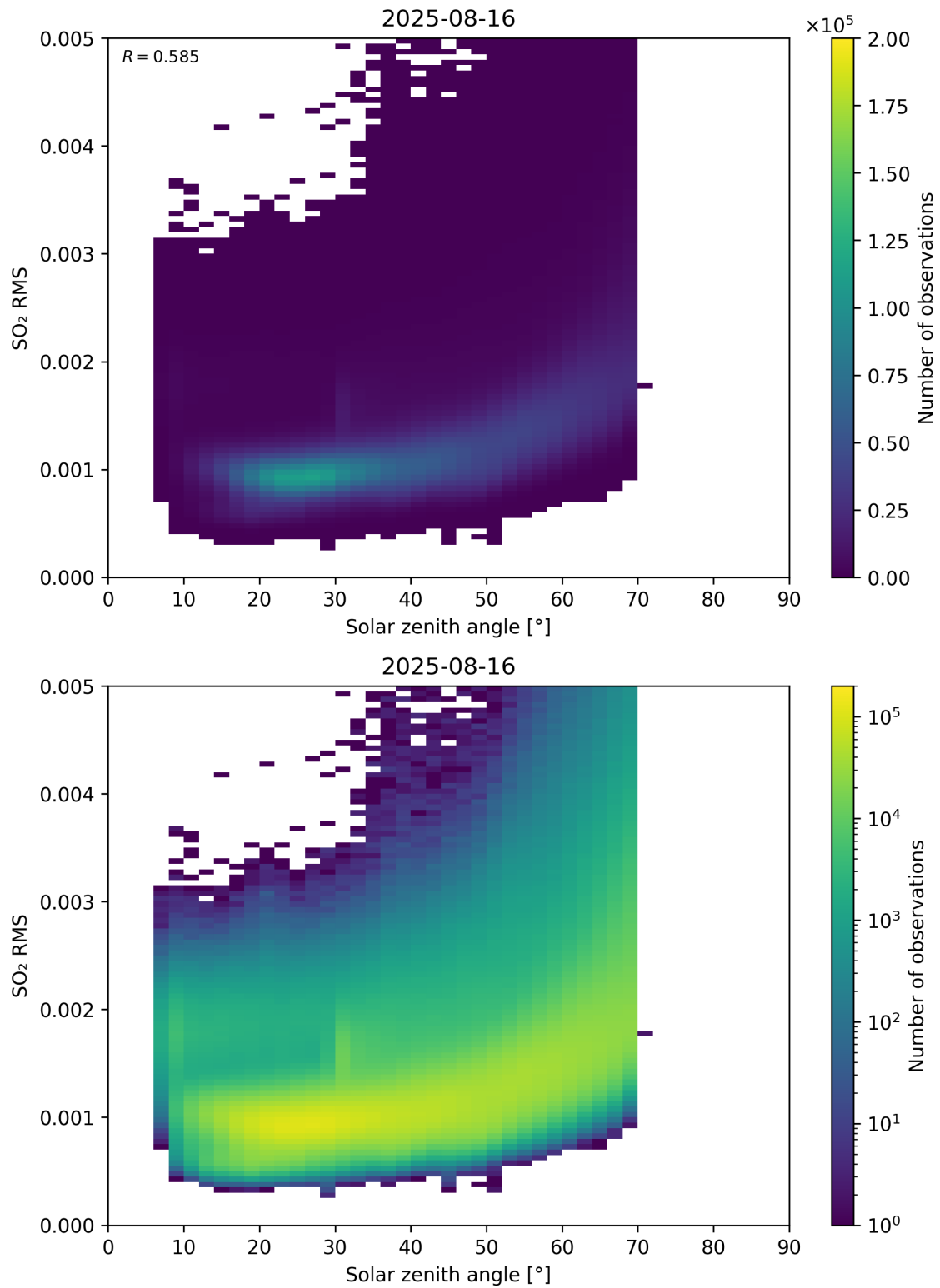
Figure 176: Scatter density plot of “Solar zenith angle” against “SO 2 RMS” for 2025-08-15 to 2025-08-17.
