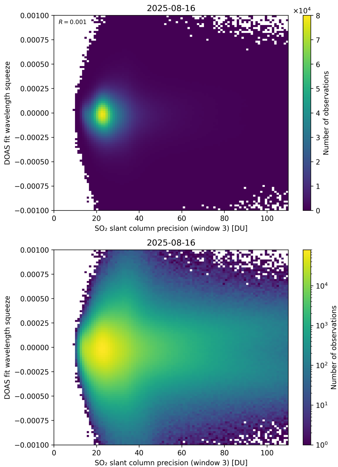
Figure 309: Scatter density plot of “SO 2 slant column precision (window 3)” against “DOAS fit wavelength squeeze” for 2025-08-15 to 2025-08-17.
