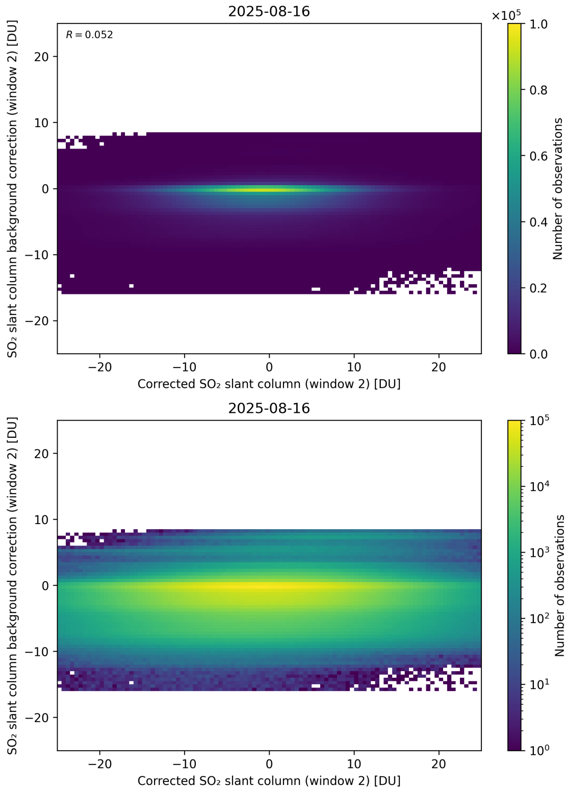
Figure 244: Scatter density plot of “Corrected SO 2 slant column (window 2)” against “SO 2 slant column background correction (window 2)” for 2025-08-15 to 2025-08-17.
