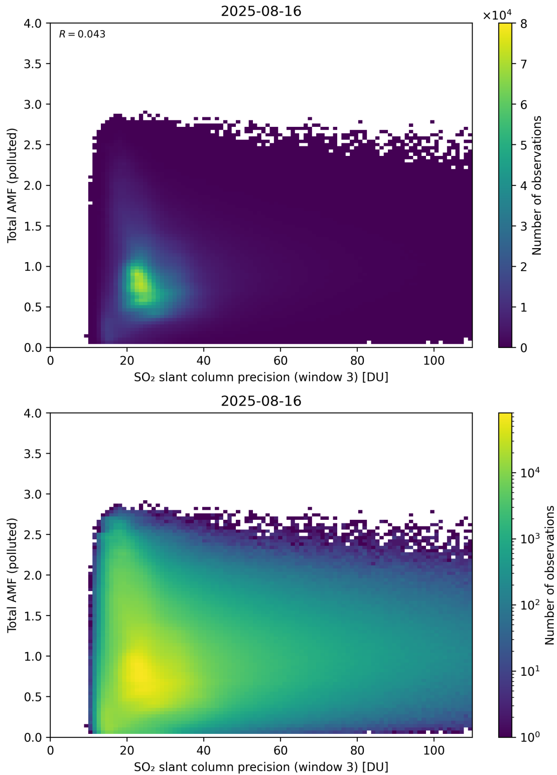
Figure 313: Scatter density plot of “SO 2 slant column precision (window 3)” against “Total AMF (polluted)” for 2025-08-15 to 2025-08-17.
