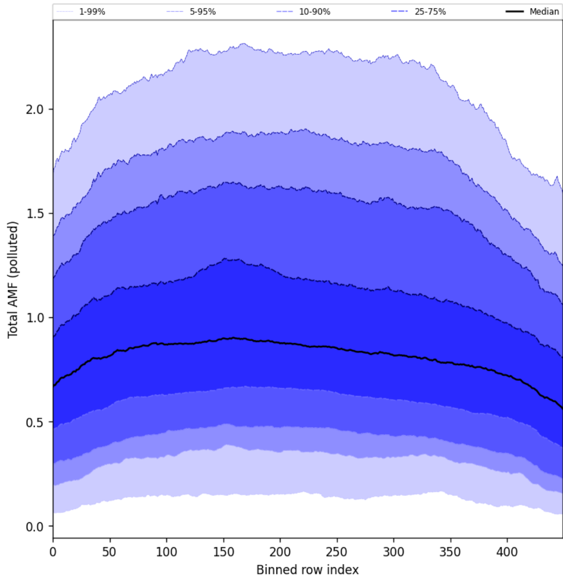
Figure 105: Along track statistics of “Total AMF (polluted)” for 2025-08-15 to 2025-08-17
