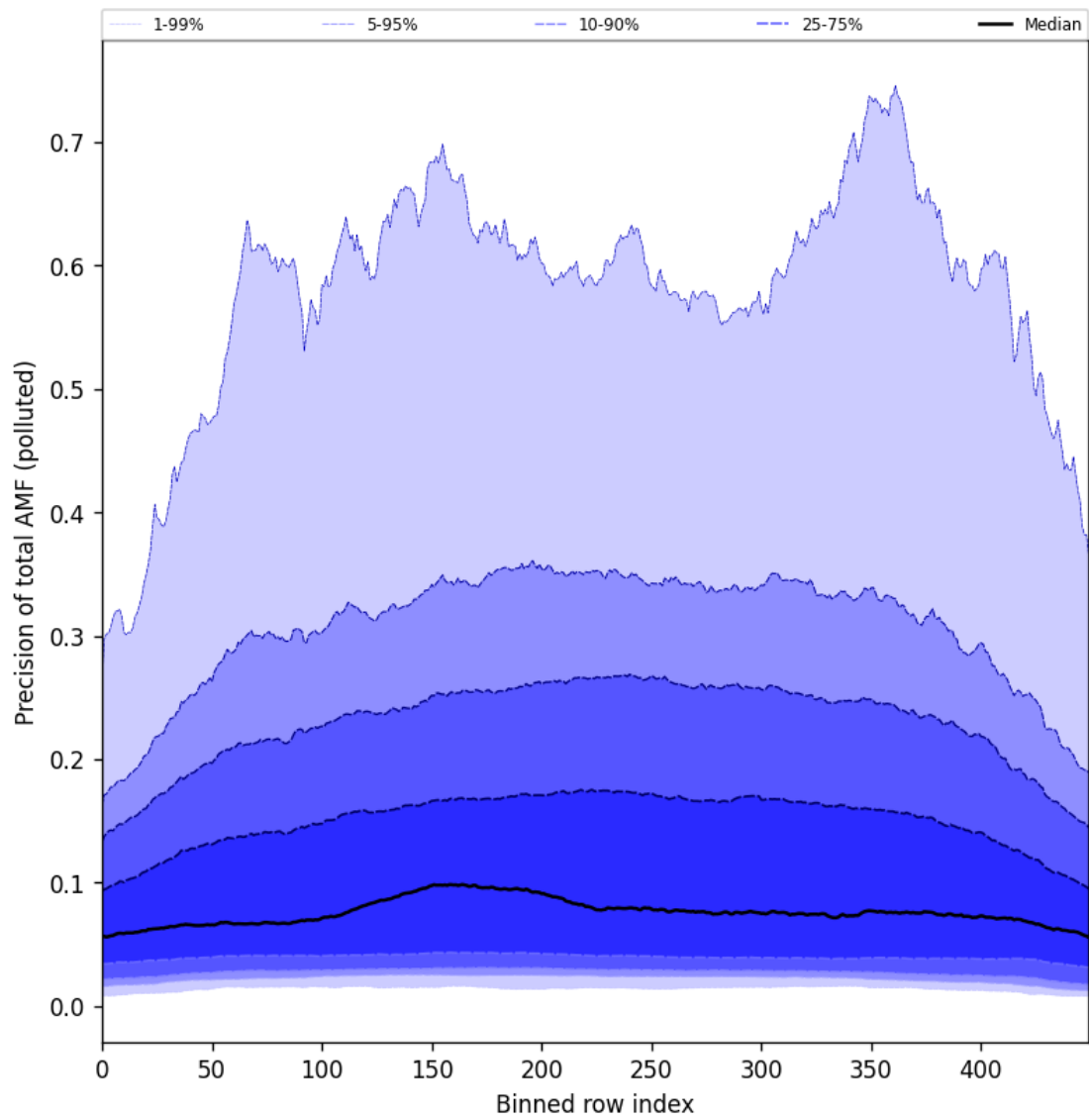
Figure 106: Along track statistics of “Precision of total AMF (polluted)” for 2025-08-15 to 2025-08-17
