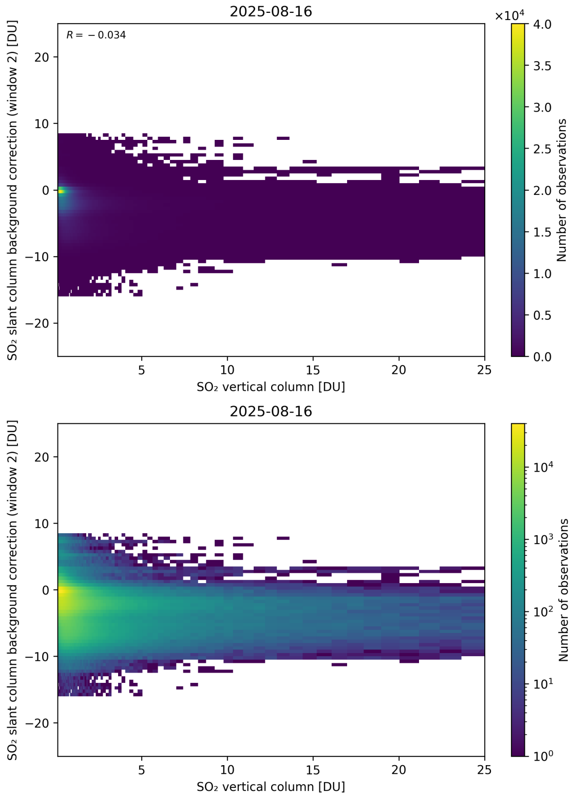
Figure 324: Scatter density plot of “SO 2 vertical column” against “SO 2 slant column background correction (window 2)” for 2025-08-15 to 2025-08-17.
