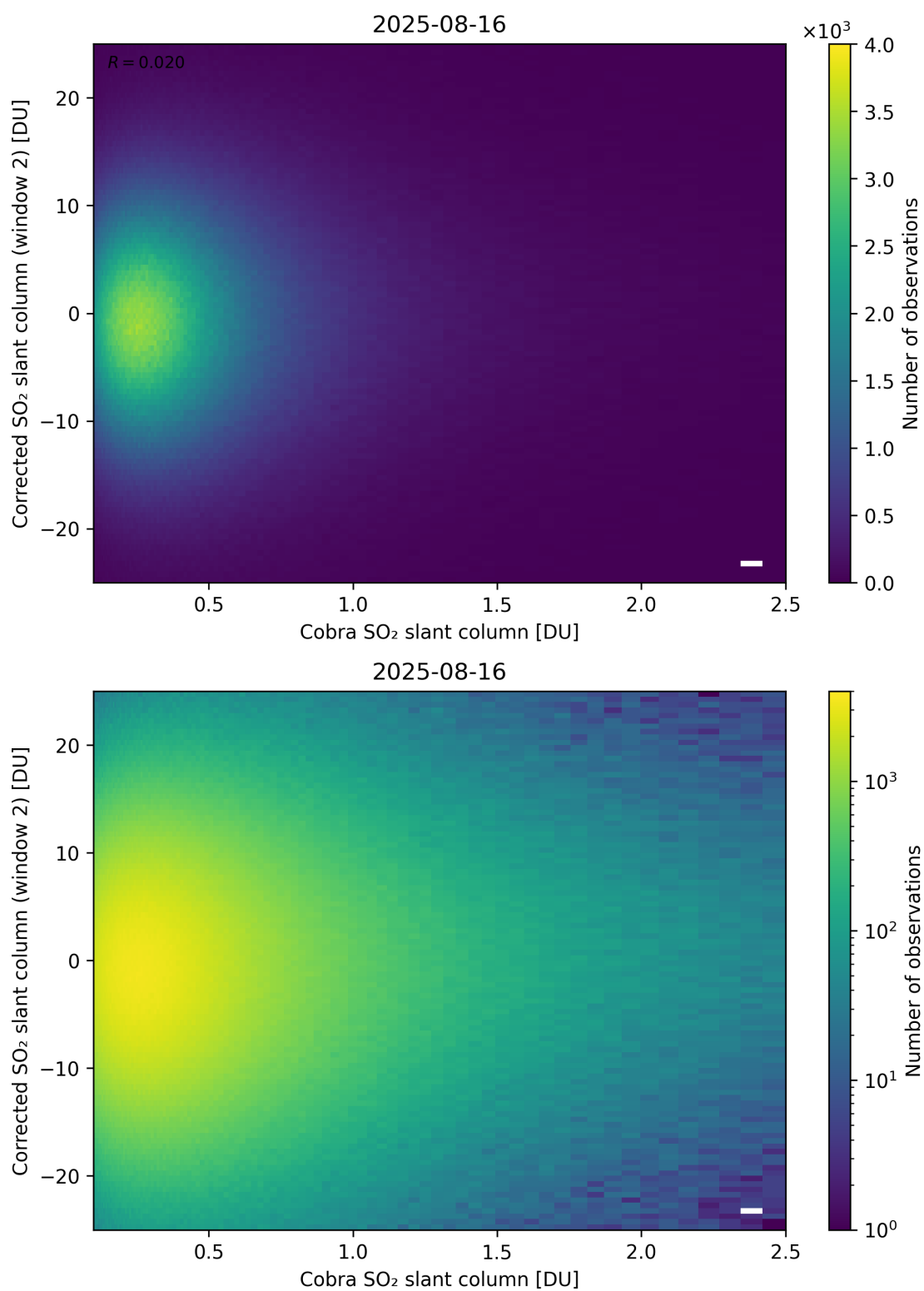
Figure 217: Scatter density plot of “Cobra SO 2 slant column” against “Corrected SO 2 slant column (window 2)” for 2025-08-15 to 2025-08-17.
