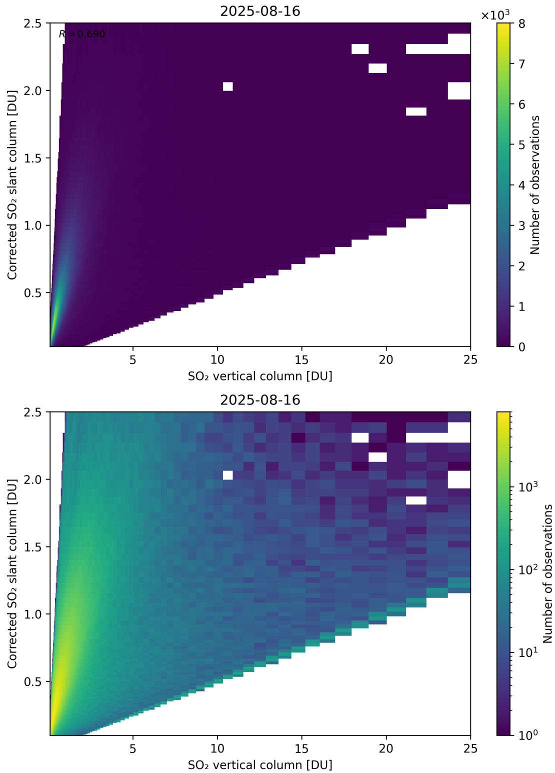
Figure 351: Scatter density plot of “SO 2 vertical column” against “Corrected SO 2 slant column” for 2025-08-15 to 2025-08-17.
