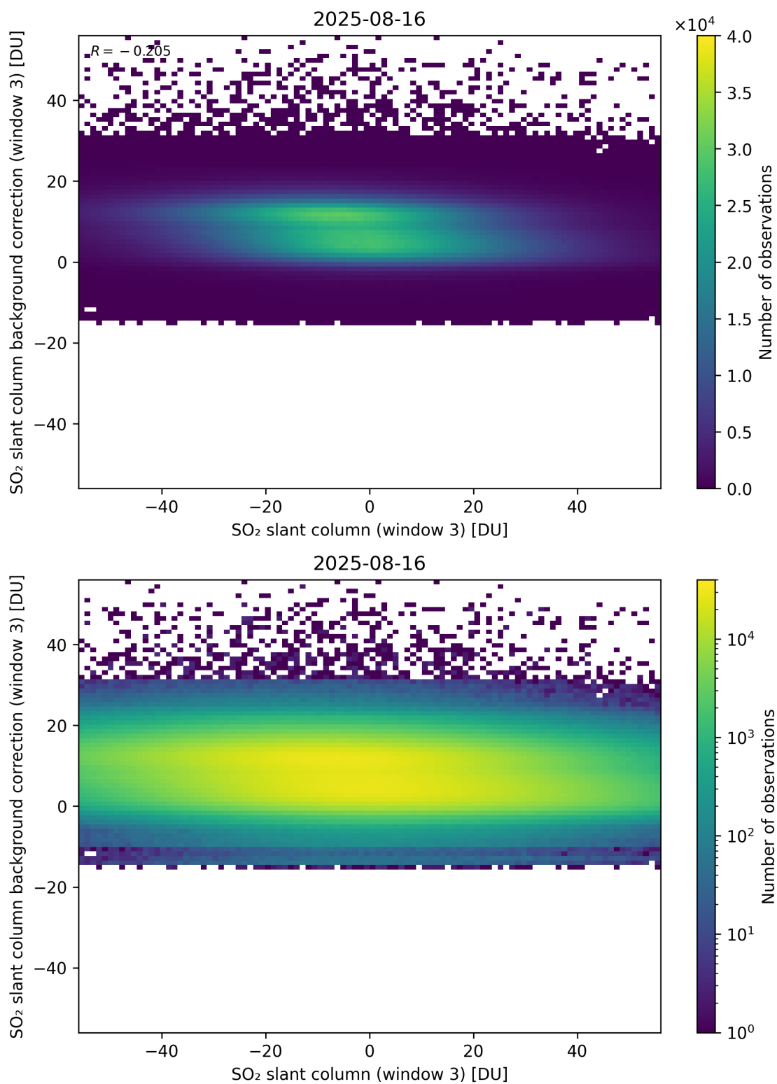
Figure 303: Scatter density plot of “SO 2 slant column (window 3)” against “SO 2 slant column background correction (window 3)” for 2025-08-15 to 2025-08-17.
