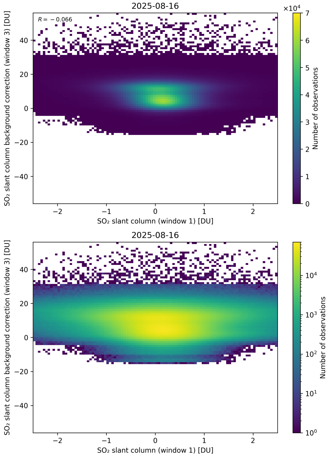
Figure 264: Scatter density plot of “SO 2 slant column (window 1)” against “SO 2 slant column background correction (window 3)” for 2025-08-15 to 2025-08-17.
