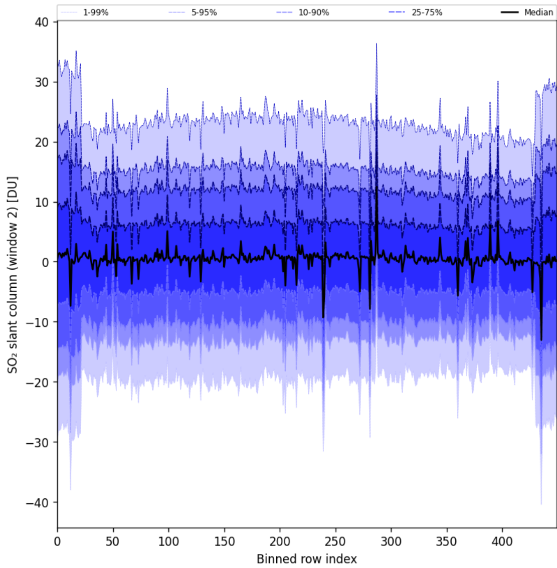
Figure 93: Along track statistics of “SO 2 slant column (window 2)” for 2025-08-15 to 2025-08-17
