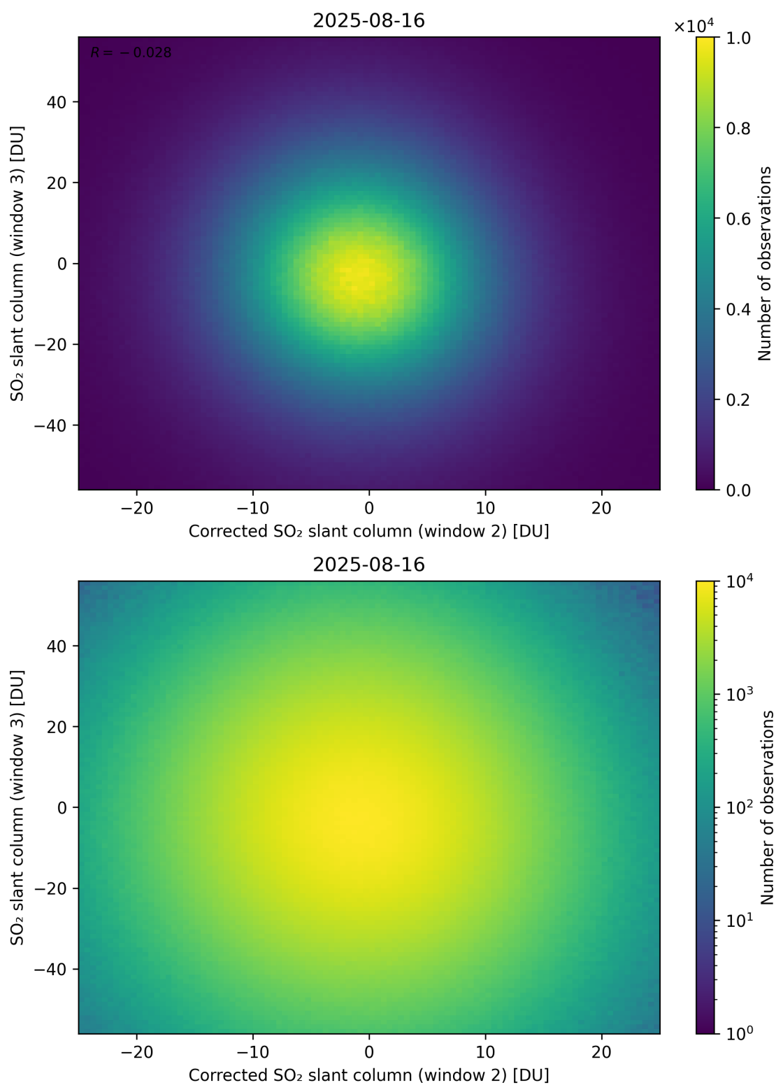
Figure 251: Scatter density plot of “Corrected SO 2 slant column (window 2)” against “SO 2 slant column (window 3)” for 2025-08-15 to 2025-08-17.
