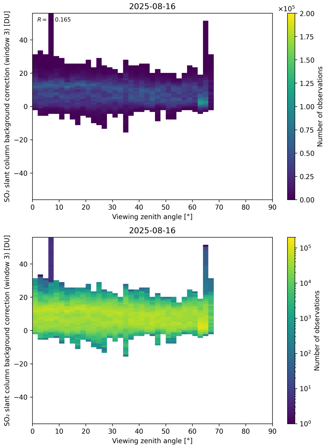
Figure 364: Scatter density plot of “Viewing zenith angle” against “SO 2 slant column background correction (window 3)” for 2025-08-15 to 2025-08-17.
