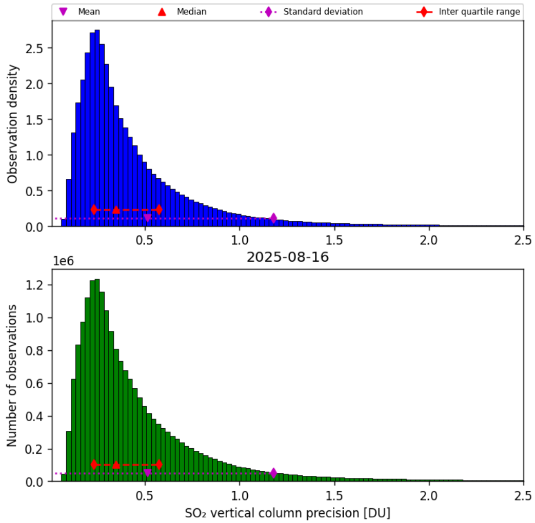
Figure 59: Histogram of “SO 2 vertical column precision” for 2025-08-15 to 2025-08-17
