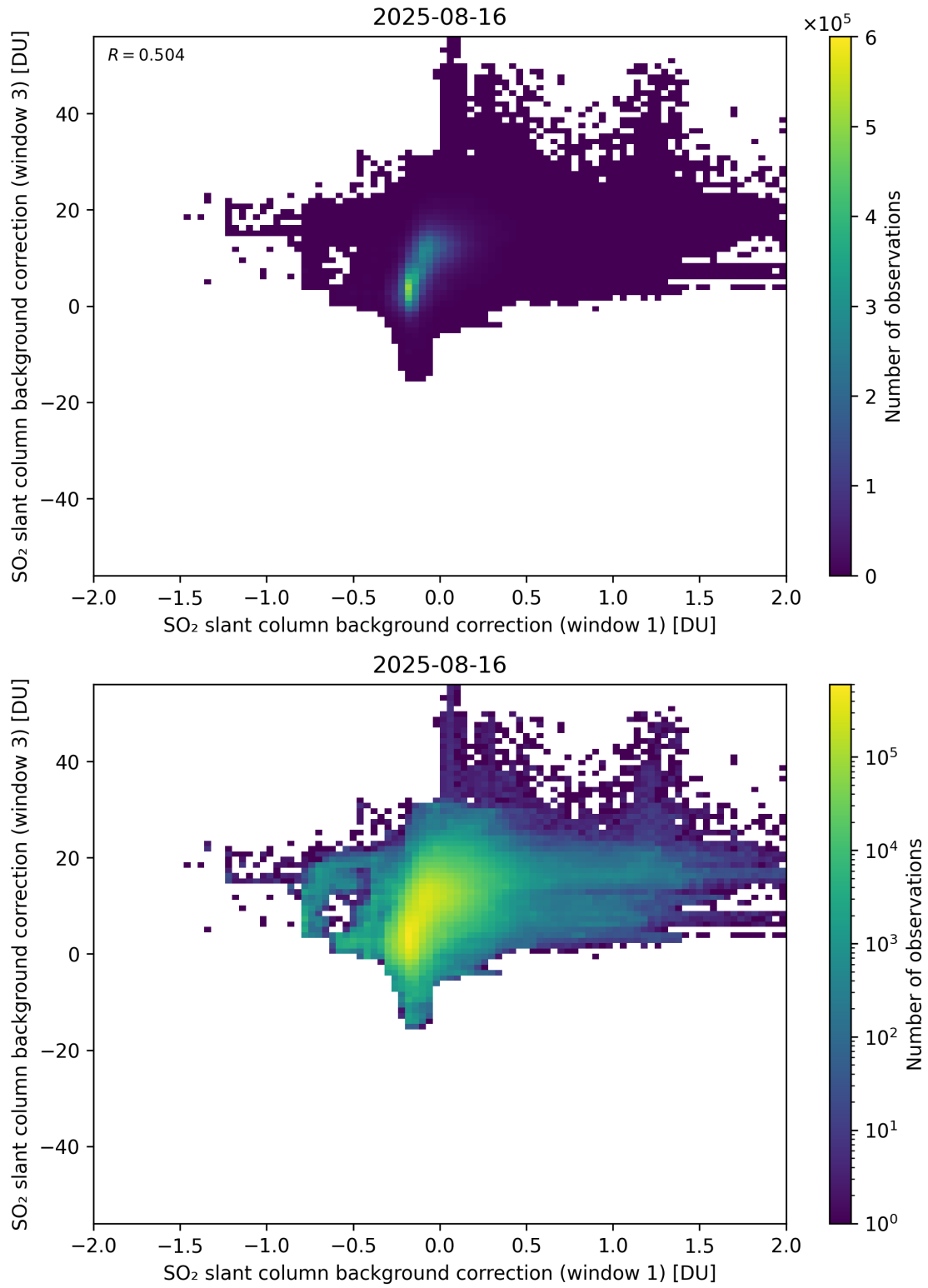
Figure 110: Scatter density plot of “SO 2 slant column background correction (window 1)” against “SO 2 slant column background correction (window 3)” for 2025-08-15 to 2025-08-17.
