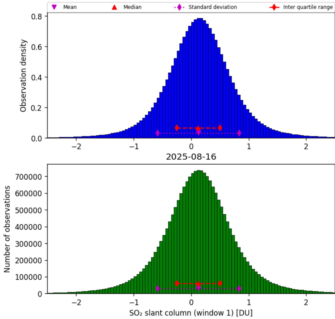
Figure 63: Histogram of “SO 2 slant column (window 1)” for 2025-08-15 to 2025-08-17
