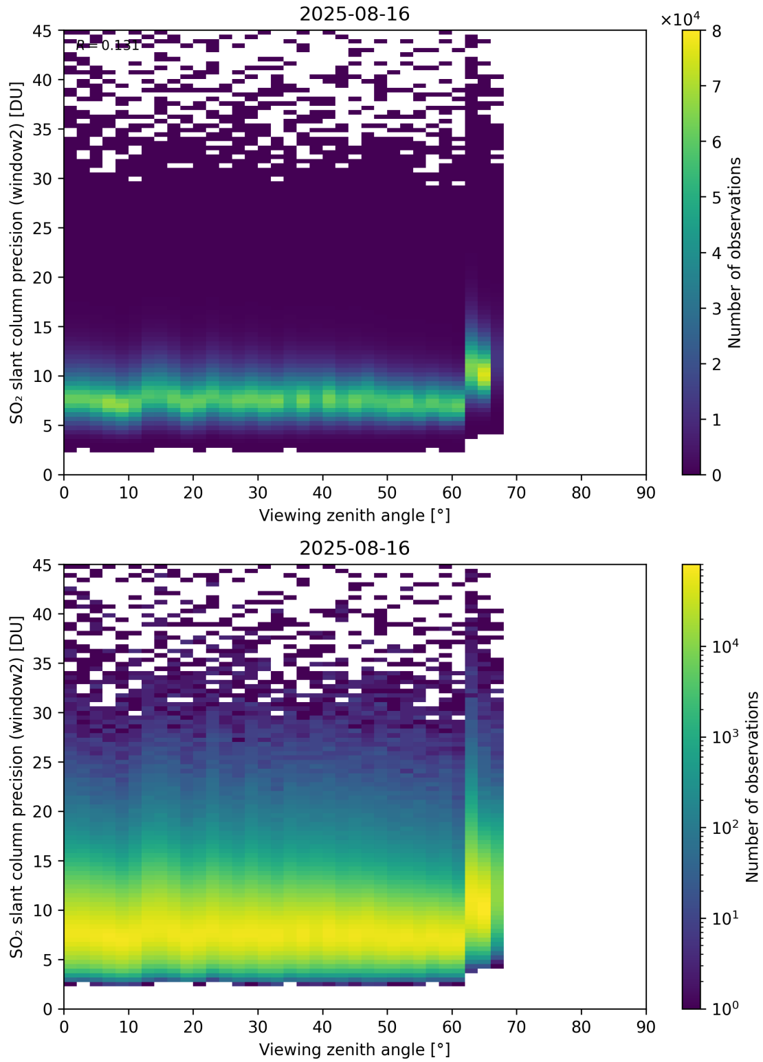
Figure 378: Scatter density plot of “Viewing zenith angle” against “SO 2 slant column precision (window2)” for 2025-08-15 to 2025-08-17.
