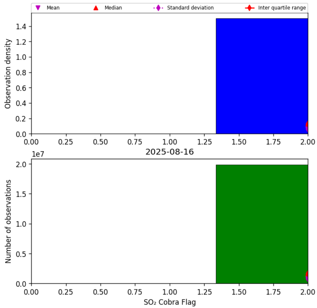
Figure 75: Histogram of “SO 2 Cobra Flag” for 2025-08-15 to 2025-08-17
