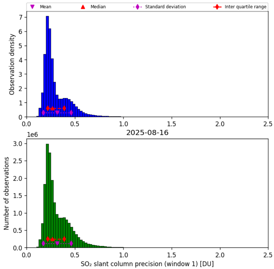
Figure 64: Histogram of “SO 2 slant column precision (window 1)” for 2025-08-15 to 2025-08-17
