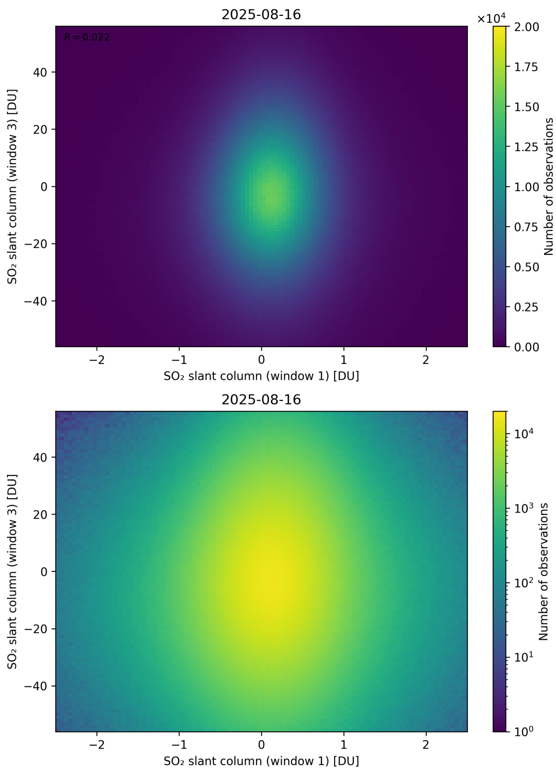
Figure 287: Scatter density plot of “SO 2 slant column (window 1)” against “SO 2 slant column (window 3)” for 2025-08-15 to 2025-08-17.
