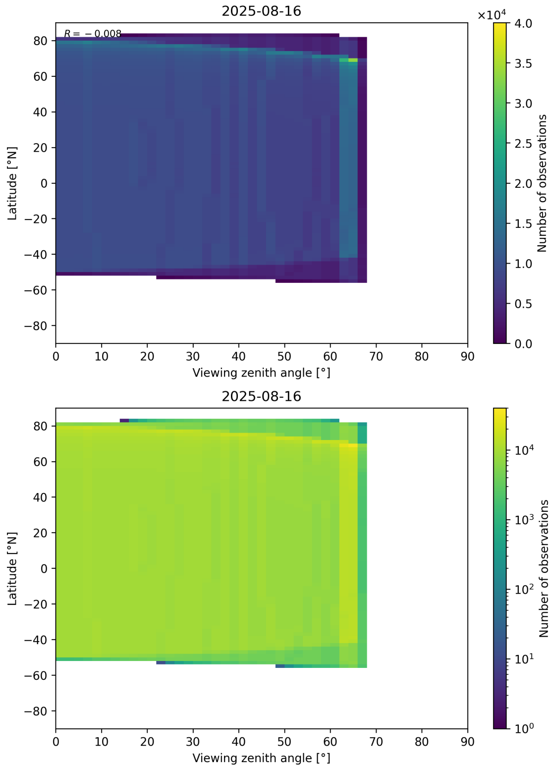
Figure 368: Scatter density plot of “Viewing zenith angle” against “Latitude” for 2025-08-15 to 2025-08-17.
