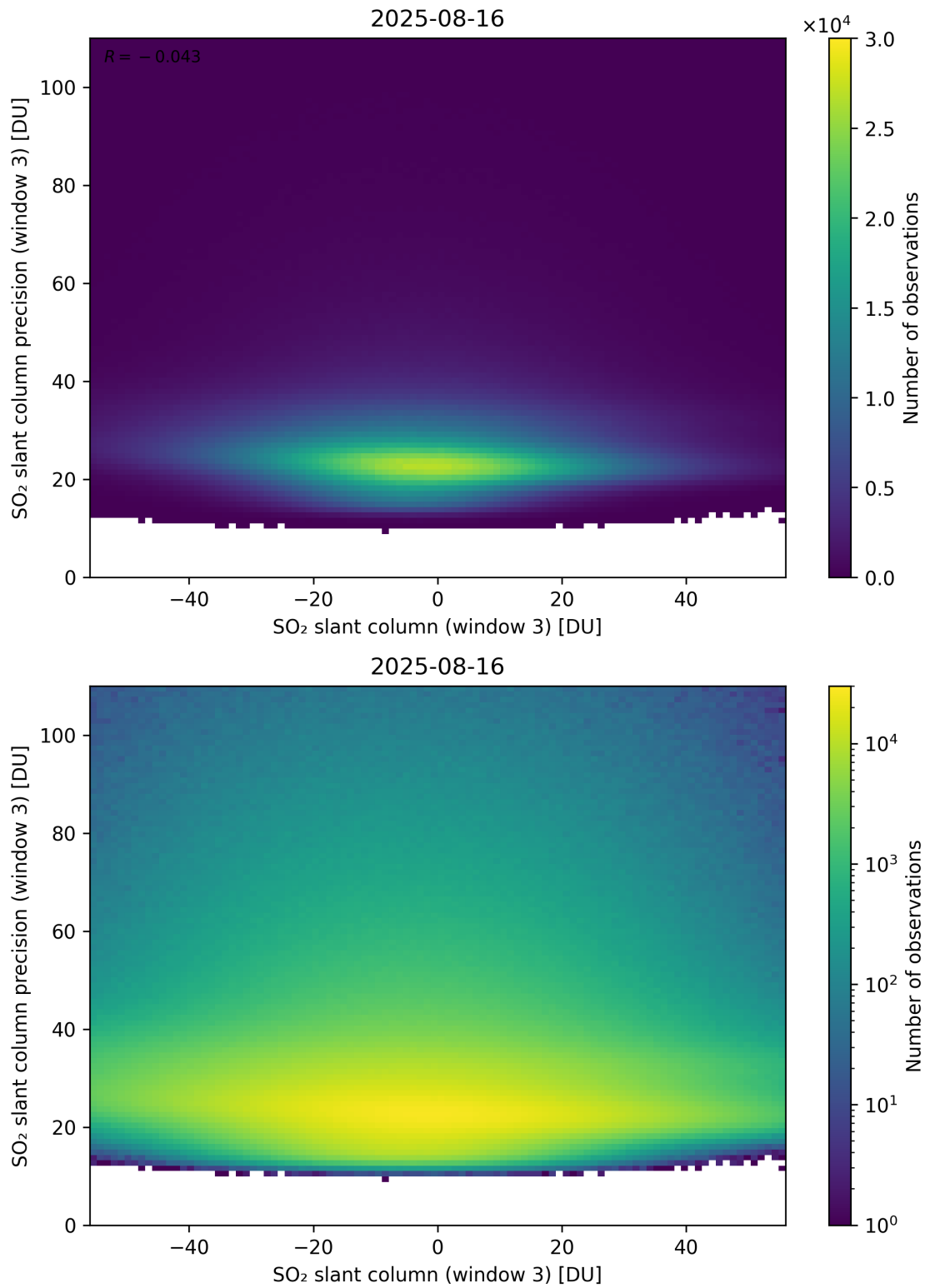
Figure 317: Scatter density plot of “SO 2 slant column (window 3)” against “SO 2 slant column precision (window 3)” for 2025-08-15 to 2025-08-17.
