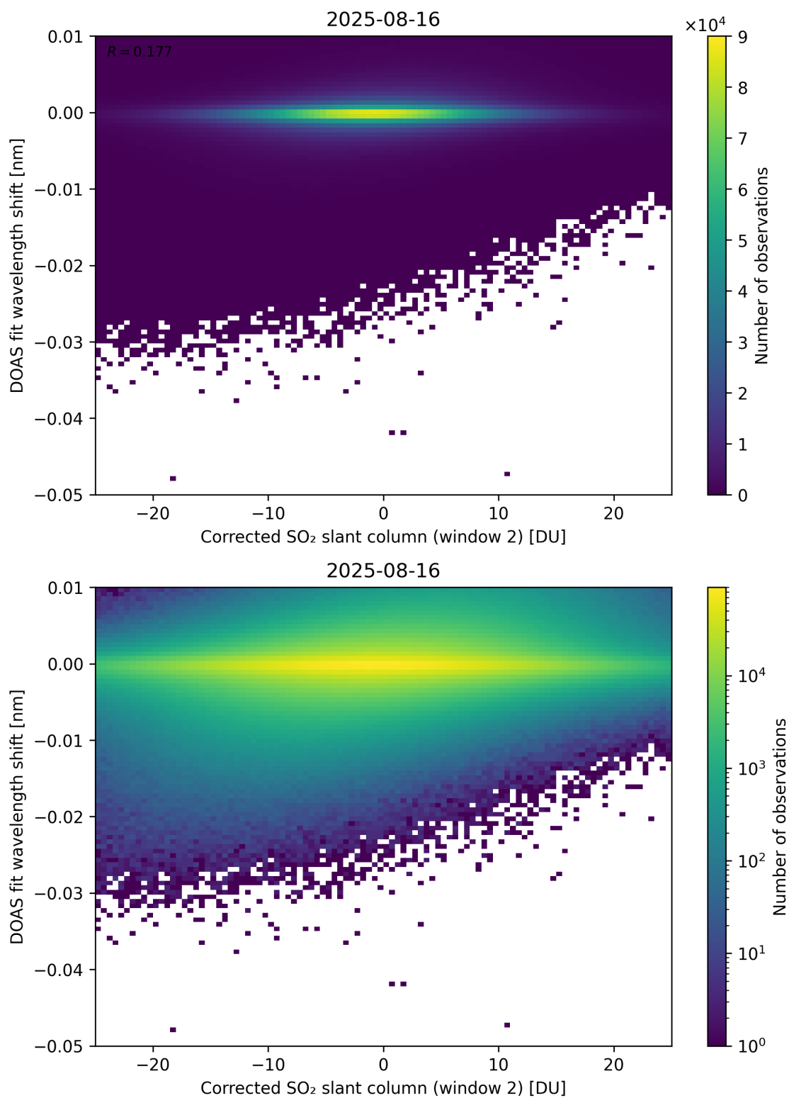
Figure 246: Scatter density plot of “Corrected SO 2 slant column (window 2)” against “DOAS fit wavelength shift” for 2025-08-15 to 2025-08-17.
