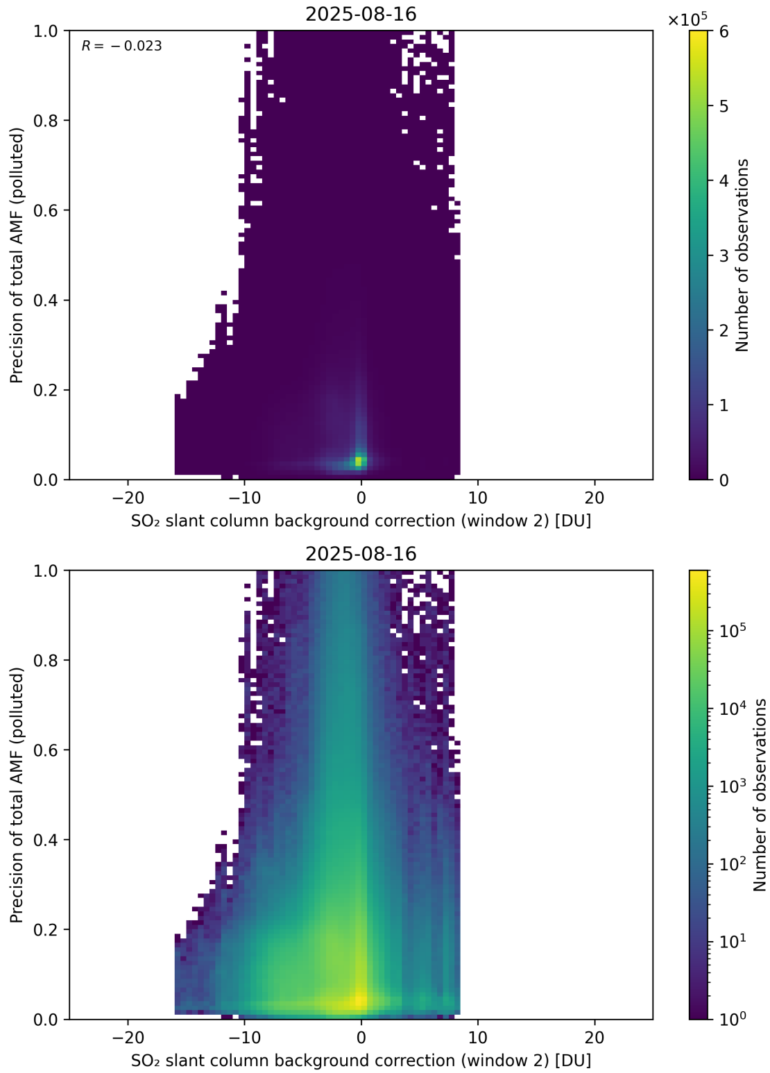
Figure 131: Scatter density plot of “SO 2 slant column background correction (window 2)” against “Precision of total AMF (polluted)” for 2025-08-15 to 2025-08-17.
