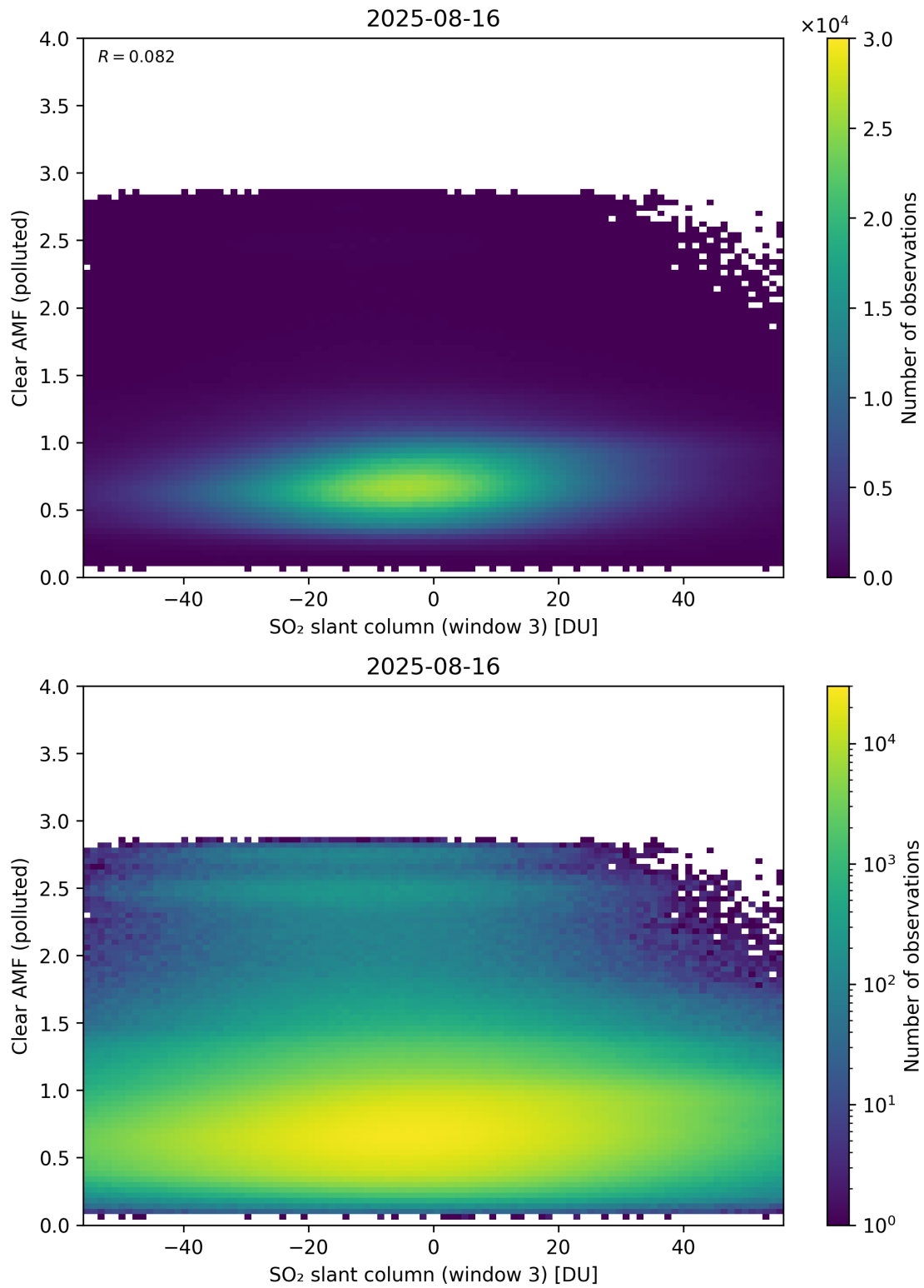
Figure 315: Scatter density plot of “SO 2 slant column (window 3)” against “Clear AMF (polluted)” for 2025-08-15 to 2025-08-17.
