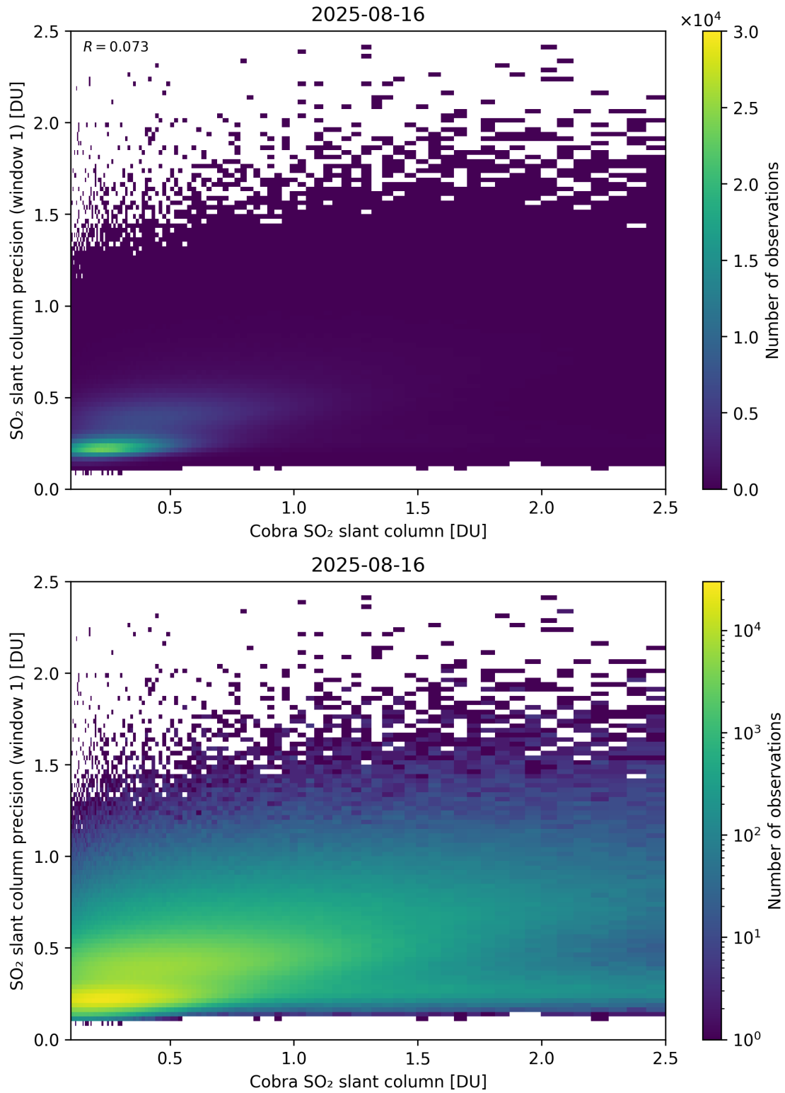
Figure 220: Scatter density plot of “Cobra SO 2 slant column” against “SO 2 slant column precision (window 1)” for 2025-08-15 to 2025-08-17.
