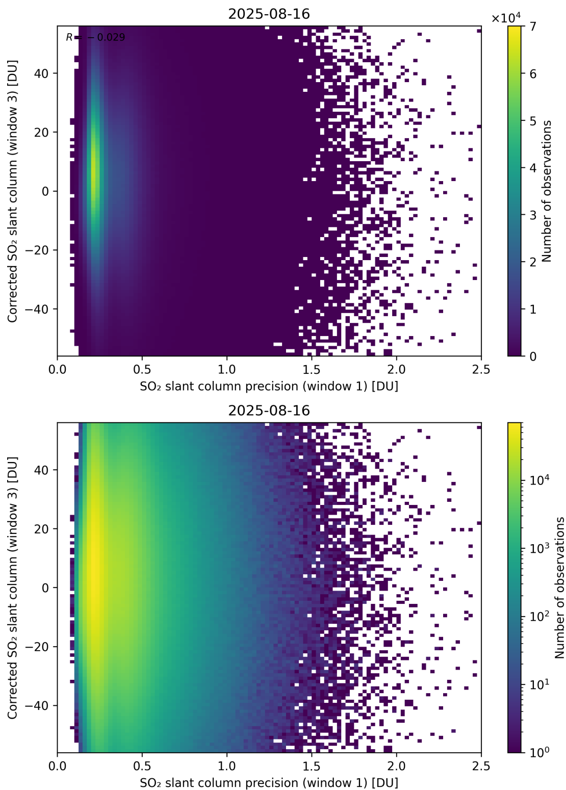
Figure 276: Scatter density plot of “SO 2 slant column precision (window 1)” against “Corrected SO 2 slant column (window 3)” for 2025-08-15 to 2025-08-17.
