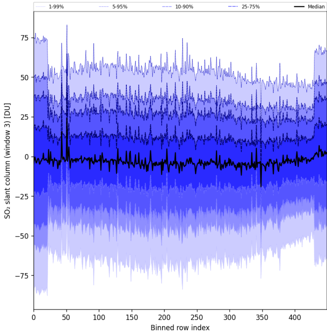
Figure 97: Along track statistics of “SO 2 slant column (window 3)” for 2025-08-15 to 2025-08-17
