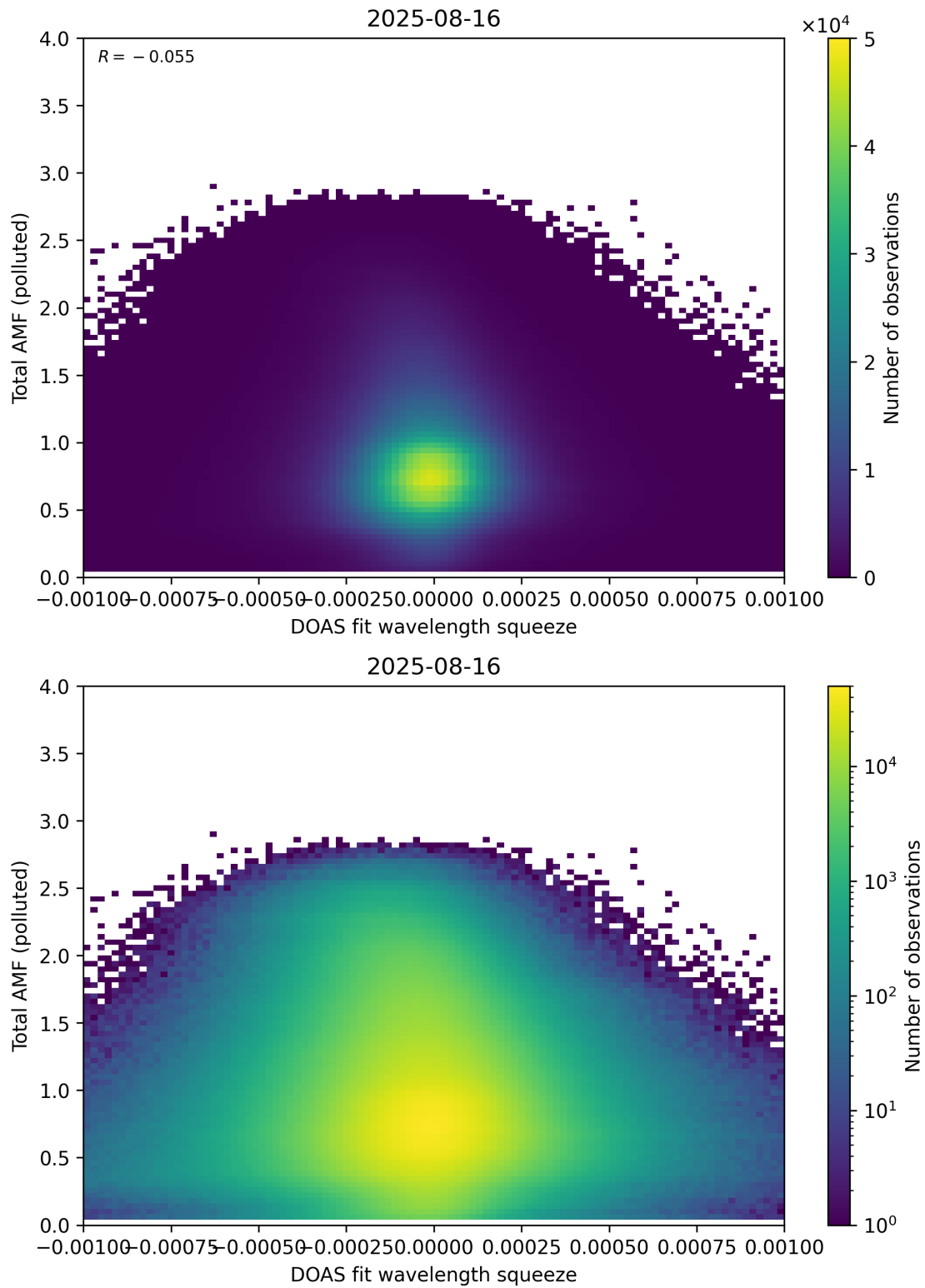
Figure 145: Scatter density plot of “DOAS fit wavelength squeeze” against “Total AMF (polluted)” for 2025-08-15 to 2025-08-17.
