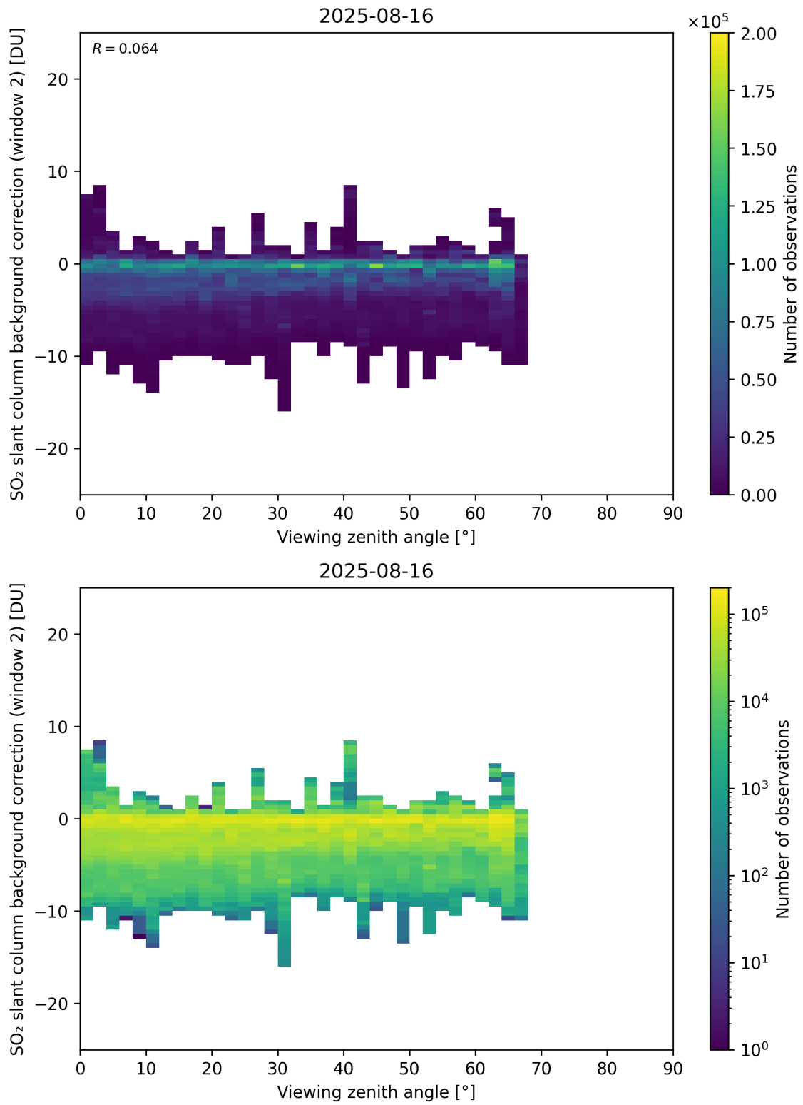
Figure 363: Scatter density plot of “Viewing zenith angle” against “SO 2 slant column background correction (window 2)” for 2025-08-15 to 2025-08-17.
