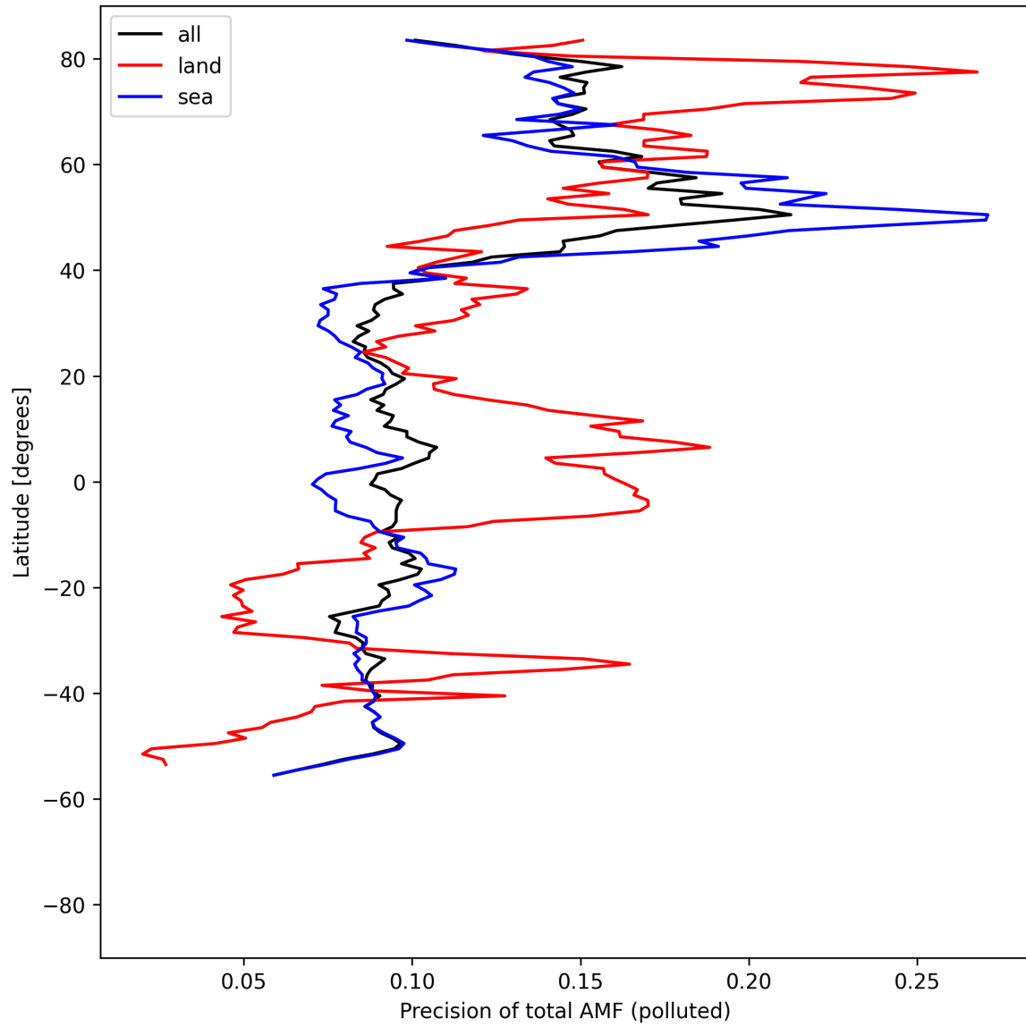
Figure 54: Zonal average of “Precision of total AMF (polluted)” for 2025-08-15 to 2025-08-17.
