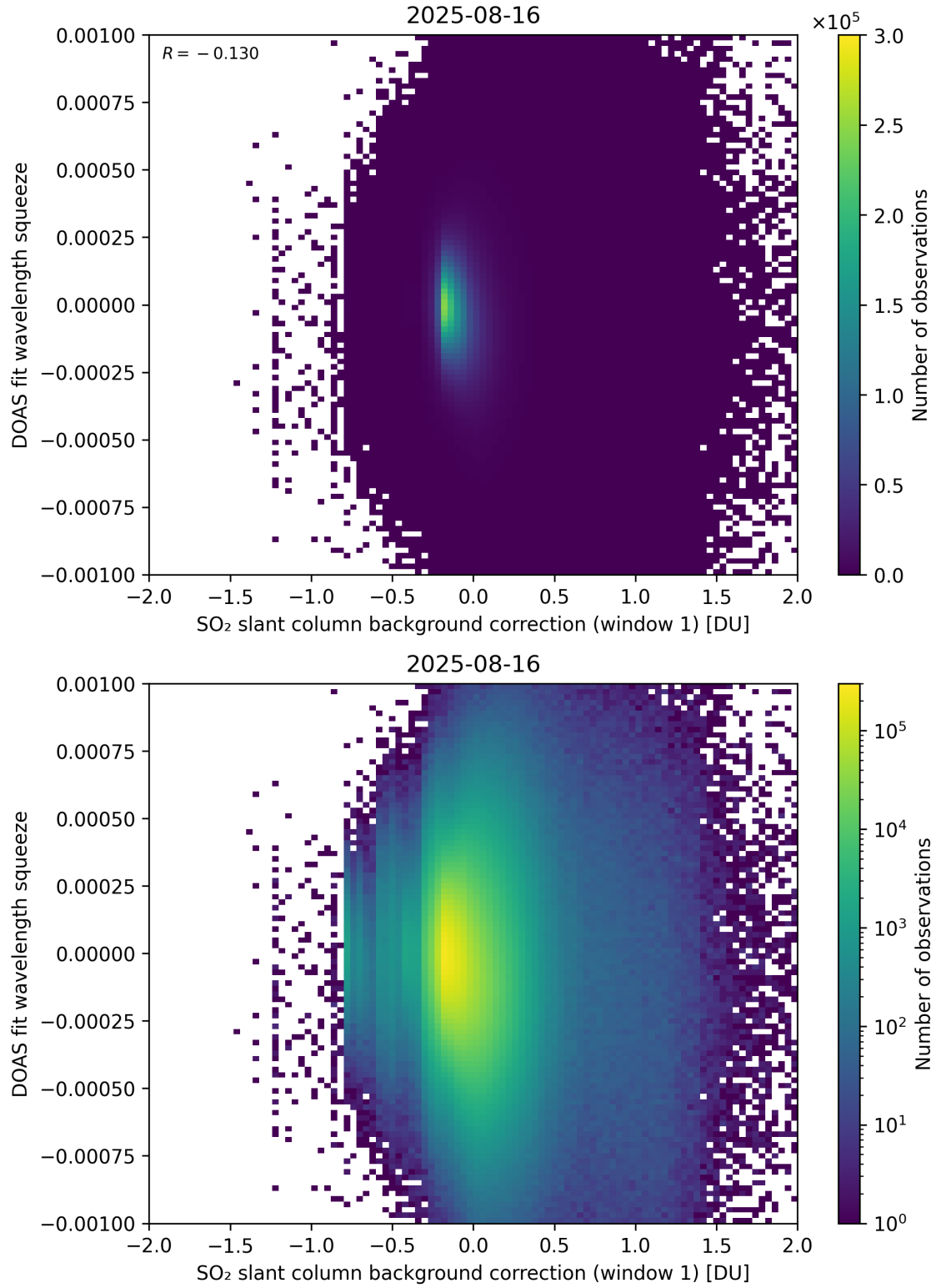
Figure 112: Scatter density plot of “SO 2 slant column background correction (window 1)” against “DOAS fit wavelength squeeze” for 2025-08-15 to 2025-08-17.
