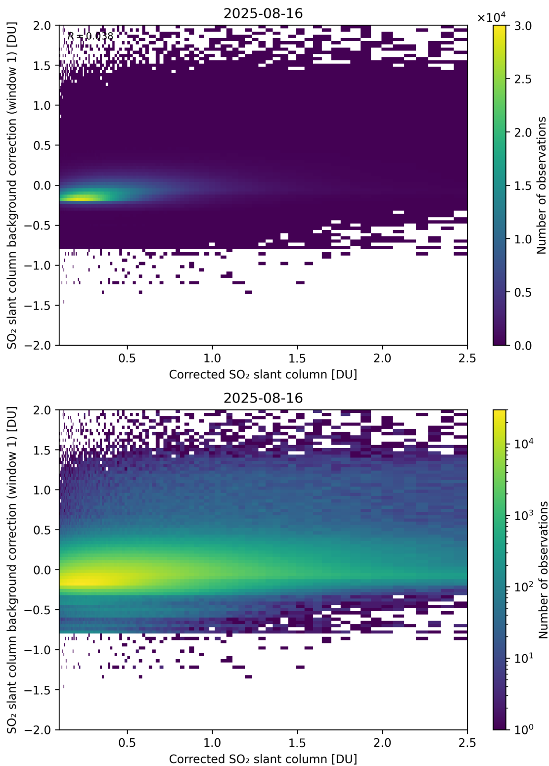
Figure 226: Scatter density plot of “Corrected SO 2 slant column” against “SO 2 slant column background correction (window 1)” for 2025-08-15 to 2025-08-17.
