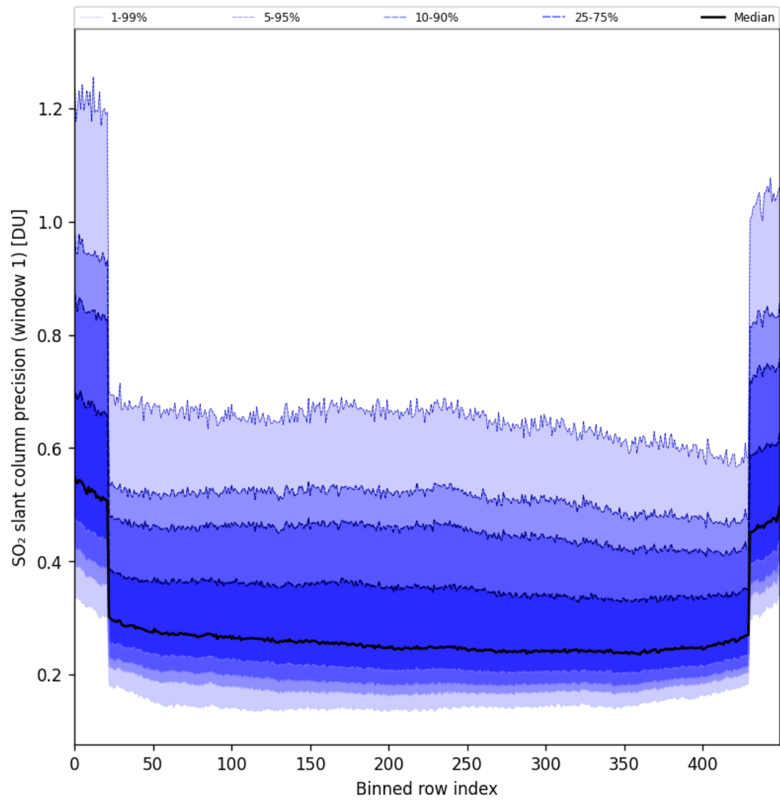
Figure 90: Along track statistics of “SO 2 slant column precision (window 1)” for 2025-08-15 to 2025-08-17
