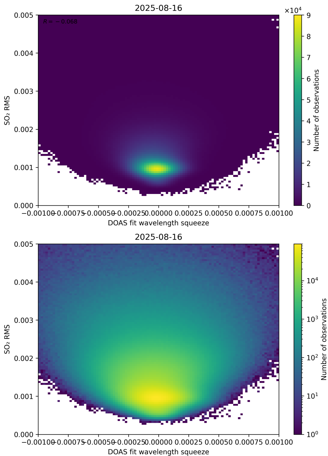
Figure 143: Scatter density plot of “DOAS fit wavelength squeeze” against “SO 2 RMS” for 2025-08-15 to 2025-08-17.
