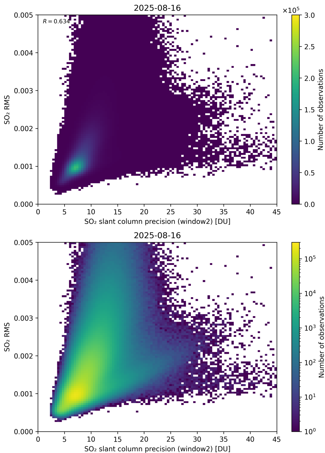
Figure 295: Scatter density plot of “SO 2 slant column precision (window2)” against “SO 2 RMS” for 2025-08-15 to 2025-08-17.
