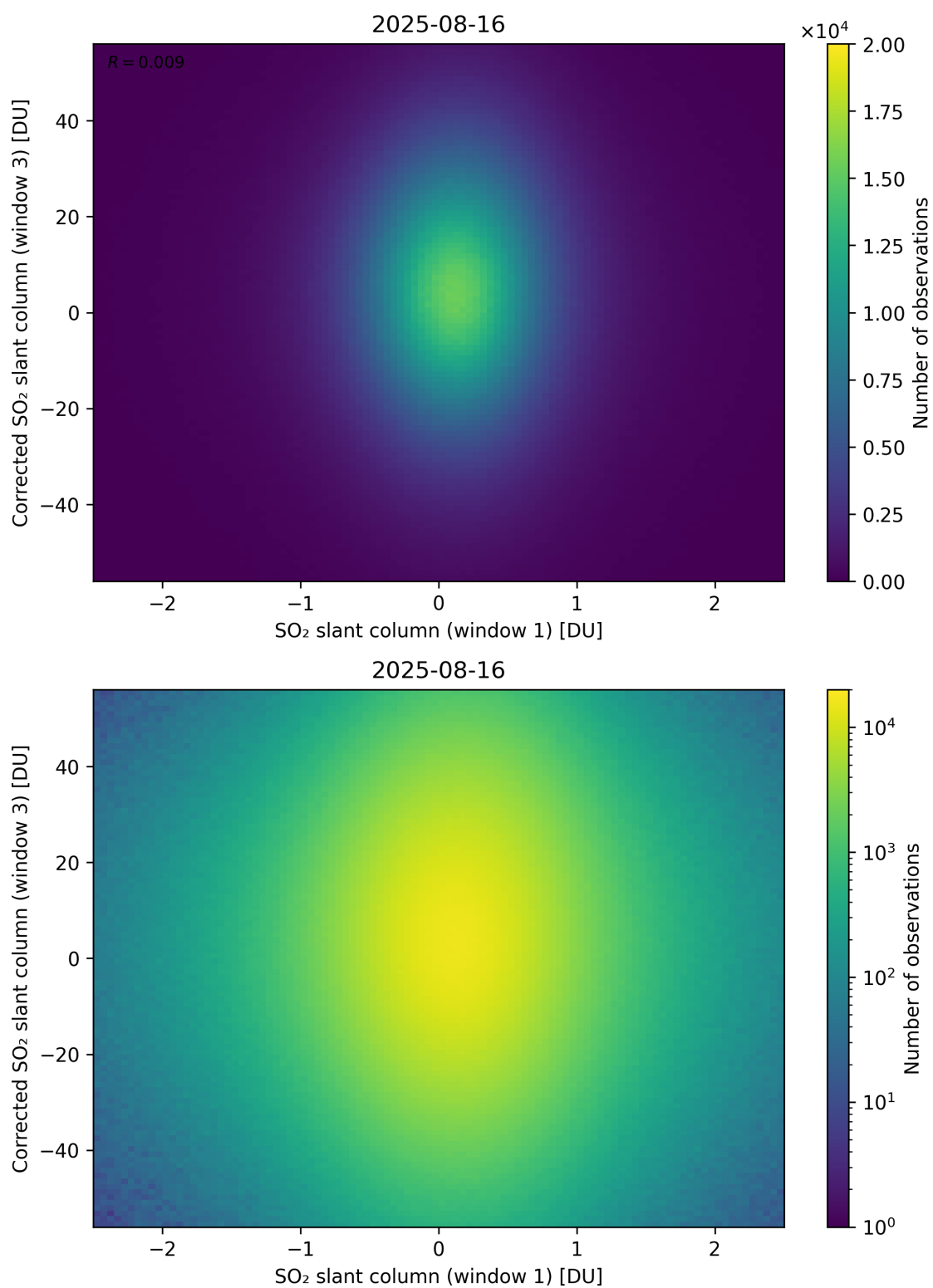
Figure 284: Scatter density plot of “SO 2 slant column (window 1)” against “Corrected SO 2 slant column (window 3)” for 2025-08-15 to 2025-08-17.
