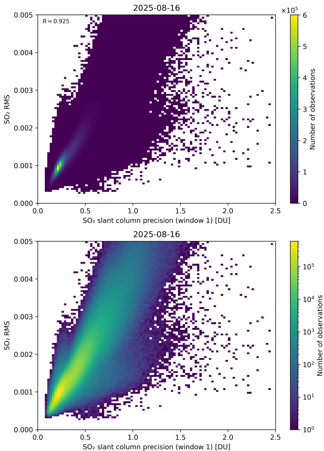
Figure 273: Scatter density plot of “SO 2 slant column precision (window 1)” against “SO 2 RMS” for 2025-08-15 to 2025-08-17.
