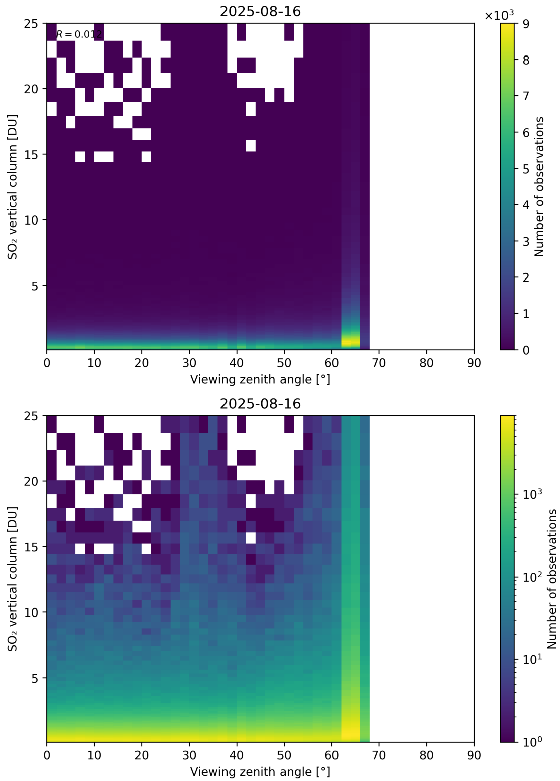
Figure 383: Scatter density plot of “Viewing zenith angle” against “SO 2 vertical column” for 2025-08-15 to 2025-08-17.
