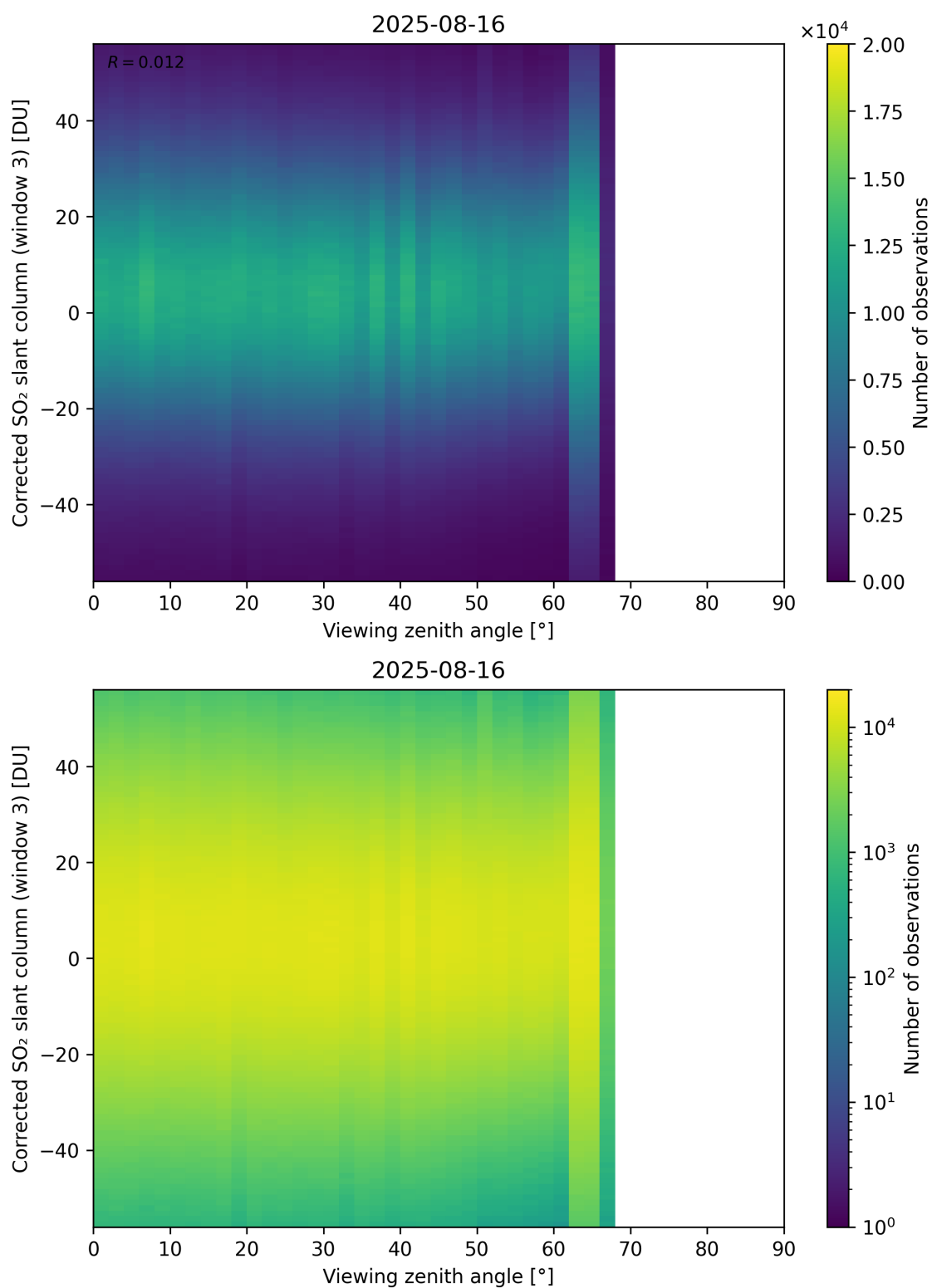
Figure 375: Scatter density plot of “Viewing zenith angle” against “Corrected SO 2 slant column (window 3)” for 2025-08-15 to 2025-08-17.
