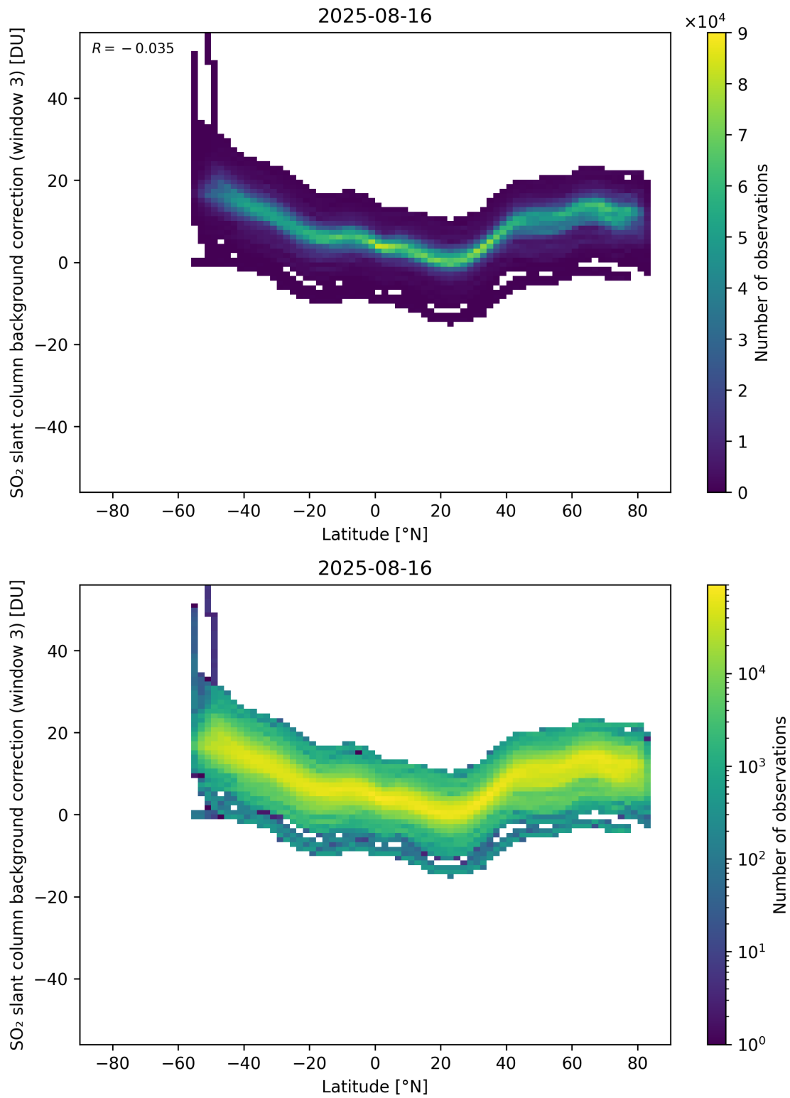
Figure 152: Scatter density plot of “Latitude” against “SO 2 slant column background correction (window 3)” for 2025-08-15 to 2025-08-17.
