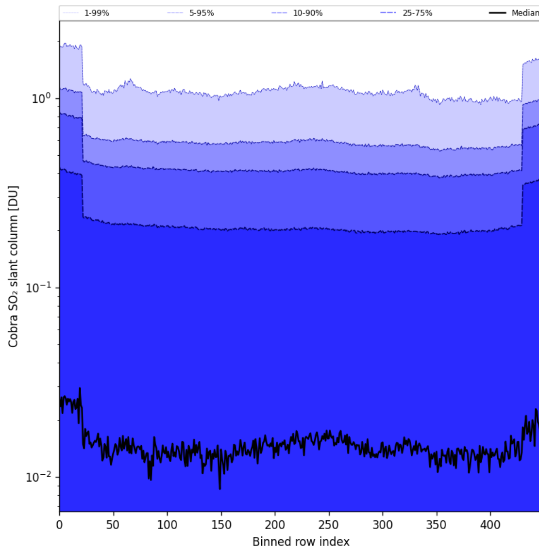
Figure 87: Along track statistics of "Cobra SO 2 slant column" for 2025-08-15 to 2025-08-17
