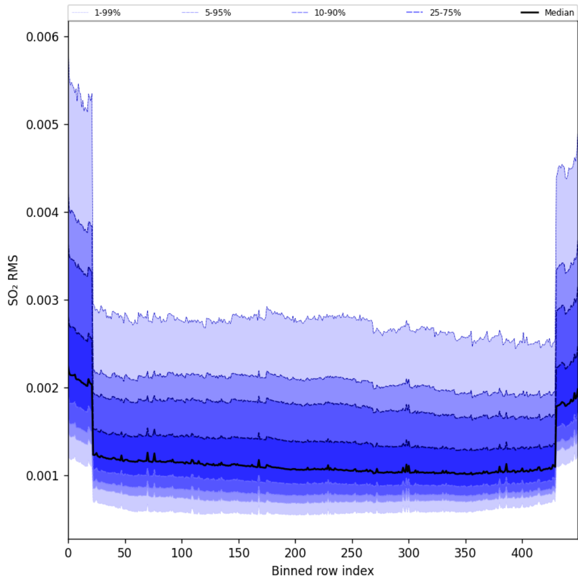
Figure 104: Along track statistics of “SO 2 RMS” for 2025-08-15 to 2025-08-17
