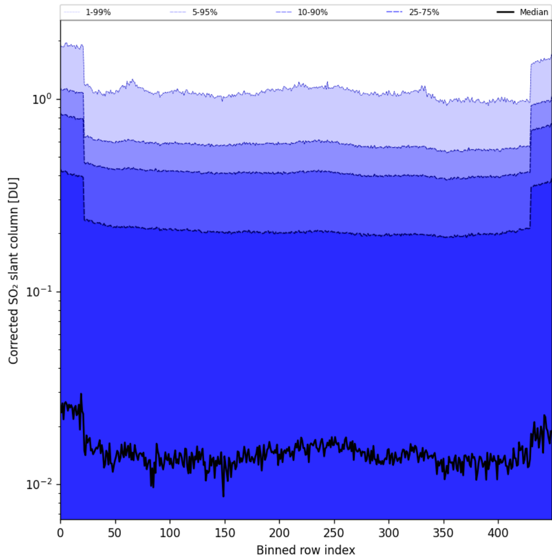
Figure 86: Along track statistics of “Corrected SO 2 slant column” for 2025-08-15 to 2025-08-17
