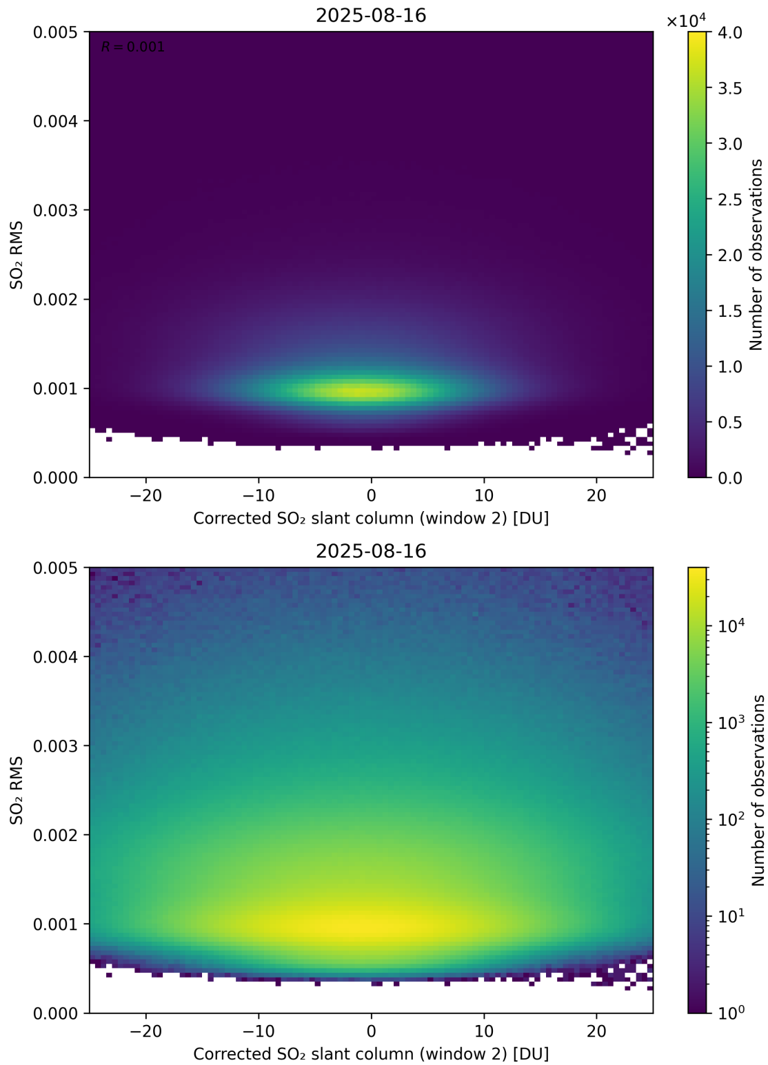
Figure 248: Scatter density plot of “Corrected SO 2 slant column (window 2)” against “SO 2 RMS” for 2025-08-15 to 2025-08-17.
