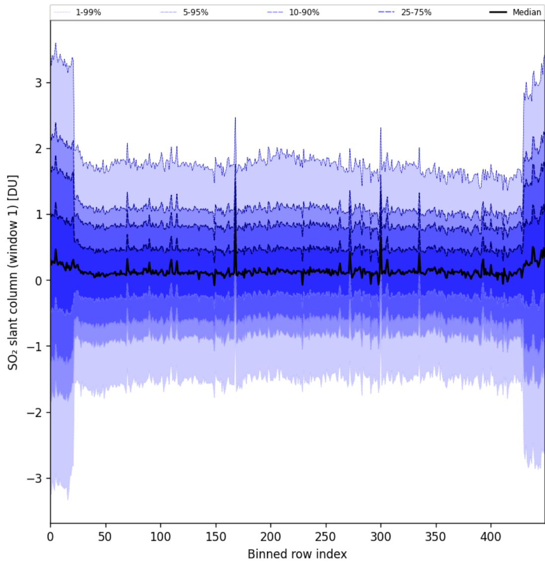
Figure 89: Along track statistics of “SO 2 slant column (window 1)” for 2025-08-15 to 2025-08-17
