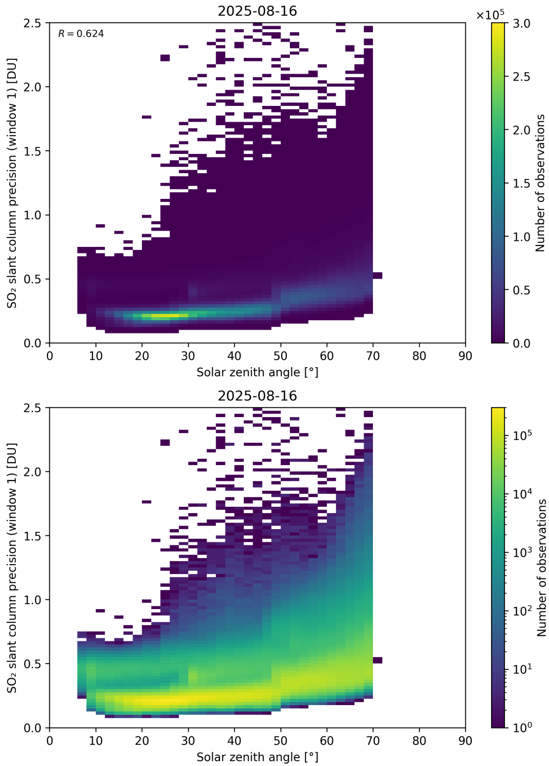
Figure 185: Scatter density plot of “Solar zenith angle” against “SO 2 slant column precision (window 1)” for 2025-08-15 to 2025-08-17.
