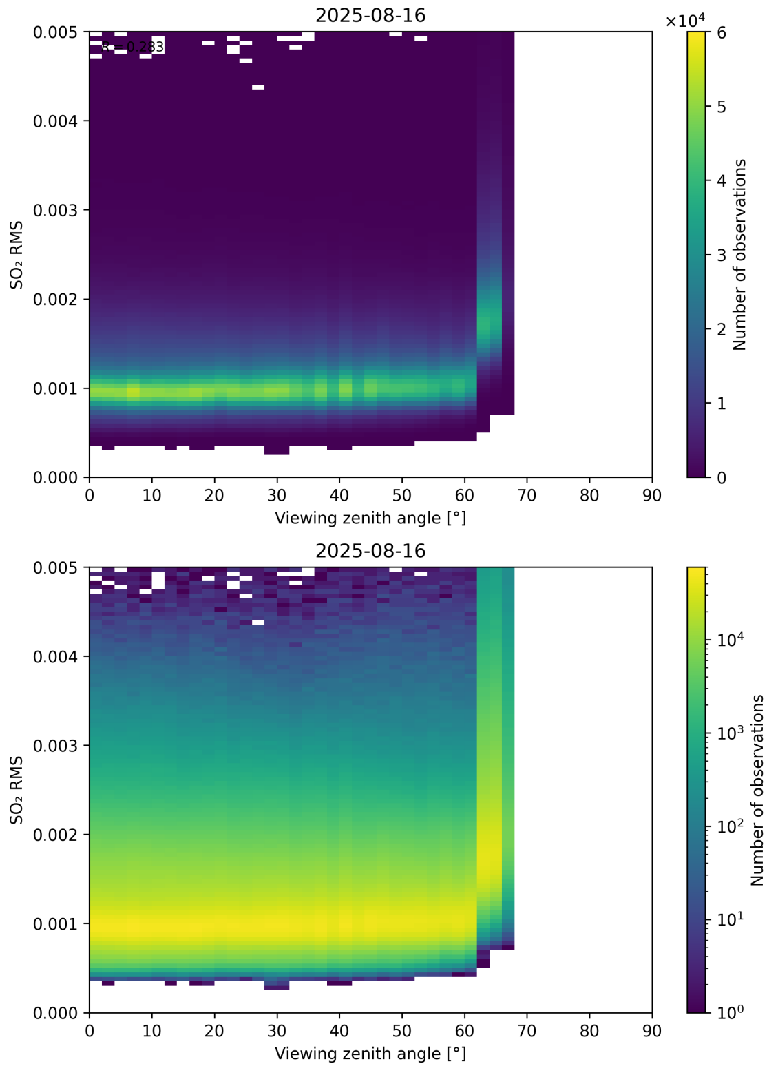
Figure 367: Scatter density plot of “Viewing zenith angle” against “SO 2 RMS” for 2025-08-15 to 2025-08-17.
