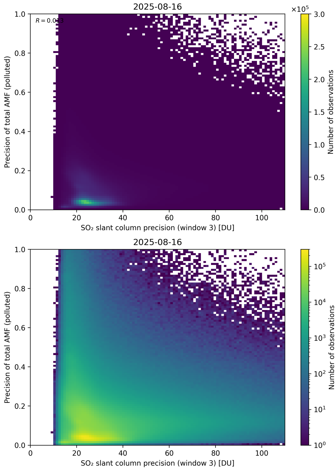
Figure 314: Scatter density plot of “SO 2 slant column precision (window 3)” against “Precision of total AMF (polluted)” for 2025-08-15 to 2025-08-17.
