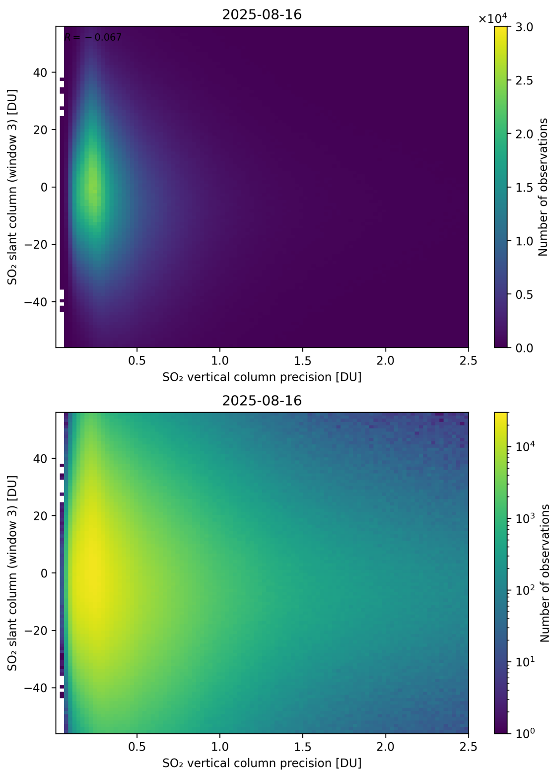
Figure 344: Scatter density plot of “SO 2 vertical column precision” against “SO 2 slant column (window 3)” for 2025-08-15 to 2025-08-17.
