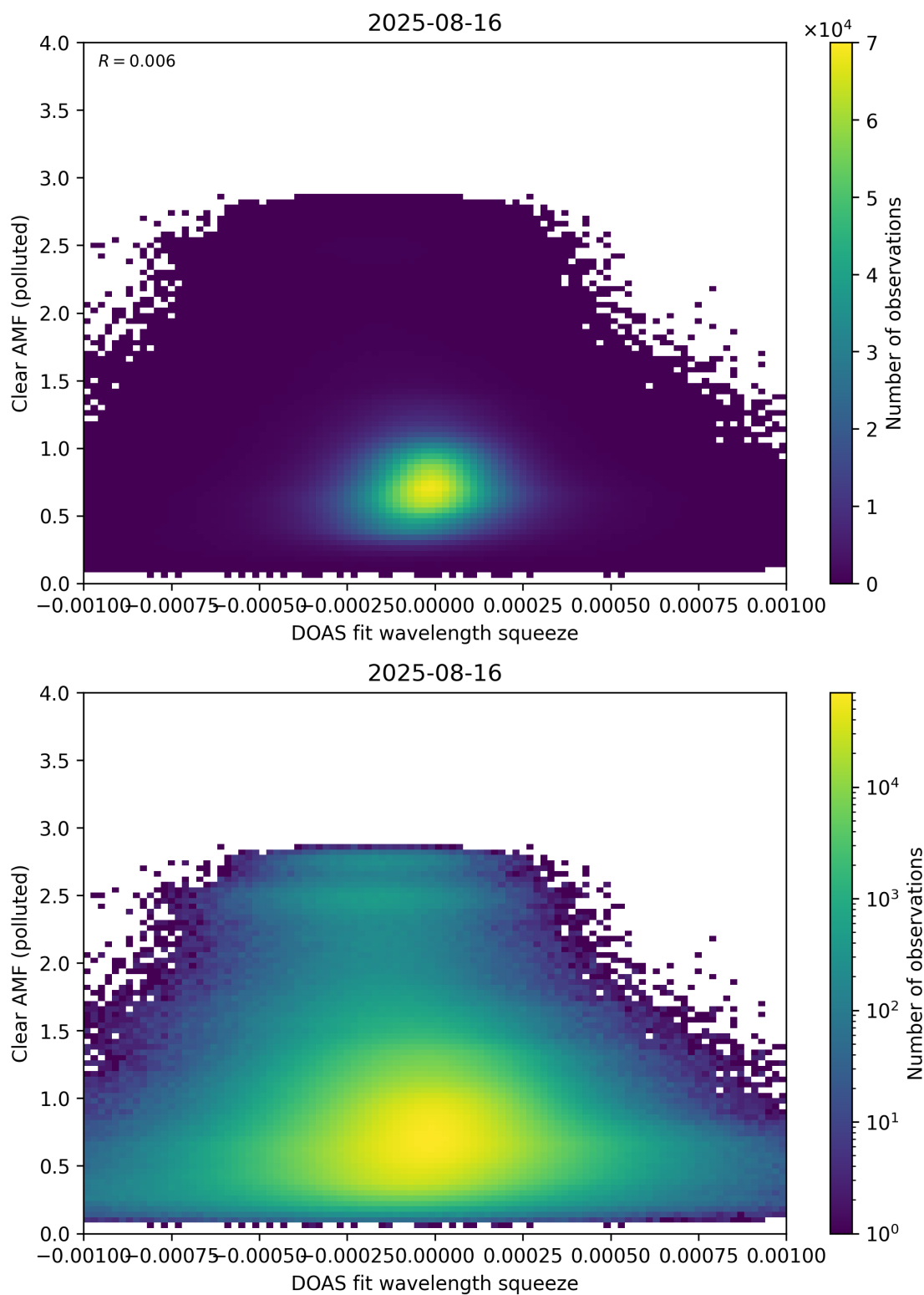
Figure 144: Scatter density plot of “DOAS fit wavelength squeeze” against “Clear AMF (polluted)” for 2025-08-15 to 2025-08-17.
