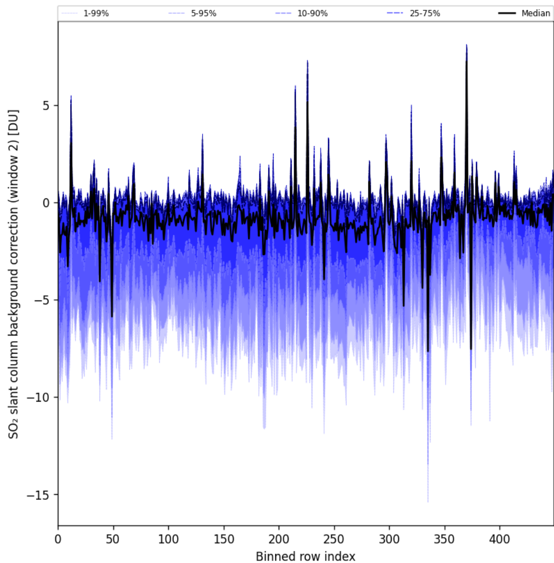
Figure 96: Along track statistics of “SO 2 slant column background correction (window 2)” for 2025-08-15 to 2025-08-17
