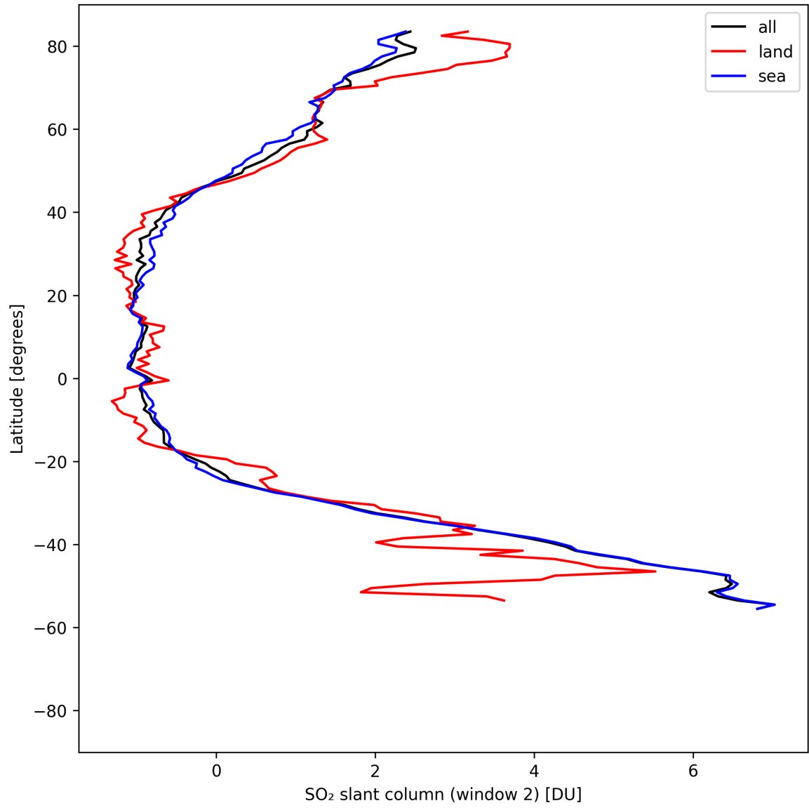
Figure 41: Zonal average of “SO 2 slant column (window 2)” for 2025-08-15 to 2025-08-17.
