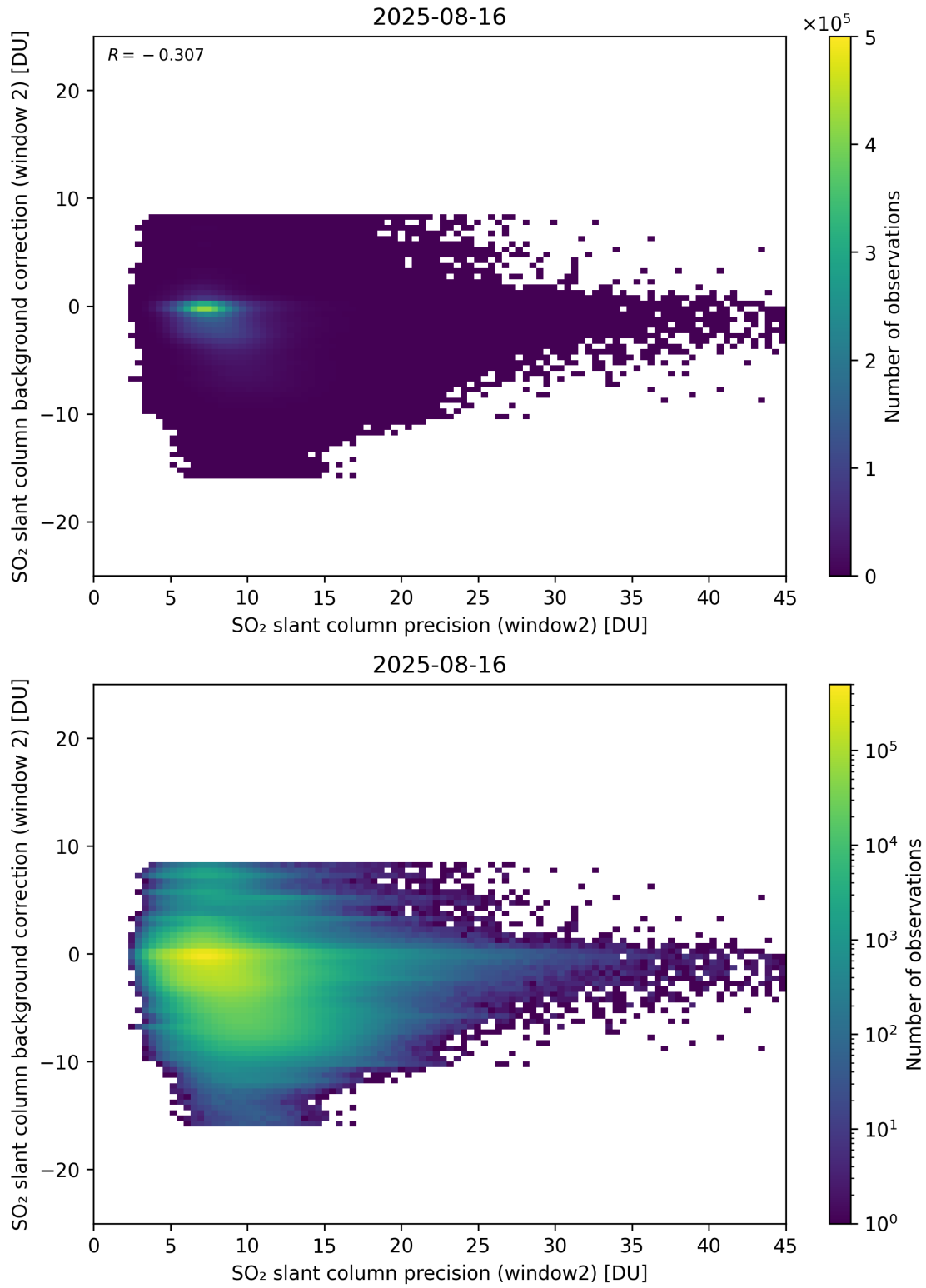
Figure 291: Scatter density plot of “SO 2 slant column precision (window2)” against “SO 2 slant column background correction (window 2)” for 2025-08-15 to 2025-08-17.
