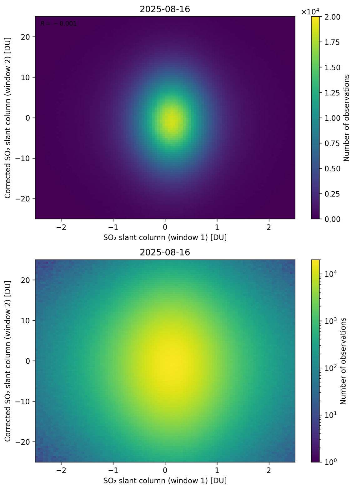
Figure 283: Scatter density plot of “SO 2 slant column (window 1)” against “Corrected SO 2 slant column (window 2)” for 2025-08-15 to 2025-08-17.
