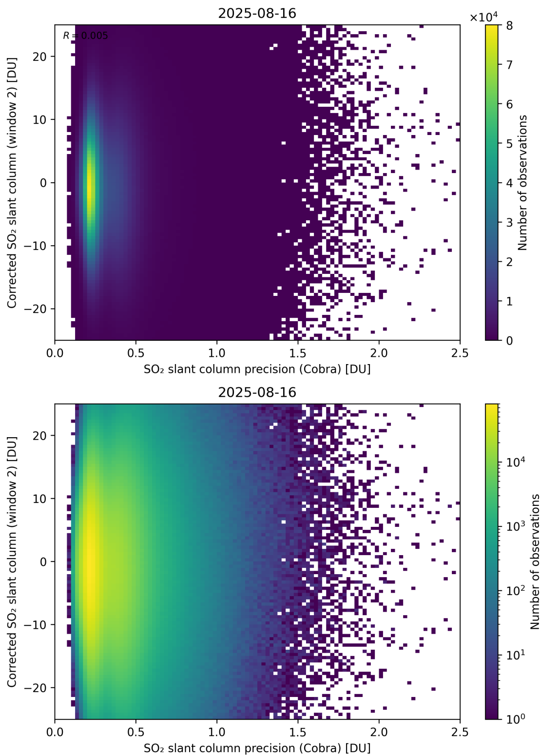
Figure 206: Scatter density plot of “SO 2 slant column precision (Cobra)” against “Corrected SO 2 slant column (window 2)” for 2025-08-15 to 2025-08-17.
