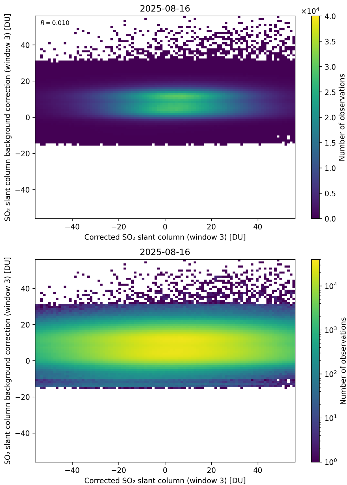
Figure 255: Scatter density plot of “Corrected SO 2 slant column (window 3)” against “SO 2 slant column background correction (window 3)” for 2025-08-15 to 2025-08-17.
