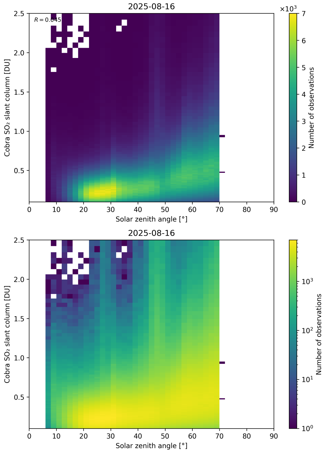
Figure 179: Scatter density plot of “Solar zenith angle” against “Cobra SO 2 slant column” for 2025-08-15 to 2025-08-17.
