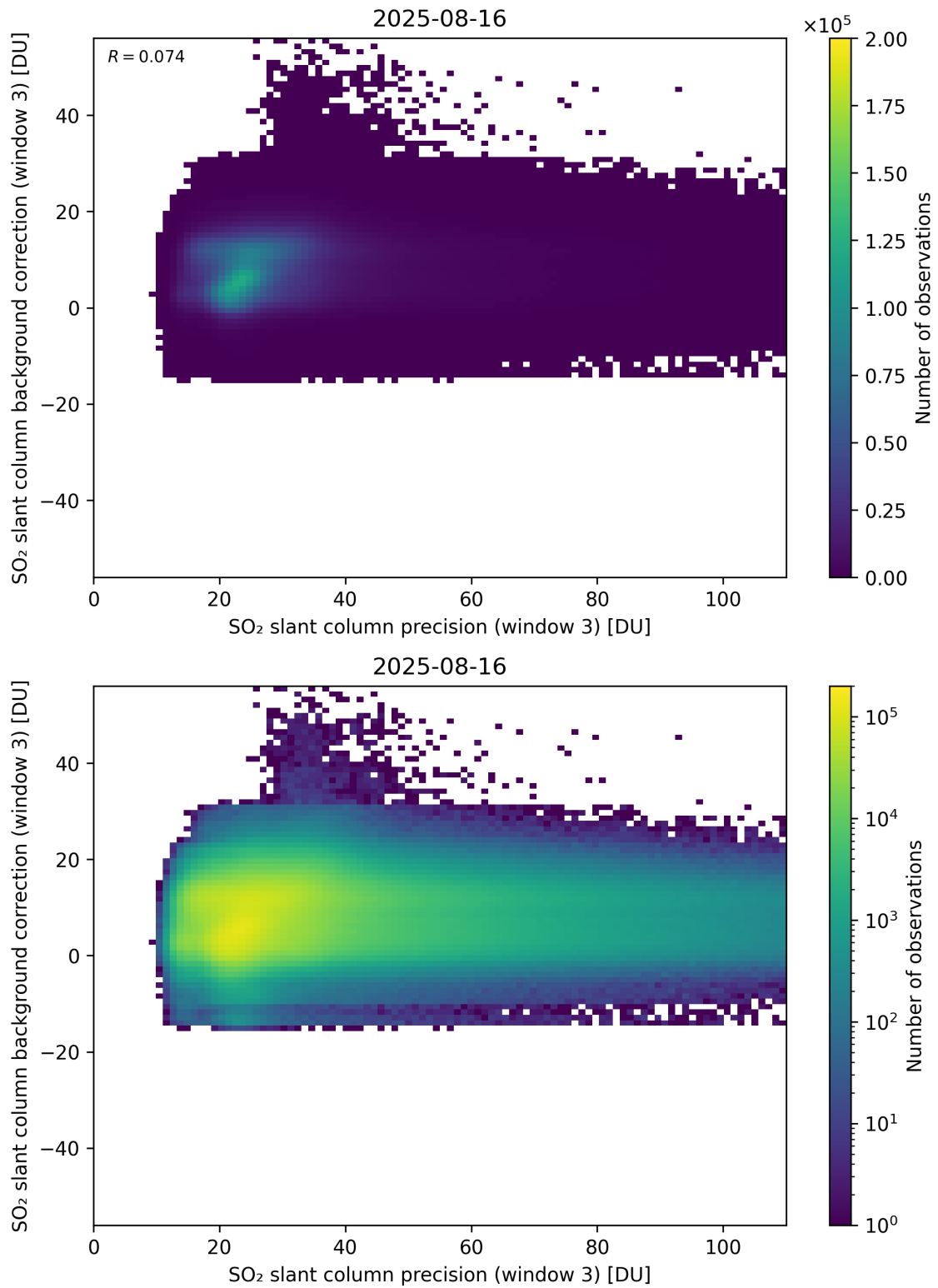
Figure 307: Scatter density plot of “SO 2 slant column precision (window 3)” against “SO 2 slant column background correction (window 3)” for 2025-08-15 to 2025-08-17.
