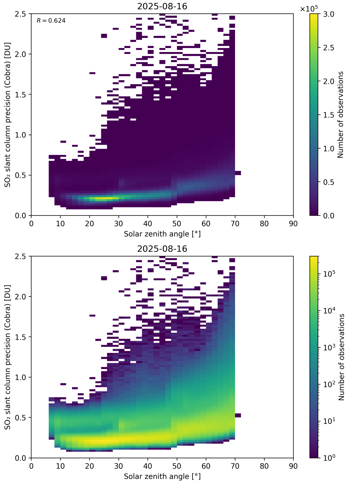
Figure 180: Scatter density plot of “Solar zenith angle” against “SO 2 slant column precision (Cobra)” for 2025-08-15 to 2025-08-17.
