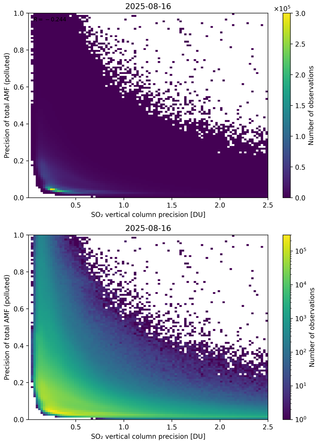
Figure 347: Scatter density plot of “SO 2 vertical column precision” against “Precision of total AMF (polluted)” for 2025-08-15 to 2025-08-17.
