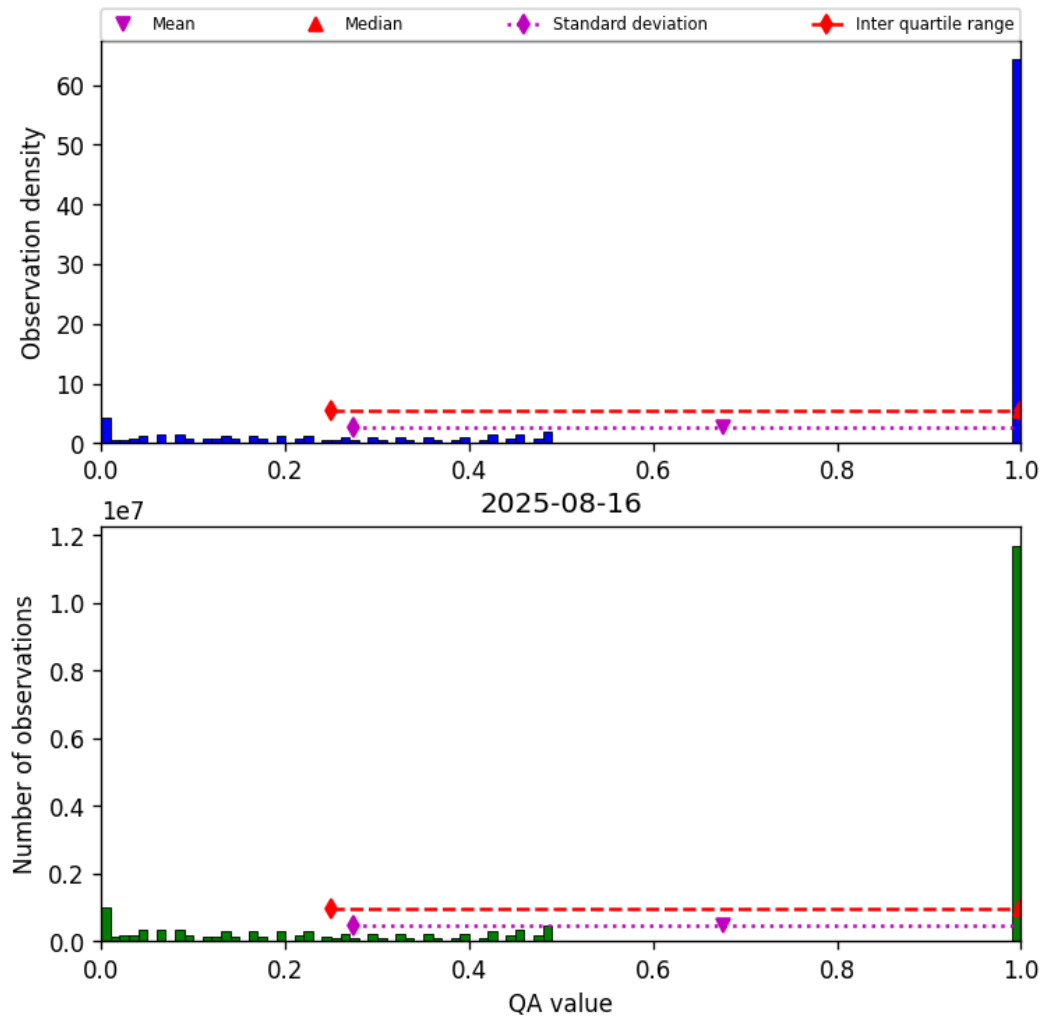
Figure 57: Histogram of “QA value” for 2025-08-15 to 2025-08-17
