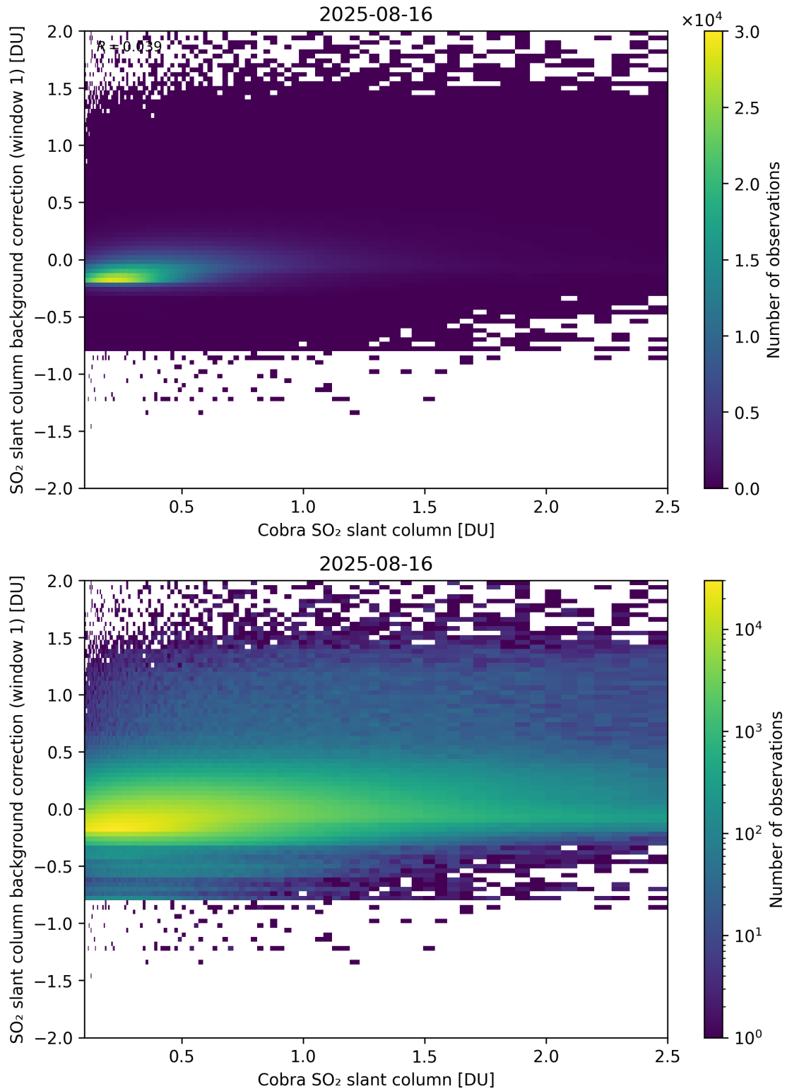
Figure 193: Scatter density plot of “Cobra SO 2 slant column” against “SO 2 slant column background correction (window 1)” for 2025-08-15 to 2025-08-17.
