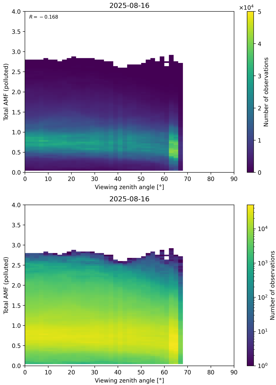
Figure 381: Scatter density plot of “Viewing zenith angle” against “Total AMF (polluted)” for 2025-08-15 to 2025-08-17.
