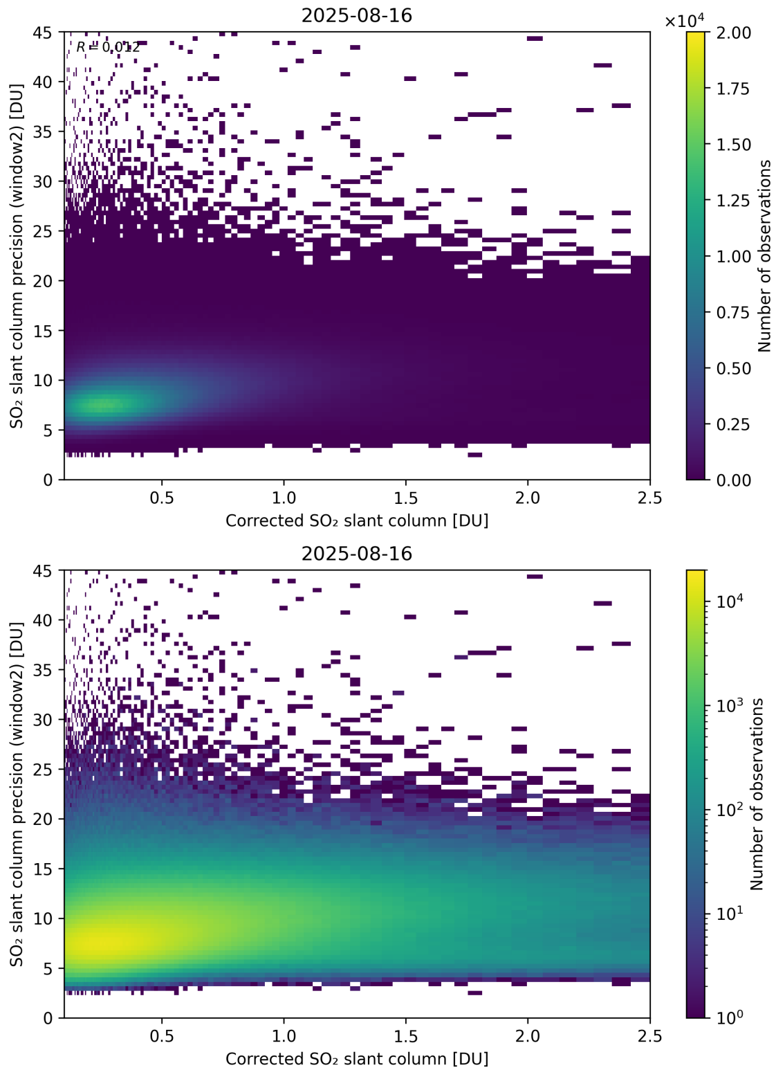
Figure 239: Scatter density plot of “Corrected SO 2 slant column” against “SO 2 slant column precision (window2)” for 2025-08-15 to 2025-08-17.
