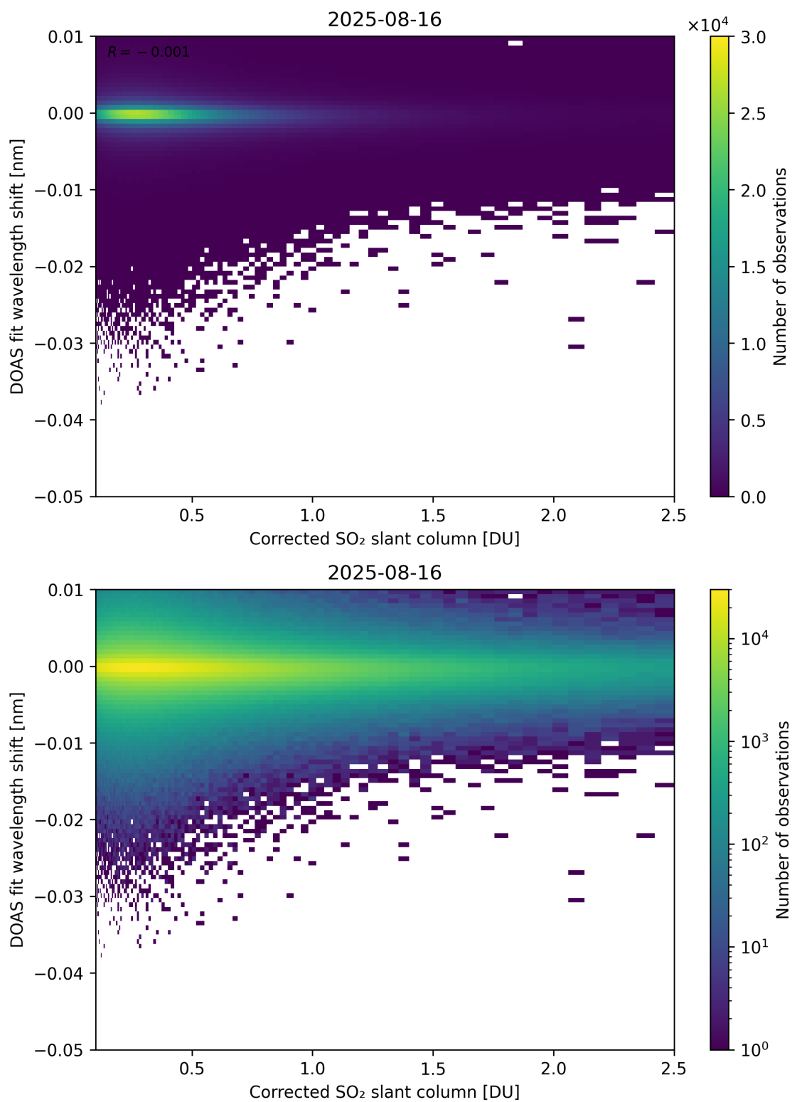
Figure 229: Scatter density plot of “Corrected SO 2 slant column” against “DOAS fit wavelength shift” for 2025-08-15 to 2025-08-17.
