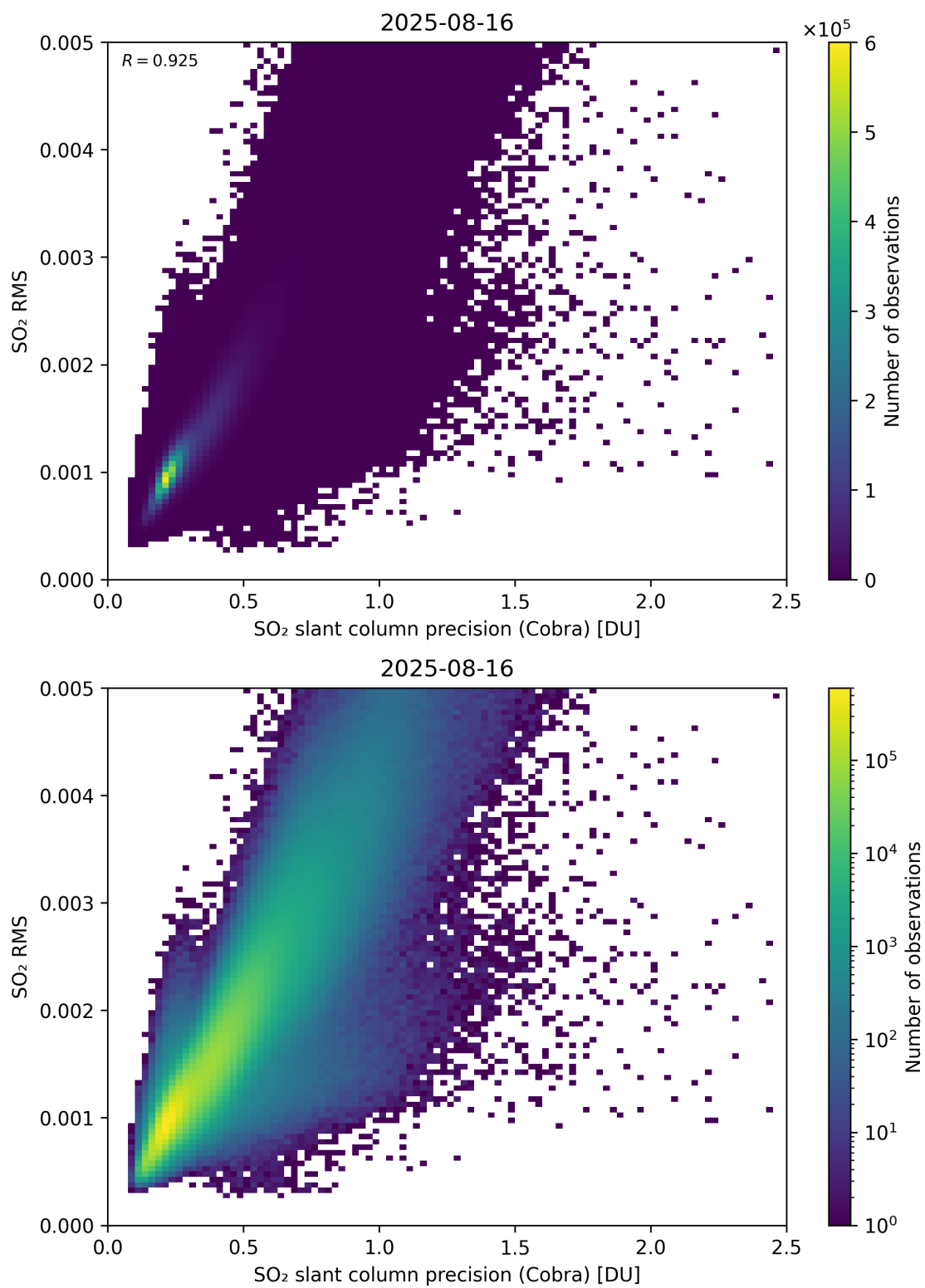
Figure 204: Scatter density plot of “SO 2 slant column precision (Cobra)” against “SO 2 RMS” for 2025-08-15 to 2025-08-17.
