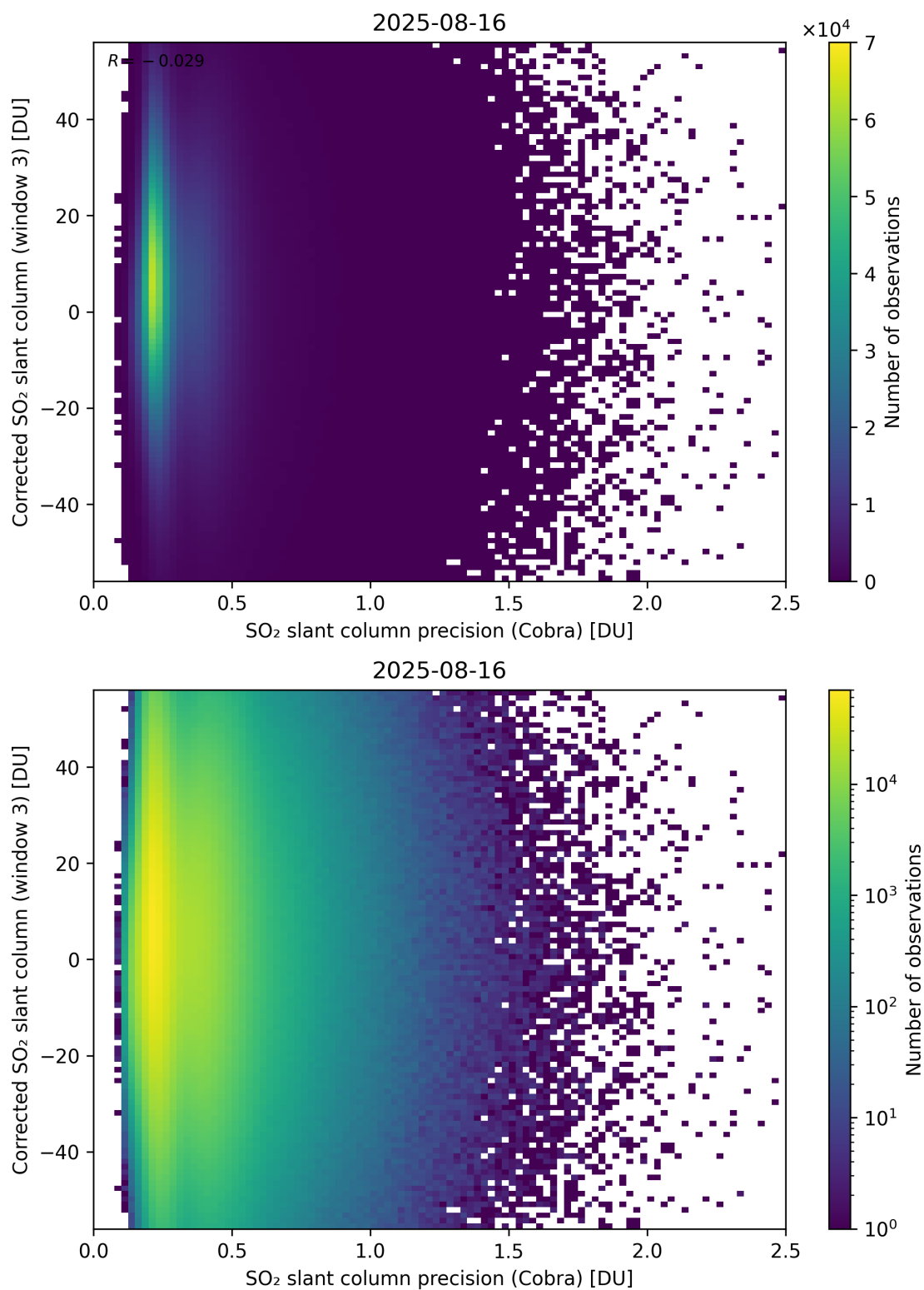
Figure 207: Scatter density plot of “SO 2 slant column precision (Cobra)” against “Corrected SO 2 slant column (window 3)” for 2025-08-15 to 2025-08-17.
