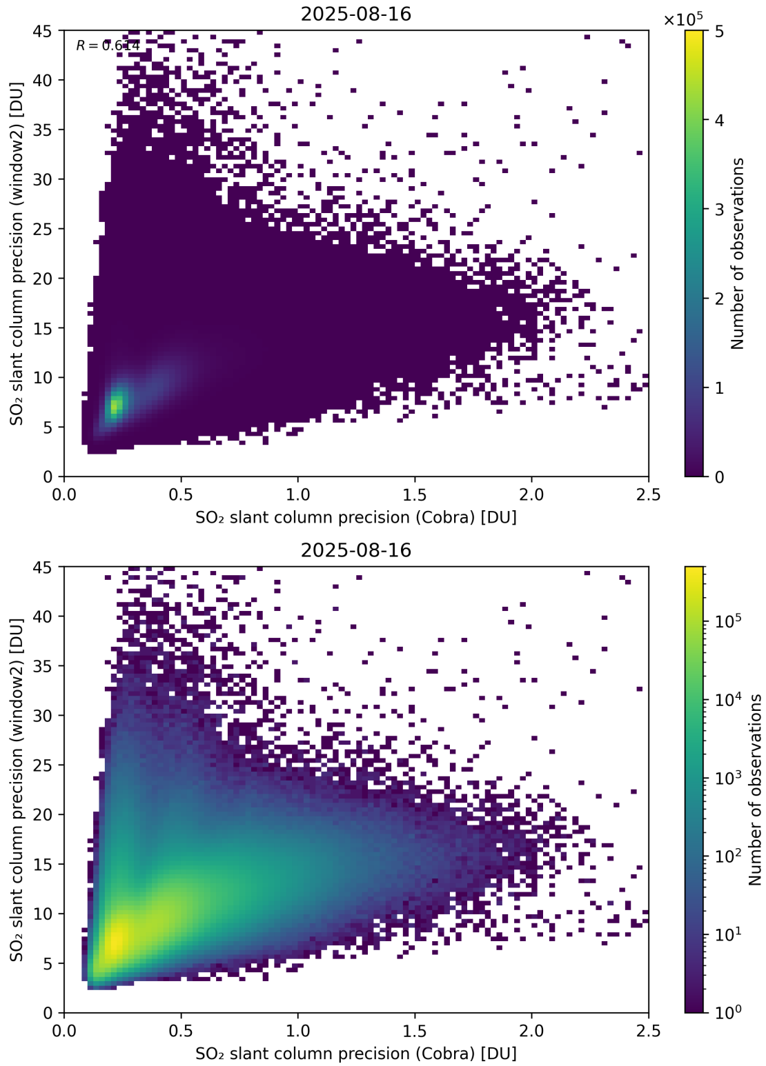
Figure 210: Scatter density plot of “SO 2 slant column precision (Cobra)” against “SO 2 slant column precision (window2)” for 2025-08-15 to 2025-08-17.
