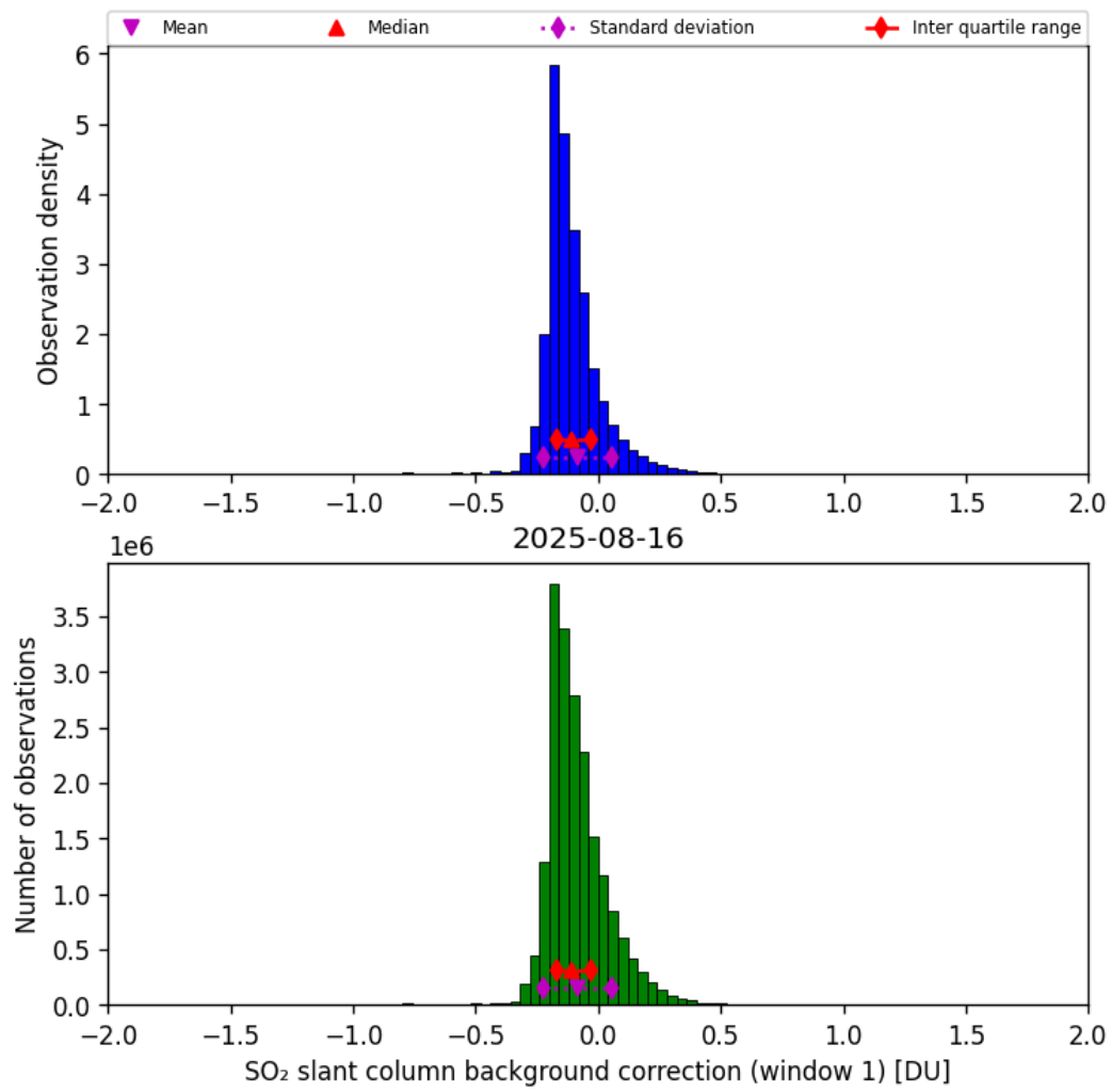
Figure 66: Histogram of “SO 2 slant column background correction (window 1)” for 2025-08-15 to 2025-08-17
