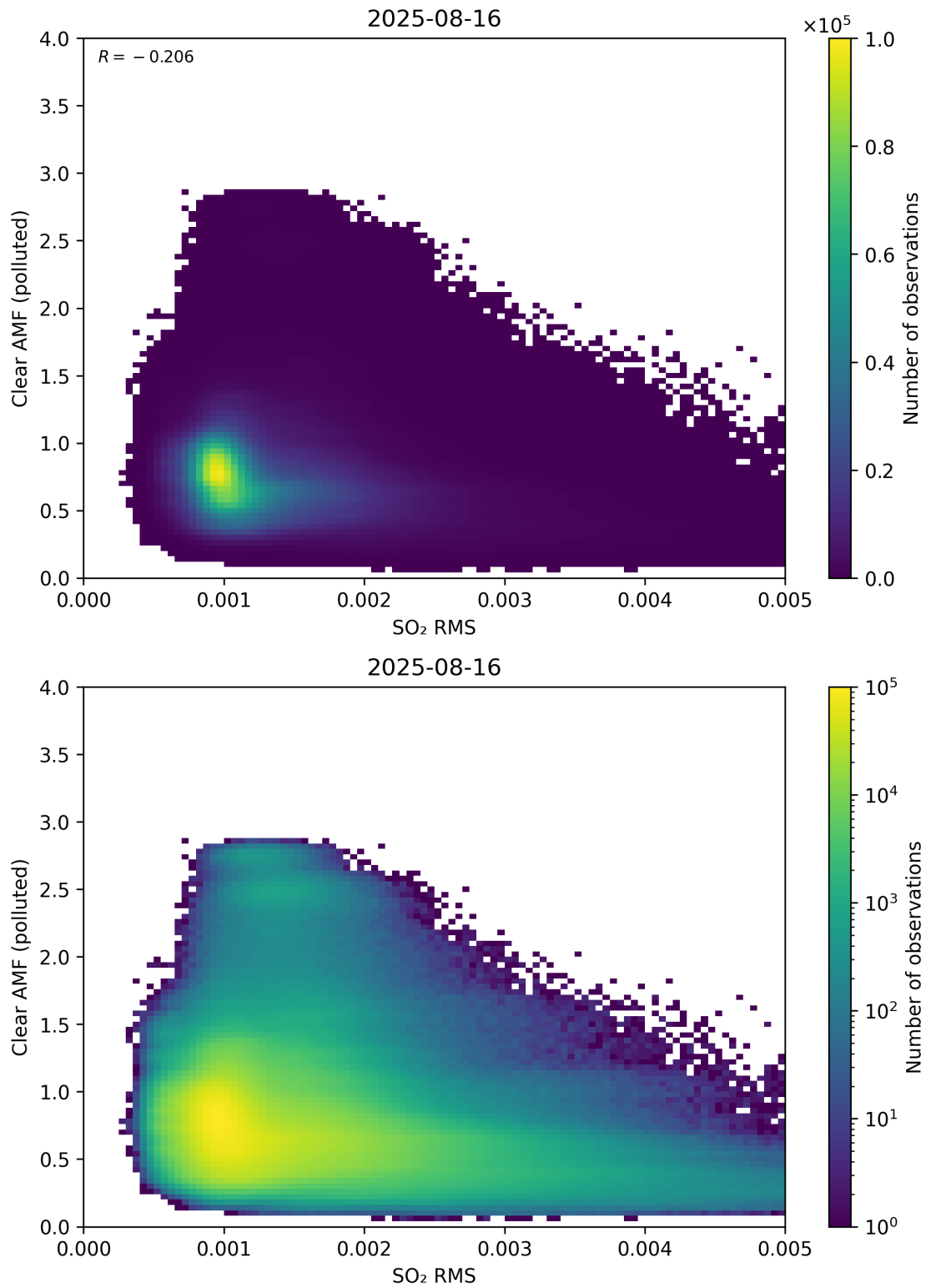
Figure 147: Scatter density plot of “SO 2 RMS” against “Clear AMF (polluted)” for 2025-08-15 to 2025-08-17.
