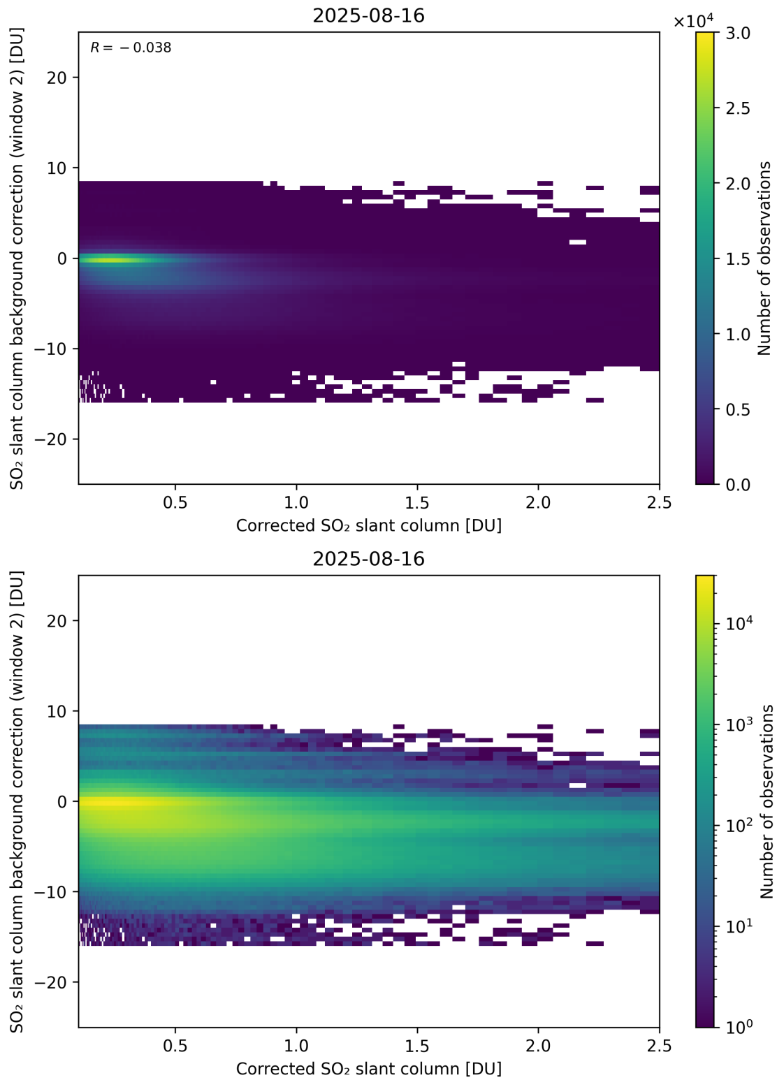
Figure 227: Scatter density plot of “Corrected SO 2 slant column” against “SO 2 slant column background correction (window 2)” for 2025-08-15 to 2025-08-17.
