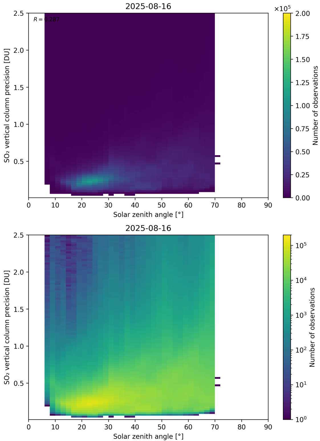
Figure 192: Scatter density plot of “Solar zenith angle” against “SO 2 vertical column precision” for 2025-08-15 to 2025-08-17.
