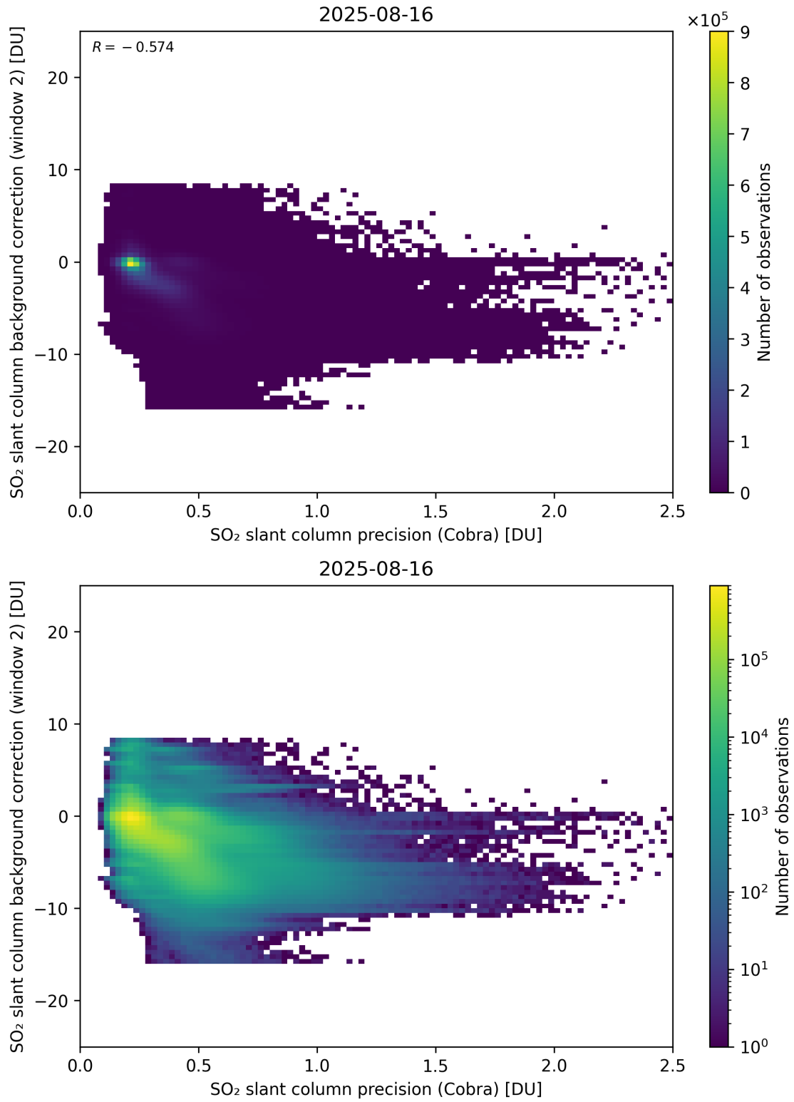
Figure 200: Scatter density plot of “SO 2 slant column precision (Cobra)” against “SO 2 slant column background correction (window 2)” for 2025-08-15 to 2025-08-17.
