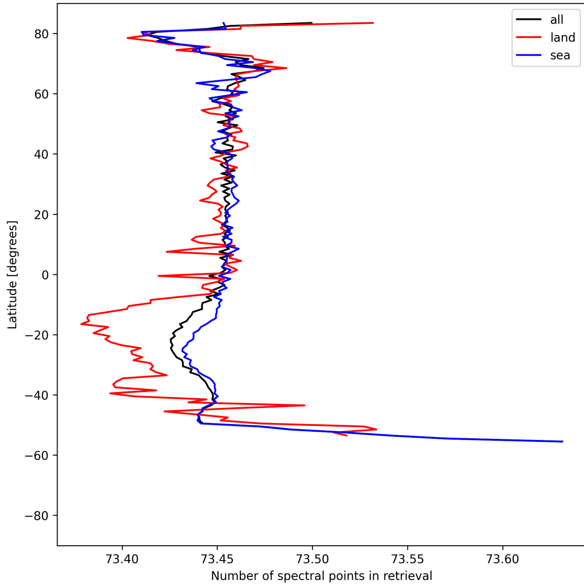
Figure 56: Zonal average of “Number of spectral points in retrieval” for 2025-08-15 to 2025-08-17.
