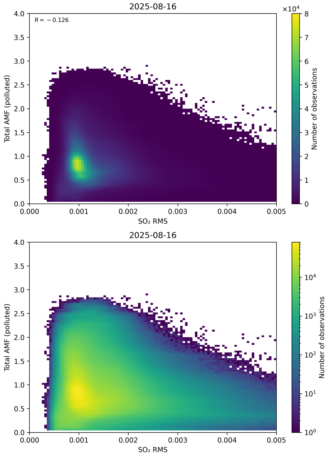
Figure 148: Scatter density plot of “SO 2 RMS” against “Total AMF (polluted)” for 2025-08-15 to 2025-08-17.
