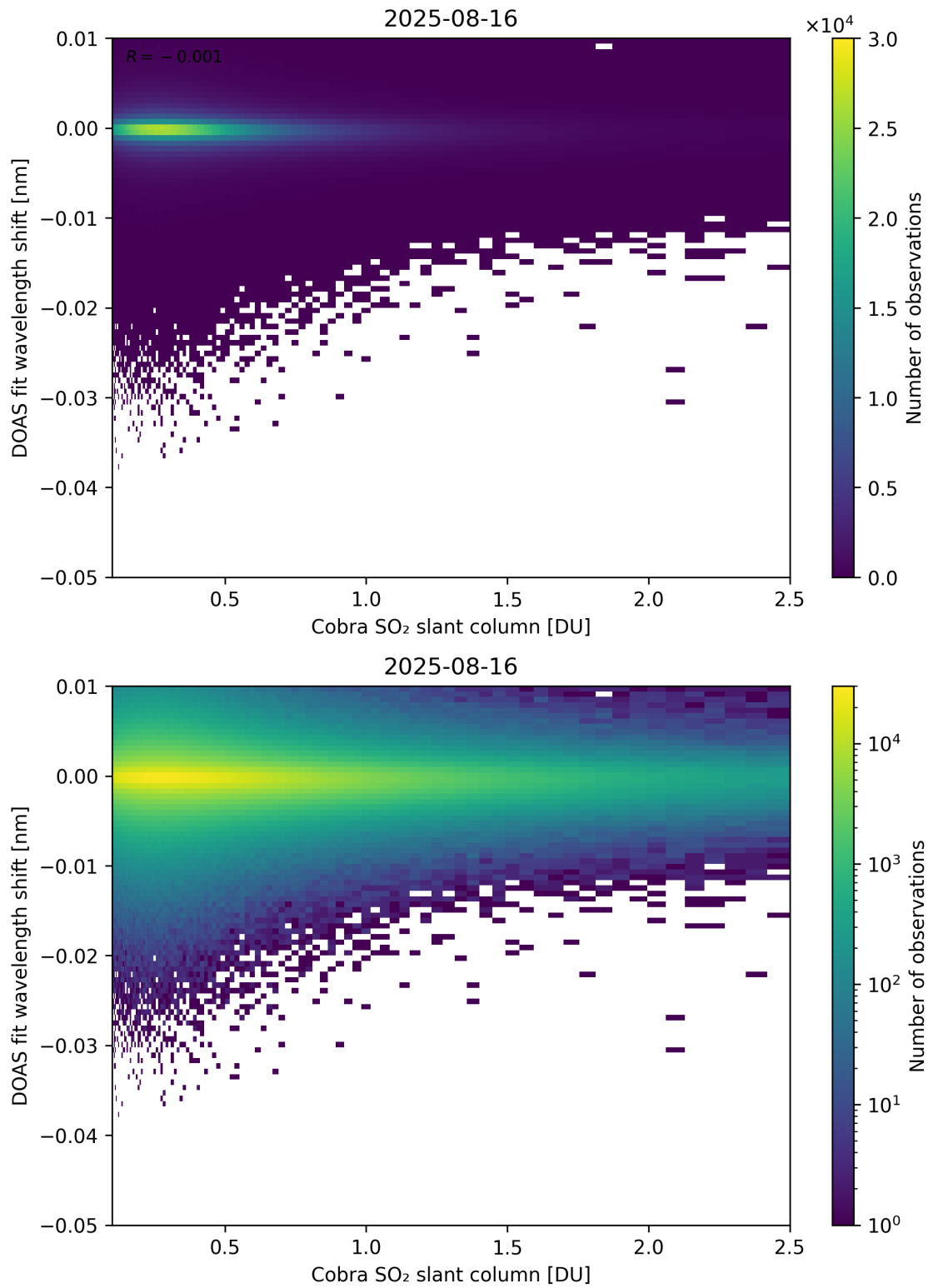
Figure 196: Scatter density plot of “Cobra SO 2 slant column” against “DOAS fit wavelength shift” for 2025-08-15 to 2025-08-17.
