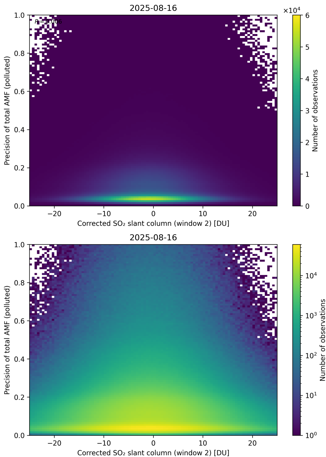
Figure 254: Scatter density plot of “Corrected SO 2 slant column (window 2)” against “Precision of total AMF (polluted)” for 2025-08-15 to 2025-08-17.
