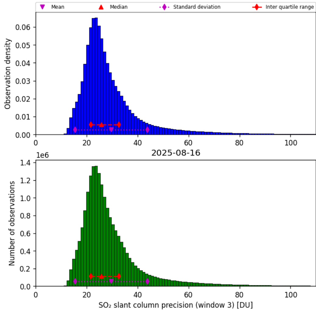
Figure 72: Histogram of “SO 2 slant column precision (window 3)” for 2025-08-15 to 2025-08-17
