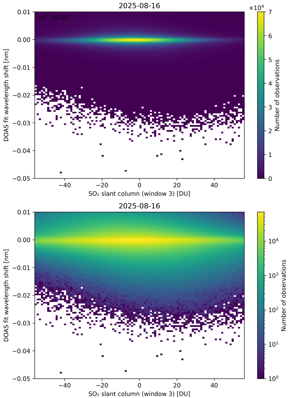
Figure 304: Scatter density plot of “SO 2 slant column (window 3)” against “DOAS fit wavelength shift” for 2025-08-15 to 2025-08-17.
