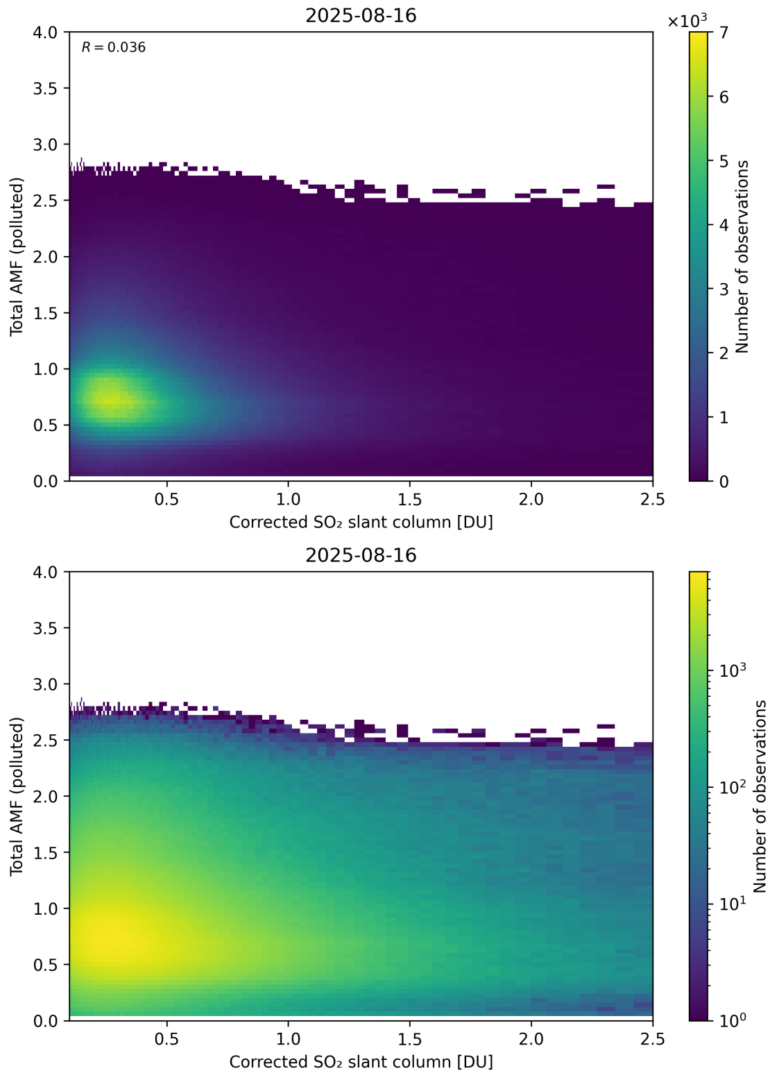
Figure 242: Scatter density plot of “Corrected SO 2 slant column” against “Total AMF (polluted)” for 2025-08-15 to 2025-08-17.
