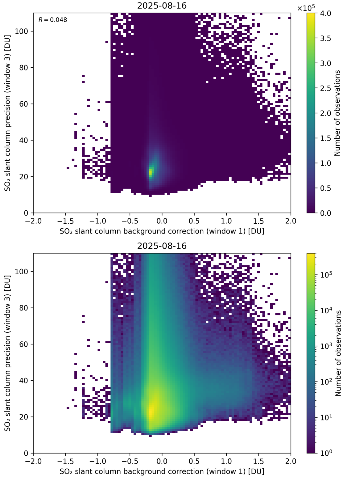
Figure 119: Scatter density plot of “SO 2 slant column background correction (window 1)” against “SO 2 slant column precision (window 3)” for 2025-08-15 to 2025-08-17.
