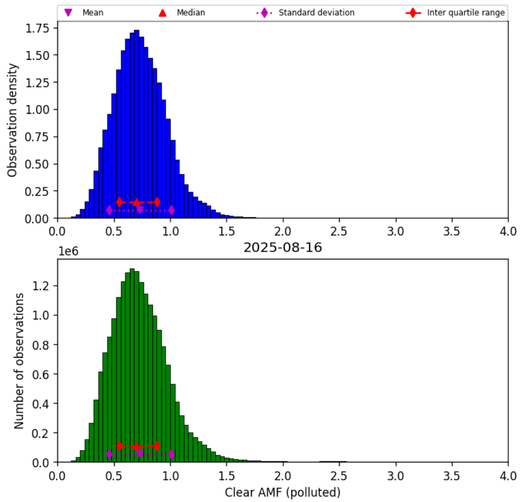
Figure 81: Histogram of “Clear AMF (polluted)” for 2025-08-15 to 2025-08-17
