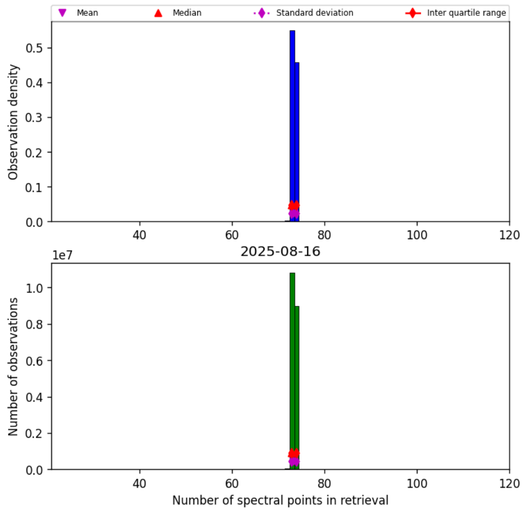
Figure 82: Histogram of “Number of spectral points in retrieval” for 2025-08-15 to 2025-08-17
