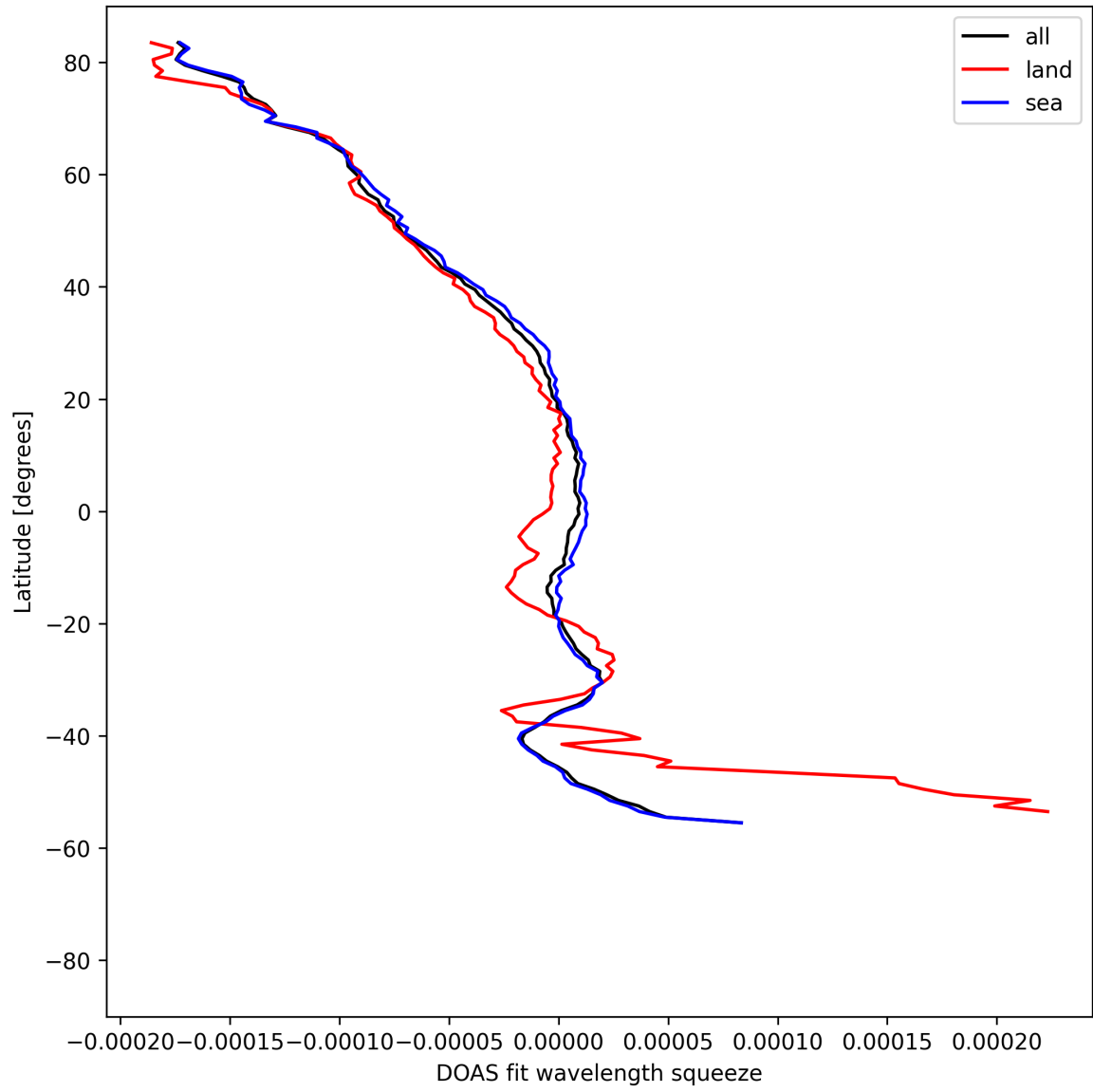
Figure 51: Zonal average of "DOAS fit wavelength squeeze" for 2025-08-15 to 2025-08-17.
