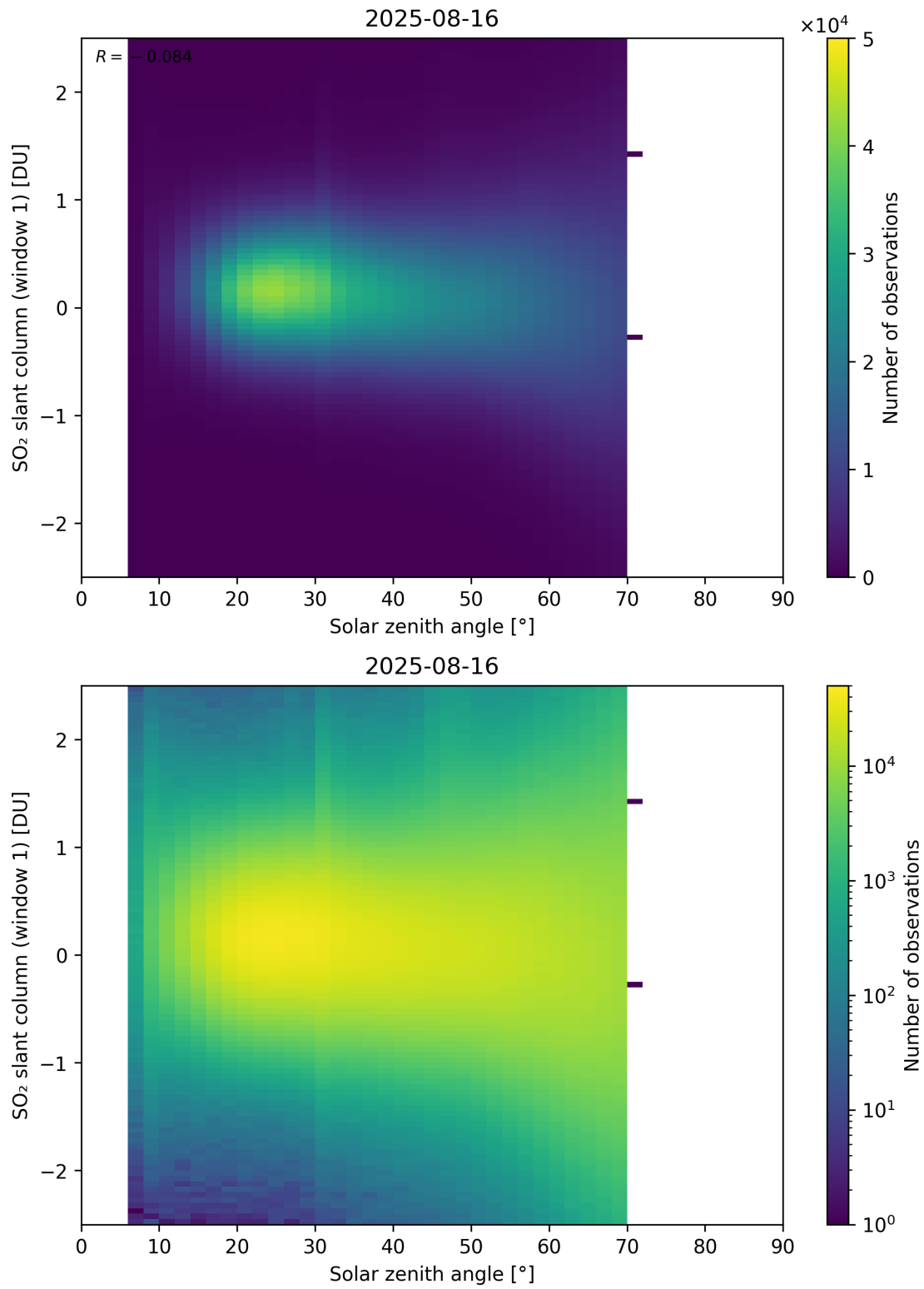
Figure 184: Scatter density plot of “Solar zenith angle” against “SO 2 slant column (window 1)” for 2025-08-15 to 2025-08-17.
