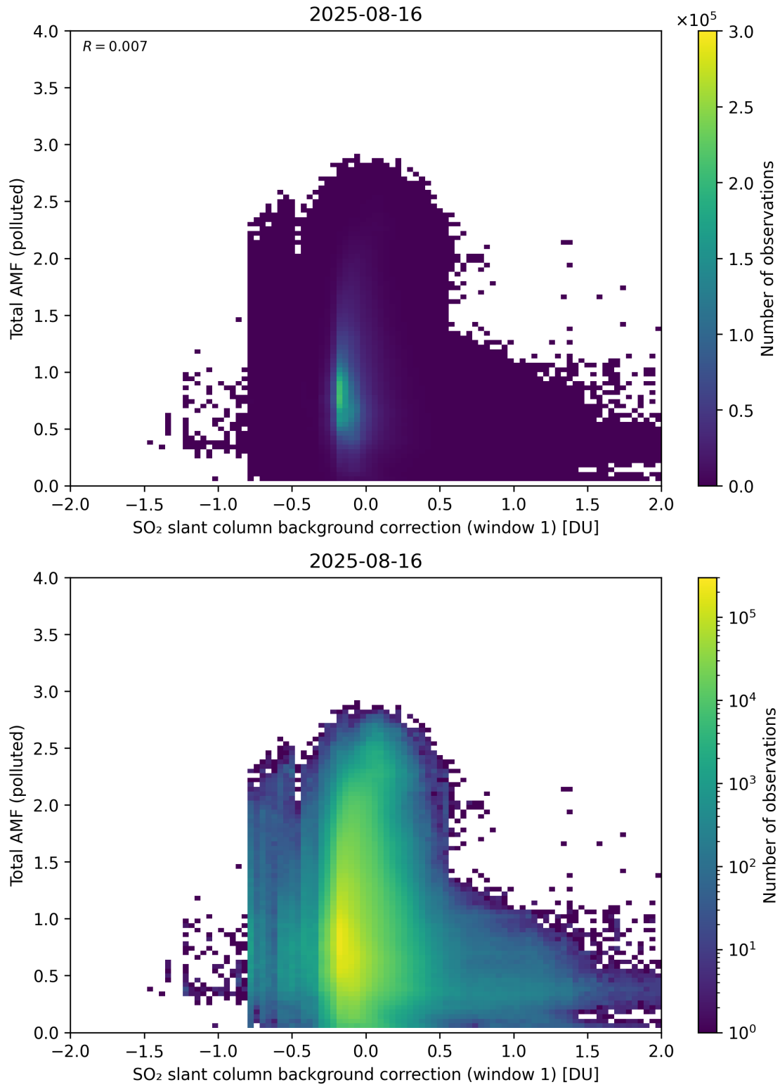
Figure 120: Scatter density plot of “SO 2 slant column background correction (window 1)” against “Total AMF (polluted)” for 2025-08-15 to 2025-08-17.
