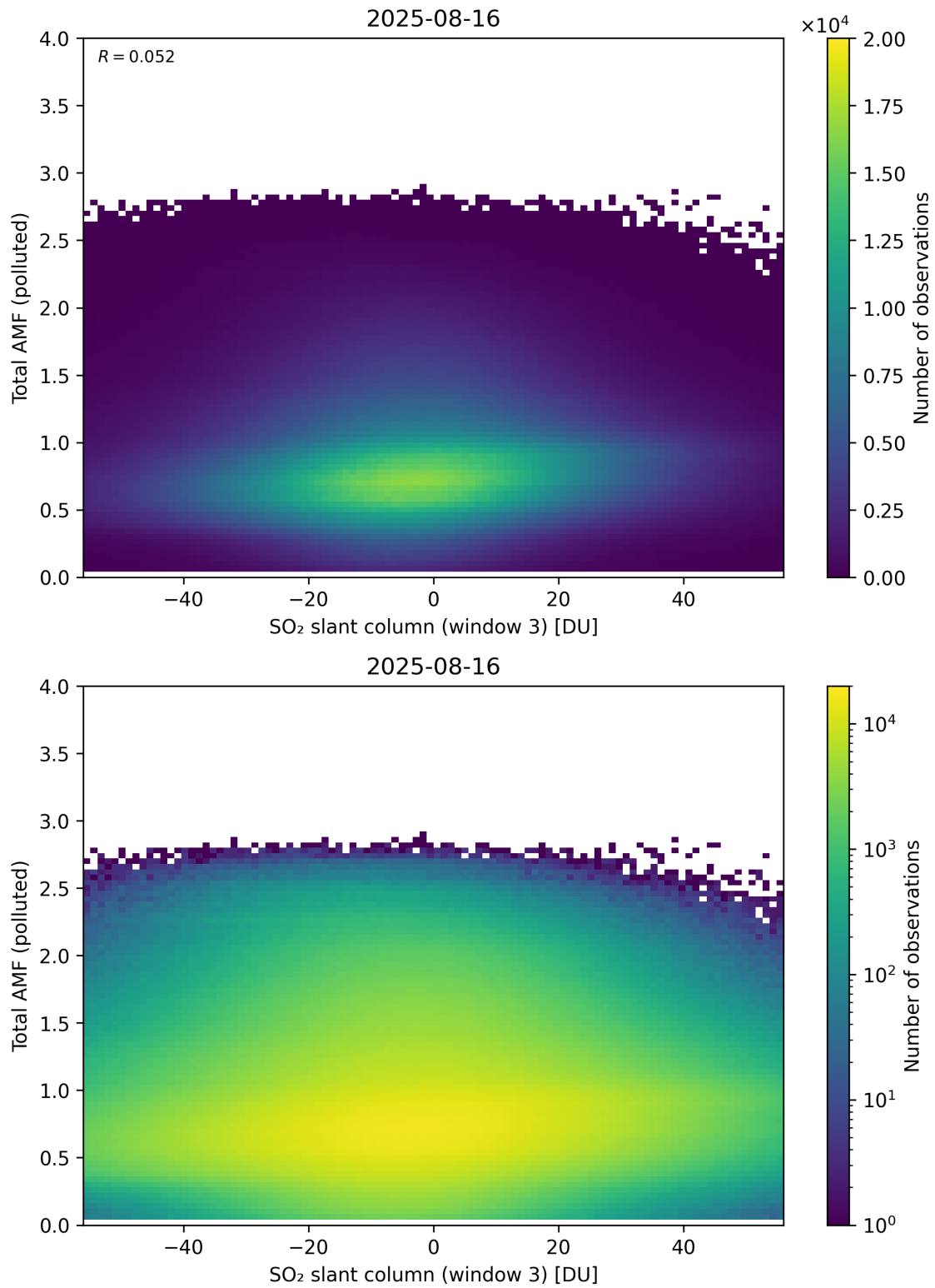
Figure 318: Scatter density plot of “SO 2 slant column (window 3)” against “Total AMF (polluted)” for 2025-08-15 to 2025-08-17.
