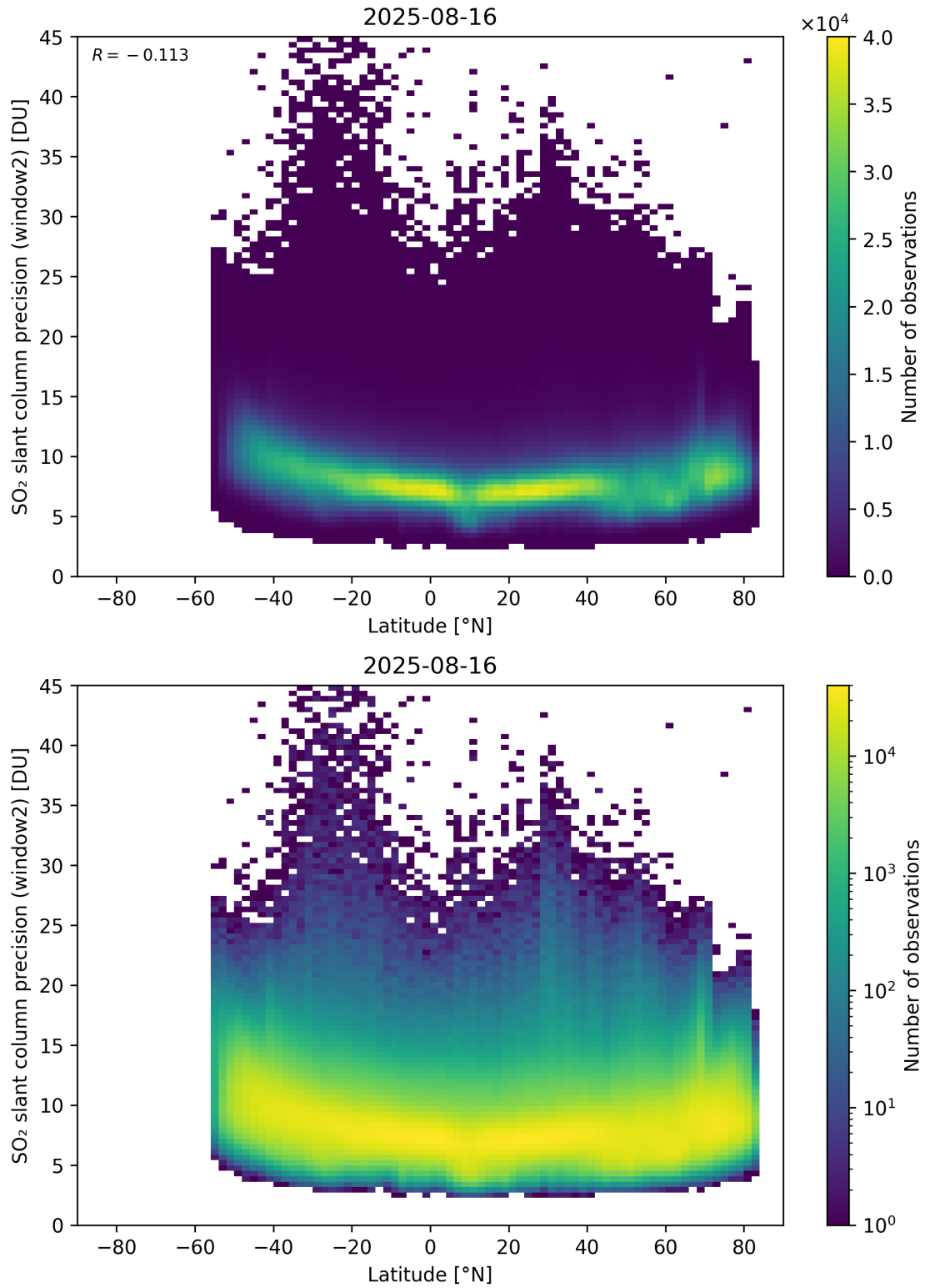
Figure 164: Scatter density plot of “Latitude” against “SO 2 slant column precision (window2)” for 2025-08-15 to 2025-08-17.
