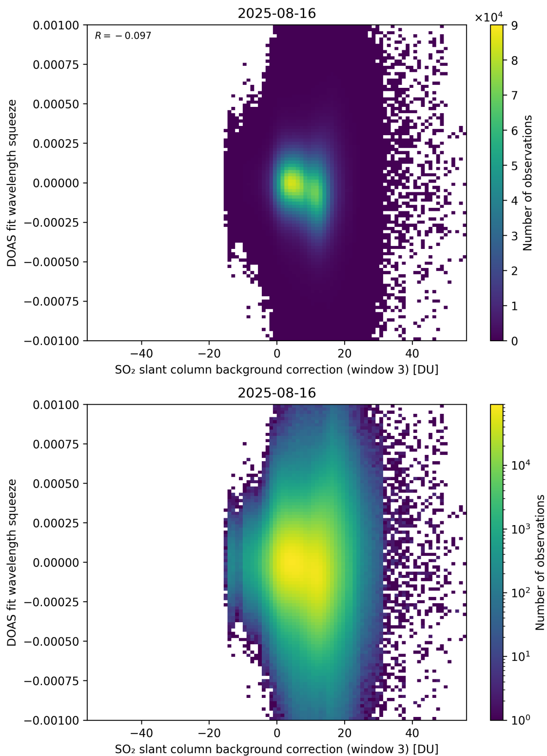
Figure 133: Scatter density plot of “SO 2 slant column background correction (window 3)” against “DOAS fit wavelength squeeze” for 2025-08-15 to 2025-08-17.
