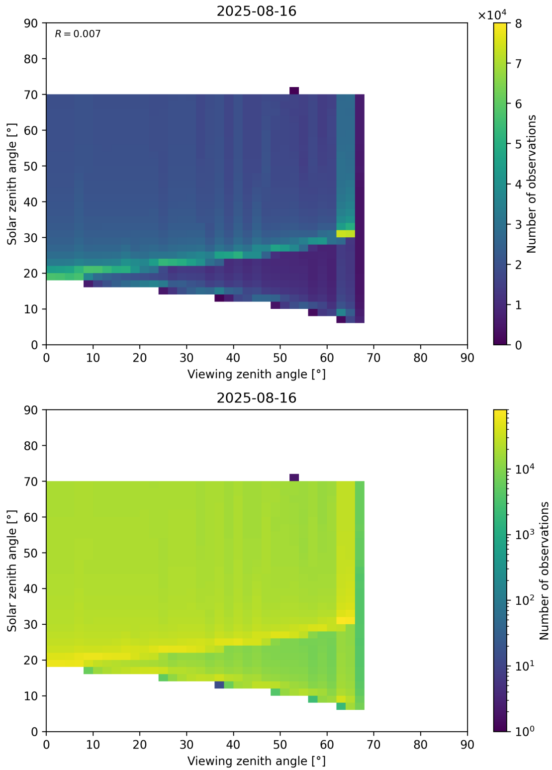
Figure 369: Scatter density plot of “Viewing zenith angle” against “Solar zenith angle” for 2025-08-15 to 2025-08-17.
