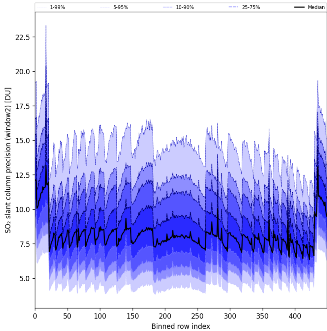
Figure 94: Along track statistics of “SO 2 slant column precision (window2)” for 2025-08-15 to 2025-08-17
