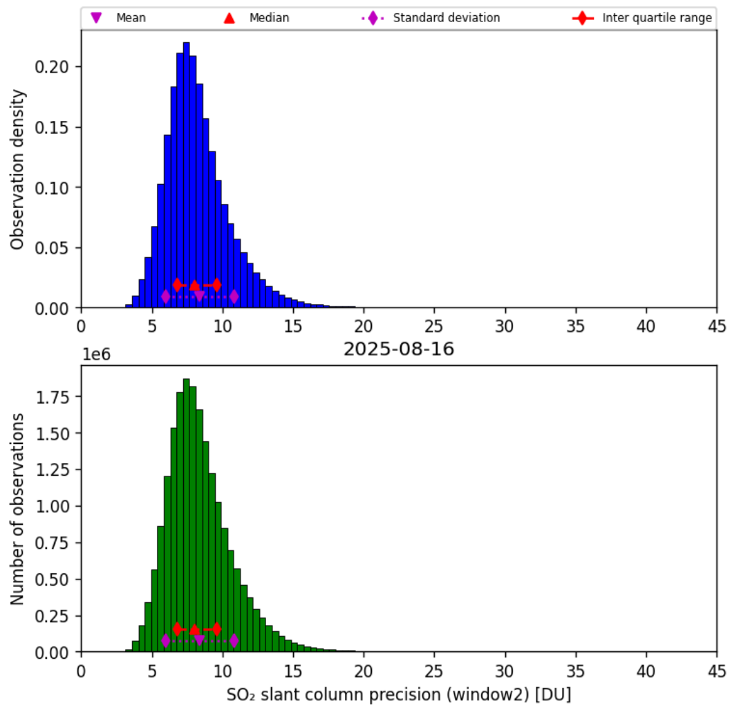
Figure 68: Histogram of “SO 2 slant column precision (window2)” for 2025-08-15 to 2025-08-17
