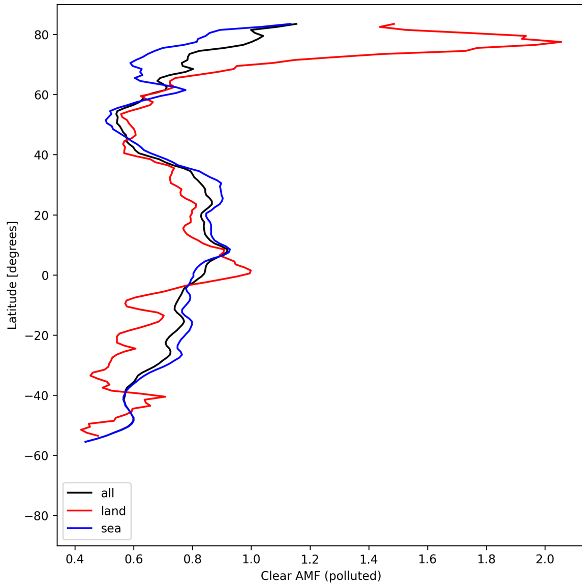
Figure 55: Zonal average of “Clear AMF (polluted)” for 2025-08-15 to 2025-08-17.
