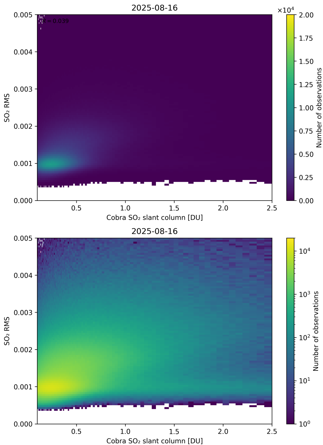
Figure 198: Scatter density plot of “Cobra SO 2 slant column” against “SO 2 RMS” for 2025-08-15 to 2025-08-17.
