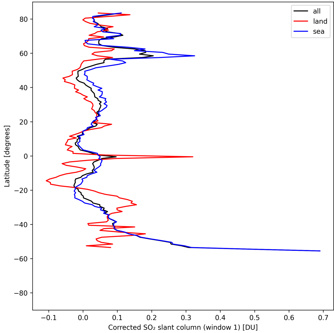
Figure 39: Zonal average of “Corrected SO 2 slant column (window 1)” for 2025-08-15 to 2025-08-17.
