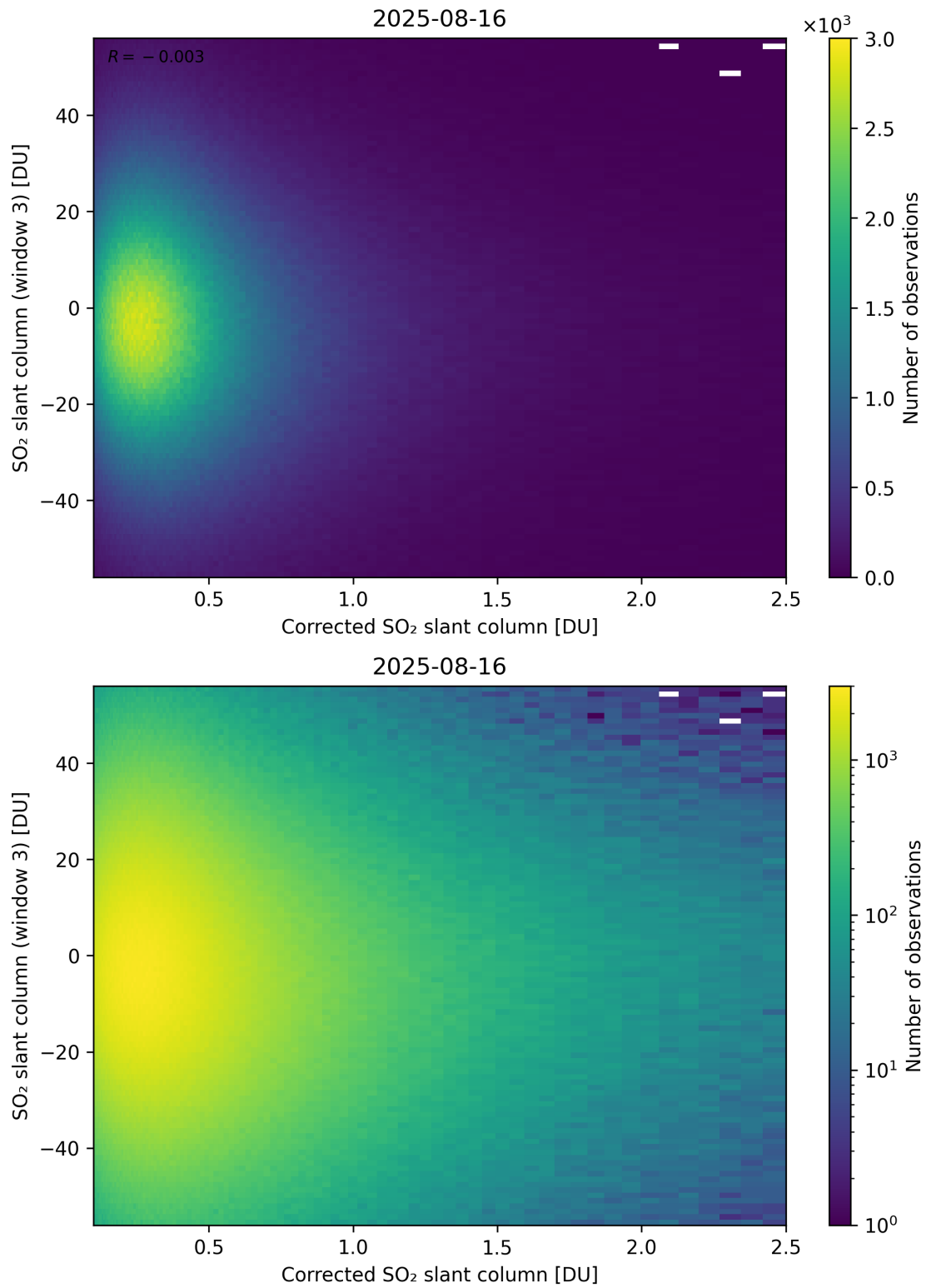
Figure 240: Scatter density plot of “Corrected SO 2 slant column” against “SO 2 slant column (window 3)” for 2025-08-15 to 2025-08-17.
