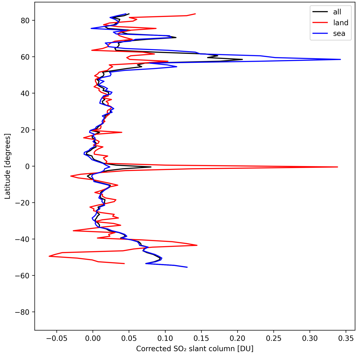
Figure 34: Zonal average of “Corrected SO 2 slant column” for 2025-08-15 to 2025-08-17.
