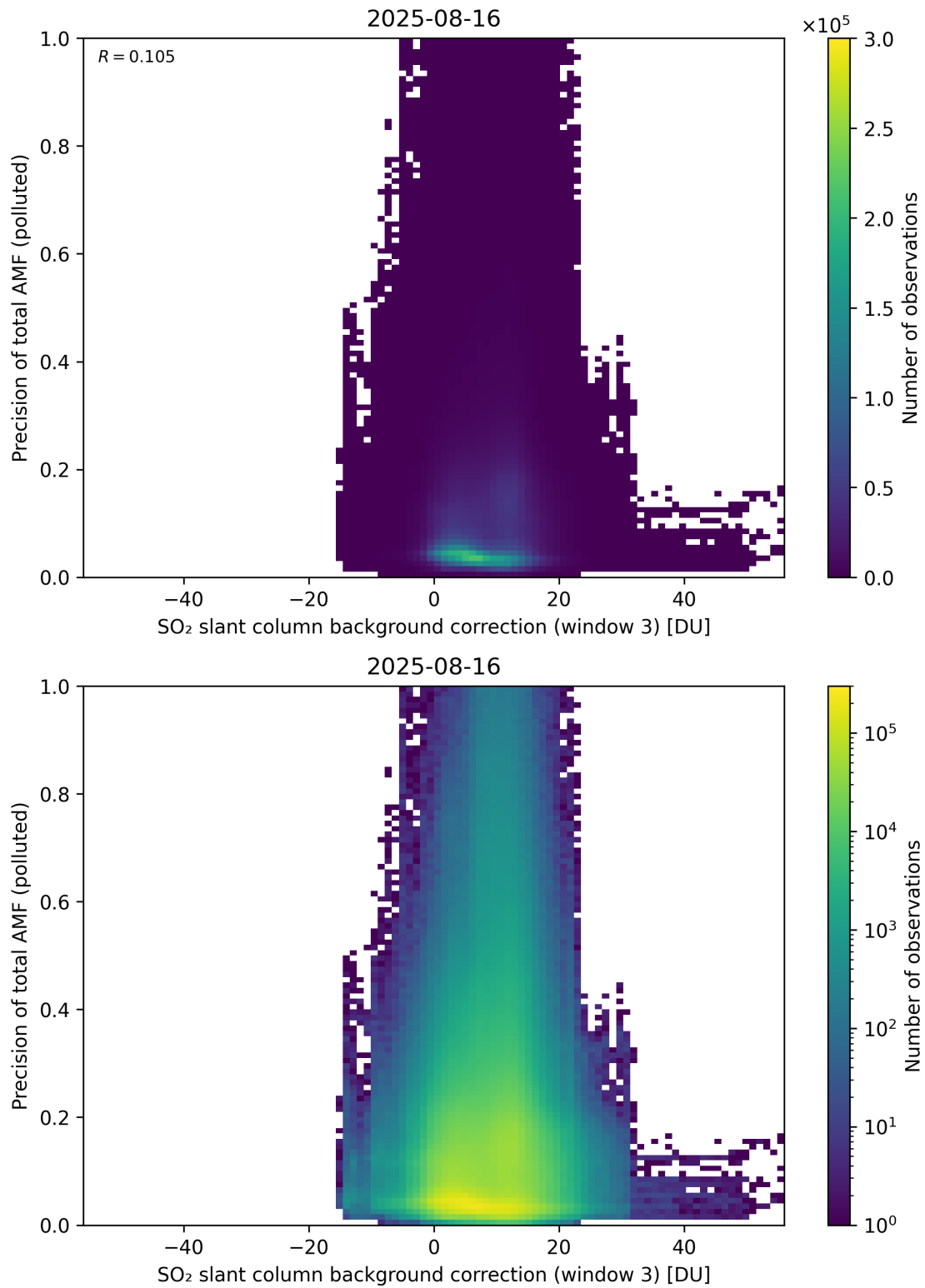
Figure 137: Scatter density plot of “SO 2 slant column background correction (window 3)” against “Precision of total AMF (polluted)” for 2025-08-15 to 2025-08-17.
