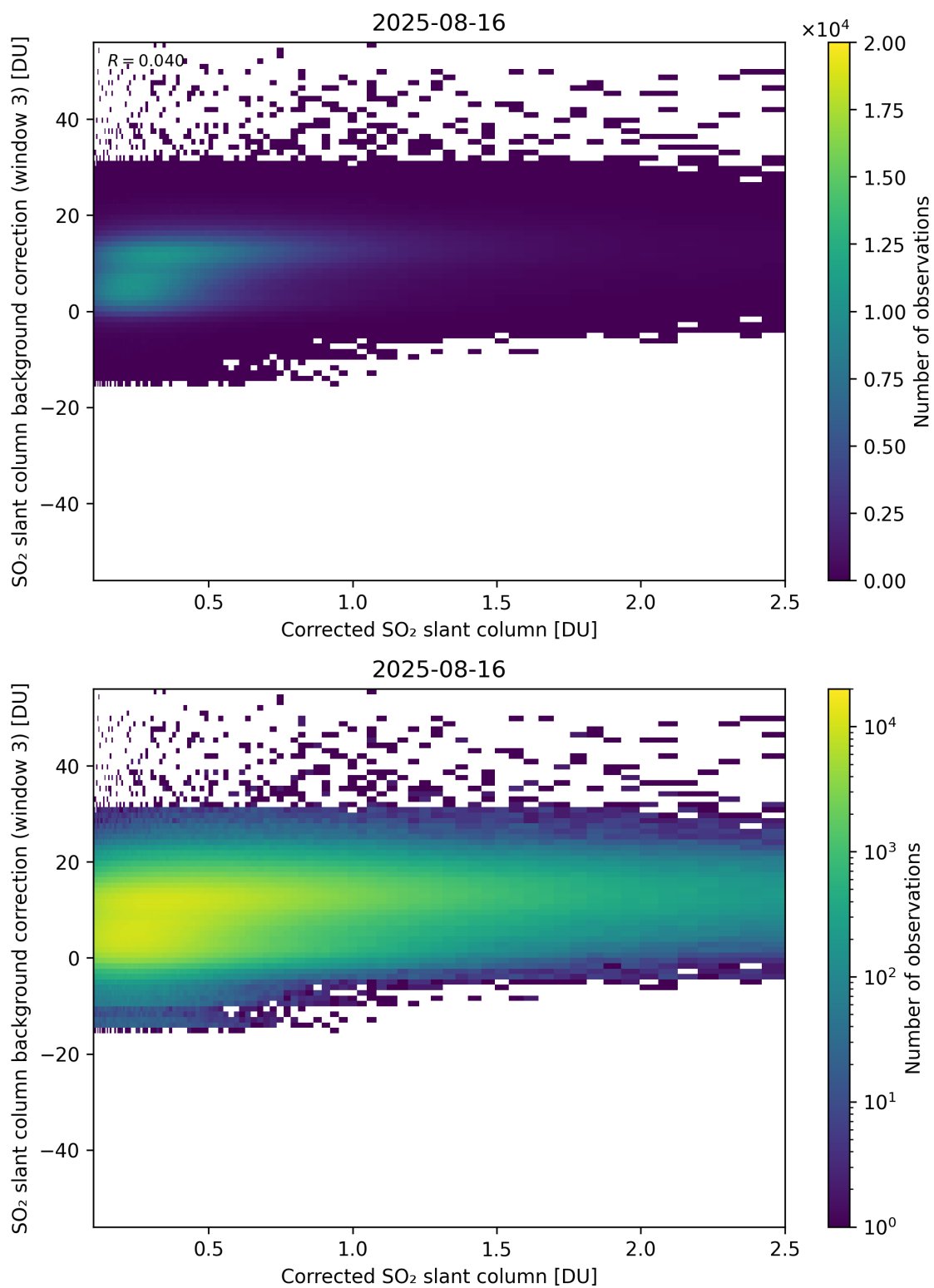
Figure 228: Scatter density plot of “Corrected SO 2 slant column” against “SO 2 slant column background correction (window 3)” for 2025-08-15 to 2025-08-17.
