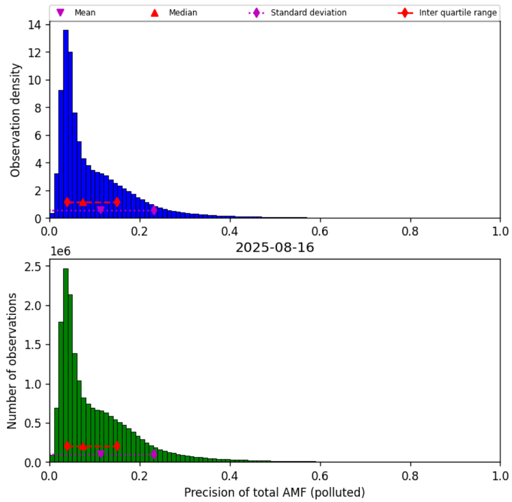
Figure 80: Histogram of “Precision of total AMF (polluted)” for 2025-08-15 to 2025-08-17
