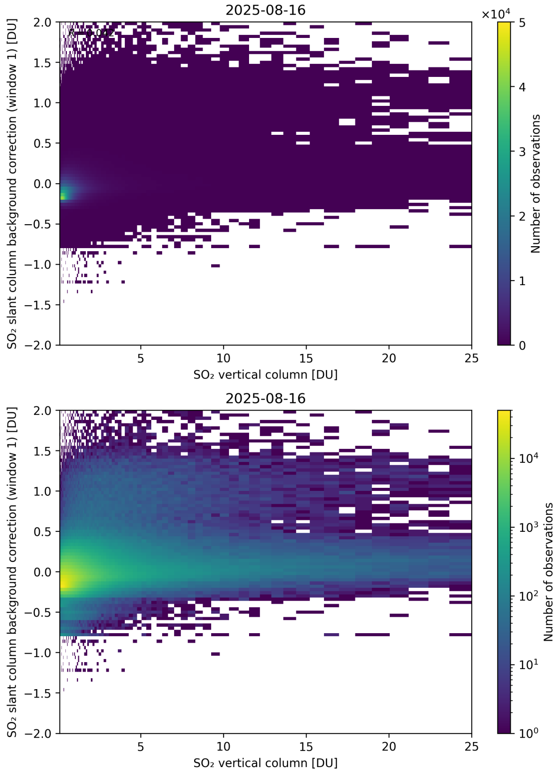
Figure 323: Scatter density plot of “SO 2 vertical column” against “SO 2 slant column background correction (window 1)” for 2025-08-15 to 2025-08-17.
