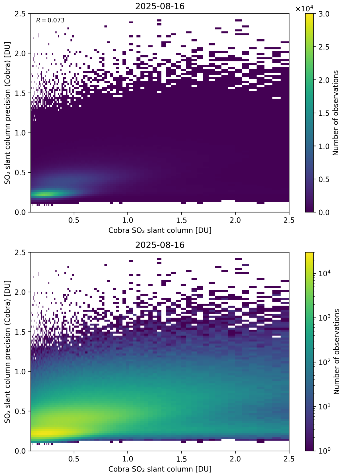
Figure 216: Scatter density plot of “Cobra SO 2 slant column” against “SO 2 slant column precision (Cobra)” for 2025-08-15 to 2025-08-17.
