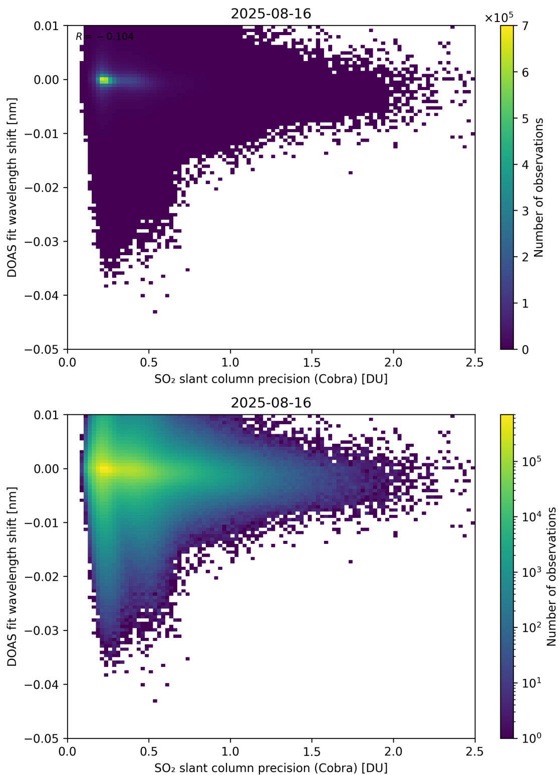
Figure 202: Scatter density plot of “SO 2 slant column precision (Cobra)” against “DOAS fit wavelength shift” for 2025-08-15 to 2025-08-17.
