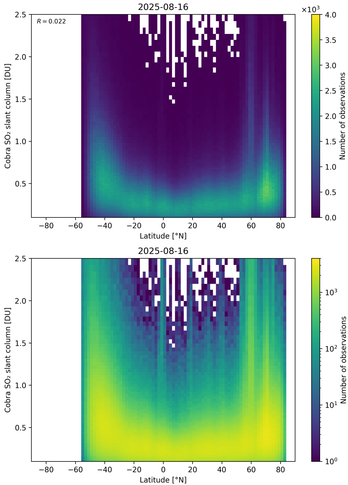
Figure 157: Scatter density plot of “Latitude” against “Cobra SO 2 slant column” for 2025-08-15 to 2025-08-17.
