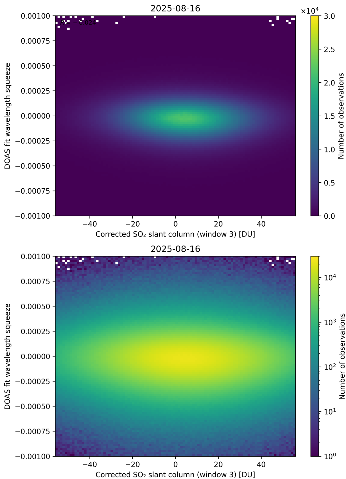
Figure 257: Scatter density plot of “Corrected SO 2 slant column (window 3)” against “DOAS fit wavelength squeeze” for 2025-08-15 to 2025-08-17.
