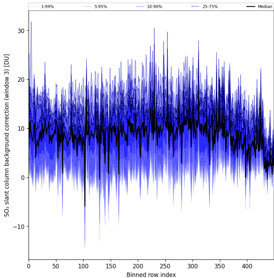
Figure 100: Along track statistics of “SO 2 slant column background correction (window 3)” for 2025-08-15 to 2025-08-17
