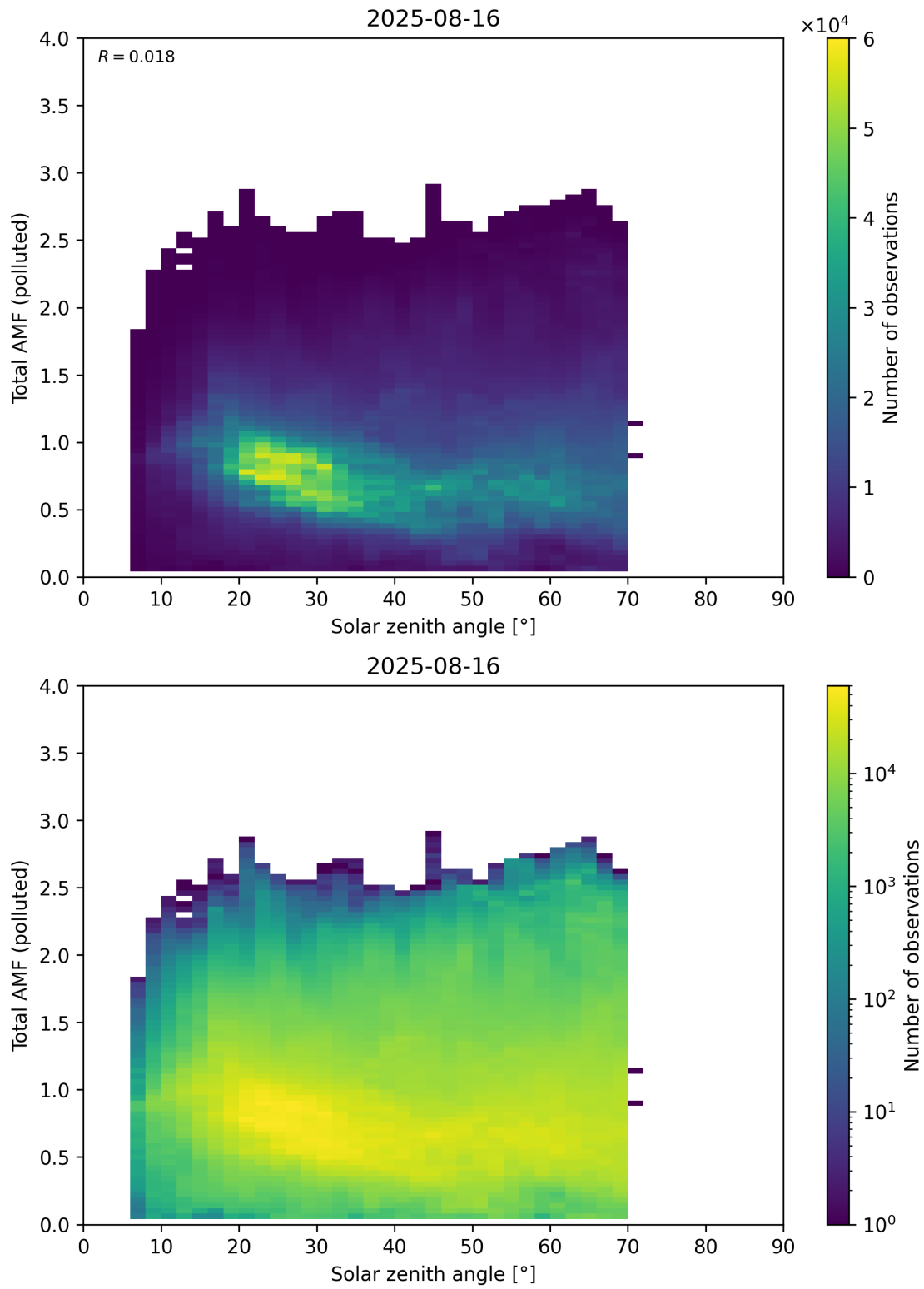
Figure 189: Scatter density plot of “Solar zenith angle” against “Total AMF (polluted)” for 2025-08-15 to 2025-08-17.
