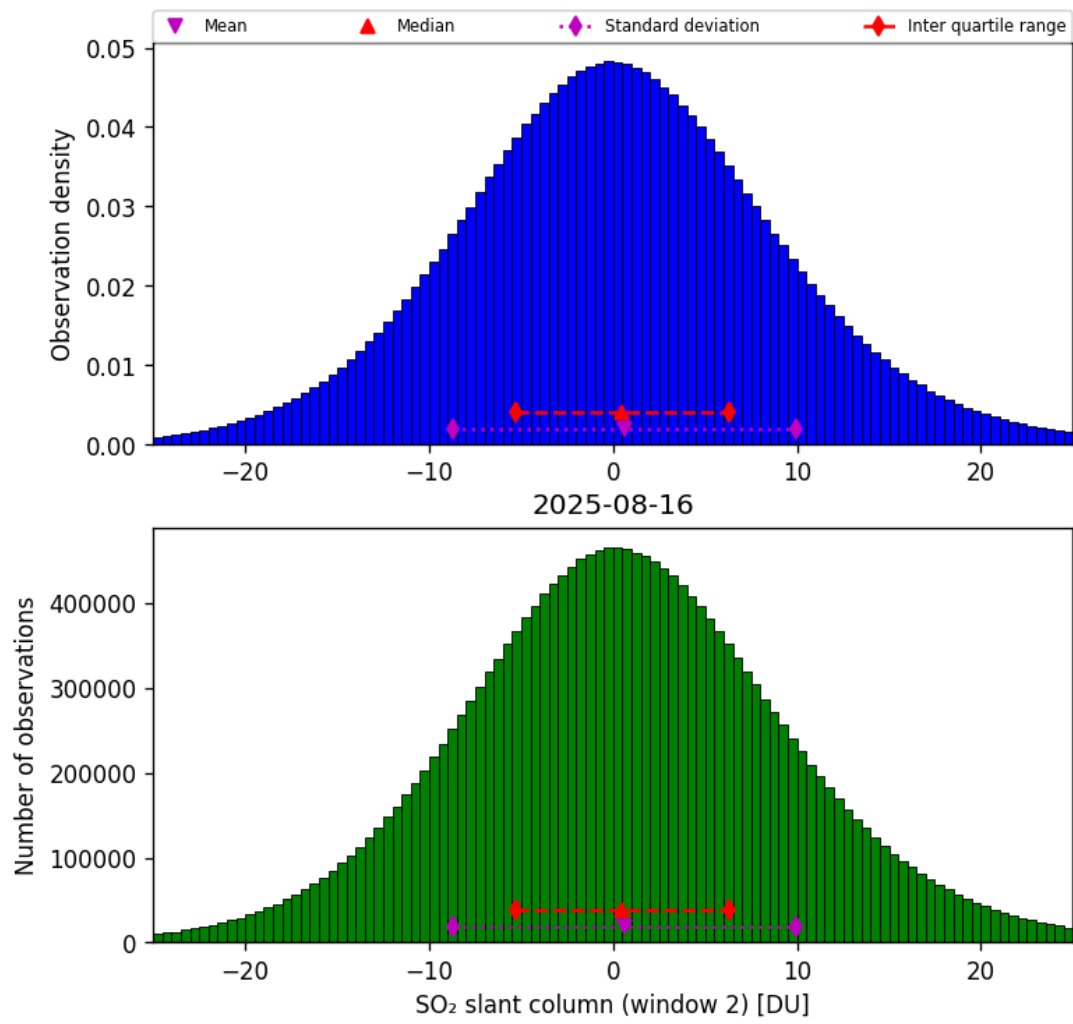
Figure 67: Histogram of “SO 2 slant column (window 2)” for 2025-08-15 to 2025-08-17
