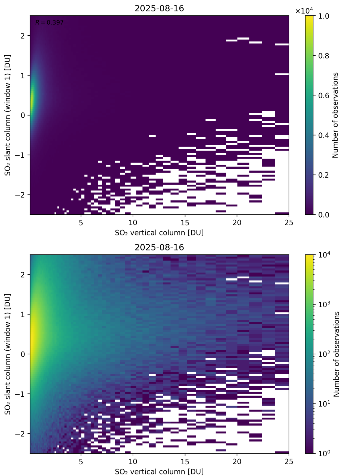
Figure 354: Scatter density plot of “SO 2 vertical column” against “SO 2 slant column (window 1)” for 2025-08-15 to 2025-08-17.
