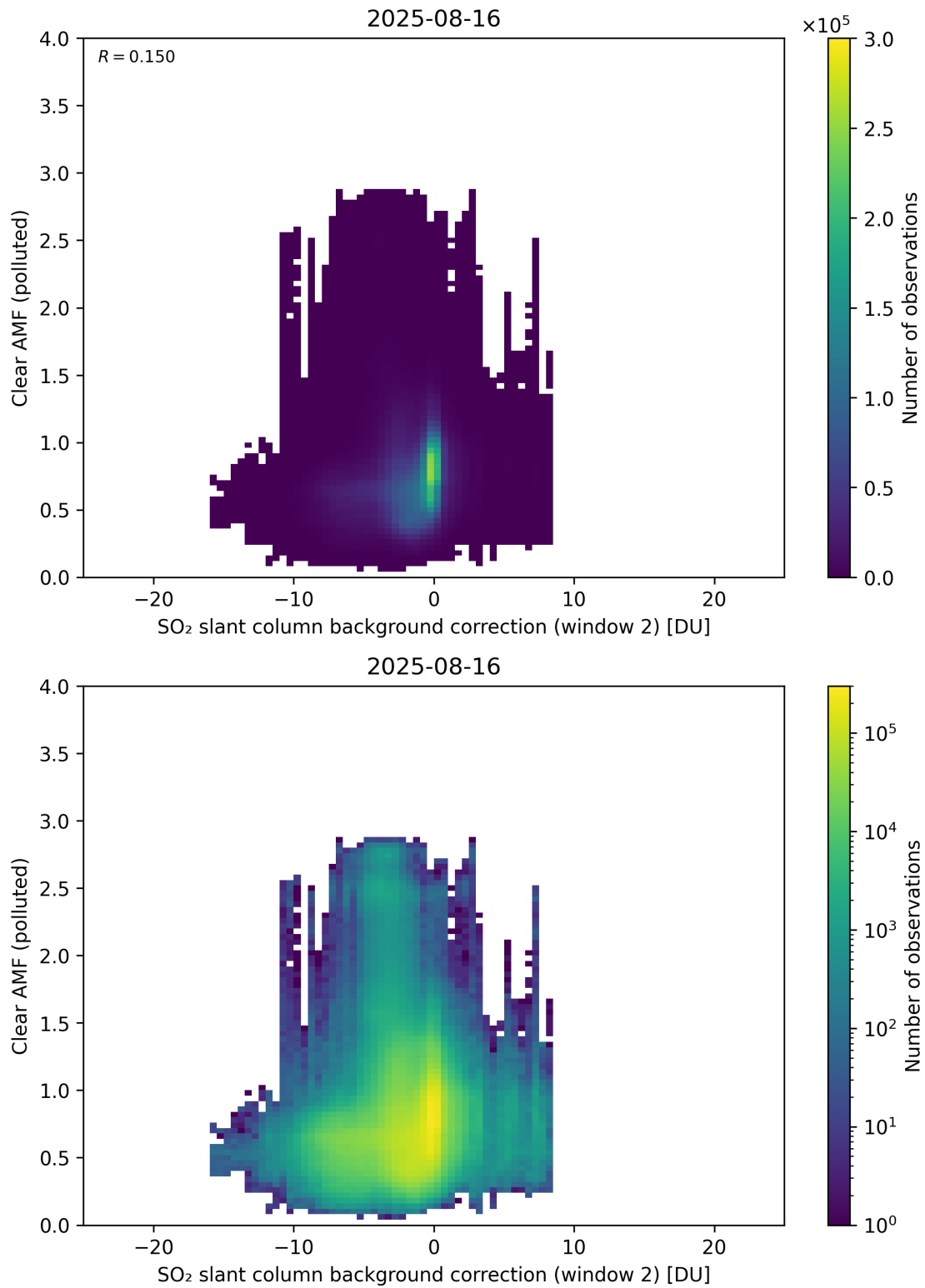
Figure 126: Scatter density plot of “SO 2 slant column background correction (window 2)” against “Clear AMF (polluted)” for 2025-08-15 to 2025-08-17.
