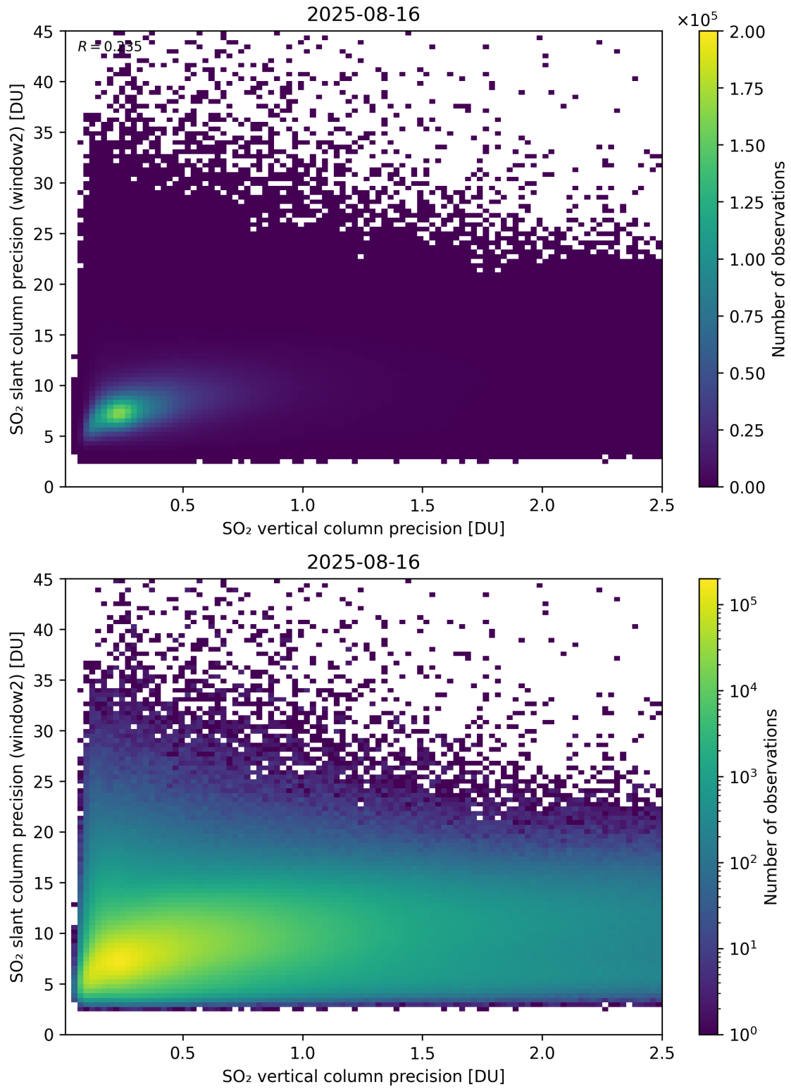
Figure 343: Scatter density plot of “SO 2 vertical column precision” against “SO 2 slant column precision (window2)” for 2025-08-15 to 2025-08-17.
