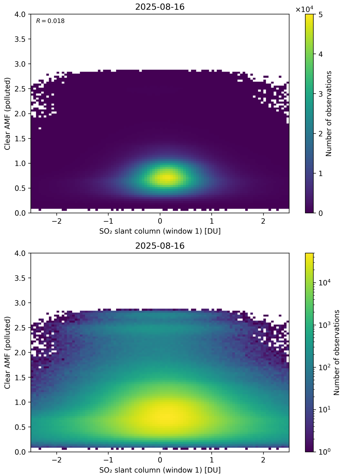
Figure 282: Scatter density plot of “SO 2 slant column (window 1)” against “Clear AMF (polluted)” for 2025-08-15 to 2025-08-17.
