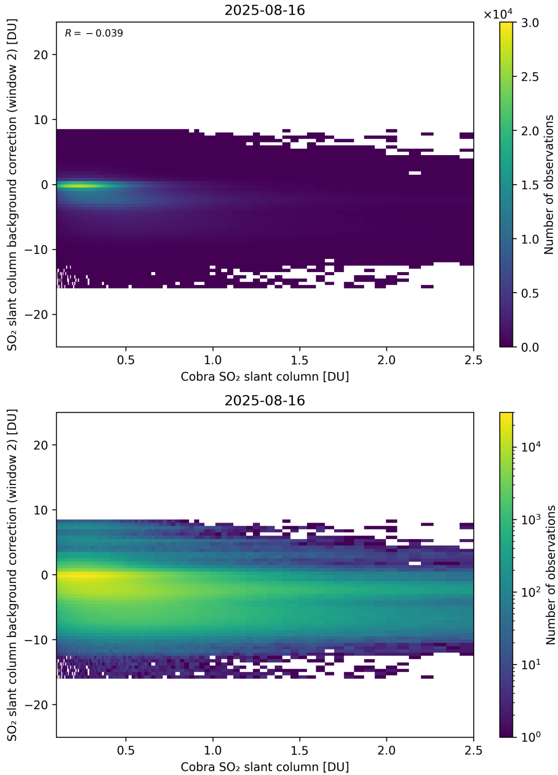
Figure 194: Scatter density plot of “Cobra SO 2 slant column” against “SO 2 slant column background correction (window 2)” for 2025-08-15 to 2025-08-17.
