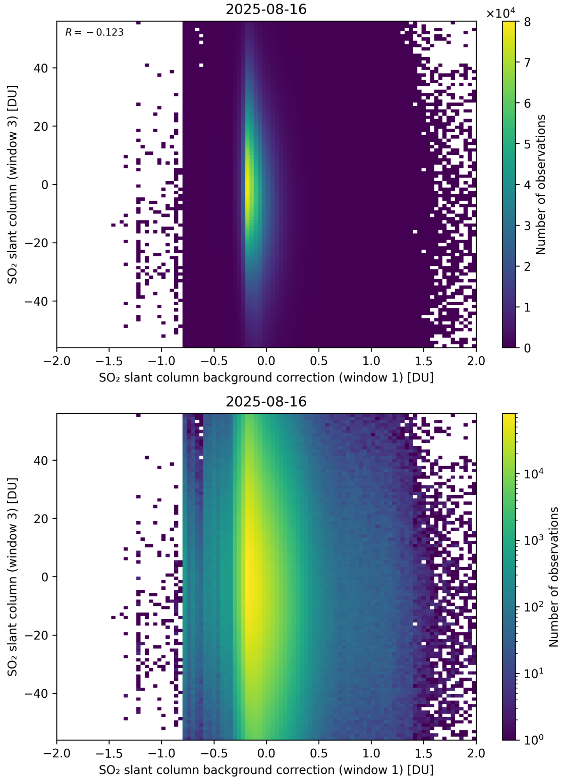
Figure 118: Scatter density plot of “SO 2 slant column background correction (window 1)” against “SO 2 slant column (window 3)” for 2025-08-15 to 2025-08-17.
