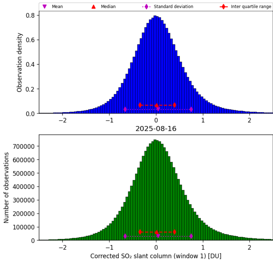
Figure 65: Histogram of “Corrected SO 2 slant column (window 1)” for 2025-08-15 to 2025-08-17
