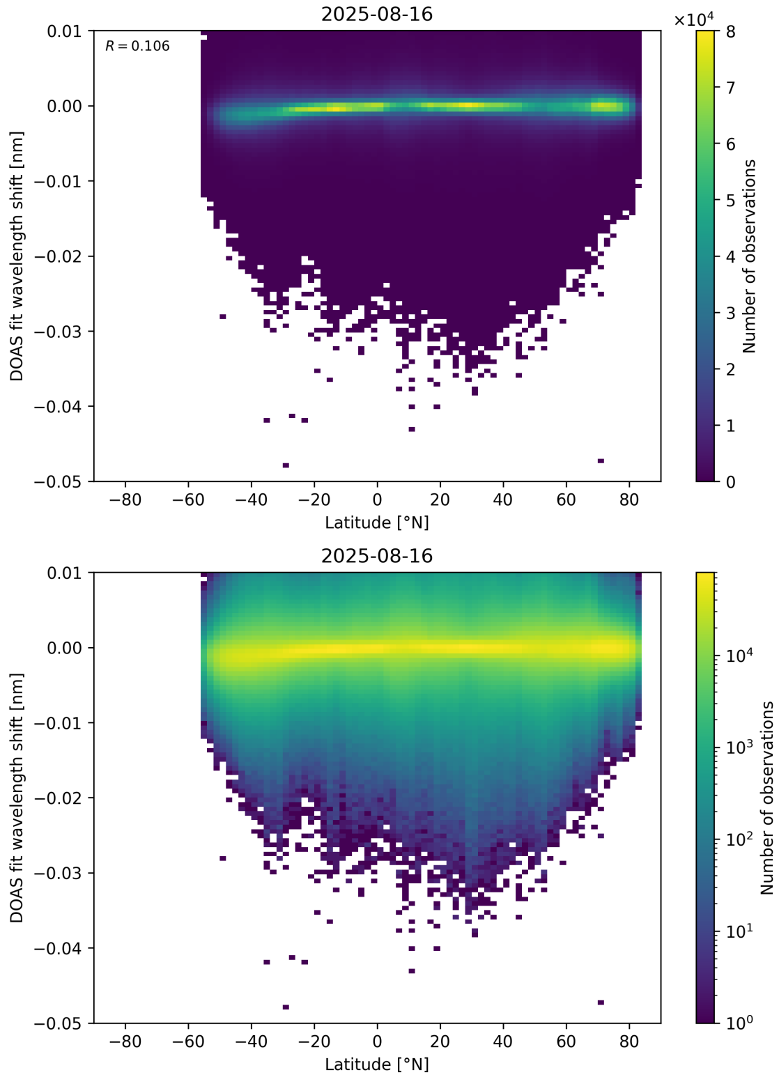
Figure 153: Scatter density plot of “Latitude” against “DOAS fit wavelength shift” for 2025-08-15 to 2025-08-17.
