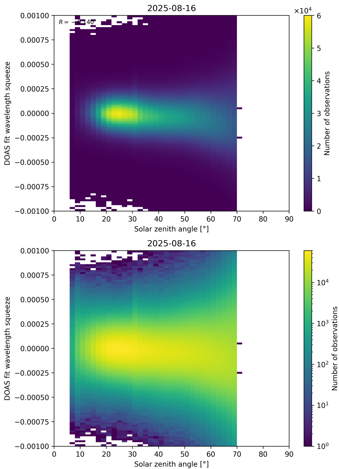
Figure 175: Scatter density plot of “Solar zenith angle” against “DOAS fit wavelength squeeze” for 2025-08-15 to 2025-08-17.
