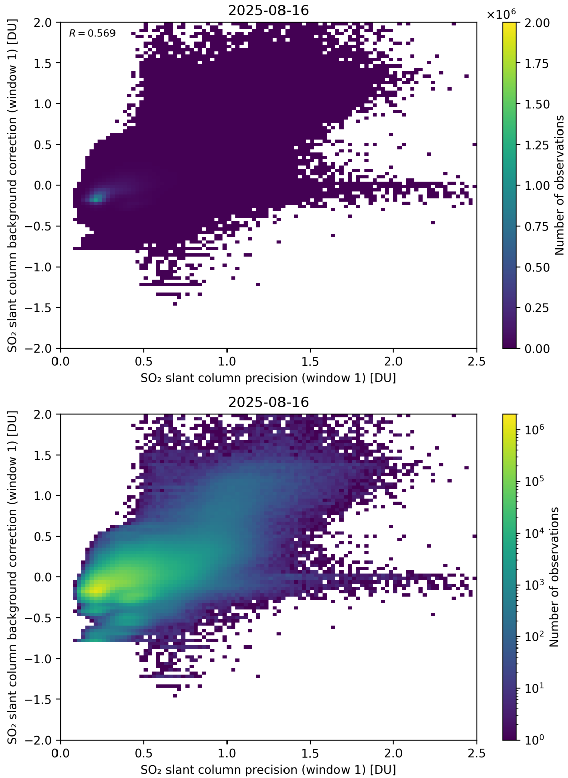
Figure 268: Scatter density plot of “SO 2 slant column precision (window 1)” against “SO 2 slant column background correction (window 1)” for 2025-08-15 to 2025-08-17.
