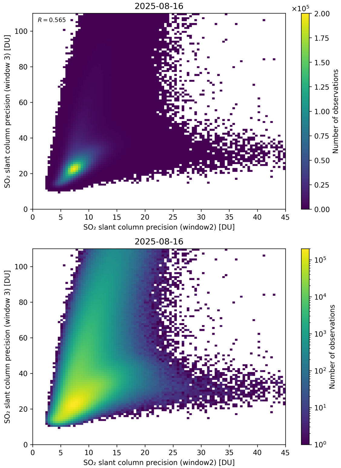
Figure 300: Scatter density plot of “SO 2 slant column precision (window2)” against “SO 2 slant column precision (window 3)” for 2025-08-15 to 2025-08-17.
