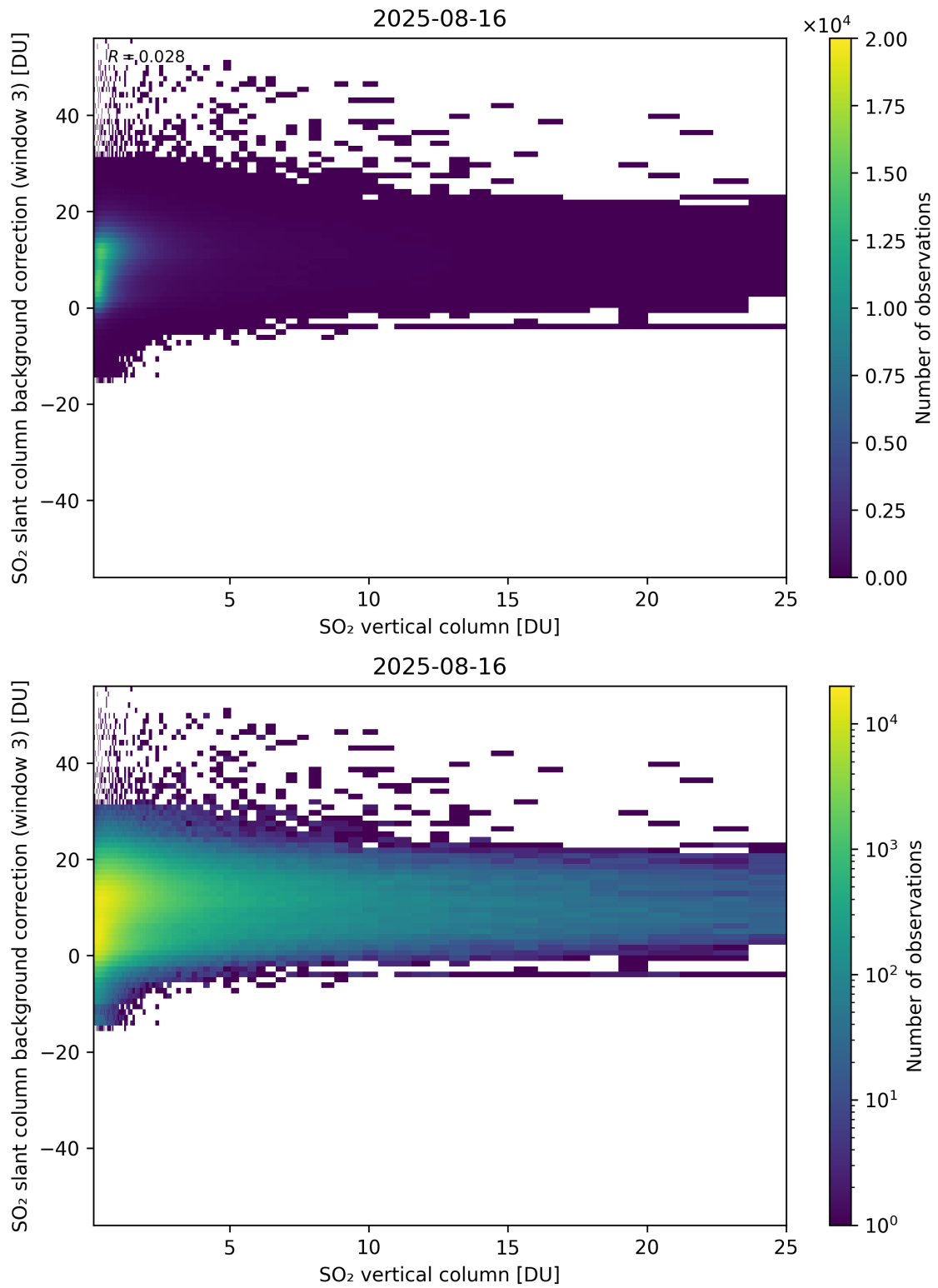
Figure 325: Scatter density plot of “SO 2 vertical column” against “SO 2 slant column background correction (window 3)” for 2025-08-15 to 2025-08-17.
