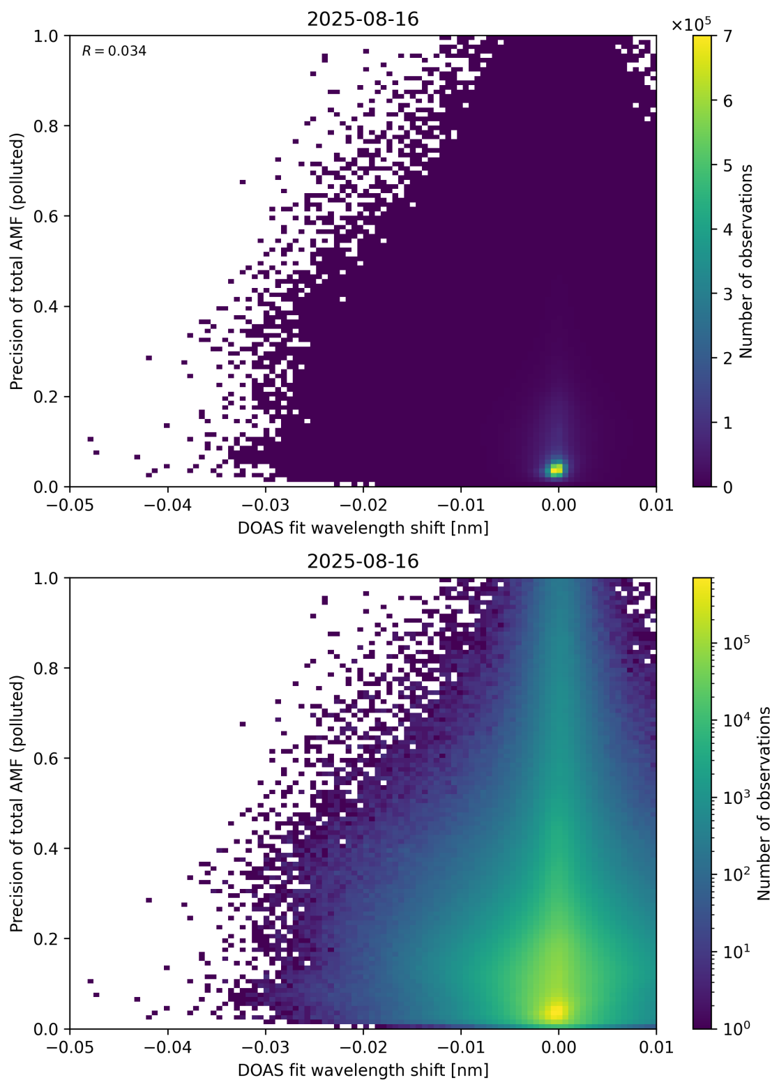
Figure 142: Scatter density plot of “DOAS fit wavelength shift” against “Precision of total AMF (polluted)” for 2025-08-15 to 2025-08-17.
