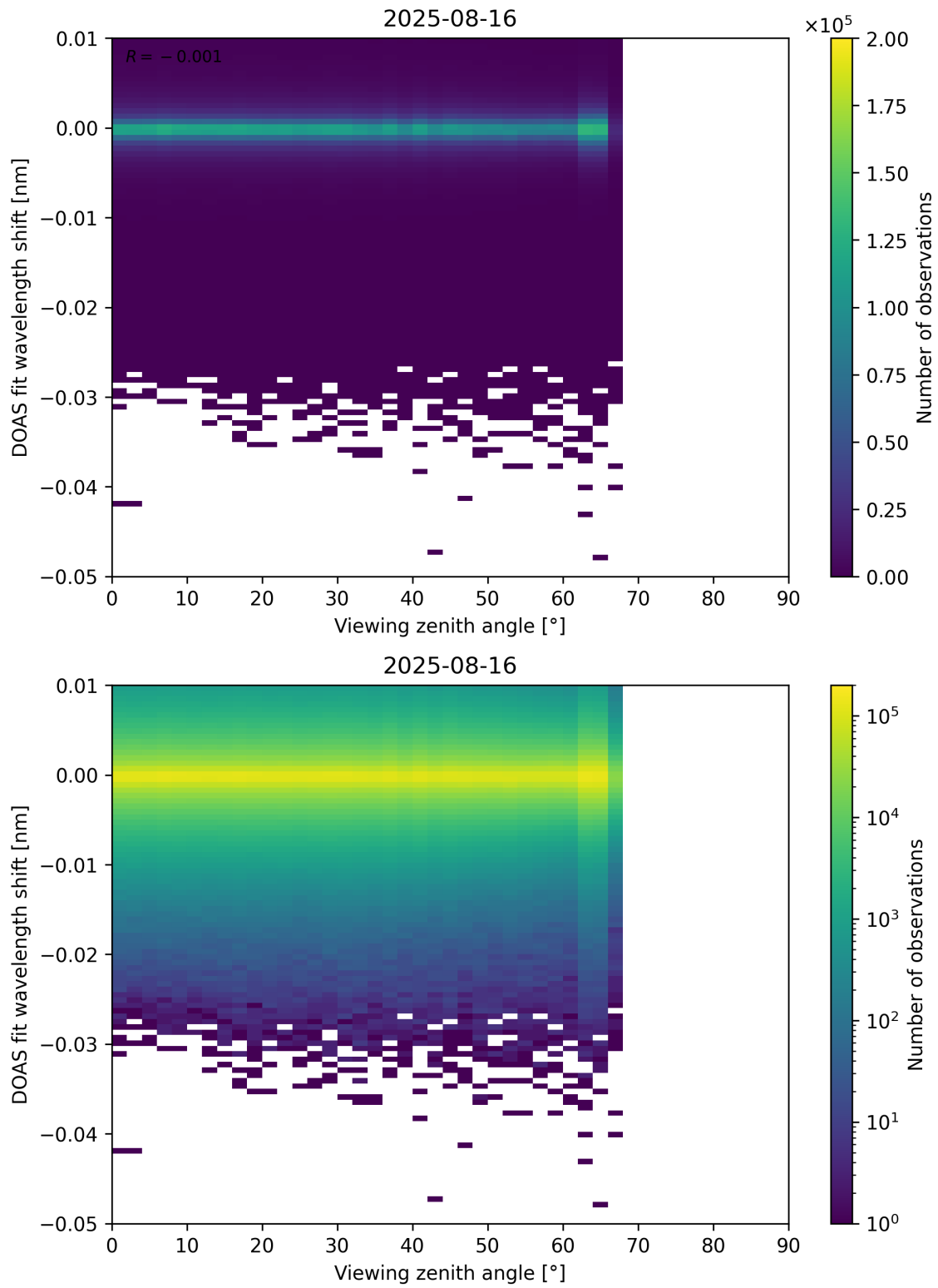
Figure 365: Scatter density plot of “Viewing zenith angle” against “DOAS fit wavelength shift” for 2025-08-15 to 2025-08-17.
