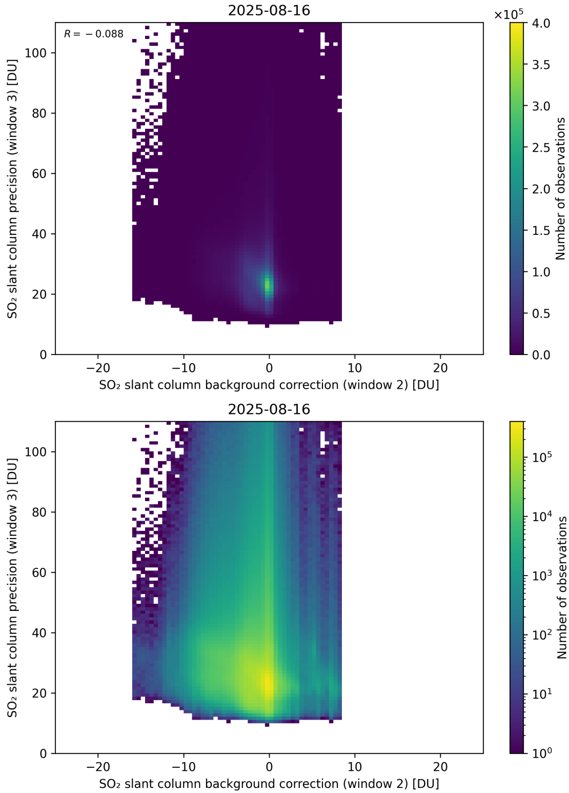
Figure 129: Scatter density plot of “SO 2 slant column background correction (window 2)” against “SO 2 slant column precision (window 3)” for 2025-08-15 to 2025-08-17.
