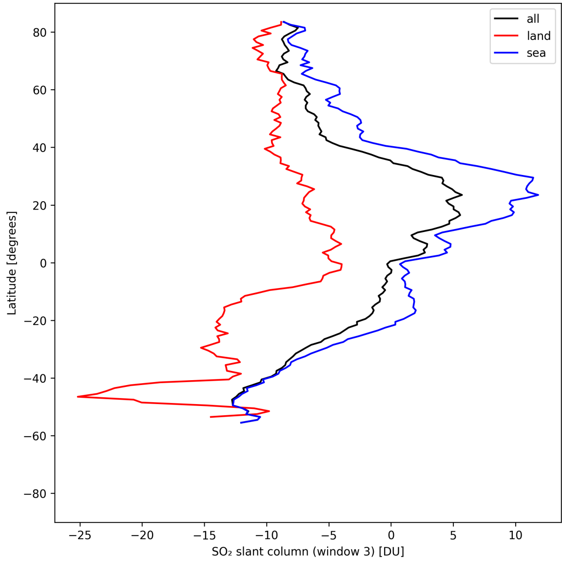
Figure 45: Zonal average of “SO 2 slant column (window 3)” for 2025-08-15 to 2025-08-17.
