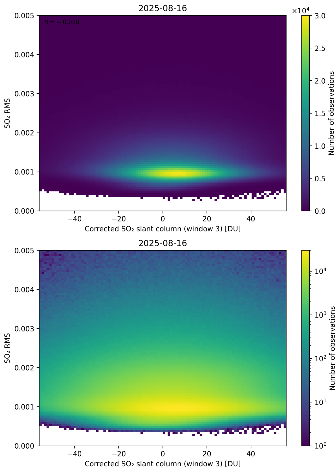
Figure 258: Scatter density plot of “Corrected SO 2 slant column (window 3)” against “SO 2 RMS” for 2025-08-15 to 2025-08-17.
