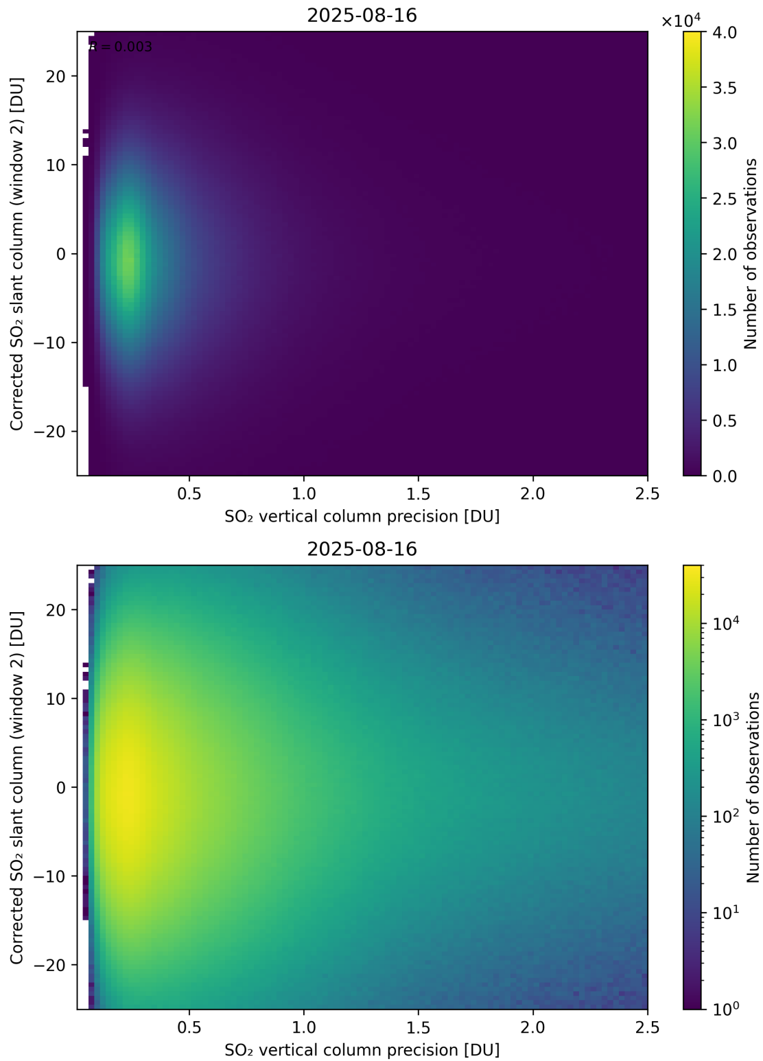
Figure 339: Scatter density plot of “SO 2 vertical column precision” against “Corrected SO 2 slant column (window 2)” for 2025-08-15 to 2025-08-17.
