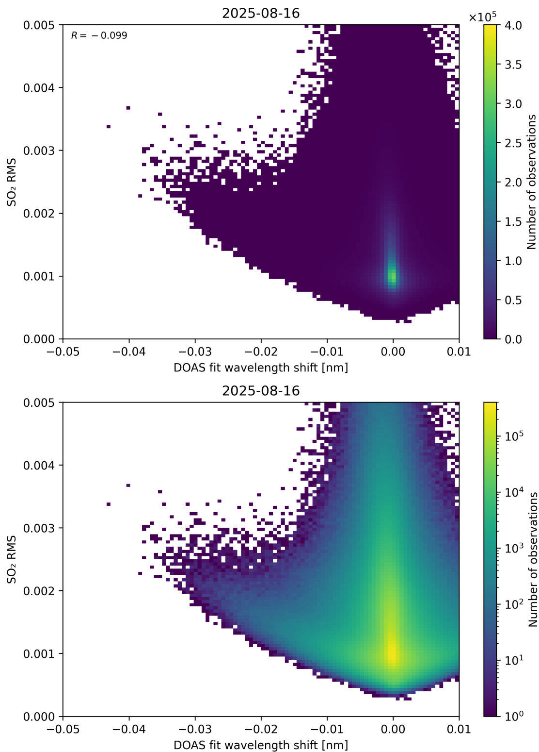
Figure 139: Scatter density plot of “DOAS fit wavelength shift” against “SO 2 RMS” for 2025-08-15 to 2025-08-17.
