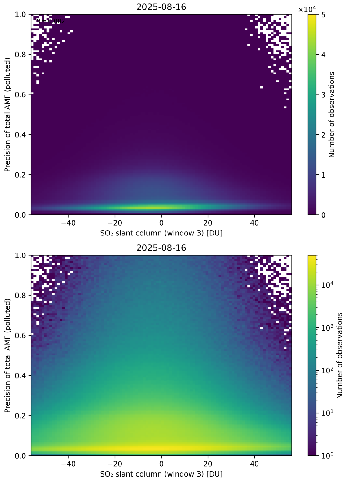
Figure 319: Scatter density plot of “SO 2 slant column (window 3)” against “Precision of total AMF (polluted)” for 2025-08-15 to 2025-08-17.
