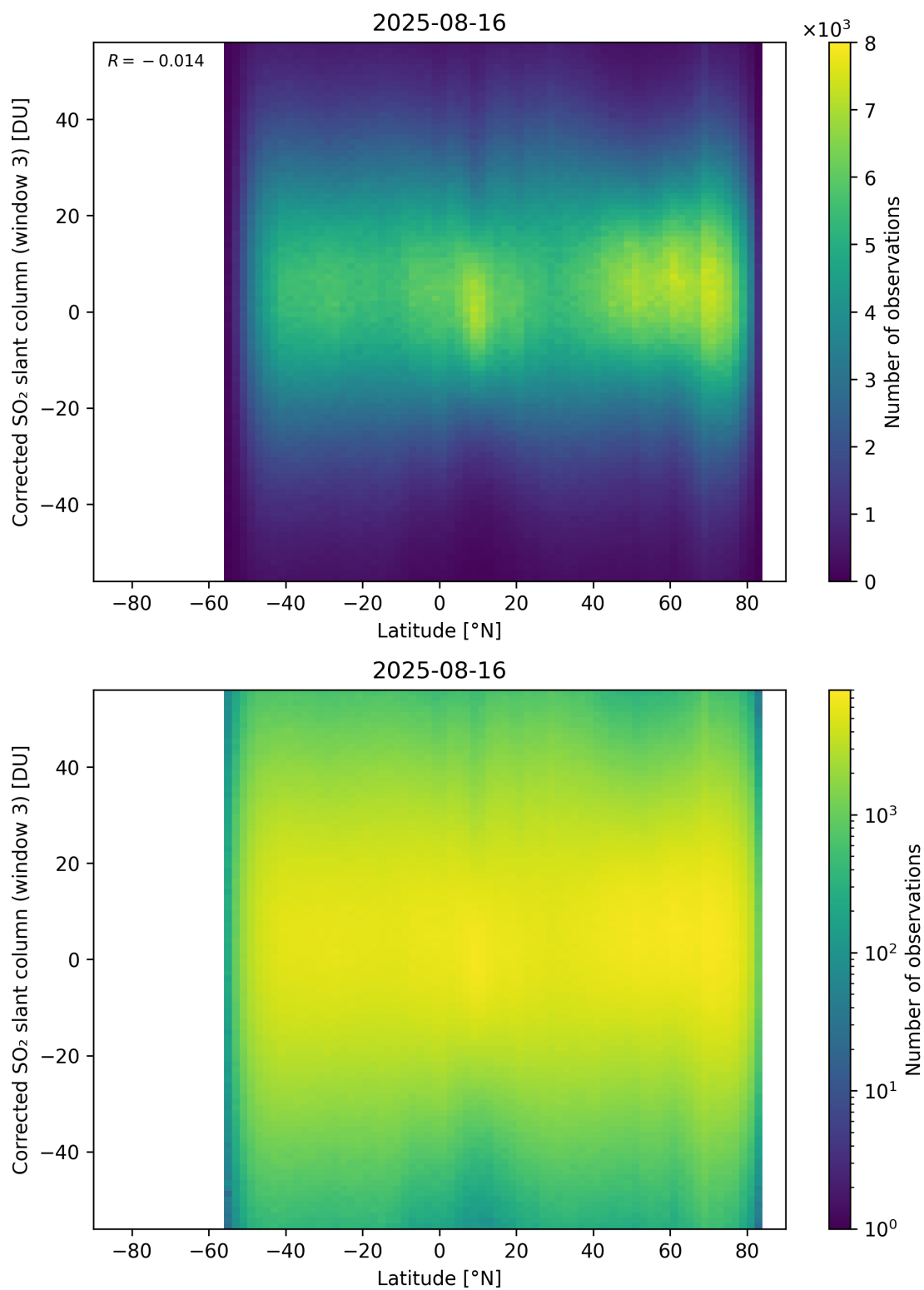
Figure 161: Scatter density plot of “Latitude” against “Corrected SO 2 slant column (window 3)” for 2025-08-15 to 2025-08-17.
