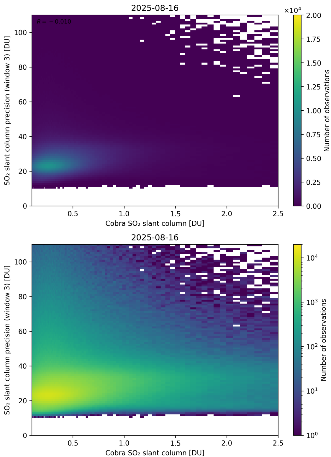
Figure 223: Scatter density plot of “Cobra SO 2 slant column” against “SO 2 slant column precision (window 3)” for 2025-08-15 to 2025-08-17.
