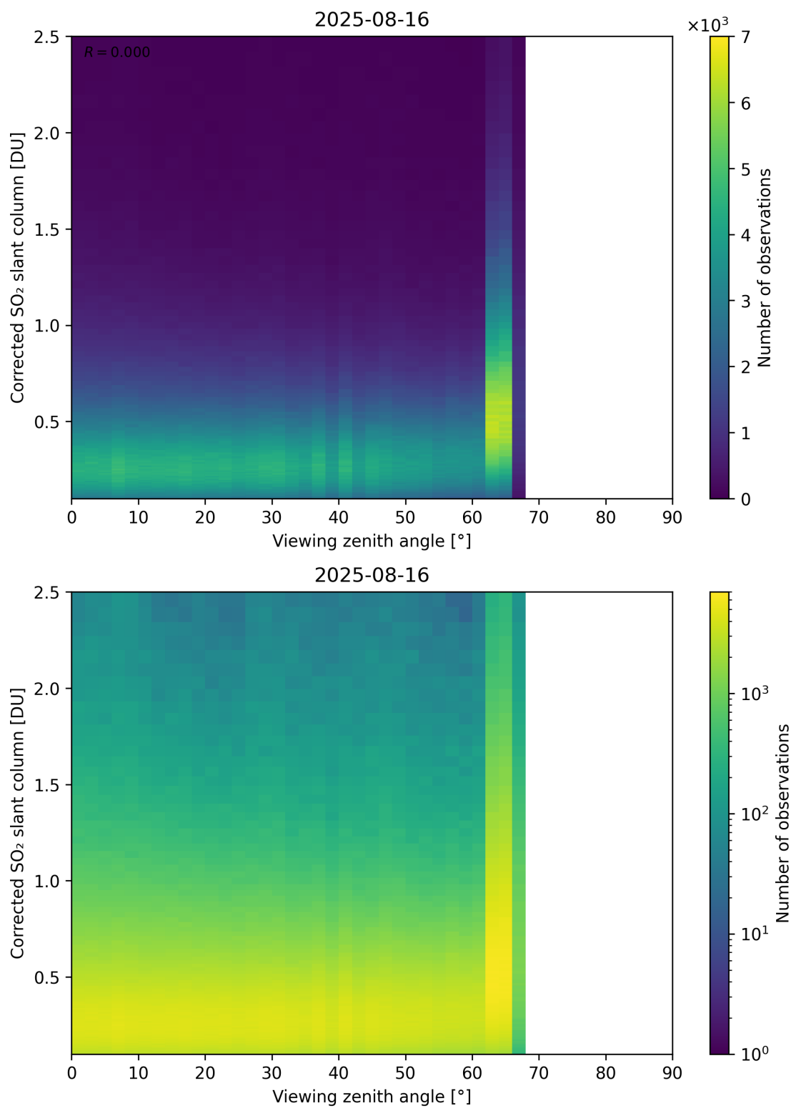
Figure 373: Scatter density plot of “Viewing zenith angle” against “Corrected SO 2 slant column” for 2025-08-15 to 2025-08-17.
