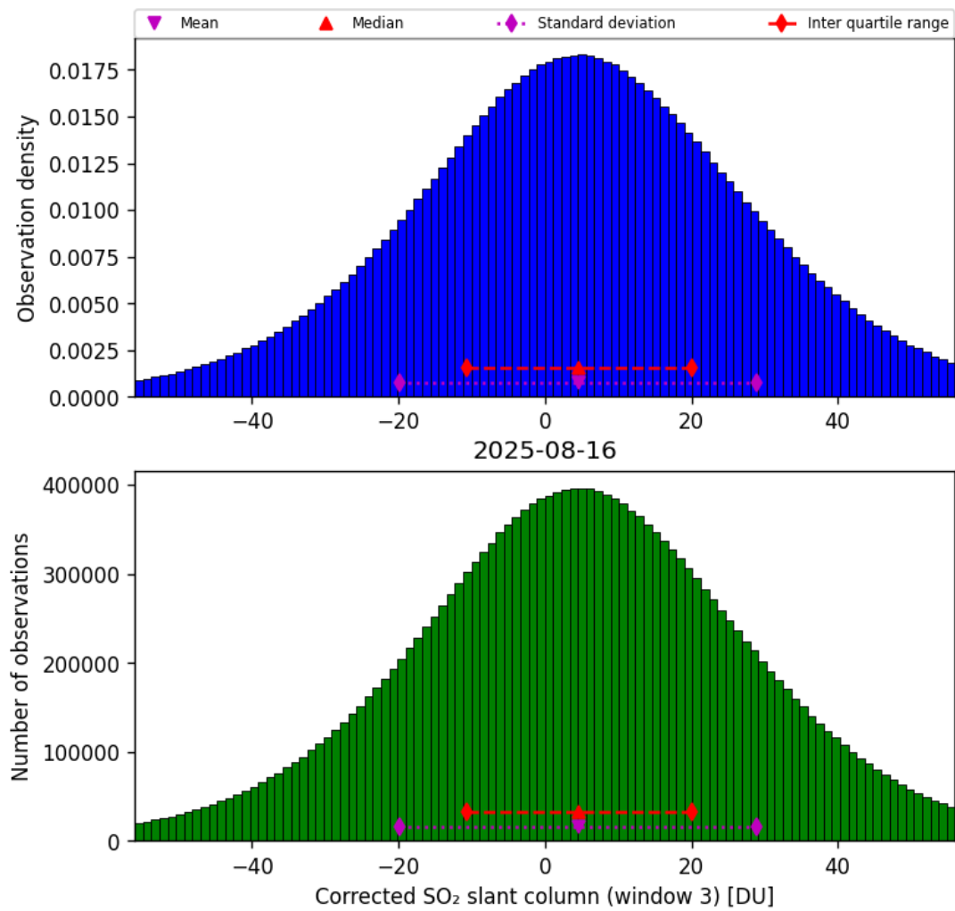
Figure 73: Histogram of “Corrected SO 2 slant column (window 3)” for 2025-08-15 to 2025-08-17
