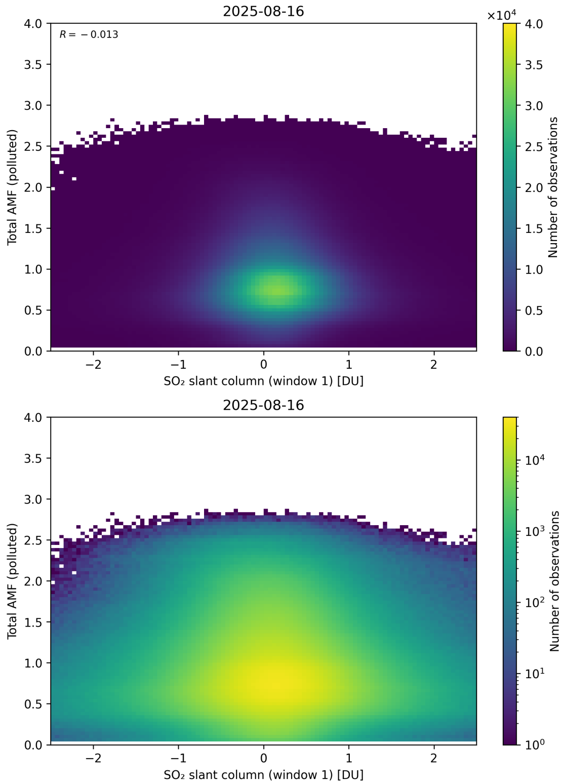
Figure 289: Scatter density plot of “SO 2 slant column (window 1)” against “Total AMF (polluted)” for 2025-08-15 to 2025-08-17.
