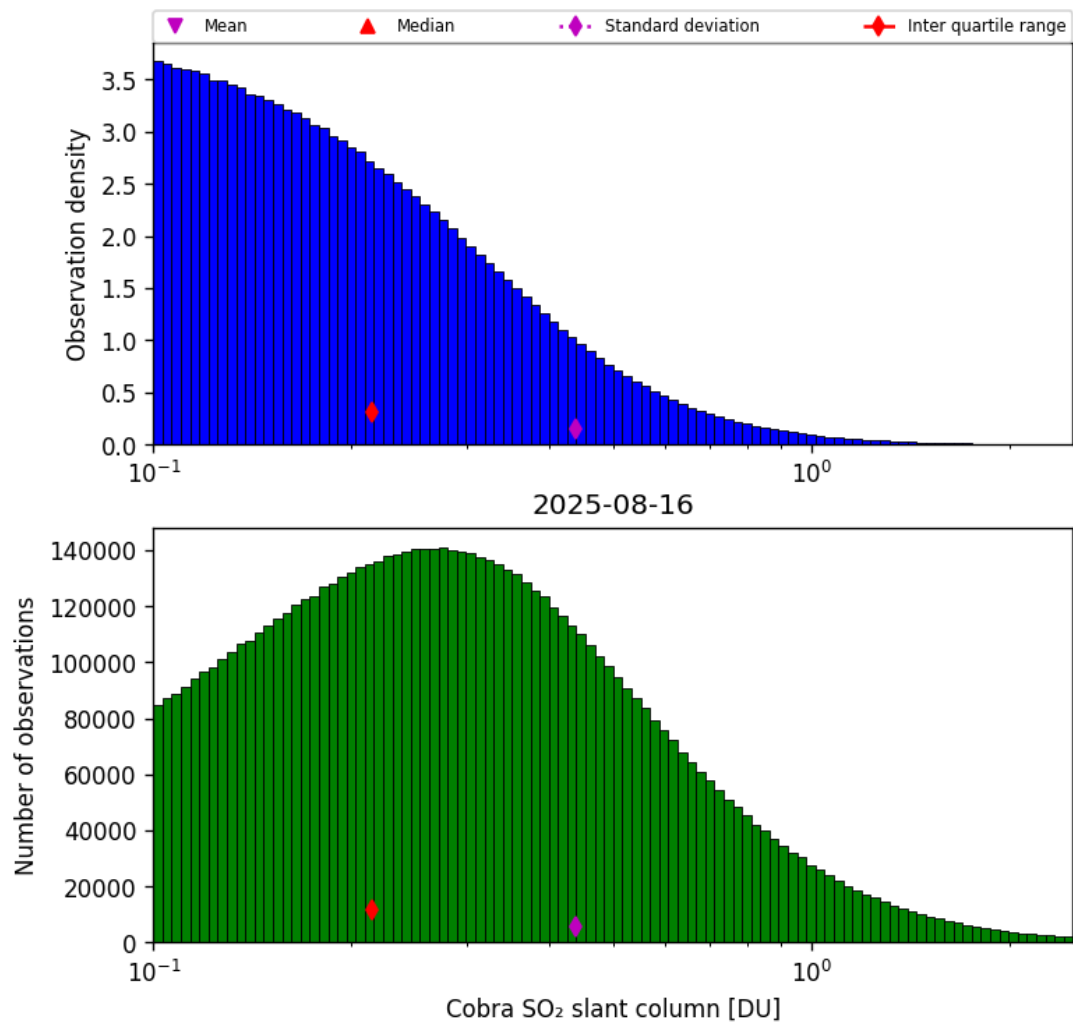
Figure 61: Histogram of “Cobra SO 2 slant column” for 2025-08-15 to 2025-08-17
