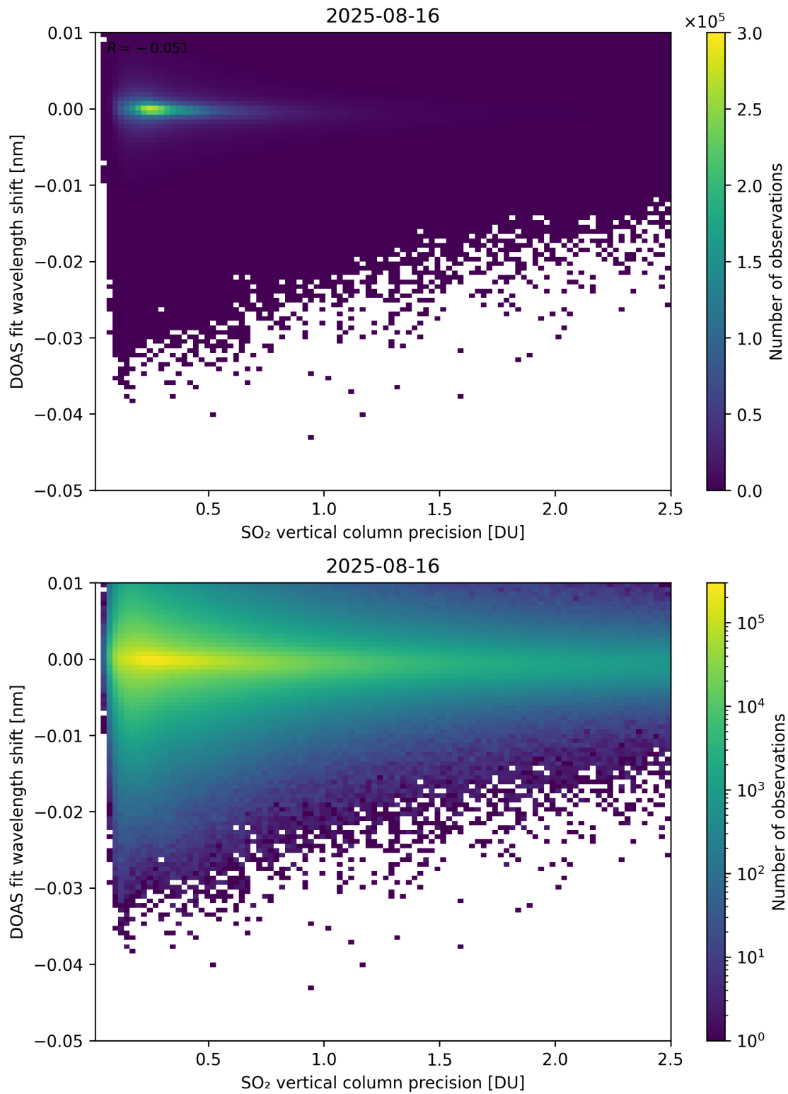
Figure 332: Scatter density plot of “SO 2 vertical column precision” against “DOAS fit wavelength shift” for 2025-08-15 to 2025-08-17.
