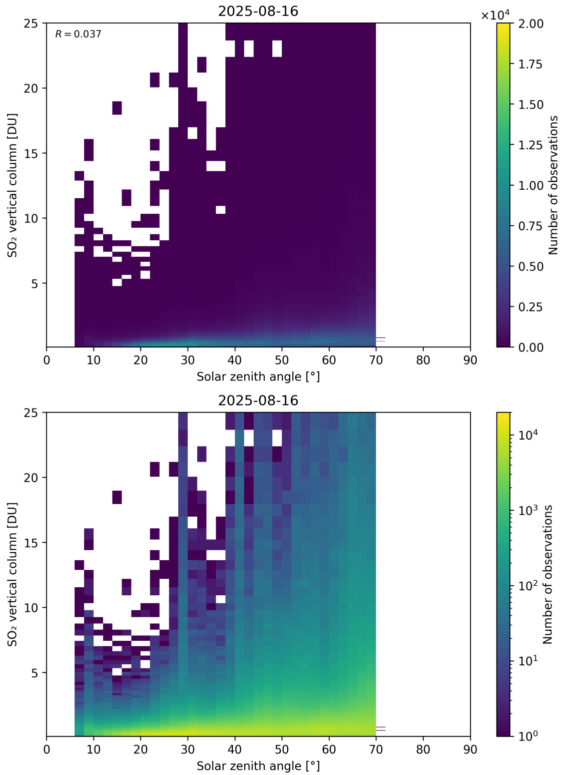
Figure 191: Scatter density plot of “Solar zenith angle” against “SO 2 vertical column” for 2025-08-15 to 2025-08-17.
