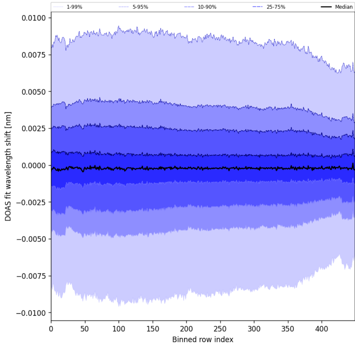
Figure 102: Along track statistics of “DOAS fit wavelength shift” for 2025-08-15 to 2025-08-17
