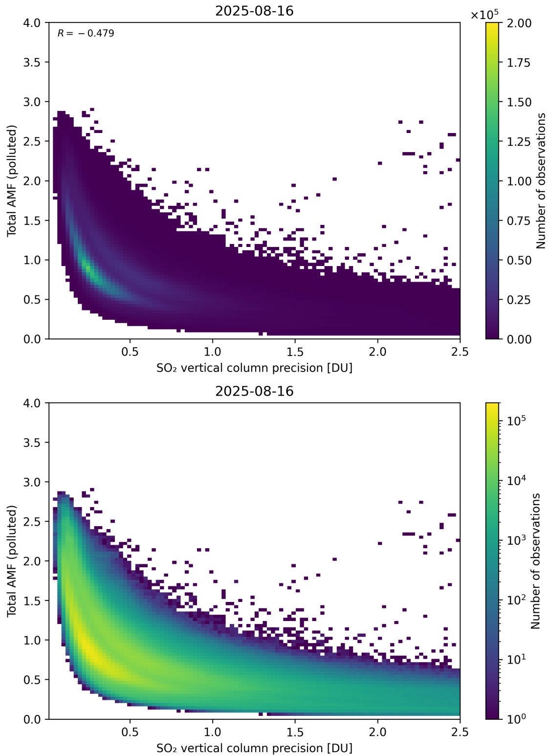
Figure 346: Scatter density plot of “SO 2 vertical column precision” against “Total AMF (polluted)” for 2025-08-15 to 2025-08-17.
