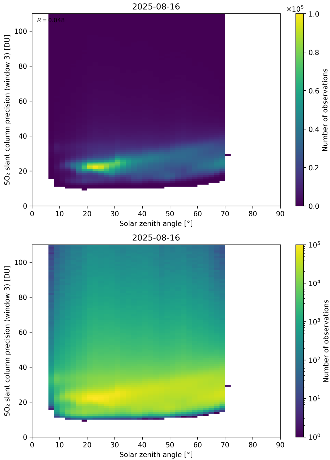
Figure 188: Scatter density plot of “Solar zenith angle” against “SO 2 slant column precision (window 3)” for 2025-08-15 to 2025-08-17.
