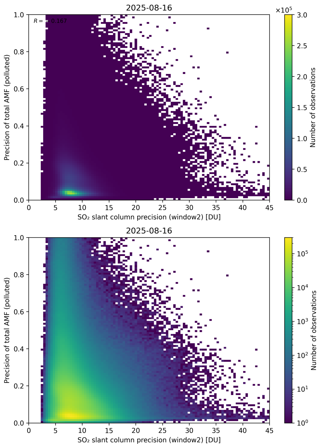
Figure 302: Scatter density plot of “SO 2 slant column precision (window2)” against “Precision of total AMF (polluted)” for 2025-08-15 to 2025-08-17.
