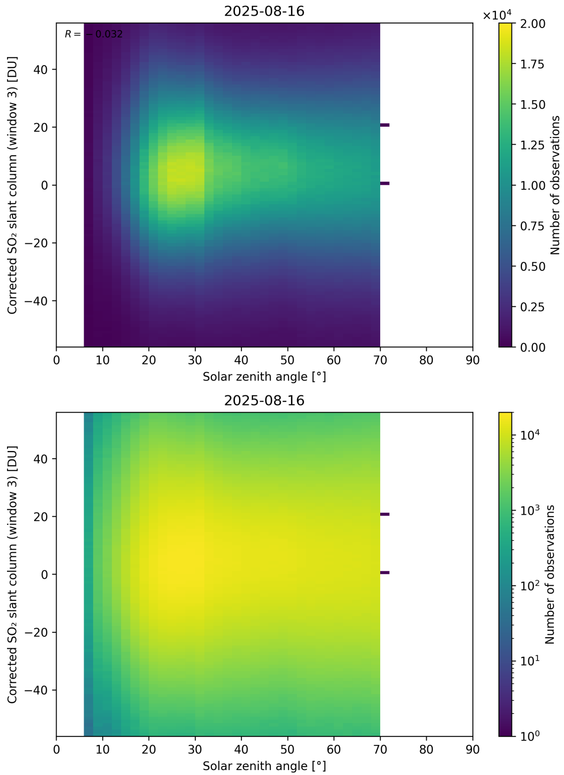
Figure 183: Scatter density plot of “Solar zenith angle” against “Corrected SO 2 slant column (window 3)” for 2025-08-15 to 2025-08-17.
