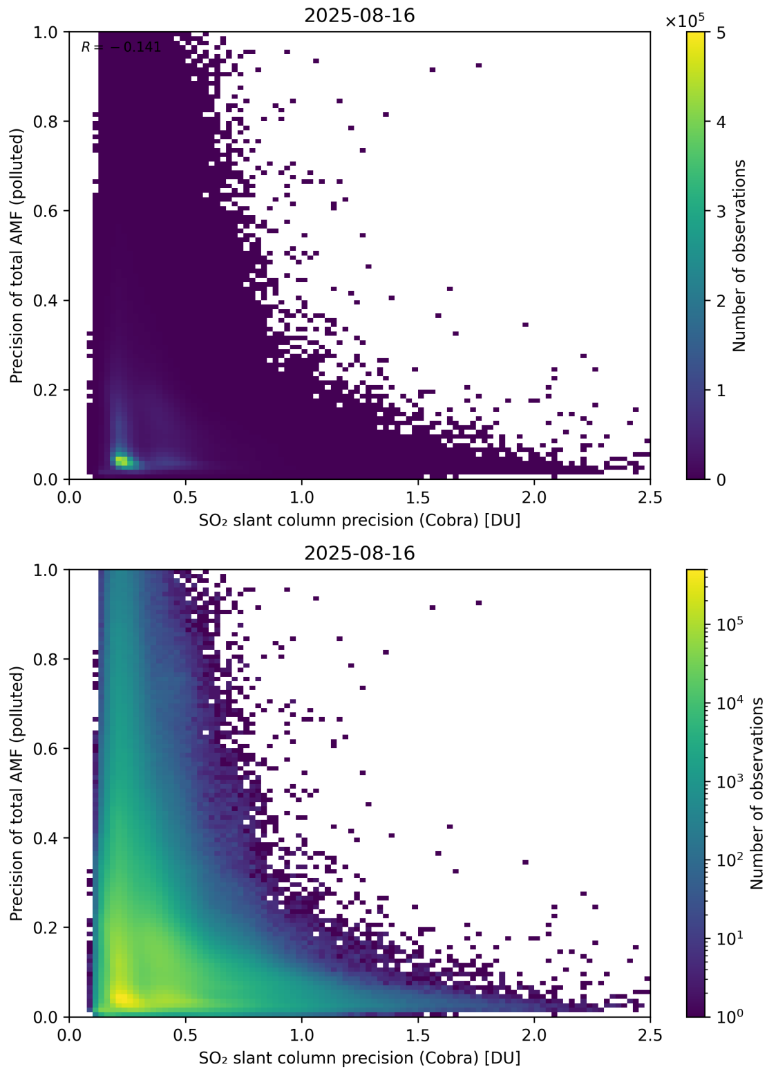
Figure 214: Scatter density plot of “SO 2 slant column precision (Cobra)” against “Precision of total AMF (polluted)” for 2025-08-15 to 2025-08-17.
