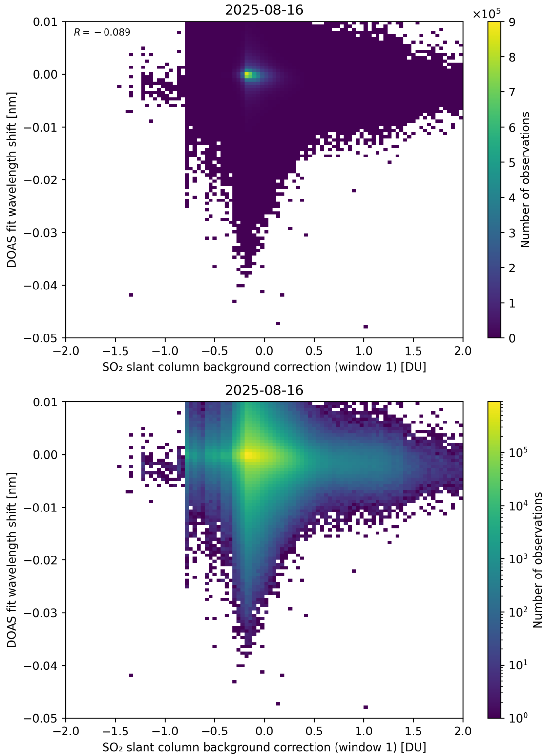
Figure 111: Scatter density plot of “SO 2 slant column background correction (window 1)” against “DOAS fit wavelength shift” for 2025-08-15 to 2025-08-17.
