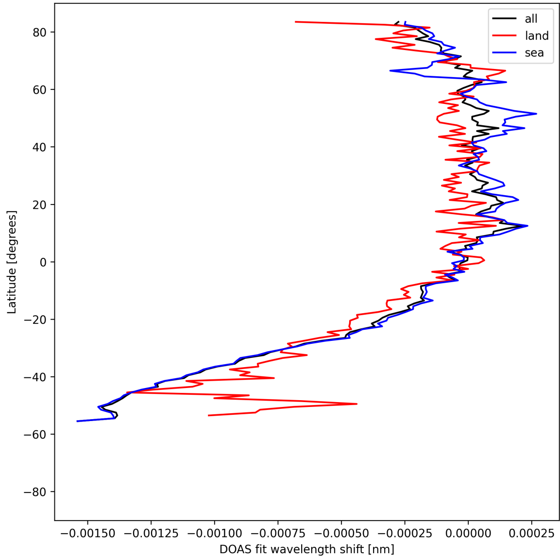
Figure 50: Zonal average of “DOAS fit wavelength shift” for 2025-08-15 to 2025-08-17.
