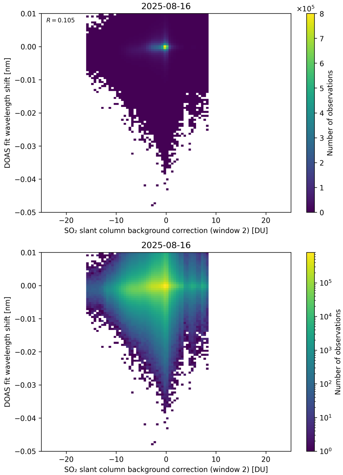
Figure 123: Scatter density plot of “SO 2 slant column background correction (window 2)” against “DOAS fit wavelength shift” for 2025-08-15 to 2025-08-17.
