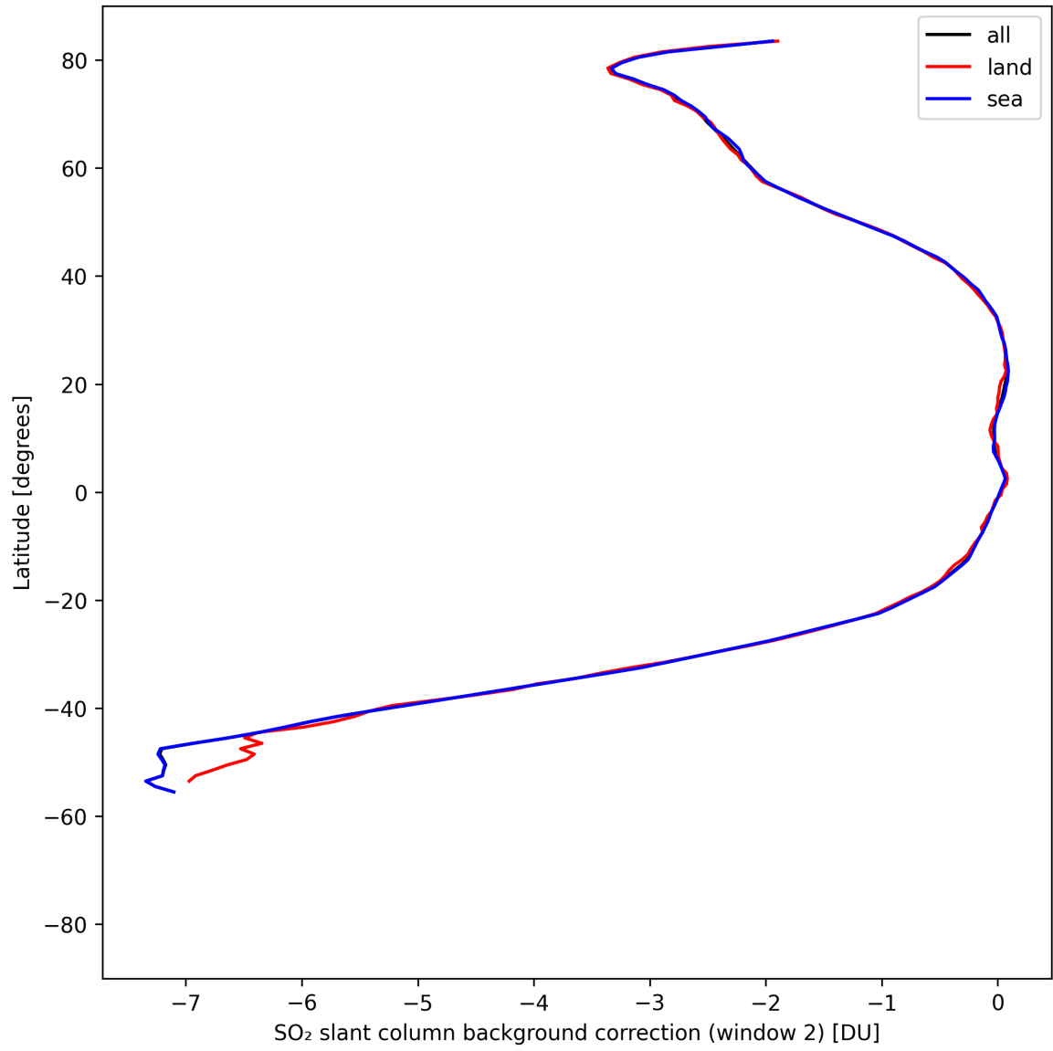
Figure 44: Zonal average of “SO 2 slant column background correction (window 2)” for 2025-08-15 to 2025-08-17.
