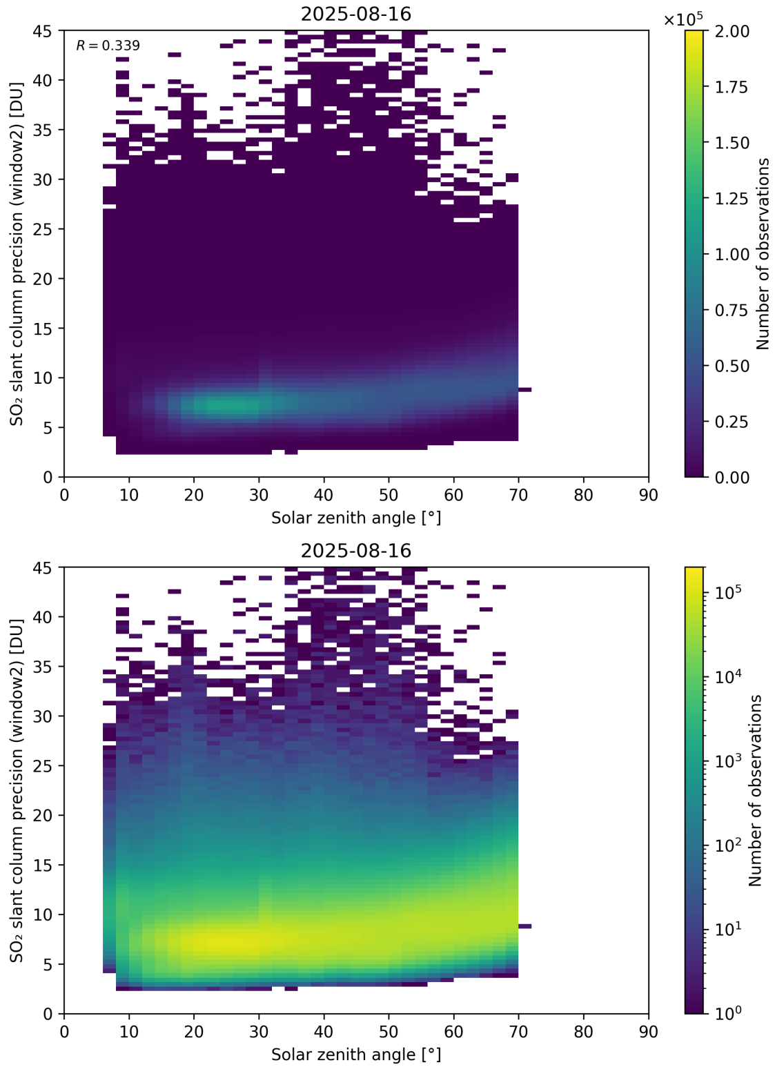
Figure 186: Scatter density plot of “Solar zenith angle” against “SO 2 slant column precision (window2)” for 2025-08-15 to 2025-08-17.
