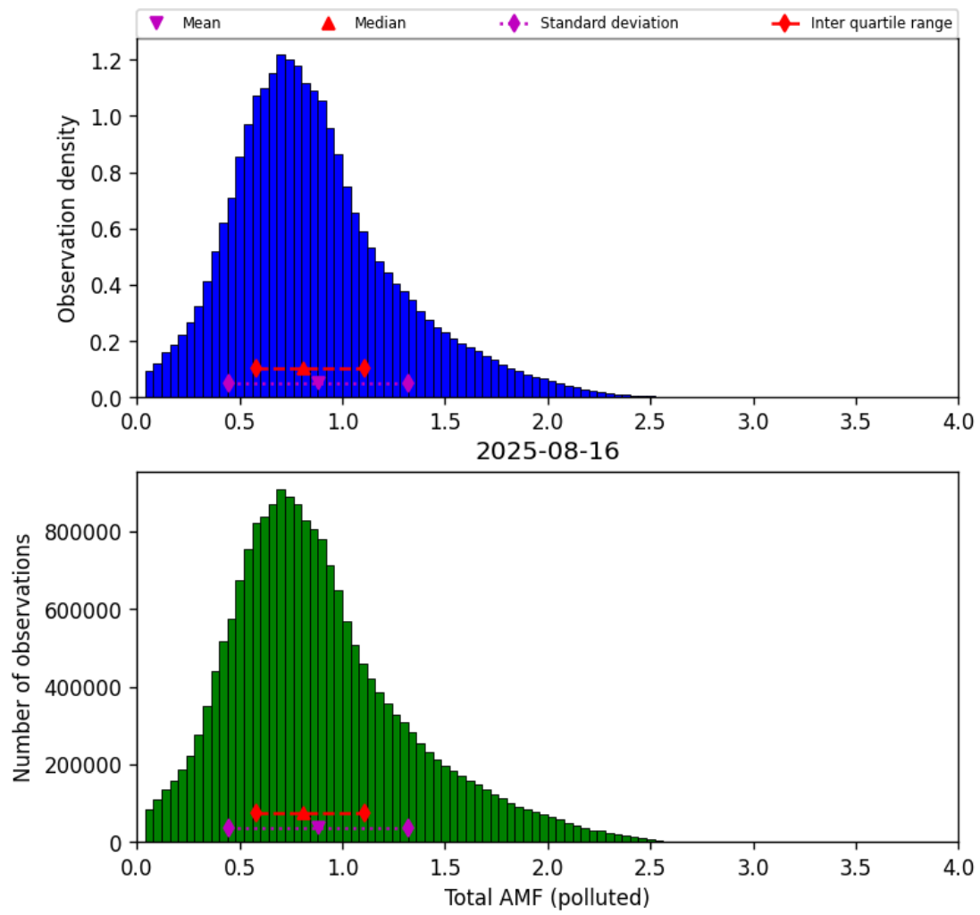
Figure 79: Histogram of “Total AMF (polluted)” for 2025-08-15 to 2025-08-17
