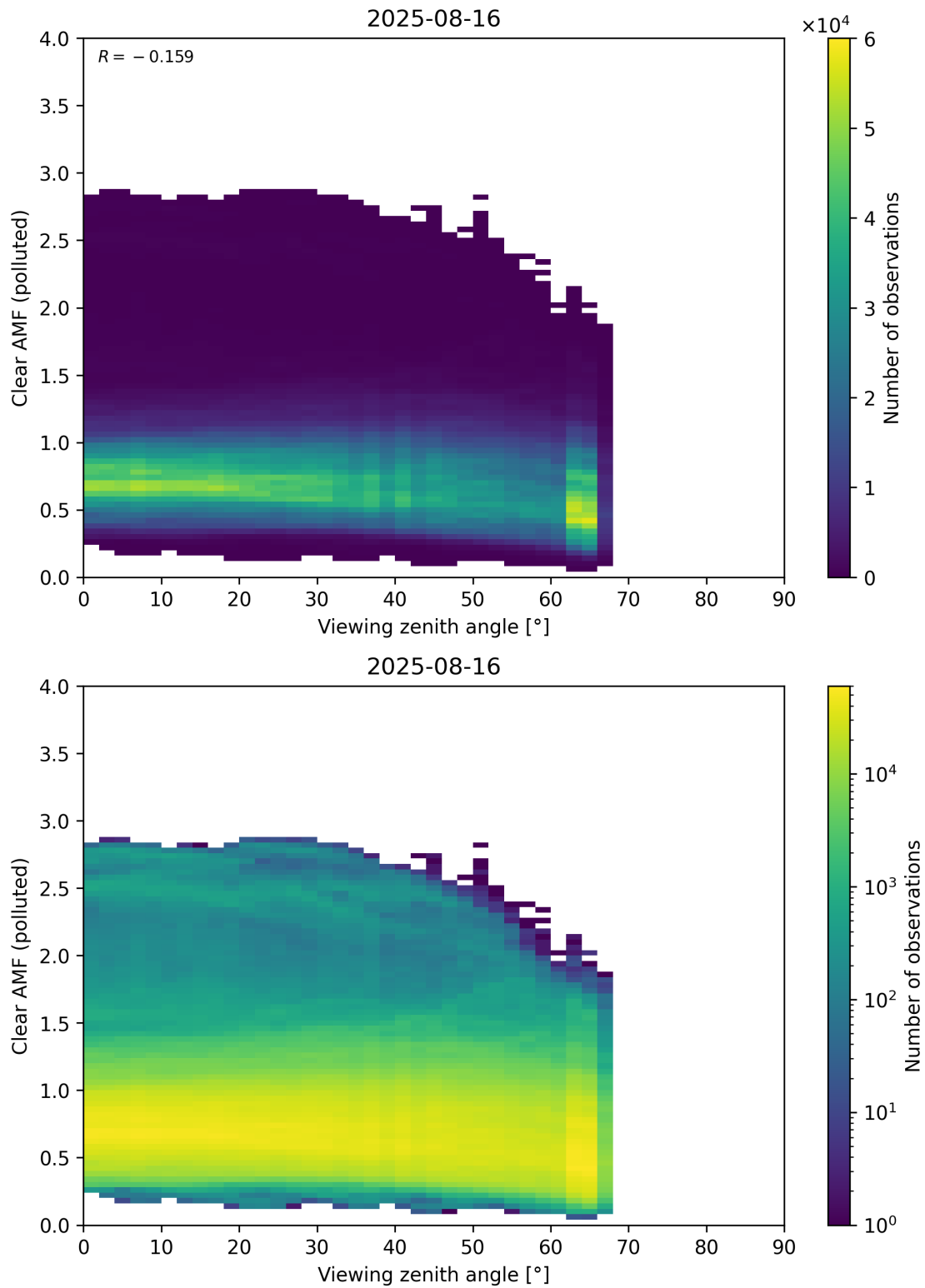
Figure 370: Scatter density plot of “Viewing zenith angle” against “Clear AMF (polluted)” for 2025-08-15 to 2025-08-17.
