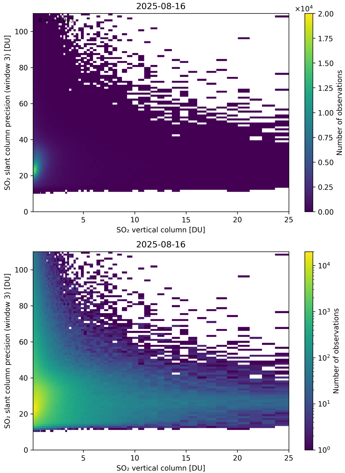
Figure 358: Scatter density plot of “SO 2 vertical column” against “SO 2 slant column precision (window 3)” for 2025-08-15 to 2025-08-17.
