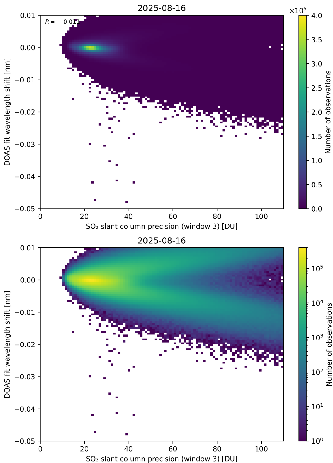
Figure 308: Scatter density plot of “SO 2 slant column precision (window 3)” against “DOAS fit wavelength shift” for 2025-08-15 to 2025-08-17.
