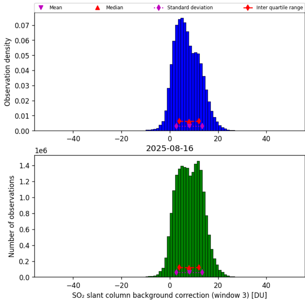
Figure 74: Histogram of “SO 2 slant column background correction (window 3)” for 2025-08-15 to 2025-08-17
