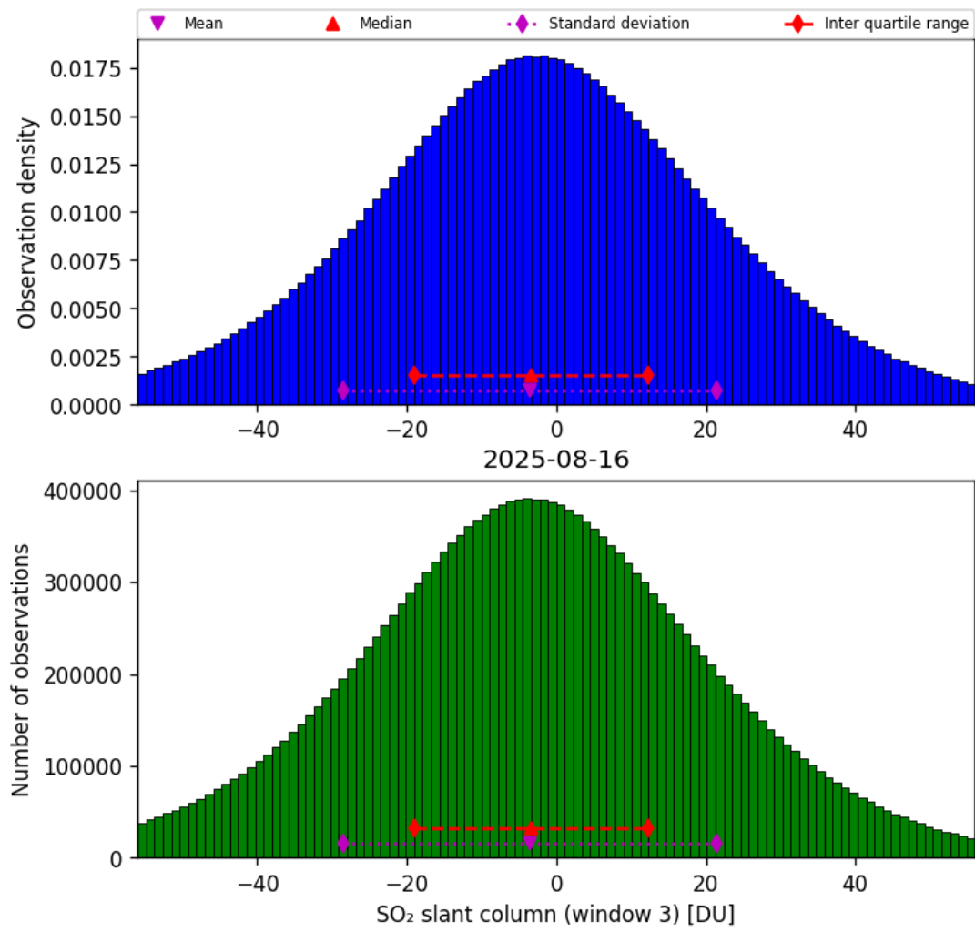
Figure 71: Histogram of “SO 2 slant column (window 3)” for 2025-08-15 to 2025-08-17
