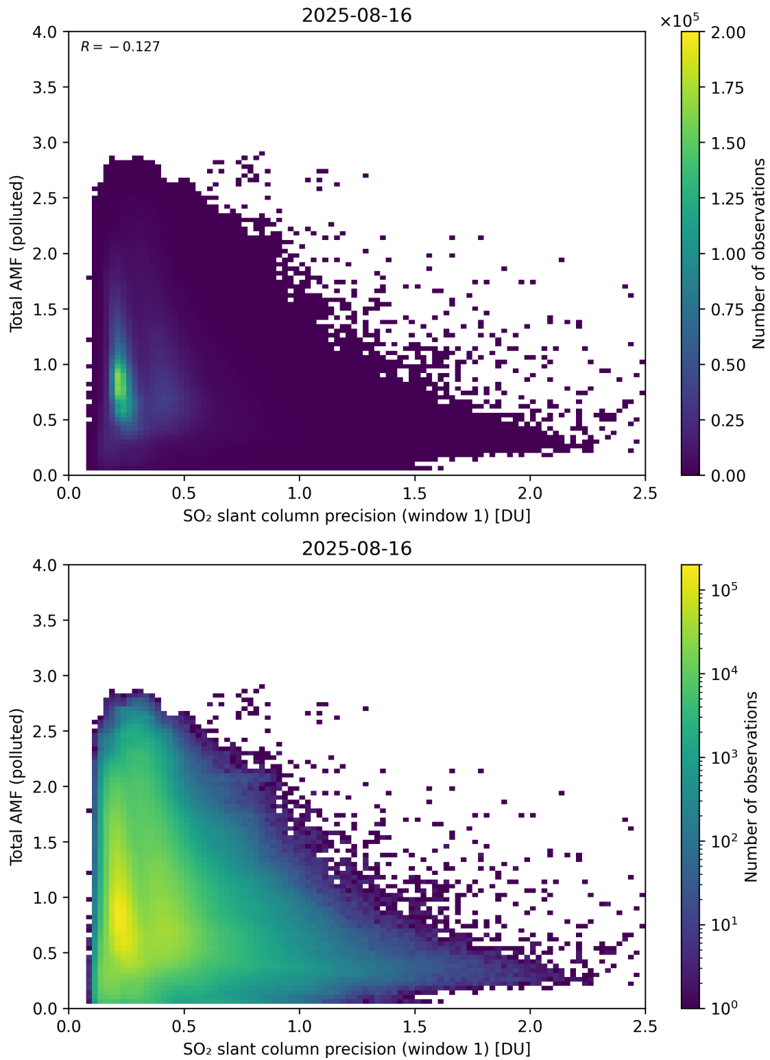
Figure 280: Scatter density plot of “SO 2 slant column precision (window 1)” against “Total AMF (polluted)” for 2025-08-15 to 2025-08-17.
