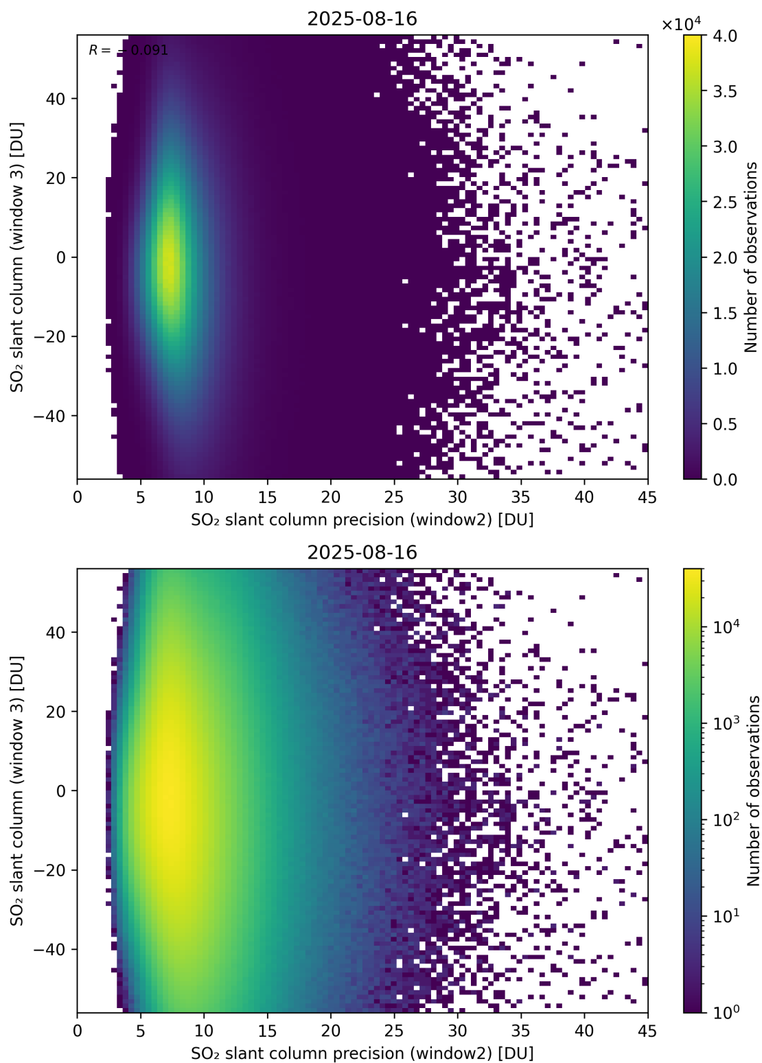
Figure 299: Scatter density plot of “SO 2 slant column precision (window2)” against “SO 2 slant column (window 3)” for 2025-08-15 to 2025-08-17.
