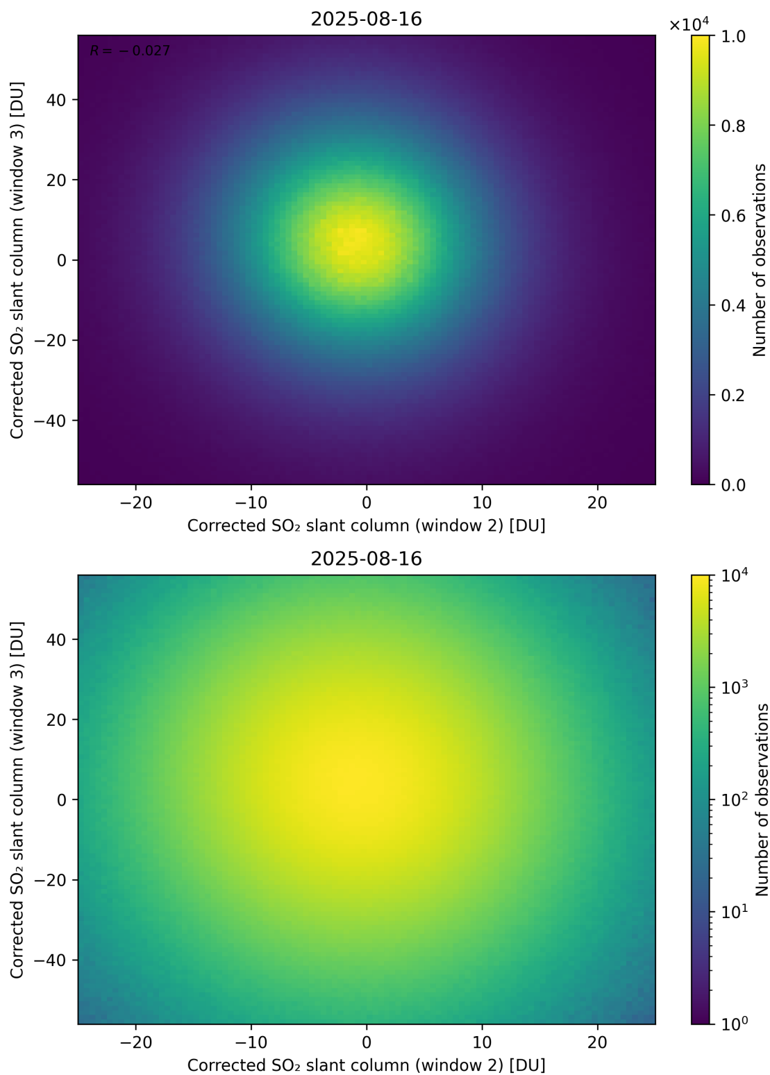
Figure 250: Scatter density plot of “Corrected SO 2 slant column (window 2)” against “Corrected SO 2 slant column (window 3)” for 2025-08-15 to 2025-08-17.
