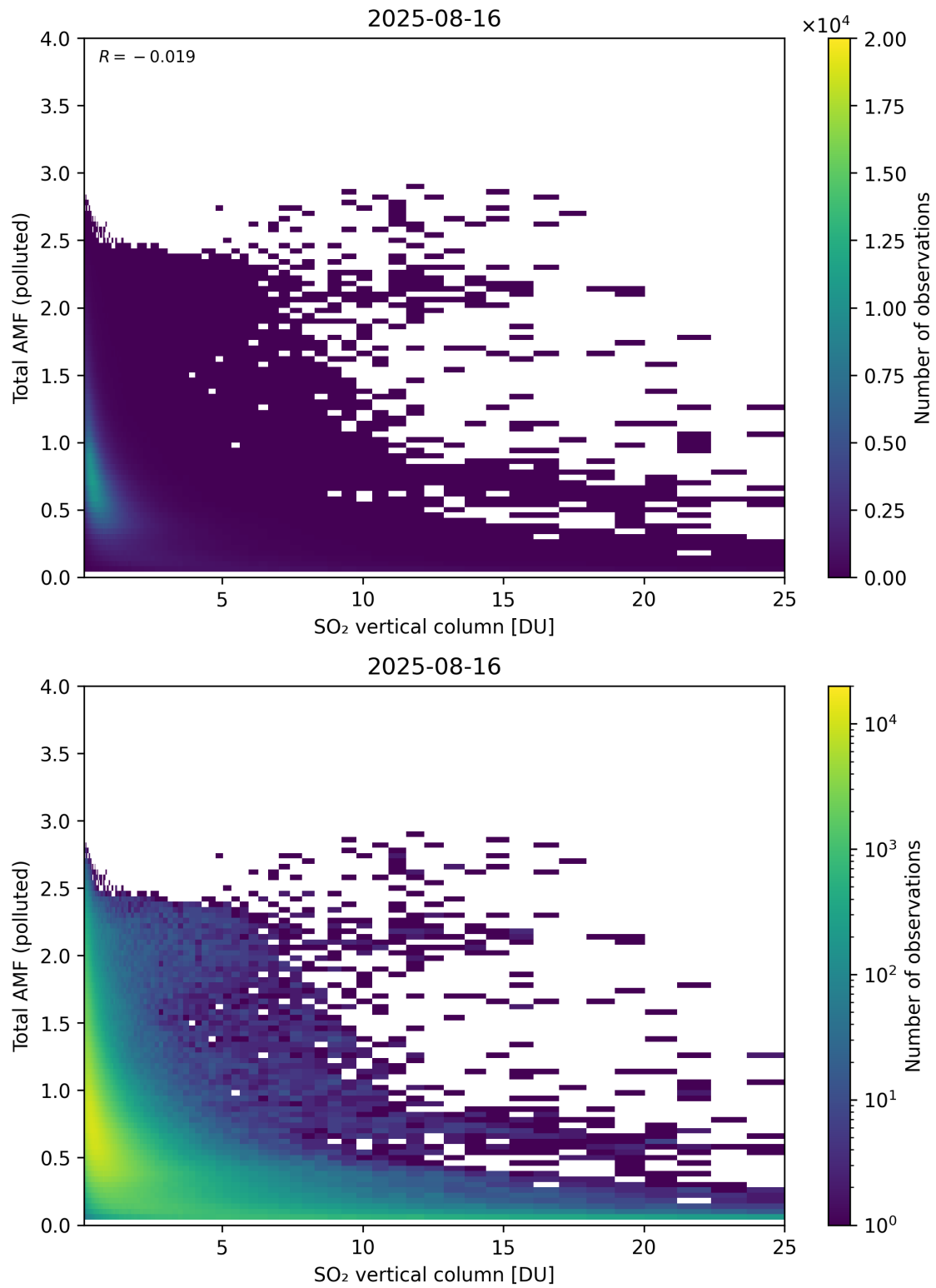
Figure 359: Scatter density plot of “SO 2 vertical column” against “Total AMF (polluted)” for 2025-08-15 to 2025-08-17.
