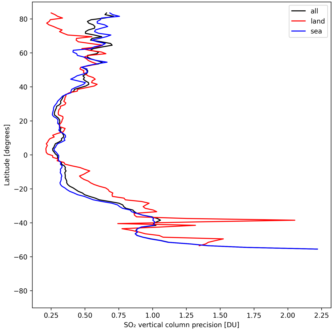
Figure 33: Zonal average of “SO 2 vertical column precision” for 2025-08-15 to 2025-08-17.
