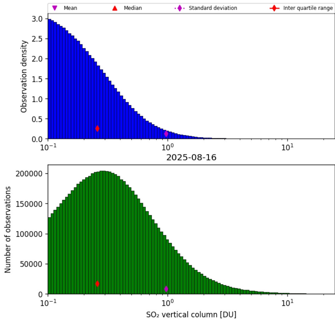
Figure 58: Histogram of “SO 2 vertical column” for 2025-08-15 to 2025-08-17
