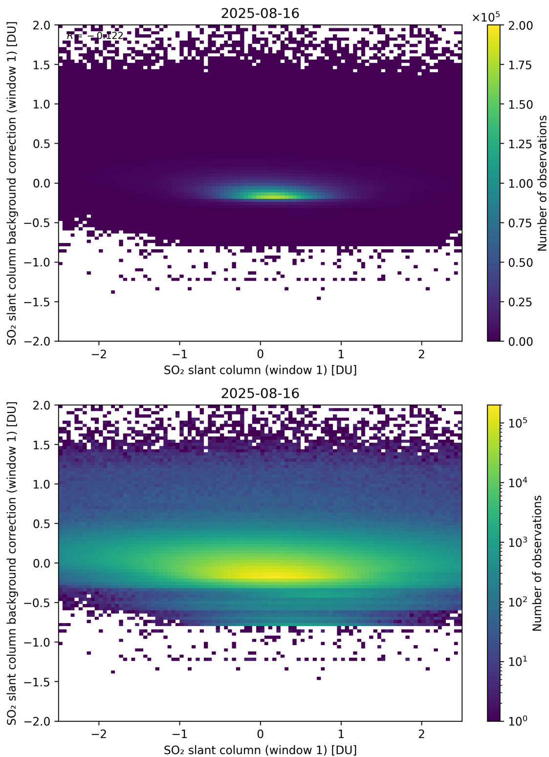
Figure 262: Scatter density plot of “SO 2 slant column (window 1)” against “SO 2 slant column background correction (window 1)” for 2025-08-15 to 2025-08-17.
