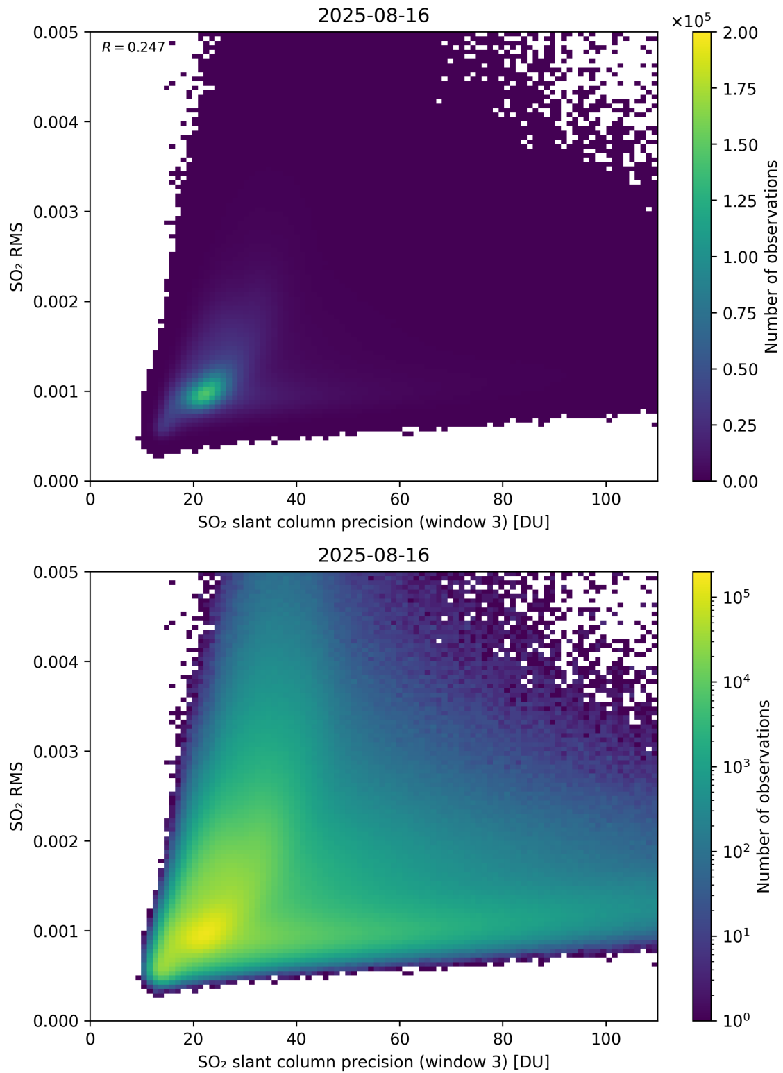
Figure 310: Scatter density plot of “SO 2 slant column precision (window 3)” against “SO 2 RMS” for 2025-08-15 to 2025-08-17.
