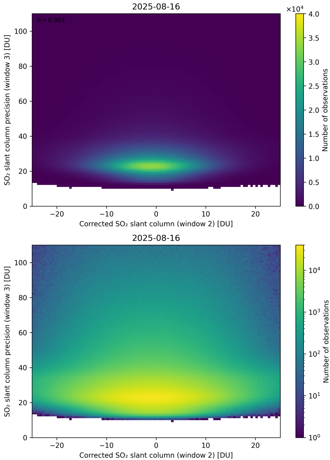
Figure 252: Scatter density plot of “Corrected SO 2 slant column (window 2)” against “SO 2 slant column precision (window 3)” for 2025-08-15 to 2025-08-17.
