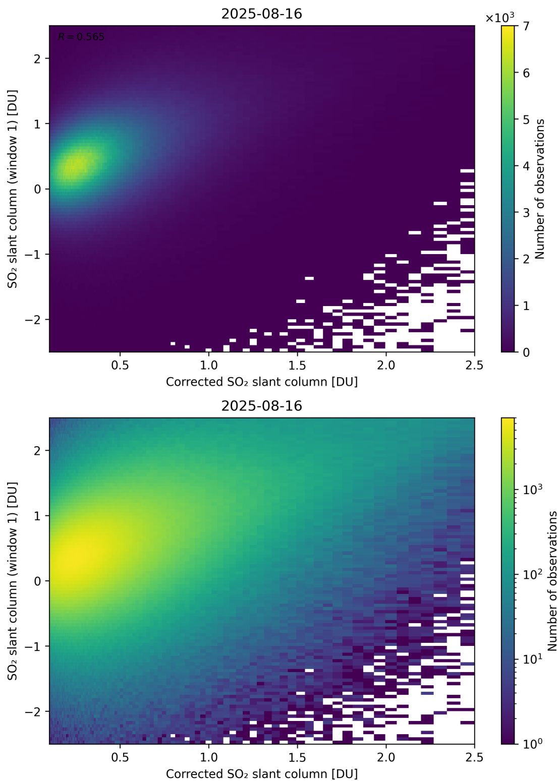
Figure 237: Scatter density plot of “Corrected SO 2 slant column” against “SO 2 slant column (window 1)” for 2025-08-15 to 2025-08-17.
