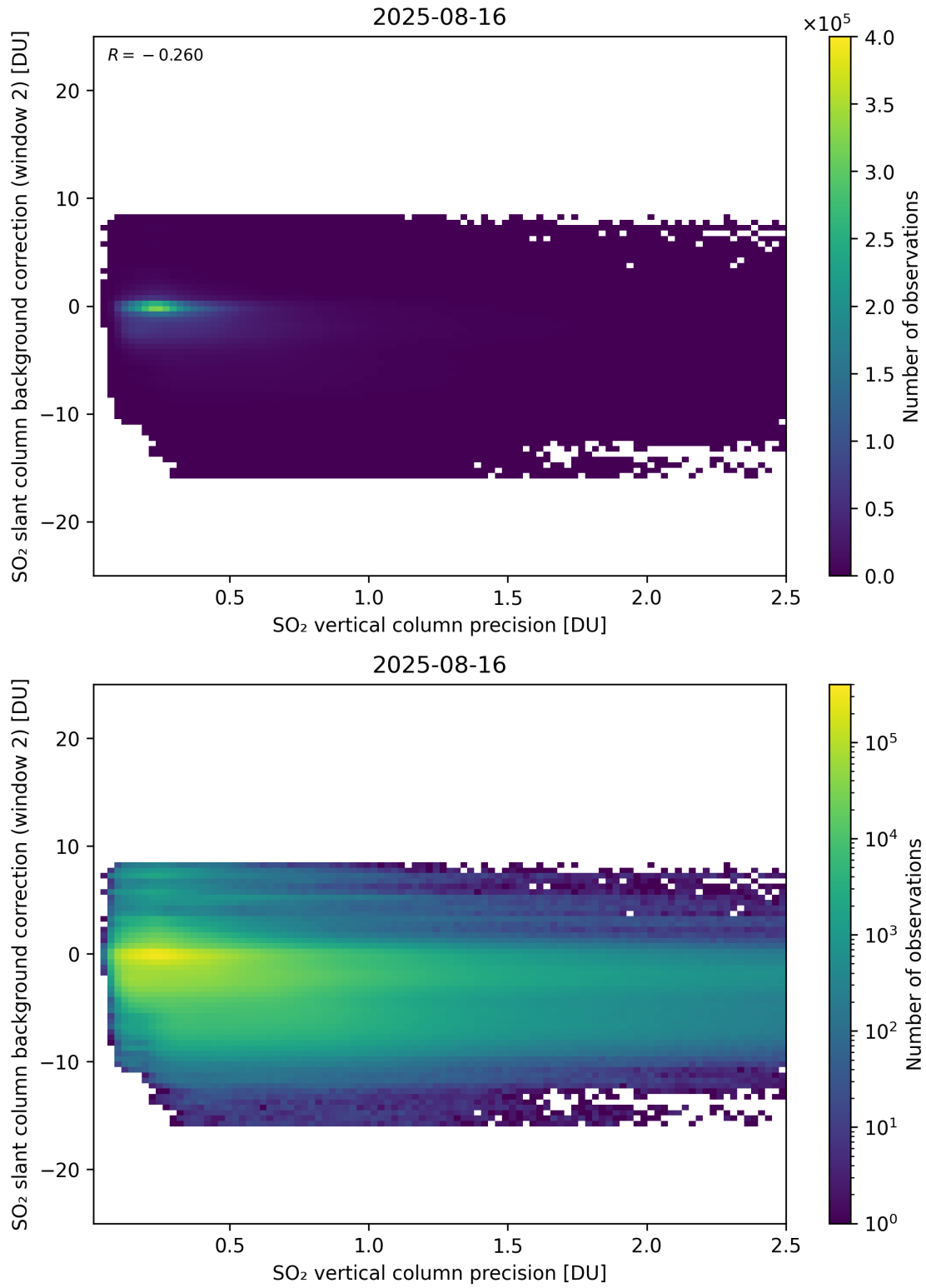
Figure 330: Scatter density plot of “SO 2 vertical column precision” against “SO 2 slant column background correction (window 2)” for 2025-08-15 to 2025-08-17.
