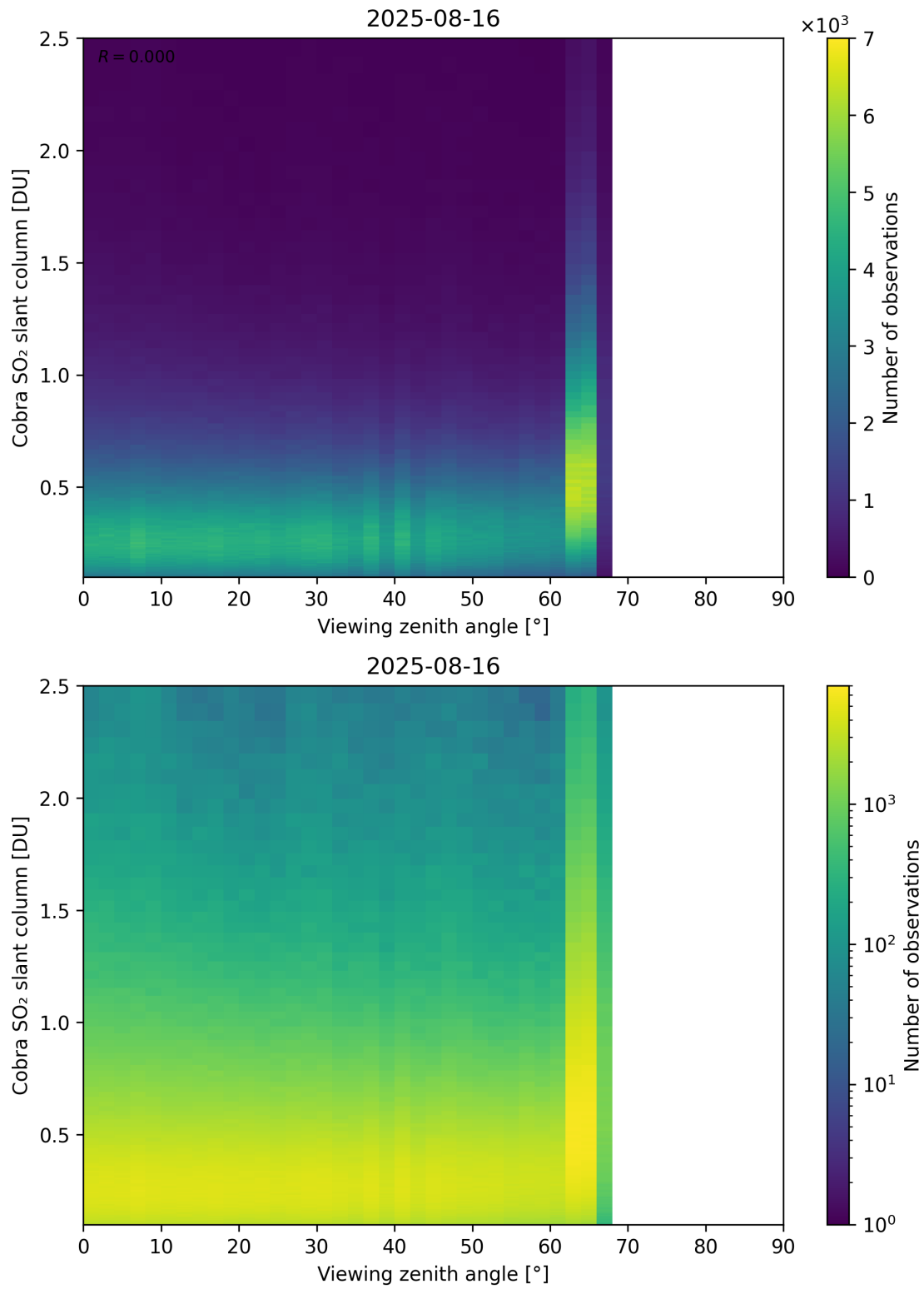
Figure 371: Scatter density plot of “Viewing zenith angle” against “Cobra SO 2 slant column” for 2025-08-15 to 2025-08-17.
