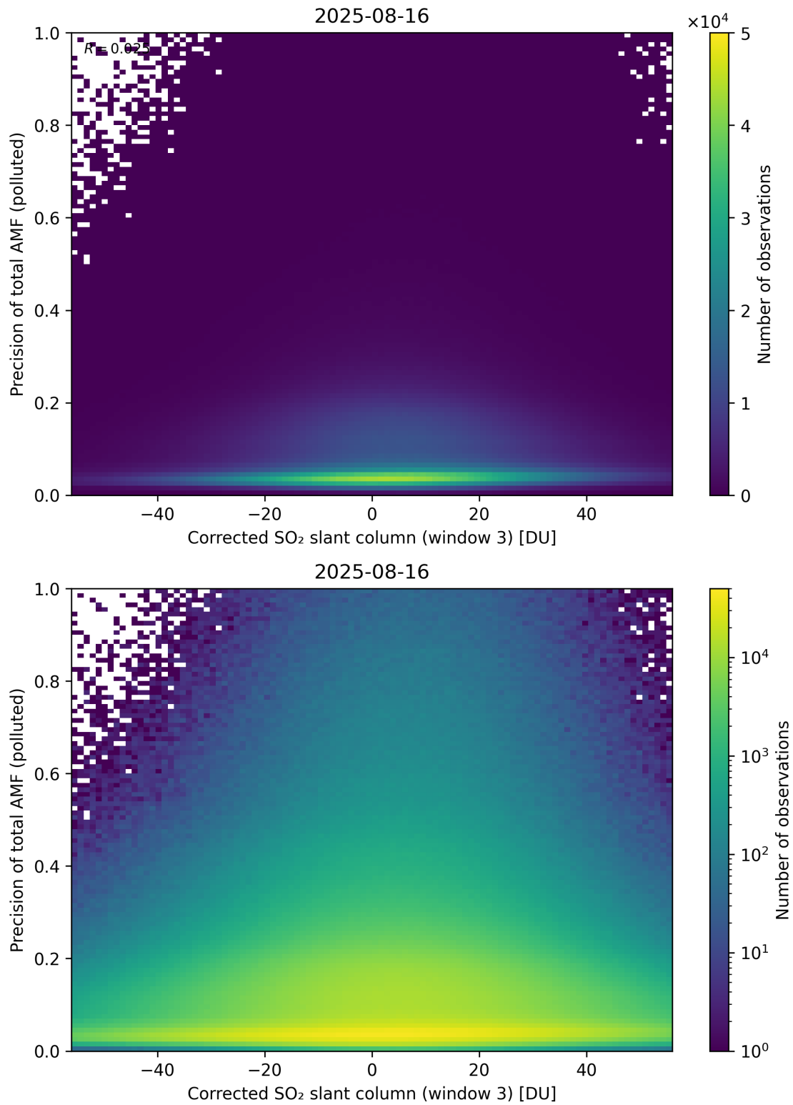
Figure 261: Scatter density plot of “Corrected SO 2 slant column (window 3)” against “Precision of total AMF (polluted)” for 2025-08-15 to 2025-08-17.
