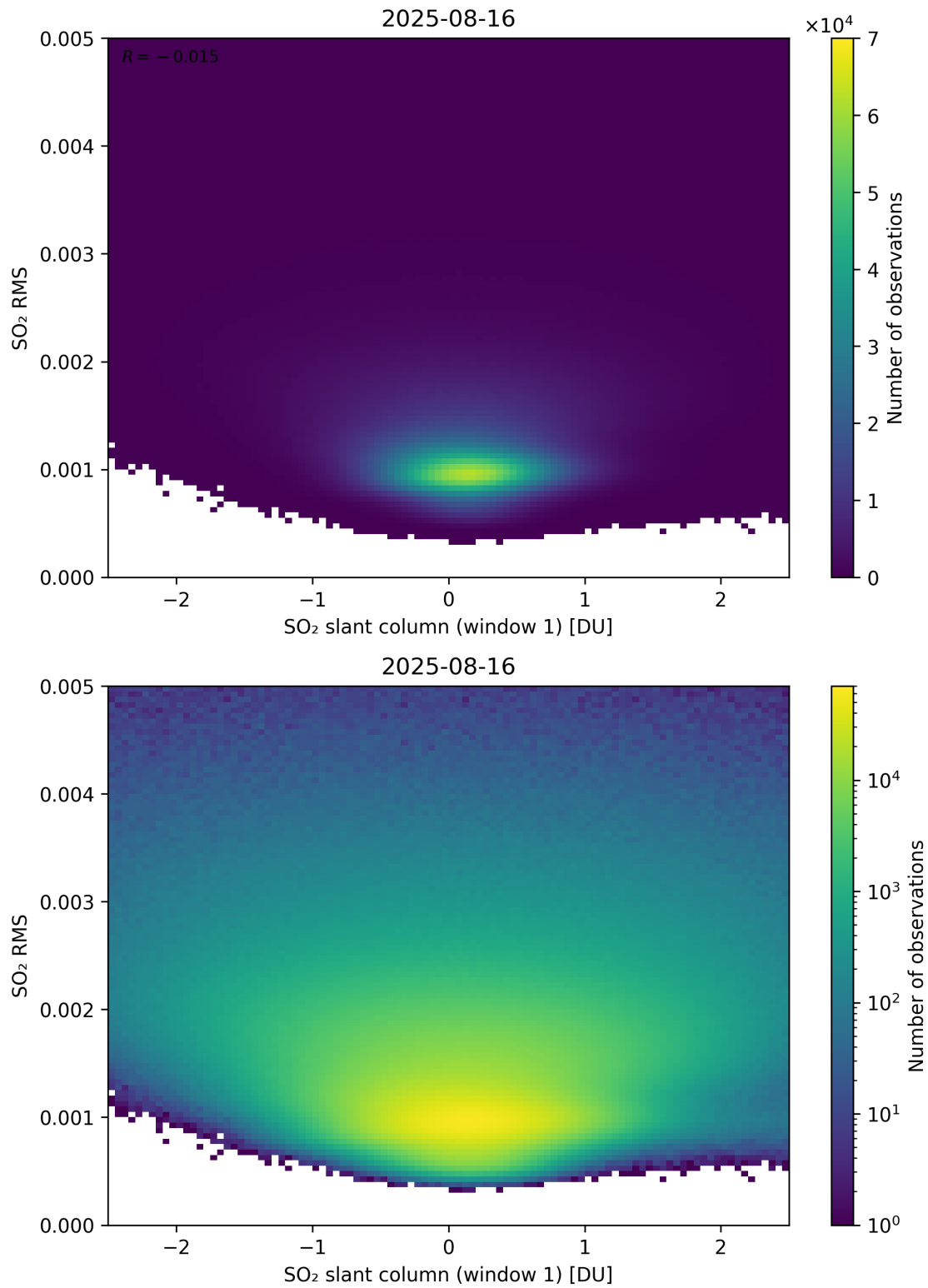
Figure 267: Scatter density plot of “SO 2 slant column (window 1)” against “SO 2 RMS” for 2025-08-15 to 2025-08-17.
