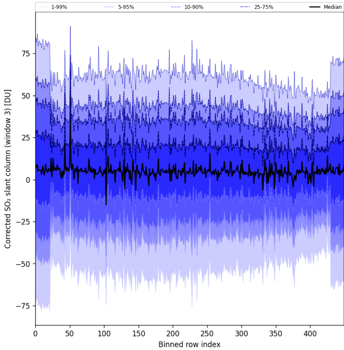
Figure 99: Along track statistics of “Corrected SO 2 slant column (window 3)” for 2025-08-15 to 2025-08-17
