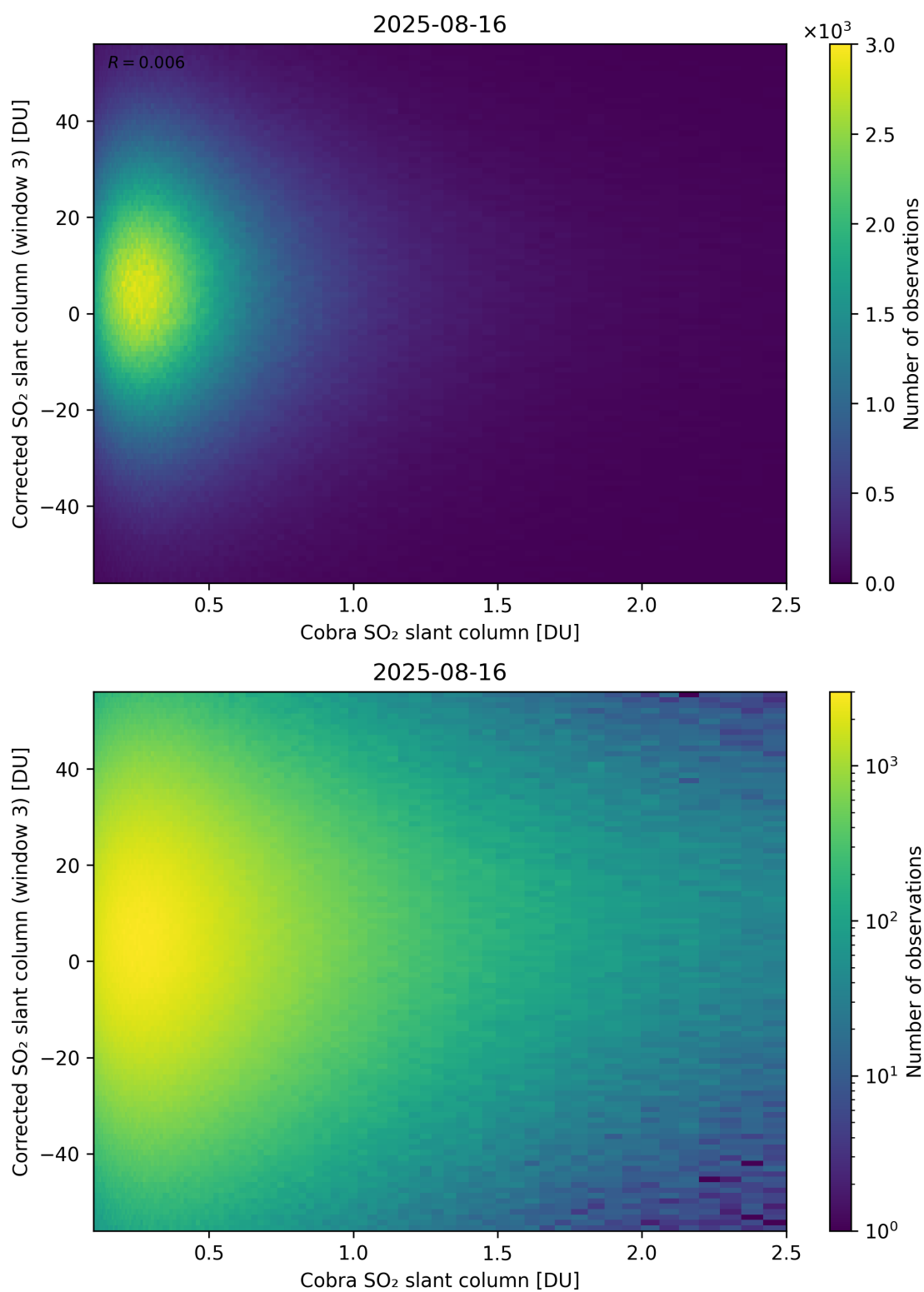
Figure 218: Scatter density plot of “Cobra SO 2 slant column” against “Corrected SO 2 slant column (window 3)” for 2025-08-15 to 2025-08-17.
