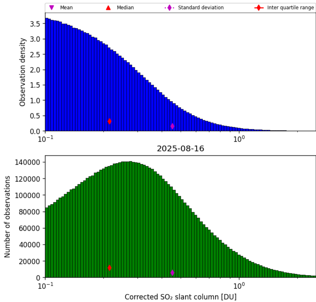
Figure 60: Histogram of "Corrected SO 2 slant column" for 2025-08-15 to 2025-08-17
