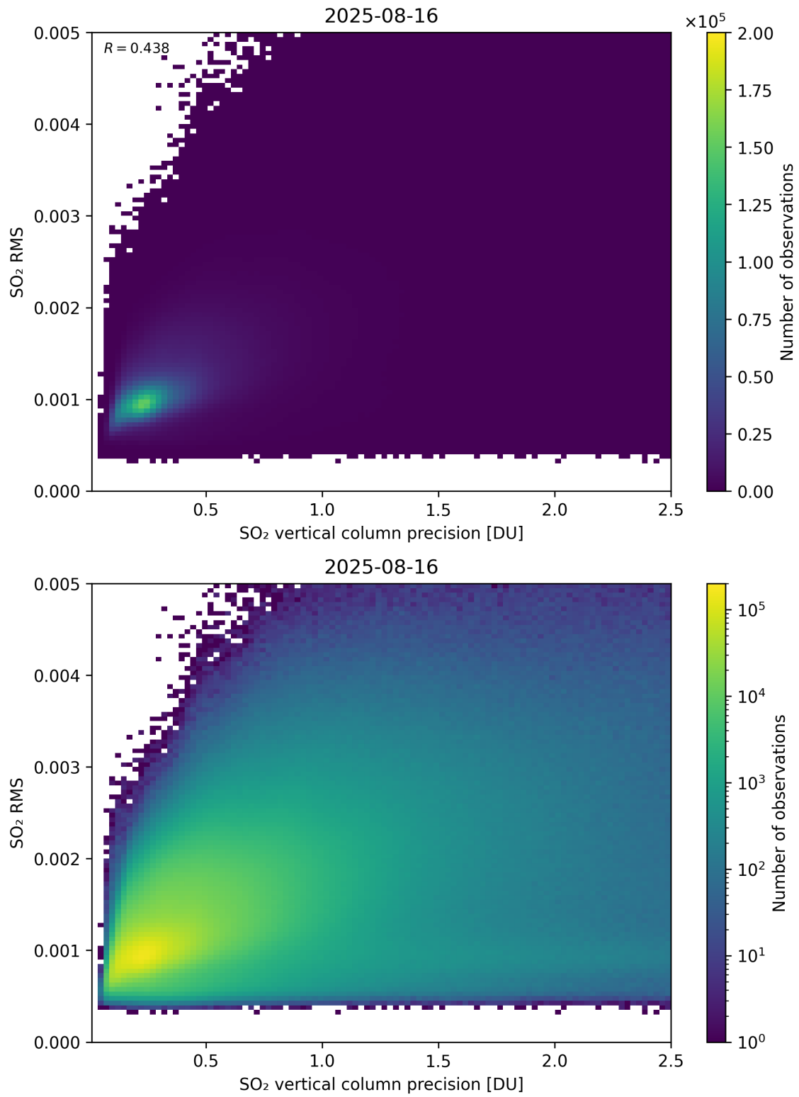
Figure 334: Scatter density plot of “SO 2 vertical column precision” against “SO 2 RMS” for 2025-08-15 to 2025-08-17.
