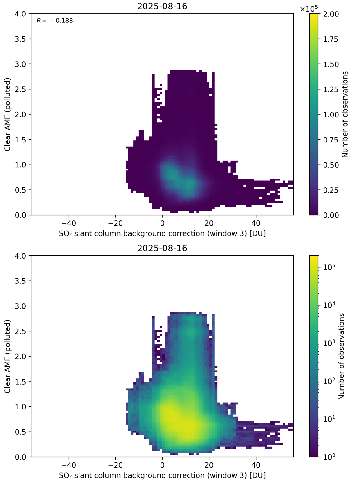
Figure 135: Scatter density plot of “SO 2 slant column background correction (window 3)” against “Clear AMF (polluted)” for 2025-08-15 to 2025-08-17.
