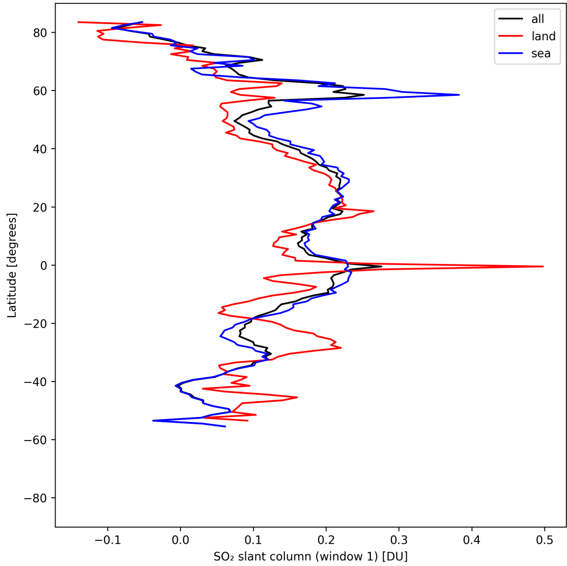
Figure 37: Zonal average of “SO 2 slant column (window 1)” for 2025-08-15 to 2025-08-17.
