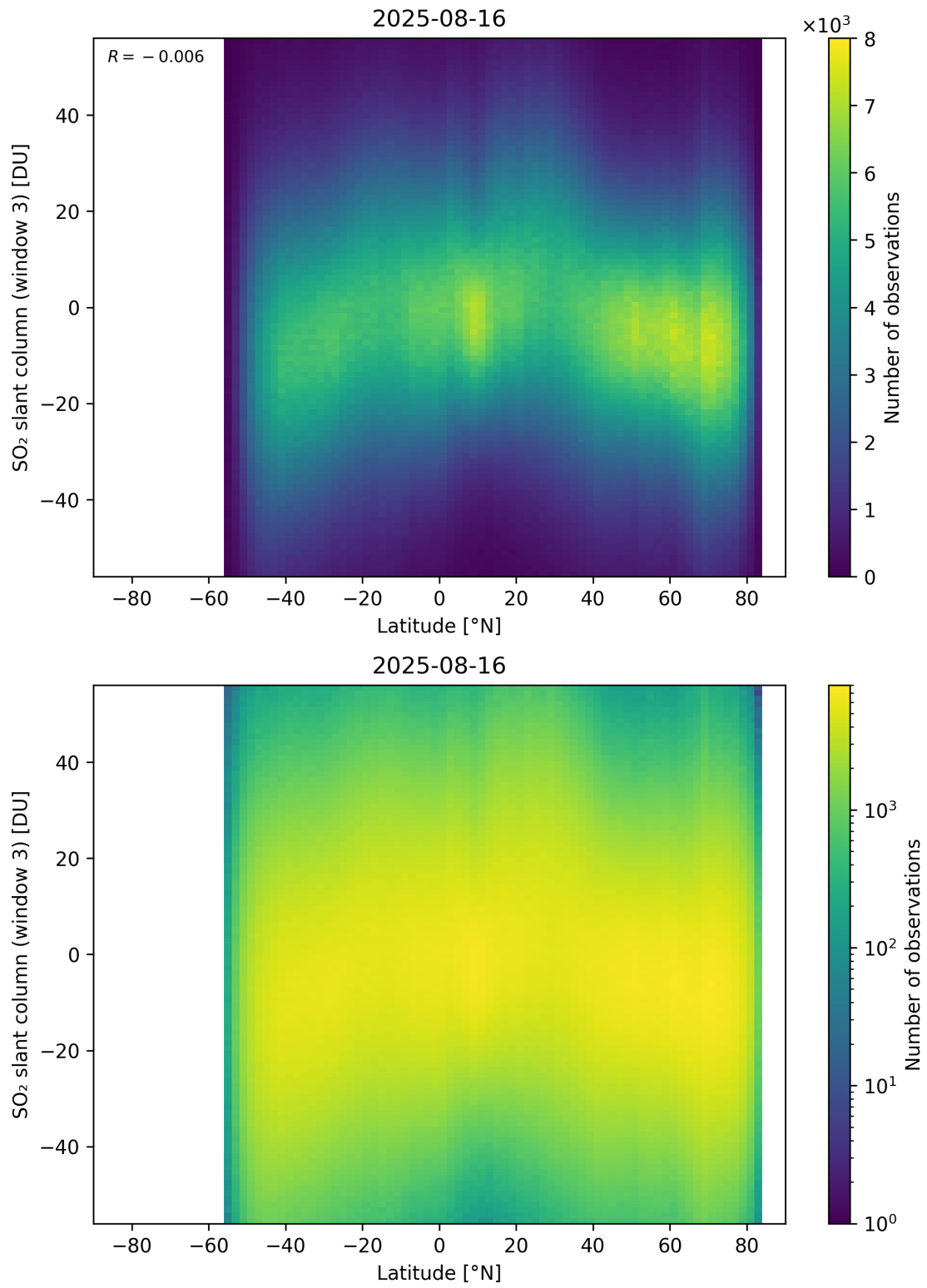
Figure 165: Scatter density plot of “Latitude” against “SO 2 slant column (window 3)” for 2025-08-15 to 2025-08-17.
