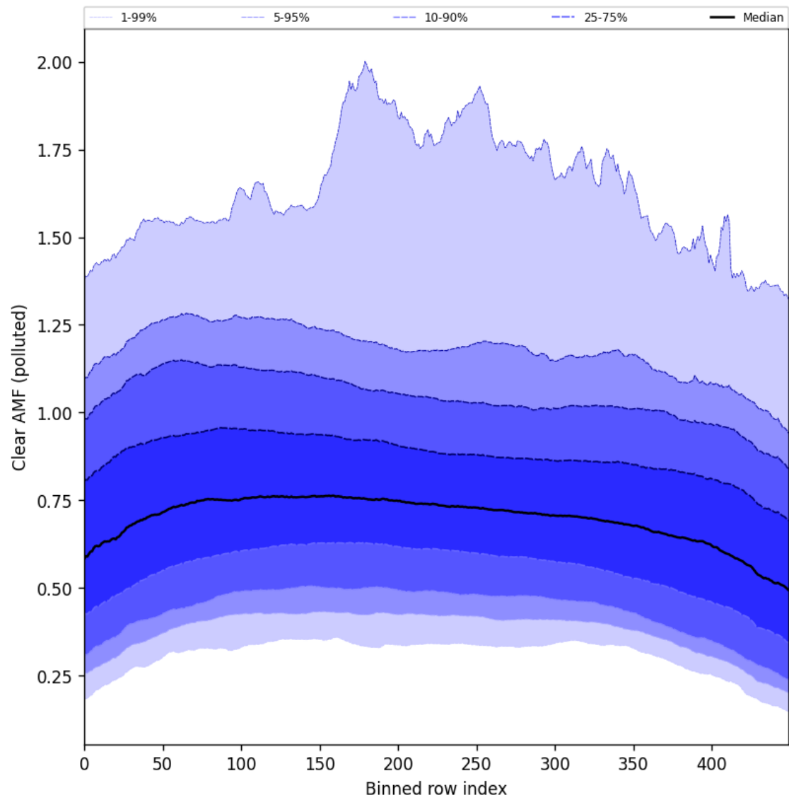
Figure 107: Along track statistics of “Clear AMF (polluted)” for 2025-08-15 to 2025-08-17
