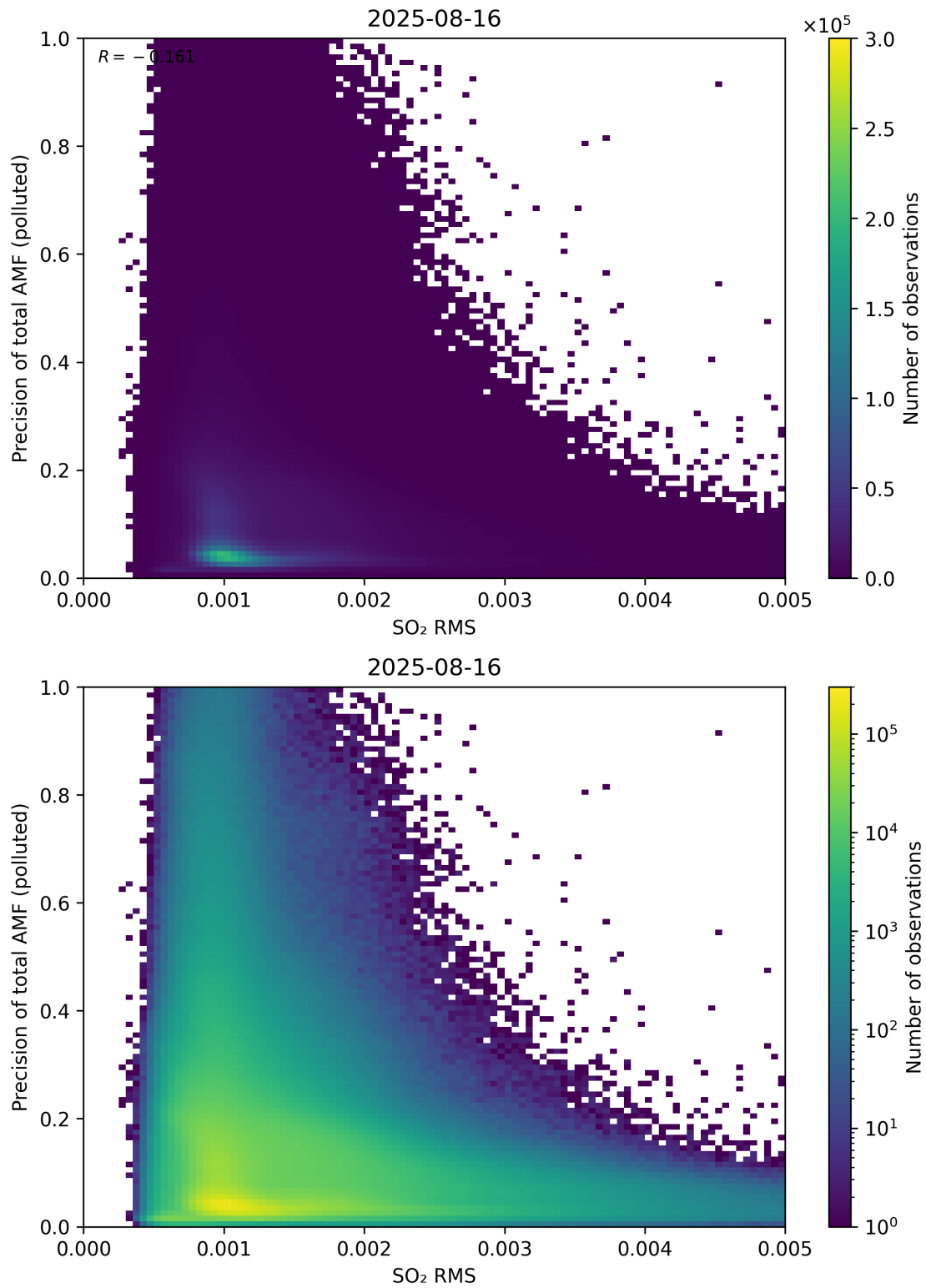
Figure 149: Scatter density plot of “SO 2 RMS” against “Precision of total AMF (polluted)” for 2025-08-15 to 2025-08-17.
