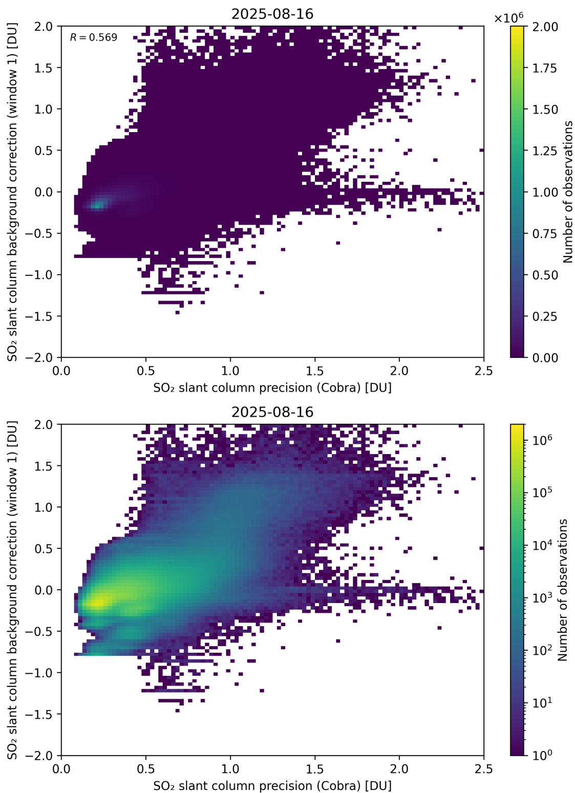
Figure 199: Scatter density plot of “SO 2 slant column precision (Cobra)” against “SO 2 slant column background correction (window 1)” for 2025-08-15 to 2025-08-17.
