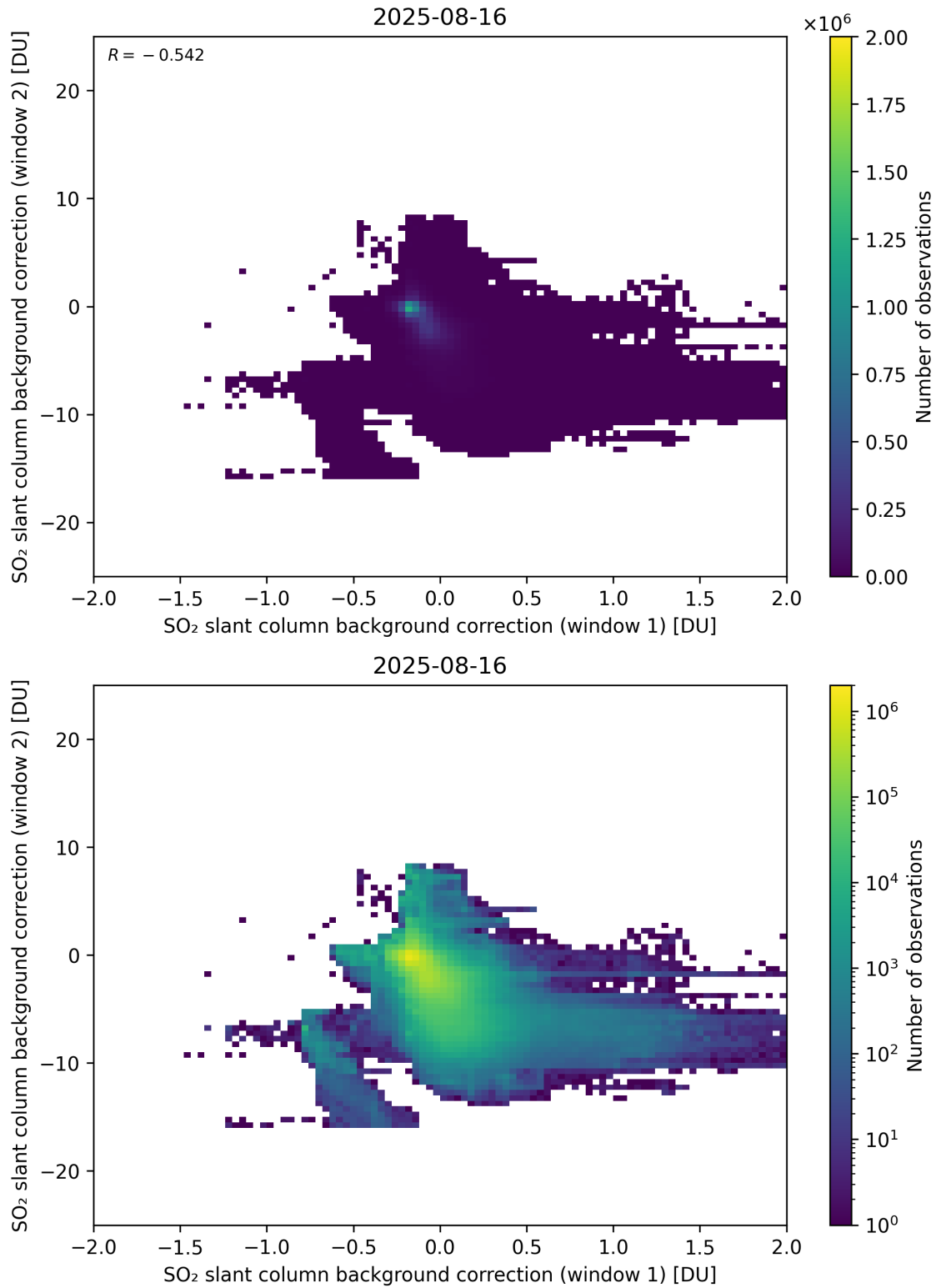
Figure 109: Scatter density plot of “SO 2 slant column background correction (window 1)” against “SO 2 slant column background correction (window 2)” for 2025-08-15 to 2025-08-17.
