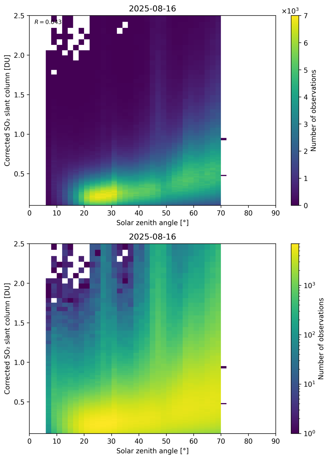
Figure 181: Scatter density plot of “Solar zenith angle” against “Corrected SO 2 slant column” for 2025-08-15 to 2025-08-17.
