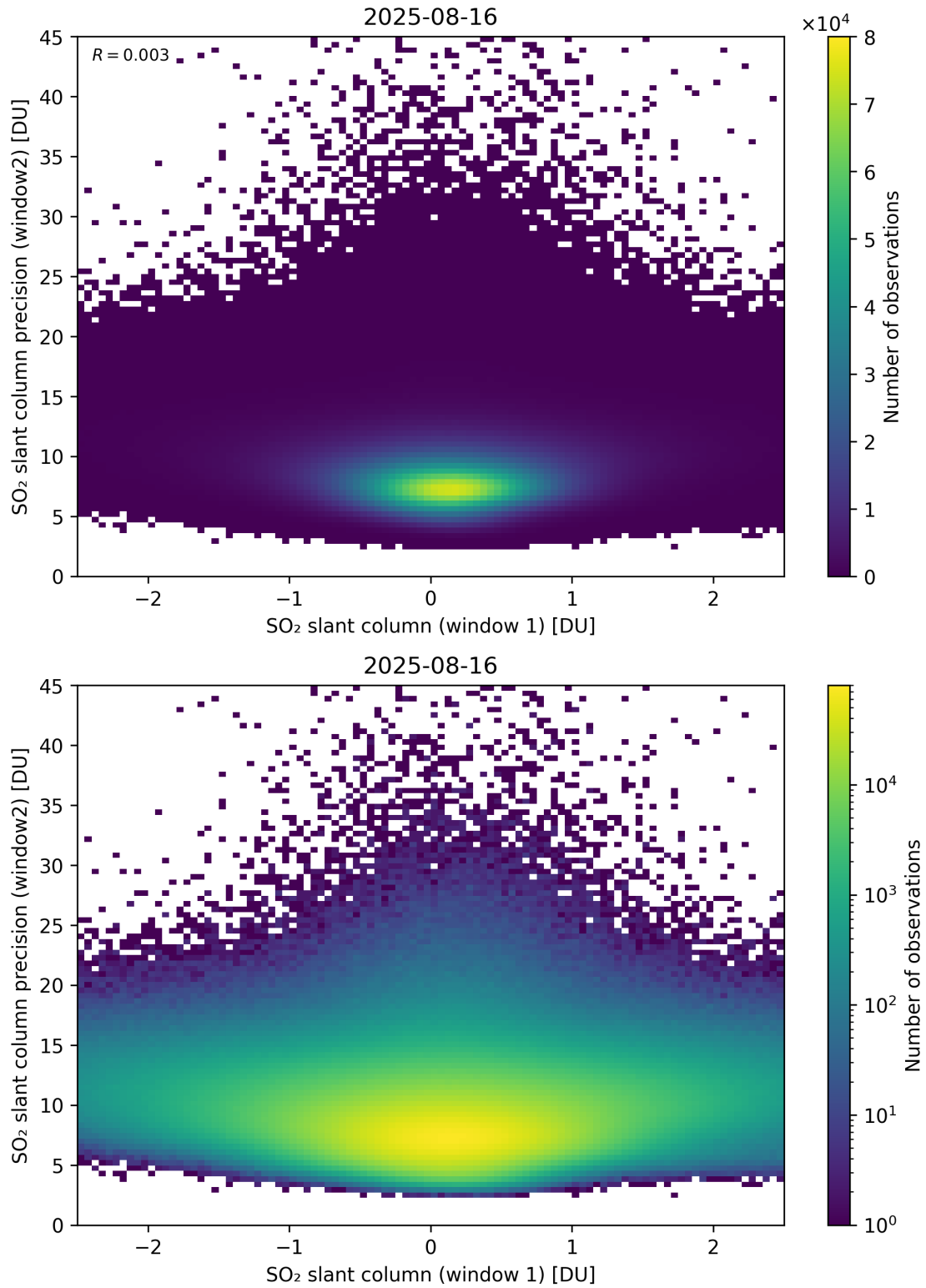
Figure 286: Scatter density plot of “SO 2 slant column (window 1)” against “SO 2 slant column precision (window2)” for 2025-08-15 to 2025-08-17.
