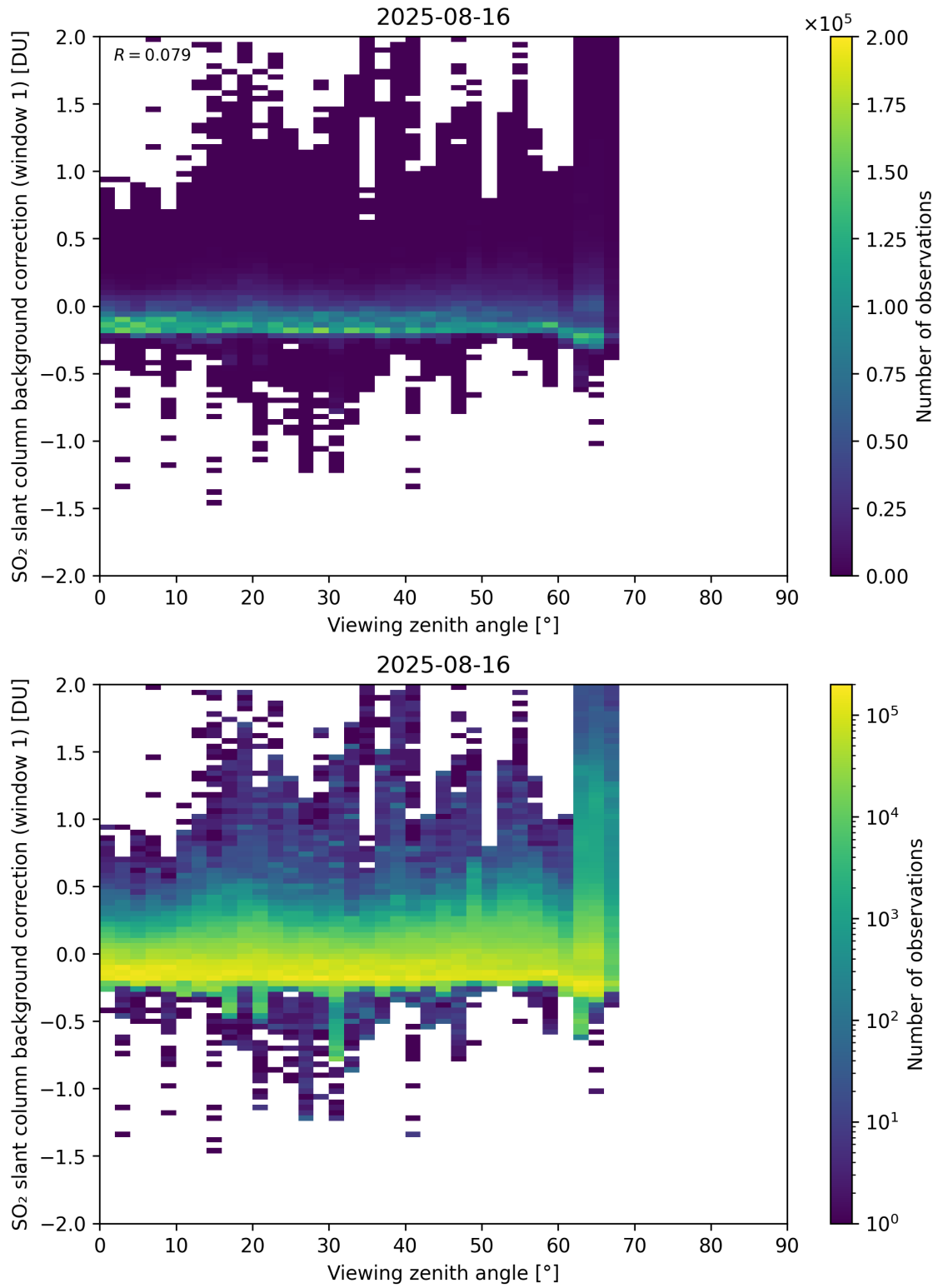
Figure 362: Scatter density plot of “Viewing zenith angle” against “SO 2 slant column background correction (window 1)” for 2025-08-15 to 2025-08-17.
