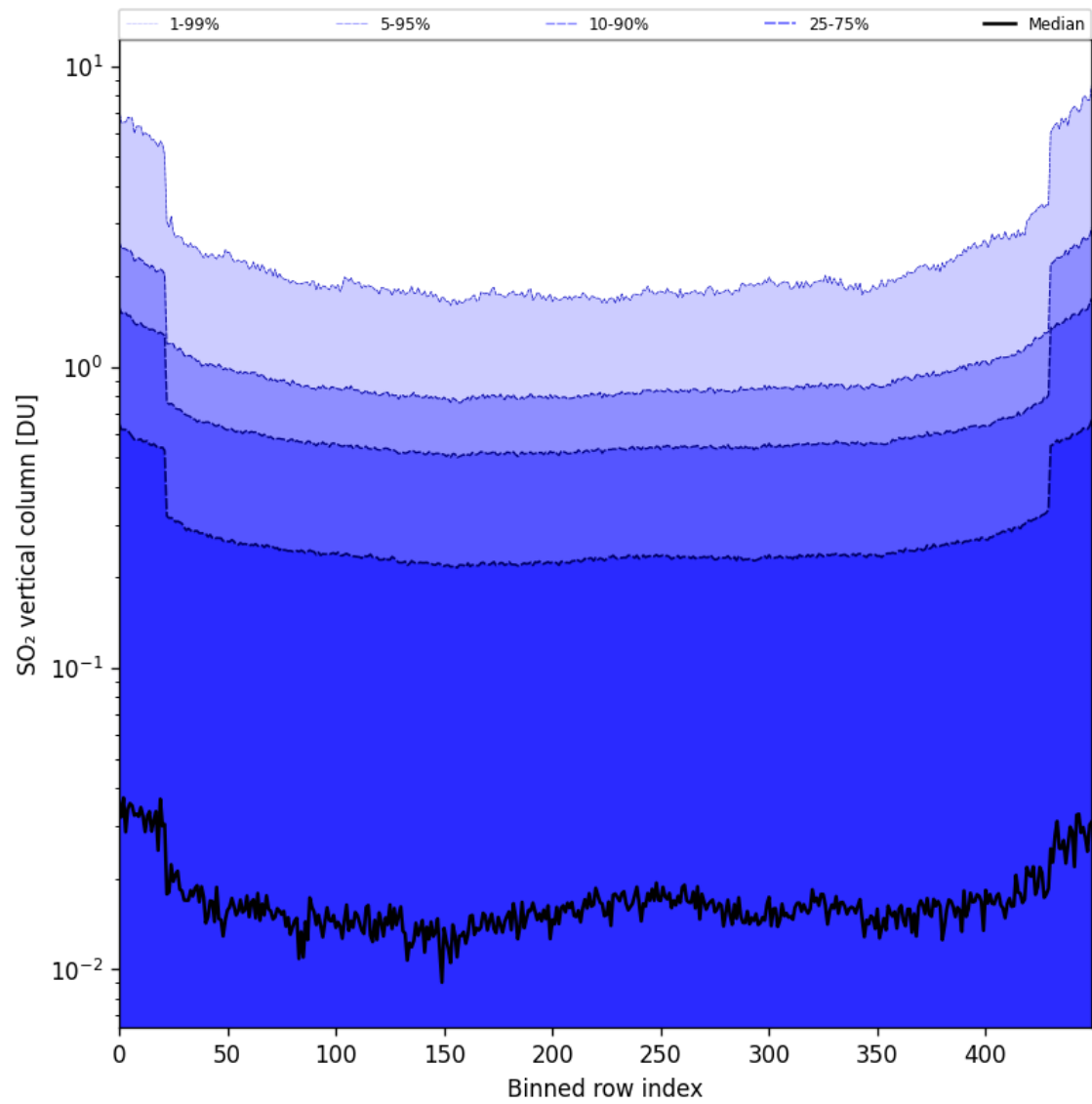
Figure 84: Along track statistics of “SO 2 vertical column” for 2025-08-15 to 2025-08-17
