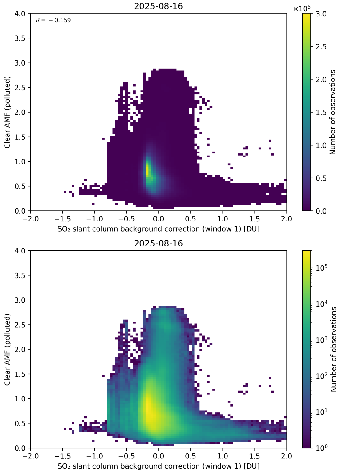
Figure 114: Scatter density plot of “SO 2 slant column background correction (window 1)” against “Clear AMF (polluted)” for 2025-08-15 to 2025-08-17.
