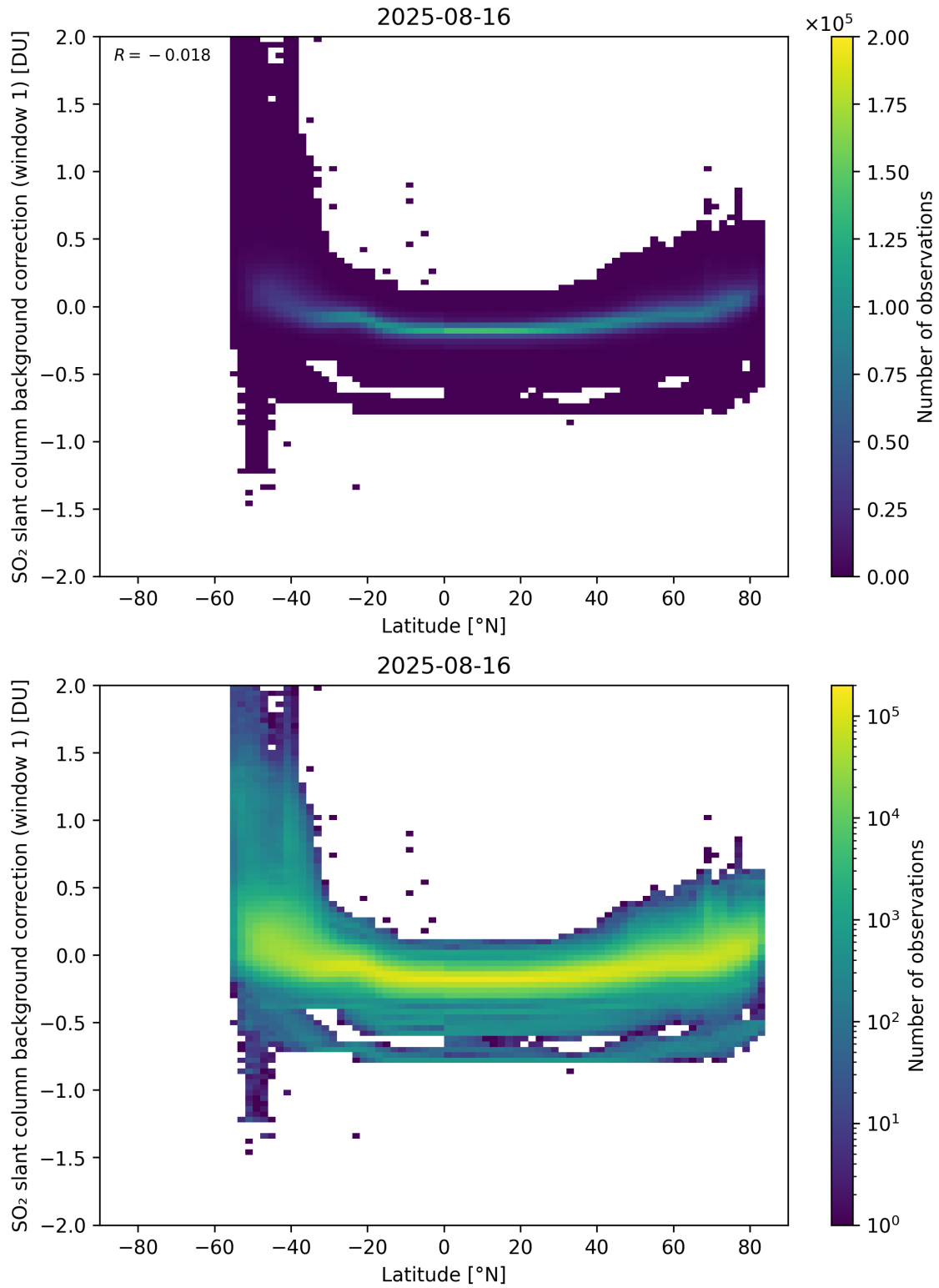
Figure 150: Scatter density plot of “Latitude” against “SO 2 slant column background correction (window 1)” for 2025-08-15 to 2025-08-17.
