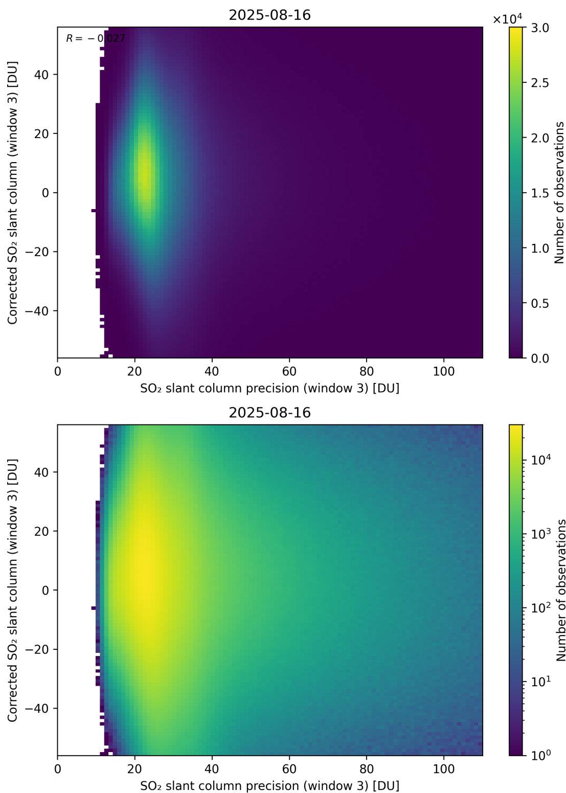
Figure 312: Scatter density plot of “SO 2 slant column precision (window 3)” against “Corrected SO 2 slant column (window 3)” for 2025-08-15 to 2025-08-17.
