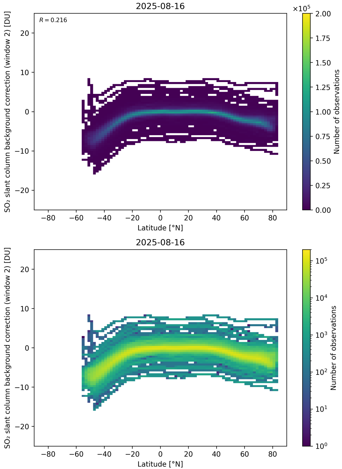
Figure 151: Scatter density plot of “Latitude” against “SO 2 slant column background correction (window 2)” for 2025-08-15 to 2025-08-17.
