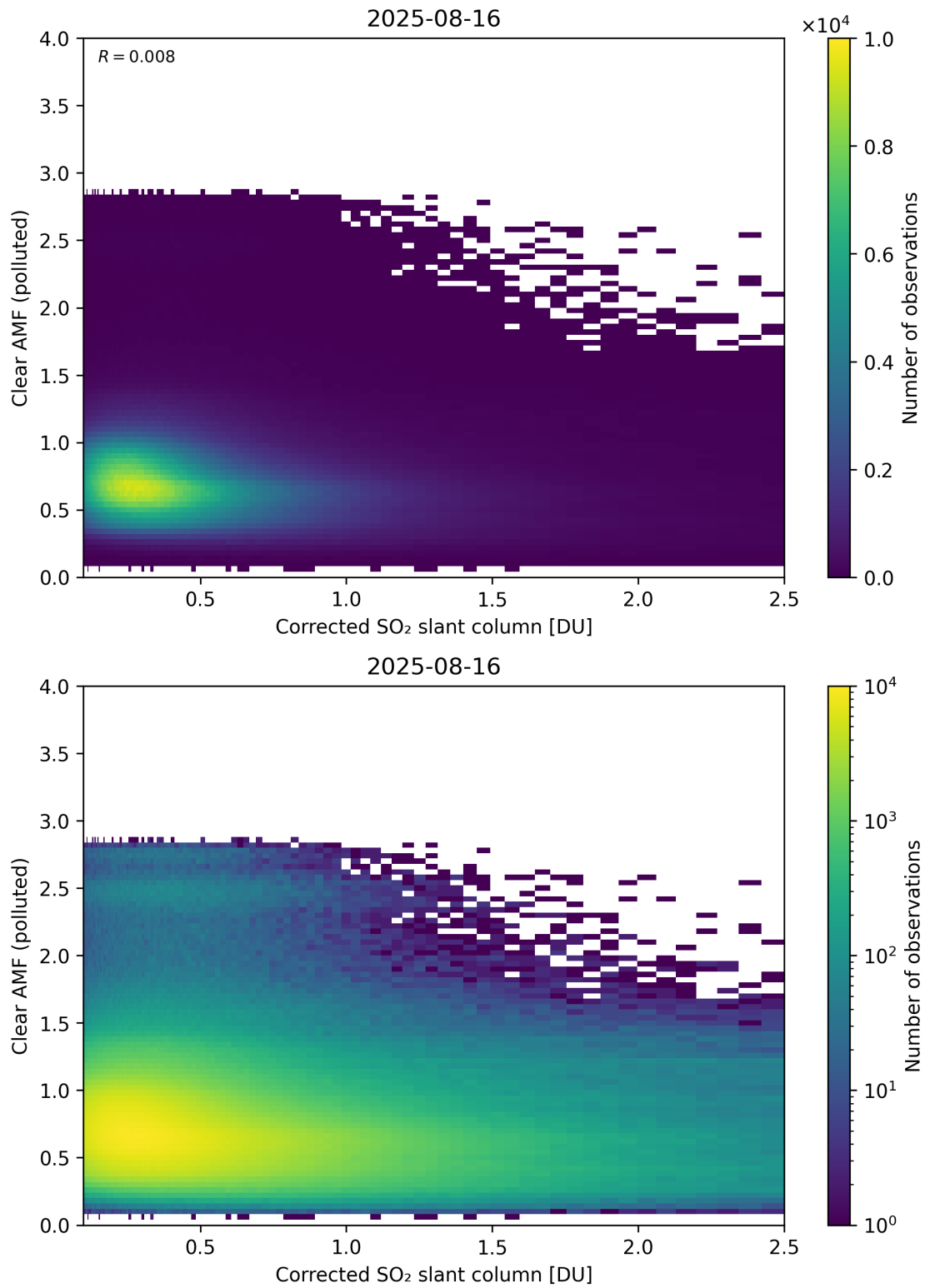
Figure 232: Scatter density plot of “Corrected SO 2 slant column” against “Clear AMF (polluted)” for 2025-08-15 to 2025-08-17.
