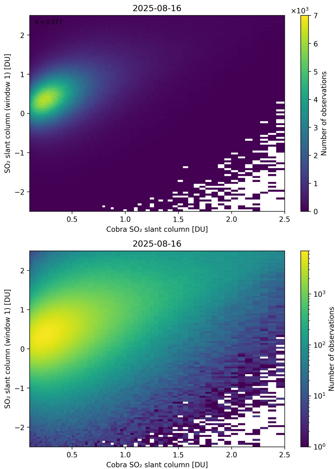
Figure 219: Scatter density plot of “Cobra SO 2 slant column” against “SO 2 slant column (window 1)” for 2025-08-15 to 2025-08-17.
