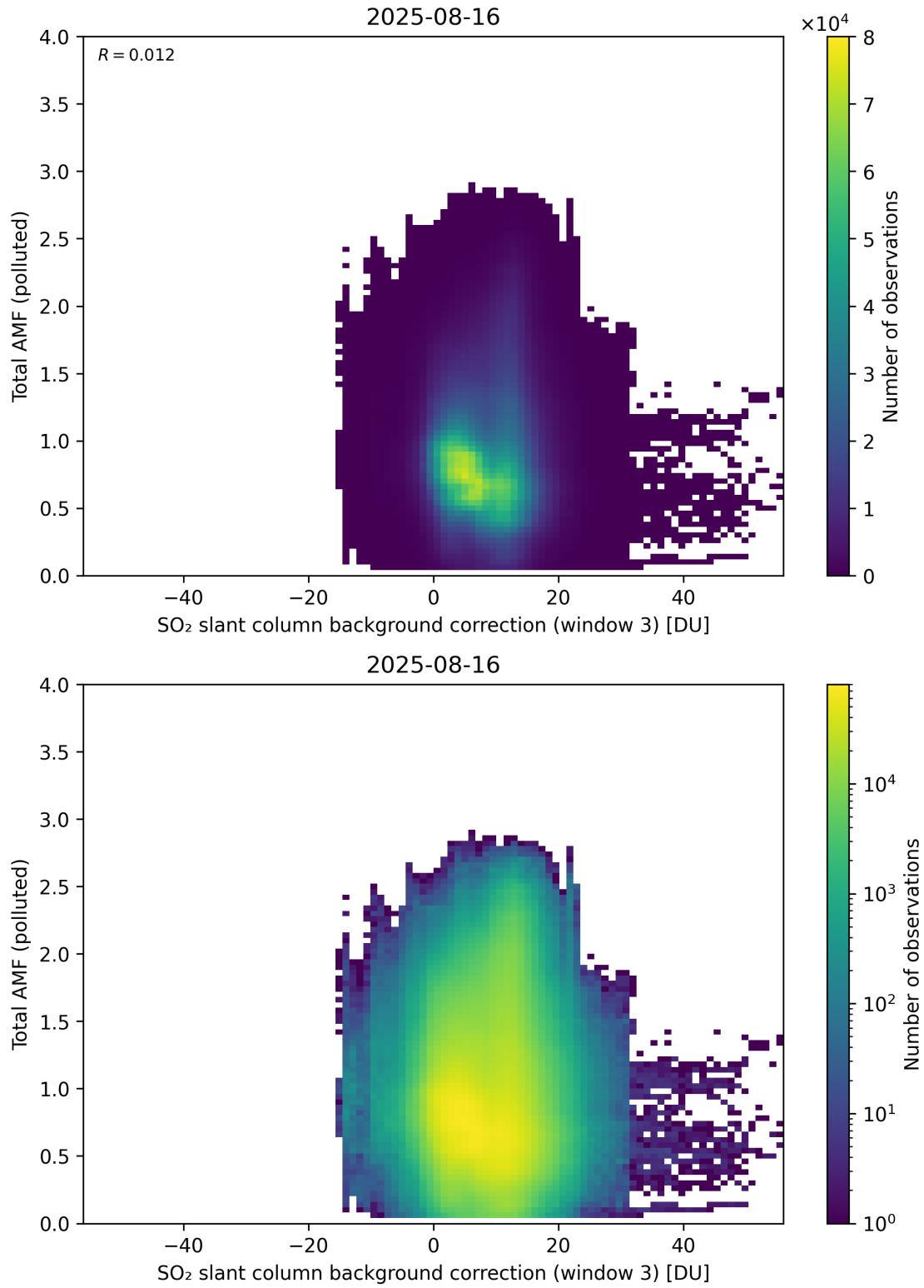
Figure 136: Scatter density plot of “SO 2 slant column background correction (window 3)” against “Total AMF (polluted)” for 2025-08-15 to 2025-08-17.
