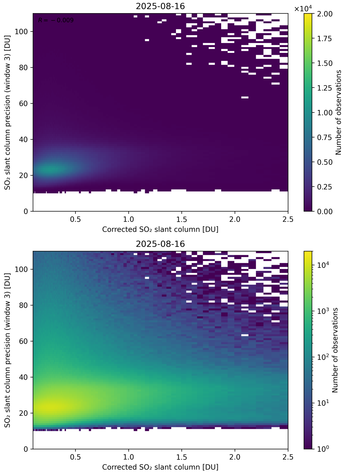
Figure 241: Scatter density plot of “Corrected SO 2 slant column” against “SO 2 slant column precision (window 3)” for 2025-08-15 to 2025-08-17.
