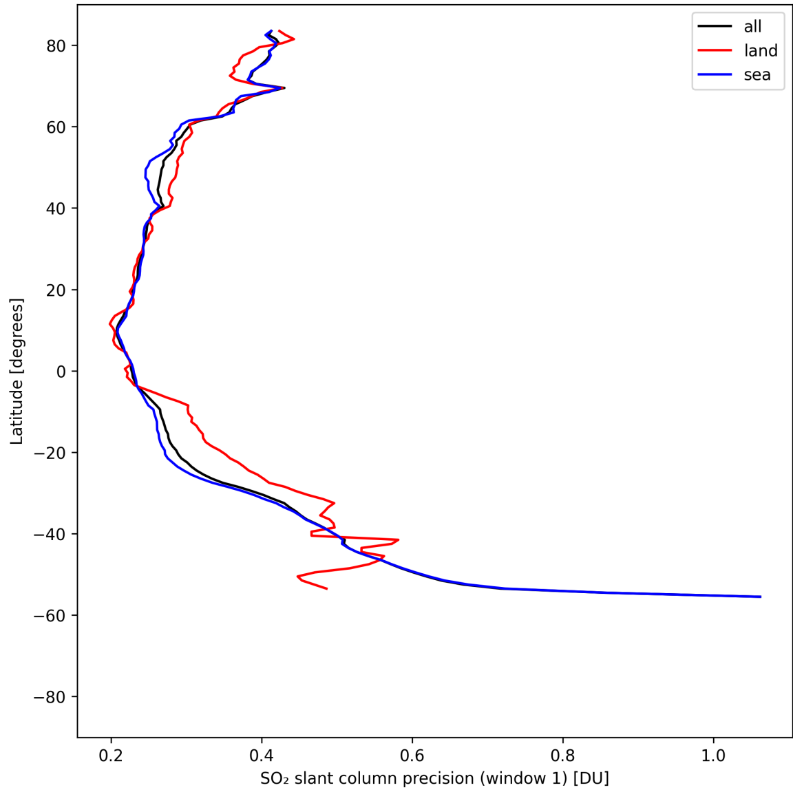
Figure 38: Zonal average of “SO 2 slant column precision (window 1)” for 2025-08-15 to 2025-08-17.
