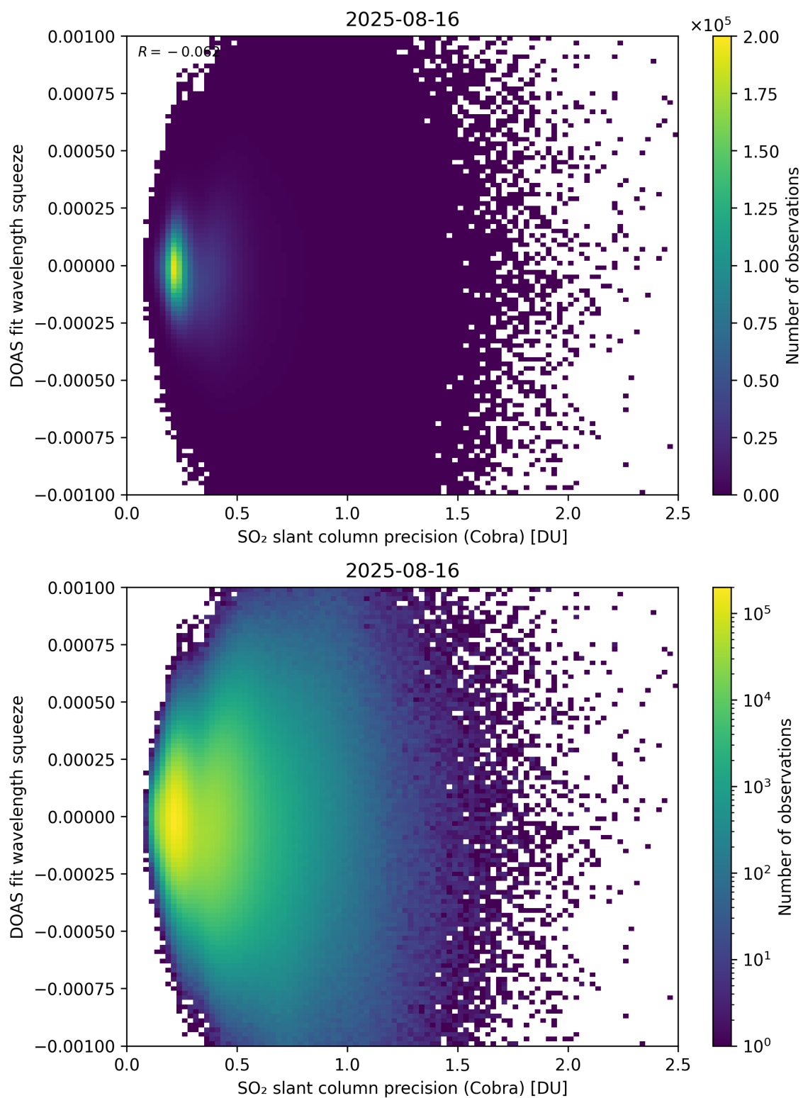
Figure 203: Scatter density plot of “SO 2 slant column precision (Cobra)” against “DOAS fit wavelength squeeze” for 2025-08-15 to 2025-08-17.
