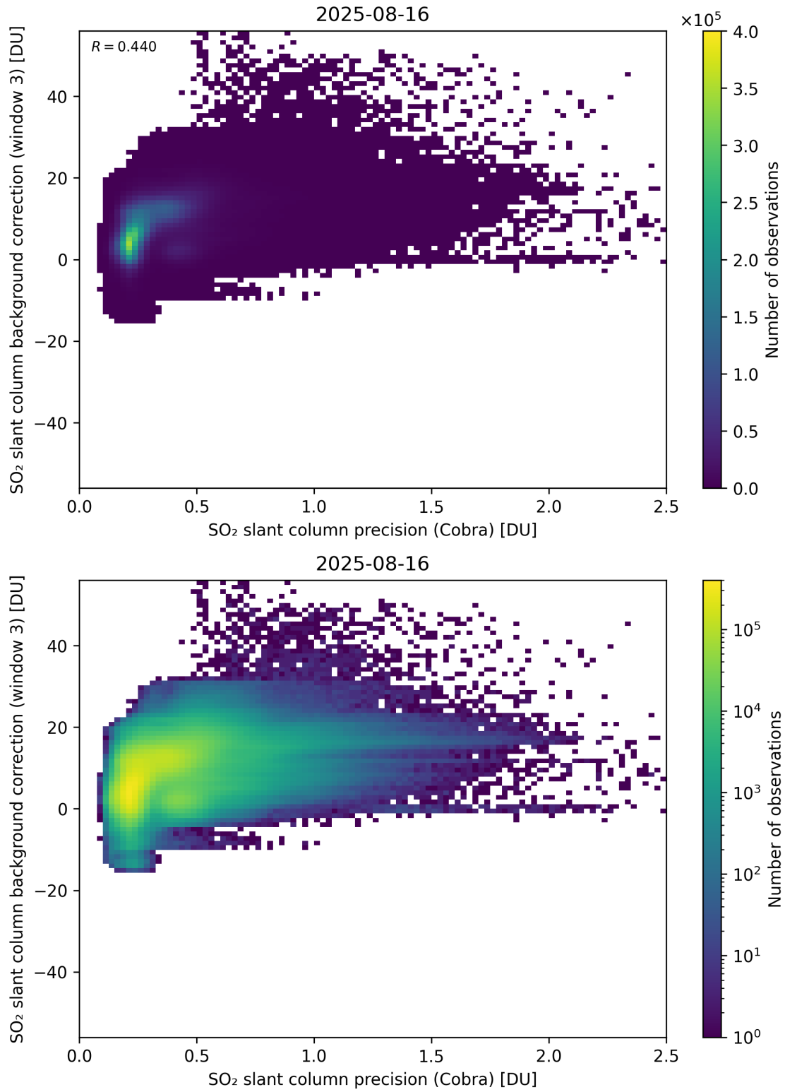
Figure 201: Scatter density plot of “SO 2 slant column precision (Cobra)” against “SO 2 slant column background correction (window 3)” for 2025-08-15 to 2025-08-17.
