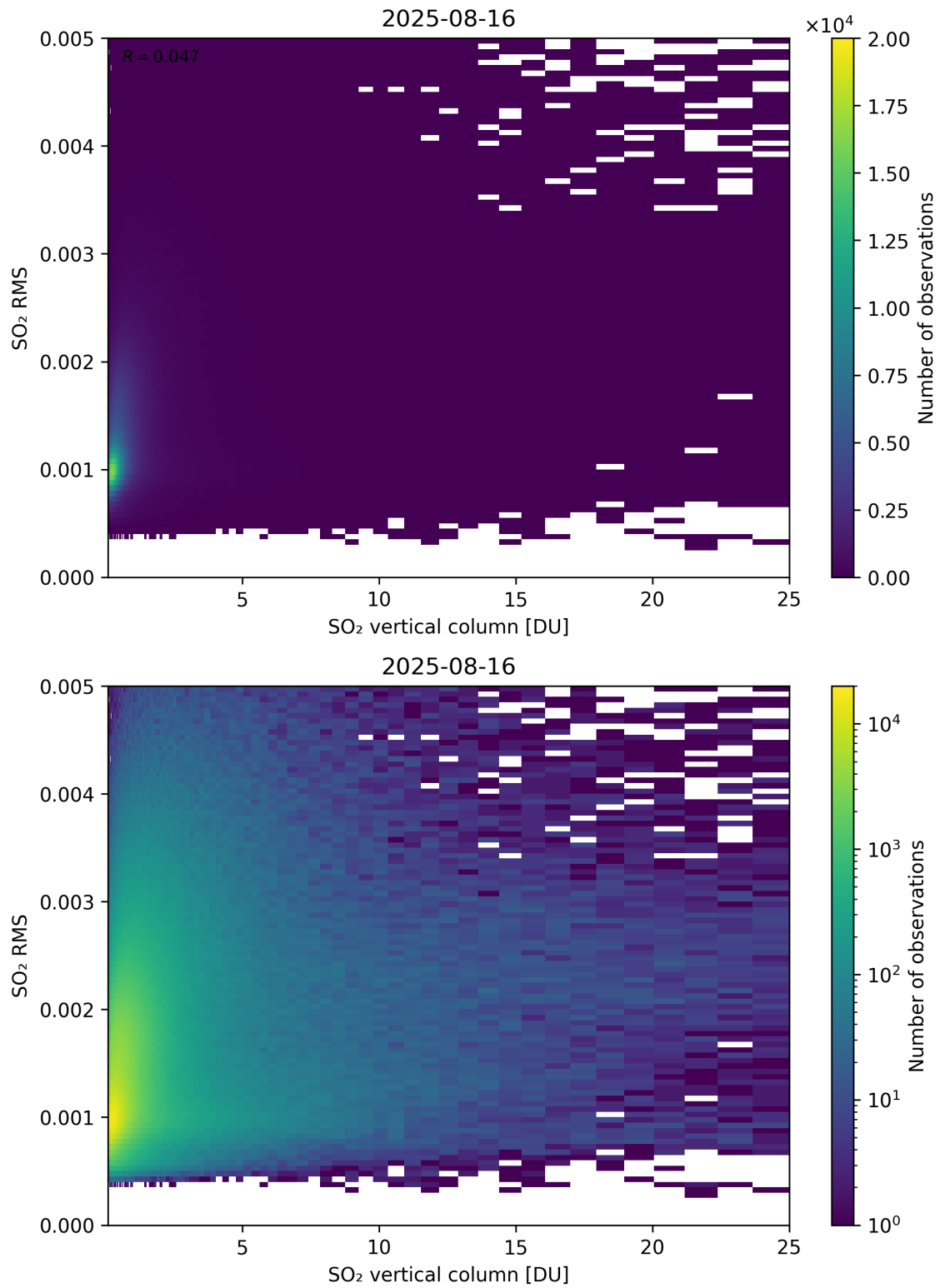
Figure 328: Scatter density plot of “SO 2 vertical column” against “SO 2 RMS” for 2025-08-15 to 2025-08-17.
