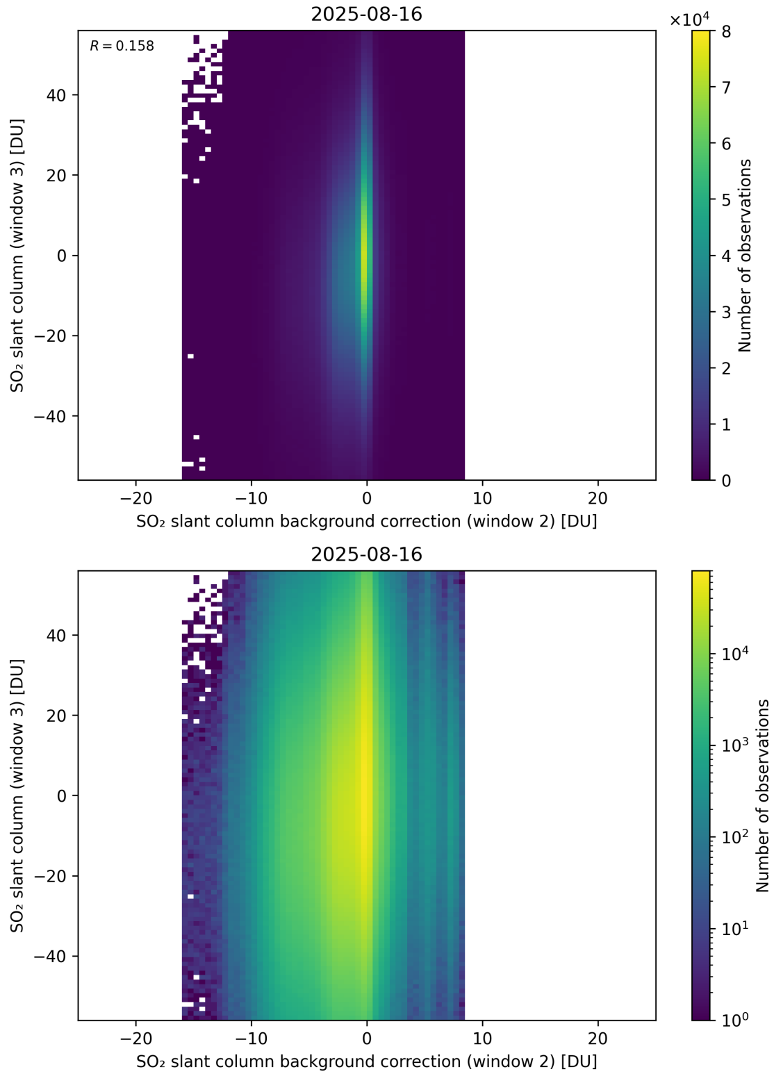
Figure 128: Scatter density plot of “SO 2 slant column background correction (window 2)” against “SO 2 slant column (window 3)” for 2025-08-15 to 2025-08-17.
