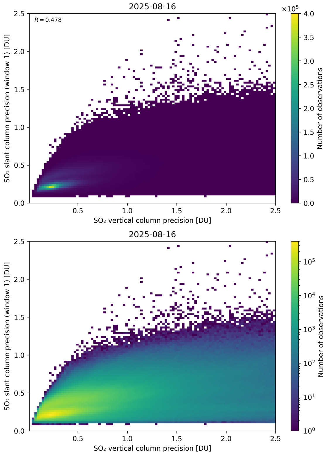
Figure 342: Scatter density plot of “SO 2 vertical column precision” against “SO 2 slant column precision (window 1)” for 2025-08-15 to 2025-08-17.
