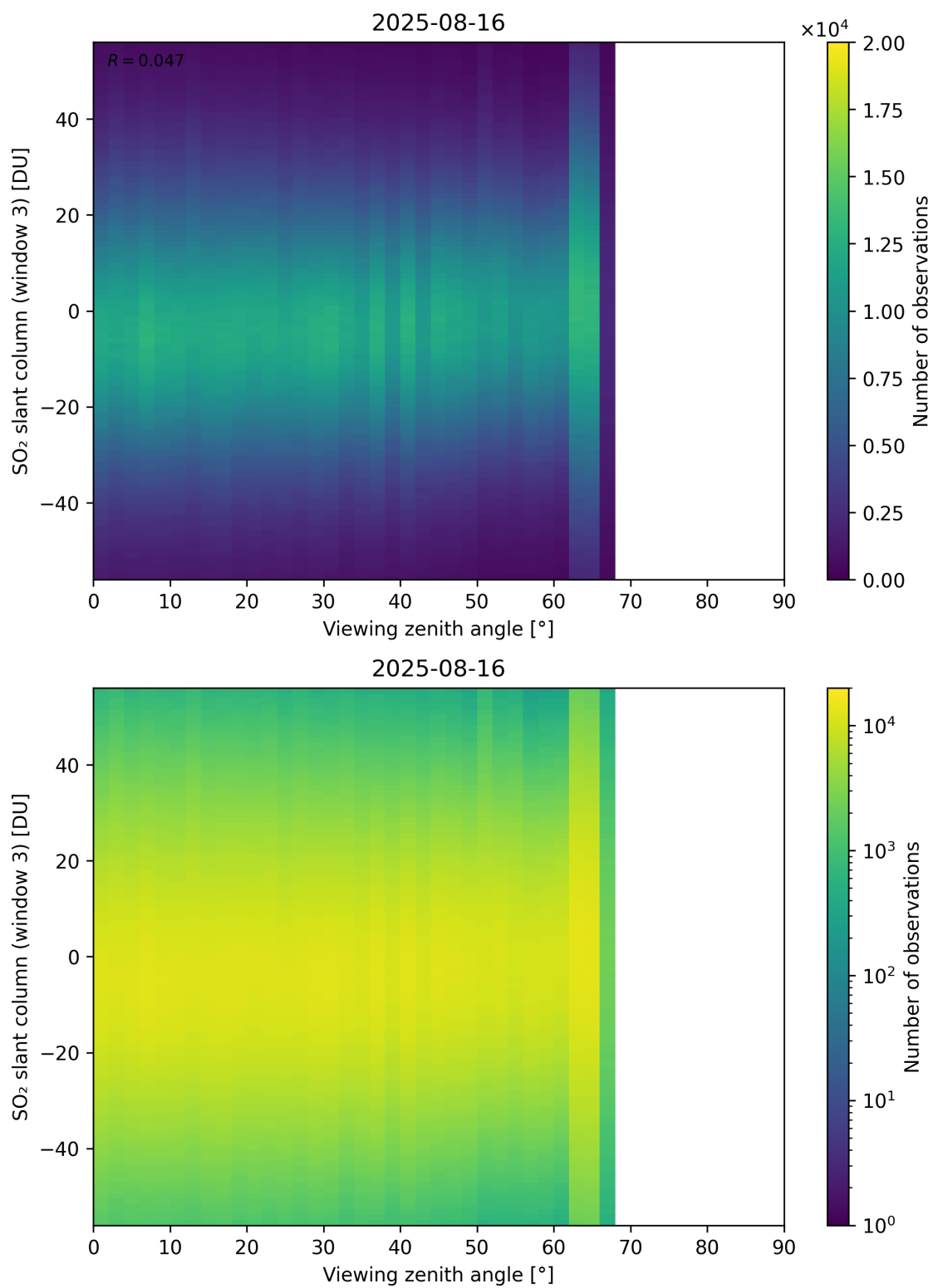
Figure 379: Scatter density plot of “Viewing zenith angle” against “SO 2 slant column (window 3)” for 2025-08-15 to 2025-08-17.
