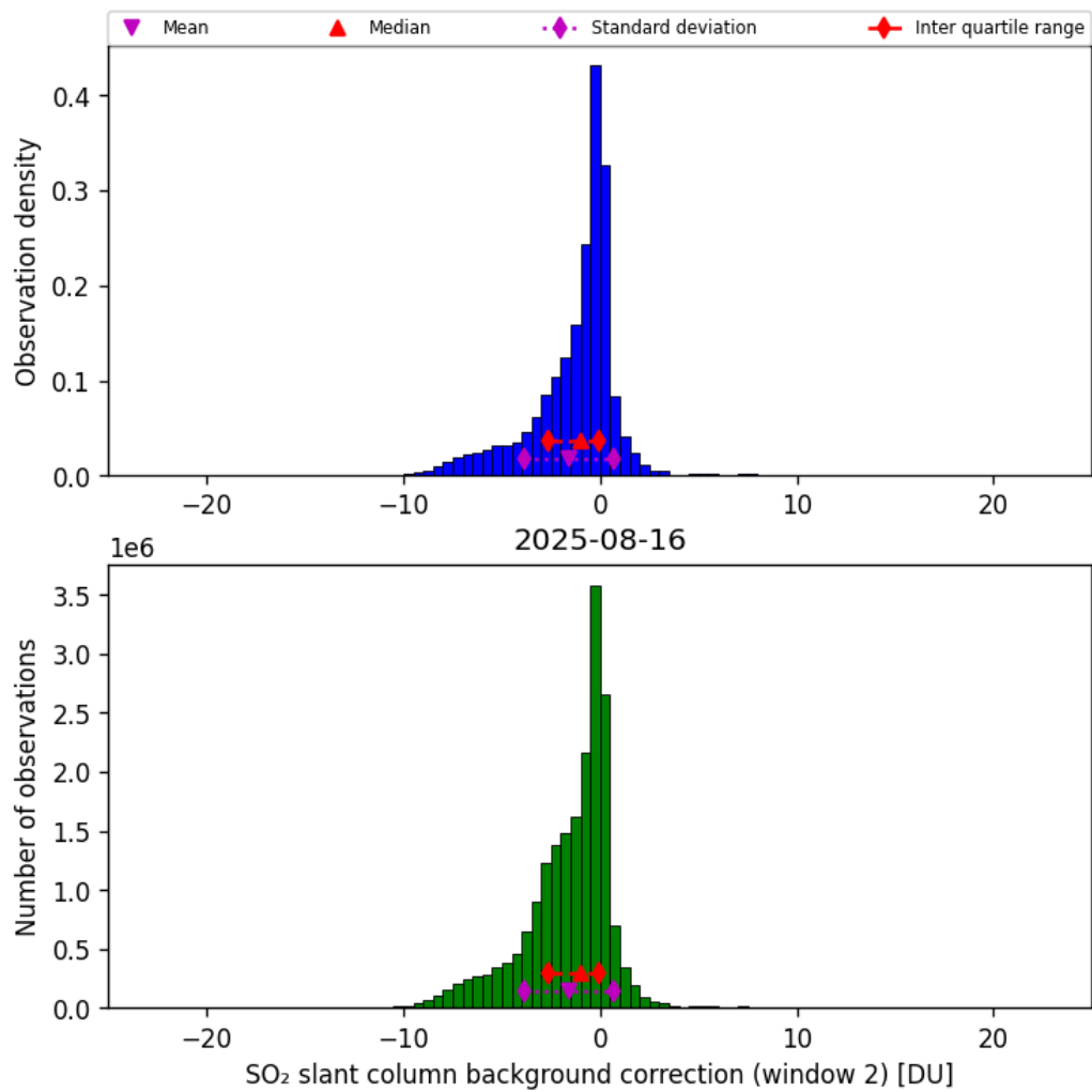
Figure 70: Histogram of “SO 2 slant column background correction (window 2)” for 2025-08-15 to 2025-08-17
