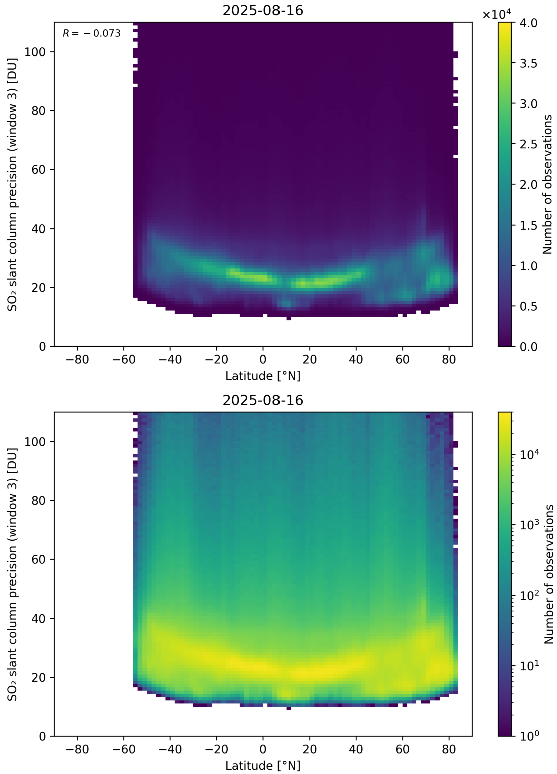
Figure 166: Scatter density plot of “Latitude” against “SO 2 slant column precision (window 3)” for 2025-08-15 to 2025-08-17.
