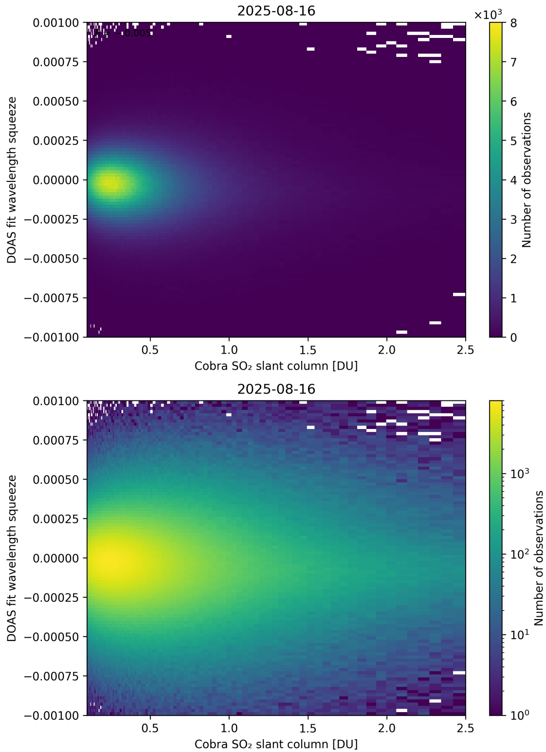
Figure 197: Scatter density plot of “Cobra SO 2 slant column” against “DOAS fit wavelength squeeze” for 2025-08-15 to 2025-08-17.
