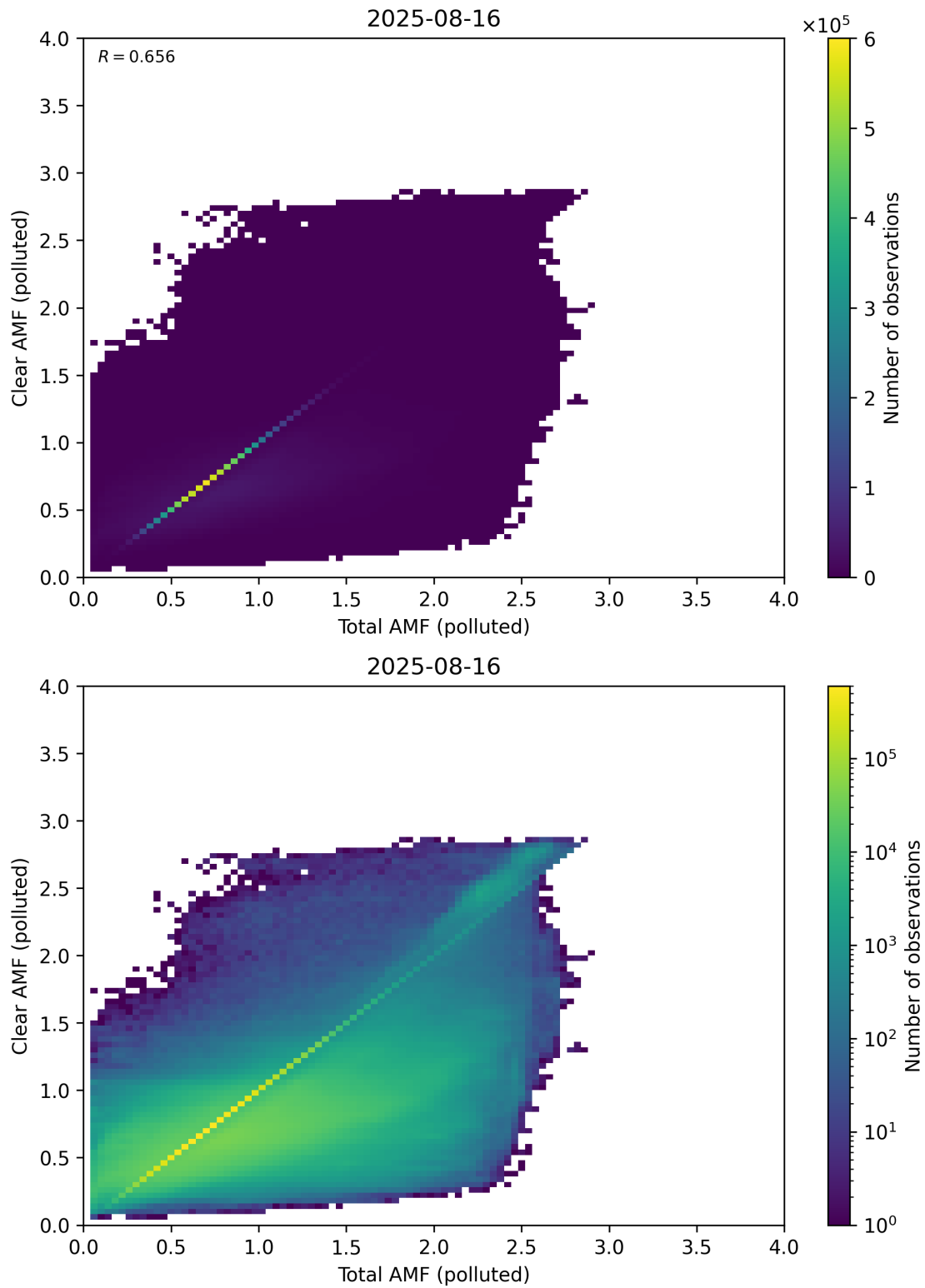
Figure 321: Scatter density plot of “Total AMF (polluted)” against “Clear AMF (polluted)” for 2025-08-15 to 2025-08-17.
