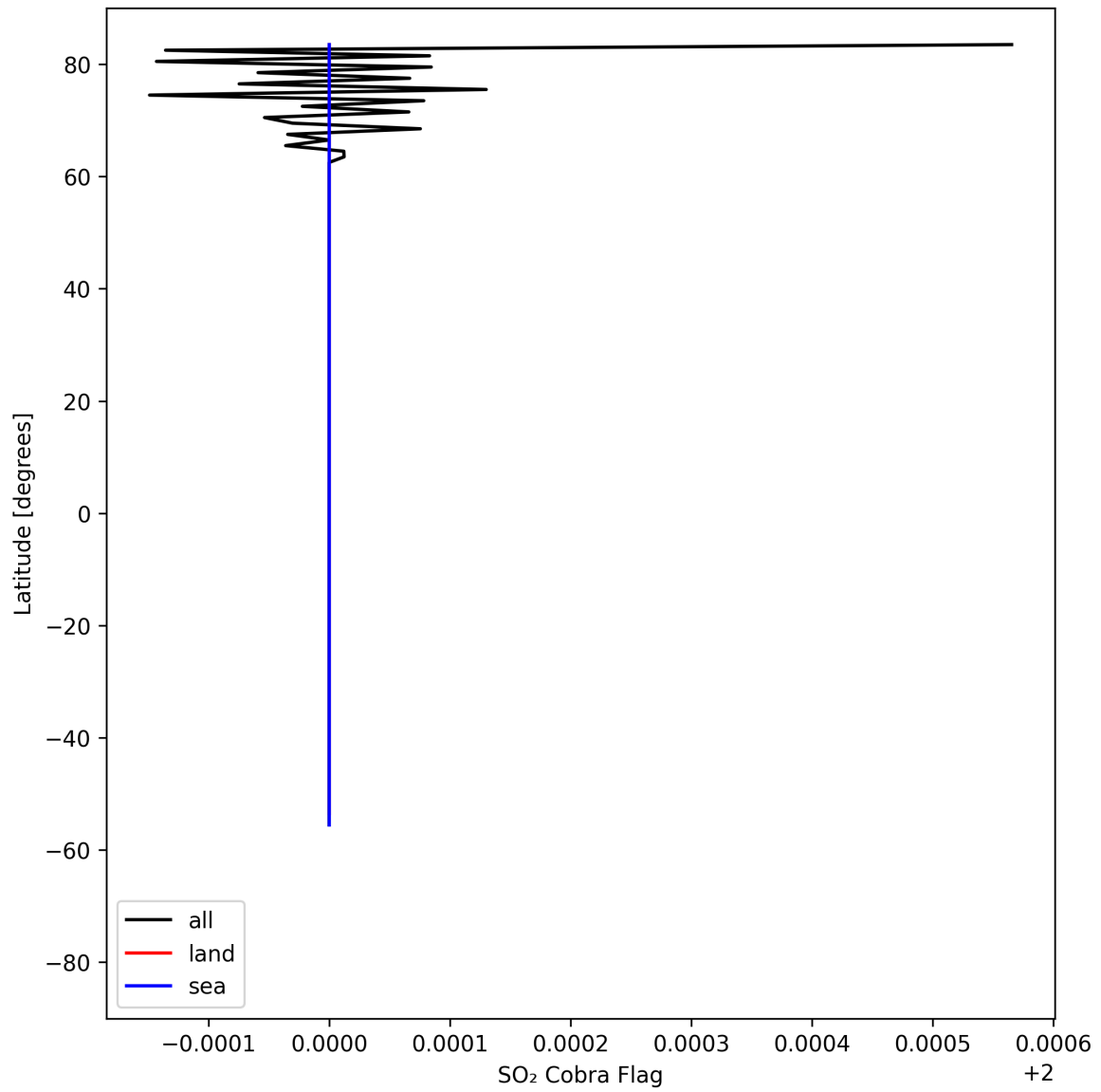
Figure 49: Zonal average of “SO 2 Cobra Flag” for 2025-08-15 to 2025-08-17.
