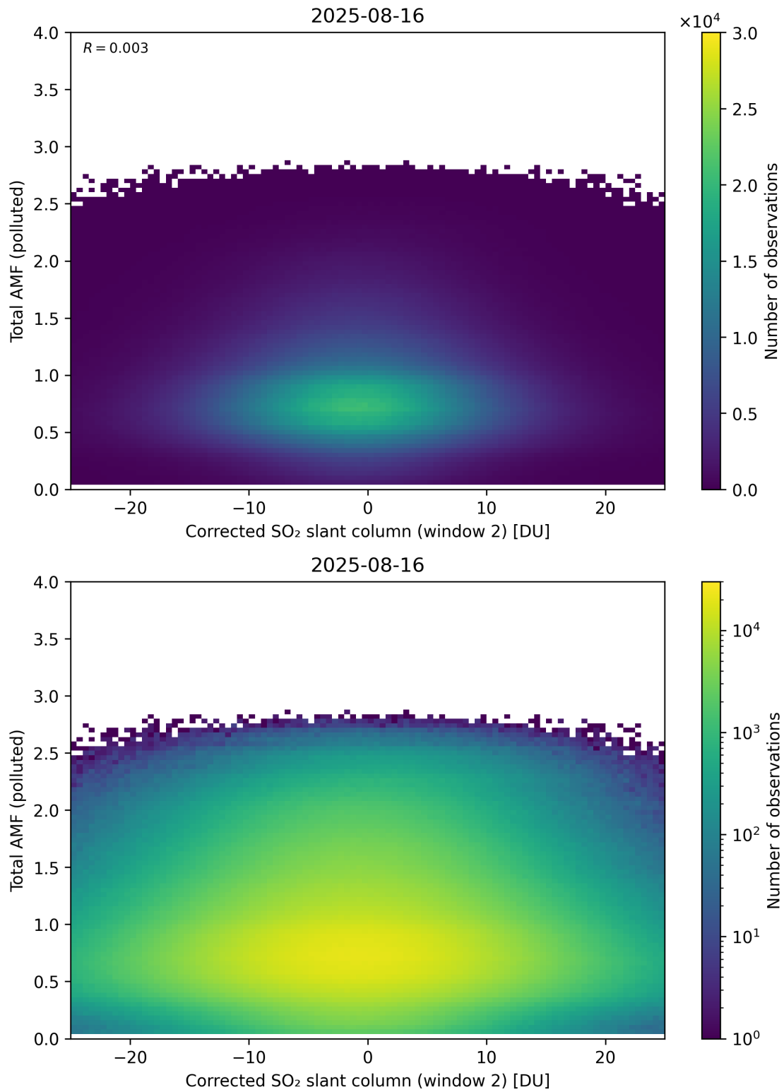
Figure 253: Scatter density plot of “Corrected SO 2 slant column (window 2)” against “Total AMF (polluted)” for 2025-08-15 to 2025-08-17.
