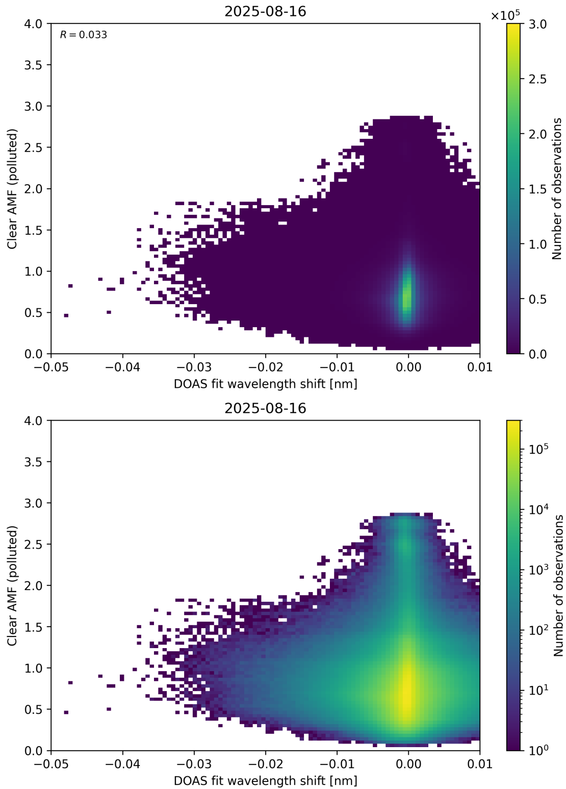
Figure 140: Scatter density plot of “DOAS fit wavelength shift” against “Clear AMF (polluted)” for 2025-08-15 to 2025-08-17.
