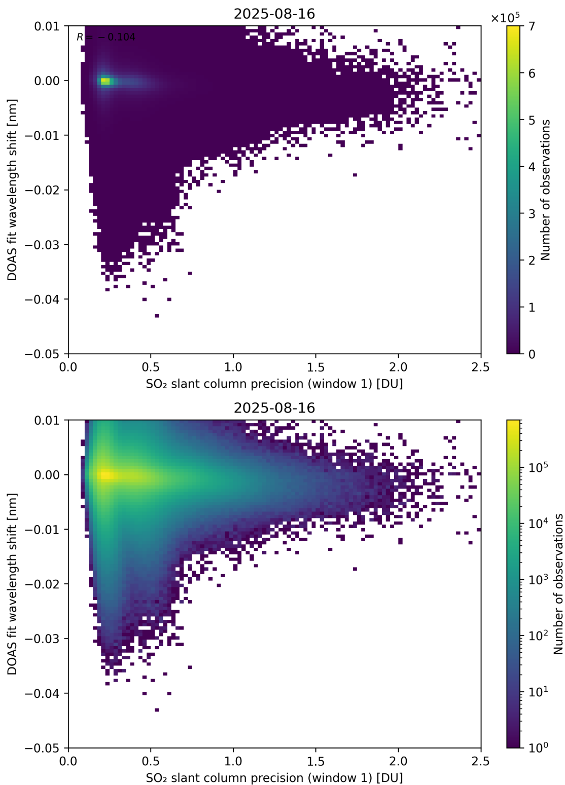
Figure 271: Scatter density plot of “SO 2 slant column precision (window 1)” against “DOAS fit wavelength shift” for 2025-08-15 to 2025-08-17.
