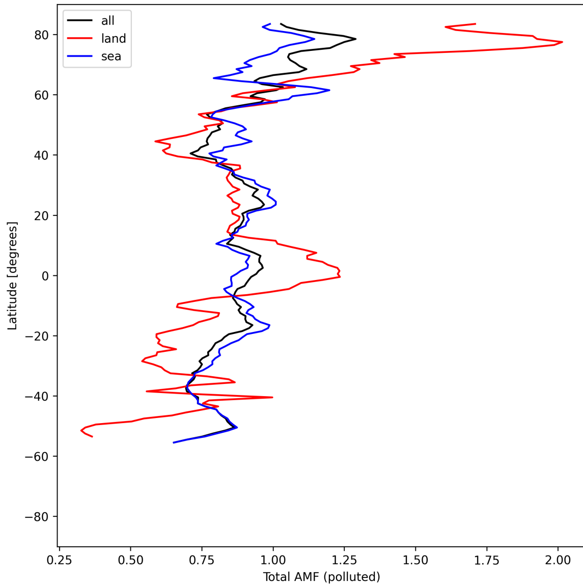
Figure 53: Zonal average of “Total AMF (polluted)” for 2025-08-15 to 2025-08-17.
