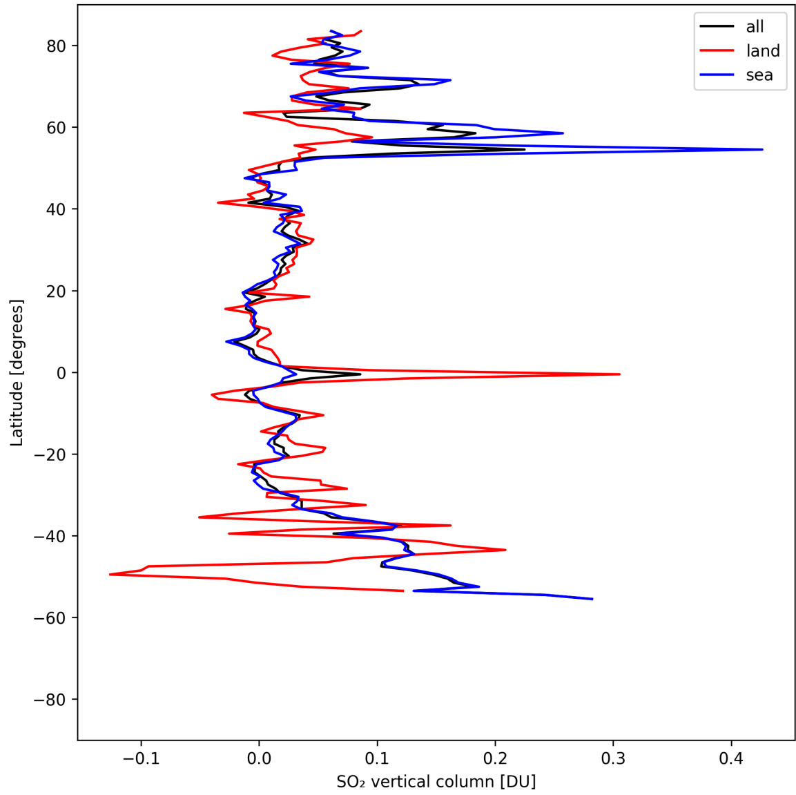
Figure 32: Zonal average of “SO 2 vertical column” for 2025-08-15 to 2025-08-17.
