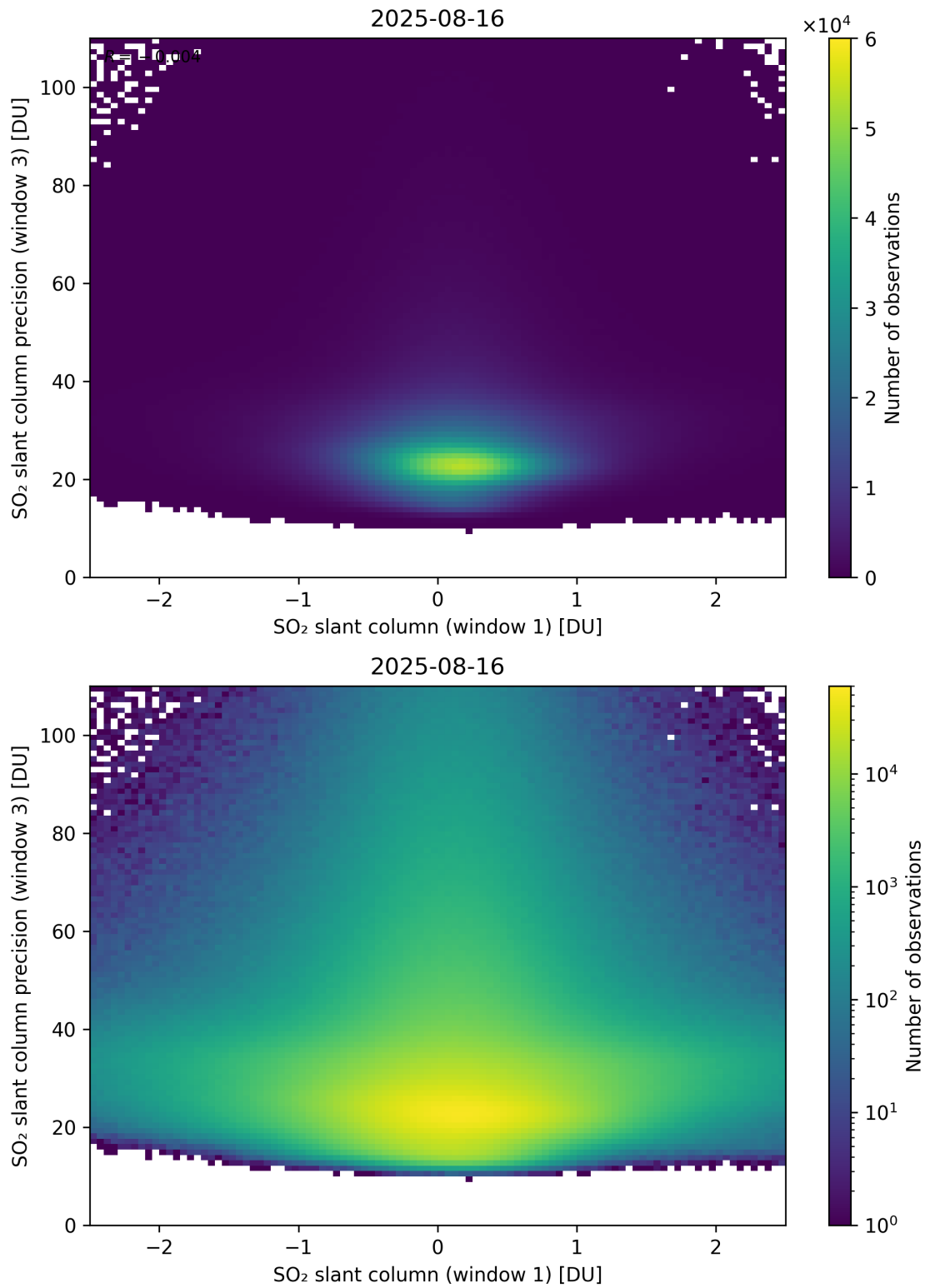
Figure 288: Scatter density plot of “SO 2 slant column (window 1)” against “SO 2 slant column precision (window 3)” for 2025-08-15 to 2025-08-17.
