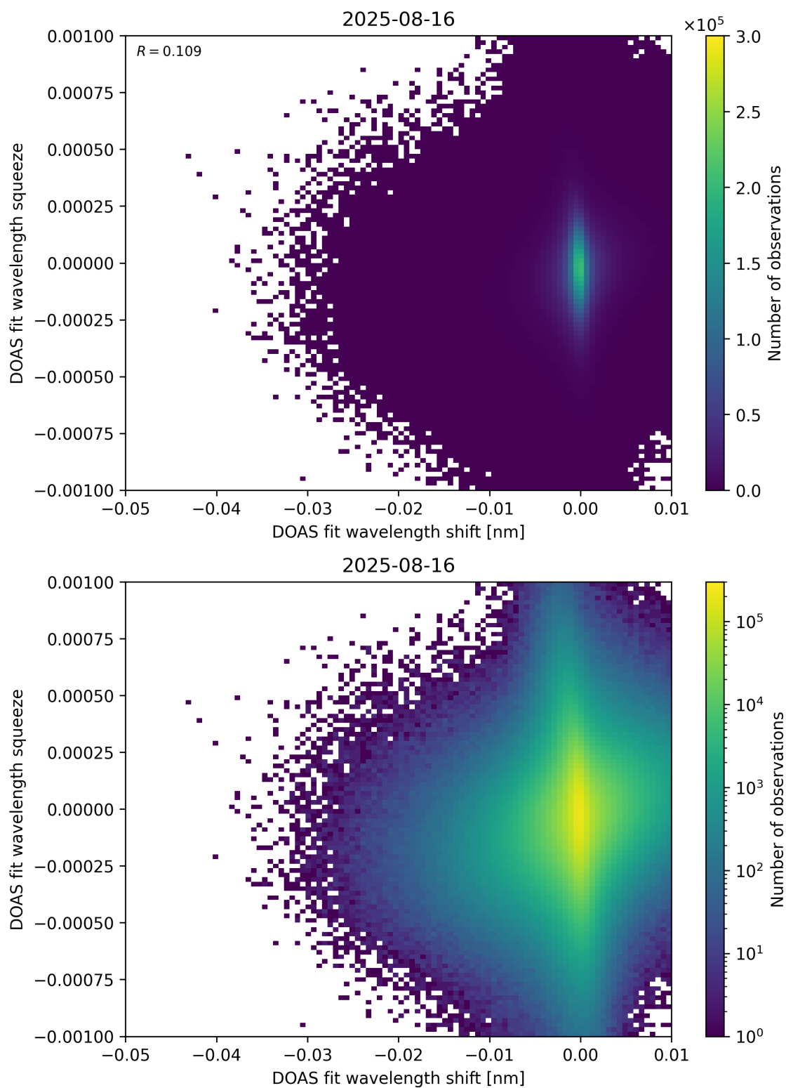
Figure 138: Scatter density plot of “DOAS fit wavelength shift” against “DOAS fit wavelength squeeze” for 2025-08-15 to 2025-08-17.
