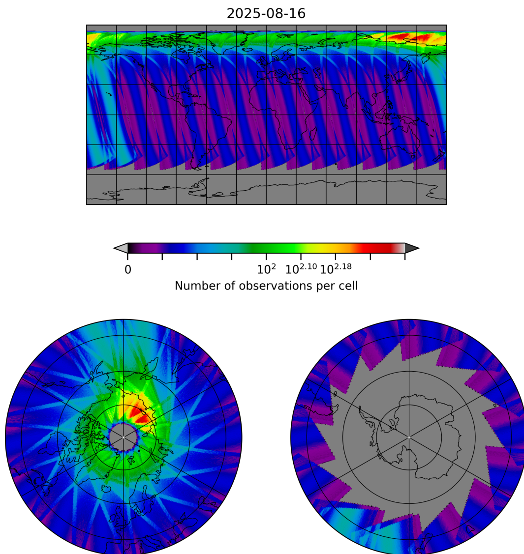
Figure 30: Map of the number of observations for 2025-08-15 to 2025-08-17
