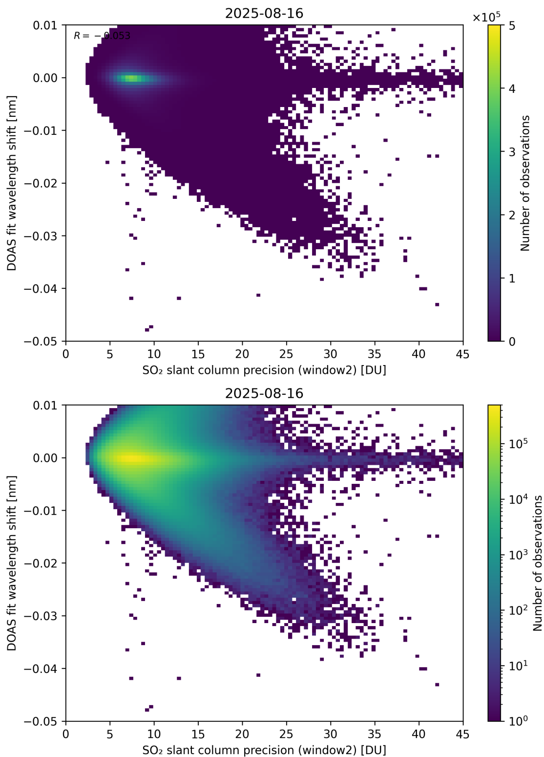
Figure 293: Scatter density plot of “SO 2 slant column precision (window2)” against “DOAS fit wavelength shift” for 2025-08-15 to 2025-08-17.
