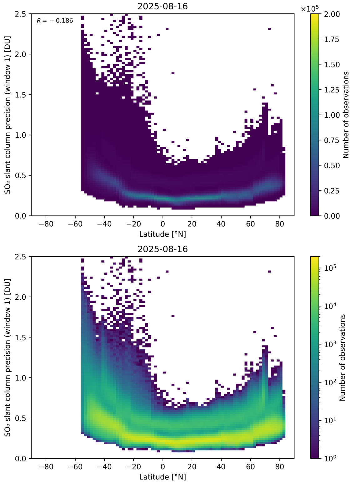
Figure 163: Scatter density plot of “Latitude” against “SO 2 slant column precision (window 1)” for 2025-08-15 to 2025-08-17.
