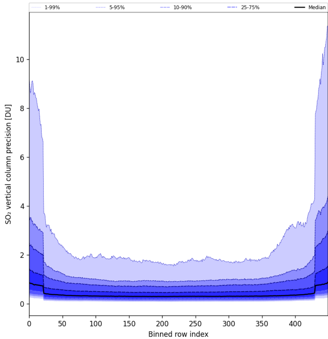
Figure 85: Along track statistics of “SO 2 vertical column precision” for 2025-08-15 to 2025-08-17
