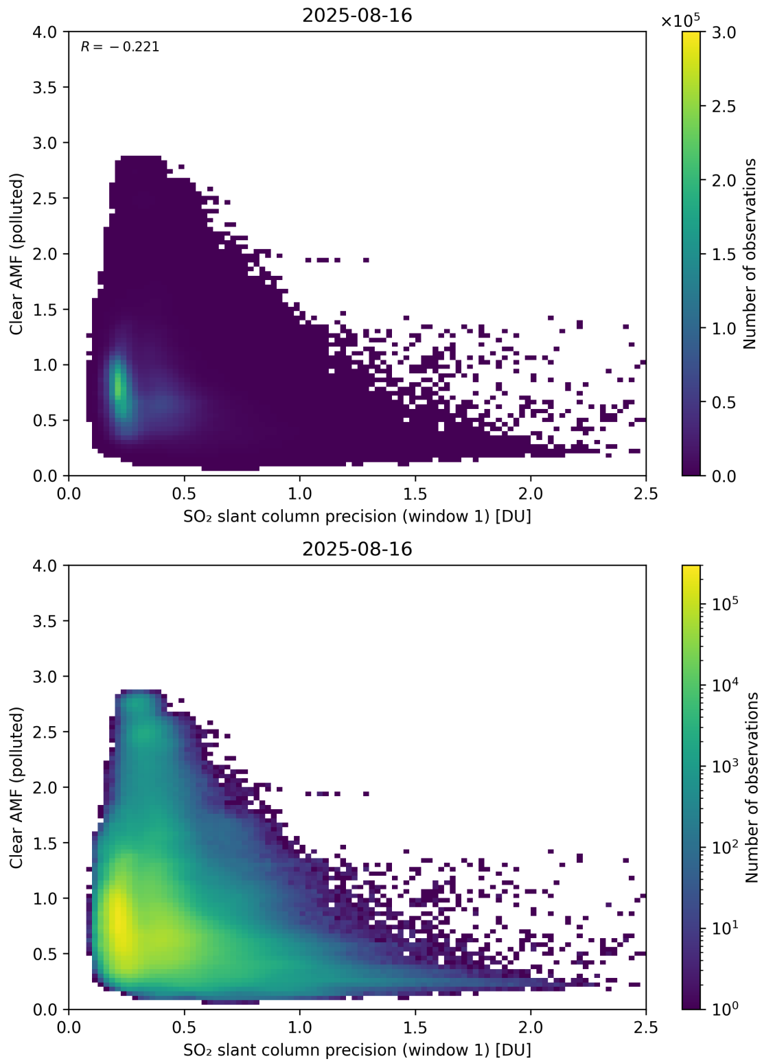
Figure 274: Scatter density plot of “SO 2 slant column precision (window 1)” against “Clear AMF (polluted)” for 2025-08-15 to 2025-08-17.
