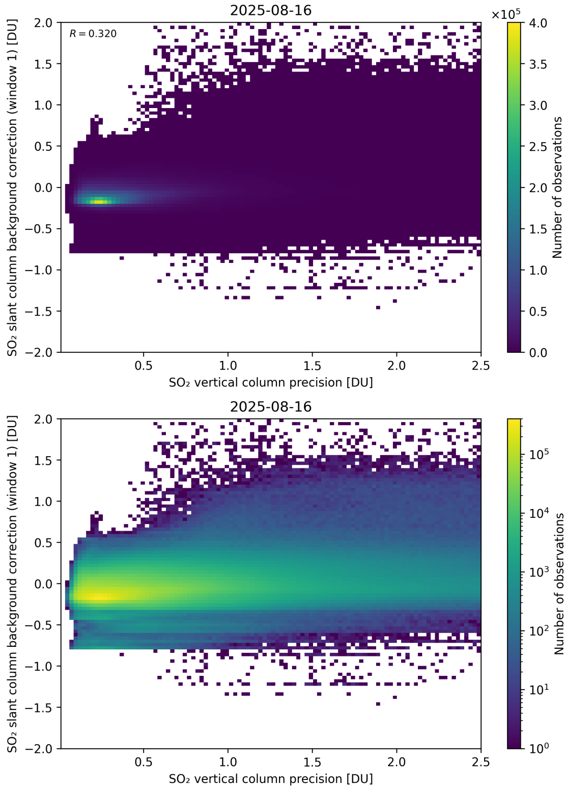
Figure 329: Scatter density plot of “SO 2 vertical column precision” against “SO 2 slant column background correction (window 1)” for 2025-08-15 to 2025-08-17.
