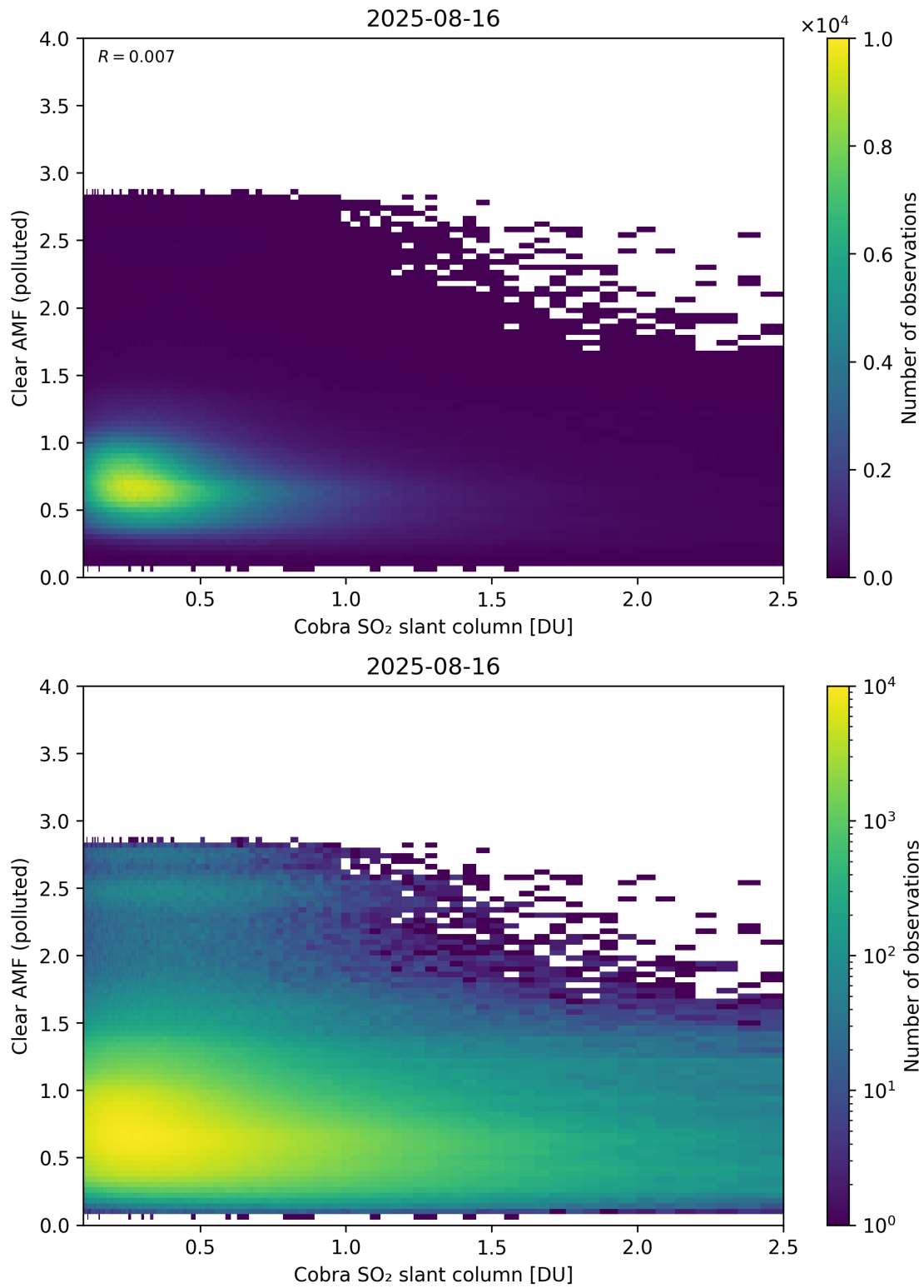
Figure 215: Scatter density plot of “Cobra SO 2 slant column” against “Clear AMF (polluted)” for 2025-08-15 to 2025-08-17.
