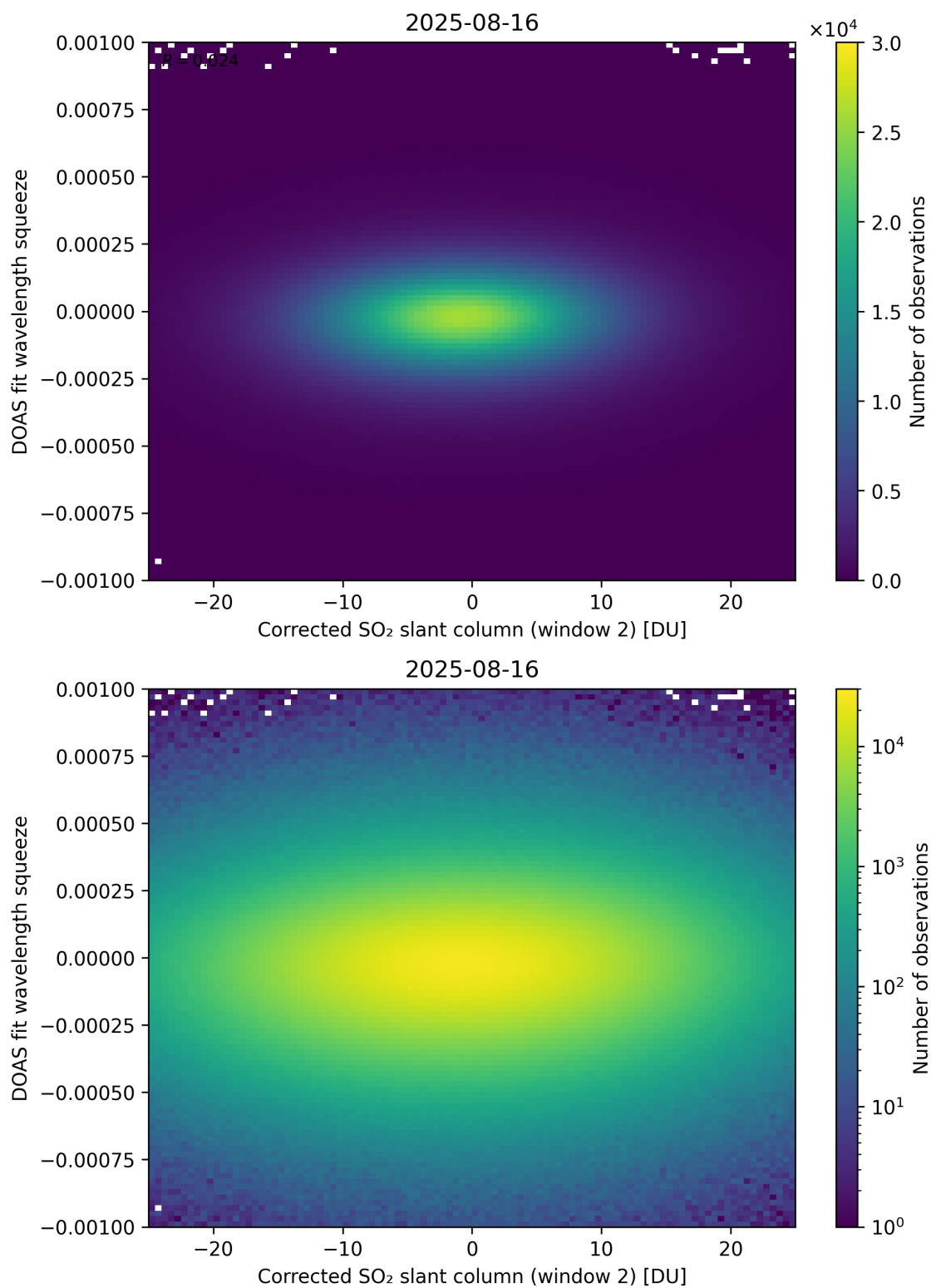
Figure 247: Scatter density plot of “Corrected SO 2 slant column (window 2)” against “DOAS fit wavelength squeeze” for 2025-08-15 to 2025-08-17.
