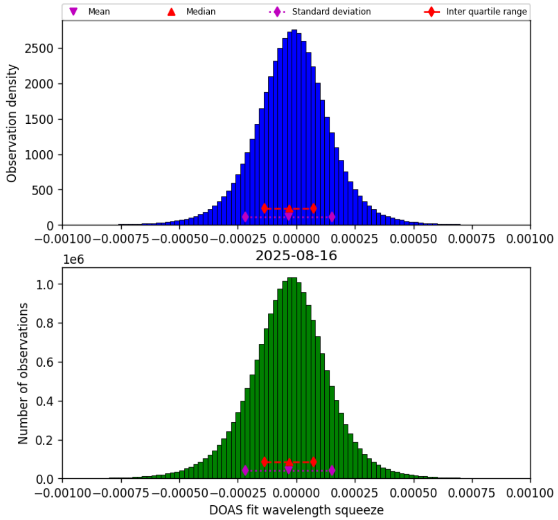
Figure 77: Histogram of “DOAS fit wavelength squeeze” for 2025-08-15 to 2025-08-17
