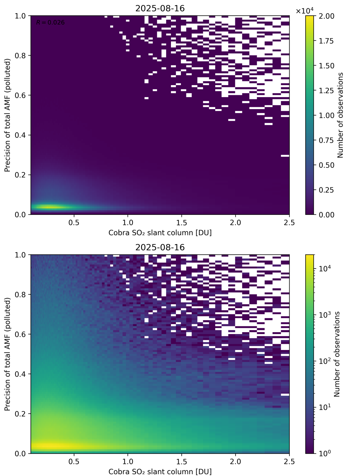
Figure 225: Scatter density plot of “Cobra SO 2 slant column” against “Precision of total AMF (polluted)” for 2025-08-15 to 2025-08-17.
