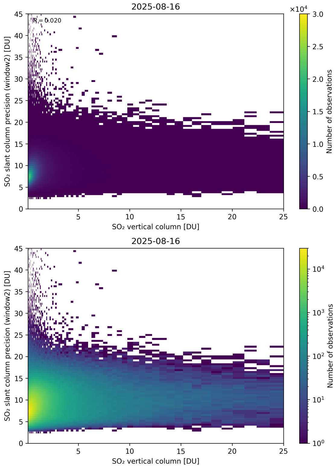
Figure 356: Scatter density plot of “SO 2 vertical column” against “SO 2 slant column precision (window2)” for 2025-08-15 to 2025-08-17.
