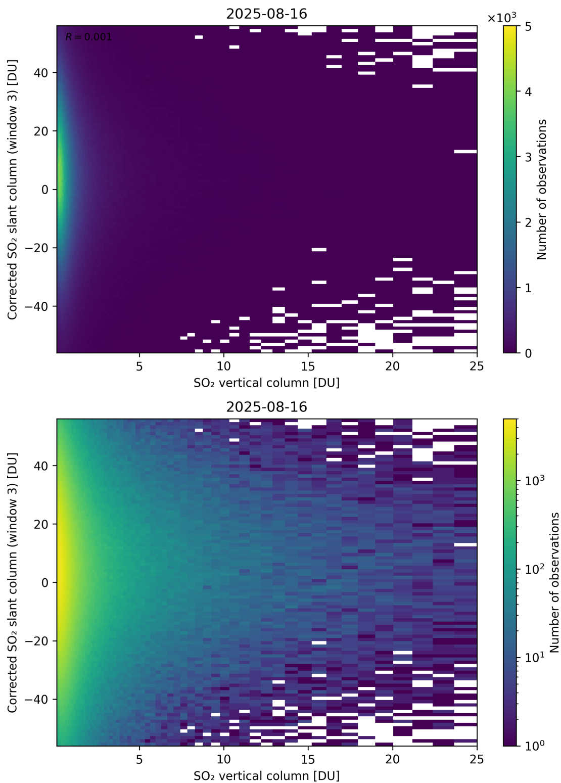
Figure 353: Scatter density plot of “SO 2 vertical column” against “Corrected SO 2 slant column (window 3)” for 2025-08-15 to 2025-08-17.
