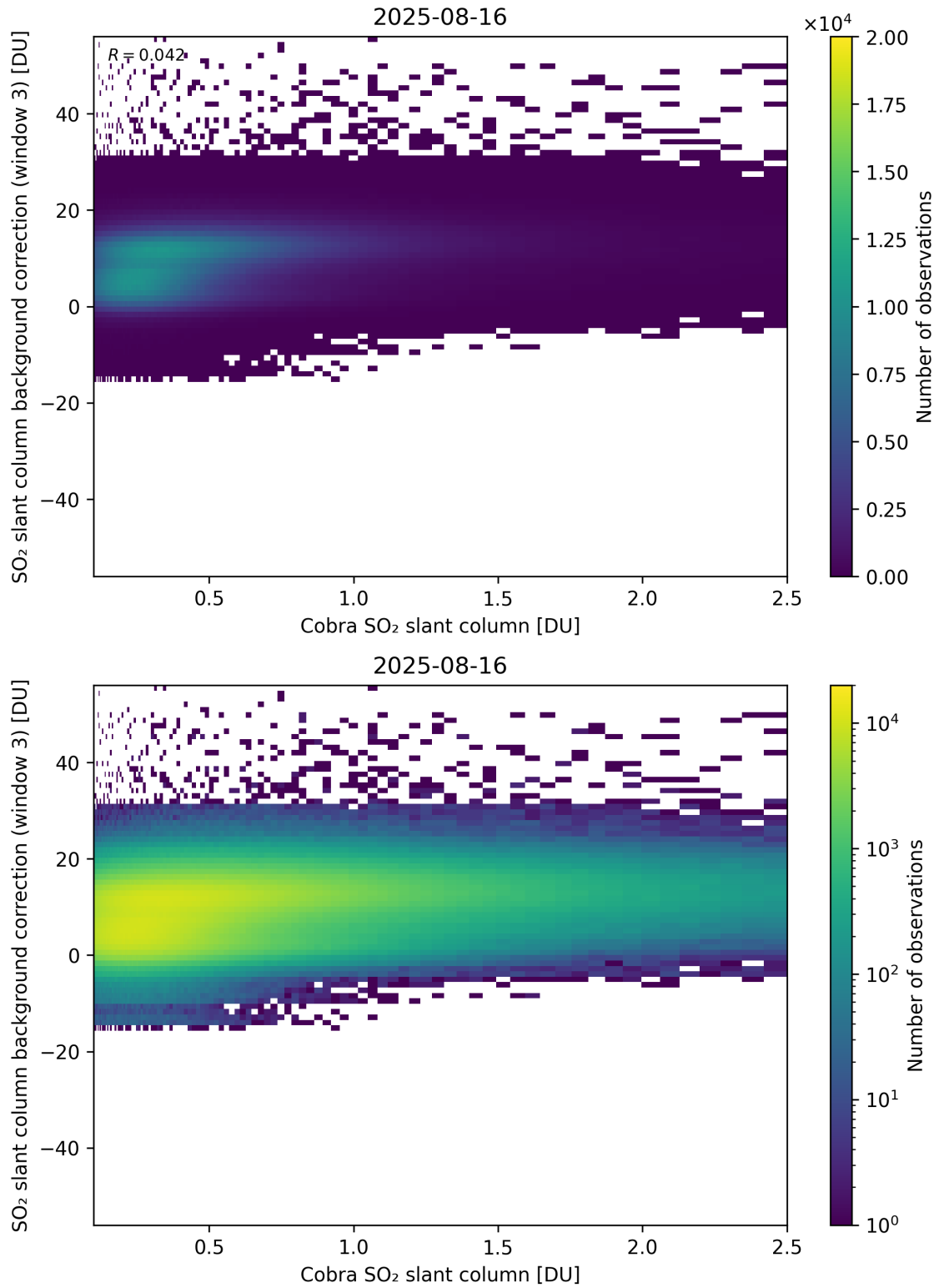
Figure 195: Scatter density plot of “Cobra SO 2 slant column” against “SO 2 slant column background correction (window 3)” for 2025-08-15 to 2025-08-17.
