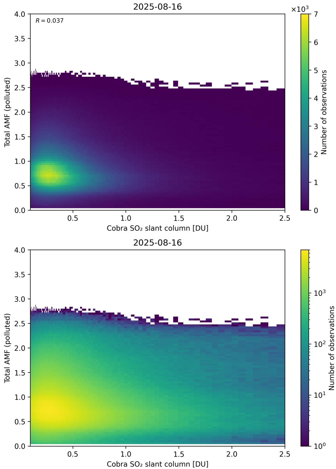
Figure 224: Scatter density plot of “Cobra SO 2 slant column” against “Total AMF (polluted)” for 2025-08-15 to 2025-08-17.
