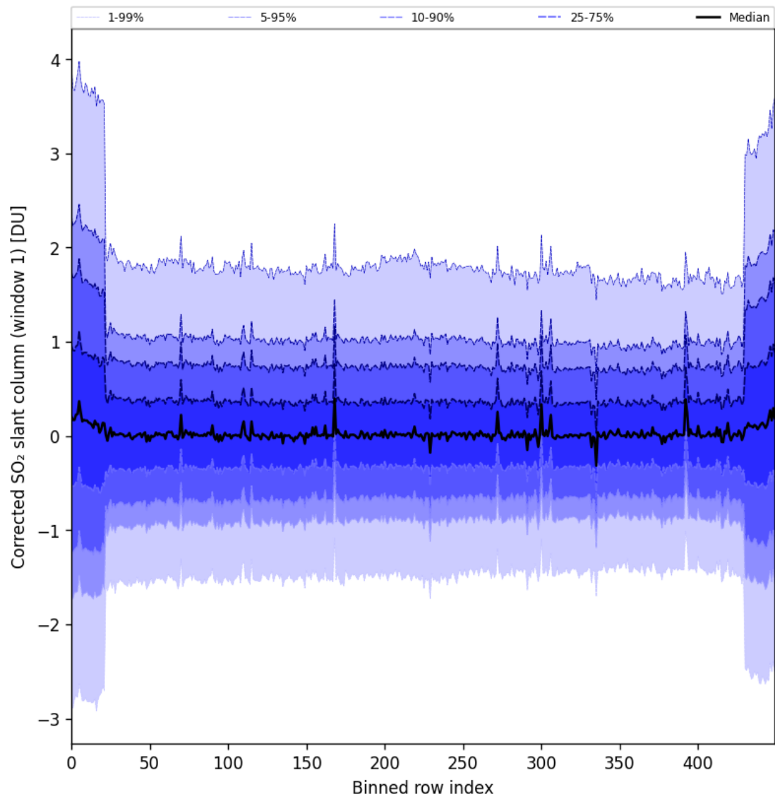
Figure 91: Along track statistics of “Corrected SO 2 slant column (window 1)” for 2025-08-15 to 2025-08-17
