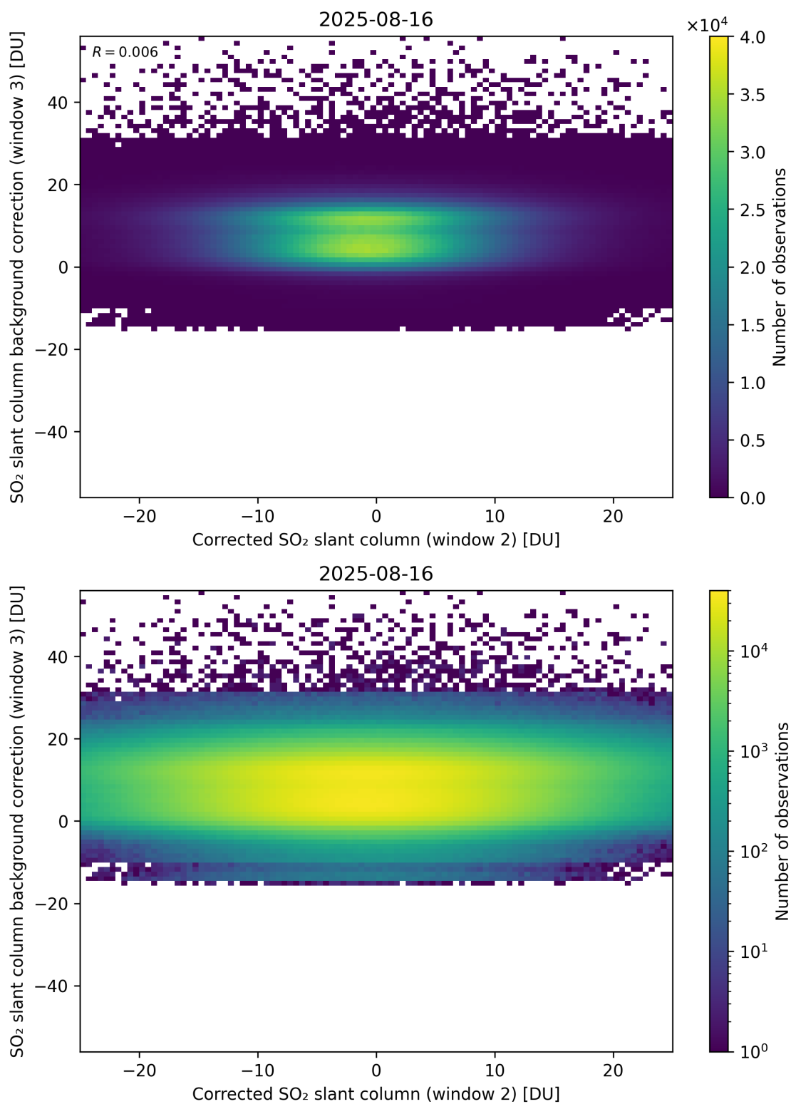
Figure 245: Scatter density plot of “Corrected SO 2 slant column (window 2)” against “SO 2 slant column background correction (window 3)” for 2025-08-15 to 2025-08-17.
