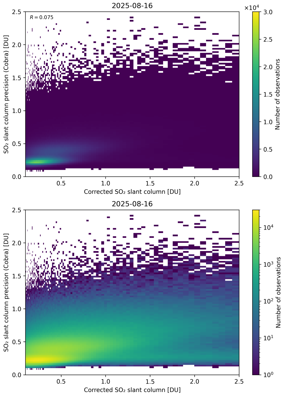
Figure 234: Scatter density plot of “Corrected SO 2 slant column” against “SO 2 slant column precision (Cobra)” for 2025-08-15 to 2025-08-17.
