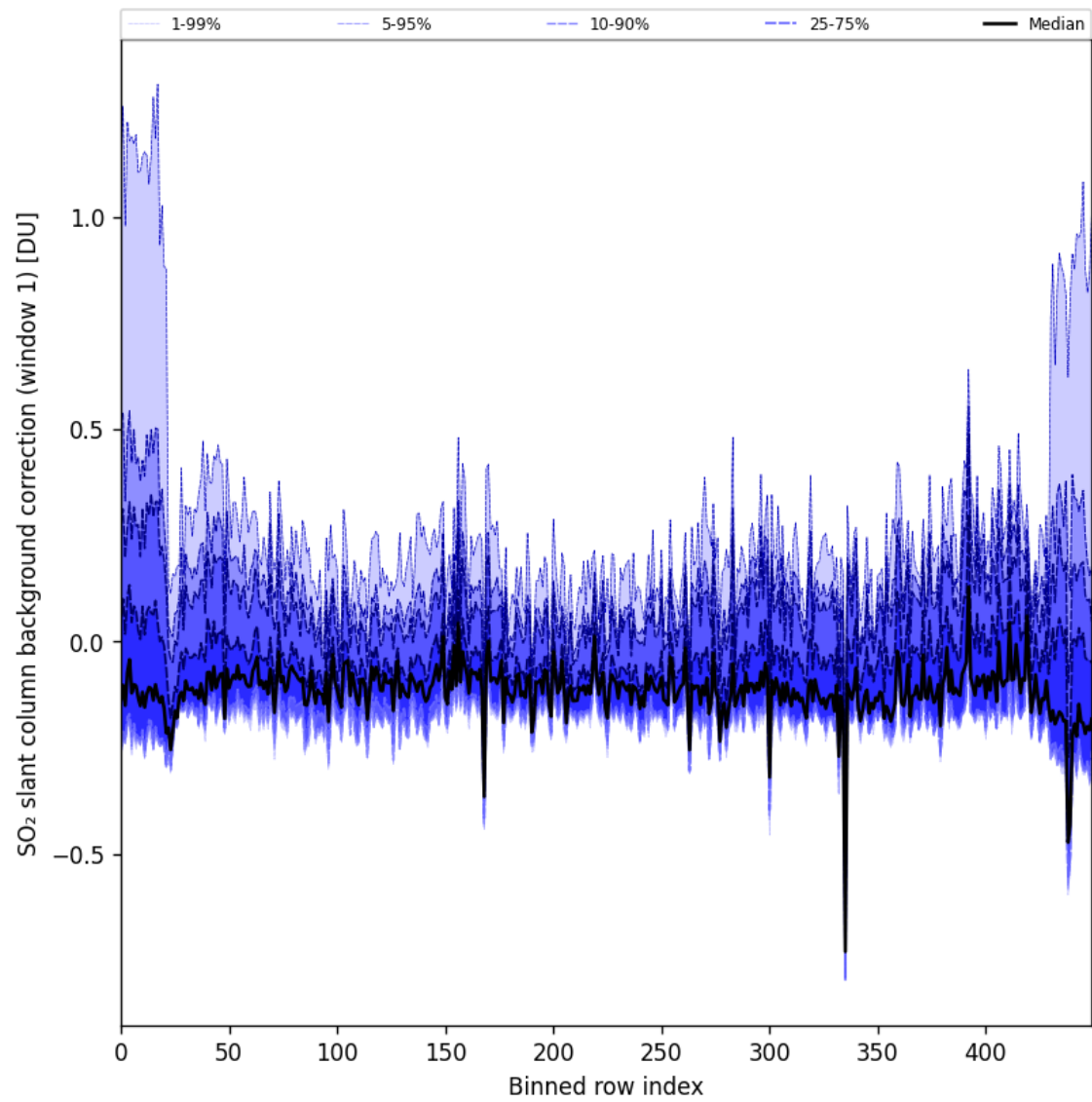
Figure 92: Along track statistics of “SO 2 slant column background correction (window 1)” for 2025-08-15 to 2025-08-17
