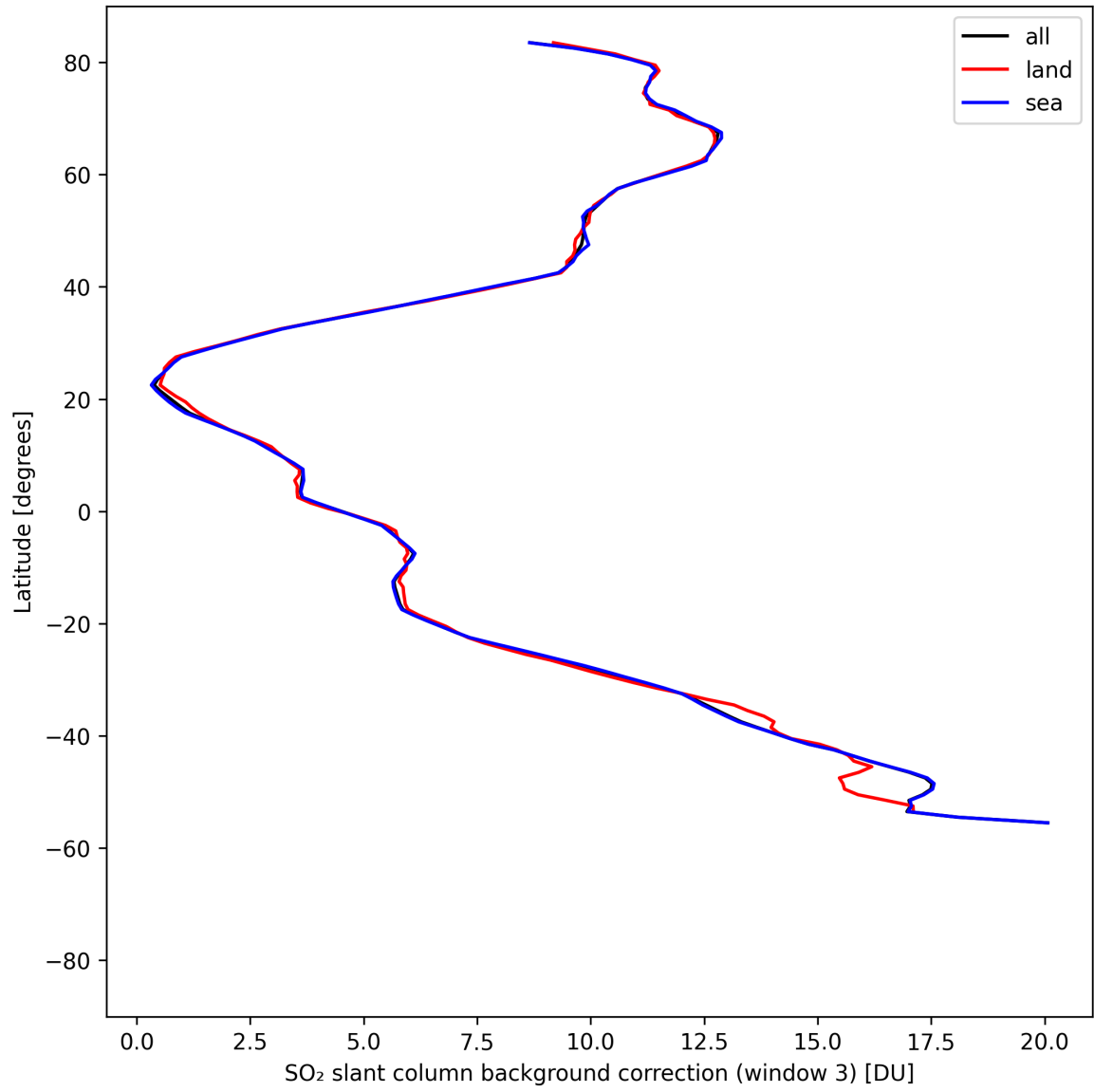
Figure 48: Zonal average of “SO 2 slant column background correction (window 3)” for 2025-08-15 to 2025-08-17.
