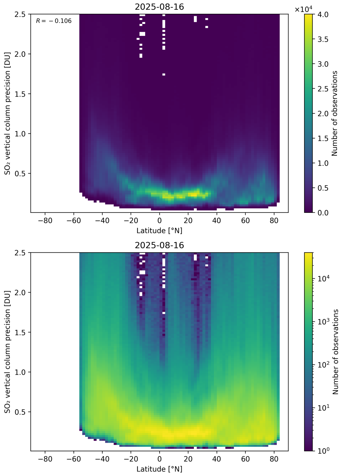
Figure 170: Scatter density plot of “Latitude” against “SO 2 vertical column precision” for 2025-08-15 to 2025-08-17.
