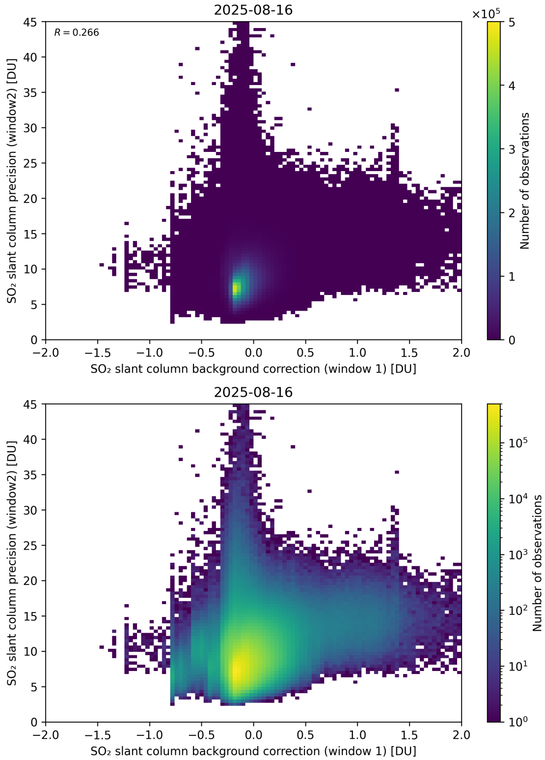
Figure 117: Scatter density plot of “SO 2 slant column background correction (window 1)” against “SO 2 slant column precision (window2)” for 2025-08-15 to 2025-08-17.
