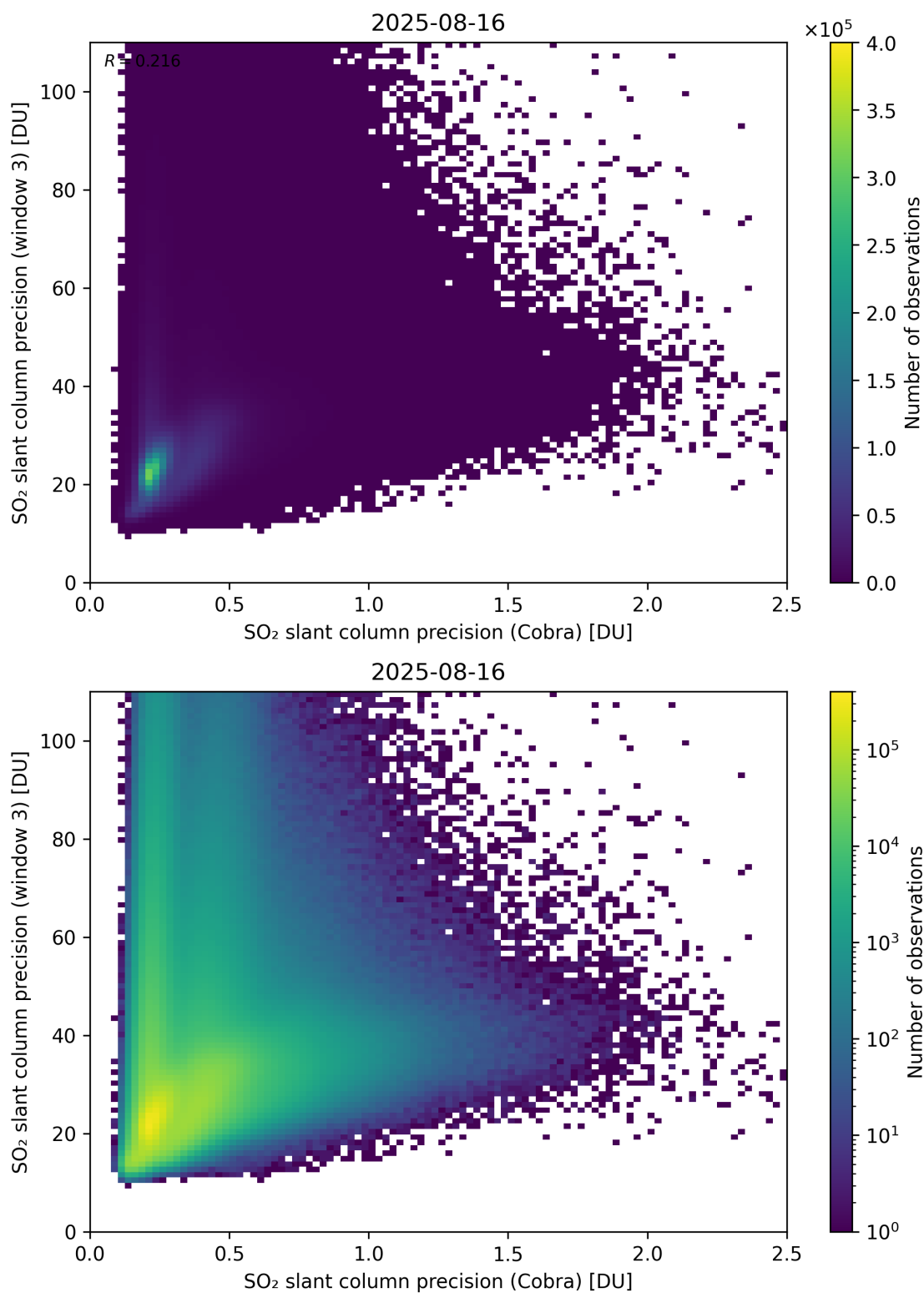
Figure 212: Scatter density plot of “SO 2 slant column precision (Cobra)” against “SO 2 slant column precision (window 3)” for 2025-08-15 to 2025-08-17.
