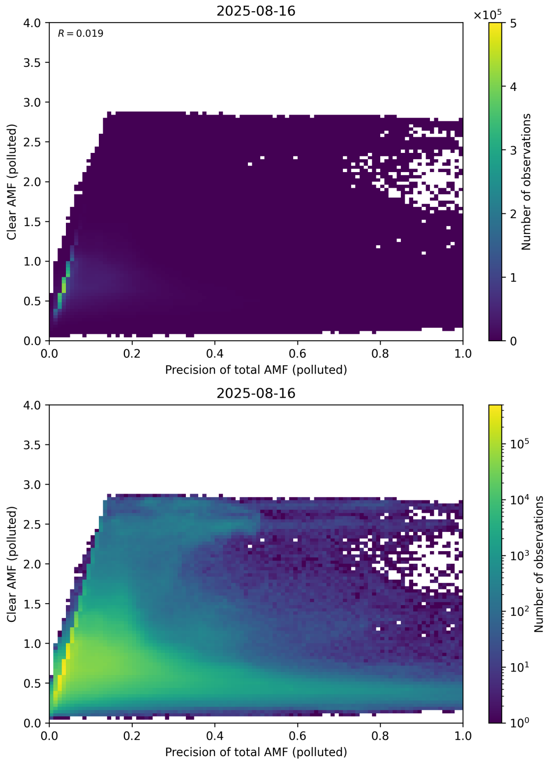
Figure 320: Scatter density plot of “Precision of total AMF (polluted)” against “Clear AMF (polluted)” for 2025-08-15 to 2025-08-17.
