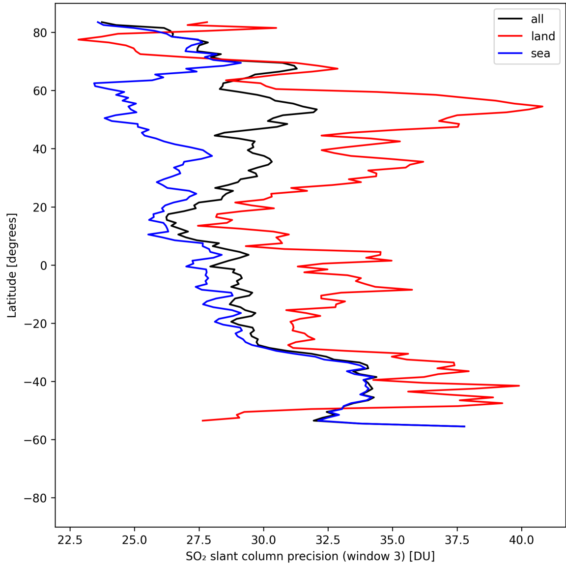
Figure 46: Zonal average of “SO 2 slant column precision (window 3)” for 2025-08-15 to 2025-08-17.
