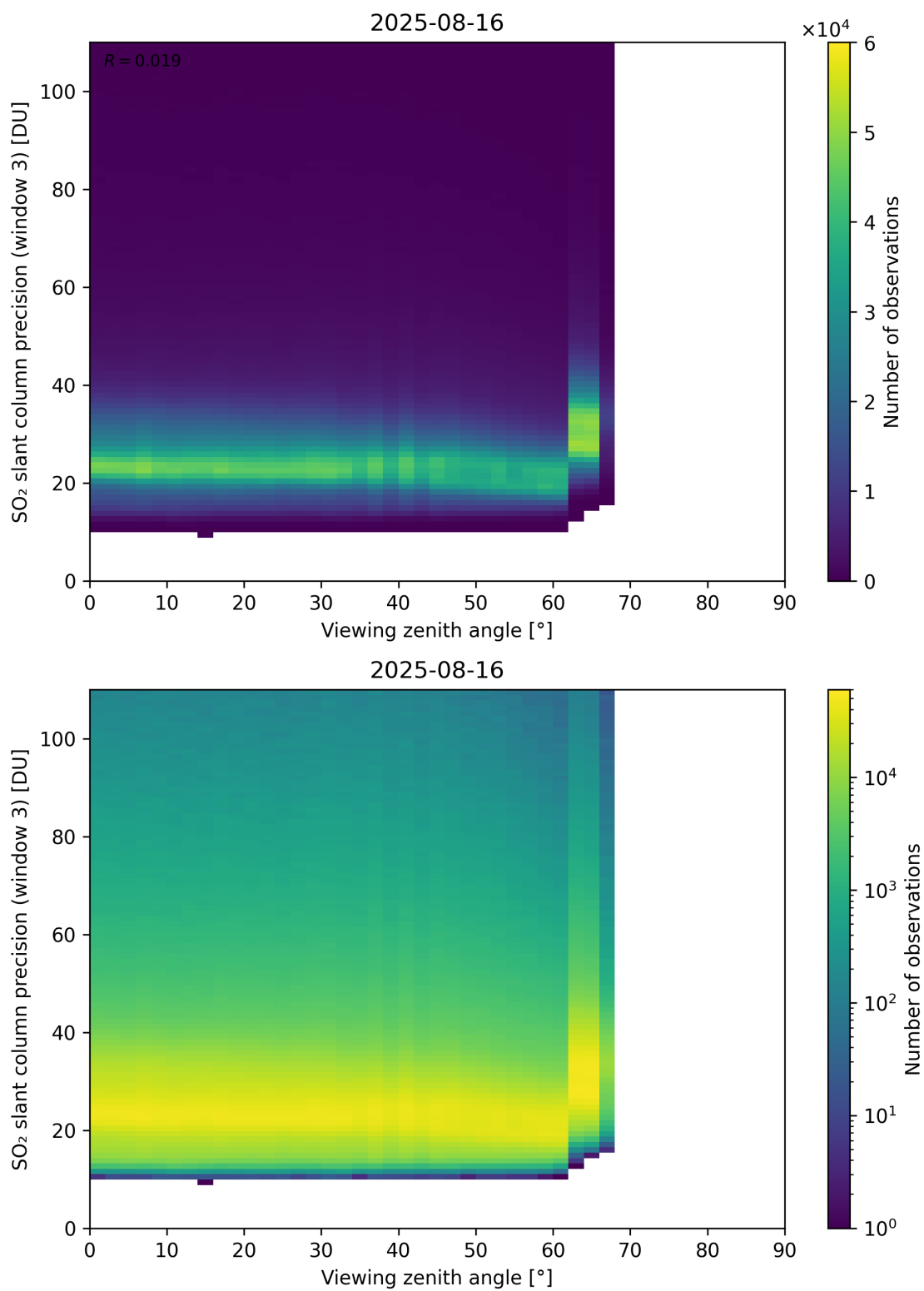
Figure 380: Scatter density plot of “Viewing zenith angle” against “SO 2 slant column precision (window 3)” for 2025-08-15 to 2025-08-17.
