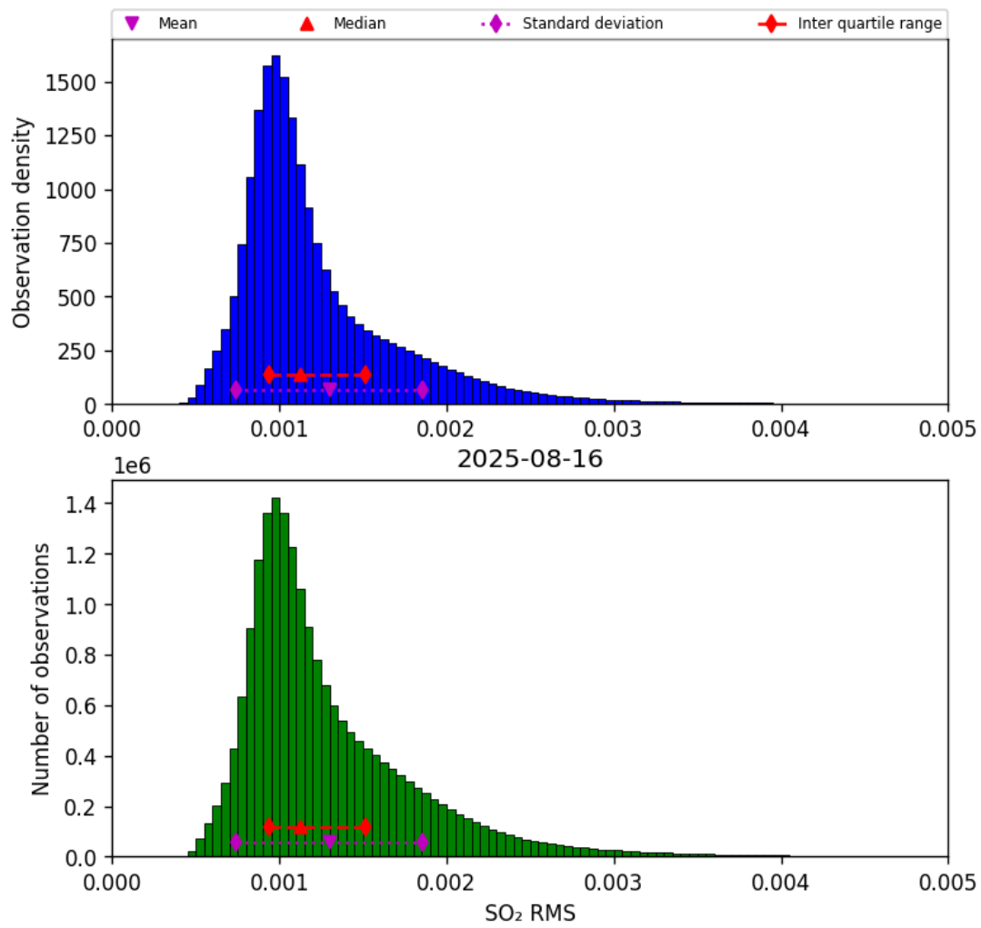
Figure 78: Histogram of “SO 2 RMS” for 2025-08-15 to 2025-08-17
