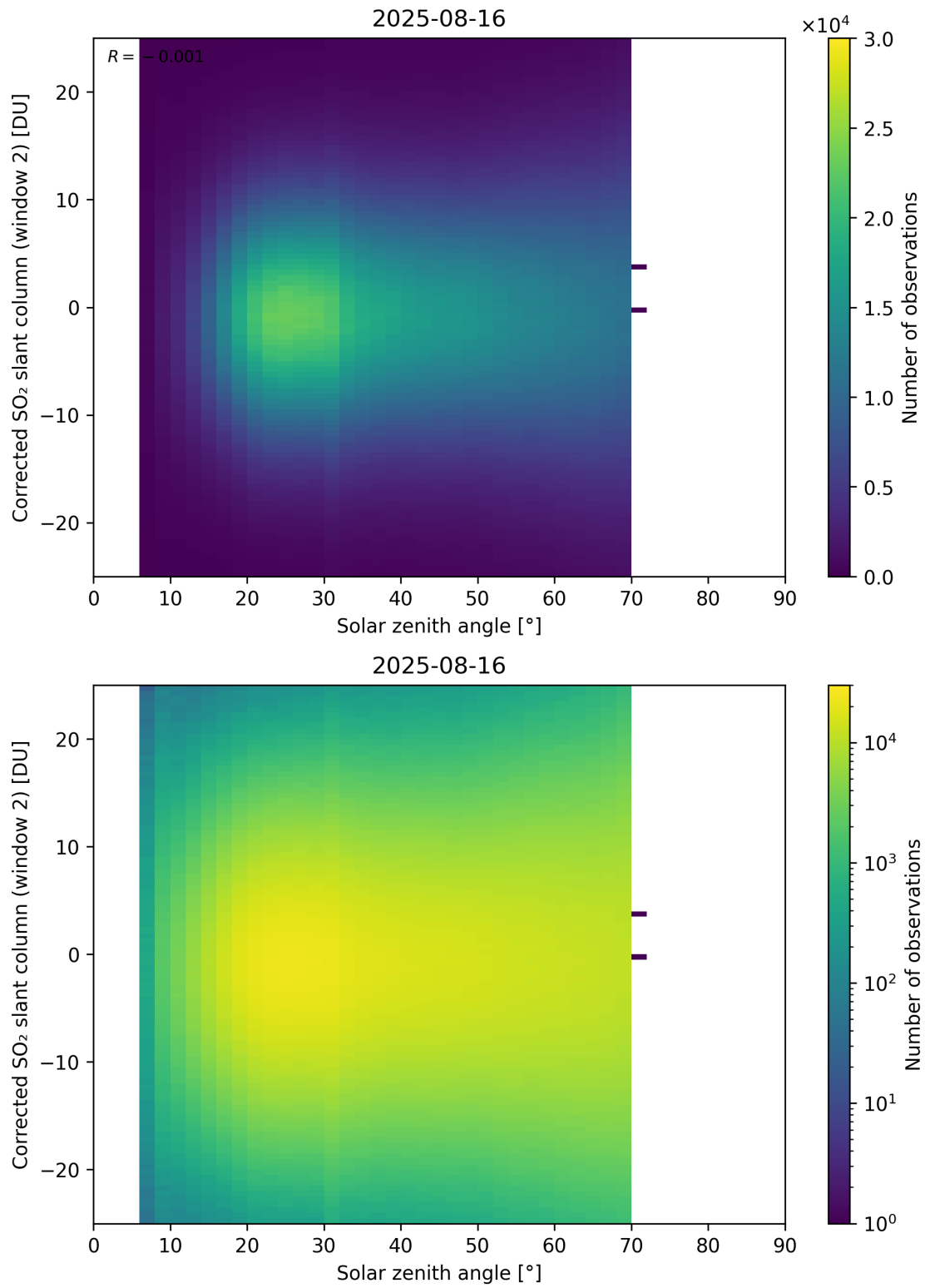
Figure 182: Scatter density plot of “Solar zenith angle” against “Corrected SO 2 slant column (window 2)” for 2025-08-15 to 2025-08-17.
