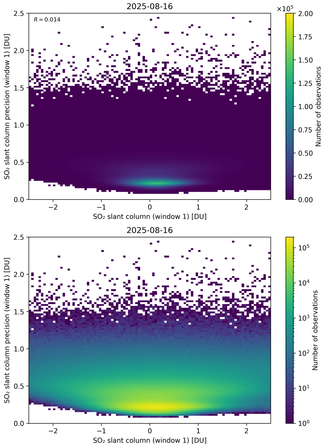
Figure 285: Scatter density plot of “SO 2 slant column (window 1)” against “SO 2 slant column precision (window 1)” for 2025-08-15 to 2025-08-17.
