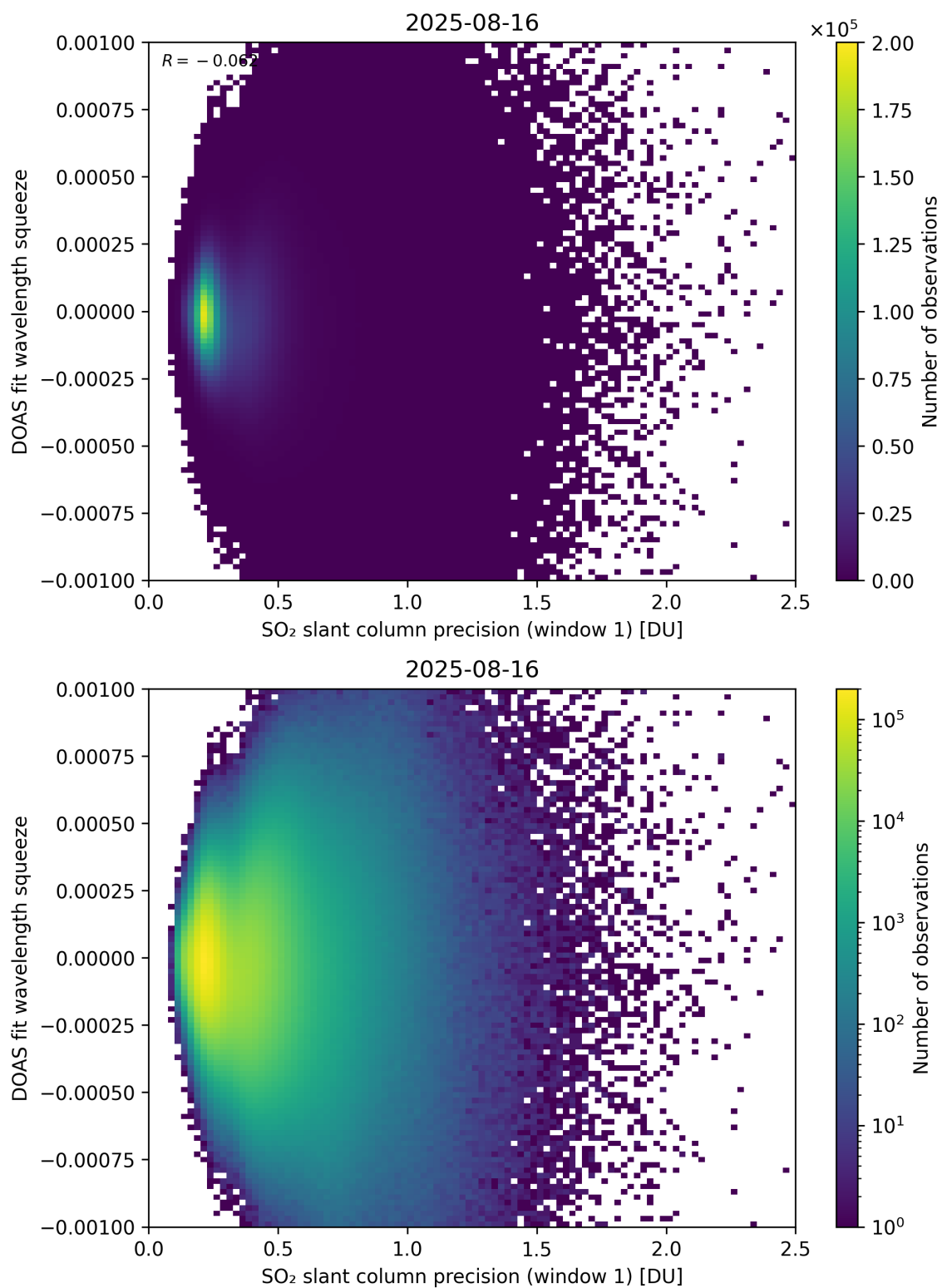
Figure 272: Scatter density plot of “SO 2 slant column precision (window 1)” against “DOAS fit wavelength squeeze” for 2025-08-15 to 2025-08-17.
