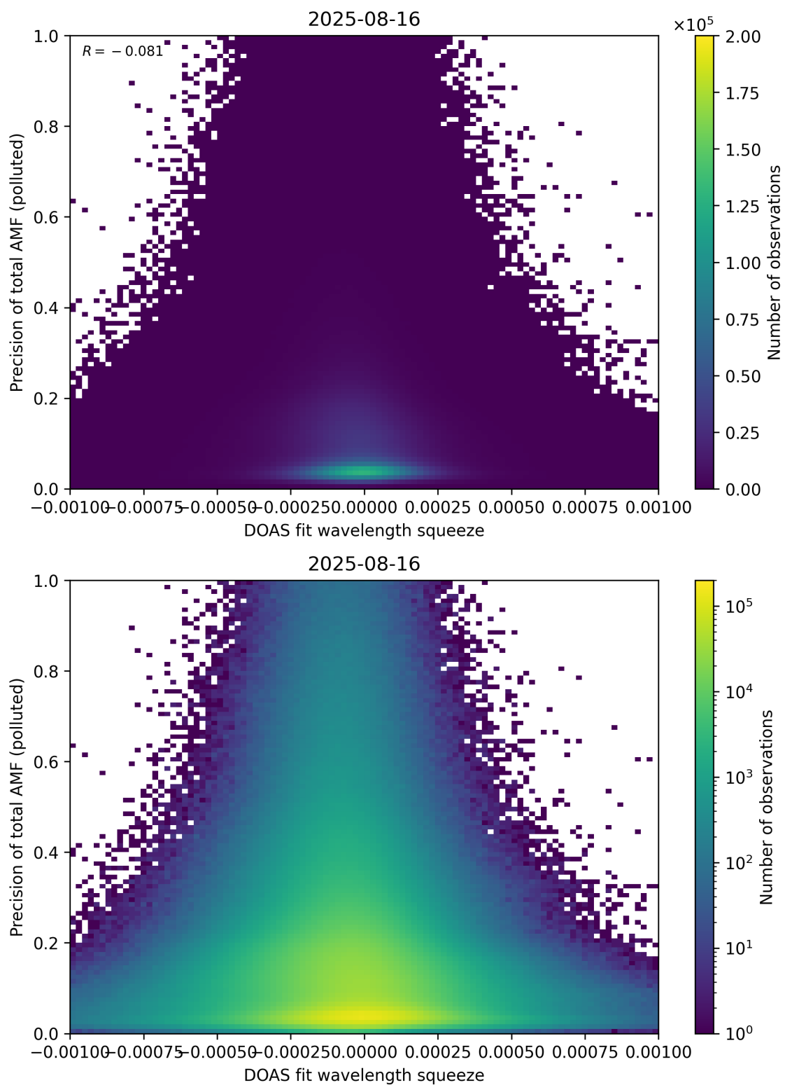
Figure 146: Scatter density plot of “DOAS fit wavelength squeeze” against “Precision of total AMF (polluted)” for 2025-08-15 to 2025-08-17.
