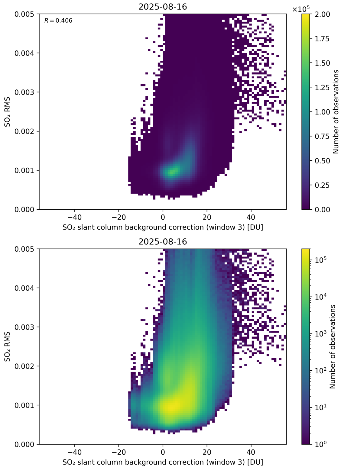
Figure 134: Scatter density plot of “SO 2 slant column background correction (window 3)” against “SO 2 RMS” for 2025-08-15 to 2025-08-17.
