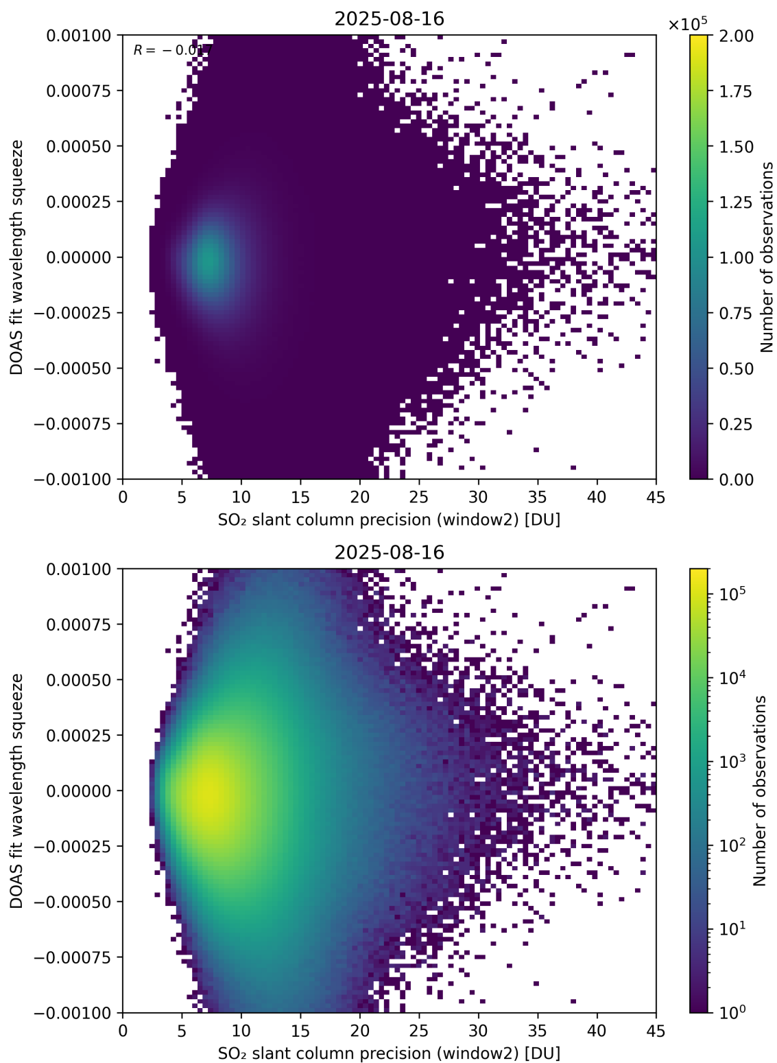
Figure 294: Scatter density plot of “SO 2 slant column precision (window2)” against “DOAS fit wavelength squeeze” for 2025-08-15 to 2025-08-17.
