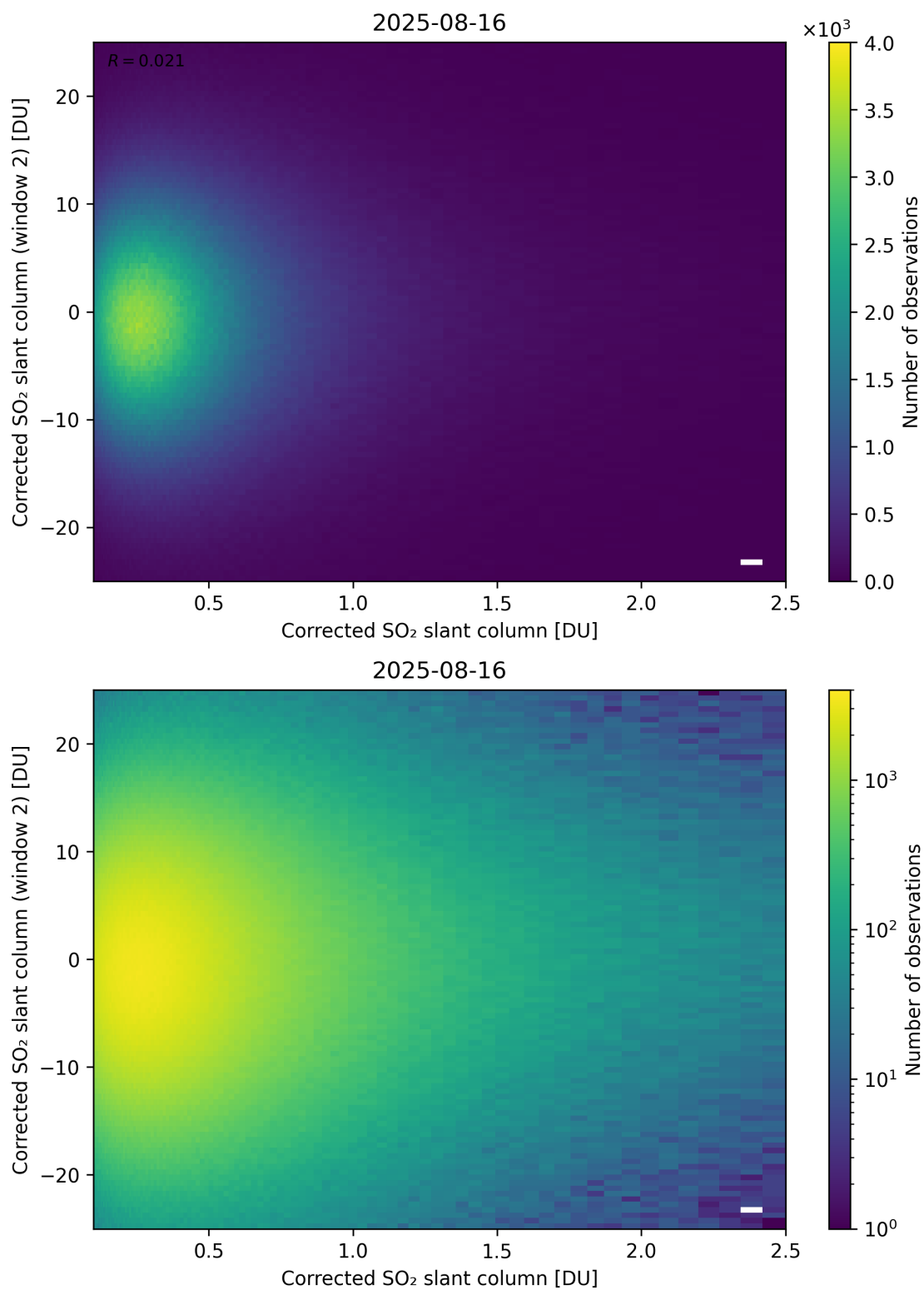
Figure 235: Scatter density plot of “Corrected SO 2 slant column” against “Corrected SO 2 slant column (window 2)” for 2025-08-15 to 2025-08-17.
