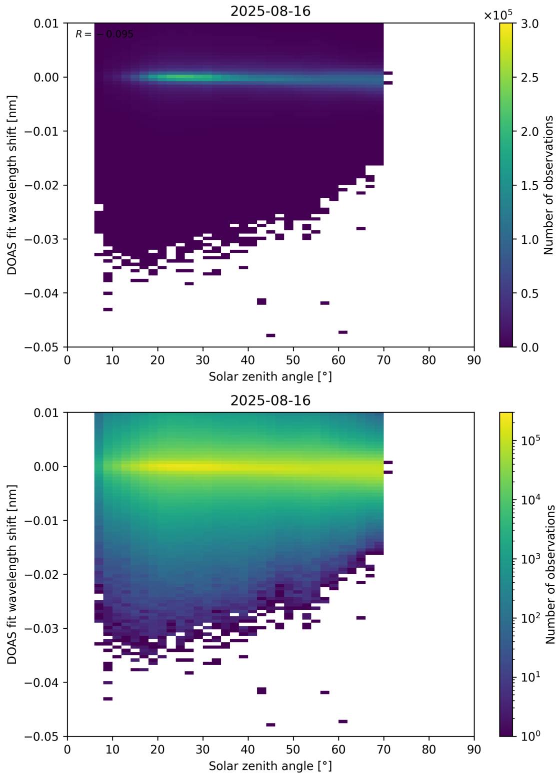
Figure 174: Scatter density plot of “Solar zenith angle” against “DOAS fit wavelength shift” for 2025-08-15 to 2025-08-17.
