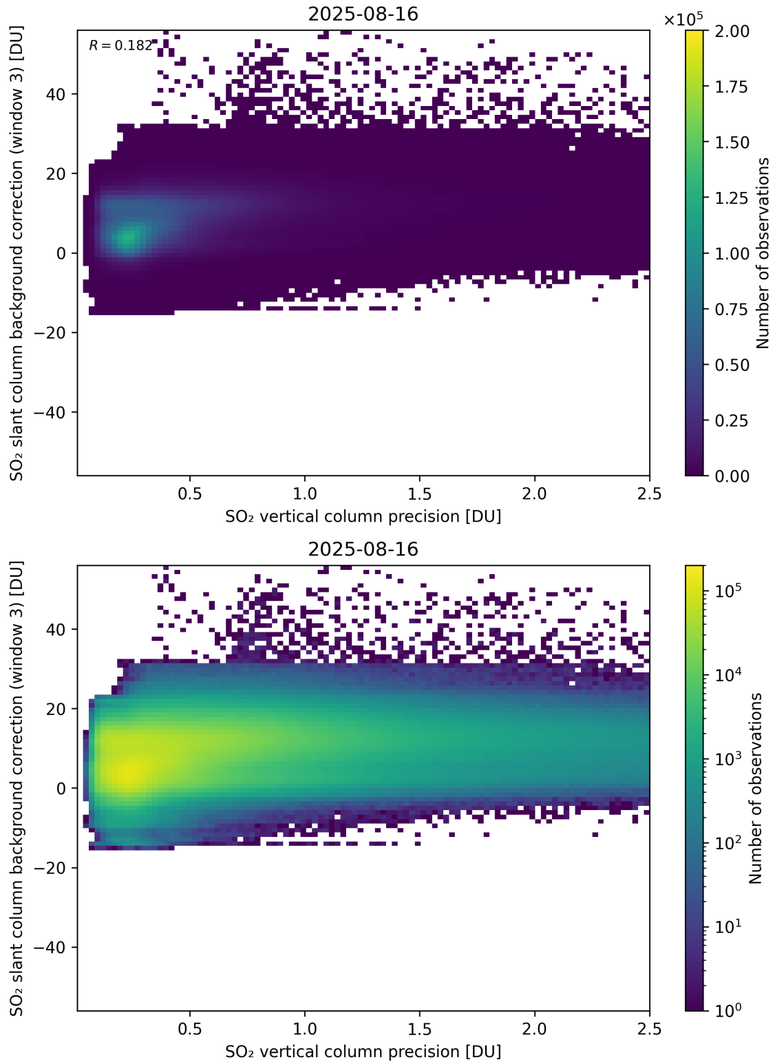
Figure 331: Scatter density plot of “SO 2 vertical column precision” against “SO 2 slant column background correction (window 3)” for 2025-08-15 to 2025-08-17.
