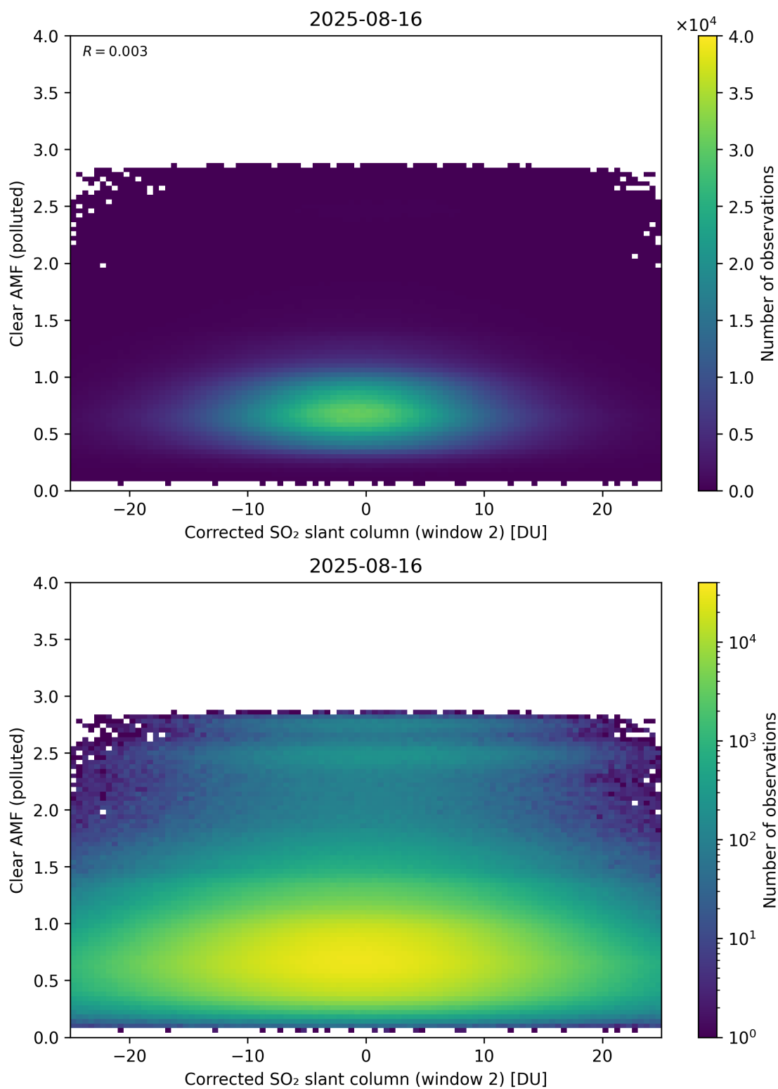
Figure 249: Scatter density plot of “Corrected SO 2 slant column (window 2)” against “Clear AMF (polluted)” for 2025-08-15 to 2025-08-17.
