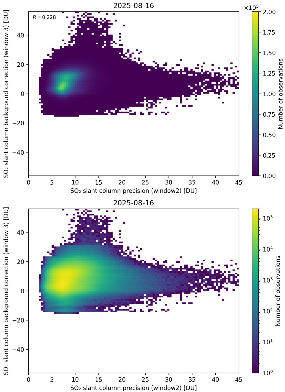
Figure 292: Scatter density plot of “SO 2 slant column precision (window2)” against “SO 2 slant column background correction (window 3)” for 2025-08-15 to 2025-08-17.
