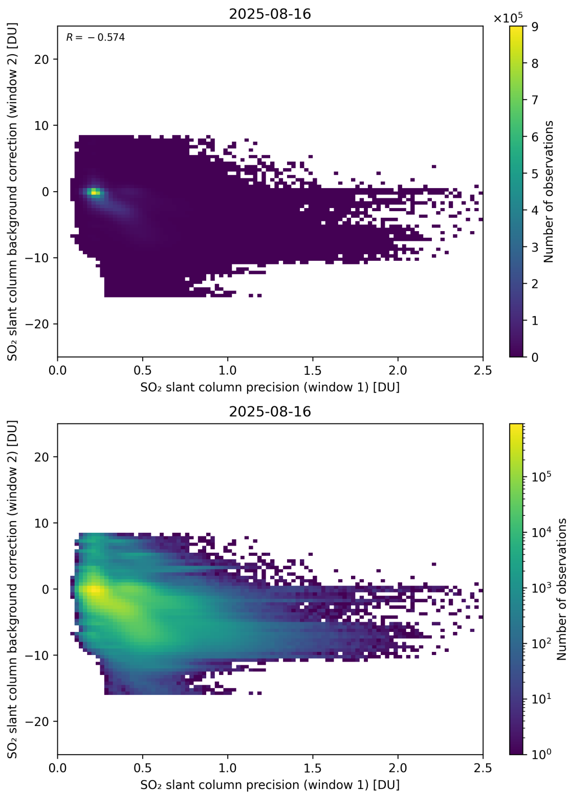
Figure 269: Scatter density plot of “SO 2 slant column precision (window 1)” against “SO 2 slant column background correction (window 2)” for 2025-08-15 to 2025-08-17.
