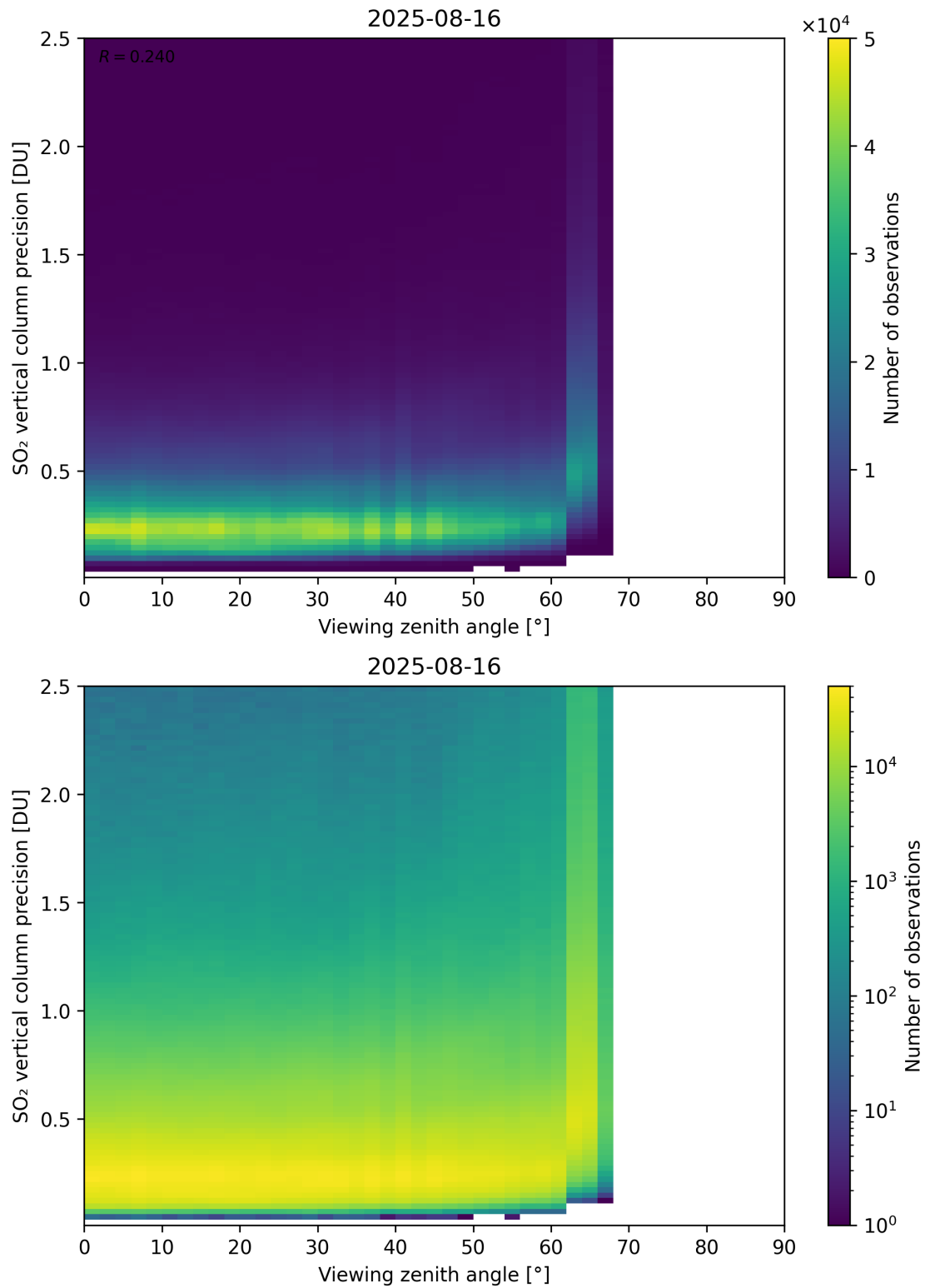
Figure 384: Scatter density plot of “Viewing zenith angle” against “SO 2 vertical column precision” for 2025-08-15 to 2025-08-17.
