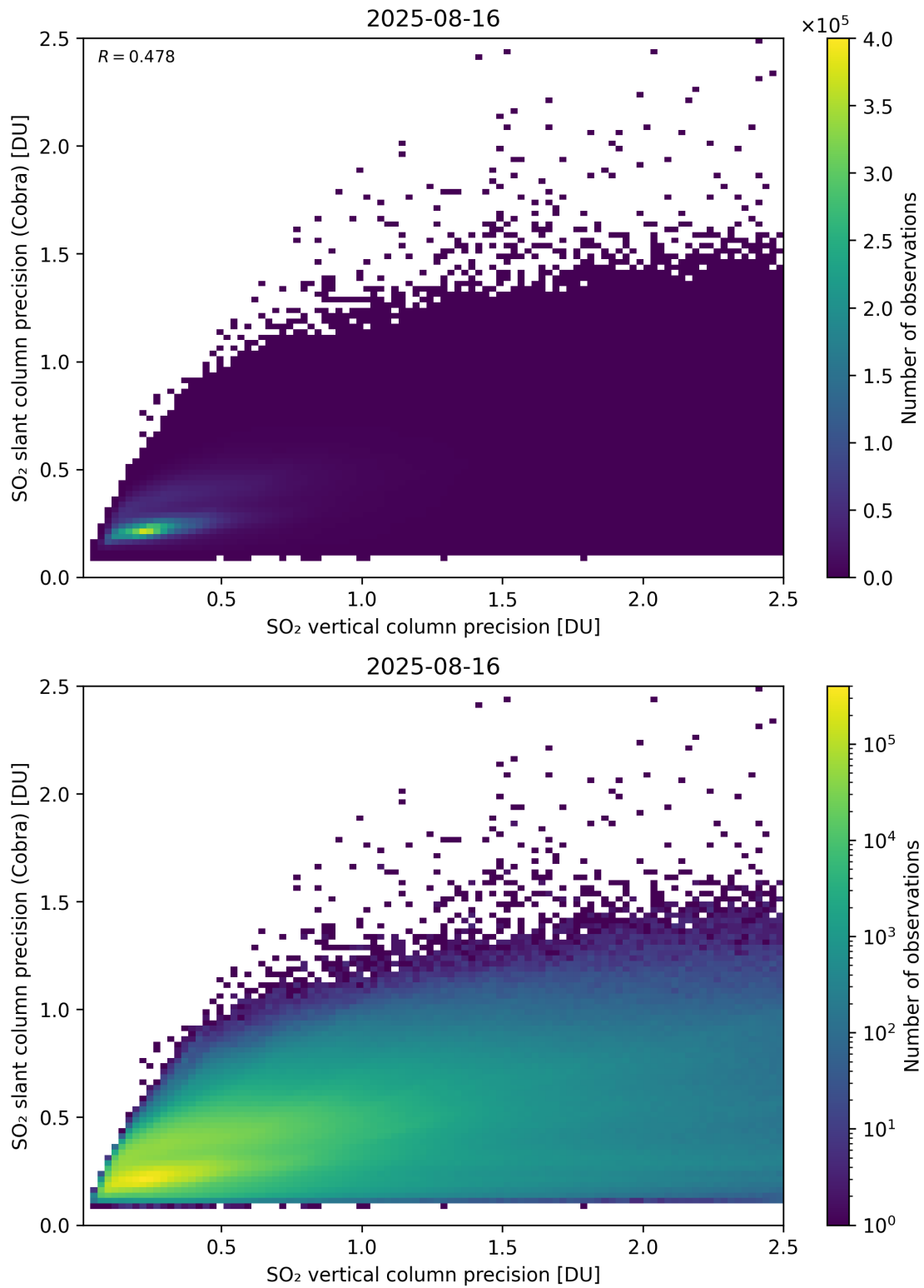
Figure 337: Scatter density plot of “SO 2 vertical column precision” against “SO 2 slant column precision (Cobra)” for 2025-08-15 to 2025-08-17.
