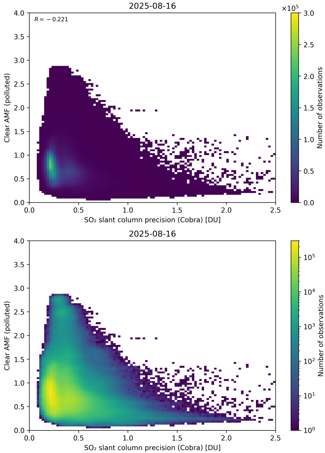
Figure 205: Scatter density plot of “SO 2 slant column precision (Cobra)” against “Clear AMF (polluted)” for 2025-08-15 to 2025-08-17.
