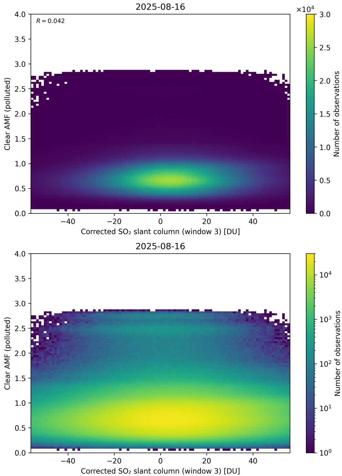
Figure 259: Scatter density plot of “Corrected SO 2 slant column (window 3)” against “Clear AMF (polluted)” for 2025-08-15 to 2025-08-17.
