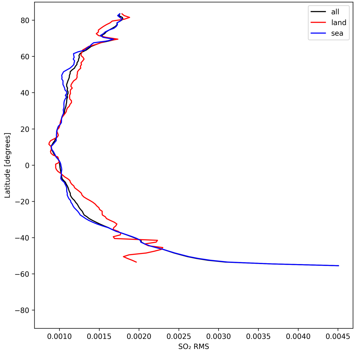
Figure 52: Zonal average of “SO 2 RMS” for 2025-08-15 to 2025-08-17.
