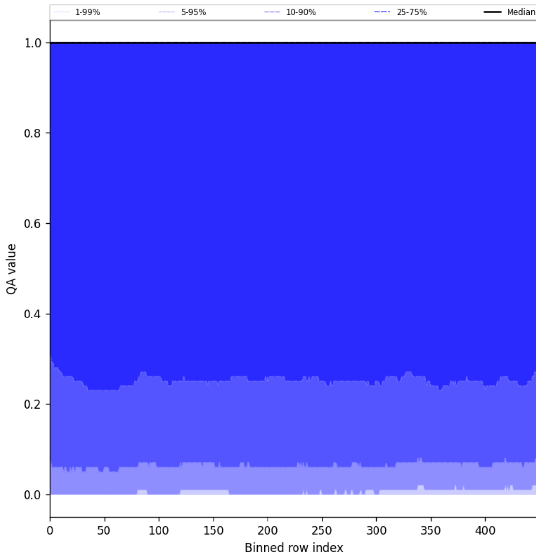
Figure 83: Along track statistics of “QA value” for 2025-08-15 to 2025-08-17
