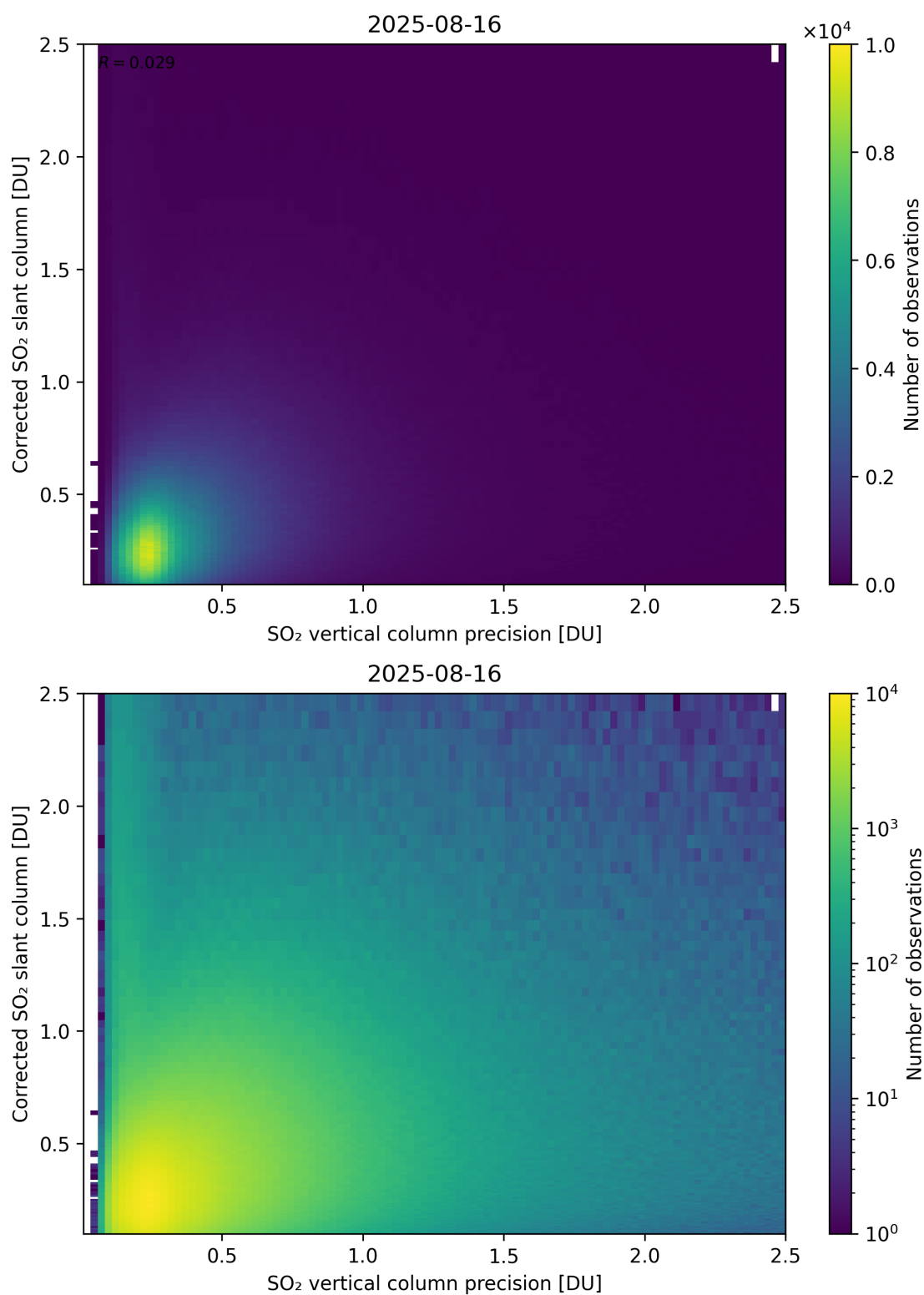
Figure 338: Scatter density plot of “SO 2 vertical column precision” against “Corrected SO 2 slant column” for 2025-08-15 to 2025-08-17.
