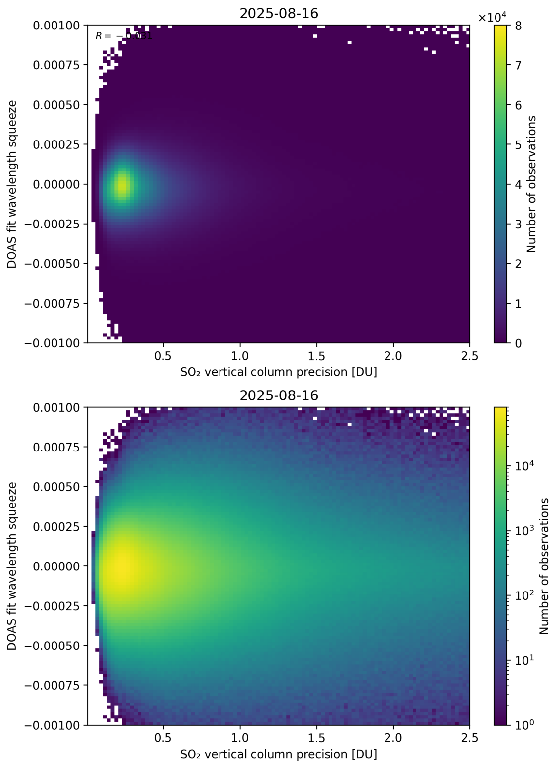
Figure 333: Scatter density plot of “SO 2 vertical column precision” against “DOAS fit wavelength squeeze” for 2025-08-15 to 2025-08-17.
