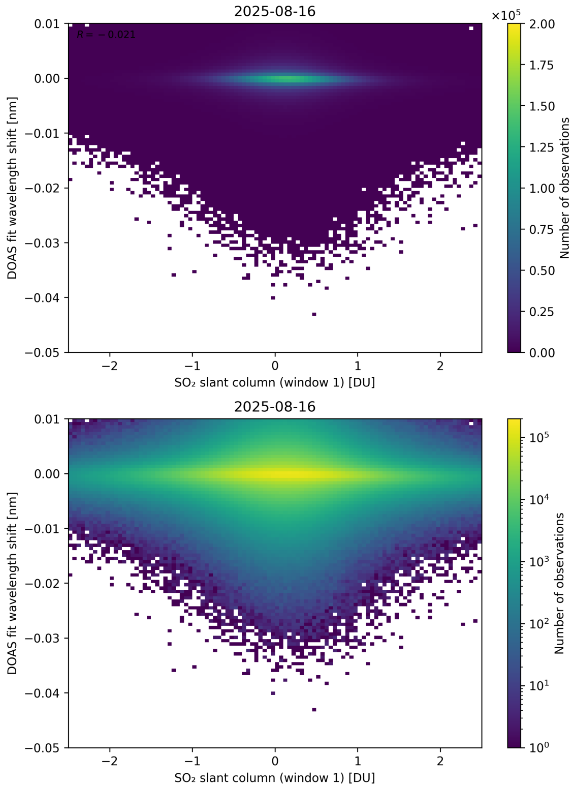
Figure 265: Scatter density plot of “SO 2 slant column (window 1)” against “DOAS fit wavelength shift” for 2025-08-15 to 2025-08-17.
