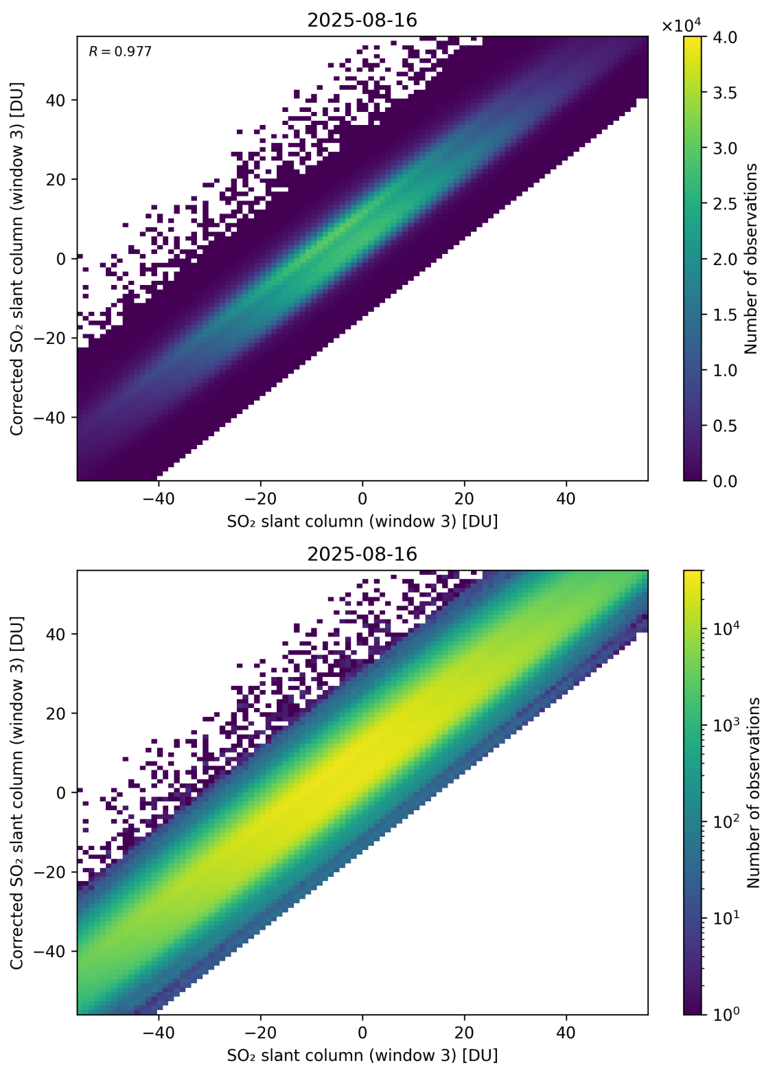
Figure 316: Scatter density plot of “SO 2 slant column (window 3)” against “Corrected SO 2 slant column (window 3)” for 2025-08-15 to 2025-08-17.
