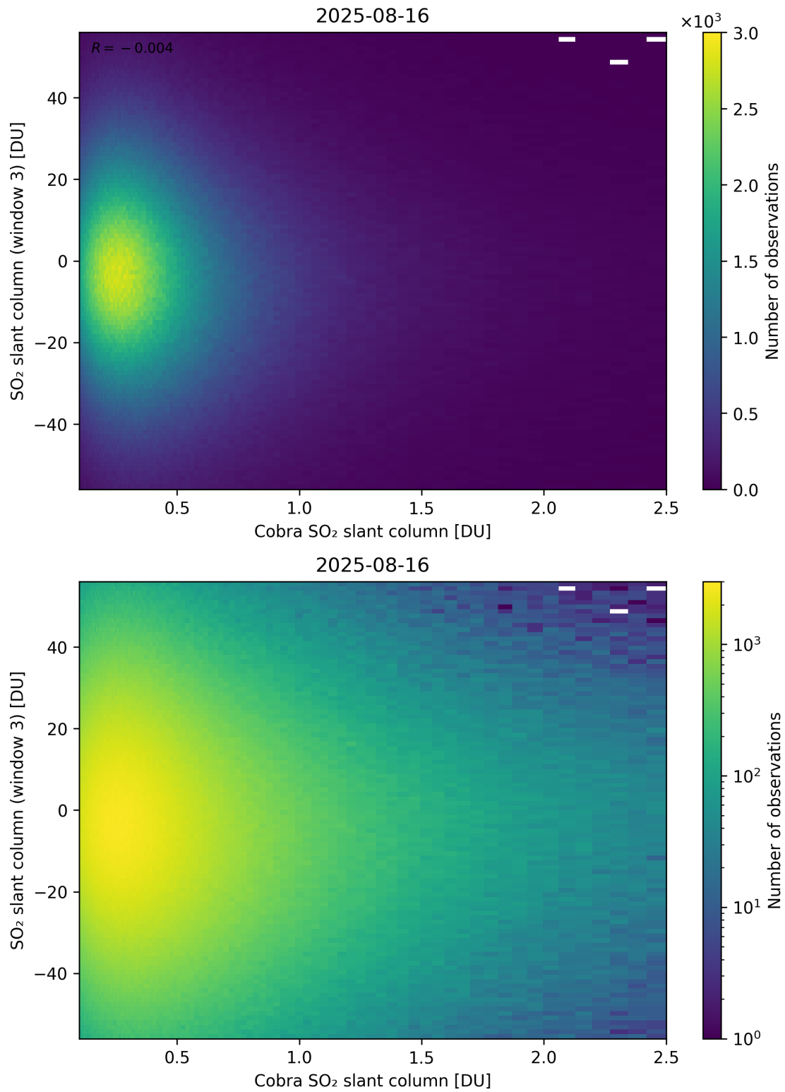
Figure 222: Scatter density plot of “Cobra SO 2 slant column” against “SO 2 slant column (window 3)” for 2025-08-15 to 2025-08-17.
