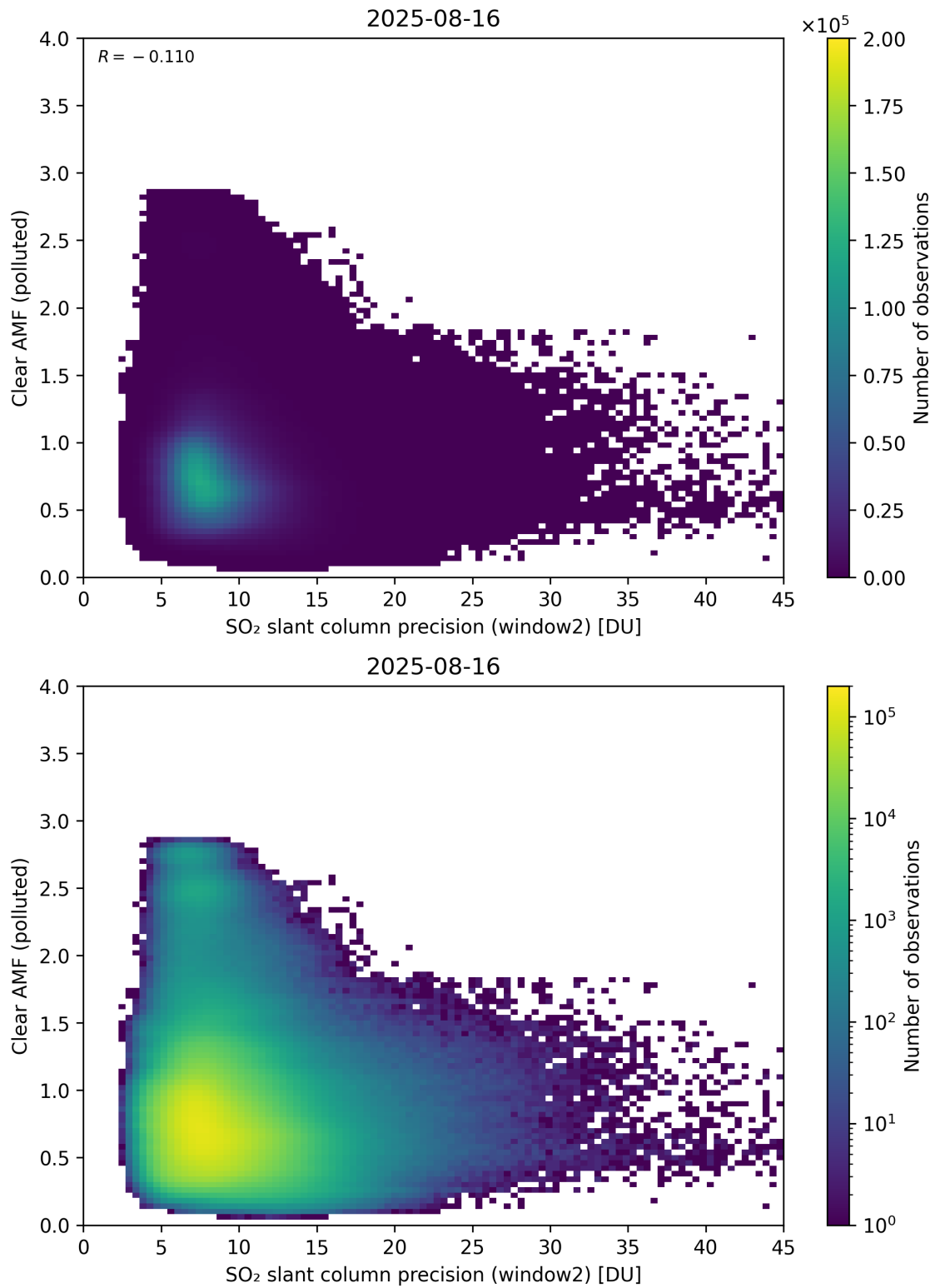
Figure 296: Scatter density plot of “SO 2 slant column precision (window2)” against “Clear AMF (polluted)” for 2025-08-15 to 2025-08-17.
