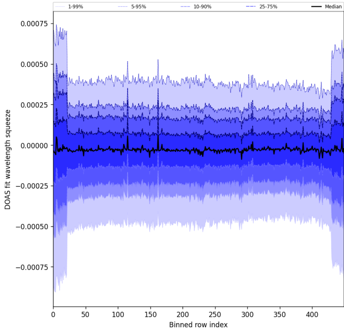
Figure 103: Along track statistics of “DOAS fit wavelength squeeze” for 2025-08-15 to 2025-08-17
