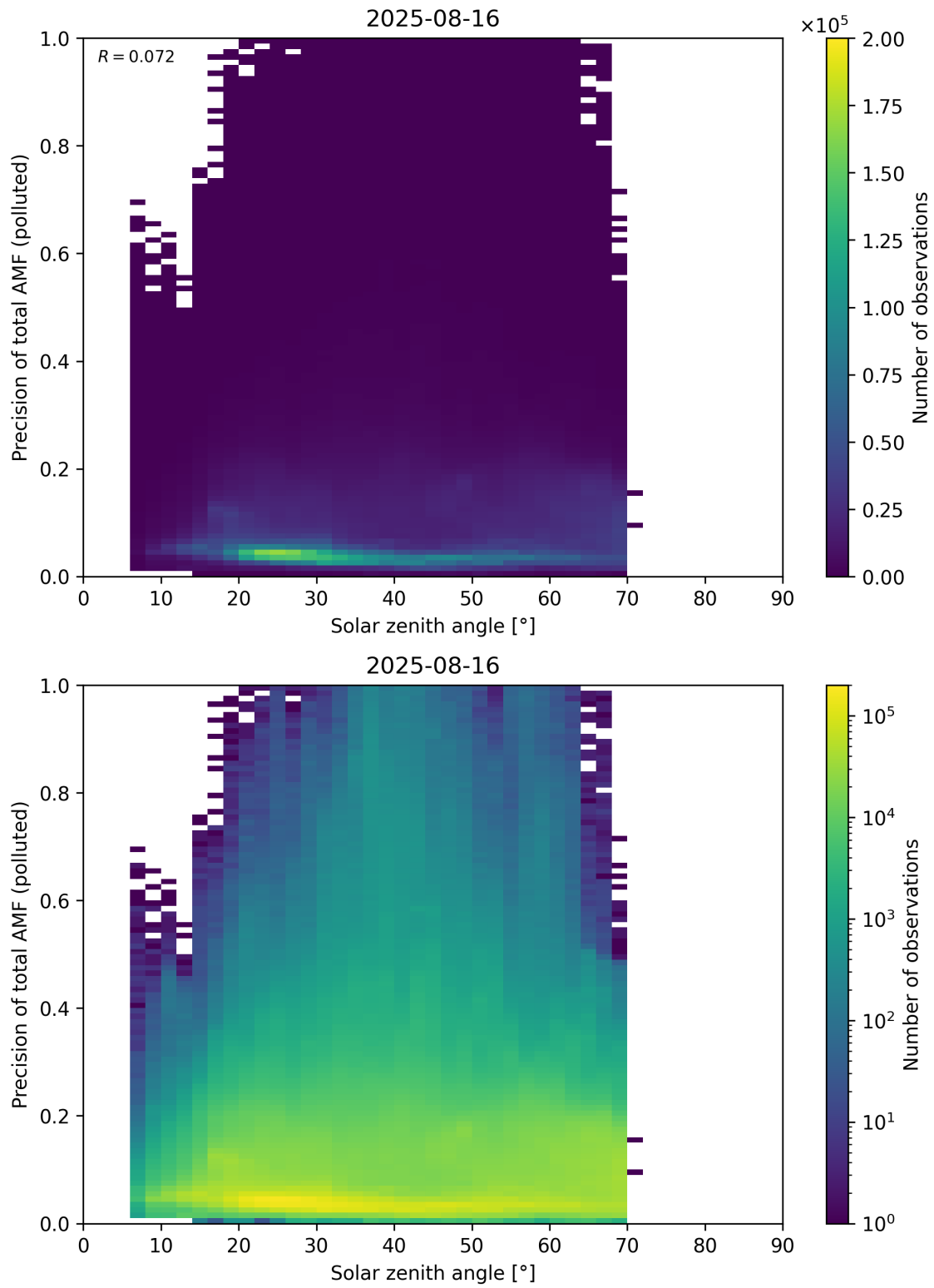
Figure 190: Scatter density plot of “Solar zenith angle” against “Precision of total AMF (polluted)” for 2025-08-15 to 2025-08-17.
