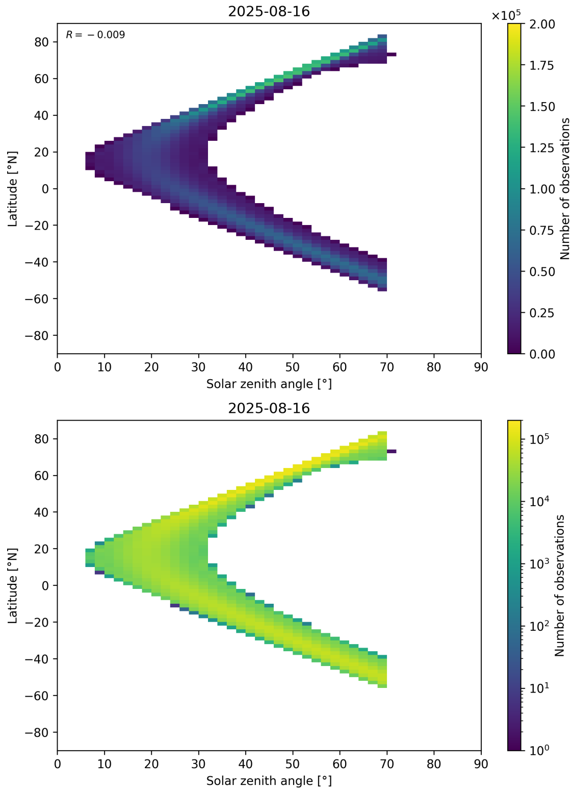
Figure 177: Scatter density plot of “Solar zenith angle” against “Latitude” for 2025-08-15 to 2025-08-17.
