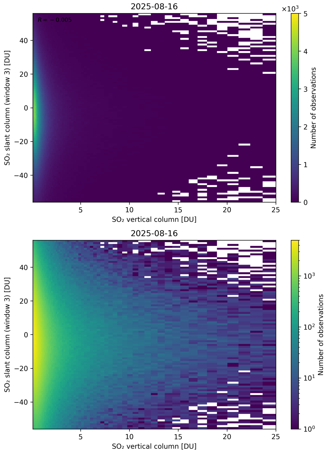
Figure 357: Scatter density plot of “SO 2 vertical column” against “SO 2 slant column (window 3)” for 2025-08-15 to 2025-08-17.
