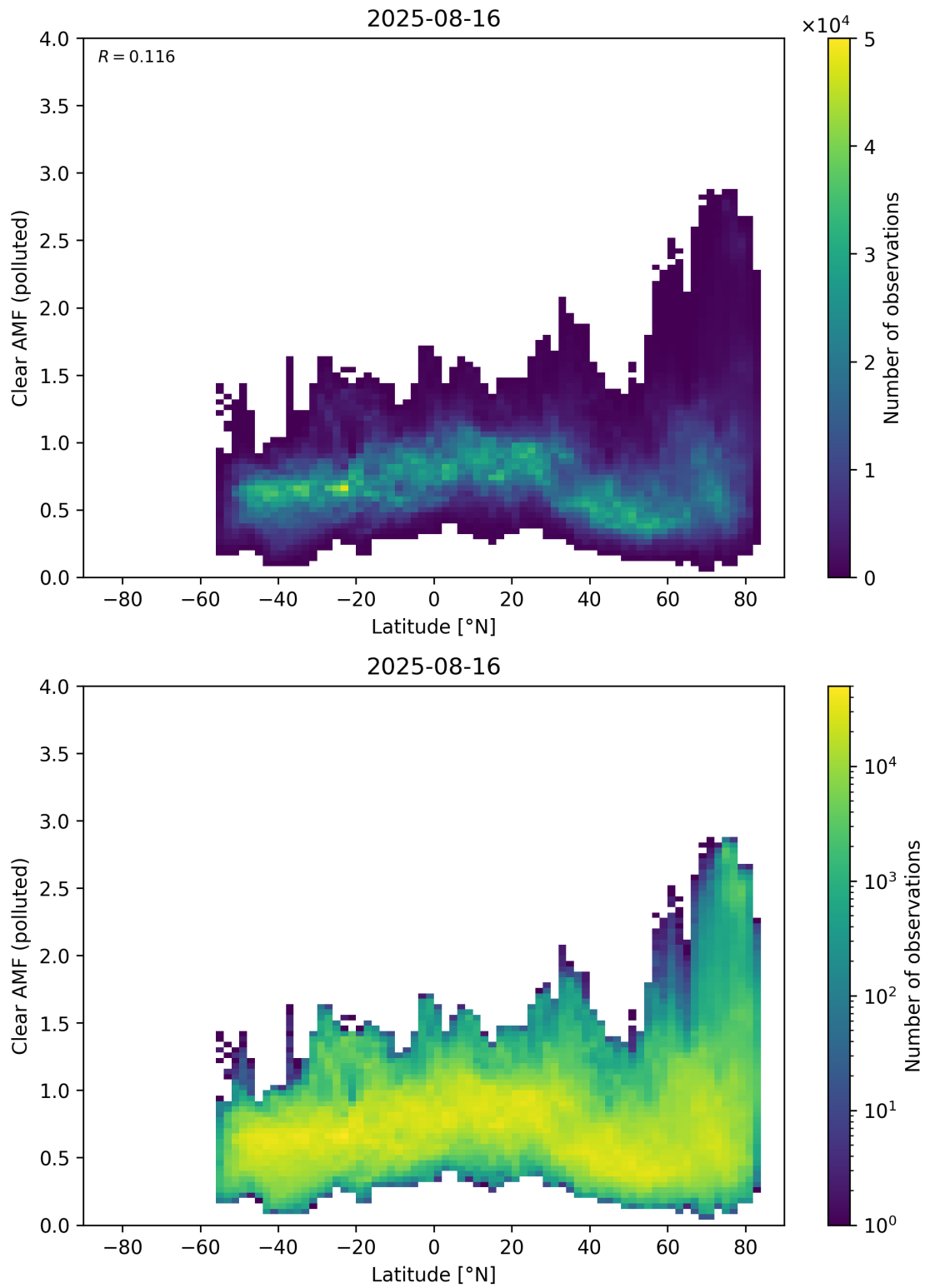
Figure 156: Scatter density plot of “Latitude” against “Clear AMF (polluted)” for 2025-08-15 to 2025-08-17.
