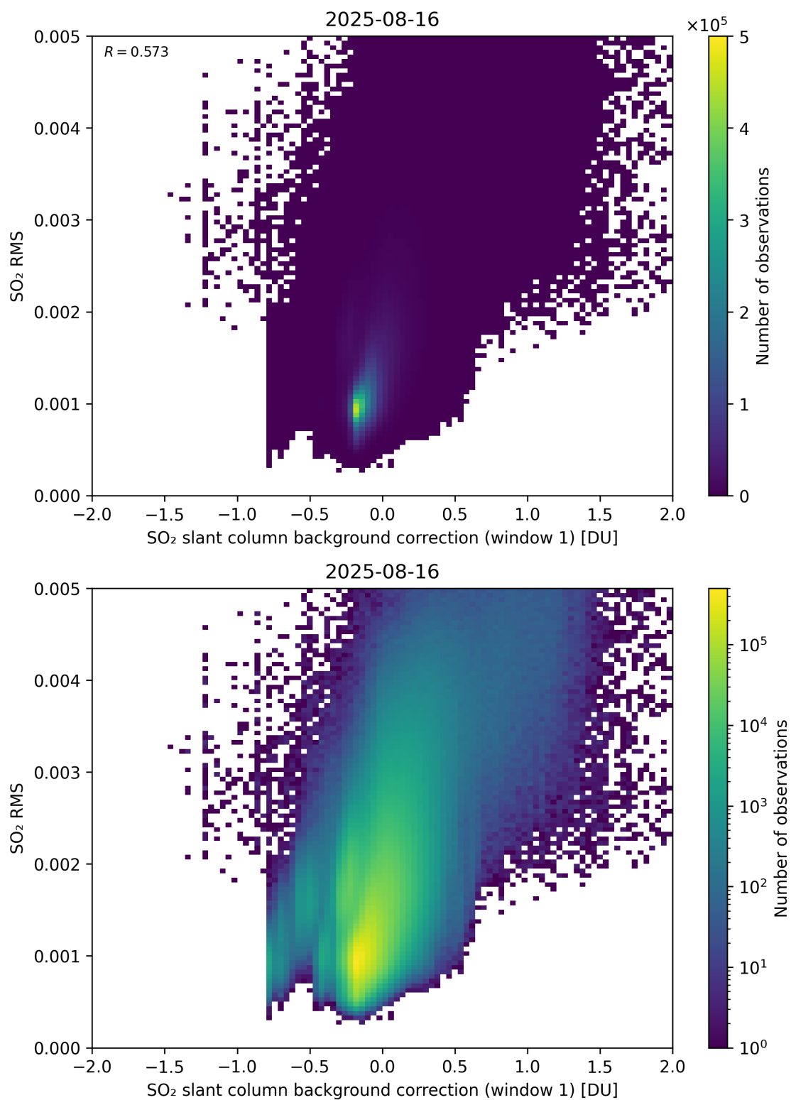
Figure 113: Scatter density plot of “SO 2 slant column background correction (window 1)” against “SO 2 RMS” for 2025-08-15 to 2025-08-17.
