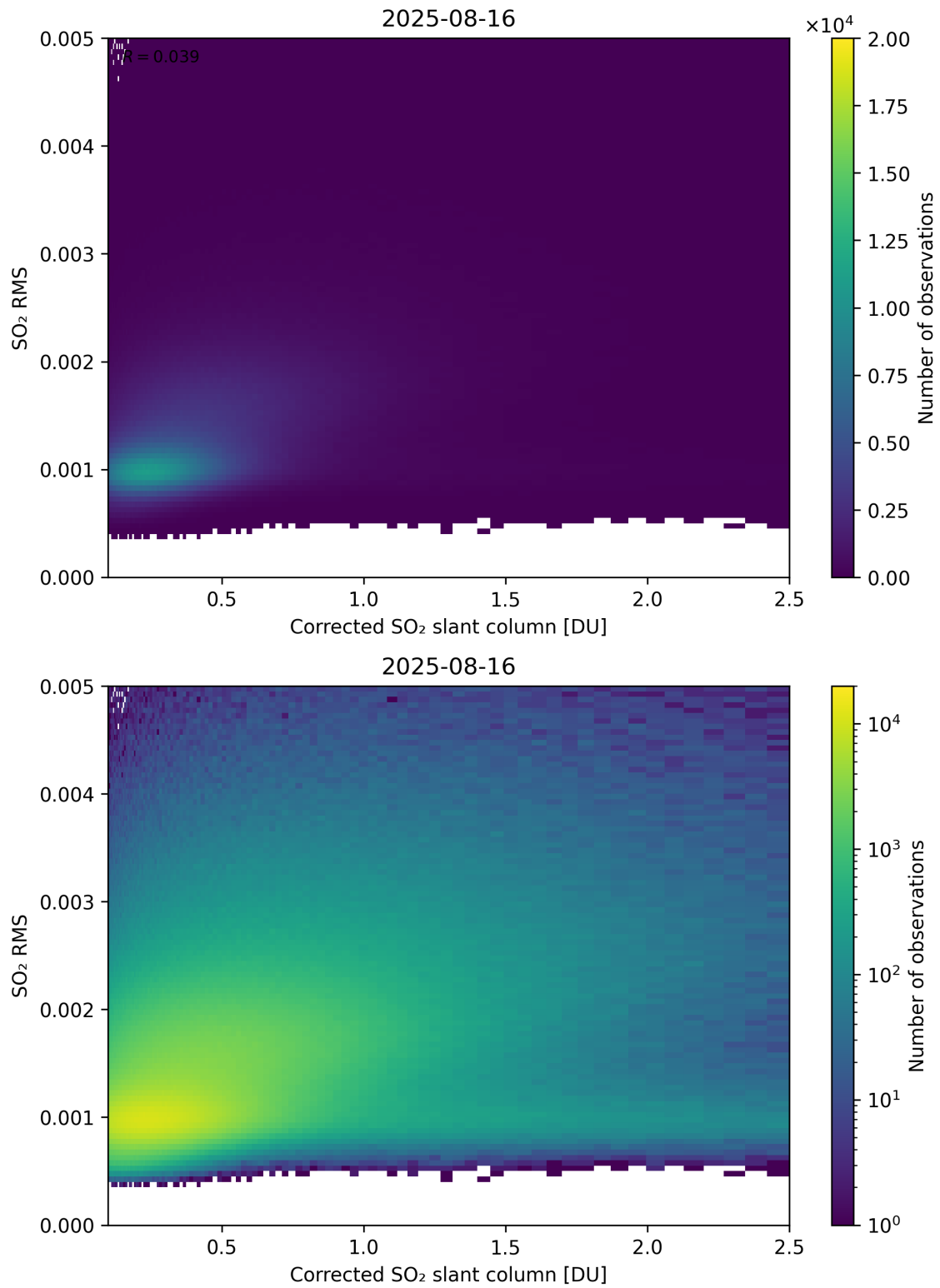
Figure 231: Scatter density plot of “Corrected SO 2 slant column” against “SO 2 RMS” for 2025-08-15 to 2025-08-17.
