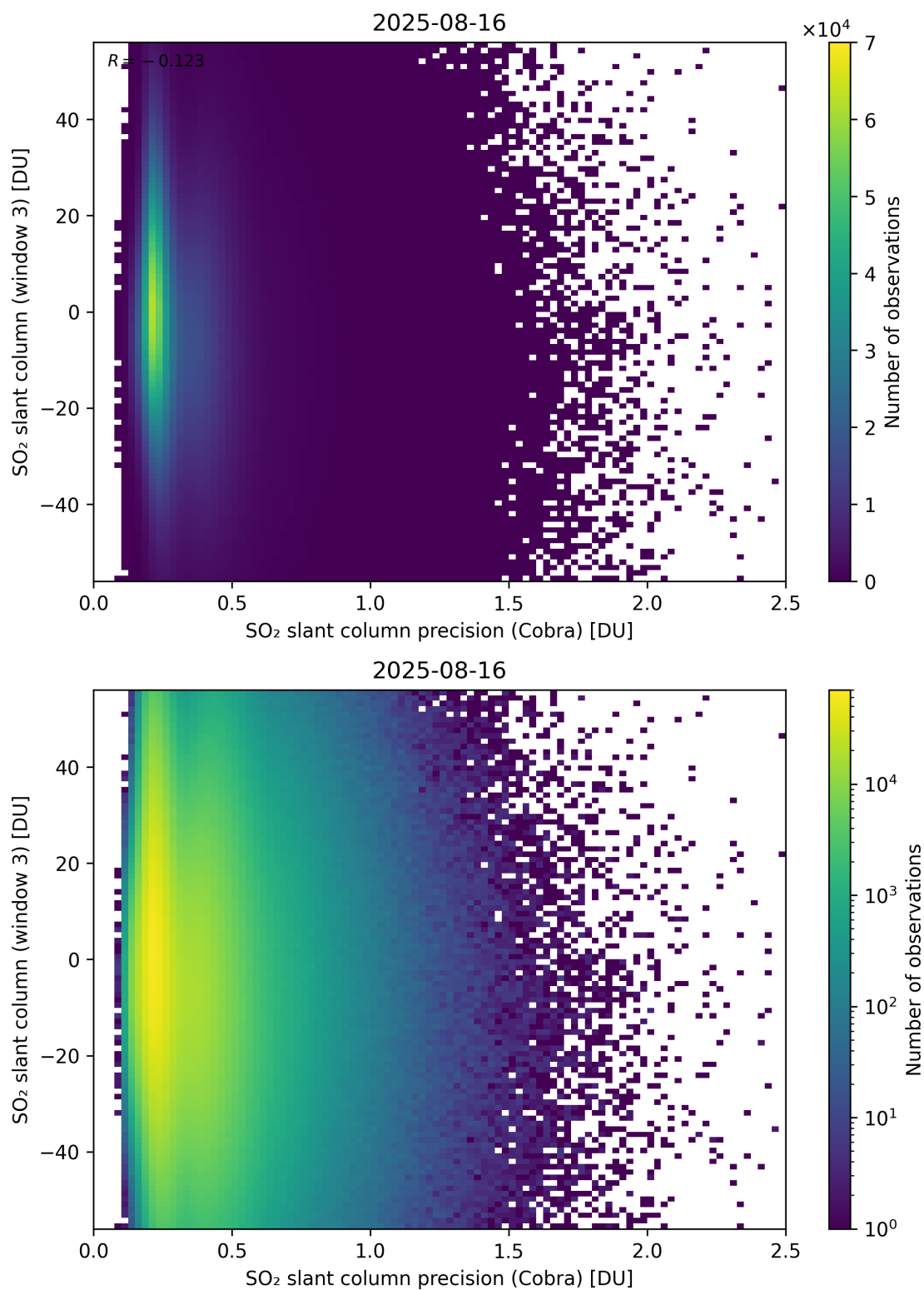
Figure 211: Scatter density plot of “SO 2 slant column precision (Cobra)” against “SO 2 slant column (window 3)” for 2025-08-15 to 2025-08-17.
