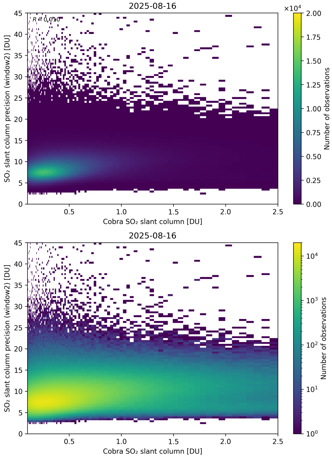
Figure 221: Scatter density plot of “Cobra SO 2 slant column” against “SO 2 slant column precision (window2)” for 2025-08-15 to 2025-08-17.
