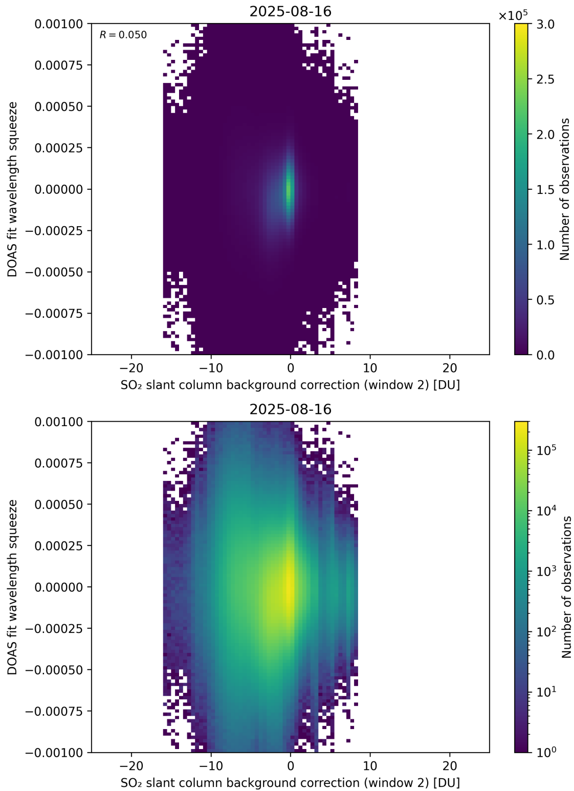
Figure 124: Scatter density plot of “SO 2 slant column background correction (window 2)” against “DOAS fit wavelength squeeze” for 2025-08-15 to 2025-08-17.
