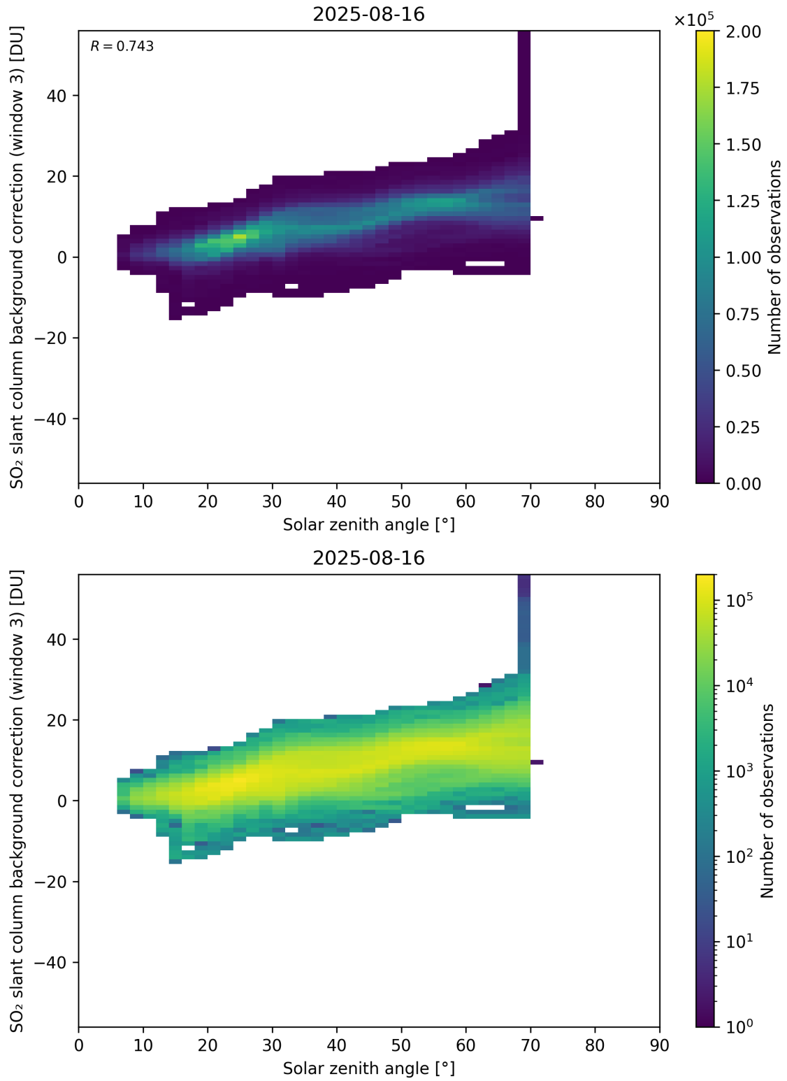
Figure 173: Scatter density plot of “Solar zenith angle” against “SO 2 slant column background correction (window 3)” for 2025-08-15 to 2025-08-17.
