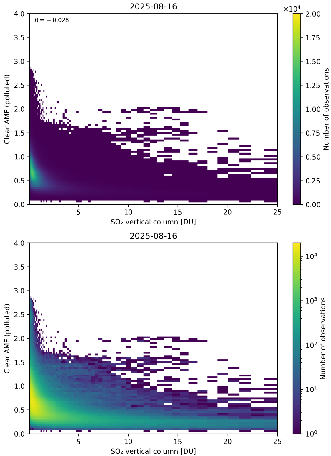
Figure 348: Scatter density plot of “SO 2 vertical column” against “Clear AMF (polluted)” for 2025-08-15 to 2025-08-17.
