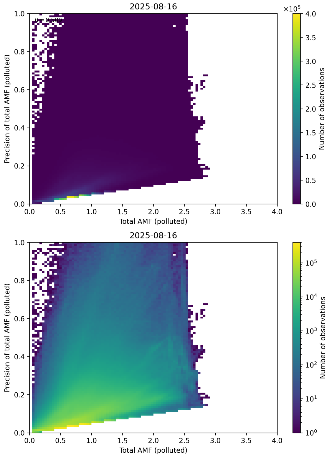
Figure 322: Scatter density plot of “Total AMF (polluted)” against “Precision of total AMF (polluted)” for 2025-08-15 to 2025-08-17.
