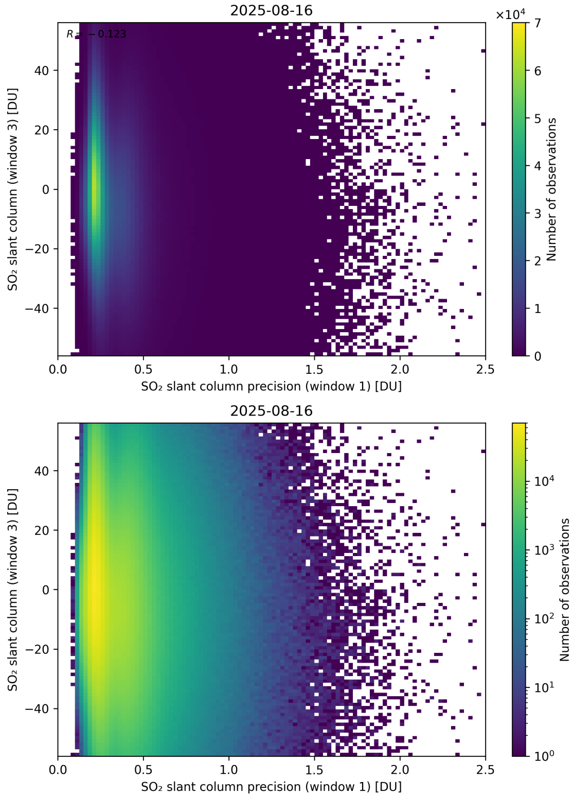
Figure 278: Scatter density plot of “SO 2 slant column precision (window 1)” against “SO 2 slant column (window 3)” for 2025-08-15 to 2025-08-17.
