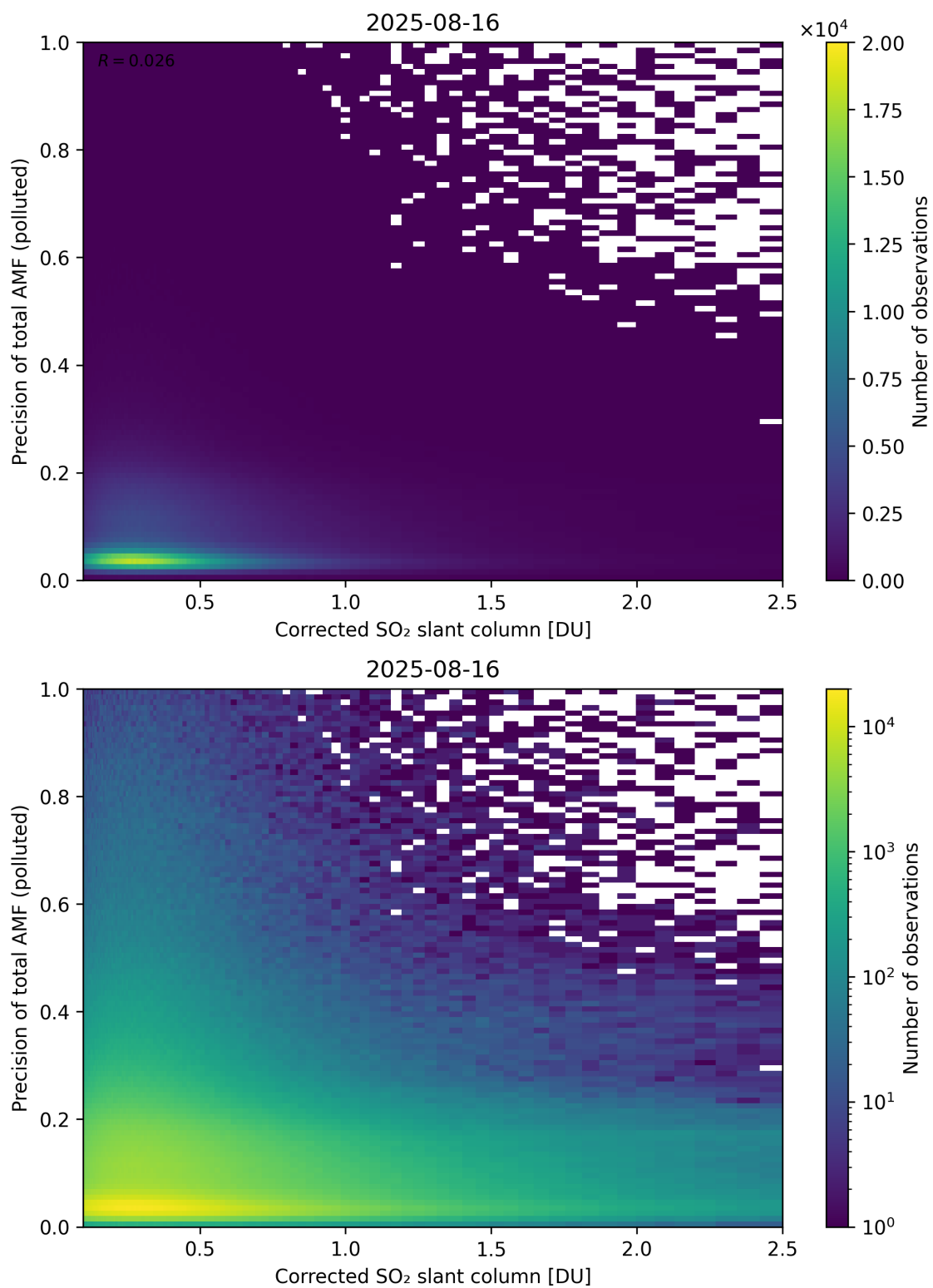
Figure 243: Scatter density plot of “Corrected SO 2 slant column” against “Precision of total AMF (polluted)” for 2025-08-15 to 2025-08-17.
