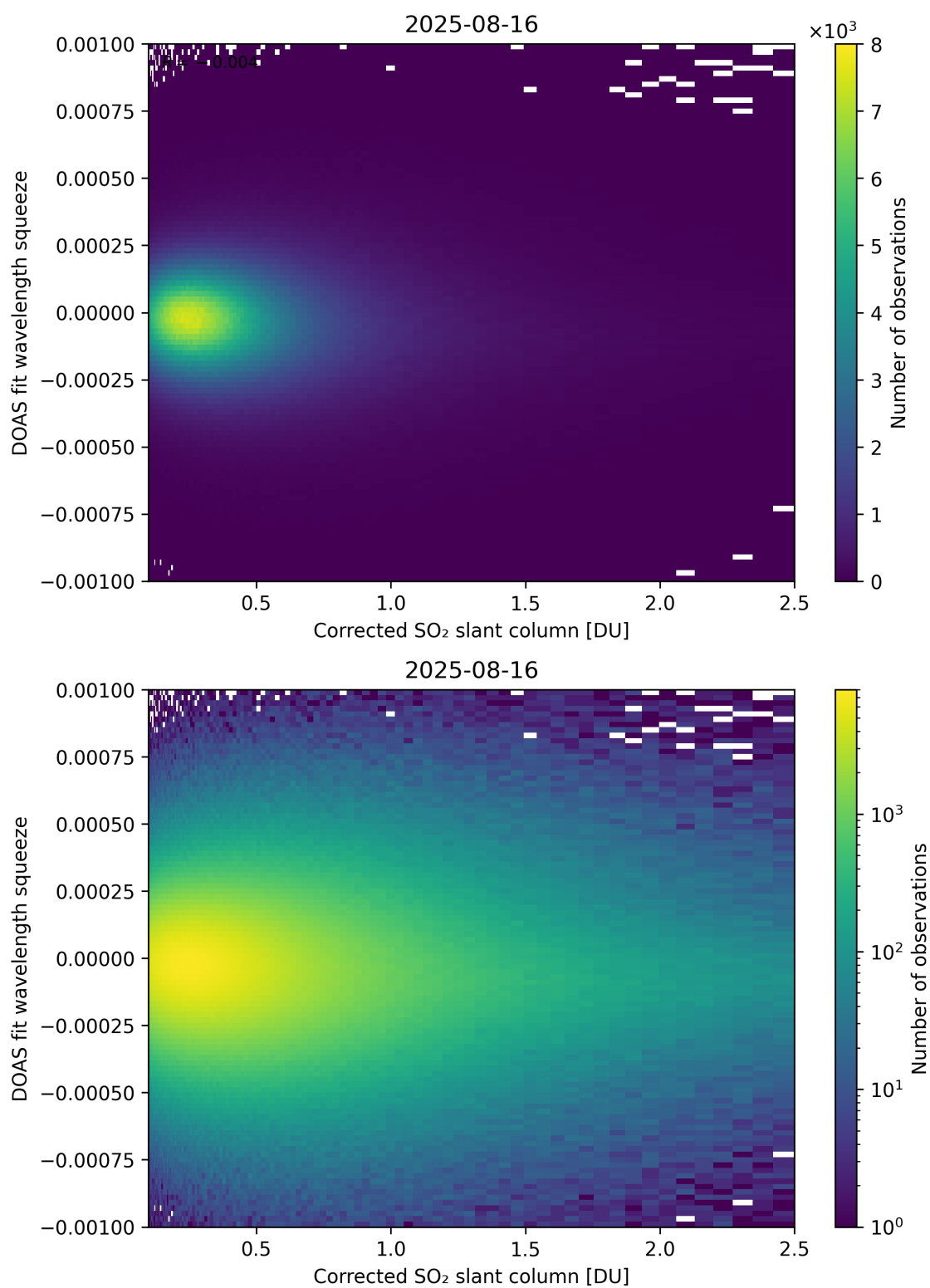
Figure 230: Scatter density plot of “Corrected SO 2 slant column” against “DOAS fit wavelength squeeze” for 2025-08-15 to 2025-08-17.
