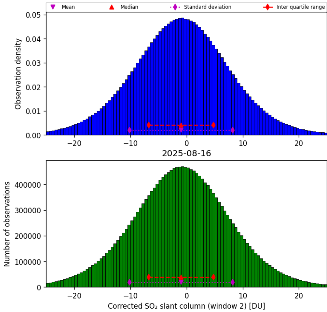
Figure 69: Histogram of “Corrected SO 2 slant column (window 2)” for 2025-08-15 to 2025-08-17
