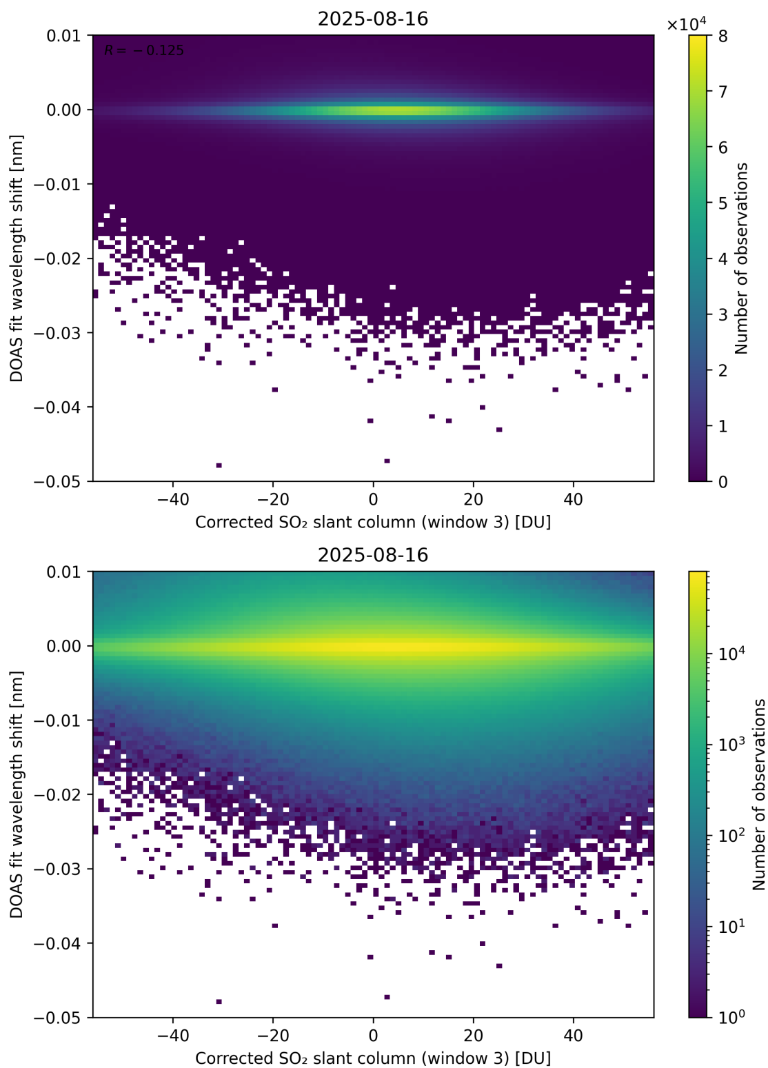
Figure 256: Scatter density plot of “Corrected SO 2 slant column (window 3)” against “DOAS fit wavelength shift” for 2025-08-15 to 2025-08-17.
