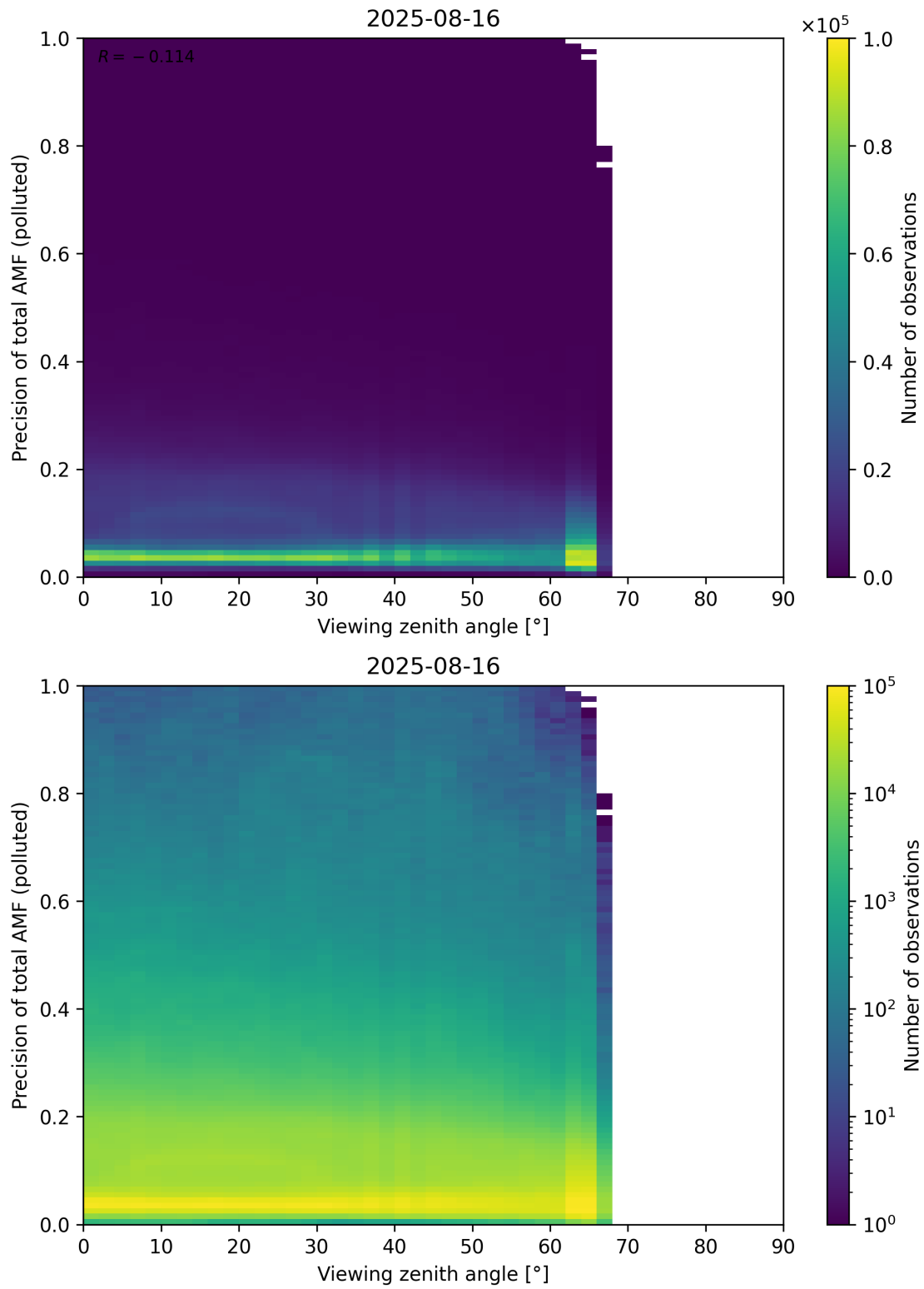
Figure 382: Scatter density plot of “Viewing zenith angle” against “Precision of total AMF (polluted)” for 2025-08-15 to 2025-08-17.
