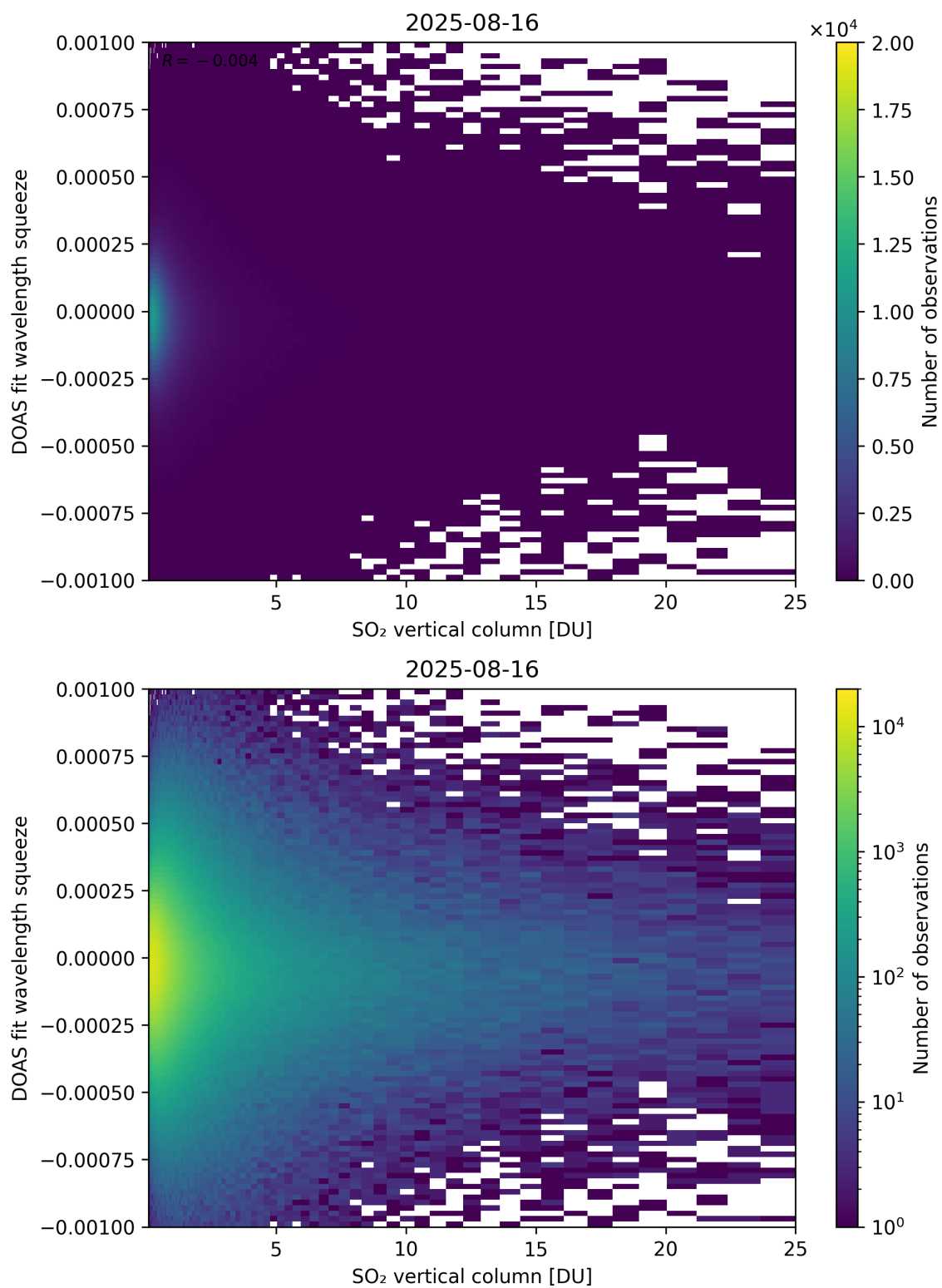
Figure 327: Scatter density plot of “SO 2 vertical column” against “DOAS fit wavelength squeeze” for 2025-08-15 to 2025-08-17.
