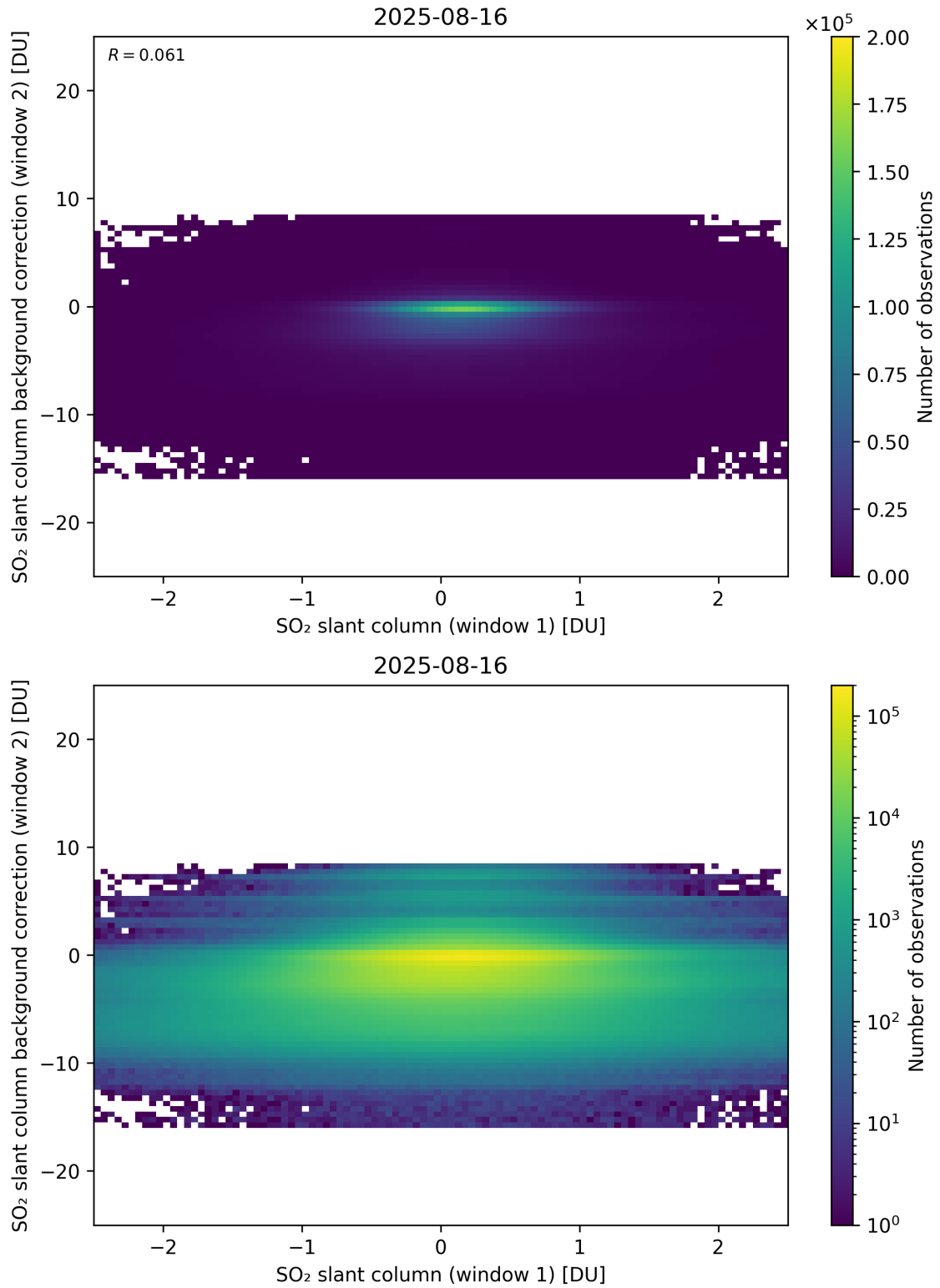
Figure 263: Scatter density plot of “SO 2 slant column (window 1)” against “SO 2 slant column background correction (window 2)” for 2025-08-15 to 2025-08-17.
