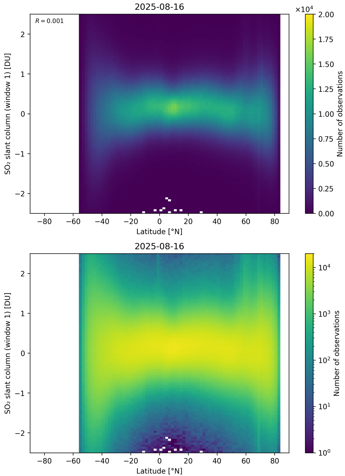
Figure 162: Scatter density plot of “Latitude” against “SO 2 slant column (window 1)” for 2025-08-15 to 2025-08-17.
