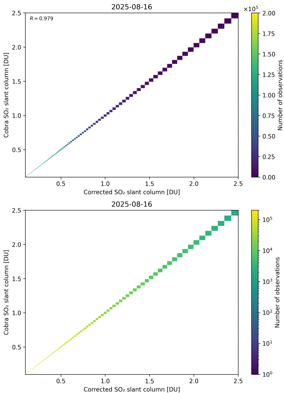
Figure 233: Scatter density plot of “Corrected SO 2 slant column” against “Cobra SO 2 slant column” for 2025-08-15 to 2025-08-17.
