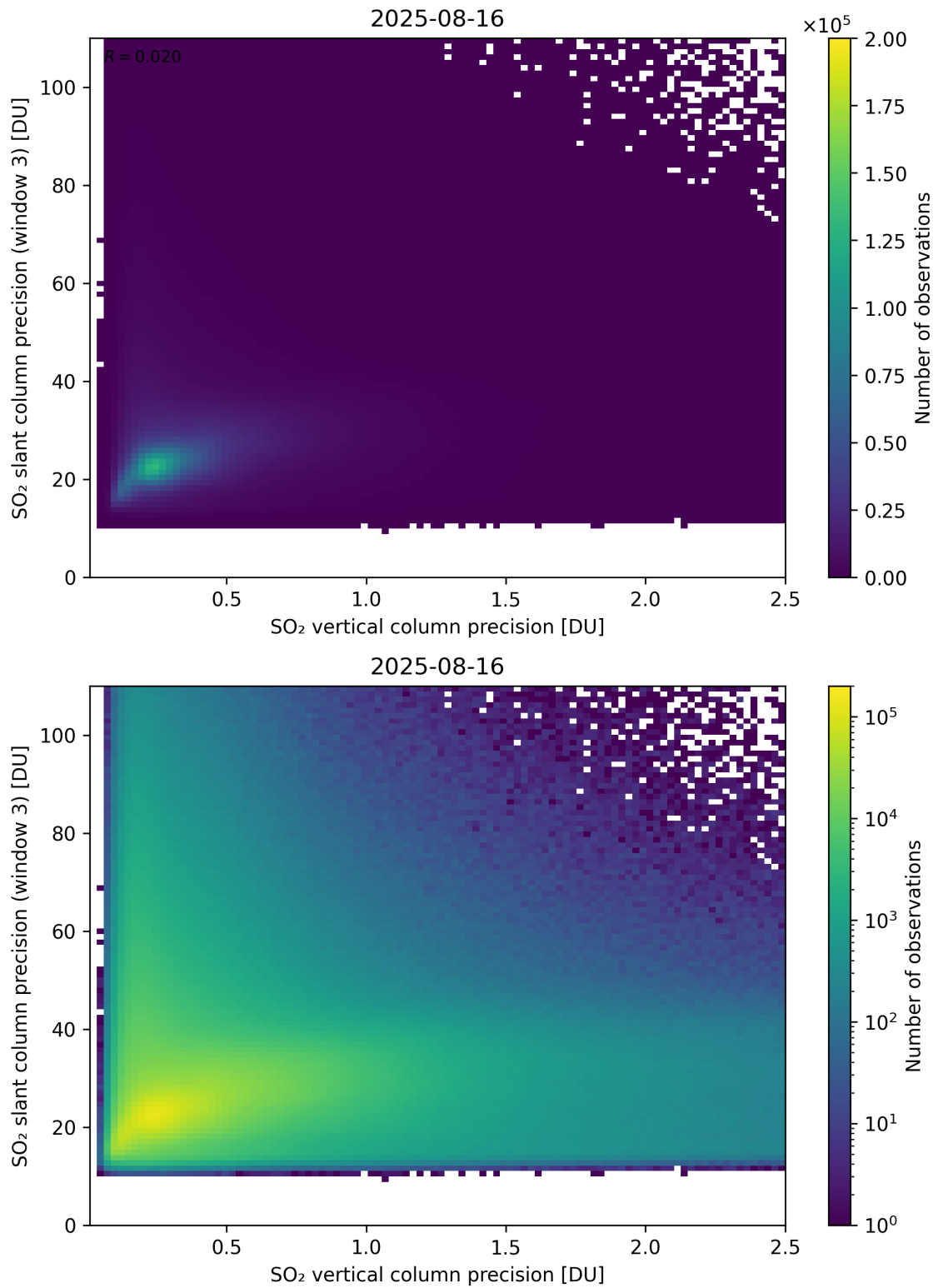
Figure 345: Scatter density plot of “SO 2 vertical column precision” against “SO 2 slant column precision (window 3)” for 2025-08-15 to 2025-08-17.
