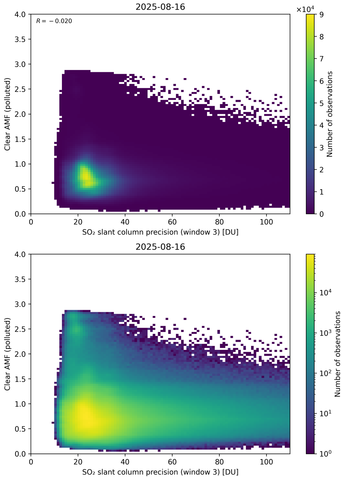
Figure 311: Scatter density plot of “SO 2 slant column precision (window 3)” against “Clear AMF (polluted)” for 2025-08-15 to 2025-08-17.
