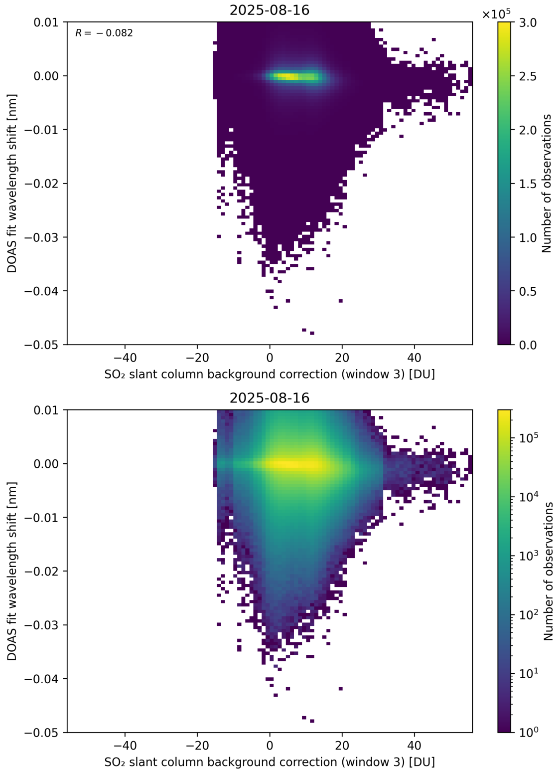
Figure 132: Scatter density plot of “SO 2 slant column background correction (window 3)” against “DOAS fit wavelength shift” for 2025-08-15 to 2025-08-17.
