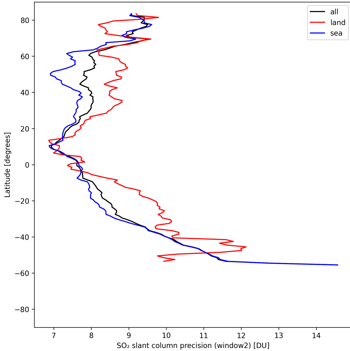
Figure 42: Zonal average of “SO 2 slant column precision (window2)” for 2025-08-15 to 2025-08-17.
