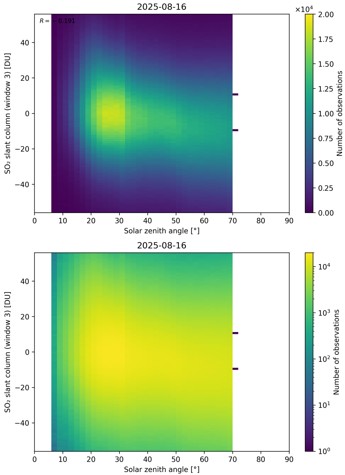
Figure 187: Scatter density plot of “Solar zenith angle” against “SO 2 slant column (window 3)” for 2025-08-15 to 2025-08-17.
