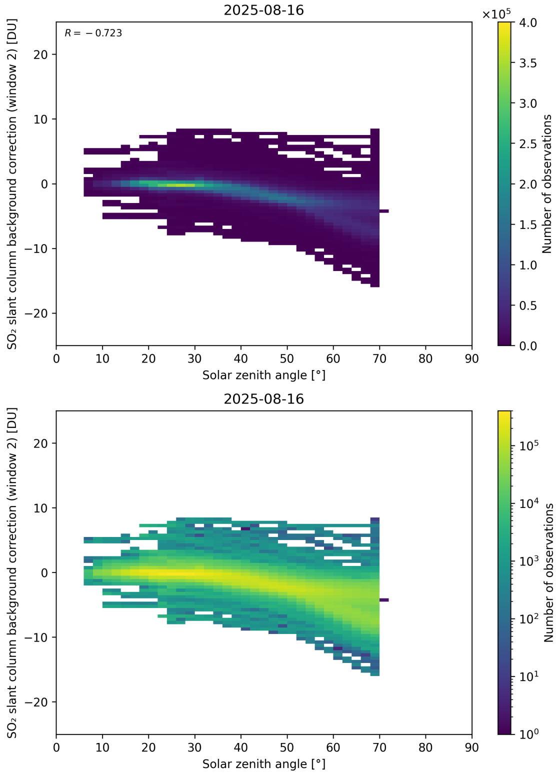
Figure 172: Scatter density plot of “Solar zenith angle” against “SO 2 slant column background correction (window 2)” for 2025-08-15 to 2025-08-17.
