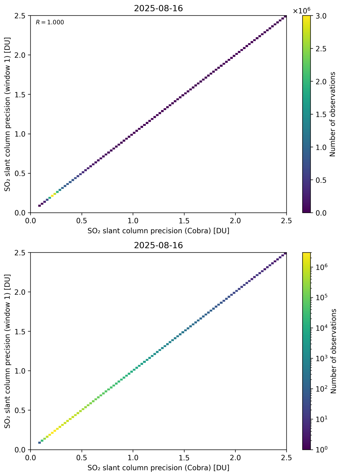
Figure 209: Scatter density plot of “SO 2 slant column precision (Cobra)” against “SO 2 slant column precision (window 1)” for 2025-08-15 to 2025-08-17.
