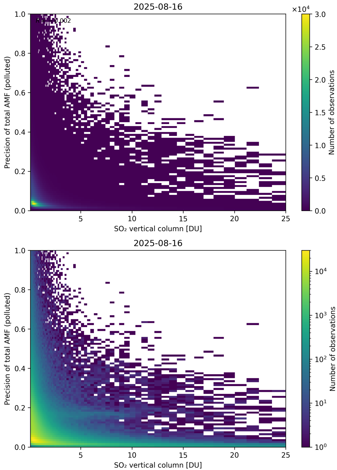
Figure 360: Scatter density plot of “SO 2 vertical column” against “Precision of total AMF (polluted)” for 2025-08-15 to 2025-08-17.
