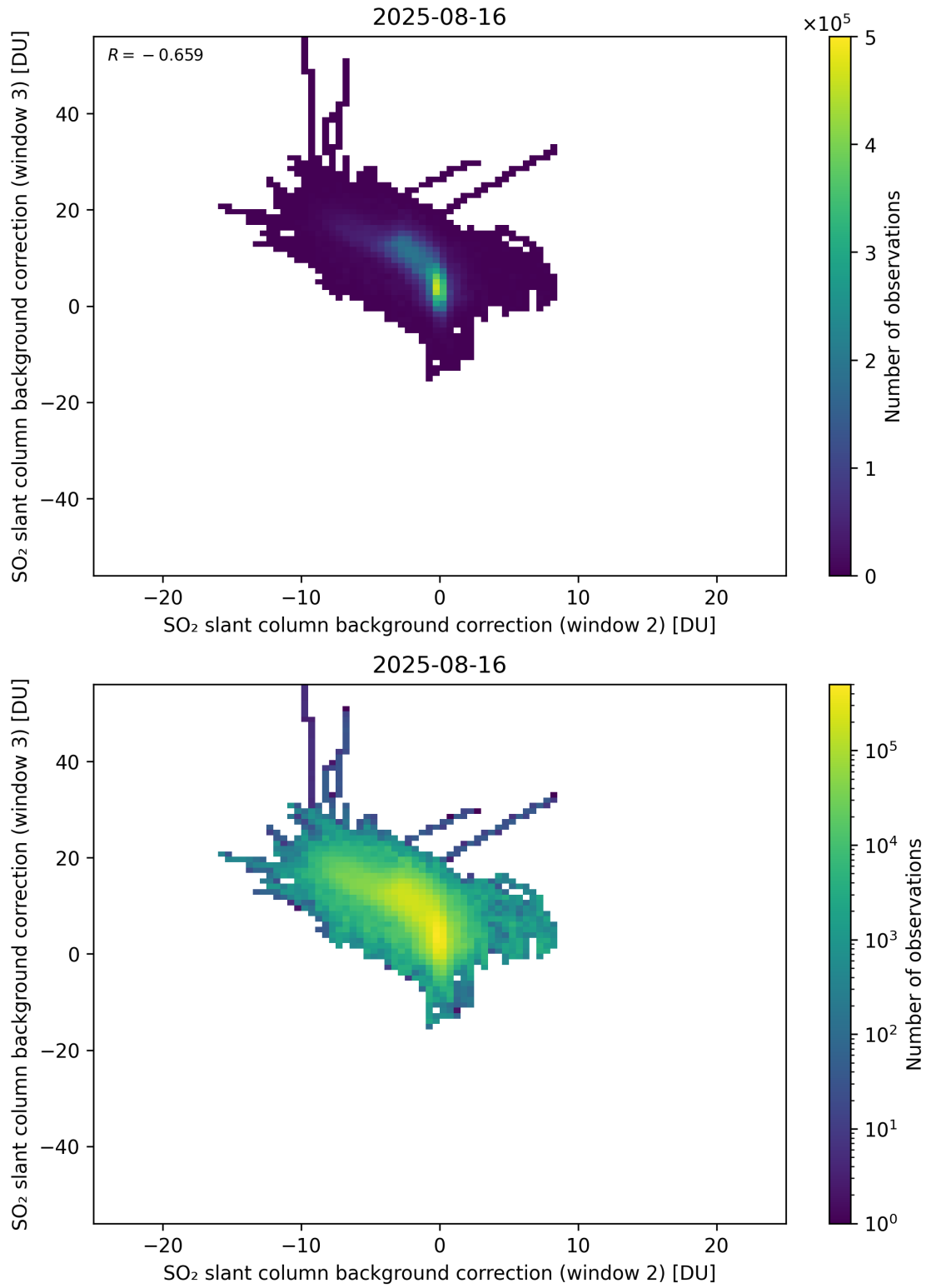
Figure 122: Scatter density plot of “SO 2 slant column background correction (window 2)” against “SO 2 slant column background correction (window 3)” for 2025-08-15 to 2025-08-17.
