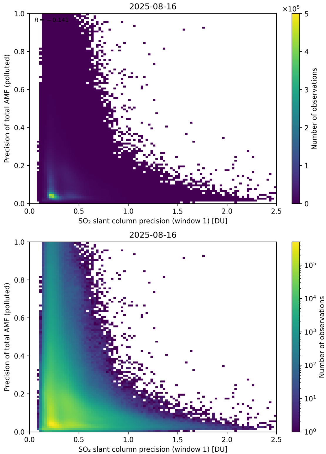
Figure 281: Scatter density plot of “SO 2 slant column precision (window 1)” against “Precision of total AMF (polluted)” for 2025-08-15 to 2025-08-17.
