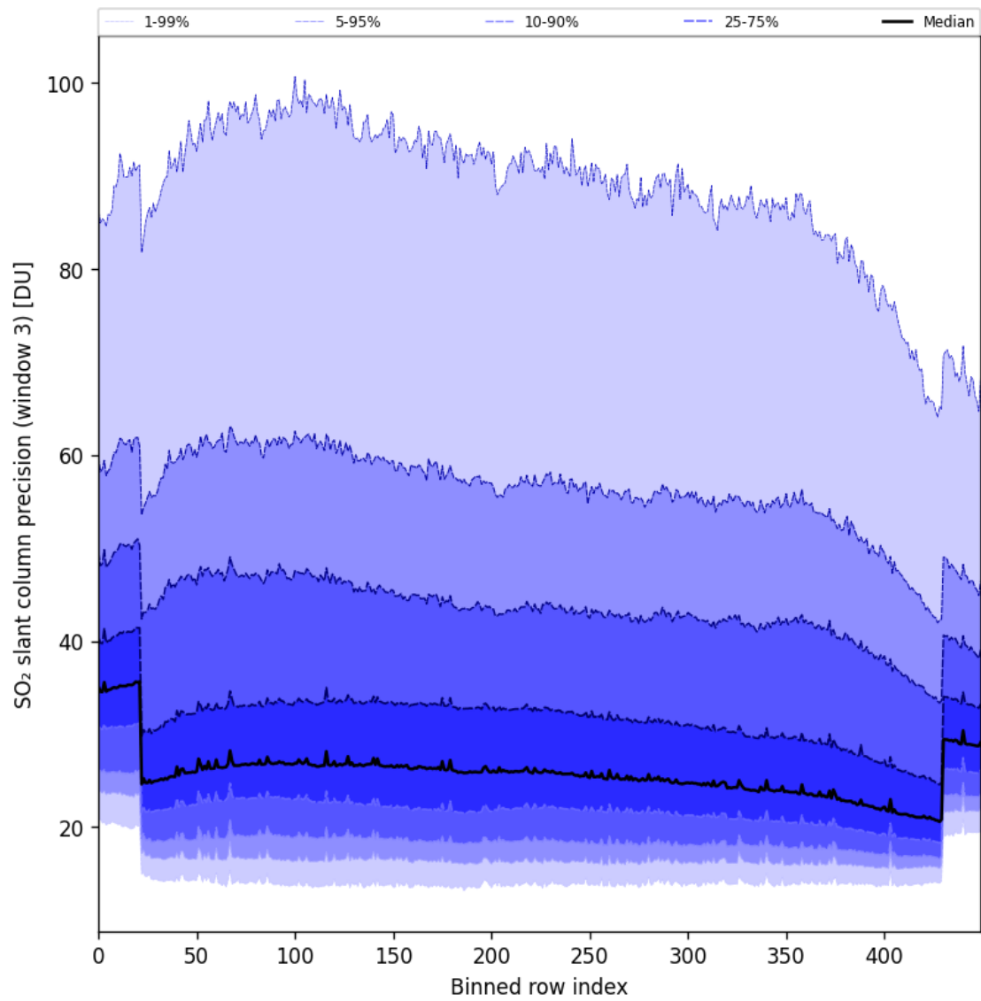
Figure 98: Along track statistics of “SO 2 slant column precision (window 3)” for 2025-08-15 to 2025-08-17
