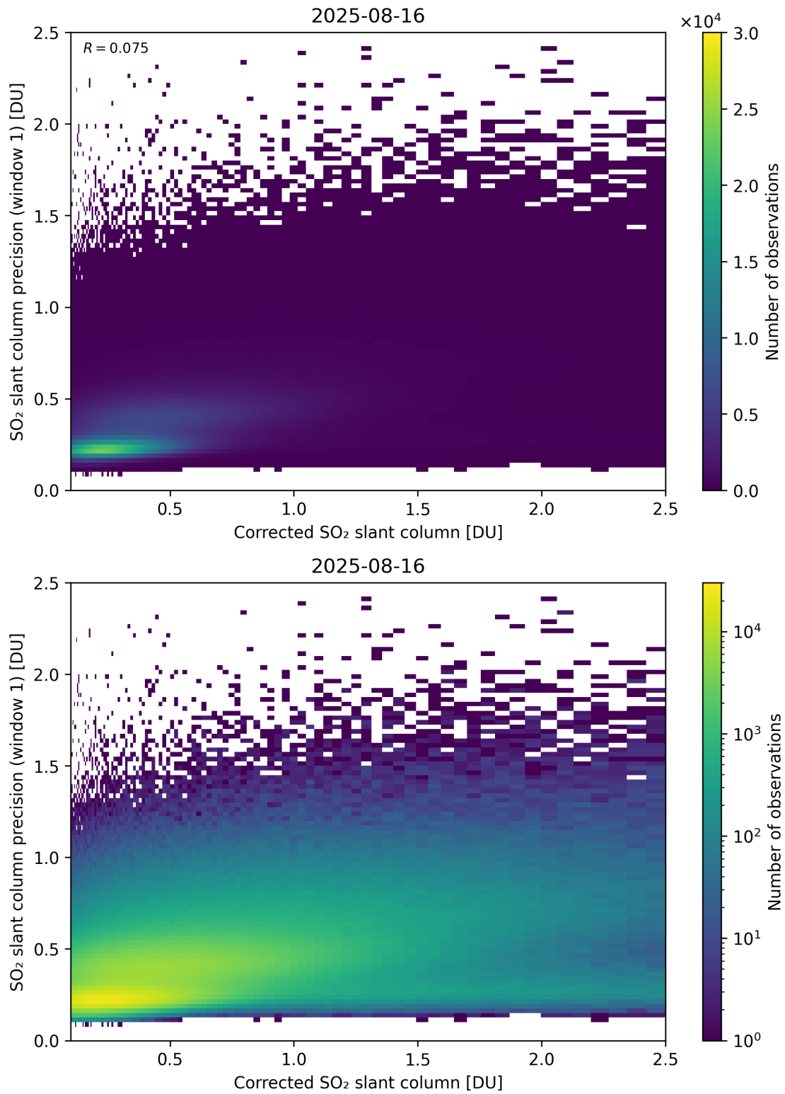
Figure 238: Scatter density plot of “Corrected SO 2 slant column” against “SO 2 slant column precision (window 1)” for 2025-08-15 to 2025-08-17.
