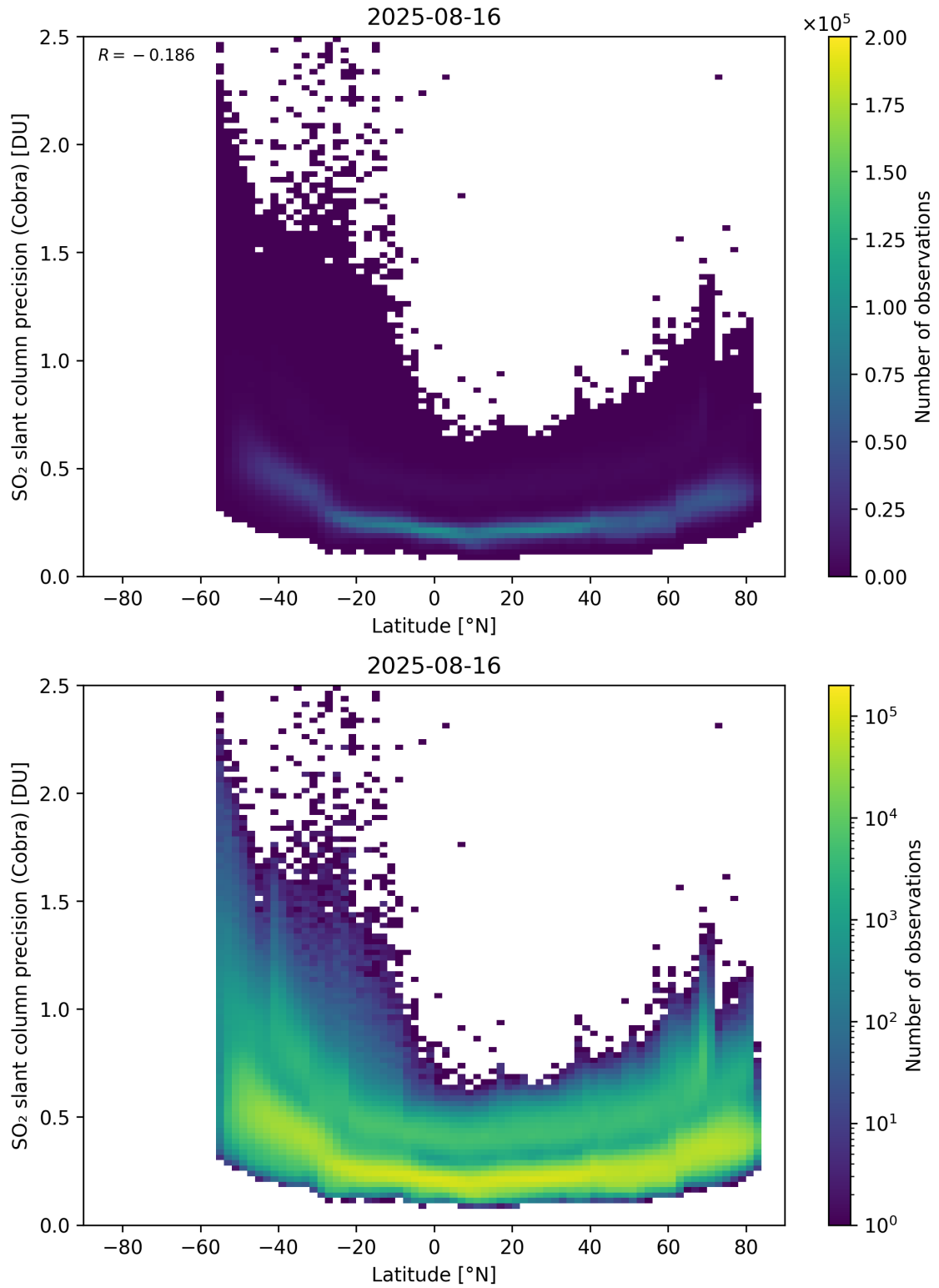
Figure 158: Scatter density plot of “Latitude” against “SO 2 slant column precision (Cobra)” for 2025-08-15 to 2025-08-17.
