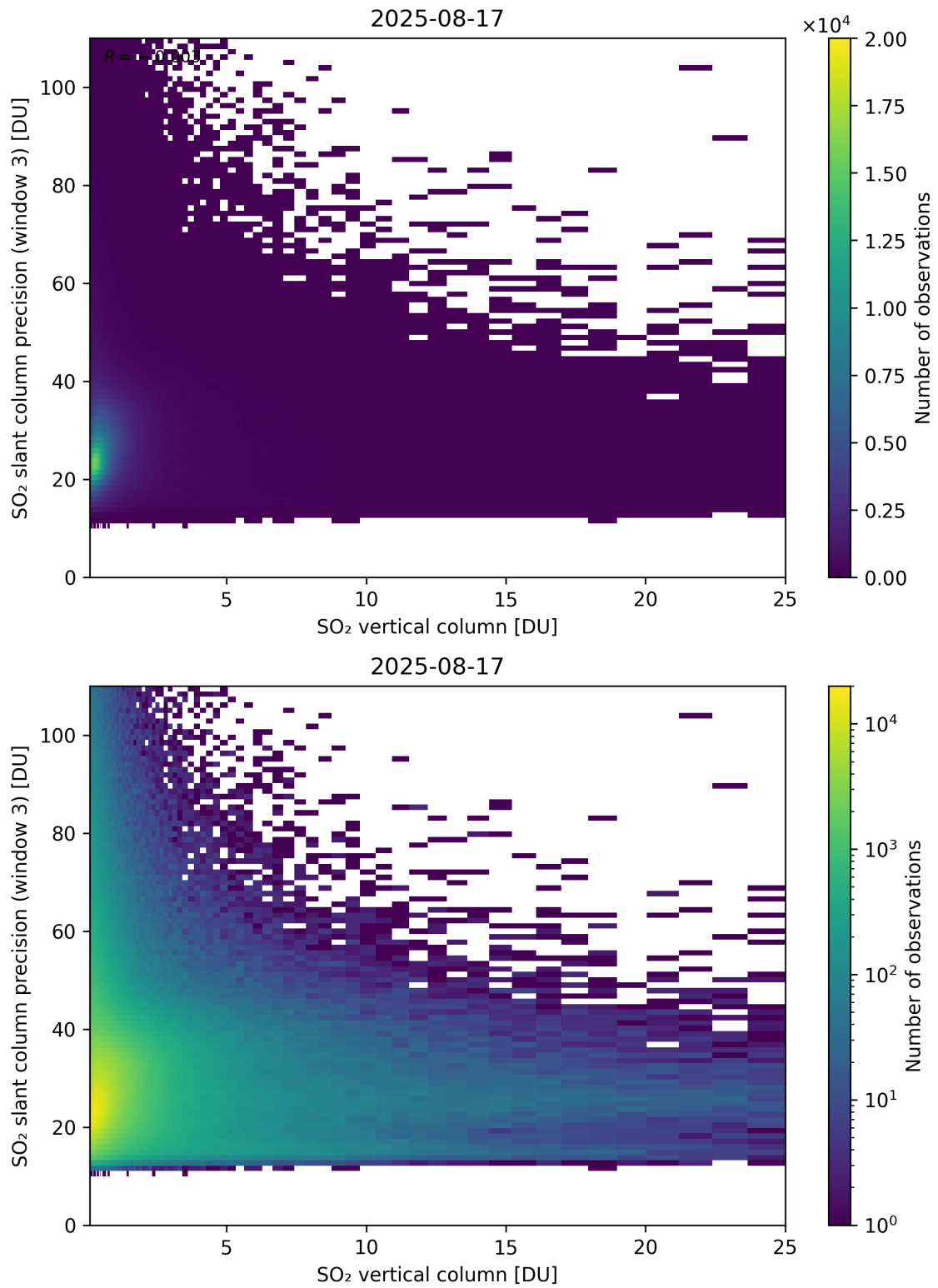
Figure 358: Scatter density plot of “SO 2 vertical column” against “SO 2 slant column precision (window 3)” for 2025-08-16 to 2025-08-18.
