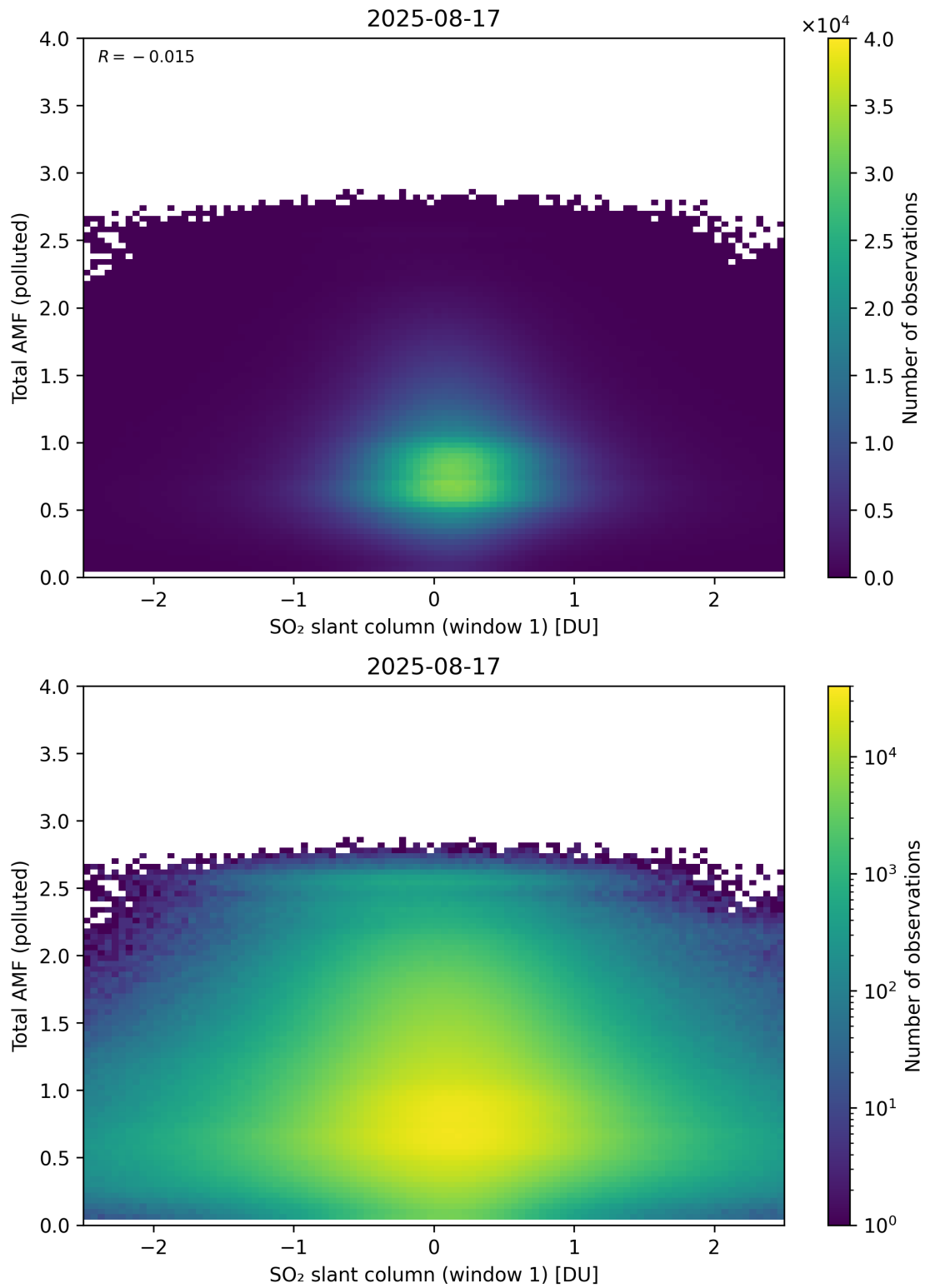
Figure 289: Scatter density plot of “SO 2 slant column (window 1)” against “Total AMF (polluted)” for 2025-08-16 to 2025-08-18.
