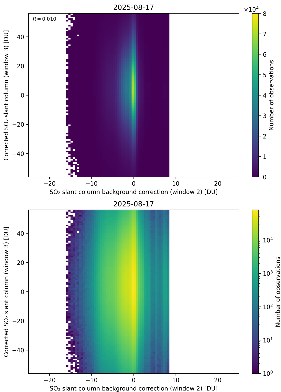
Figure 127: Scatter density plot of “SO 2 slant column background correction (window 2)” against “Corrected SO 2 slant column (window 3)” for 2025-08-16 to 2025-08-18.
