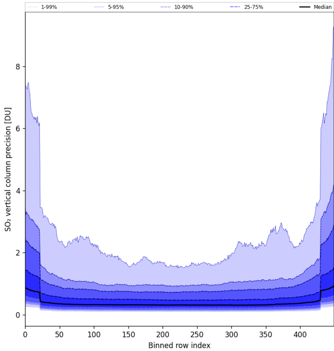
Figure 85: Along track statistics of “SO 2 vertical column precision” for 2025-08-16 to 2025-08-18
