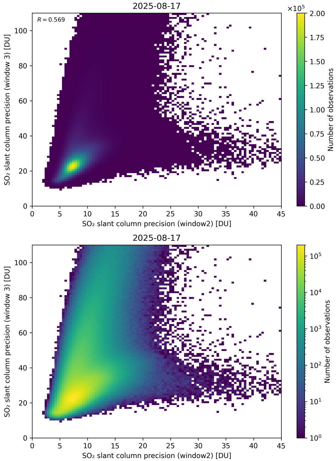
Figure 300: Scatter density plot of “SO 2 slant column precision (window2)” against “SO 2 slant column precision (window 3)” for 2025-08-16 to 2025-08-18.
