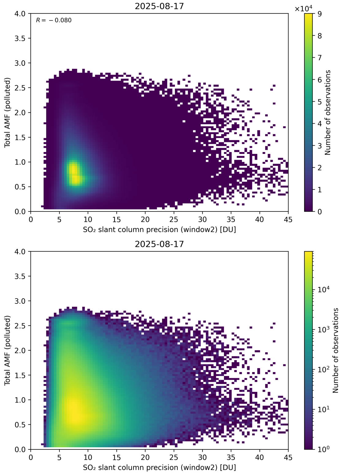
Figure 301: Scatter density plot of “SO 2 slant column precision (window2)” against “Total AMF (polluted)” for 2025-08-16 to 2025-08-18.
