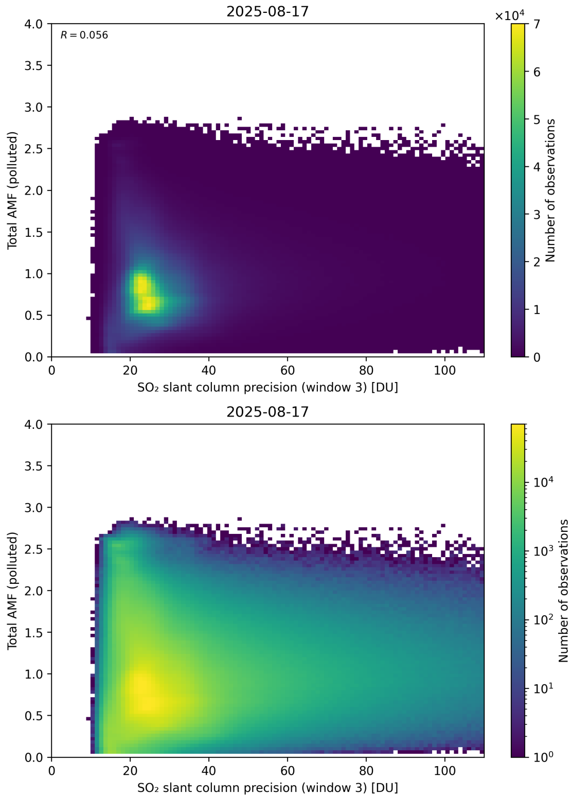
Figure 313: Scatter density plot of “SO 2 slant column precision (window 3)” against “Total AMF (polluted)” for 2025-08-16 to 2025-08-18.
