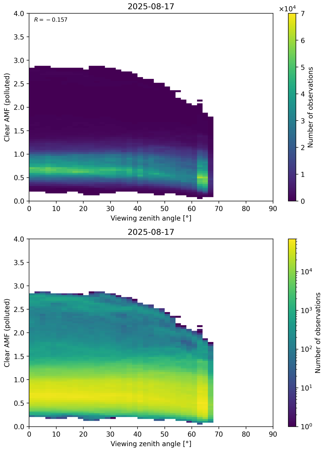
Figure 370: Scatter density plot of “Viewing zenith angle” against “Clear AMF (polluted)” for 2025-08-16 to 2025-08-18.
