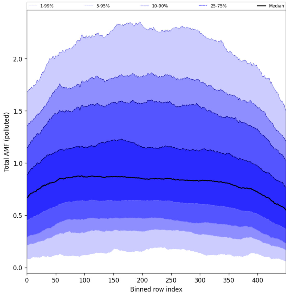
Figure 105: Along track statistics of “Total AMF (polluted)” for 2025-08-16 to 2025-08-18
