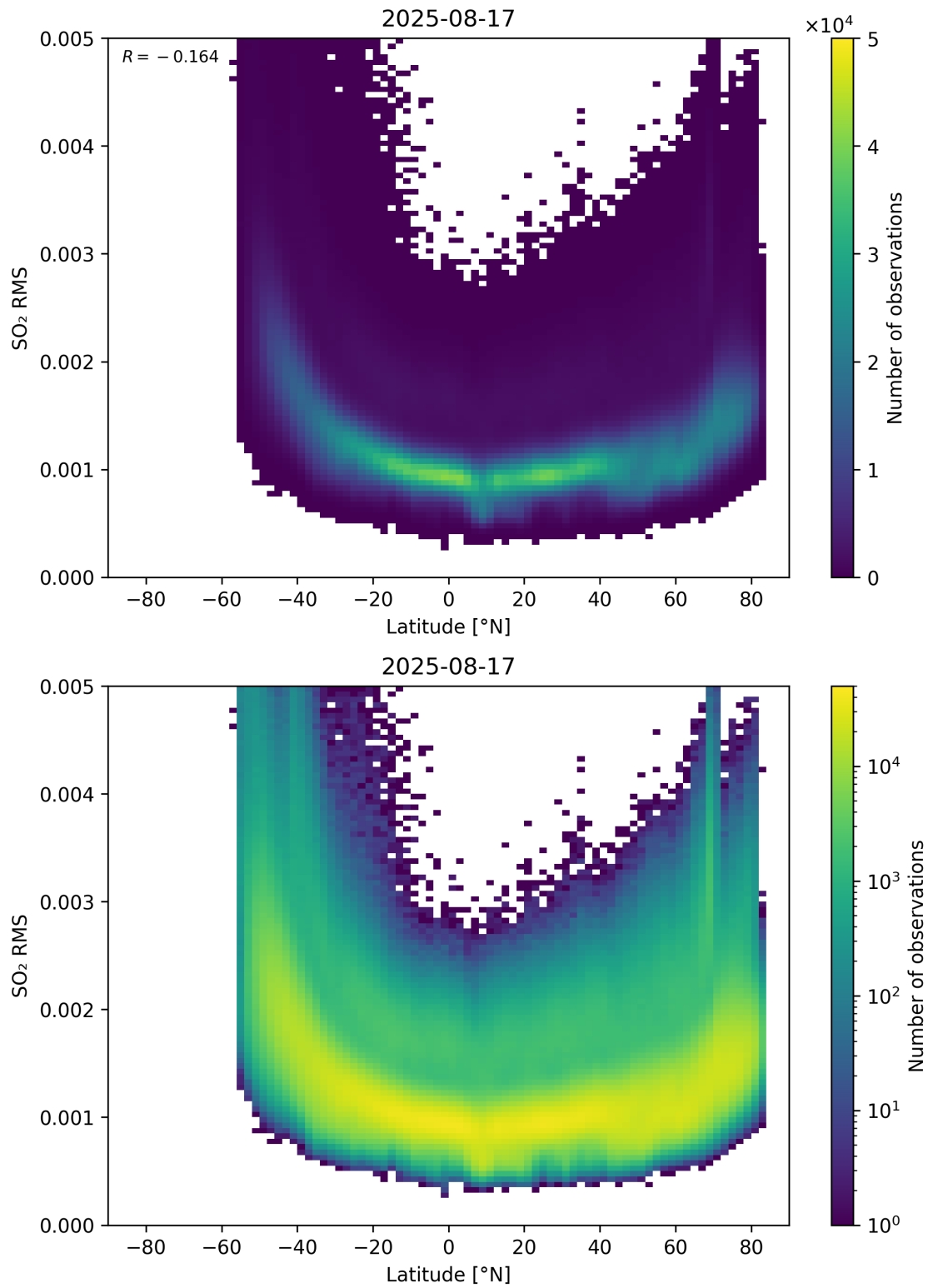
Figure 155: Scatter density plot of “Latitude” against “SO 2 RMS” for 2025-08-16 to 2025-08-18.
