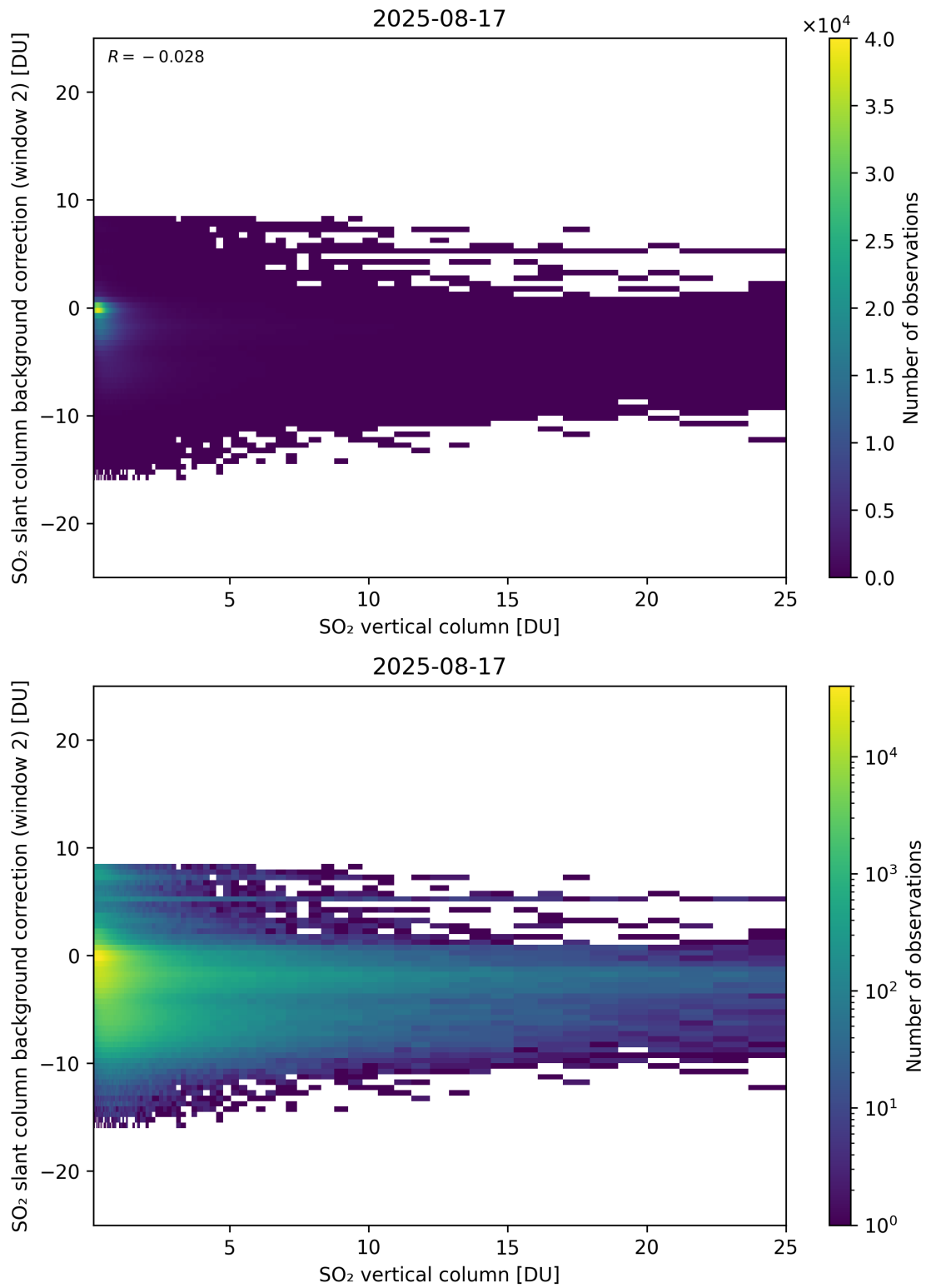
Figure 324: Scatter density plot of “SO 2 vertical column” against “SO 2 slant column background correction (window 2)” for 2025-08-16 to 2025-08-18.
