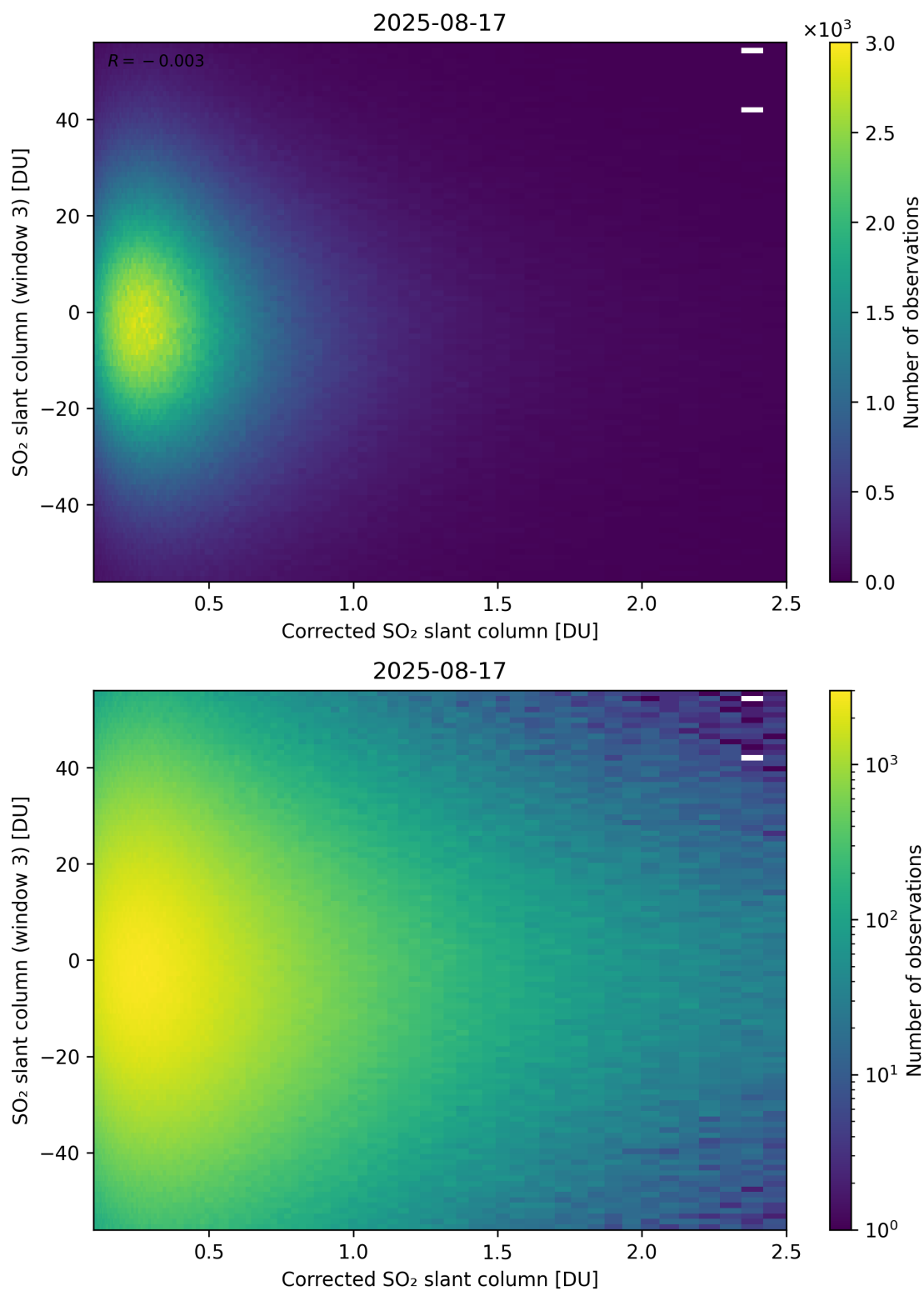
Figure 240: Scatter density plot of “Corrected SO 2 slant column” against “SO 2 slant column (window 3)” for 2025-08-16 to 2025-08-18.
