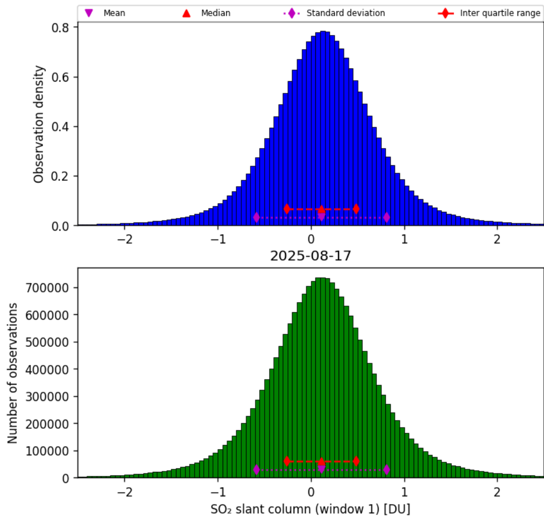
Figure 63: Histogram of “SO 2 slant column (window 1)” for 2025-08-16 to 2025-08-18
