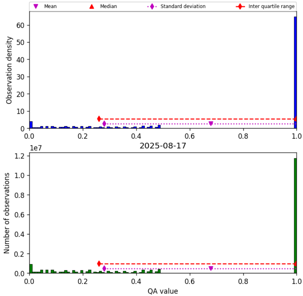
Figure 57: Histogram of “QA value” for 2025-08-16 to 2025-08-18
