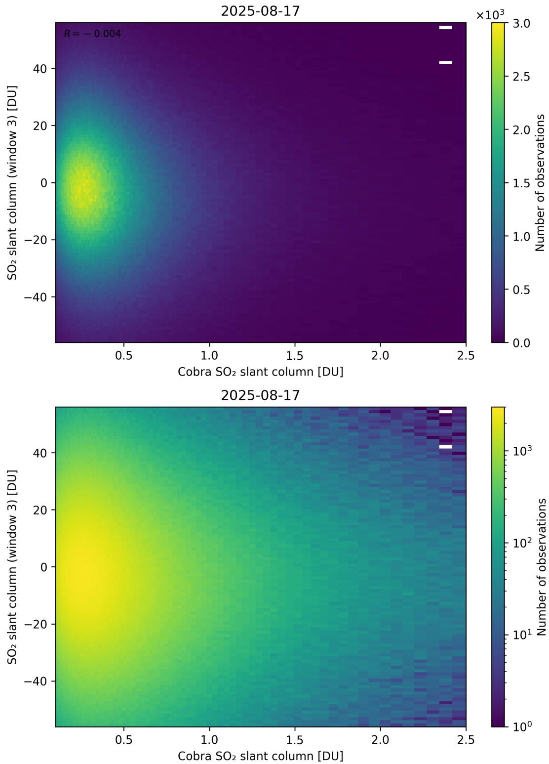
Figure 222: Scatter density plot of “Cobra SO 2 slant column” against “SO 2 slant column (window 3)” for 2025-08-16 to 2025-08-18.
