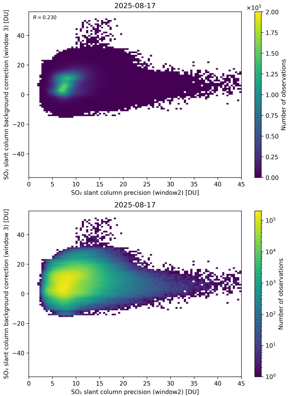
Figure 292: Scatter density plot of “SO 2 slant column precision (window2)” against “SO 2 slant column background correction (window 3)” for 2025-08-16 to 2025-08-18.
