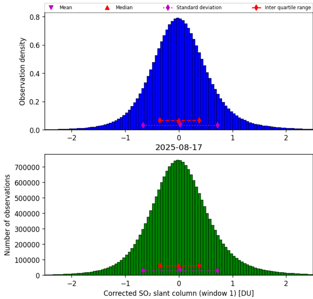
Figure 65: Histogram of “Corrected SO 2 slant column (window 1)” for 2025-08-16 to 2025-08-18
