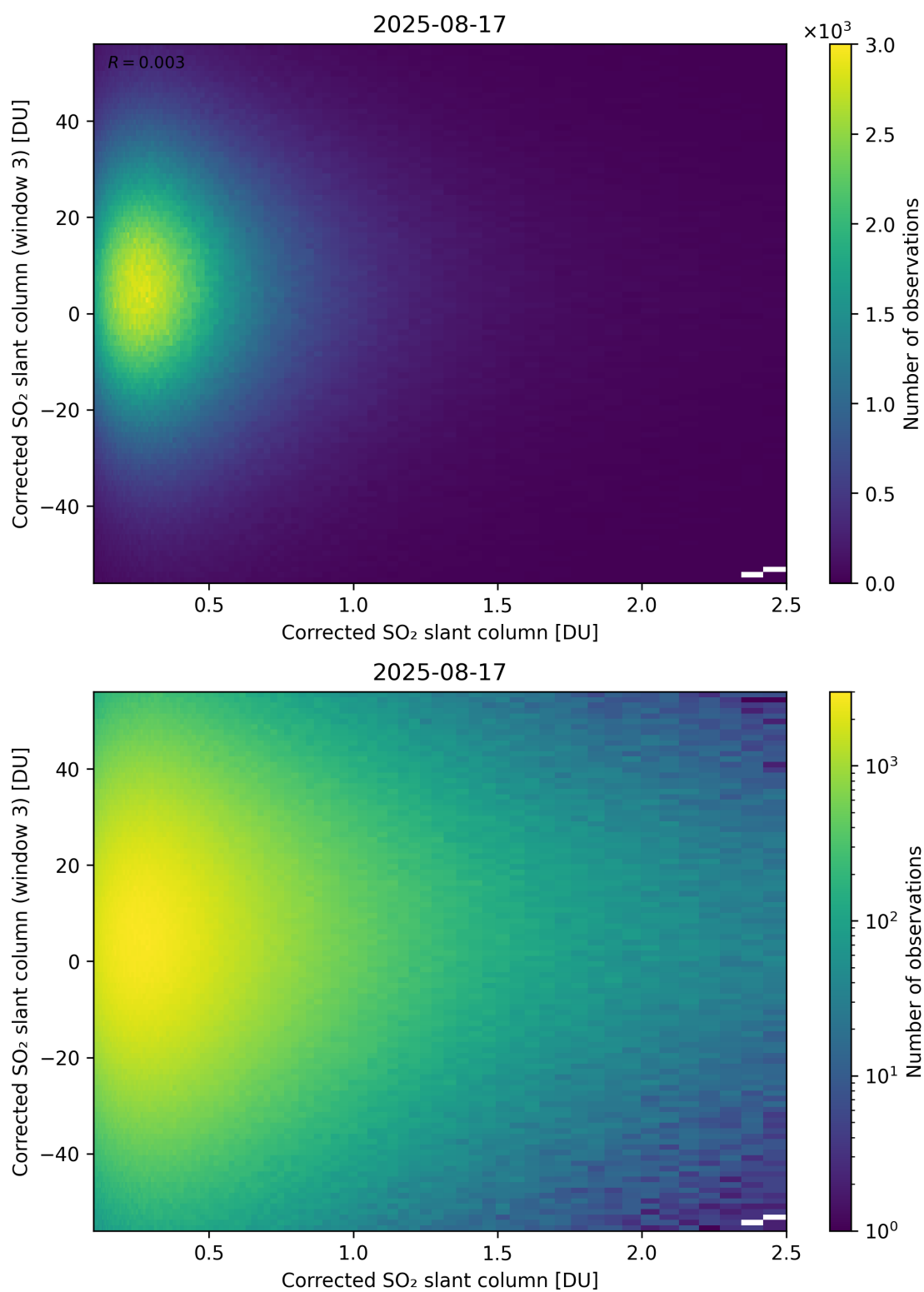
Figure 236: Scatter density plot of “Corrected SO 2 slant column” against “Corrected SO 2 slant column (window 3)” for 2025-08-16 to 2025-08-18.
