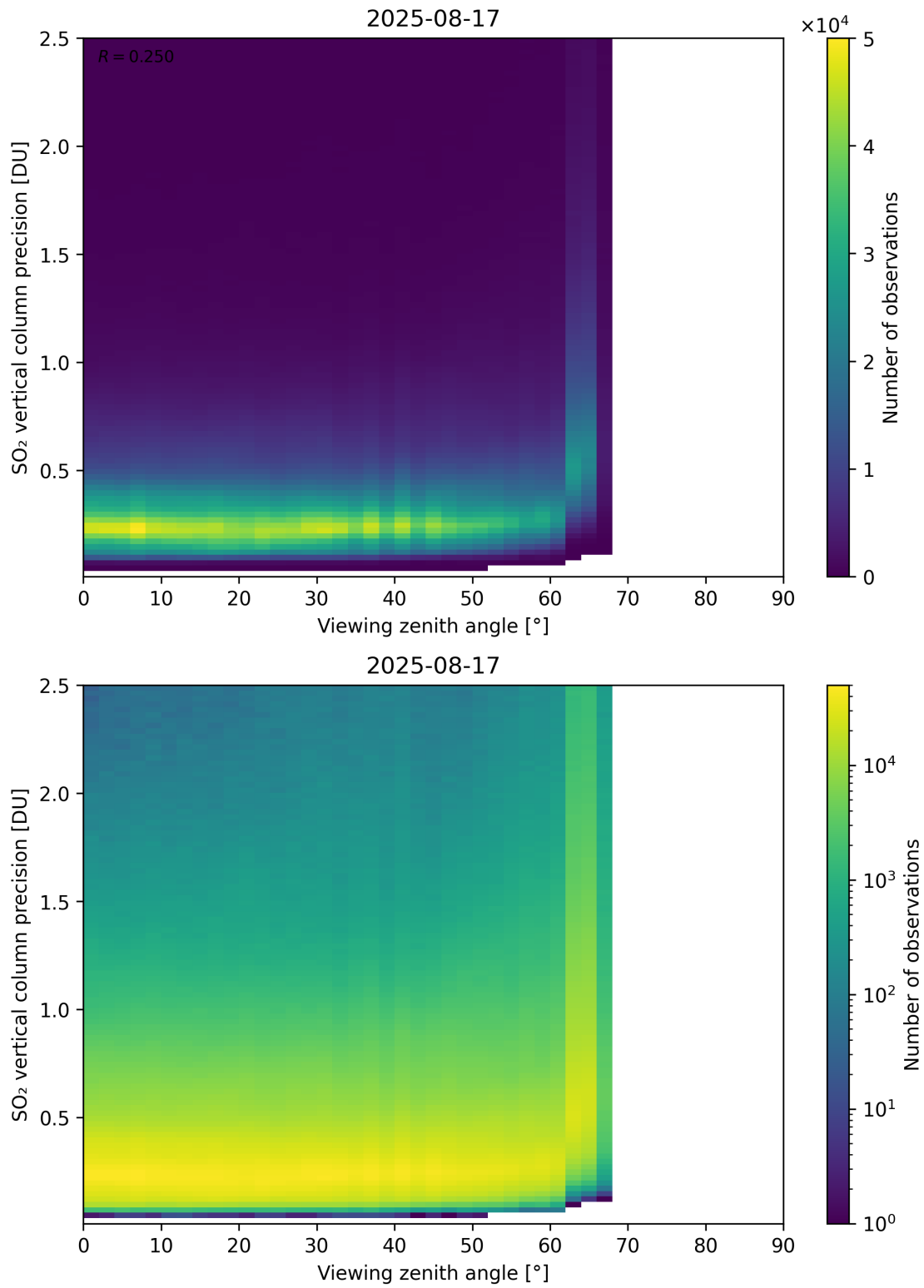
Figure 384: Scatter density plot of “Viewing zenith angle” against “SO 2 vertical column precision” for 2025-08-16 to 2025-08-18.
