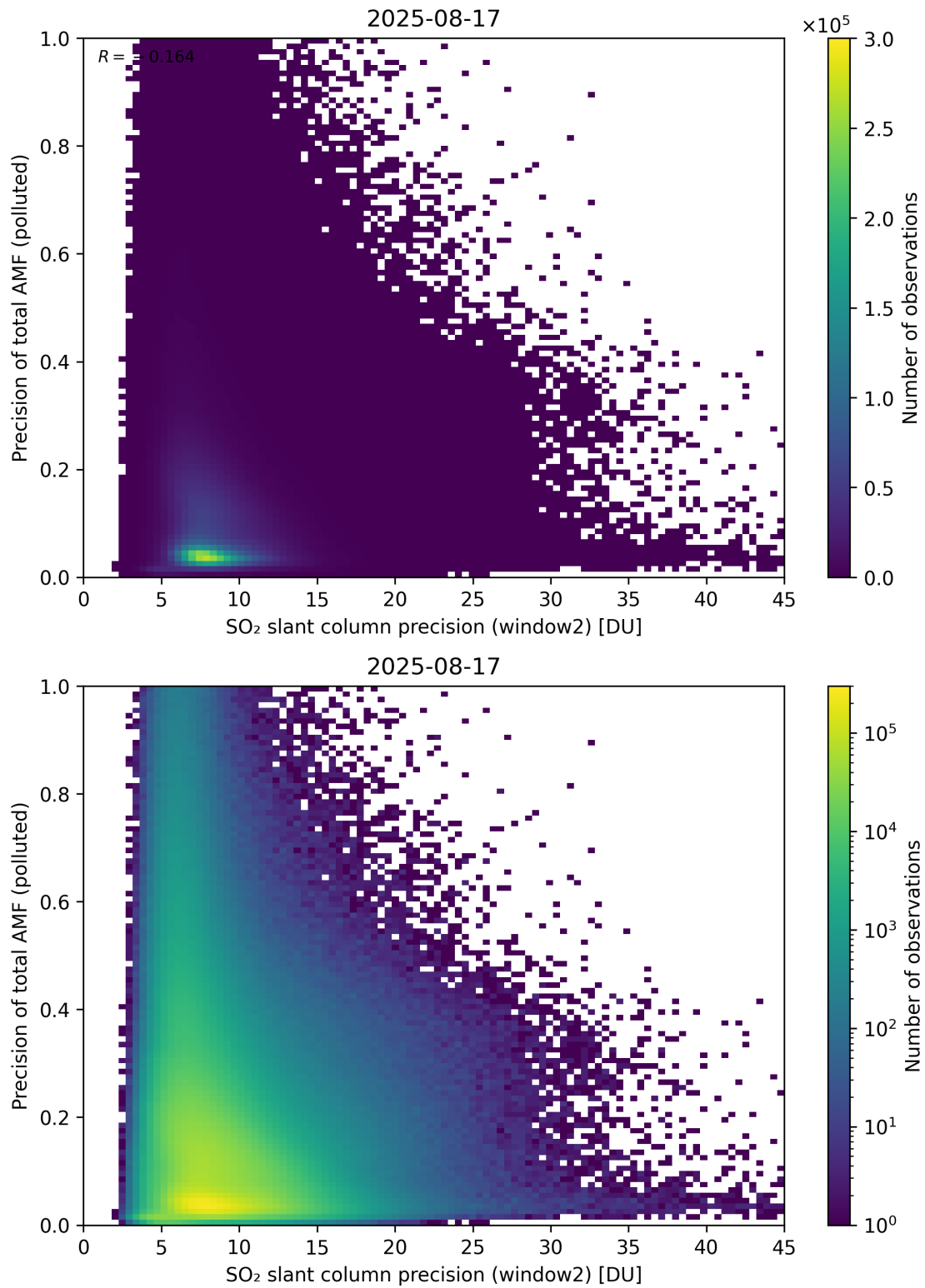
Figure 302: Scatter density plot of “SO 2 slant column precision (window2)” against “Precision of total AMF (polluted)” for 2025-08-16 to 2025-08-18.
