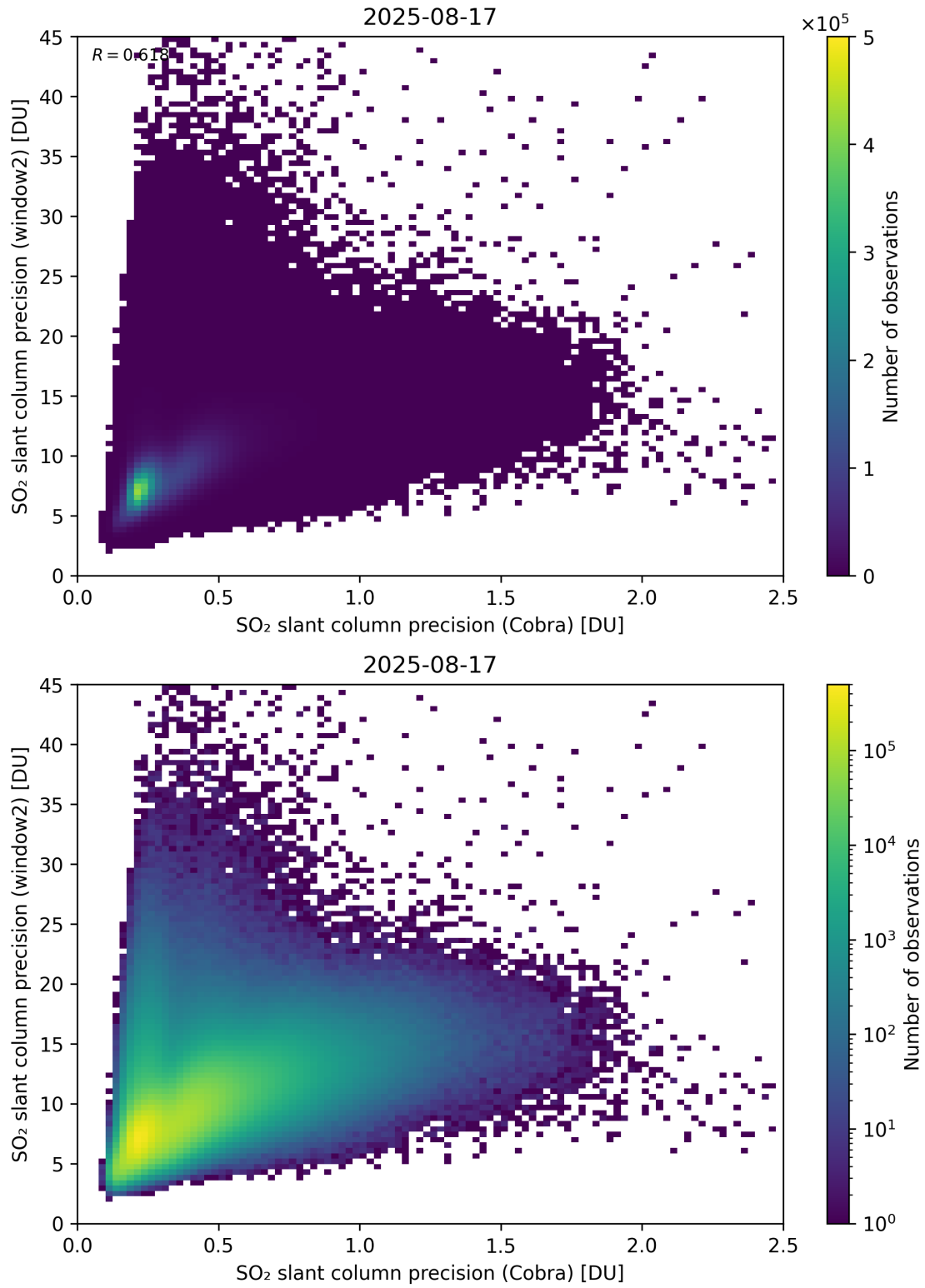
Figure 210: Scatter density plot of “SO 2 slant column precision (Cobra)” against “SO 2 slant column precision (window2)” for 2025-08-16 to 2025-08-18.
