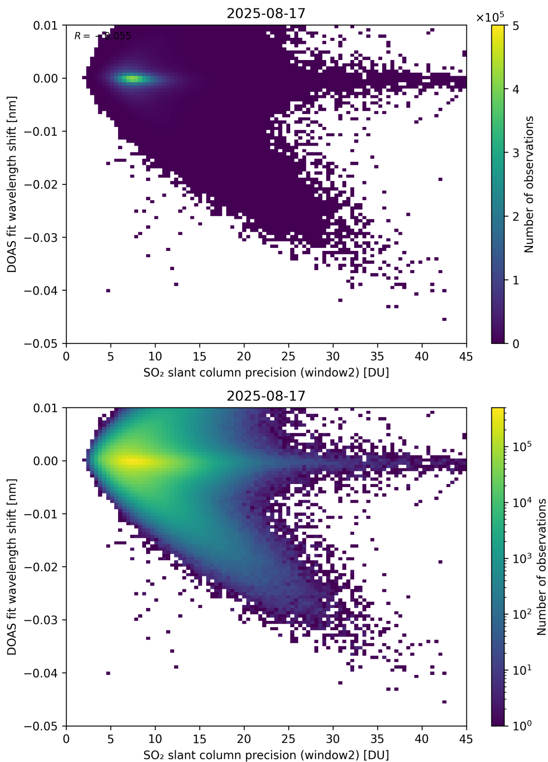
Figure 293: Scatter density plot of “SO 2 slant column precision (window2)” against “DOAS fit wavelength shift” for 2025-08-16 to 2025-08-18.
