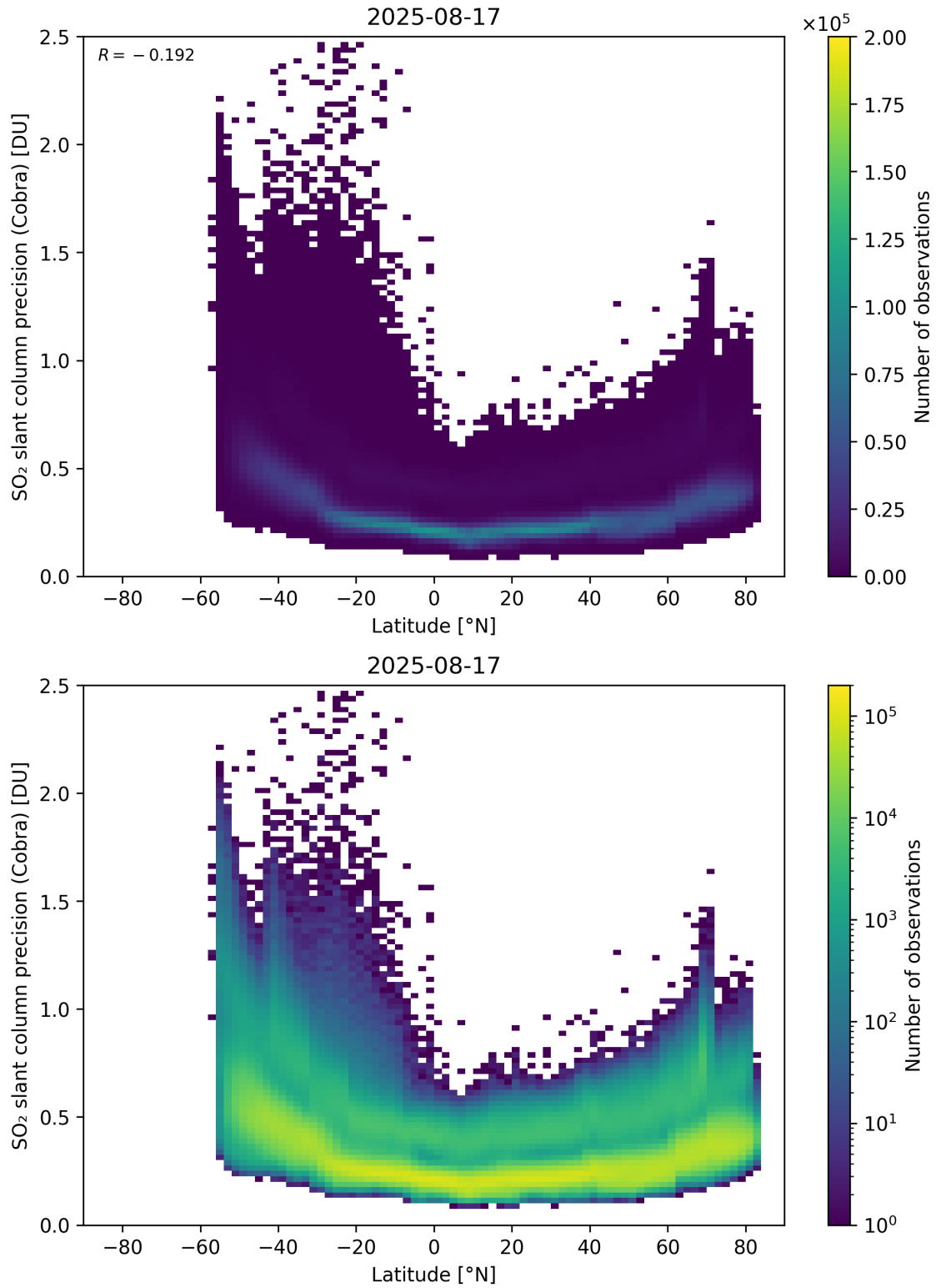
Figure 158: Scatter density plot of “Latitude” against “SO 2 slant column precision (Cobra)” for 2025-08-16 to 2025-08-18.
