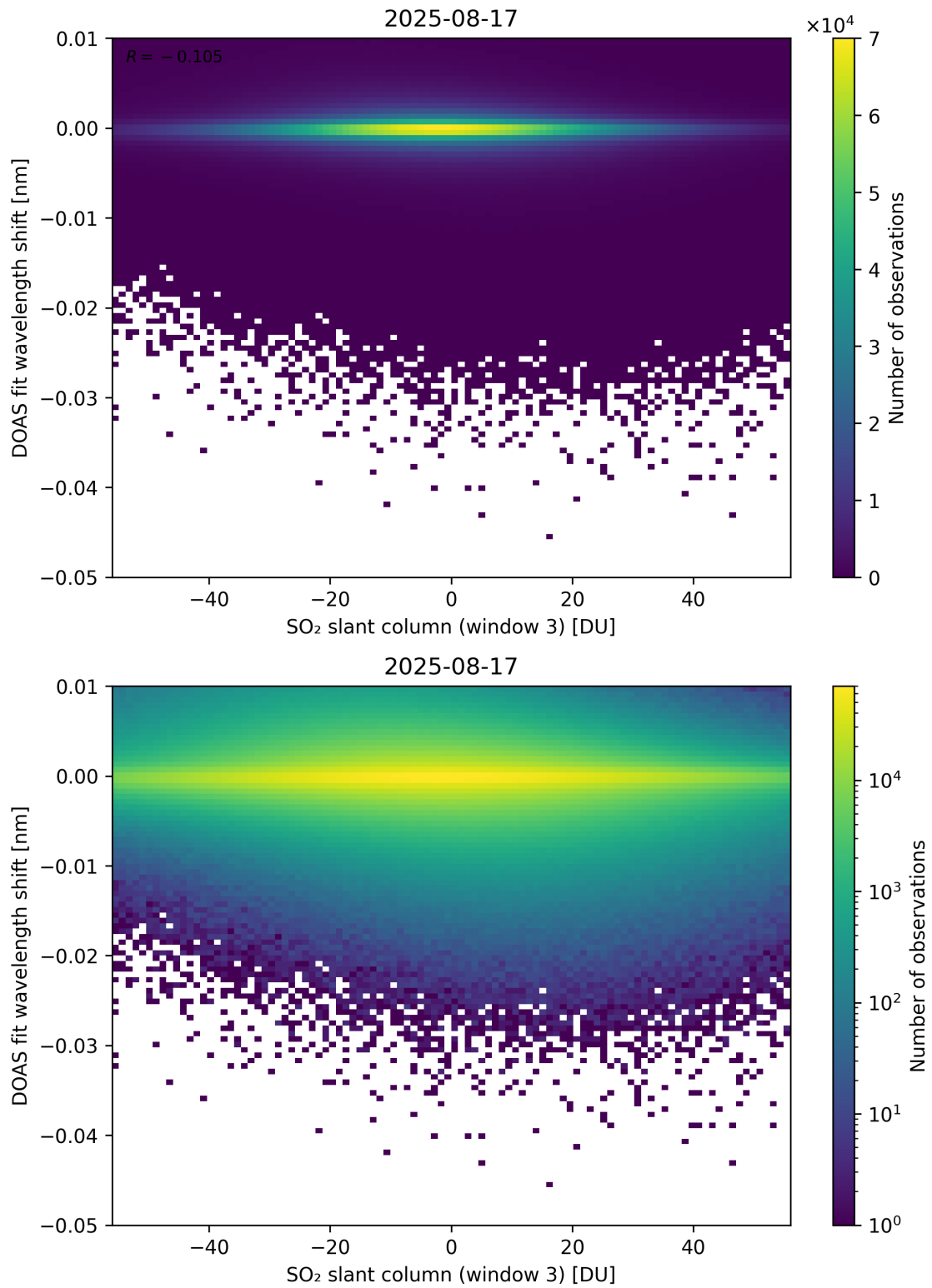
Figure 304: Scatter density plot of “SO 2 slant column (window 3)” against “DOAS fit wavelength shift” for 2025-08-16 to 2025-08-18.
