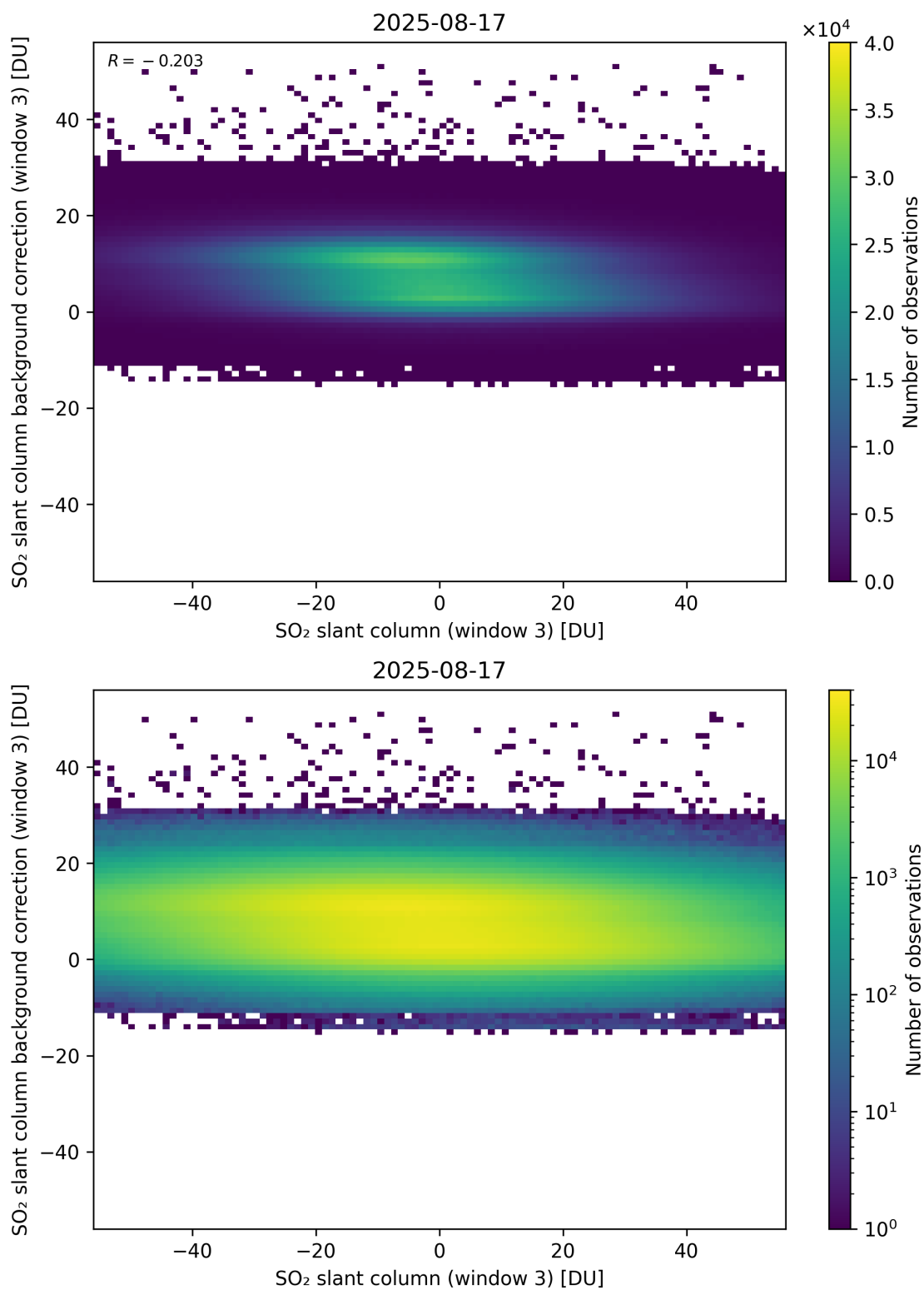
Figure 303: Scatter density plot of “SO 2 slant column (window 3)” against “SO 2 slant column background correction (window 3)” for 2025-08-16 to 2025-08-18.
