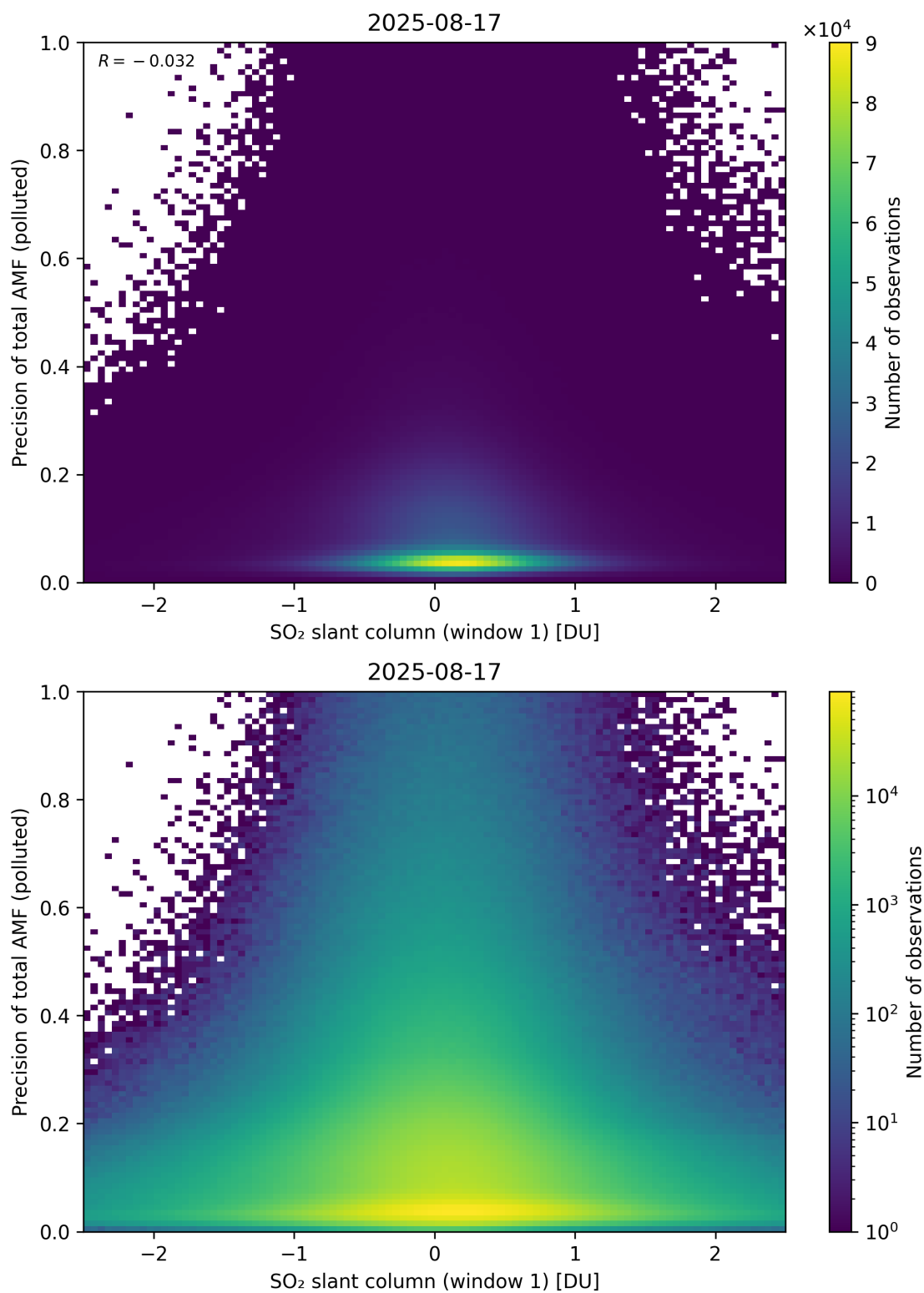
Figure 290: Scatter density plot of “SO 2 slant column (window 1)” against “Precision of total AMF (polluted)” for 2025-08-16 to 2025-08-18.
