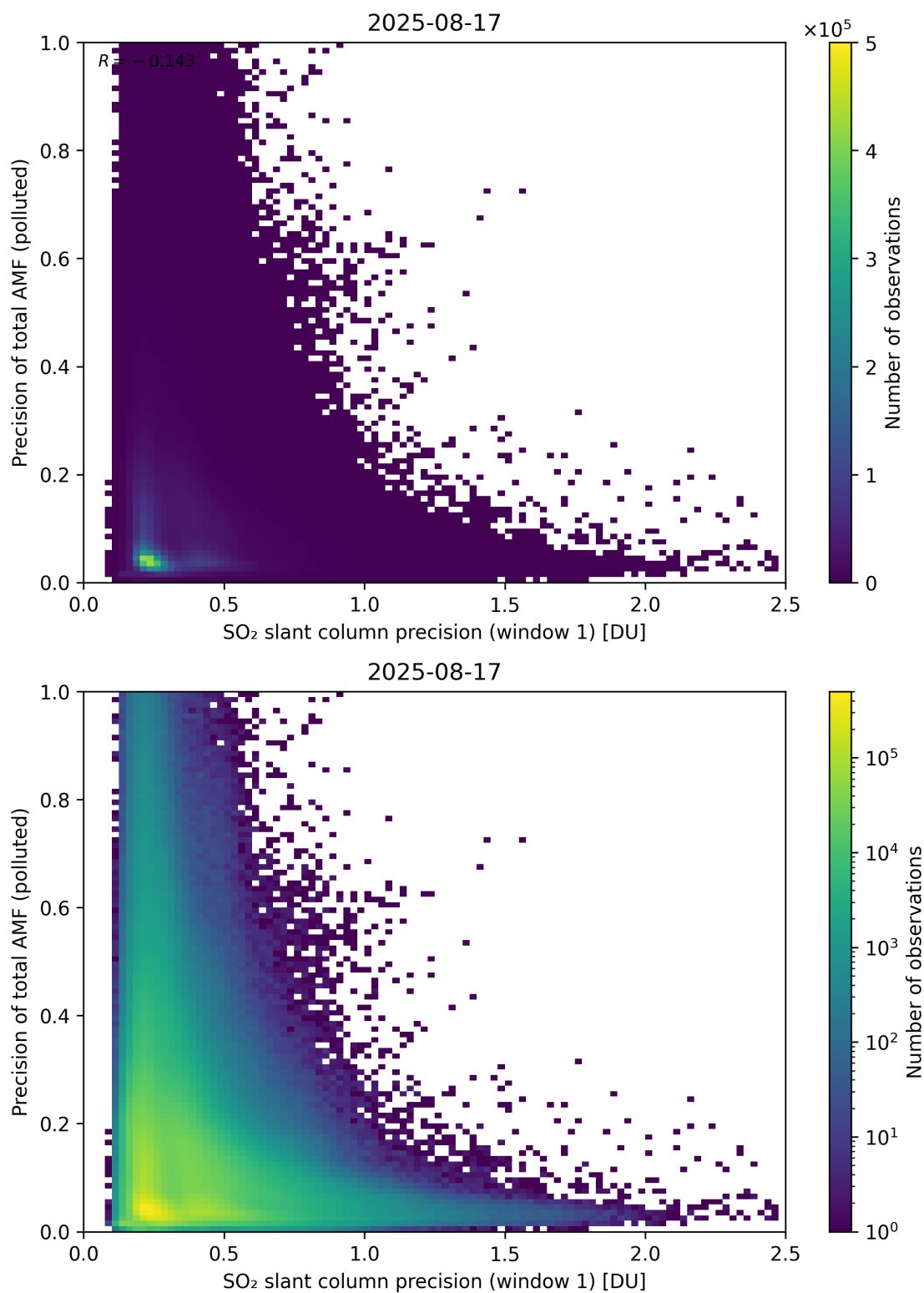
Figure 281: Scatter density plot of “SO 2 slant column precision (window 1)” against “Precision of total AMF (polluted)” for 2025-08-16 to 2025-08-18.
