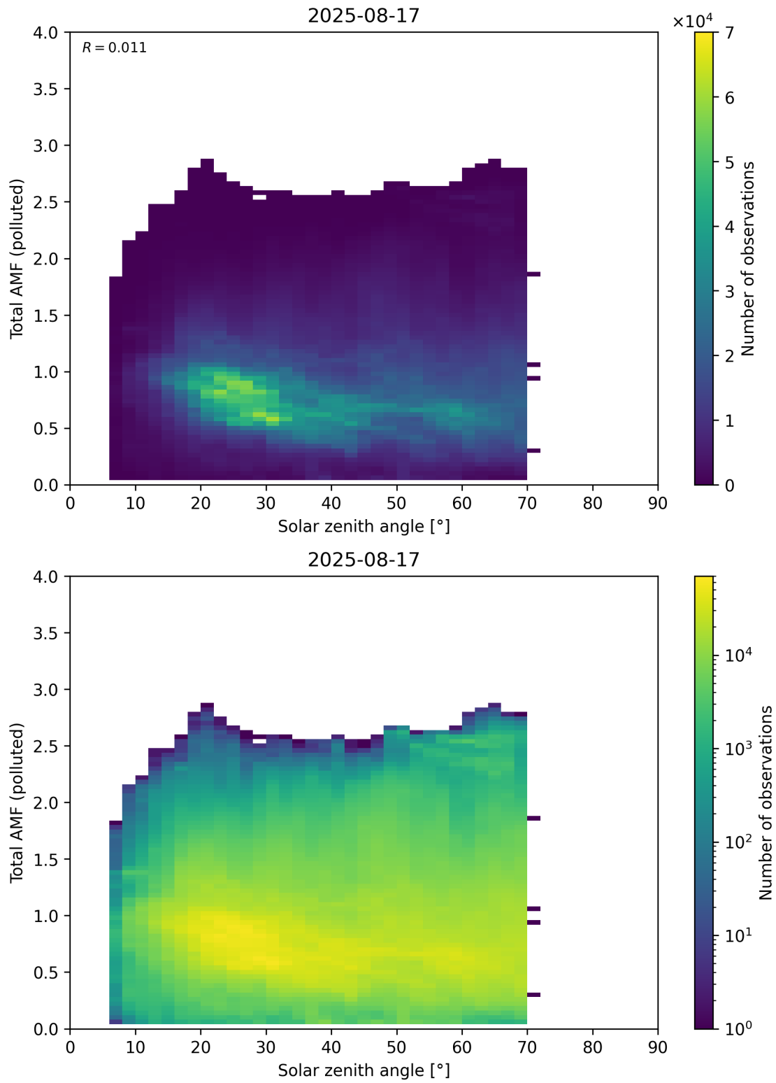
Figure 189: Scatter density plot of “Solar zenith angle” against “Total AMF (polluted)” for 2025-08-16 to 2025-08-18.
