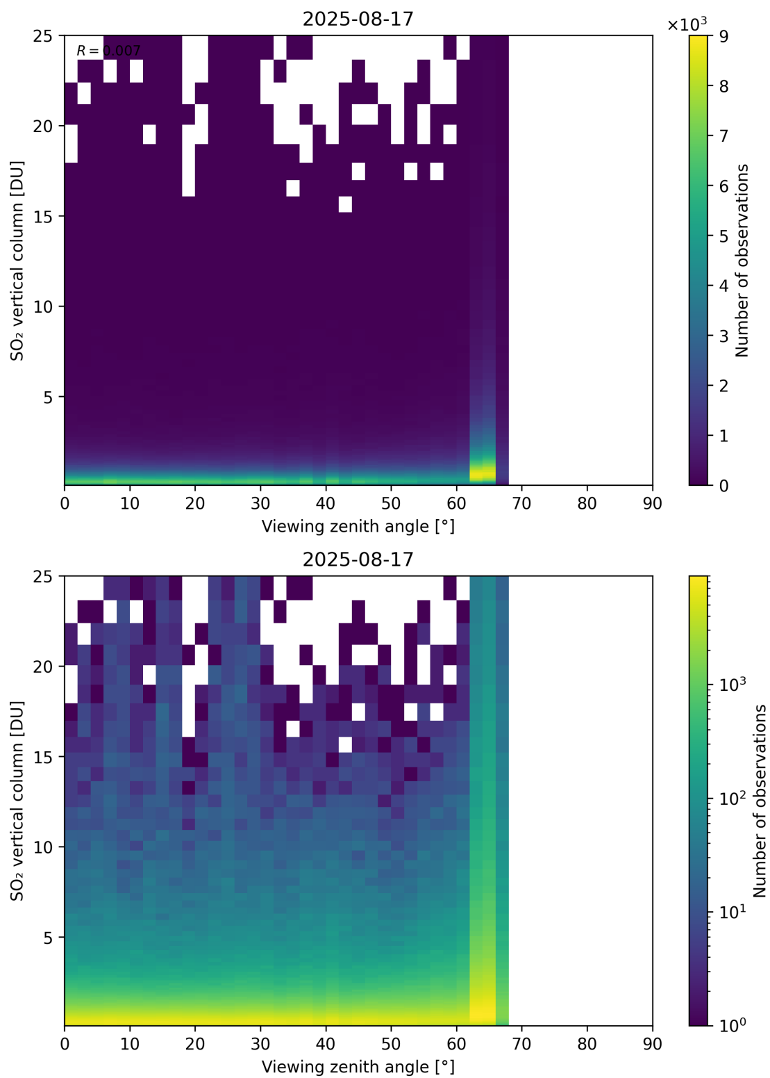
Figure 383: Scatter density plot of “Viewing zenith angle” against “SO 2 vertical column” for 2025-08-16 to 2025-08-18.
