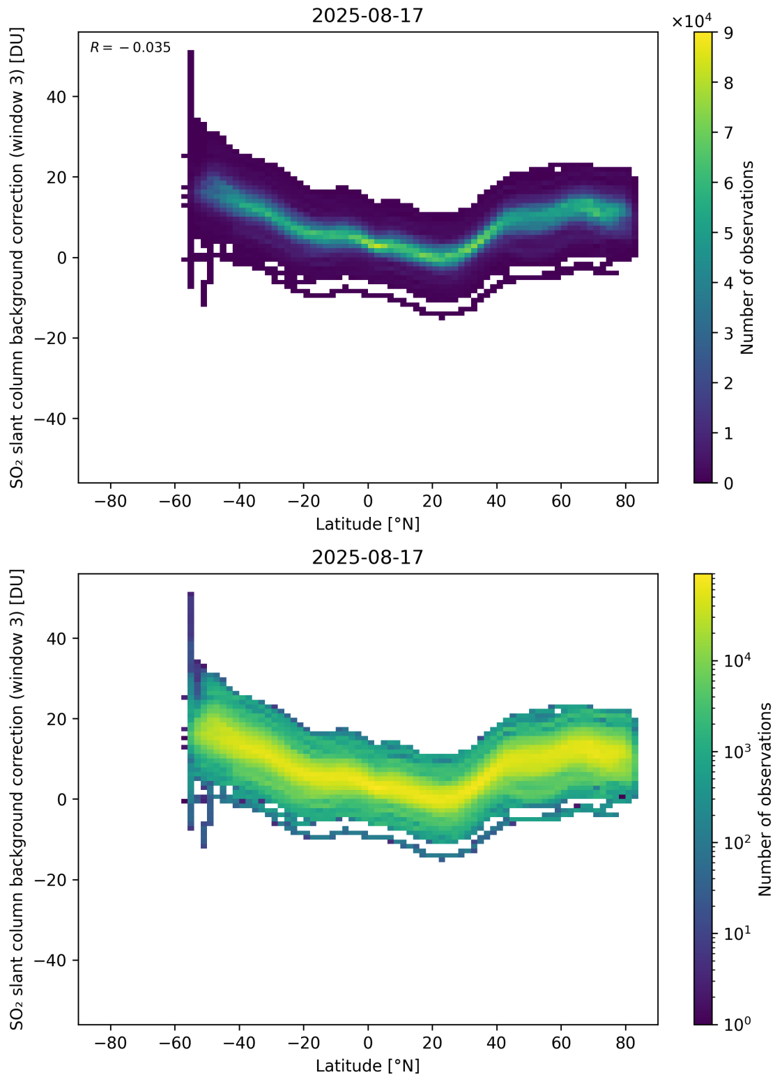
Figure 152: Scatter density plot of “Latitude” against “SO 2 slant column background correction (window 3)” for 2025-08-16 to 2025-08-18.
