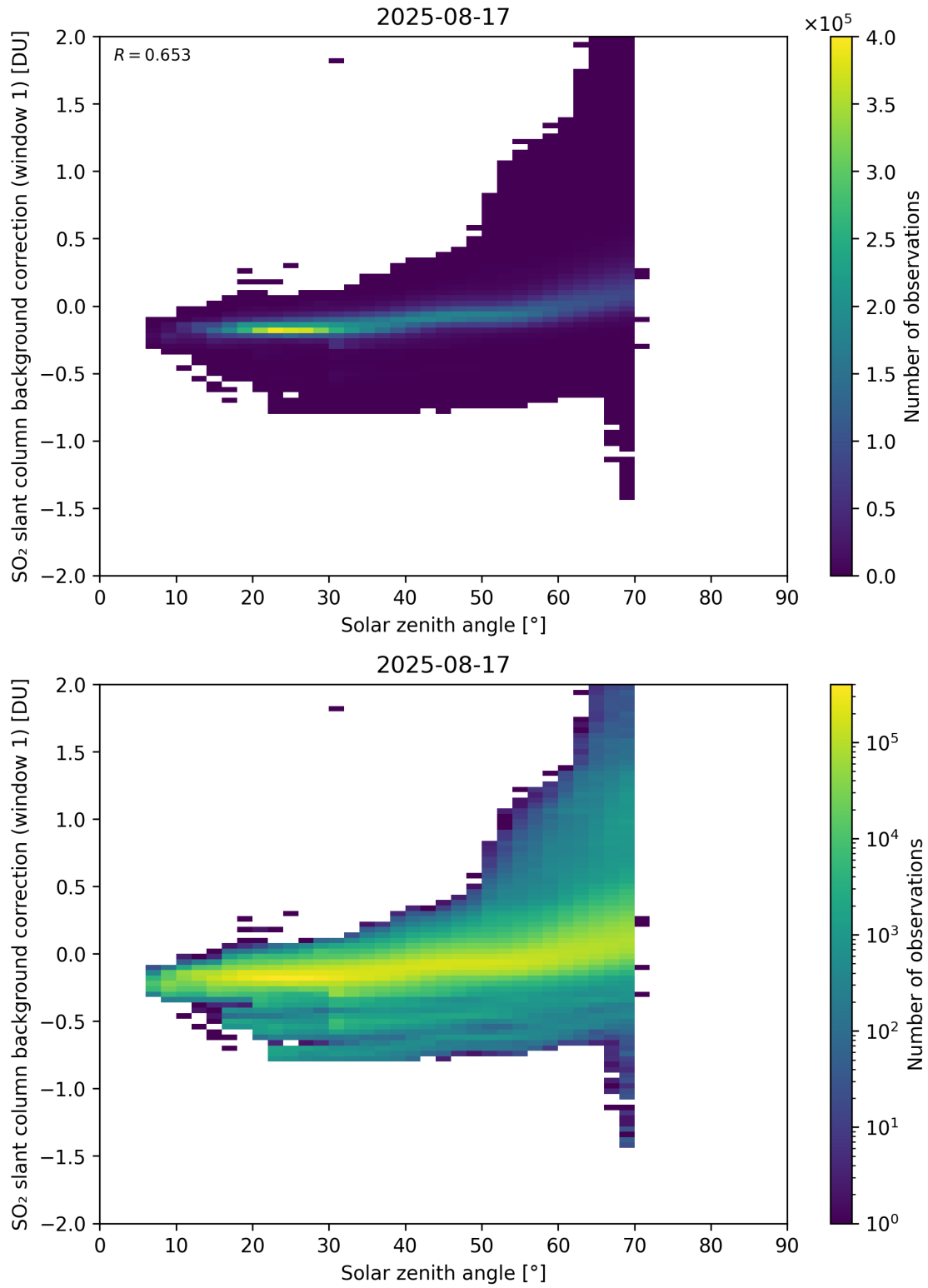
Figure 171: Scatter density plot of “Solar zenith angle” against “SO 2 slant column background correction (window 1)” for 2025-08-16 to 2025-08-18.
