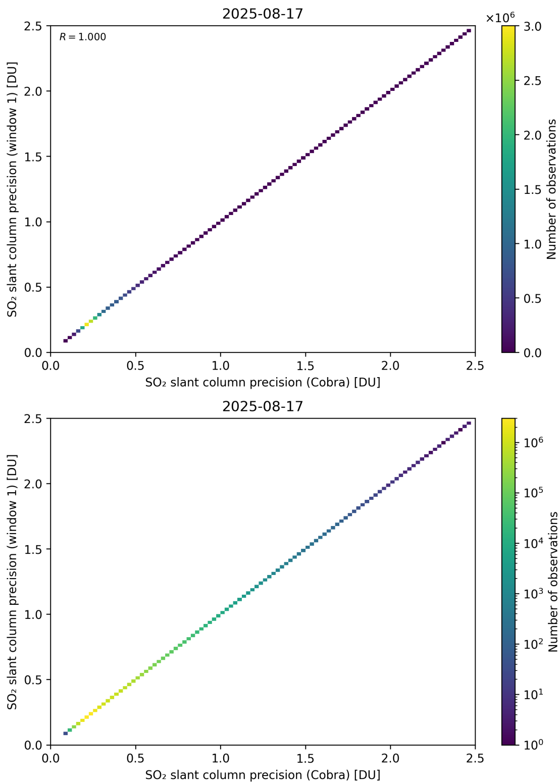
Figure 209: Scatter density plot of “SO 2 slant column precision (Cobra)” against “SO 2 slant column precision (window 1)” for 2025-08-16 to 2025-08-18.
