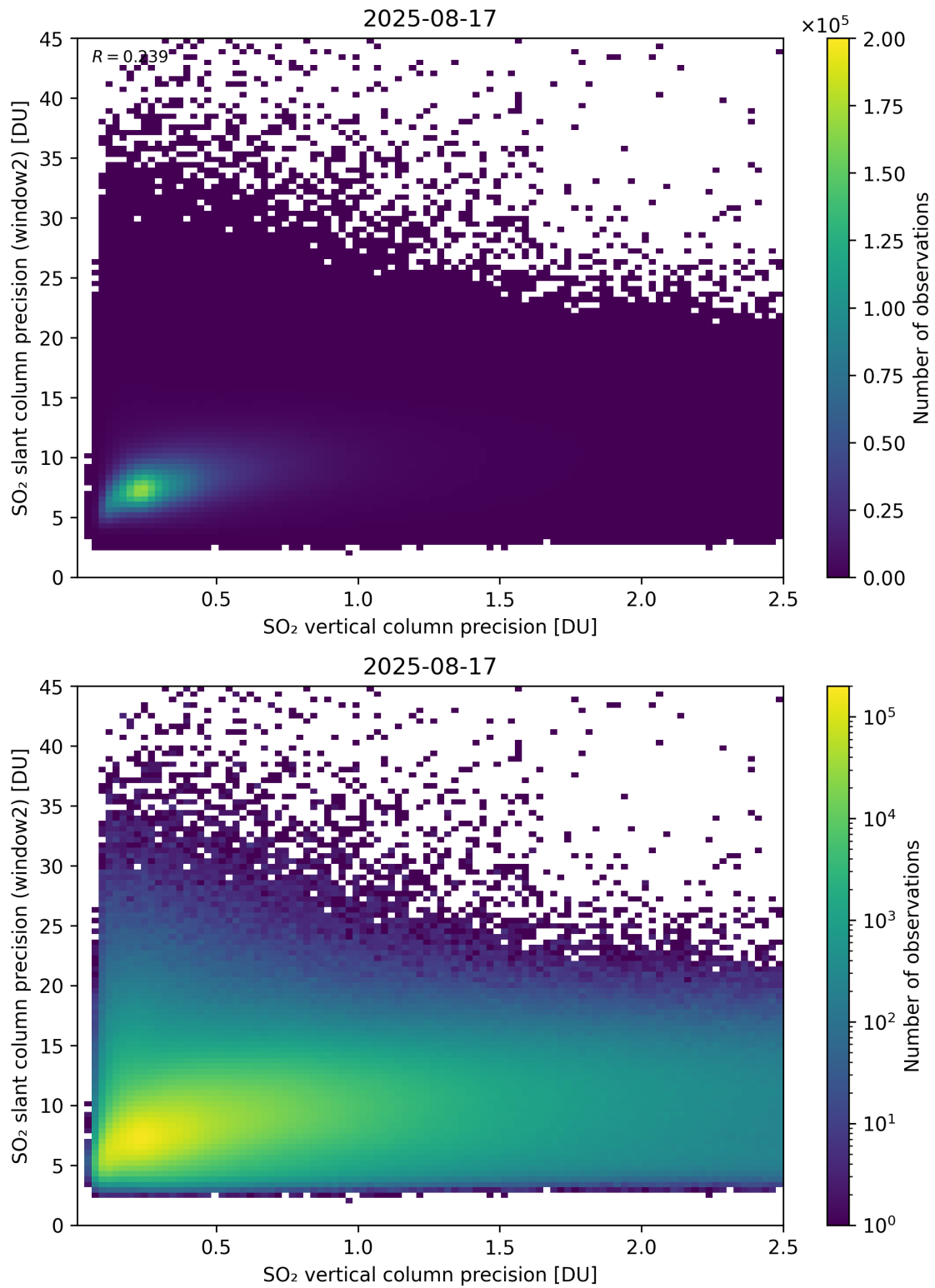
Figure 343: Scatter density plot of “SO 2 vertical column precision” against “SO 2 slant column precision (window2)” for 2025-08-16 to 2025-08-18.
