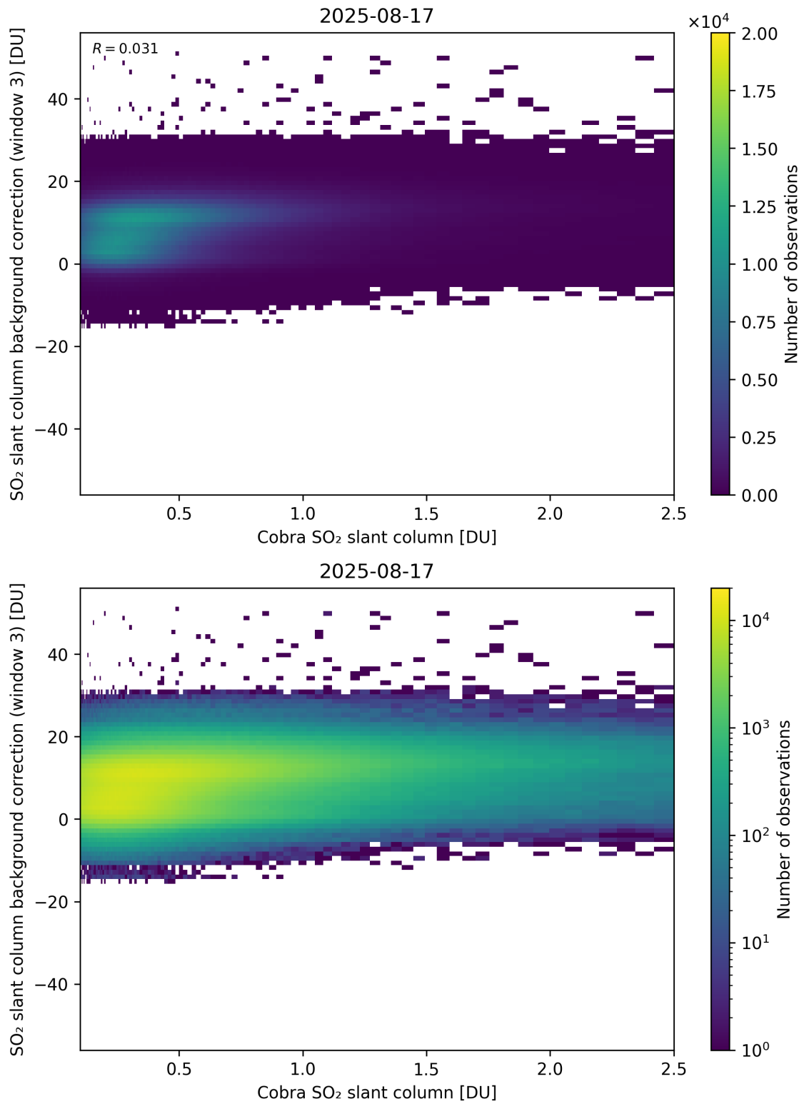
Figure 195: Scatter density plot of “Cobra SO 2 slant column” against “SO 2 slant column background correction (window 3)” for 2025-08-16 to 2025-08-18.
