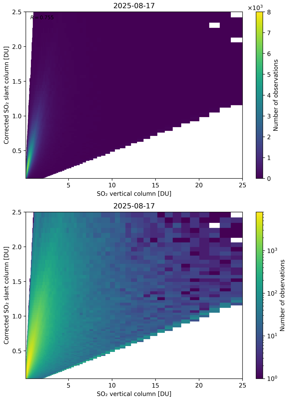
Figure 351: Scatter density plot of “SO 2 vertical column” against “Corrected SO 2 slant column” for 2025-08-16 to 2025-08-18.
