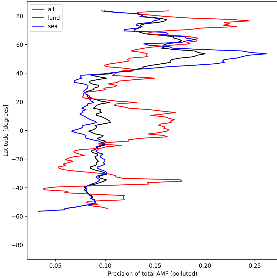
Figure 54: Zonal average of “Precision of total AMF (polluted)” for 2025-08-16 to 2025-08-18.
