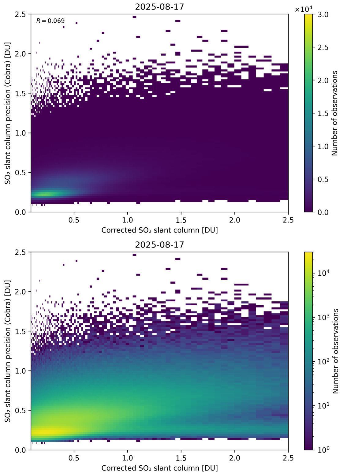
Figure 234: Scatter density plot of “Corrected SO 2 slant column” against “SO 2 slant column precision (Cobra)” for 2025-08-16 to 2025-08-18.
