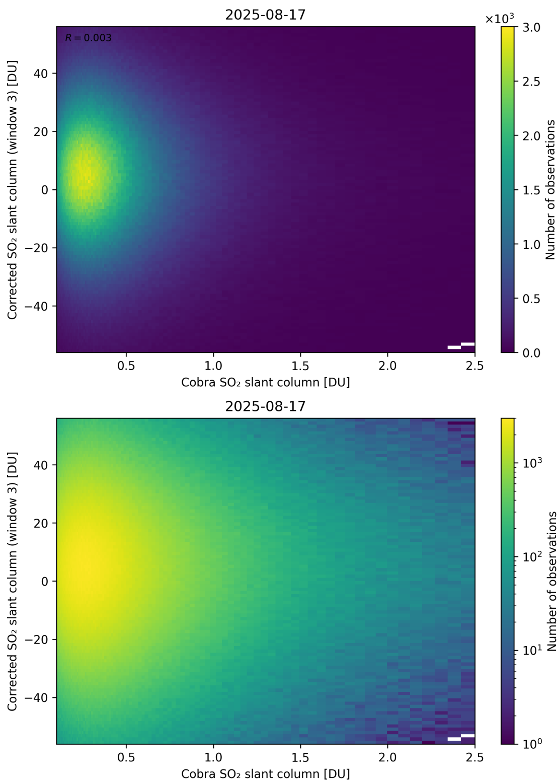
Figure 218: Scatter density plot of “Cobra SO 2 slant column” against “Corrected SO 2 slant column (window 3)” for 2025-08-16 to 2025-08-18.
