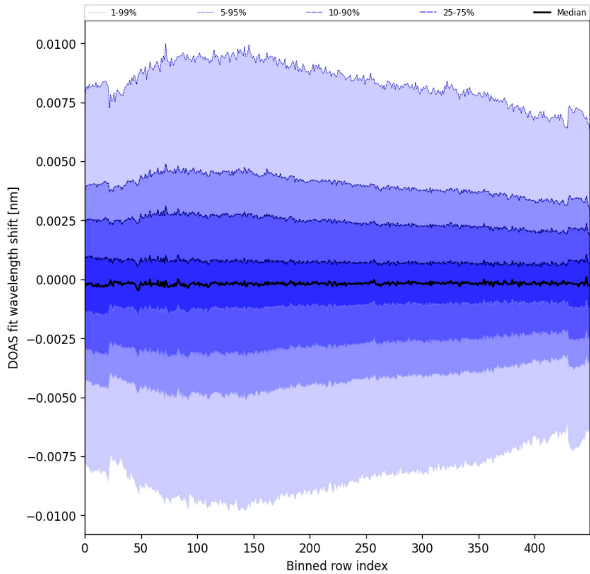
Figure 102: Along track statistics of “DOAS fit wavelength shift” for 2025-08-16 to 2025-08-18
