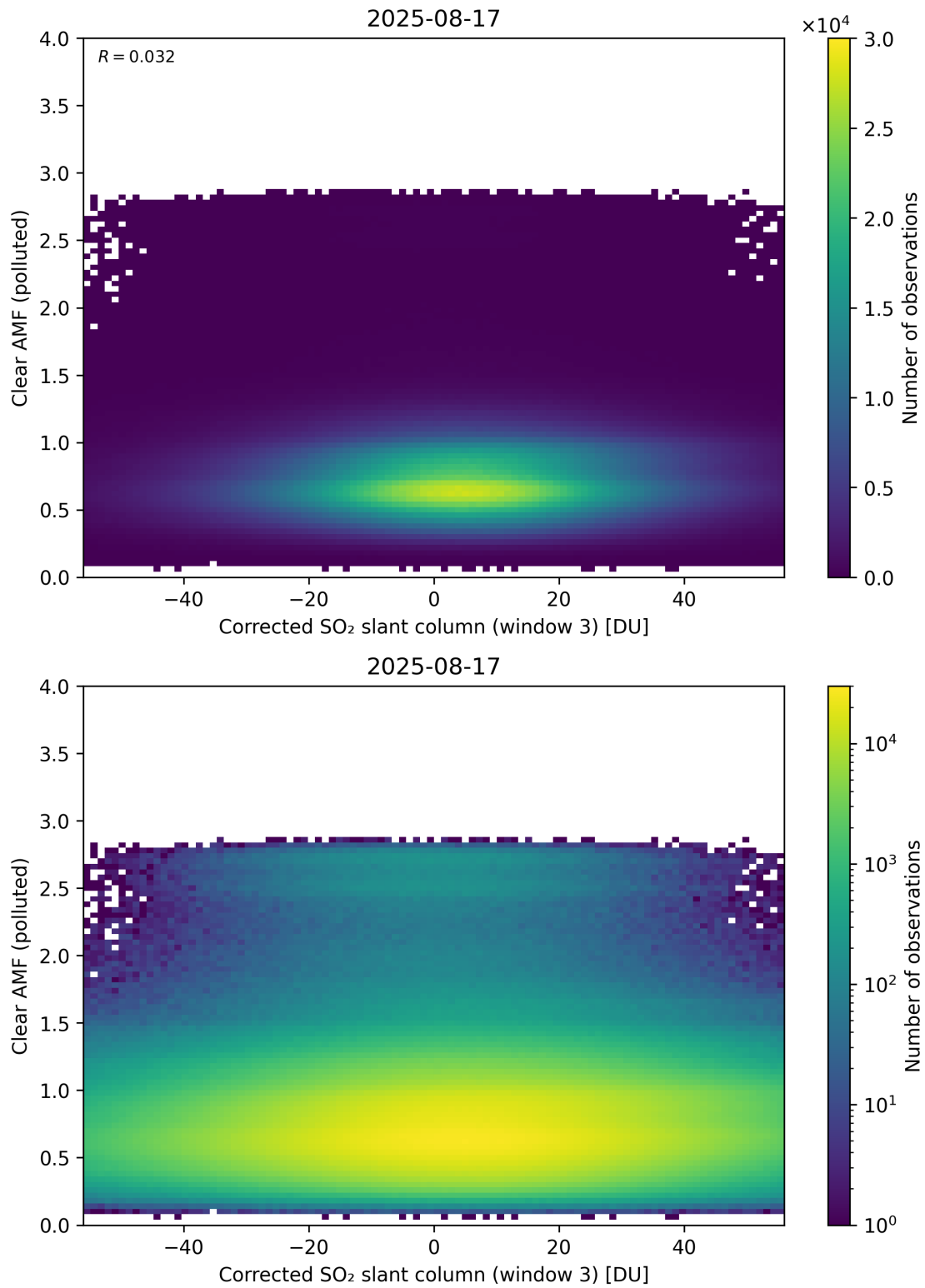
Figure 259: Scatter density plot of “Corrected SO 2 slant column (window 3)” against “Clear AMF (polluted)” for 2025-08-16 to 2025-08-18.
