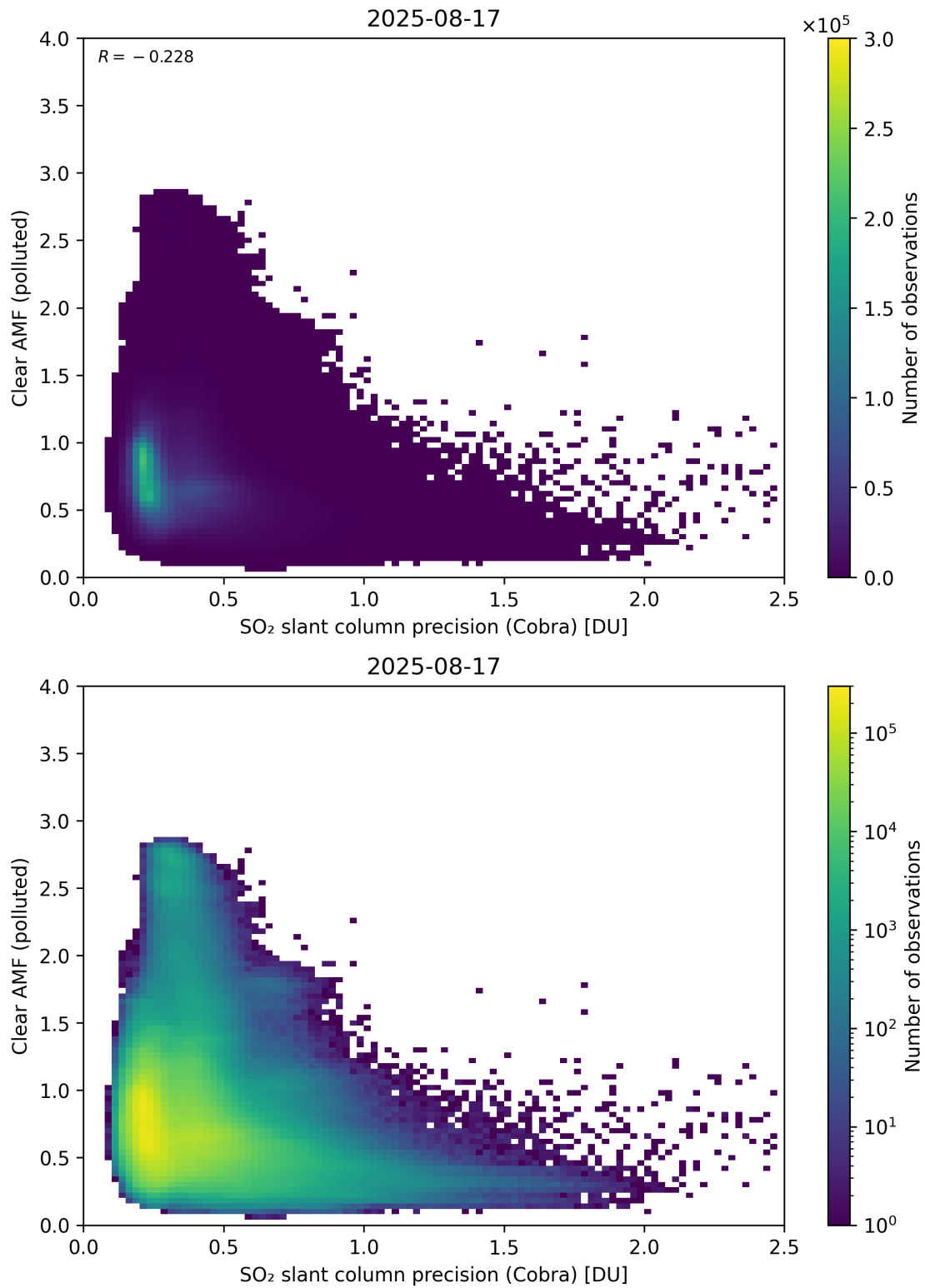
Figure 205: Scatter density plot of “SO 2 slant column precision (Cobra)” against “Clear AMF (polluted)” for 2025-08-16 to 2025-08-18.
