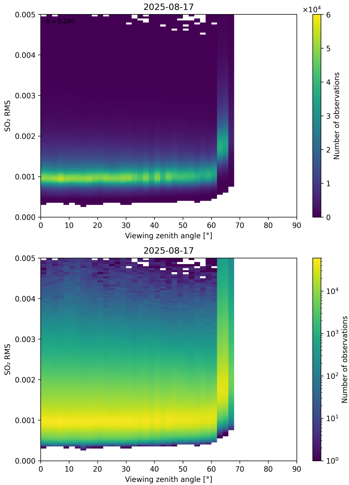
Figure 367: Scatter density plot of “Viewing zenith angle” against “SO 2 RMS” for 2025-08-16 to 2025-08-18.
