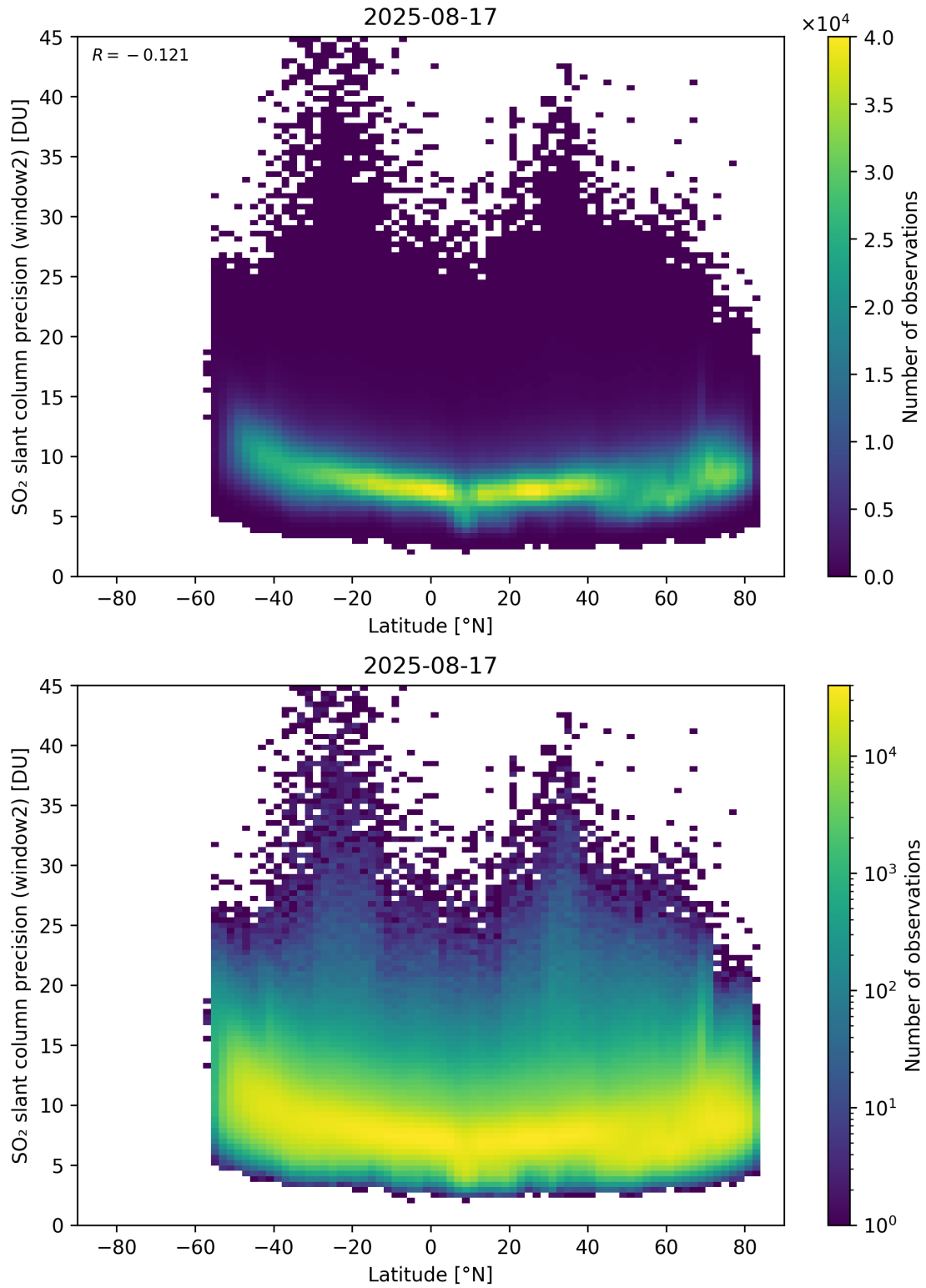
Figure 164: Scatter density plot of “Latitude” against “SO 2 slant column precision (window2)” for 2025-08-16 to 2025-08-18.
