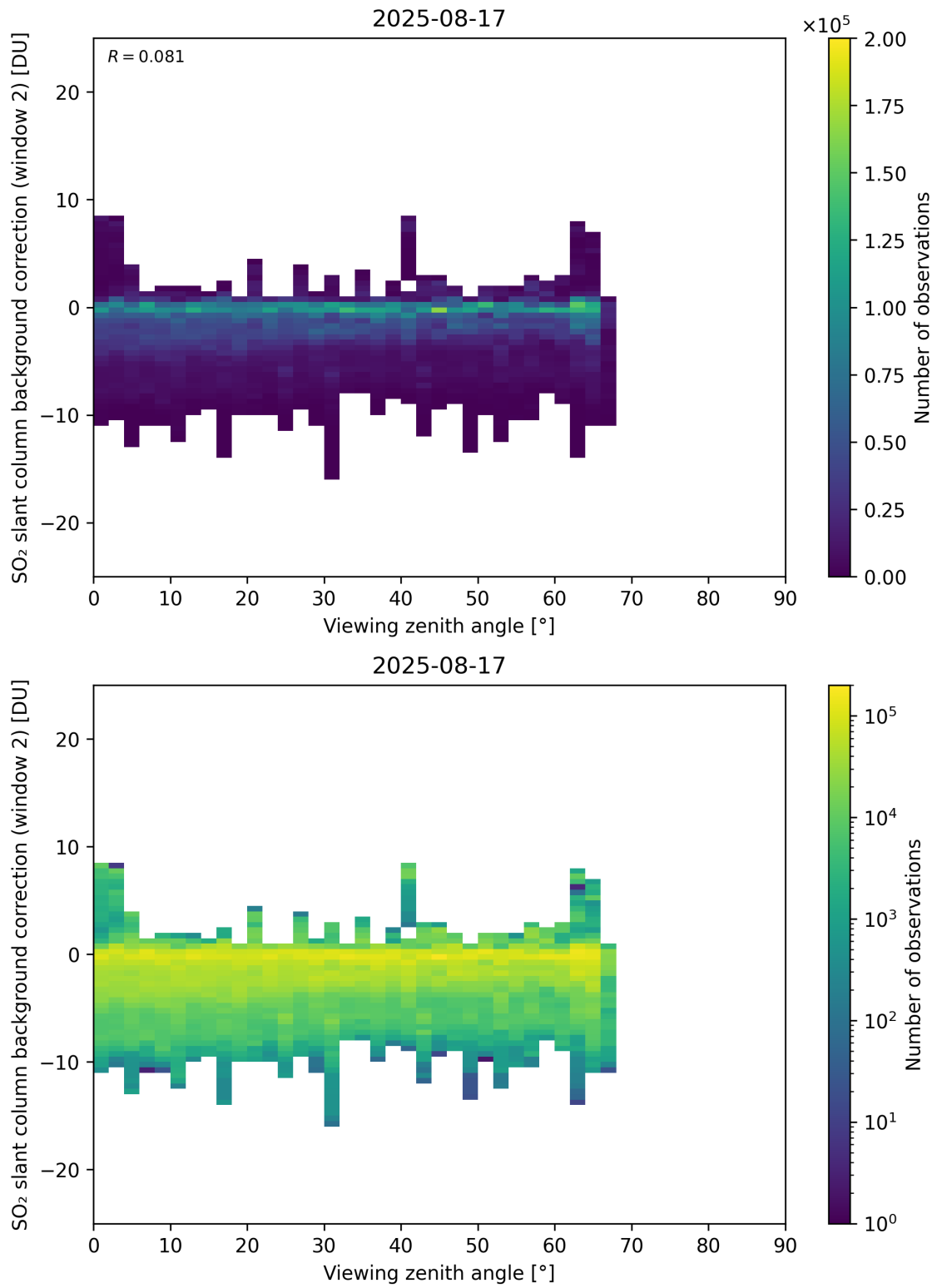
Figure 363: Scatter density plot of “Viewing zenith angle” against “SO 2 slant column background correction (window 2)” for 2025-08-16 to 2025-08-18.
