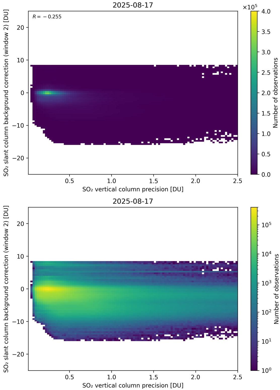
Figure 330: Scatter density plot of “SO 2 vertical column precision” against “SO 2 slant column background correction (window 2)” for 2025-08-16 to 2025-08-18.
