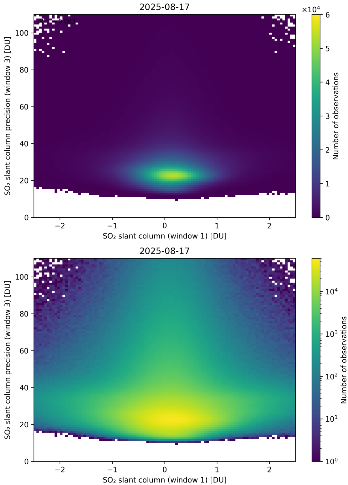
Figure 288: Scatter density plot of “SO 2 slant column (window 1)” against “SO 2 slant column precision (window 3)” for 2025-08-16 to 2025-08-18.
