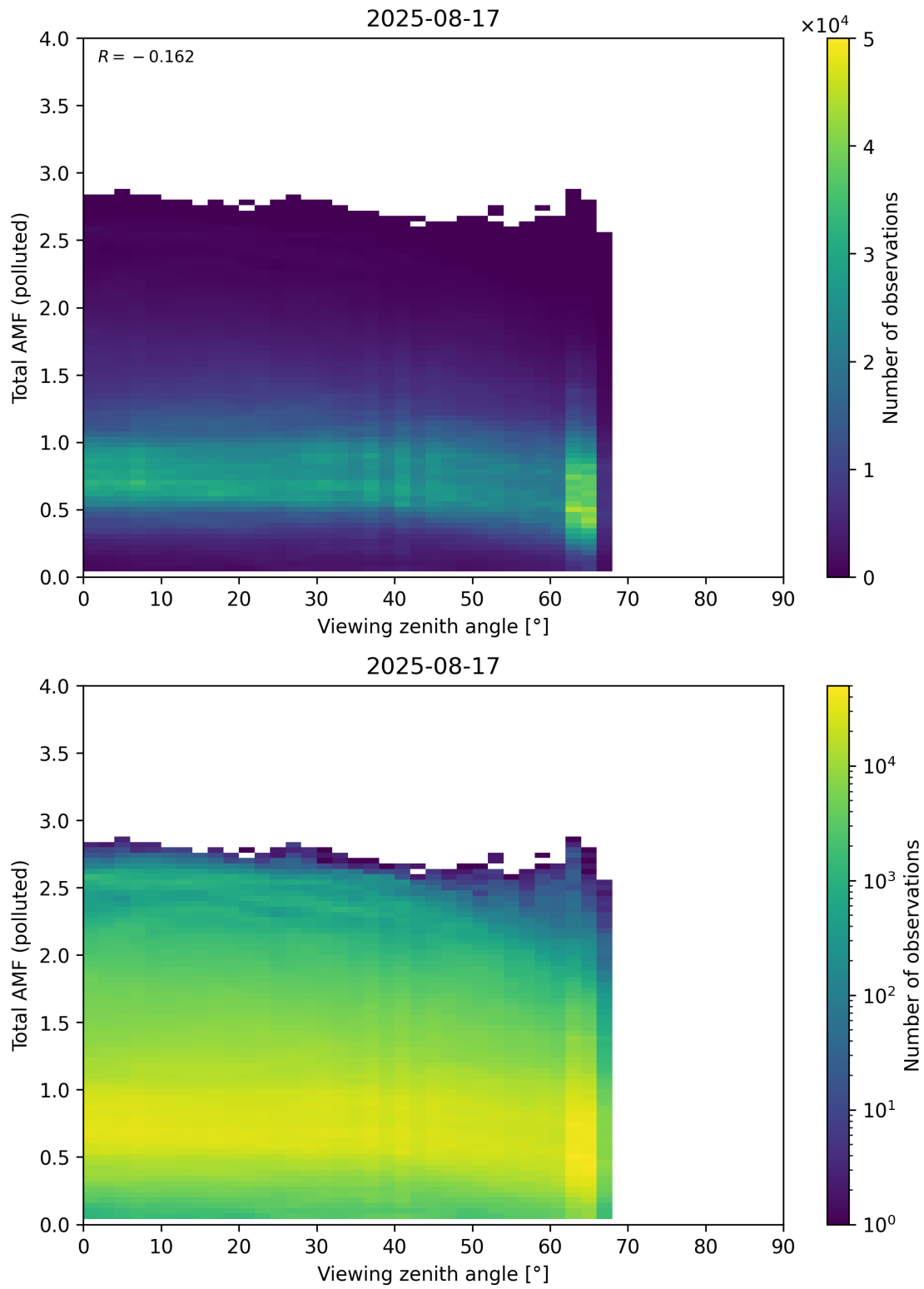
Figure 381: Scatter density plot of “Viewing zenith angle” against “Total AMF (polluted)” for 2025-08-16 to 2025-08-18.
