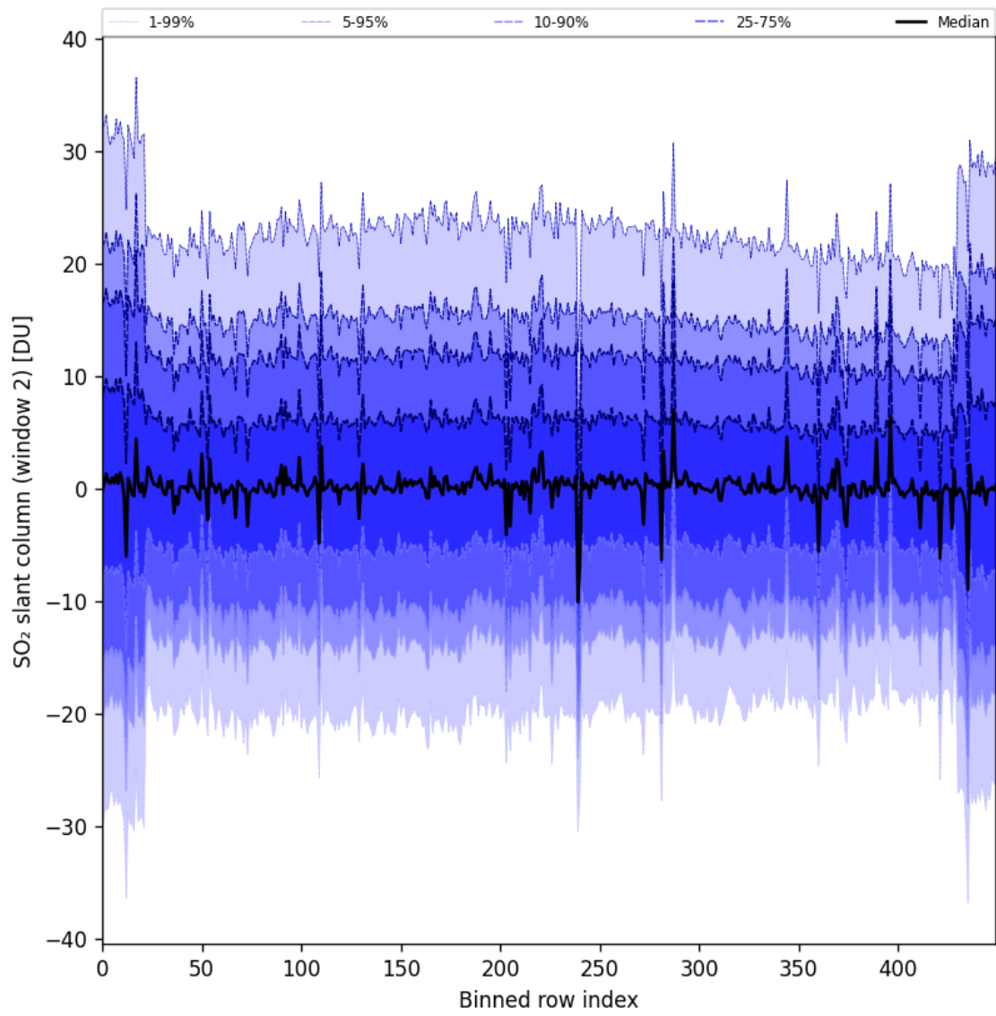
Figure 93: Along track statistics of “SO 2 slant column (window 2)” for 2025-08-16 to 2025-08-18
