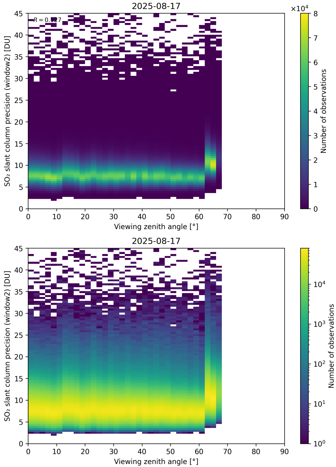
Figure 378: Scatter density plot of “Viewing zenith angle” against “SO 2 slant column precision (window2)” for 2025-08-16 to 2025-08-18.
