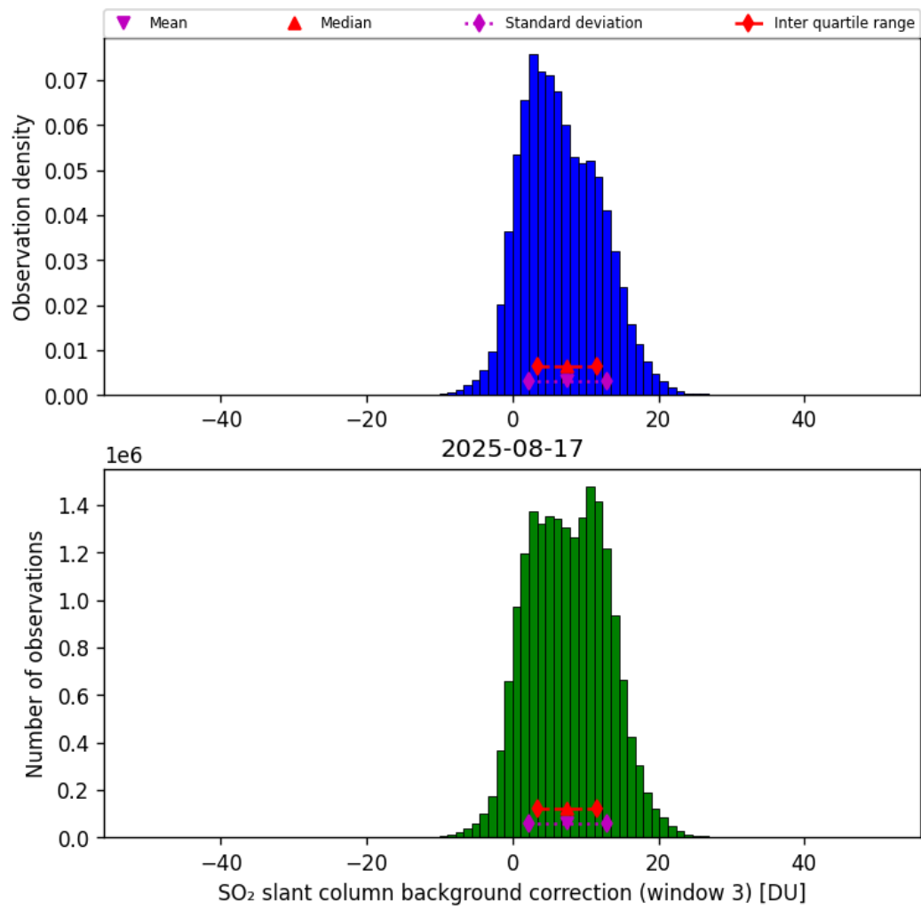
Figure 74: Histogram of “SO 2 slant column background correction (window 3)” for 2025-08-16 to 2025-08-18
