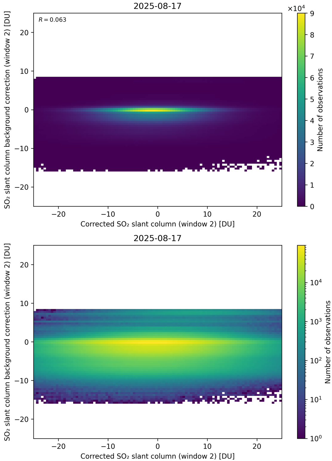
Figure 244: Scatter density plot of “Corrected SO 2 slant column (window 2)” against “SO 2 slant column background correction (window 2)” for 2025-08-16 to 2025-08-18.
