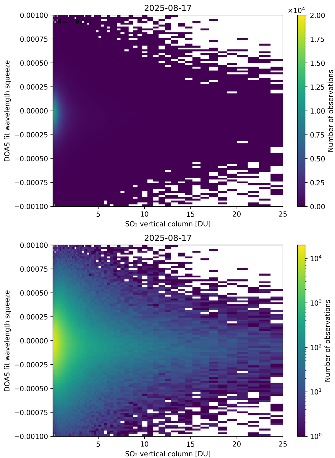
Figure 327: Scatter density plot of “SO 2 vertical column” against “DOAS fit wavelength squeeze” for 2025-08-16 to 2025-08-18.
