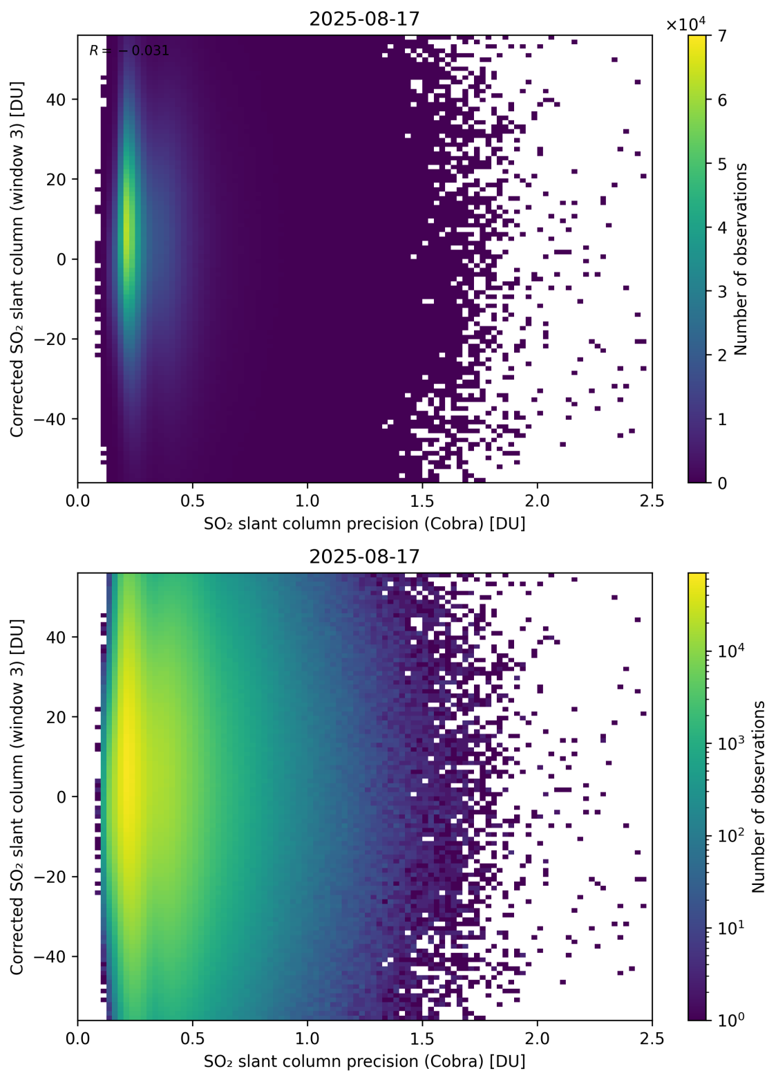
Figure 207: Scatter density plot of “SO 2 slant column precision (Cobra)” against “Corrected SO 2 slant column (window 3)” for 2025-08-16 to 2025-08-18.
