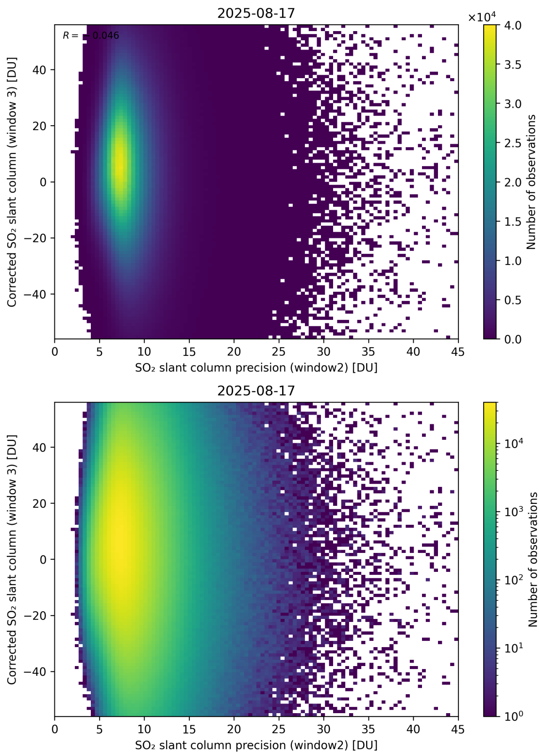
Figure 298: Scatter density plot of “SO 2 slant column precision (window2)” against “Corrected SO 2 slant column (window 3)” for 2025-08-16 to 2025-08-18.
