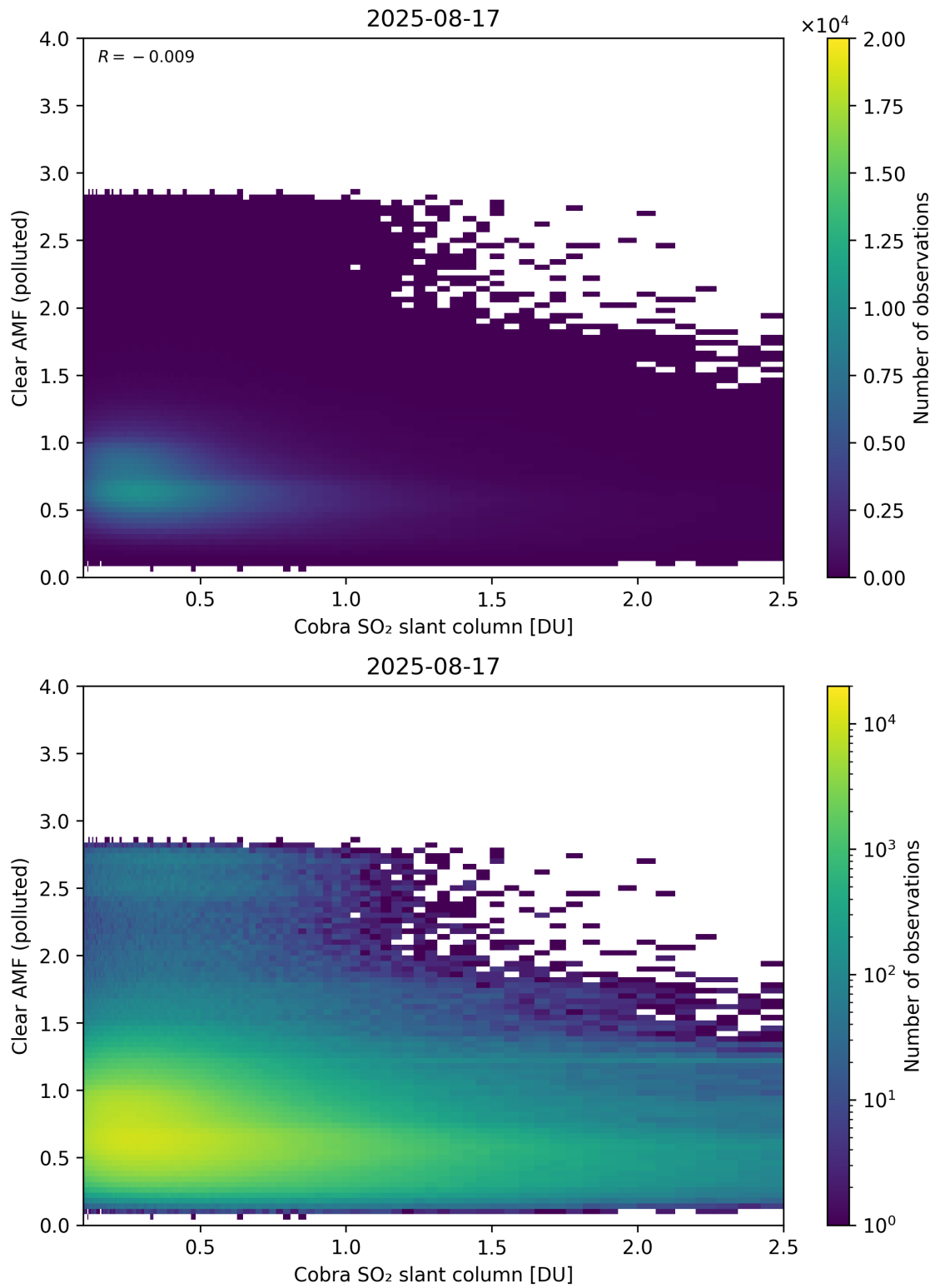
Figure 215: Scatter density plot of “Cobra SO 2 slant column” against “Clear AMF (polluted)” for 2025-08-16 to 2025-08-18.
