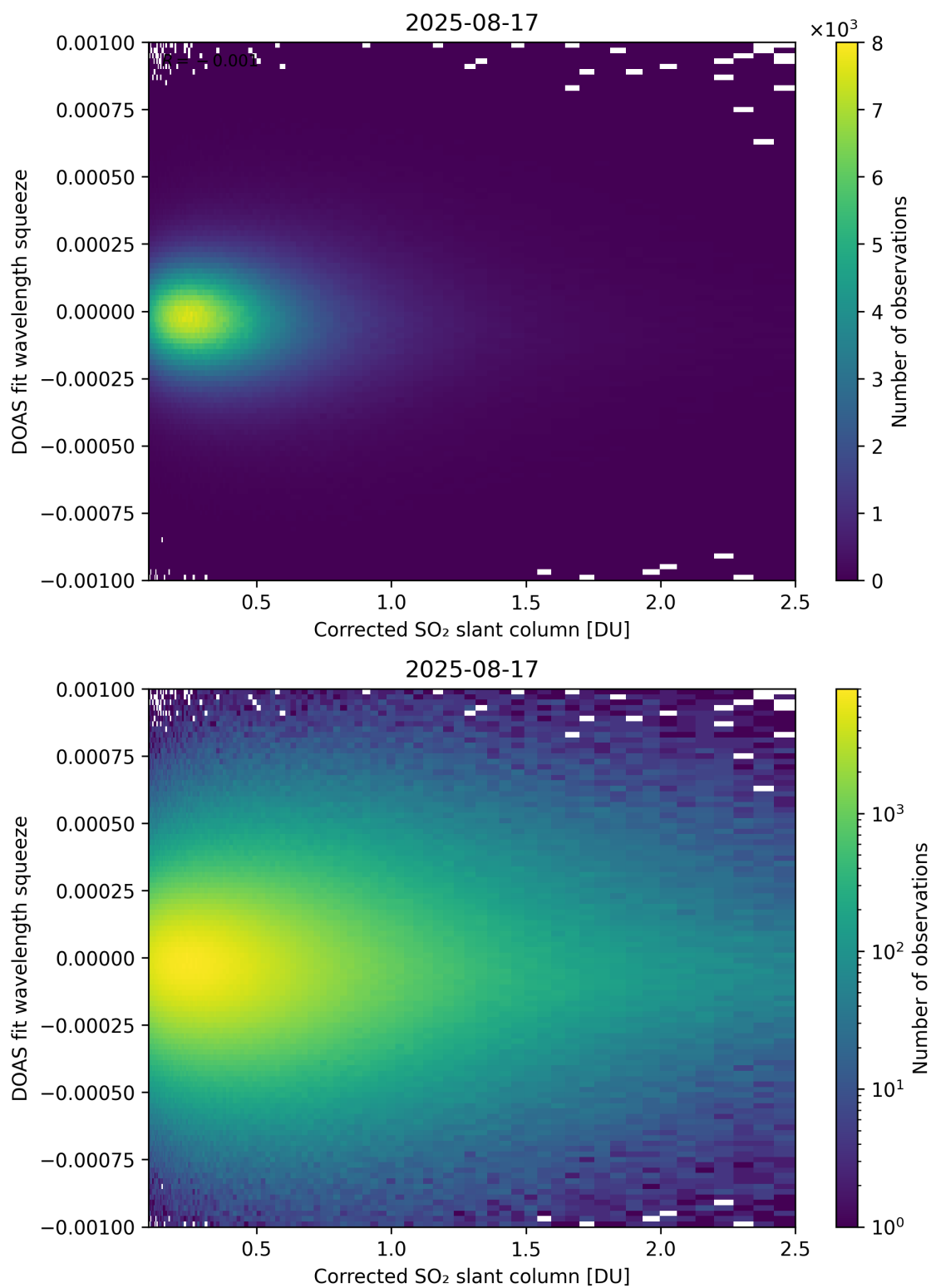
Figure 230: Scatter density plot of “Corrected SO 2 slant column” against “DOAS fit wavelength squeeze” for 2025-08-16 to 2025-08-18.
