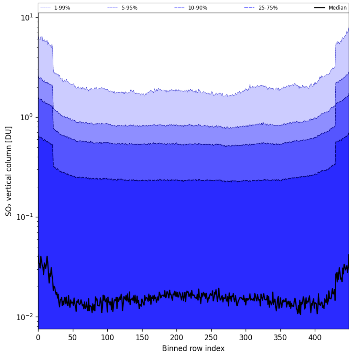
Figure 84: Along track statistics of “SO 2 vertical column” for 2025-08-16 to 2025-08-18
