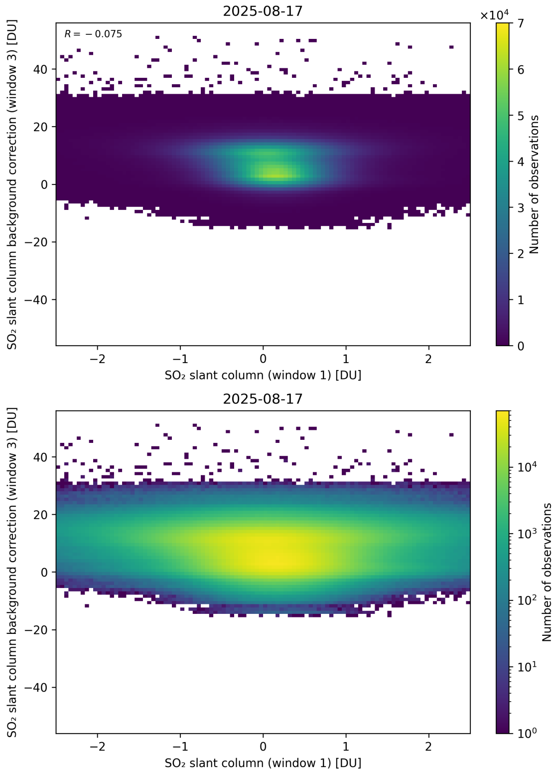
Figure 264: Scatter density plot of “SO 2 slant column (window 1)” against “SO 2 slant column background correction (window 3)” for 2025-08-16 to 2025-08-18.
