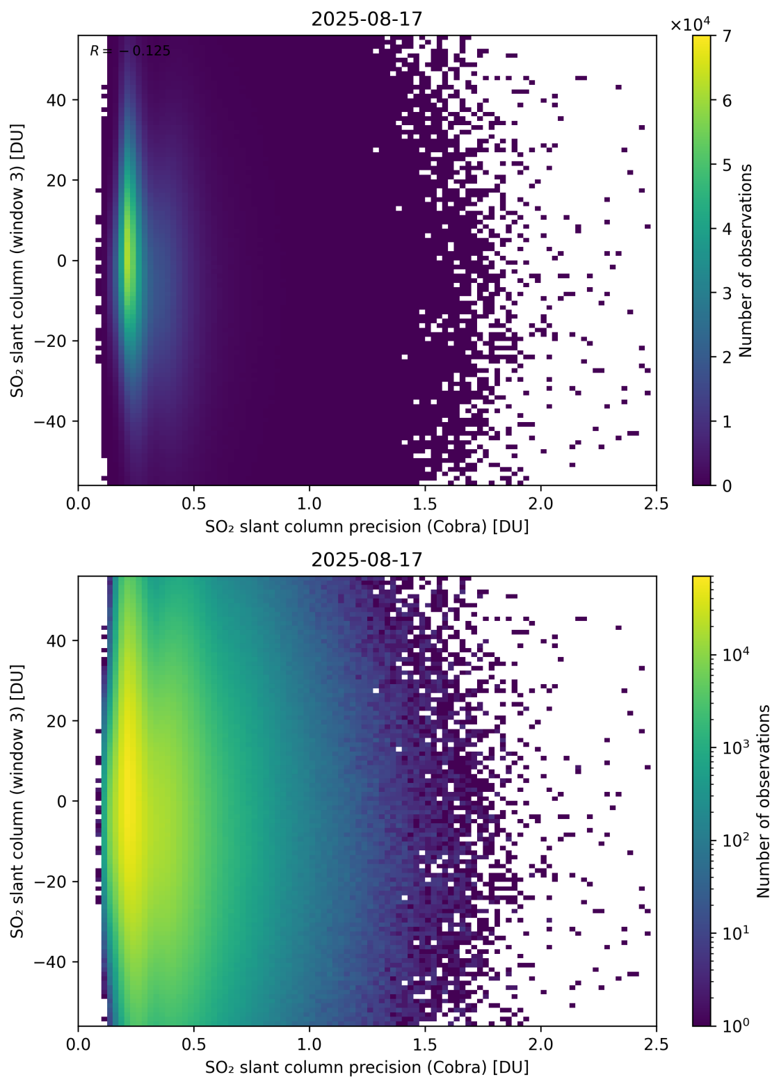
Figure 211: Scatter density plot of “SO 2 slant column precision (Cobra)” against “SO 2 slant column (window 3)” for 2025-08-16 to 2025-08-18.
