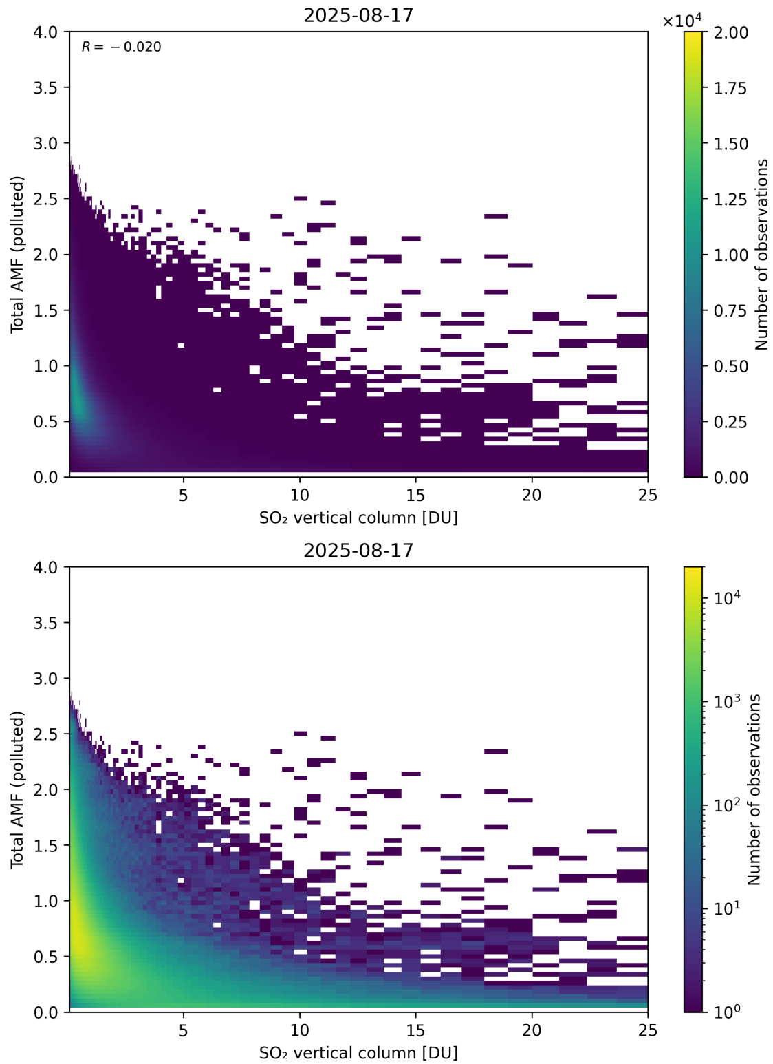
Figure 359: Scatter density plot of “SO 2 vertical column” against “Total AMF (polluted)” for 2025-08-16 to 2025-08-18.
