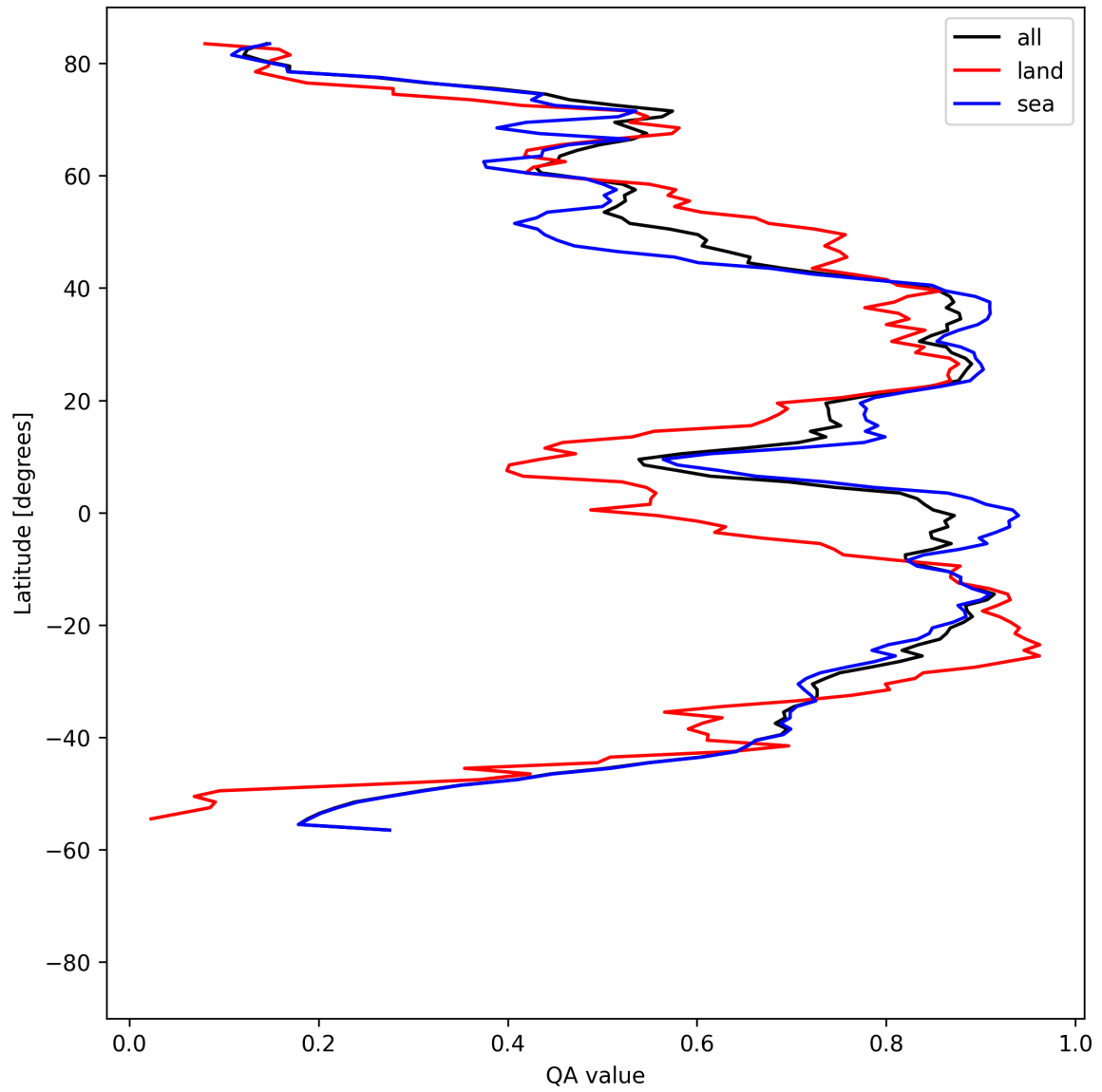
Figure 31: Zonal average of “QA value” for 2025-08-16 to 2025-08-18.
