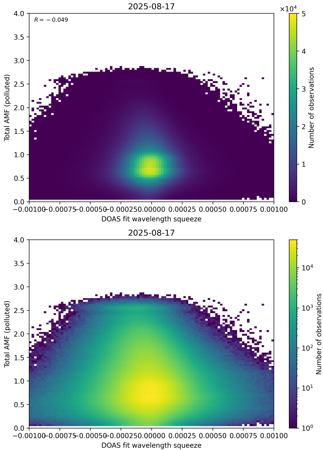
Figure 145: Scatter density plot of “DOAS fit wavelength squeeze” against “Total AMF (polluted)” for 2025-08-16 to 2025-08-18.
