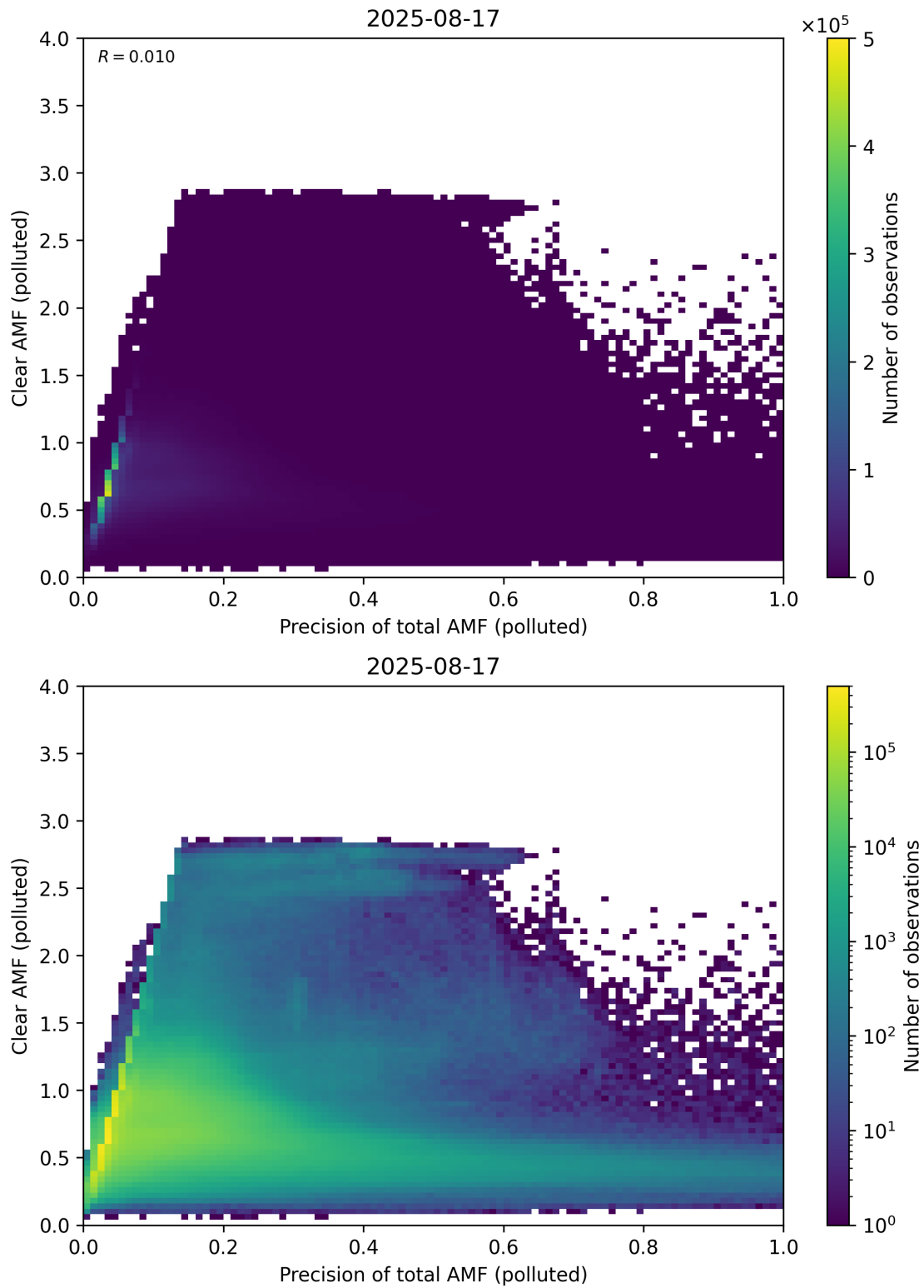
Figure 320: Scatter density plot of “Precision of total AMF (polluted)” against “Clear AMF (polluted)” for 2025-08-16 to 2025-08-18.
