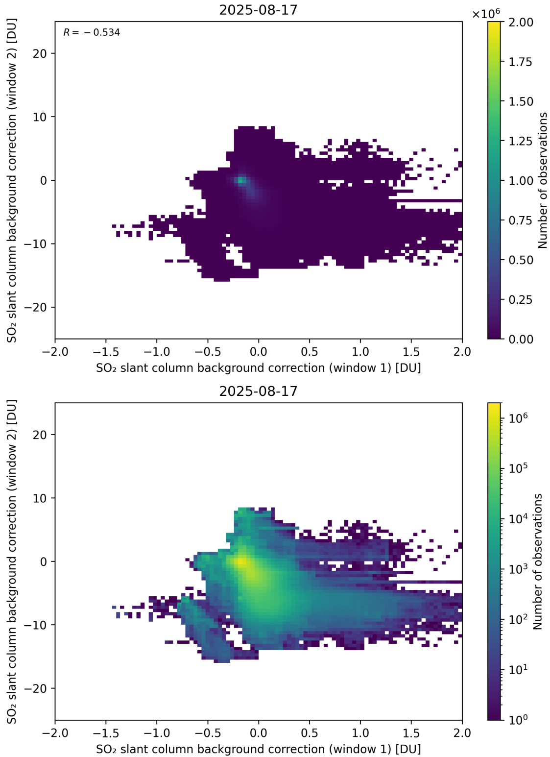
Figure 109: Scatter density plot of “SO 2 slant column background correction (window 1)” against “SO 2 slant column background correction (window 2)” for 2025-08-16 to 2025-08-18.
