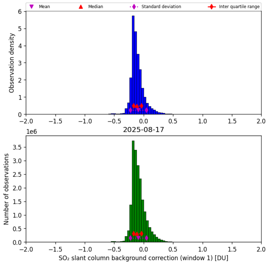
Figure 66: Histogram of “SO 2 slant column background correction (window 1)” for 2025-08-16 to 2025-08-18
