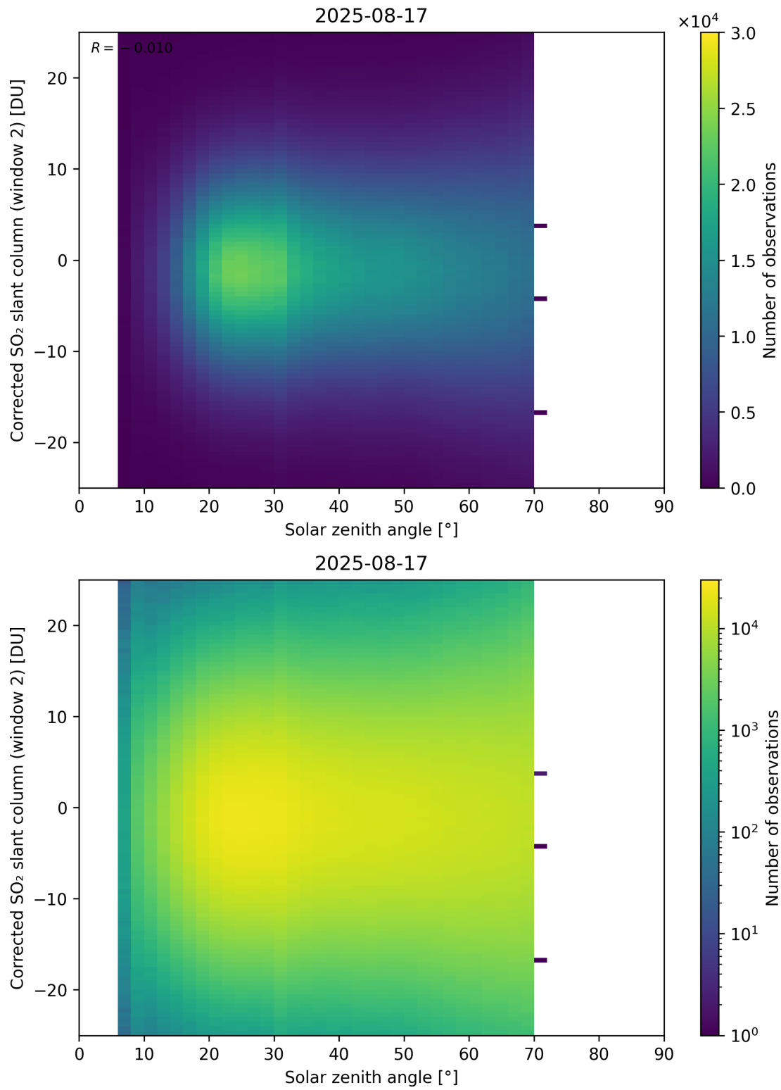
Figure 182: Scatter density plot of “Solar zenith angle” against “Corrected SO 2 slant column (window 2)” for 2025-08-16 to 2025-08-18.
