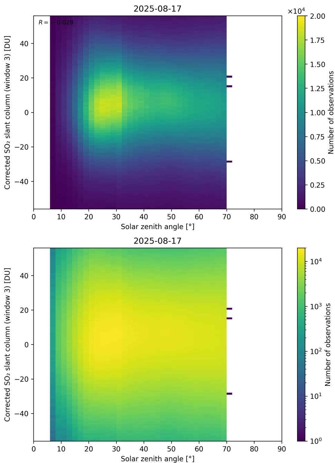
Figure 183: Scatter density plot of “Solar zenith angle” against “Corrected SO 2 slant column (window 3)” for 2025-08-16 to 2025-08-18.
