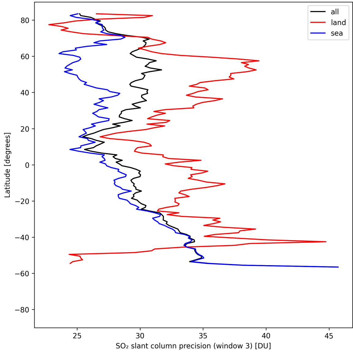
Figure 46: Zonal average of “SO 2 slant column precision (window 3)” for 2025-08-16 to 2025-08-18.
