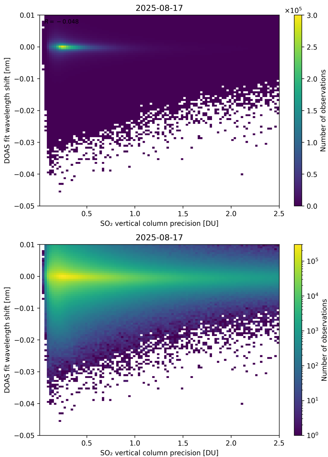
Figure 332: Scatter density plot of “SO 2 vertical column precision” against “DOAS fit wavelength shift” for 2025-08-16 to 2025-08-18.
