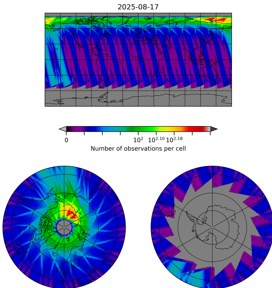
Figure 30: Map of the number of observations for 2025-08-16 to 2025-08-18
