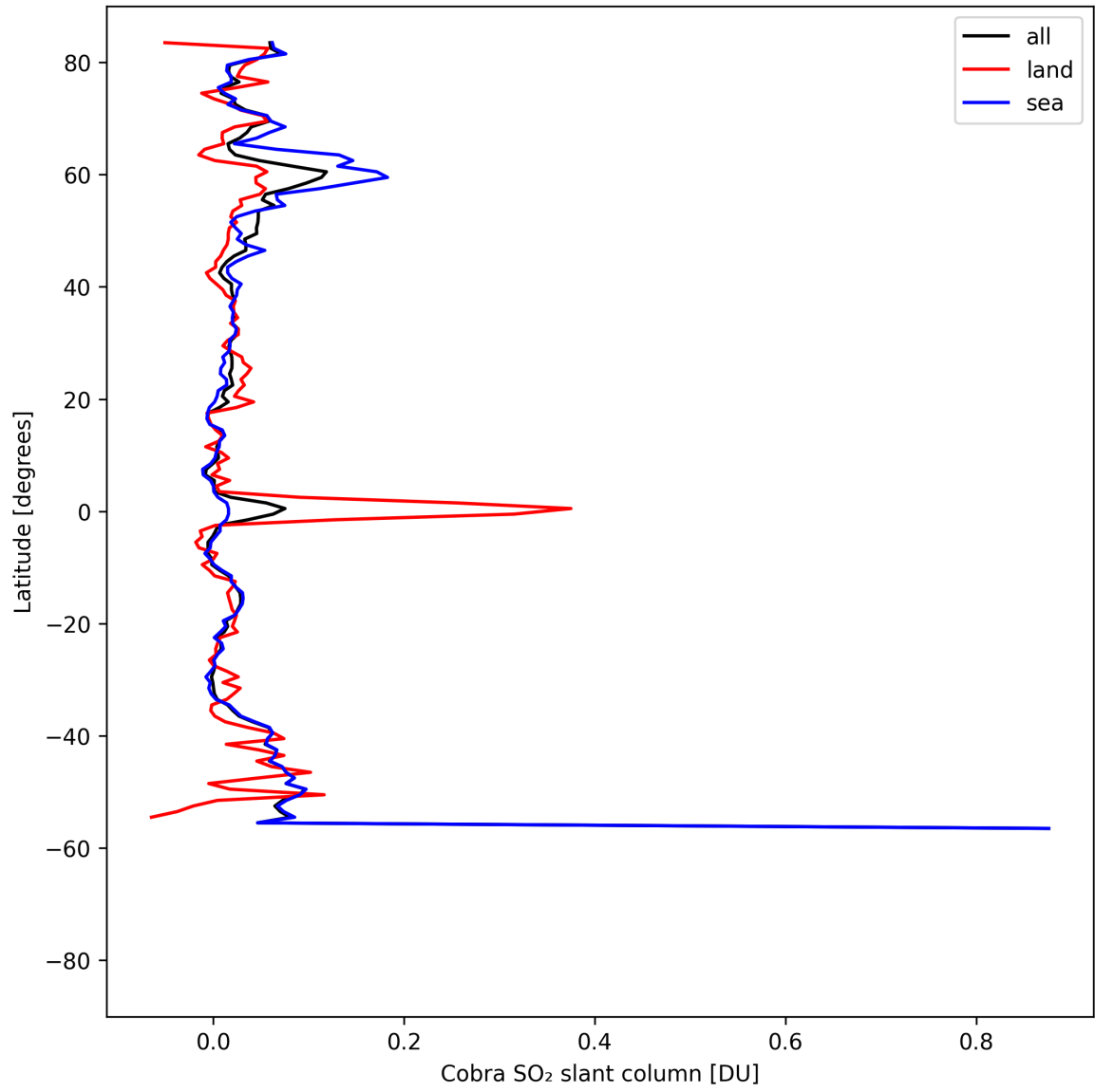
Figure 35: Zonal average of “Cobra SO 2 slant column” for 2025-08-16 to 2025-08-18.
