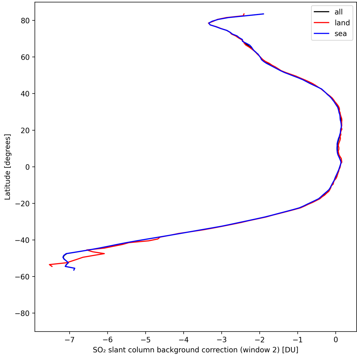
Figure 44: Zonal average of “SO 2 slant column background correction (window 2)” for 2025-08-16 to 2025-08-18.
