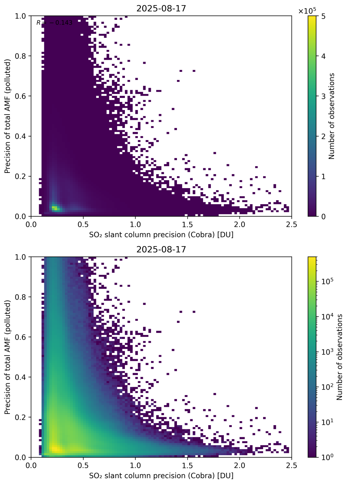
Figure 214: Scatter density plot of “SO 2 slant column precision (Cobra)” against “Precision of total AMF (polluted)” for 2025-08-16 to 2025-08-18.
