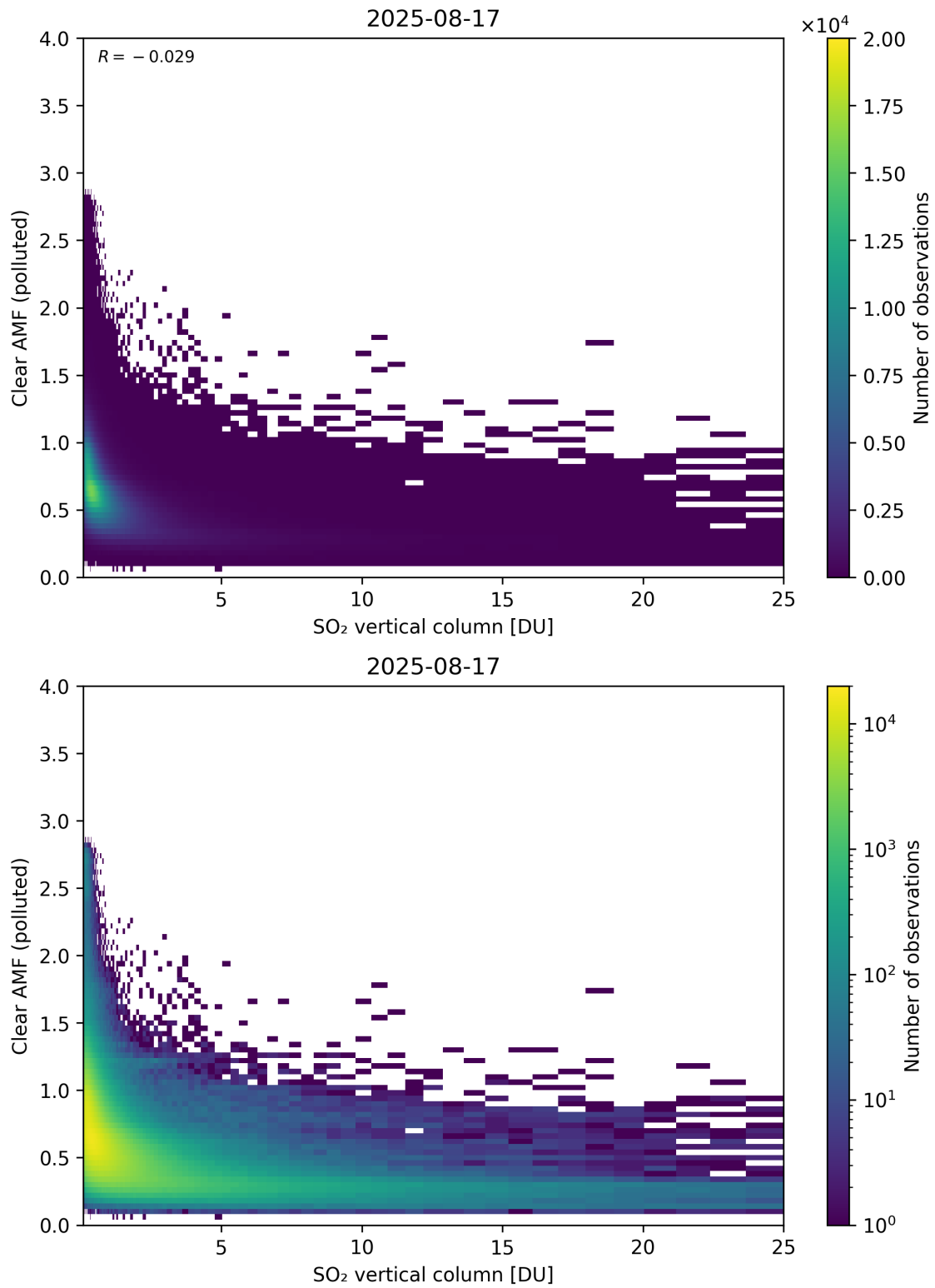
Figure 348: Scatter density plot of “SO 2 vertical column” against “Clear AMF (polluted)” for 2025-08-16 to 2025-08-18.
