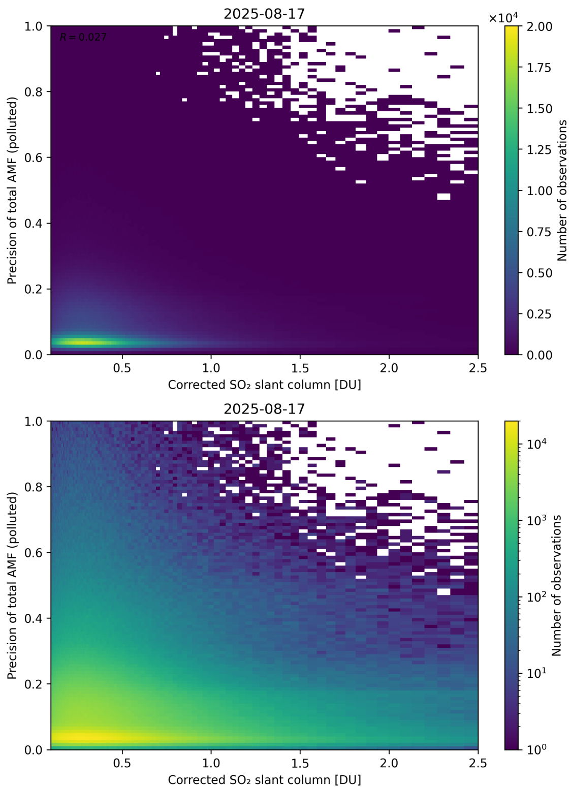
Figure 243: Scatter density plot of “Corrected SO 2 slant column” against “Precision of total AMF (polluted)” for 2025-08-16 to 2025-08-18.
