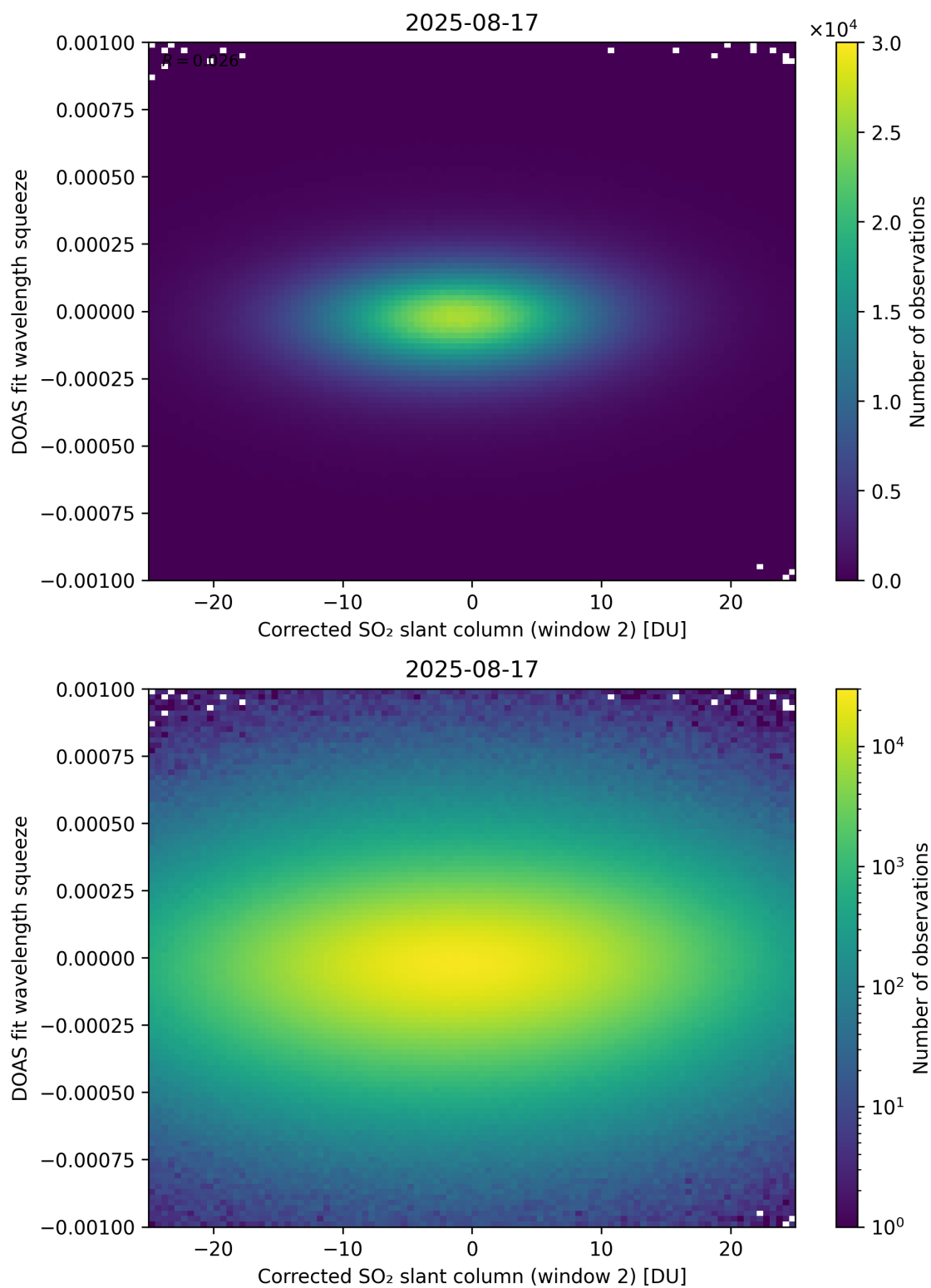
Figure 247: Scatter density plot of “Corrected SO 2 slant column (window 2)” against “DOAS fit wavelength squeeze” for 2025-08-16 to 2025-08-18.
