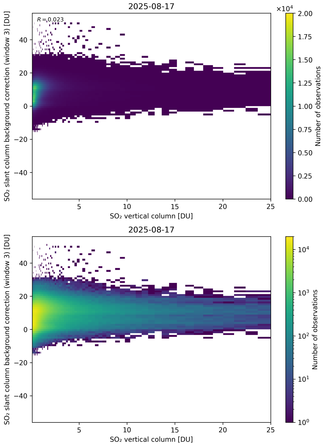
Figure 325: Scatter density plot of “SO 2 vertical column” against “SO 2 slant column background correction (window 3)” for 2025-08-16 to 2025-08-18.
