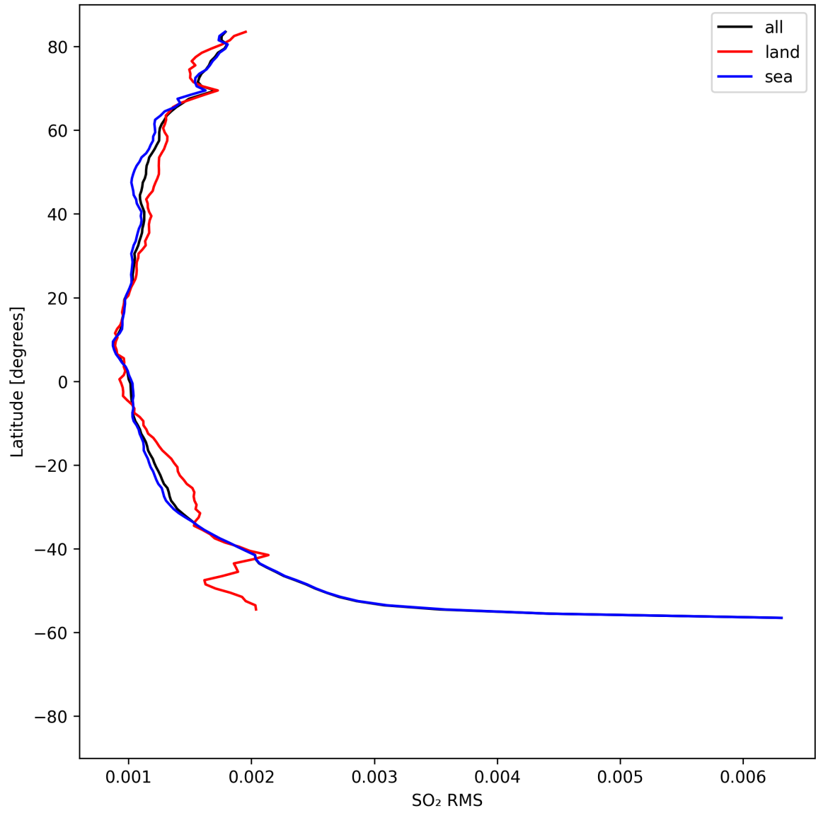
Figure 52: Zonal average of “SO 2 RMS” for 2025-08-16 to 2025-08-18.
