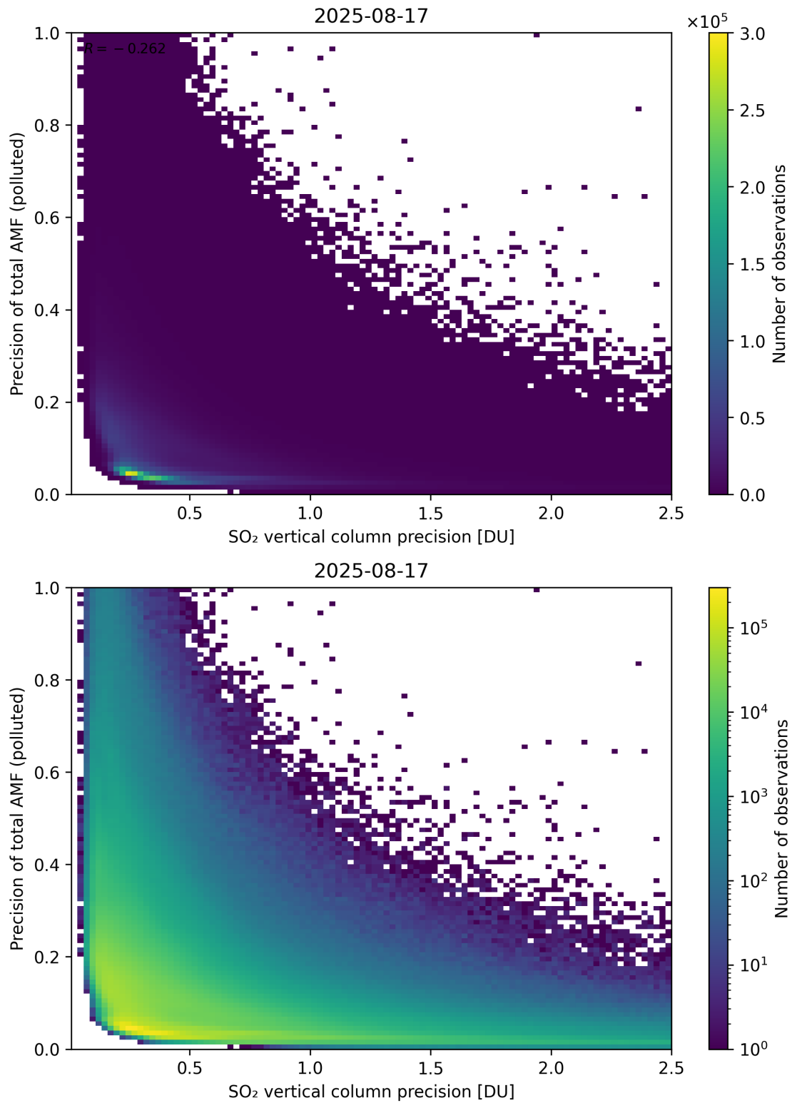
Figure 347: Scatter density plot of “SO 2 vertical column precision” against “Precision of total AMF (polluted)” for 2025-08-16 to 2025-08-18.
