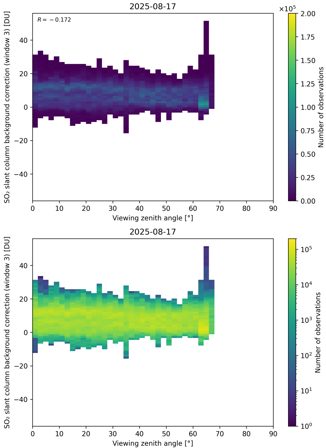
Figure 364: Scatter density plot of “Viewing zenith angle” against “SO 2 slant column background correction (window 3)” for 2025-08-16 to 2025-08-18.
