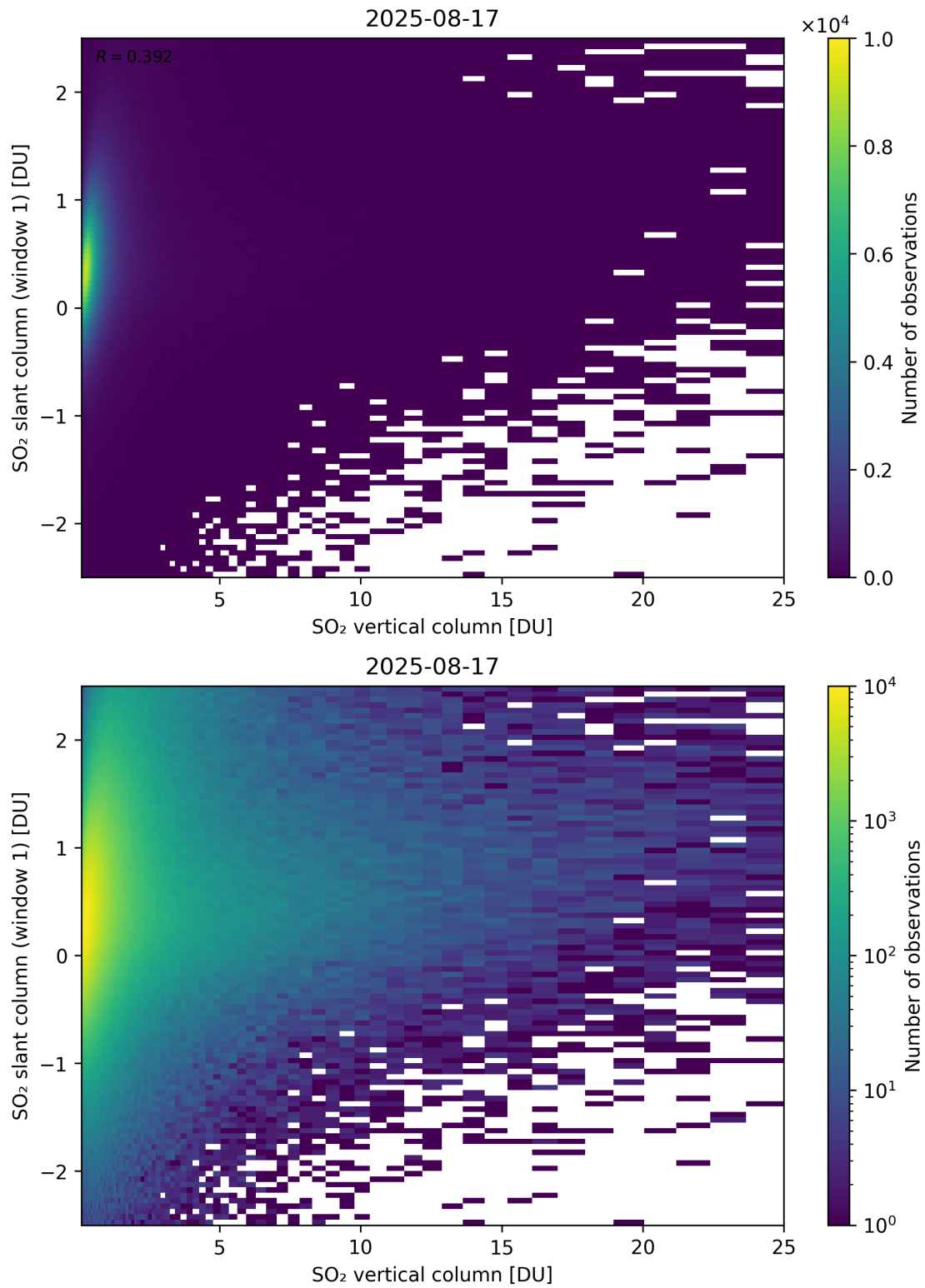
Figure 354: Scatter density plot of “SO 2 vertical column” against “SO 2 slant column (window 1)” for 2025-08-16 to 2025-08-18.
