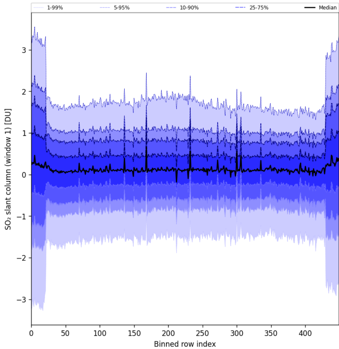
Figure 89: Along track statistics of “SO 2 slant column (window 1)” for 2025-08-16 to 2025-08-18
