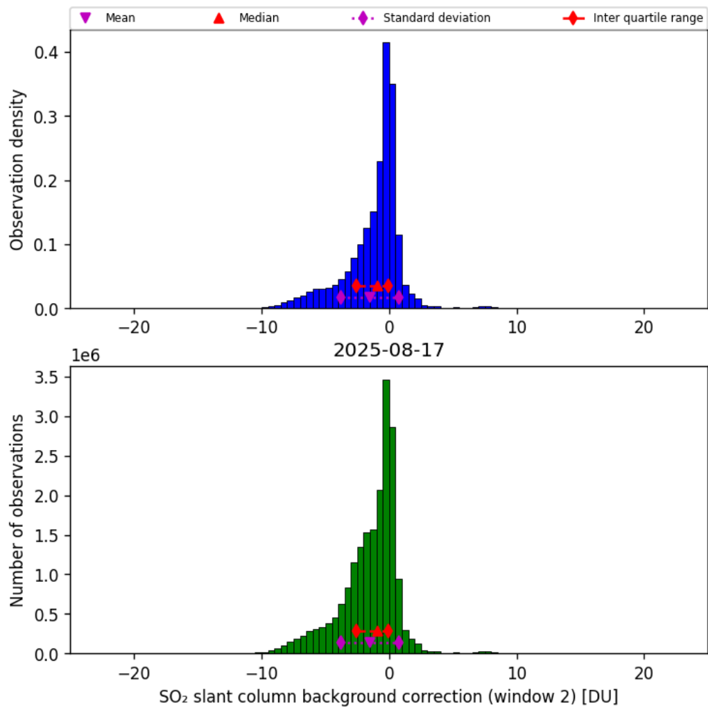
Figure 70: Histogram of “SO 2 slant column background correction (window 2)” for 2025-08-16 to 2025-08-18
