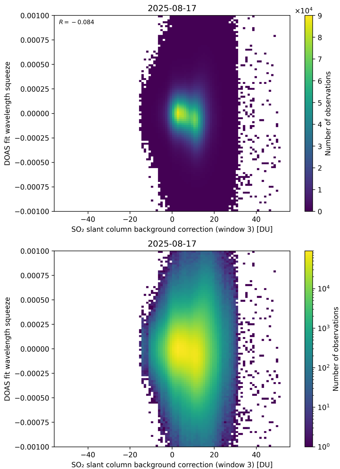
Figure 133: Scatter density plot of “SO 2 slant column background correction (window 3)” against “DOAS fit wavelength squeeze” for 2025-08-16 to 2025-08-18.
