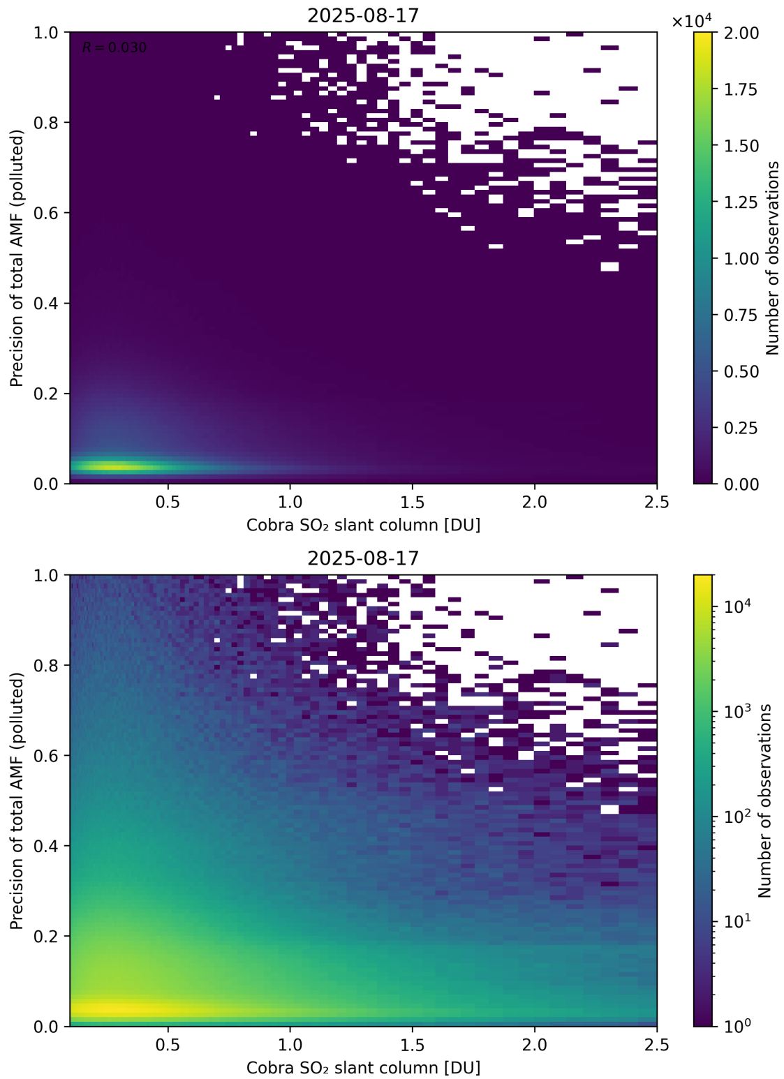
Figure 225: Scatter density plot of “Cobra SO 2 slant column” against “Precision of total AMF (polluted)” for 2025-08-16 to 2025-08-18.
