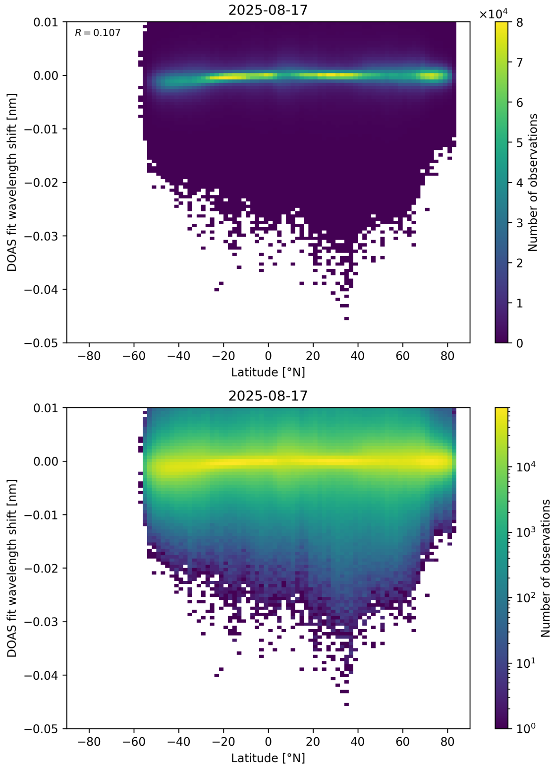
Figure 153: Scatter density plot of “Latitude” against “DOAS fit wavelength shift” for 2025-08-16 to 2025-08-18.
