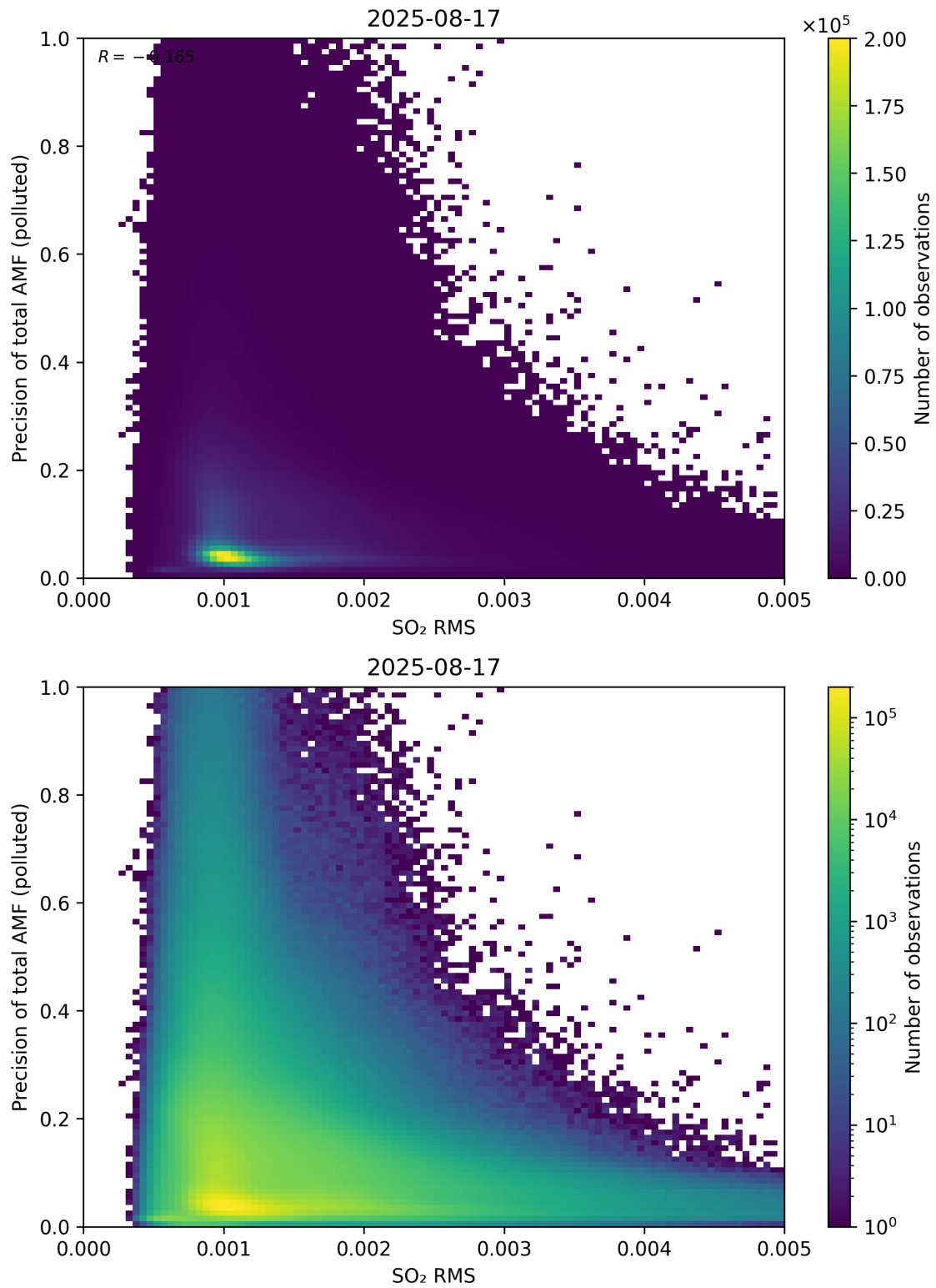
Figure 149: Scatter density plot of “SO 2 RMS” against “Precision of total AMF (polluted)” for 2025-08-16 to 2025-08-18.
