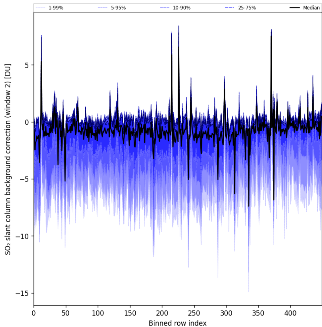
Figure 96: Along track statistics of “SO 2 slant column background correction (window 2)” for 2025-08-16 to 2025-08-18
