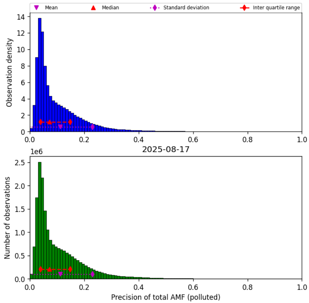
Figure 80: Histogram of “Precision of total AMF (polluted)” for 2025-08-16 to 2025-08-18
