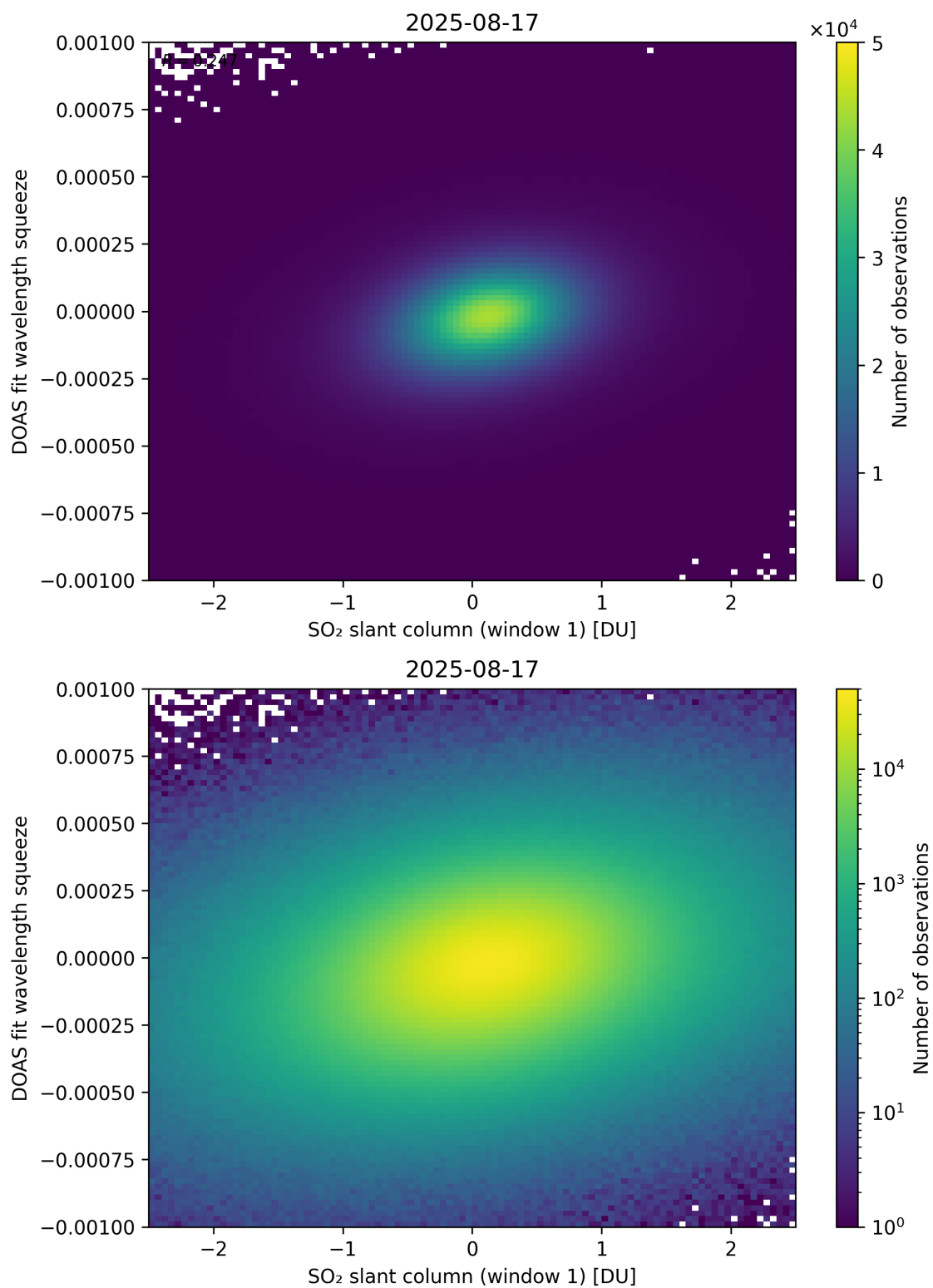
Figure 266: Scatter density plot of “SO 2 slant column (window 1)” against “DOAS fit wavelength squeeze” for 2025-08-16 to 2025-08-18.
