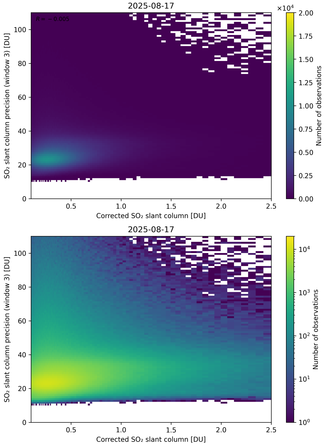
Figure 241: Scatter density plot of “Corrected SO 2 slant column” against “SO 2 slant column precision (window 3)” for 2025-08-16 to 2025-08-18.
