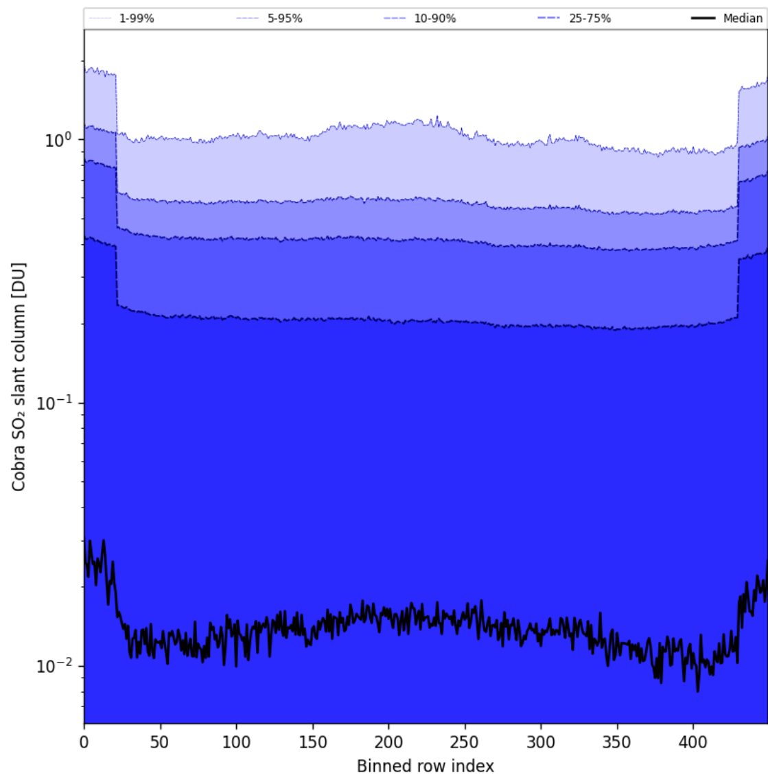
Figure 87: Along track statistics of “Cobra SO 2 slant column” for 2025-08-16 to 2025-08-18
