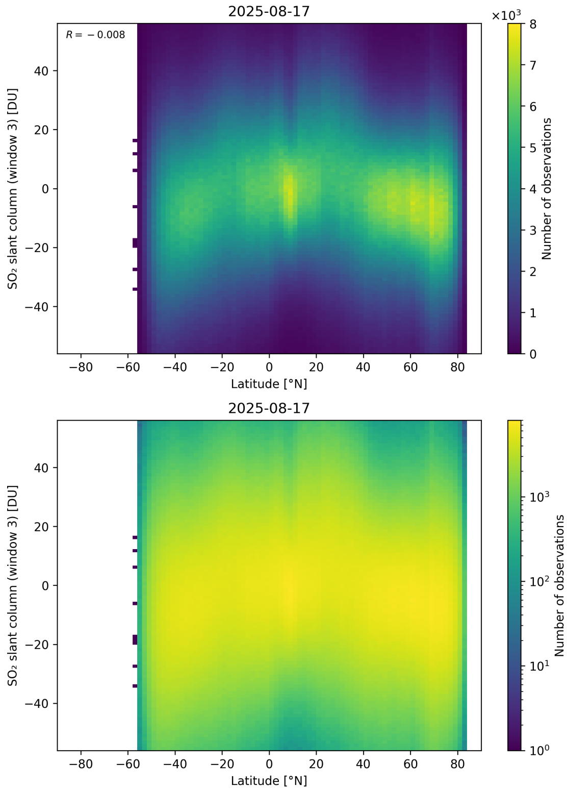
Figure 165: Scatter density plot of “Latitude” against “SO 2 slant column (window 3)” for 2025-08-16 to 2025-08-18.
