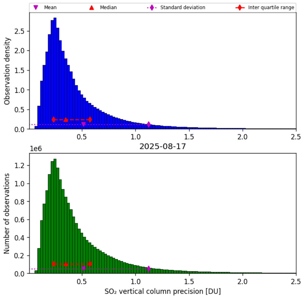
Figure 59: Histogram of “SO 2 vertical column precision” for 2025-08-16 to 2025-08-18
