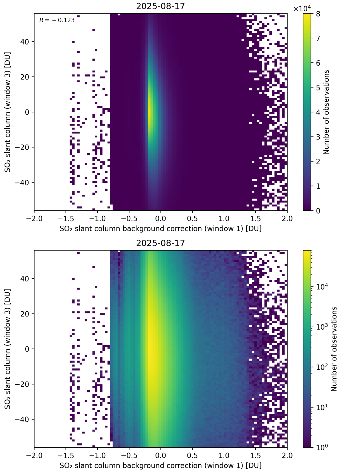
Figure 118: Scatter density plot of “SO 2 slant column background correction (window 1)” against “SO 2 slant column (window 3)” for 2025-08-16 to 2025-08-18.
