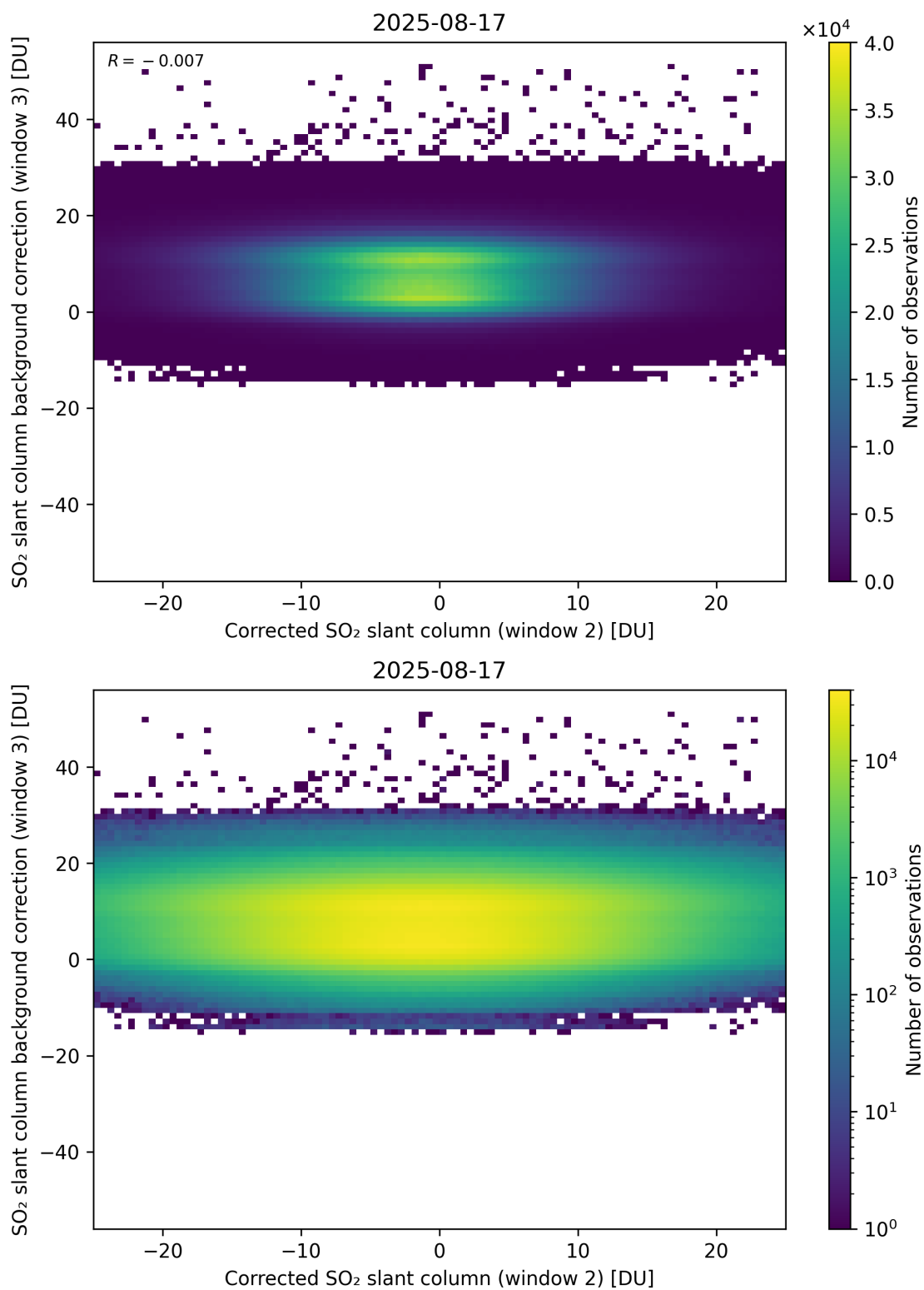
Figure 245: Scatter density plot of “Corrected SO 2 slant column (window 2)” against “SO 2 slant column background correction (window 3)” for 2025-08-16 to 2025-08-18.
