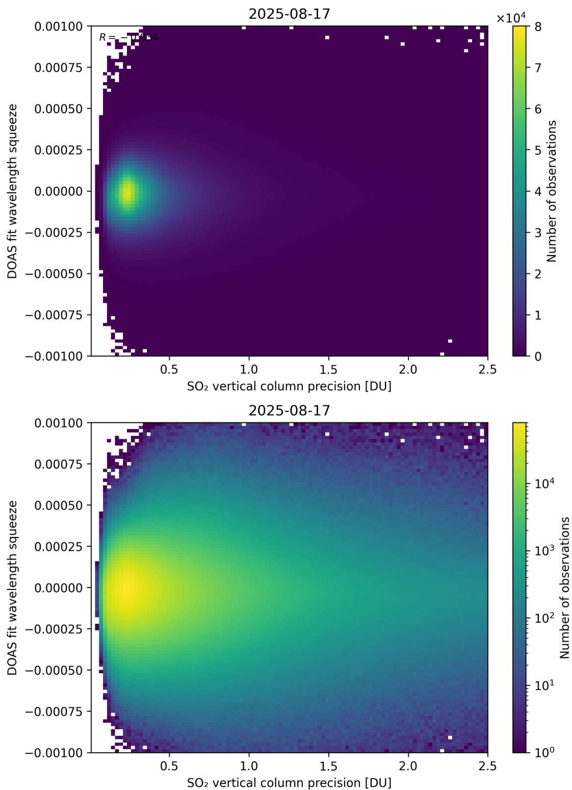
Figure 333: Scatter density plot of “SO 2 vertical column precision” against “DOAS fit wavelength squeeze” for 2025-08-16 to 2025-08-18.
