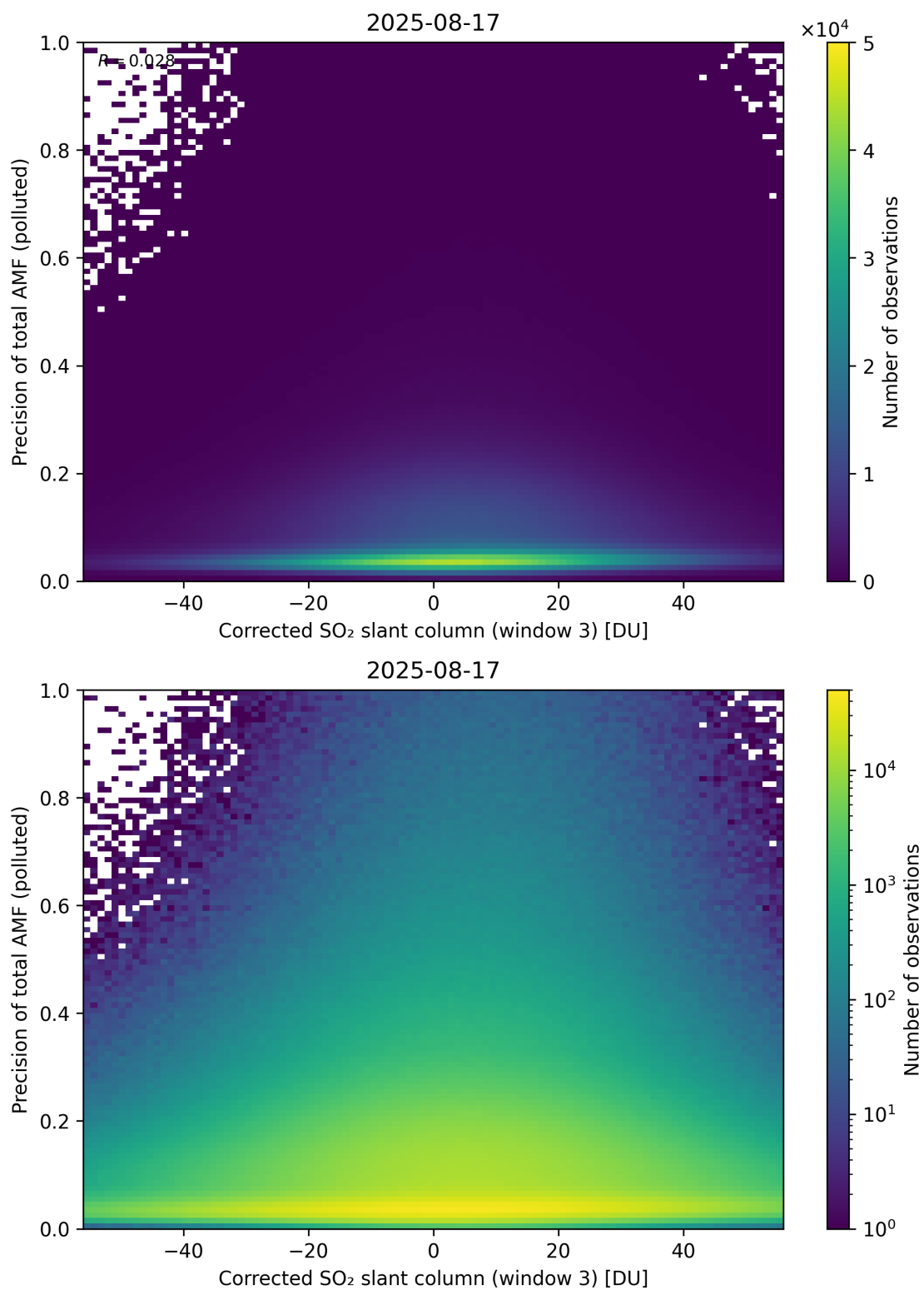
Figure 261: Scatter density plot of “Corrected SO 2 slant column (window 3)” against “Precision of total AMF (polluted)” for 2025-08-16 to 2025-08-18.
