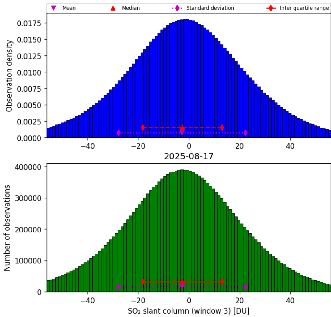
Figure 71: Histogram of “SO 2 slant column (window 3)” for 2025-08-16 to 2025-08-18
