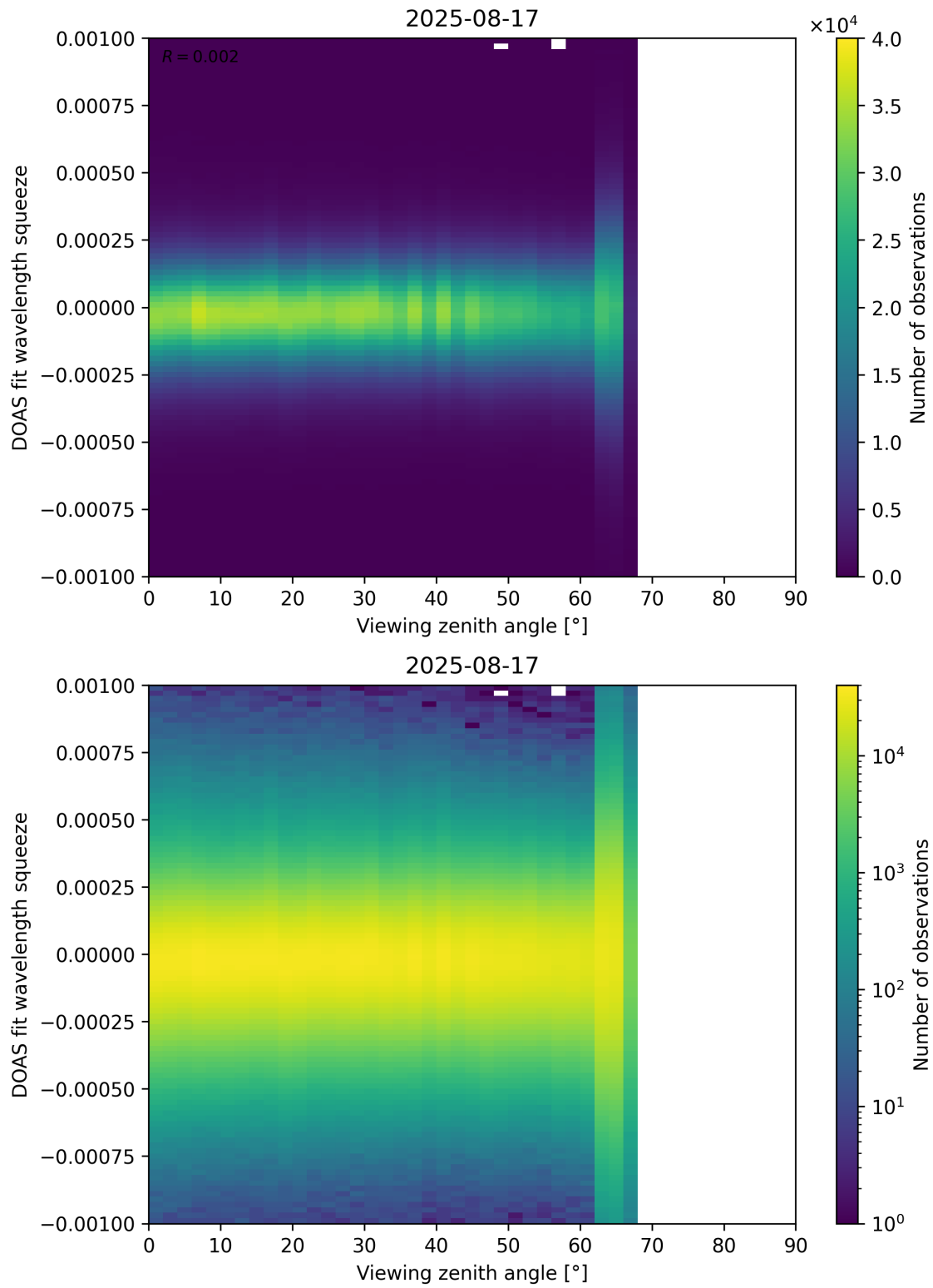
Figure 366: Scatter density plot of “Viewing zenith angle” against “DOAS fit wavelength squeeze” for 2025-08-16 to 2025-08-18.
