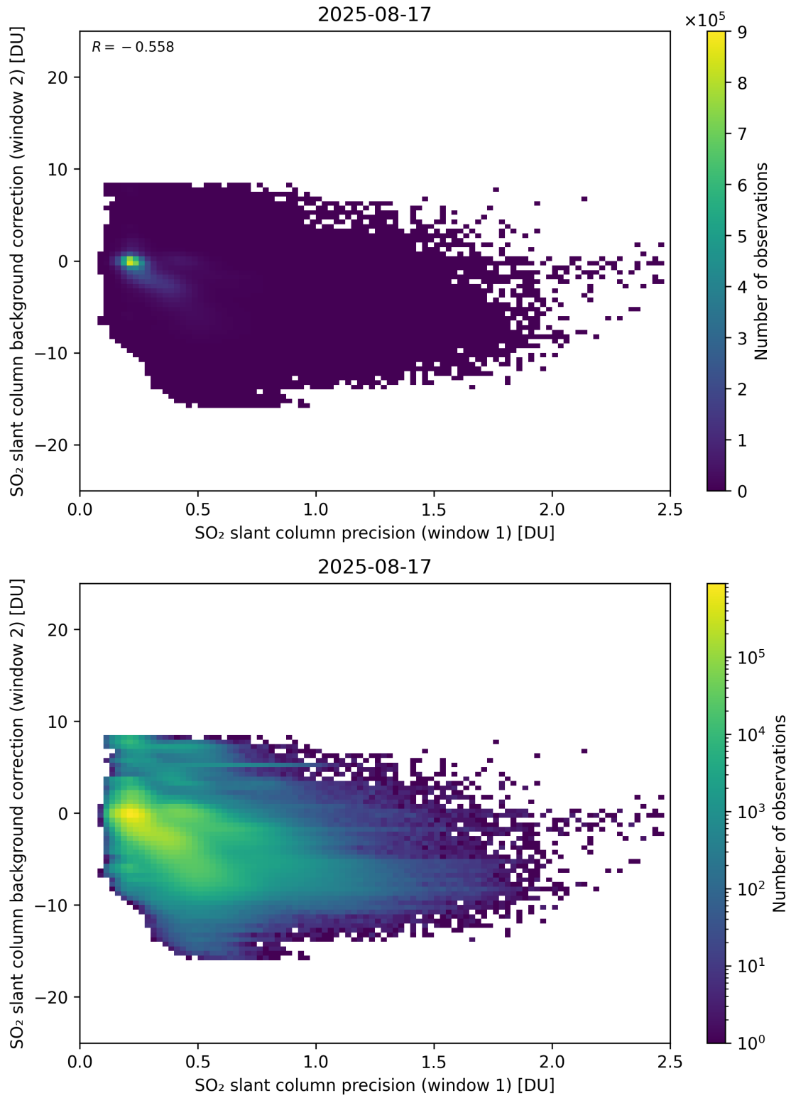
Figure 269: Scatter density plot of “SO 2 slant column precision (window 1)” against “SO 2 slant column background correction (window 2)” for 2025-08-16 to 2025-08-18.
