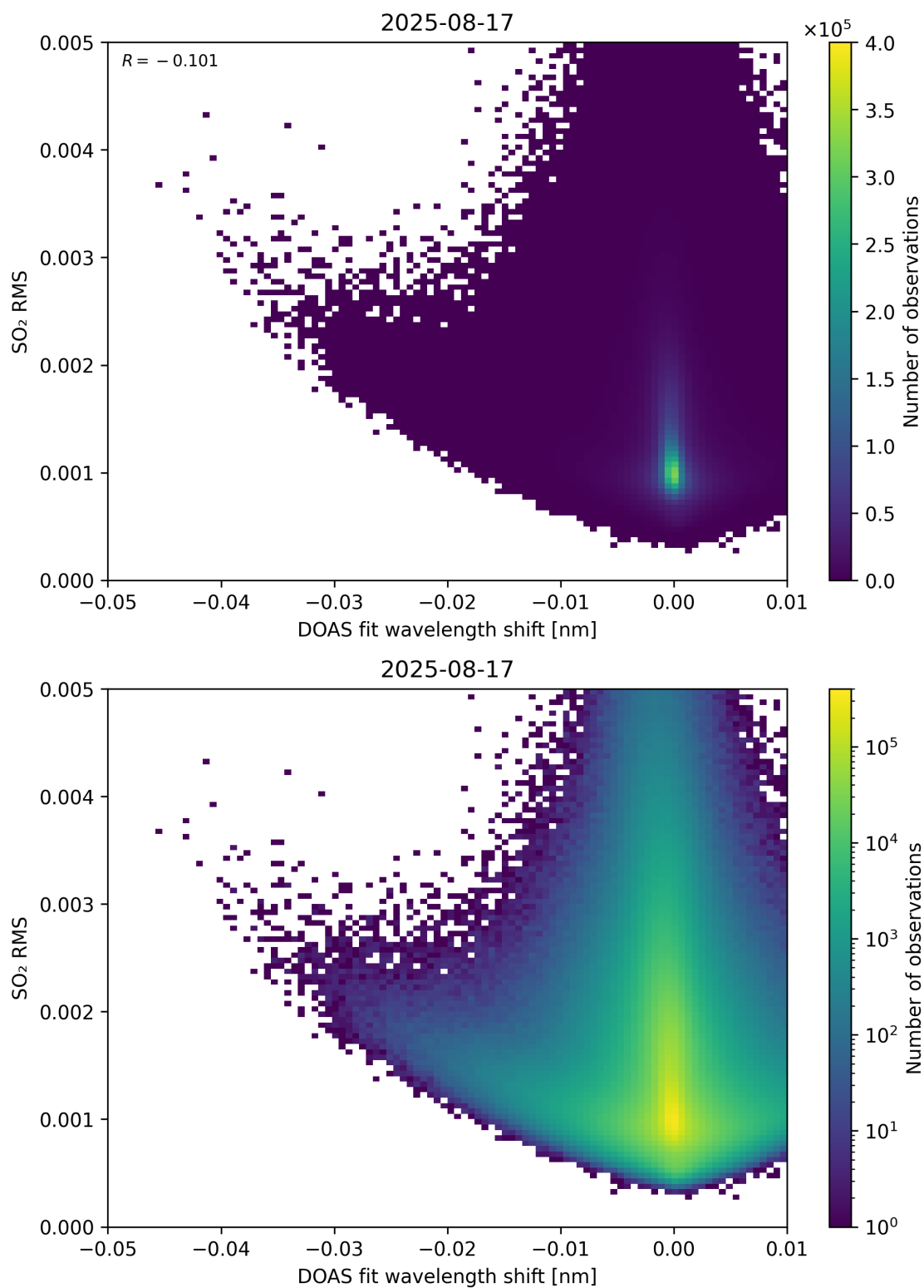
Figure 139: Scatter density plot of “DOAS fit wavelength shift” against “SO 2 RMS” for 2025-08-16 to 2025-08-18.
