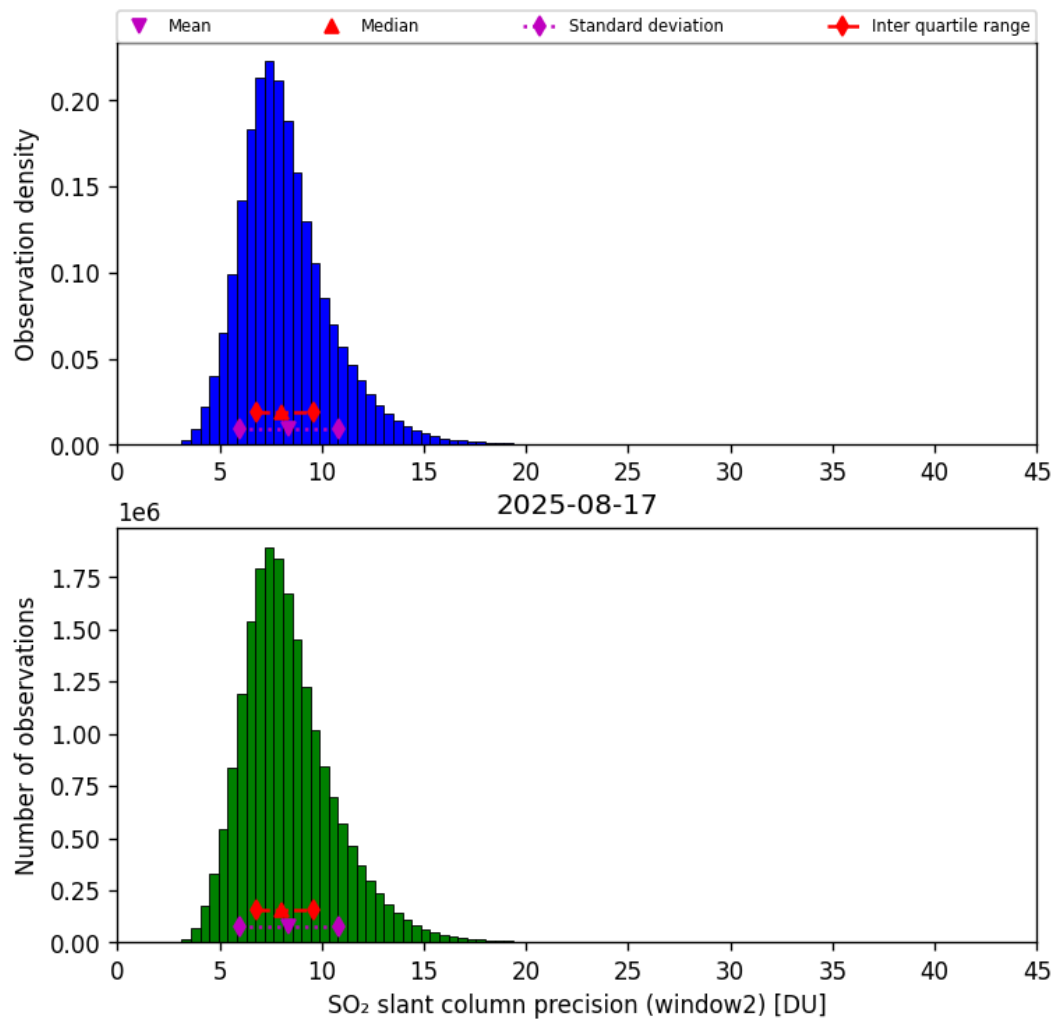
Figure 68: Histogram of “SO 2 slant column precision (window2)” for 2025-08-16 to 2025-08-18
