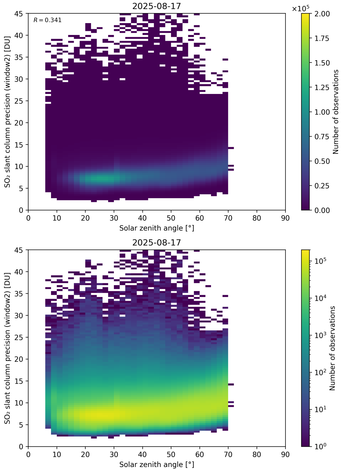
Figure 186: Scatter density plot of “Solar zenith angle” against “SO 2 slant column precision (window2)” for 2025-08-16 to 2025-08-18.
