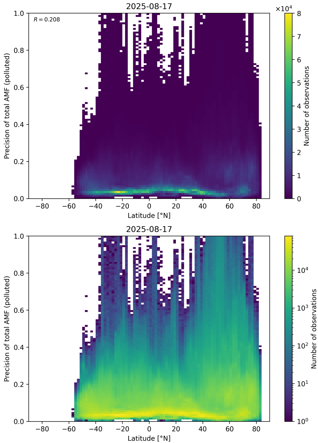
Figure 168: Scatter density plot of “Latitude” against “Precision of total AMF (polluted)” for 2025-08-16 to 2025-08-18.
