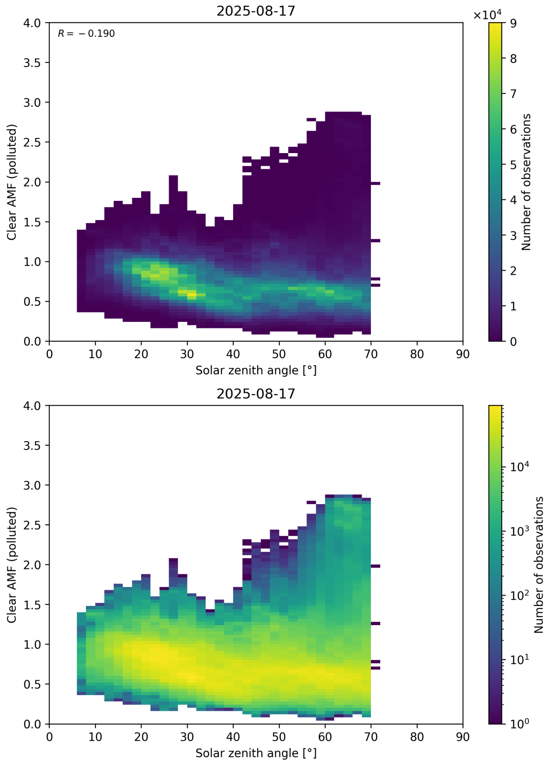
Figure 178: Scatter density plot of “Solar zenith angle” against “Clear AMF (polluted)” for 2025-08-16 to 2025-08-18.
