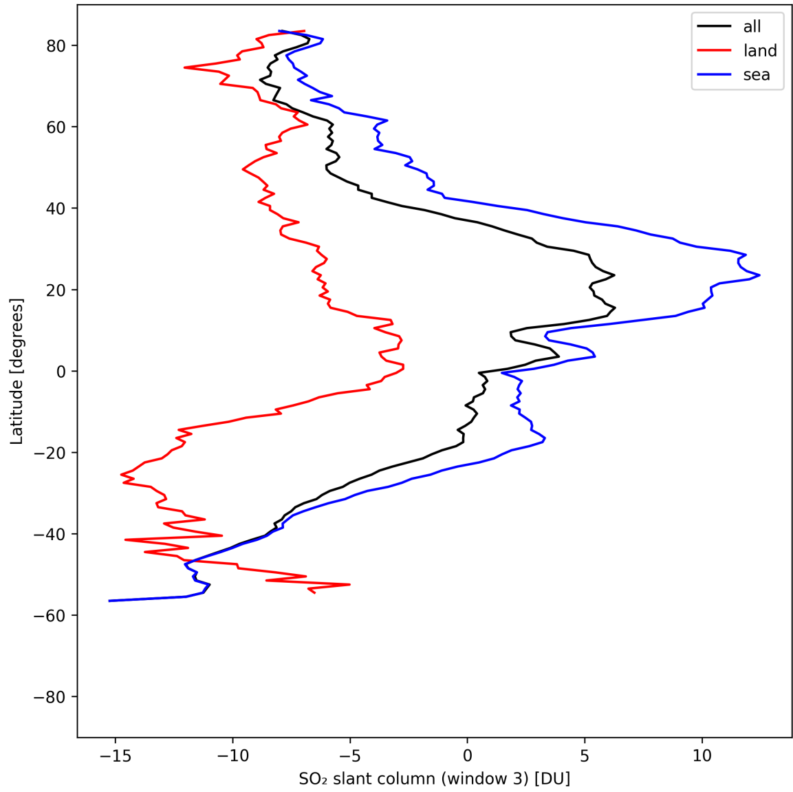
Figure 45: Zonal average of “SO 2 slant column (window 3)” for 2025-08-16 to 2025-08-18.
