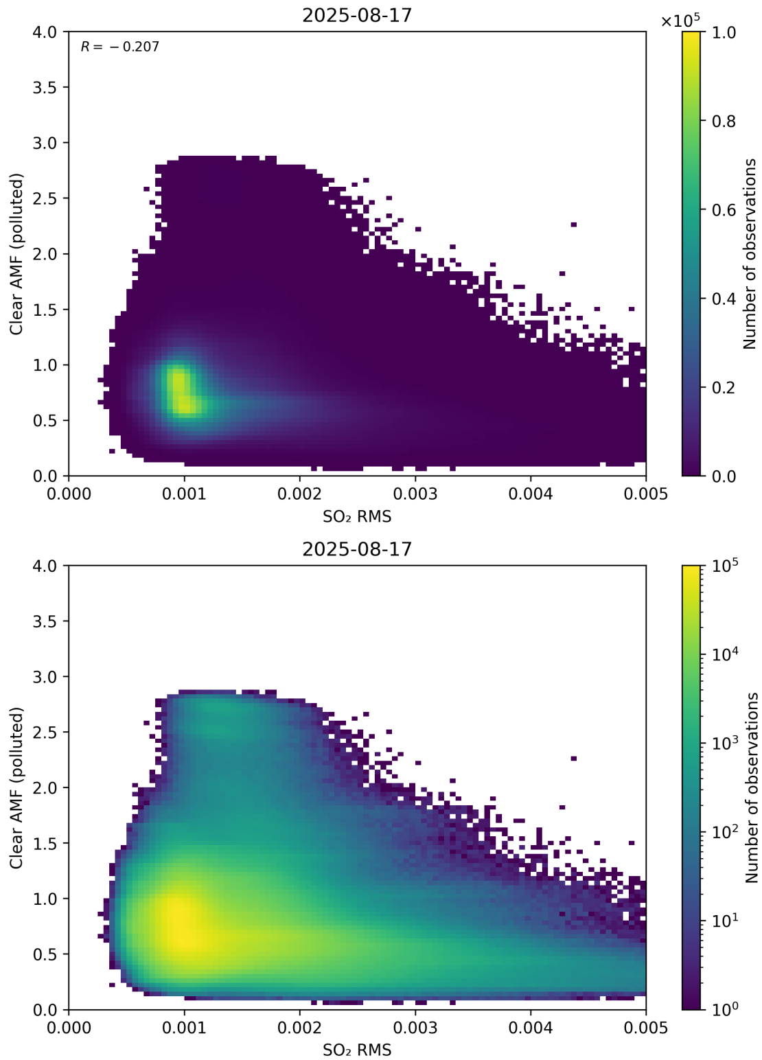
Figure 147: Scatter density plot of “SO 2 RMS” against “Clear AMF (polluted)” for 2025-08-16 to 2025-08-18.
