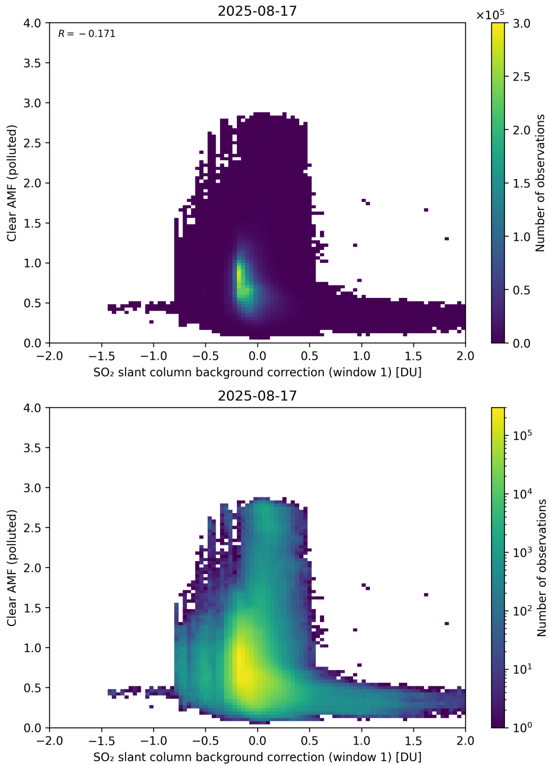
Figure 114: Scatter density plot of “SO 2 slant column background correction (window 1)” against “Clear AMF (polluted)” for 2025-08-16 to 2025-08-18.
