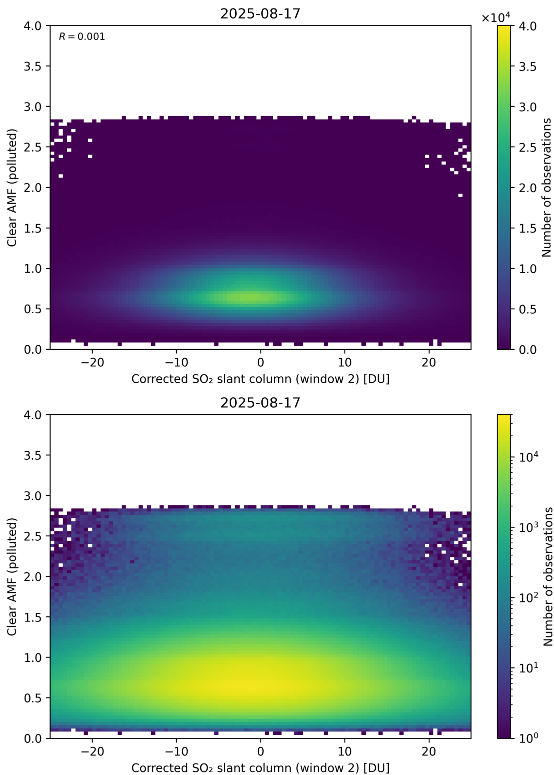
Figure 249: Scatter density plot of “Corrected SO 2 slant column (window 2)” against “Clear AMF (polluted)” for 2025-08-16 to 2025-08-18.
