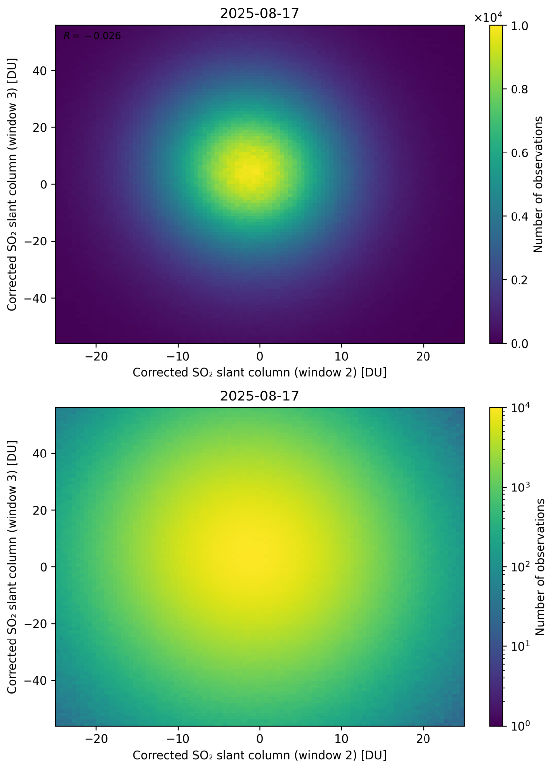
Figure 250: Scatter density plot of “Corrected SO 2 slant column (window 2)” against “Corrected SO 2 slant column (window 3)” for 2025-08-16 to 2025-08-18.
