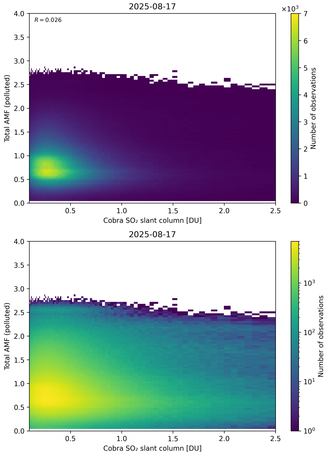
Figure 224: Scatter density plot of “Cobra SO 2 slant column” against “Total AMF (polluted)” for 2025-08-16 to 2025-08-18.
