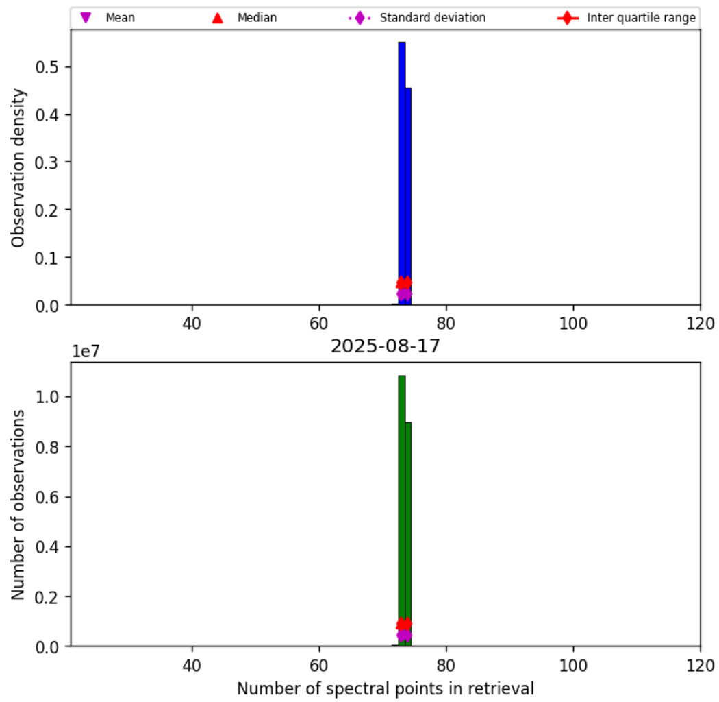
Figure 82: Histogram of “Number of spectral points in retrieval” for 2025-08-16 to 2025-08-18
