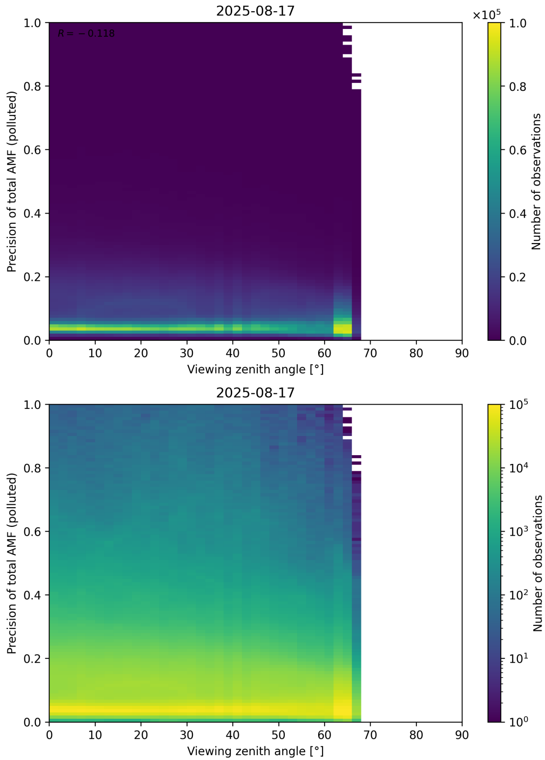
Figure 382: Scatter density plot of “Viewing zenith angle” against “Precision of total AMF (polluted)” for 2025-08-16 to 2025-08-18.
