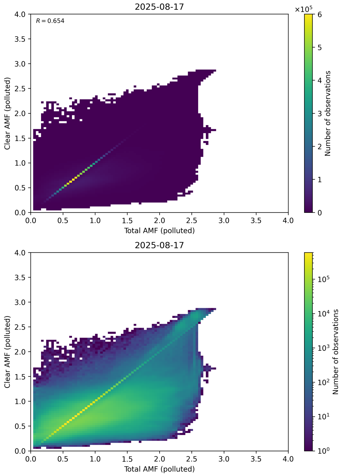
Figure 321: Scatter density plot of “Total AMF (polluted)” against “Clear AMF (polluted)” for 2025-08-16 to 2025-08-18.
