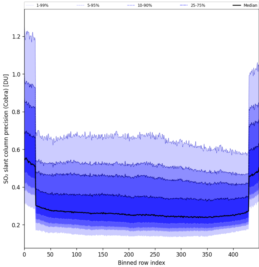
Figure 88: Along track statistics of “SO 2 slant column precision (Cobra)” for 2025-08-16 to 2025-08-18
