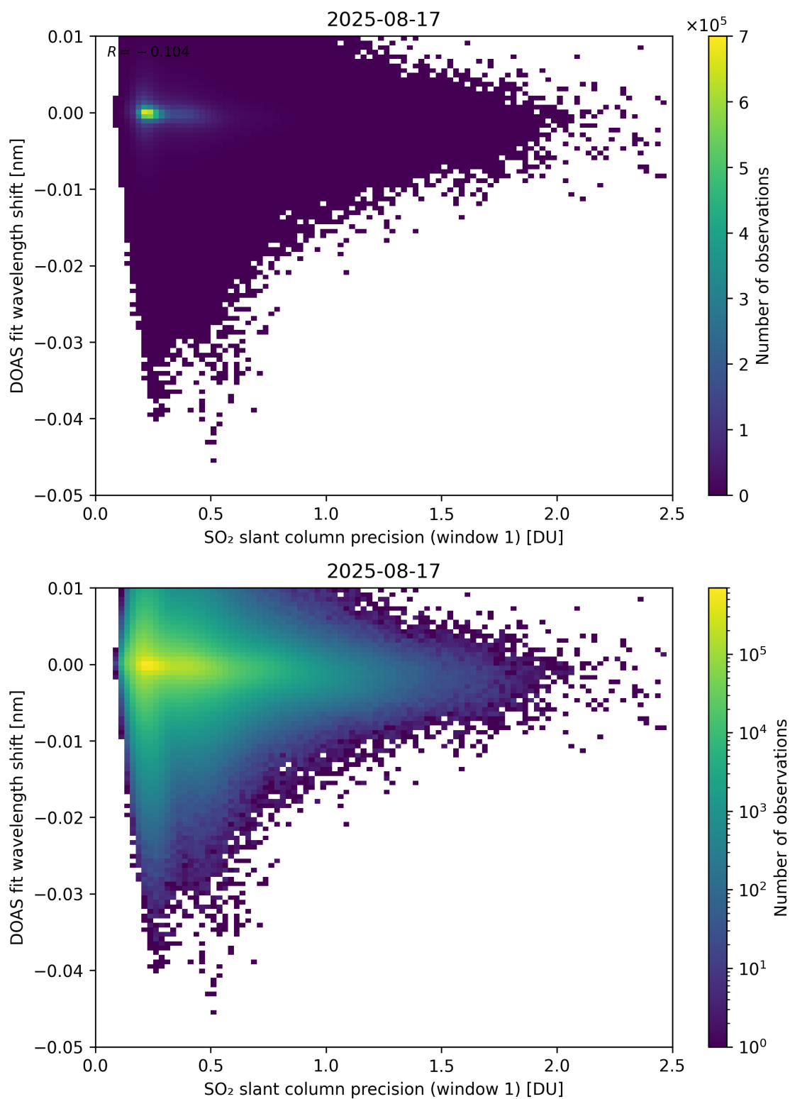
Figure 271: Scatter density plot of “SO 2 slant column precision (window 1)” against “DOAS fit wavelength shift” for 2025-08-16 to 2025-08-18.
