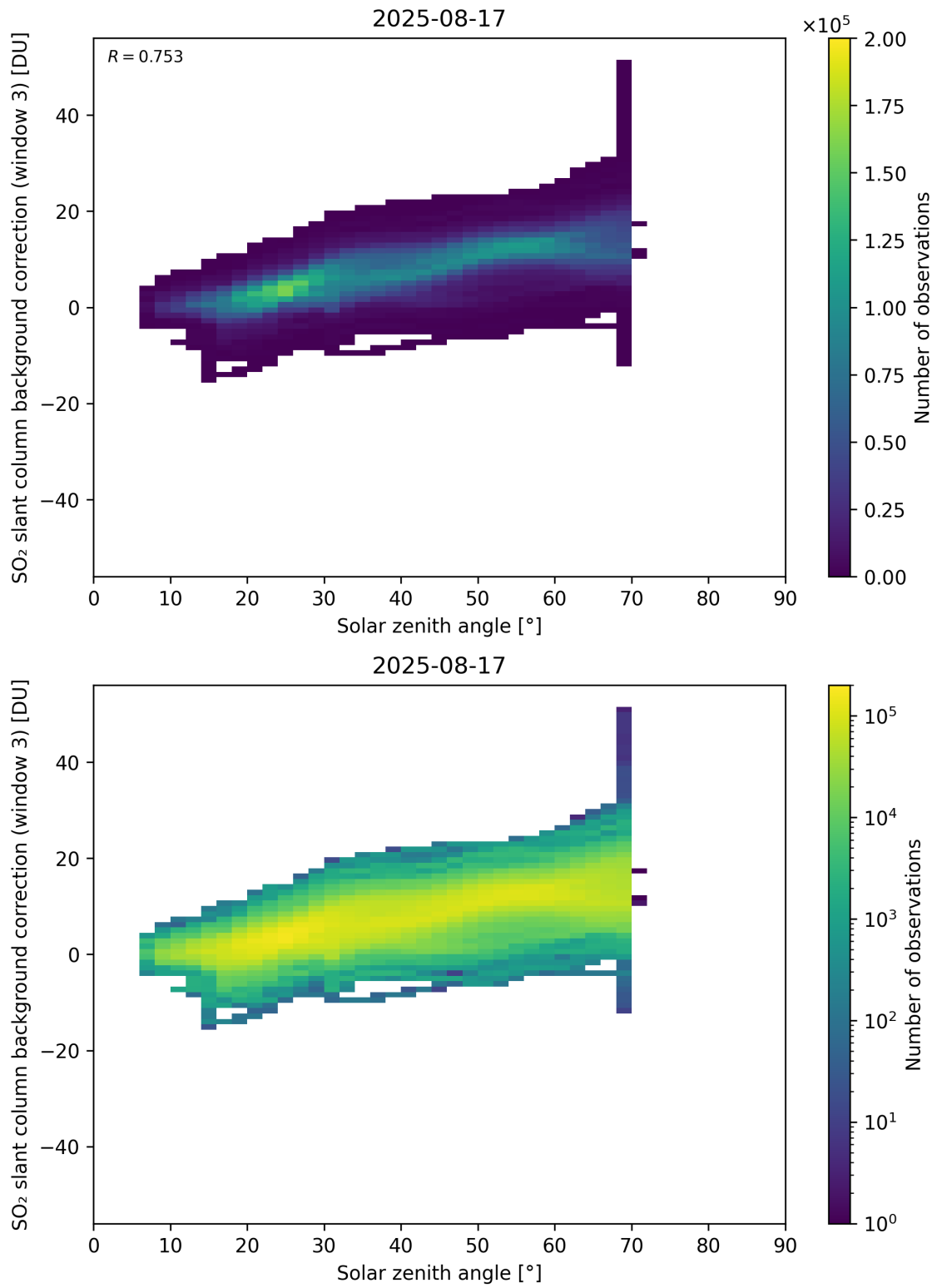
Figure 173: Scatter density plot of “Solar zenith angle” against “SO 2 slant column background correction (window 3)” for 2025-08-16 to 2025-08-18.
