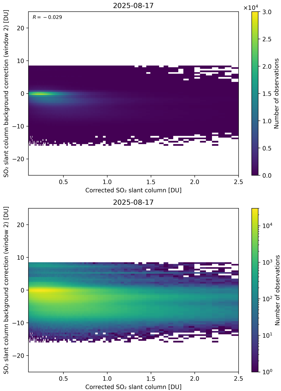
Figure 227: Scatter density plot of “Corrected SO 2 slant column” against “SO 2 slant column background correction (window 2)” for 2025-08-16 to 2025-08-18.
