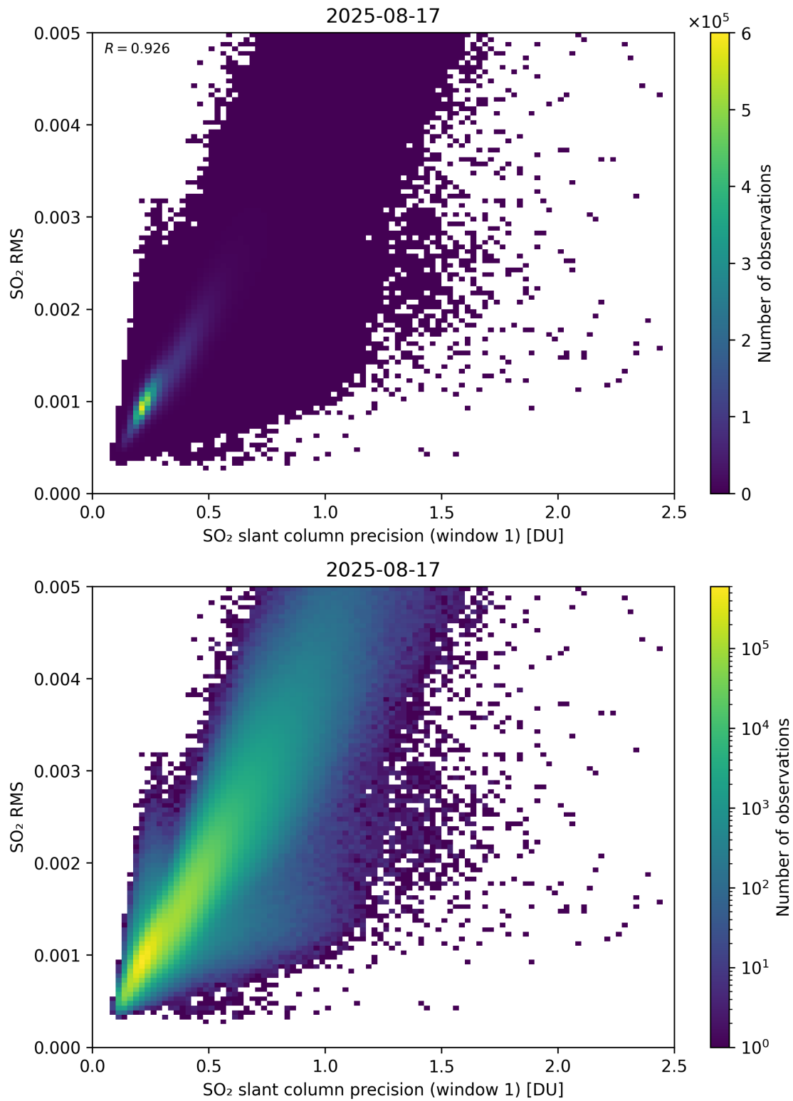
Figure 273: Scatter density plot of “SO 2 slant column precision (window 1)” against “SO 2 RMS” for 2025-08-16 to 2025-08-18.
