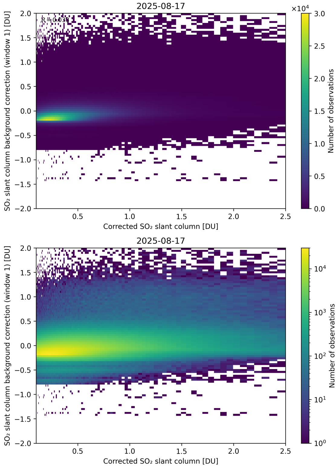
Figure 226: Scatter density plot of “Corrected SO 2 slant column” against “SO 2 slant column background correction (window 1)” for 2025-08-16 to 2025-08-18.
