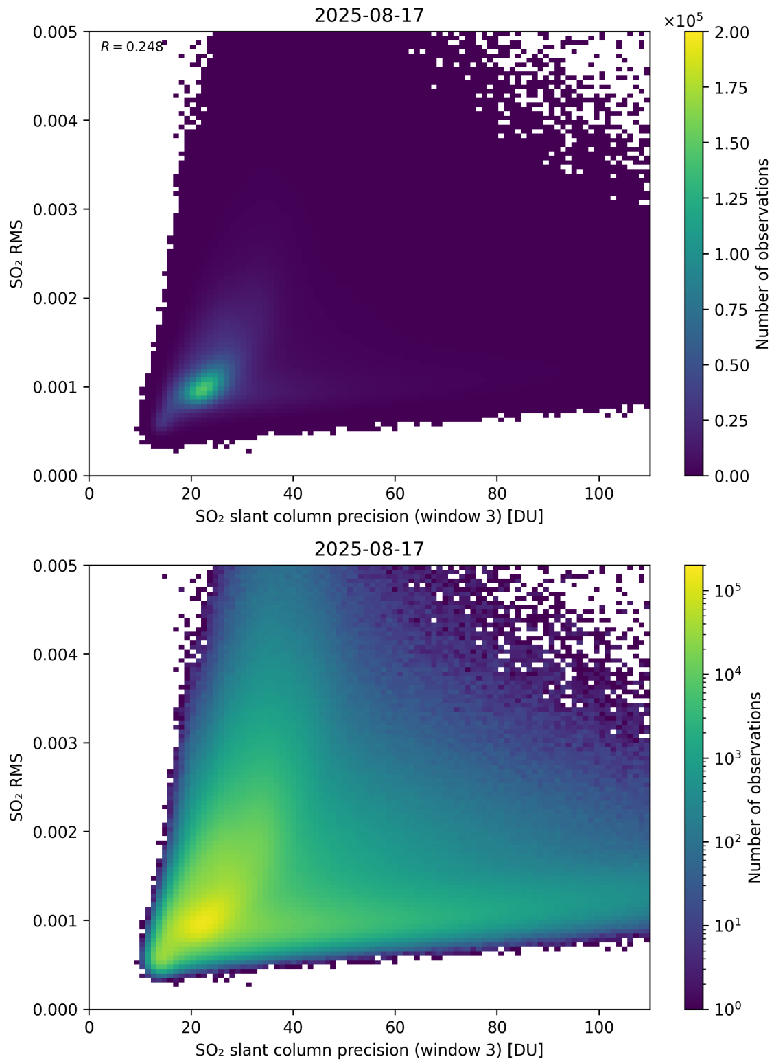
Figure 310: Scatter density plot of “SO 2 slant column precision (window 3)” against “SO 2 RMS” for 2025-08-16 to 2025-08-18.
