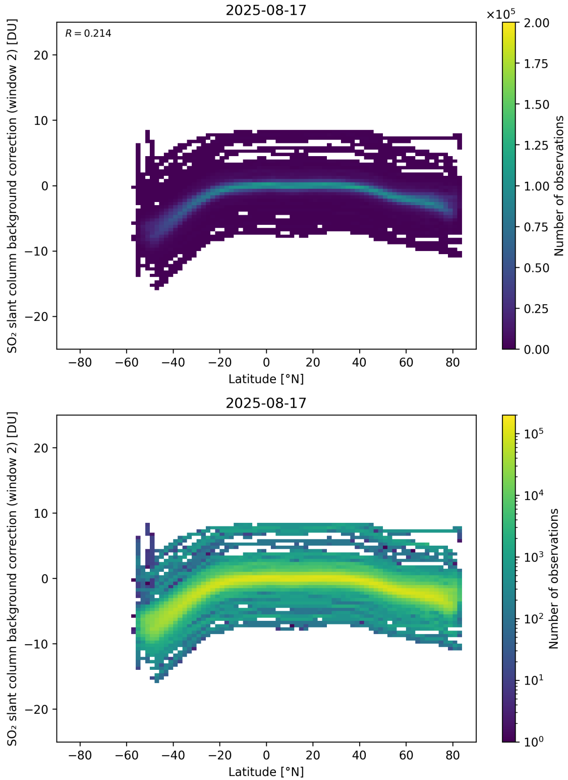
Figure 151: Scatter density plot of “Latitude” against “SO 2 slant column background correction (window 2)” for 2025-08-16 to 2025-08-18.
