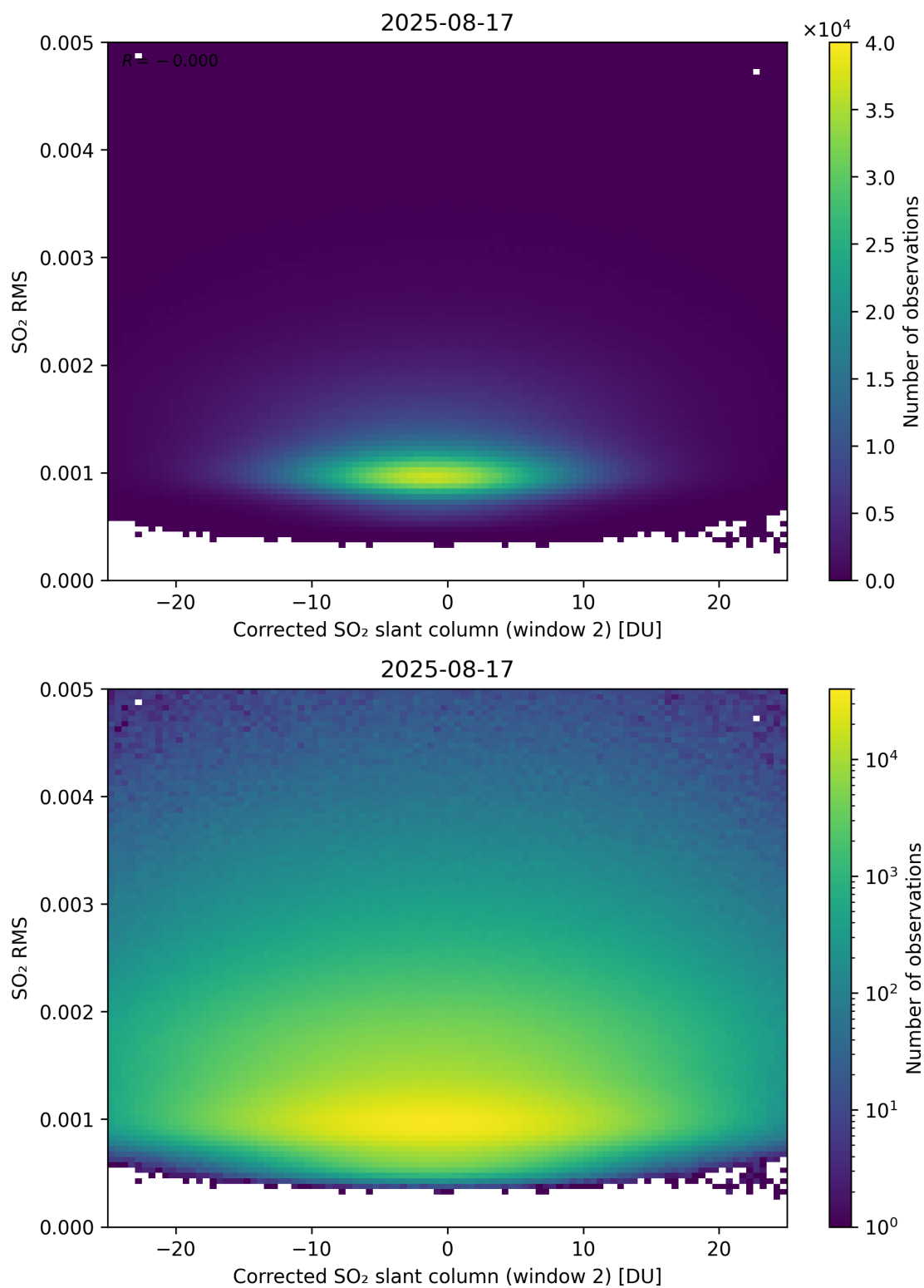
Figure 248: Scatter density plot of “Corrected SO 2 slant column (window 2)” against “SO 2 RMS” for 2025-08-16 to 2025-08-18.
