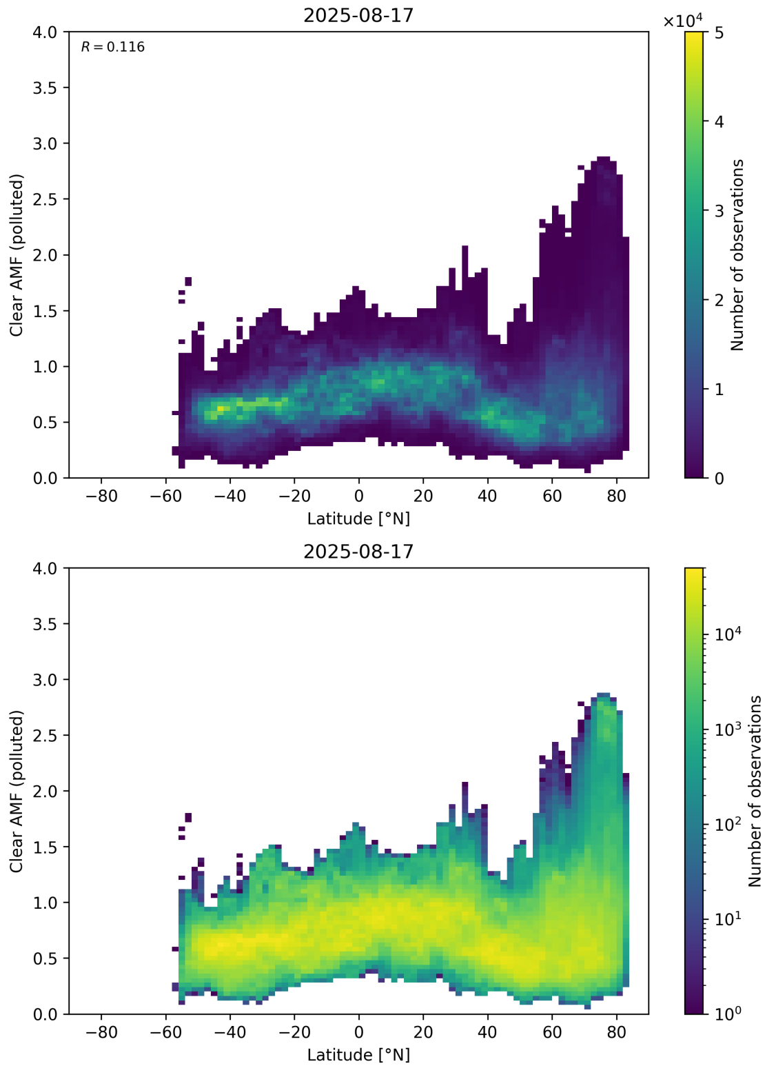
Figure 156: Scatter density plot of “Latitude” against “Clear AMF (polluted)” for 2025-08-16 to 2025-08-18.
