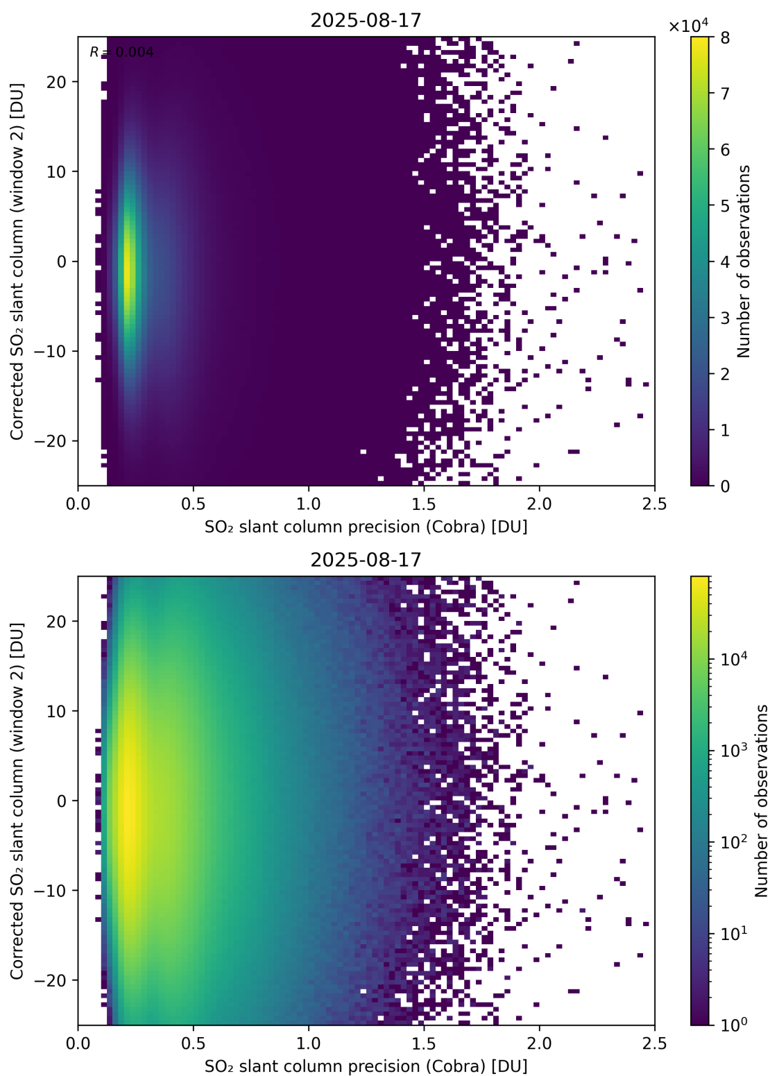
Figure 206: Scatter density plot of “SO 2 slant column precision (Cobra)” against “Corrected SO 2 slant column (window 2)” for 2025-08-16 to 2025-08-18.
