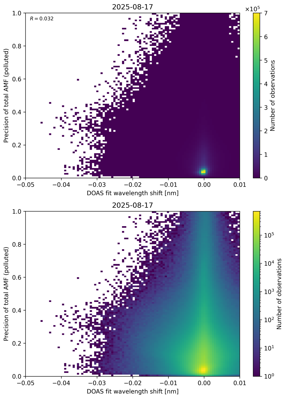
Figure 142: Scatter density plot of “DOAS fit wavelength shift” against “Precision of total AMF (polluted)” for 2025-08-16 to 2025-08-18.
