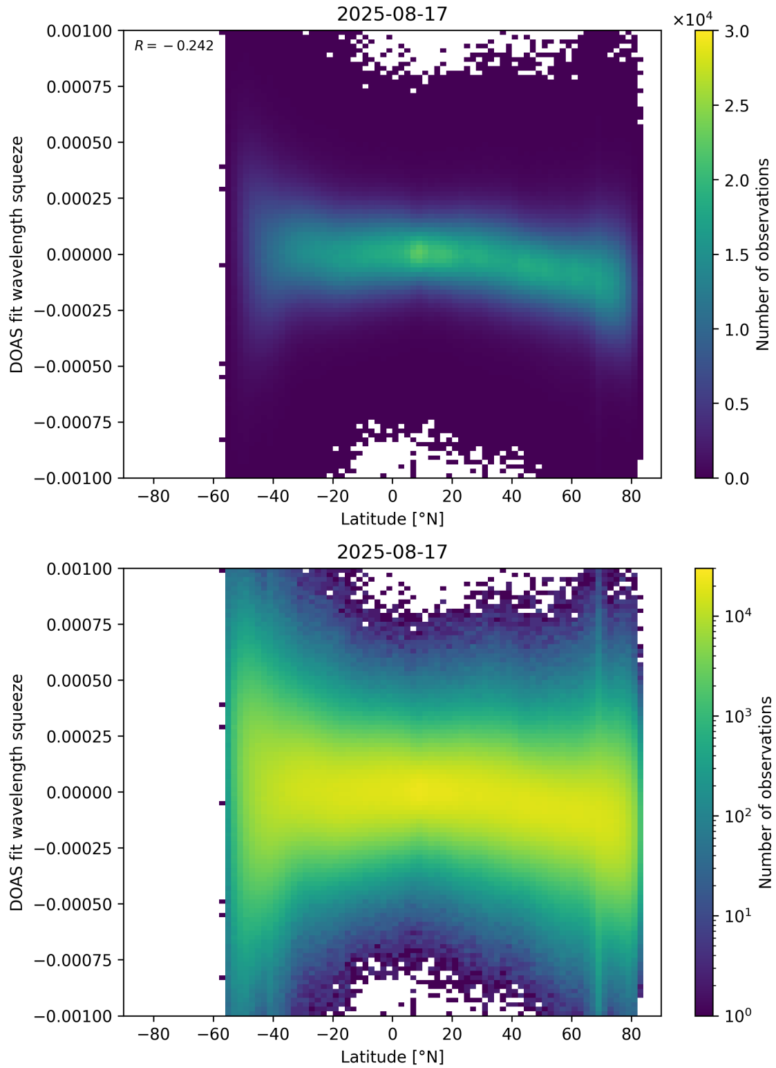
Figure 154: Scatter density plot of “Latitude” against “DOAS fit wavelength squeeze” for 2025-08-16 to 2025-08-18.
