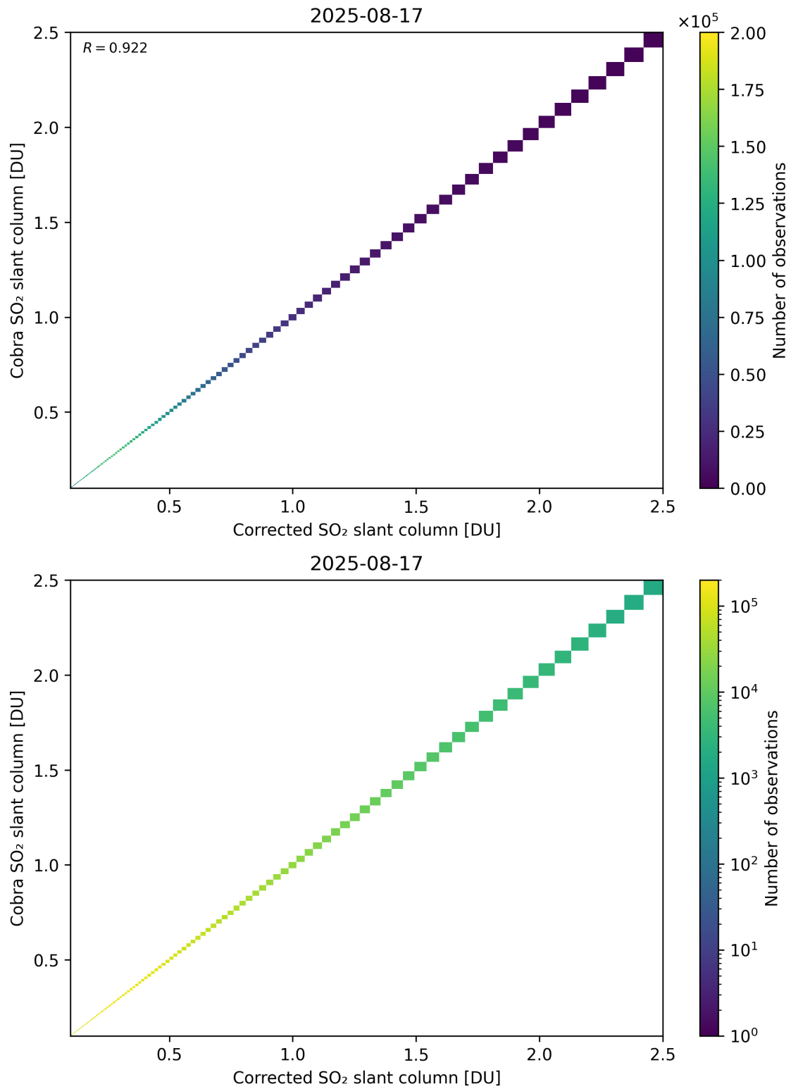
Figure 233: Scatter density plot of “Corrected SO 2 slant column” against “Cobra SO 2 slant column” for 2025-08-16 to 2025-08-18.
