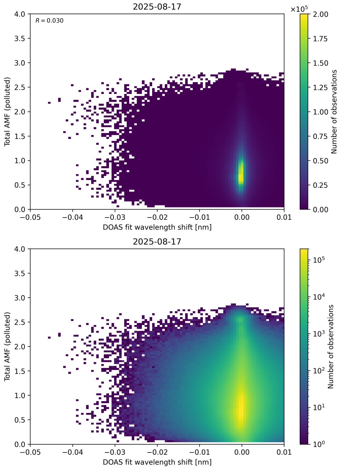
Figure 141: Scatter density plot of “DOAS fit wavelength shift” against “Total AMF (polluted)” for 2025-08-16 to 2025-08-18.
