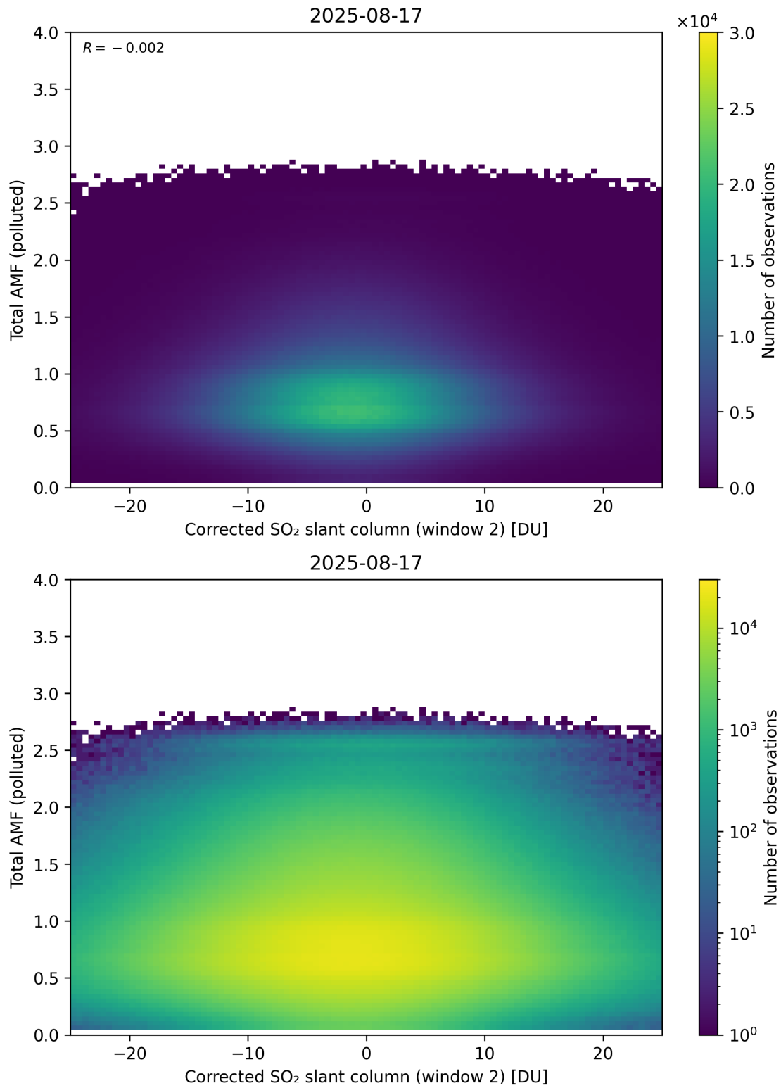
Figure 253: Scatter density plot of “Corrected SO 2 slant column (window 2)” against “Total AMF (polluted)” for 2025-08-16 to 2025-08-18.
