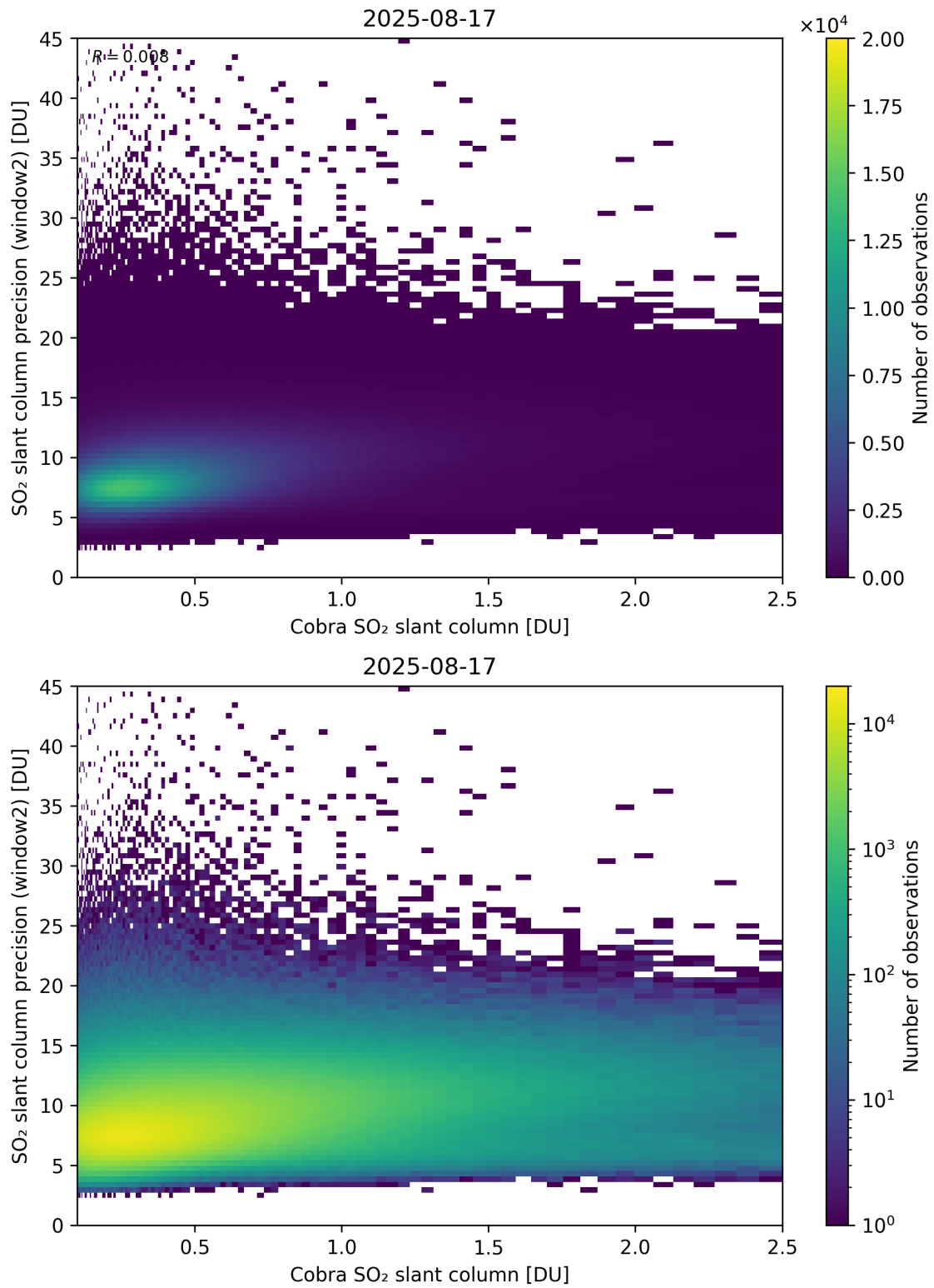
Figure 221: Scatter density plot of “Cobra SO 2 slant column” against “SO 2 slant column precision (window2)” for 2025-08-16 to 2025-08-18.
