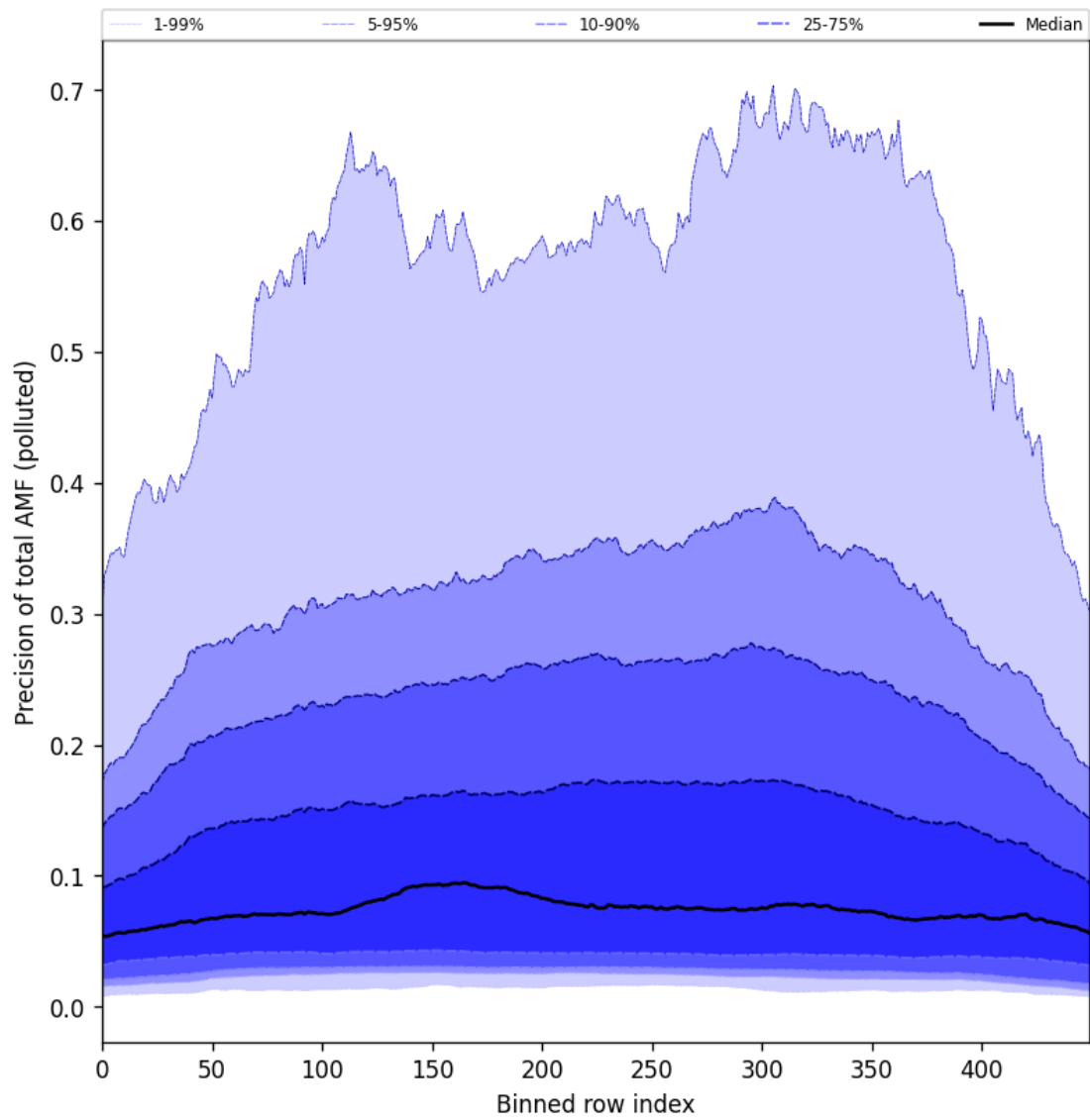
Figure 106: Along track statistics of “Precision of total AMF (polluted)” for 2025-08-16 to 2025-08-18
