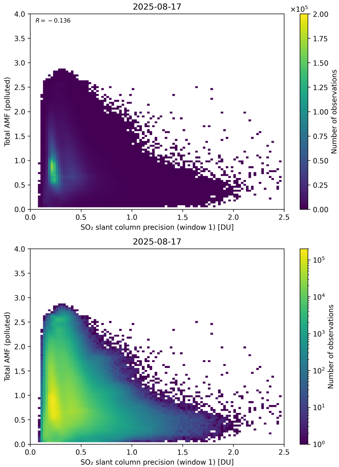
Figure 280: Scatter density plot of “SO 2 slant column precision (window 1)” against “Total AMF (polluted)” for 2025-08-16 to 2025-08-18.
