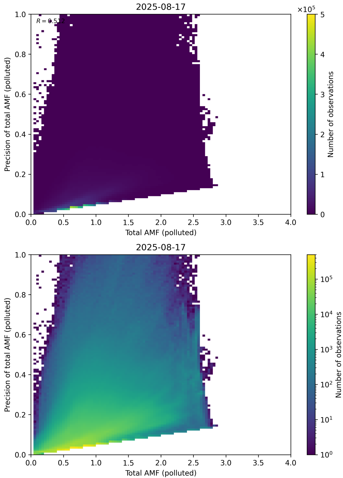
Figure 322: Scatter density plot of “Total AMF (polluted)” against “Precision of total AMF (polluted)” for 2025-08-16 to 2025-08-18.
