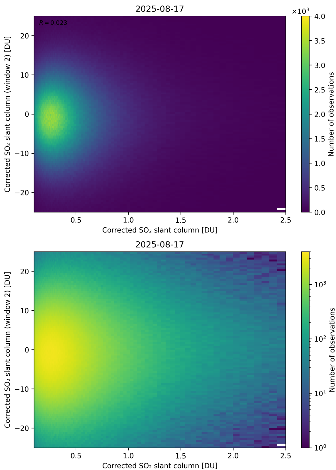
Figure 235: Scatter density plot of “Corrected SO 2 slant column” against “Corrected SO 2 slant column (window 2)” for 2025-08-16 to 2025-08-18.
