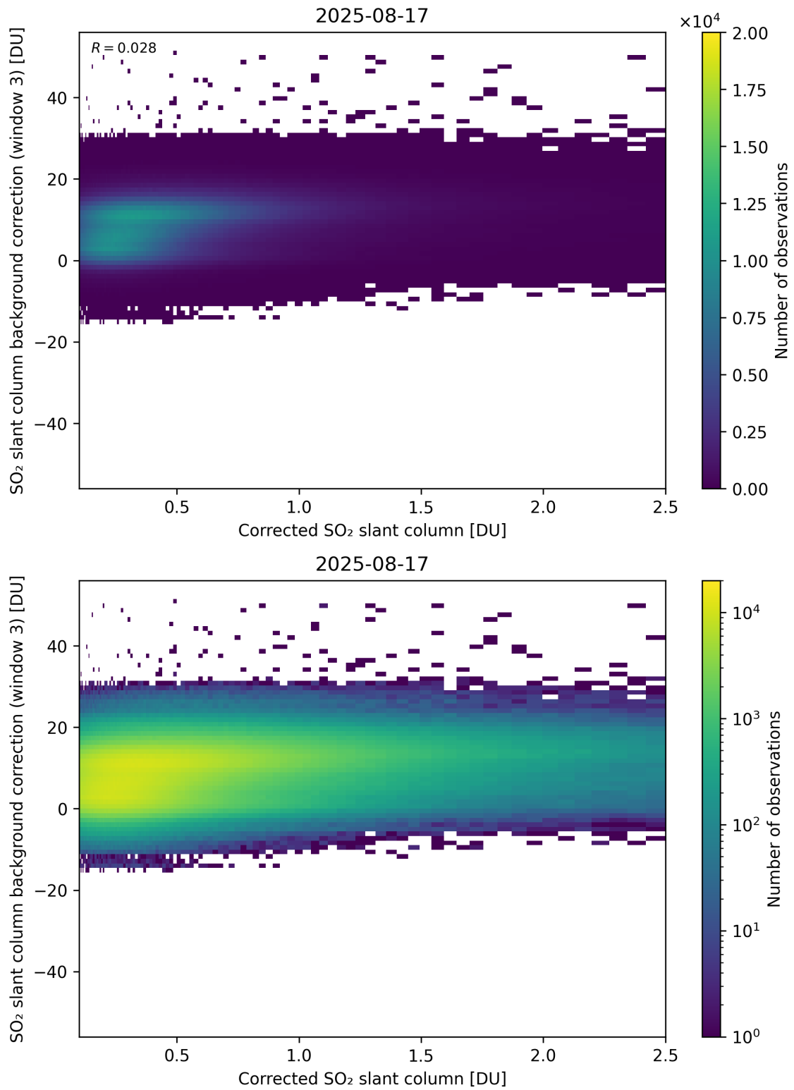
Figure 228: Scatter density plot of “Corrected SO 2 slant column” against “SO 2 slant column background correction (window 3)” for 2025-08-16 to 2025-08-18.
