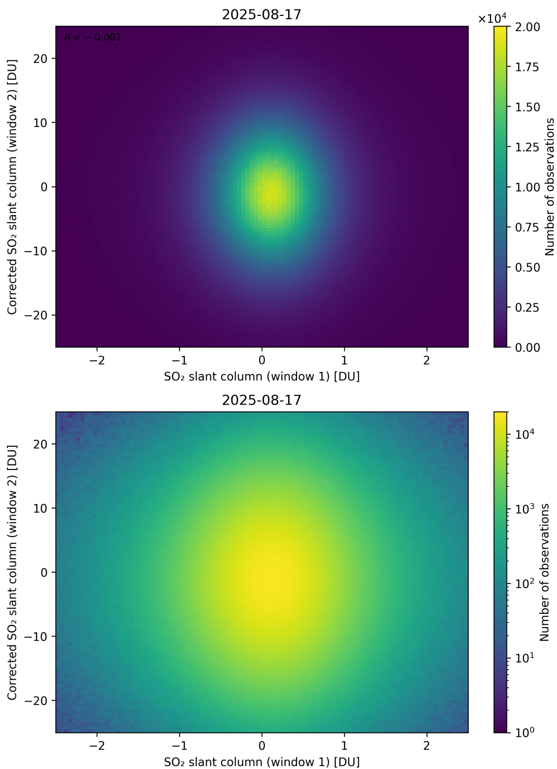
Figure 283: Scatter density plot of “SO 2 slant column (window 1)” against “Corrected SO 2 slant column (window 2)” for 2025-08-16 to 2025-08-18.
