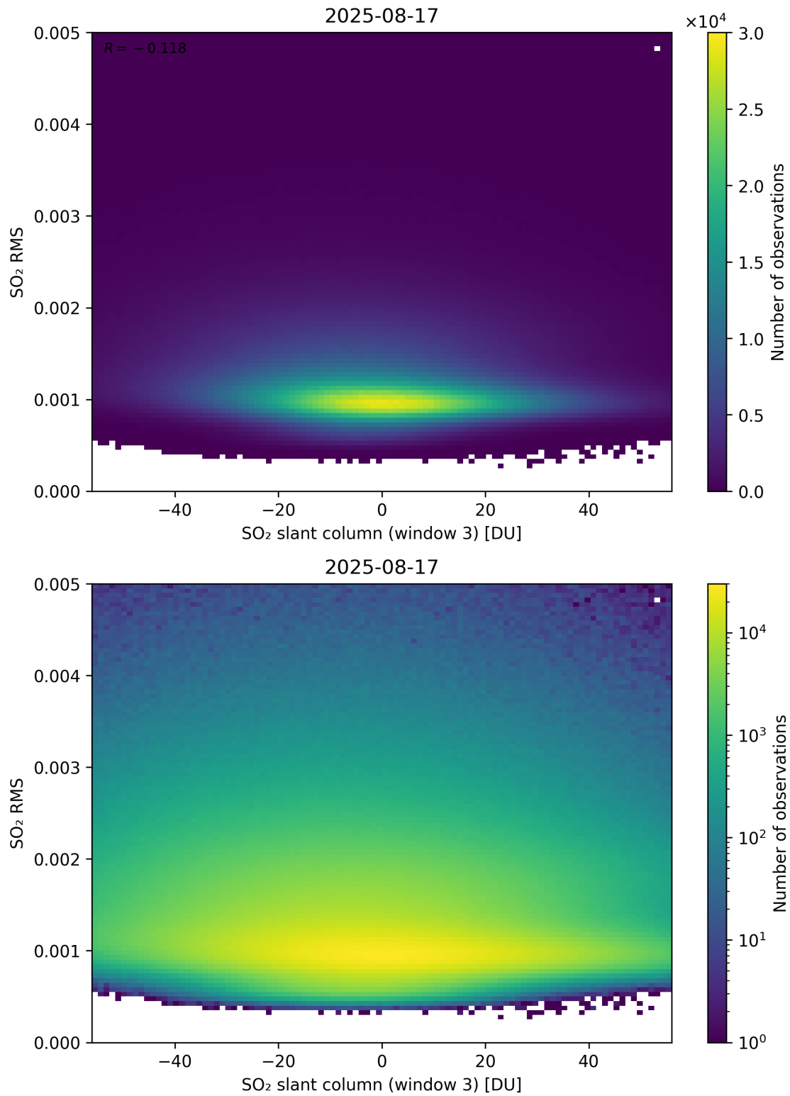
Figure 306: Scatter density plot of “SO 2 slant column (window 3)” against “SO 2 RMS” for 2025-08-16 to 2025-08-18.
