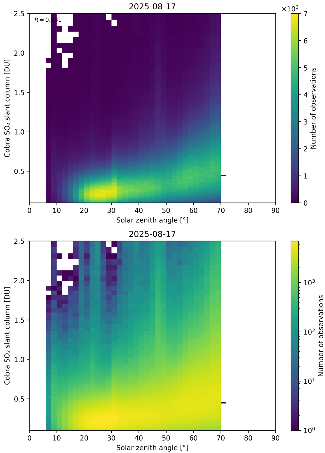
Figure 179: Scatter density plot of “Solar zenith angle” against “Cobra SO 2 slant column” for 2025-08-16 to 2025-08-18.
