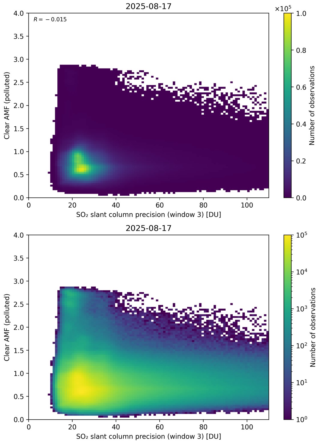
Figure 311: Scatter density plot of “SO 2 slant column precision (window 3)” against “Clear AMF (polluted)” for 2025-08-16 to 2025-08-18.
