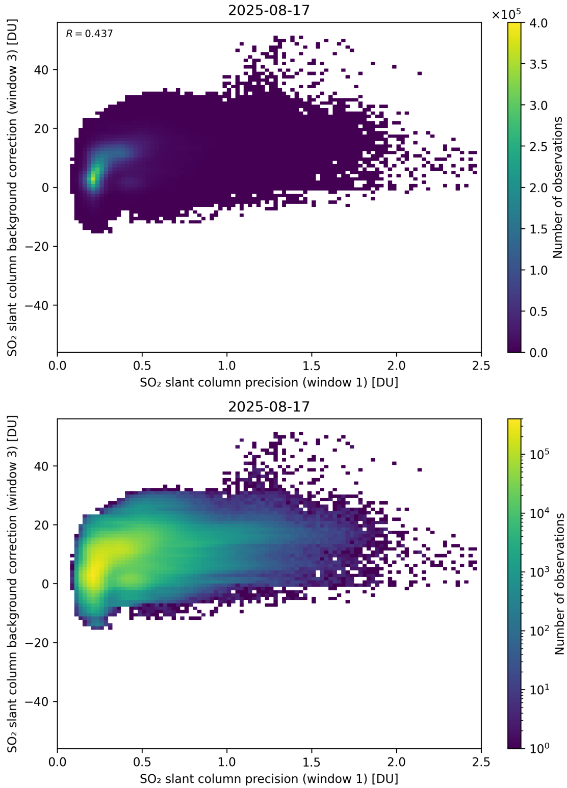
Figure 270: Scatter density plot of “SO 2 slant column precision (window 1)” against “SO 2 slant column background correction (window 3)” for 2025-08-16 to 2025-08-18.
