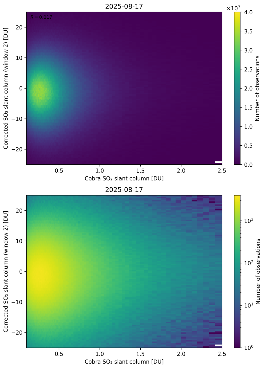
Figure 217: Scatter density plot of “Cobra SO 2 slant column” against “Corrected SO 2 slant column (window 2)” for 2025-08-16 to 2025-08-18.
