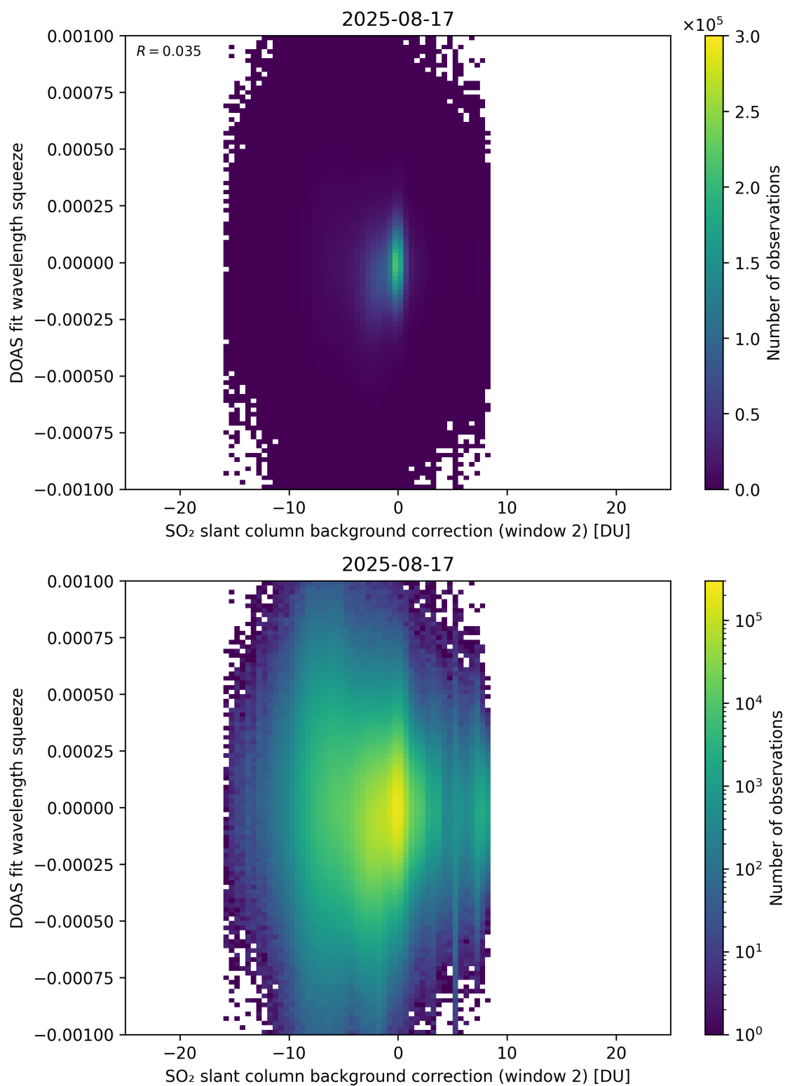
Figure 124: Scatter density plot of “SO 2 slant column background correction (window 2)” against “DOAS fit wavelength squeeze” for 2025-08-16 to 2025-08-18.
