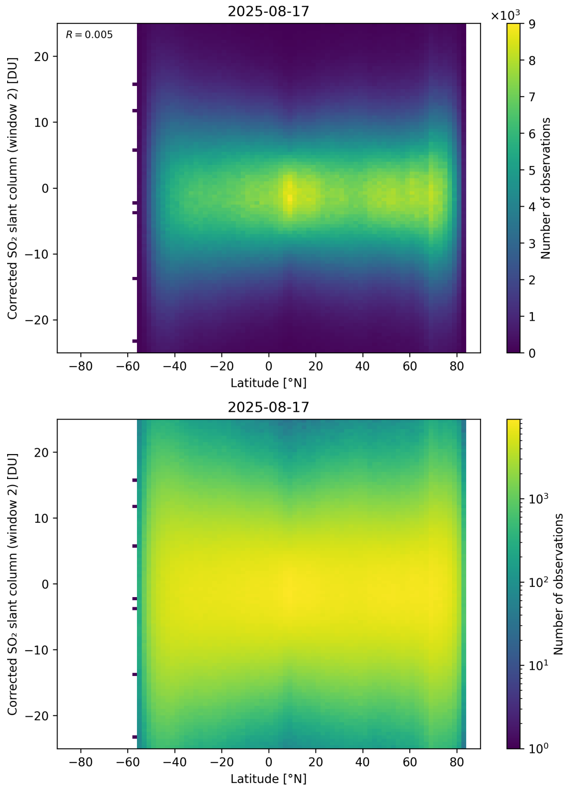
Figure 160: Scatter density plot of “Latitude” against “Corrected SO 2 slant column (window 2)” for 2025-08-16 to 2025-08-18.
