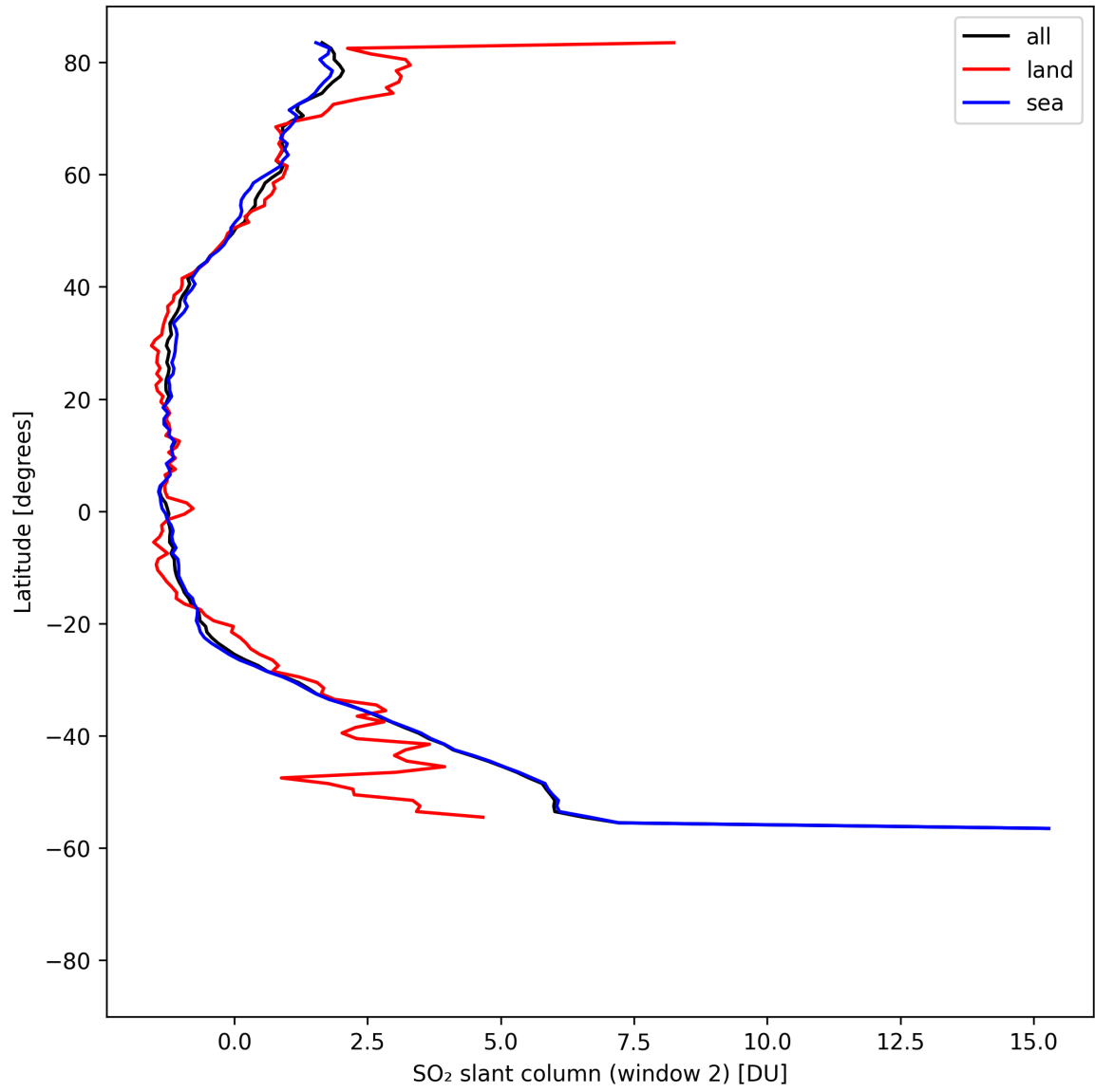
Figure 41: Zonal average of “SO 2 slant column (window 2)” for 2025-08-16 to 2025-08-18.
