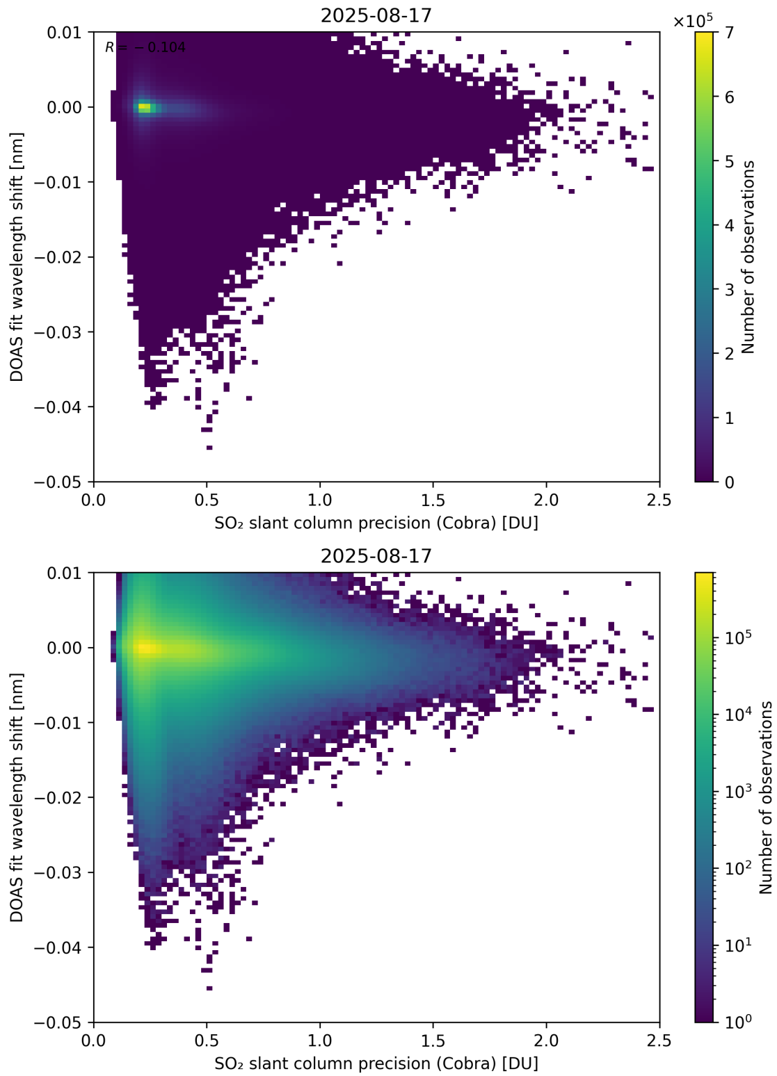
Figure 202: Scatter density plot of “SO 2 slant column precision (Cobra)” against “DOAS fit wavelength shift” for 2025-08-16 to 2025-08-18.
