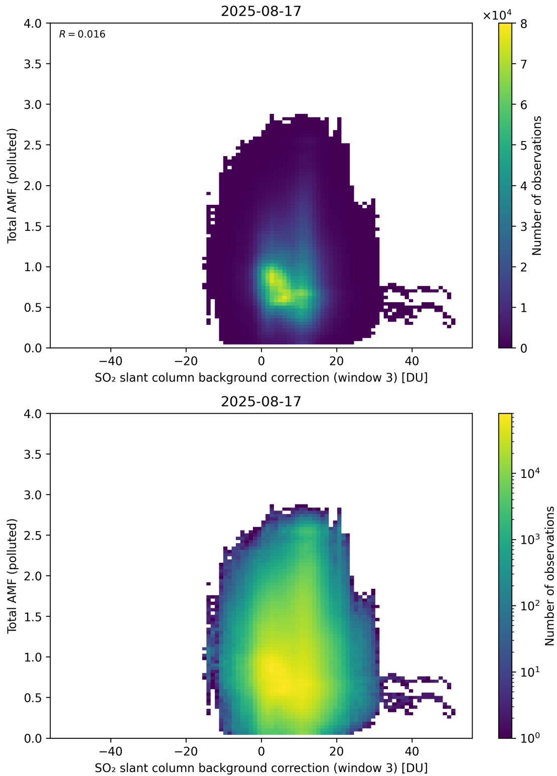
Figure 136: Scatter density plot of “SO 2 slant column background correction (window 3)” against “Total AMF (polluted)” for 2025-08-16 to 2025-08-18.
