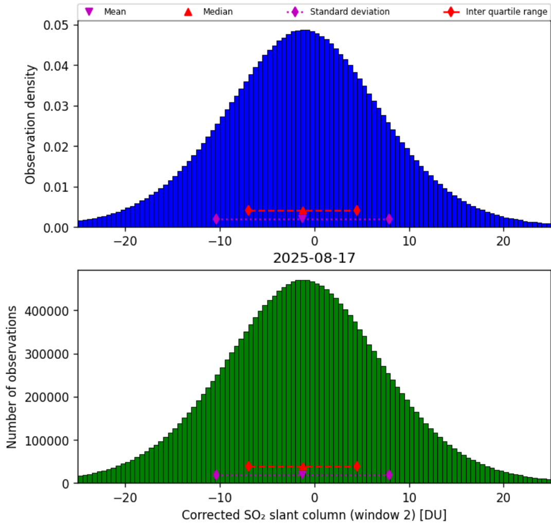
Figure 69: Histogram of “Corrected SO 2 slant column (window 2)” for 2025-08-16 to 2025-08-18
