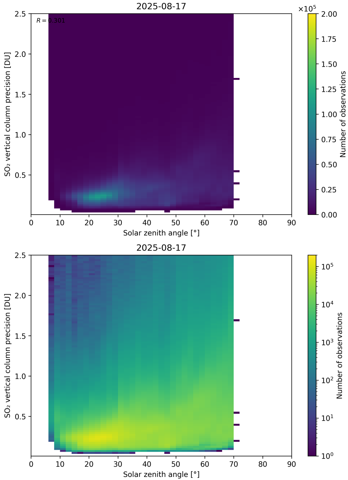
Figure 192: Scatter density plot of “Solar zenith angle” against “SO 2 vertical column precision” for 2025-08-16 to 2025-08-18.
