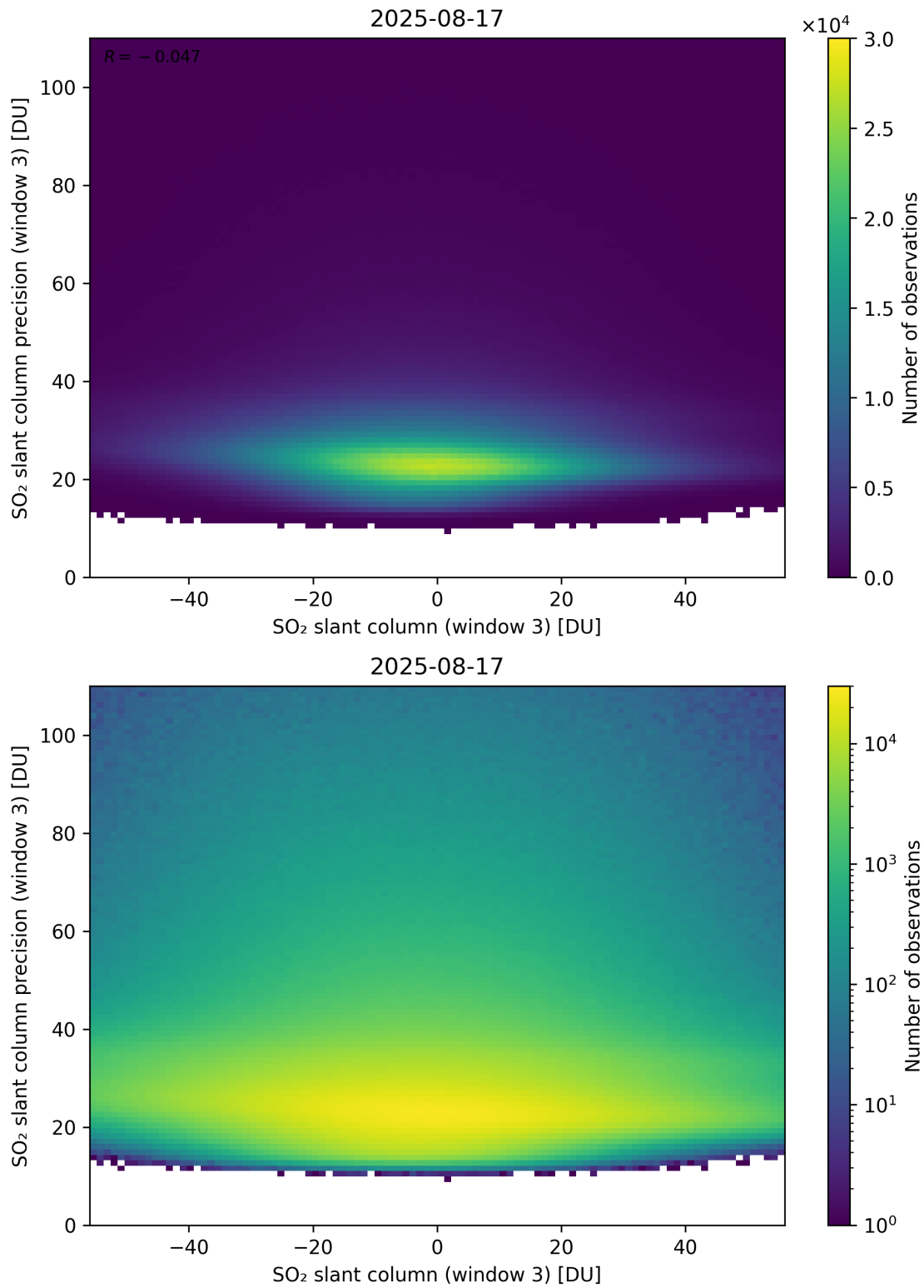
Figure 317: Scatter density plot of “SO 2 slant column (window 3)” against “SO 2 slant column precision (window 3)” for 2025-08-16 to 2025-08-18.
