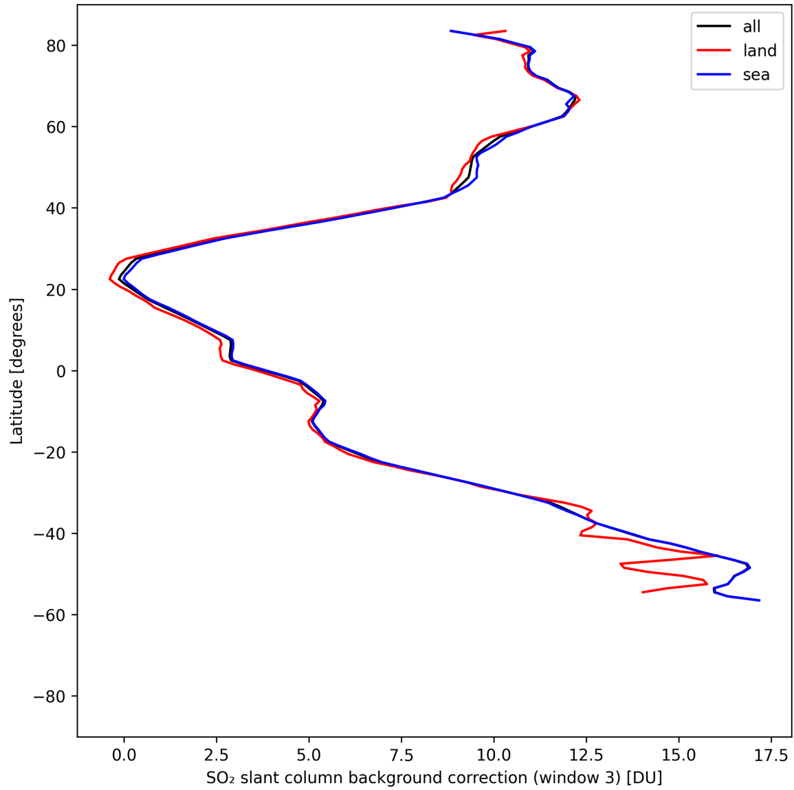
Figure 48: Zonal average of “SO 2 slant column background correction (window 3)” for 2025-08-16 to 2025-08-18.
