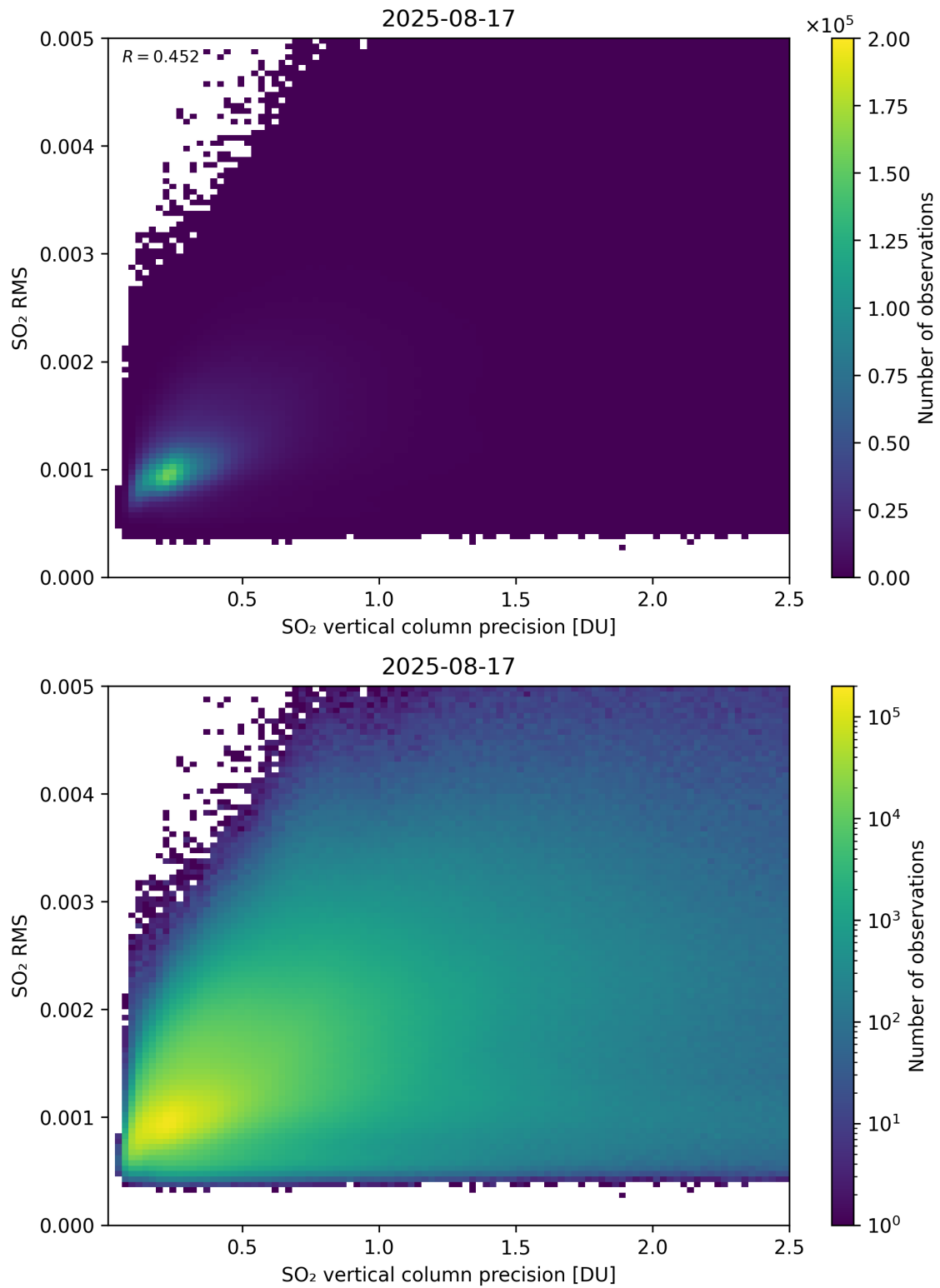
Figure 334: Scatter density plot of “SO 2 vertical column precision” against “SO 2 RMS” for 2025-08-16 to 2025-08-18.
