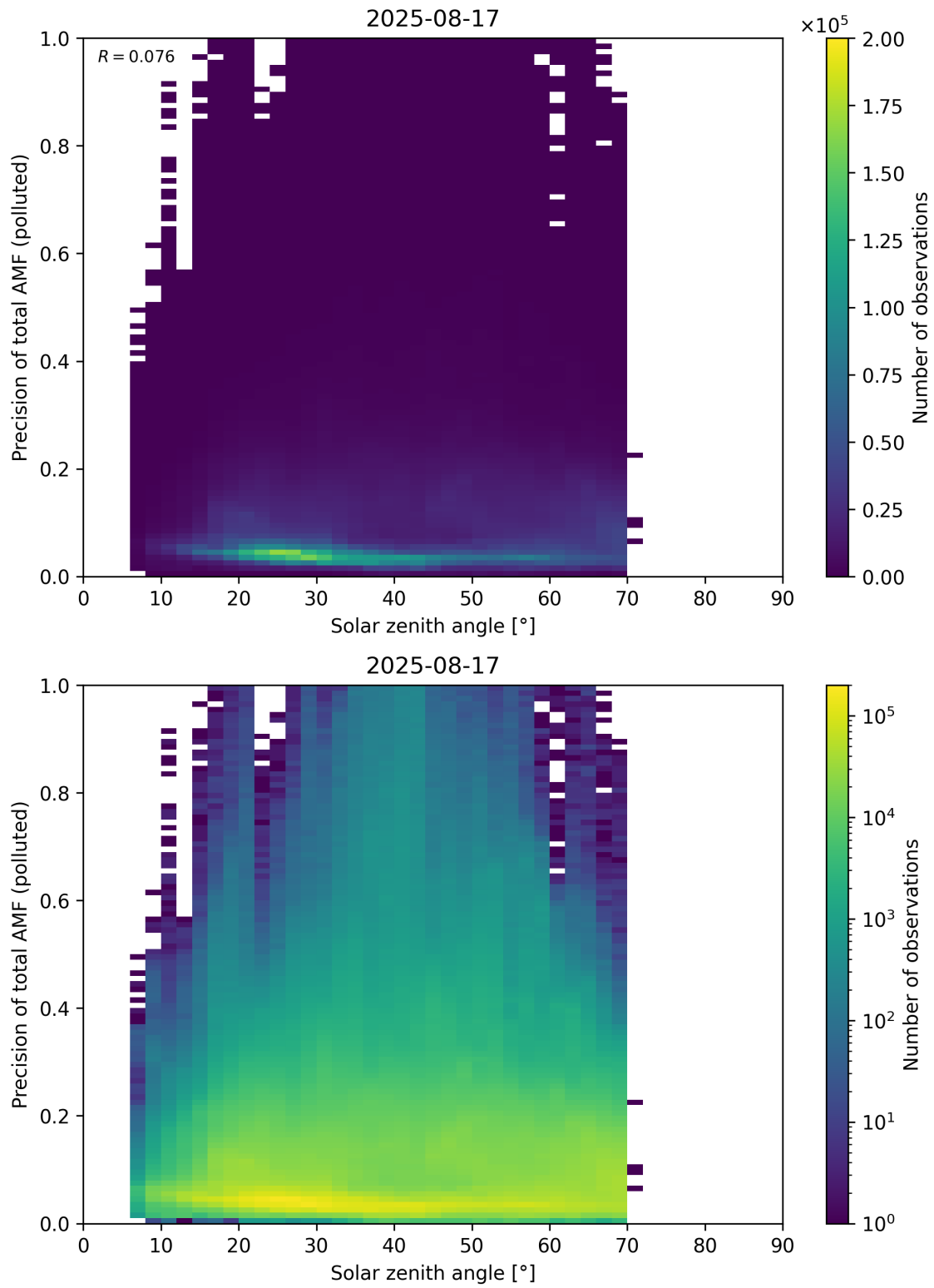
Figure 190: Scatter density plot of “Solar zenith angle” against “Precision of total AMF (polluted)” for 2025-08-16 to 2025-08-18.
