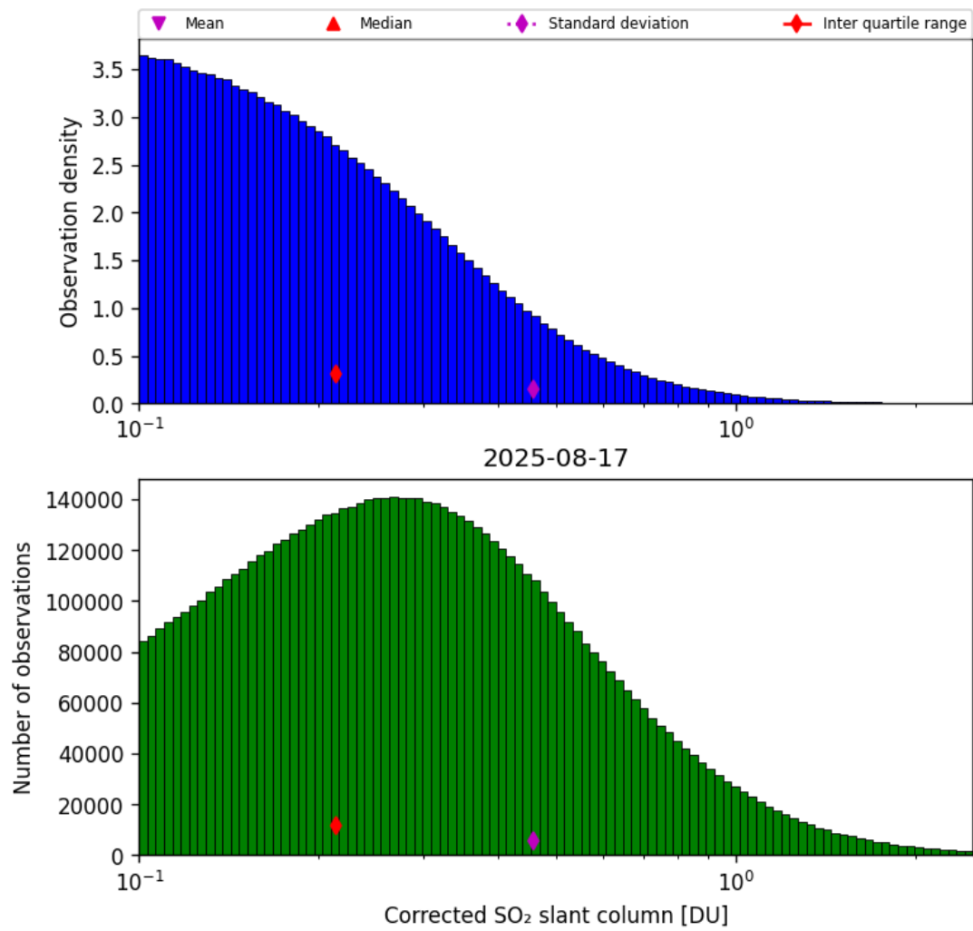
Figure 60: Histogram of “Corrected SO 2 slant column” for 2025-08-16 to 2025-08-18
