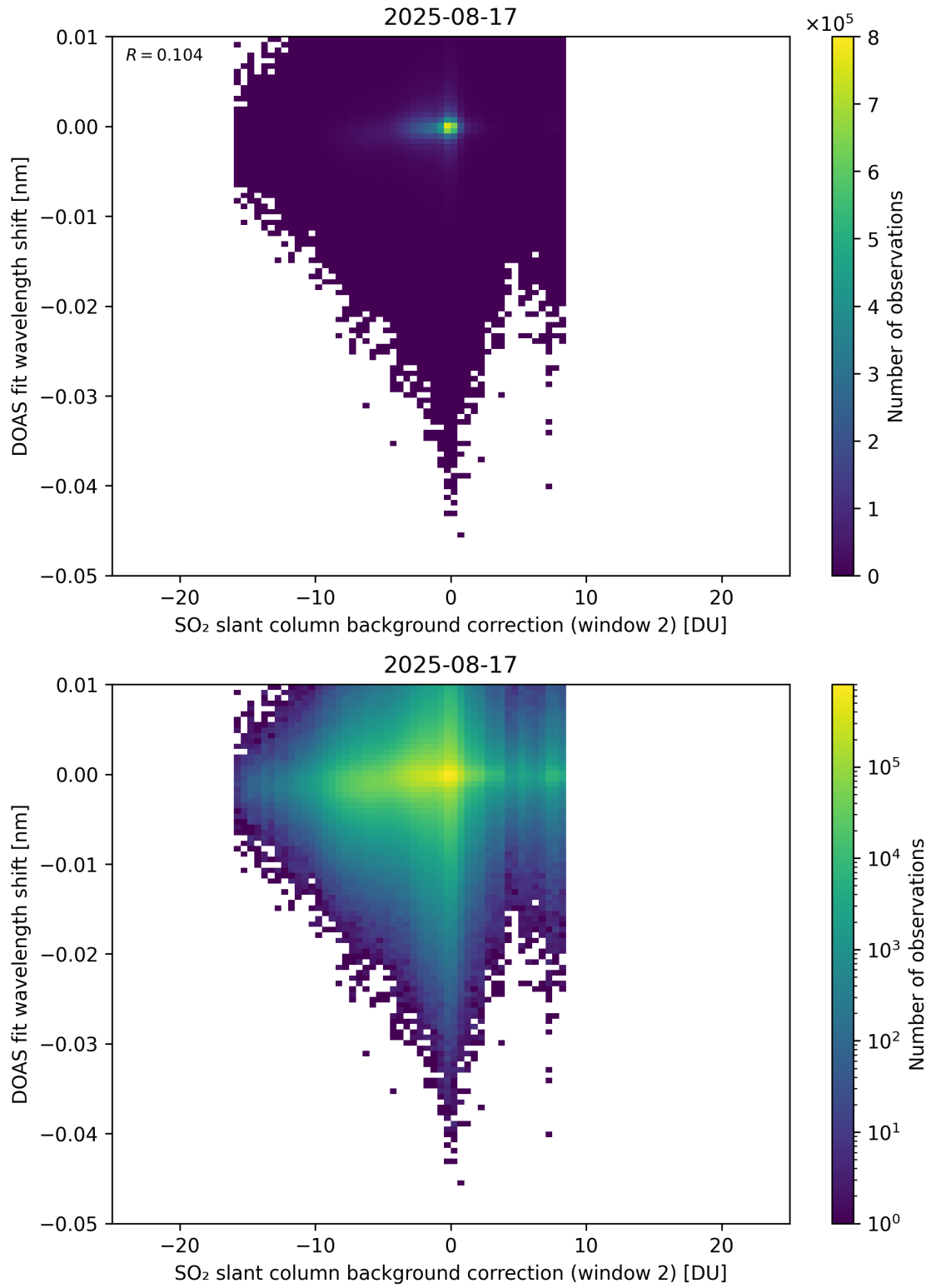
Figure 123: Scatter density plot of “SO 2 slant column background correction (window 2)” against “DOAS fit wavelength shift” for 2025-08-16 to 2025-08-18.
