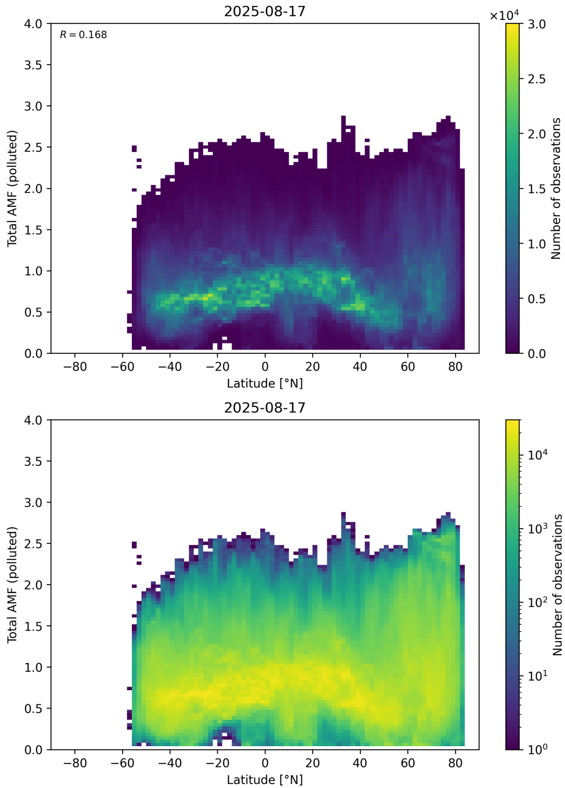
Figure 167: Scatter density plot of “Latitude” against “Total AMF (polluted)” for 2025-08-16 to 2025-08-18.
