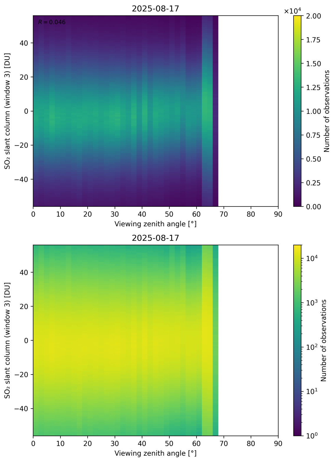
Figure 379: Scatter density plot of “Viewing zenith angle” against “SO 2 slant column (window 3)” for 2025-08-16 to 2025-08-18.
