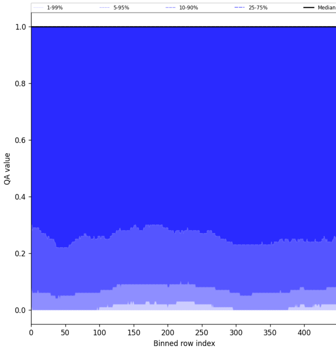
Figure 83: Along track statistics of “QA value” for 2025-08-16 to 2025-08-18
