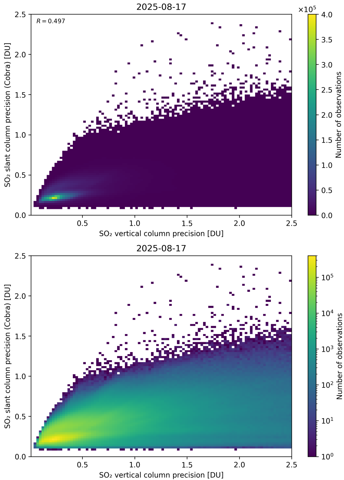
Figure 337: Scatter density plot of “SO 2 vertical column precision” against “SO 2 slant column precision (Cobra)” for 2025-08-16 to 2025-08-18.
