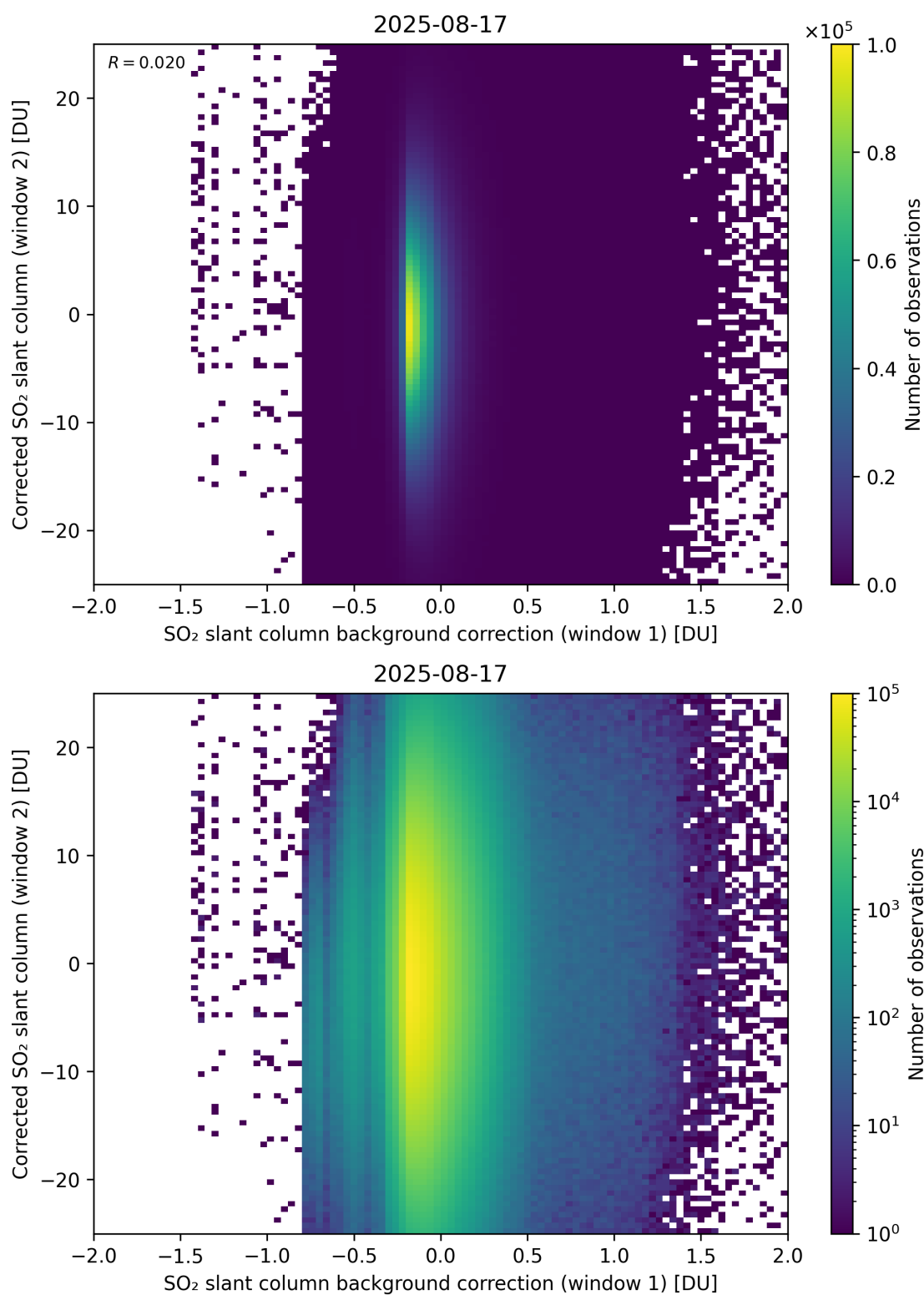
Figure 115: Scatter density plot of “SO 2 slant column background correction (window 1)” against “Corrected SO 2 slant column (window 2)” for 2025-08-16 to 2025-08-18.
