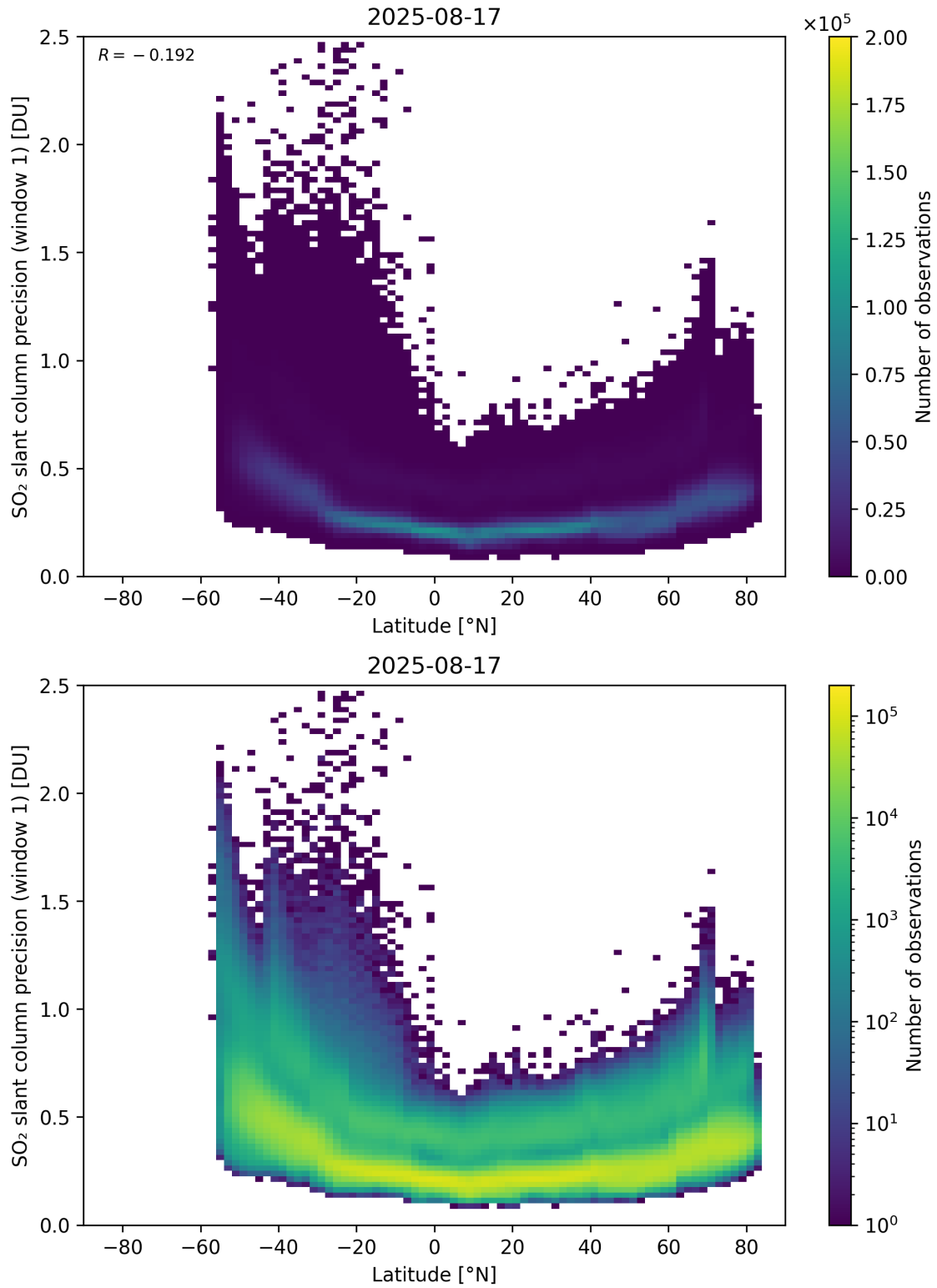
Figure 163: Scatter density plot of “Latitude” against “SO 2 slant column precision (window 1)” for 2025-08-16 to 2025-08-18.
