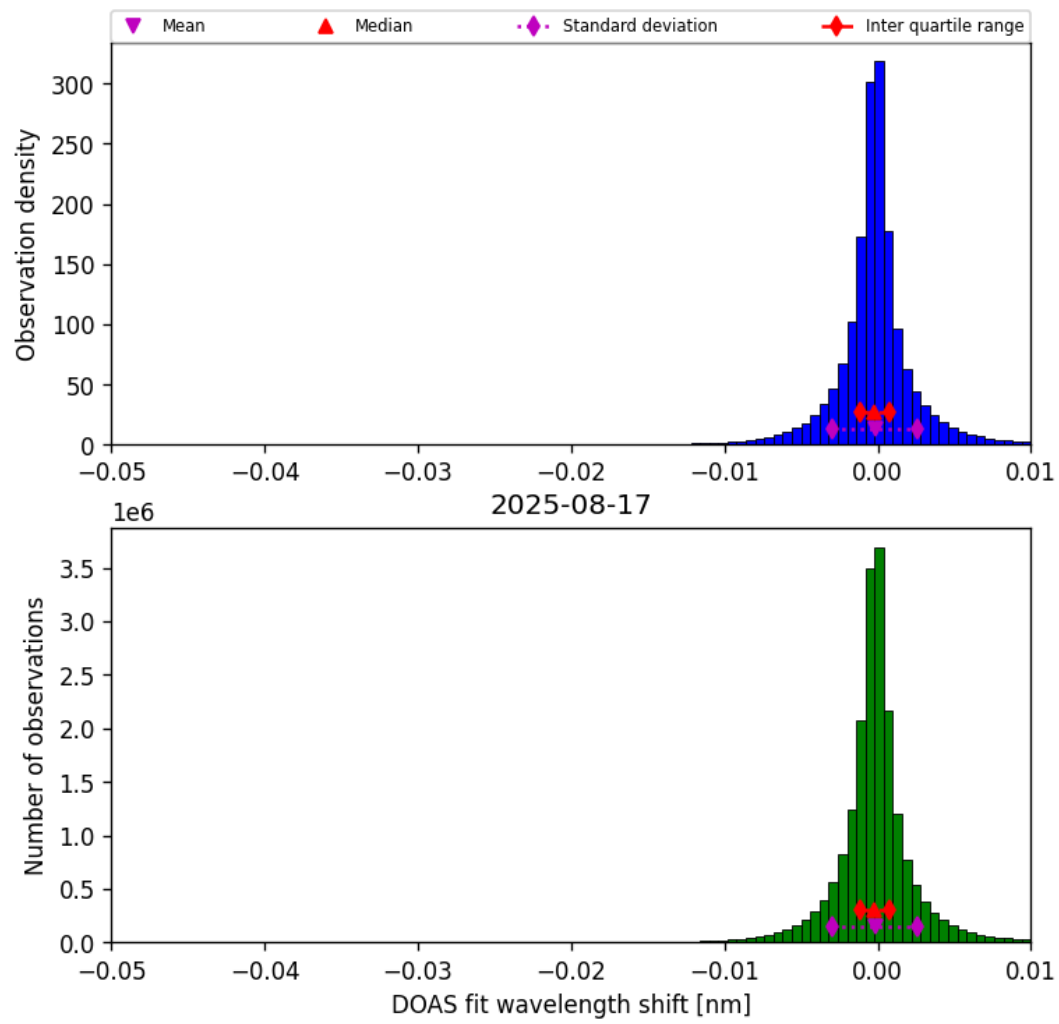
Figure 76: Histogram of “DOAS fit wavelength shift” for 2025-08-16 to 2025-08-18
