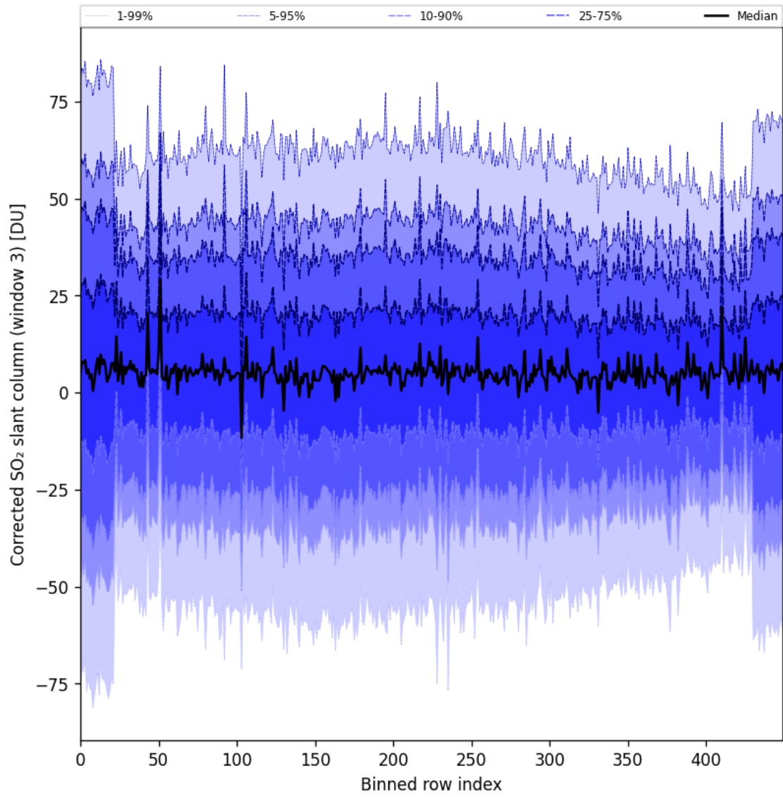
Figure 99: Along track statistics of “Corrected SO 2 slant column (window 3)” for 2025-08-16 to 2025-08-18
