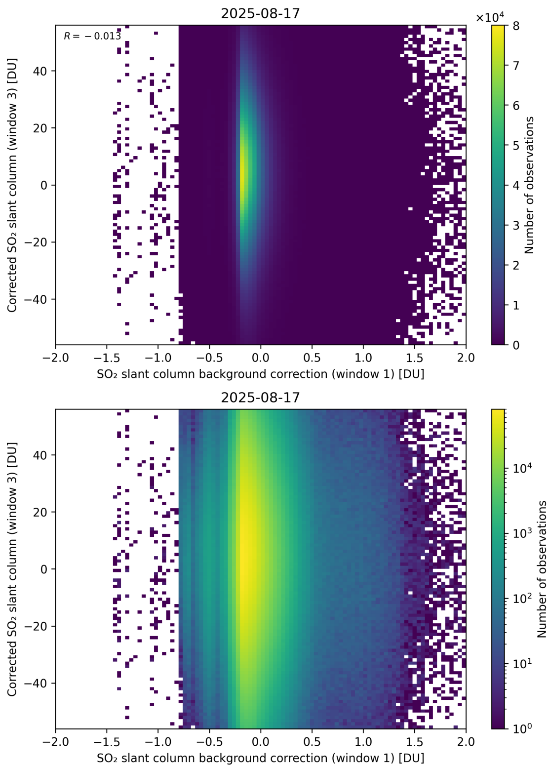
Figure 116: Scatter density plot of “SO 2 slant column background correction (window 1)” against “Corrected SO 2 slant column (window 3)” for 2025-08-16 to 2025-08-18.
