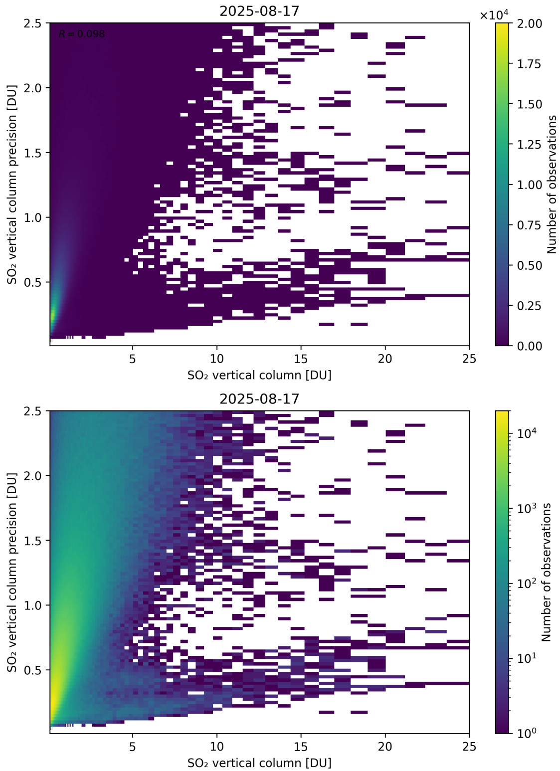
Figure 361: Scatter density plot of “SO 2 vertical column” against “SO 2 vertical column precision” for 2025-08-16 to 2025-08-18.
