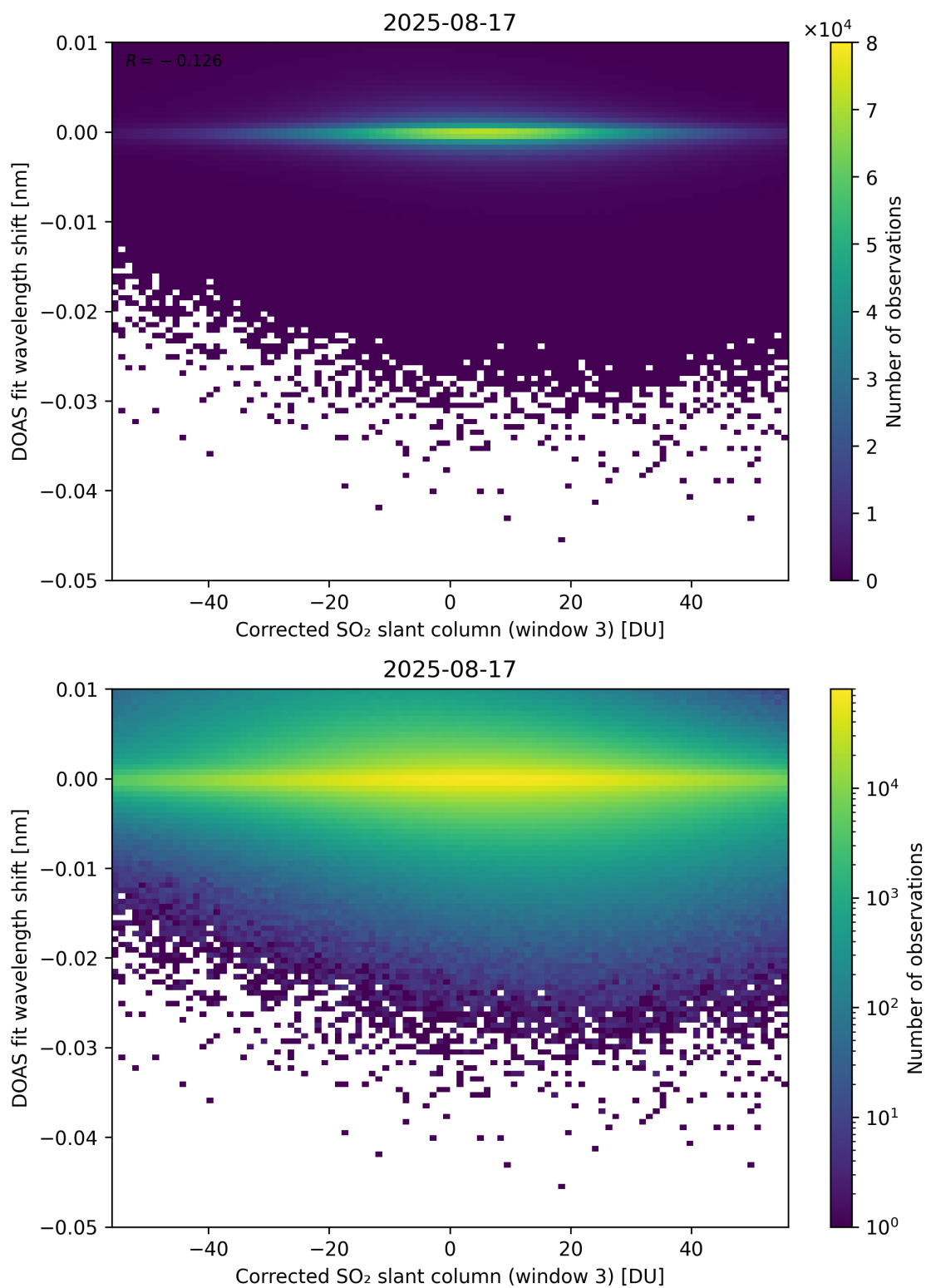
Figure 256: Scatter density plot of “Corrected SO 2 slant column (window 3)” against “DOAS fit wavelength shift” for 2025-08-16 to 2025-08-18.
