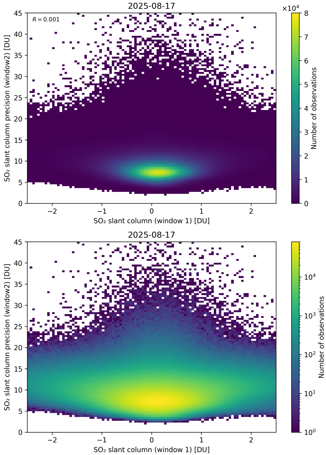
Figure 286: Scatter density plot of “SO 2 slant column (window 1)” against “SO 2 slant column precision (window2)” for 2025-08-16 to 2025-08-18.
