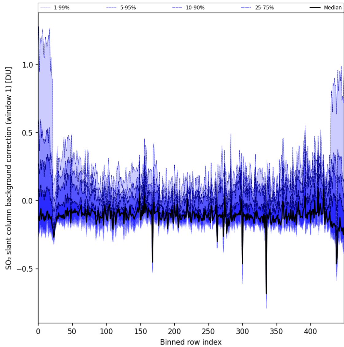
Figure 92: Along track statistics of “SO 2 slant column background correction (window 1)” for 2025-08-16 to 2025-08-18
