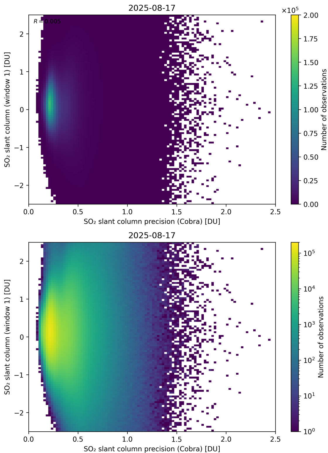
Figure 208: Scatter density plot of “SO 2 slant column precision (Cobra)” against “SO 2 slant column (window 1)” for 2025-08-16 to 2025-08-18.
