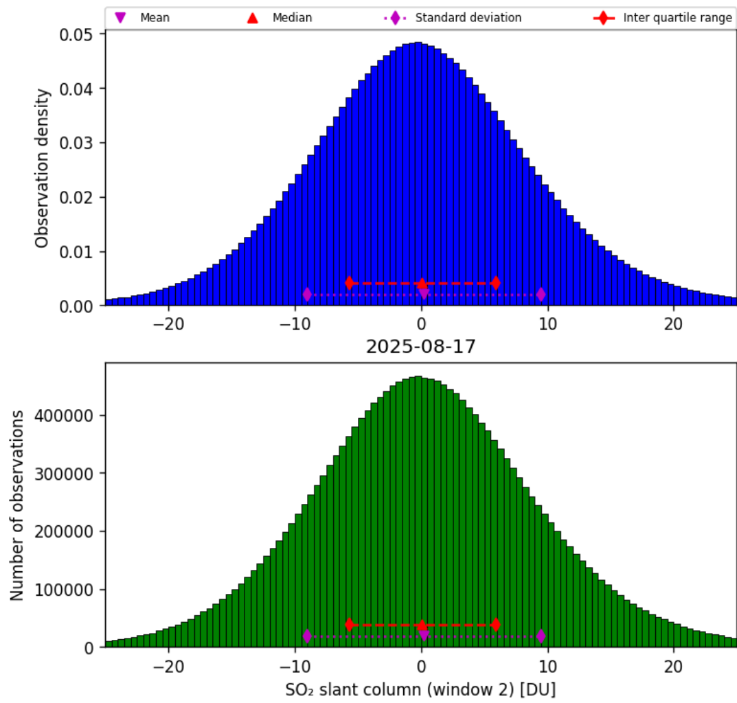
Figure 67: Histogram of “SO 2 slant column (window 2)” for 2025-08-16 to 2025-08-18
