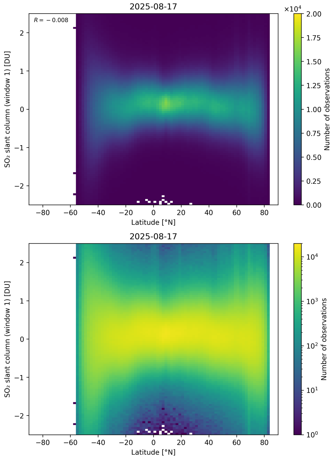
Figure 162: Scatter density plot of “Latitude” against “SO 2 slant column (window 1)” for 2025-08-16 to 2025-08-18.
