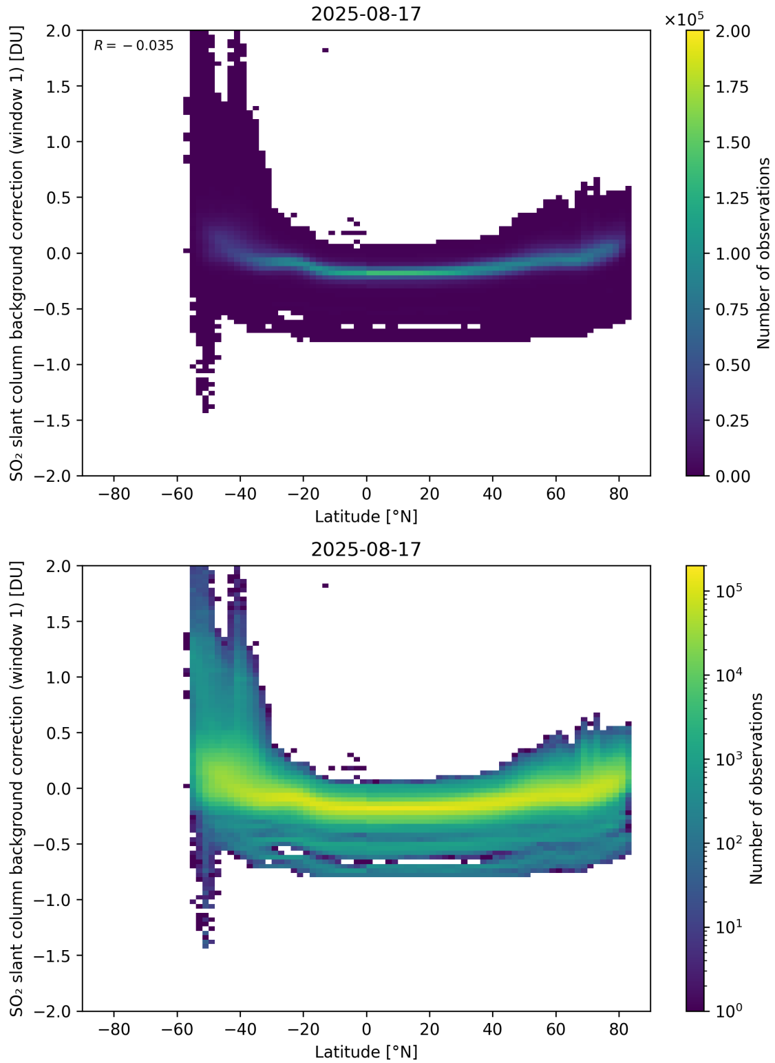
Figure 150: Scatter density plot of “Latitude” against “SO 2 slant column background correction (window 1)” for 2025-08-16 to 2025-08-18.
