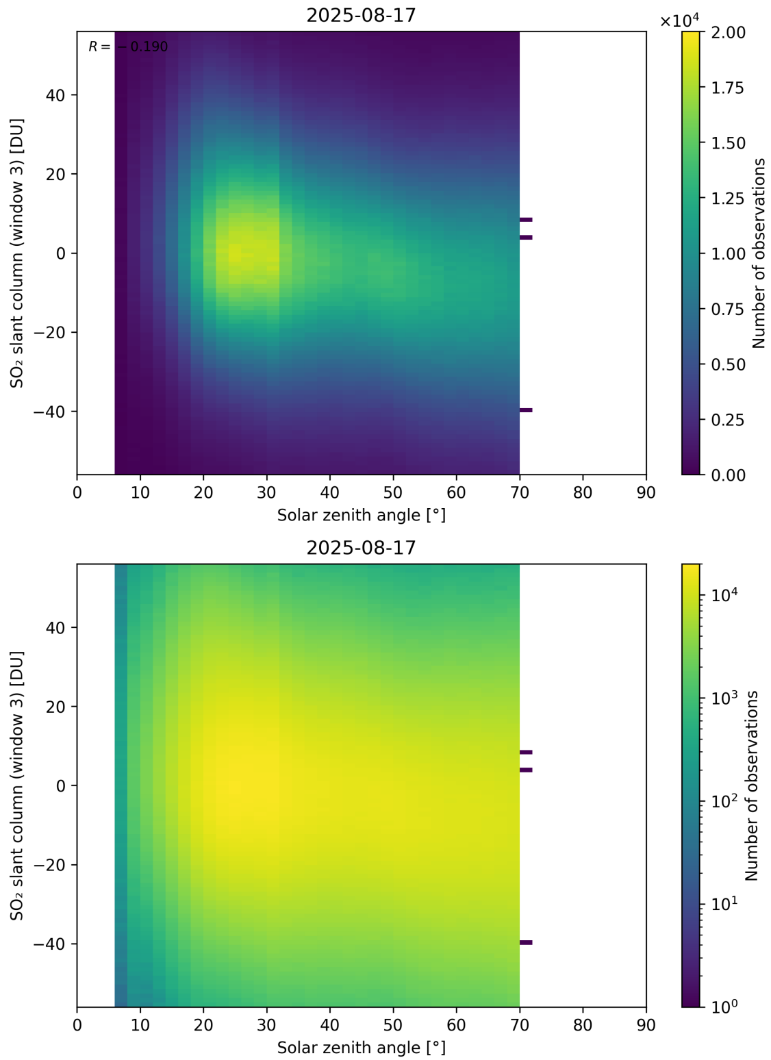
Figure 187: Scatter density plot of “Solar zenith angle” against “SO 2 slant column (window 3)” for 2025-08-16 to 2025-08-18.
