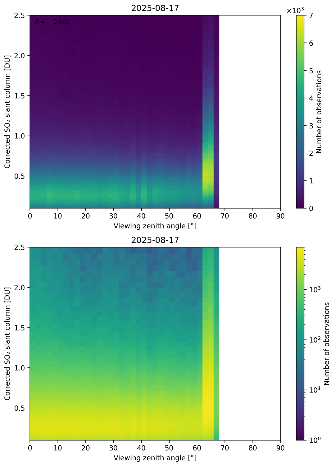
Figure 373: Scatter density plot of “Viewing zenith angle” against “Corrected SO 2 slant column” for 2025-08-16 to 2025-08-18.
