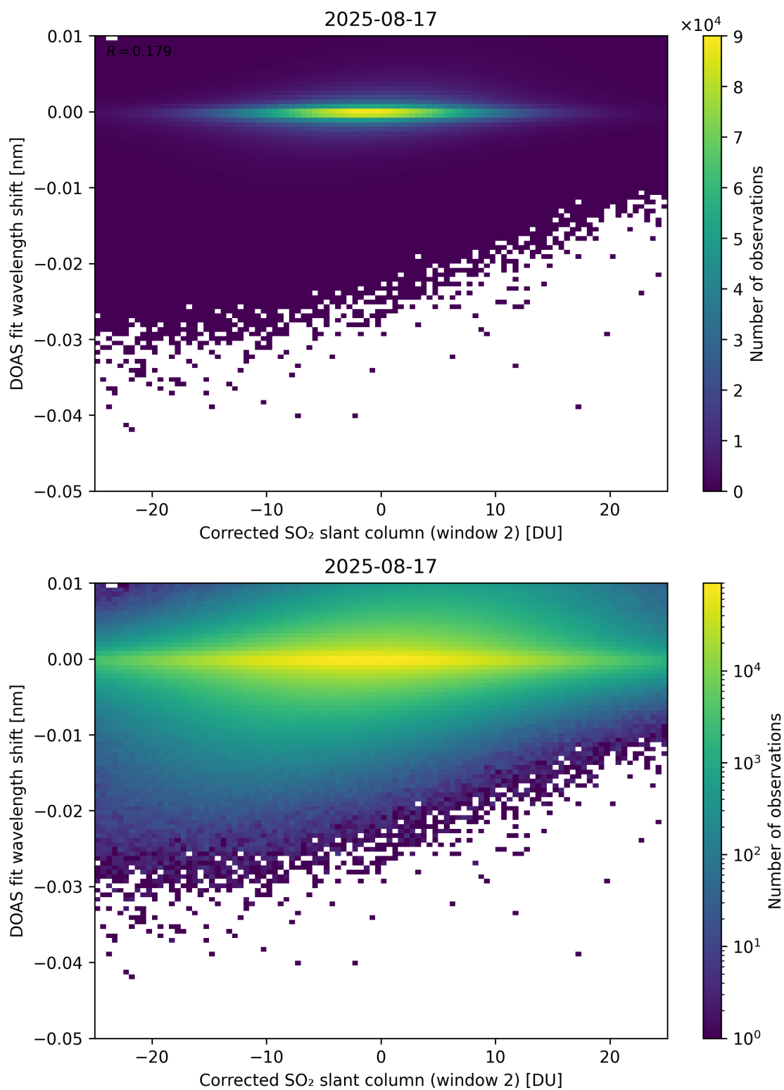
Figure 246: Scatter density plot of “Corrected SO 2 slant column (window 2)” against “DOAS fit wavelength shift” for 2025-08-16 to 2025-08-18.
