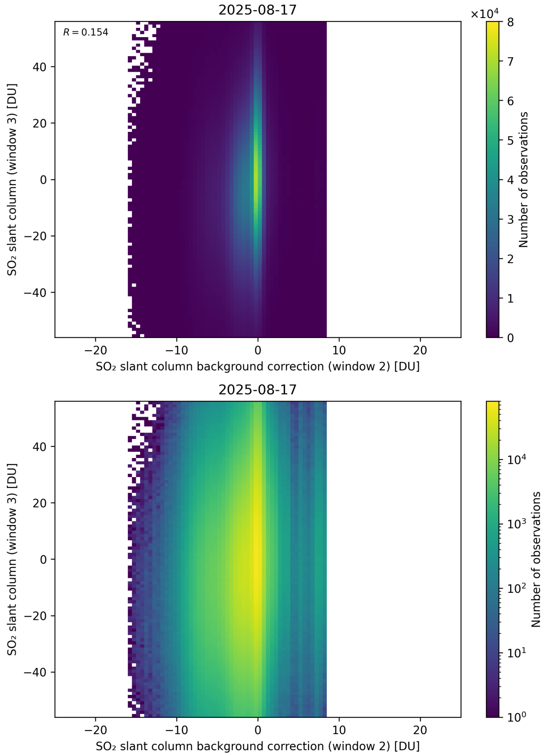
Figure 128: Scatter density plot of “SO 2 slant column background correction (window 2)” against “SO 2 slant column (window 3)” for 2025-08-16 to 2025-08-18.
