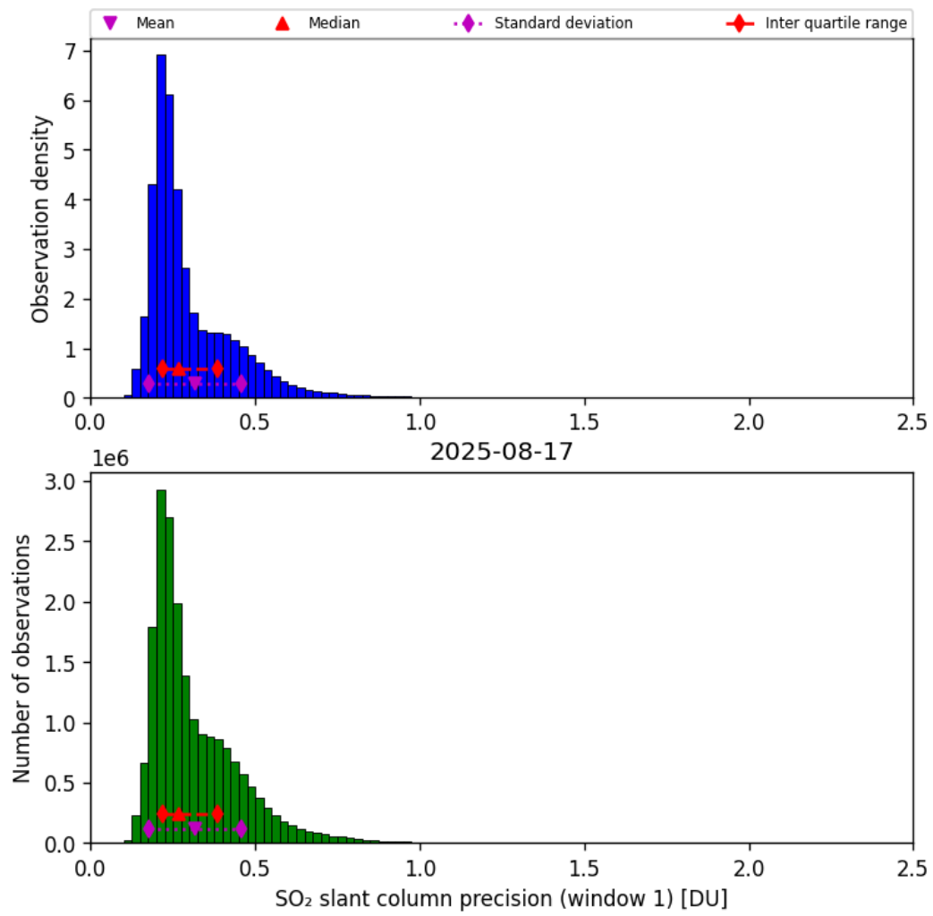
Figure 64: Histogram of “SO 2 slant column precision (window 1)” for 2025-08-16 to 2025-08-18
