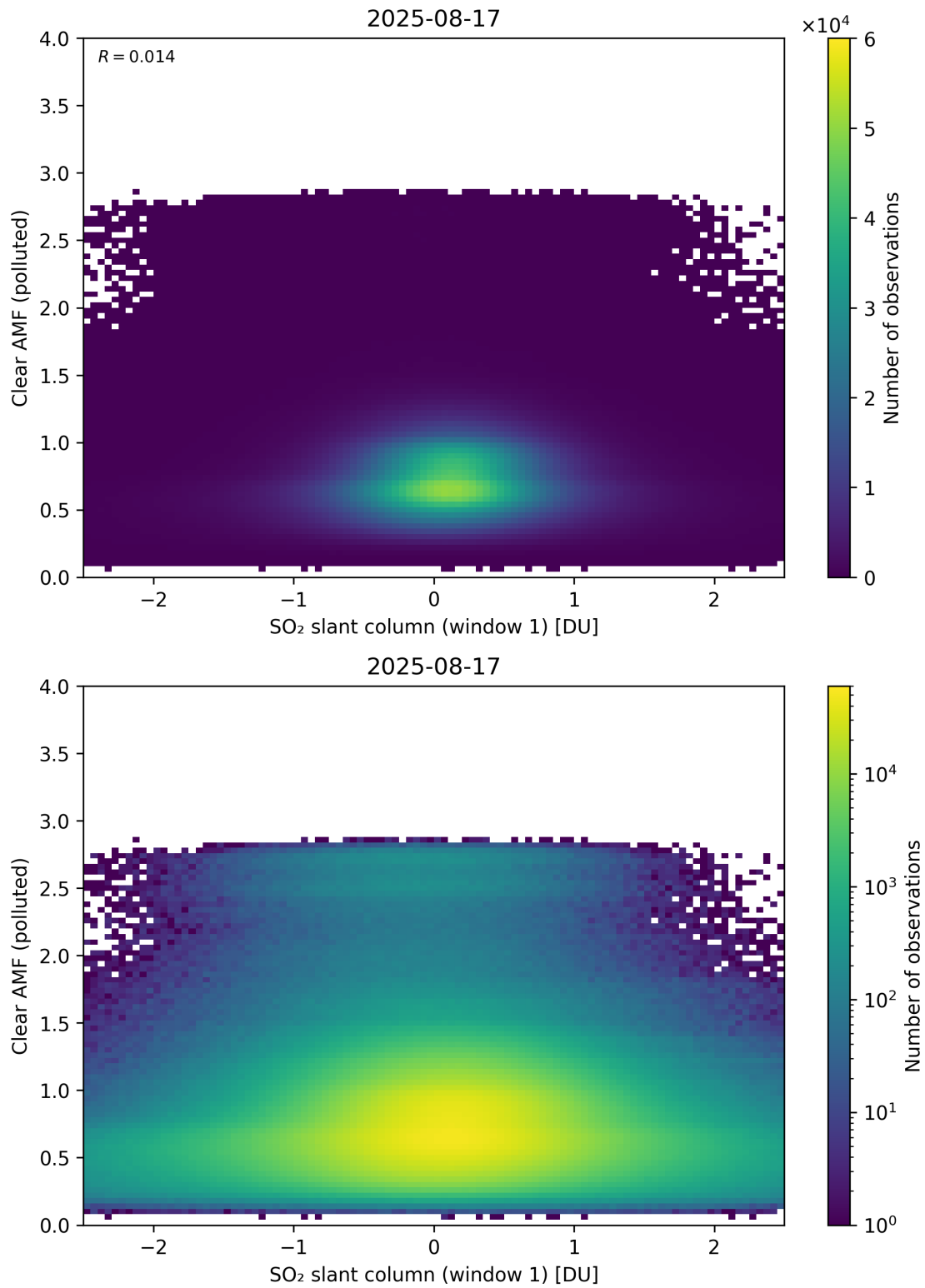
Figure 282: Scatter density plot of “SO 2 slant column (window 1)” against “Clear AMF (polluted)” for 2025-08-16 to 2025-08-18.
