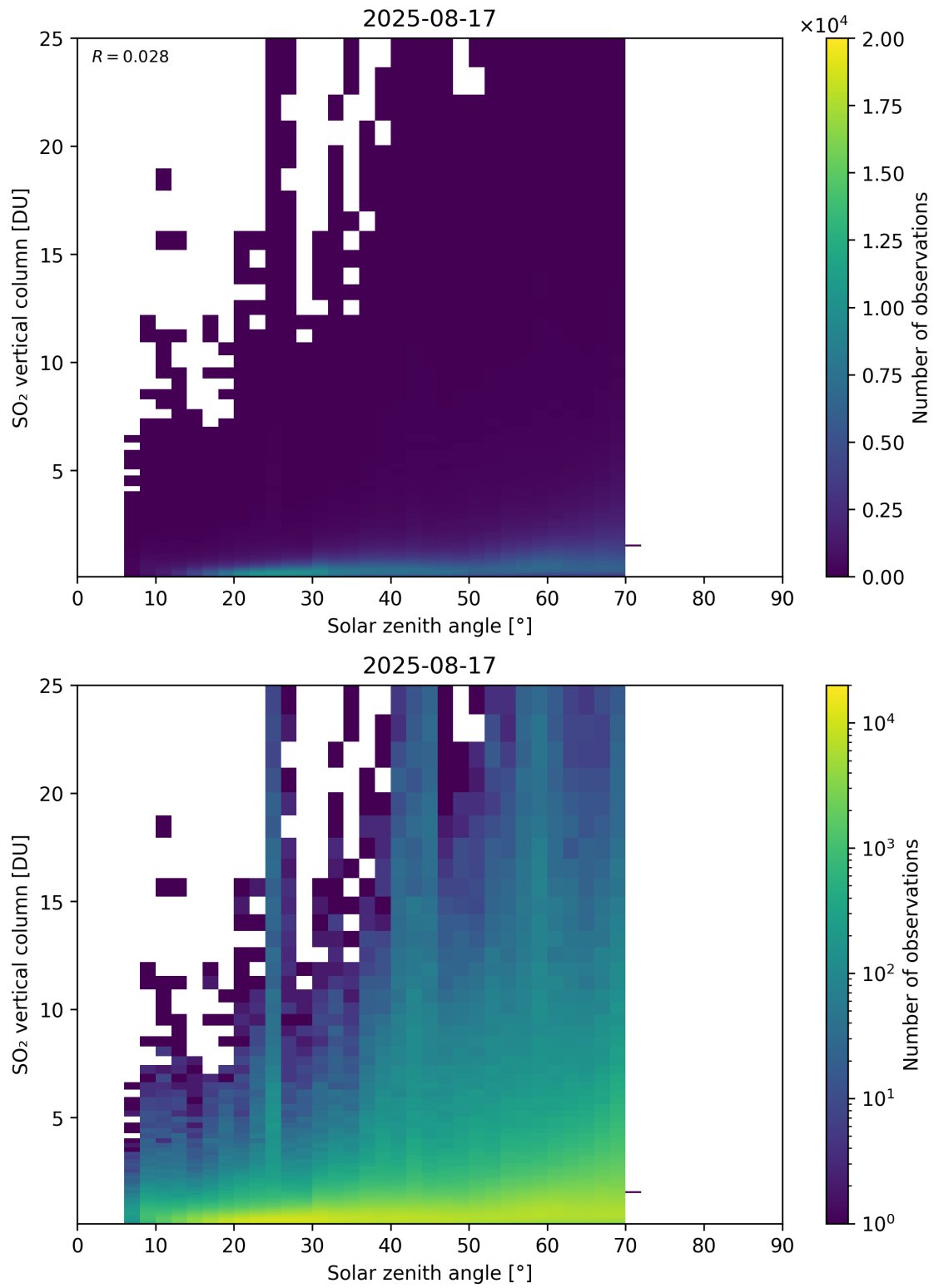
Figure 191: Scatter density plot of “Solar zenith angle” against “SO 2 vertical column” for 2025-08-16 to 2025-08-18.
