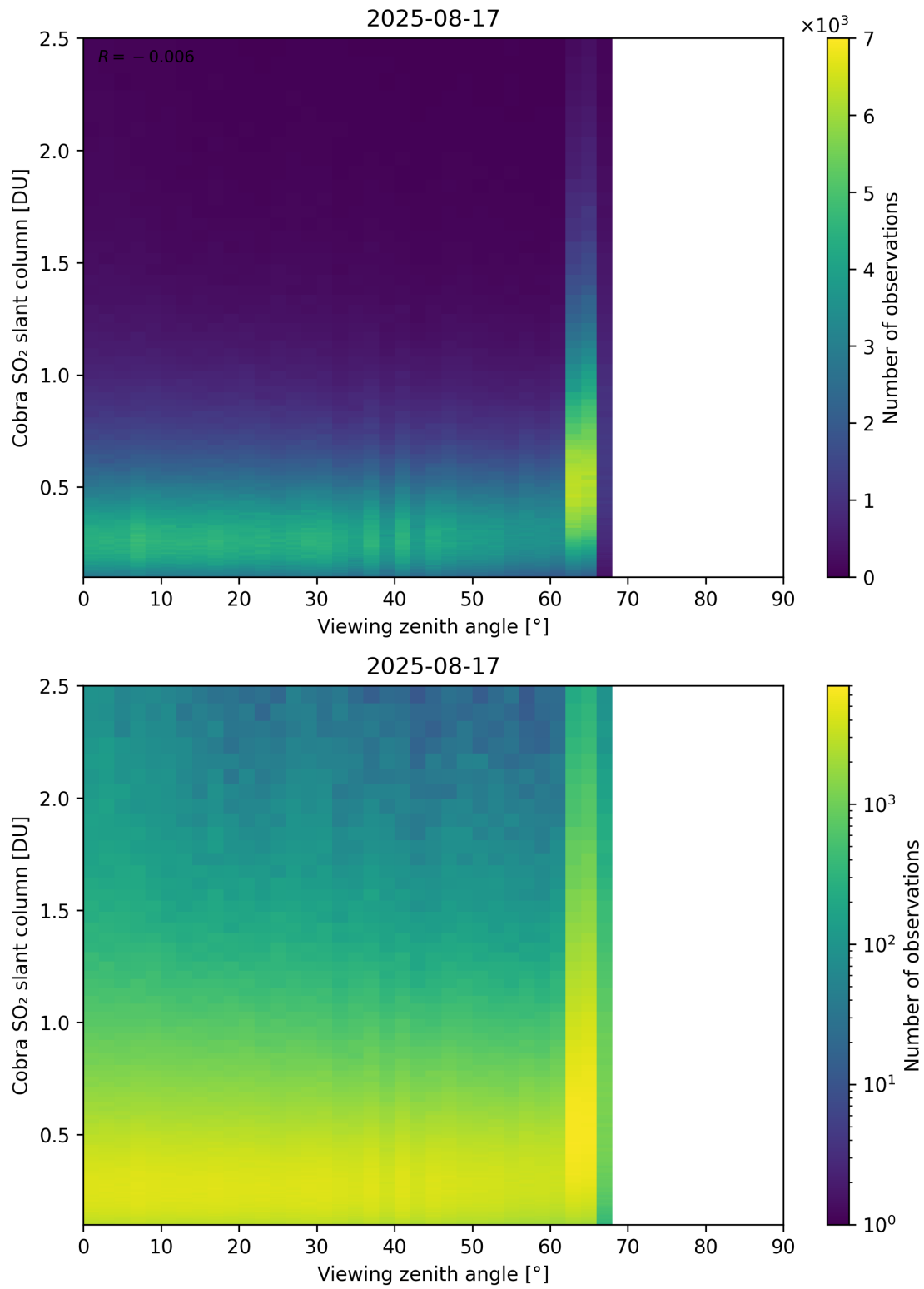
Figure 371: Scatter density plot of “Viewing zenith angle” against “Cobra SO 2 slant column” for 2025-08-16 to 2025-08-18.
