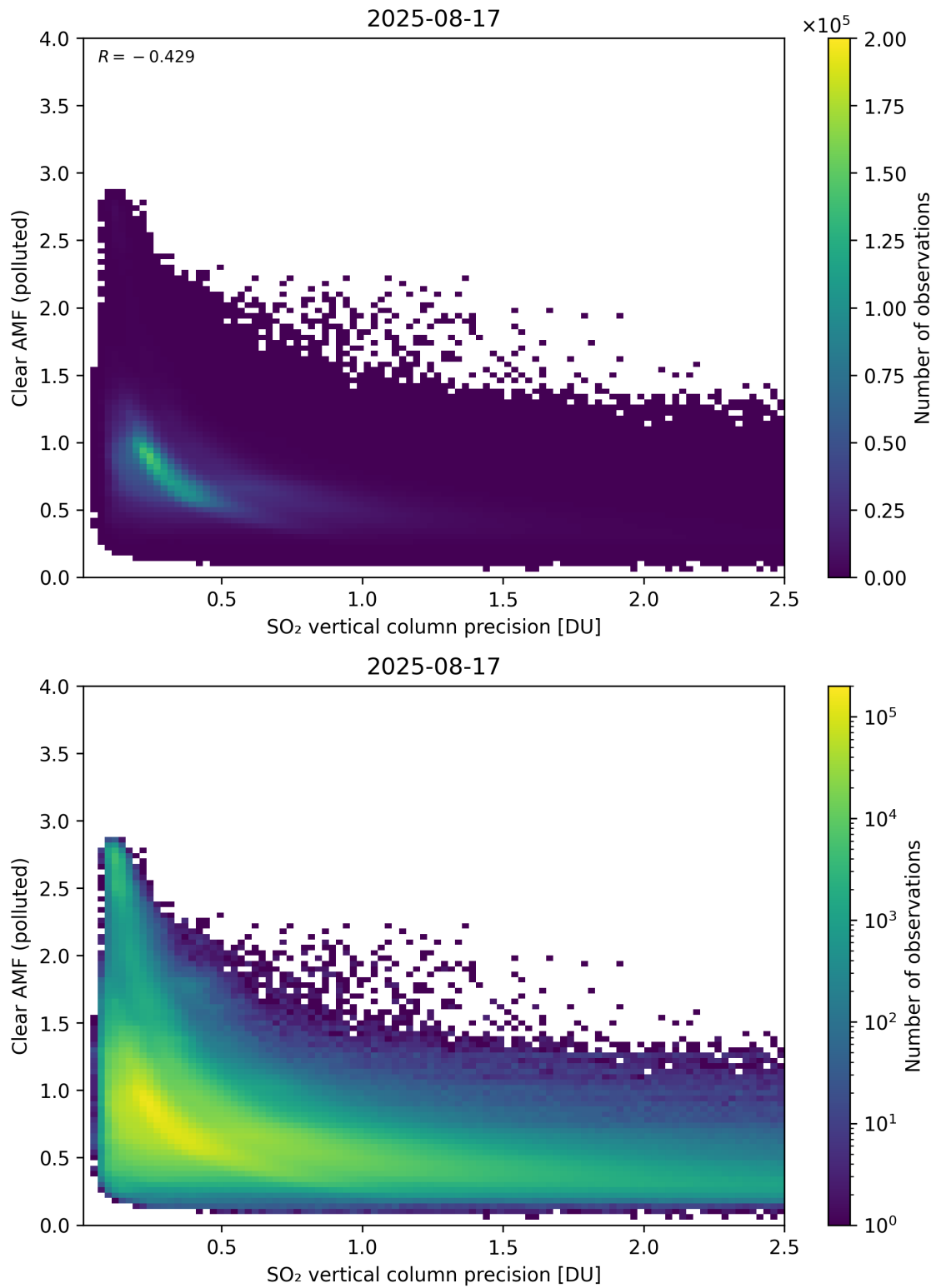
Figure 335: Scatter density plot of “SO 2 vertical column precision” against “Clear AMF (polluted)” for 2025-08-16 to 2025-08-18.
