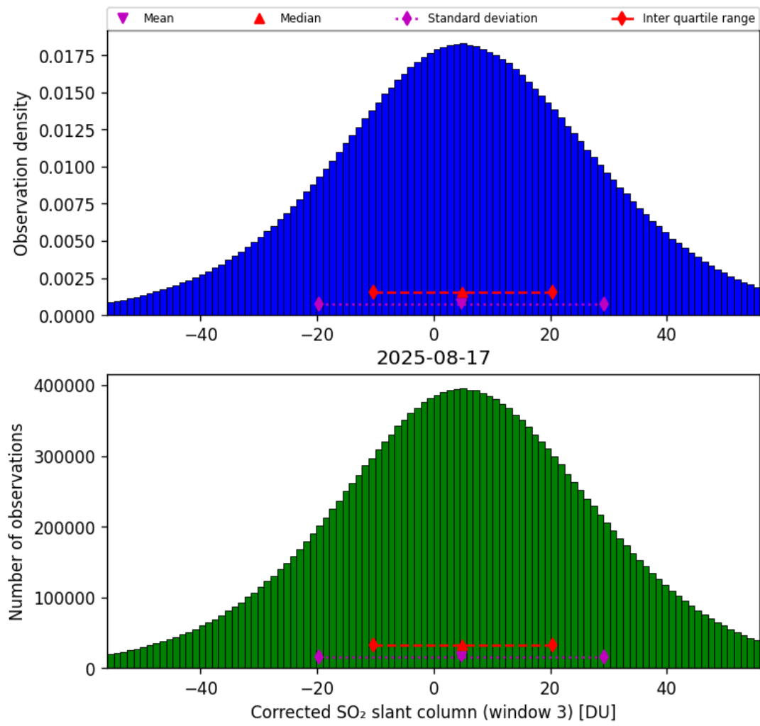
Figure 73: Histogram of “Corrected SO 2 slant column (window 3)” for 2025-08-16 to 2025-08-18
