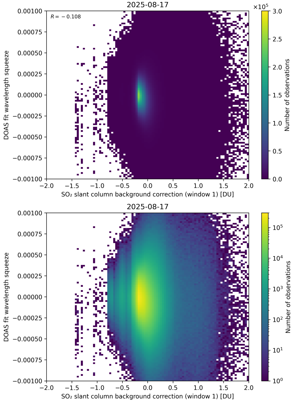
Figure 112: Scatter density plot of “SO 2 slant column background correction (window 1)” against “DOAS fit wavelength squeeze” for 2025-08-16 to 2025-08-18.
