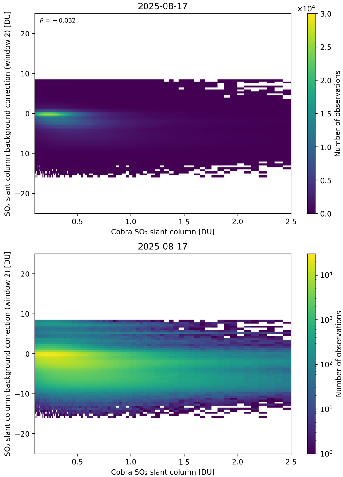
Figure 194: Scatter density plot of “Cobra SO 2 slant column” against “SO 2 slant column background correction (window 2)” for 2025-08-16 to 2025-08-18.
