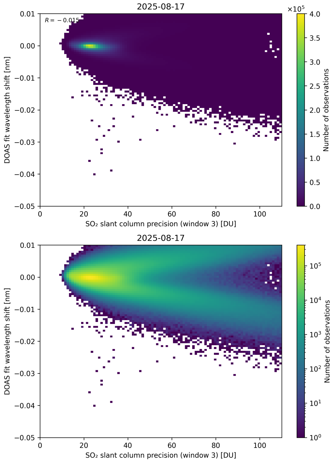
Figure 308: Scatter density plot of “SO 2 slant column precision (window 3)” against “DOAS fit wavelength shift” for 2025-08-16 to 2025-08-18.
