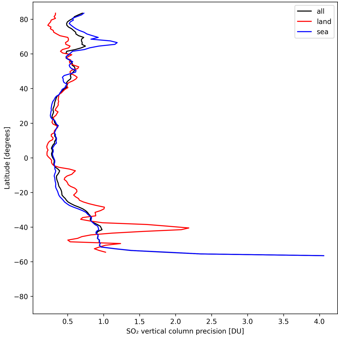
Figure 33: Zonal average of “SO 2 vertical column precision” for 2025-08-16 to 2025-08-18.
