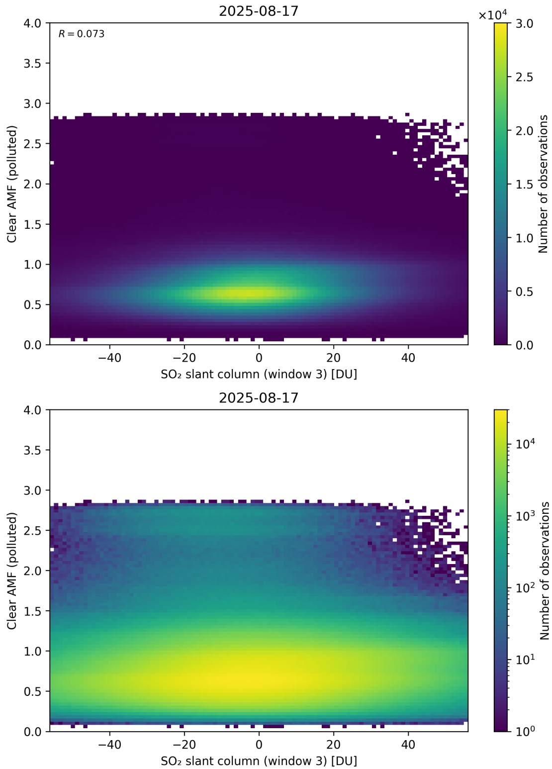
Figure 315: Scatter density plot of “SO 2 slant column (window 3)” against “Clear AMF (polluted)” for 2025-08-16 to 2025-08-18.
