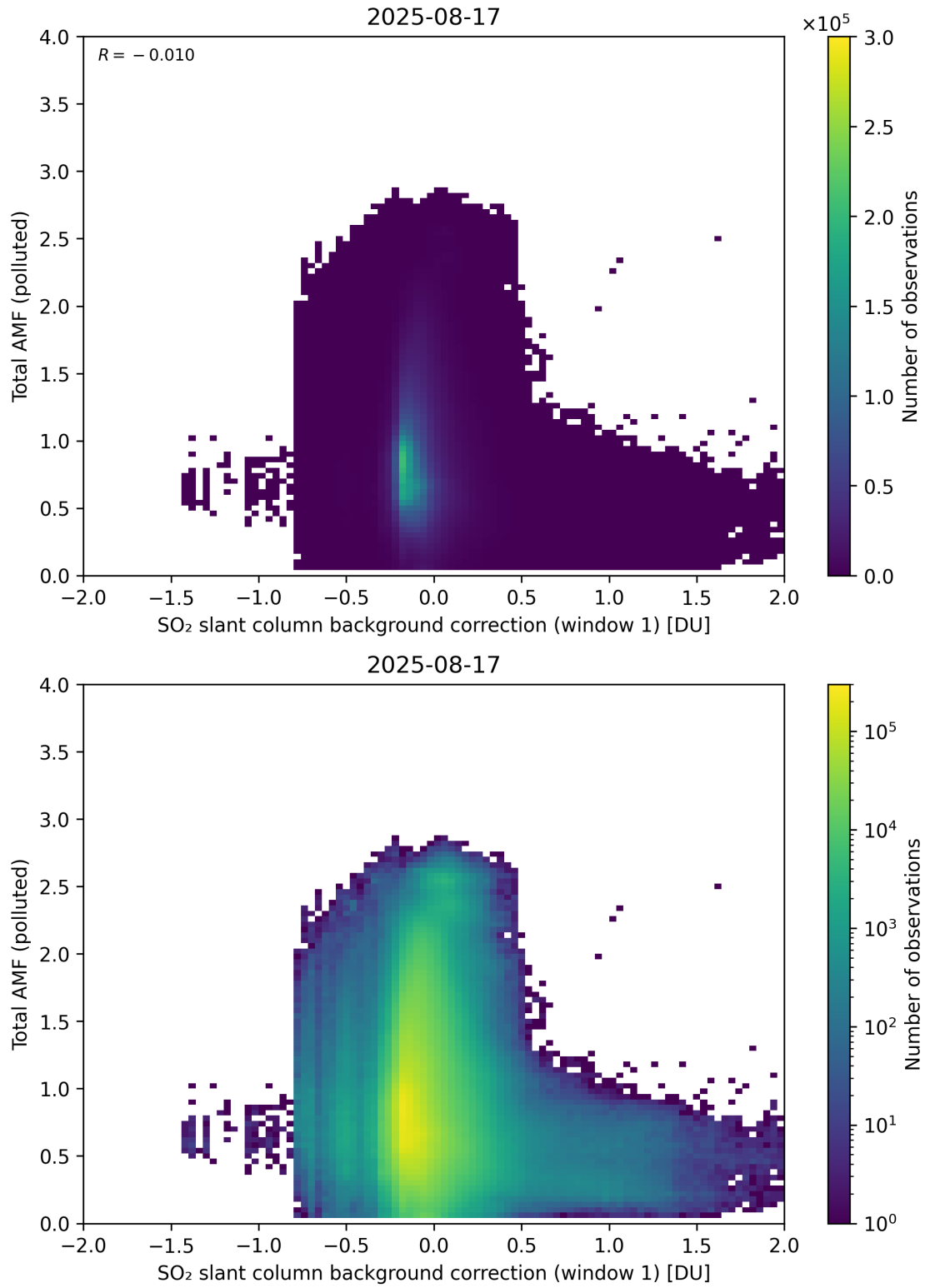
Figure 120: Scatter density plot of “SO 2 slant column background correction (window 1)” against “Total AMF (polluted)” for 2025-08-16 to 2025-08-18.
