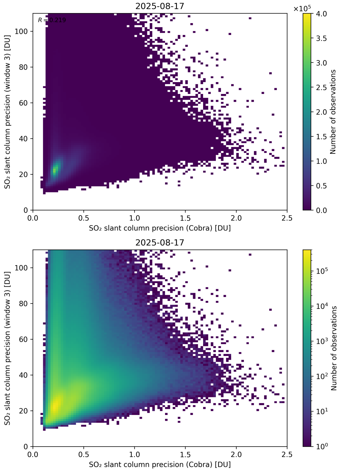
Figure 212: Scatter density plot of “SO 2 slant column precision (Cobra)” against “SO 2 slant column precision (window 3)” for 2025-08-16 to 2025-08-18.
