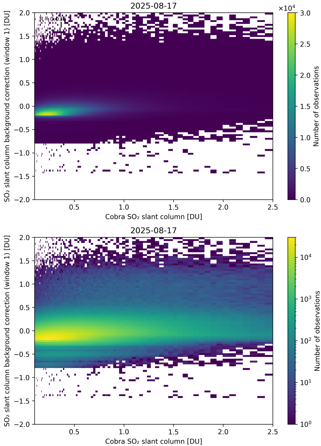
Figure 193: Scatter density plot of “Cobra SO 2 slant column” against “SO 2 slant column background correction (window 1)” for 2025-08-16 to 2025-08-18.
