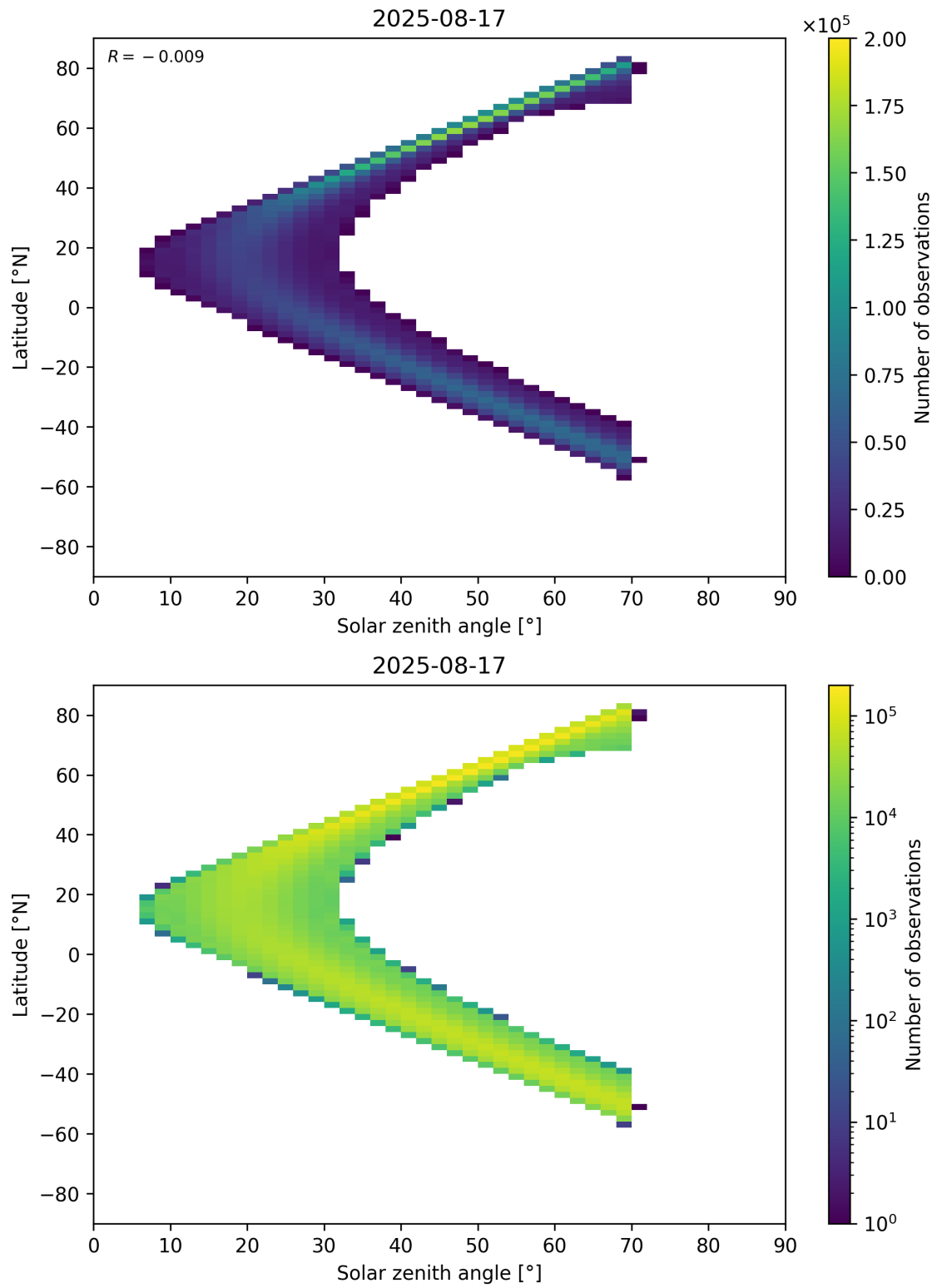
Figure 177: Scatter density plot of “Solar zenith angle” against “Latitude” for 2025-08-16 to 2025-08-18.
