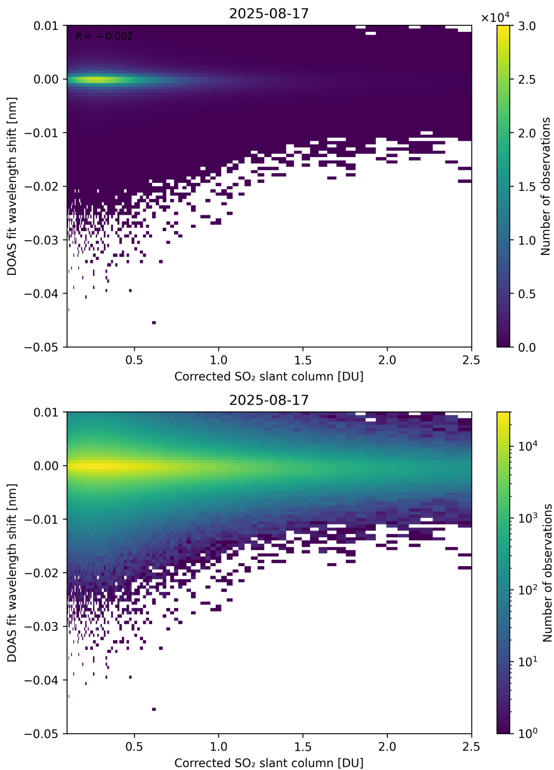
Figure 229: Scatter density plot of “Corrected SO 2 slant column” against “DOAS fit wavelength shift” for 2025-08-16 to 2025-08-18.
