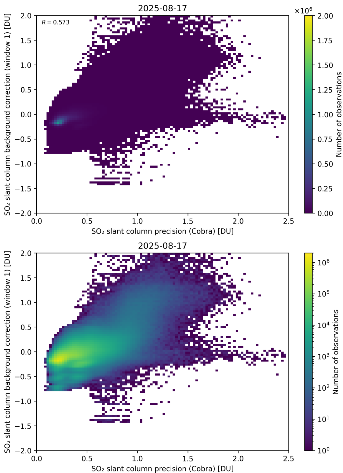
Figure 199: Scatter density plot of “SO 2 slant column precision (Cobra)” against “SO 2 slant column background correction (window 1)” for 2025-08-16 to 2025-08-18.
