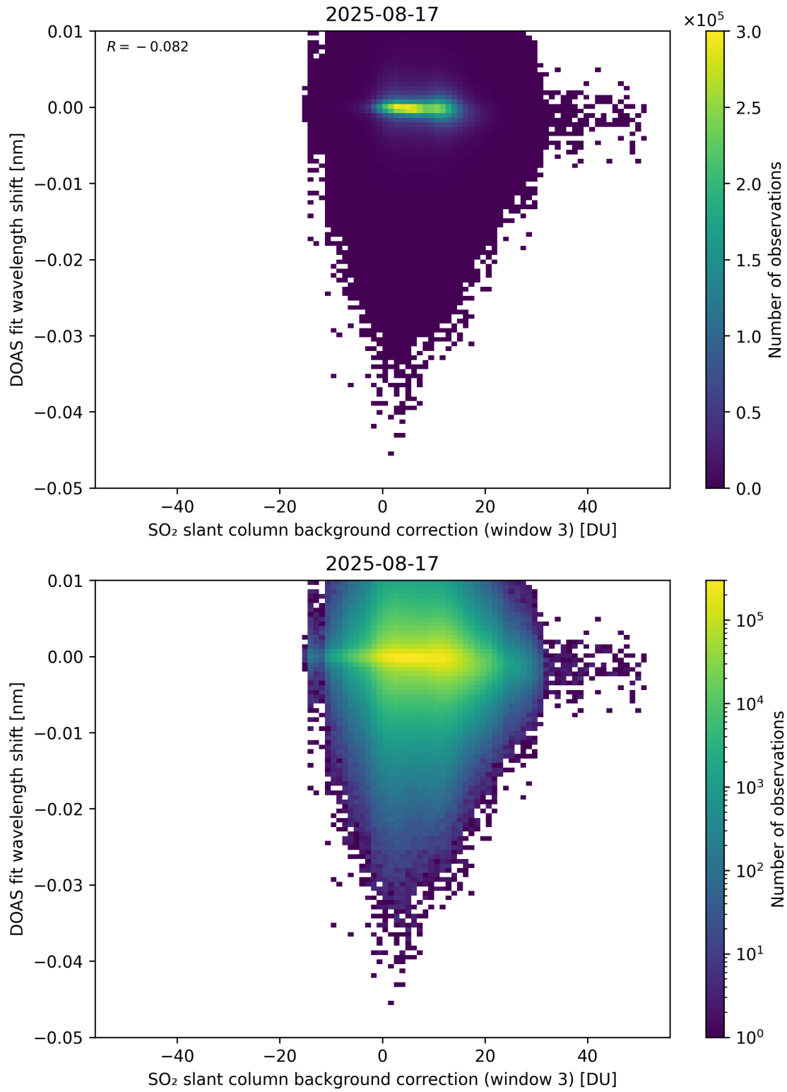
Figure 132: Scatter density plot of “SO 2 slant column background correction (window 3)” against “DOAS fit wavelength shift” for 2025-08-16 to 2025-08-18.
