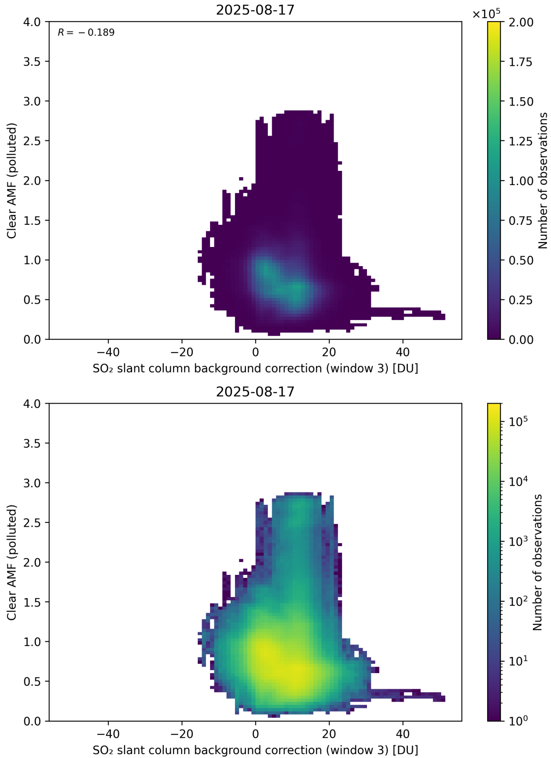
Figure 135: Scatter density plot of “SO 2 slant column background correction (window 3)” against “Clear AMF (polluted)” for 2025-08-16 to 2025-08-18.
