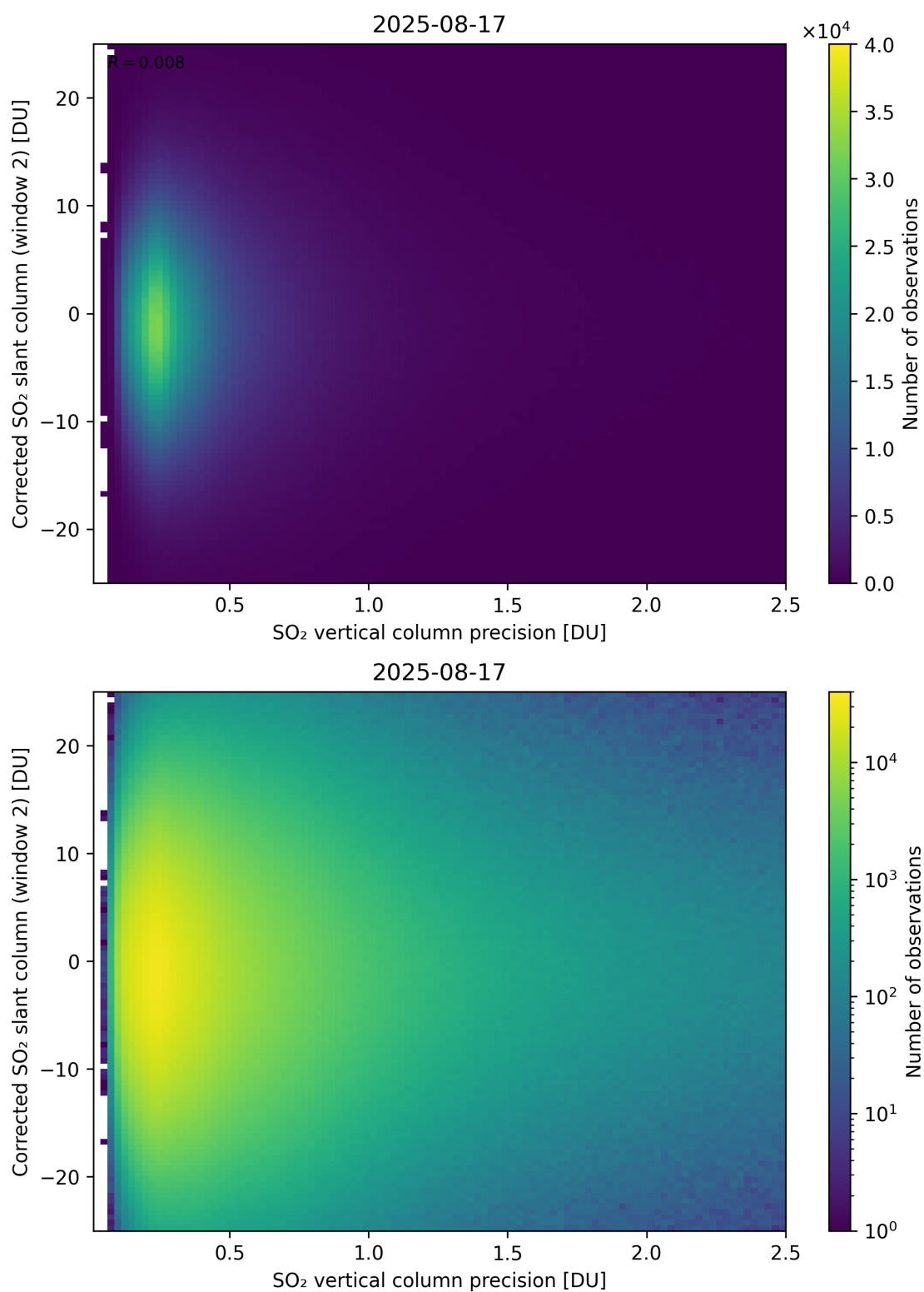
Figure 339: Scatter density plot of “SO 2 vertical column precision” against “Corrected SO 2 slant column (window 2)” for 2025-08-16 to 2025-08-18.
