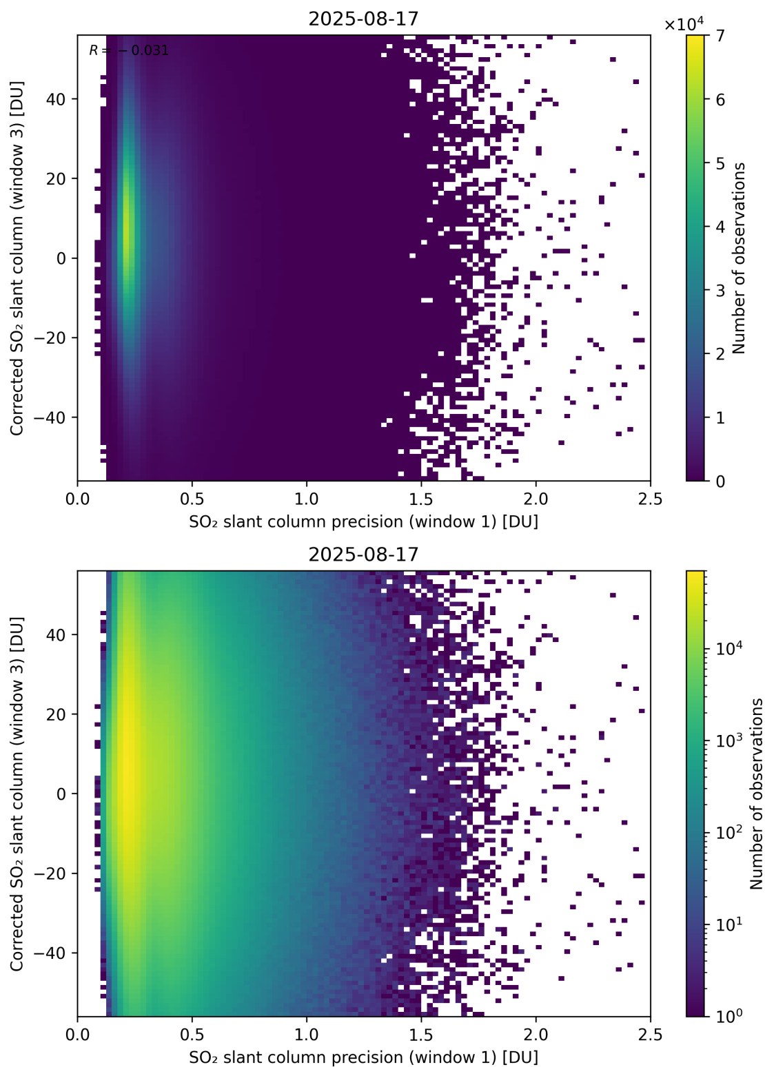
Figure 276: Scatter density plot of “SO 2 slant column precision (window 1)” against “Corrected SO 2 slant column (window 3)” for 2025-08-16 to 2025-08-18.
