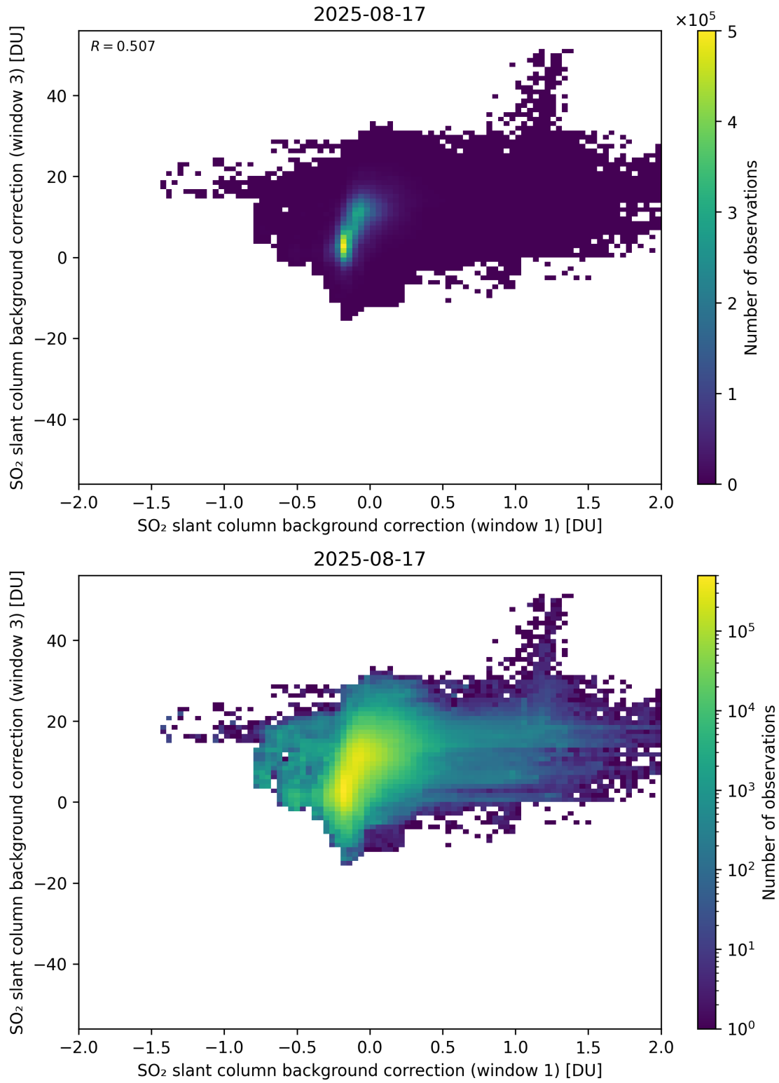
Figure 110: Scatter density plot of “SO 2 slant column background correction (window 1)” against “SO 2 slant column background correction (window 3)” for 2025-08-16 to 2025-08-18.
