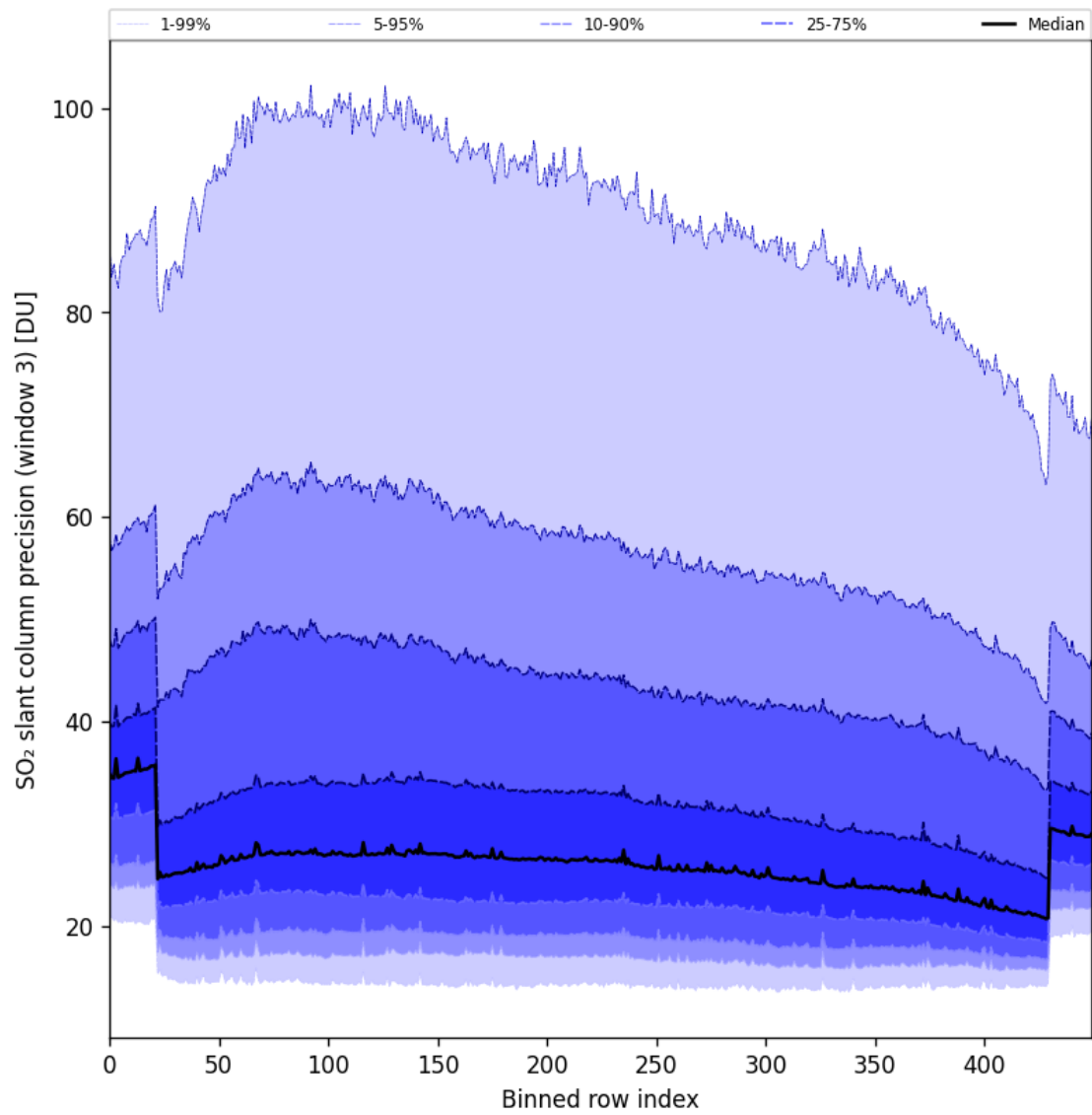
Figure 98: Along track statistics of “SO 2 slant column precision (window 3)” for 2025-08-16 to 2025-08-18
