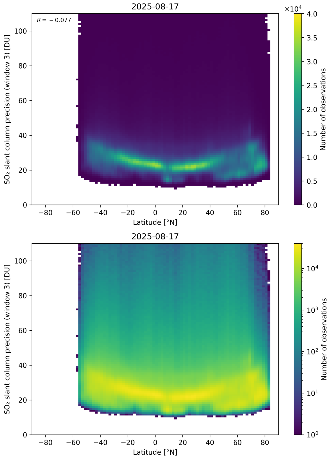
Figure 166: Scatter density plot of “Latitude” against “SO 2 slant column precision (window 3)” for 2025-08-16 to 2025-08-18.
