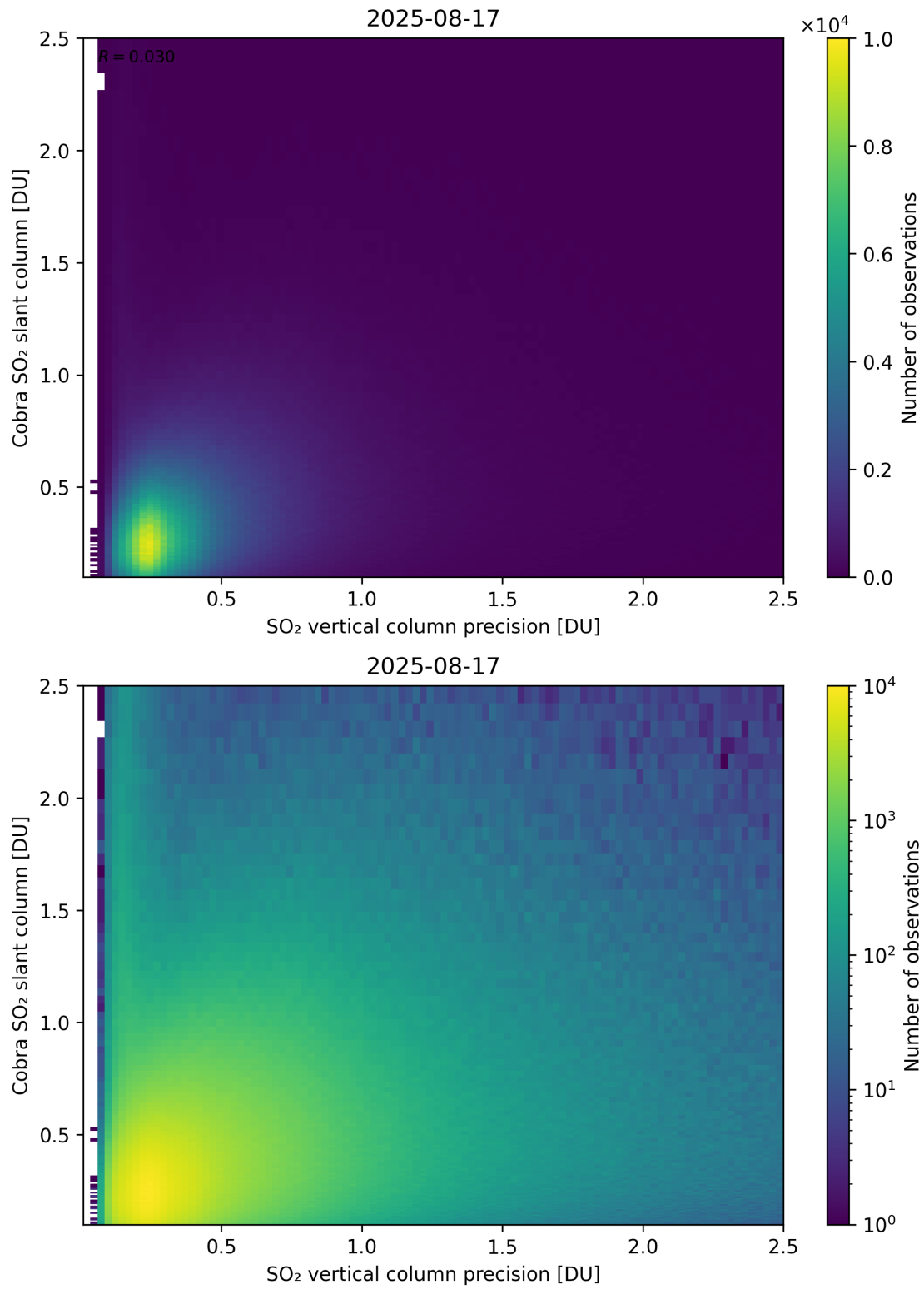
Figure 336: Scatter density plot of “SO 2 vertical column precision” against “Cobra SO 2 slant column” for 2025-08-16 to 2025-08-18.
