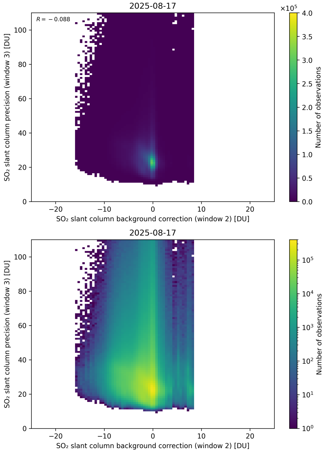
Figure 129: Scatter density plot of “SO 2 slant column background correction (window 2)” against “SO 2 slant column precision (window 3)” for 2025-08-16 to 2025-08-18.
