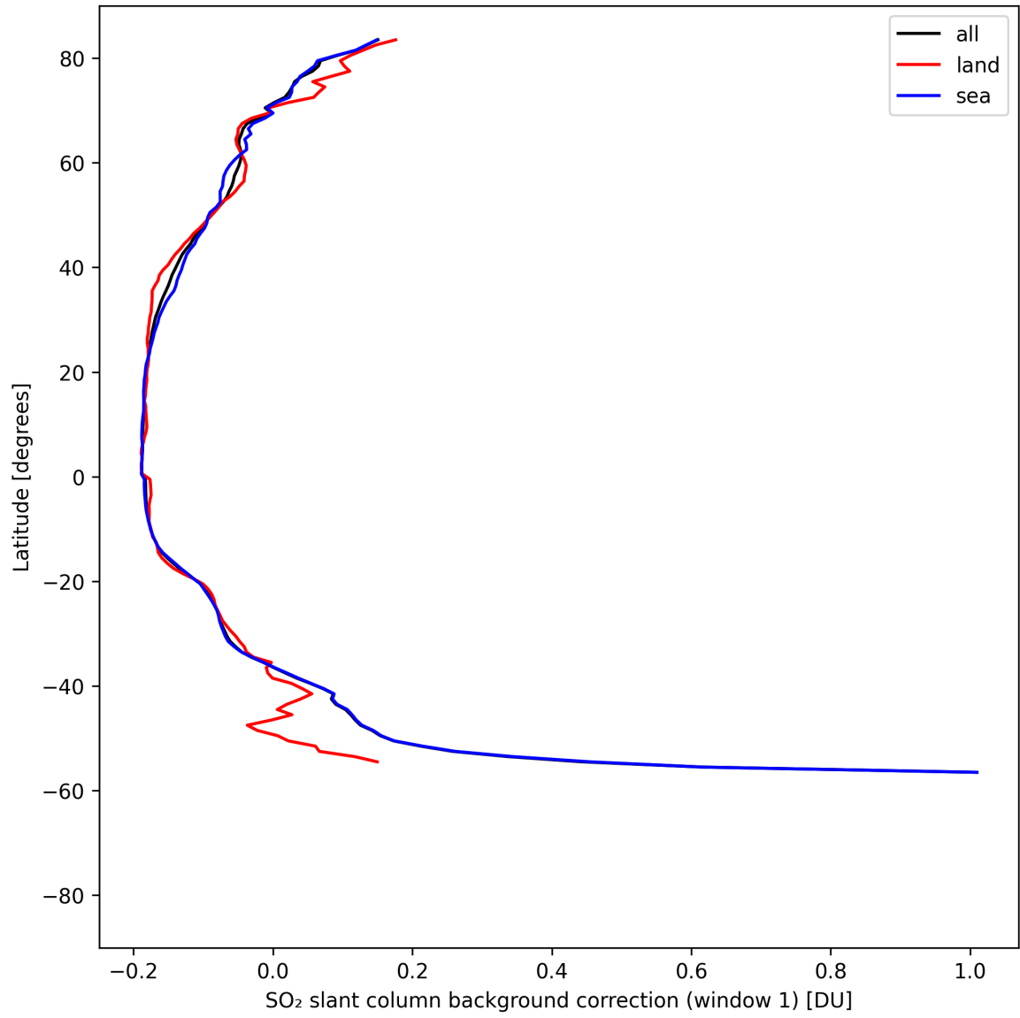
Figure 40: Zonal average of “SO 2 slant column background correction (window 1)” for 2025-08-16 to 2025-08-18.
