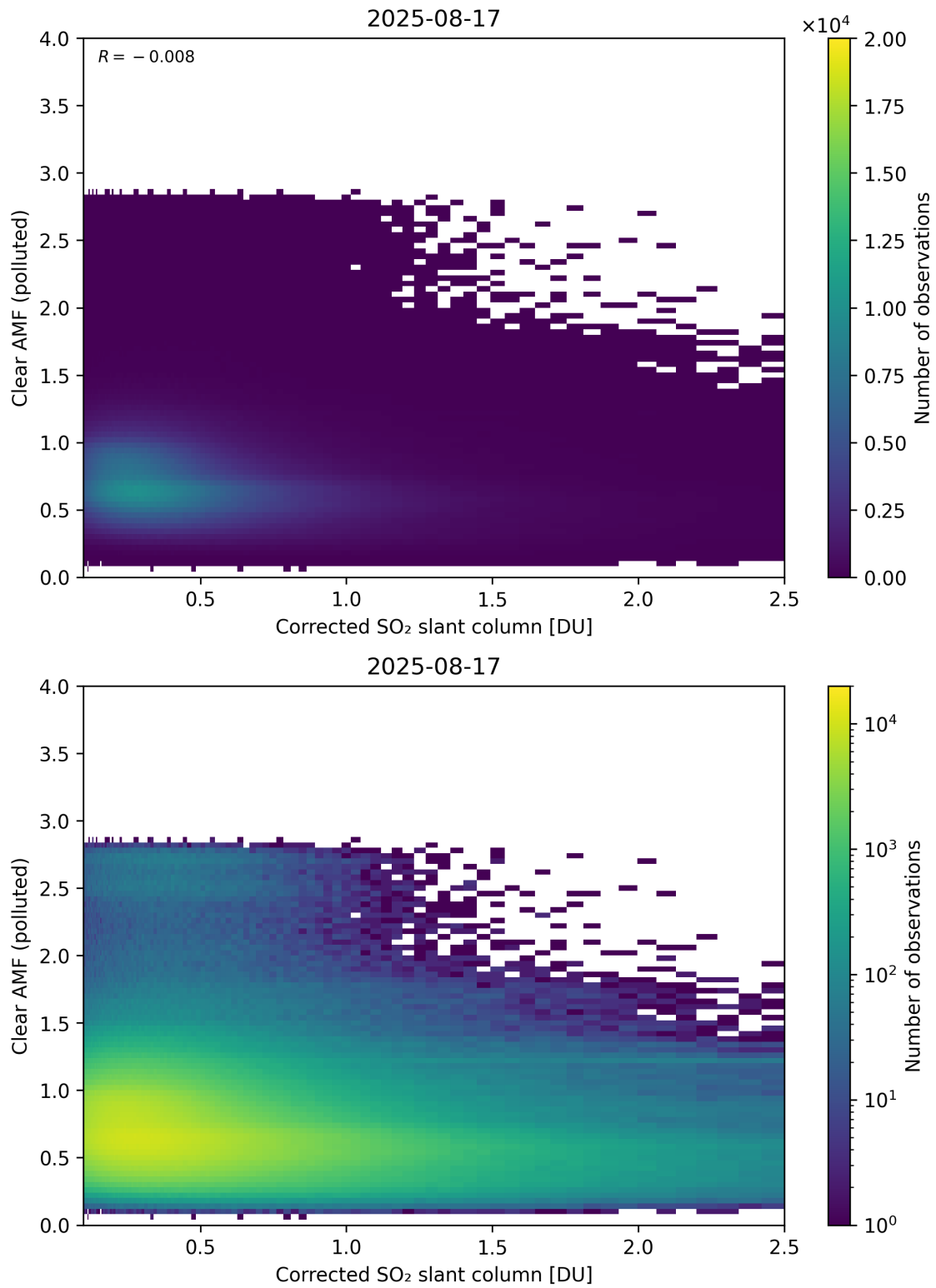
Figure 232: Scatter density plot of “Corrected SO 2 slant column” against “Clear AMF (polluted)” for 2025-08-16 to 2025-08-18.
