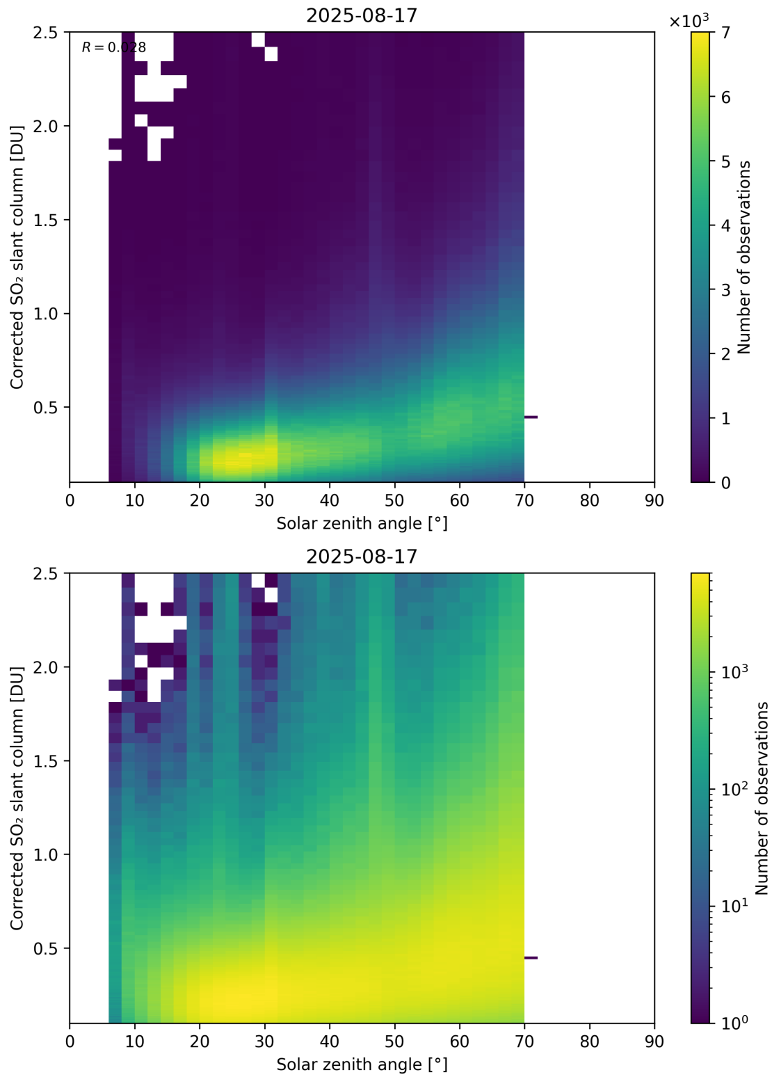
Figure 181: Scatter density plot of “Solar zenith angle” against “Corrected SO 2 slant column” for 2025-08-16 to 2025-08-18.
