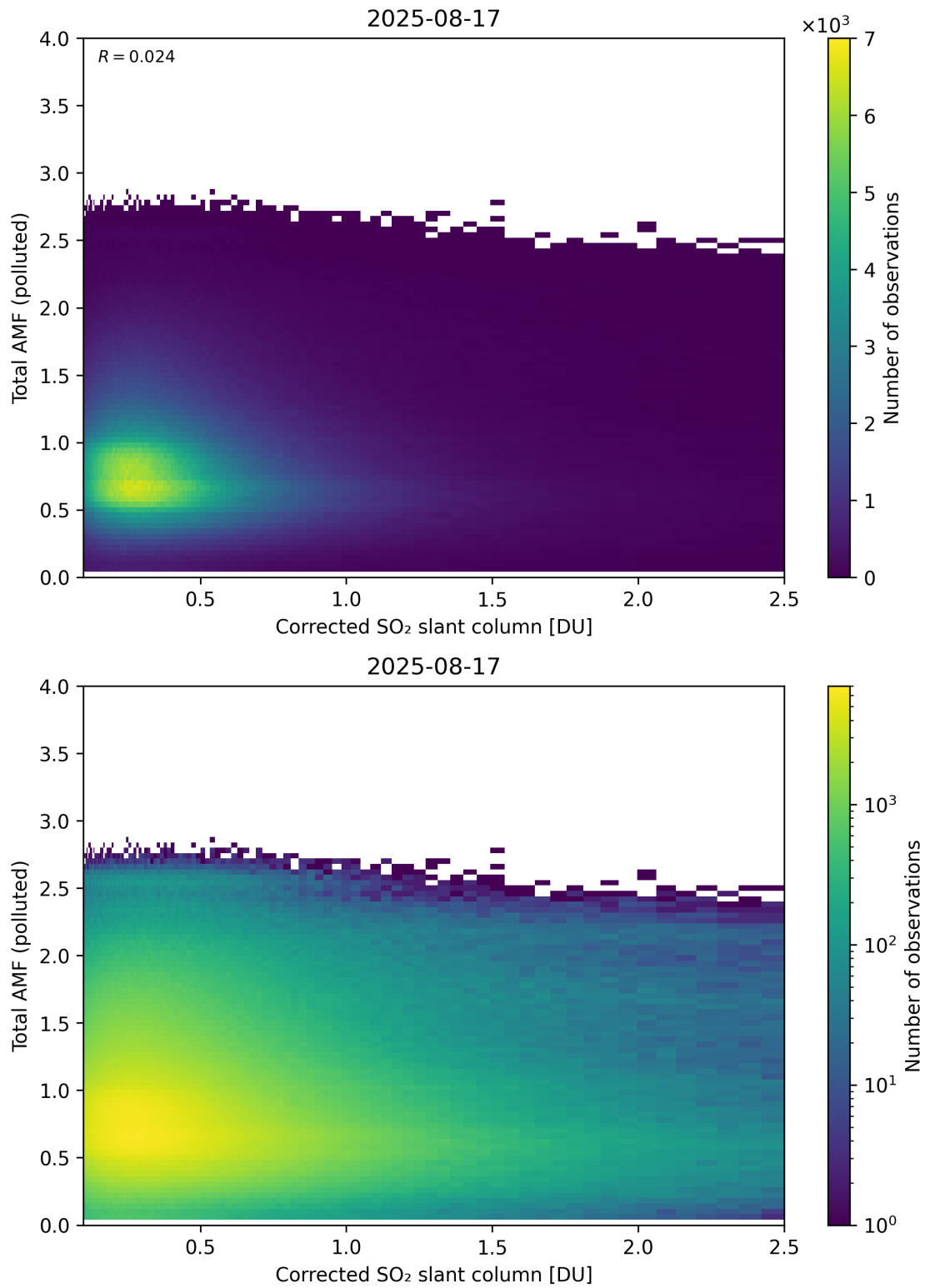
Figure 242: Scatter density plot of “Corrected SO 2 slant column” against “Total AMF (polluted)” for 2025-08-16 to 2025-08-18.
