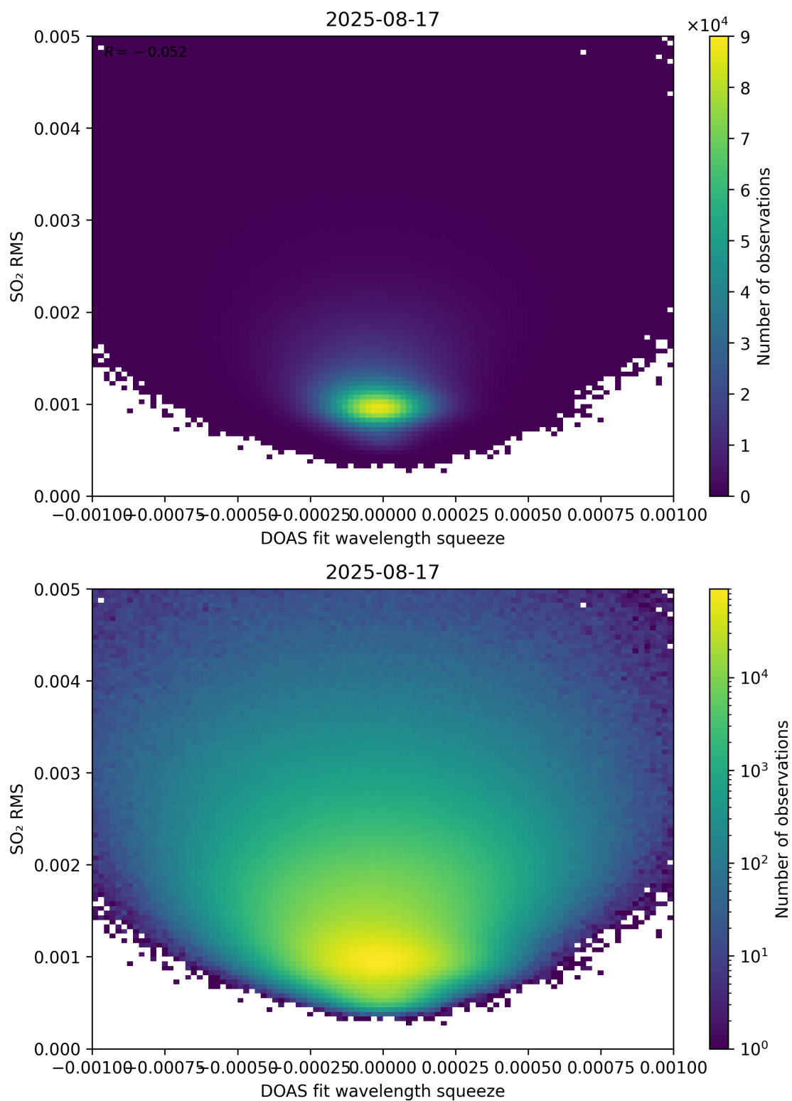
Figure 143: Scatter density plot of “DOAS fit wavelength squeeze” against “SO 2 RMS” for 2025-08-16 to 2025-08-18.
