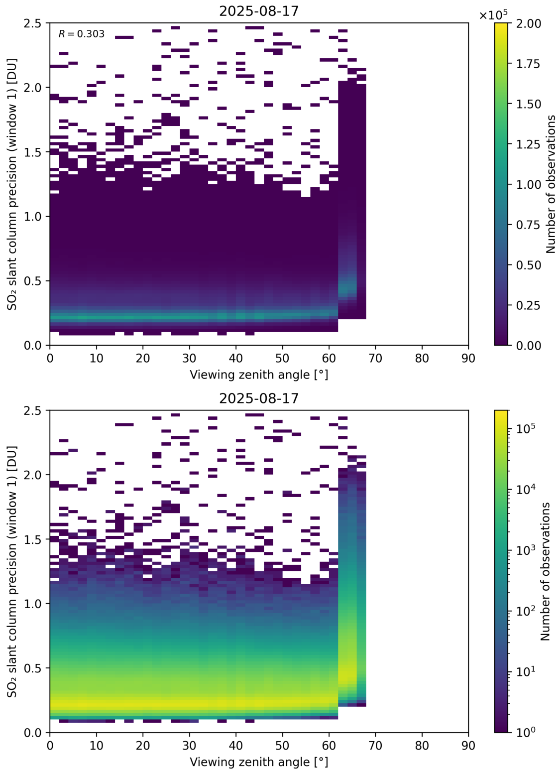
Figure 377: Scatter density plot of “Viewing zenith angle” against “SO 2 slant column precision (window 1)” for 2025-08-16 to 2025-08-18.
