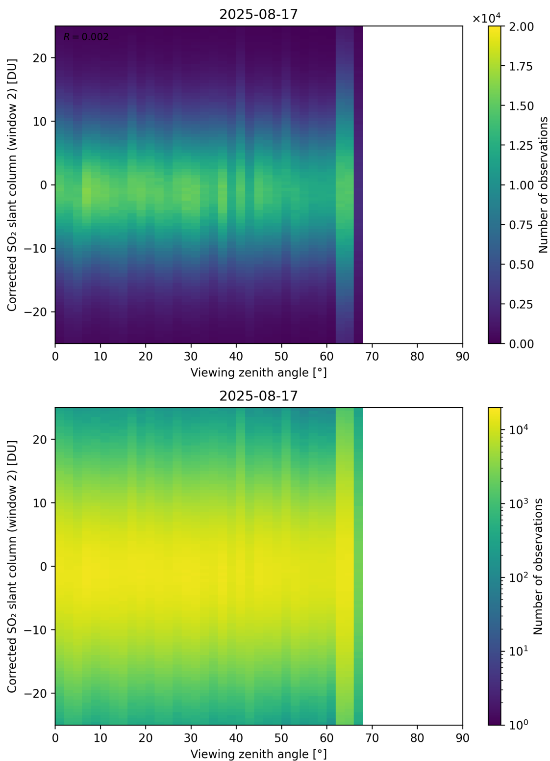
Figure 374: Scatter density plot of “Viewing zenith angle” against “Corrected SO 2 slant column (window 2)” for 2025-08-16 to 2025-08-18.
