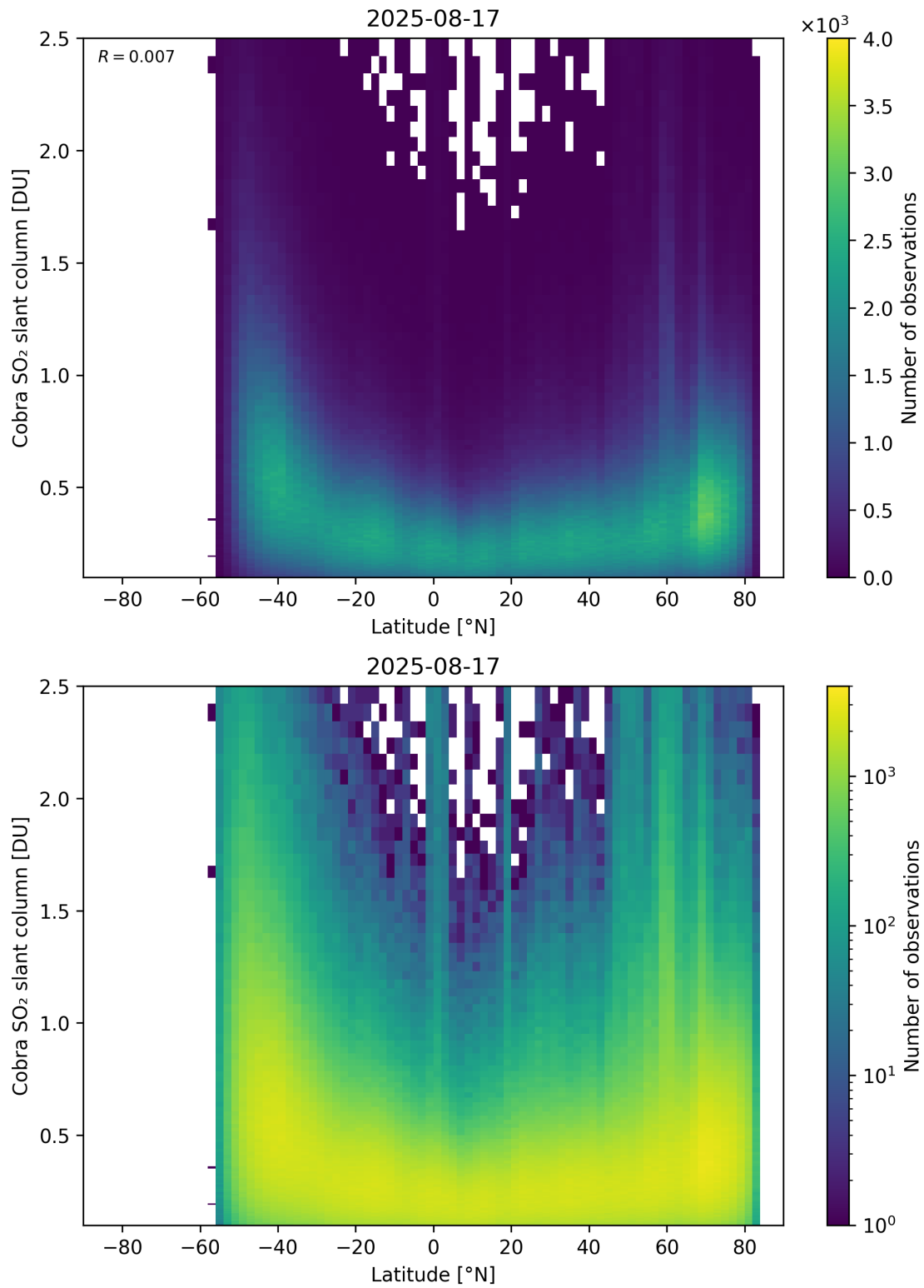
Figure 157: Scatter density plot of “Latitude” against “Cobra SO 2 slant column” for 2025-08-16 to 2025-08-18.
