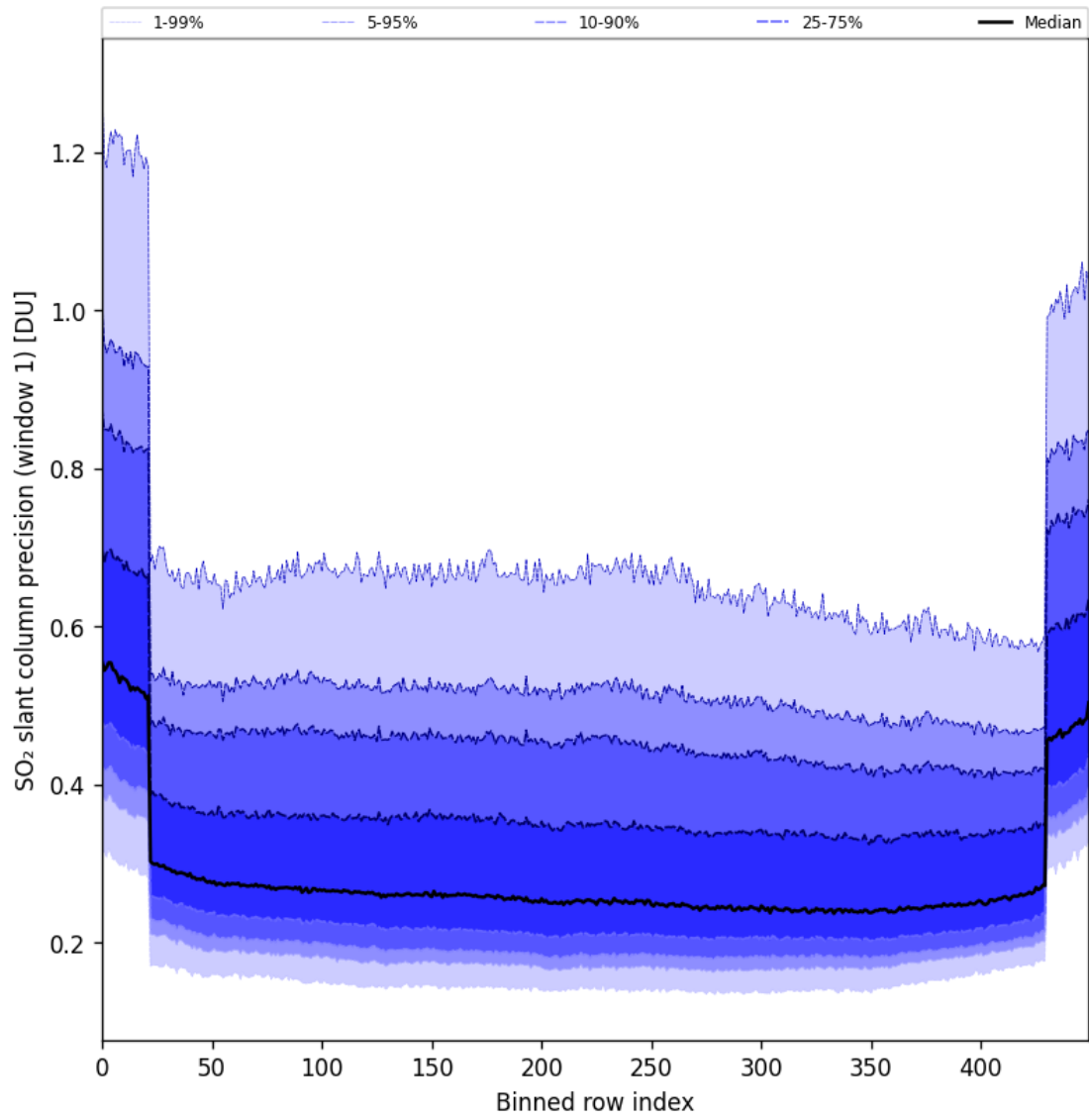
Figure 90: Along track statistics of “SO 2 slant column precision (window 1)” for 2025-08-16 to 2025-08-18
