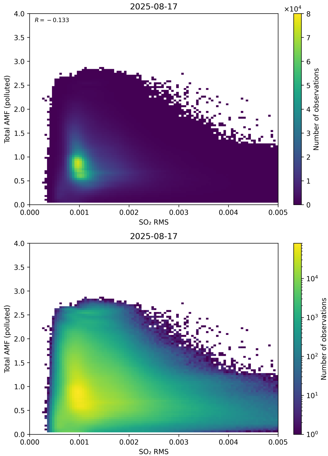
Figure 148: Scatter density plot of “SO 2 RMS” against “Total AMF (polluted)” for 2025-08-16 to 2025-08-18.
