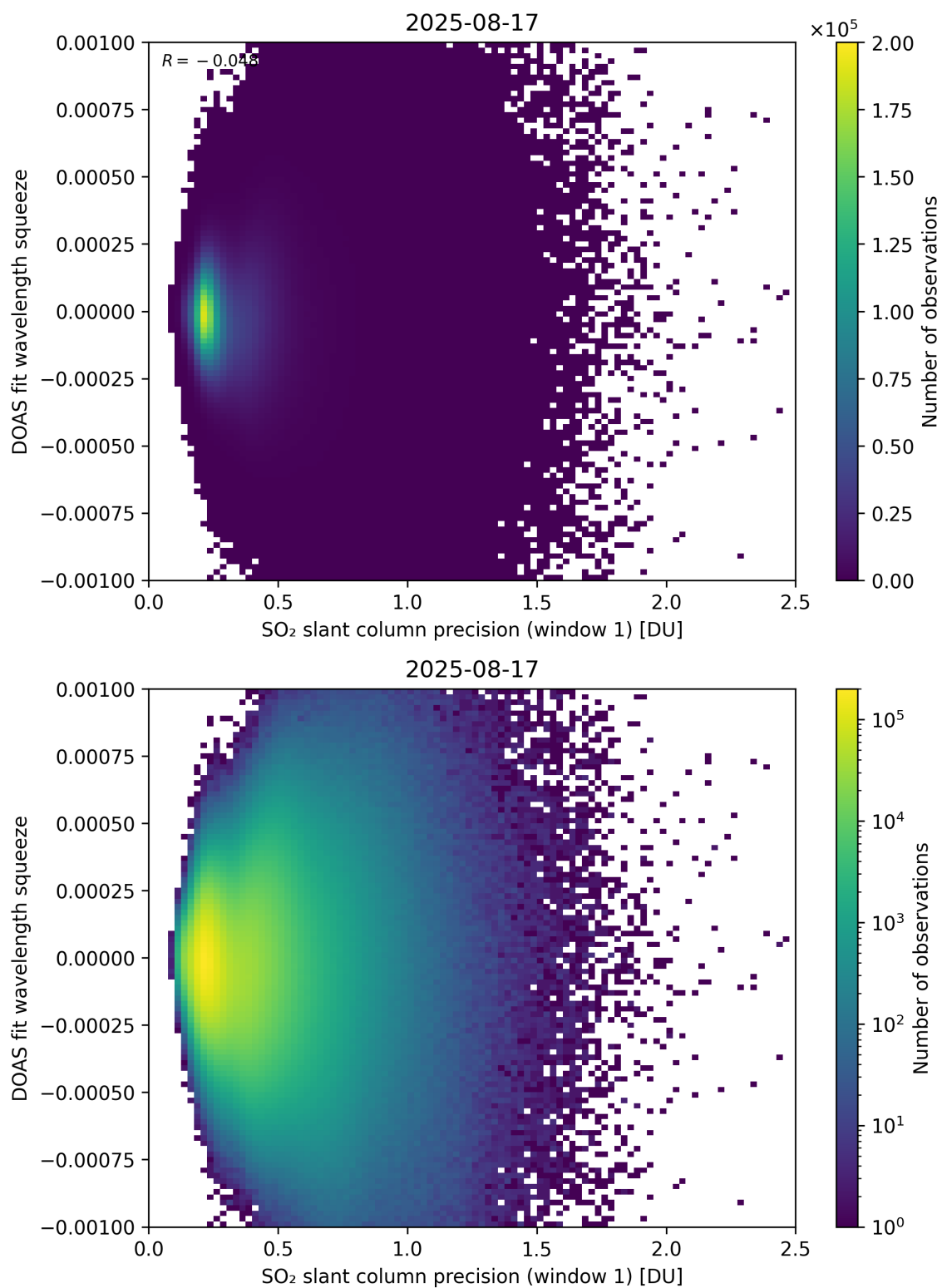
Figure 272: Scatter density plot of “SO 2 slant column precision (window 1)” against “DOAS fit wavelength squeeze” for 2025-08-16 to 2025-08-18.
