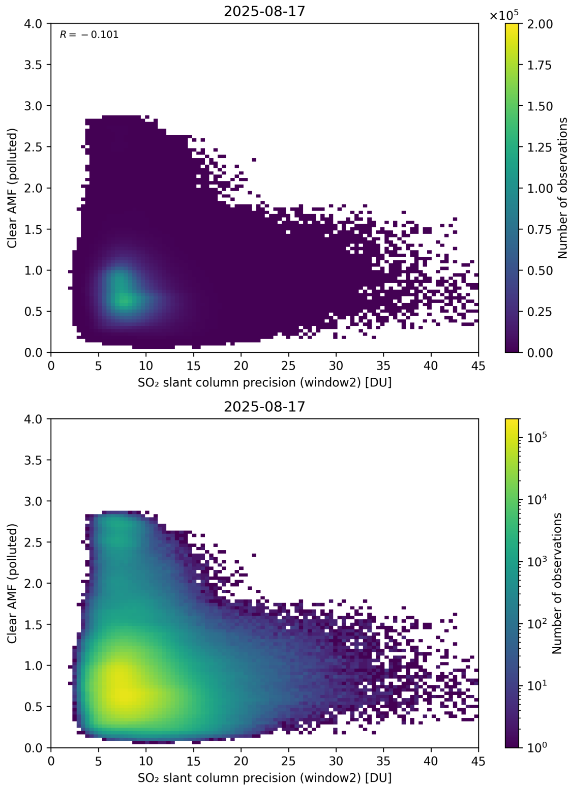
Figure 296: Scatter density plot of “SO 2 slant column precision (window2)” against “Clear AMF (polluted)” for 2025-08-16 to 2025-08-18.
