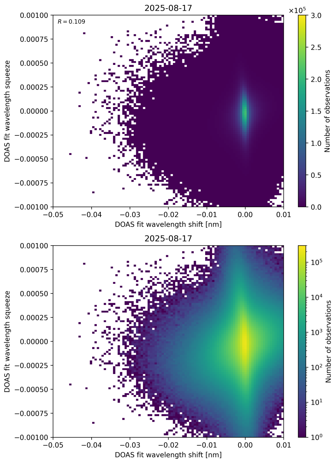
Figure 138: Scatter density plot of “DOAS fit wavelength shift” against “DOAS fit wavelength squeeze” for 2025-08-16 to 2025-08-18.
