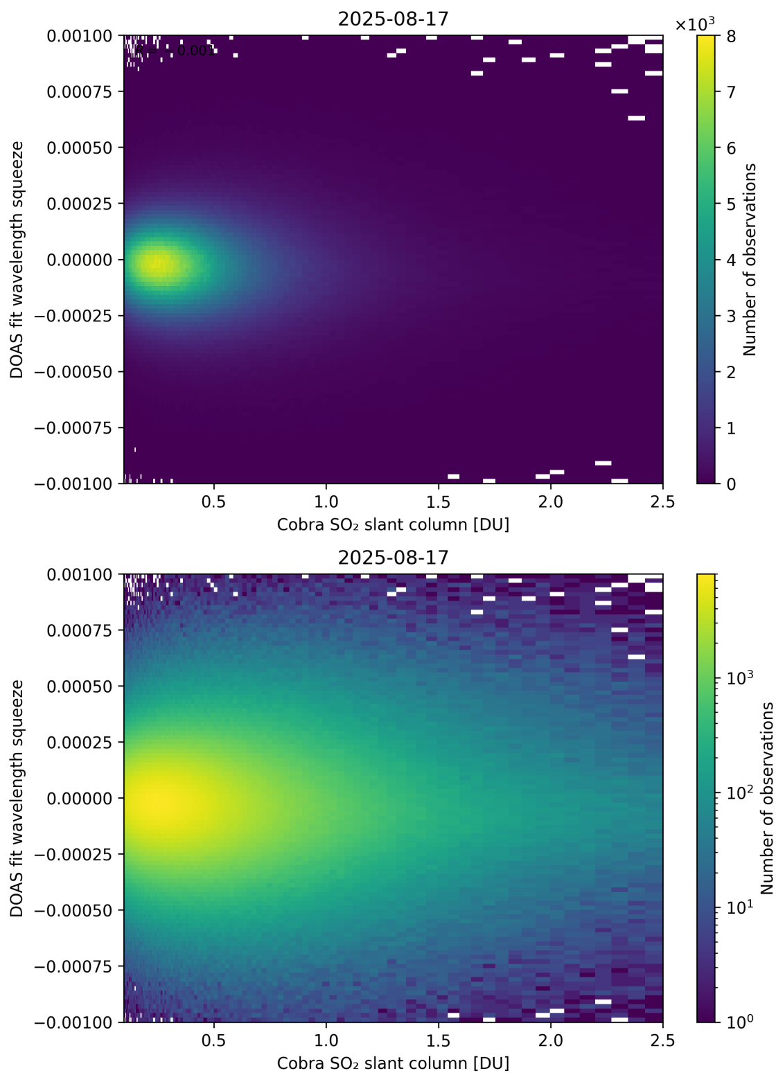
Figure 197: Scatter density plot of “Cobra SO 2 slant column” against “DOAS fit wavelength squeeze” for 2025-08-16 to 2025-08-18.
