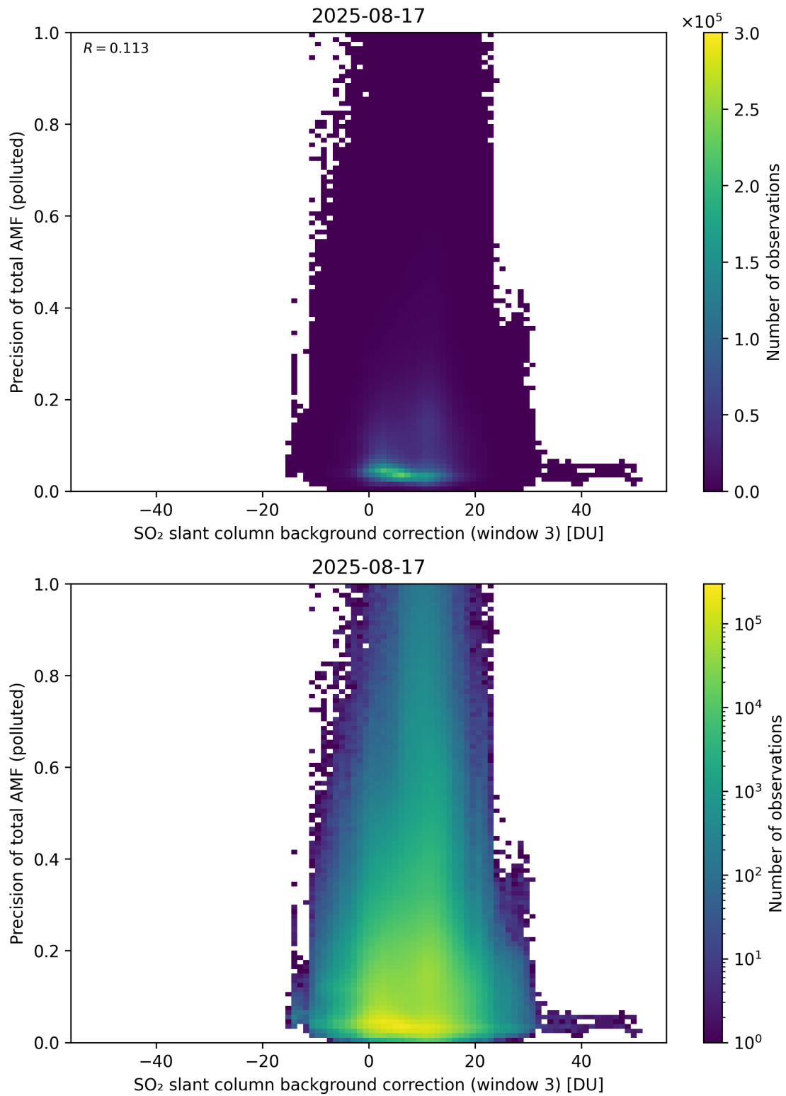
Figure 137: Scatter density plot of “SO 2 slant column background correction (window 3)” against “Precision of total AMF (polluted)” for 2025-08-16 to 2025-08-18.
