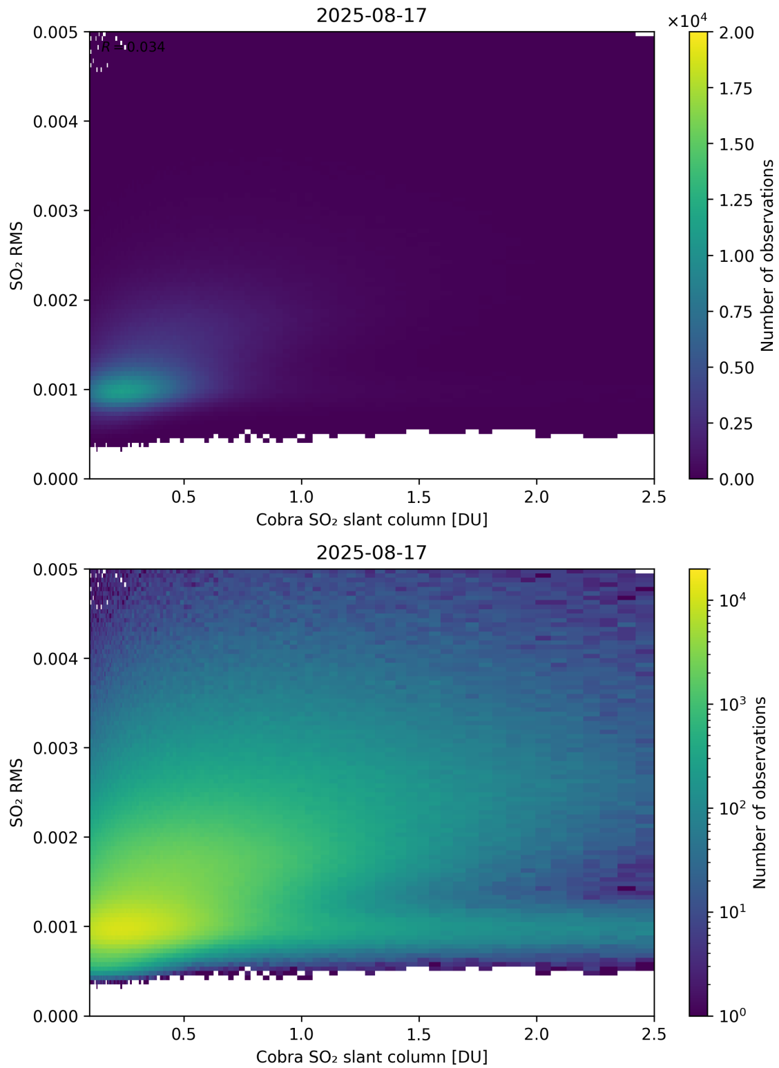
Figure 198: Scatter density plot of “Cobra SO 2 slant column” against “SO 2 RMS” for 2025-08-16 to 2025-08-18.
