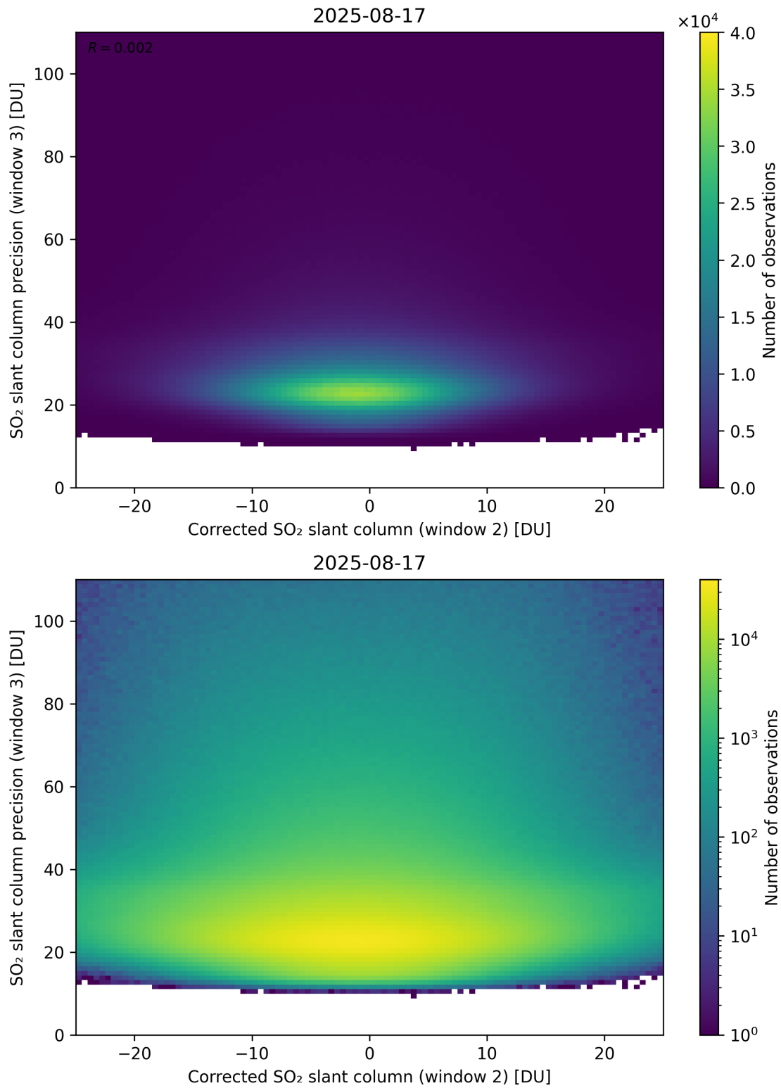
Figure 252: Scatter density plot of “Corrected SO 2 slant column (window 2)” against “SO 2 slant column precision (window 3)” for 2025-08-16 to 2025-08-18.
