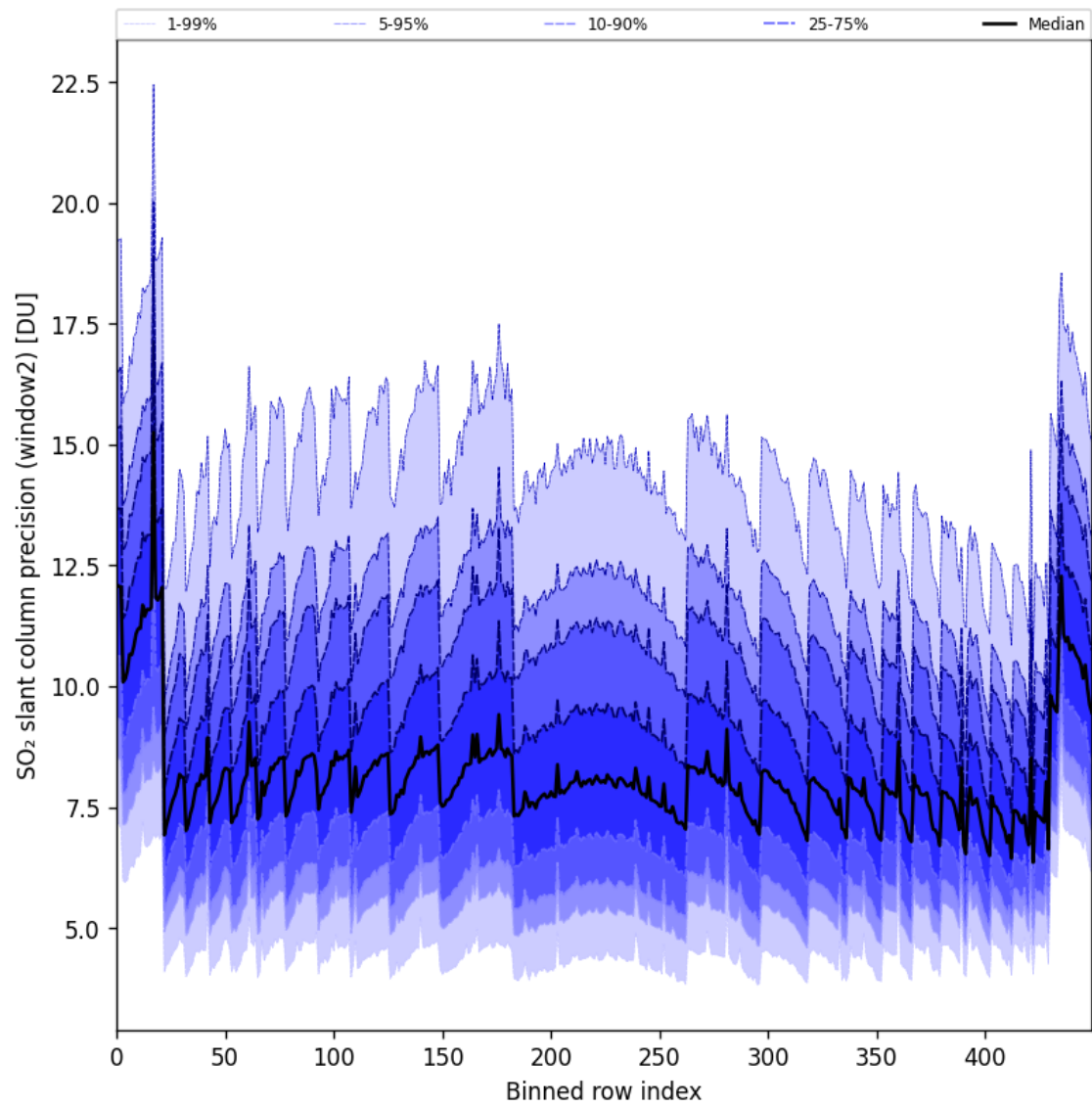
Figure 94: Along track statistics of “SO 2 slant column precision (window2)” for 2025-08-16 to 2025-08-18
