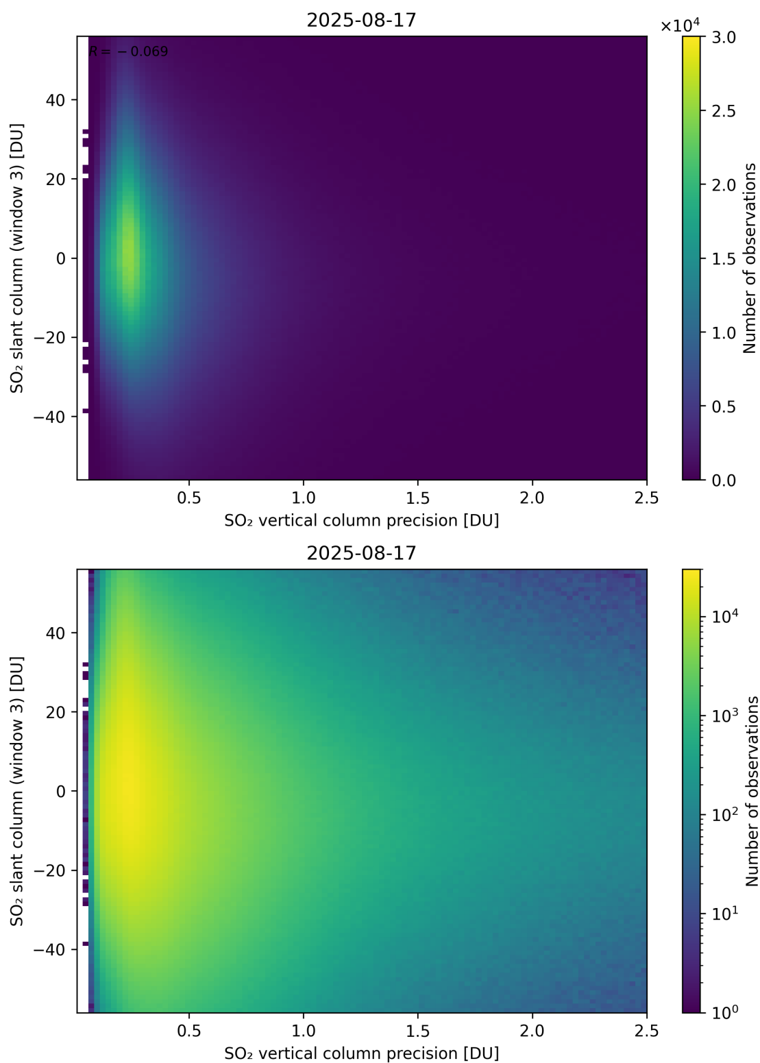
Figure 344: Scatter density plot of “SO 2 vertical column precision” against “SO 2 slant column (window 3)” for 2025-08-16 to 2025-08-18.
