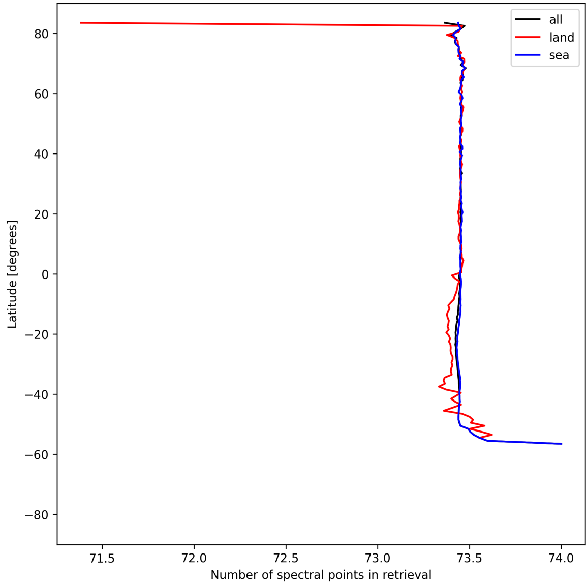
Figure 56: Zonal average of “Number of spectral points in retrieval” for 2025-08-16 to 2025-08-18.
