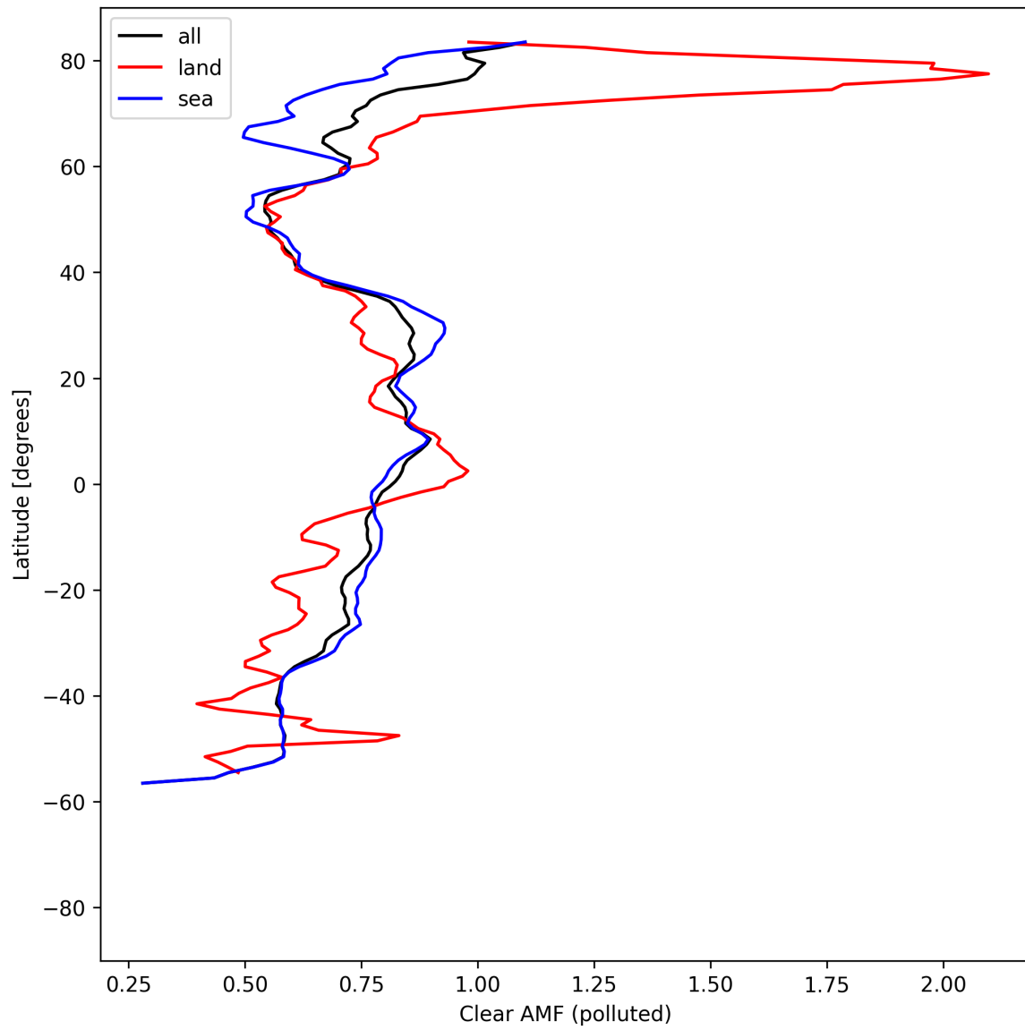
Figure 55: Zonal average of “Clear AMF (polluted)” for 2025-08-16 to 2025-08-18.
