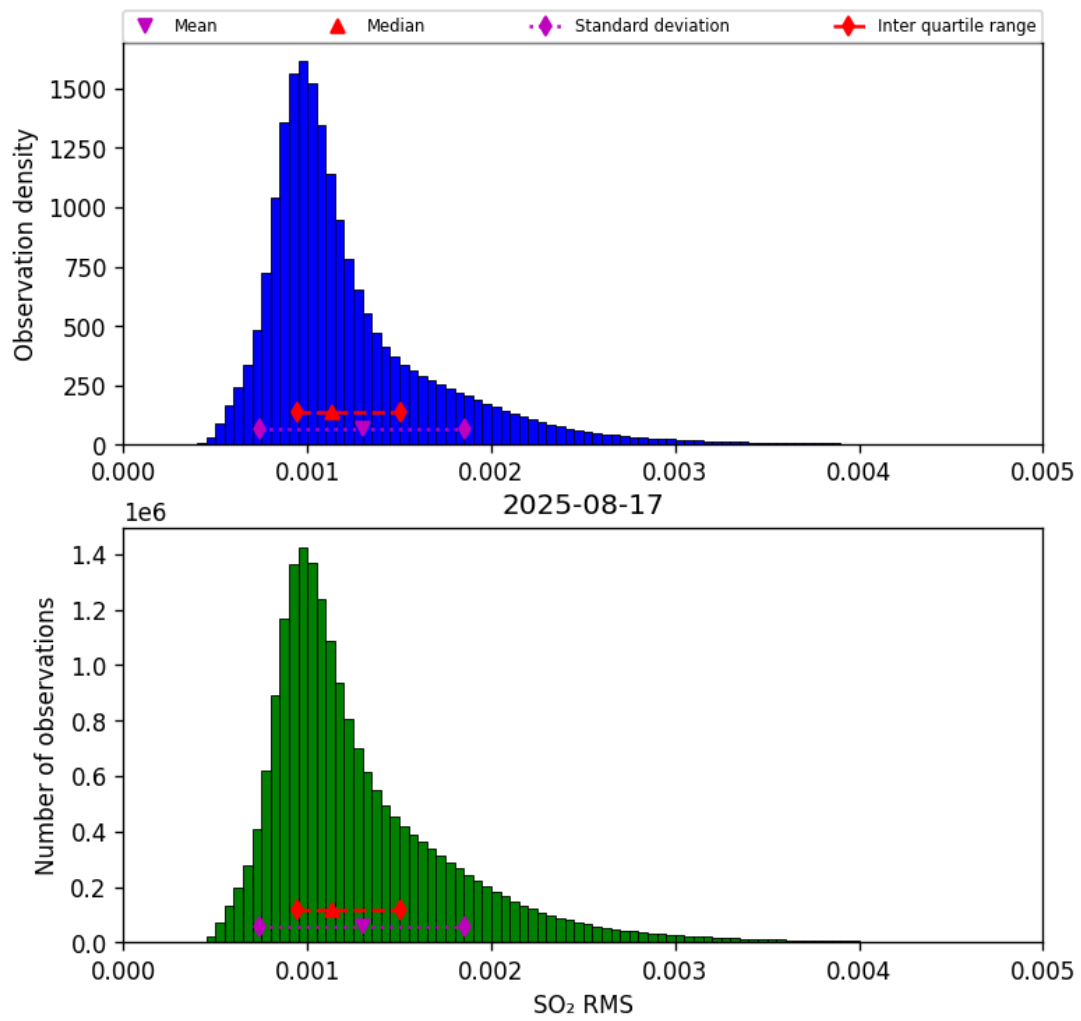
Figure 78: Histogram of “SO 2 RMS” for 2025-08-16 to 2025-08-18
