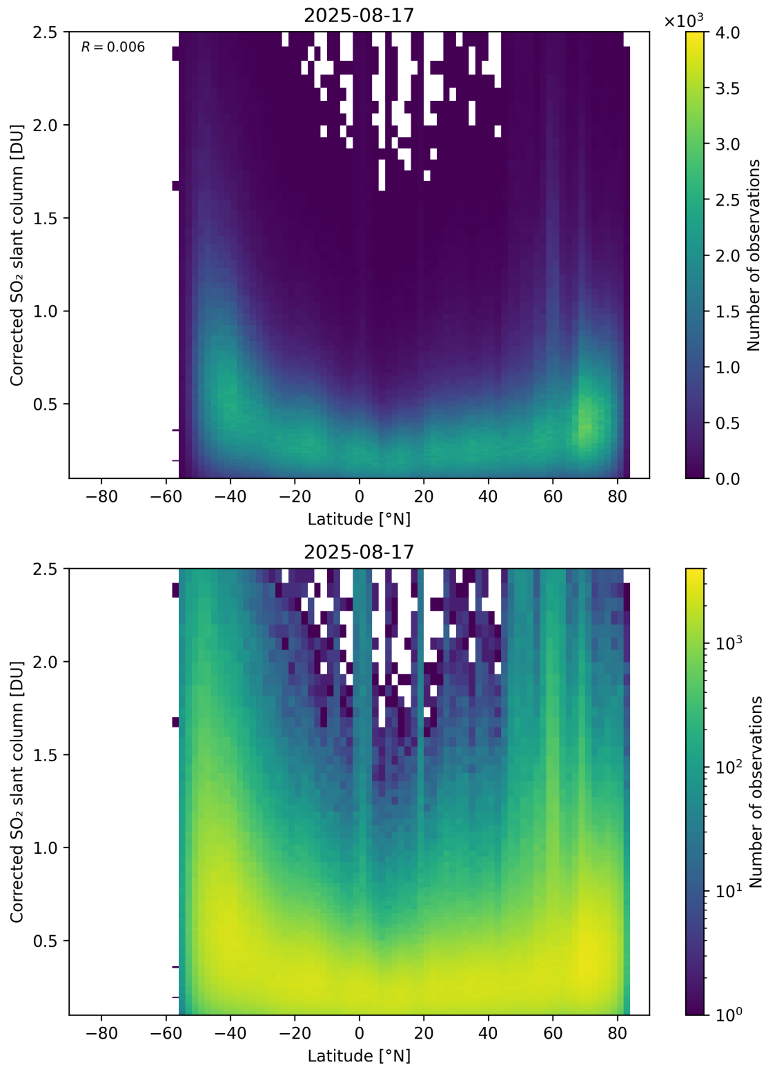
Figure 159: Scatter density plot of “Latitude” against “Corrected SO 2 slant column” for 2025-08-16 to 2025-08-18.
