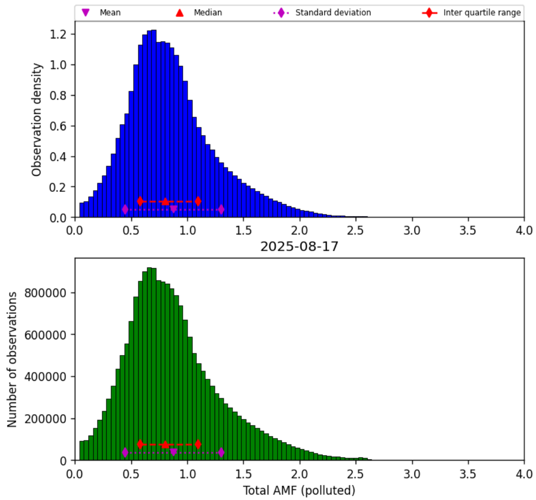
Figure 79: Histogram of “Total AMF (polluted)” for 2025-08-16 to 2025-08-18
