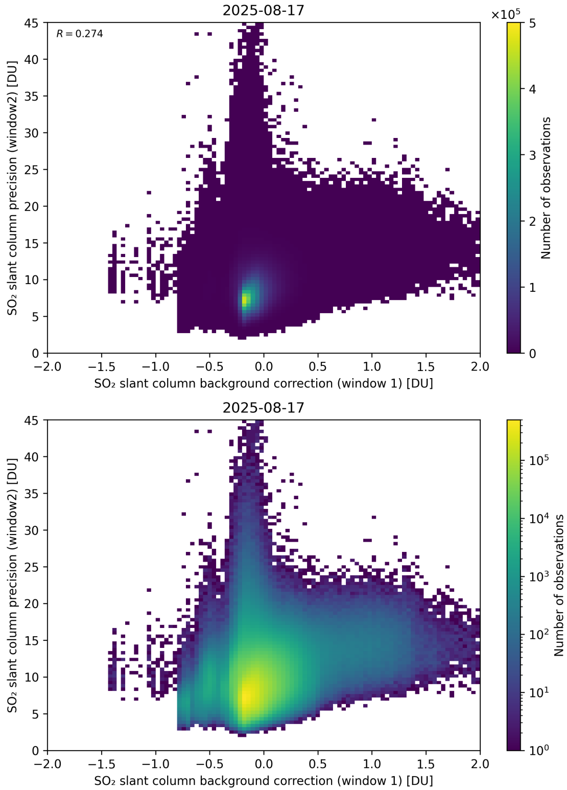
Figure 117: Scatter density plot of “SO 2 slant column background correction (window 1)” against “SO 2 slant column precision (window2)” for 2025-08-16 to 2025-08-18.
