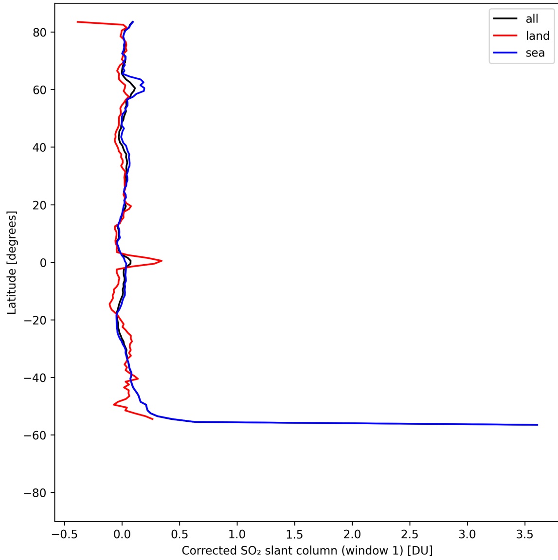
Figure 39: Zonal average of “Corrected SO 2 slant column (window 1)” for 2025-08-16 to 2025-08-18.
