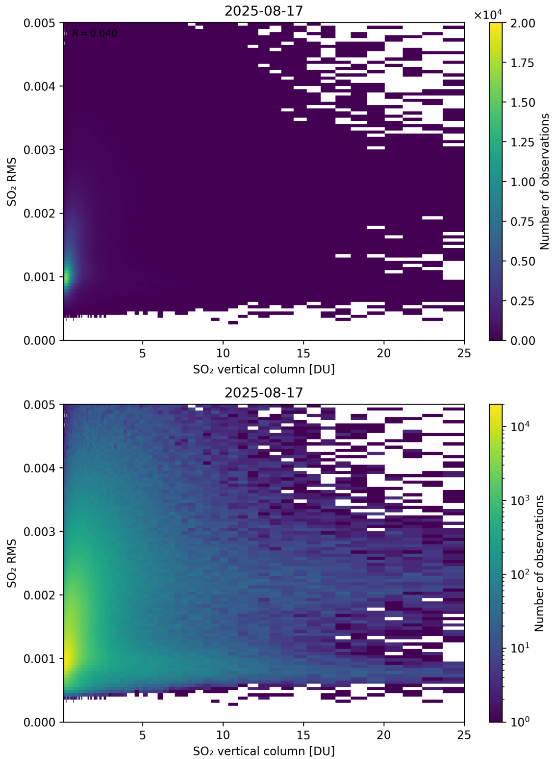
Figure 328: Scatter density plot of “SO 2 vertical column” against “SO 2 RMS” for 2025-08-16 to 2025-08-18.
