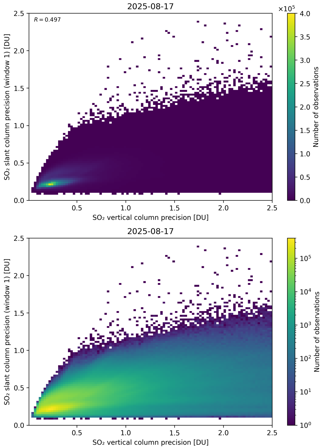
Figure 342: Scatter density plot of “SO 2 vertical column precision” against “SO 2 slant column precision (window 1)” for 2025-08-16 to 2025-08-18.
