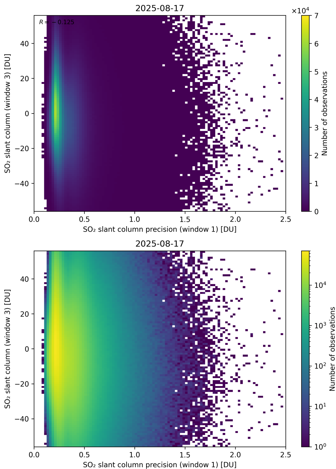
Figure 278: Scatter density plot of “SO 2 slant column precision (window 1)” against “SO 2 slant column (window 3)” for 2025-08-16 to 2025-08-18.
