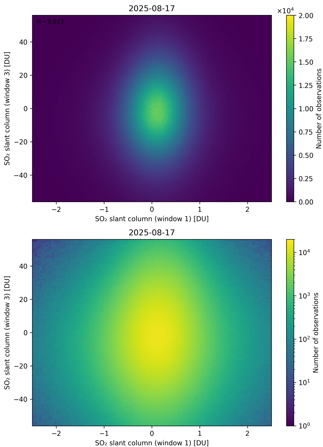
Figure 287: Scatter density plot of “SO 2 slant column (window 1)” against “SO 2 slant column (window 3)” for 2025-08-16 to 2025-08-18.
