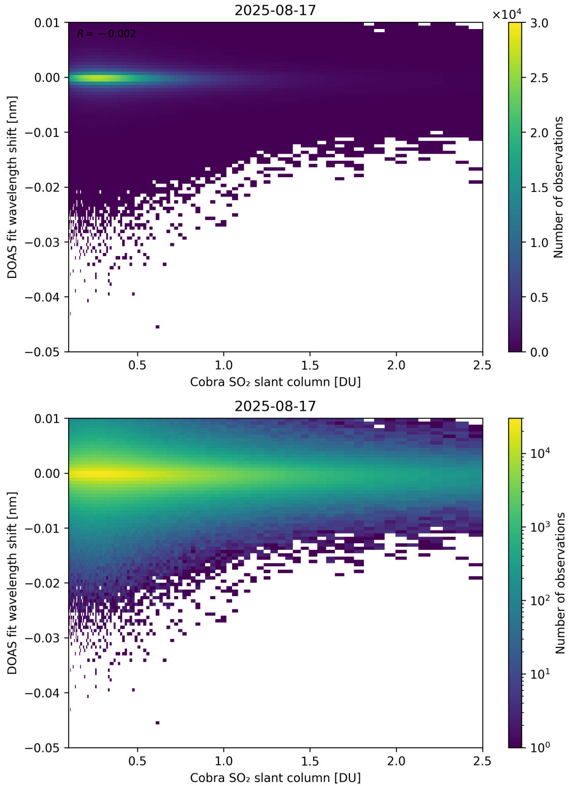
Figure 196: Scatter density plot of “Cobra SO 2 slant column” against “DOAS fit wavelength shift” for 2025-08-16 to 2025-08-18.
