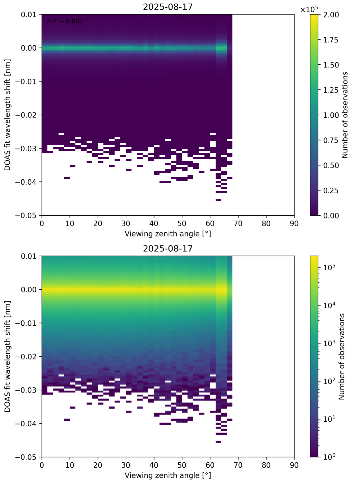
Figure 365: Scatter density plot of “Viewing zenith angle” against “DOAS fit wavelength shift” for 2025-08-16 to 2025-08-18.
