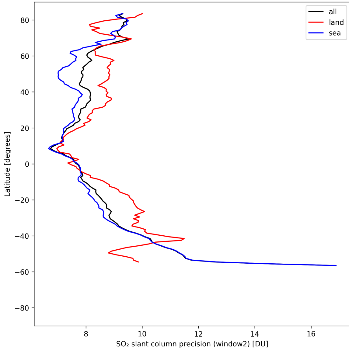
Figure 42: Zonal average of “SO 2 slant column precision (window2)” for 2025-08-16 to 2025-08-18.
