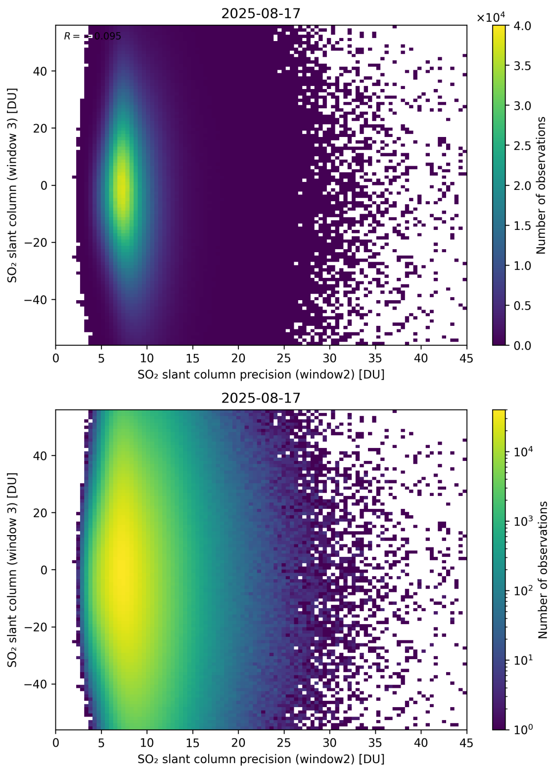
Figure 299: Scatter density plot of “SO 2 slant column precision (window2)” against “SO 2 slant column (window 3)” for 2025-08-16 to 2025-08-18.
