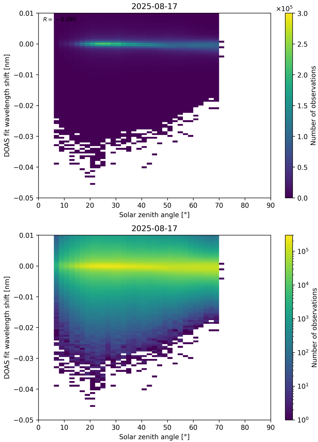
Figure 174: Scatter density plot of “Solar zenith angle” against “DOAS fit wavelength shift” for 2025-08-16 to 2025-08-18.
