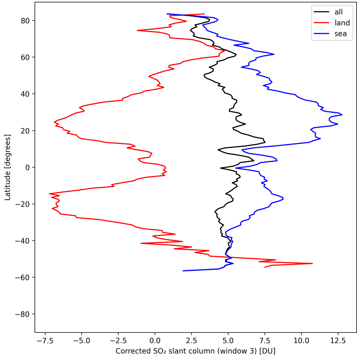
Figure 47: Zonal average of “Corrected SO 2 slant column (window 3)” for 2025-08-16 to 2025-08-18.
