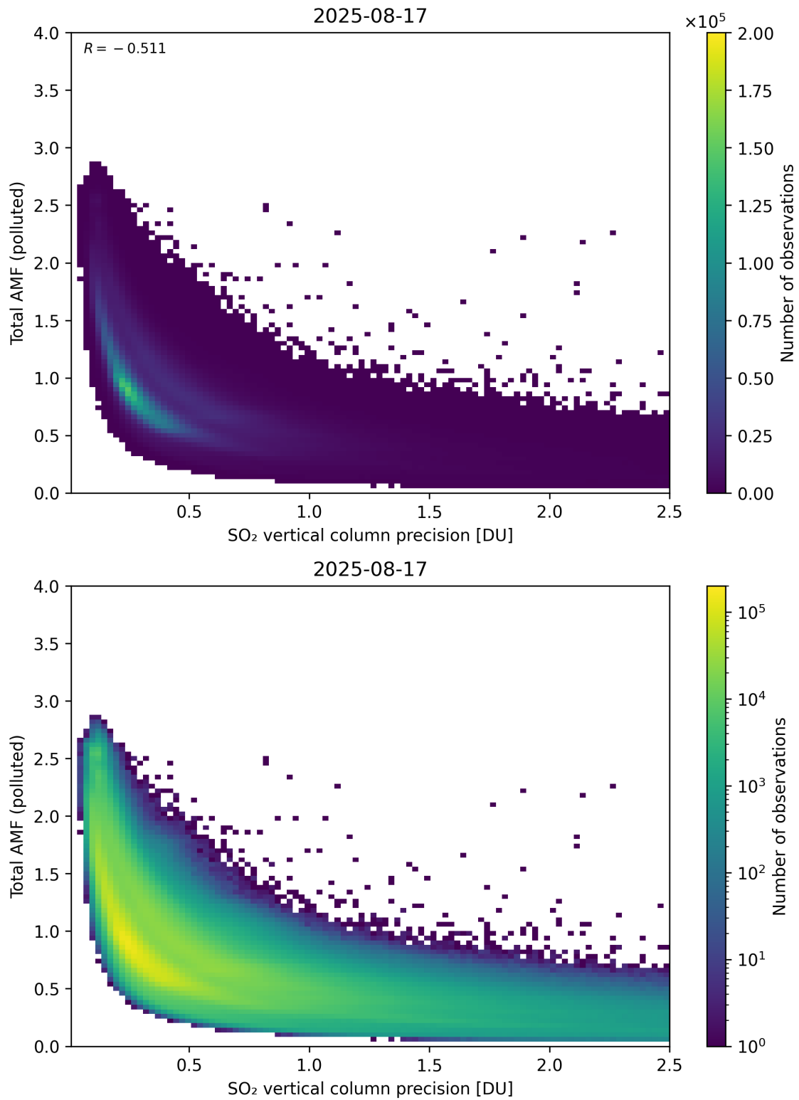
Figure 346: Scatter density plot of “SO 2 vertical column precision” against “Total AMF (polluted)” for 2025-08-16 to 2025-08-18.
