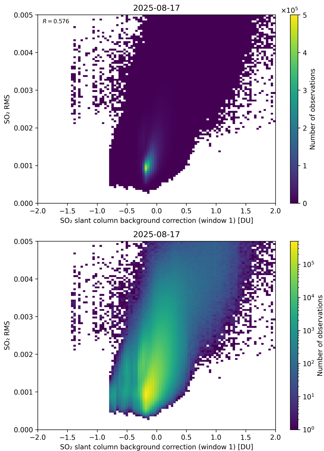
Figure 113: Scatter density plot of “SO 2 slant column background correction (window 1)” against “SO 2 RMS” for 2025-08-16 to 2025-08-18.
