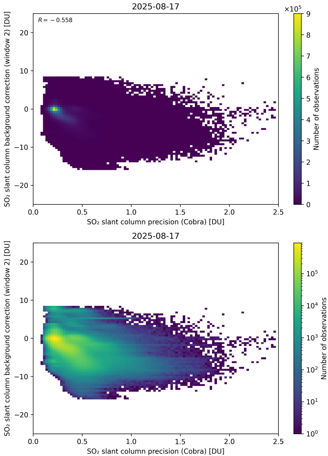
Figure 200: Scatter density plot of “SO 2 slant column precision (Cobra)” against “SO 2 slant column background correction (window 2)” for 2025-08-16 to 2025-08-18.
