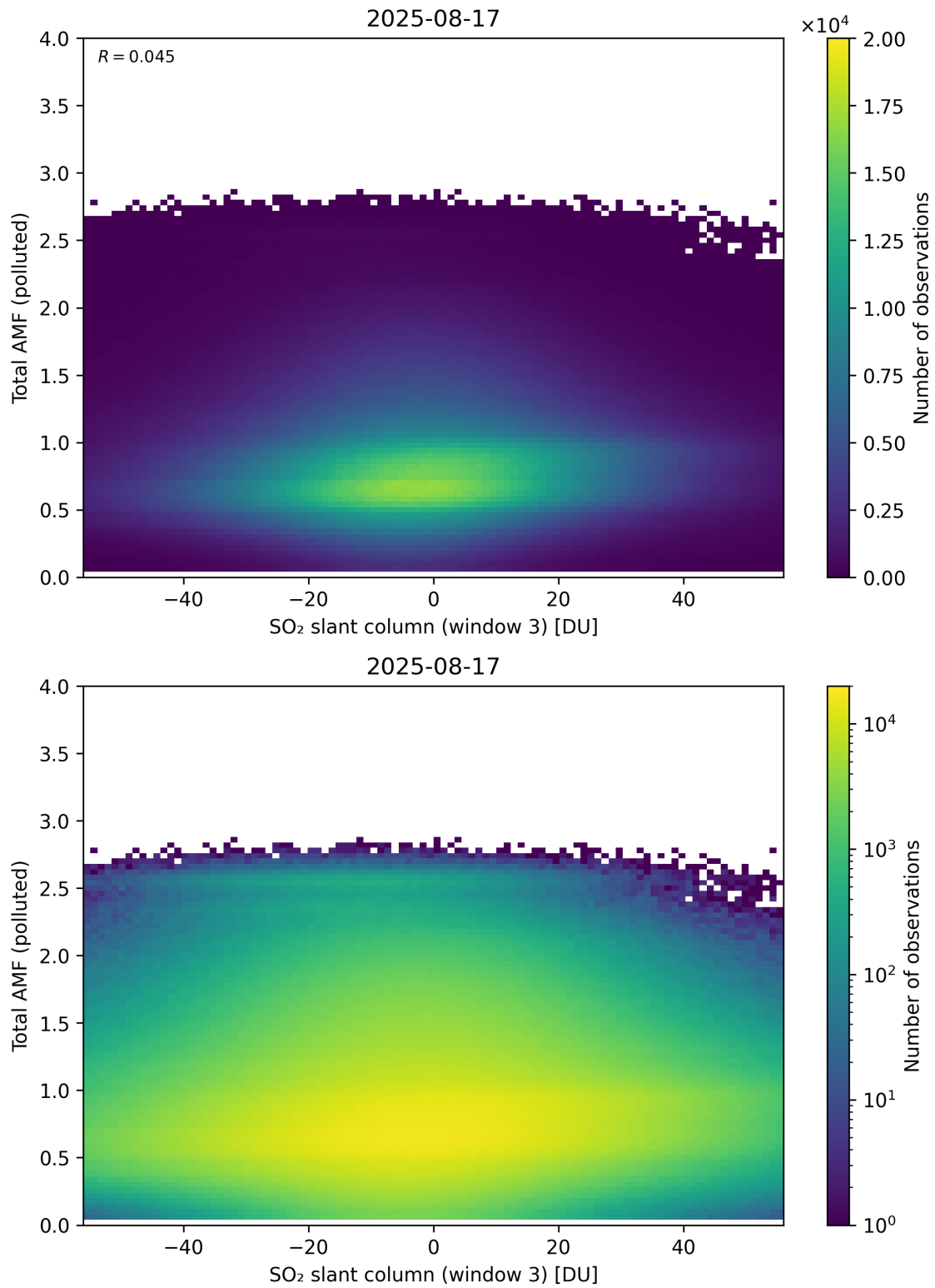
Figure 318: Scatter density plot of “SO 2 slant column (window 3)” against “Total AMF (polluted)” for 2025-08-16 to 2025-08-18.
