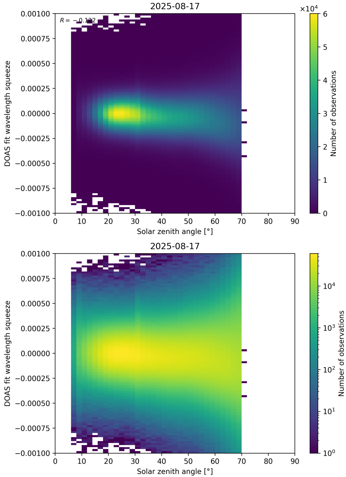
Figure 175: Scatter density plot of “Solar zenith angle” against “DOAS fit wavelength squeeze” for 2025-08-16 to 2025-08-18.
