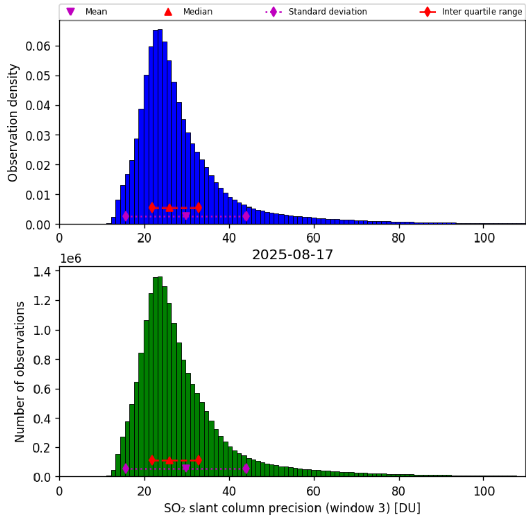
Figure 72: Histogram of “SO 2 slant column precision (window 3)” for 2025-08-16 to 2025-08-18
