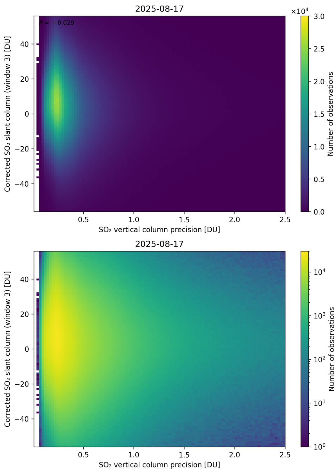
Figure 340: Scatter density plot of “SO 2 vertical column precision” against “Corrected SO 2 slant column (window 3)” for 2025-08-16 to 2025-08-18.
