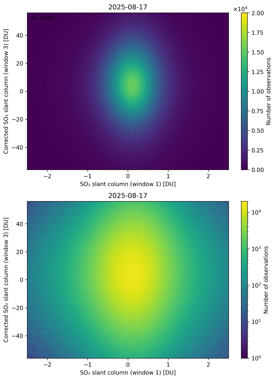
Figure 284: Scatter density plot of “SO 2 slant column (window 1)” against “Corrected SO 2 slant column (window 3)” for 2025-08-16 to 2025-08-18.
