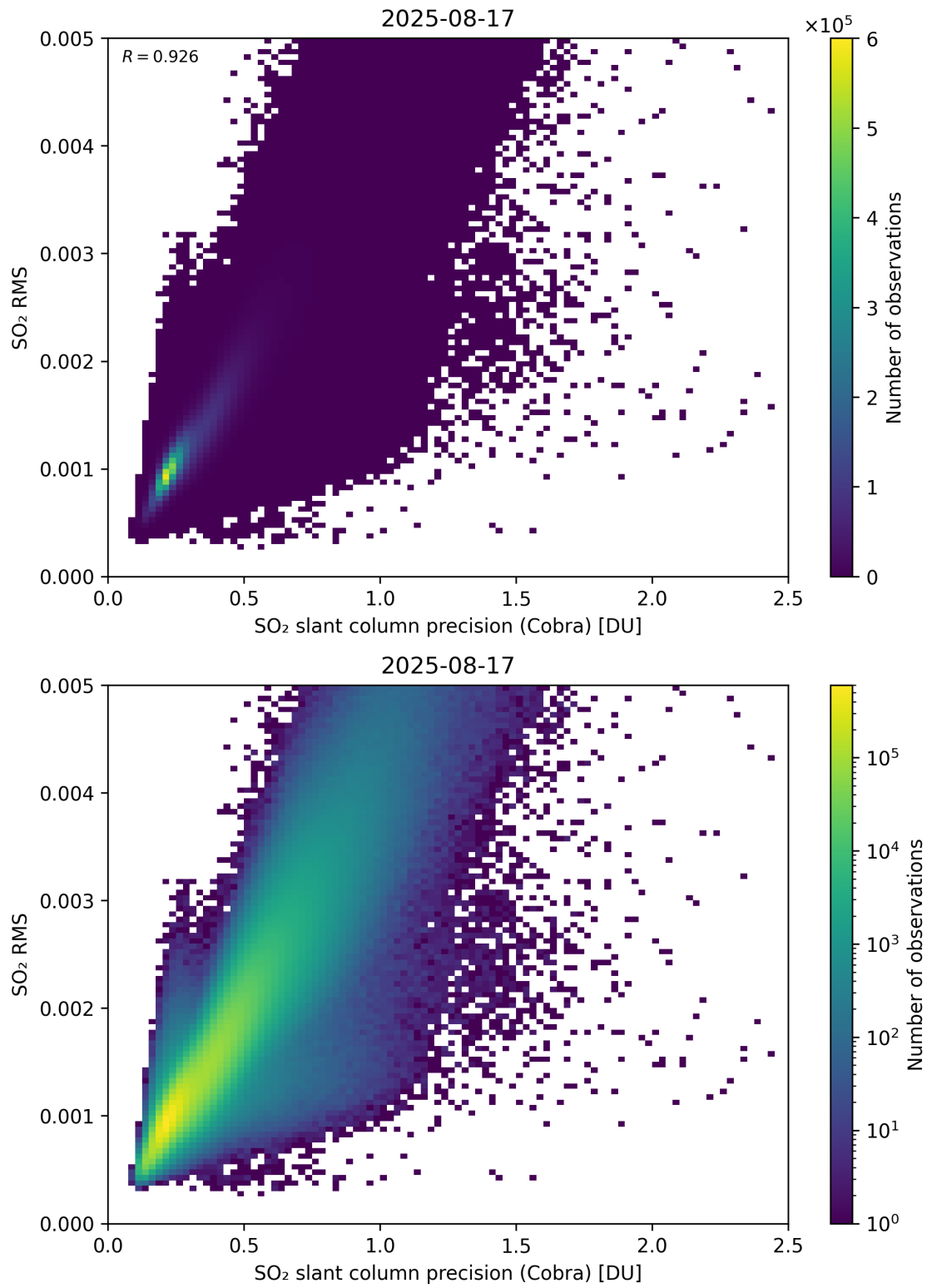
Figure 204: Scatter density plot of “SO 2 slant column precision (Cobra)” against “SO 2 RMS” for 2025-08-16 to 2025-08-18.
