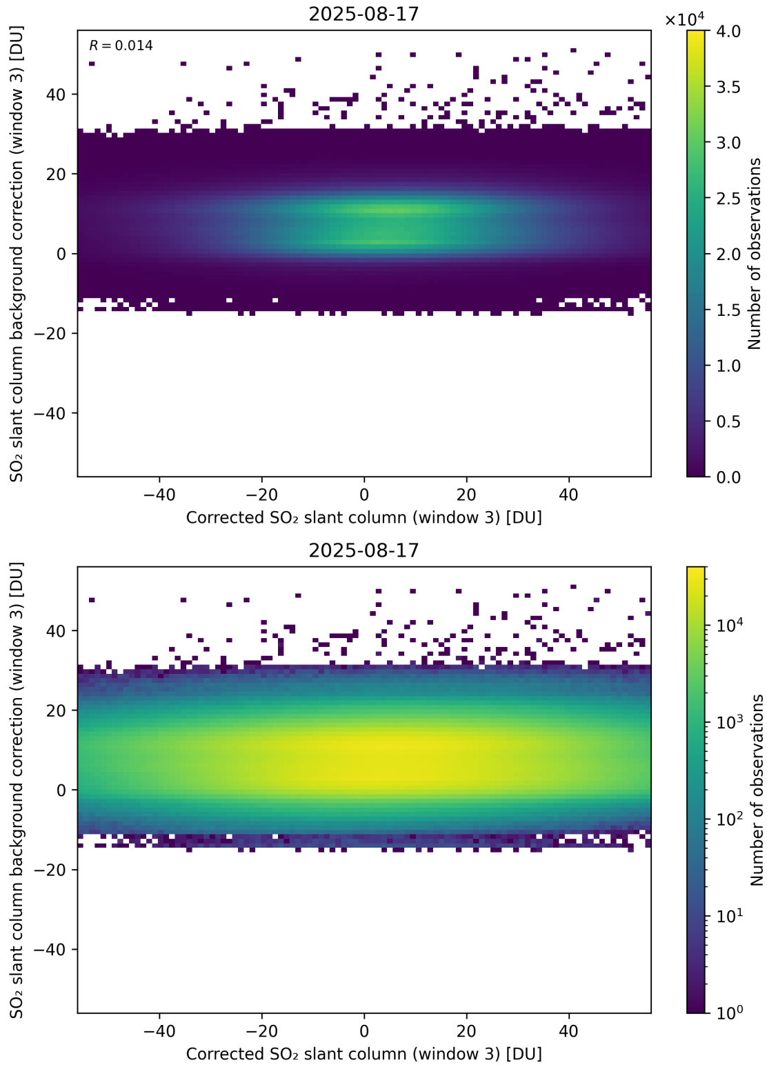
Figure 255: Scatter density plot of “Corrected SO 2 slant column (window 3)” against “SO 2 slant column background correction (window 3)” for 2025-08-16 to 2025-08-18.
