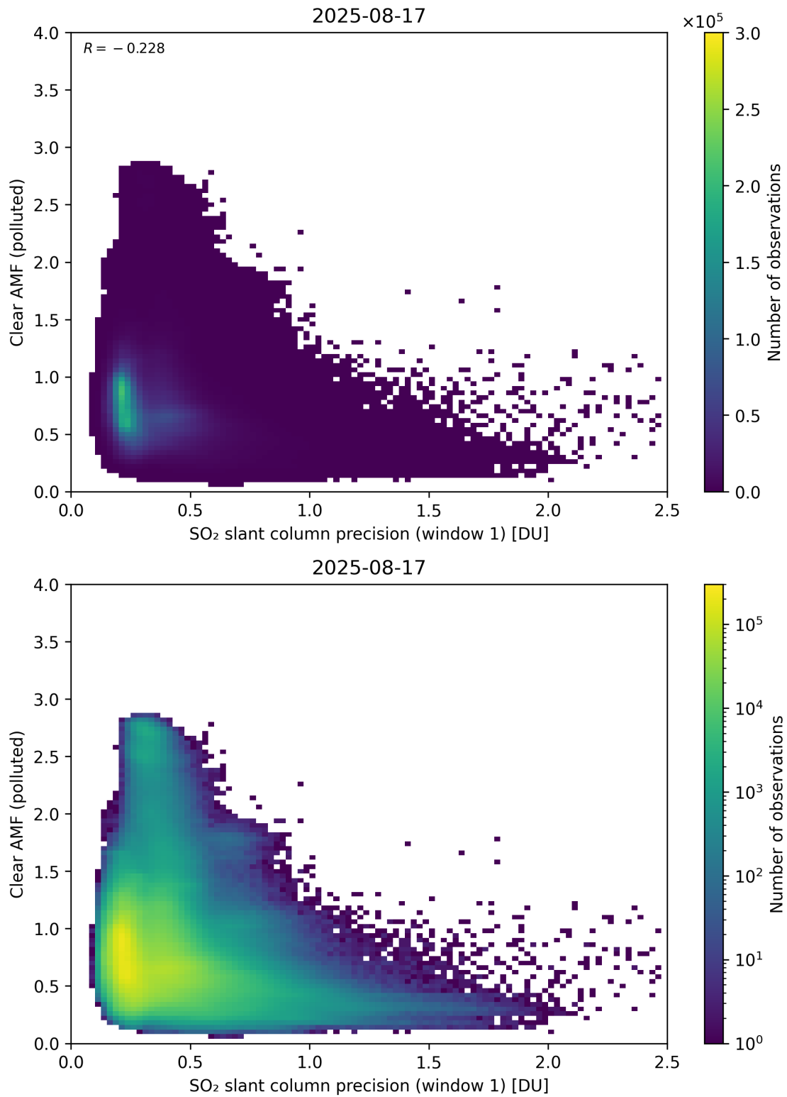
Figure 274: Scatter density plot of “SO 2 slant column precision (window 1)” against “Clear AMF (polluted)” for 2025-08-16 to 2025-08-18.
