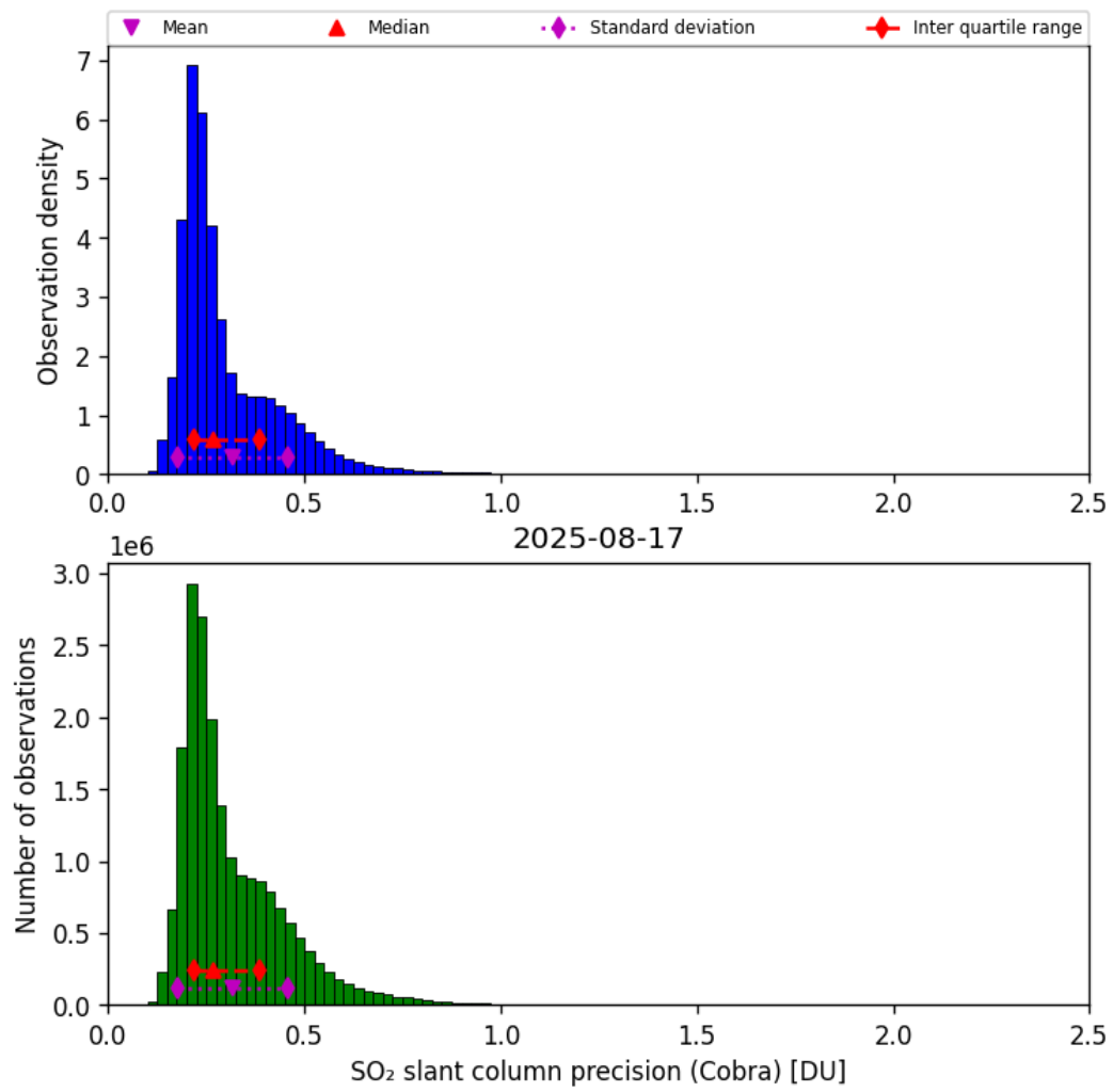
Figure 62: Histogram of “SO 2 slant column precision (Cobra)” for 2025-08-16 to 2025-08-18
