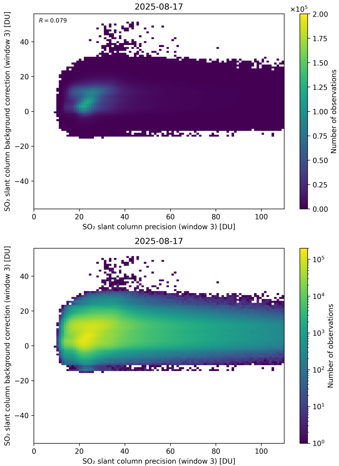
Figure 307: Scatter density plot of “SO 2 slant column precision (window 3)” against “SO 2 slant column background correction (window 3)” for 2025-08-16 to 2025-08-18.
