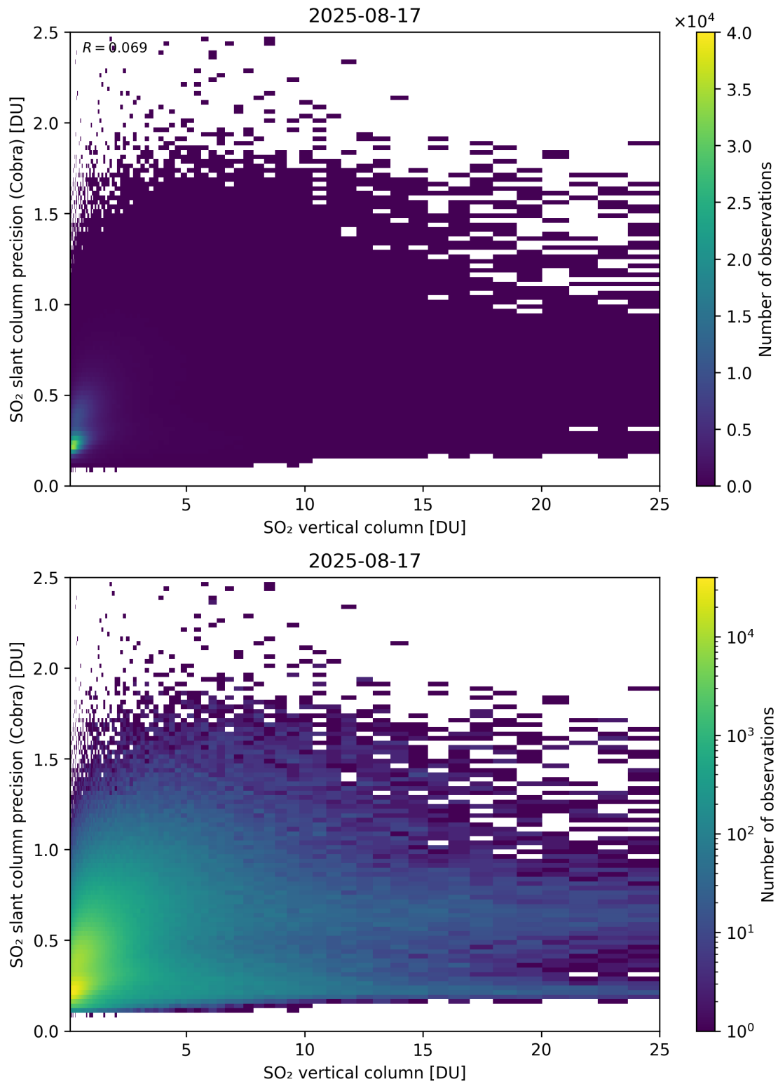
Figure 350: Scatter density plot of “SO 2 vertical column” against “SO 2 slant column precision (Cobra)” for 2025-08-16 to 2025-08-18.
