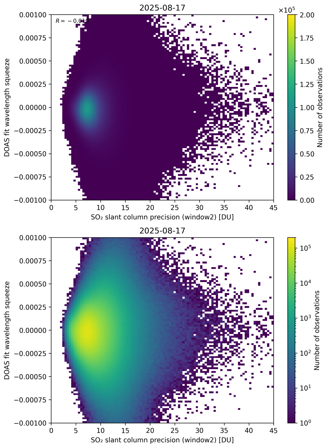
Figure 294: Scatter density plot of “SO 2 slant column precision (window2)” against “DOAS fit wavelength squeeze” for 2025-08-16 to 2025-08-18.
