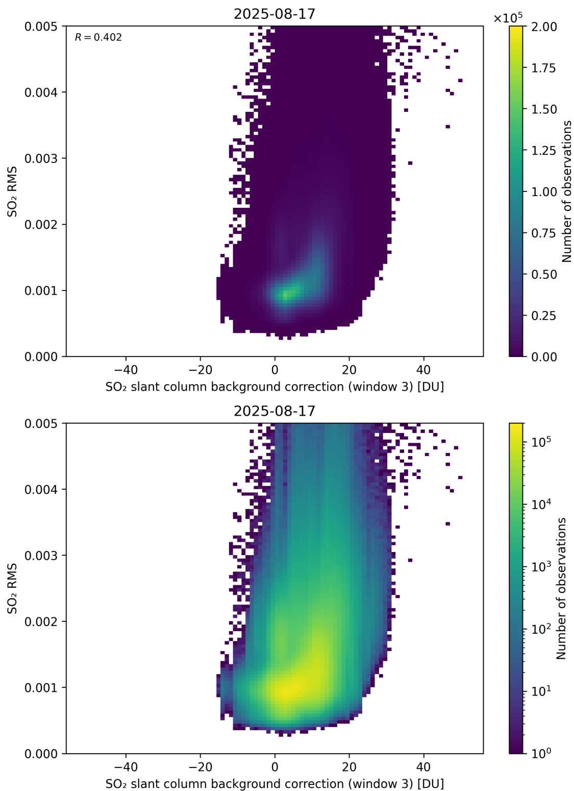
Figure 134: Scatter density plot of “SO 2 slant column background correction (window 3)” against “SO 2 RMS” for 2025-08-16 to 2025-08-18.
