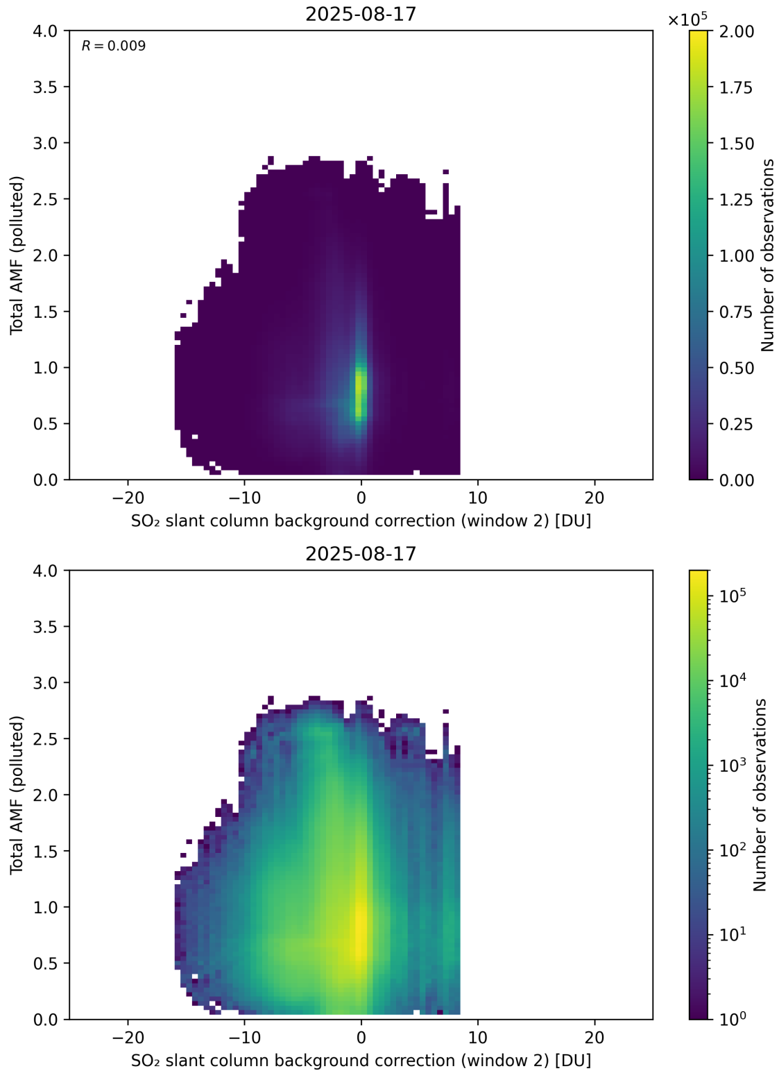
Figure 130: Scatter density plot of “SO 2 slant column background correction (window 2)” against “Total AMF (polluted)” for 2025-08-16 to 2025-08-18.
