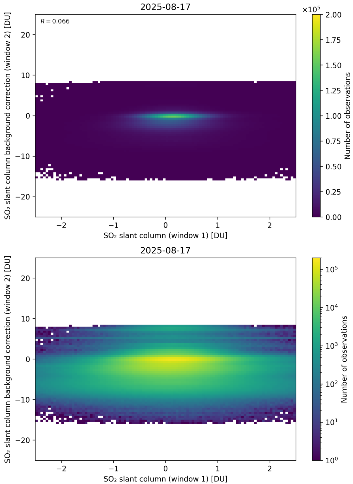
Figure 263: Scatter density plot of “SO 2 slant column (window 1)” against “SO 2 slant column background correction (window 2)” for 2025-08-16 to 2025-08-18.
