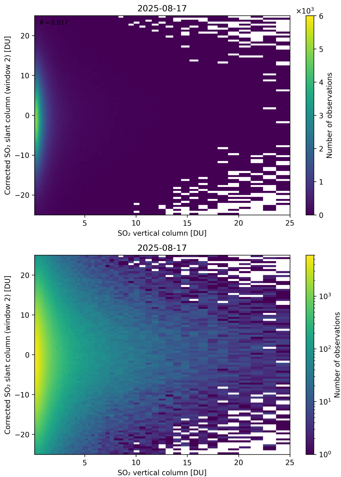
Figure 352: Scatter density plot of “SO 2 vertical column” against “Corrected SO 2 slant column (window 2)” for 2025-08-16 to 2025-08-18.
