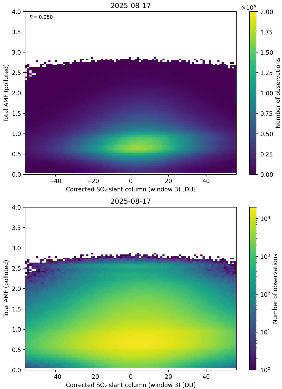
Figure 260: Scatter density plot of “Corrected SO 2 slant column (window 3)” against “Total AMF (polluted)” for 2025-08-16 to 2025-08-18.
