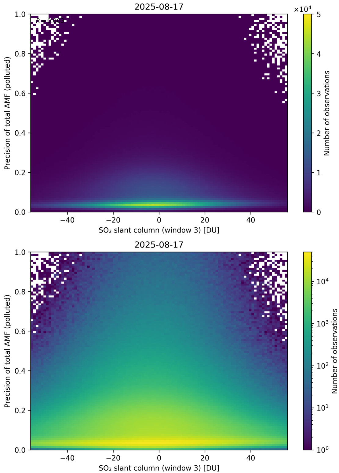
Figure 319: Scatter density plot of “SO 2 slant column (window 3)” against “Precision of total AMF (polluted)” for 2025-08-16 to 2025-08-18.
