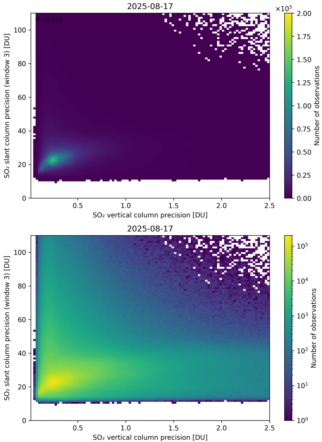
Figure 345: Scatter density plot of “SO 2 vertical column precision” against “SO 2 slant column precision (window 3)” for 2025-08-16 to 2025-08-18.
