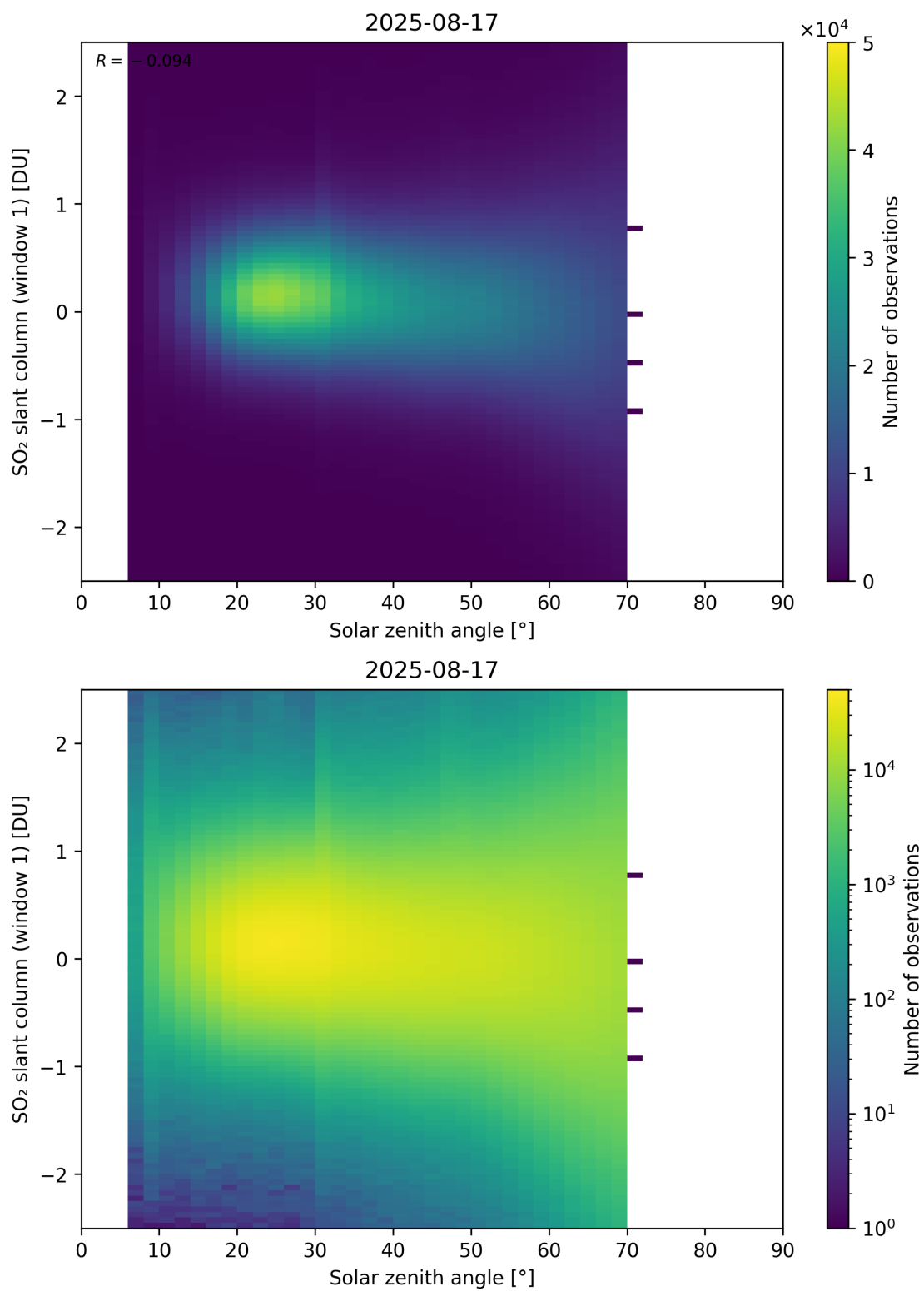
Figure 184: Scatter density plot of “Solar zenith angle” against “SO 2 slant column (window 1)” for 2025-08-16 to 2025-08-18.
