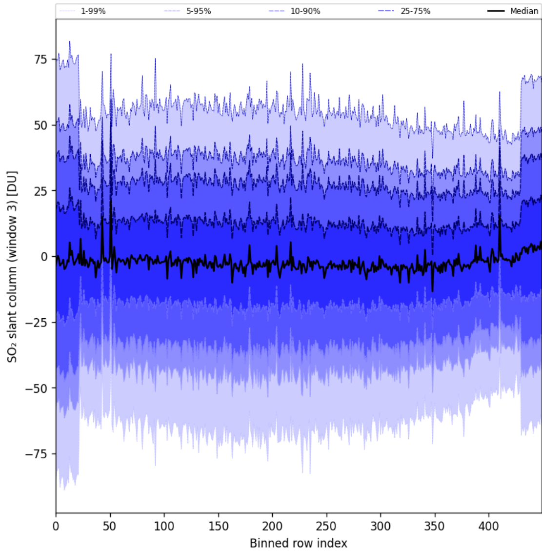
Figure 97: Along track statistics of “SO 2 slant column (window 3)” for 2025-08-16 to 2025-08-18
