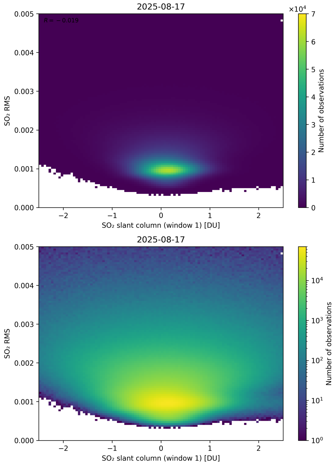
Figure 267: Scatter density plot of “SO 2 slant column (window 1)” against “SO 2 RMS” for 2025-08-16 to 2025-08-18.
