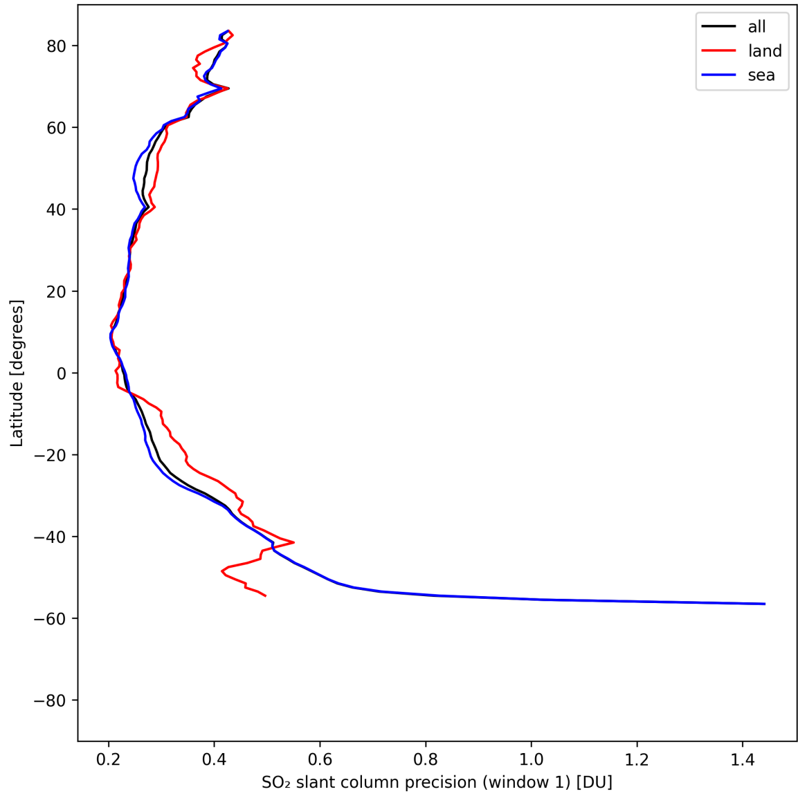
Figure 38: Zonal average of “SO 2 slant column precision (window 1)” for 2025-08-16 to 2025-08-18.
