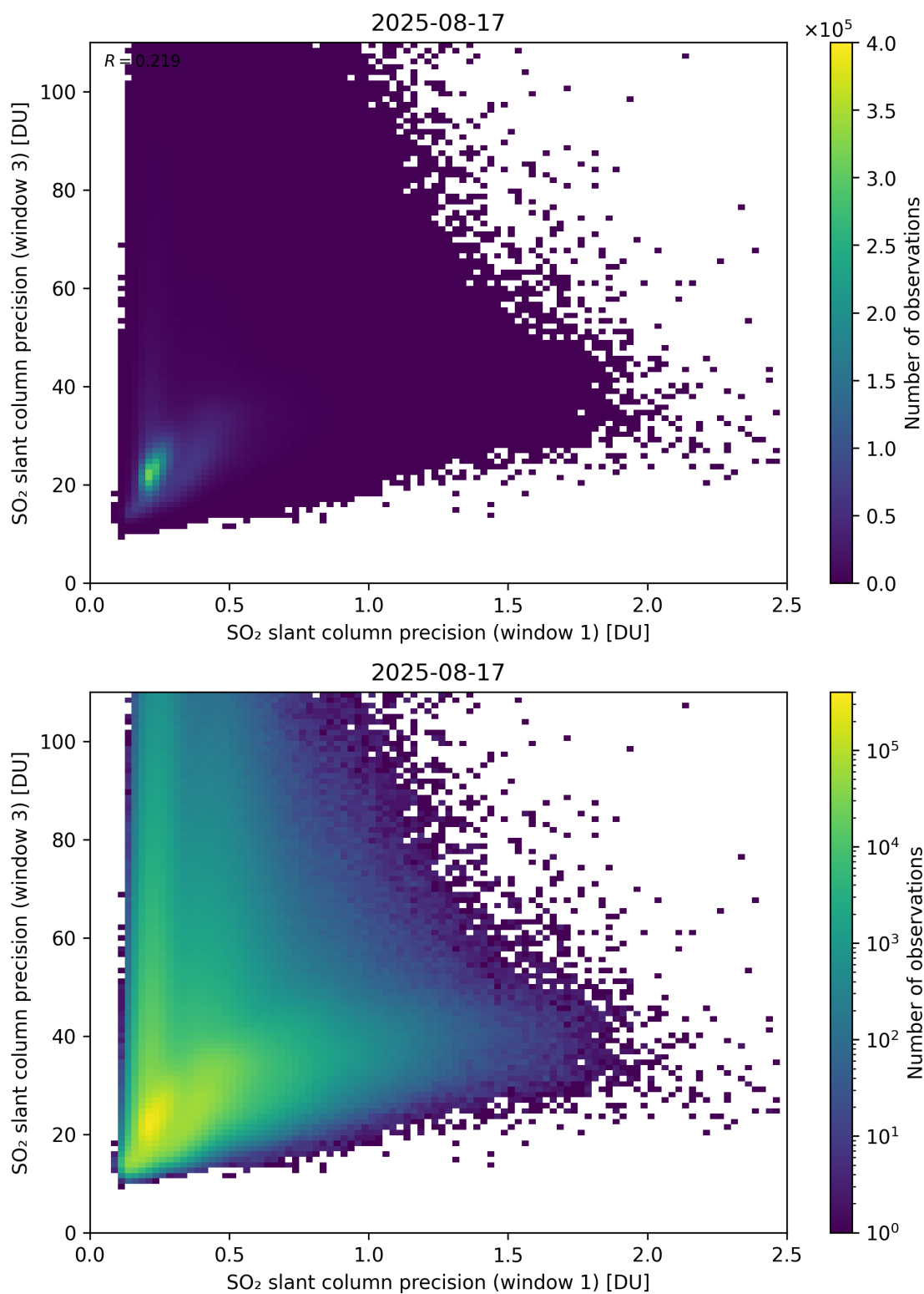
Figure 279: Scatter density plot of “SO 2 slant column precision (window 1)” against “SO 2 slant column precision (window 3)” for 2025-08-16 to 2025-08-18.
