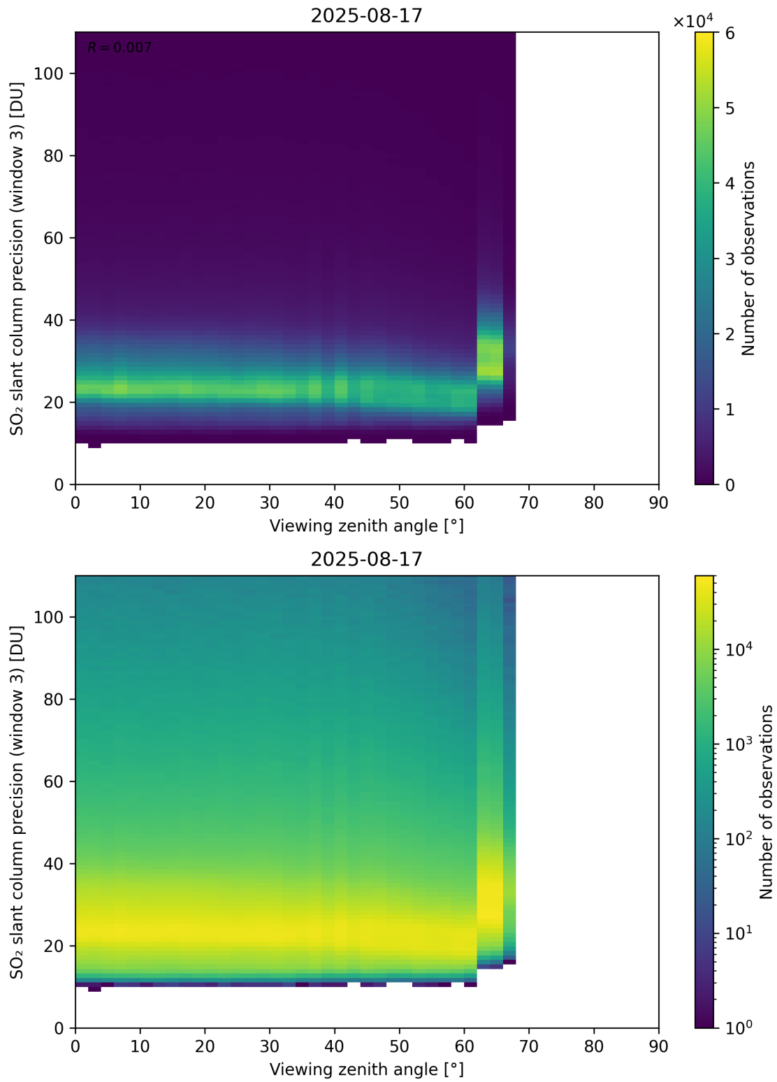
Figure 380: Scatter density plot of “Viewing zenith angle” against “SO 2 slant column precision (window 3)” for 2025-08-16 to 2025-08-18.
