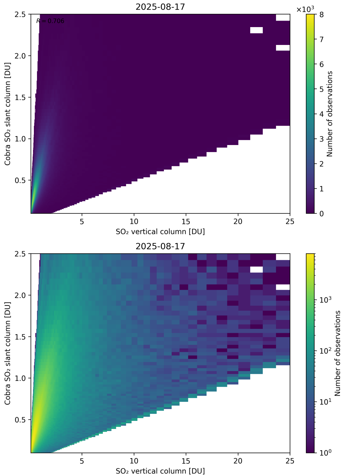
Figure 349: Scatter density plot of “SO 2 vertical column” against “Cobra SO 2 slant column” for 2025-08-16 to 2025-08-18.
