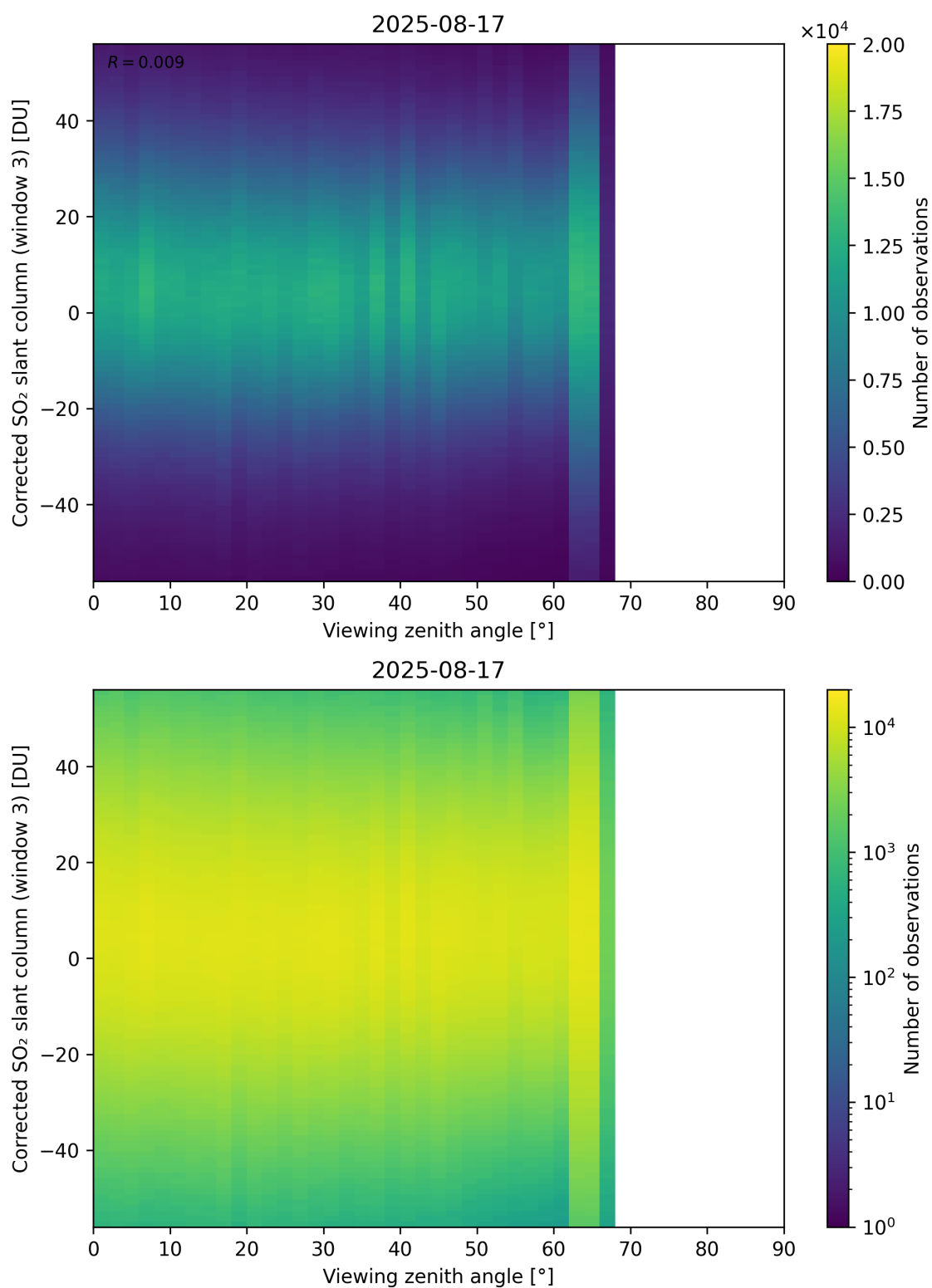
Figure 375: Scatter density plot of “Viewing zenith angle” against “Corrected SO 2 slant column (window 3)” for 2025-08-16 to 2025-08-18.
