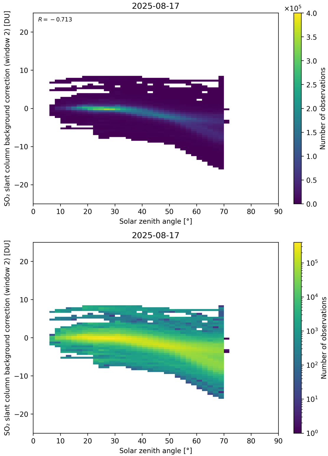
Figure 172: Scatter density plot of “Solar zenith angle” against “SO 2 slant column background correction (window 2)” for 2025-08-16 to 2025-08-18.
