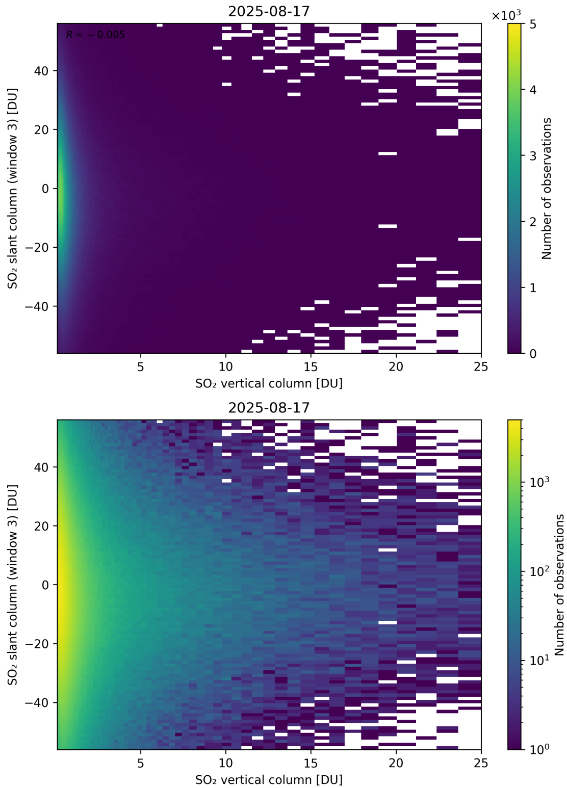
Figure 357: Scatter density plot of “SO 2 vertical column” against “SO 2 slant column (window 3)” for 2025-08-16 to 2025-08-18.
