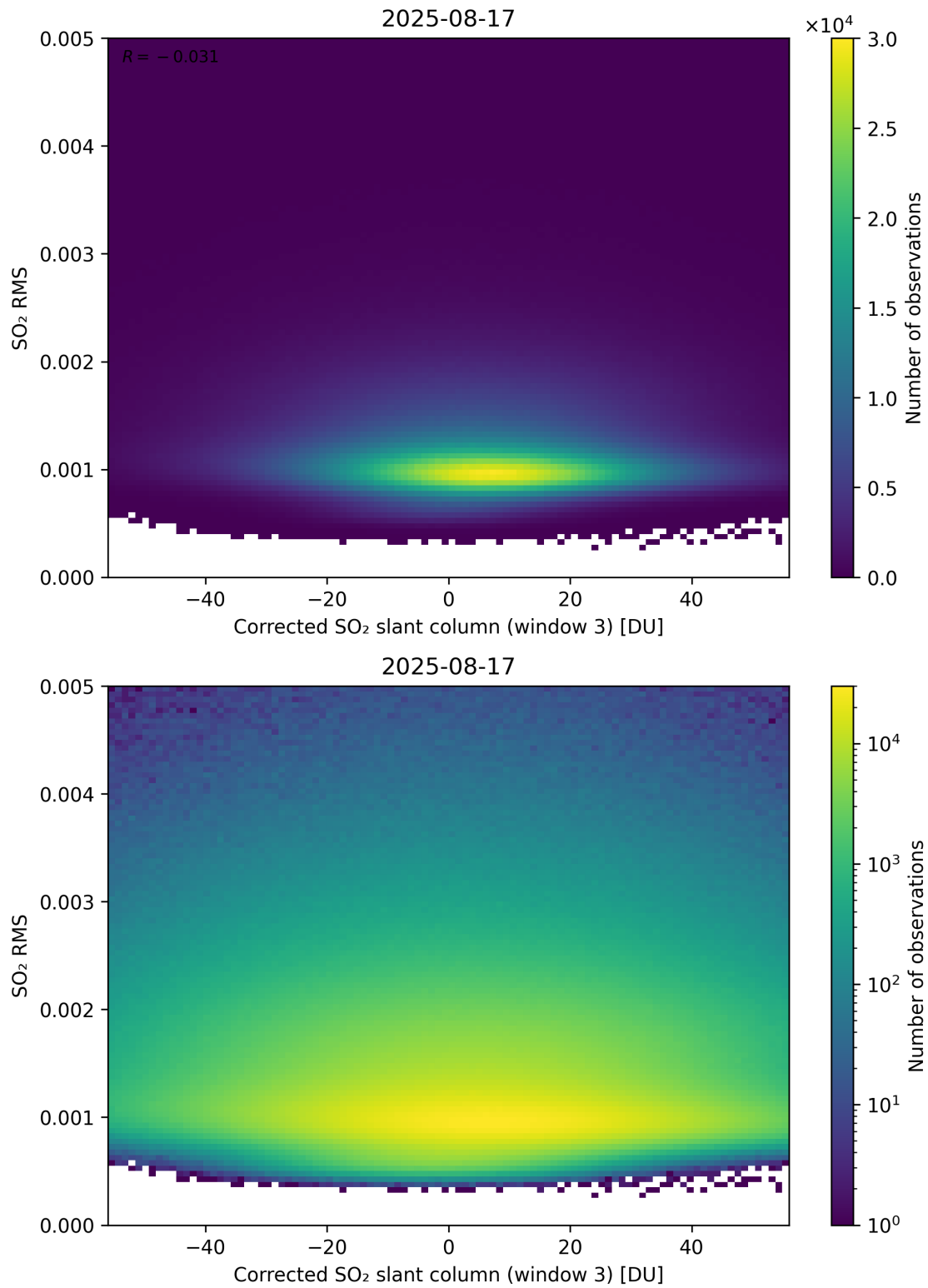
Figure 258: Scatter density plot of “Corrected SO 2 slant column (window 3)” against “SO 2 RMS” for 2025-08-16 to 2025-08-18.
