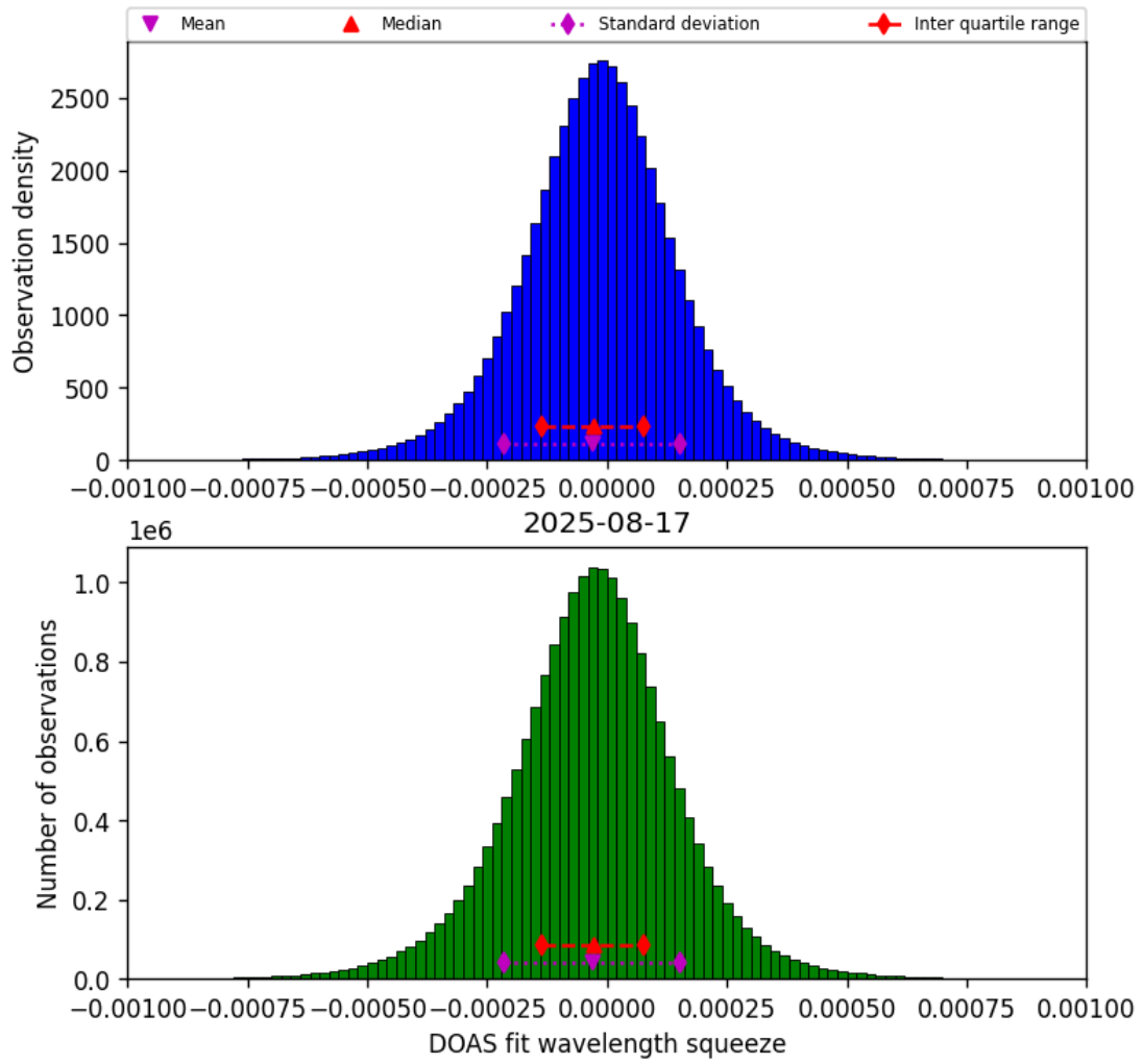
Figure 77: Histogram of “DOAS fit wavelength squeeze” for 2025-08-16 to 2025-08-18
