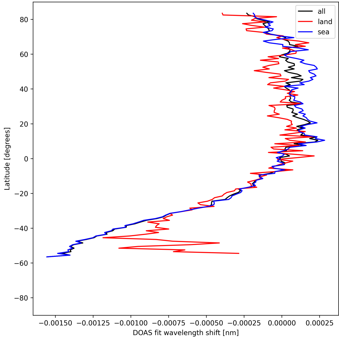
Figure 50: Zonal average of "DOAS fit wavelength shift" for 2025-08-16 to 2025-08-18.
