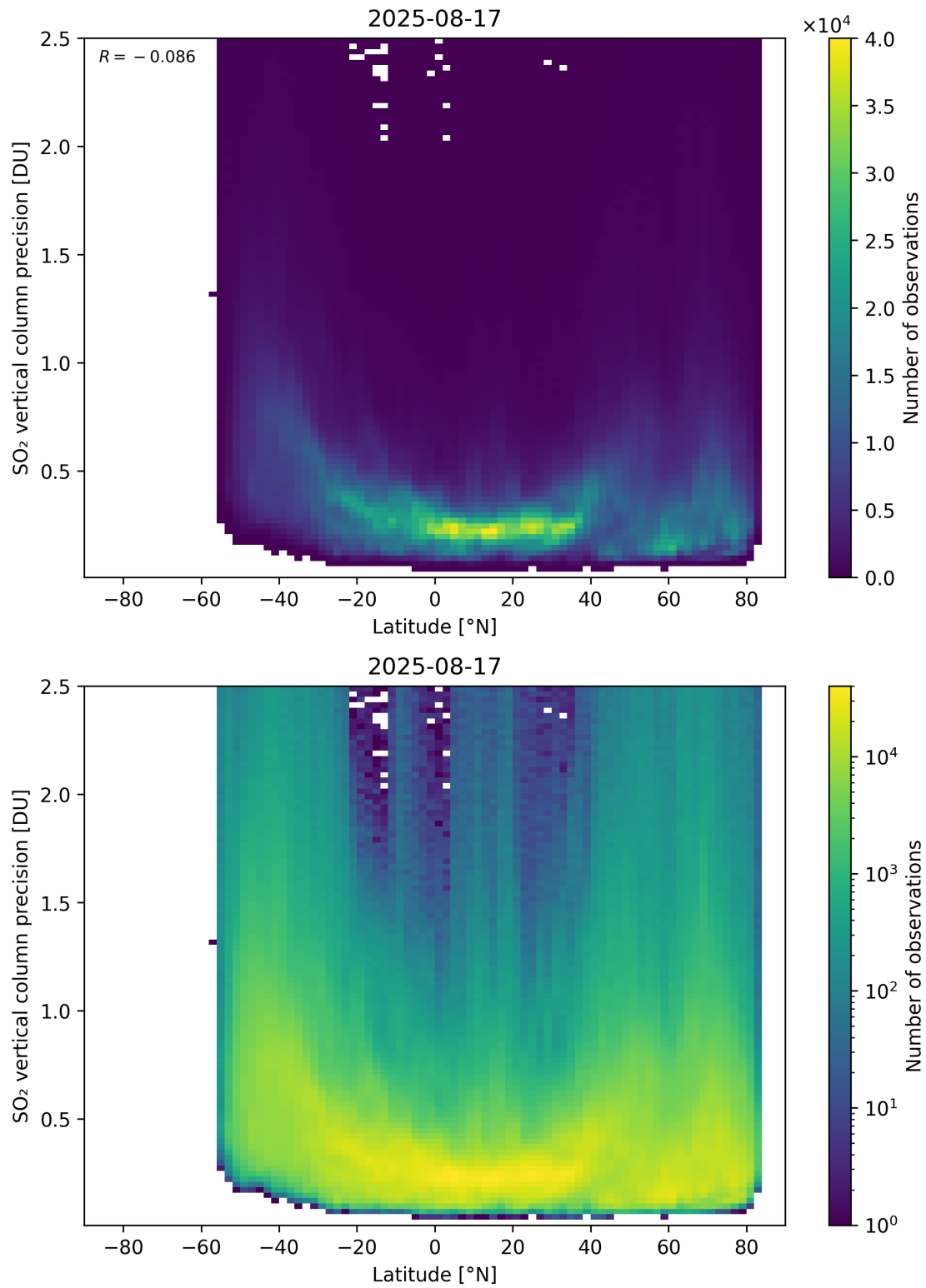
Figure 170: Scatter density plot of “Latitude” against “SO 2 vertical column precision” for 2025-08-16 to 2025-08-18.
