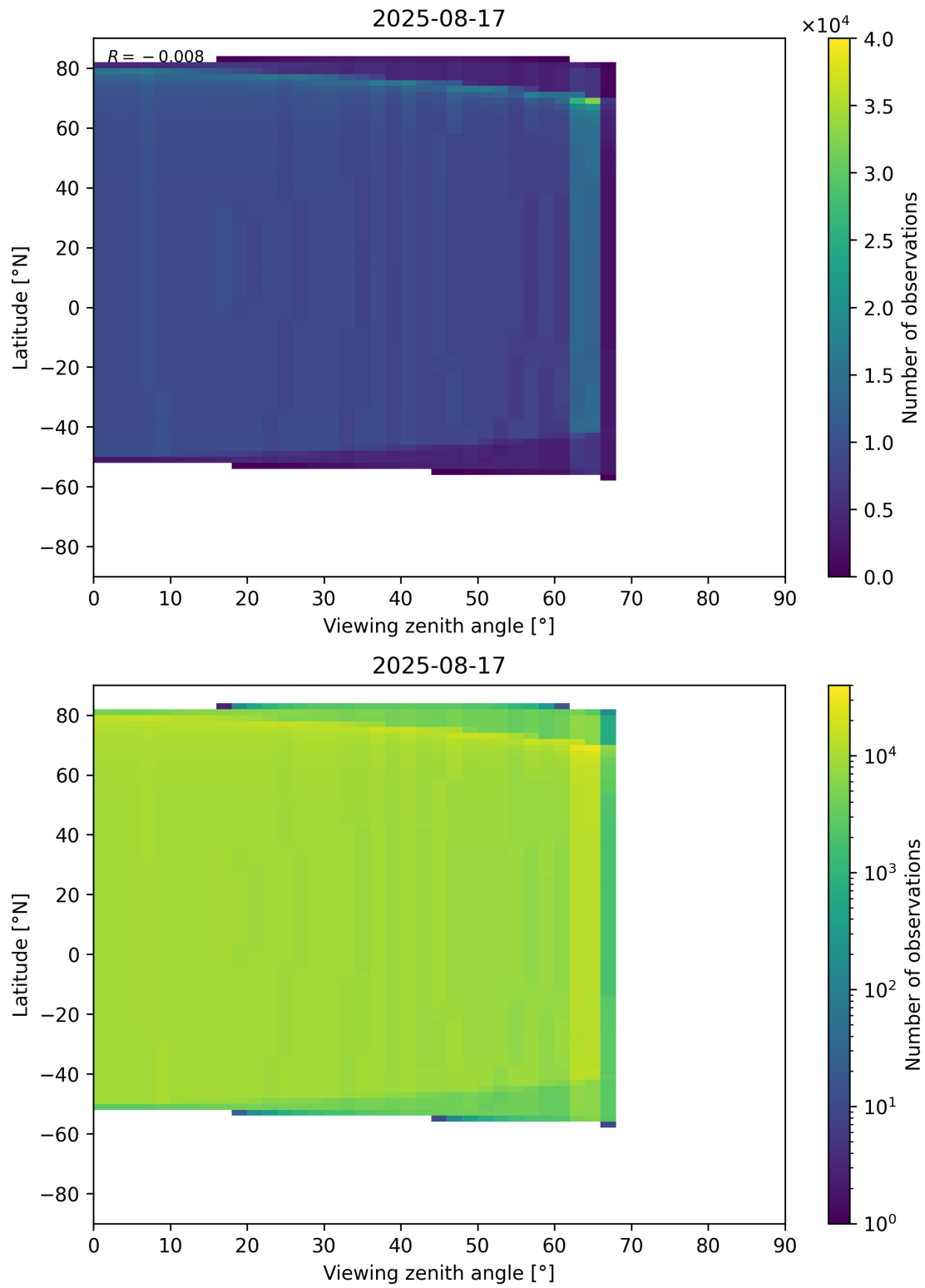
Figure 368: Scatter density plot of “Viewing zenith angle” against “Latitude” for 2025-08-16 to 2025-08-18.
