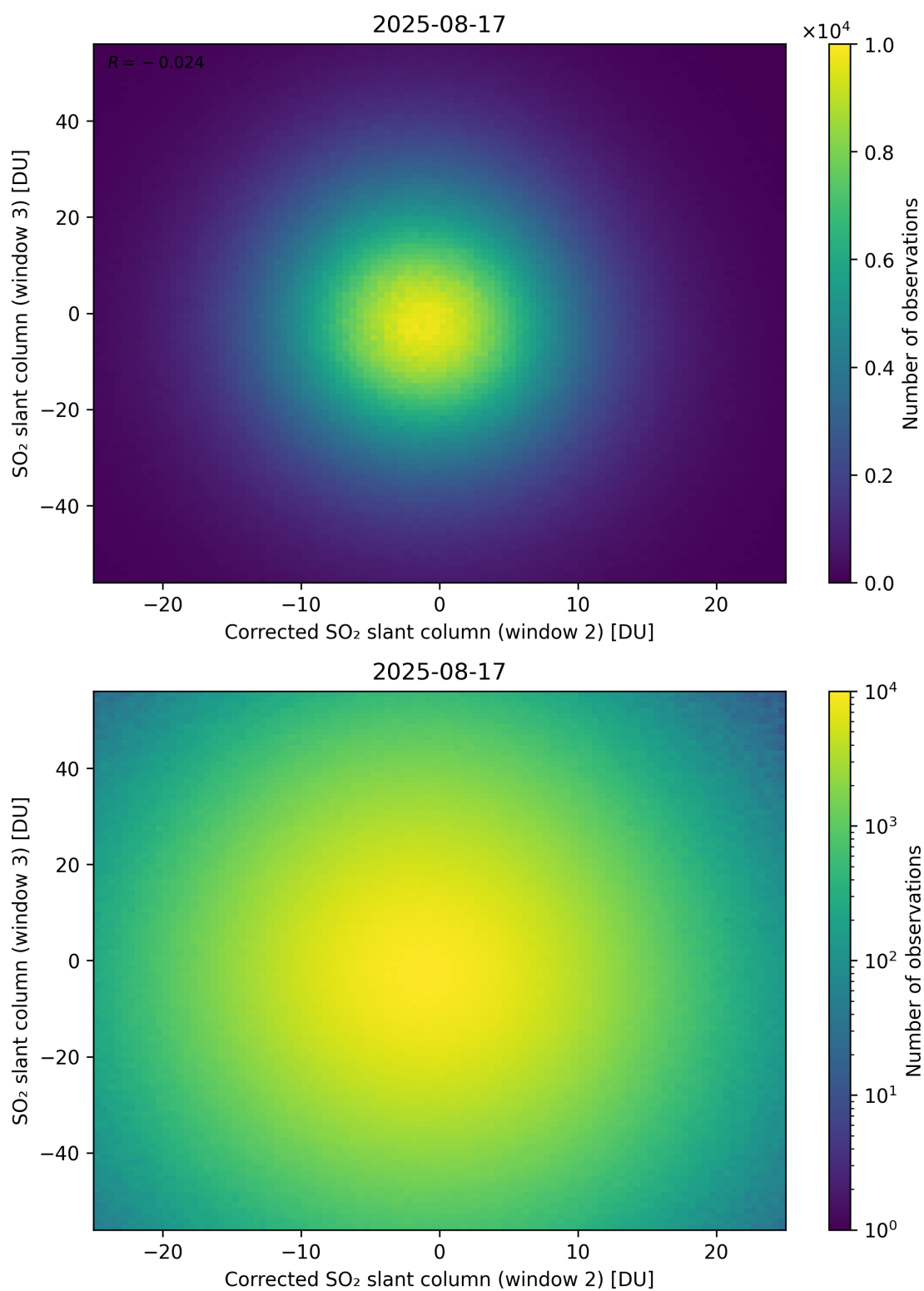
Figure 251: Scatter density plot of “Corrected SO 2 slant column (window 2)” against “SO 2 slant column (window 3)” for 2025-08-16 to 2025-08-18.
