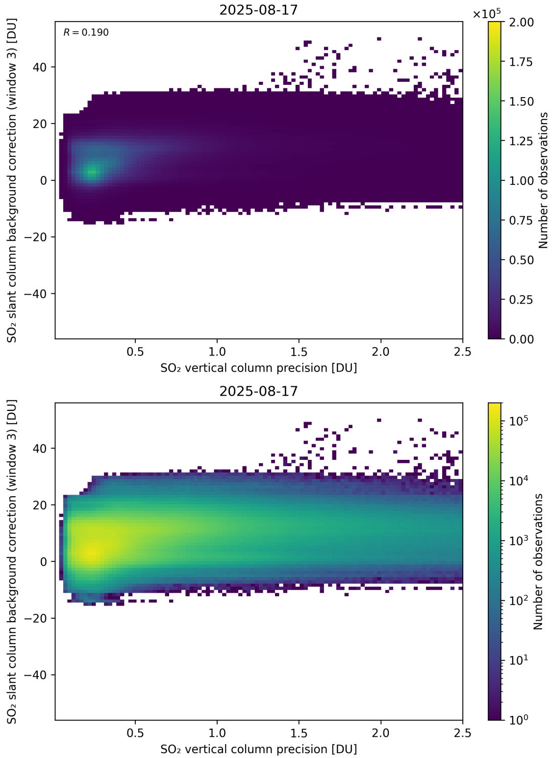
Figure 331: Scatter density plot of “SO 2 vertical column precision” against “SO 2 slant column background correction (window 3)” for 2025-08-16 to 2025-08-18.
