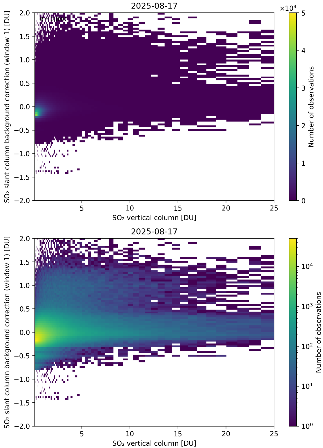
Figure 323: Scatter density plot of “SO 2 vertical column” against “SO 2 slant column background correction (window 1)” for 2025-08-16 to 2025-08-18.
