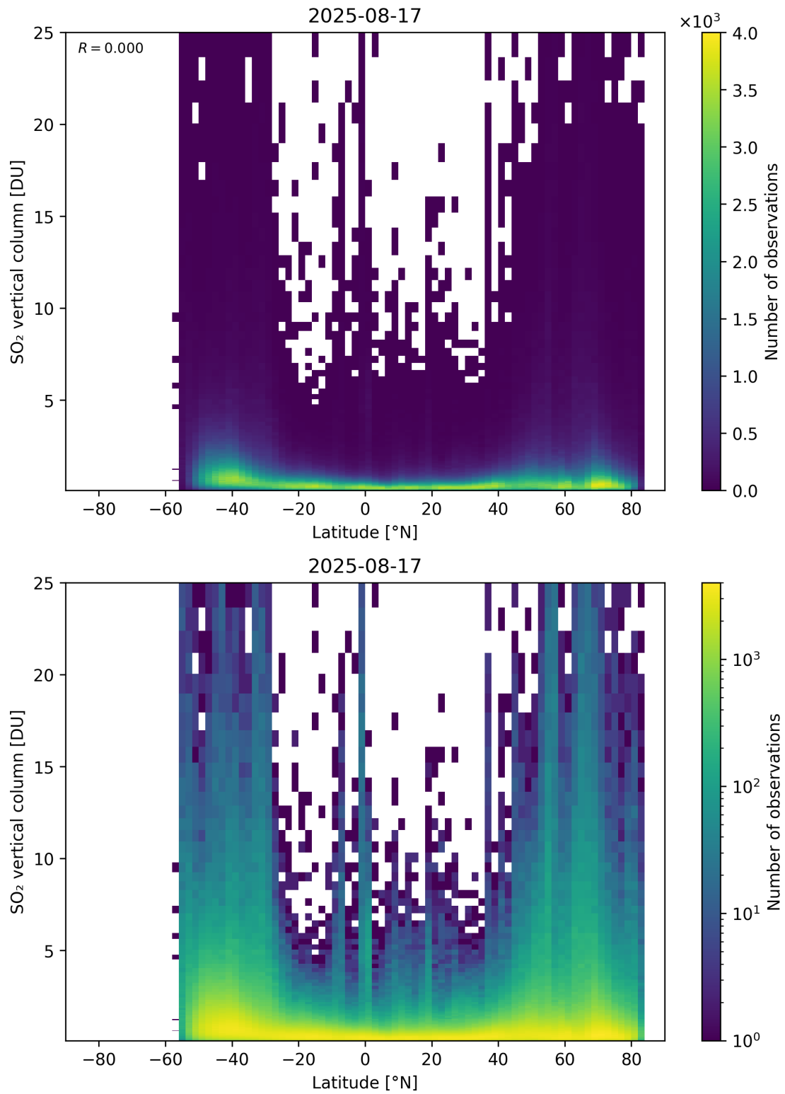
Figure 169: Scatter density plot of “Latitude” against “SO 2 vertical column” for 2025-08-16 to 2025-08-18.
