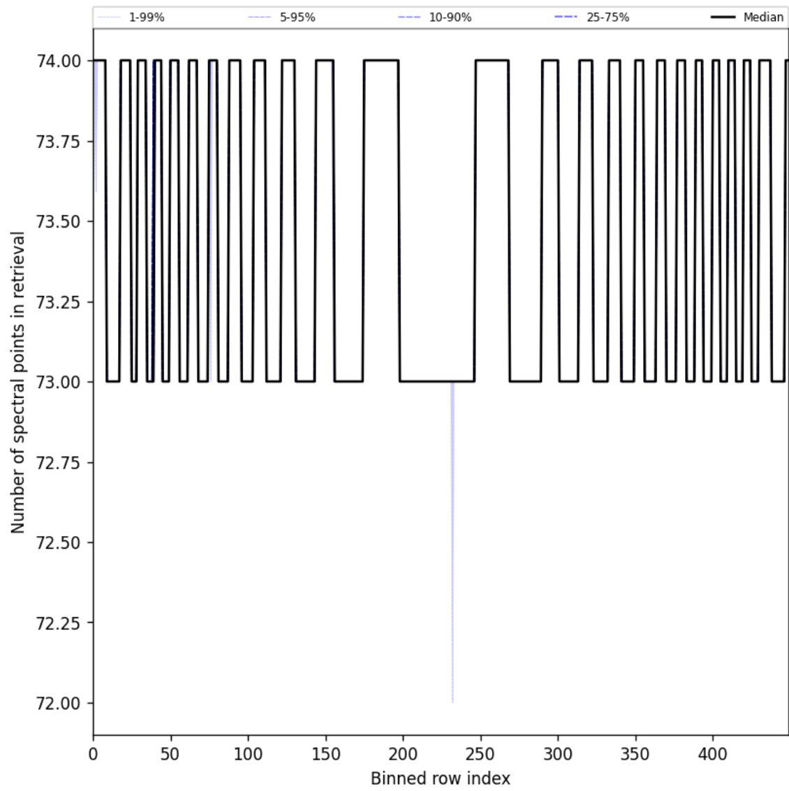
Figure 108: Along track statistics of “Number of spectral points in retrieval” for 2025-08-16 to 2025-08-18
