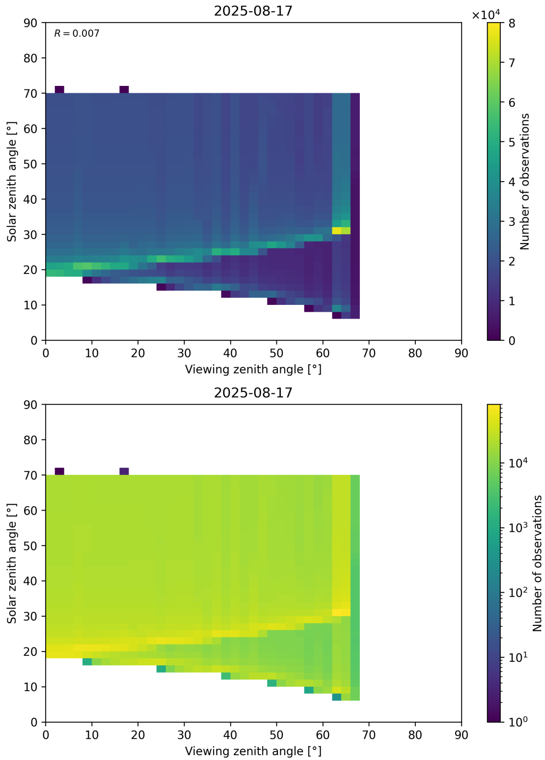
Figure 369: Scatter density plot of “Viewing zenith angle” against “Solar zenith angle” for 2025-08-16 to 2025-08-18.
