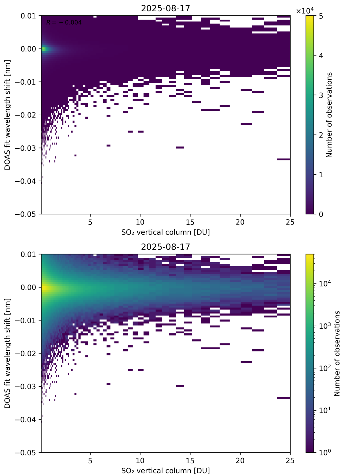
Figure 326: Scatter density plot of “SO 2 vertical column” against “DOAS fit wavelength shift” for 2025-08-16 to 2025-08-18.
