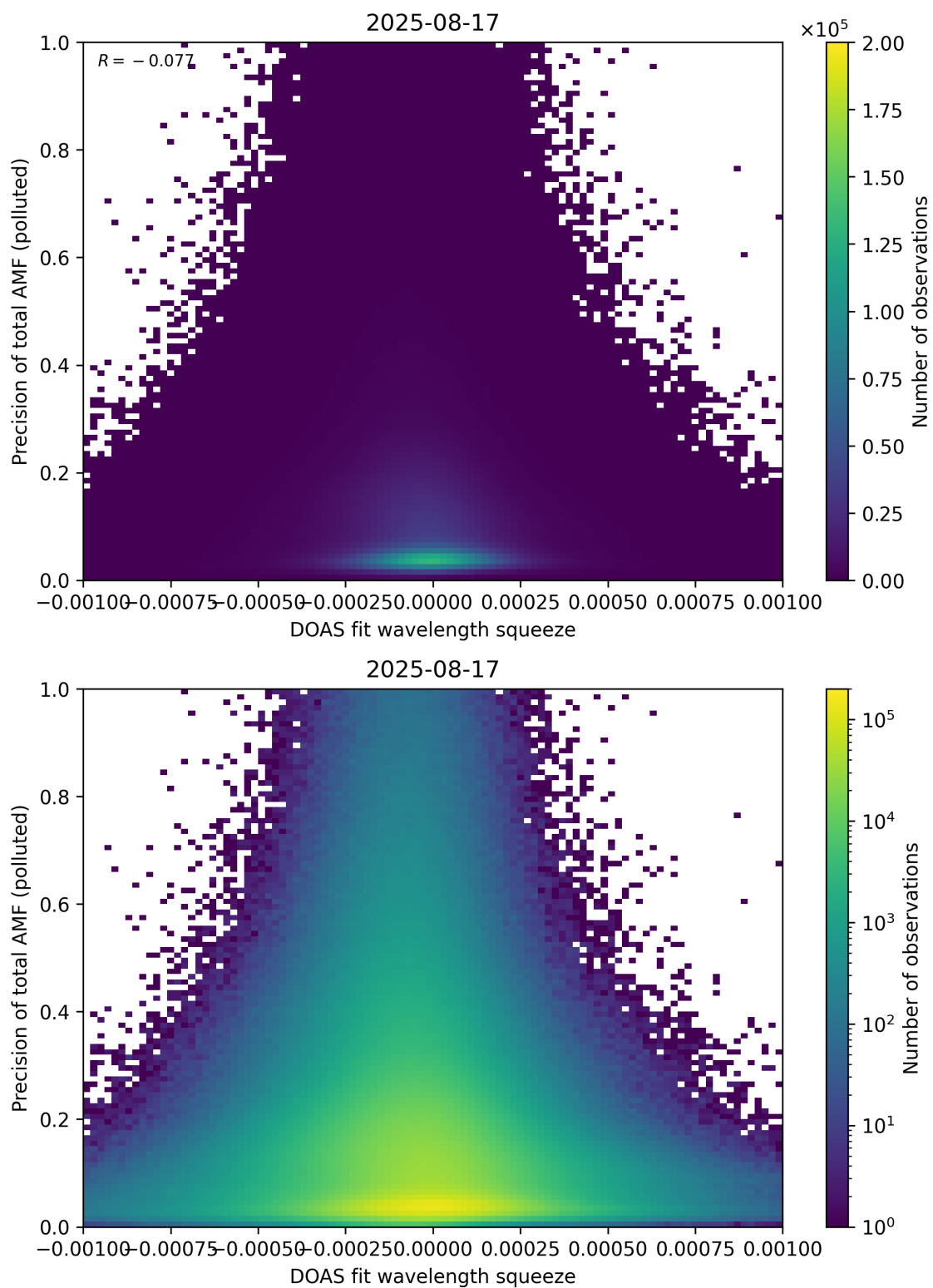
Figure 146: Scatter density plot of “DOAS fit wavelength squeeze” against “Precision of total AMF (polluted)” for 2025-08-16 to 2025-08-18.
