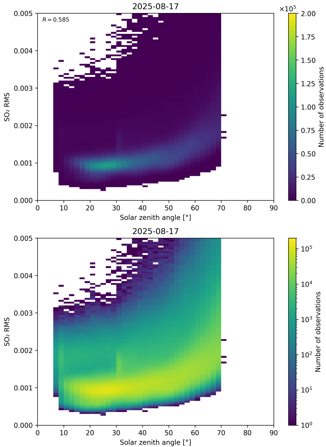
Figure 176: Scatter density plot of “Solar zenith angle” against “SO 2 RMS” for 2025-08-16 to 2025-08-18.
