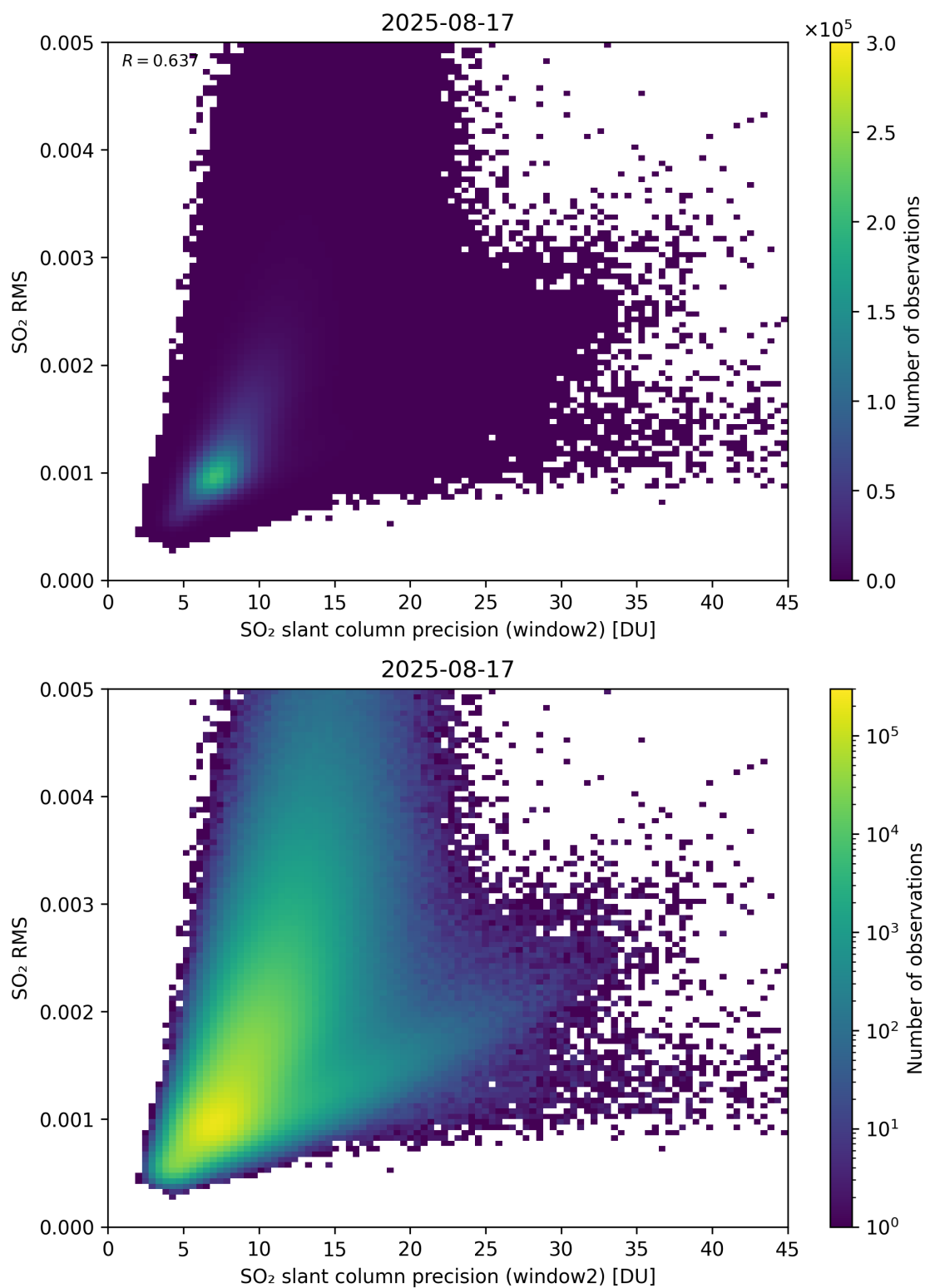
Figure 295: Scatter density plot of “SO 2 slant column precision (window2)” against “SO 2 RMS” for 2025-08-16 to 2025-08-18.
