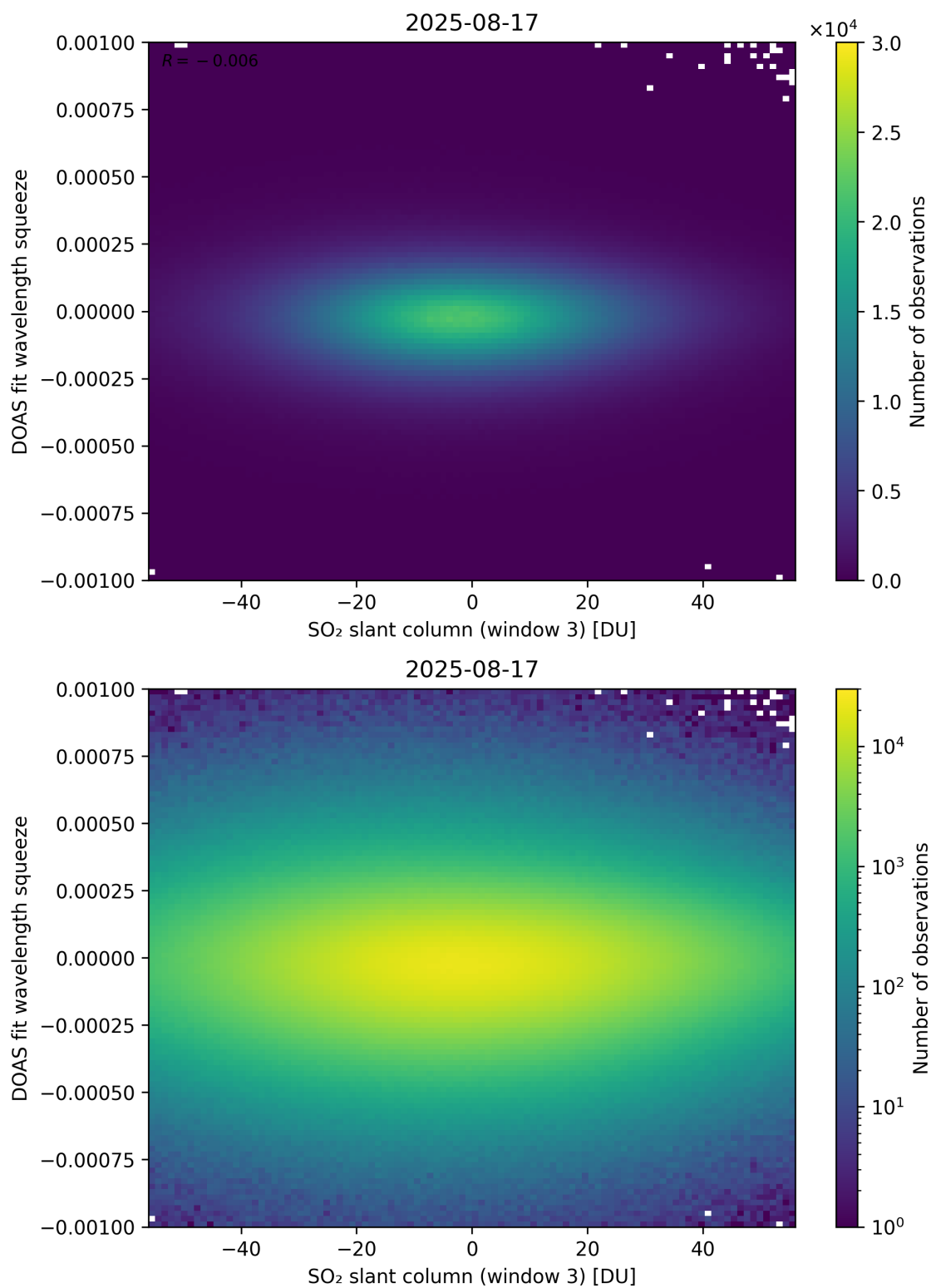
Figure 305: Scatter density plot of “SO 2 slant column (window 3)” against “DOAS fit wavelength squeeze” for 2025-08-16 to 2025-08-18.
