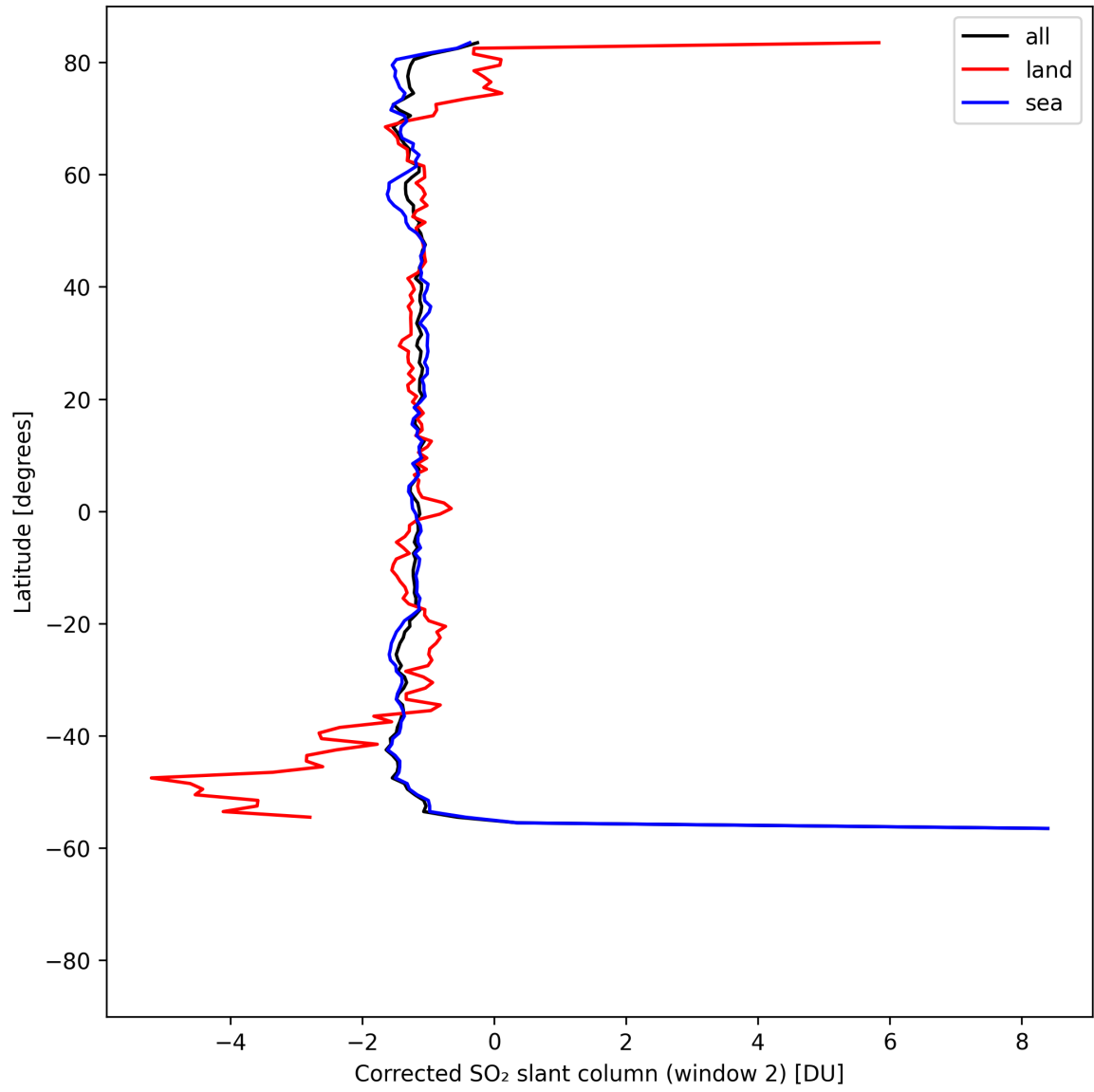
Figure 43: Zonal average of “Corrected SO 2 slant column (window 2)” for 2025-08-16 to 2025-08-18.
