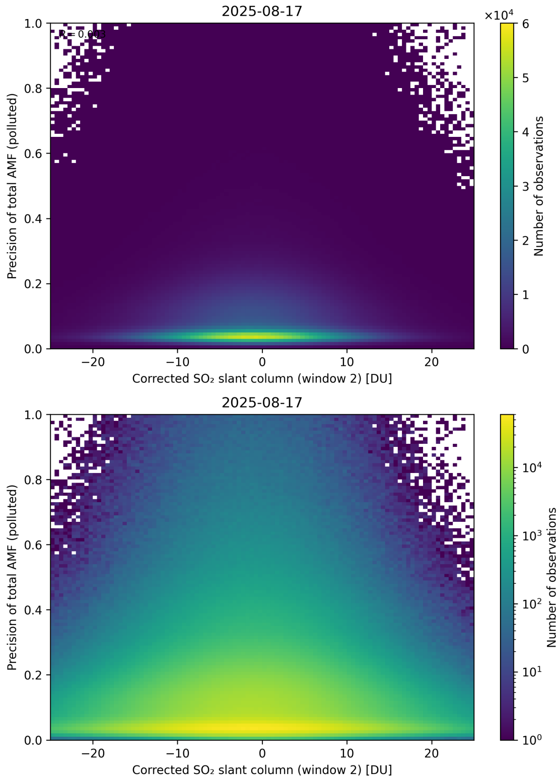
Figure 254: Scatter density plot of “Corrected SO 2 slant column (window 2)” against “Precision of total AMF (polluted)” for 2025-08-16 to 2025-08-18.
