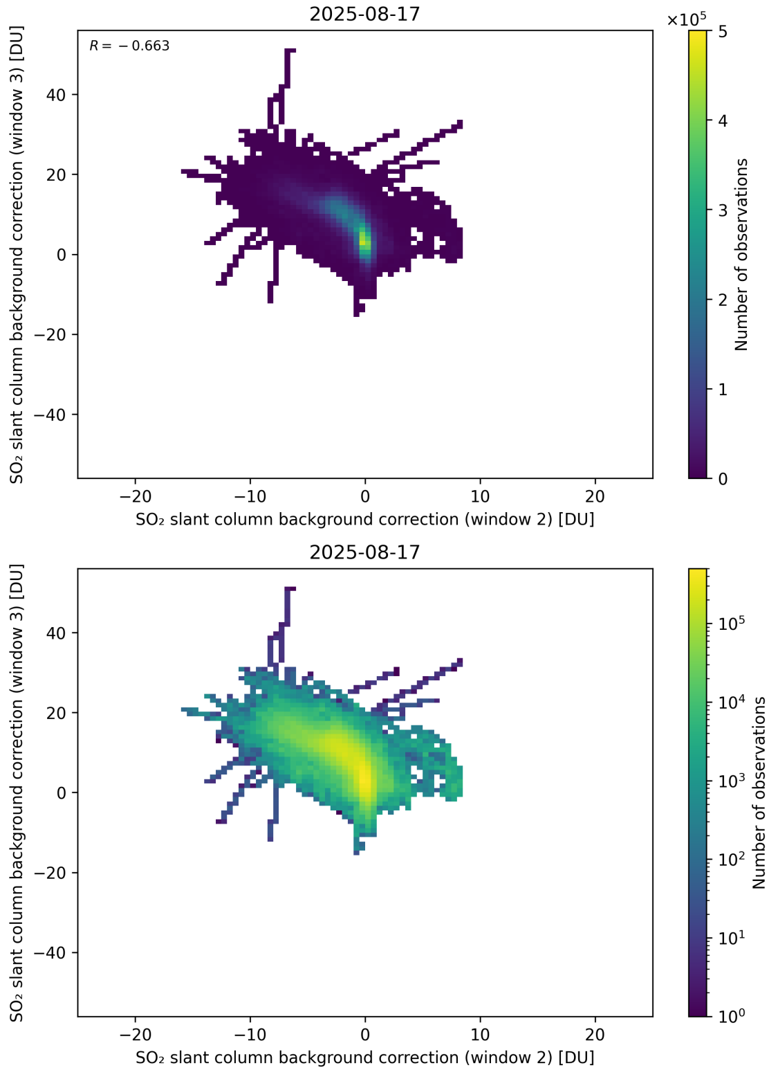
Figure 122: Scatter density plot of “SO 2 slant column background correction (window 2)” against “SO 2 slant column background correction (window 3)” for 2025-08-16 to 2025-08-18.
