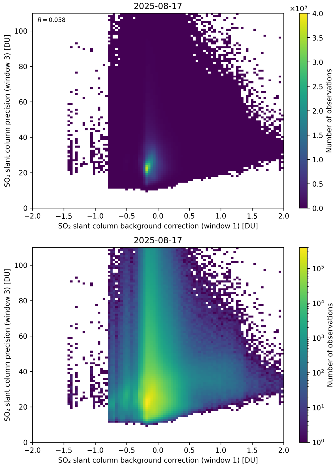
Figure 119: Scatter density plot of “SO 2 slant column background correction (window 1)” against “SO 2 slant column precision (window 3)” for 2025-08-16 to 2025-08-18.
