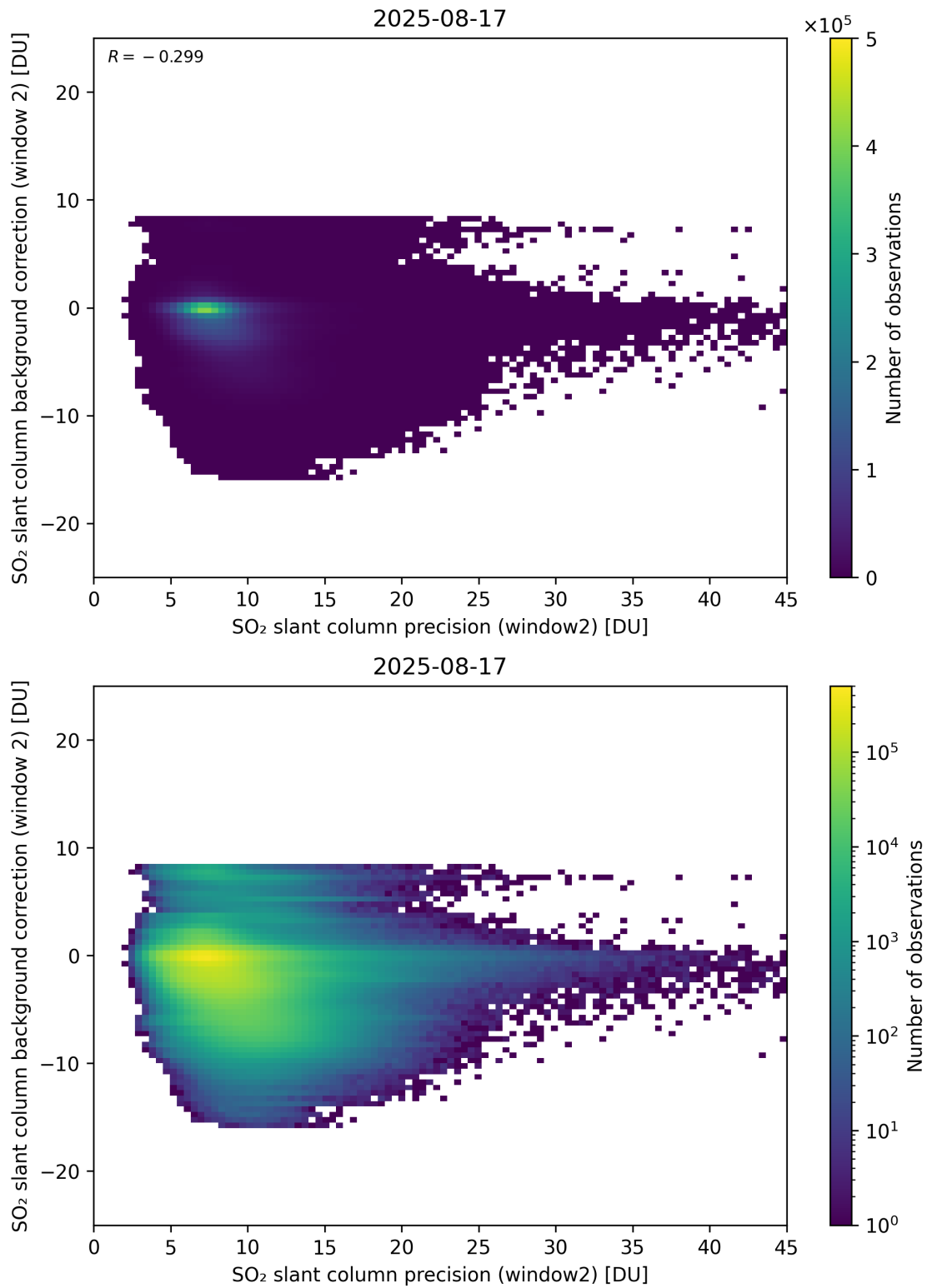
Figure 291: Scatter density plot of “SO 2 slant column precision (window2)” against “SO 2 slant column background correction (window 2)” for 2025-08-16 to 2025-08-18.
