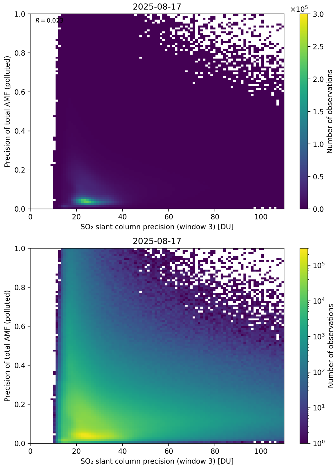
Figure 314: Scatter density plot of “SO 2 slant column precision (window 3)” against “Precision of total AMF (polluted)” for 2025-08-16 to 2025-08-18.
