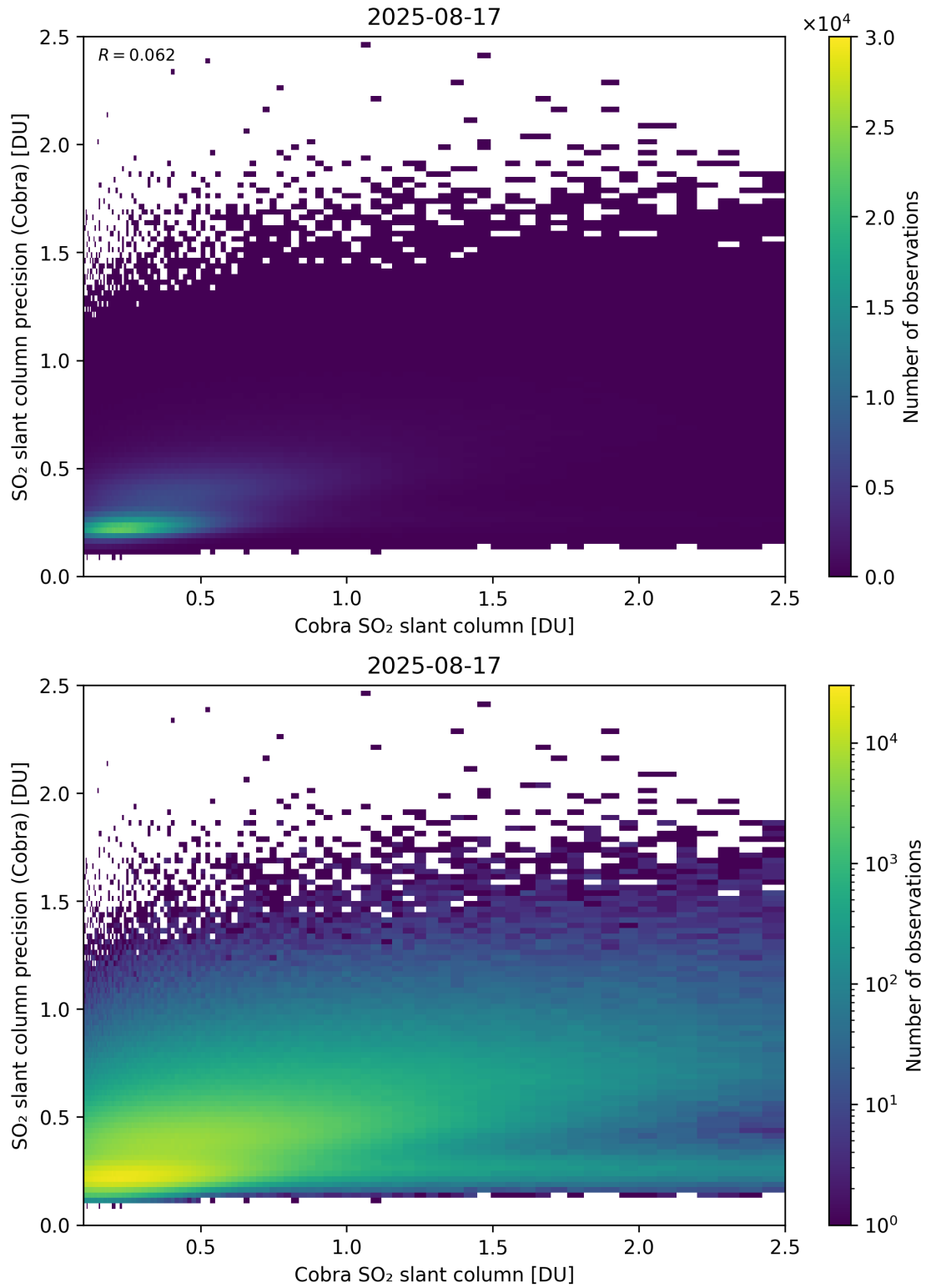
Figure 216: Scatter density plot of “Cobra SO 2 slant column” against “SO 2 slant column precision (Cobra)” for 2025-08-16 to 2025-08-18.
