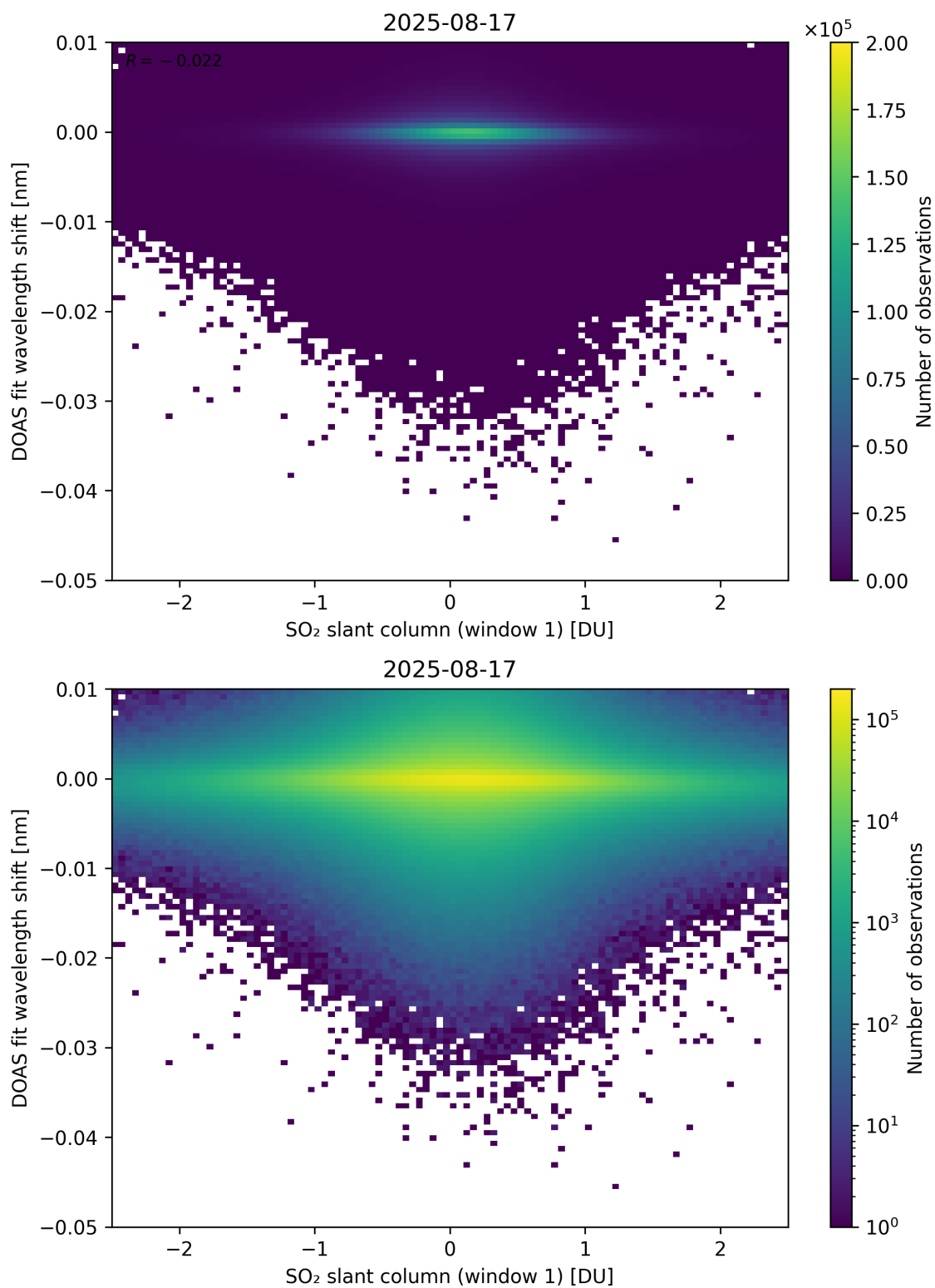
Figure 265: Scatter density plot of “SO 2 slant column (window 1)” against “DOAS fit wavelength shift” for 2025-08-16 to 2025-08-18.
