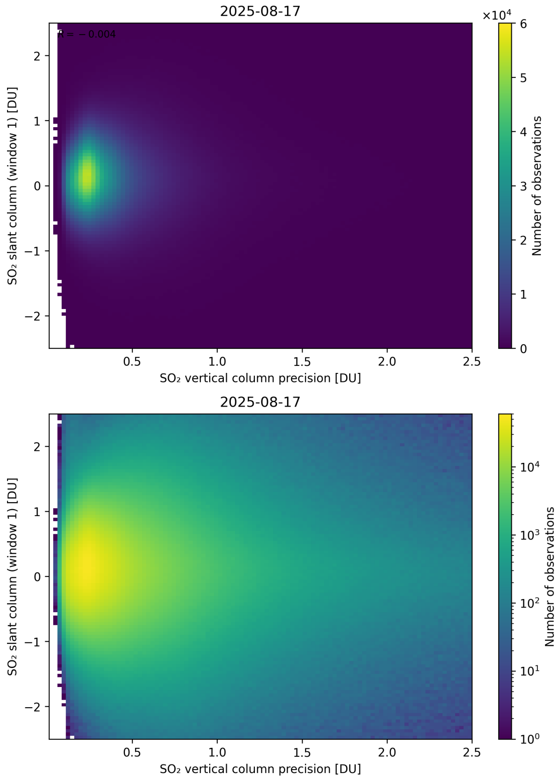
Figure 341: Scatter density plot of “SO 2 vertical column precision” against “SO 2 slant column (window 1)” for 2025-08-16 to 2025-08-18.
