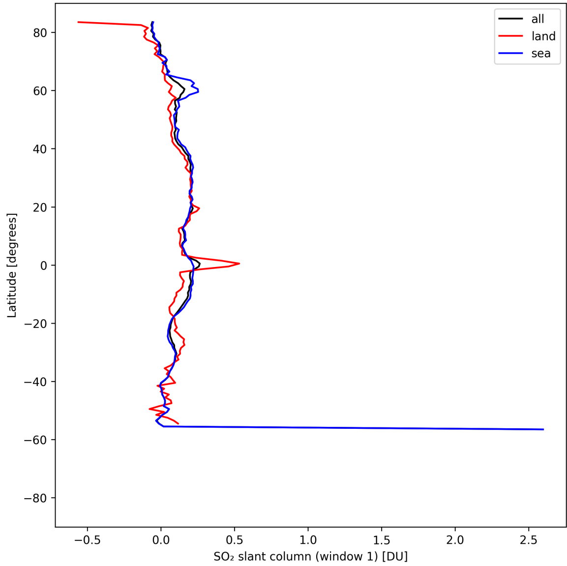
Figure 37: Zonal average of “SO 2 slant column (window 1)” for 2025-08-16 to 2025-08-18.
