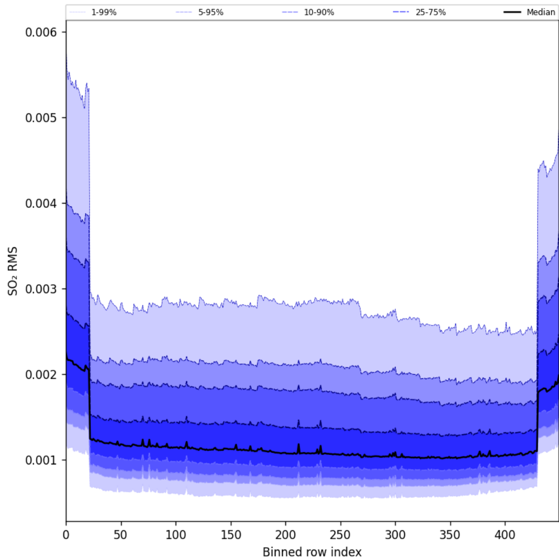
Figure 104: Along track statistics of “SO 2 RMS” for 2025-08-16 to 2025-08-18
