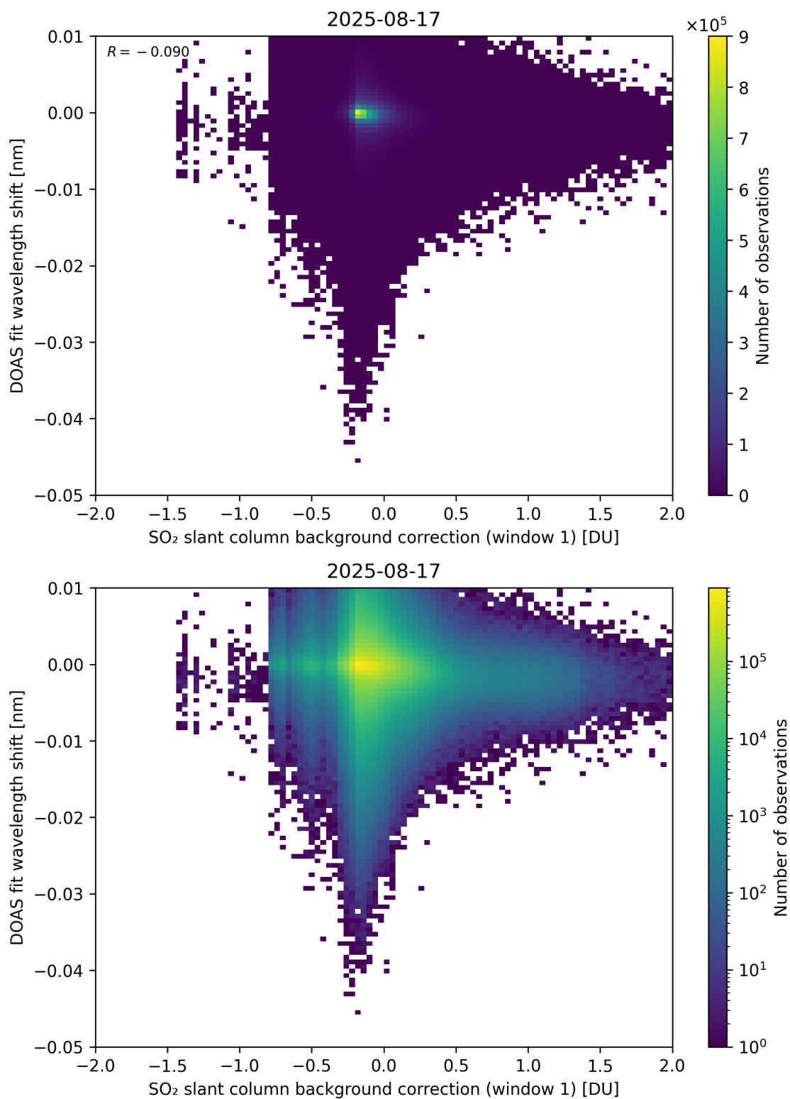
Figure 111: Scatter density plot of “SO 2 slant column background correction (window 1)” against “DOAS fit wavelength shift” for 2025-08-16 to 2025-08-18.
