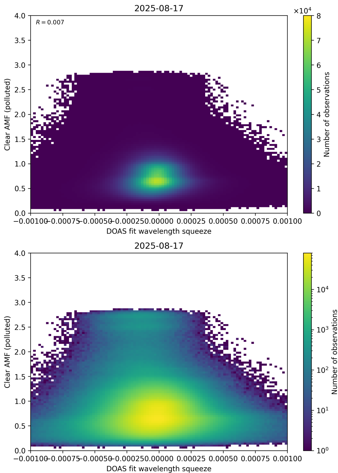
Figure 144: Scatter density plot of “DOAS fit wavelength squeeze” against “Clear AMF (polluted)” for 2025-08-16 to 2025-08-18.
