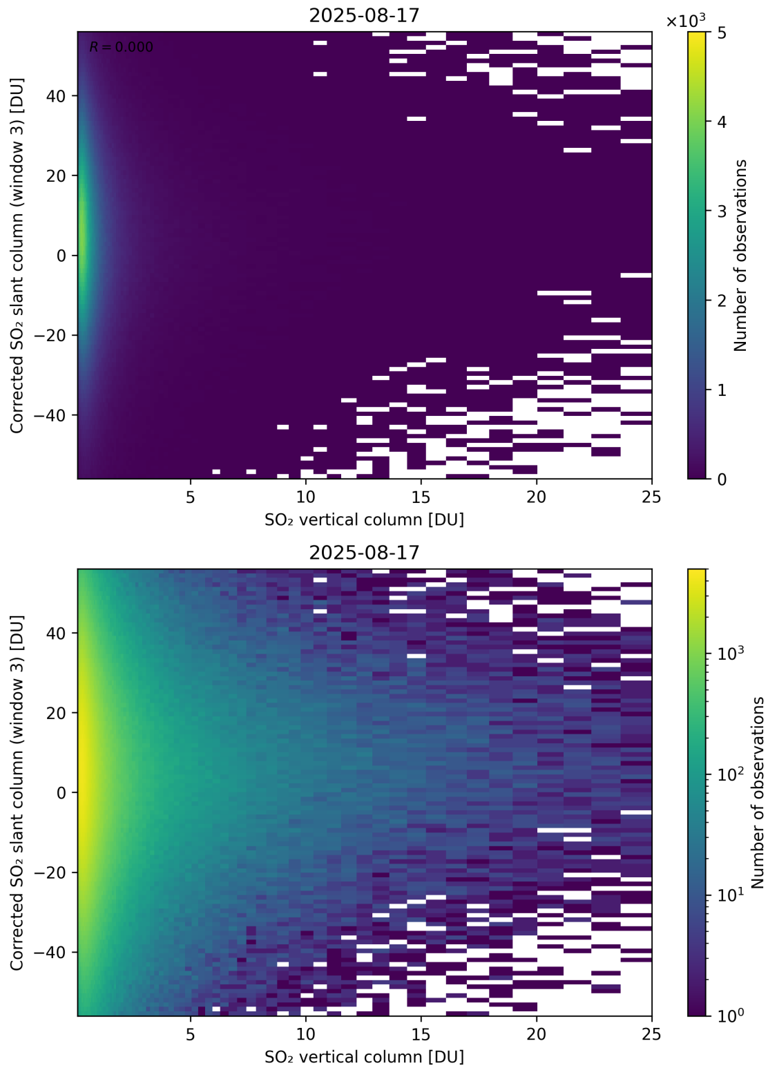
Figure 353: Scatter density plot of “SO 2 vertical column” against “Corrected SO 2 slant column (window 3)” for 2025-08-16 to 2025-08-18.
