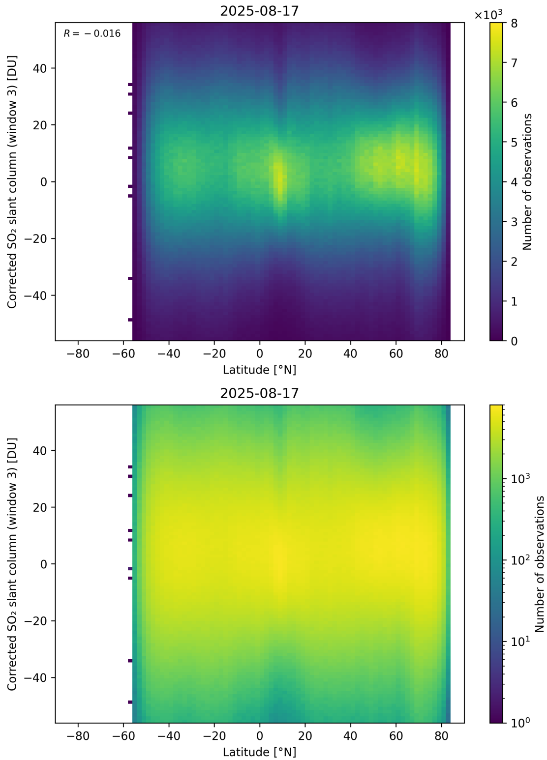
Figure 161: Scatter density plot of “Latitude” against “Corrected SO 2 slant column (window 3)” for 2025-08-16 to 2025-08-18.
