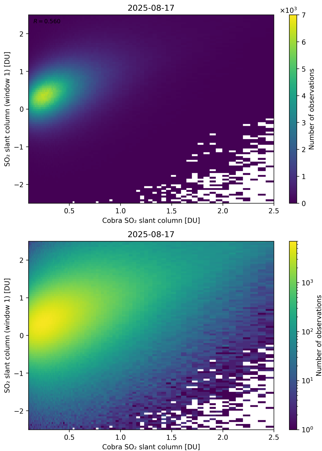
Figure 219: Scatter density plot of “Cobra SO 2 slant column” against “SO 2 slant column (window 1)” for 2025-08-16 to 2025-08-18.
