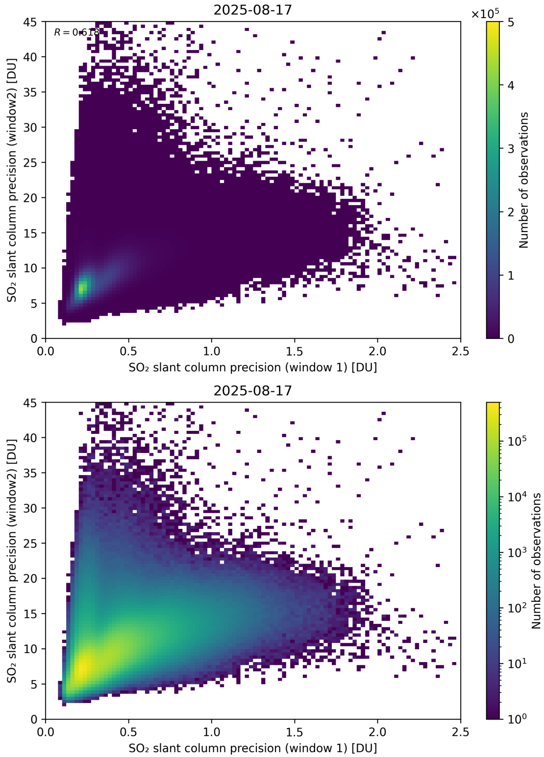
Figure 277: Scatter density plot of “SO 2 slant column precision (window 1)” against “SO 2 slant column precision (window2)” for 2025-08-16 to 2025-08-18.
