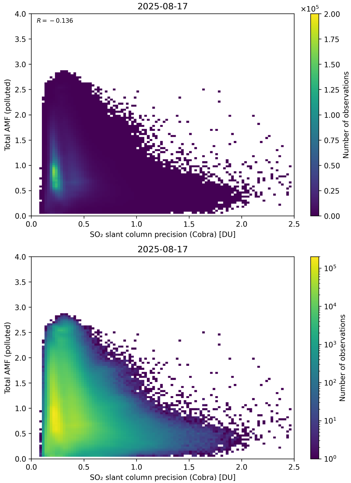
Figure 213: Scatter density plot of “SO 2 slant column precision (Cobra)” against “Total AMF (polluted)” for 2025-08-16 to 2025-08-18.
