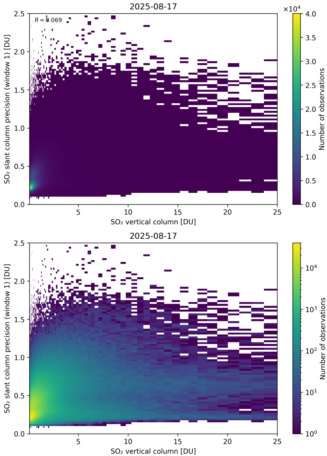
Figure 355: Scatter density plot of “SO 2 vertical column” against “SO 2 slant column precision (window 1)” for 2025-08-16 to 2025-08-18.
