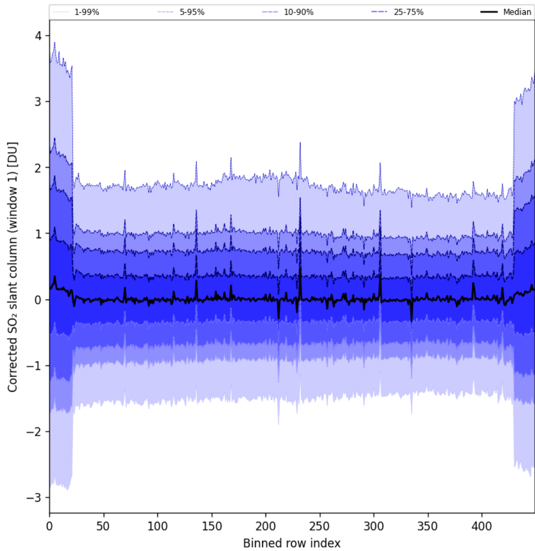
Figure 91: Along track statistics of “Corrected SO 2 slant column (window 1)” for 2025-08-16 to 2025-08-18
