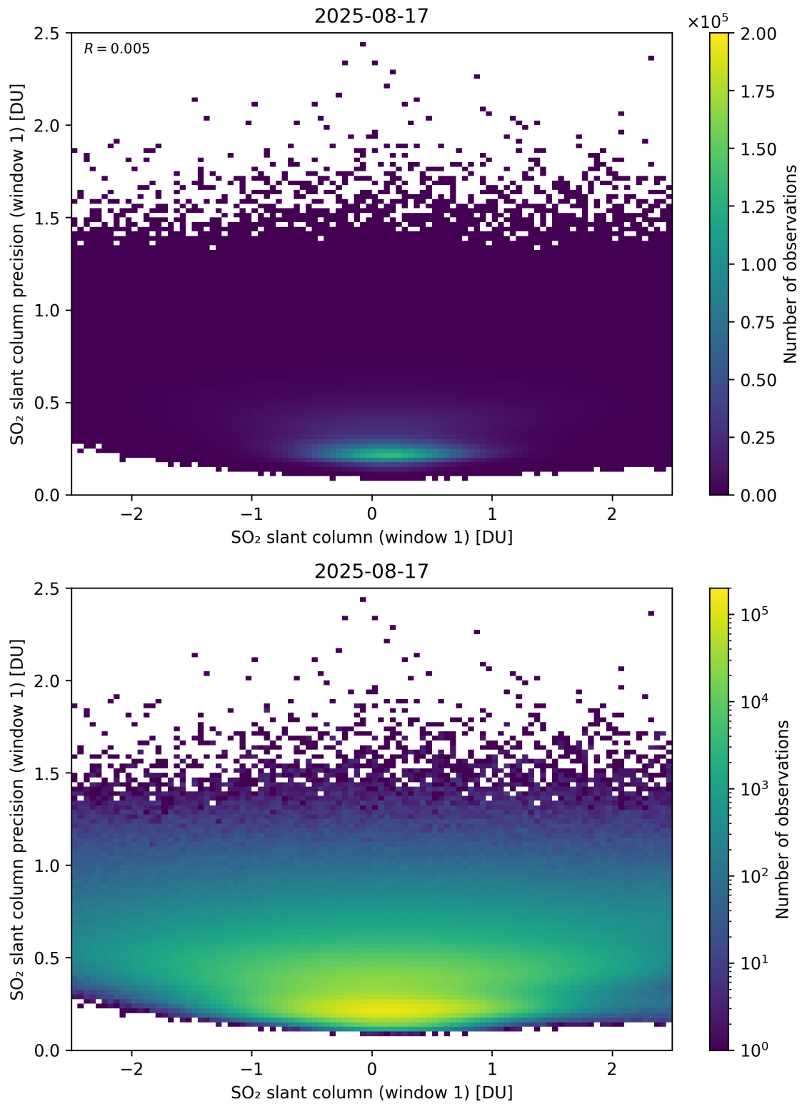
Figure 285: Scatter density plot of “SO 2 slant column (window 1)” against “SO 2 slant column precision (window 1)” for 2025-08-16 to 2025-08-18.
