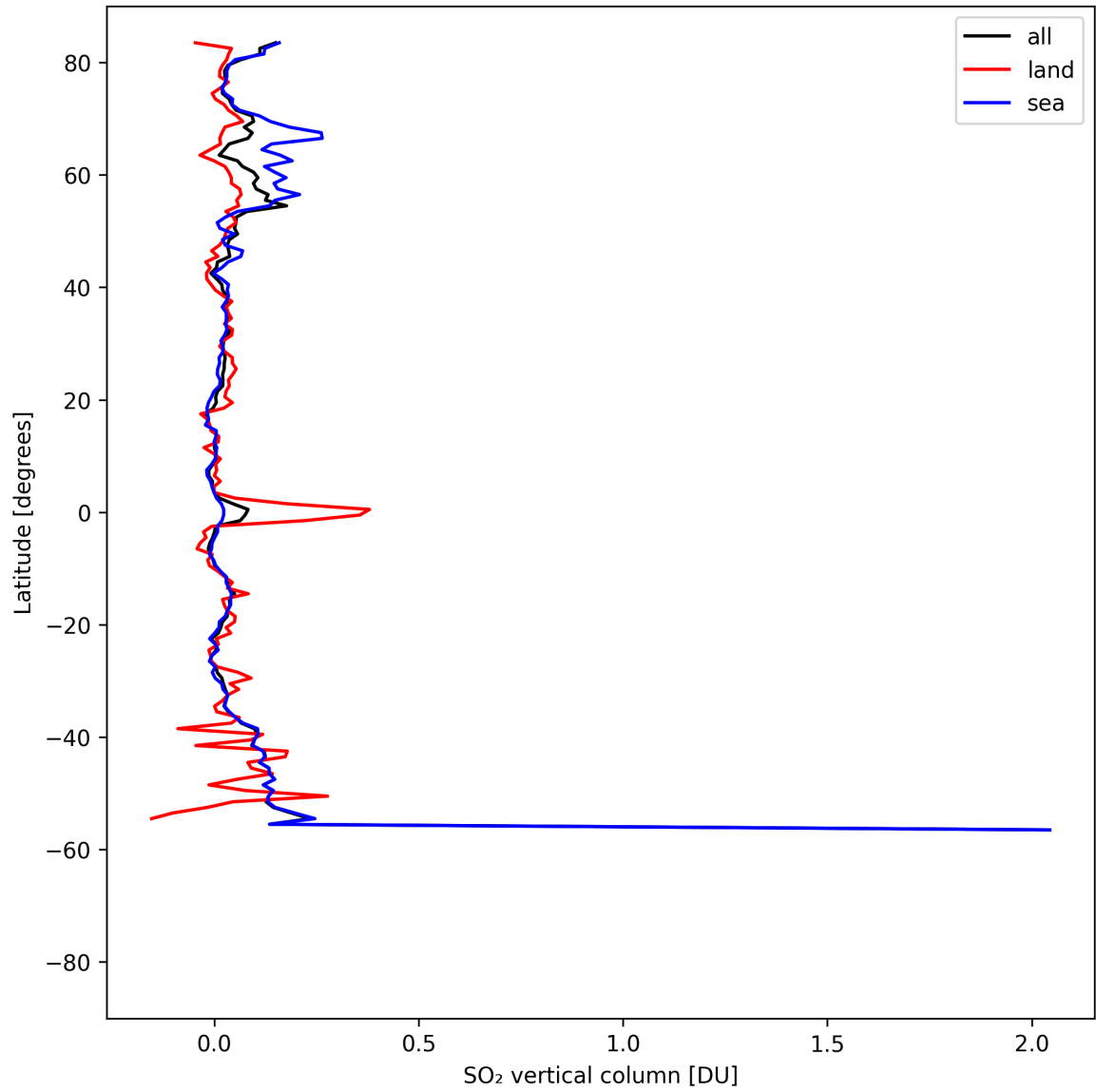
Figure 32: Zonal average of “SO 2 vertical column” for 2025-08-16 to 2025-08-18.
