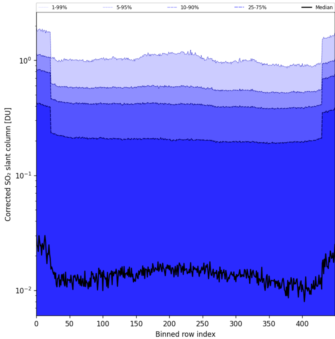
Figure 86: Along track statistics of “Corrected SO 2 slant column” for 2025-08-16 to 2025-08-18
