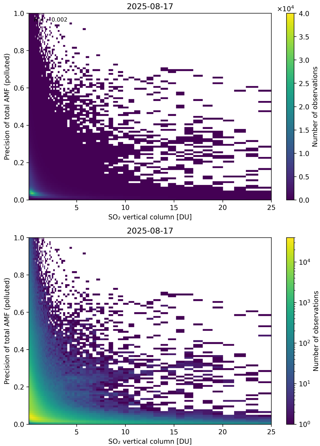
Figure 360: Scatter density plot of “SO 2 vertical column” against “Precision of total AMF (polluted)” for 2025-08-16 to 2025-08-18.
