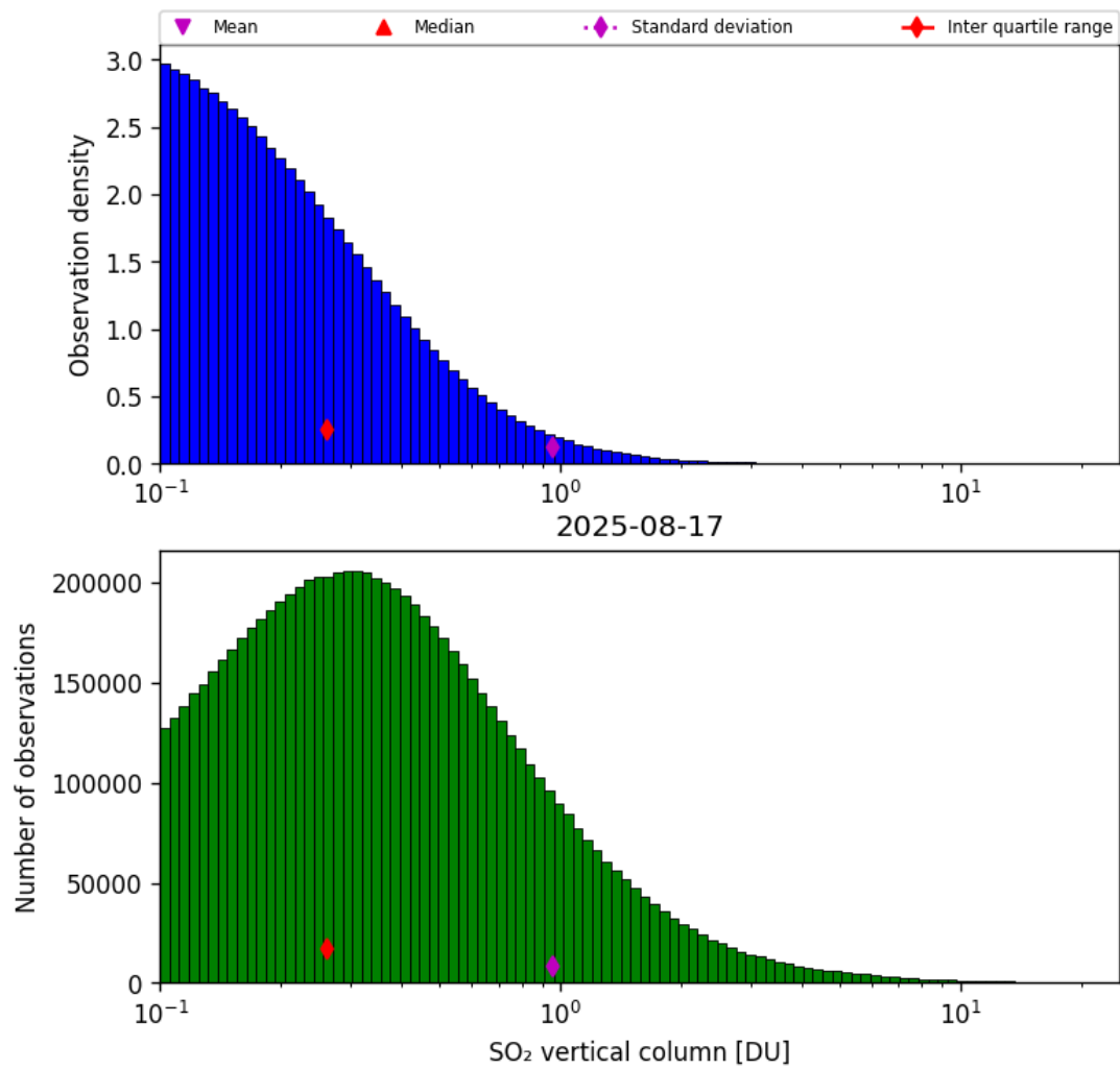
Figure 58: Histogram of “SO 2 vertical column” for 2025-08-16 to 2025-08-18
