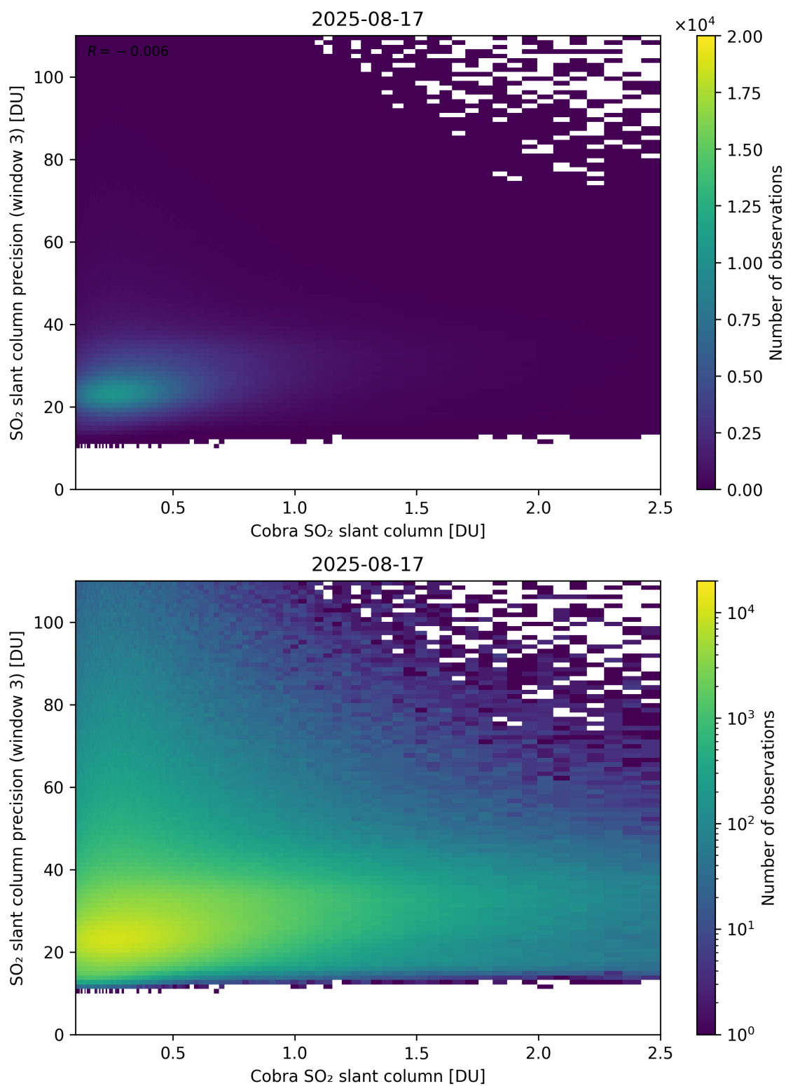
Figure 223: Scatter density plot of “Cobra SO 2 slant column” against “SO 2 slant column precision (window 3)” for 2025-08-16 to 2025-08-18.
