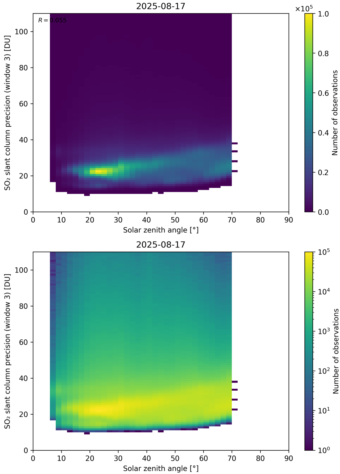
Figure 188: Scatter density plot of “Solar zenith angle” against “SO 2 slant column precision (window 3)” for 2025-08-16 to 2025-08-18.
