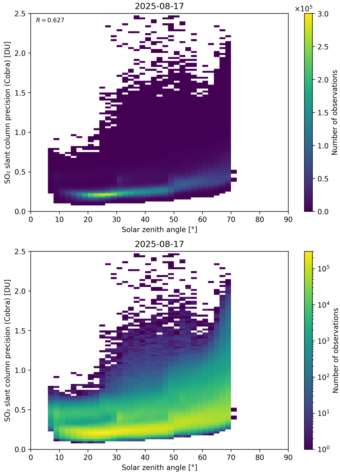
Figure 180: Scatter density plot of “Solar zenith angle” against “SO 2 slant column precision (Cobra)” for 2025-08-16 to 2025-08-18.
