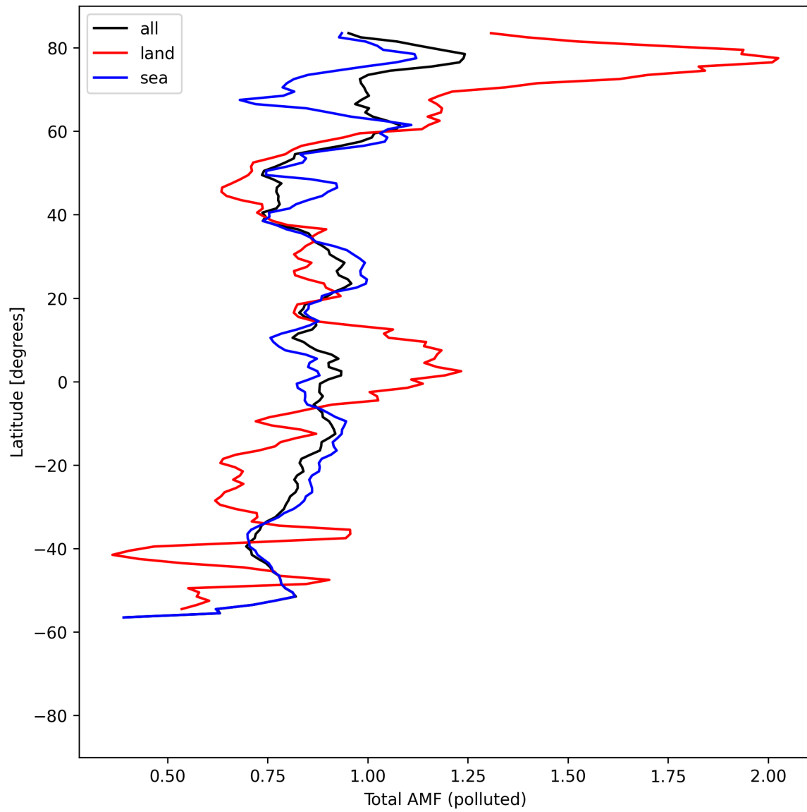
Figure 53: Zonal average of “Total AMF (polluted)” for 2025-08-16 to 2025-08-18.
