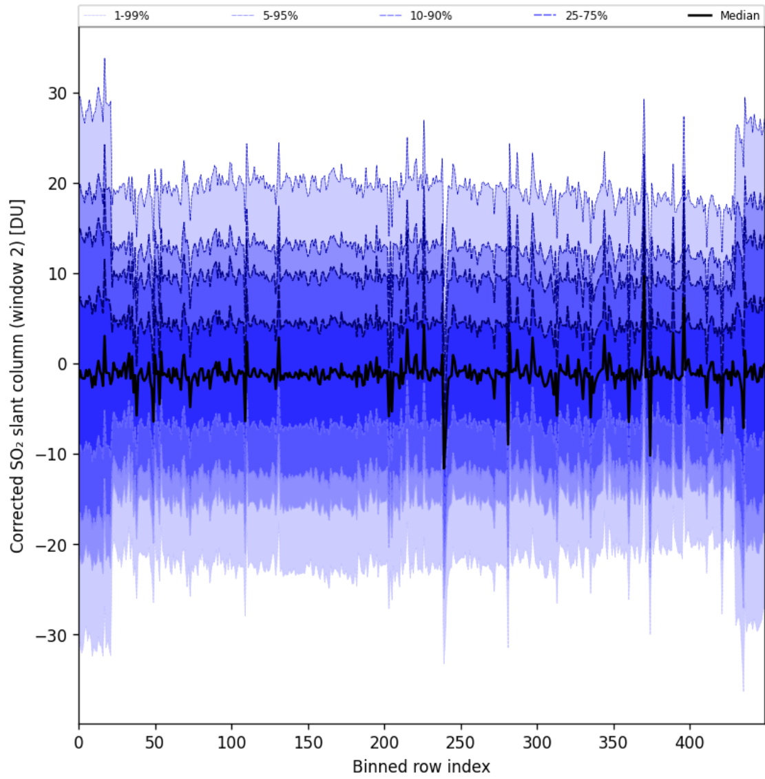
Figure 95: Along track statistics of “Corrected SO 2 slant column (window 2)” for 2025-08-16 to 2025-08-18
