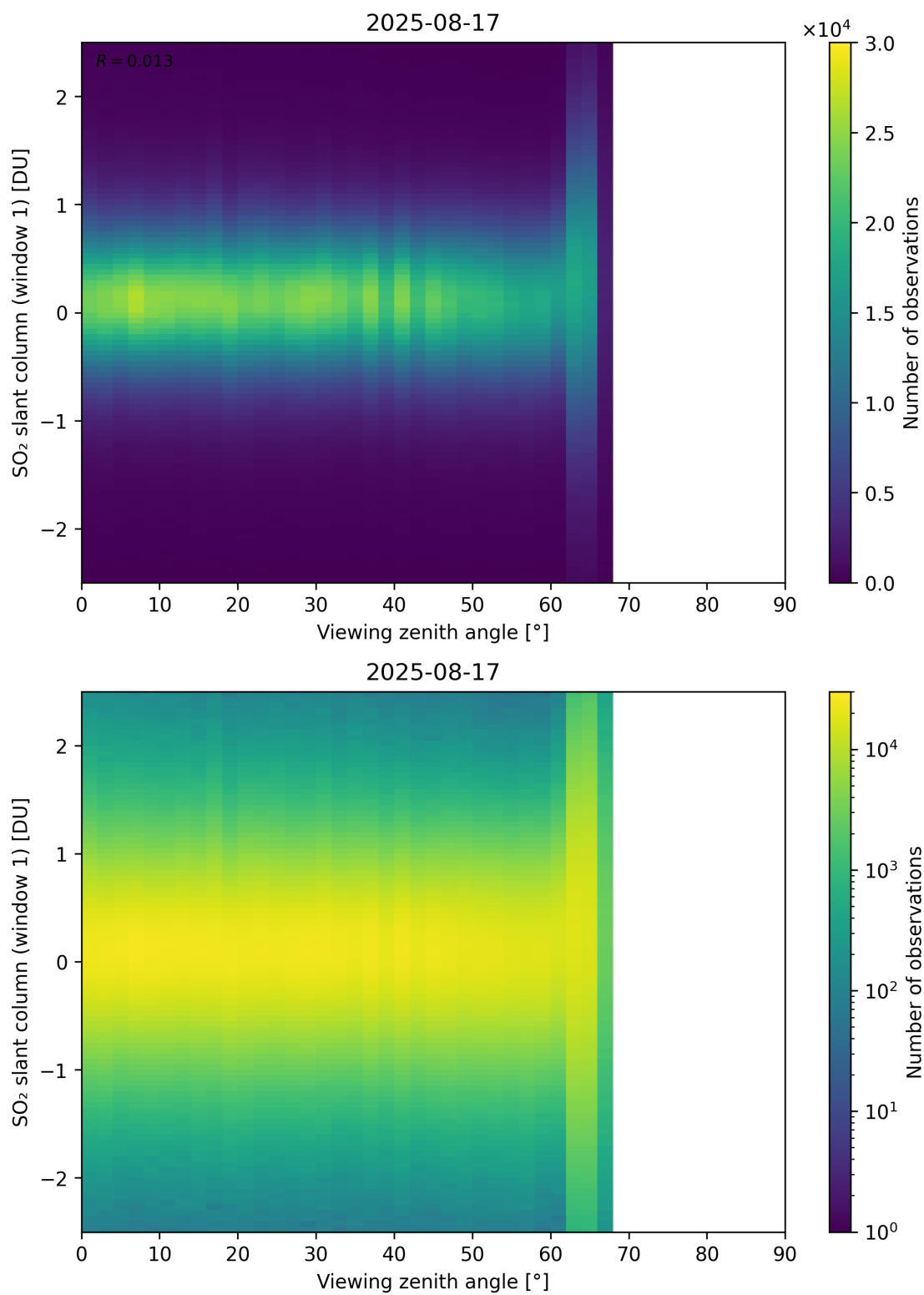
Figure 376: Scatter density plot of “Viewing zenith angle” against “SO 2 slant column (window 1)” for 2025-08-16 to 2025-08-18.
