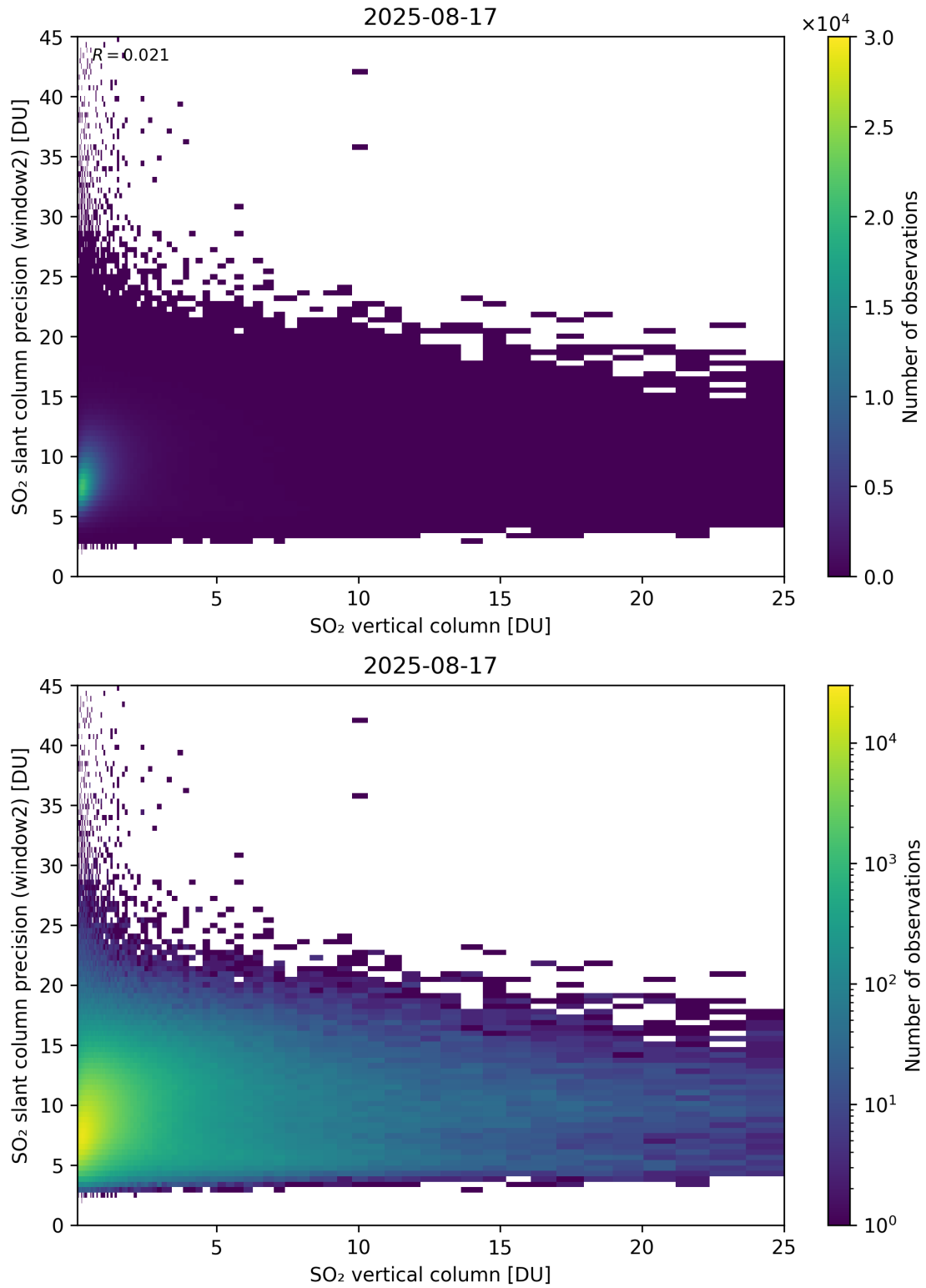
Figure 356: Scatter density plot of “SO 2 vertical column” against “SO 2 slant column precision (window2)” for 2025-08-16 to 2025-08-18.
