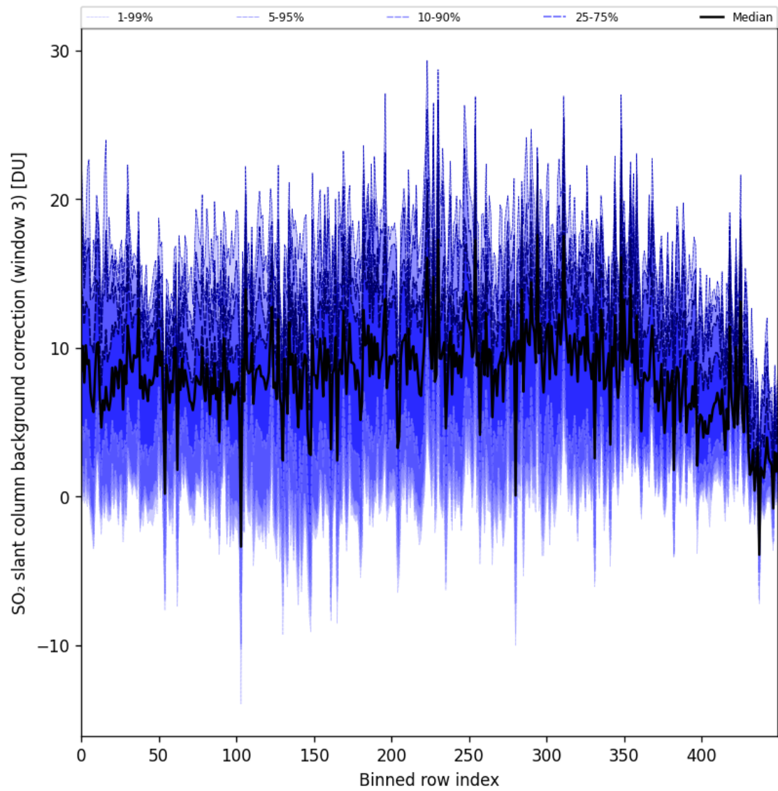
Figure 100: Along track statistics of “SO 2 slant column background correction (window 3)” for 2025-08-16 to 2025-08-18
