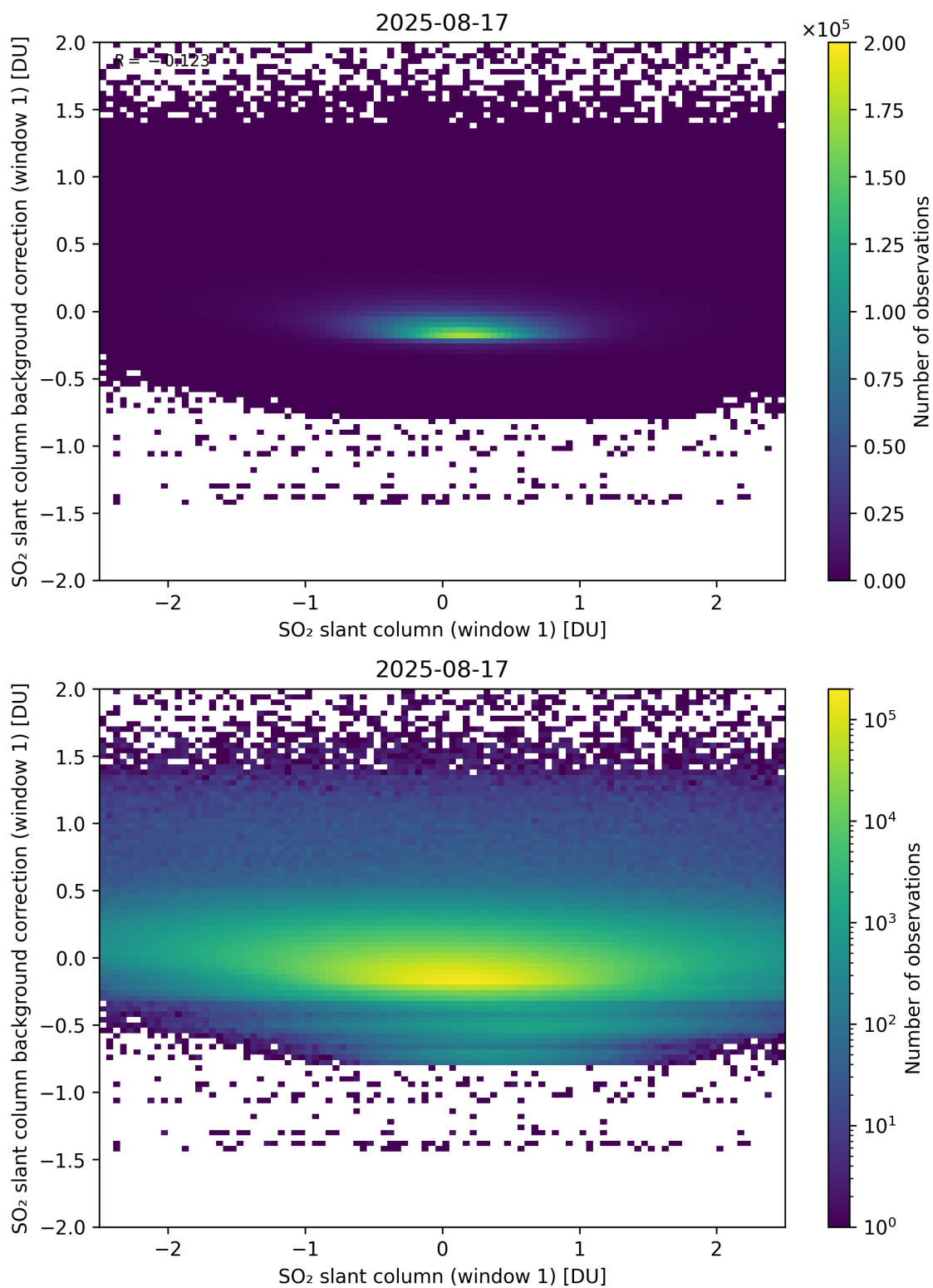
Figure 262: Scatter density plot of “SO 2 slant column (window 1)” against “SO 2 slant column background correction (window 1)” for 2025-08-16 to 2025-08-18.
