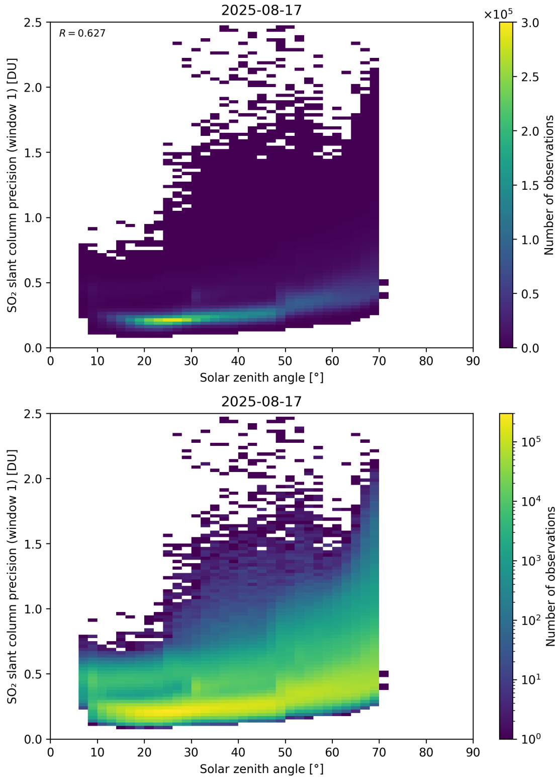
Figure 185: Scatter density plot of “Solar zenith angle” against “SO 2 slant column precision (window 1)” for 2025-08-16 to 2025-08-18.
