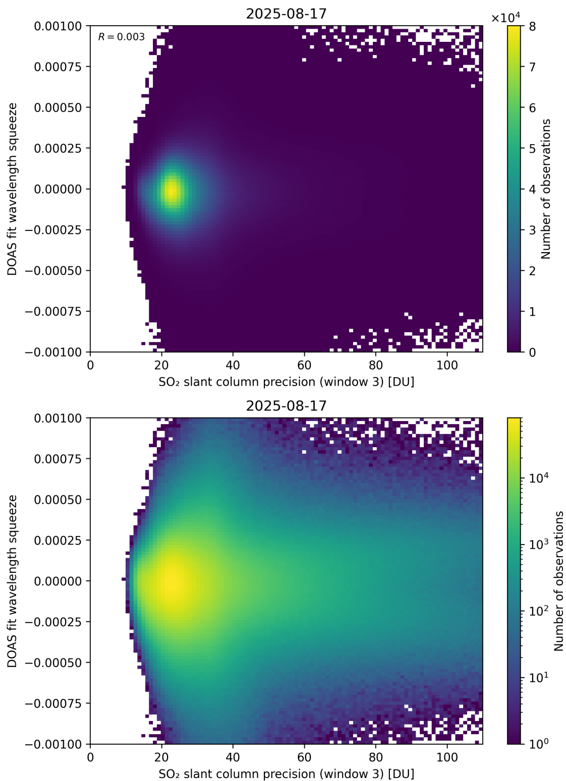
Figure 309: Scatter density plot of “SO 2 slant column precision (window 3)” against “DOAS fit wavelength squeeze” for 2025-08-16 to 2025-08-18.
