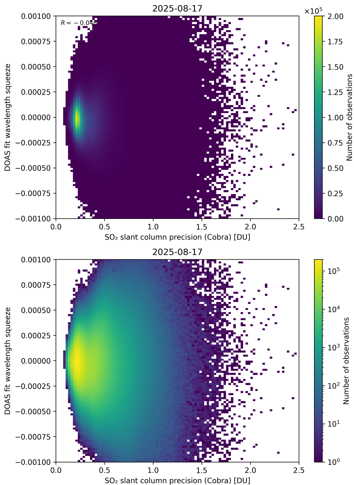
Figure 203: Scatter density plot of “SO 2 slant column precision (Cobra)” against “DOAS fit wavelength squeeze” for 2025-08-16 to 2025-08-18.
