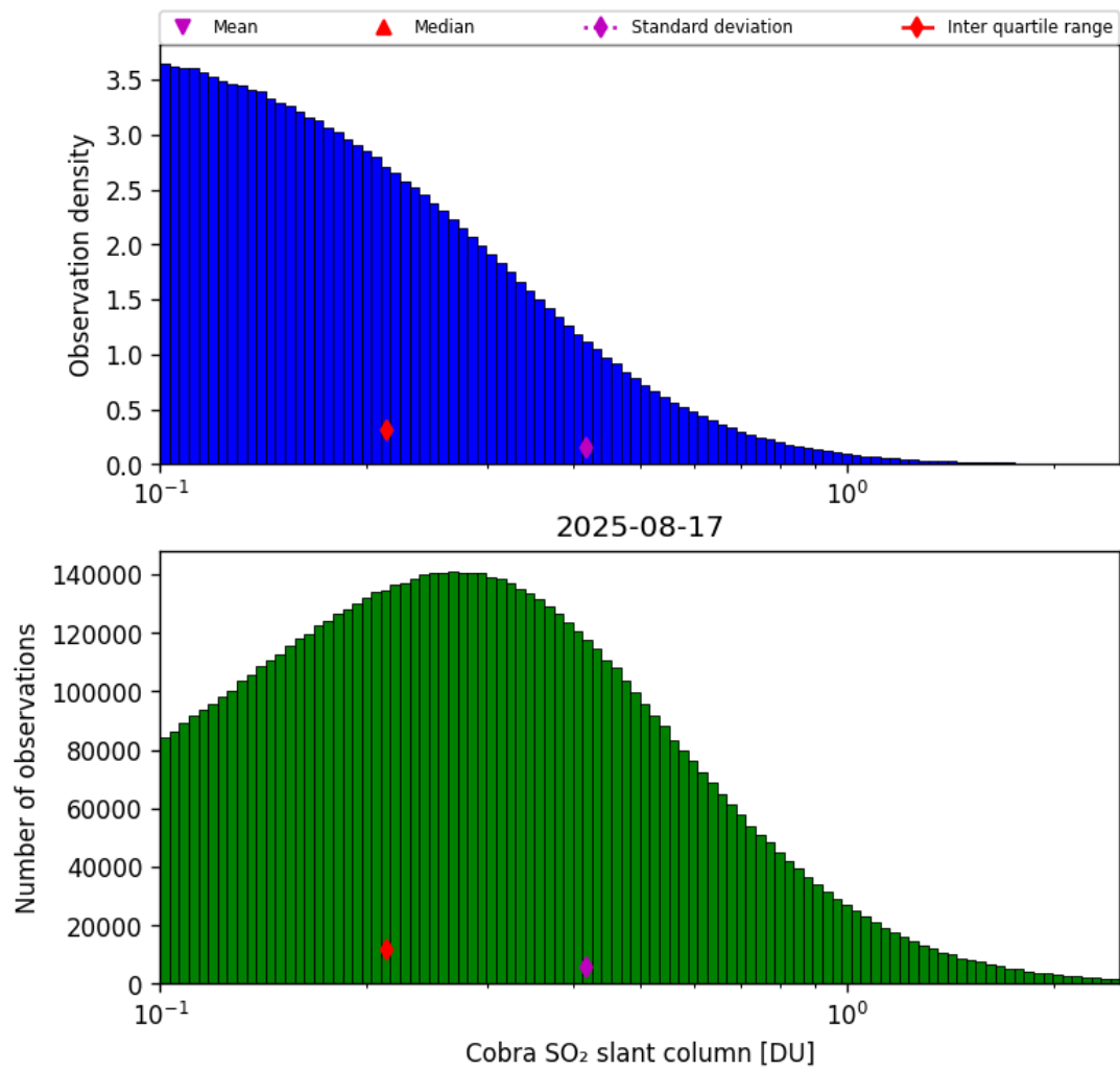
Figure 61: Histogram of “Cobra SO 2 slant column” for 2025-08-16 to 2025-08-18
