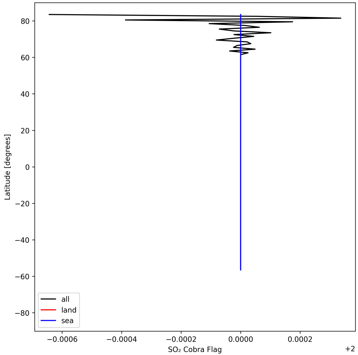
Figure 49: Zonal average of “SO 2 Cobra Flag” for 2025-08-16 to 2025-08-18.
