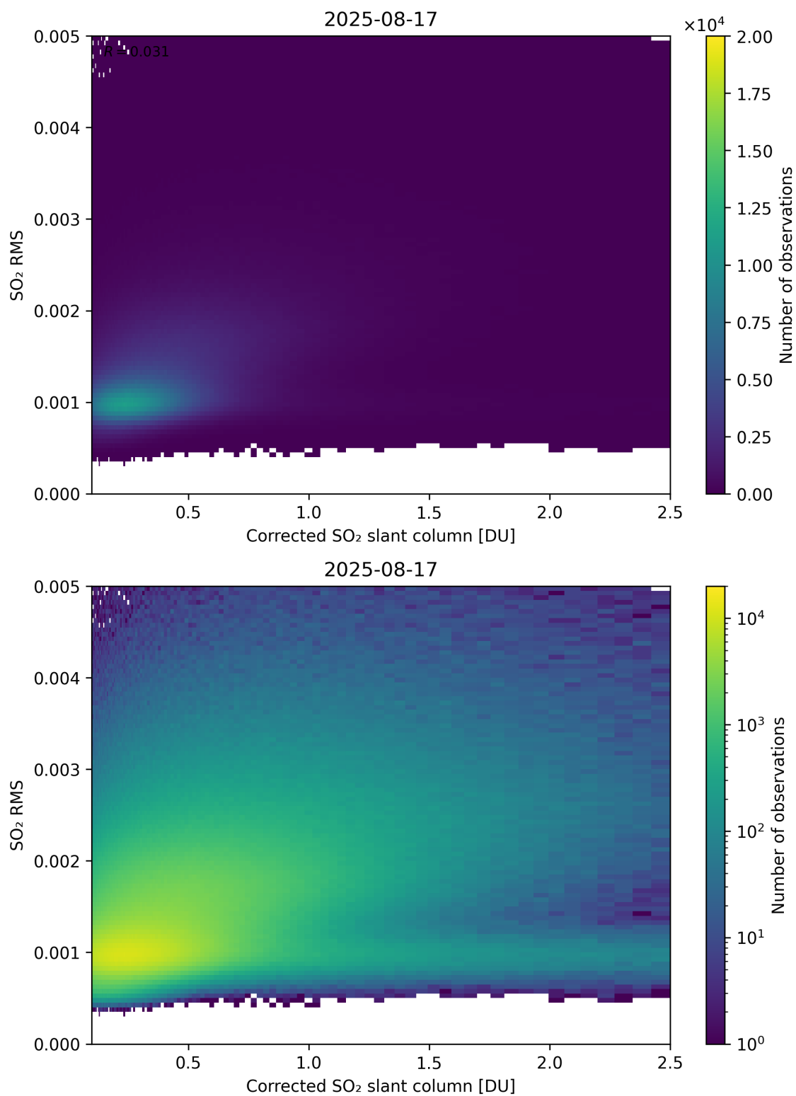
Figure 231: Scatter density plot of “Corrected SO 2 slant column” against “SO 2 RMS” for 2025-08-16 to 2025-08-18.
