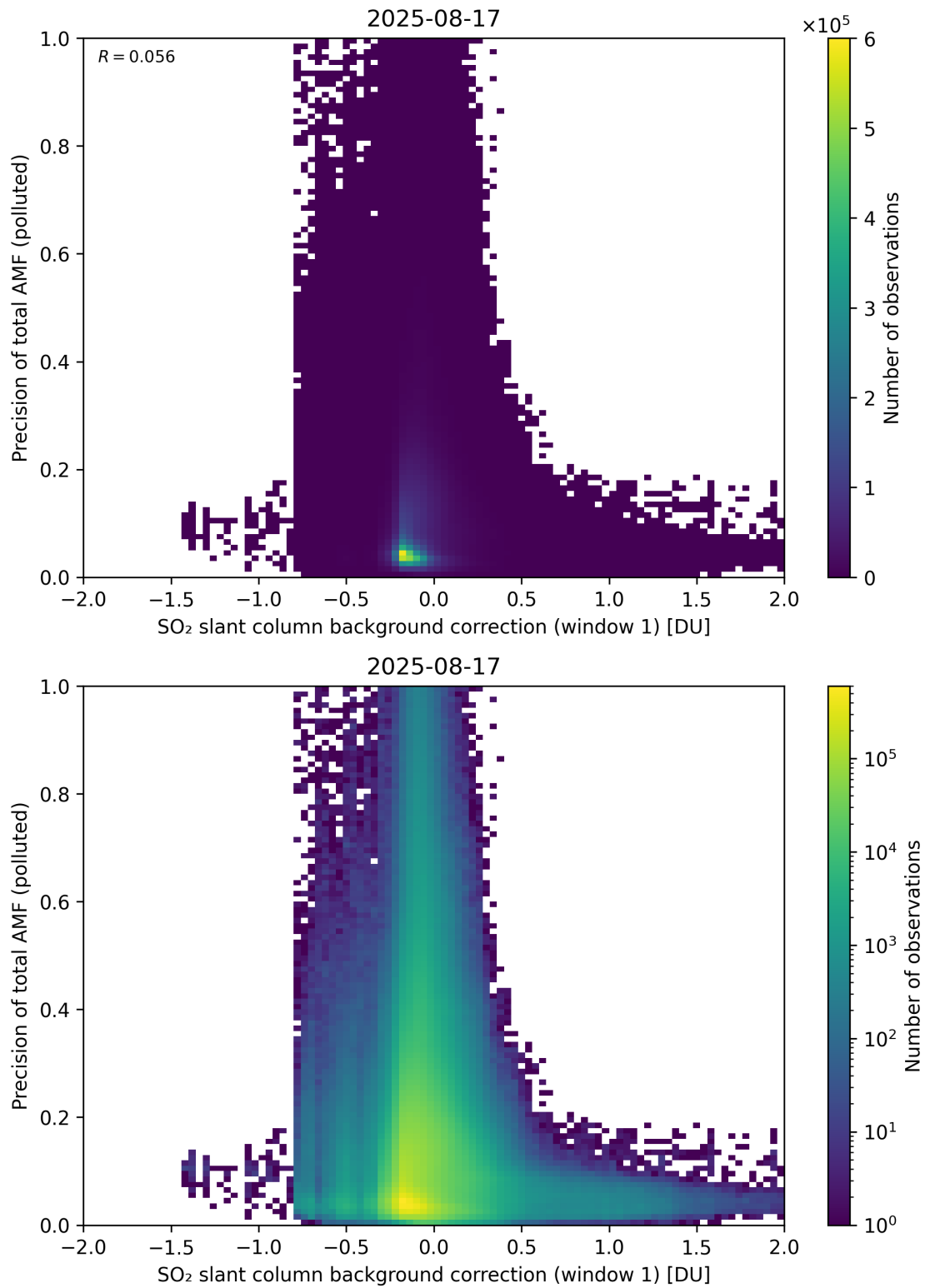
Figure 121: Scatter density plot of “SO 2 slant column background correction (window 1)” against “Precision of total AMF (polluted)” for 2025-08-16 to 2025-08-18.
