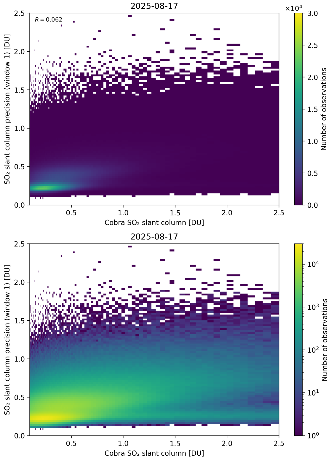
Figure 220: Scatter density plot of “Cobra SO 2 slant column” against “SO 2 slant column precision (window 1)” for 2025-08-16 to 2025-08-18.
