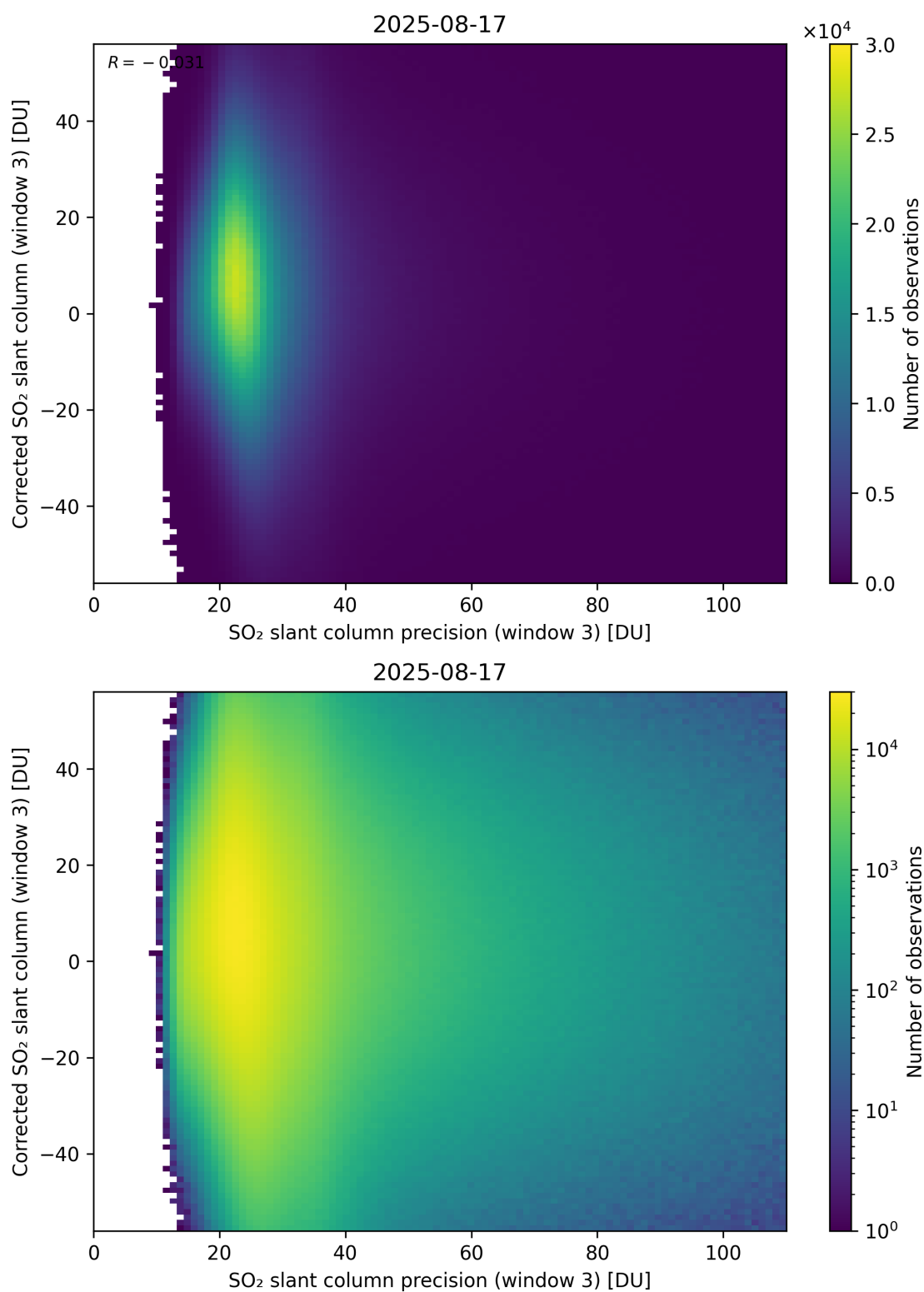
Figure 312: Scatter density plot of “SO 2 slant column precision (window 3)” against “Corrected SO 2 slant column (window 3)” for 2025-08-16 to 2025-08-18.
