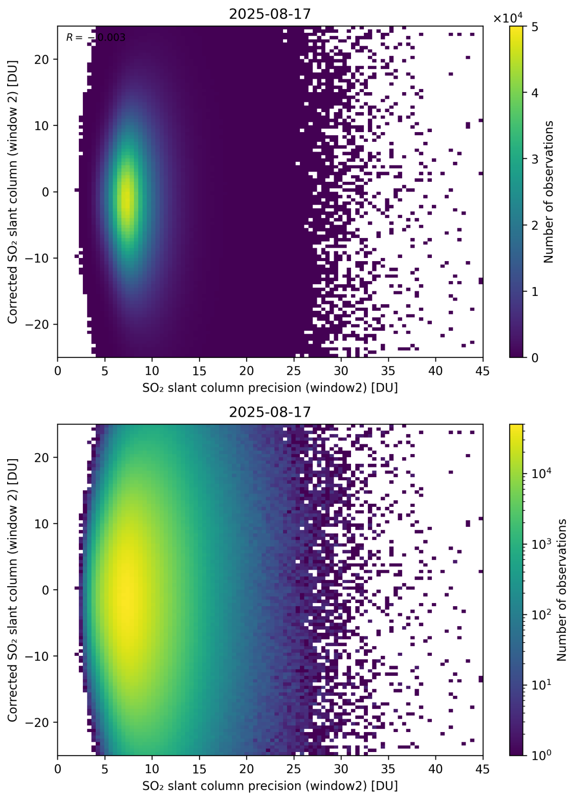
Figure 297: Scatter density plot of “SO 2 slant column precision (window2)” against “Corrected SO 2 slant column (window 2)” for 2025-08-16 to 2025-08-18.
