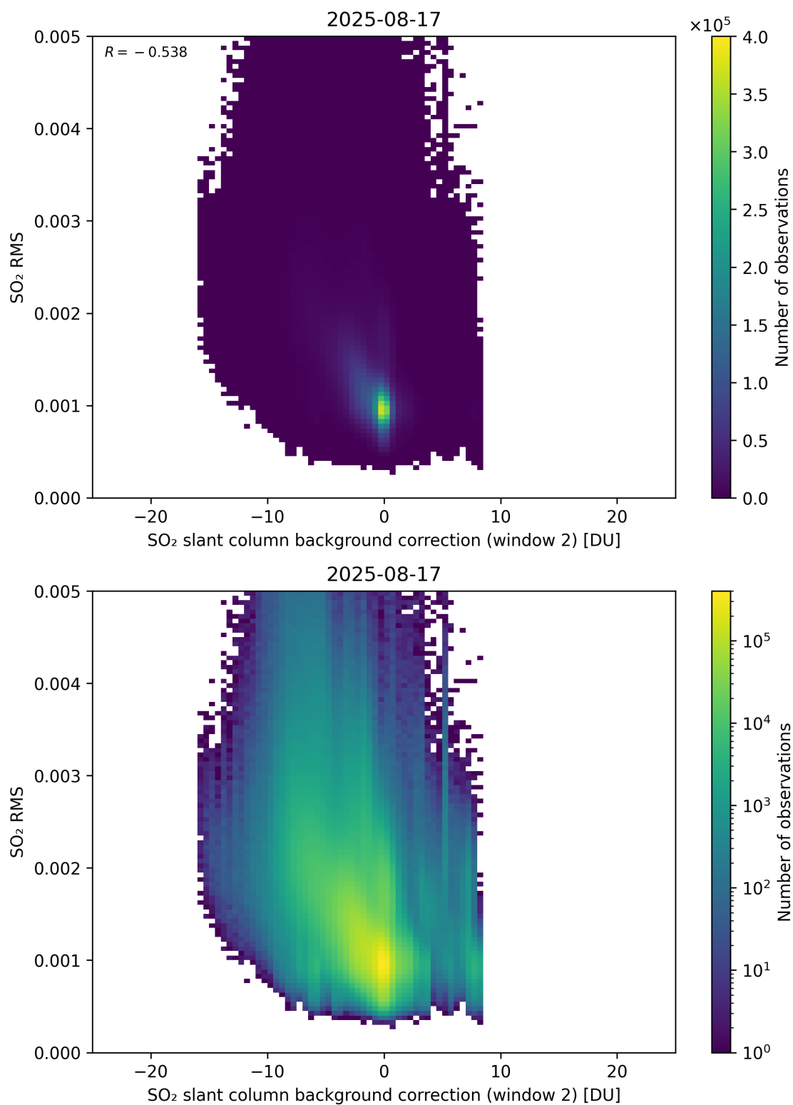
Figure 125: Scatter density plot of “SO 2 slant column background correction (window 2)” against “SO 2 RMS” for 2025-08-16 to 2025-08-18.
