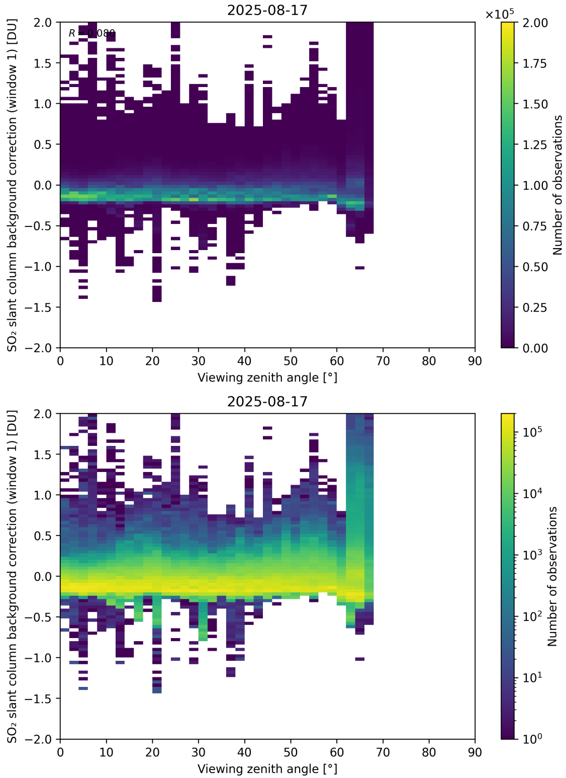
Figure 362: Scatter density plot of “Viewing zenith angle” against “SO 2 slant column background correction (window 1)” for 2025-08-16 to 2025-08-18.
