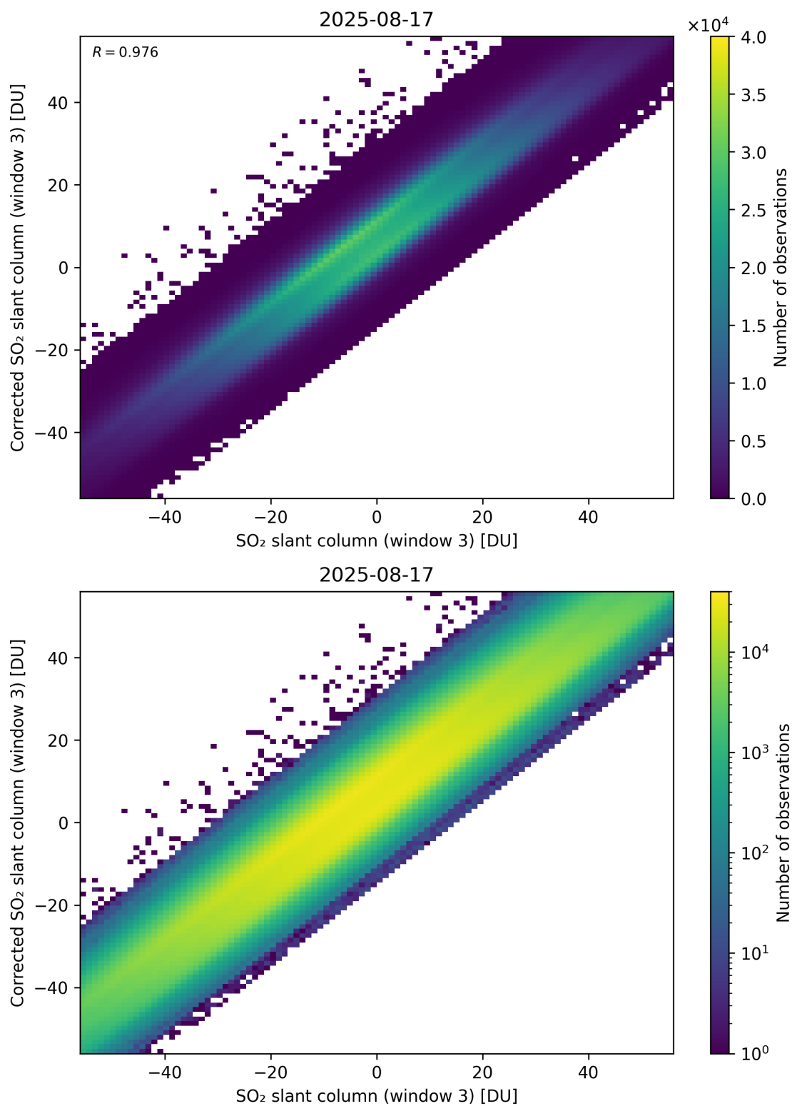
Figure 316: Scatter density plot of “SO 2 slant column (window 3)” against “Corrected SO 2 slant column (window 3)” for 2025-08-16 to 2025-08-18.
