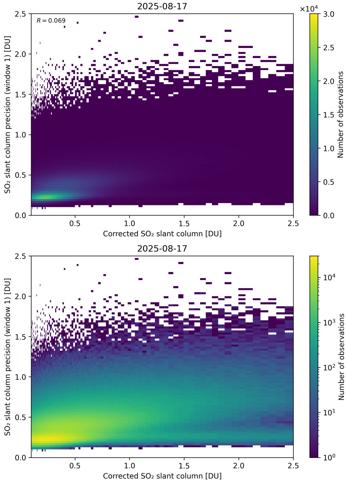
Figure 238: Scatter density plot of “Corrected SO 2 slant column” against “SO 2 slant column precision (window 1)” for 2025-08-16 to 2025-08-18.
