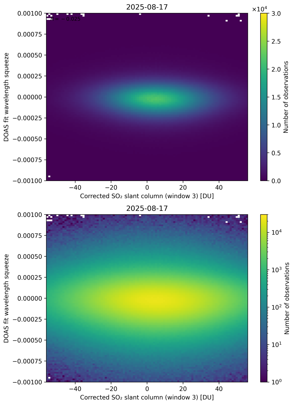
Figure 257: Scatter density plot of “Corrected SO 2 slant column (window 3)” against “DOAS fit wavelength squeeze” for 2025-08-16 to 2025-08-18.
