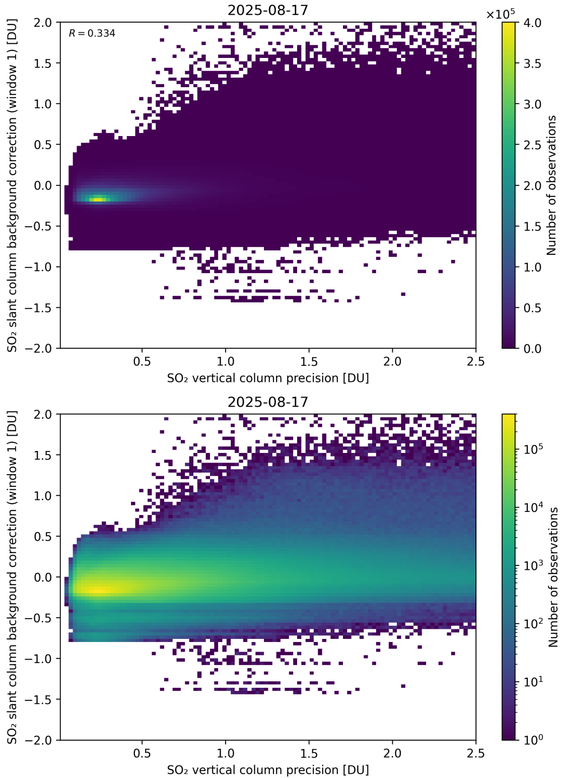
Figure 329: Scatter density plot of “SO 2 vertical column precision” against “SO 2 slant column background correction (window 1)” for 2025-08-16 to 2025-08-18.
