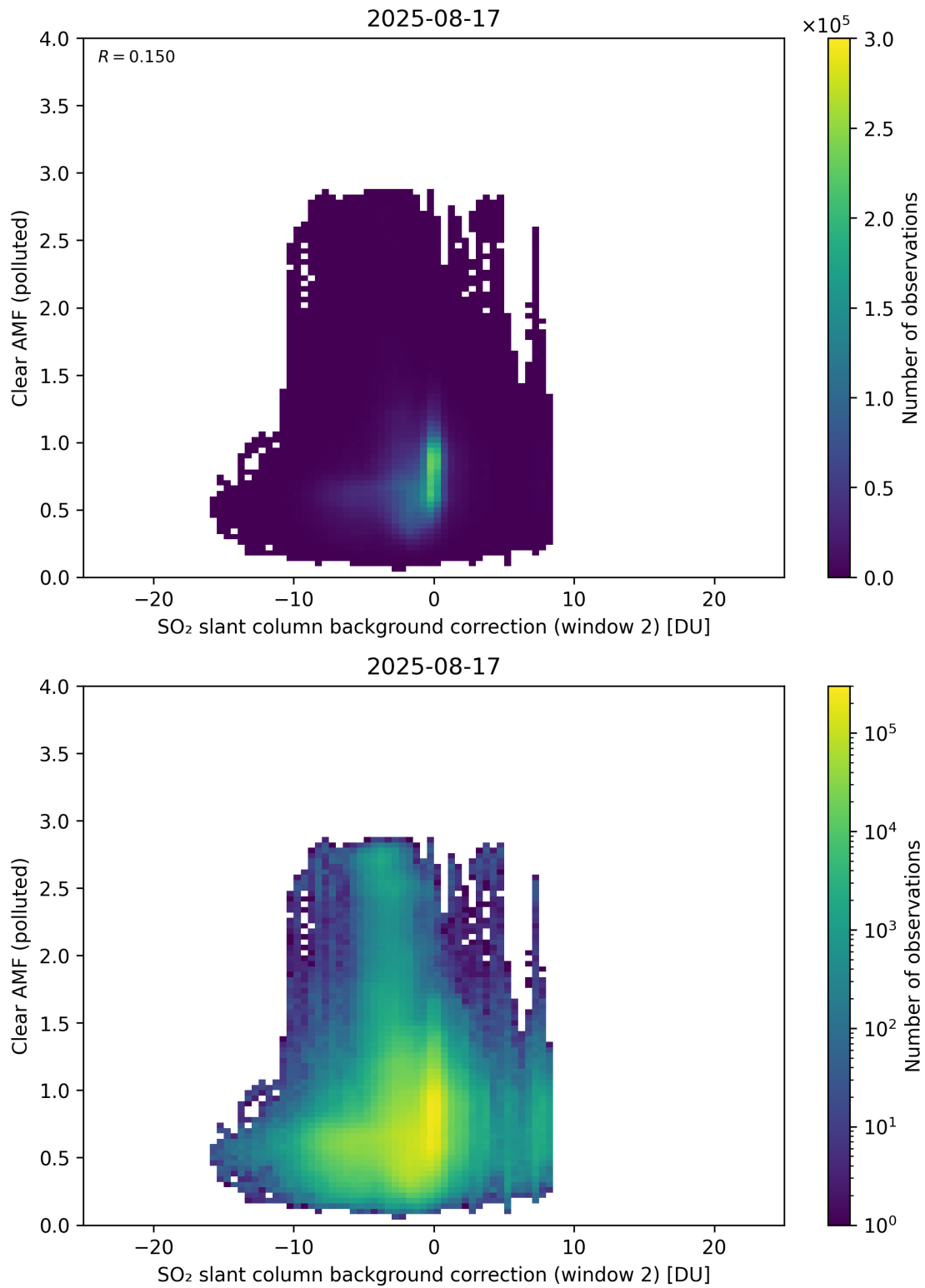
Figure 126: Scatter density plot of “SO 2 slant column background correction (window 2)” against “Clear AMF (polluted)” for 2025-08-16 to 2025-08-18.
