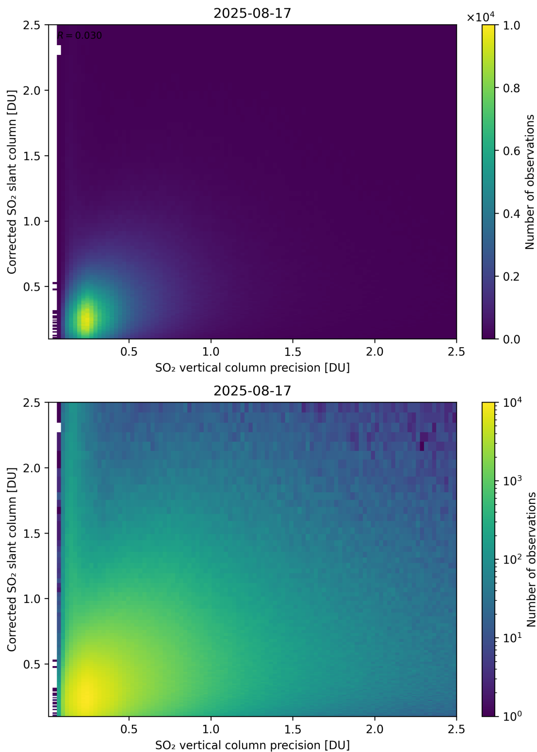
Figure 338: Scatter density plot of “SO 2 vertical column precision” against “Corrected SO 2 slant column” for 2025-08-16 to 2025-08-18.
