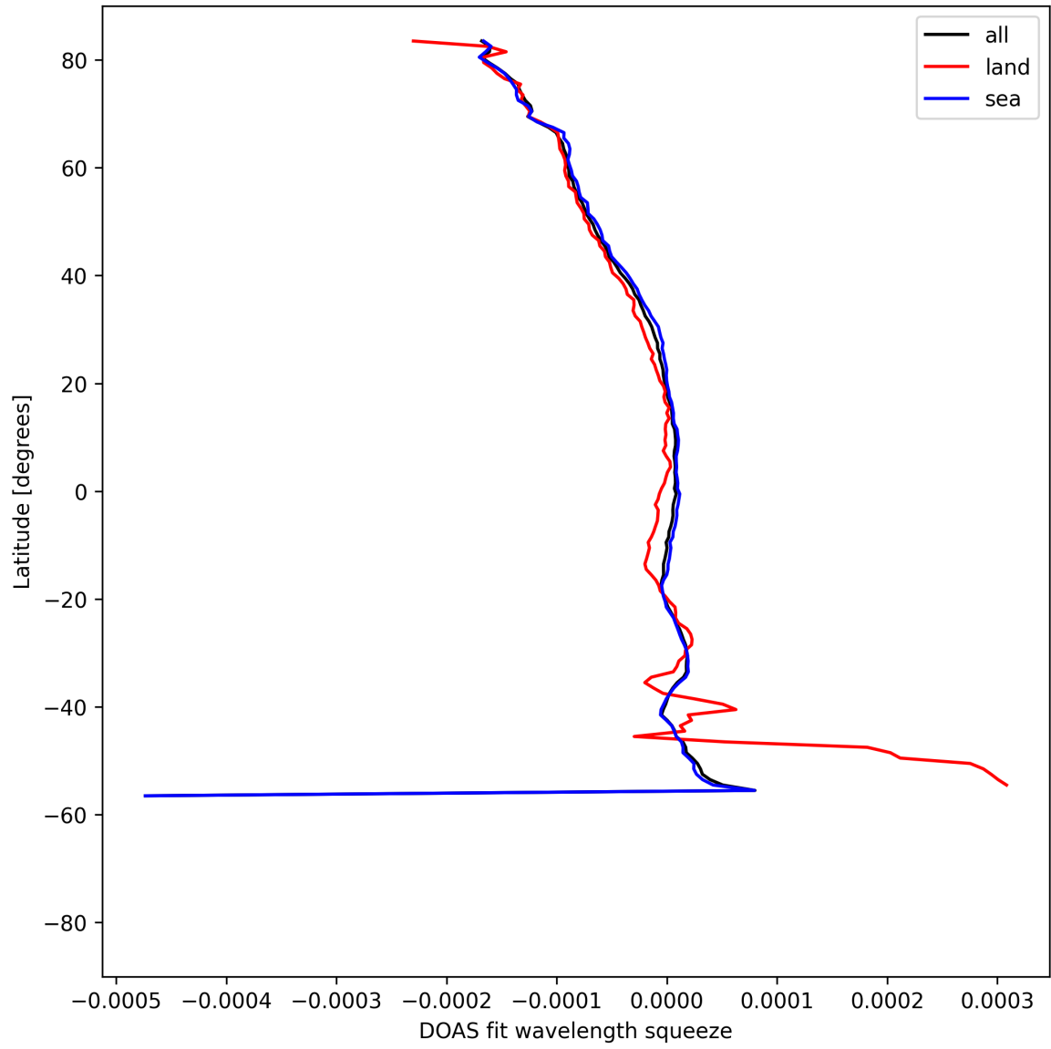
Figure 51: Zonal average of “DOAS fit wavelength squeeze” for 2025-08-16 to 2025-08-18.
