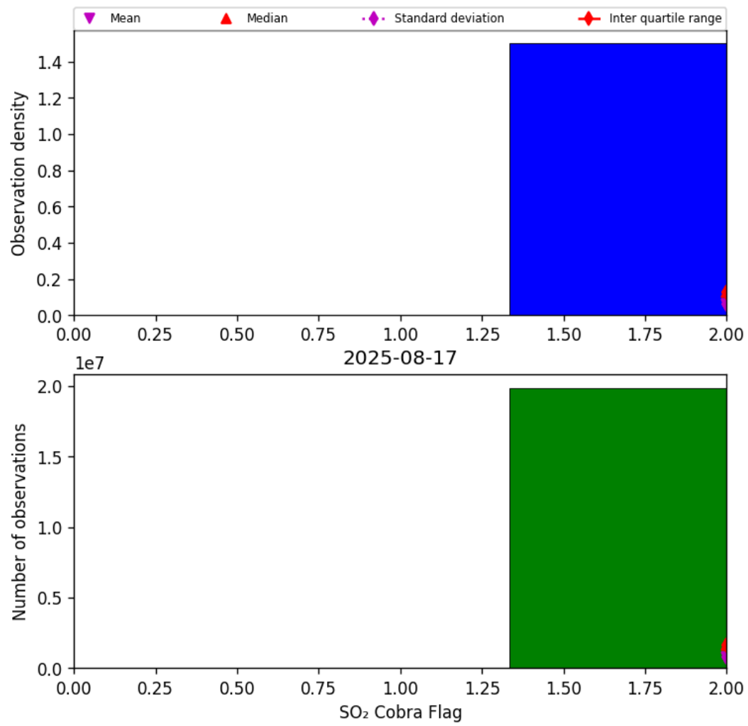
Figure 75: Histogram of “SO 2 Cobra Flag” for 2025-08-16 to 2025-08-18
