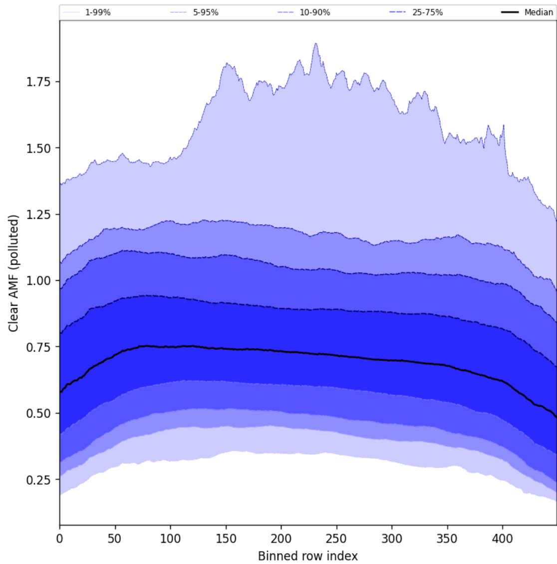
Figure 107: Along track statistics of “Clear AMF (polluted)” for 2025-08-16 to 2025-08-18
