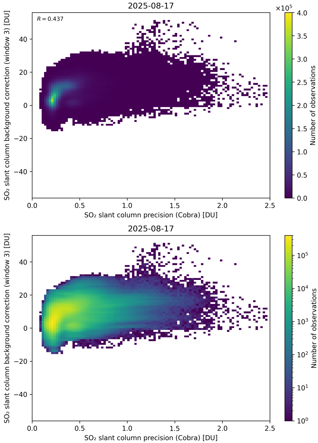
Figure 201: Scatter density plot of “SO 2 slant column precision (Cobra)” against “SO 2 slant column background correction (window 3)” for 2025-08-16 to 2025-08-18.
