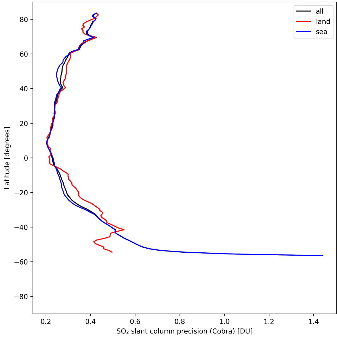
Figure 36: Zonal average of “SO 2 slant column precision (Cobra)” for 2025-08-16 to 2025-08-18.
