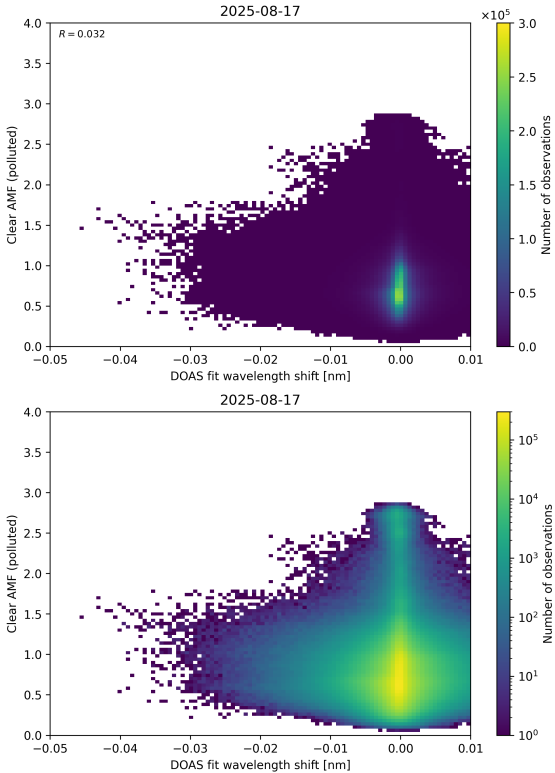
Figure 140: Scatter density plot of “DOAS fit wavelength shift” against “Clear AMF (polluted)” for 2025-08-16 to 2025-08-18.
