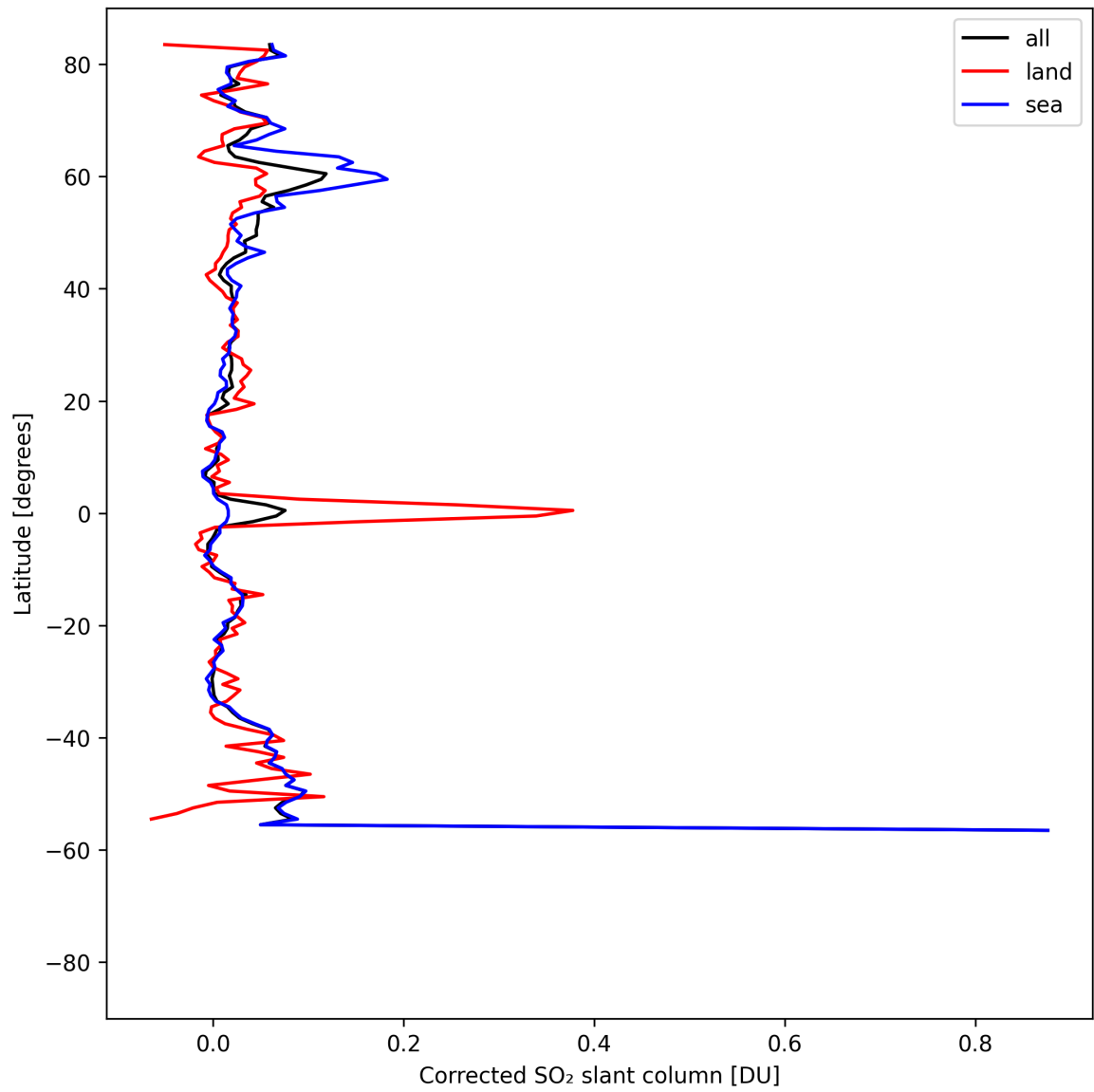
Figure 34: Zonal average of “Corrected SO 2 slant column” for 2025-08-16 to 2025-08-18.
