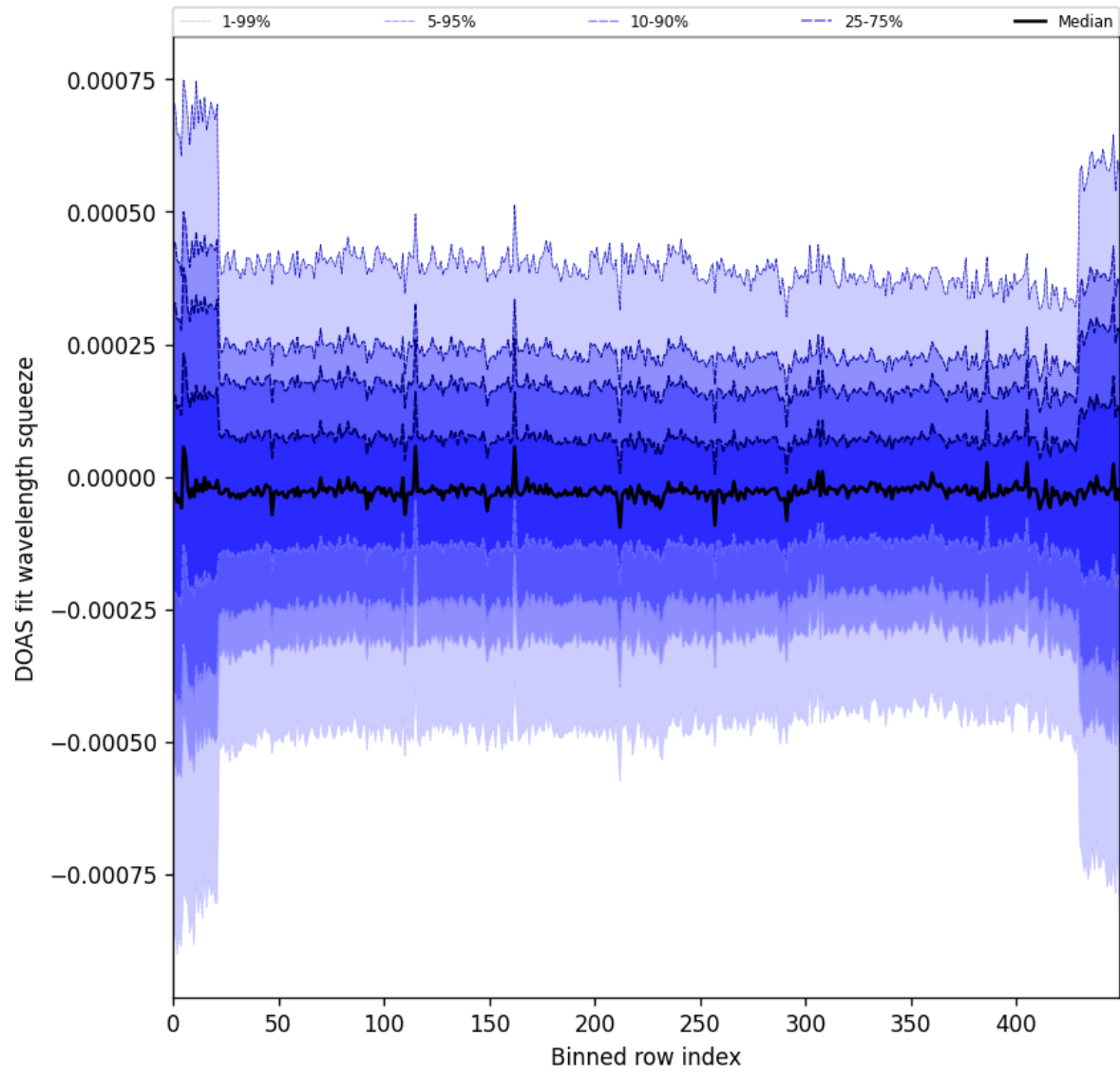
Figure 103: Along track statistics of “DOAS fit wavelength squeeze” for 2025-08-16 to 2025-08-18
