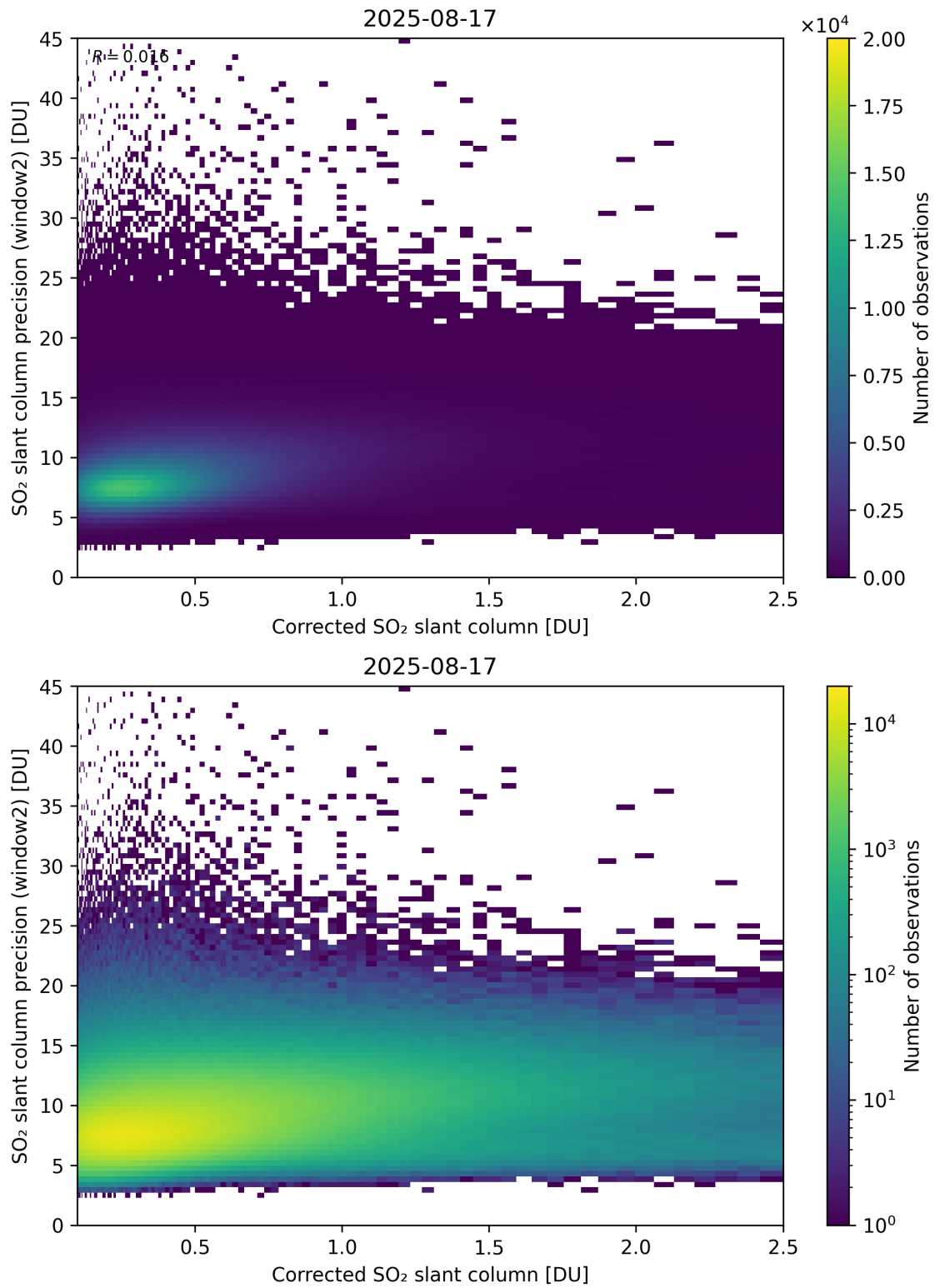
Figure 239: Scatter density plot of “Corrected SO 2 slant column” against “SO 2 slant column precision (window2)” for 2025-08-16 to 2025-08-18.
