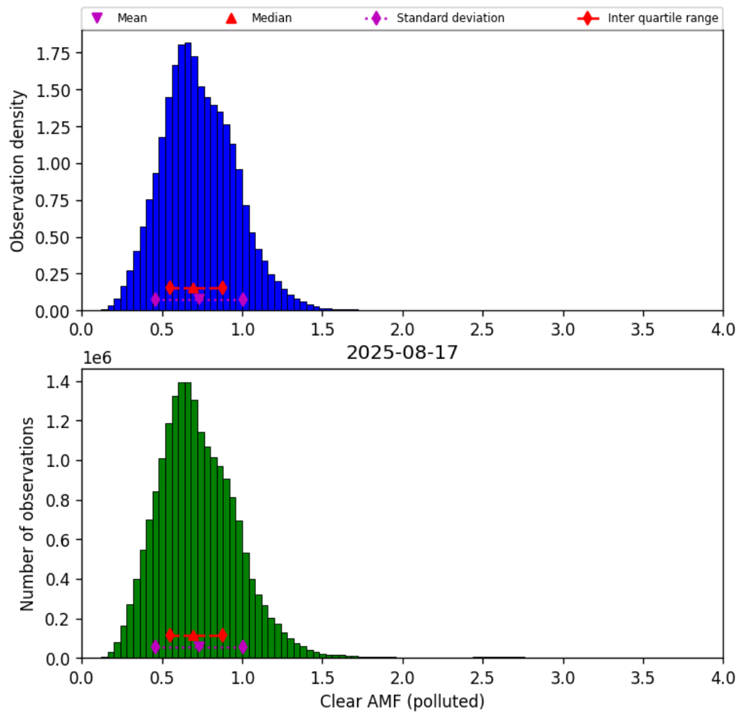
Figure 81: Histogram of “Clear AMF (polluted)” for 2025-08-16 to 2025-08-18
