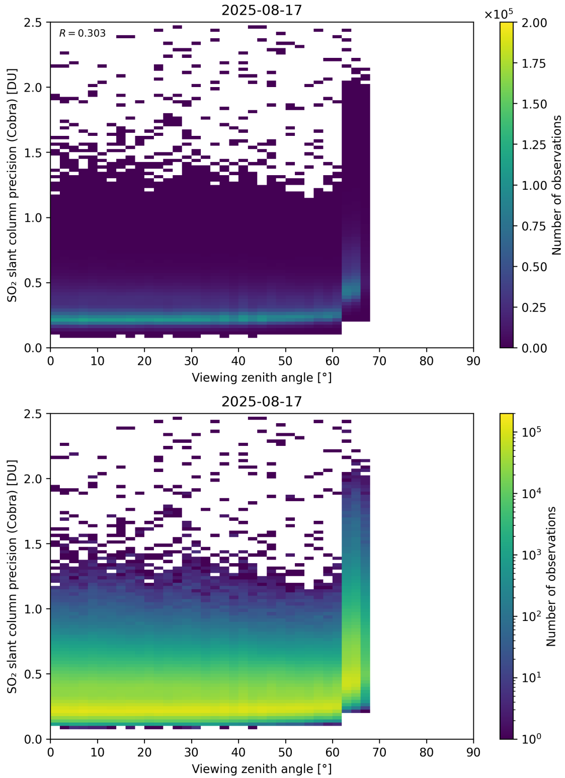
Figure 372: Scatter density plot of “Viewing zenith angle” against “SO 2 slant column precision (Cobra)” for 2025-08-16 to 2025-08-18.
