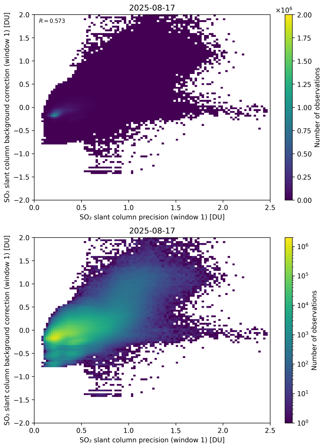
Figure 268: Scatter density plot of “SO 2 slant column precision (window 1)” against “SO 2 slant column background correction (window 1)” for 2025-08-16 to 2025-08-18.
