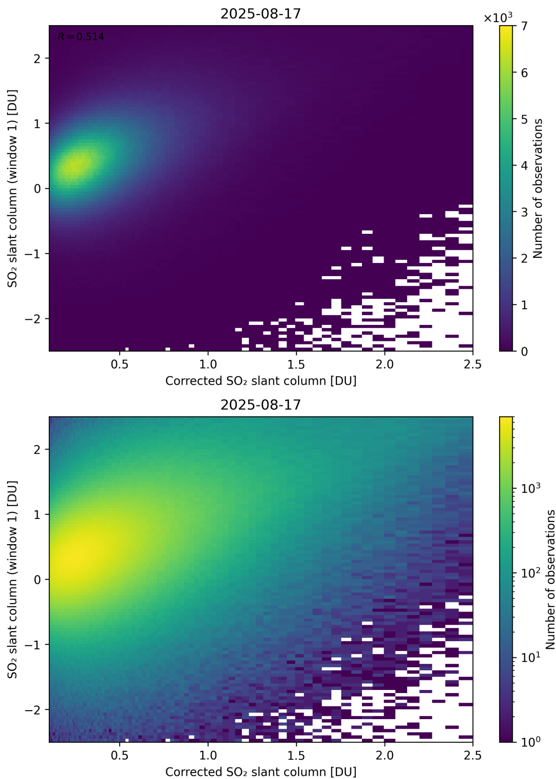
Figure 237: Scatter density plot of “Corrected SO 2 slant column” against “SO 2 slant column (window 1)” for 2025-08-16 to 2025-08-18.
