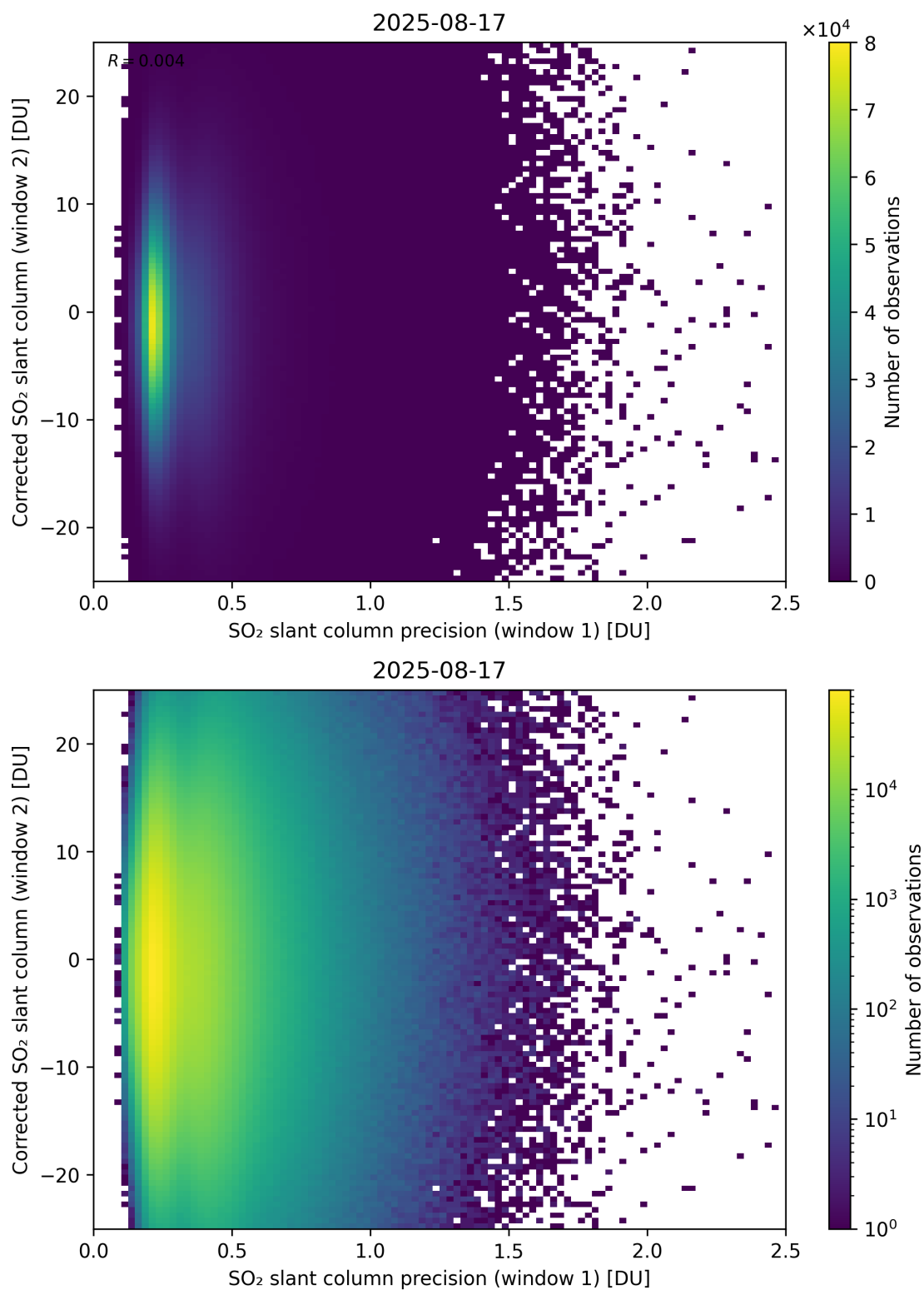
Figure 275: Scatter density plot of “SO 2 slant column precision (window 1)” against “Corrected SO 2 slant column (window 2)” for 2025-08-16 to 2025-08-18.
