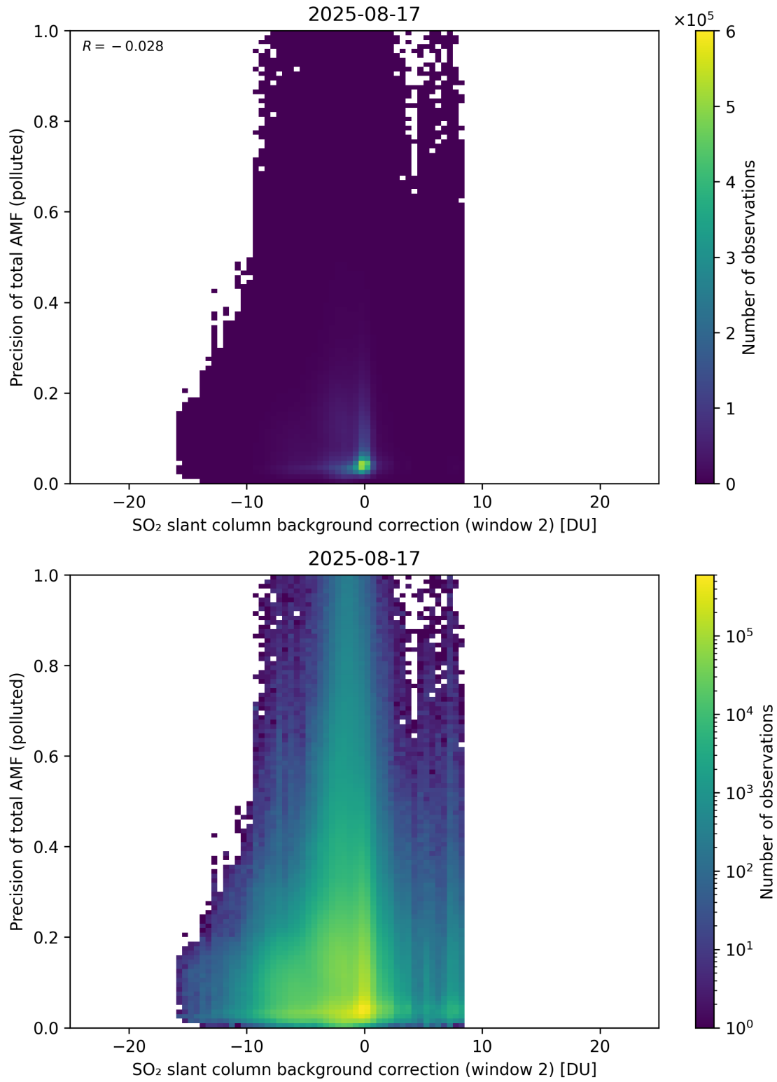
Figure 131: Scatter density plot of “SO 2 slant column background correction (window 2)” against “Precision of total AMF (polluted)” for 2025-08-16 to 2025-08-18.
