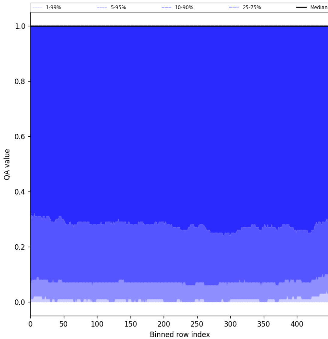
Figure 83: Along track statistics of “QA value” for 2025-08-17 to 2025-08-19
