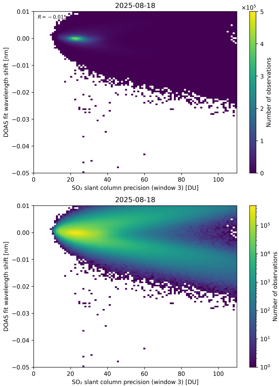
Figure 308: Scatter density plot of “SO 2 slant column precision (window 3)” against “DOAS fit wavelength shift” for 2025-08-17 to 2025-08-19.
