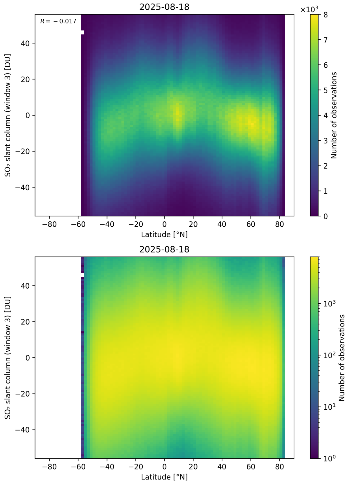
Figure 165: Scatter density plot of “Latitude” against “SO 2 slant column (window 3)” for 2025-08-17 to 2025-08-19.
