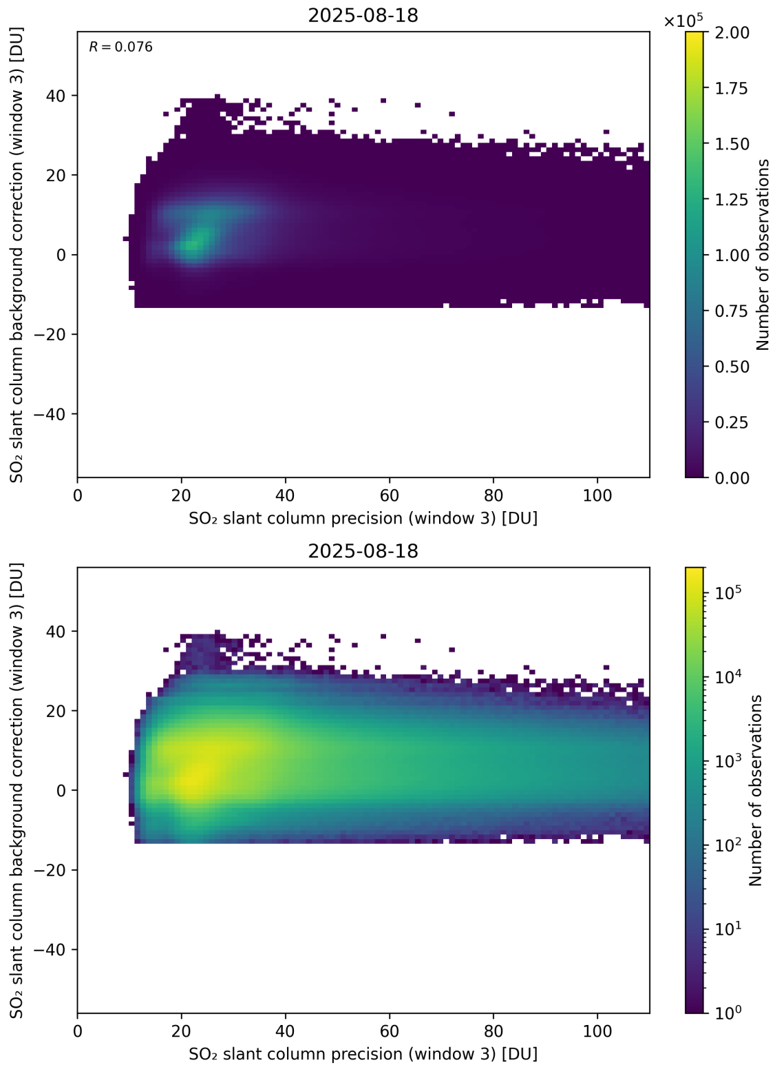
Figure 307: Scatter density plot of “SO 2 slant column precision (window 3)” against “SO 2 slant column background correction (window 3)” for 2025-08-17 to 2025-08-19.
