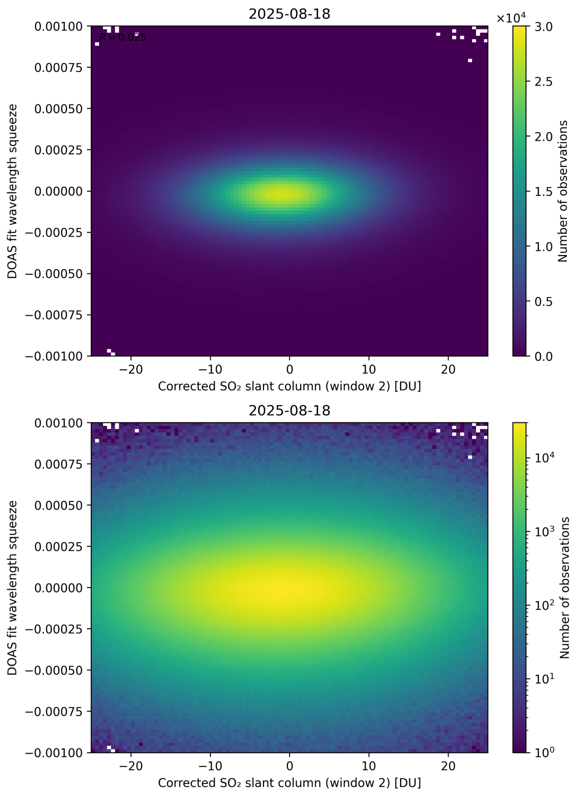
Figure 247: Scatter density plot of “Corrected SO 2 slant column (window 2)” against “DOAS fit wavelength squeeze” for 2025-08-17 to 2025-08-19.
