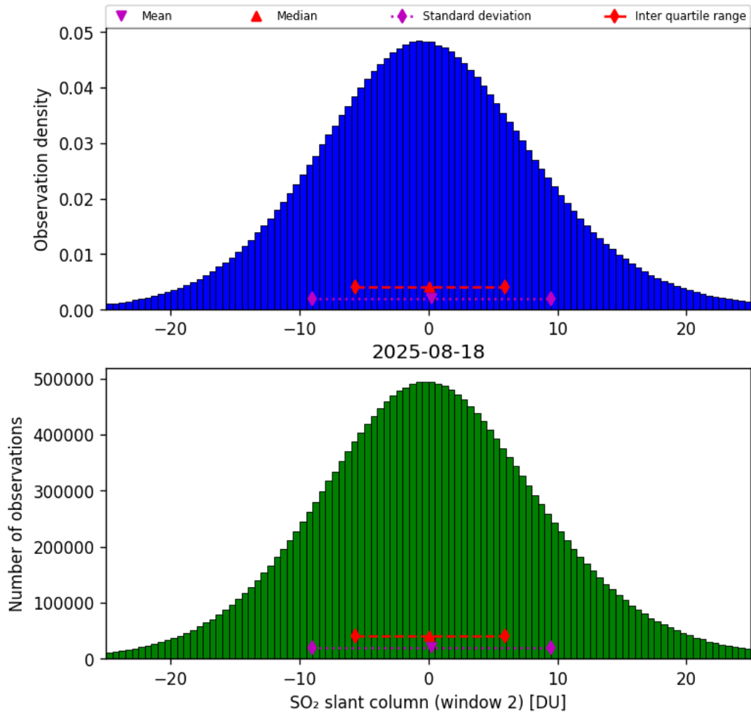
Figure 67: Histogram of “SO 2 slant column (window 2)” for 2025-08-17 to 2025-08-19
