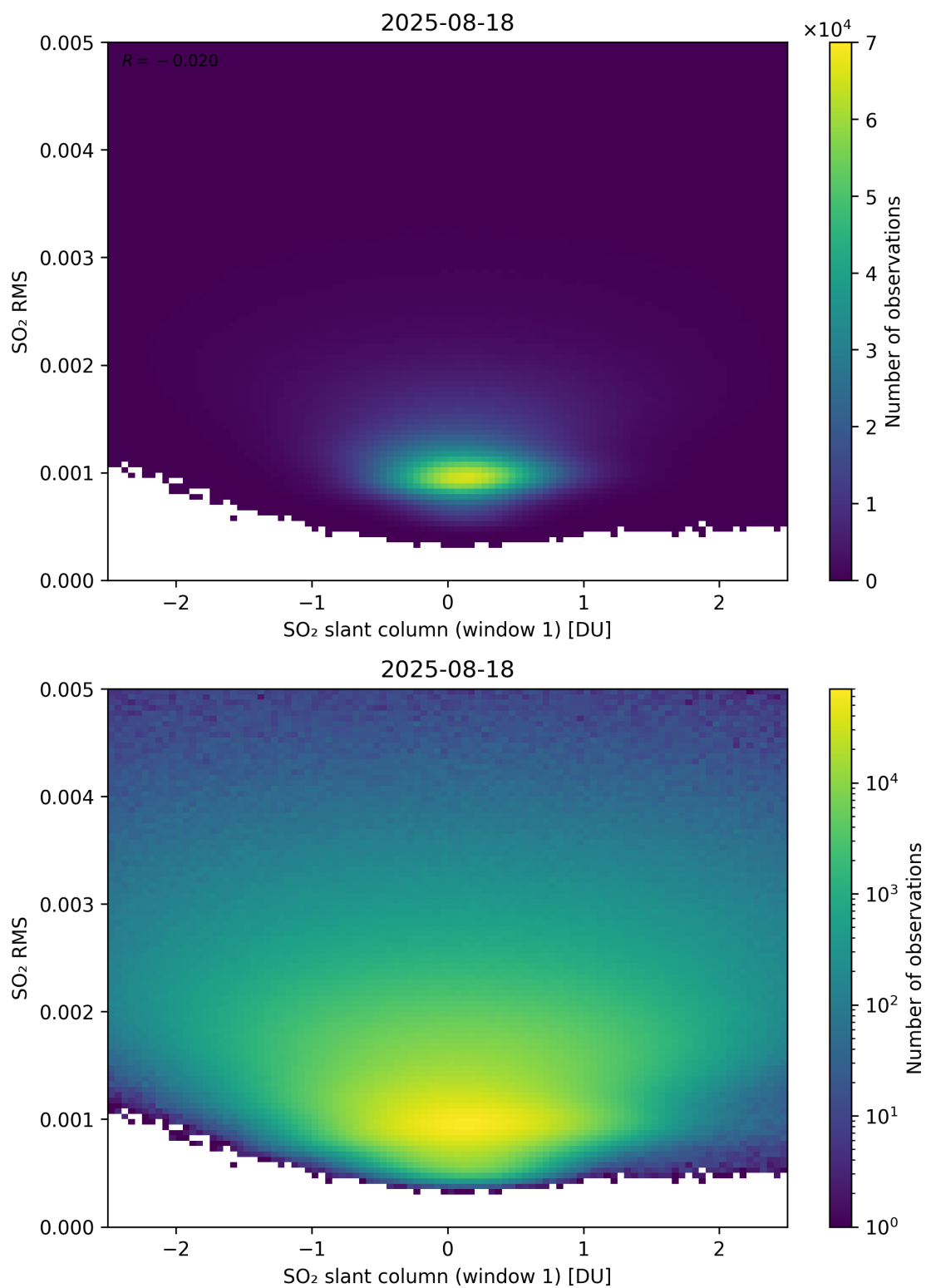
Figure 267: Scatter density plot of “SO 2 slant column (window 1)” against “SO 2 RMS” for 2025-08-17 to 2025-08-19.
