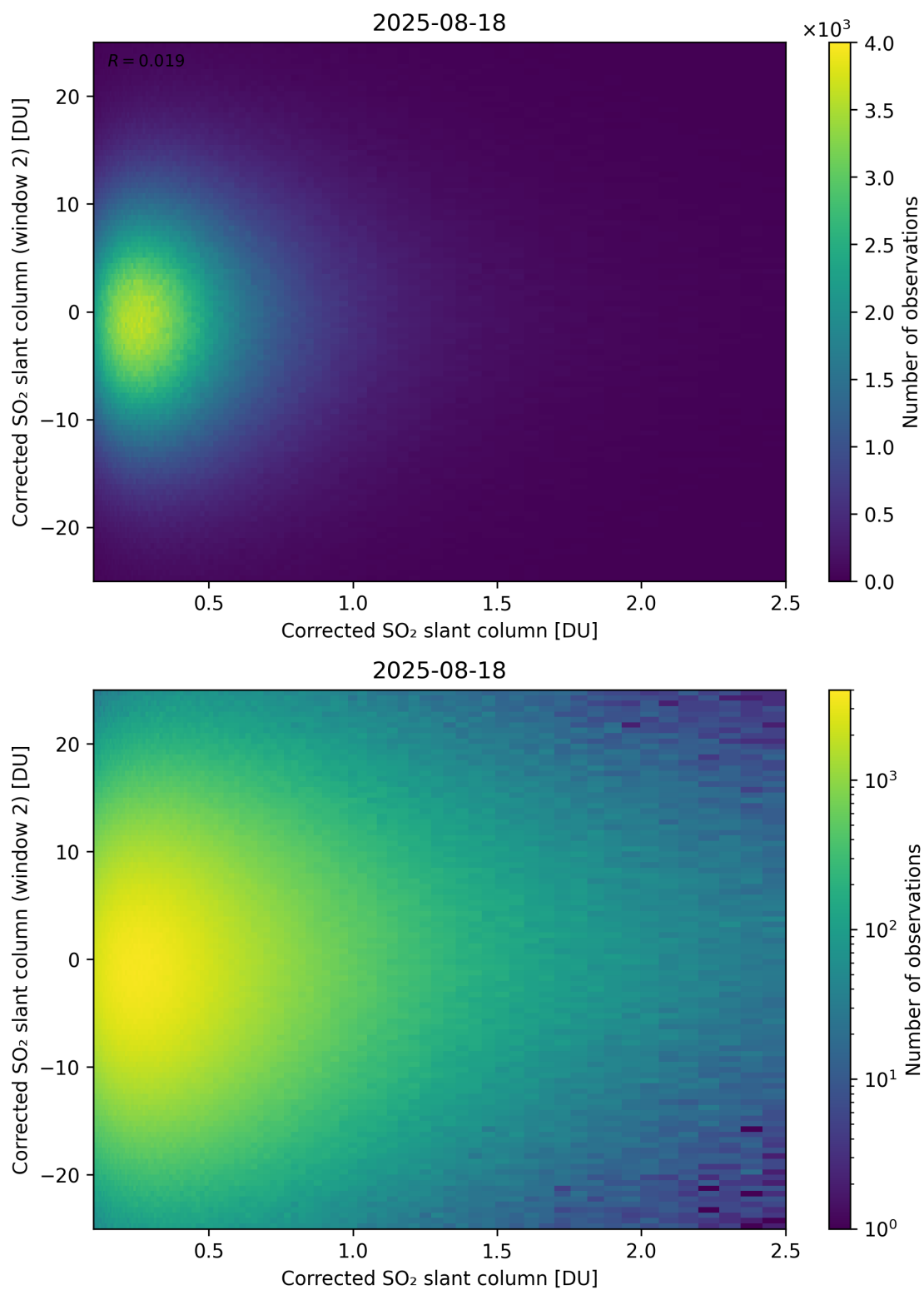
Figure 235: Scatter density plot of “Corrected SO 2 slant column” against “Corrected SO 2 slant column (window 2)” for 2025-08-17 to 2025-08-19.
