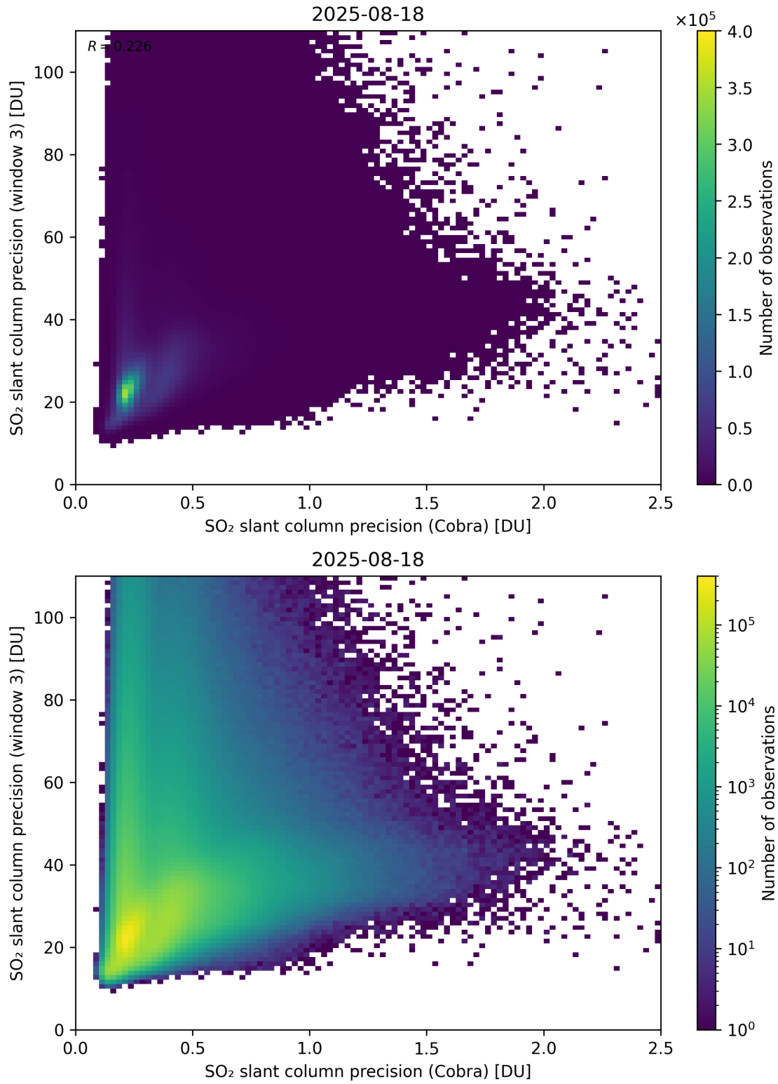
Figure 212: Scatter density plot of “SO 2 slant column precision (Cobra)” against “SO 2 slant column precision (window 3)” for 2025-08-17 to 2025-08-19.
