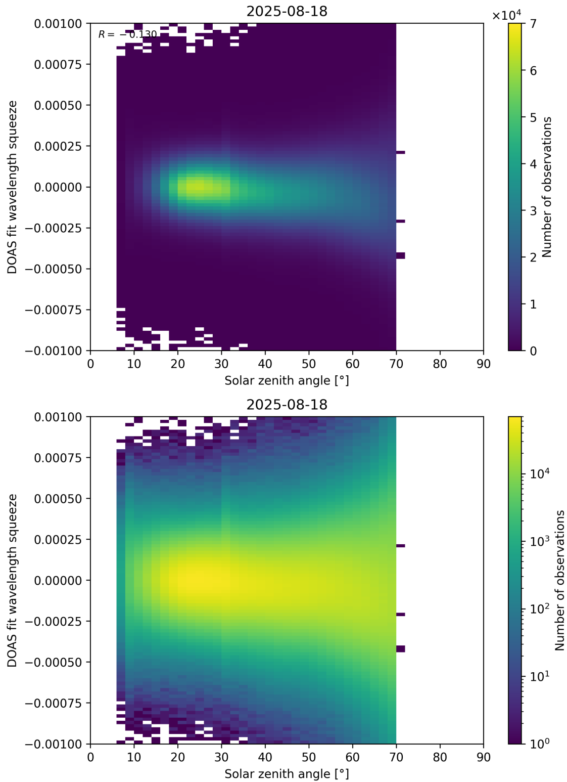
Figure 175: Scatter density plot of “Solar zenith angle” against “DOAS fit wavelength squeeze” for 2025-08-17 to 2025-08-19.
