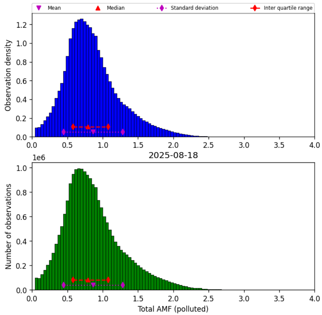
Figure 79: Histogram of “Total AMF (polluted)” for 2025-08-17 to 2025-08-19
