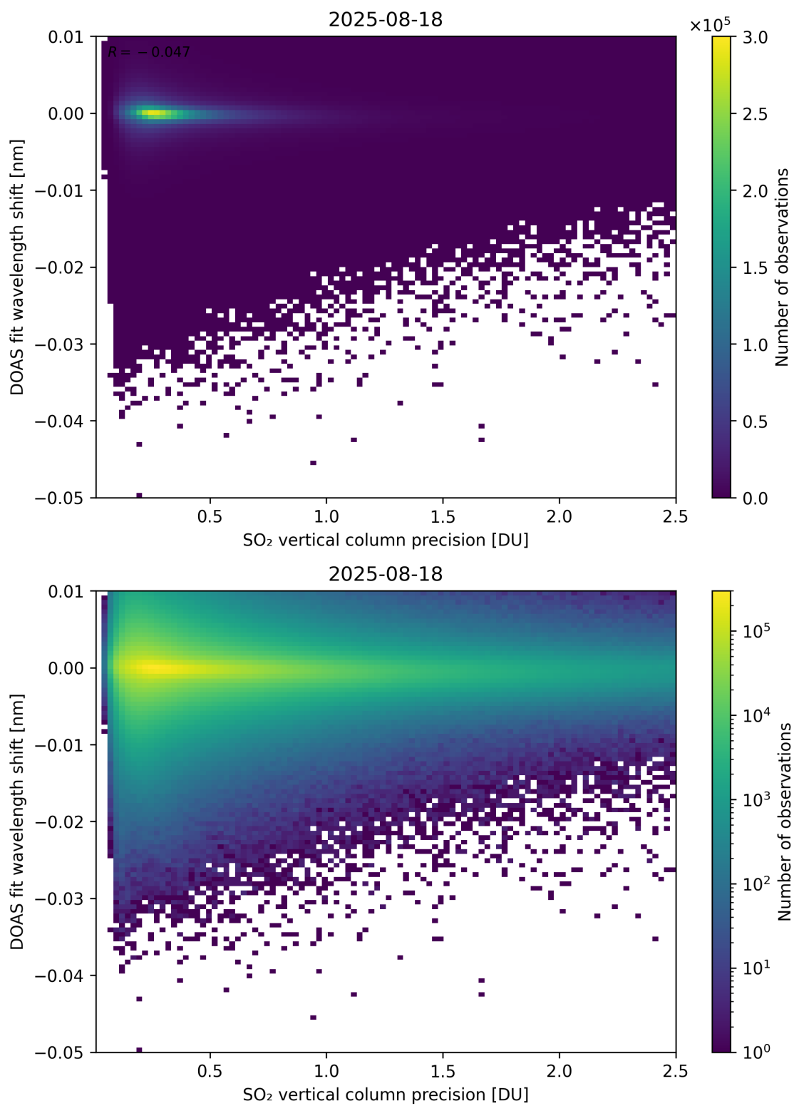
Figure 332: Scatter density plot of “SO 2 vertical column precision” against “DOAS fit wavelength shift” for 2025-08-17 to 2025-08-19.
