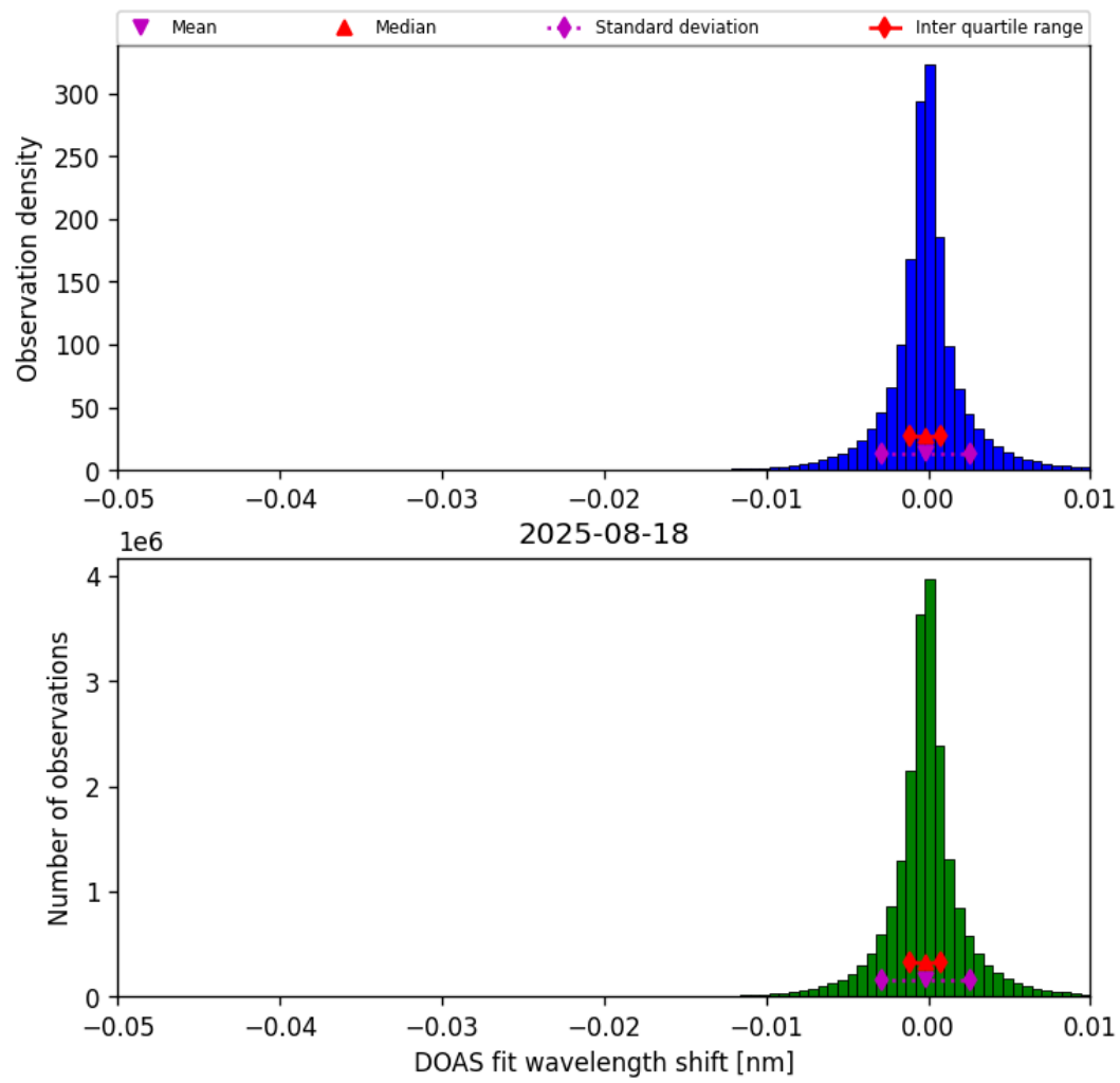
Figure 76: Histogram of “DOAS fit wavelength shift” for 2025-08-17 to 2025-08-19
