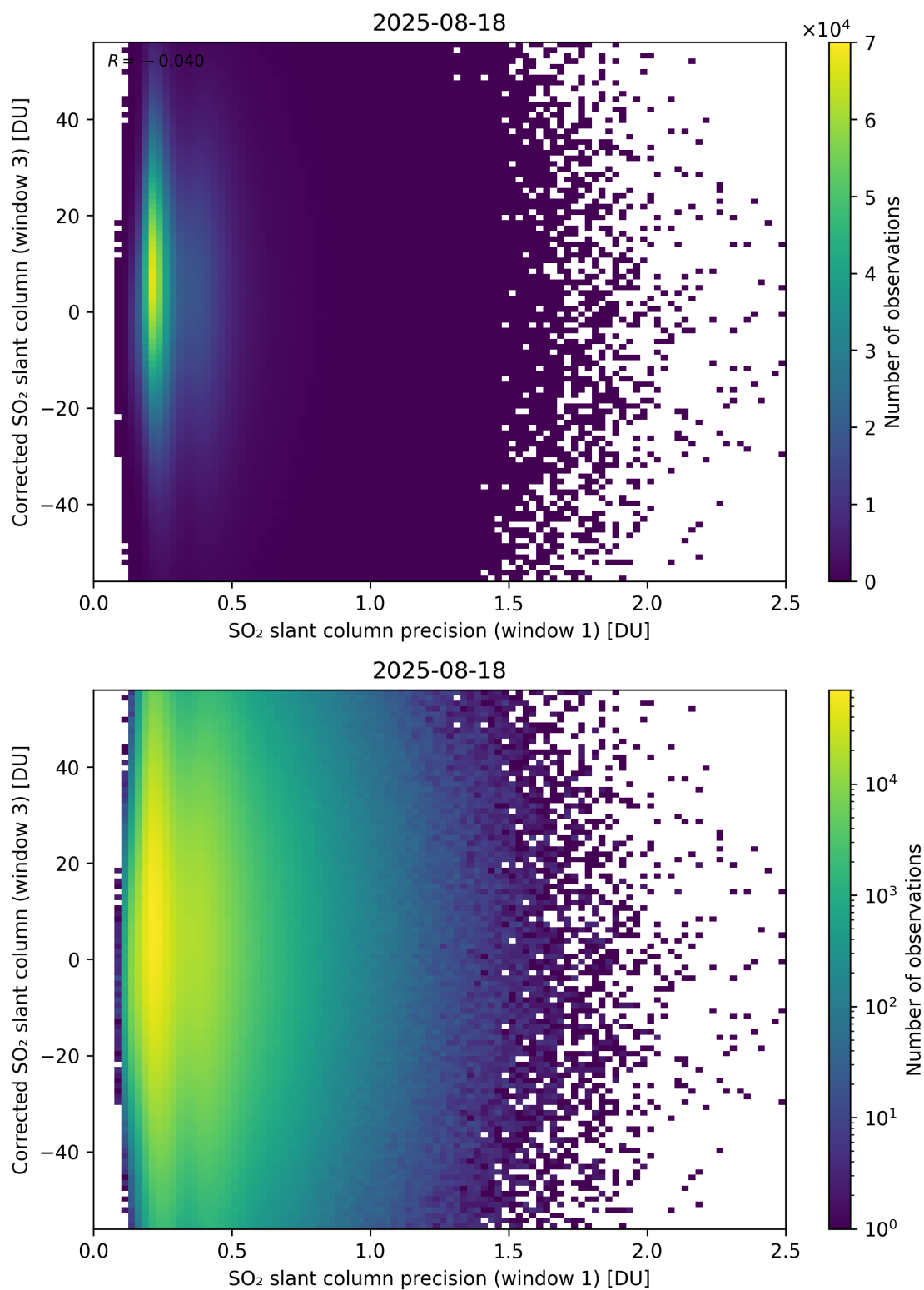
Figure 276: Scatter density plot of “SO 2 slant column precision (window 1)” against “Corrected SO 2 slant column (window 3)” for 2025-08-17 to 2025-08-19.
