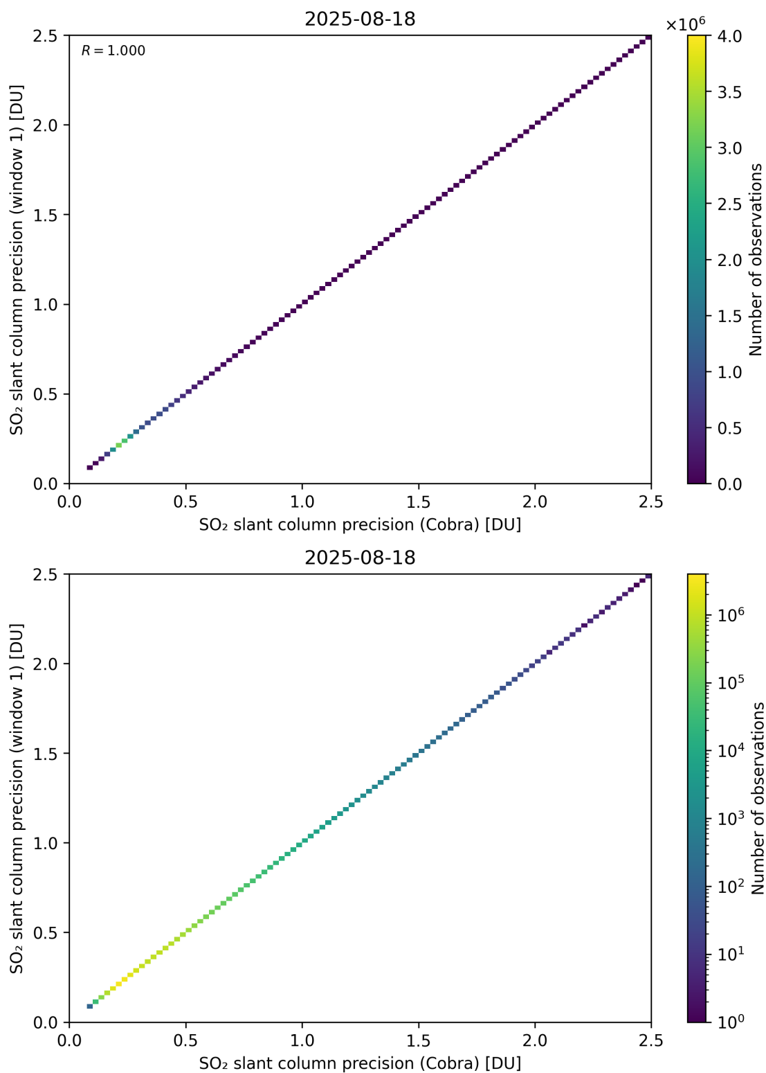
Figure 209: Scatter density plot of “SO 2 slant column precision (Cobra)” against “SO 2 slant column precision (window 1)” for 2025-08-17 to 2025-08-19.
