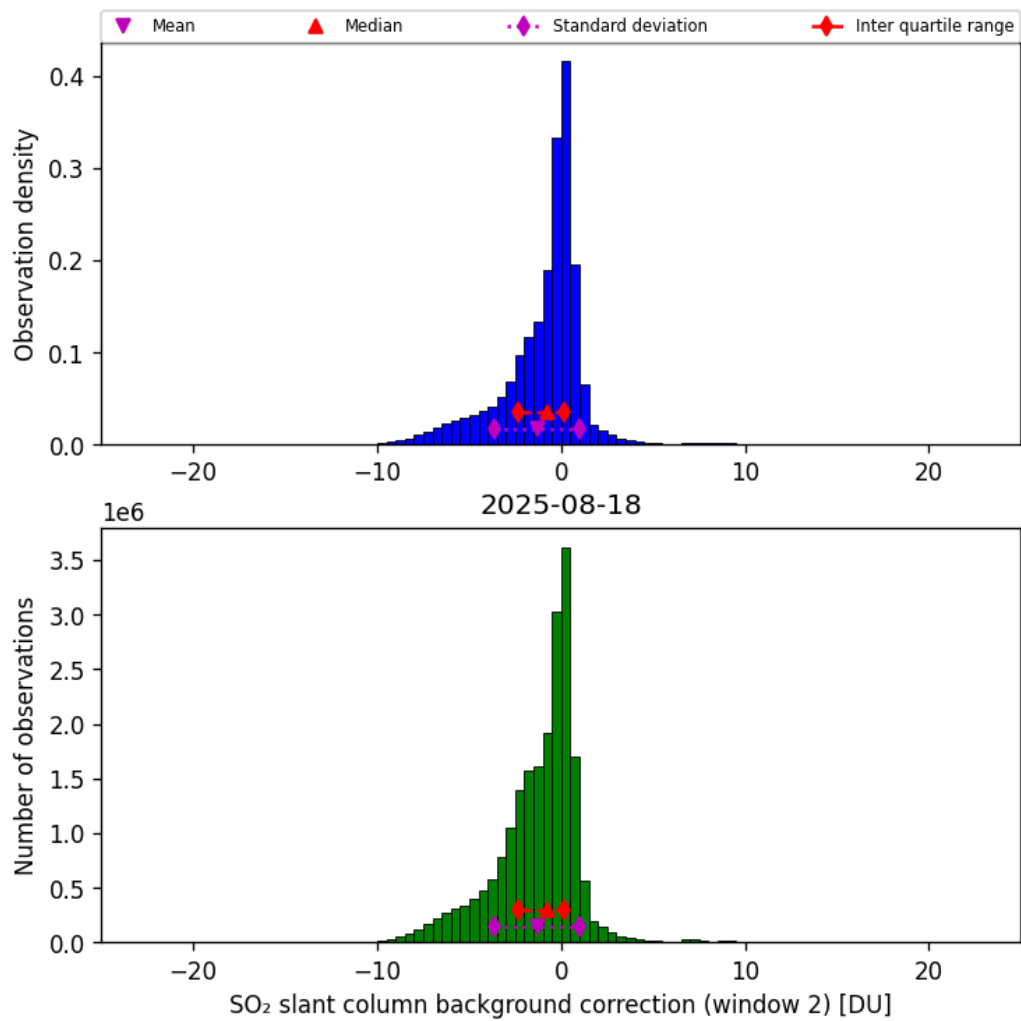
Figure 70: Histogram of “SO 2 slant column background correction (window 2)” for 2025-08-17 to 2025-08-19
