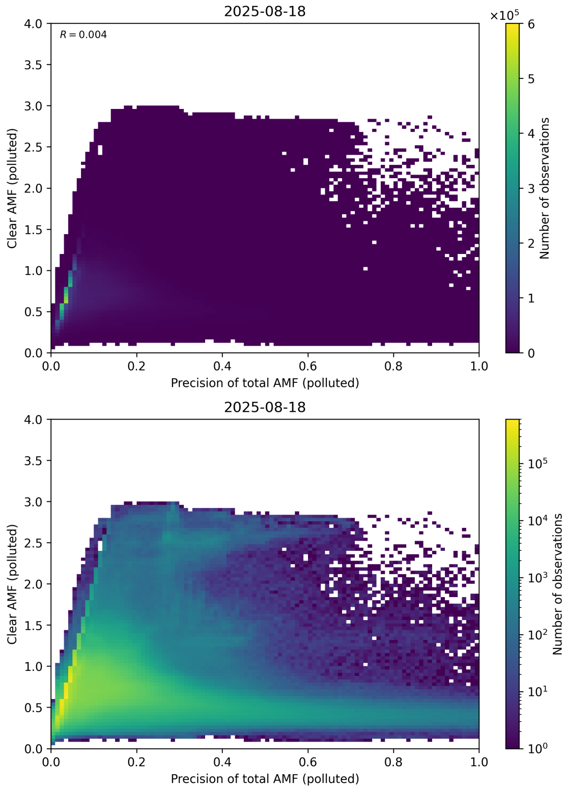
Figure 320: Scatter density plot of “Precision of total AMF (polluted)” against “Clear AMF (polluted)” for 2025-08-17 to 2025-08-19.
