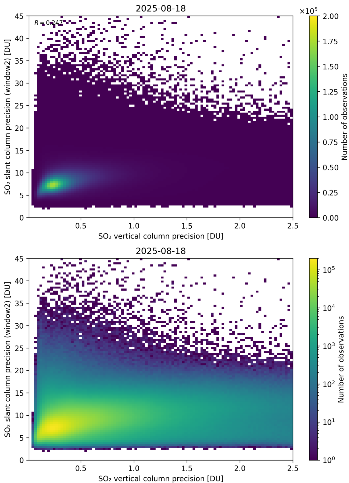
Figure 343: Scatter density plot of “SO 2 vertical column precision” against “SO 2 slant column precision (window2)” for 2025-08-17 to 2025-08-19.
