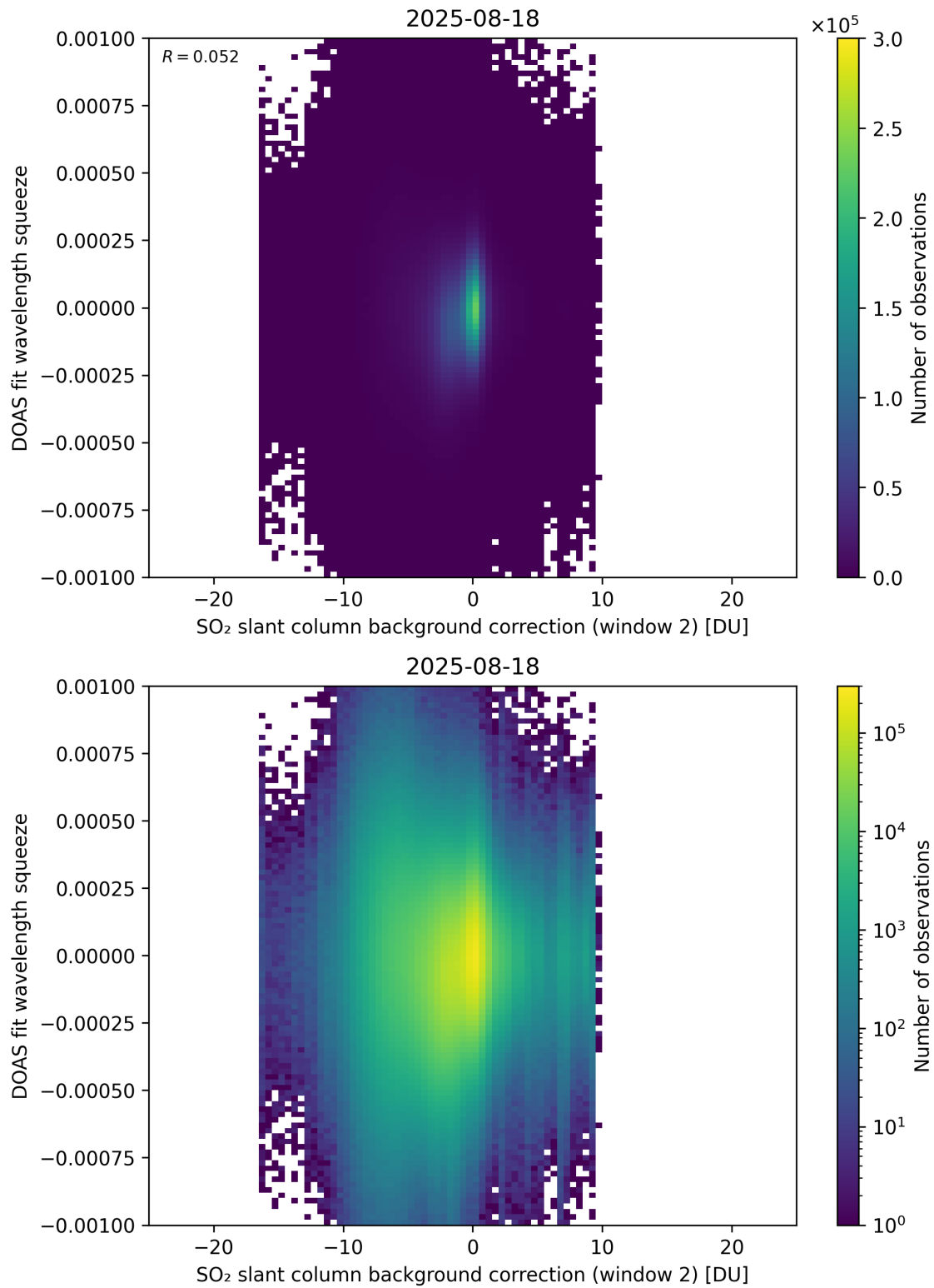
Figure 124: Scatter density plot of “SO 2 slant column background correction (window 2)” against “DOAS fit wavelength squeeze” for 2025-08-17 to 2025-08-19.
