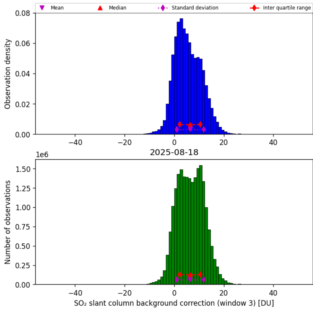
Figure 74: Histogram of “SO 2 slant column background correction (window 3)” for 2025-08-17 to 2025-08-19
