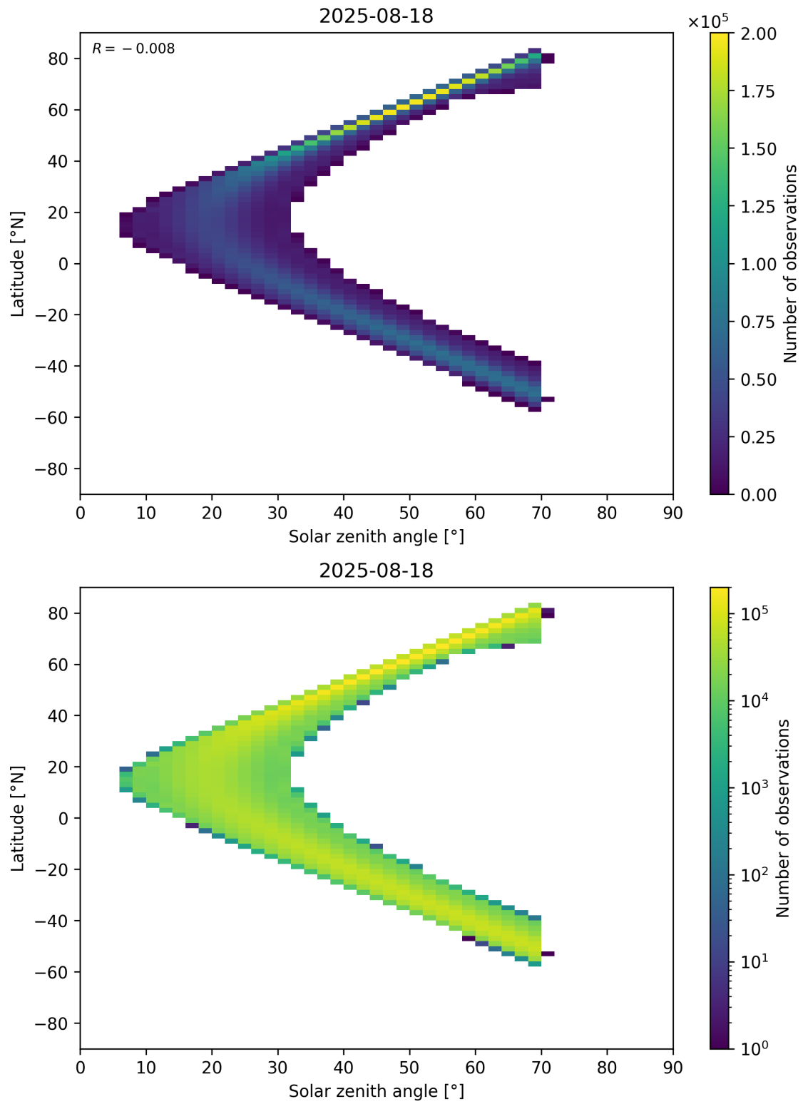
Figure 177: Scatter density plot of “Solar zenith angle” against “Latitude” for 2025-08-17 to 2025-08-19.
