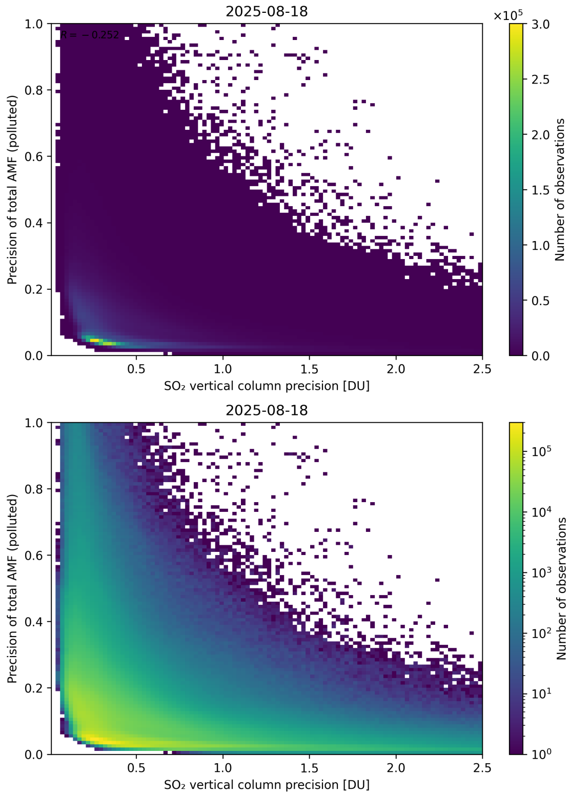
Figure 347: Scatter density plot of “SO 2 vertical column precision” against “Precision of total AMF (polluted)” for 2025-08-17 to 2025-08-19.
