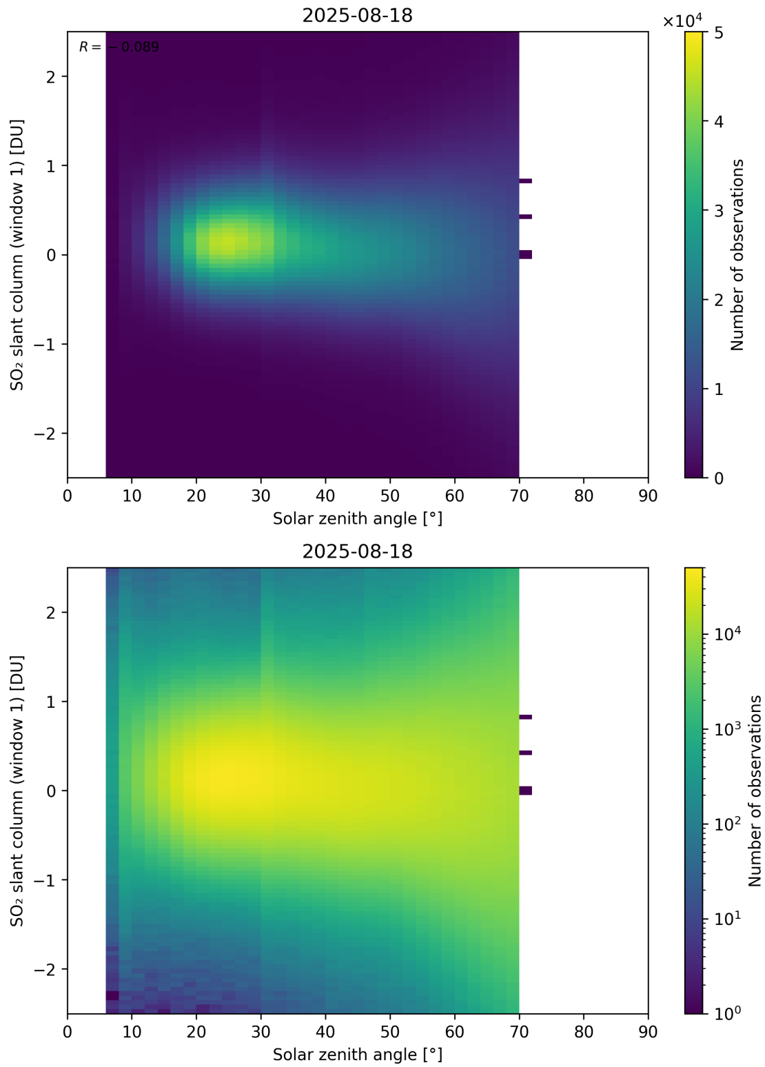
Figure 184: Scatter density plot of “Solar zenith angle” against “SO 2 slant column (window 1)” for 2025-08-17 to 2025-08-19.
