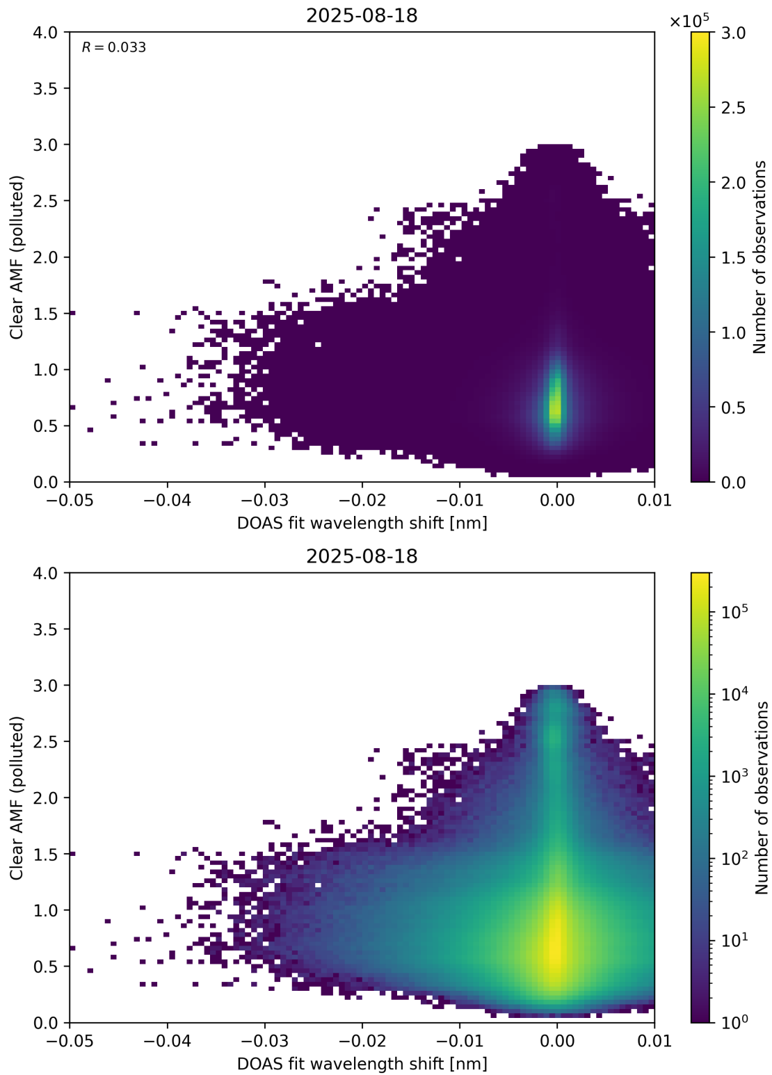
Figure 140: Scatter density plot of “DOAS fit wavelength shift” against “Clear AMF (polluted)” for 2025-08-17 to 2025-08-19.
