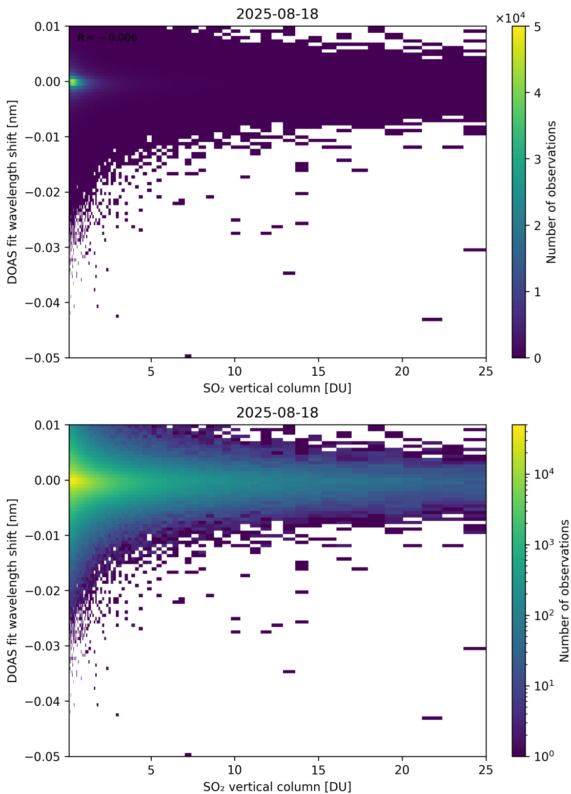
Figure 326: Scatter density plot of “SO 2 vertical column” against “DOAS fit wavelength shift” for 2025-08-17 to 2025-08-19.
