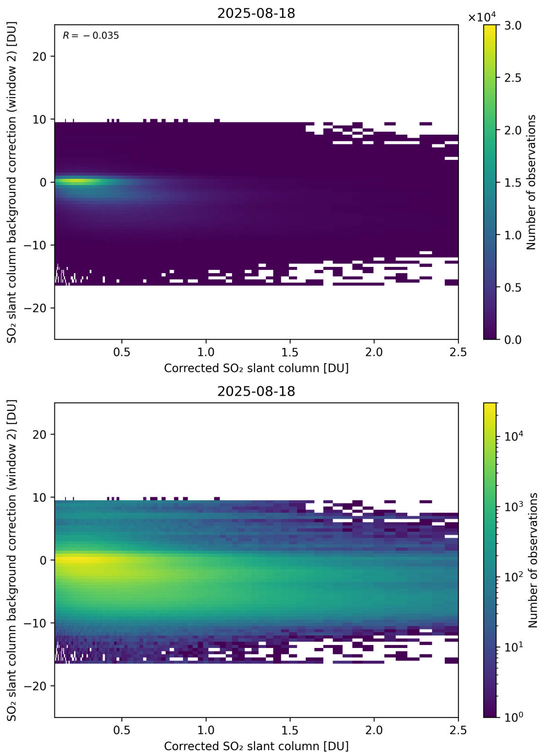
Figure 227: Scatter density plot of “Corrected SO 2 slant column” against “SO 2 slant column background correction (window 2)” for 2025-08-17 to 2025-08-19.
