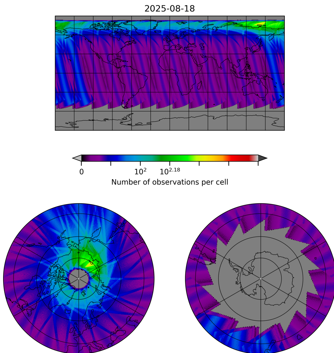
Figure 30: Map of the number of observations for 2025-08-17 to 2025-08-19
