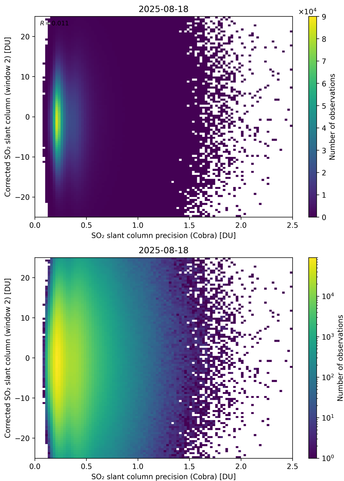
Figure 206: Scatter density plot of “SO 2 slant column precision (Cobra)” against “Corrected SO 2 slant column (window 2)” for 2025-08-17 to 2025-08-19.
