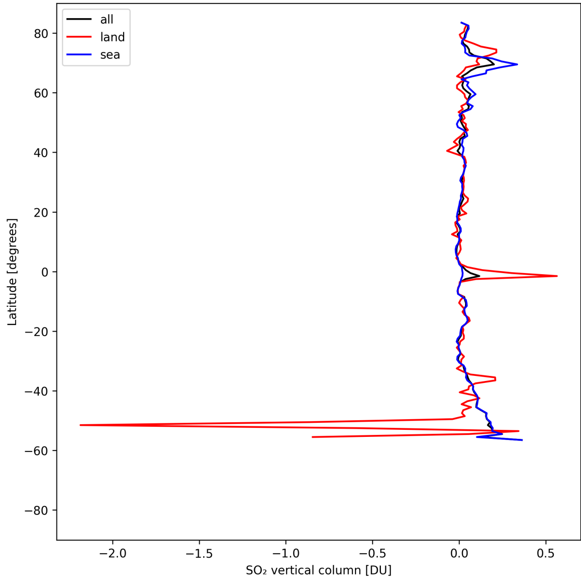
Figure 32: Zonal average of “SO 2 vertical column” for 2025-08-17 to 2025-08-19.
