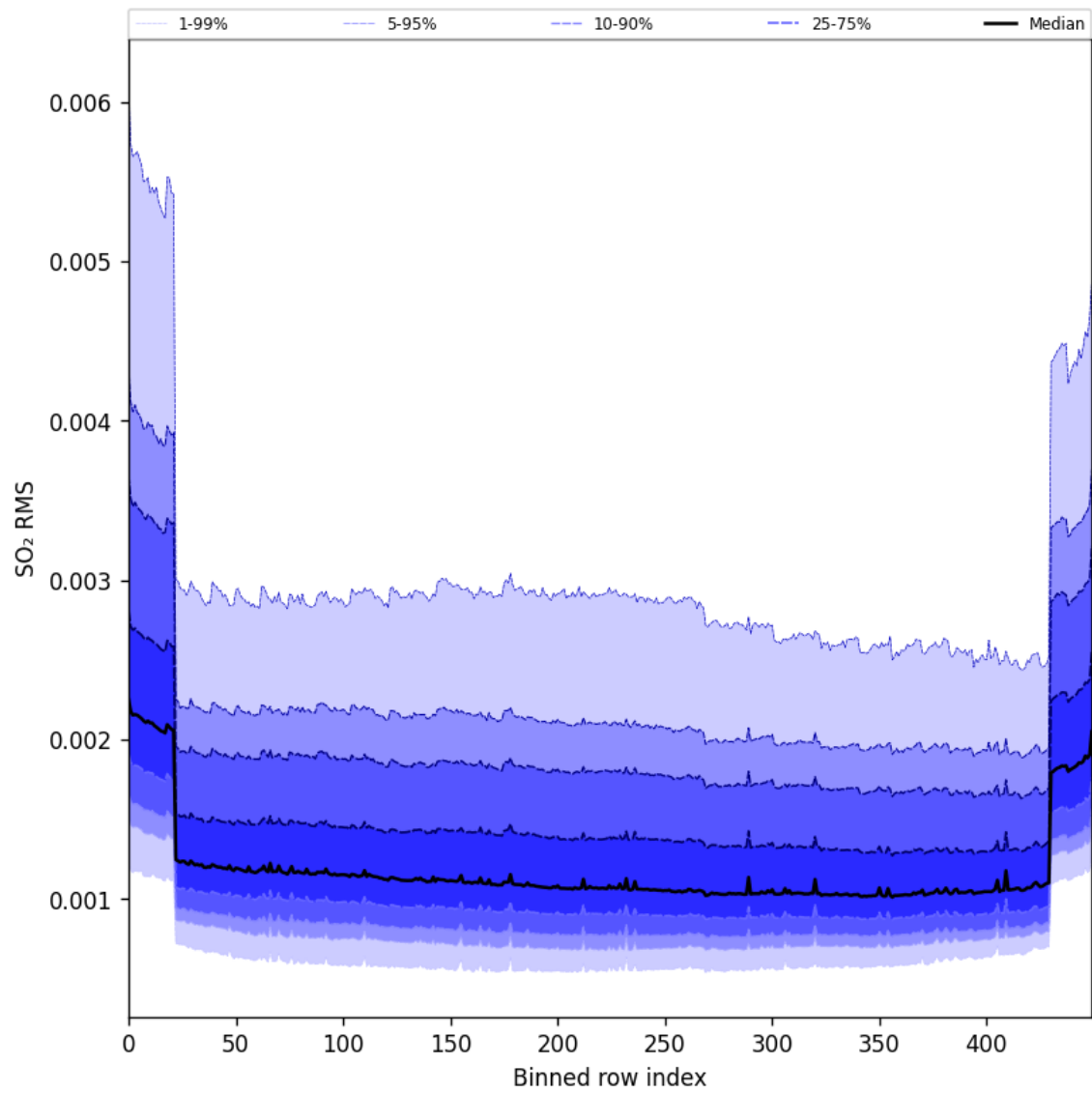
Figure 104: Along track statistics of “SO 2 RMS” for 2025-08-17 to 2025-08-19
