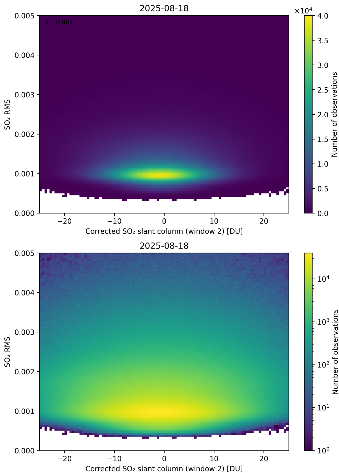
Figure 248: Scatter density plot of “Corrected SO 2 slant column (window 2)” against “SO 2 RMS” for 2025-08-17 to 2025-08-19.
