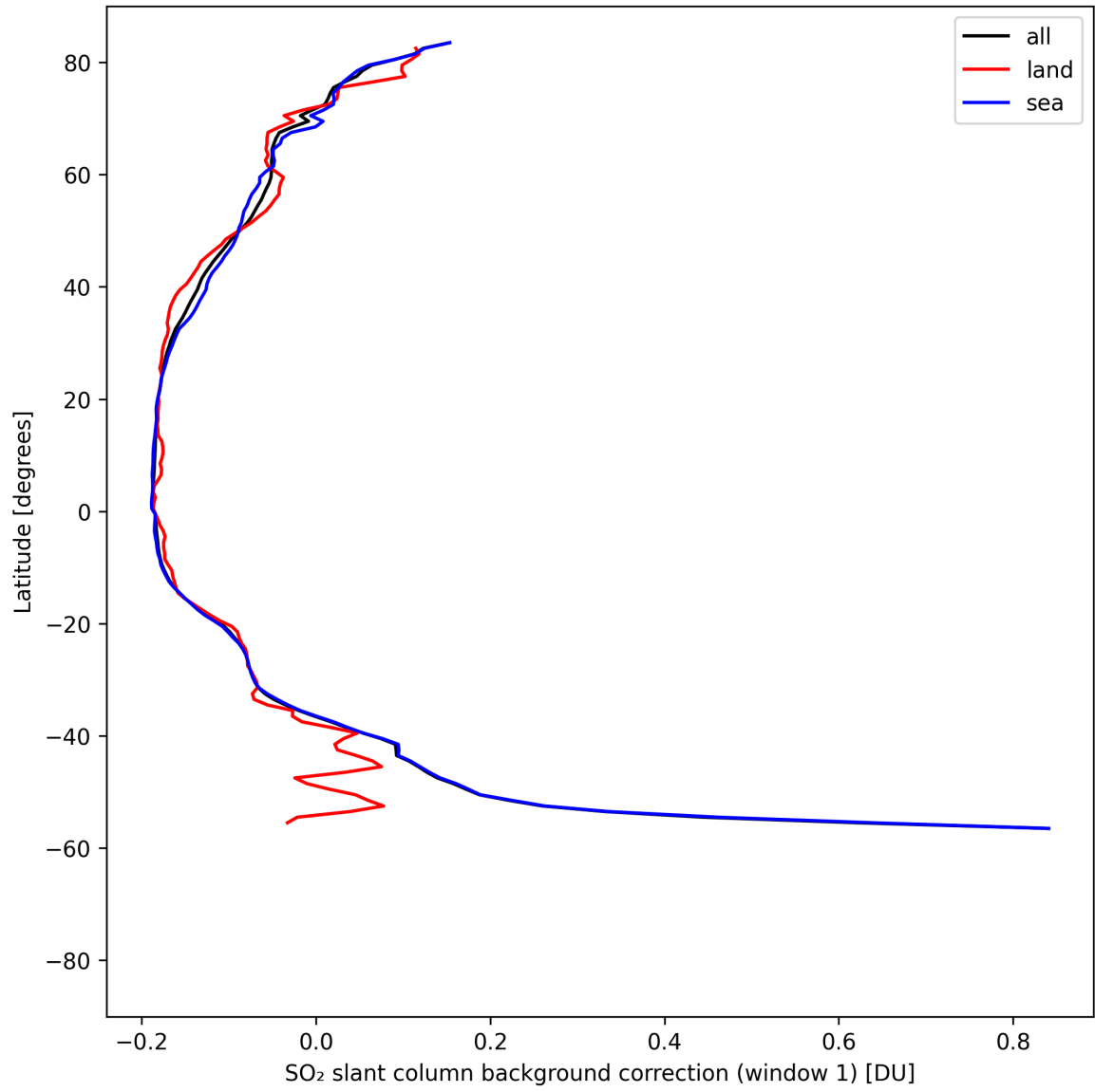
Figure 40: Zonal average of “SO 2 slant column background correction (window 1)” for 2025-08-17 to 2025-08-19.
