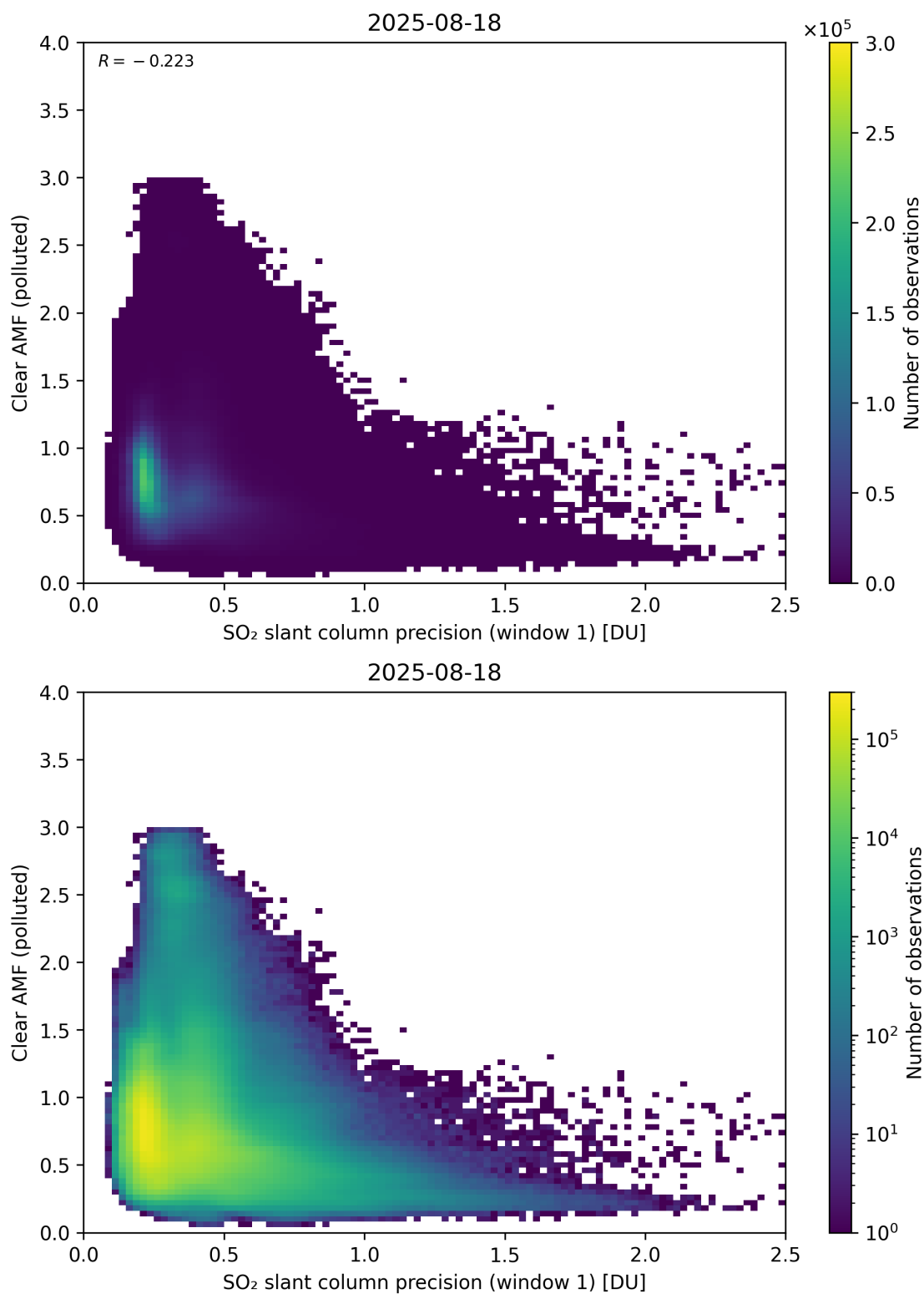
Figure 274: Scatter density plot of “SO 2 slant column precision (window 1)” against “Clear AMF (polluted)” for 2025-08-17 to 2025-08-19.
