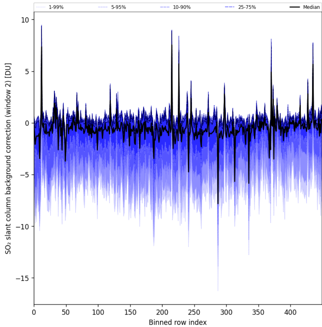
Figure 96: Along track statistics of “SO 2 slant column background correction (window 2)” for 2025-08-17 to 2025-08-19
