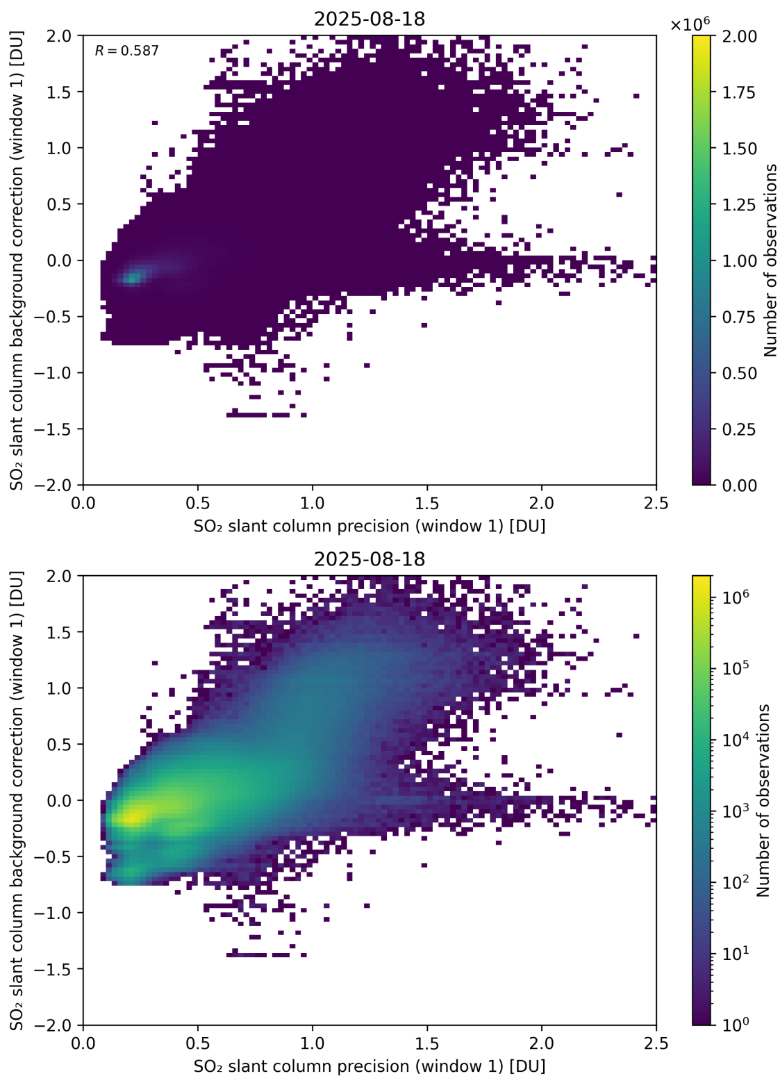
Figure 268: Scatter density plot of “SO 2 slant column precision (window 1)” against “SO 2 slant column background correction (window 1)” for 2025-08-17 to 2025-08-19.
