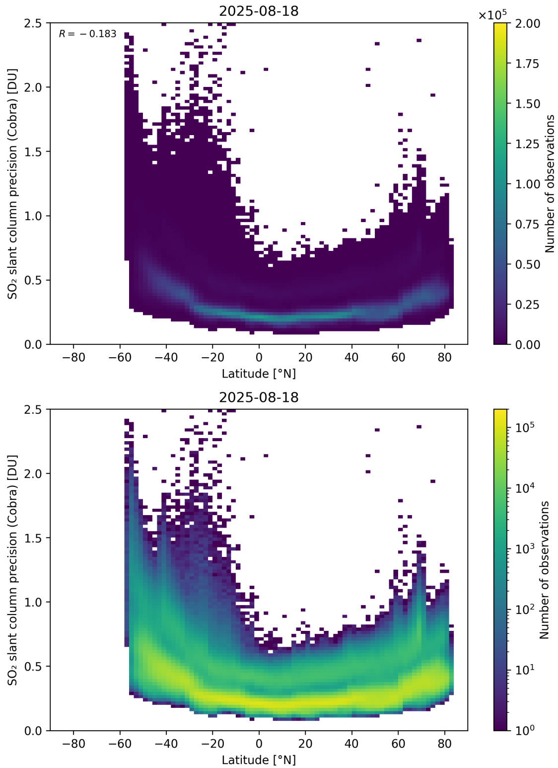
Figure 158: Scatter density plot of “Latitude” against “SO 2 slant column precision (Cobra)” for 2025-08-17 to 2025-08-19.
