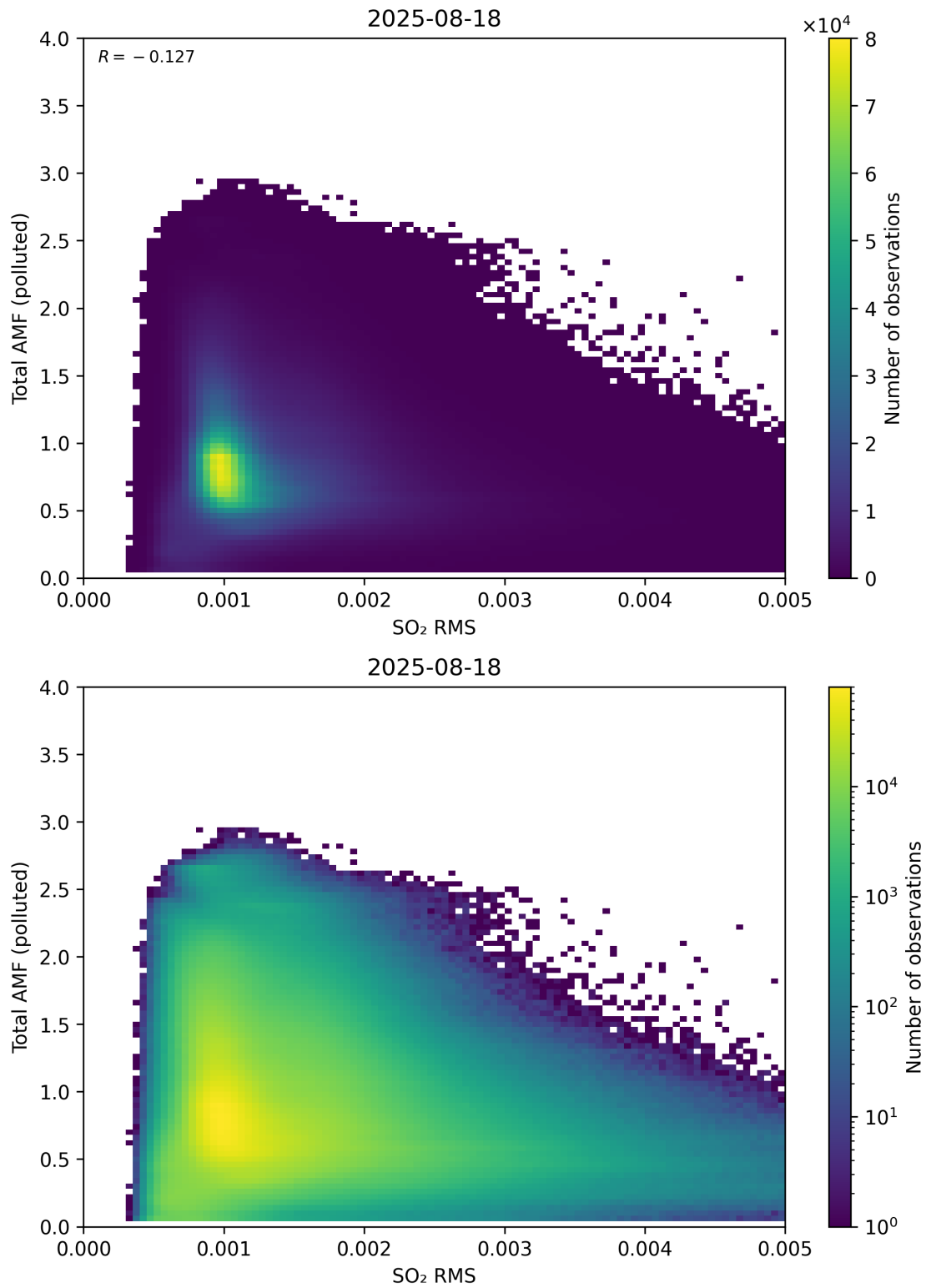
Figure 148: Scatter density plot of “SO 2 RMS” against “Total AMF (polluted)” for 2025-08-17 to 2025-08-19.
