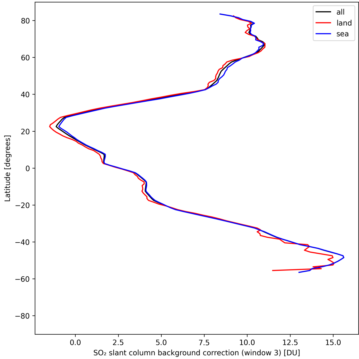
Figure 48: Zonal average of “SO 2 slant column background correction (window 3)” for 2025-08-17 to 2025-08-19.
