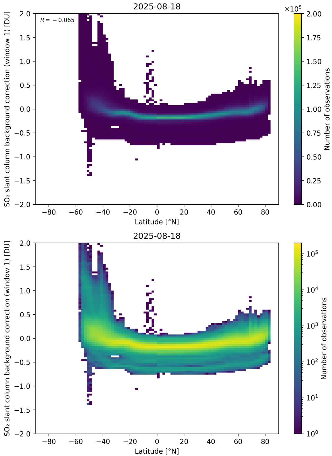
Figure 150: Scatter density plot of “Latitude” against “SO 2 slant column background correction (window 1)” for 2025-08-17 to 2025-08-19.
