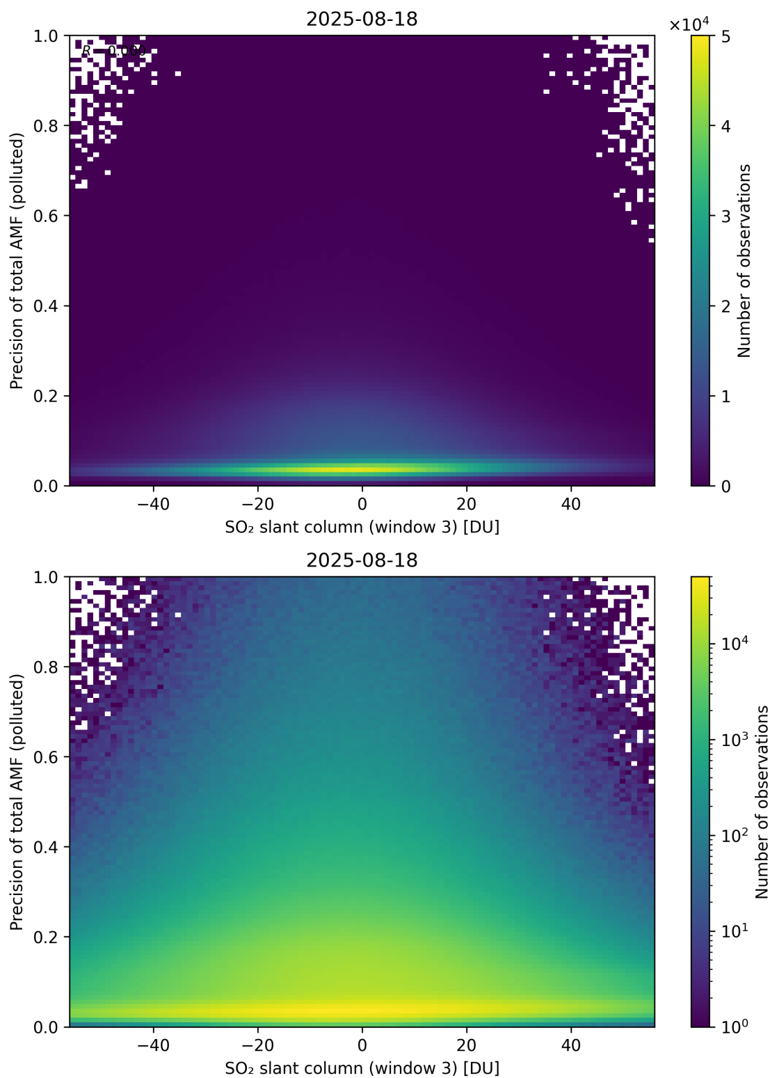
Figure 319: Scatter density plot of “SO 2 slant column (window 3)” against “Precision of total AMF (polluted)” for 2025-08-17 to 2025-08-19.
