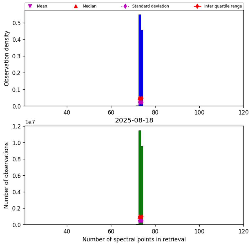
Figure 82: Histogram of “Number of spectral points in retrieval” for 2025-08-17 to 2025-08-19
