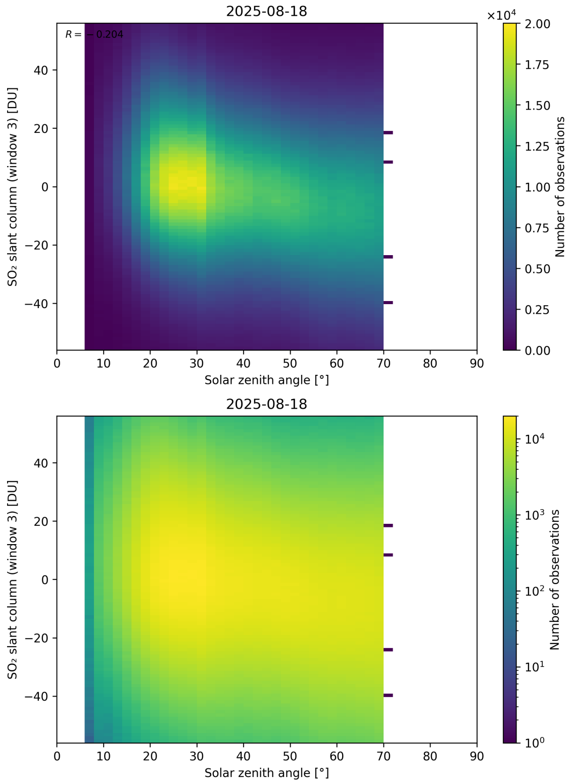
Figure 187: Scatter density plot of “Solar zenith angle” against “SO 2 slant column (window 3)” for 2025-08-17 to 2025-08-19.
