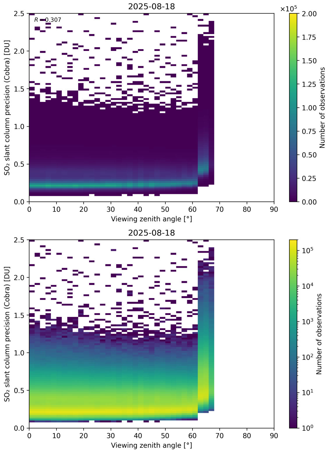
Figure 372: Scatter density plot of “Viewing zenith angle” against “SO 2 slant column precision (Cobra)” for 2025-08-17 to 2025-08-19.
