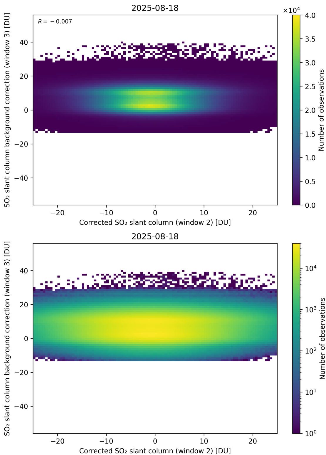
Figure 245: Scatter density plot of “Corrected SO 2 slant column (window 2)” against “SO 2 slant column background correction (window 3)” for 2025-08-17 to 2025-08-19.
