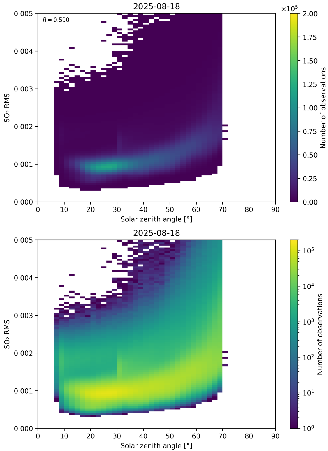
Figure 176: Scatter density plot of “Solar zenith angle” against “SO 2 RMS” for 2025-08-17 to 2025-08-19.
