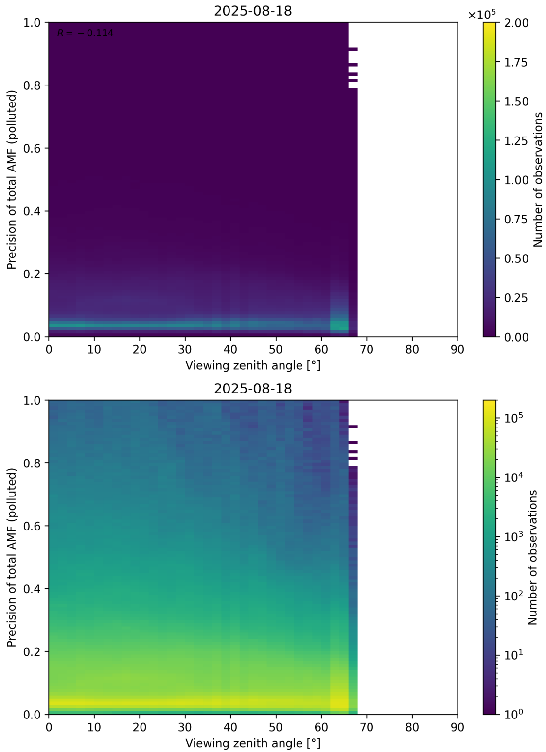
Figure 382: Scatter density plot of “Viewing zenith angle” against “Precision of total AMF (polluted)” for 2025-08-17 to 2025-08-19.
