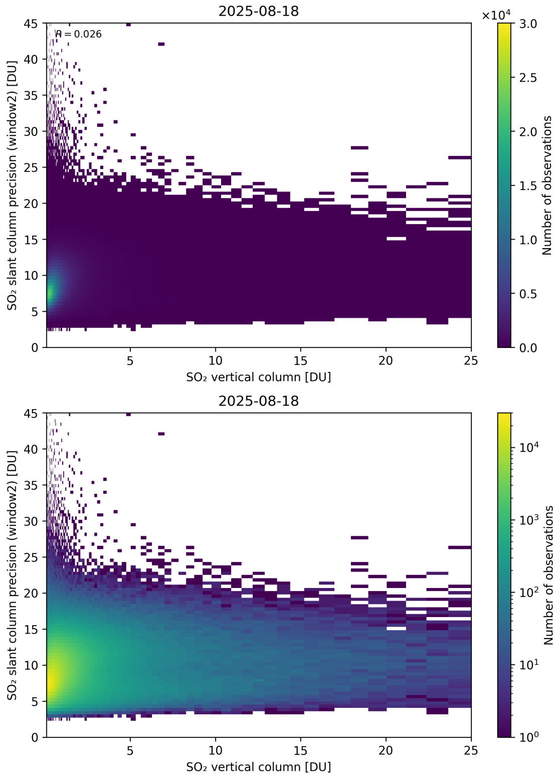
Figure 356: Scatter density plot of “SO 2 vertical column” against “SO 2 slant column precision (window2)” for 2025-08-17 to 2025-08-19.
