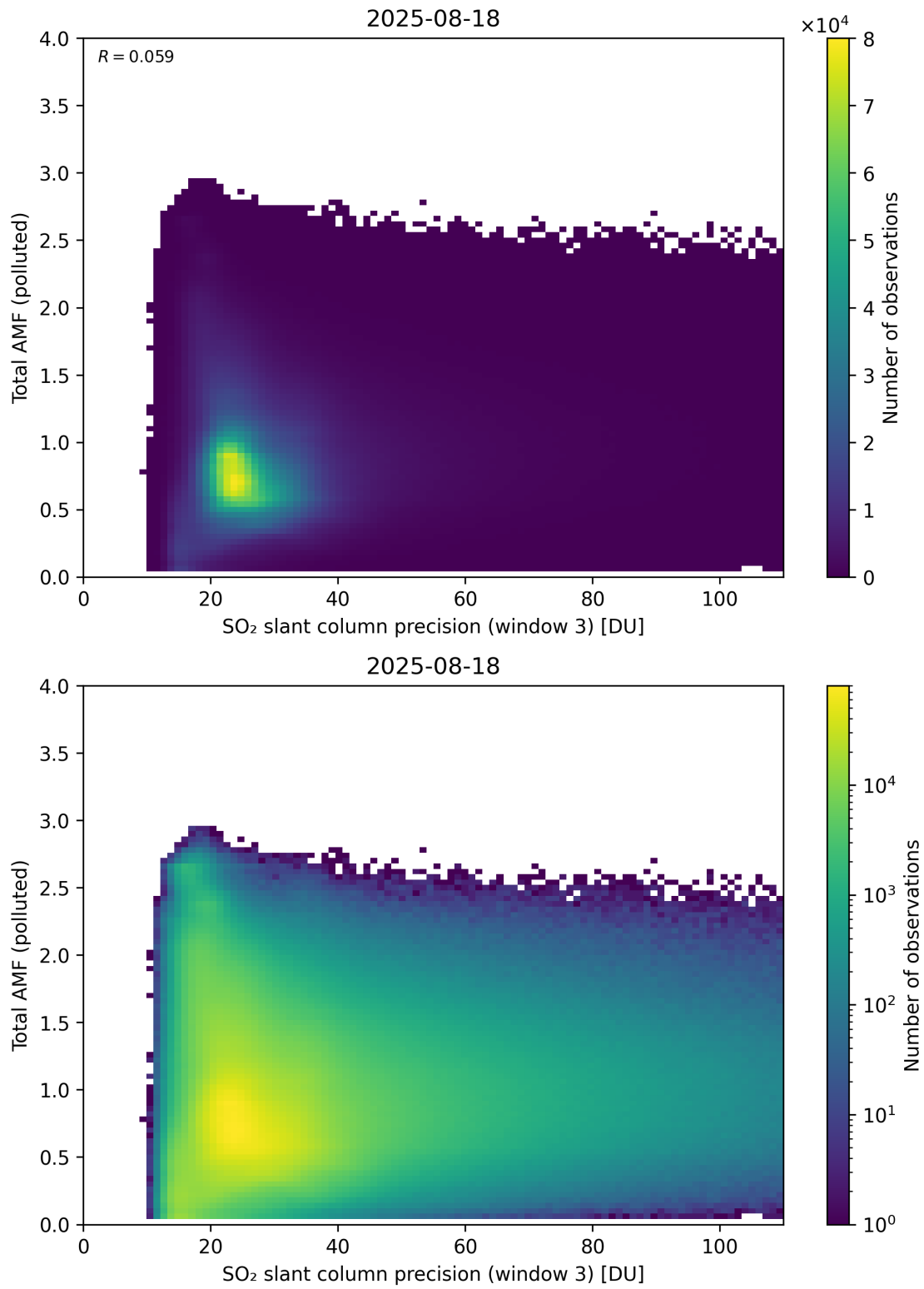
Figure 313: Scatter density plot of “SO 2 slant column precision (window 3)” against “Total AMF (polluted)” for 2025-08-17 to 2025-08-19.
