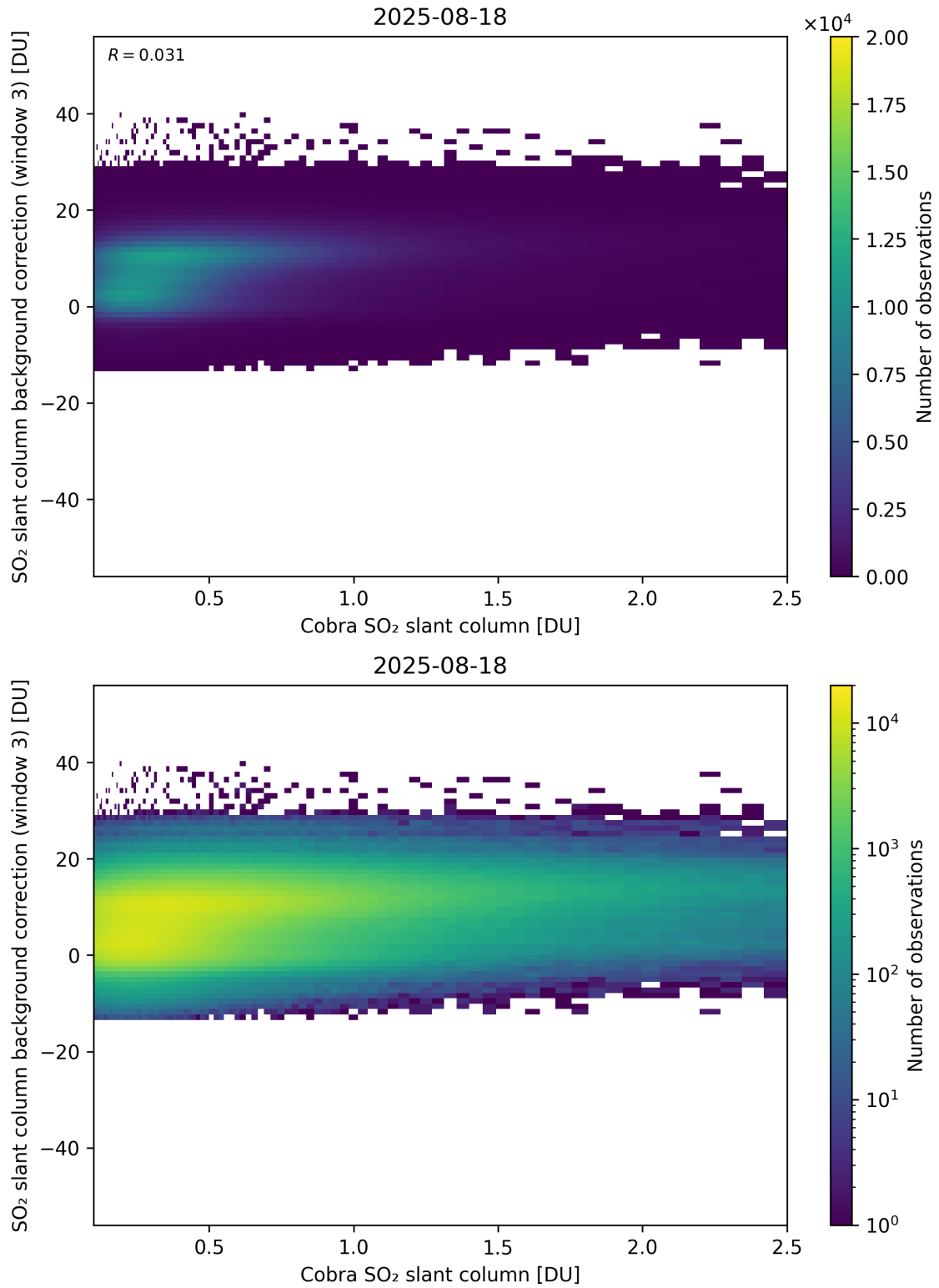
Figure 195: Scatter density plot of “Cobra SO 2 slant column” against “SO 2 slant column background correction (window 3)” for 2025-08-17 to 2025-08-19.
