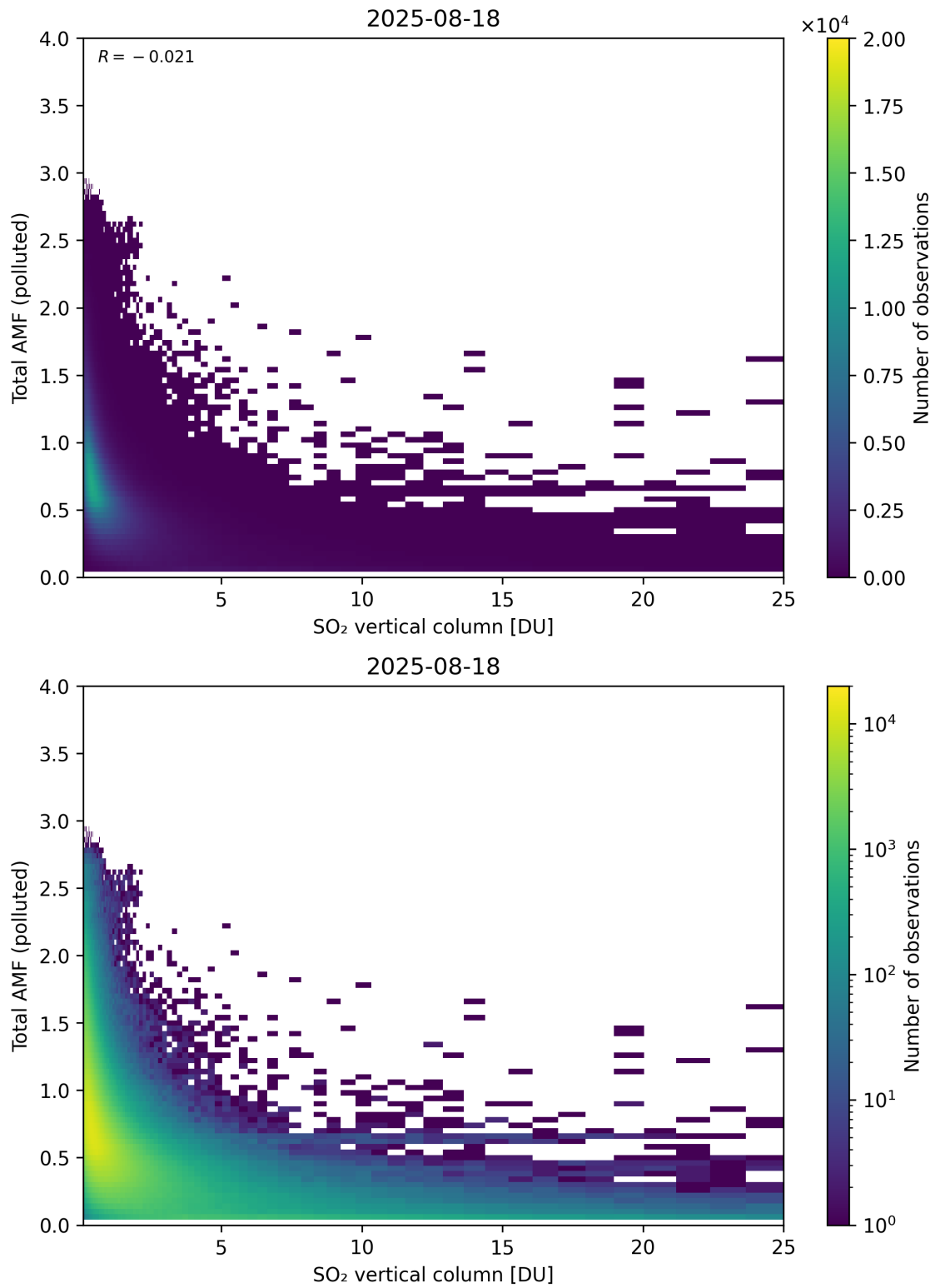
Figure 359: Scatter density plot of “SO 2 vertical column” against “Total AMF (polluted)” for 2025-08-17 to 2025-08-19.
