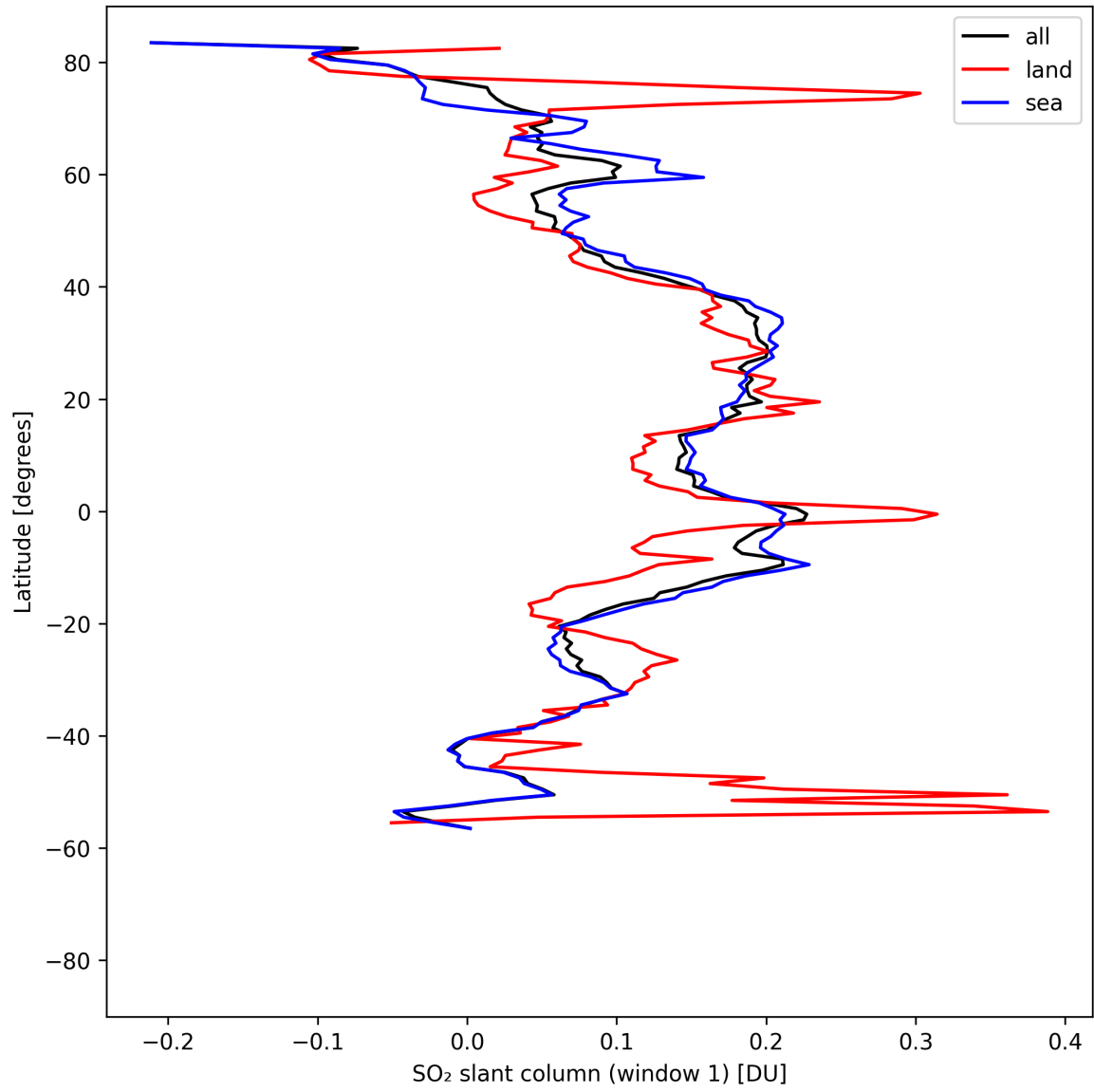
Figure 37: Zonal average of “SO 2 slant column (window 1)” for 2025-08-17 to 2025-08-19.
