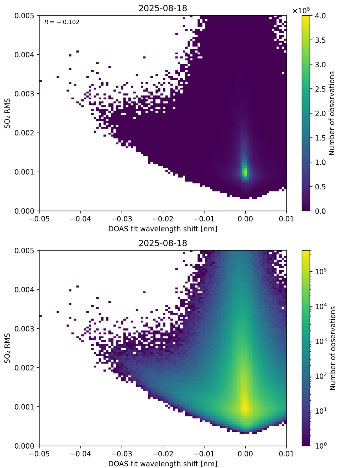
Figure 139: Scatter density plot of “DOAS fit wavelength shift” against “SO 2 RMS” for 2025-08-17 to 2025-08-19.
