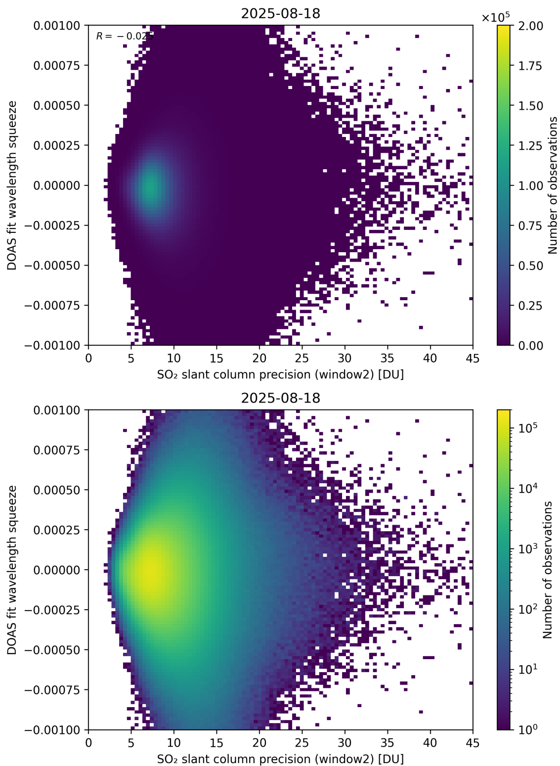
Figure 294: Scatter density plot of “SO 2 slant column precision (window2)” against “DOAS fit wavelength squeeze” for 2025-08-17 to 2025-08-19.
