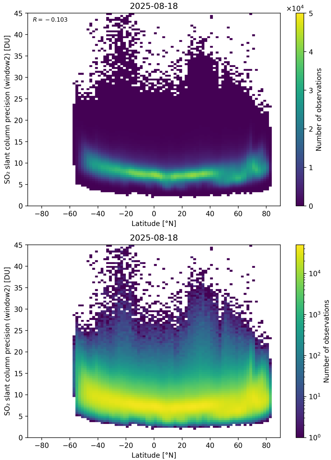
Figure 164: Scatter density plot of “Latitude” against “SO 2 slant column precision (window2)” for 2025-08-17 to 2025-08-19.
