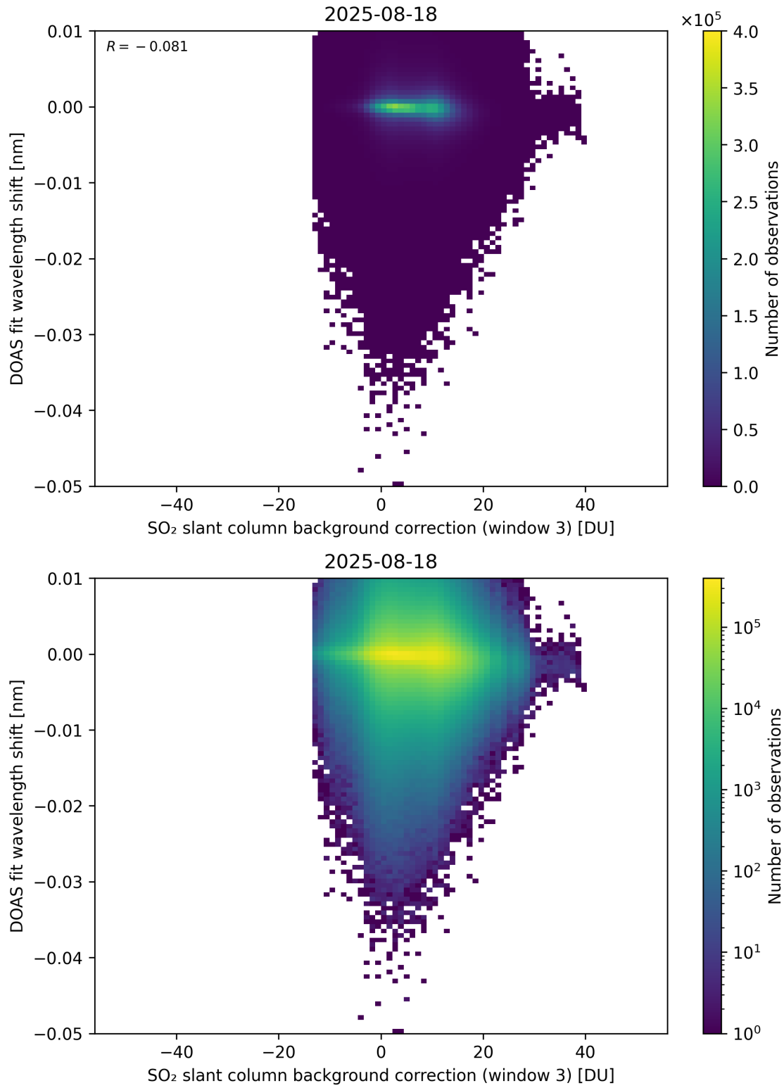
Figure 132: Scatter density plot of “SO 2 slant column background correction (window 3)” against “DOAS fit wavelength shift” for 2025-08-17 to 2025-08-19.
