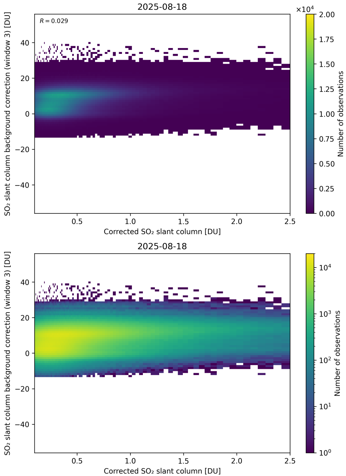
Figure 228: Scatter density plot of “Corrected SO 2 slant column” against “SO 2 slant column background correction (window 3)” for 2025-08-17 to 2025-08-19.
