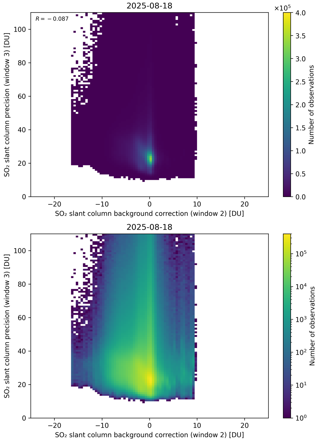
Figure 129: Scatter density plot of “SO 2 slant column background correction (window 2)” against “SO 2 slant column precision (window 3)” for 2025-08-17 to 2025-08-19.
