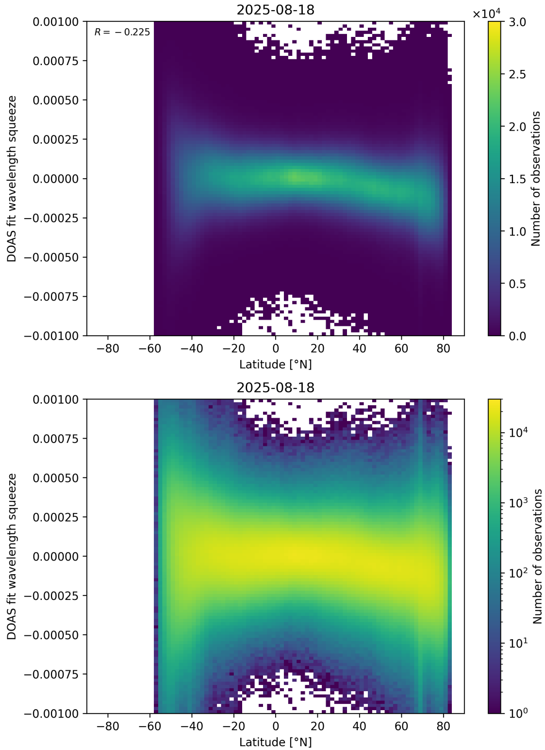
Figure 154: Scatter density plot of “Latitude” against “DOAS fit wavelength squeeze” for 2025-08-17 to 2025-08-19.
