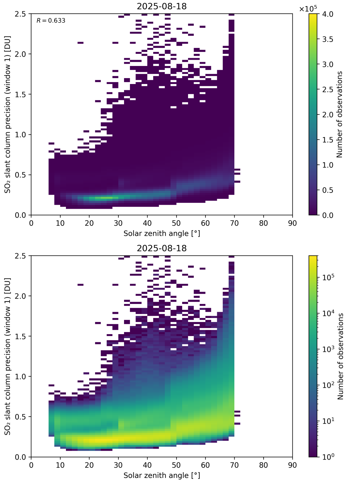
Figure 185: Scatter density plot of “Solar zenith angle” against “SO 2 slant column precision (window 1)” for 2025-08-17 to 2025-08-19.
