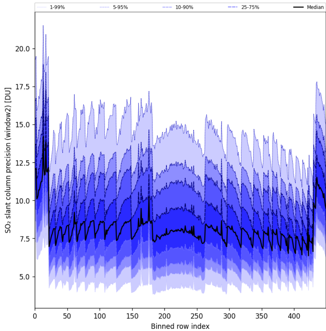
Figure 94: Along track statistics of “SO 2 slant column precision (window2)” for 2025-08-17 to 2025-08-19
