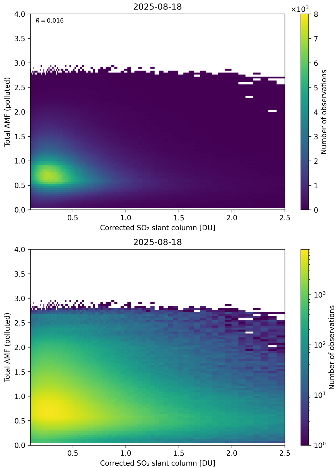
Figure 242: Scatter density plot of “Corrected SO 2 slant column” against “Total AMF (polluted)” for 2025-08-17 to 2025-08-19.
