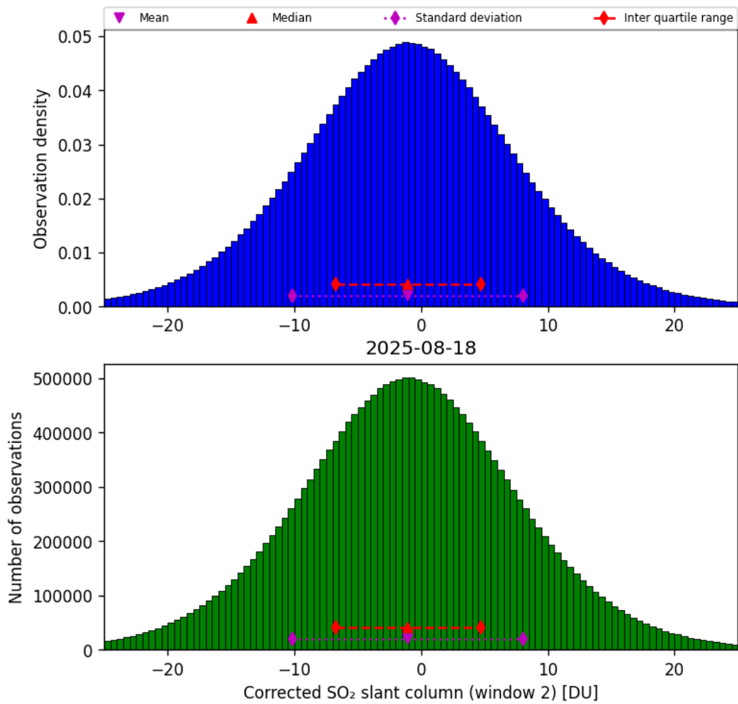
Figure 69: Histogram of “Corrected SO 2 slant column (window 2)” for 2025-08-17 to 2025-08-19
