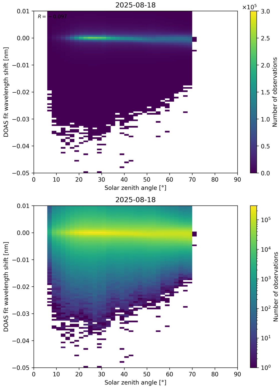
Figure 174: Scatter density plot of “Solar zenith angle” against “DOAS fit wavelength shift” for 2025-08-17 to 2025-08-19.
