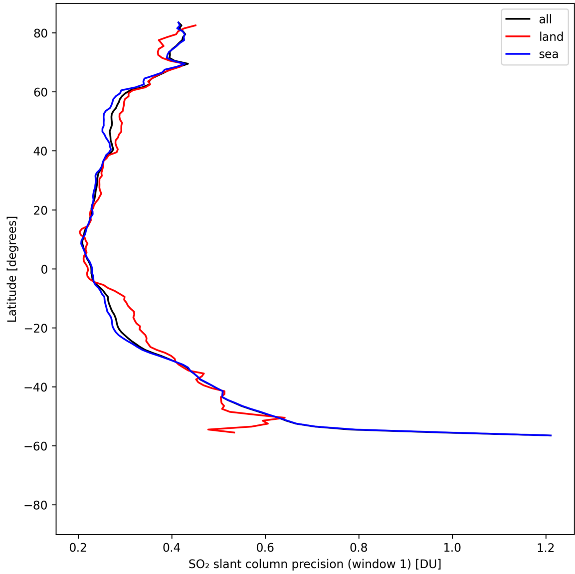
Figure 38: Zonal average of “SO 2 slant column precision (window 1)” for 2025-08-17 to 2025-08-19.
