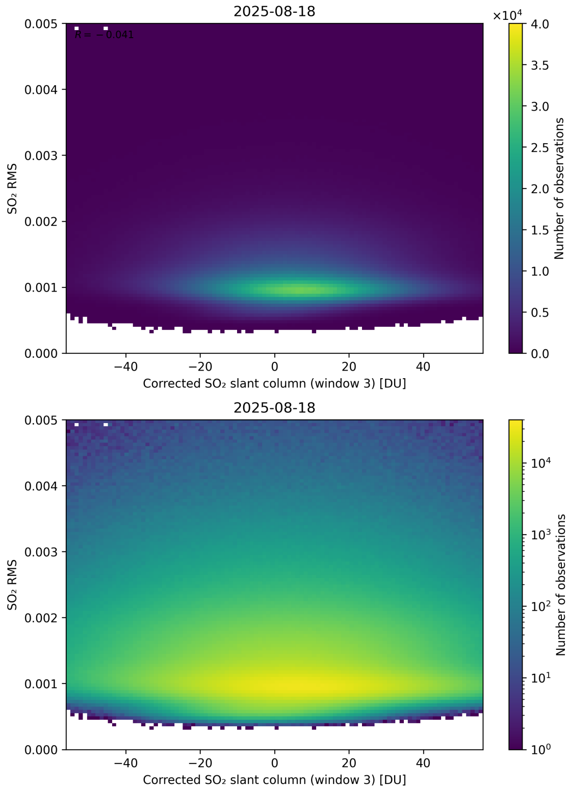
Figure 258: Scatter density plot of “Corrected SO 2 slant column (window 3)” against “SO 2 RMS” for 2025-08-17 to 2025-08-19.
