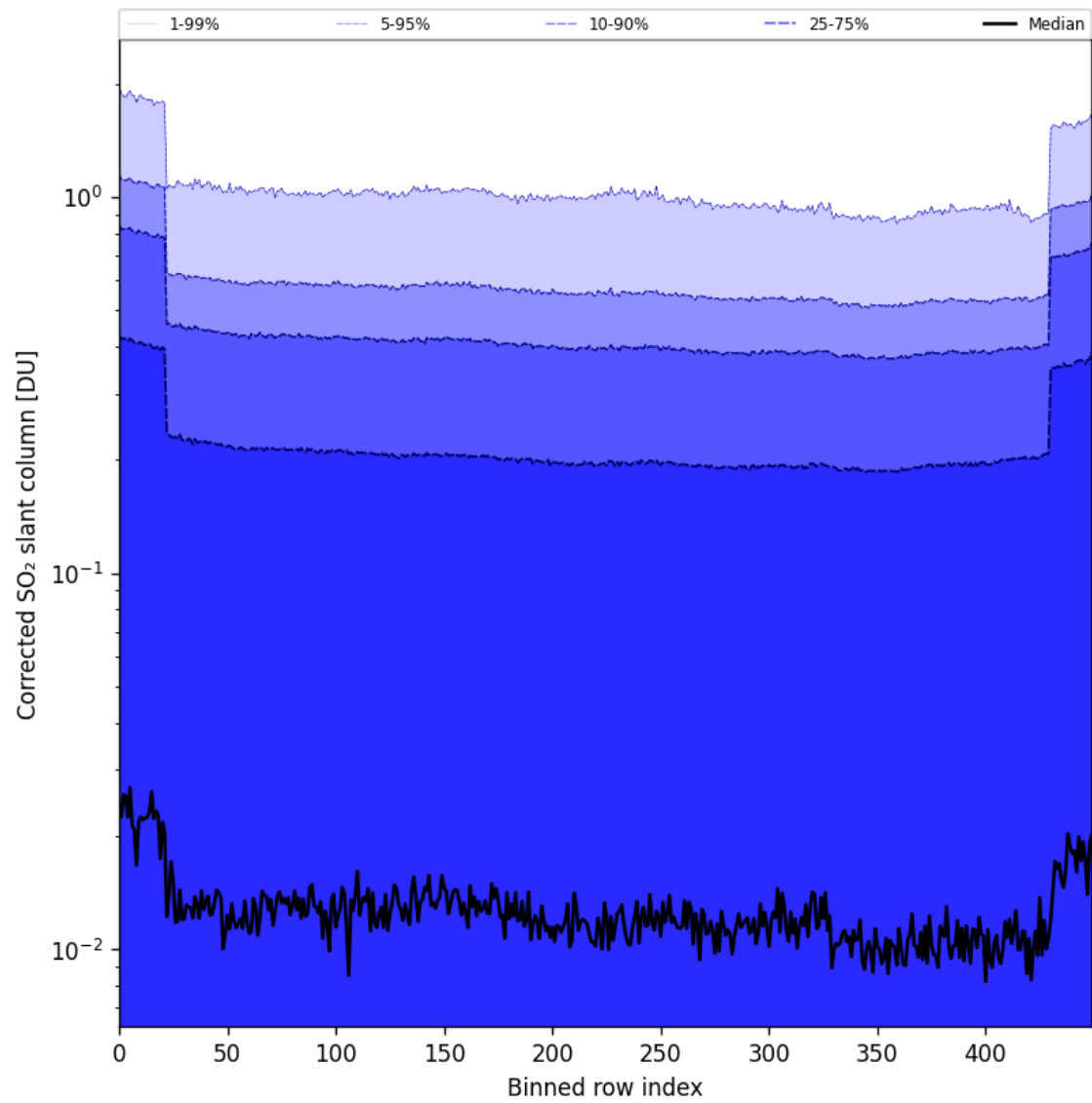
Figure 86: Along track statistics of “Corrected SO 2 slant column” for 2025-08-17 to 2025-08-19
