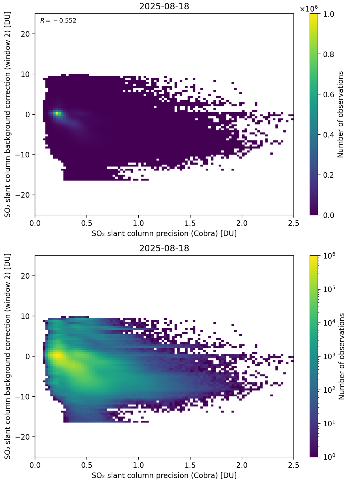
Figure 200: Scatter density plot of “SO 2 slant column precision (Cobra)” against “SO 2 slant column background correction (window 2)” for 2025-08-17 to 2025-08-19.
