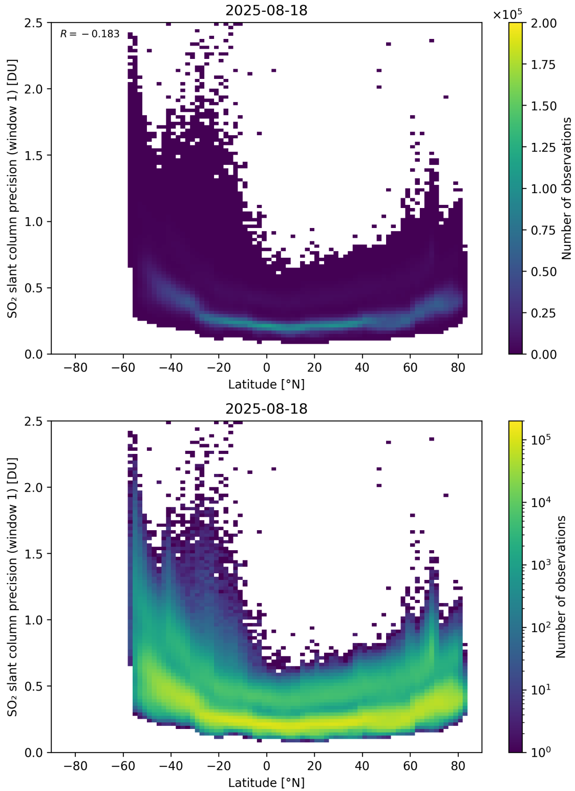
Figure 163: Scatter density plot of “Latitude” against “SO 2 slant column precision (window 1)” for 2025-08-17 to 2025-08-19.
