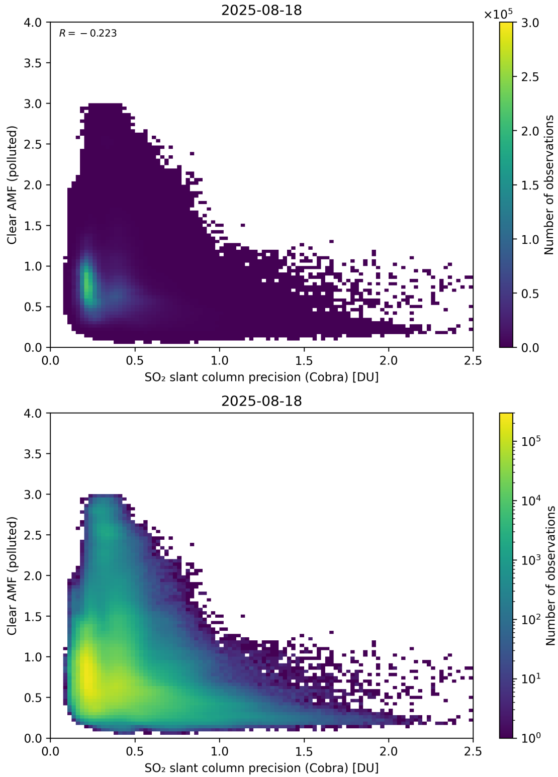
Figure 205: Scatter density plot of “SO 2 slant column precision (Cobra)” against “Clear AMF (polluted)” for 2025-08-17 to 2025-08-19.
