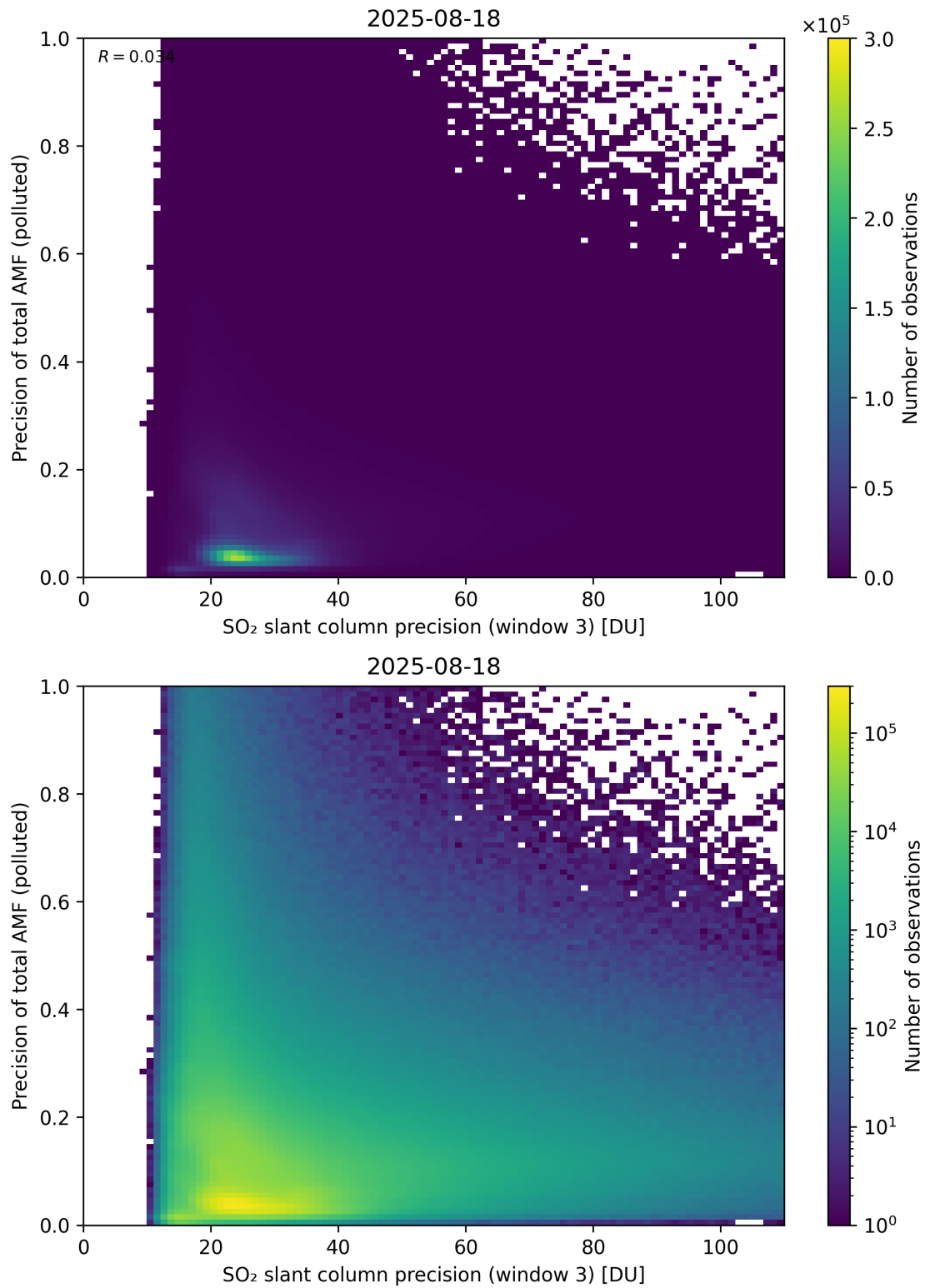
Figure 314: Scatter density plot of “SO 2 slant column precision (window 3)” against “Precision of total AMF (polluted)” for 2025-08-17 to 2025-08-19.
