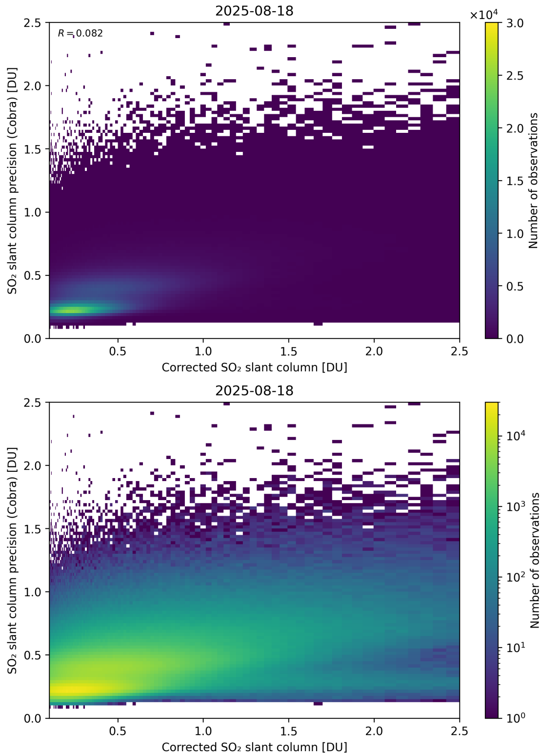
Figure 234: Scatter density plot of “Corrected SO 2 slant column” against “SO 2 slant column precision (Cobra)” for 2025-08-17 to 2025-08-19.
