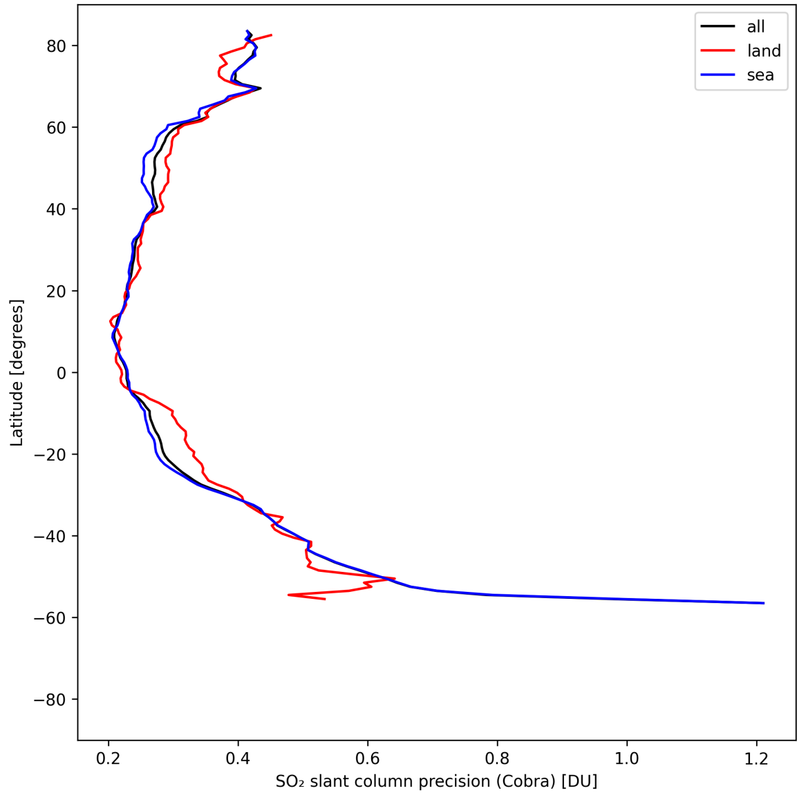
Figure 36: Zonal average of “SO 2 slant column precision (Cobra)” for 2025-08-17 to 2025-08-19.
