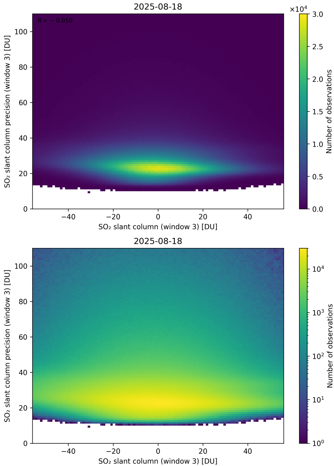
Figure 317: Scatter density plot of “SO 2 slant column (window 3)” against “SO 2 slant column precision (window 3)” for 2025-08-17 to 2025-08-19.
