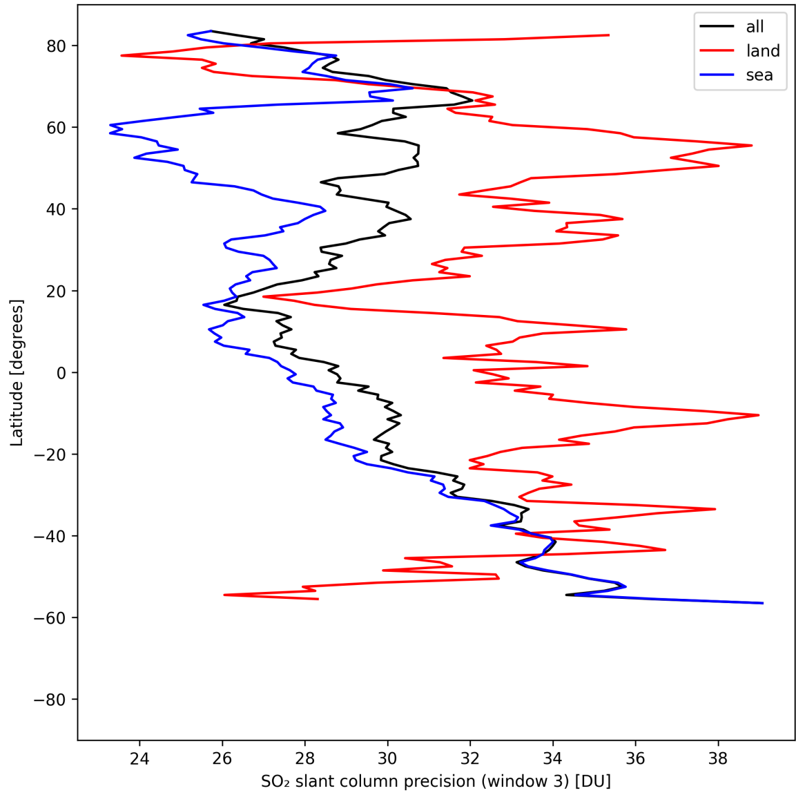
Figure 46: Zonal average of “SO 2 slant column precision (window 3)” for 2025-08-17 to 2025-08-19.
