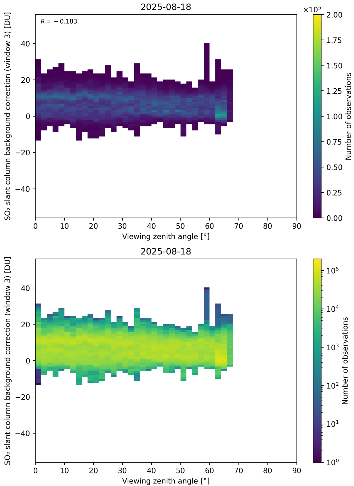
Figure 364: Scatter density plot of “Viewing zenith angle” against “SO 2 slant column background correction (window 3)” for 2025-08-17 to 2025-08-19.
