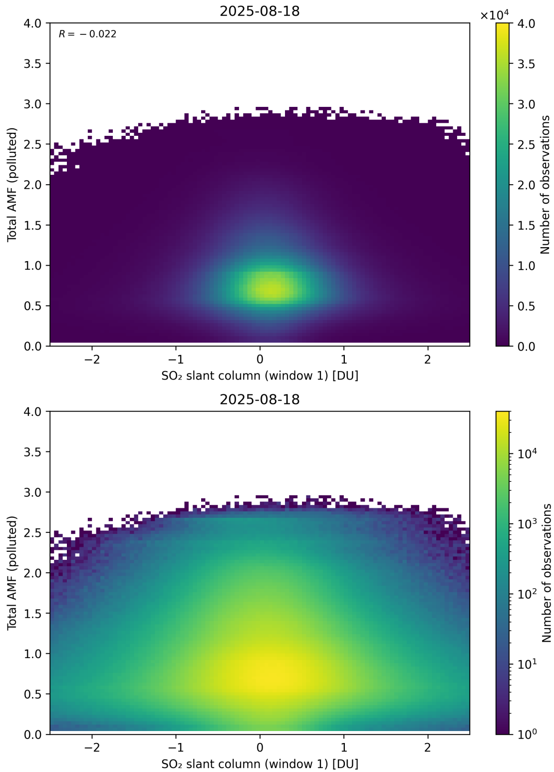
Figure 289: Scatter density plot of “SO 2 slant column (window 1)” against “Total AMF (polluted)” for 2025-08-17 to 2025-08-19.
