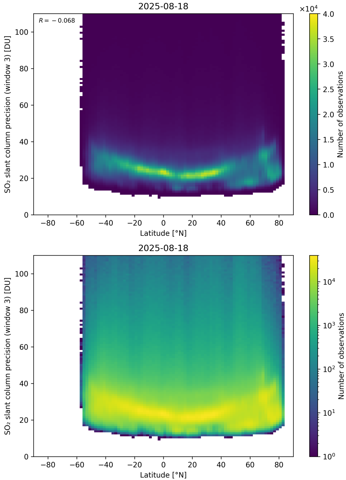
Figure 166: Scatter density plot of “Latitude” against “SO 2 slant column precision (window 3)” for 2025-08-17 to 2025-08-19.
