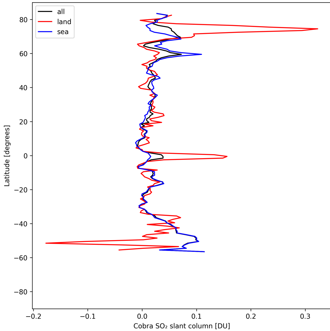
Figure 35: Zonal average of “Cobra SO 2 slant column” for 2025-08-17 to 2025-08-19.
