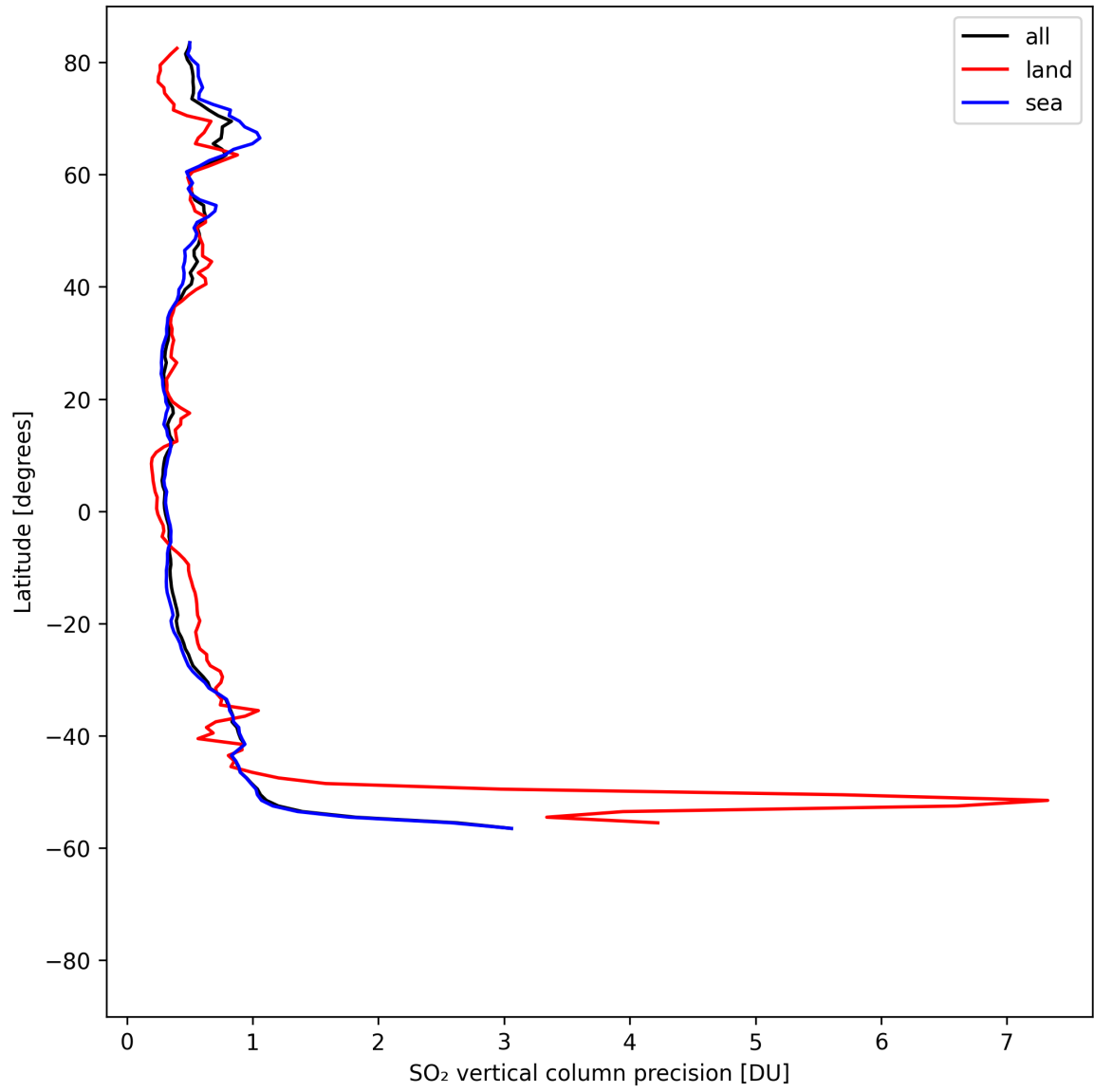
Figure 33: Zonal average of “SO 2 vertical column precision” for 2025-08-17 to 2025-08-19.
