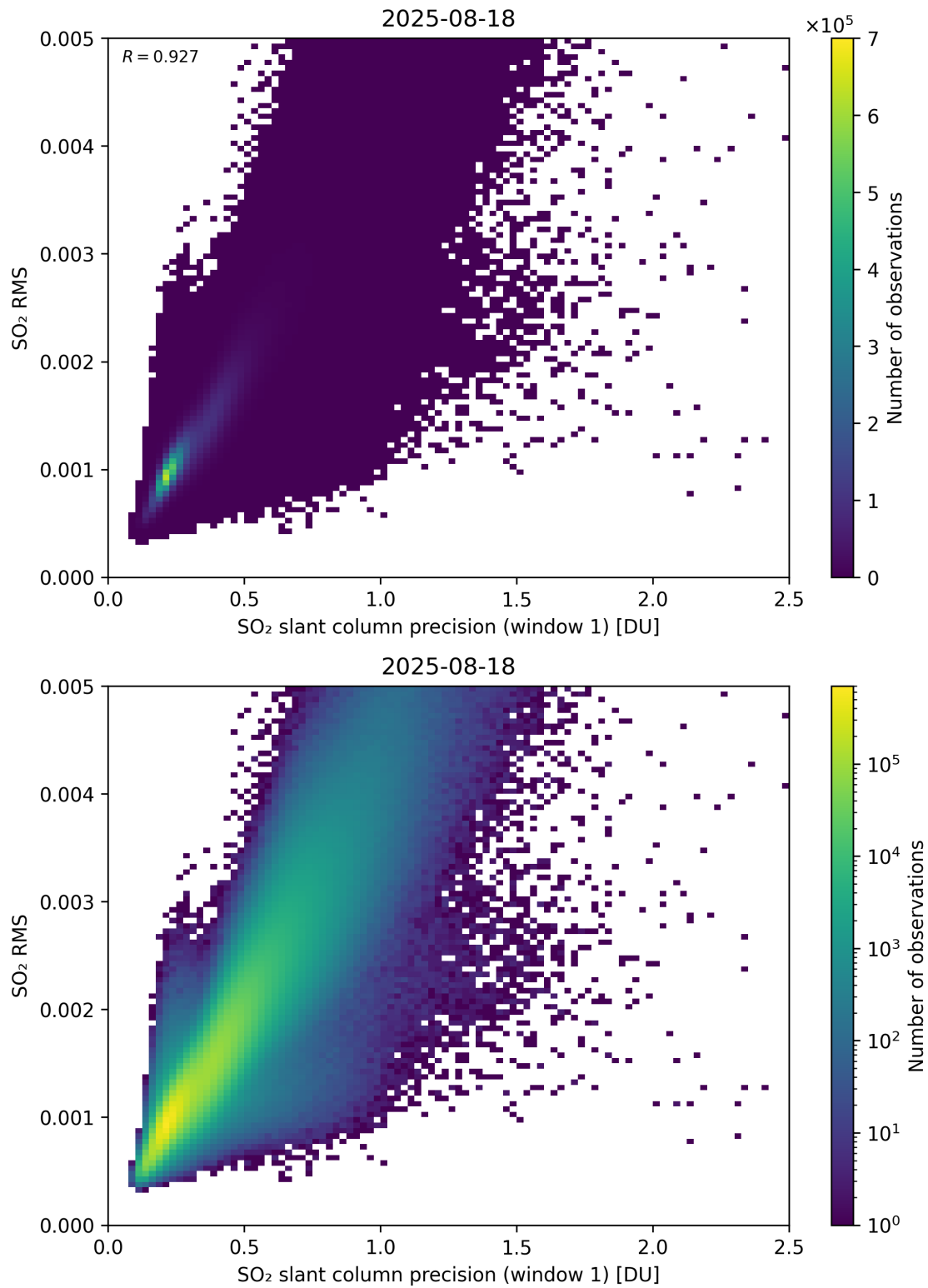
Figure 273: Scatter density plot of “SO 2 slant column precision (window 1)” against “SO 2 RMS” for 2025-08-17 to 2025-08-19.
