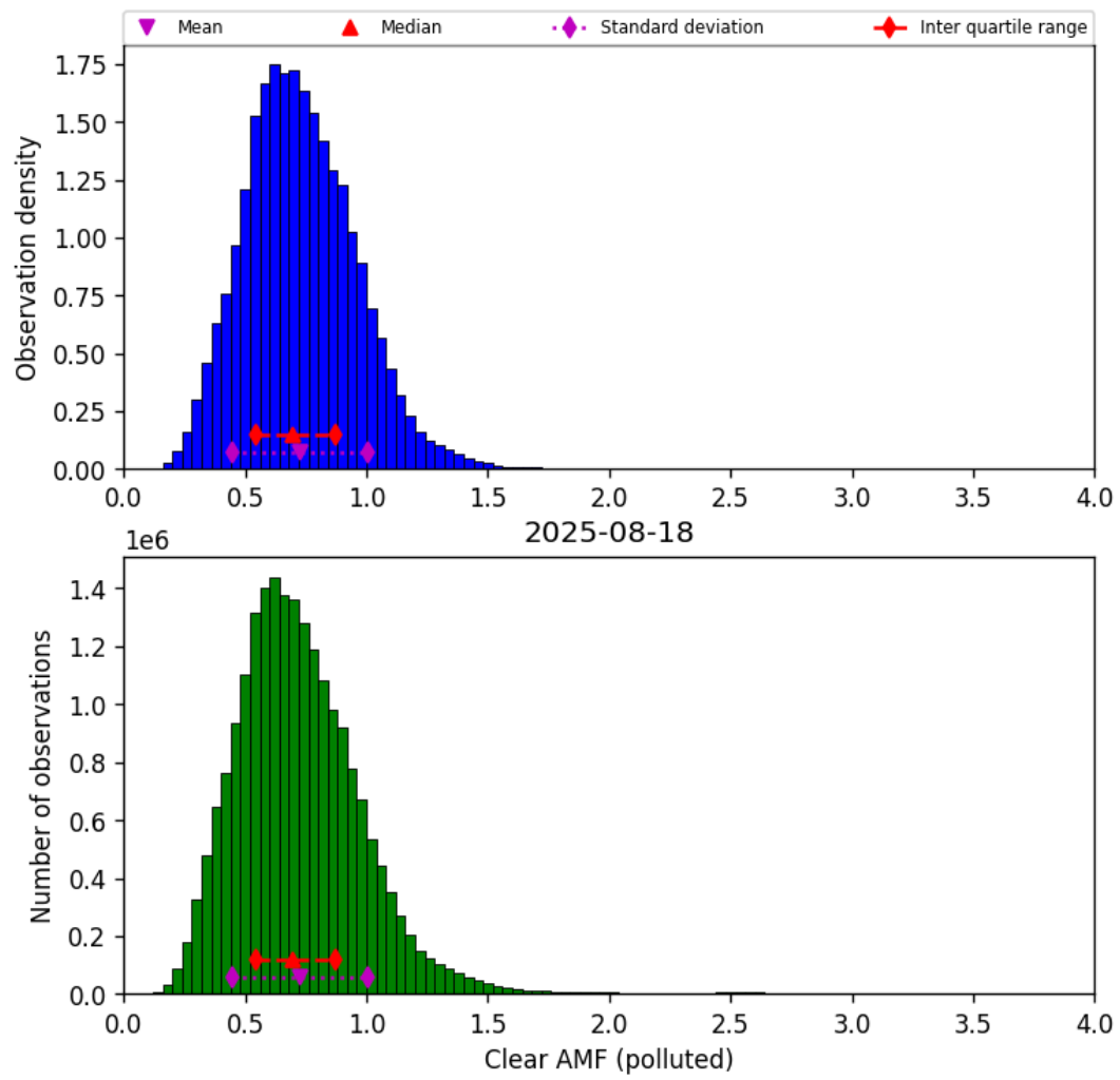
Figure 81: Histogram of “Clear AMF (polluted)” for 2025-08-17 to 2025-08-19
