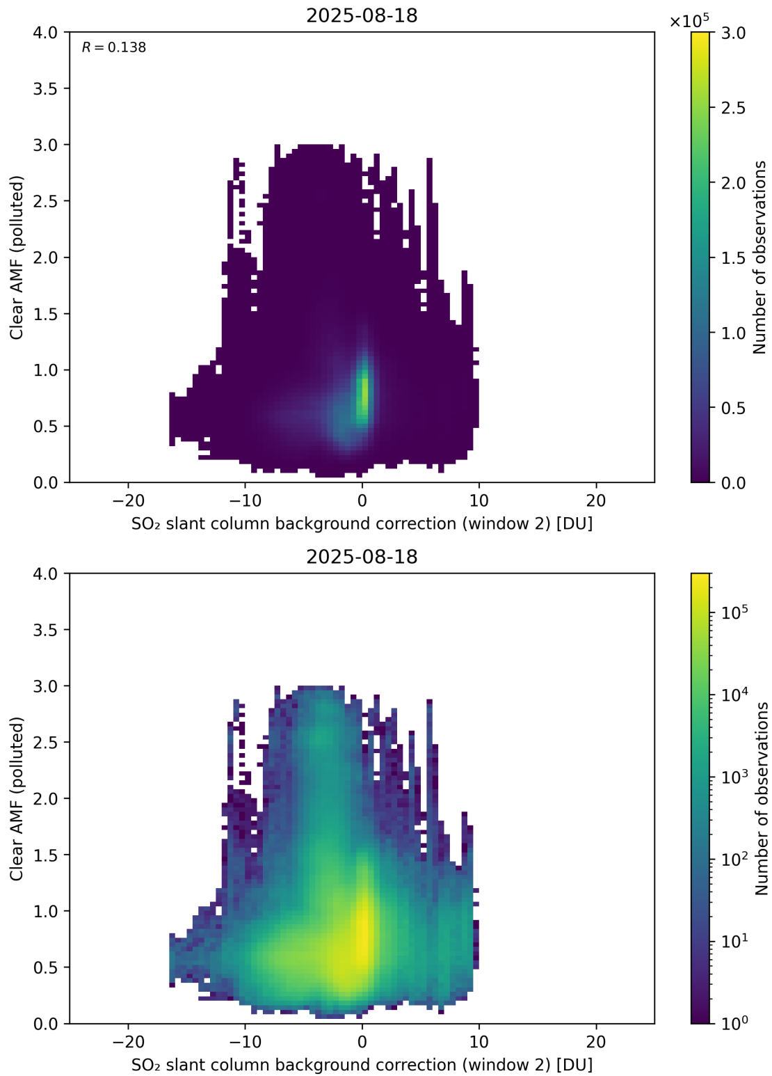
Figure 126: Scatter density plot of “SO 2 slant column background correction (window 2)” against “Clear AMF (polluted)” for 2025-08-17 to 2025-08-19.
