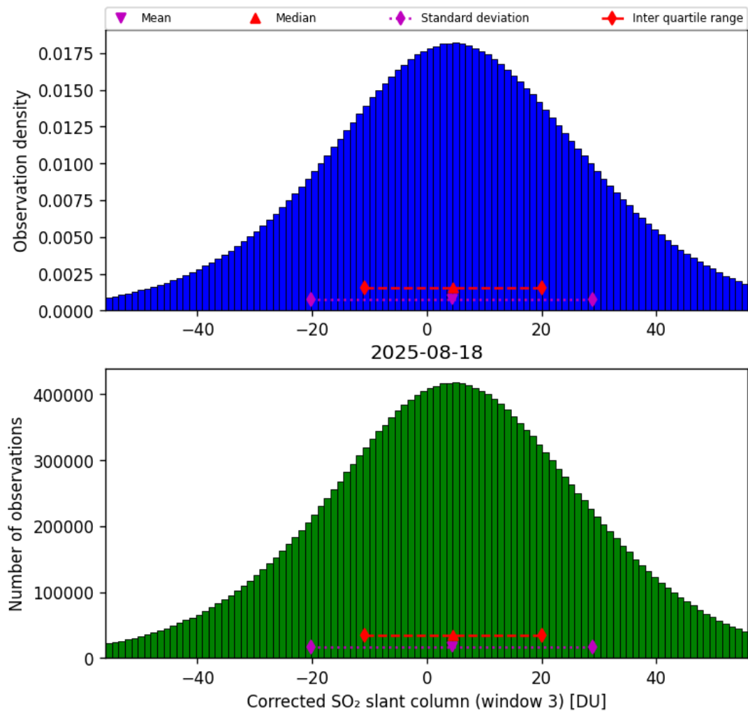
Figure 73: Histogram of “Corrected SO 2 slant column (window 3)” for 2025-08-17 to 2025-08-19
