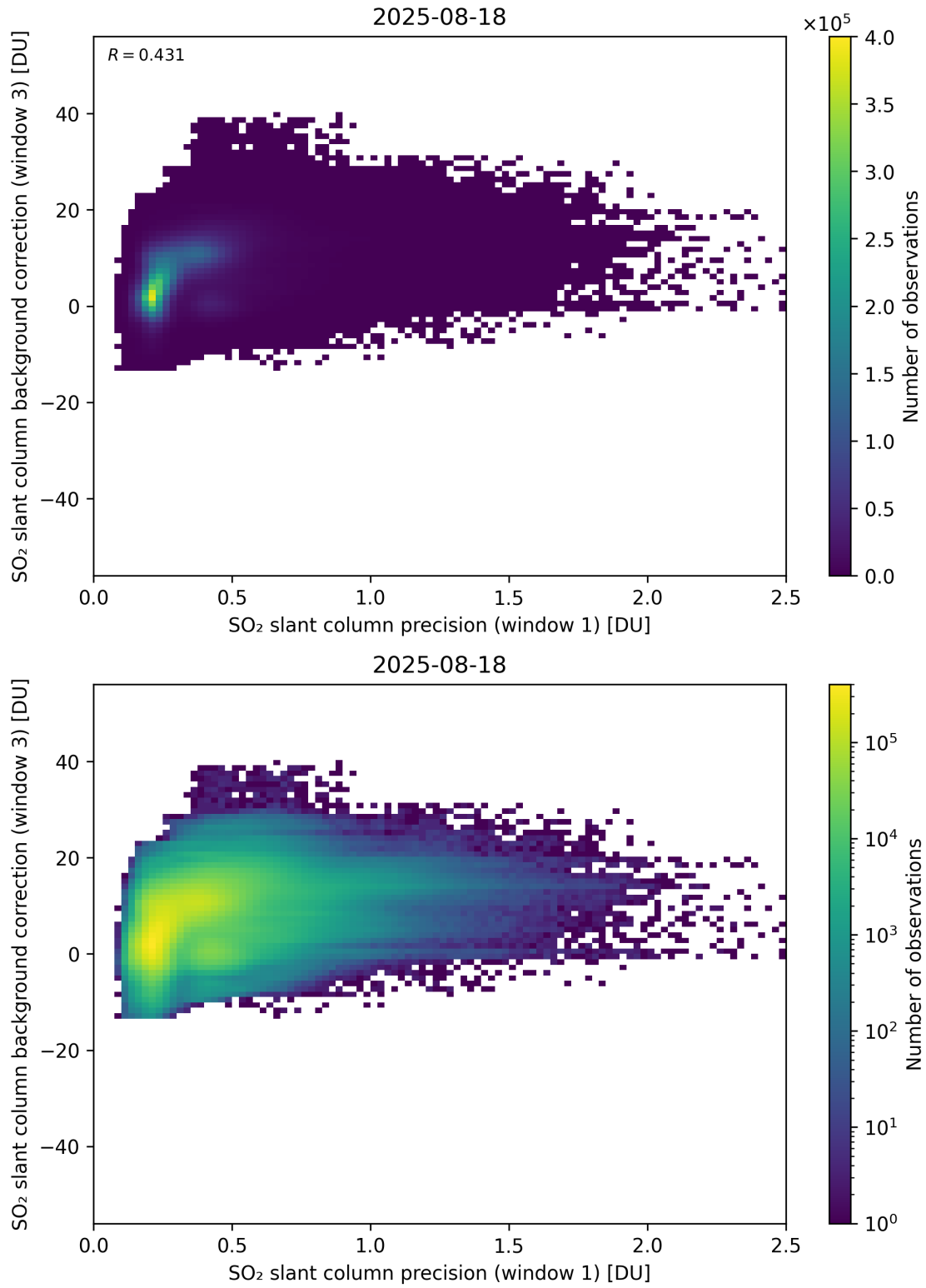
Figure 270: Scatter density plot of “SO 2 slant column precision (window 1)” against “SO 2 slant column background correction (window 3)” for 2025-08-17 to 2025-08-19.
