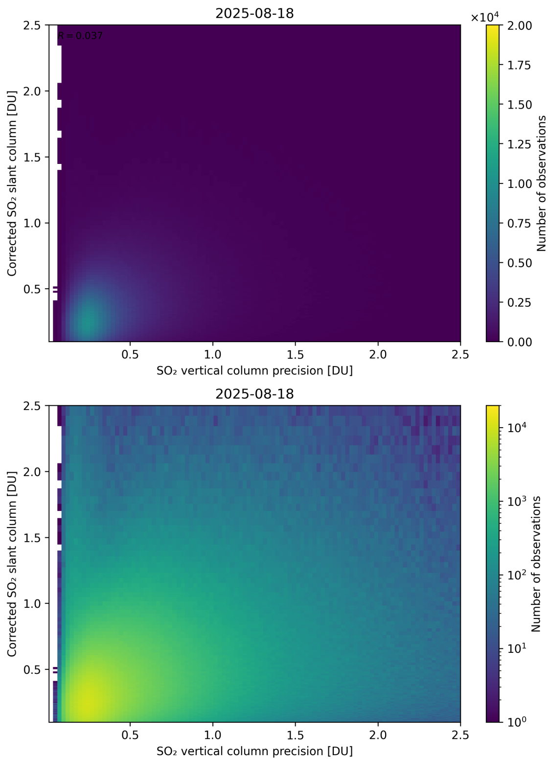
Figure 338: Scatter density plot of “SO 2 vertical column precision” against “Corrected SO 2 slant column” for 2025-08-17 to 2025-08-19.
