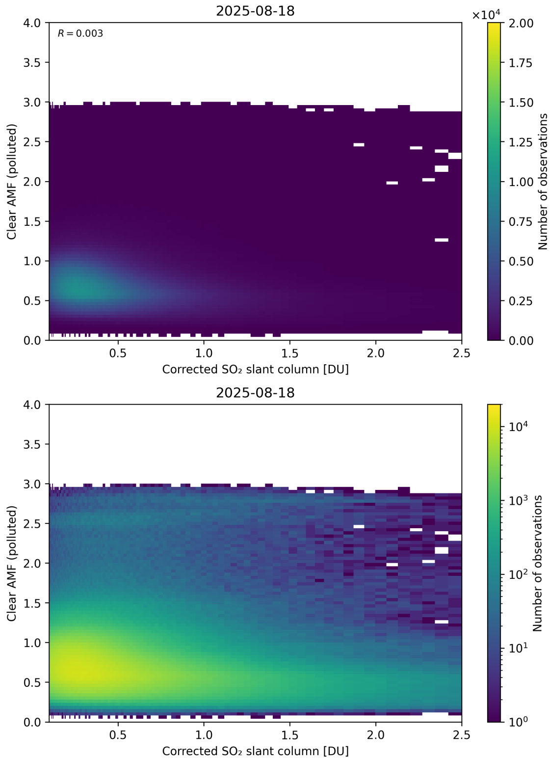
Figure 232: Scatter density plot of “Corrected SO 2 slant column” against “Clear AMF (polluted)” for 2025-08-17 to 2025-08-19.
