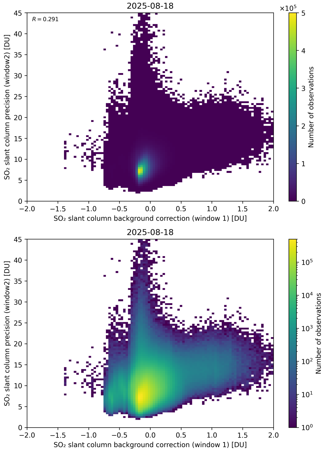
Figure 117: Scatter density plot of “SO 2 slant column background correction (window 1)” against “SO 2 slant column precision (window2)” for 2025-08-17 to 2025-08-19.
