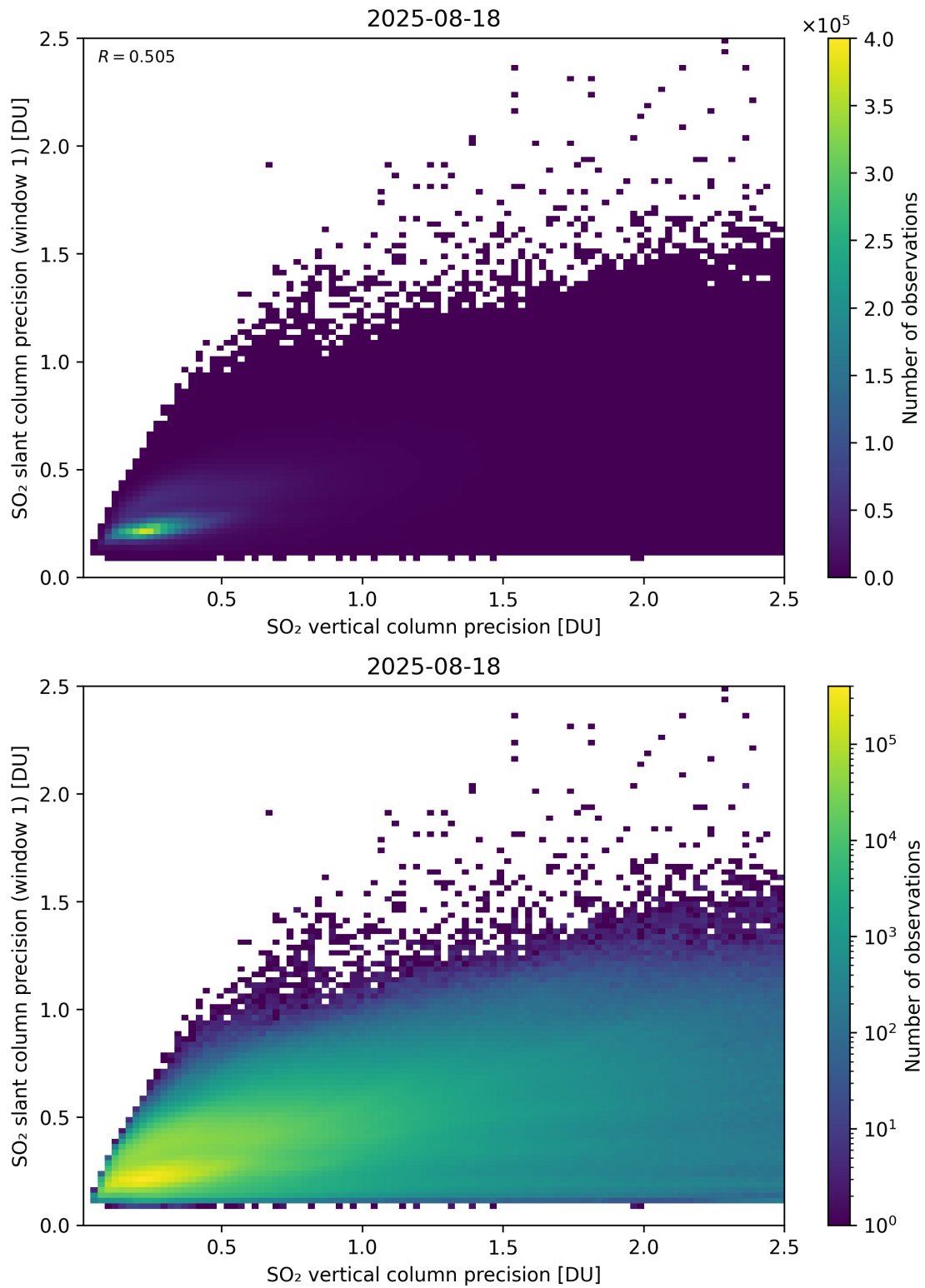
Figure 342: Scatter density plot of “SO 2 vertical column precision” against “SO 2 slant column precision (window 1)” for 2025-08-17 to 2025-08-19.
