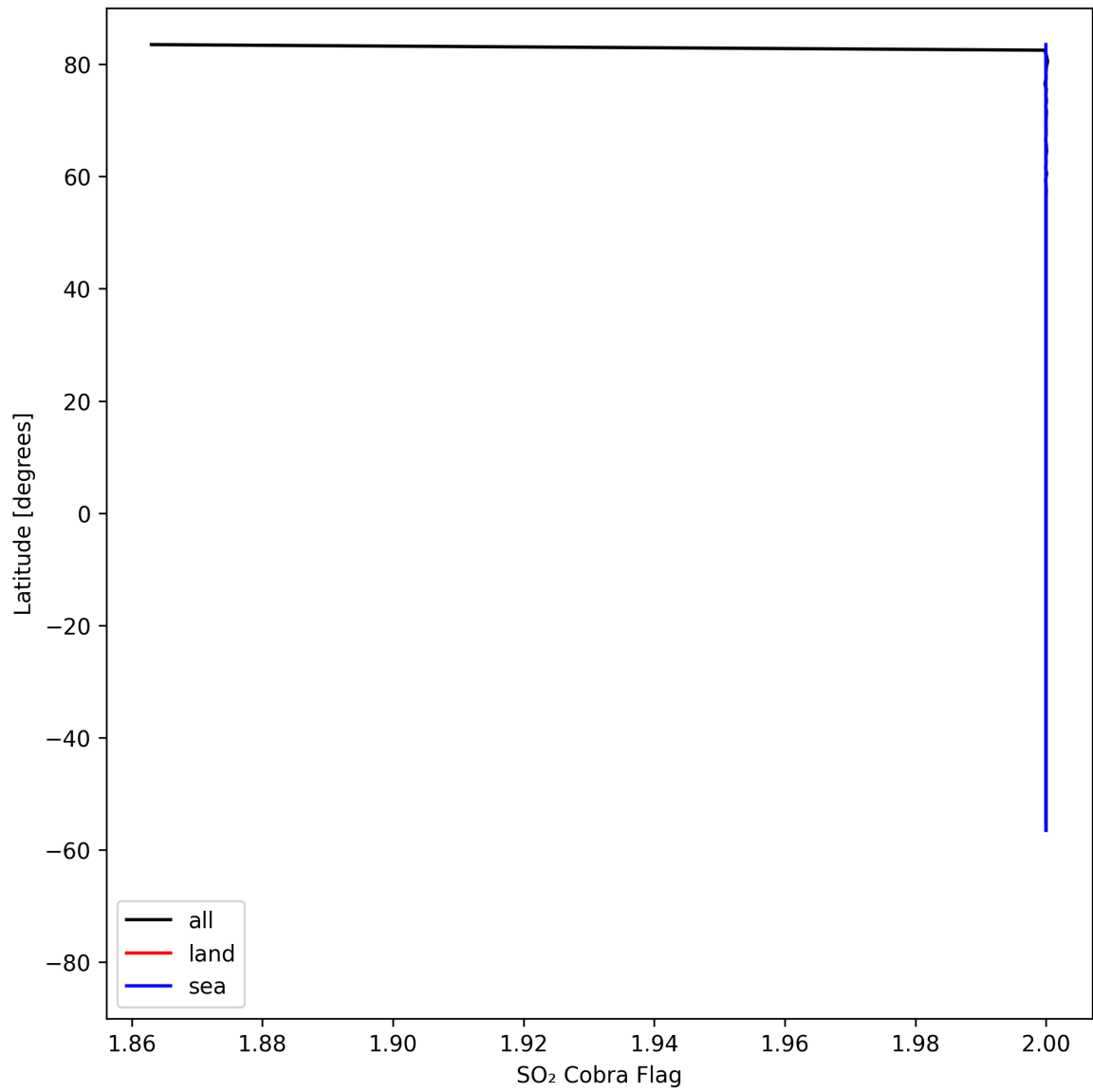
Figure 49: Zonal average of "SO 2 Cobra Flag" for 2025-08-17 to 2025-08-19.
