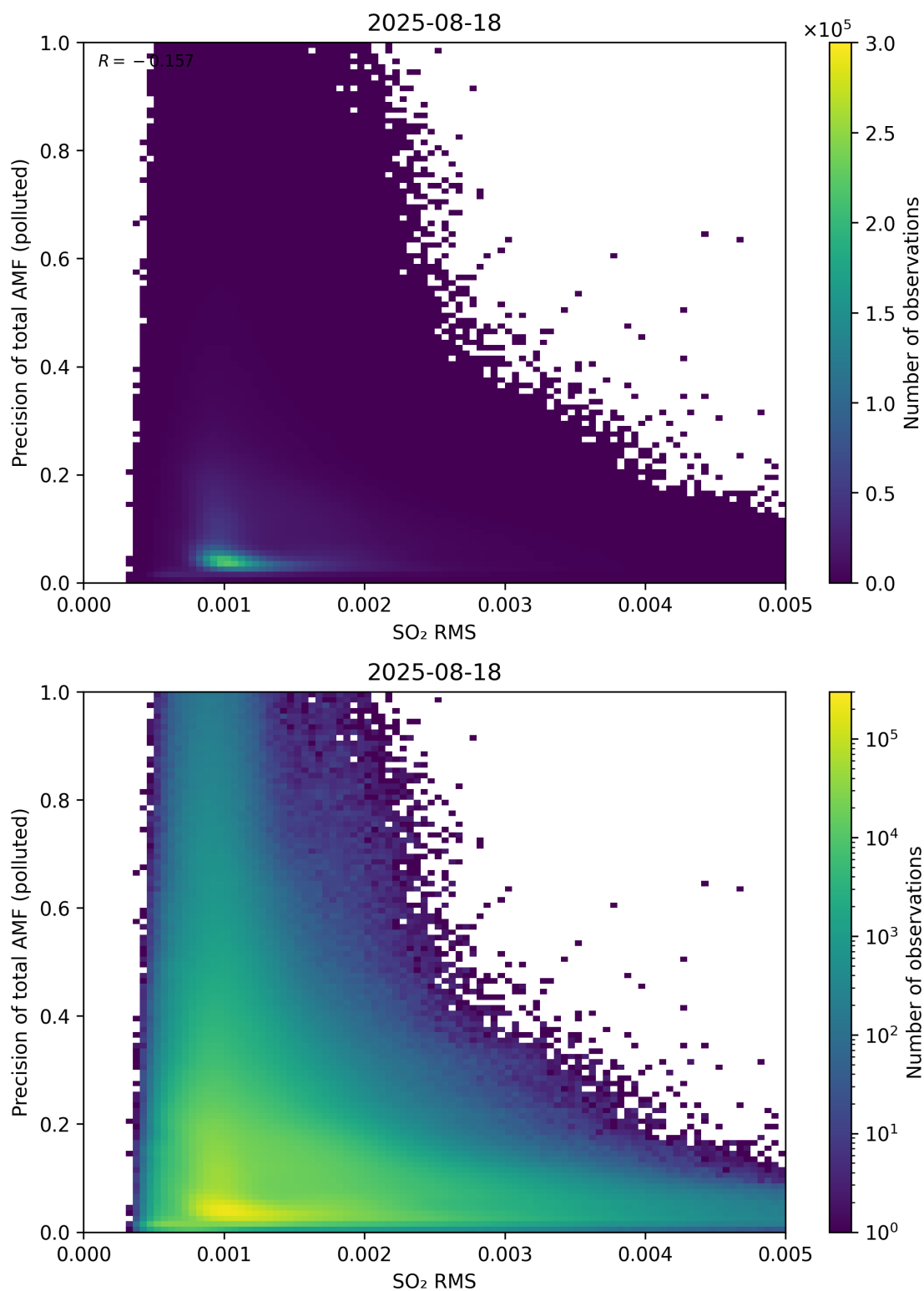
Figure 149: Scatter density plot of “SO 2 RMS” against “Precision of total AMF (polluted)” for 2025-08-17 to 2025-08-19.
