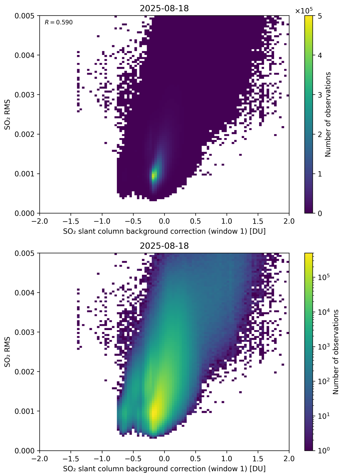
Figure 113: Scatter density plot of “SO 2 slant column background correction (window 1)” against “SO 2 RMS” for 2025-08-17 to 2025-08-19.
