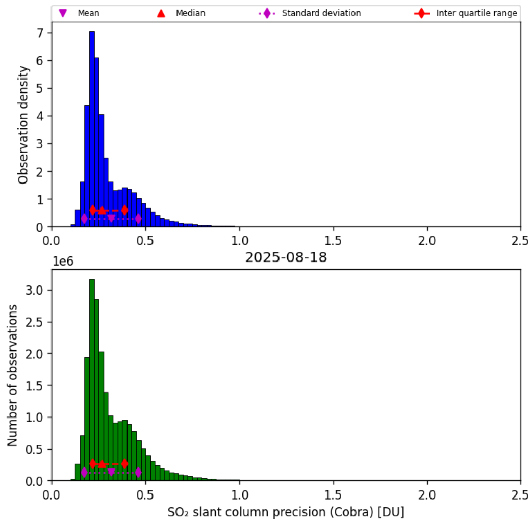
Figure 62: Histogram of “SO 2 slant column precision (Cobra)” for 2025-08-17 to 2025-08-19
