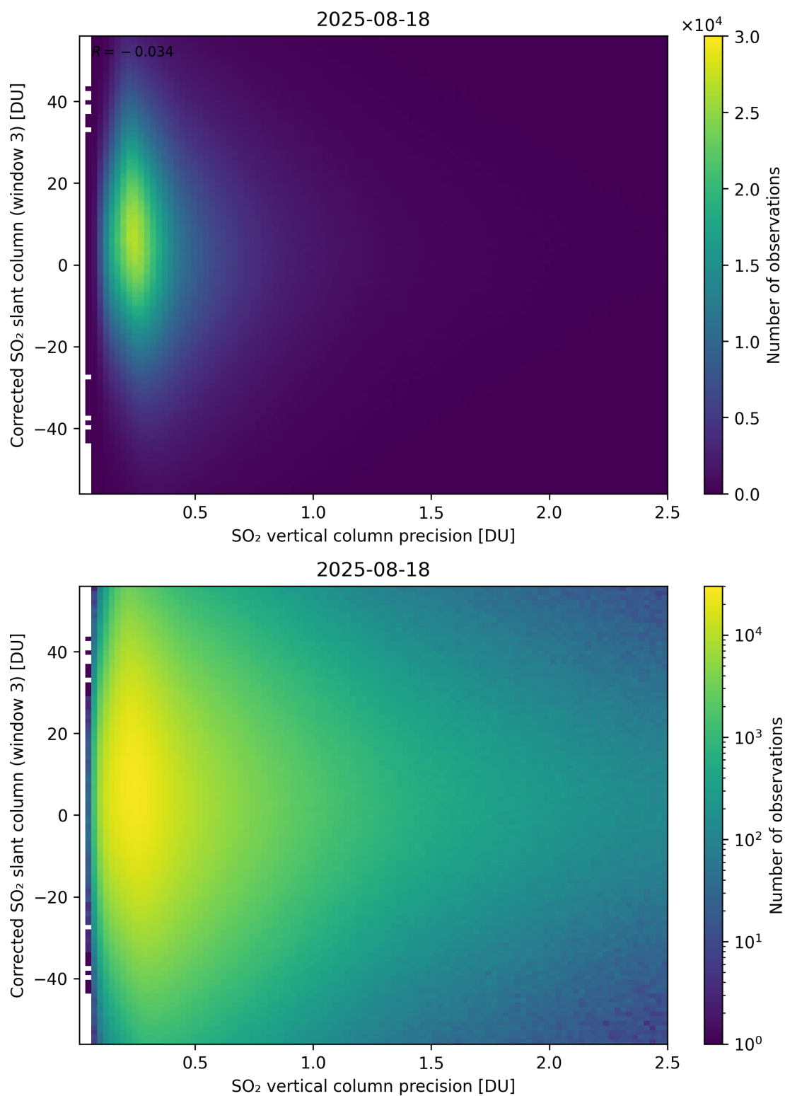
Figure 340: Scatter density plot of “SO 2 vertical column precision” against “Corrected SO 2 slant column (window 3)” for 2025-08-17 to 2025-08-19.
