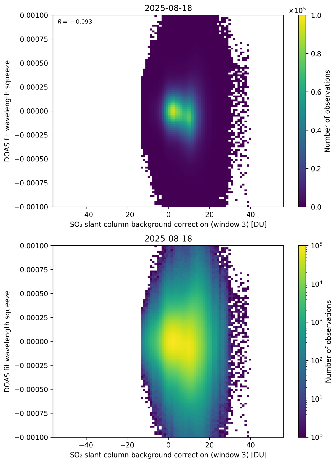
Figure 133: Scatter density plot of “SO 2 slant column background correction (window 3)” against “DOAS fit wavelength squeeze” for 2025-08-17 to 2025-08-19.
