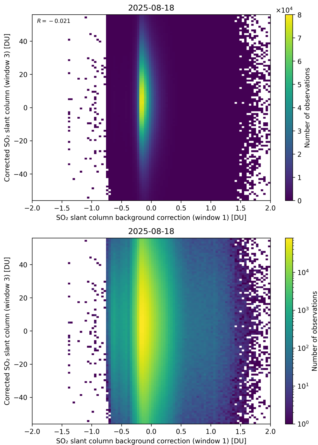
Figure 116: Scatter density plot of “SO 2 slant column background correction (window 1)” against “Corrected SO 2 slant column (window 3)” for 2025-08-17 to 2025-08-19.
