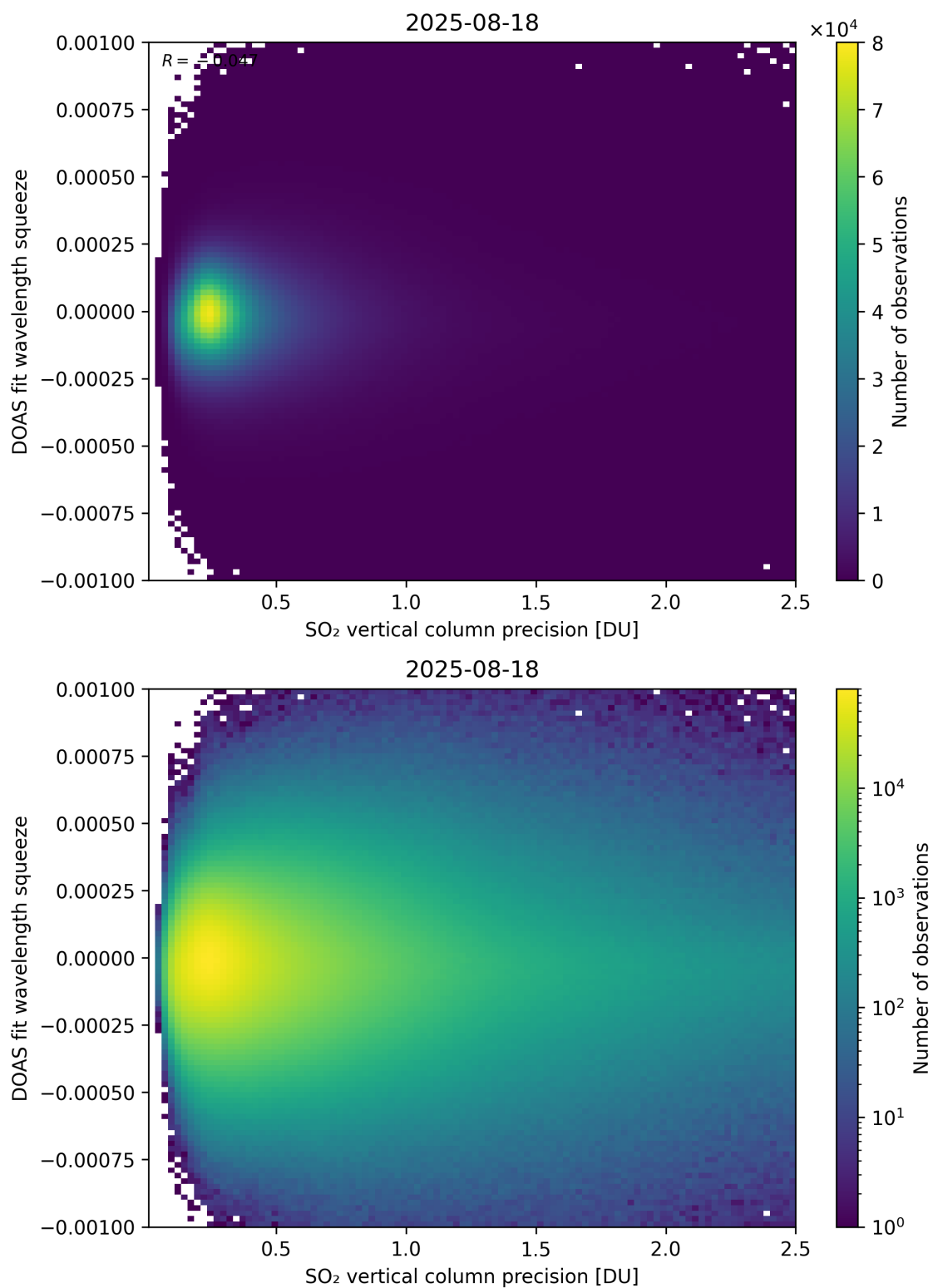
Figure 333: Scatter density plot of “SO 2 vertical column precision” against “DOAS fit wavelength squeeze” for 2025-08-17 to 2025-08-19.
