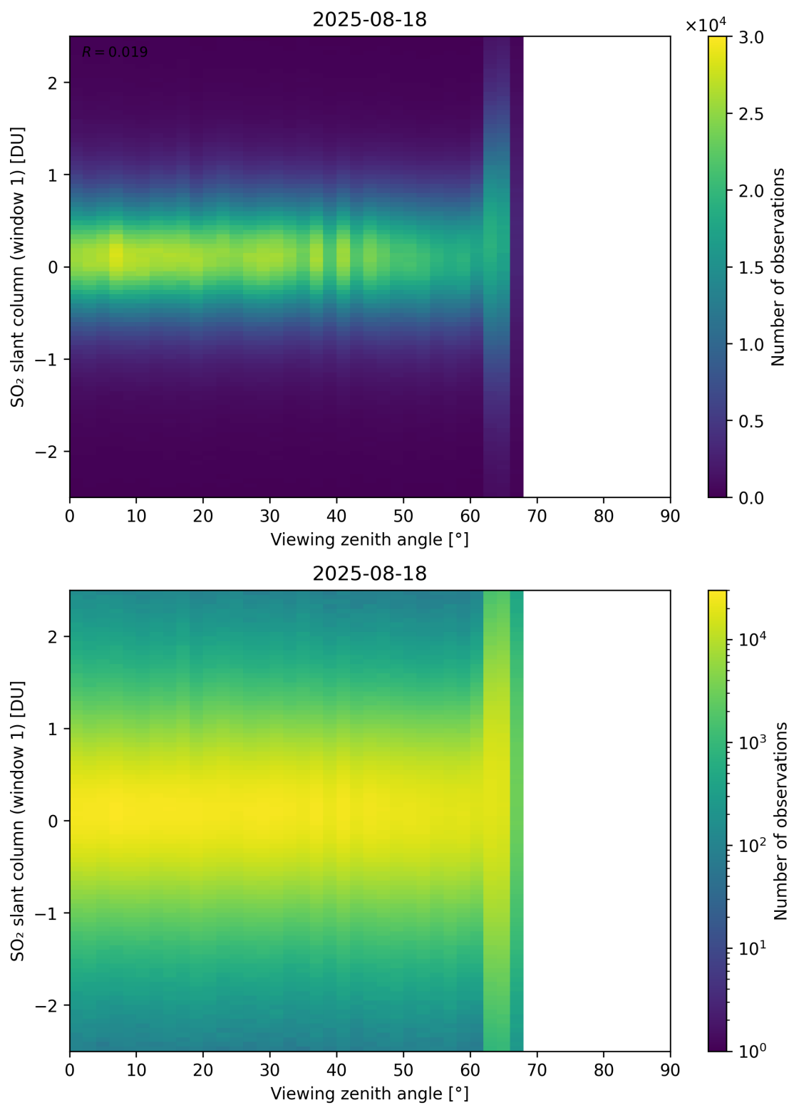
Figure 376: Scatter density plot of “Viewing zenith angle” against “SO 2 slant column (window 1)” for 2025-08-17 to 2025-08-19.
