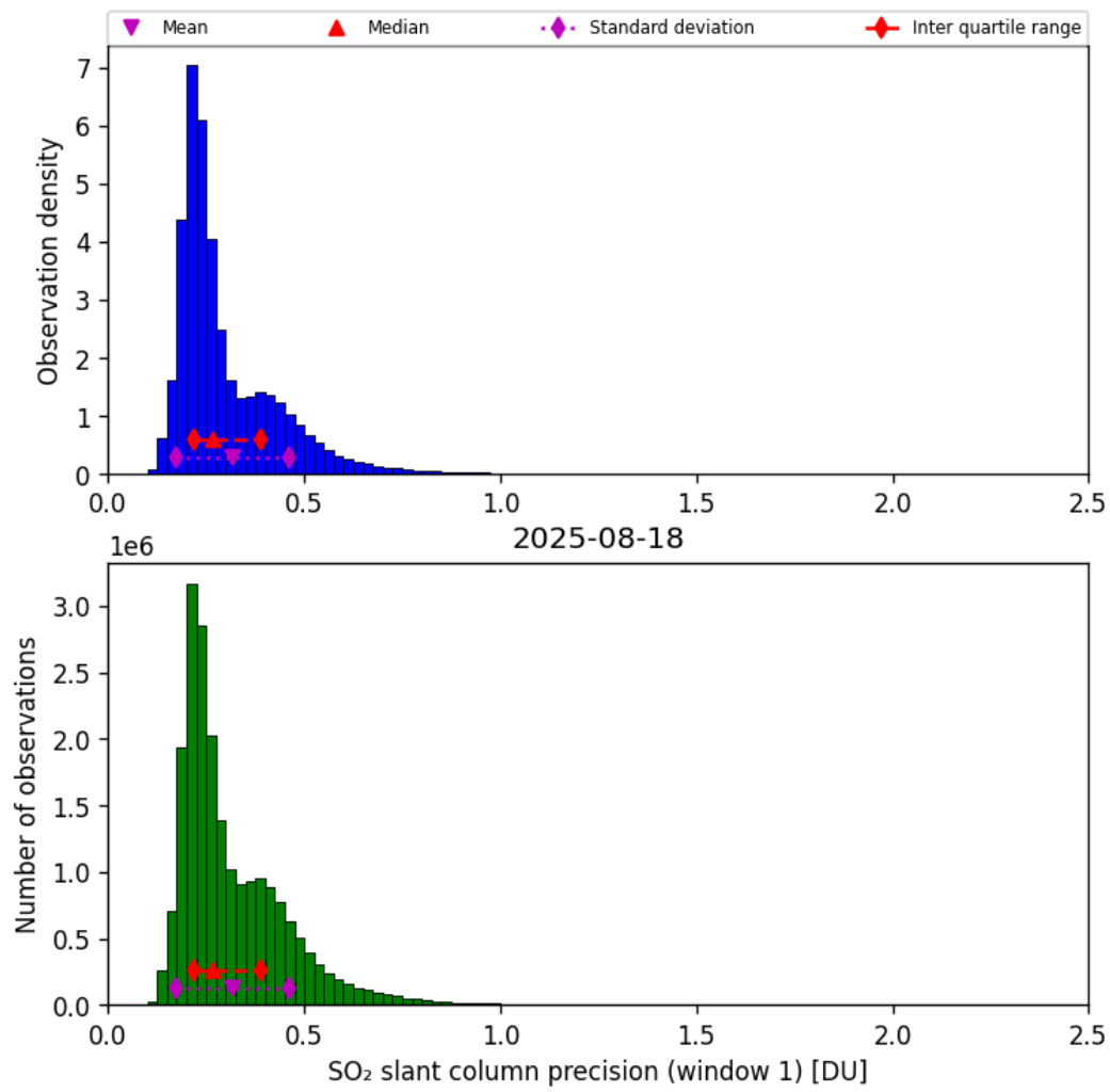
Figure 64: Histogram of “SO 2 slant column precision (window 1)” for 2025-08-17 to 2025-08-19
