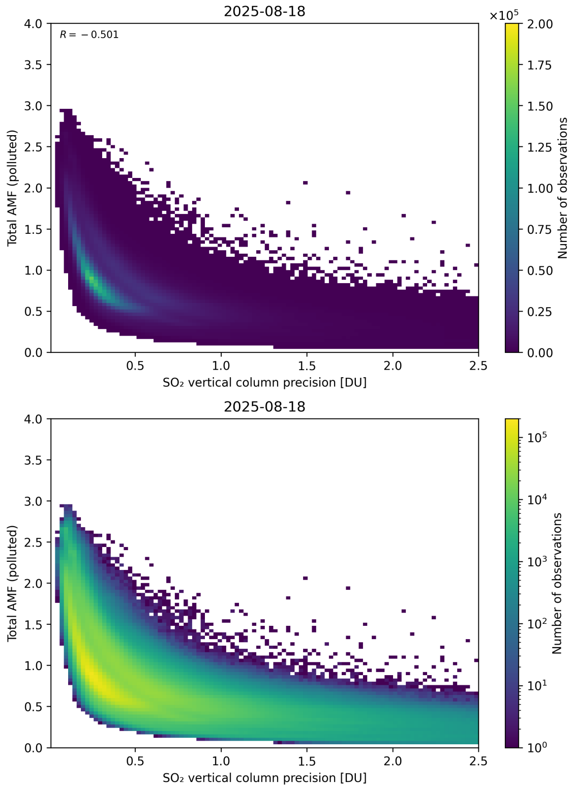
Figure 346: Scatter density plot of “SO 2 vertical column precision” against “Total AMF (polluted)” for 2025-08-17 to 2025-08-19.
