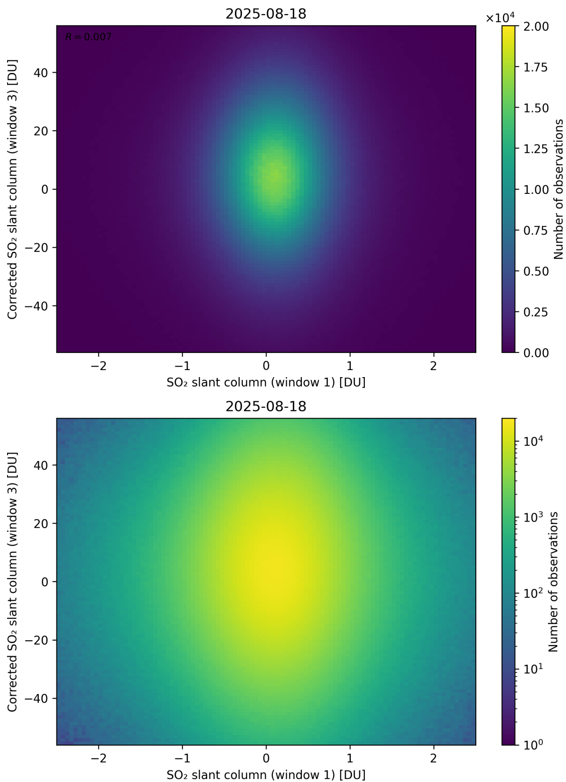
Figure 284: Scatter density plot of “SO 2 slant column (window 1)” against “Corrected SO 2 slant column (window 3)” for 2025-08-17 to 2025-08-19.
