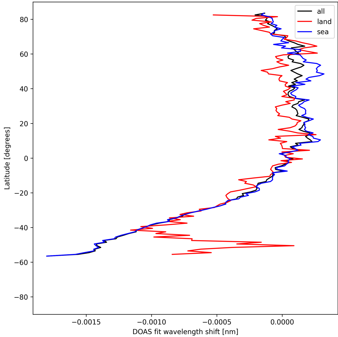
Figure 50: Zonal average of “DOAS fit wavelength shift” for 2025-08-17 to 2025-08-19.
