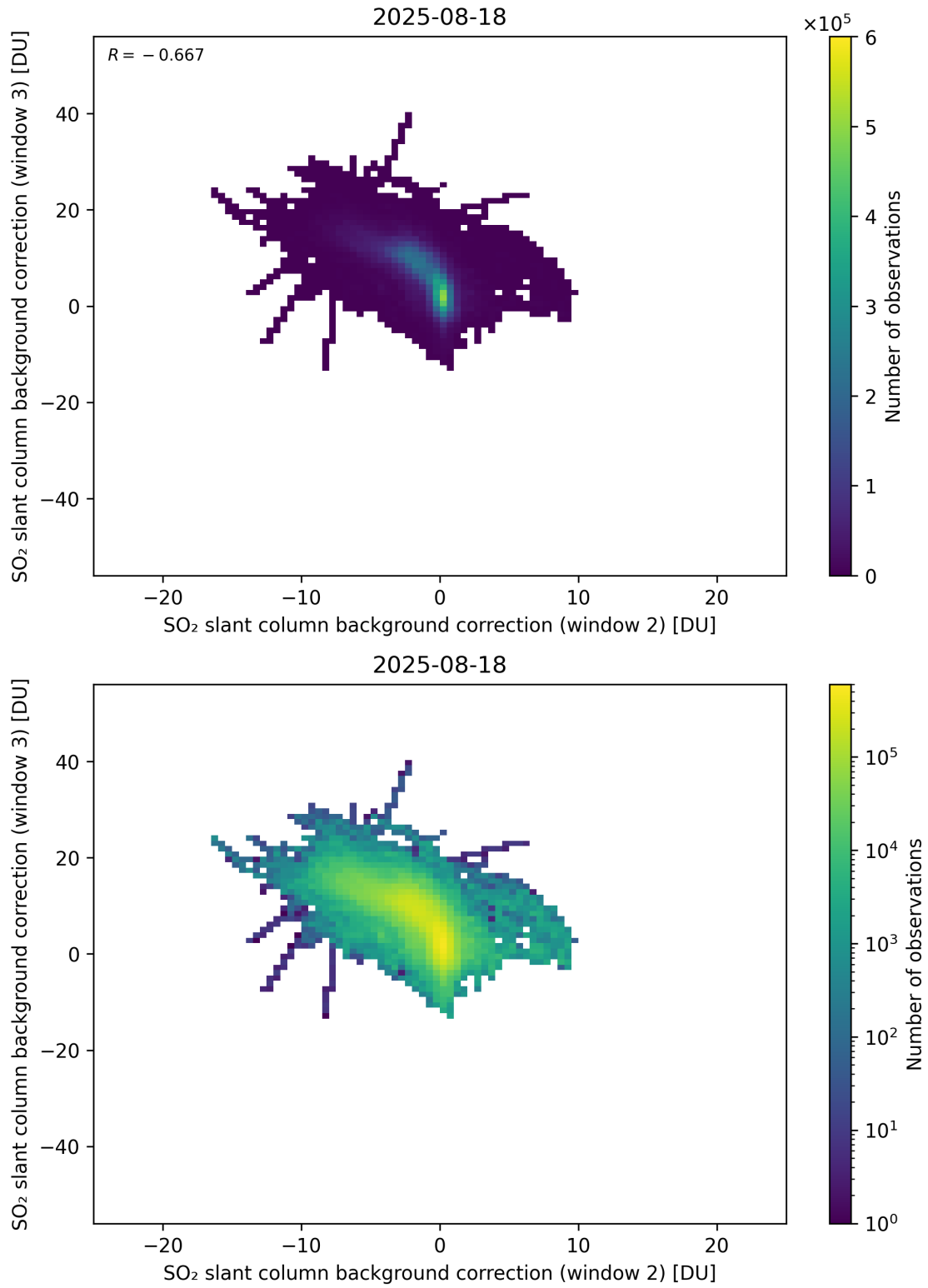
Figure 122: Scatter density plot of “SO 2 slant column background correction (window 2)” against “SO 2 slant column background correction (window 3)” for 2025-08-17 to 2025-08-19.
