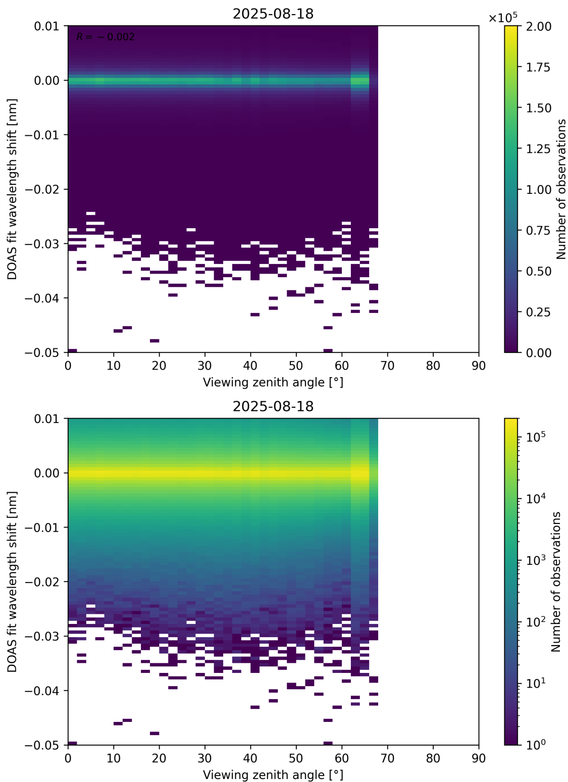
Figure 365: Scatter density plot of “Viewing zenith angle” against “DOAS fit wavelength shift” for 2025-08-17 to 2025-08-19.
