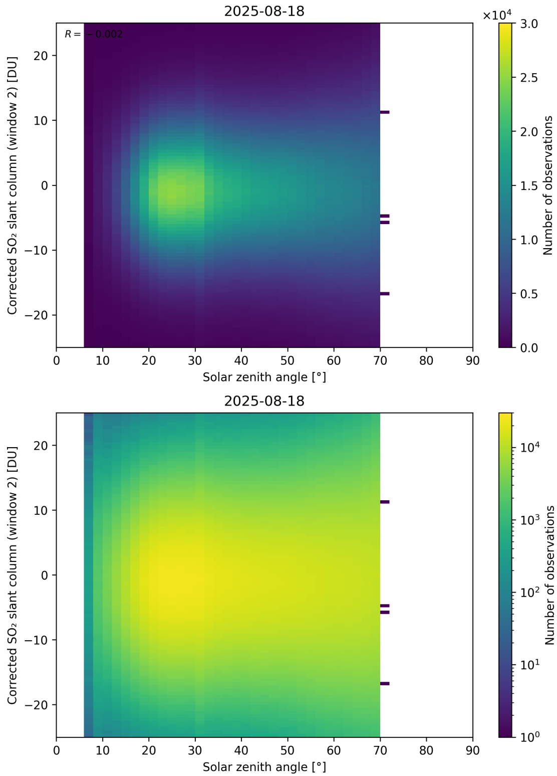
Figure 182: Scatter density plot of “Solar zenith angle” against “Corrected SO 2 slant column (window 2)” for 2025-08-17 to 2025-08-19.
