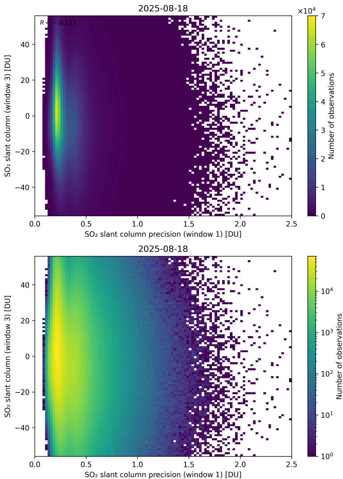
Figure 278: Scatter density plot of “SO 2 slant column precision (window 1)” against “SO 2 slant column (window 3)” for 2025-08-17 to 2025-08-19.
