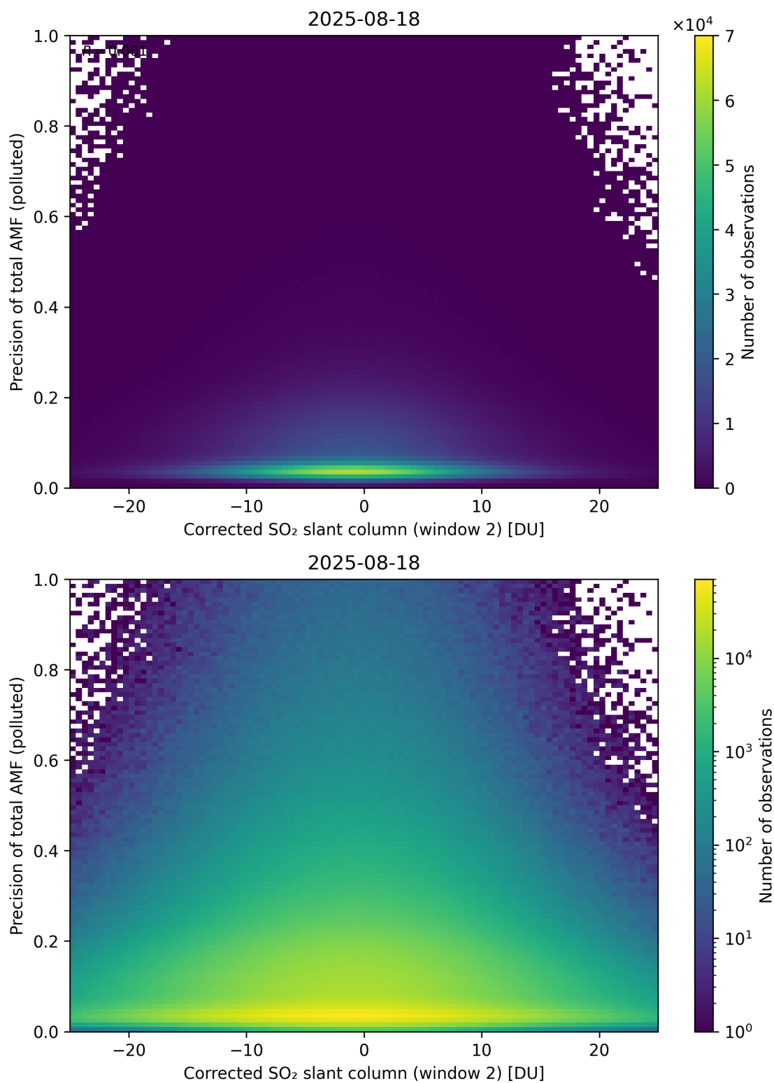
Figure 254: Scatter density plot of “Corrected SO 2 slant column (window 2)” against “Precision of total AMF (polluted)” for 2025-08-17 to 2025-08-19.
