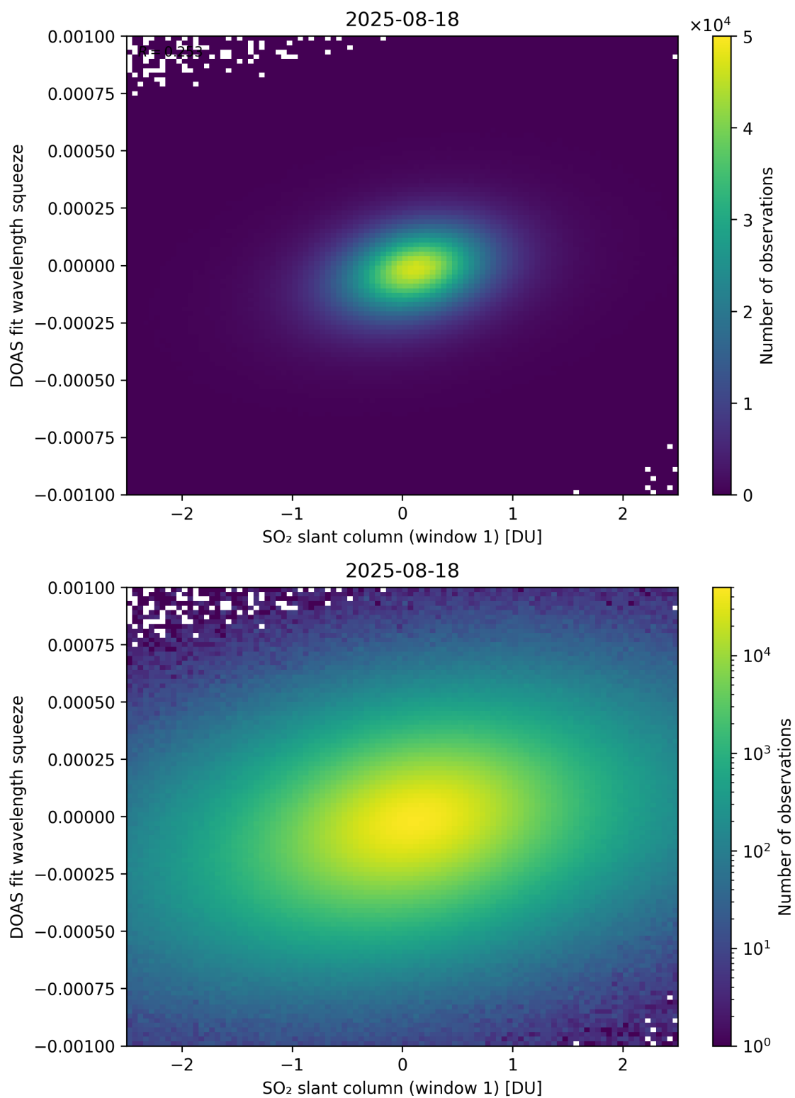
Figure 266: Scatter density plot of “SO 2 slant column (window 1)” against “DOAS fit wavelength squeeze” for 2025-08-17 to 2025-08-19.
