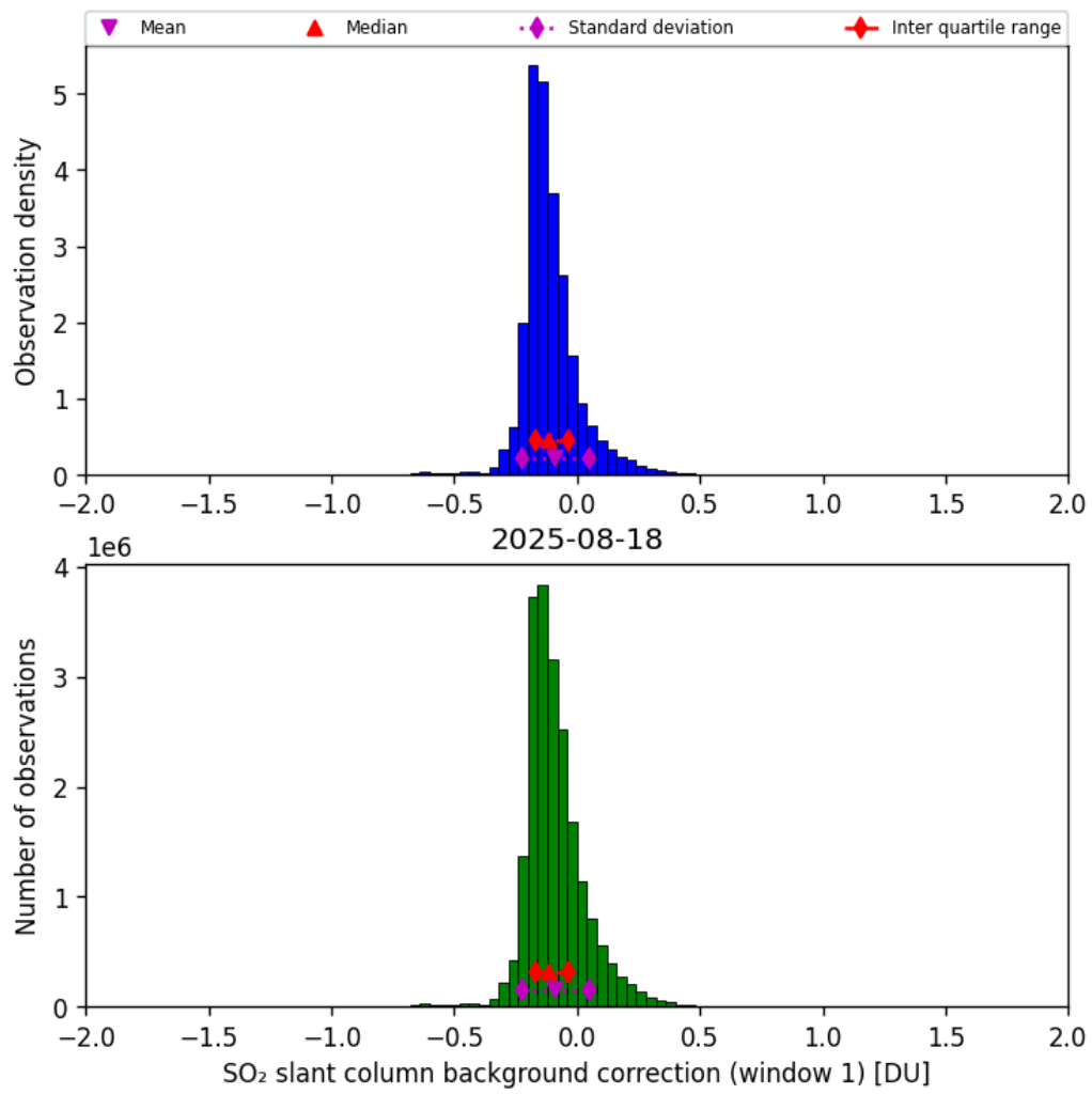
Figure 66: Histogram of “SO 2 slant column background correction (window 1)” for 2025-08-17 to 2025-08-19
