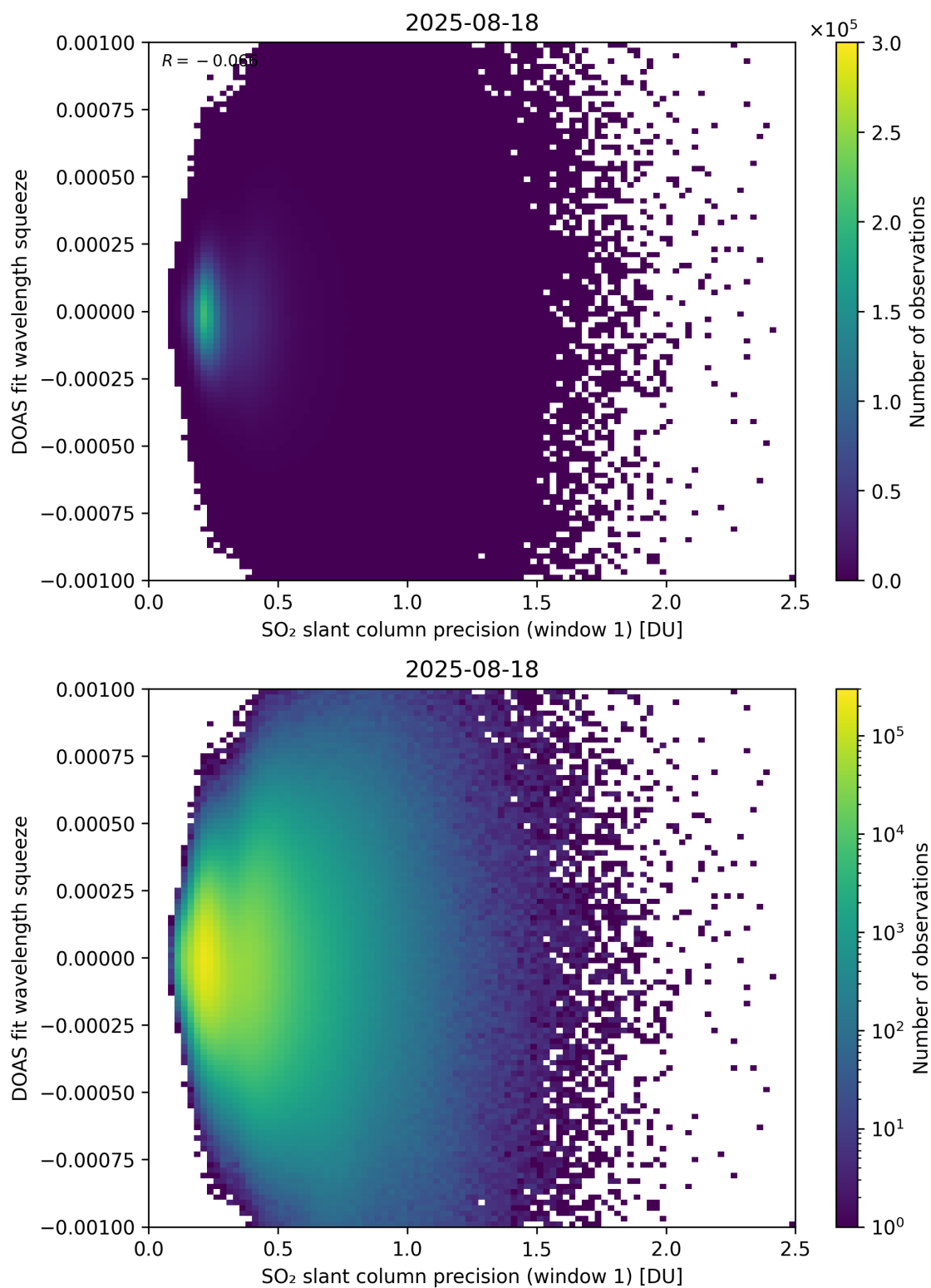
Figure 272: Scatter density plot of “SO 2 slant column precision (window 1)” against “DOAS fit wavelength squeeze” for 2025-08-17 to 2025-08-19.
