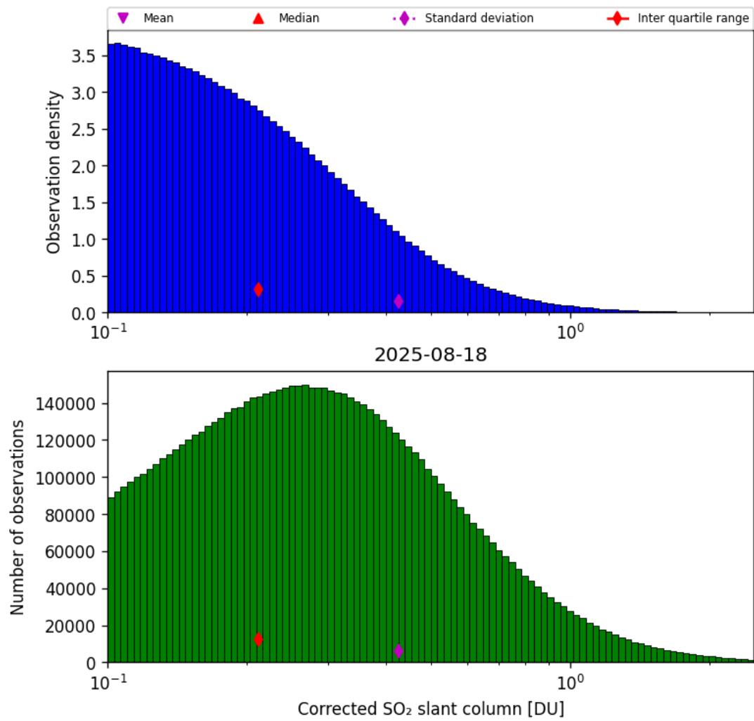
Figure 60: Histogram of “Corrected SO 2 slant column” for 2025-08-17 to 2025-08-19
