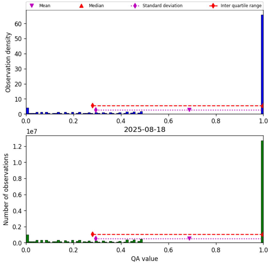
Figure 57: Histogram of “QA value” for 2025-08-17 to 2025-08-19
