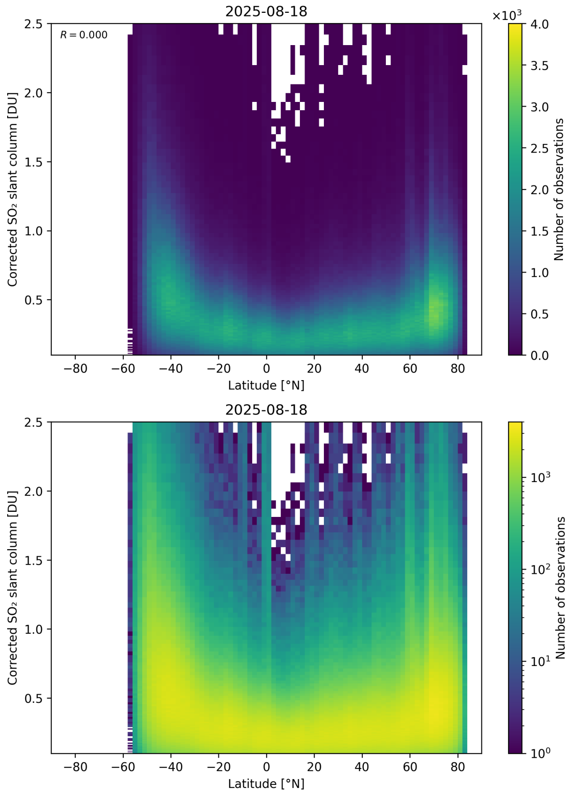
Figure 159: Scatter density plot of “Latitude” against “Corrected SO 2 slant column” for 2025-08-17 to 2025-08-19.
