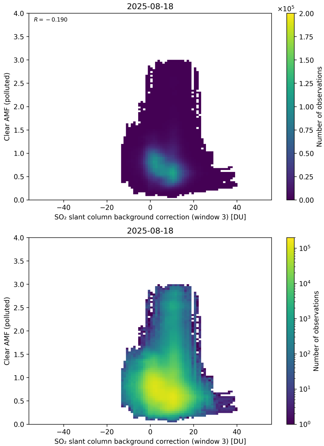
Figure 135: Scatter density plot of “SO 2 slant column background correction (window 3)” against “Clear AMF (polluted)” for 2025-08-17 to 2025-08-19.
