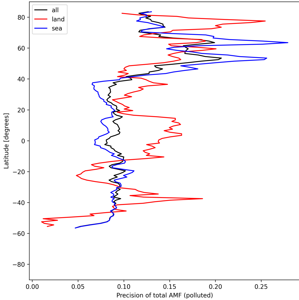
Figure 54: Zonal average of “Precision of total AMF (polluted)” for 2025-08-17 to 2025-08-19.
