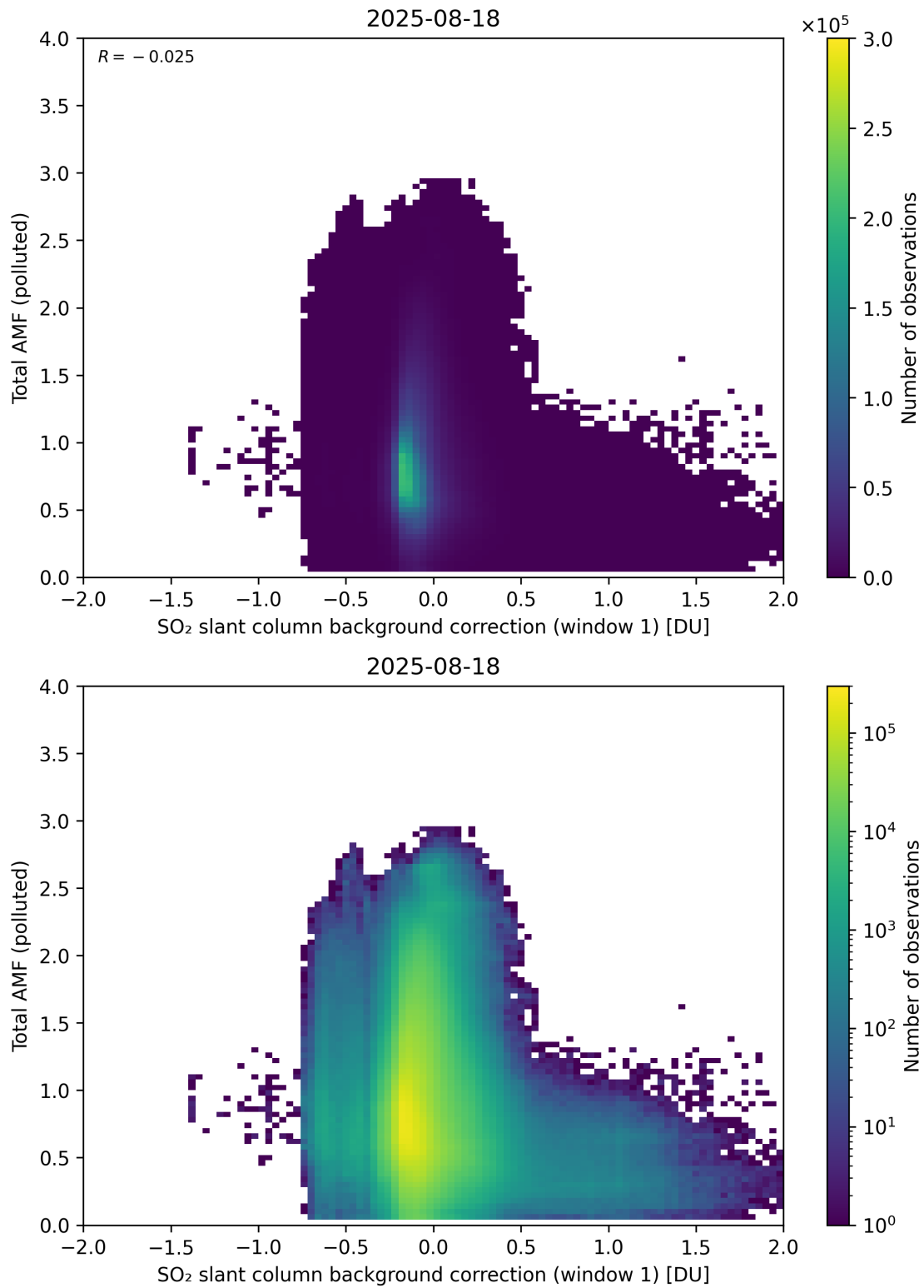
Figure 120: Scatter density plot of “SO 2 slant column background correction (window 1)” against “Total AMF (polluted)” for 2025-08-17 to 2025-08-19.
