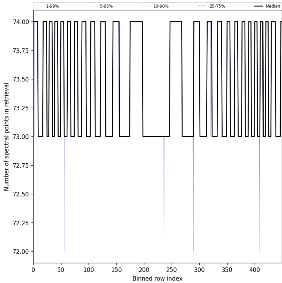
Figure 108: Along track statistics of “Number of spectral points in retrieval” for 2025-08-17 to 2025-08-19
