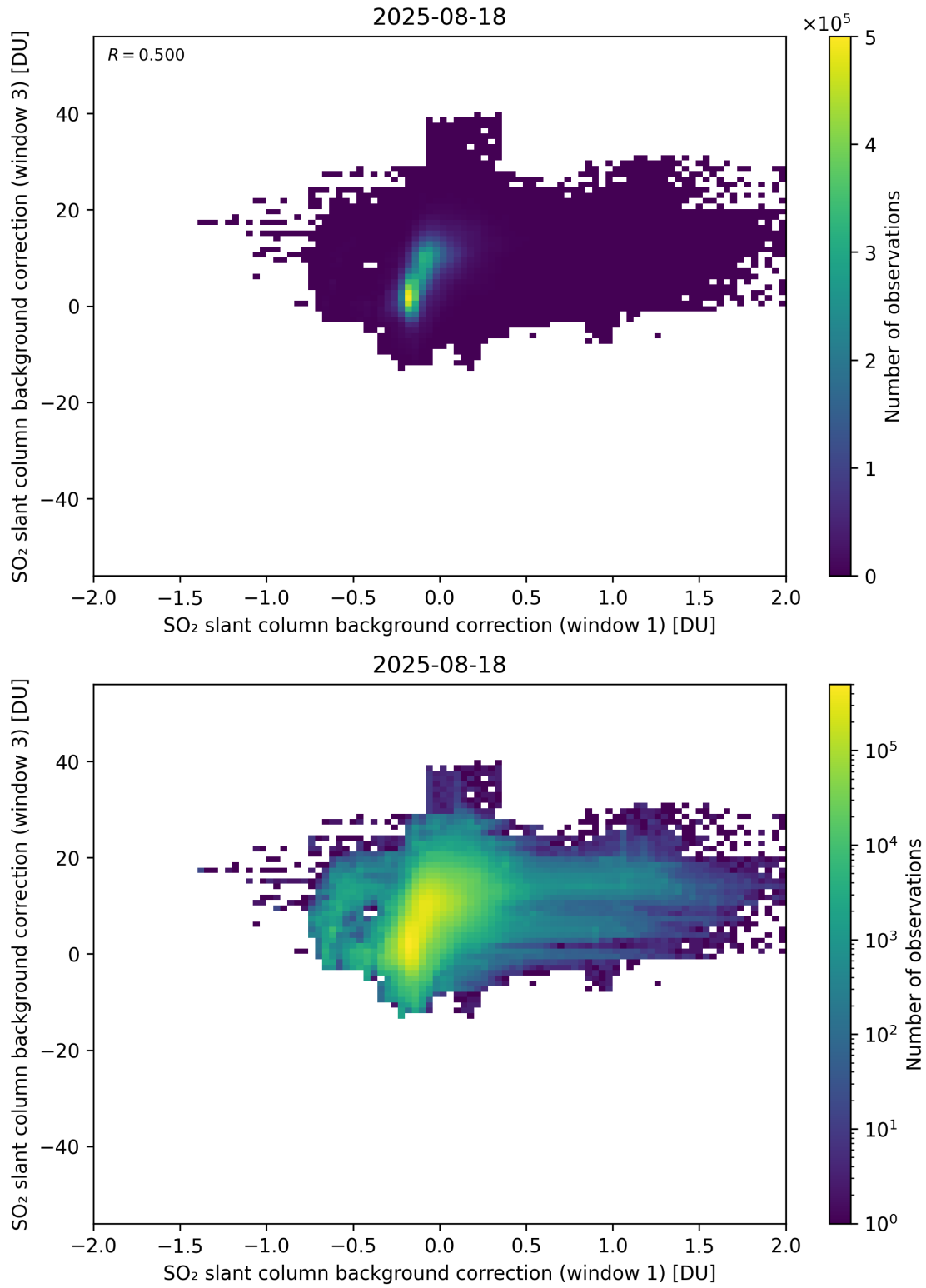
Figure 110: Scatter density plot of “SO 2 slant column background correction (window 1)” against “SO 2 slant column background correction (window 3)” for 2025-08-17 to 2025-08-19.
