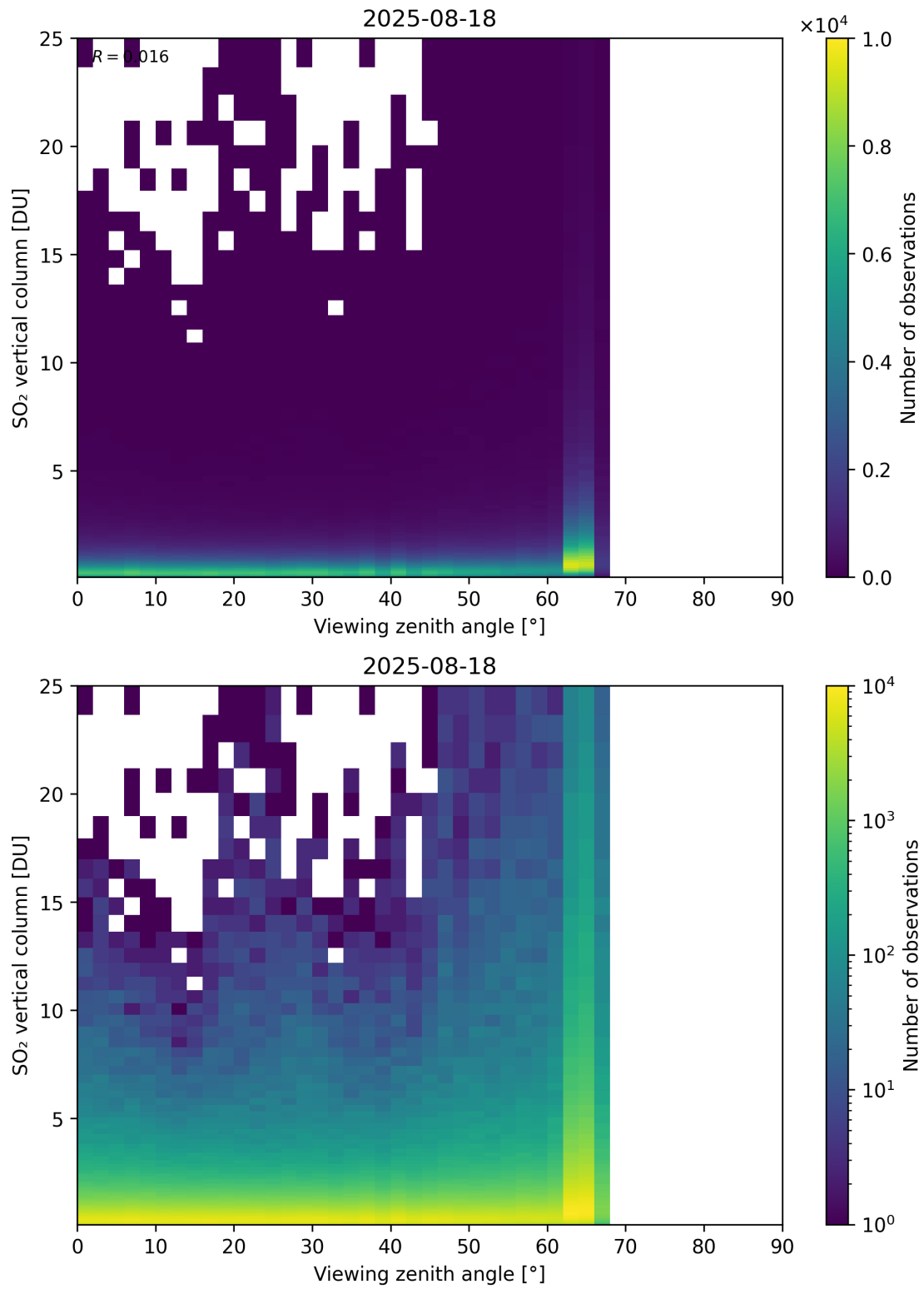
Figure 383: Scatter density plot of “Viewing zenith angle” against “SO 2 vertical column” for 2025-08-17 to 2025-08-19.
