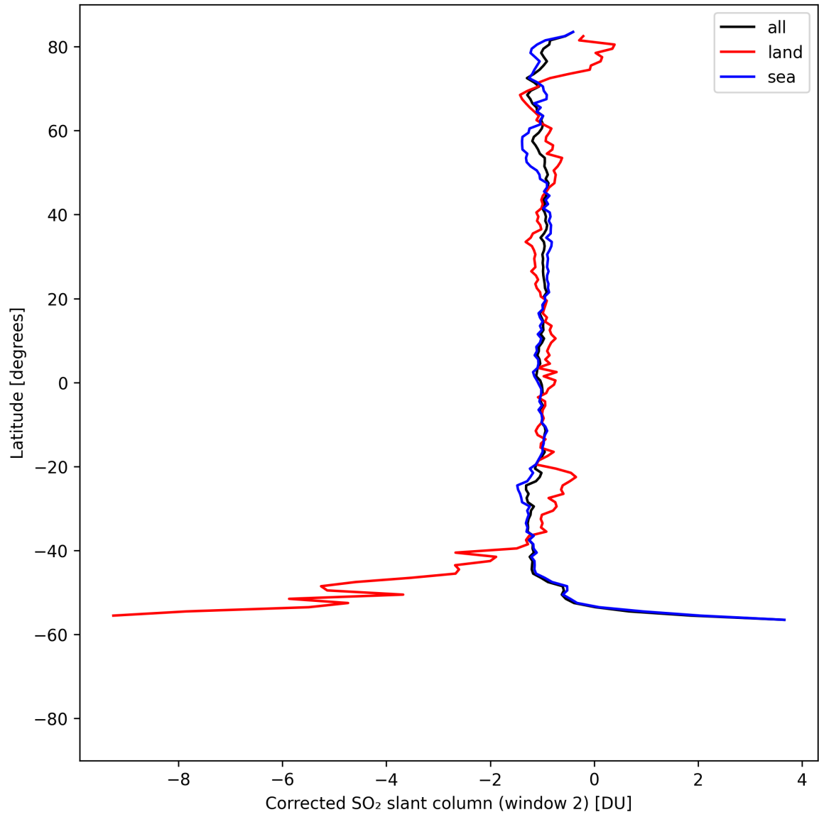
Figure 43: Zonal average of “Corrected SO 2 slant column (window 2)” for 2025-08-17 to 2025-08-19.
