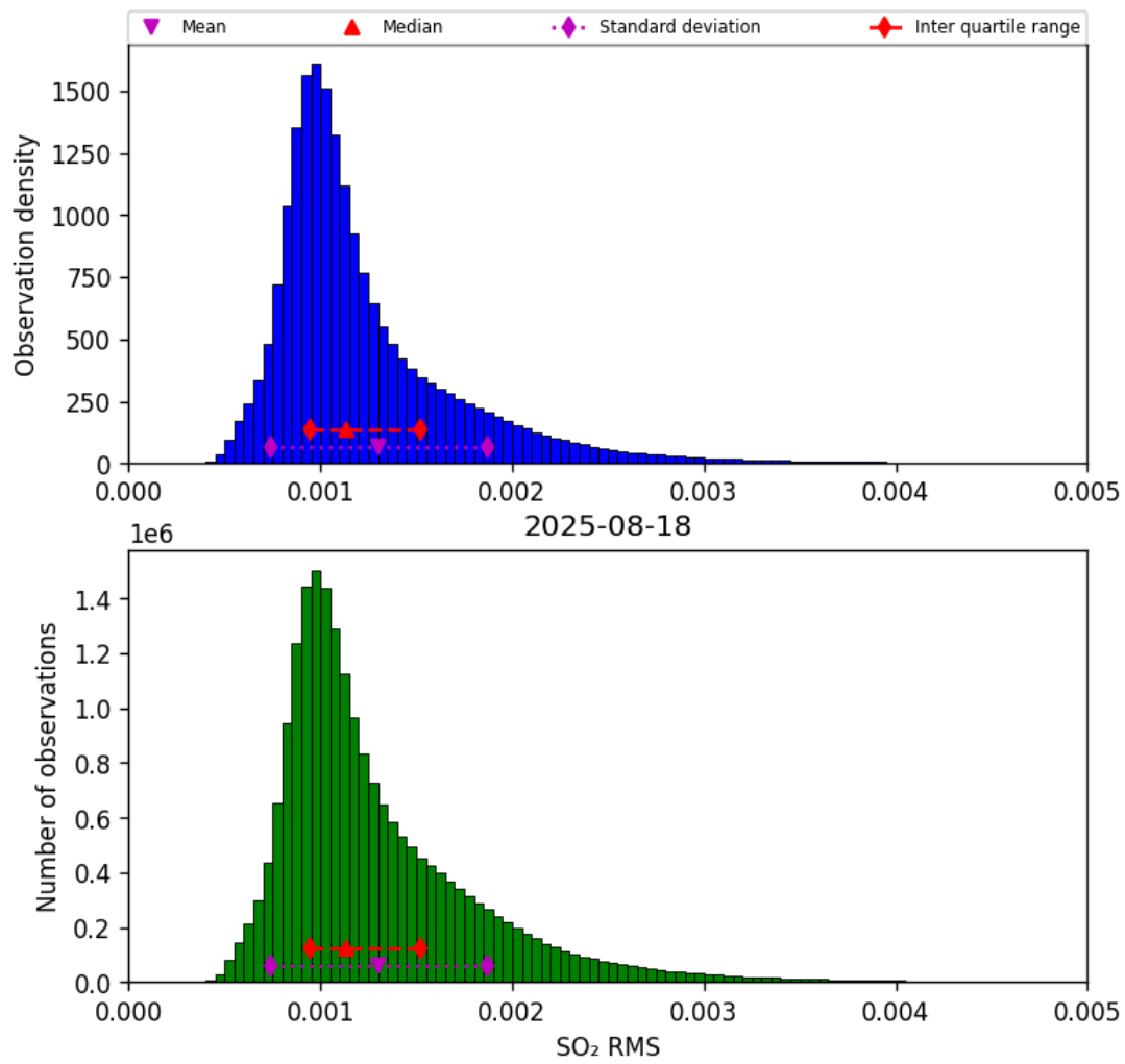
Figure 78: Histogram of “SO 2 RMS” for 2025-08-17 to 2025-08-19
