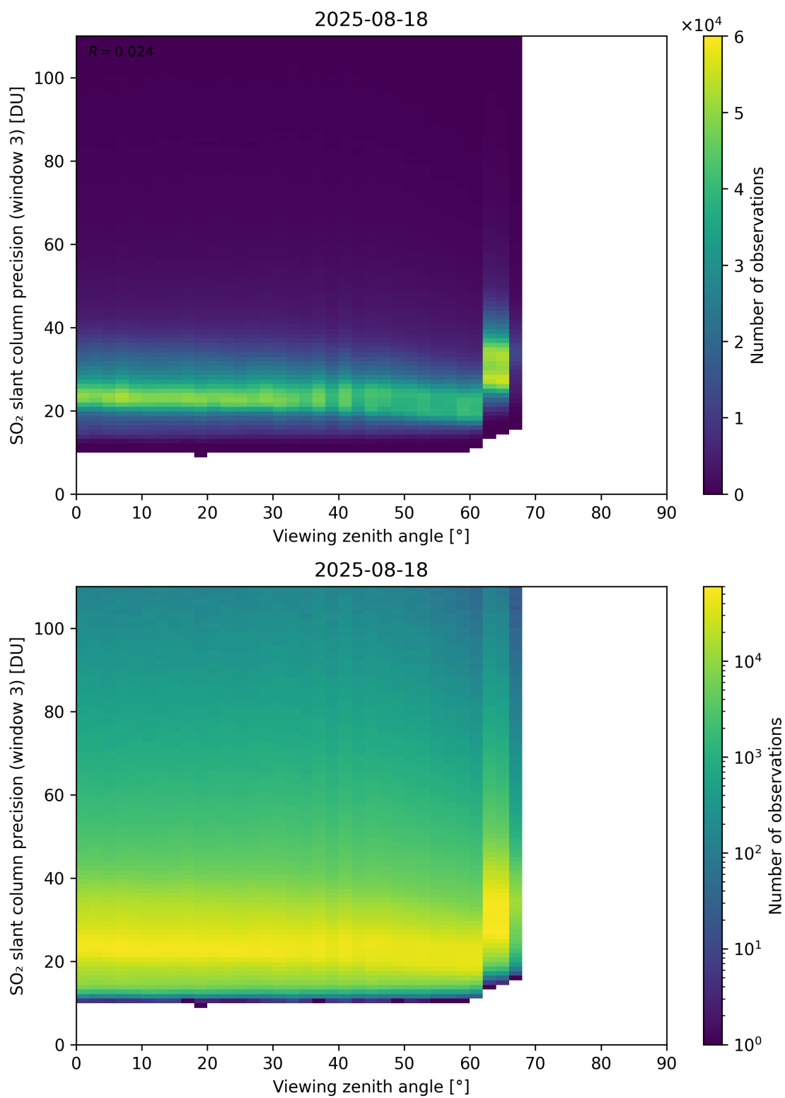
Figure 380: Scatter density plot of “Viewing zenith angle” against “SO 2 slant column precision (window 3)” for 2025-08-17 to 2025-08-19.
