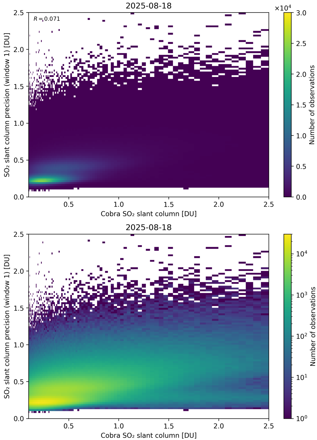
Figure 220: Scatter density plot of “Cobra SO 2 slant column” against “SO 2 slant column precision (window 1)” for 2025-08-17 to 2025-08-19.
