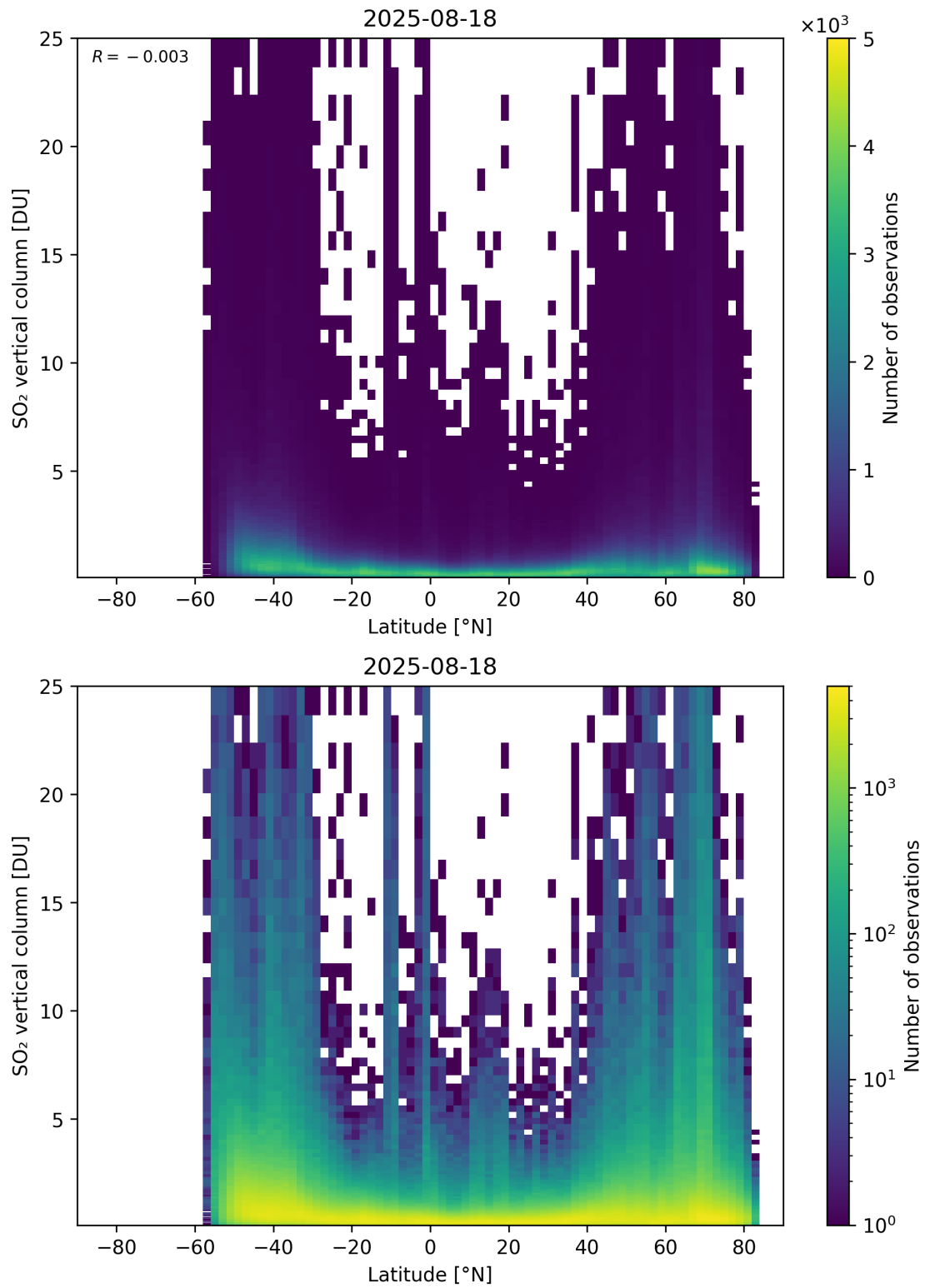
Figure 169: Scatter density plot of “Latitude” against “SO 2 vertical column” for 2025-08-17 to 2025-08-19.
