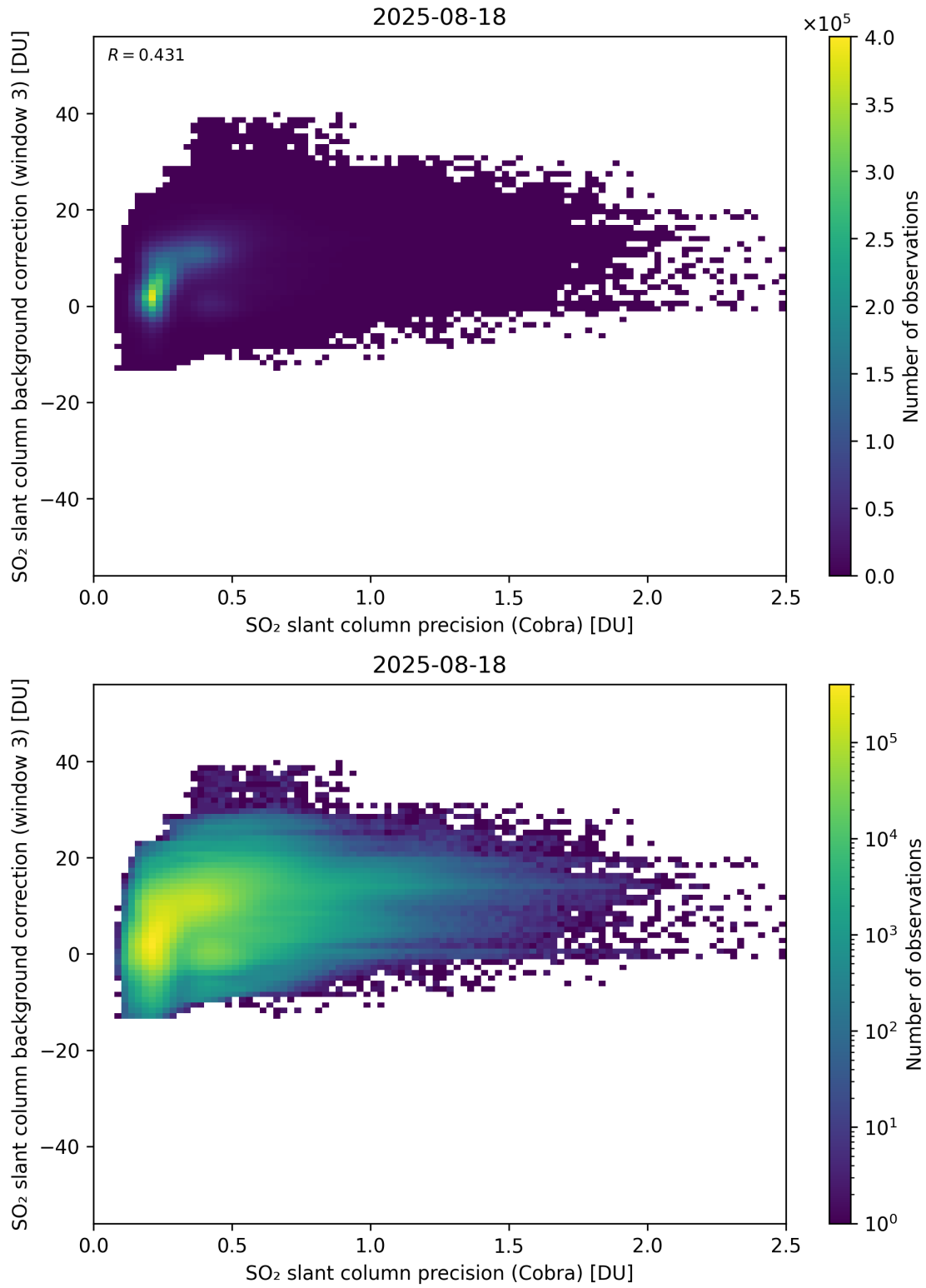
Figure 201: Scatter density plot of “SO 2 slant column precision (Cobra)” against “SO 2 slant column background correction (window 3)” for 2025-08-17 to 2025-08-19.
