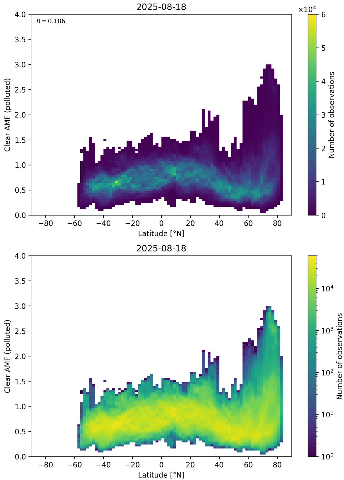
Figure 156: Scatter density plot of “Latitude” against “Clear AMF (polluted)” for 2025-08-17 to 2025-08-19.
