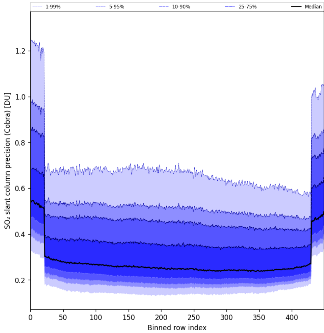
Figure 88: Along track statistics of “SO 2 slant column precision (Cobra)” for 2025-08-17 to 2025-08-19
