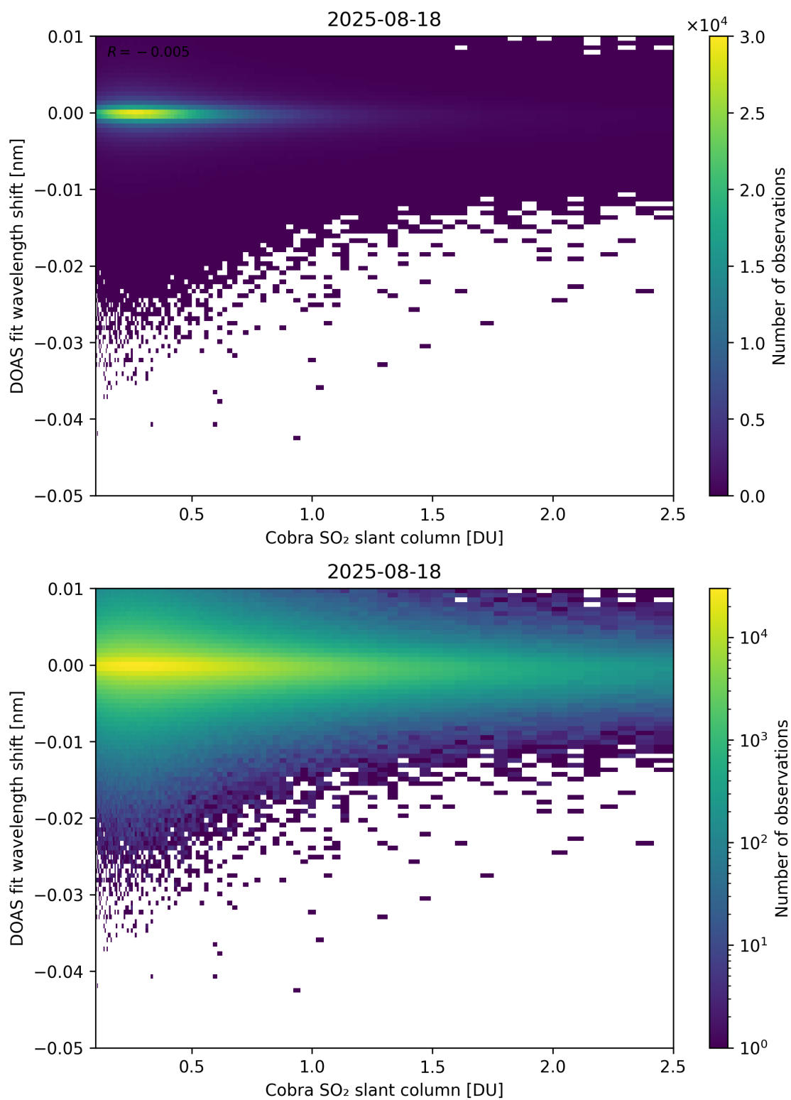
Figure 196: Scatter density plot of “Cobra SO 2 slant column” against “DOAS fit wavelength shift” for 2025-08-17 to 2025-08-19.
