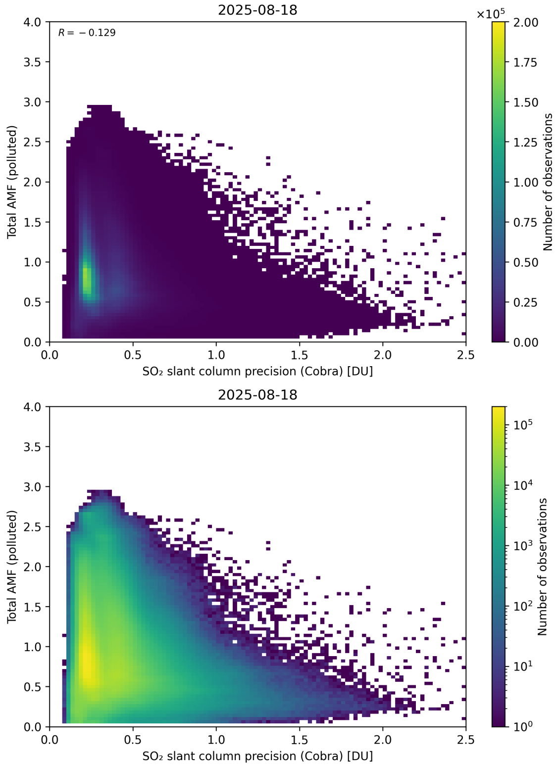
Figure 213: Scatter density plot of “SO 2 slant column precision (Cobra)” against “Total AMF (polluted)” for 2025-08-17 to 2025-08-19.
