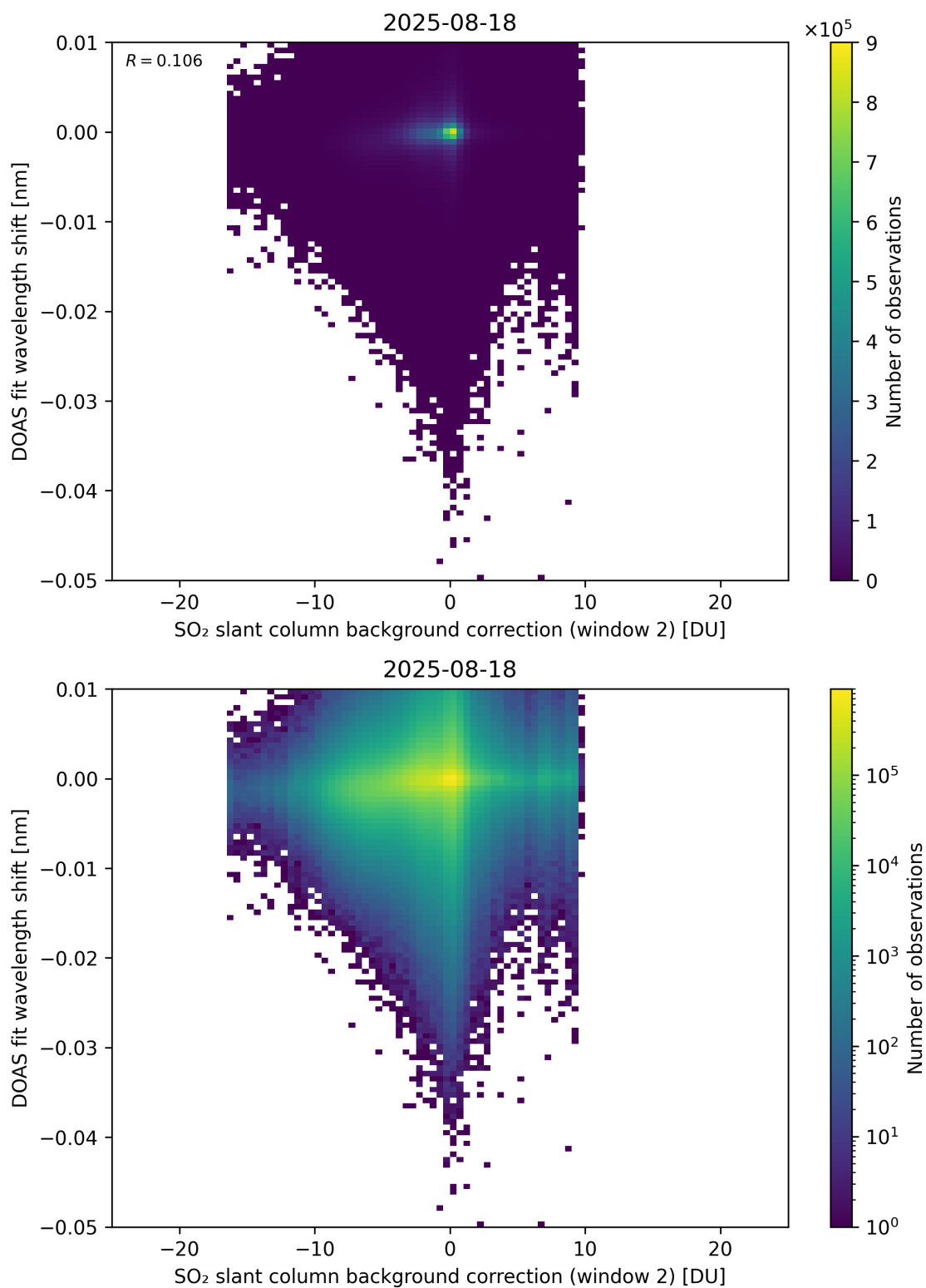
Figure 123: Scatter density plot of “SO 2 slant column background correction (window 2)” against “DOAS fit wavelength shift” for 2025-08-17 to 2025-08-19.
