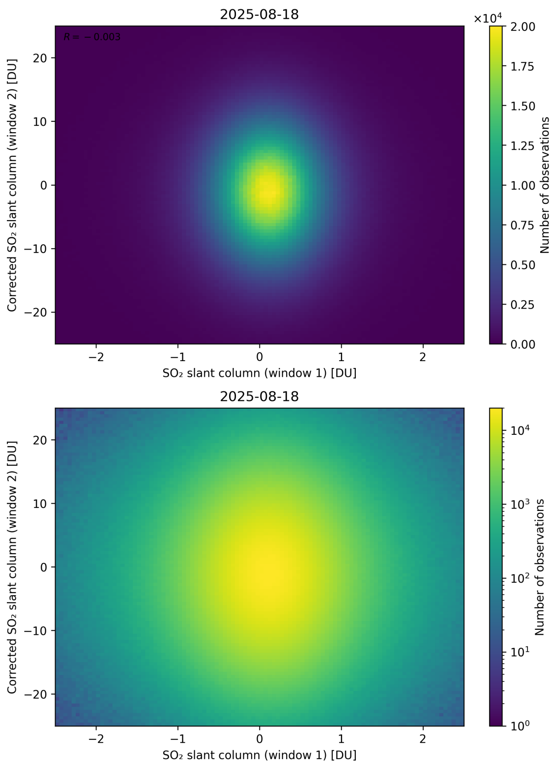
Figure 283: Scatter density plot of “SO 2 slant column (window 1)” against “Corrected SO 2 slant column (window 2)” for 2025-08-17 to 2025-08-19.
