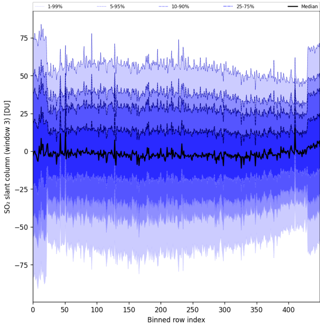
Figure 97: Along track statistics of “SO 2 slant column (window 3)” for 2025-08-17 to 2025-08-19
