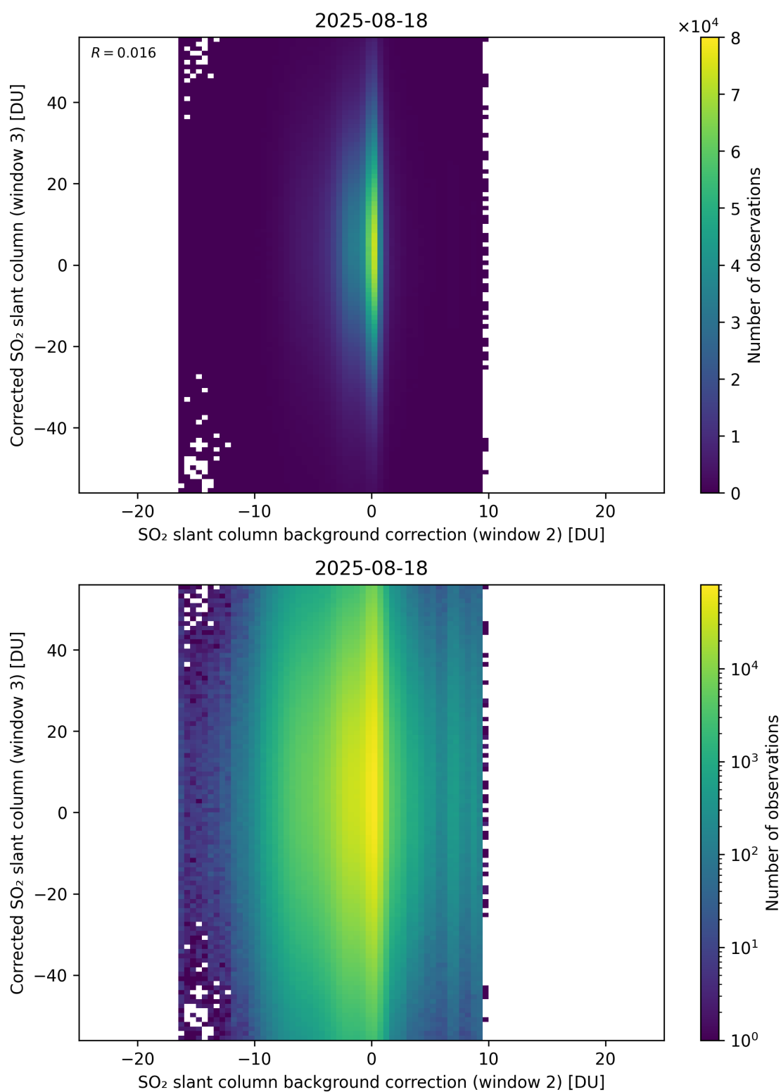
Figure 127: Scatter density plot of “SO 2 slant column background correction (window 2)” against “Corrected SO 2 slant column (window 3)” for 2025-08-17 to 2025-08-19.
