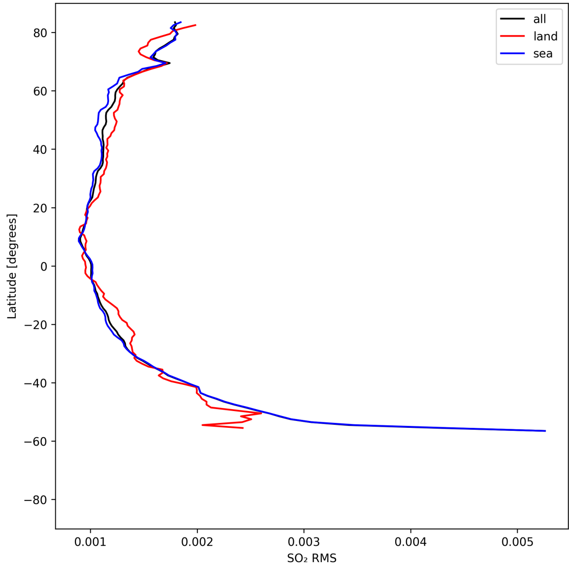
Figure 52: Zonal average of “SO 2 RMS” for 2025-08-17 to 2025-08-19.
