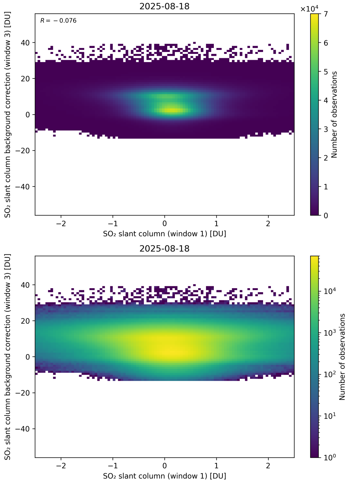
Figure 264: Scatter density plot of “SO 2 slant column (window 1)” against “SO 2 slant column background correction (window 3)” for 2025-08-17 to 2025-08-19.
