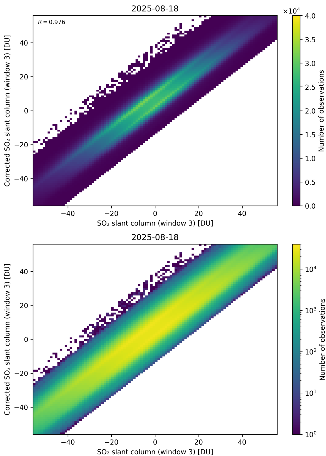
Figure 316: Scatter density plot of “SO 2 slant column (window 3)” against “Corrected SO 2 slant column (window 3)” for 2025-08-17 to 2025-08-19.
