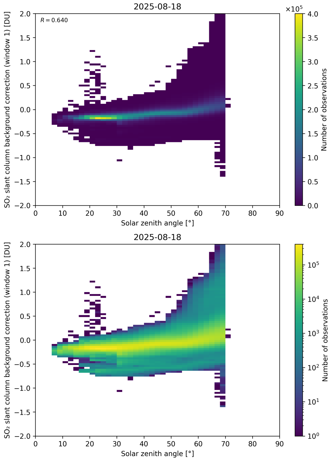
Figure 171: Scatter density plot of “Solar zenith angle” against “SO 2 slant column background correction (window 1)” for 2025-08-17 to 2025-08-19.
