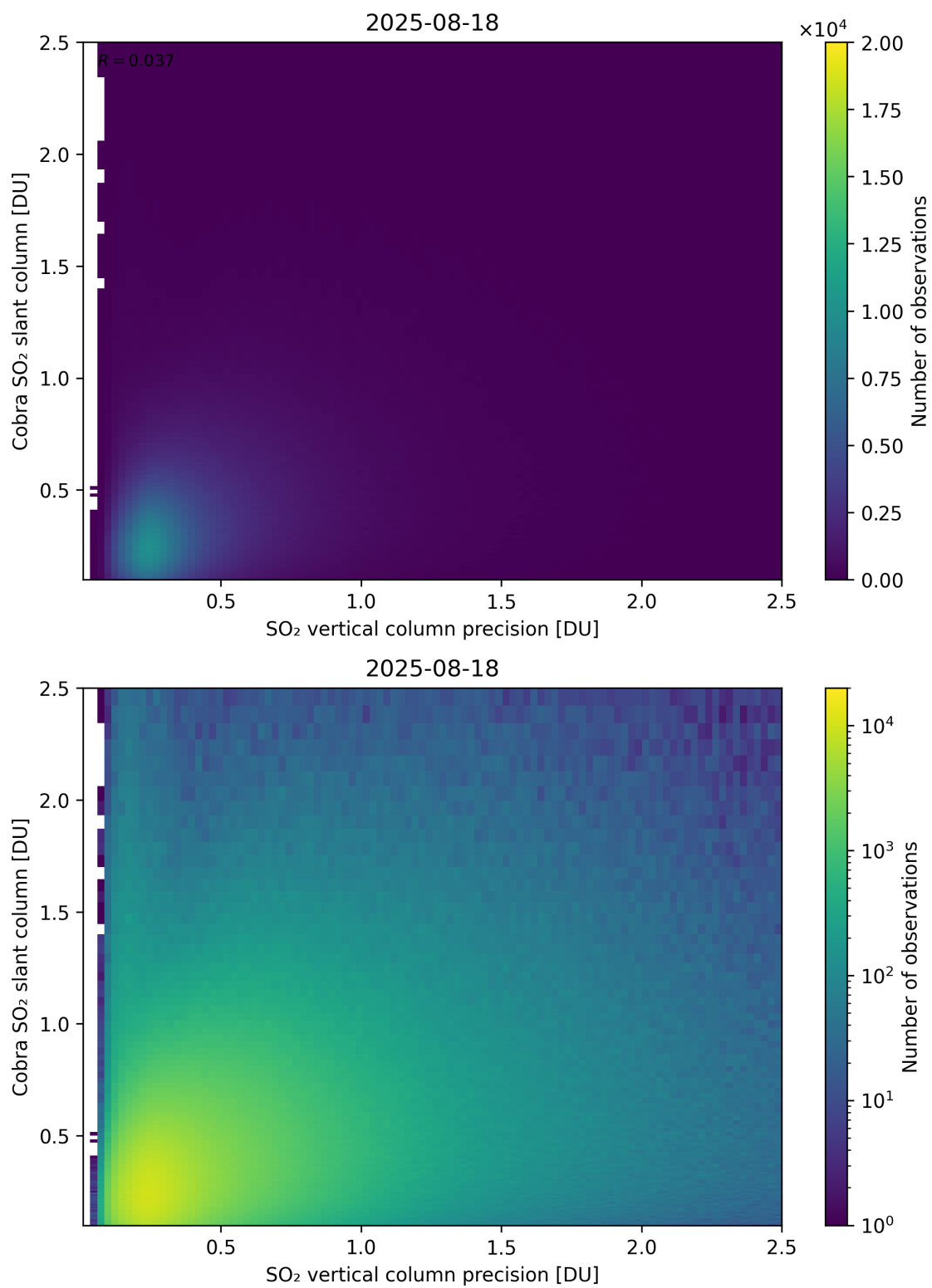
Figure 336: Scatter density plot of “SO 2 vertical column precision” against “Cobra SO 2 slant column” for 2025-08-17 to 2025-08-19.
