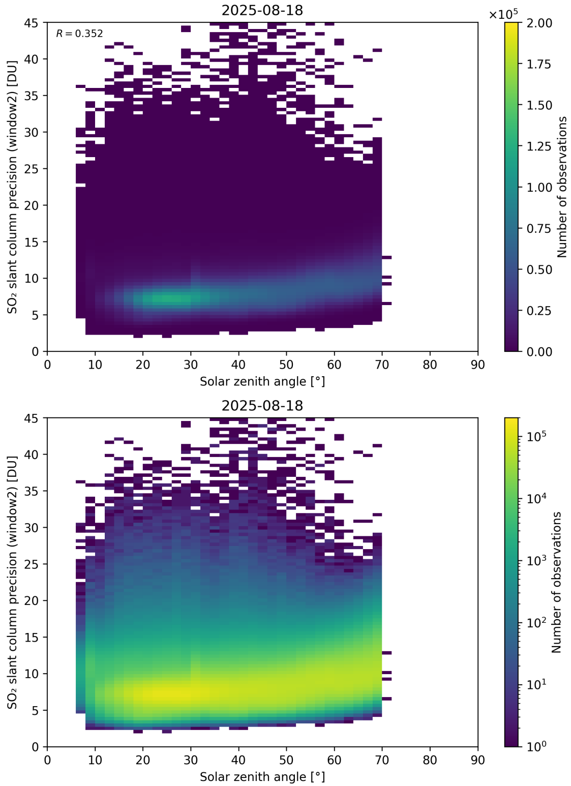
Figure 186: Scatter density plot of “Solar zenith angle” against “SO 2 slant column precision (window2)” for 2025-08-17 to 2025-08-19.
