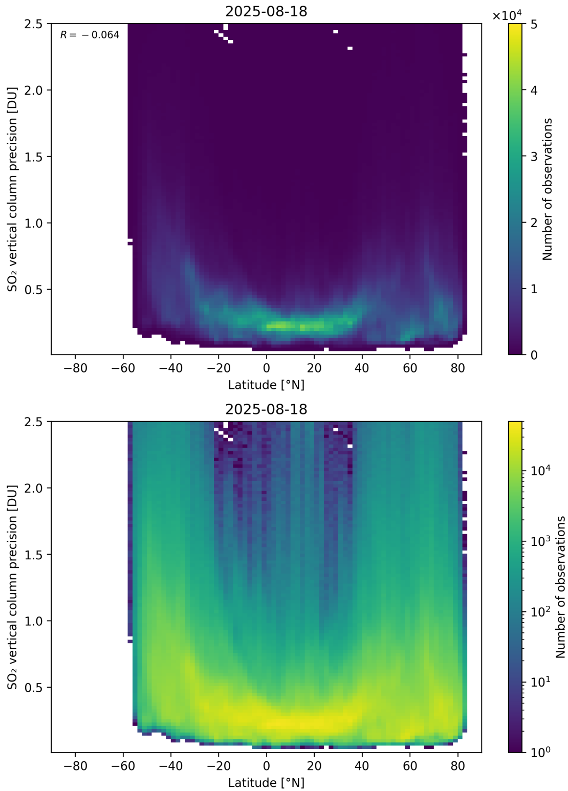
Figure 170: Scatter density plot of “Latitude” against “SO 2 vertical column precision” for 2025-08-17 to 2025-08-19.
