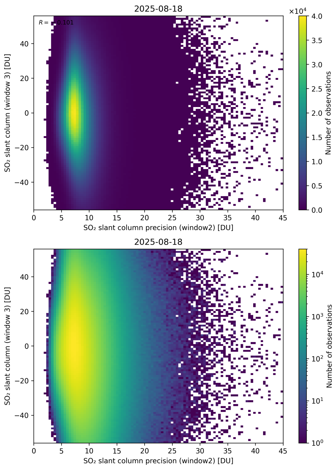
Figure 299: Scatter density plot of “SO 2 slant column precision (window2)” against “SO 2 slant column (window 3)” for 2025-08-17 to 2025-08-19.
