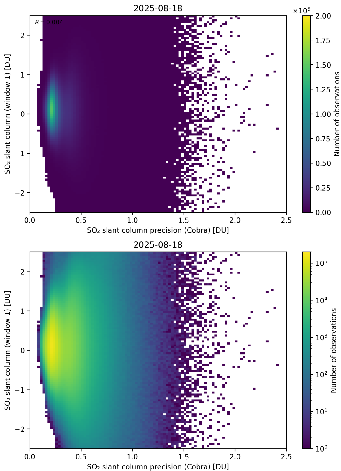
Figure 208: Scatter density plot of “SO 2 slant column precision (Cobra)” against “SO 2 slant column (window 1)” for 2025-08-17 to 2025-08-19.
