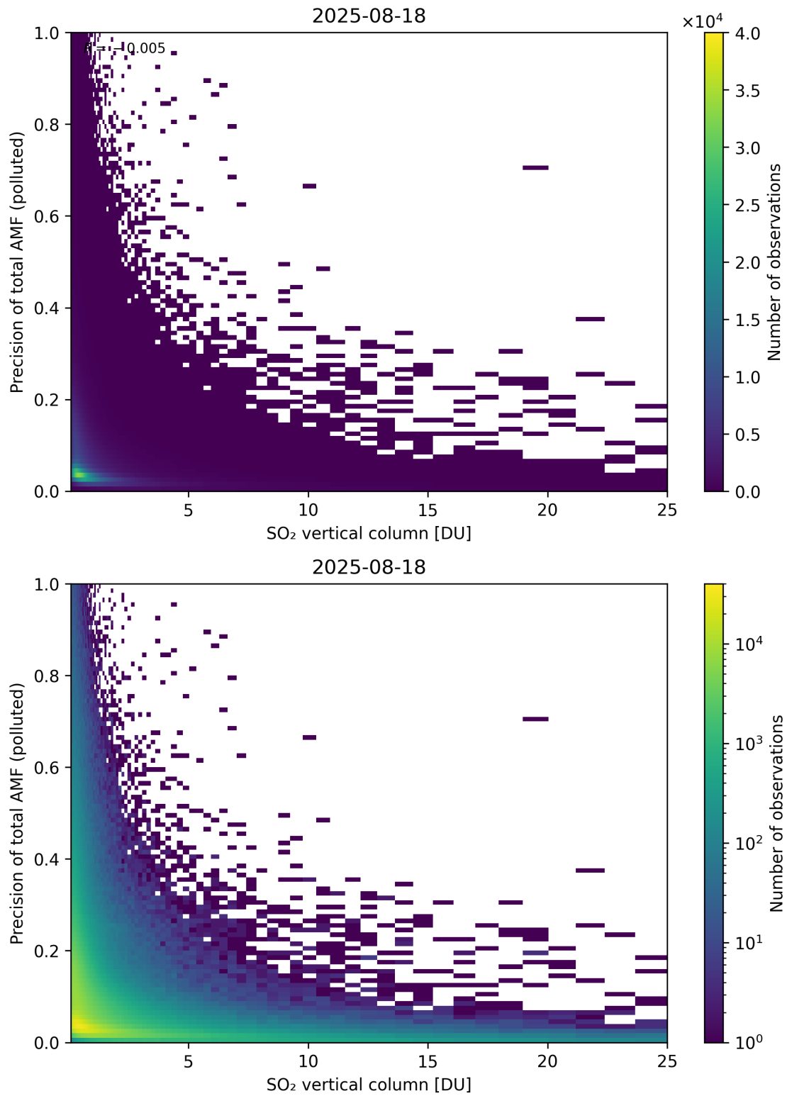
Figure 360: Scatter density plot of “SO 2 vertical column” against “Precision of total AMF (polluted)” for 2025-08-17 to 2025-08-19.
