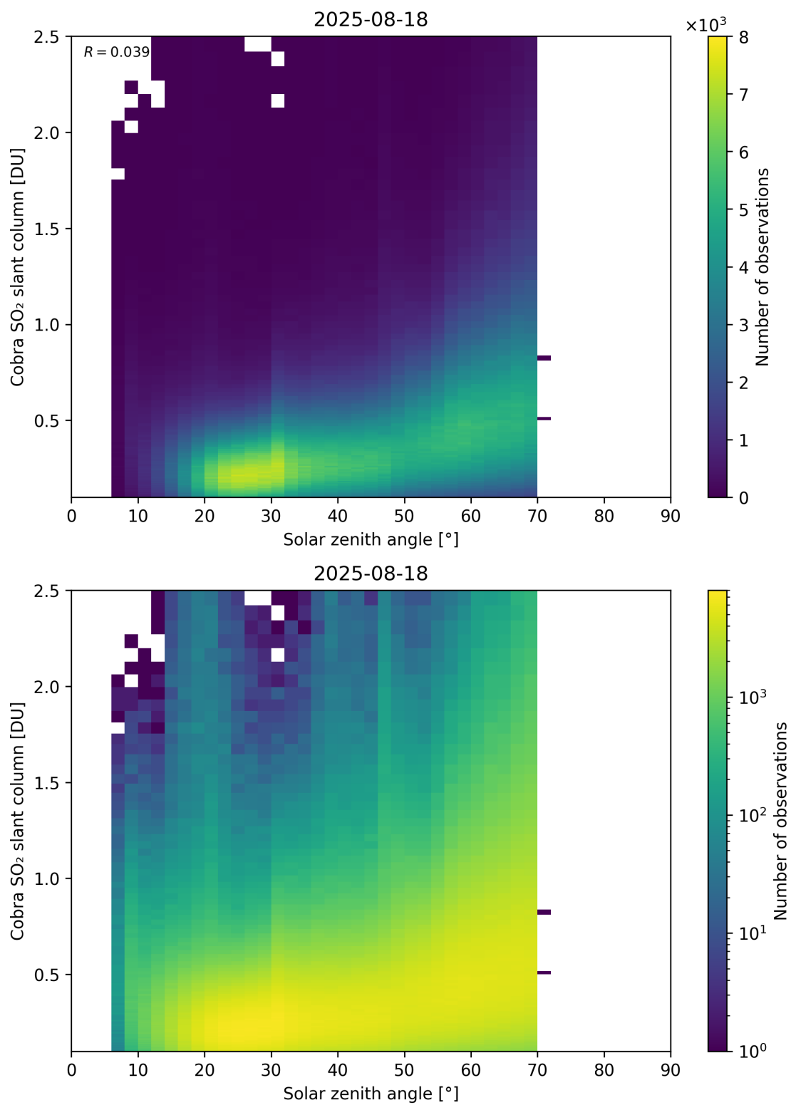
Figure 179: Scatter density plot of “Solar zenith angle” against “Cobra SO 2 slant column” for 2025-08-17 to 2025-08-19.
