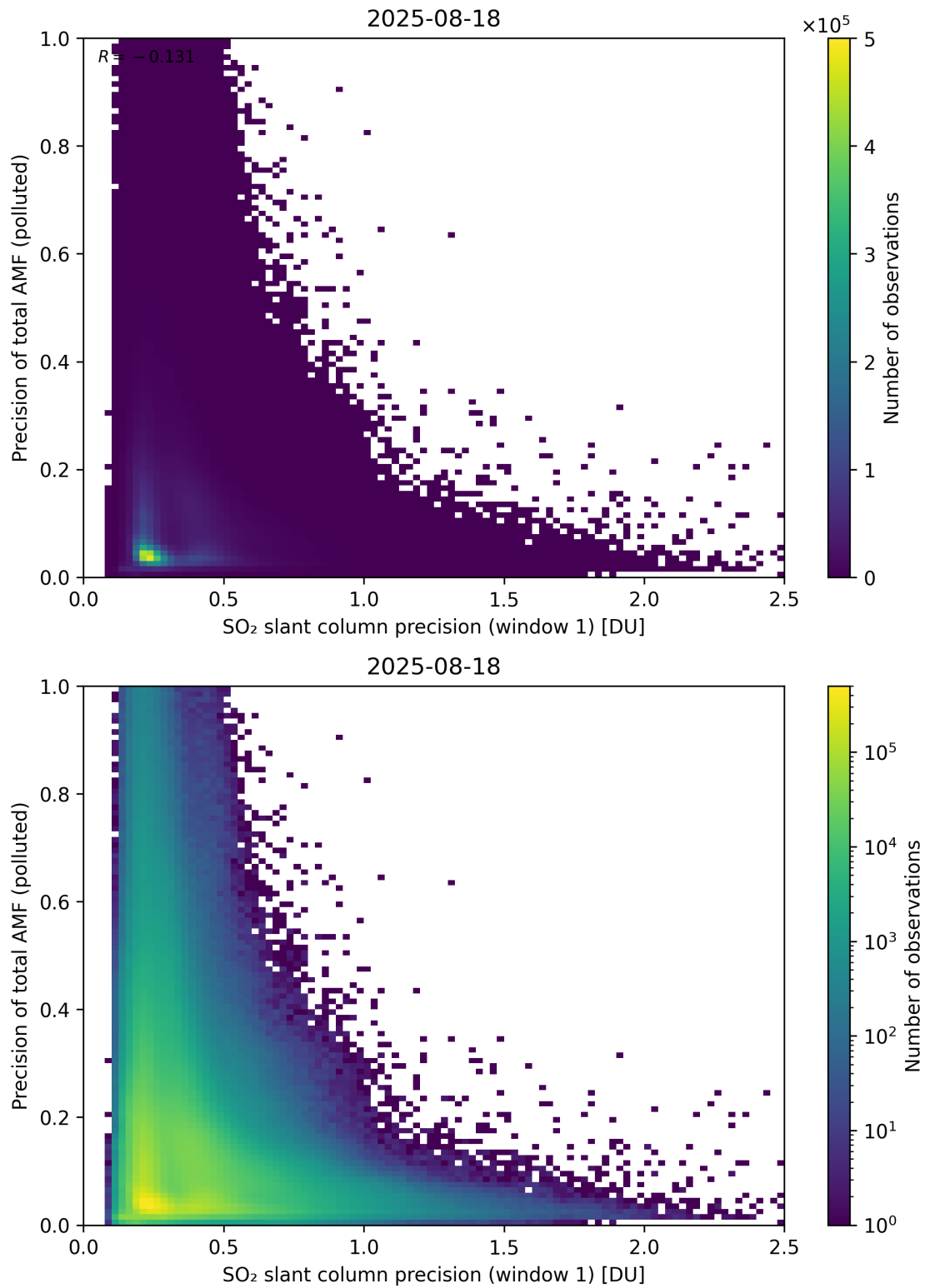
Figure 281: Scatter density plot of “SO 2 slant column precision (window 1)” against “Precision of total AMF (polluted)” for 2025-08-17 to 2025-08-19.
