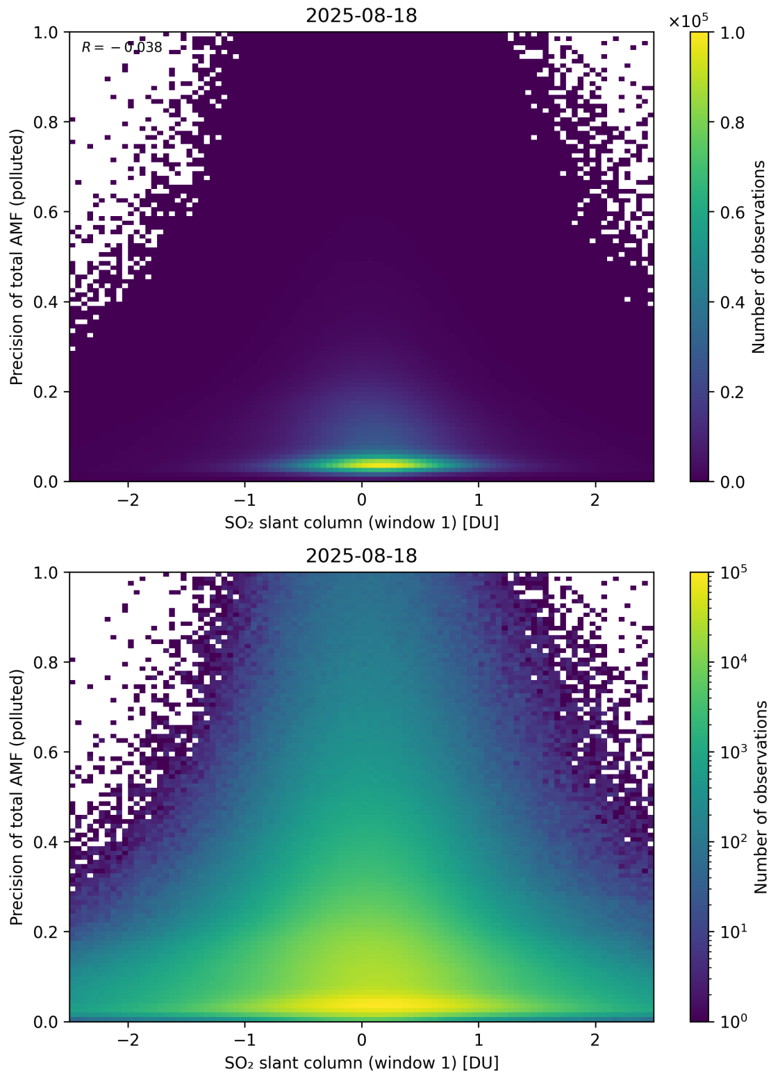
Figure 290: Scatter density plot of “SO 2 slant column (window 1)” against “Precision of total AMF (polluted)” for 2025-08-17 to 2025-08-19.
