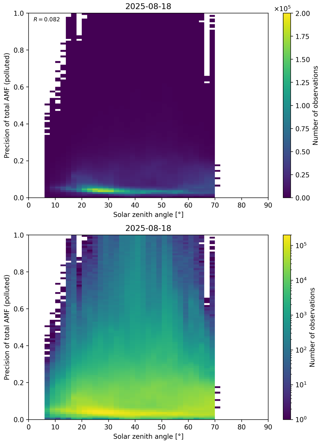
Figure 190: Scatter density plot of “Solar zenith angle” against “Precision of total AMF (polluted)” for 2025-08-17 to 2025-08-19.
