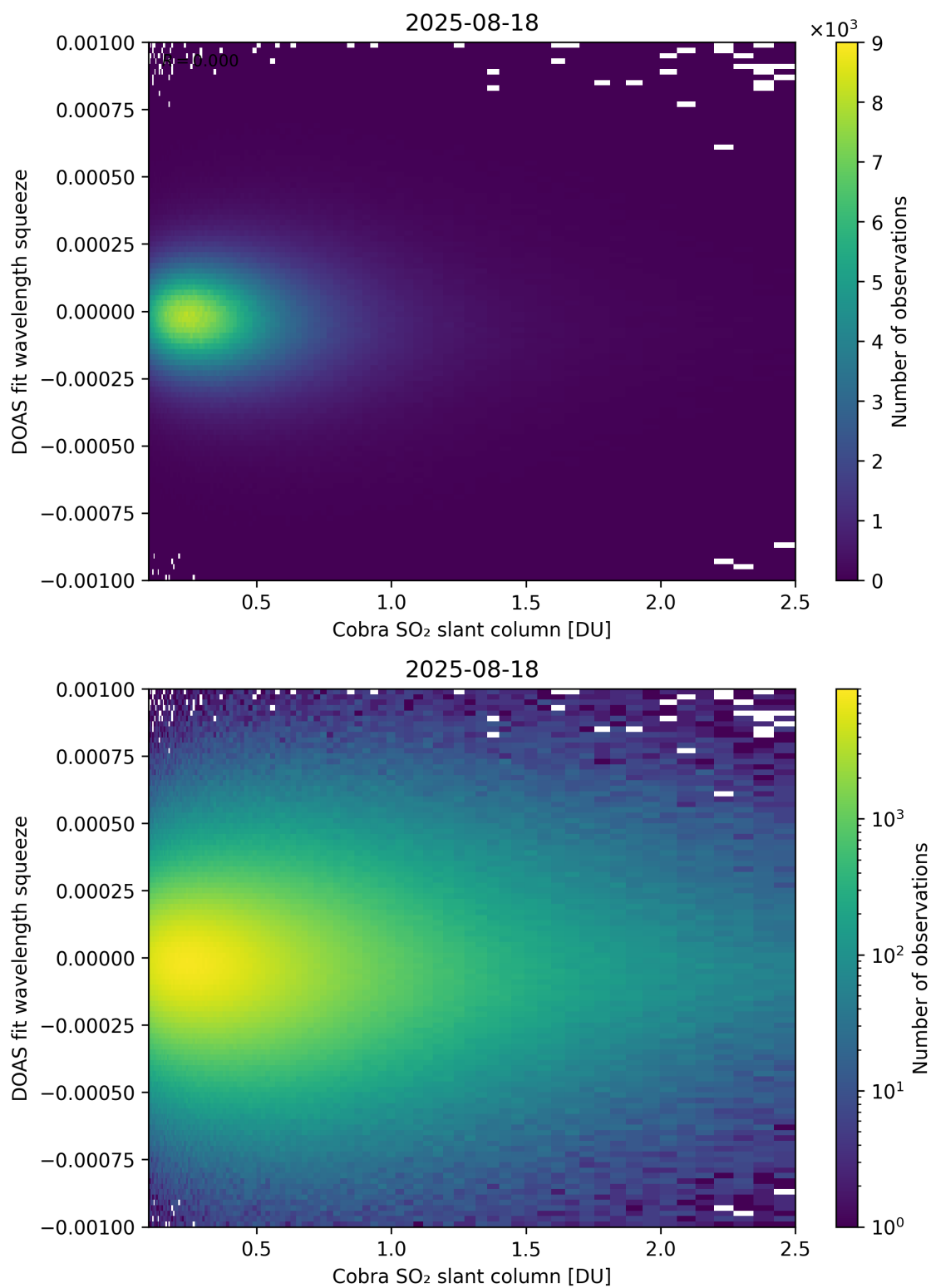
Figure 197: Scatter density plot of “Cobra SO 2 slant column” against “DOAS fit wavelength squeeze” for 2025-08-17 to 2025-08-19.
