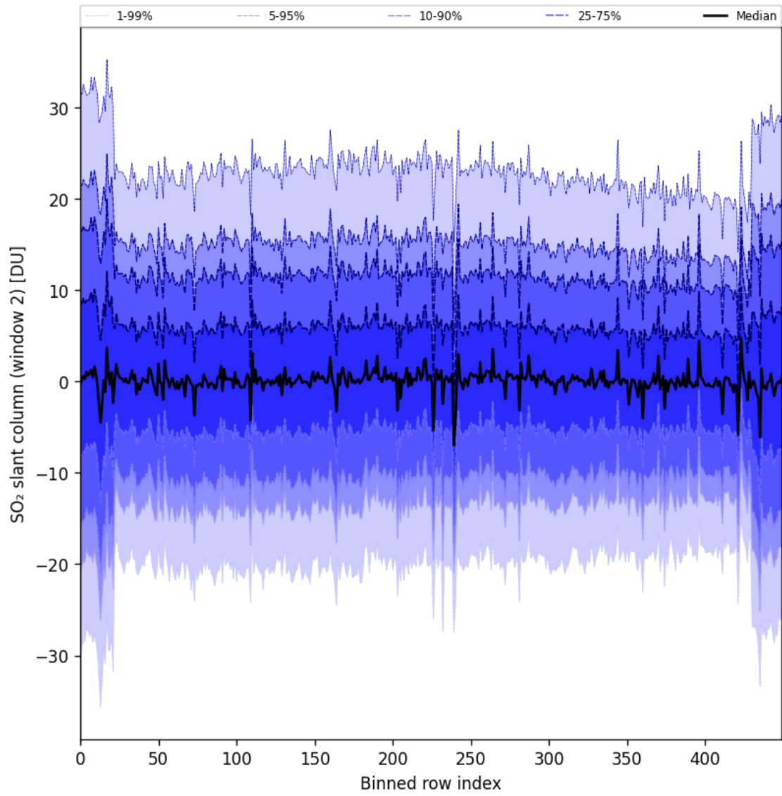
Figure 93: Along track statistics of “SO 2 slant column (window 2)” for 2025-08-17 to 2025-08-19
