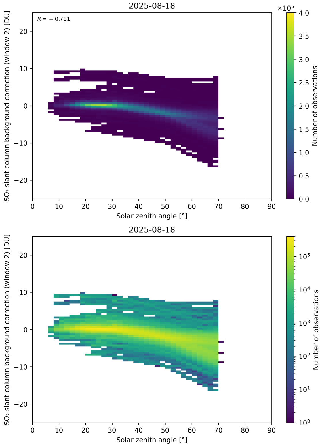
Figure 172: Scatter density plot of “Solar zenith angle” against “SO 2 slant column background correction (window 2)” for 2025-08-17 to 2025-08-19.
