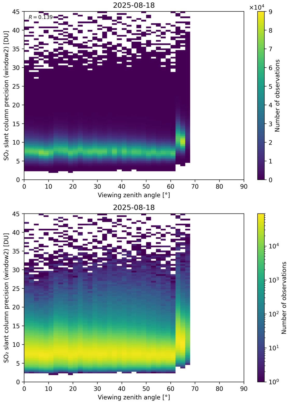
Figure 378: Scatter density plot of “Viewing zenith angle” against “SO 2 slant column precision (window2)” for 2025-08-17 to 2025-08-19.
