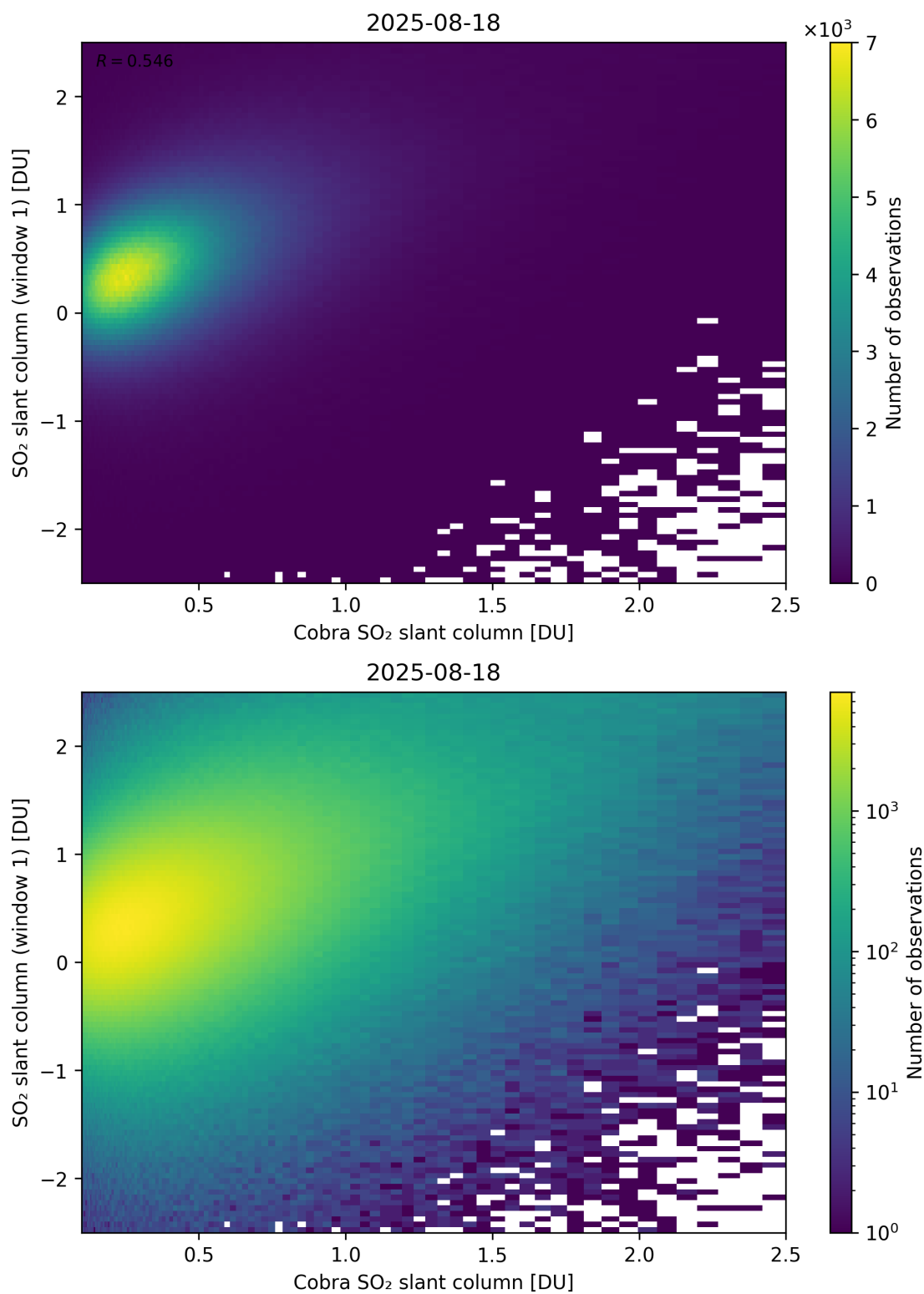
Figure 219: Scatter density plot of “Cobra SO 2 slant column” against “SO 2 slant column (window 1)” for 2025-08-17 to 2025-08-19.
