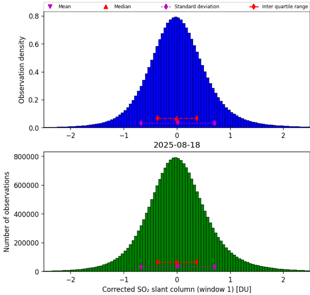
Figure 65: Histogram of “Corrected SO 2 slant column (window 1)” for 2025-08-17 to 2025-08-19
