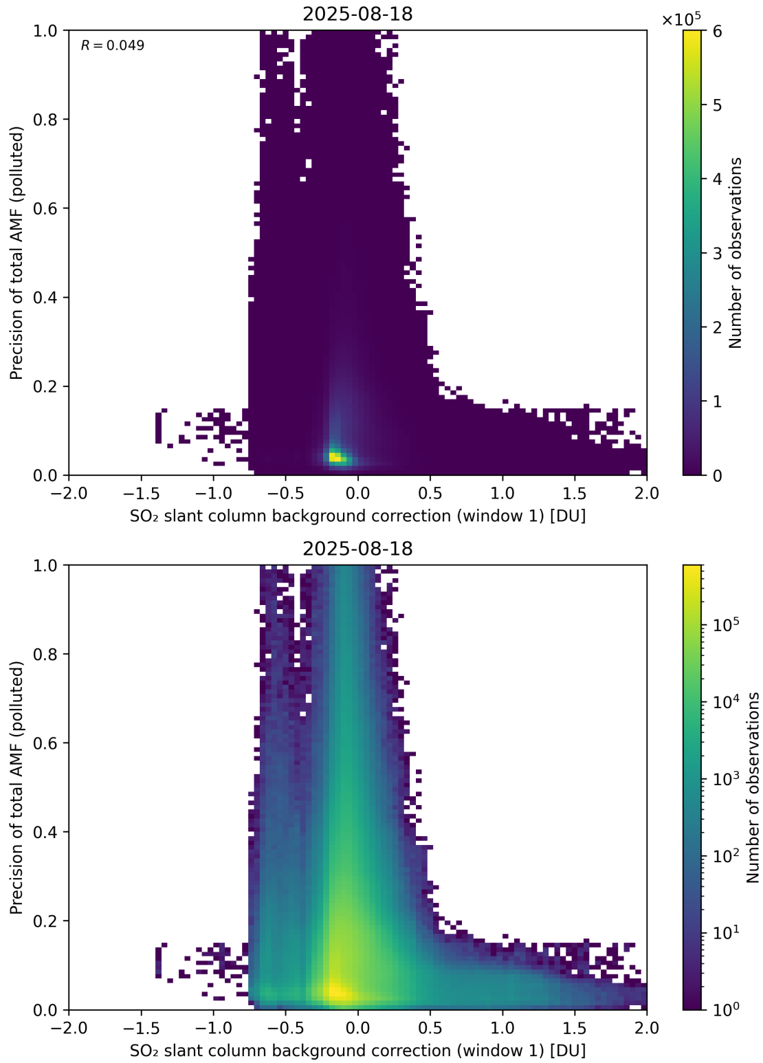
Figure 121: Scatter density plot of “SO 2 slant column background correction (window 1)” against “Precision of total AMF (polluted)” for 2025-08-17 to 2025-08-19.
