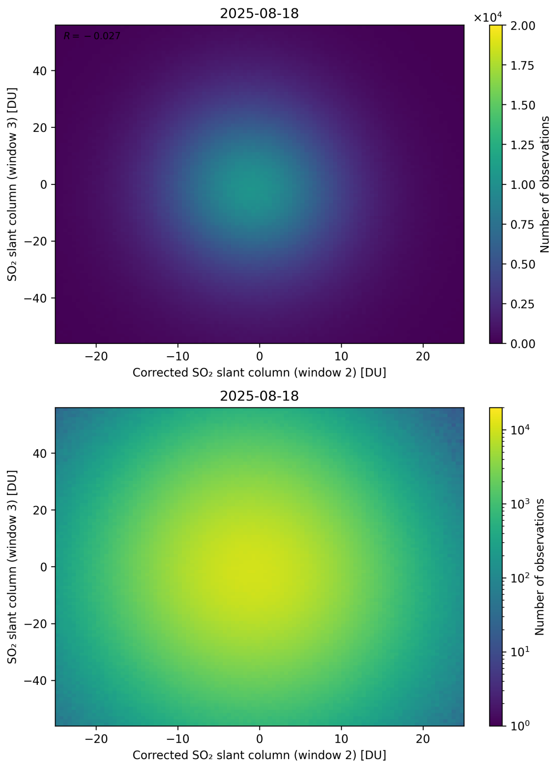
Figure 251: Scatter density plot of “Corrected SO 2 slant column (window 2)” against “SO 2 slant column (window 3)” for 2025-08-17 to 2025-08-19.
