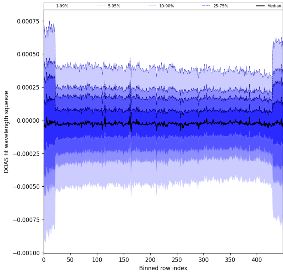
Figure 103: Along track statistics of “DOAS fit wavelength squeeze” for 2025-08-17 to 2025-08-19
