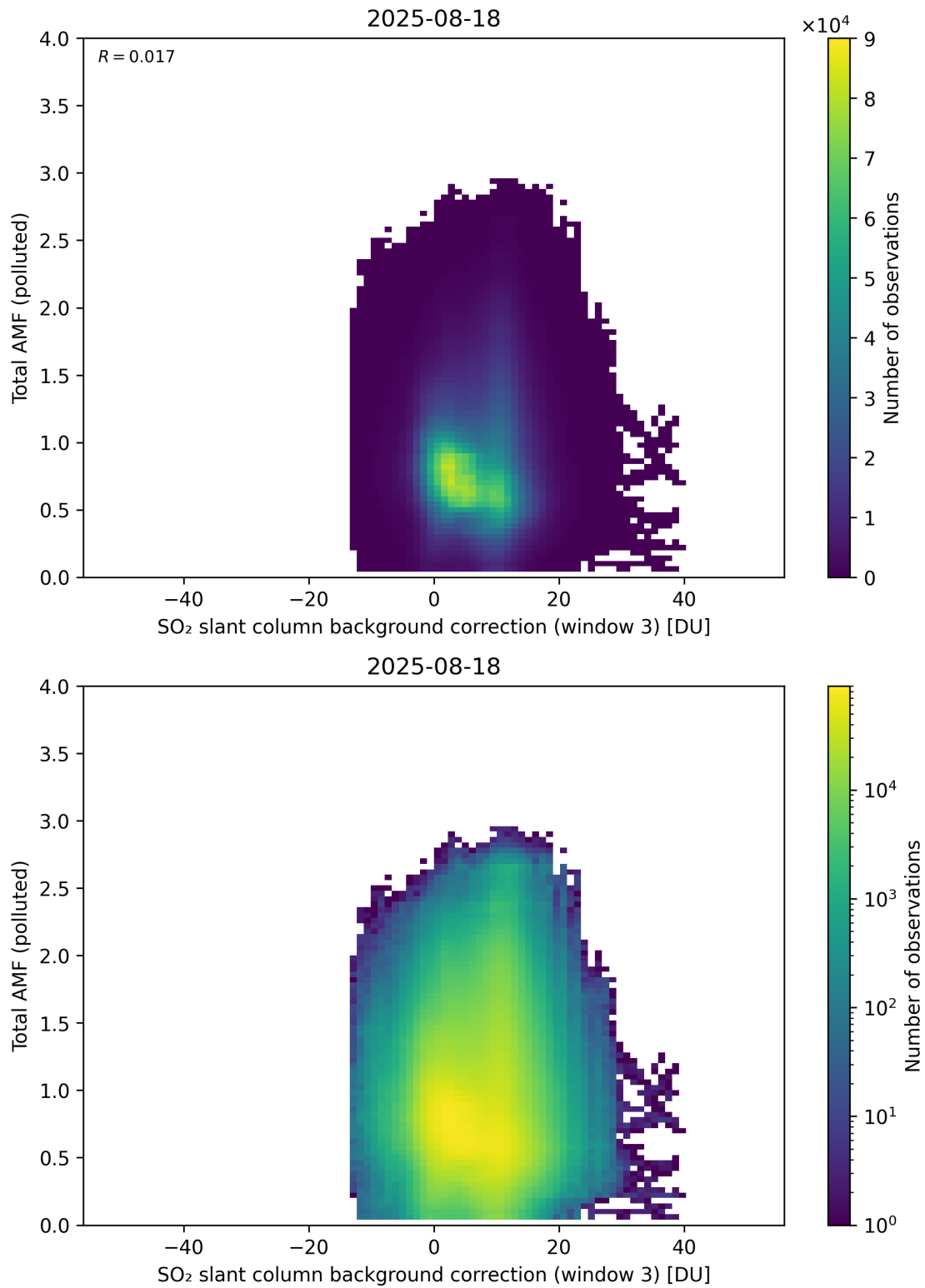
Figure 136: Scatter density plot of “SO 2 slant column background correction (window 3)” against “Total AMF (polluted)” for 2025-08-17 to 2025-08-19.
