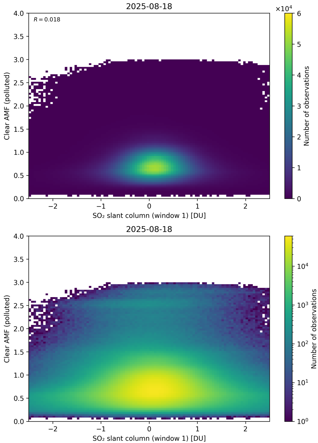
Figure 282: Scatter density plot of “SO 2 slant column (window 1)” against “Clear AMF (polluted)” for 2025-08-17 to 2025-08-19.
