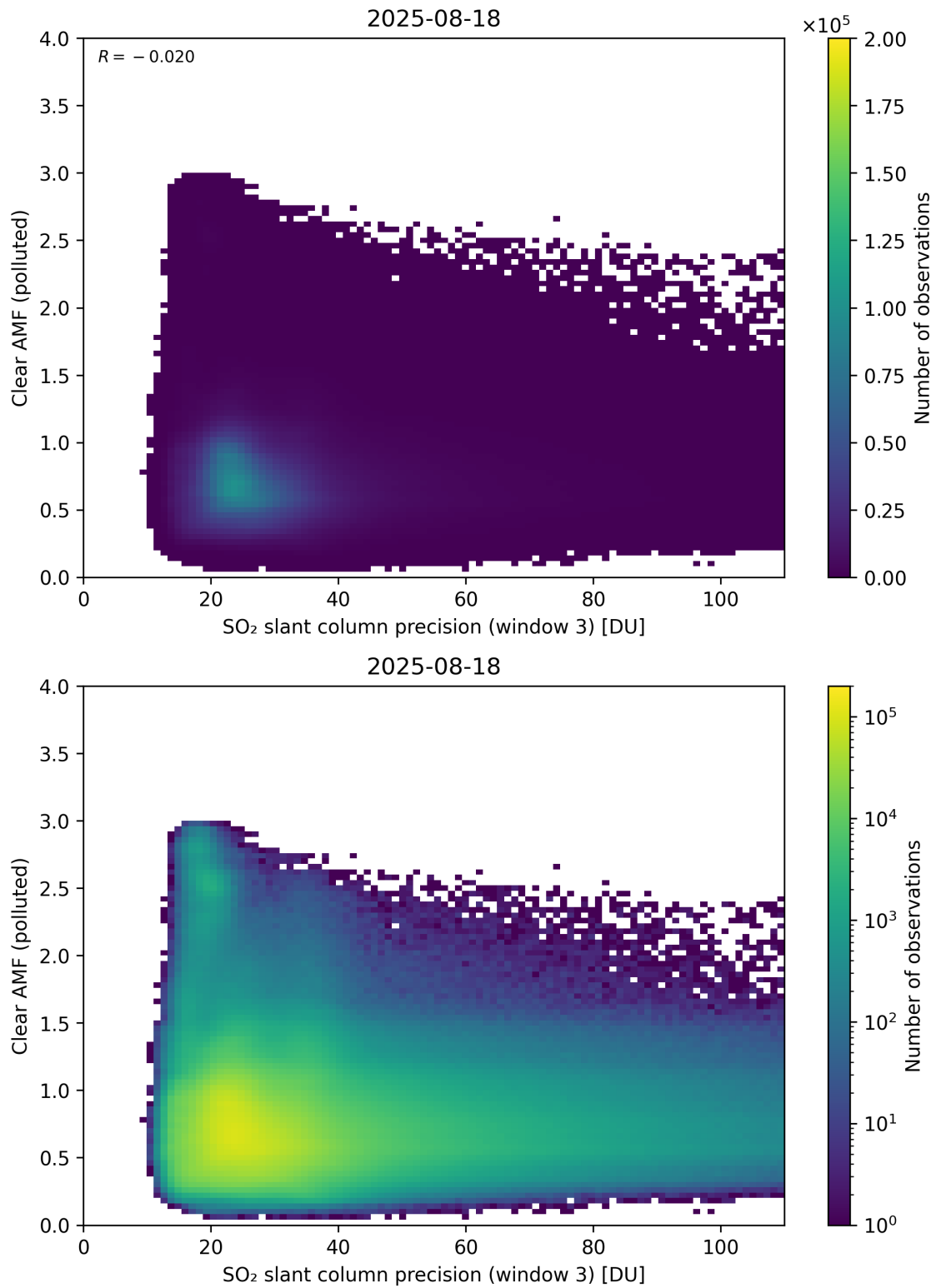
Figure 311: Scatter density plot of “SO 2 slant column precision (window 3)” against “Clear AMF (polluted)” for 2025-08-17 to 2025-08-19.
