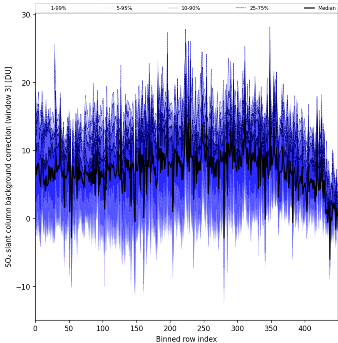
Figure 100: Along track statistics of “SO 2 slant column background correction (window 3)” for 2025-08-17 to 2025-08-19
