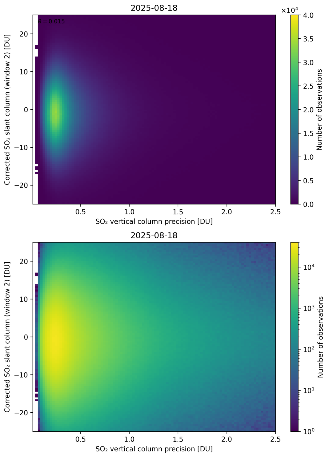
Figure 339: Scatter density plot of “SO 2 vertical column precision” against “Corrected SO 2 slant column (window 2)” for 2025-08-17 to 2025-08-19.
