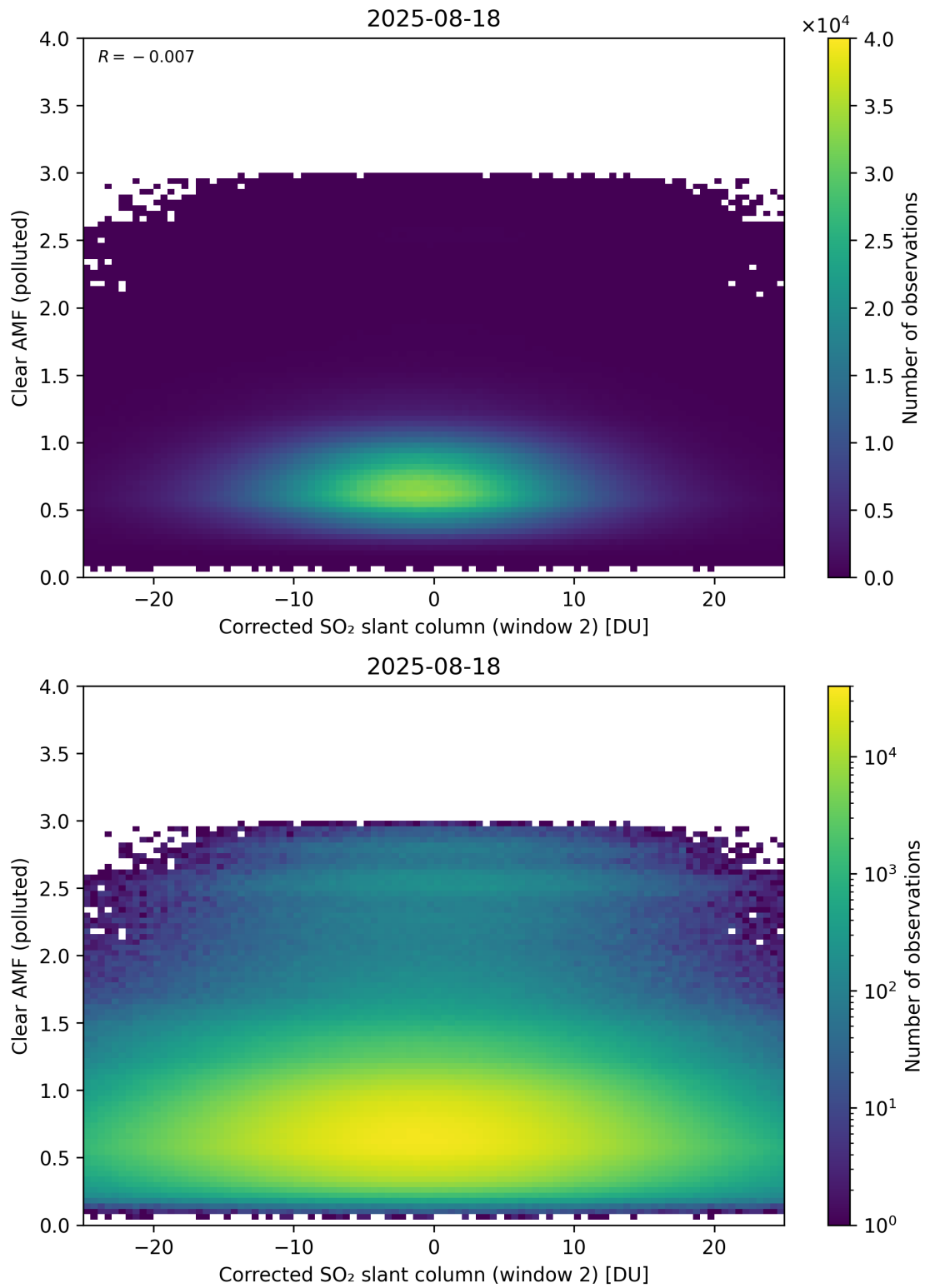
Figure 249: Scatter density plot of “Corrected SO 2 slant column (window 2)” against “Clear AMF (polluted)” for 2025-08-17 to 2025-08-19.
