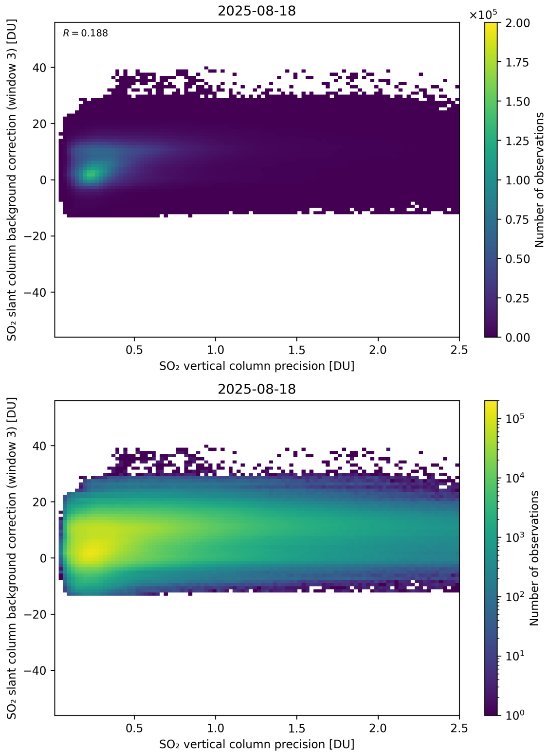
Figure 331: Scatter density plot of “SO 2 vertical column precision” against “SO 2 slant column background correction (window 3)” for 2025-08-17 to 2025-08-19.
