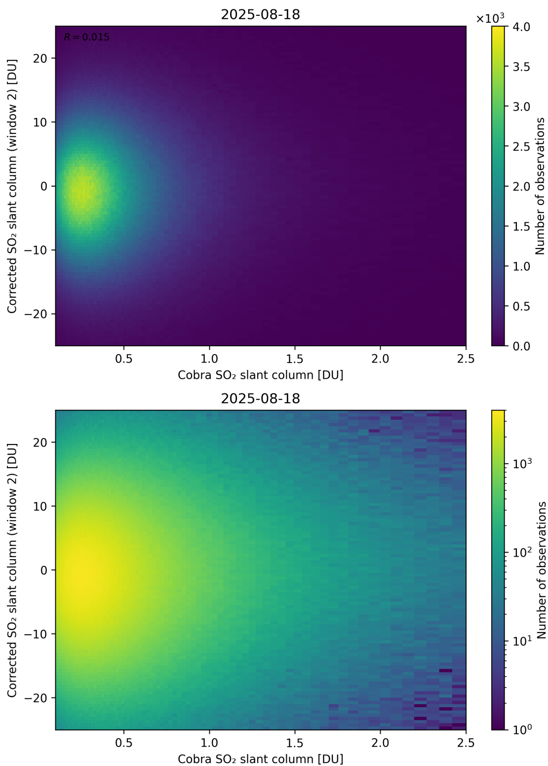
Figure 217: Scatter density plot of “Cobra SO 2 slant column” against “Corrected SO 2 slant column (window 2)” for 2025-08-17 to 2025-08-19.
