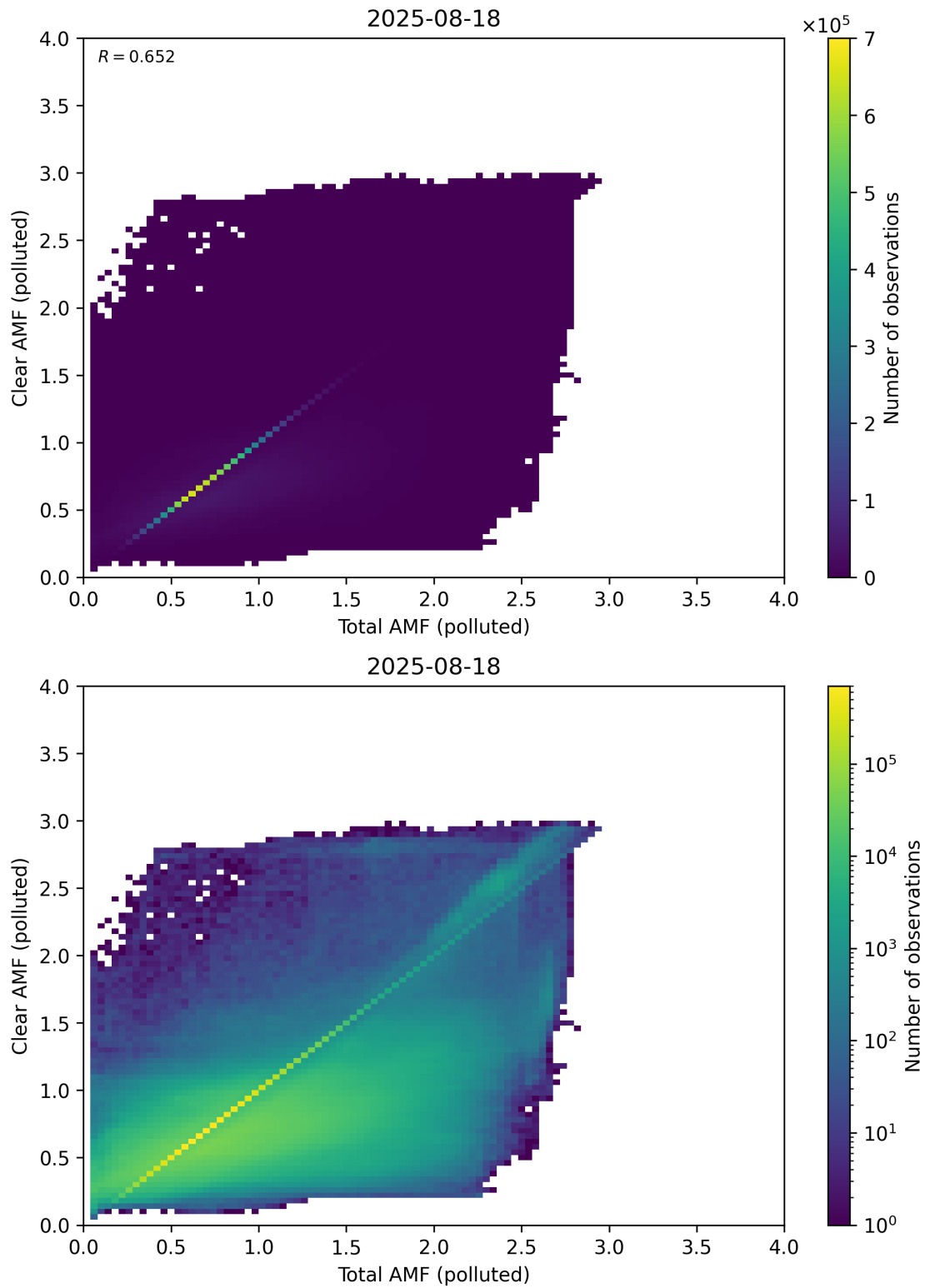
Figure 321: Scatter density plot of “Total AMF (polluted)” against “Clear AMF (polluted)” for 2025-08-17 to 2025-08-19.
