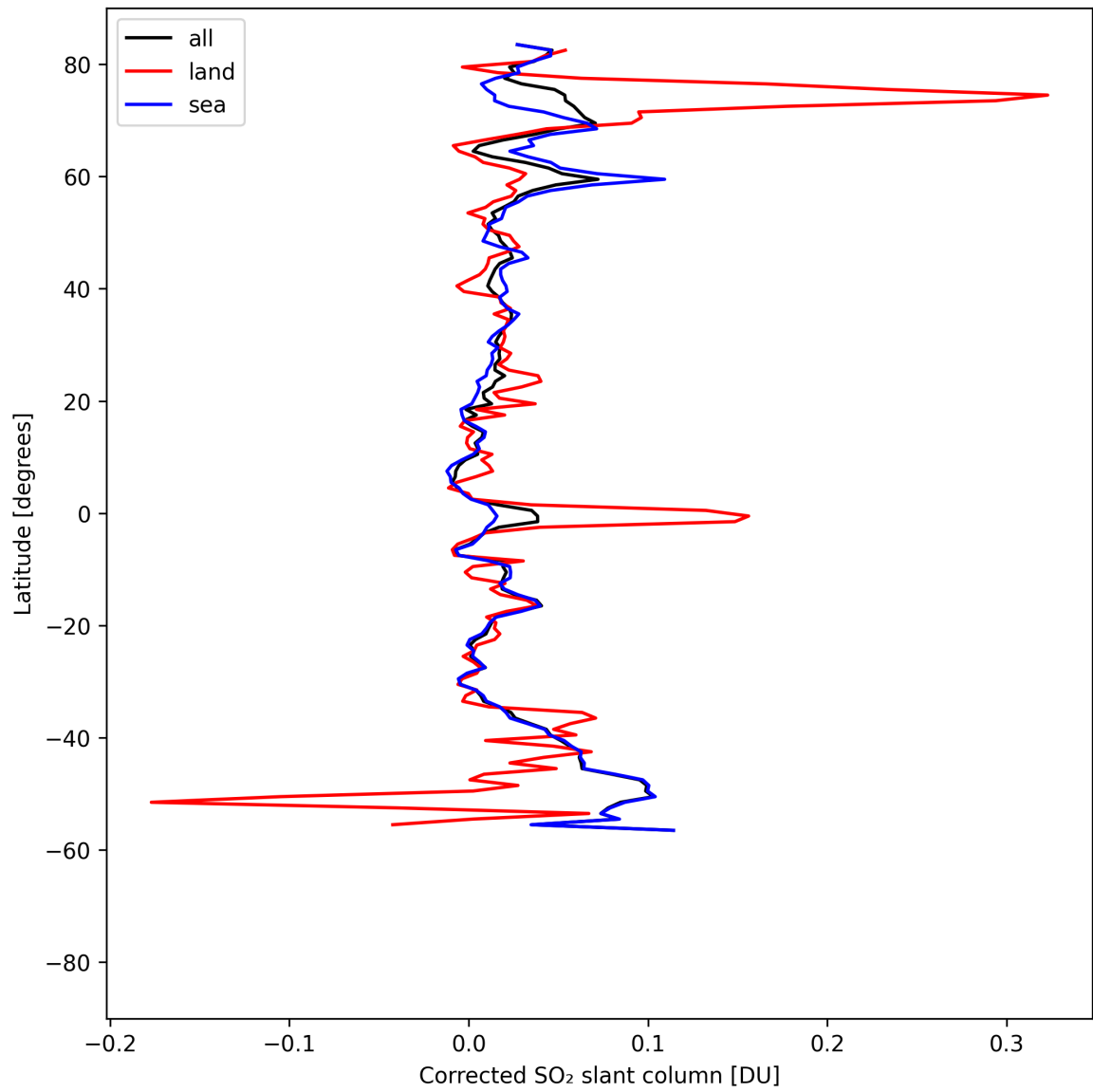
Figure 34: Zonal average of “Corrected SO 2 slant column” for 2025-08-17 to 2025-08-19.
