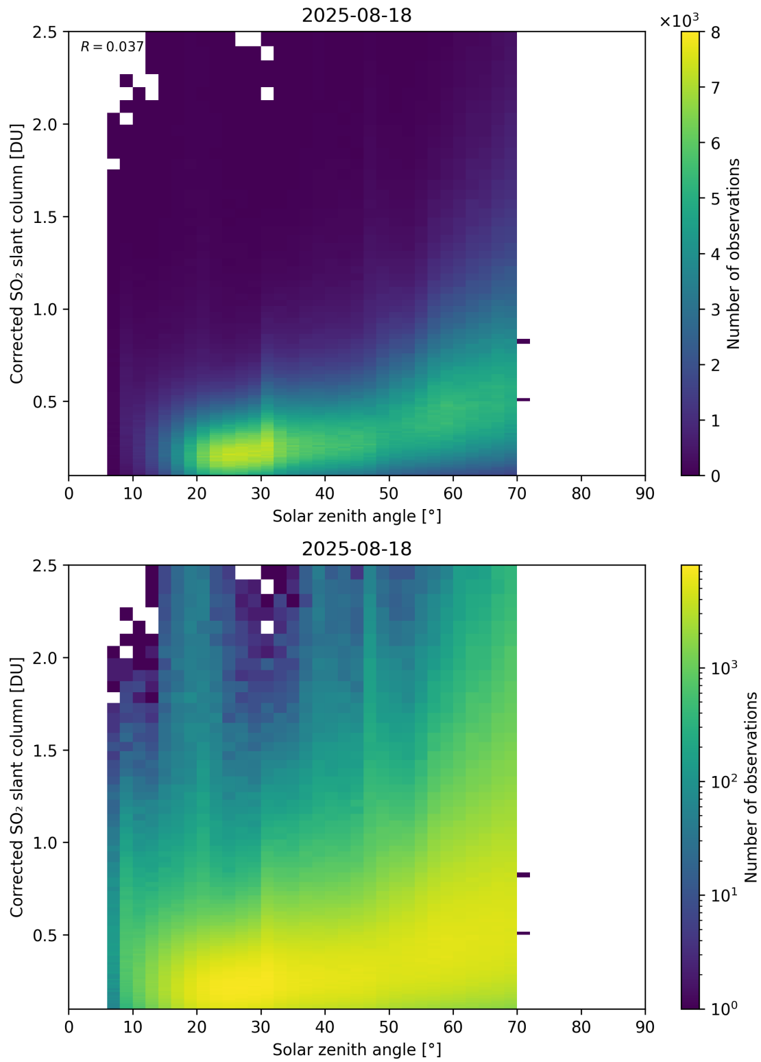
Figure 181: Scatter density plot of “Solar zenith angle” against “Corrected SO 2 slant column” for 2025-08-17 to 2025-08-19.
