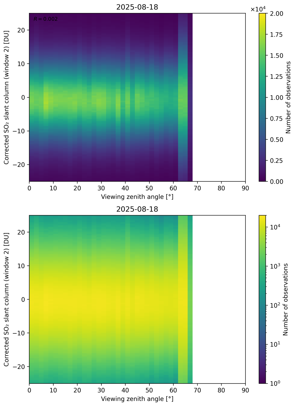
Figure 374: Scatter density plot of “Viewing zenith angle” against “Corrected SO 2 slant column (window 2)” for 2025-08-17 to 2025-08-19.
