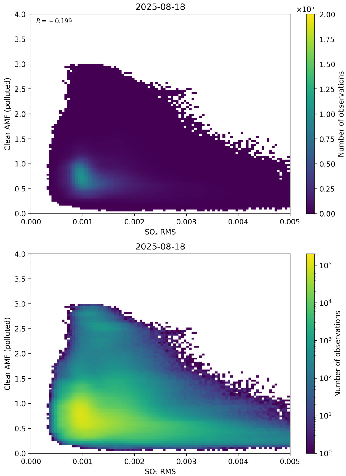
Figure 147: Scatter density plot of “SO 2 RMS” against “Clear AMF (polluted)” for 2025-08-17 to 2025-08-19.
