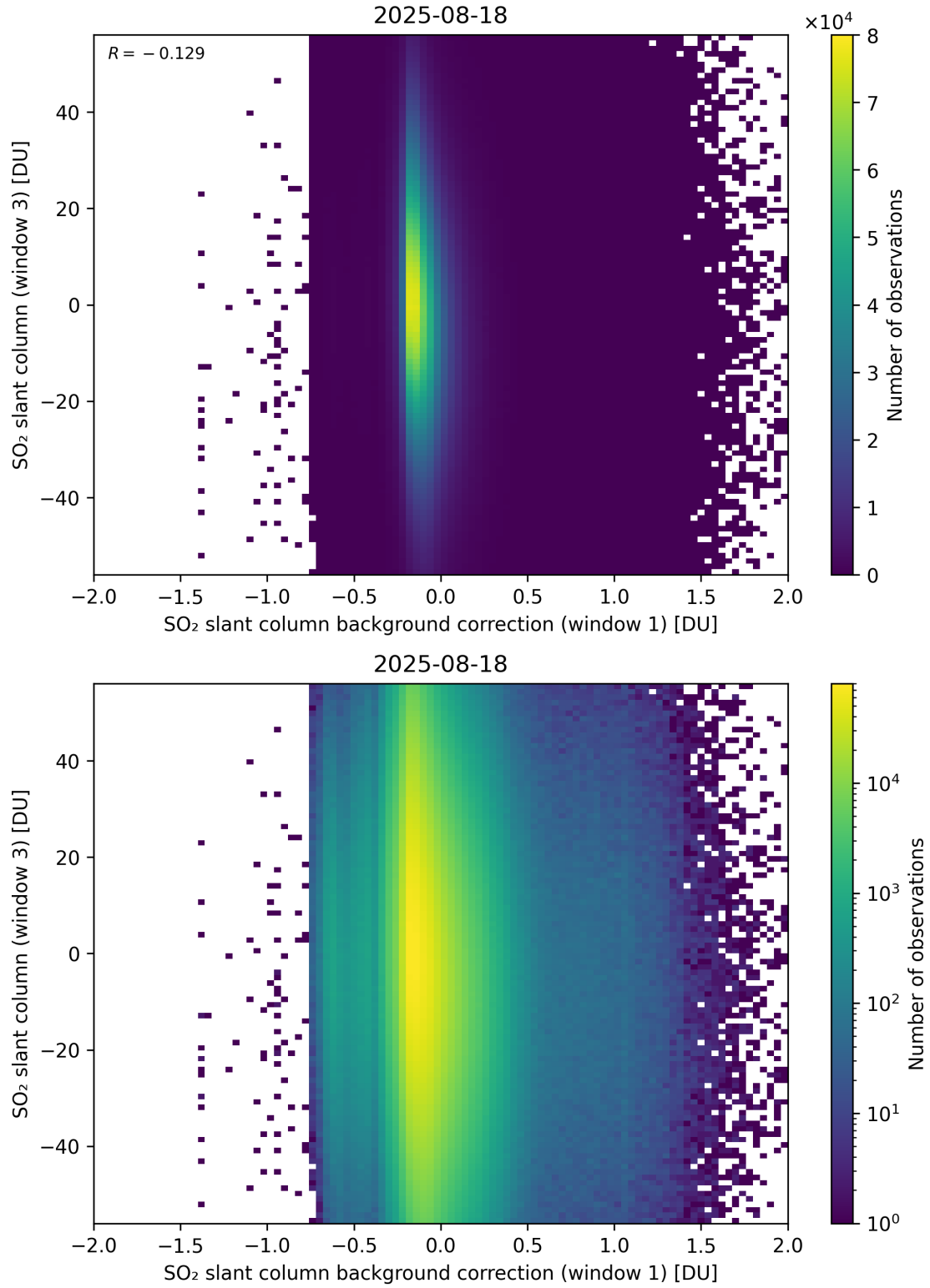
Figure 118: Scatter density plot of “SO 2 slant column background correction (window 1)” against “SO 2 slant column (window 3)” for 2025-08-17 to 2025-08-19.
