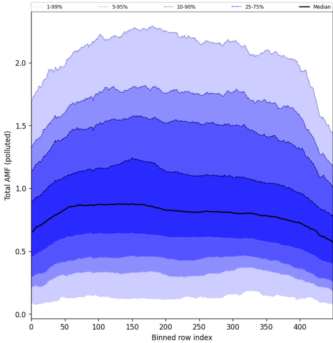
Figure 105: Along track statistics of “Total AMF (polluted)” for 2025-08-17 to 2025-08-19
