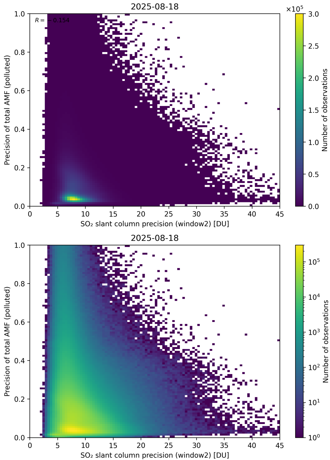
Figure 302: Scatter density plot of “SO 2 slant column precision (window2)” against “Precision of total AMF (polluted)” for 2025-08-17 to 2025-08-19.
