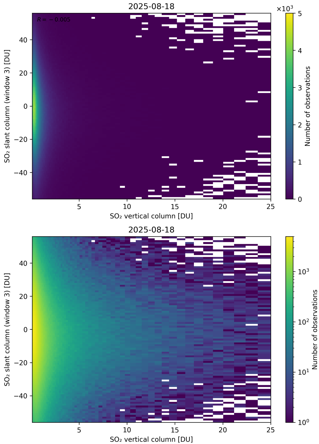
Figure 357: Scatter density plot of “SO 2 vertical column” against “SO 2 slant column (window 3)” for 2025-08-17 to 2025-08-19.
