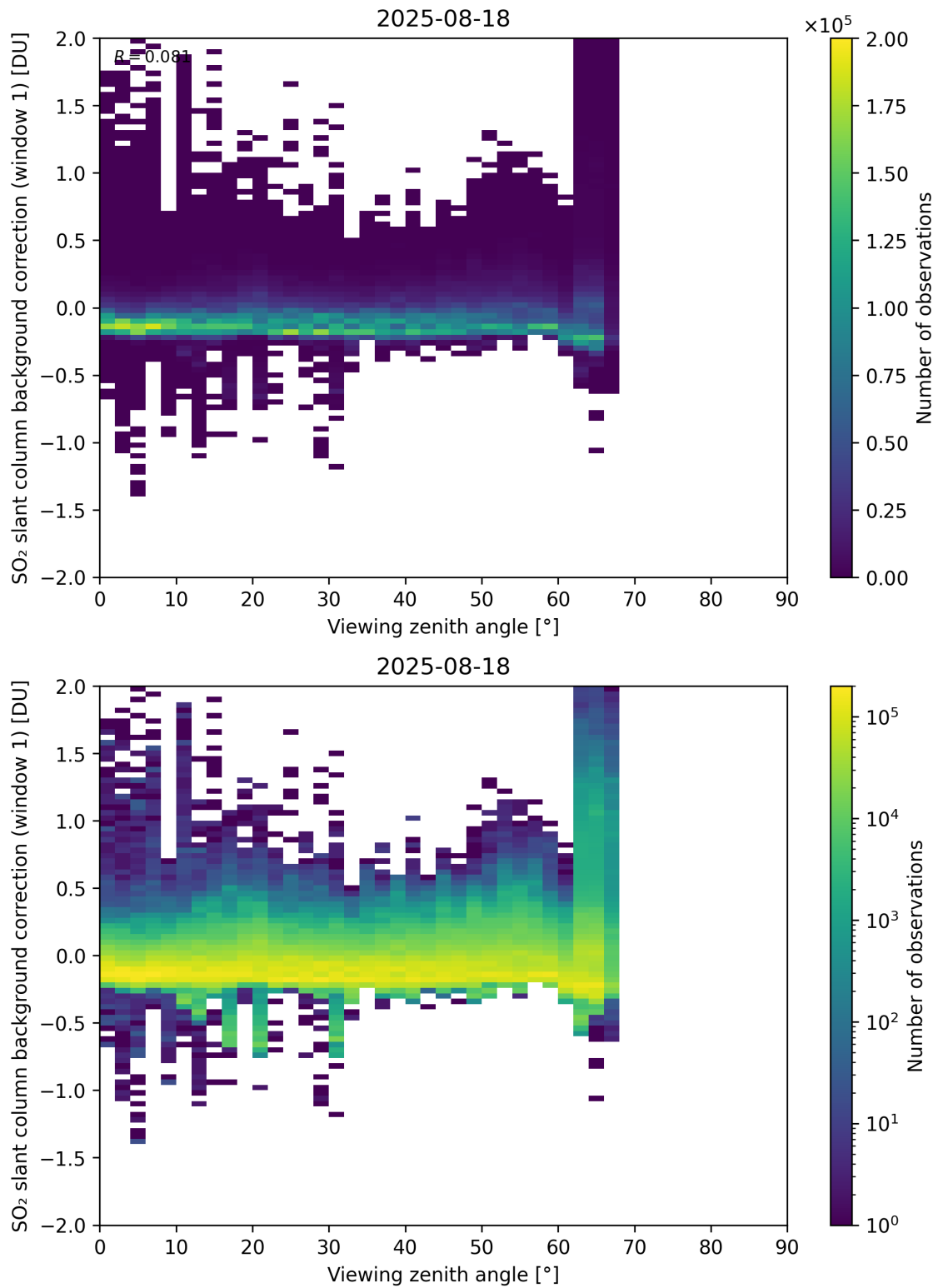
Figure 362: Scatter density plot of “Viewing zenith angle” against “SO 2 slant column background correction (window 1)” for 2025-08-17 to 2025-08-19.
