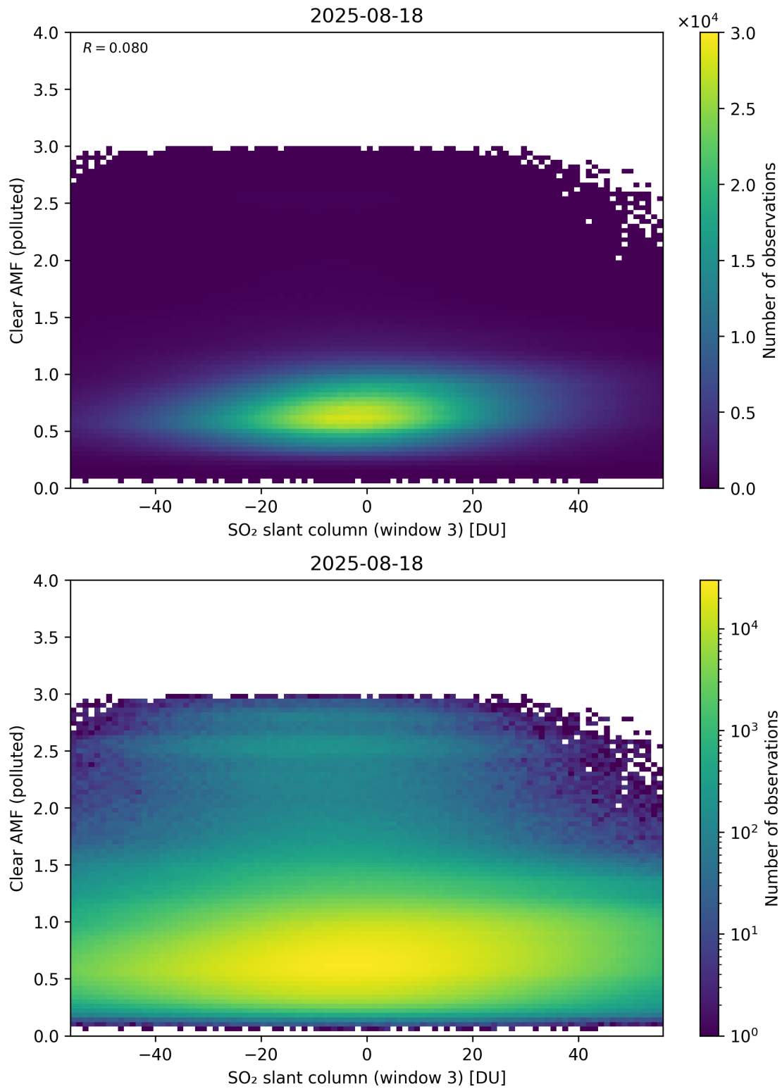
Figure 315: Scatter density plot of “SO 2 slant column (window 3)” against “Clear AMF (polluted)” for 2025-08-17 to 2025-08-19.
