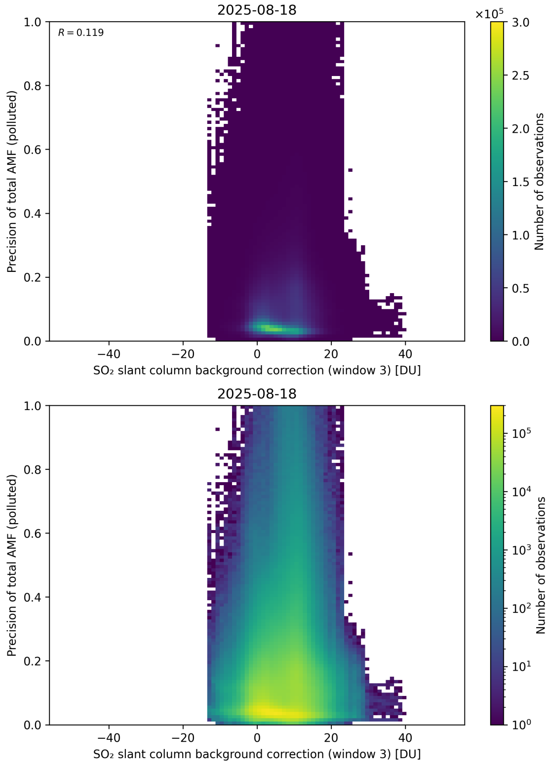
Figure 137: Scatter density plot of “SO 2 slant column background correction (window 3)” against “Precision of total AMF (polluted)” for 2025-08-17 to 2025-08-19.
