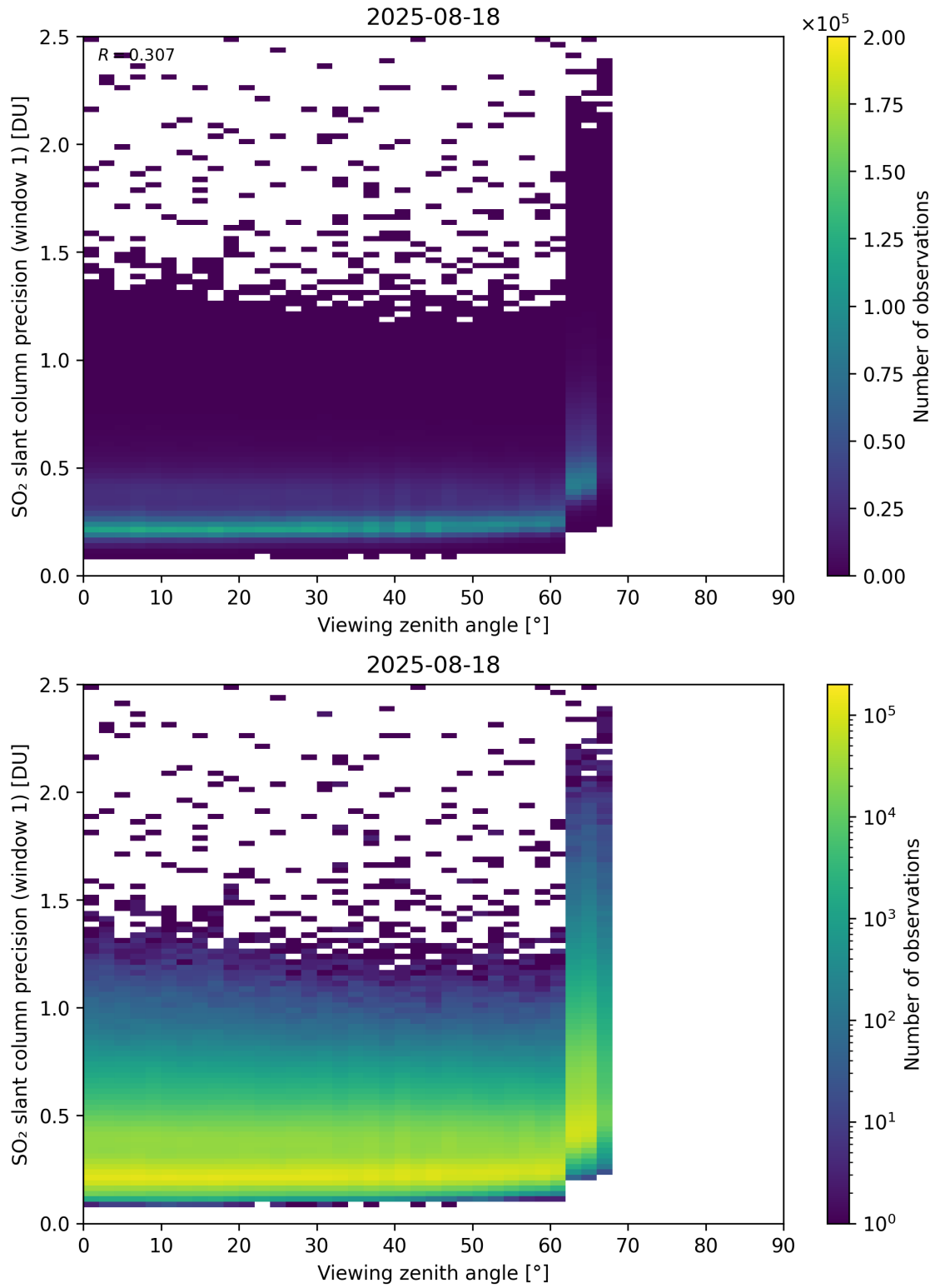
Figure 377: Scatter density plot of “Viewing zenith angle” against “SO 2 slant column precision (window 1)” for 2025-08-17 to 2025-08-19.
