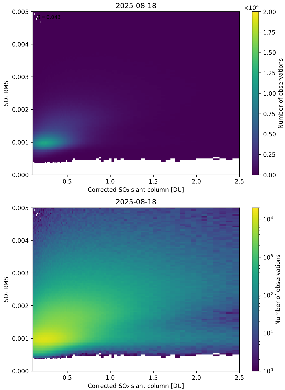
Figure 231: Scatter density plot of “Corrected SO 2 slant column” against “SO 2 RMS” for 2025-08-17 to 2025-08-19.
