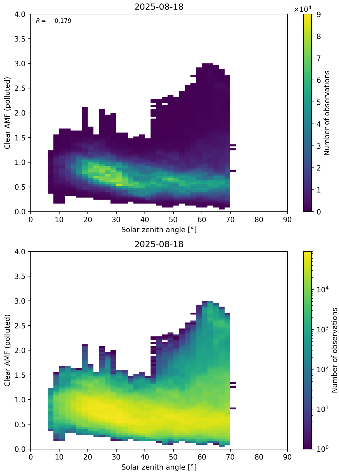
Figure 178: Scatter density plot of “Solar zenith angle” against “Clear AMF (polluted)” for 2025-08-17 to 2025-08-19.
