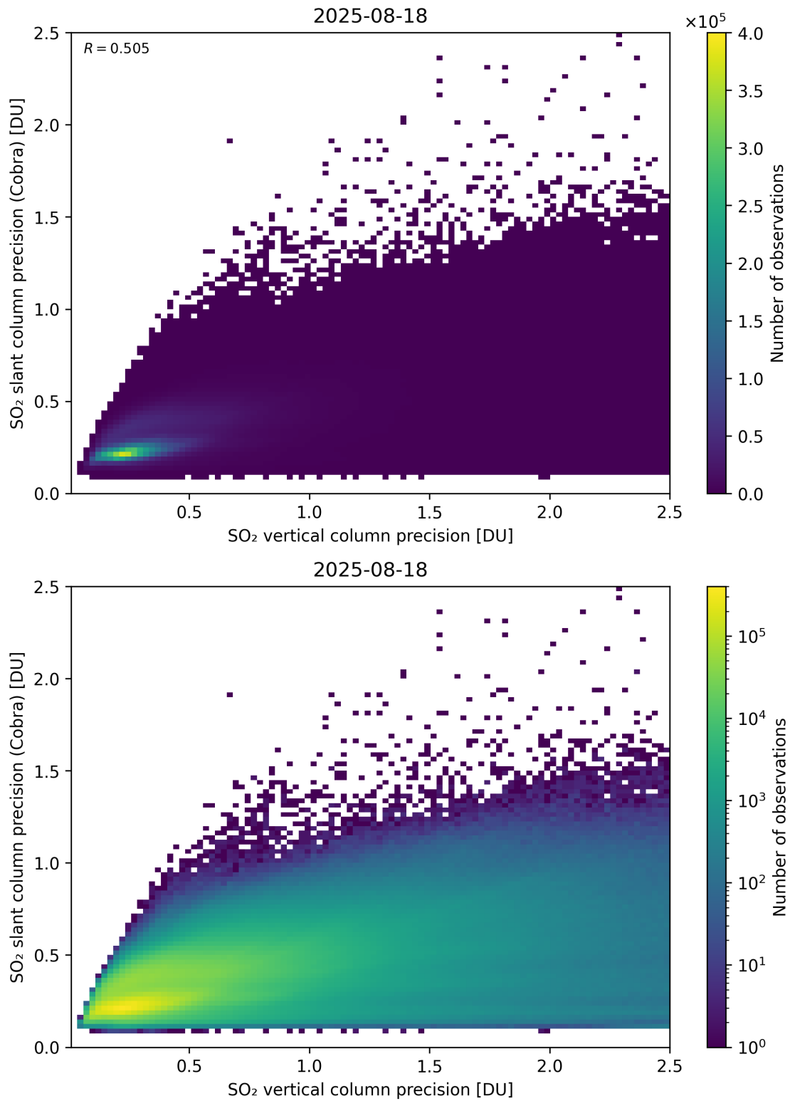
Figure 337: Scatter density plot of “SO 2 vertical column precision” against “SO 2 slant column precision (Cobra)” for 2025-08-17 to 2025-08-19.
