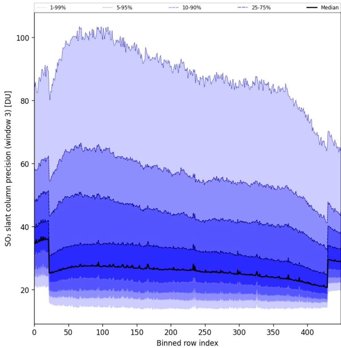
Figure 98: Along track statistics of “SO 2 slant column precision (window 3)” for 2025-08-17 to 2025-08-19
