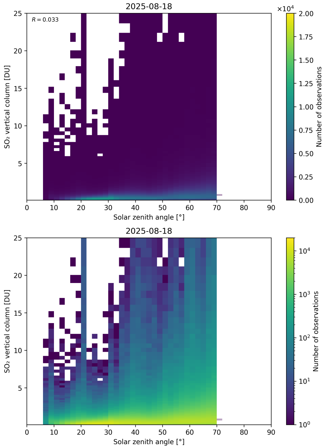
Figure 191: Scatter density plot of “Solar zenith angle” against “SO 2 vertical column” for 2025-08-17 to 2025-08-19.
