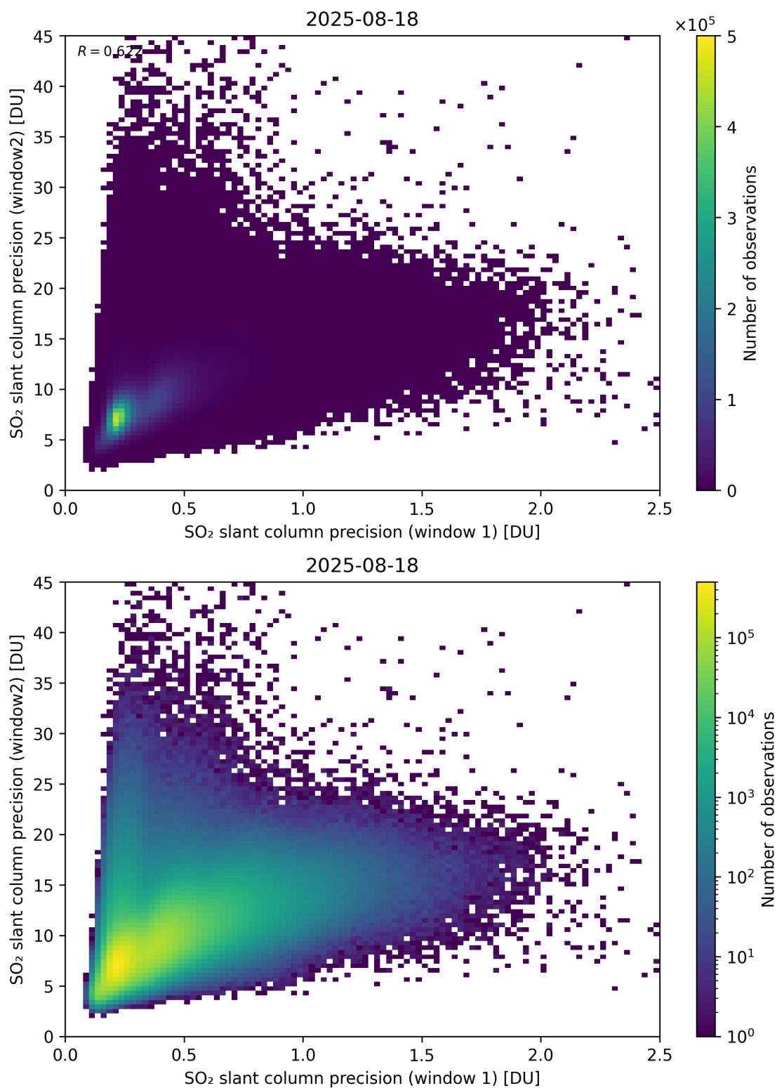
Figure 277: Scatter density plot of “SO 2 slant column precision (window 1)” against “SO 2 slant column precision (window2)” for 2025-08-17 to 2025-08-19.
