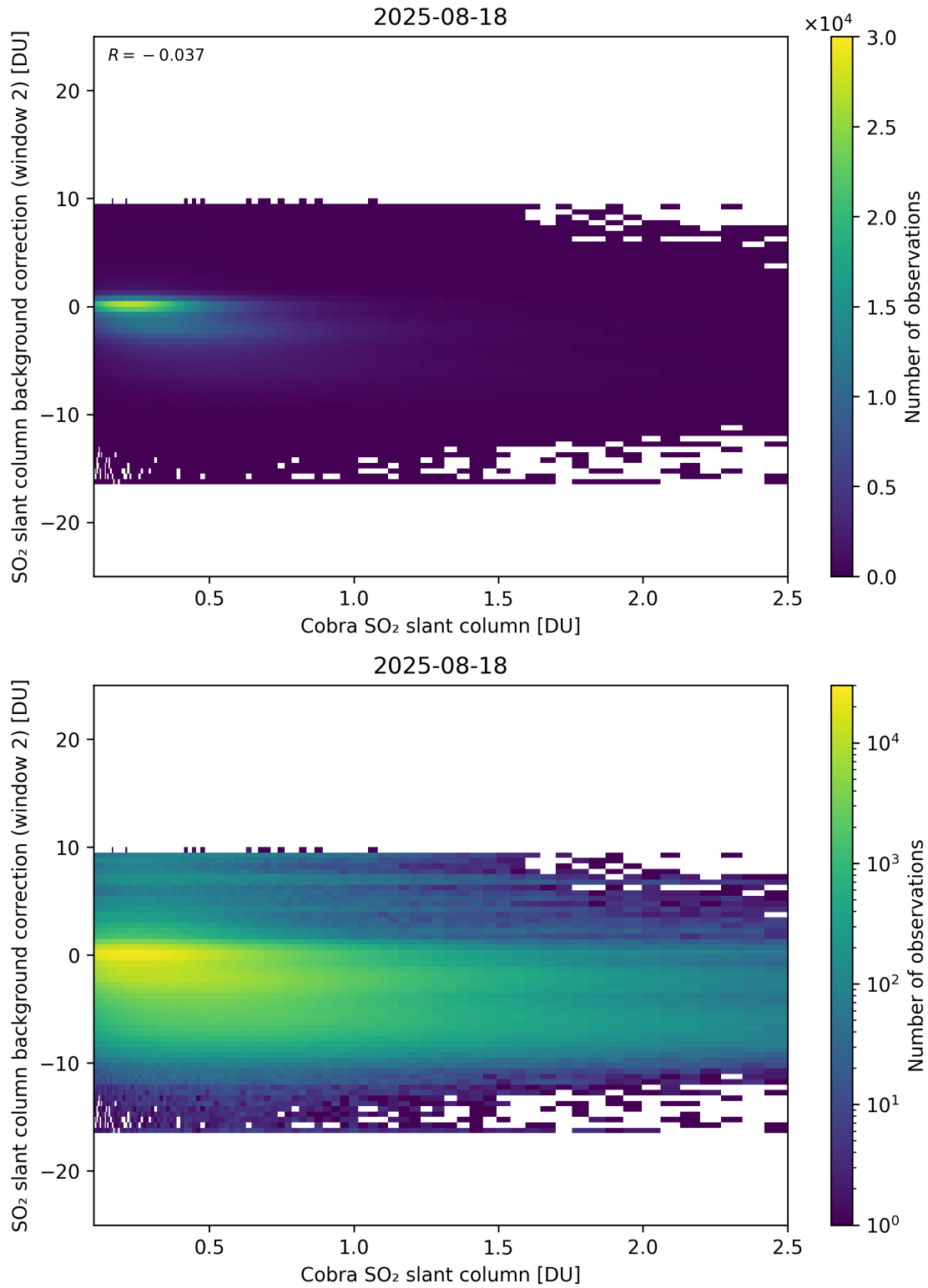
Figure 194: Scatter density plot of “Cobra SO 2 slant column” against “SO 2 slant column background correction (window 2)” for 2025-08-17 to 2025-08-19.
