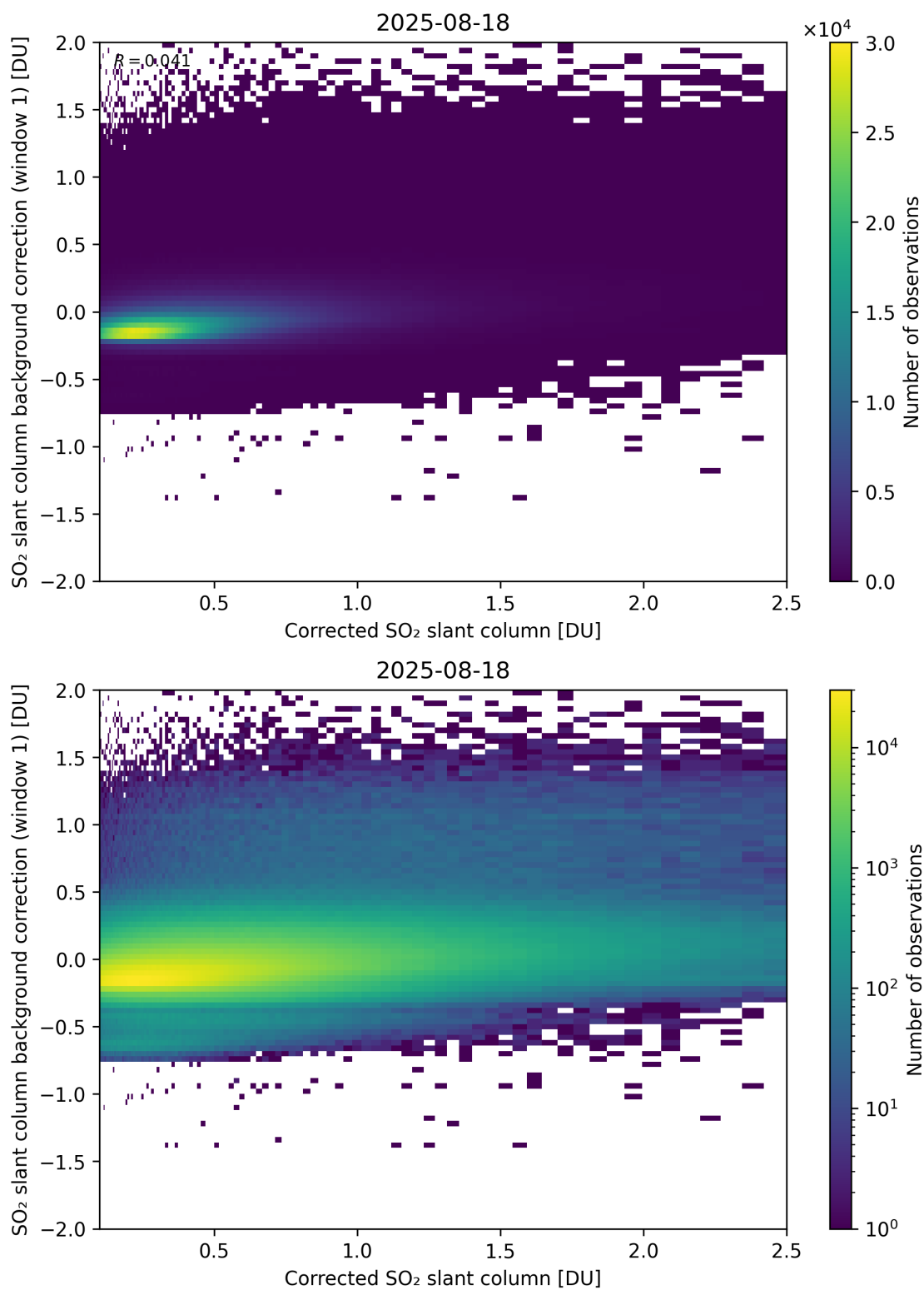
Figure 226: Scatter density plot of “Corrected SO 2 slant column” against “SO 2 slant column background correction (window 1)” for 2025-08-17 to 2025-08-19.
