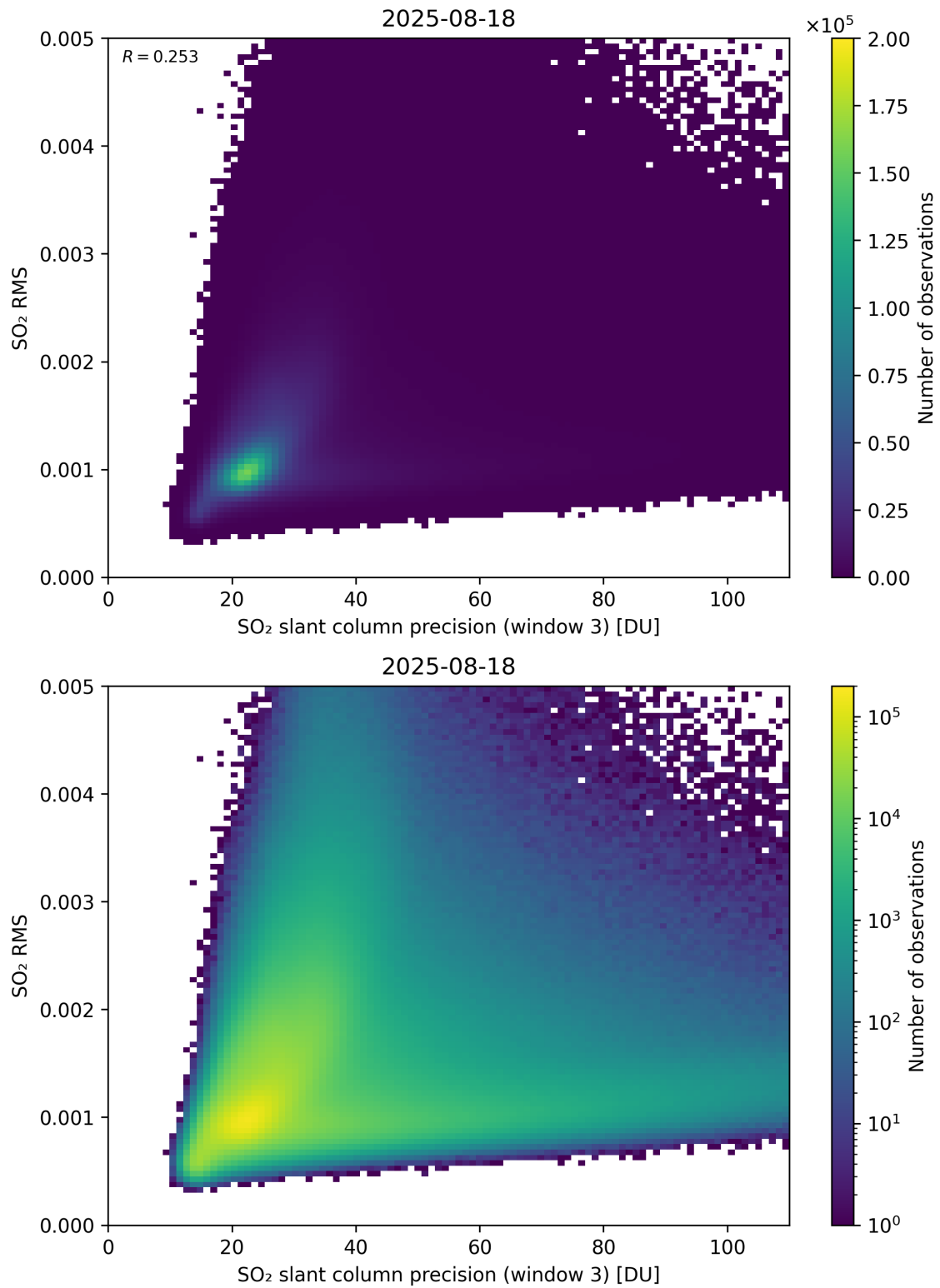
Figure 310: Scatter density plot of “SO 2 slant column precision (window 3)” against “SO 2 RMS” for 2025-08-17 to 2025-08-19.
