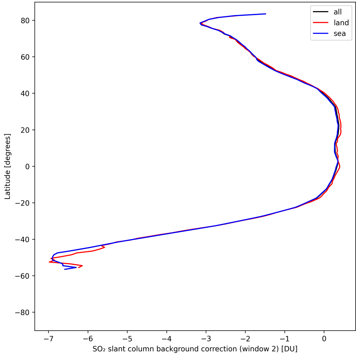
Figure 44: Zonal average of “SO 2 slant column background correction (window 2)” for 2025-08-17 to 2025-08-19.
