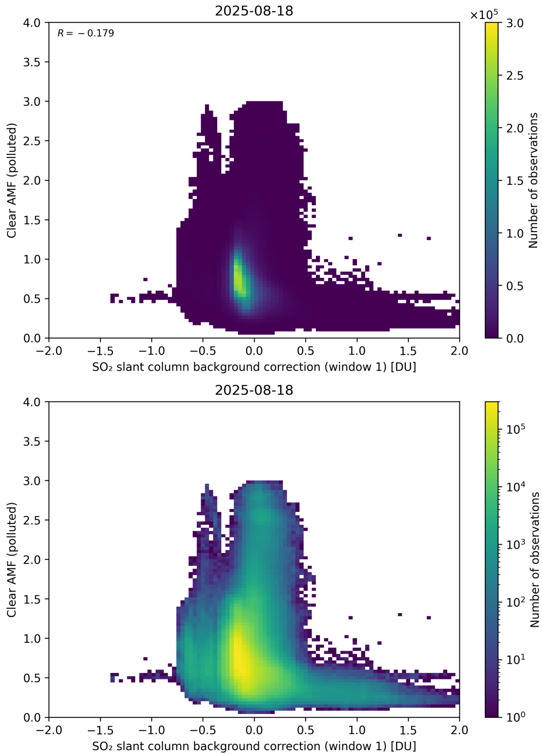
Figure 114: Scatter density plot of “SO 2 slant column background correction (window 1)” against “Clear AMF (polluted)” for 2025-08-17 to 2025-08-19.
