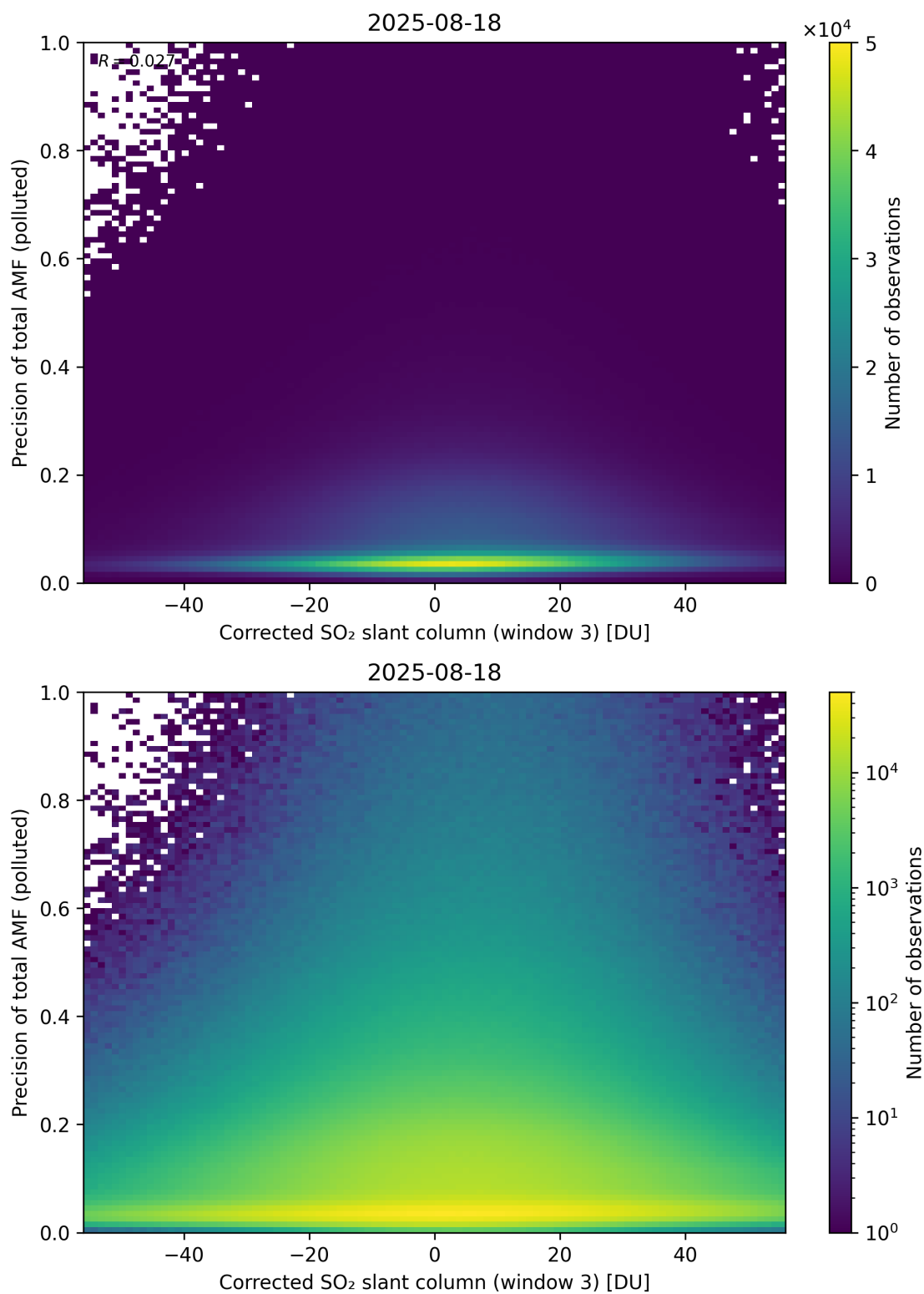
Figure 261: Scatter density plot of “Corrected SO 2 slant column (window 3)” against “Precision of total AMF (polluted)” for 2025-08-17 to 2025-08-19.
