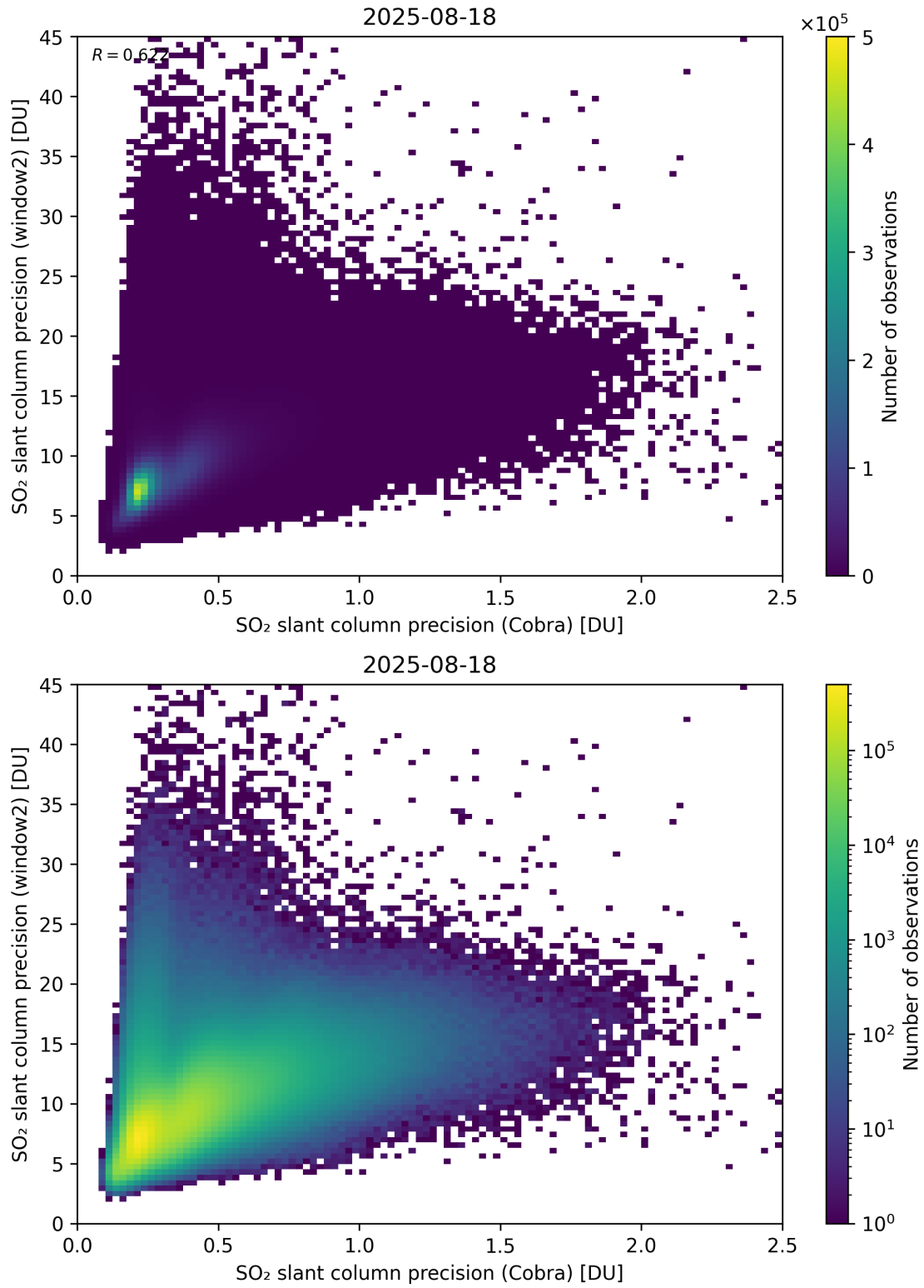
Figure 210: Scatter density plot of “SO 2 slant column precision (Cobra)” against “SO 2 slant column precision (window2)” for 2025-08-17 to 2025-08-19.
