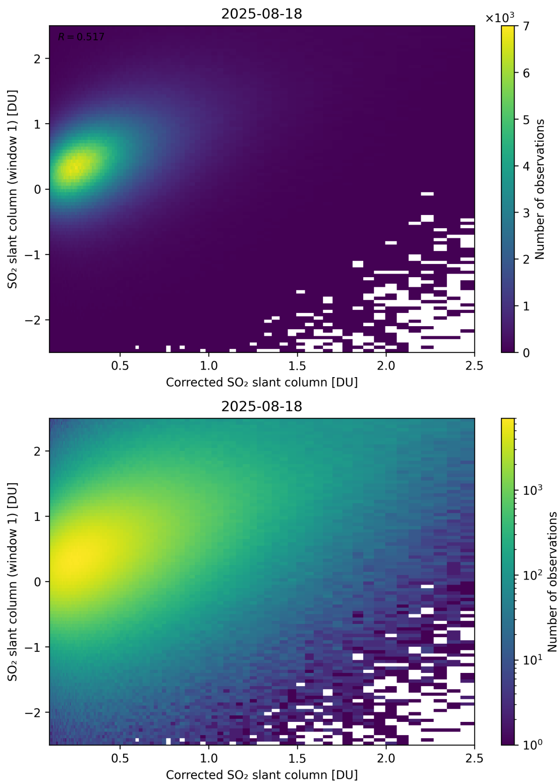
Figure 237: Scatter density plot of “Corrected SO 2 slant column” against “SO 2 slant column (window 1)” for 2025-08-17 to 2025-08-19.
