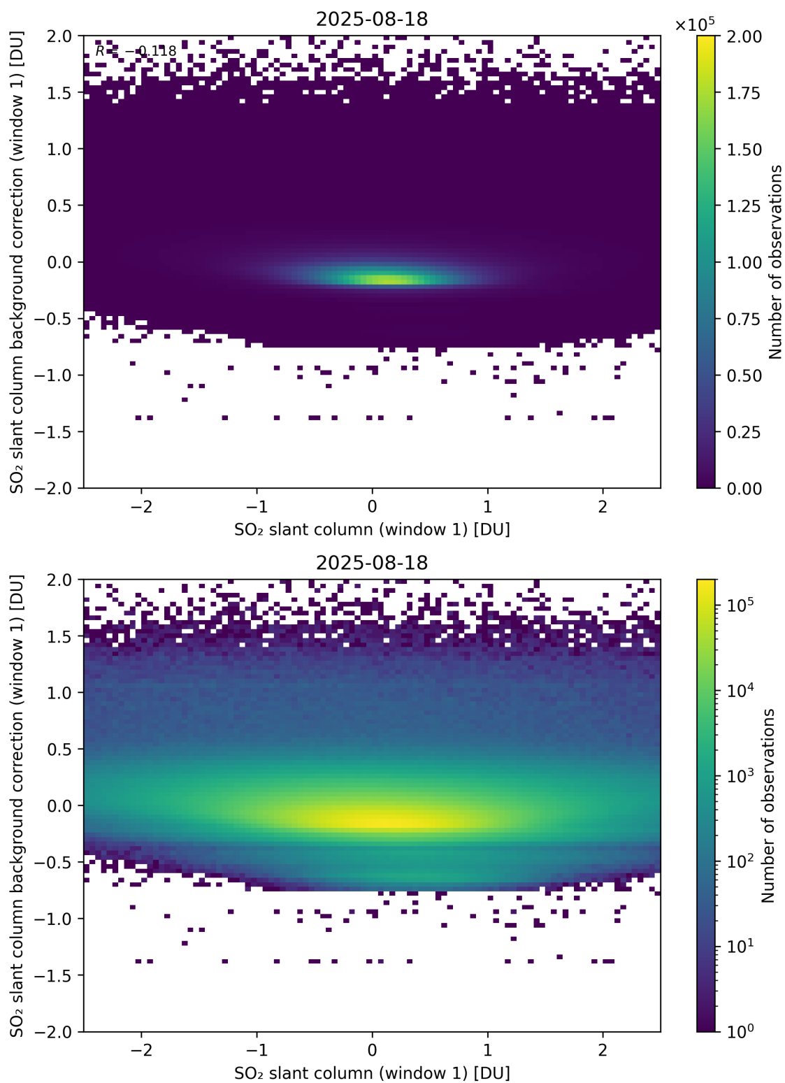
Figure 262: Scatter density plot of “SO 2 slant column (window 1)” against “SO 2 slant column background correction (window 1)” for 2025-08-17 to 2025-08-19.
