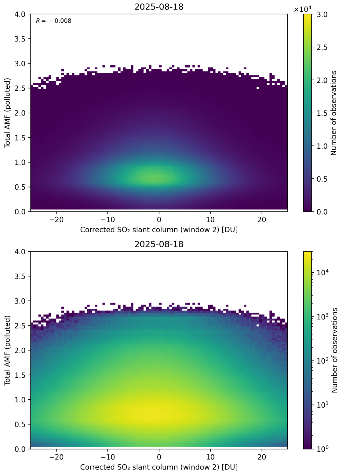
Figure 253: Scatter density plot of “Corrected SO 2 slant column (window 2)” against “Total AMF (polluted)” for 2025-08-17 to 2025-08-19.
