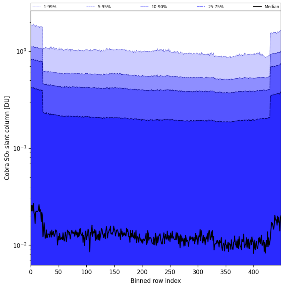
Figure 87: Along track statistics of "Cobra SO 2 slant column" for 2025-08-17 to 2025-08-19
