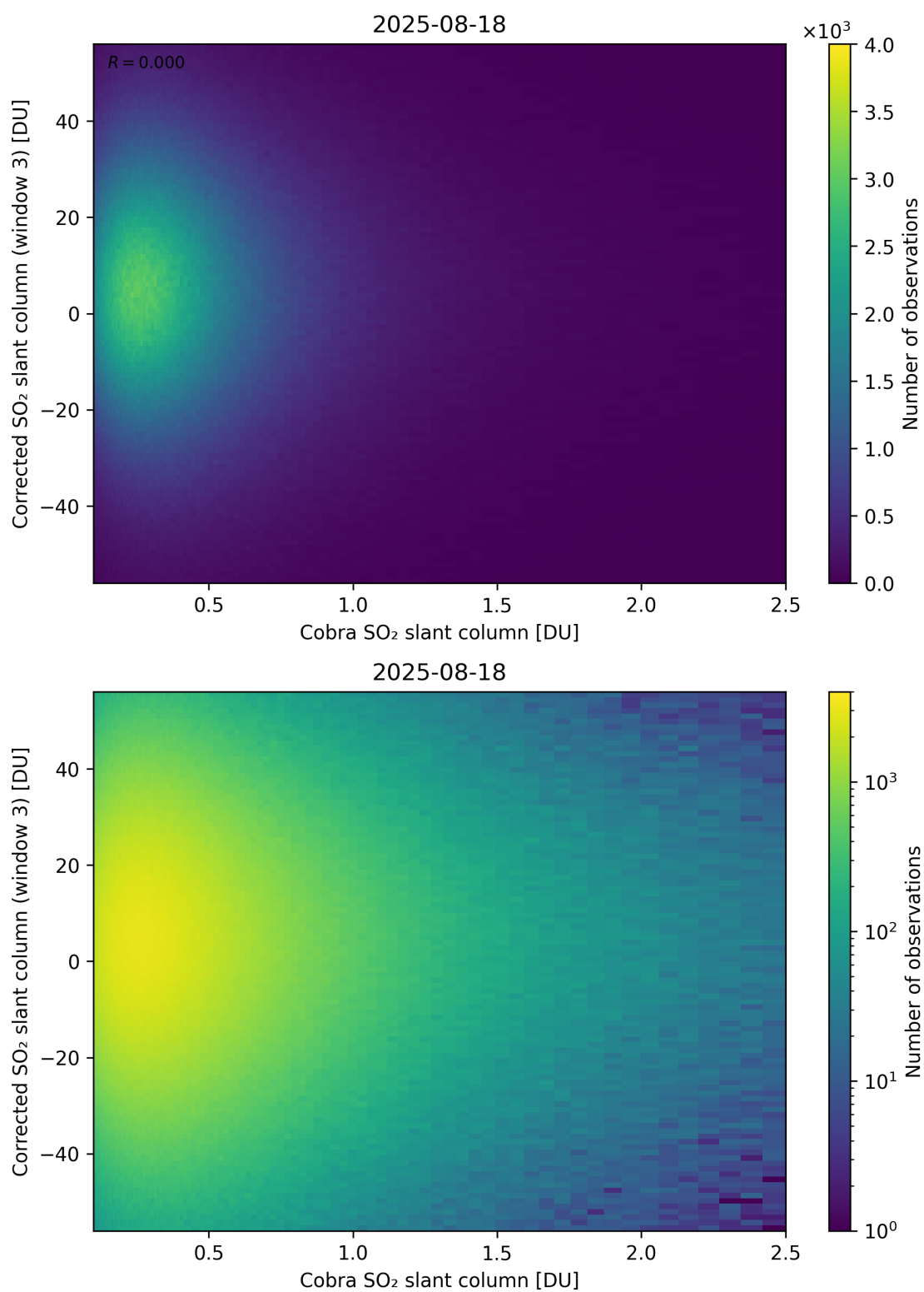
Figure 218: Scatter density plot of “Cobra SO 2 slant column” against “Corrected SO 2 slant column (window 3)” for 2025-08-17 to 2025-08-19.
