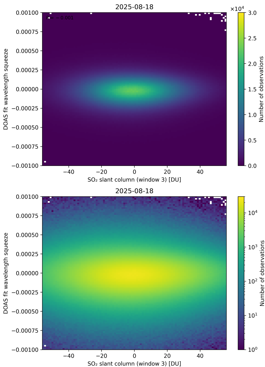
Figure 305: Scatter density plot of “SO 2 slant column (window 3)” against “DOAS fit wavelength squeeze” for 2025-08-17 to 2025-08-19.
