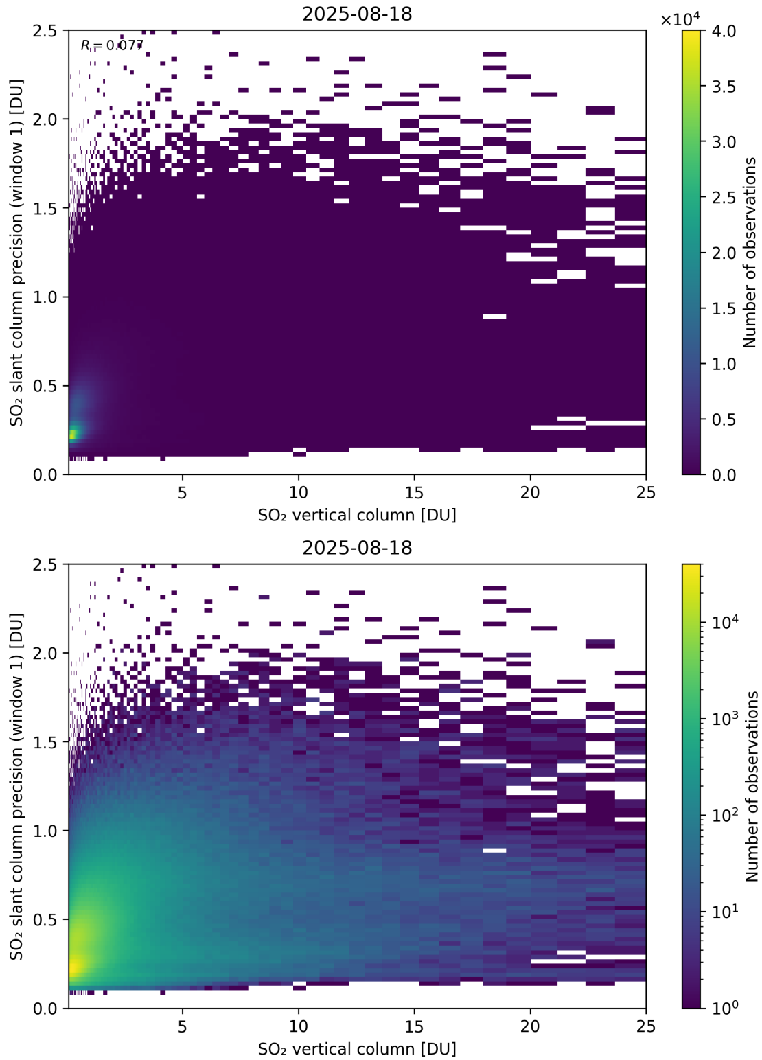
Figure 355: Scatter density plot of “SO 2 vertical column” against “SO 2 slant column precision (window 1)” for 2025-08-17 to 2025-08-19.
