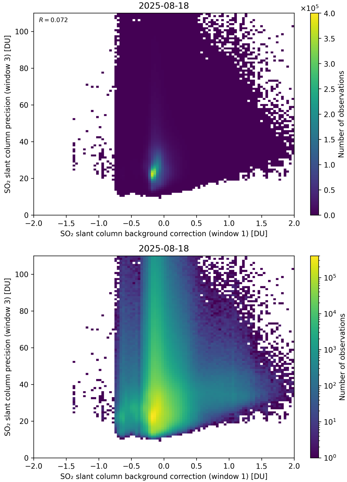
Figure 119: Scatter density plot of “SO 2 slant column background correction (window 1)” against “SO 2 slant column precision (window 3)” for 2025-08-17 to 2025-08-19.
