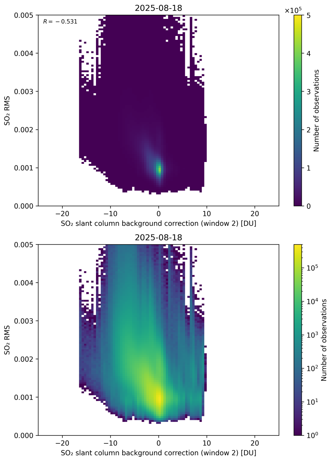
Figure 125: Scatter density plot of “SO 2 slant column background correction (window 2)” against “SO 2 RMS” for 2025-08-17 to 2025-08-19.
