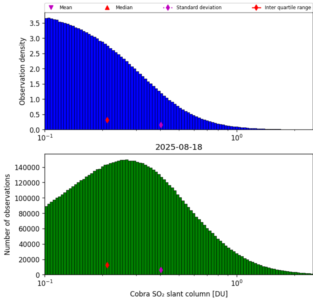
Figure 61: Histogram of “Cobra SO 2 slant column” for 2025-08-17 to 2025-08-19
