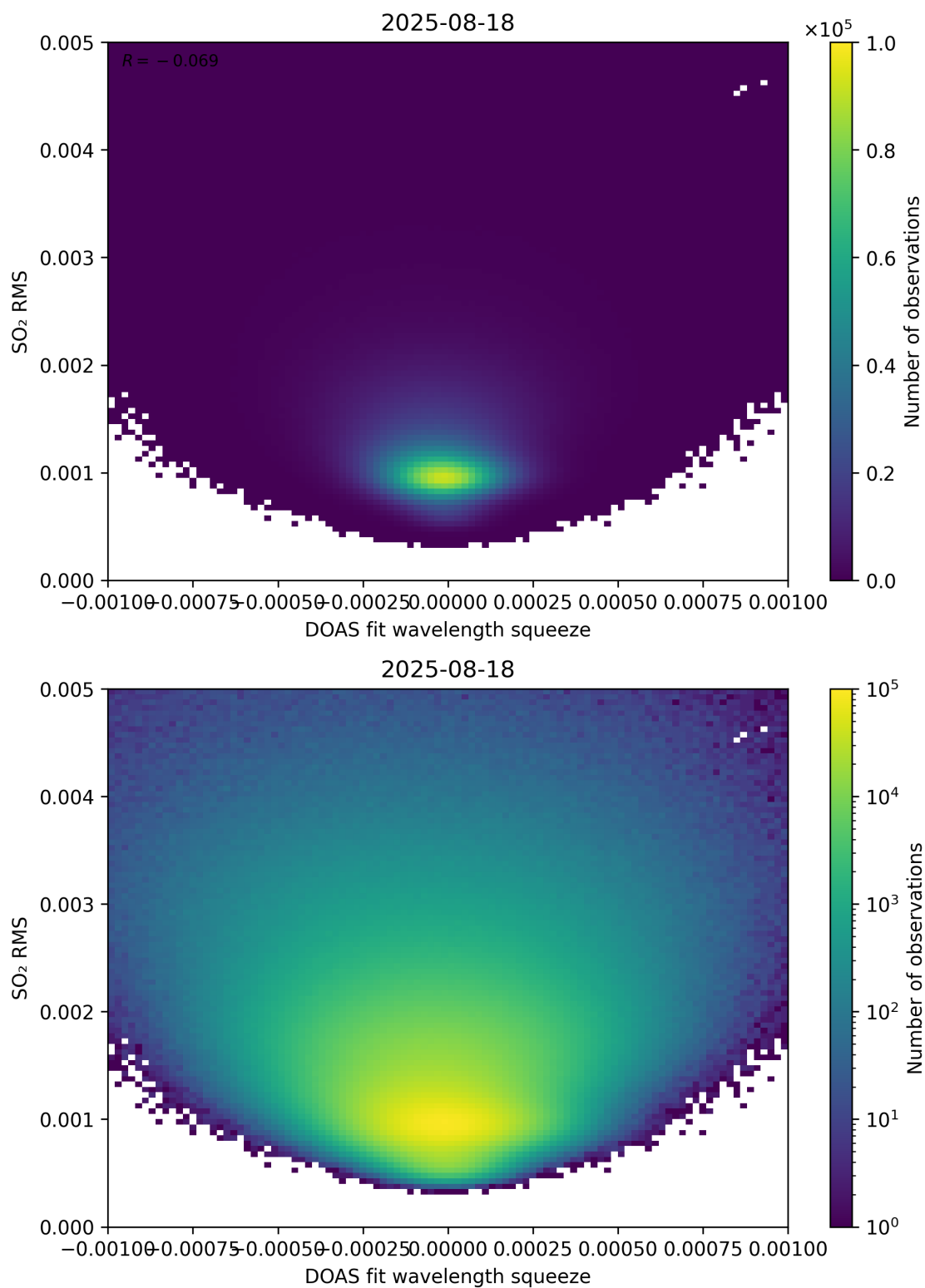
Figure 143: Scatter density plot of “DOAS fit wavelength squeeze” against “SO 2 RMS” for 2025-08-17 to 2025-08-19.
