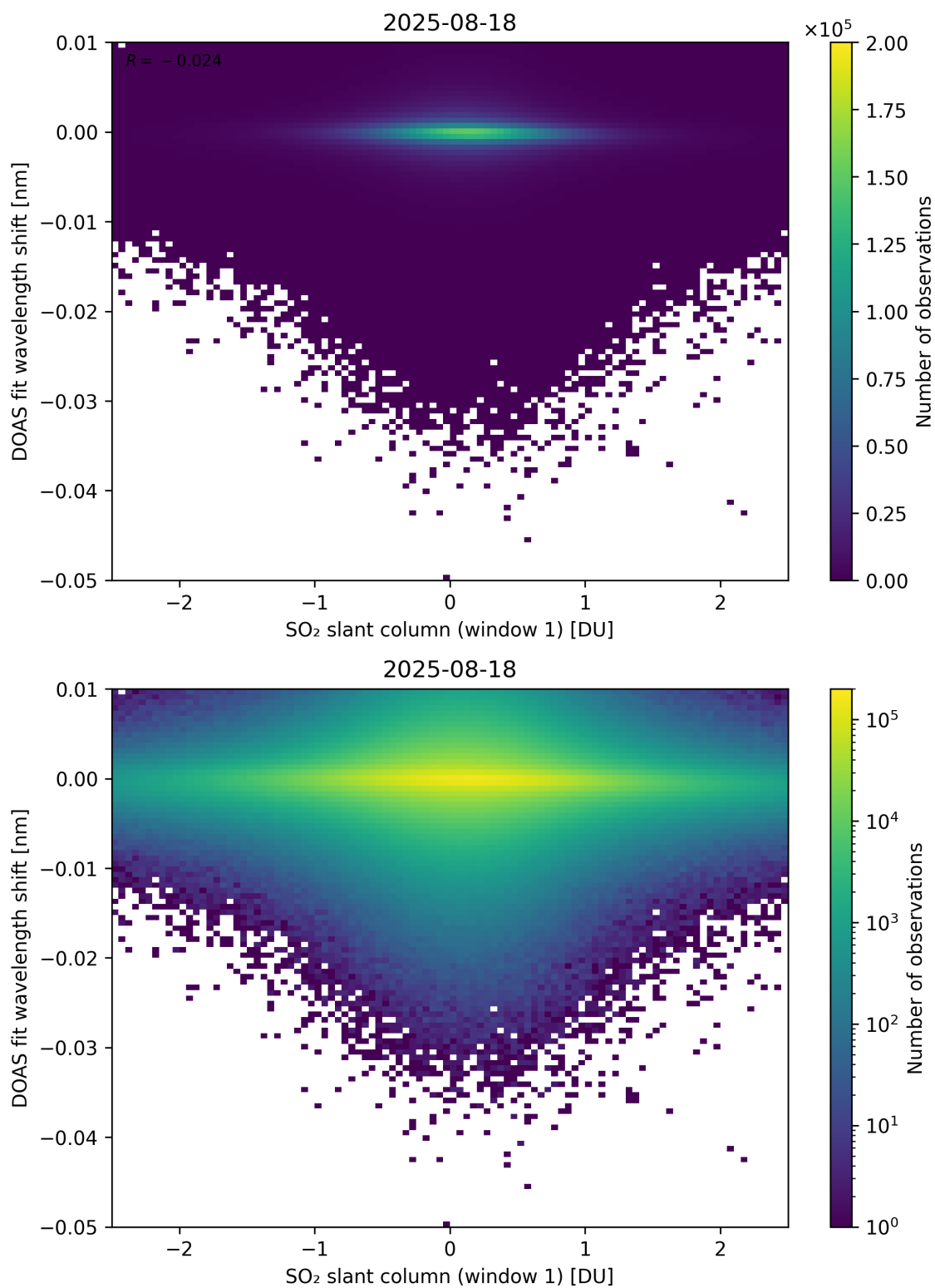
Figure 265: Scatter density plot of “SO 2 slant column (window 1)” against “DOAS fit wavelength shift” for 2025-08-17 to 2025-08-19.
