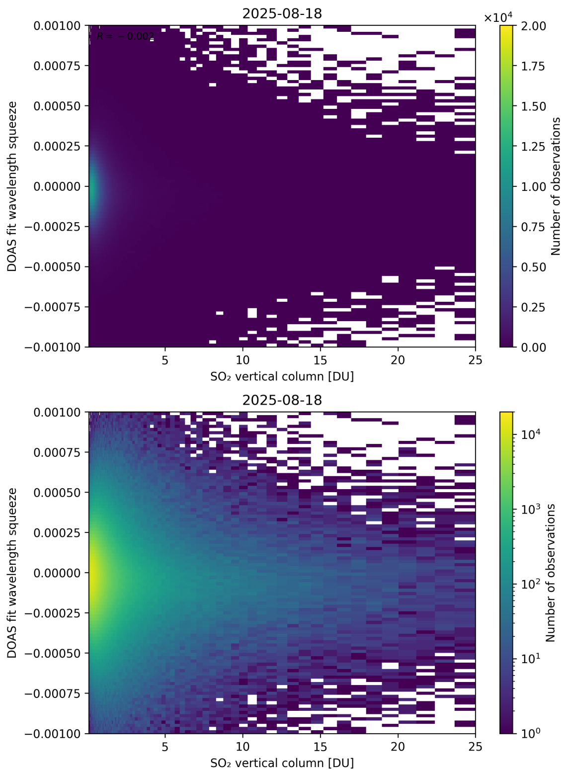
Figure 327: Scatter density plot of “SO 2 vertical column” against “DOAS fit wavelength squeeze” for 2025-08-17 to 2025-08-19.
