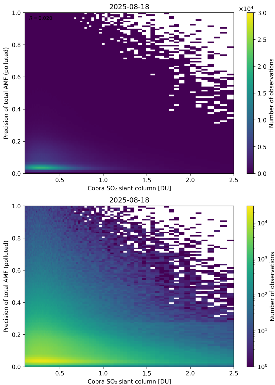
Figure 225: Scatter density plot of “Cobra SO 2 slant column” against “Precision of total AMF (polluted)” for 2025-08-17 to 2025-08-19.
