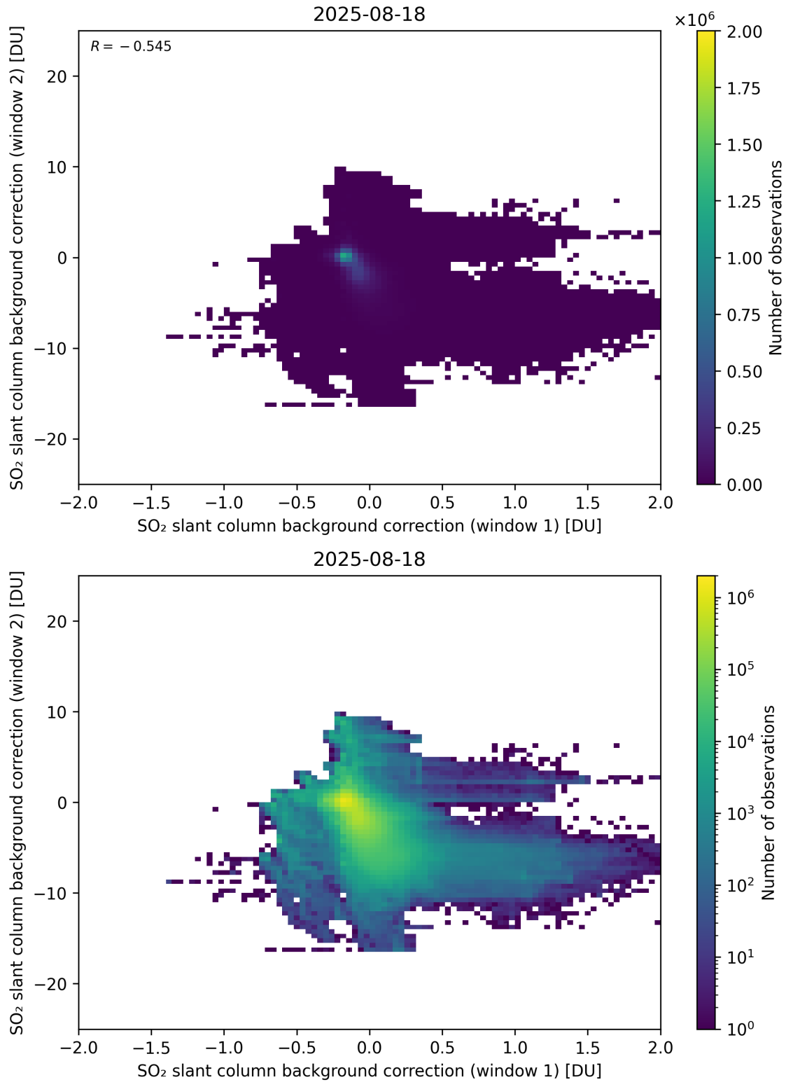
Figure 109: Scatter density plot of “SO 2 slant column background correction (window 1)” against “SO 2 slant column background correction (window 2)” for 2025-08-17 to 2025-08-19.
