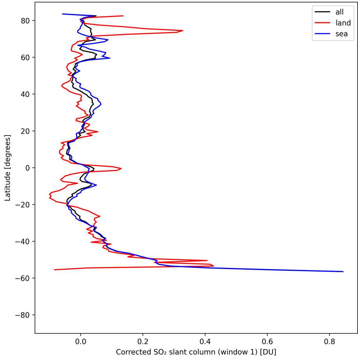
Figure 39: Zonal average of “Corrected SO 2 slant column (window 1)” for 2025-08-17 to 2025-08-19.
