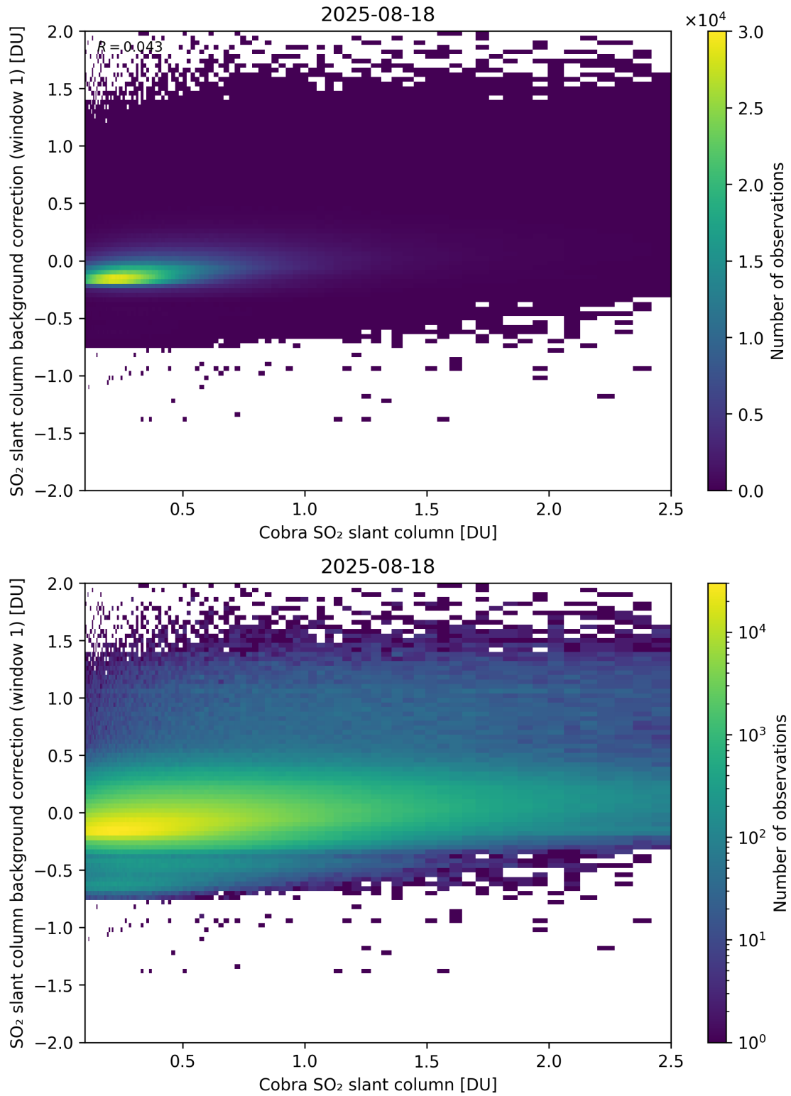
Figure 193: Scatter density plot of “Cobra SO 2 slant column” against “SO 2 slant column background correction (window 1)” for 2025-08-17 to 2025-08-19.
