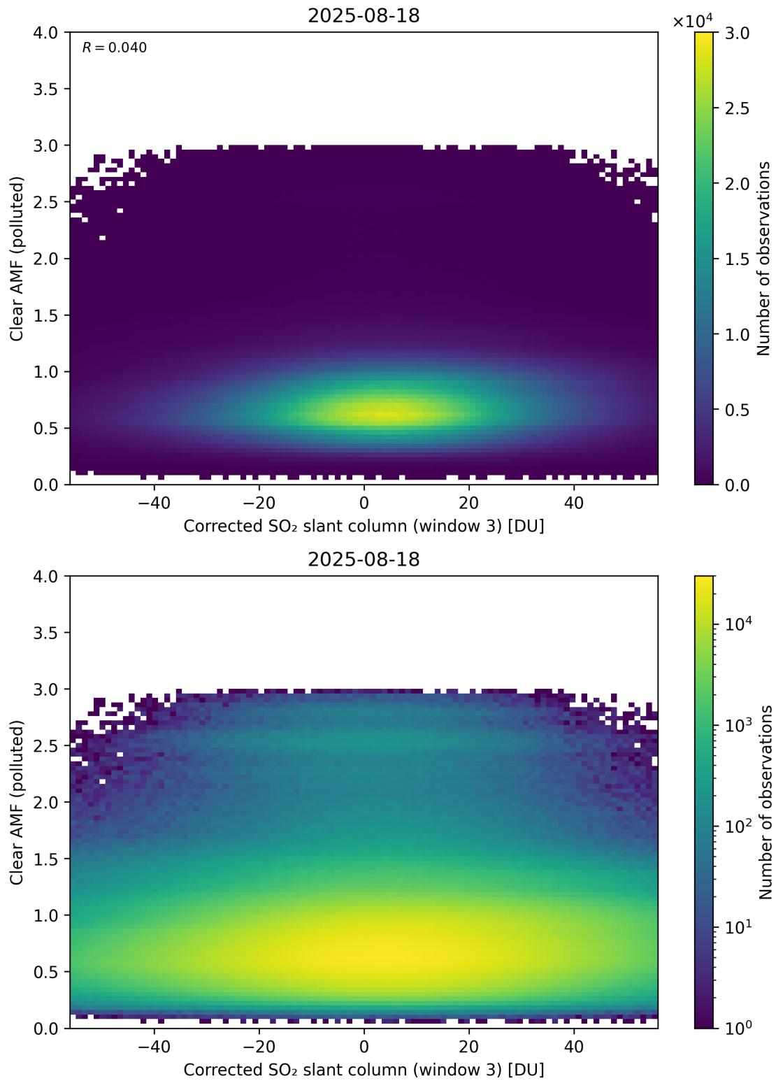
Figure 259: Scatter density plot of “Corrected SO 2 slant column (window 3)” against “Clear AMF (polluted)” for 2025-08-17 to 2025-08-19.
