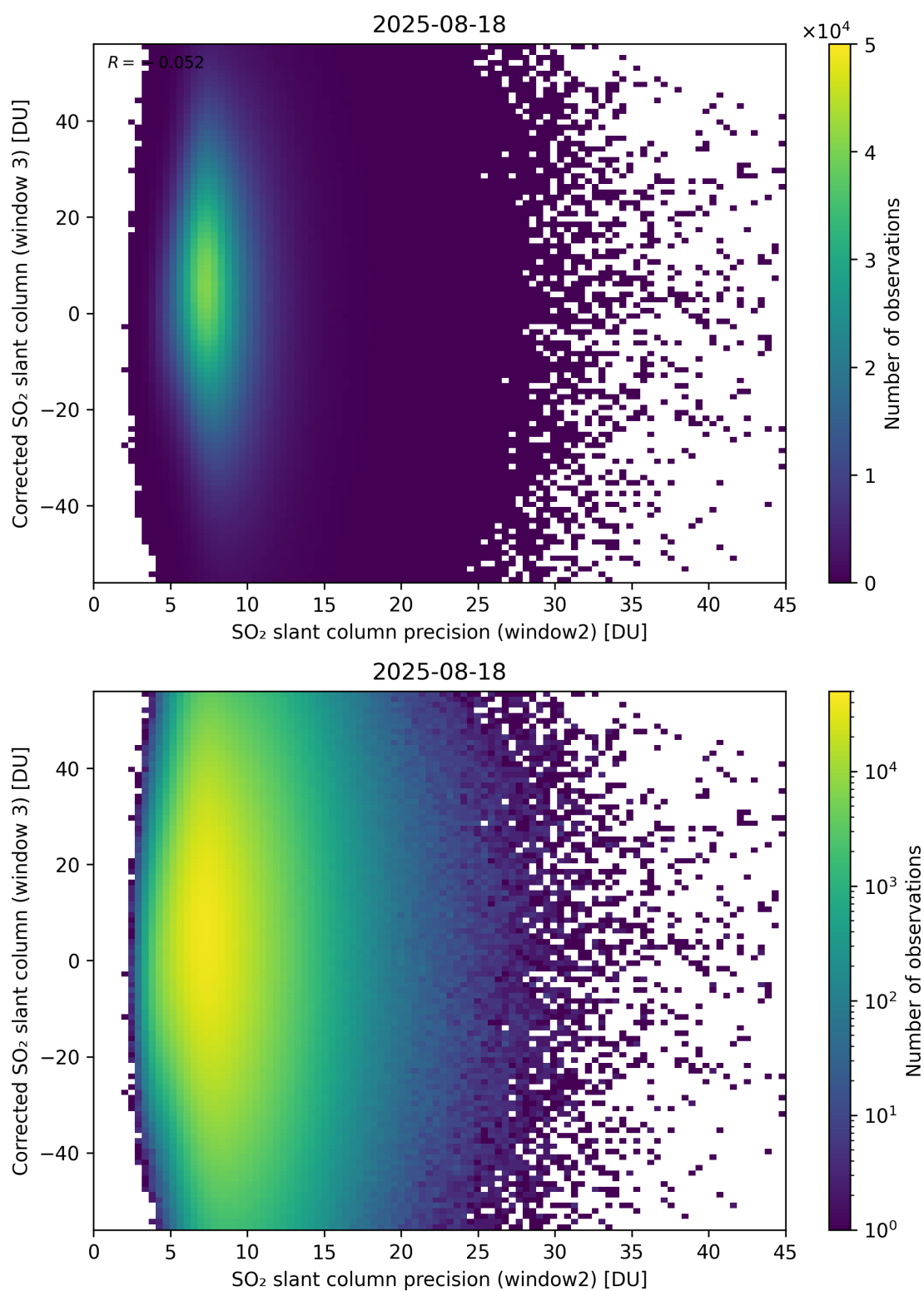
Figure 298: Scatter density plot of “SO 2 slant column precision (window2)” against “Corrected SO 2 slant column (window 3)” for 2025-08-17 to 2025-08-19.
