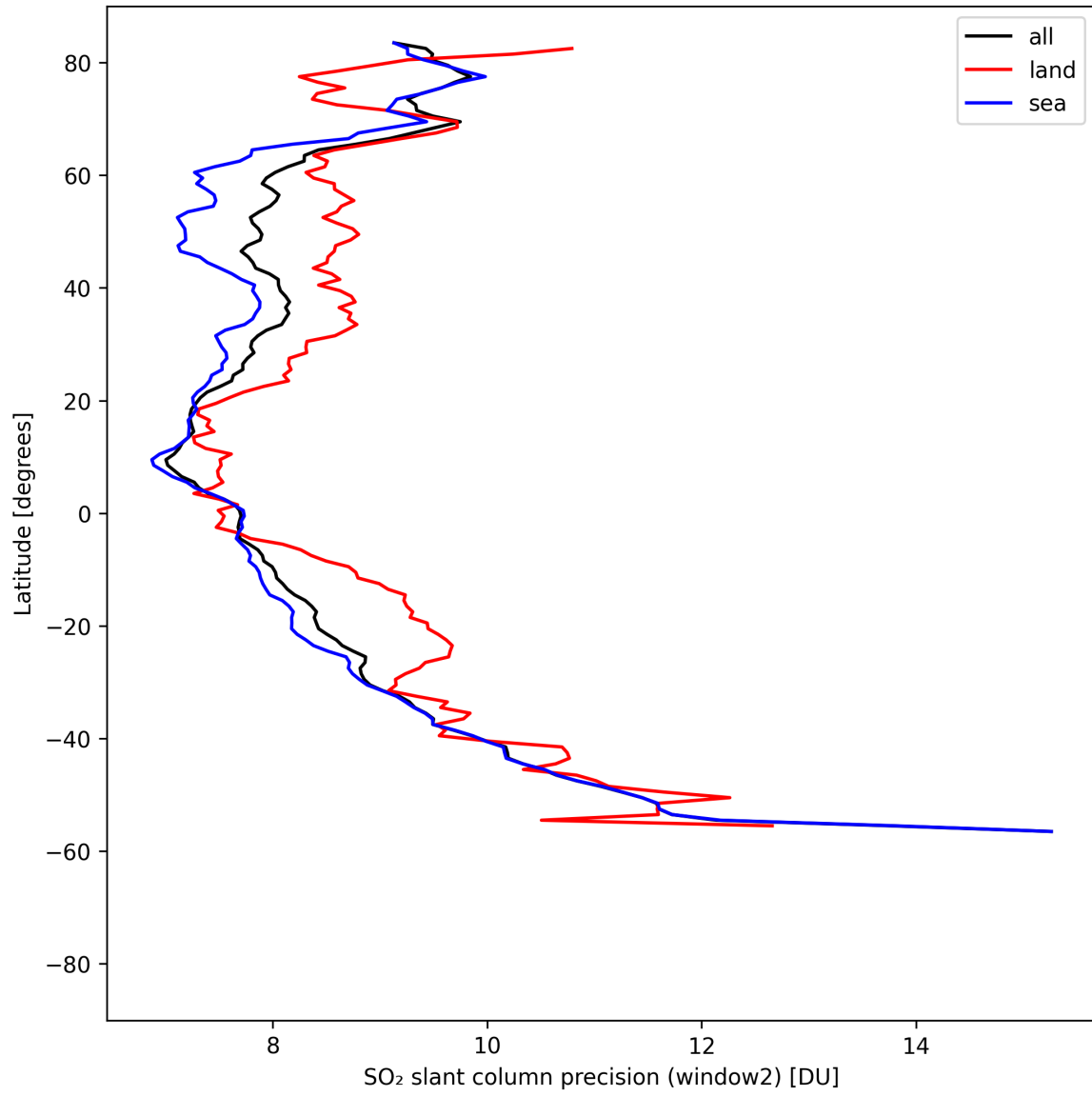
Figure 42: Zonal average of "SO 2 slant column precision (window2)" for 2025-08-17 to 2025-08-19.
