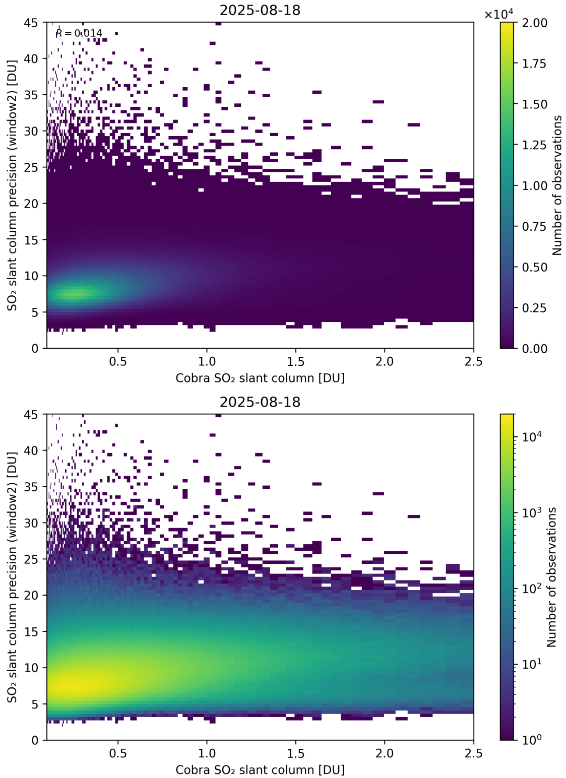
Figure 221: Scatter density plot of “Cobra SO 2 slant column” against “SO 2 slant column precision (window2)” for 2025-08-17 to 2025-08-19.
