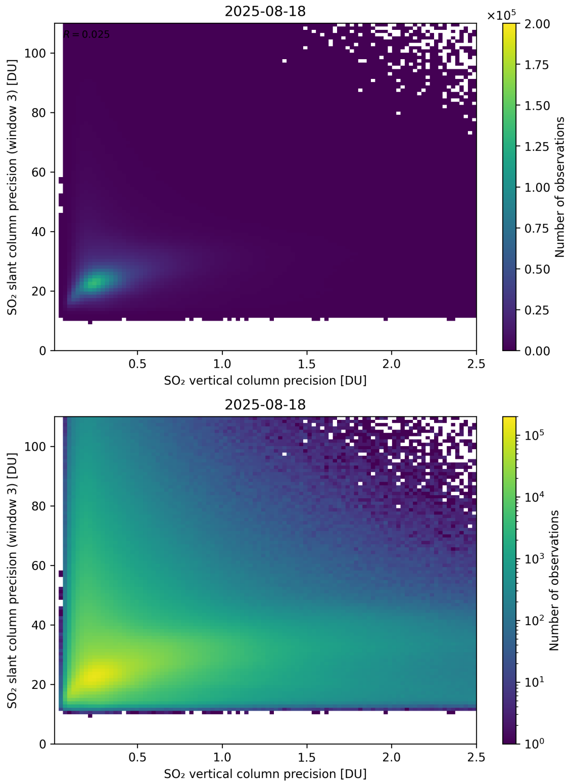
Figure 345: Scatter density plot of “SO 2 vertical column precision” against “SO 2 slant column precision (window 3)” for 2025-08-17 to 2025-08-19.
