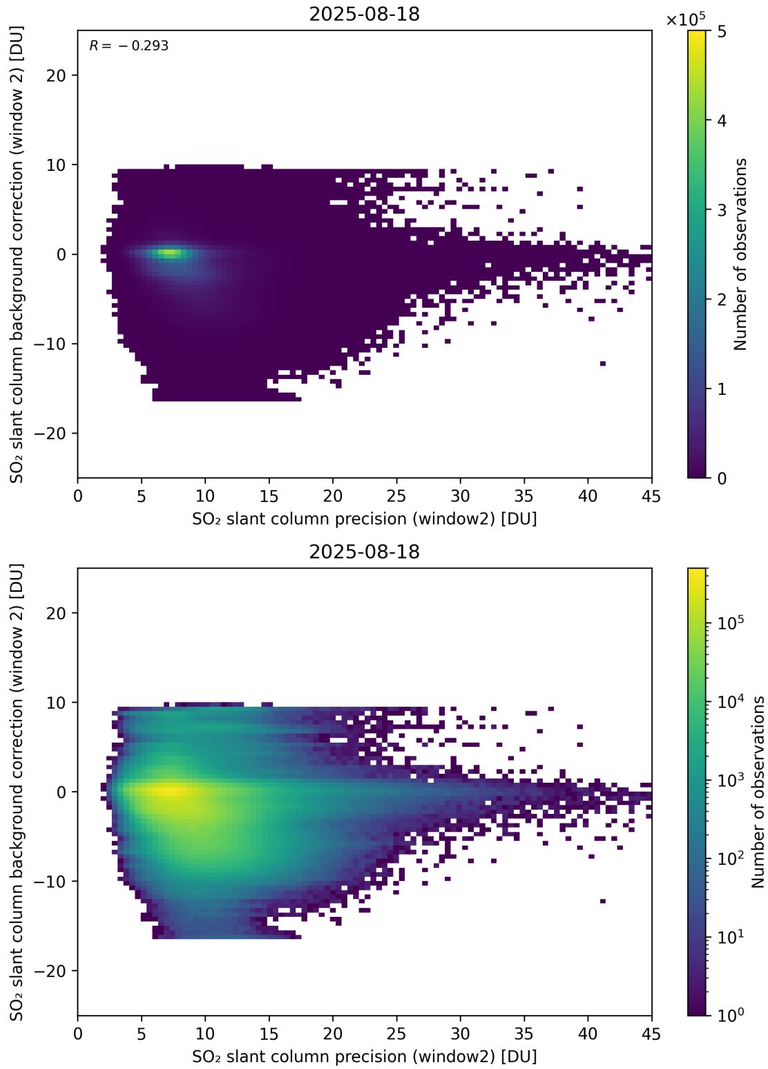
Figure 291: Scatter density plot of “SO 2 slant column precision (window2)” against “SO 2 slant column background correction (window 2)” for 2025-08-17 to 2025-08-19.
