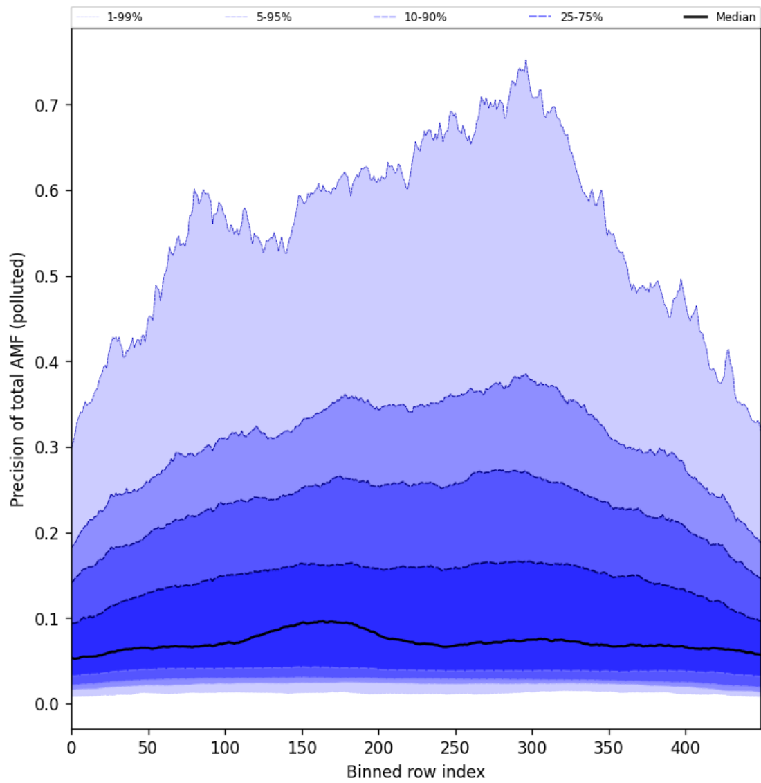
Figure 106: Along track statistics of “Precision of total AMF (polluted)” for 2025-08-17 to 2025-08-19
