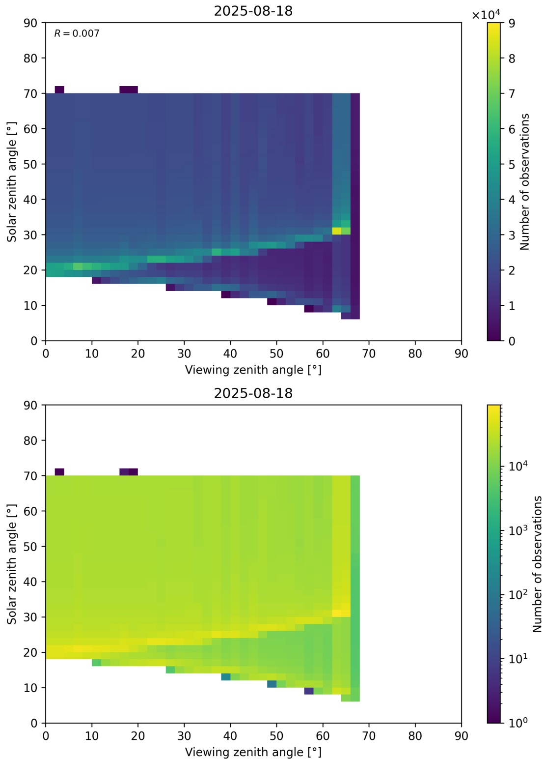
Figure 369: Scatter density plot of “Viewing zenith angle” against “Solar zenith angle” for 2025-08-17 to 2025-08-19.
