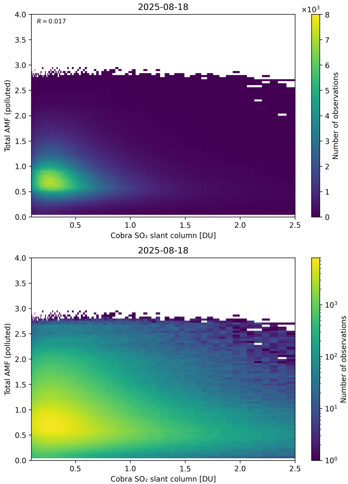
Figure 224: Scatter density plot of “Cobra SO 2 slant column” against “Total AMF (polluted)” for 2025-08-17 to 2025-08-19.
