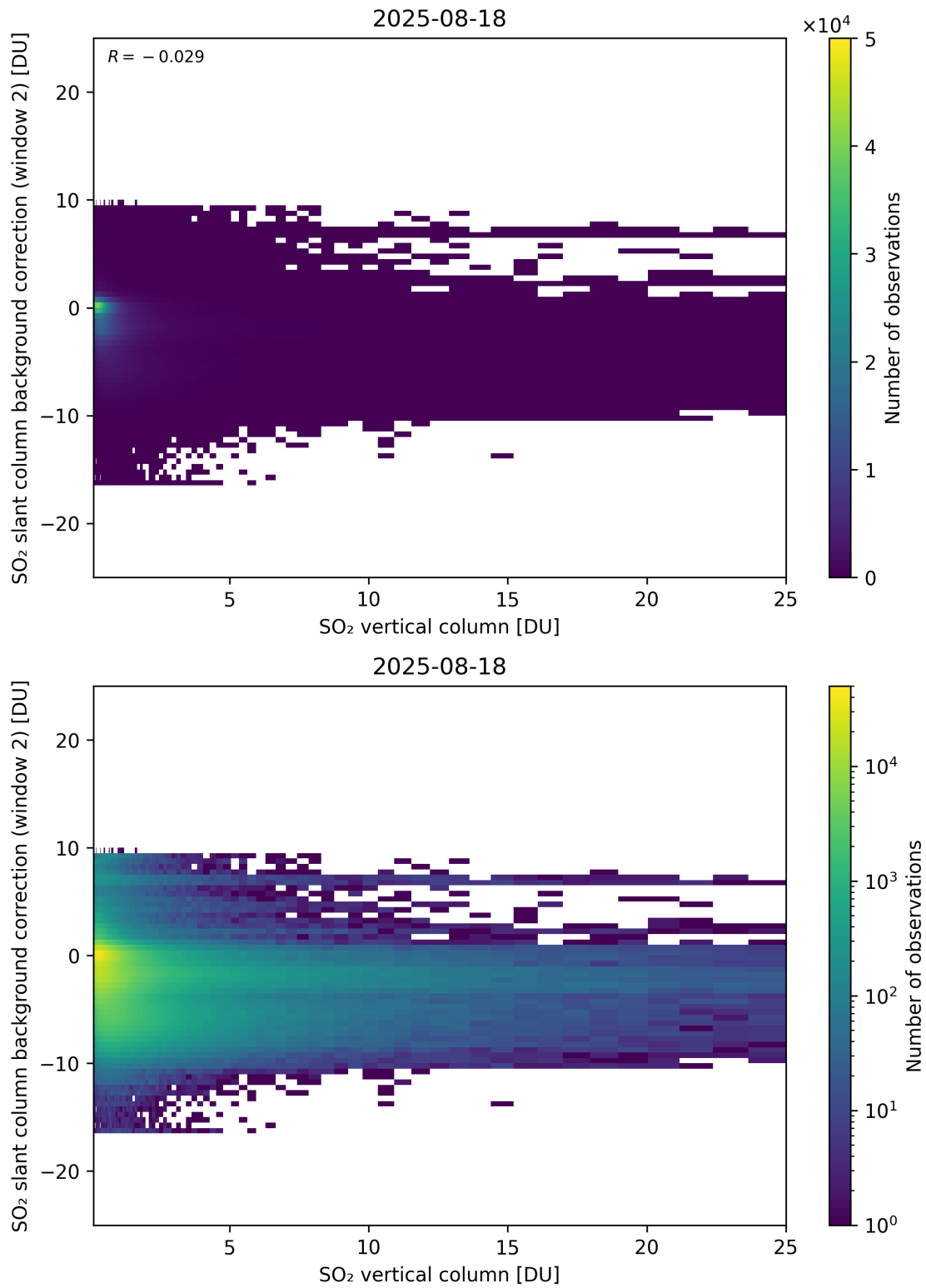
Figure 324: Scatter density plot of “SO 2 vertical column” against “SO 2 slant column background correction (window 2)” for 2025-08-17 to 2025-08-19.
