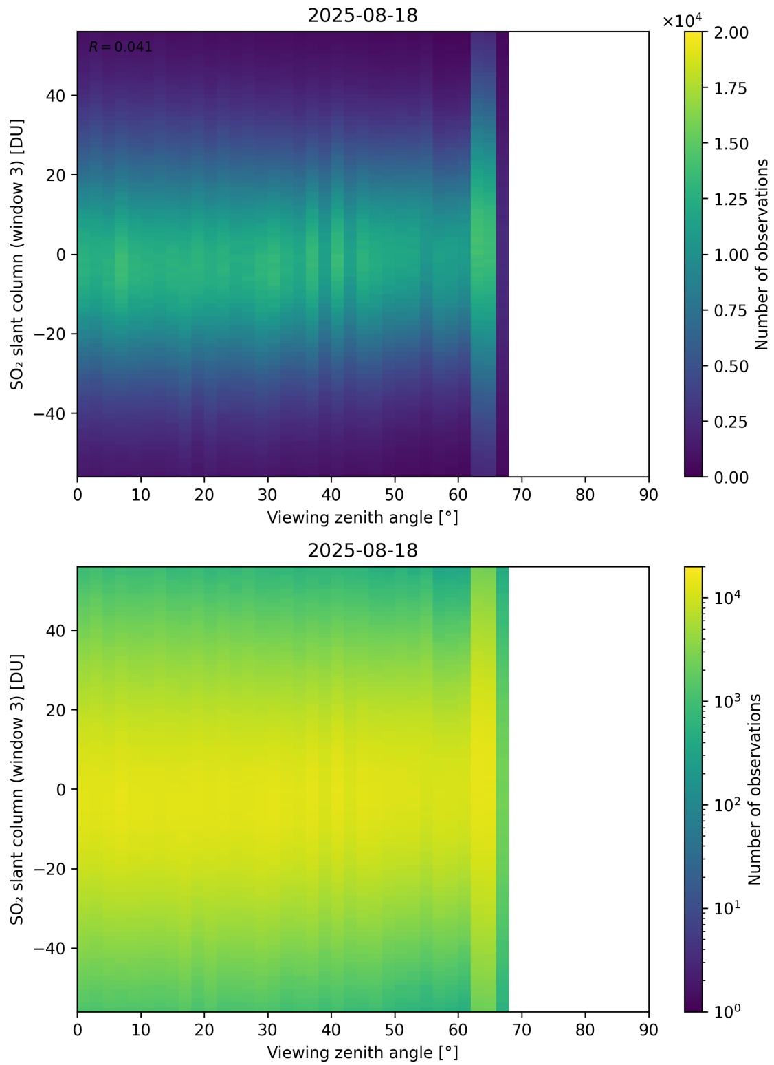
Figure 379: Scatter density plot of “Viewing zenith angle” against “SO 2 slant column (window 3)” for 2025-08-17 to 2025-08-19.
