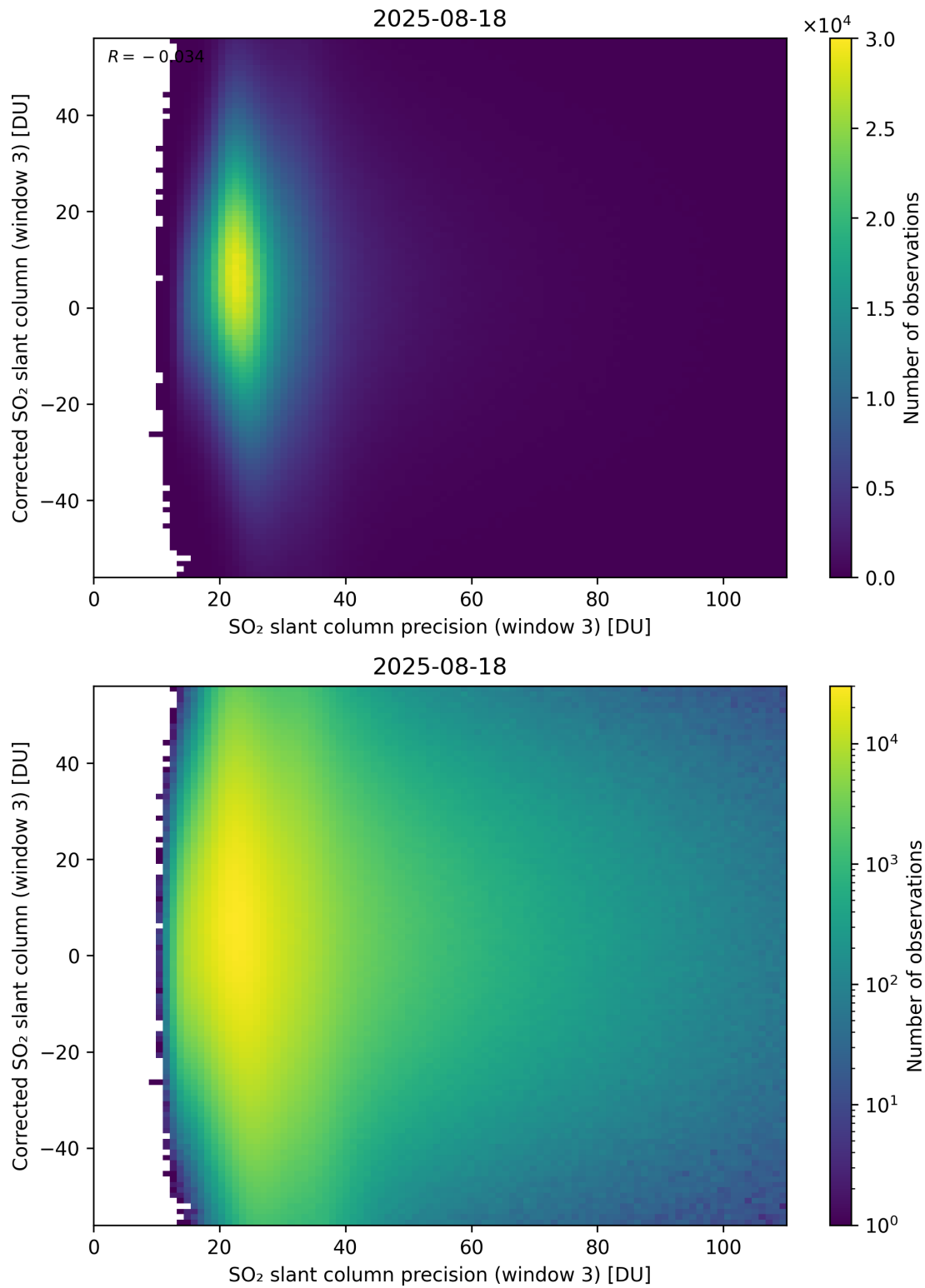
Figure 312: Scatter density plot of “SO 2 slant column precision (window 3)” against “Corrected SO 2 slant column (window 3)” for 2025-08-17 to 2025-08-19.
