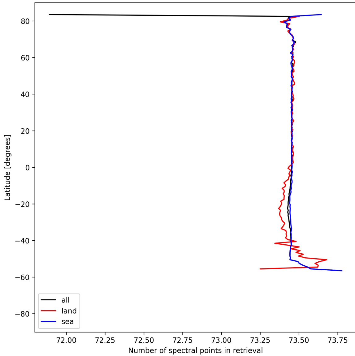
Figure 56: Zonal average of “Number of spectral points in retrieval” for 2025-08-17 to 2025-08-19.
