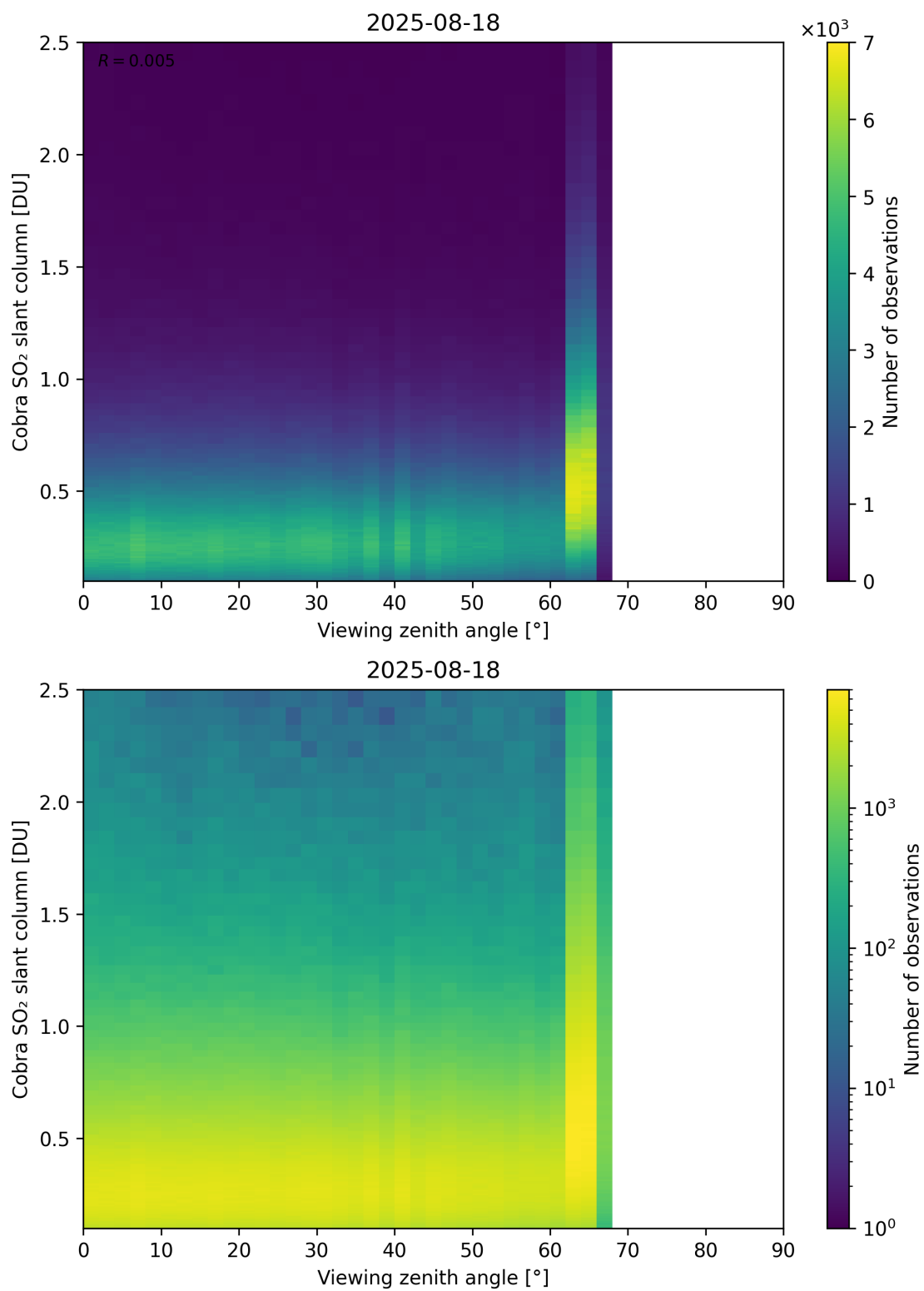
Figure 371: Scatter density plot of “Viewing zenith angle” against “Cobra SO 2 slant column” for 2025-08-17 to 2025-08-19.
