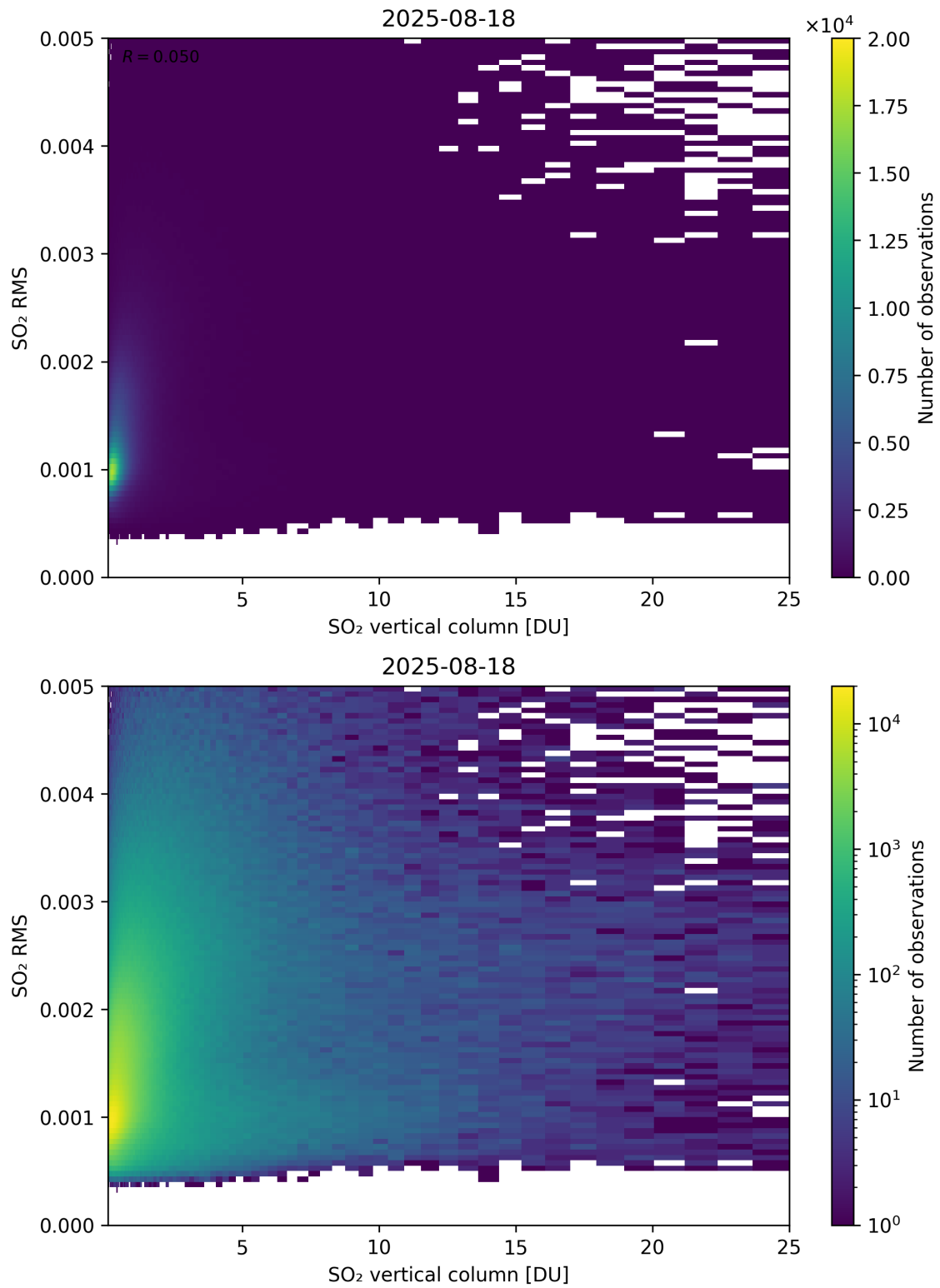
Figure 328: Scatter density plot of “SO 2 vertical column” against “SO 2 RMS” for 2025-08-17 to 2025-08-19.
