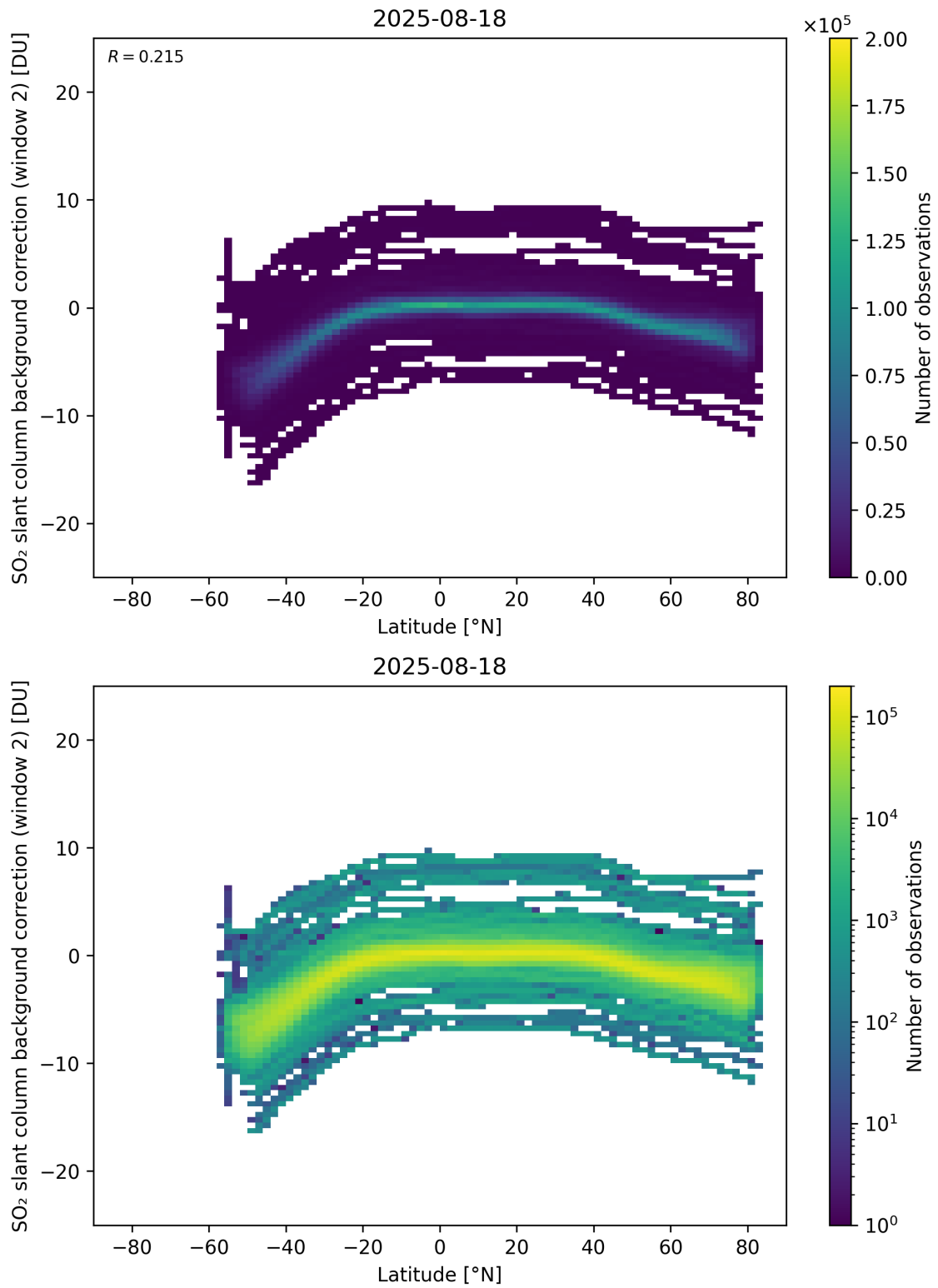
Figure 151: Scatter density plot of “Latitude” against “SO 2 slant column background correction (window 2)” for 2025-08-17 to 2025-08-19.
