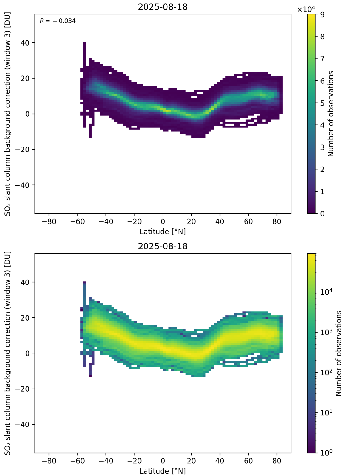
Figure 152: Scatter density plot of “Latitude” against “SO 2 slant column background correction (window 3)” for 2025-08-17 to 2025-08-19.
