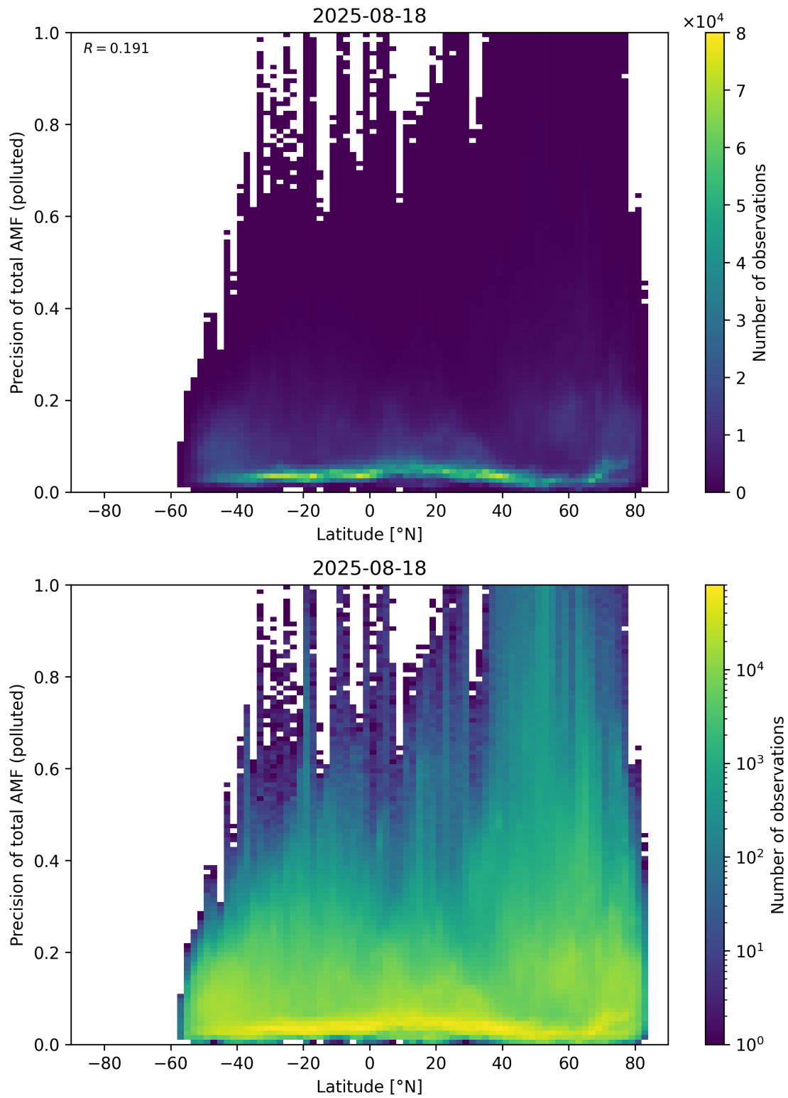
Figure 168: Scatter density plot of “Latitude” against “Precision of total AMF (polluted)” for 2025-08-17 to 2025-08-19.
