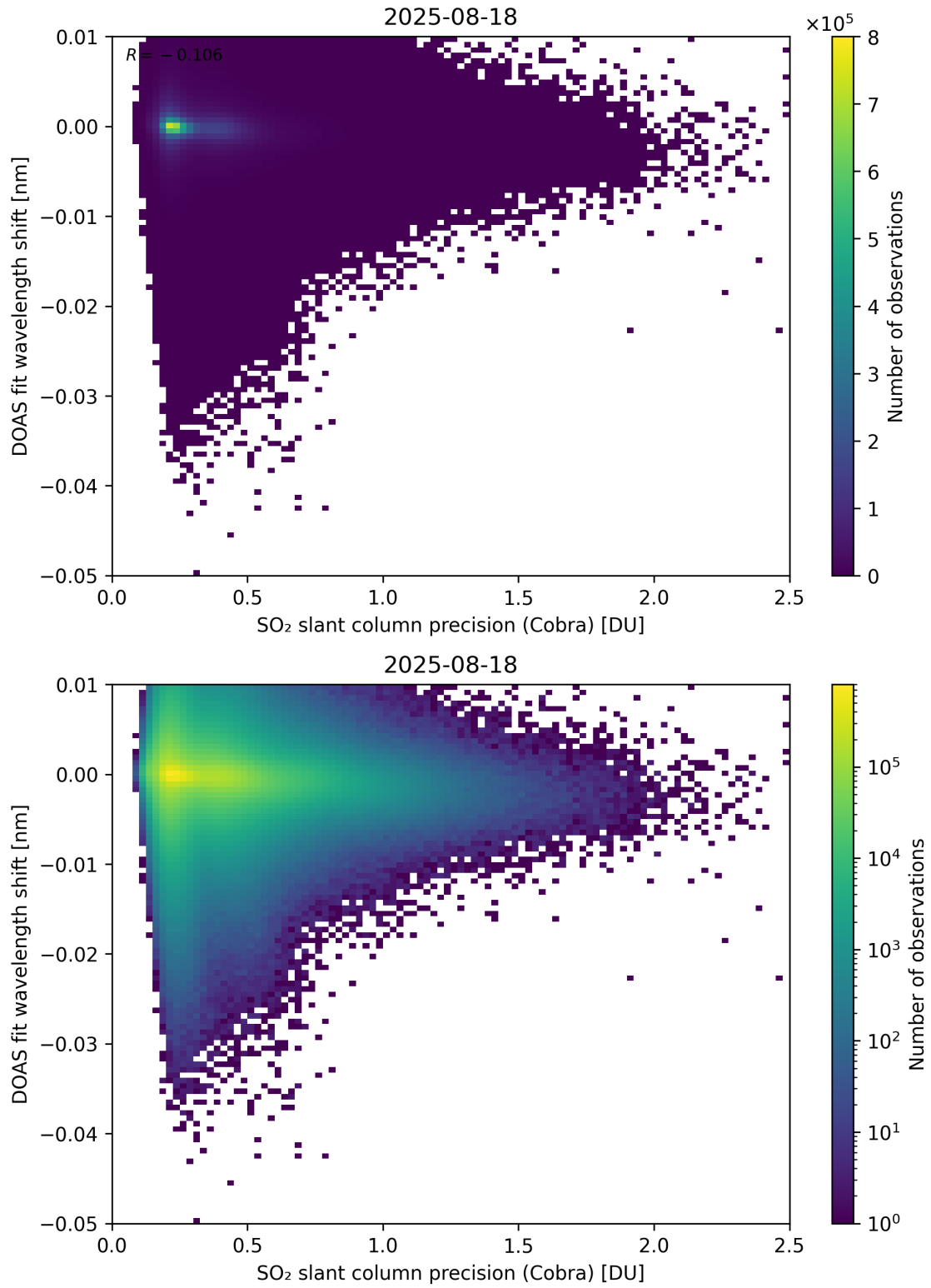
Figure 202: Scatter density plot of “SO 2 slant column precision (Cobra)” against “DOAS fit wavelength shift” for 2025-08-17 to 2025-08-19.
