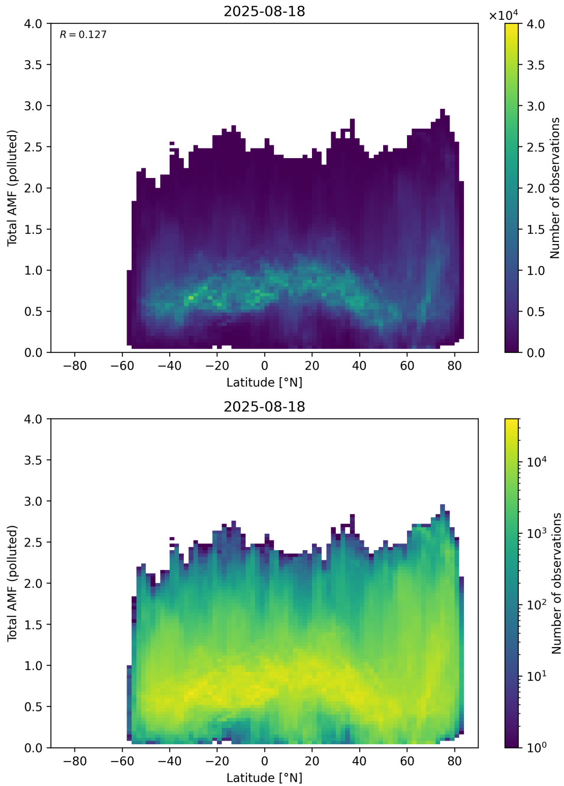
Figure 167: Scatter density plot of “Latitude” against “Total AMF (polluted)” for 2025-08-17 to 2025-08-19.
