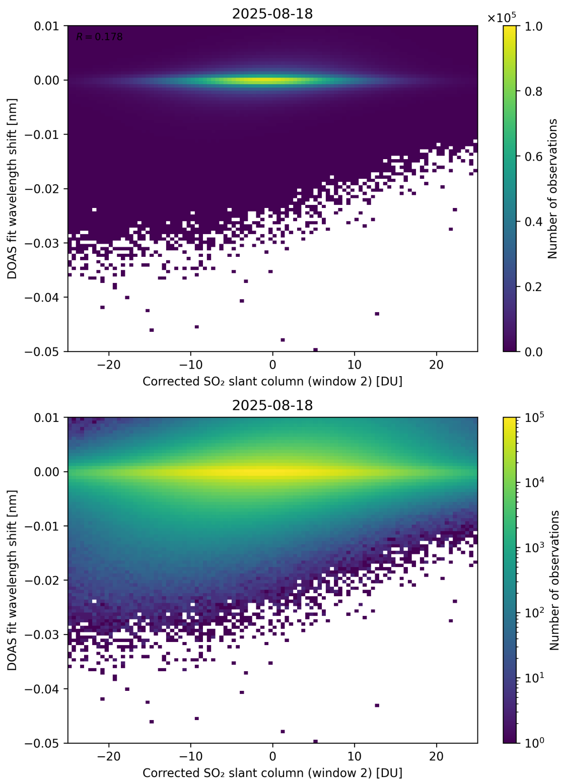
Figure 246: Scatter density plot of “Corrected SO 2 slant column (window 2)” against “DOAS fit wavelength shift” for 2025-08-17 to 2025-08-19.
