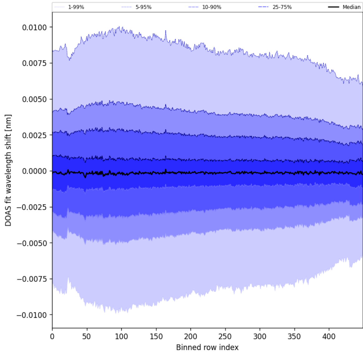
Figure 102: Along track statistics of “DOAS fit wavelength shift” for 2025-08-17 to 2025-08-19
