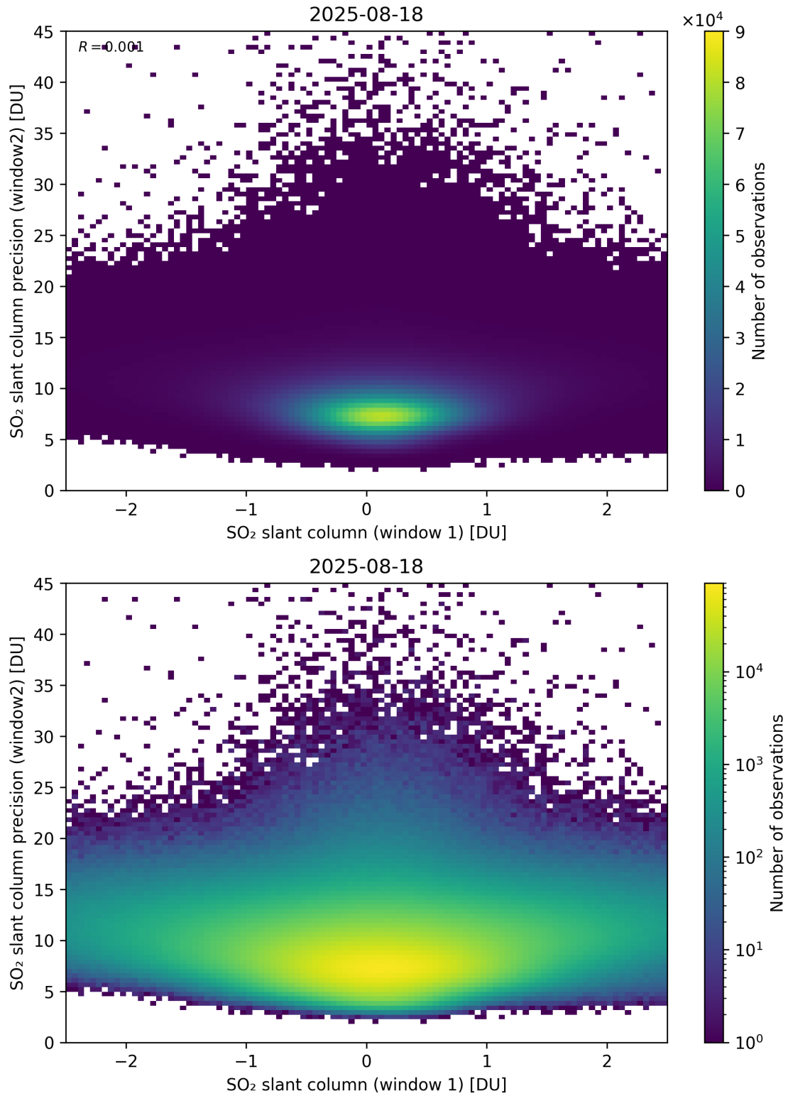
Figure 286: Scatter density plot of “SO 2 slant column (window 1)” against “SO 2 slant column precision (window2)” for 2025-08-17 to 2025-08-19.
