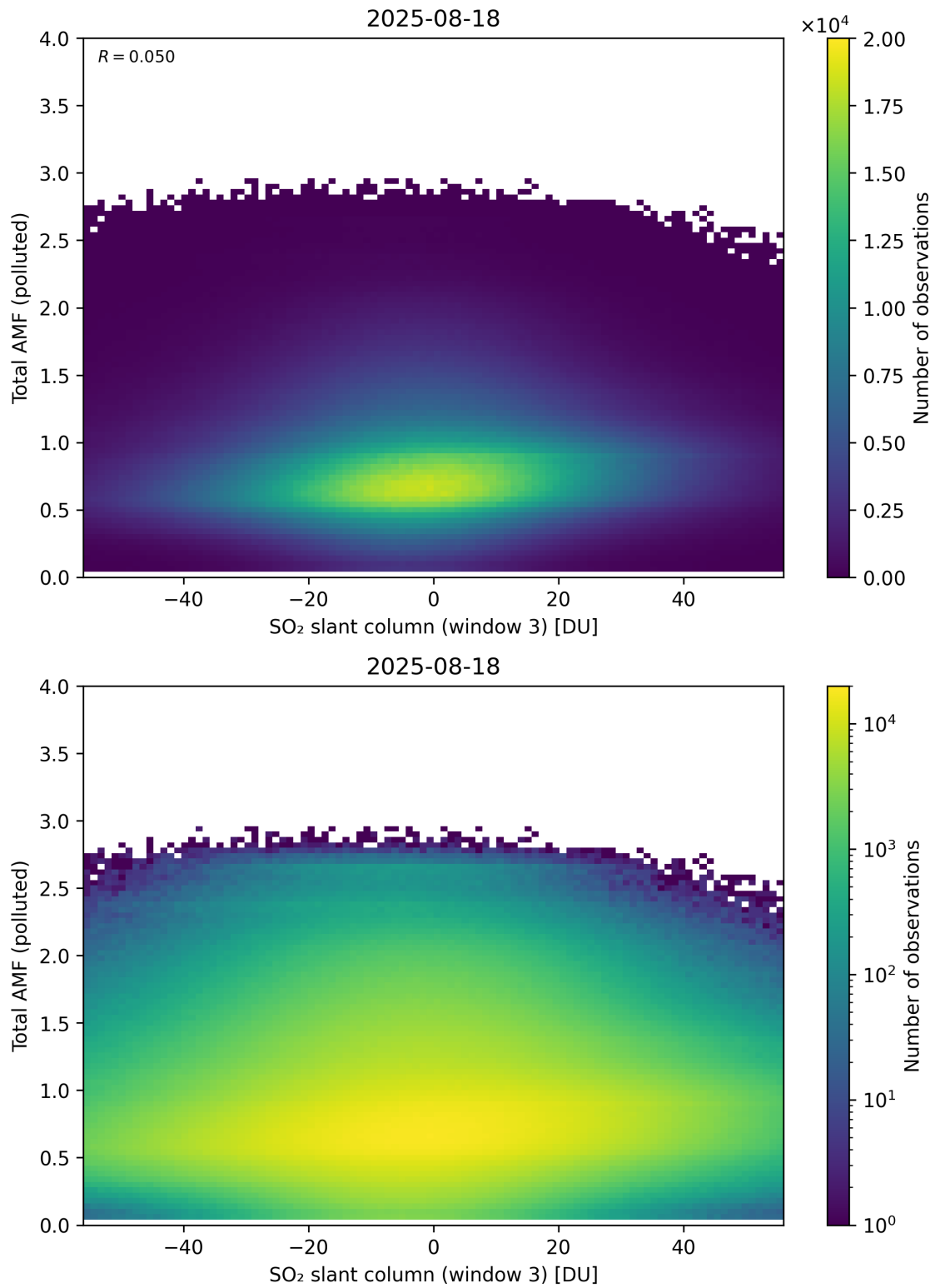
Figure 318: Scatter density plot of “SO 2 slant column (window 3)” against “Total AMF (polluted)” for 2025-08-17 to 2025-08-19.
