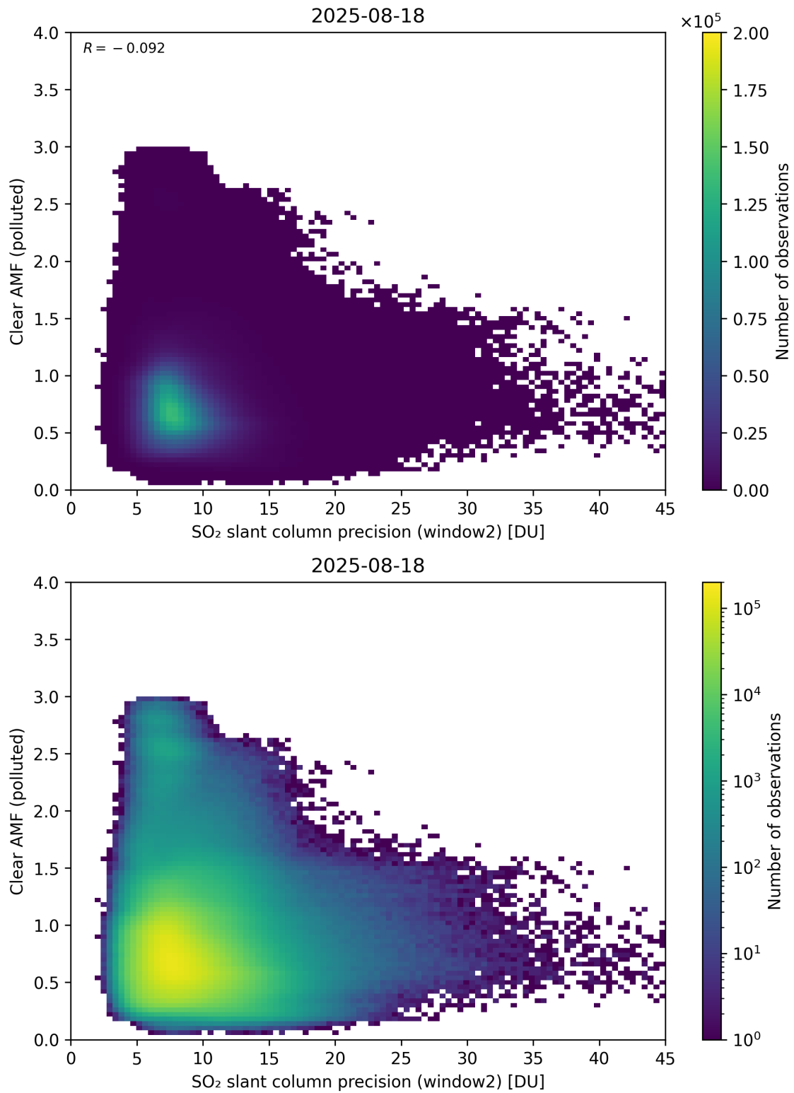
Figure 296: Scatter density plot of “SO 2 slant column precision (window2)” against “Clear AMF (polluted)” for 2025-08-17 to 2025-08-19.
