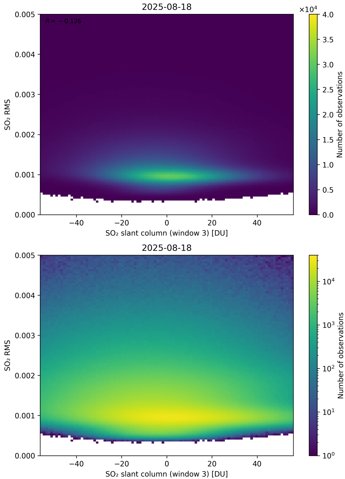
Figure 306: Scatter density plot of “SO 2 slant column (window 3)” against “SO 2 RMS” for 2025-08-17 to 2025-08-19.
