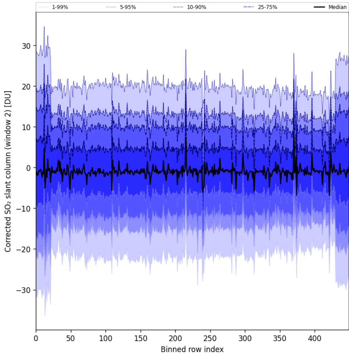
Figure 95: Along track statistics of “Corrected SO 2 slant column (window 2)” for 2025-08-17 to 2025-08-19
