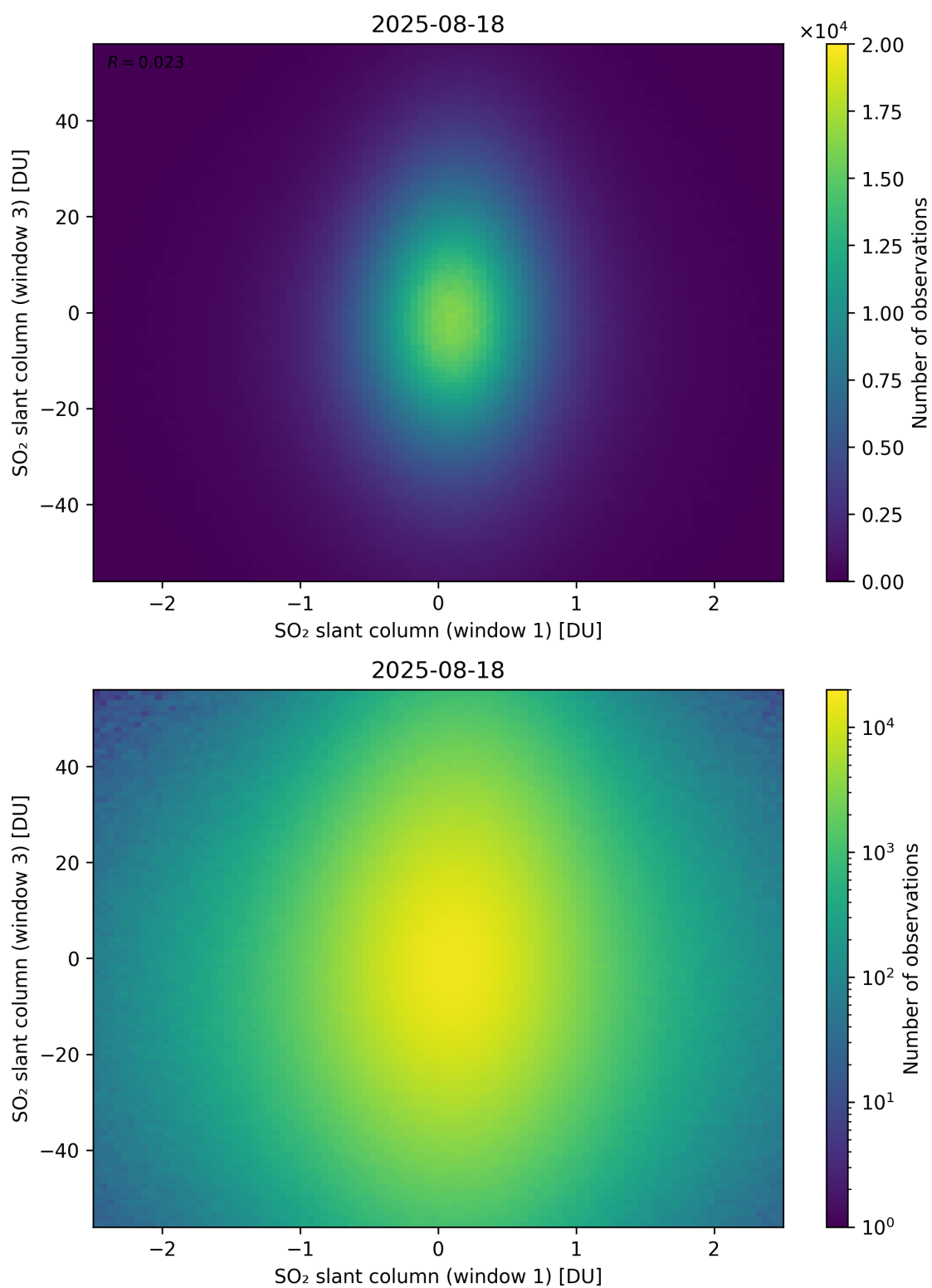
Figure 287: Scatter density plot of “SO 2 slant column (window 1)” against “SO 2 slant column (window 3)” for 2025-08-17 to 2025-08-19.
