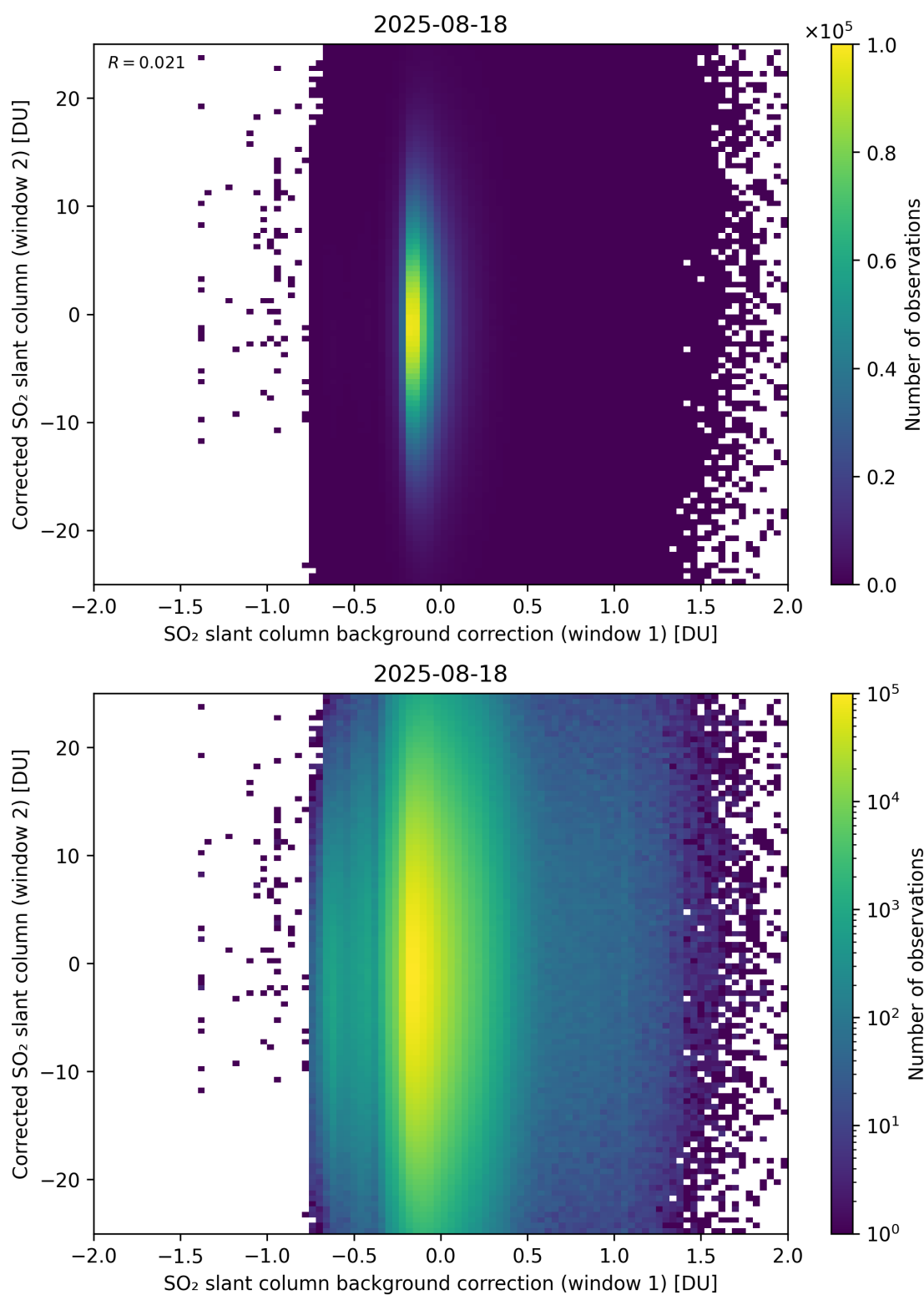
Figure 115: Scatter density plot of “SO 2 slant column background correction (window 1)” against “Corrected SO 2 slant column (window 2)” for 2025-08-17 to 2025-08-19.
