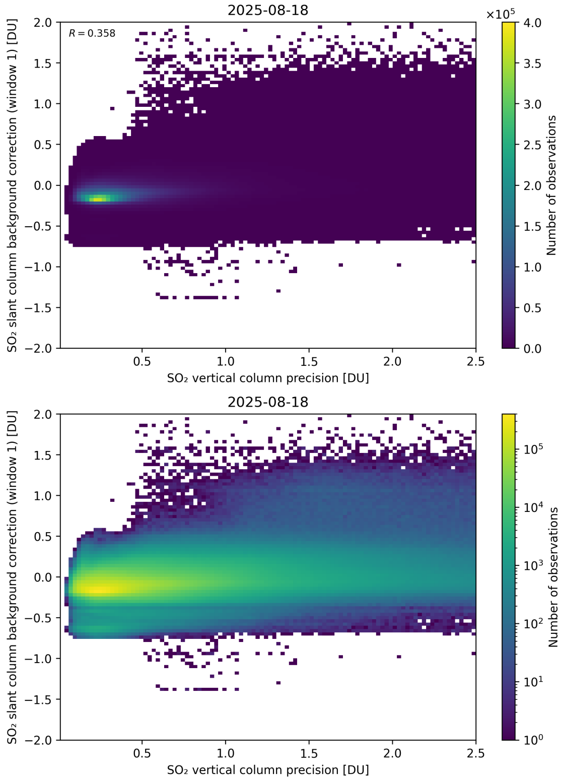
Figure 329: Scatter density plot of “SO 2 vertical column precision” against “SO 2 slant column background correction (window 1)” for 2025-08-17 to 2025-08-19.
