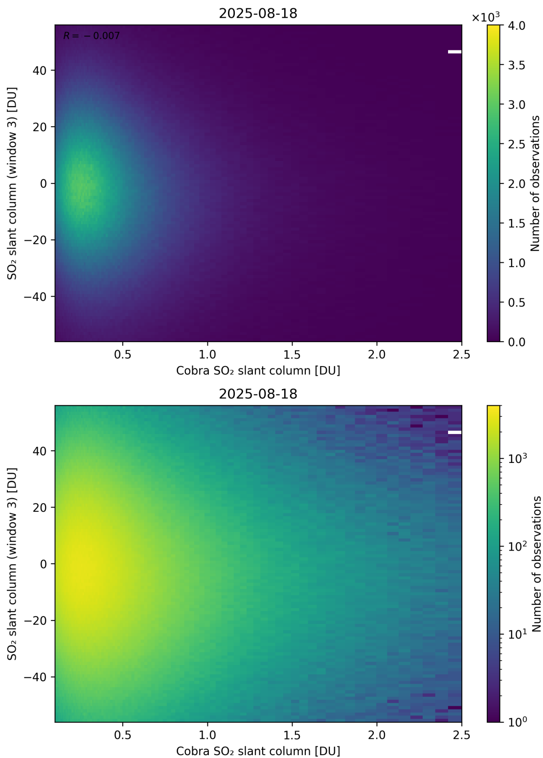
Figure 222: Scatter density plot of “Cobra SO 2 slant column” against “SO 2 slant column (window 3)” for 2025-08-17 to 2025-08-19.
