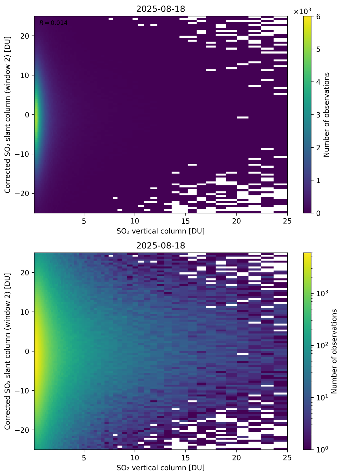
Figure 352: Scatter density plot of “SO 2 vertical column” against “Corrected SO 2 slant column (window 2)” for 2025-08-17 to 2025-08-19.
