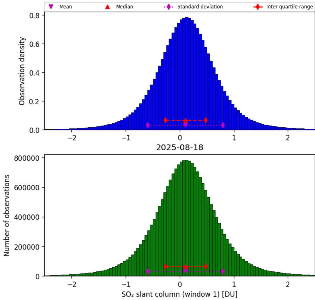
Figure 63: Histogram of “SO 2 slant column (window 1)” for 2025-08-17 to 2025-08-19
