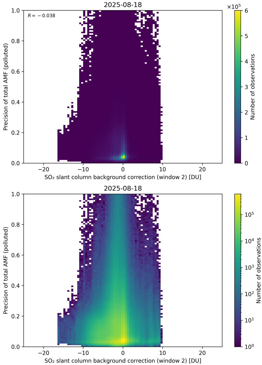
Figure 131: Scatter density plot of “SO 2 slant column background correction (window 2)” against “Precision of total AMF (polluted)” for 2025-08-17 to 2025-08-19.
