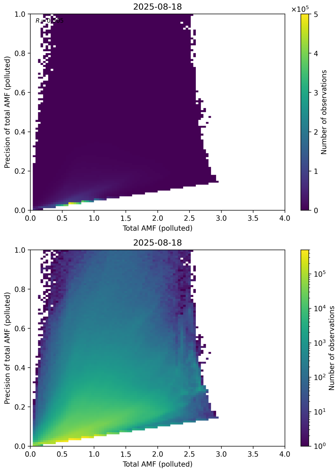
Figure 322: Scatter density plot of “Total AMF (polluted)” against “Precision of total AMF (polluted)” for 2025-08-17 to 2025-08-19.
