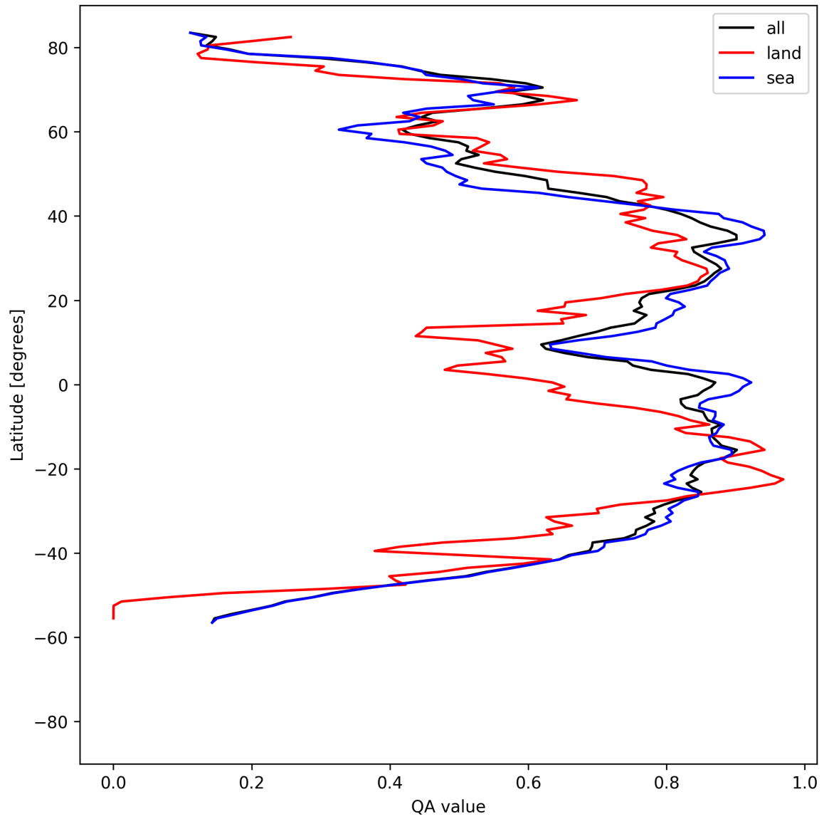
Figure 31: Zonal average of “QA value” for 2025-08-17 to 2025-08-19.
