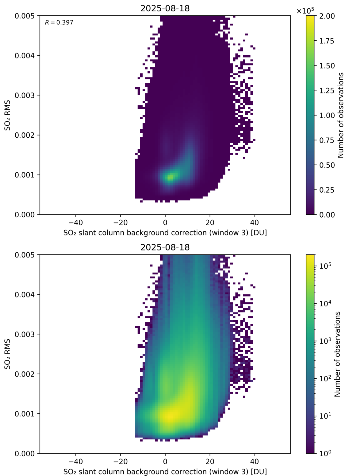
Figure 134: Scatter density plot of “SO 2 slant column background correction (window 3)” against “SO 2 RMS” for 2025-08-17 to 2025-08-19.
