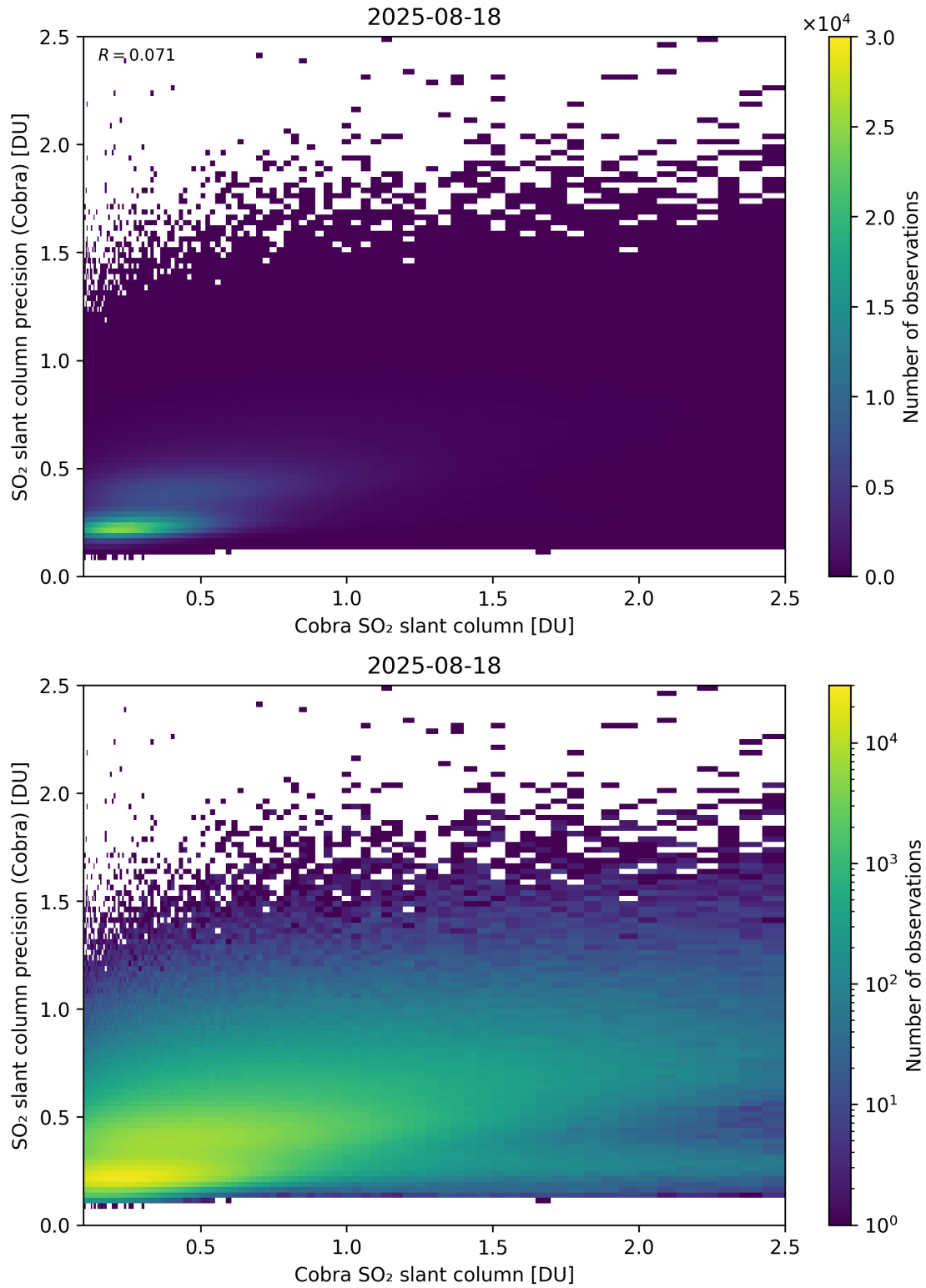
Figure 216: Scatter density plot of “Cobra SO 2 slant column” against “SO 2 slant column precision (Cobra)” for 2025-08-17 to 2025-08-19.
