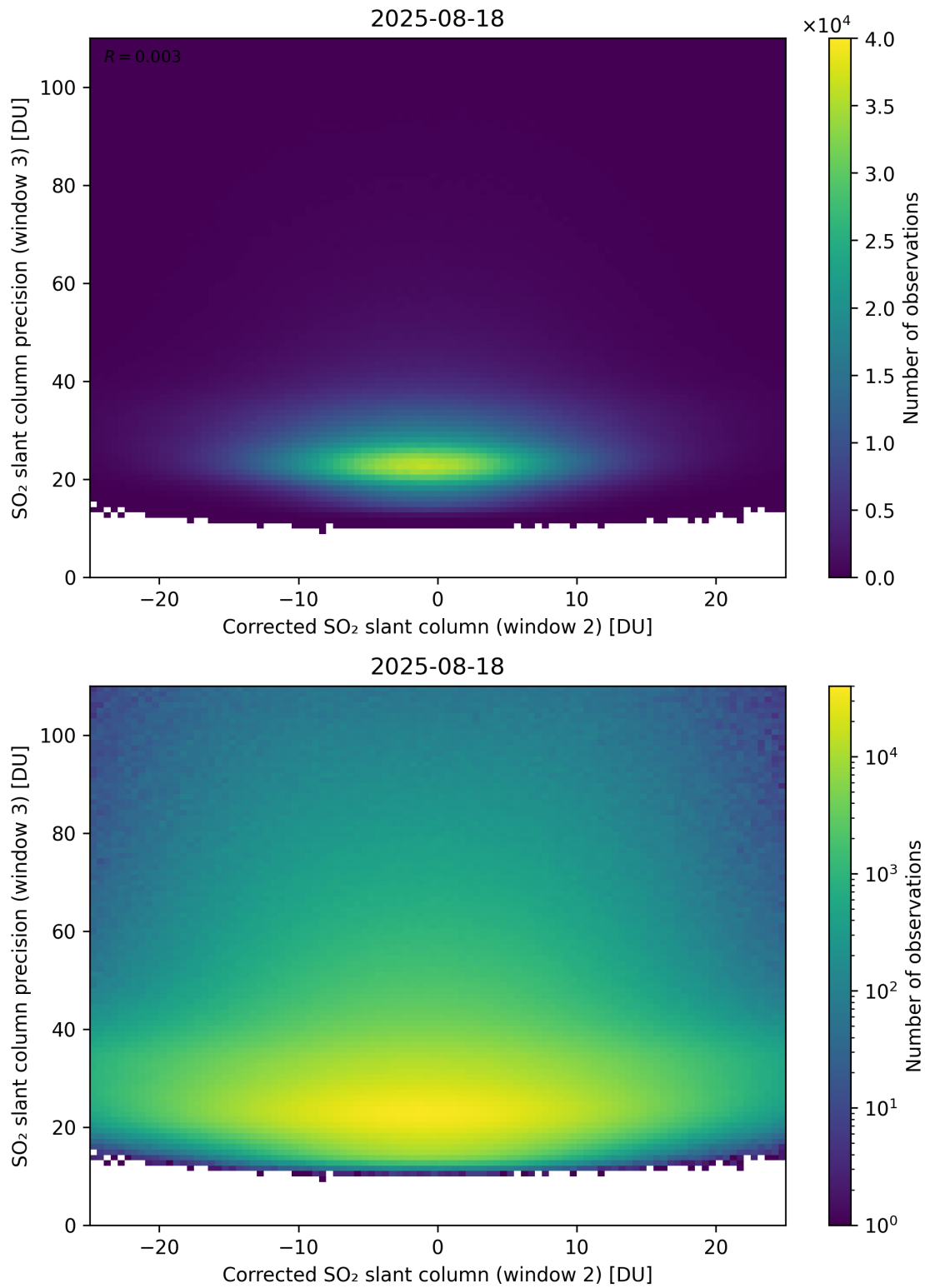
Figure 252: Scatter density plot of “Corrected SO 2 slant column (window 2)” against “SO 2 slant column precision (window 3)” for 2025-08-17 to 2025-08-19.
