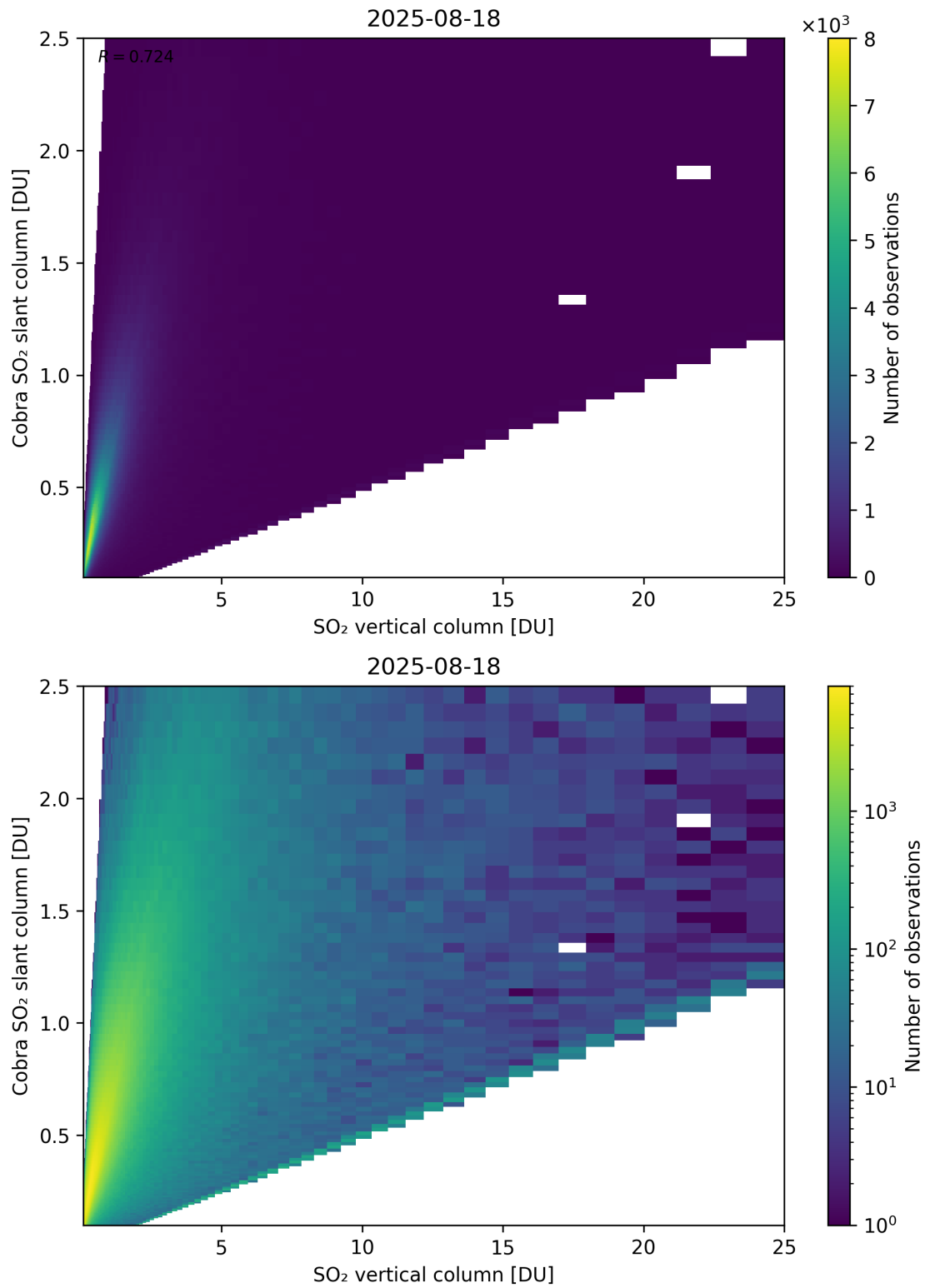
Figure 349: Scatter density plot of “SO 2 vertical column” against “Cobra SO 2 slant column” for 2025-08-17 to 2025-08-19.
