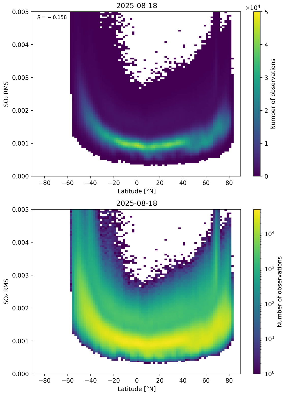
Figure 155: Scatter density plot of “Latitude” against “SO 2 RMS” for 2025-08-17 to 2025-08-19.
