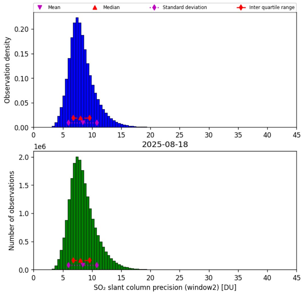
Figure 68: Histogram of “SO 2 slant column precision (window2)” for 2025-08-17 to 2025-08-19
