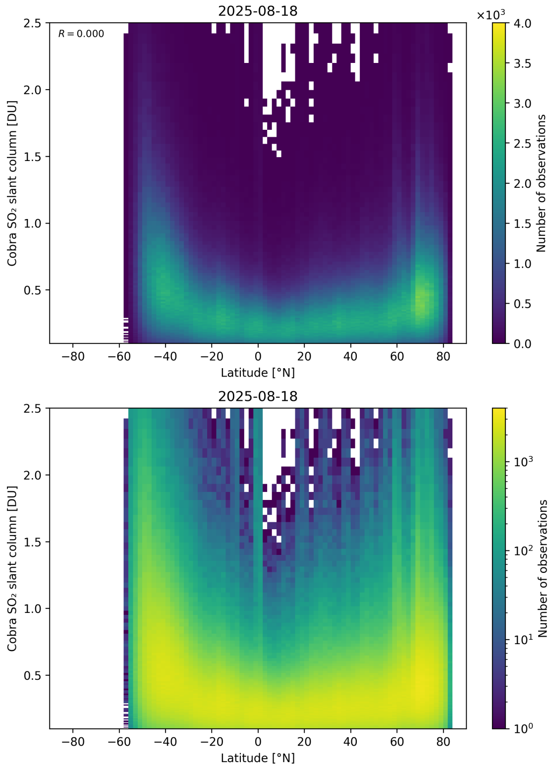
Figure 157: Scatter density plot of “Latitude” against “Cobra SO 2 slant column” for 2025-08-17 to 2025-08-19.
