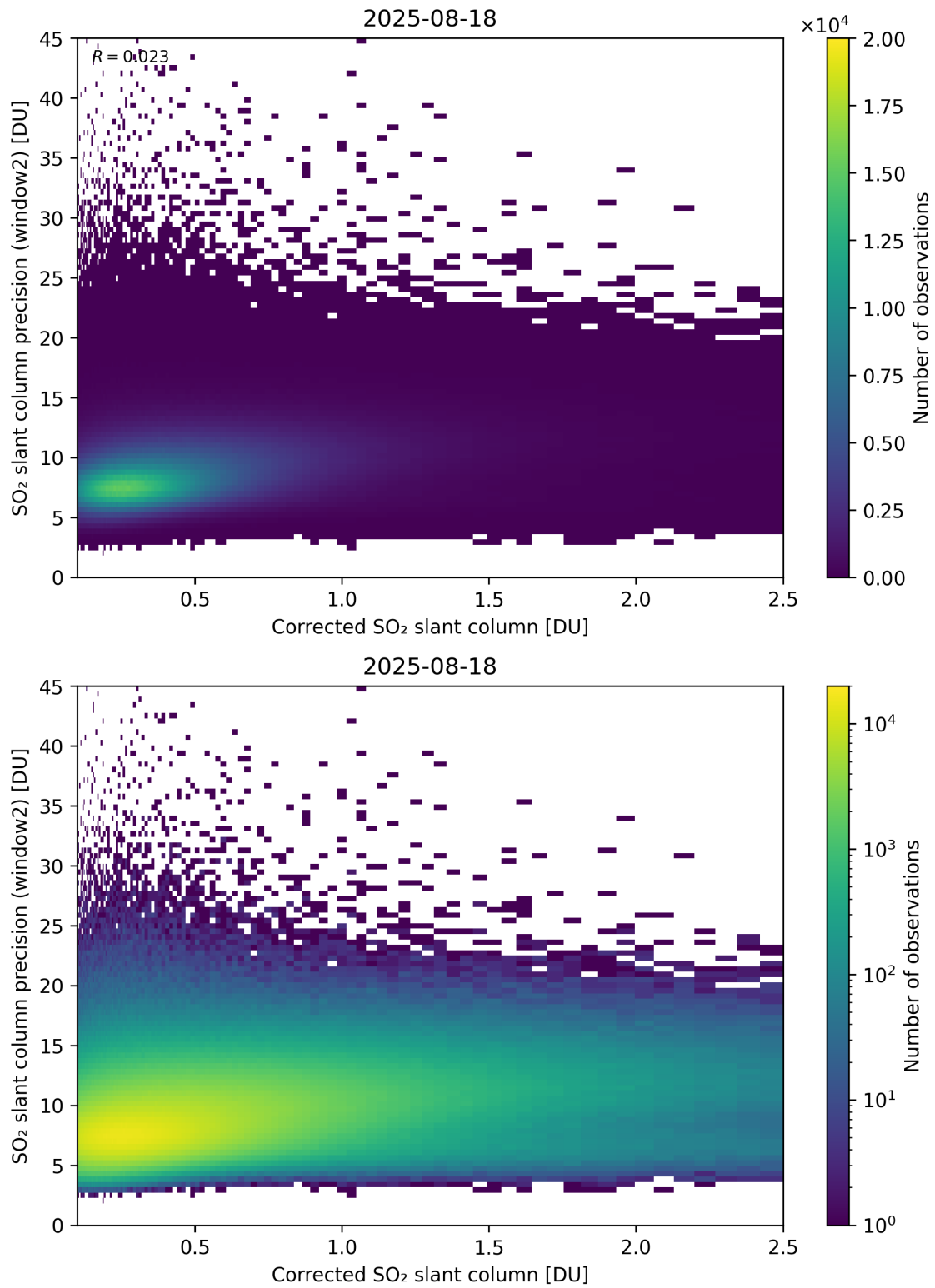
Figure 239: Scatter density plot of “Corrected SO 2 slant column” against “SO 2 slant column precision (window2)” for 2025-08-17 to 2025-08-19.
