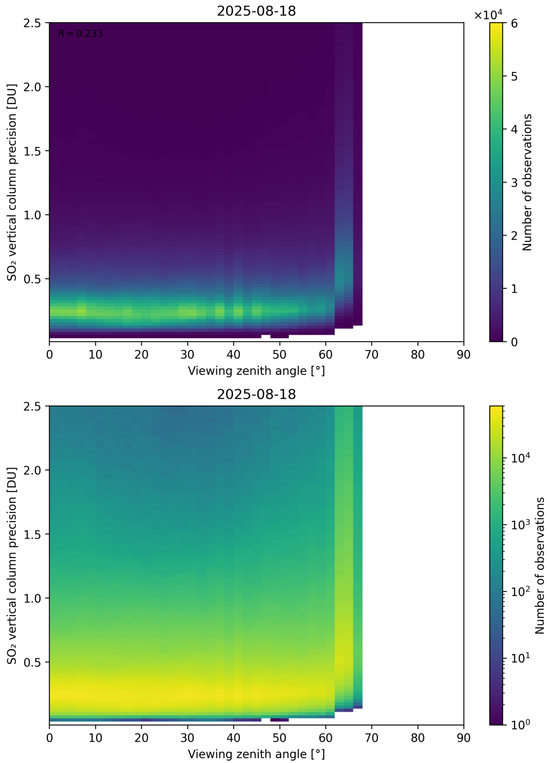
Figure 384: Scatter density plot of “Viewing zenith angle” against “SO 2 vertical column precision” for 2025-08-17 to 2025-08-19.
