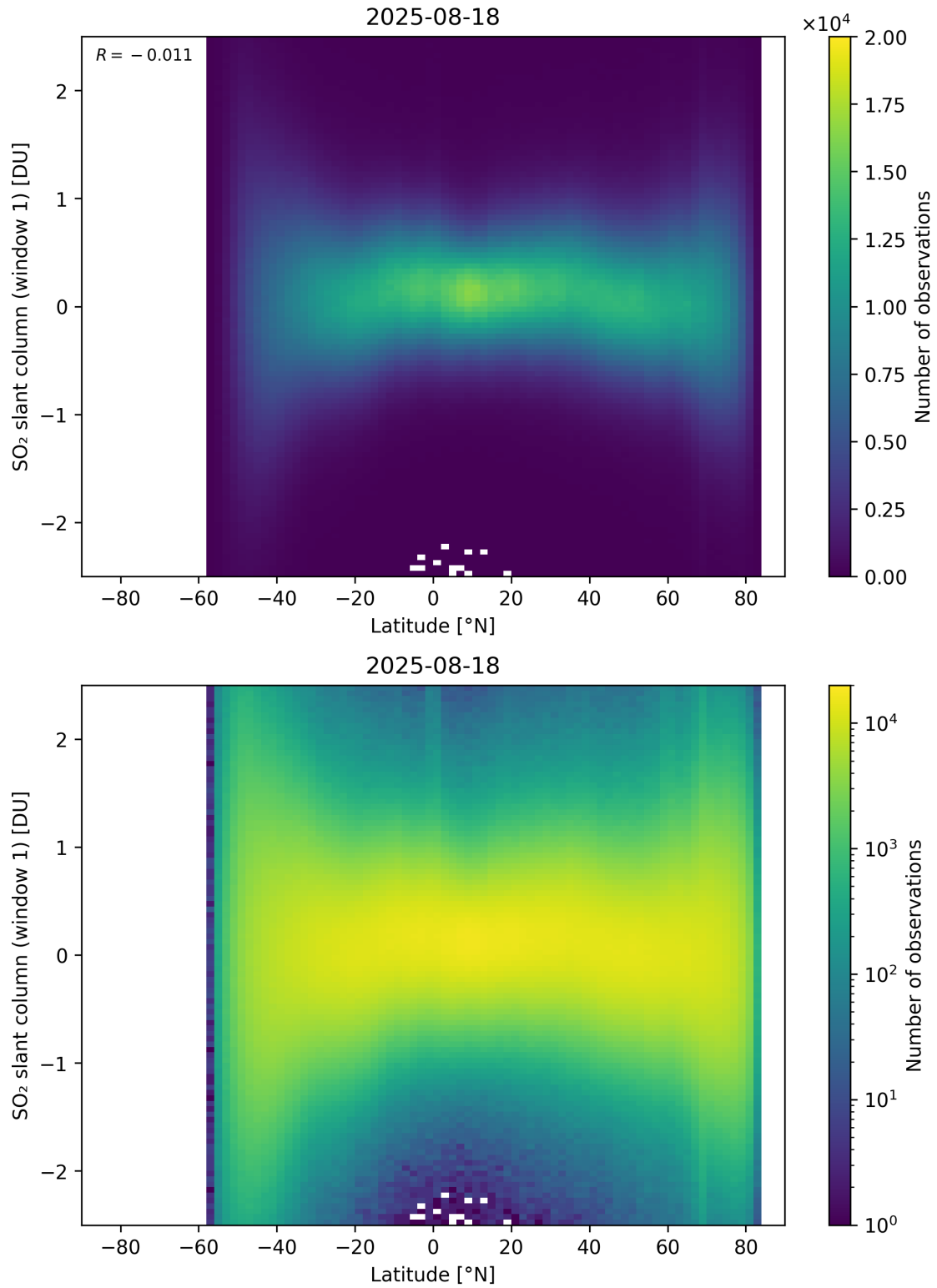
Figure 162: Scatter density plot of “Latitude” against “SO 2 slant column (window 1)” for 2025-08-17 to 2025-08-19.
