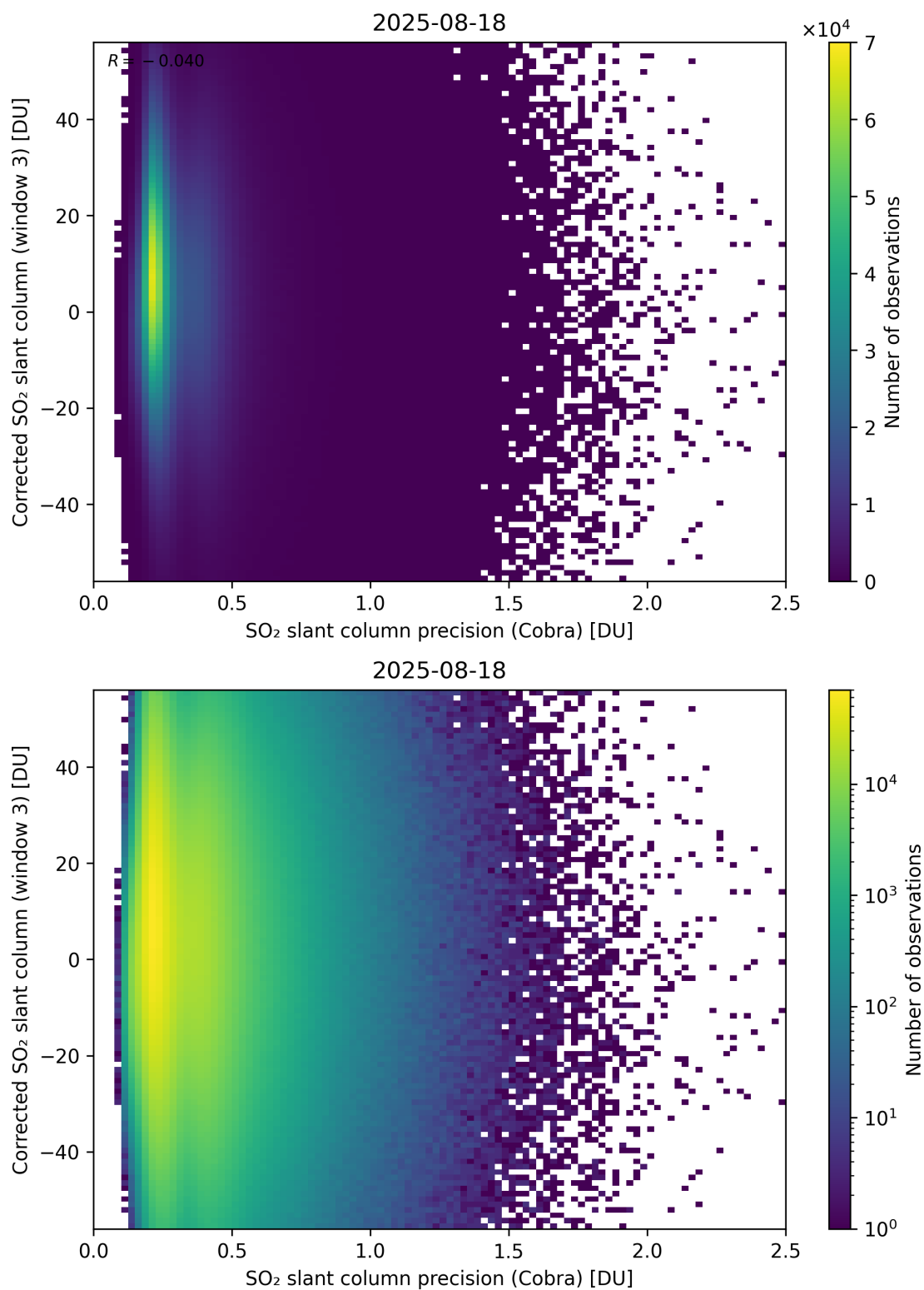
Figure 207: Scatter density plot of “SO 2 slant column precision (Cobra)” against “Corrected SO 2 slant column (window 3)” for 2025-08-17 to 2025-08-19.
