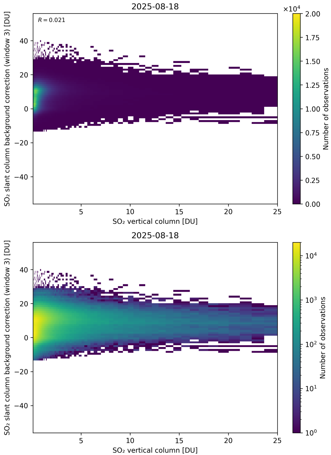
Figure 325: Scatter density plot of “SO 2 vertical column” against “SO 2 slant column background correction (window 3)” for 2025-08-17 to 2025-08-19.
