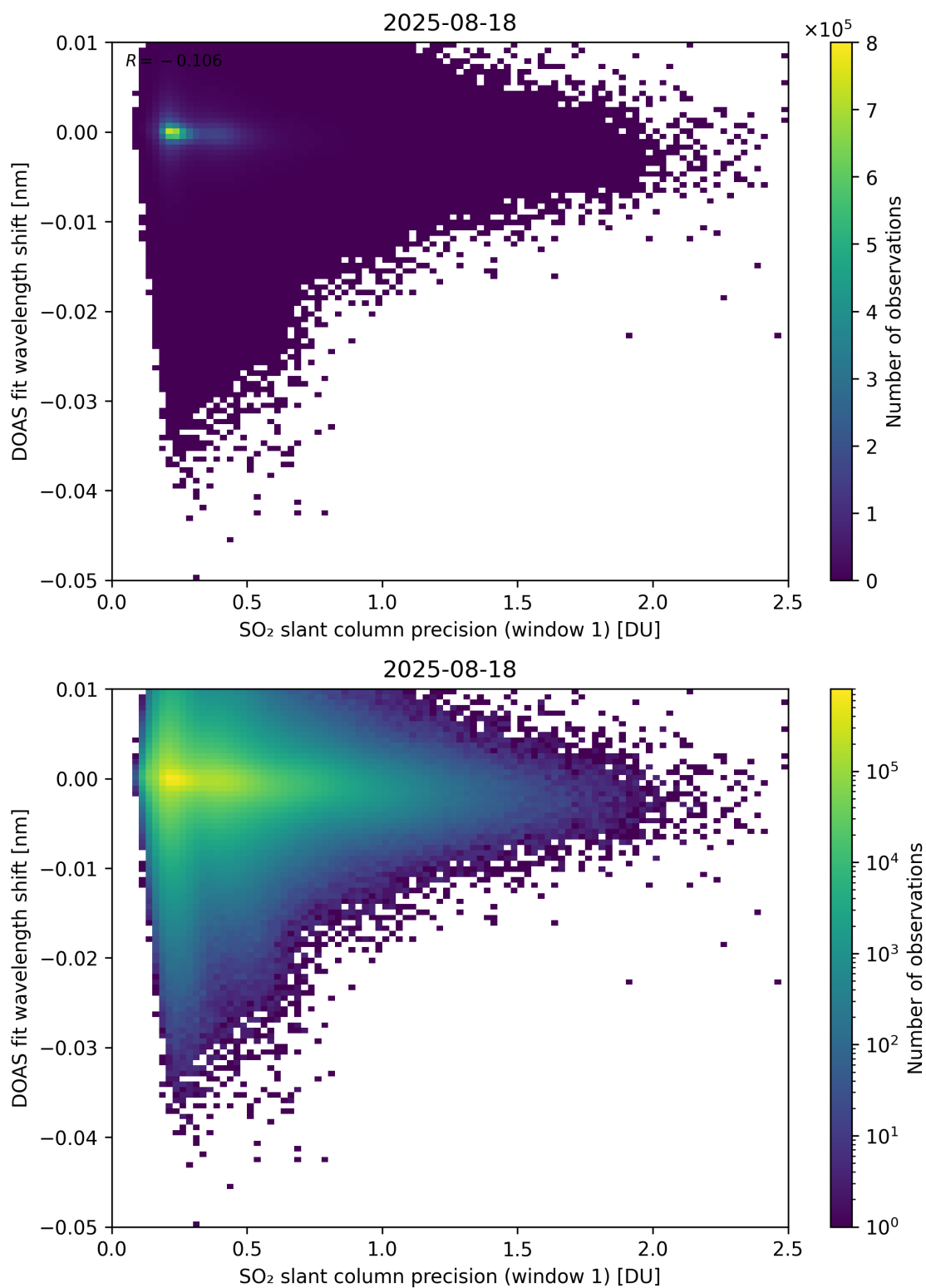
Figure 271: Scatter density plot of “SO 2 slant column precision (window 1)” against “DOAS fit wavelength shift” for 2025-08-17 to 2025-08-19.
