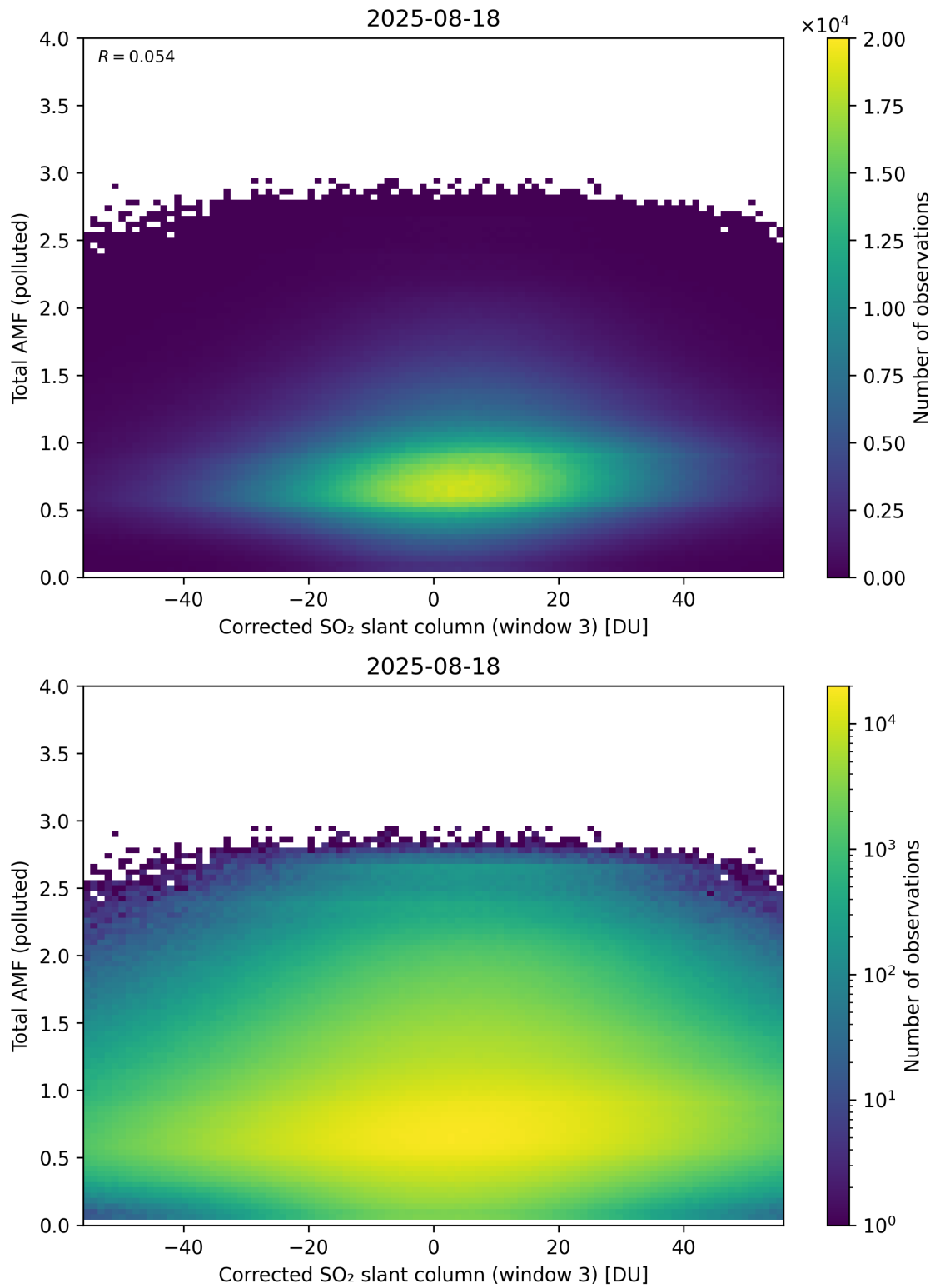
Figure 260: Scatter density plot of “Corrected SO 2 slant column (window 3)” against “Total AMF (polluted)” for 2025-08-17 to 2025-08-19.
