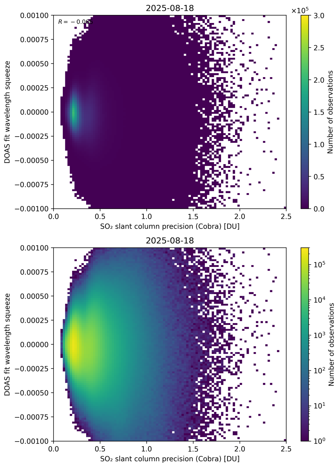
Figure 203: Scatter density plot of “SO 2 slant column precision (Cobra)” against “DOAS fit wavelength squeeze” for 2025-08-17 to 2025-08-19.
