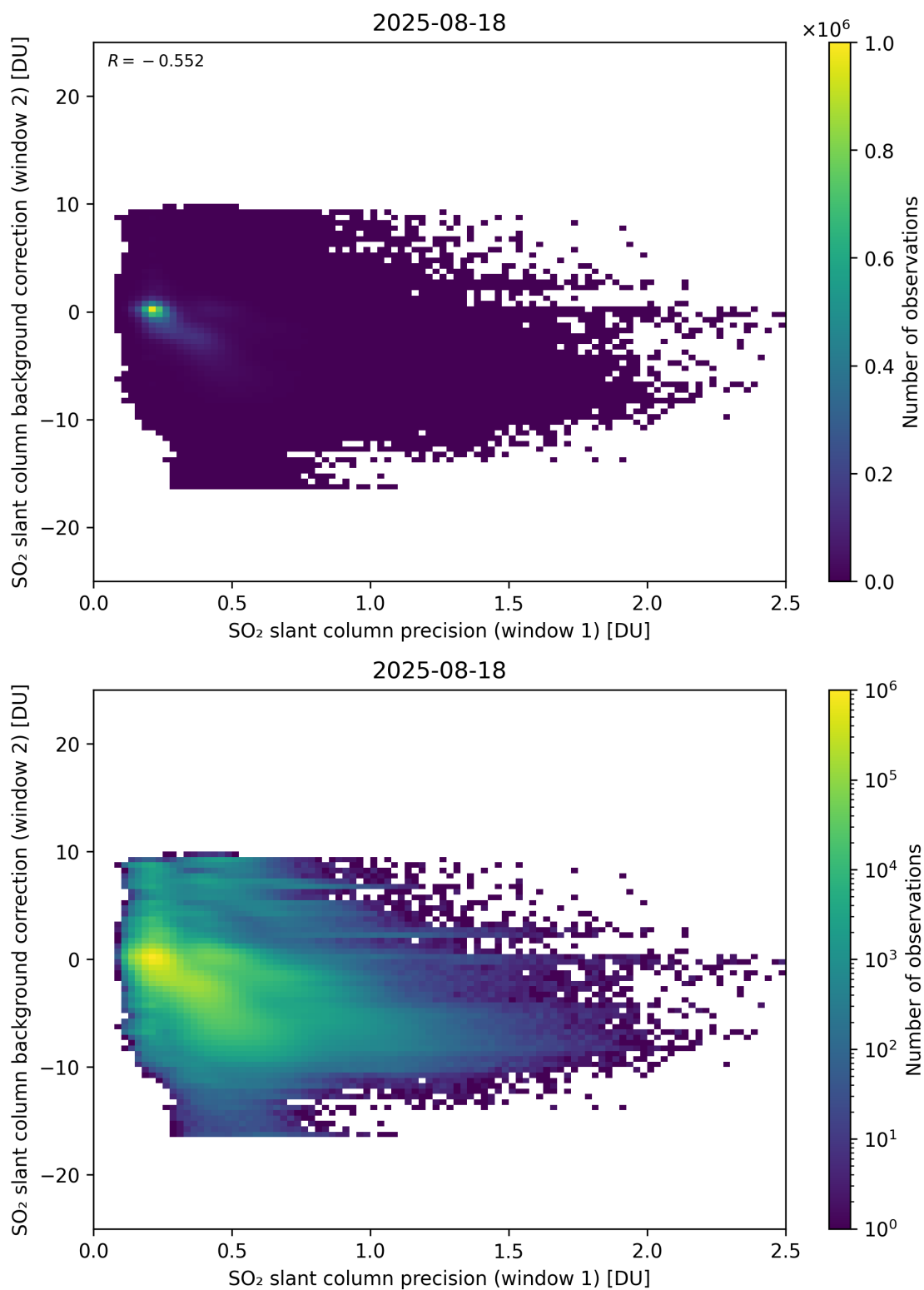
Figure 269: Scatter density plot of “SO 2 slant column precision (window 1)” against “SO 2 slant column background correction (window 2)” for 2025-08-17 to 2025-08-19.
