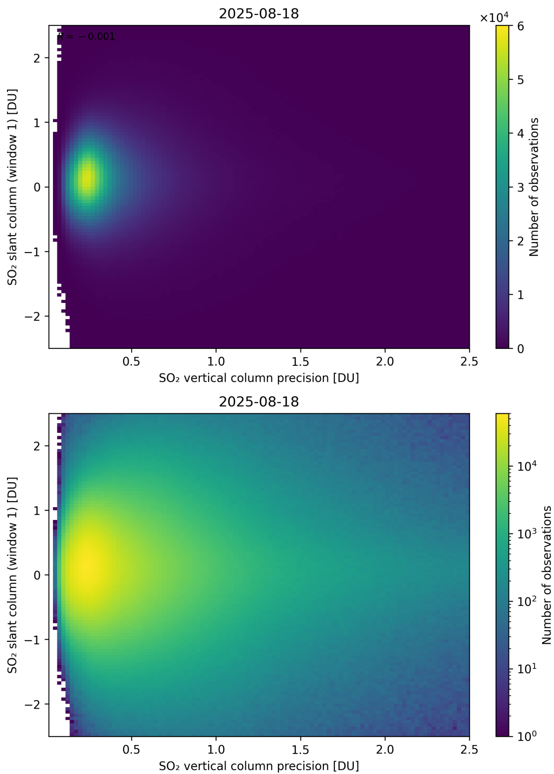
Figure 341: Scatter density plot of “SO 2 vertical column precision” against “SO 2 slant column (window 1)” for 2025-08-17 to 2025-08-19.
