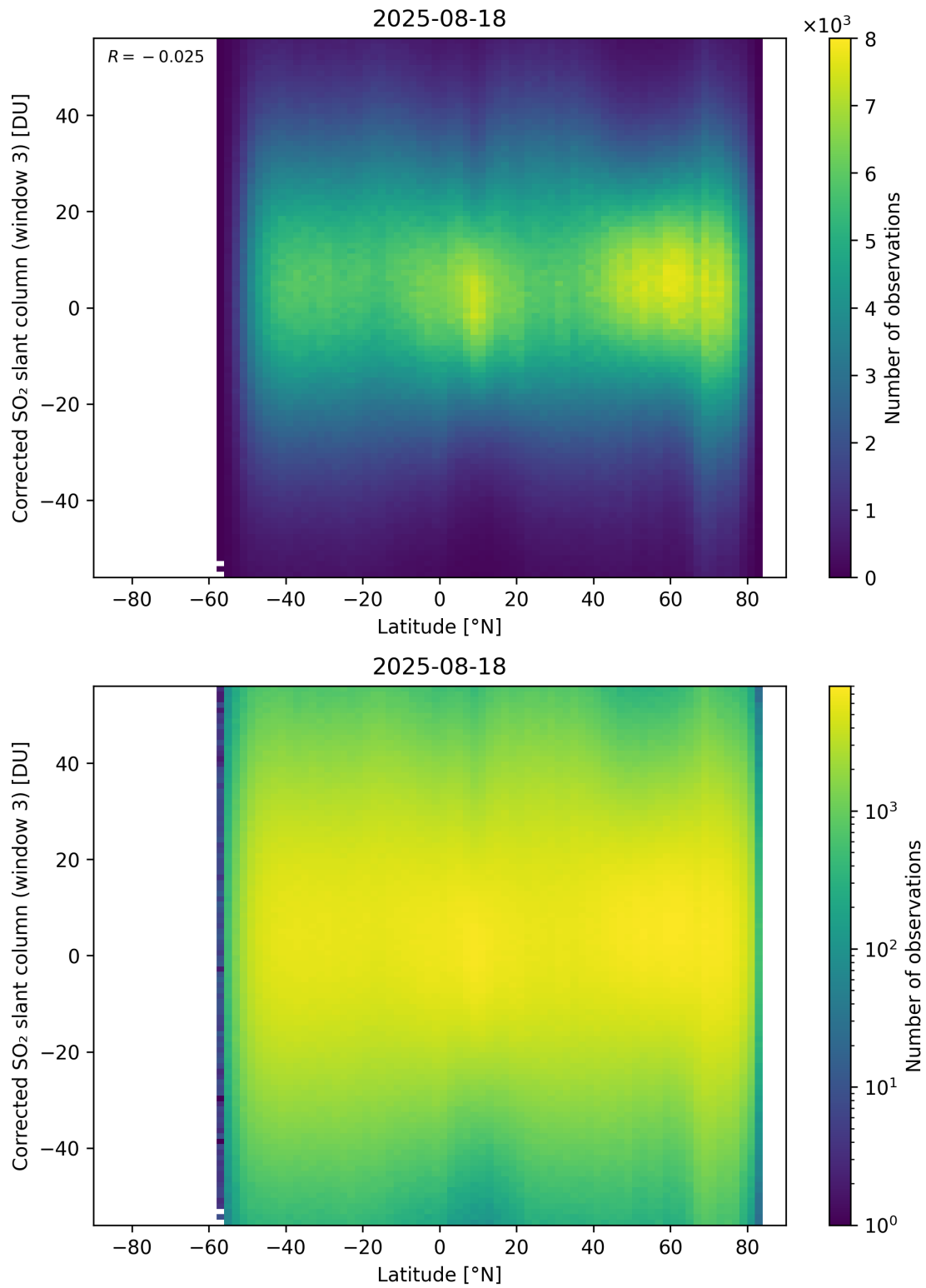
Figure 161: Scatter density plot of “Latitude” against “Corrected SO 2 slant column (window 3)” for 2025-08-17 to 2025-08-19.
