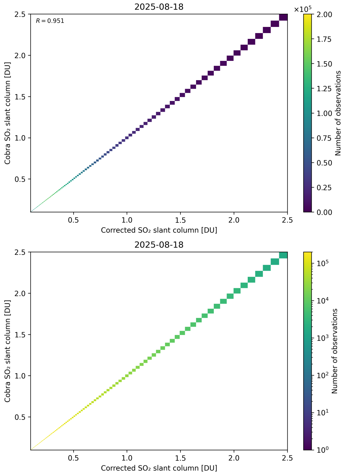
Figure 233: Scatter density plot of “Corrected SO 2 slant column” against “Cobra SO 2 slant column” for 2025-08-17 to 2025-08-19.
