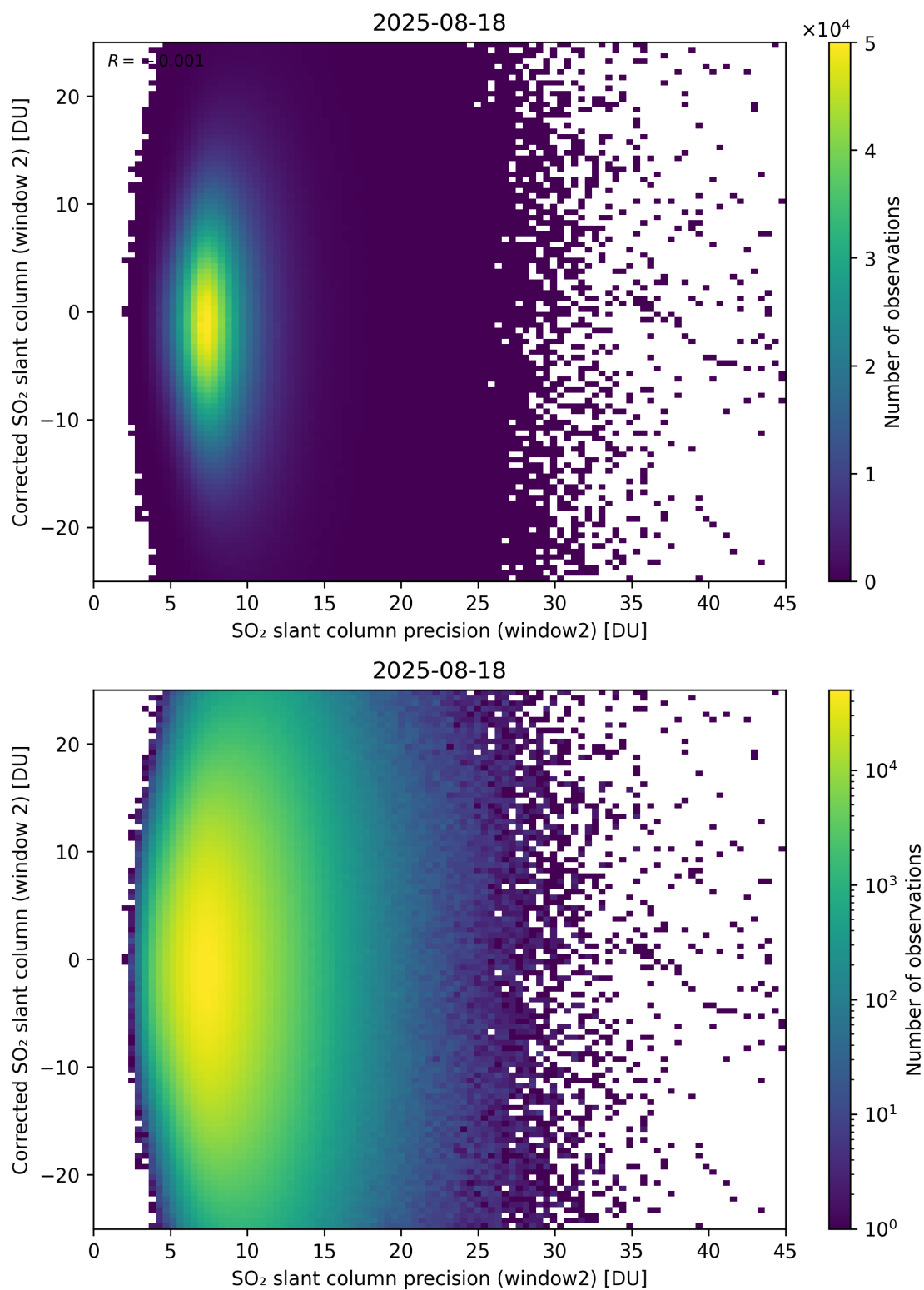
Figure 297: Scatter density plot of “SO 2 slant column precision (window2)” against “Corrected SO 2 slant column (window 2)” for 2025-08-17 to 2025-08-19.
