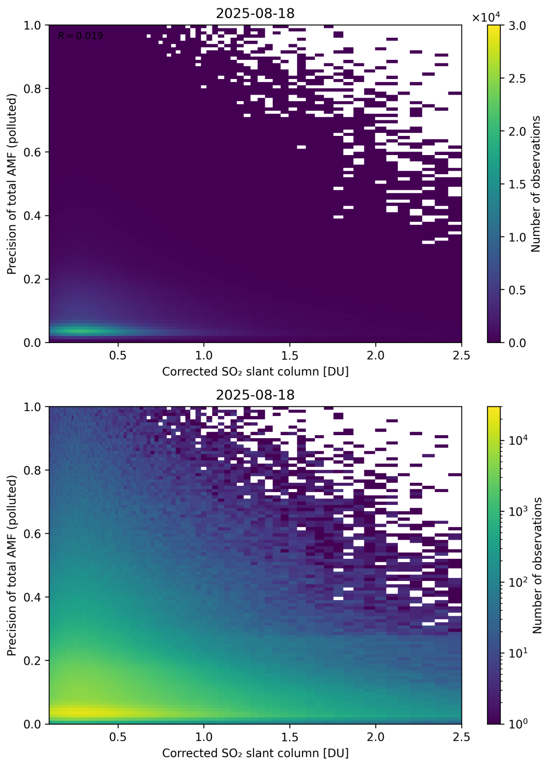
Figure 243: Scatter density plot of “Corrected SO 2 slant column” against “Precision of total AMF (polluted)” for 2025-08-17 to 2025-08-19.
