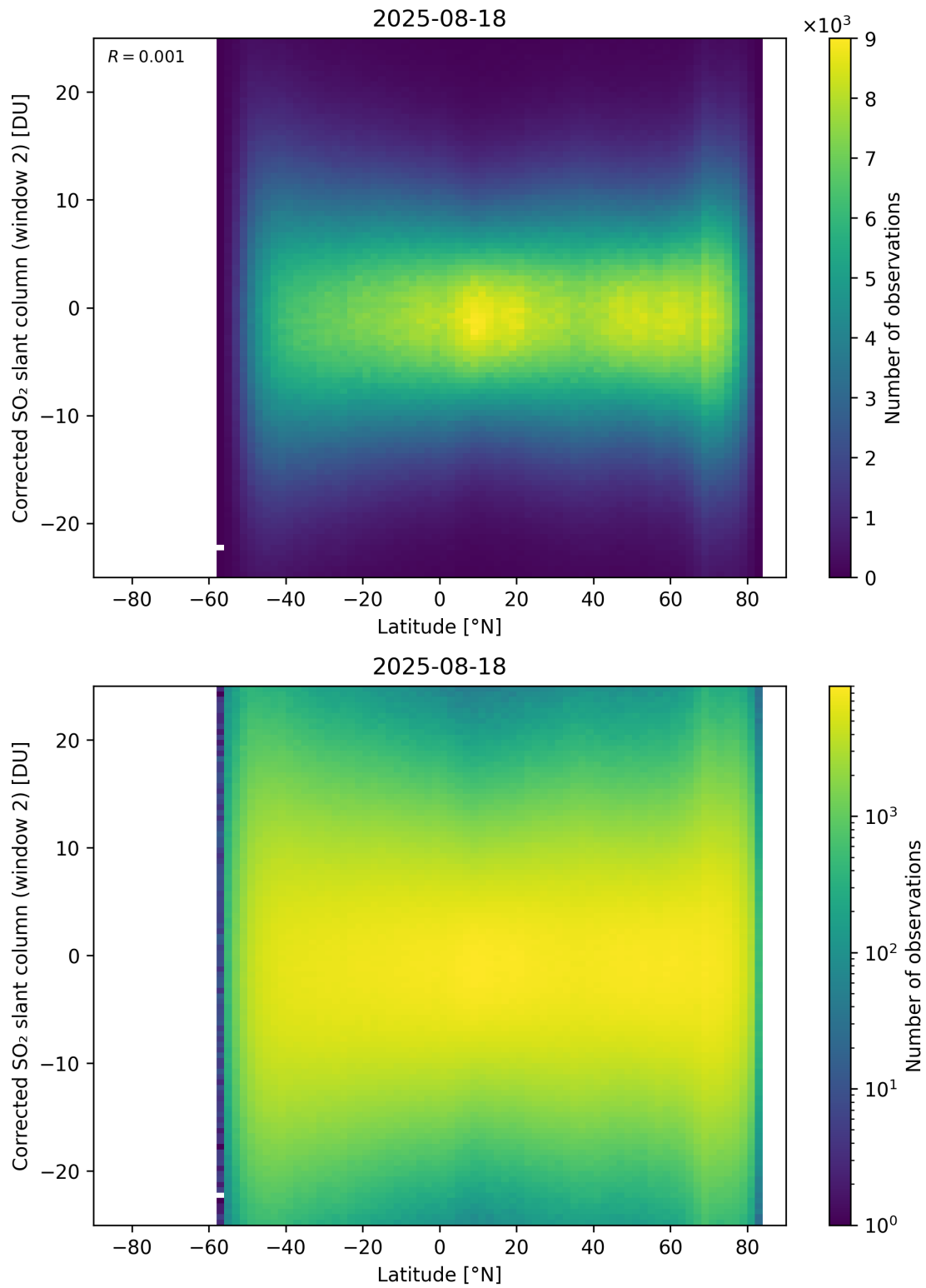
Figure 160: Scatter density plot of “Latitude” against “Corrected SO 2 slant column (window 2)” for 2025-08-17 to 2025-08-19.
