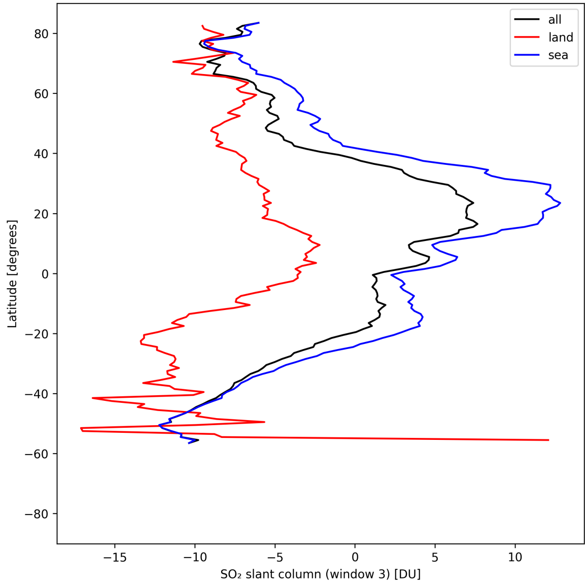
Figure 45: Zonal average of “SO 2 slant column (window 3)” for 2025-08-17 to 2025-08-19.
