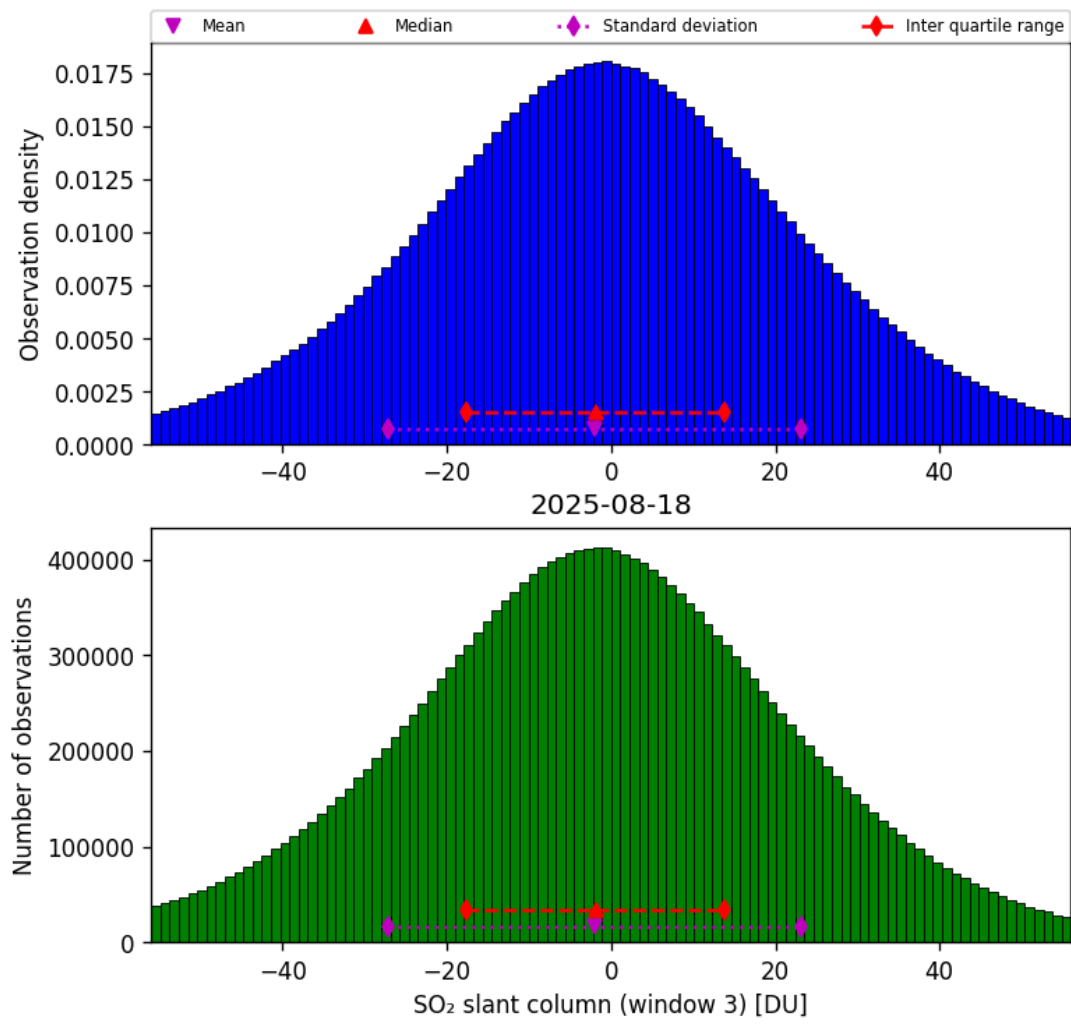
Figure 71: Histogram of “SO 2 slant column (window 3)” for 2025-08-17 to 2025-08-19
