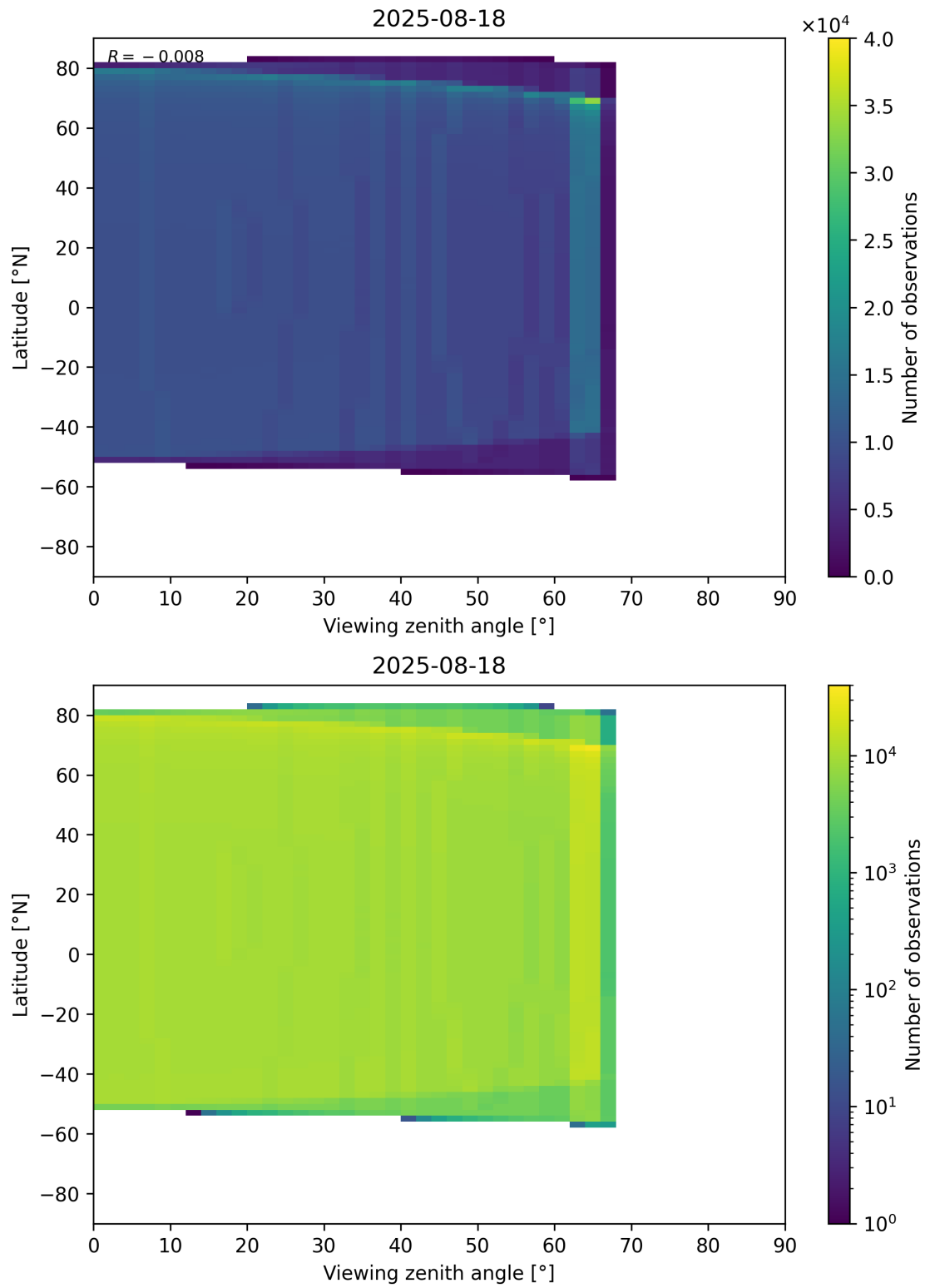
Figure 368: Scatter density plot of “Viewing zenith angle” against “Latitude” for 2025-08-17 to 2025-08-19.
