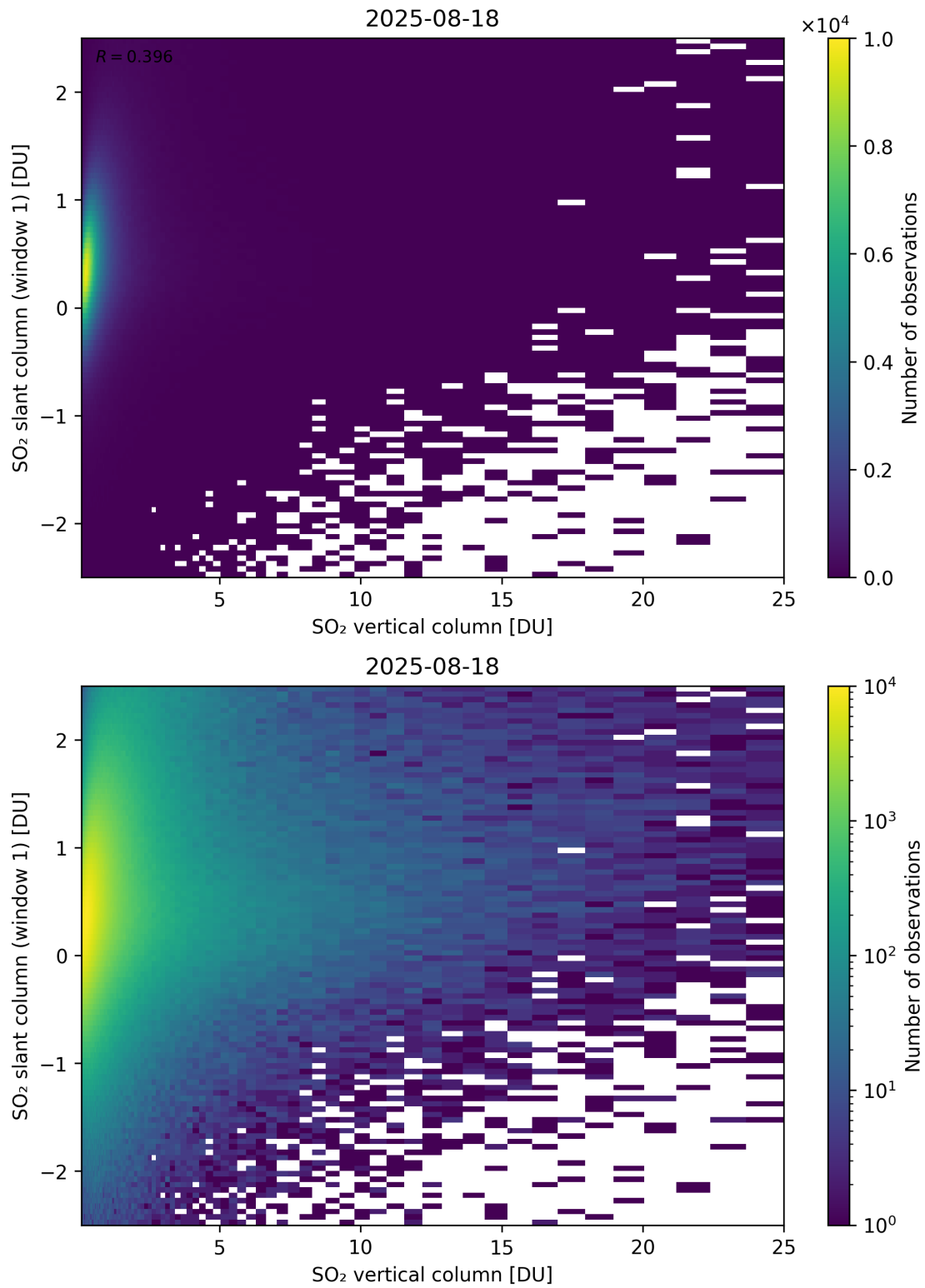
Figure 354: Scatter density plot of “SO 2 vertical column” against “SO 2 slant column (window 1)” for 2025-08-17 to 2025-08-19.
