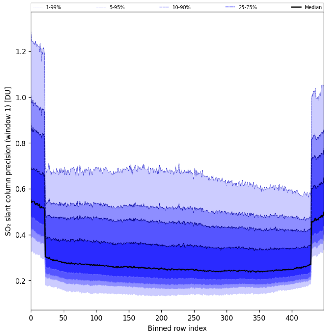
Figure 90: Along track statistics of “SO 2 slant column precision (window 1)” for 2025-08-17 to 2025-08-19
