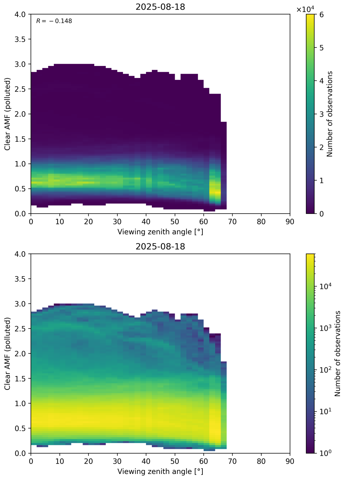
Figure 370: Scatter density plot of “Viewing zenith angle” against “Clear AMF (polluted)” for 2025-08-17 to 2025-08-19.
