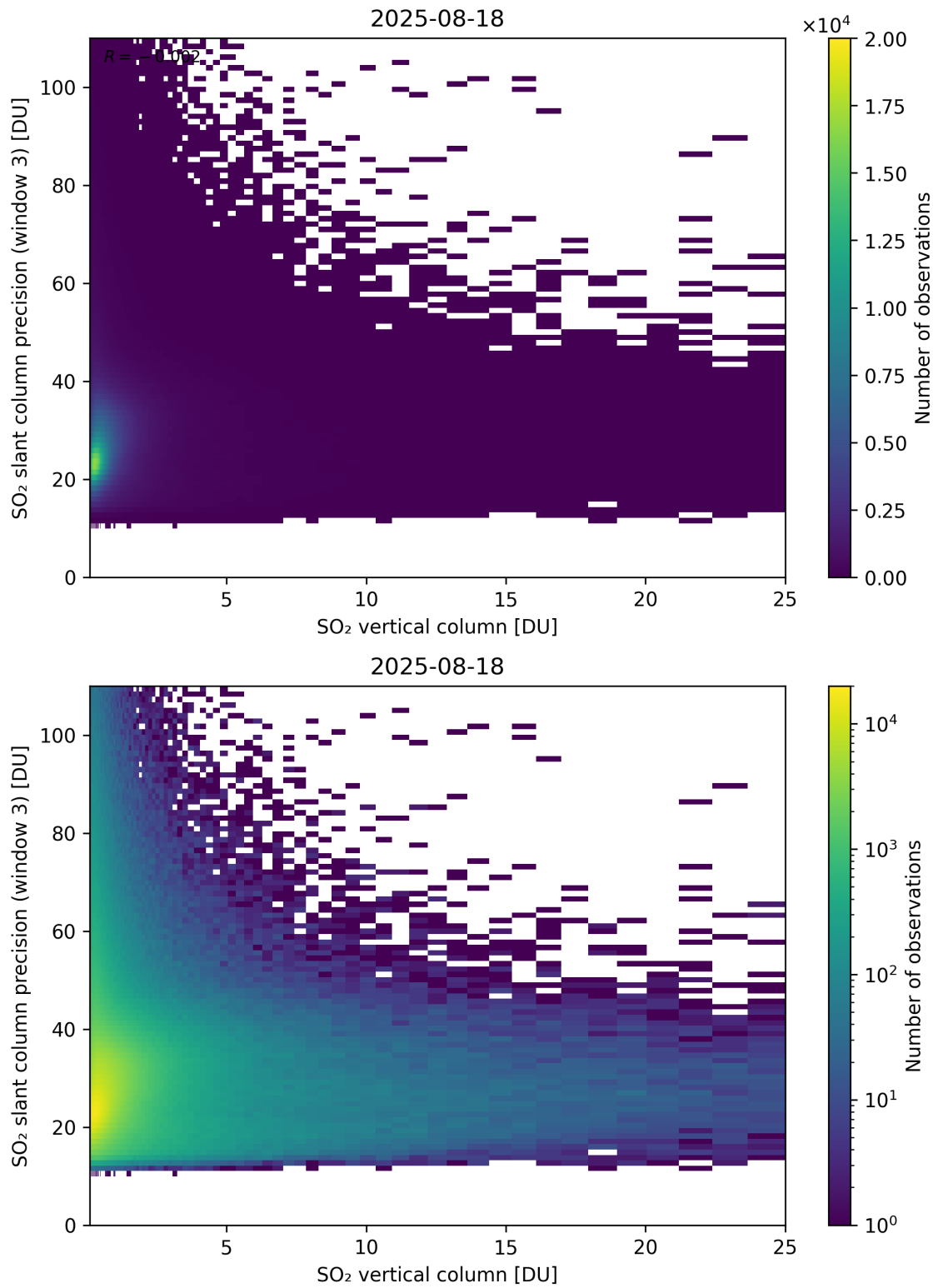
Figure 358: Scatter density plot of “SO 2 vertical column” against “SO 2 slant column precision (window 3)” for 2025-08-17 to 2025-08-19.
