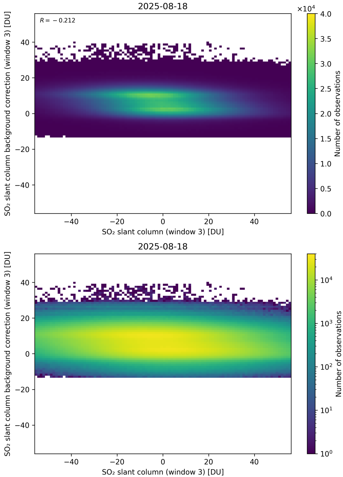
Figure 303: Scatter density plot of “SO 2 slant column (window 3)” against “SO 2 slant column background correction (window 3)” for 2025-08-17 to 2025-08-19.
