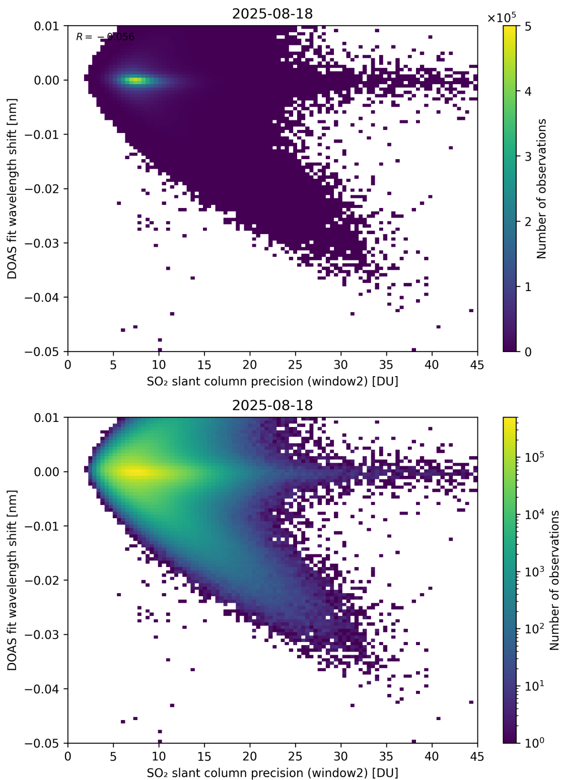
Figure 293: Scatter density plot of “SO 2 slant column precision (window2)” against “DOAS fit wavelength shift” for 2025-08-17 to 2025-08-19.
