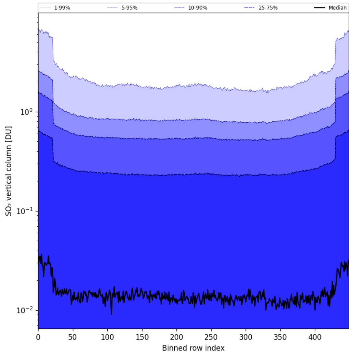
Figure 84: Along track statistics of “SO 2 vertical column” for 2025-08-17 to 2025-08-19
