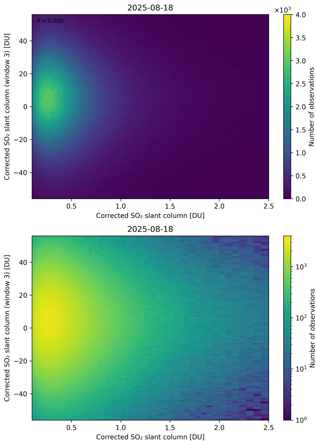
Figure 236: Scatter density plot of “Corrected SO 2 slant column” against “Corrected SO 2 slant column (window 3)” for 2025-08-17 to 2025-08-19.
