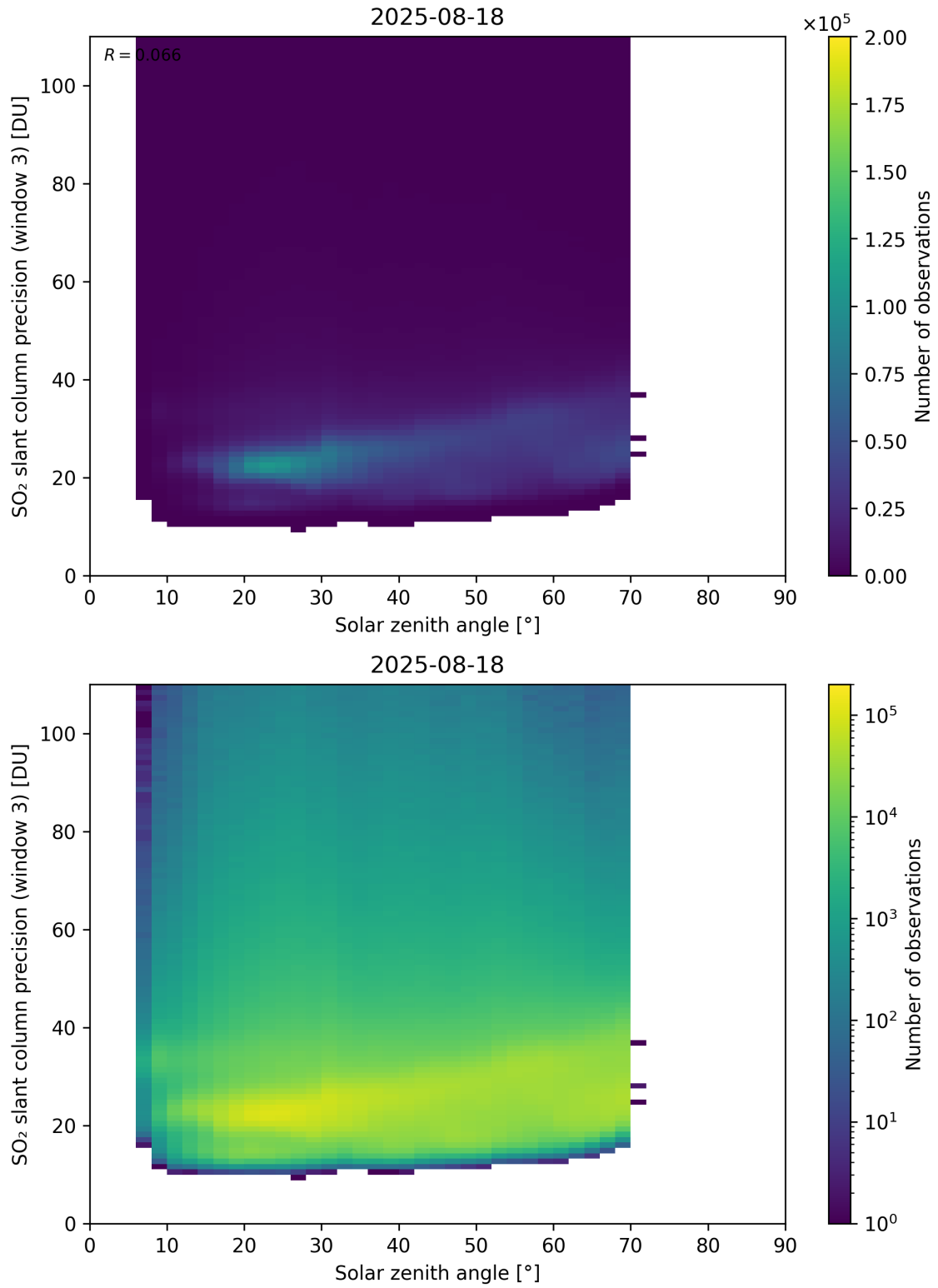
Figure 188: Scatter density plot of “Solar zenith angle” against “SO 2 slant column precision (window 3)” for 2025-08-17 to 2025-08-19.
