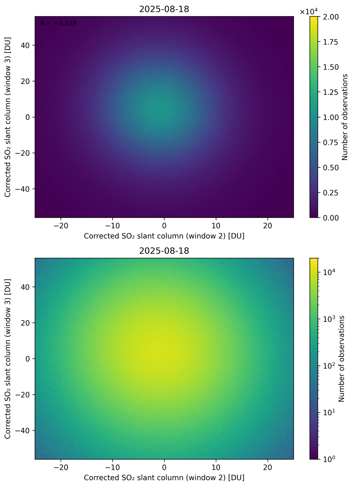
Figure 250: Scatter density plot of “Corrected SO 2 slant column (window 2)” against “Corrected SO 2 slant column (window 3)” for 2025-08-17 to 2025-08-19.
