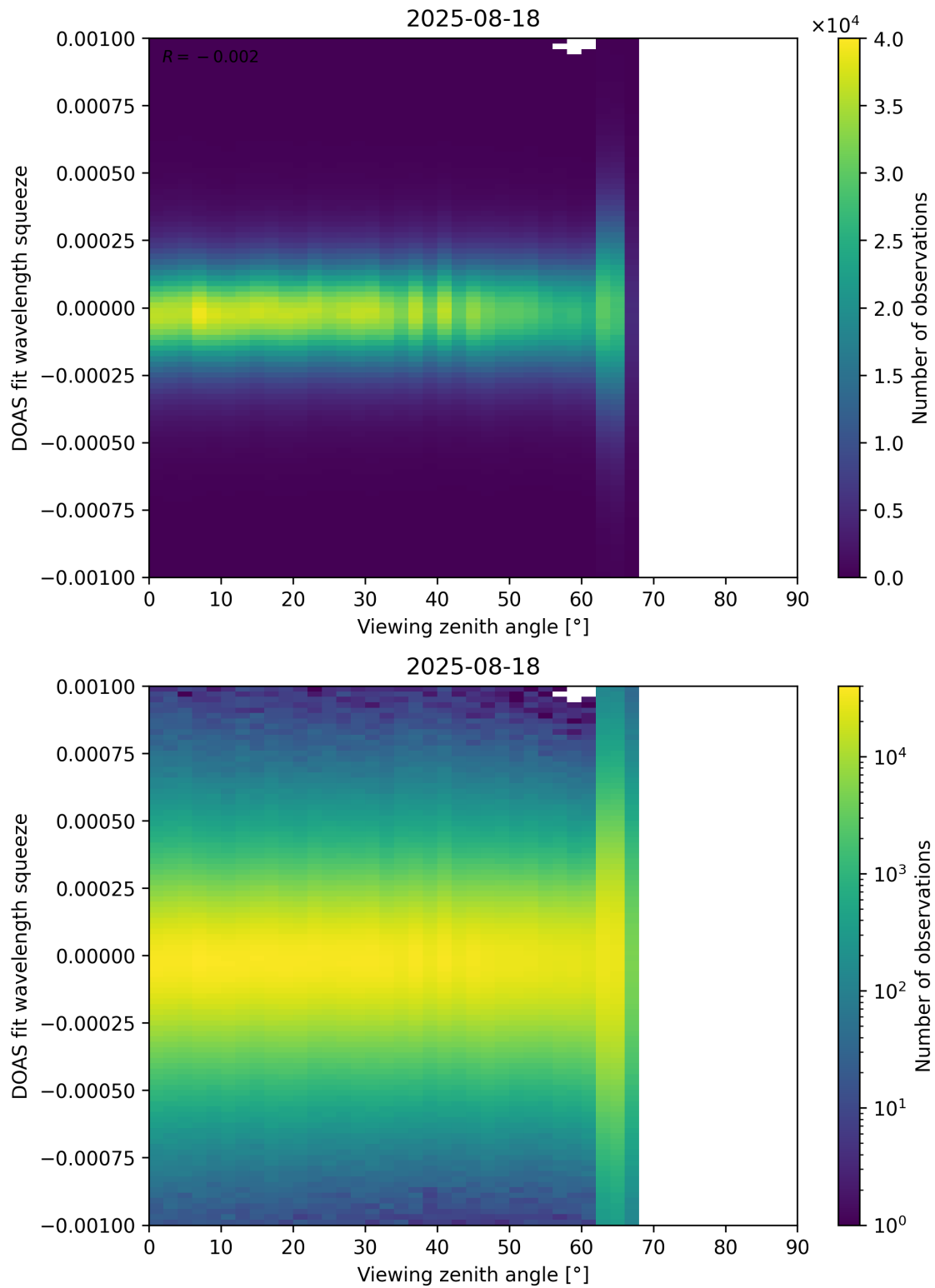
Figure 366: Scatter density plot of “Viewing zenith angle” against “DOAS fit wavelength squeeze” for 2025-08-17 to 2025-08-19.
