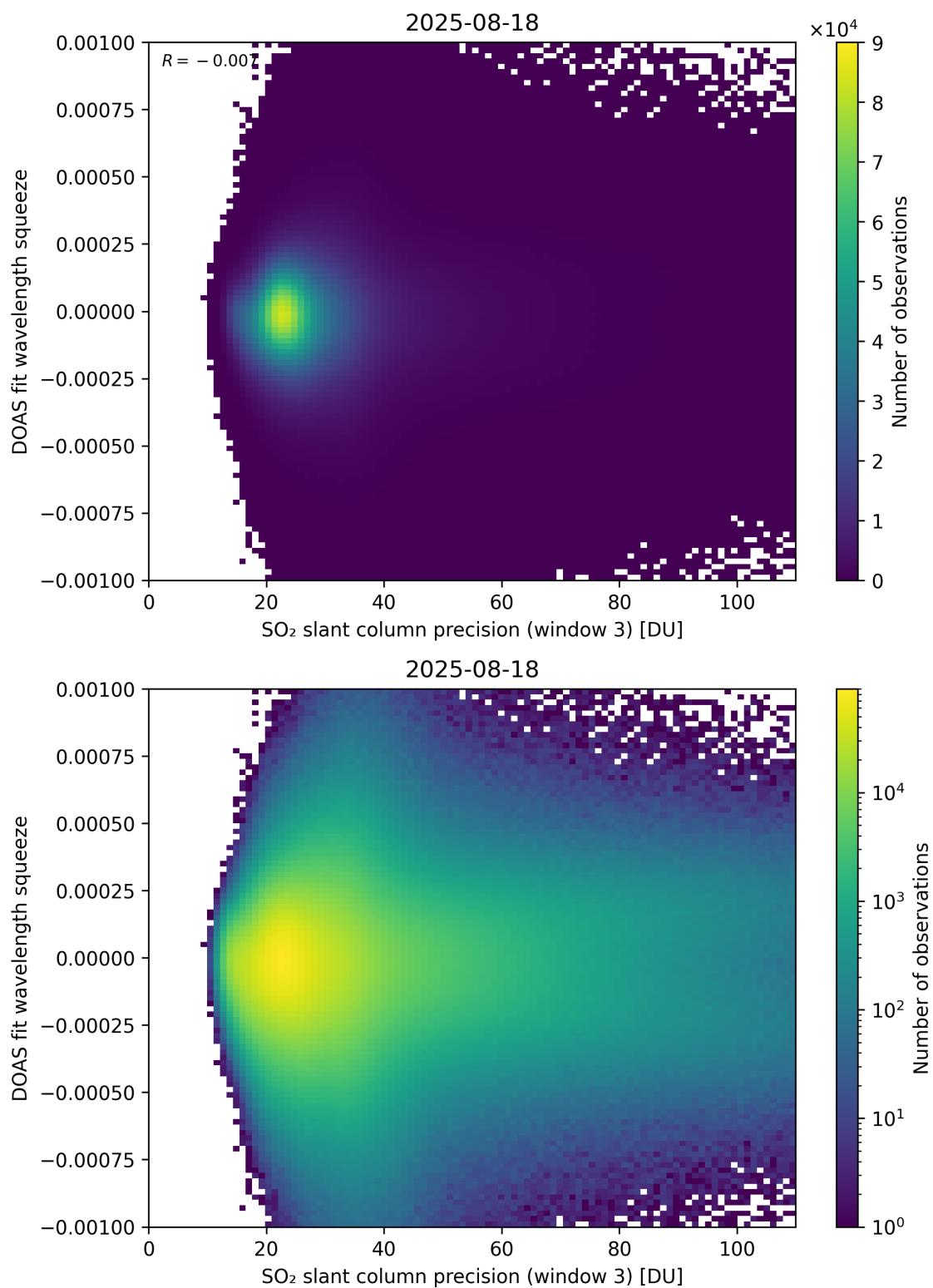
Figure 309: Scatter density plot of “SO 2 slant column precision (window 3)” against “DOAS fit wavelength squeeze” for 2025-08-17 to 2025-08-19.
