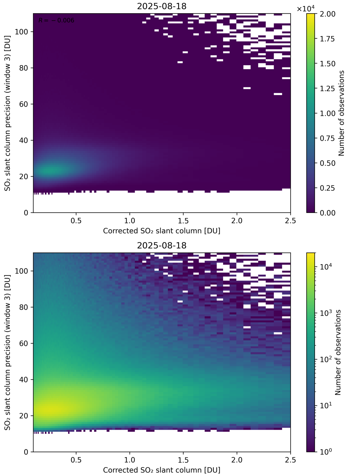
Figure 241: Scatter density plot of “Corrected SO 2 slant column” against “SO 2 slant column precision (window 3)” for 2025-08-17 to 2025-08-19.
