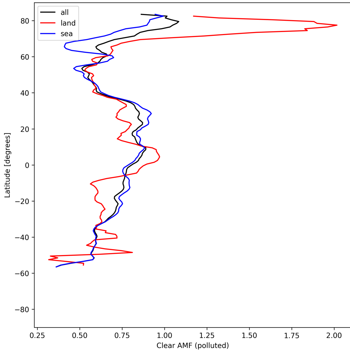
Figure 55: Zonal average of “Clear AMF (polluted)” for 2025-08-17 to 2025-08-19.
