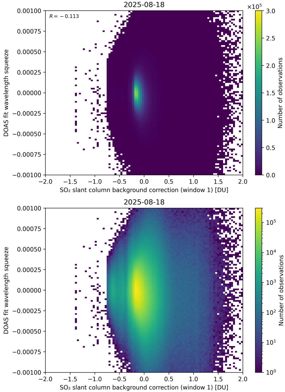
Figure 112: Scatter density plot of “SO 2 slant column background correction (window 1)” against “DOAS fit wavelength squeeze” for 2025-08-17 to 2025-08-19.
