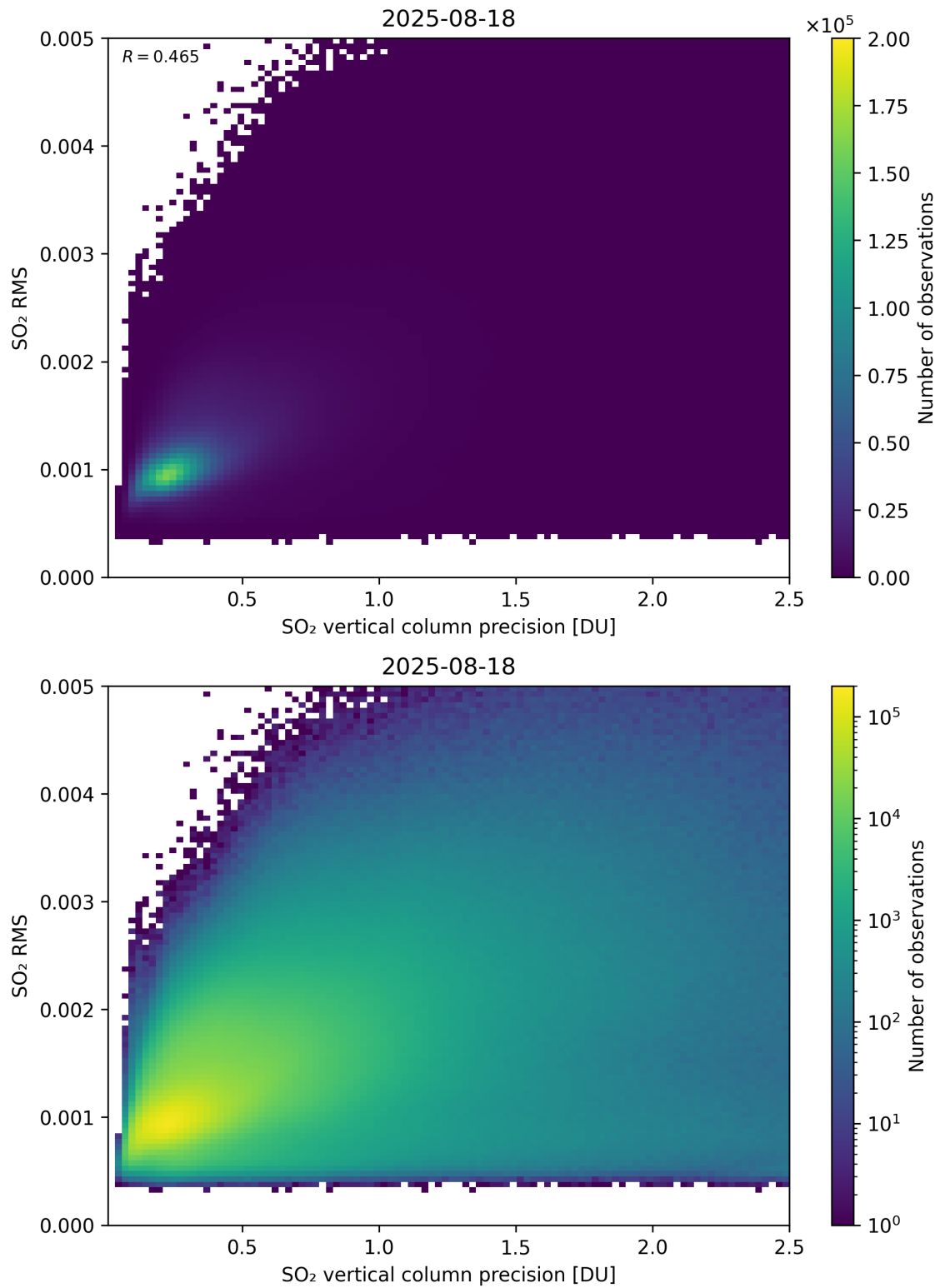
Figure 334: Scatter density plot of “SO 2 vertical column precision” against “SO 2 RMS” for 2025-08-17 to 2025-08-19.
