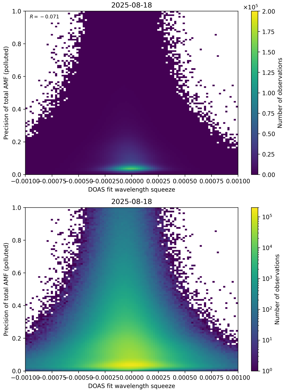
Figure 146: Scatter density plot of “DOAS fit wavelength squeeze” against “Precision of total AMF (polluted)” for 2025-08-17 to 2025-08-19.
