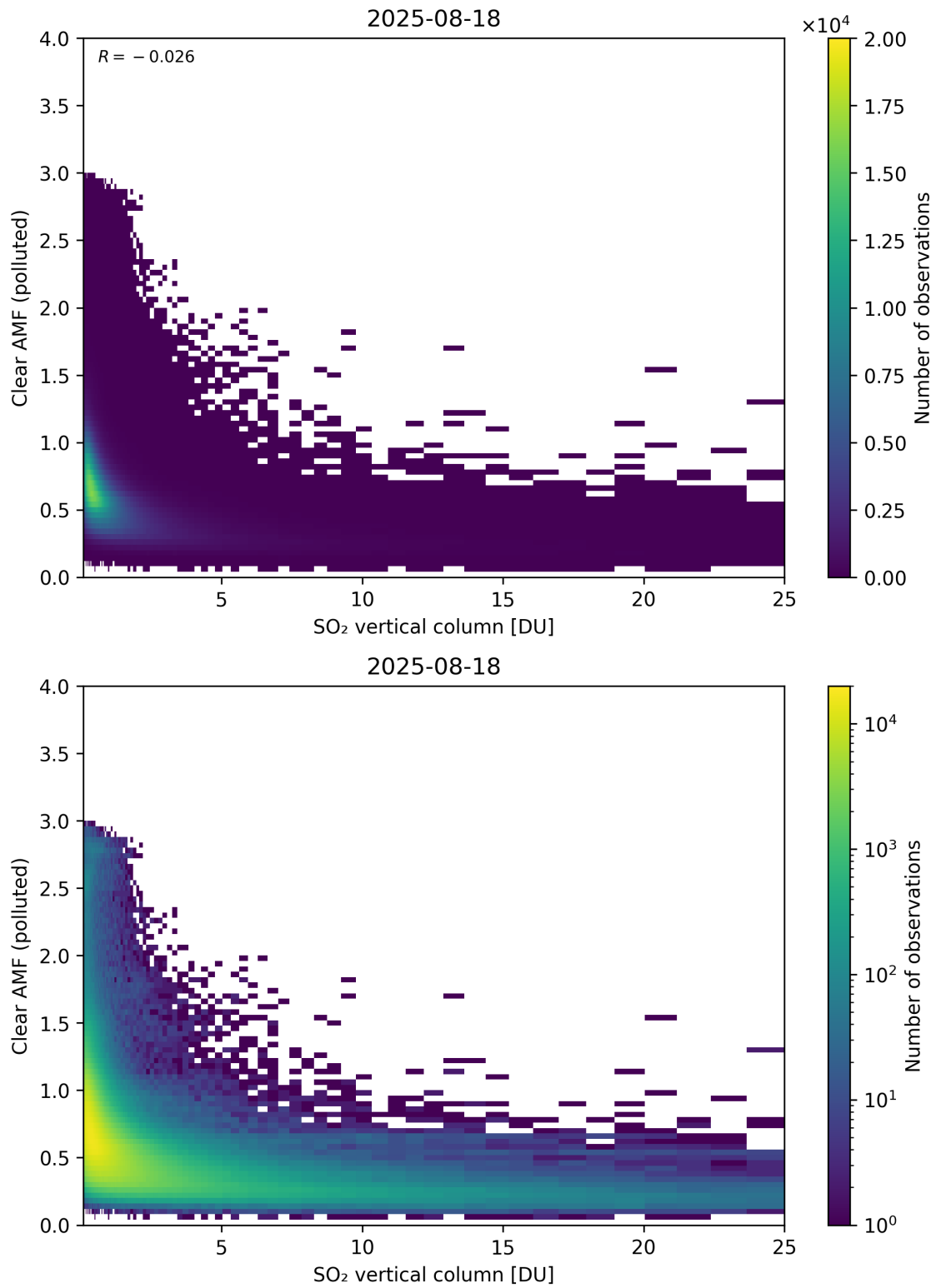
Figure 348: Scatter density plot of “SO 2 vertical column” against “Clear AMF (polluted)” for 2025-08-17 to 2025-08-19.
