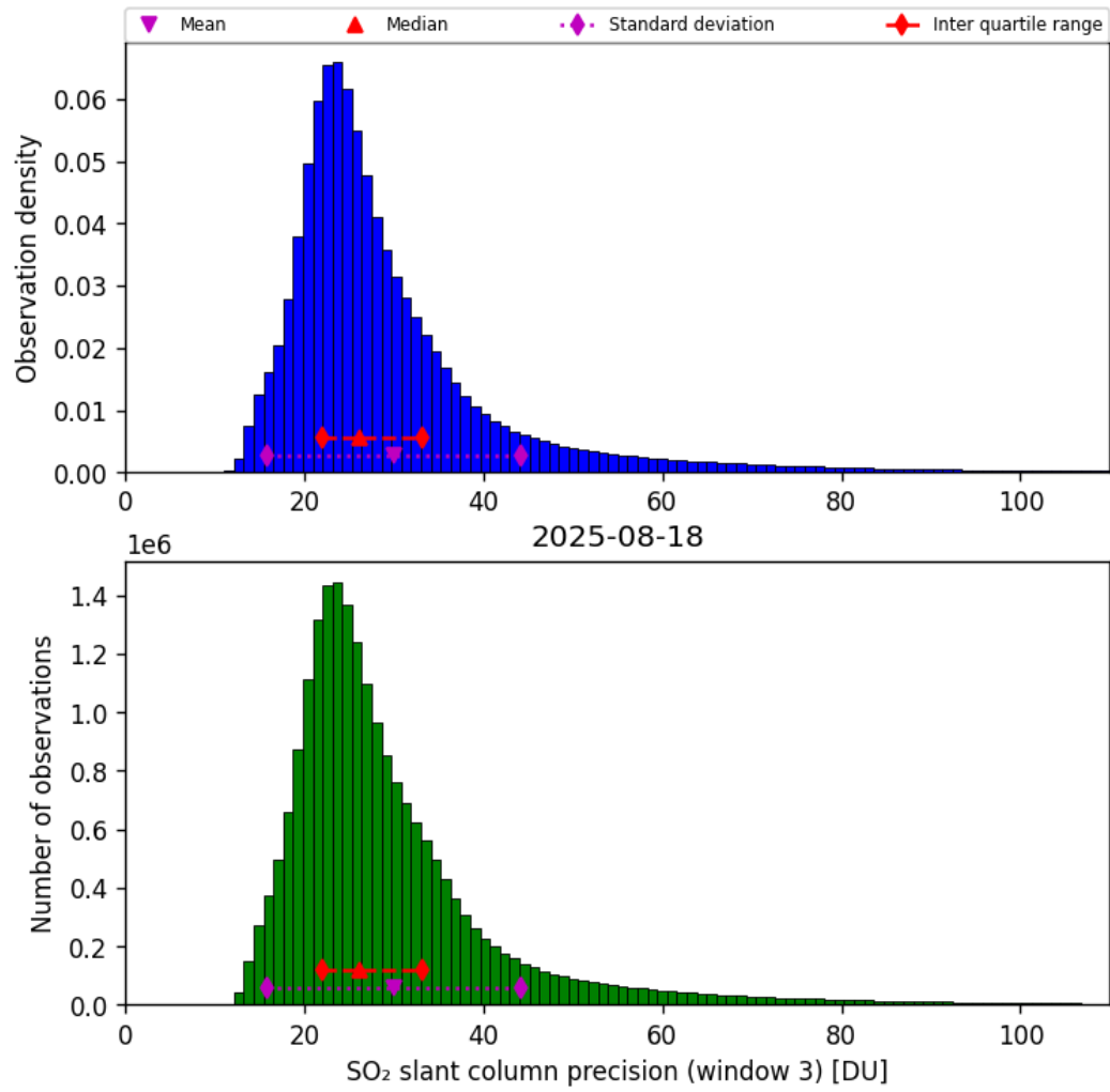
Figure 72: Histogram of “SO 2 slant column precision (window 3)” for 2025-08-17 to 2025-08-19
