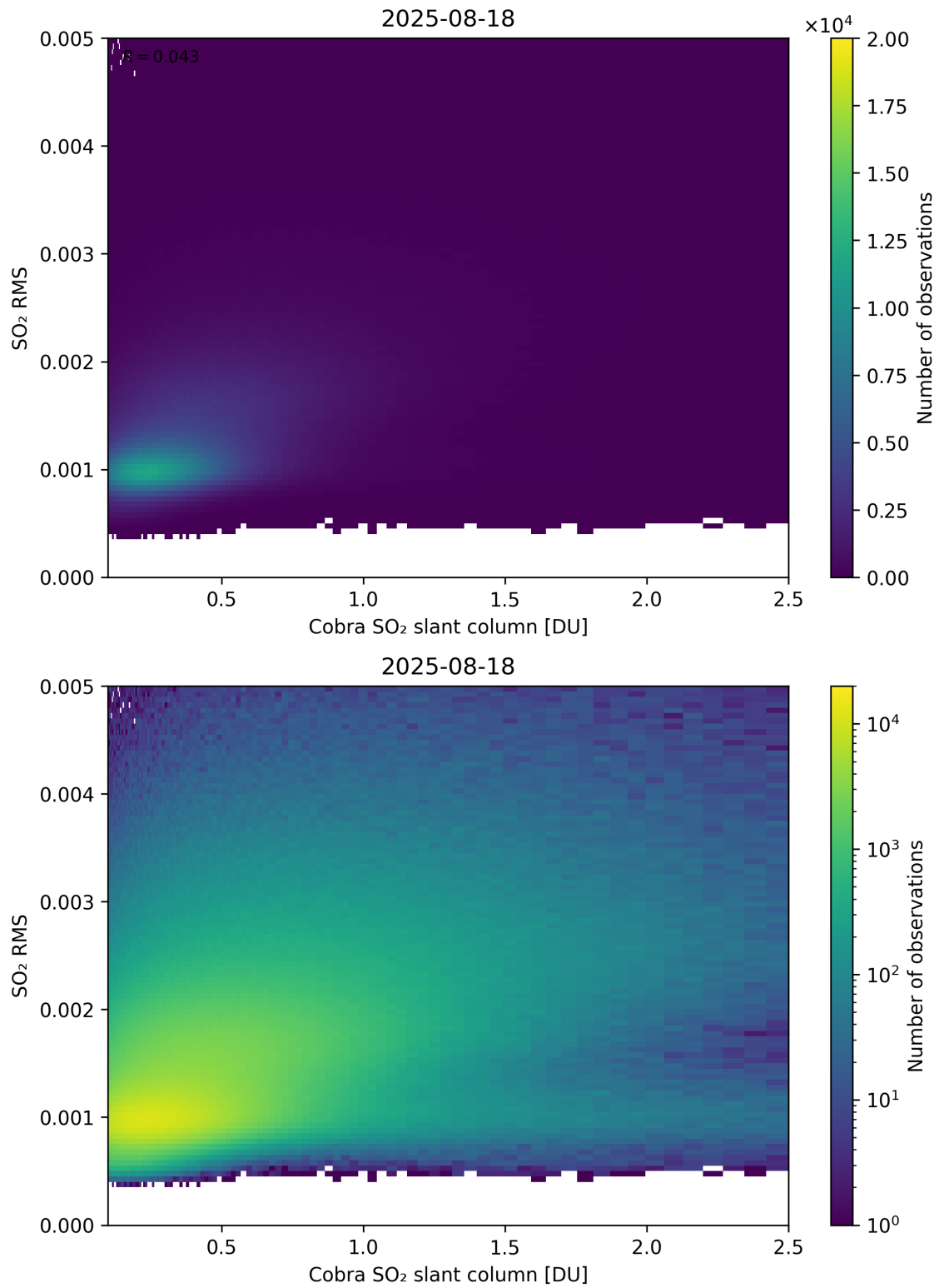
Figure 198: Scatter density plot of “Cobra SO 2 slant column” against “SO 2 RMS” for 2025-08-17 to 2025-08-19.
