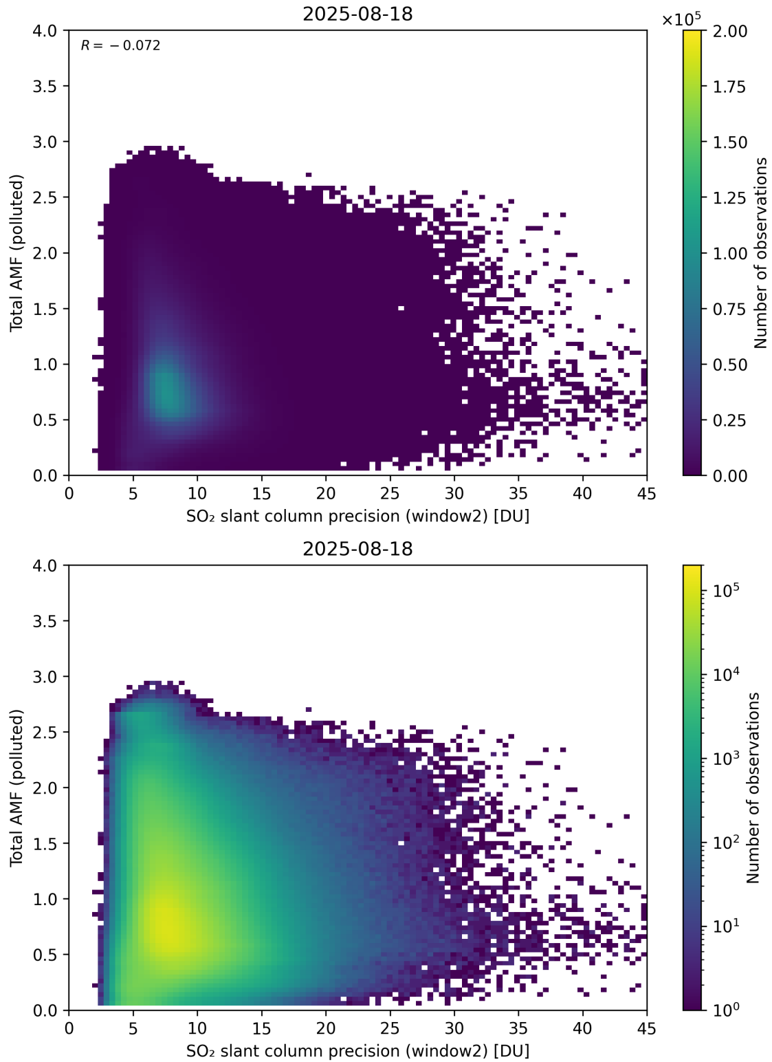
Figure 301: Scatter density plot of “SO 2 slant column precision (window2)” against “Total AMF (polluted)” for 2025-08-17 to 2025-08-19.
