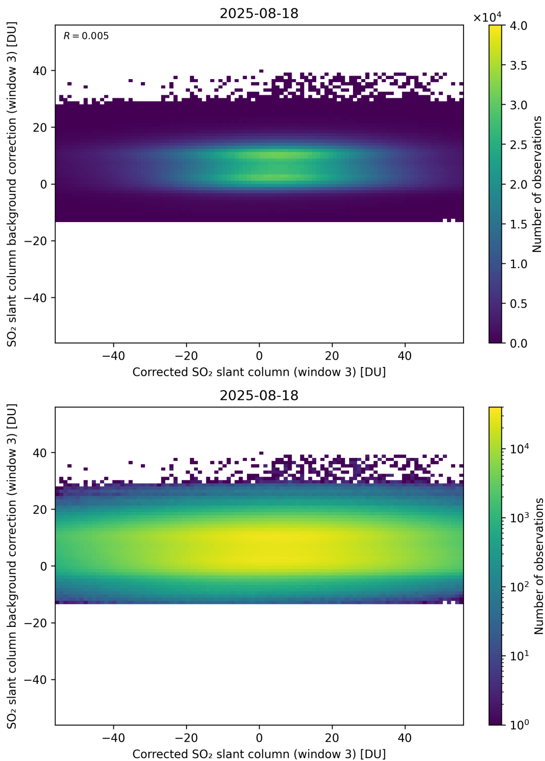
Figure 255: Scatter density plot of “Corrected SO 2 slant column (window 3)” against “SO 2 slant column background correction (window 3)” for 2025-08-17 to 2025-08-19.
