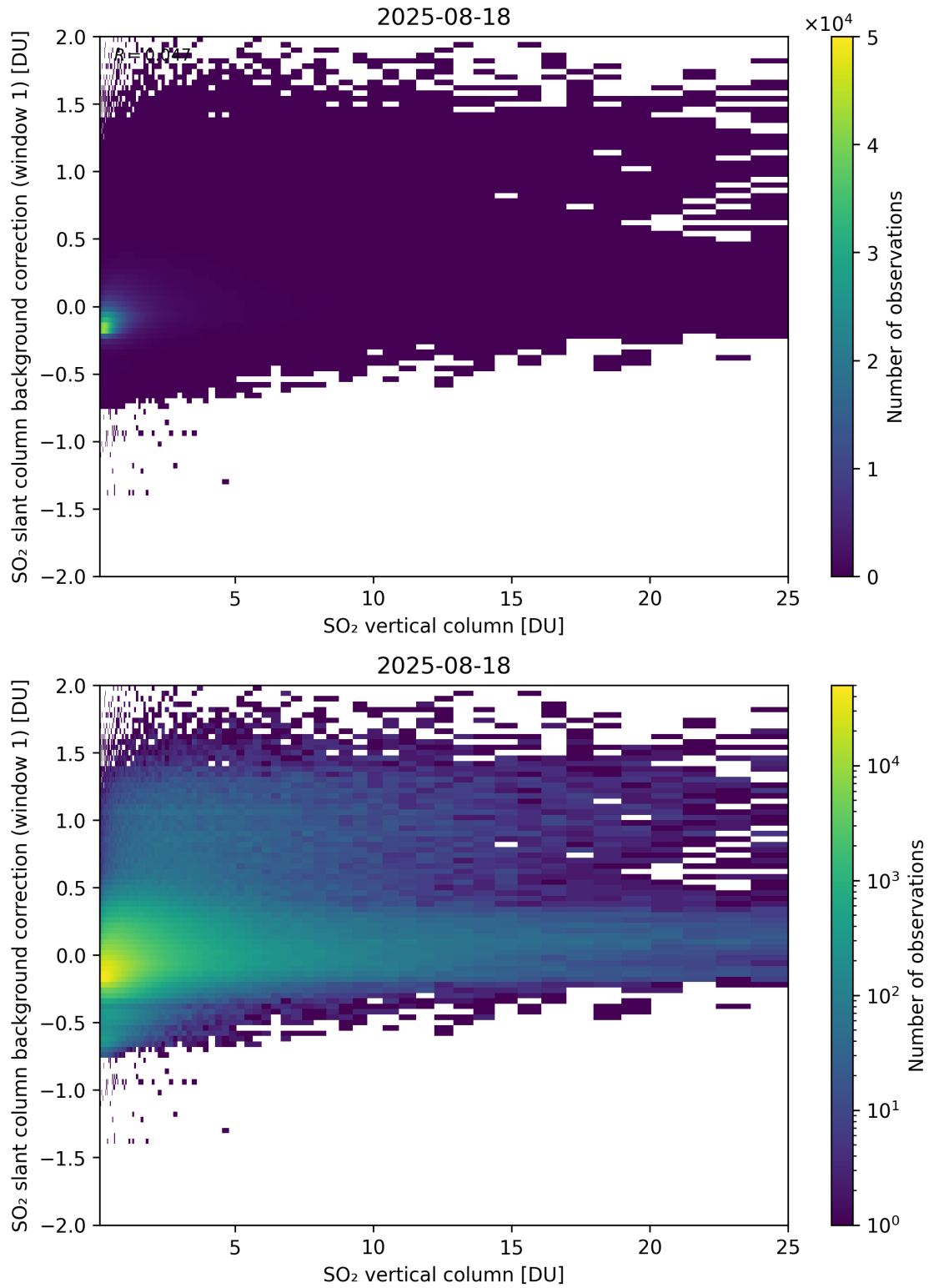
Figure 323: Scatter density plot of “SO 2 vertical column” against “SO 2 slant column background correction (window 1)” for 2025-08-17 to 2025-08-19.
