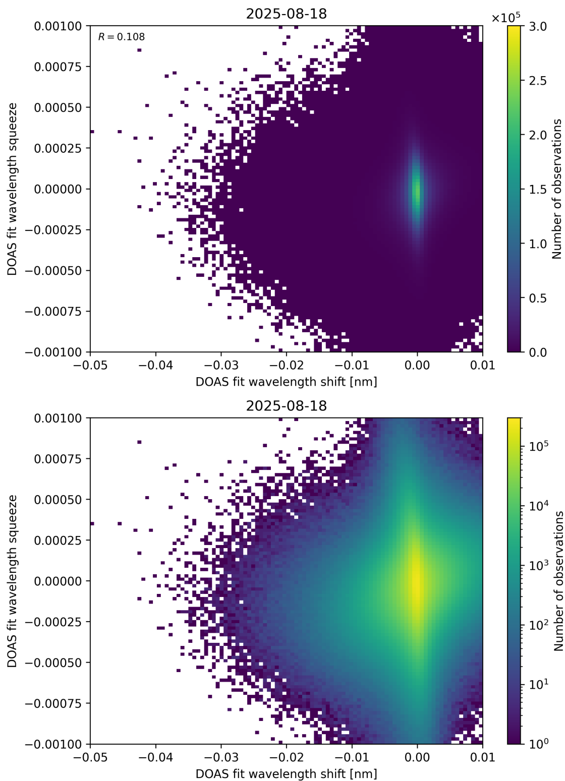
Figure 138: Scatter density plot of “DOAS fit wavelength shift” against “DOAS fit wavelength squeeze” for 2025-08-17 to 2025-08-19.
