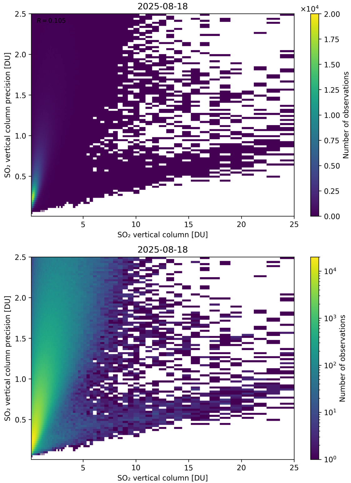
Figure 361: Scatter density plot of “SO 2 vertical column” against “SO 2 vertical column precision” for 2025-08-17 to 2025-08-19.
