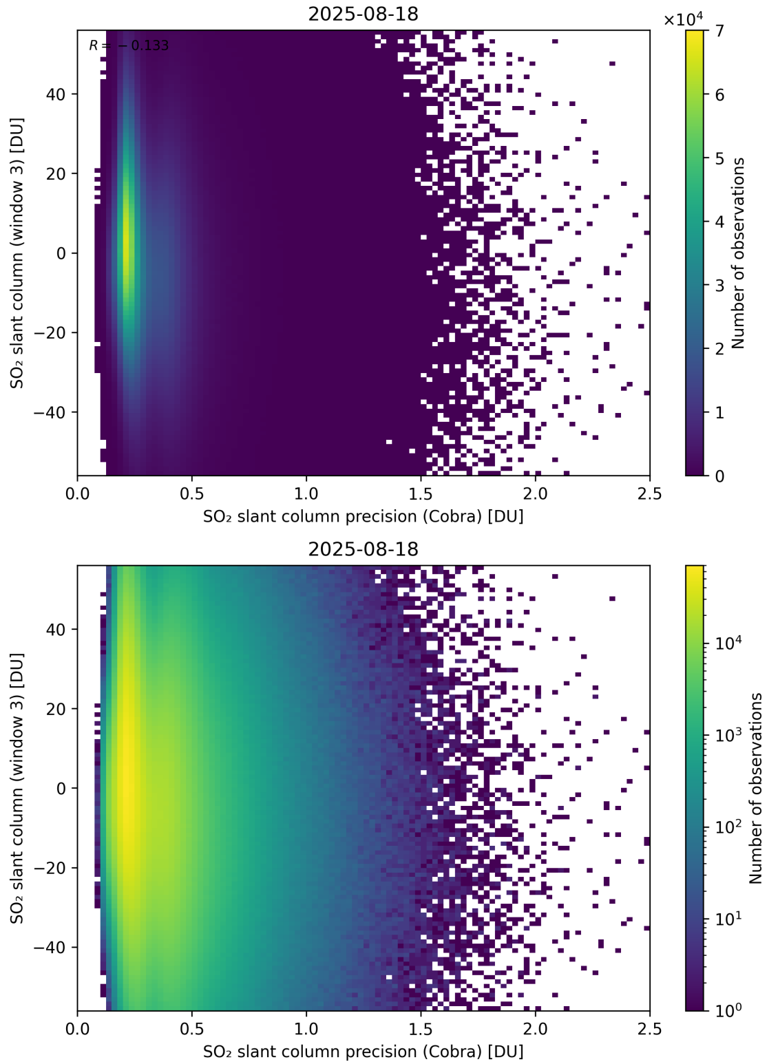
Figure 211: Scatter density plot of “SO 2 slant column precision (Cobra)” against “SO 2 slant column (window 3)” for 2025-08-17 to 2025-08-19.
