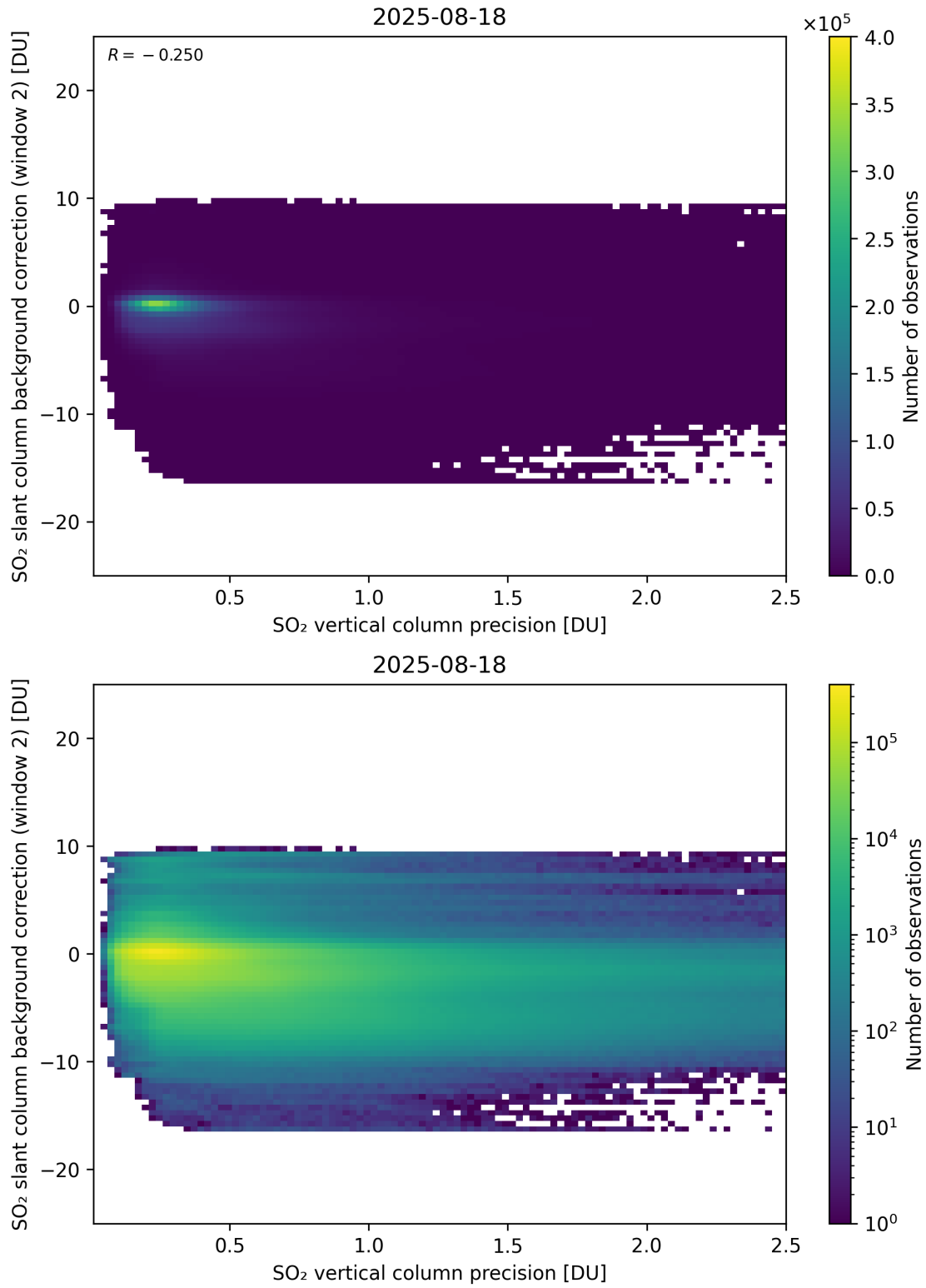
Figure 330: Scatter density plot of “SO 2 vertical column precision” against “SO 2 slant column background correction (window 2)” for 2025-08-17 to 2025-08-19.
