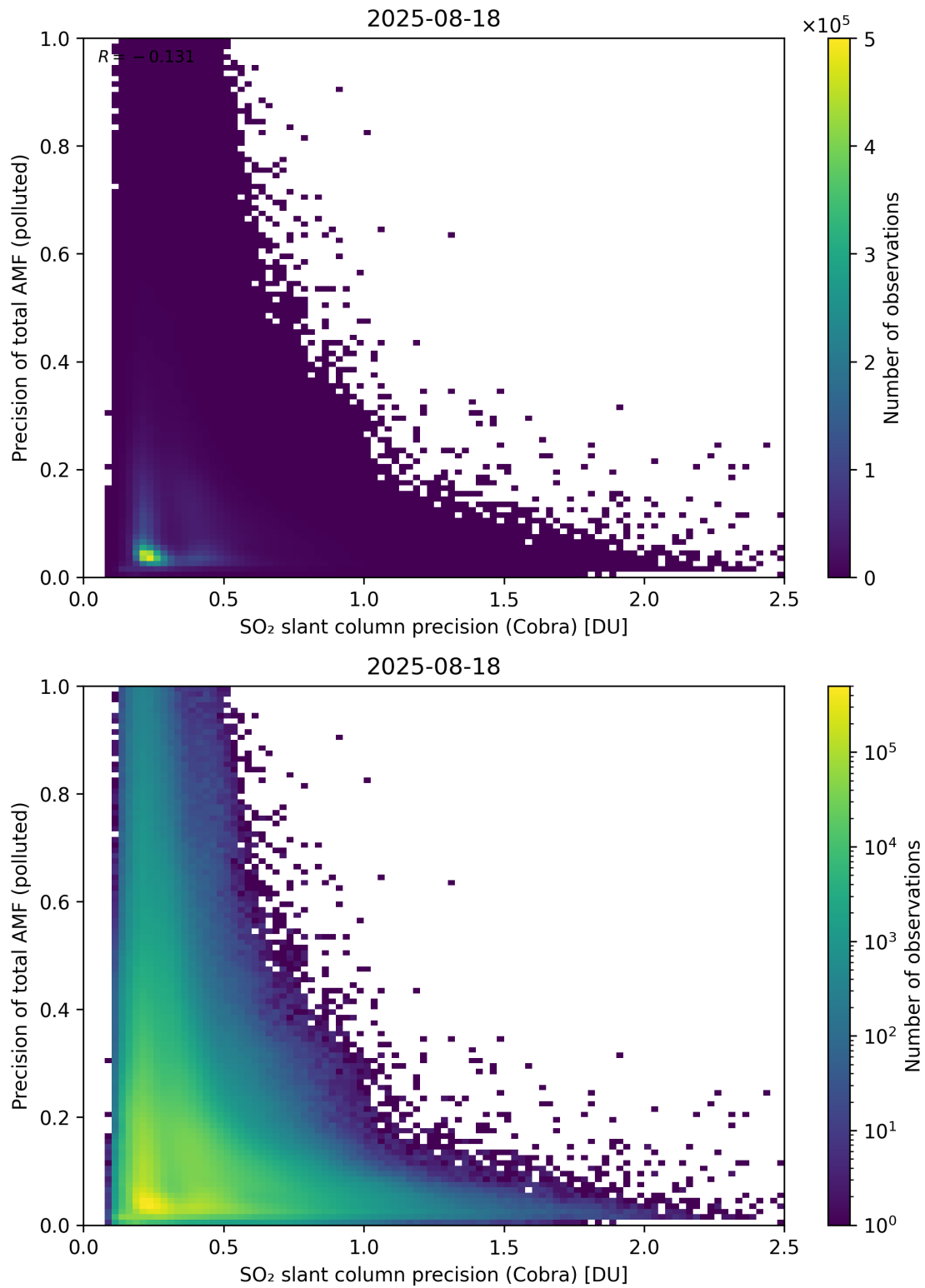
Figure 214: Scatter density plot of “SO 2 slant column precision (Cobra)” against “Precision of total AMF (polluted)” for 2025-08-17 to 2025-08-19.
