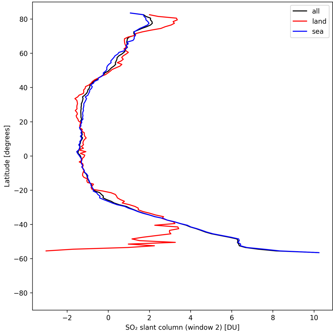
Figure 41: Zonal average of “SO 2 slant column (window 2)” for 2025-08-17 to 2025-08-19.
