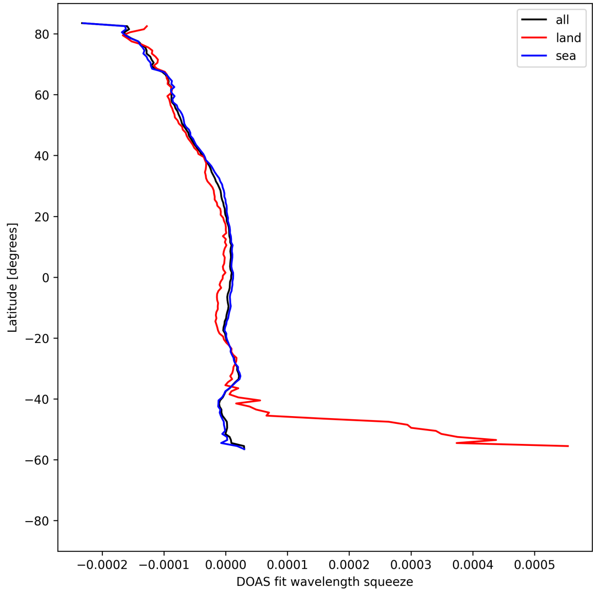
Figure 51: Zonal average of “DOAS fit wavelength squeeze” for 2025-08-17 to 2025-08-19.
