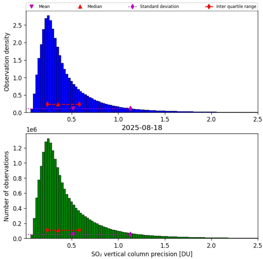
Figure 59: Histogram of “SO 2 vertical column precision” for 2025-08-17 to 2025-08-19
