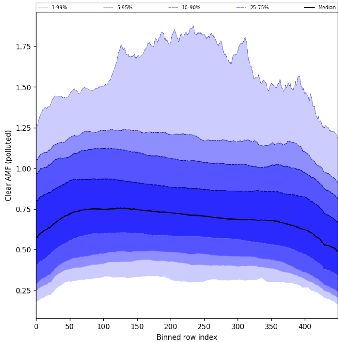
Figure 107: Along track statistics of “Clear AMF (polluted)” for 2025-08-17 to 2025-08-19
