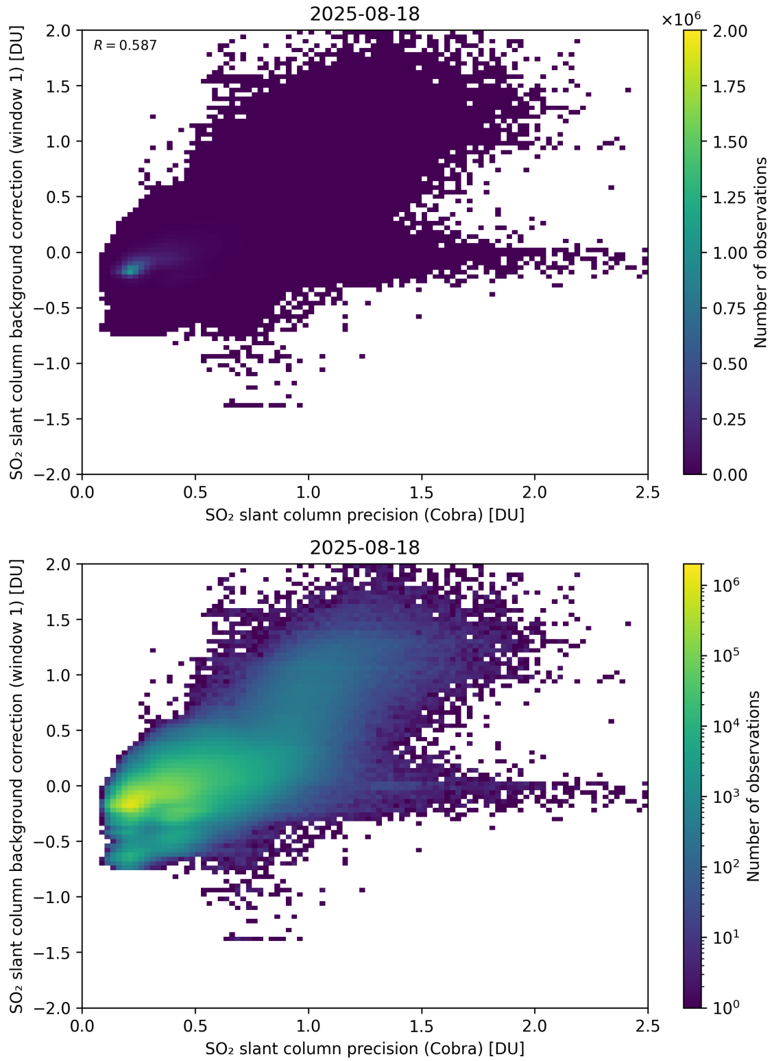
Figure 199: Scatter density plot of “SO 2 slant column precision (Cobra)” against “SO 2 slant column background correction (window 1)” for 2025-08-17 to 2025-08-19.
