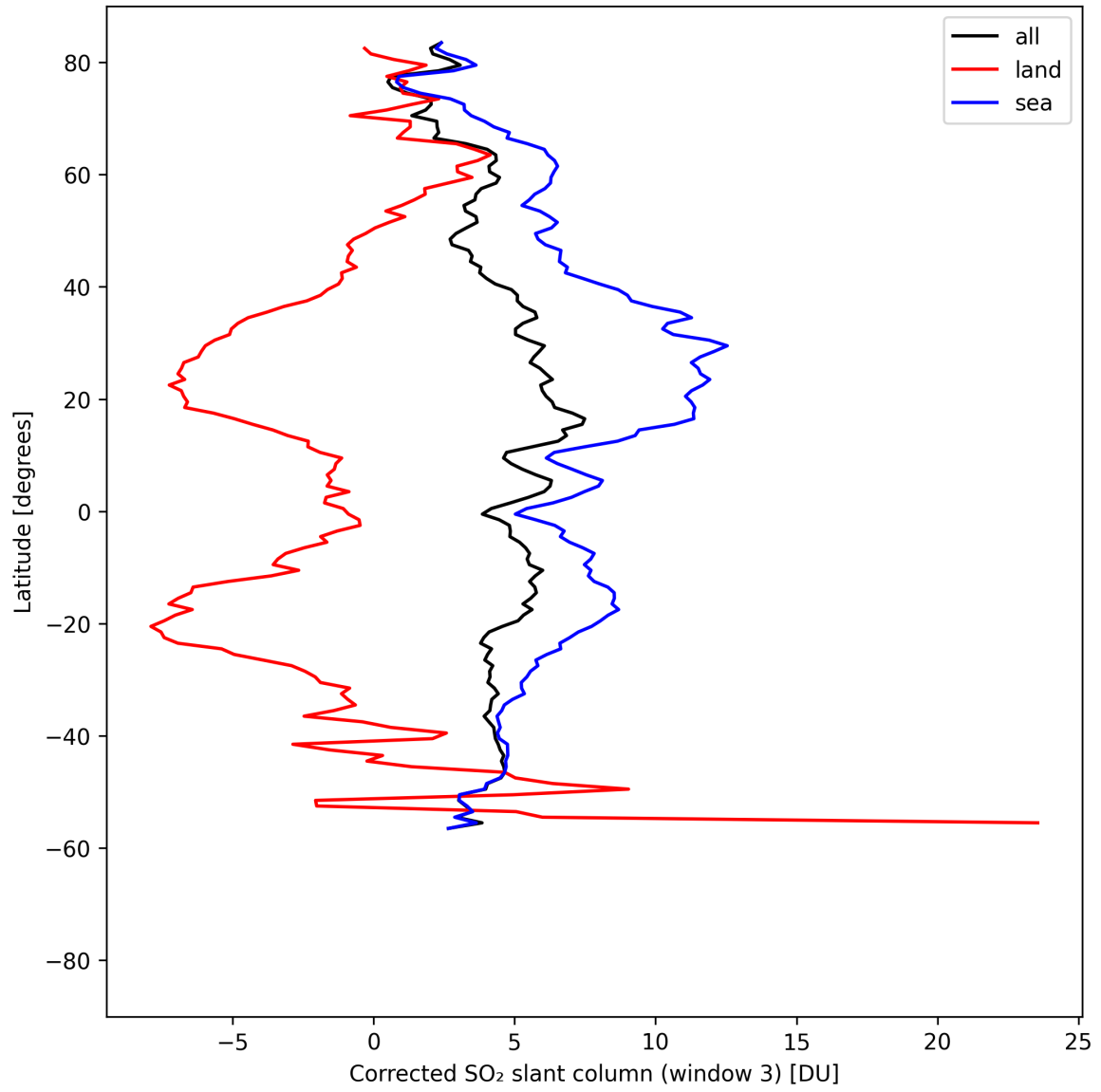
Figure 47: Zonal average of “Corrected SO 2 slant column (window 3)” for 2025-08-17 to 2025-08-19.
