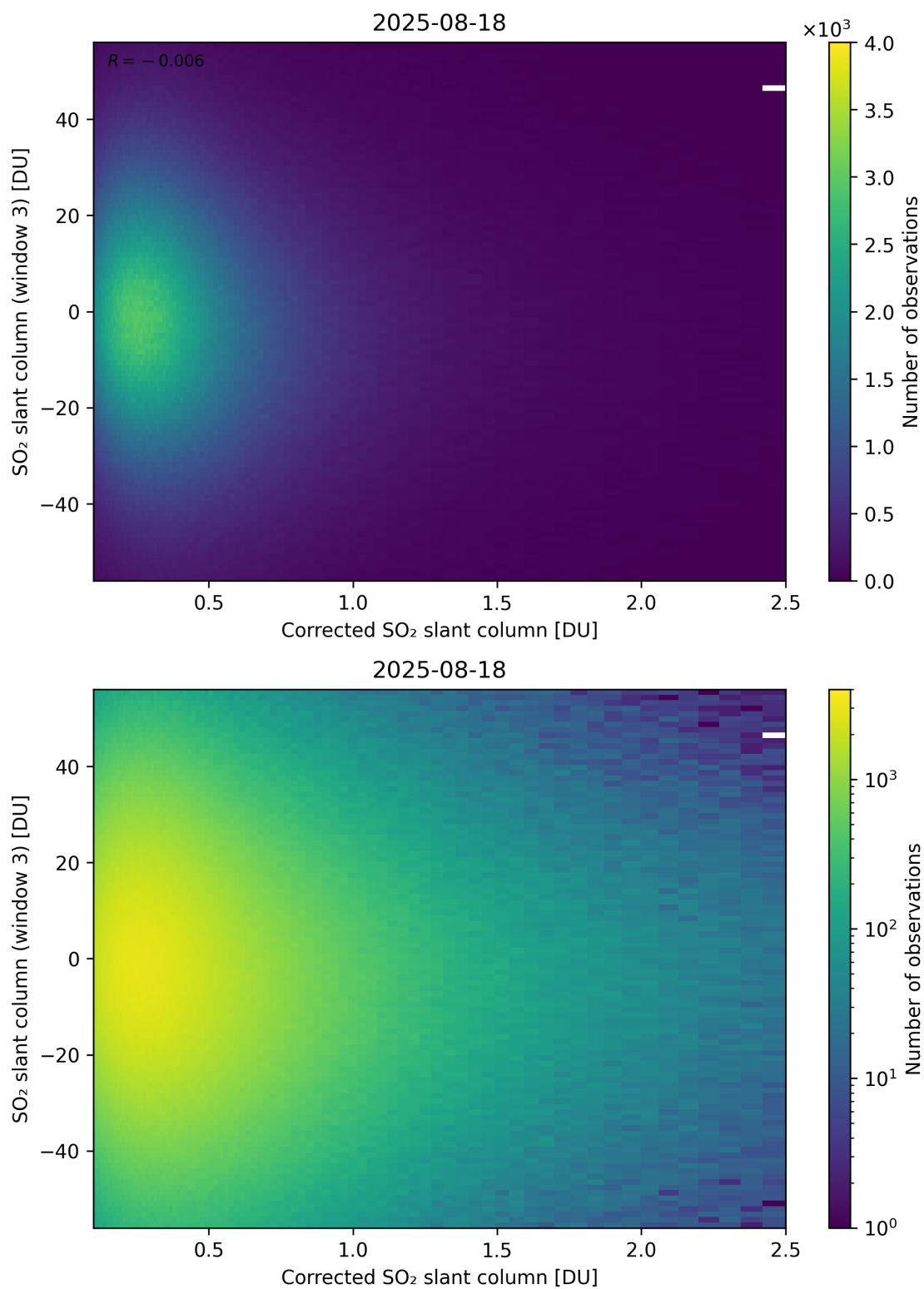
Figure 240: Scatter density plot of “Corrected SO 2 slant column” against “SO 2 slant column (window 3)” for 2025-08-17 to 2025-08-19.
