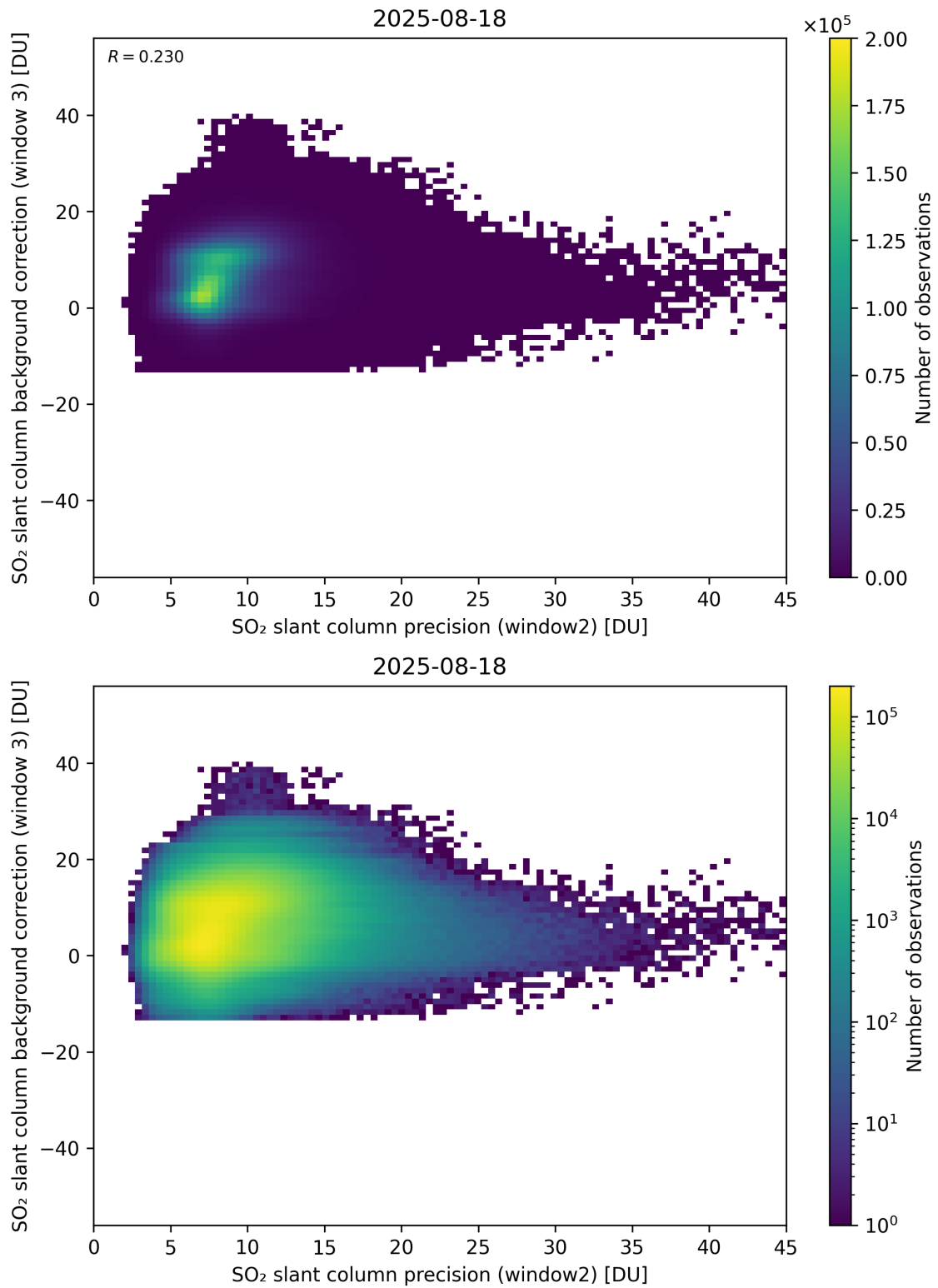
Figure 292: Scatter density plot of “SO 2 slant column precision (window2)” against “SO 2 slant column background correction (window 3)” for 2025-08-17 to 2025-08-19.
