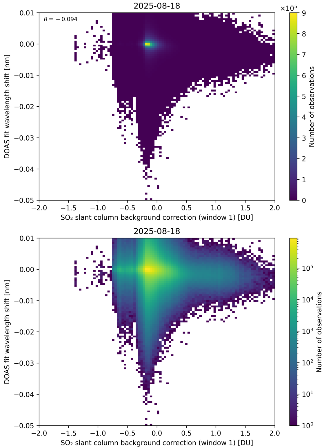
Figure 111: Scatter density plot of “SO 2 slant column background correction (window 1)” against “DOAS fit wavelength shift” for 2025-08-17 to 2025-08-19.
