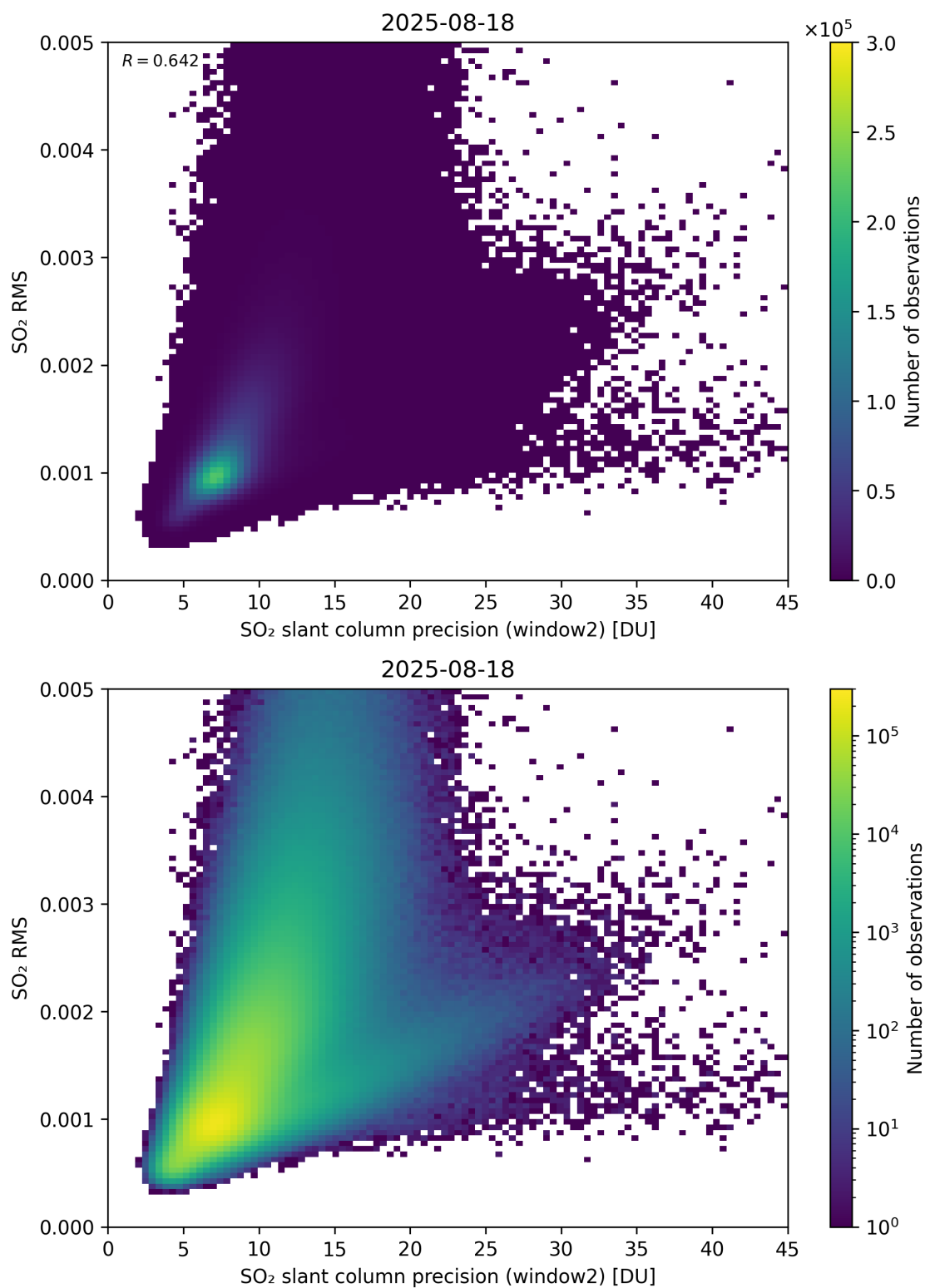
Figure 295: Scatter density plot of “SO 2 slant column precision (window2)” against “SO 2 RMS” for 2025-08-17 to 2025-08-19.
