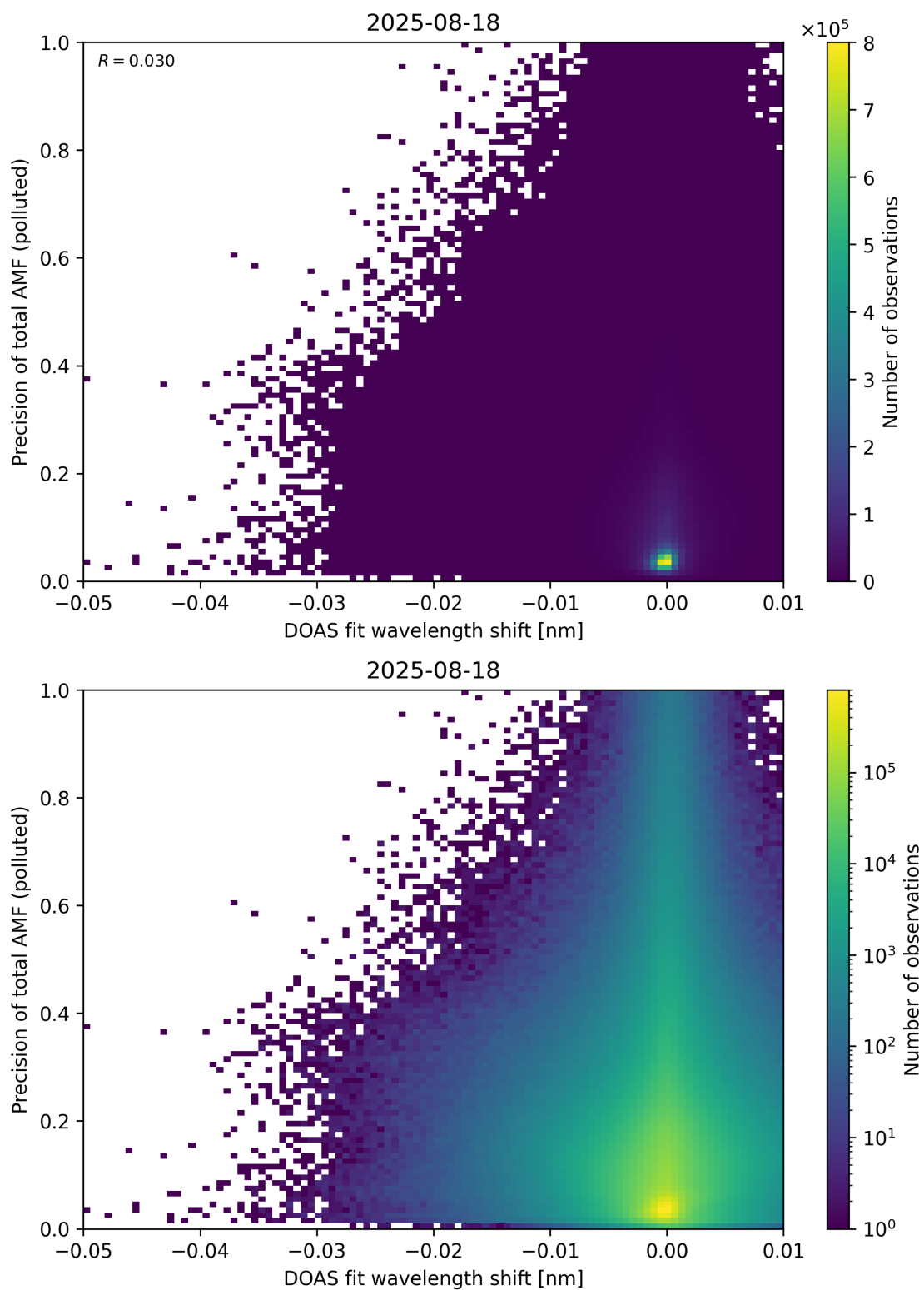
Figure 142: Scatter density plot of “DOAS fit wavelength shift” against “Precision of total AMF (polluted)” for 2025-08-17 to 2025-08-19.
