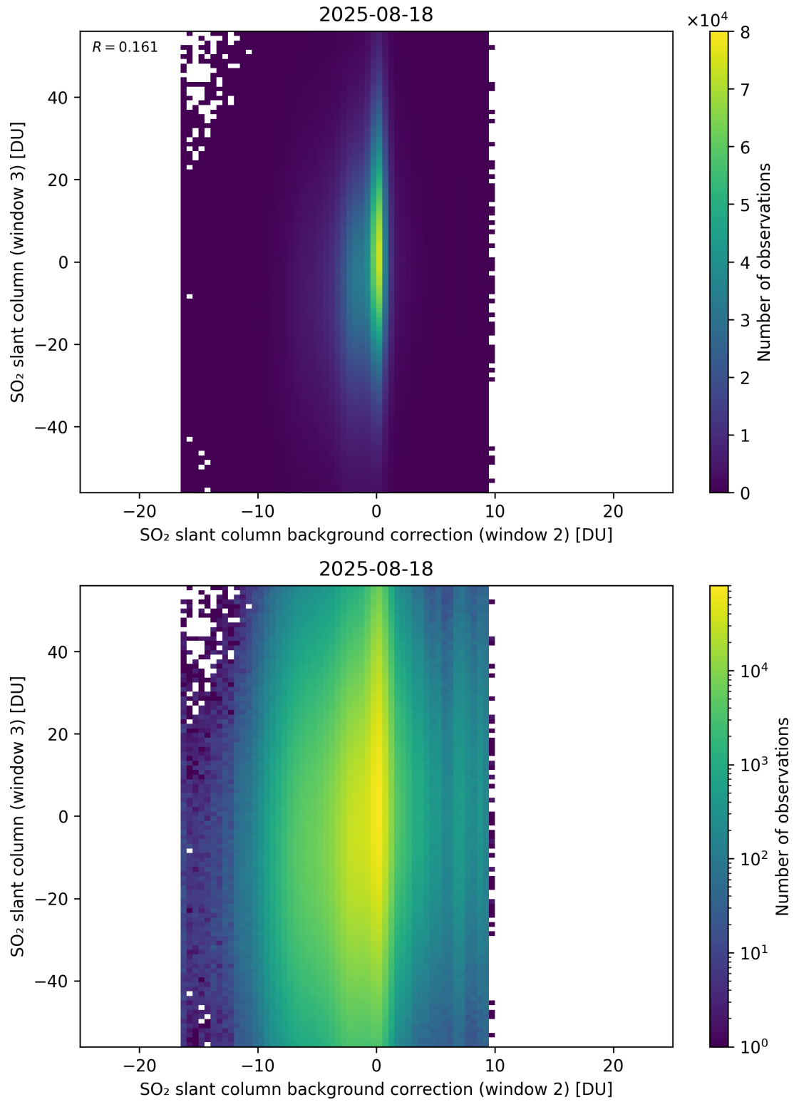
Figure 128: Scatter density plot of “SO 2 slant column background correction (window 2)” against “SO 2 slant column (window 3)” for 2025-08-17 to 2025-08-19.
