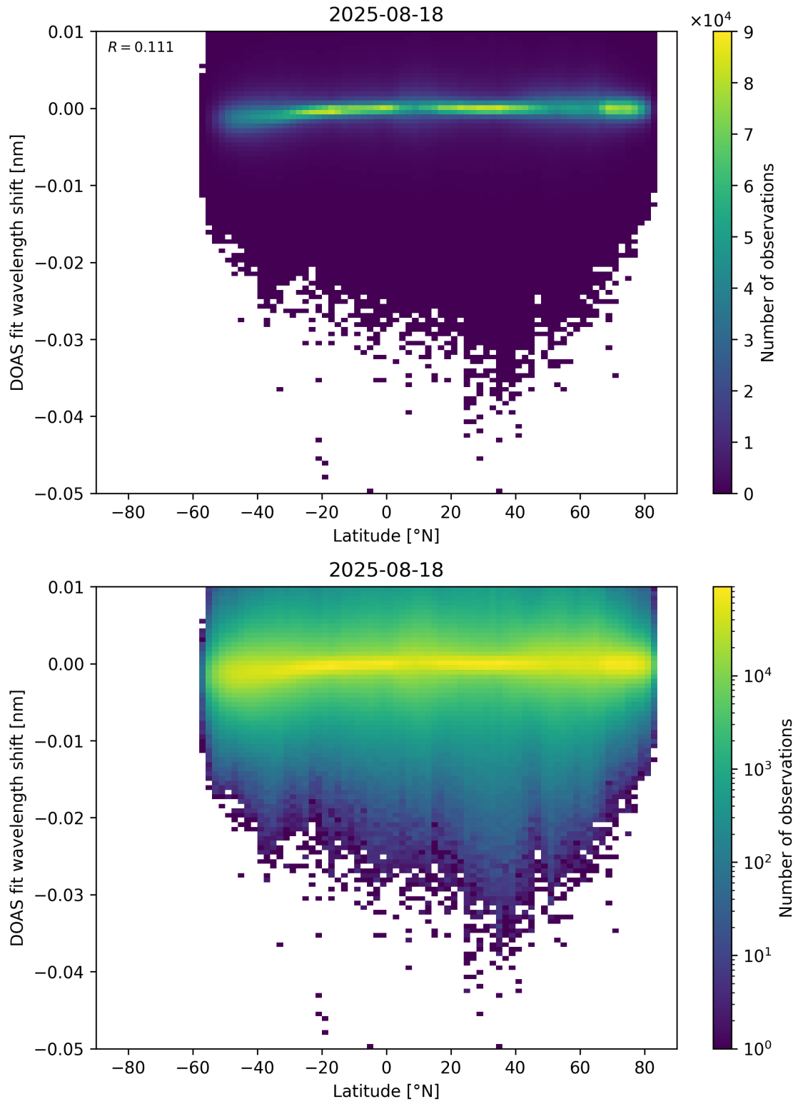
Figure 153: Scatter density plot of “Latitude” against “DOAS fit wavelength shift” for 2025-08-17 to 2025-08-19.
