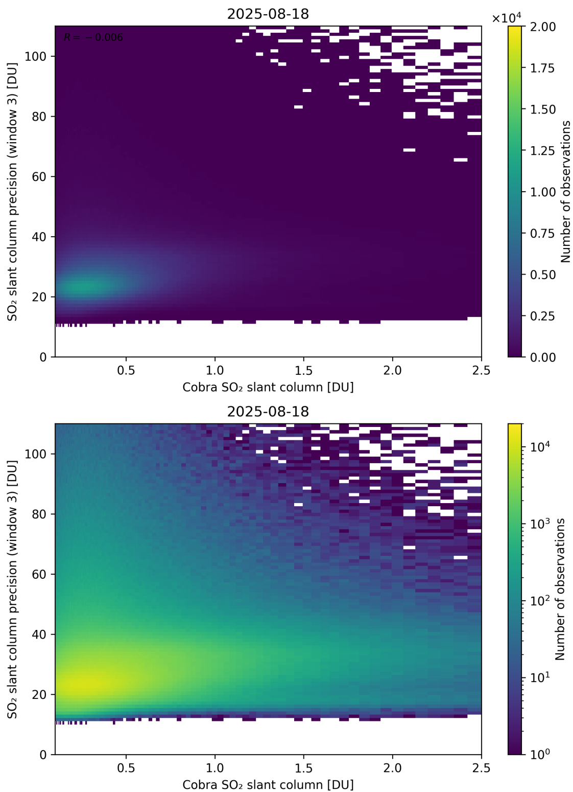
Figure 223: Scatter density plot of “Cobra SO 2 slant column” against “SO 2 slant column precision (window 3)” for 2025-08-17 to 2025-08-19.
