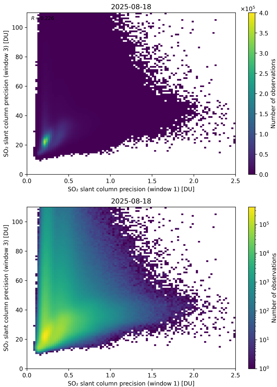
Figure 279: Scatter density plot of “SO 2 slant column precision (window 1)” against “SO 2 slant column precision (window 3)” for 2025-08-17 to 2025-08-19.
