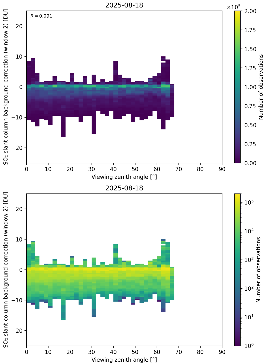
Figure 363: Scatter density plot of “Viewing zenith angle” against “SO 2 slant column background correction (window 2)” for 2025-08-17 to 2025-08-19.
