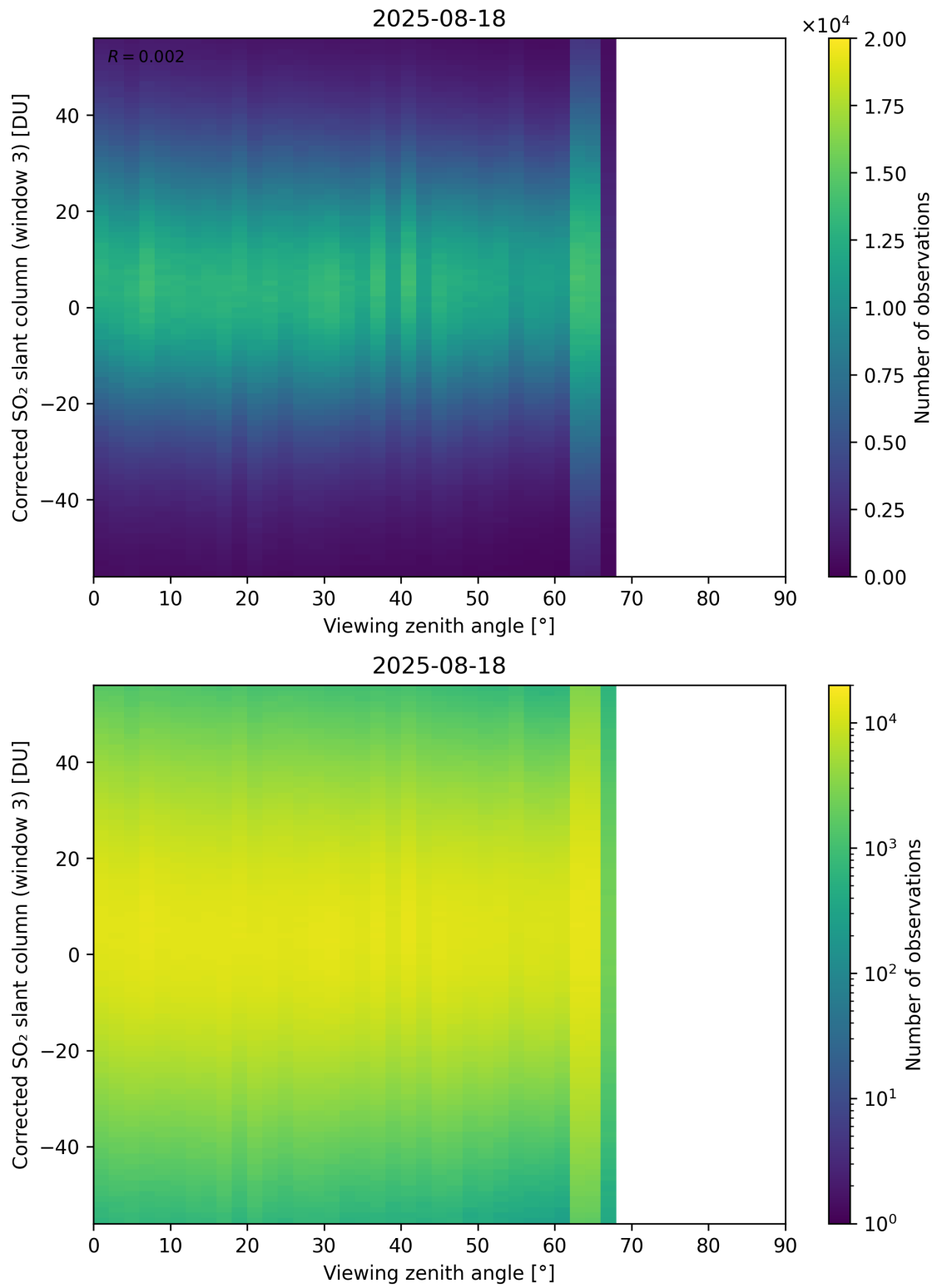
Figure 375: Scatter density plot of “Viewing zenith angle” against “Corrected SO 2 slant column (window 3)” for 2025-08-17 to 2025-08-19.
