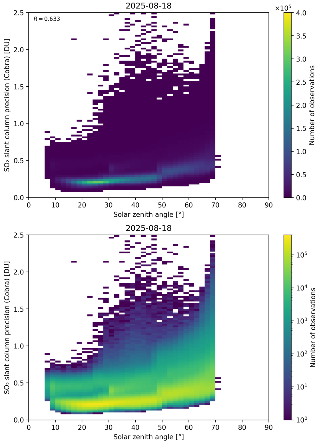
Figure 180: Scatter density plot of “Solar zenith angle” against “SO 2 slant column precision (Cobra)” for 2025-08-17 to 2025-08-19.
