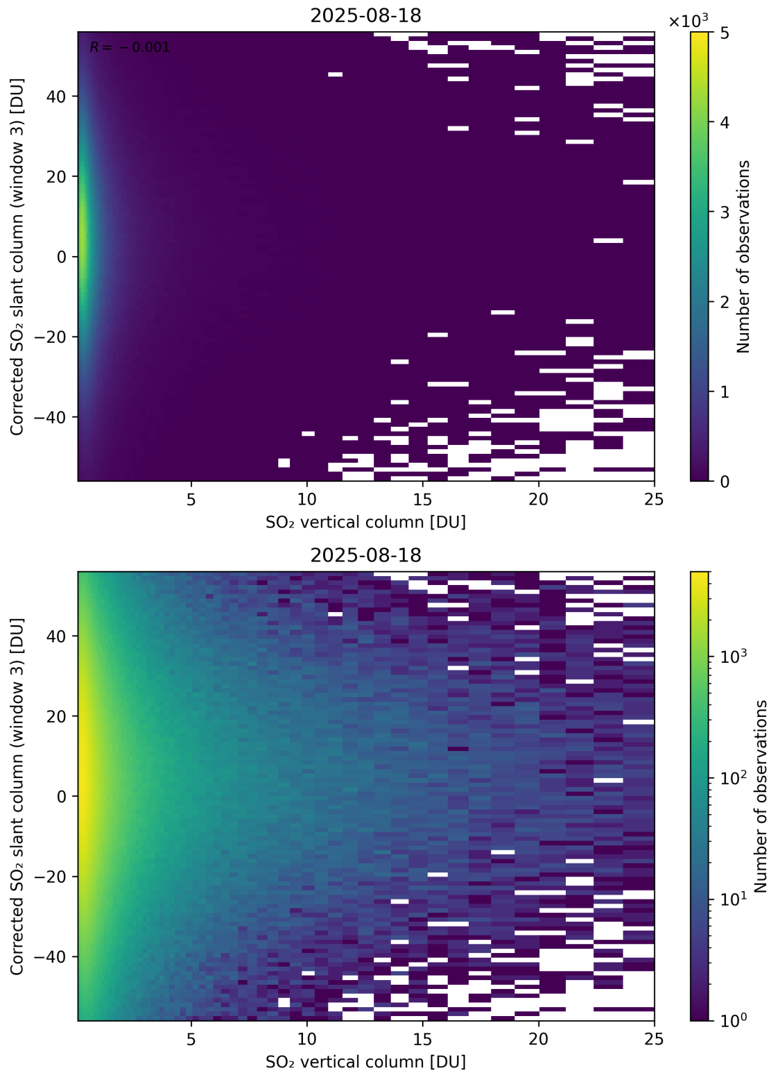
Figure 353: Scatter density plot of “SO 2 vertical column” against “Corrected SO 2 slant column (window 3)” for 2025-08-17 to 2025-08-19.
