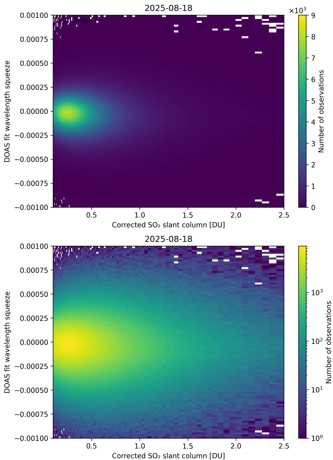
Figure 230: Scatter density plot of “Corrected SO 2 slant column” against “DOAS fit wavelength squeeze” for 2025-08-17 to 2025-08-19.
