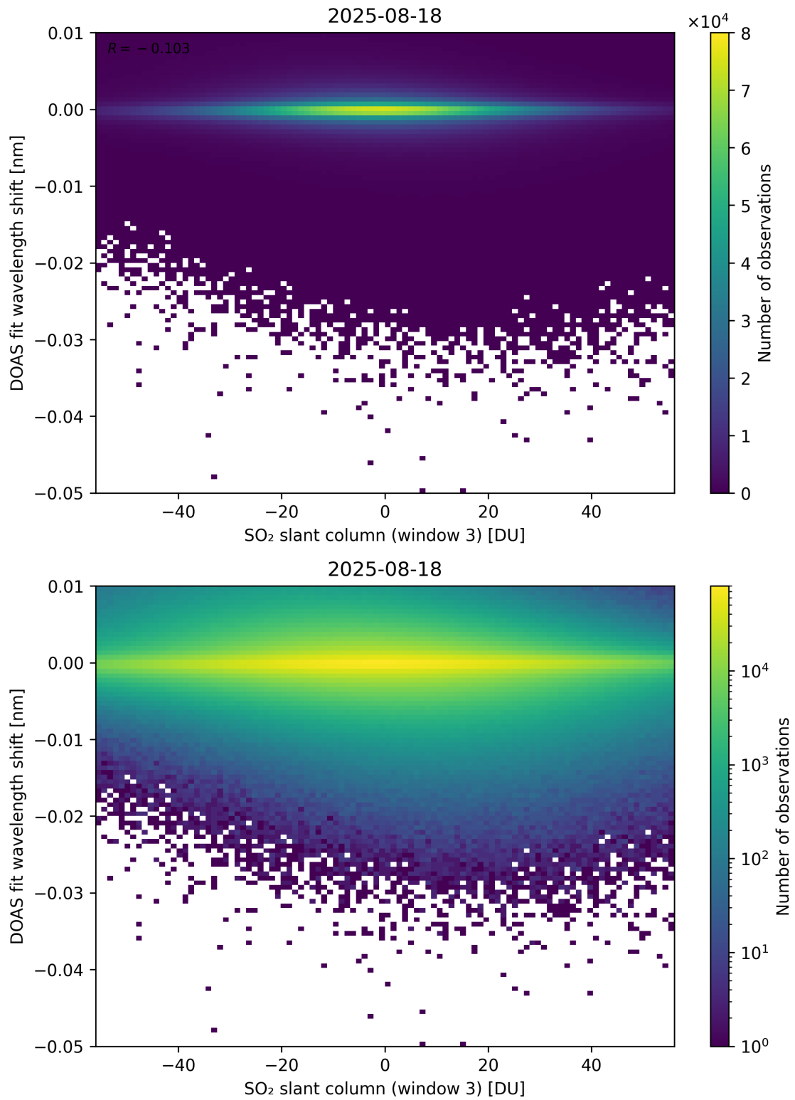
Figure 304: Scatter density plot of “SO 2 slant column (window 3)” against “DOAS fit wavelength shift” for 2025-08-17 to 2025-08-19.
