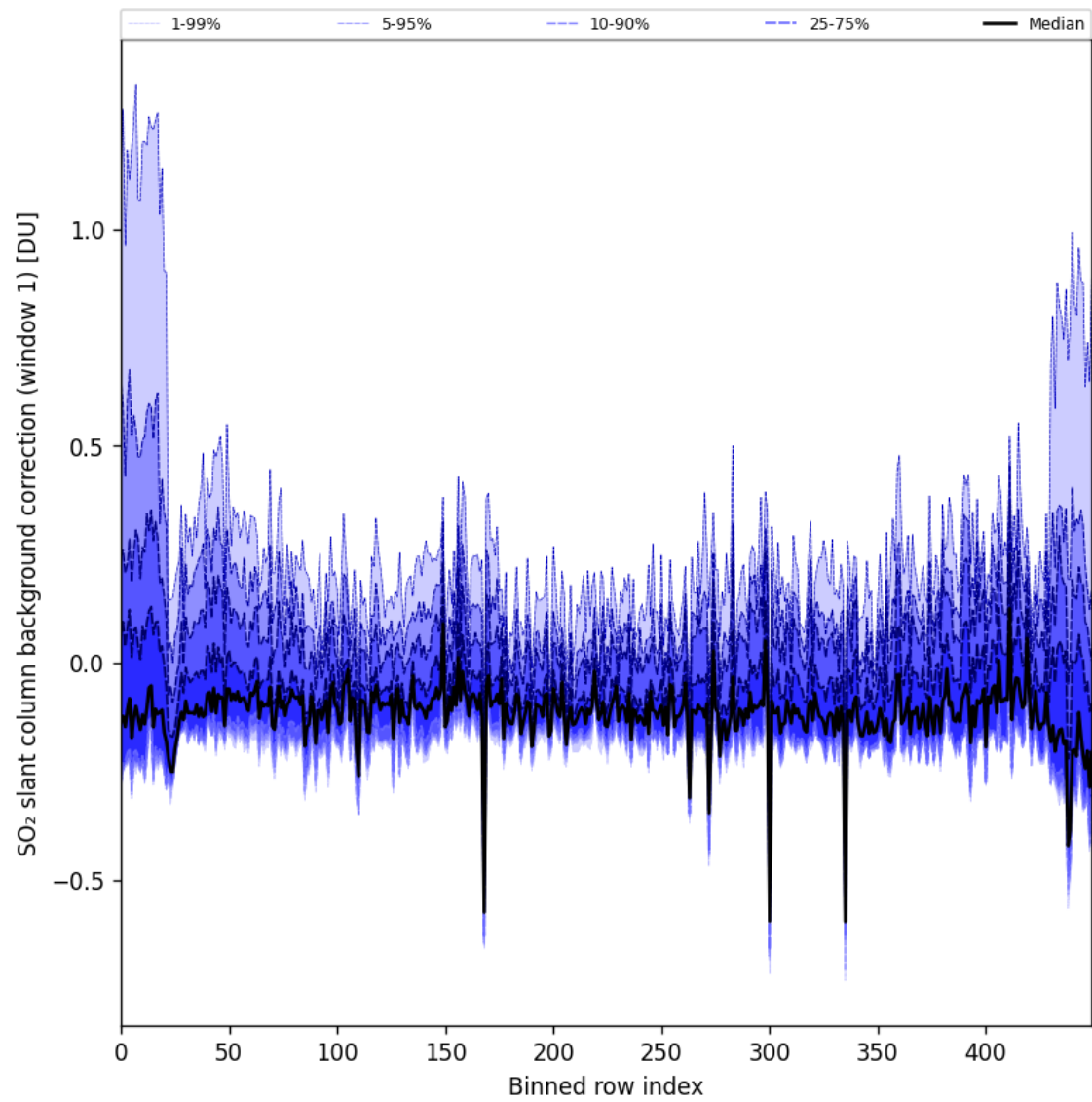
Figure 92: Along track statistics of “SO 2 slant column background correction (window 1)” for 2025-08-17 to 2025-08-19
