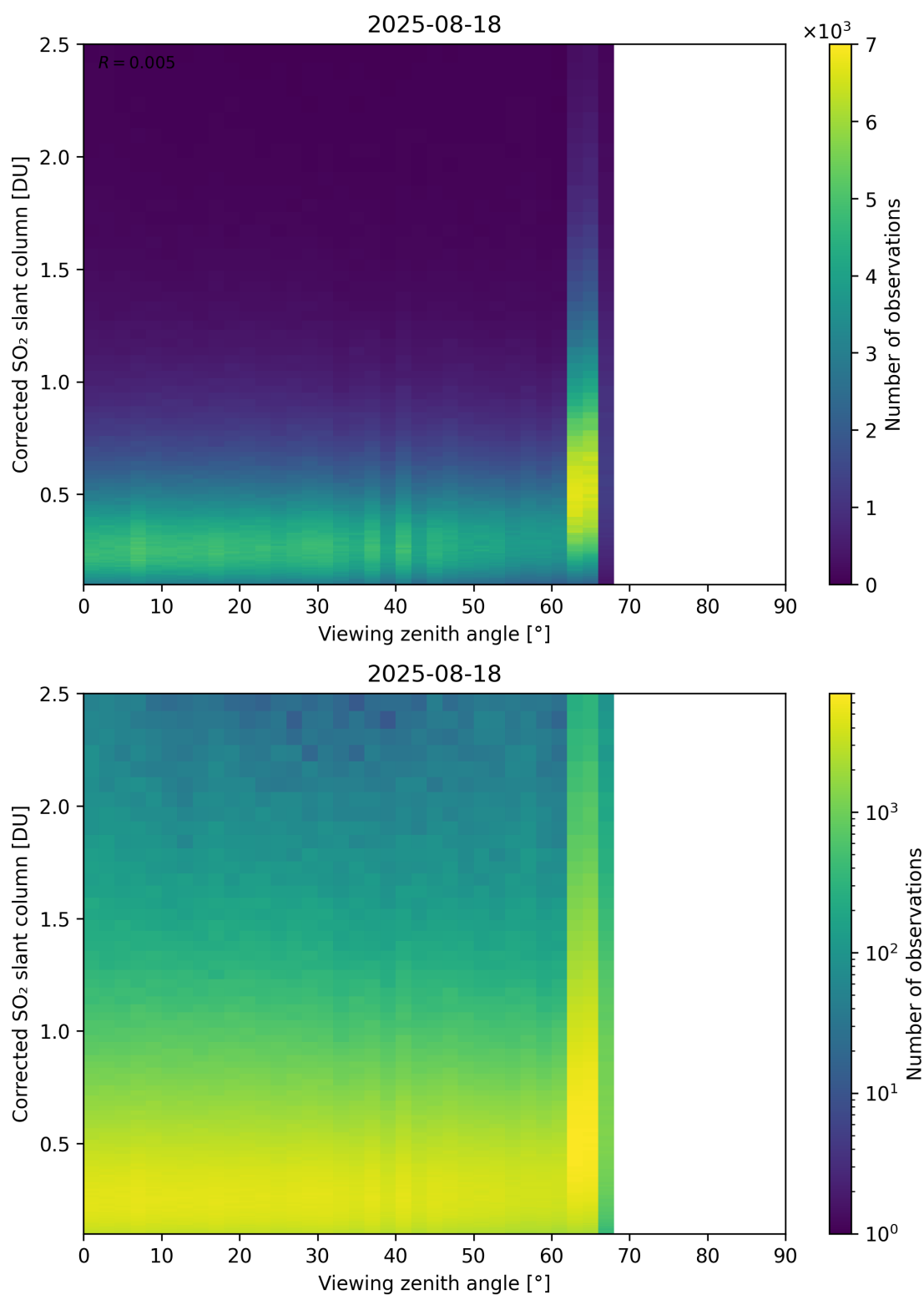
Figure 373: Scatter density plot of “Viewing zenith angle” against “Corrected SO 2 slant column” for 2025-08-17 to 2025-08-19.
