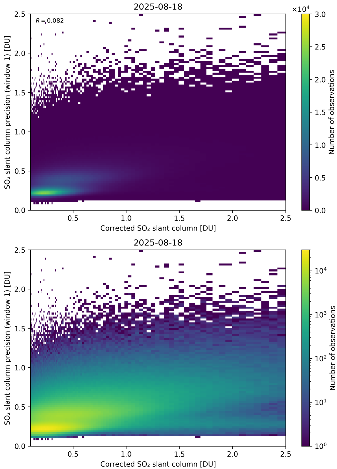
Figure 238: Scatter density plot of “Corrected SO 2 slant column” against “SO 2 slant column precision (window 1)” for 2025-08-17 to 2025-08-19.
