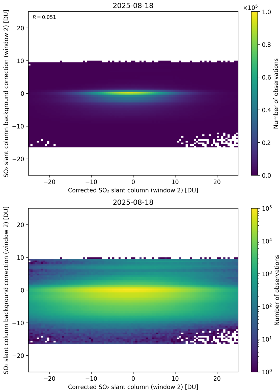
Figure 244: Scatter density plot of “Corrected SO 2 slant column (window 2)” against “SO 2 slant column background correction (window 2)” for 2025-08-17 to 2025-08-19.
