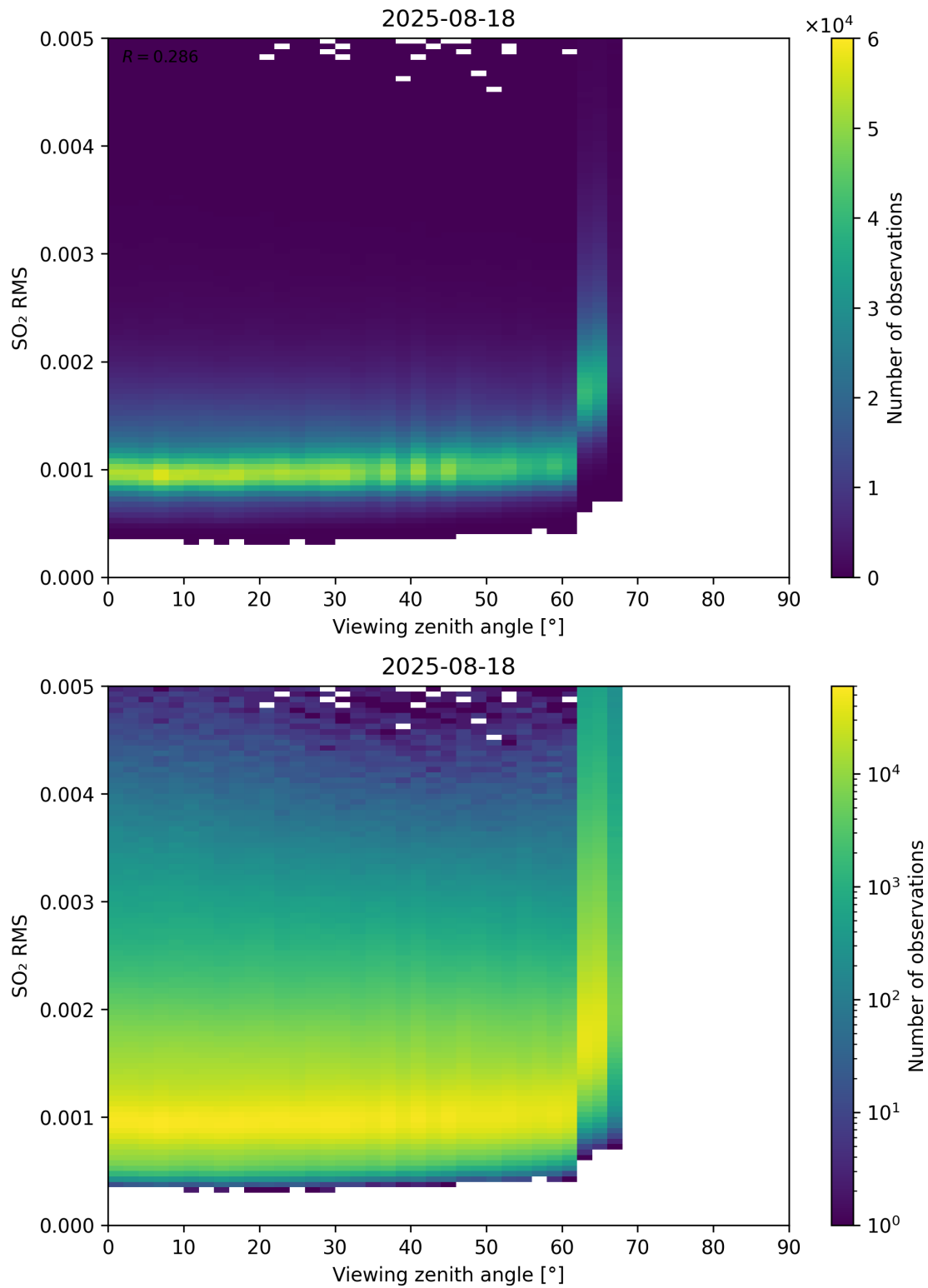
Figure 367: Scatter density plot of “Viewing zenith angle” against “SO 2 RMS” for 2025-08-17 to 2025-08-19.
