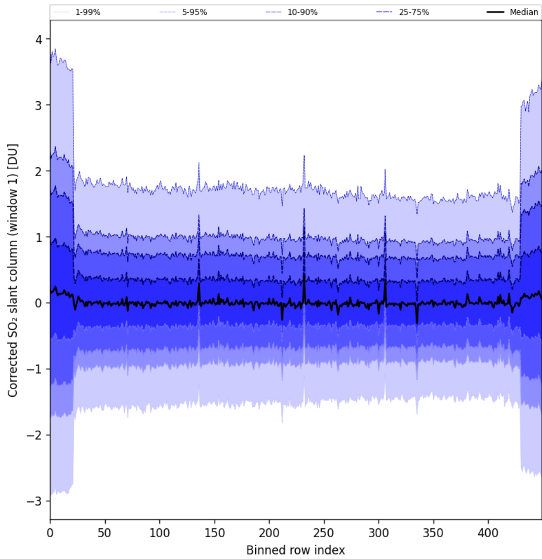
Figure 91: Along track statistics of “Corrected SO 2 slant column (window 1)” for 2025-08-17 to 2025-08-19
