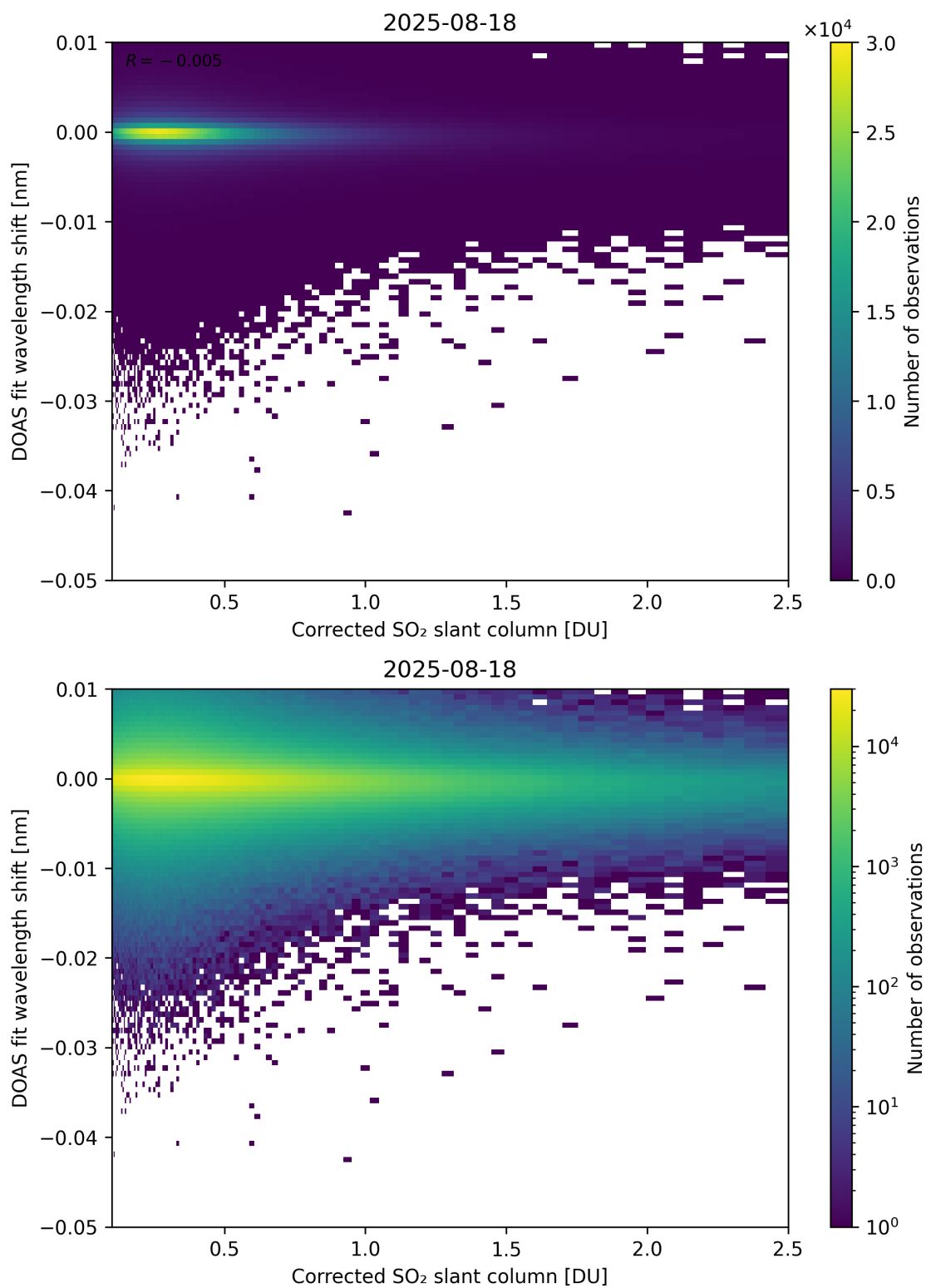
Figure 229: Scatter density plot of “Corrected SO 2 slant column” against “DOAS fit wavelength shift” for 2025-08-17 to 2025-08-19.
