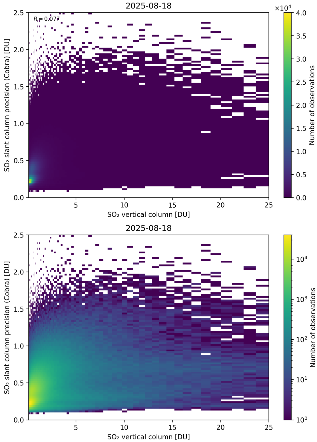
Figure 350: Scatter density plot of “SO 2 vertical column” against “SO 2 slant column precision (Cobra)” for 2025-08-17 to 2025-08-19.
