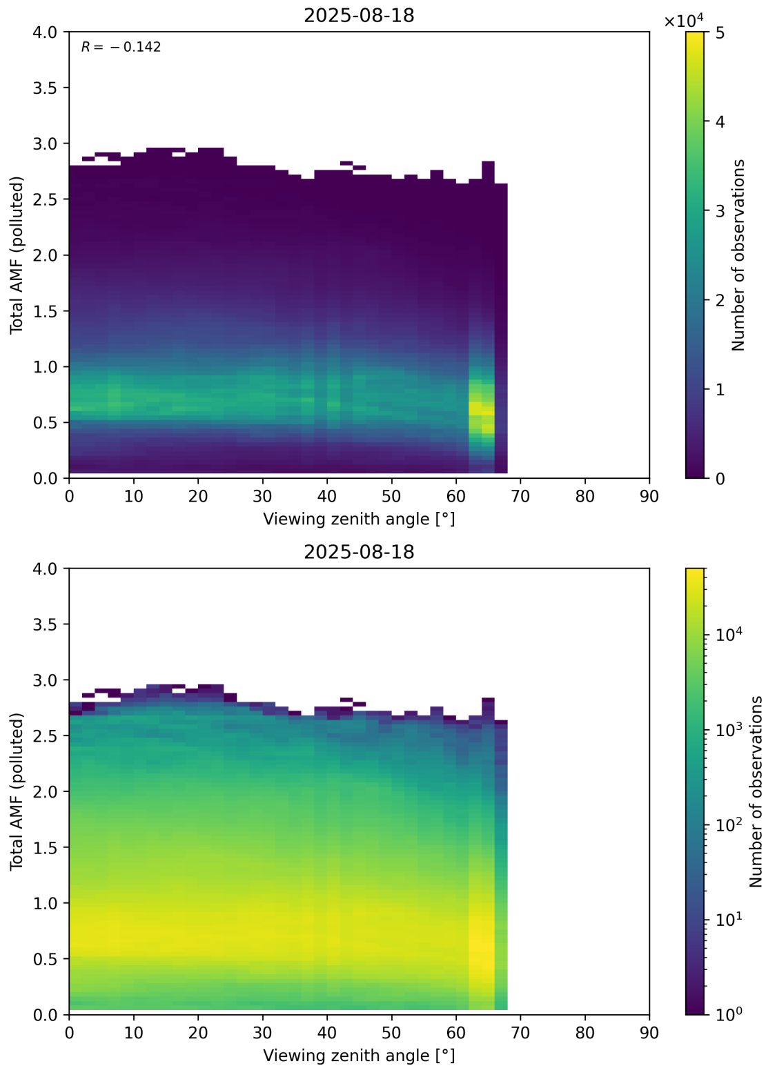
Figure 381: Scatter density plot of “Viewing zenith angle” against “Total AMF (polluted)” for 2025-08-17 to 2025-08-19.
