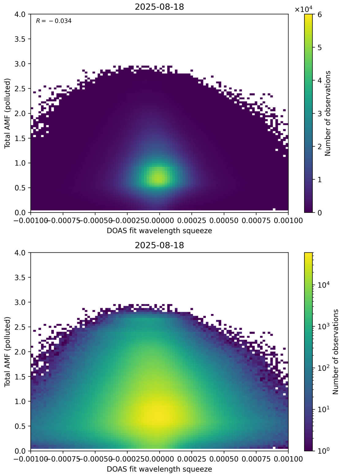
Figure 145: Scatter density plot of “DOAS fit wavelength squeeze” against “Total AMF (polluted)” for 2025-08-17 to 2025-08-19.
