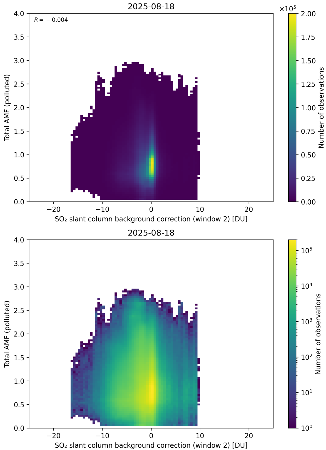
Figure 130: Scatter density plot of “SO 2 slant column background correction (window 2)” against “Total AMF (polluted)” for 2025-08-17 to 2025-08-19.
