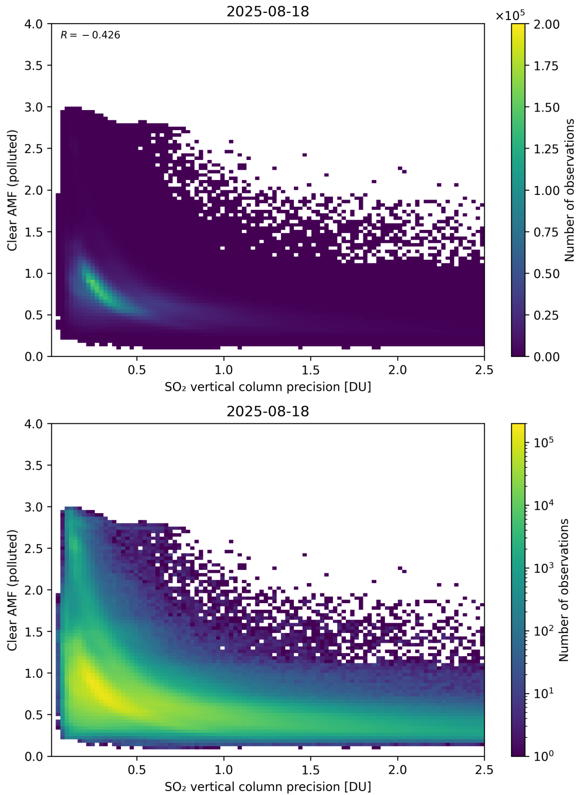
Figure 335: Scatter density plot of “SO 2 vertical column precision” against “Clear AMF (polluted)” for 2025-08-17 to 2025-08-19.
