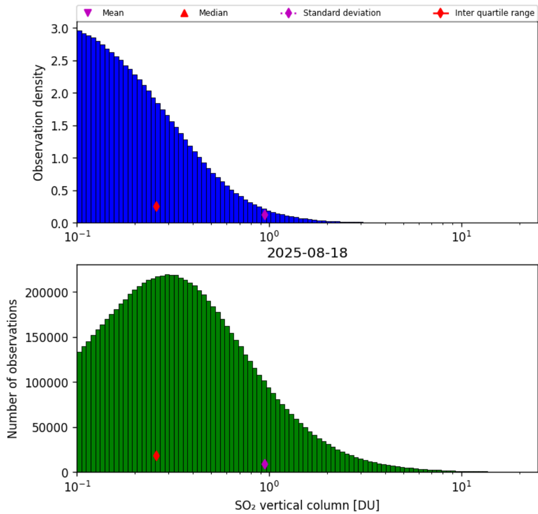
Figure 58: Histogram of “SO 2 vertical column” for 2025-08-17 to 2025-08-19
