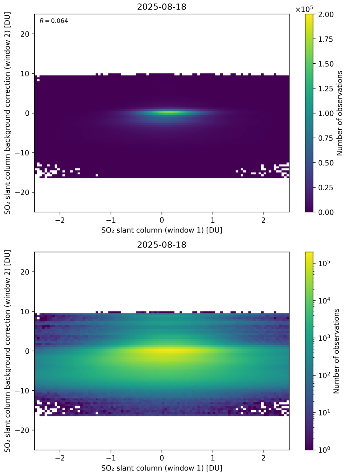
Figure 263: Scatter density plot of “SO 2 slant column (window 1)” against “SO 2 slant column background correction (window 2)” for 2025-08-17 to 2025-08-19.
