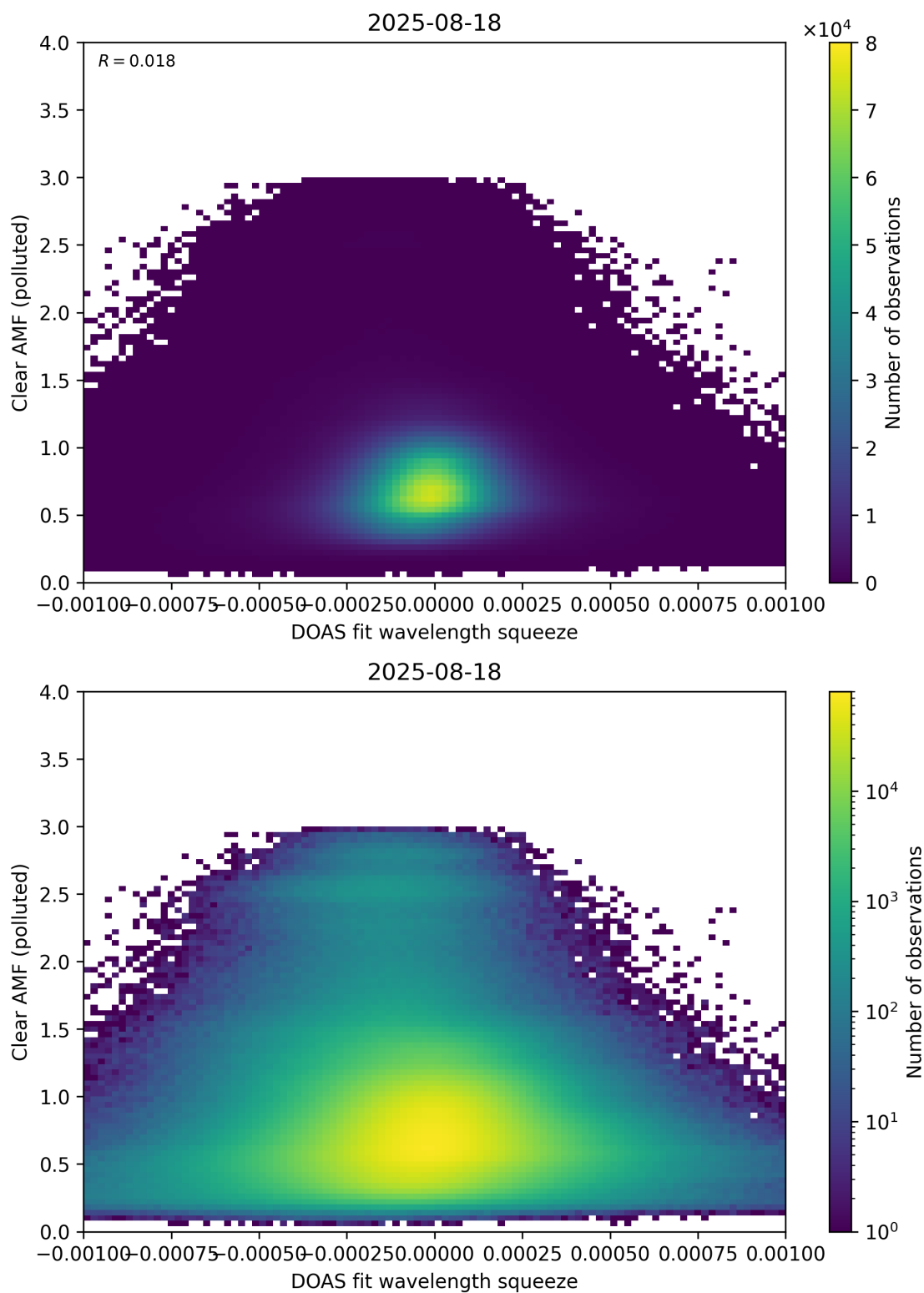
Figure 144: Scatter density plot of “DOAS fit wavelength squeeze” against “Clear AMF (polluted)” for 2025-08-17 to 2025-08-19.
