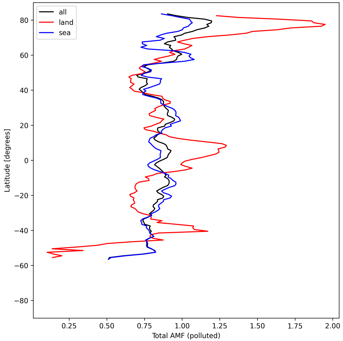
Figure 53: Zonal average of “Total AMF (polluted)” for 2025-08-17 to 2025-08-19.
