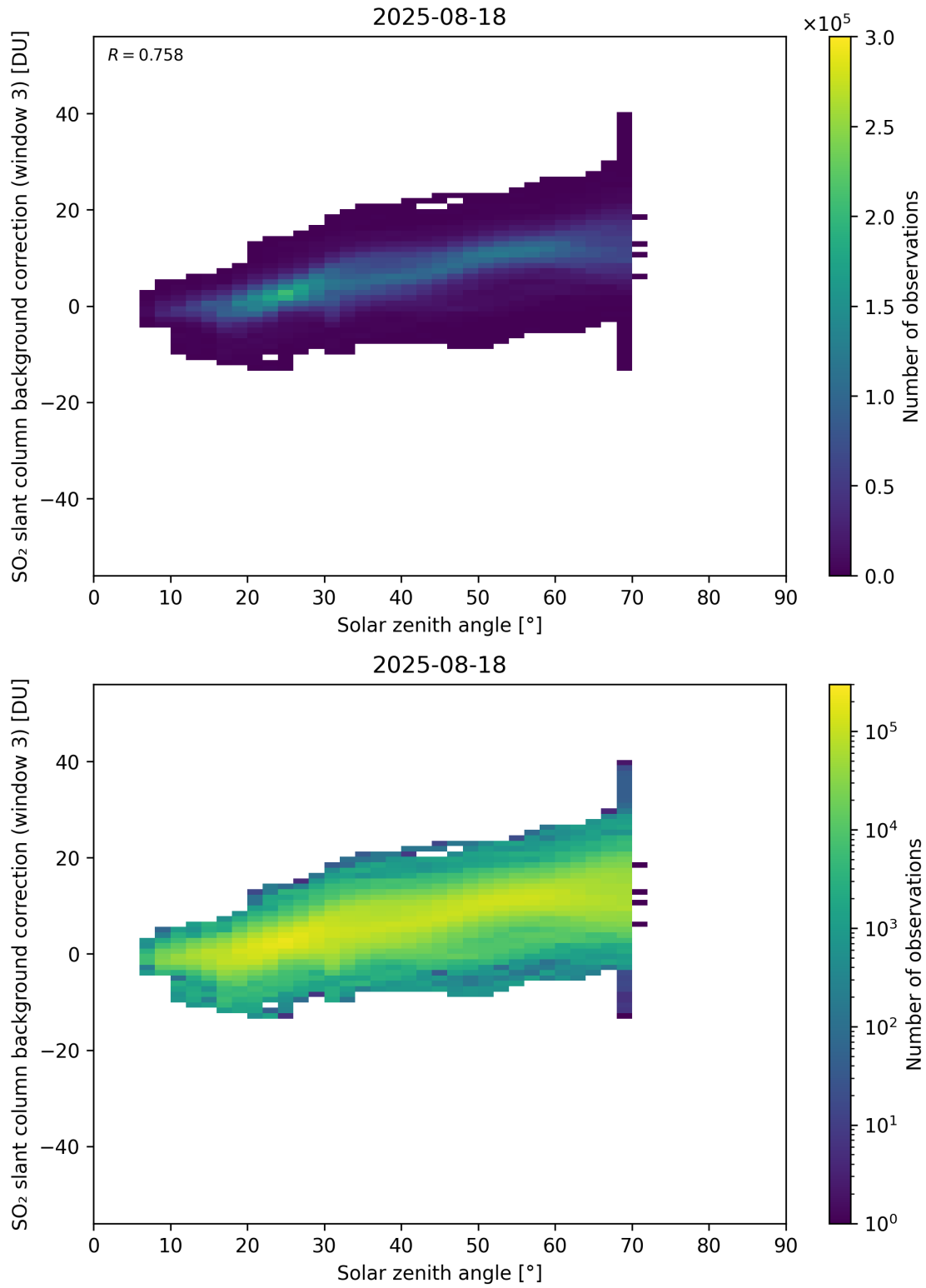
Figure 173: Scatter density plot of “Solar zenith angle” against “SO 2 slant column background correction (window 3)” for 2025-08-17 to 2025-08-19.
