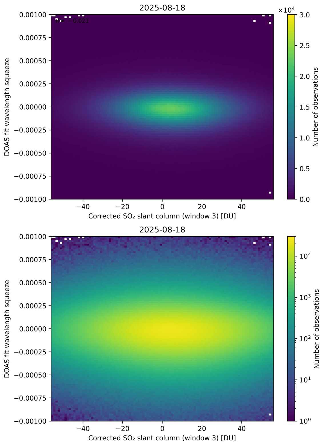
Figure 257: Scatter density plot of “Corrected SO 2 slant column (window 3)” against “DOAS fit wavelength squeeze” for 2025-08-17 to 2025-08-19.
