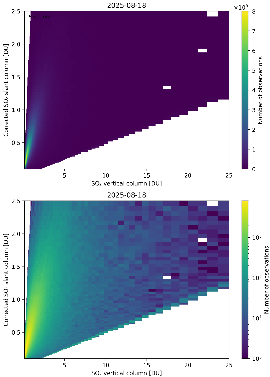
Figure 351: Scatter density plot of “SO 2 vertical column” against “Corrected SO 2 slant column” for 2025-08-17 to 2025-08-19.
