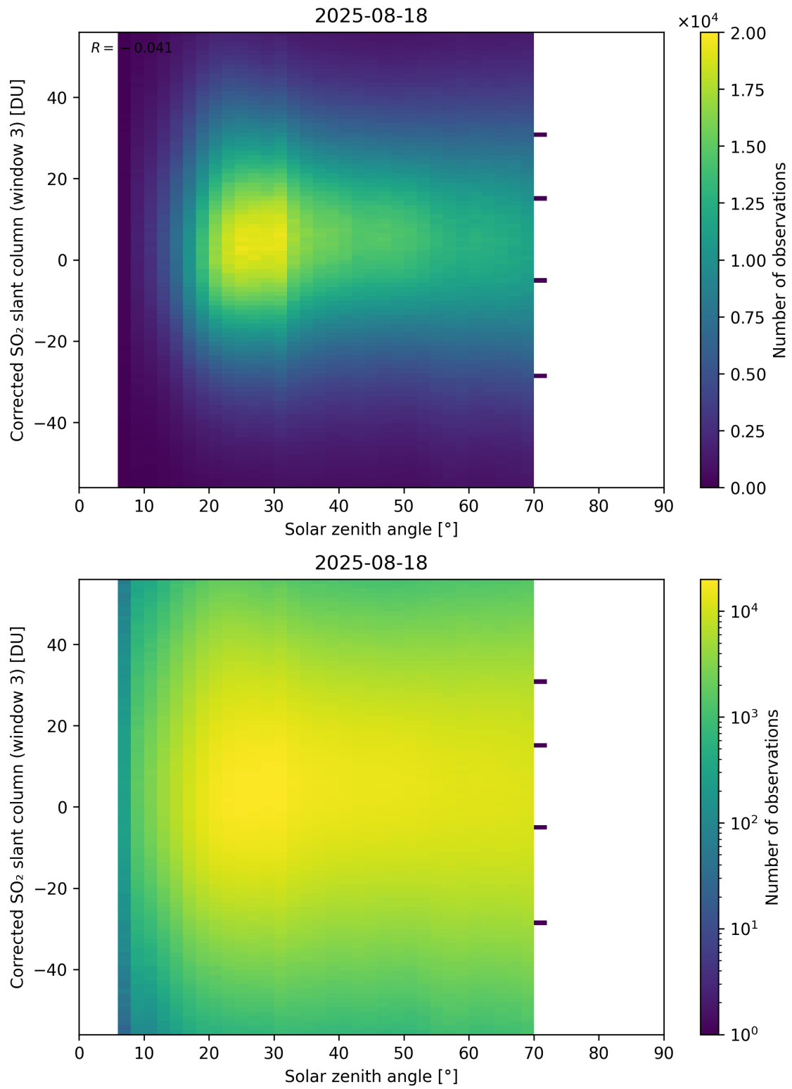
Figure 183: Scatter density plot of “Solar zenith angle” against “Corrected SO 2 slant column (window 3)” for 2025-08-17 to 2025-08-19.
