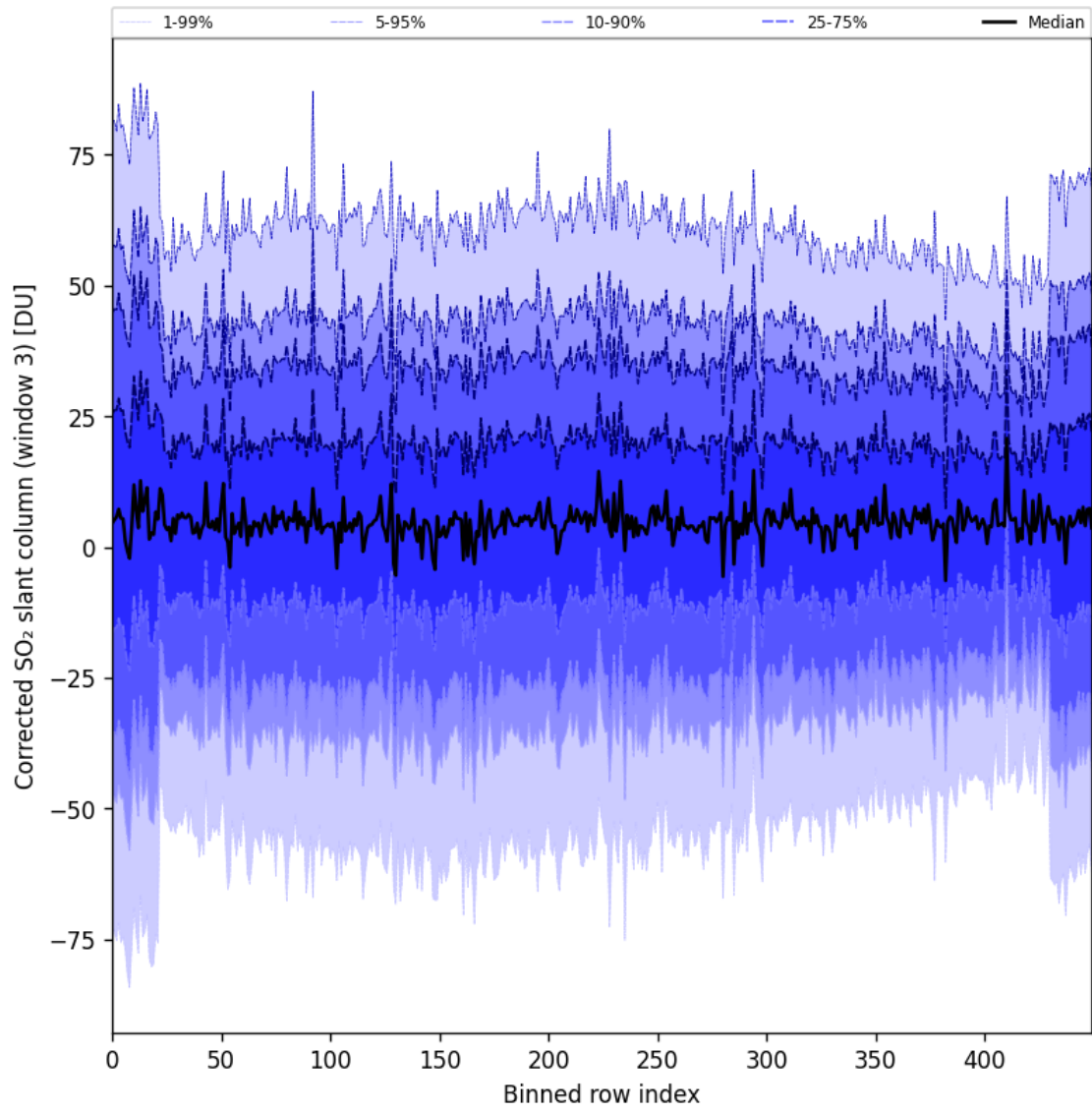
Figure 99: Along track statistics of “Corrected SO 2 slant column (window 3)” for 2025-08-17 to 2025-08-19
