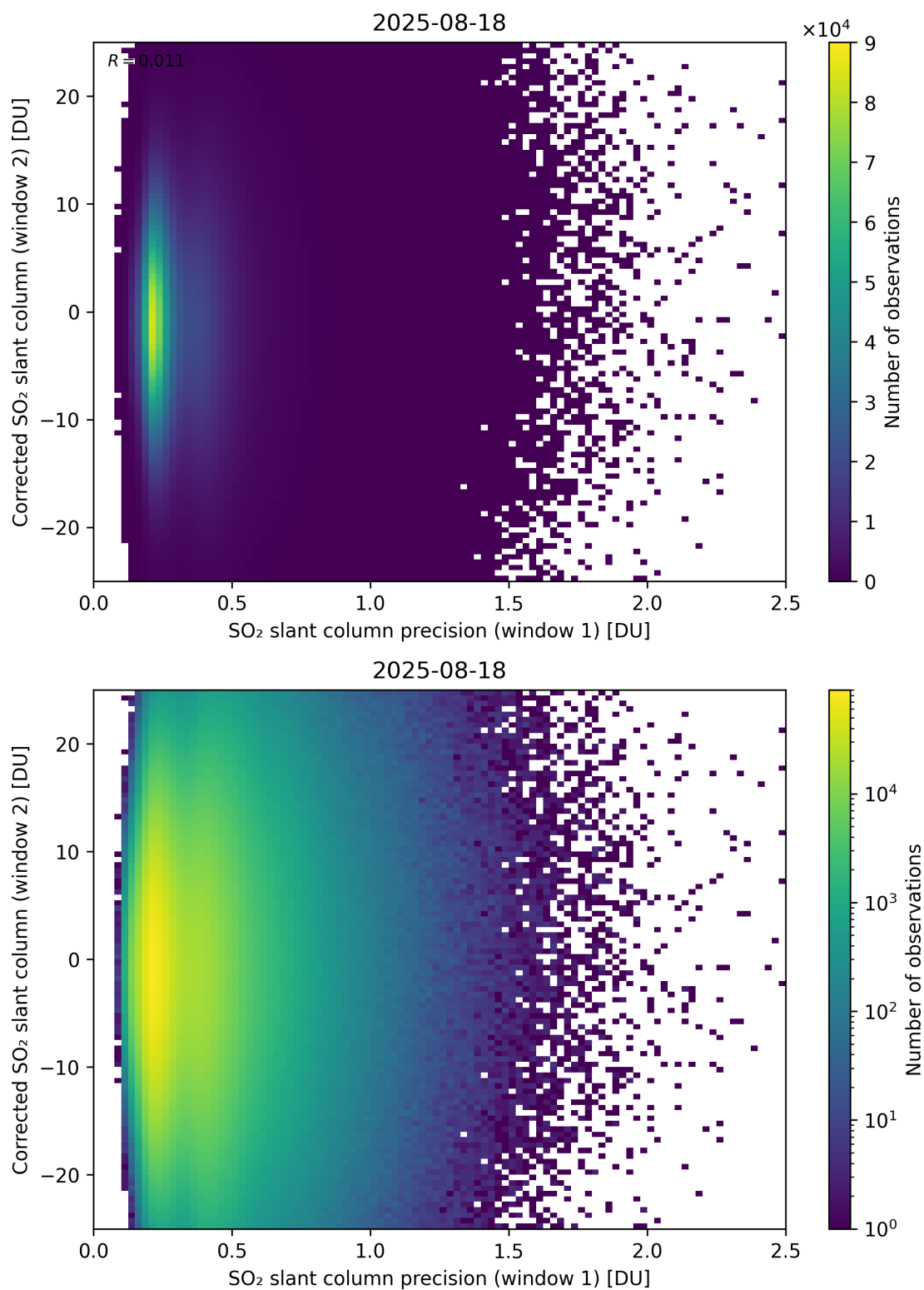
Figure 275: Scatter density plot of “SO 2 slant column precision (window 1)” against “Corrected SO 2 slant column (window 2)” for 2025-08-17 to 2025-08-19.
