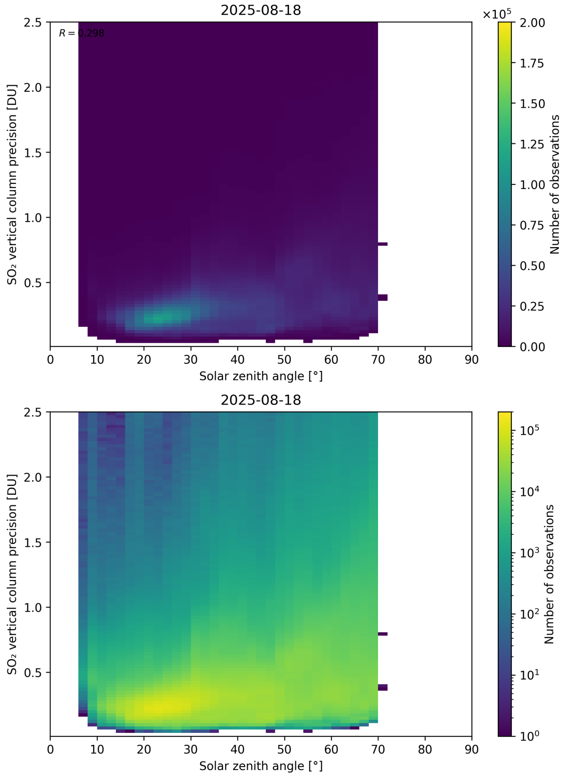
Figure 192: Scatter density plot of “Solar zenith angle” against “SO 2 vertical column precision” for 2025-08-17 to 2025-08-19.
