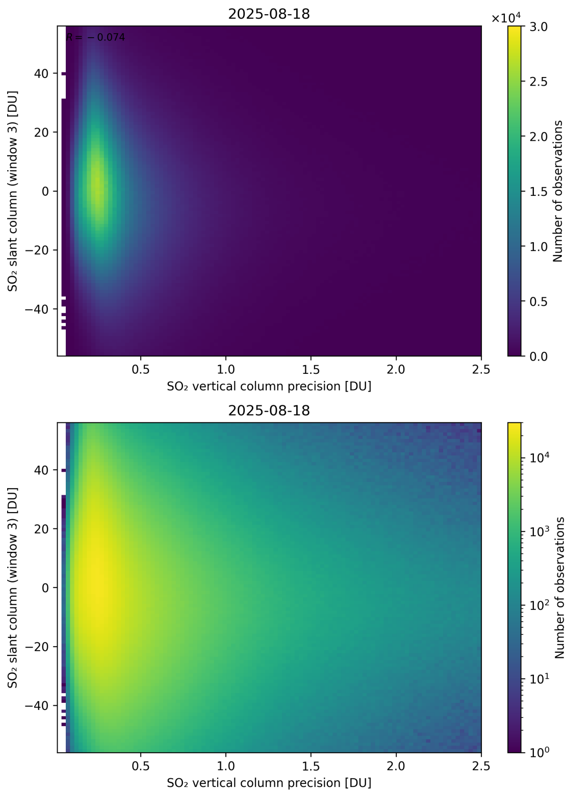
Figure 344: Scatter density plot of “SO 2 vertical column precision” against “SO 2 slant column (window 3)” for 2025-08-17 to 2025-08-19.
