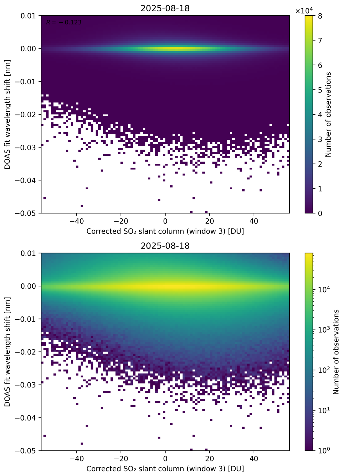
Figure 256: Scatter density plot of “Corrected SO 2 slant column (window 3)” against “DOAS fit wavelength shift” for 2025-08-17 to 2025-08-19.
