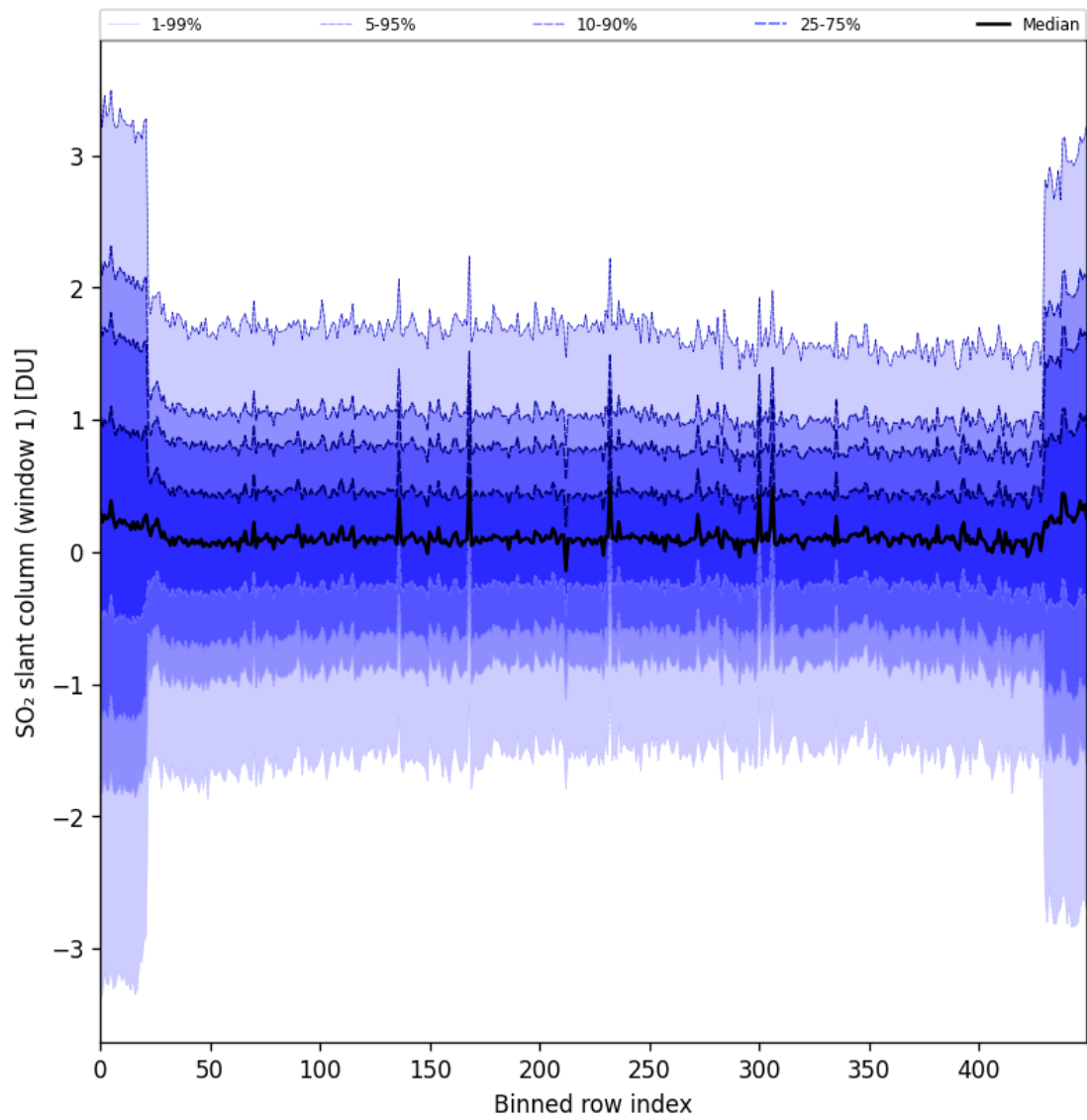
Figure 89: Along track statistics of “SO 2 slant column (window 1)” for 2025-08-17 to 2025-08-19
