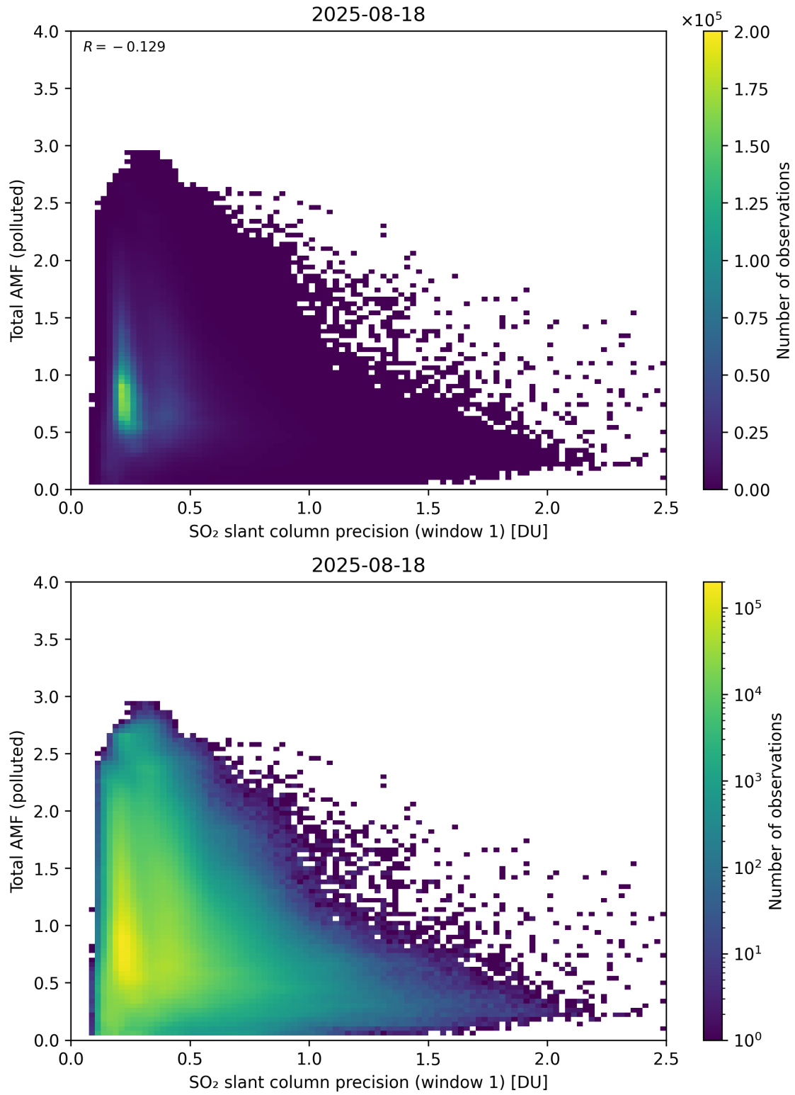
Figure 280: Scatter density plot of “SO 2 slant column precision (window 1)” against “Total AMF (polluted)” for 2025-08-17 to 2025-08-19.
