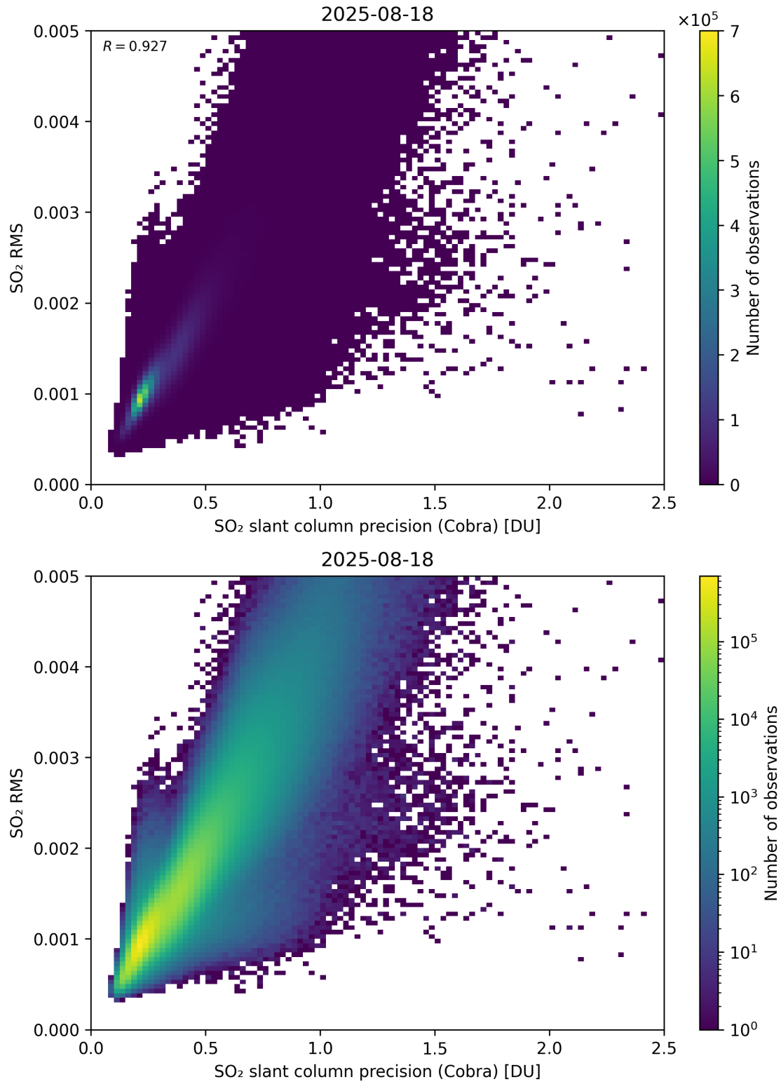
Figure 204: Scatter density plot of “SO 2 slant column precision (Cobra)” against “SO 2 RMS” for 2025-08-17 to 2025-08-19.
