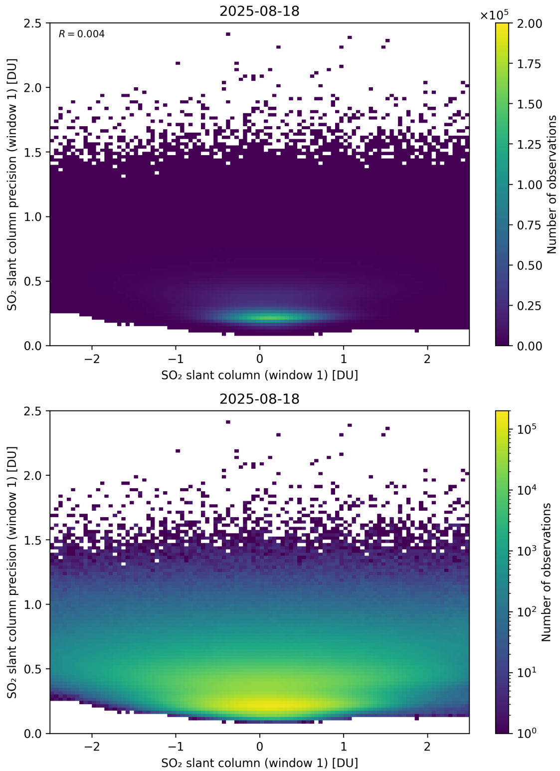
Figure 285: Scatter density plot of “SO 2 slant column (window 1)” against “SO 2 slant column precision (window 1)” for 2025-08-17 to 2025-08-19.
