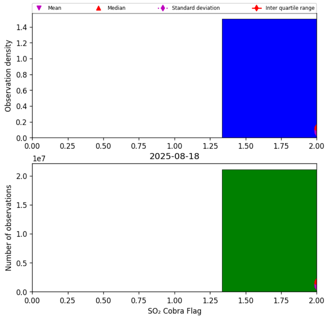
Figure 75: Histogram of “SO 2 Cobra Flag” for 2025-08-17 to 2025-08-19
