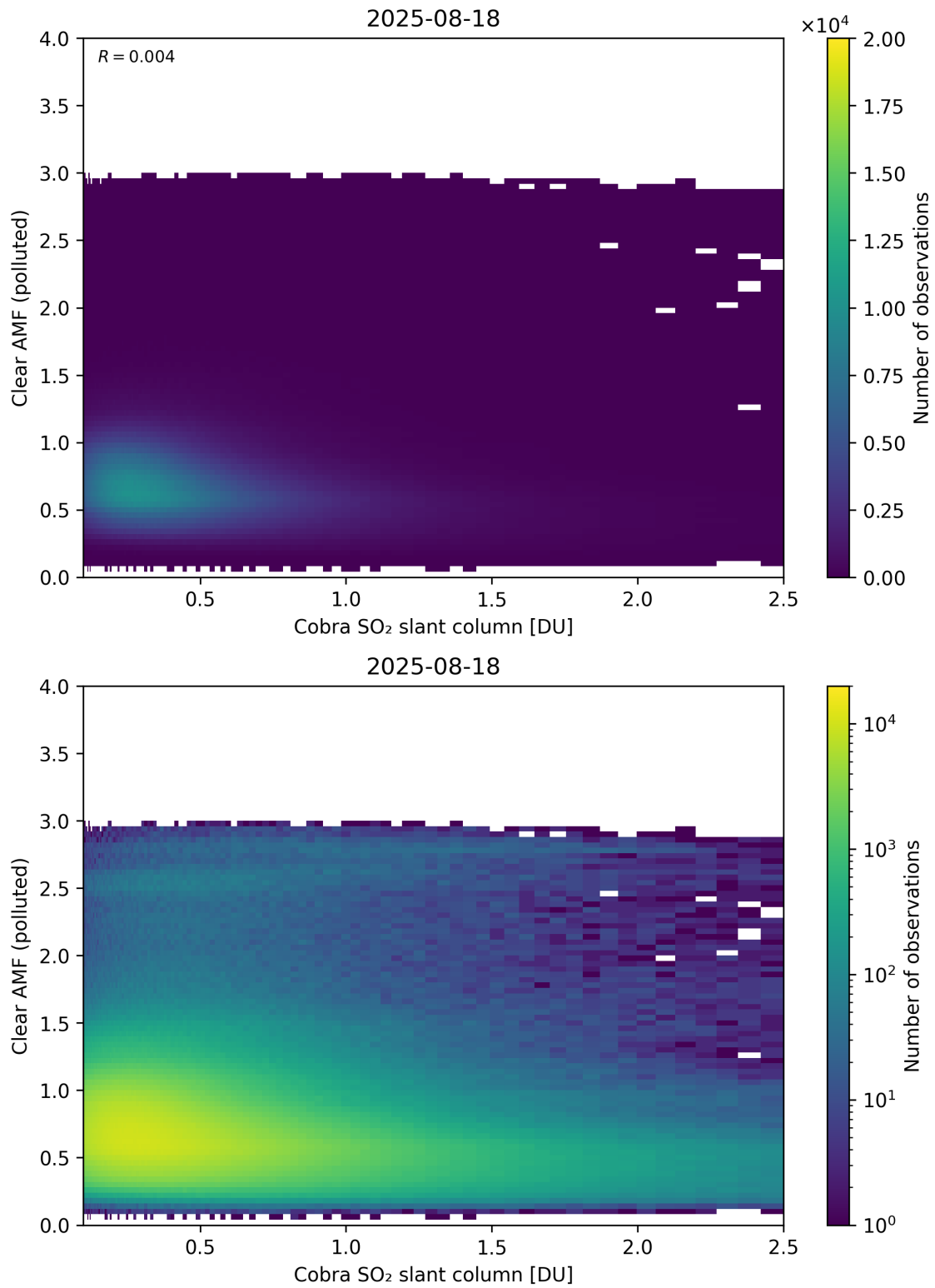
Figure 215: Scatter density plot of “Cobra SO 2 slant column” against “Clear AMF (polluted)” for 2025-08-17 to 2025-08-19.
