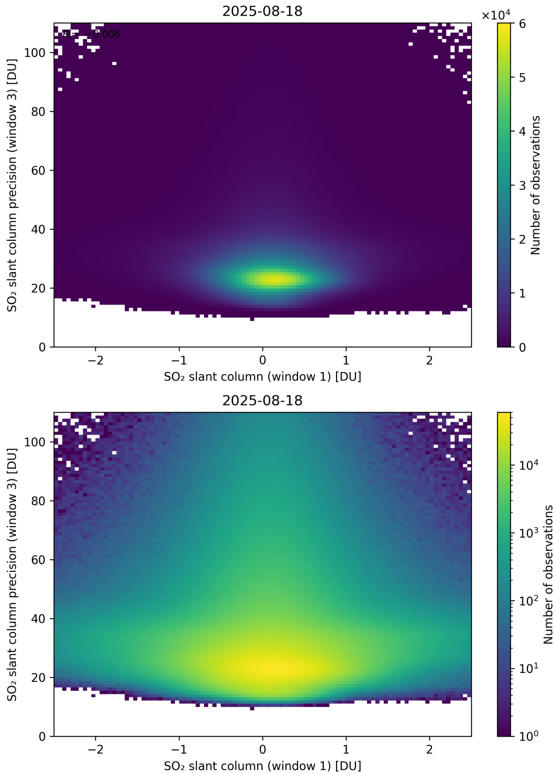
Figure 288: Scatter density plot of “SO 2 slant column (window 1)” against “SO 2 slant column precision (window 3)” for 2025-08-17 to 2025-08-19.
