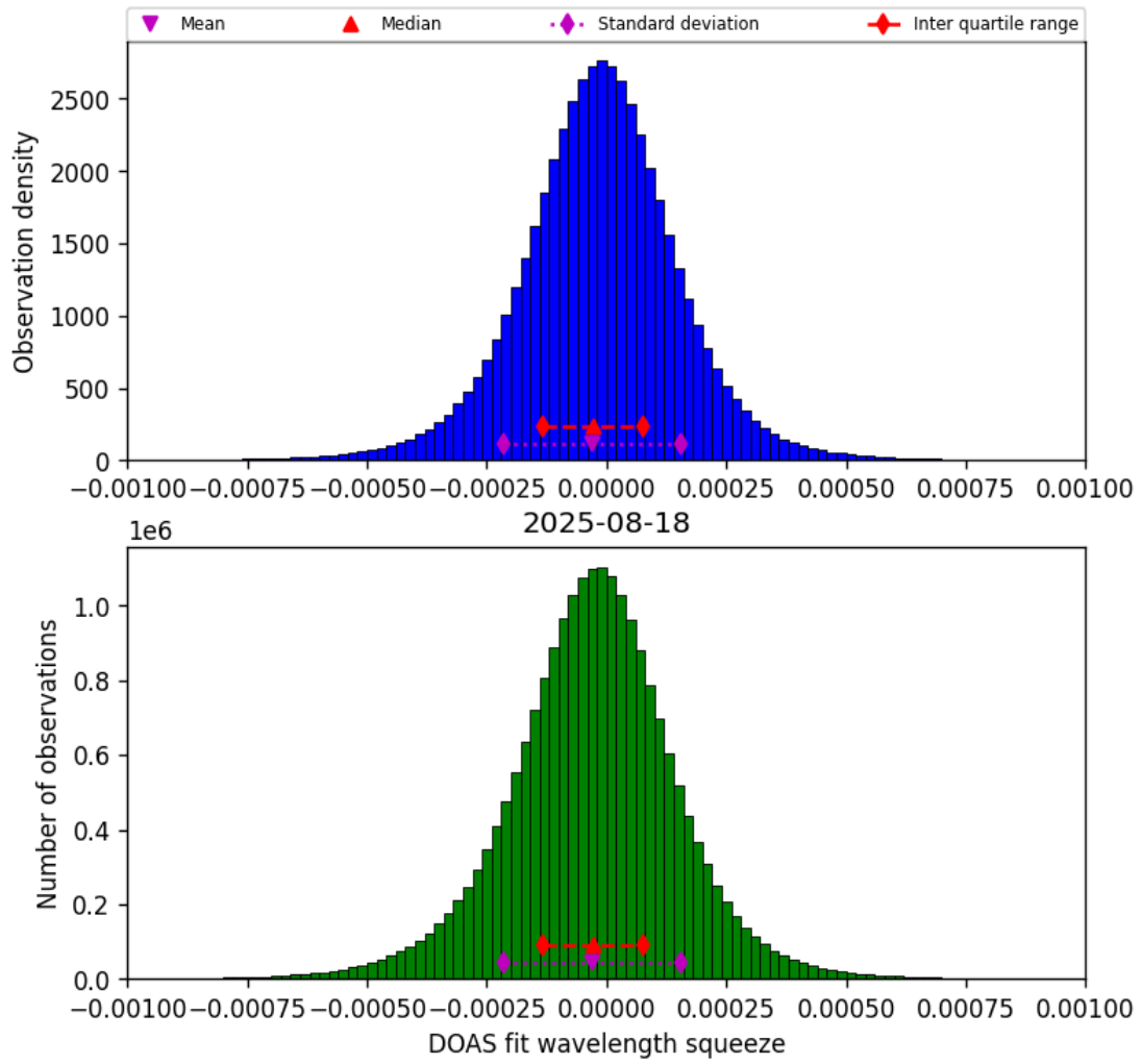
Figure 77: Histogram of “DOAS fit wavelength squeeze” for 2025-08-17 to 2025-08-19
