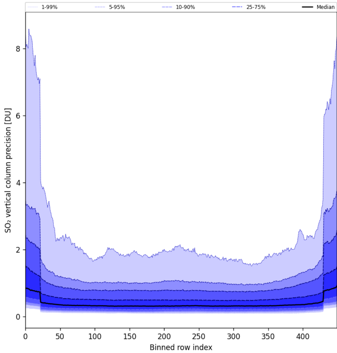
Figure 85: Along track statistics of “SO 2 vertical column precision” for 2025-08-17 to 2025-08-19
