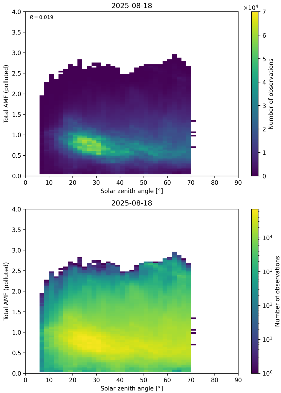
Figure 189: Scatter density plot of “Solar zenith angle” against “Total AMF (polluted)” for 2025-08-17 to 2025-08-19.
