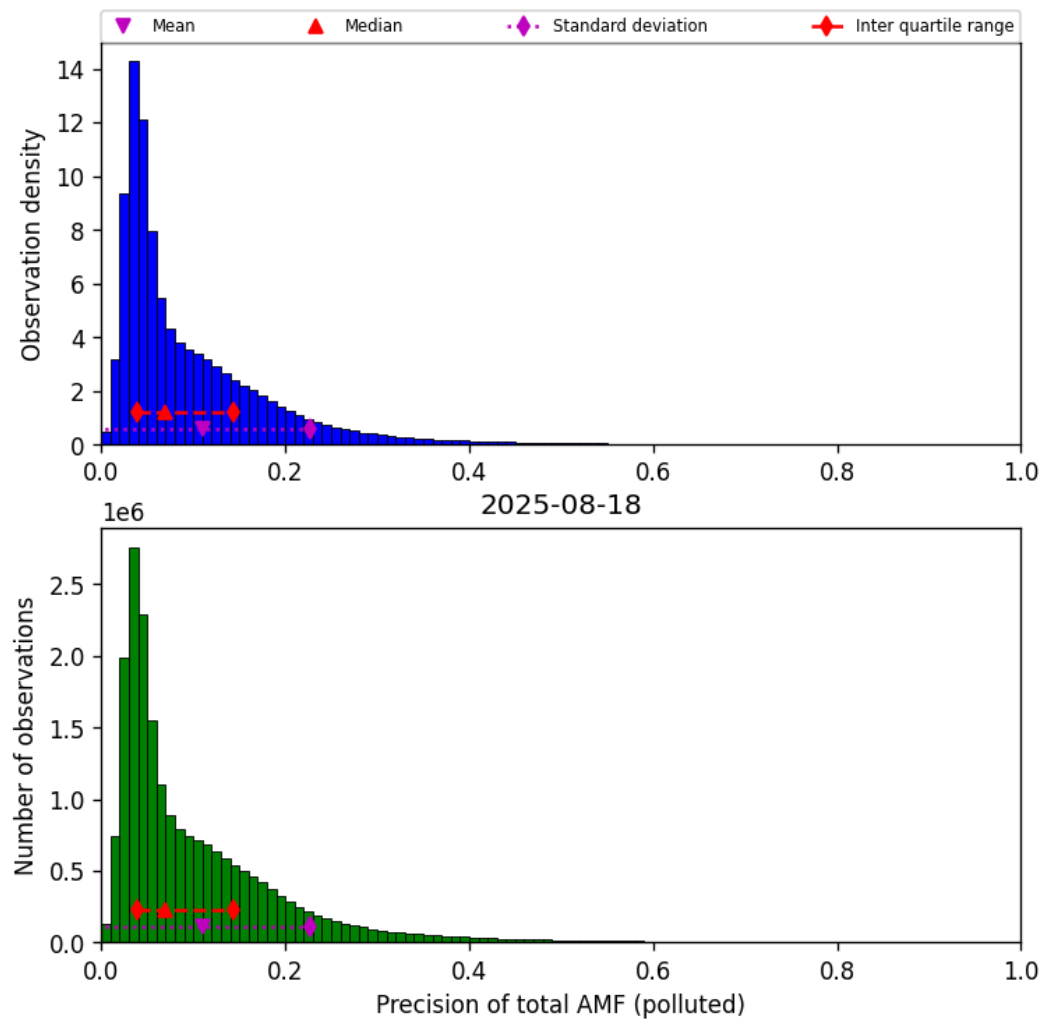
Figure 80: Histogram of “Precision of total AMF (polluted)” for 2025-08-17 to 2025-08-19
