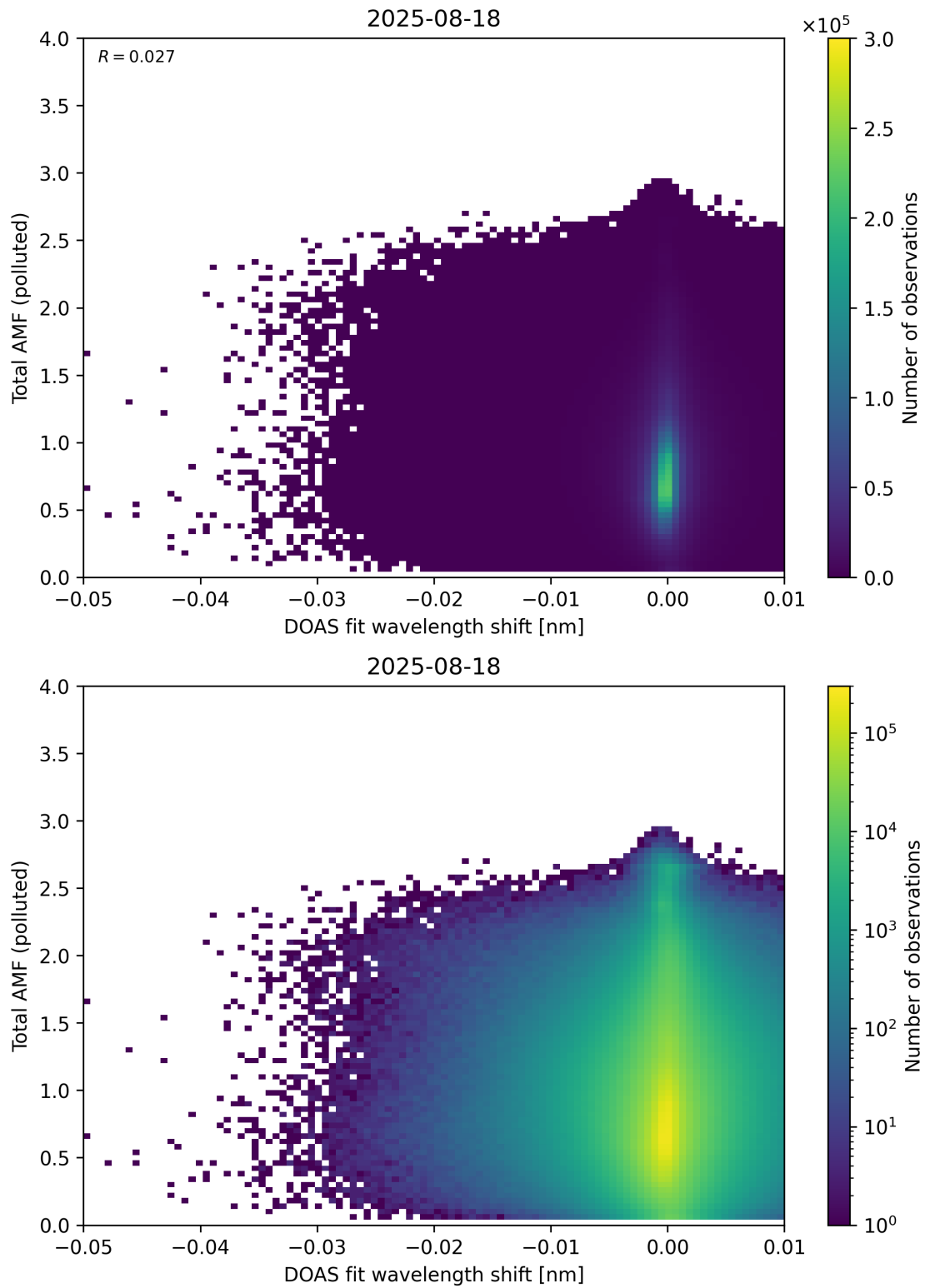
Figure 141: Scatter density plot of “DOAS fit wavelength shift” against “Total AMF (polluted)” for 2025-08-17 to 2025-08-19.
