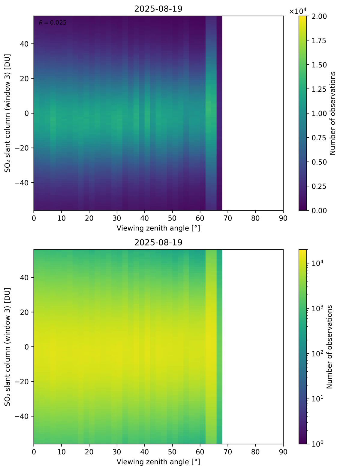
Figure 379: Scatter density plot of “Viewing zenith angle” against “SO 2 slant column (window 3)” for 2025-08-19 to 2025-08-20.
