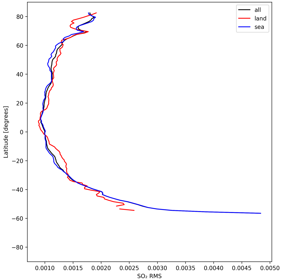
Figure 52: Zonal average of “SO 2 RMS” for 2025-08-19 to 2025-08-20.
