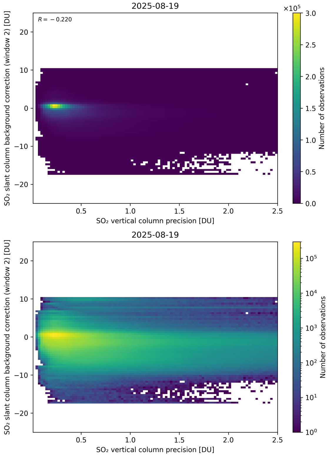
Figure 330: Scatter density plot of “SO 2 vertical column precision” against “SO 2 slant column background correction (window 2)” for 2025-08-19 to 2025-08-20.
