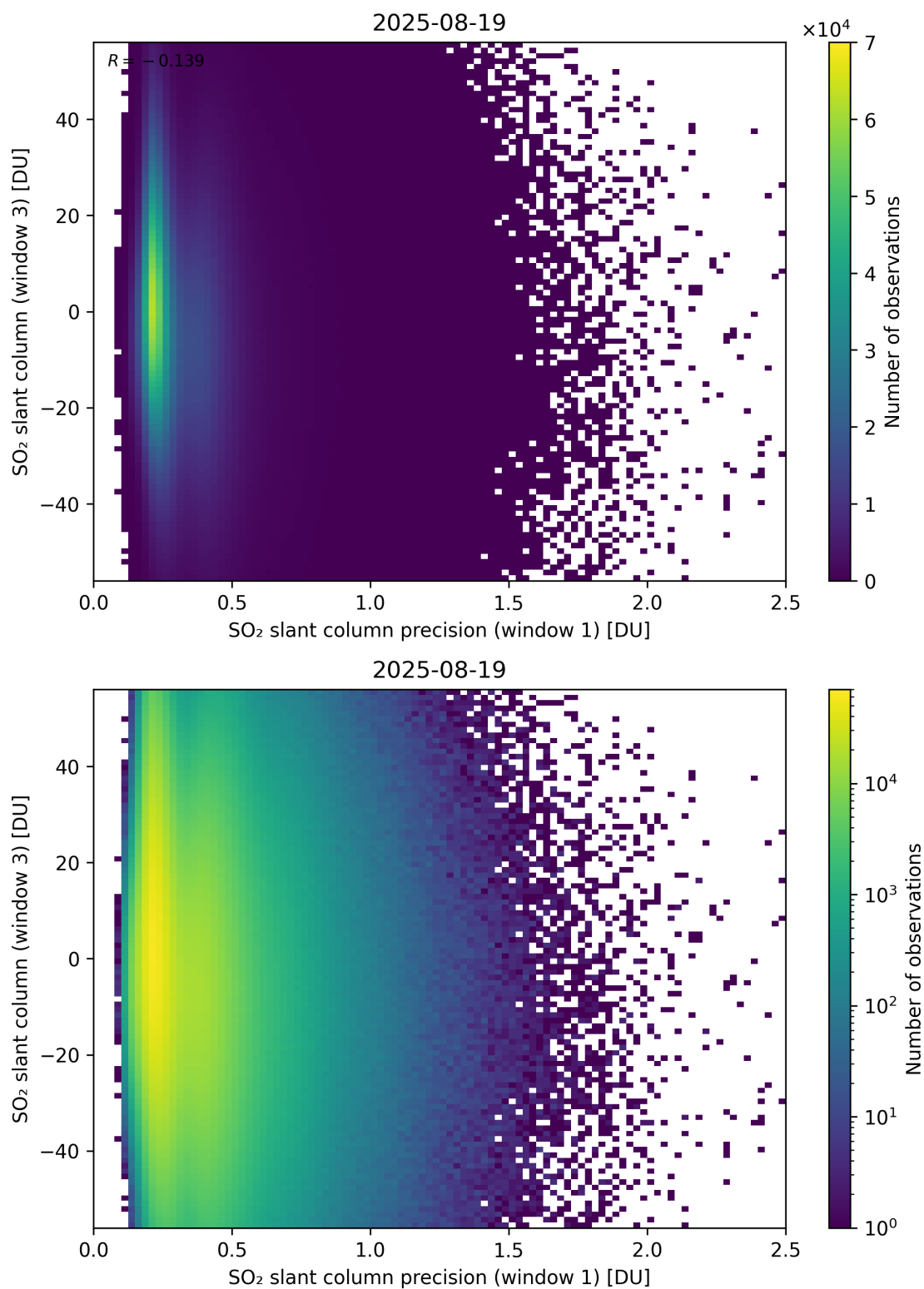
Figure 278: Scatter density plot of “SO 2 slant column precision (window 1)” against “SO 2 slant column (window 3)” for 2025-08-19 to 2025-08-20.
