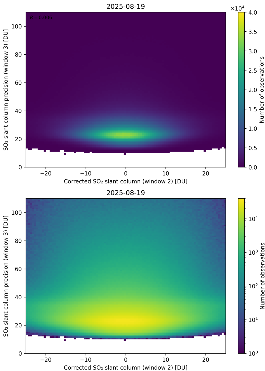
Figure 252: Scatter density plot of “Corrected SO 2 slant column (window 2)” against “SO 2 slant column precision (window 3)” for 2025-08-19 to 2025-08-20.
