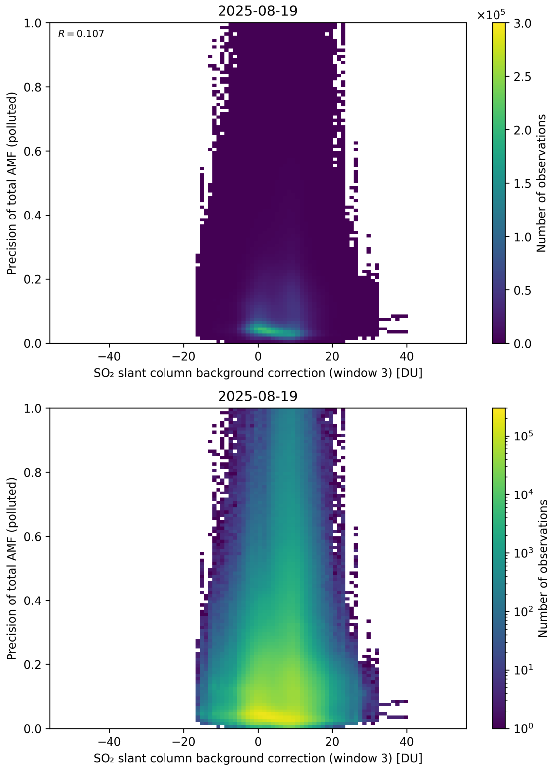
Figure 137: Scatter density plot of “SO 2 slant column background correction (window 3)” against “Precision of total AMF (polluted)” for 2025-08-19 to 2025-08-20.
