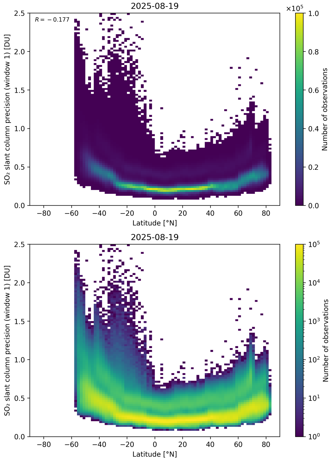
Figure 163: Scatter density plot of “Latitude” against “SO 2 slant column precision (window 1)” for 2025-08-19 to 2025-08-20.
