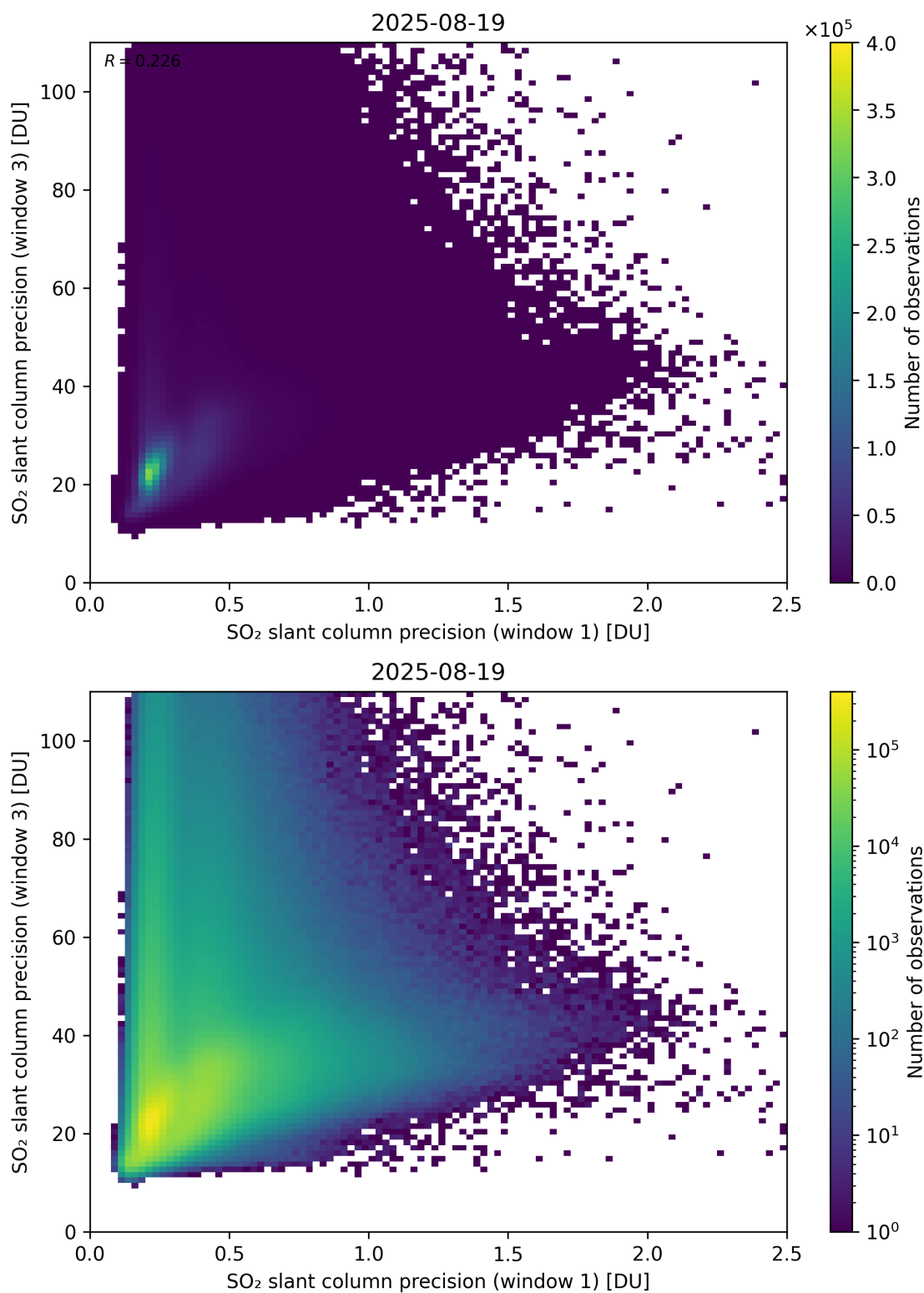
Figure 279: Scatter density plot of “SO 2 slant column precision (window 1)” against “SO 2 slant column precision (window 3)” for 2025-08-19 to 2025-08-20.
