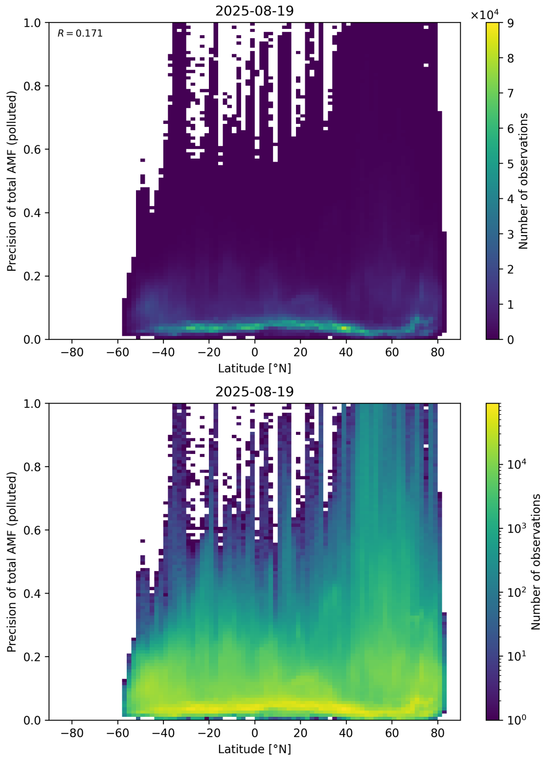
Figure 168: Scatter density plot of “Latitude” against “Precision of total AMF (polluted)” for 2025-08-19 to 2025-08-20.
