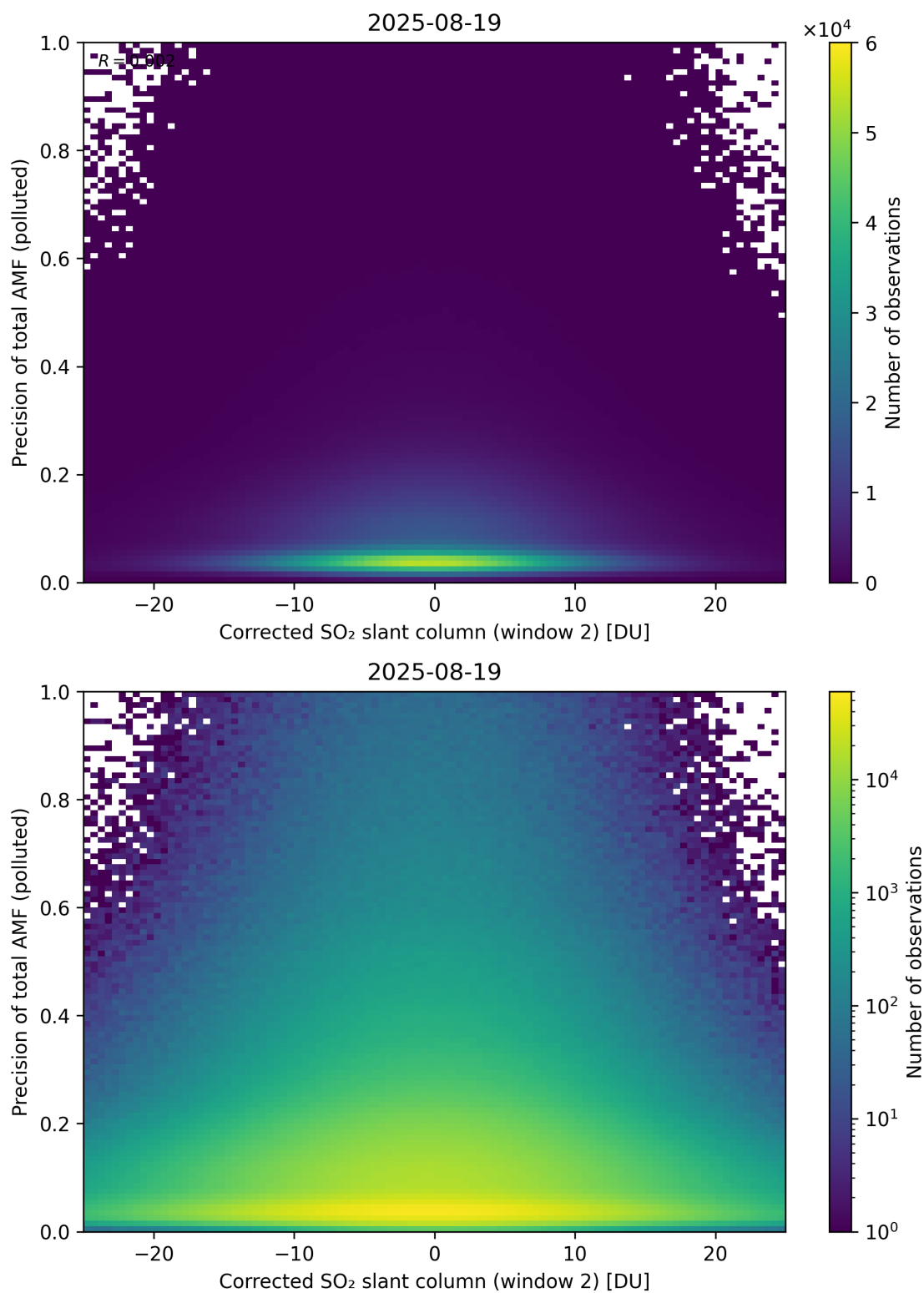
Figure 254: Scatter density plot of “Corrected SO 2 slant column (window 2)” against “Precision of total AMF (polluted)” for 2025-08-19 to 2025-08-20.
