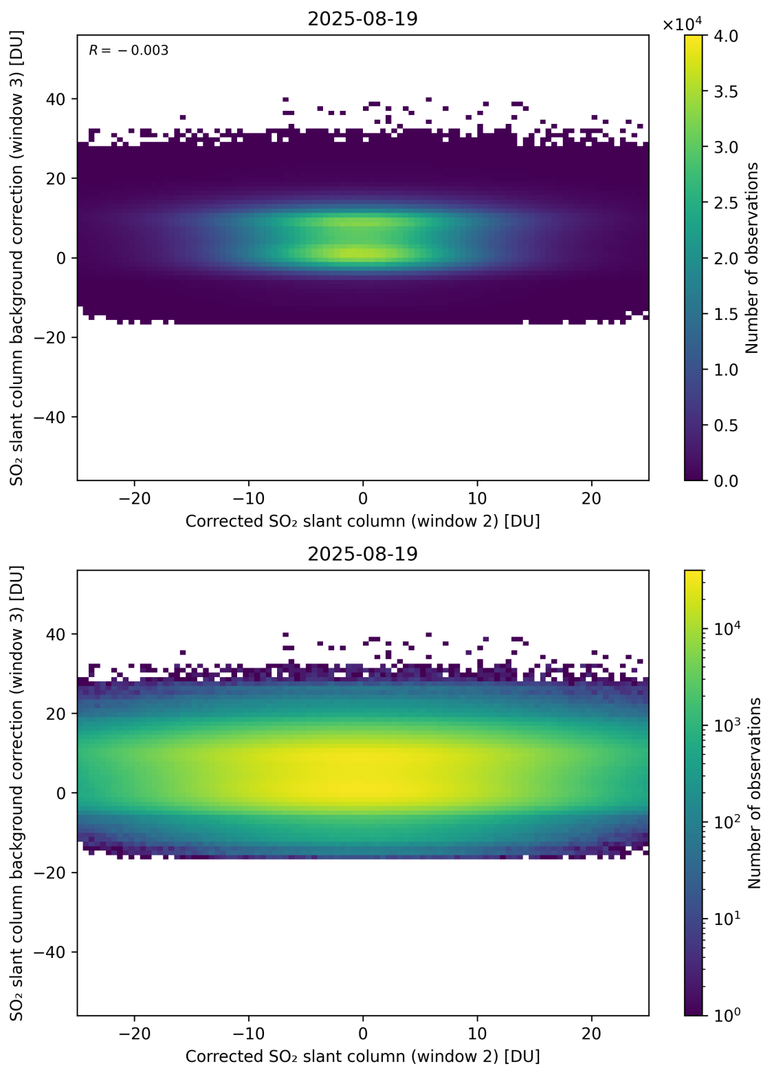
Figure 245: Scatter density plot of “Corrected SO 2 slant column (window 2)” against “SO 2 slant column background correction (window 3)” for 2025-08-19 to 2025-08-20.
