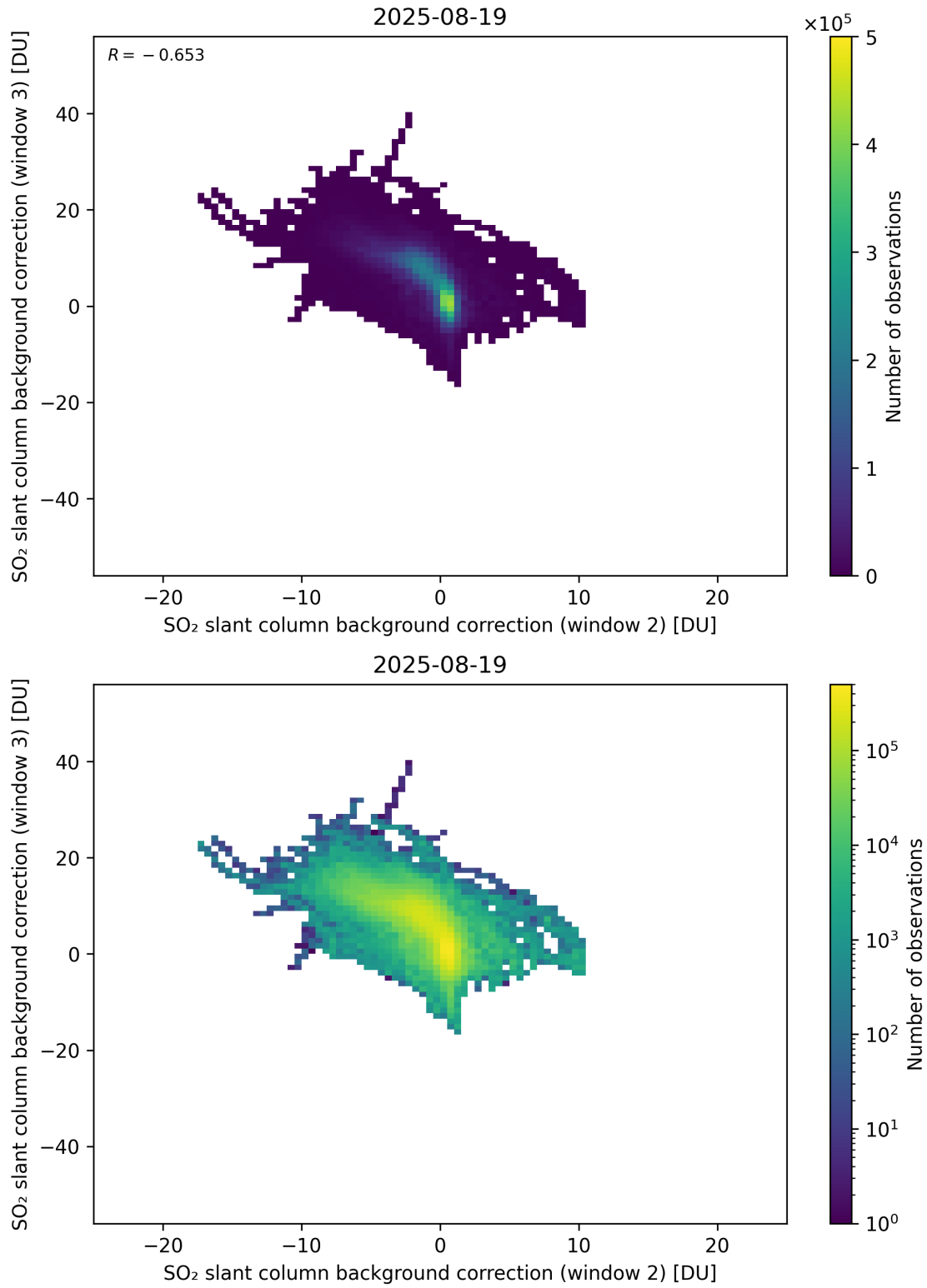
Figure 122: Scatter density plot of “SO 2 slant column background correction (window 2)” against “SO 2 slant column background correction (window 3)” for 2025-08-19 to 2025-08-20.
