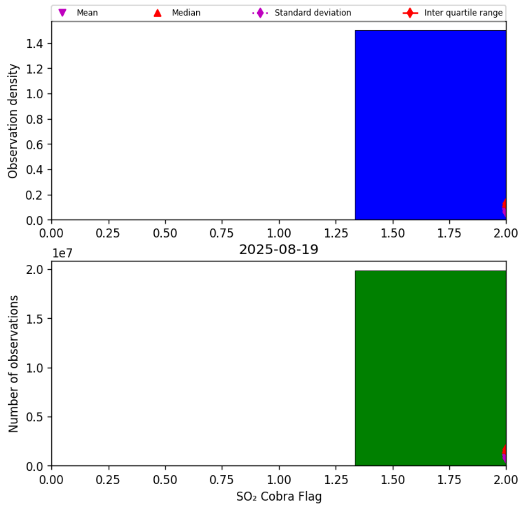
Figure 75: Histogram of “SO 2 Cobra Flag” for 2025-08-19 to 2025-08-20
