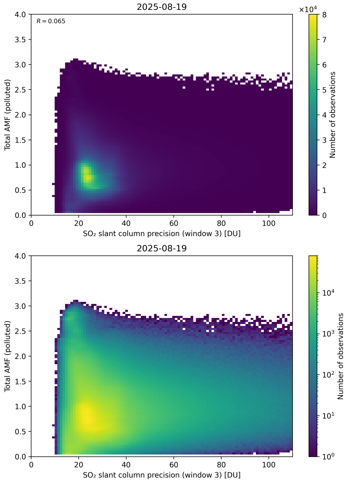
Figure 313: Scatter density plot of “SO 2 slant column precision (window 3)” against “Total AMF (polluted)” for 2025-08-19 to 2025-08-20.
