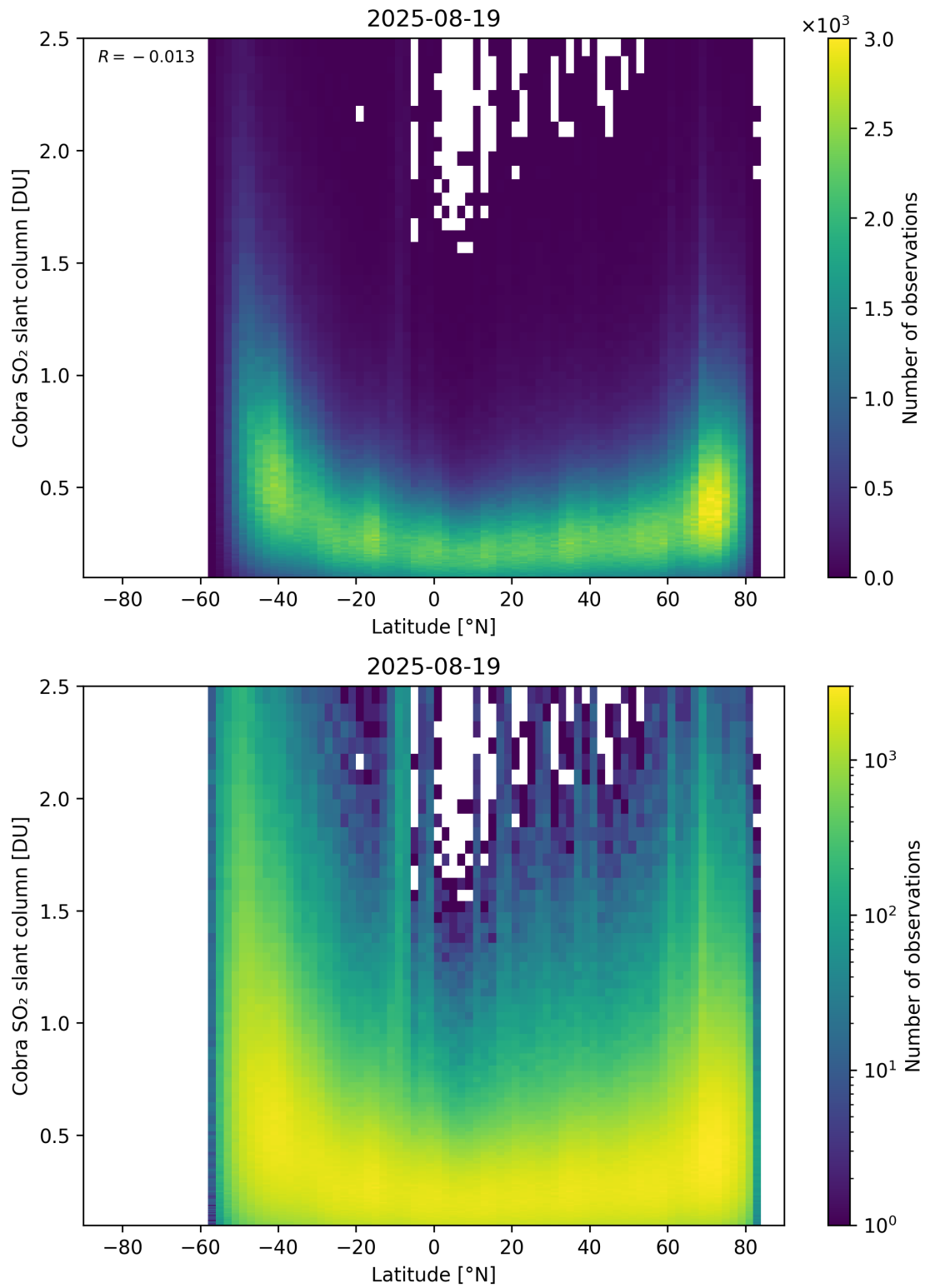
Figure 157: Scatter density plot of “Latitude” against “Cobra SO 2 slant column” for 2025-08-19 to 2025-08-20.
