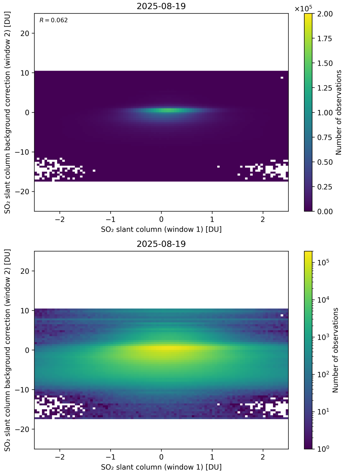
Figure 263: Scatter density plot of “SO 2 slant column (window 1)” against “SO 2 slant column background correction (window 2)” for 2025-08-19 to 2025-08-20.
