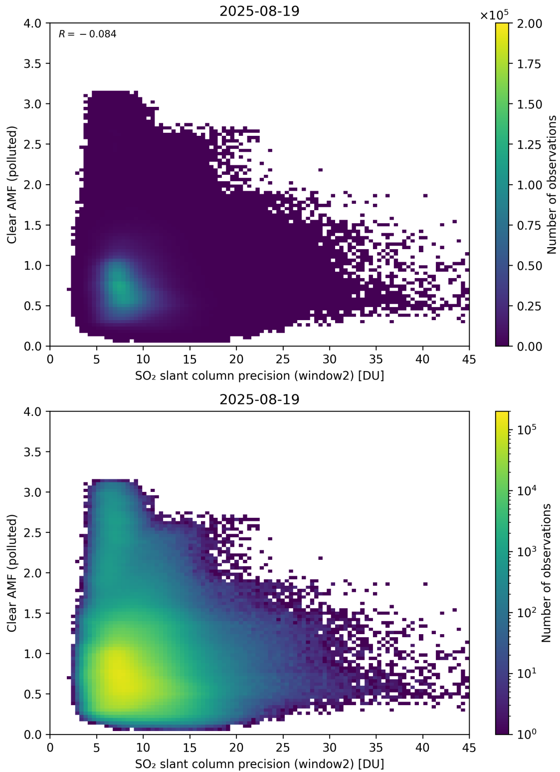
Figure 296: Scatter density plot of “SO 2 slant column precision (window2)” against “Clear AMF (polluted)” for 2025-08-19 to 2025-08-20.
