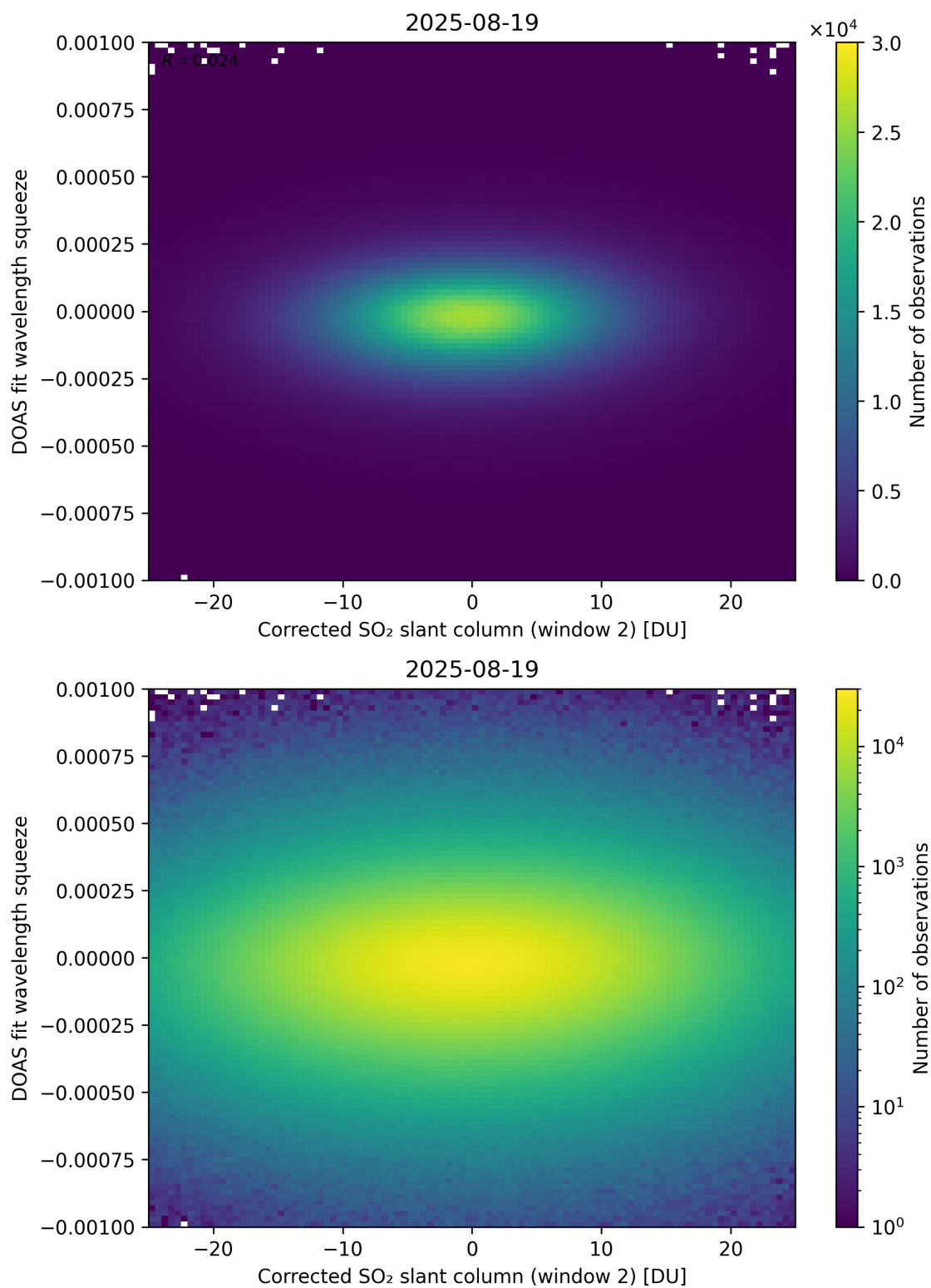
Figure 247: Scatter density plot of “Corrected SO 2 slant column (window 2)” against “DOAS fit wavelength squeeze” for 2025-08-19 to 2025-08-20.
