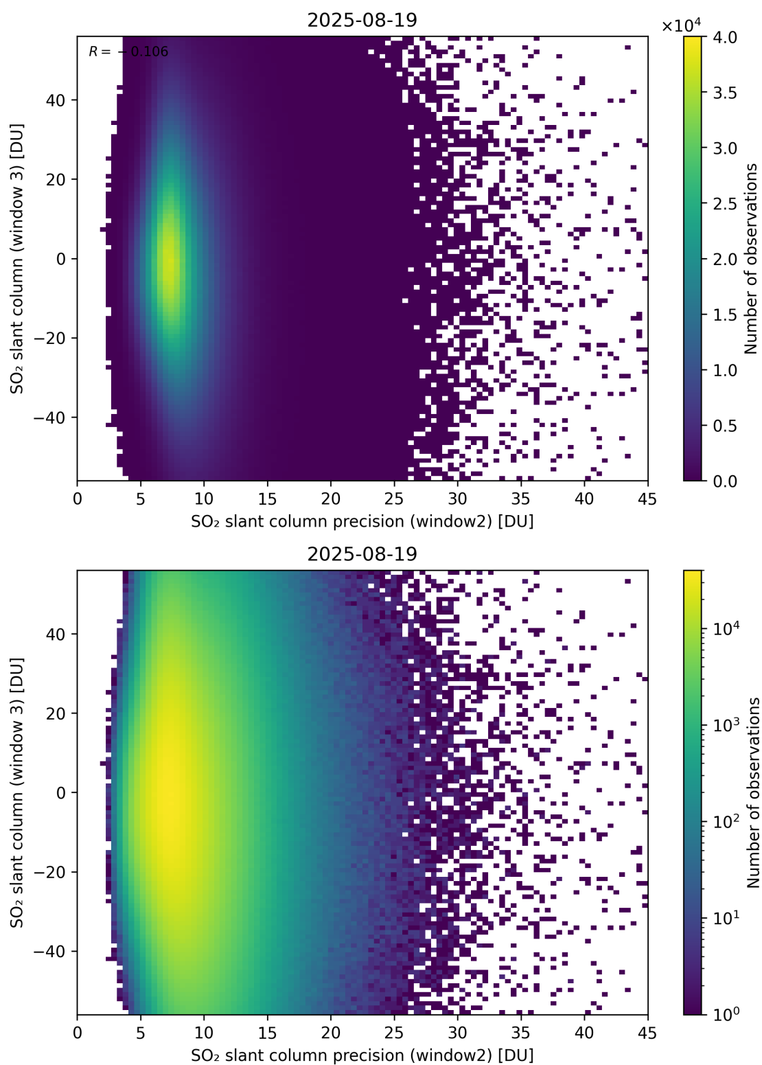
Figure 299: Scatter density plot of “SO 2 slant column precision (window2)” against “SO 2 slant column (window 3)” for 2025-08-19 to 2025-08-20.
