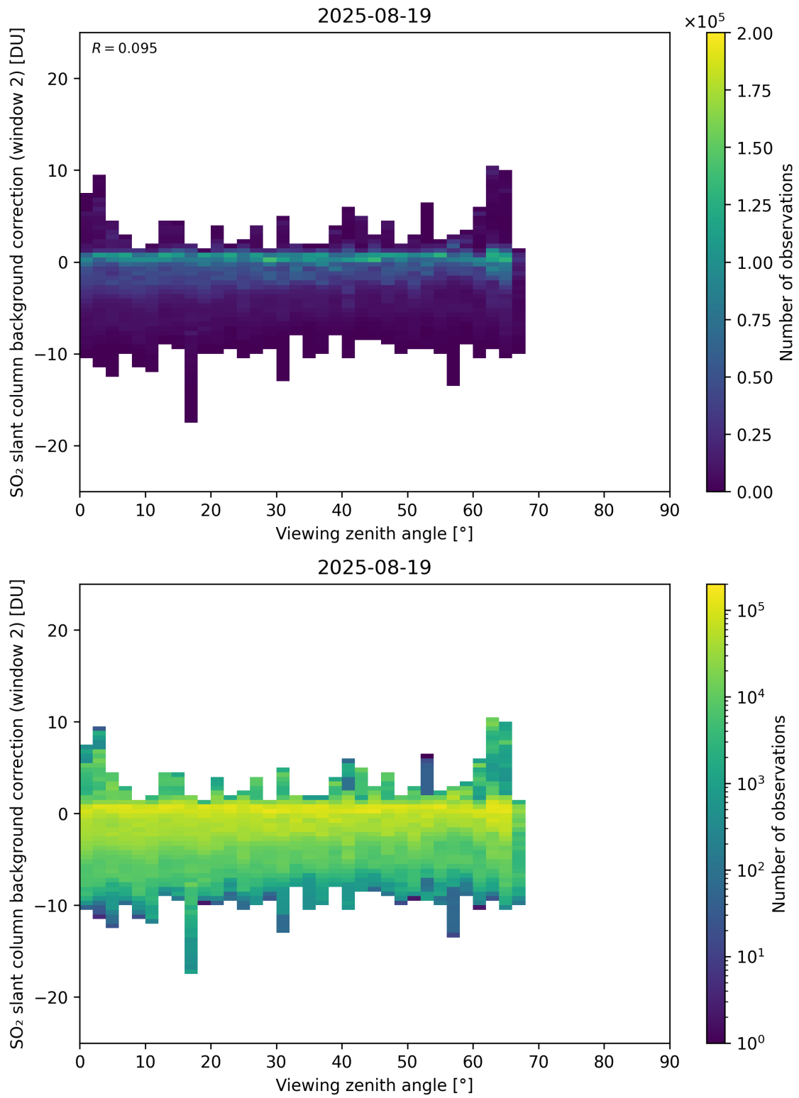
Figure 363: Scatter density plot of “Viewing zenith angle” against “SO 2 slant column background correction (window 2)” for 2025-08-19 to 2025-08-20.
