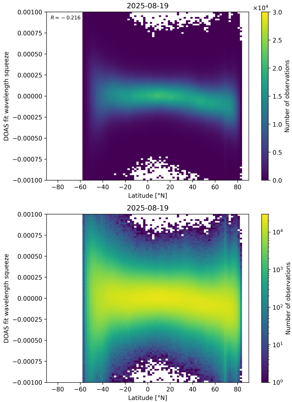
Figure 154: Scatter density plot of “Latitude” against “DOAS fit wavelength squeeze” for 2025-08-19 to 2025-08-20.
