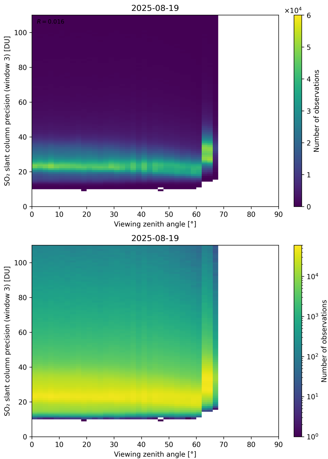
Figure 380: Scatter density plot of “Viewing zenith angle” against “SO 2 slant column precision (window 3)” for 2025-08-19 to 2025-08-20.
