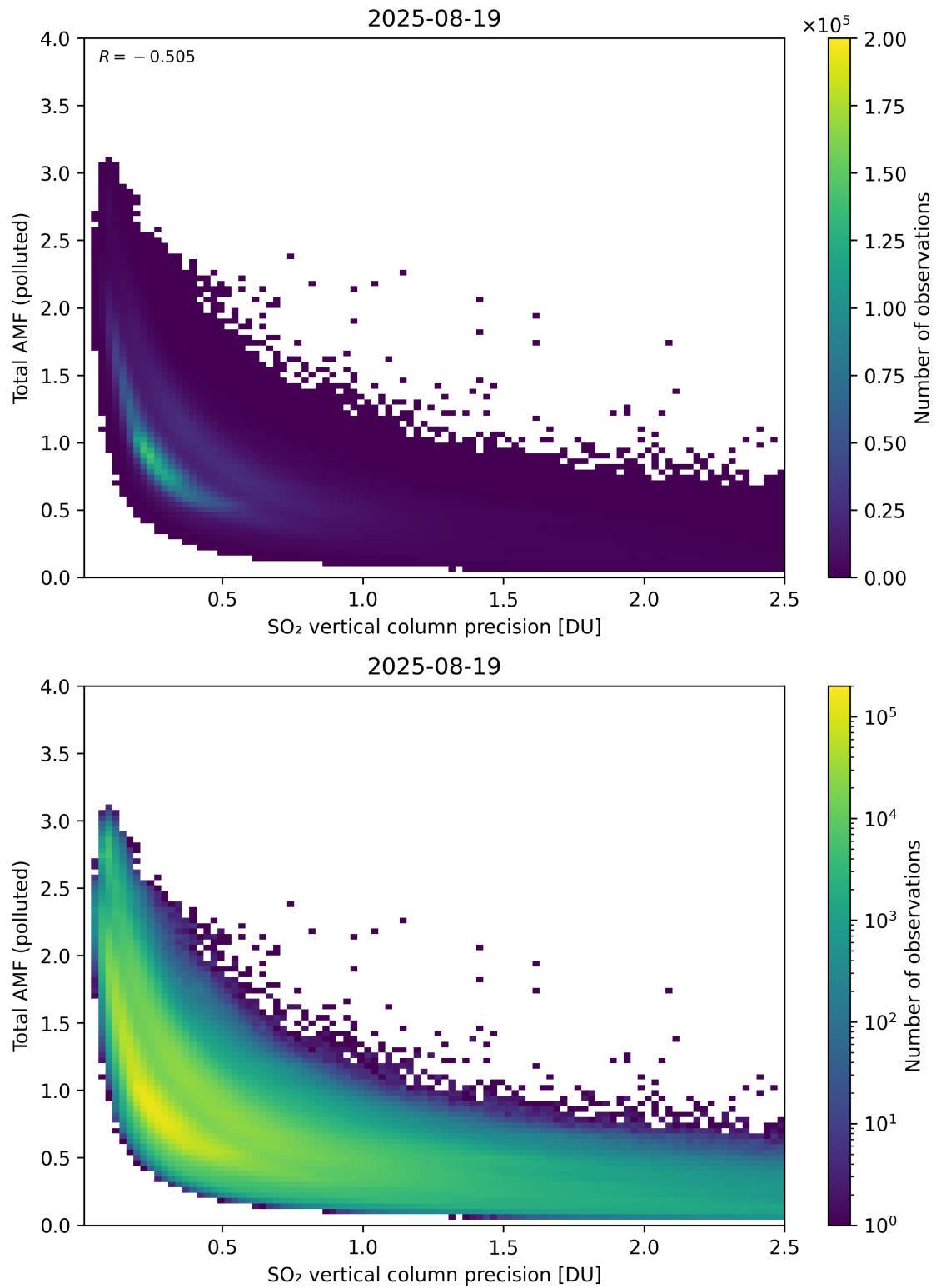
Figure 346: Scatter density plot of “SO 2 vertical column precision” against “Total AMF (polluted)” for 2025-08-19 to 2025-08-20.
