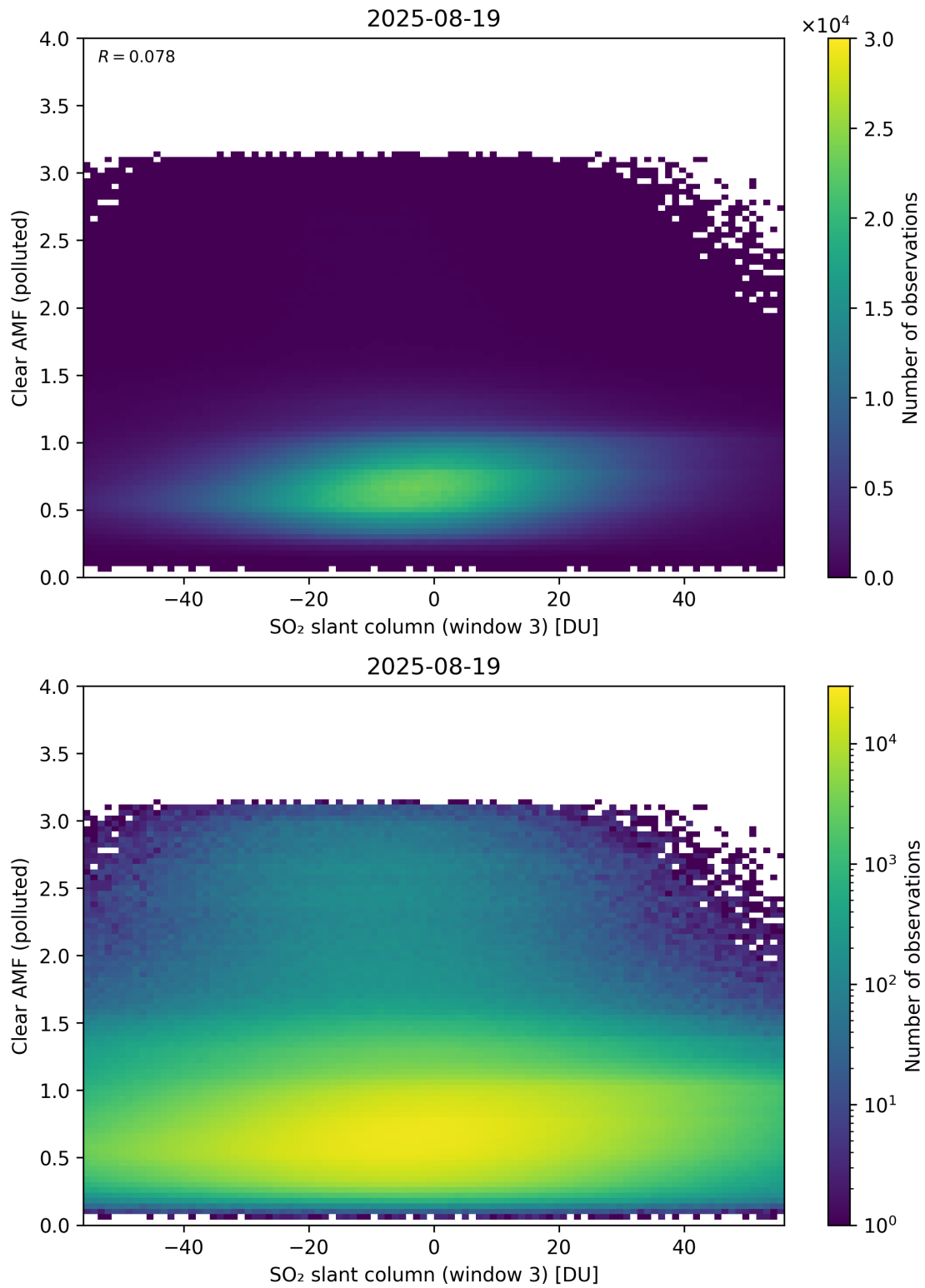
Figure 315: Scatter density plot of “SO 2 slant column (window 3)” against “Clear AMF (polluted)” for 2025-08-19 to 2025-08-20.
