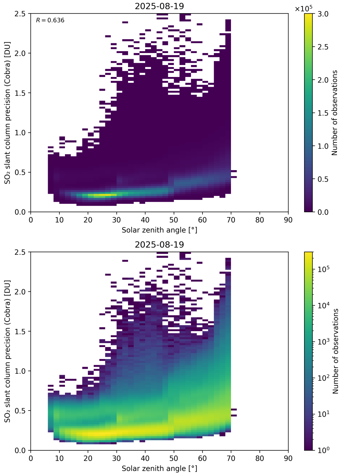
Figure 180: Scatter density plot of “Solar zenith angle” against “SO 2 slant column precision (Cobra)” for 2025-08-19 to 2025-08-20.
