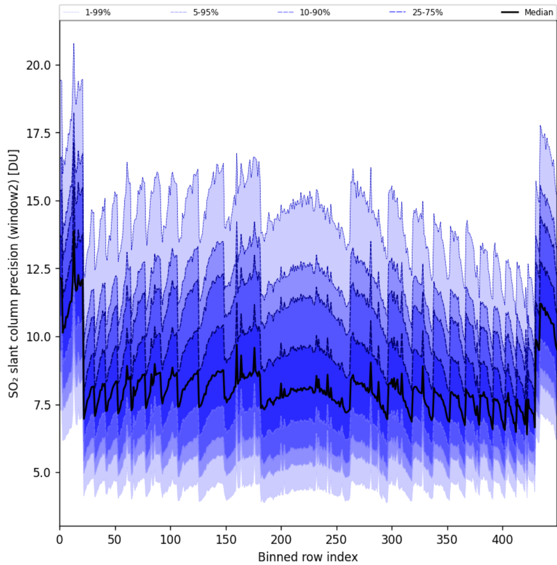
Figure 94: Along track statistics of “SO 2 slant column precision (window2)” for 2025-08-19 to 2025-08-20
