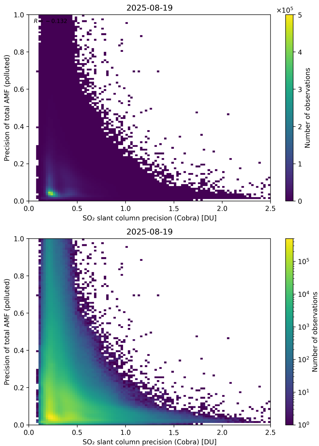
Figure 214: Scatter density plot of “SO 2 slant column precision (Cobra)” against “Precision of total AMF (polluted)” for 2025-08-19 to 2025-08-20.
