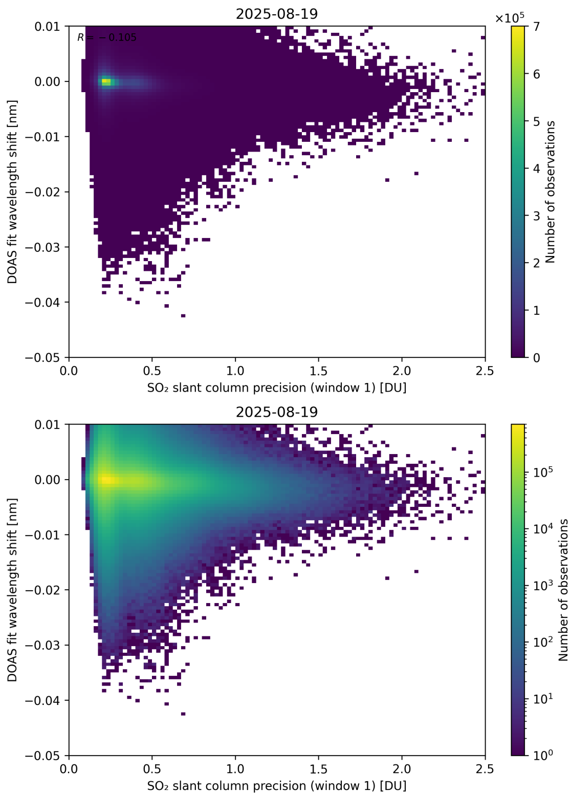
Figure 271: Scatter density plot of “SO 2 slant column precision (window 1)” against “DOAS fit wavelength shift” for 2025-08-19 to 2025-08-20.
