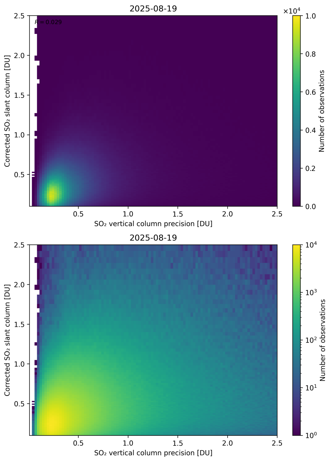
Figure 338: Scatter density plot of “SO 2 vertical column precision” against “Corrected SO 2 slant column” for 2025-08-19 to 2025-08-20.
