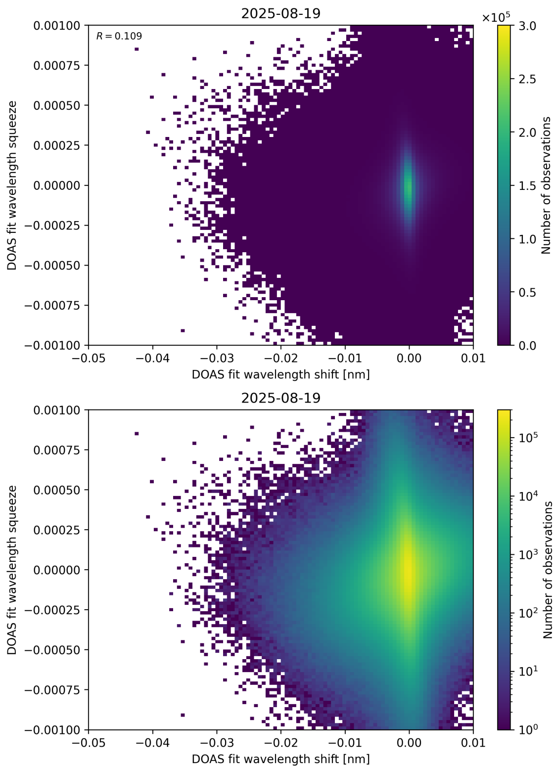
Figure 138: Scatter density plot of “DOAS fit wavelength shift” against “DOAS fit wavelength squeeze” for 2025-08-19 to 2025-08-20.
