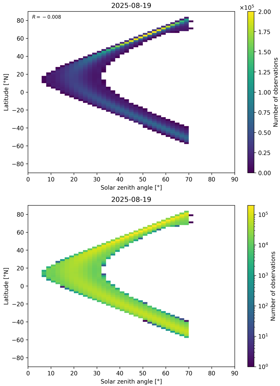
Figure 177: Scatter density plot of “Solar zenith angle” against “Latitude” for 2025-08-19 to 2025-08-20.
