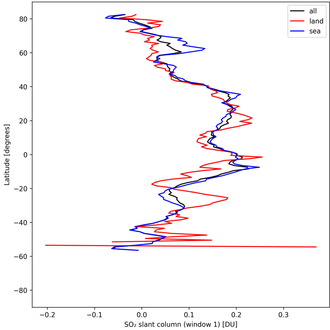
Figure 37: Zonal average of “SO 2 slant column (window 1)” for 2025-08-19 to 2025-08-20.
