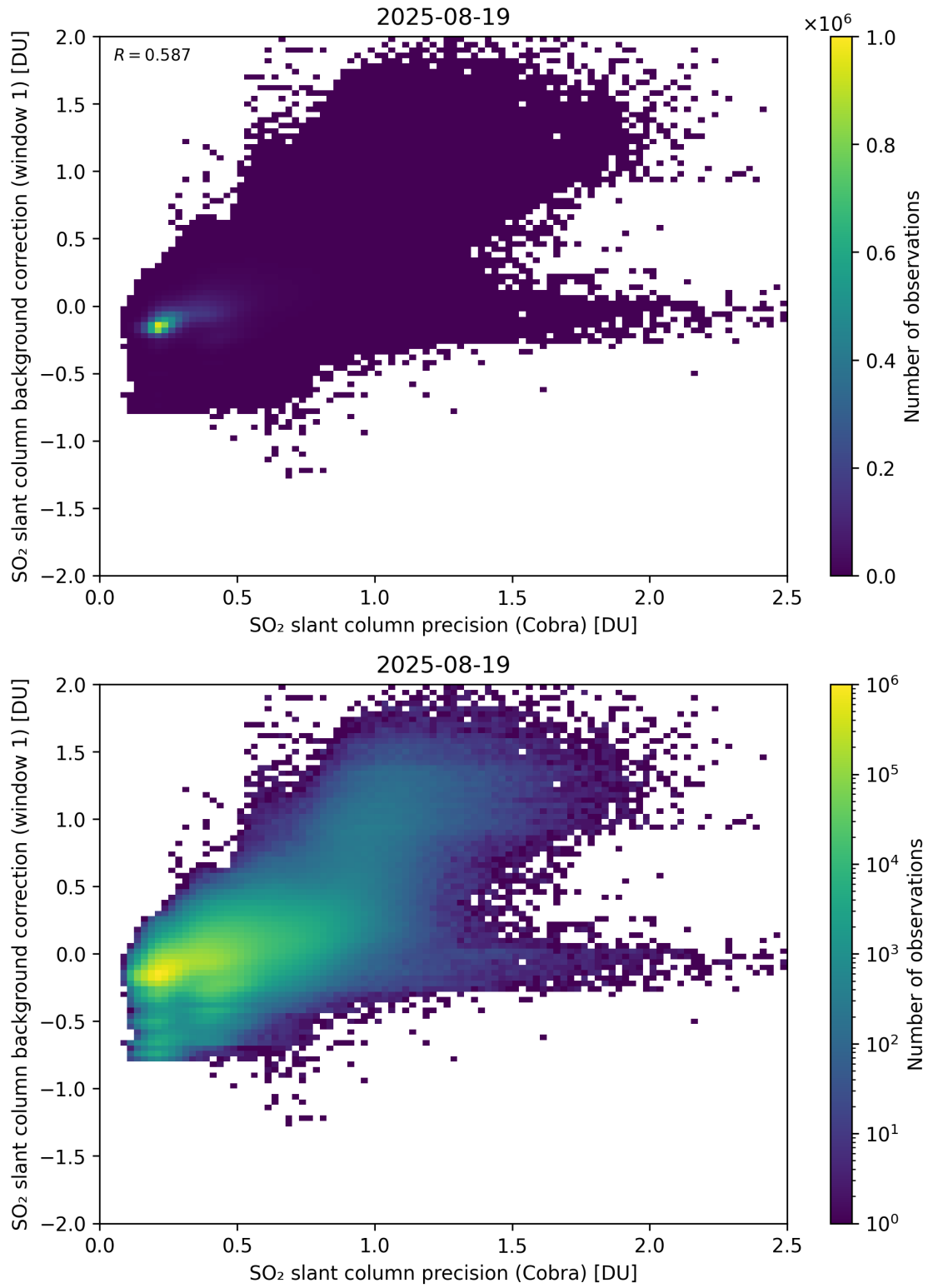
Figure 199: Scatter density plot of “SO 2 slant column precision (Cobra)” against “SO 2 slant column background correction (window 1)” for 2025-08-19 to 2025-08-20.
