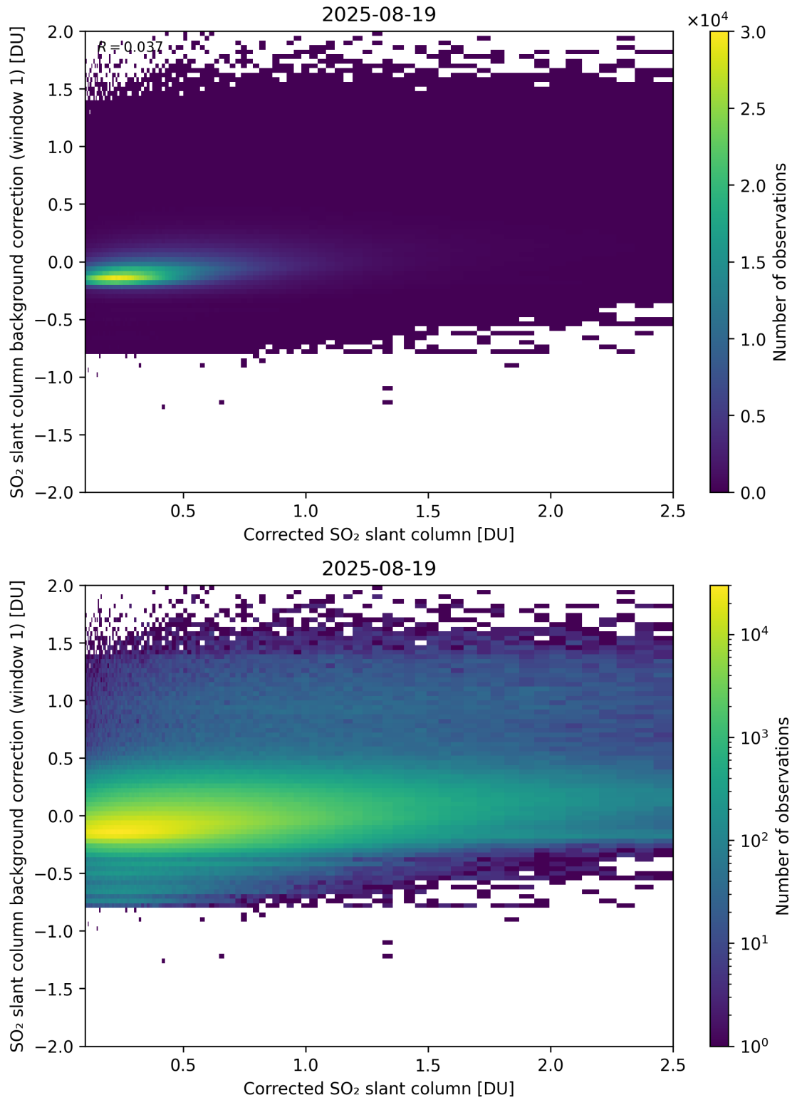
Figure 226: Scatter density plot of “Corrected SO 2 slant column” against “SO 2 slant column background correction (window 1)” for 2025-08-19 to 2025-08-20.
