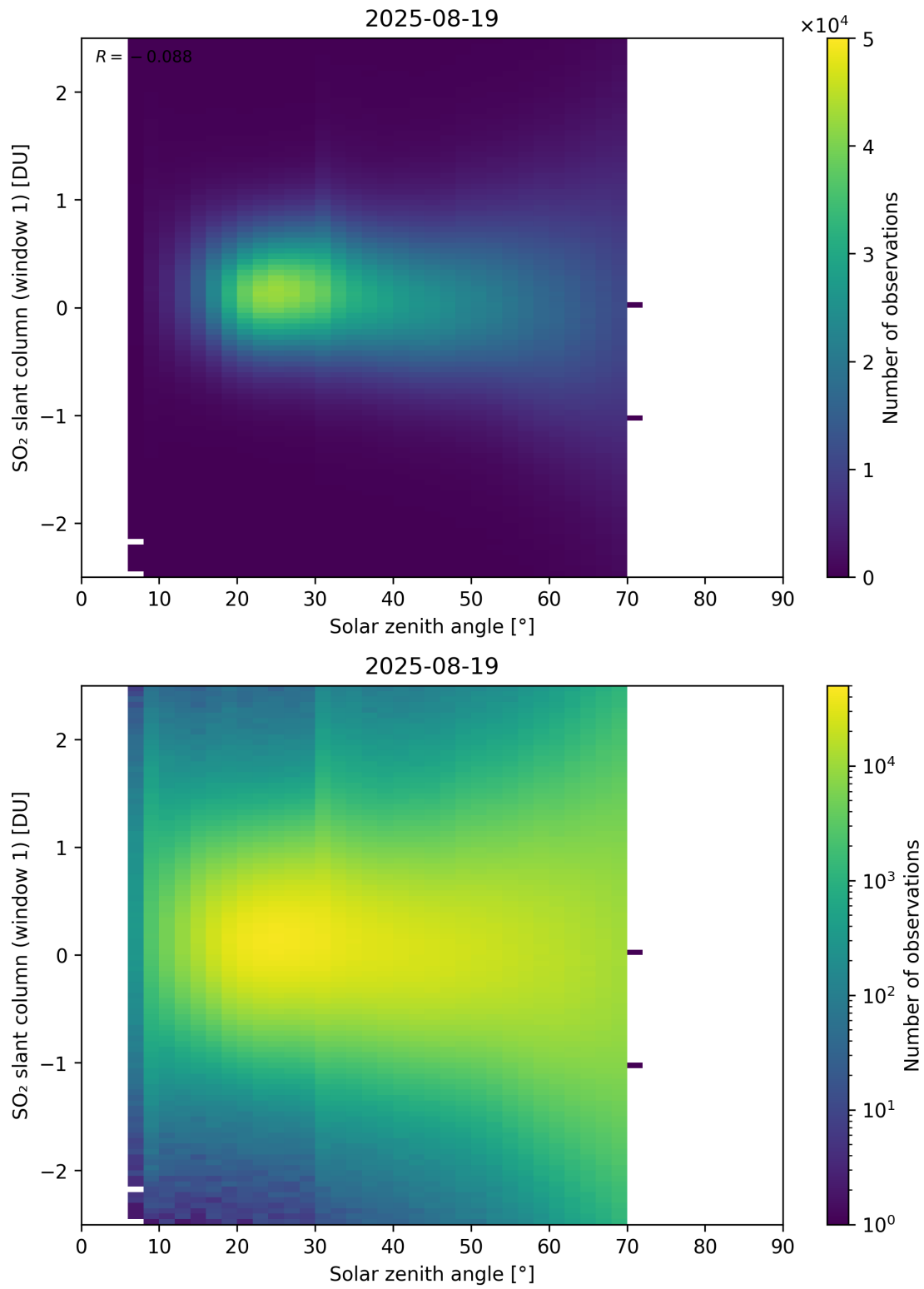
Figure 184: Scatter density plot of “Solar zenith angle” against “SO 2 slant column (window 1)” for 2025-08-19 to 2025-08-20.
