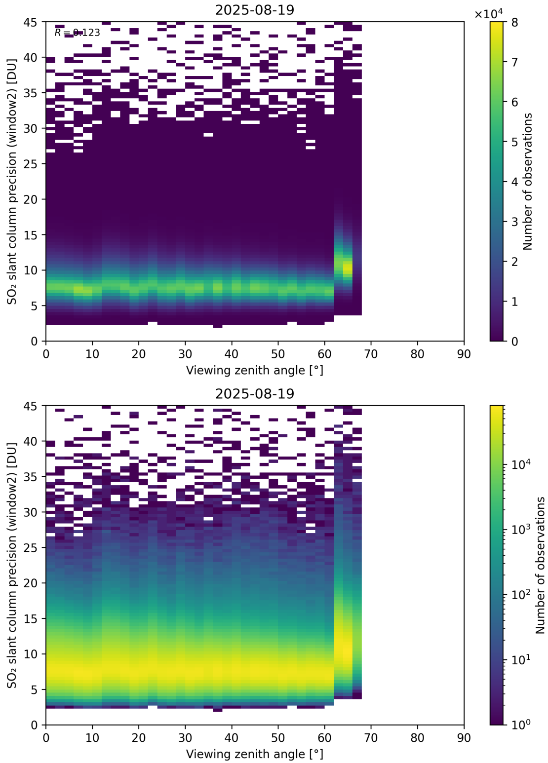
Figure 378: Scatter density plot of “Viewing zenith angle” against “SO 2 slant column precision (window2)” for 2025-08-19 to 2025-08-20.
