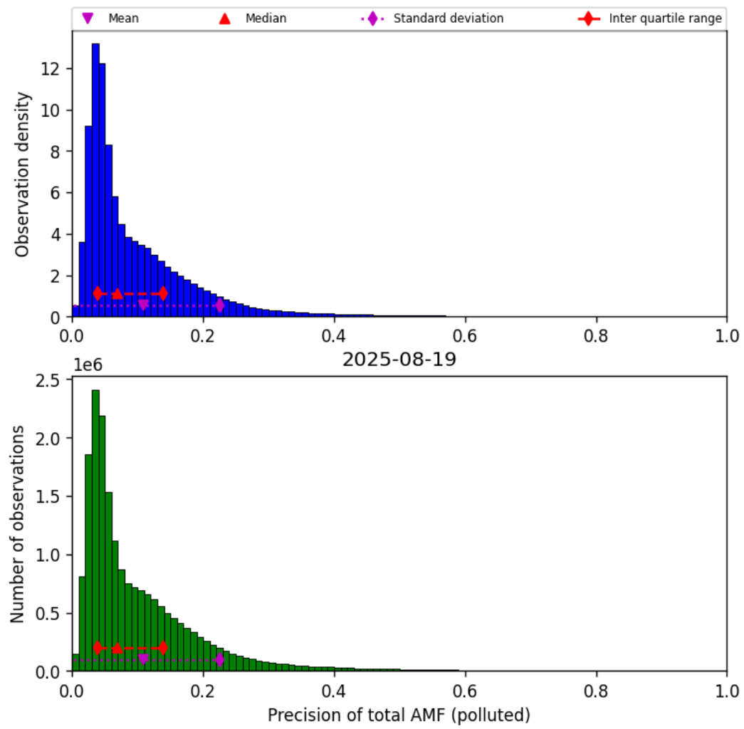
Figure 80: Histogram of “Precision of total AMF (polluted)” for 2025-08-19 to 2025-08-20
