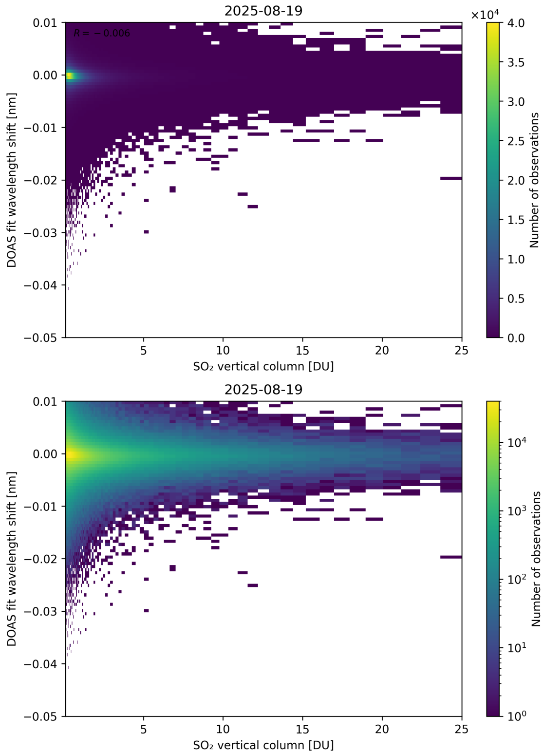
Figure 326: Scatter density plot of “SO 2 vertical column” against “DOAS fit wavelength shift” for 2025-08-19 to 2025-08-20.
