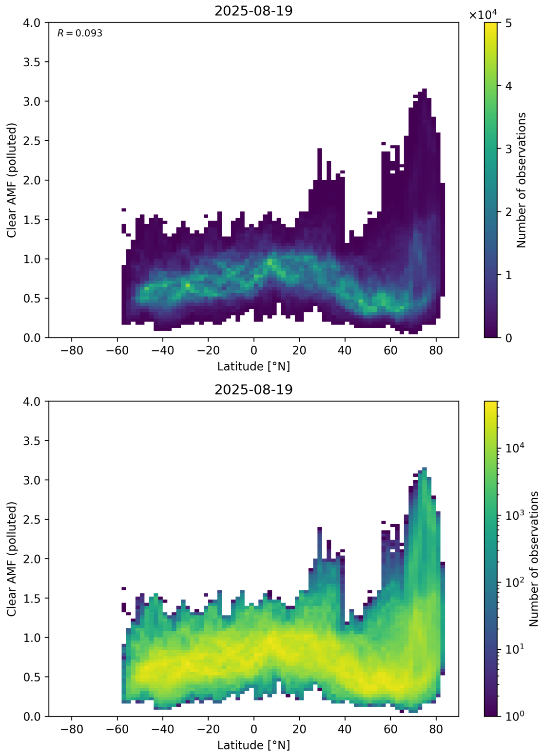
Figure 156: Scatter density plot of “Latitude” against “Clear AMF (polluted)” for 2025-08-19 to 2025-08-20.
