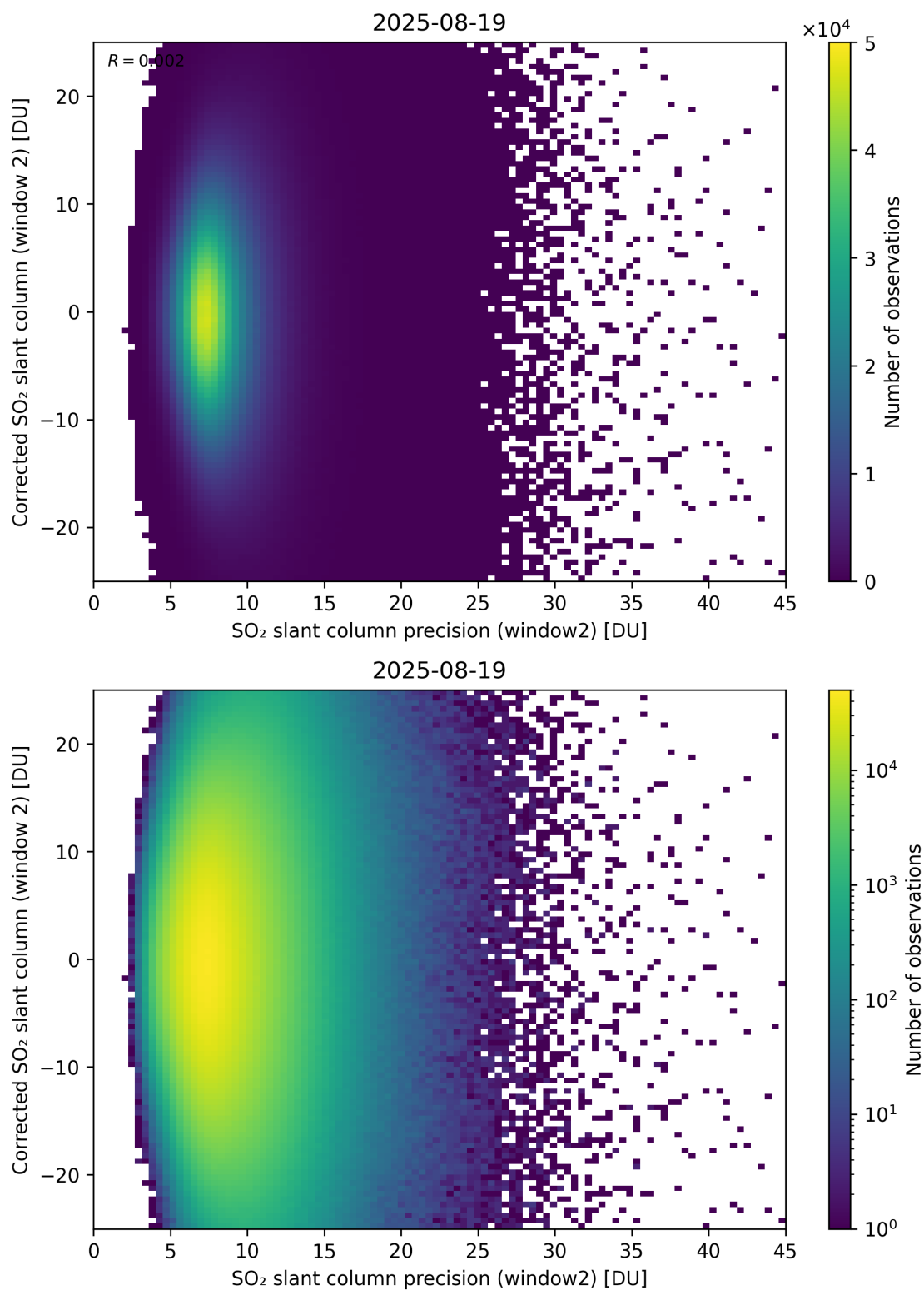
Figure 297: Scatter density plot of “SO 2 slant column precision (window2)” against “Corrected SO 2 slant column (window 2)” for 2025-08-19 to 2025-08-20.
