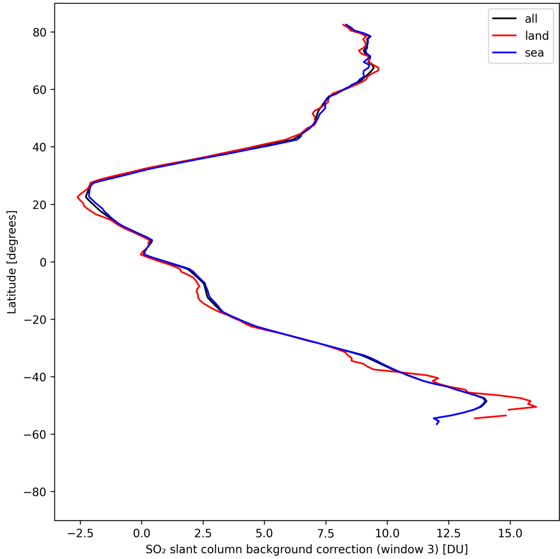
Figure 48: Zonal average of “SO 2 slant column background correction (window 3)” for 2025-08-19 to 2025-08-20.
