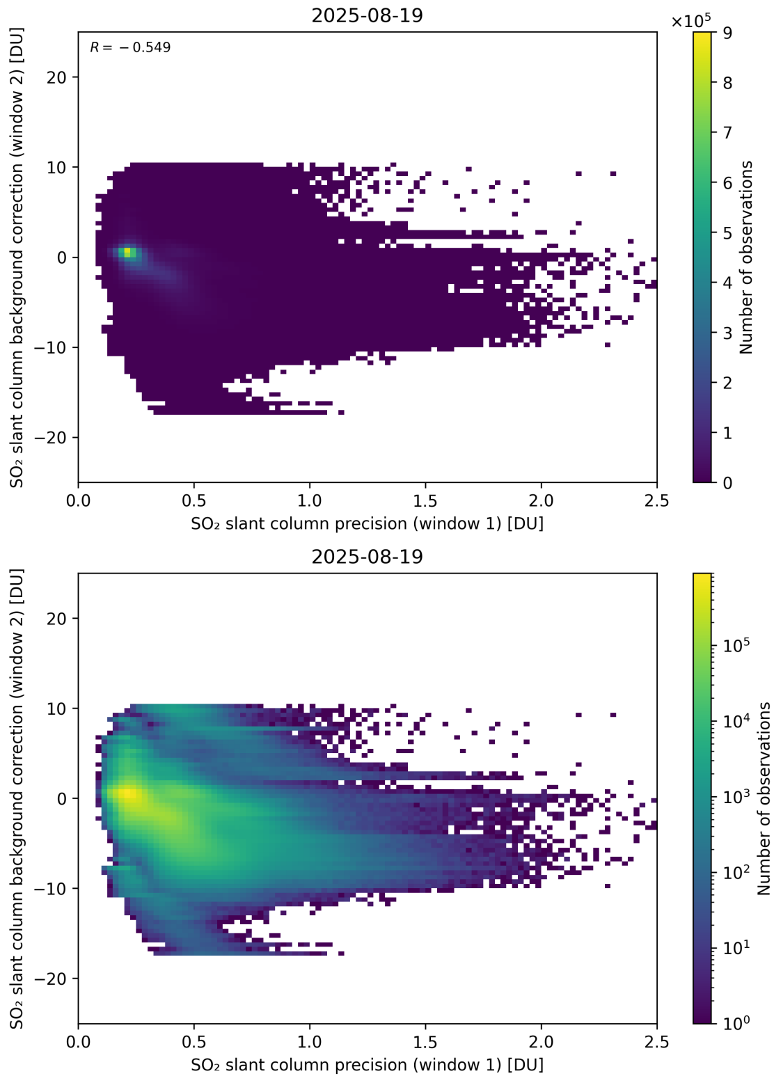
Figure 269: Scatter density plot of “SO 2 slant column precision (window 1)” against “SO 2 slant column background correction (window 2)” for 2025-08-19 to 2025-08-20.
