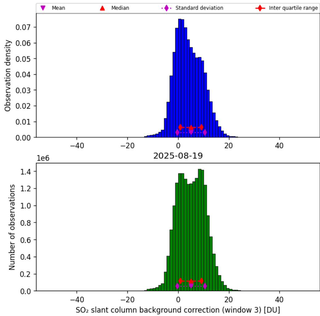
Figure 74: Histogram of “SO 2 slant column background correction (window 3)” for 2025-08-19 to 2025-08-20
