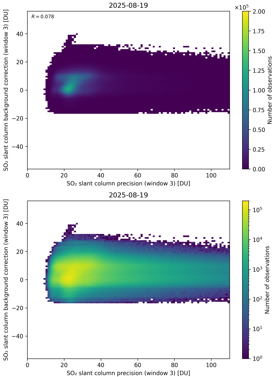
Figure 307: Scatter density plot of “SO 2 slant column precision (window 3)” against “SO 2 slant column background correction (window 3)” for 2025-08-19 to 2025-08-20.
