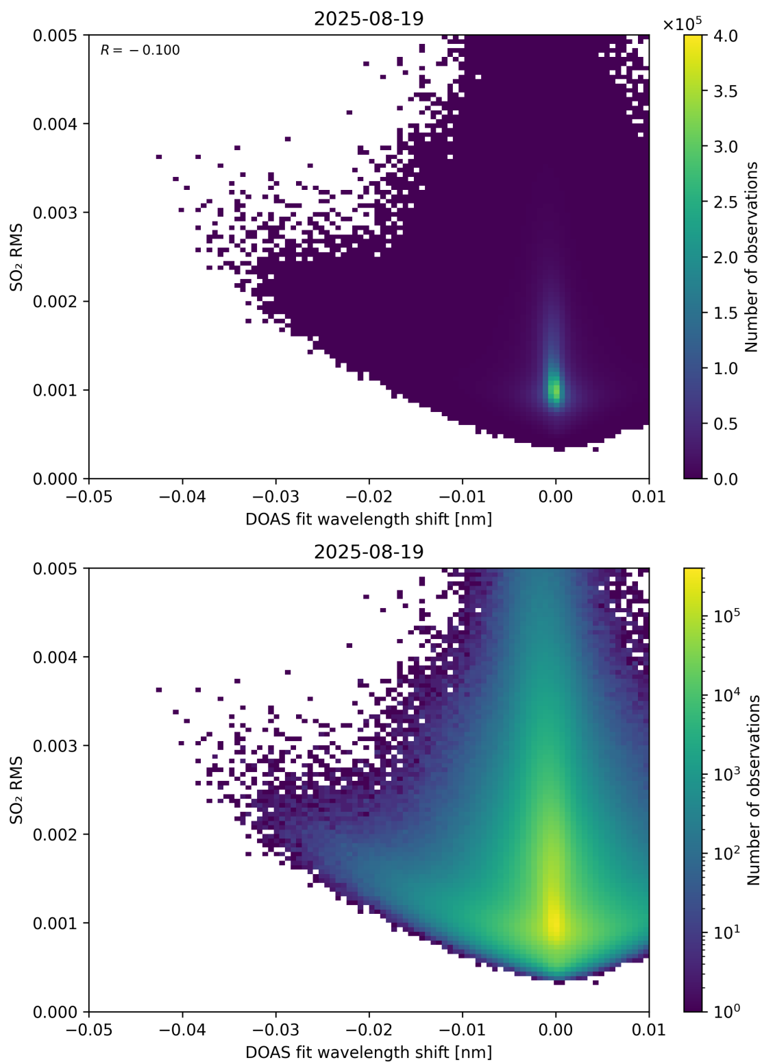
Figure 139: Scatter density plot of “DOAS fit wavelength shift” against “SO 2 RMS” for 2025-08-19 to 2025-08-20.
