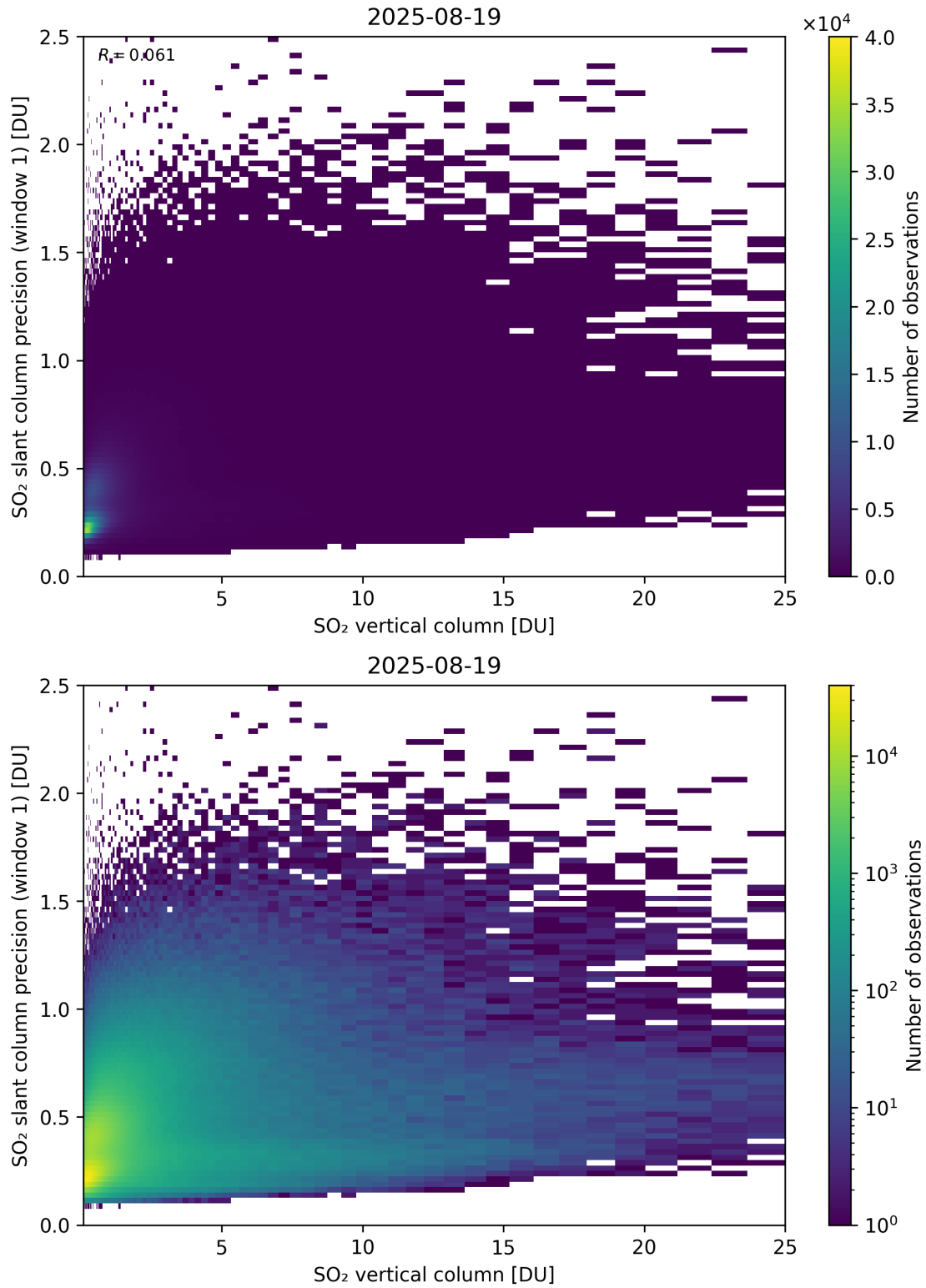
Figure 355: Scatter density plot of “SO 2 vertical column” against “SO 2 slant column precision (window 1)” for 2025-08-19 to 2025-08-20.
