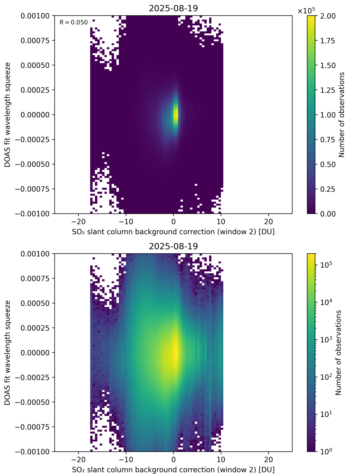
Figure 124: Scatter density plot of “SO 2 slant column background correction (window 2)” against “DOAS fit wavelength squeeze” for 2025-08-19 to 2025-08-20.
