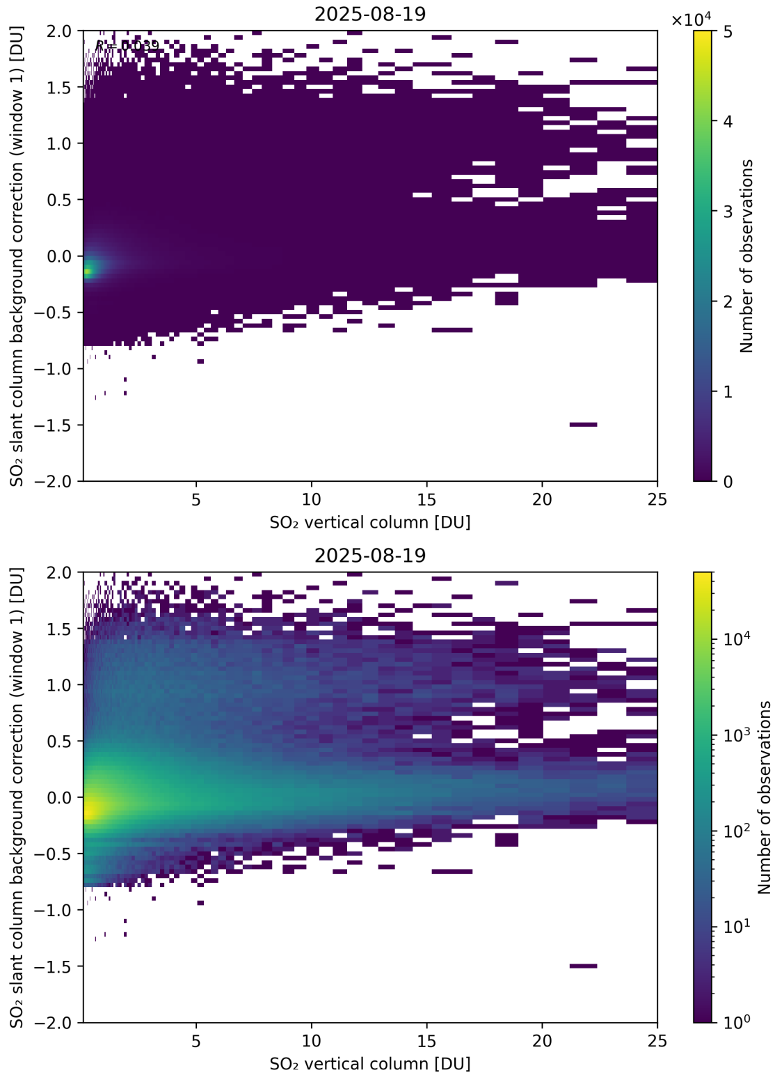
Figure 323: Scatter density plot of “SO 2 vertical column” against “SO 2 slant column background correction (window 1)” for 2025-08-19 to 2025-08-20.
