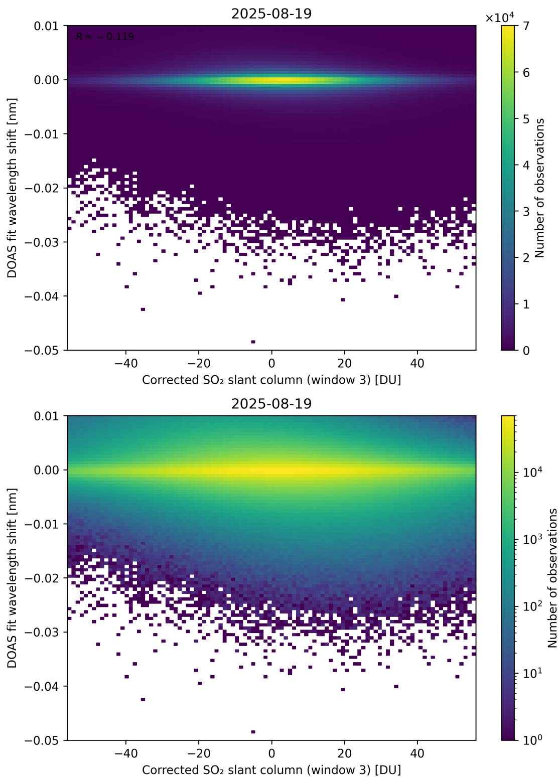
Figure 256: Scatter density plot of “Corrected SO 2 slant column (window 3)” against “DOAS fit wavelength shift” for 2025-08-19 to 2025-08-20.
