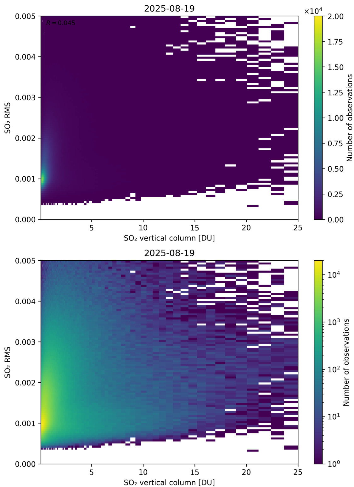
Figure 328: Scatter density plot of “SO 2 vertical column” against “SO 2 RMS” for 2025-08-19 to 2025-08-20.
