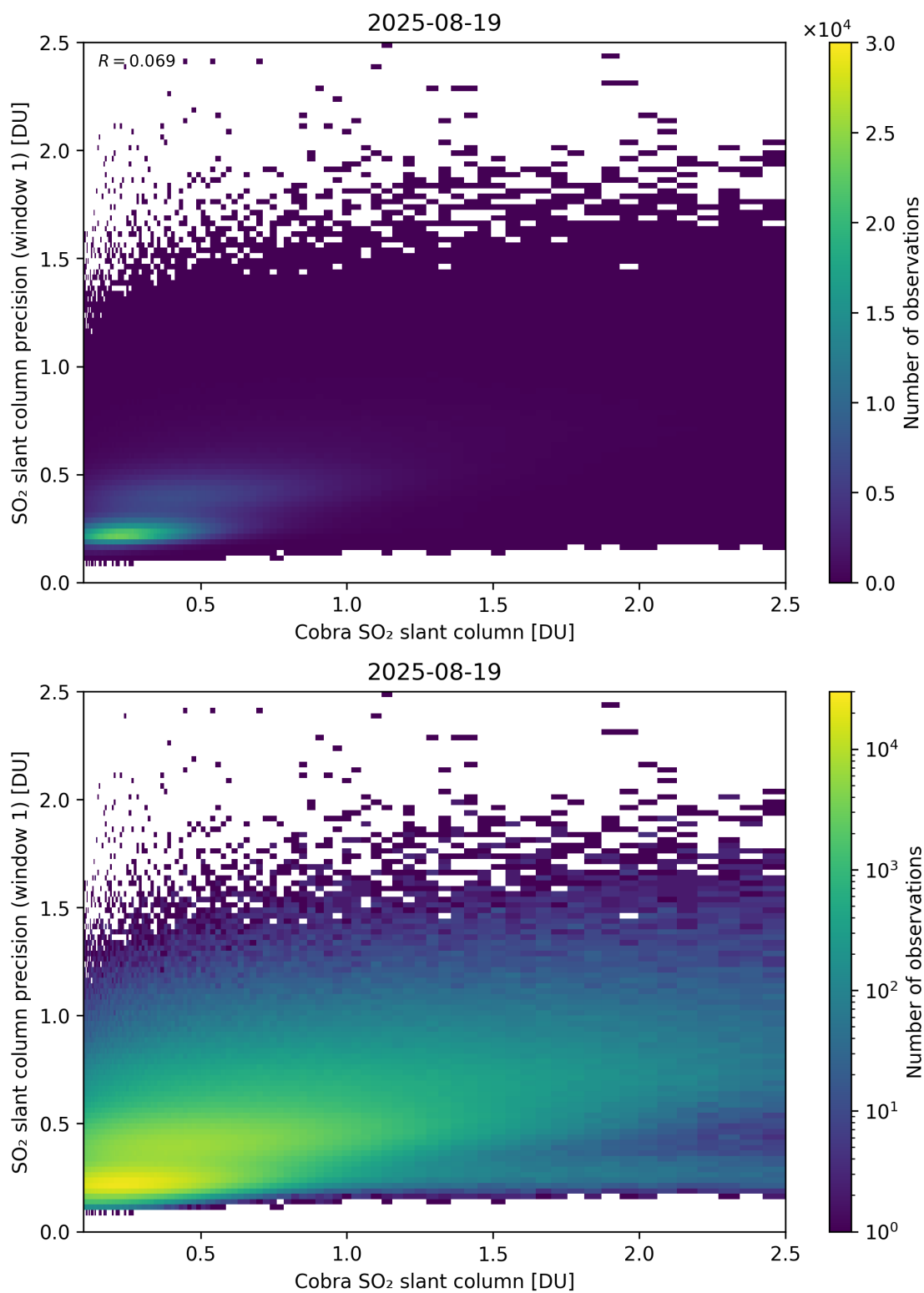
Figure 220: Scatter density plot of “Cobra SO 2 slant column” against “SO 2 slant column precision (window 1)” for 2025-08-19 to 2025-08-20.
