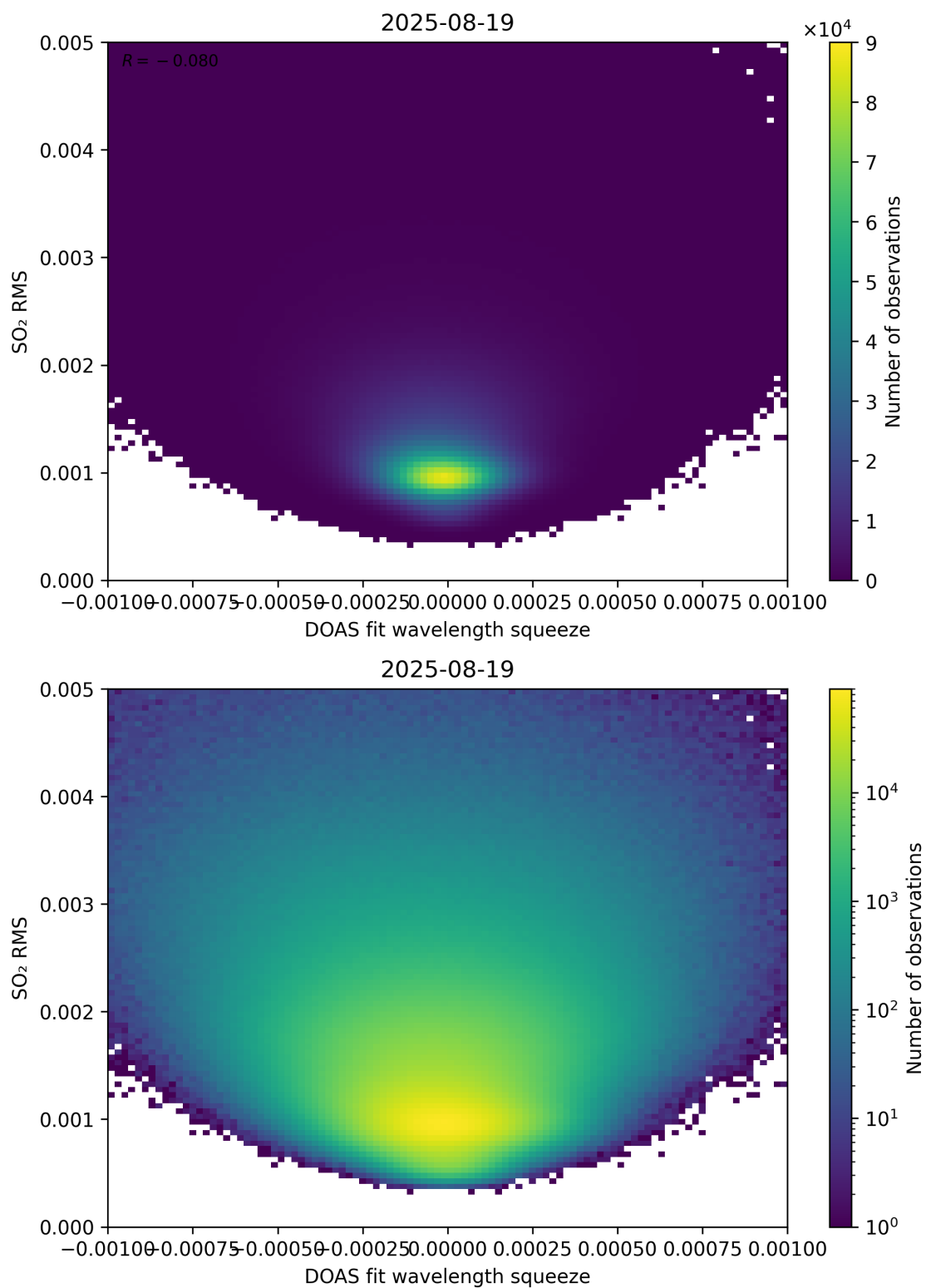
Figure 143: Scatter density plot of “DOAS fit wavelength squeeze” against “SO 2 RMS” for 2025-08-19 to 2025-08-20.
