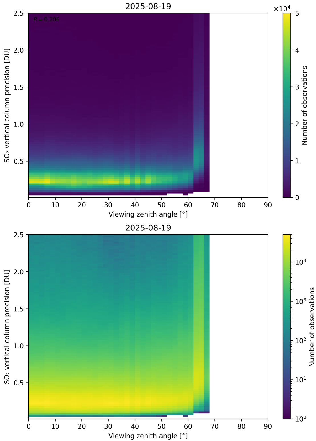
Figure 384: Scatter density plot of “Viewing zenith angle” against “SO 2 vertical column precision” for 2025-08-19 to 2025-08-20.
