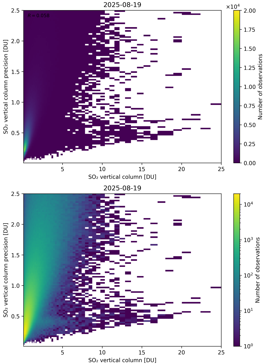
Figure 361: Scatter density plot of “SO 2 vertical column” against “SO 2 vertical column precision” for 2025-08-19 to 2025-08-20.
