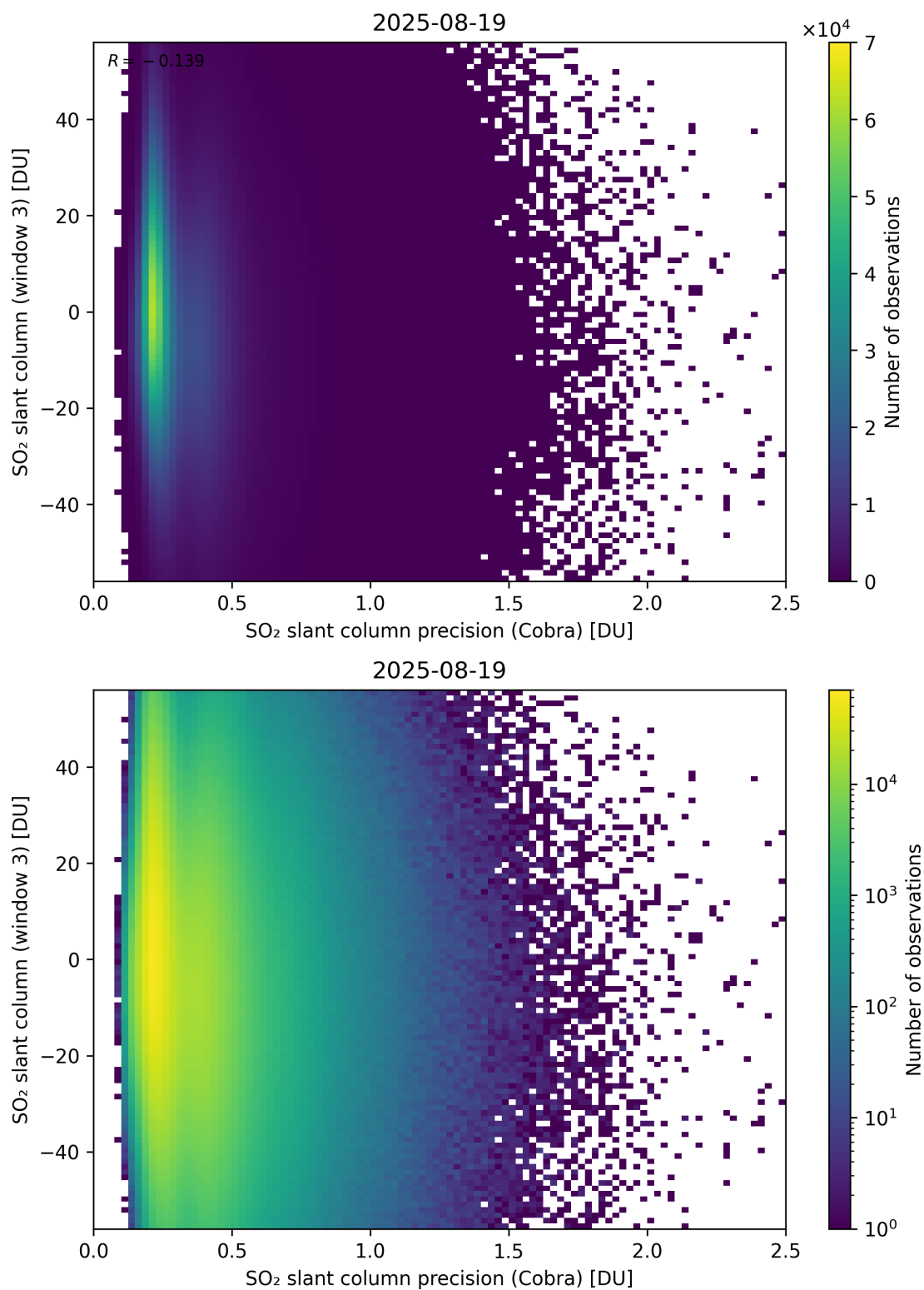
Figure 211: Scatter density plot of “SO 2 slant column precision (Cobra)” against “SO 2 slant column (window 3)” for 2025-08-19 to 2025-08-20.
