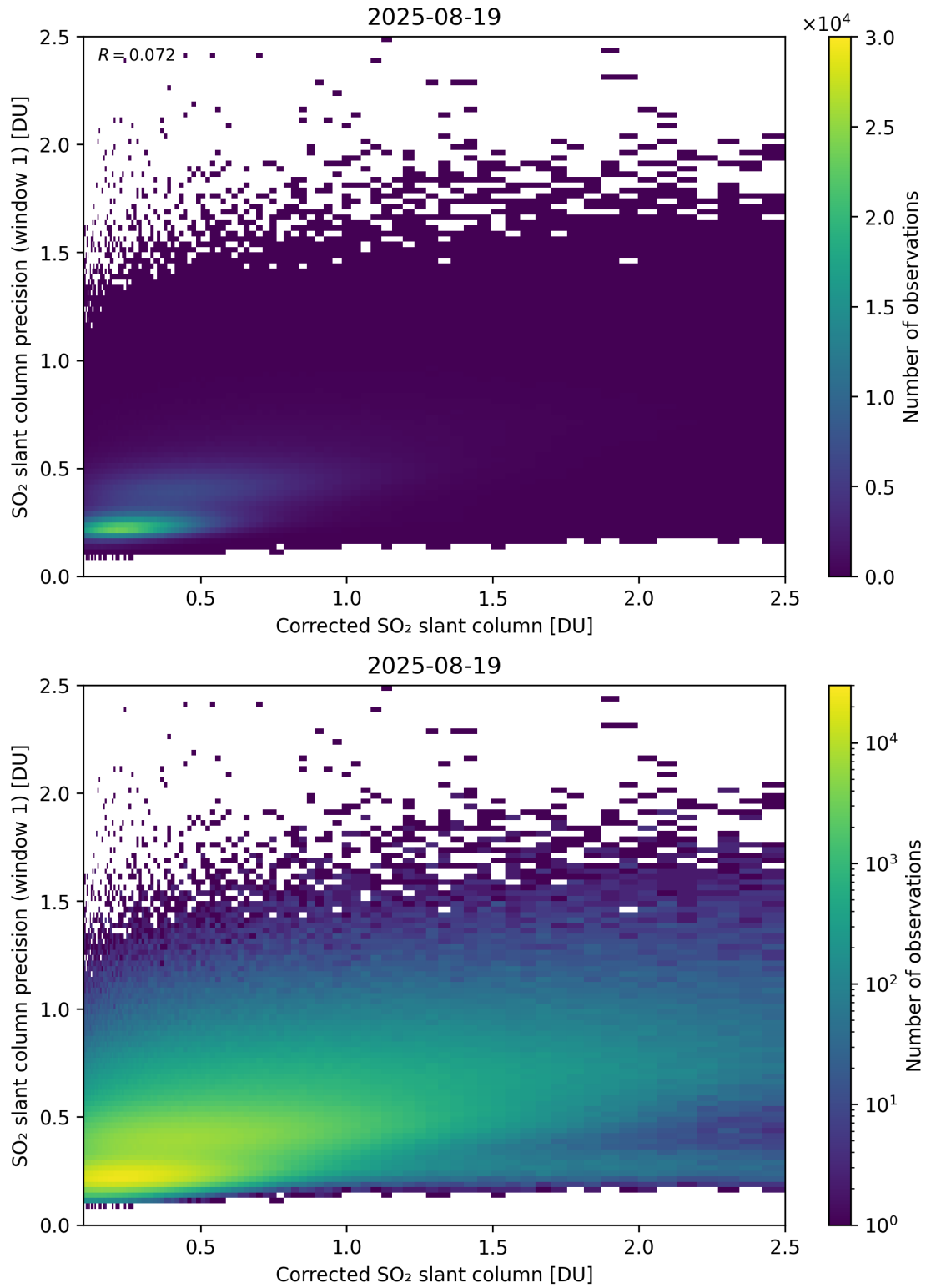
Figure 238: Scatter density plot of “Corrected SO 2 slant column” against “SO 2 slant column precision (window 1)” for 2025-08-19 to 2025-08-20.
