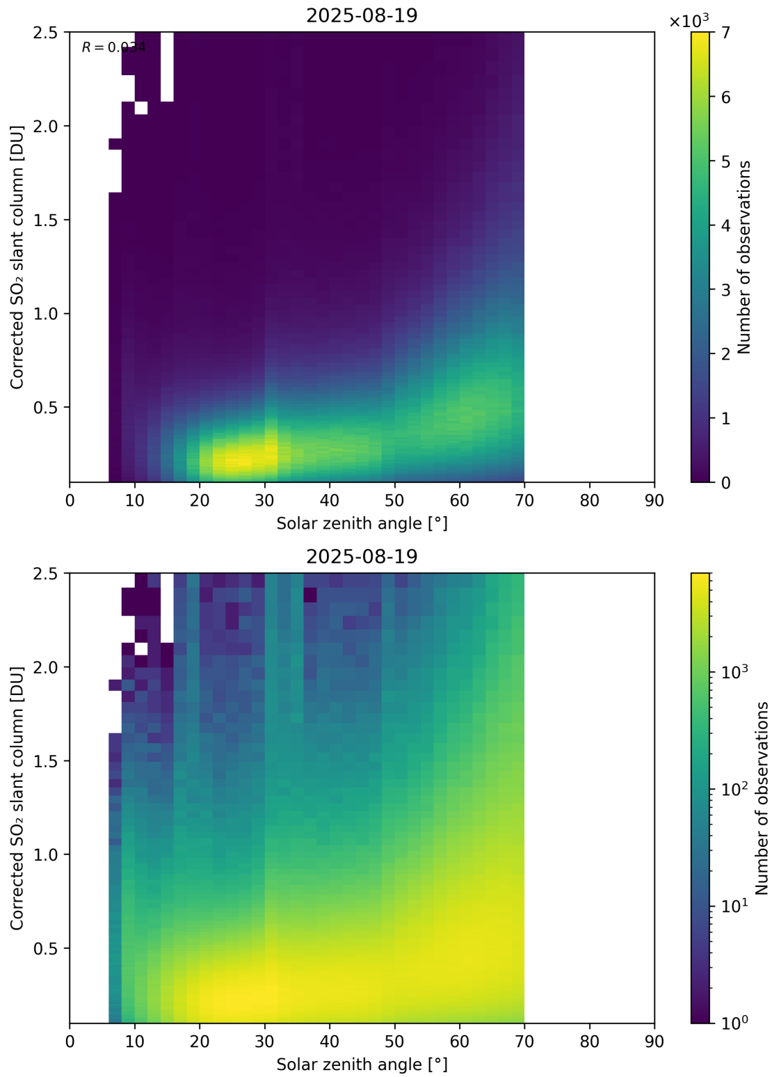
Figure 181: Scatter density plot of “Solar zenith angle” against “Corrected SO 2 slant column” for 2025-08-19 to 2025-08-20.
