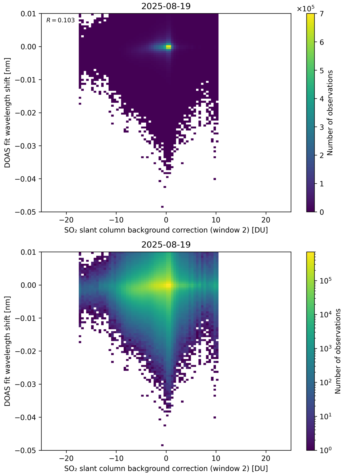
Figure 123: Scatter density plot of “SO 2 slant column background correction (window 2)” against “DOAS fit wavelength shift” for 2025-08-19 to 2025-08-20.
