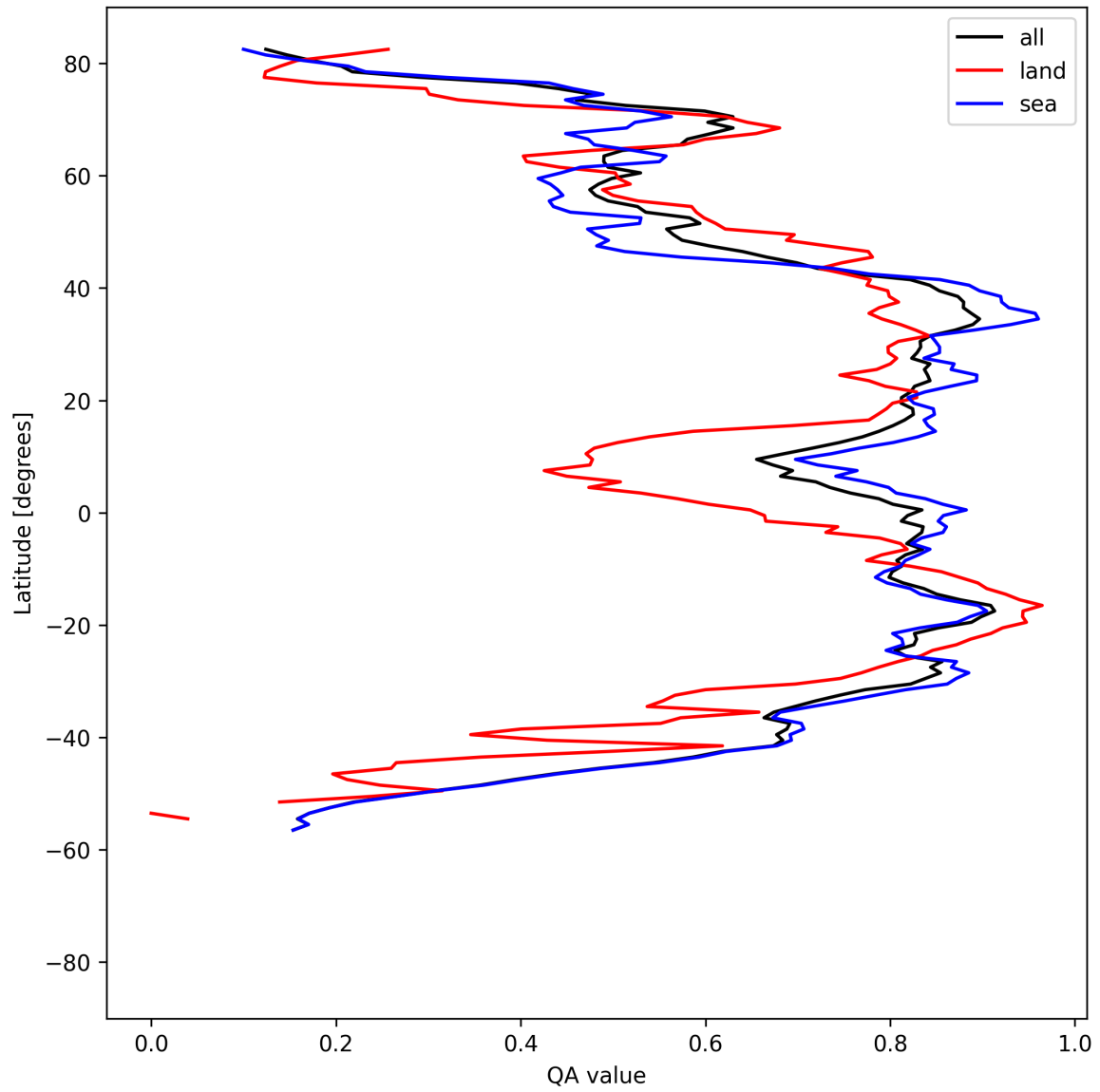
Figure 31: Zonal average of “QA value” for 2025-08-19 to 2025-08-20.
