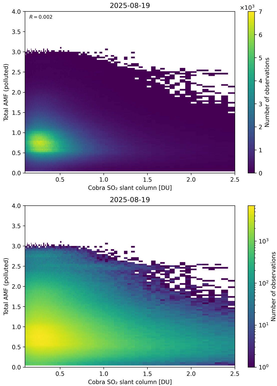
Figure 224: Scatter density plot of “Cobra SO 2 slant column” against “Total AMF (polluted)” for 2025-08-19 to 2025-08-20.
