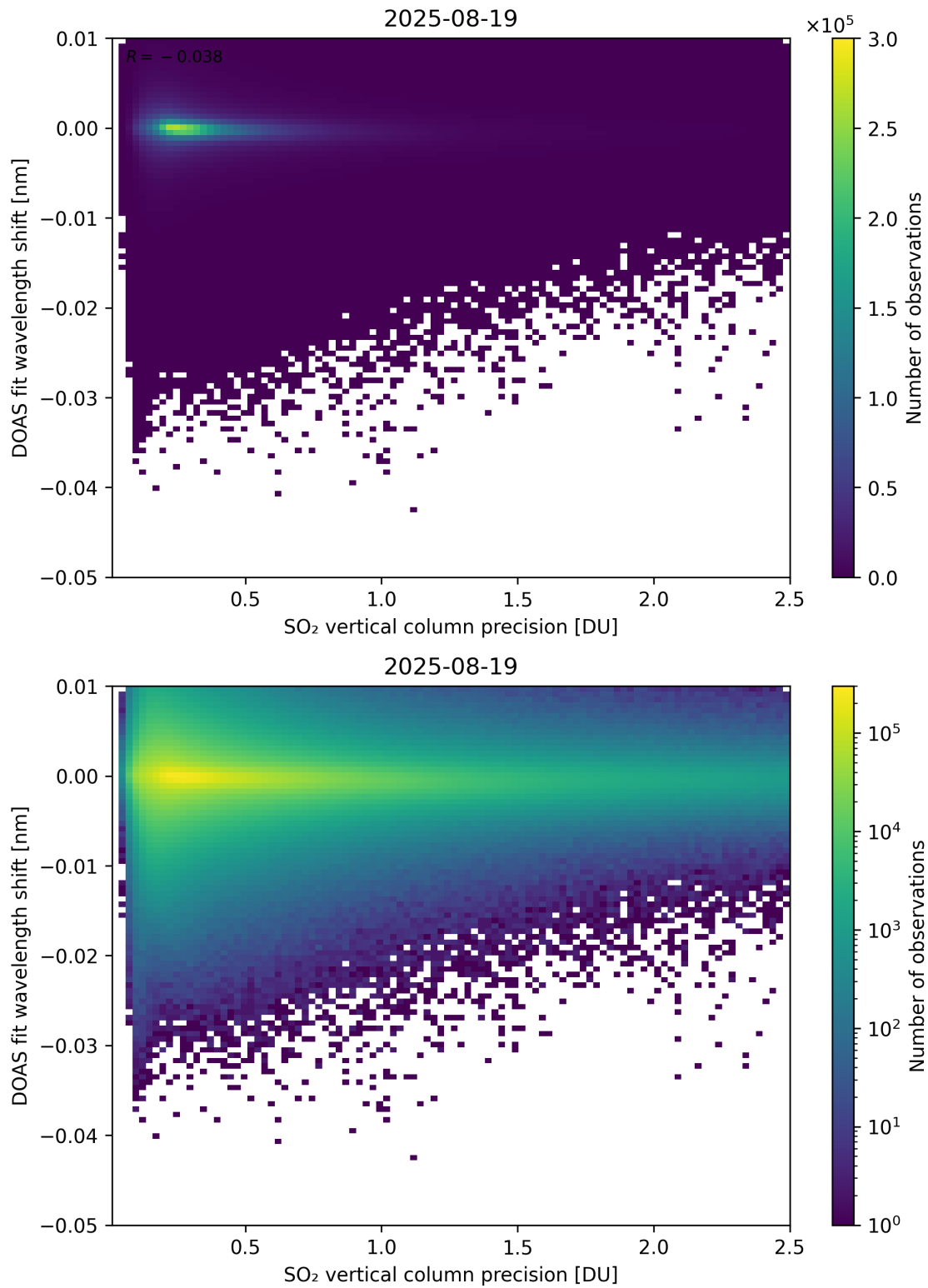
Figure 332: Scatter density plot of “SO 2 vertical column precision” against “DOAS fit wavelength shift” for 2025-08-19 to 2025-08-20.
