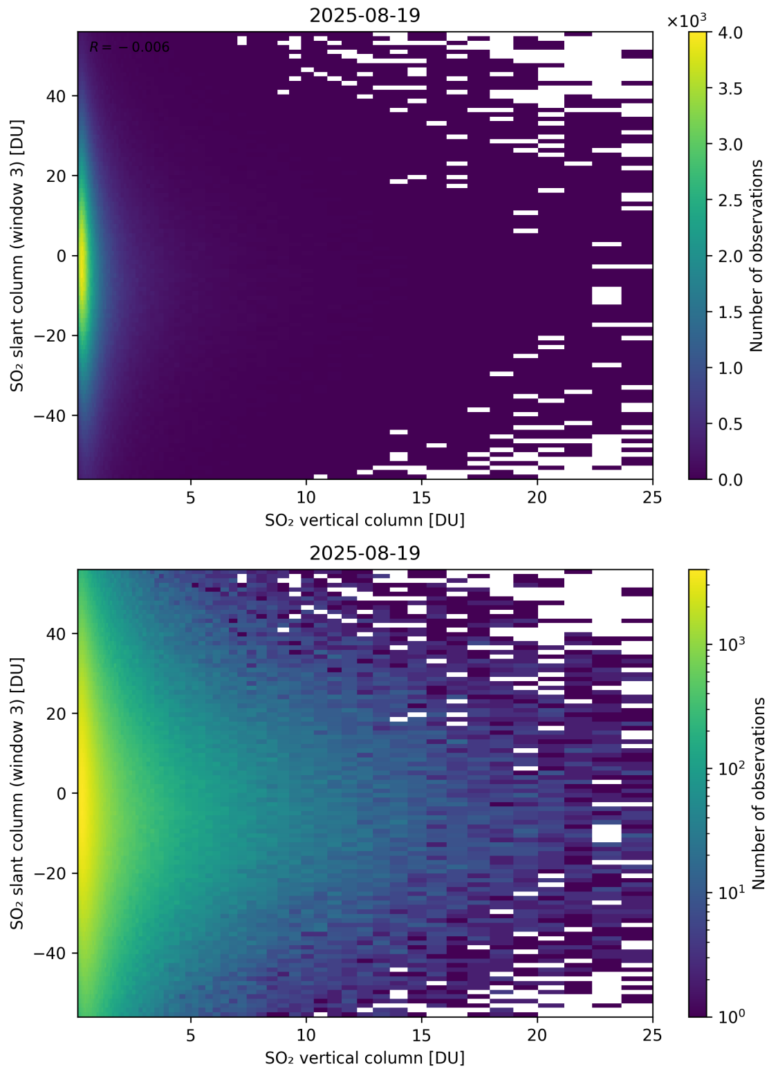
Figure 357: Scatter density plot of “SO 2 vertical column” against “SO 2 slant column (window 3)” for 2025-08-19 to 2025-08-20.
