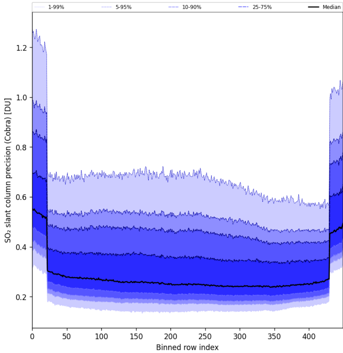
Figure 88: Along track statistics of “SO 2 slant column precision (Cobra)” for 2025-08-19 to 2025-08-20
