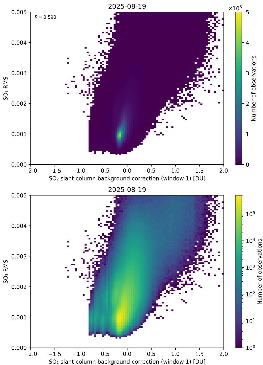
Figure 113: Scatter density plot of “SO 2 slant column background correction (window 1)” against “SO 2 RMS” for 2025-08-19 to 2025-08-20.
