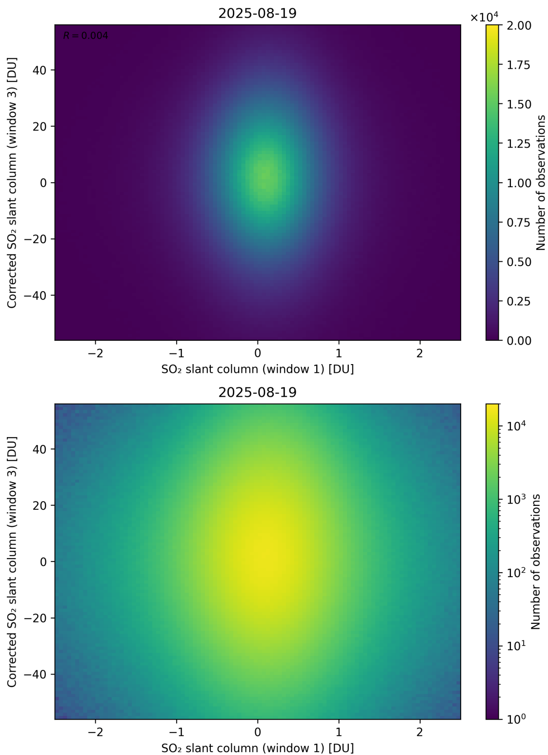
Figure 284: Scatter density plot of “SO 2 slant column (window 1)” against “Corrected SO 2 slant column (window 3)” for 2025-08-19 to 2025-08-20.
