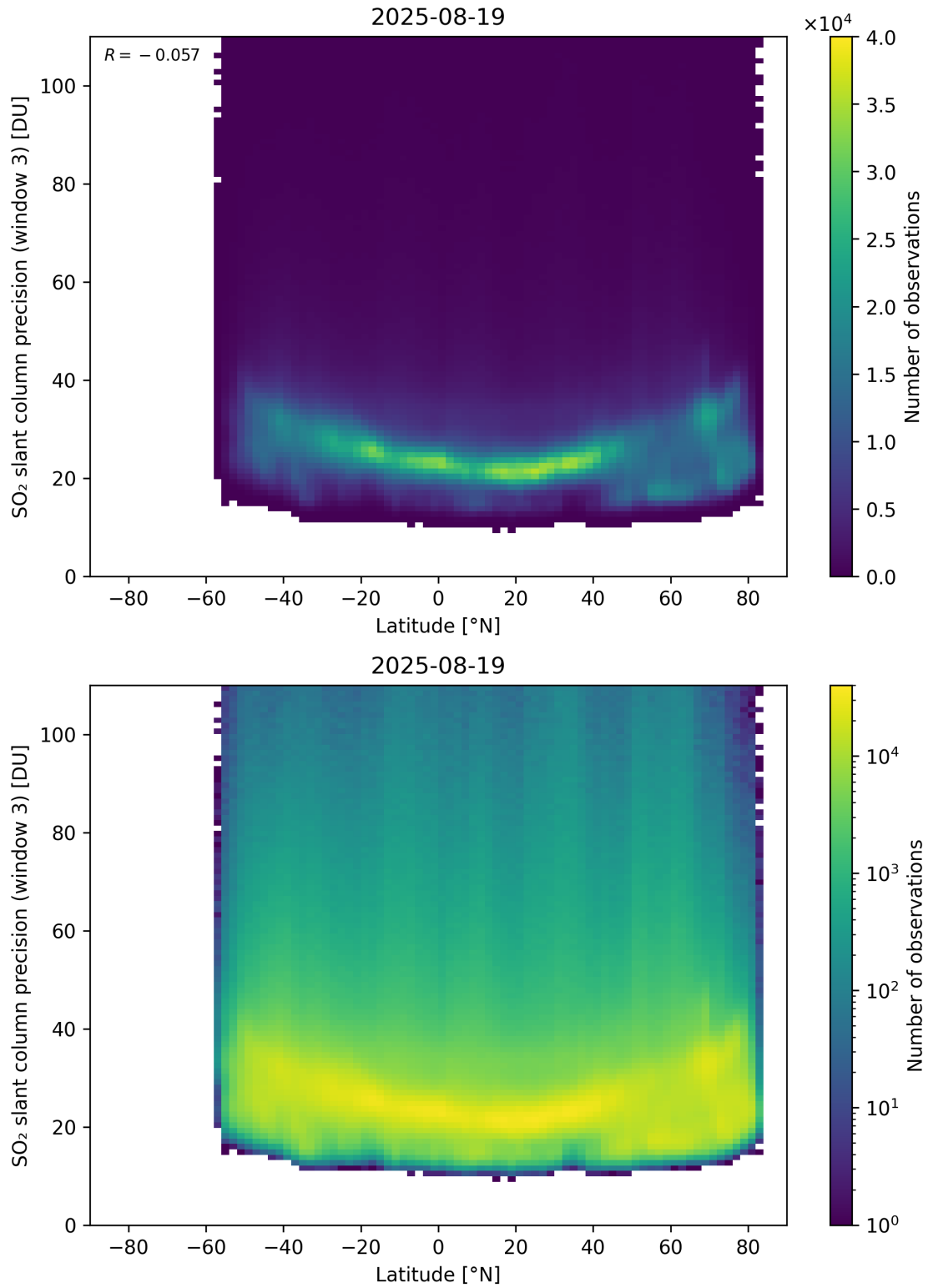
Figure 166: Scatter density plot of “Latitude” against “SO 2 slant column precision (window 3)” for 2025-08-19 to 2025-08-20.
