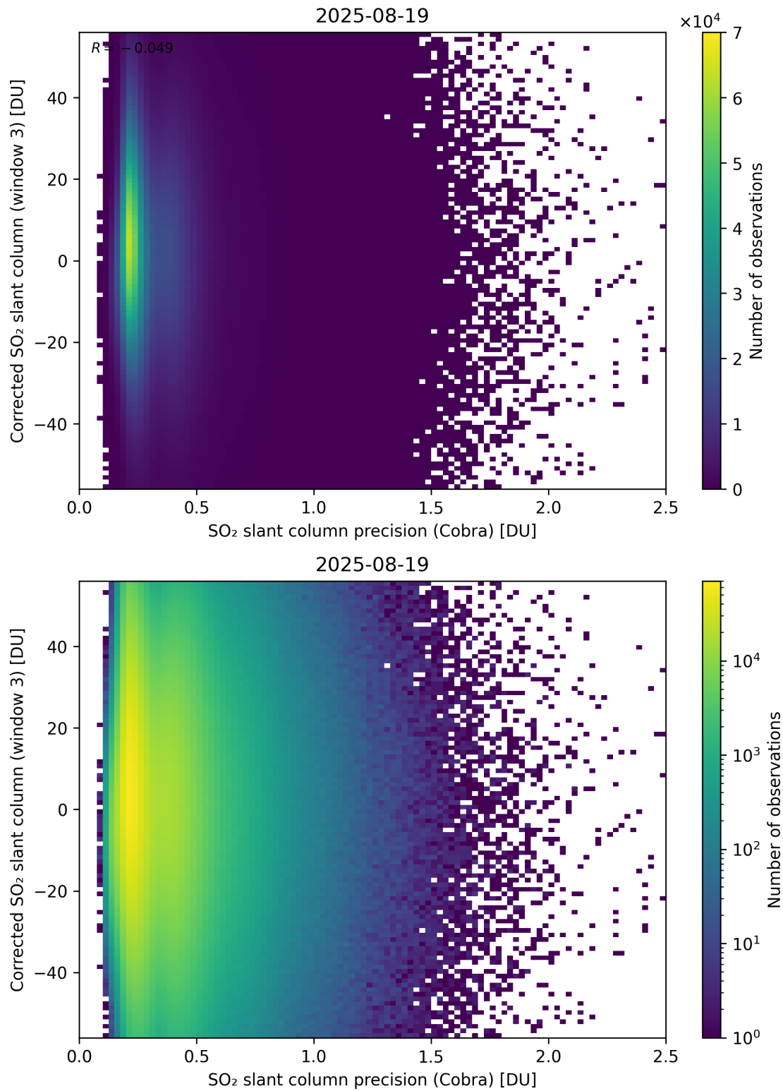
Figure 207: Scatter density plot of “SO 2 slant column precision (Cobra)” against “Corrected SO 2 slant column (window 3)” for 2025-08-19 to 2025-08-20.
