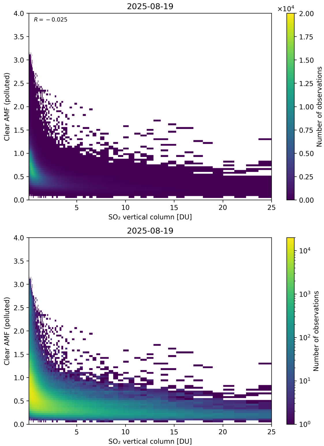
Figure 348: Scatter density plot of “SO 2 vertical column” against “Clear AMF (polluted)” for 2025-08-19 to 2025-08-20.
