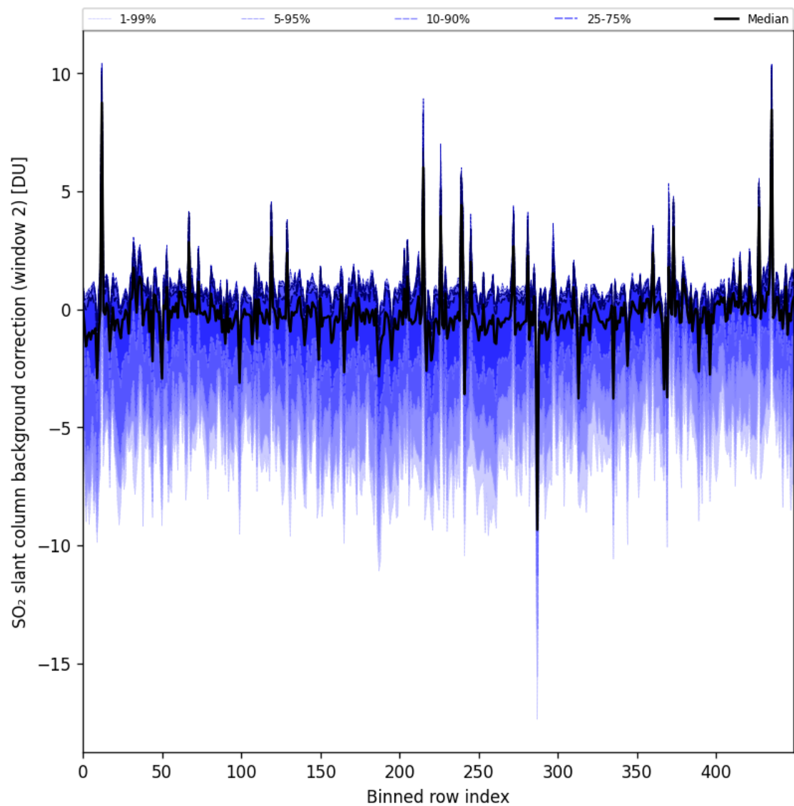
Figure 96: Along track statistics of “SO 2 slant column background correction (window 2)” for 2025-08-19 to 2025-08-20
