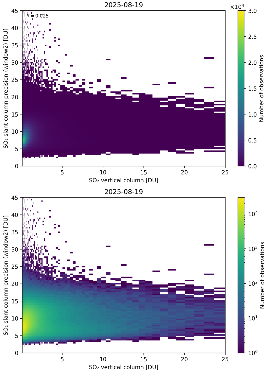
Figure 356: Scatter density plot of “SO 2 vertical column” against “SO 2 slant column precision (window2)” for 2025-08-19 to 2025-08-20.
