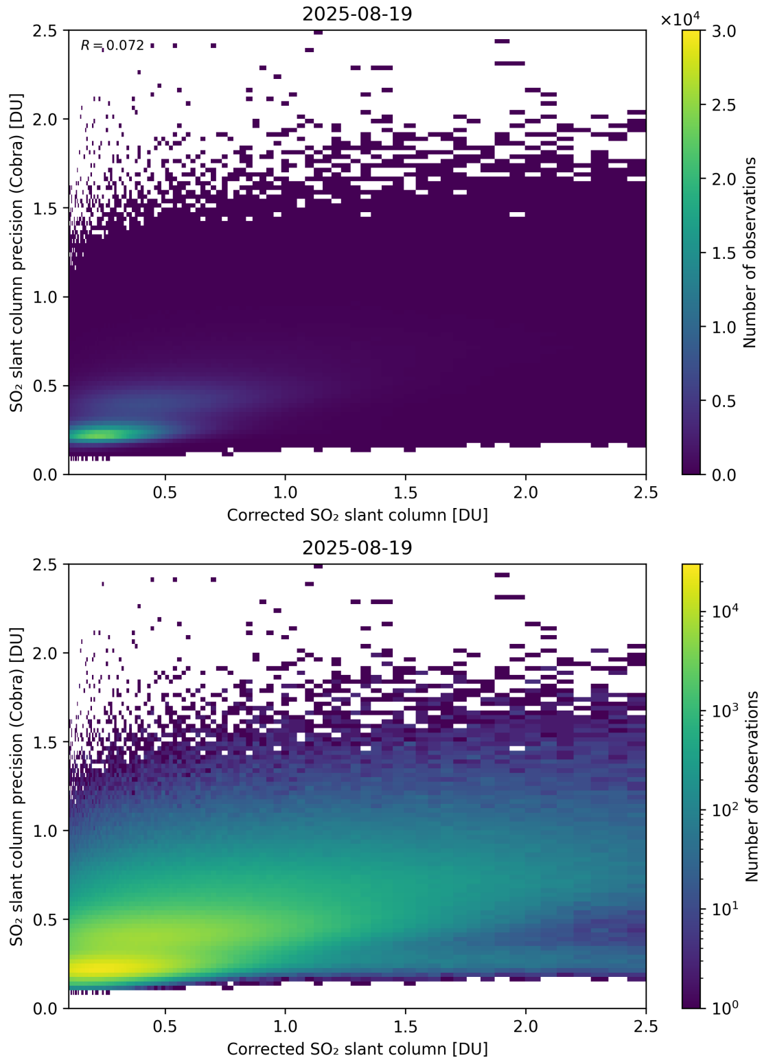
Figure 234: Scatter density plot of “Corrected SO 2 slant column” against “SO 2 slant column precision (Cobra)” for 2025-08-19 to 2025-08-20.
