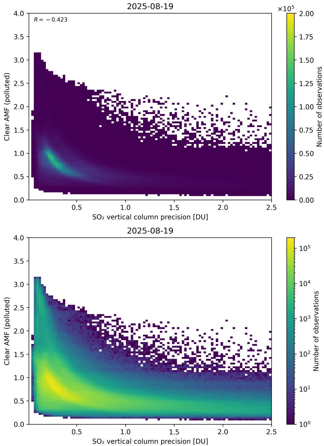
Figure 335: Scatter density plot of “SO 2 vertical column precision” against “Clear AMF (polluted)” for 2025-08-19 to 2025-08-20.
