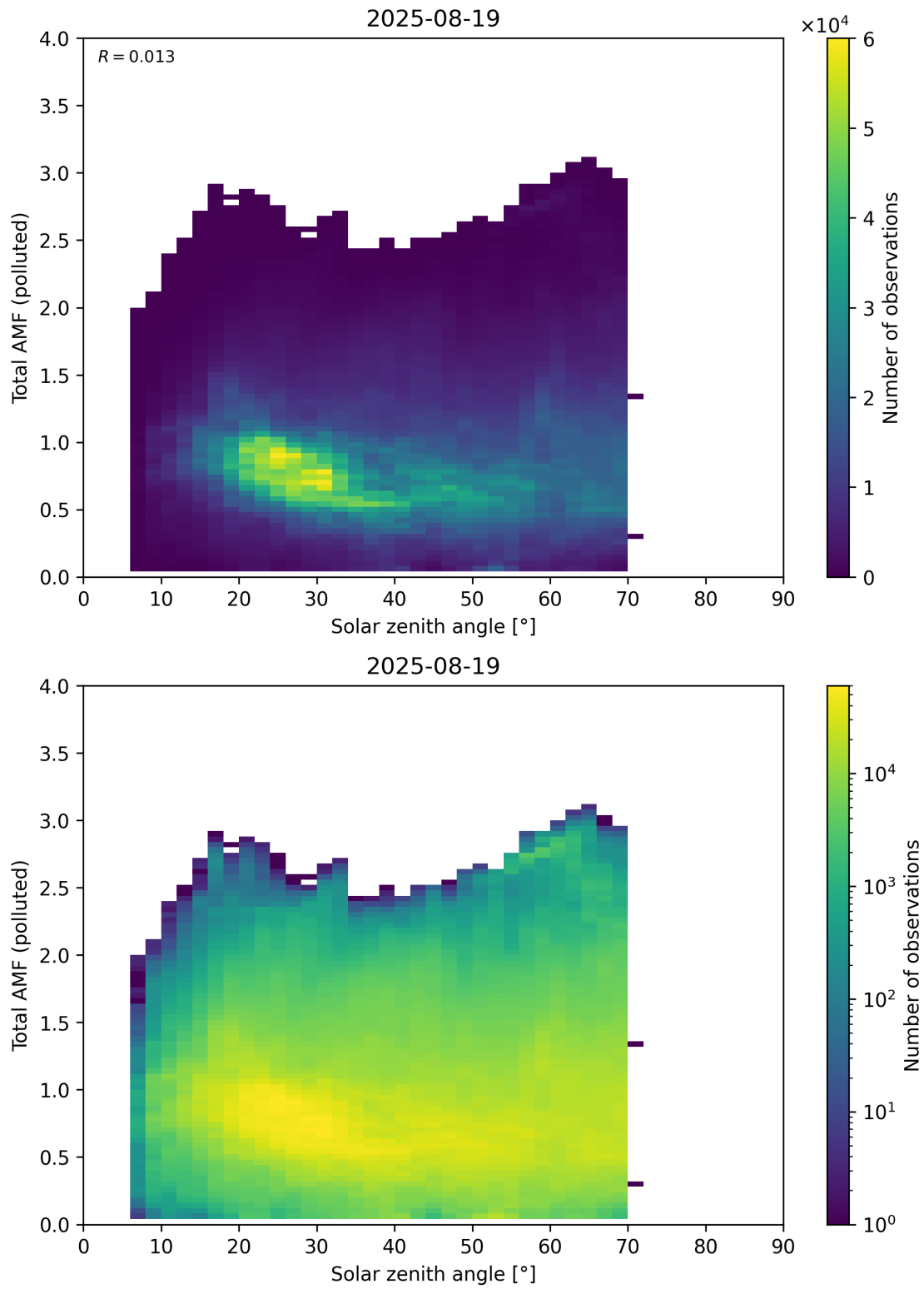
Figure 189: Scatter density plot of “Solar zenith angle” against “Total AMF (polluted)” for 2025-08-19 to 2025-08-20.
