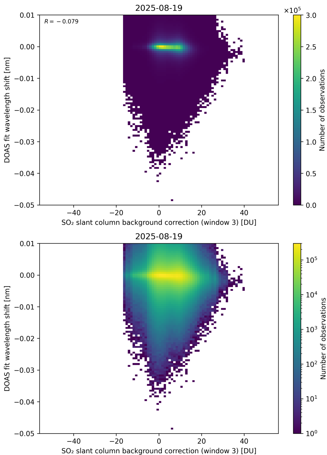
Figure 132: Scatter density plot of “SO 2 slant column background correction (window 3)” against “DOAS fit wavelength shift” for 2025-08-19 to 2025-08-20.
