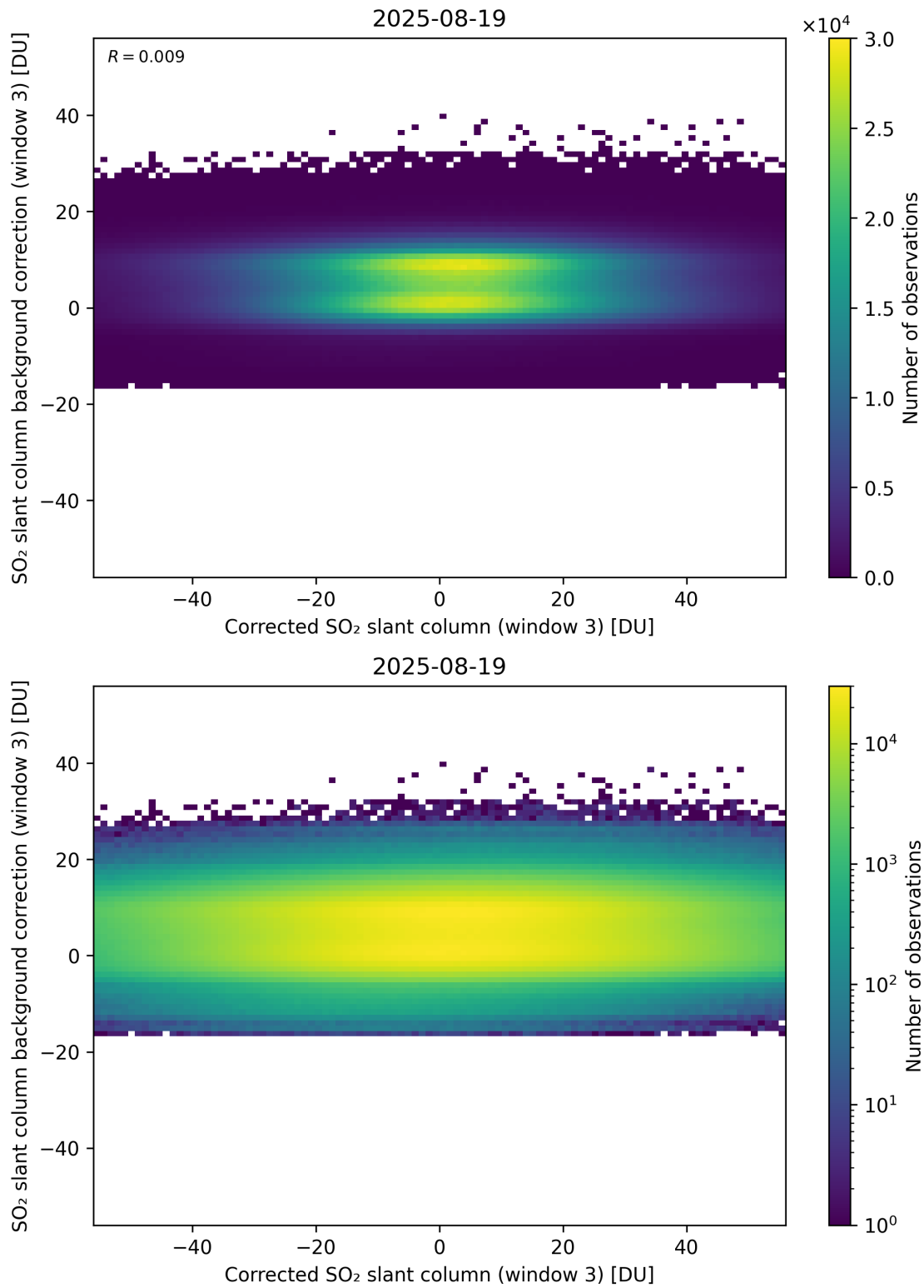
Figure 255: Scatter density plot of “Corrected SO 2 slant column (window 3)” against “SO 2 slant column background correction (window 3)” for 2025-08-19 to 2025-08-20.
