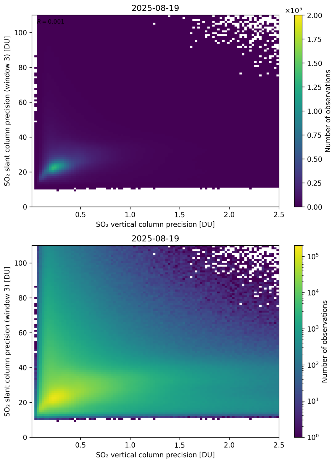
Figure 345: Scatter density plot of “SO 2 vertical column precision” against “SO 2 slant column precision (window 3)” for 2025-08-19 to 2025-08-20.
