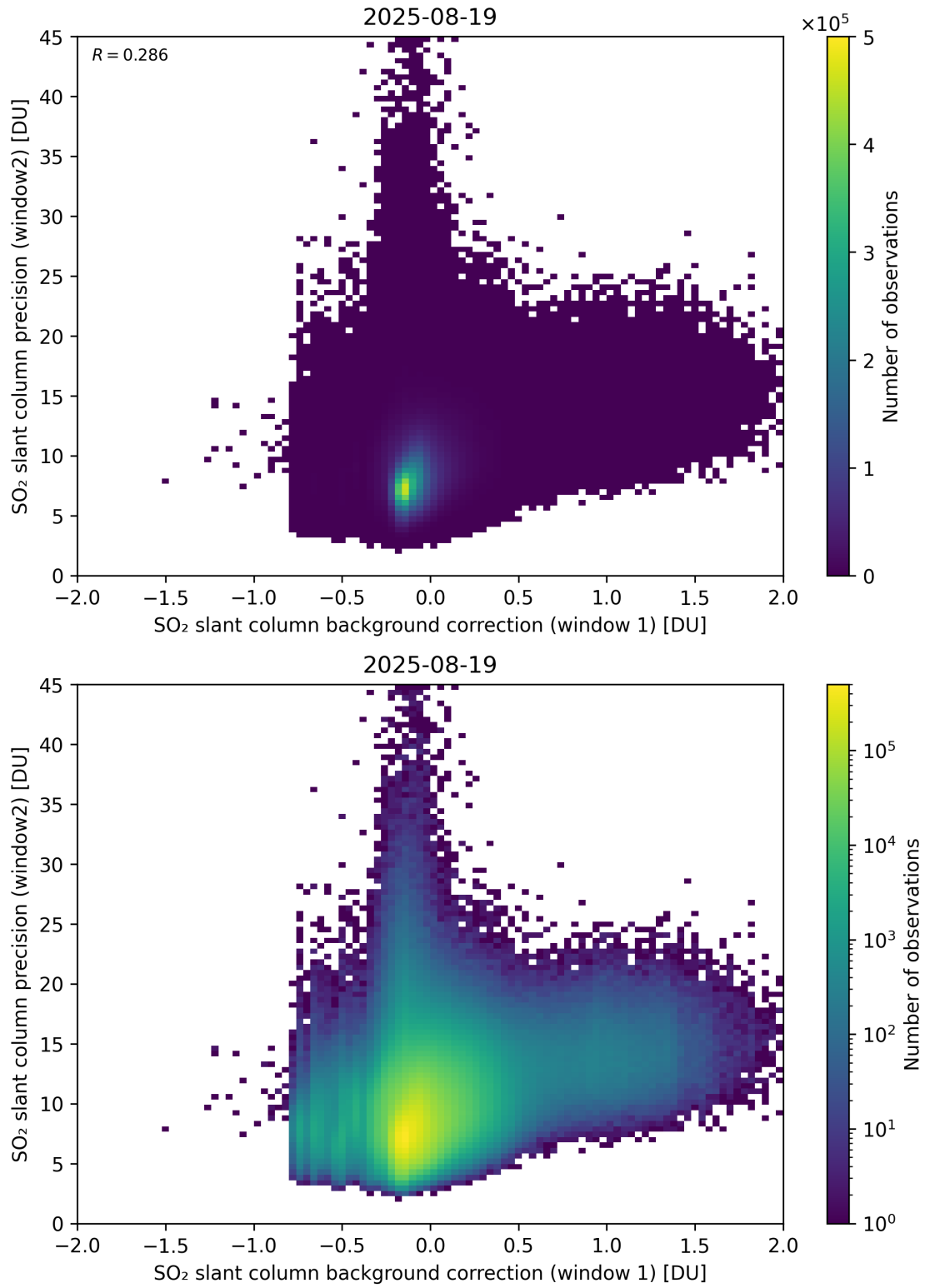
Figure 117: Scatter density plot of “SO 2 slant column background correction (window 1)” against “SO 2 slant column precision (window2)” for 2025-08-19 to 2025-08-20.
