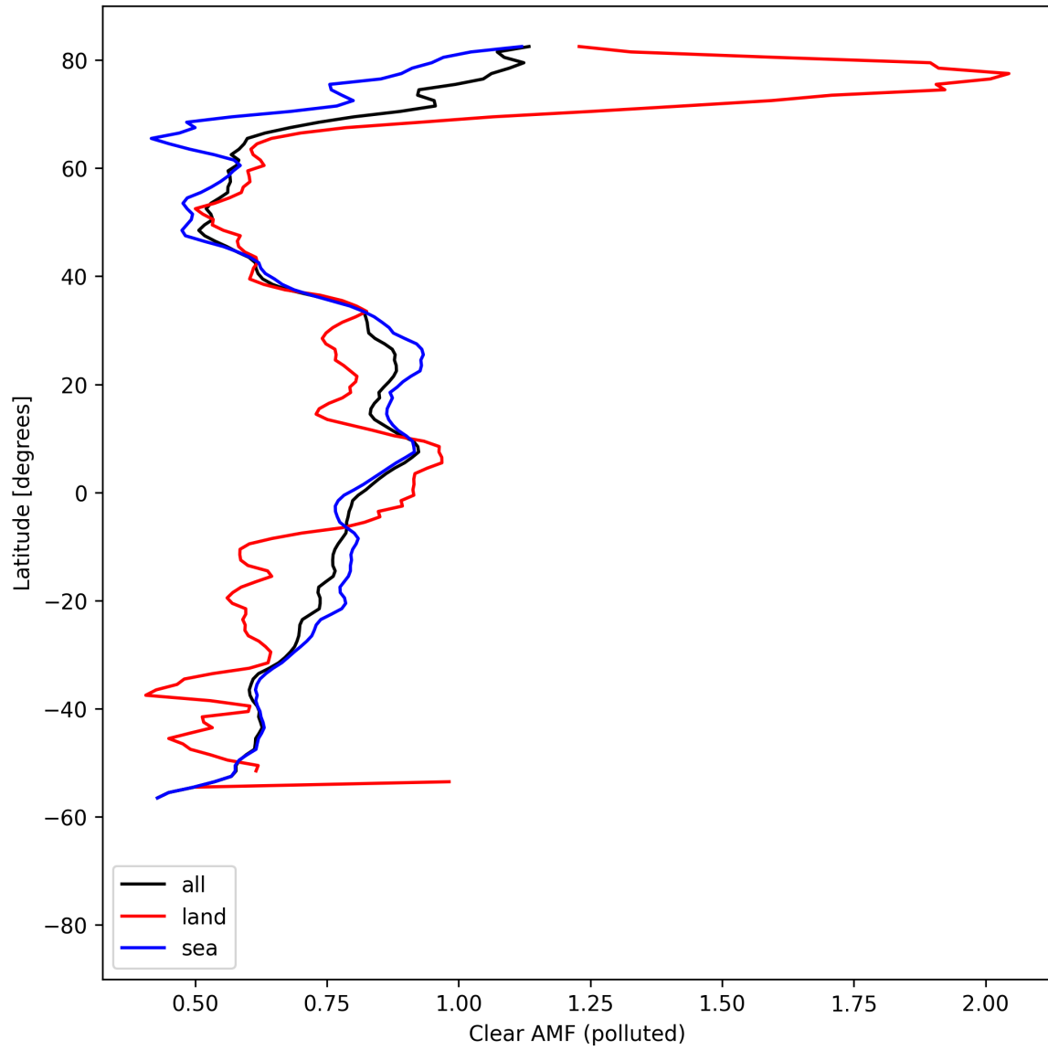
Figure 55: Zonal average of “Clear AMF (polluted)” for 2025-08-19 to 2025-08-20.
