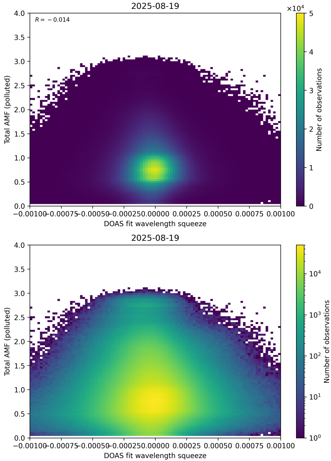
Figure 145: Scatter density plot of “DOAS fit wavelength squeeze” against “Total AMF (polluted)” for 2025-08-19 to 2025-08-20.
