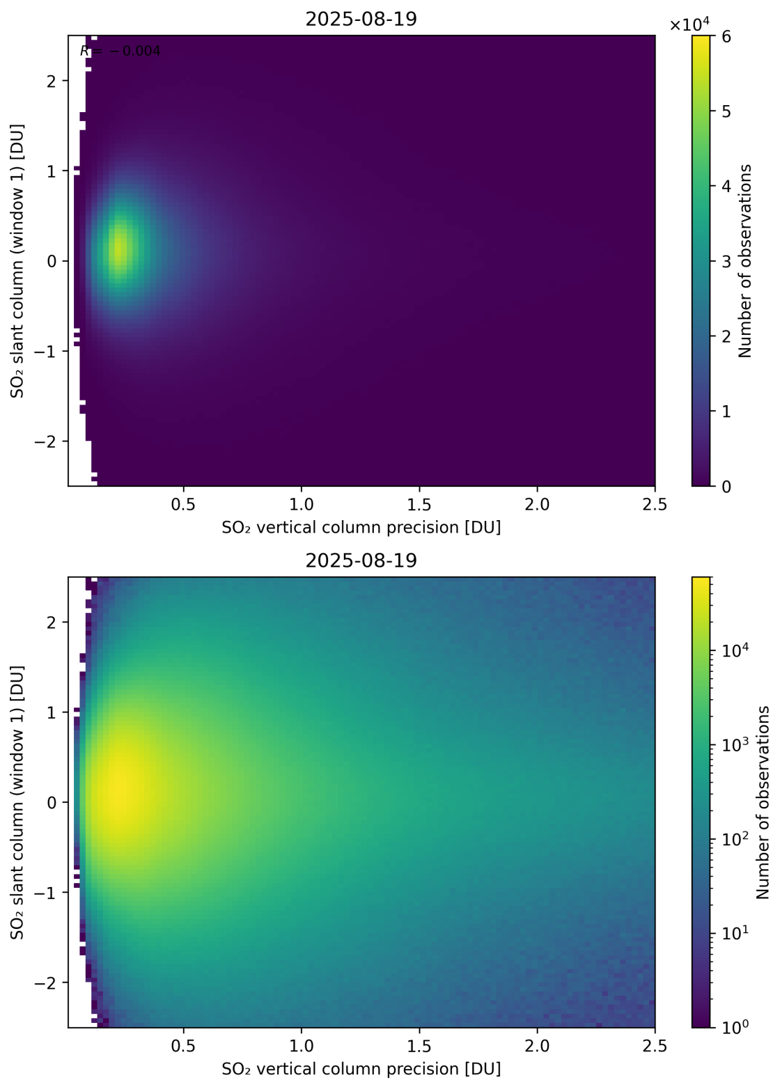
Figure 341: Scatter density plot of “SO 2 vertical column precision” against “SO 2 slant column (window 1)” for 2025-08-19 to 2025-08-20.
