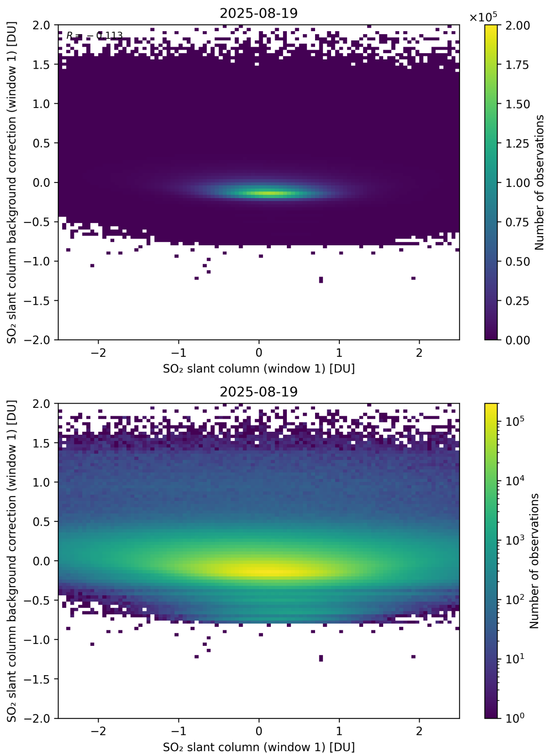
Figure 262: Scatter density plot of “SO 2 slant column (window 1)” against “SO 2 slant column background correction (window 1)” for 2025-08-19 to 2025-08-20.
