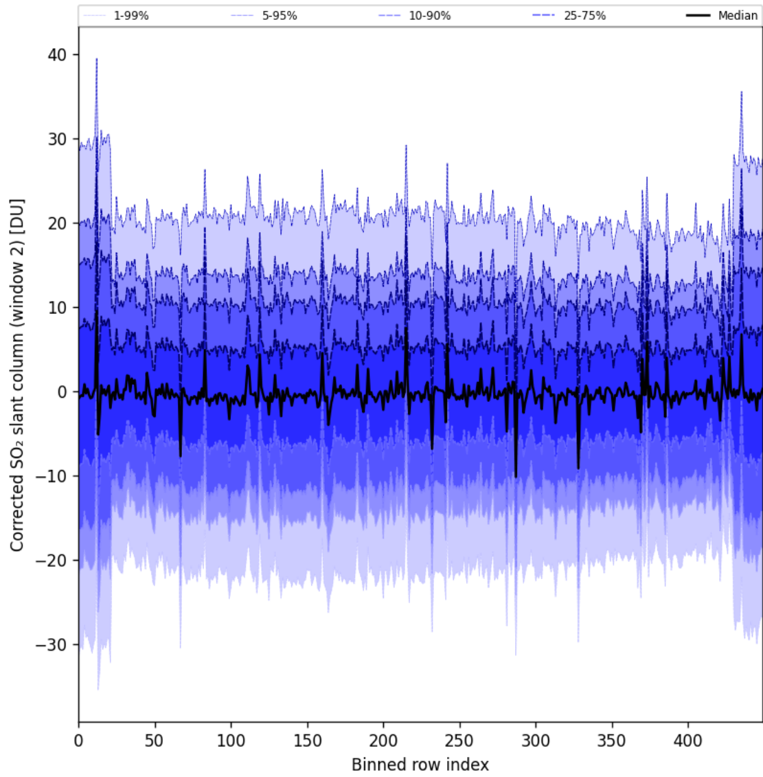
Figure 95: Along track statistics of “Corrected SO 2 slant column (window 2)” for 2025-08-19 to 2025-08-20
