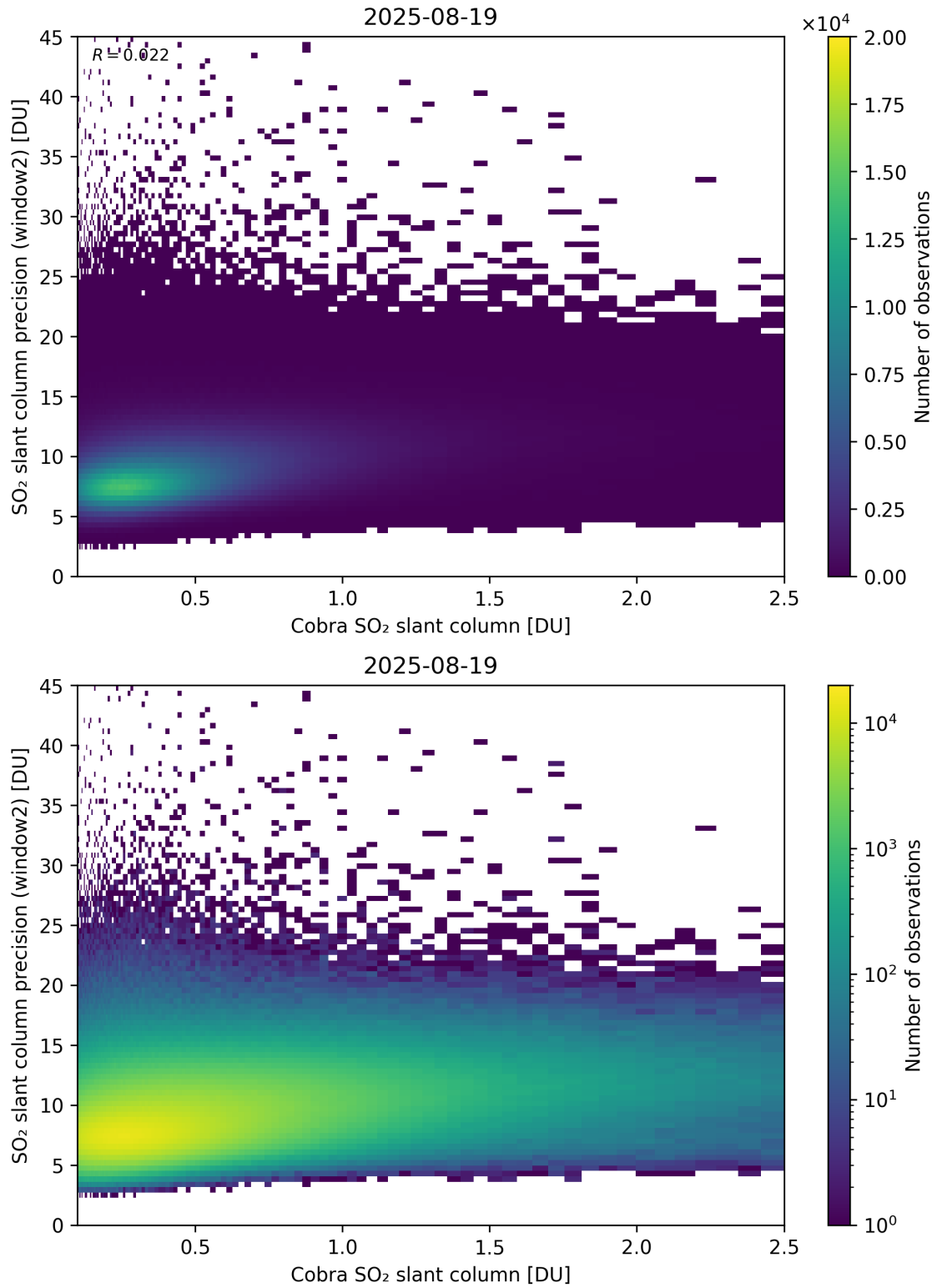
Figure 221: Scatter density plot of “Cobra SO 2 slant column” against “SO 2 slant column precision (window2)” for 2025-08-19 to 2025-08-20.
