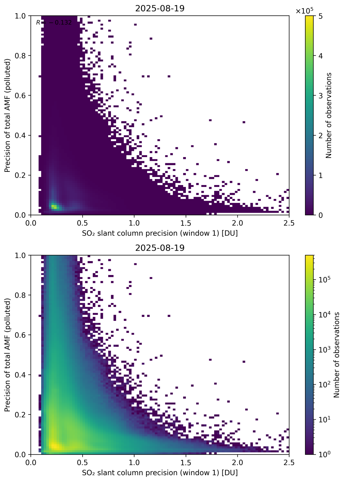
Figure 281: Scatter density plot of “SO 2 slant column precision (window 1)” against “Precision of total AMF (polluted)” for 2025-08-19 to 2025-08-20.
