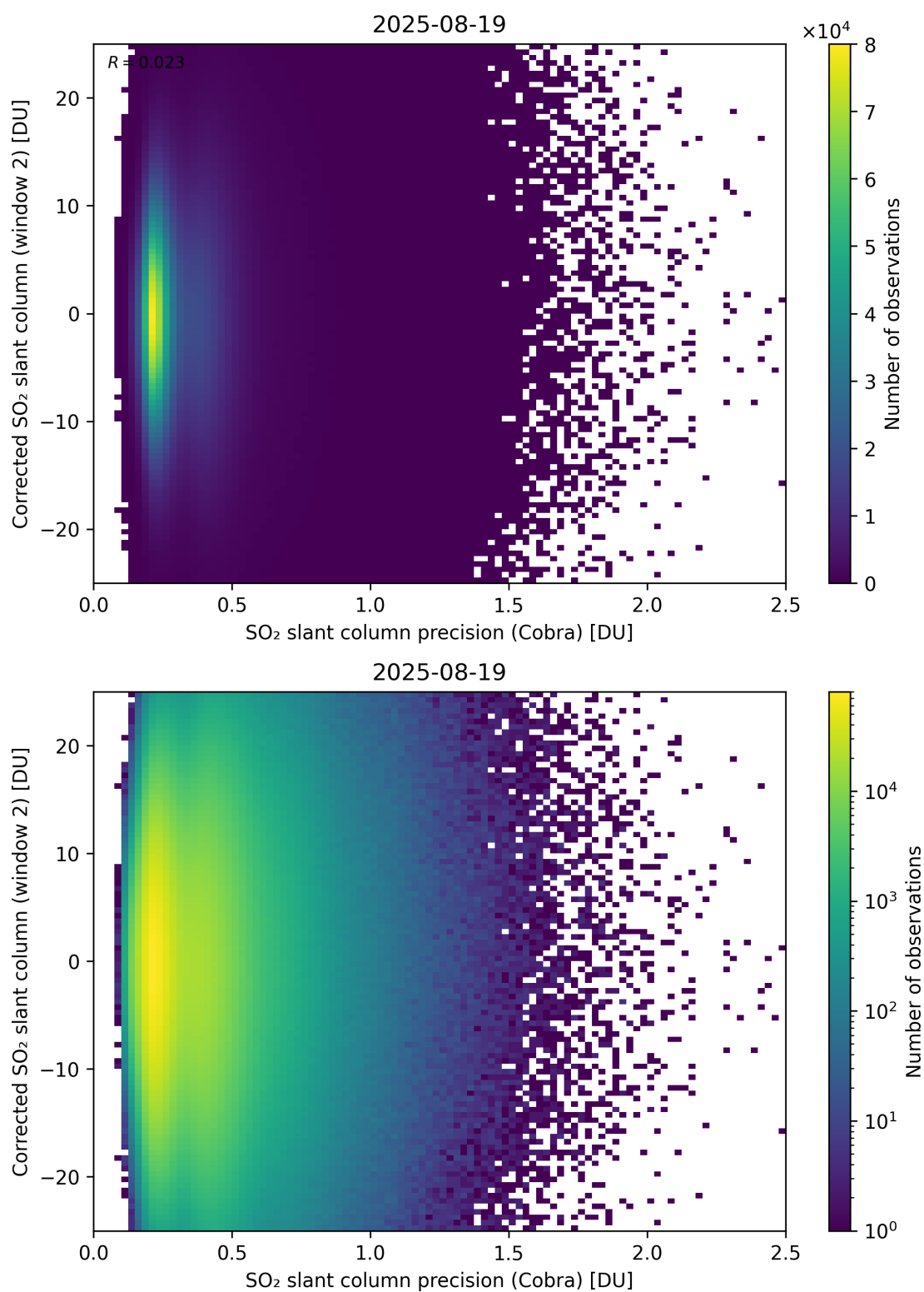
Figure 206: Scatter density plot of “SO 2 slant column precision (Cobra)” against “Corrected SO 2 slant column (window 2)” for 2025-08-19 to 2025-08-20.
