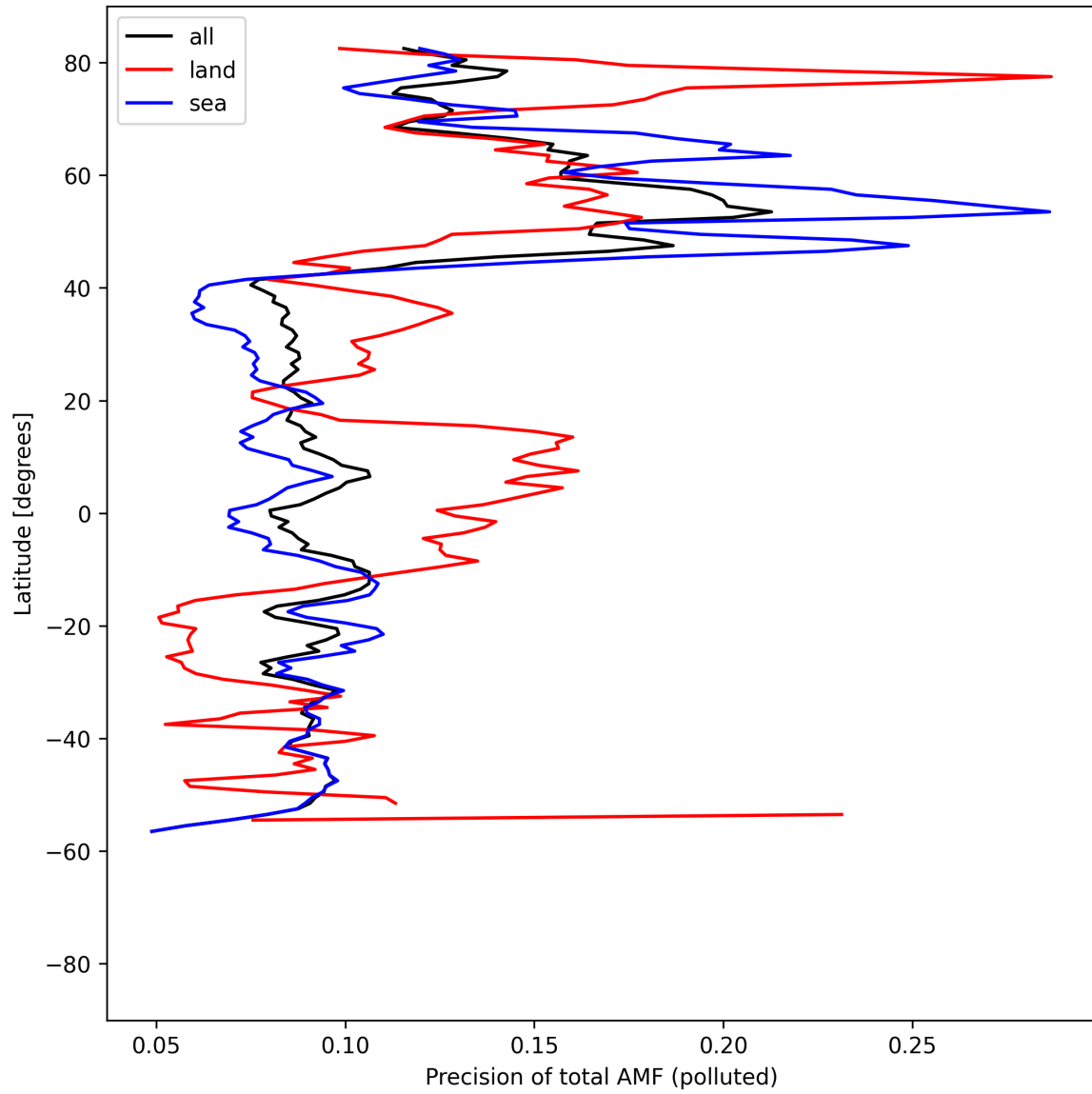
Figure 54: Zonal average of “Precision of total AMF (polluted)” for 2025-08-19 to 2025-08-20.
