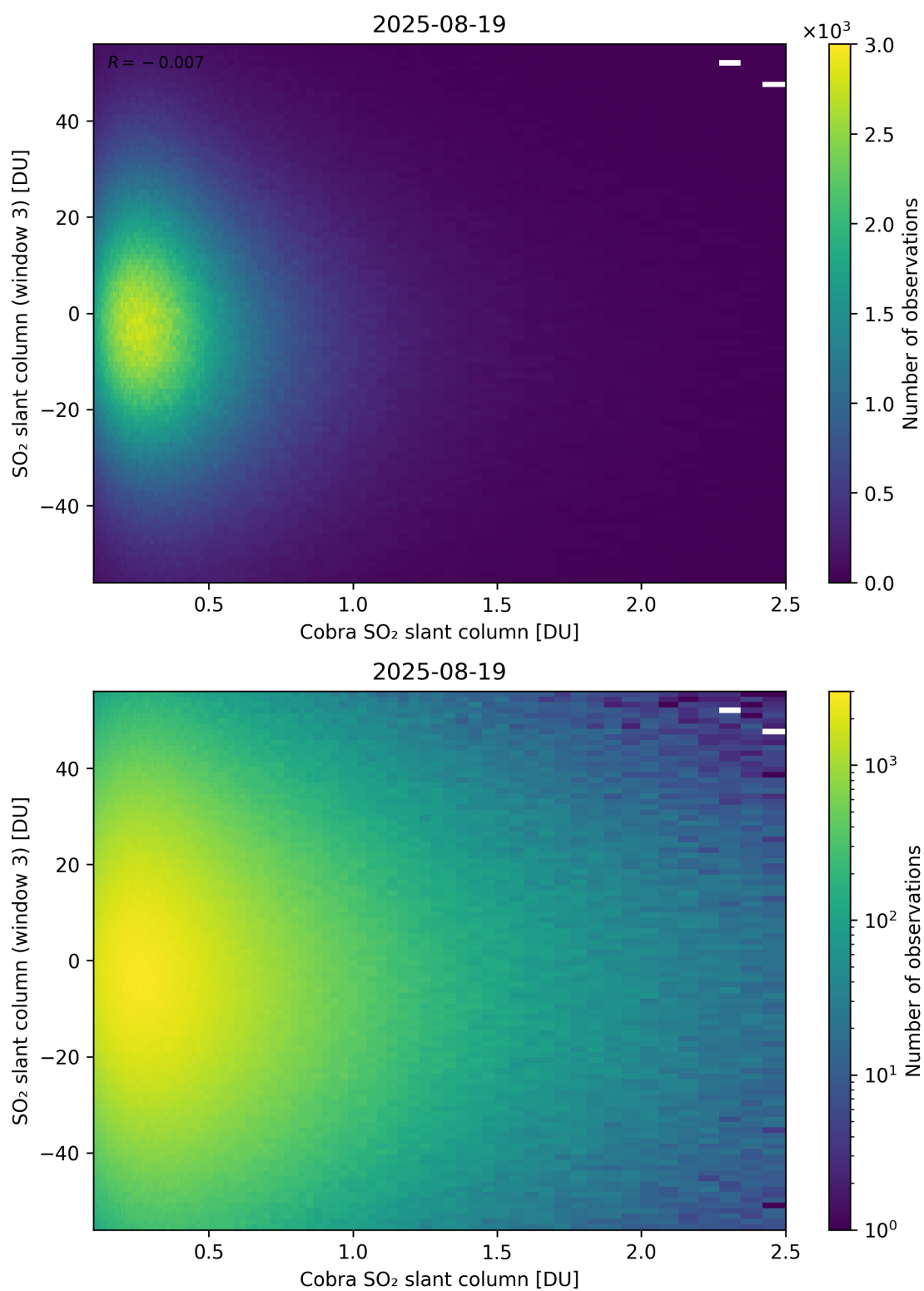
Figure 222: Scatter density plot of “Cobra SO 2 slant column” against “SO 2 slant column (window 3)” for 2025-08-19 to 2025-08-20.
