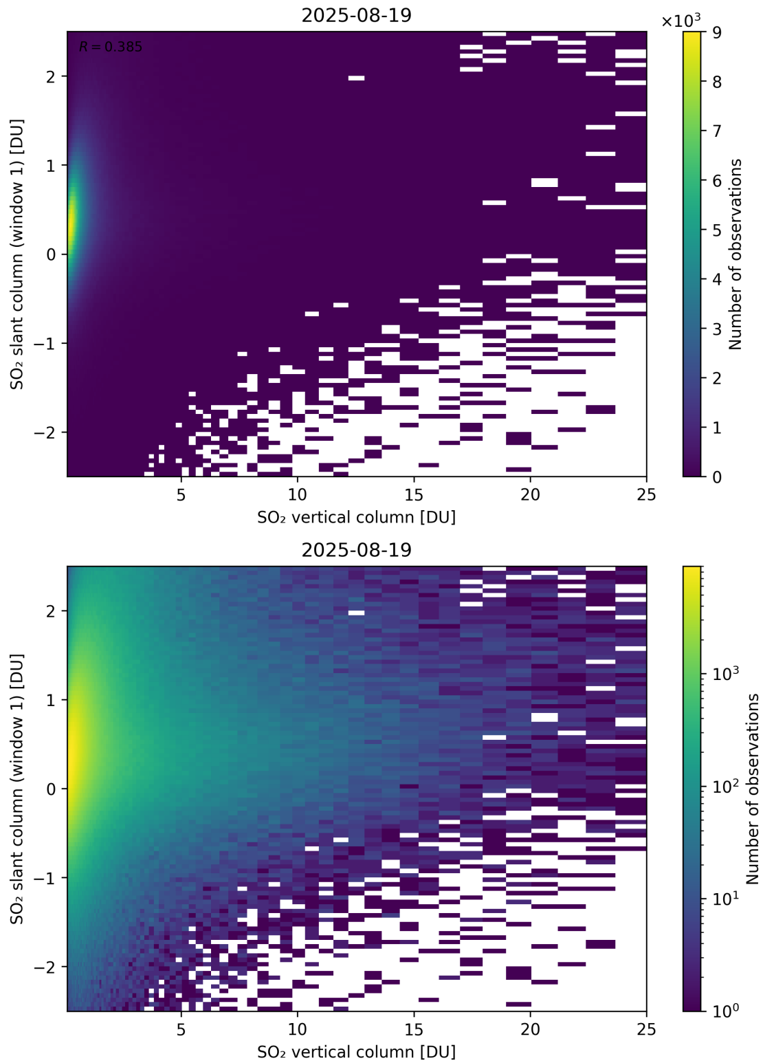
Figure 354: Scatter density plot of “SO 2 vertical column” against “SO 2 slant column (window 1)” for 2025-08-19 to 2025-08-20.
