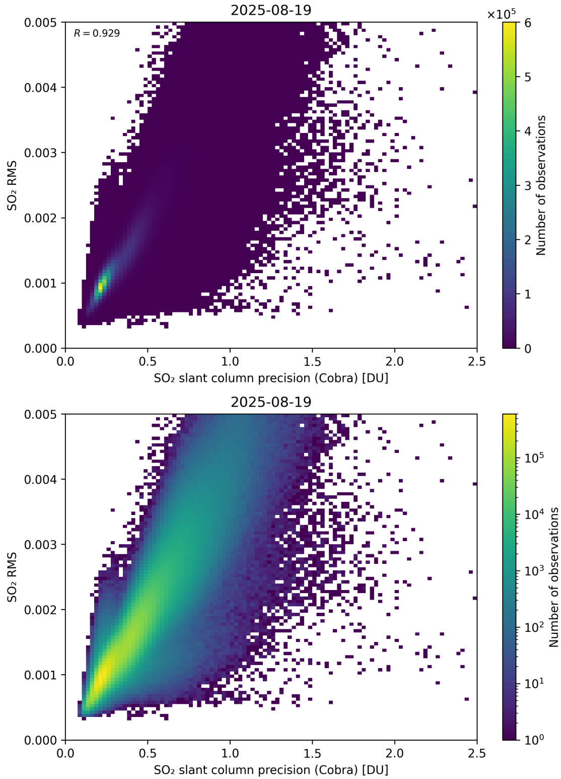
Figure 204: Scatter density plot of “SO 2 slant column precision (Cobra)” against “SO 2 RMS” for 2025-08-19 to 2025-08-20.
