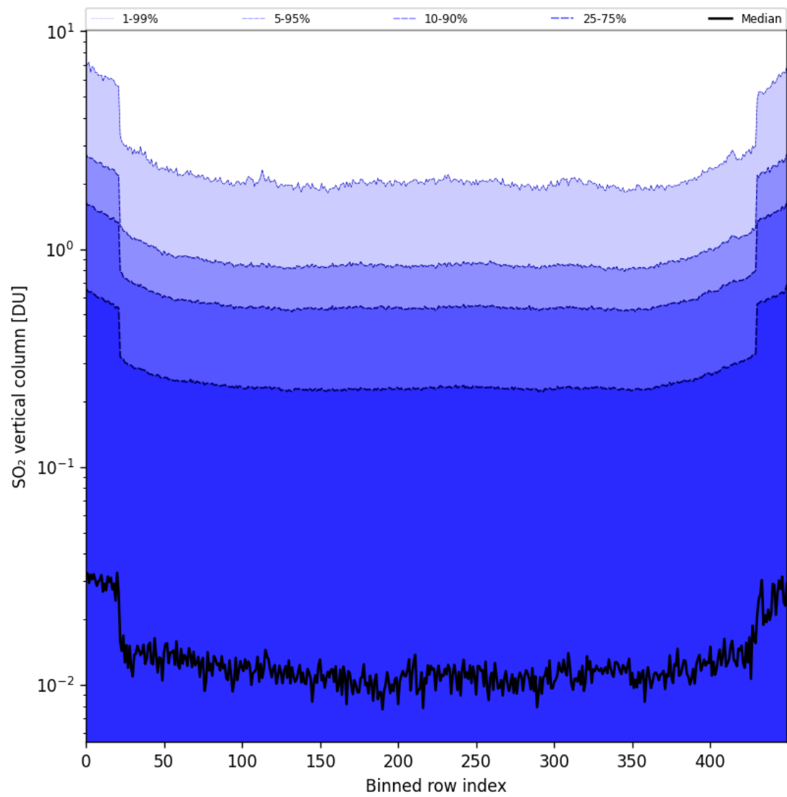
Figure 84: Along track statistics of “SO 2 vertical column” for 2025-08-19 to 2025-08-20
