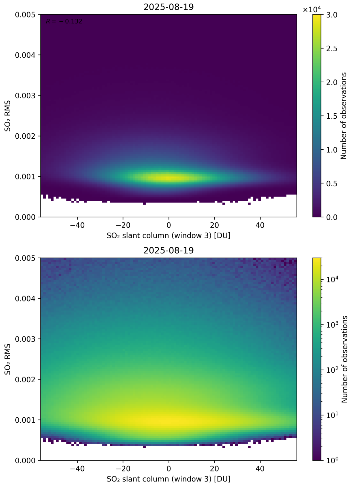
Figure 306: Scatter density plot of “SO 2 slant column (window 3)” against “SO 2 RMS” for 2025-08-19 to 2025-08-20.
