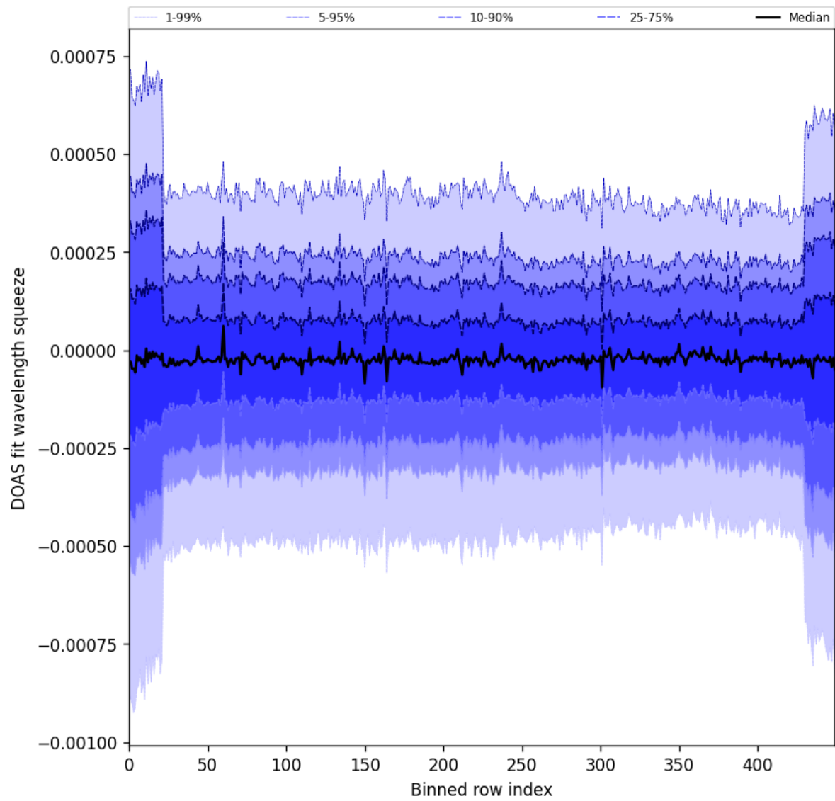
Figure 103: Along track statistics of “DOAS fit wavelength squeeze” for 2025-08-19 to 2025-08-20
