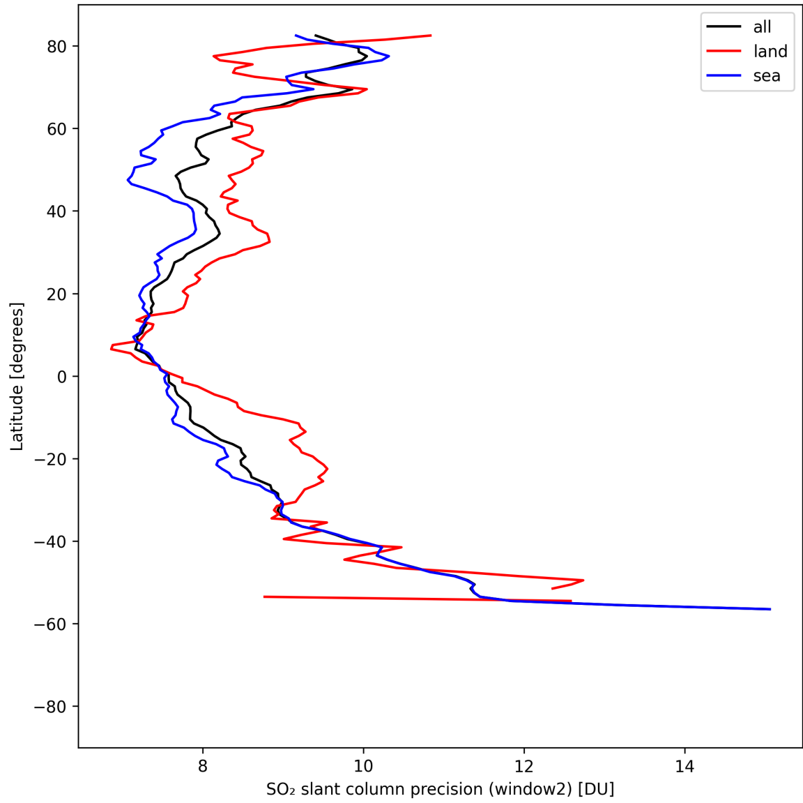
Figure 42: Zonal average of “SO 2 slant column precision (window2)” for 2025-08-19 to 2025-08-20.
