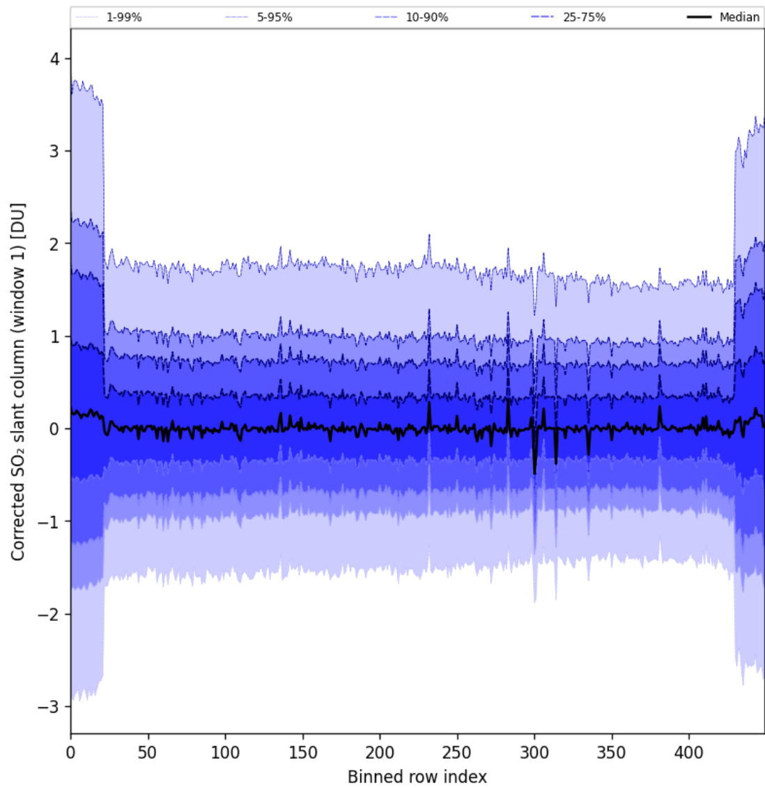
Figure 91: Along track statistics of “Corrected SO 2 slant column (window 1)” for 2025-08-19 to 2025-08-20
