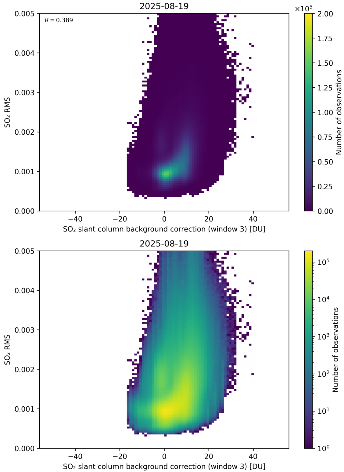
Figure 134: Scatter density plot of “SO 2 slant column background correction (window 3)” against “SO 2 RMS” for 2025-08-19 to 2025-08-20.
