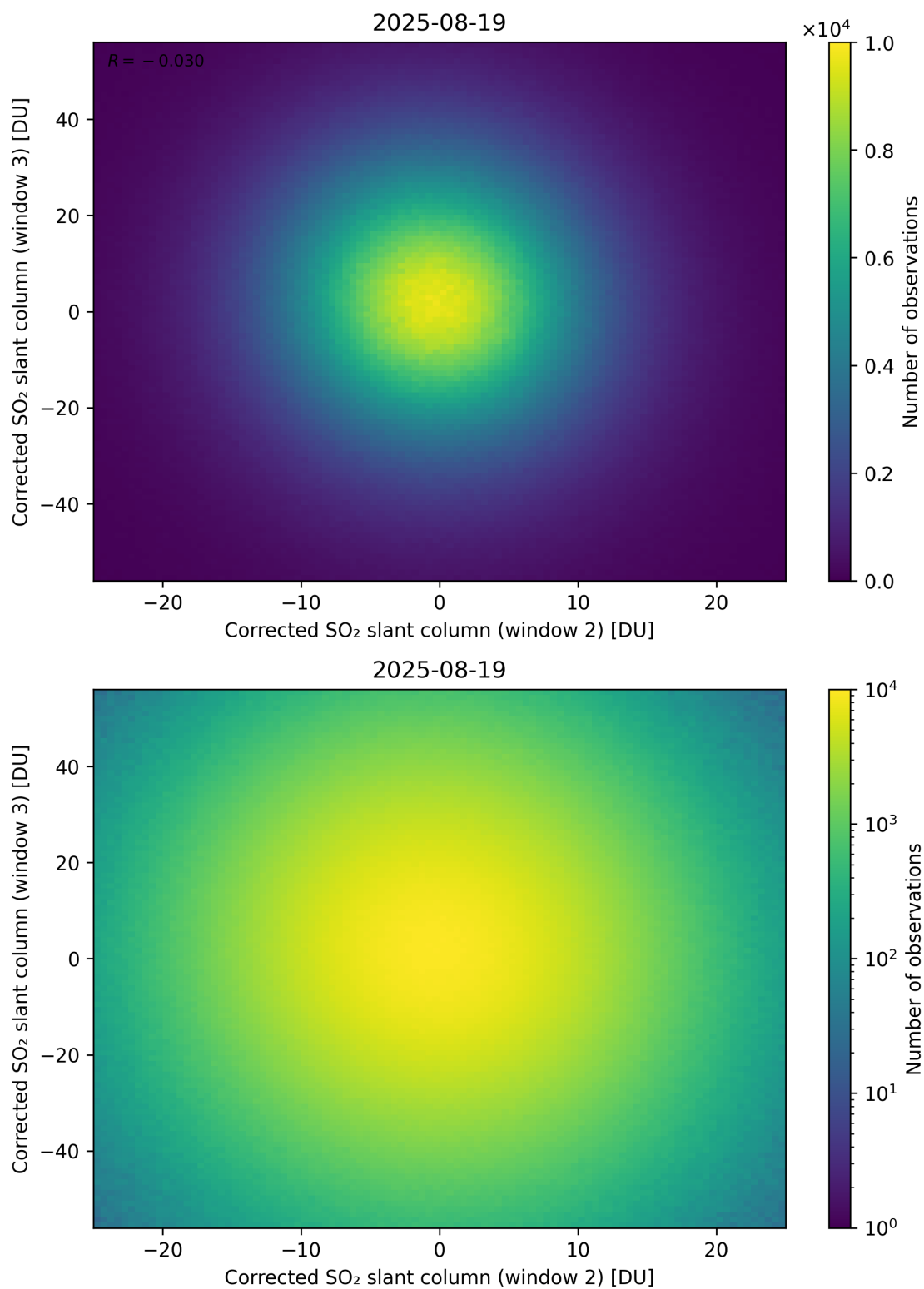
Figure 250: Scatter density plot of “Corrected SO 2 slant column (window 2)” against “Corrected SO 2 slant column (window 3)” for 2025-08-19 to 2025-08-20.
