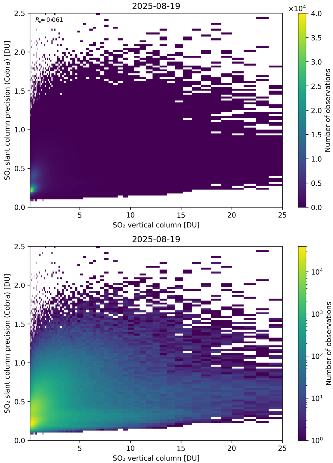
Figure 350: Scatter density plot of “SO 2 vertical column” against “SO 2 slant column precision (Cobra)” for 2025-08-19 to 2025-08-20.
