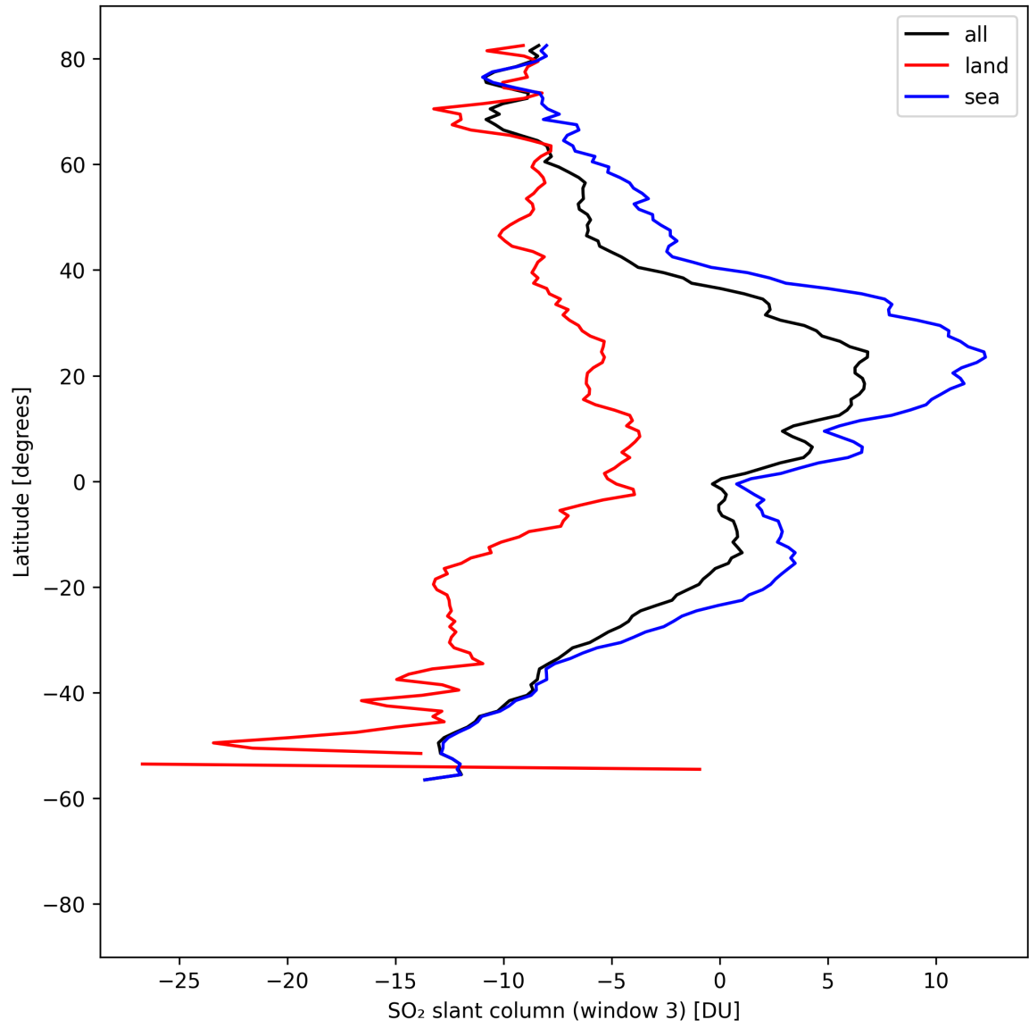
Figure 45: Zonal average of “SO 2 slant column (window 3)” for 2025-08-19 to 2025-08-20.
