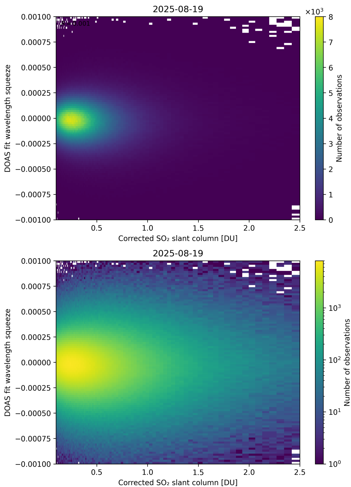
Figure 230: Scatter density plot of “Corrected SO 2 slant column” against “DOAS fit wavelength squeeze” for 2025-08-19 to 2025-08-20.
