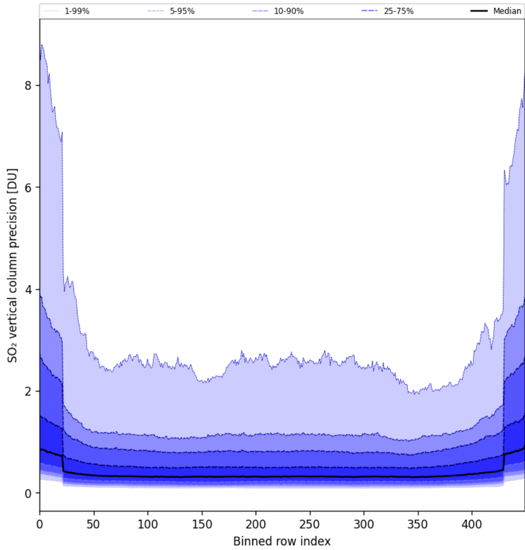
Figure 85: Along track statistics of “SO 2 vertical column precision” for 2025-08-19 to 2025-08-20
