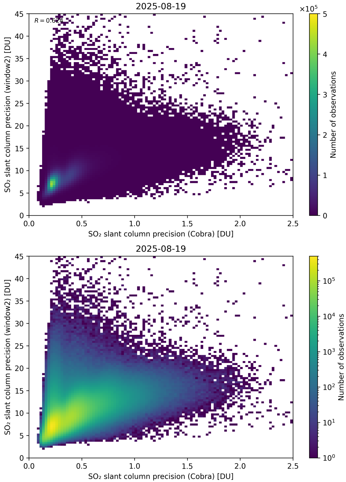
Figure 210: Scatter density plot of “SO 2 slant column precision (Cobra)” against “SO 2 slant column precision (window2)” for 2025-08-19 to 2025-08-20.
