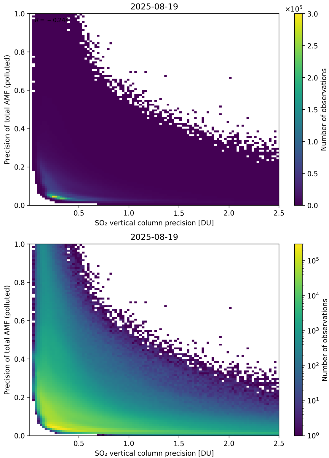
Figure 347: Scatter density plot of “SO 2 vertical column precision” against “Precision of total AMF (polluted)” for 2025-08-19 to 2025-08-20.
