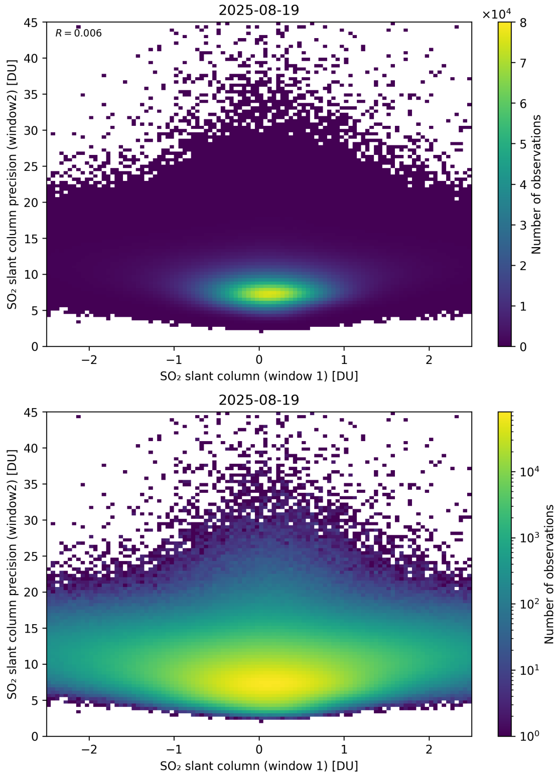
Figure 286: Scatter density plot of “SO 2 slant column (window 1)” against “SO 2 slant column precision (window2)” for 2025-08-19 to 2025-08-20.
