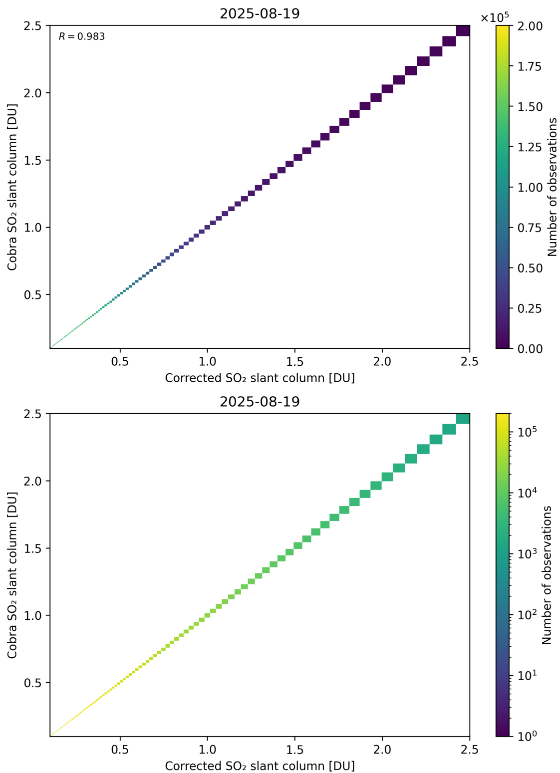
Figure 233: Scatter density plot of “Corrected SO 2 slant column” against “Cobra SO 2 slant column” for 2025-08-19 to 2025-08-20.
