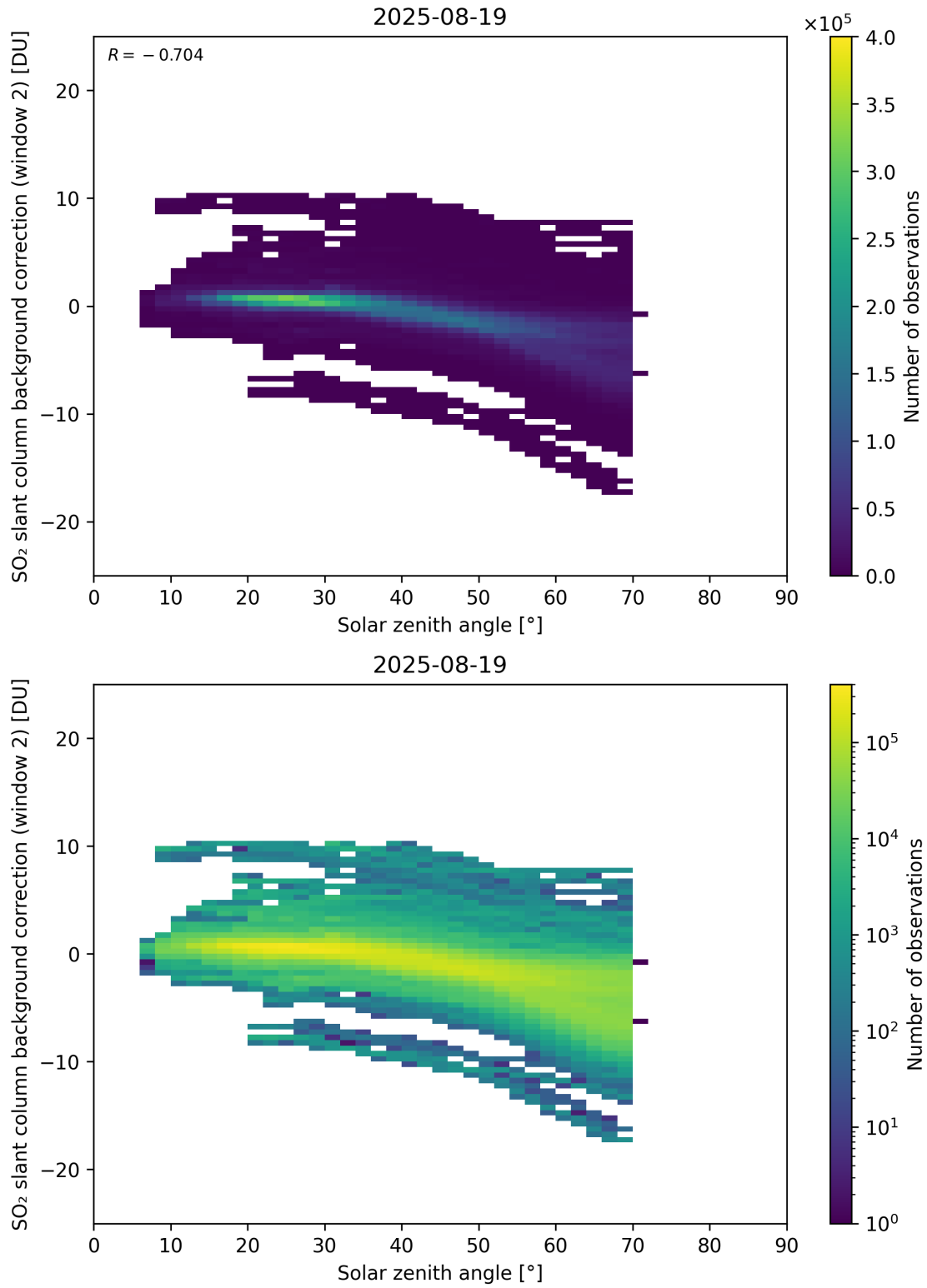
Figure 172: Scatter density plot of “Solar zenith angle” against “SO 2 slant column background correction (window 2)” for 2025-08-19 to 2025-08-20.
