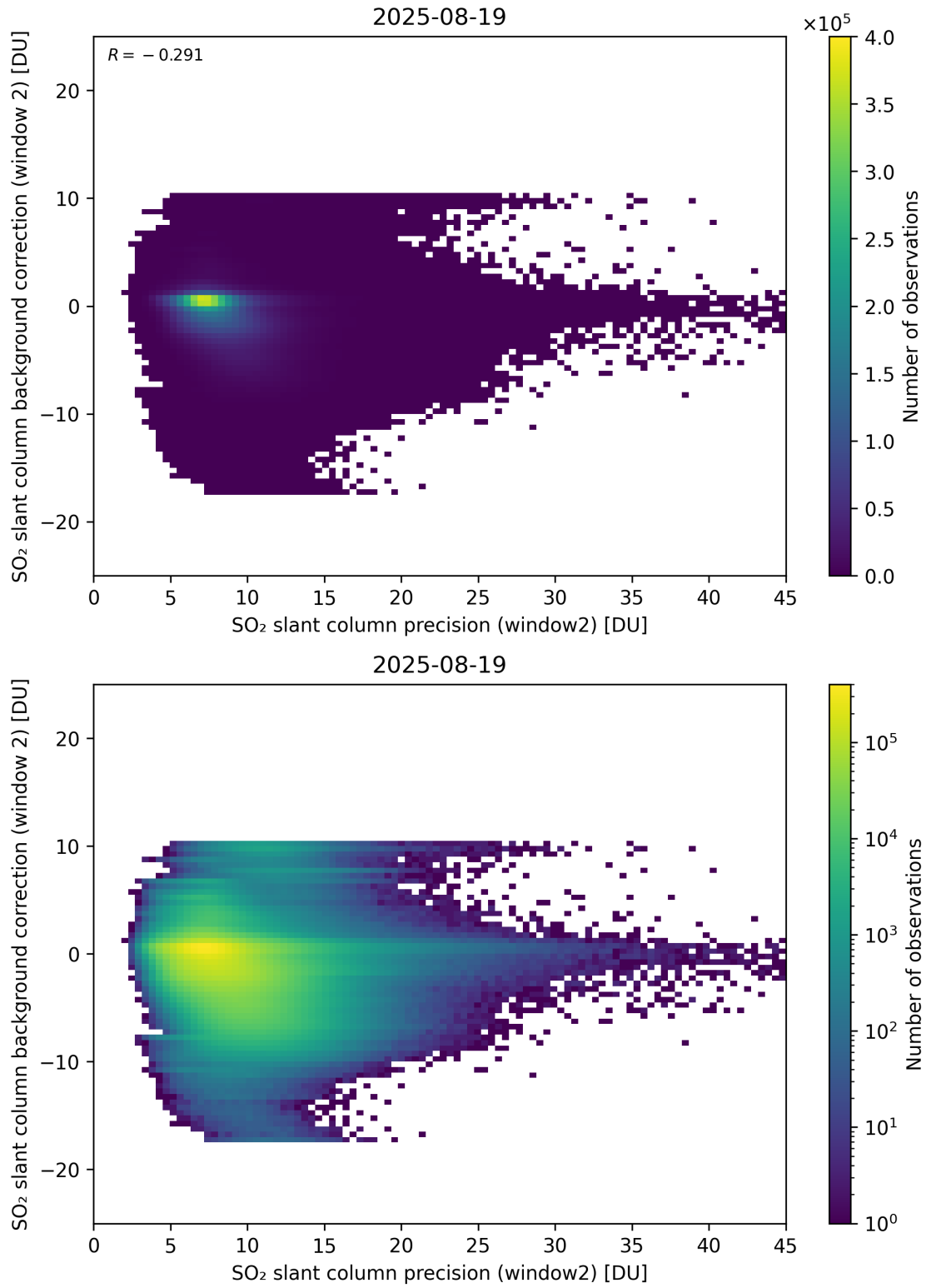
Figure 291: Scatter density plot of “SO 2 slant column precision (window2)” against “SO 2 slant column background correction (window 2)” for 2025-08-19 to 2025-08-20.
