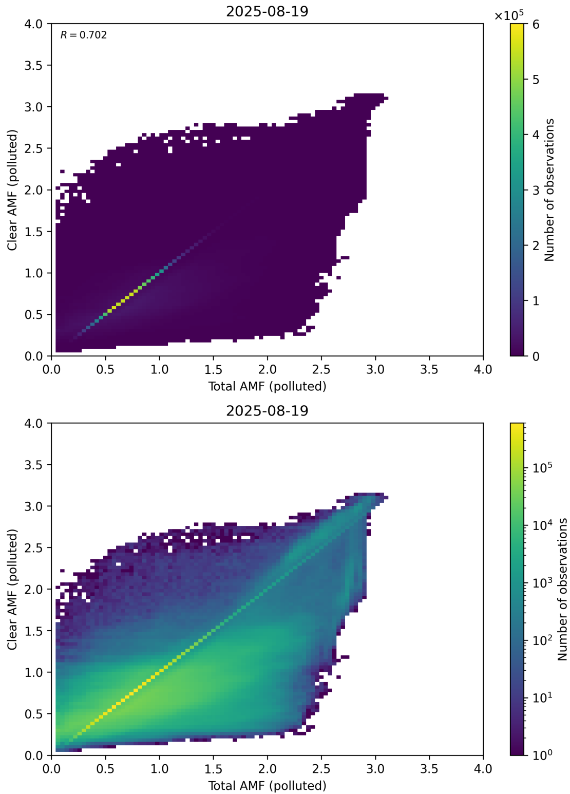
Figure 321: Scatter density plot of “Total AMF (polluted)” against “Clear AMF (polluted)” for 2025-08-19 to 2025-08-20.
