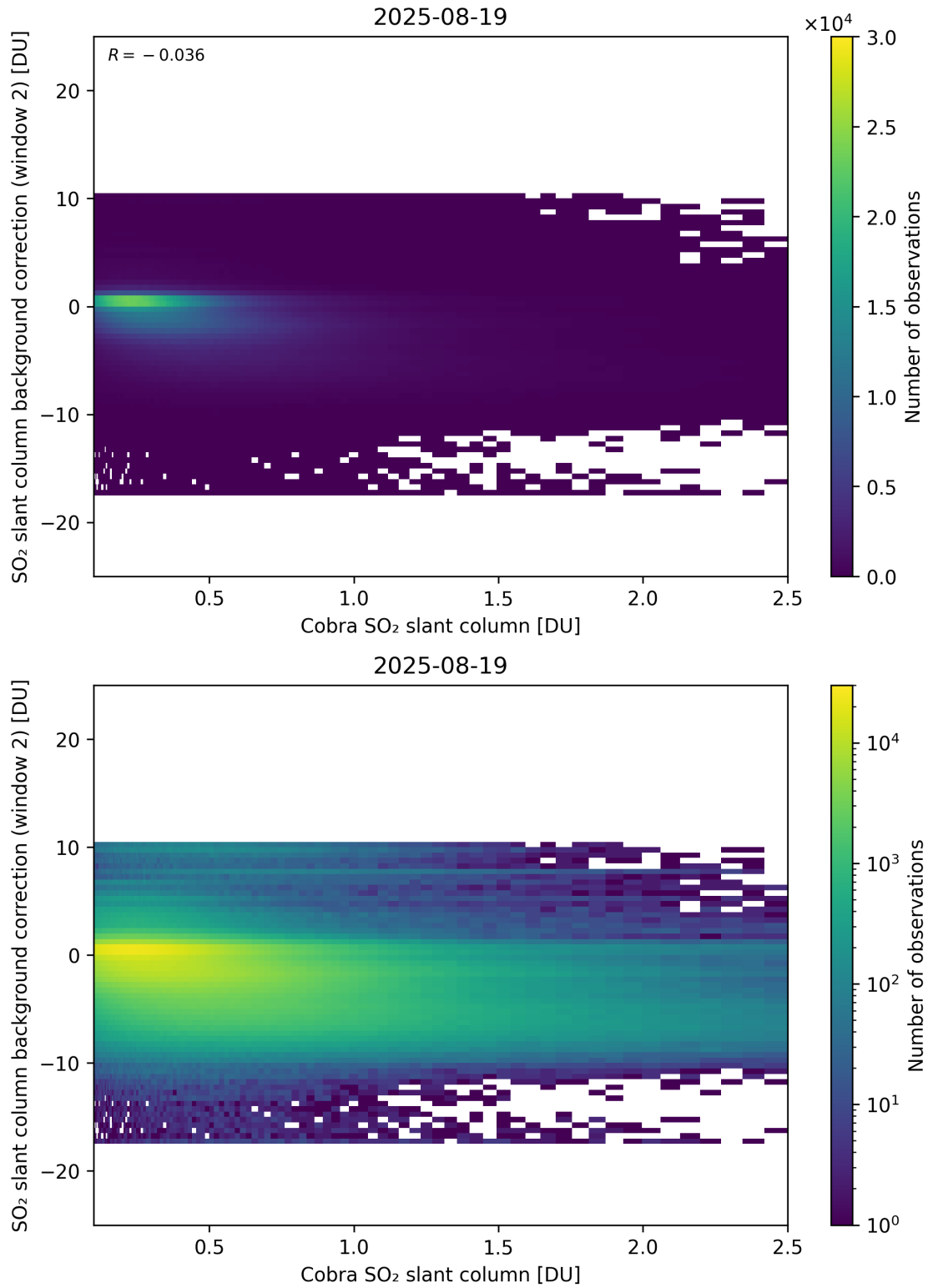
Figure 194: Scatter density plot of “Cobra SO 2 slant column” against “SO 2 slant column background correction (window 2)” for 2025-08-19 to 2025-08-20.
