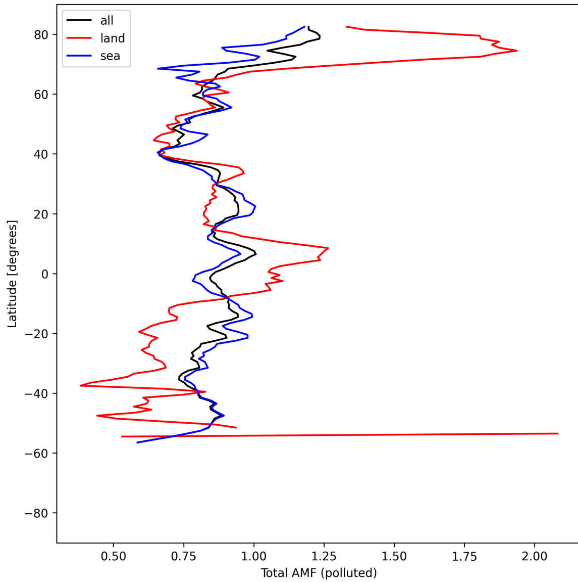
Figure 53: Zonal average of “Total AMF (polluted)” for 2025-08-19 to 2025-08-20.
