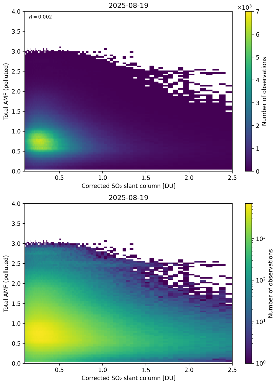
Figure 242: Scatter density plot of “Corrected SO 2 slant column” against “Total AMF (polluted)” for 2025-08-19 to 2025-08-20.
