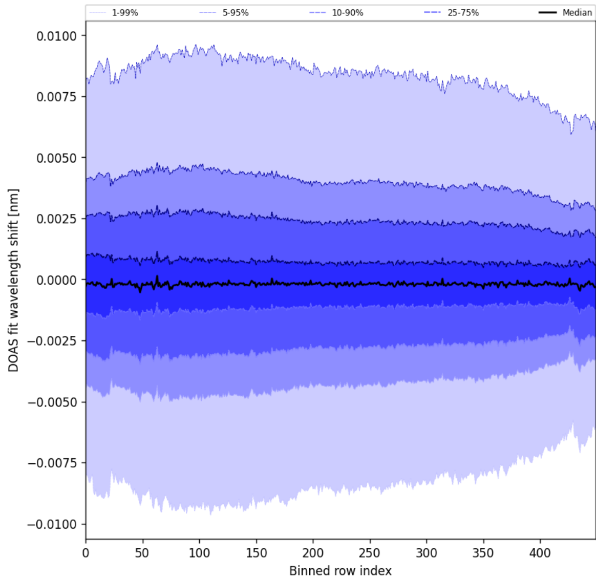
Figure 102: Along track statistics of “DOAS fit wavelength shift” for 2025-08-19 to 2025-08-20
