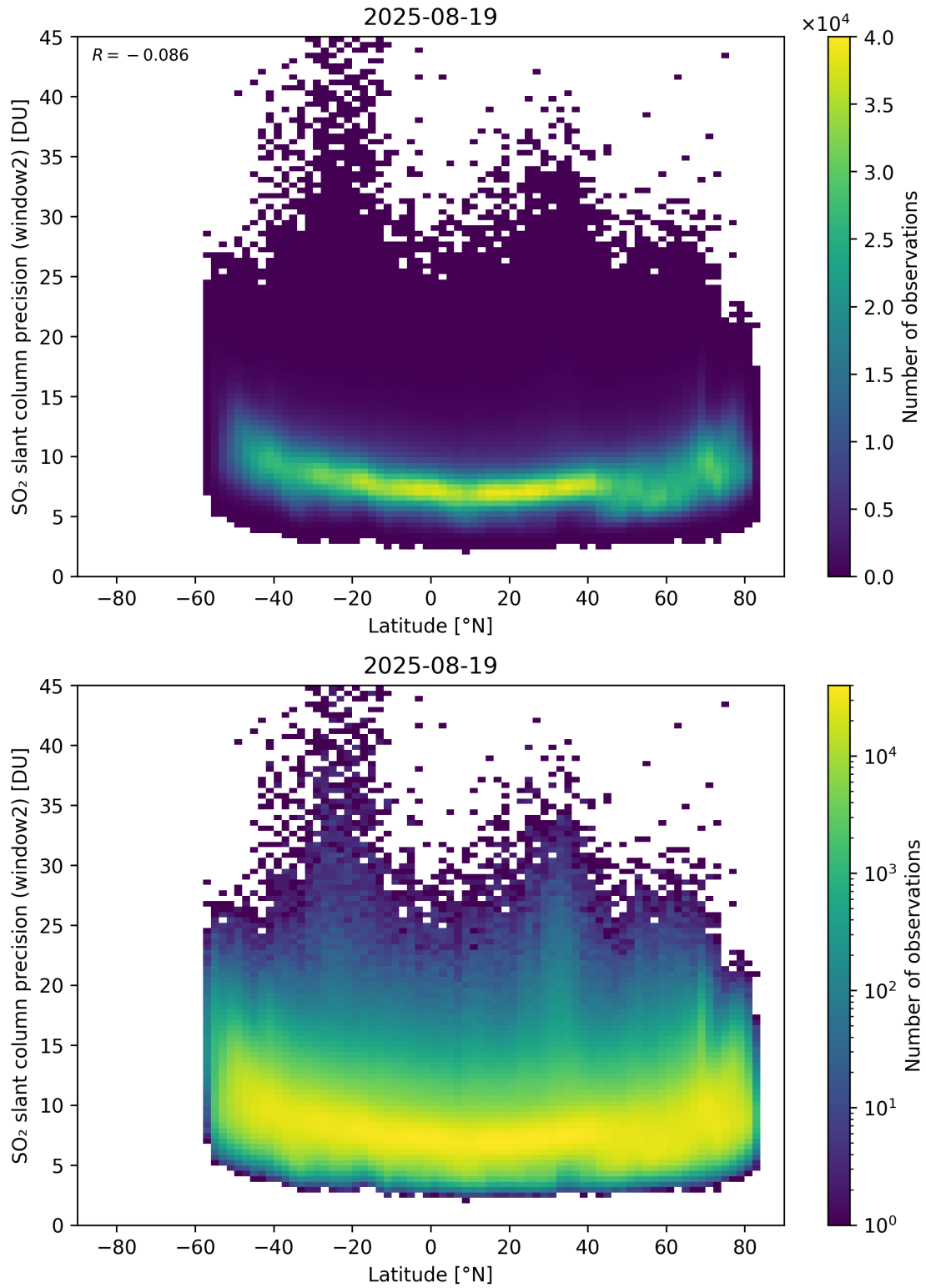
Figure 164: Scatter density plot of “Latitude” against “SO 2 slant column precision (window2)” for 2025-08-19 to 2025-08-20.
