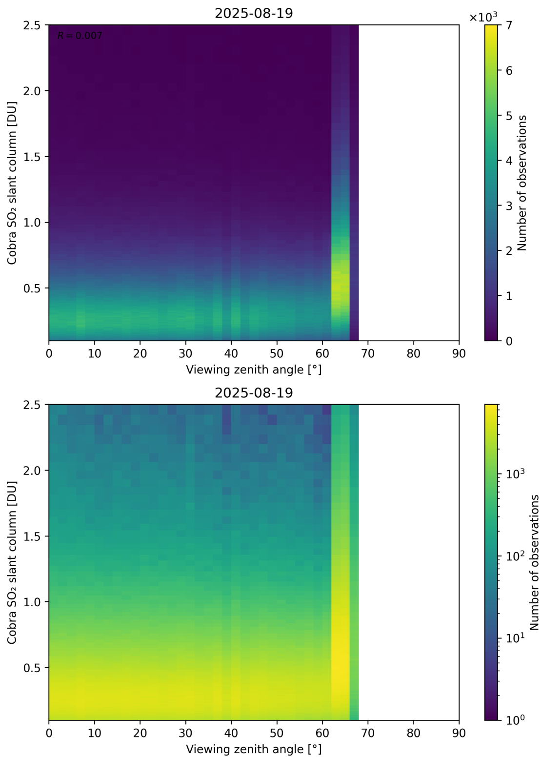
Figure 371: Scatter density plot of “Viewing zenith angle” against “Cobra SO 2 slant column” for 2025-08-19 to 2025-08-20.
