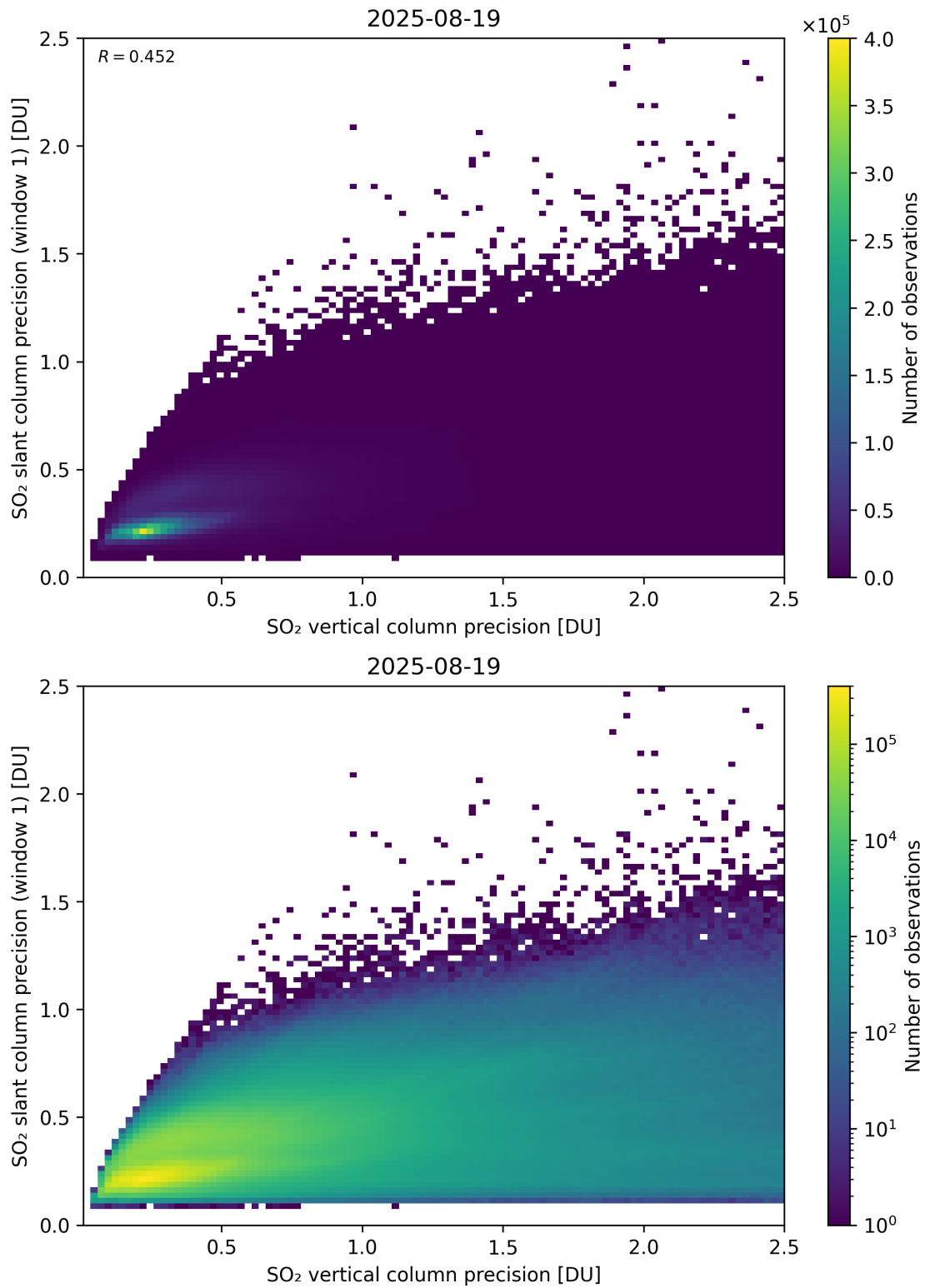
Figure 342: Scatter density plot of “SO 2 vertical column precision” against “SO 2 slant column precision (window 1)” for 2025-08-19 to 2025-08-20.
