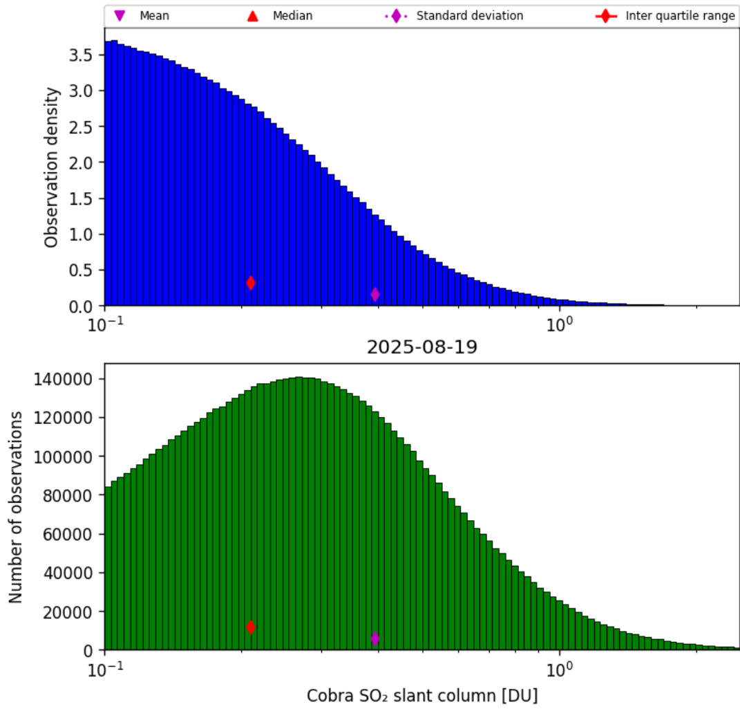
Figure 61: Histogram of “Cobra SO 2 slant column” for 2025-08-19 to 2025-08-20
