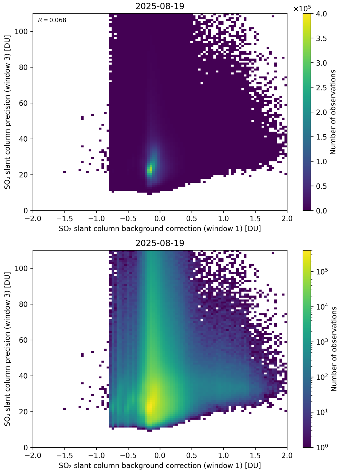
Figure 119: Scatter density plot of “SO 2 slant column background correction (window 1)” against “SO 2 slant column precision (window 3)” for 2025-08-19 to 2025-08-20.
