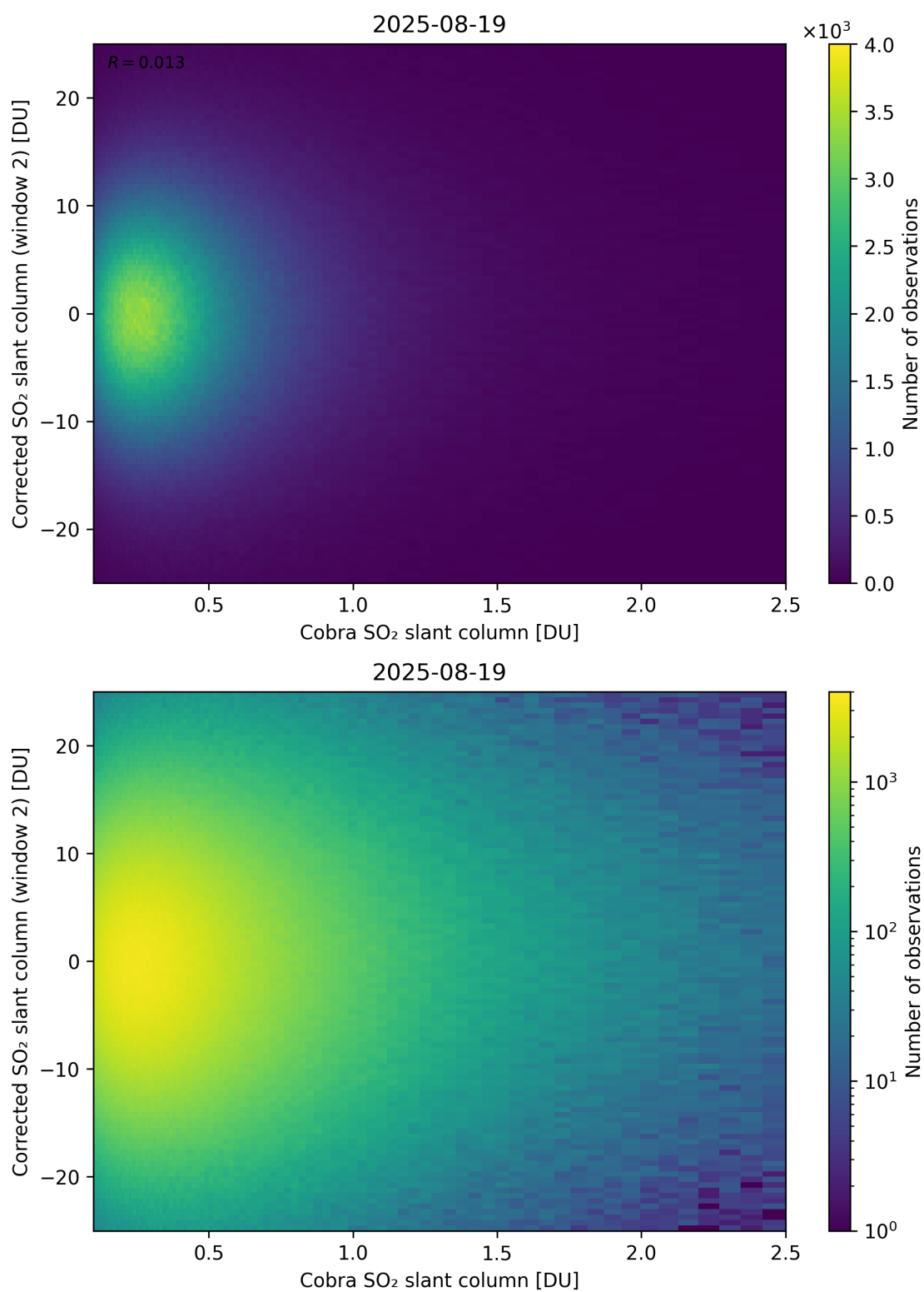
Figure 217: Scatter density plot of “Cobra SO 2 slant column” against “Corrected SO 2 slant column (window 2)” for 2025-08-19 to 2025-08-20.
