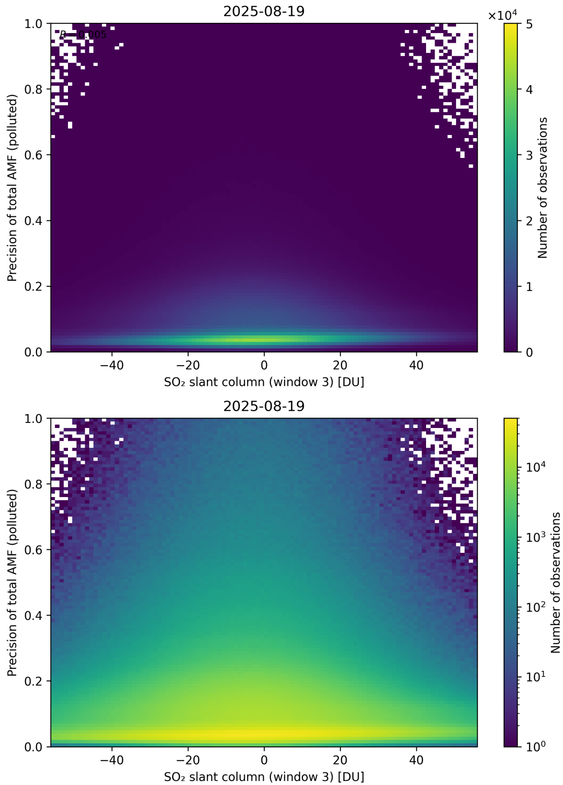
Figure 319: Scatter density plot of “SO 2 slant column (window 3)” against “Precision of total AMF (polluted)” for 2025-08-19 to 2025-08-20.
