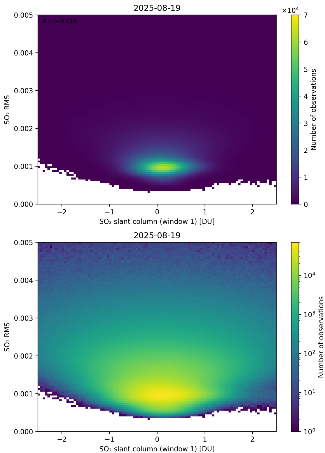
Figure 267: Scatter density plot of “SO 2 slant column (window 1)” against “SO 2 RMS” for 2025-08-19 to 2025-08-20.
