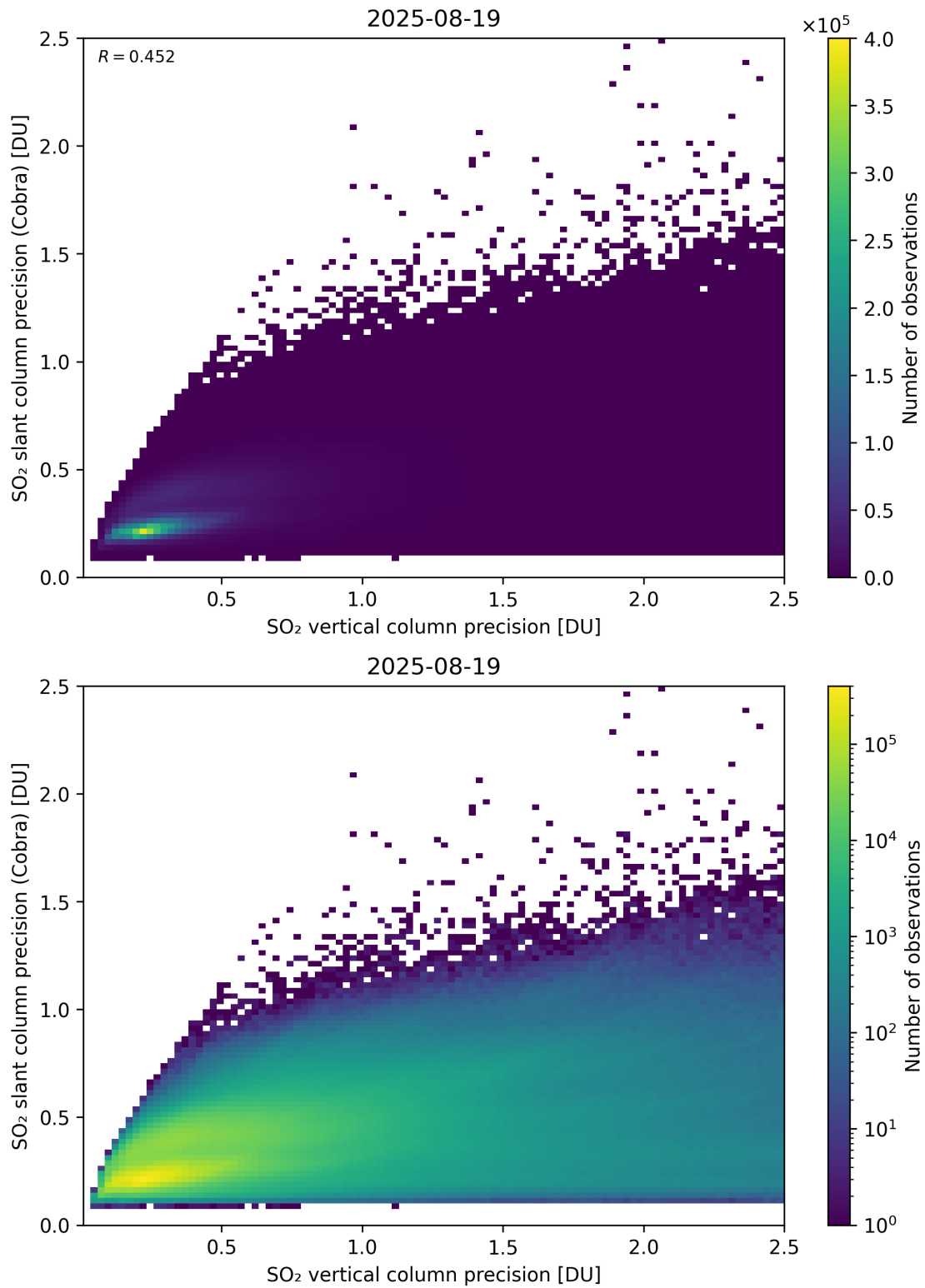
Figure 337: Scatter density plot of “SO 2 vertical column precision” against “SO 2 slant column precision (Cobra)” for 2025-08-19 to 2025-08-20.
