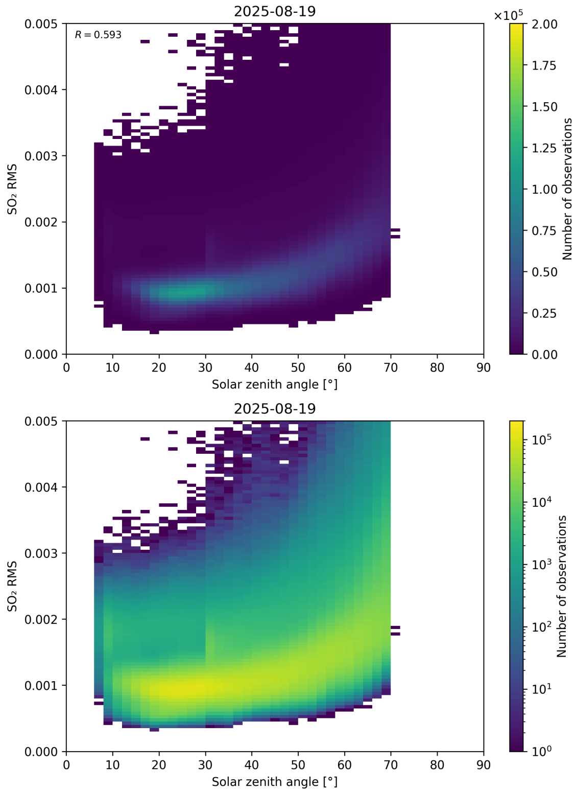
Figure 176: Scatter density plot of “Solar zenith angle” against “SO 2 RMS” for 2025-08-19 to 2025-08-20.
