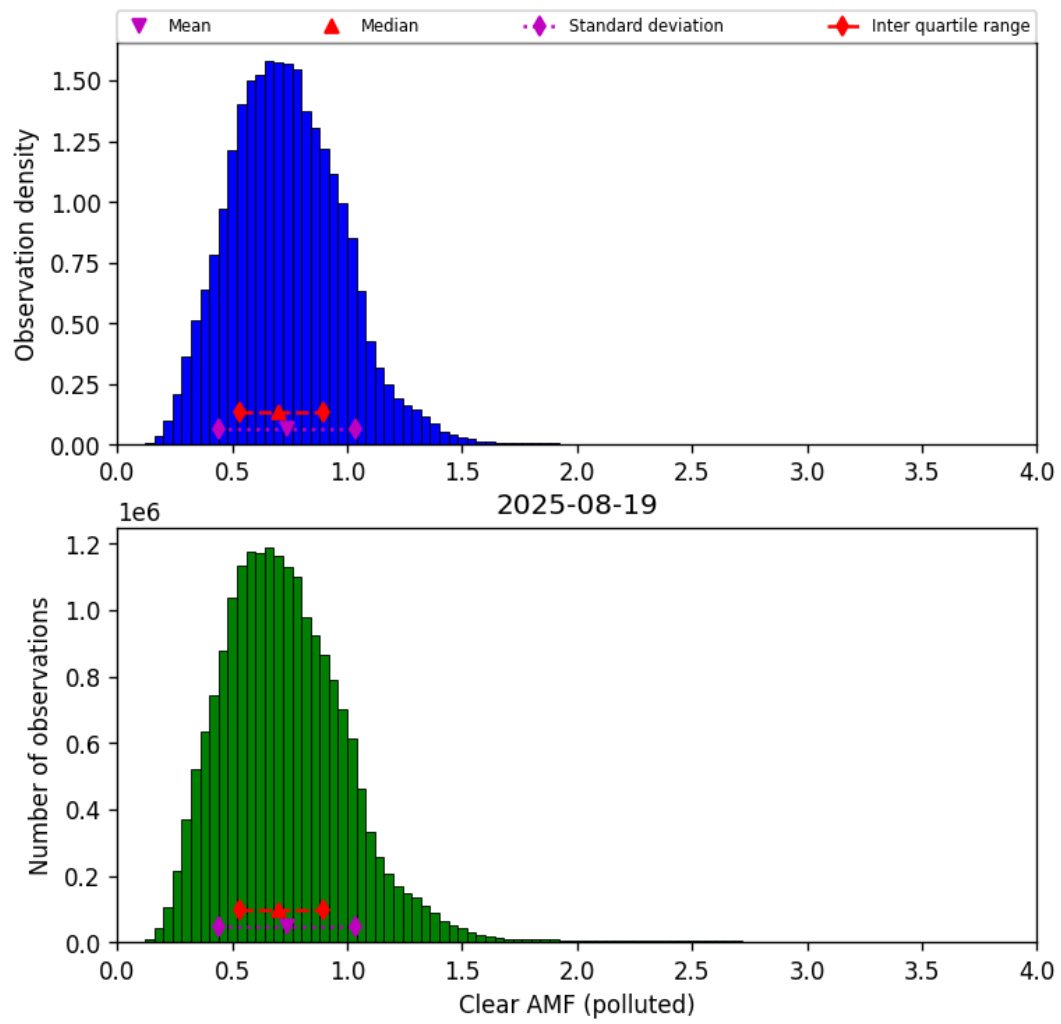
Figure 81: Histogram of “Clear AMF (polluted)” for 2025-08-19 to 2025-08-20
