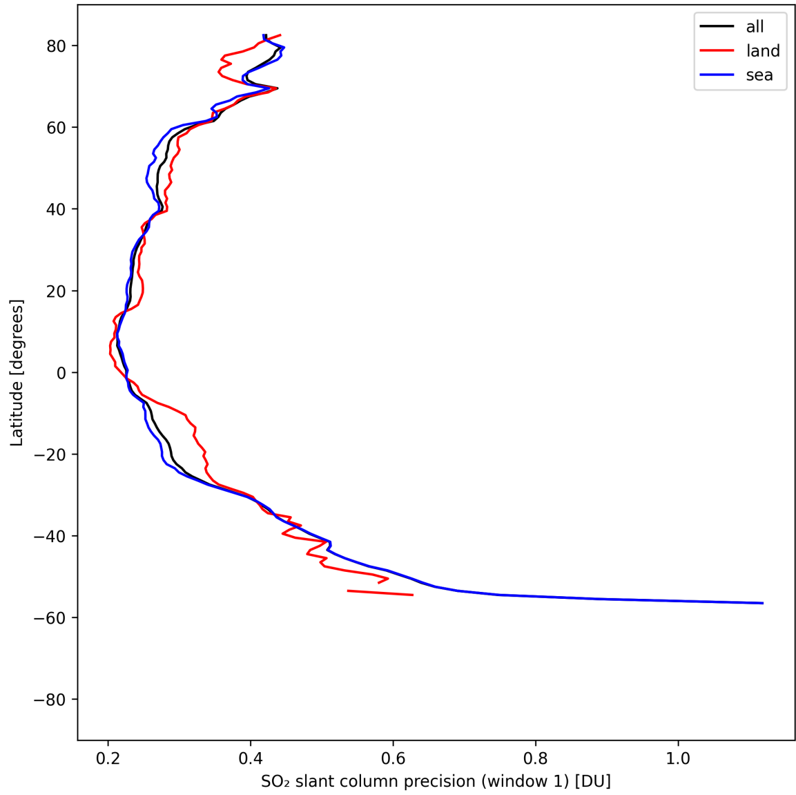
Figure 38: Zonal average of “SO 2 slant column precision (window 1)” for 2025-08-19 to 2025-08-20.
