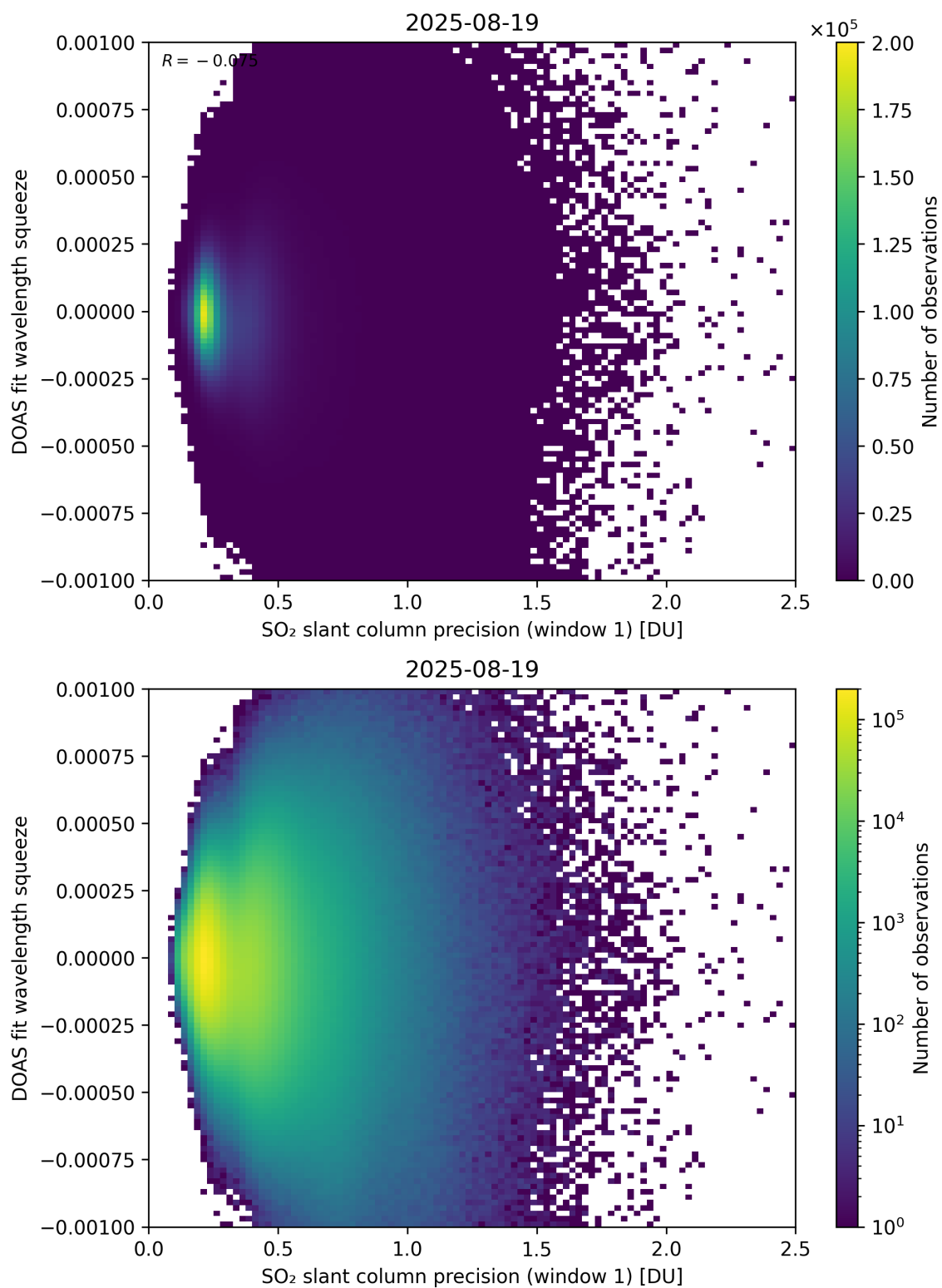
Figure 272: Scatter density plot of “SO 2 slant column precision (window 1)” against “DOAS fit wavelength squeeze” for 2025-08-19 to 2025-08-20.
