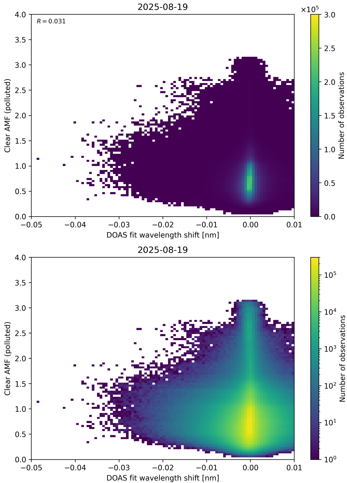
Figure 140: Scatter density plot of “DOAS fit wavelength shift” against “Clear AMF (polluted)” for 2025-08-19 to 2025-08-20.
