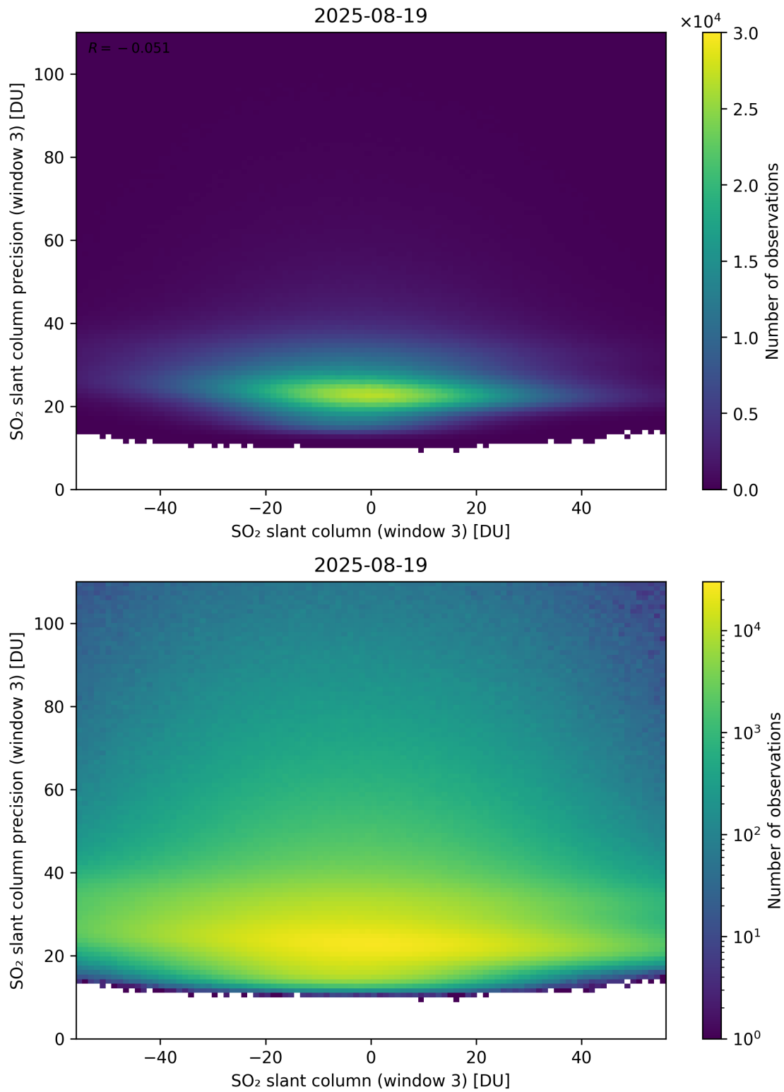
Figure 317: Scatter density plot of “SO 2 slant column (window 3)” against “SO 2 slant column precision (window 3)” for 2025-08-19 to 2025-08-20.
