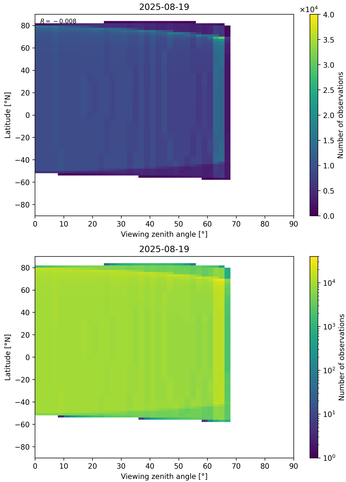
Figure 368: Scatter density plot of “Viewing zenith angle” against “Latitude” for 2025-08-19 to 2025-08-20.
