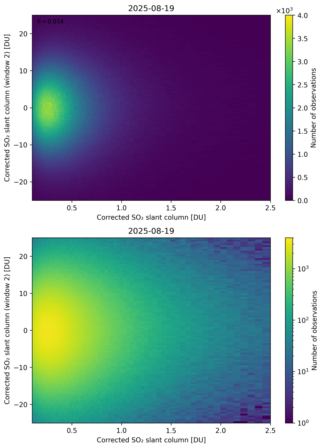
Figure 235: Scatter density plot of “Corrected SO 2 slant column” against “Corrected SO 2 slant column (window 2)” for 2025-08-19 to 2025-08-20.
