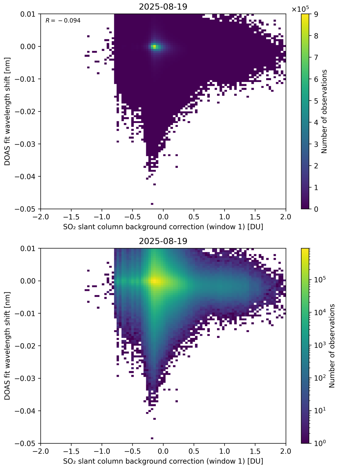
Figure 111: Scatter density plot of “SO 2 slant column background correction (window 1)” against “DOAS fit wavelength shift” for 2025-08-19 to 2025-08-20.
