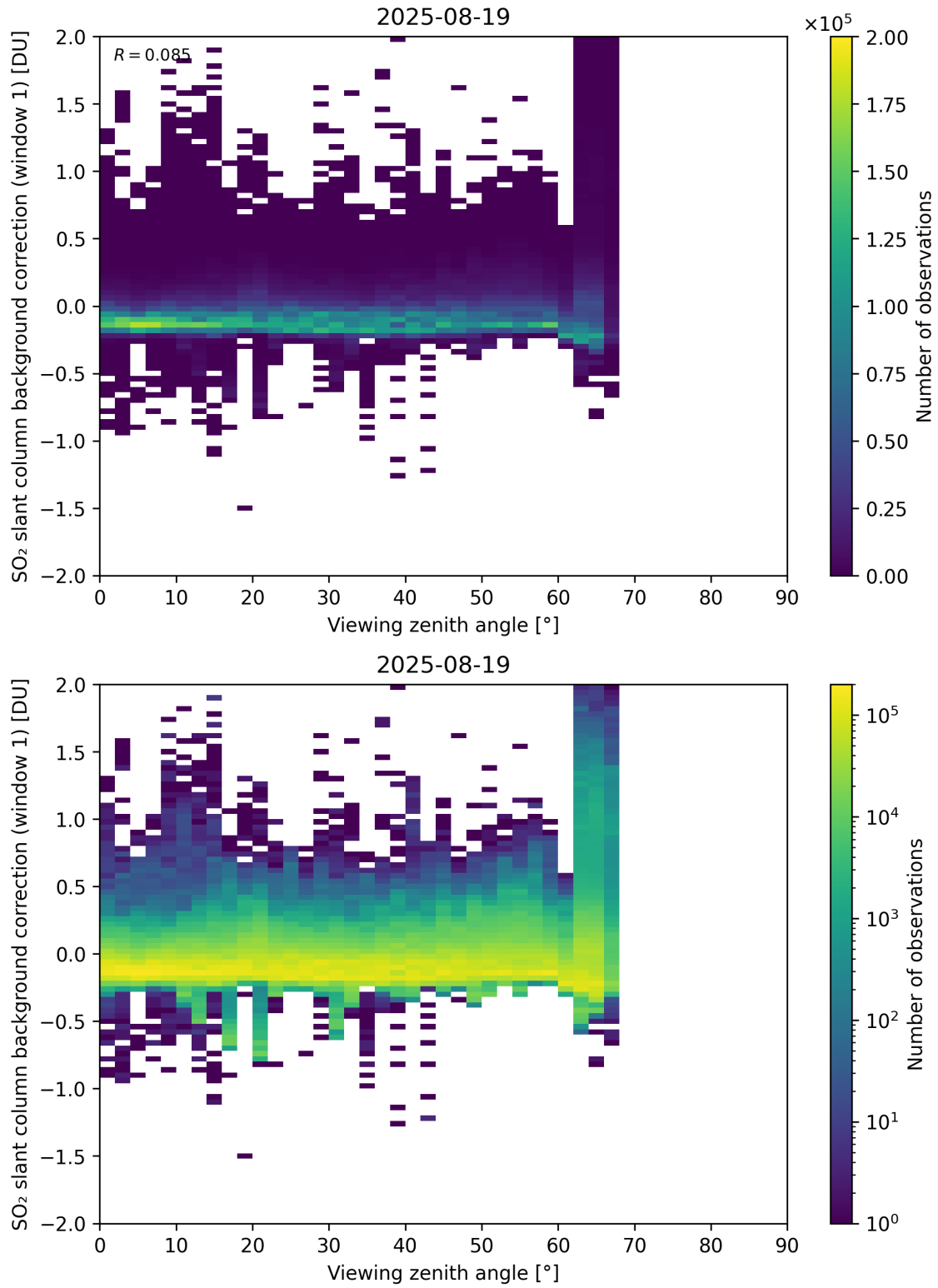
Figure 362: Scatter density plot of “Viewing zenith angle” against “SO 2 slant column background correction (window 1)” for 2025-08-19 to 2025-08-20.
