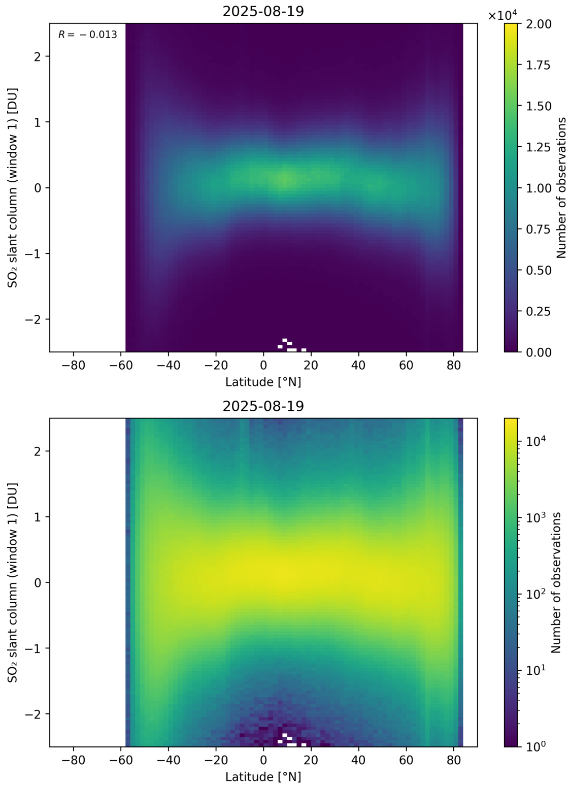
Figure 162: Scatter density plot of “Latitude” against “SO 2 slant column (window 1)” for 2025-08-19 to 2025-08-20.
