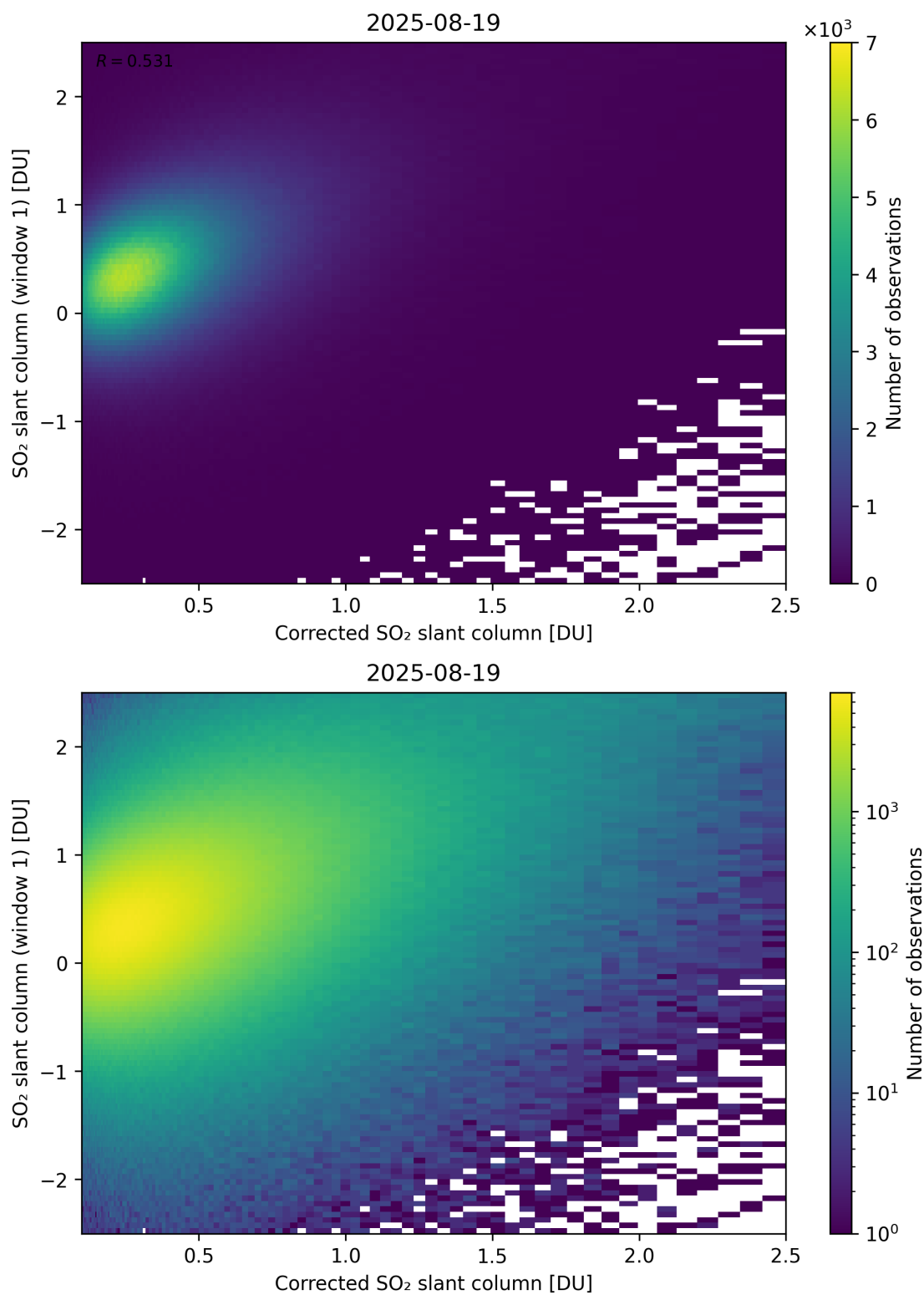
Figure 237: Scatter density plot of “Corrected SO 2 slant column” against “SO 2 slant column (window 1)” for 2025-08-19 to 2025-08-20.
