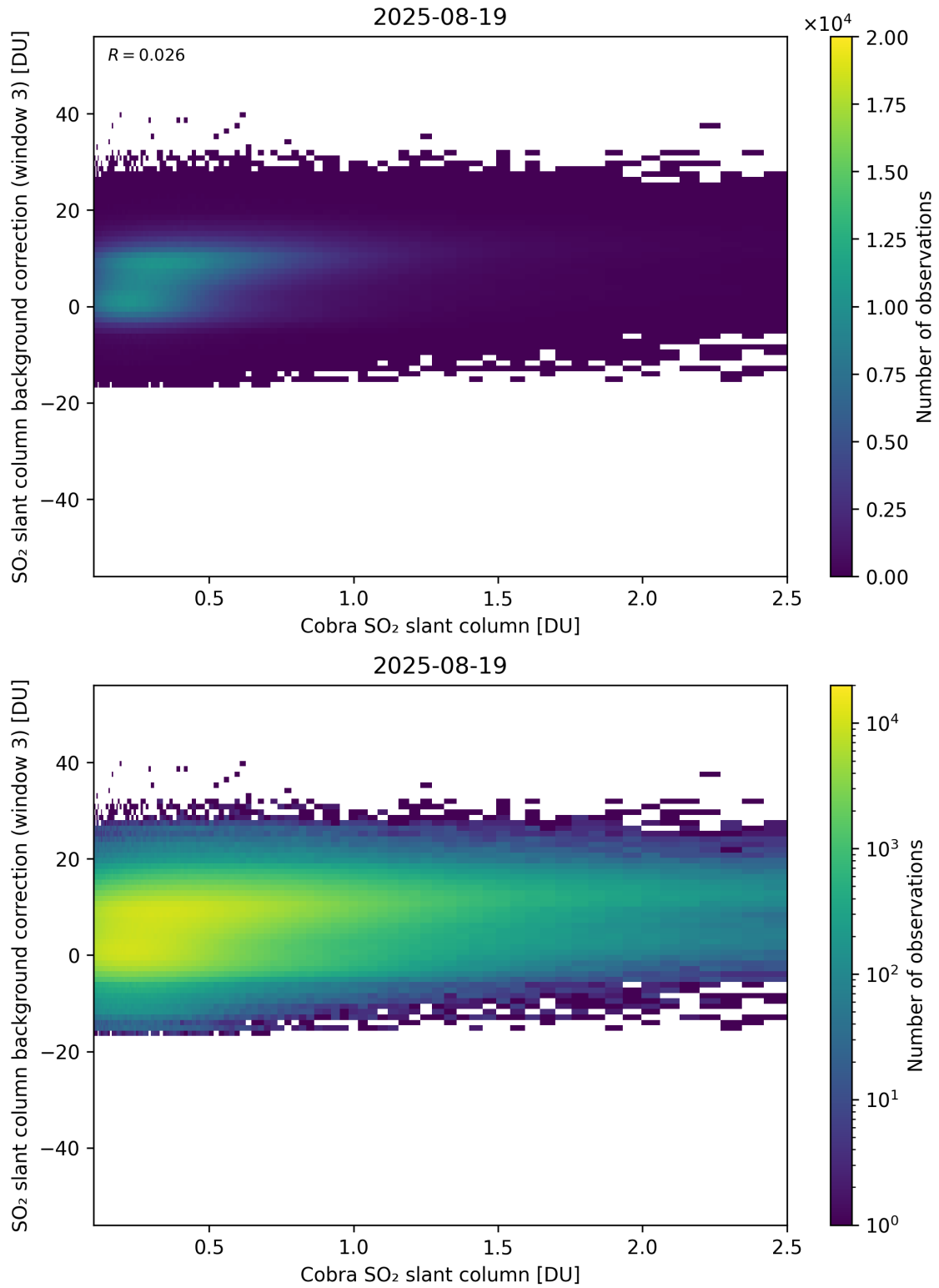
Figure 195: Scatter density plot of “Cobra SO 2 slant column” against “SO 2 slant column background correction (window 3)” for 2025-08-19 to 2025-08-20.
