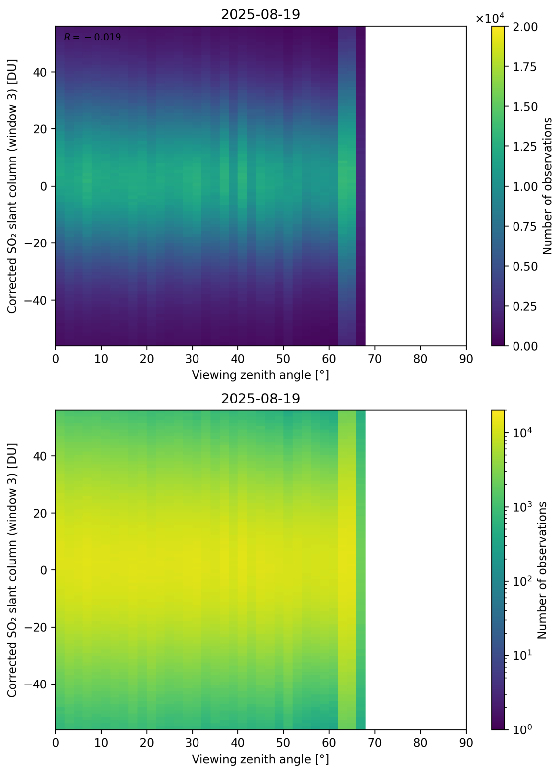
Figure 375: Scatter density plot of “Viewing zenith angle” against “Corrected SO 2 slant column (window 3)” for 2025-08-19 to 2025-08-20.
