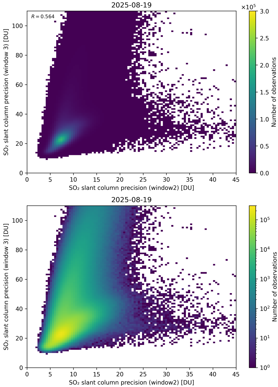
Figure 300: Scatter density plot of “SO 2 slant column precision (window2)” against “SO 2 slant column precision (window 3)” for 2025-08-19 to 2025-08-20.
