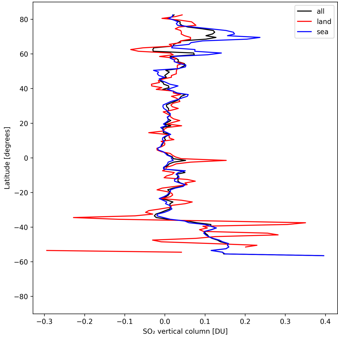
Figure 32: Zonal average of “SO 2 vertical column” for 2025-08-19 to 2025-08-20.
