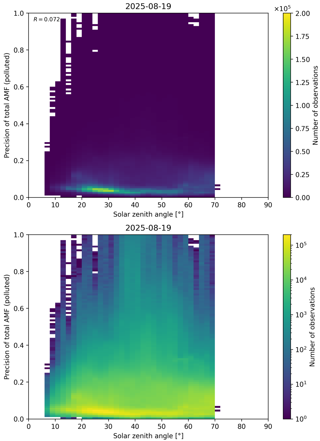
Figure 190: Scatter density plot of “Solar zenith angle” against “Precision of total AMF (polluted)” for 2025-08-19 to 2025-08-20.
