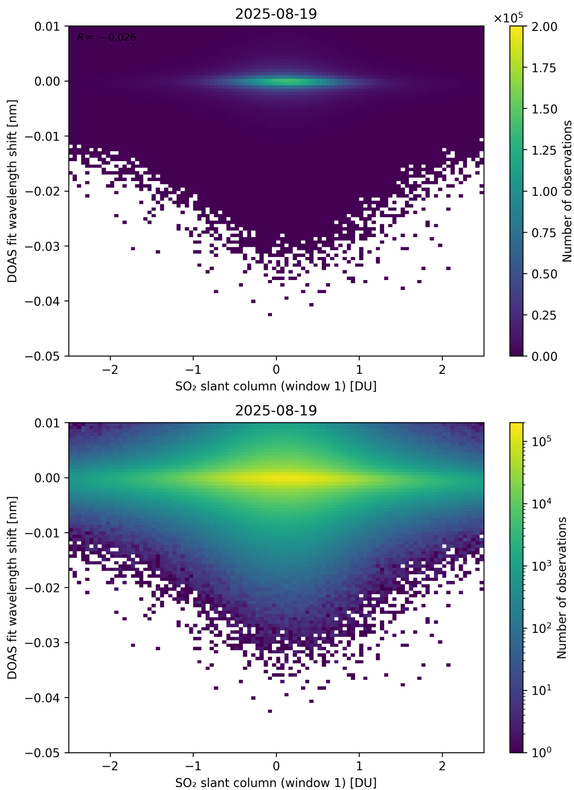
Figure 265: Scatter density plot of “SO 2 slant column (window 1)” against “DOAS fit wavelength shift” for 2025-08-19 to 2025-08-20.
