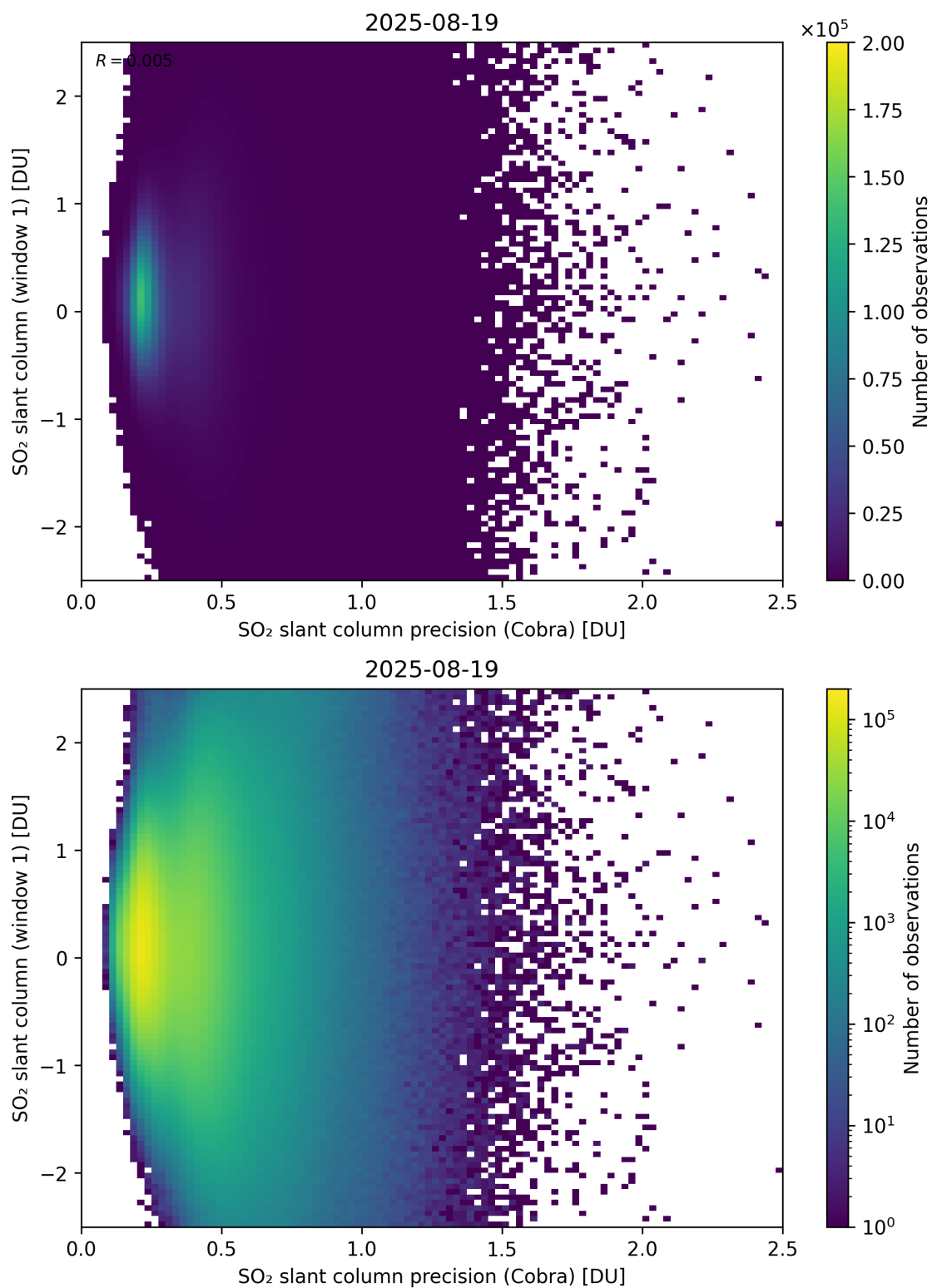
Figure 208: Scatter density plot of “SO 2 slant column precision (Cobra)” against “SO 2 slant column (window 1)” for 2025-08-19 to 2025-08-20.
