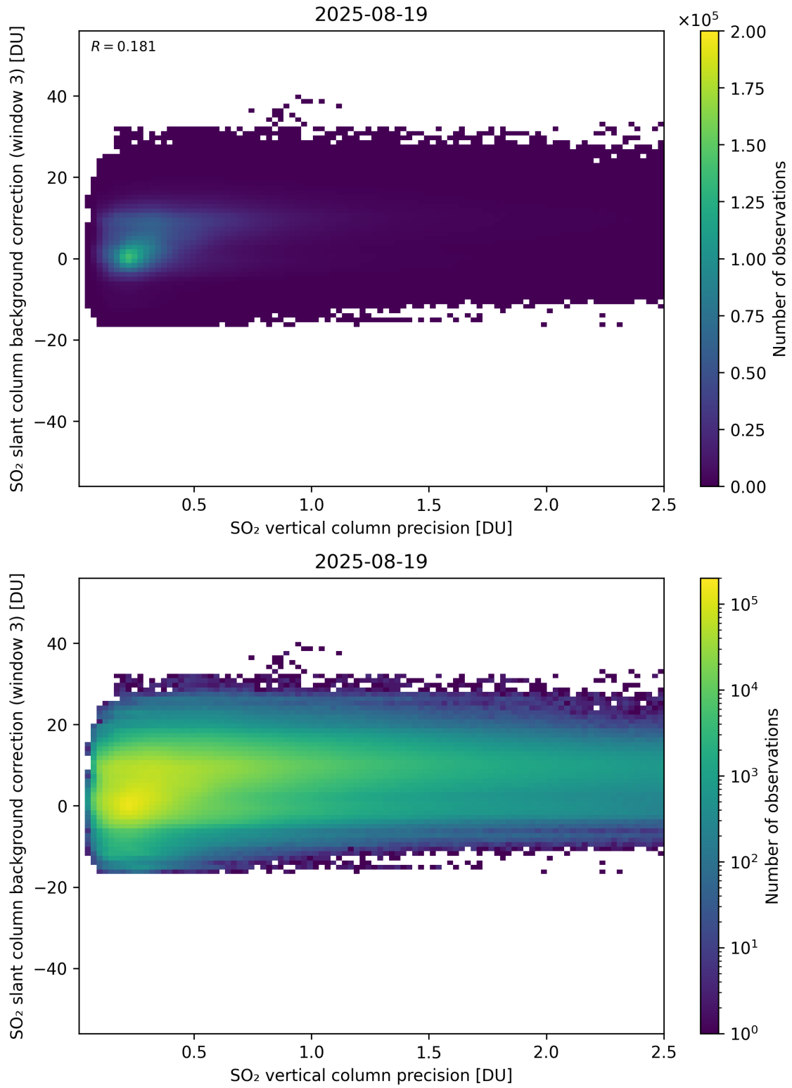
Figure 331: Scatter density plot of “SO 2 vertical column precision” against “SO 2 slant column background correction (window 3)” for 2025-08-19 to 2025-08-20.
