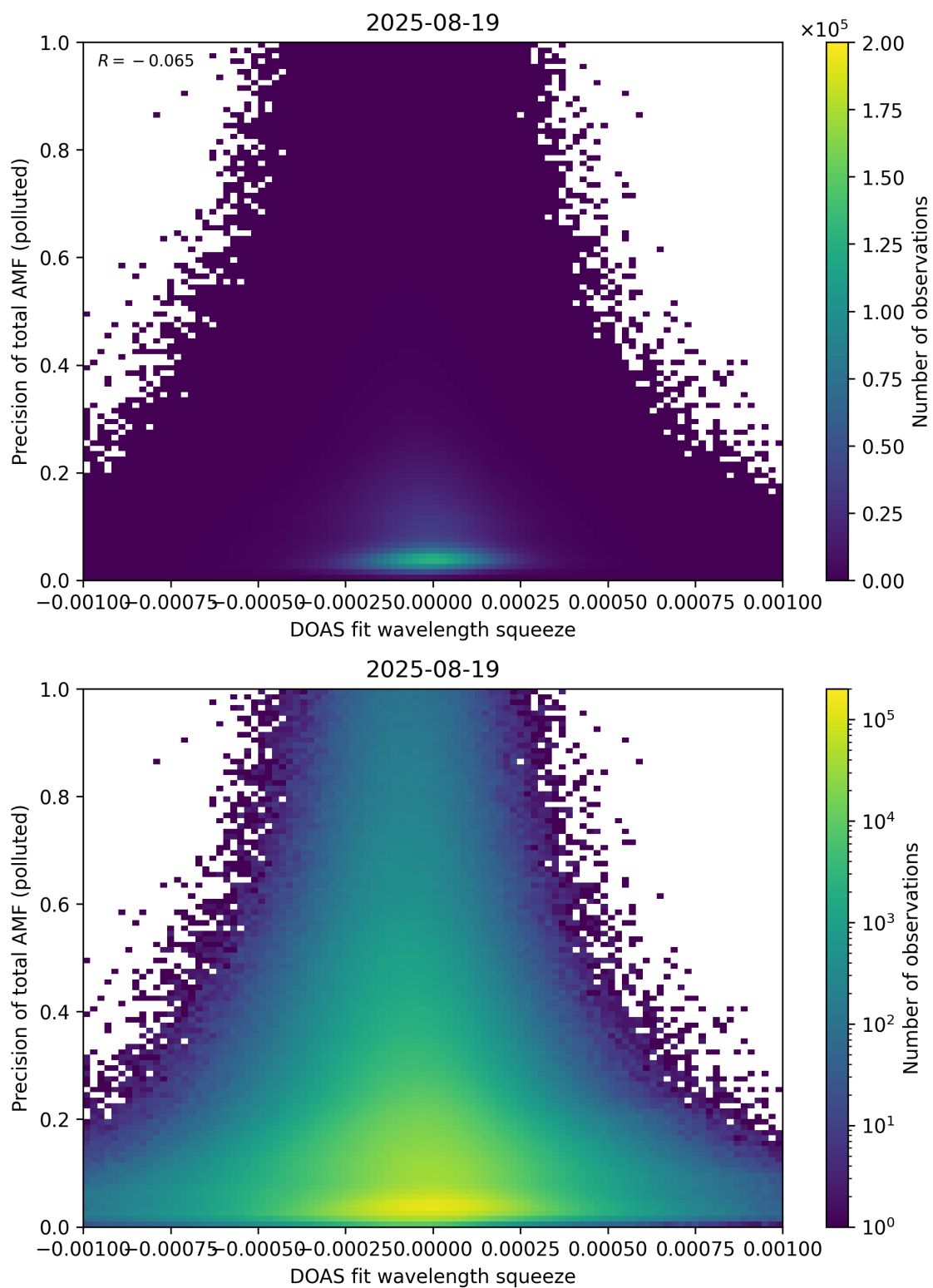
Figure 146: Scatter density plot of “DOAS fit wavelength squeeze” against “Precision of total AMF (polluted)” for 2025-08-19 to 2025-08-20.
