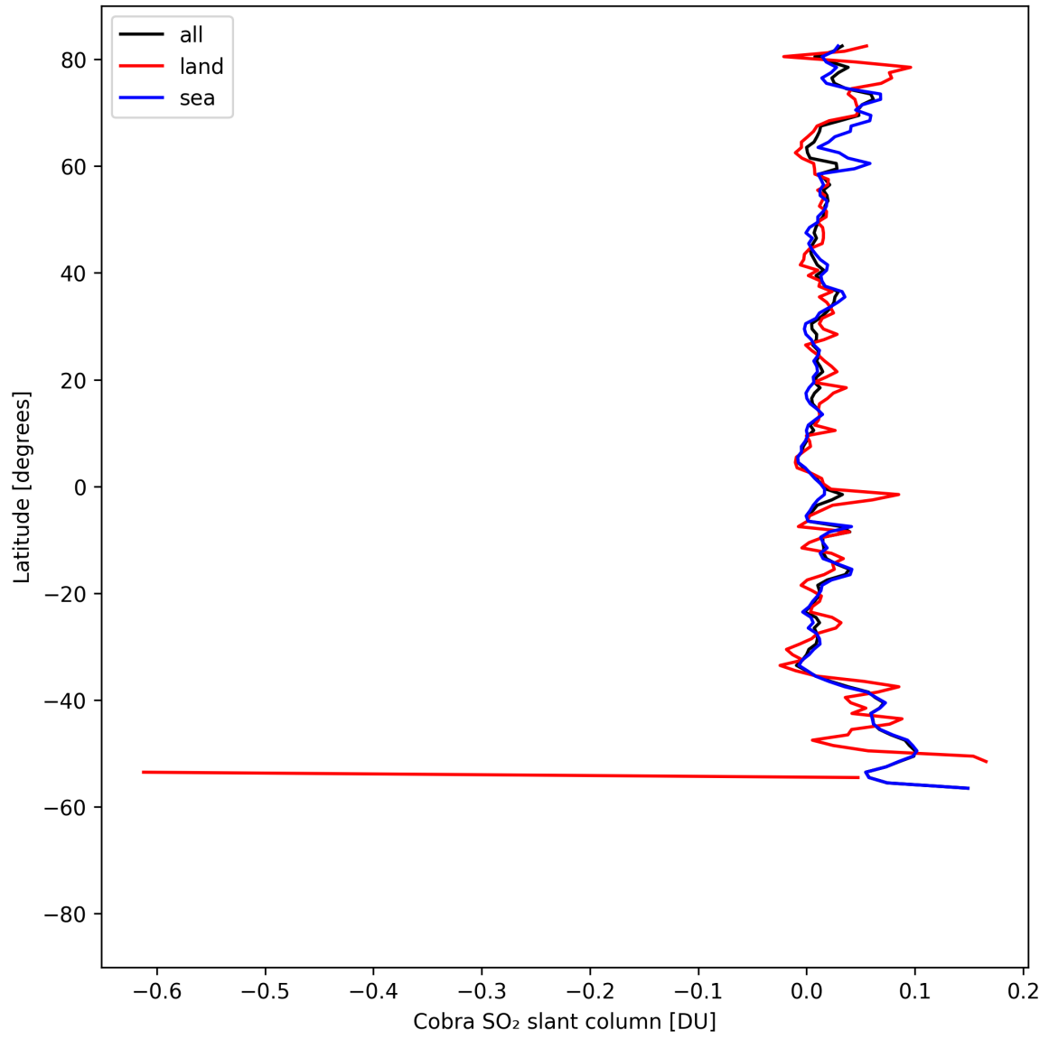
Figure 35: Zonal average of “Cobra SO 2 slant column” for 2025-08-19 to 2025-08-20.
