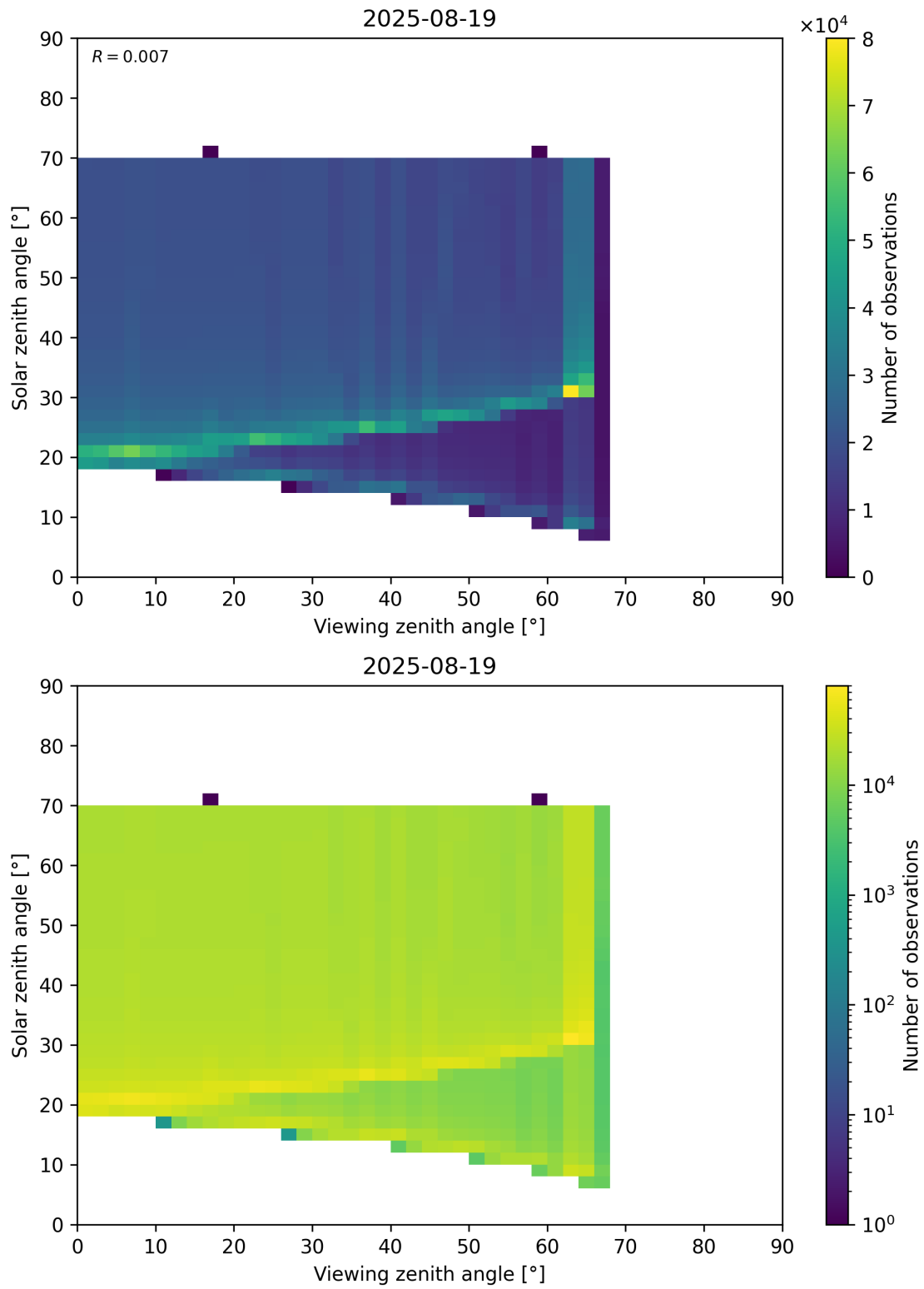
Figure 369: Scatter density plot of “Viewing zenith angle” against “Solar zenith angle” for 2025-08-19 to 2025-08-20.
