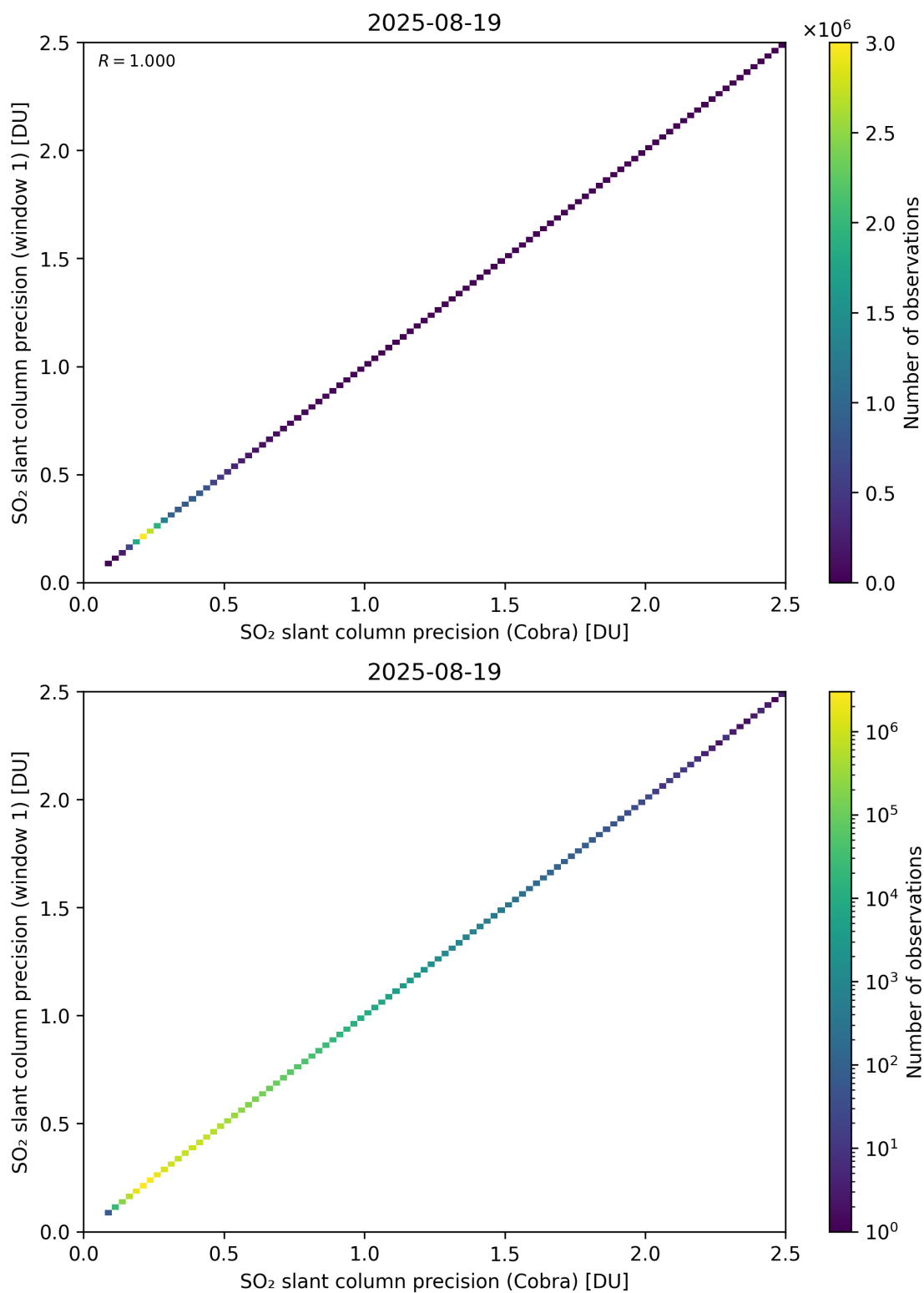
Figure 209: Scatter density plot of “SO 2 slant column precision (Cobra)” against “SO 2 slant column precision (window 1)” for 2025-08-19 to 2025-08-20.
