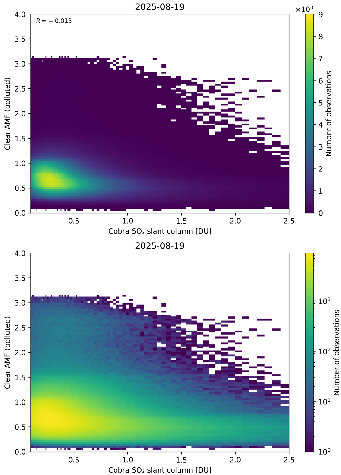
Figure 215: Scatter density plot of “Cobra SO 2 slant column” against “Clear AMF (polluted)” for 2025-08-19 to 2025-08-20.
