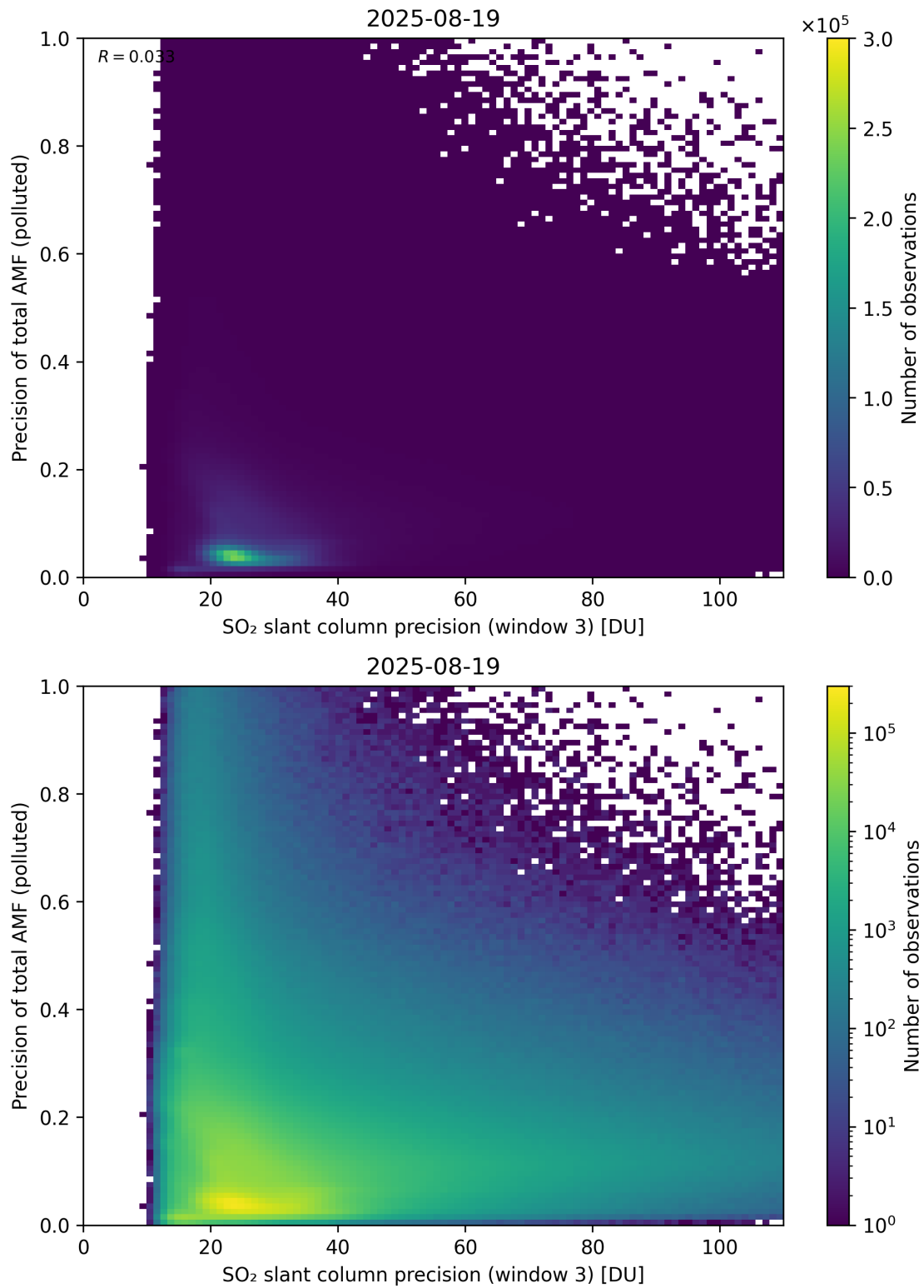
Figure 314: Scatter density plot of “SO 2 slant column precision (window 3)” against “Precision of total AMF (polluted)” for 2025-08-19 to 2025-08-20.
