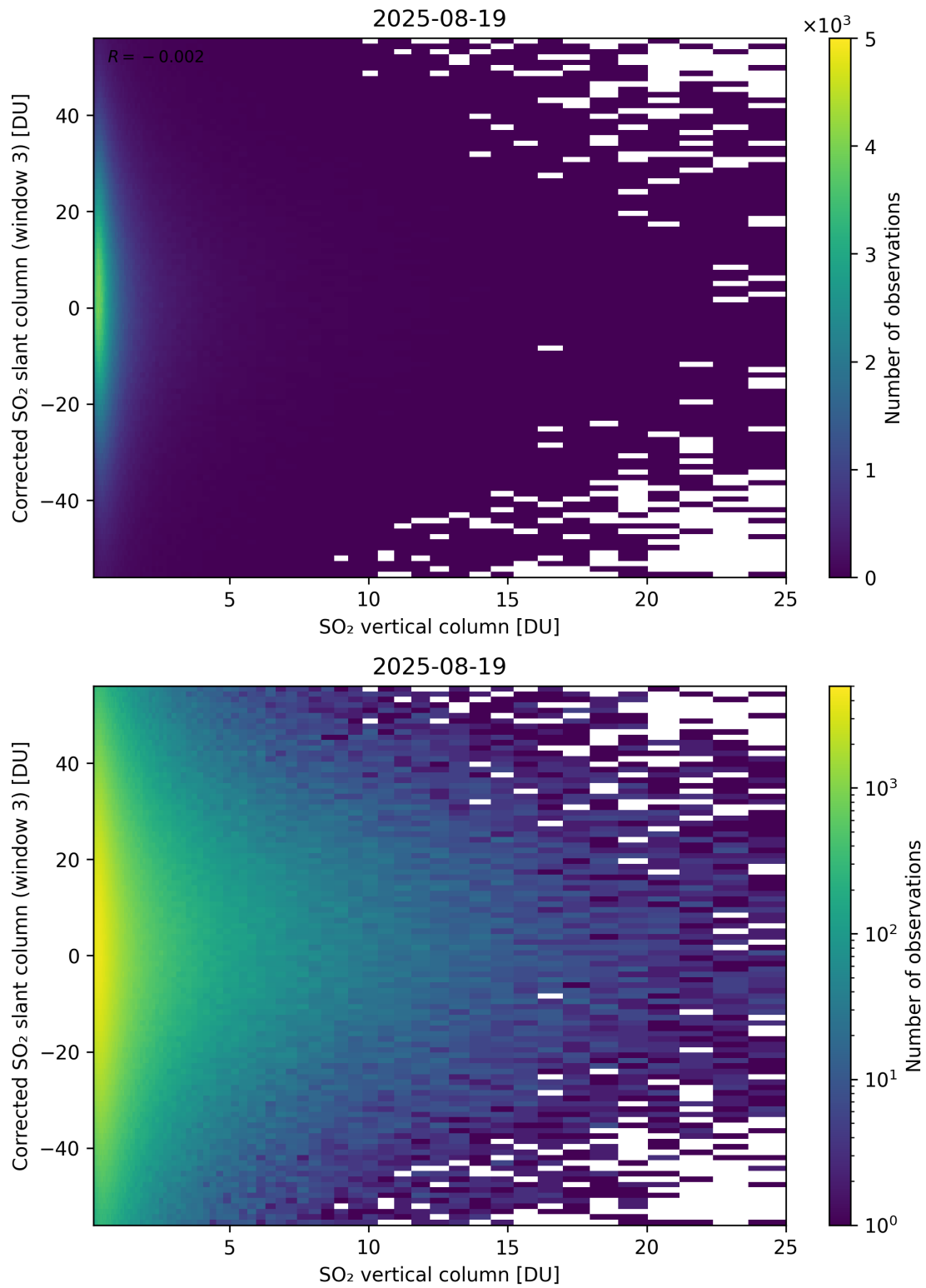
Figure 353: Scatter density plot of “SO 2 vertical column” against “Corrected SO 2 slant column (window 3)” for 2025-08-19 to 2025-08-20.
