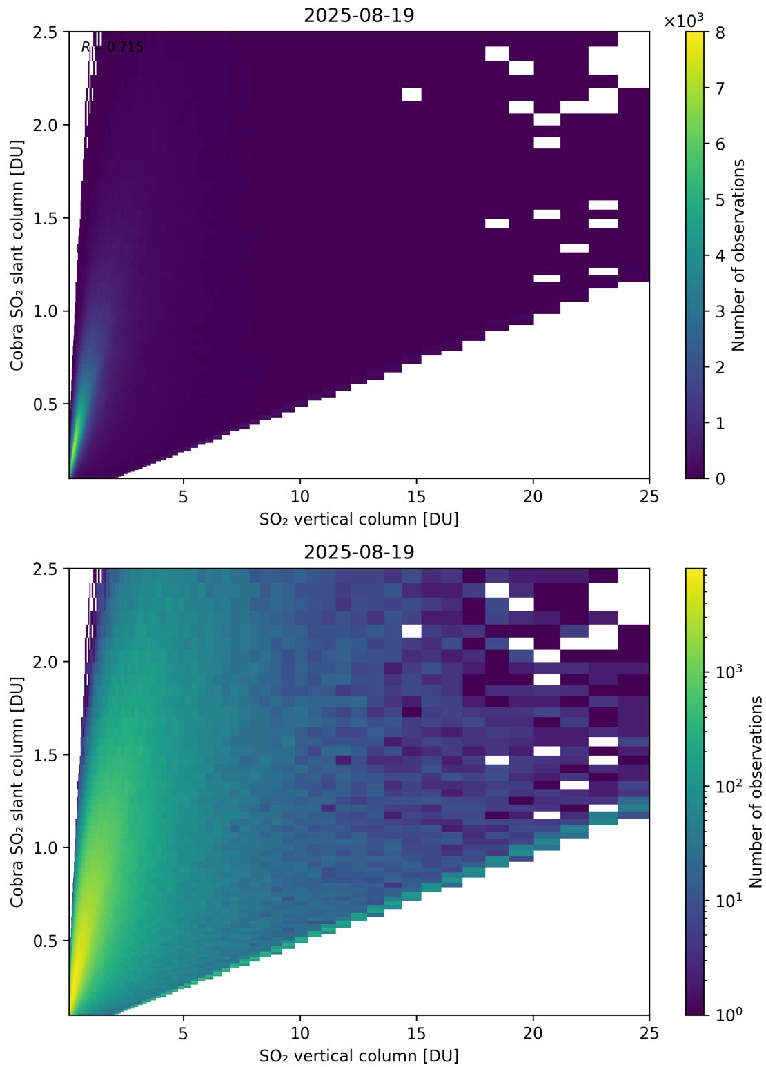
Figure 349: Scatter density plot of “SO 2 vertical column” against “Cobra SO 2 slant column” for 2025-08-19 to 2025-08-20.
