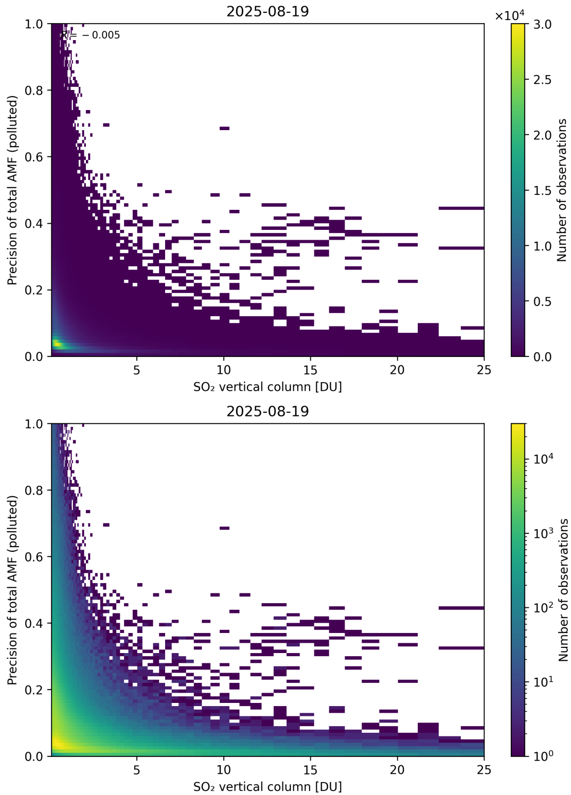
Figure 360: Scatter density plot of “SO 2 vertical column” against “Precision of total AMF (polluted)” for 2025-08-19 to 2025-08-20.
