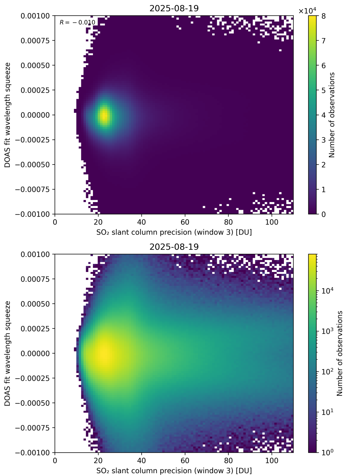
Figure 309: Scatter density plot of “SO 2 slant column precision (window 3)” against “DOAS fit wavelength squeeze” for 2025-08-19 to 2025-08-20.
