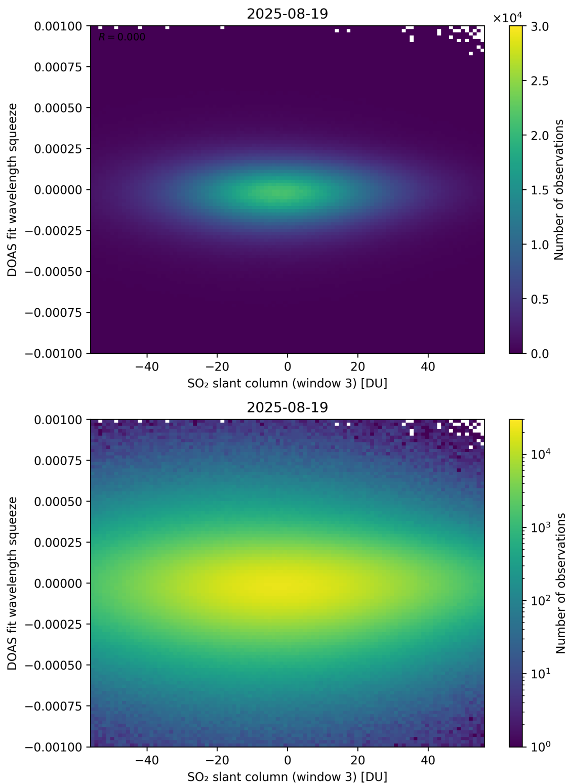
Figure 305: Scatter density plot of “SO 2 slant column (window 3)” against “DOAS fit wavelength squeeze” for 2025-08-19 to 2025-08-20.
