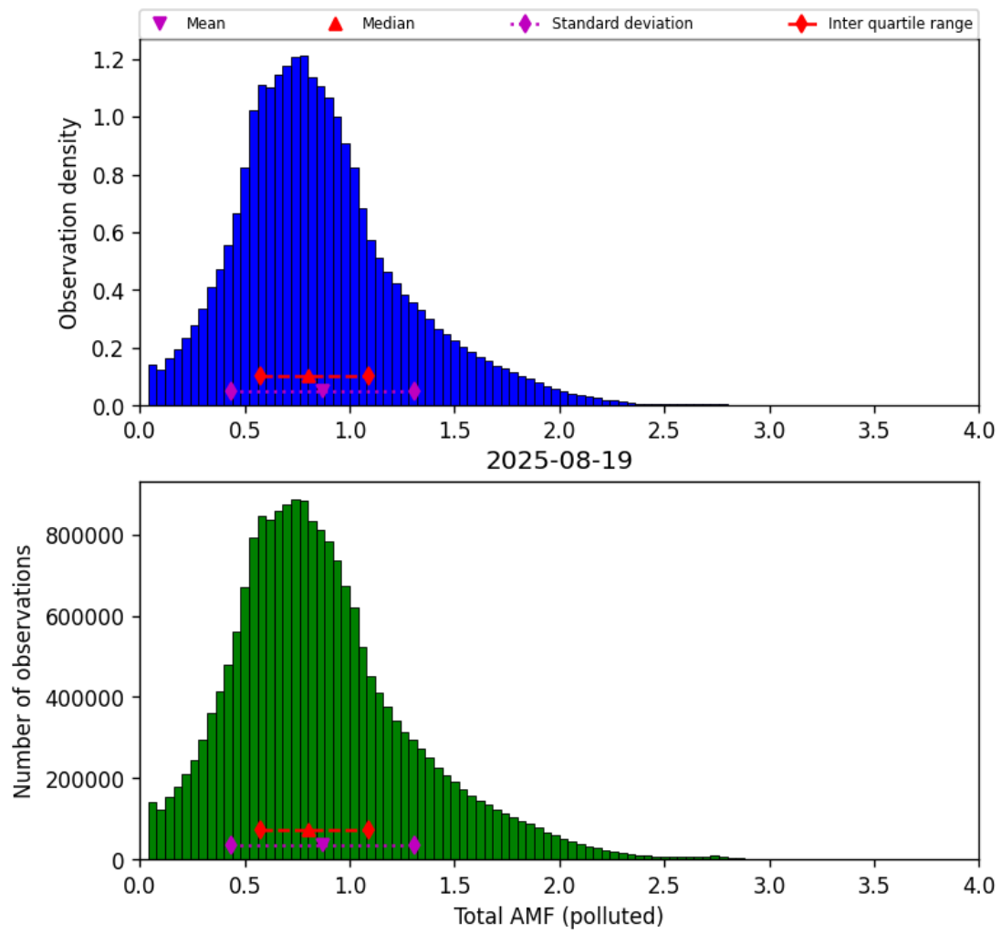
Figure 79: Histogram of “Total AMF (polluted)” for 2025-08-19 to 2025-08-20
