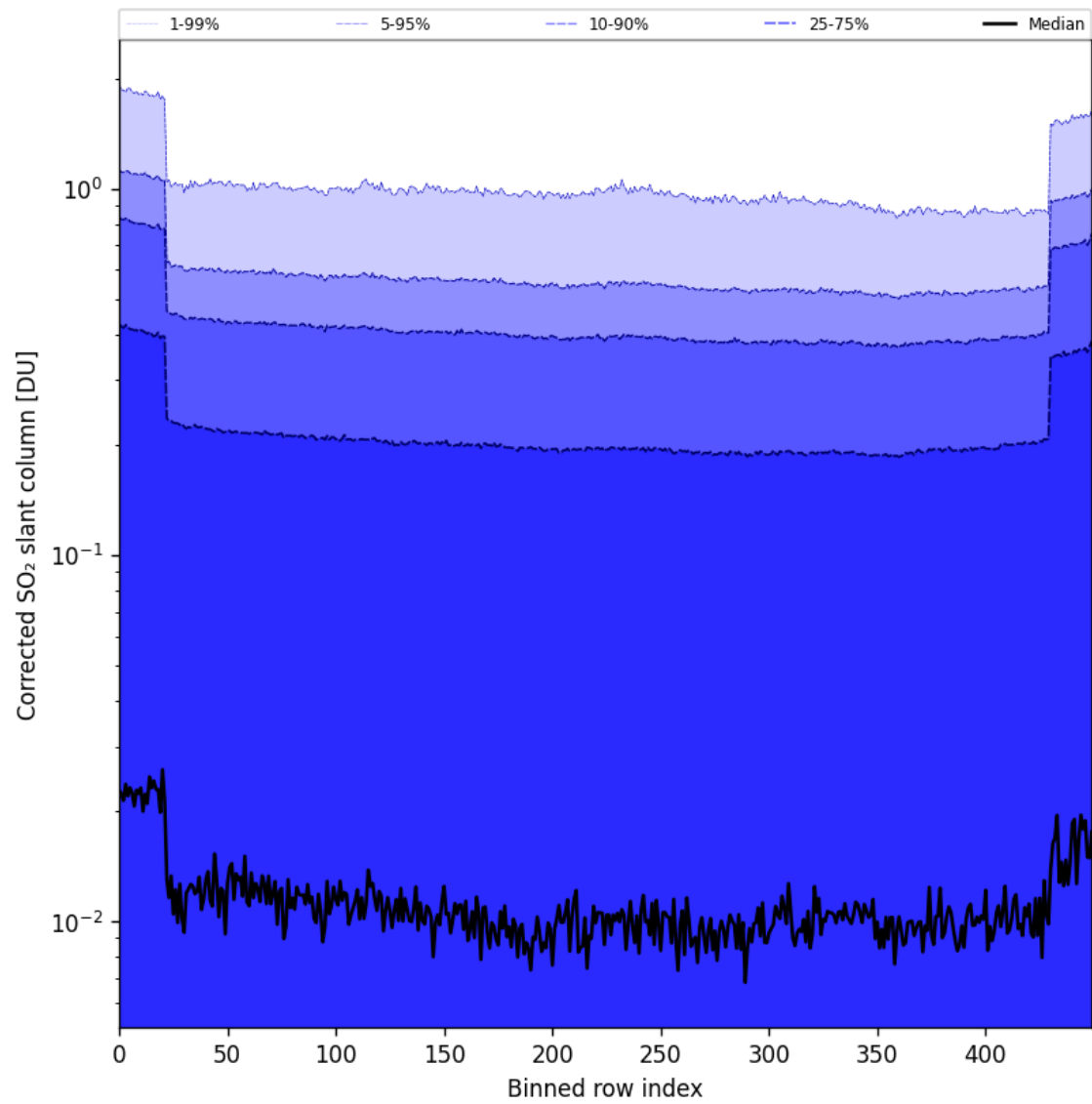
Figure 86: Along track statistics of “Corrected SO 2 slant column” for 2025-08-19 to 2025-08-20
