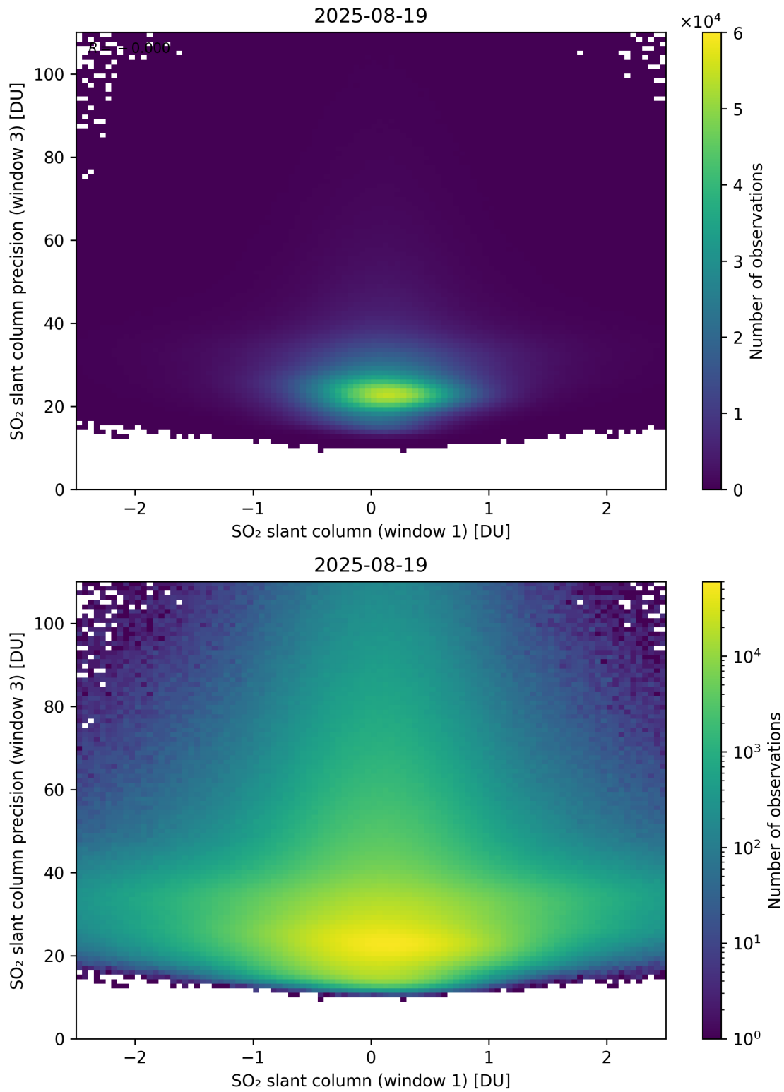
Figure 288: Scatter density plot of “SO 2 slant column (window 1)” against “SO 2 slant column precision (window 3)” for 2025-08-19 to 2025-08-20.
