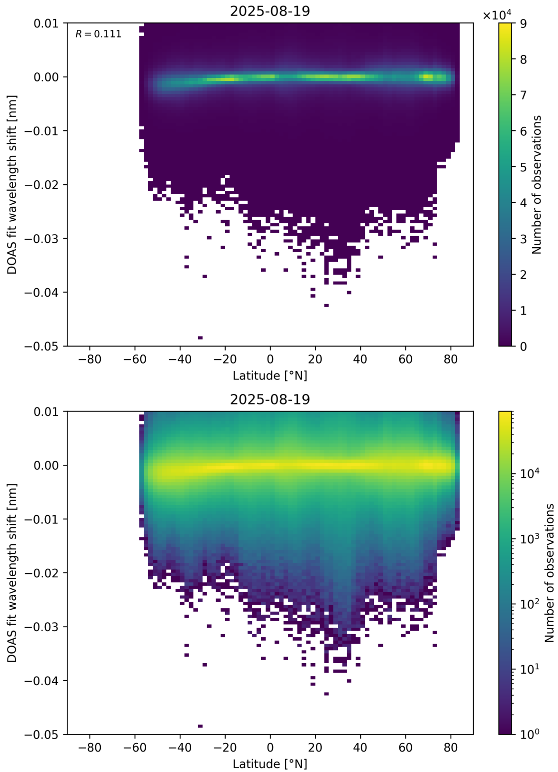
Figure 153: Scatter density plot of “Latitude” against “DOAS fit wavelength shift” for 2025-08-19 to 2025-08-20.
