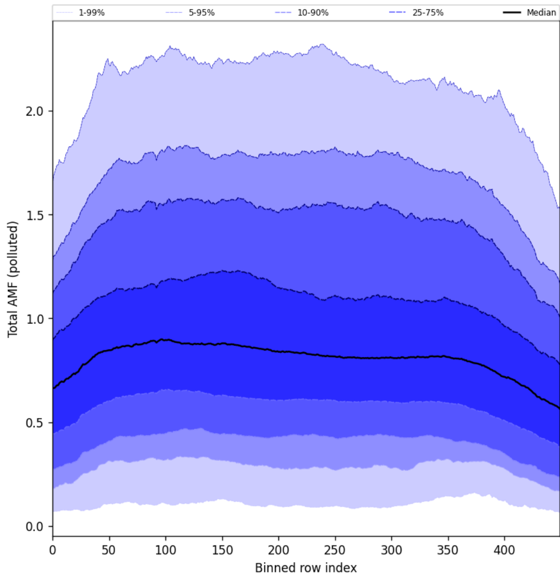
Figure 105: Along track statistics of “Total AMF (polluted)” for 2025-08-19 to 2025-08-20
