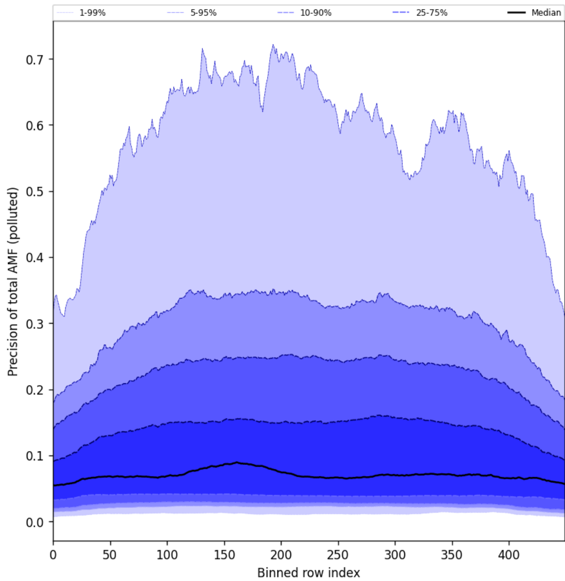
Figure 106: Along track statistics of “Precision of total AMF (polluted)” for 2025-08-19 to 2025-08-20
