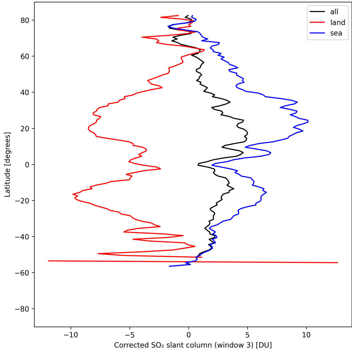
Figure 47: Zonal average of “Corrected SO 2 slant column (window 3)” for 2025-08-19 to 2025-08-20.
