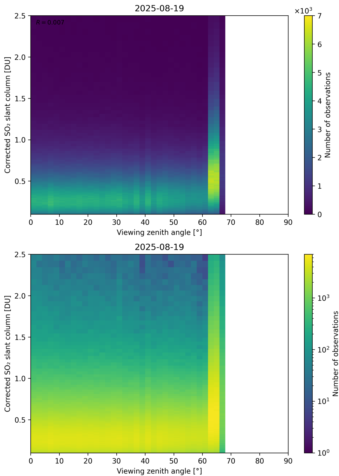
Figure 373: Scatter density plot of “Viewing zenith angle” against “Corrected SO 2 slant column” for 2025-08-19 to 2025-08-20.
