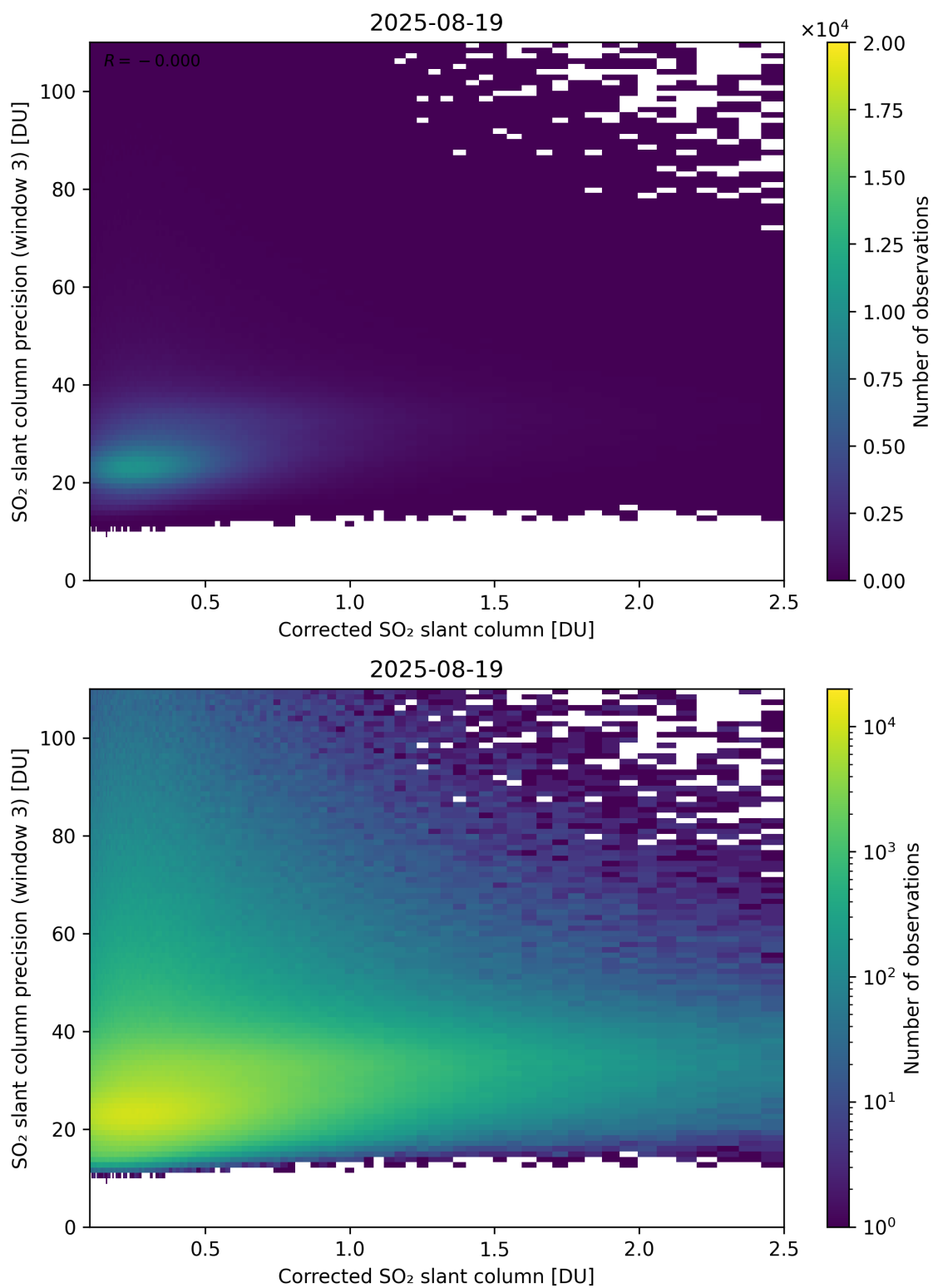
Figure 241: Scatter density plot of “Corrected SO 2 slant column” against “SO 2 slant column precision (window 3)” for 2025-08-19 to 2025-08-20.
