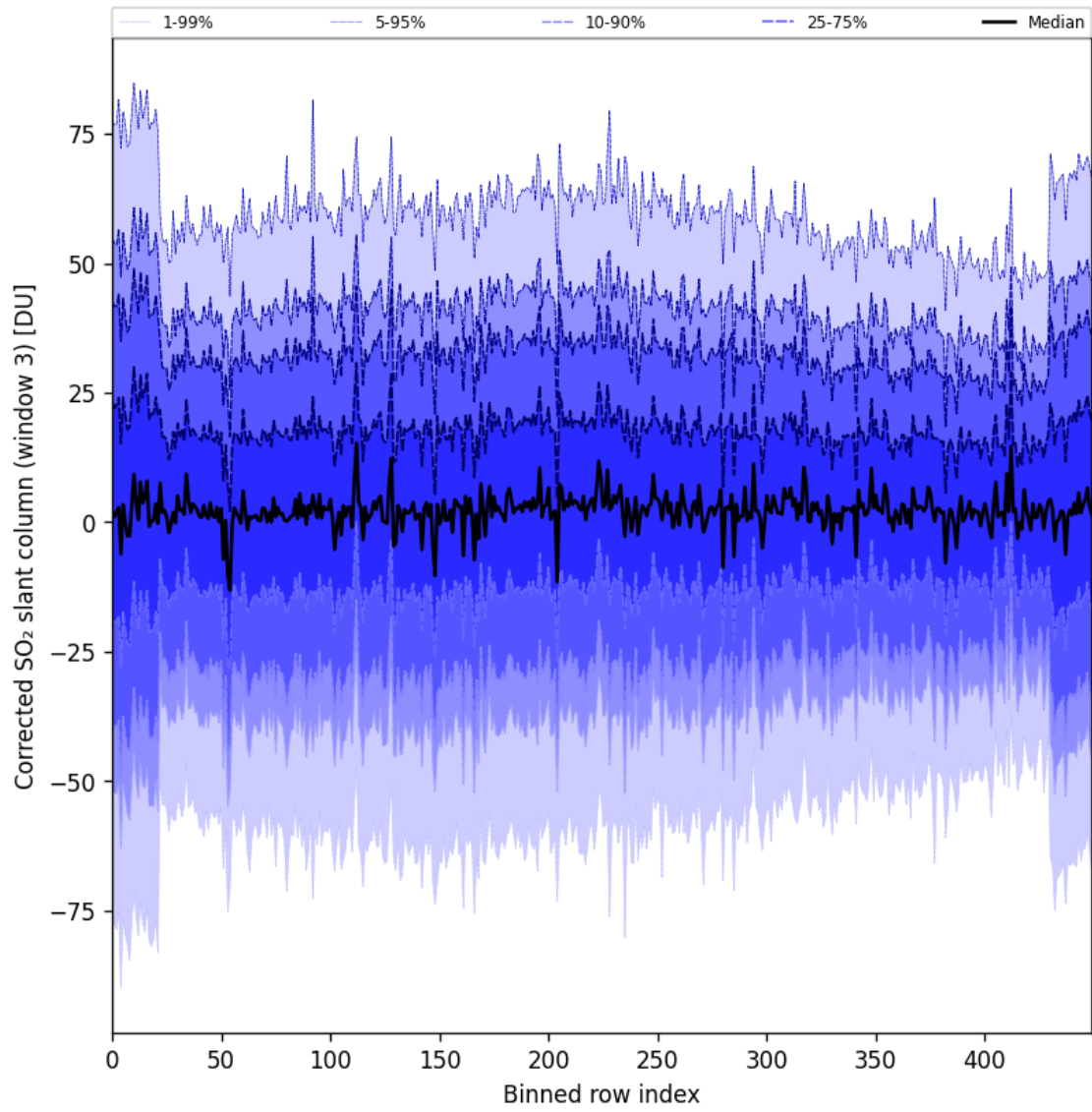
Figure 99: Along track statistics of “Corrected SO 2 slant column (window 3)” for 2025-08-19 to 2025-08-20
