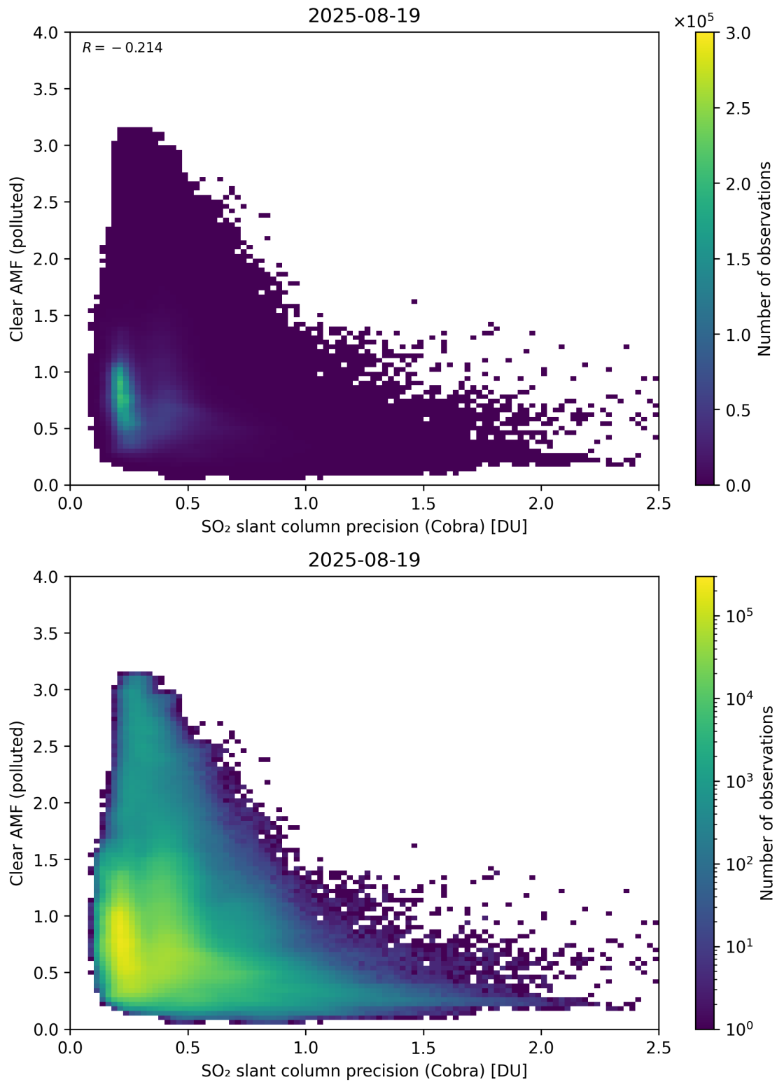
Figure 205: Scatter density plot of “SO 2 slant column precision (Cobra)” against “Clear AMF (polluted)” for 2025-08-19 to 2025-08-20.
