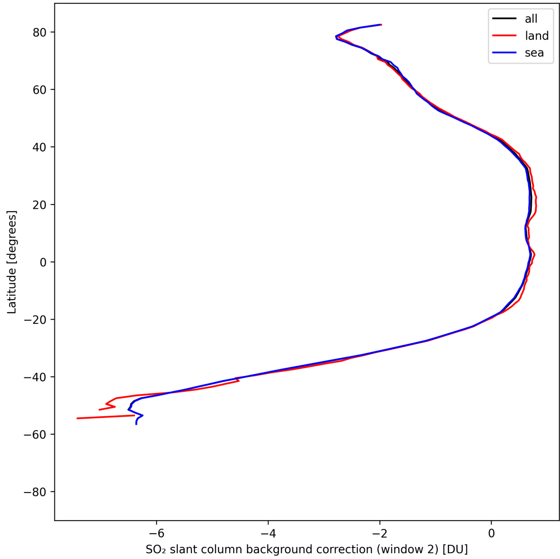
Figure 44: Zonal average of “SO 2 slant column background correction (window 2)” for 2025-08-19 to 2025-08-20.
