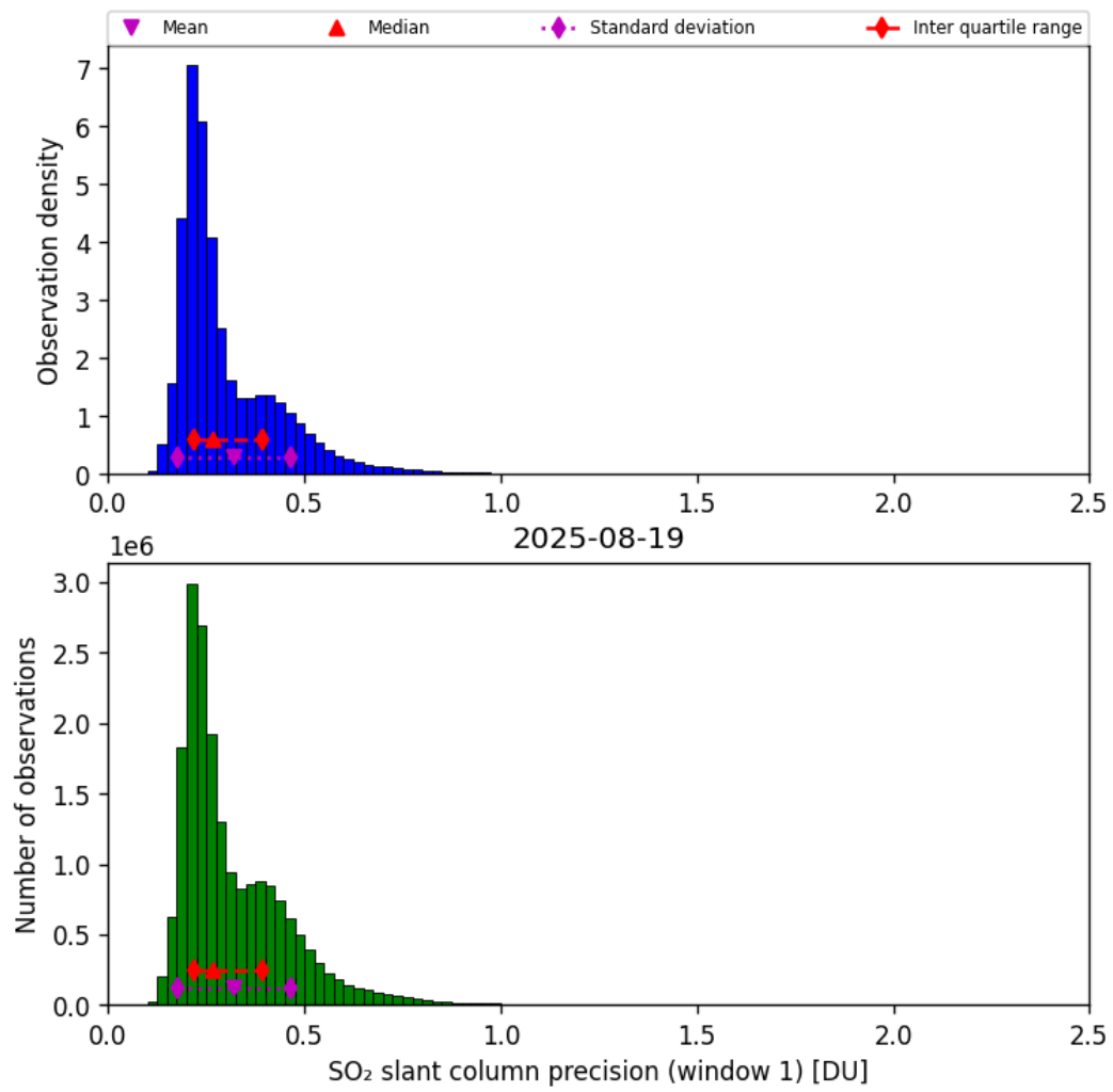
Figure 64: Histogram of “SO 2 slant column precision (window 1)” for 2025-08-19 to 2025-08-20
