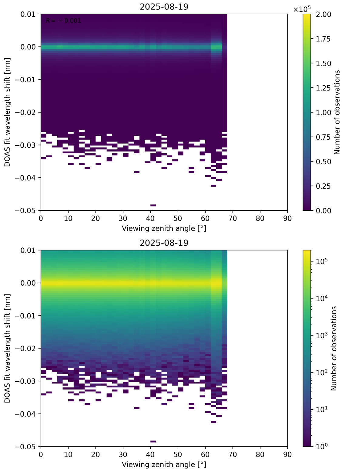
Figure 365: Scatter density plot of “Viewing zenith angle” against “DOAS fit wavelength shift” for 2025-08-19 to 2025-08-20.
