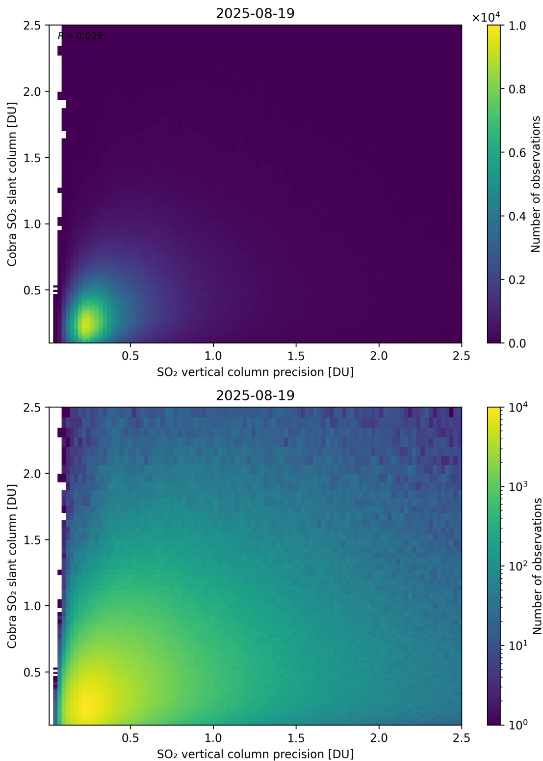
Figure 336: Scatter density plot of “SO 2 vertical column precision” against “Cobra SO 2 slant column” for 2025-08-19 to 2025-08-20.
