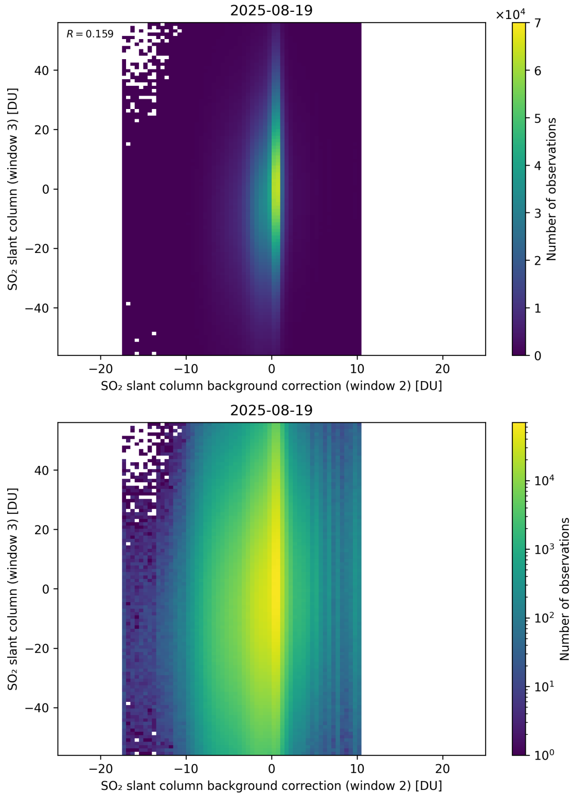
Figure 128: Scatter density plot of “SO 2 slant column background correction (window 2)” against “SO 2 slant column (window 3)” for 2025-08-19 to 2025-08-20.
