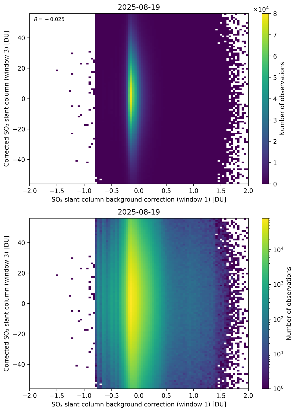
Figure 116: Scatter density plot of “SO 2 slant column background correction (window 1)” against “Corrected SO 2 slant column (window 3)” for 2025-08-19 to 2025-08-20.
