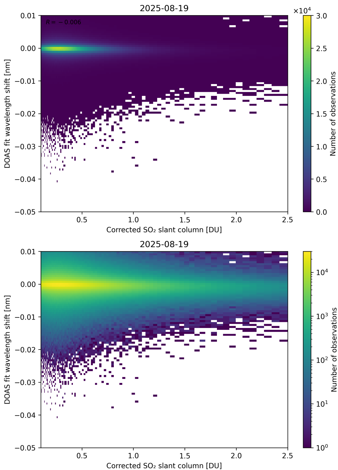
Figure 229: Scatter density plot of “Corrected SO 2 slant column” against “DOAS fit wavelength shift” for 2025-08-19 to 2025-08-20.
