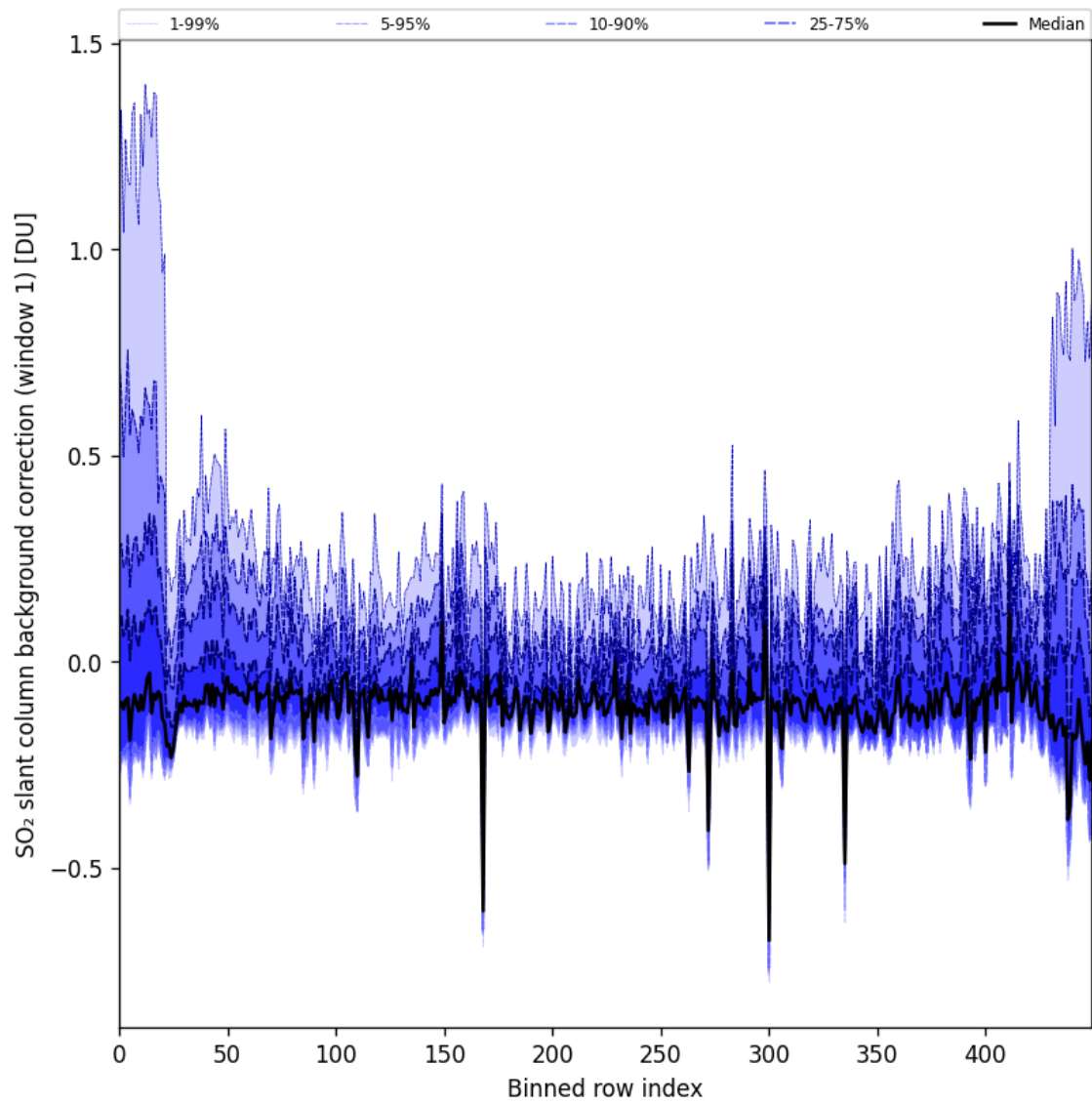
Figure 92: Along track statistics of “SO 2 slant column background correction (window 1)” for 2025-08-19 to 2025-08-20
