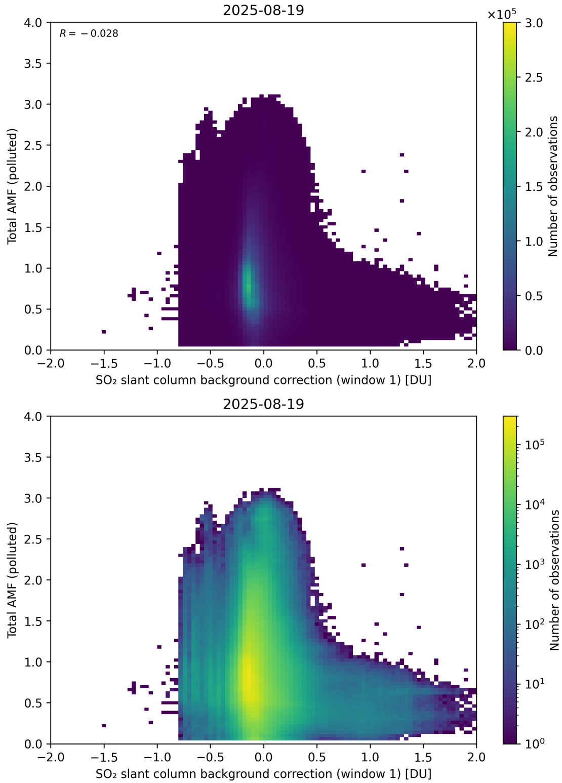
Figure 120: Scatter density plot of “SO 2 slant column background correction (window 1)” against “Total AMF (polluted)” for 2025-08-19 to 2025-08-20.
