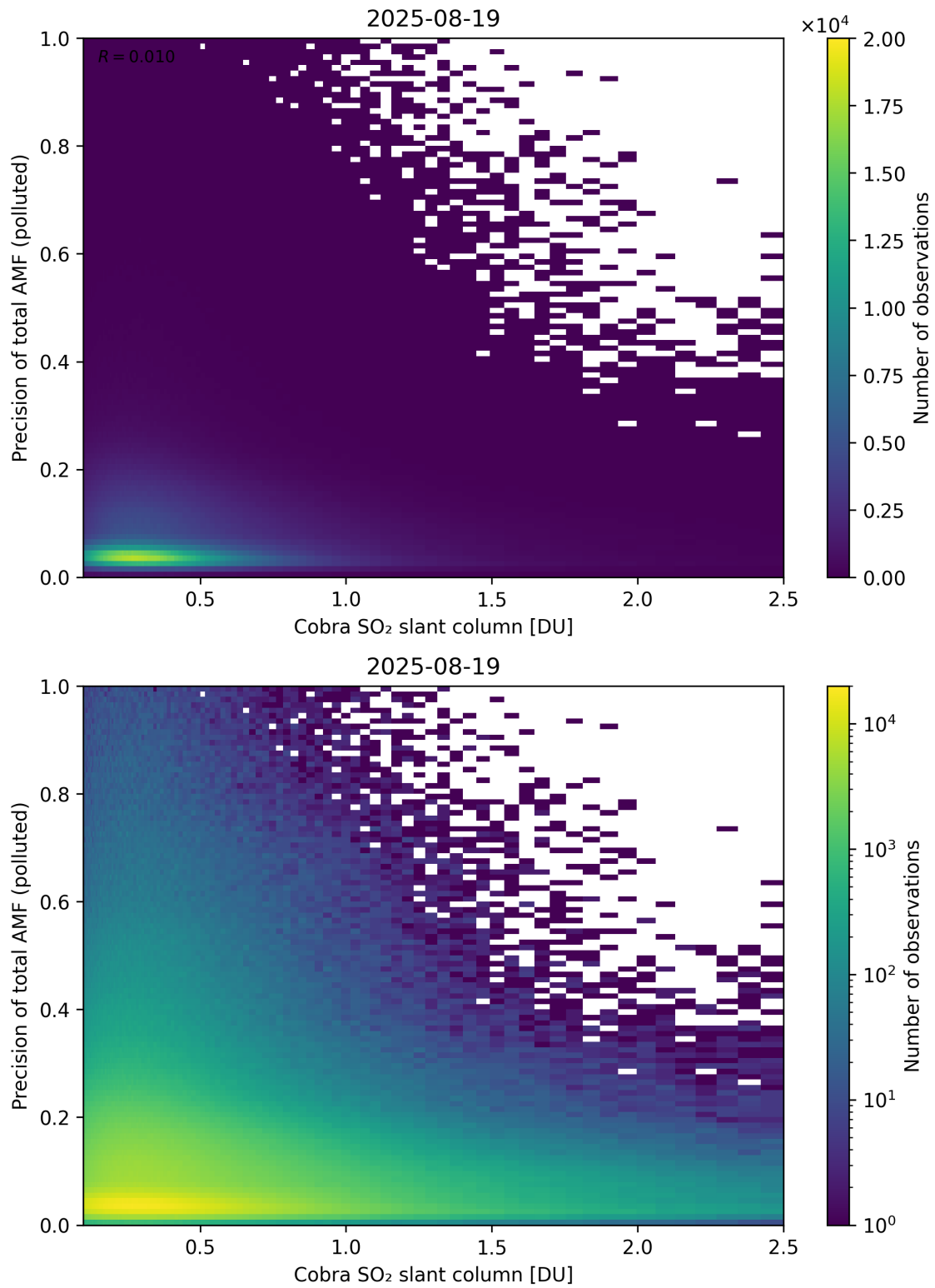
Figure 225: Scatter density plot of “Cobra SO 2 slant column” against “Precision of total AMF (polluted)” for 2025-08-19 to 2025-08-20.
