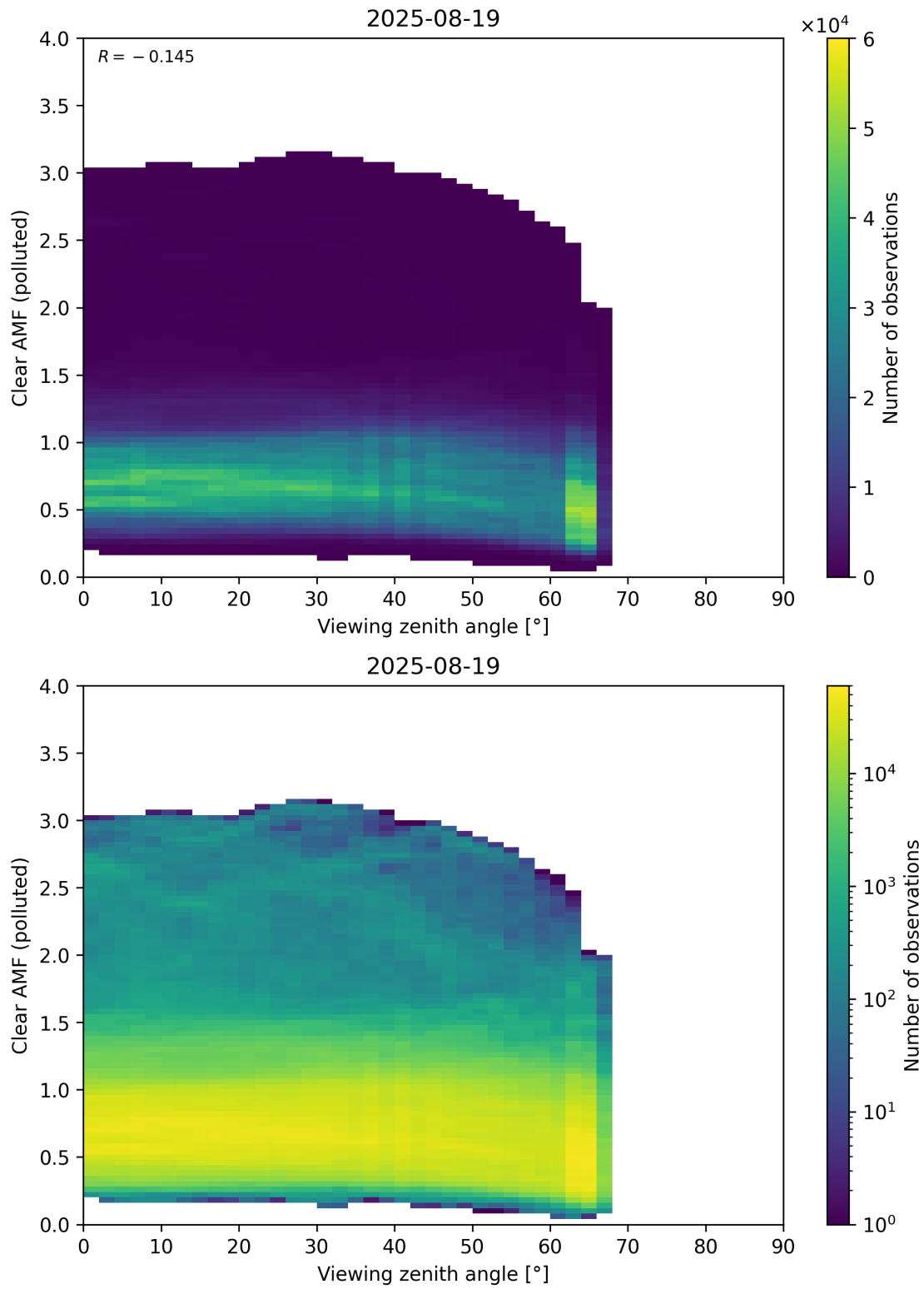
Figure 370: Scatter density plot of “Viewing zenith angle” against “Clear AMF (polluted)” for 2025-08-19 to 2025-08-20.
