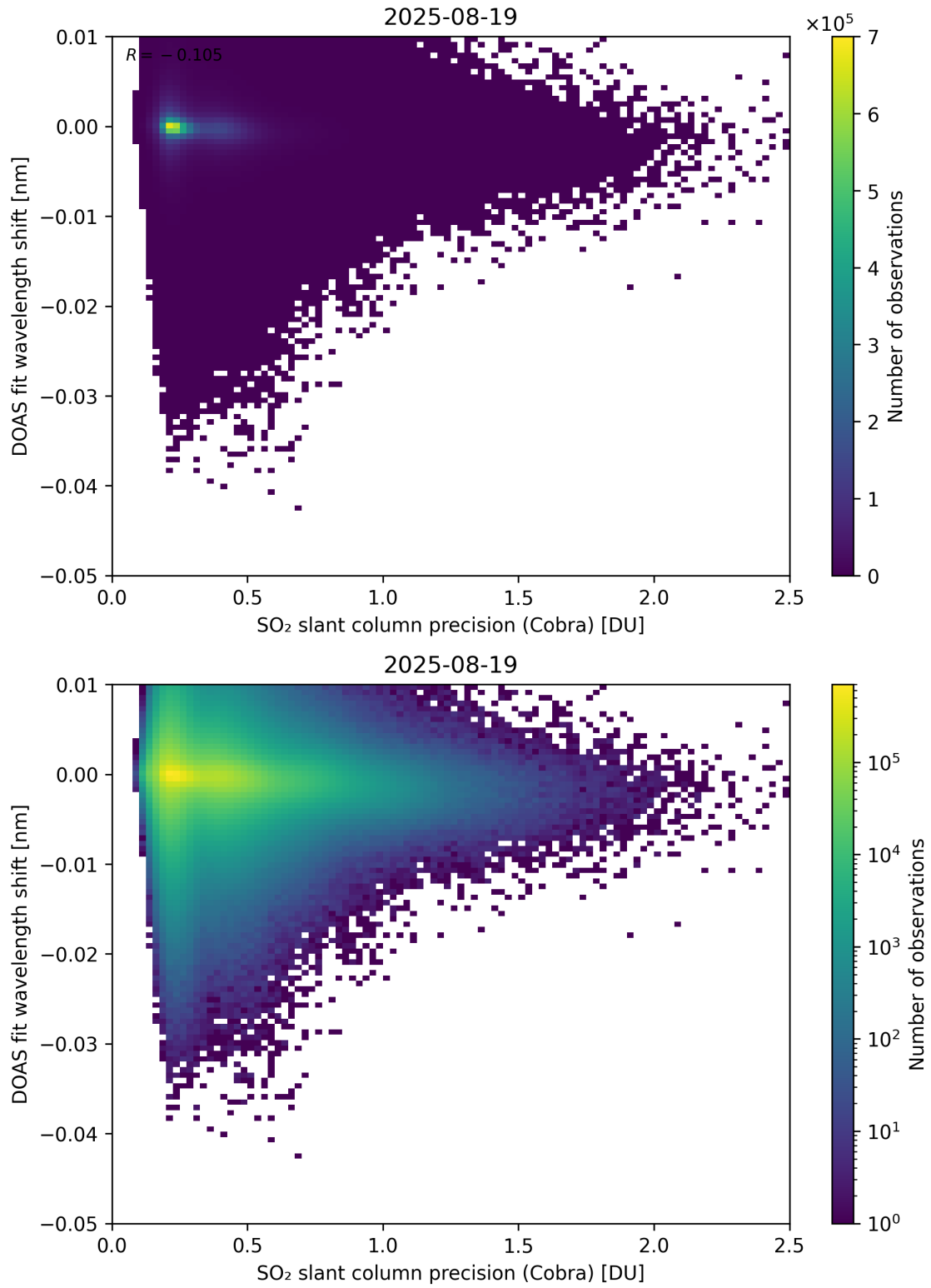
Figure 202: Scatter density plot of “SO 2 slant column precision (Cobra)” against “DOAS fit wavelength shift” for 2025-08-19 to 2025-08-20.
