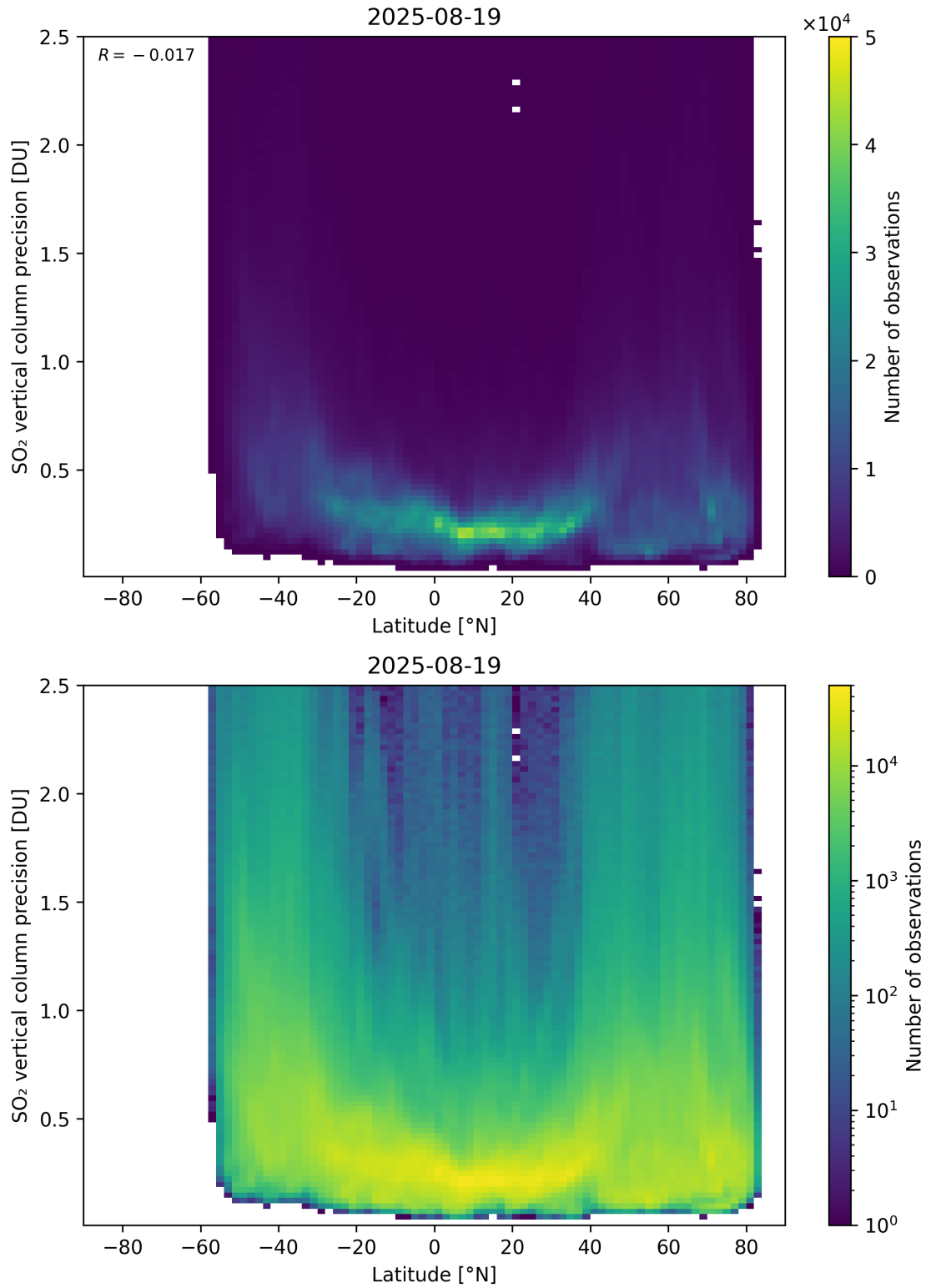
Figure 170: Scatter density plot of “Latitude” against “SO 2 vertical column precision” for 2025-08-19 to 2025-08-20.
