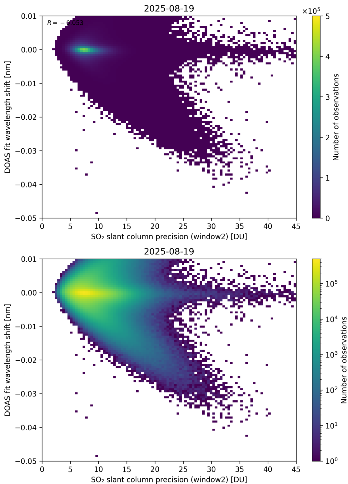
Figure 293: Scatter density plot of “SO 2 slant column precision (window2)” against “DOAS fit wavelength shift” for 2025-08-19 to 2025-08-20.
