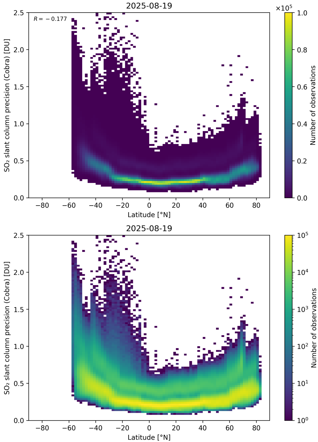
Figure 158: Scatter density plot of “Latitude” against “SO 2 slant column precision (Cobra)” for 2025-08-19 to 2025-08-20.
