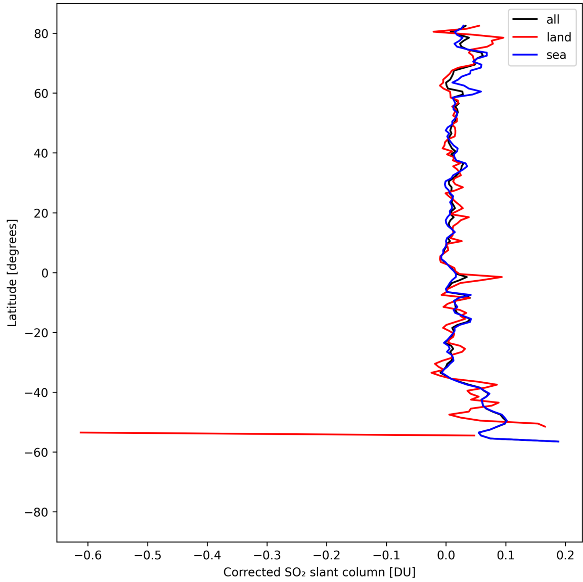
Figure 34: Zonal average of “Corrected SO 2 slant column” for 2025-08-19 to 2025-08-20.
