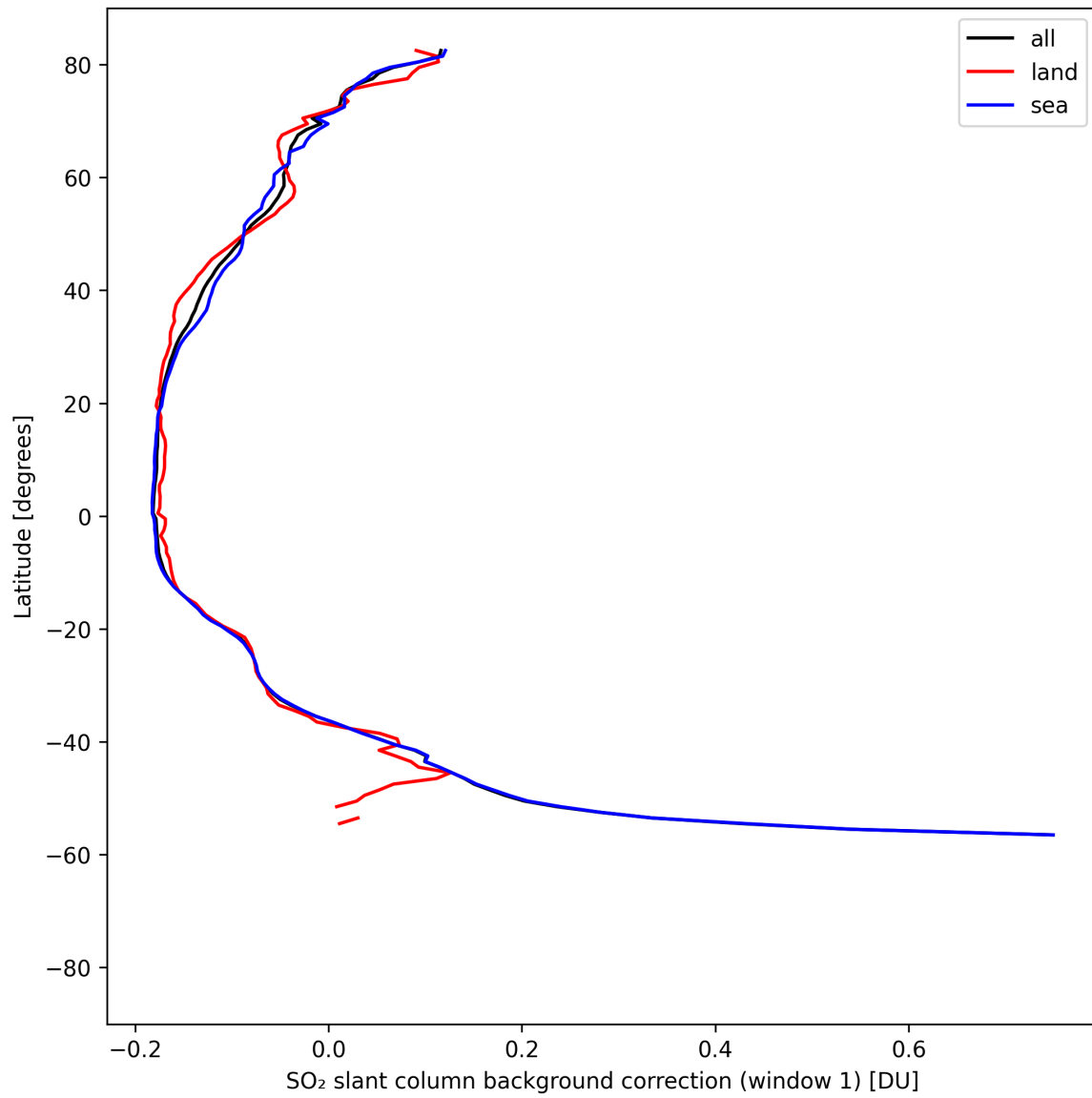
Figure 40: Zonal average of “SO 2 slant column background correction (window 1)” for 2025-08-19 to 2025-08-20.
