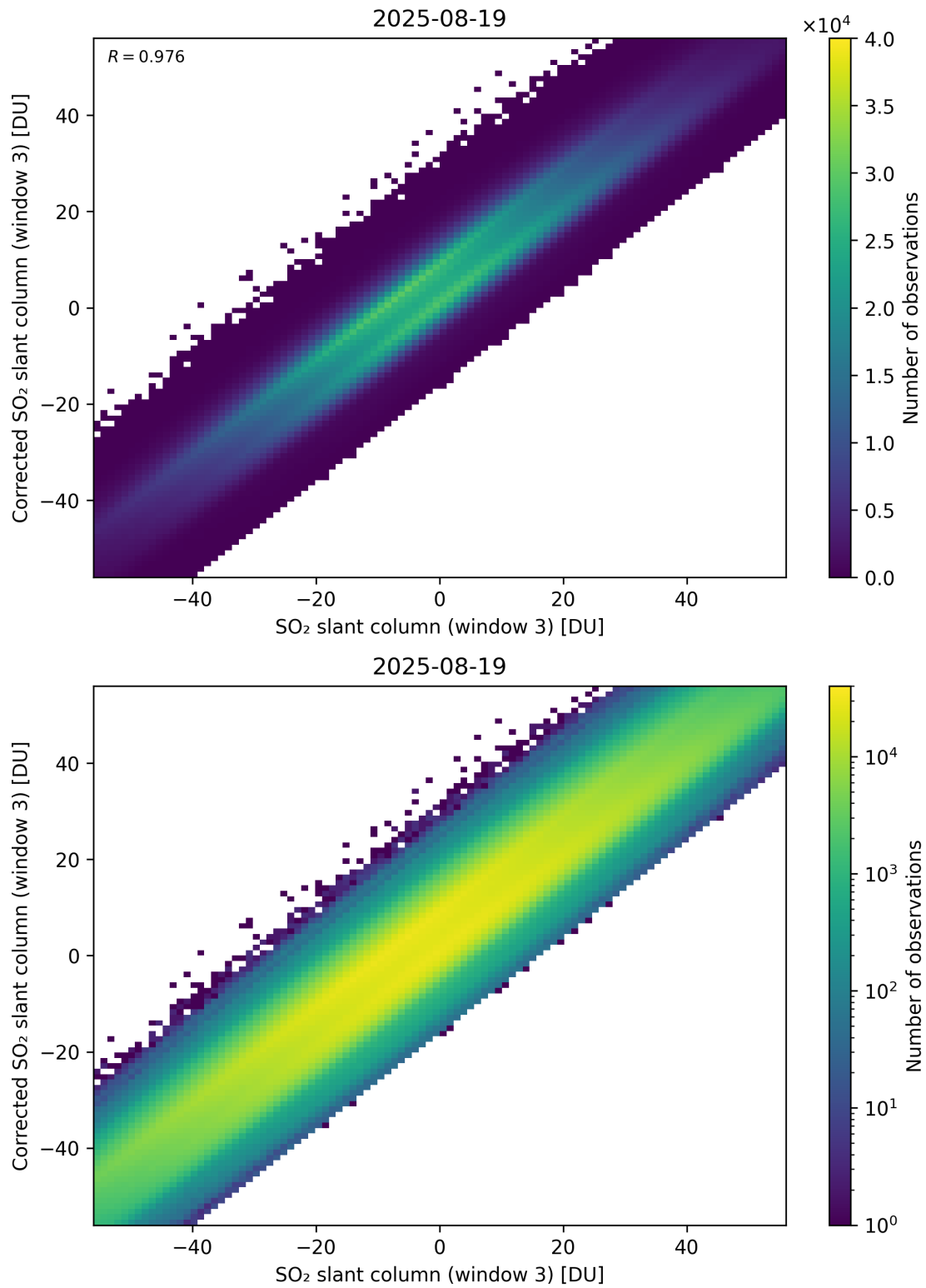
Figure 316: Scatter density plot of “SO 2 slant column (window 3)” against “Corrected SO 2 slant column (window 3)” for 2025-08-19 to 2025-08-20.
