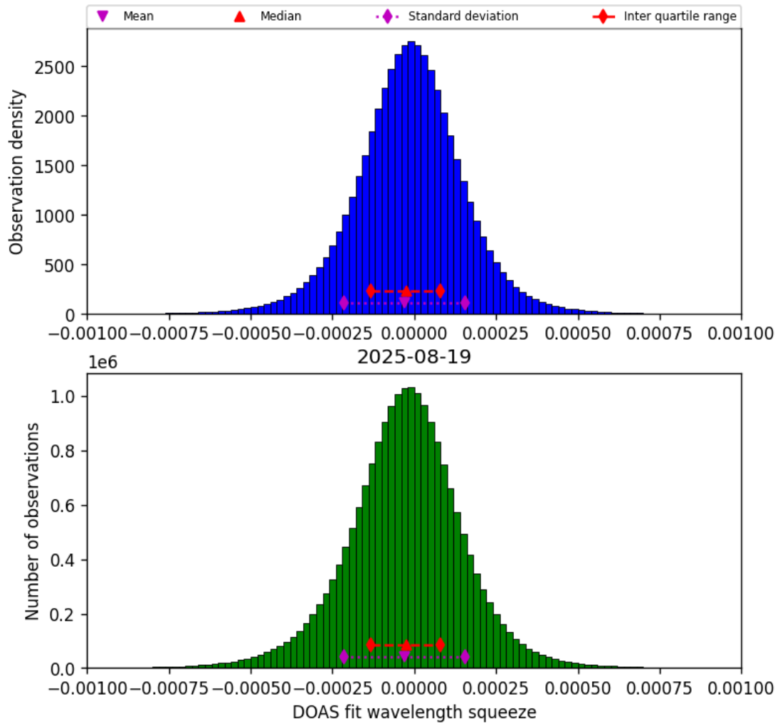
Figure 77: Histogram of “DOAS fit wavelength squeeze” for 2025-08-19 to 2025-08-20
