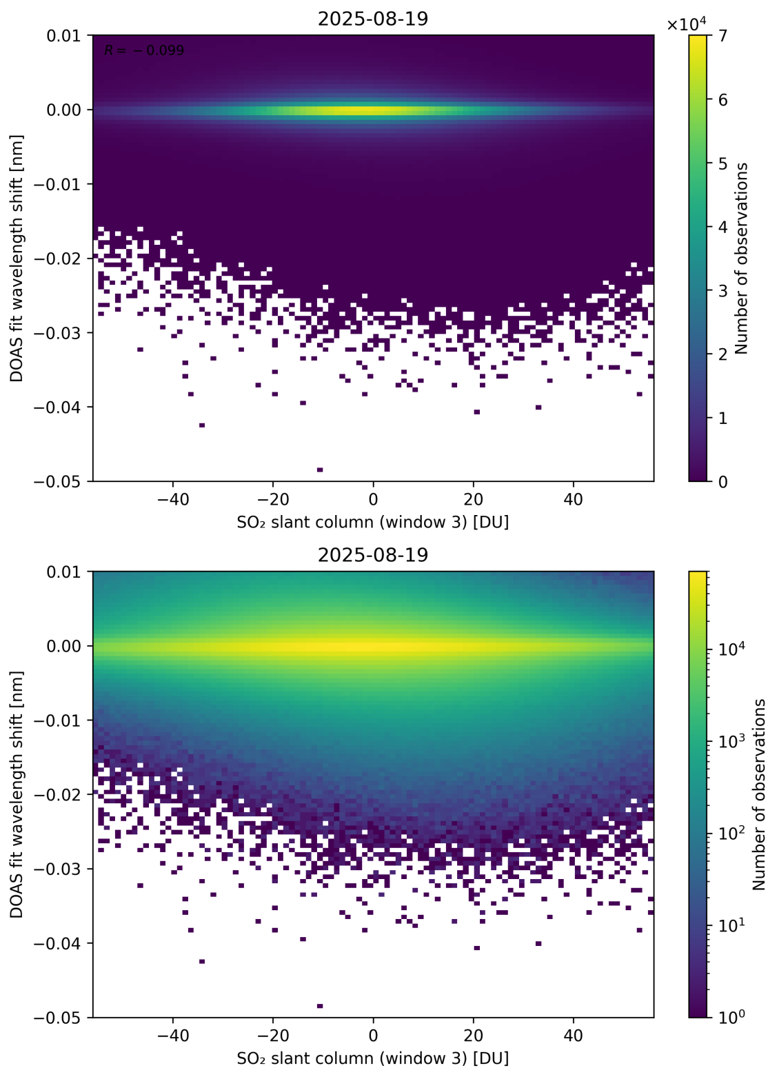
Figure 304: Scatter density plot of “SO 2 slant column (window 3)” against “DOAS fit wavelength shift” for 2025-08-19 to 2025-08-20.
