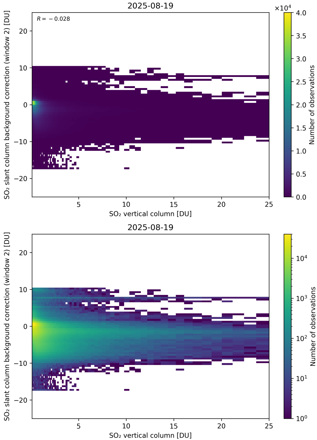
Figure 324: Scatter density plot of “SO 2 vertical column” against “SO 2 slant column background correction (window 2)” for 2025-08-19 to 2025-08-20.
