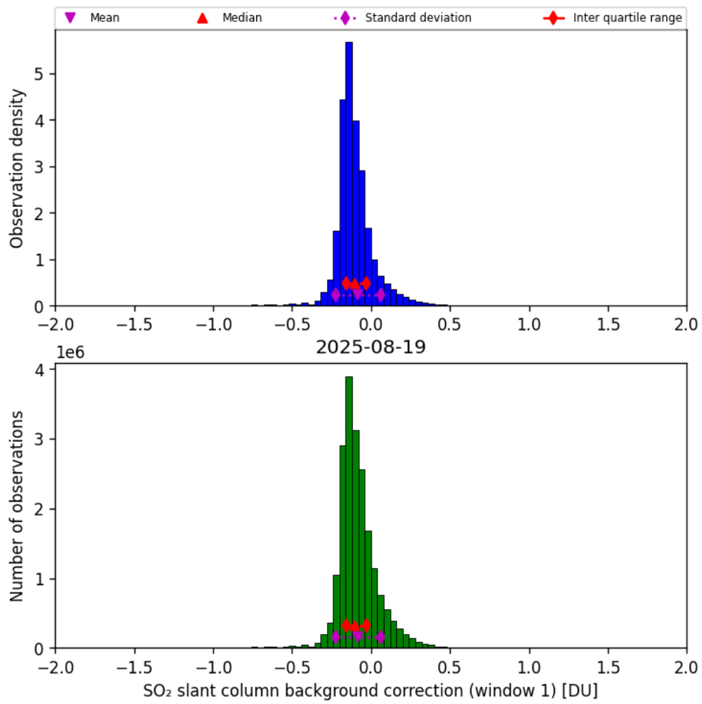
Figure 66: Histogram of “SO 2 slant column background correction (window 1)” for 2025-08-19 to 2025-08-20
