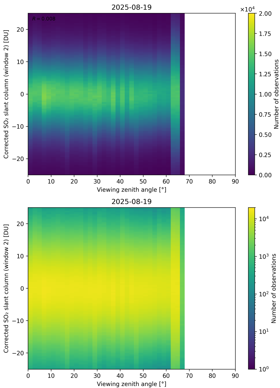
Figure 374: Scatter density plot of “Viewing zenith angle” against “Corrected SO 2 slant column (window 2)” for 2025-08-19 to 2025-08-20.
