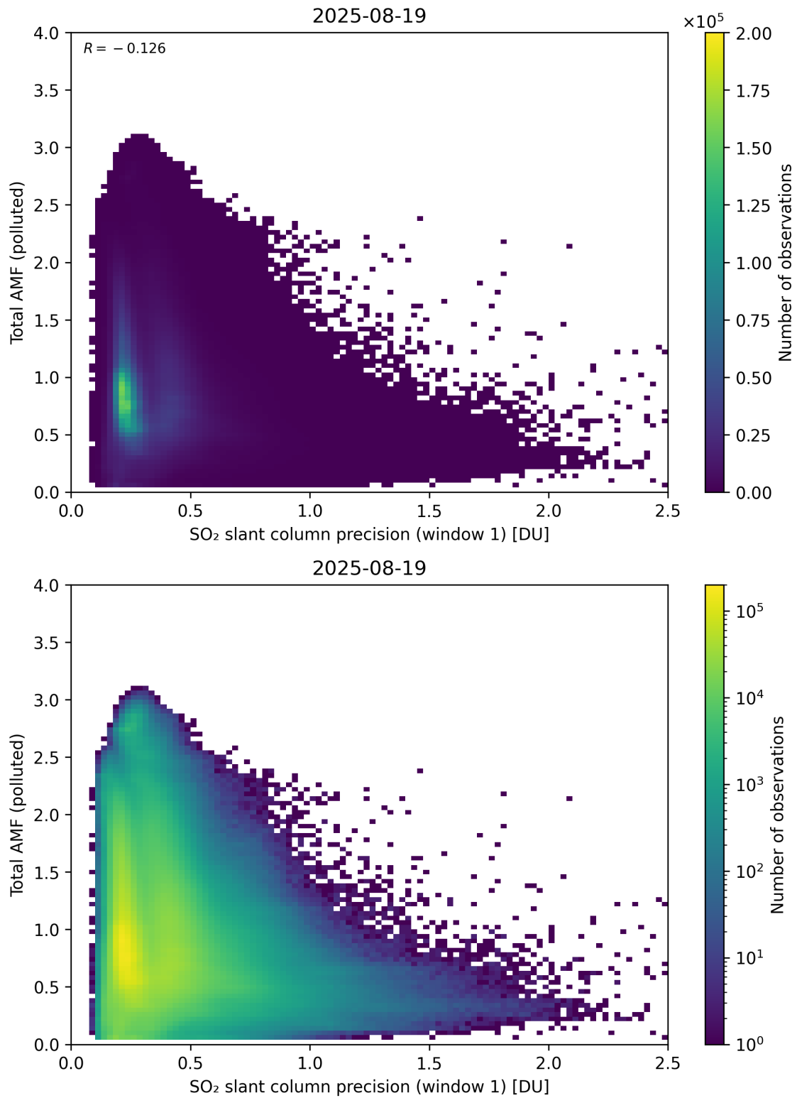
Figure 280: Scatter density plot of “SO 2 slant column precision (window 1)” against “Total AMF (polluted)” for 2025-08-19 to 2025-08-20.
