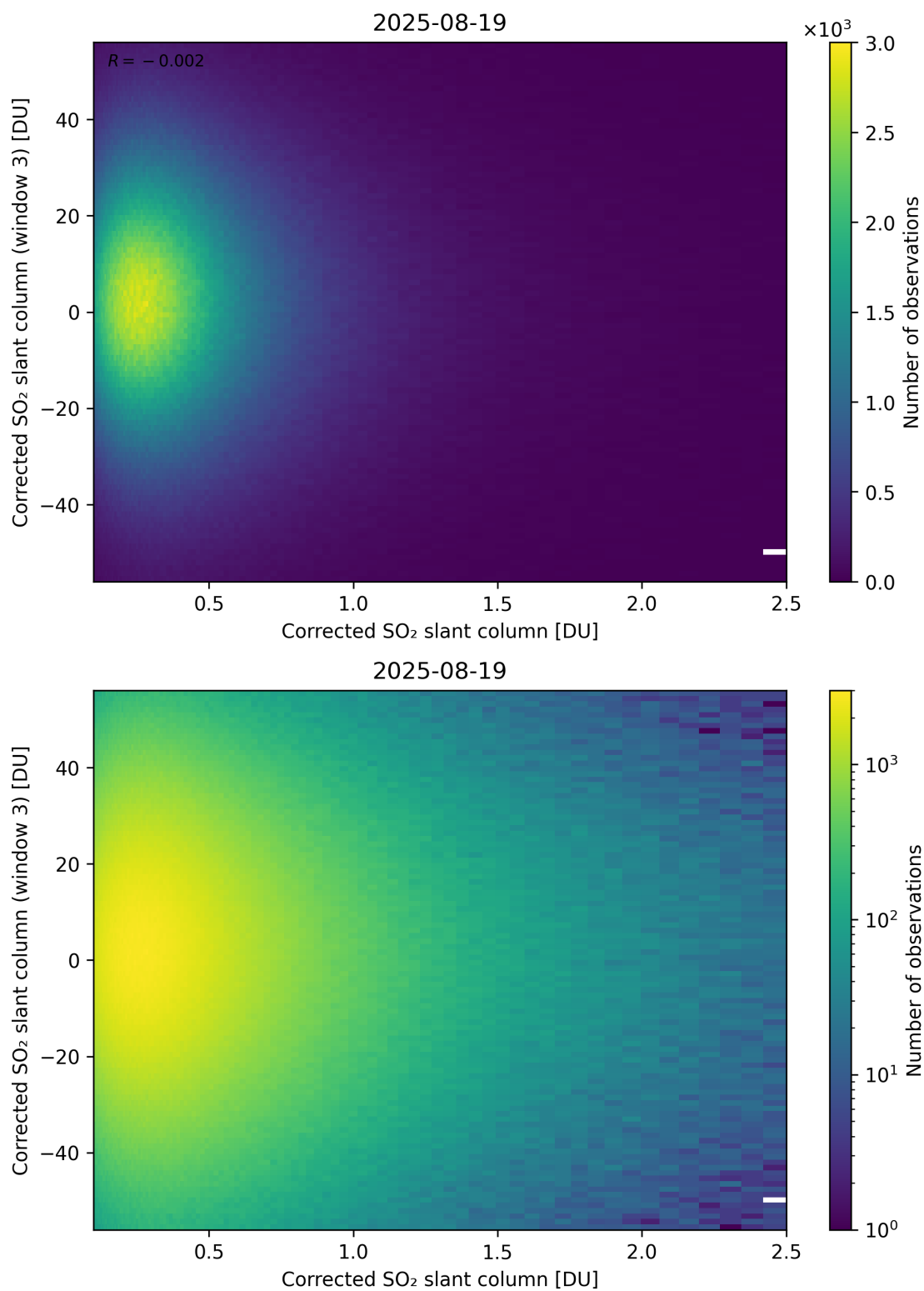
Figure 236: Scatter density plot of “Corrected SO 2 slant column” against “Corrected SO 2 slant column (window 3)” for 2025-08-19 to 2025-08-20.
