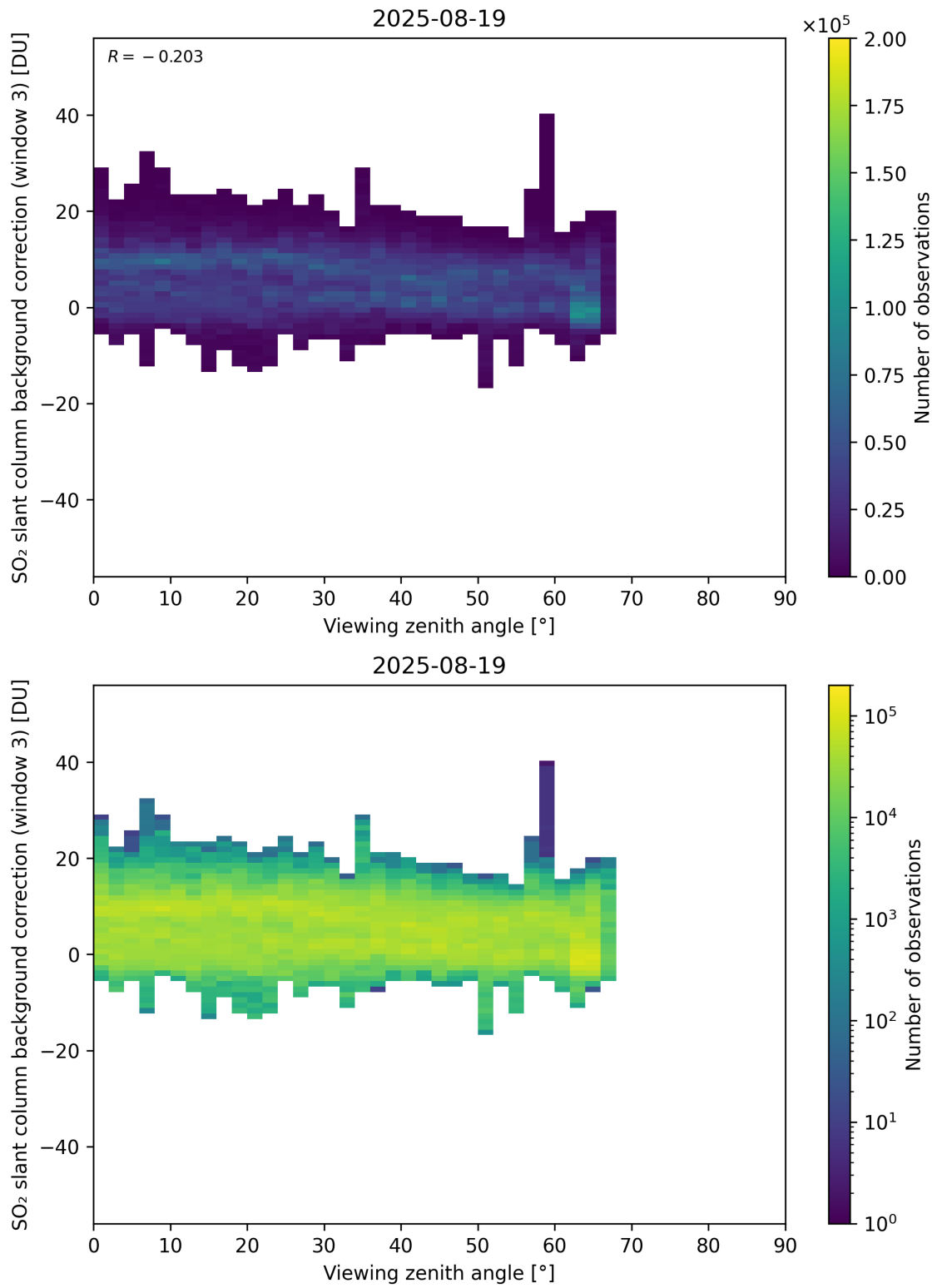
Figure 364: Scatter density plot of “Viewing zenith angle” against “SO 2 slant column background correction (window 3)” for 2025-08-19 to 2025-08-20.
