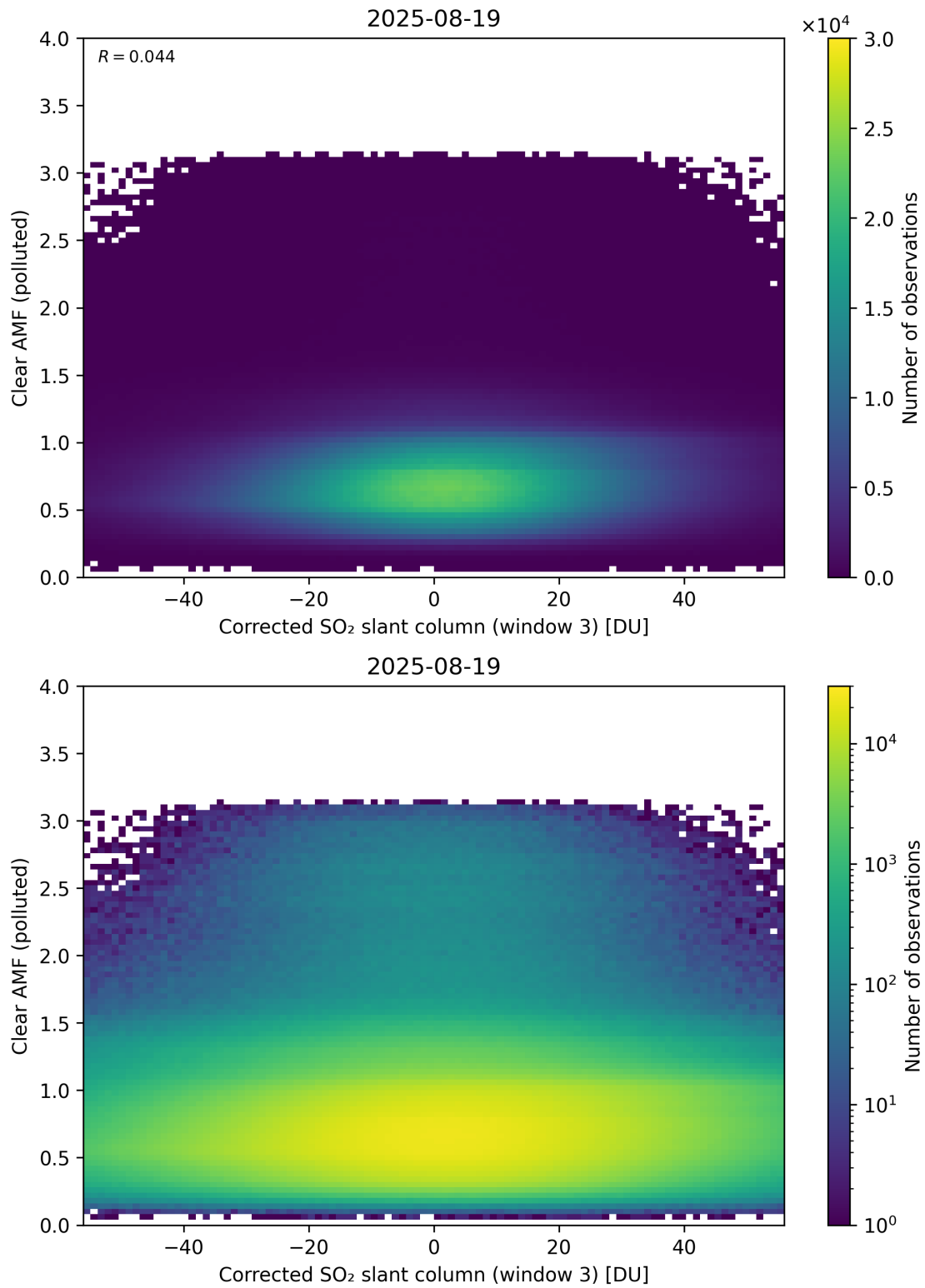
Figure 259: Scatter density plot of “Corrected SO 2 slant column (window 3)” against “Clear AMF (polluted)” for 2025-08-19 to 2025-08-20.
