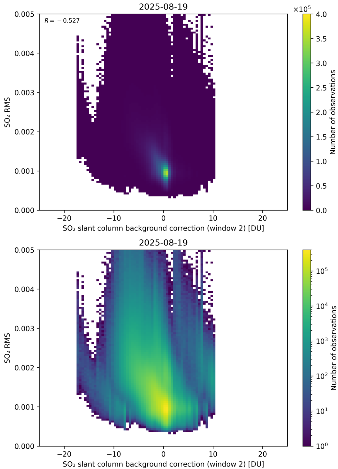
Figure 125: Scatter density plot of “SO 2 slant column background correction (window 2)” against “SO 2 RMS” for 2025-08-19 to 2025-08-20.
