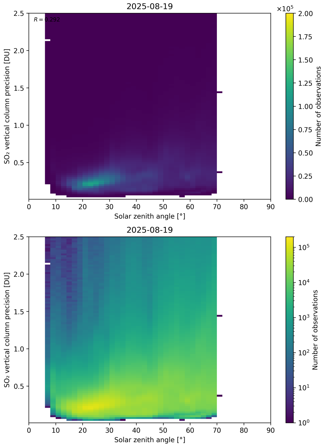
Figure 192: Scatter density plot of “Solar zenith angle” against “SO 2 vertical column precision” for 2025-08-19 to 2025-08-20.
