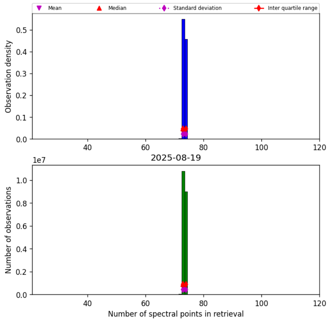
Figure 82: Histogram of “Number of spectral points in retrieval” for 2025-08-19 to 2025-08-20
