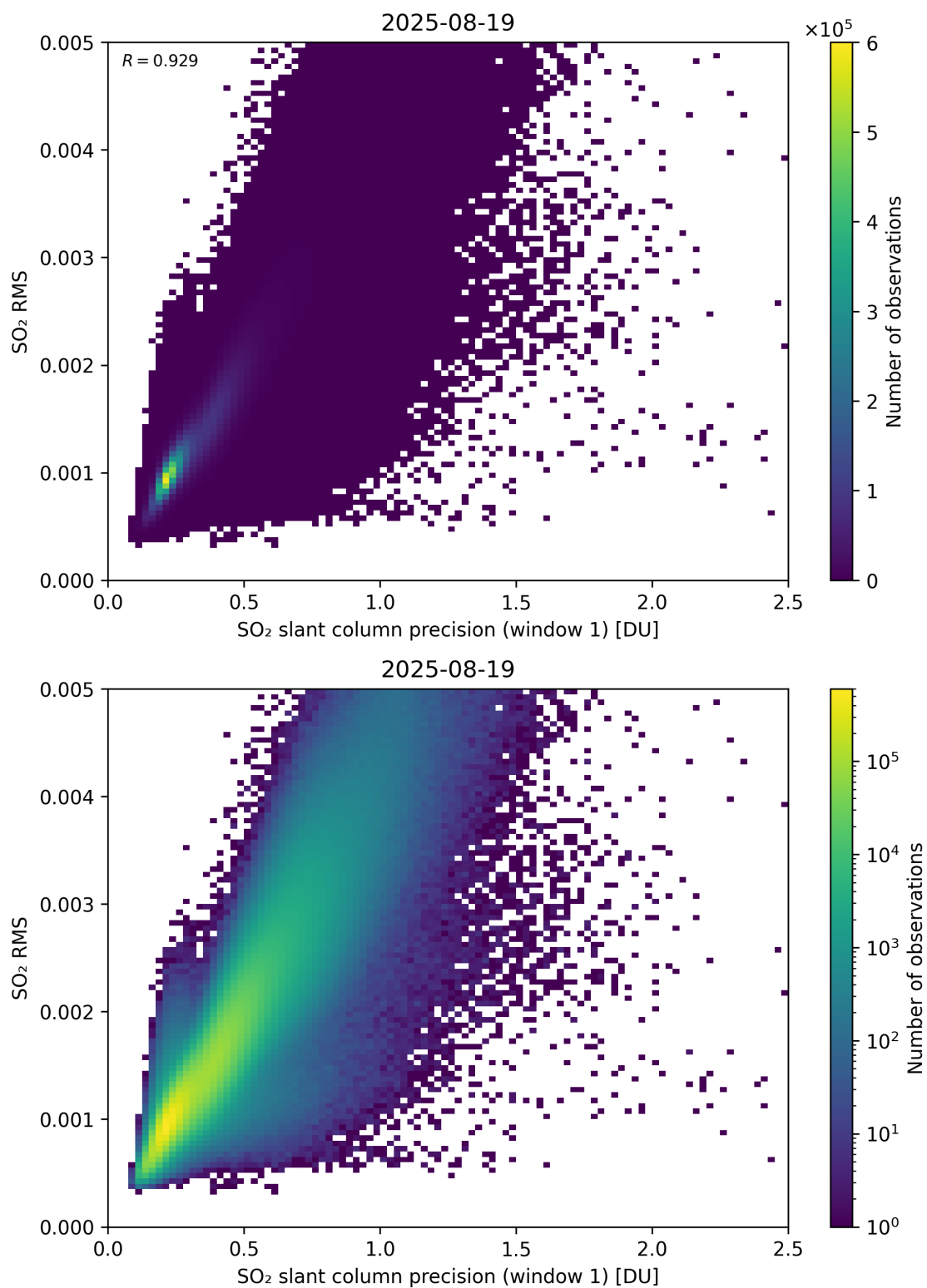
Figure 273: Scatter density plot of “SO 2 slant column precision (window 1)” against “SO 2 RMS” for 2025-08-19 to 2025-08-20.
