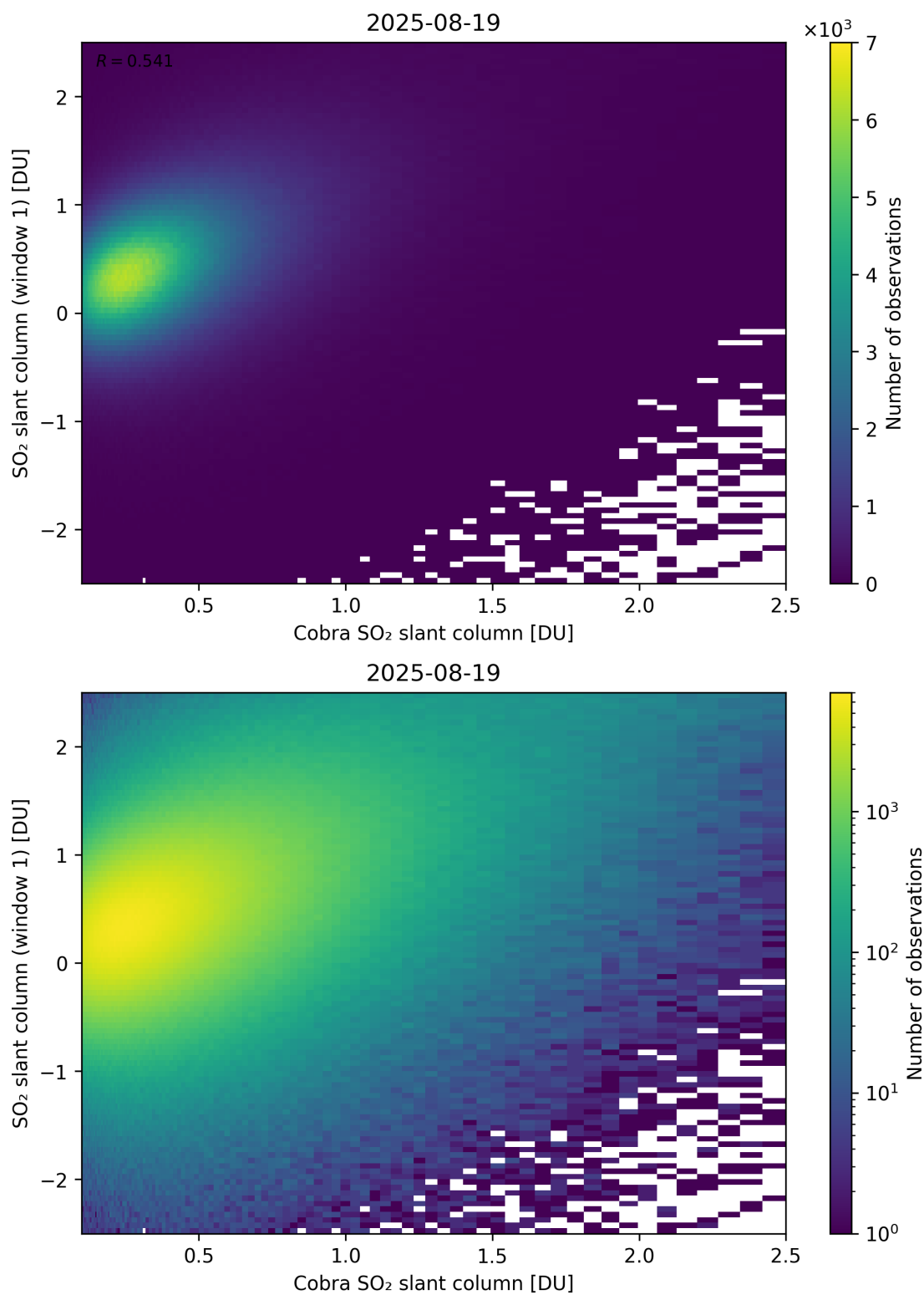
Figure 219: Scatter density plot of “Cobra SO 2 slant column” against “SO 2 slant column (window 1)” for 2025-08-19 to 2025-08-20.
