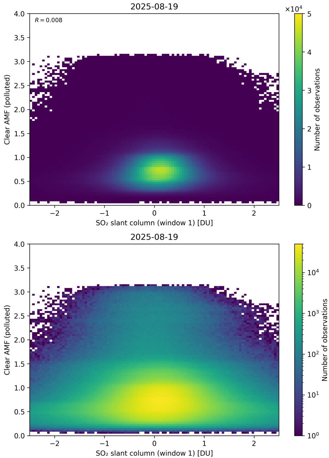
Figure 282: Scatter density plot of “SO 2 slant column (window 1)” against “Clear AMF (polluted)” for 2025-08-19 to 2025-08-20.
