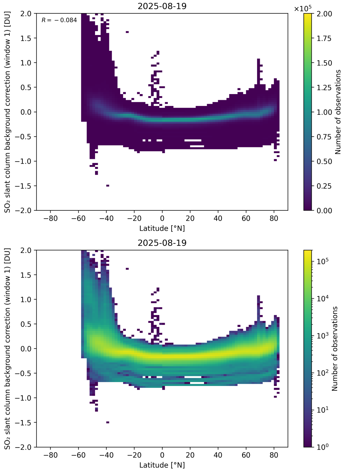
Figure 150: Scatter density plot of “Latitude” against “SO 2 slant column background correction (window 1)” for 2025-08-19 to 2025-08-20.
