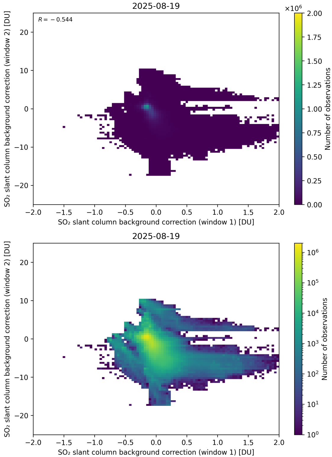
Figure 109: Scatter density plot of “SO 2 slant column background correction (window 1)” against “SO 2 slant column background correction (window 2)” for 2025-08-19 to 2025-08-20.
