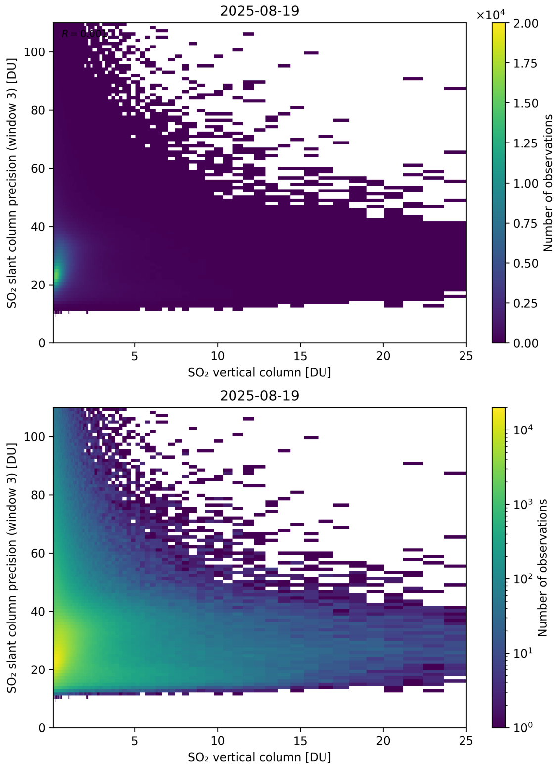
Figure 358: Scatter density plot of “SO 2 vertical column” against “SO 2 slant column precision (window 3)” for 2025-08-19 to 2025-08-20.
