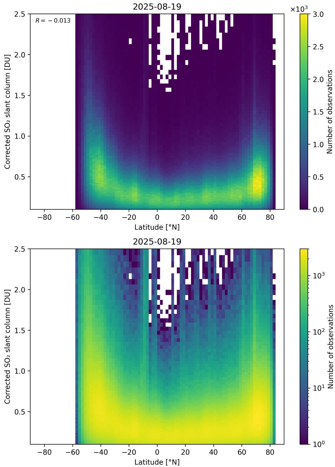
Figure 159: Scatter density plot of “Latitude” against “Corrected SO 2 slant column” for 2025-08-19 to 2025-08-20.
