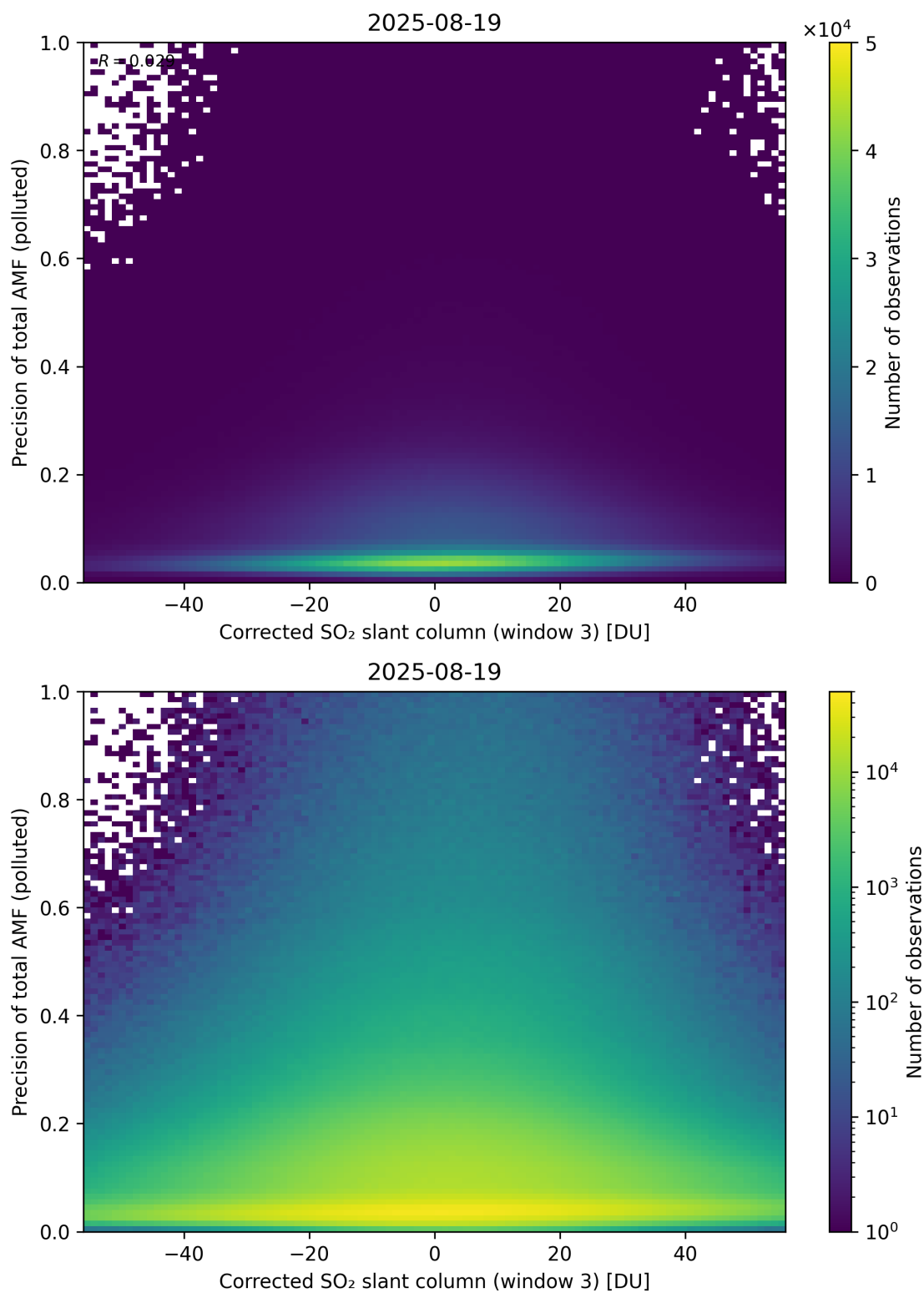
Figure 261: Scatter density plot of “Corrected SO 2 slant column (window 3)” against “Precision of total AMF (polluted)” for 2025-08-19 to 2025-08-20.
