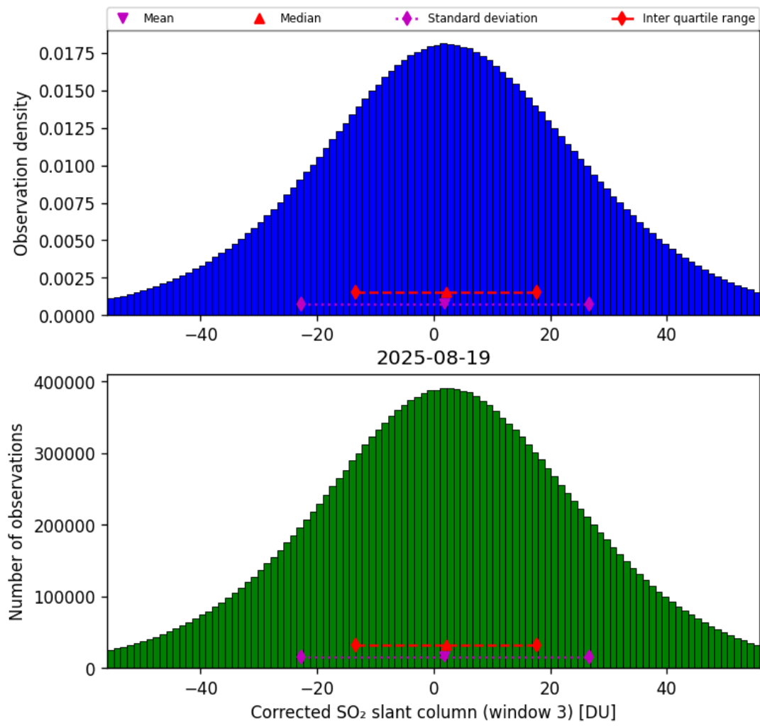
Figure 73: Histogram of “Corrected SO 2 slant column (window 3)” for 2025-08-19 to 2025-08-20
