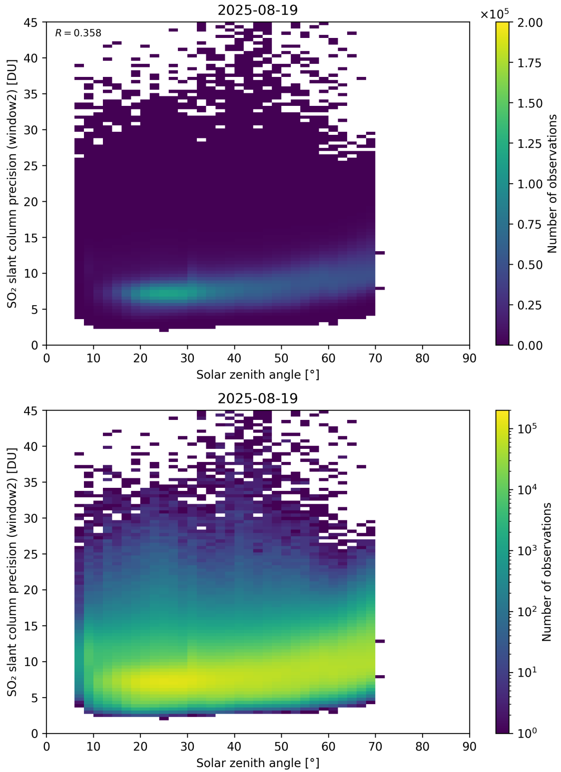
Figure 186: Scatter density plot of “Solar zenith angle” against “SO 2 slant column precision (window2)” for 2025-08-19 to 2025-08-20.
