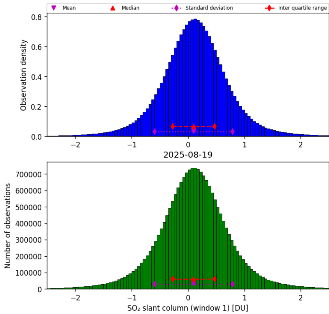
Figure 63: Histogram of “SO 2 slant column (window 1)” for 2025-08-19 to 2025-08-20
