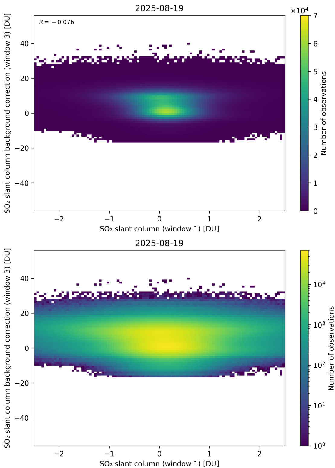
Figure 264: Scatter density plot of “SO 2 slant column (window 1)” against “SO 2 slant column background correction (window 3)” for 2025-08-19 to 2025-08-20.
