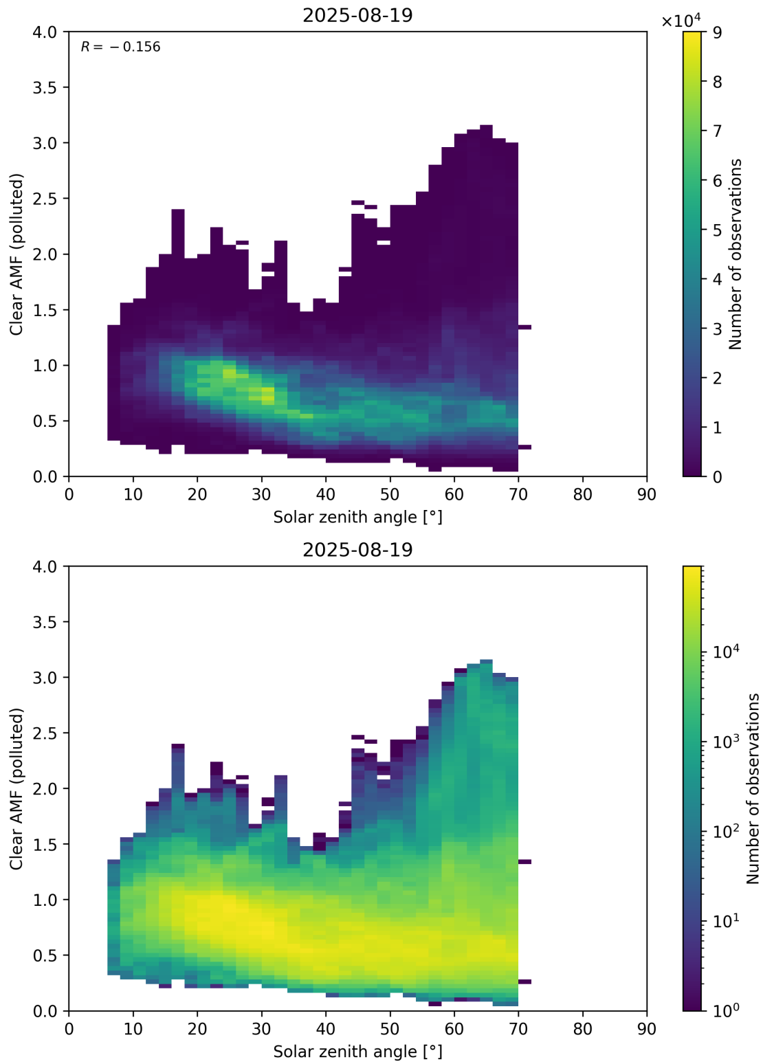
Figure 178: Scatter density plot of “Solar zenith angle” against “Clear AMF (polluted)” for 2025-08-19 to 2025-08-20.
