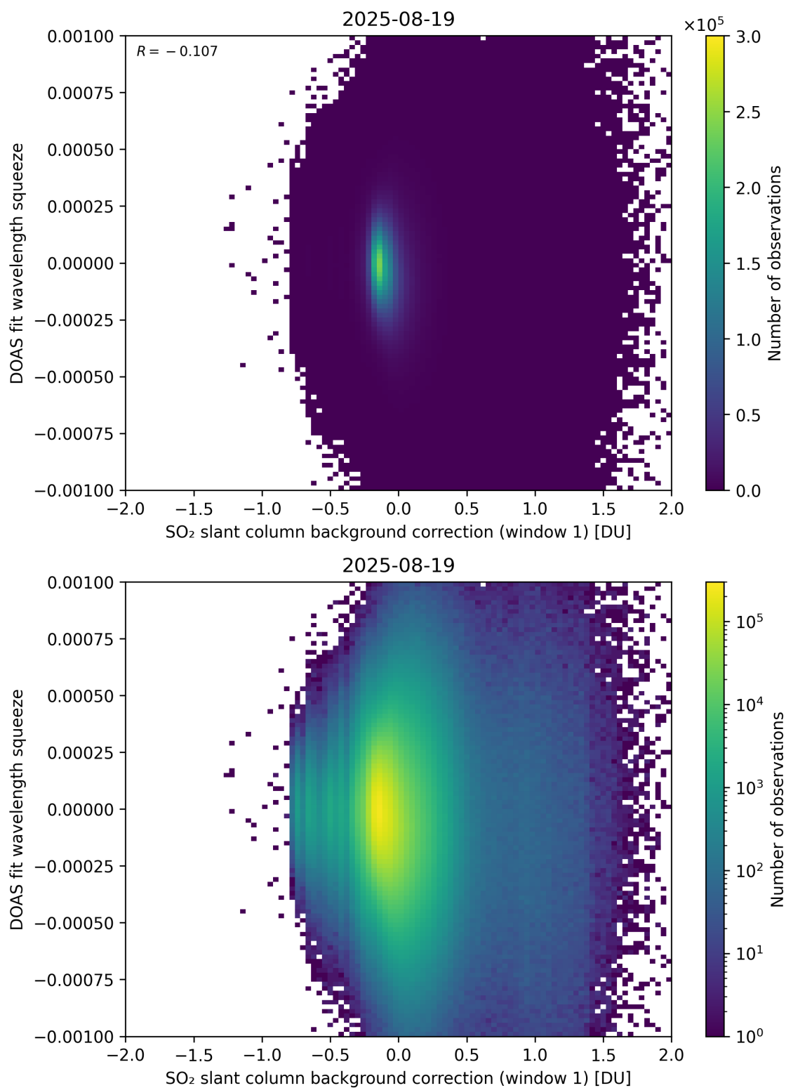
Figure 112: Scatter density plot of “SO 2 slant column background correction (window 1)” against “DOAS fit wavelength squeeze” for 2025-08-19 to 2025-08-20.
