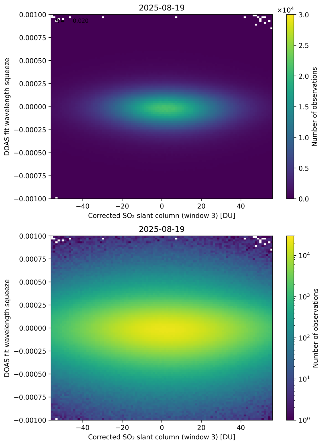
Figure 257: Scatter density plot of “Corrected SO 2 slant column (window 3)” against “DOAS fit wavelength squeeze” for 2025-08-19 to 2025-08-20.
