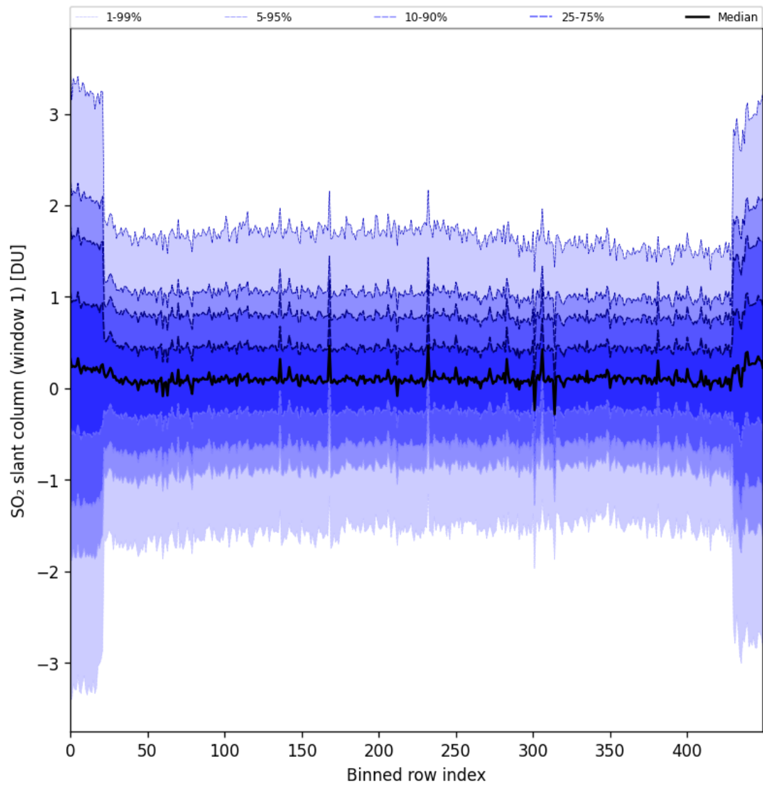
Figure 89: Along track statistics of “SO 2 slant column (window 1)” for 2025-08-19 to 2025-08-20
