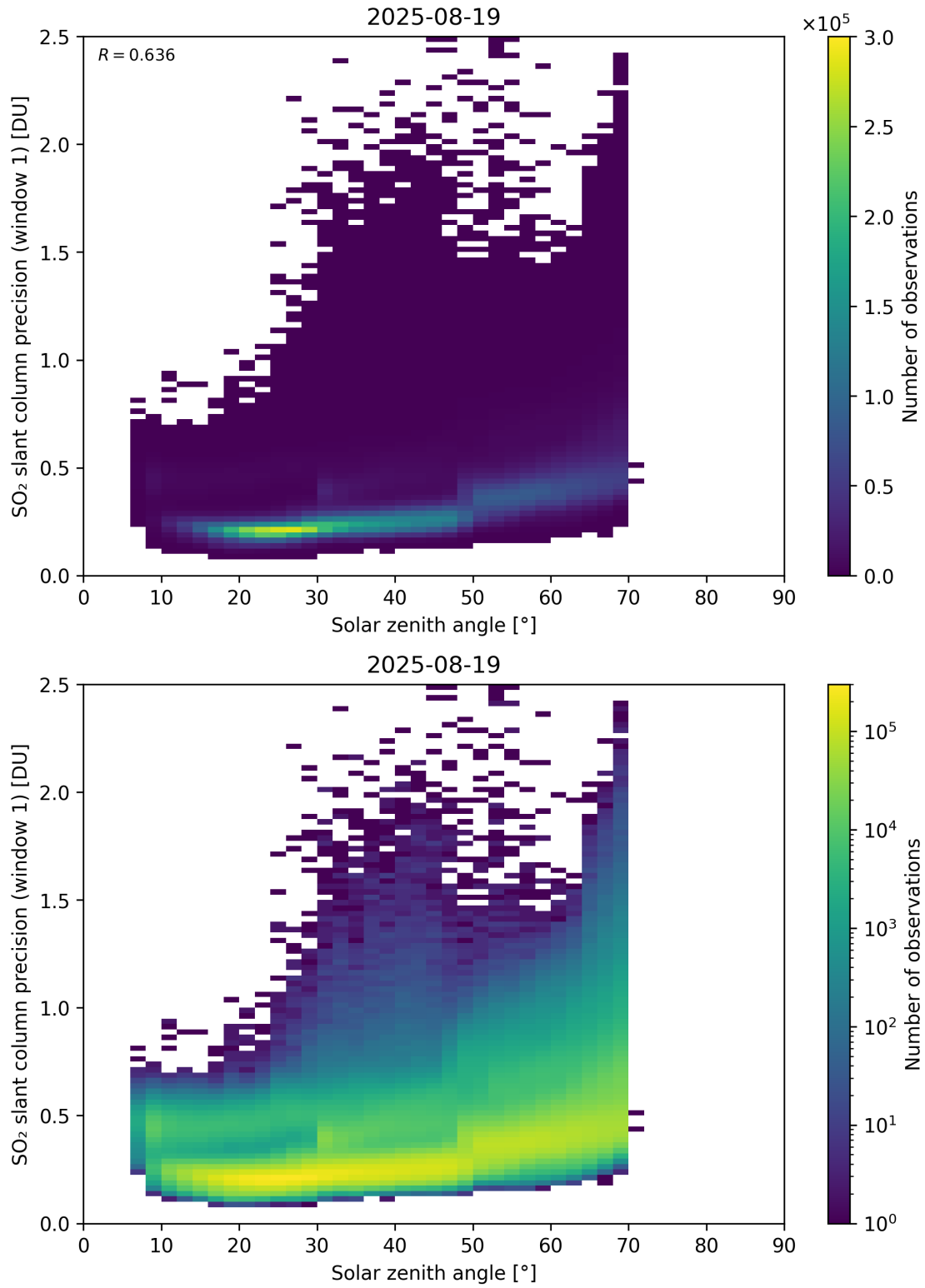
Figure 185: Scatter density plot of “Solar zenith angle” against “SO 2 slant column precision (window 1)” for 2025-08-19 to 2025-08-20.
