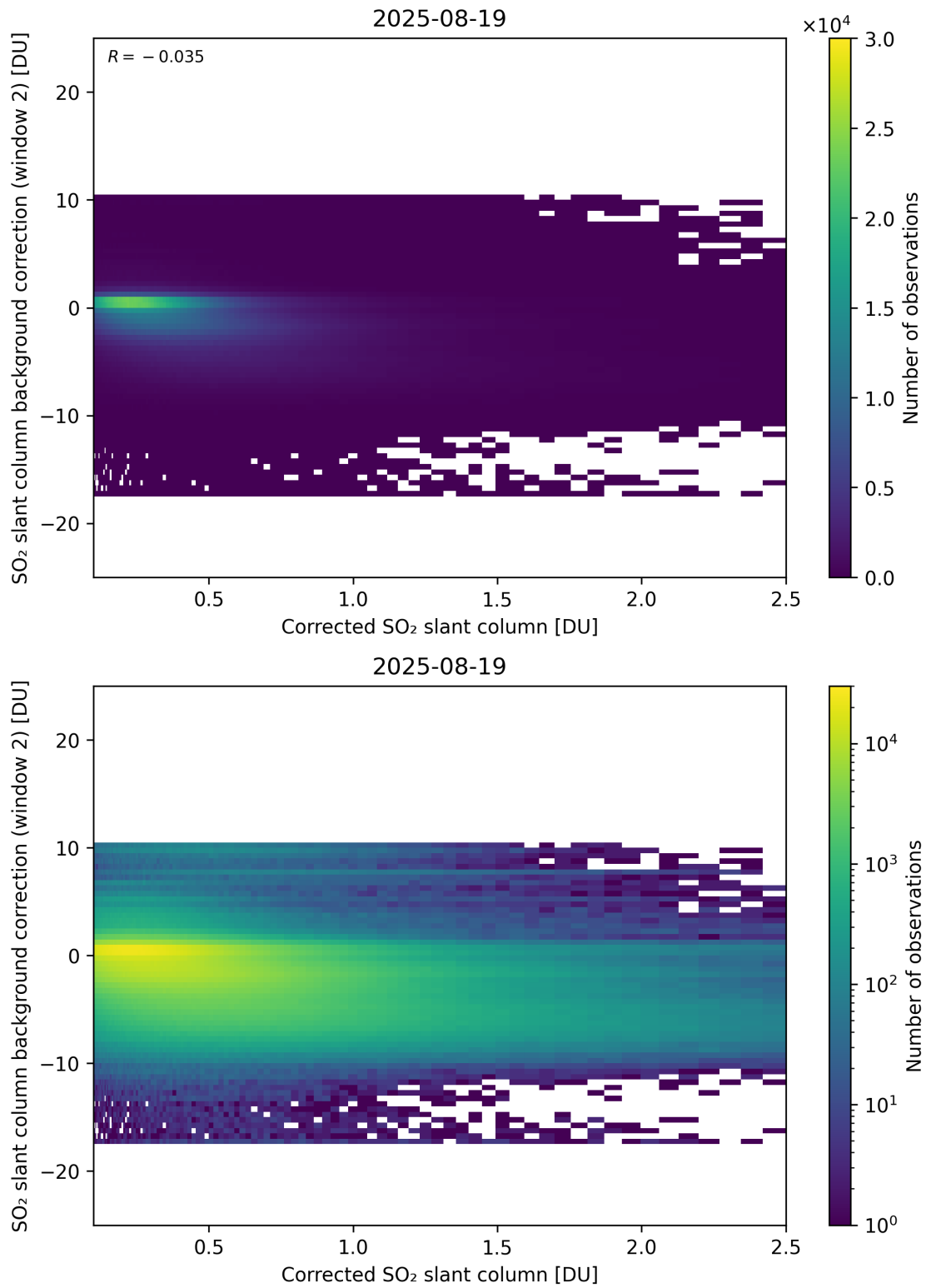
Figure 227: Scatter density plot of “Corrected SO 2 slant column” against “SO 2 slant column background correction (window 2)” for 2025-08-19 to 2025-08-20.
