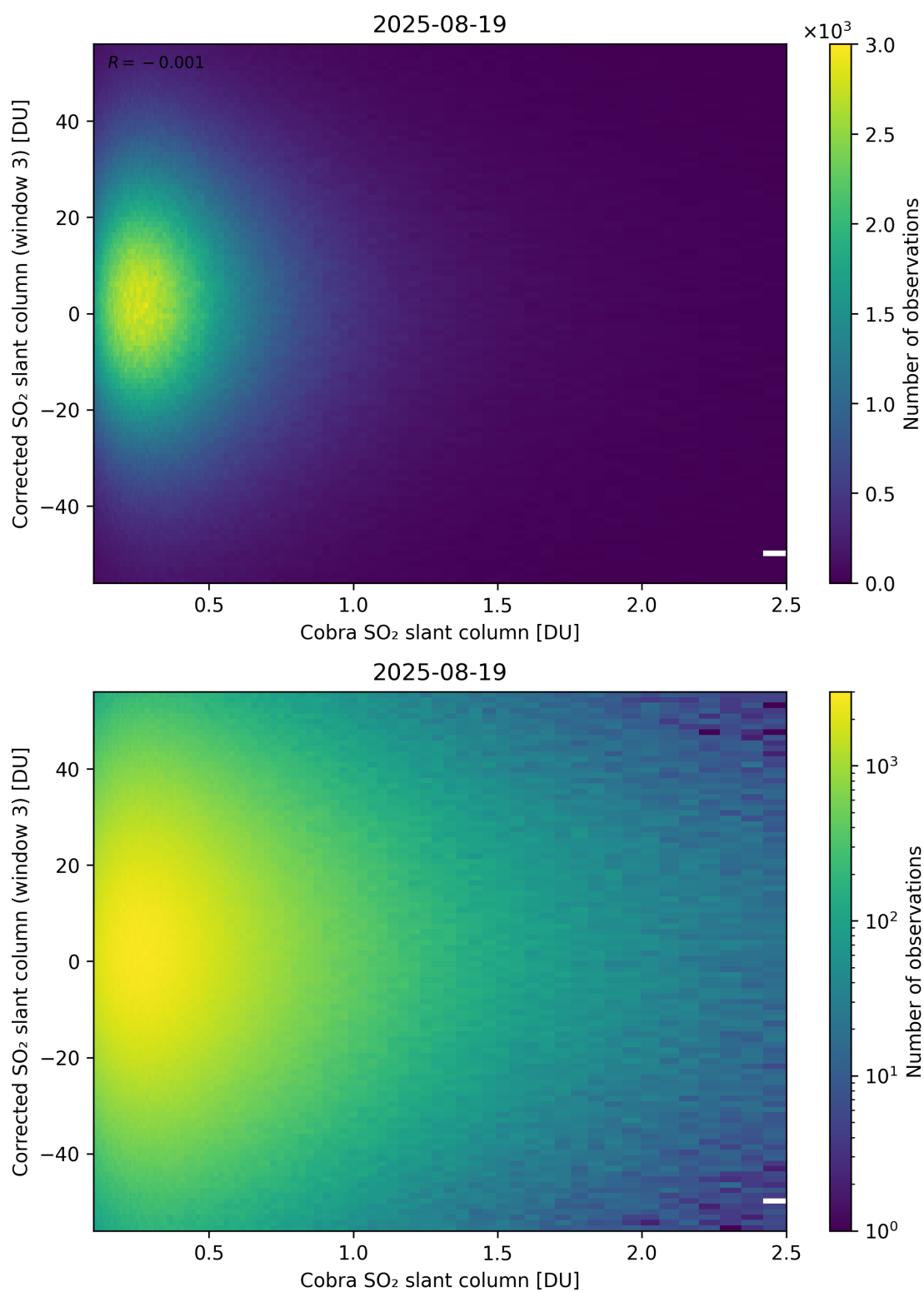
Figure 218: Scatter density plot of “Cobra SO 2 slant column” against “Corrected SO 2 slant column (window 3)” for 2025-08-19 to 2025-08-20.
