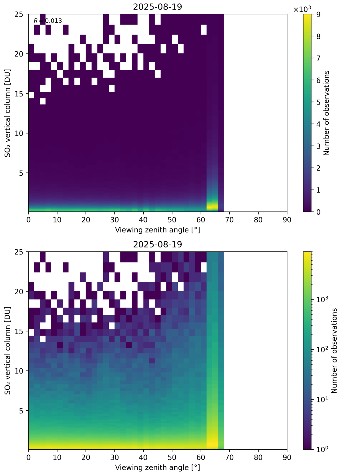
Figure 383: Scatter density plot of “Viewing zenith angle” against “SO 2 vertical column” for 2025-08-19 to 2025-08-20.
