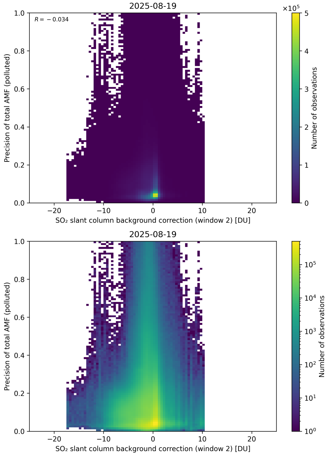
Figure 131: Scatter density plot of “SO 2 slant column background correction (window 2)” against “Precision of total AMF (polluted)” for 2025-08-19 to 2025-08-20.
