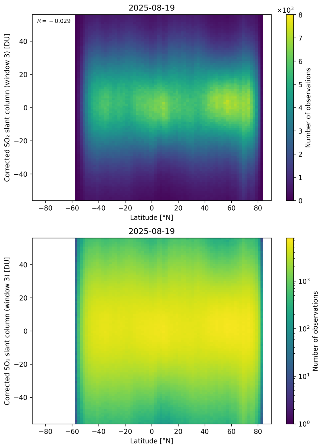
Figure 161: Scatter density plot of “Latitude” against “Corrected SO 2 slant column (window 3)” for 2025-08-19 to 2025-08-20.
