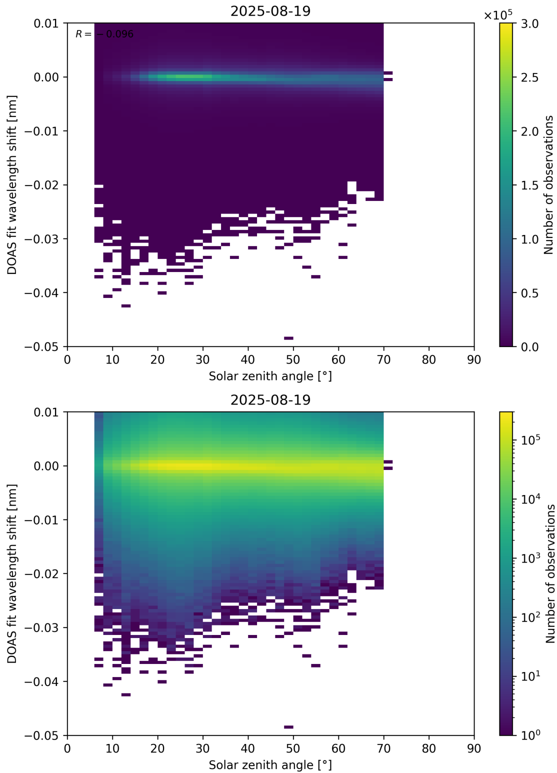
Figure 174: Scatter density plot of “Solar zenith angle” against “DOAS fit wavelength shift” for 2025-08-19 to 2025-08-20.
