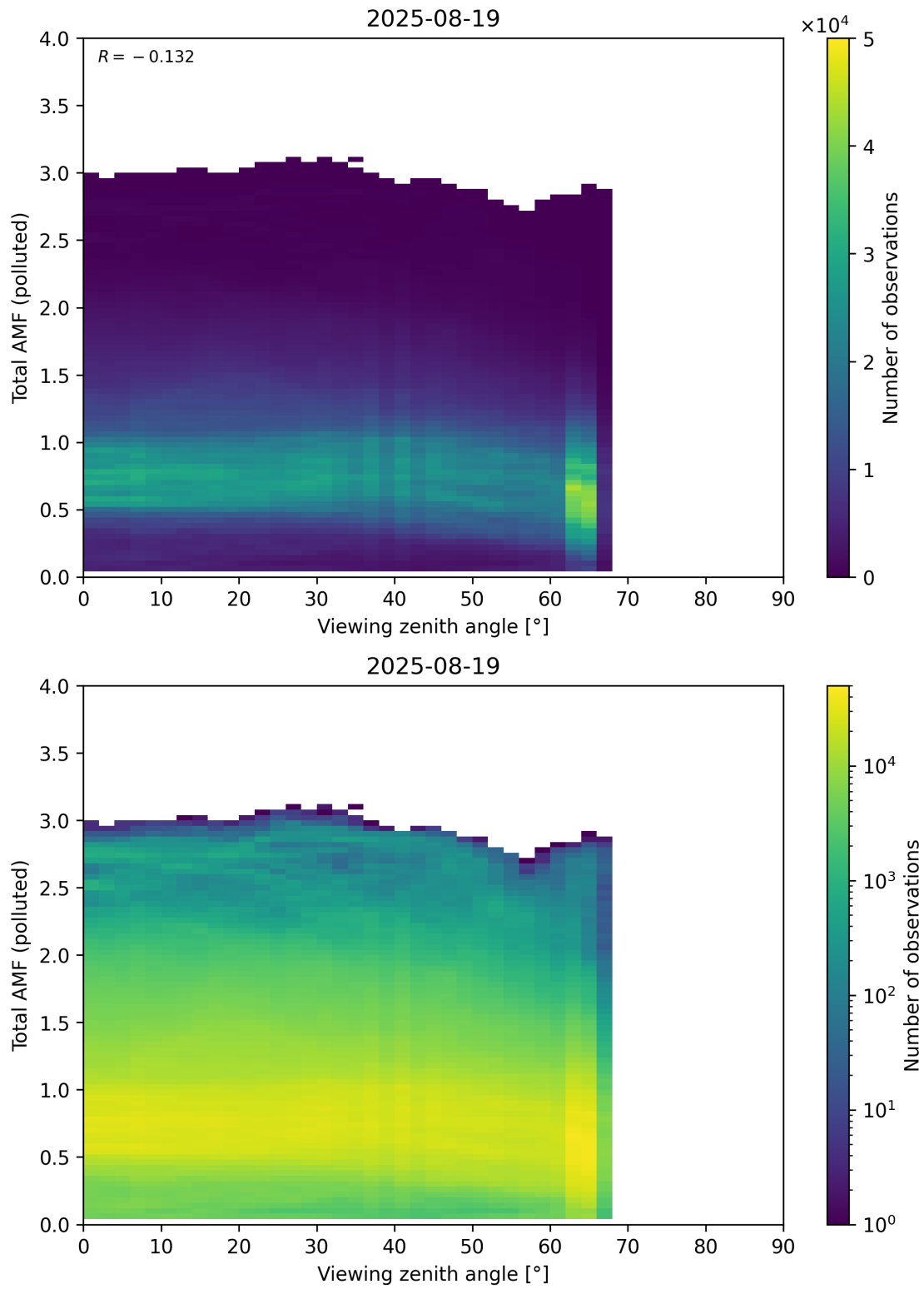
Figure 381: Scatter density plot of “Viewing zenith angle” against “Total AMF (polluted)” for 2025-08-19 to 2025-08-20.
