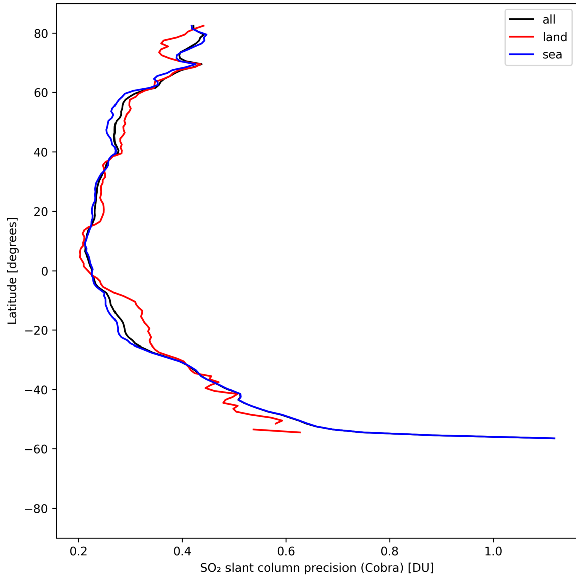
Figure 36: Zonal average of “SO 2 slant column precision (Cobra)” for 2025-08-19 to 2025-08-20.
