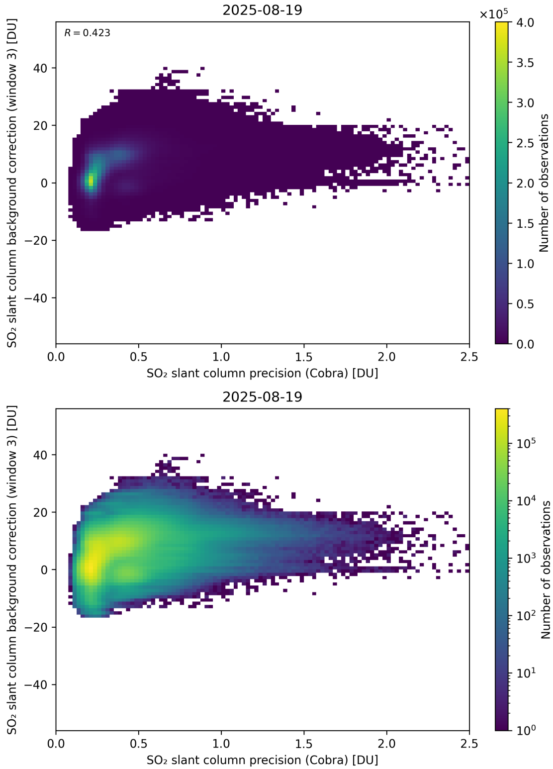
Figure 201: Scatter density plot of “SO 2 slant column precision (Cobra)” against “SO 2 slant column background correction (window 3)” for 2025-08-19 to 2025-08-20.
