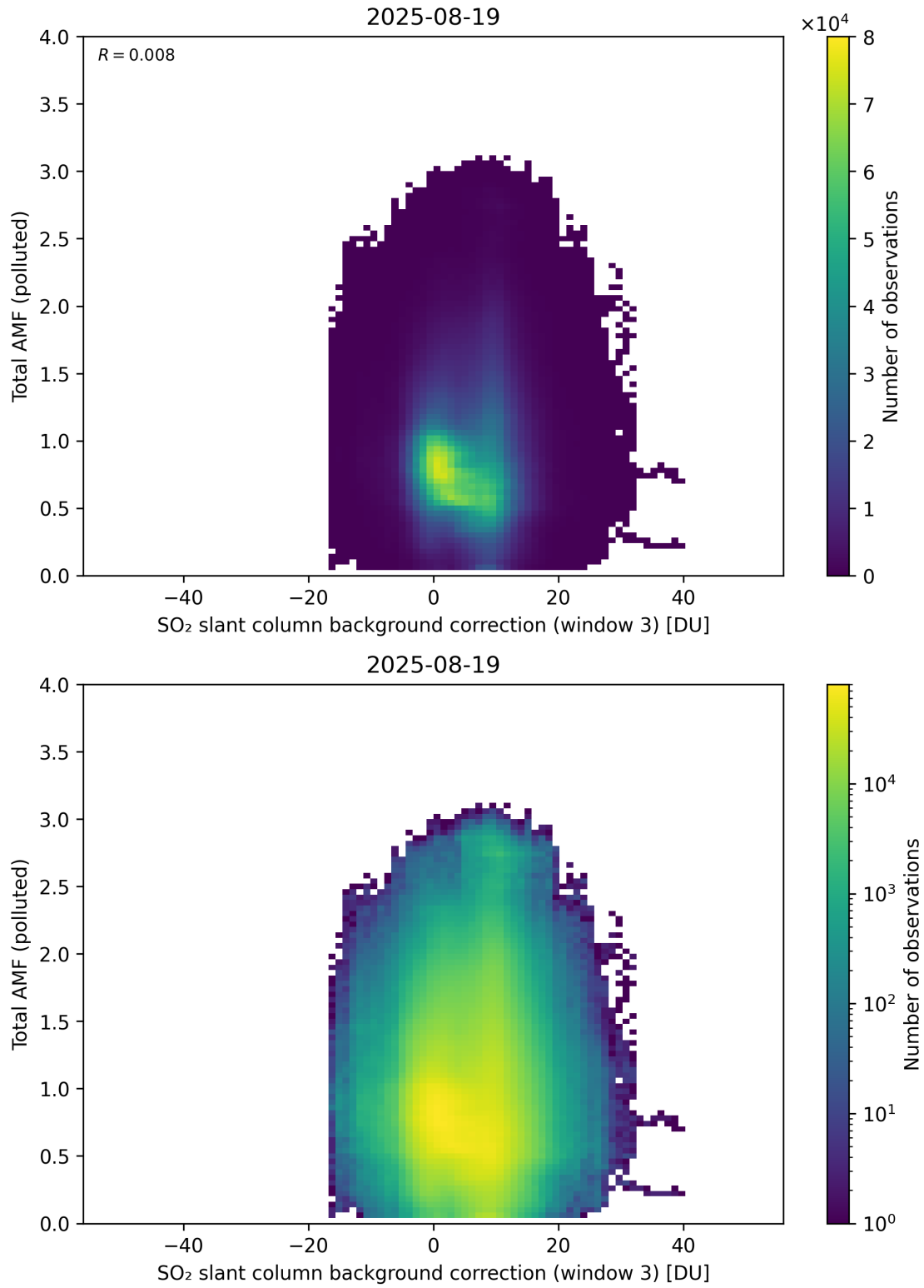
Figure 136: Scatter density plot of “SO 2 slant column background correction (window 3)” against “Total AMF (polluted)” for 2025-08-19 to 2025-08-20.
