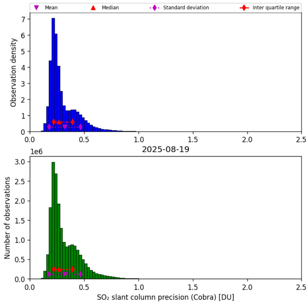
Figure 62: Histogram of “SO 2 slant column precision (Cobra)” for 2025-08-19 to 2025-08-20
