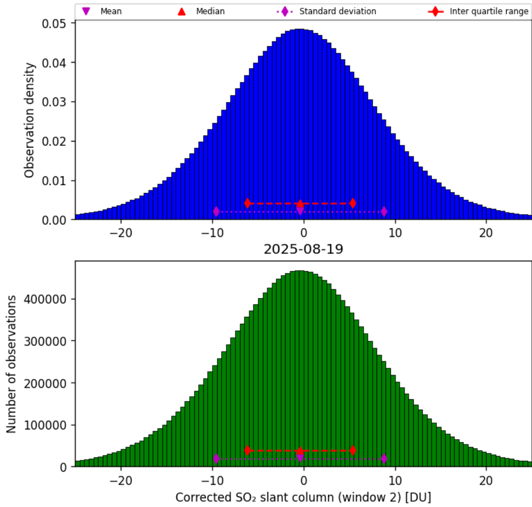
Figure 69: Histogram of “Corrected SO 2 slant column (window 2)” for 2025-08-19 to 2025-08-20
