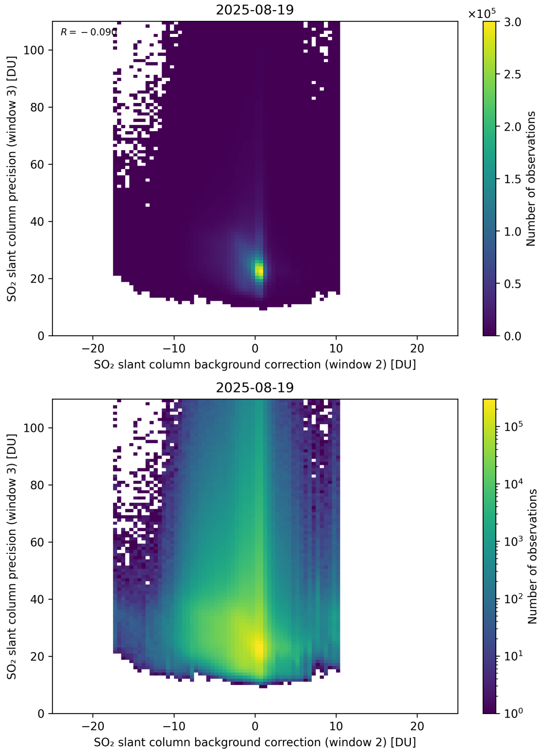
Figure 129: Scatter density plot of “SO 2 slant column background correction (window 2)” against “SO 2 slant column precision (window 3)” for 2025-08-19 to 2025-08-20.
