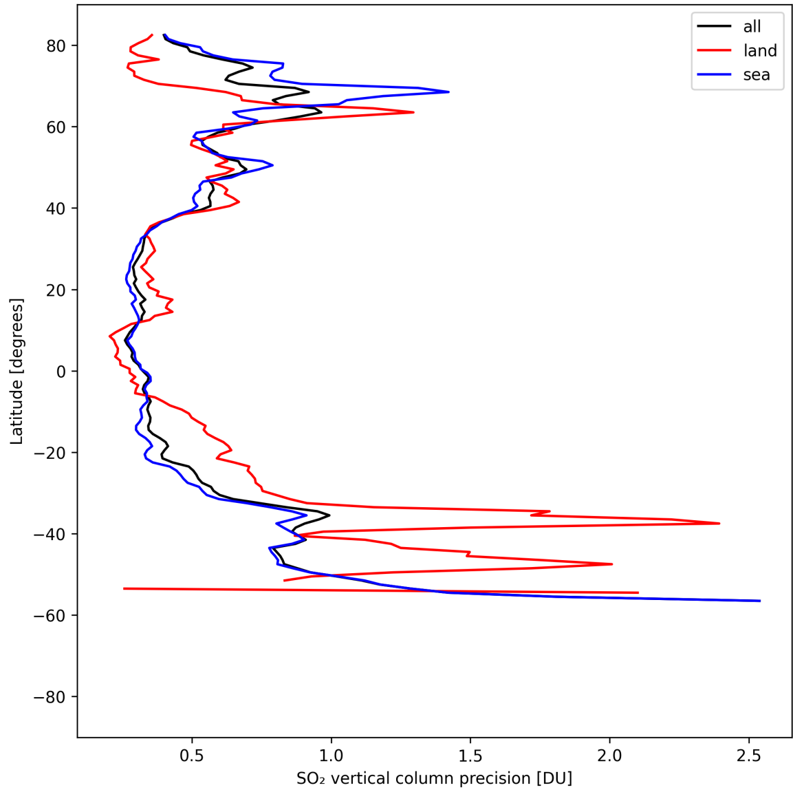
Figure 33: Zonal average of “SO 2 vertical column precision” for 2025-08-19 to 2025-08-20.
