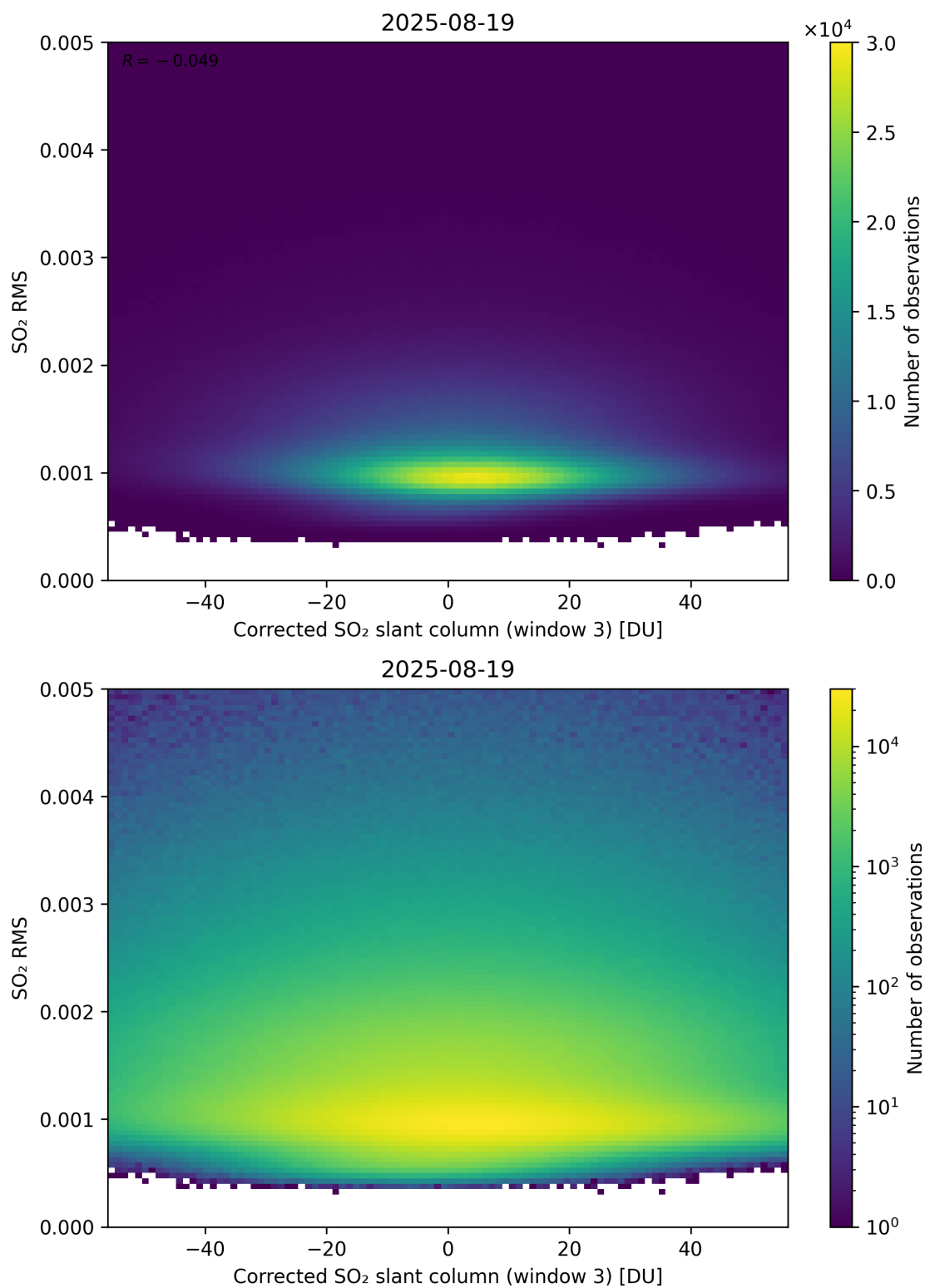
Figure 258: Scatter density plot of “Corrected SO 2 slant column (window 3)” against “SO 2 RMS” for 2025-08-19 to 2025-08-20.
