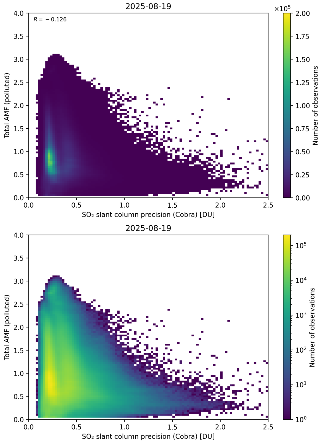
Figure 213: Scatter density plot of “SO 2 slant column precision (Cobra)” against “Total AMF (polluted)” for 2025-08-19 to 2025-08-20.
