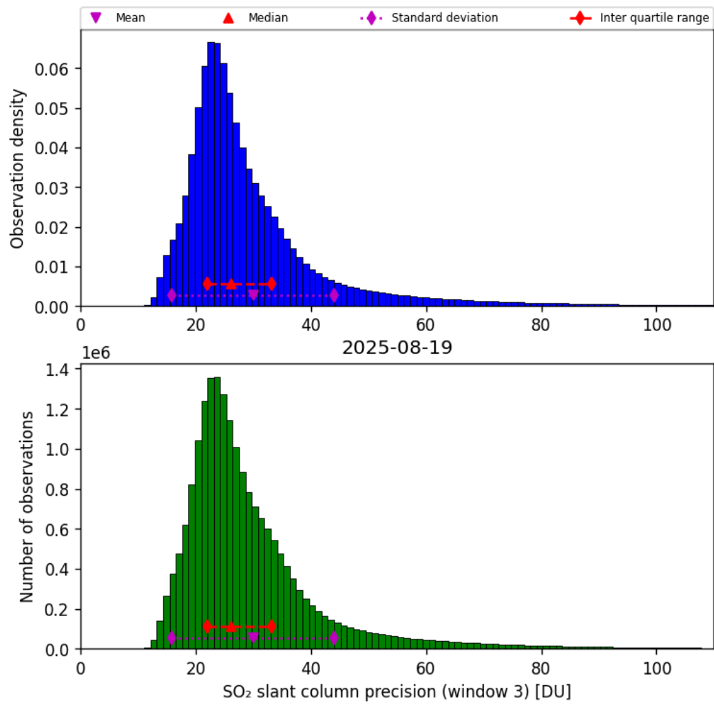
Figure 72: Histogram of “SO 2 slant column precision (window 3)” for 2025-08-19 to 2025-08-20
