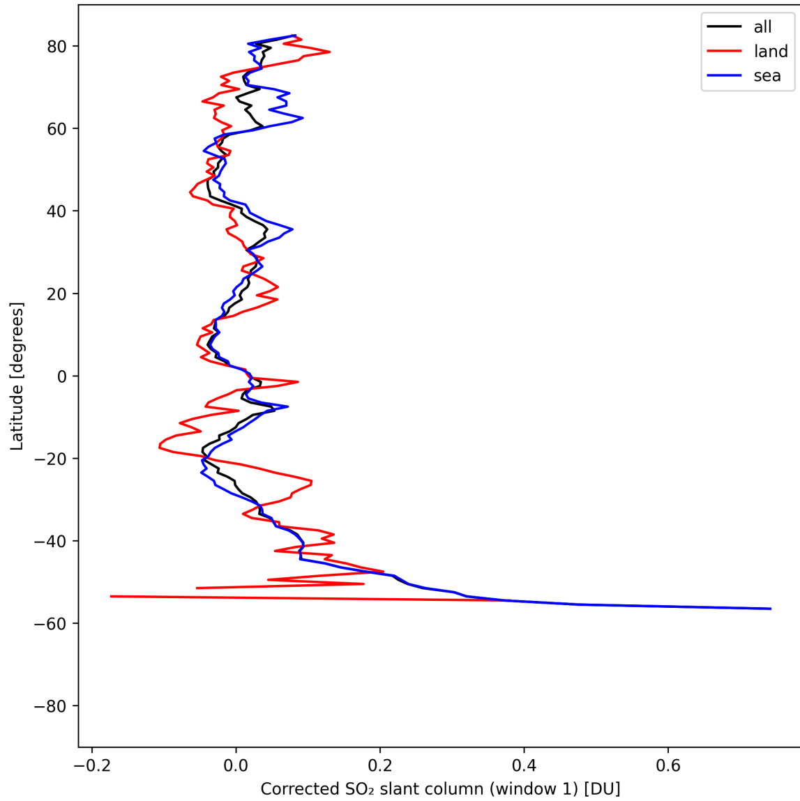
Figure 39: Zonal average of “Corrected SO 2 slant column (window 1)” for 2025-08-19 to 2025-08-20.
