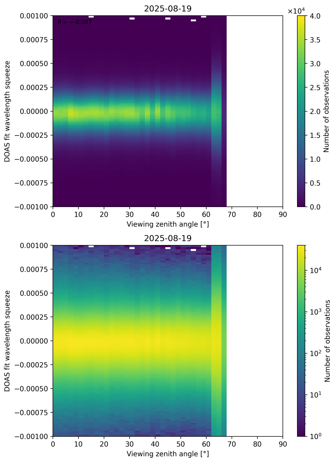
Figure 366: Scatter density plot of “Viewing zenith angle” against “DOAS fit wavelength squeeze” for 2025-08-19 to 2025-08-20.
