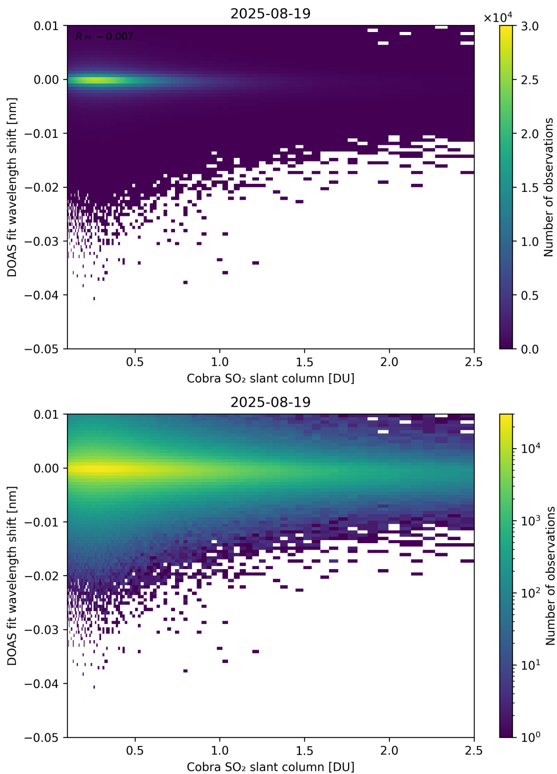
Figure 196: Scatter density plot of “Cobra SO 2 slant column” against “DOAS fit wavelength shift” for 2025-08-19 to 2025-08-20.
