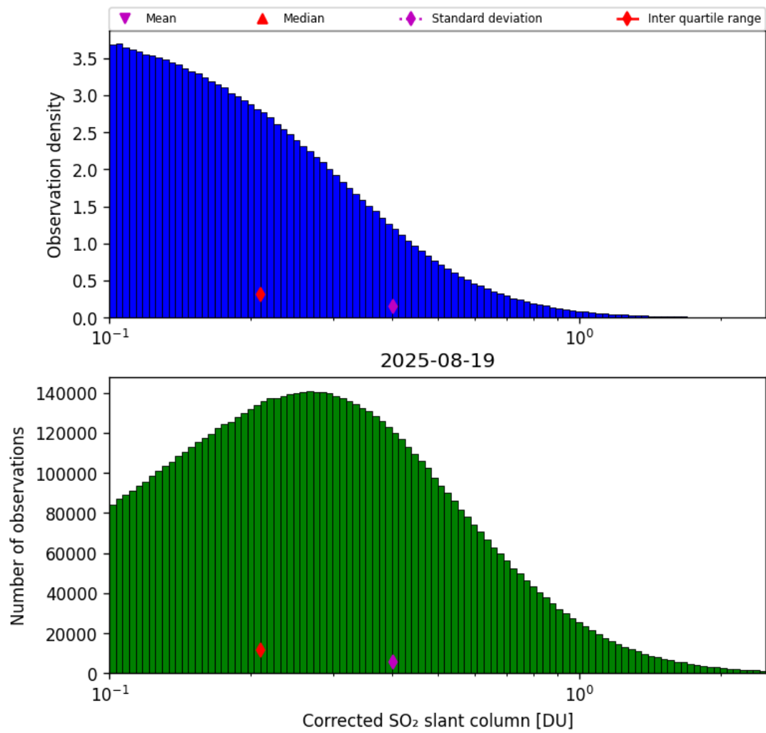
Figure 60: Histogram of “Corrected SO 2 slant column” for 2025-08-19 to 2025-08-20
