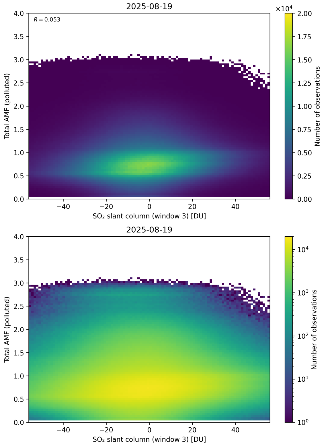
Figure 318: Scatter density plot of “SO 2 slant column (window 3)” against “Total AMF (polluted)” for 2025-08-19 to 2025-08-20.
