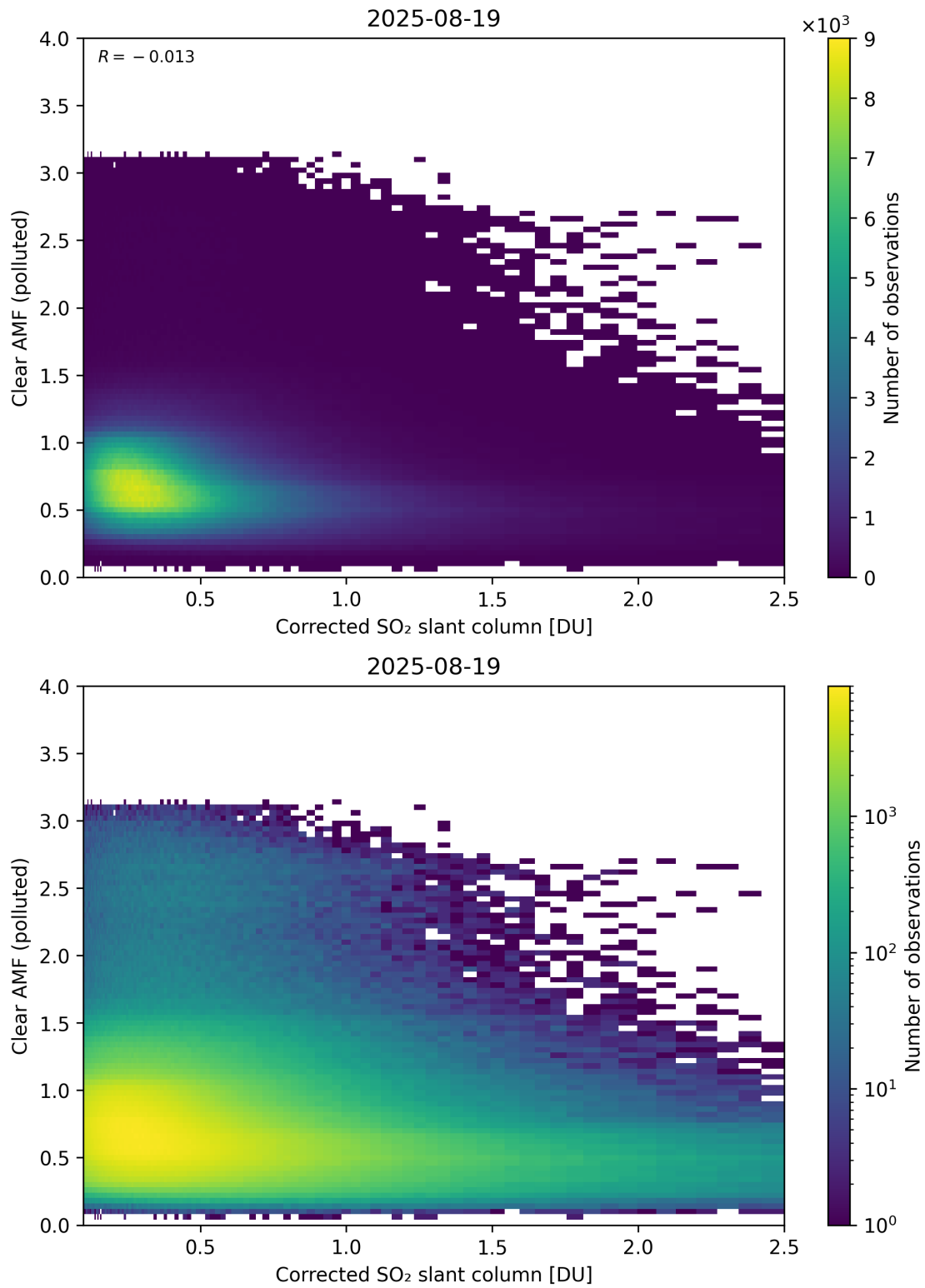
Figure 232: Scatter density plot of “Corrected SO 2 slant column” against “Clear AMF (polluted)” for 2025-08-19 to 2025-08-20.
