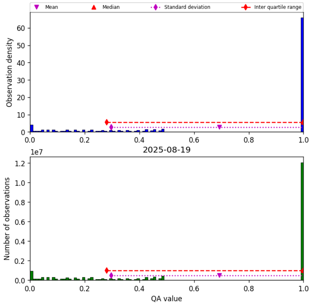
Figure 57: Histogram of “QA value” for 2025-08-19 to 2025-08-20
