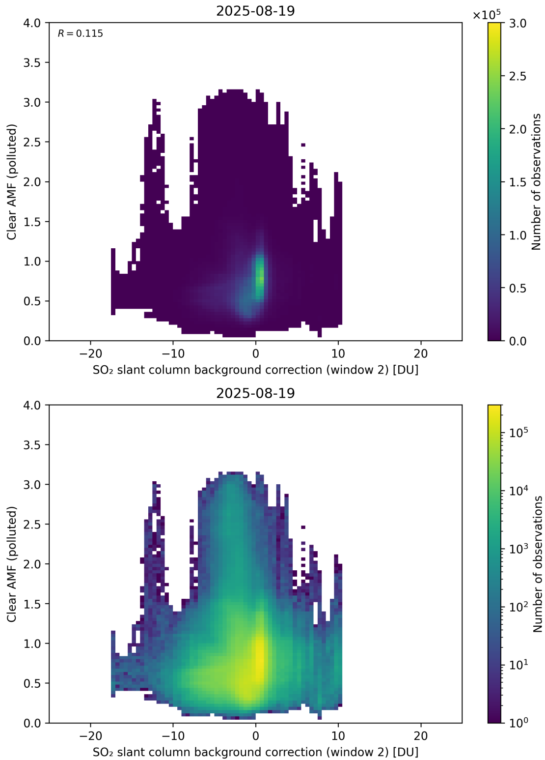
Figure 126: Scatter density plot of “SO 2 slant column background correction (window 2)” against “Clear AMF (polluted)” for 2025-08-19 to 2025-08-20.
