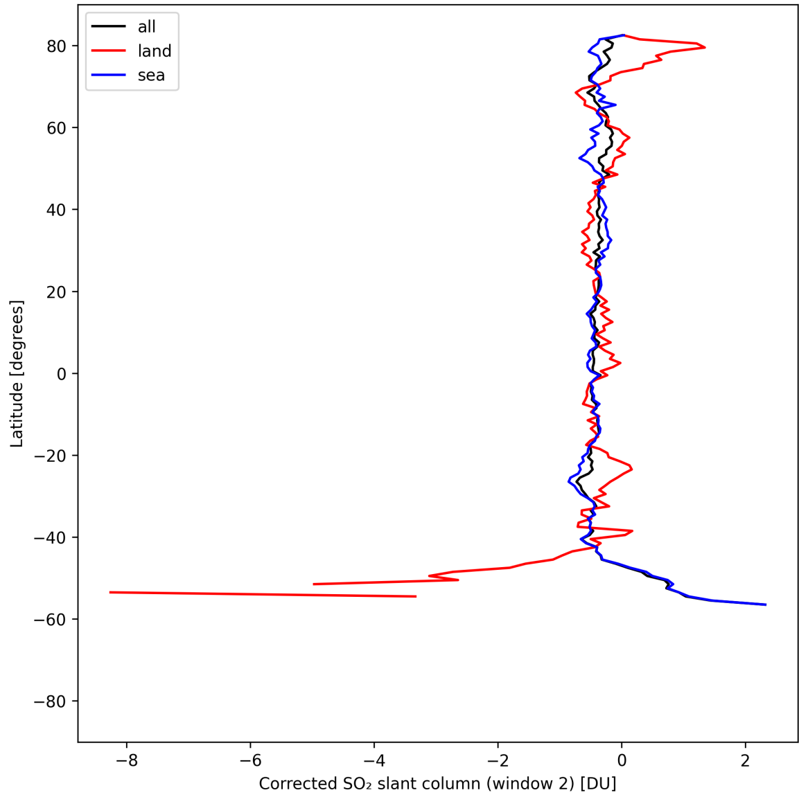
Figure 43: Zonal average of “Corrected SO 2 slant column (window 2)” for 2025-08-19 to 2025-08-20.
