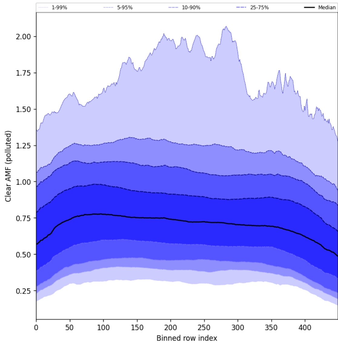
Figure 107: Along track statistics of “Clear AMF (polluted)” for 2025-08-19 to 2025-08-20
