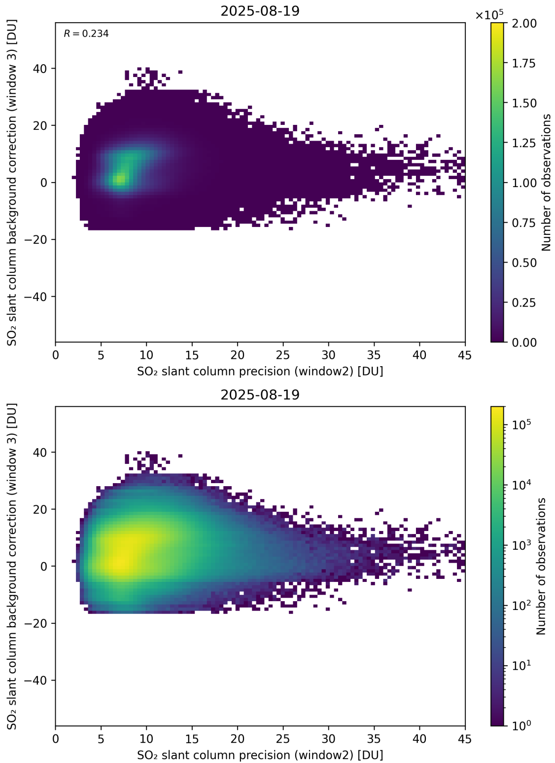
Figure 292: Scatter density plot of “SO 2 slant column precision (window2)” against “SO 2 slant column background correction (window 3)” for 2025-08-19 to 2025-08-20.
