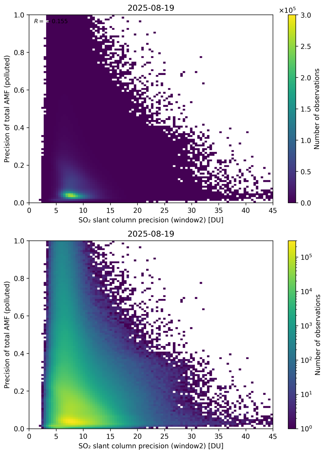
Figure 302: Scatter density plot of “SO 2 slant column precision (window2)” against “Precision of total AMF (polluted)” for 2025-08-19 to 2025-08-20.
