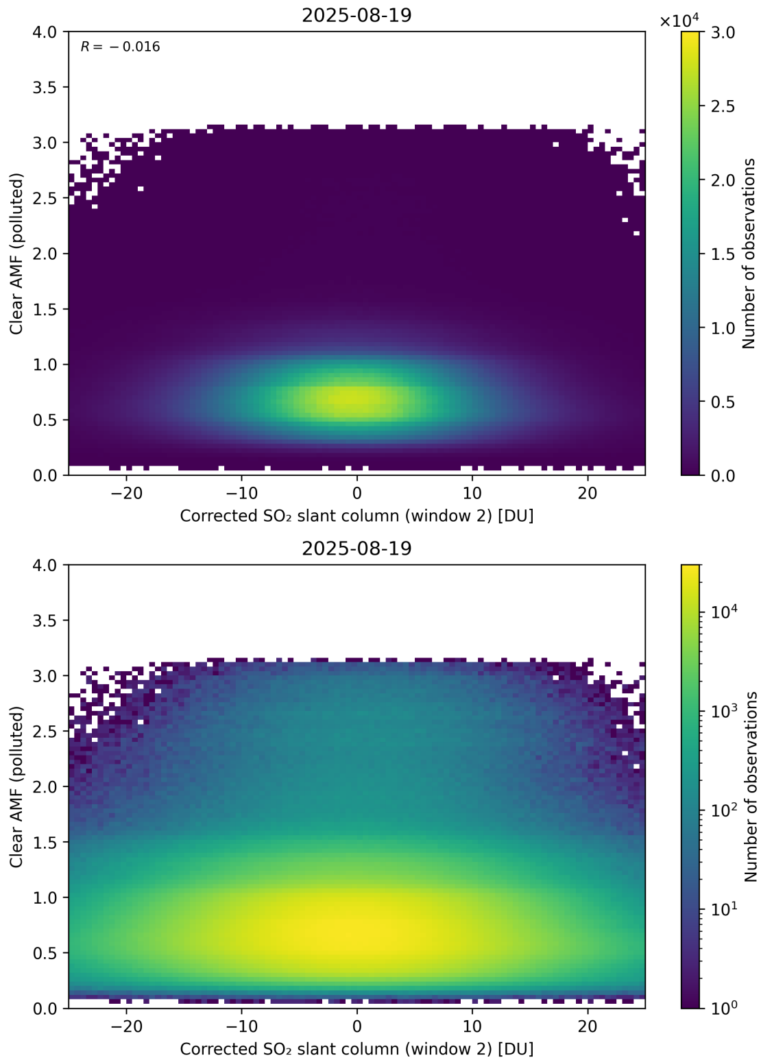
Figure 249: Scatter density plot of “Corrected SO 2 slant column (window 2)” against “Clear AMF (polluted)” for 2025-08-19 to 2025-08-20.
