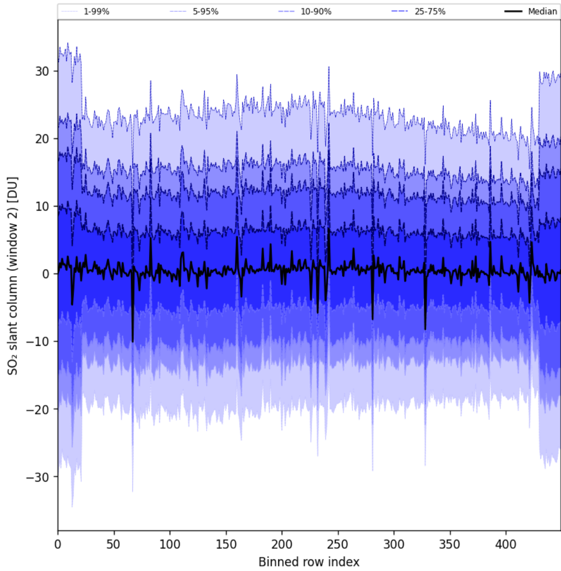
Figure 93: Along track statistics of “SO 2 slant column (window 2)” for 2025-08-19 to 2025-08-20
