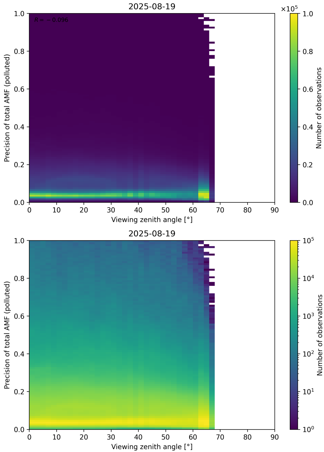
Figure 382: Scatter density plot of “Viewing zenith angle” against “Precision of total AMF (polluted)” for 2025-08-19 to 2025-08-20.
