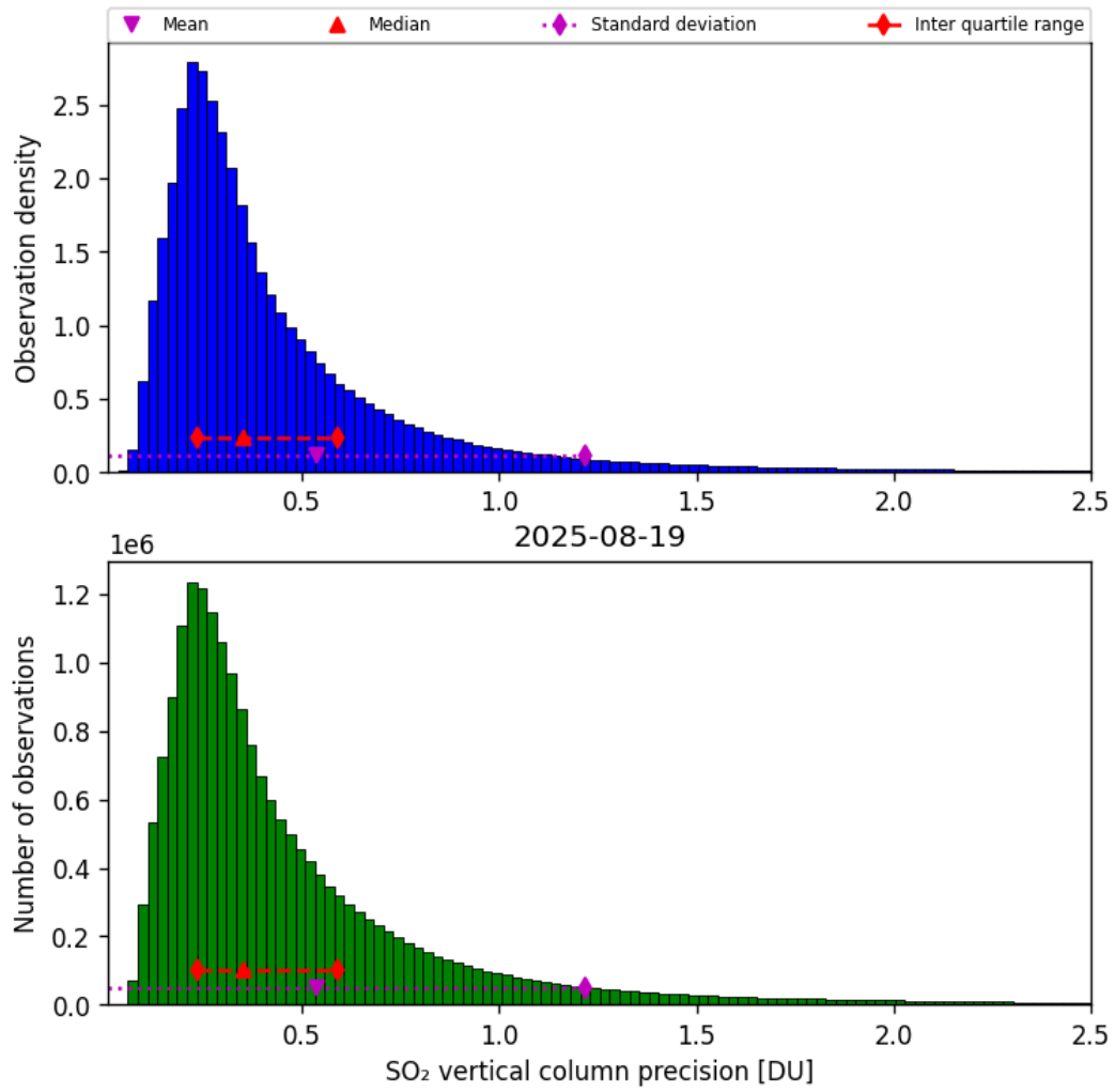
Figure 59: Histogram of “SO 2 vertical column precision” for 2025-08-19 to 2025-08-20
