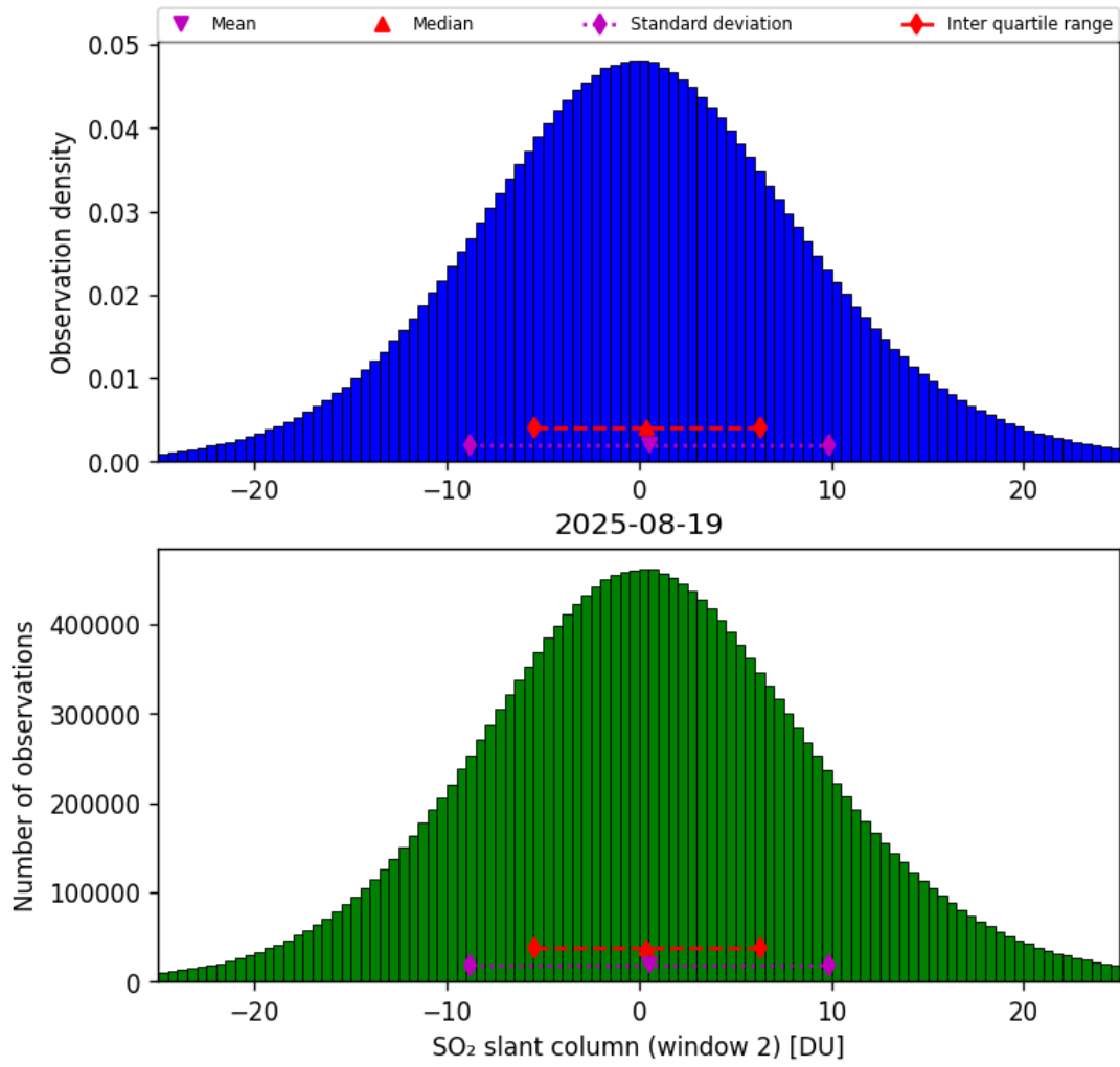
Figure 67: Histogram of “SO 2 slant column (window 2)” for 2025-08-19 to 2025-08-20
