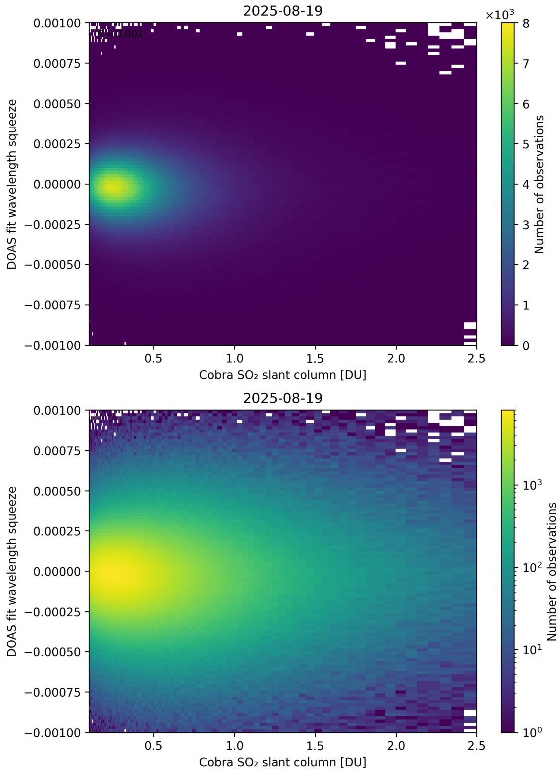
Figure 197: Scatter density plot of “Cobra SO 2 slant column” against “DOAS fit wavelength squeeze” for 2025-08-19 to 2025-08-20.
