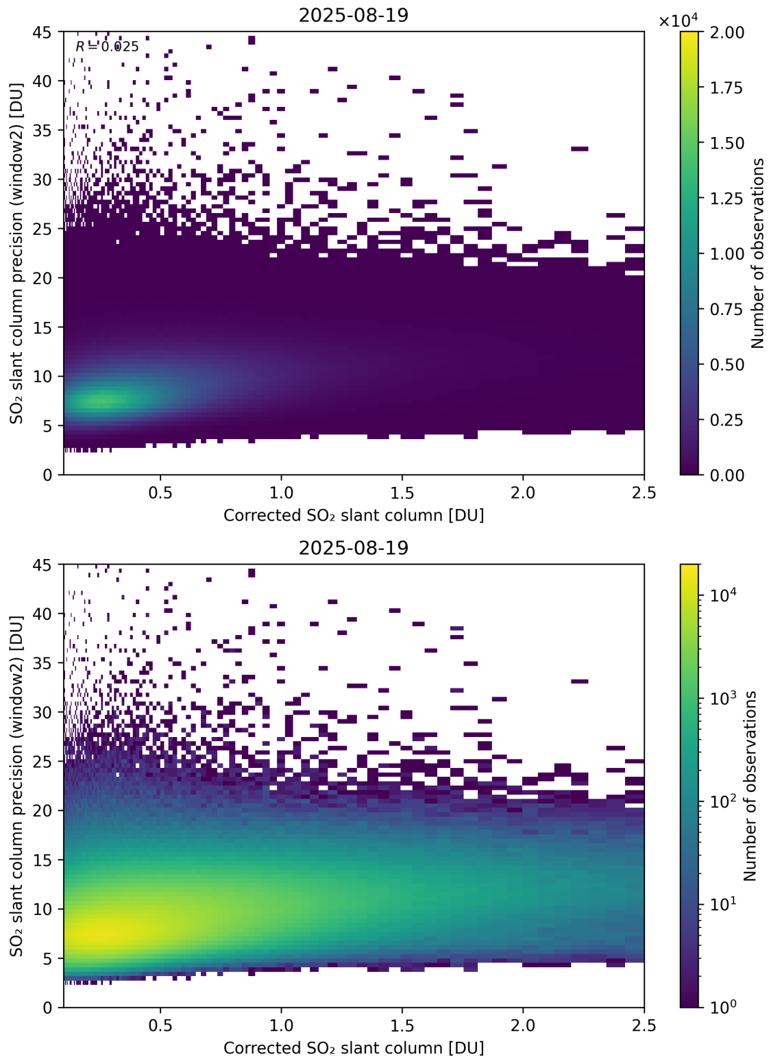
Figure 239: Scatter density plot of “Corrected SO 2 slant column” against “SO 2 slant column precision (window2)” for 2025-08-19 to 2025-08-20.
