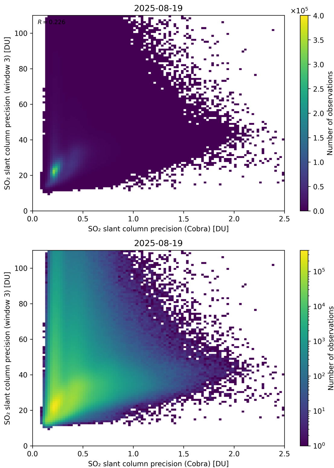
Figure 212: Scatter density plot of “SO 2 slant column precision (Cobra)” against “SO 2 slant column precision (window 3)” for 2025-08-19 to 2025-08-20.
