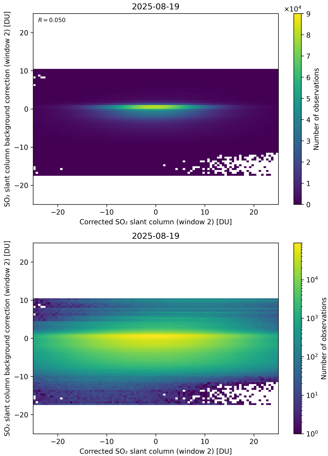
Figure 244: Scatter density plot of “Corrected SO 2 slant column (window 2)” against “SO 2 slant column background correction (window 2)” for 2025-08-19 to 2025-08-20.
