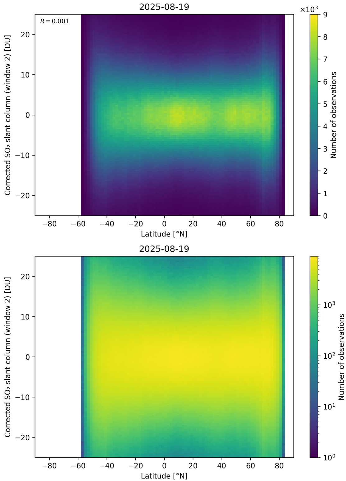
Figure 160: Scatter density plot of “Latitude” against “Corrected SO 2 slant column (window 2)” for 2025-08-19 to 2025-08-20.
