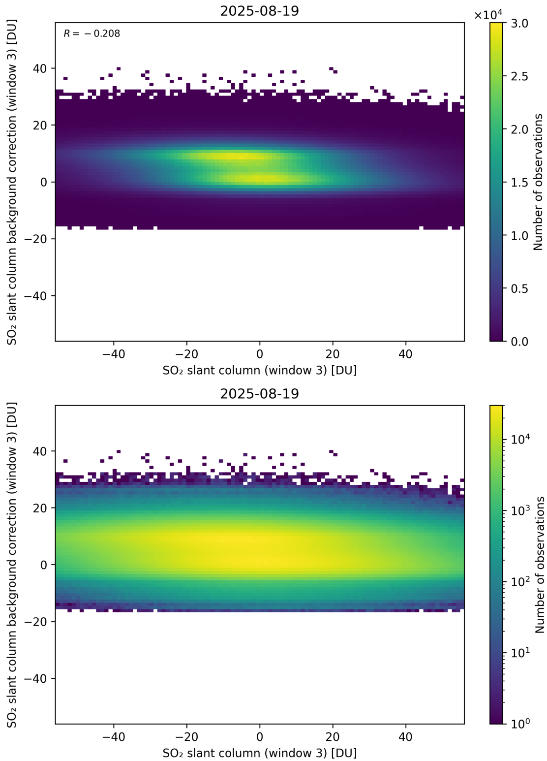
Figure 303: Scatter density plot of “SO 2 slant column (window 3)” against “SO 2 slant column background correction (window 3)” for 2025-08-19 to 2025-08-20.
