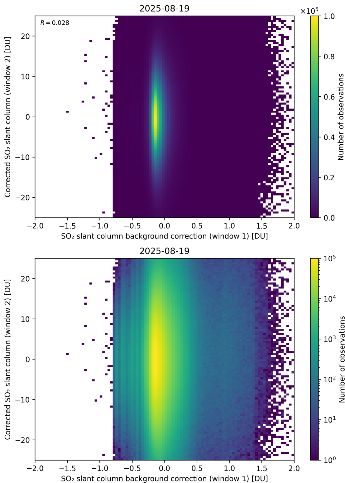
Figure 115: Scatter density plot of “SO 2 slant column background correction (window 1)” against “Corrected SO 2 slant column (window 2)” for 2025-08-19 to 2025-08-20.
