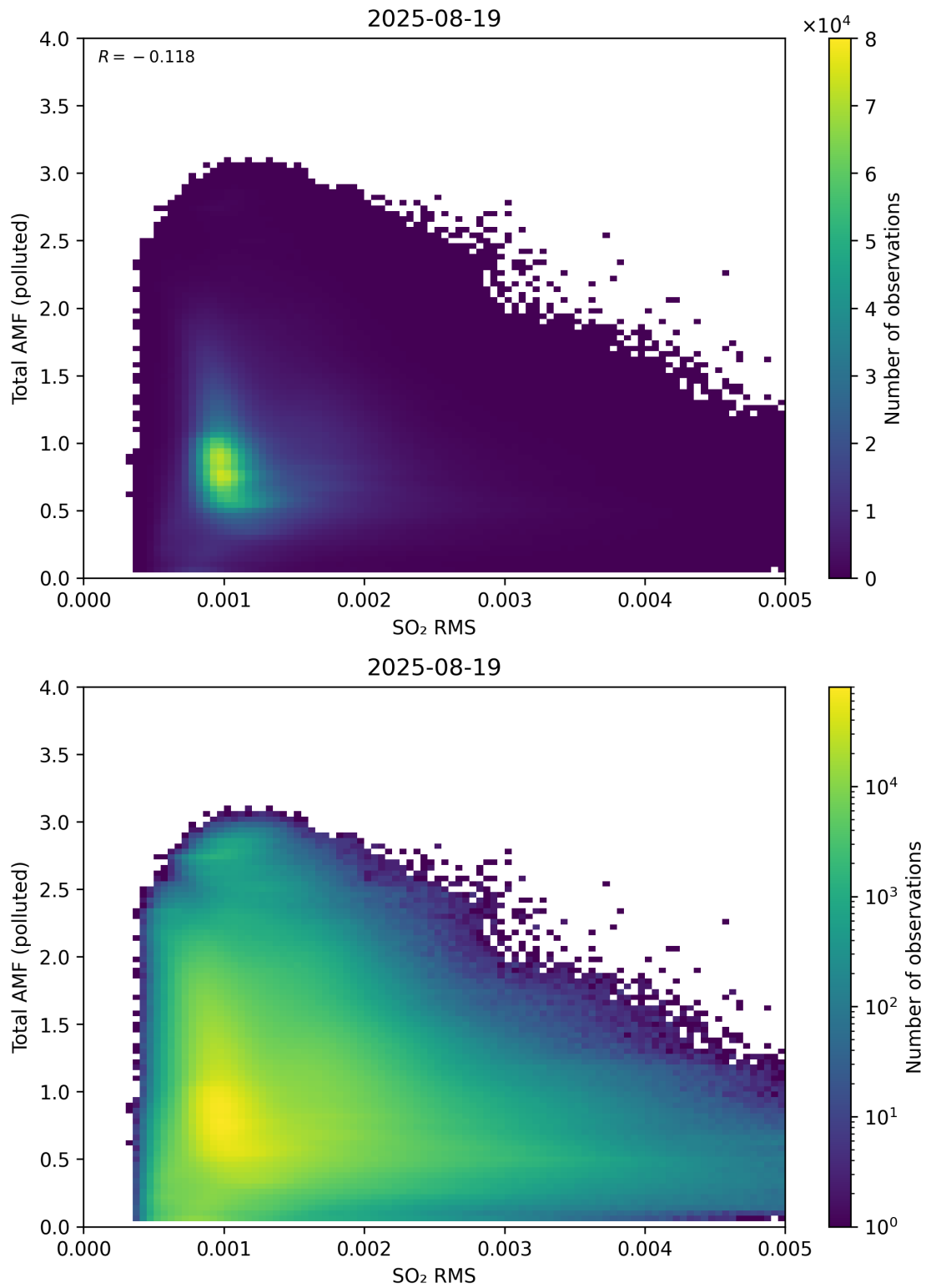
Figure 148: Scatter density plot of “SO 2 RMS” against “Total AMF (polluted)” for 2025-08-19 to 2025-08-20.
