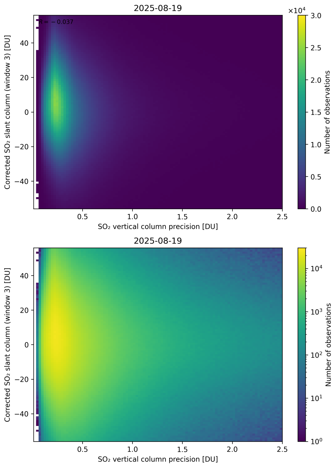
Figure 340: Scatter density plot of “SO 2 vertical column precision” against “Corrected SO 2 slant column (window 3)” for 2025-08-19 to 2025-08-20.
