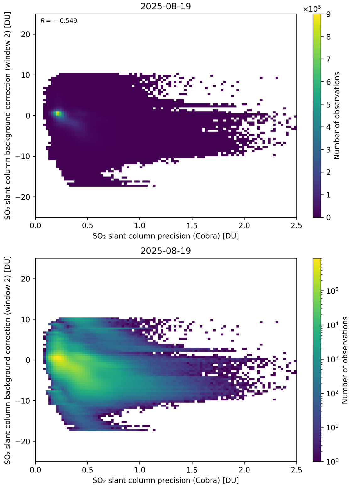
Figure 200: Scatter density plot of “SO 2 slant column precision (Cobra)” against “SO 2 slant column background correction (window 2)” for 2025-08-19 to 2025-08-20.
