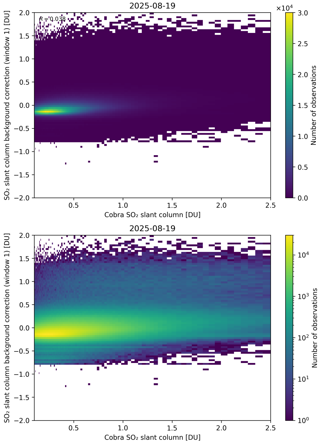
Figure 193: Scatter density plot of “Cobra SO 2 slant column” against “SO 2 slant column background correction (window 1)” for 2025-08-19 to 2025-08-20.
