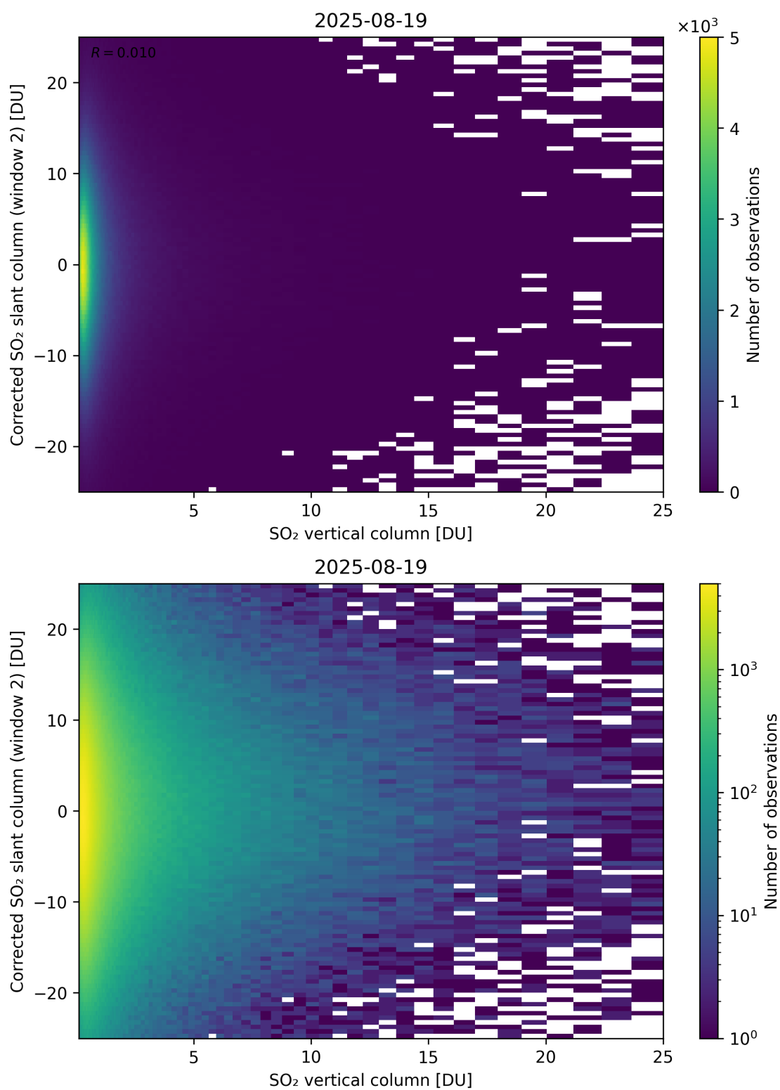
Figure 352: Scatter density plot of “SO 2 vertical column” against “Corrected SO 2 slant column (window 2)” for 2025-08-19 to 2025-08-20.
