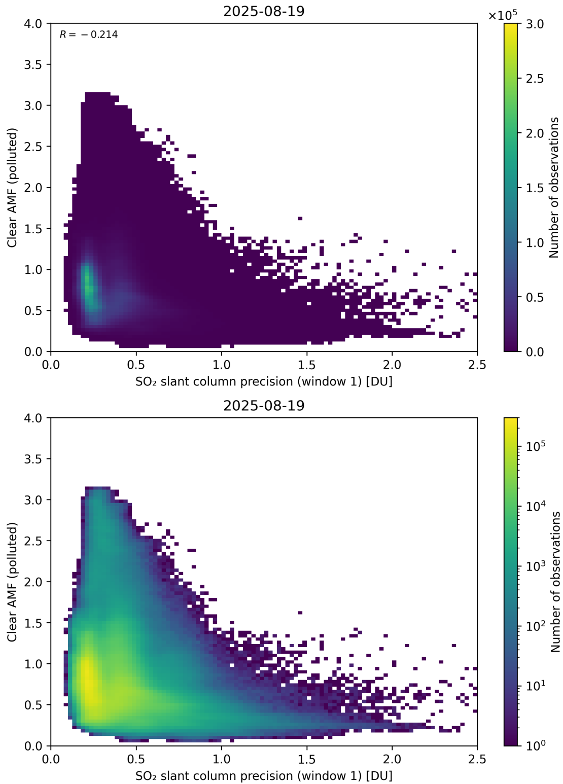
Figure 274: Scatter density plot of “SO 2 slant column precision (window 1)” against “Clear AMF (polluted)” for 2025-08-19 to 2025-08-20.
