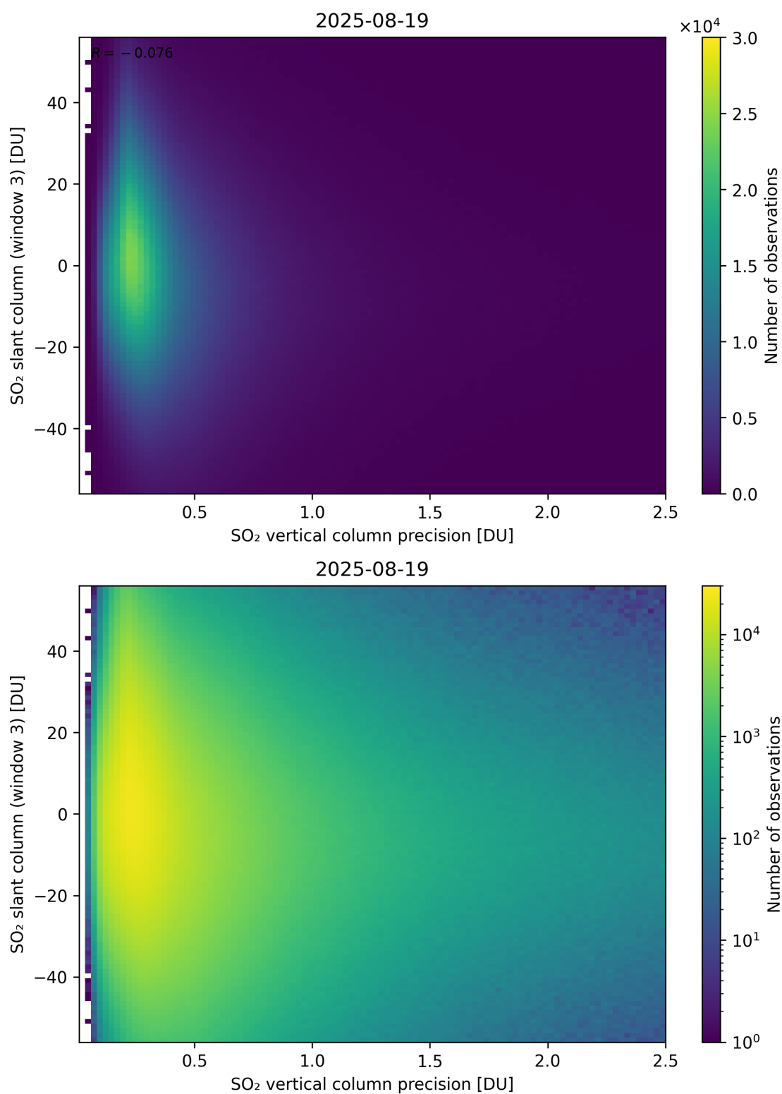
Figure 344: Scatter density plot of “SO 2 vertical column precision” against “SO 2 slant column (window 3)” for 2025-08-19 to 2025-08-20.
