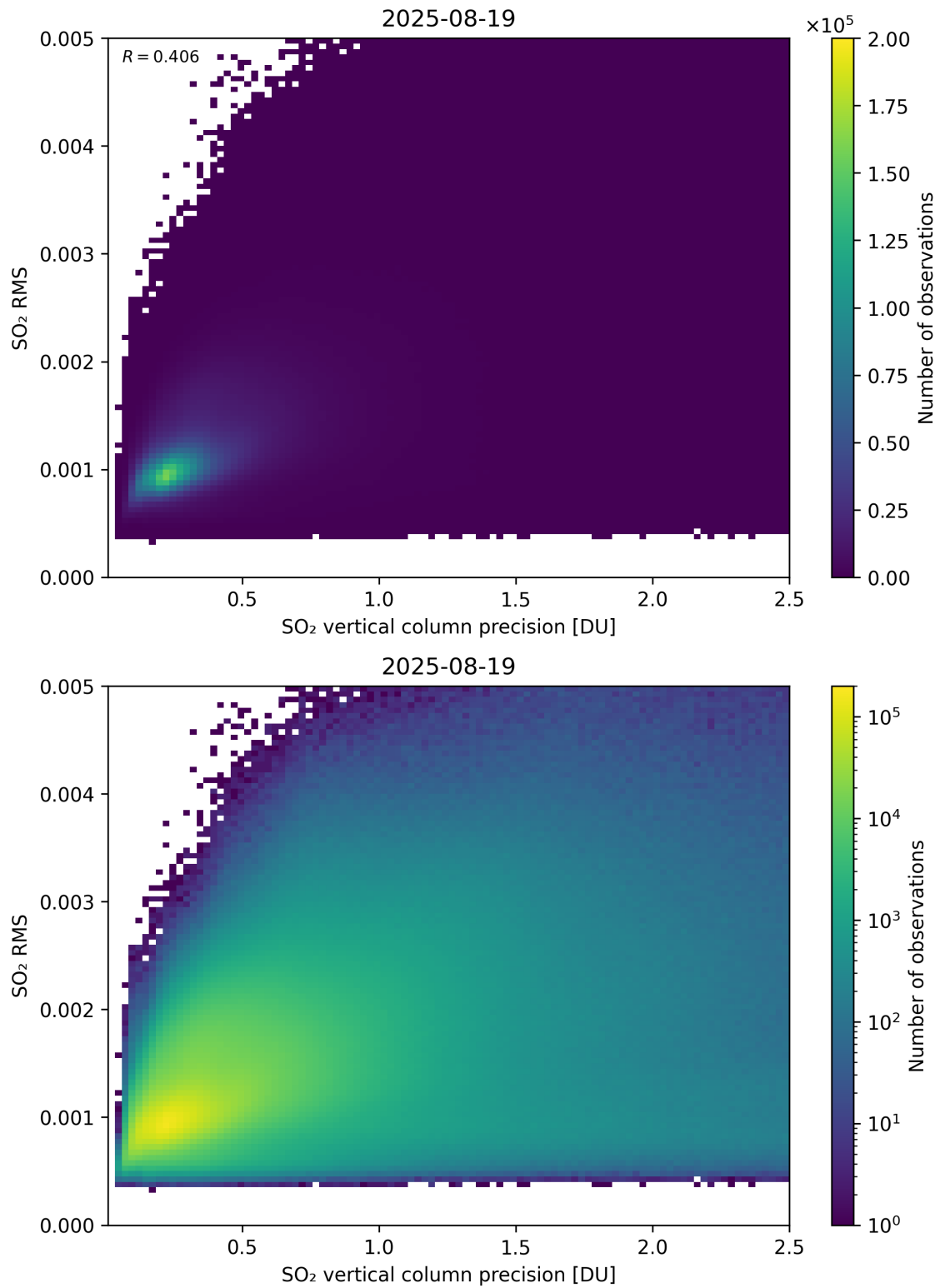
Figure 334: Scatter density plot of “SO 2 vertical column precision” against “SO 2 RMS” for 2025-08-19 to 2025-08-20.
