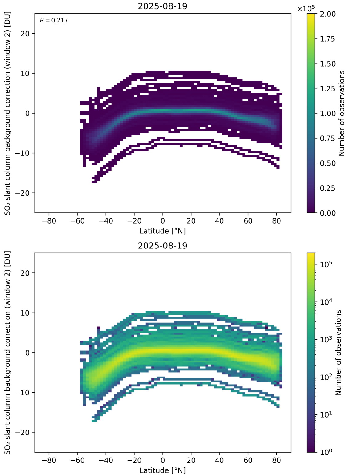
Figure 151: Scatter density plot of “Latitude” against “SO 2 slant column background correction (window 2)” for 2025-08-19 to 2025-08-20.
