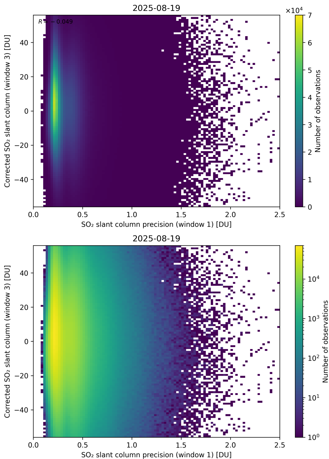
Figure 276: Scatter density plot of “SO 2 slant column precision (window 1)” against “Corrected SO 2 slant column (window 3)” for 2025-08-19 to 2025-08-20.
