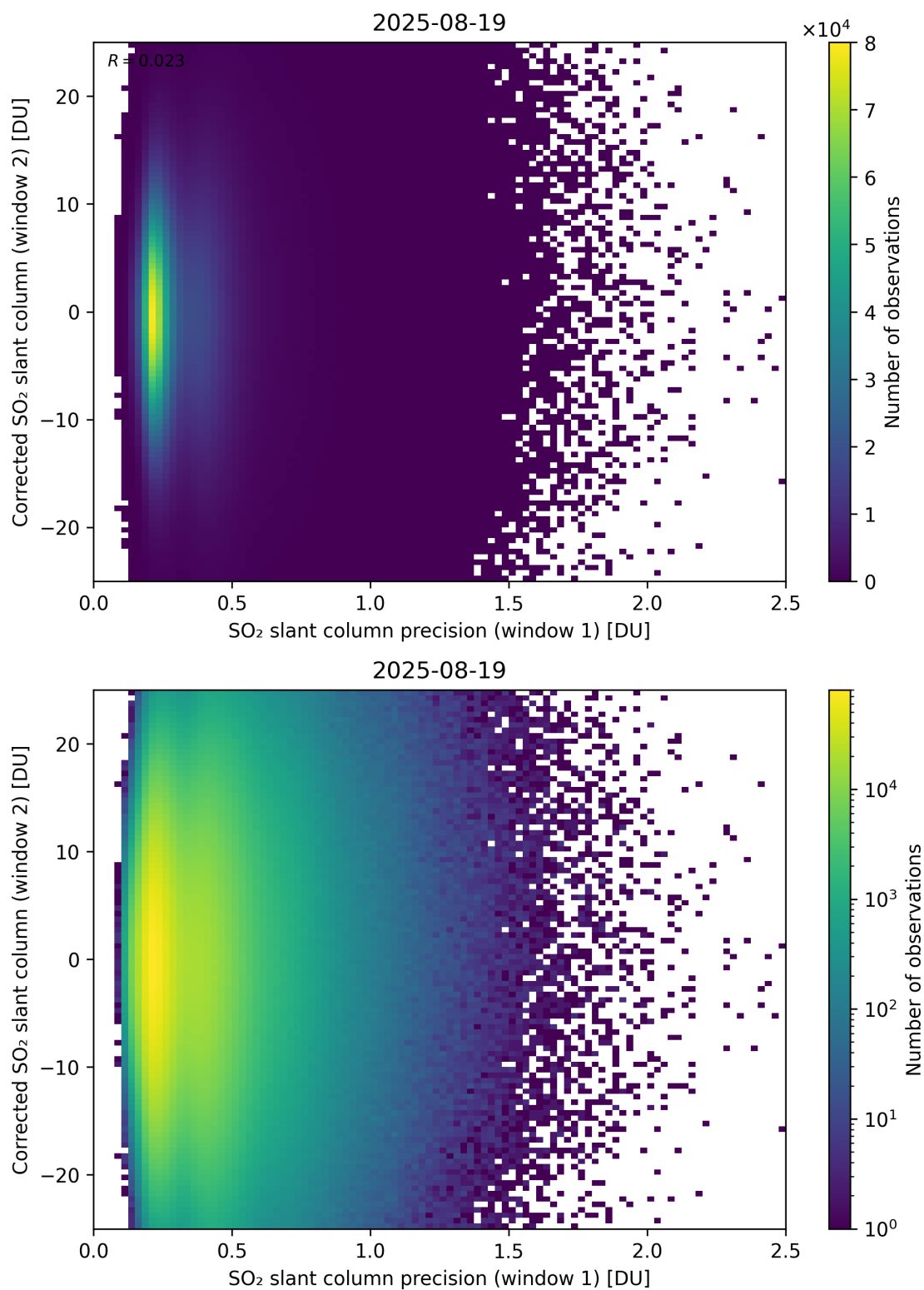
Figure 275: Scatter density plot of “SO 2 slant column precision (window 1)” against “Corrected SO 2 slant column (window 2)” for 2025-08-19 to 2025-08-20.
