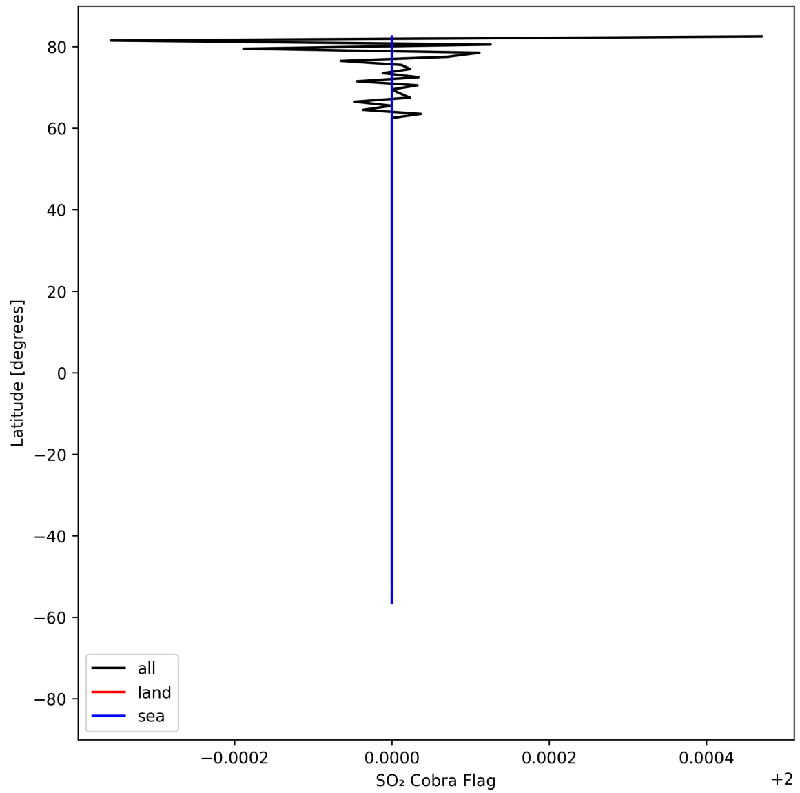
Figure 49: Zonal average of "SO 2 Cobra Flag" for 2025-08-19 to 2025-08-20.
