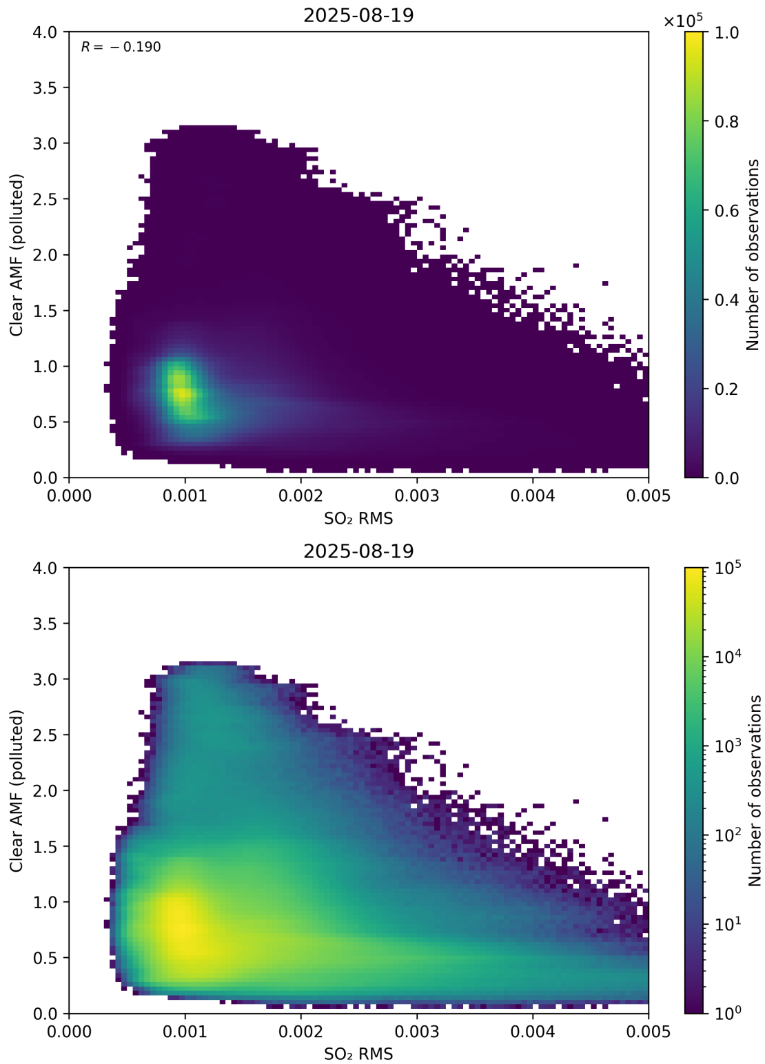
Figure 147: Scatter density plot of “SO 2 RMS” against “Clear AMF (polluted)” for 2025-08-19 to 2025-08-20.
