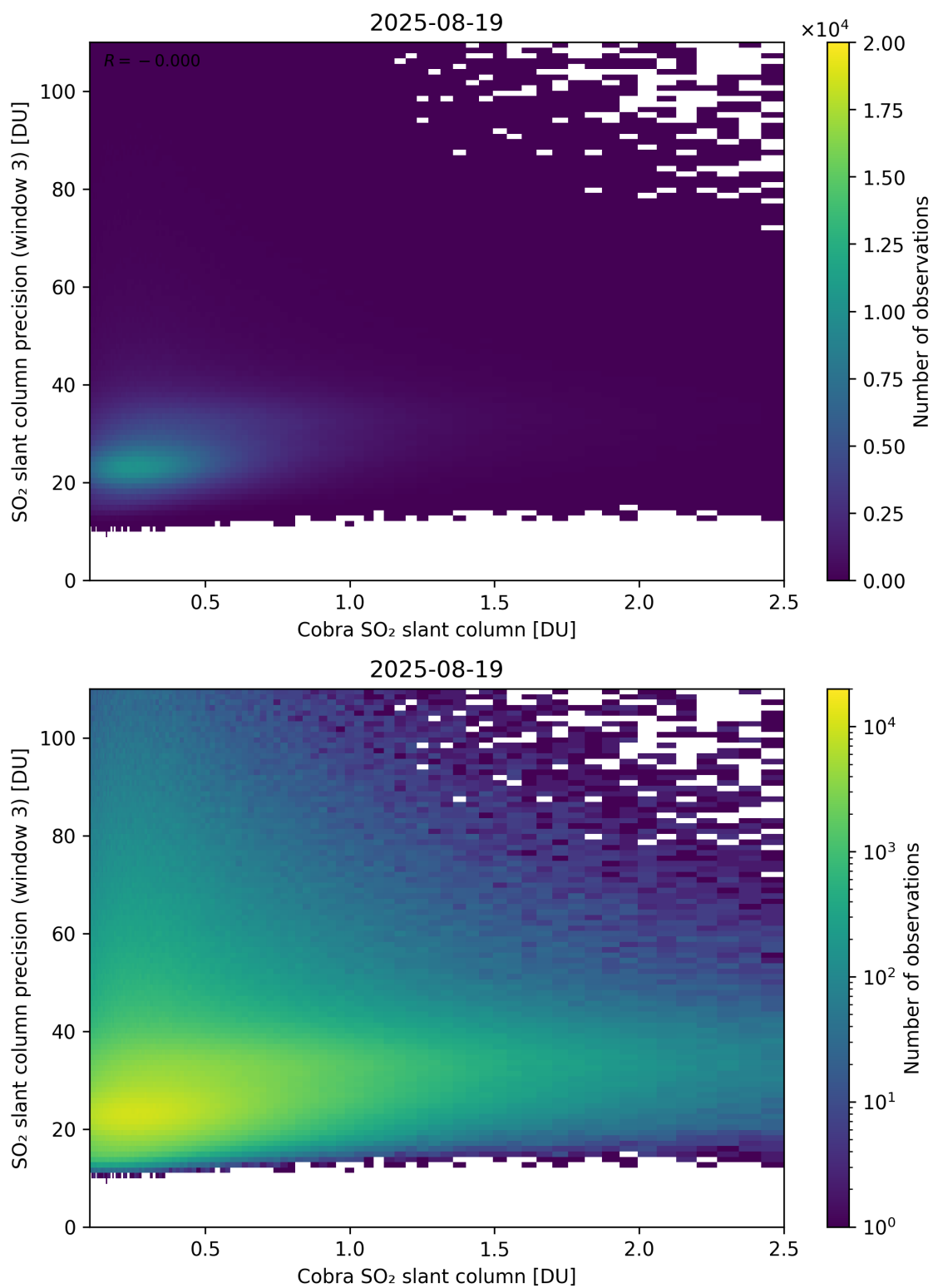
Figure 223: Scatter density plot of “Cobra SO 2 slant column” against “SO 2 slant column precision (window 3)” for 2025-08-19 to 2025-08-20.
