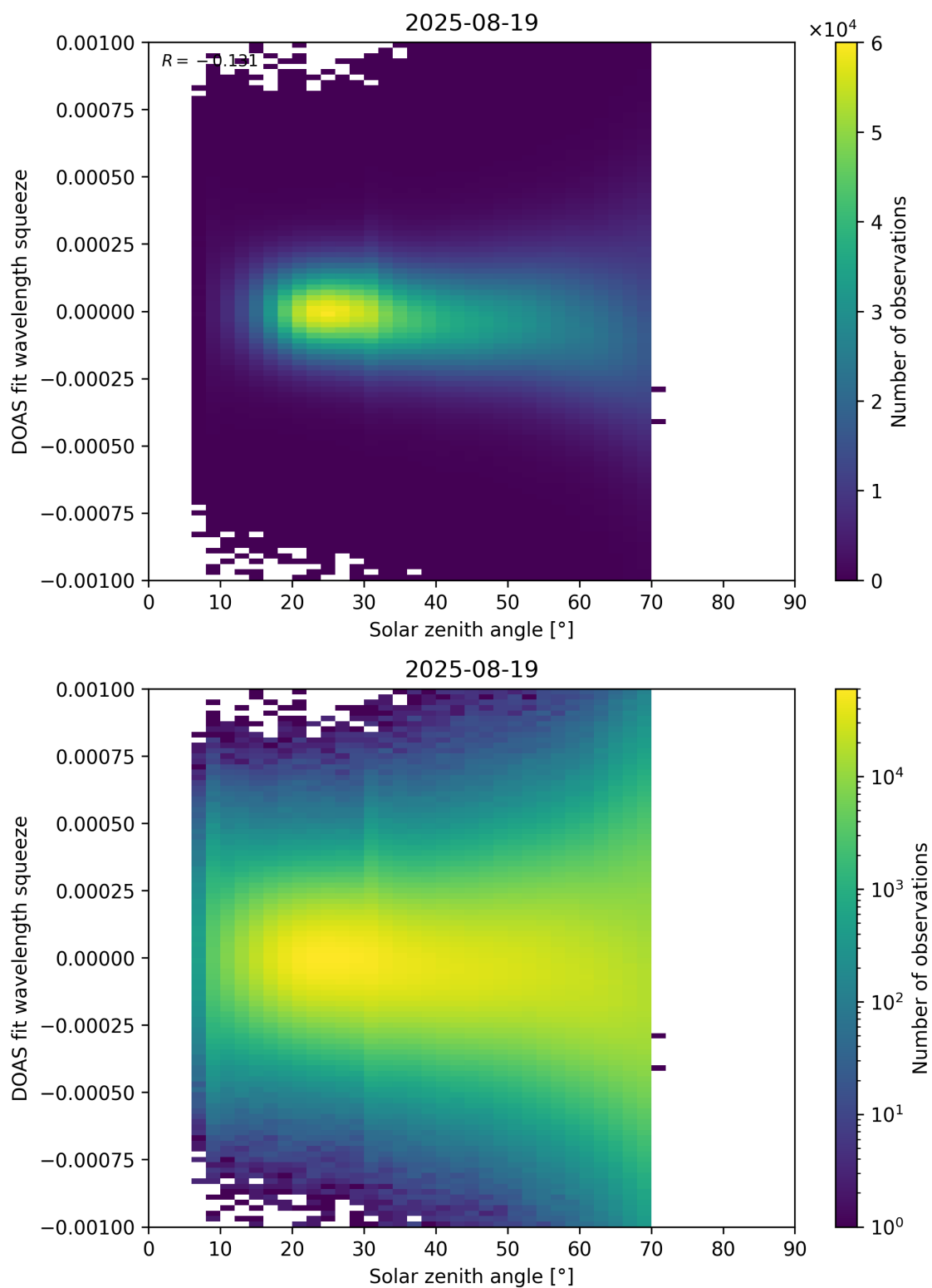
Figure 175: Scatter density plot of “Solar zenith angle” against “DOAS fit wavelength squeeze” for 2025-08-19 to 2025-08-20.
