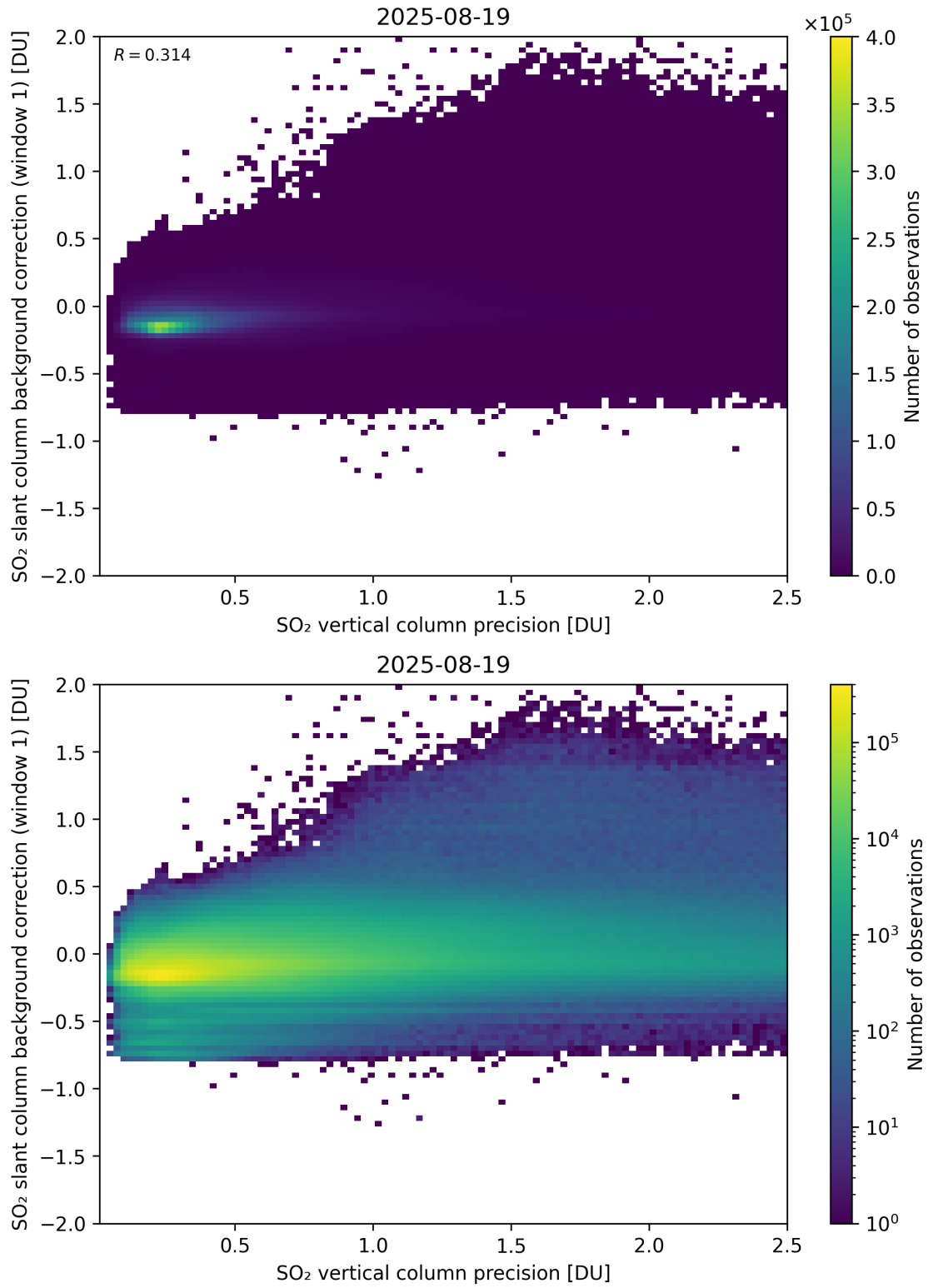
Figure 329: Scatter density plot of “SO 2 vertical column precision” against “SO 2 slant column background correction (window 1)” for 2025-08-19 to 2025-08-20.
