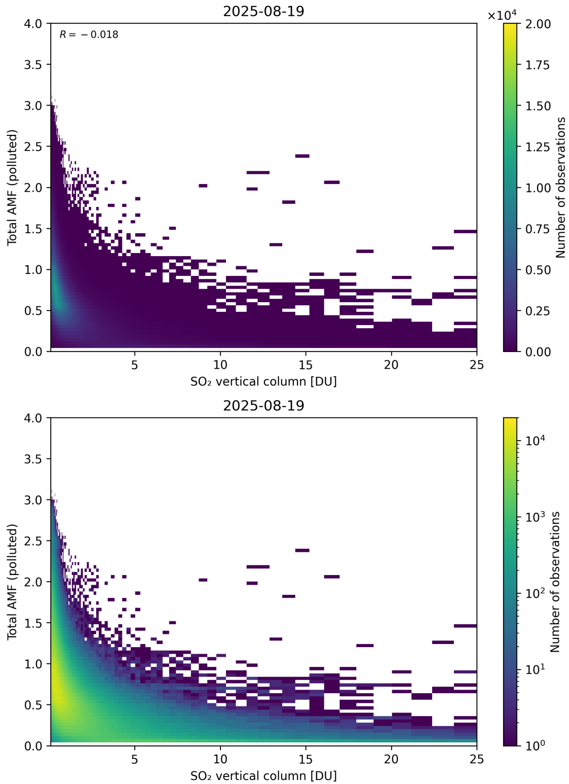
Figure 359: Scatter density plot of “SO 2 vertical column” against “Total AMF (polluted)” for 2025-08-19 to 2025-08-20.
