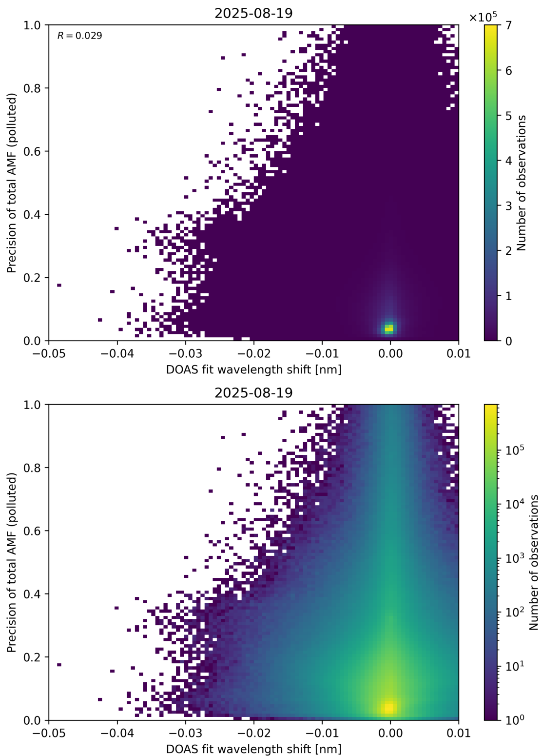
Figure 142: Scatter density plot of “DOAS fit wavelength shift” against “Precision of total AMF (polluted)” for 2025-08-19 to 2025-08-20.
