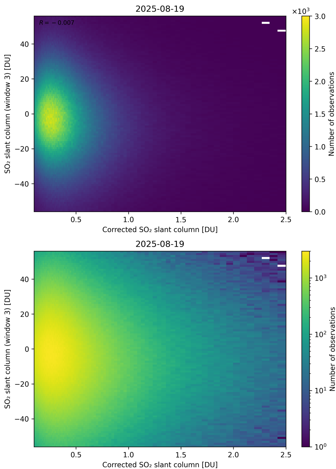
Figure 240: Scatter density plot of “Corrected SO 2 slant column” against “SO 2 slant column (window 3)” for 2025-08-19 to 2025-08-20.
