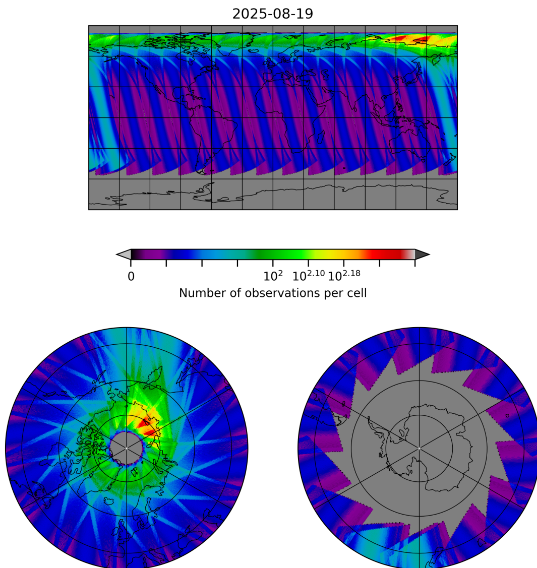
Figure 30: Map of the number of observations for 2025-08-19 to 2025-08-20
