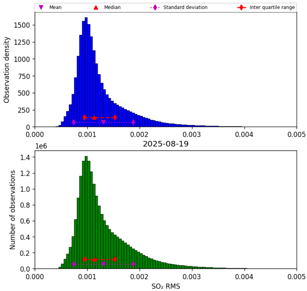
Figure 78: Histogram of “SO 2 RMS” for 2025-08-19 to 2025-08-20
