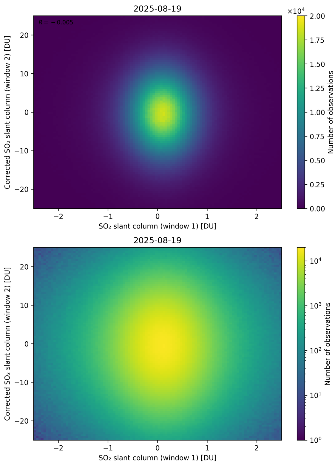
Figure 283: Scatter density plot of “SO 2 slant column (window 1)” against “Corrected SO 2 slant column (window 2)” for 2025-08-19 to 2025-08-20.
