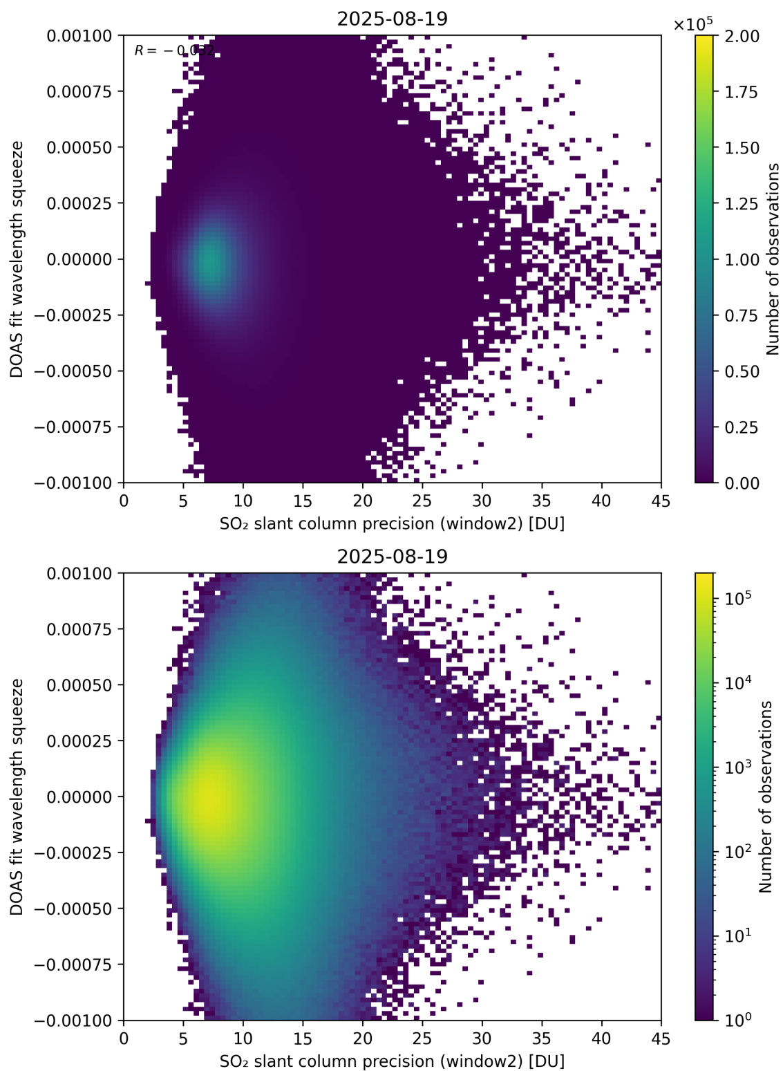
Figure 294: Scatter density plot of “SO 2 slant column precision (window2)” against “DOAS fit wavelength squeeze” for 2025-08-19 to 2025-08-20.
