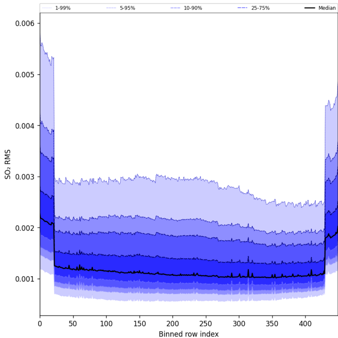
Figure 104: Along track statistics of “SO 2 RMS” for 2025-08-19 to 2025-08-20
