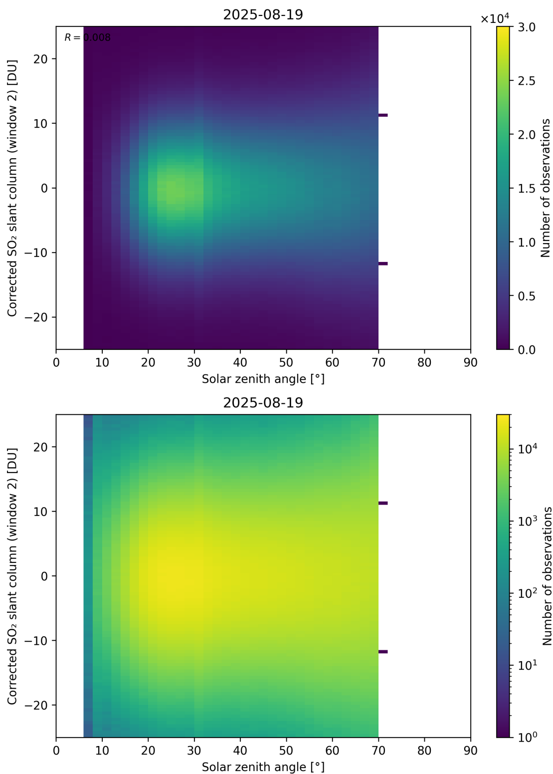
Figure 182: Scatter density plot of “Solar zenith angle” against “Corrected SO 2 slant column (window 2)” for 2025-08-19 to 2025-08-20.
