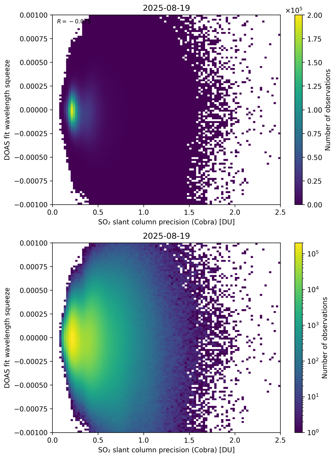
Figure 203: Scatter density plot of “SO 2 slant column precision (Cobra)” against “DOAS fit wavelength squeeze” for 2025-08-19 to 2025-08-20.
