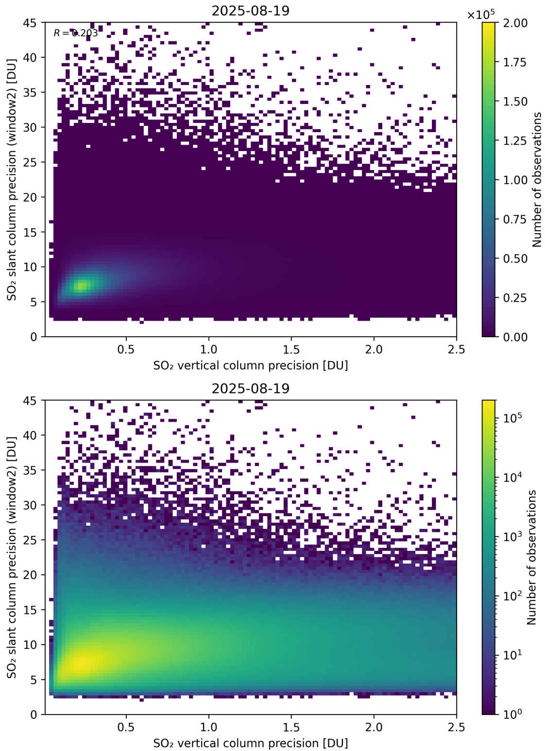
Figure 343: Scatter density plot of “SO 2 vertical column precision” against “SO 2 slant column precision (window2)” for 2025-08-19 to 2025-08-20.
