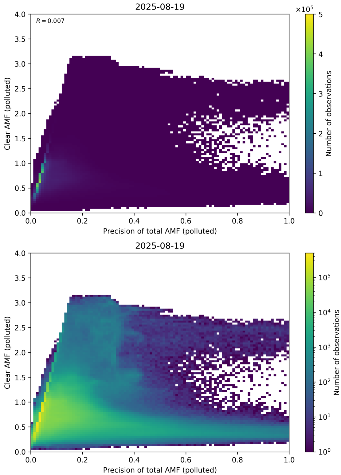
Figure 320: Scatter density plot of “Precision of total AMF (polluted)” against “Clear AMF (polluted)” for 2025-08-19 to 2025-08-20.
