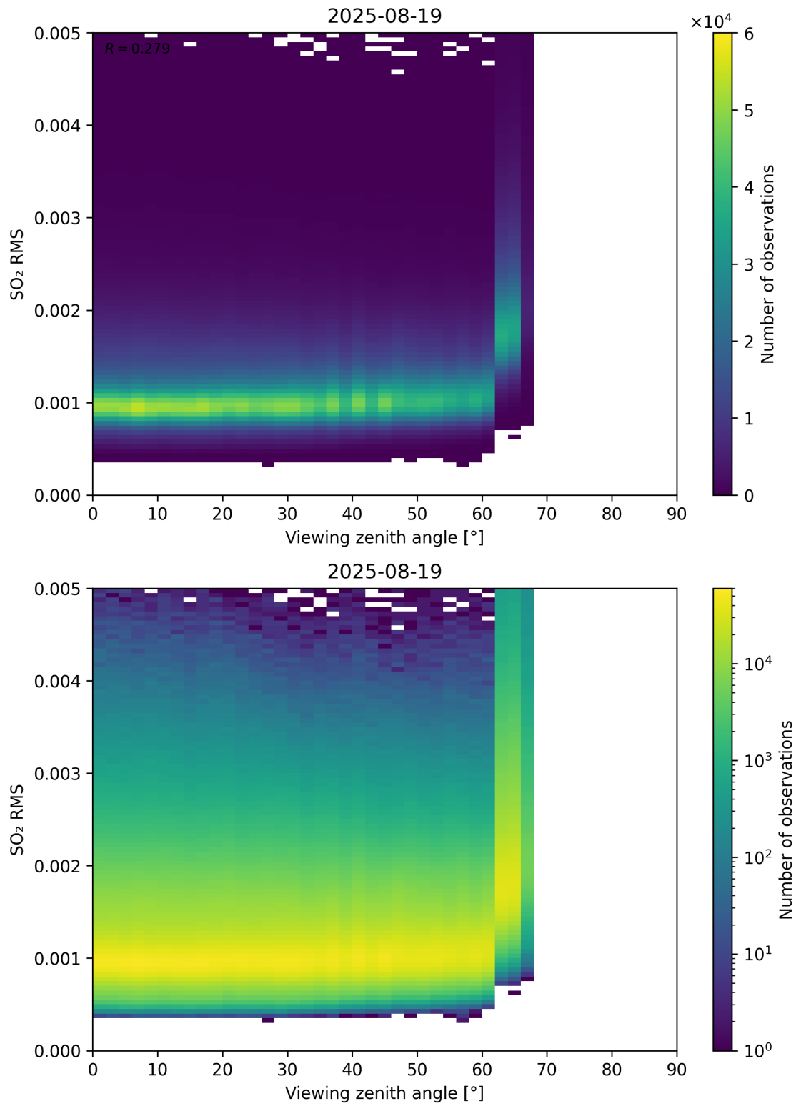
Figure 367: Scatter density plot of “Viewing zenith angle” against “SO 2 RMS” for 2025-08-19 to 2025-08-20.
