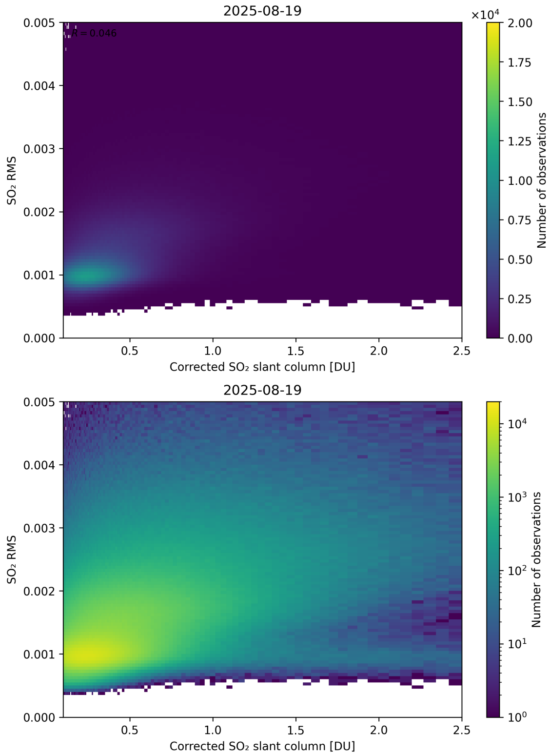
Figure 231: Scatter density plot of “Corrected SO 2 slant column” against “SO 2 RMS” for 2025-08-19 to 2025-08-20.
