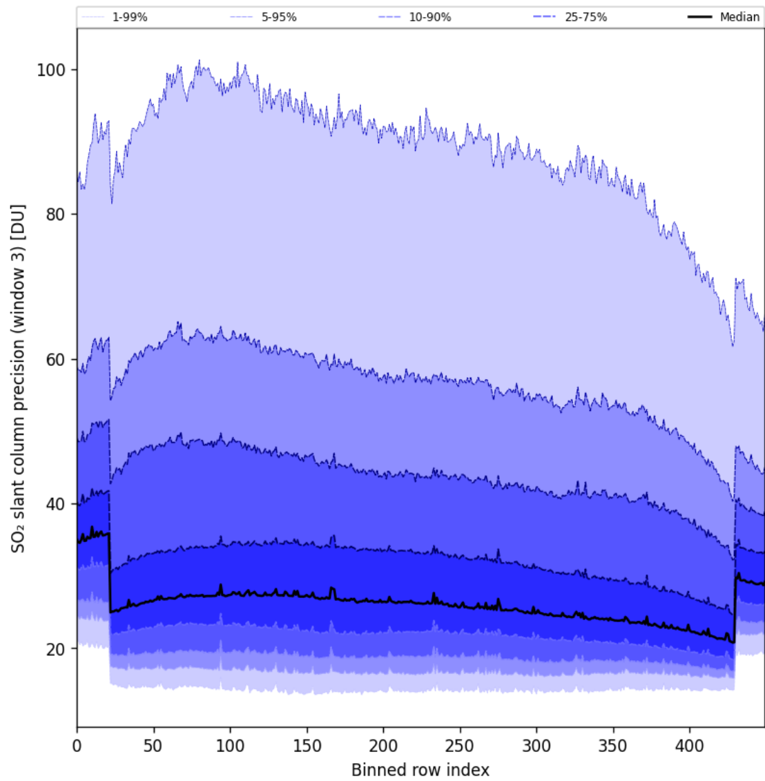
Figure 98: Along track statistics of “SO 2 slant column precision (window 3)” for 2025-08-19 to 2025-08-20
