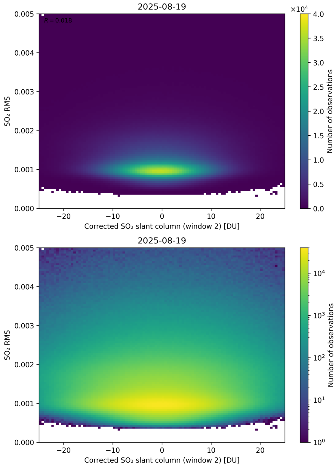
Figure 248: Scatter density plot of “Corrected SO 2 slant column (window 2)” against “SO 2 RMS” for 2025-08-19 to 2025-08-20.
