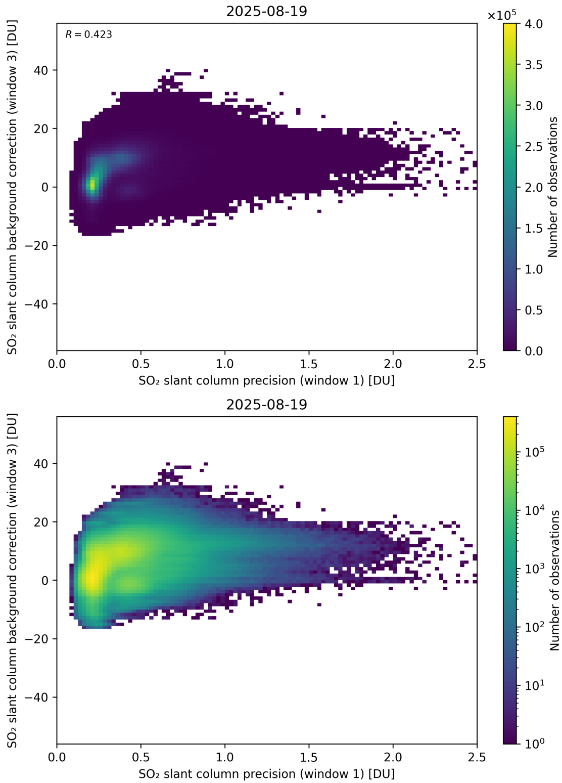
Figure 270: Scatter density plot of “SO 2 slant column precision (window 1)” against “SO 2 slant column background correction (window 3)” for 2025-08-19 to 2025-08-20.
