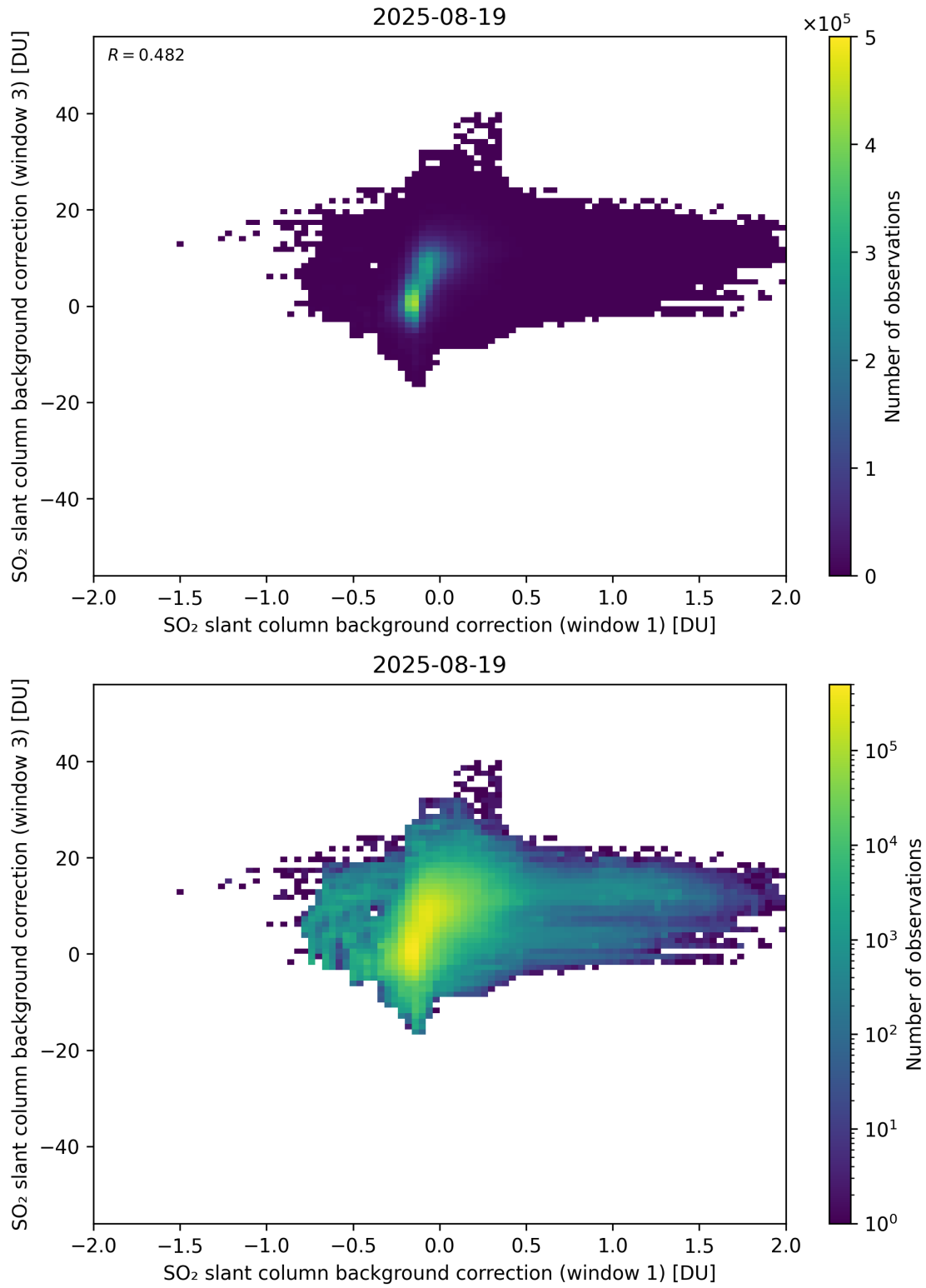
Figure 110: Scatter density plot of “SO 2 slant column background correction (window 1)” against “SO 2 slant column background correction (window 3)” for 2025-08-19 to 2025-08-20.
