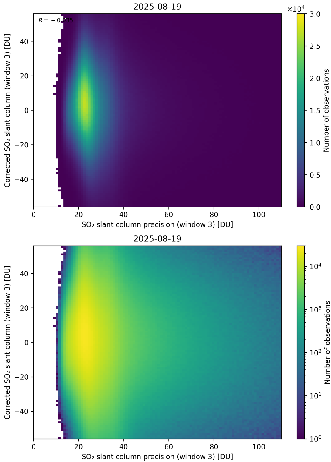
Figure 312: Scatter density plot of “SO 2 slant column precision (window 3)” against “Corrected SO 2 slant column (window 3)” for 2025-08-19 to 2025-08-20.
