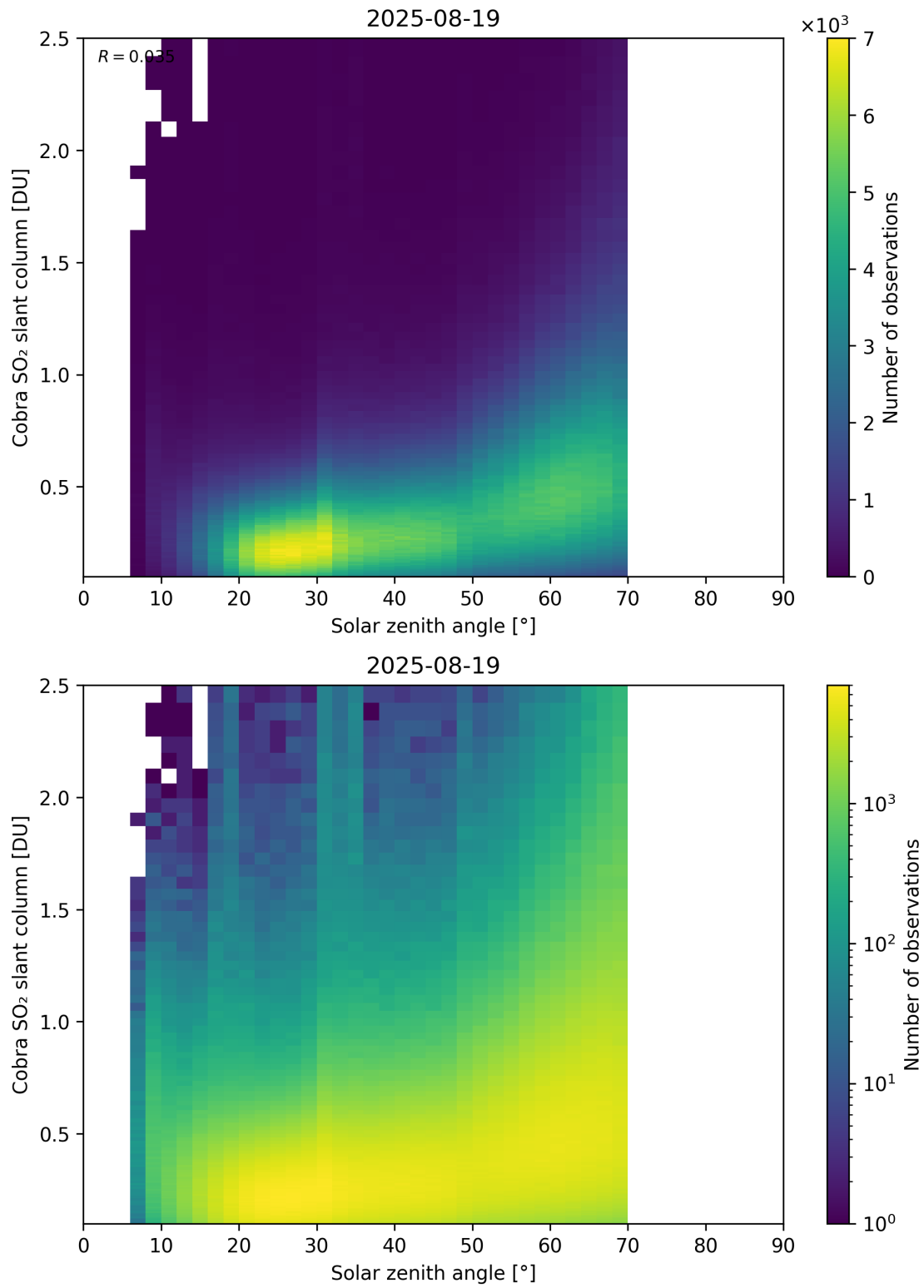
Figure 179: Scatter density plot of “Solar zenith angle” against “Cobra SO 2 slant column” for 2025-08-19 to 2025-08-20.
