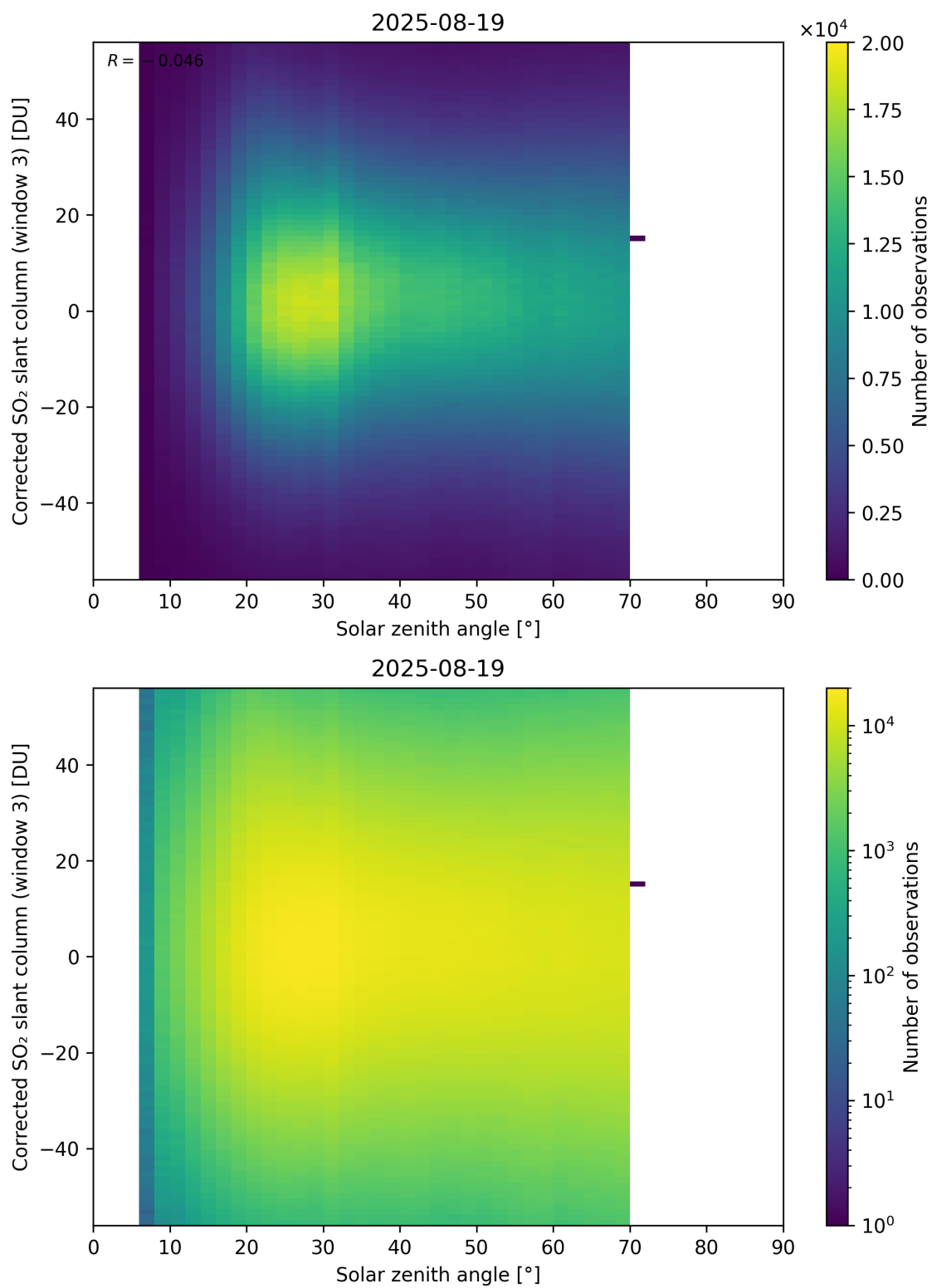
Figure 183: Scatter density plot of “Solar zenith angle” against “Corrected SO 2 slant column (window 3)” for 2025-08-19 to 2025-08-20.
