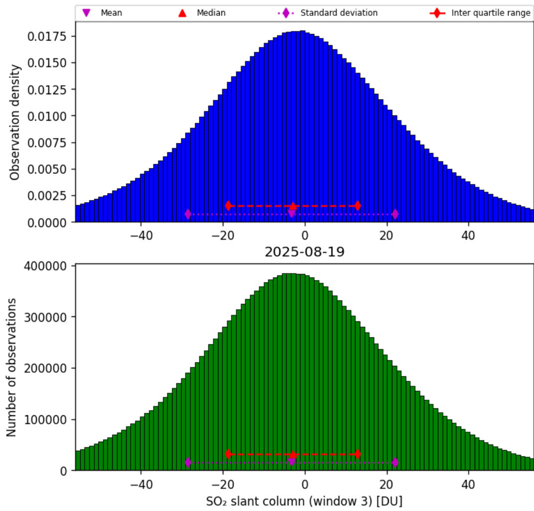
Figure 71: Histogram of “SO 2 slant column (window 3)” for 2025-08-19 to 2025-08-20
