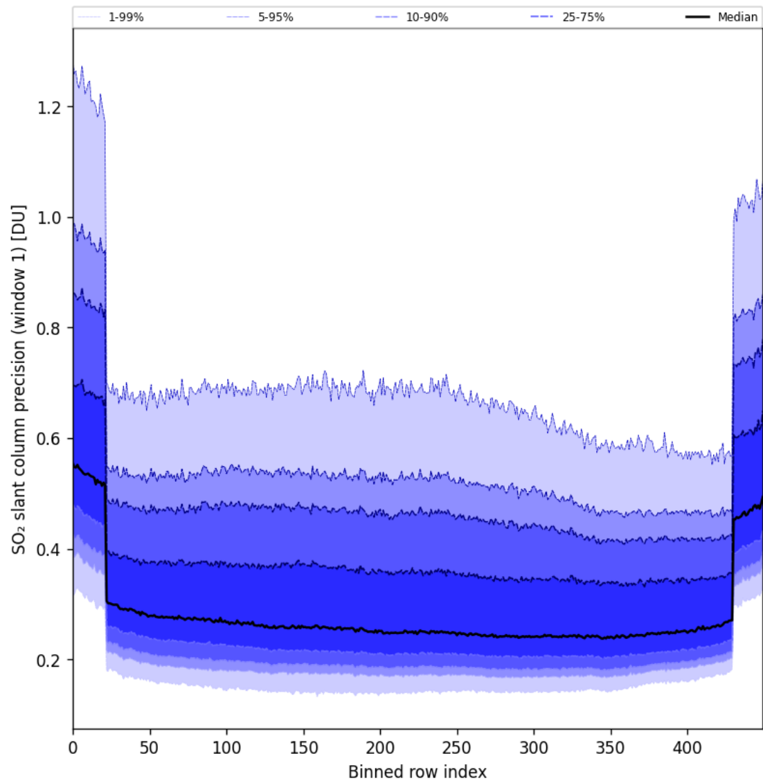
Figure 90: Along track statistics of “SO 2 slant column precision (window 1)” for 2025-08-19 to 2025-08-20
