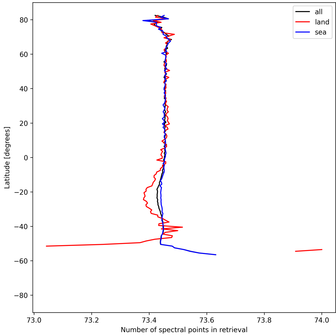
Figure 56: Zonal average of “Number of spectral points in retrieval” for 2025-08-19 to 2025-08-20.
