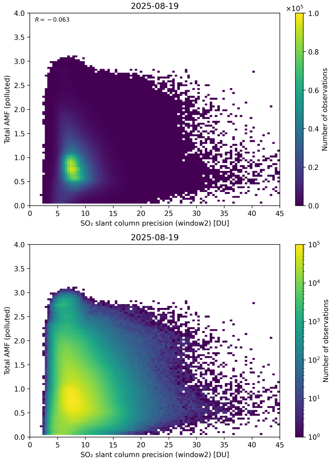
Figure 301: Scatter density plot of “SO 2 slant column precision (window2)” against “Total AMF (polluted)” for 2025-08-19 to 2025-08-20.
