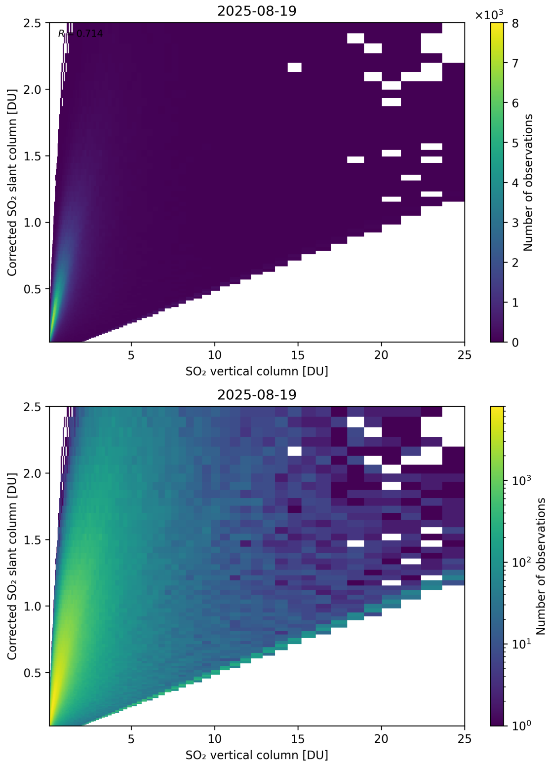
Figure 351: Scatter density plot of “SO 2 vertical column” against “Corrected SO 2 slant column” for 2025-08-19 to 2025-08-20.
