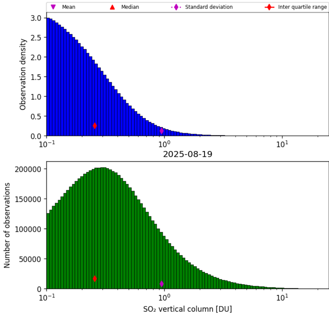
Figure 58: Histogram of “SO 2 vertical column” for 2025-08-19 to 2025-08-20
