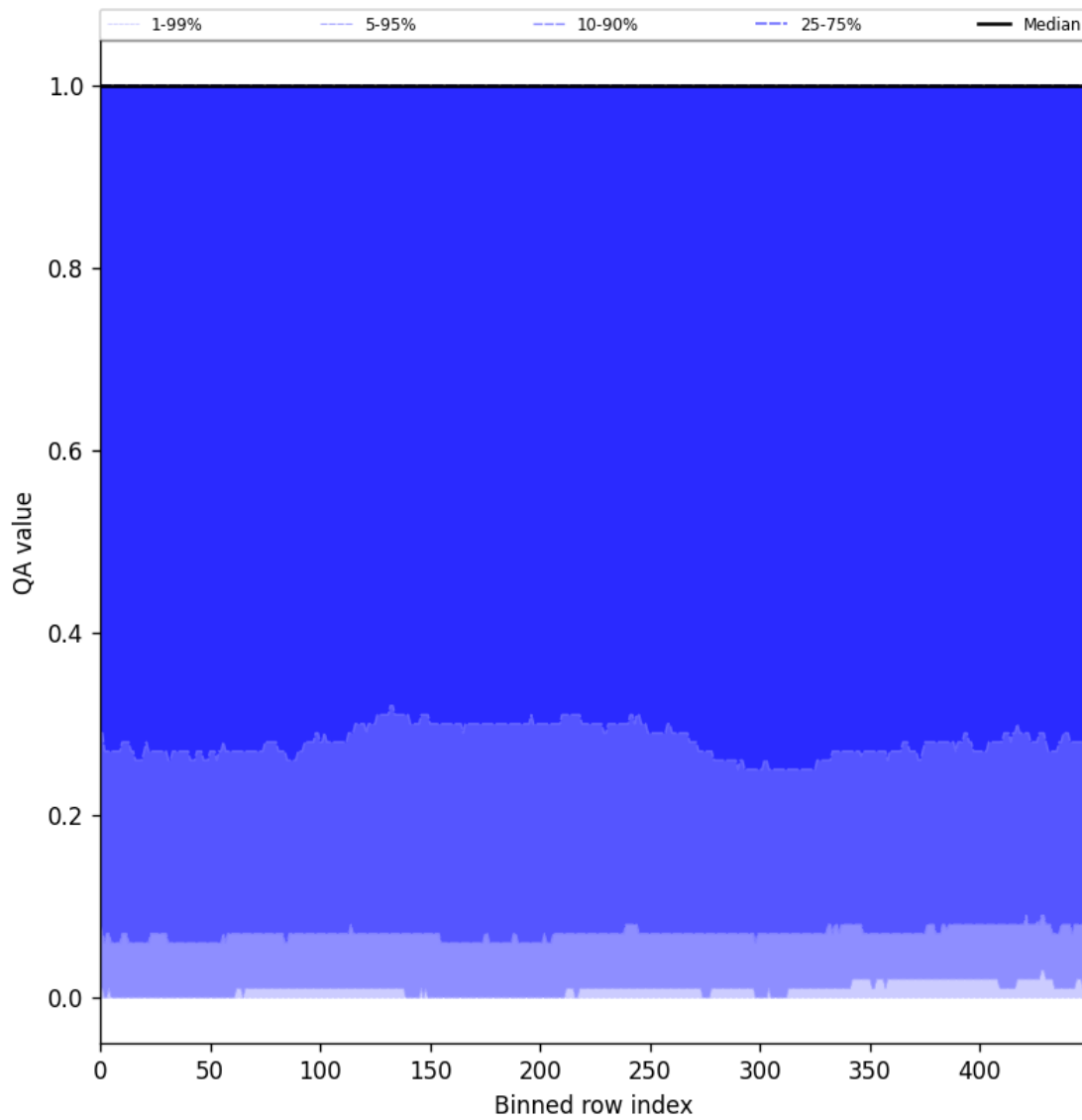
Figure 83: Along track statistics of “QA value” for 2025-08-19 to 2025-08-20
