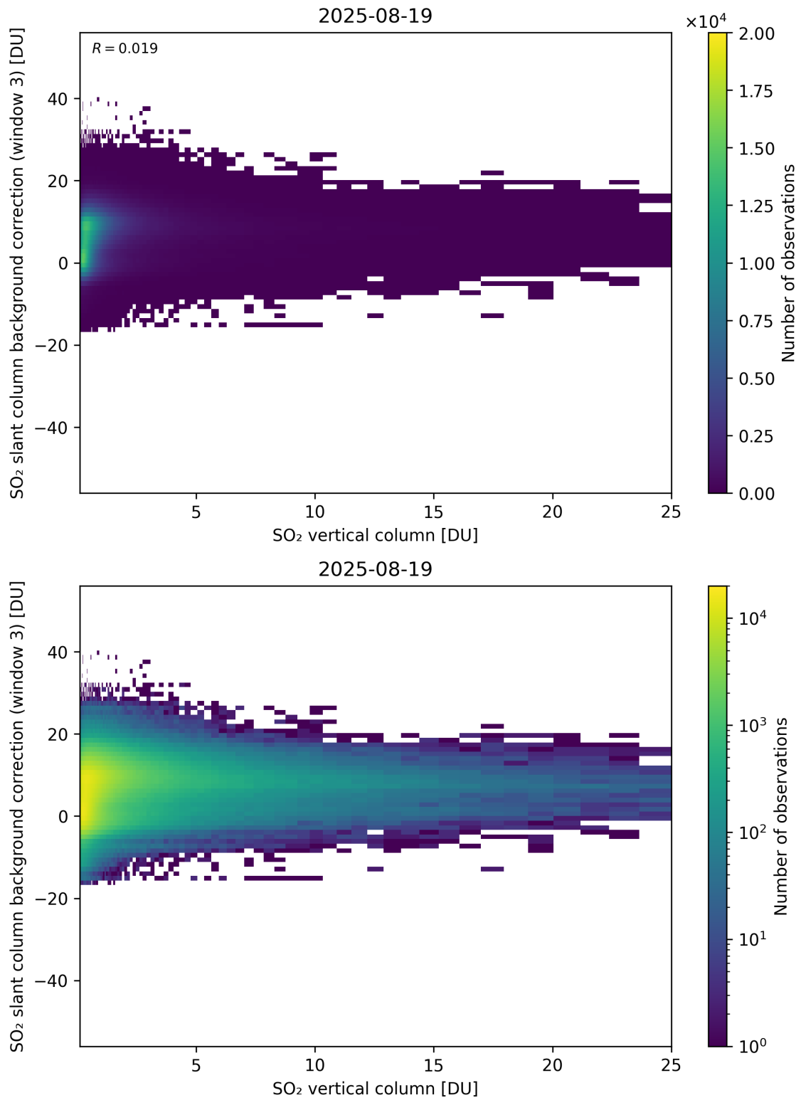
Figure 325: Scatter density plot of “SO 2 vertical column” against “SO 2 slant column background correction (window 3)” for 2025-08-19 to 2025-08-20.
