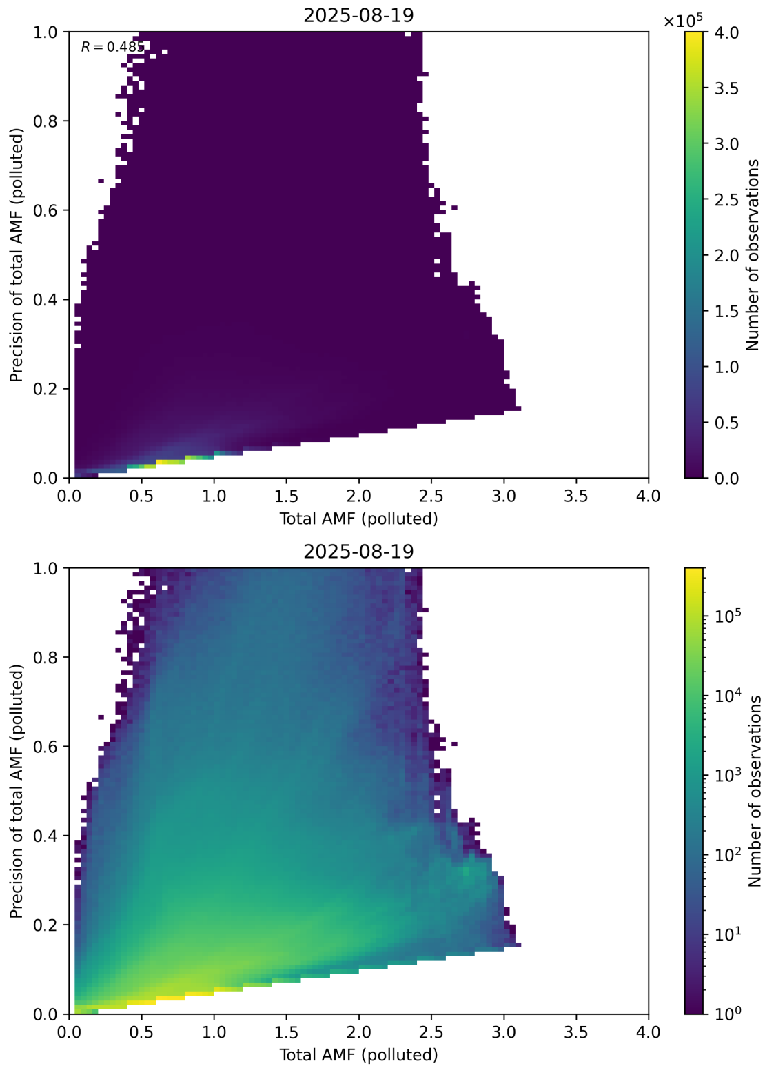
Figure 322: Scatter density plot of “Total AMF (polluted)” against “Precision of total AMF (polluted)” for 2025-08-19 to 2025-08-20.
