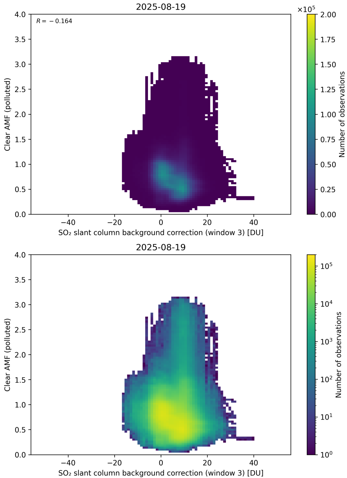
Figure 135: Scatter density plot of “SO 2 slant column background correction (window 3)” against “Clear AMF (polluted)” for 2025-08-19 to 2025-08-20.
