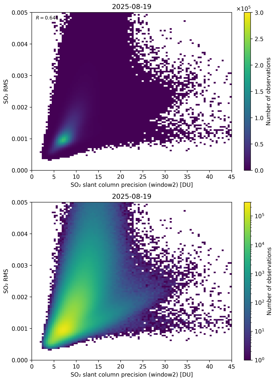
Figure 295: Scatter density plot of “SO 2 slant column precision (window2)” against “SO 2 RMS” for 2025-08-19 to 2025-08-20.
