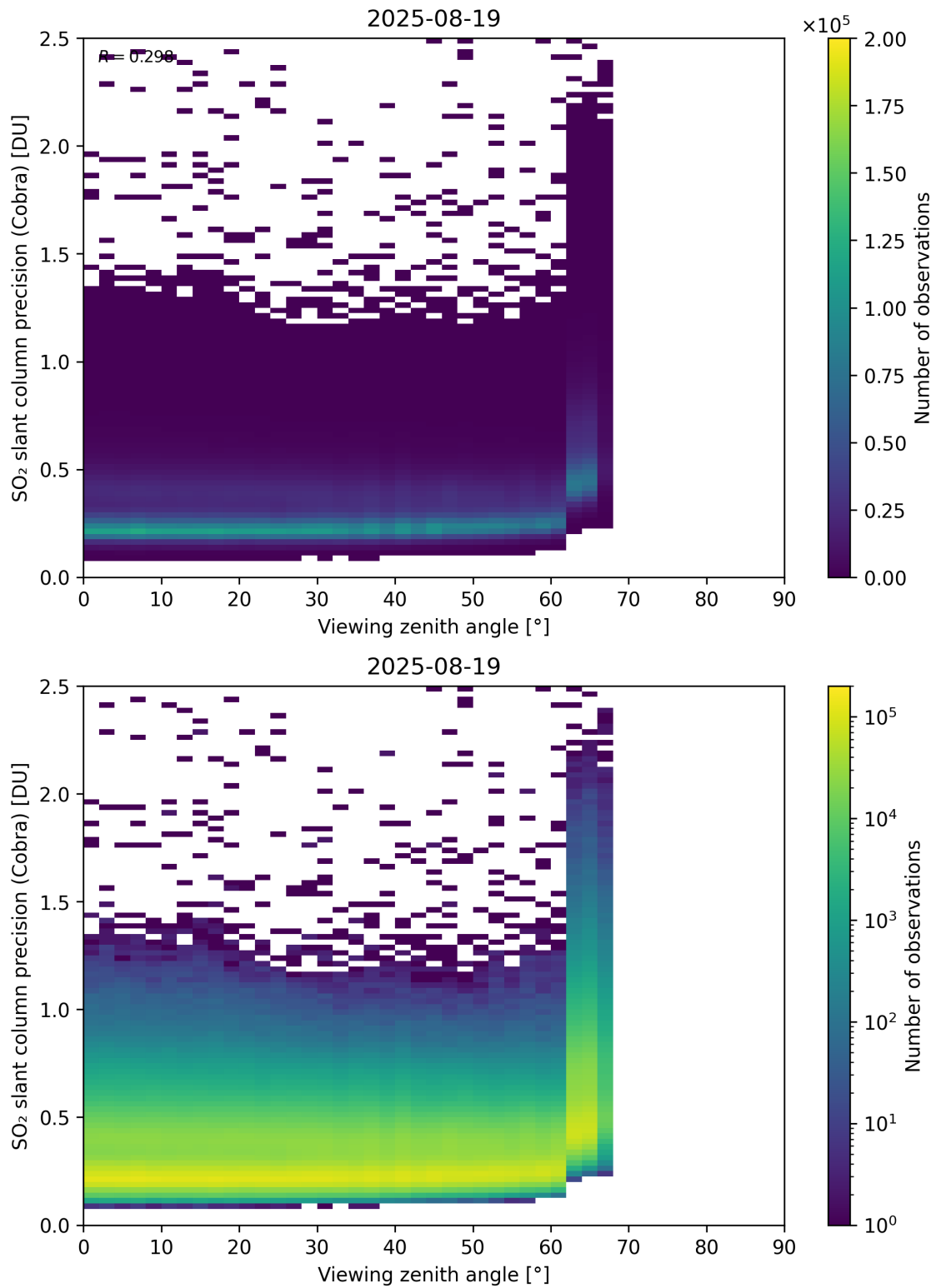
Figure 372: Scatter density plot of “Viewing zenith angle” against “SO 2 slant column precision (Cobra)” for 2025-08-19 to 2025-08-20.
