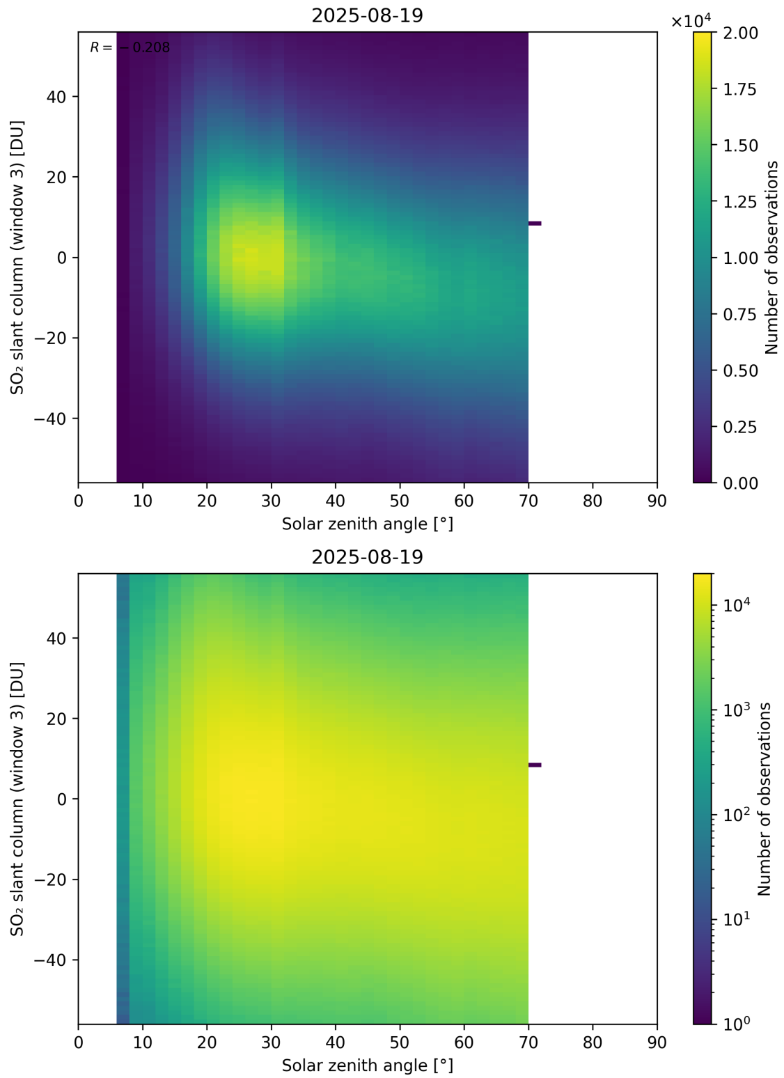
Figure 187: Scatter density plot of “Solar zenith angle” against “SO 2 slant column (window 3)” for 2025-08-19 to 2025-08-20.
