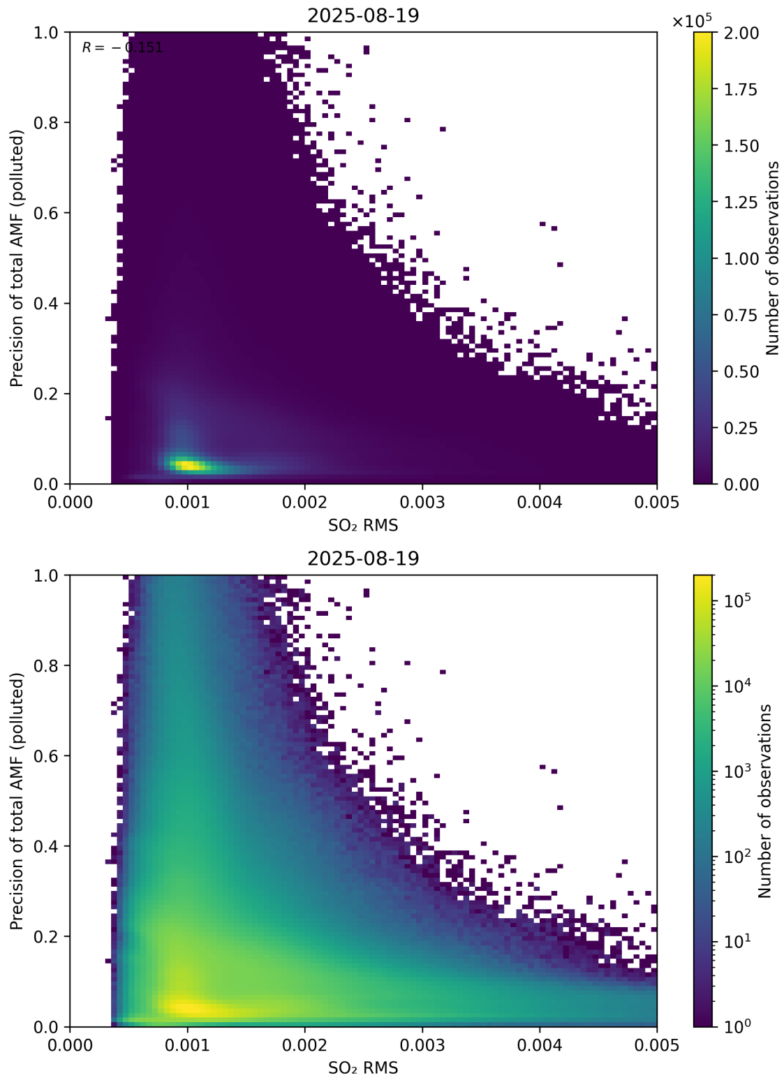
Figure 149: Scatter density plot of “SO 2 RMS” against “Precision of total AMF (polluted)” for 2025-08-19 to 2025-08-20.
