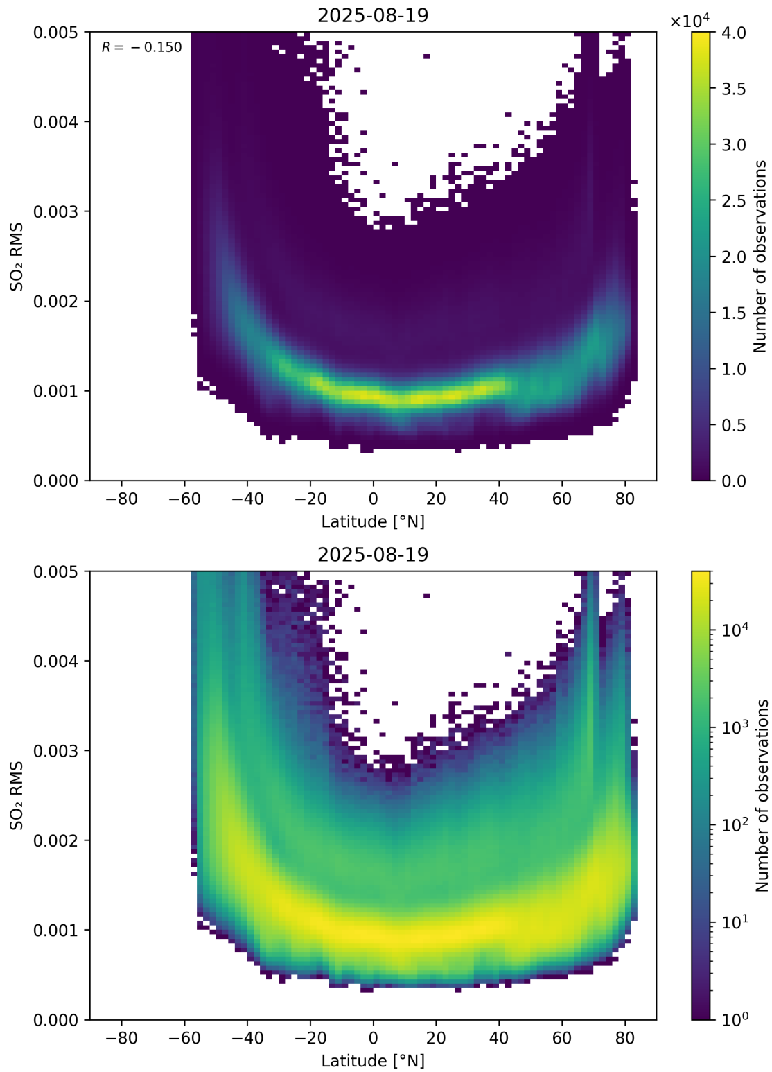
Figure 155: Scatter density plot of “Latitude” against “SO 2 RMS” for 2025-08-19 to 2025-08-20.
