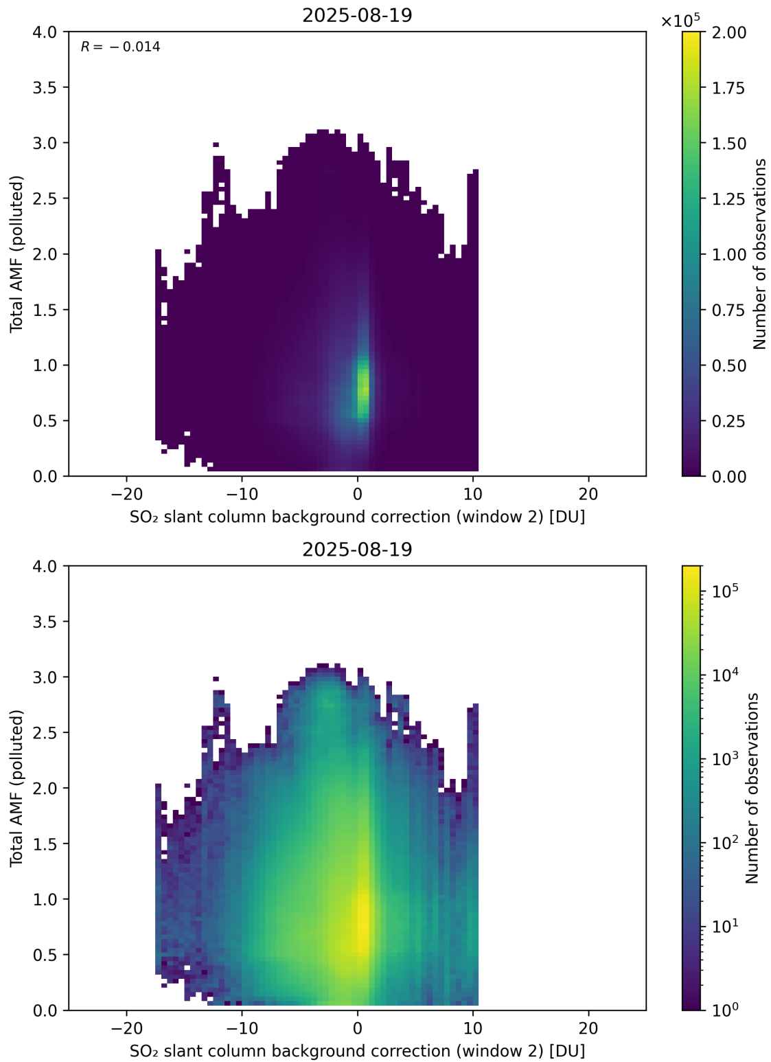
Figure 130: Scatter density plot of “SO 2 slant column background correction (window 2)” against “Total AMF (polluted)” for 2025-08-19 to 2025-08-20.
