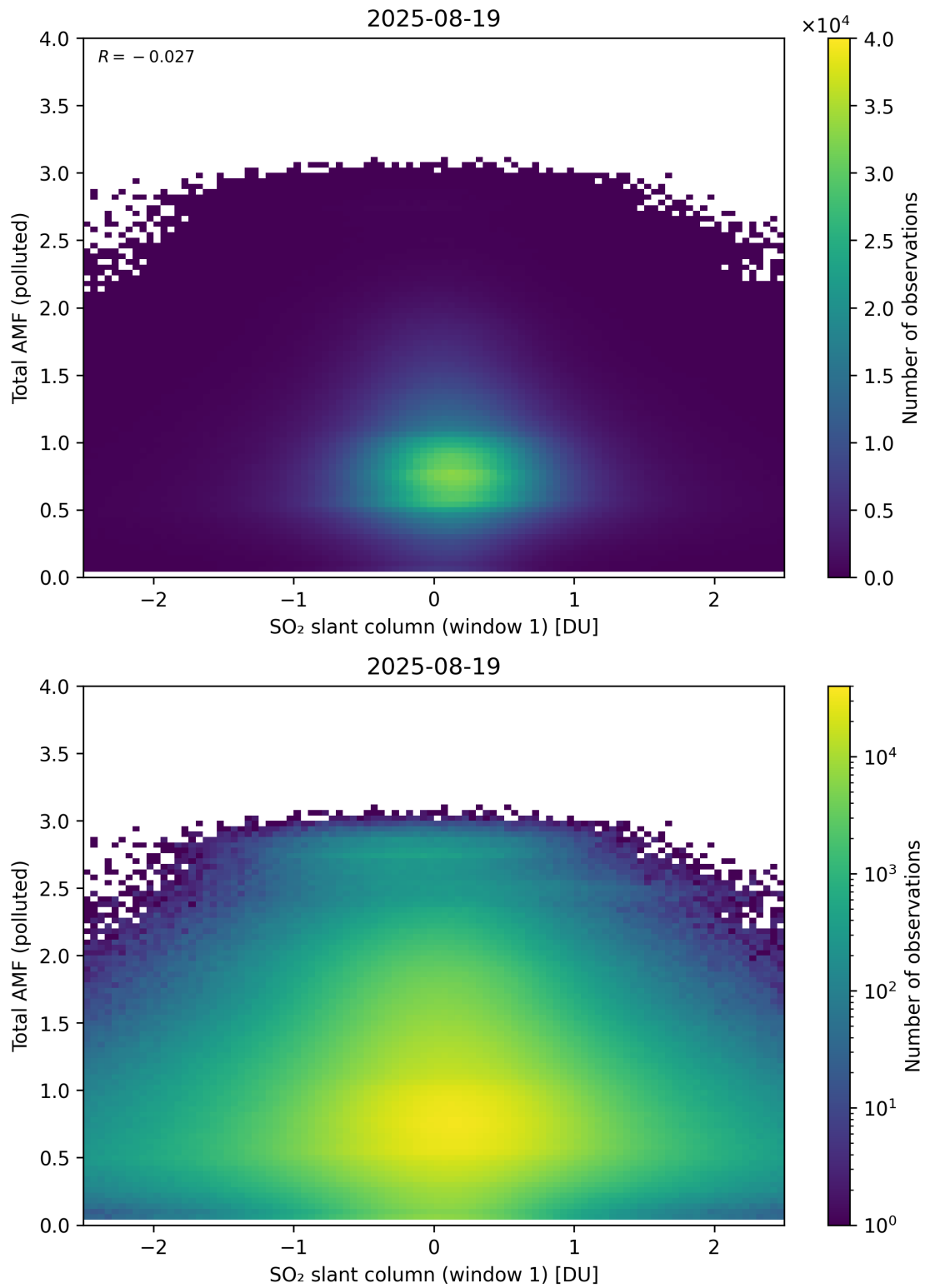
Figure 289: Scatter density plot of “SO 2 slant column (window 1)” against “Total AMF (polluted)” for 2025-08-19 to 2025-08-20.
