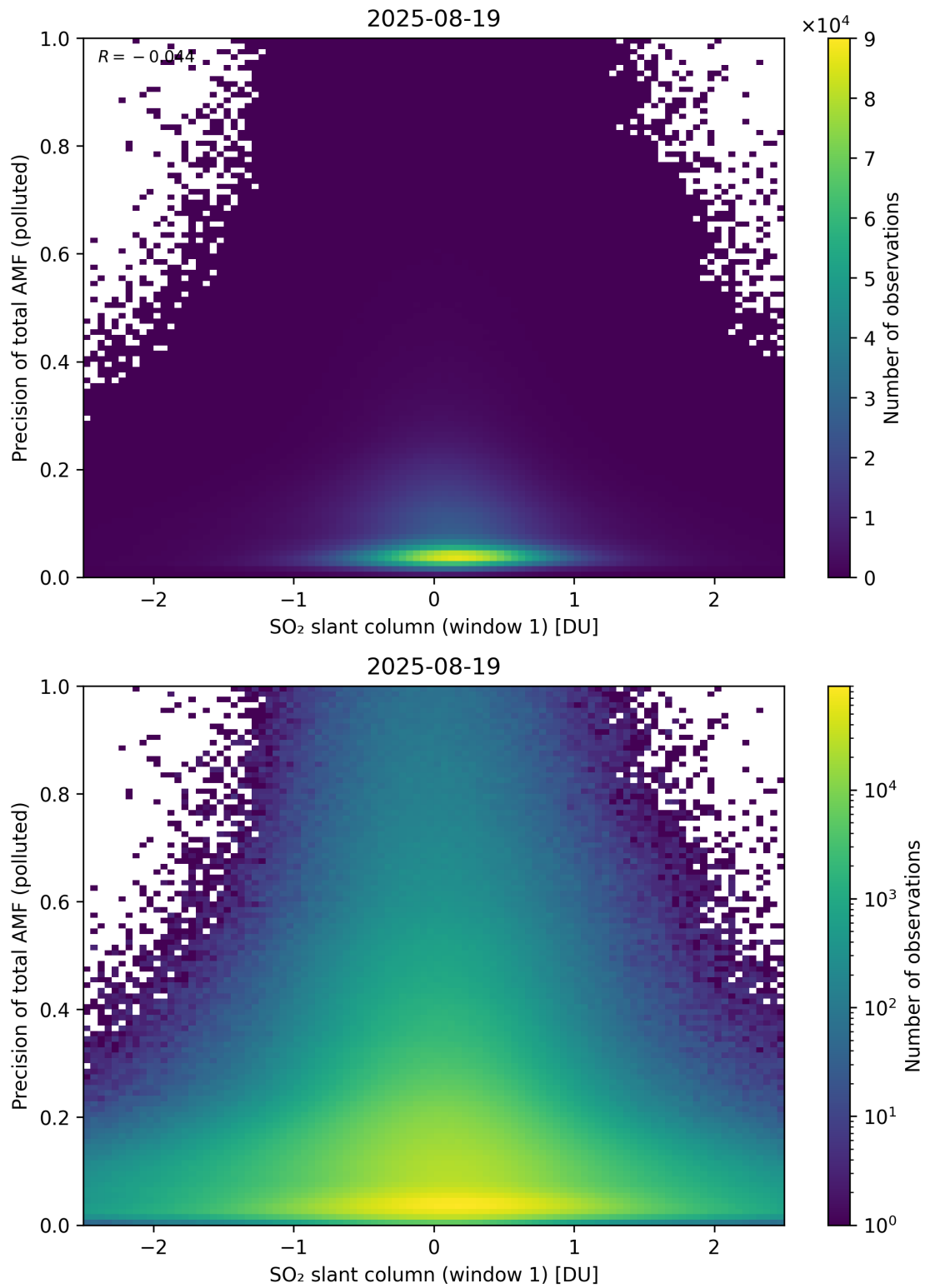
Figure 290: Scatter density plot of “SO 2 slant column (window 1)” against “Precision of total AMF (polluted)” for 2025-08-19 to 2025-08-20.
