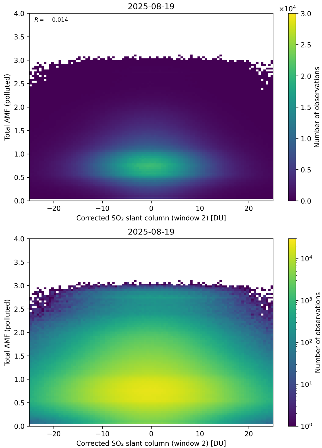
Figure 253: Scatter density plot of “Corrected SO 2 slant column (window 2)” against “Total AMF (polluted)” for 2025-08-19 to 2025-08-20.
