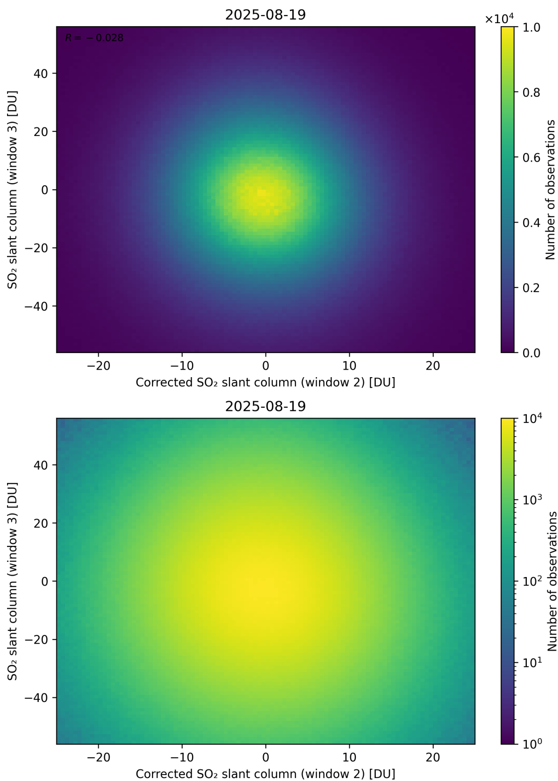
Figure 251: Scatter density plot of “Corrected SO 2 slant column (window 2)” against “SO 2 slant column (window 3)” for 2025-08-19 to 2025-08-20.
