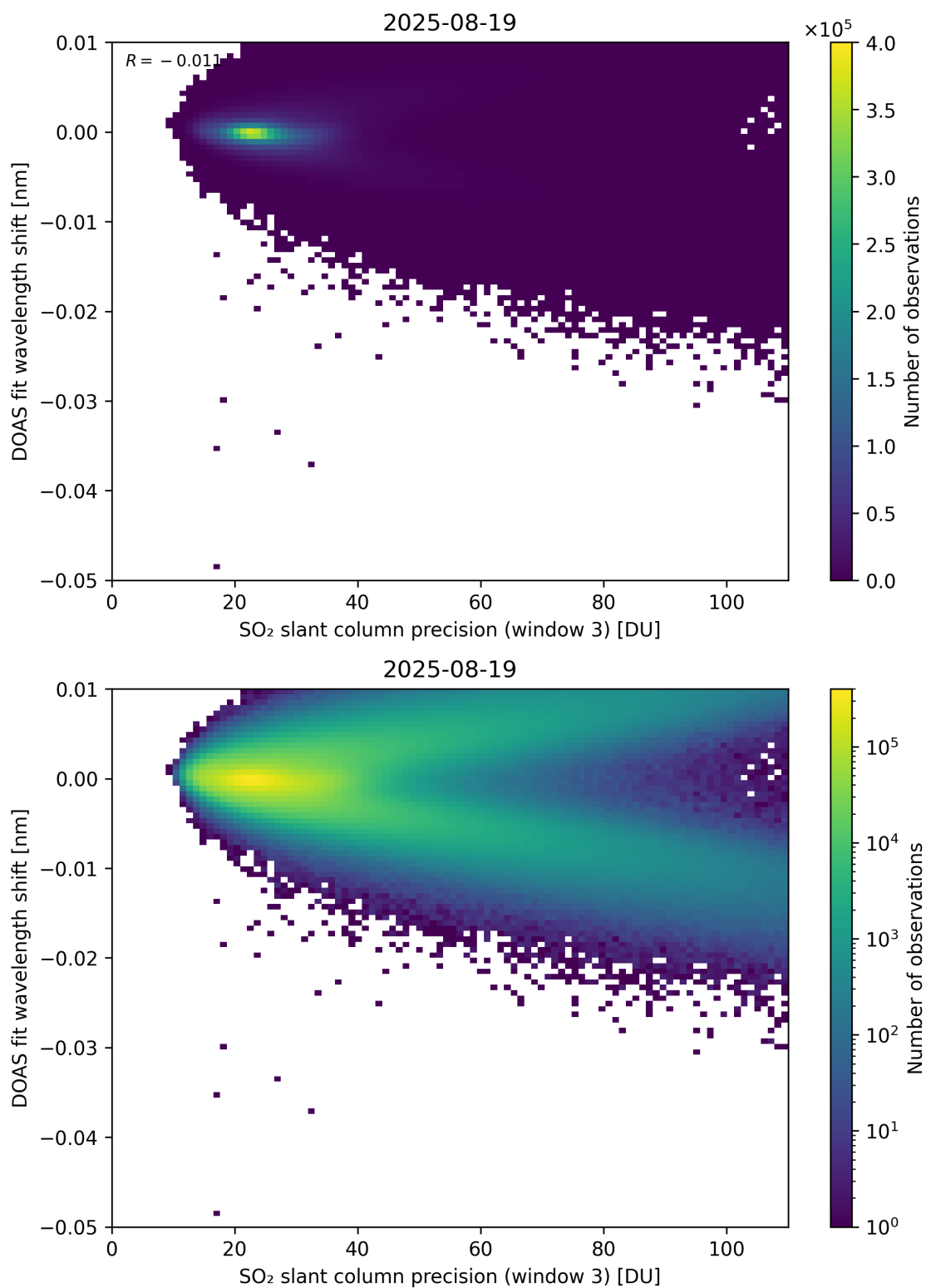
Figure 308: Scatter density plot of “SO 2 slant column precision (window 3)” against “DOAS fit wavelength shift” for 2025-08-19 to 2025-08-20.
