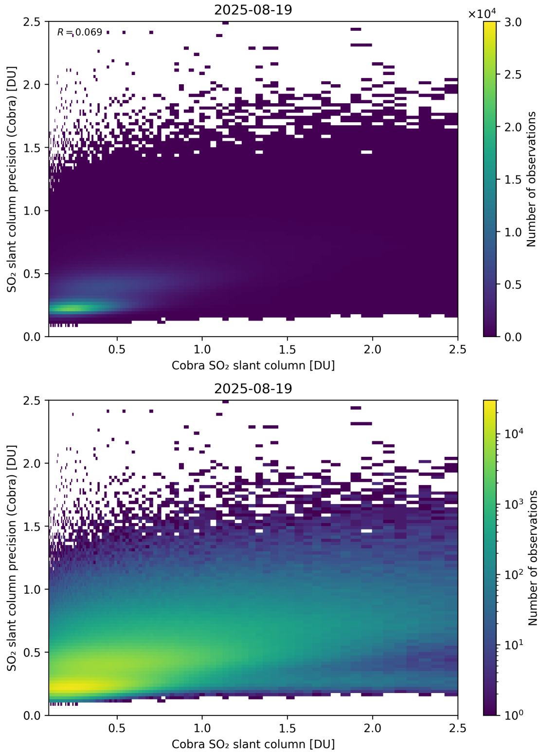
Figure 216: Scatter density plot of “Cobra SO 2 slant column” against “SO 2 slant column precision (Cobra)” for 2025-08-19 to 2025-08-20.
