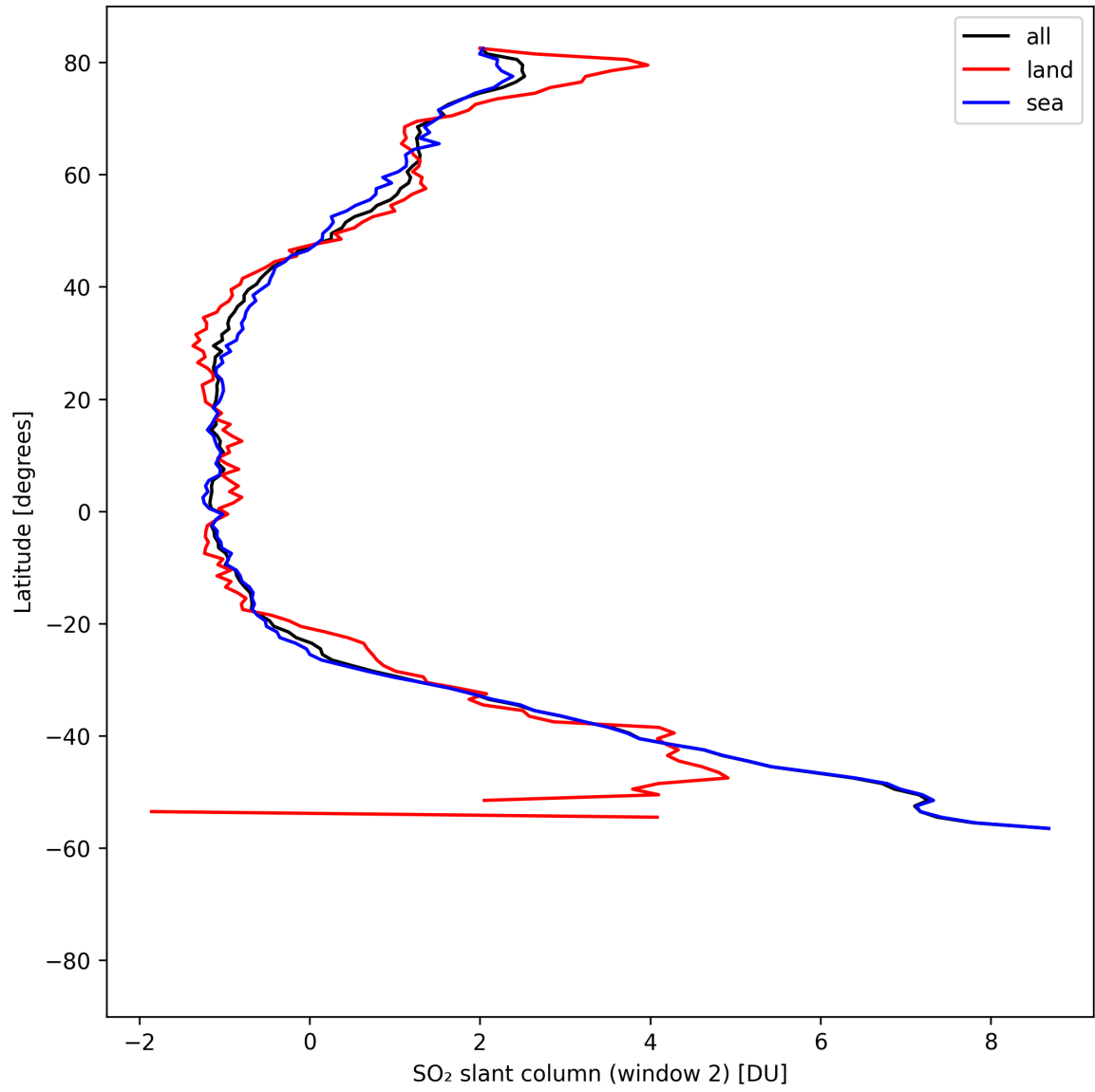
Figure 41: Zonal average of “SO 2 slant column (window 2)” for 2025-08-19 to 2025-08-20.
