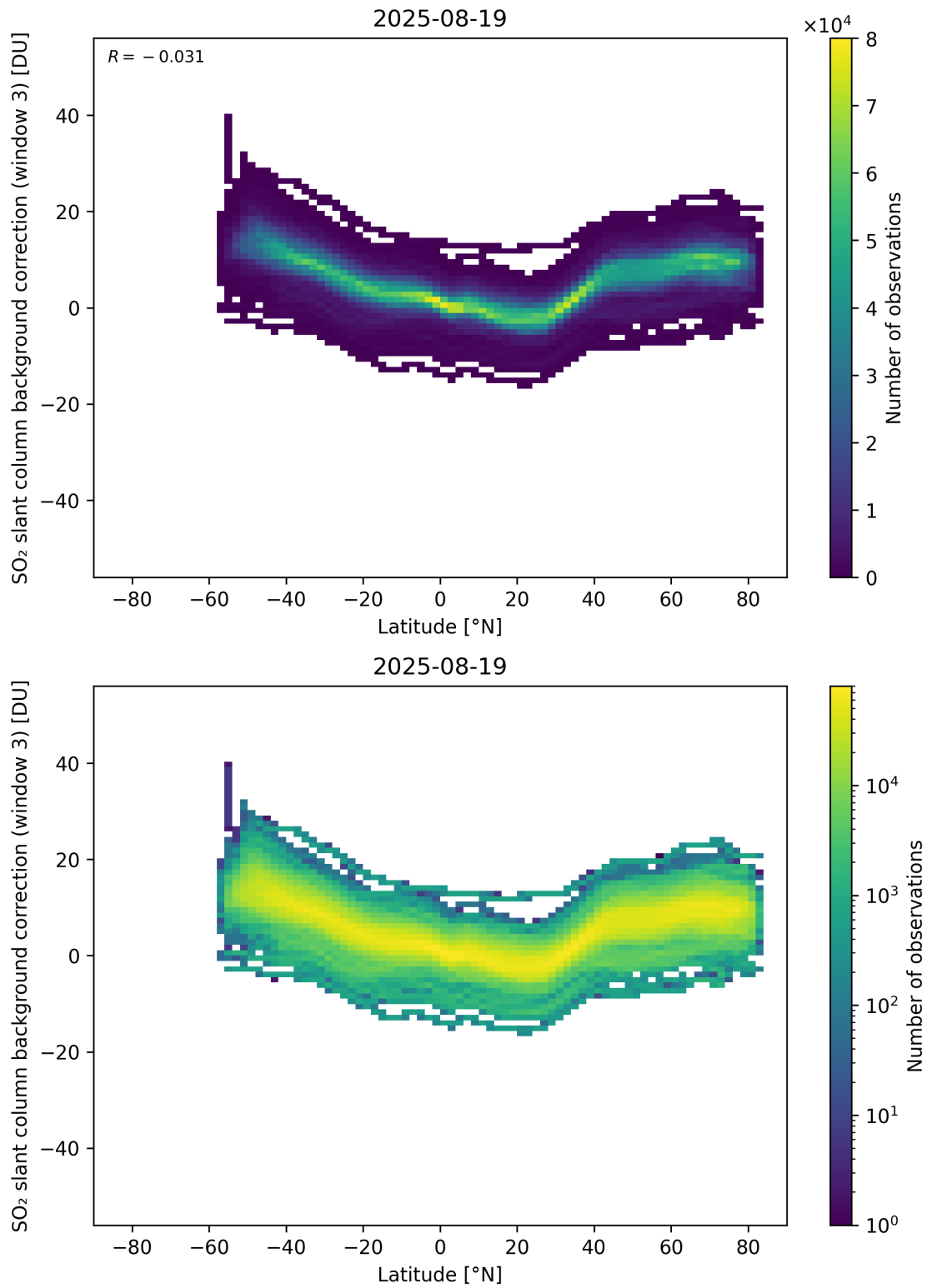
Figure 152: Scatter density plot of “Latitude” against “SO 2 slant column background correction (window 3)” for 2025-08-19 to 2025-08-20.
