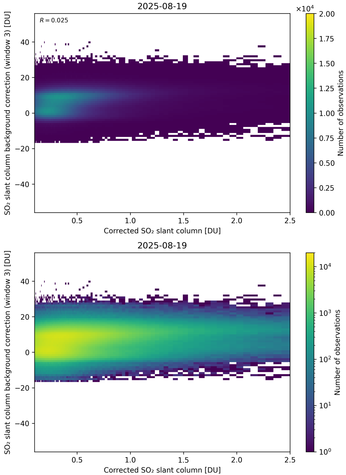
Figure 228: Scatter density plot of “Corrected SO 2 slant column” against “SO 2 slant column background correction (window 3)” for 2025-08-19 to 2025-08-20.
