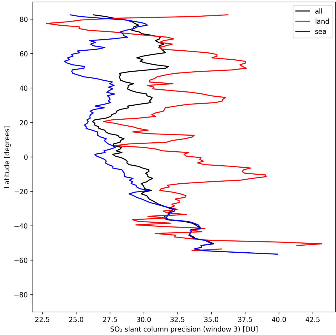
Figure 46: Zonal average of “SO 2 slant column precision (window 3)” for 2025-08-19 to 2025-08-20.
