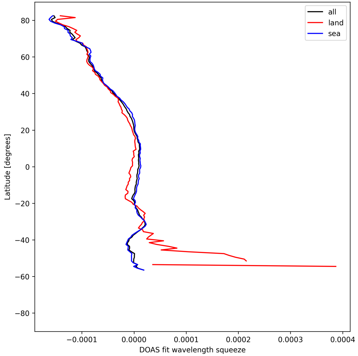
Figure 51: Zonal average of “DOAS fit wavelength squeeze” for 2025-08-19 to 2025-08-20.
