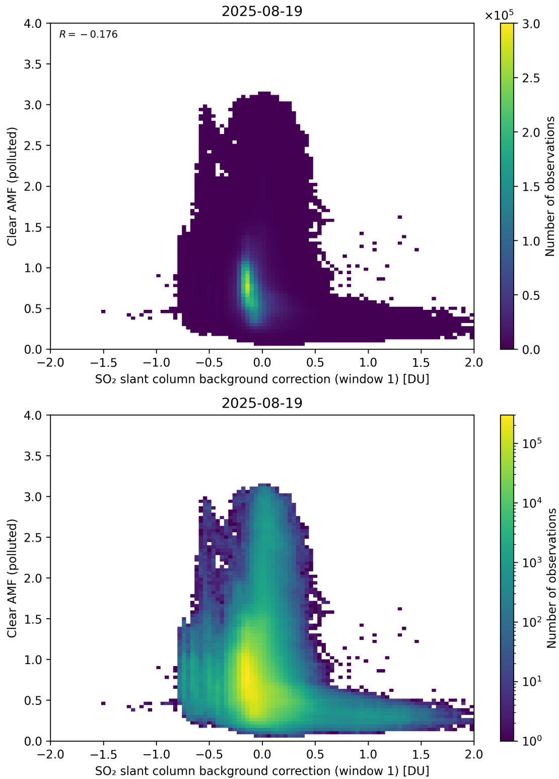
Figure 114: Scatter density plot of “SO 2 slant column background correction (window 1)” against “Clear AMF (polluted)” for 2025-08-19 to 2025-08-20.
