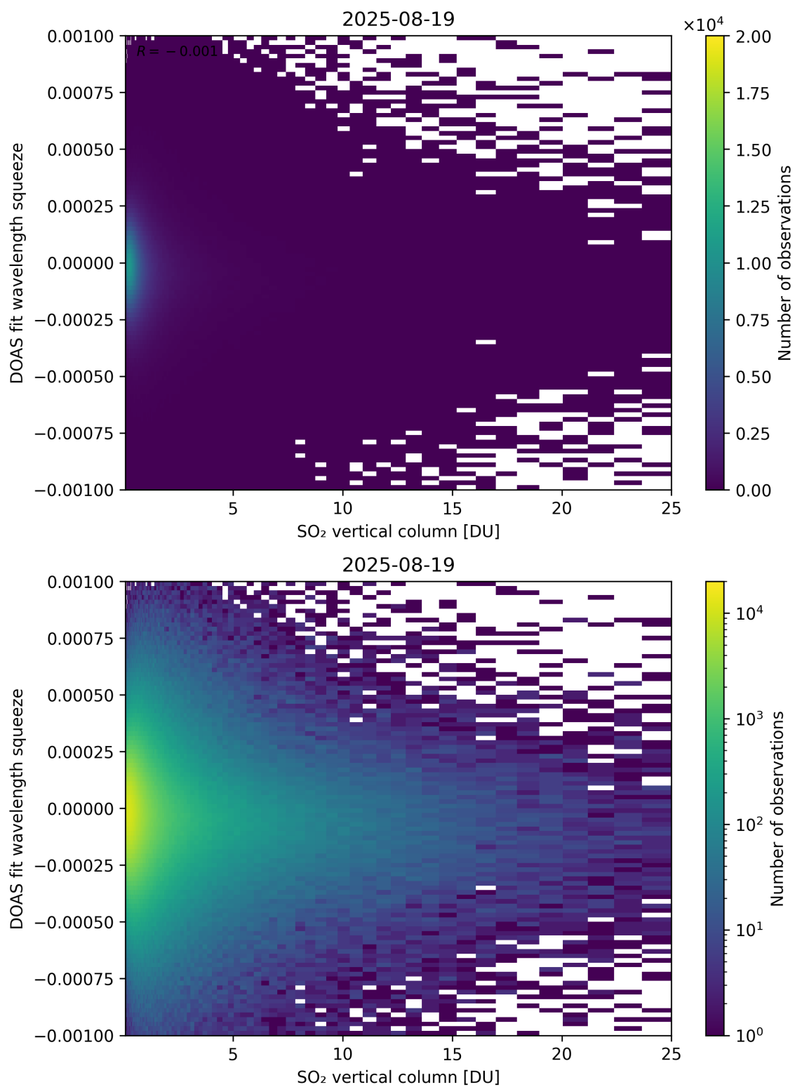
Figure 327: Scatter density plot of “SO 2 vertical column” against “DOAS fit wavelength squeeze” for 2025-08-19 to 2025-08-20.
