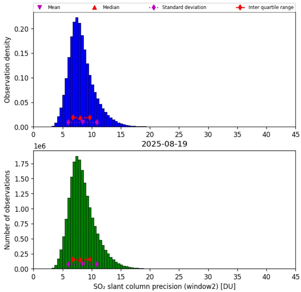
Figure 68: Histogram of “SO 2 slant column precision (window2)” for 2025-08-19 to 2025-08-20
