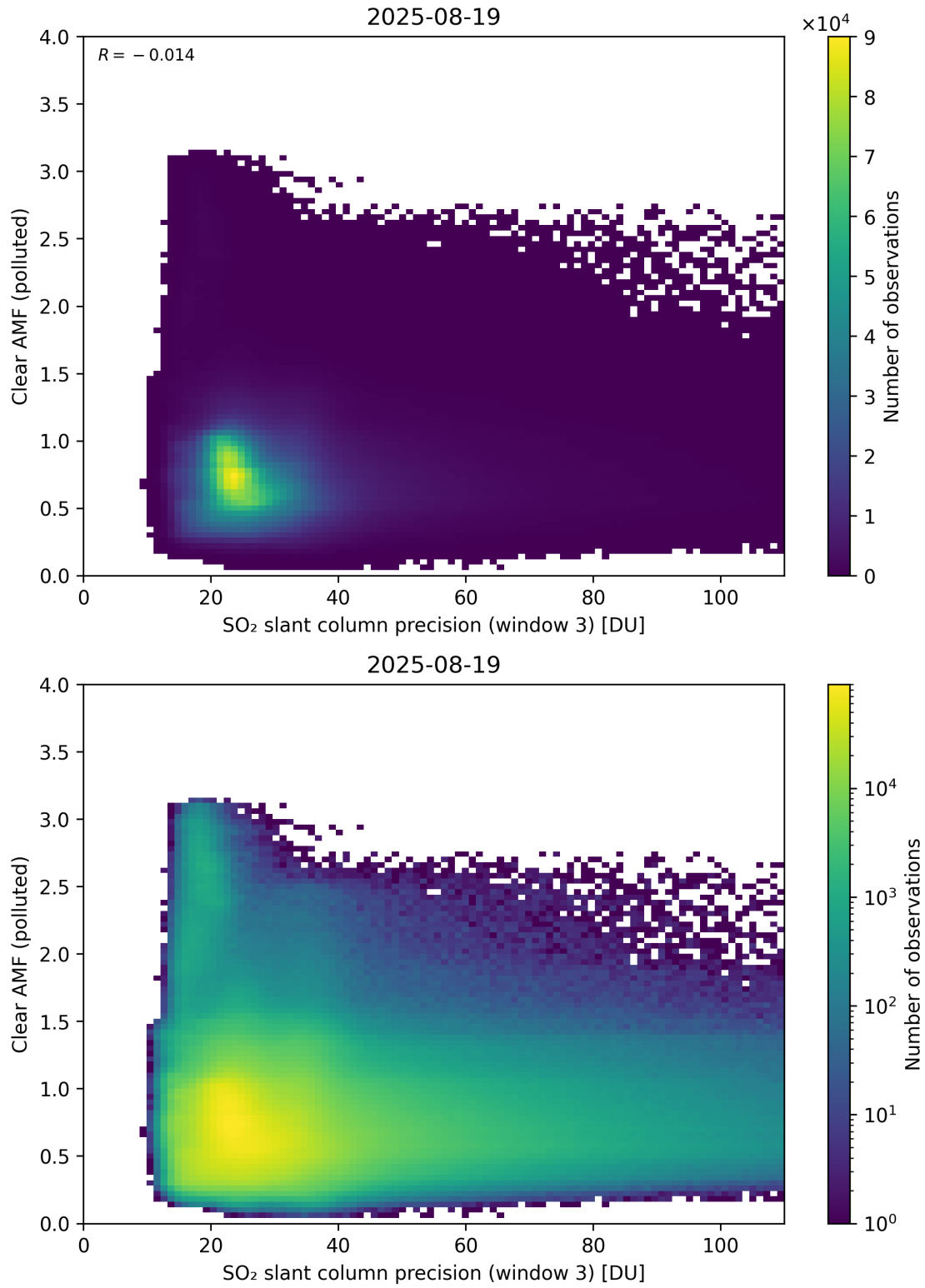
Figure 311: Scatter density plot of “SO 2 slant column precision (window 3)” against “Clear AMF (polluted)” for 2025-08-19 to 2025-08-20.
