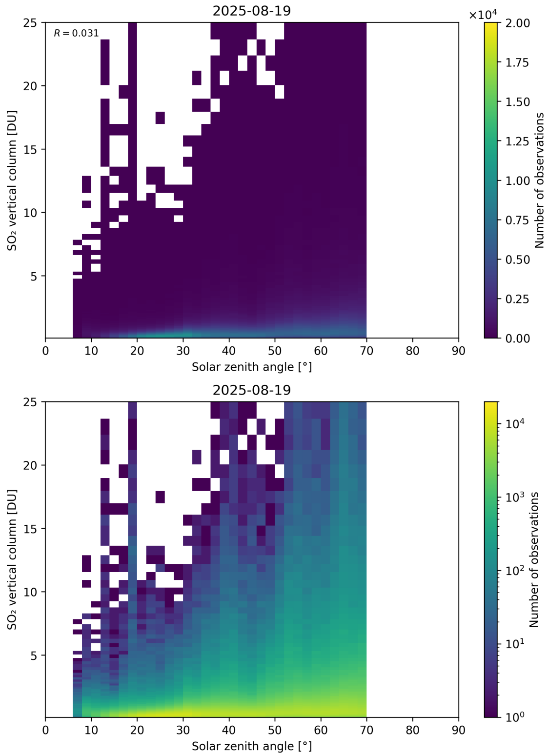
Figure 191: Scatter density plot of “Solar zenith angle” against “SO 2 vertical column” for 2025-08-19 to 2025-08-20.
