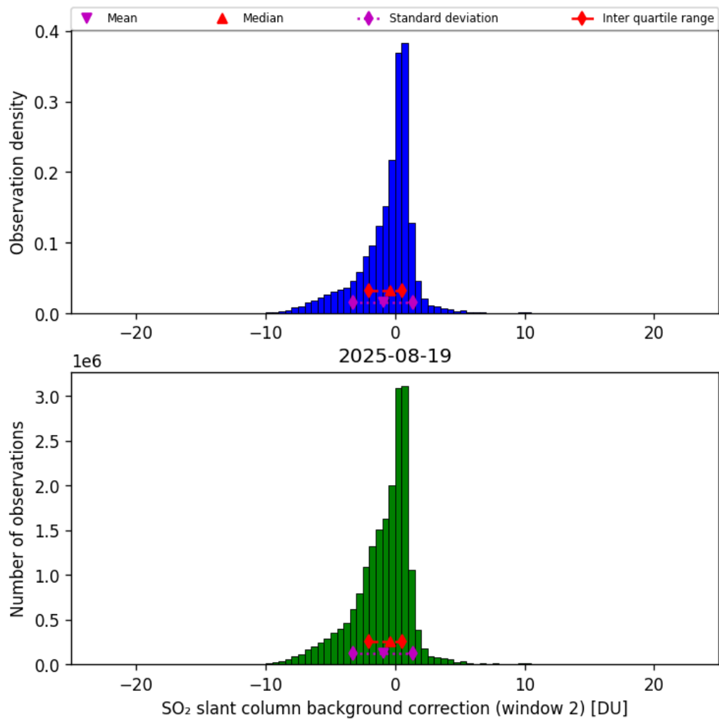
Figure 70: Histogram of “SO 2 slant column background correction (window 2)” for 2025-08-19 to 2025-08-20
