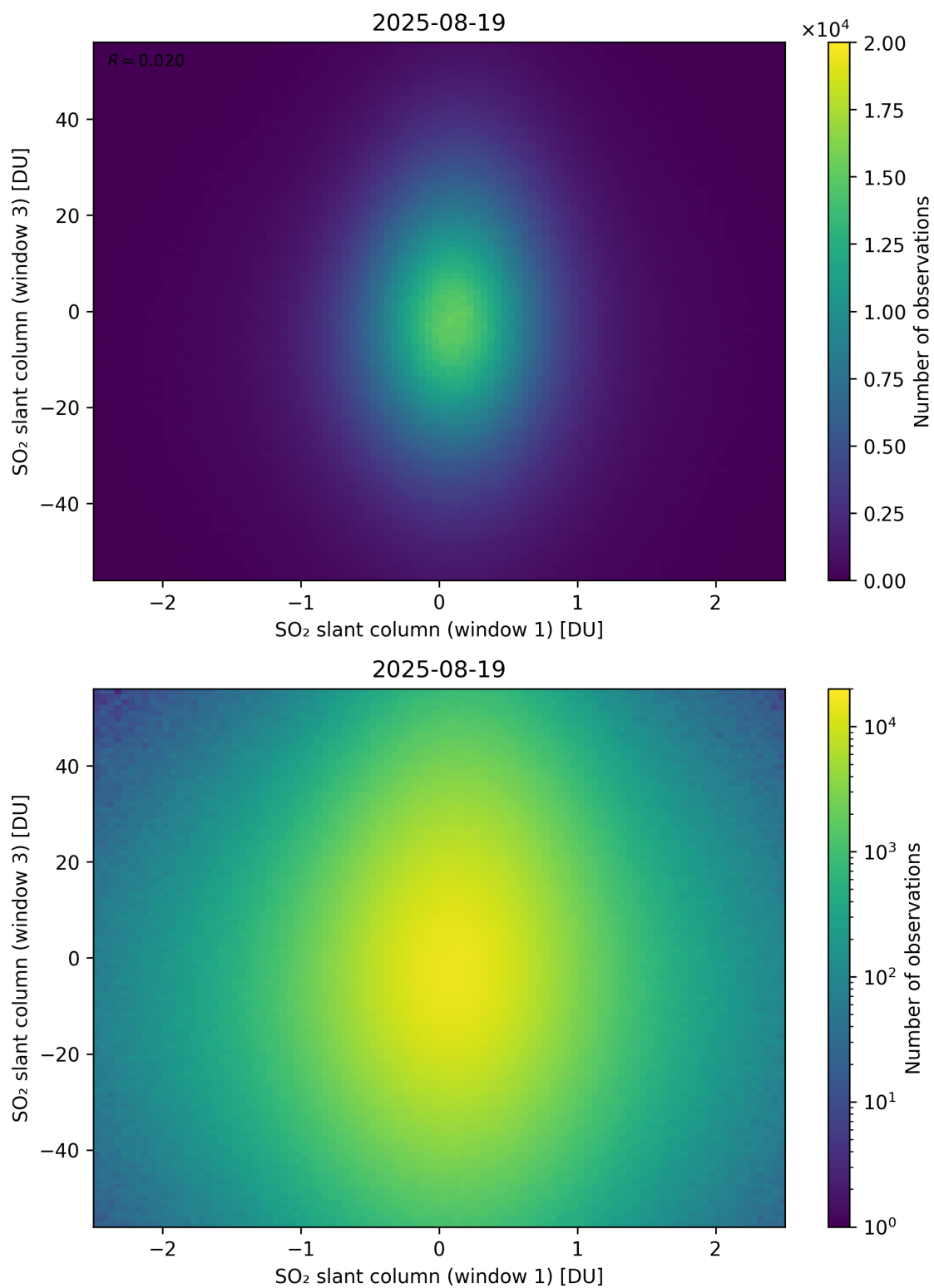
Figure 287: Scatter density plot of “SO 2 slant column (window 1)” against “SO 2 slant column (window 3)” for 2025-08-19 to 2025-08-20.
