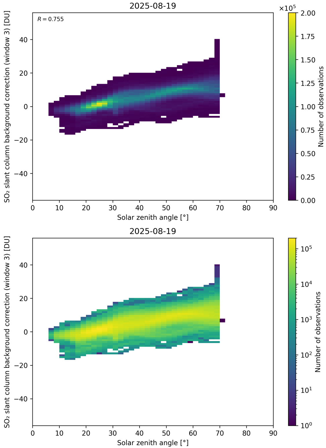
Figure 173: Scatter density plot of “Solar zenith angle” against “SO 2 slant column background correction (window 3)” for 2025-08-19 to 2025-08-20.
