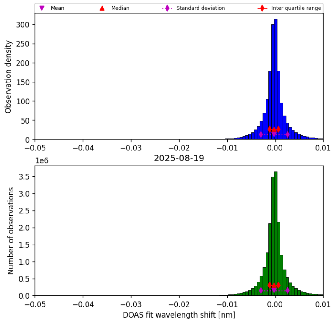
Figure 76: Histogram of “DOAS fit wavelength shift” for 2025-08-19 to 2025-08-20
