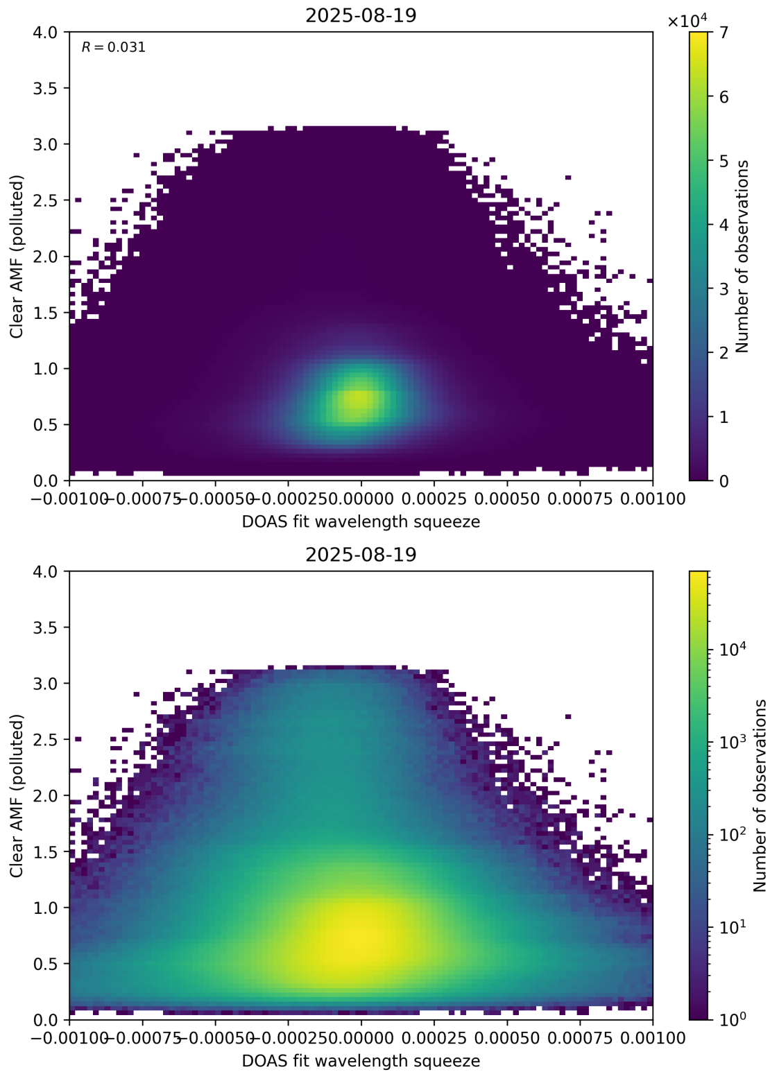
Figure 144: Scatter density plot of “DOAS fit wavelength squeeze” against “Clear AMF (polluted)” for 2025-08-19 to 2025-08-20.
