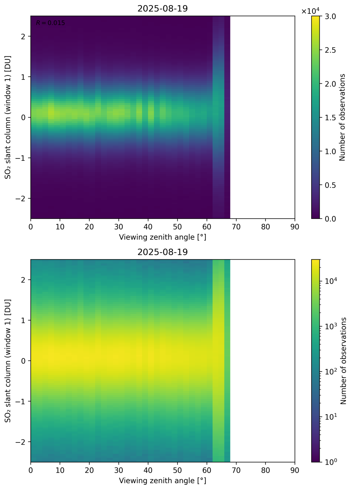
Figure 376: Scatter density plot of “Viewing zenith angle” against “SO 2 slant column (window 1)” for 2025-08-19 to 2025-08-20.
