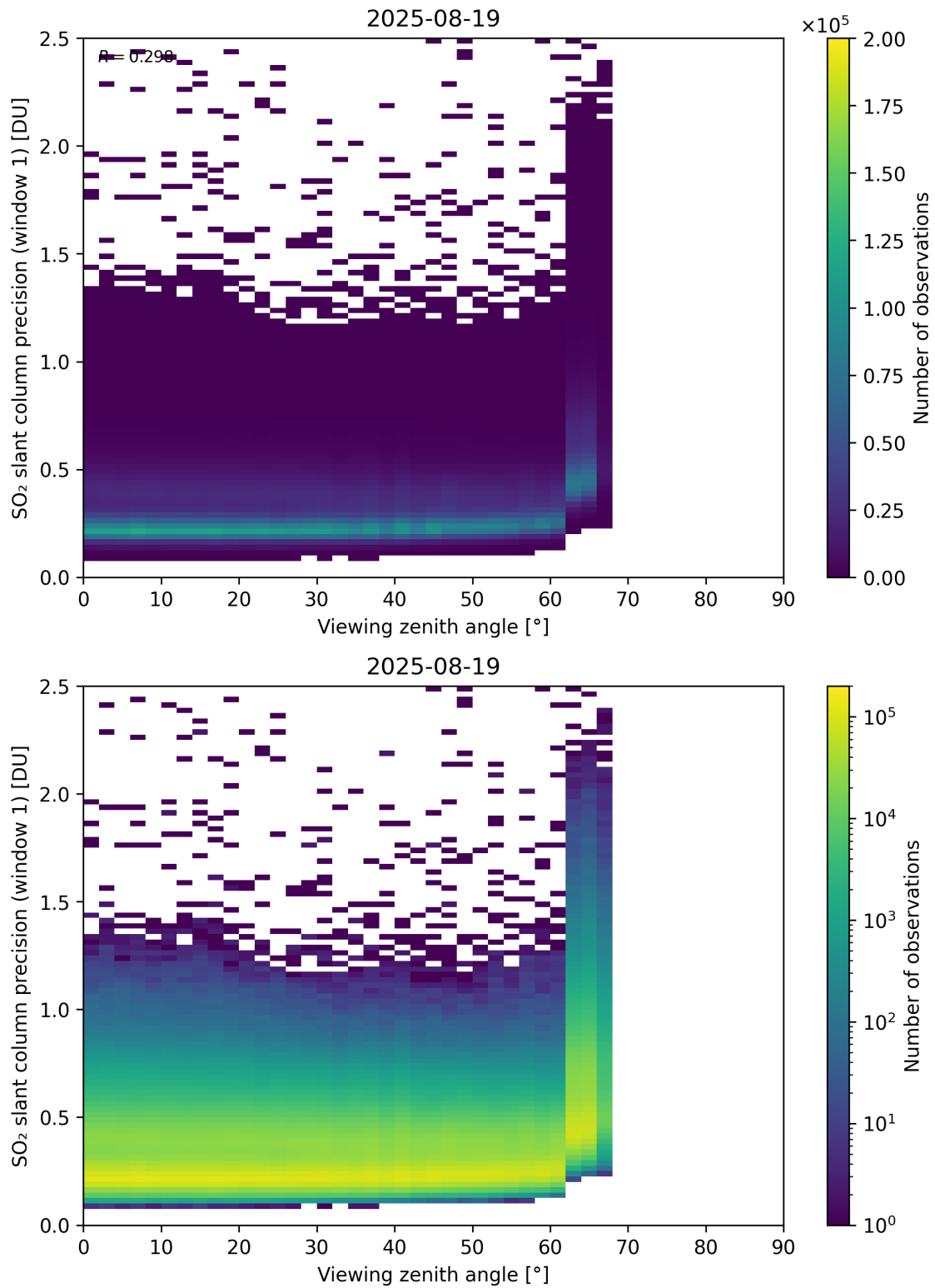
Figure 377: Scatter density plot of “Viewing zenith angle” against “SO 2 slant column precision (window 1)” for 2025-08-19 to 2025-08-20.
