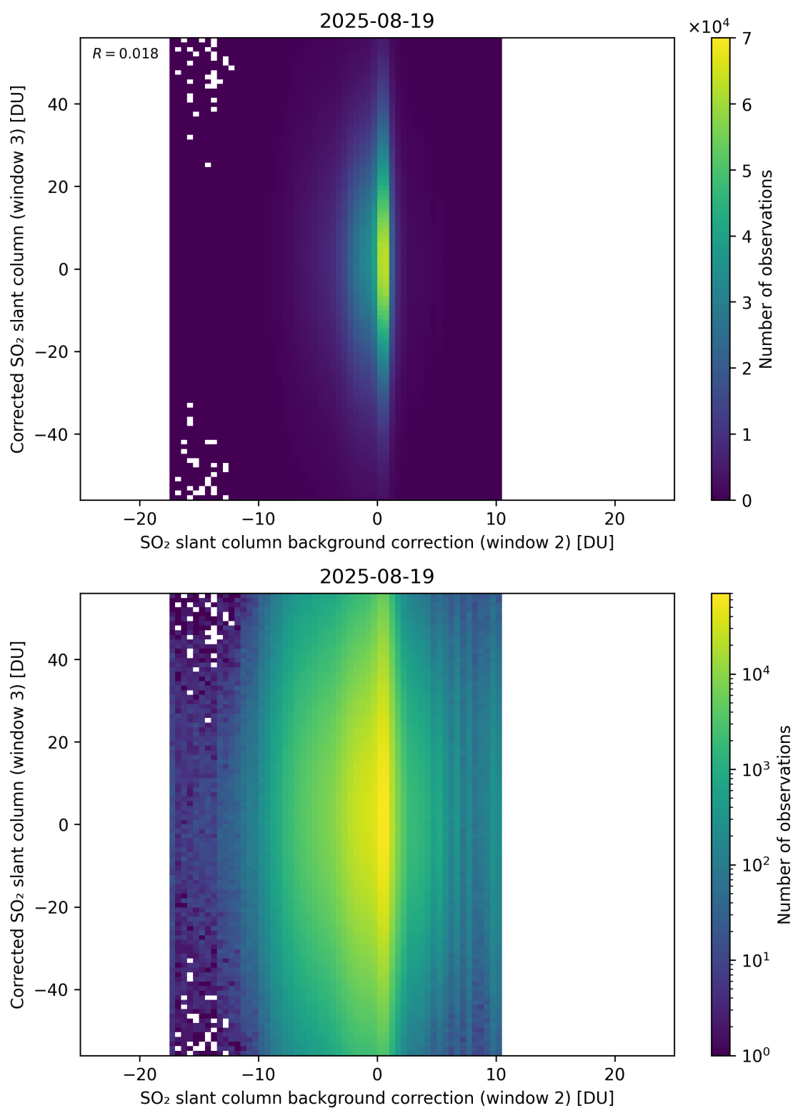
Figure 127: Scatter density plot of “SO 2 slant column background correction (window 2)” against “Corrected SO 2 slant column (window 3)” for 2025-08-19 to 2025-08-20.
