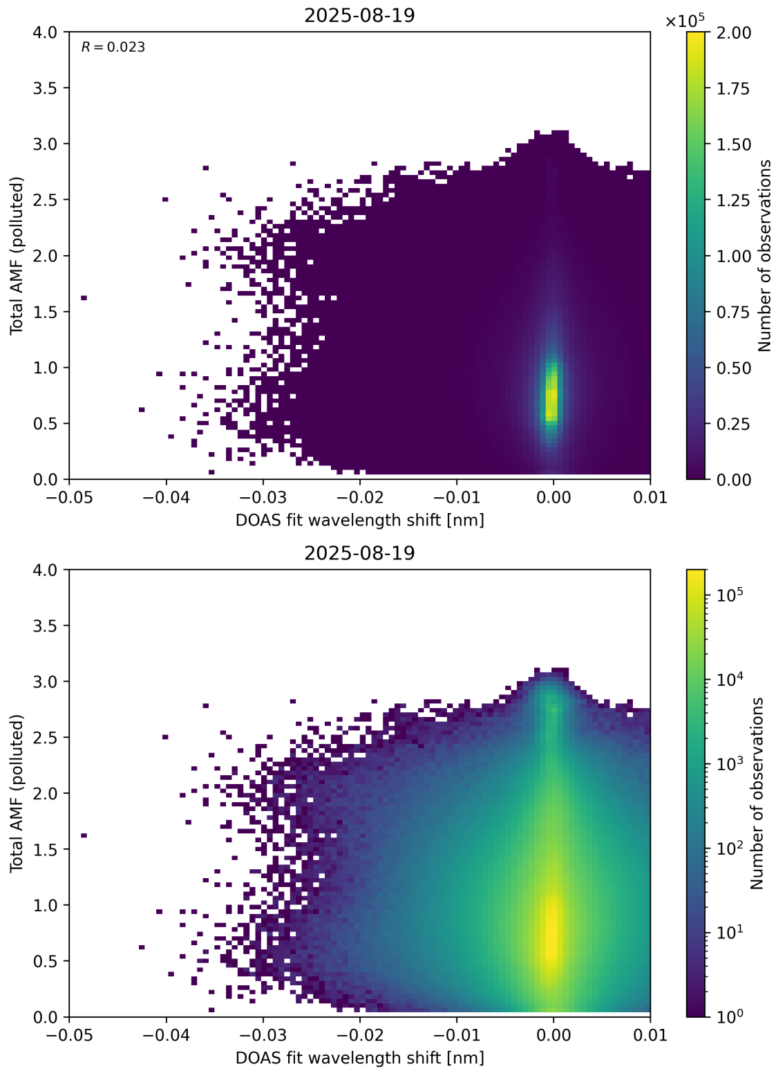
Figure 141: Scatter density plot of “DOAS fit wavelength shift” against “Total AMF (polluted)” for 2025-08-19 to 2025-08-20.
