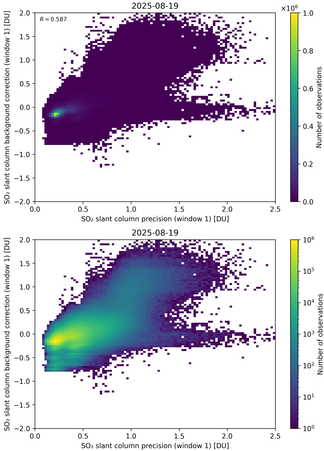
Figure 268: Scatter density plot of “SO 2 slant column precision (window 1)” against “SO 2 slant column background correction (window 1)” for 2025-08-19 to 2025-08-20.
