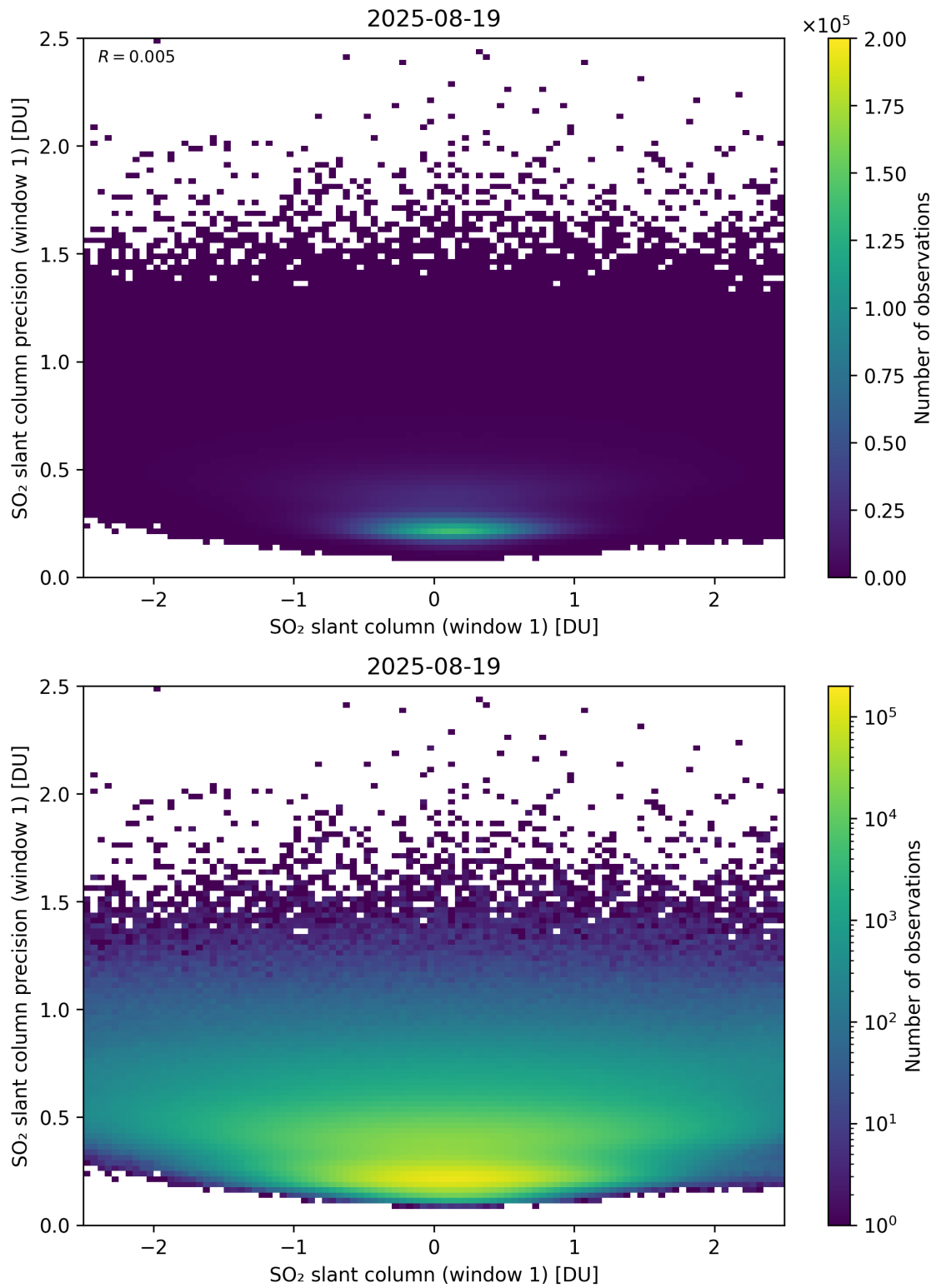
Figure 285: Scatter density plot of “SO 2 slant column (window 1)” against “SO 2 slant column precision (window 1)” for 2025-08-19 to 2025-08-20.
