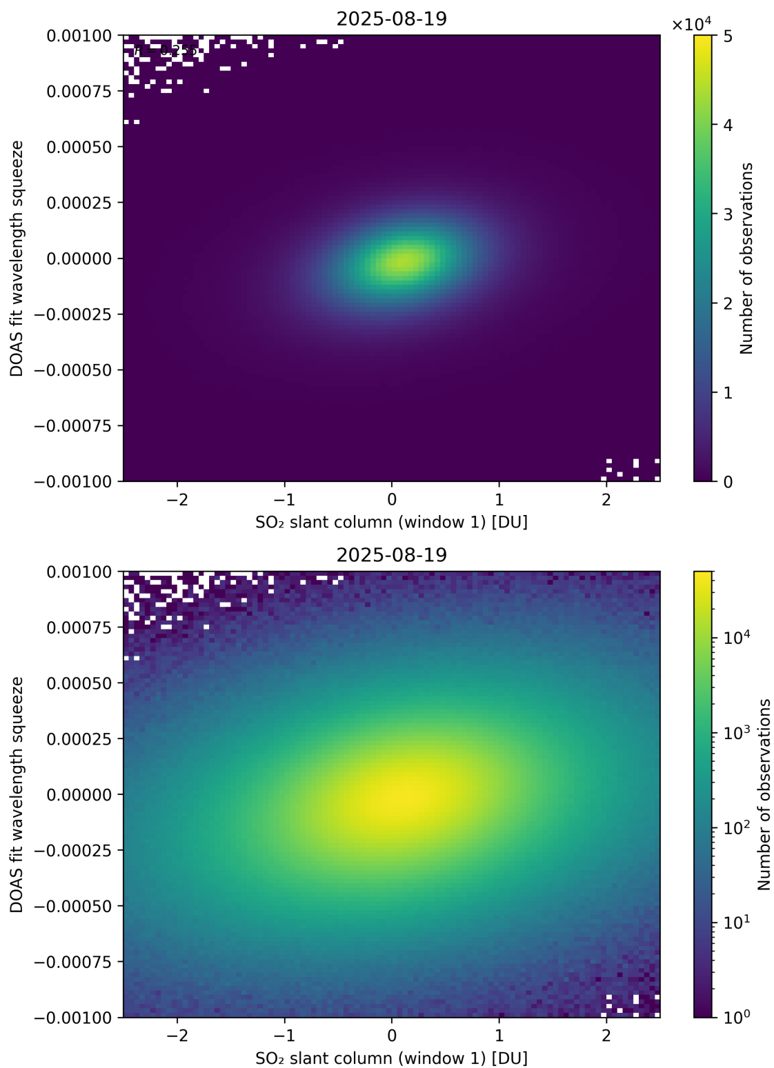
Figure 266: Scatter density plot of “SO 2 slant column (window 1)” against “DOAS fit wavelength squeeze” for 2025-08-19 to 2025-08-20.
