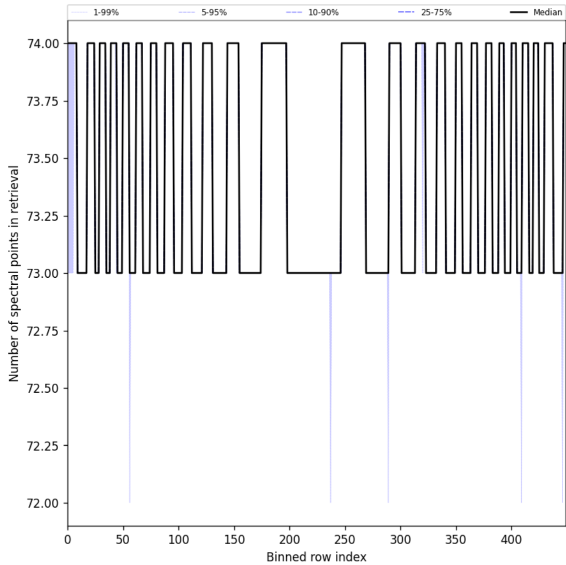
Figure 108: Along track statistics of “Number of spectral points in retrieval” for 2025-08-19 to 2025-08-20
