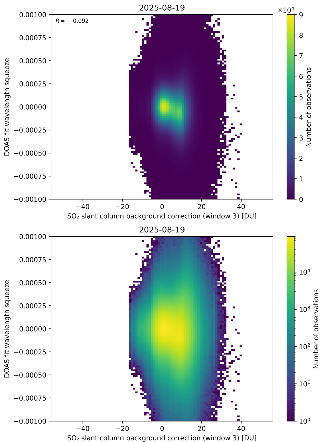
Figure 133: Scatter density plot of “SO 2 slant column background correction (window 3)” against “DOAS fit wavelength squeeze” for 2025-08-19 to 2025-08-20.
