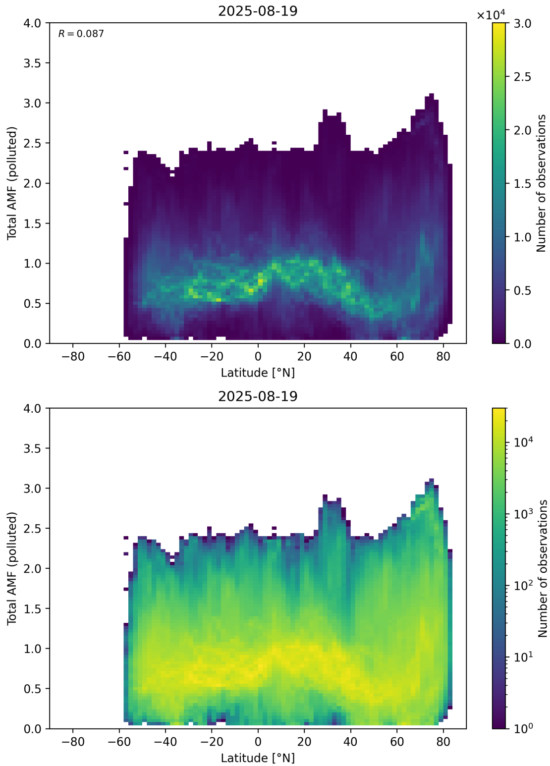
Figure 167: Scatter density plot of “Latitude” against “Total AMF (polluted)” for 2025-08-19 to 2025-08-20.
