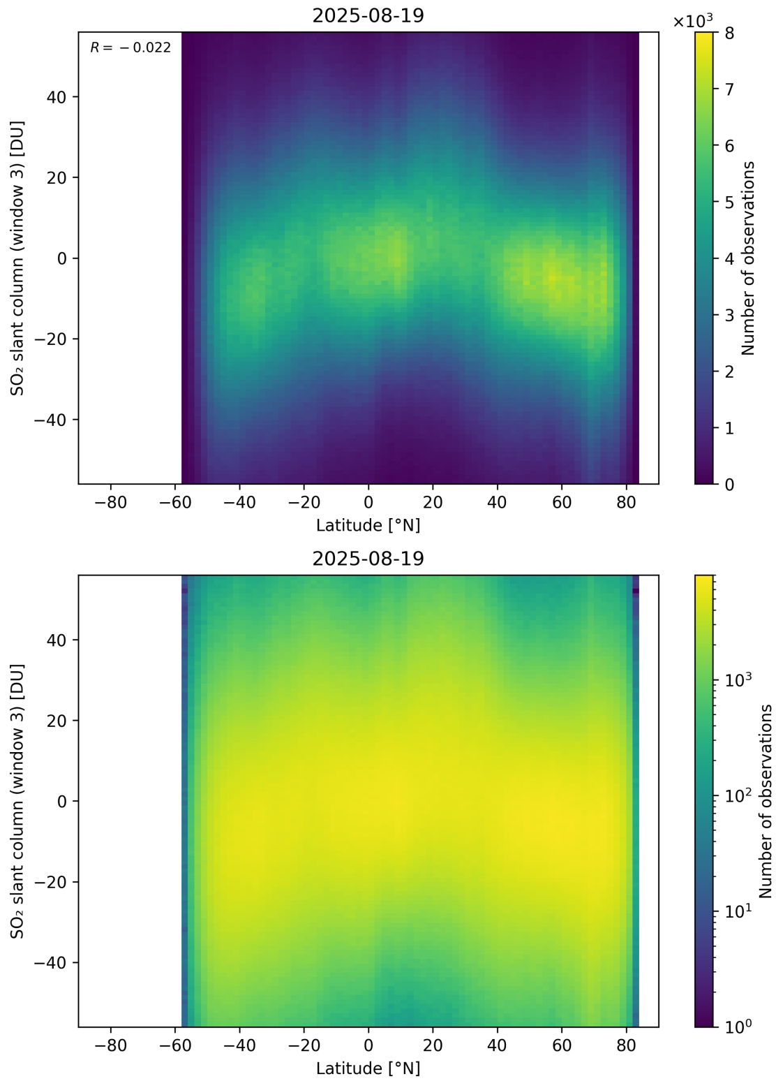
Figure 165: Scatter density plot of “Latitude” against “SO 2 slant column (window 3)” for 2025-08-19 to 2025-08-20.
