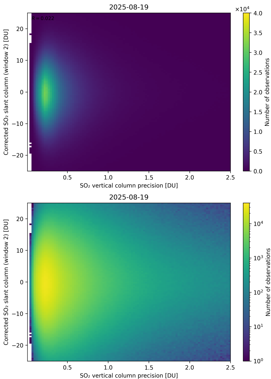
Figure 339: Scatter density plot of “SO 2 vertical column precision” against “Corrected SO 2 slant column (window 2)” for 2025-08-19 to 2025-08-20.
