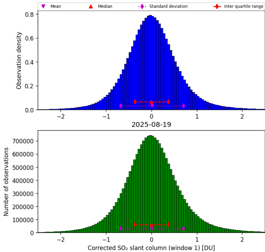
Figure 65: Histogram of “Corrected SO 2 slant column (window 1)” for 2025-08-19 to 2025-08-20
