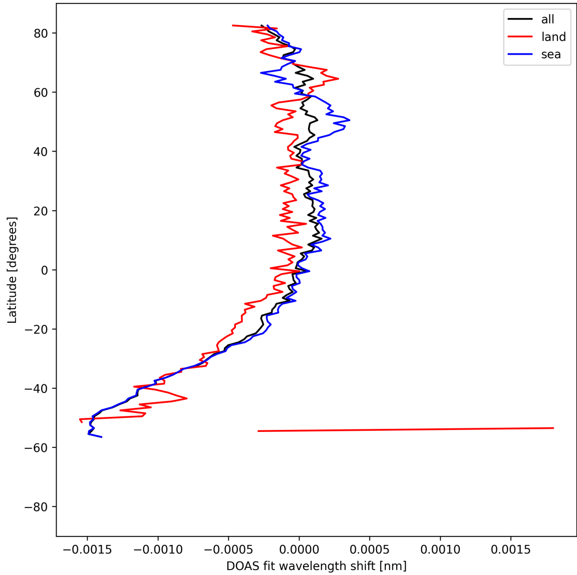
Figure 50: Zonal average of “DOAS fit wavelength shift” for 2025-08-19 to 2025-08-20.
