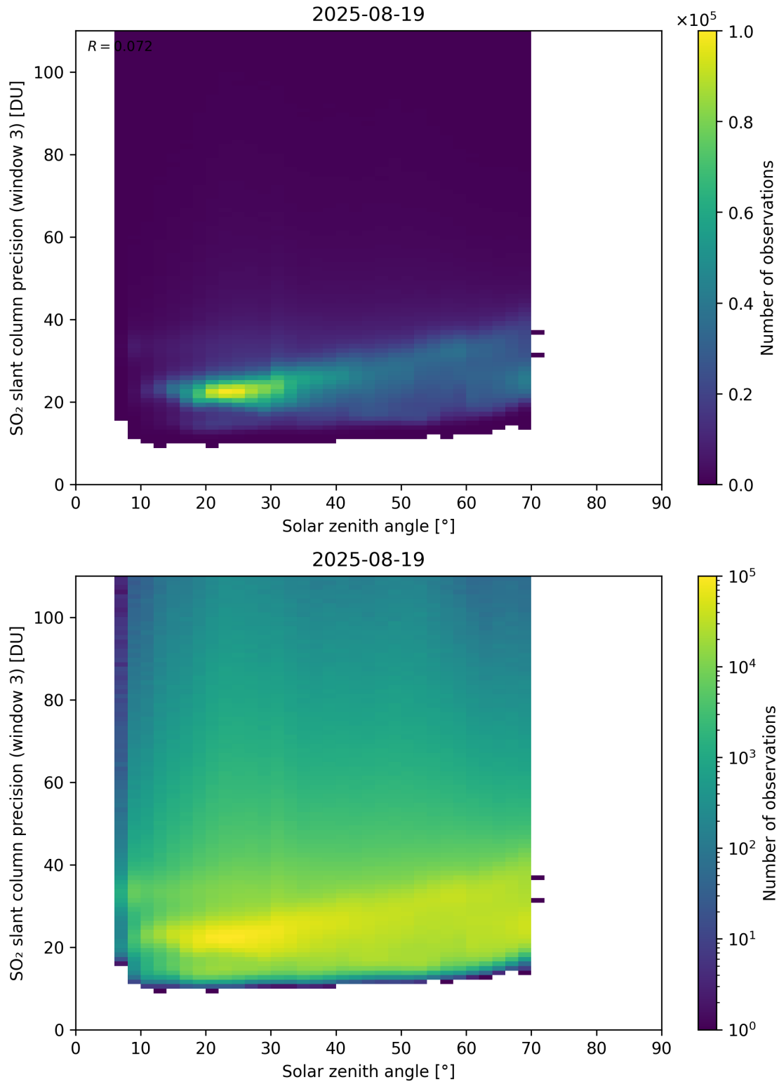
Figure 188: Scatter density plot of “Solar zenith angle” against “SO 2 slant column precision (window 3)” for 2025-08-19 to 2025-08-20.
