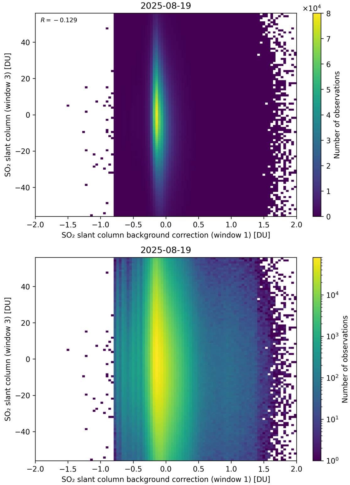
Figure 118: Scatter density plot of “SO 2 slant column background correction (window 1)” against “SO 2 slant column (window 3)” for 2025-08-19 to 2025-08-20.
