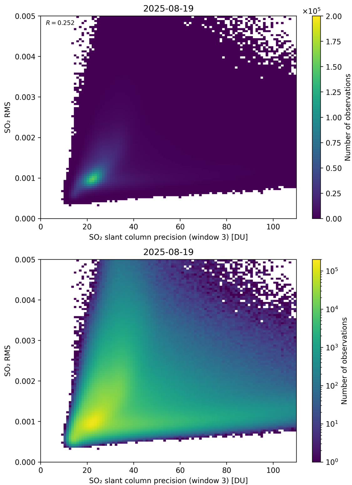
Figure 310: Scatter density plot of “SO 2 slant column precision (window 3)” against “SO 2 RMS” for 2025-08-19 to 2025-08-20.
