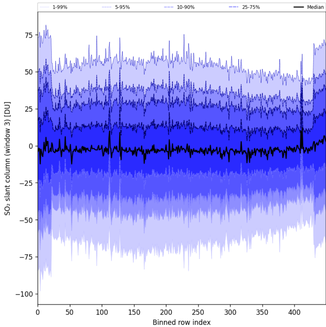
Figure 97: Along track statistics of “SO 2 slant column (window 3)” for 2025-08-19 to 2025-08-20
