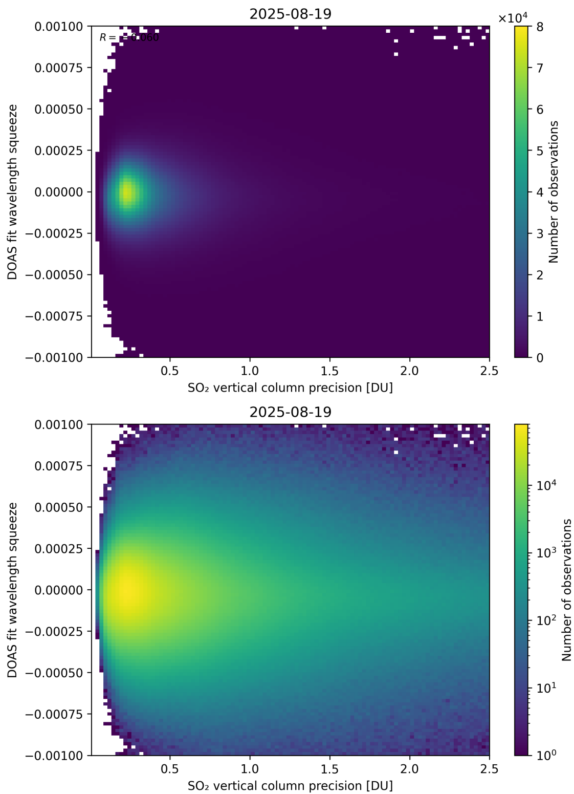
Figure 333: Scatter density plot of “SO 2 vertical column precision” against “DOAS fit wavelength squeeze” for 2025-08-19 to 2025-08-20.
