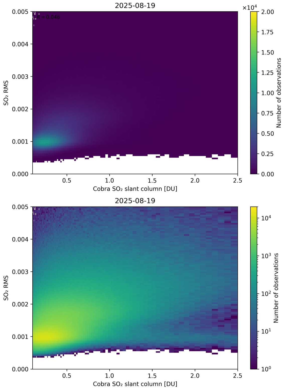
Figure 198: Scatter density plot of “Cobra SO 2 slant column” against “SO 2 RMS” for 2025-08-19 to 2025-08-20.
