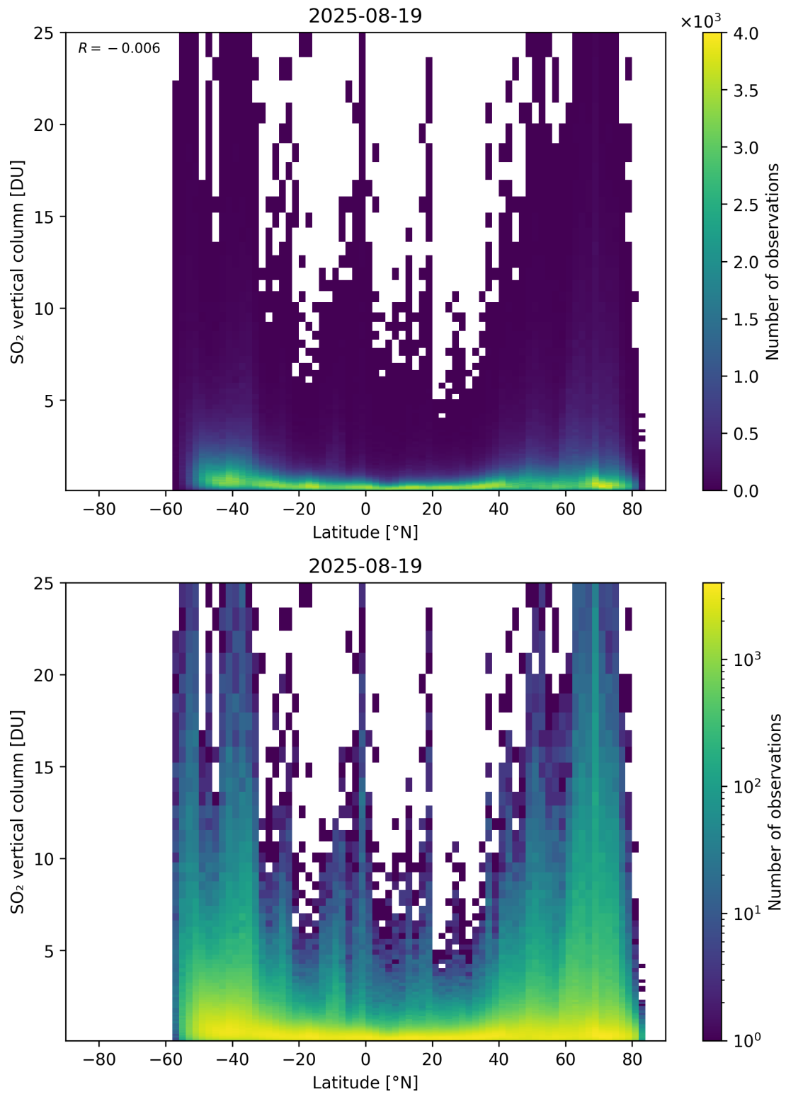
Figure 169: Scatter density plot of “Latitude” against “SO 2 vertical column” for 2025-08-19 to 2025-08-20.
