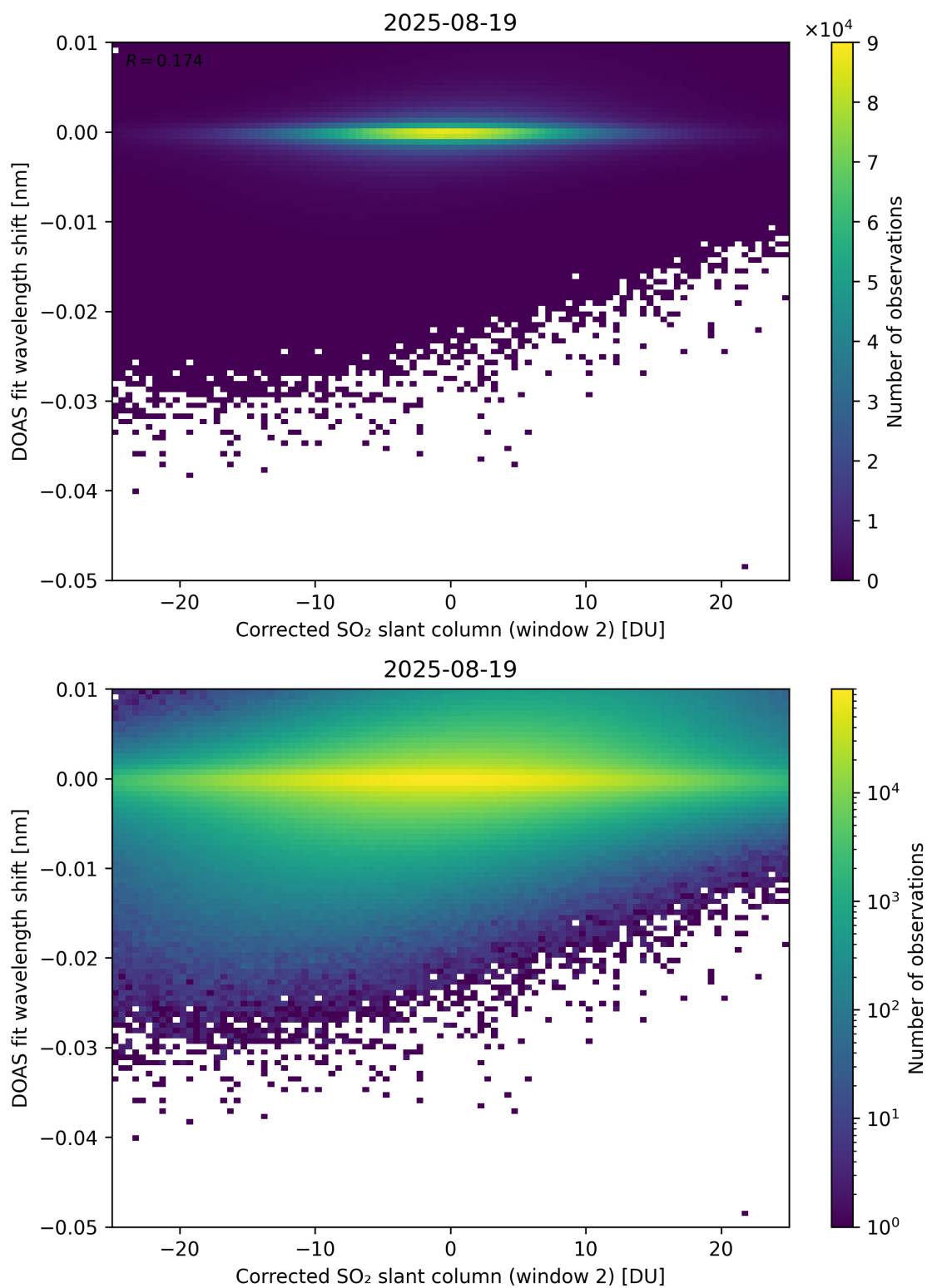
Figure 246: Scatter density plot of “Corrected SO 2 slant column (window 2)” against “DOAS fit wavelength shift” for 2025-08-19 to 2025-08-20.
