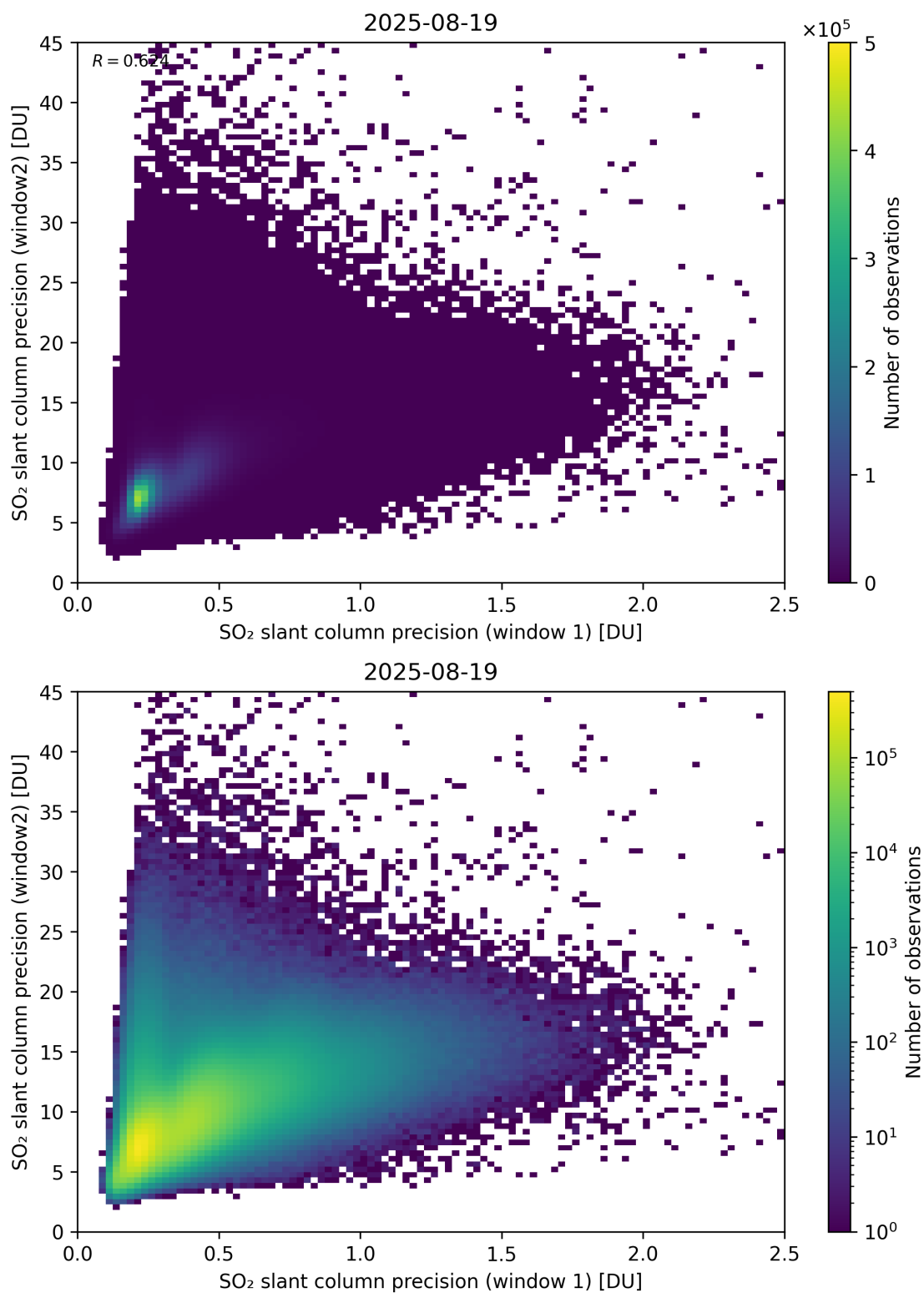
Figure 277: Scatter density plot of “SO 2 slant column precision (window 1)” against “SO 2 slant column precision (window2)” for 2025-08-19 to 2025-08-20.
