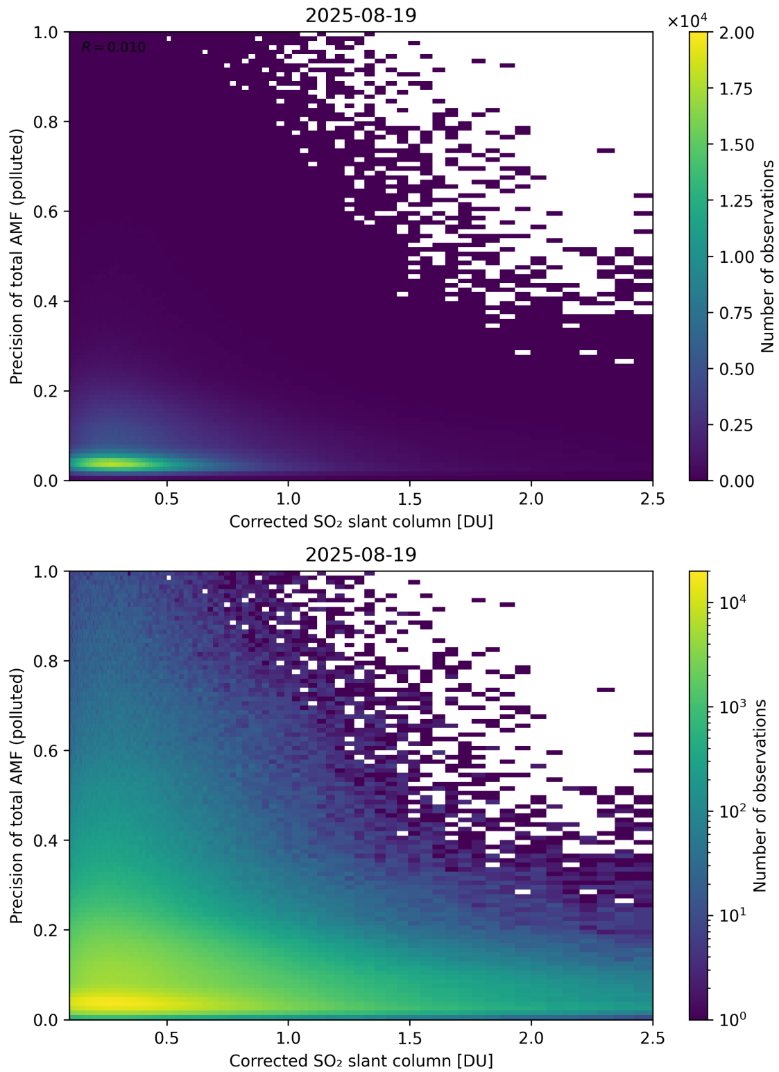
Figure 243: Scatter density plot of “Corrected SO 2 slant column” against “Precision of total AMF (polluted)” for 2025-08-19 to 2025-08-20.
