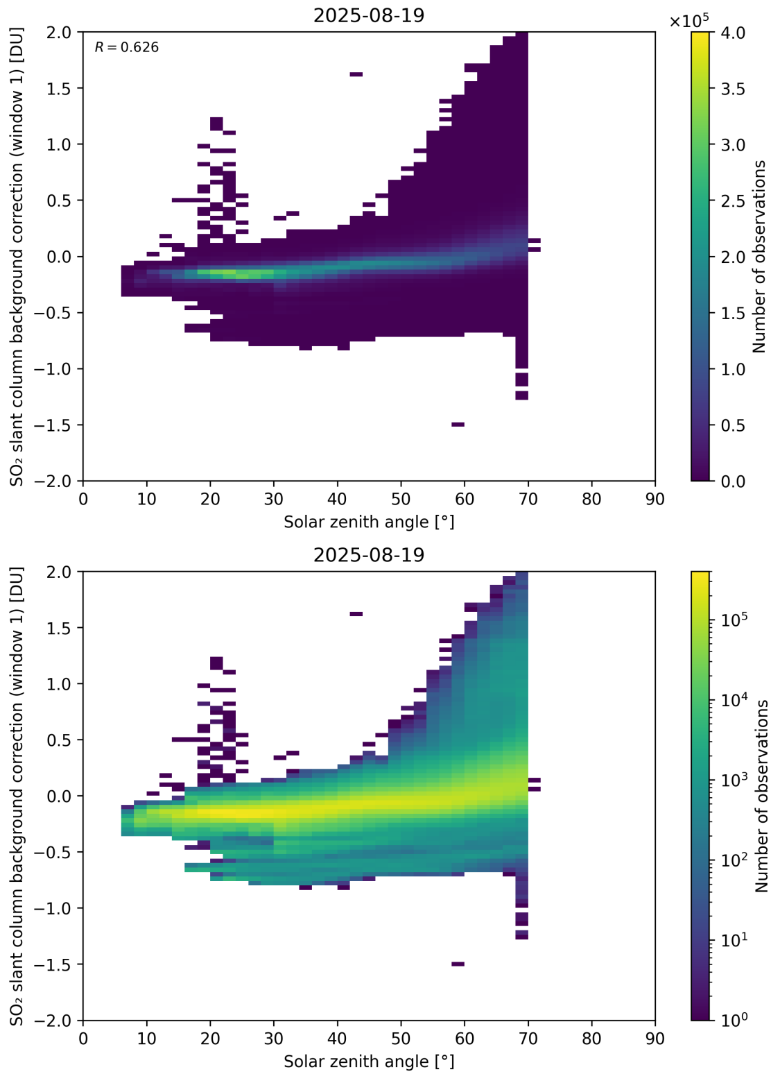
Figure 171: Scatter density plot of “Solar zenith angle” against “SO 2 slant column background correction (window 1)” for 2025-08-19 to 2025-08-20.
