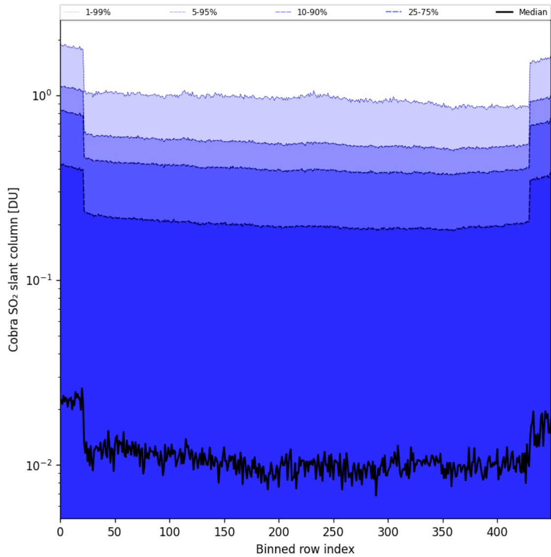
Figure 87: Along track statistics of “Cobra SO 2 slant column” for 2025-08-19 to 2025-08-20
