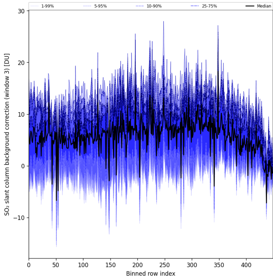
Figure 100: Along track statistics of “SO 2 slant column background correction (window 3)” for 2025-08-19 to 2025-08-20
