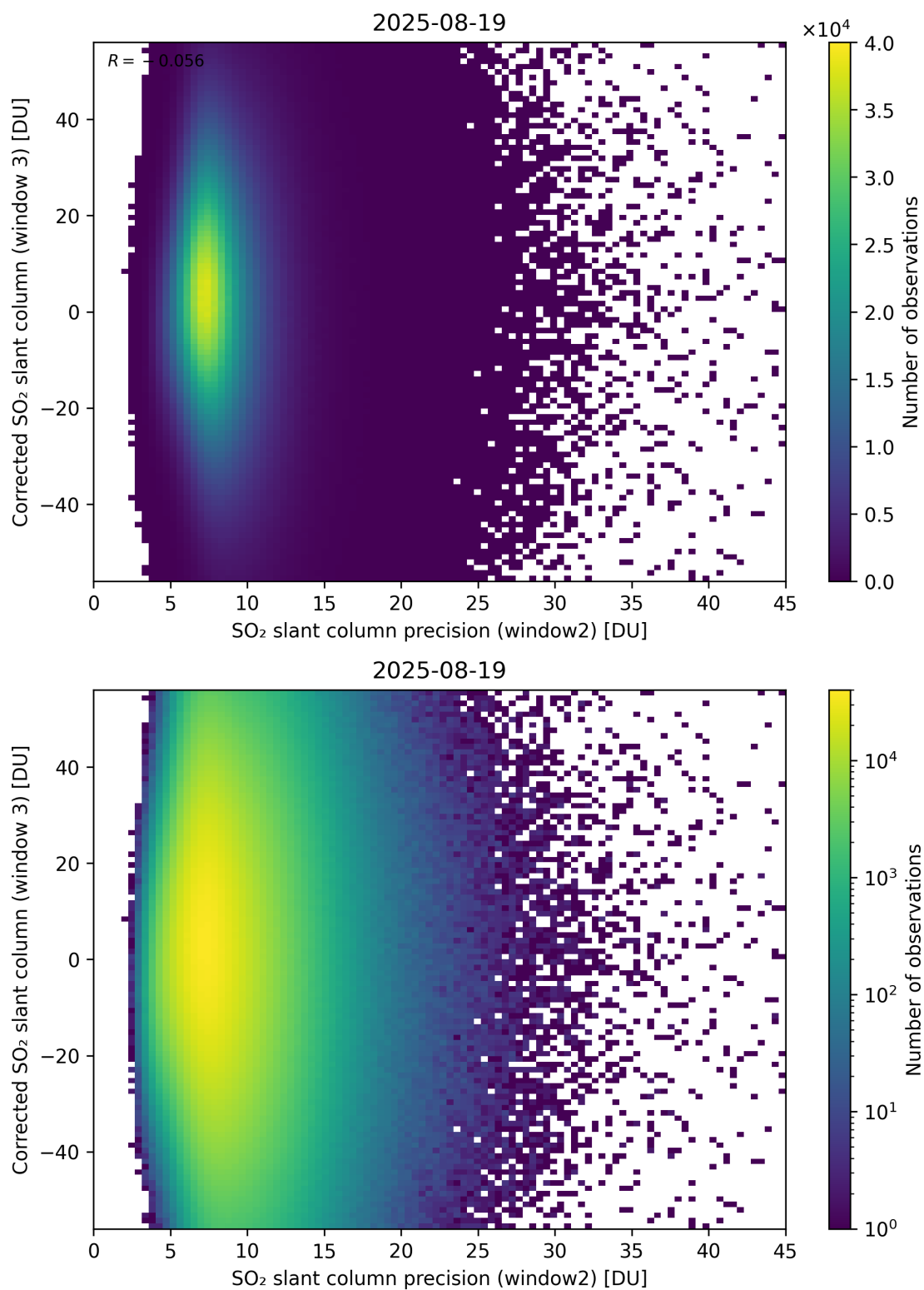
Figure 298: Scatter density plot of “SO 2 slant column precision (window2)” against “Corrected SO 2 slant column (window 3)” for 2025-08-19 to 2025-08-20.
