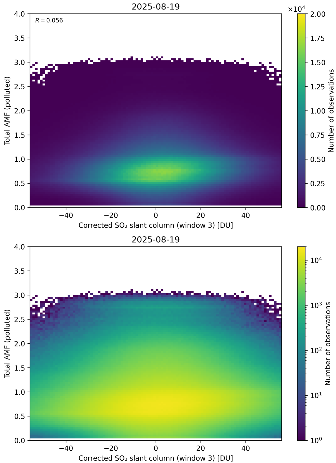
Figure 260: Scatter density plot of “Corrected SO 2 slant column (window 3)” against “Total AMF (polluted)” for 2025-08-19 to 2025-08-20.
