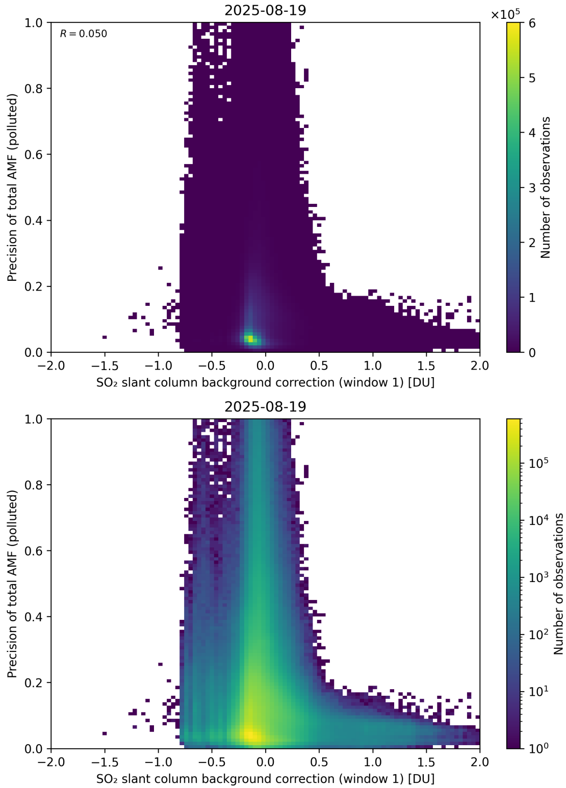
Figure 121: Scatter density plot of “SO 2 slant column background correction (window 1)” against “Precision of total AMF (polluted)” for 2025-08-19 to 2025-08-20.
