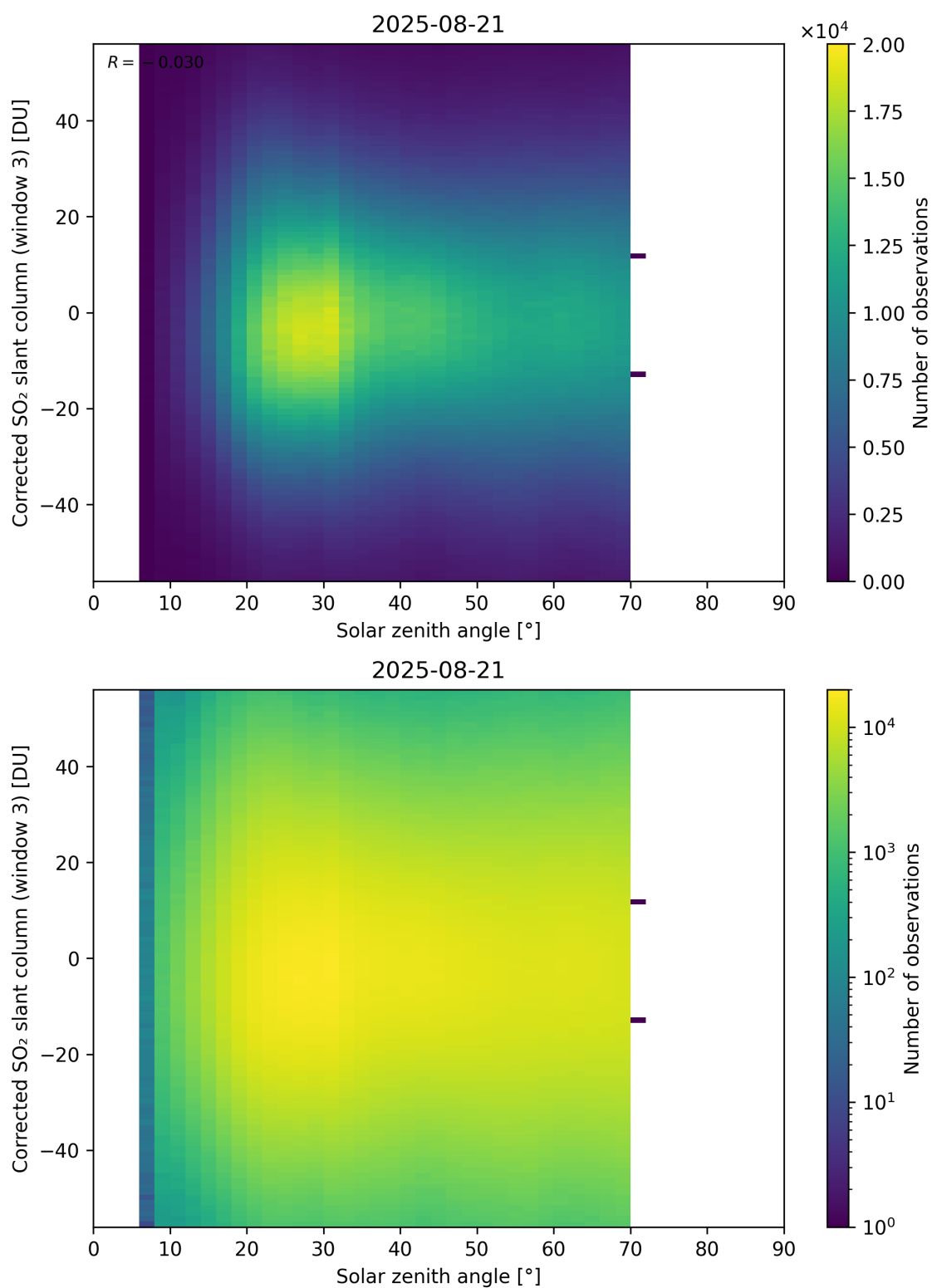
Figure 183: Scatter density plot of “Solar zenith angle” against “Corrected SO 2 slant column (window 3)” for 2025-08-20 to 2025-08-22.
