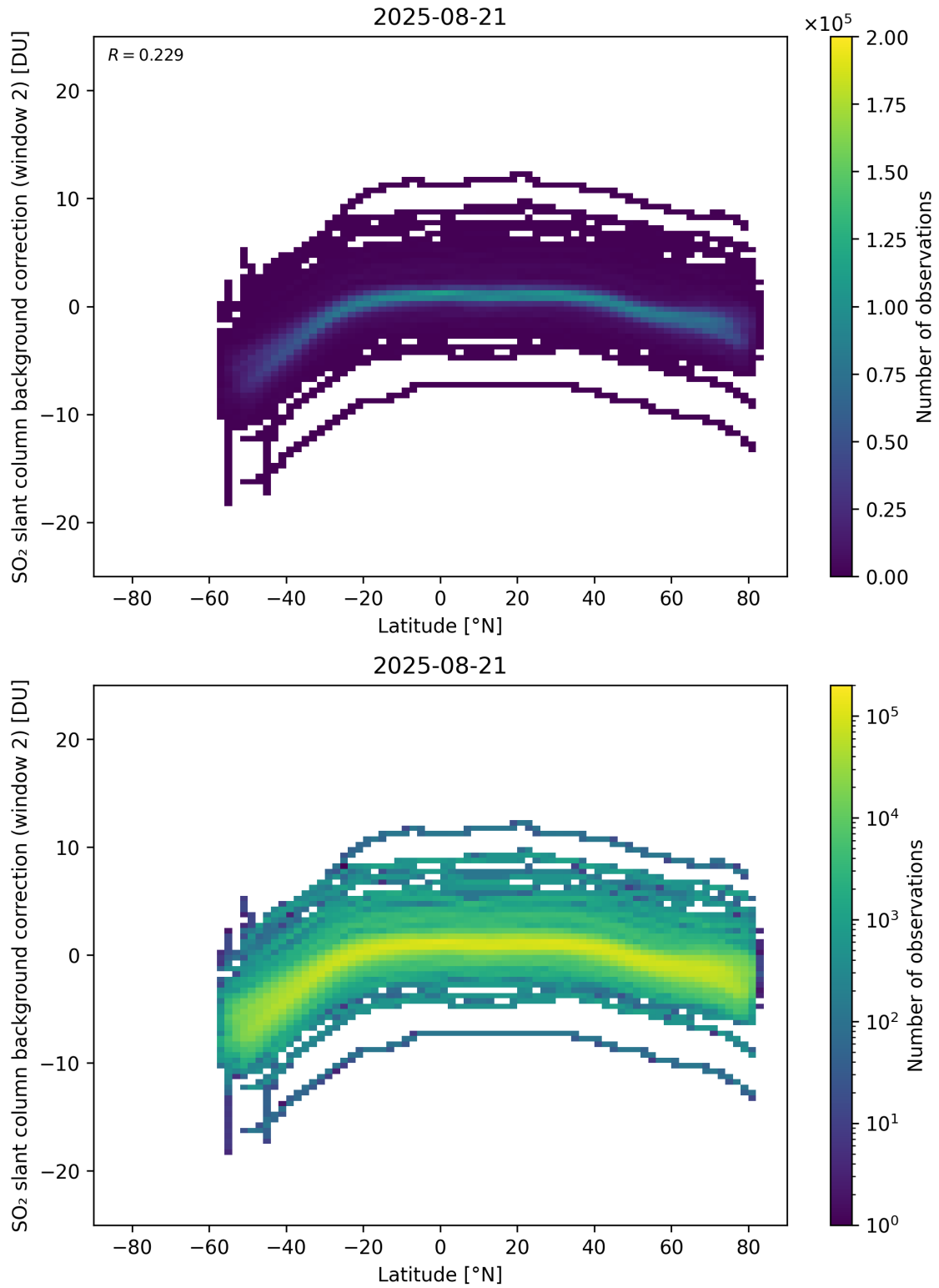
Figure 151: Scatter density plot of “Latitude” against “SO 2 slant column background correction (window 2)” for 2025-08-20 to 2025-08-22.
