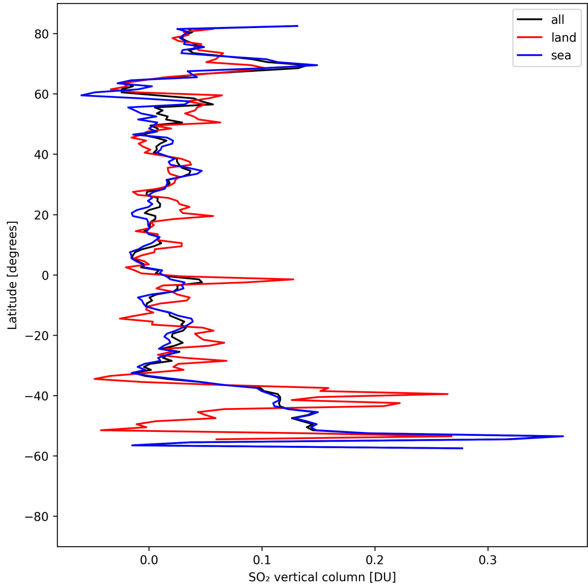
Figure 32: Zonal average of “SO 2 vertical column” for 2025-08-20 to 2025-08-22.
