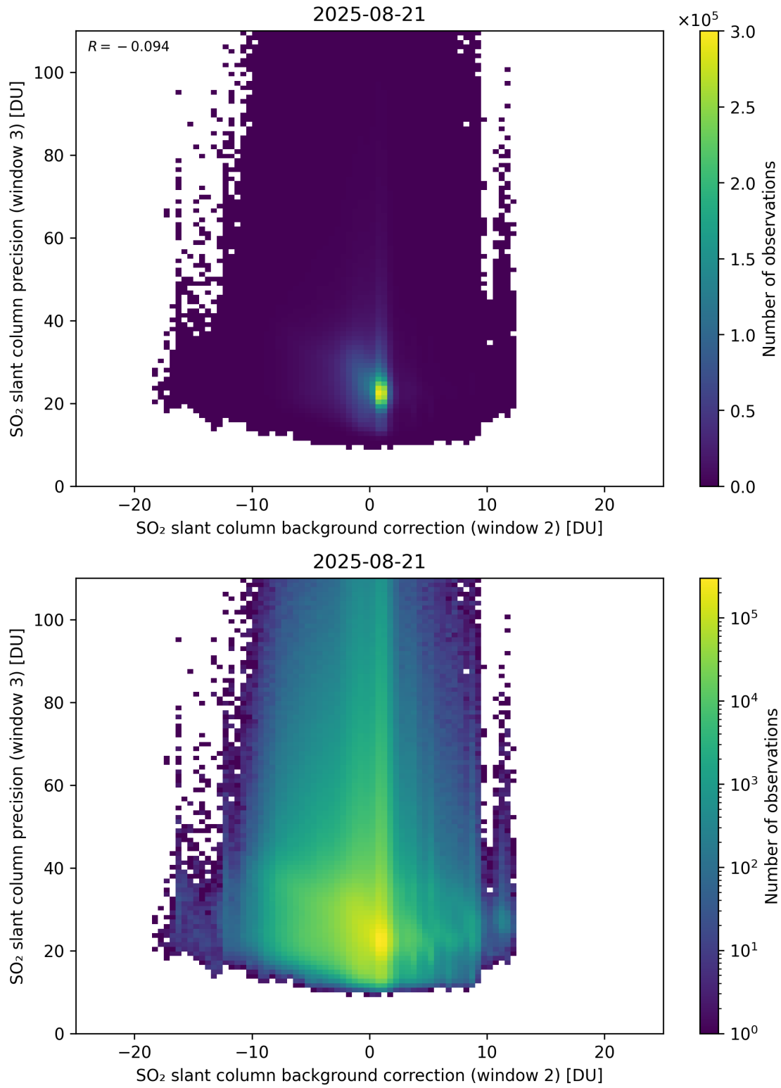
Figure 129: Scatter density plot of “SO 2 slant column background correction (window 2)” against “SO 2 slant column precision (window 3)” for 2025-08-20 to 2025-08-22.
