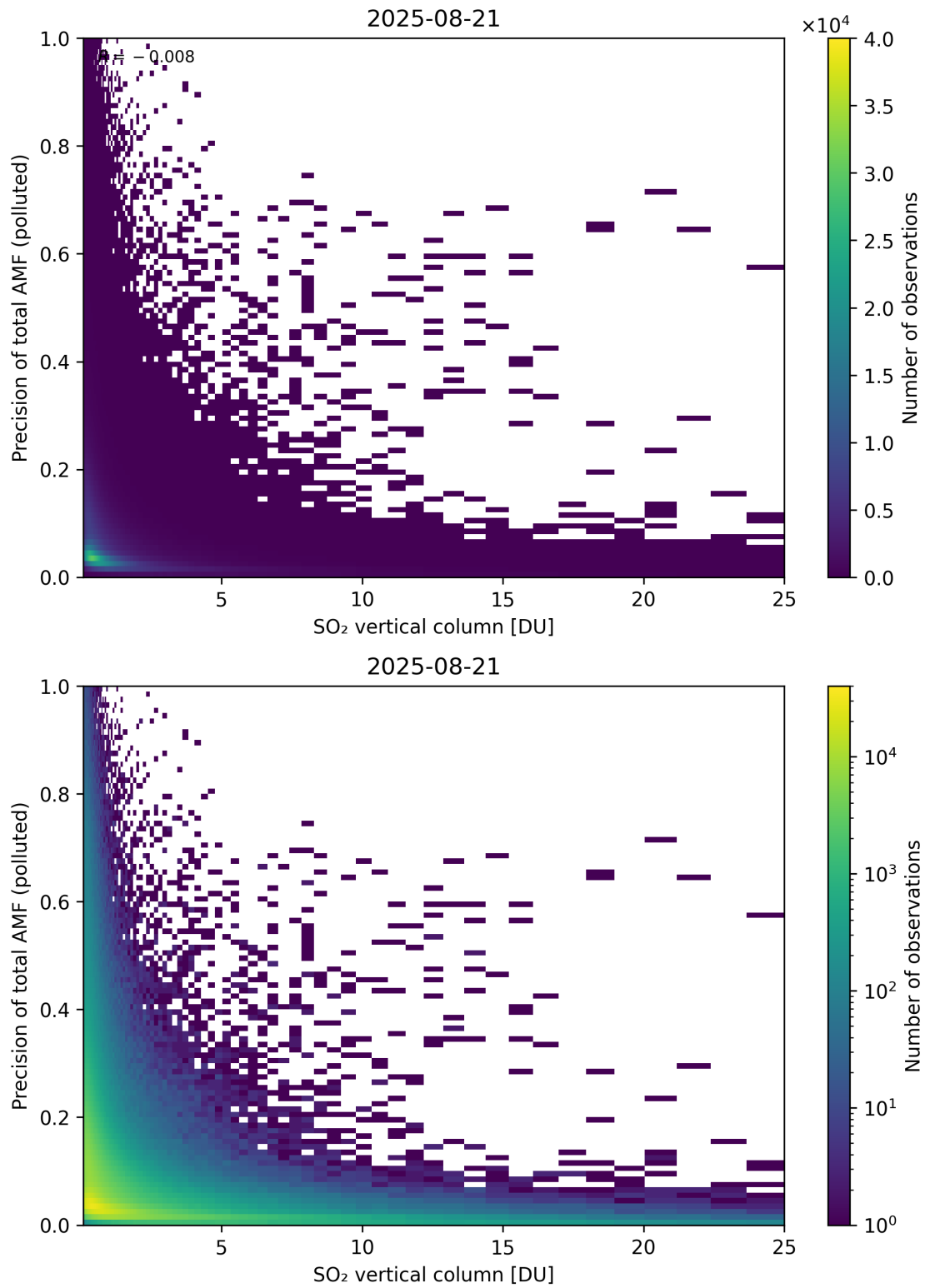
Figure 360: Scatter density plot of “SO 2 vertical column” against “Precision of total AMF (polluted)” for 2025-08-20 to 2025-08-22.
