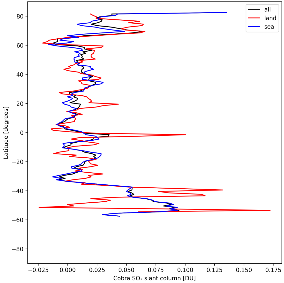
Figure 35: Zonal average of “Cobra SO 2 slant column” for 2025-08-20 to 2025-08-22.
