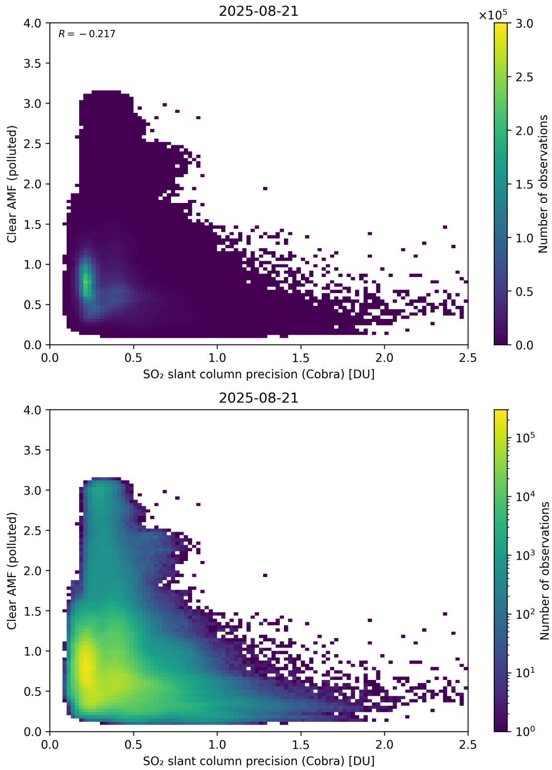
Figure 205: Scatter density plot of “SO 2 slant column precision (Cobra)” against “Clear AMF (polluted)” for 2025-08-20 to 2025-08-22.
