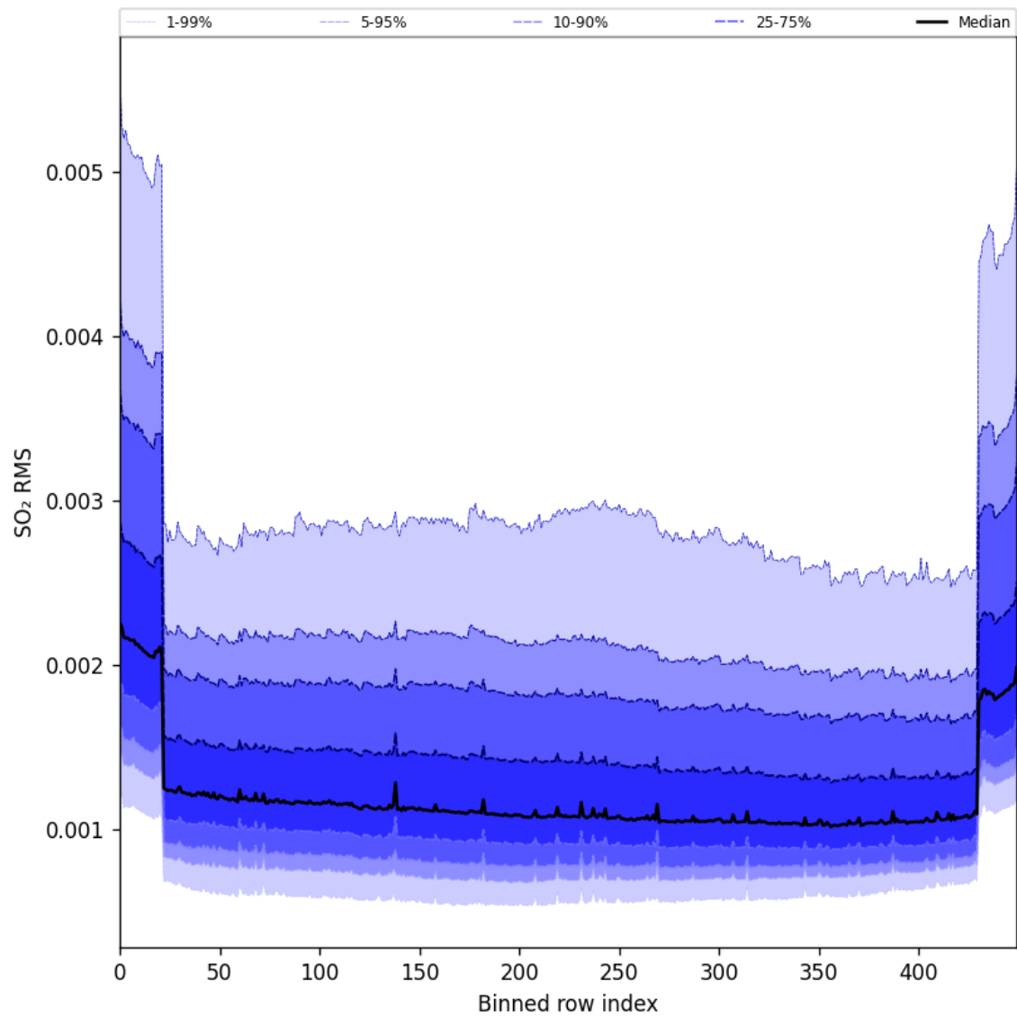
Figure 104: Along track statistics of “SO 2 RMS” for 2025-08-20 to 2025-08-22
