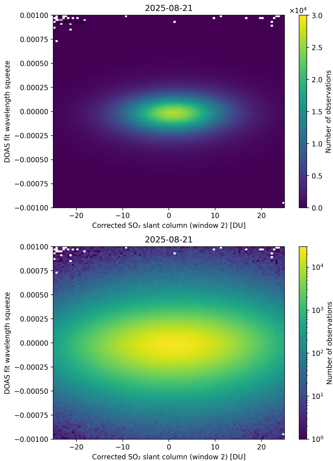
Figure 247: Scatter density plot of “Corrected SO 2 slant column (window 2)” against “DOAS fit wavelength squeeze” for 2025-08-20 to 2025-08-22.
