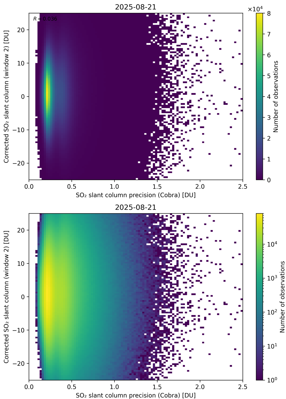
Figure 206: Scatter density plot of “SO 2 slant column precision (Cobra)” against “Corrected SO 2 slant column (window 2)” for 2025-08-20 to 2025-08-22.
