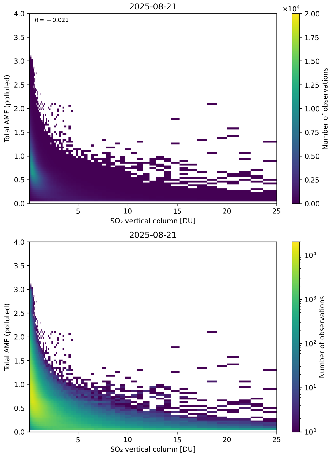
Figure 359: Scatter density plot of “SO 2 vertical column” against “Total AMF (polluted)” for 2025-08-20 to 2025-08-22.
