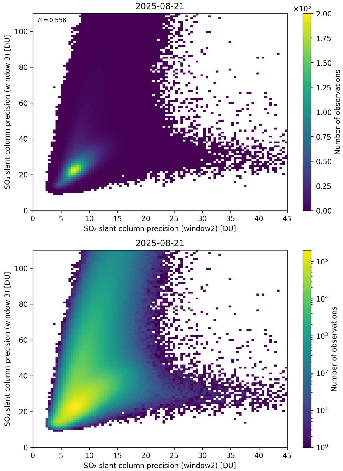
Figure 300: Scatter density plot of “SO 2 slant column precision (window2)” against “SO 2 slant column precision (window 3)” for 2025-08-20 to 2025-08-22.
