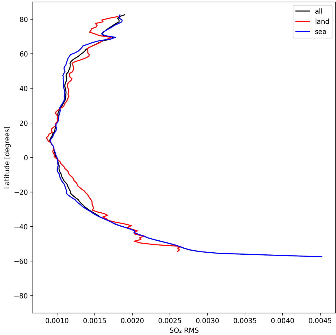
Figure 52: Zonal average of “SO 2 RMS” for 2025-08-20 to 2025-08-22.
