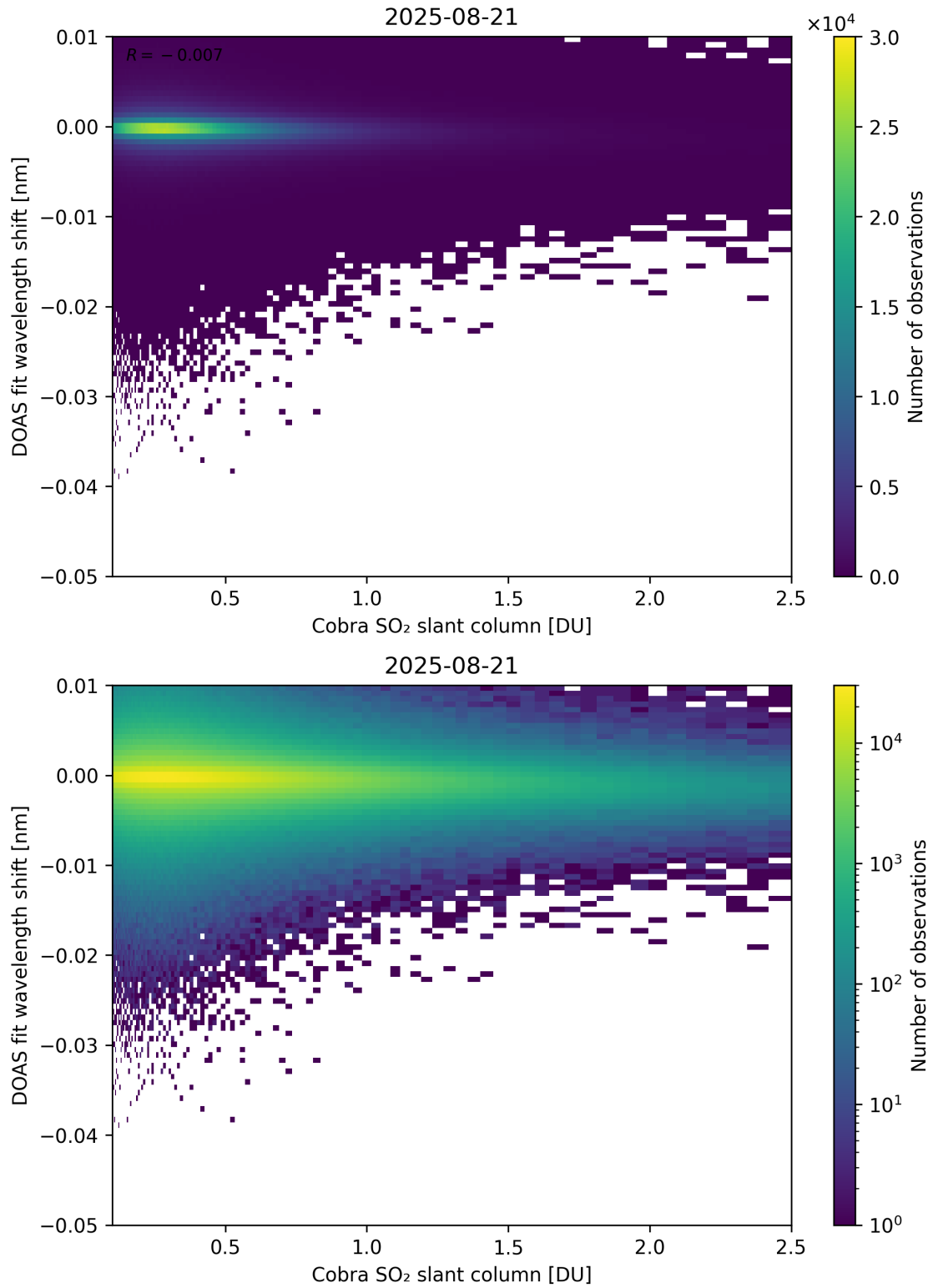
Figure 196: Scatter density plot of “Cobra SO 2 slant column” against “DOAS fit wavelength shift” for 2025-08-20 to 2025-08-22.
