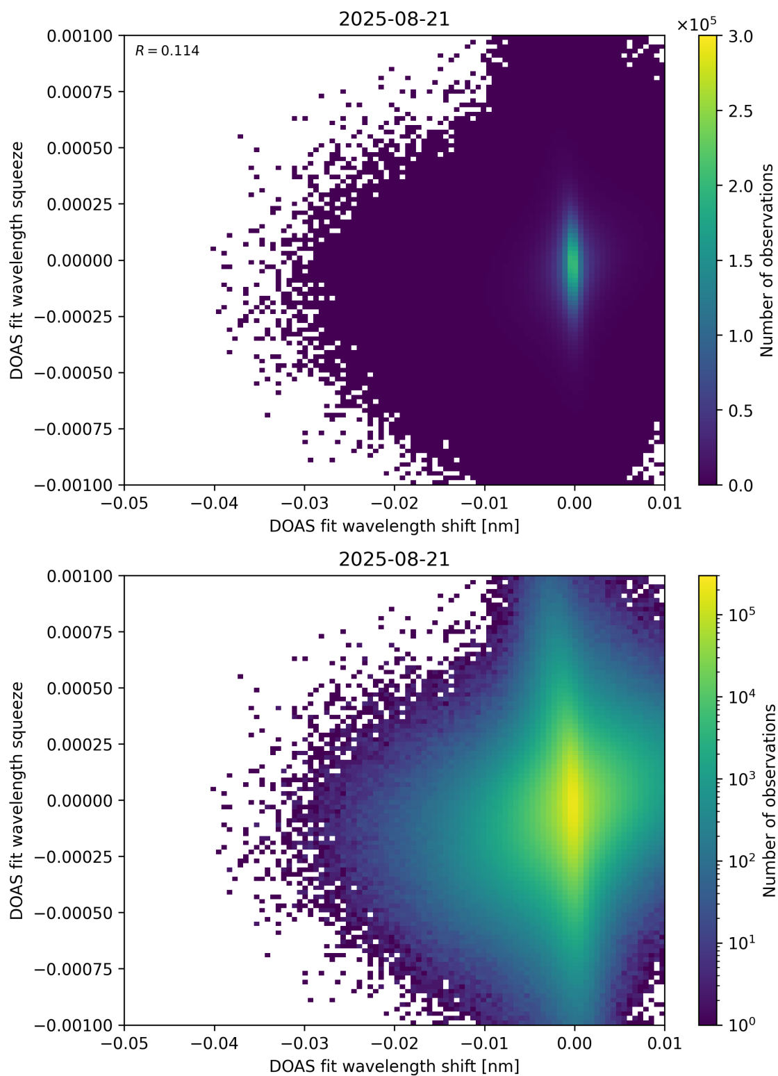
Figure 138: Scatter density plot of “DOAS fit wavelength shift” against “DOAS fit wavelength squeeze” for 2025-08-20 to 2025-08-22.
