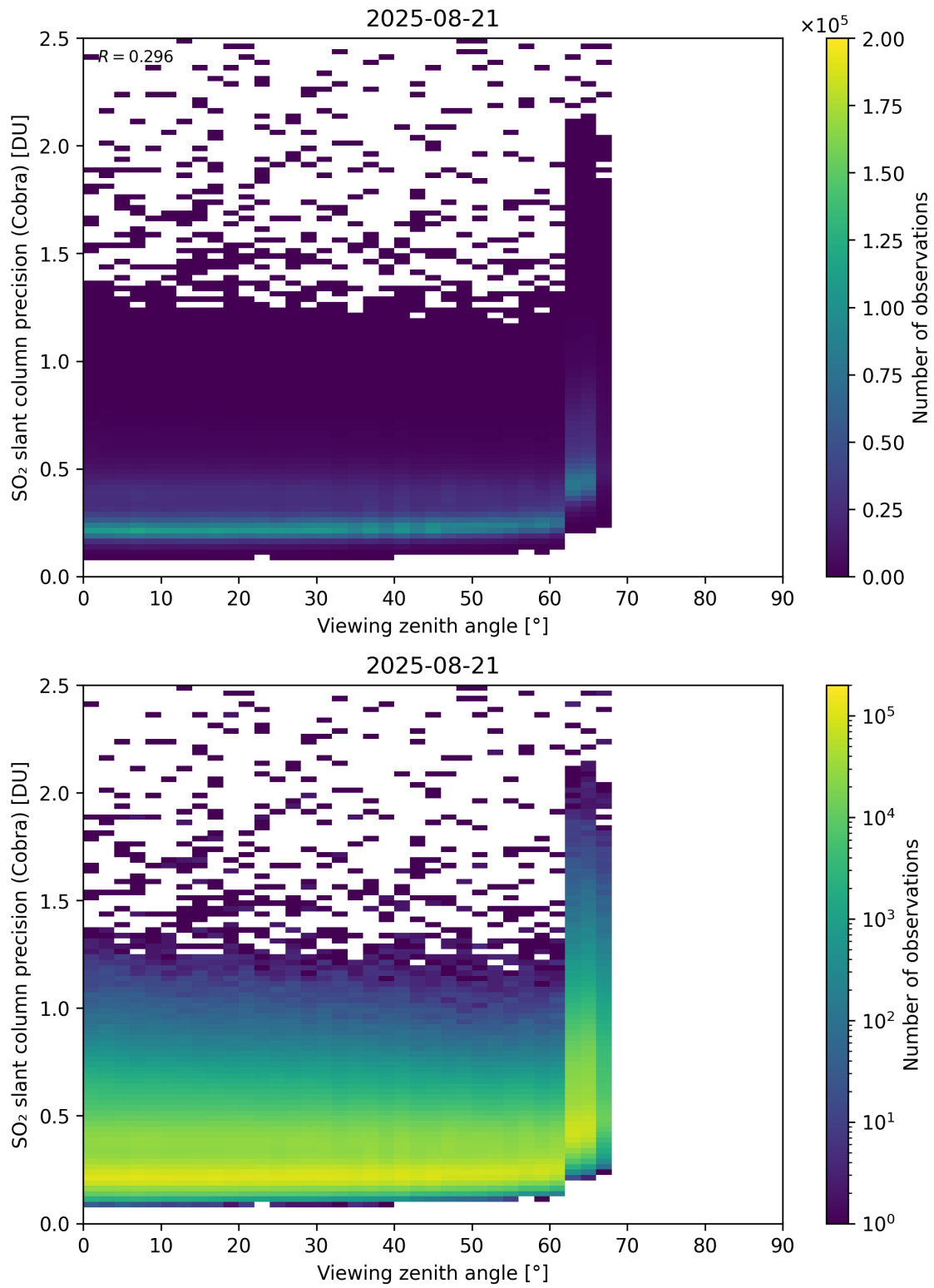
Figure 372: Scatter density plot of “Viewing zenith angle” against “SO 2 slant column precision (Cobra)” for 2025-08-20 to 2025-08-22.
