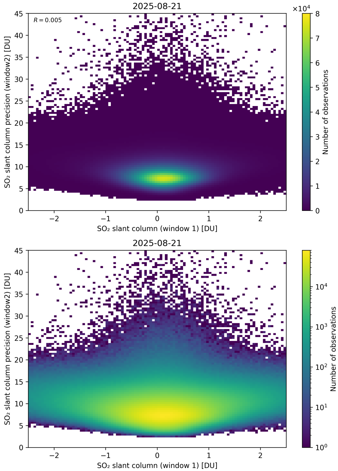
Figure 286: Scatter density plot of “SO 2 slant column (window 1)” against “SO 2 slant column precision (window2)” for 2025-08-20 to 2025-08-22.
