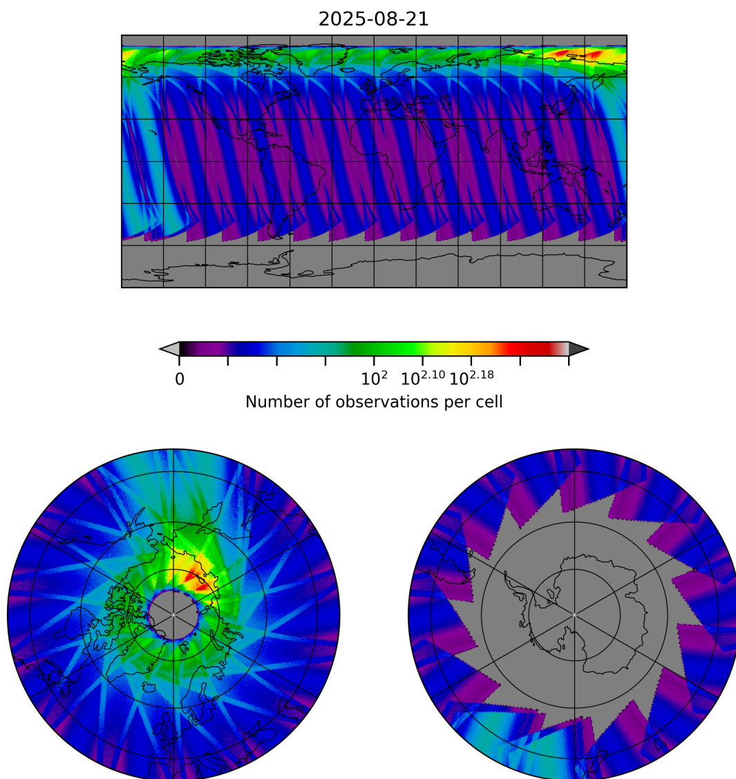
Figure 30: Map of the number of observations for 2025-08-20 to 2025-08-22
