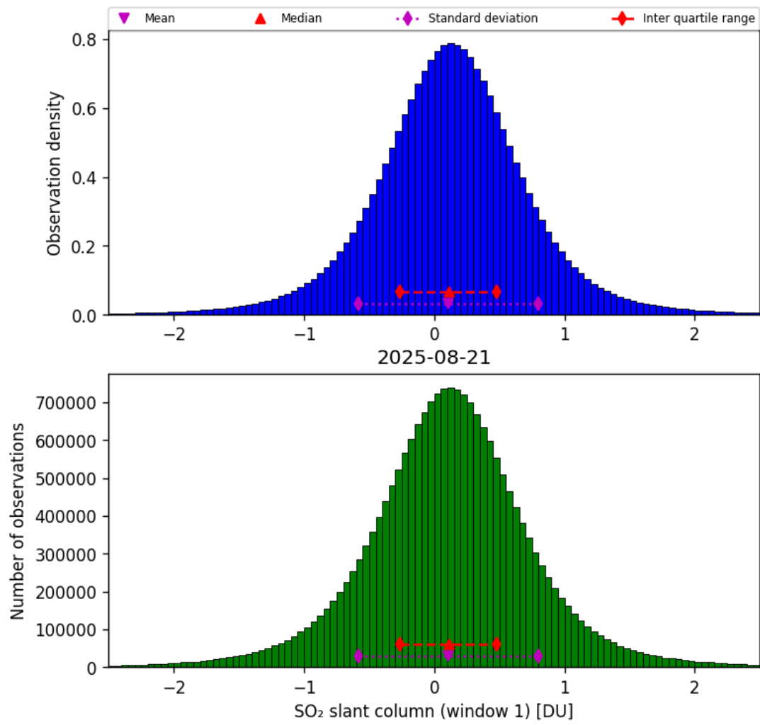
Figure 63: Histogram of “SO 2 slant column (window 1)” for 2025-08-20 to 2025-08-22
