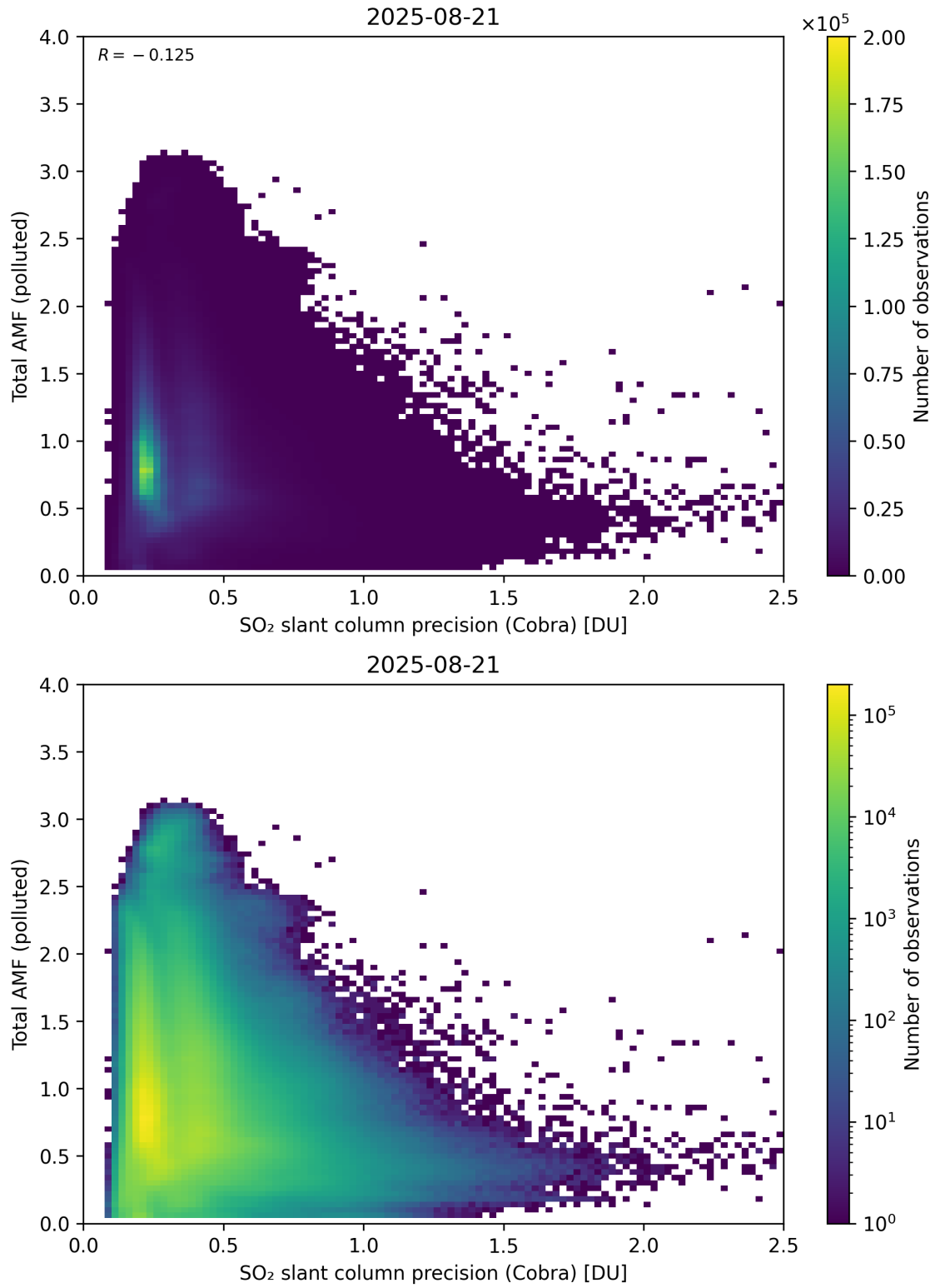
Figure 213: Scatter density plot of “SO 2 slant column precision (Cobra)” against “Total AMF (polluted)” for 2025-08-20 to 2025-08-22.
