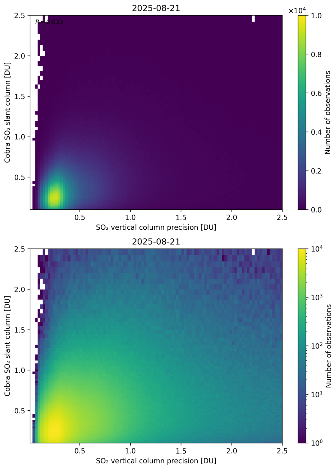
Figure 336: Scatter density plot of “SO 2 vertical column precision” against “Cobra SO 2 slant column” for 2025-08-20 to 2025-08-22.
