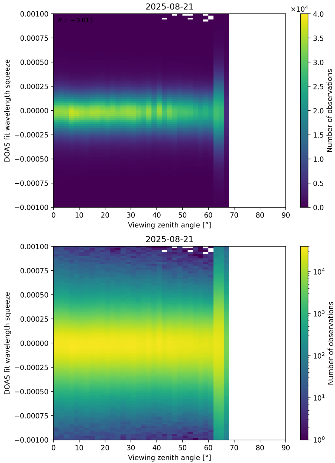
Figure 366: Scatter density plot of “Viewing zenith angle” against “DOAS fit wavelength squeeze” for 2025-08-20 to 2025-08-22.
