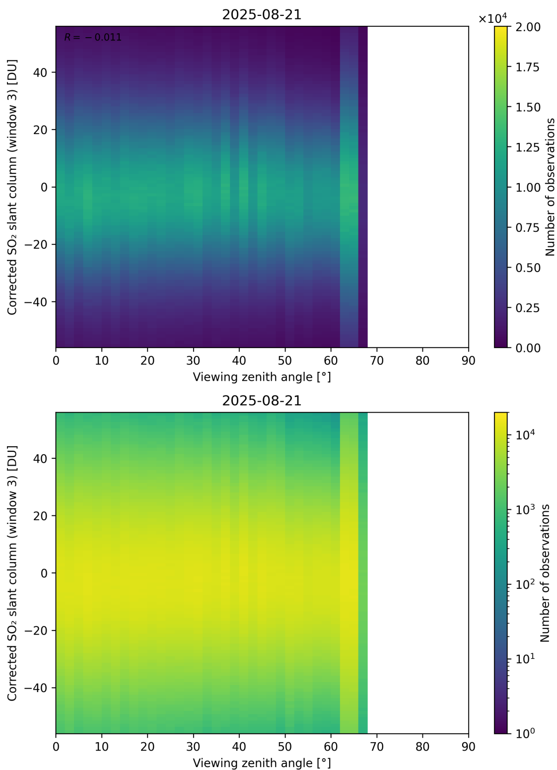
Figure 375: Scatter density plot of “Viewing zenith angle” against “Corrected SO 2 slant column (window 3)” for 2025-08-20 to 2025-08-22.
