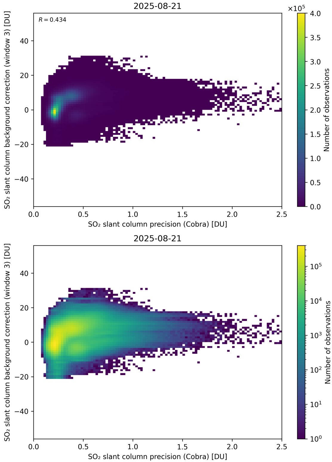
Figure 201: Scatter density plot of “SO 2 slant column precision (Cobra)” against “SO 2 slant column background correction (window 3)” for 2025-08-20 to 2025-08-22.
