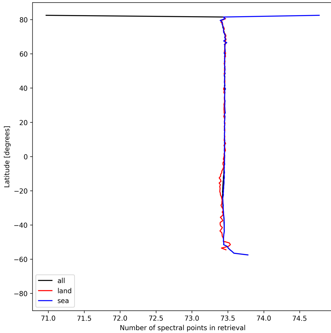
Figure 56: Zonal average of “Number of spectral points in retrieval” for 2025-08-20 to 2025-08-22.
