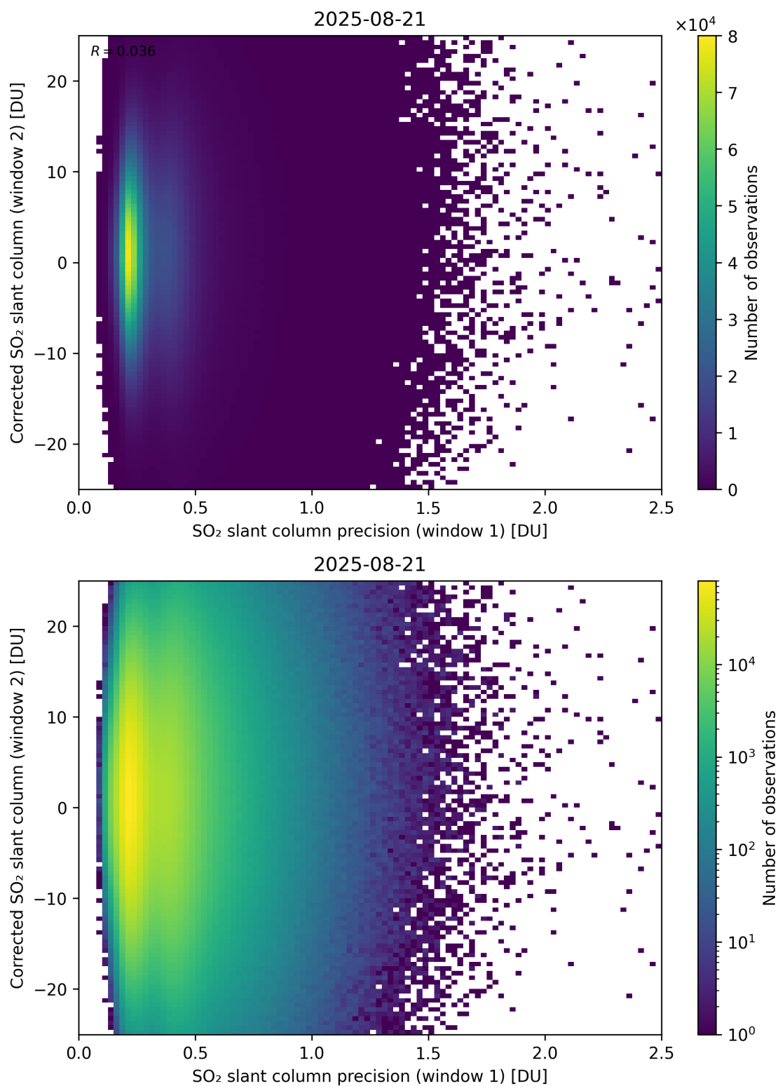
Figure 275: Scatter density plot of “SO 2 slant column precision (window 1)” against “Corrected SO 2 slant column (window 2)” for 2025-08-20 to 2025-08-22.
