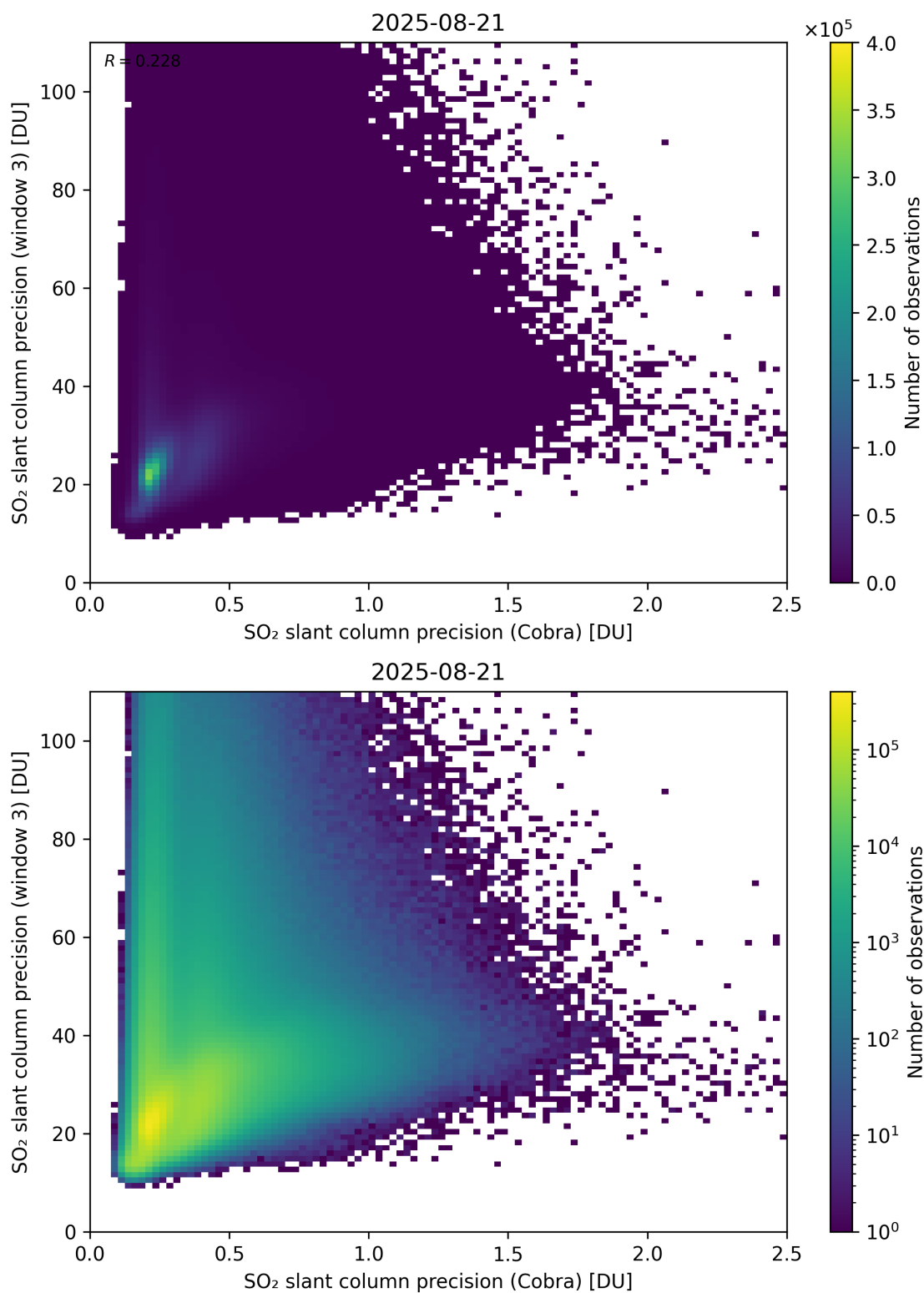
Figure 212: Scatter density plot of “SO 2 slant column precision (Cobra)” against “SO 2 slant column precision (window 3)” for 2025-08-20 to 2025-08-22.
