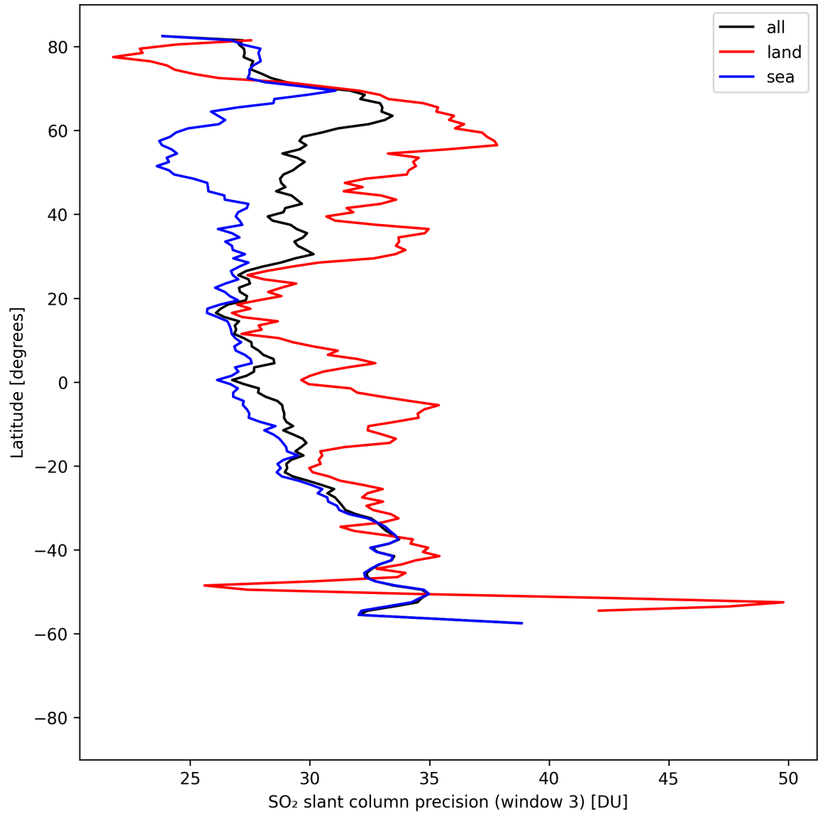
Figure 46: Zonal average of “SO 2 slant column precision (window 3)” for 2025-08-20 to 2025-08-22.
