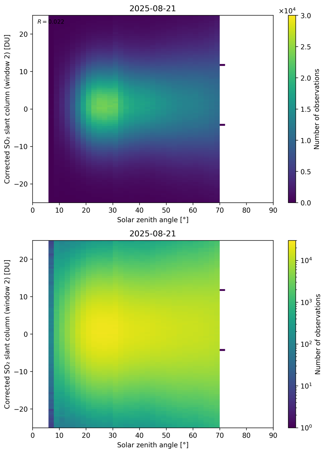
Figure 182: Scatter density plot of “Solar zenith angle” against “Corrected SO 2 slant column (window 2)” for 2025-08-20 to 2025-08-22.
