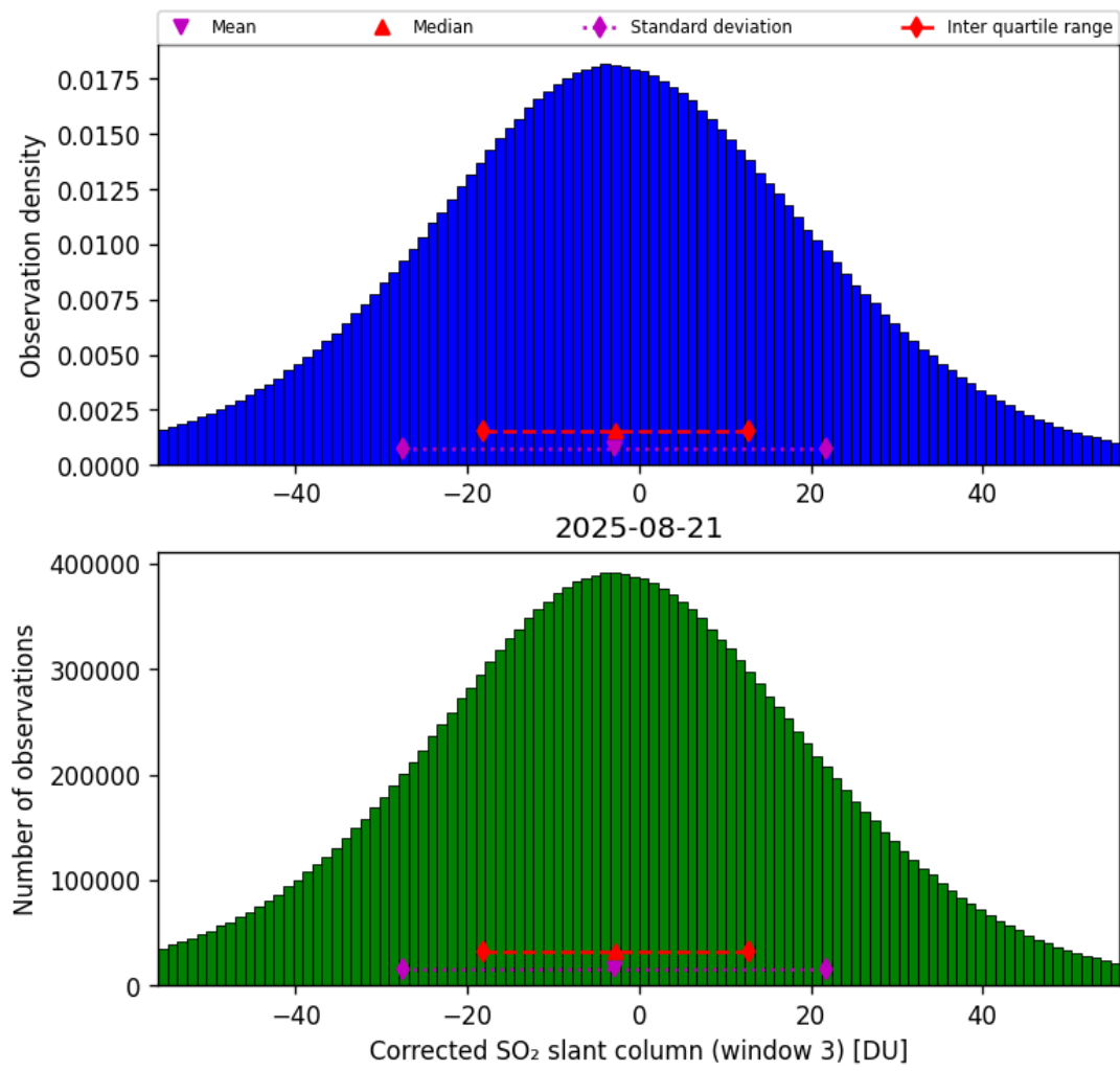
Figure 73: Histogram of “Corrected SO 2 slant column (window 3)” for 2025-08-20 to 2025-08-22
