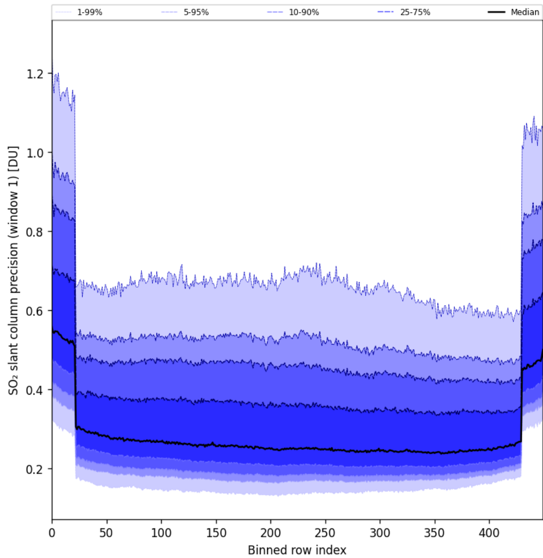
Figure 90: Along track statistics of “SO 2 slant column precision (window 1)” for 2025-08-20 to 2025-08-22
