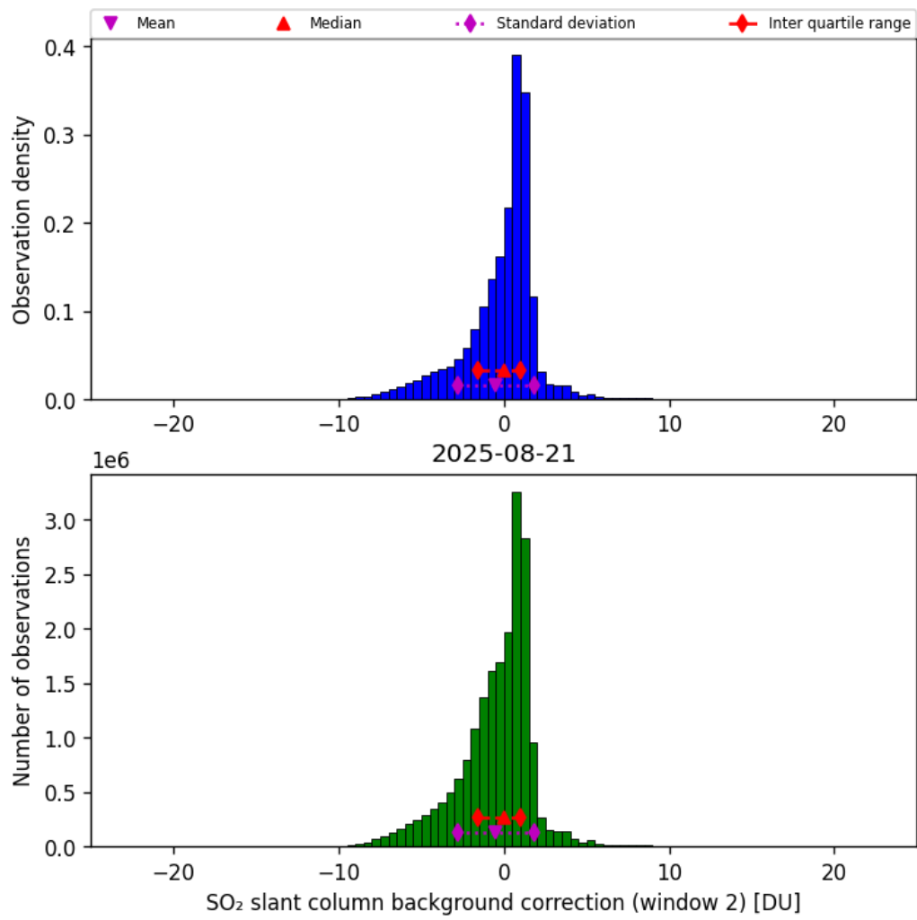
Figure 70: Histogram of “SO 2 slant column background correction (window 2)” for 2025-08-20 to 2025-08-22
