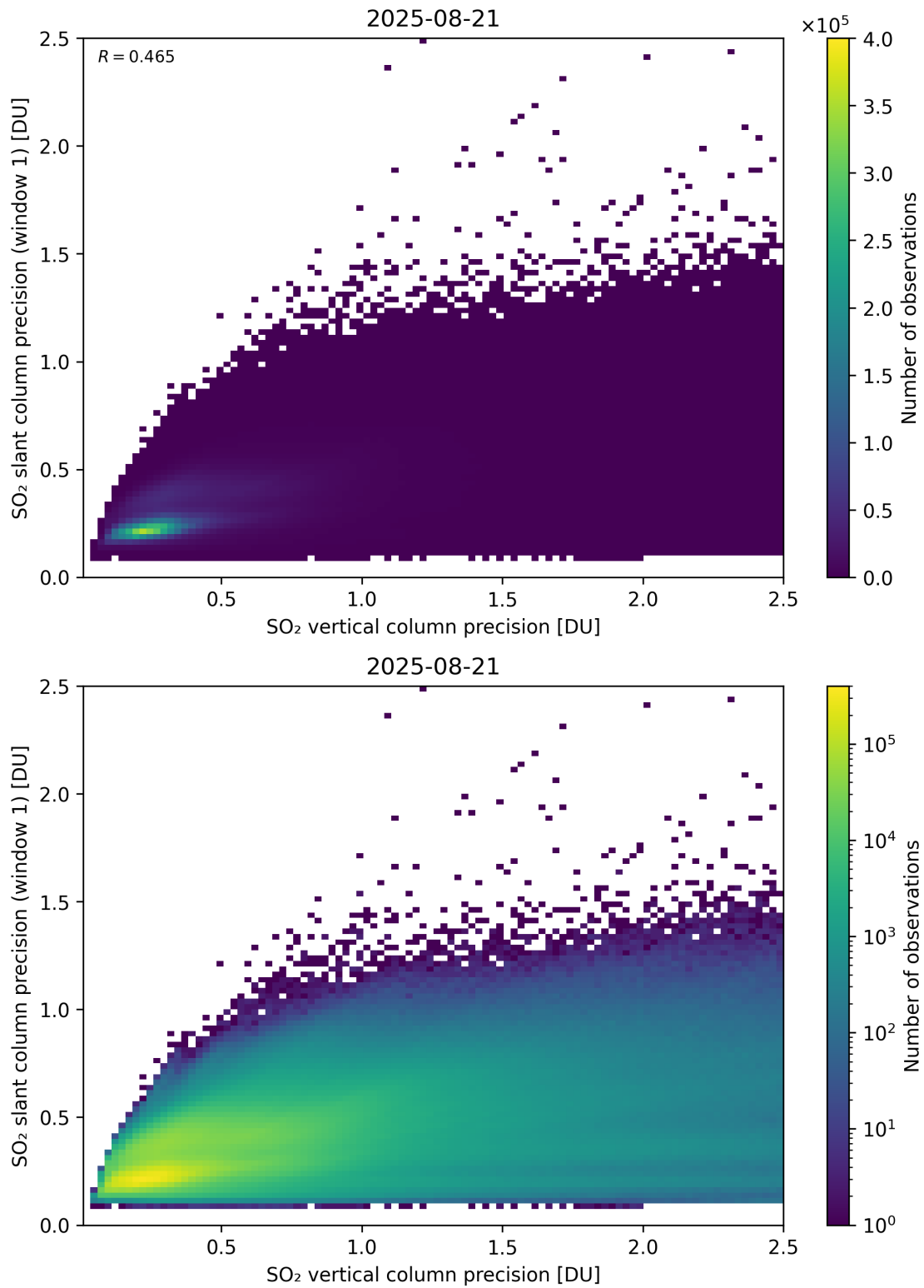
Figure 342: Scatter density plot of “SO 2 vertical column precision” against “SO 2 slant column precision (window 1)” for 2025-08-20 to 2025-08-22.
