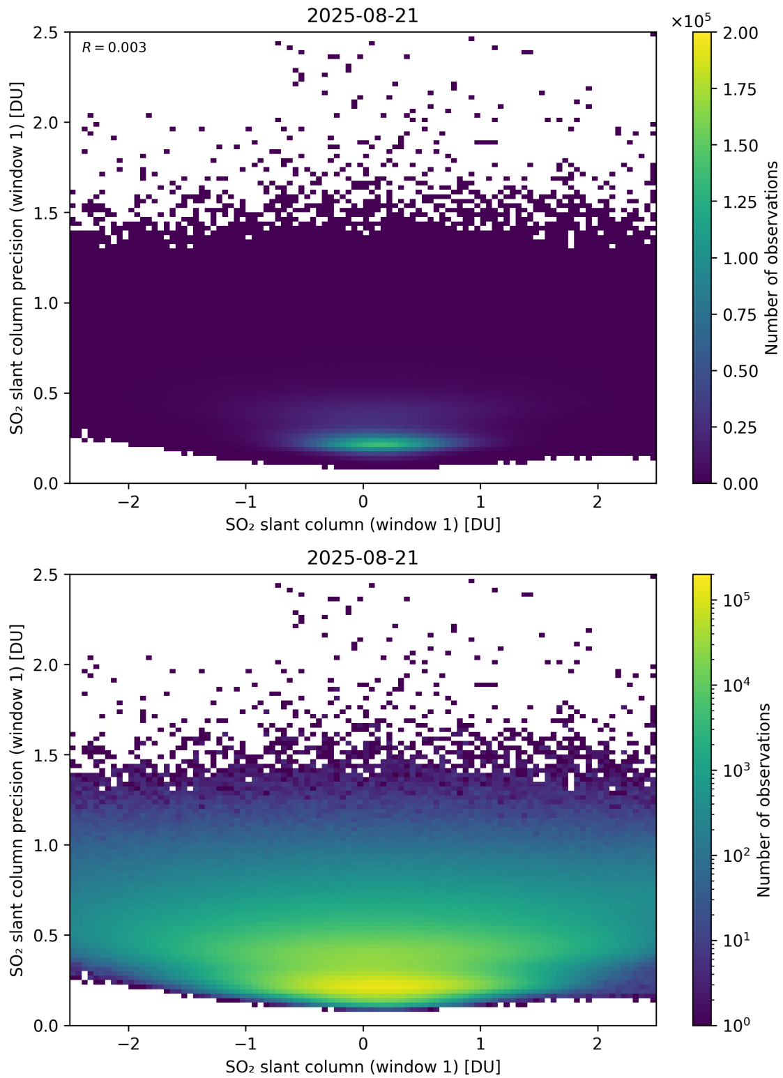
Figure 285: Scatter density plot of “SO 2 slant column (window 1)” against “SO 2 slant column precision (window 1)” for 2025-08-20 to 2025-08-22.
