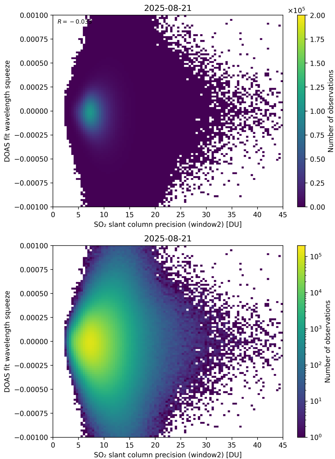
Figure 294: Scatter density plot of “SO 2 slant column precision (window2)” against “DOAS fit wavelength squeeze” for 2025-08-20 to 2025-08-22.
