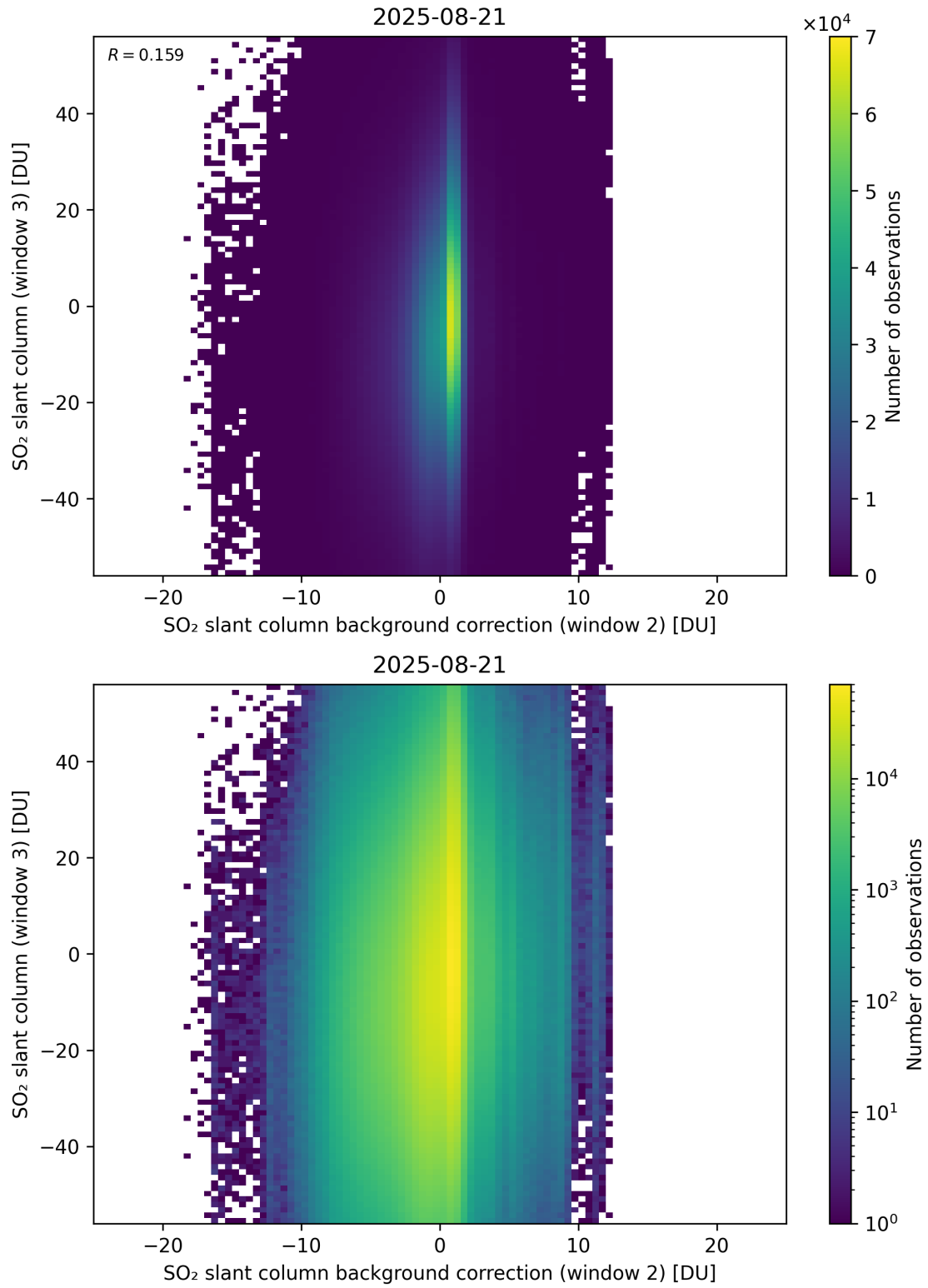
Figure 128: Scatter density plot of “SO 2 slant column background correction (window 2)” against “SO 2 slant column (window 3)” for 2025-08-20 to 2025-08-22.
