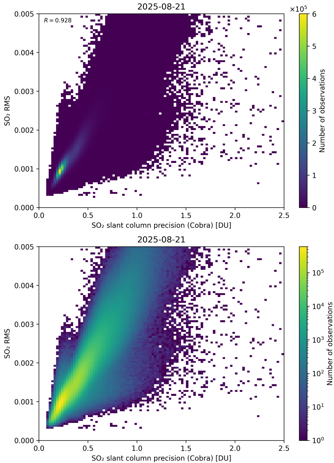
Figure 204: Scatter density plot of “SO 2 slant column precision (Cobra)” against “SO 2 RMS” for 2025-08-20 to 2025-08-22.
