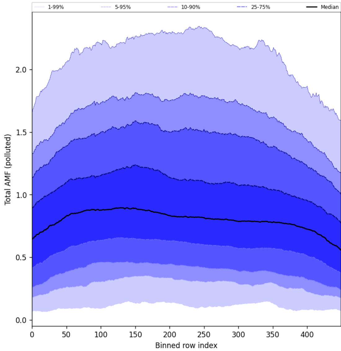
Figure 105: Along track statistics of “Total AMF (polluted)” for 2025-08-20 to 2025-08-22
