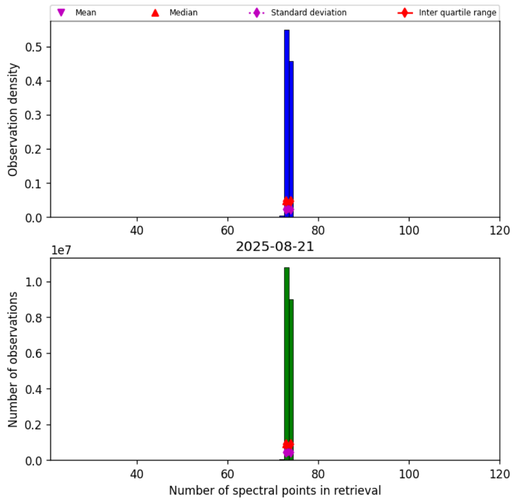
Figure 82: Histogram of "Number of spectral points in retrieval" for 2025-08-20 to 2025-08-22
