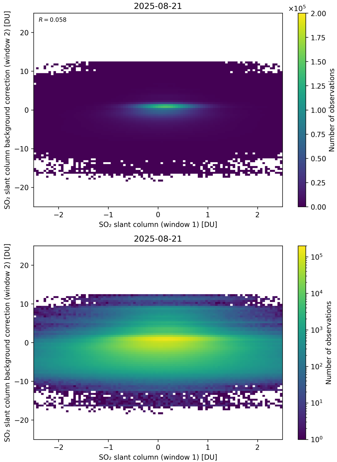
Figure 263: Scatter density plot of “SO 2 slant column (window 1)” against “SO 2 slant column background correction (window 2)” for 2025-08-20 to 2025-08-22.
