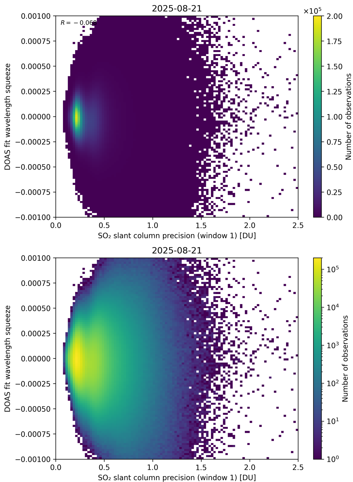
Figure 272: Scatter density plot of “SO 2 slant column precision (window 1)” against “DOAS fit wavelength squeeze” for 2025-08-20 to 2025-08-22.
