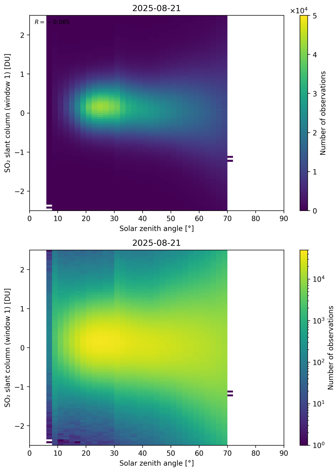
Figure 184: Scatter density plot of “Solar zenith angle” against “SO 2 slant column (window 1)” for 2025-08-20 to 2025-08-22.
