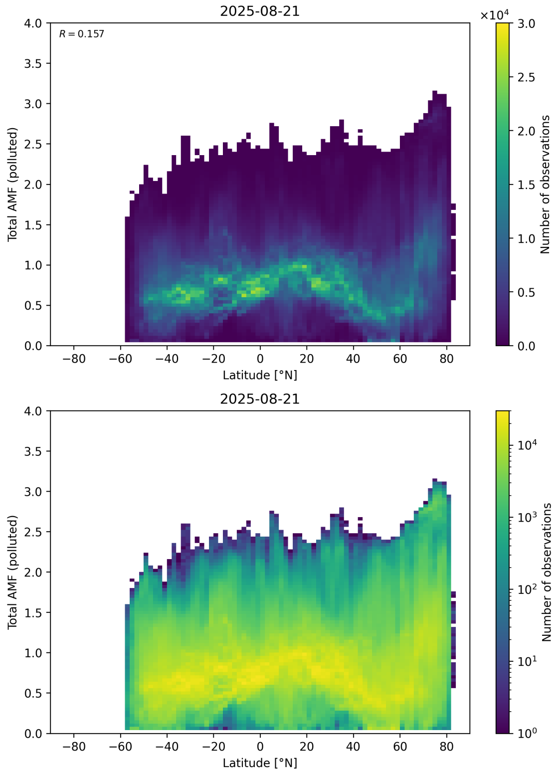
Figure 167: Scatter density plot of “Latitude” against “Total AMF (polluted)” for 2025-08-20 to 2025-08-22.
