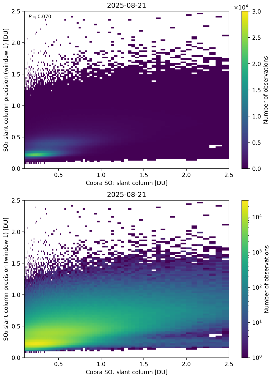
Figure 220: Scatter density plot of “Cobra SO 2 slant column” against “SO 2 slant column precision (window 1)” for 2025-08-20 to 2025-08-22.
