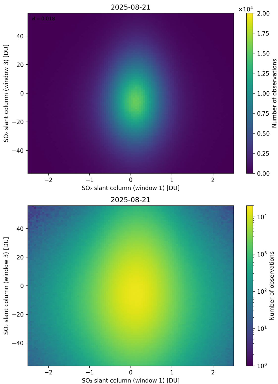
Figure 287: Scatter density plot of “SO 2 slant column (window 1)” against “SO 2 slant column (window 3)” for 2025-08-20 to 2025-08-22.
