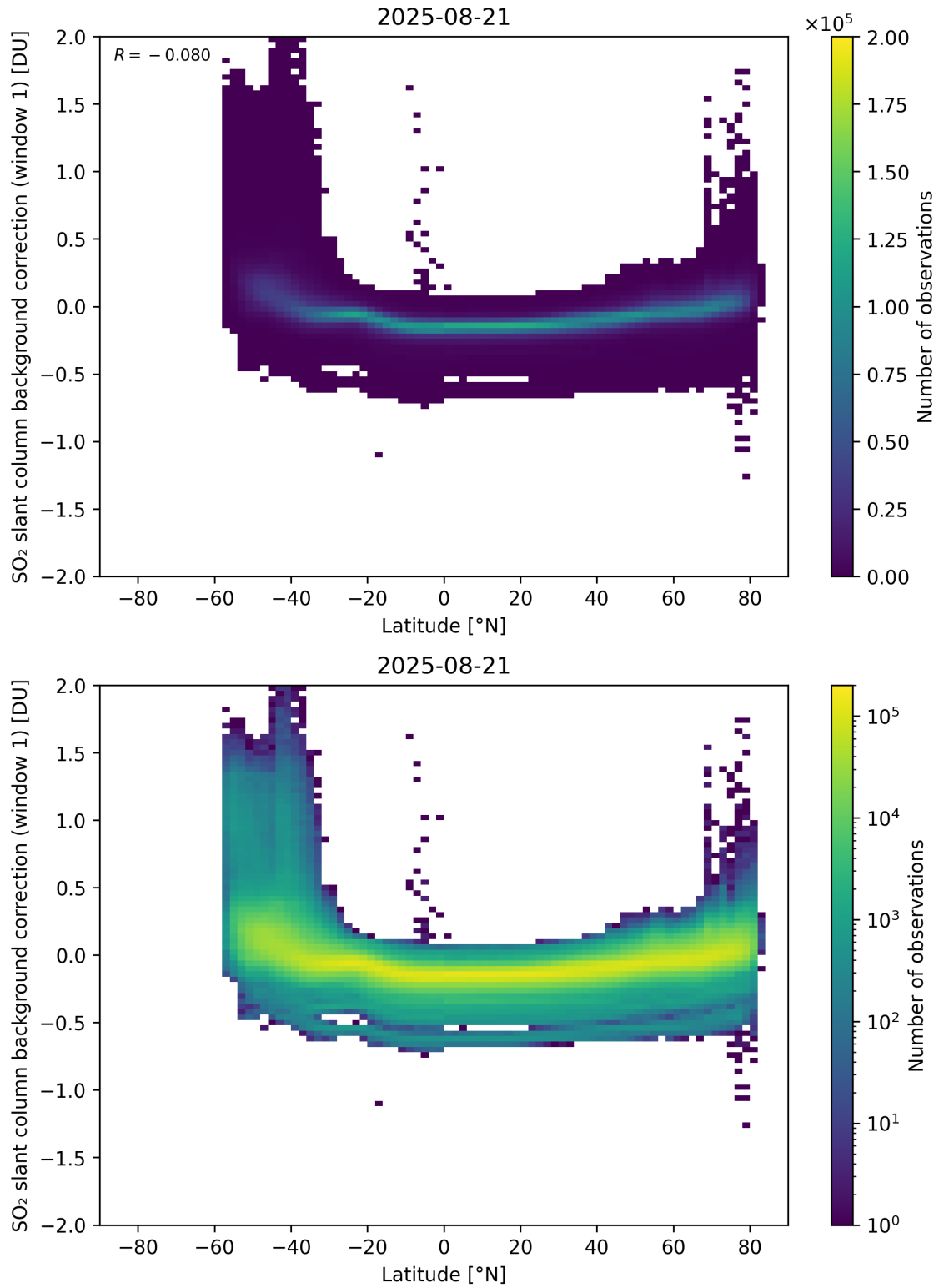
Figure 150: Scatter density plot of “Latitude” against “SO 2 slant column background correction (window 1)” for 2025-08-20 to 2025-08-22.
