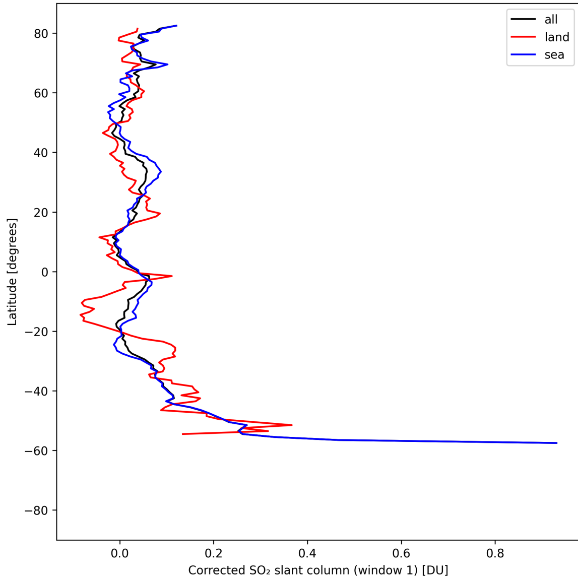
Figure 39: Zonal average of “Corrected SO 2 slant column (window 1)” for 2025-08-20 to 2025-08-22.
