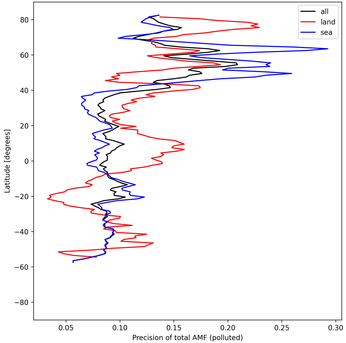
Figure 54: Zonal average of “Precision of total AMF (polluted)” for 2025-08-20 to 2025-08-22.
