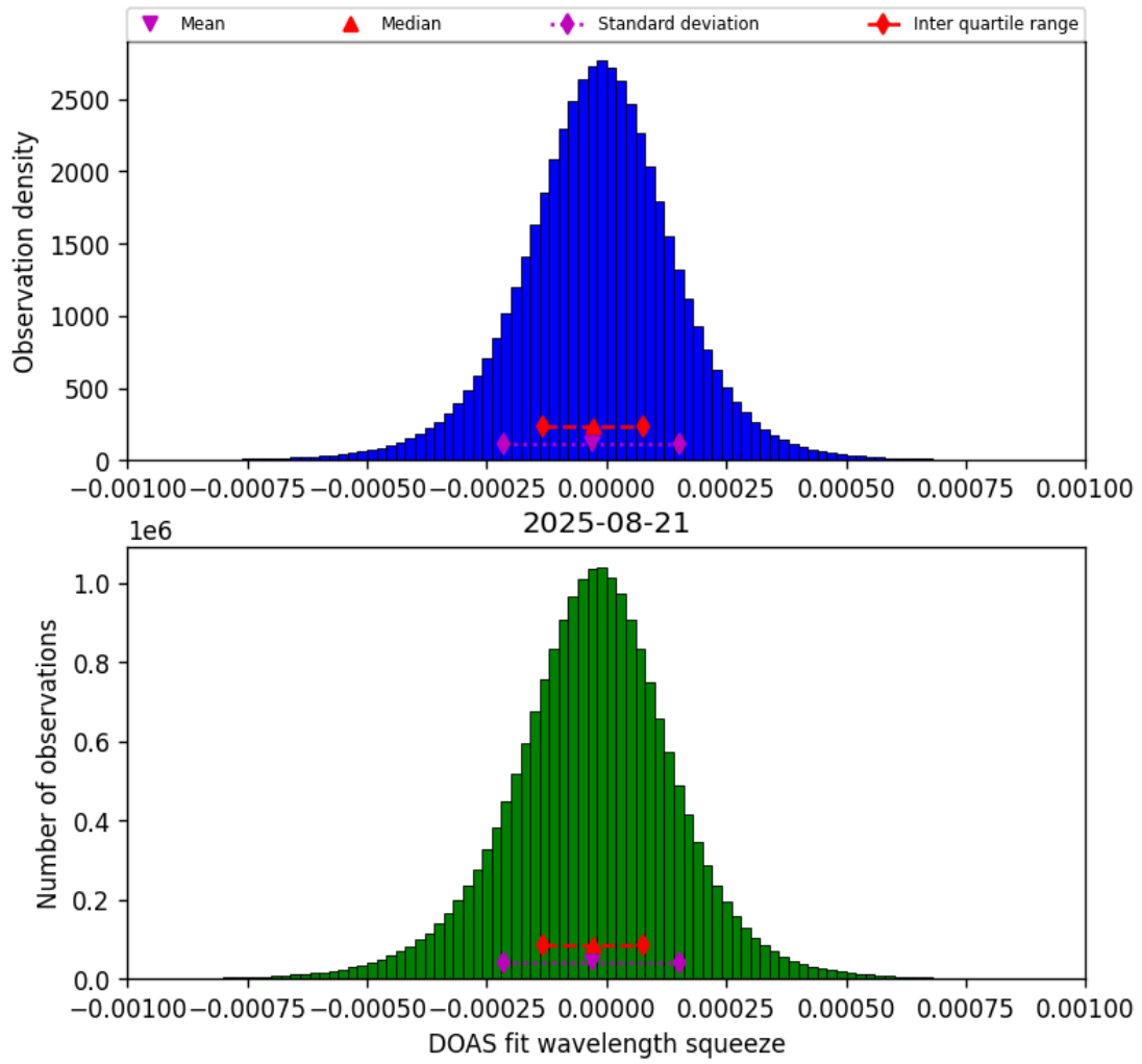
Figure 77: Histogram of “DOAS fit wavelength squeeze” for 2025-08-20 to 2025-08-22
