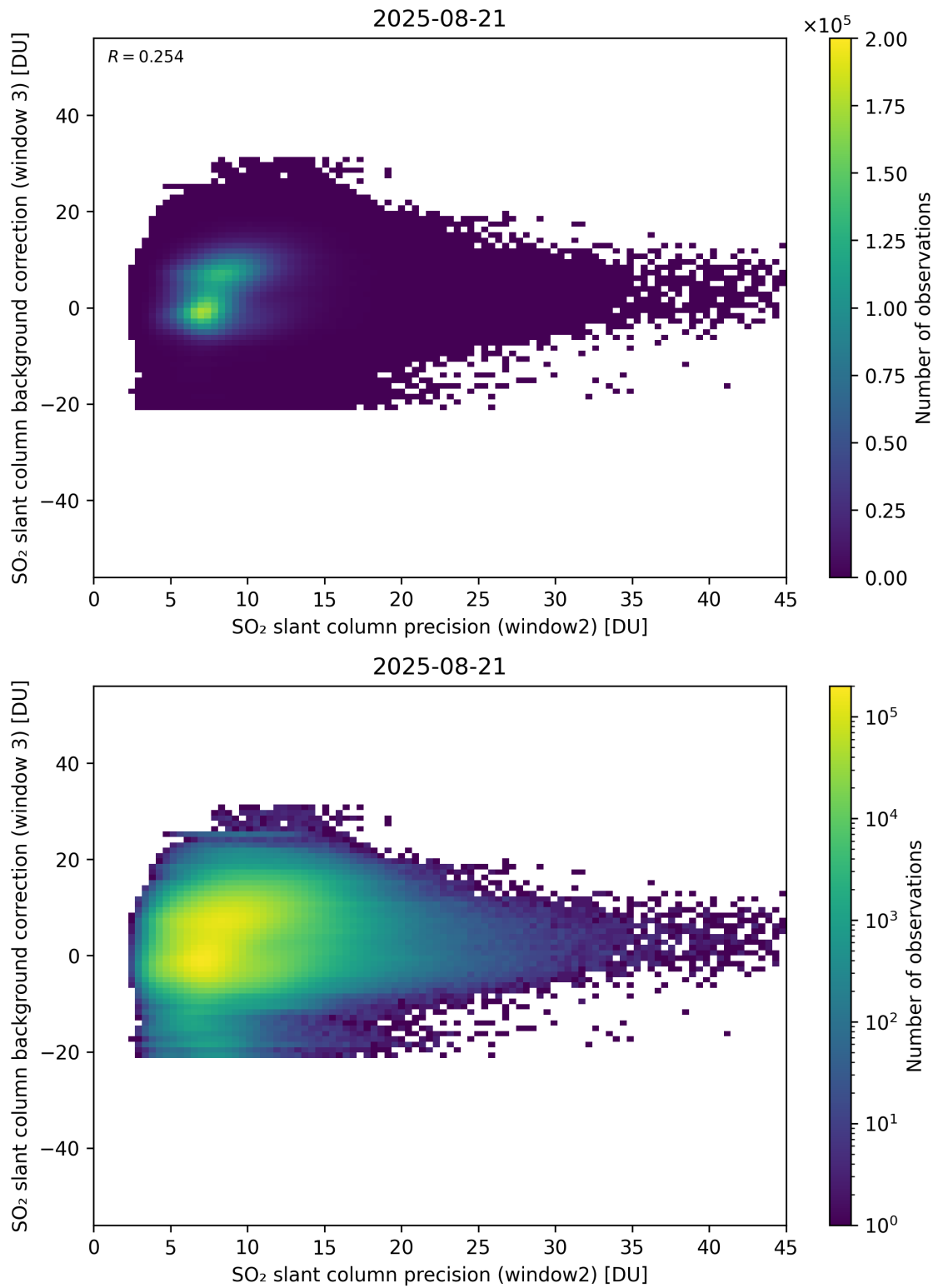
Figure 292: Scatter density plot of “SO 2 slant column precision (window2)” against “SO 2 slant column background correction (window 3)” for 2025-08-20 to 2025-08-22.
