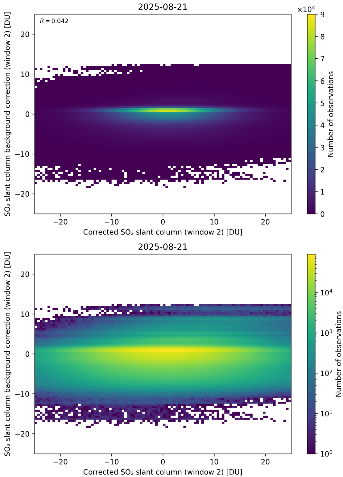
Figure 244: Scatter density plot of “Corrected SO 2 slant column (window 2)” against “SO 2 slant column background correction (window 2)” for 2025-08-20 to 2025-08-22.
