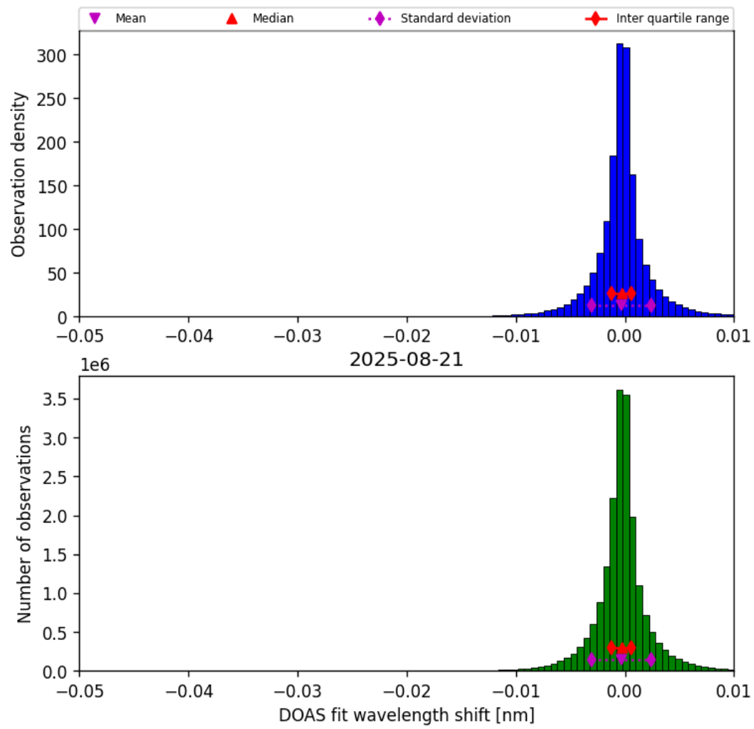
Figure 76: Histogram of “DOAS fit wavelength shift” for 2025-08-20 to 2025-08-22
