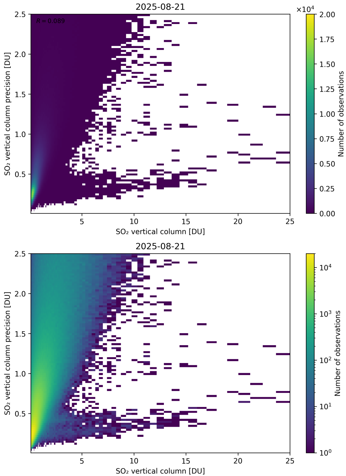
Figure 361: Scatter density plot of “SO 2 vertical column” against “SO 2 vertical column precision” for 2025-08-20 to 2025-08-22.
