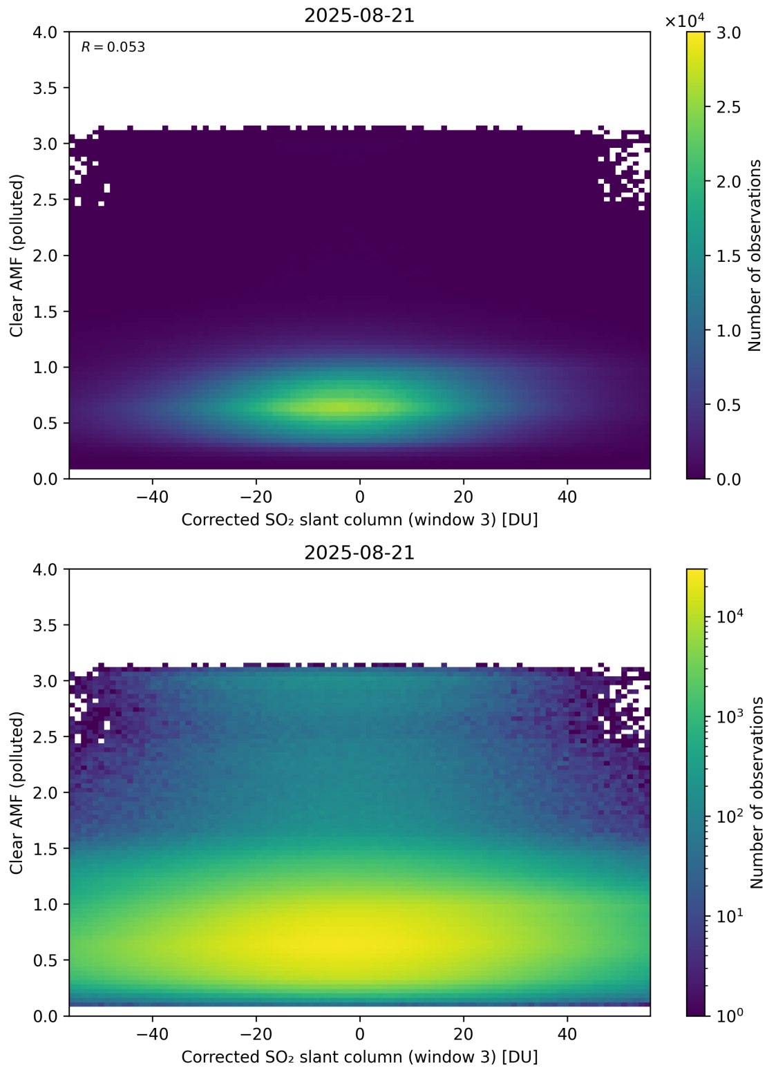
Figure 259: Scatter density plot of “Corrected SO 2 slant column (window 3)” against “Clear AMF (polluted)” for 2025-08-20 to 2025-08-22.
