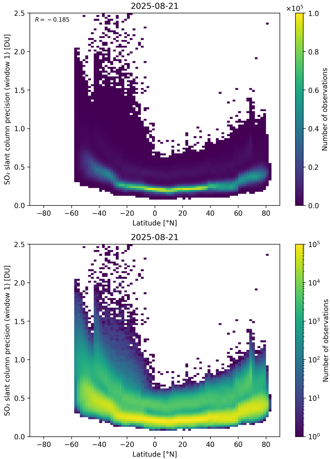
Figure 163: Scatter density plot of “Latitude” against “SO 2 slant column precision (window 1)” for 2025-08-20 to 2025-08-22.
