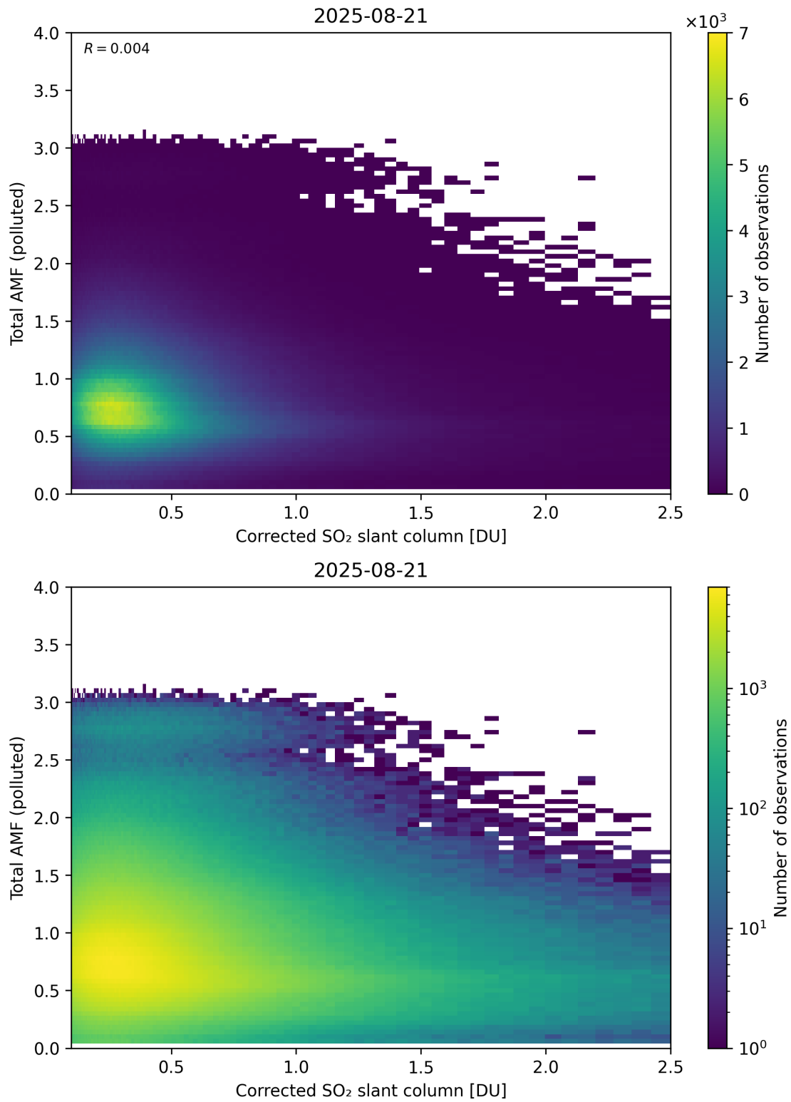
Figure 242: Scatter density plot of “Corrected SO 2 slant column” against “Total AMF (polluted)” for 2025-08-20 to 2025-08-22.
