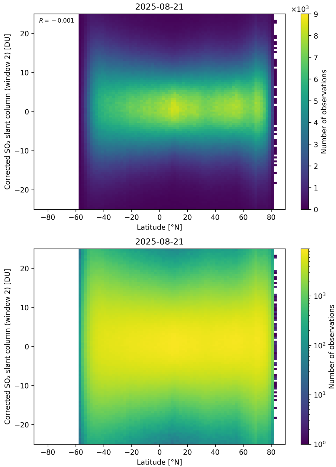
Figure 160: Scatter density plot of “Latitude” against “Corrected SO 2 slant column (window 2)” for 2025-08-20 to 2025-08-22.
