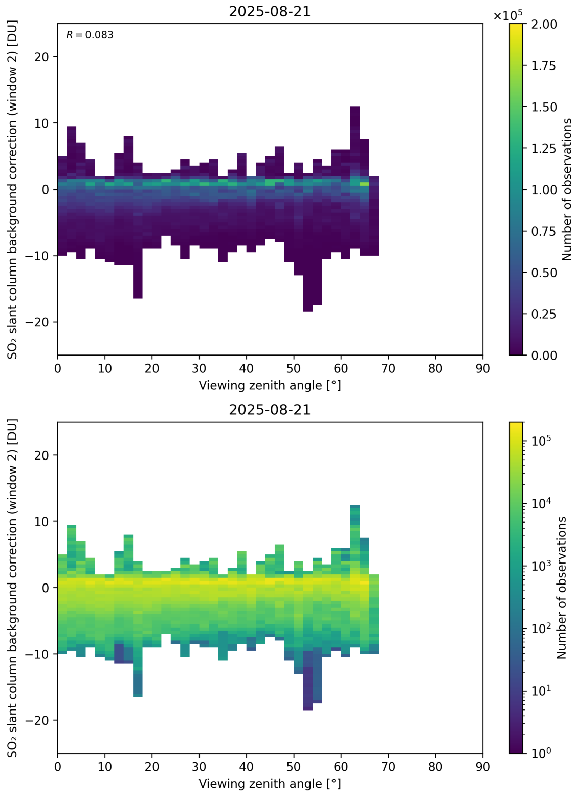
Figure 363: Scatter density plot of “Viewing zenith angle” against “SO 2 slant column background correction (window 2)” for 2025-08-20 to 2025-08-22.
