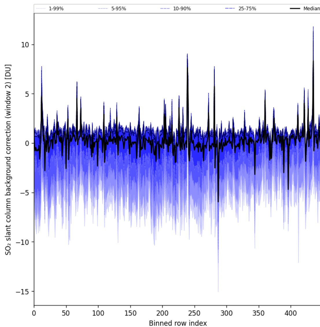
Figure 96: Along track statistics of “SO 2 slant column background correction (window 2)” for 2025-08-20 to 2025-08-22
