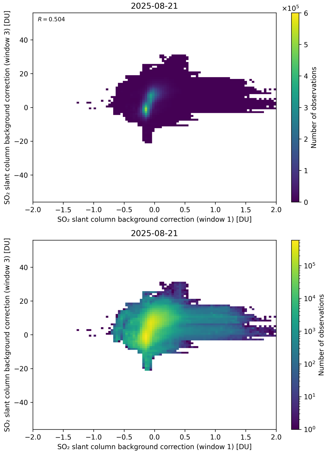
Figure 110: Scatter density plot of “SO 2 slant column background correction (window 1)” against “SO 2 slant column background correction (window 3)” for 2025-08-20 to 2025-08-22.
