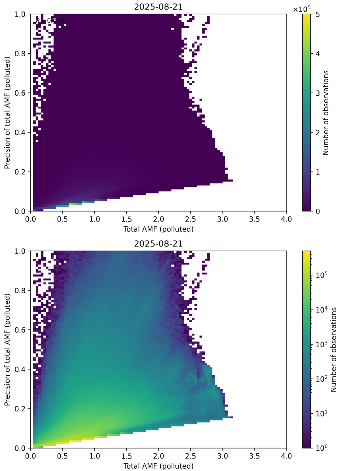
Figure 322: Scatter density plot of “Total AMF (polluted)” against “Precision of total AMF (polluted)” for 2025-08-20 to 2025-08-22.
