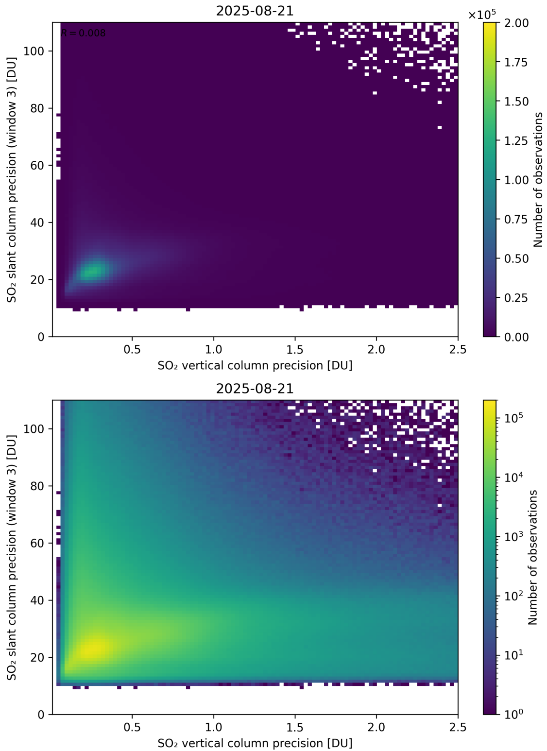
Figure 345: Scatter density plot of “SO 2 vertical column precision” against “SO 2 slant column precision (window 3)” for 2025-08-20 to 2025-08-22.
