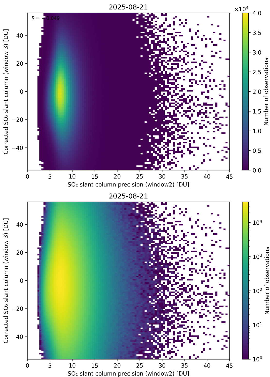
Figure 298: Scatter density plot of “SO 2 slant column precision (window2)” against “Corrected SO 2 slant column (window 3)” for 2025-08-20 to 2025-08-22.
