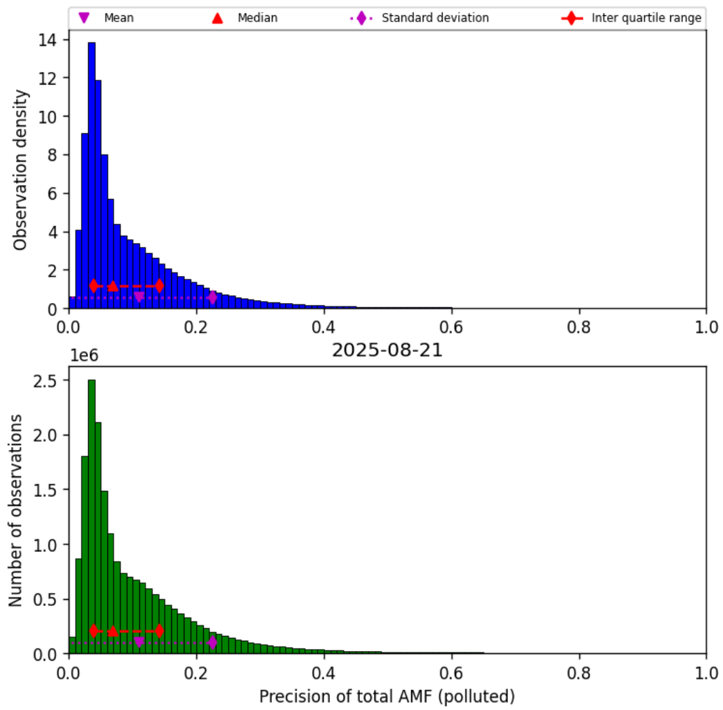
Figure 80: Histogram of “Precision of total AMF (polluted)” for 2025-08-20 to 2025-08-22
