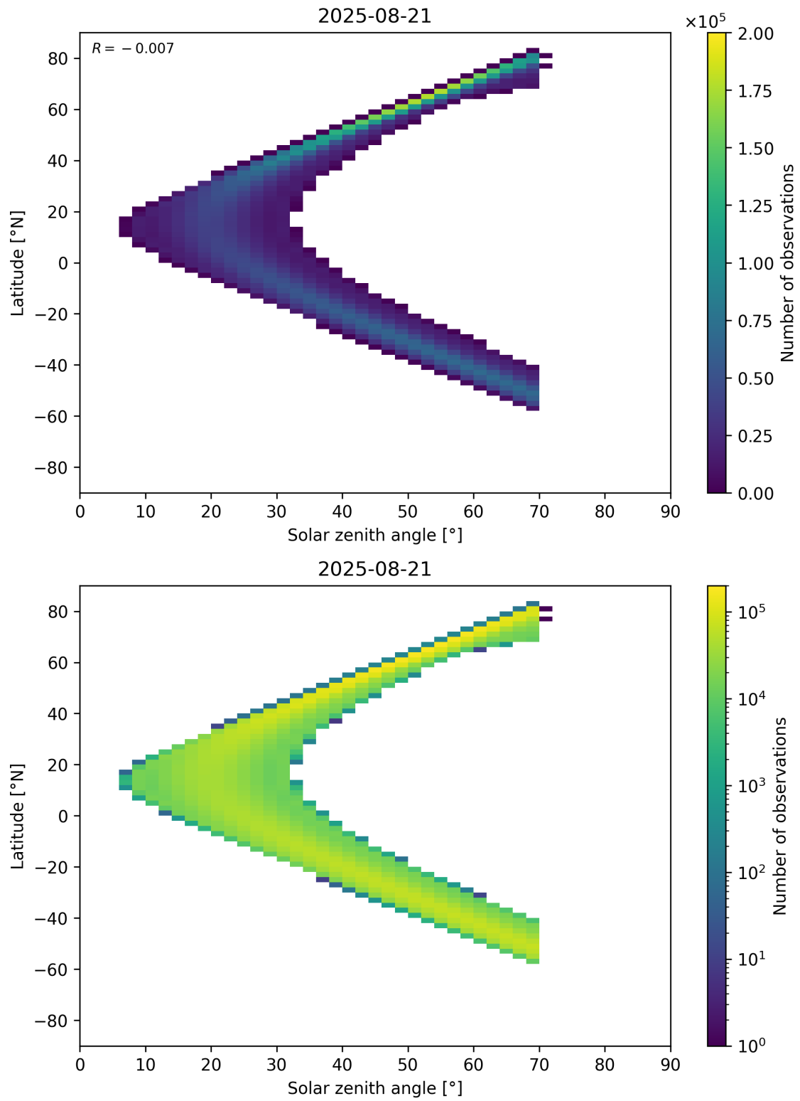
Figure 177: Scatter density plot of “Solar zenith angle” against “Latitude” for 2025-08-20 to 2025-08-22.
