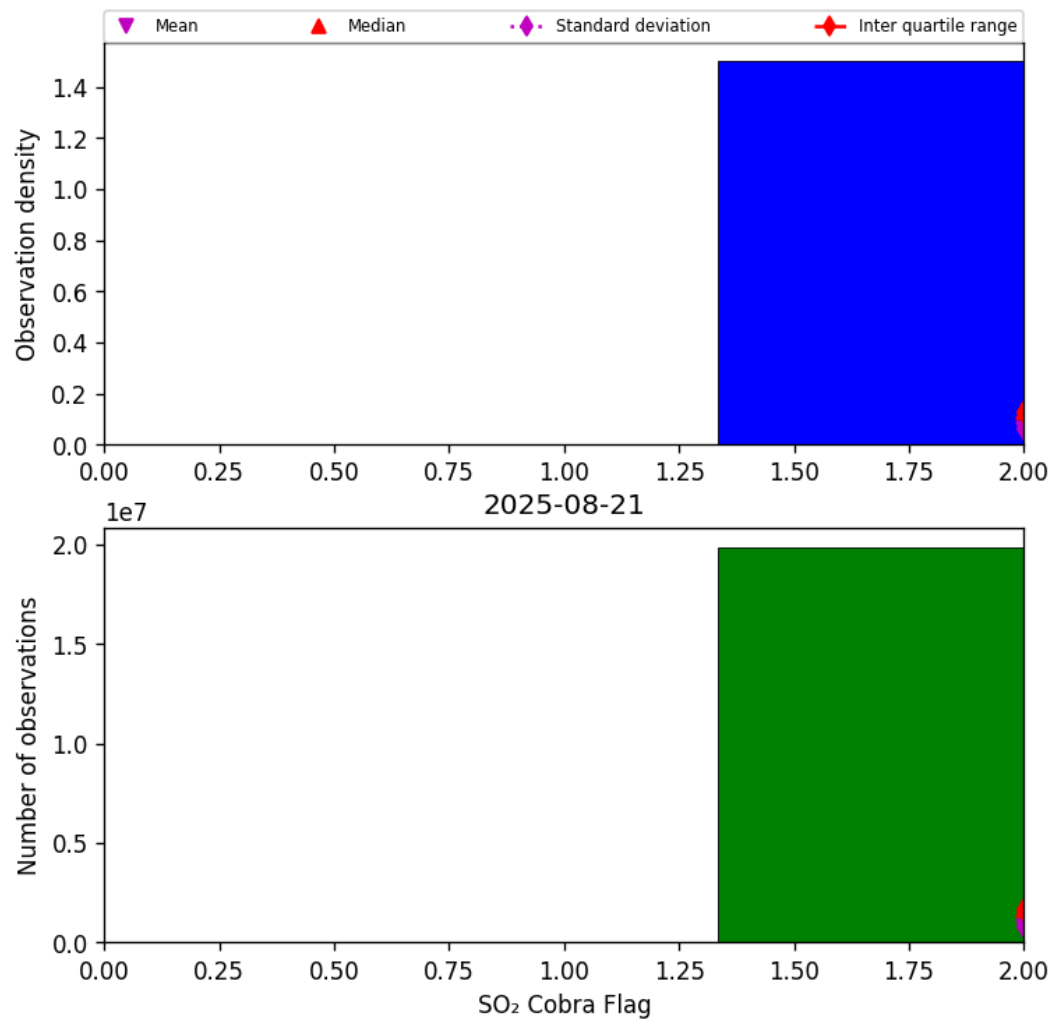
Figure 75: Histogram of “SO 2 Cobra Flag” for 2025-08-20 to 2025-08-22
