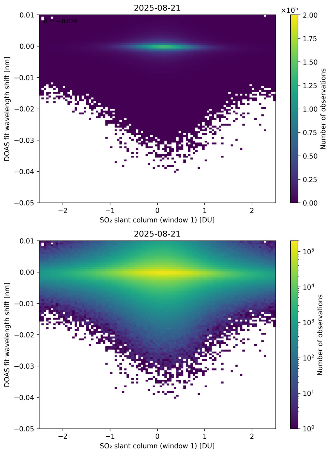
Figure 265: Scatter density plot of “SO 2 slant column (window 1)” against “DOAS fit wavelength shift” for 2025-08-20 to 2025-08-22.
