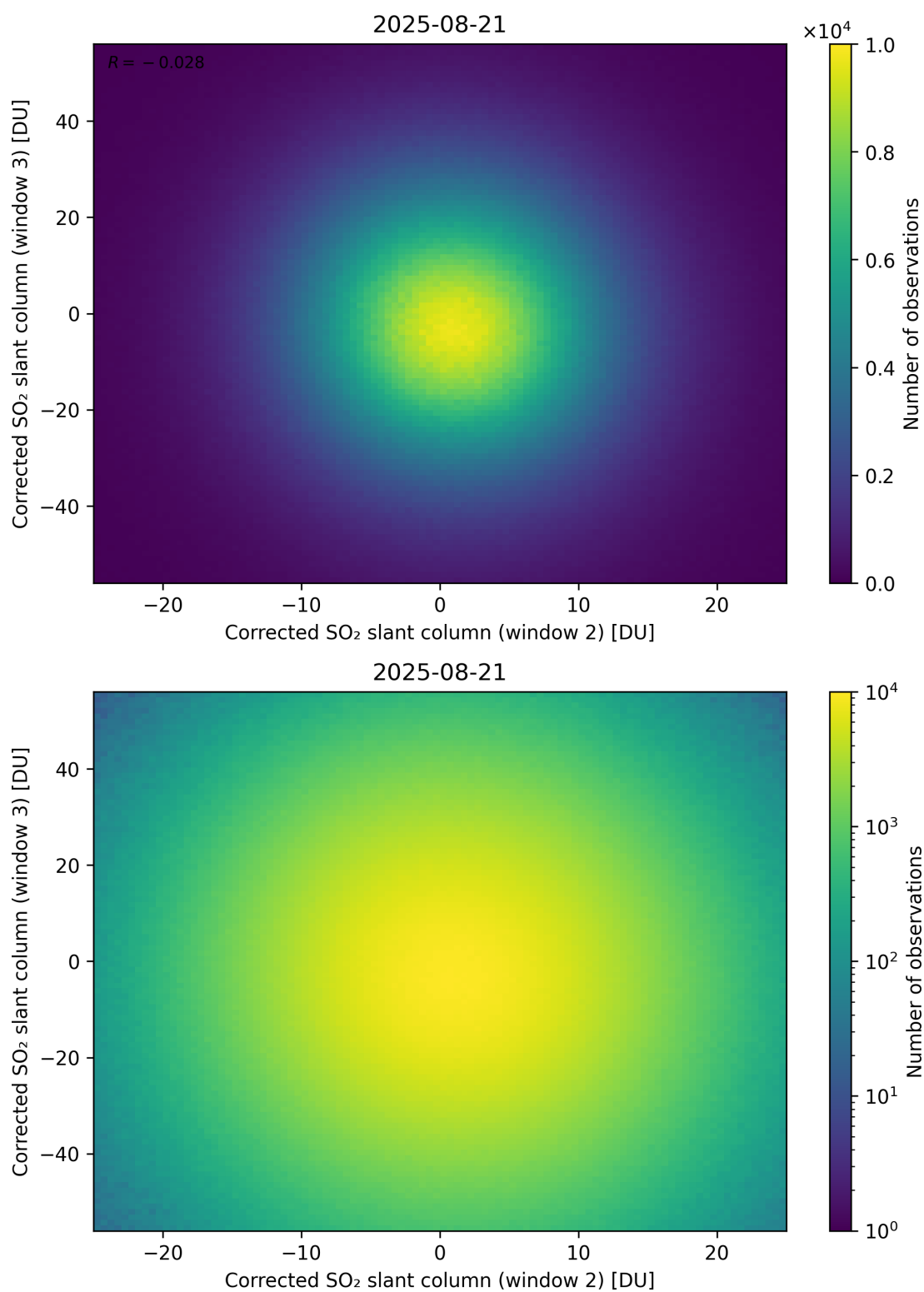
Figure 250: Scatter density plot of “Corrected SO 2 slant column (window 2)” against “Corrected SO 2 slant column (window 3)” for 2025-08-20 to 2025-08-22.
