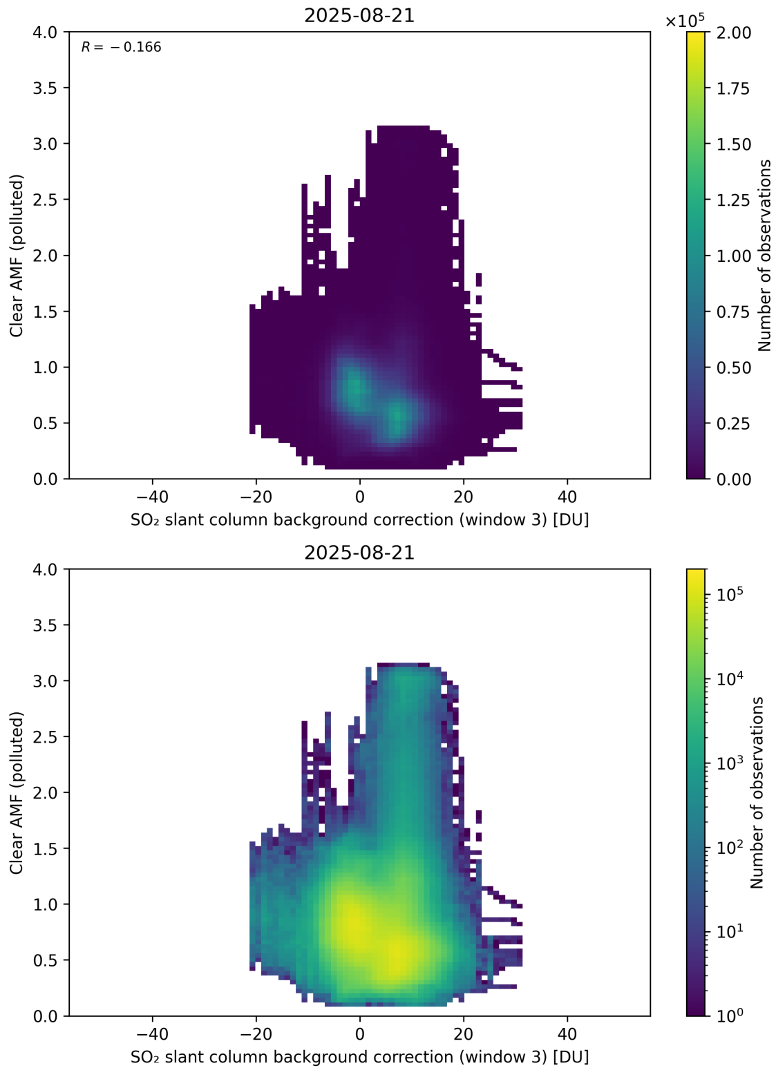
Figure 135: Scatter density plot of “SO 2 slant column background correction (window 3)” against “Clear AMF (polluted)” for 2025-08-20 to 2025-08-22.
