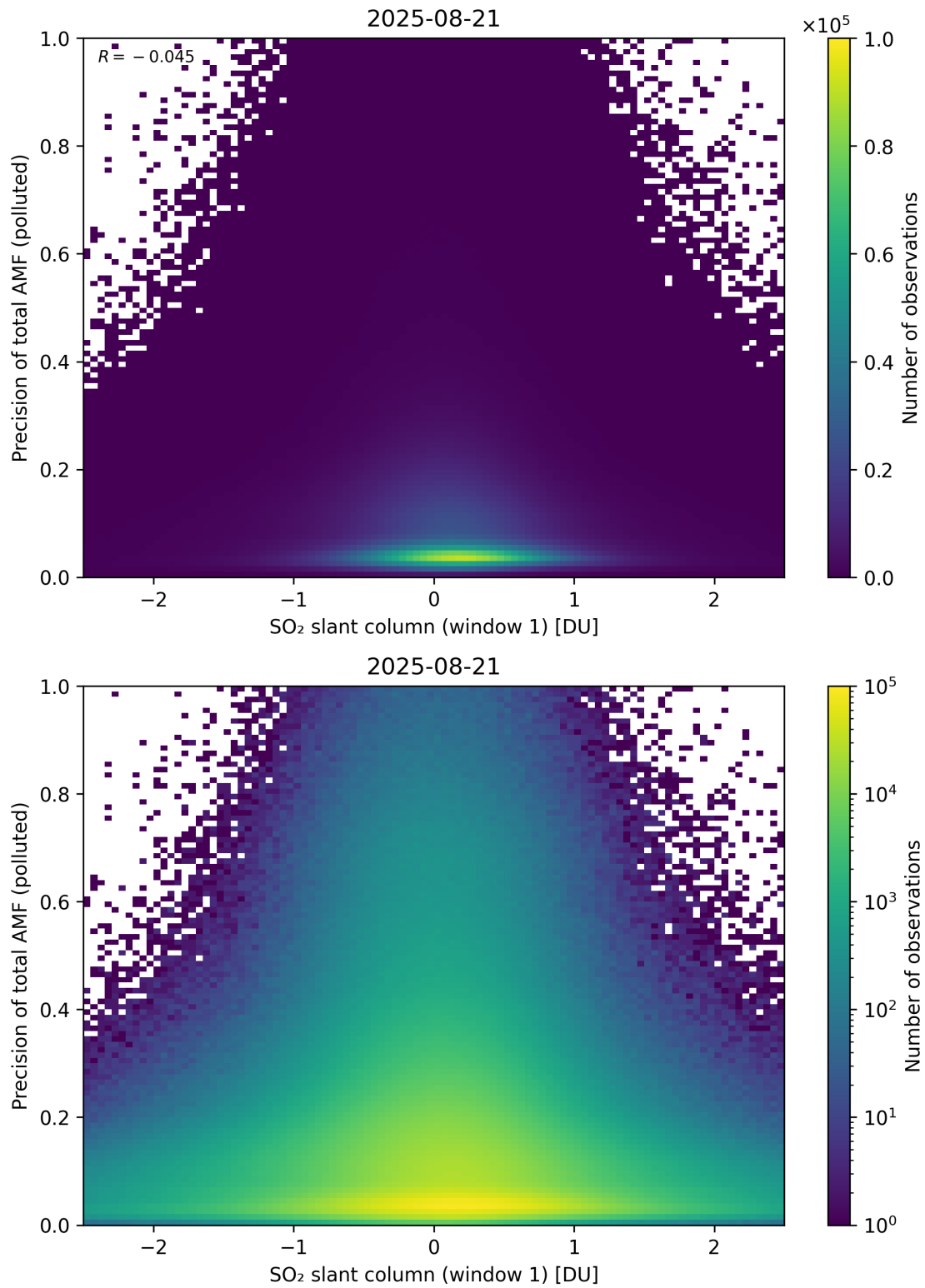
Figure 290: Scatter density plot of “SO 2 slant column (window 1)” against “Precision of total AMF (polluted)” for 2025-08-20 to 2025-08-22.
