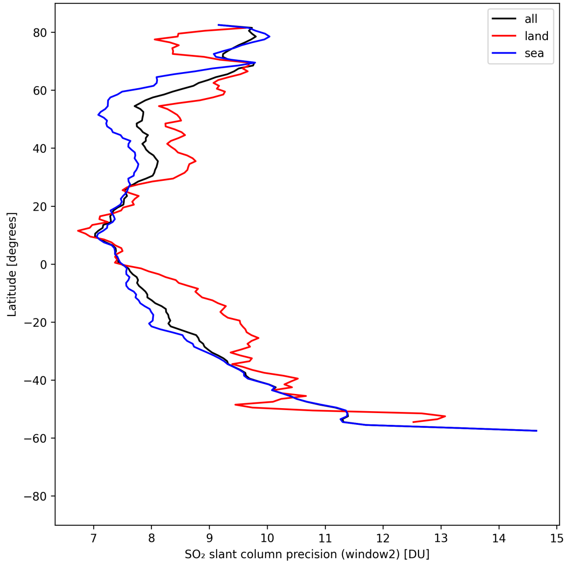
Figure 42: Zonal average of “SO 2 slant column precision (window2)” for 2025-08-20 to 2025-08-22.
