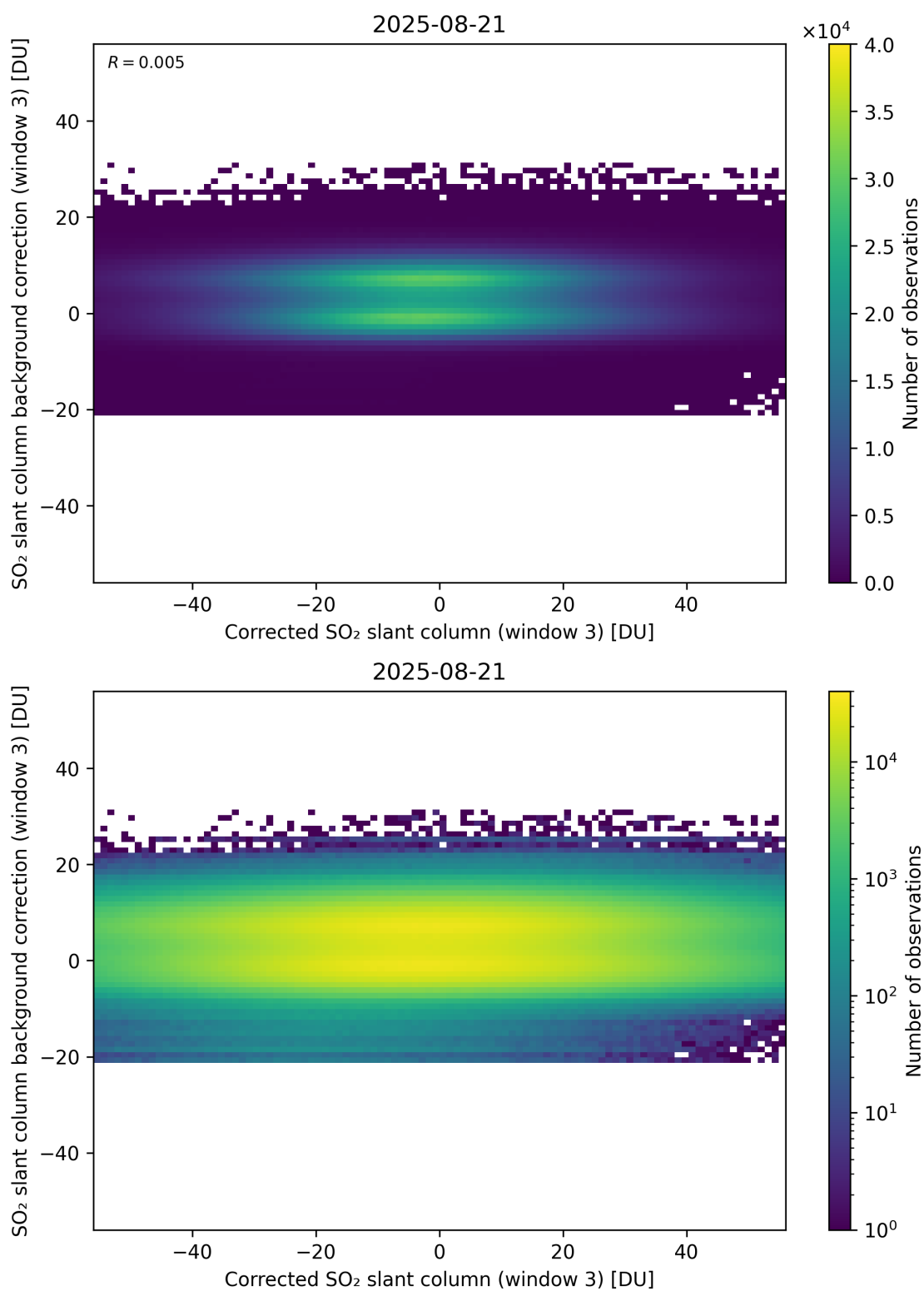
Figure 255: Scatter density plot of “Corrected SO 2 slant column (window 3)” against “SO 2 slant column background correction (window 3)” for 2025-08-20 to 2025-08-22.
