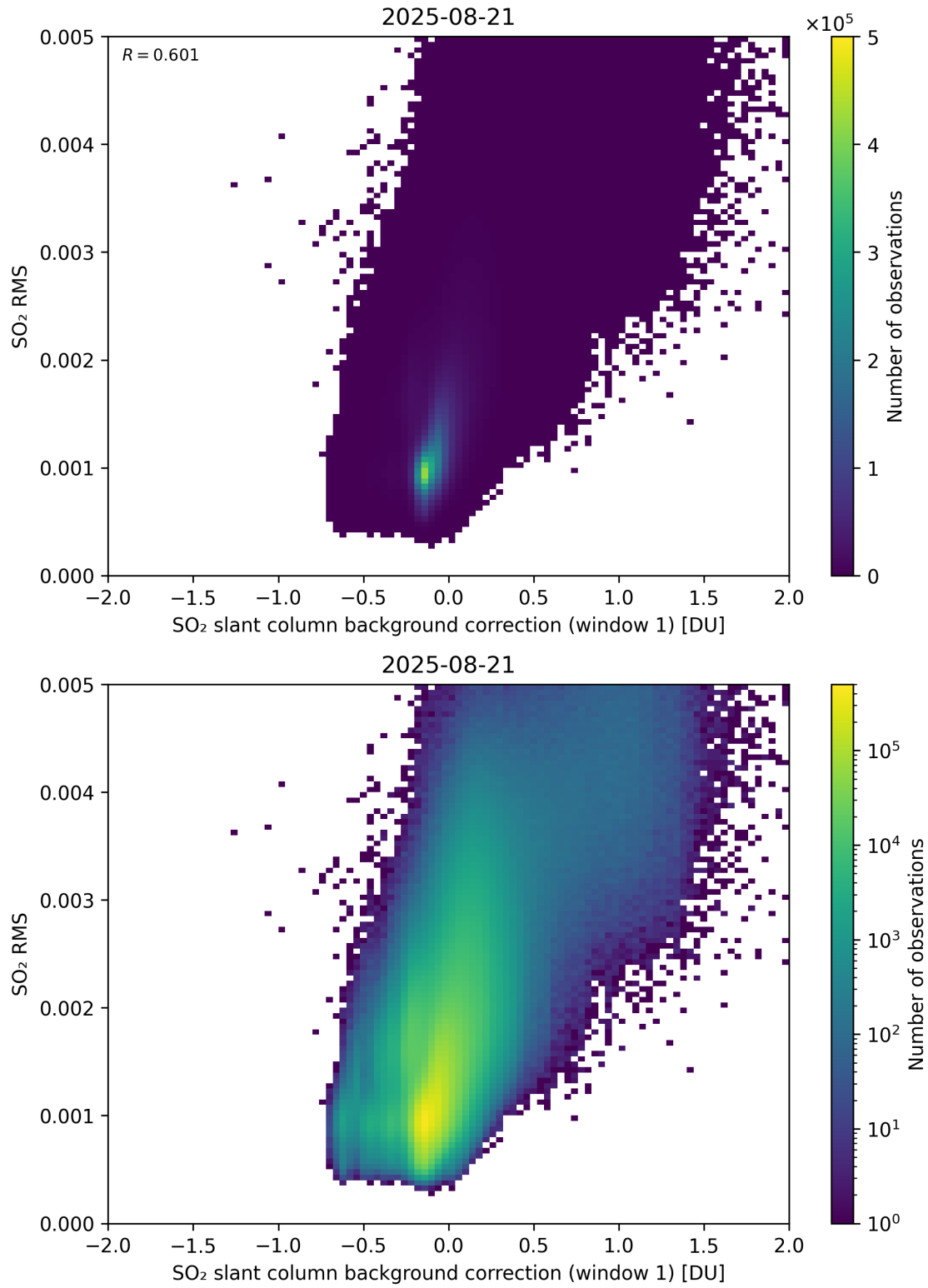
Figure 113: Scatter density plot of “SO 2 slant column background correction (window 1)” against “SO 2 RMS” for 2025-08-20 to 2025-08-22.
