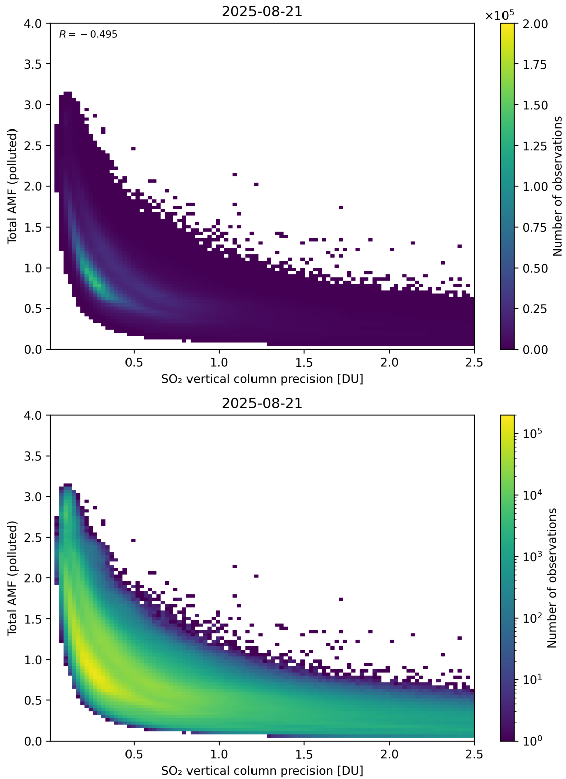
Figure 346: Scatter density plot of “SO 2 vertical column precision” against “Total AMF (polluted)” for 2025-08-20 to 2025-08-22.
