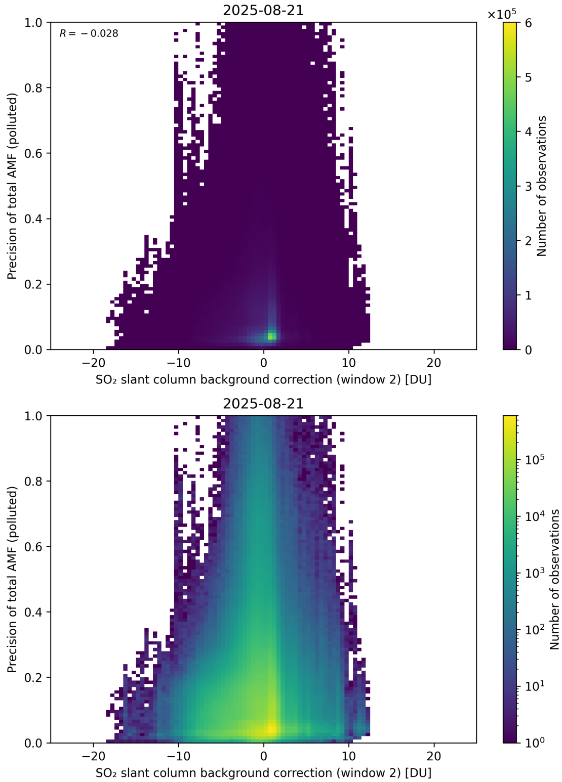
Figure 131: Scatter density plot of “SO 2 slant column background correction (window 2)” against “Precision of total AMF (polluted)” for 2025-08-20 to 2025-08-22.
