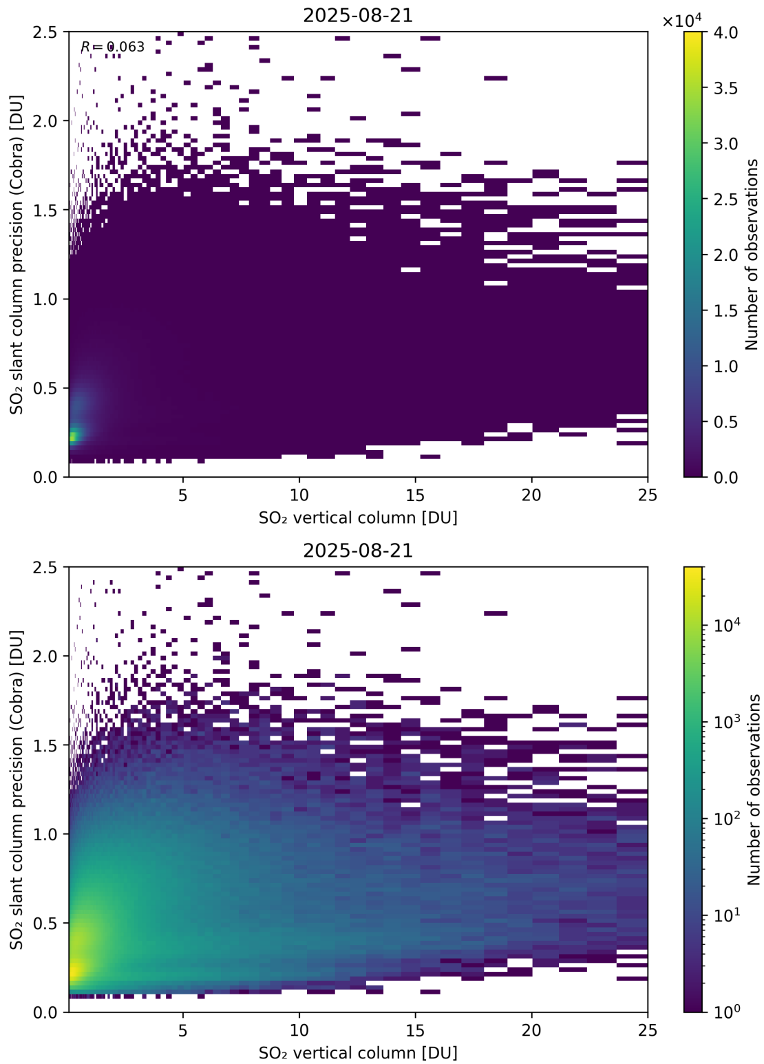
Figure 350: Scatter density plot of “SO 2 vertical column” against “SO 2 slant column precision (Cobra)” for 2025-08-20 to 2025-08-22.
