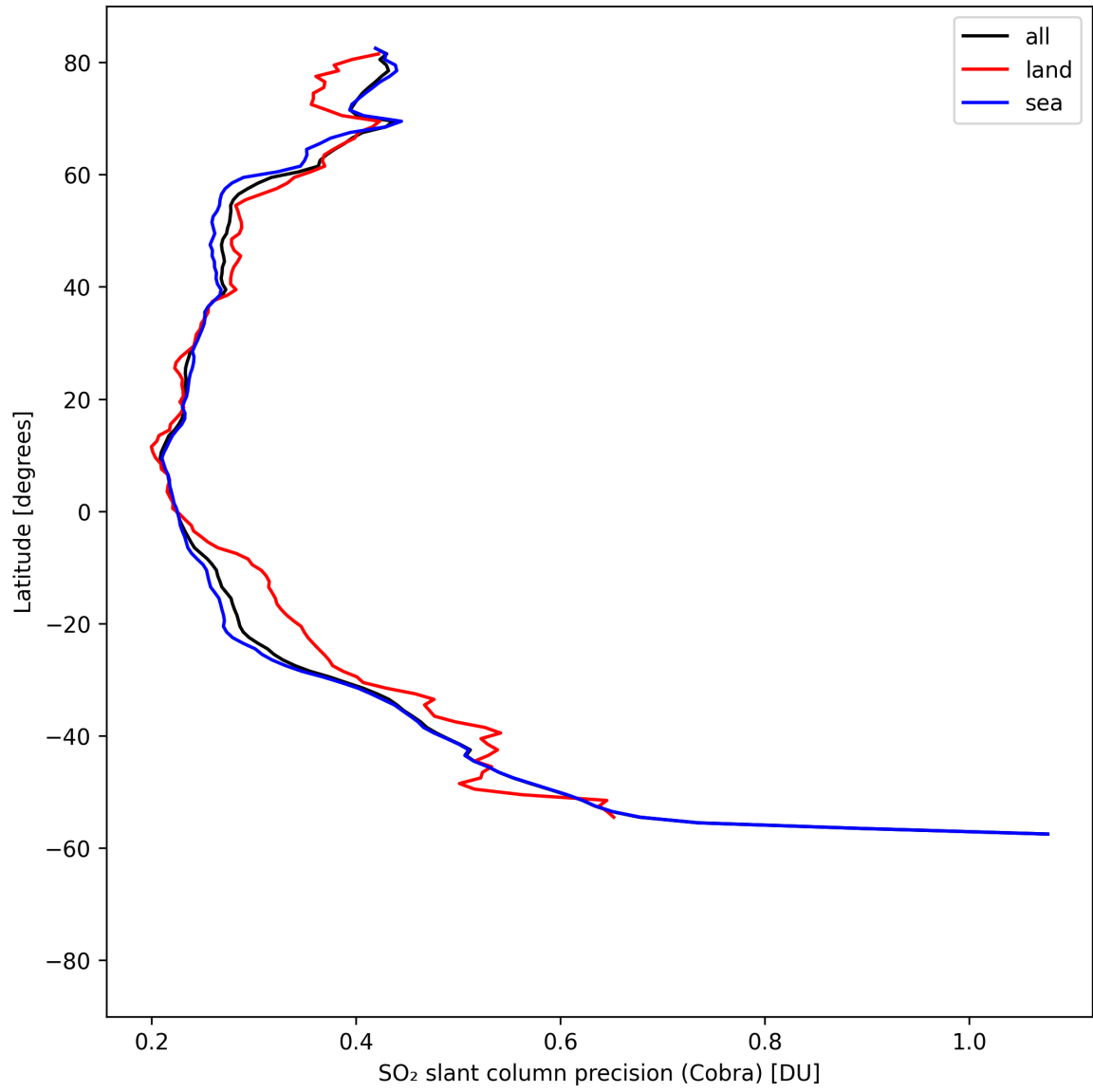
Figure 36: Zonal average of “SO 2 slant column precision (Cobra)” for 2025-08-20 to 2025-08-22.
