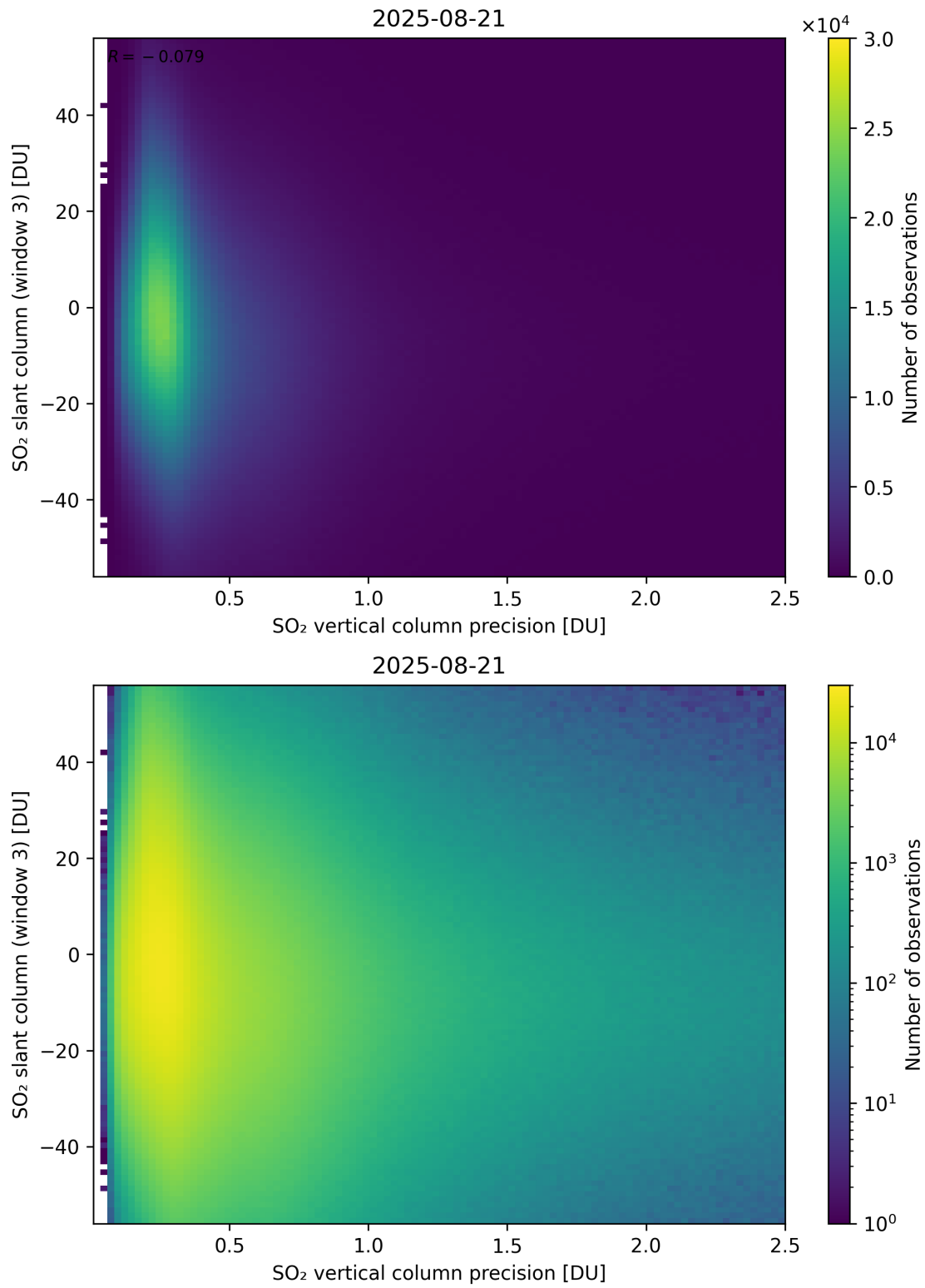
Figure 344: Scatter density plot of “SO 2 vertical column precision” against “SO 2 slant column (window 3)” for 2025-08-20 to 2025-08-22.
