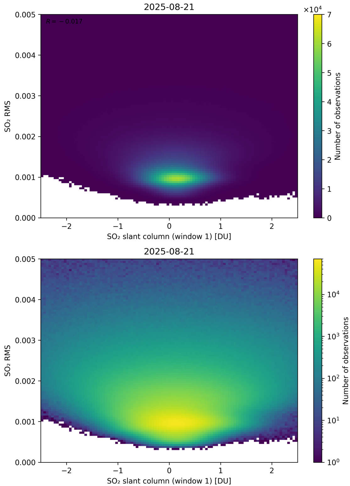
Figure 267: Scatter density plot of “SO 2 slant column (window 1)” against “SO 2 RMS” for 2025-08-20 to 2025-08-22.
