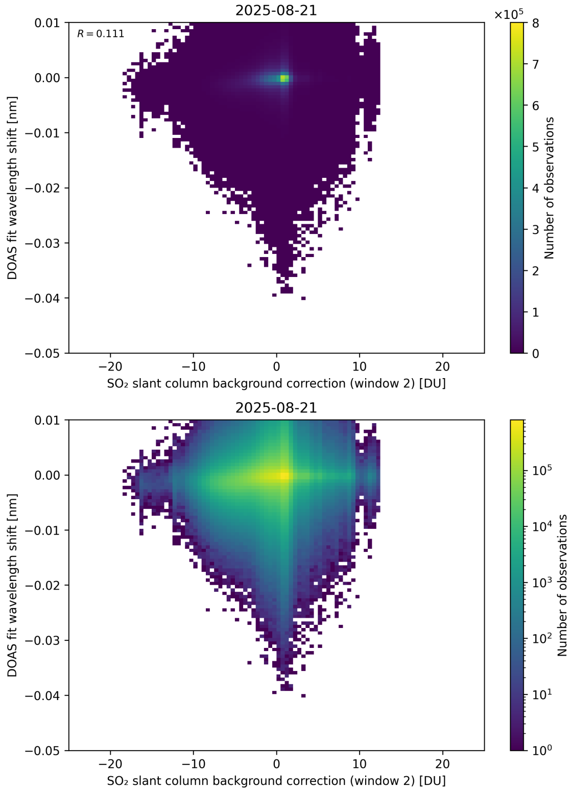
Figure 123: Scatter density plot of “SO 2 slant column background correction (window 2)” against “DOAS fit wavelength shift” for 2025-08-20 to 2025-08-22.
