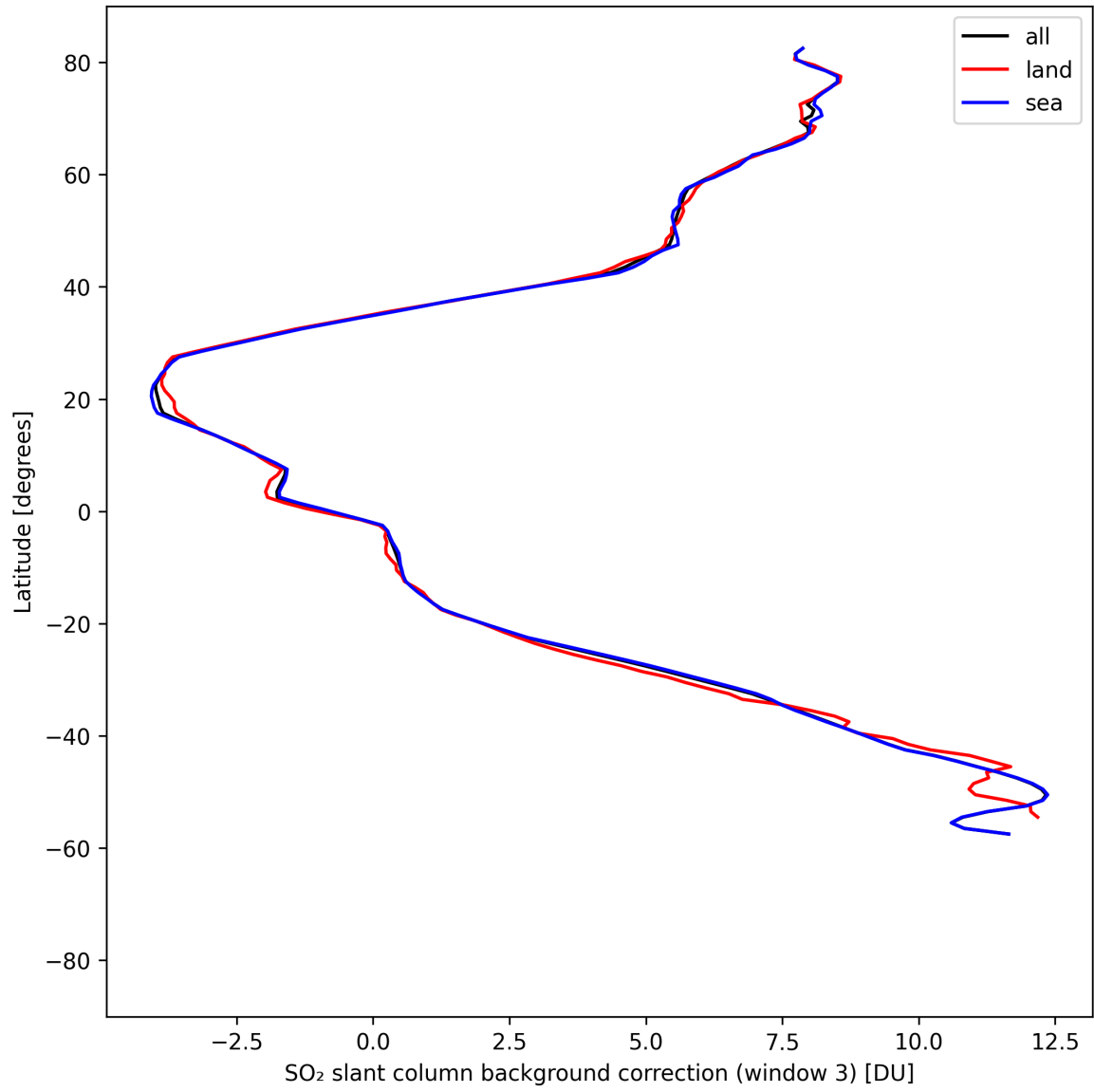
Figure 48: Zonal average of “SO 2 slant column background correction (window 3)” for 2025-08-20 to 2025-08-22.
