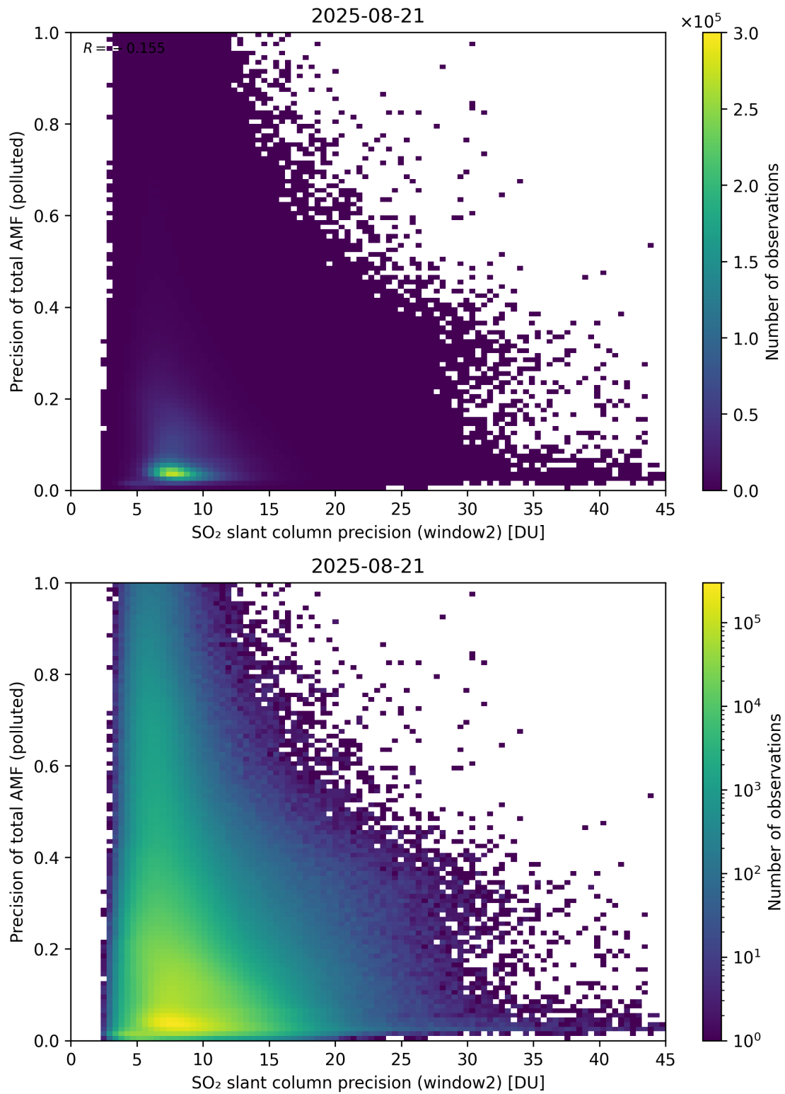
Figure 302: Scatter density plot of “SO 2 slant column precision (window2)” against “Precision of total AMF (polluted)” for 2025-08-20 to 2025-08-22.
