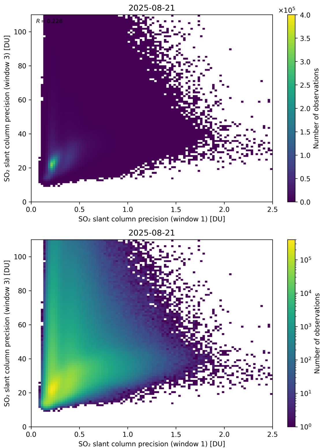
Figure 279: Scatter density plot of “SO 2 slant column precision (window 1)” against “SO 2 slant column precision (window 3)” for 2025-08-20 to 2025-08-22.
