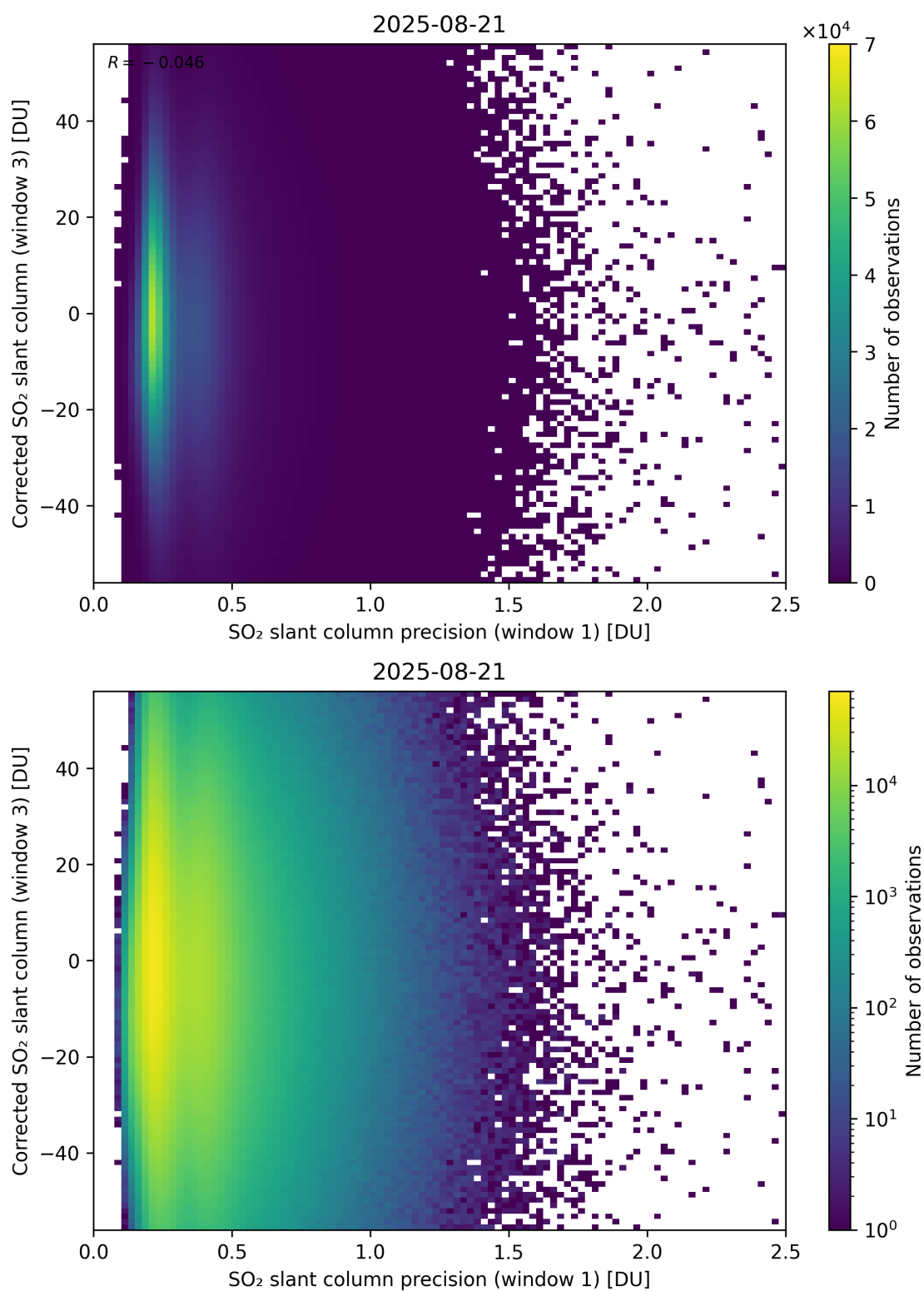
Figure 276: Scatter density plot of “SO 2 slant column precision (window 1)” against “Corrected SO 2 slant column (window 3)” for 2025-08-20 to 2025-08-22.
