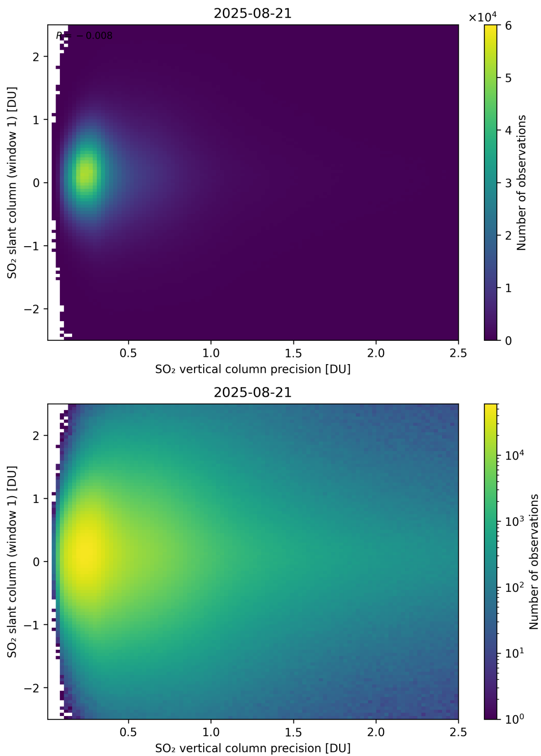
Figure 341: Scatter density plot of “SO 2 vertical column precision” against “SO 2 slant column (window 1)” for 2025-08-20 to 2025-08-22.
