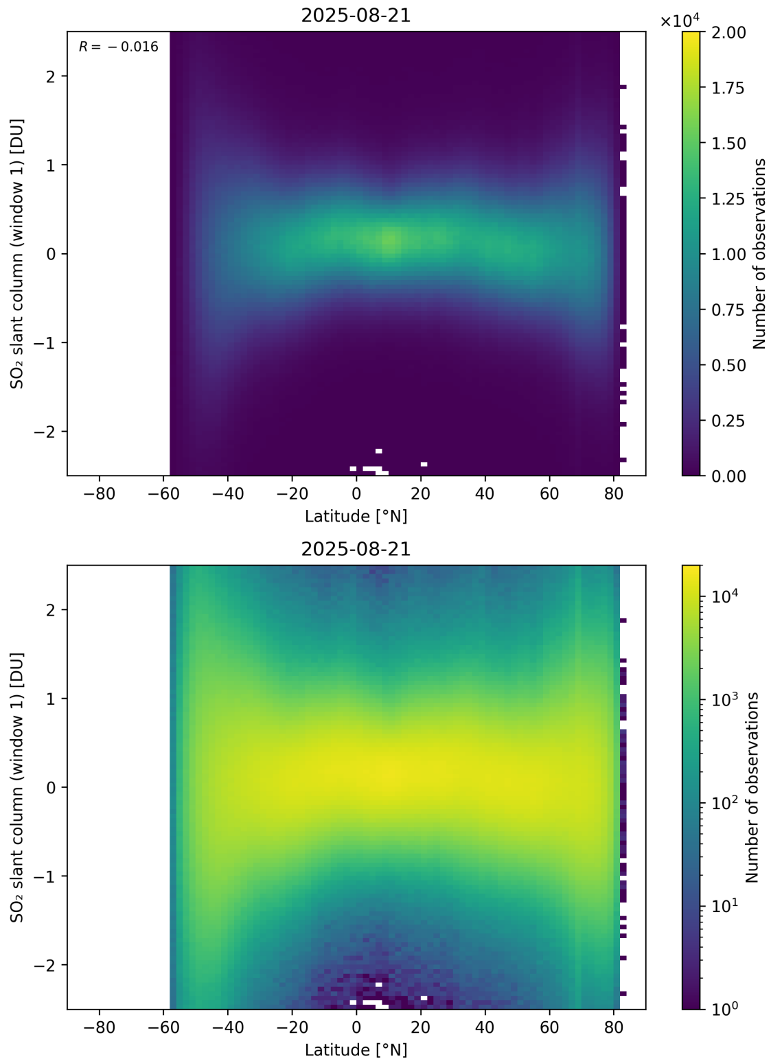
Figure 162: Scatter density plot of “Latitude” against “SO 2 slant column (window 1)” for 2025-08-20 to 2025-08-22.
