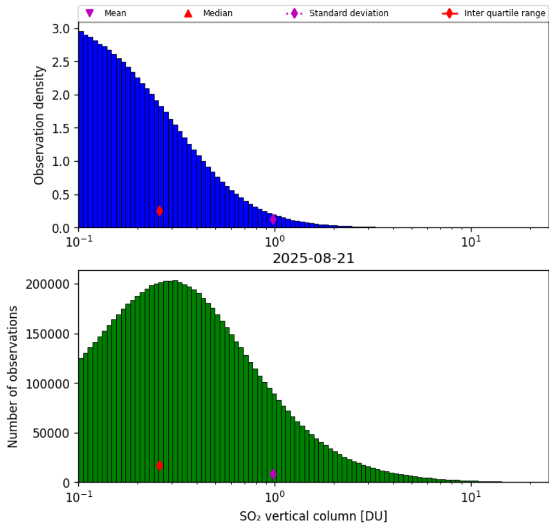
Figure 58: Histogram of “SO 2 vertical column” for 2025-08-20 to 2025-08-22
