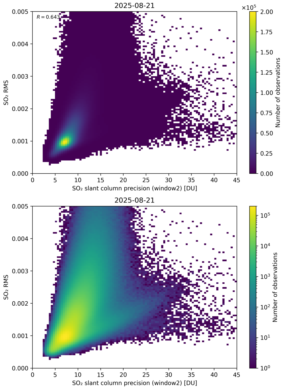
Figure 295: Scatter density plot of “SO 2 slant column precision (window2)” against “SO 2 RMS” for 2025-08-20 to 2025-08-22.
