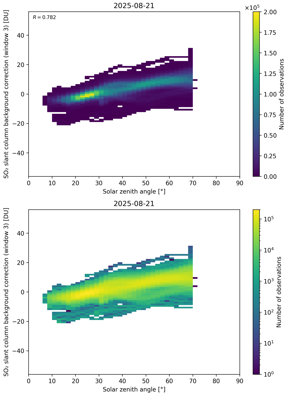
Figure 173: Scatter density plot of “Solar zenith angle” against “SO 2 slant column background correction (window 3)” for 2025-08-20 to 2025-08-22.
