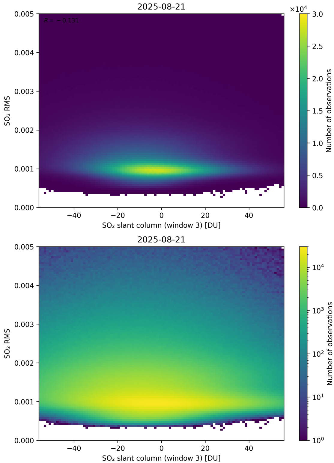
Figure 306: Scatter density plot of “SO 2 slant column (window 3)” against “SO 2 RMS” for 2025-08-20 to 2025-08-22.
