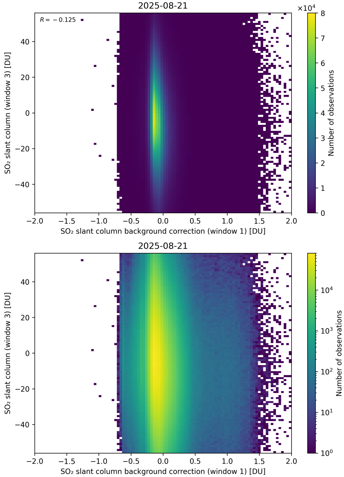
Figure 118: Scatter density plot of “SO 2 slant column background correction (window 1)” against “SO 2 slant column (window 3)” for 2025-08-20 to 2025-08-22.
