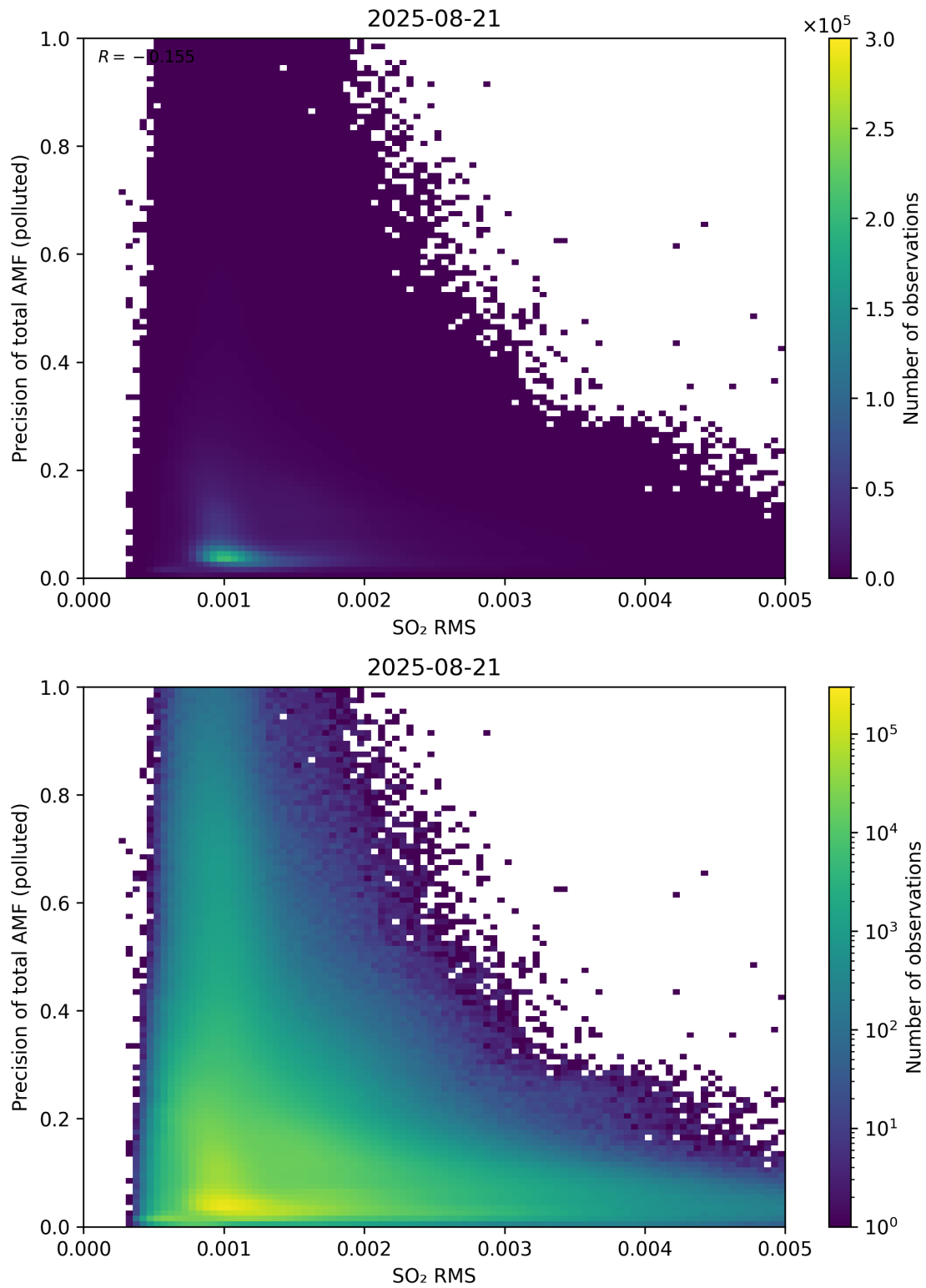
Figure 149: Scatter density plot of “SO 2 RMS” against “Precision of total AMF (polluted)” for 2025-08-20 to 2025-08-22.
