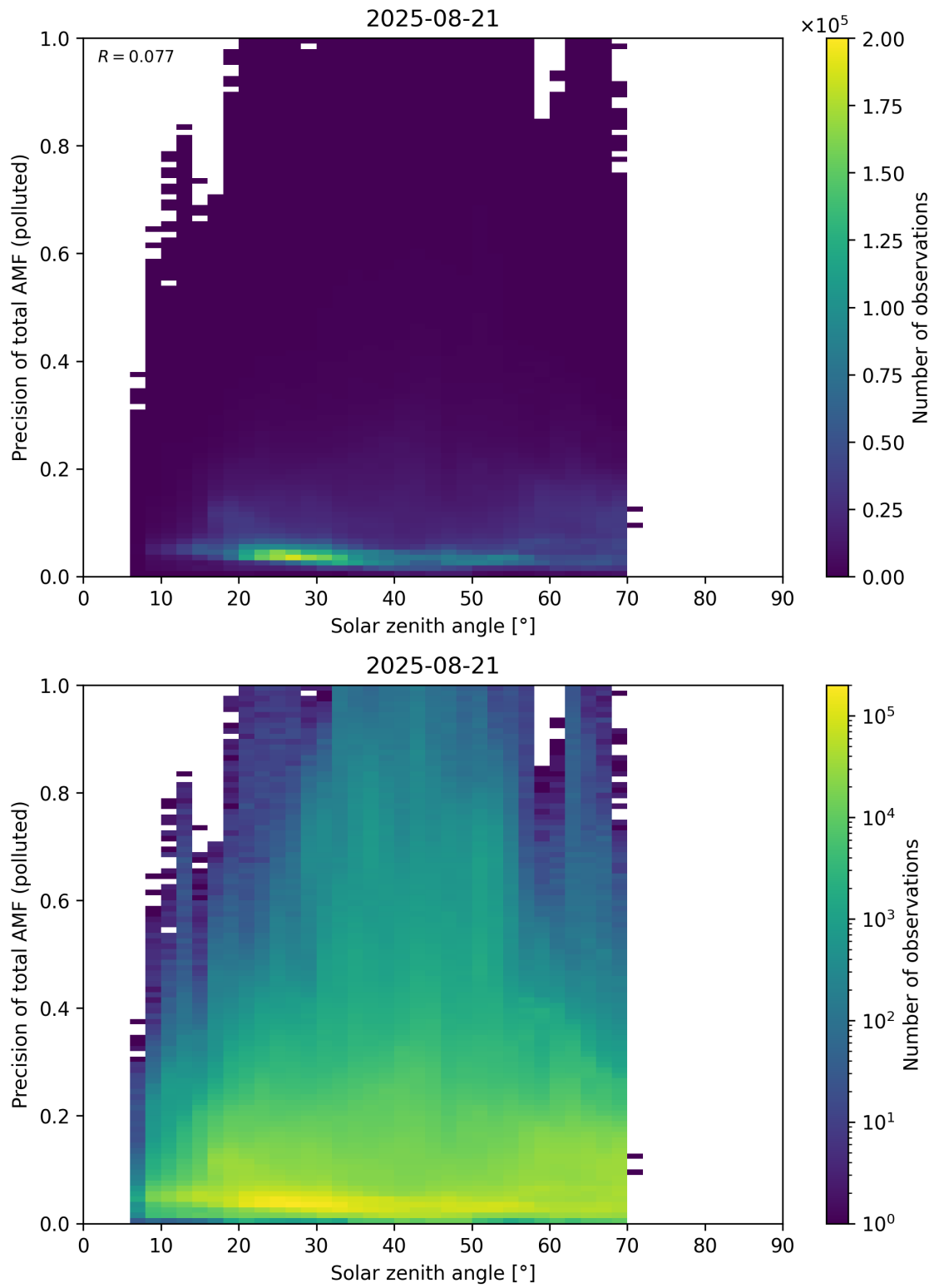
Figure 190: Scatter density plot of “Solar zenith angle” against “Precision of total AMF (polluted)” for 2025-08-20 to 2025-08-22.
