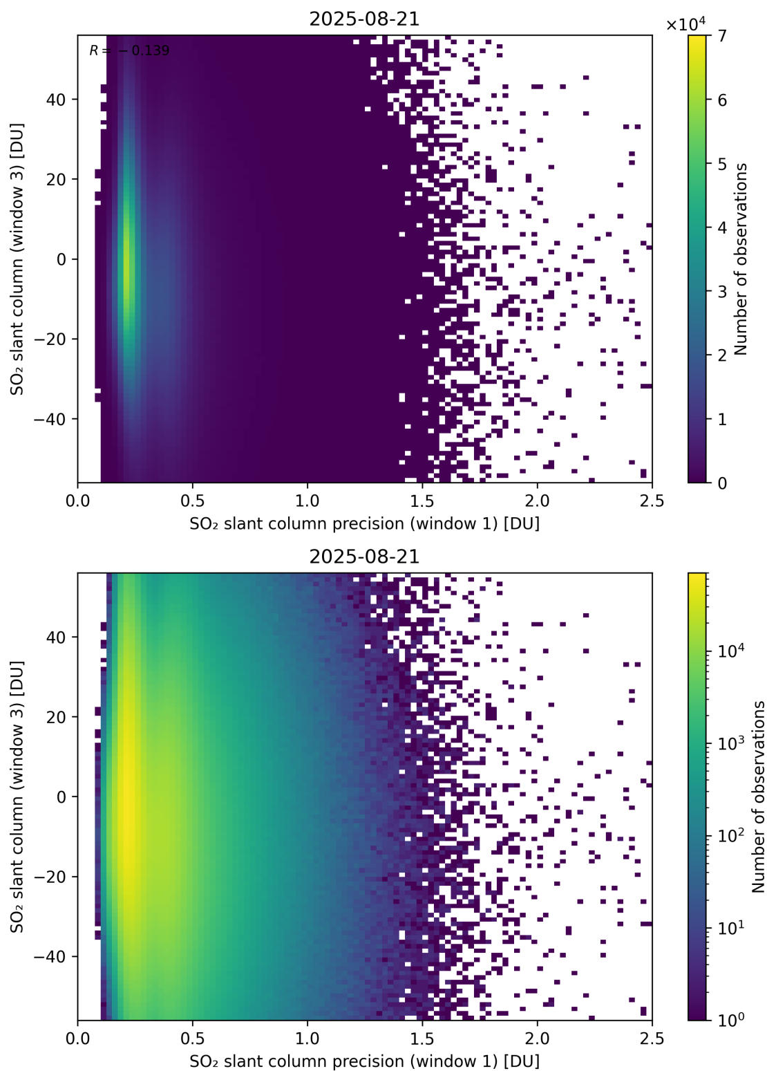
Figure 278: Scatter density plot of “SO 2 slant column precision (window 1)” against “SO 2 slant column (window 3)” for 2025-08-20 to 2025-08-22.
