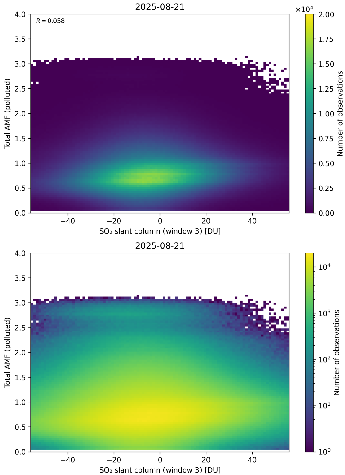
Figure 318: Scatter density plot of “SO 2 slant column (window 3)” against “Total AMF (polluted)” for 2025-08-20 to 2025-08-22.
