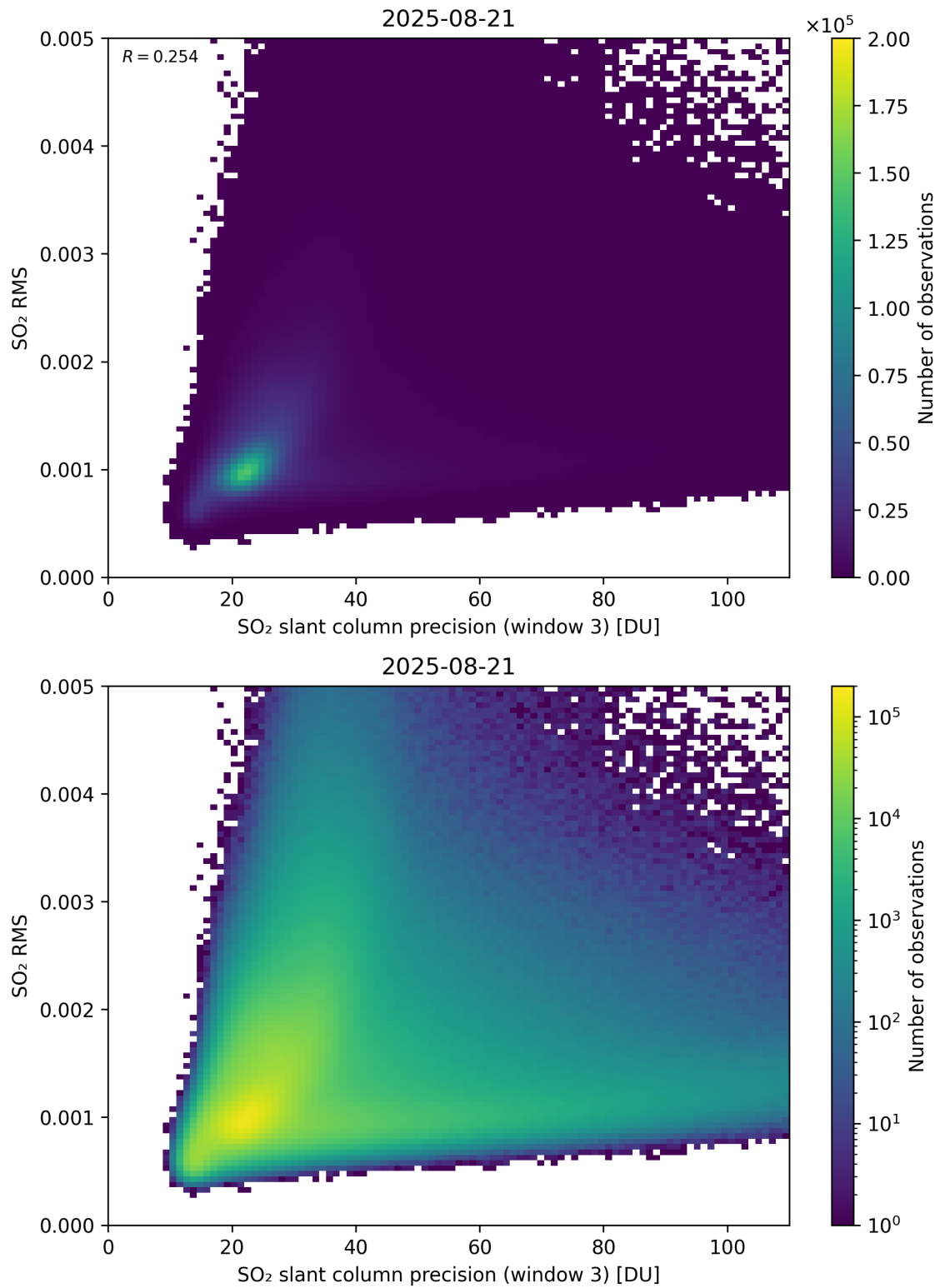
Figure 310: Scatter density plot of “SO 2 slant column precision (window 3)” against “SO 2 RMS” for 2025-08-20 to 2025-08-22.
