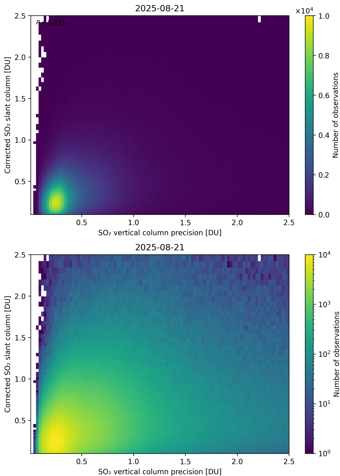
Figure 338: Scatter density plot of “SO 2 vertical column precision” against “Corrected SO 2 slant column” for 2025-08-20 to 2025-08-22.
