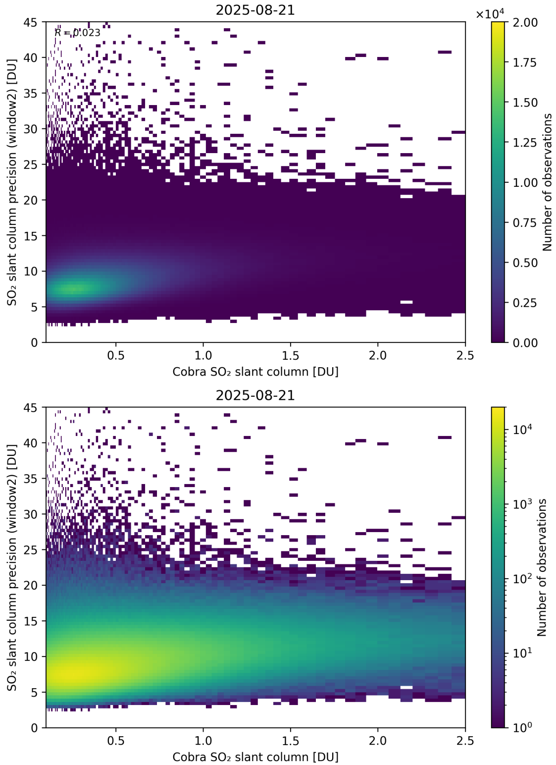
Figure 221: Scatter density plot of “Cobra SO 2 slant column” against “SO 2 slant column precision (window2)” for 2025-08-20 to 2025-08-22.
