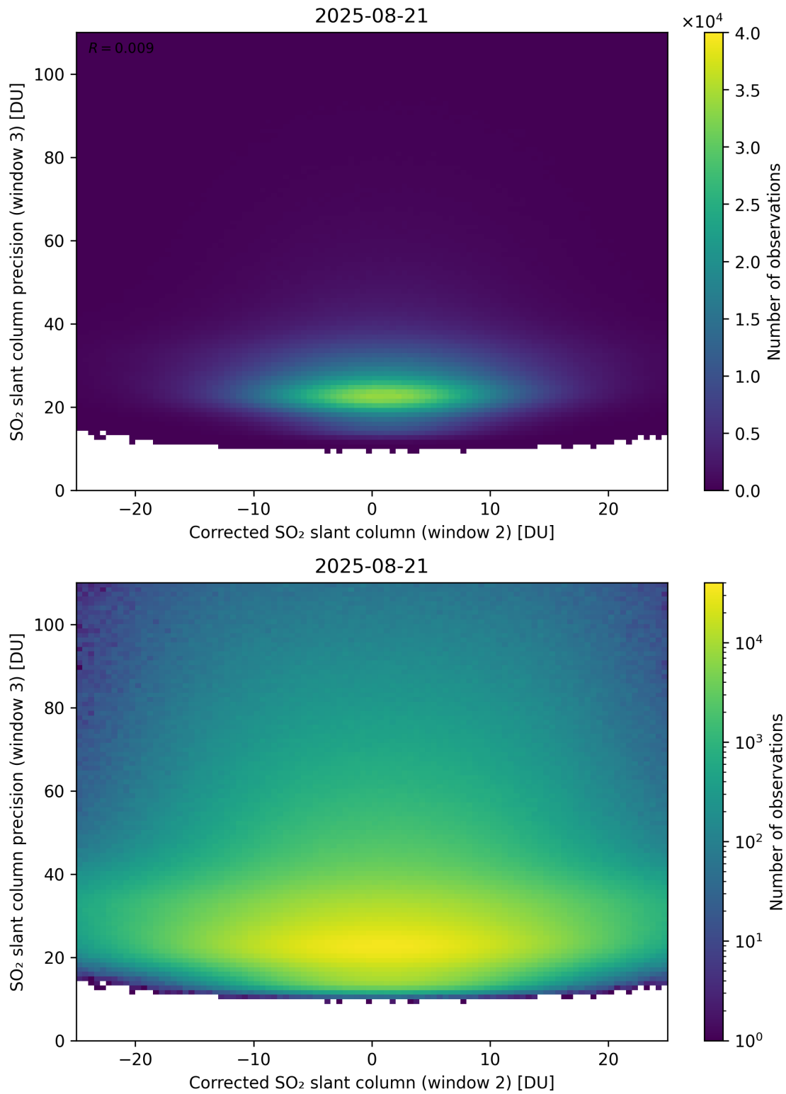
Figure 252: Scatter density plot of “Corrected SO 2 slant column (window 2)” against “SO 2 slant column precision (window 3)” for 2025-08-20 to 2025-08-22.
