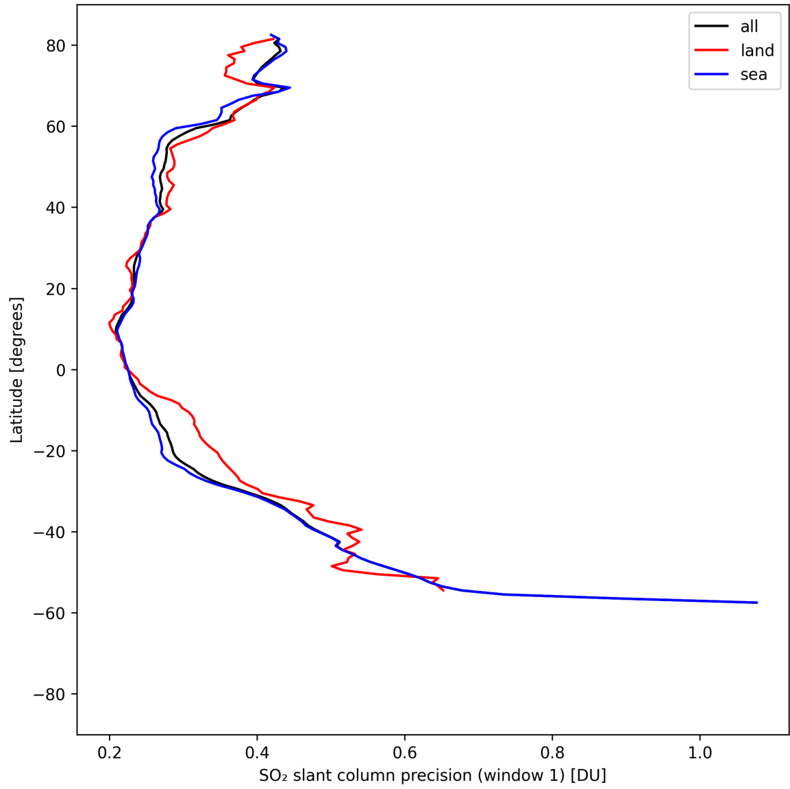
Figure 38: Zonal average of “SO 2 slant column precision (window 1)” for 2025-08-20 to 2025-08-22.
