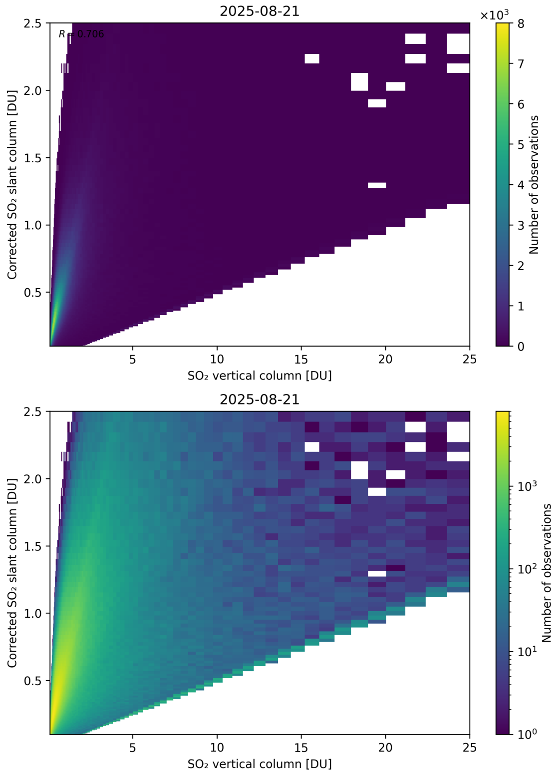
Figure 351: Scatter density plot of “SO 2 vertical column” against “Corrected SO 2 slant column” for 2025-08-20 to 2025-08-22.
