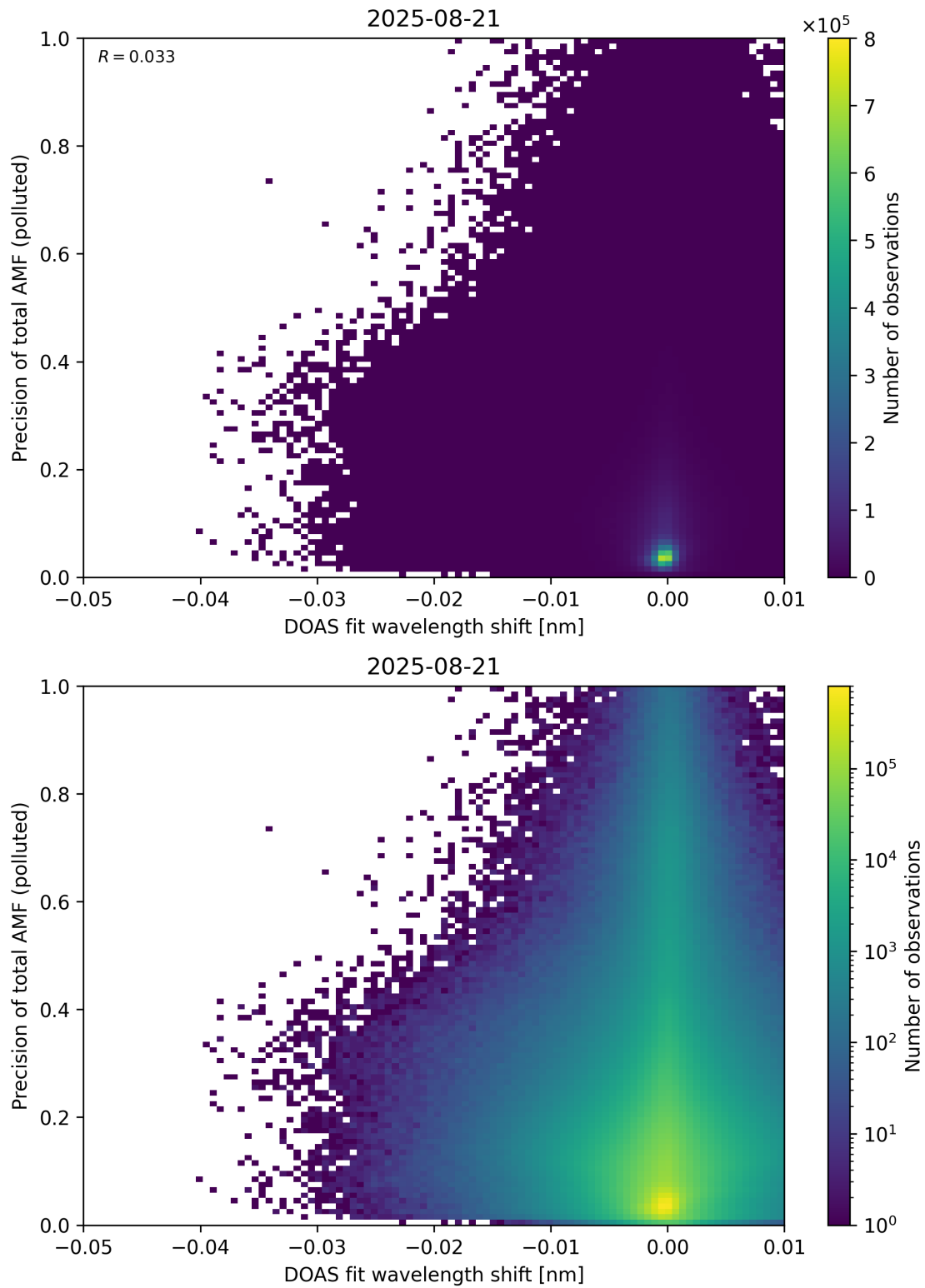
Figure 142: Scatter density plot of “DOAS fit wavelength shift” against “Precision of total AMF (polluted)” for 2025-08-20 to 2025-08-22.
