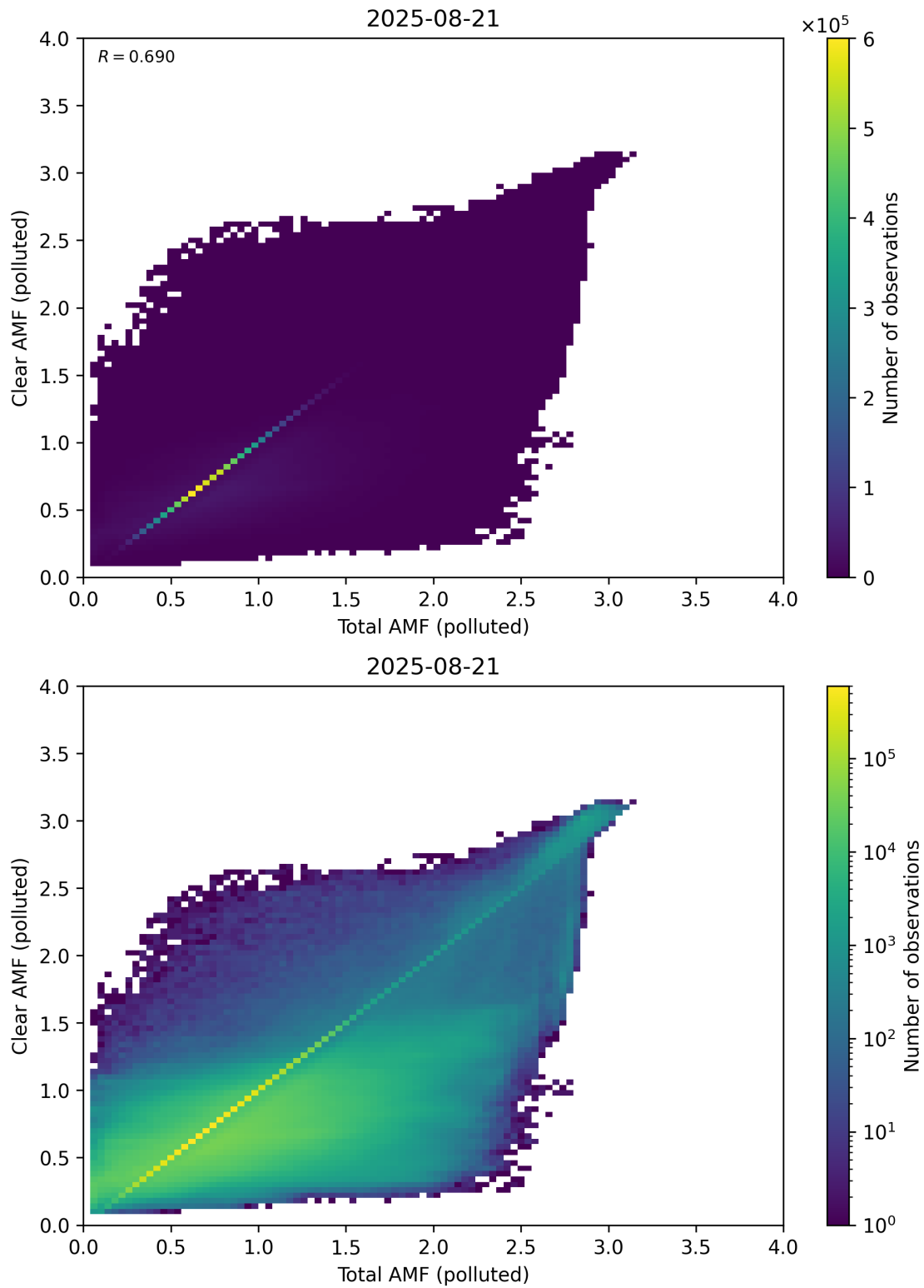
Figure 321: Scatter density plot of “Total AMF (polluted)” against “Clear AMF (polluted)” for 2025-08-20 to 2025-08-22.
