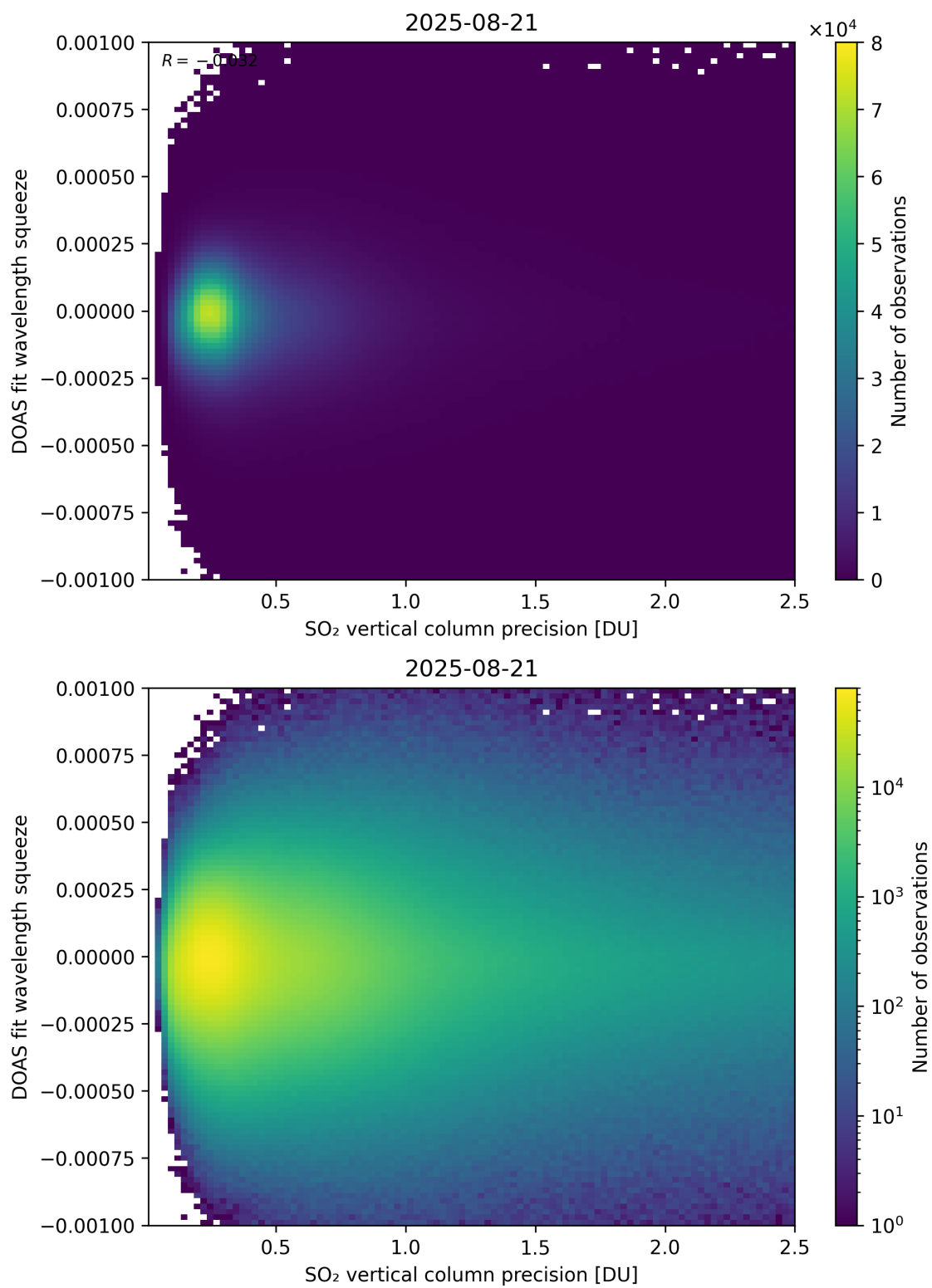
Figure 333: Scatter density plot of “SO 2 vertical column precision” against “DOAS fit wavelength squeeze” for 2025-08-20 to 2025-08-22.
