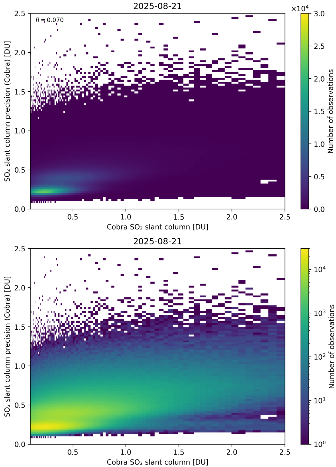
Figure 216: Scatter density plot of “Cobra SO 2 slant column” against “SO 2 slant column precision (Cobra)” for 2025-08-20 to 2025-08-22.
