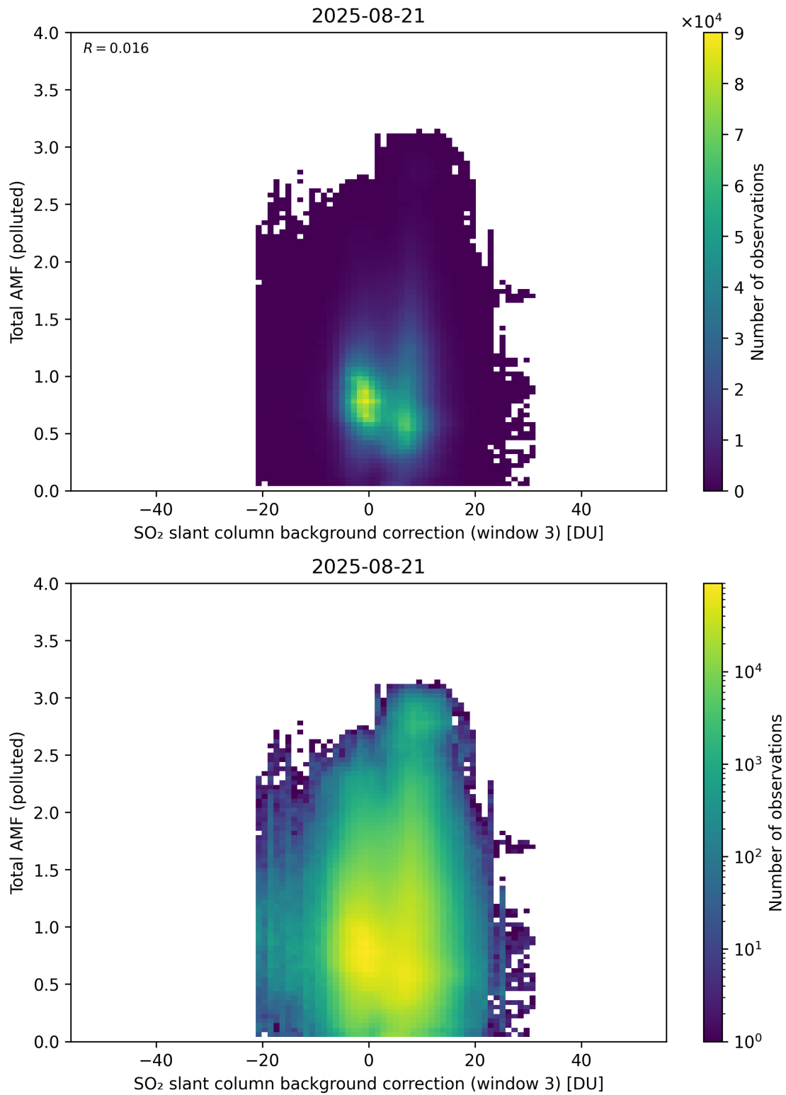
Figure 136: Scatter density plot of “SO 2 slant column background correction (window 3)” against “Total AMF (polluted)” for 2025-08-20 to 2025-08-22.
