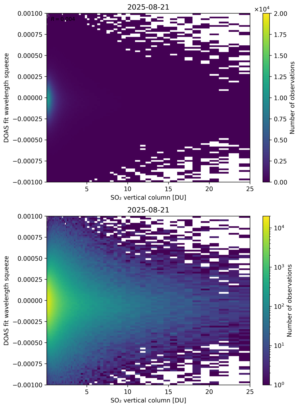
Figure 327: Scatter density plot of “SO 2 vertical column” against “DOAS fit wavelength squeeze” for 2025-08-20 to 2025-08-22.
