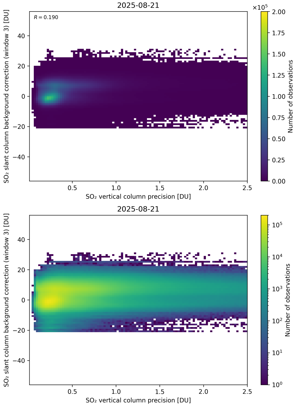
Figure 331: Scatter density plot of “SO 2 vertical column precision” against “SO 2 slant column background correction (window 3)” for 2025-08-20 to 2025-08-22.
