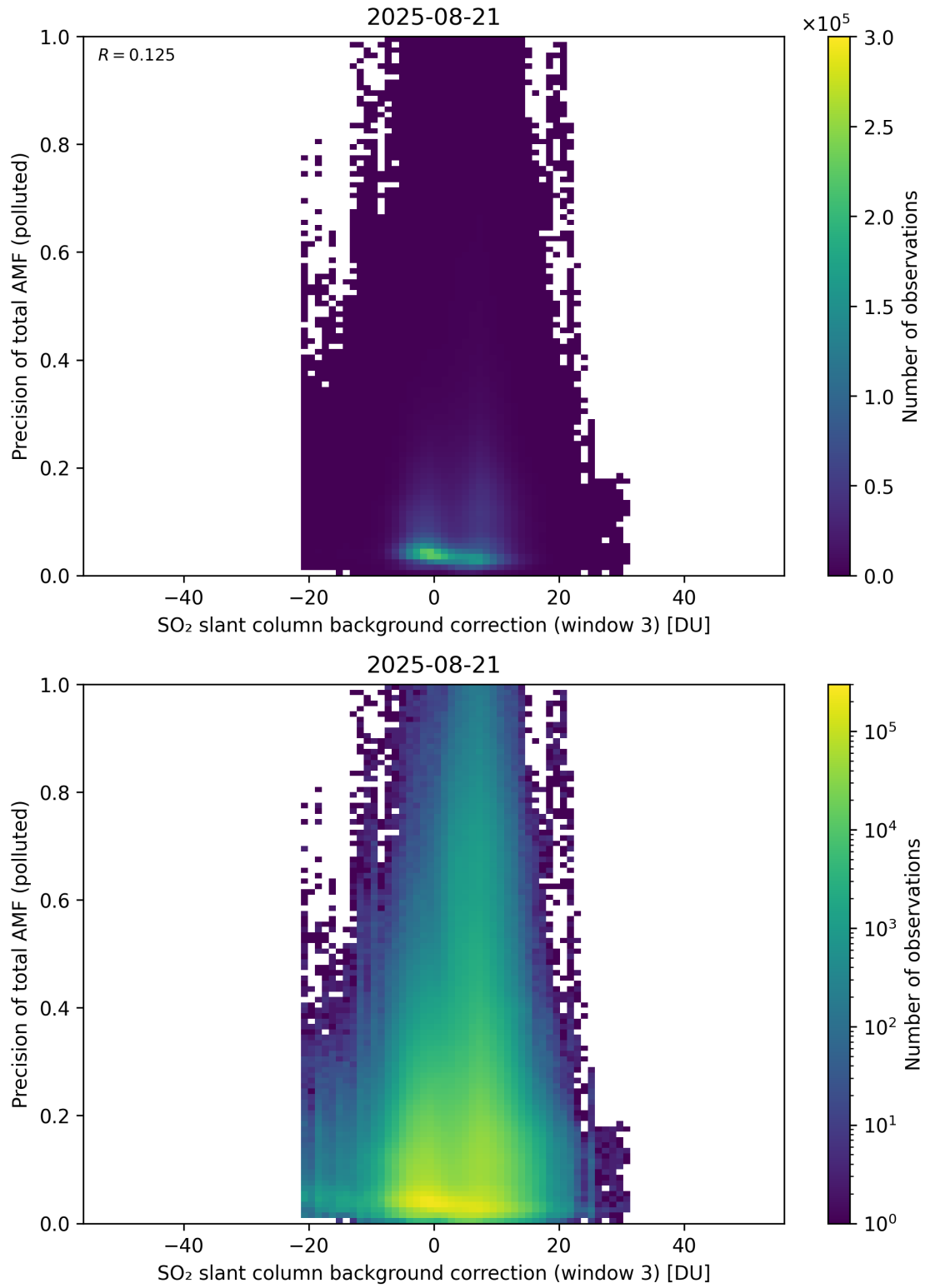
Figure 137: Scatter density plot of “SO 2 slant column background correction (window 3)” against “Precision of total AMF (polluted)” for 2025-08-20 to 2025-08-22.
