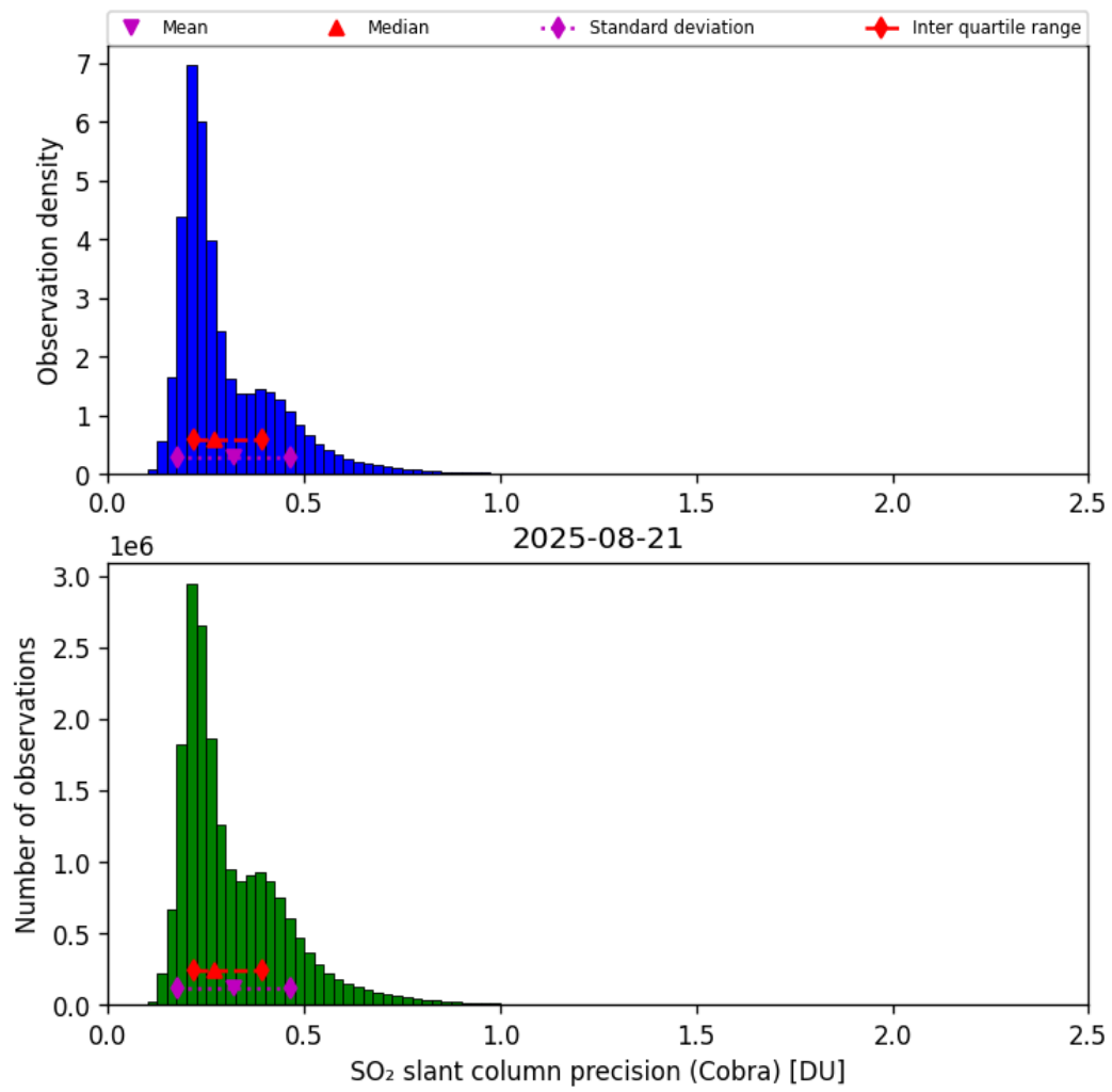
Figure 62: Histogram of “SO 2 slant column precision (Cobra)” for 2025-08-20 to 2025-08-22
