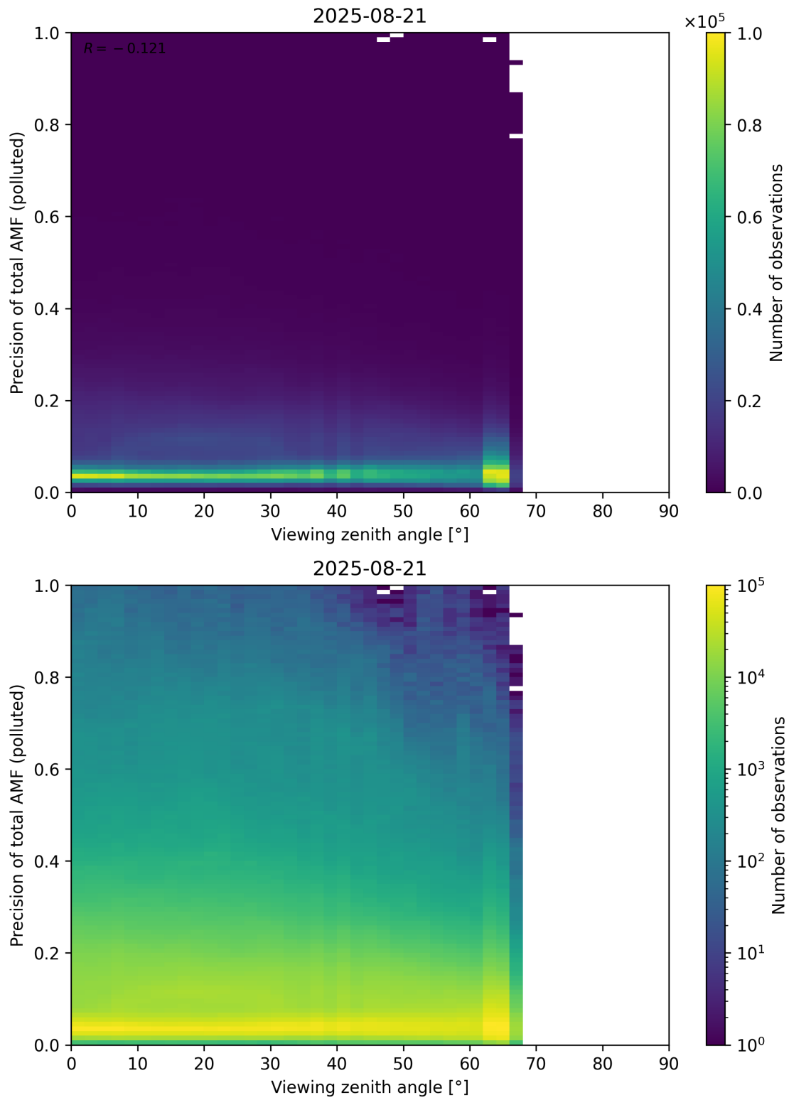
Figure 382: Scatter density plot of “Viewing zenith angle” against “Precision of total AMF (polluted)” for 2025-08-20 to 2025-08-22.
