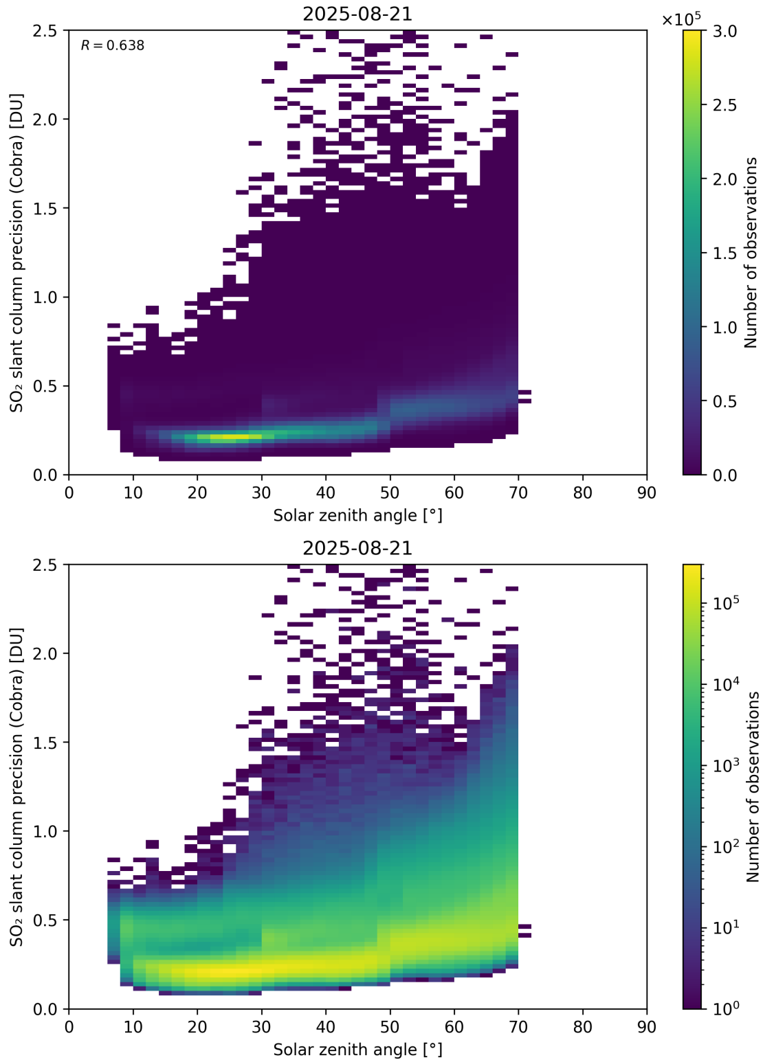
Figure 180: Scatter density plot of “Solar zenith angle” against “SO 2 slant column precision (Cobra)” for 2025-08-20 to 2025-08-22.
