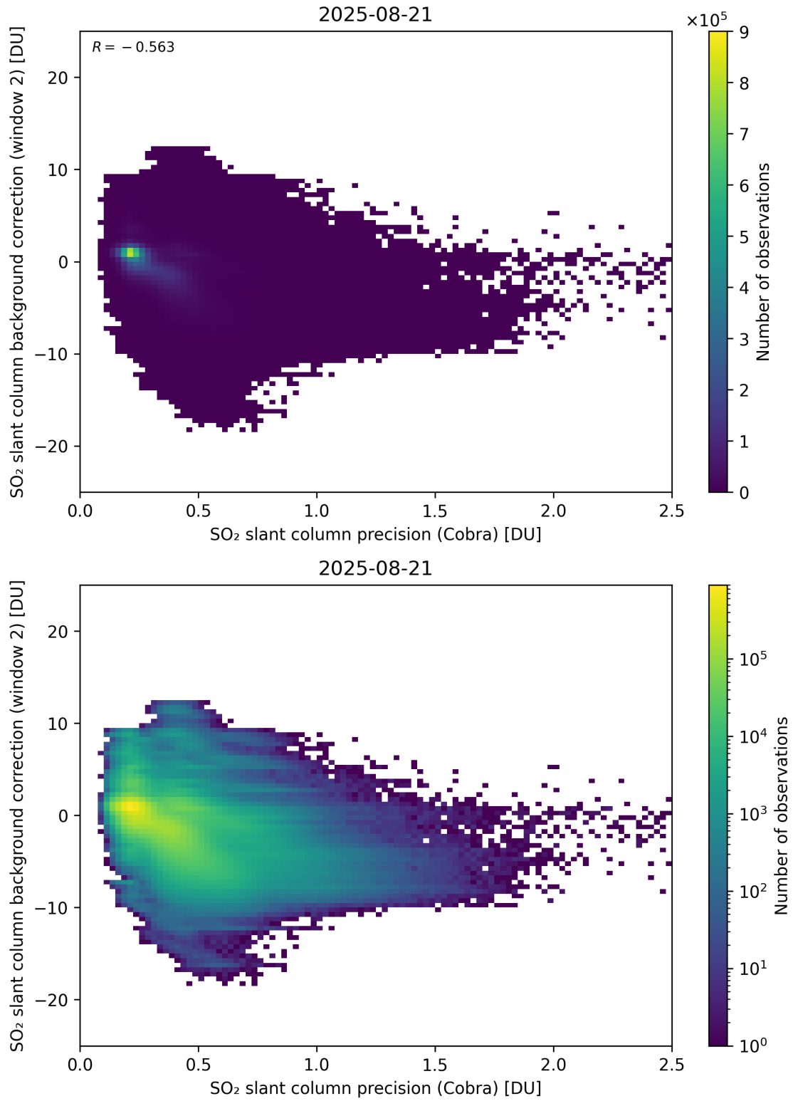
Figure 200: Scatter density plot of “SO 2 slant column precision (Cobra)” against “SO 2 slant column background correction (window 2)” for 2025-08-20 to 2025-08-22.
