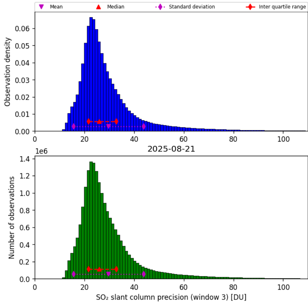
Figure 72: Histogram of “SO 2 slant column precision (window 3)” for 2025-08-20 to 2025-08-22
