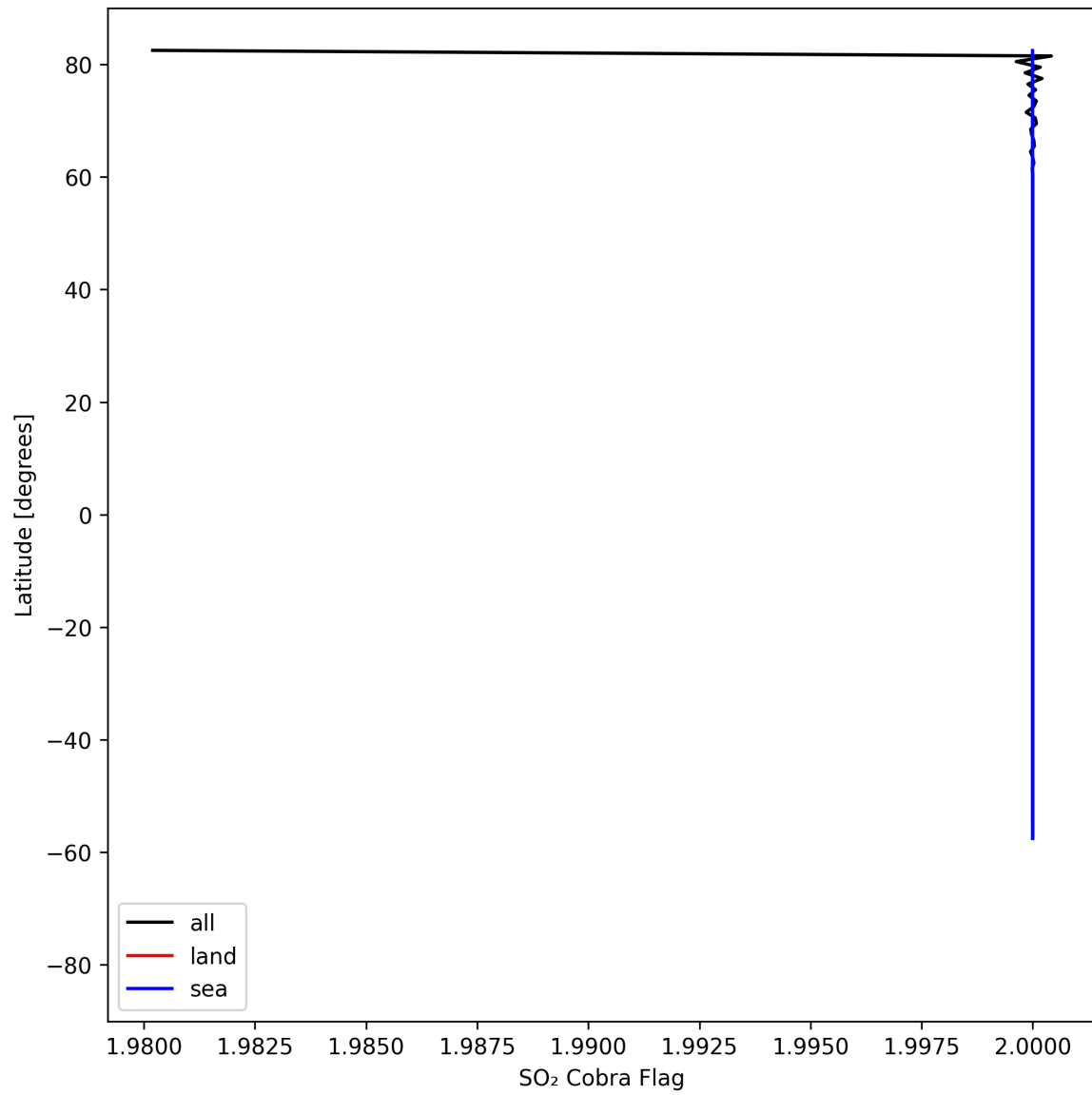
Figure 49: Zonal average of “SO 2 Cobra Flag” for 2025-08-20 to 2025-08-22.
