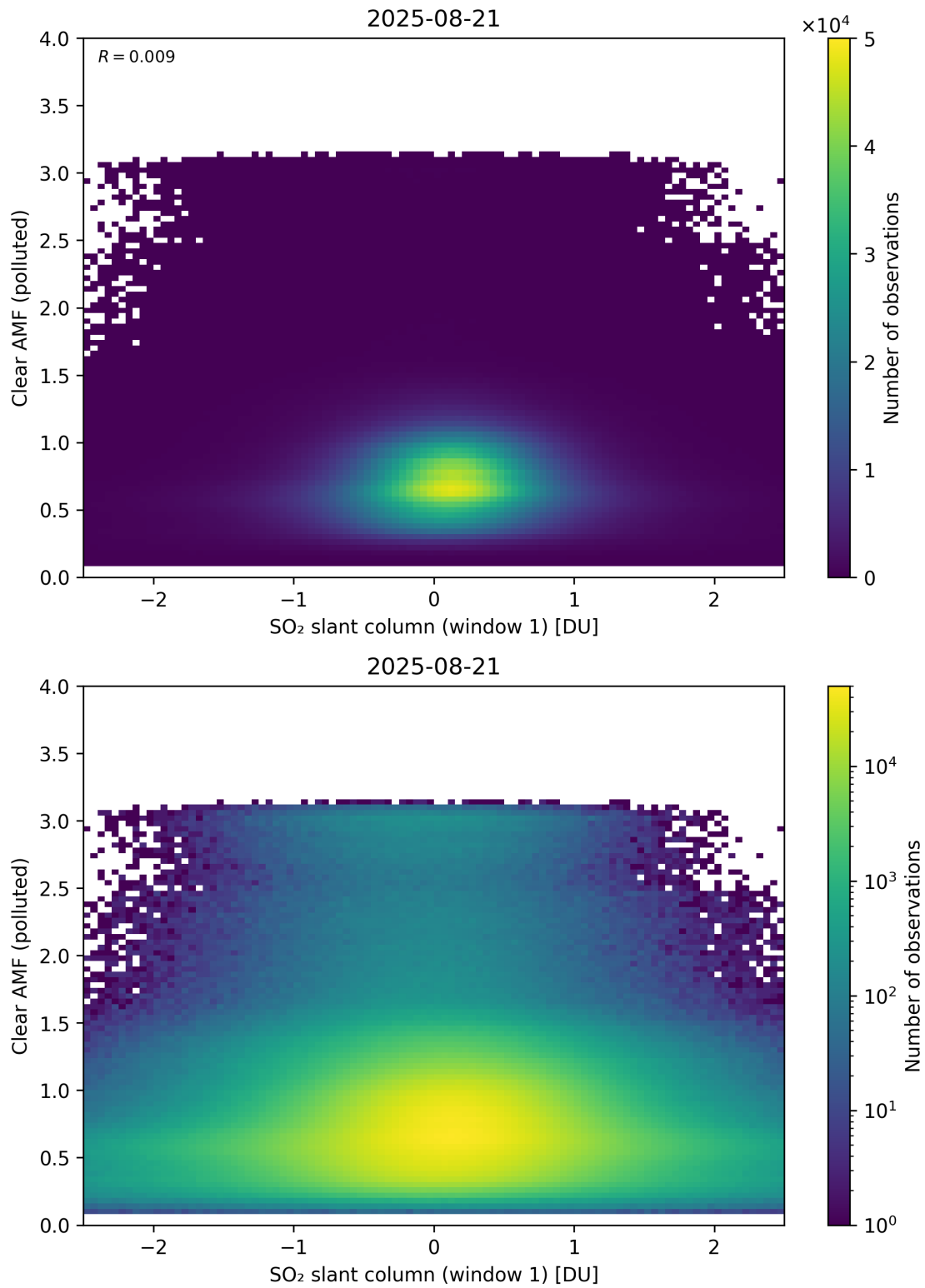
Figure 282: Scatter density plot of “SO 2 slant column (window 1)” against “Clear AMF (polluted)” for 2025-08-20 to 2025-08-22.
