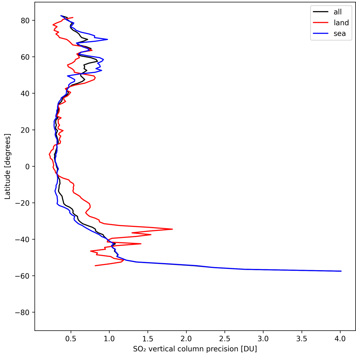
Figure 33: Zonal average of “SO 2 vertical column precision” for 2025-08-20 to 2025-08-22.
