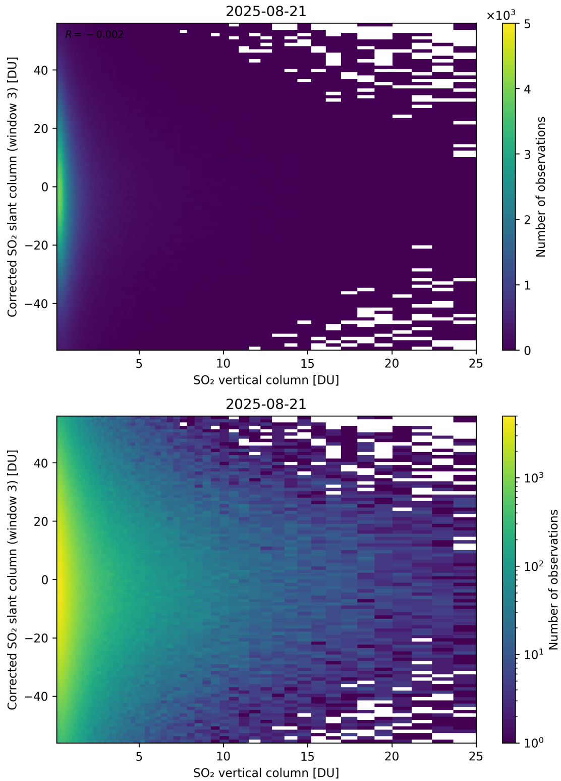
Figure 353: Scatter density plot of “SO 2 vertical column” against “Corrected SO 2 slant column (window 3)” for 2025-08-20 to 2025-08-22.
