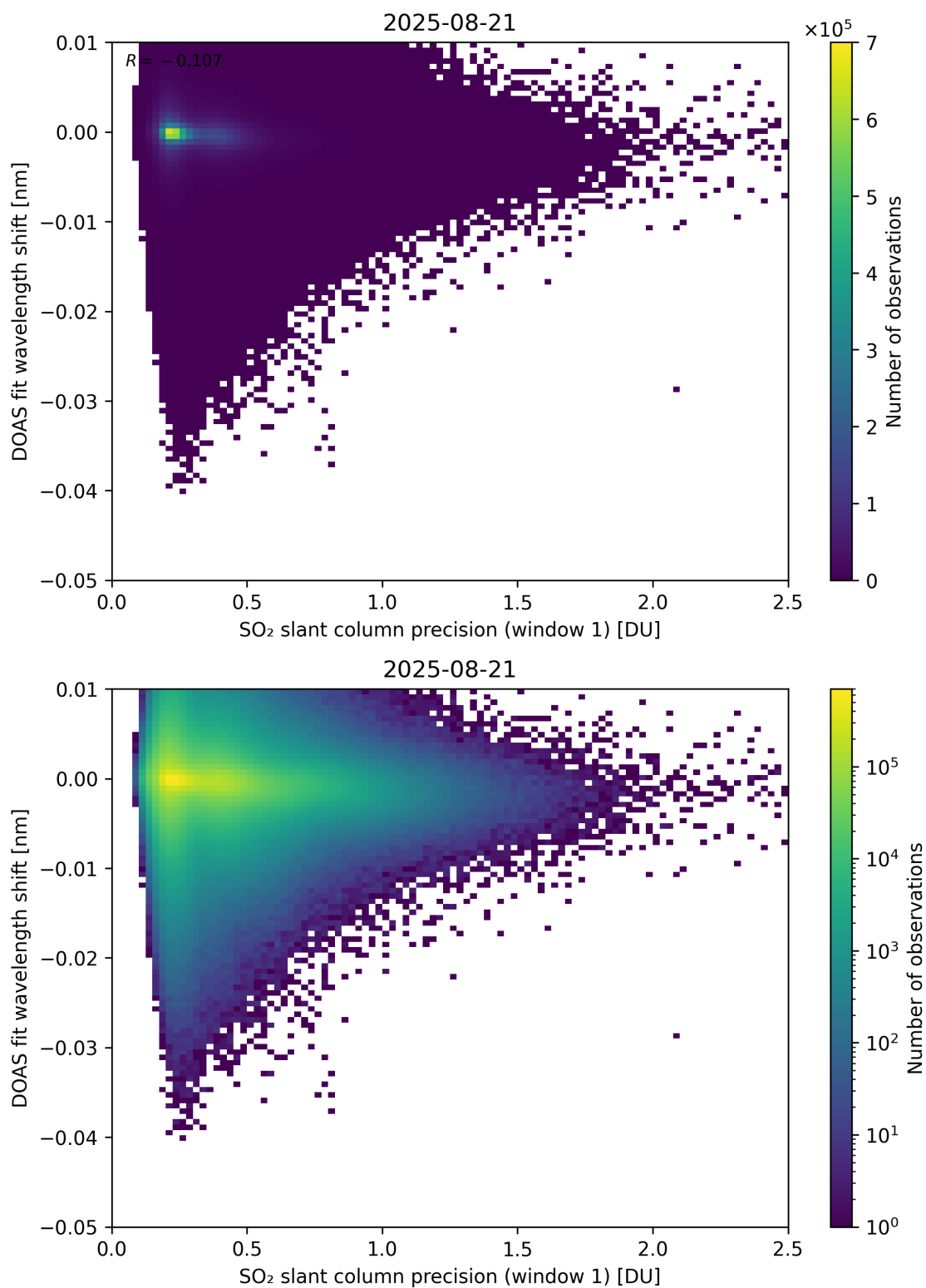
Figure 271: Scatter density plot of “SO 2 slant column precision (window 1)” against “DOAS fit wavelength shift” for 2025-08-20 to 2025-08-22.
