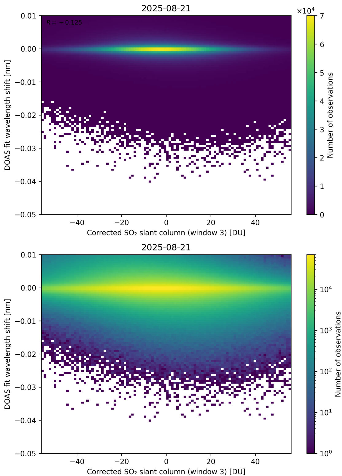
Figure 256: Scatter density plot of “Corrected SO 2 slant column (window 3)” against “DOAS fit wavelength shift” for 2025-08-20 to 2025-08-22.
