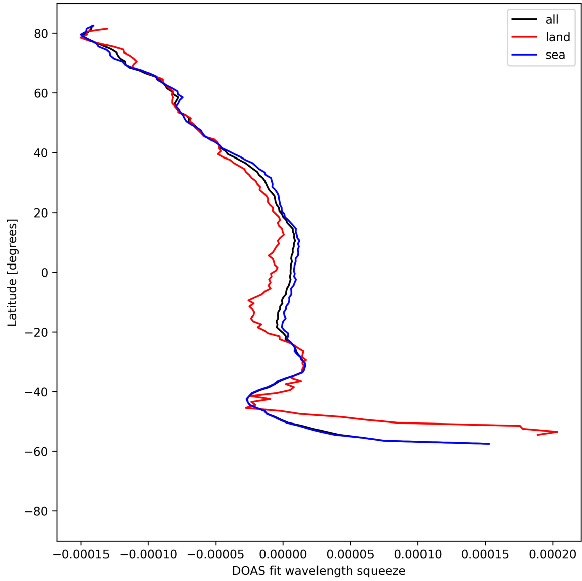
Figure 51: Zonal average of “DOAS fit wavelength squeeze” for 2025-08-20 to 2025-08-22.
