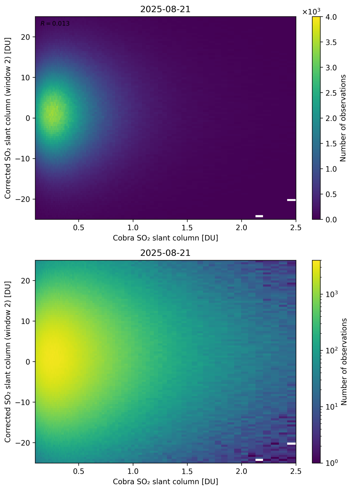
Figure 217: Scatter density plot of “Cobra SO 2 slant column” against “Corrected SO 2 slant column (window 2)” for 2025-08-20 to 2025-08-22.
