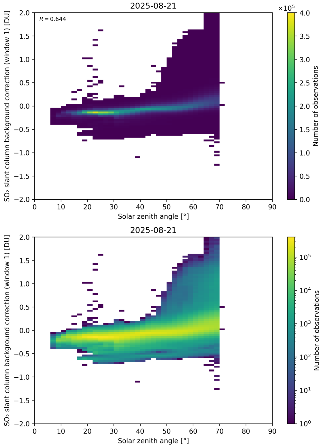
Figure 171: Scatter density plot of “Solar zenith angle” against “SO 2 slant column background correction (window 1)” for 2025-08-20 to 2025-08-22.
