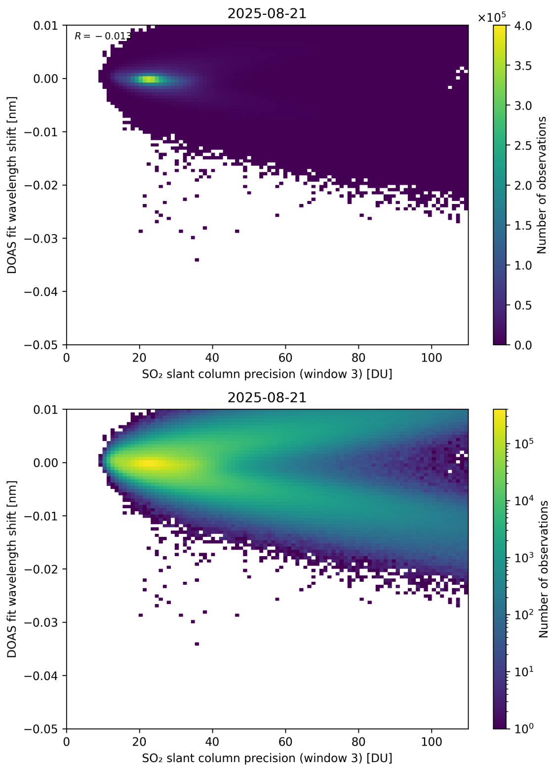
Figure 308: Scatter density plot of “SO 2 slant column precision (window 3)” against “DOAS fit wavelength shift” for 2025-08-20 to 2025-08-22.
