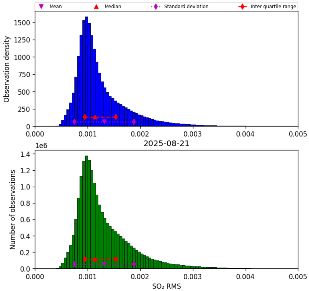
Figure 78: Histogram of “SO 2 RMS” for 2025-08-20 to 2025-08-22
