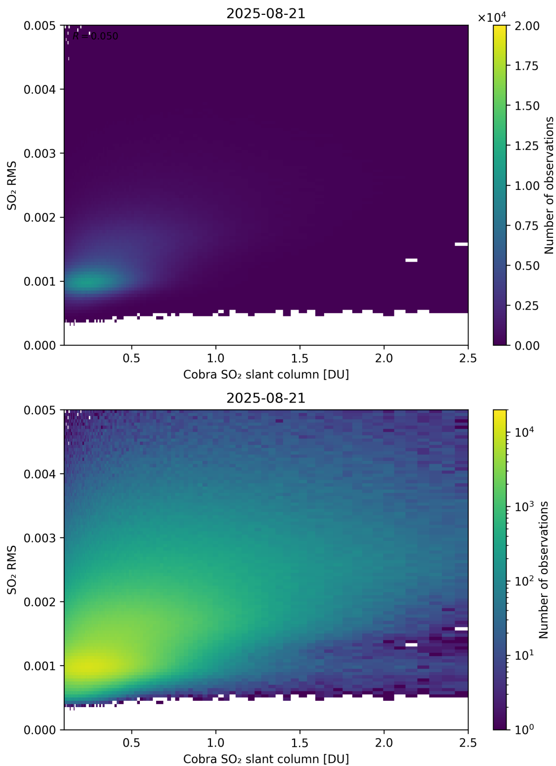
Figure 198: Scatter density plot of “Cobra SO 2 slant column” against “SO 2 RMS” for 2025-08-20 to 2025-08-22.
