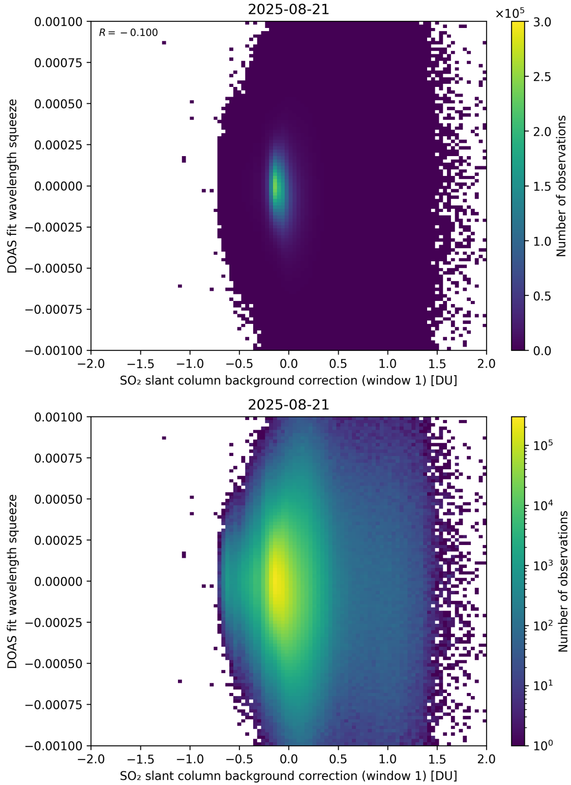
Figure 112: Scatter density plot of “SO 2 slant column background correction (window 1)” against “DOAS fit wavelength squeeze” for 2025-08-20 to 2025-08-22.
