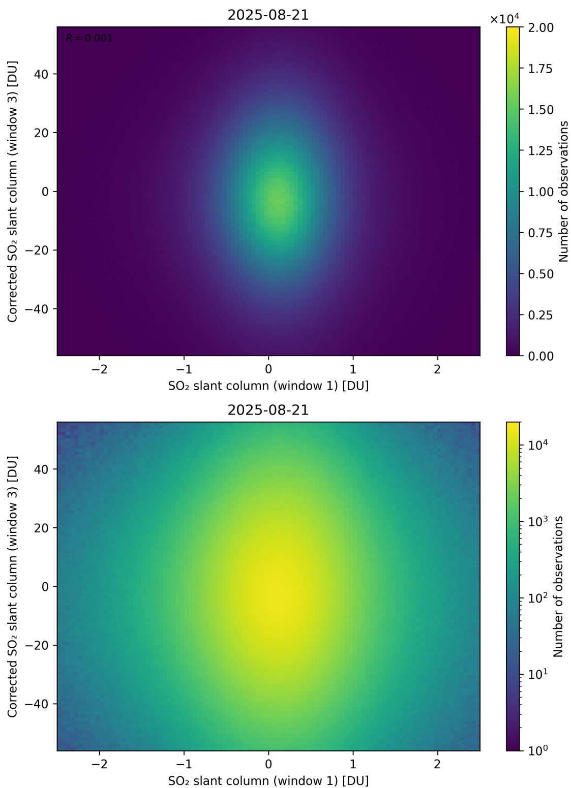
Figure 284: Scatter density plot of “SO 2 slant column (window 1)” against “Corrected SO 2 slant column (window 3)” for 2025-08-20 to 2025-08-22.
