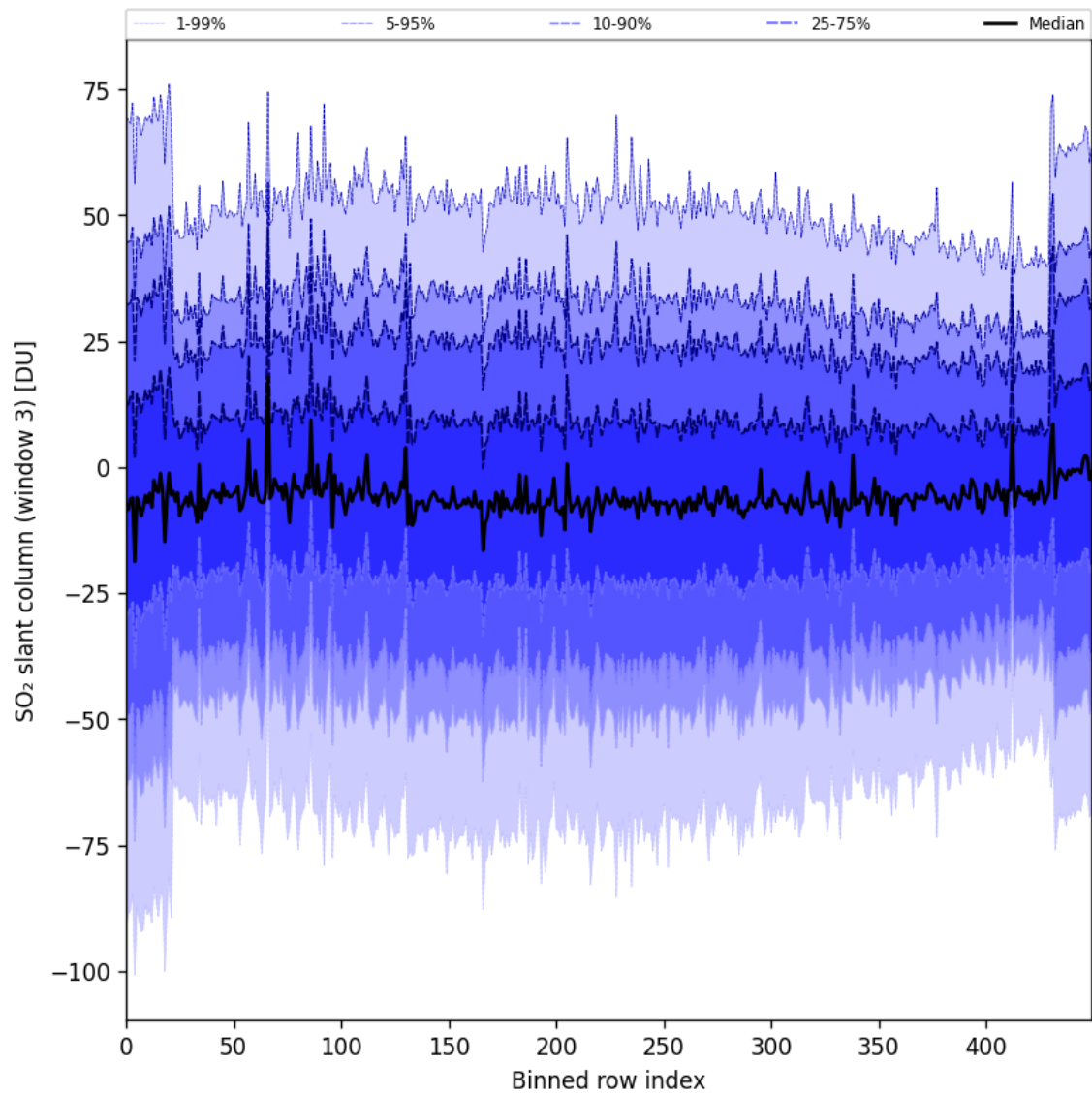
Figure 97: Along track statistics of “SO 2 slant column (window 3)” for 2025-08-20 to 2025-08-22
