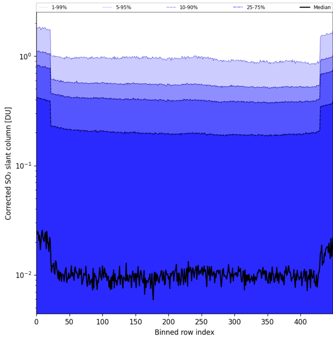
Figure 86: Along track statistics of “Corrected SO 2 slant column” for 2025-08-20 to 2025-08-22
