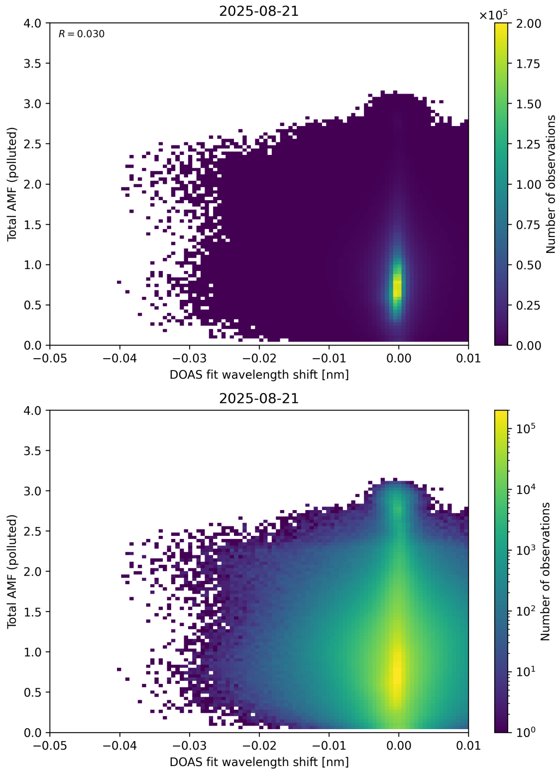
Figure 141: Scatter density plot of “DOAS fit wavelength shift” against “Total AMF (polluted)” for 2025-08-20 to 2025-08-22.
