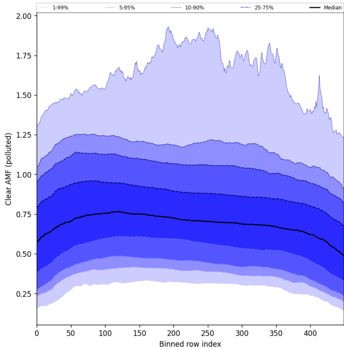
Figure 107: Along track statistics of “Clear AMF (polluted)” for 2025-08-20 to 2025-08-22
