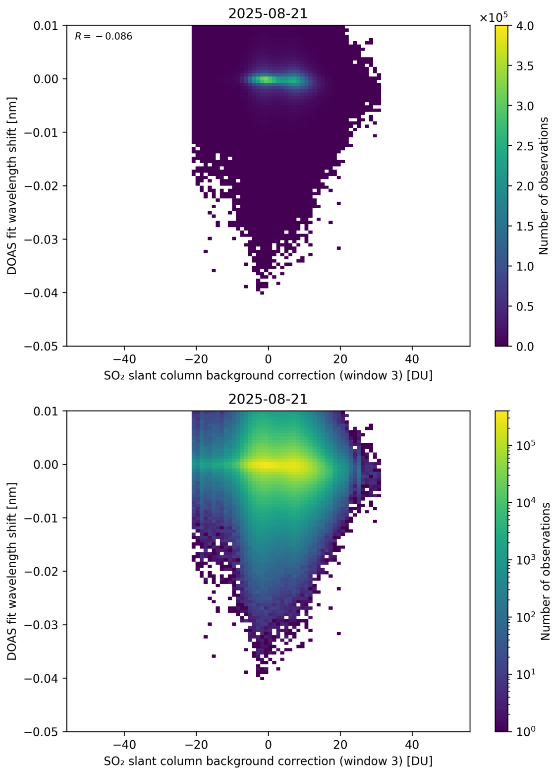
Figure 132: Scatter density plot of “SO 2 slant column background correction (window 3)” against “DOAS fit wavelength shift” for 2025-08-20 to 2025-08-22.
