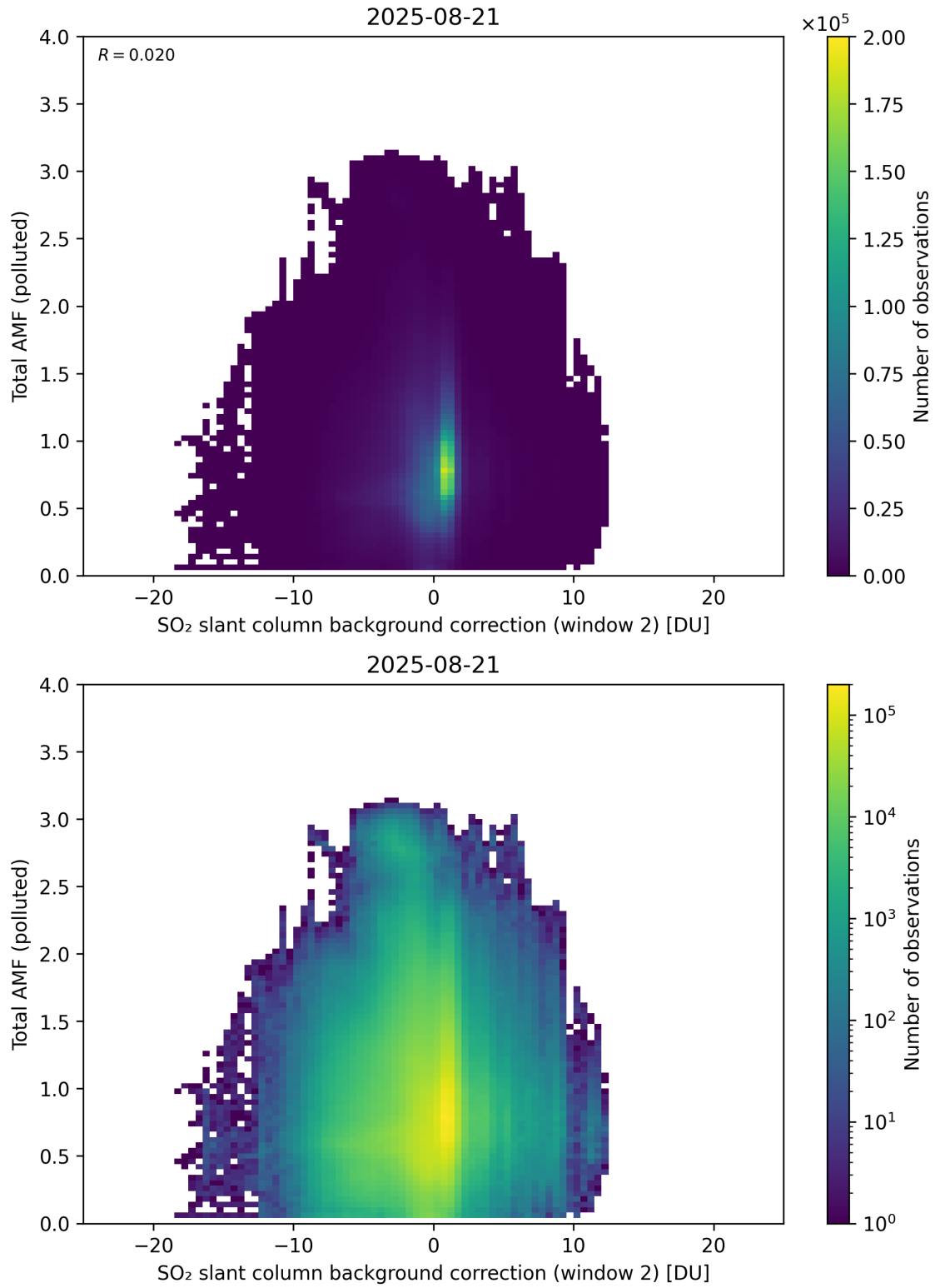
Figure 130: Scatter density plot of “SO 2 slant column background correction (window 2)” against “Total AMF (polluted)” for 2025-08-20 to 2025-08-22.
