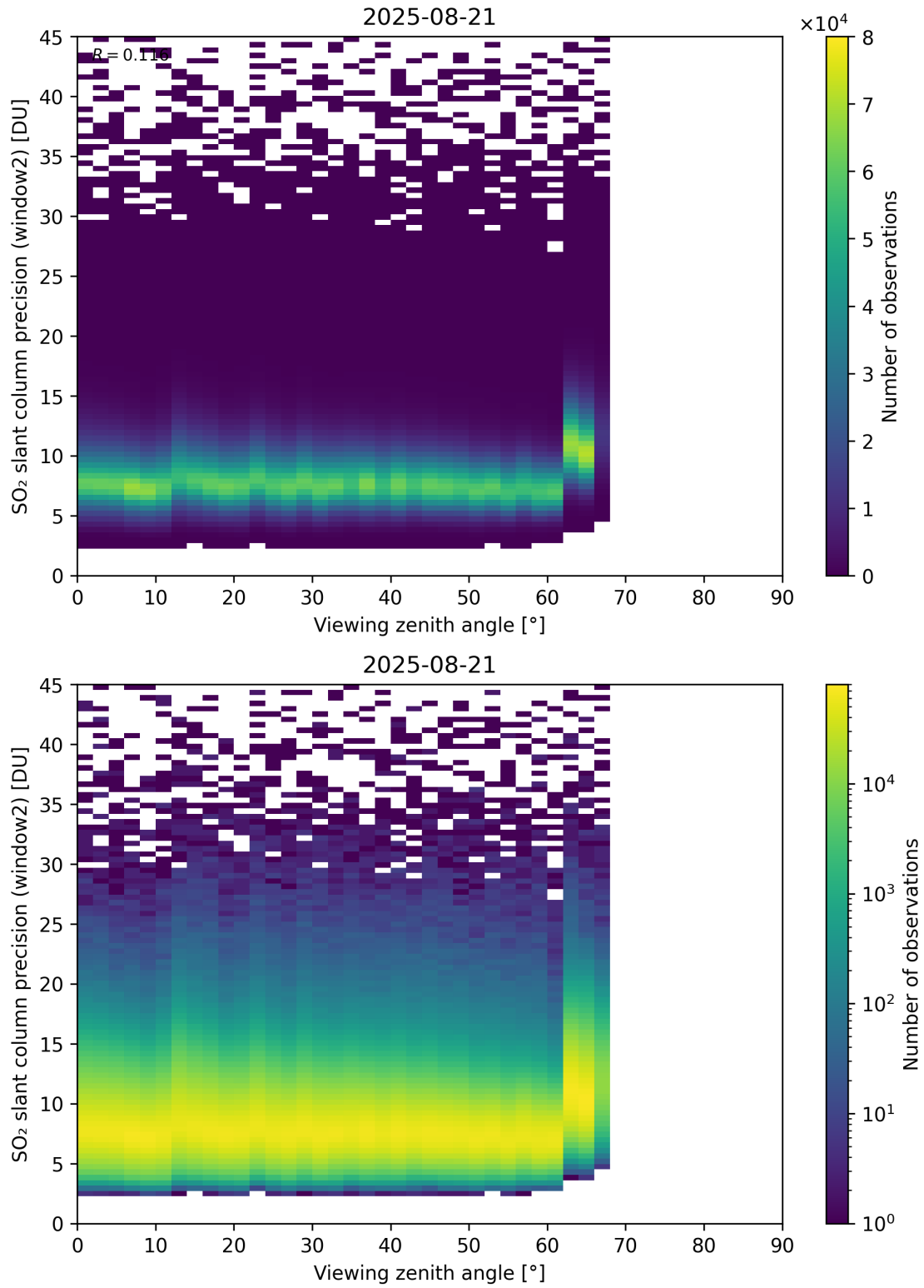
Figure 378: Scatter density plot of “Viewing zenith angle” against “SO 2 slant column precision (window2)” for 2025-08-20 to 2025-08-22.
