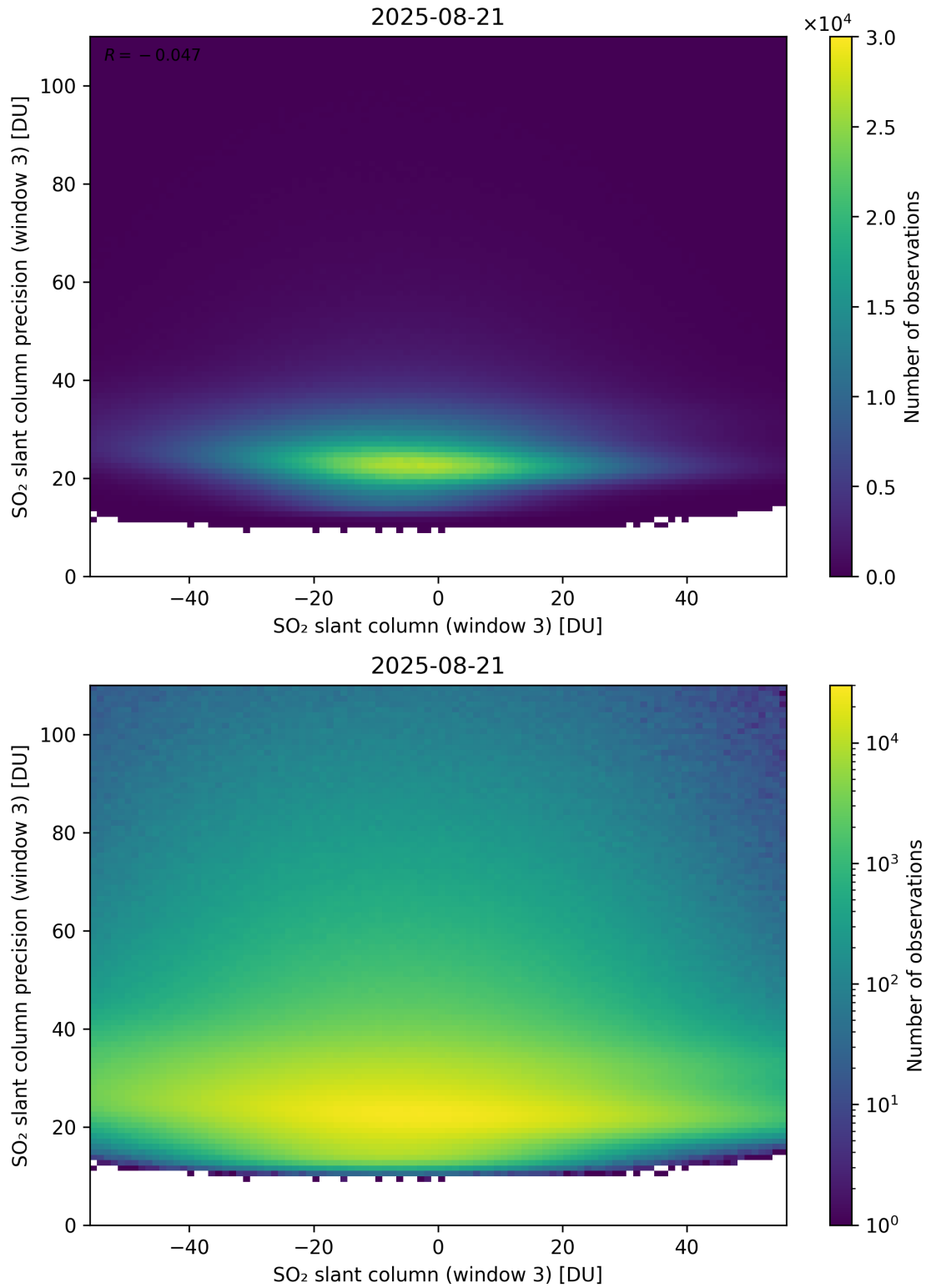
Figure 317: Scatter density plot of “SO 2 slant column (window 3)” against “SO 2 slant column precision (window 3)” for 2025-08-20 to 2025-08-22.
