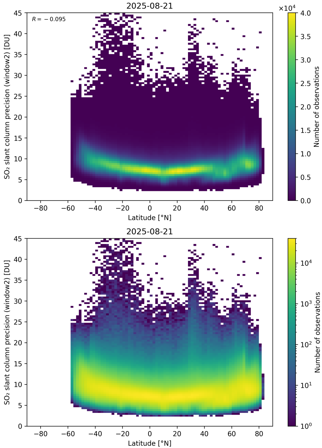
Figure 164: Scatter density plot of “Latitude” against “SO 2 slant column precision (window2)” for 2025-08-20 to 2025-08-22.
