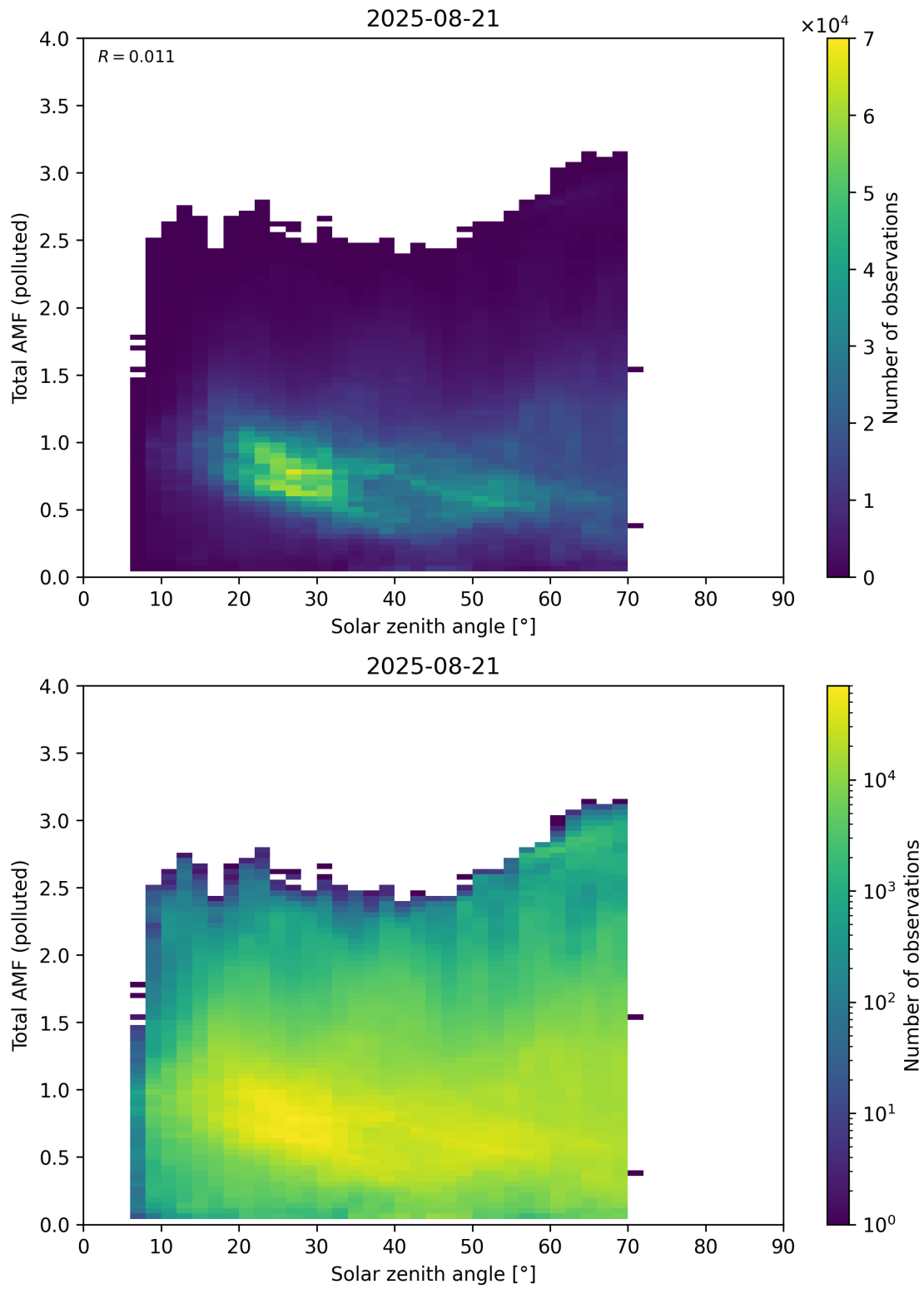
Figure 189: Scatter density plot of “Solar zenith angle” against “Total AMF (polluted)” for 2025-08-20 to 2025-08-22.
