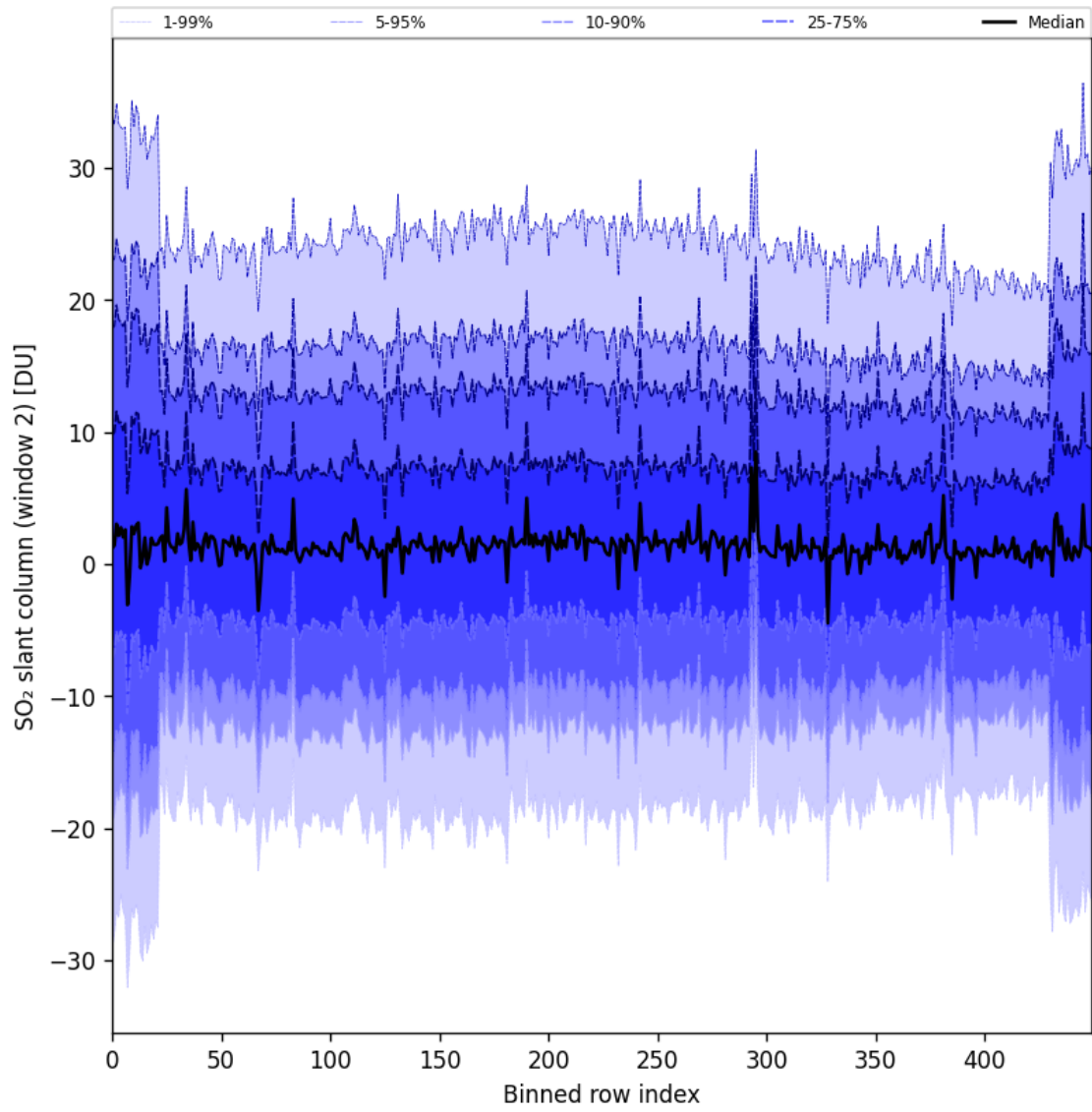
Figure 93: Along track statistics of “SO 2 slant column (window 2)” for 2025-08-20 to 2025-08-22
