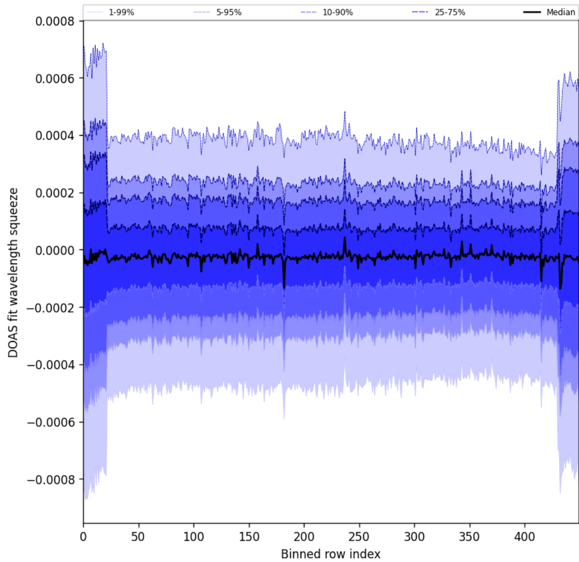
Figure 103: Along track statistics of “DOAS fit wavelength squeeze” for 2025-08-20 to 2025-08-22
