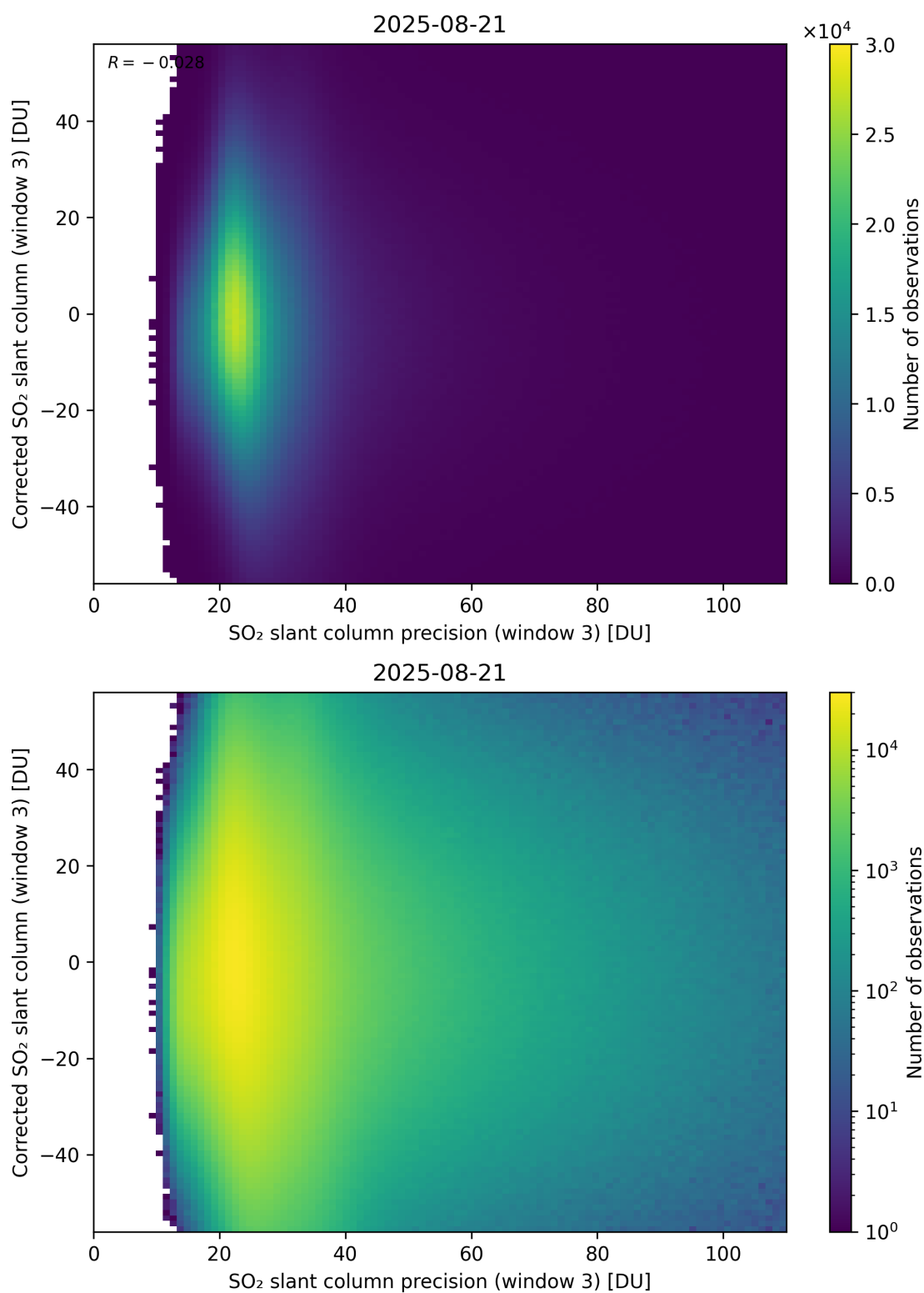
Figure 312: Scatter density plot of “SO 2 slant column precision (window 3)” against “Corrected SO 2 slant column (window 3)” for 2025-08-20 to 2025-08-22.
