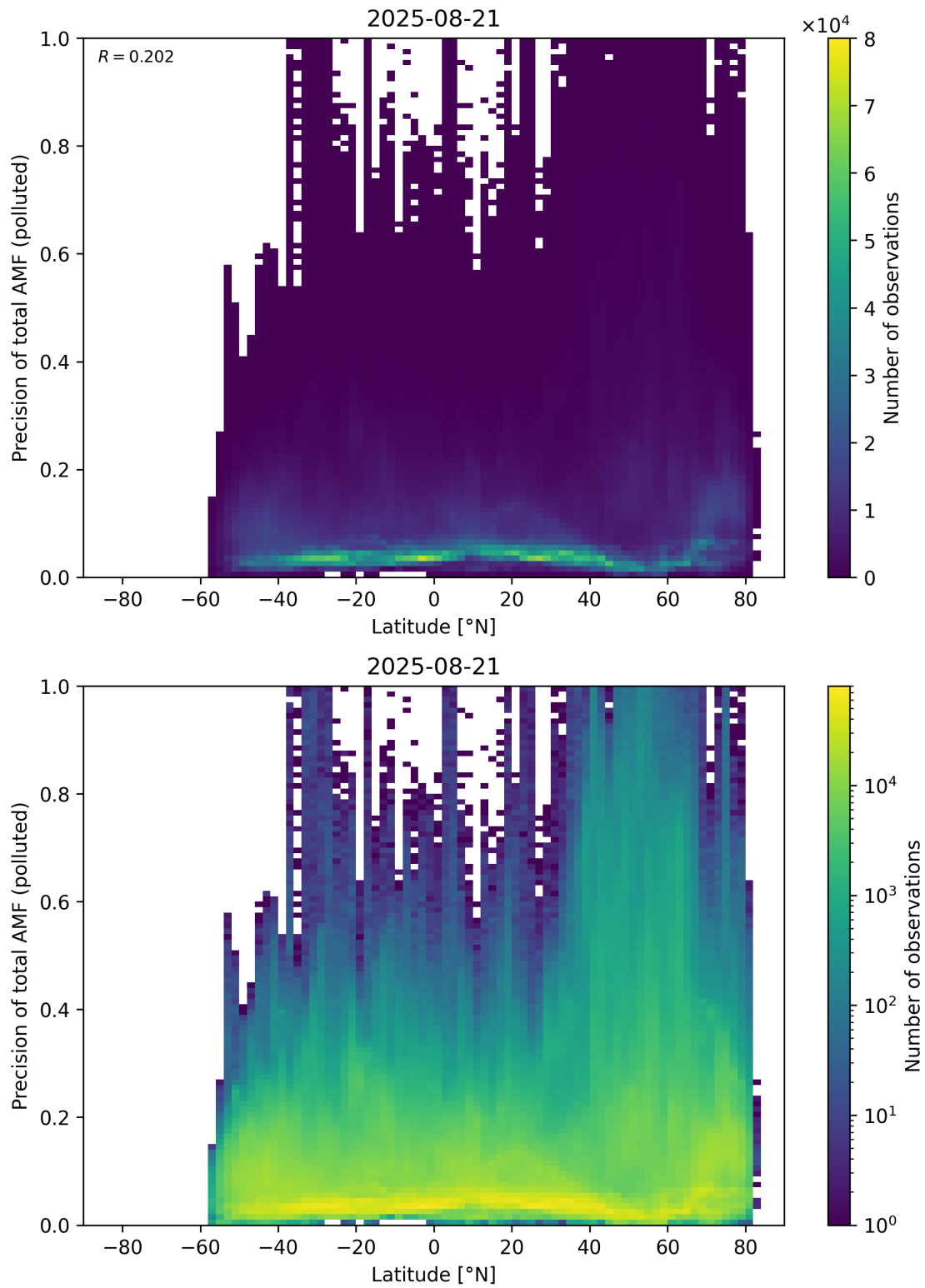
Figure 168: Scatter density plot of “Latitude” against “Precision of total AMF (polluted)” for 2025-08-20 to 2025-08-22.
