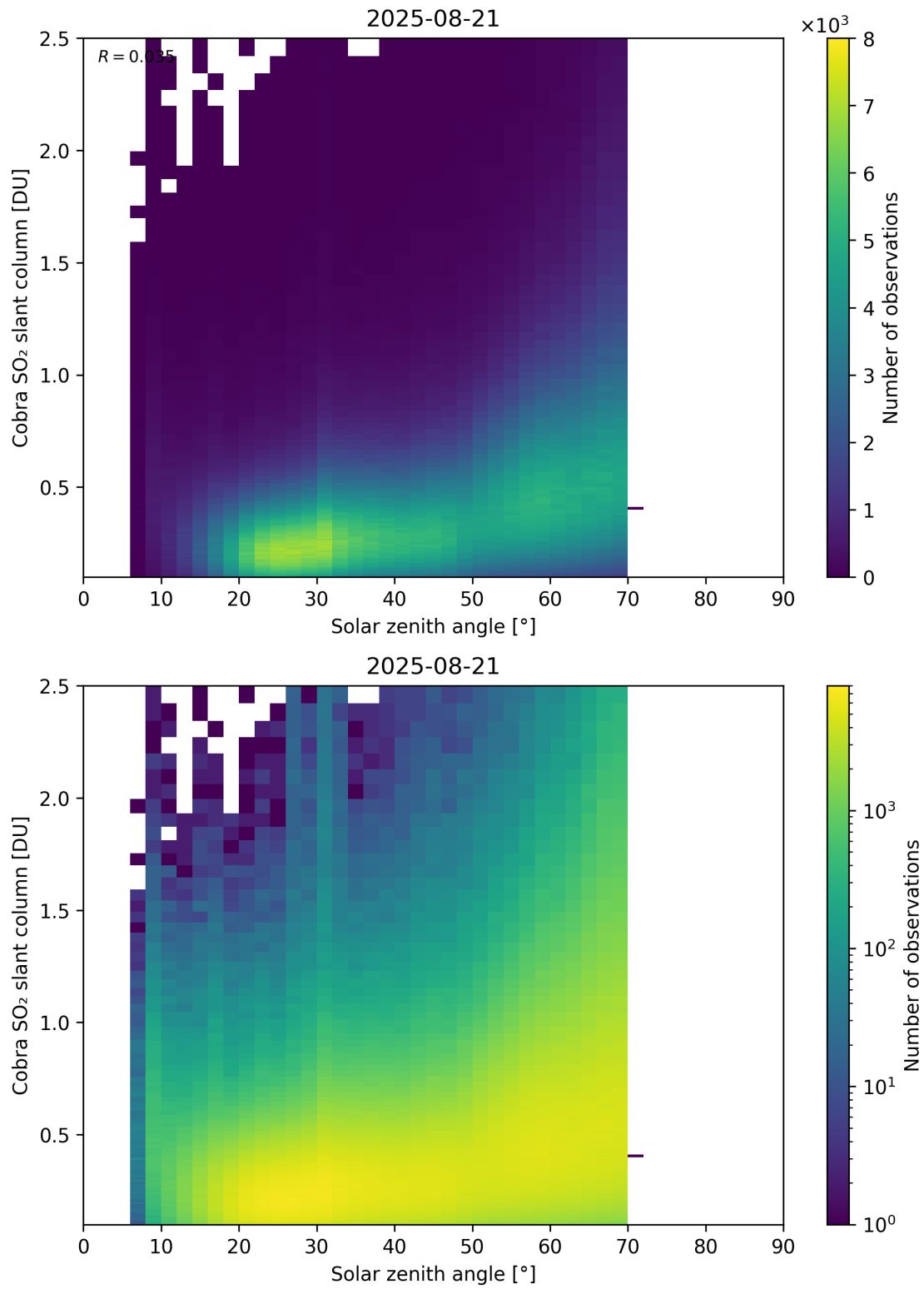
Figure 179: Scatter density plot of “Solar zenith angle” against “Cobra SO 2 slant column” for 2025-08-20 to 2025-08-22.
