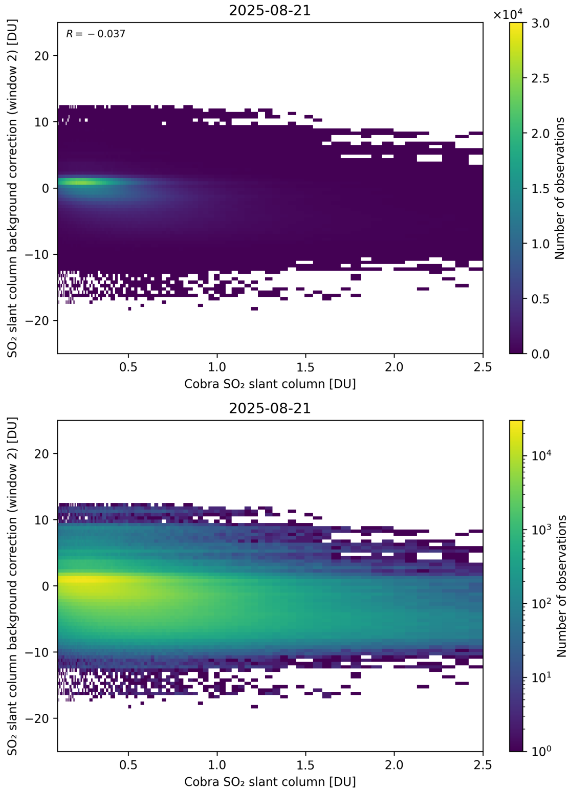
Figure 194: Scatter density plot of “Cobra SO 2 slant column” against “SO 2 slant column background correction (window 2)” for 2025-08-20 to 2025-08-22.
