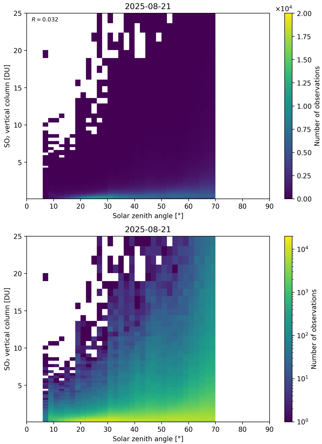
Figure 191: Scatter density plot of “Solar zenith angle” against “SO 2 vertical column” for 2025-08-20 to 2025-08-22.
