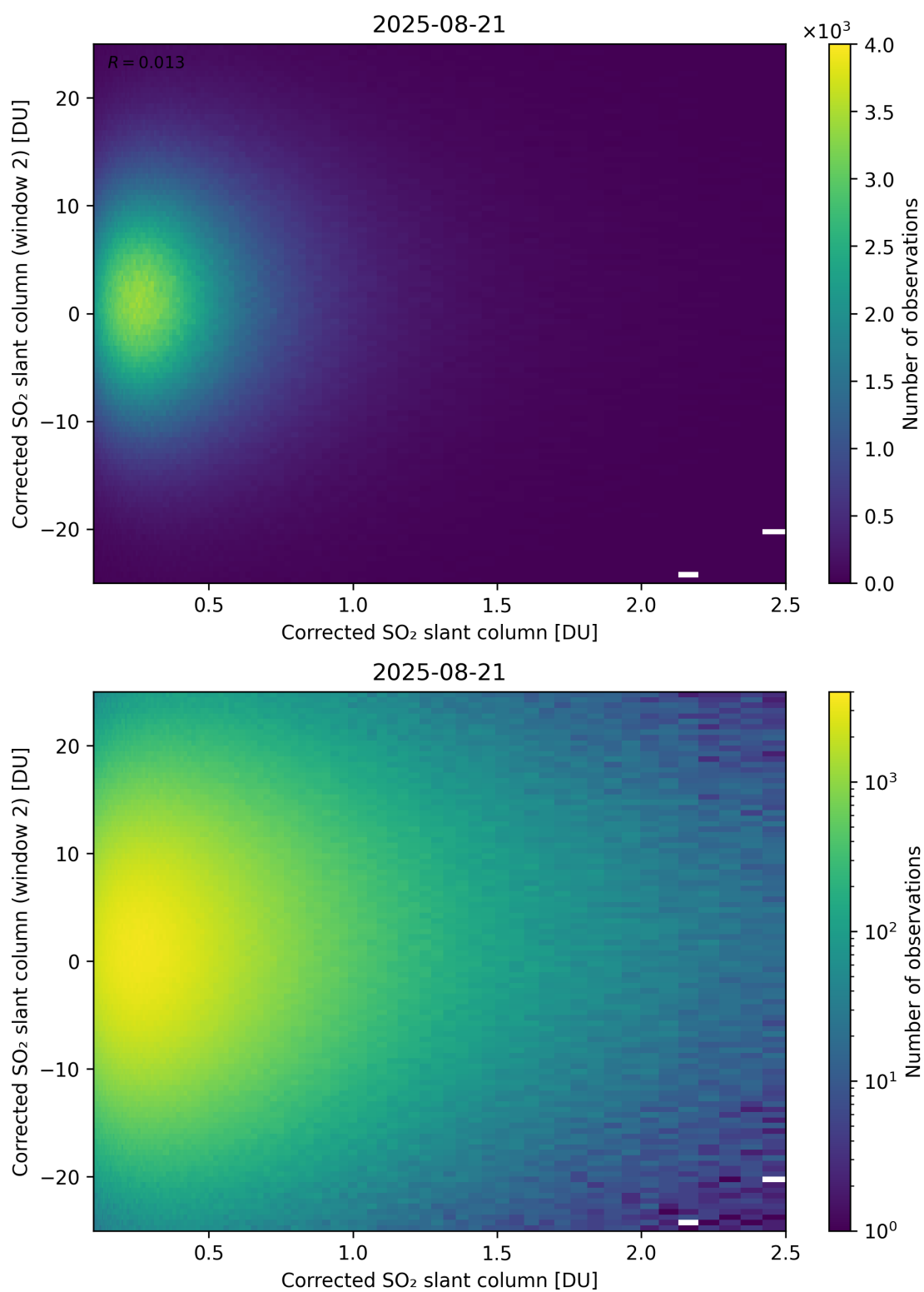
Figure 235: Scatter density plot of “Corrected SO 2 slant column” against “Corrected SO 2 slant column (window 2)” for 2025-08-20 to 2025-08-22.
