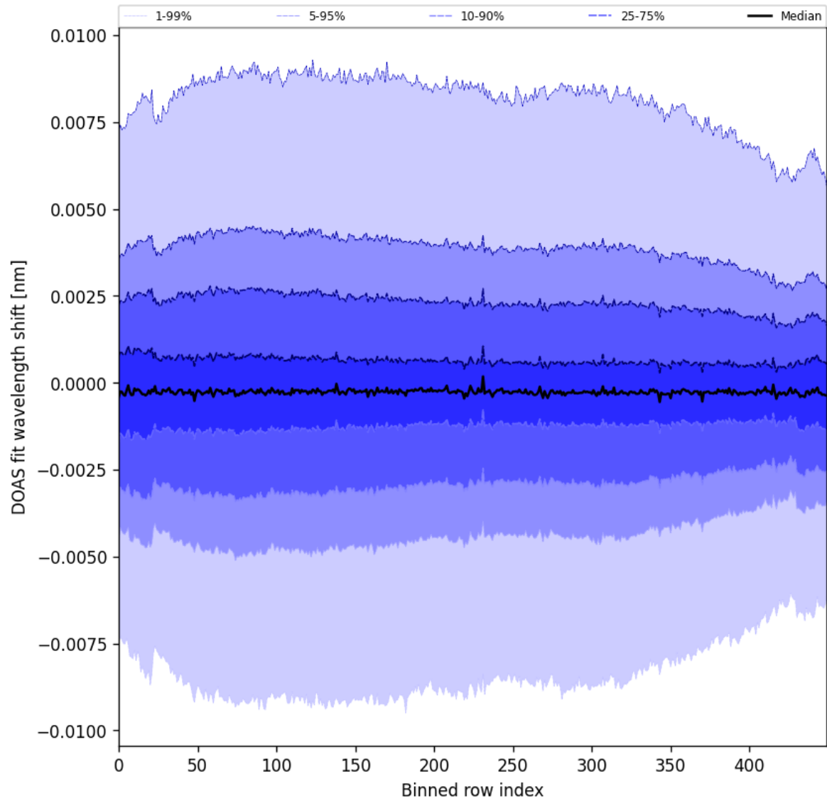
Figure 102: Along track statistics of “DOAS fit wavelength shift” for 2025-08-20 to 2025-08-22
