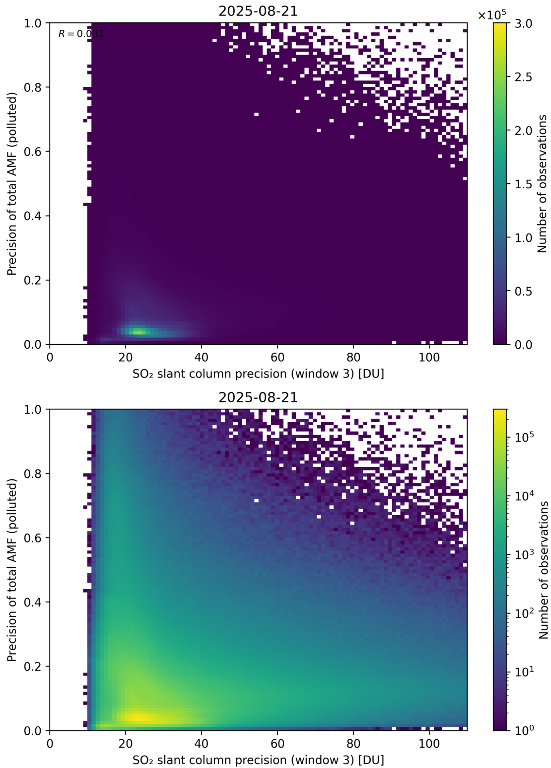
Figure 314: Scatter density plot of “SO 2 slant column precision (window 3)” against “Precision of total AMF (polluted)” for 2025-08-20 to 2025-08-22.
