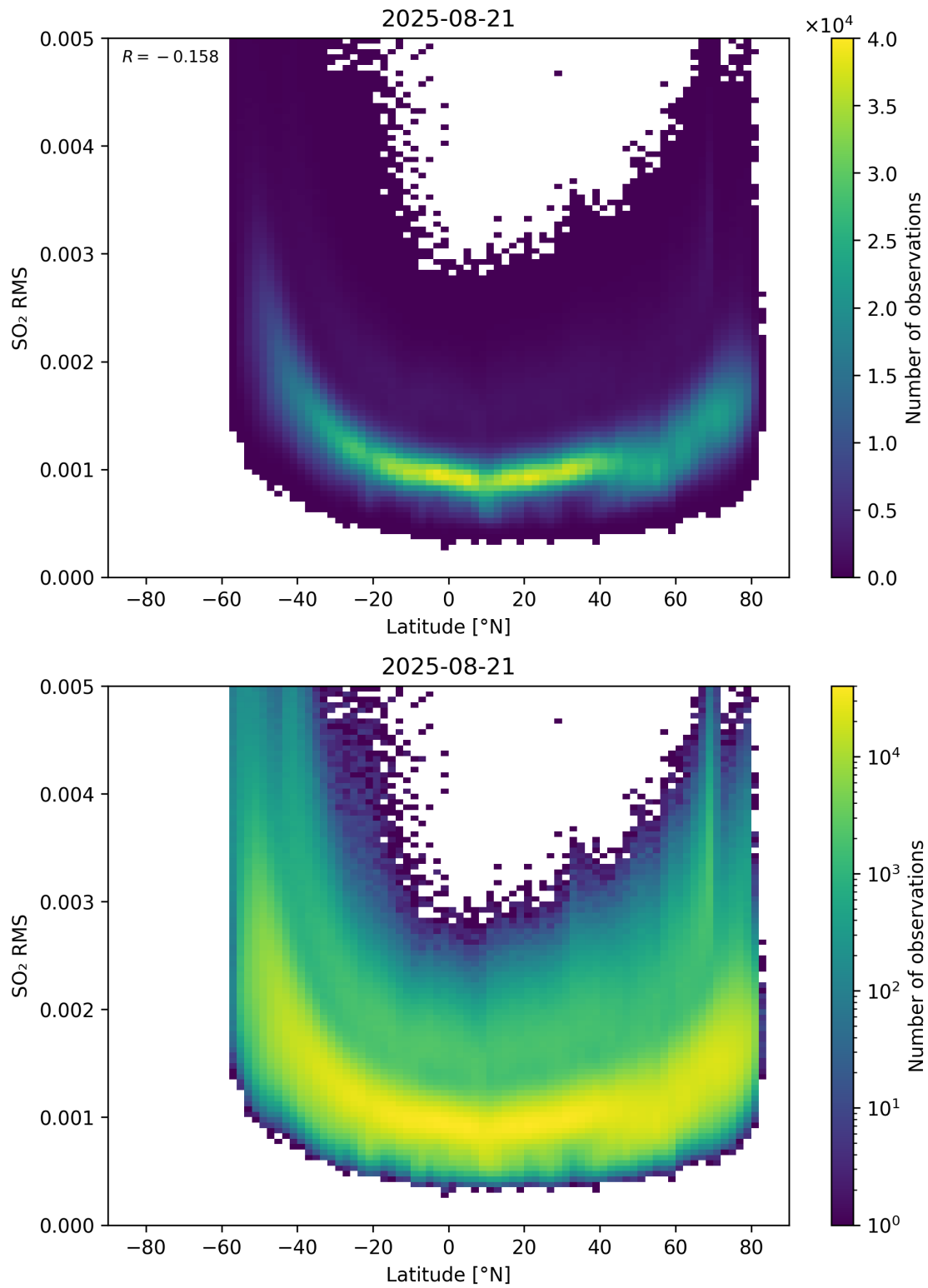
Figure 155: Scatter density plot of “Latitude” against “SO 2 RMS” for 2025-08-20 to 2025-08-22.
