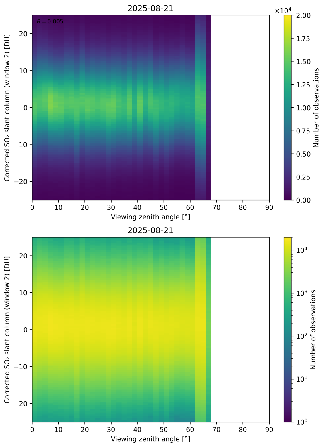
Figure 374: Scatter density plot of “Viewing zenith angle” against “Corrected SO 2 slant column (window 2)” for 2025-08-20 to 2025-08-22.
