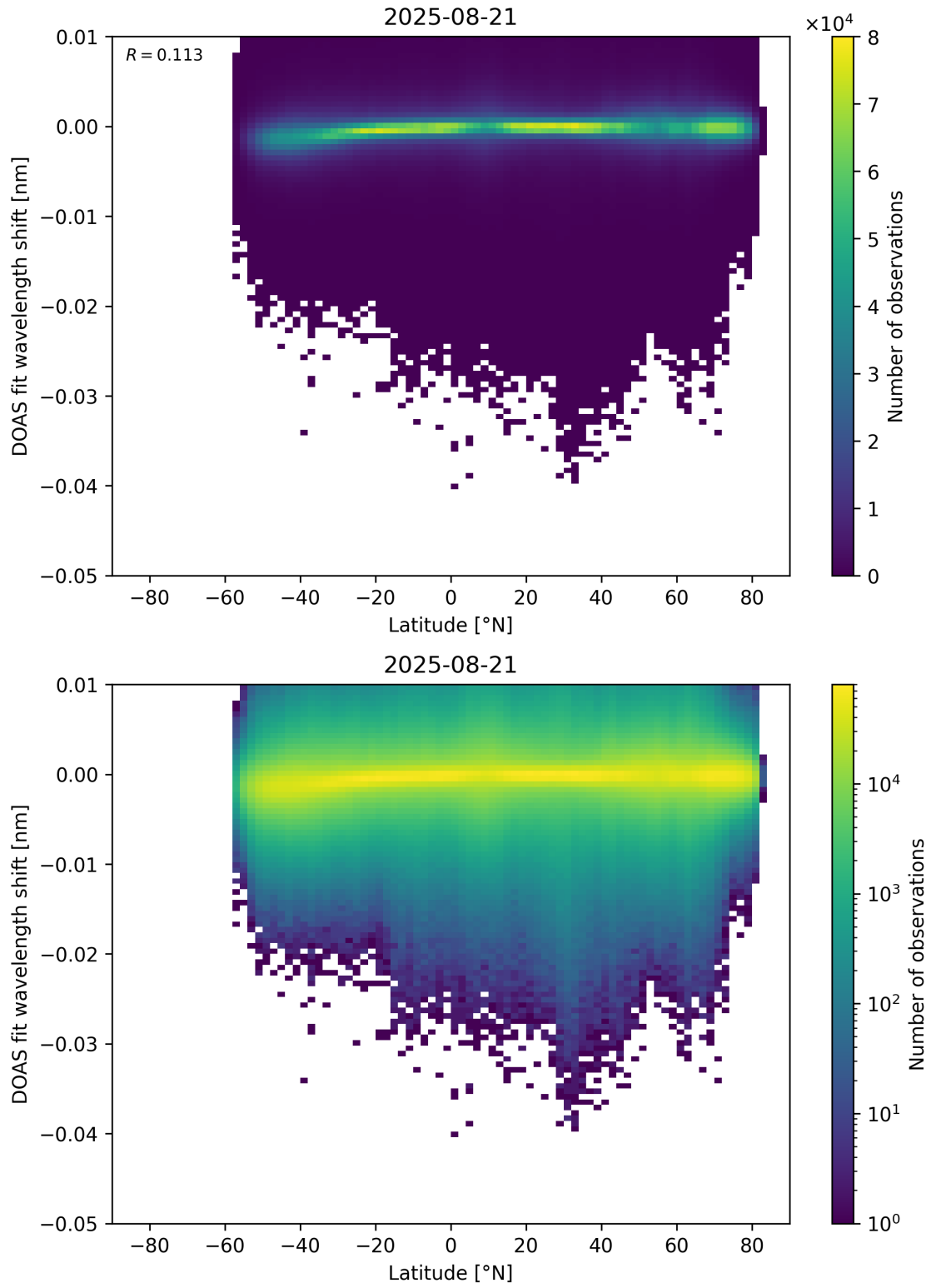
Figure 153: Scatter density plot of “Latitude” against “DOAS fit wavelength shift” for 2025-08-20 to 2025-08-22.
