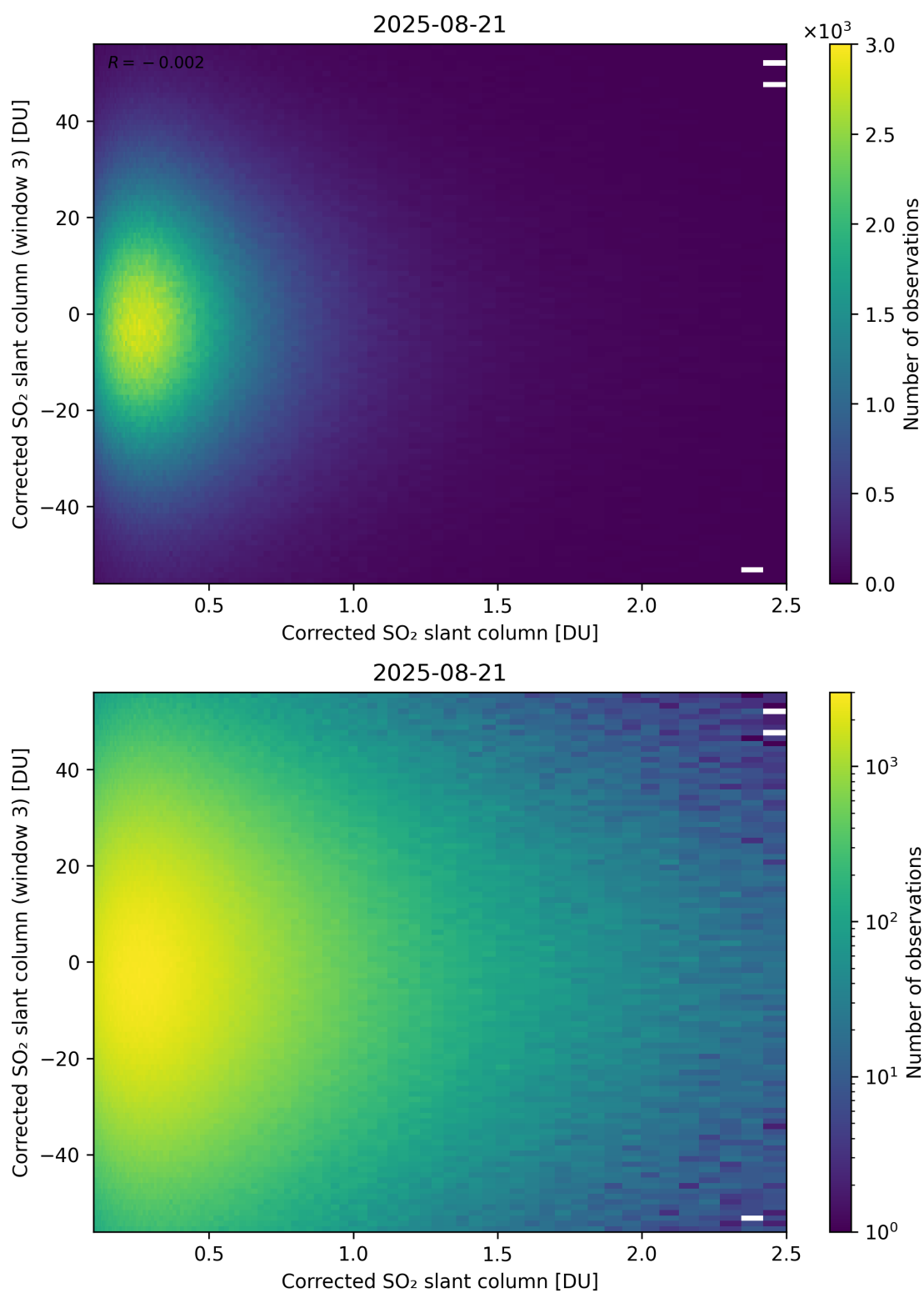
Figure 236: Scatter density plot of “Corrected SO 2 slant column” against “Corrected SO 2 slant column (window 3)” for 2025-08-20 to 2025-08-22.
