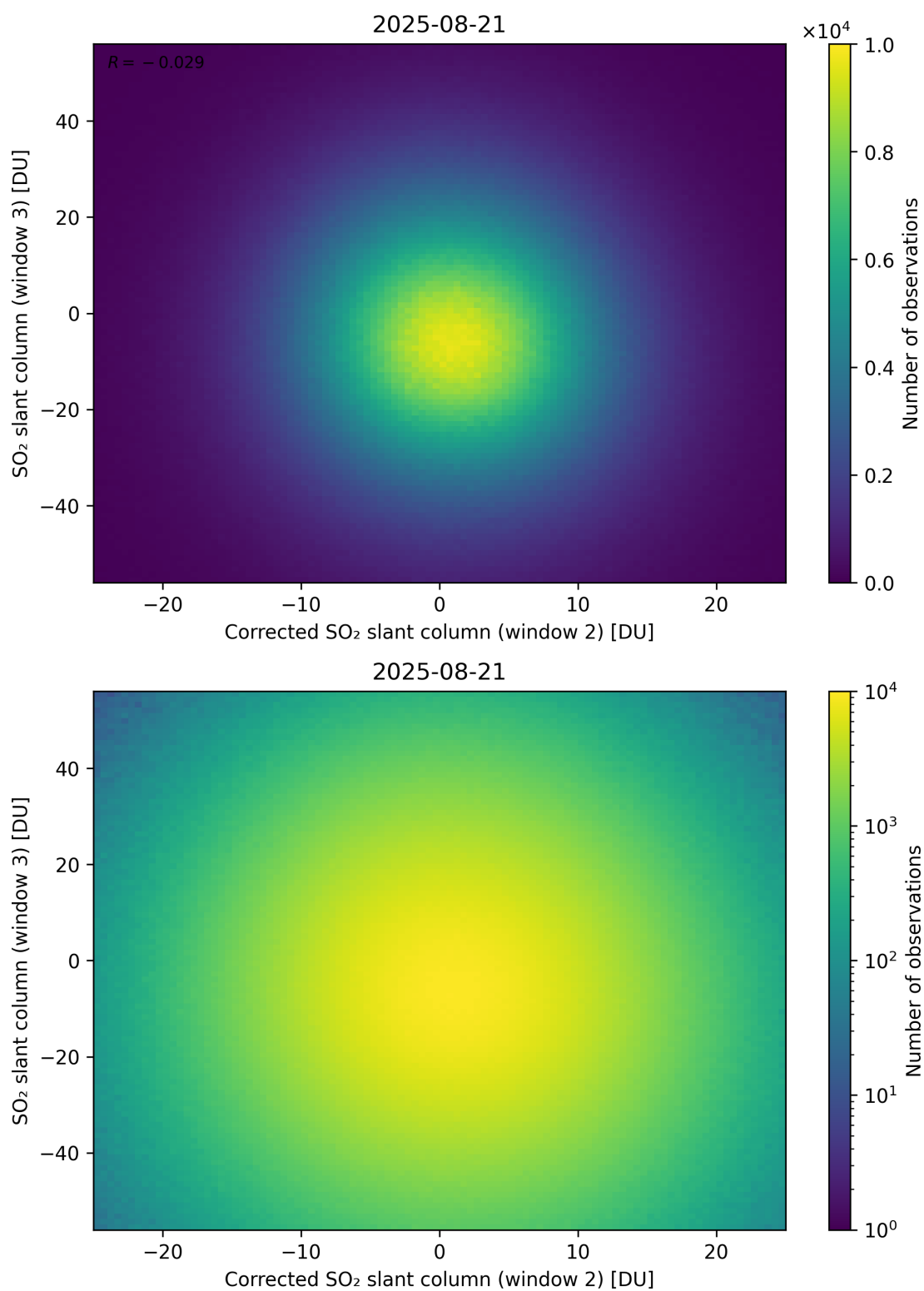
Figure 251: Scatter density plot of “Corrected SO 2 slant column (window 2)” against “SO 2 slant column (window 3)” for 2025-08-20 to 2025-08-22.
