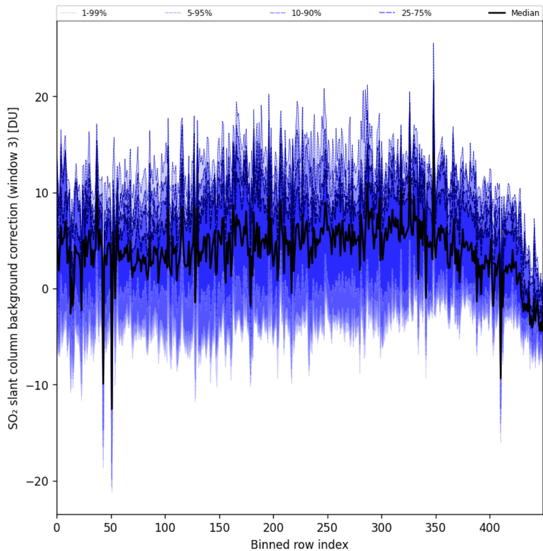
Figure 100: Along track statistics of “SO 2 slant column background correction (window 3)” for 2025-08-20 to 2025-08-22
