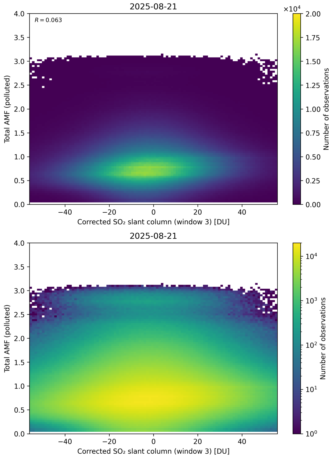
Figure 260: Scatter density plot of “Corrected SO 2 slant column (window 3)” against “Total AMF (polluted)” for 2025-08-20 to 2025-08-22.
