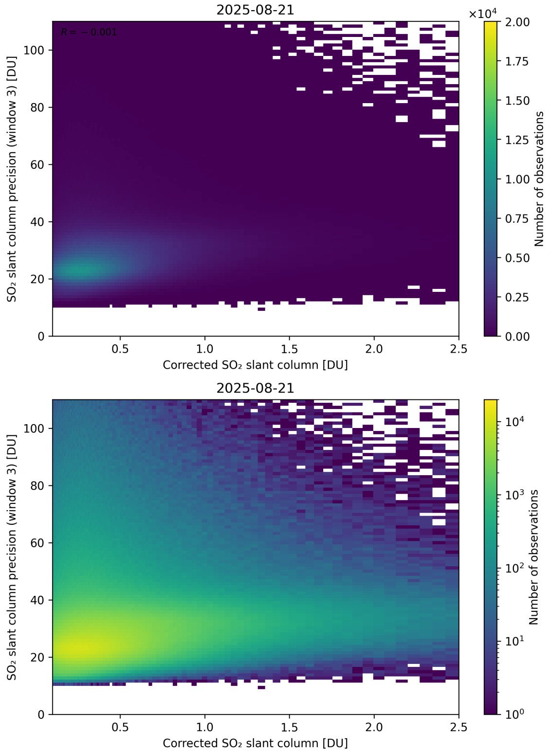
Figure 241: Scatter density plot of “Corrected SO 2 slant column” against “SO 2 slant column precision (window 3)” for 2025-08-20 to 2025-08-22.
