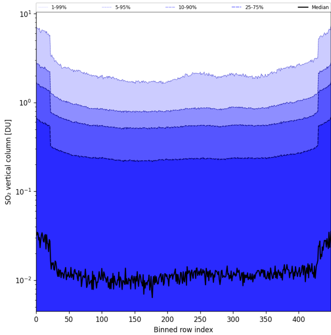
Figure 84: Along track statistics of “SO 2 vertical column” for 2025-08-20 to 2025-08-22
