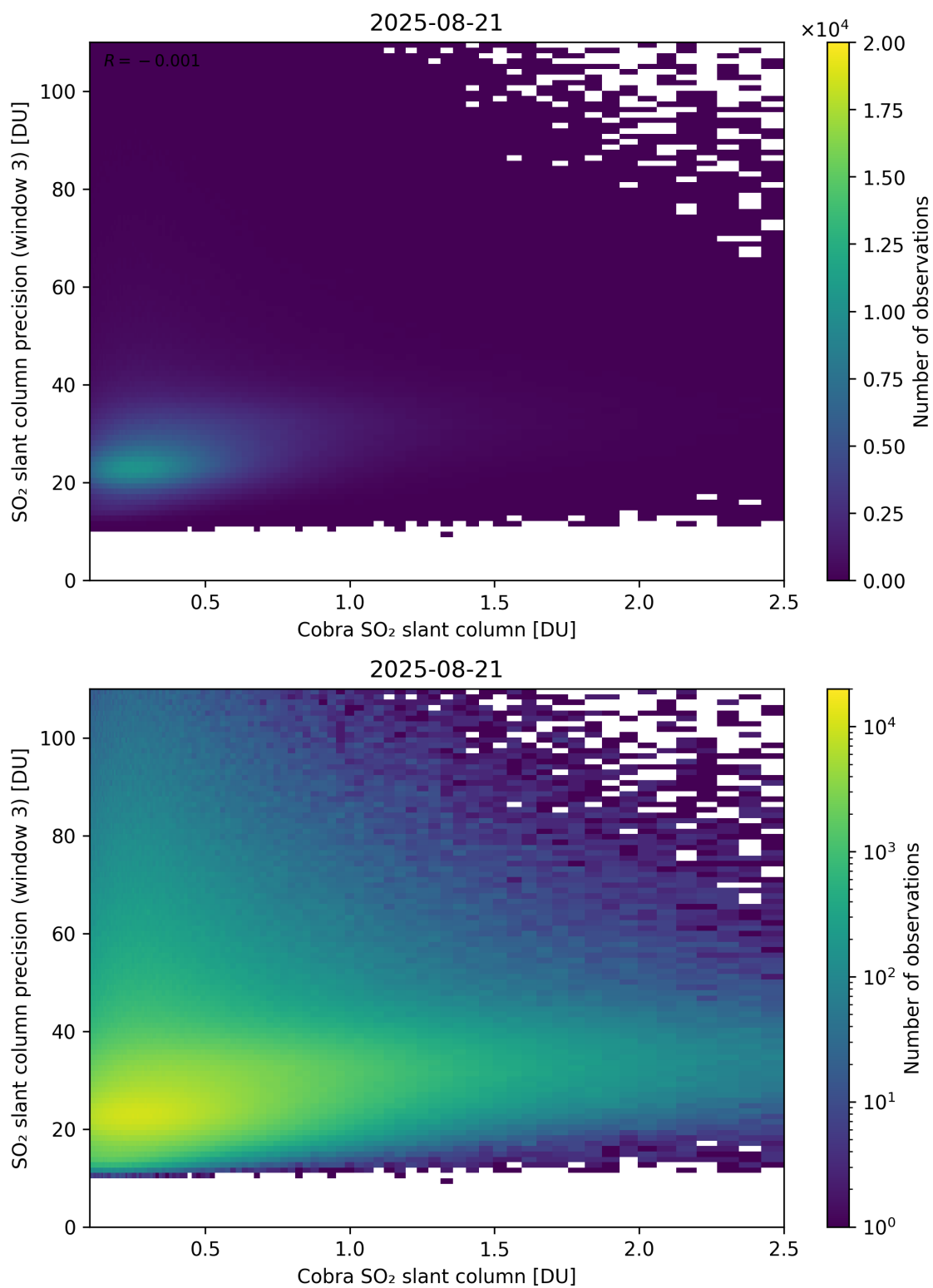
Figure 223: Scatter density plot of “Cobra SO 2 slant column” against “SO 2 slant column precision (window 3)” for 2025-08-20 to 2025-08-22.
