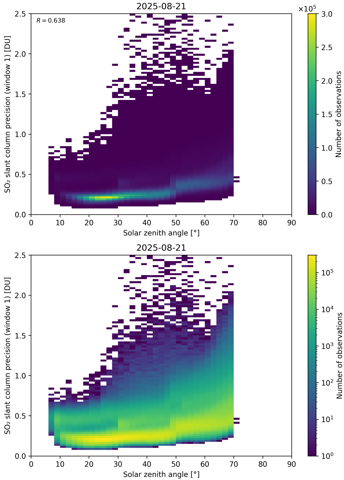
Figure 185: Scatter density plot of “Solar zenith angle” against “SO 2 slant column precision (window 1)” for 2025-08-20 to 2025-08-22.
