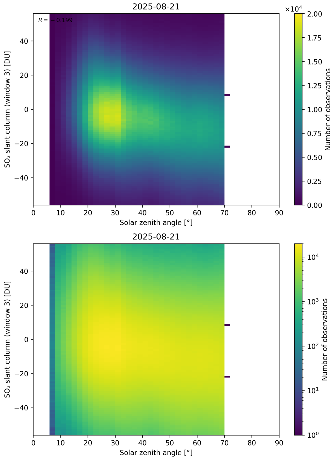
Figure 187: Scatter density plot of “Solar zenith angle” against “SO 2 slant column (window 3)” for 2025-08-20 to 2025-08-22.
