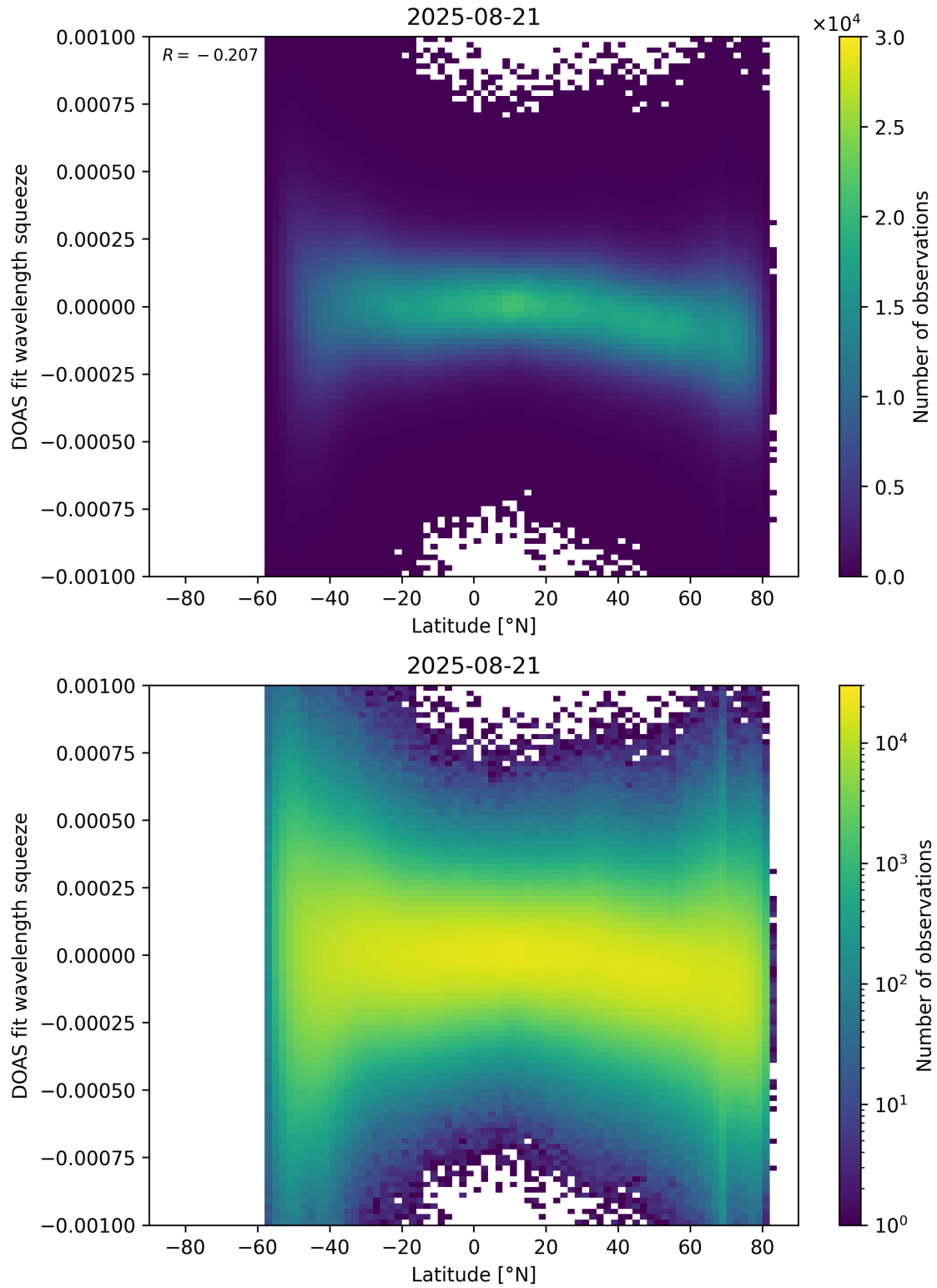
Figure 154: Scatter density plot of “Latitude” against “DOAS fit wavelength squeeze” for 2025-08-20 to 2025-08-22.
