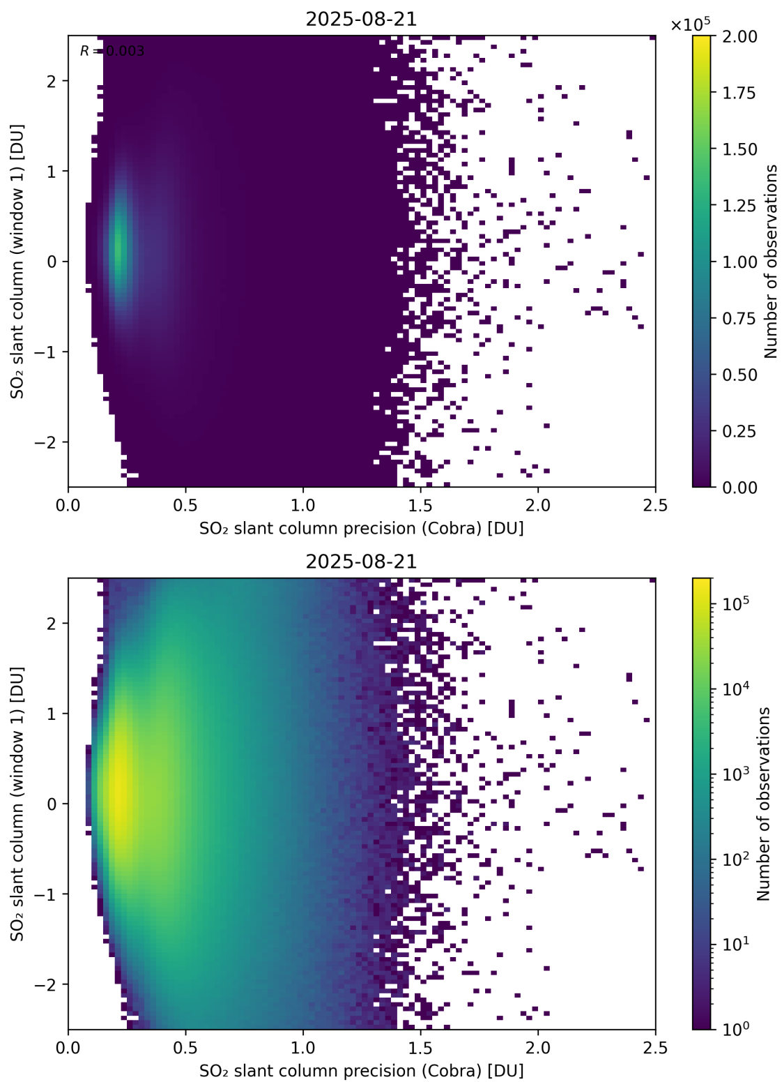
Figure 208: Scatter density plot of “SO 2 slant column precision (Cobra)” against “SO 2 slant column (window 1)” for 2025-08-20 to 2025-08-22.
