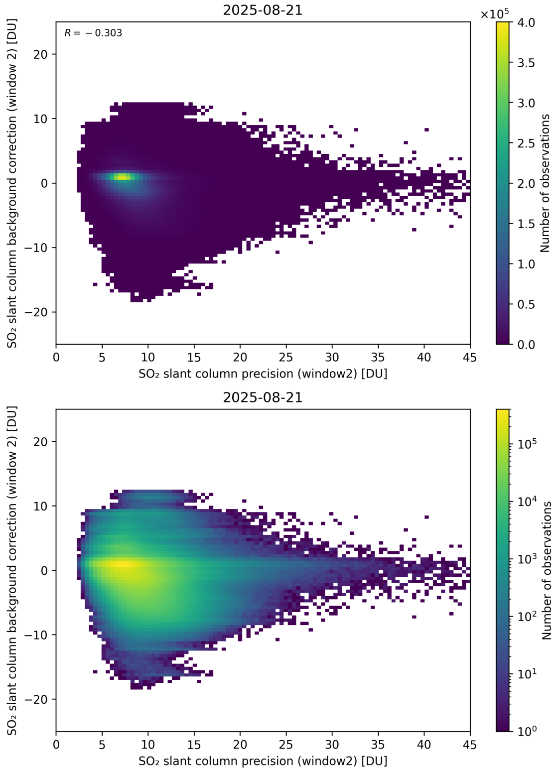
Figure 291: Scatter density plot of “SO 2 slant column precision (window2)” against “SO 2 slant column background correction (window 2)” for 2025-08-20 to 2025-08-22.
