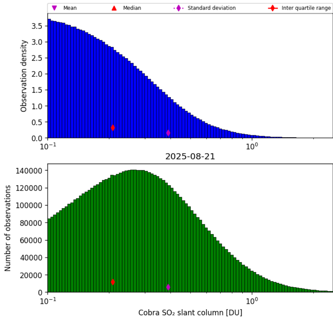
Figure 61: Histogram of “Cobra SO 2 slant column” for 2025-08-20 to 2025-08-22
