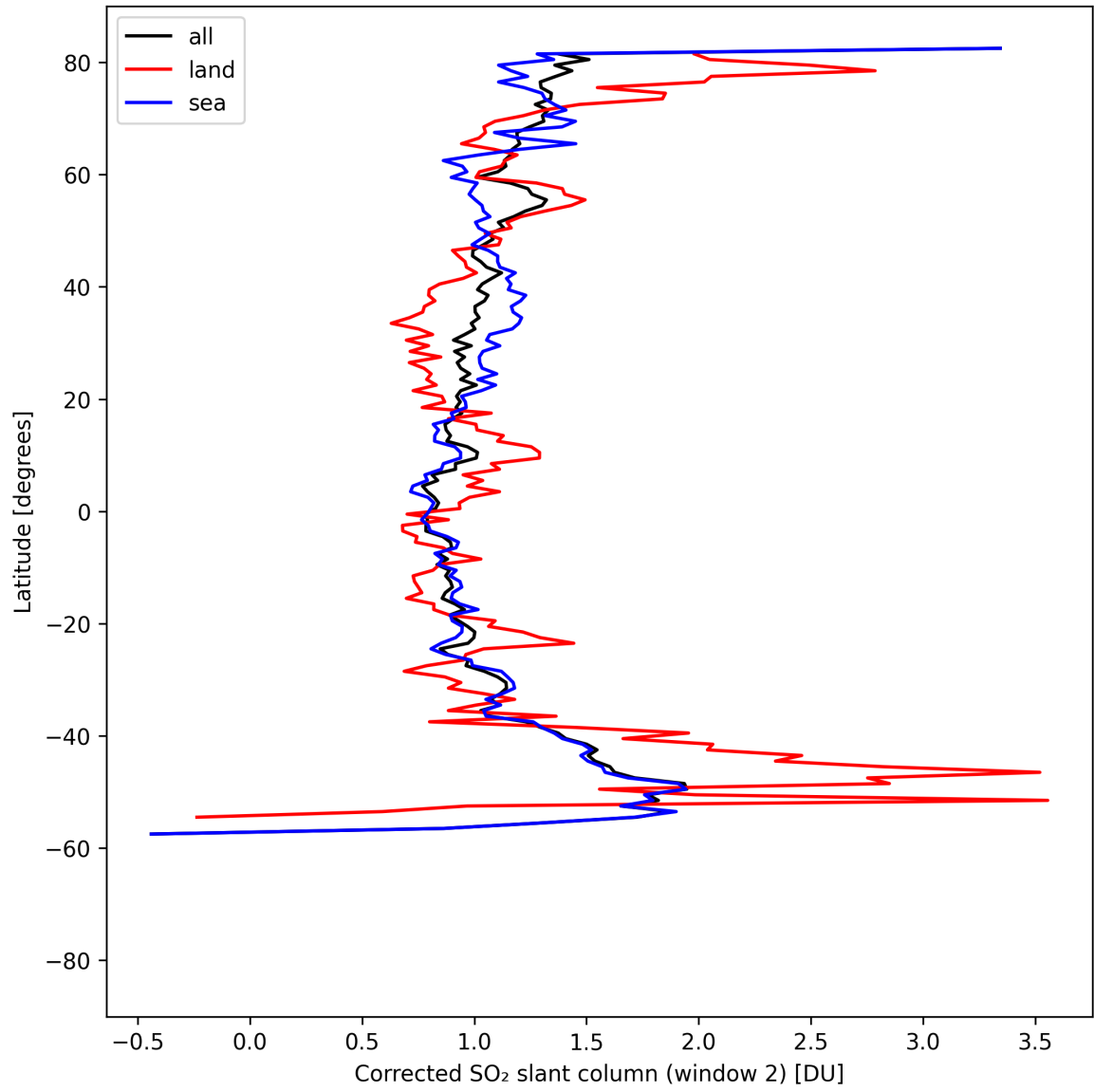
Figure 43: Zonal average of “Corrected SO 2 slant column (window 2)” for 2025-08-20 to 2025-08-22.
