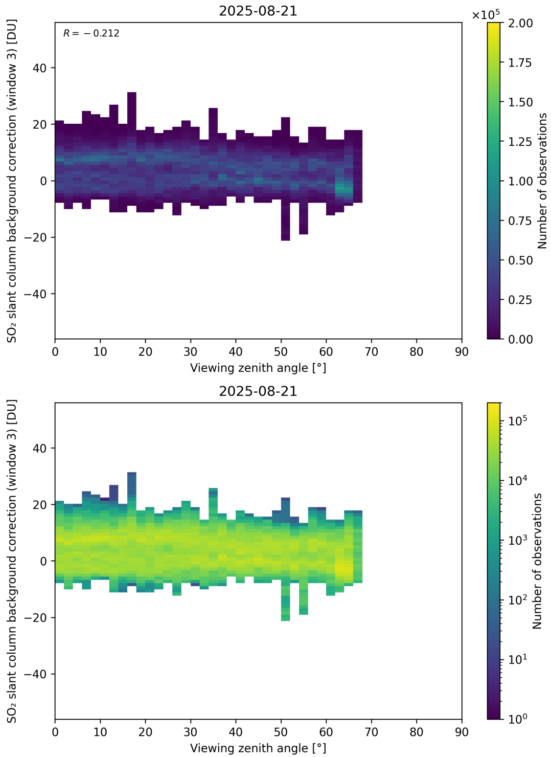
Figure 364: Scatter density plot of “Viewing zenith angle” against “SO 2 slant column background correction (window 3)” for 2025-08-20 to 2025-08-22.
