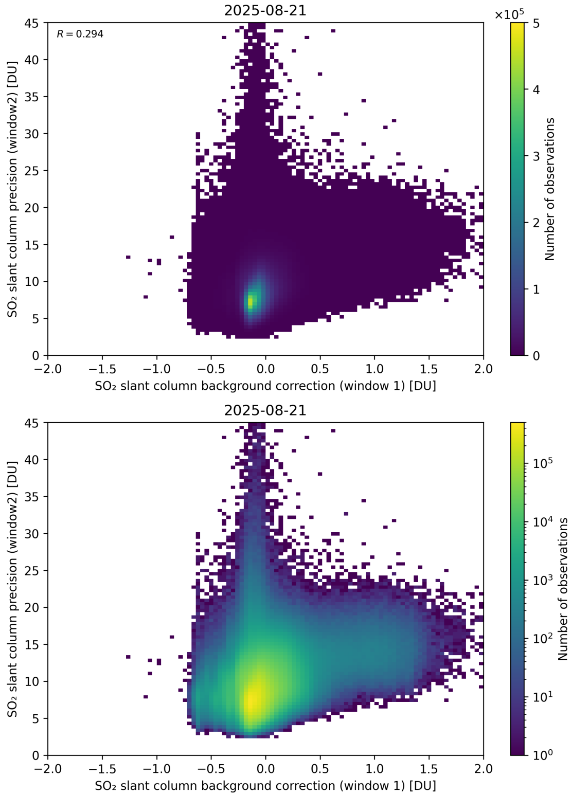
Figure 117: Scatter density plot of “SO 2 slant column background correction (window 1)” against “SO 2 slant column precision (window2)” for 2025-08-20 to 2025-08-22.
