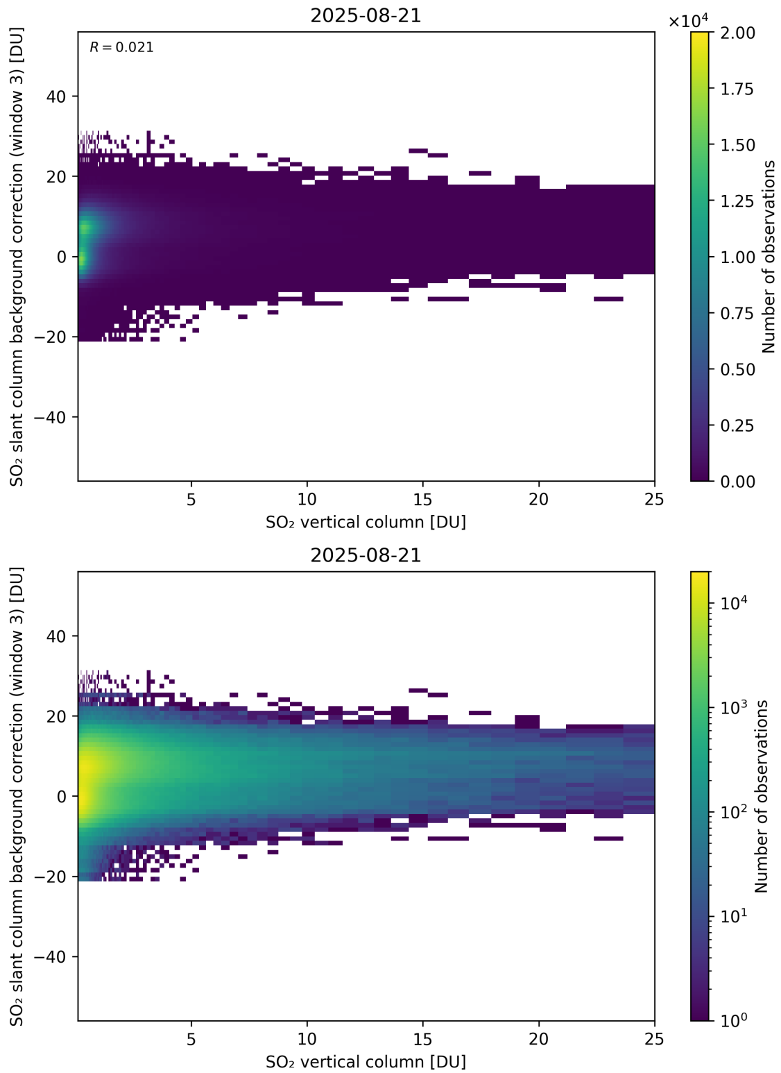
Figure 325: Scatter density plot of “SO 2 vertical column” against “SO 2 slant column background correction (window 3)” for 2025-08-20 to 2025-08-22.
