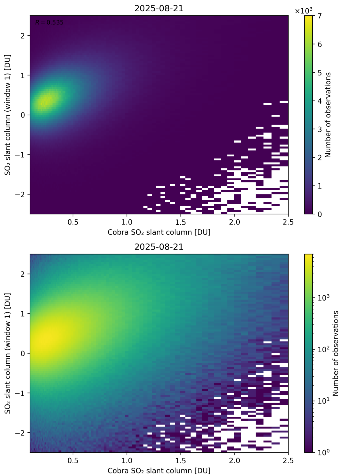
Figure 219: Scatter density plot of “Cobra SO 2 slant column” against “SO 2 slant column (window 1)” for 2025-08-20 to 2025-08-22.
