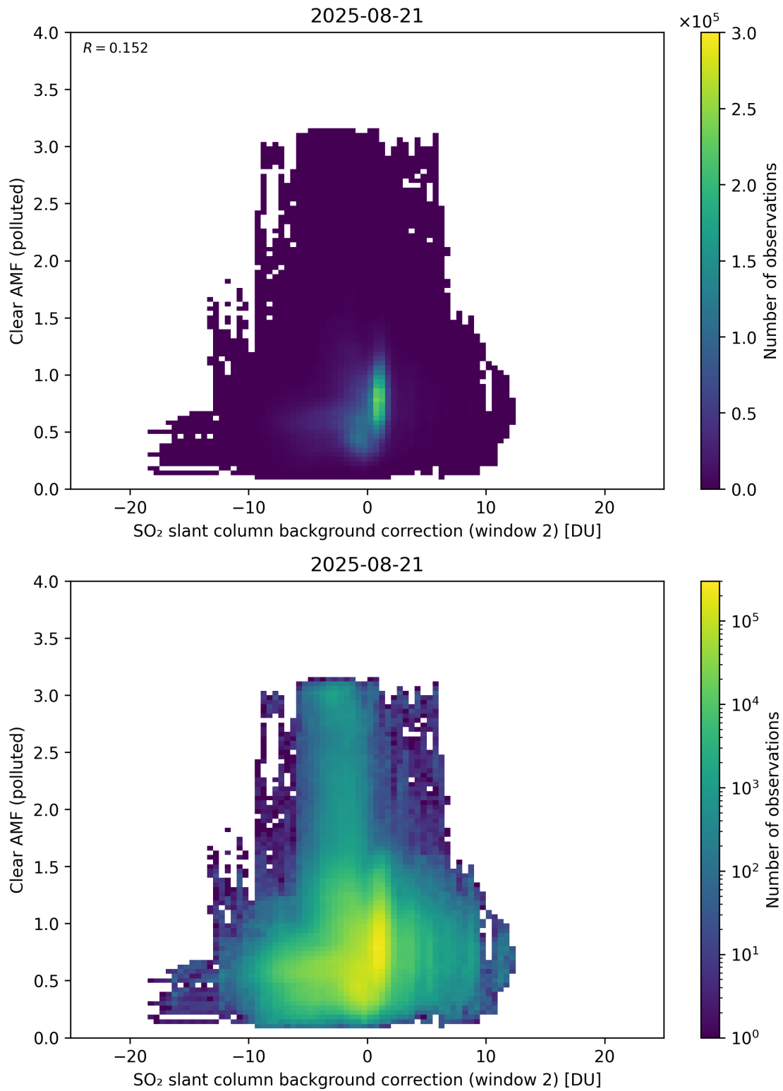
Figure 126: Scatter density plot of “SO 2 slant column background correction (window 2)” against “Clear AMF (polluted)” for 2025-08-20 to 2025-08-22.
