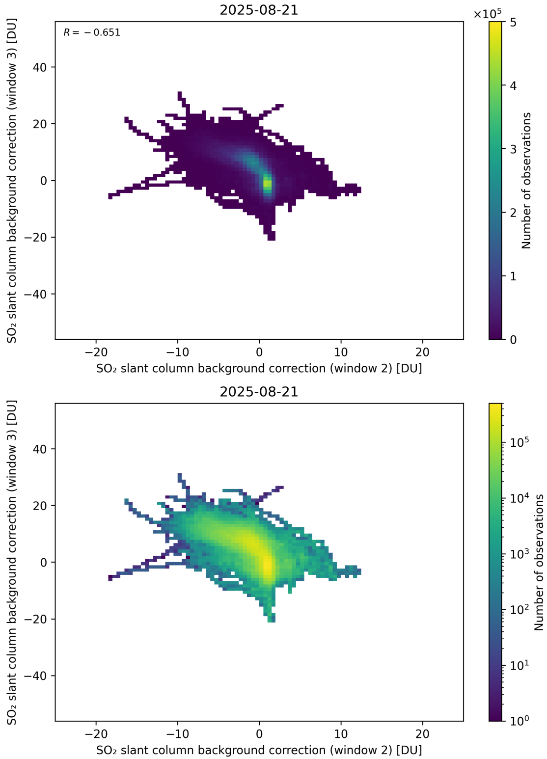
Figure 122: Scatter density plot of “SO 2 slant column background correction (window 2)” against “SO 2 slant column background correction (window 3)” for 2025-08-20 to 2025-08-22.
