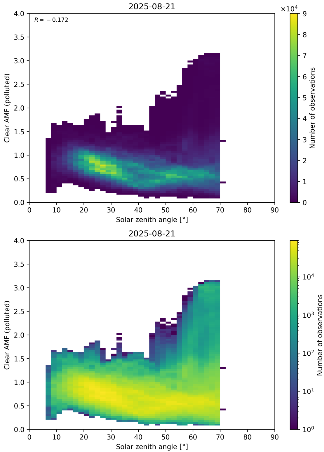
Figure 178: Scatter density plot of “Solar zenith angle” against “Clear AMF (polluted)” for 2025-08-20 to 2025-08-22.
