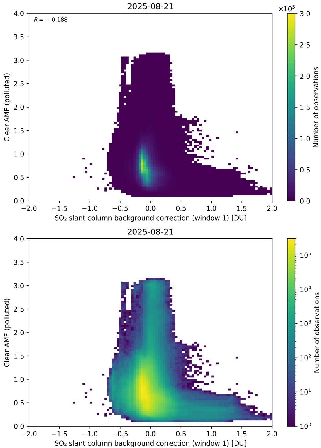
Figure 114: Scatter density plot of “SO 2 slant column background correction (window 1)” against “Clear AMF (polluted)” for 2025-08-20 to 2025-08-22.
