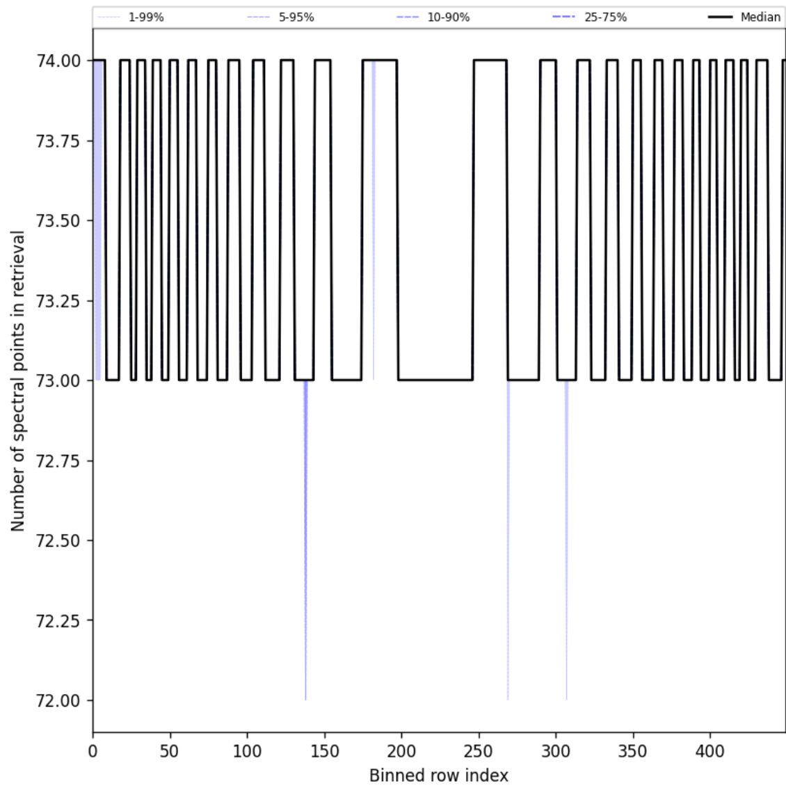
Figure 108: Along track statistics of “Number of spectral points in retrieval” for 2025-08-20 to 2025-08-22
