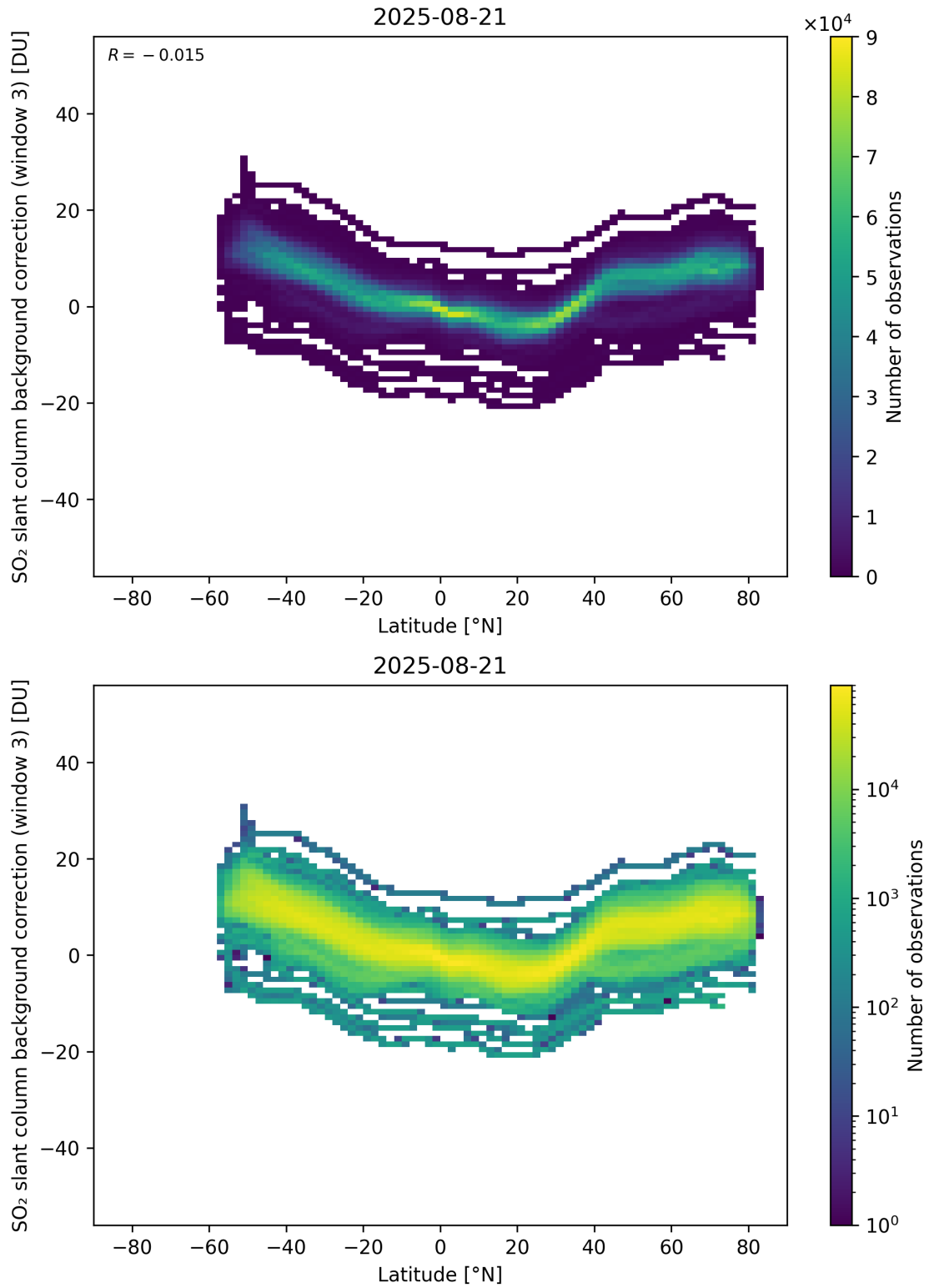
Figure 152: Scatter density plot of “Latitude” against “SO 2 slant column background correction (window 3)” for 2025-08-20 to 2025-08-22.
