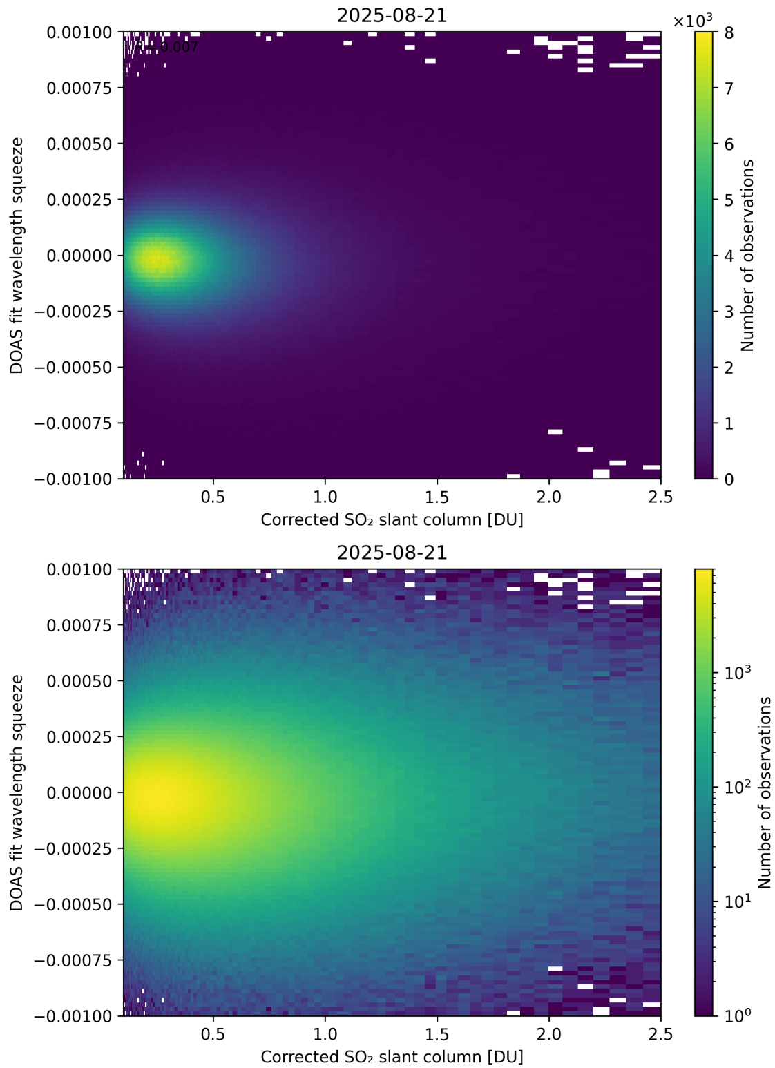
Figure 230: Scatter density plot of "Corrected SO 2 slant column" against "DOAS fit wavelength squeeze" for 2025-08-20 to 2025-08-22.
