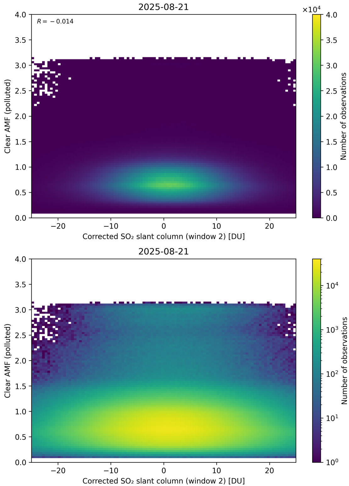
Figure 249: Scatter density plot of “Corrected SO 2 slant column (window 2)” against “Clear AMF (polluted)” for 2025-08-20 to 2025-08-22.
