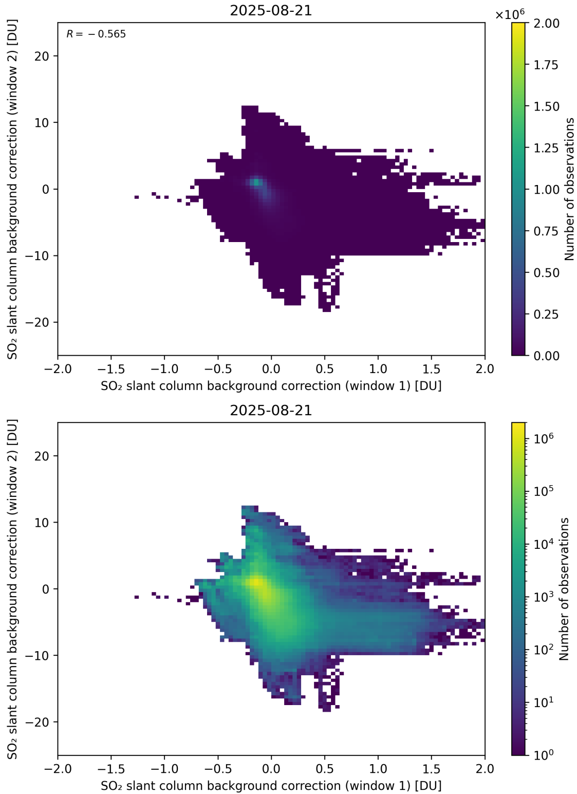
Figure 109: Scatter density plot of “SO 2 slant column background correction (window 1)” against “SO 2 slant column background correction (window 2)” for 2025-08-20 to 2025-08-22.
