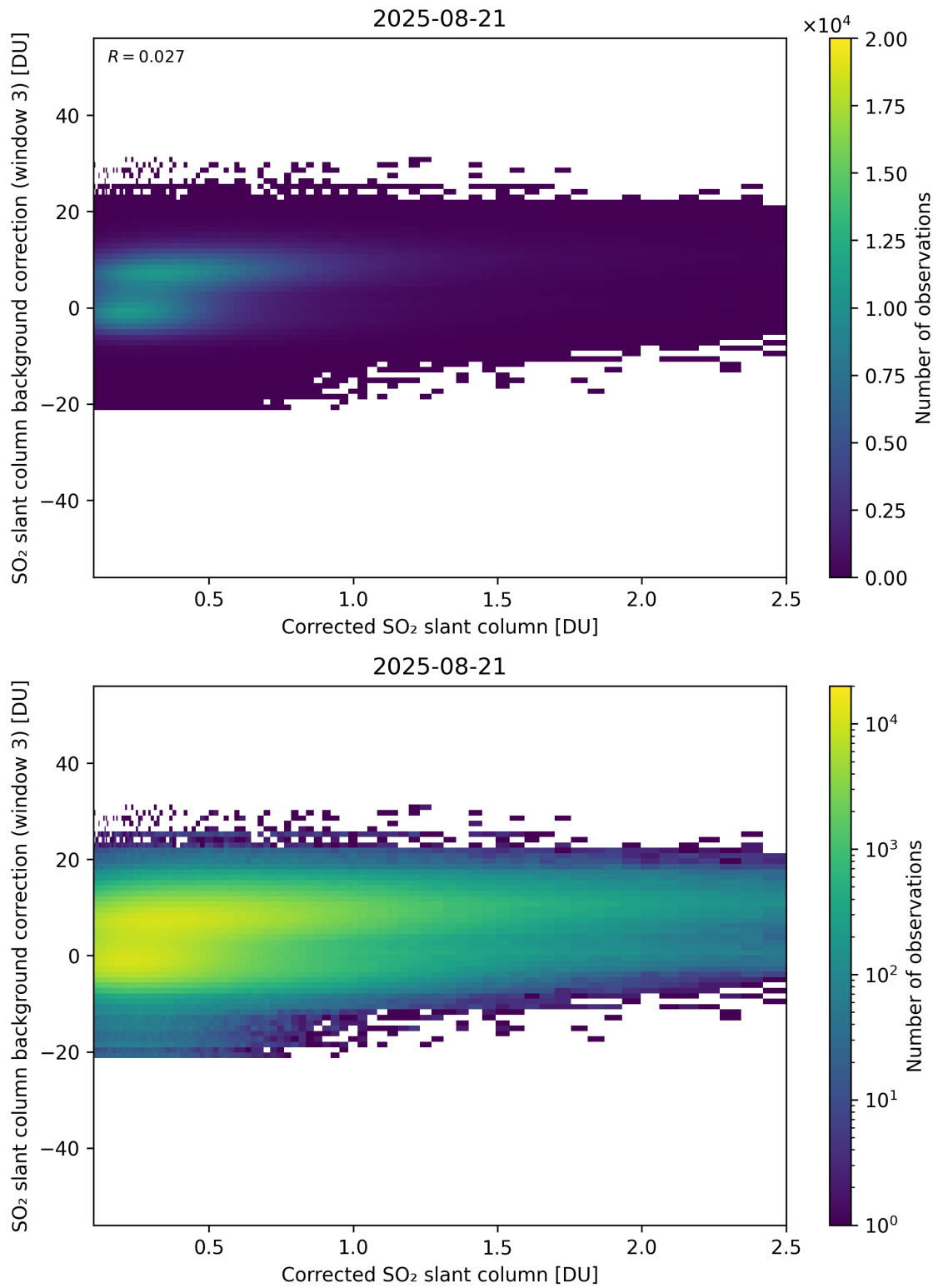
Figure 228: Scatter density plot of “Corrected SO 2 slant column” against “SO 2 slant column background correction (window 3)” for 2025-08-20 to 2025-08-22.
