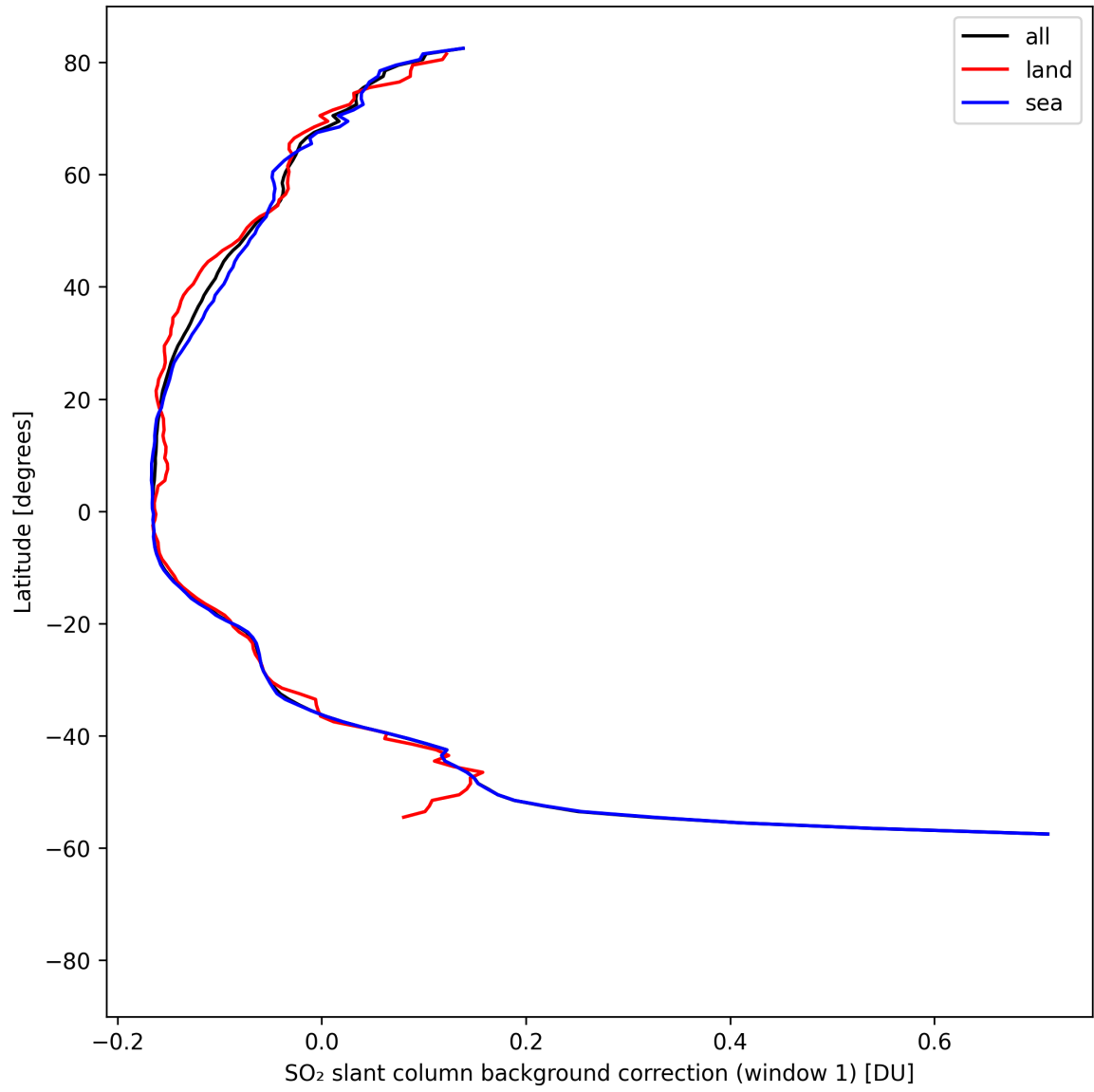
Figure 40: Zonal average of “SO 2 slant column background correction (window 1)” for 2025-08-20 to 2025-08-22.
