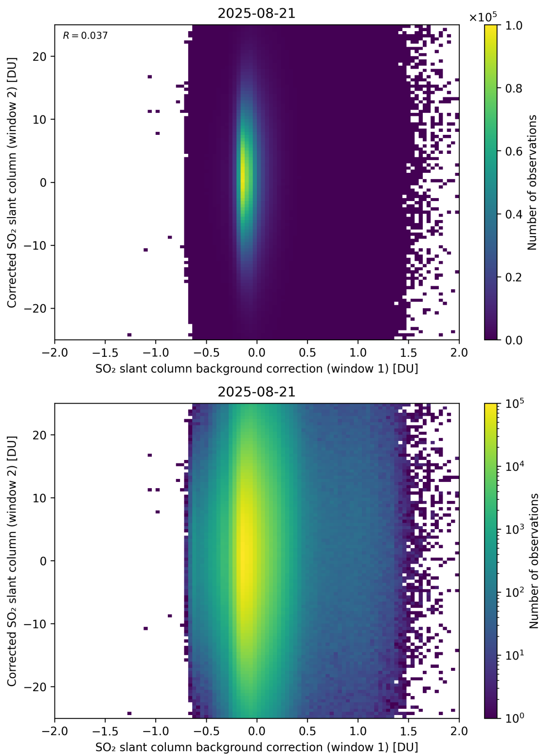
Figure 115: Scatter density plot of “SO 2 slant column background correction (window 1)” against “Corrected SO 2 slant column (window 2)” for 2025-08-20 to 2025-08-22.
