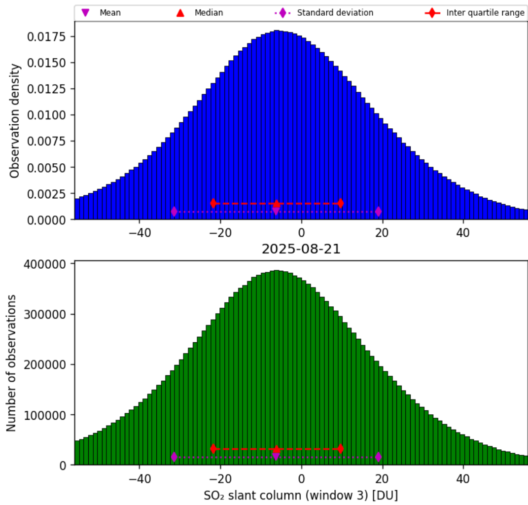
Figure 71: Histogram of “SO 2 slant column (window 3)” for 2025-08-20 to 2025-08-22
