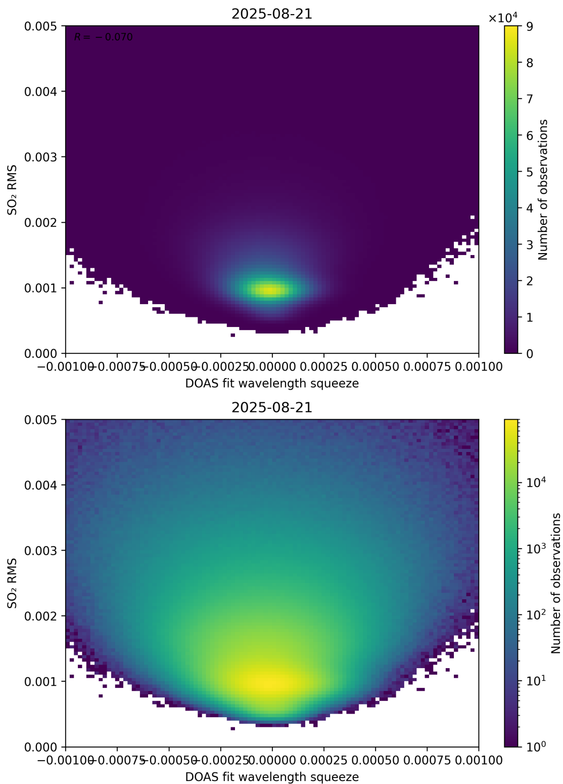
Figure 143: Scatter density plot of “DOAS fit wavelength squeeze” against “SO 2 RMS” for 2025-08-20 to 2025-08-22.
