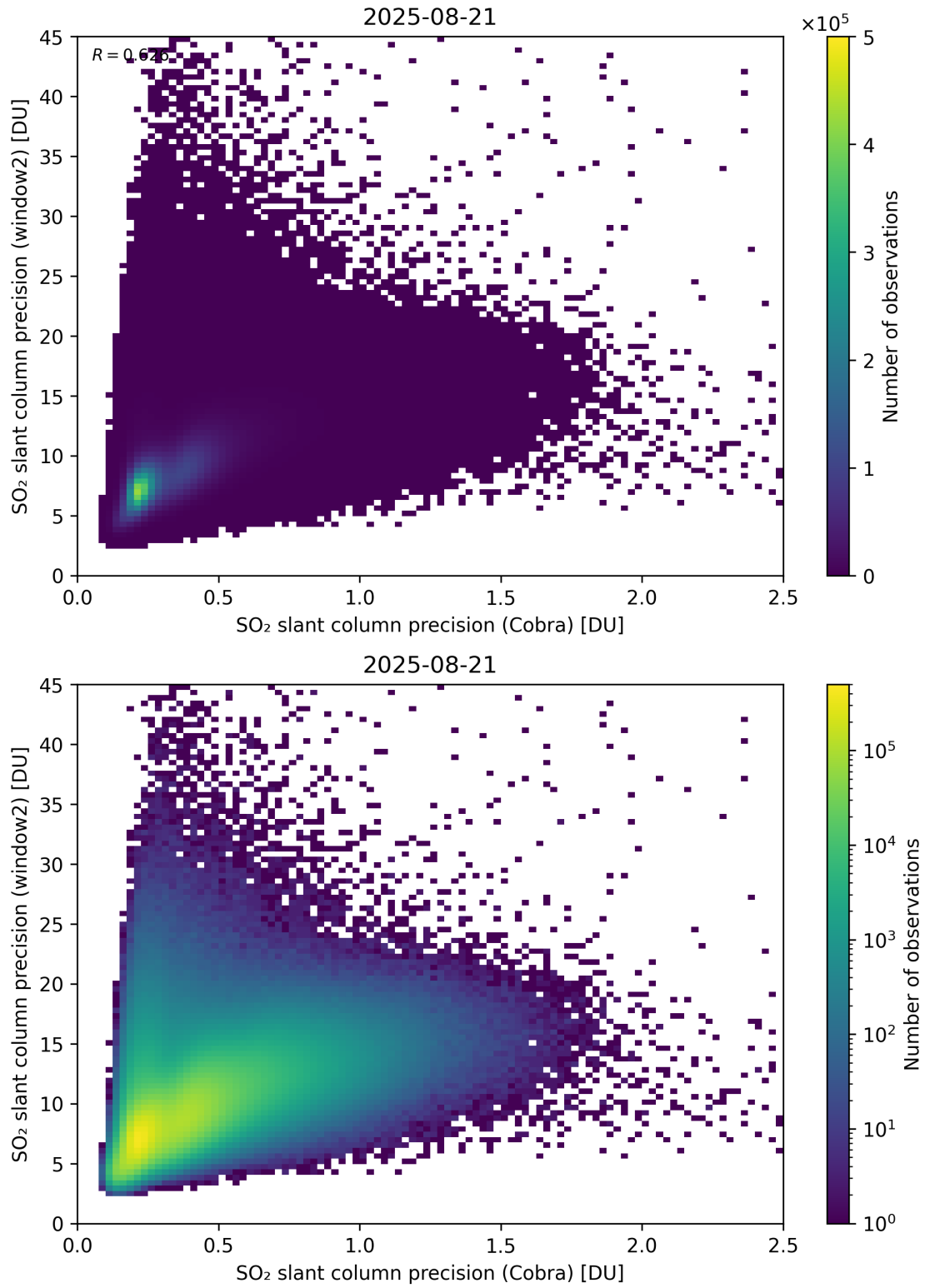
Figure 210: Scatter density plot of “SO 2 slant column precision (Cobra)” against “SO 2 slant column precision (window2)” for 2025-08-20 to 2025-08-22.
