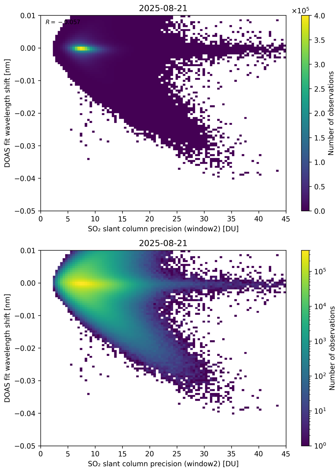
Figure 293: Scatter density plot of “SO 2 slant column precision (window2)” against “DOAS fit wavelength shift” for 2025-08-20 to 2025-08-22.
