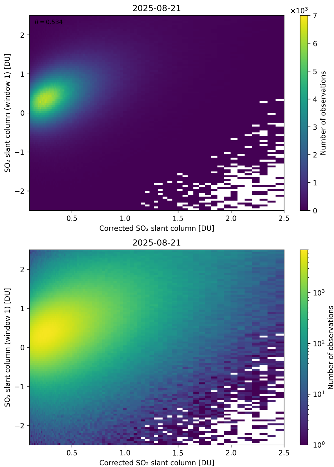
Figure 237: Scatter density plot of “Corrected SO 2 slant column” against “SO 2 slant column (window 1)” for 2025-08-20 to 2025-08-22.
