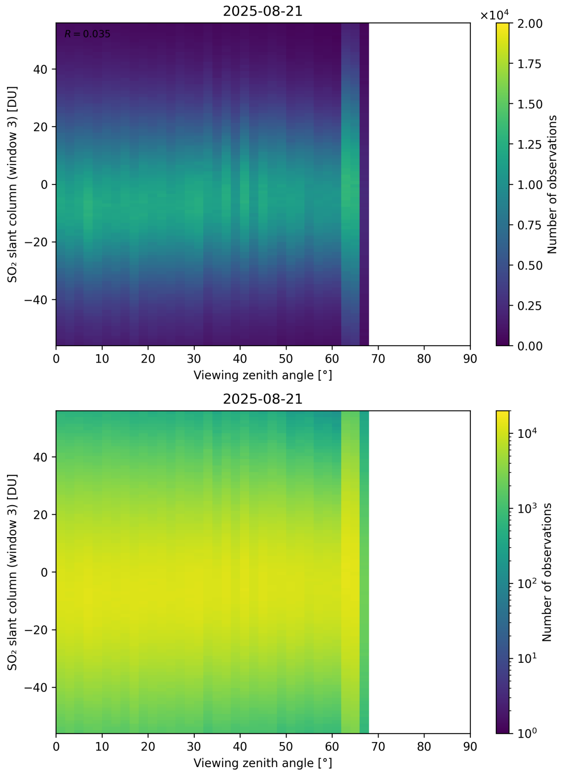
Figure 379: Scatter density plot of “Viewing zenith angle” against “SO 2 slant column (window 3)” for 2025-08-20 to 2025-08-22.
