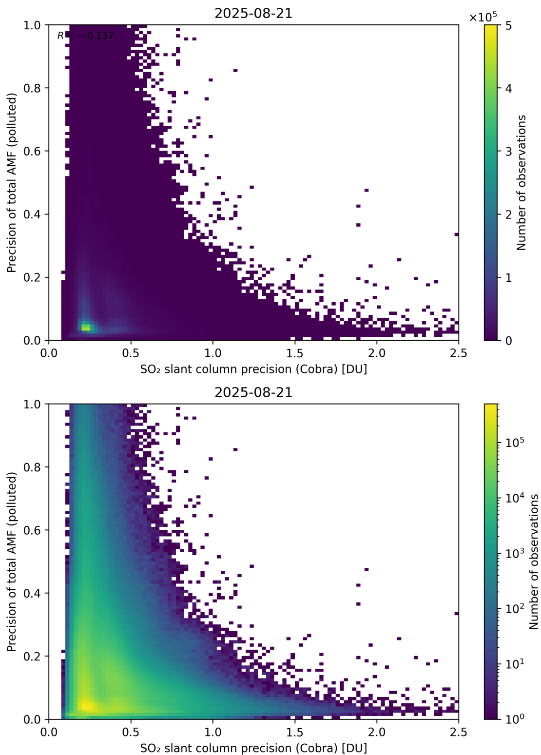
Figure 214: Scatter density plot of “SO 2 slant column precision (Cobra)” against “Precision of total AMF (polluted)” for 2025-08-20 to 2025-08-22.
