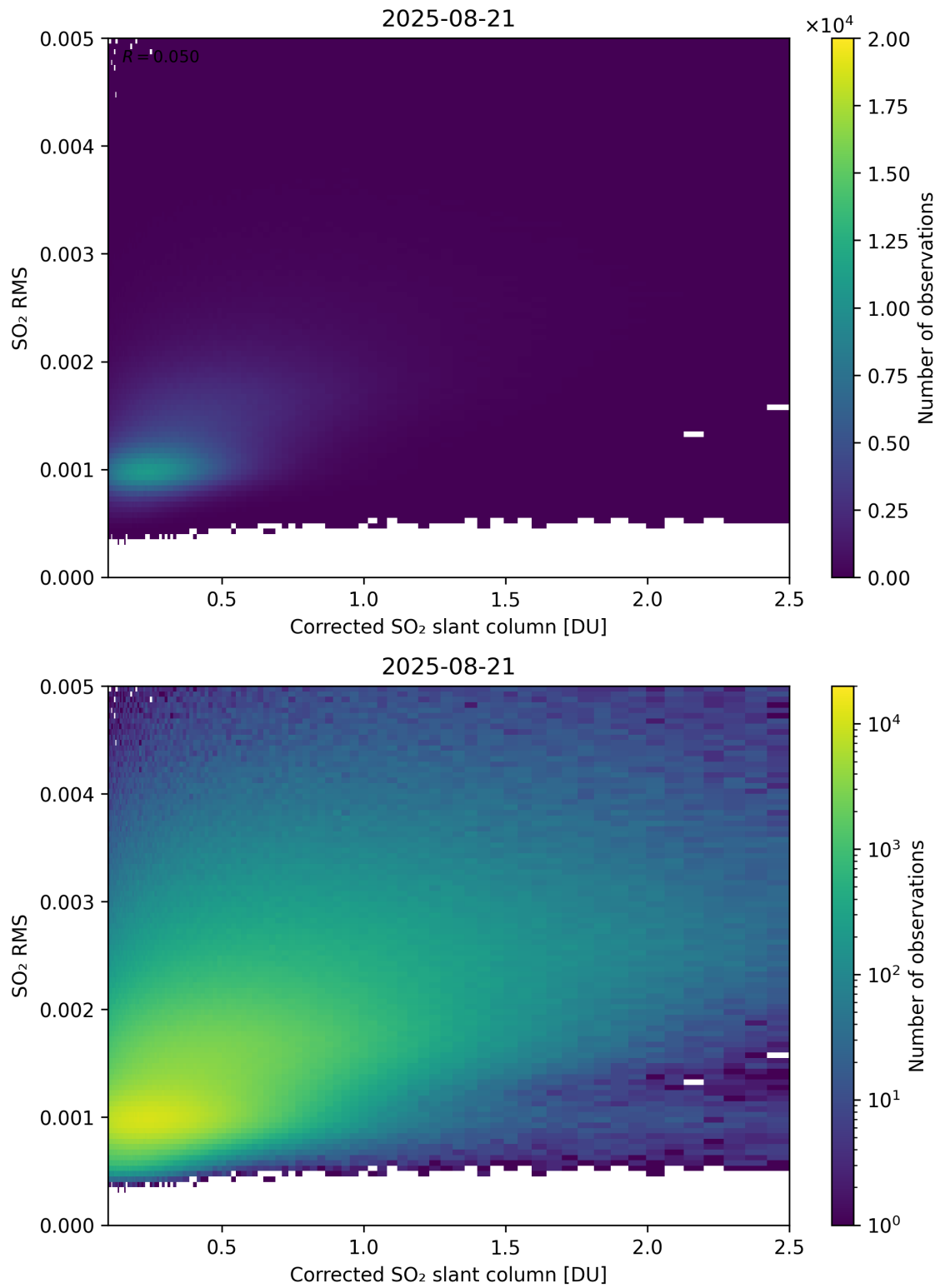
Figure 231: Scatter density plot of “Corrected SO 2 slant column” against “SO 2 RMS” for 2025-08-20 to 2025-08-22.
