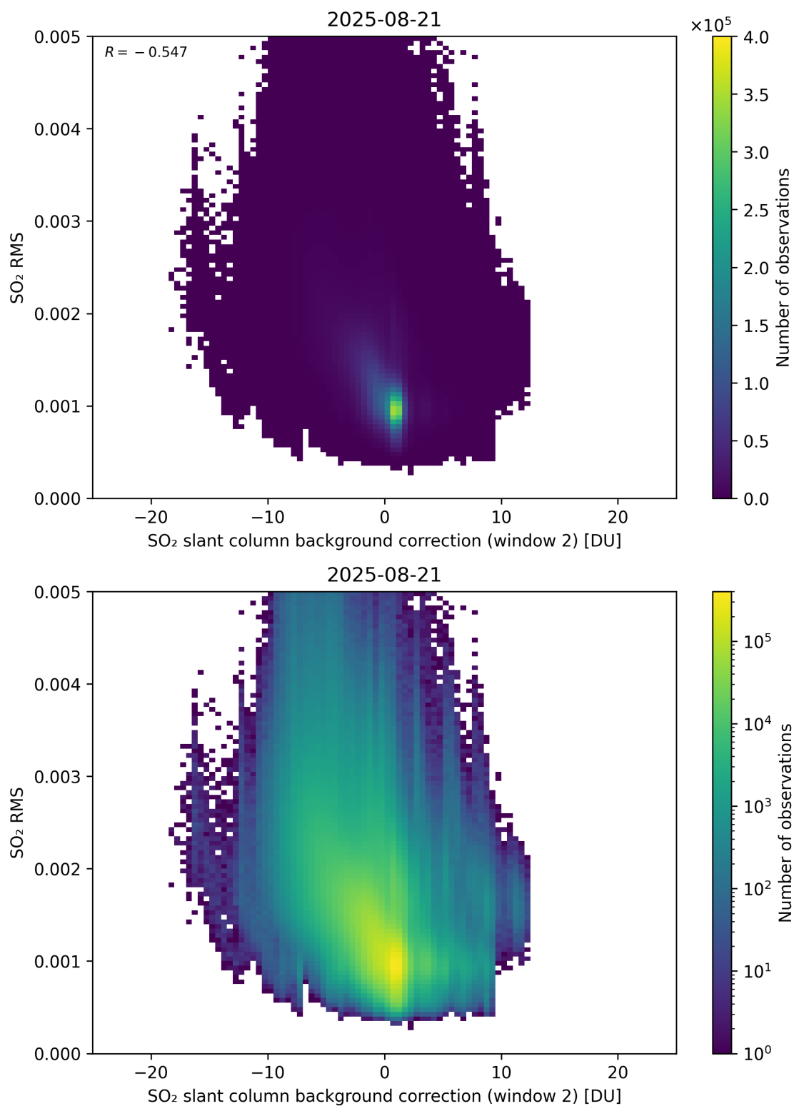
Figure 125: Scatter density plot of “SO 2 slant column background correction (window 2)” against “SO 2 RMS” for 2025-08-20 to 2025-08-22.
