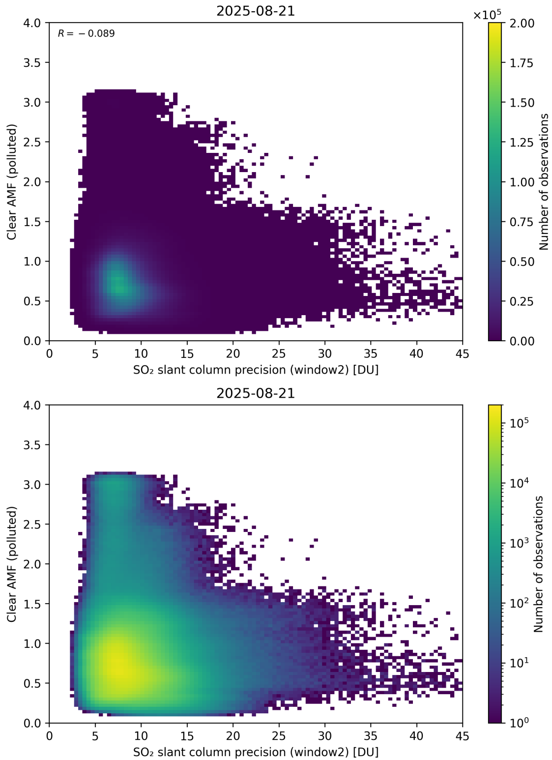
Figure 296: Scatter density plot of “SO 2 slant column precision (window2)” against “Clear AMF (polluted)” for 2025-08-20 to 2025-08-22.
