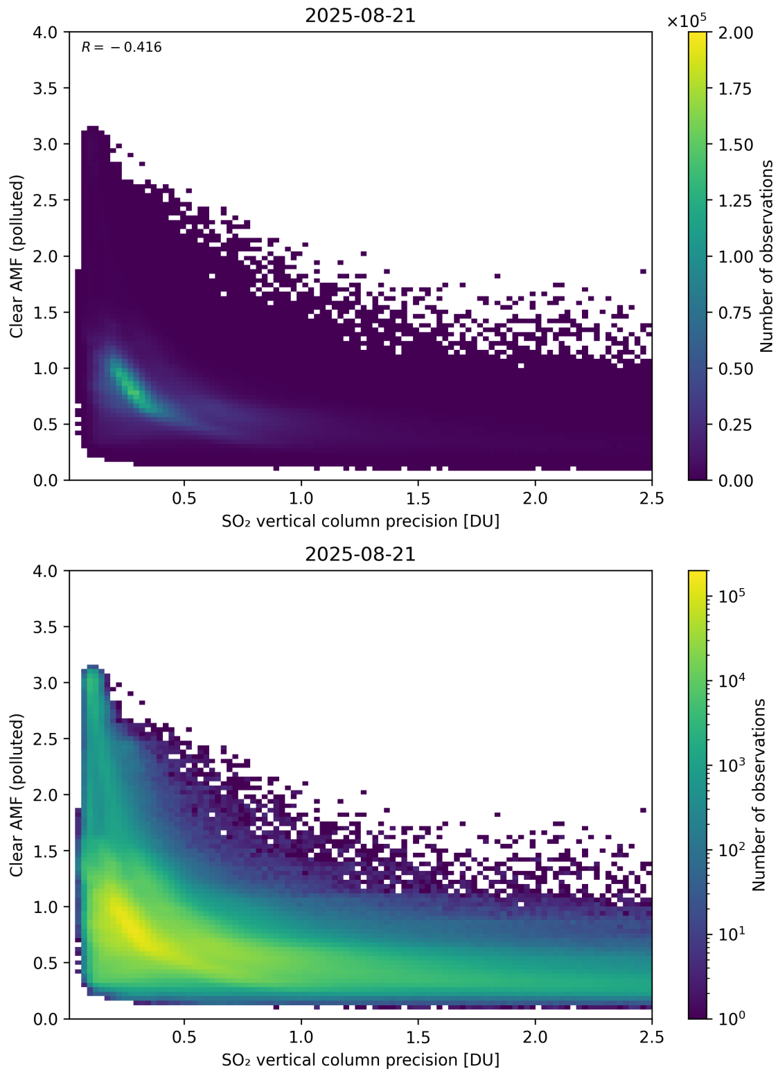
Figure 335: Scatter density plot of “SO 2 vertical column precision” against “Clear AMF (polluted)” for 2025-08-20 to 2025-08-22.
