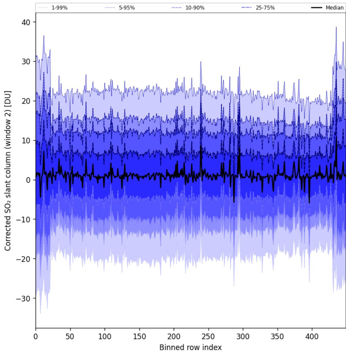
Figure 95: Along track statistics of “Corrected SO 2 slant column (window 2)” for 2025-08-20 to 2025-08-22
