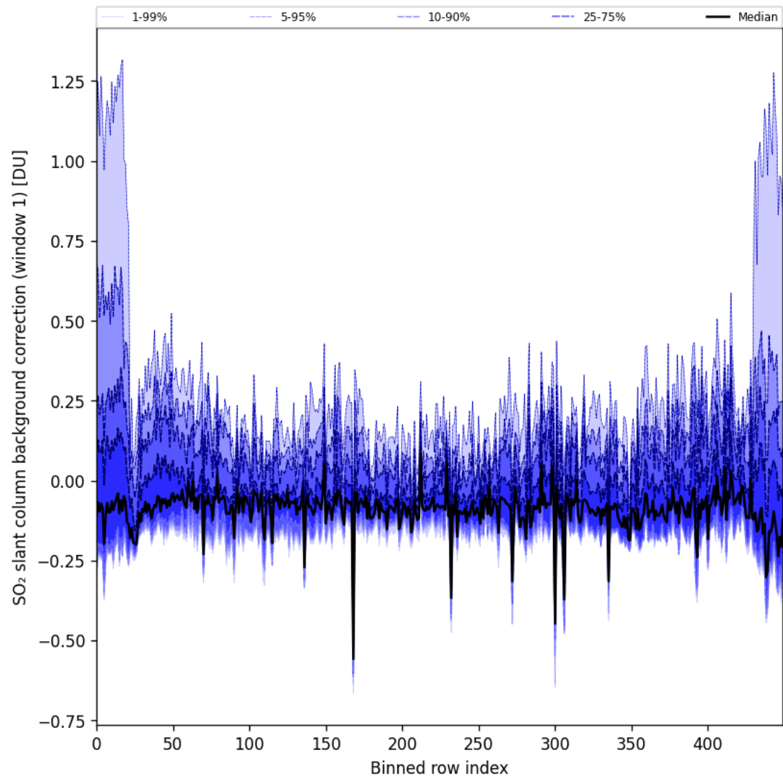
Figure 92: Along track statistics of “SO 2 slant column background correction (window 1)” for 2025-08-20 to 2025-08-22
