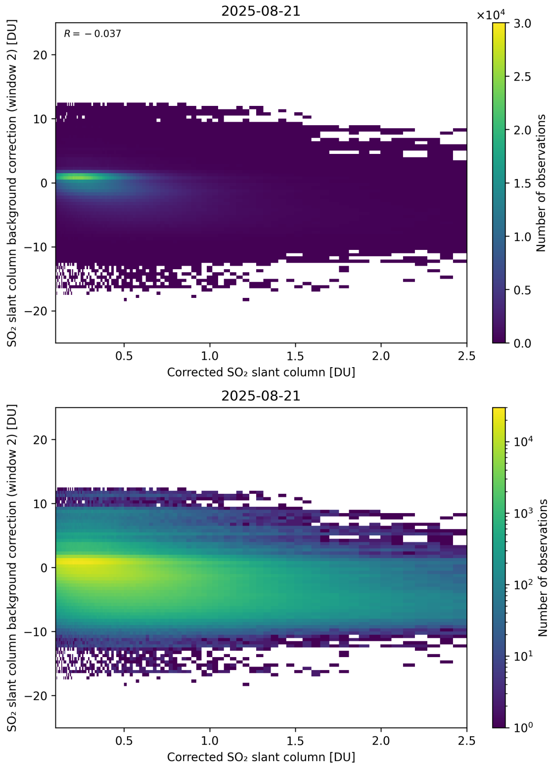
Figure 227: Scatter density plot of “Corrected SO 2 slant column” against “SO 2 slant column background correction (window 2)” for 2025-08-20 to 2025-08-22.
