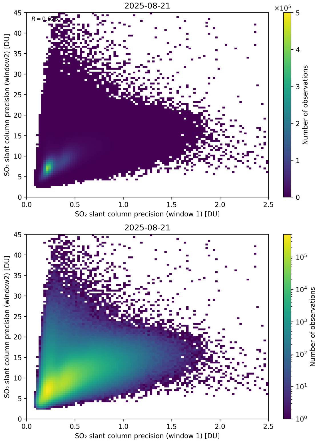
Figure 277: Scatter density plot of “SO 2 slant column precision (window 1)” against “SO 2 slant column precision (window2)” for 2025-08-20 to 2025-08-22.
