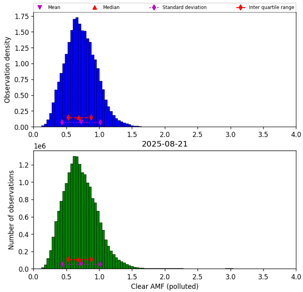
Figure 81: Histogram of “Clear AMF (polluted)” for 2025-08-20 to 2025-08-22
