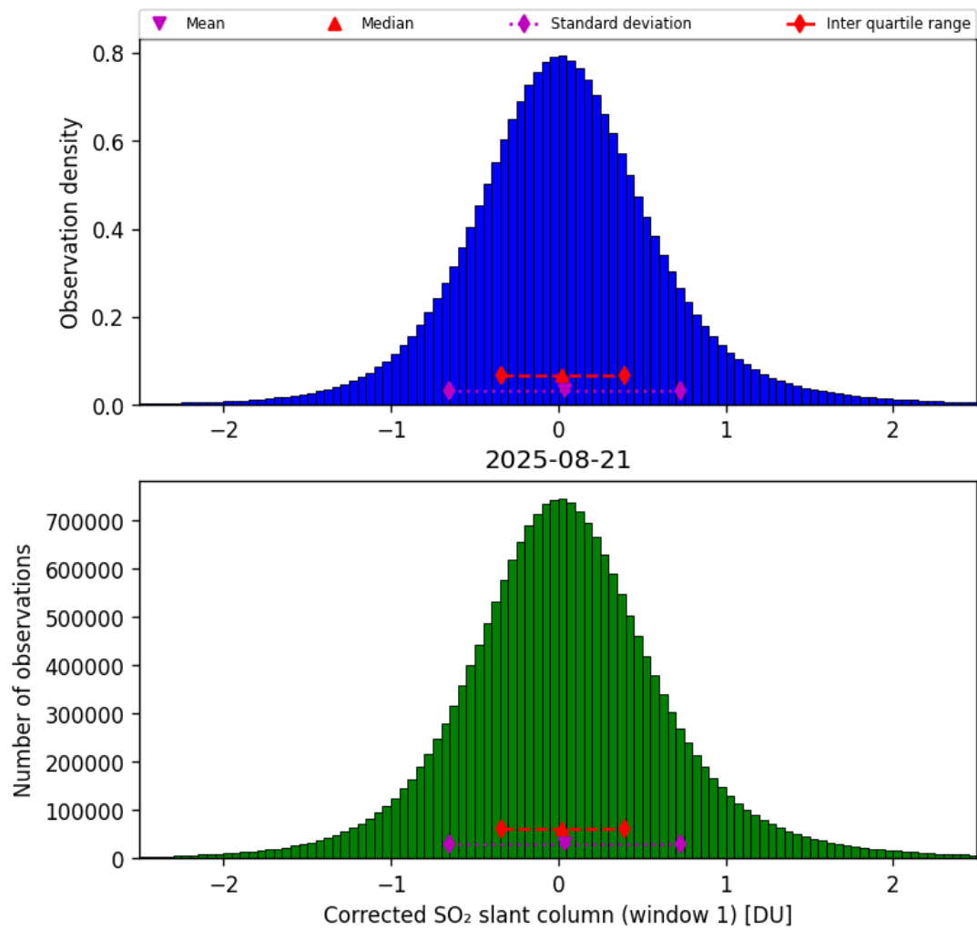
Figure 65: Histogram of “Corrected SO 2 slant column (window 1)” for 2025-08-20 to 2025-08-22
