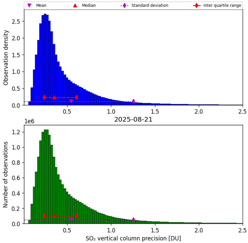
Figure 59: Histogram of “SO 2 vertical column precision” for 2025-08-20 to 2025-08-22
