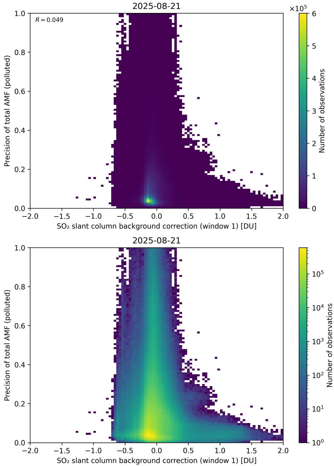
Figure 121: Scatter density plot of “SO 2 slant column background correction (window 1)” against “Precision of total AMF (polluted)” for 2025-08-20 to 2025-08-22.
