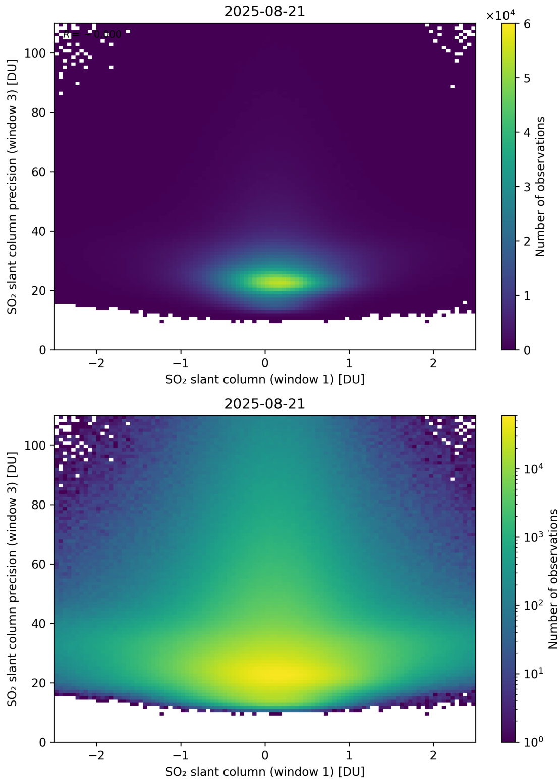
Figure 288: Scatter density plot of “SO 2 slant column (window 1)” against “SO 2 slant column precision (window 3)” for 2025-08-20 to 2025-08-22.
