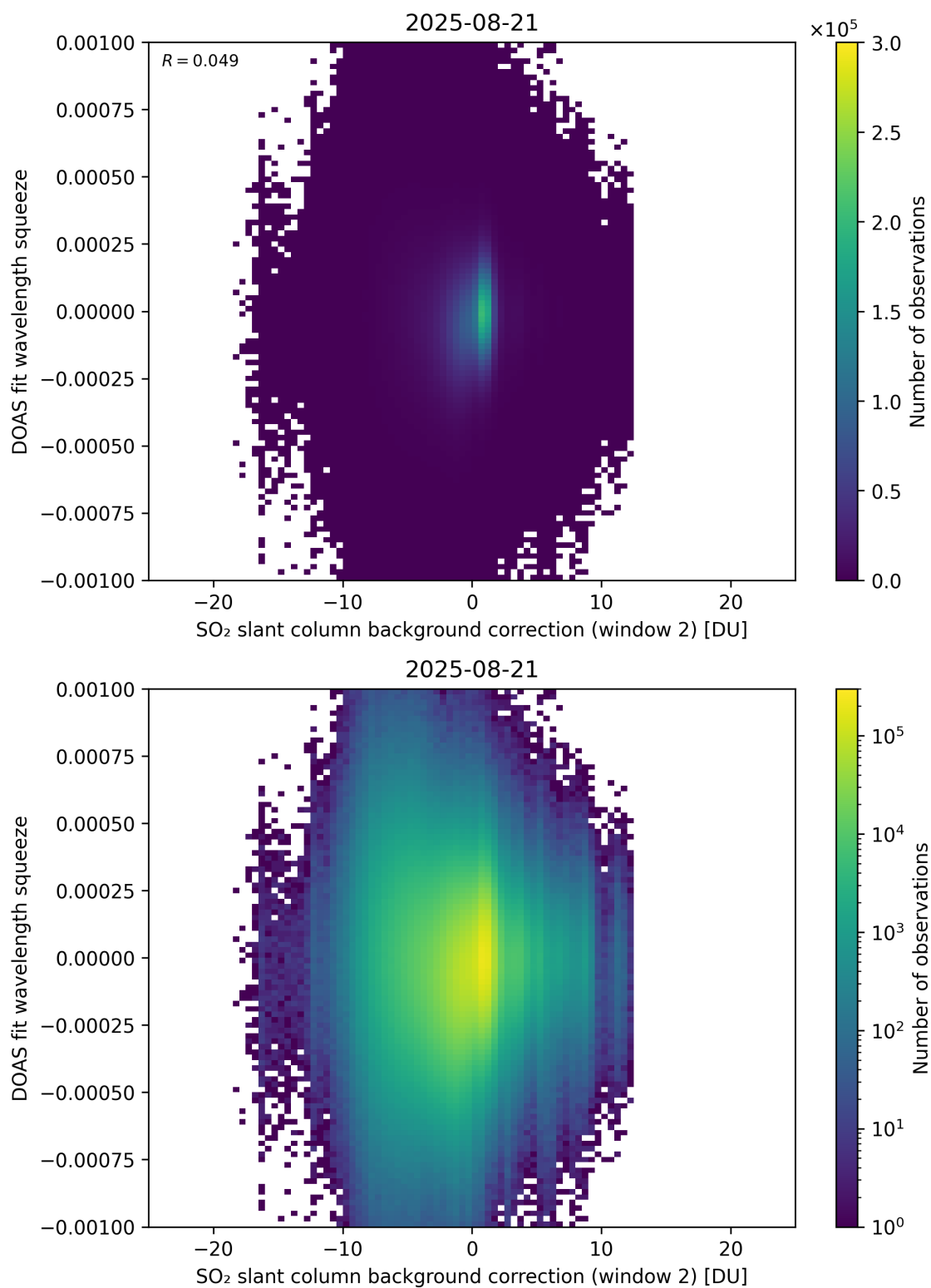
Figure 124: Scatter density plot of “SO 2 slant column background correction (window 2)” against “DOAS fit wavelength squeeze” for 2025-08-20 to 2025-08-22.
