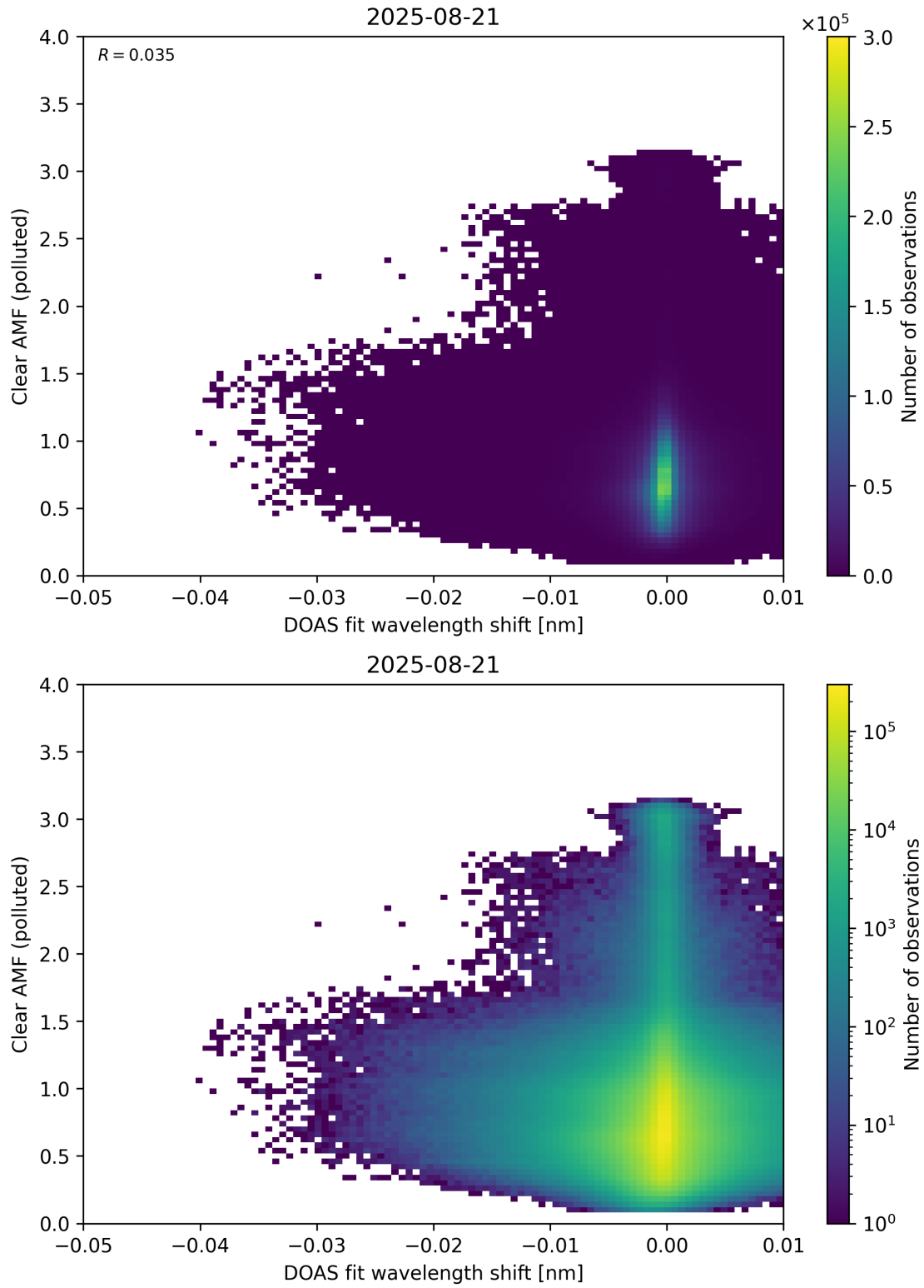
Figure 140: Scatter density plot of “DOAS fit wavelength shift” against “Clear AMF (polluted)” for 2025-08-20 to 2025-08-22.
