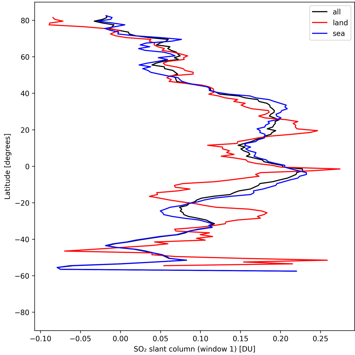
Figure 37: Zonal average of “SO 2 slant column (window 1)” for 2025-08-20 to 2025-08-22.
