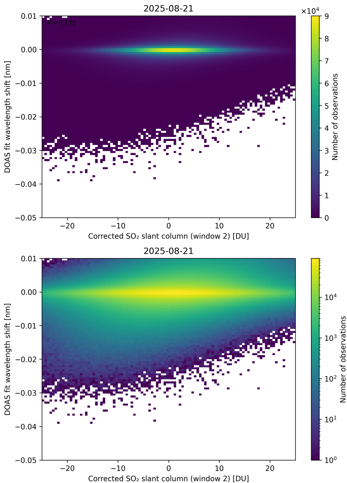
Figure 246: Scatter density plot of “Corrected SO 2 slant column (window 2)” against “DOAS fit wavelength shift” for 2025-08-20 to 2025-08-22.
