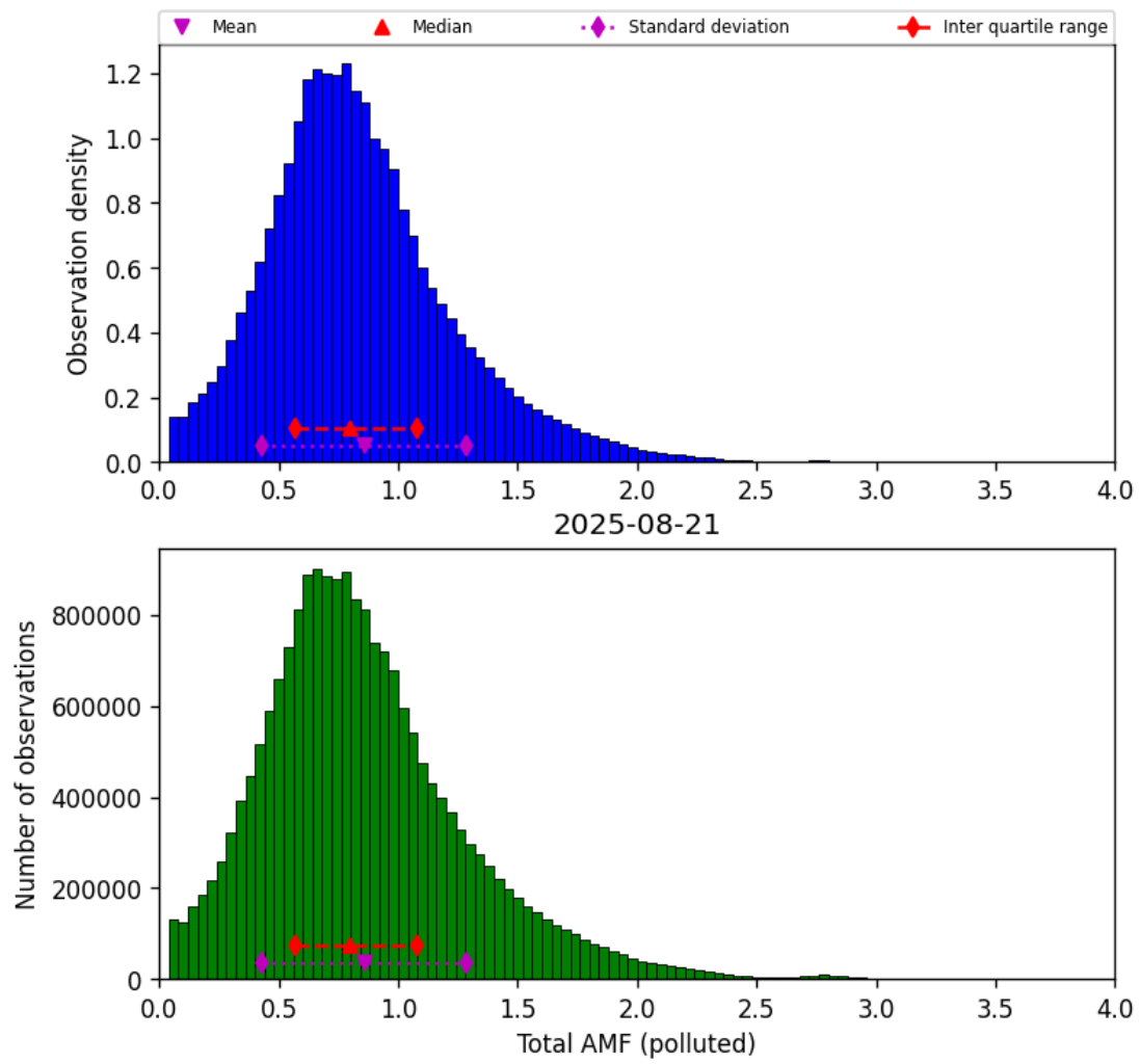
Figure 79: Histogram of “Total AMF (polluted)” for 2025-08-20 to 2025-08-22
