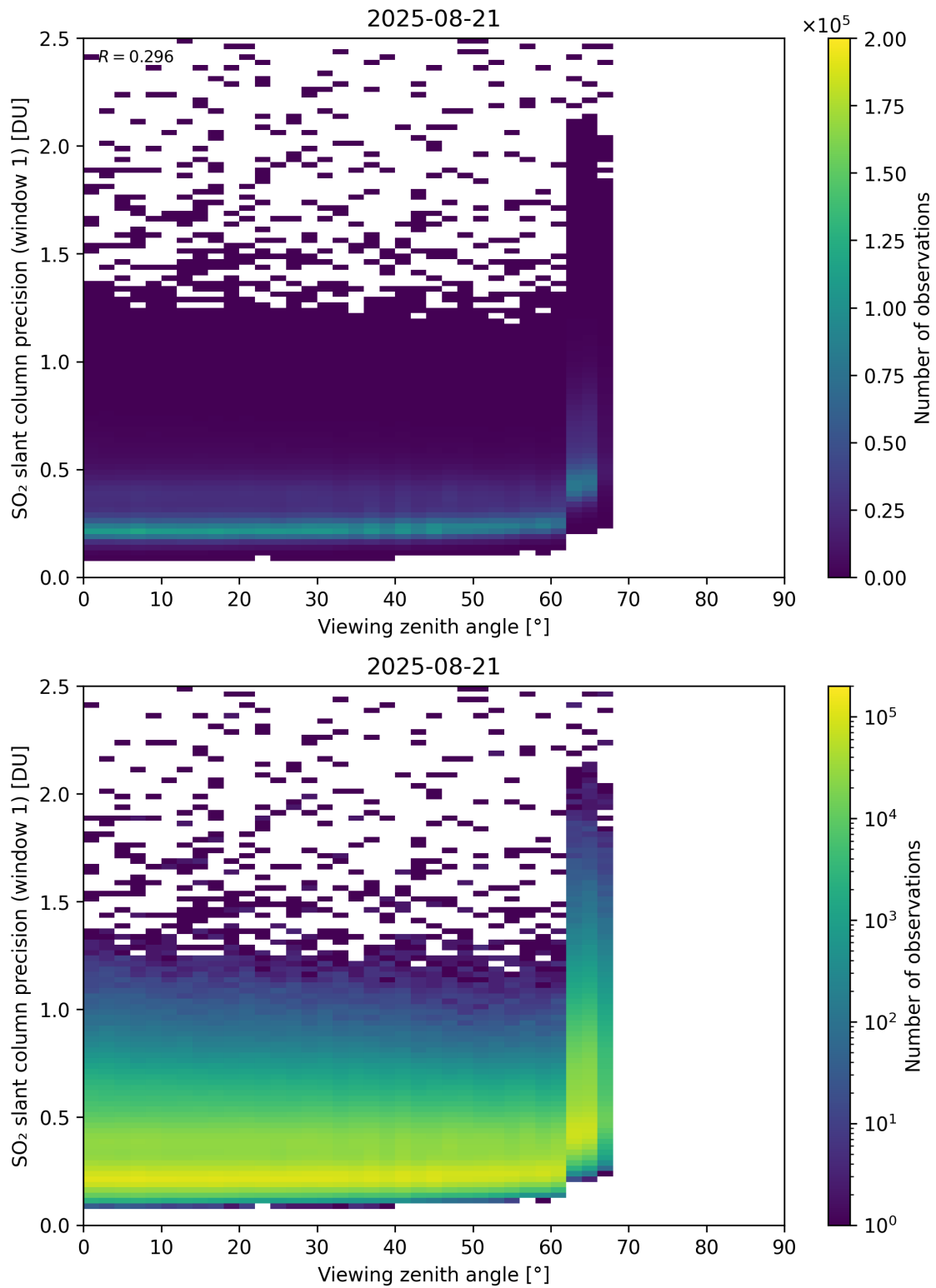
Figure 377: Scatter density plot of “Viewing zenith angle” against “SO 2 slant column precision (window 1)” for 2025-08-20 to 2025-08-22.
