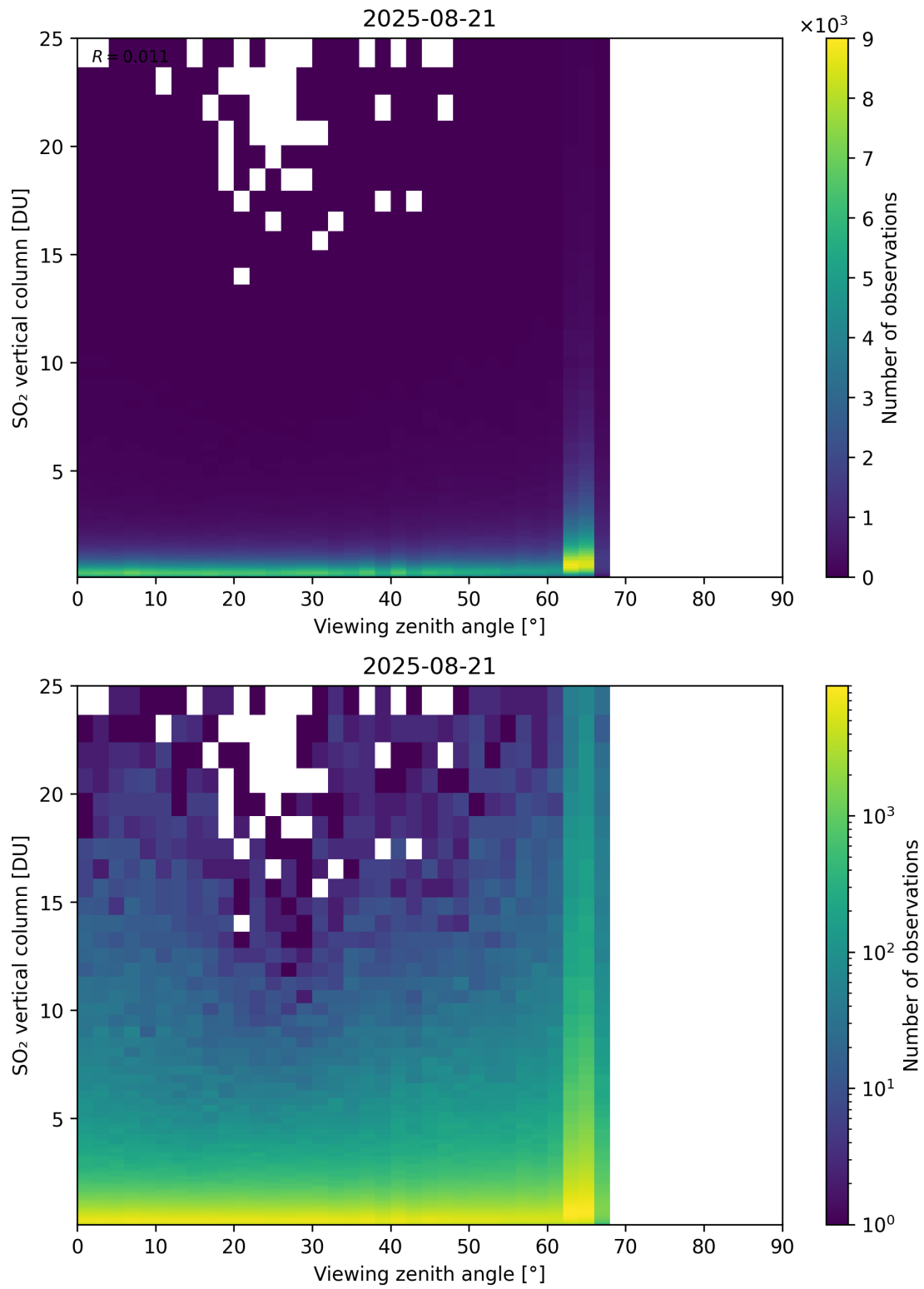
Figure 383: Scatter density plot of “Viewing zenith angle” against “SO 2 vertical column” for 2025-08-20 to 2025-08-22.
