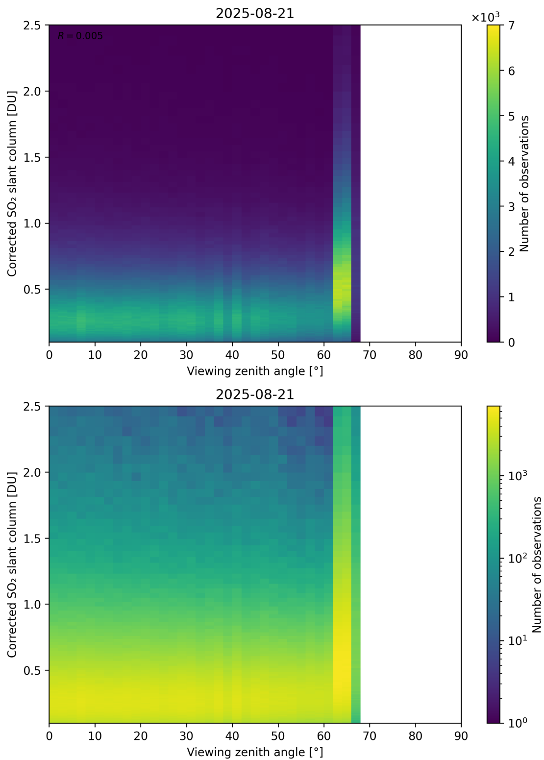
Figure 373: Scatter density plot of “Viewing zenith angle” against “Corrected SO 2 slant column” for 2025-08-20 to 2025-08-22.
