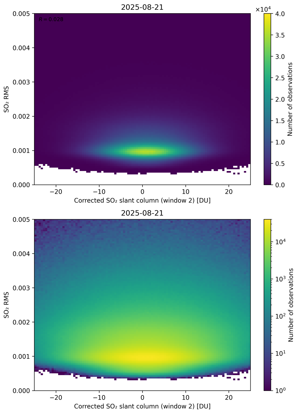
Figure 248: Scatter density plot of “Corrected SO 2 slant column (window 2)” against “SO 2 RMS” for 2025-08-20 to 2025-08-22.
