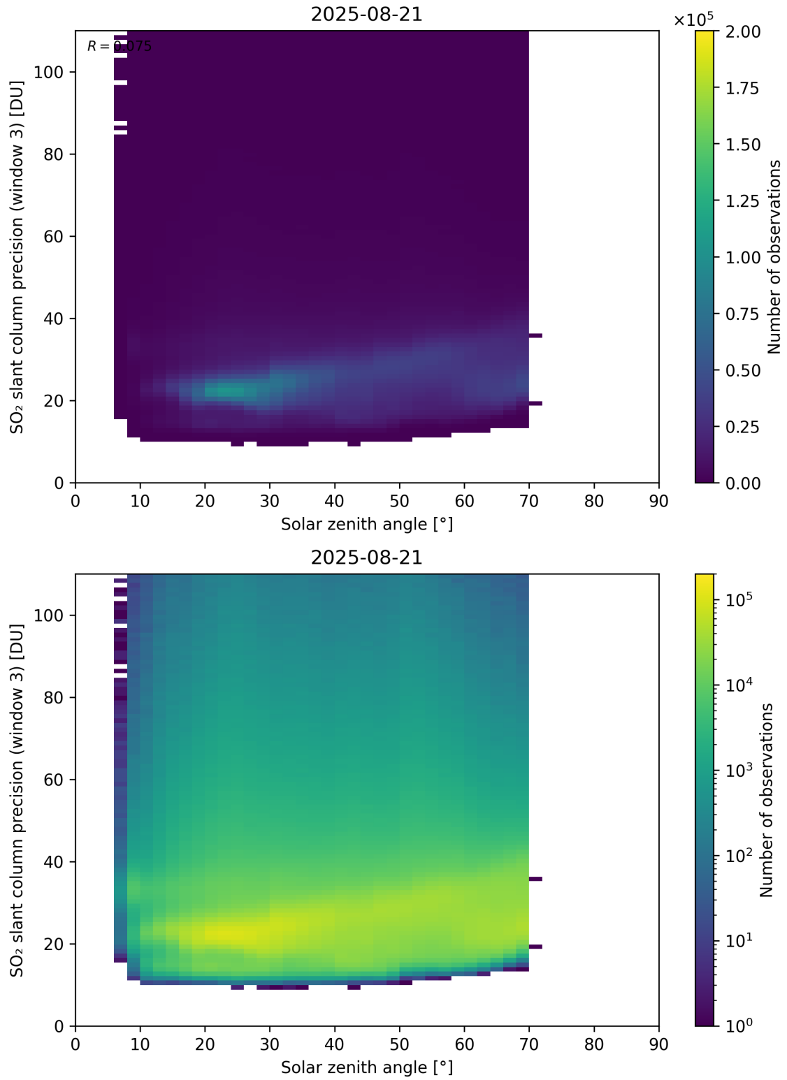
Figure 188: Scatter density plot of “Solar zenith angle” against “SO 2 slant column precision (window 3)” for 2025-08-20 to 2025-08-22.
