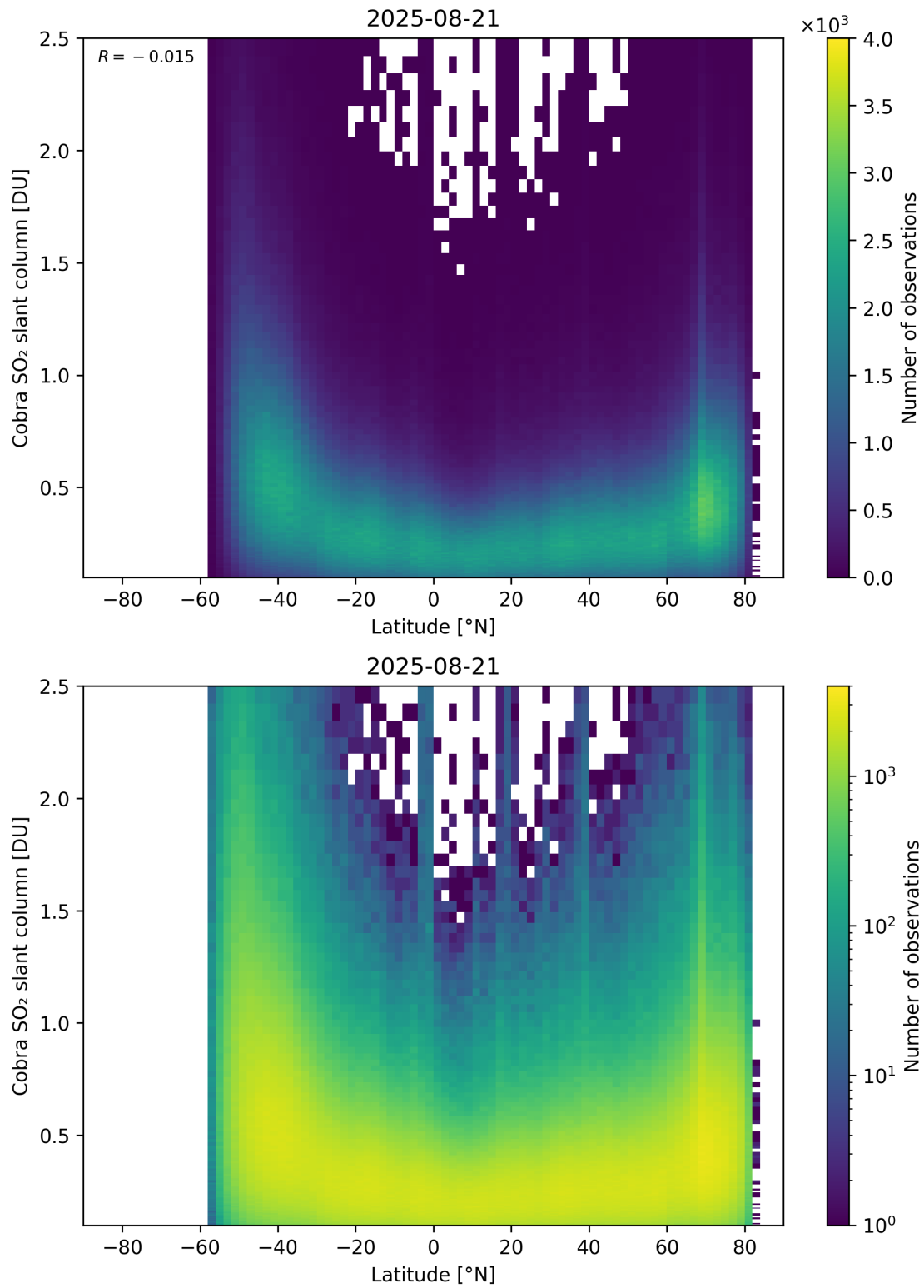
Figure 157: Scatter density plot of “Latitude” against “Cobra SO 2 slant column” for 2025-08-20 to 2025-08-22.
