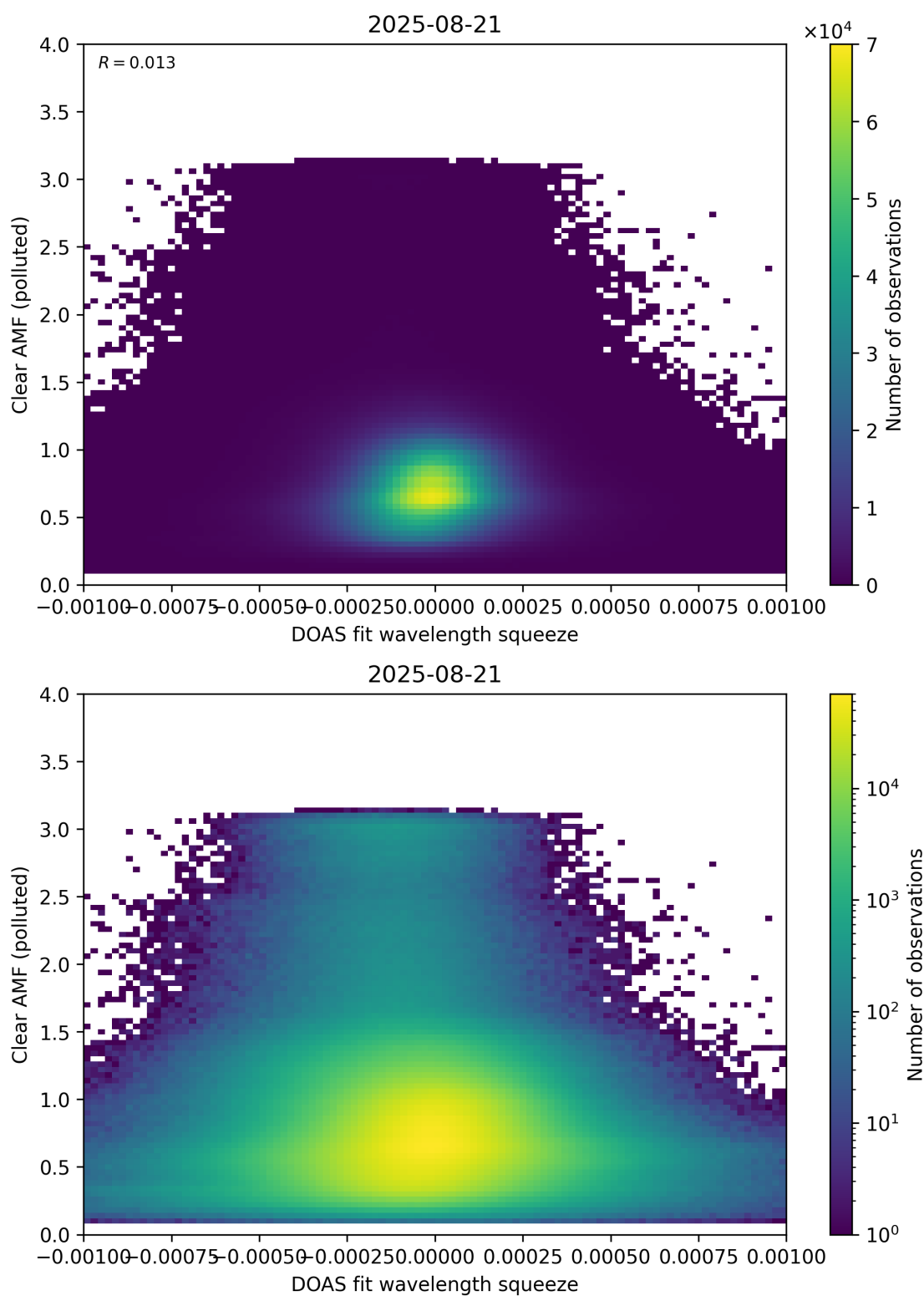
Figure 144: Scatter density plot of “DOAS fit wavelength squeeze” against “Clear AMF (polluted)” for 2025-08-20 to 2025-08-22.
