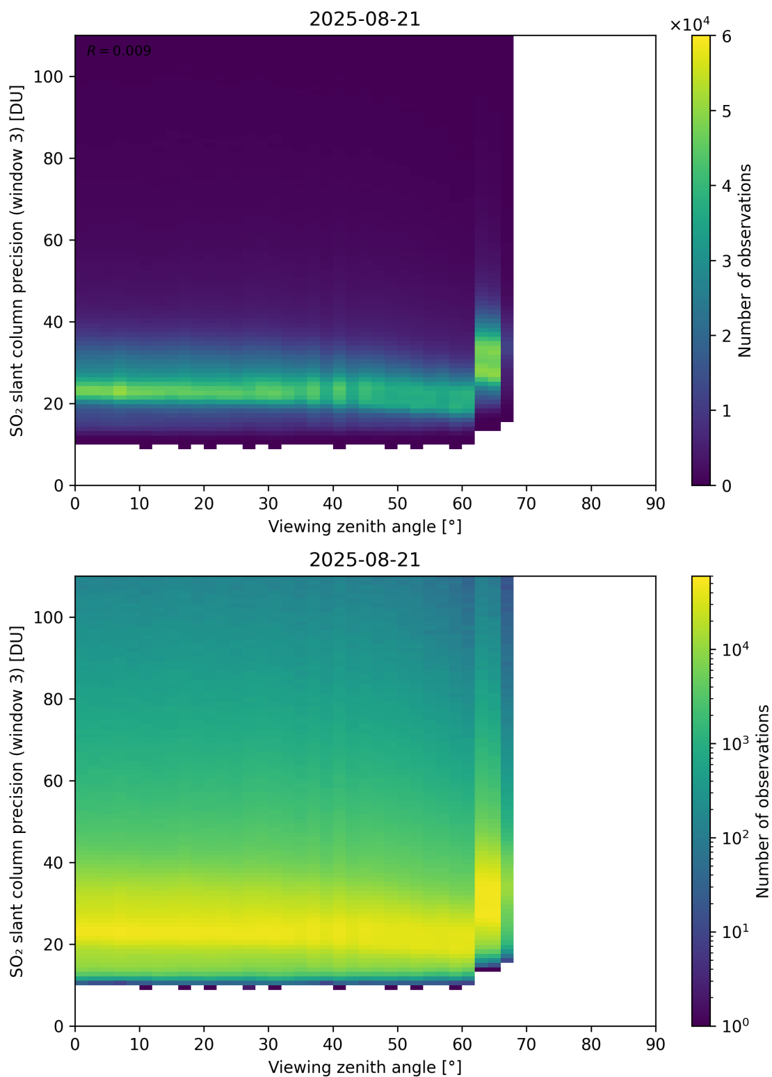
Figure 380: Scatter density plot of “Viewing zenith angle” against “SO 2 slant column precision (window 3)” for 2025-08-20 to 2025-08-22.
