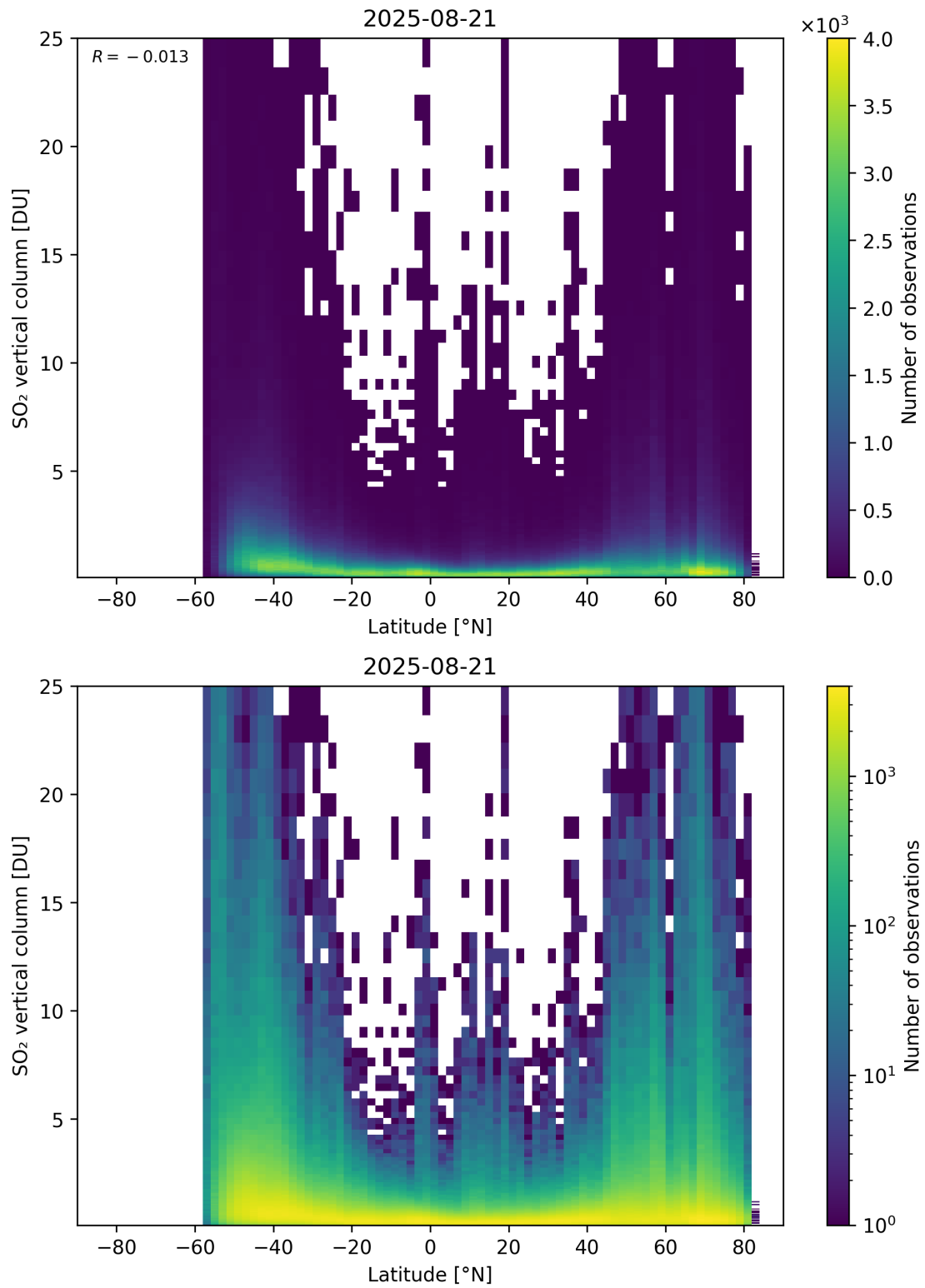
Figure 169: Scatter density plot of “Latitude” against “SO 2 vertical column” for 2025-08-20 to 2025-08-22.
