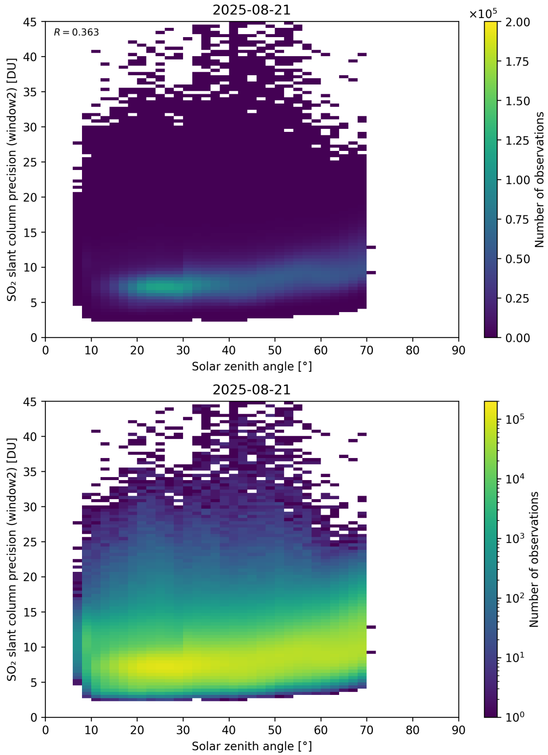
Figure 186: Scatter density plot of “Solar zenith angle” against “SO 2 slant column precision (window2)” for 2025-08-20 to 2025-08-22.
