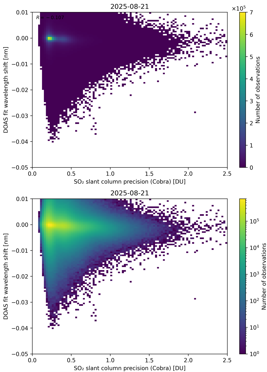
Figure 202: Scatter density plot of “SO 2 slant column precision (Cobra)” against “DOAS fit wavelength shift” for 2025-08-20 to 2025-08-22.
