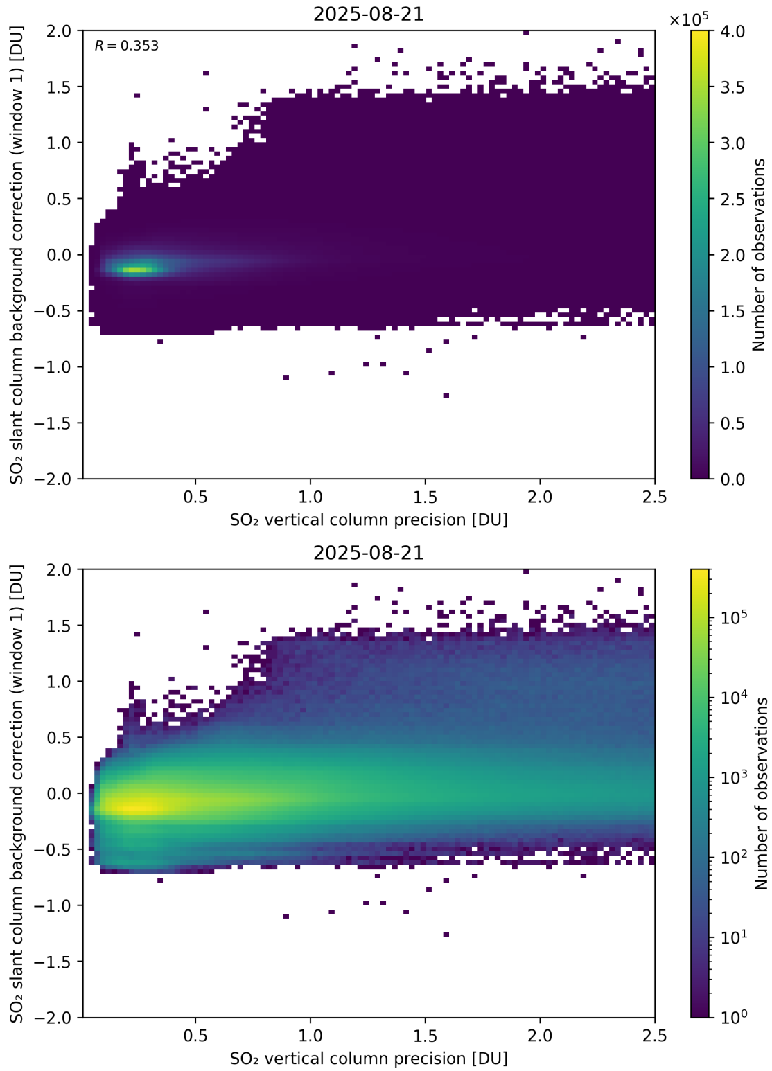
Figure 329: Scatter density plot of “SO 2 vertical column precision” against “SO 2 slant column background correction (window 1)” for 2025-08-20 to 2025-08-22.
