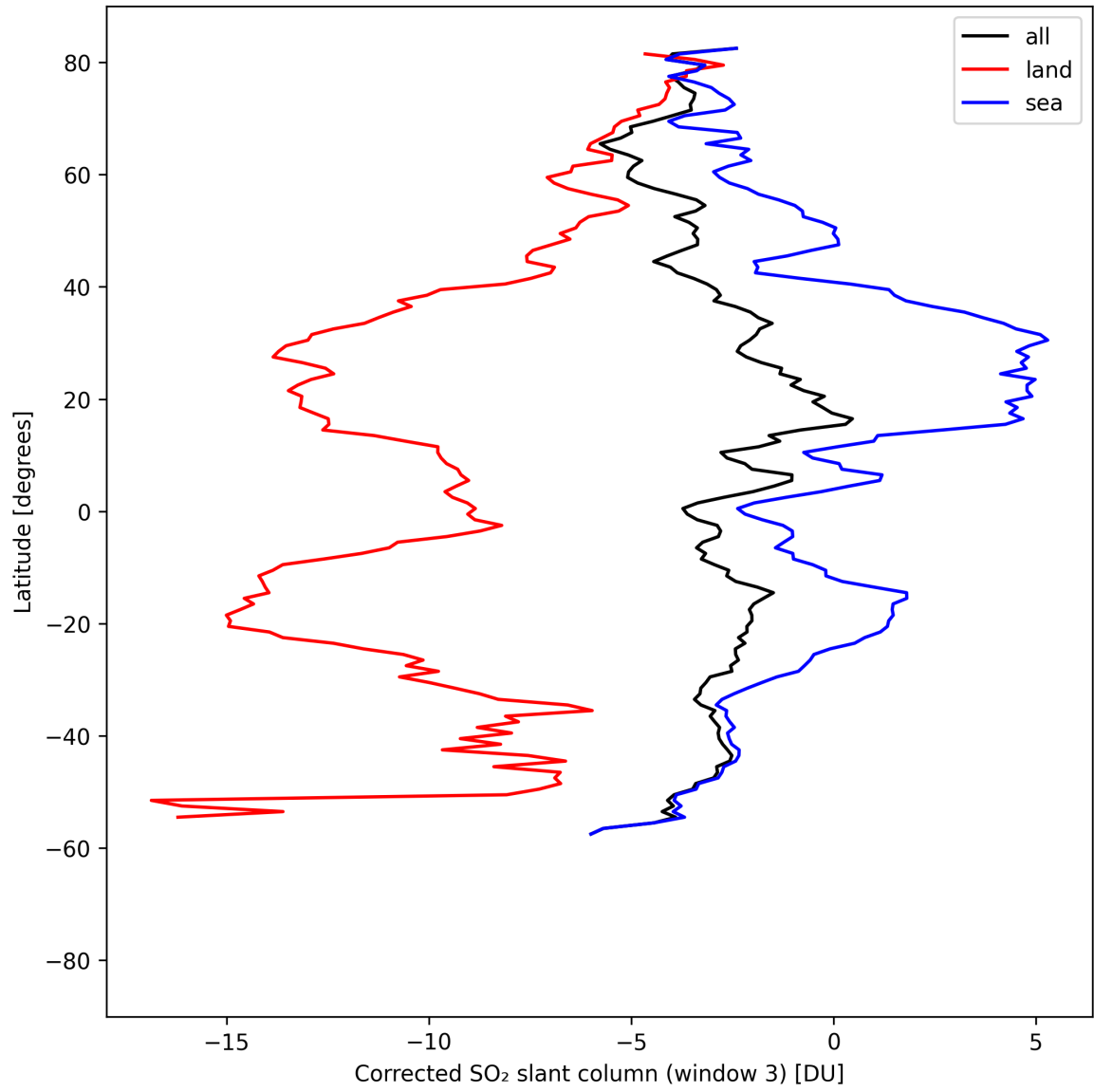
Figure 47: Zonal average of “Corrected SO 2 slant column (window 3)” for 2025-08-20 to 2025-08-22.
