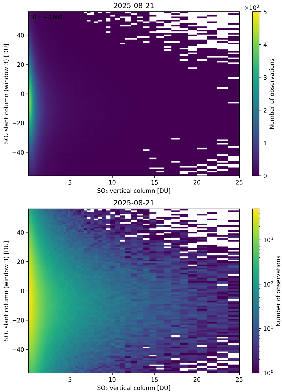
Figure 357: Scatter density plot of “SO 2 vertical column” against “SO 2 slant column (window 3)” for 2025-08-20 to 2025-08-22.
