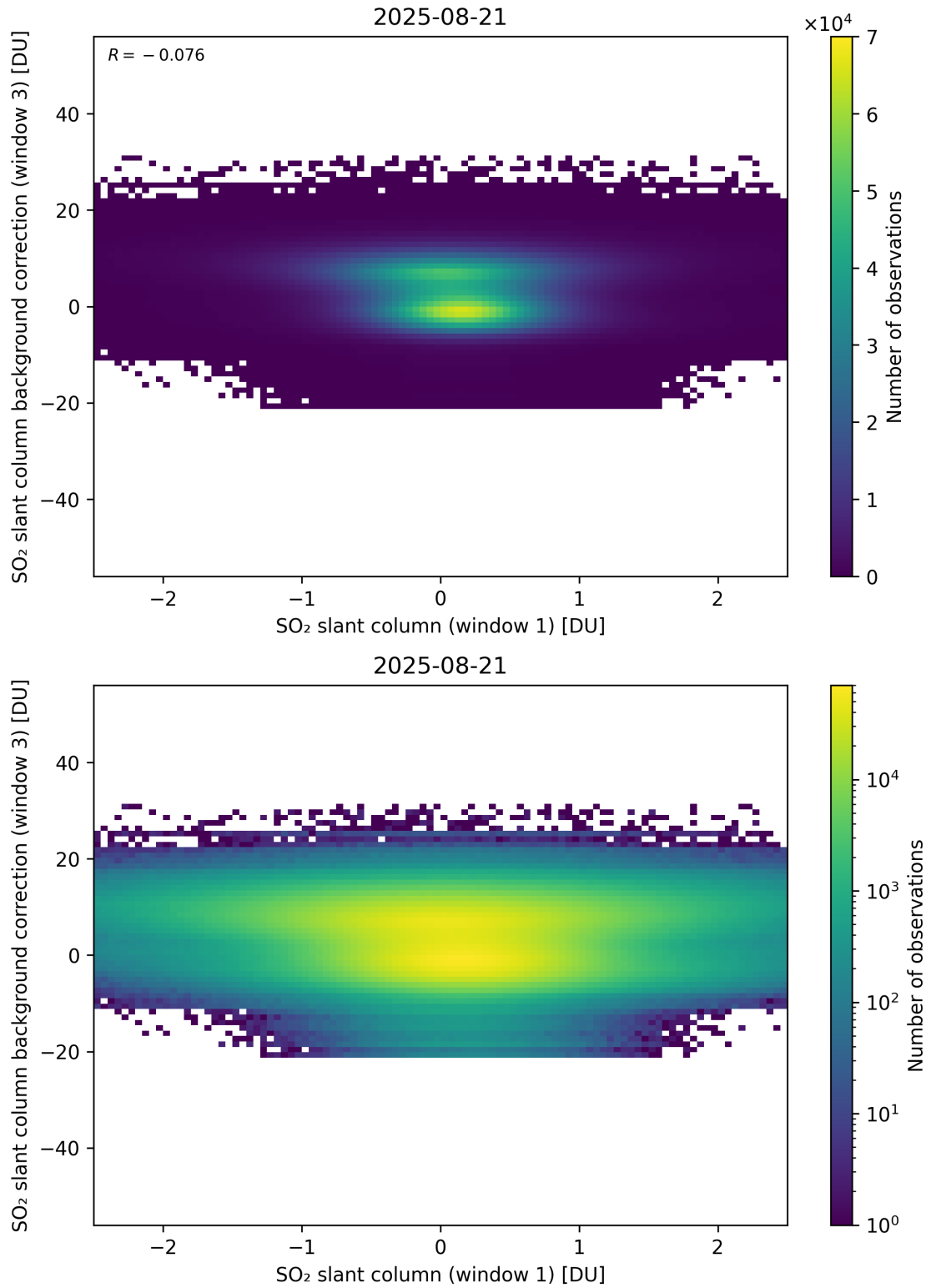
Figure 264: Scatter density plot of “SO 2 slant column (window 1)” against “SO 2 slant column background correction (window 3)” for 2025-08-20 to 2025-08-22.
