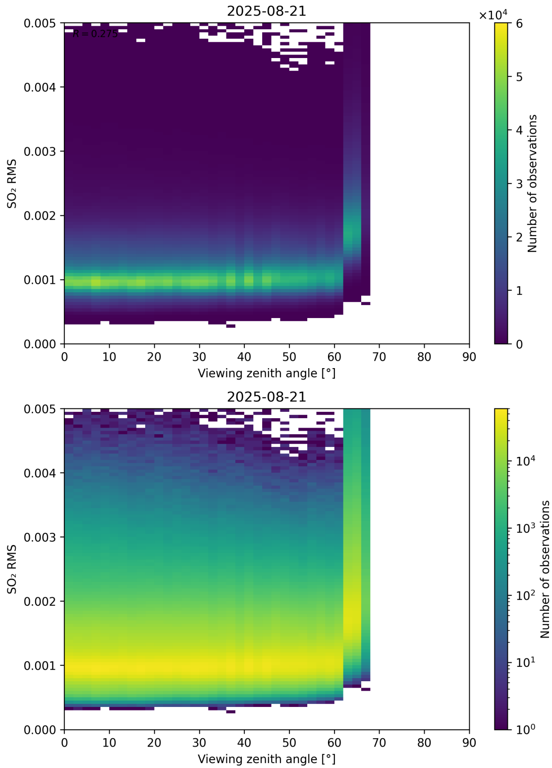
Figure 367: Scatter density plot of “Viewing zenith angle” against “SO 2 RMS” for 2025-08-20 to 2025-08-22.
