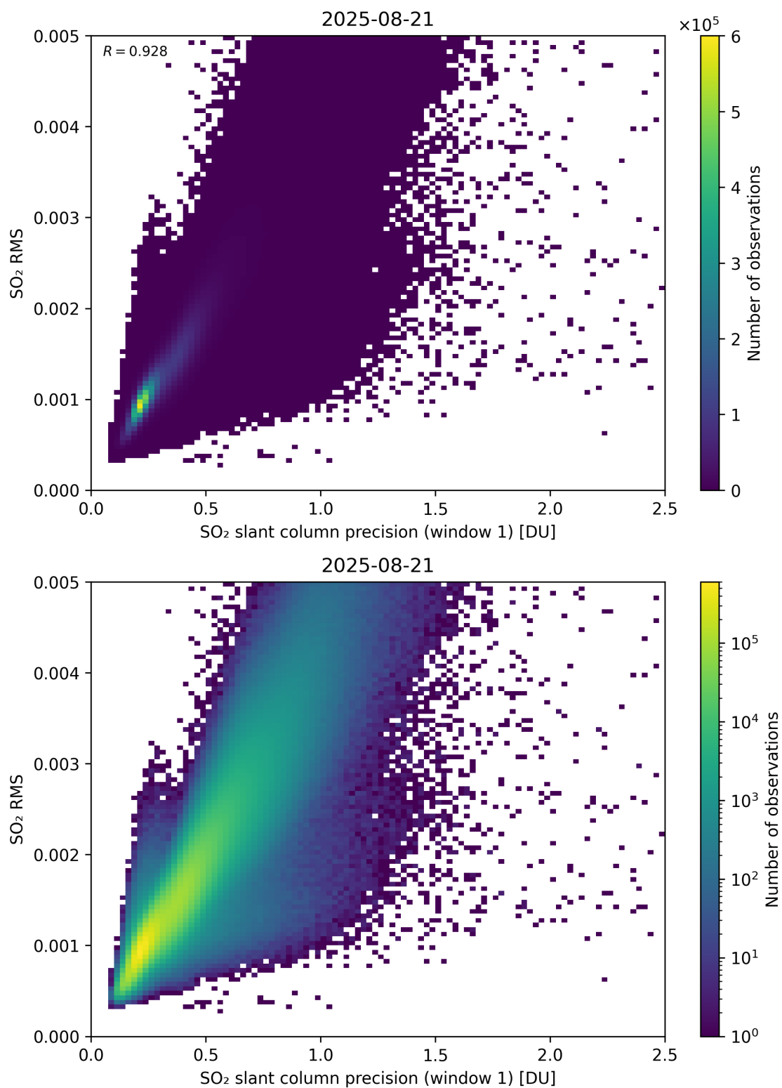
Figure 273: Scatter density plot of “SO 2 slant column precision (window 1)” against “SO 2 RMS” for 2025-08-20 to 2025-08-22.
