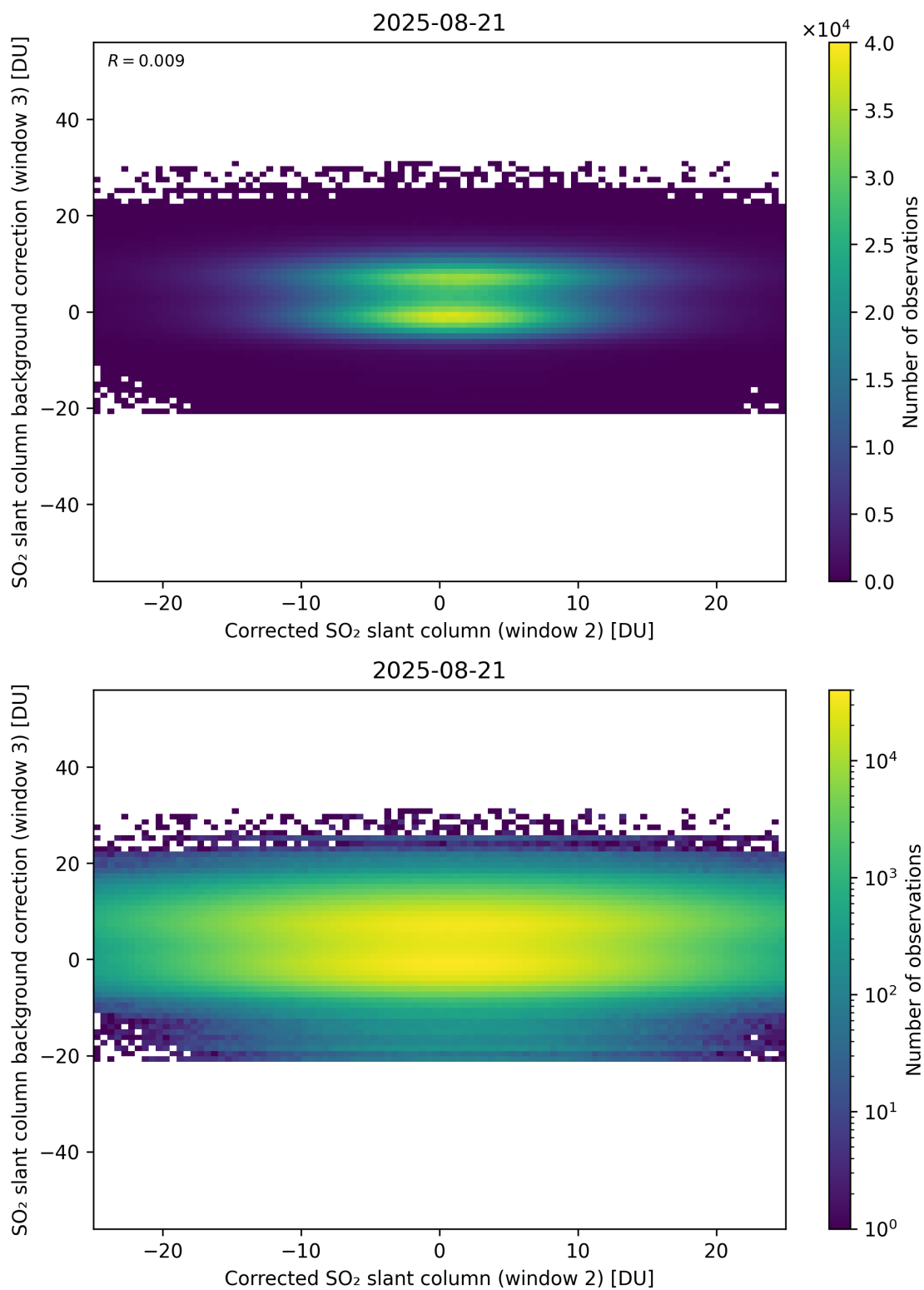
Figure 245: Scatter density plot of “Corrected SO 2 slant column (window 2)” against “SO 2 slant column background correction (window 3)” for 2025-08-20 to 2025-08-22.
