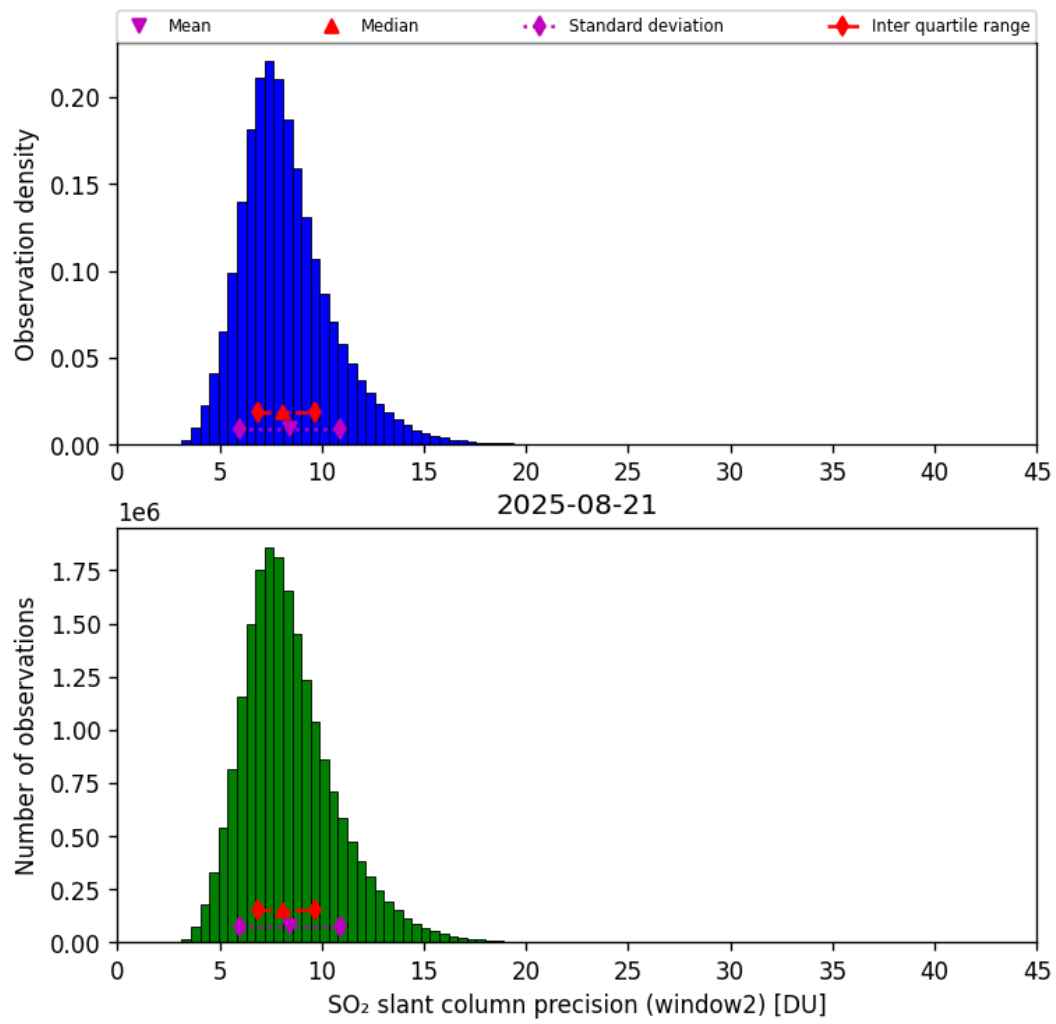
Figure 68: Histogram of “SO 2 slant column precision (window2)” for 2025-08-20 to 2025-08-22
