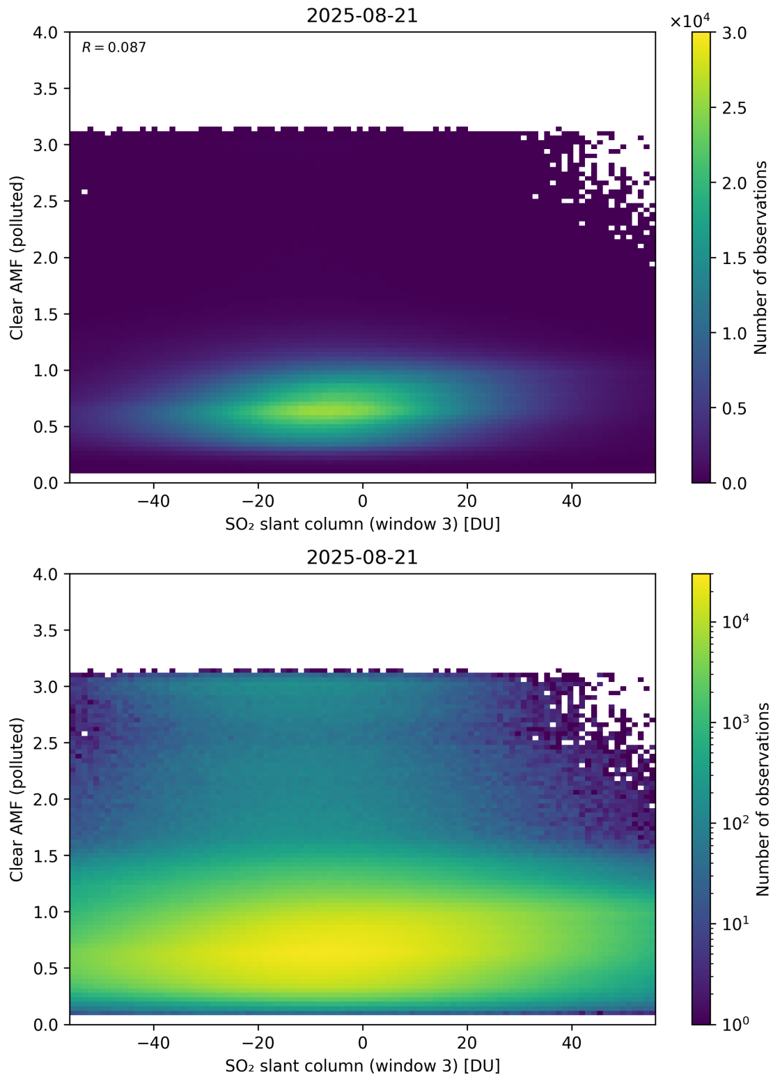
Figure 315: Scatter density plot of “SO 2 slant column (window 3)” against “Clear AMF (polluted)” for 2025-08-20 to 2025-08-22.
