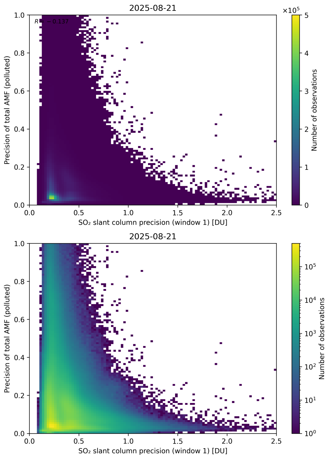
Figure 281: Scatter density plot of “SO 2 slant column precision (window 1)” against “Precision of total AMF (polluted)” for 2025-08-20 to 2025-08-22.
