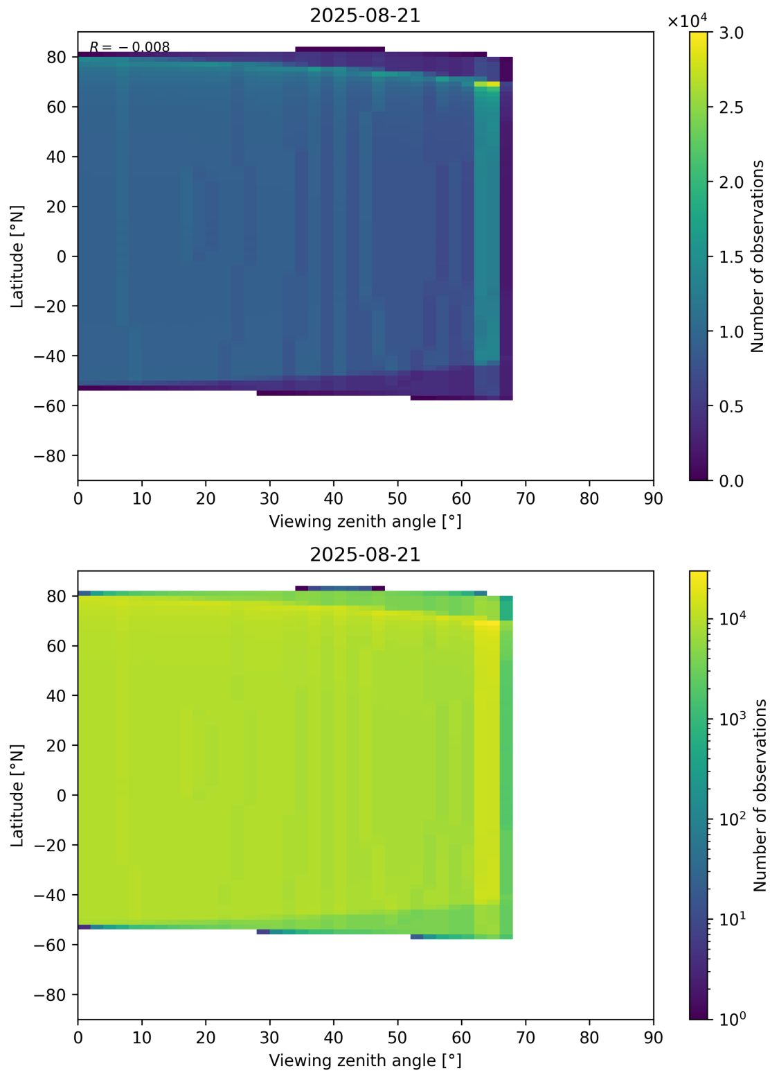
Figure 368: Scatter density plot of “Viewing zenith angle” against “Latitude” for 2025-08-20 to 2025-08-22.
