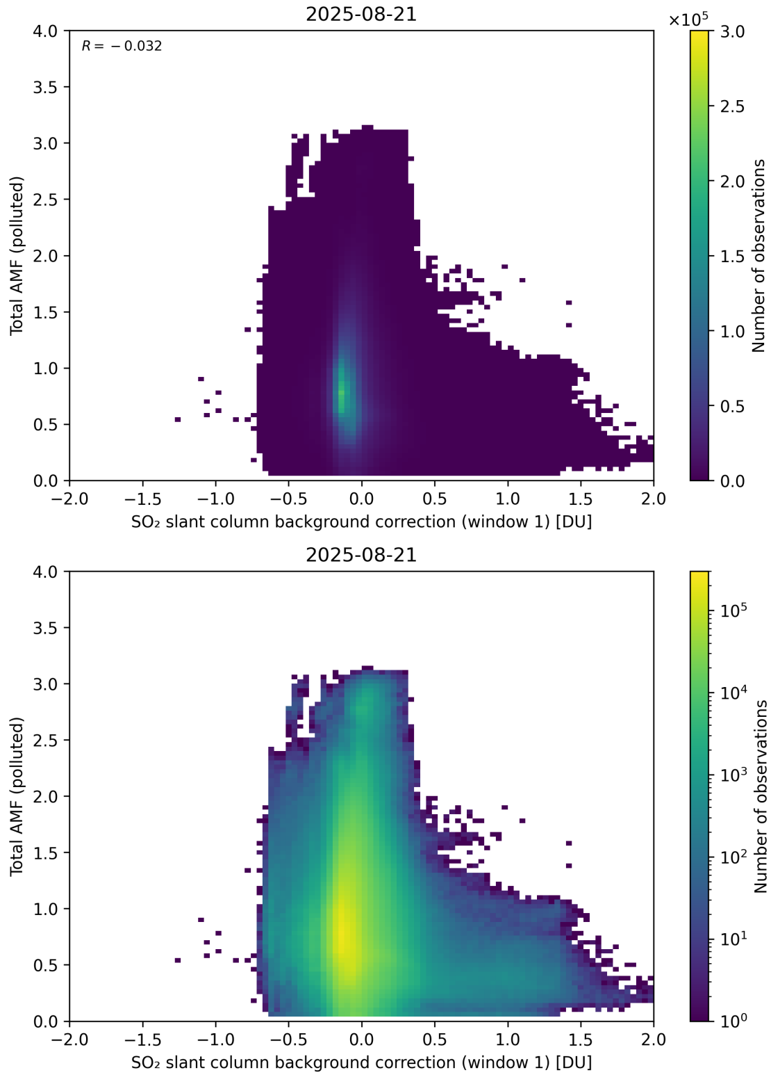
Figure 120: Scatter density plot of “SO 2 slant column background correction (window 1)” against “Total AMF (polluted)” for 2025-08-20 to 2025-08-22.
