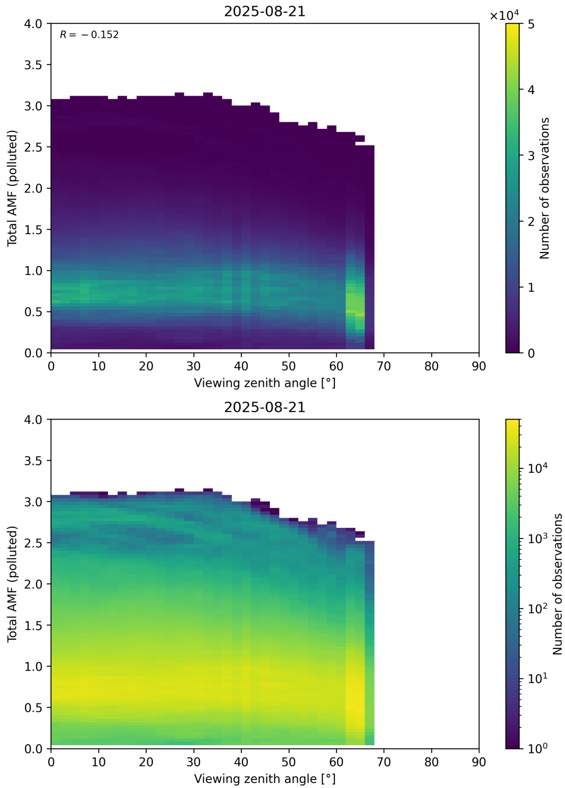
Figure 381: Scatter density plot of “Viewing zenith angle” against “Total AMF (polluted)” for 2025-08-20 to 2025-08-22.
