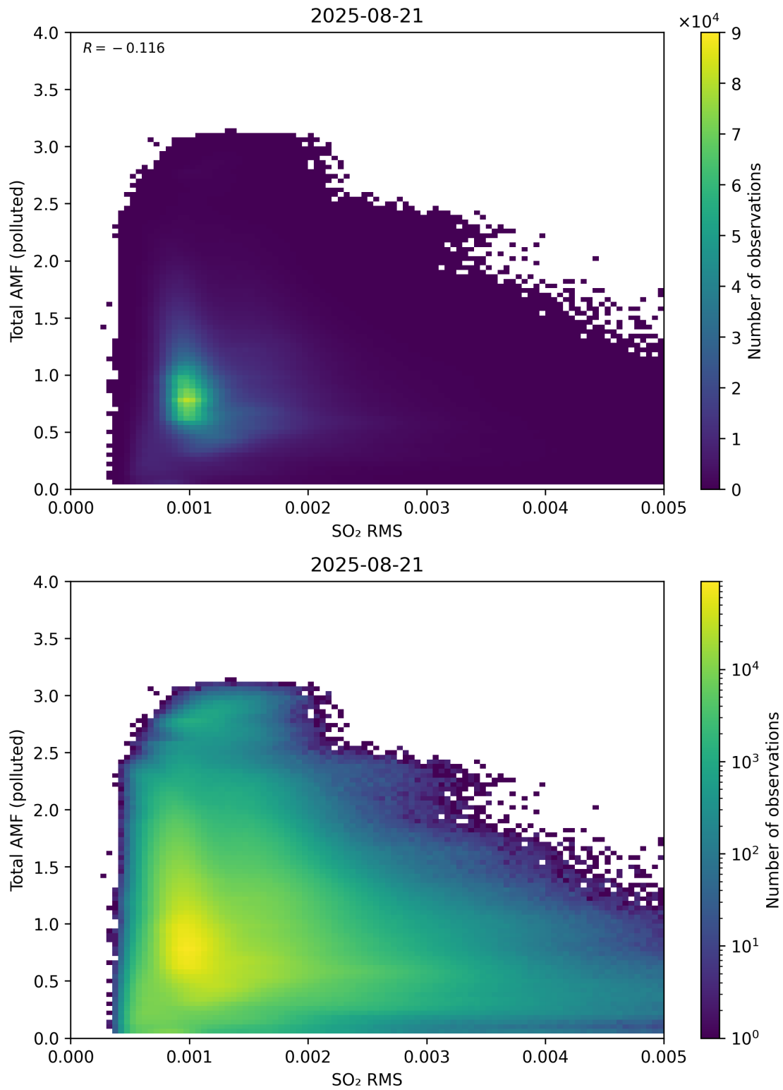
Figure 148: Scatter density plot of “SO 2 RMS” against “Total AMF (polluted)” for 2025-08-20 to 2025-08-22.
