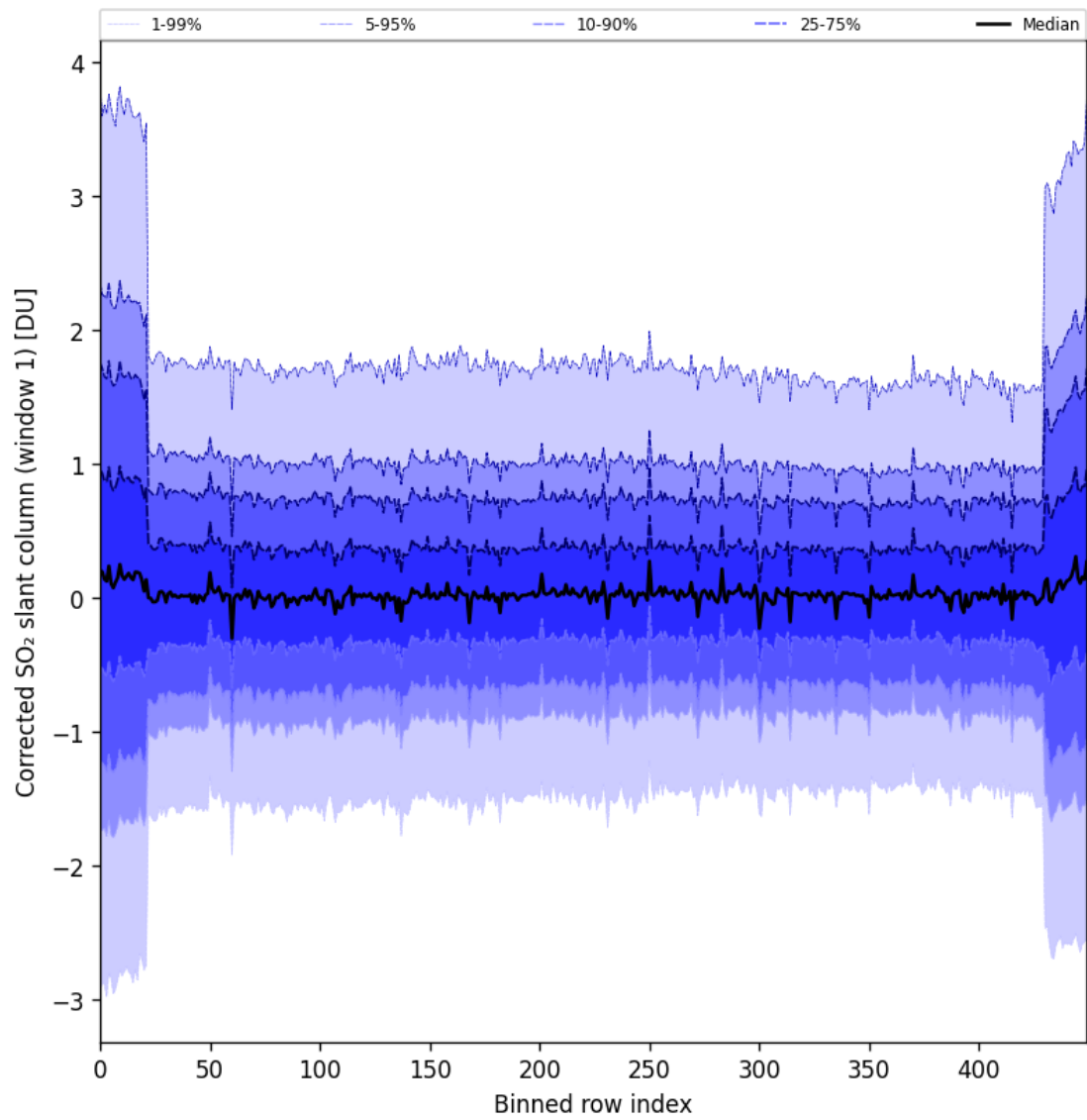
Figure 91: Along track statistics of “Corrected SO 2 slant column (window 1)” for 2025-08-20 to 2025-08-22
