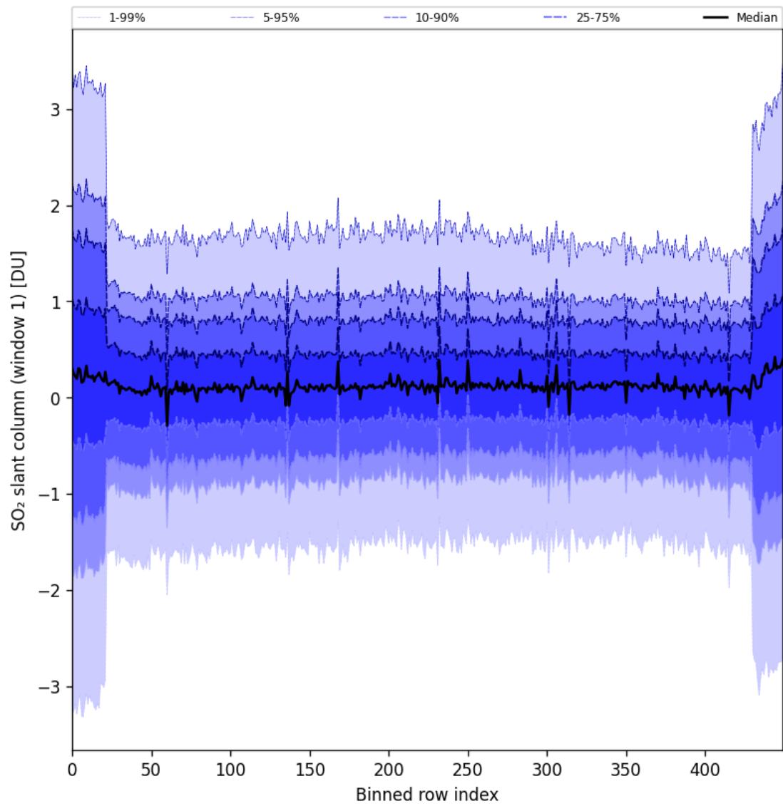
Figure 89: Along track statistics of “SO 2 slant column (window 1)” for 2025-08-20 to 2025-08-22
