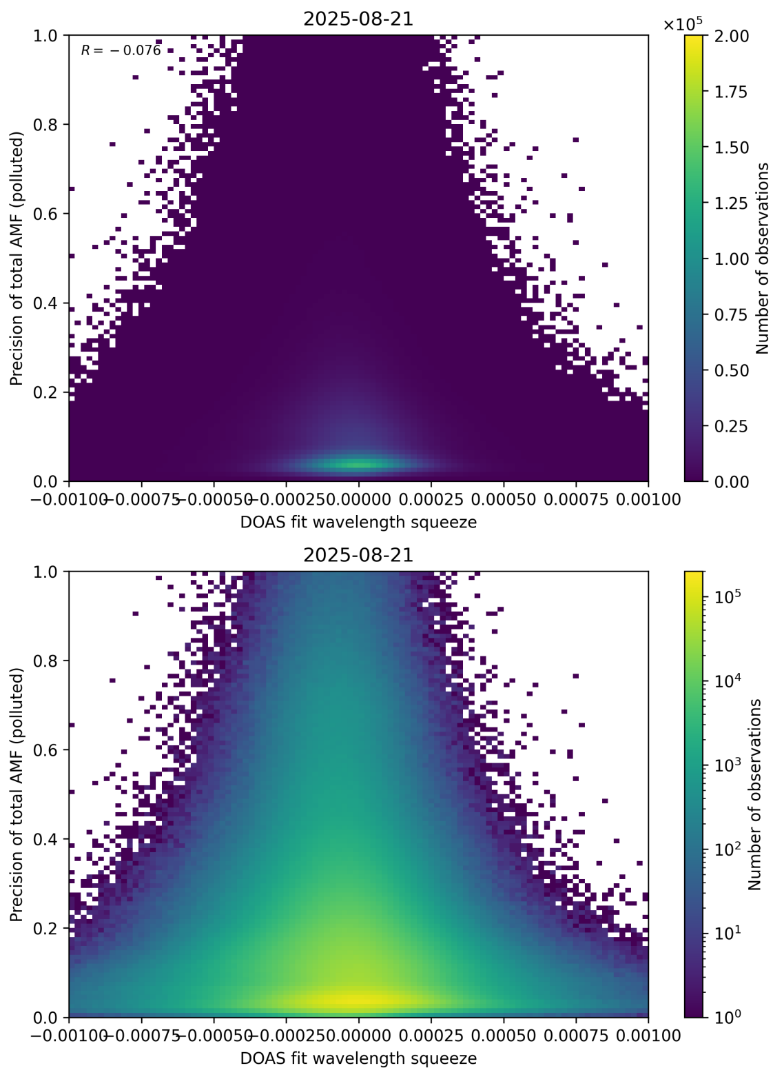
Figure 146: Scatter density plot of “DOAS fit wavelength squeeze” against “Precision of total AMF (polluted)” for 2025-08-20 to 2025-08-22.
