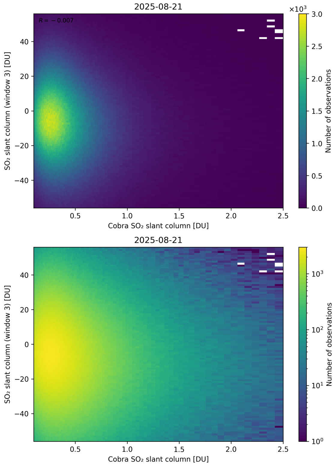
Figure 222: Scatter density plot of “Cobra SO 2 slant column” against “SO 2 slant column (window 3)” for 2025-08-20 to 2025-08-22.
