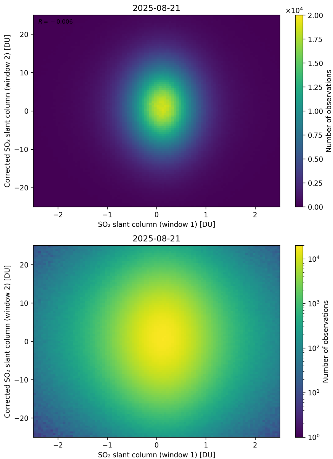
Figure 283: Scatter density plot of “SO 2 slant column (window 1)” against “Corrected SO 2 slant column (window 2)” for 2025-08-20 to 2025-08-22.
