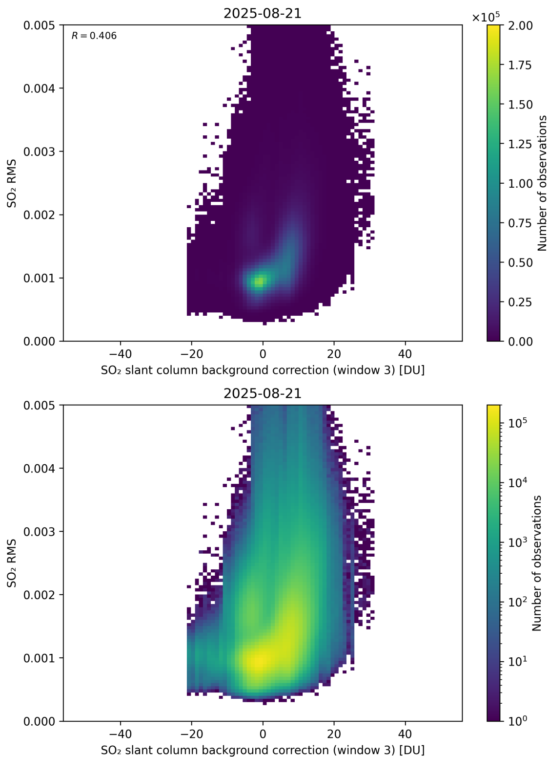
Figure 134: Scatter density plot of “SO 2 slant column background correction (window 3)” against “SO 2 RMS” for 2025-08-20 to 2025-08-22.
