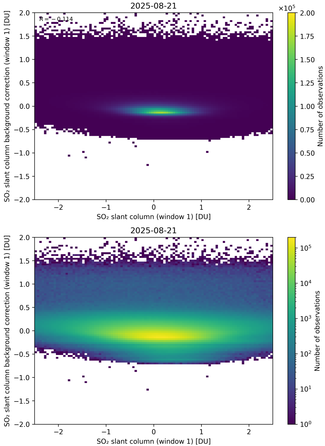
Figure 262: Scatter density plot of “SO 2 slant column (window 1)” against “SO 2 slant column background correction (window 1)” for 2025-08-20 to 2025-08-22.
