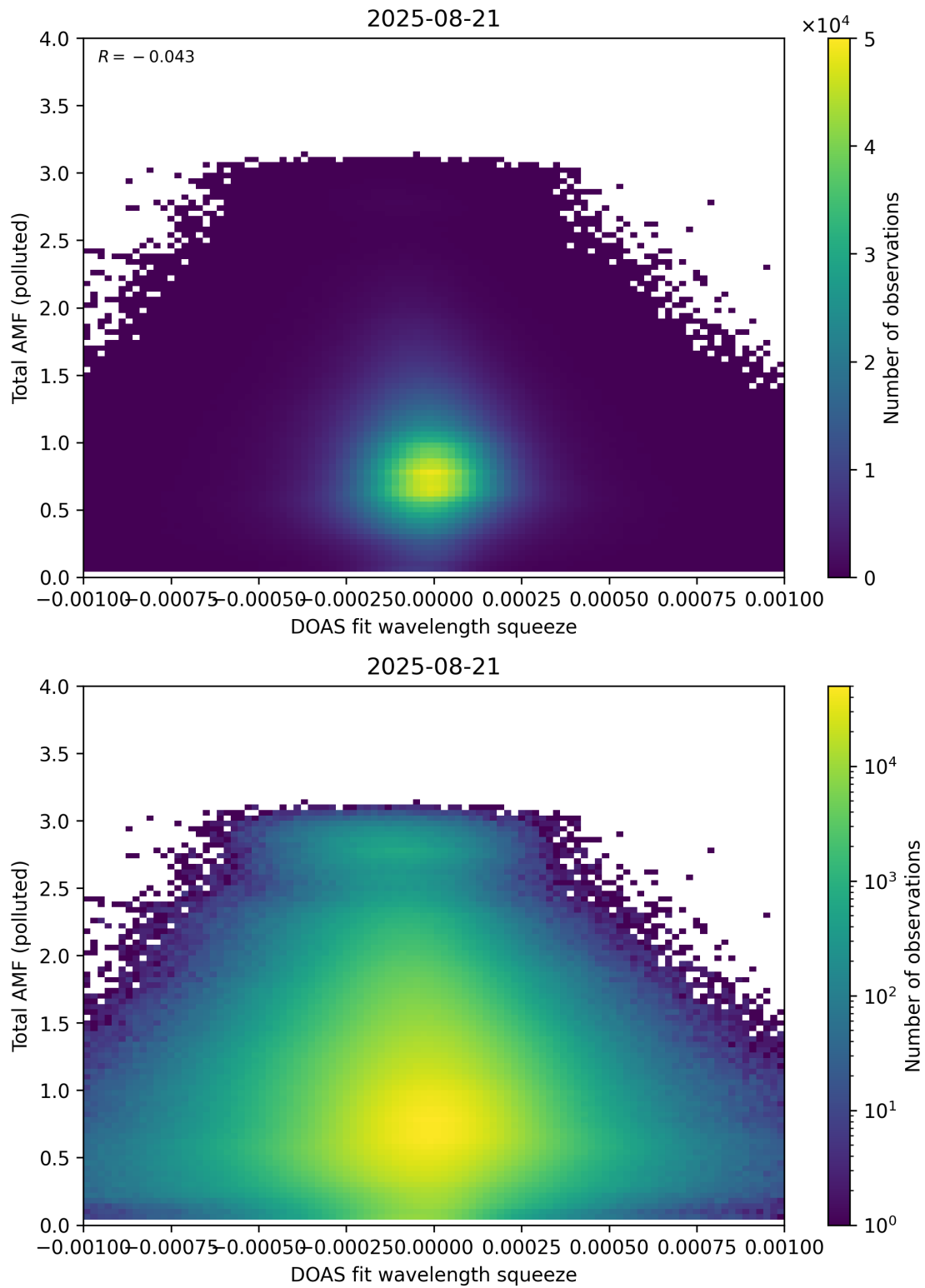
Figure 145: Scatter density plot of “DOAS fit wavelength squeeze” against “Total AMF (polluted)” for 2025-08-20 to 2025-08-22.
