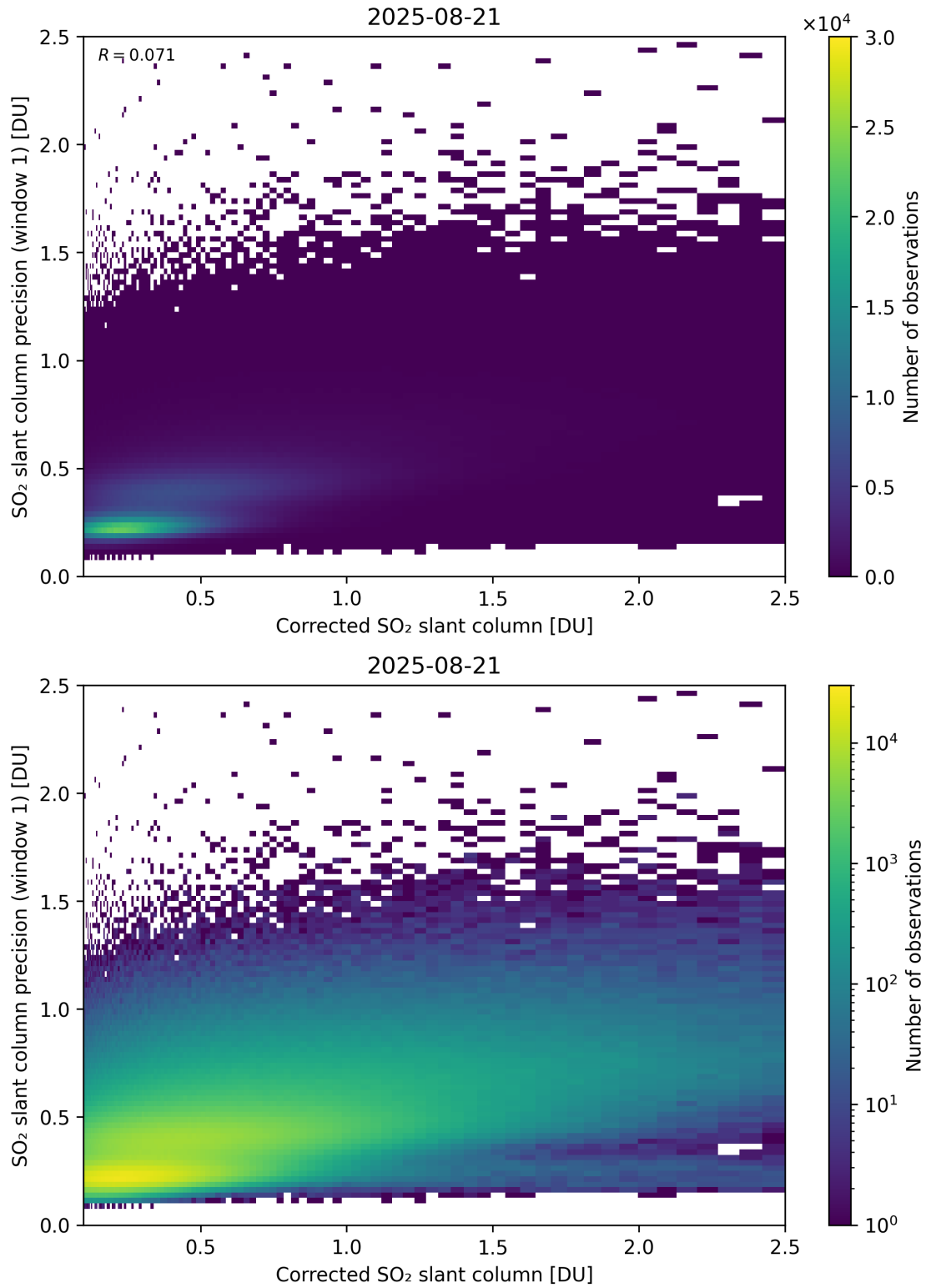
Figure 238: Scatter density plot of “Corrected SO 2 slant column” against “SO 2 slant column precision (window 1)” for 2025-08-20 to 2025-08-22.
