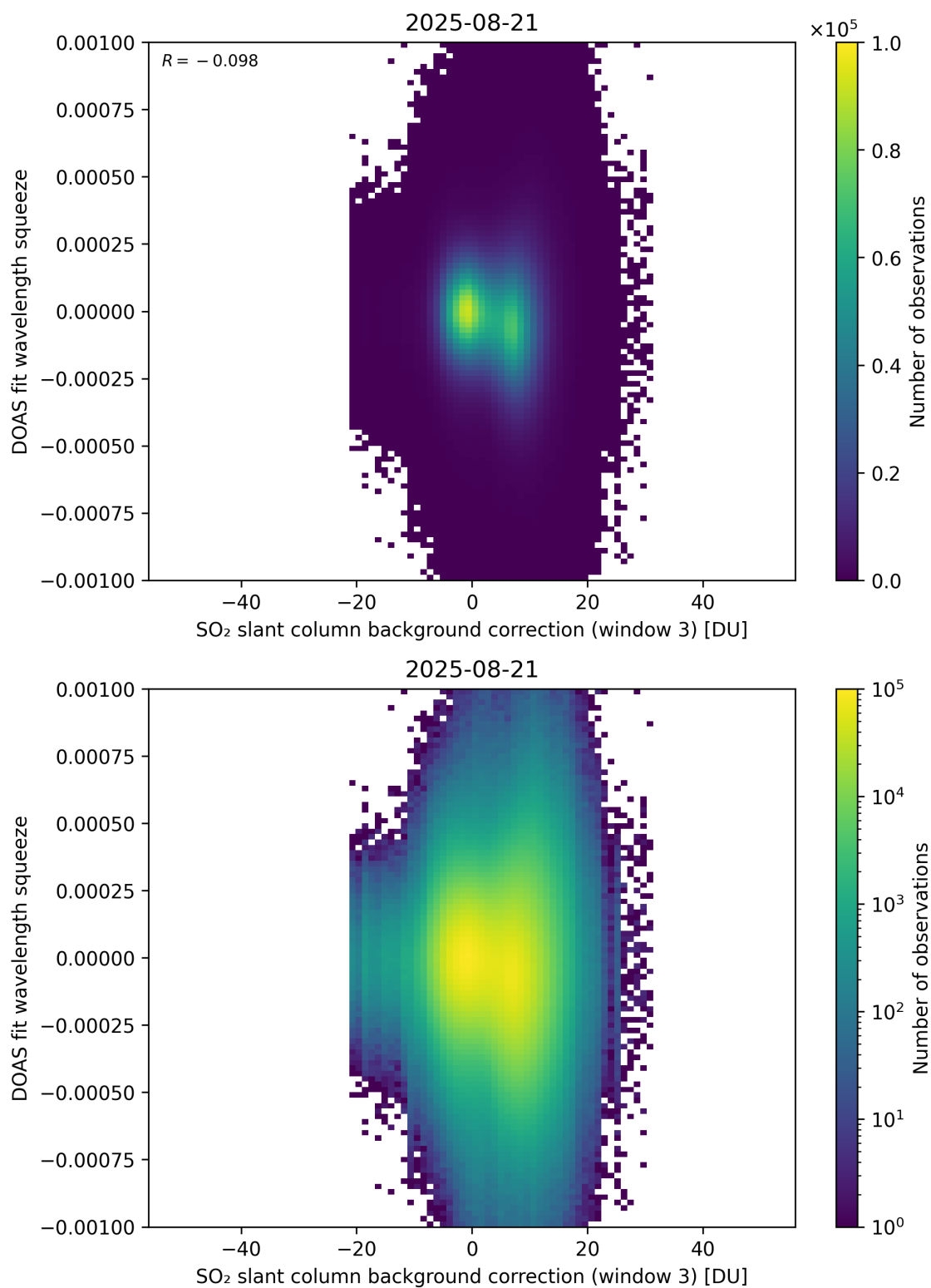
Figure 133: Scatter density plot of “SO 2 slant column background correction (window 3)” against “DOAS fit wavelength squeeze” for 2025-08-20 to 2025-08-22.
