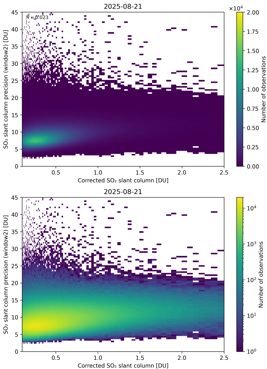
Figure 239: Scatter density plot of “Corrected SO 2 slant column” against “SO 2 slant column precision (window2)” for 2025-08-20 to 2025-08-22.
