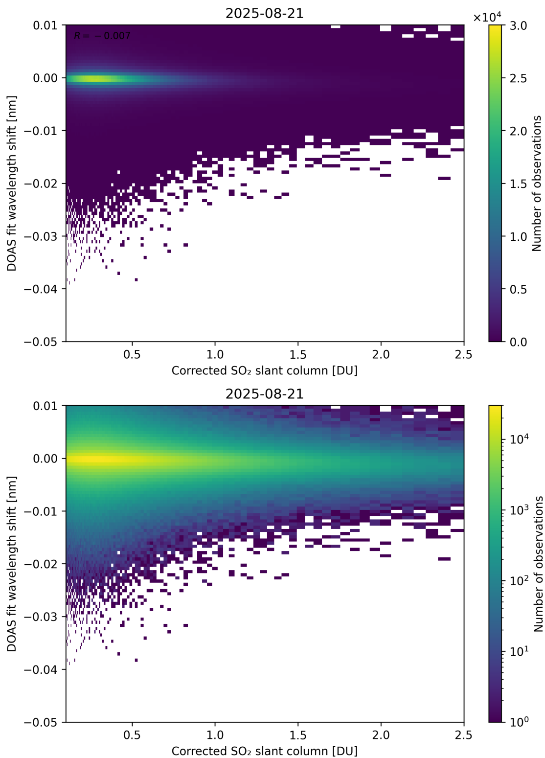
Figure 229: Scatter density plot of “Corrected SO 2 slant column” against “DOAS fit wavelength shift” for 2025-08-20 to 2025-08-22.
