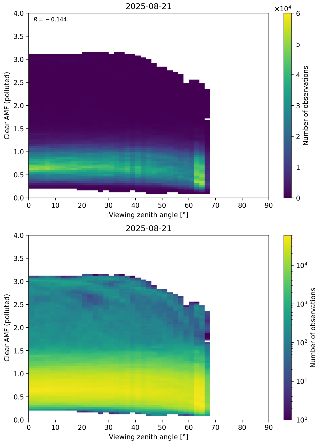
Figure 370: Scatter density plot of “Viewing zenith angle” against “Clear AMF (polluted)” for 2025-08-20 to 2025-08-22.
