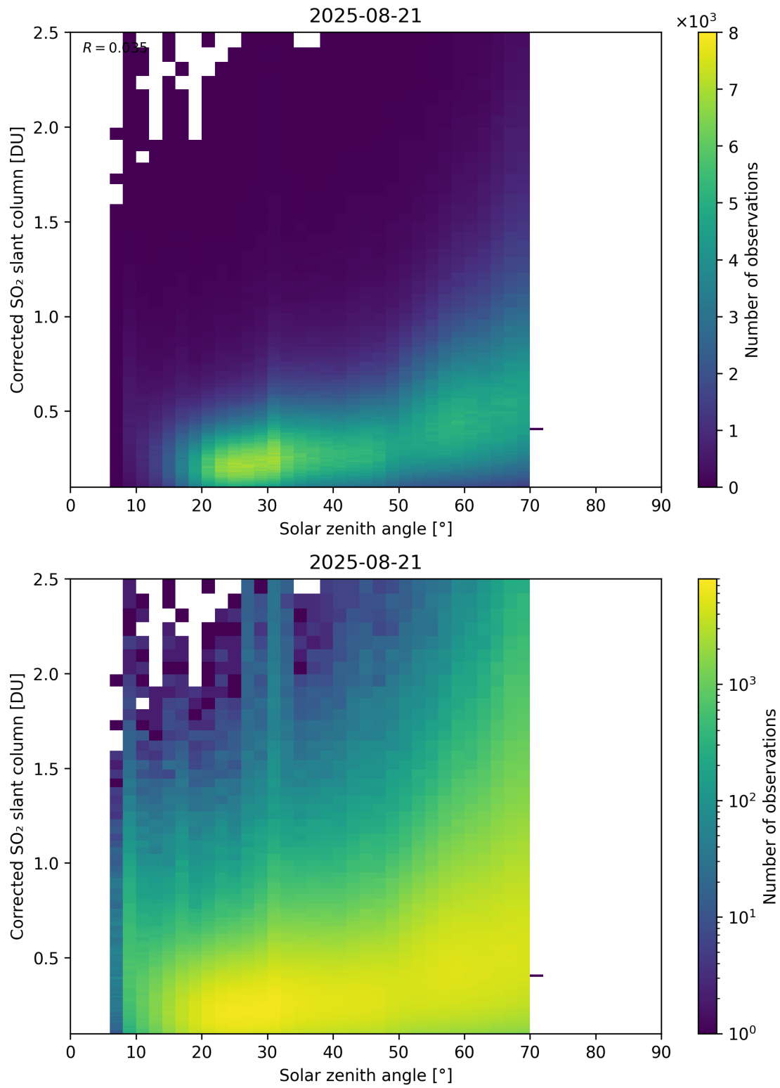
Figure 181: Scatter density plot of “Solar zenith angle” against “Corrected SO 2 slant column” for 2025-08-20 to 2025-08-22.
