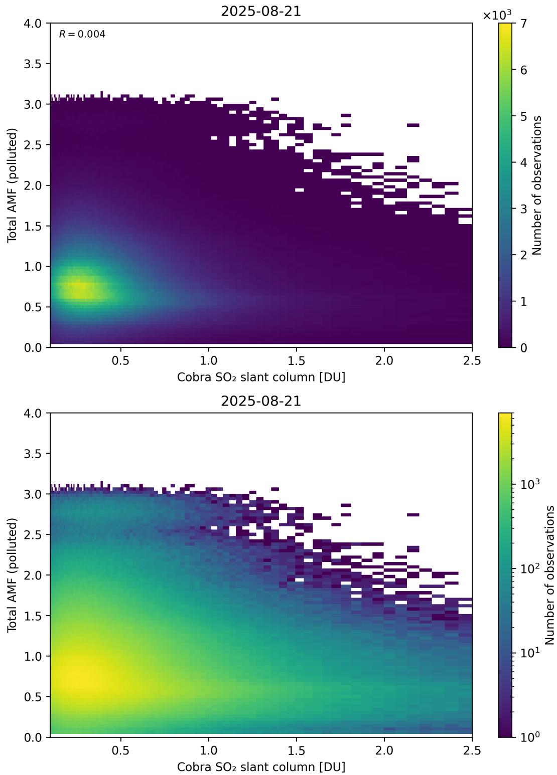
Figure 224: Scatter density plot of “Cobra SO 2 slant column” against “Total AMF (polluted)” for 2025-08-20 to 2025-08-22.
