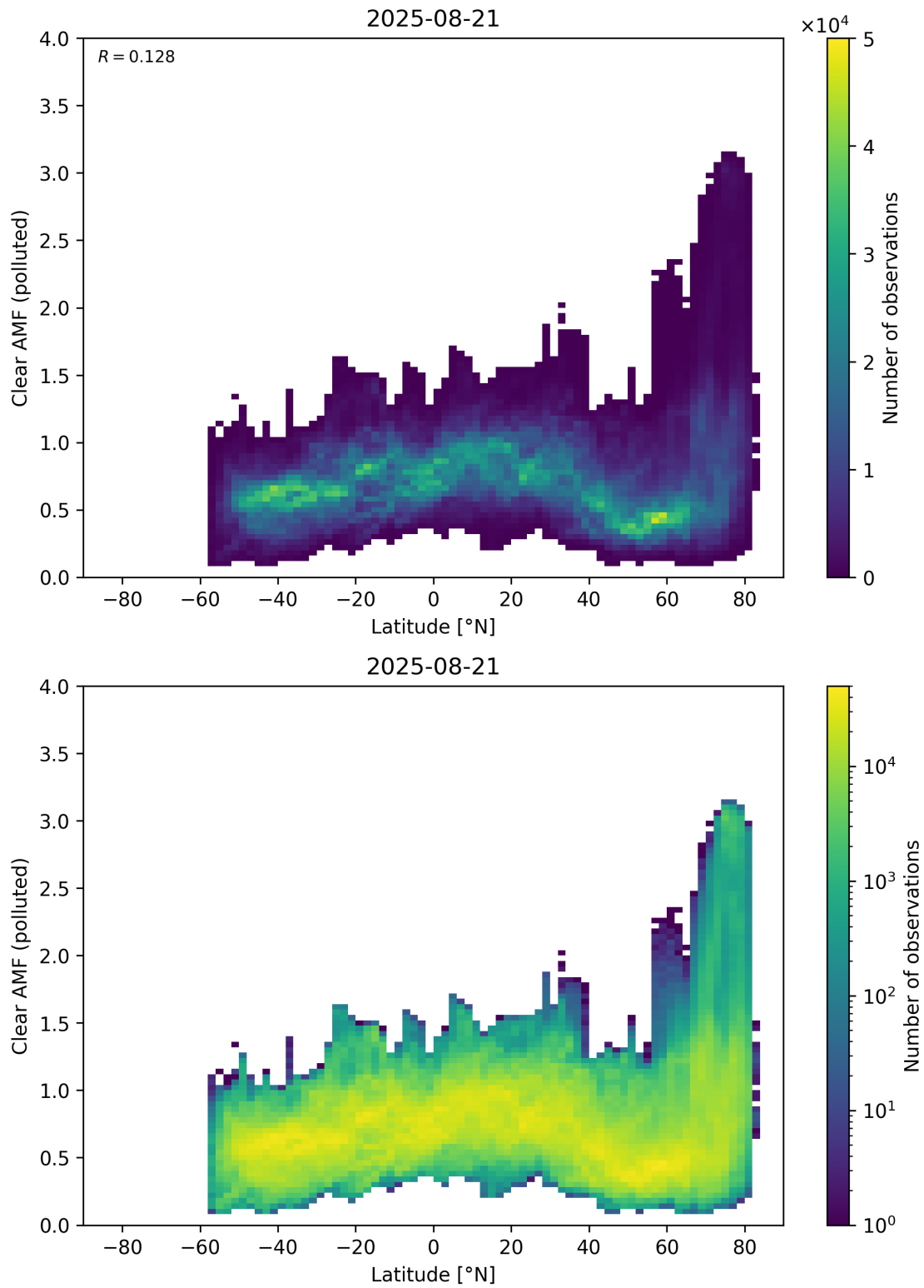
Figure 156: Scatter density plot of “Latitude” against “Clear AMF (polluted)” for 2025-08-20 to 2025-08-22.
