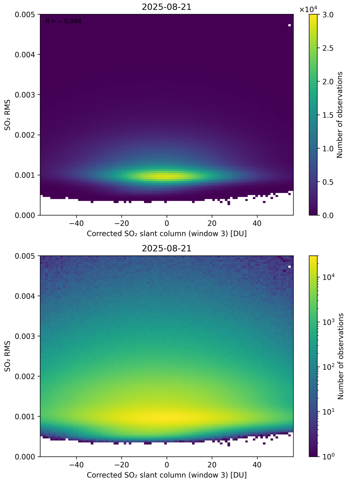
Figure 258: Scatter density plot of “Corrected SO 2 slant column (window 3)” against “SO 2 RMS” for 2025-08-20 to 2025-08-22.
