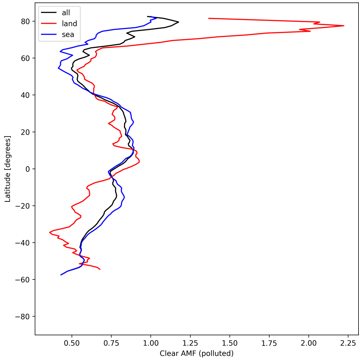
Figure 55: Zonal average of “Clear AMF (polluted)” for 2025-08-20 to 2025-08-22.
