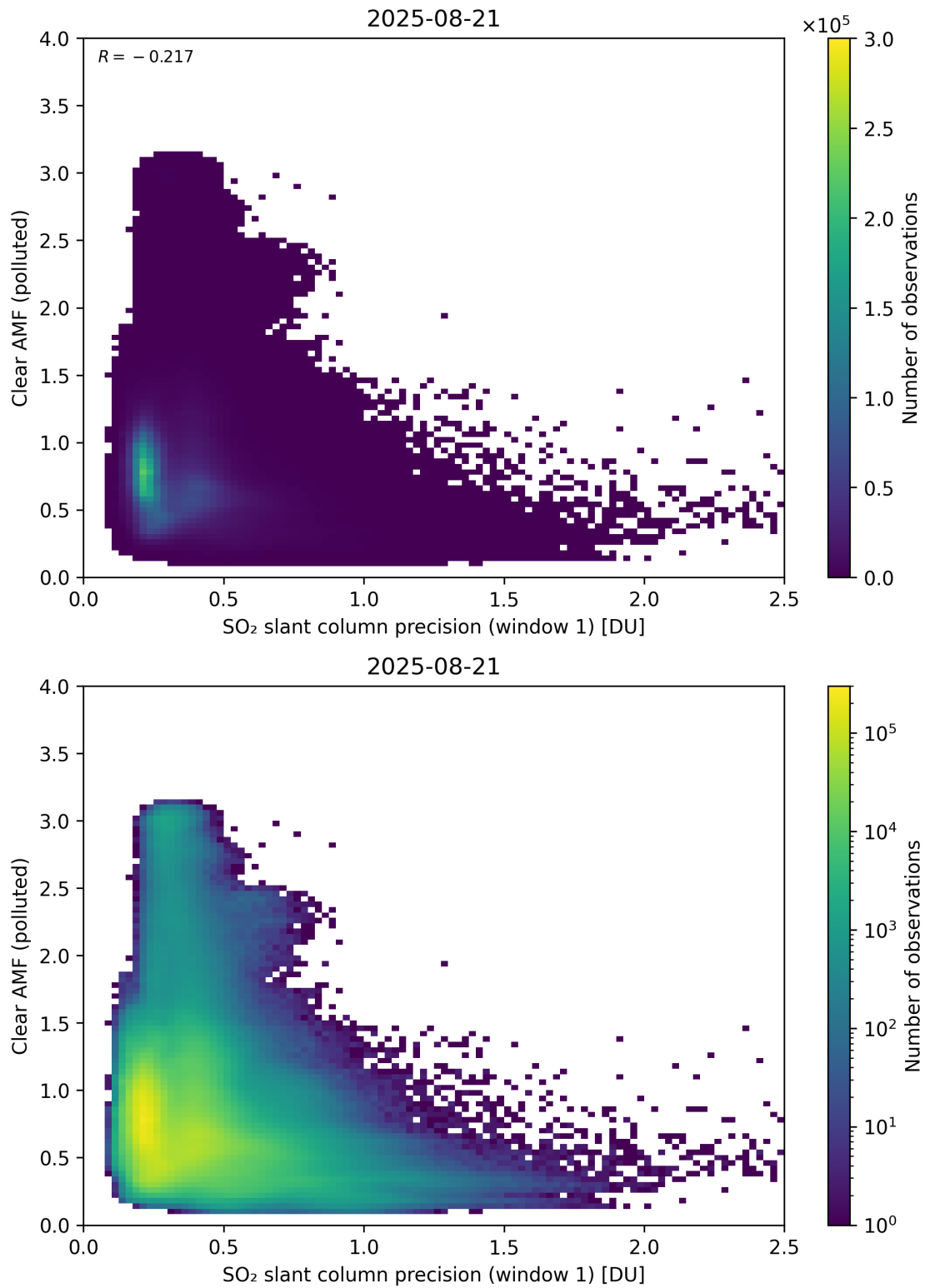
Figure 274: Scatter density plot of “SO 2 slant column precision (window 1)” against “Clear AMF (polluted)” for 2025-08-20 to 2025-08-22.
