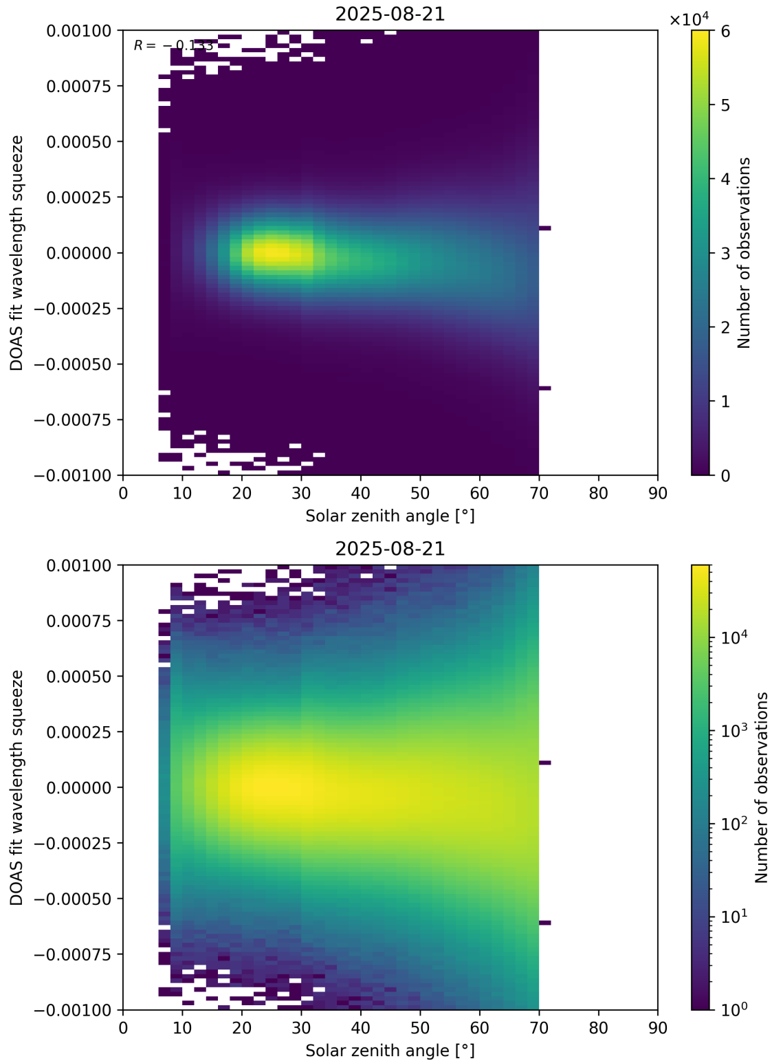
Figure 175: Scatter density plot of “Solar zenith angle” against “DOAS fit wavelength squeeze” for 2025-08-20 to 2025-08-22.
