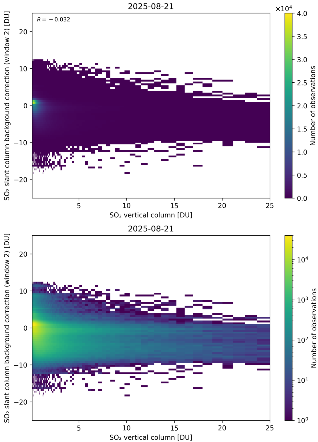
Figure 324: Scatter density plot of “SO 2 vertical column” against “SO 2 slant column background correction (window 2)” for 2025-08-20 to 2025-08-22.
