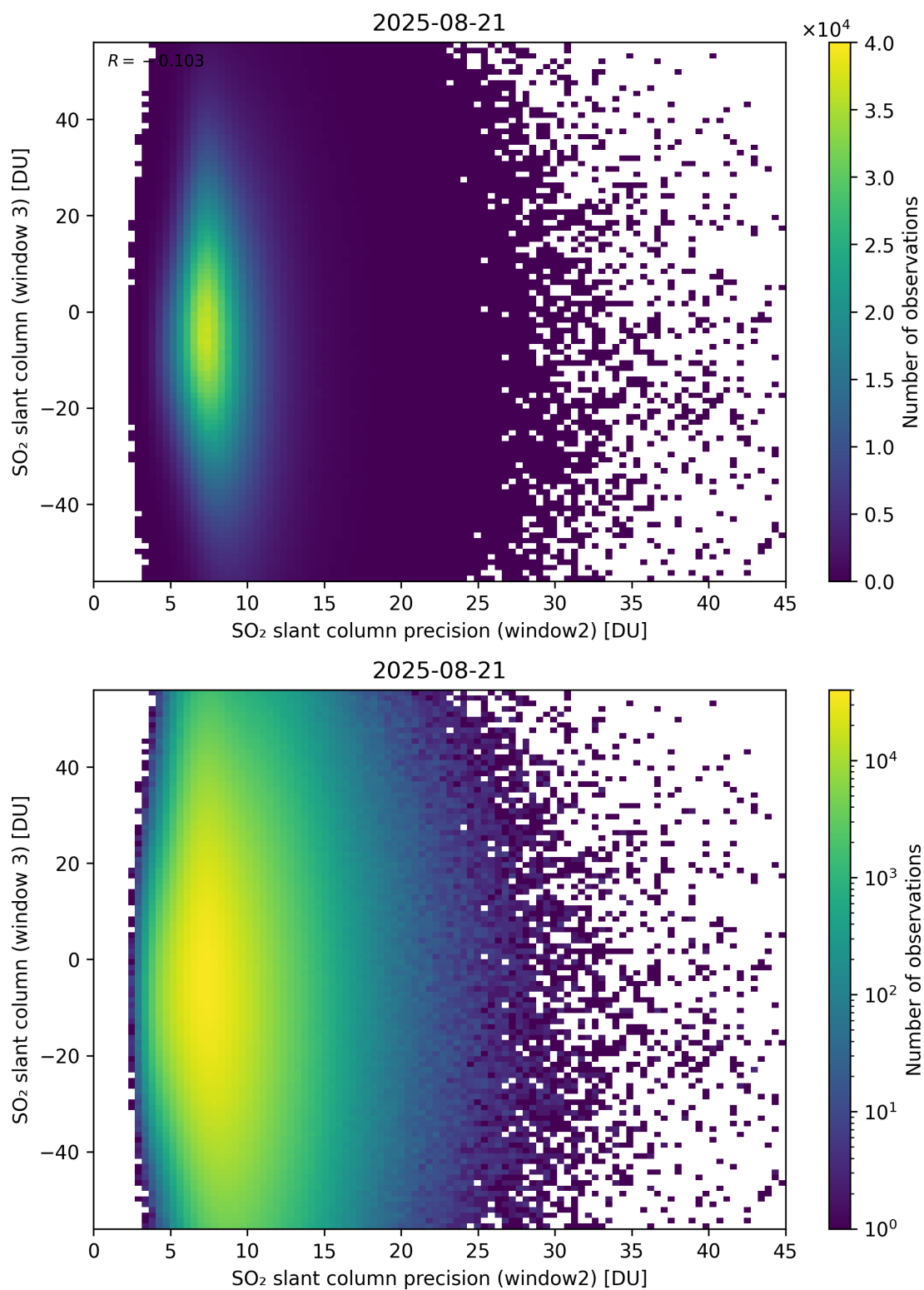
Figure 299: Scatter density plot of “SO 2 slant column precision (window2)” against “SO 2 slant column (window 3)” for 2025-08-20 to 2025-08-22.
