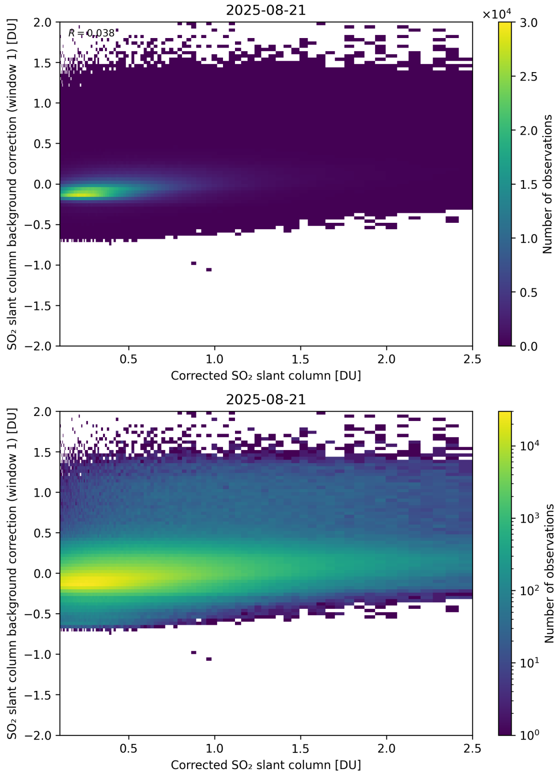
Figure 226: Scatter density plot of “Corrected SO 2 slant column” against “SO 2 slant column background correction (window 1)” for 2025-08-20 to 2025-08-22.
