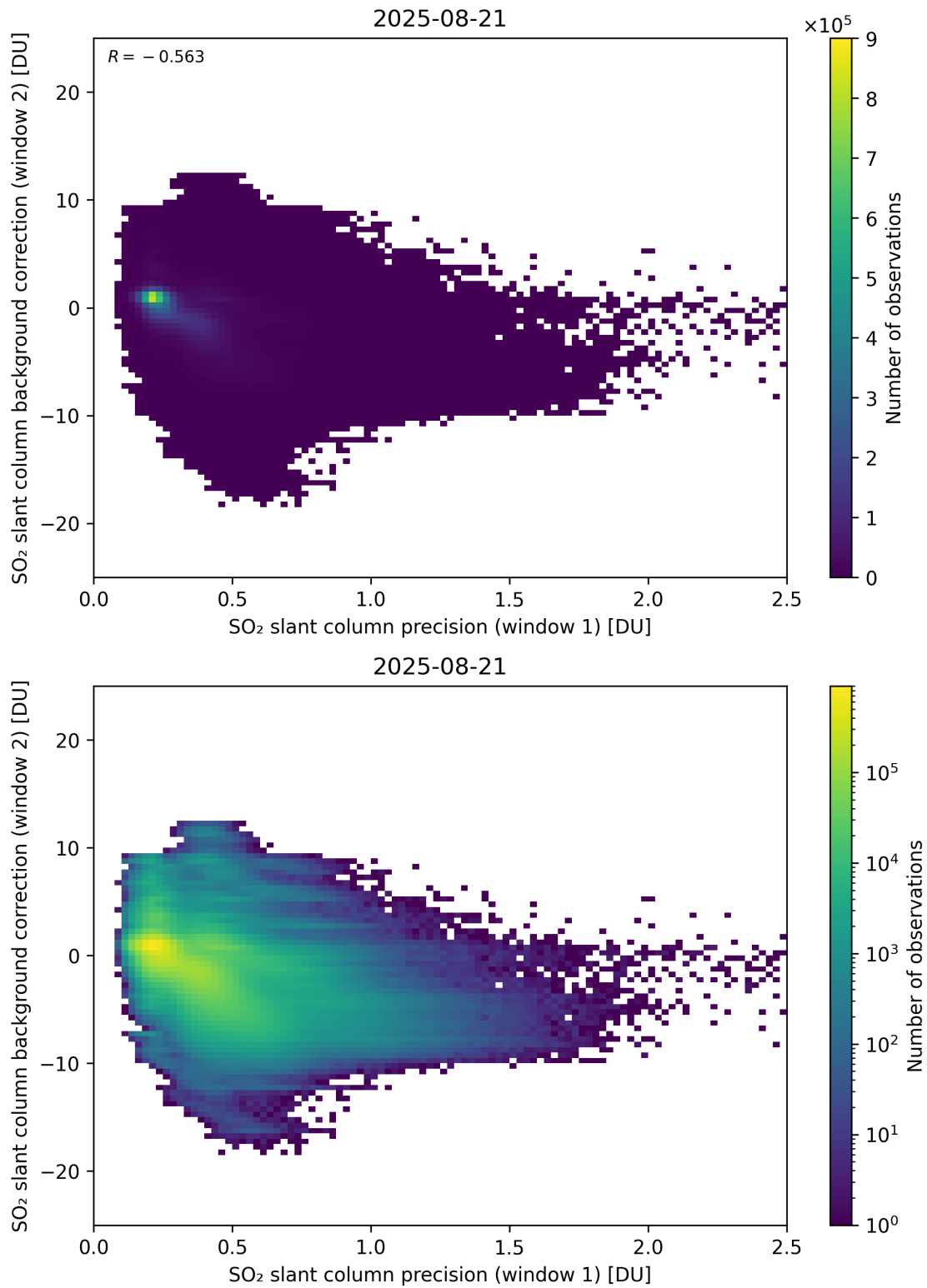
Figure 269: Scatter density plot of “SO 2 slant column precision (window 1)” against “SO 2 slant column background correction (window 2)” for 2025-08-20 to 2025-08-22.
