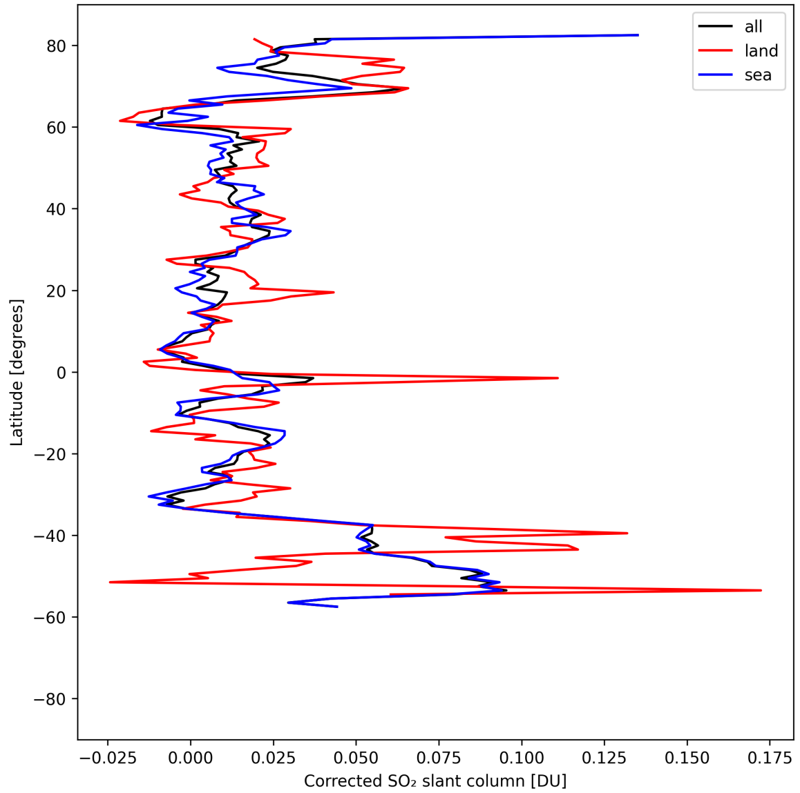
Figure 34: Zonal average of “Corrected SO 2 slant column” for 2025-08-20 to 2025-08-22.
