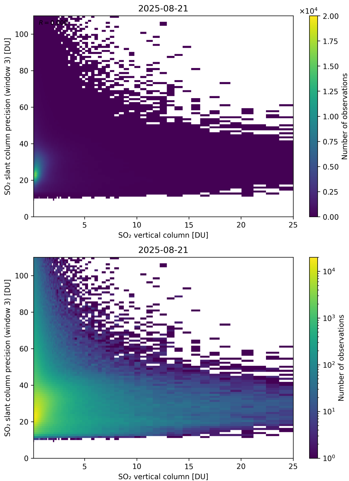
Figure 358: Scatter density plot of “SO 2 vertical column” against “SO 2 slant column precision (window 3)” for 2025-08-20 to 2025-08-22.
