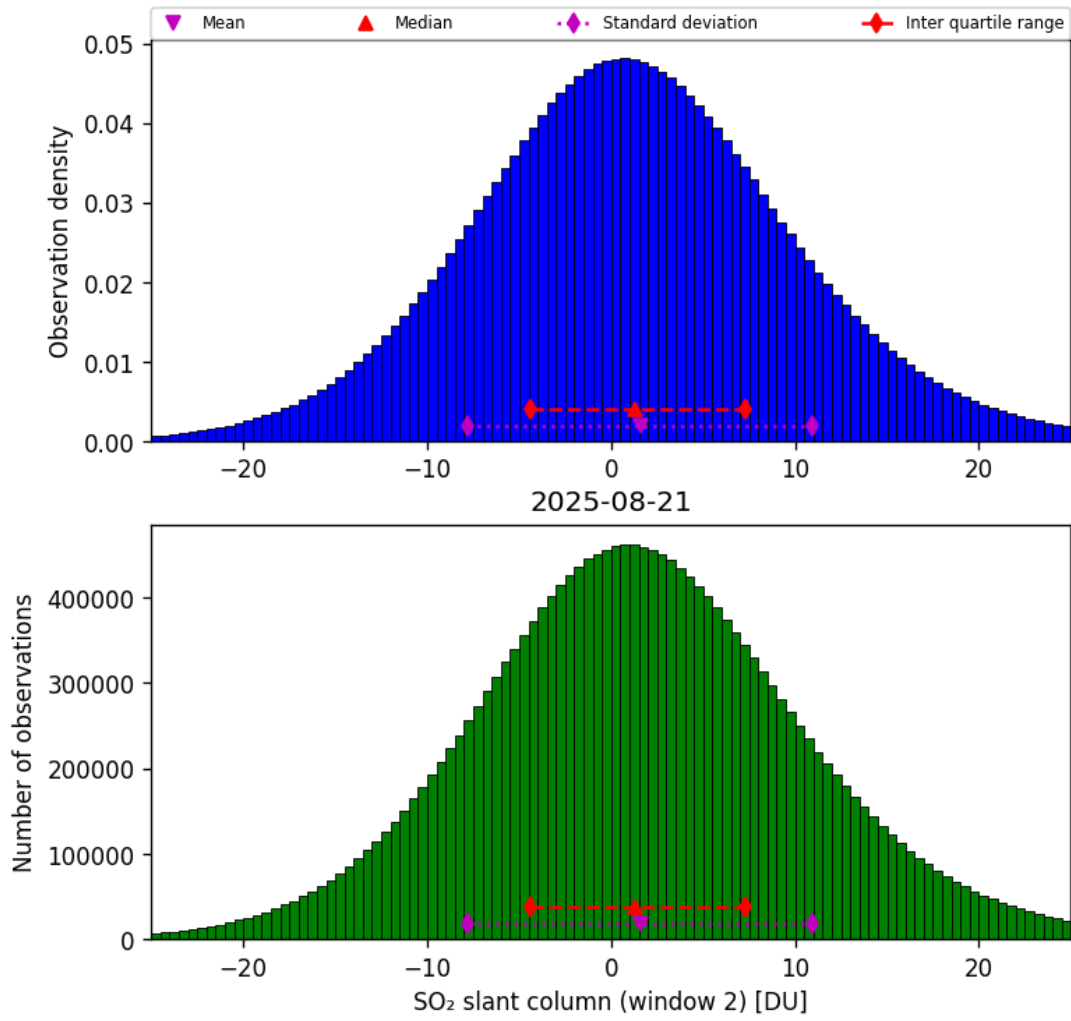
Figure 67: Histogram of “SO 2 slant column (window 2)” for 2025-08-20 to 2025-08-22
