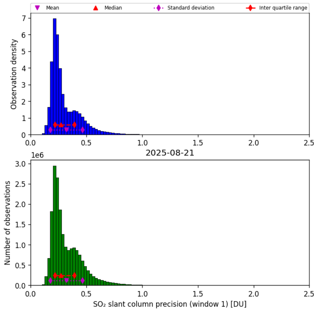
Figure 64: Histogram of “SO 2 slant column precision (window 1)” for 2025-08-20 to 2025-08-22
