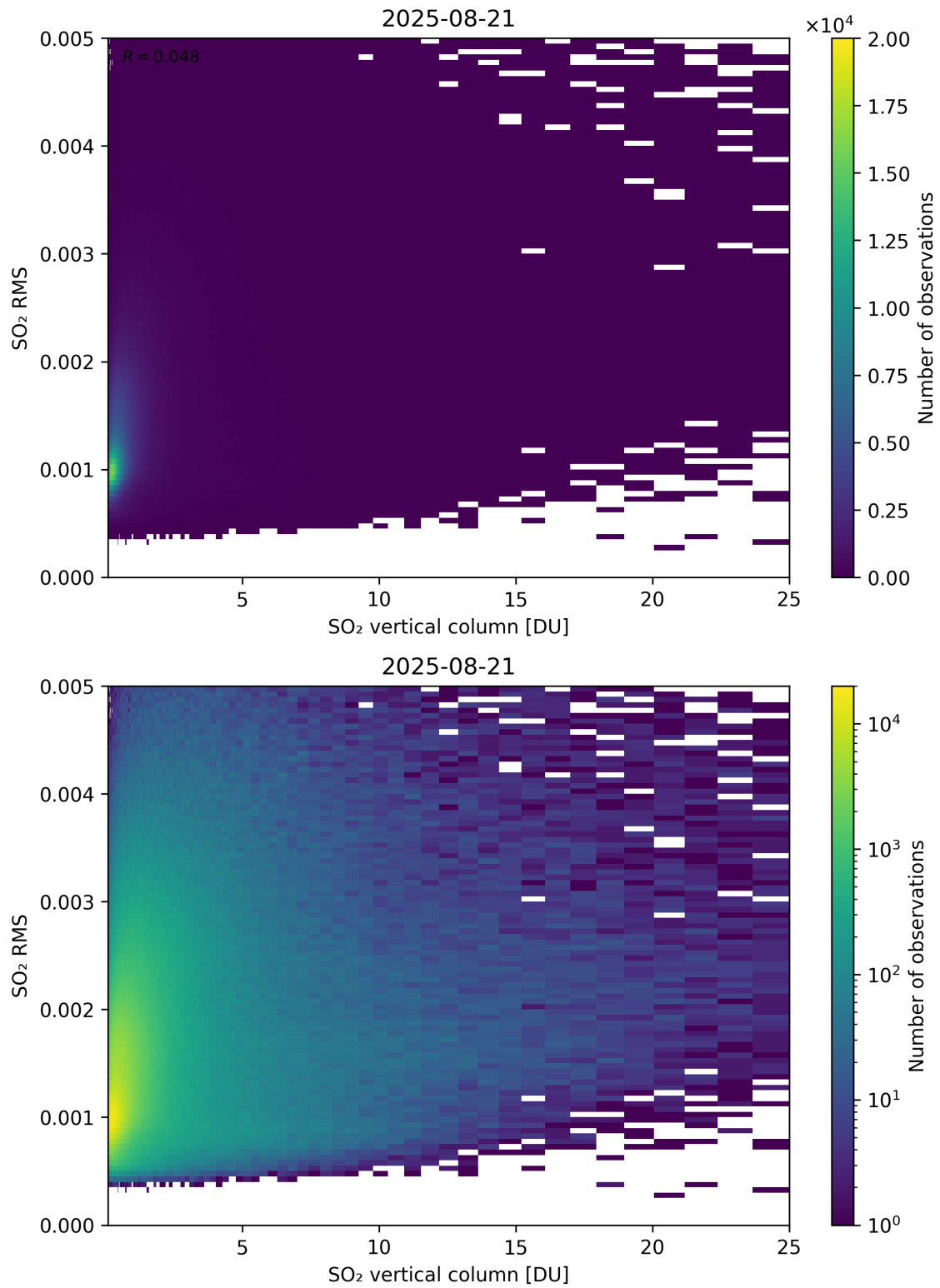
Figure 328: Scatter density plot of “SO 2 vertical column” against “SO 2 RMS” for 2025-08-20 to 2025-08-22.
