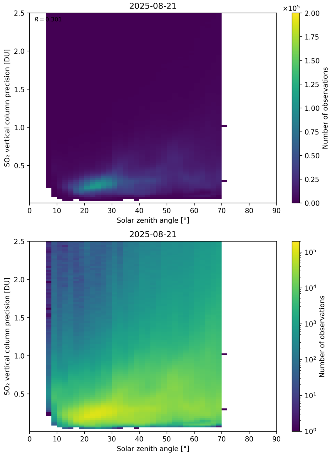
Figure 192: Scatter density plot of “Solar zenith angle” against “SO 2 vertical column precision” for 2025-08-20 to 2025-08-22.
