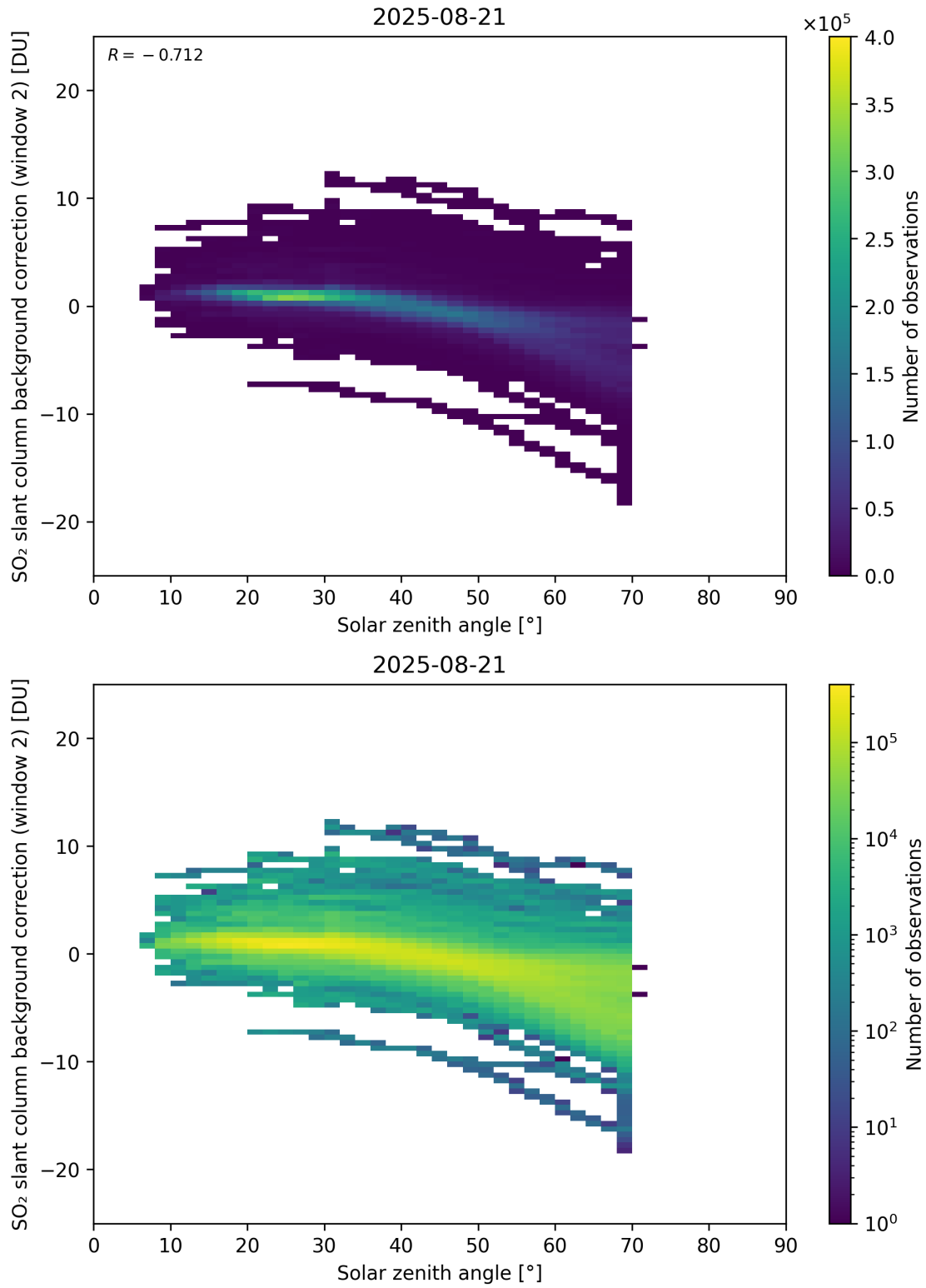
Figure 172: Scatter density plot of “Solar zenith angle” against “SO 2 slant column background correction (window 2)” for 2025-08-20 to 2025-08-22.
