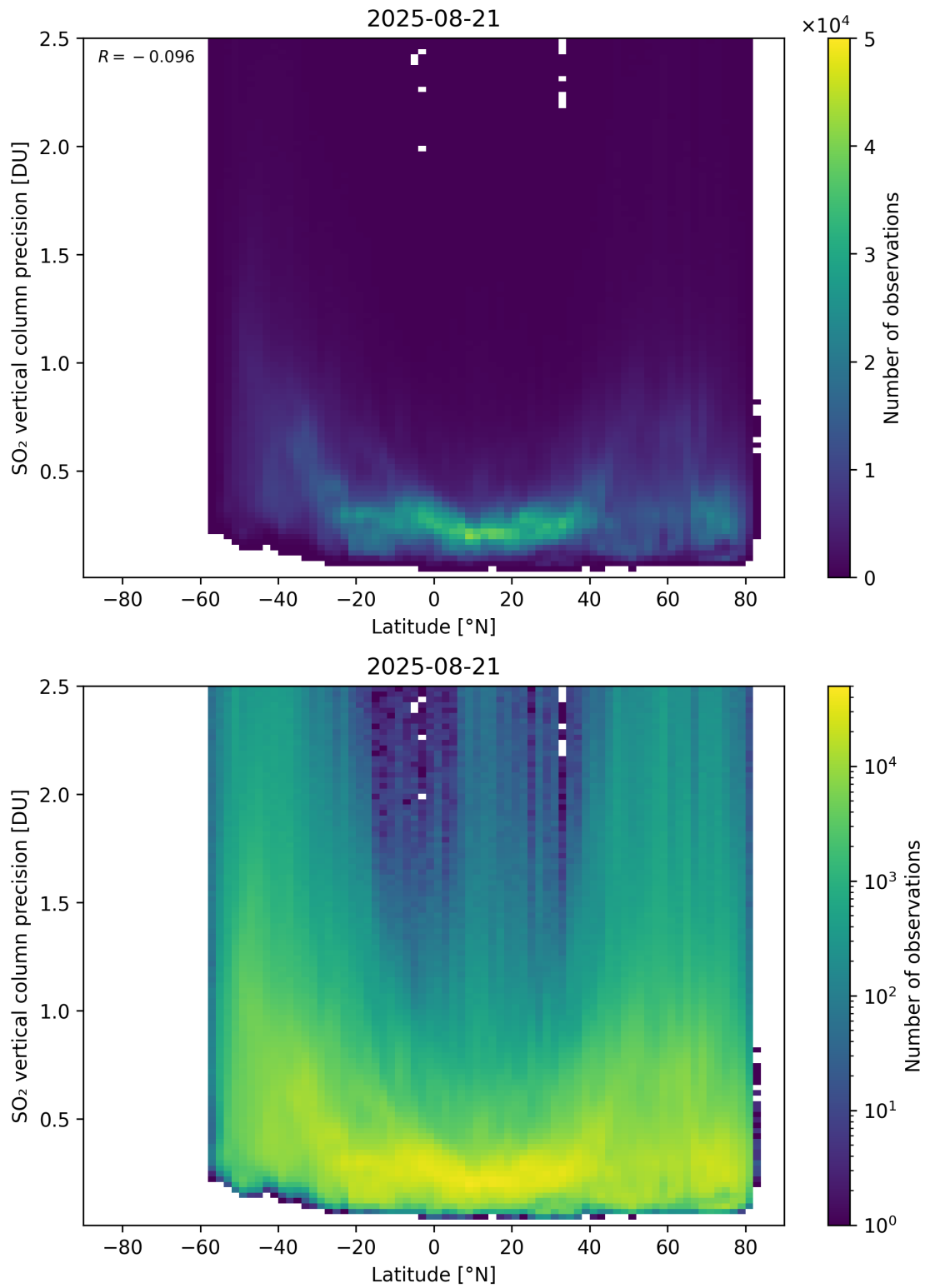
Figure 170: Scatter density plot of “Latitude” against “SO 2 vertical column precision” for 2025-08-20 to 2025-08-22.
