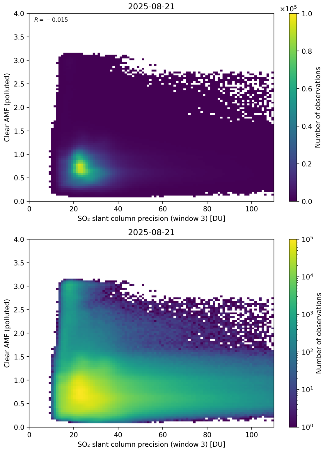
Figure 311: Scatter density plot of “SO 2 slant column precision (window 3)” against “Clear AMF (polluted)” for 2025-08-20 to 2025-08-22.
