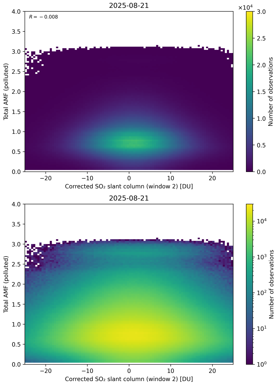
Figure 253: Scatter density plot of “Corrected SO 2 slant column (window 2)” against “Total AMF (polluted)” for 2025-08-20 to 2025-08-22.
