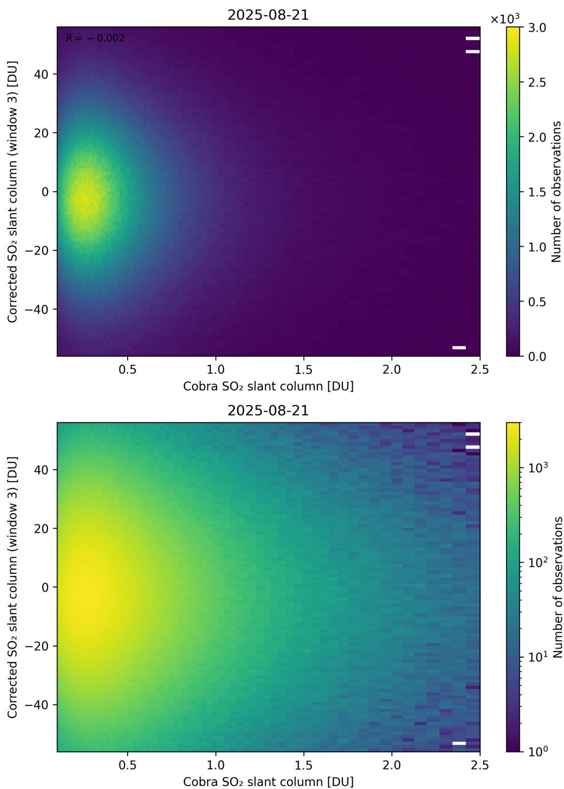
Figure 218: Scatter density plot of “Cobra SO 2 slant column” against “Corrected SO 2 slant column (window 3)” for 2025-08-20 to 2025-08-22.
