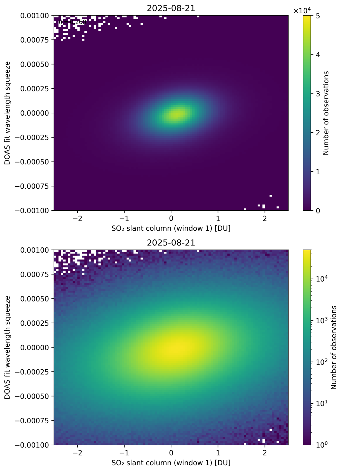
Figure 266: Scatter density plot of “SO 2 slant column (window 1)” against “DOAS fit wavelength squeeze” for 2025-08-20 to 2025-08-22.
