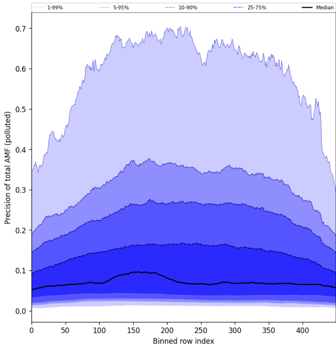
Figure 106: Along track statistics of “Precision of total AMF (polluted)” for 2025-08-20 to 2025-08-22
