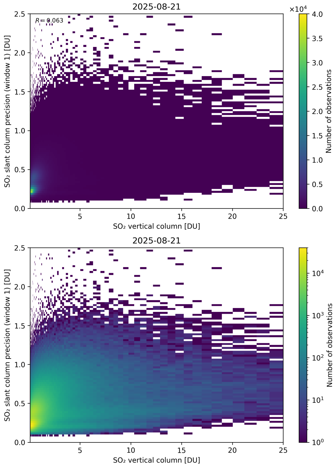
Figure 355: Scatter density plot of “SO 2 vertical column” against “SO 2 slant column precision (window 1)” for 2025-08-20 to 2025-08-22.
