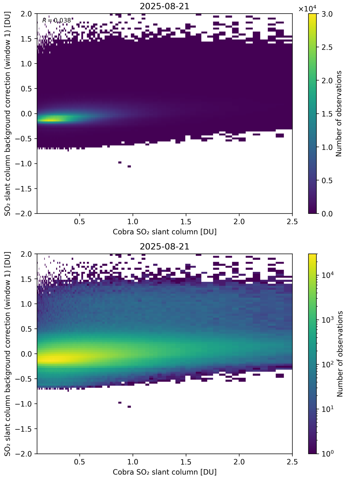
Figure 193: Scatter density plot of “Cobra SO 2 slant column” against “SO 2 slant column background correction (window 1)” for 2025-08-20 to 2025-08-22.
