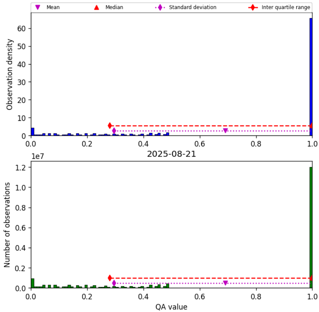
Figure 57: Histogram of “QA value” for 2025-08-20 to 2025-08-22
