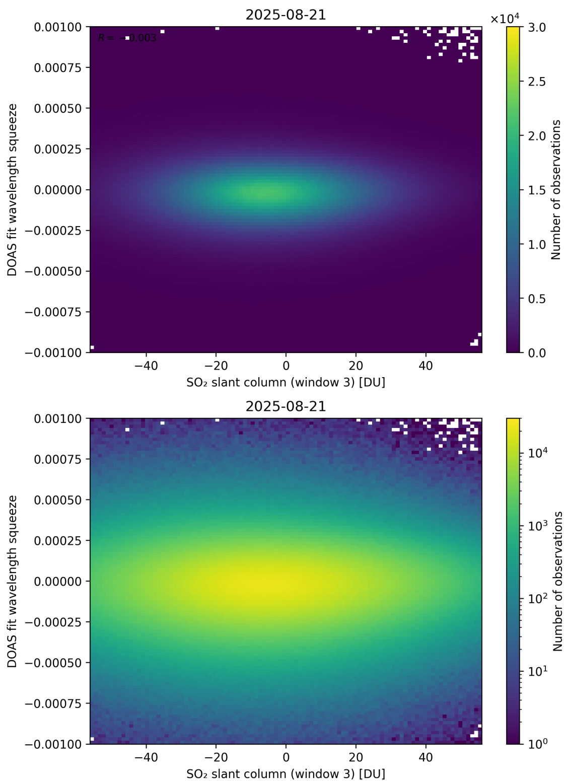
Figure 305: Scatter density plot of “SO 2 slant column (window 3)” against “DOAS fit wavelength squeeze” for 2025-08-20 to 2025-08-22.
