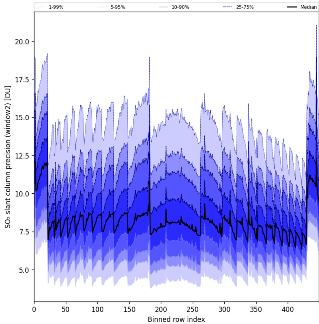
Figure 94: Along track statistics of “SO 2 slant column precision (window2)” for 2025-08-20 to 2025-08-22
