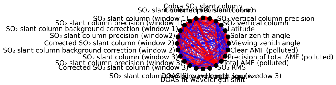
Figure 1: Map of correlation graph for 2025-08-20 to 2025-08-22.
