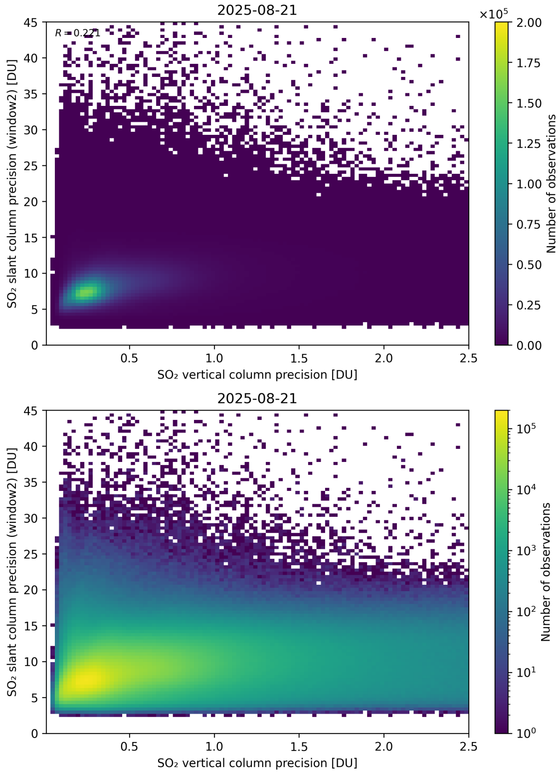
Figure 343: Scatter density plot of “SO 2 vertical column precision” against “SO 2 slant column precision (window2)” for 2025-08-20 to 2025-08-22.
