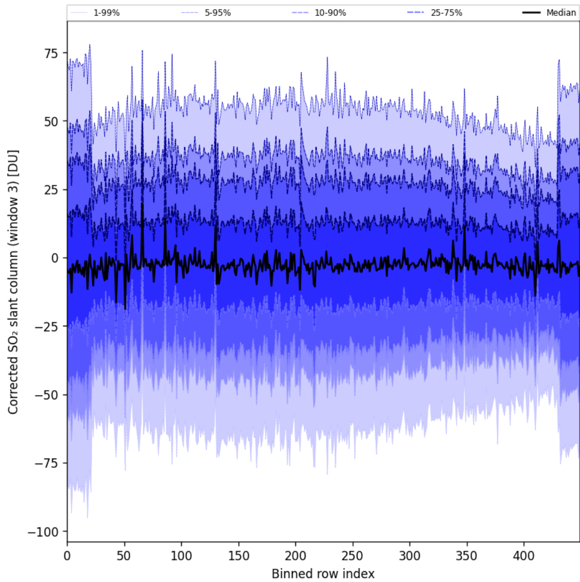
Figure 99: Along track statistics of “Corrected SO 2 slant column (window 3)” for 2025-08-20 to 2025-08-22
