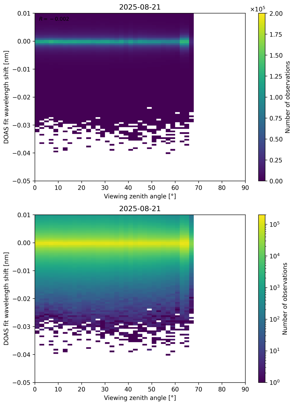
Figure 365: Scatter density plot of “Viewing zenith angle” against “DOAS fit wavelength shift” for 2025-08-20 to 2025-08-22.
