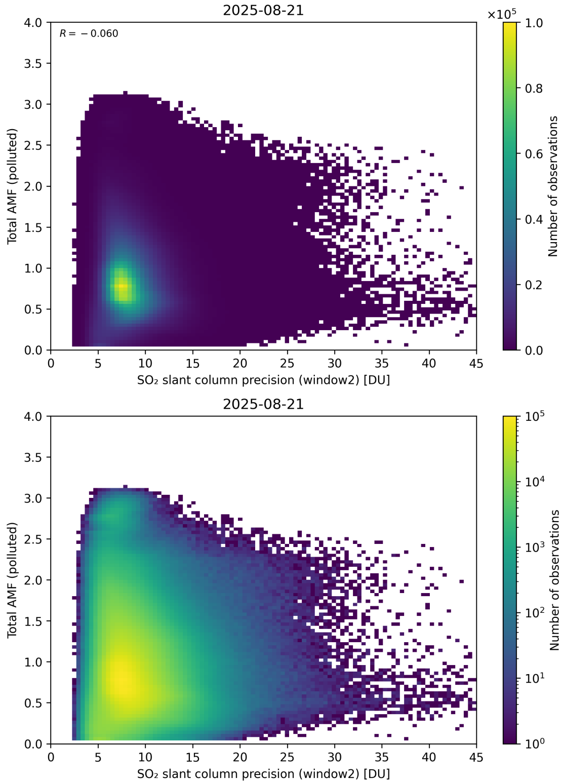
Figure 301: Scatter density plot of “SO 2 slant column precision (window2)” against “Total AMF (polluted)” for 2025-08-20 to 2025-08-22.
