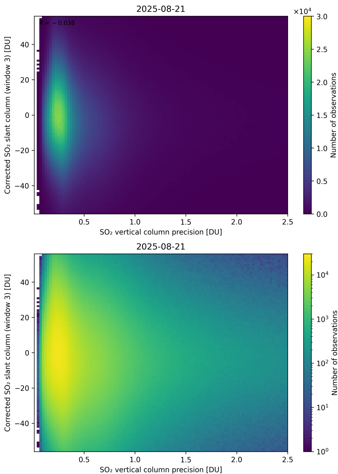
Figure 340: Scatter density plot of “SO 2 vertical column precision” against “Corrected SO 2 slant column (window 3)” for 2025-08-20 to 2025-08-22.
