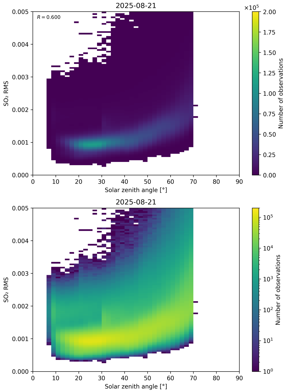
Figure 176: Scatter density plot of “Solar zenith angle” against “SO 2 RMS” for 2025-08-20 to 2025-08-22.
