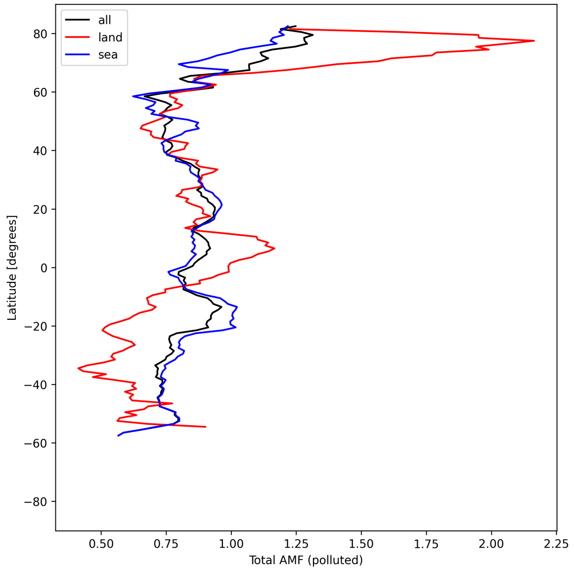
Figure 53: Zonal average of “Total AMF (polluted)” for 2025-08-20 to 2025-08-22.
