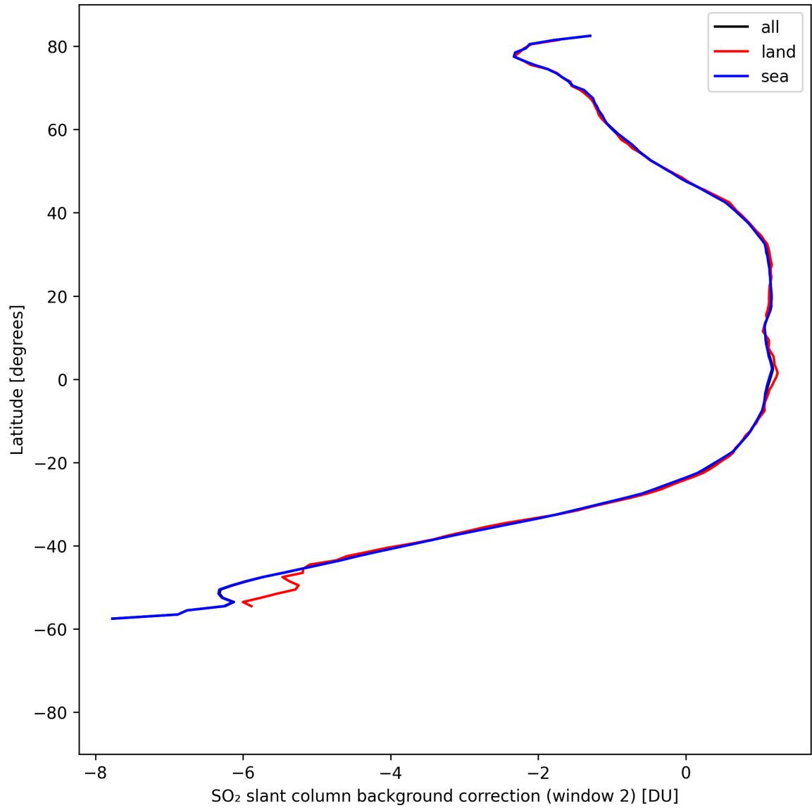
Figure 44: Zonal average of “SO 2 slant column background correction (window 2)” for 2025-08-20 to 2025-08-22.
