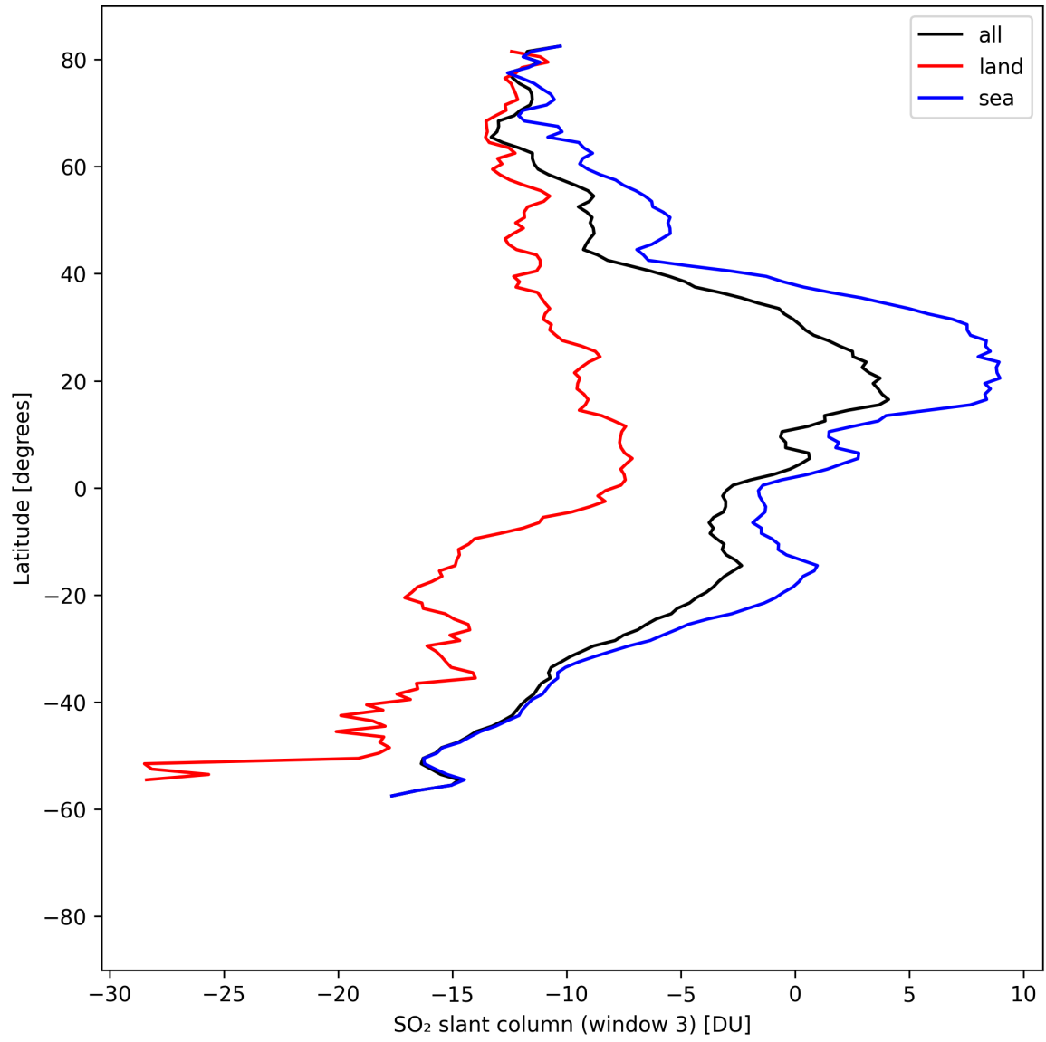
Figure 45: Zonal average of “SO 2 slant column (window 3)” for 2025-08-20 to 2025-08-22.
