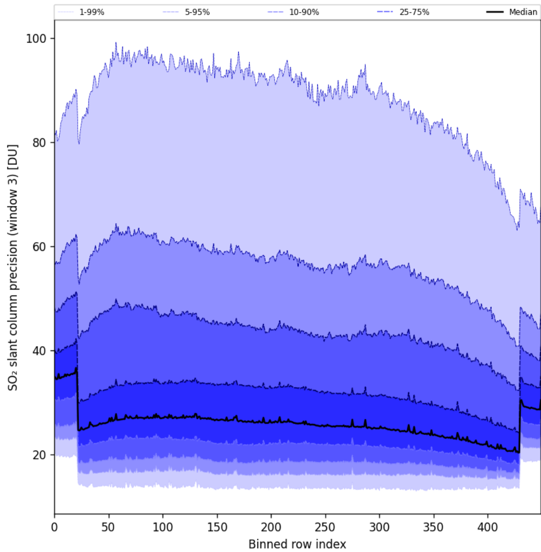
Figure 98: Along track statistics of “SO 2 slant column precision (window 3)” for 2025-08-20 to 2025-08-22
