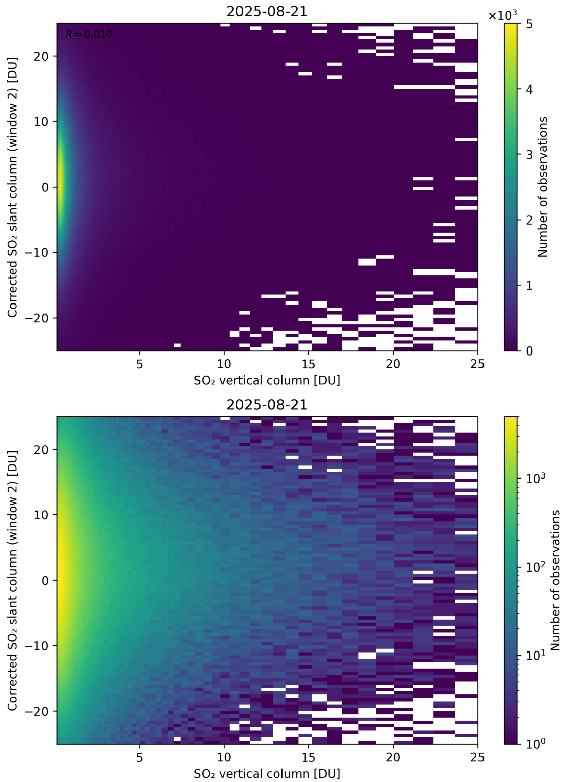
Figure 352: Scatter density plot of “SO 2 vertical column” against “Corrected SO 2 slant column (window 2)” for 2025-08-20 to 2025-08-22.
