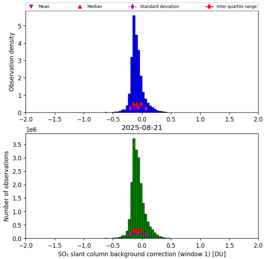
Figure 66: Histogram of “SO 2 slant column background correction (window 1)” for 2025-08-20 to 2025-08-22
