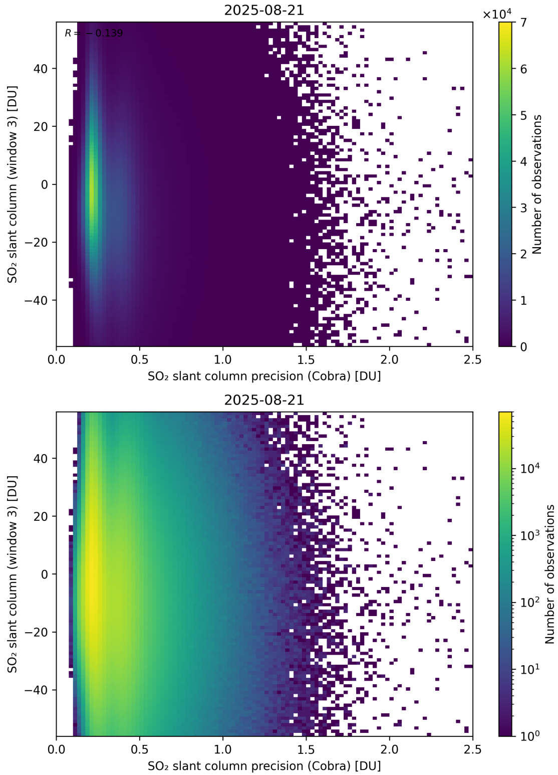
Figure 211: Scatter density plot of “SO 2 slant column precision (Cobra)” against “SO 2 slant column (window 3)” for 2025-08-20 to 2025-08-22.
