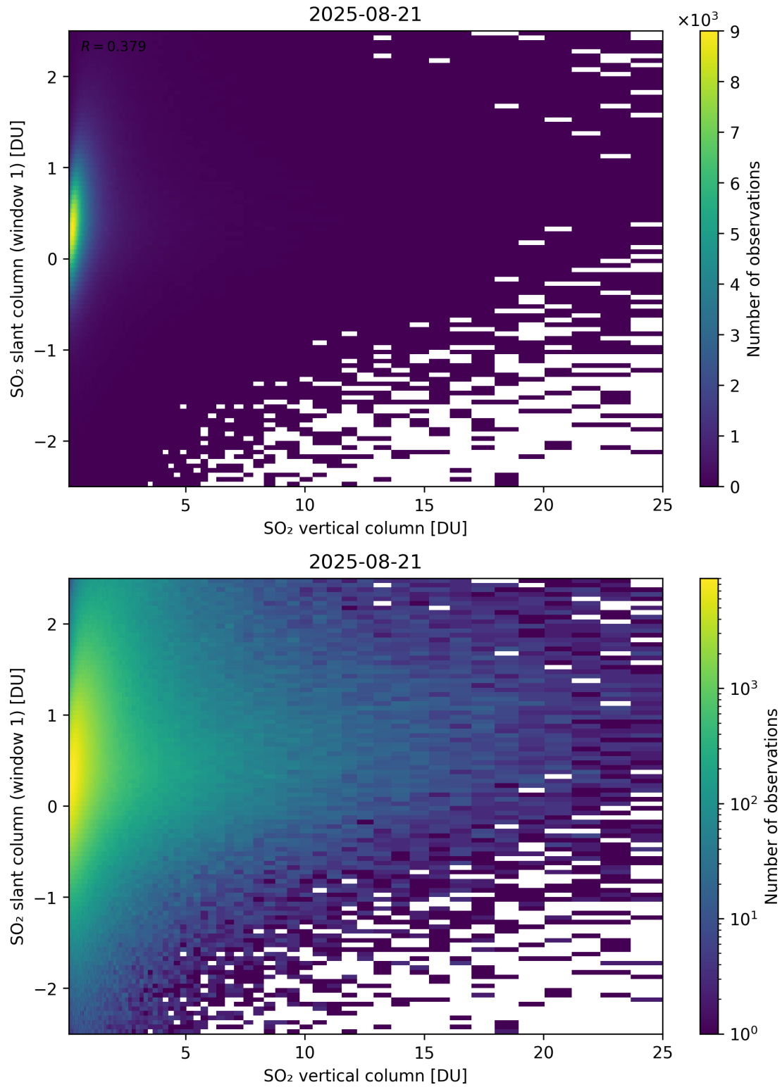
Figure 354: Scatter density plot of “SO 2 vertical column” against “SO 2 slant column (window 1)” for 2025-08-20 to 2025-08-22.
