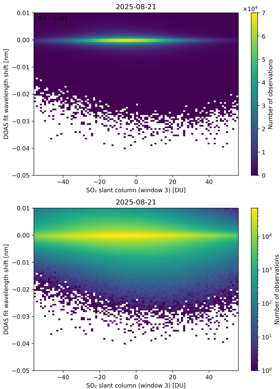
Figure 304: Scatter density plot of “SO 2 slant column (window 3)” against “DOAS fit wavelength shift” for 2025-08-20 to 2025-08-22.
