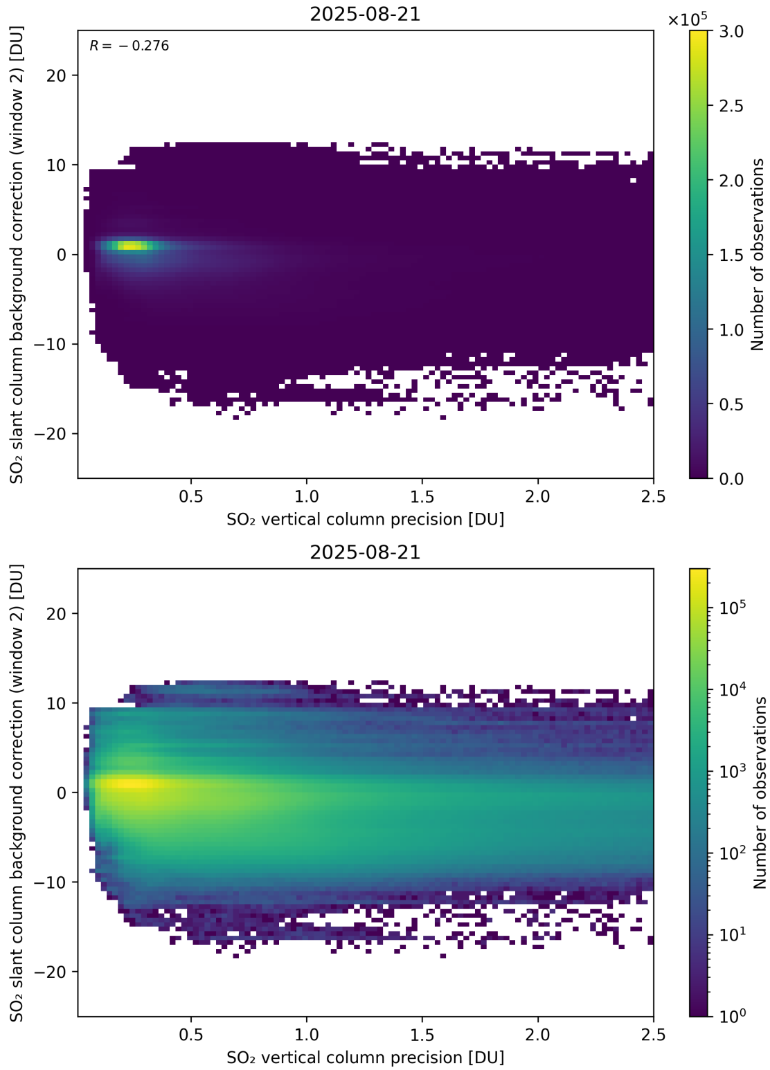
Figure 330: Scatter density plot of “SO 2 vertical column precision” against “SO 2 slant column background correction (window 2)” for 2025-08-20 to 2025-08-22.
