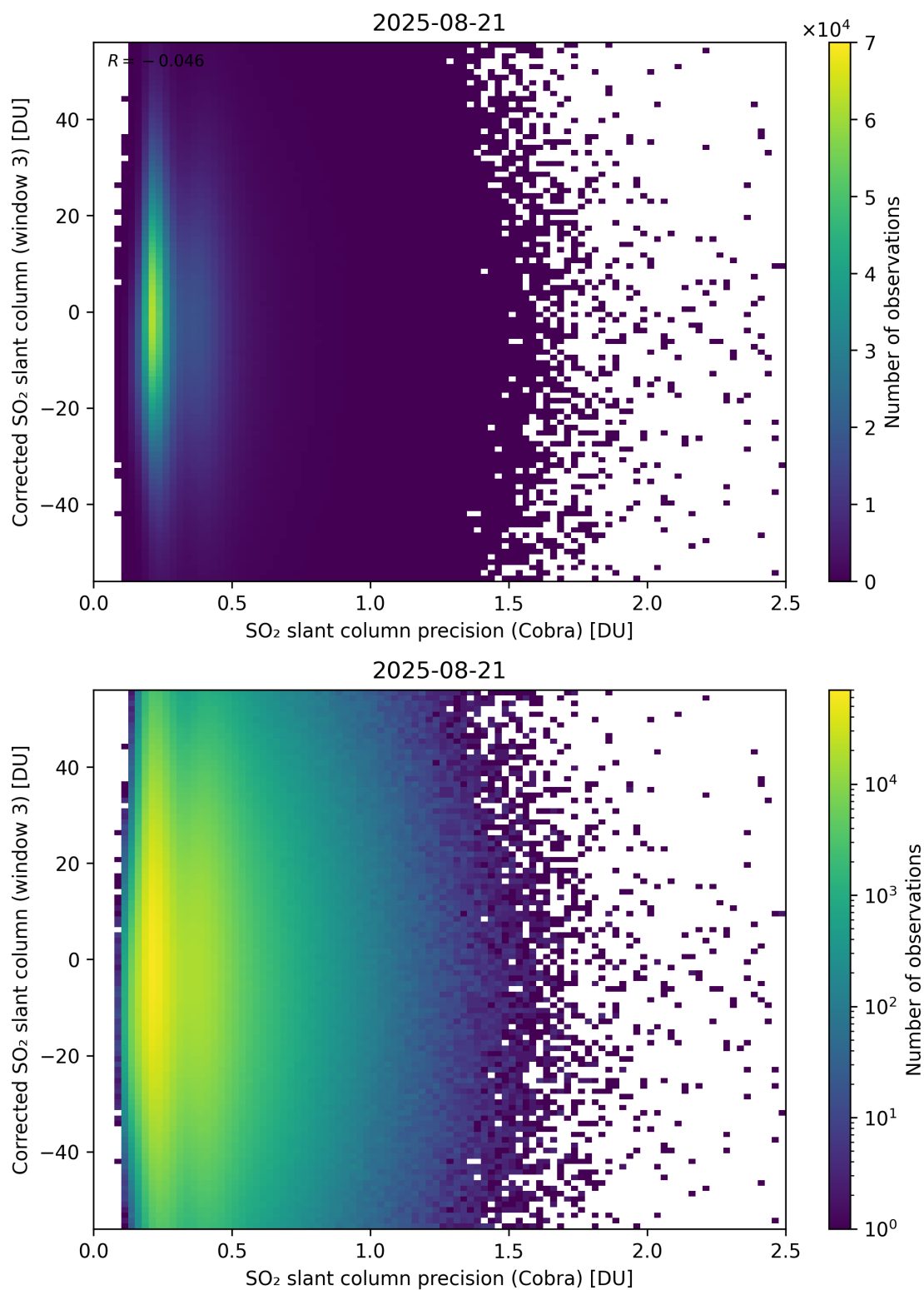
Figure 207: Scatter density plot of “SO 2 slant column precision (Cobra)” against “Corrected SO 2 slant column (window 3)” for 2025-08-20 to 2025-08-22.
