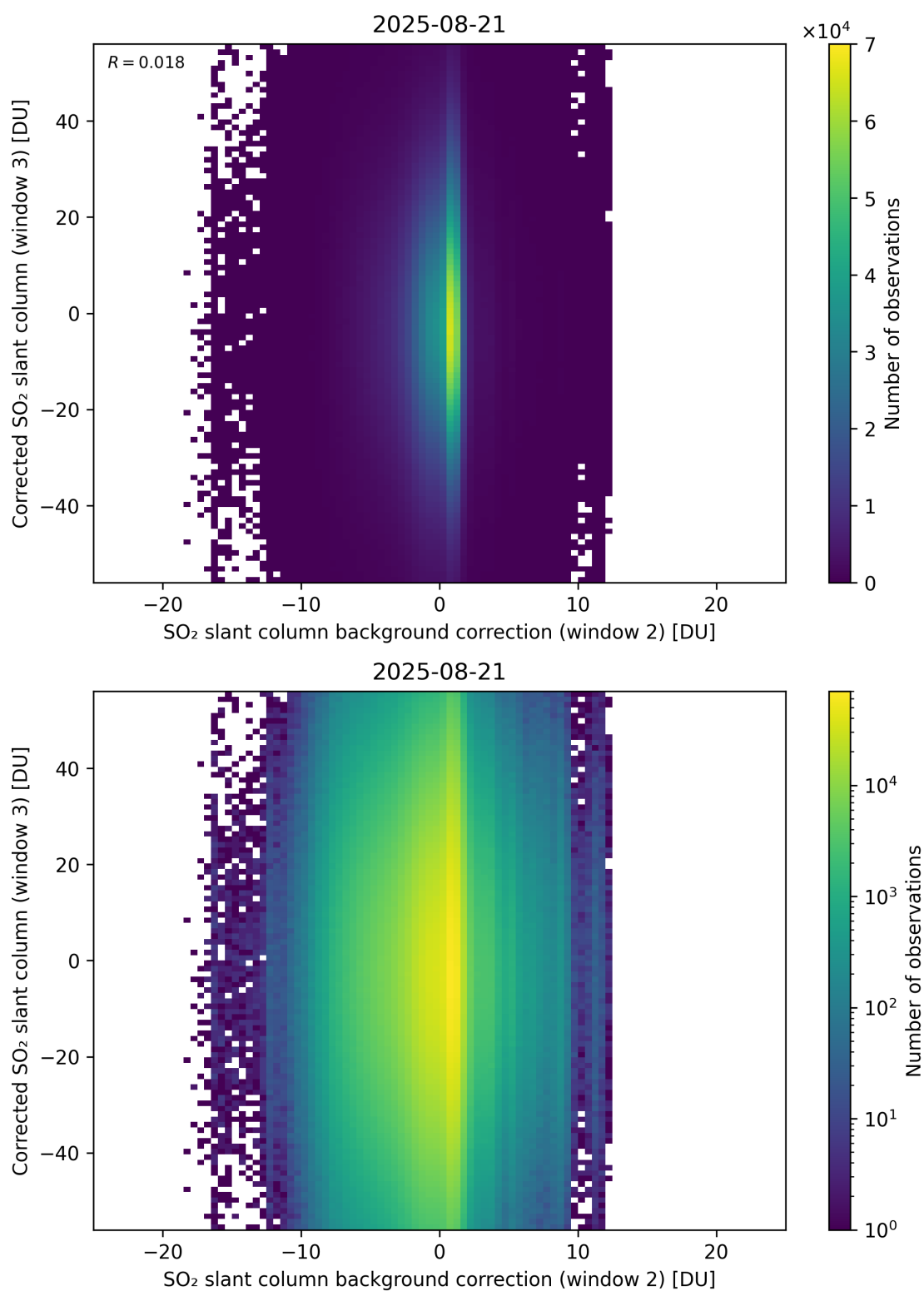
Figure 127: Scatter density plot of “SO 2 slant column background correction (window 2)” against “Corrected SO 2 slant column (window 3)” for 2025-08-20 to 2025-08-22.
