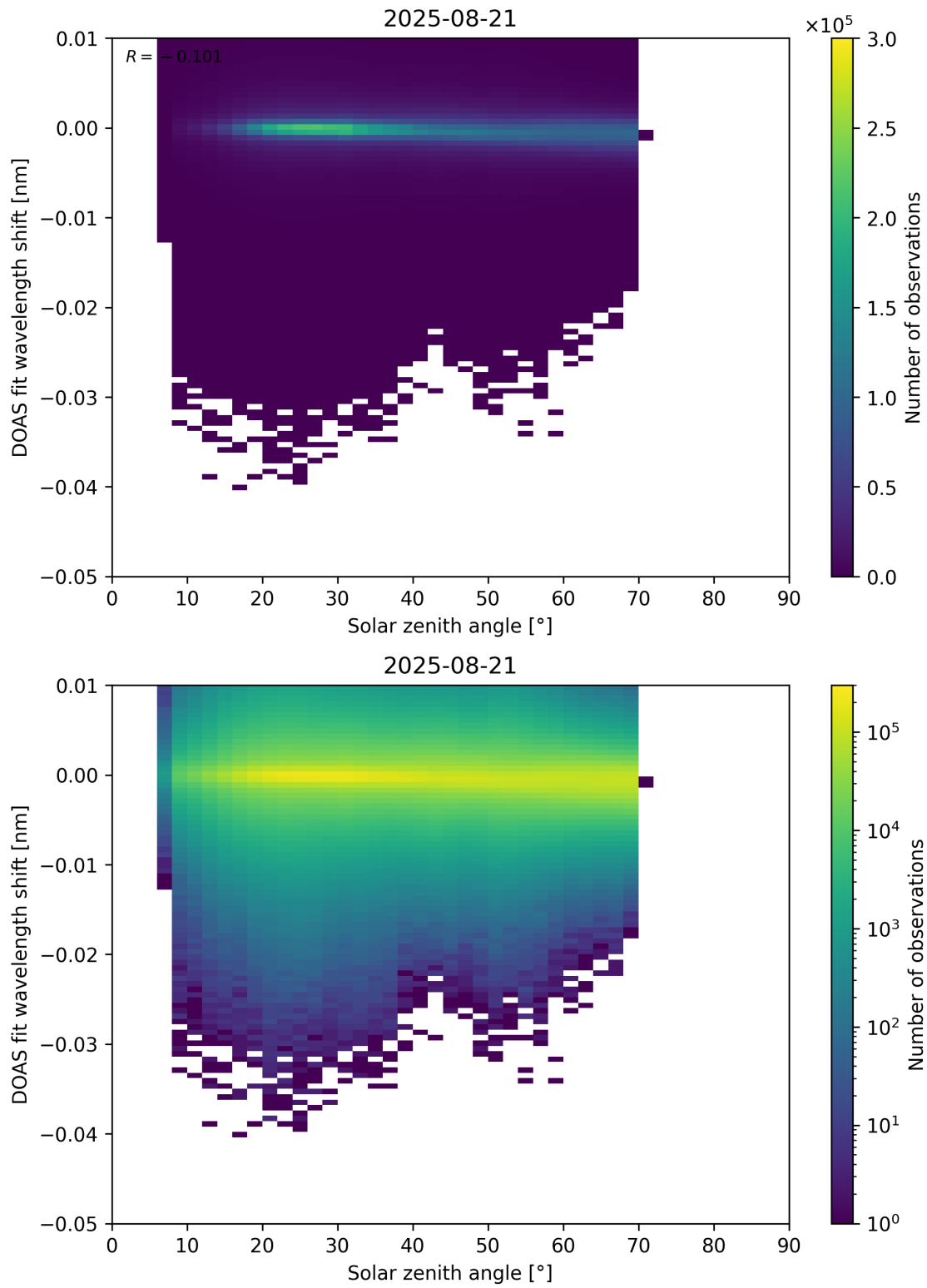
Figure 174: Scatter density plot of “Solar zenith angle” against “DOAS fit wavelength shift” for 2025-08-20 to 2025-08-22.
