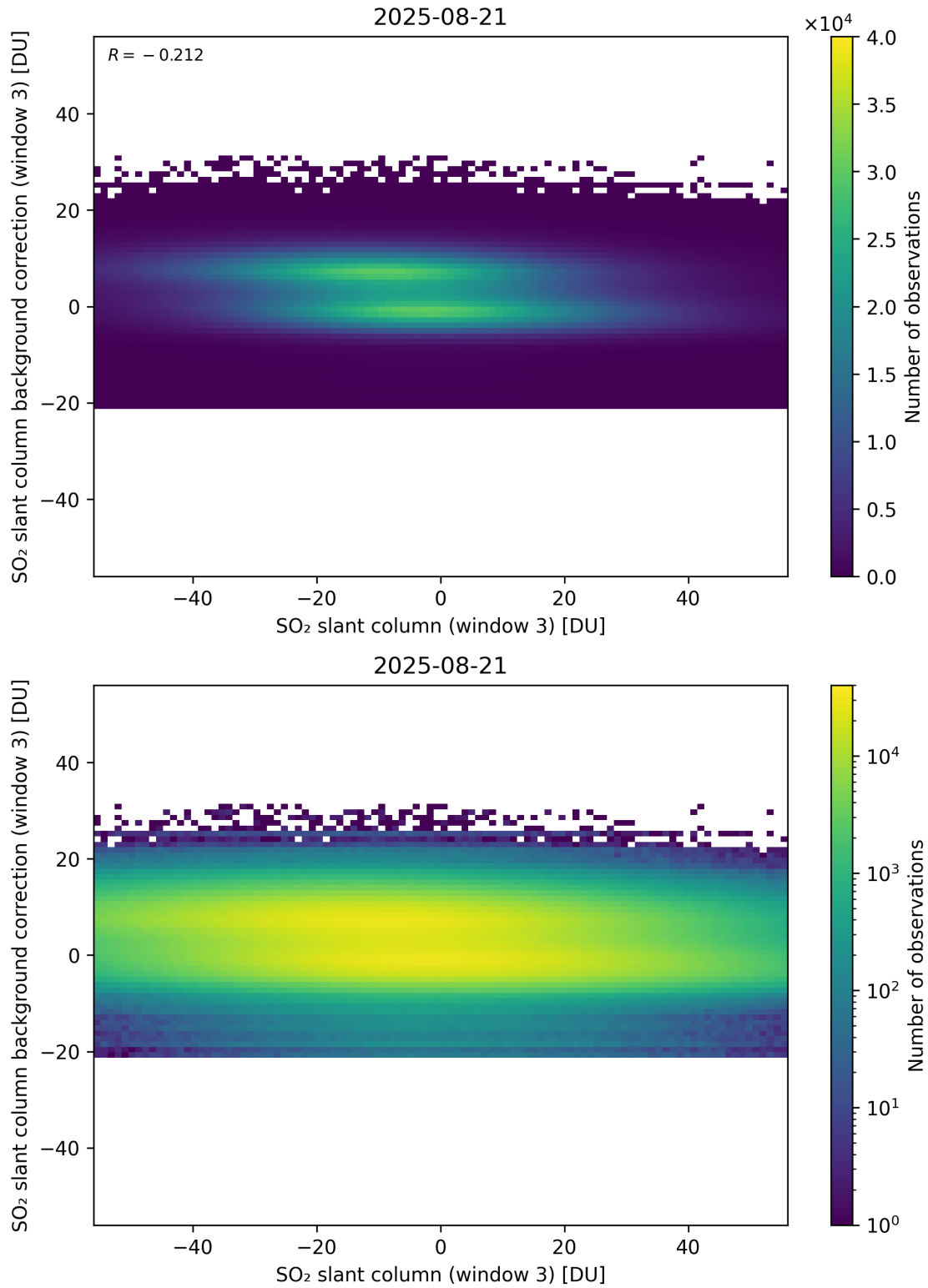
Figure 303: Scatter density plot of “SO 2 slant column (window 3)” against “SO 2 slant column background correction (window 3)” for 2025-08-20 to 2025-08-22.
