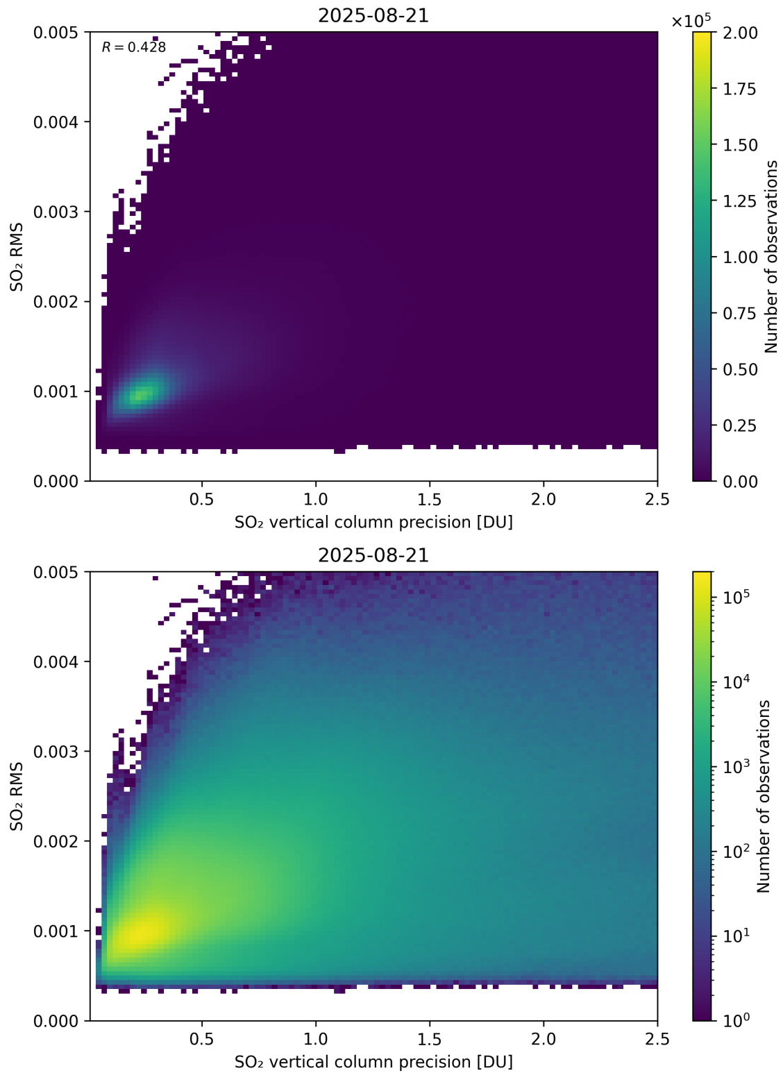
Figure 334: Scatter density plot of “SO 2 vertical column precision” against “SO 2 RMS” for 2025-08-20 to 2025-08-22.
