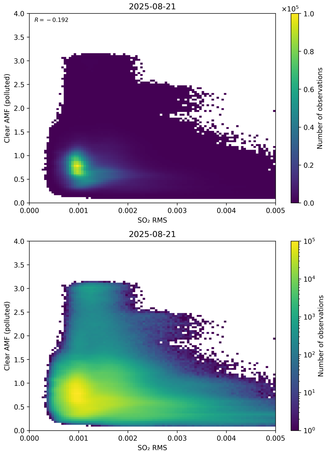
Figure 147: Scatter density plot of “SO 2 RMS” against “Clear AMF (polluted)” for 2025-08-20 to 2025-08-22.
