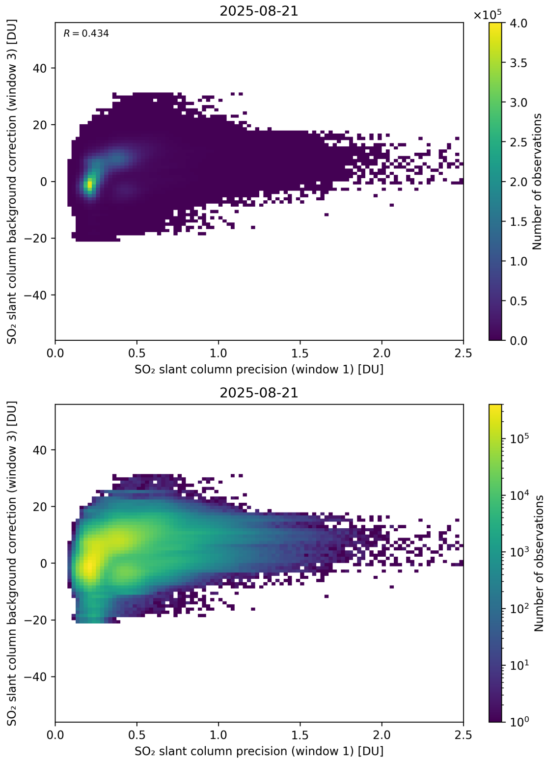
Figure 270: Scatter density plot of “SO 2 slant column precision (window 1)” against “SO 2 slant column background correction (window 3)” for 2025-08-20 to 2025-08-22.
