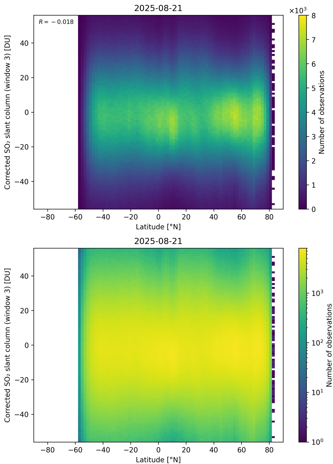
Figure 161: Scatter density plot of “Latitude” against “Corrected SO 2 slant column (window 3)” for 2025-08-20 to 2025-08-22.
