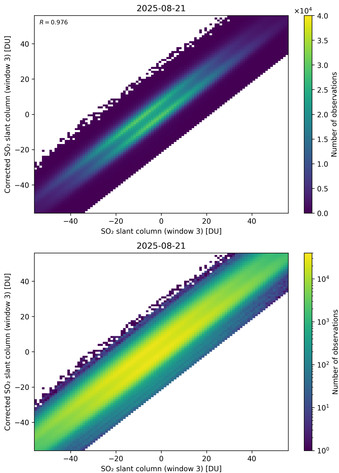
Figure 316: Scatter density plot of “SO 2 slant column (window 3)” against “Corrected SO 2 slant column (window 3)” for 2025-08-20 to 2025-08-22.
