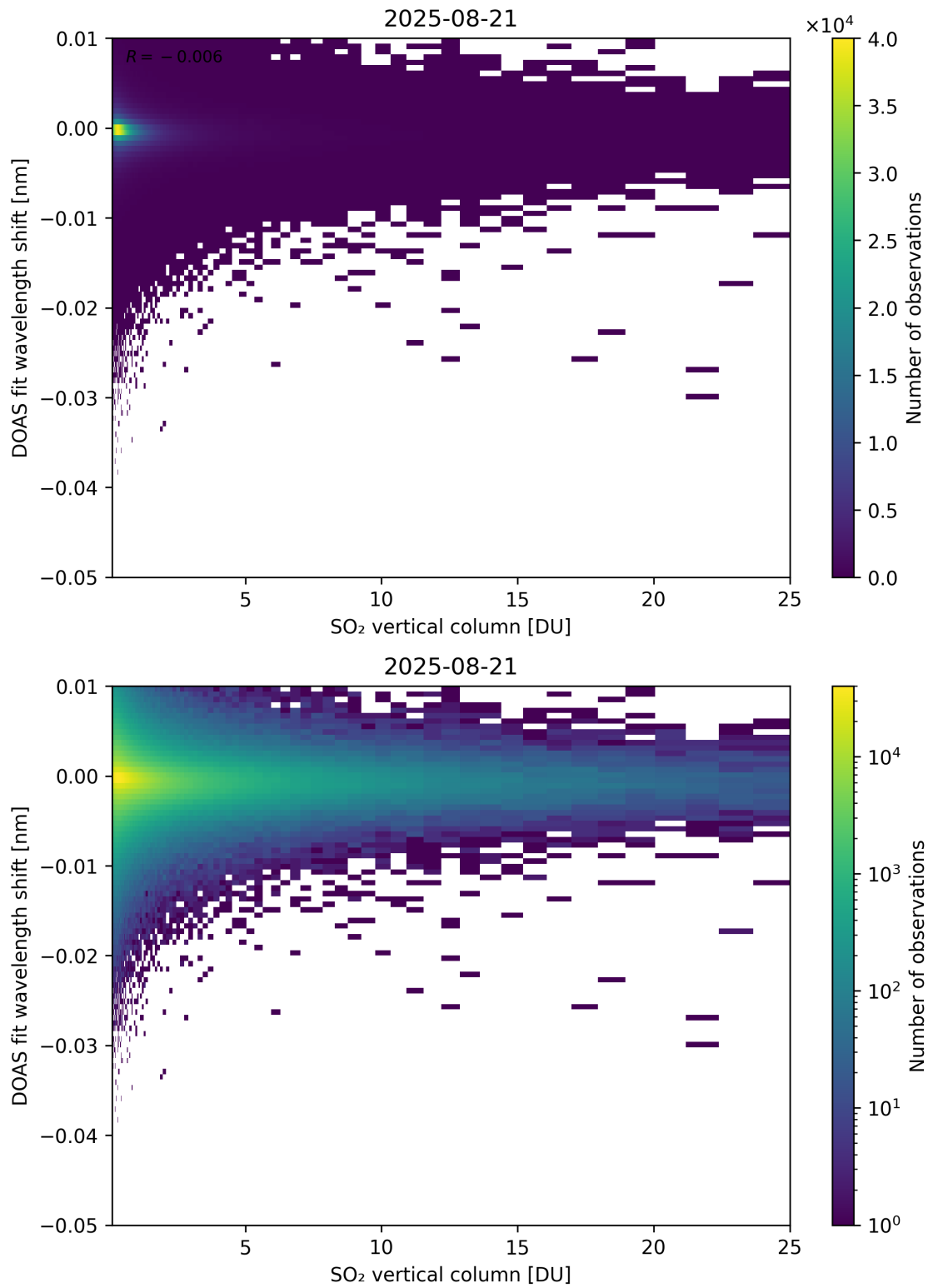
Figure 326: Scatter density plot of “SO 2 vertical column” against “DOAS fit wavelength shift” for 2025-08-20 to 2025-08-22.
