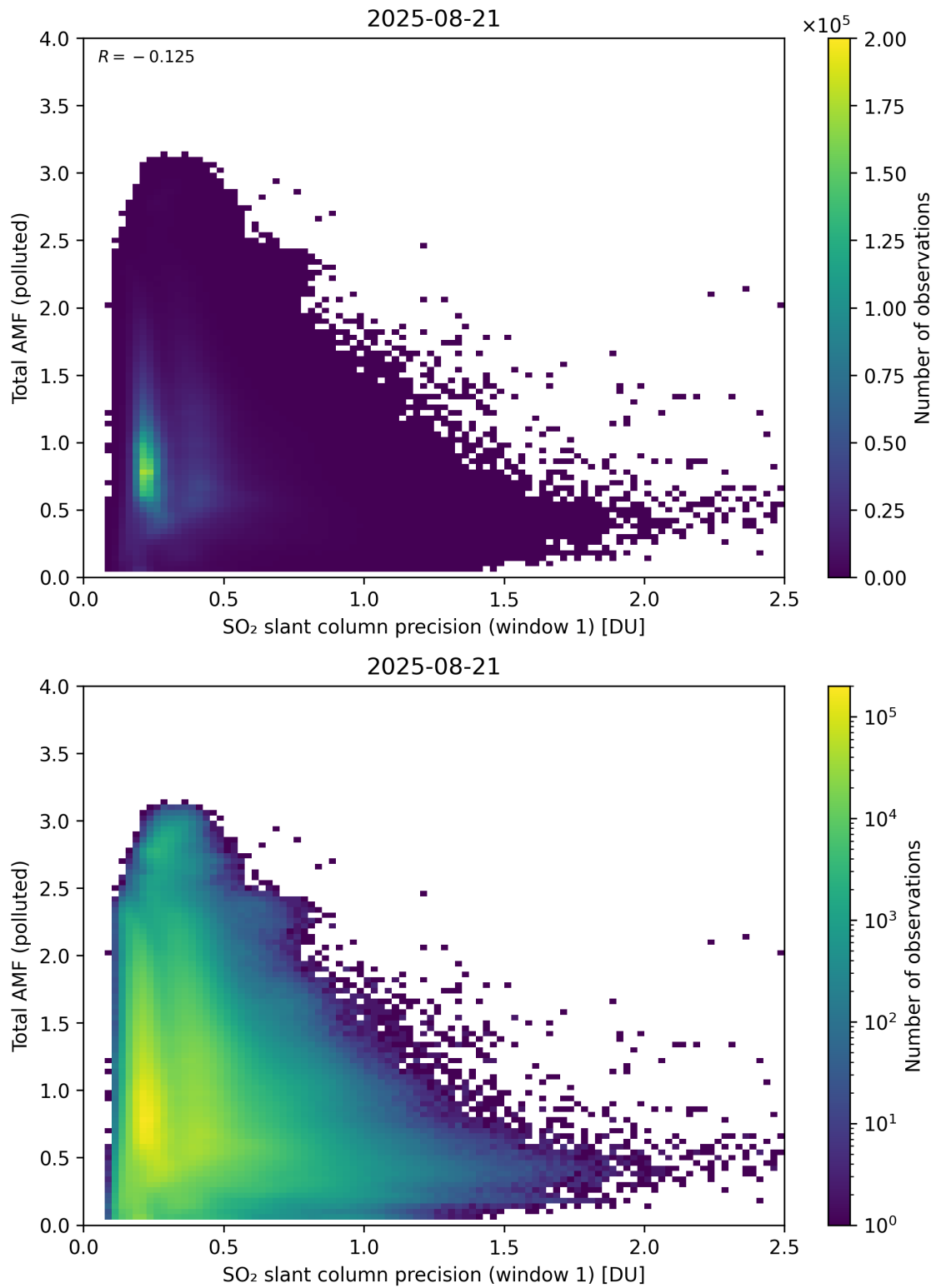
Figure 280: Scatter density plot of “SO 2 slant column precision (window 1)” against “Total AMF (polluted)” for 2025-08-20 to 2025-08-22.
