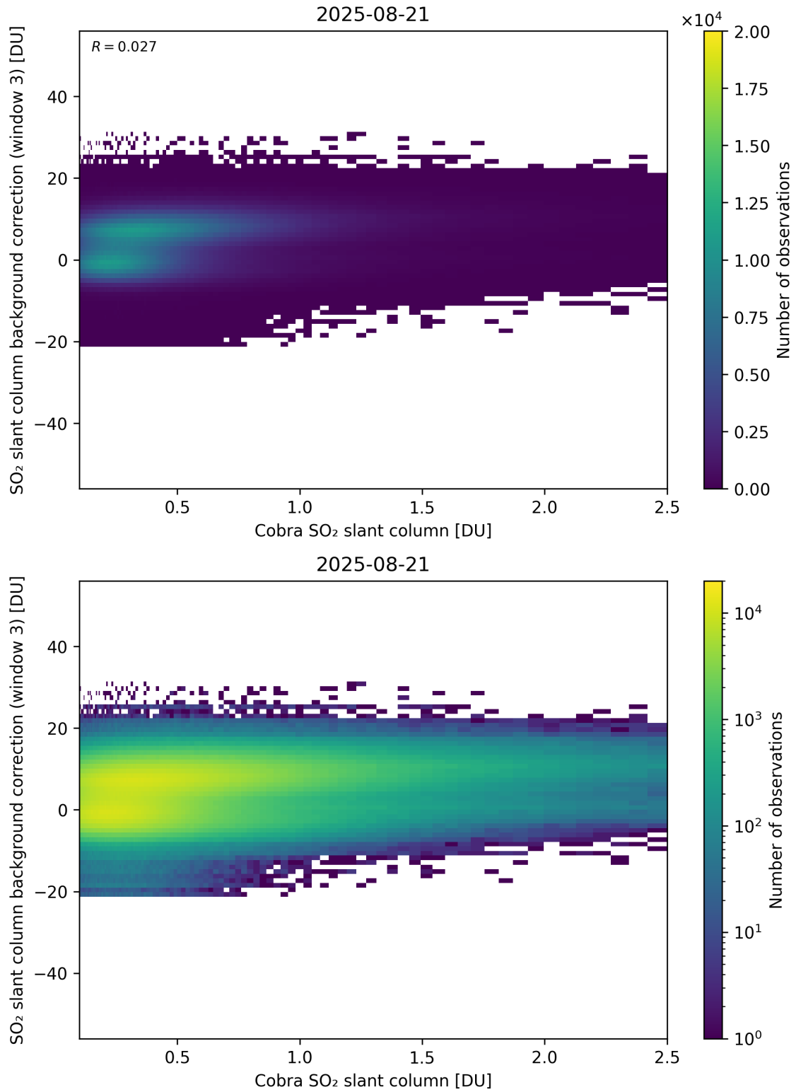
Figure 195: Scatter density plot of “Cobra SO 2 slant column” against “SO 2 slant column background correction (window 3)” for 2025-08-20 to 2025-08-22.
