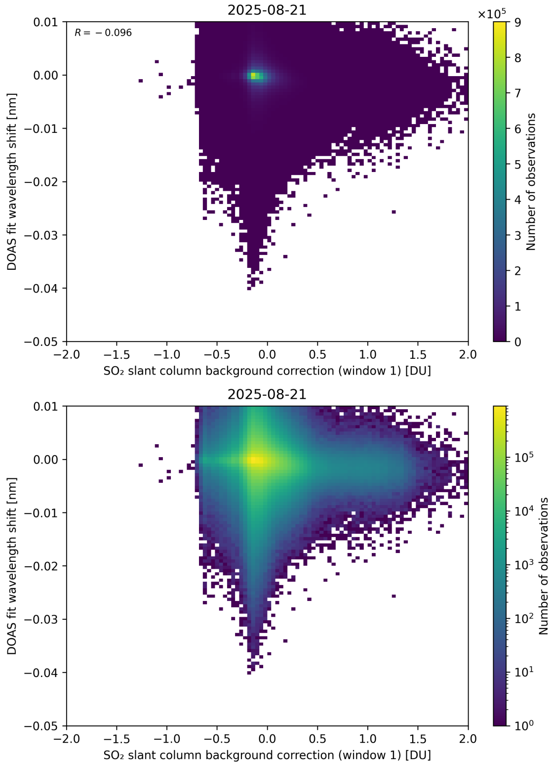
Figure 111: Scatter density plot of “SO 2 slant column background correction (window 1)” against “DOAS fit wavelength shift” for 2025-08-20 to 2025-08-22.
