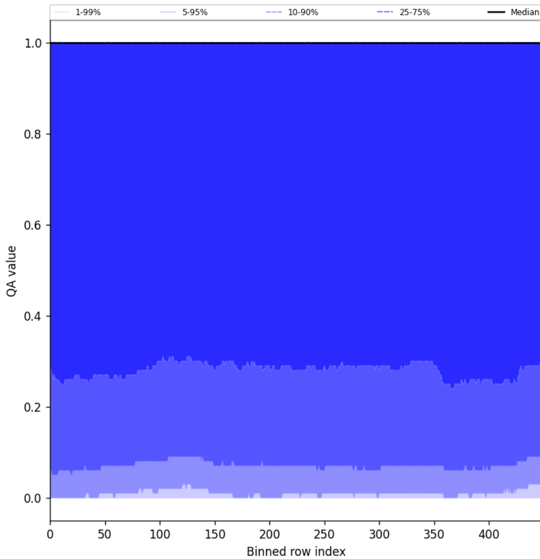
Figure 83: Along track statistics of “QA value” for 2025-08-20 to 2025-08-22
