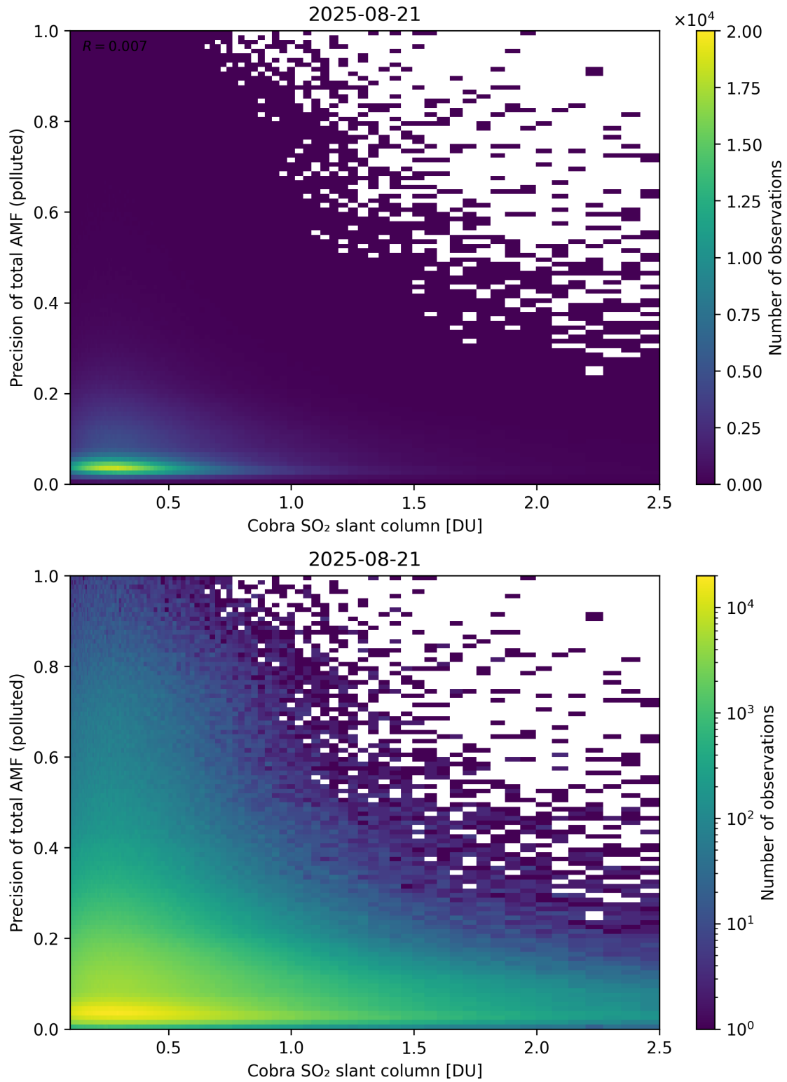
Figure 225: Scatter density plot of “Cobra SO 2 slant column” against “Precision of total AMF (polluted)” for 2025-08-20 to 2025-08-22.
