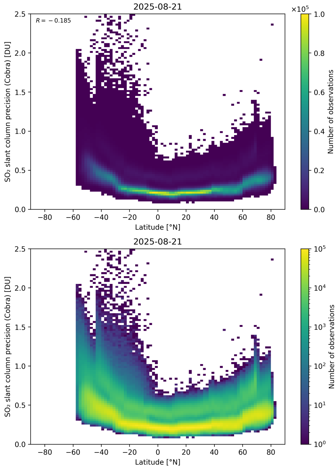
Figure 158: Scatter density plot of “Latitude” against “SO 2 slant column precision (Cobra)” for 2025-08-20 to 2025-08-22.
