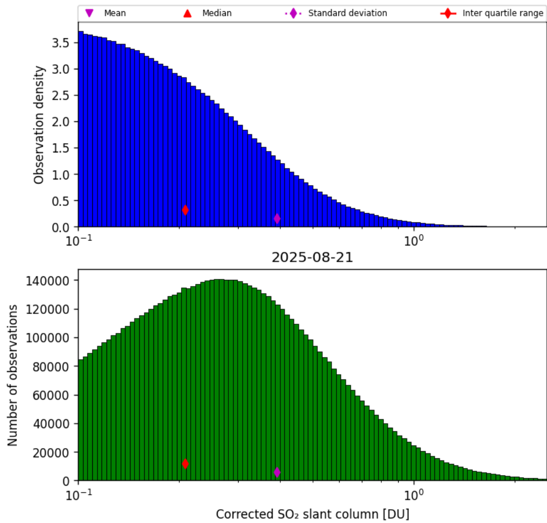
Figure 60: Histogram of "Corrected SO 2 slant column" for 2025-08-20 to 2025-08-22
