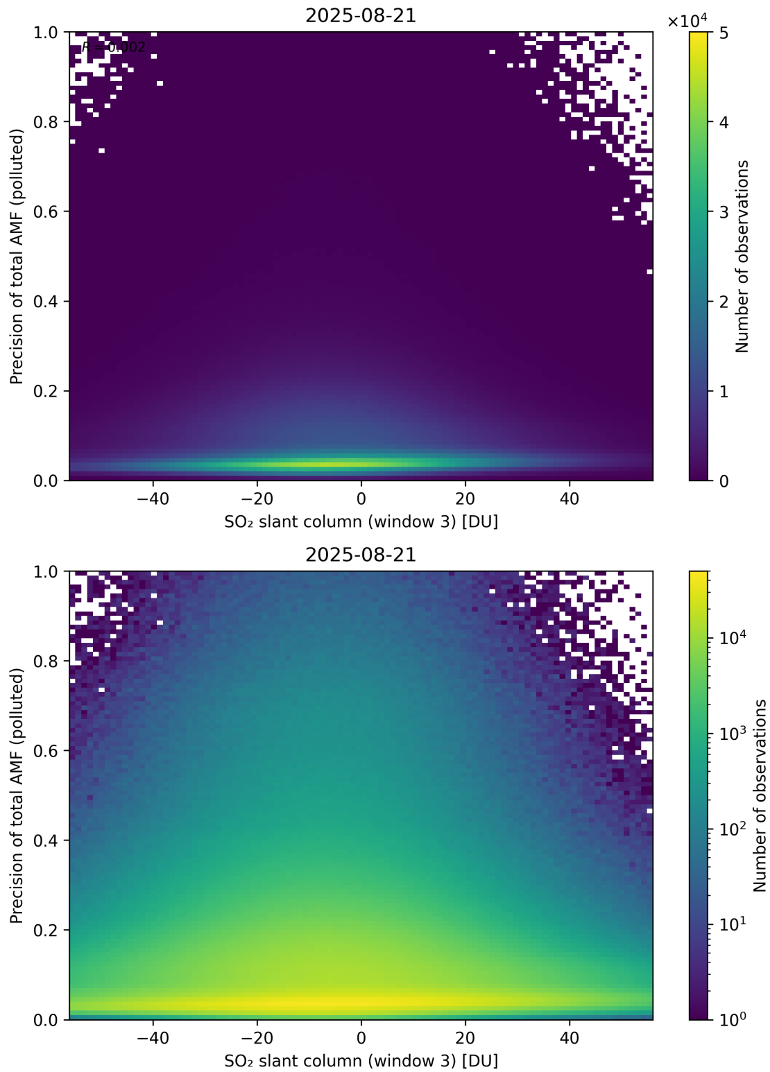
Figure 319: Scatter density plot of “SO 2 slant column (window 3)” against “Precision of total AMF (polluted)” for 2025-08-20 to 2025-08-22.
