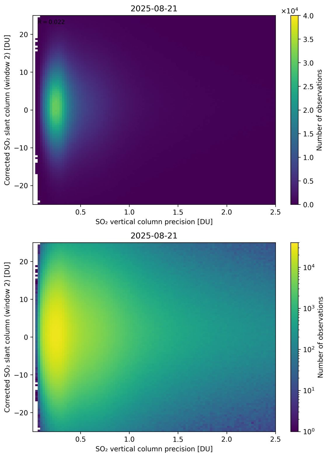
Figure 339: Scatter density plot of “SO 2 vertical column precision” against “Corrected SO 2 slant column (window 2)” for 2025-08-20 to 2025-08-22.
