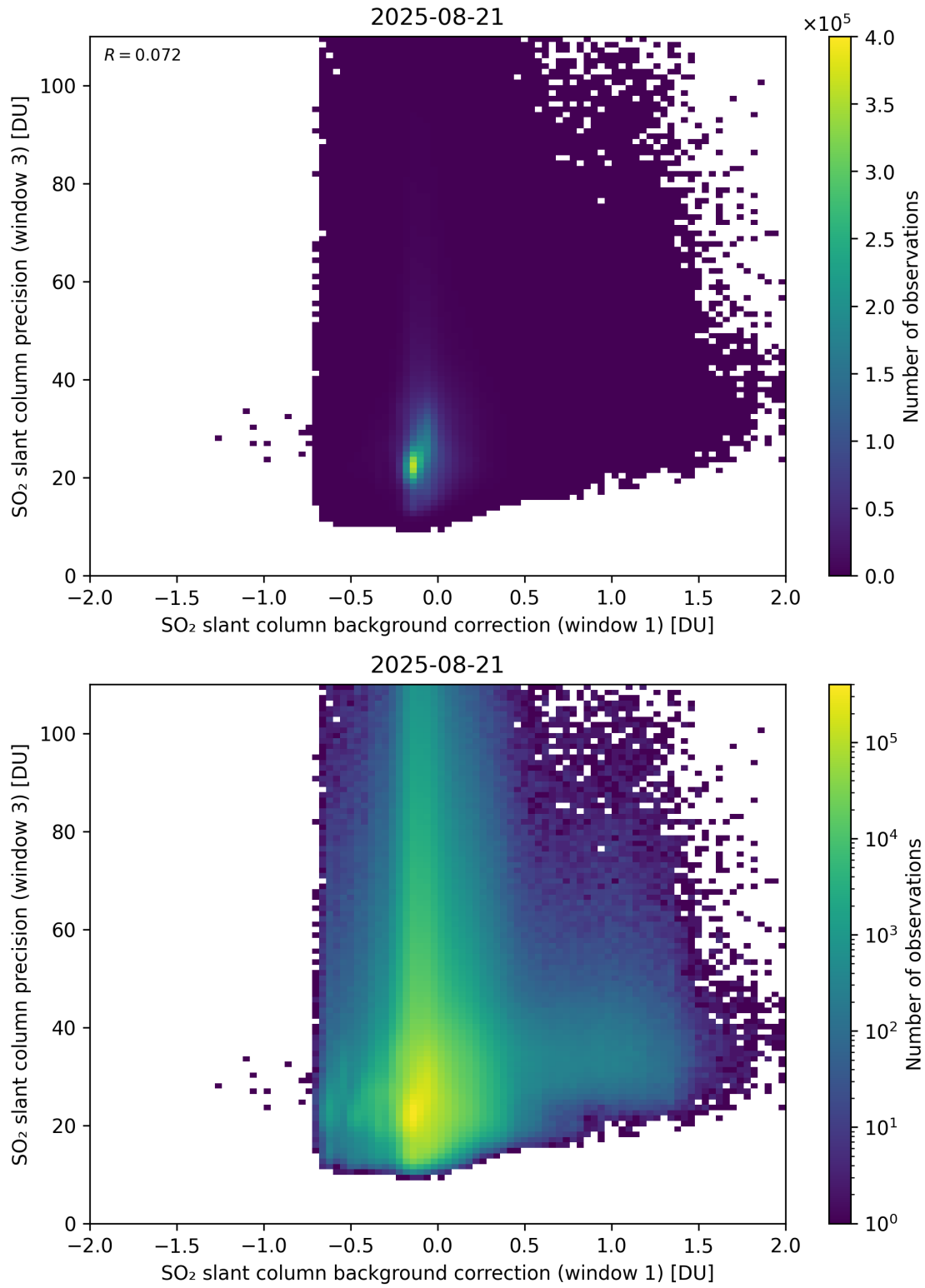
Figure 119: Scatter density plot of “SO 2 slant column background correction (window 1)” against “SO 2 slant column precision (window 3)” for 2025-08-20 to 2025-08-22.
