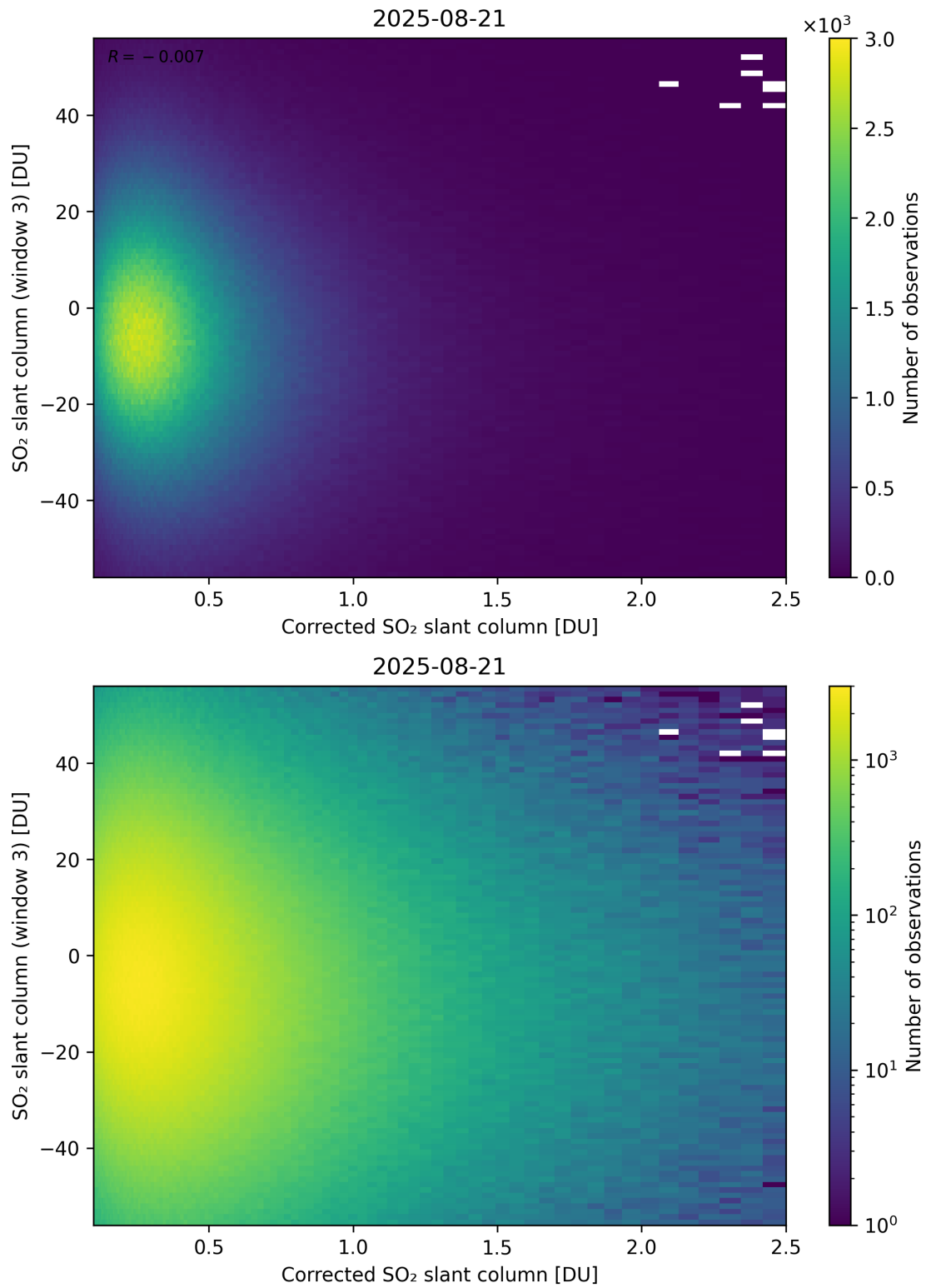
Figure 240: Scatter density plot of “Corrected SO 2 slant column” against “SO 2 slant column (window 3)” for 2025-08-20 to 2025-08-22.
