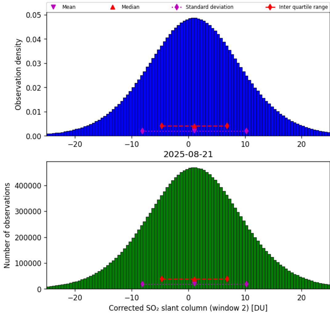
Figure 69: Histogram of “Corrected SO 2 slant column (window 2)” for 2025-08-20 to 2025-08-22
