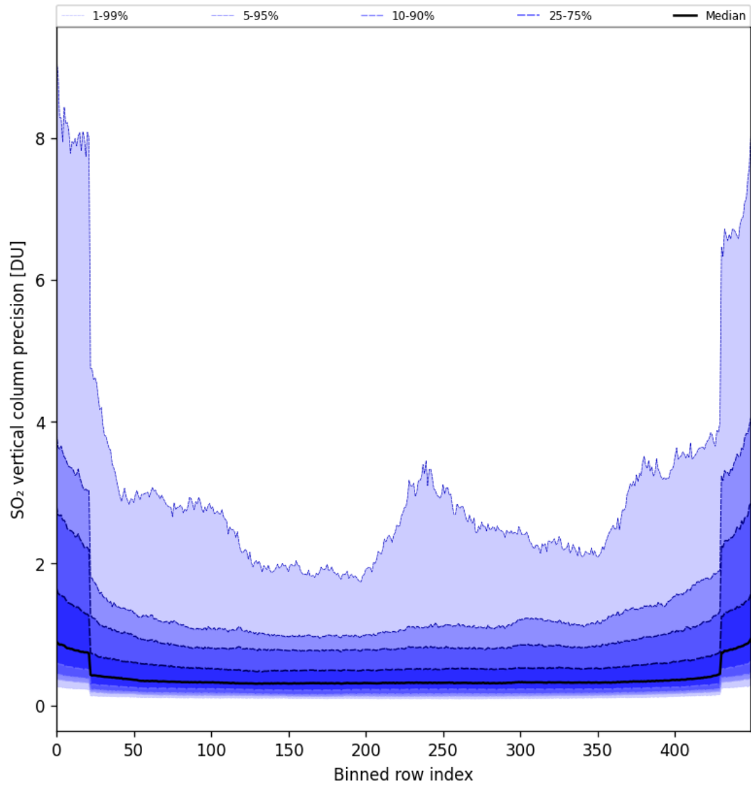
Figure 85: Along track statistics of “SO 2 vertical column precision” for 2025-08-20 to 2025-08-22
