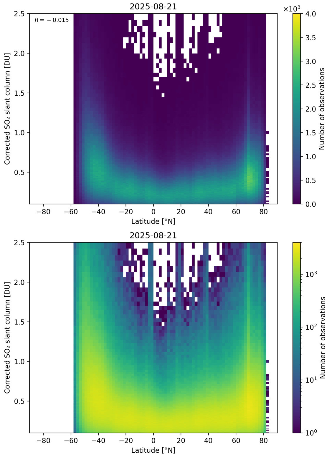
Figure 159: Scatter density plot of “Latitude” against “Corrected SO 2 slant column” for 2025-08-20 to 2025-08-22.
