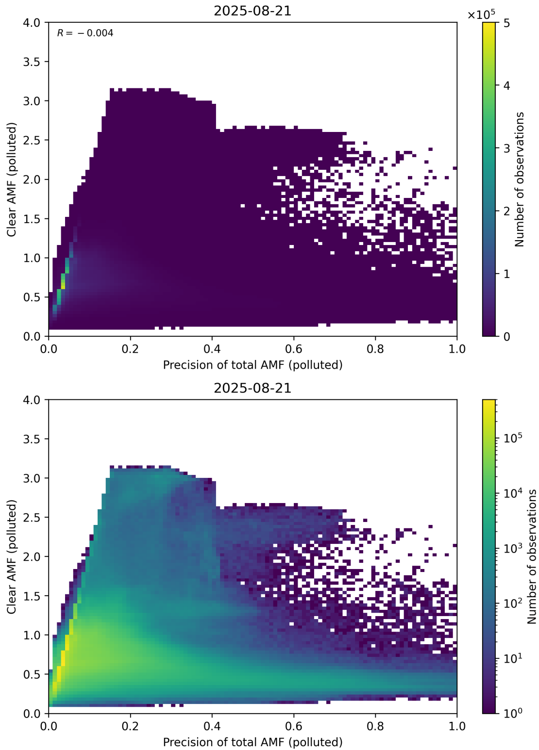
Figure 320: Scatter density plot of “Precision of total AMF (polluted)” against “Clear AMF (polluted)” for 2025-08-20 to 2025-08-22.
