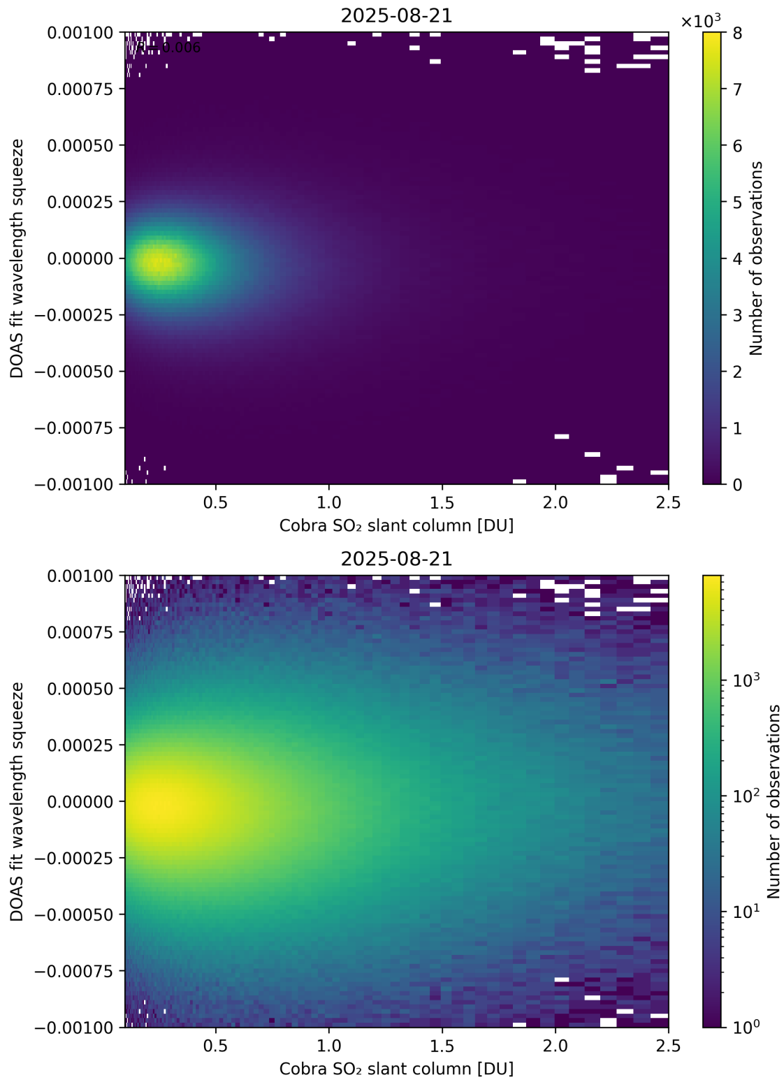
Figure 197: Scatter density plot of “Cobra SO 2 slant column” against “DOAS fit wavelength squeeze” for 2025-08-20 to 2025-08-22.
