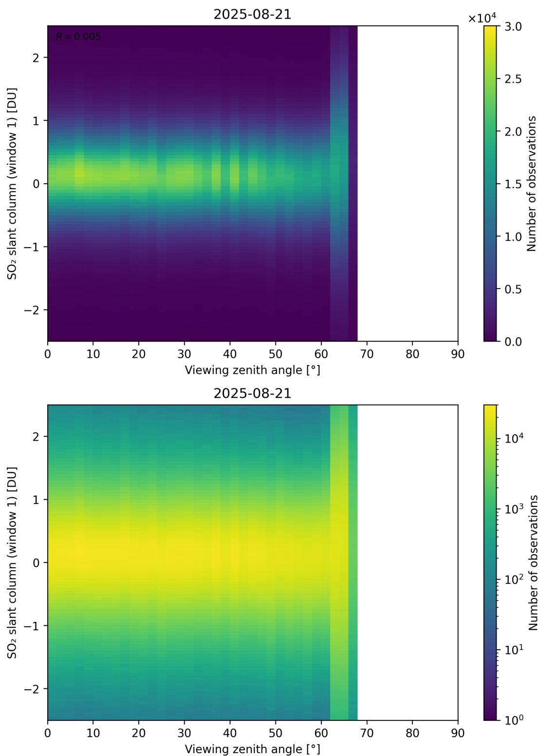
Figure 376: Scatter density plot of “Viewing zenith angle” against “SO 2 slant column (window 1)” for 2025-08-20 to 2025-08-22.
