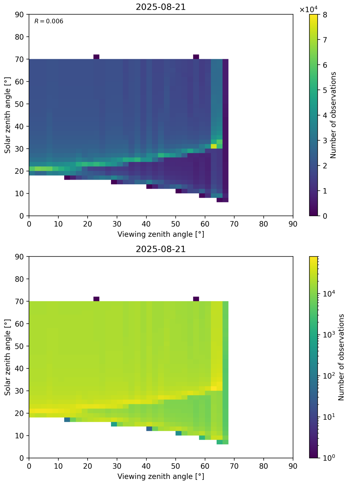
Figure 369: Scatter density plot of “Viewing zenith angle” against “Solar zenith angle” for 2025-08-20 to 2025-08-22.
