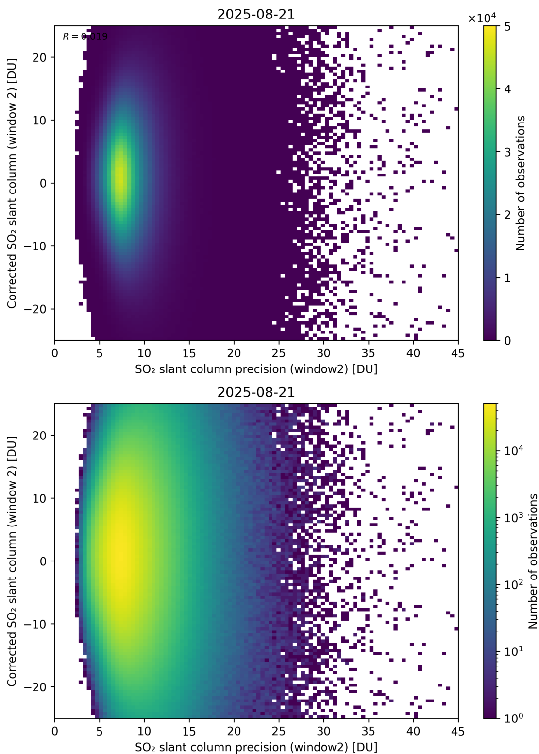
Figure 297: Scatter density plot of “SO 2 slant column precision (window2)” against “Corrected SO 2 slant column (window 2)” for 2025-08-20 to 2025-08-22.
