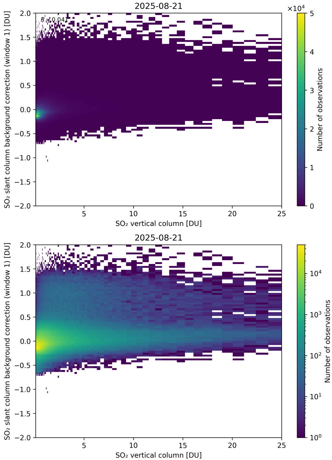
Figure 323: Scatter density plot of “SO 2 vertical column” against “SO 2 slant column background correction (window 1)” for 2025-08-20 to 2025-08-22.
