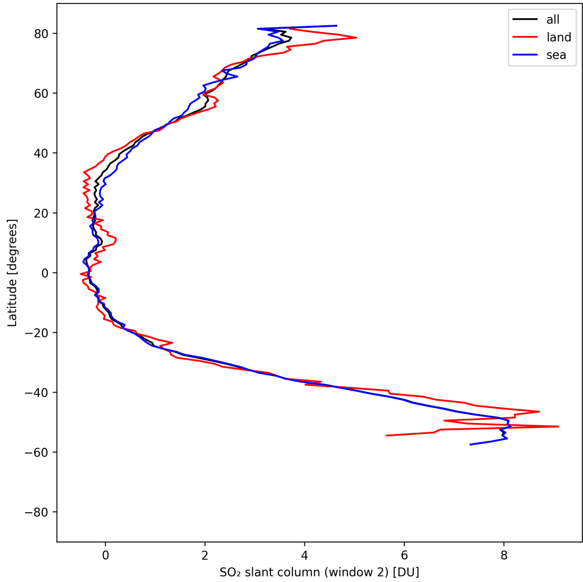
Figure 41: Zonal average of “SO 2 slant column (window 2)” for 2025-08-20 to 2025-08-22.
