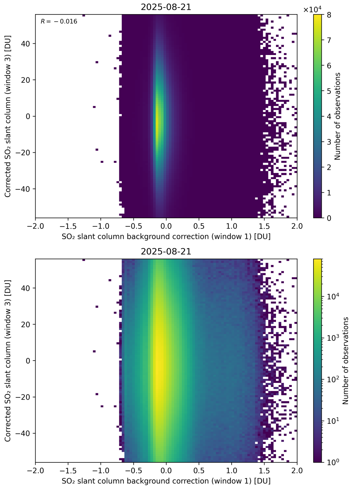
Figure 116: Scatter density plot of “SO 2 slant column background correction (window 1)” against “Corrected SO 2 slant column (window 3)” for 2025-08-20 to 2025-08-22.
