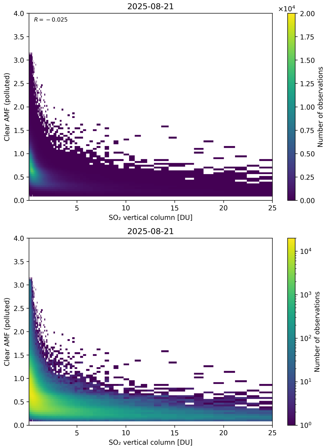
Figure 348: Scatter density plot of “SO 2 vertical column” against “Clear AMF (polluted)” for 2025-08-20 to 2025-08-22.
