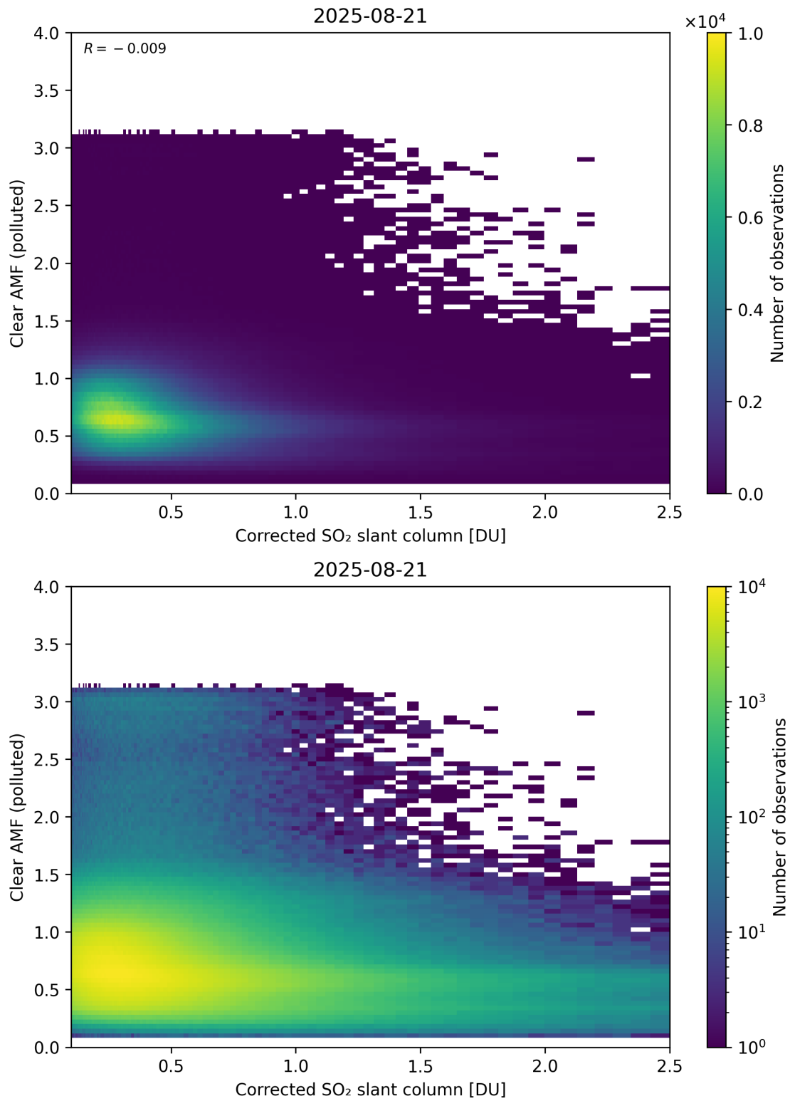
Figure 232: Scatter density plot of “Corrected SO 2 slant column” against “Clear AMF (polluted)” for 2025-08-20 to 2025-08-22.
