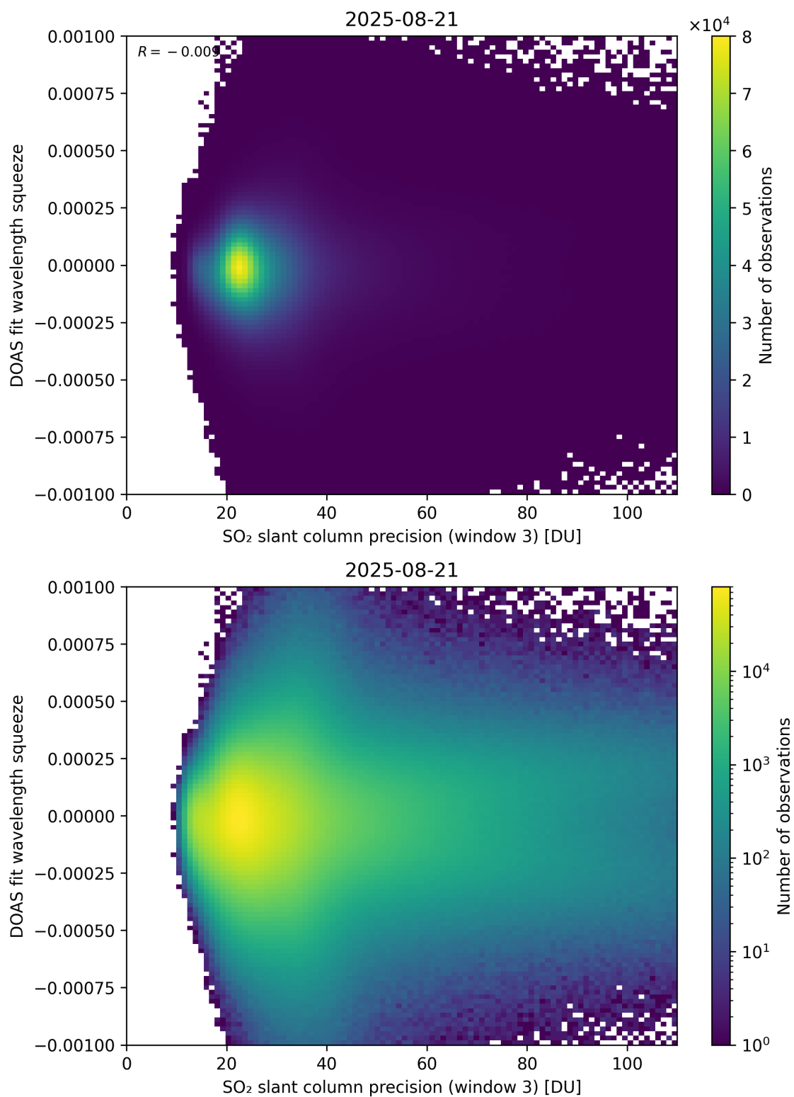
Figure 309: Scatter density plot of “SO 2 slant column precision (window 3)” against “DOAS fit wavelength squeeze” for 2025-08-20 to 2025-08-22.
