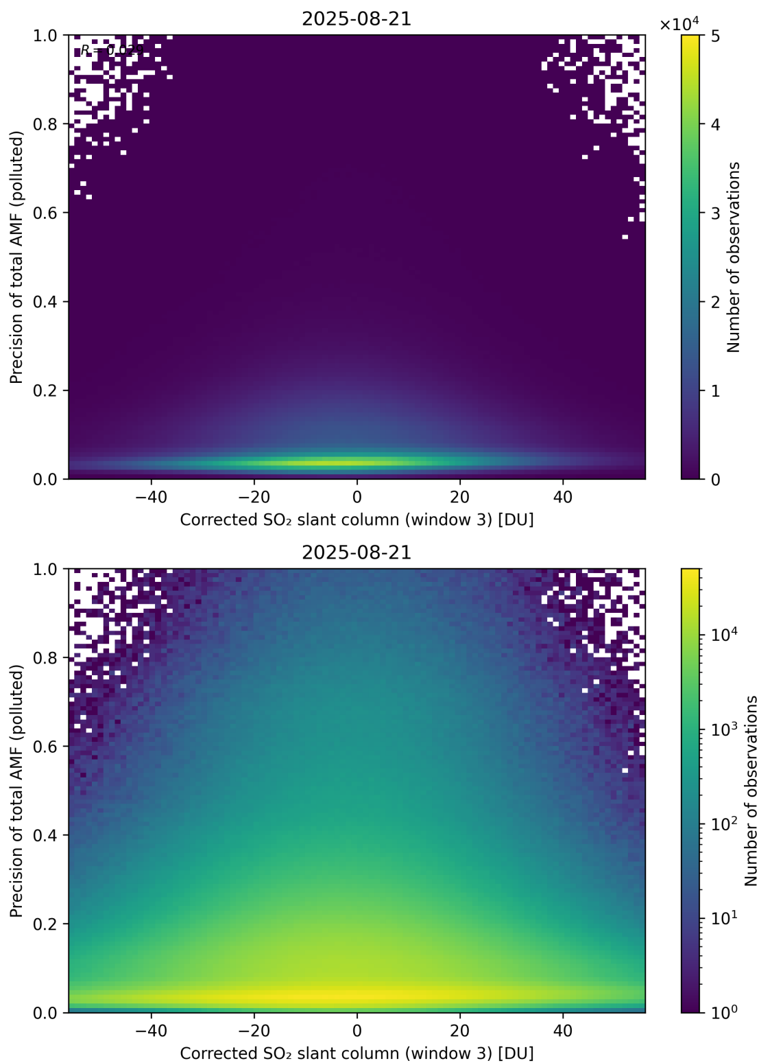
Figure 261: Scatter density plot of “Corrected SO 2 slant column (window 3)” against “Precision of total AMF (polluted)” for 2025-08-20 to 2025-08-22.
