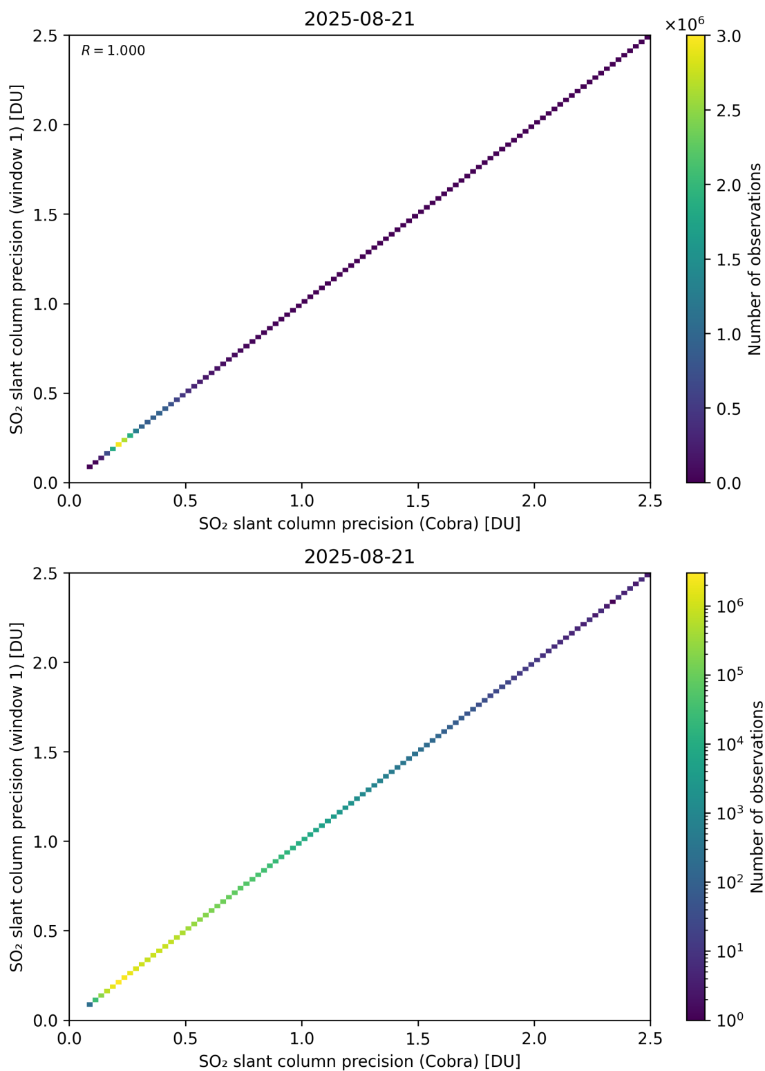
Figure 209: Scatter density plot of “SO 2 slant column precision (Cobra)” against “SO 2 slant column precision (window 1)” for 2025-08-20 to 2025-08-22.
