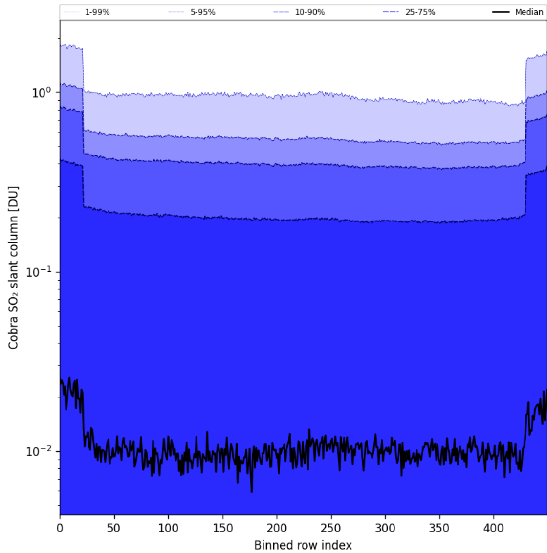
Figure 87: Along track statistics of “Cobra SO 2 slant column” for 2025-08-20 to 2025-08-22
