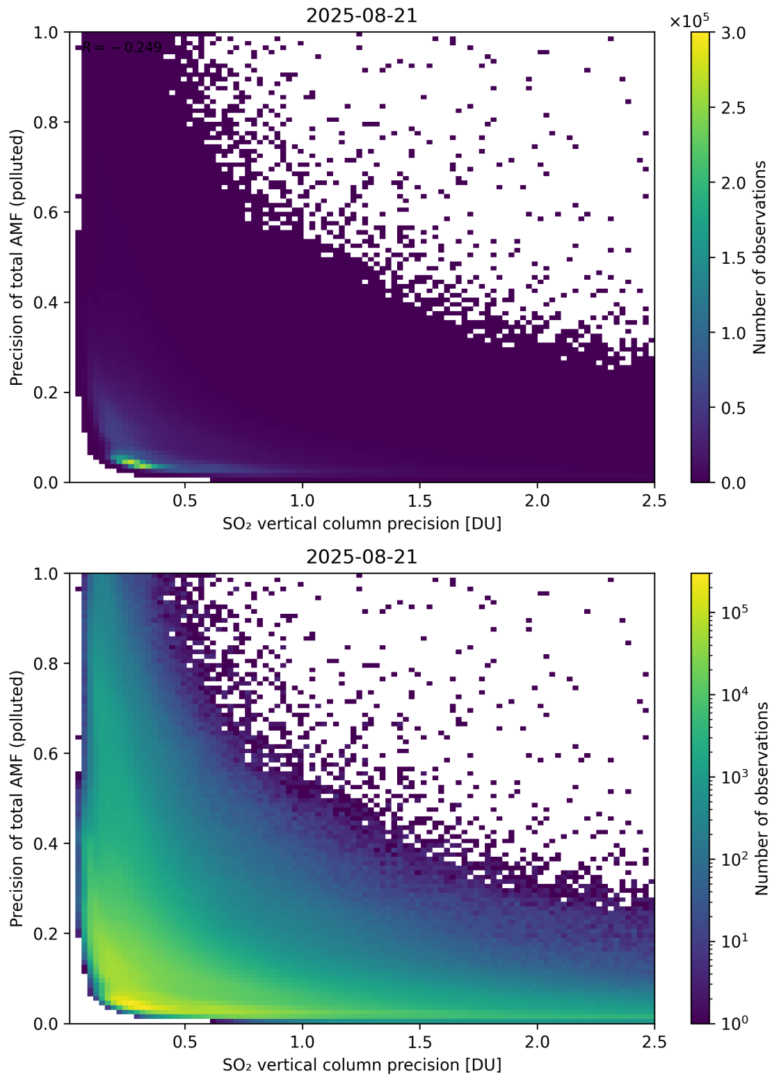
Figure 347: Scatter density plot of “SO 2 vertical column precision” against “Precision of total AMF (polluted)” for 2025-08-20 to 2025-08-22.
