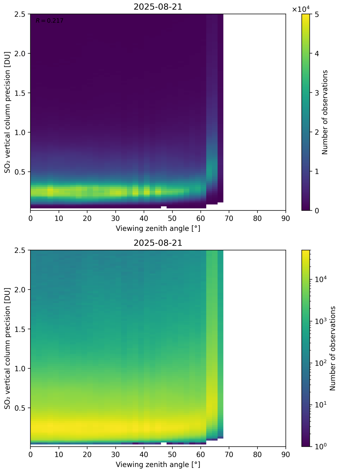
Figure 384: Scatter density plot of “Viewing zenith angle” against “SO 2 vertical column precision” for 2025-08-20 to 2025-08-22.
