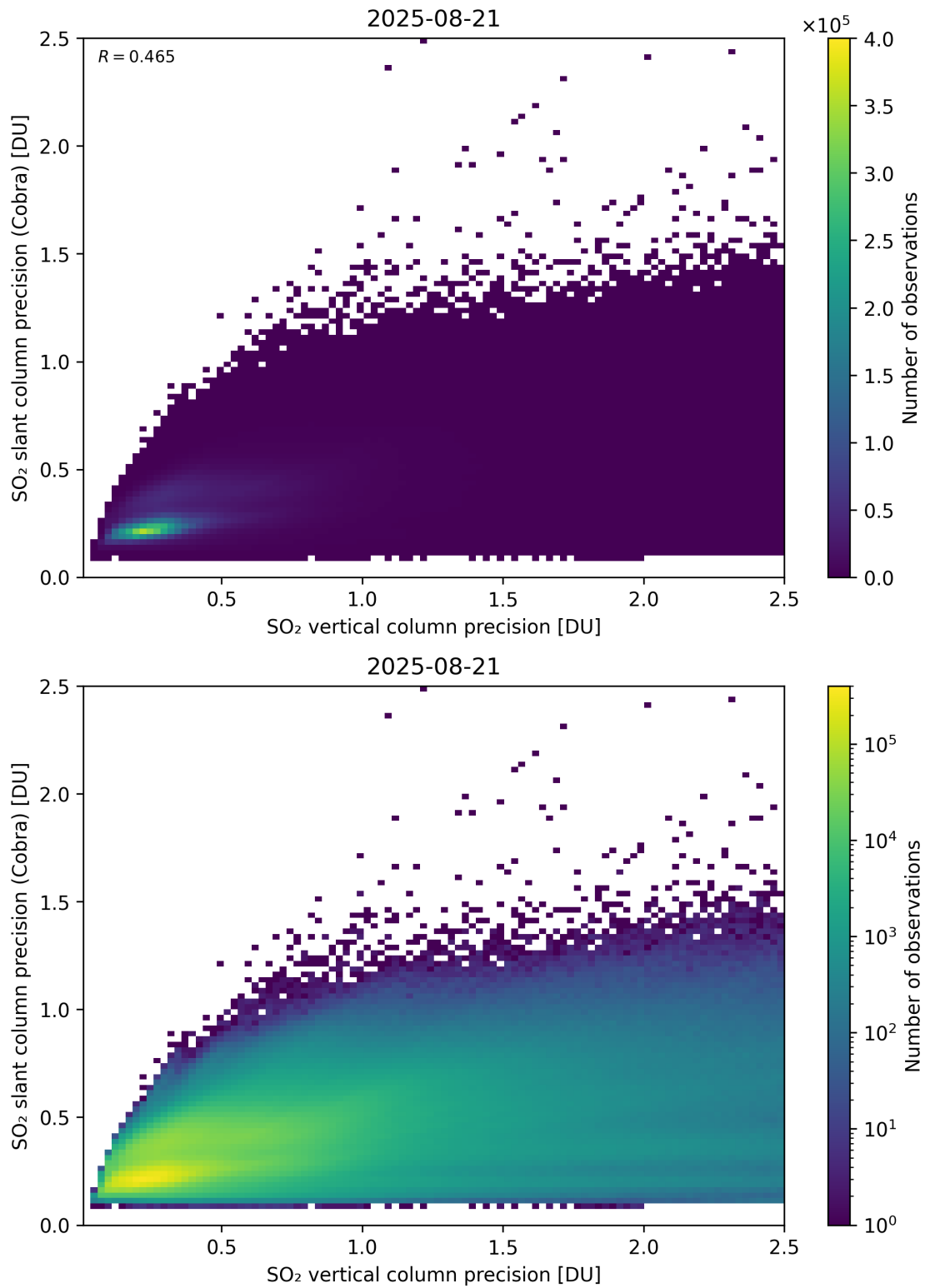
Figure 337: Scatter density plot of “SO 2 vertical column precision” against “SO 2 slant column precision (Cobra)” for 2025-08-20 to 2025-08-22.
