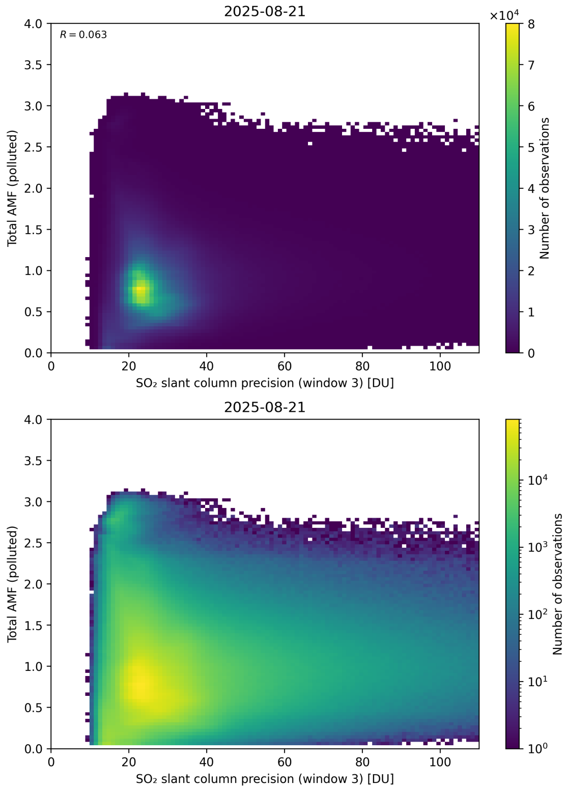
Figure 313: Scatter density plot of “SO 2 slant column precision (window 3)” against “Total AMF (polluted)” for 2025-08-20 to 2025-08-22.
