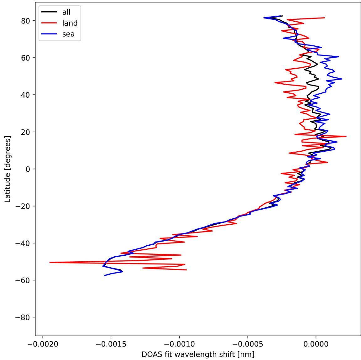
Figure 50: Zonal average of “DOAS fit wavelength shift” for 2025-08-20 to 2025-08-22.
