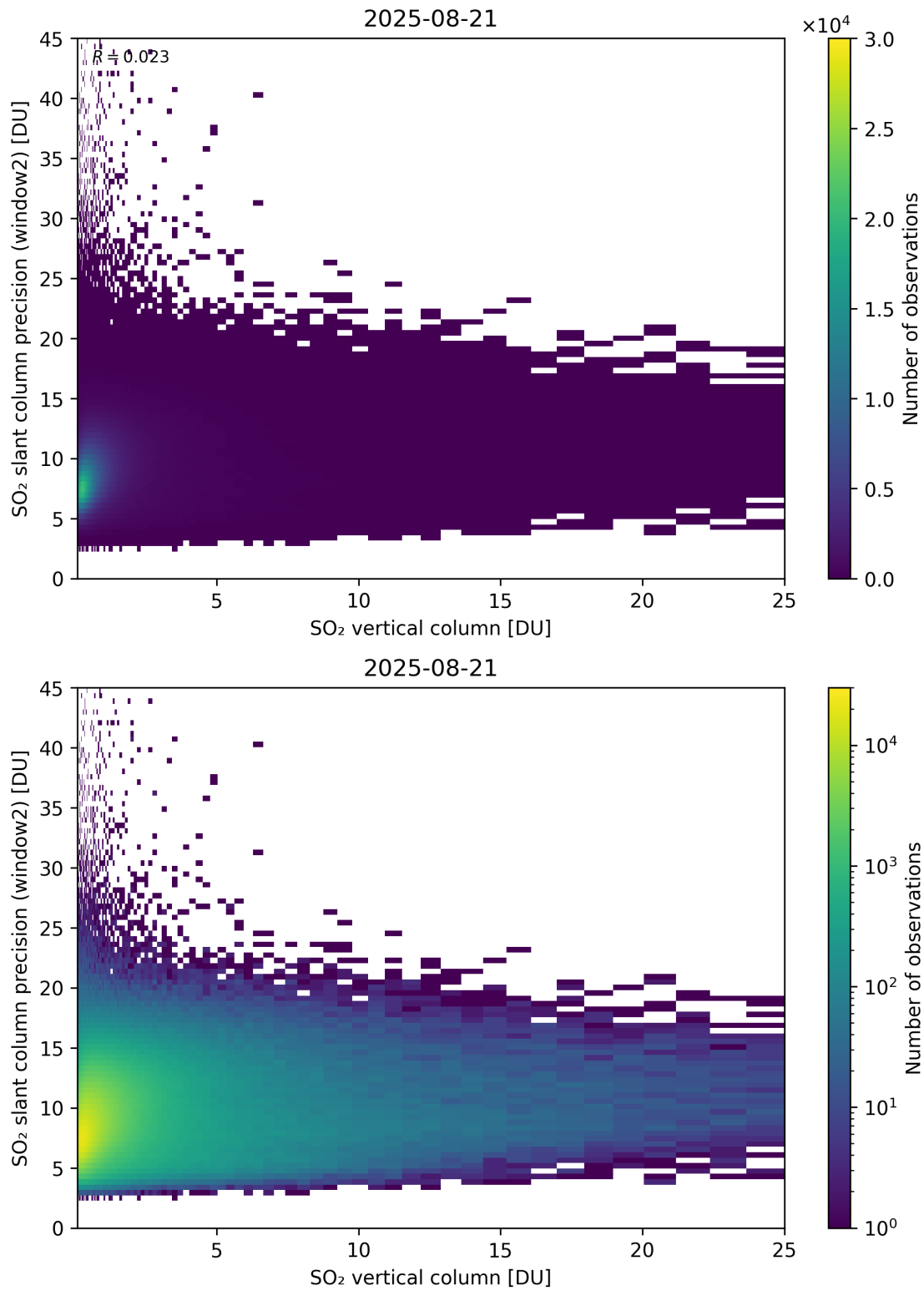
Figure 356: Scatter density plot of “SO 2 vertical column” against “SO 2 slant column precision (window2)” for 2025-08-20 to 2025-08-22.
