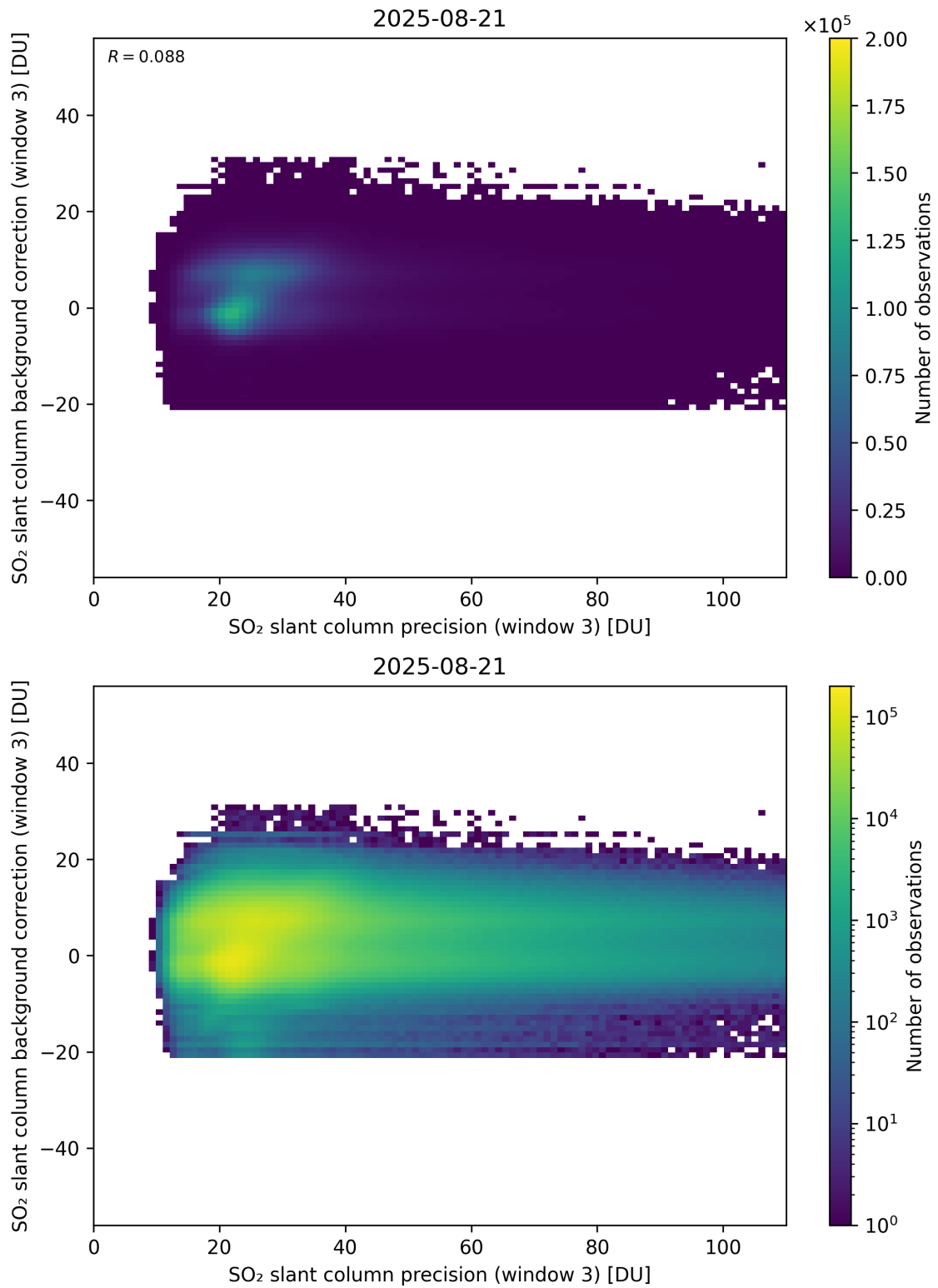
Figure 307: Scatter density plot of “SO 2 slant column precision (window 3)” against “SO 2 slant column background correction (window 3)” for 2025-08-20 to 2025-08-22.
