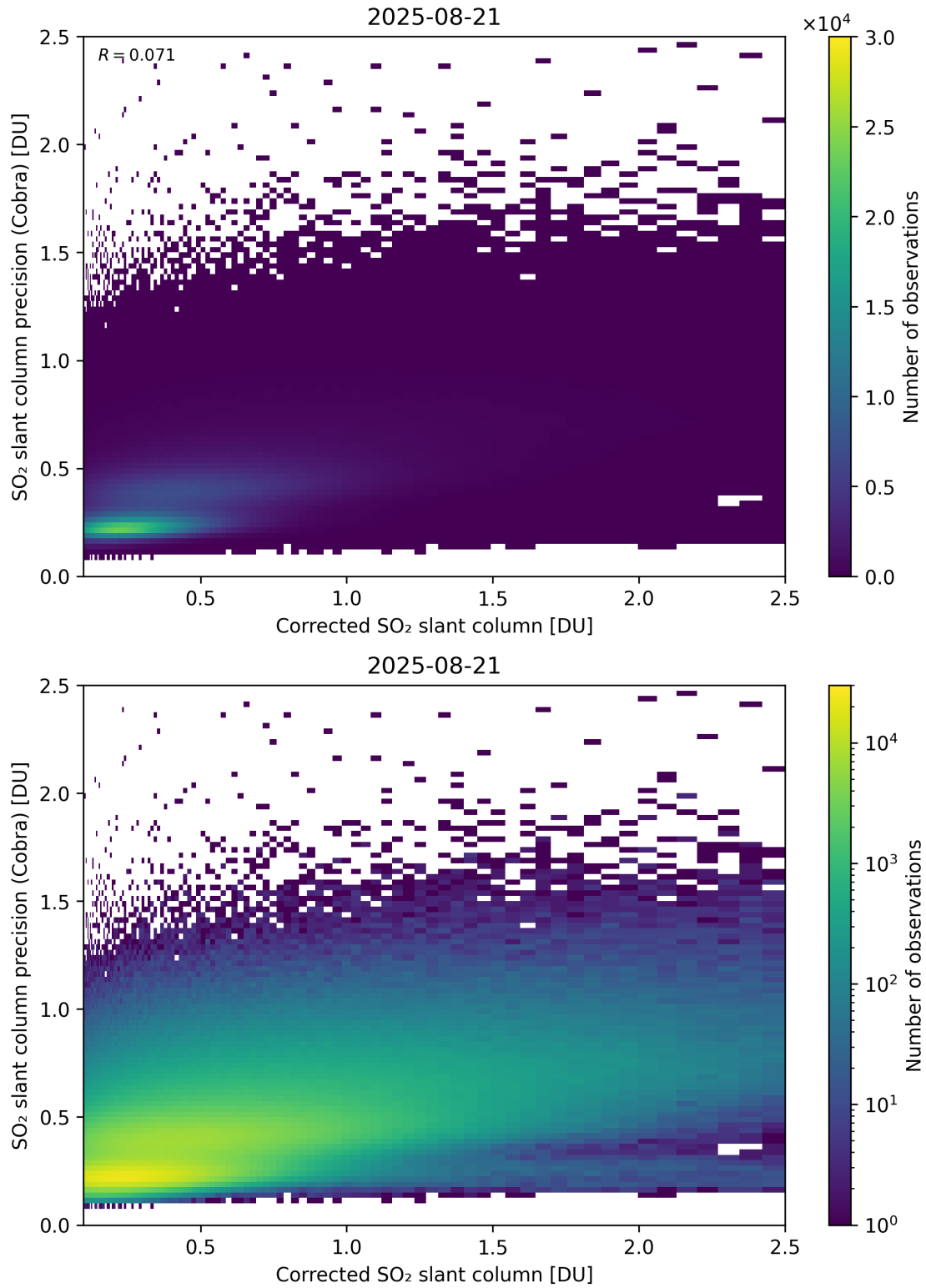
Figure 234: Scatter density plot of “Corrected SO 2 slant column” against “SO 2 slant column precision (Cobra)” for 2025-08-20 to 2025-08-22.
