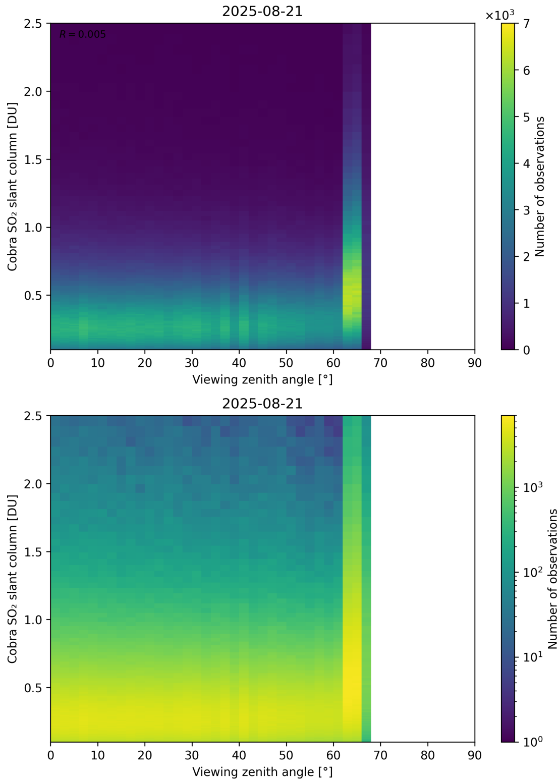
Figure 371: Scatter density plot of “Viewing zenith angle” against “Cobra SO 2 slant column” for 2025-08-20 to 2025-08-22.
