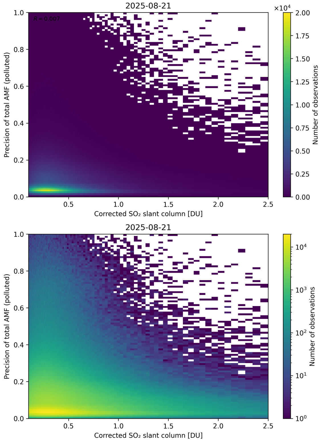
Figure 243: Scatter density plot of “Corrected SO 2 slant column” against “Precision of total AMF (polluted)” for 2025-08-20 to 2025-08-22.
