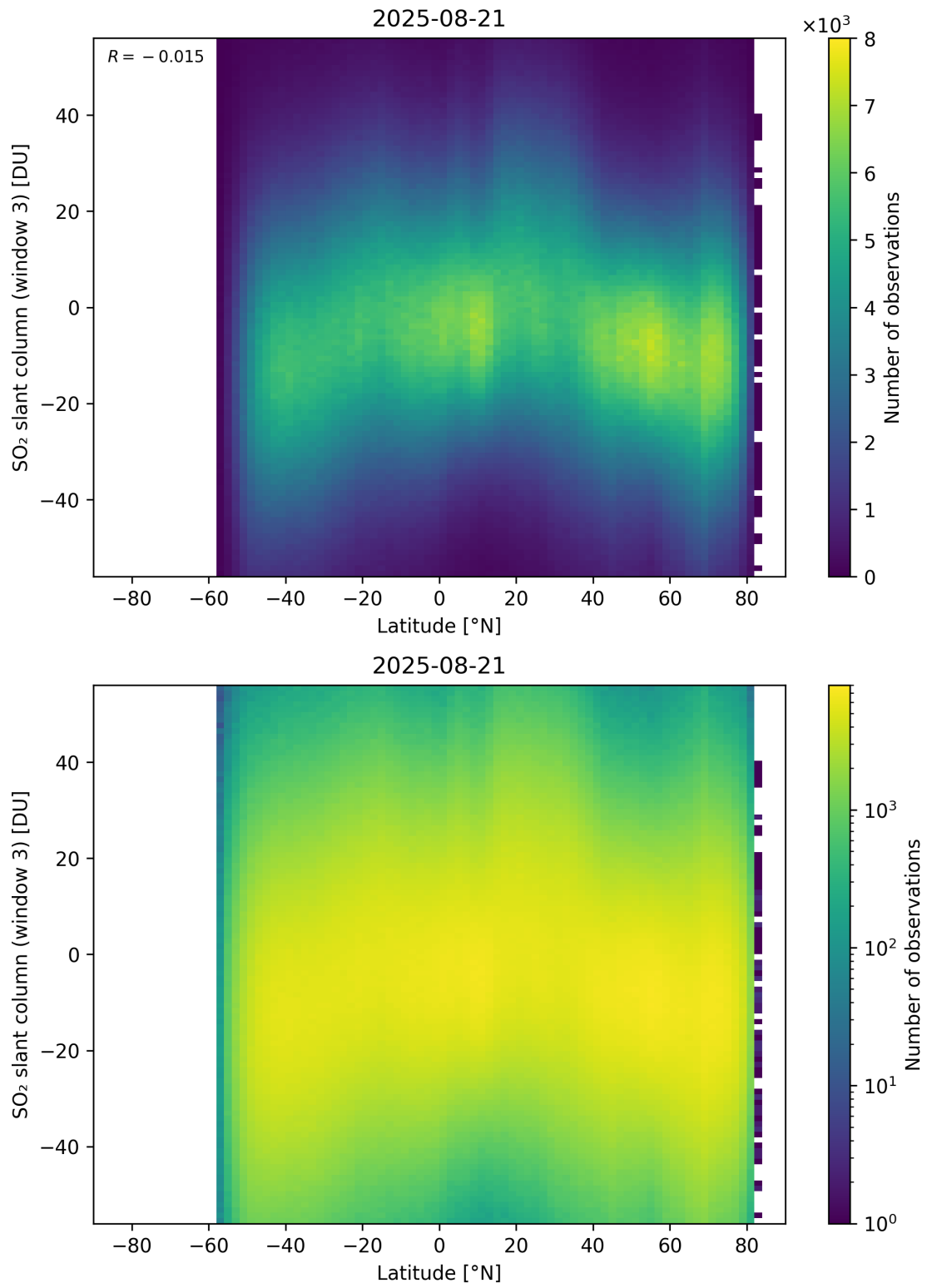
Figure 165: Scatter density plot of “Latitude” against “SO 2 slant column (window 3)” for 2025-08-20 to 2025-08-22.
