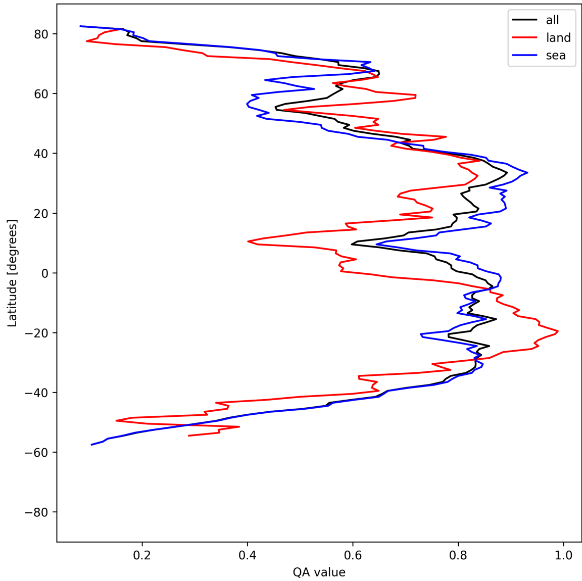
Figure 31: Zonal average of “QA value” for 2025-08-20 to 2025-08-22.
