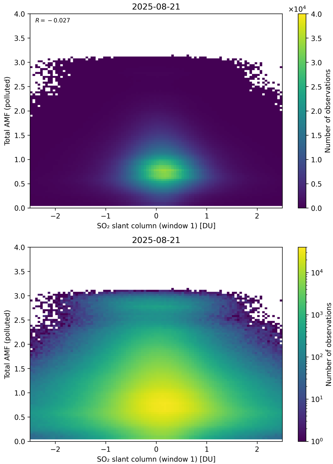
Figure 289: Scatter density plot of “SO 2 slant column (window 1)” against “Total AMF (polluted)” for 2025-08-20 to 2025-08-22.
