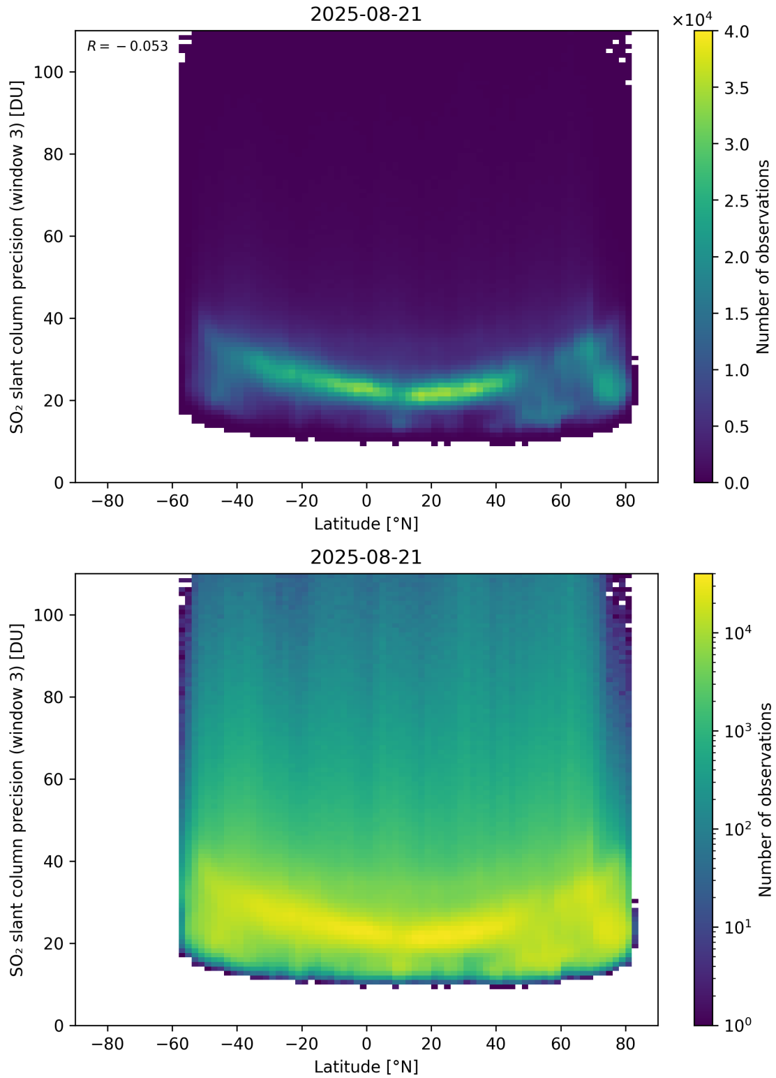
Figure 166: Scatter density plot of “Latitude” against “SO 2 slant column precision (window 3)” for 2025-08-20 to 2025-08-22.
