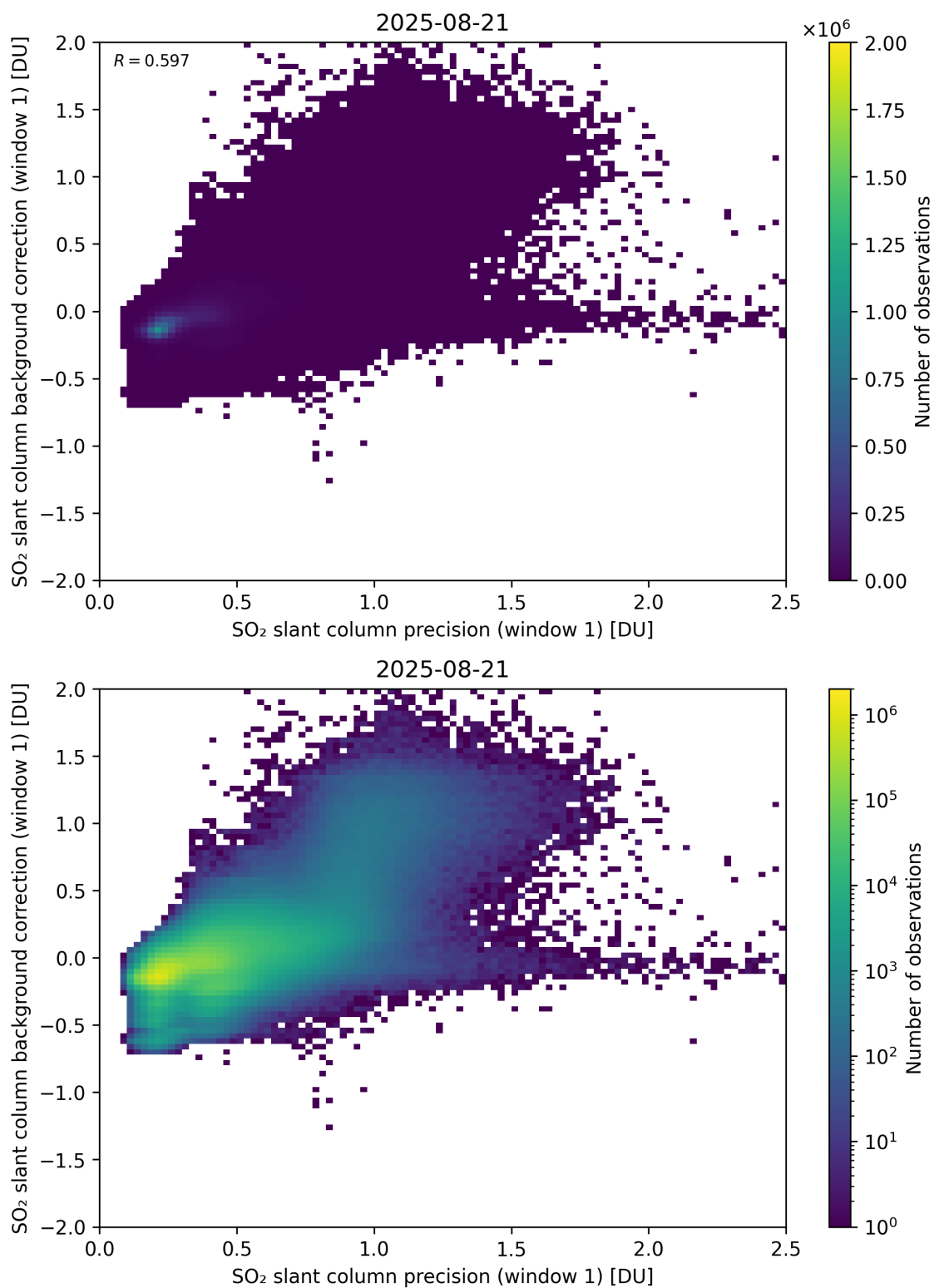
Figure 268: Scatter density plot of “SO 2 slant column precision (window 1)” against “SO 2 slant column background correction (window 1)” for 2025-08-20 to 2025-08-22.
