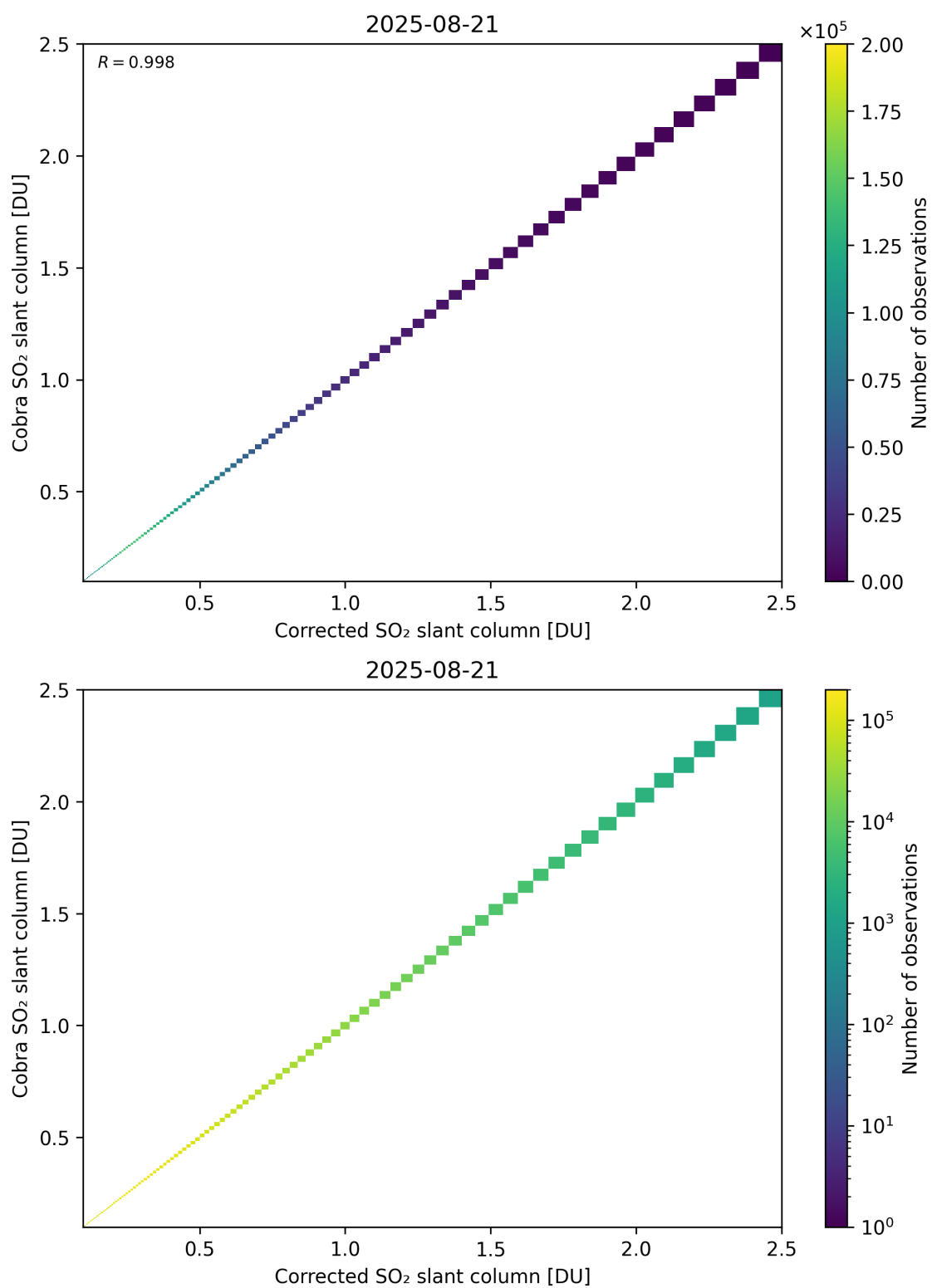
Figure 233: Scatter density plot of “Corrected SO 2 slant column” against “Cobra SO 2 slant column” for 2025-08-20 to 2025-08-22.
