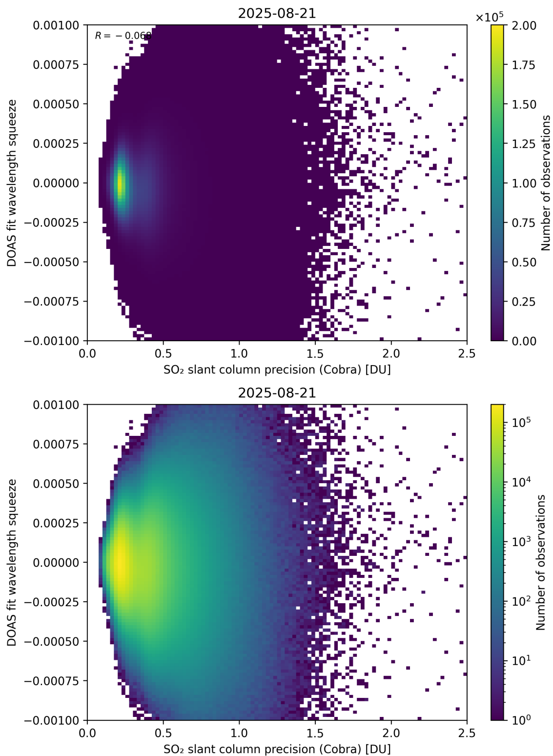
Figure 203: Scatter density plot of “SO 2 slant column precision (Cobra)” against “DOAS fit wavelength squeeze” for 2025-08-20 to 2025-08-22.
