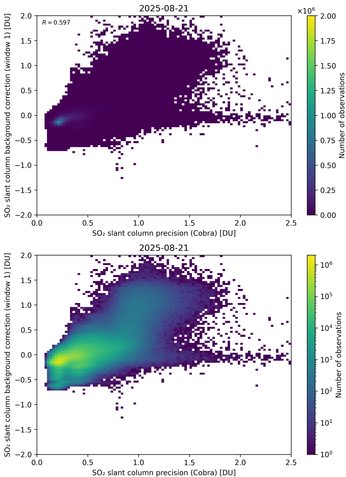
Figure 199: Scatter density plot of “SO 2 slant column precision (Cobra)” against “SO 2 slant column background correction (window 1)” for 2025-08-20 to 2025-08-22.
