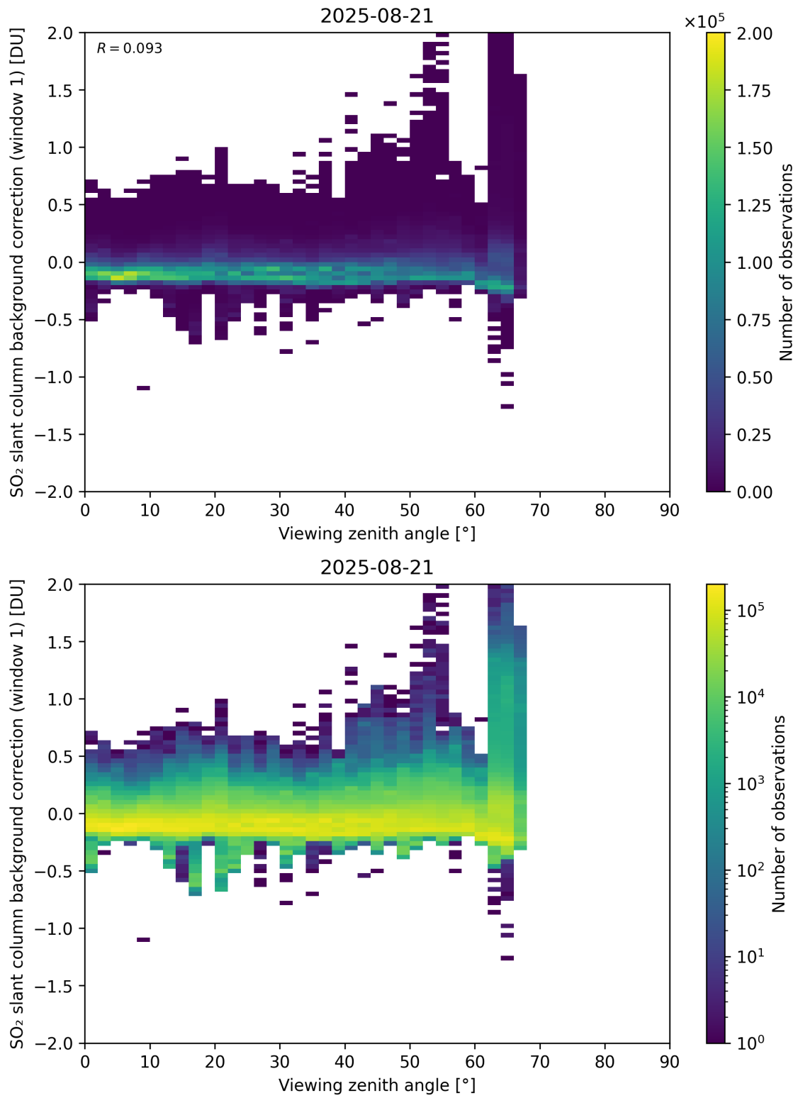
Figure 362: Scatter density plot of “Viewing zenith angle” against “SO 2 slant column background correction (window 1)” for 2025-08-20 to 2025-08-22.
