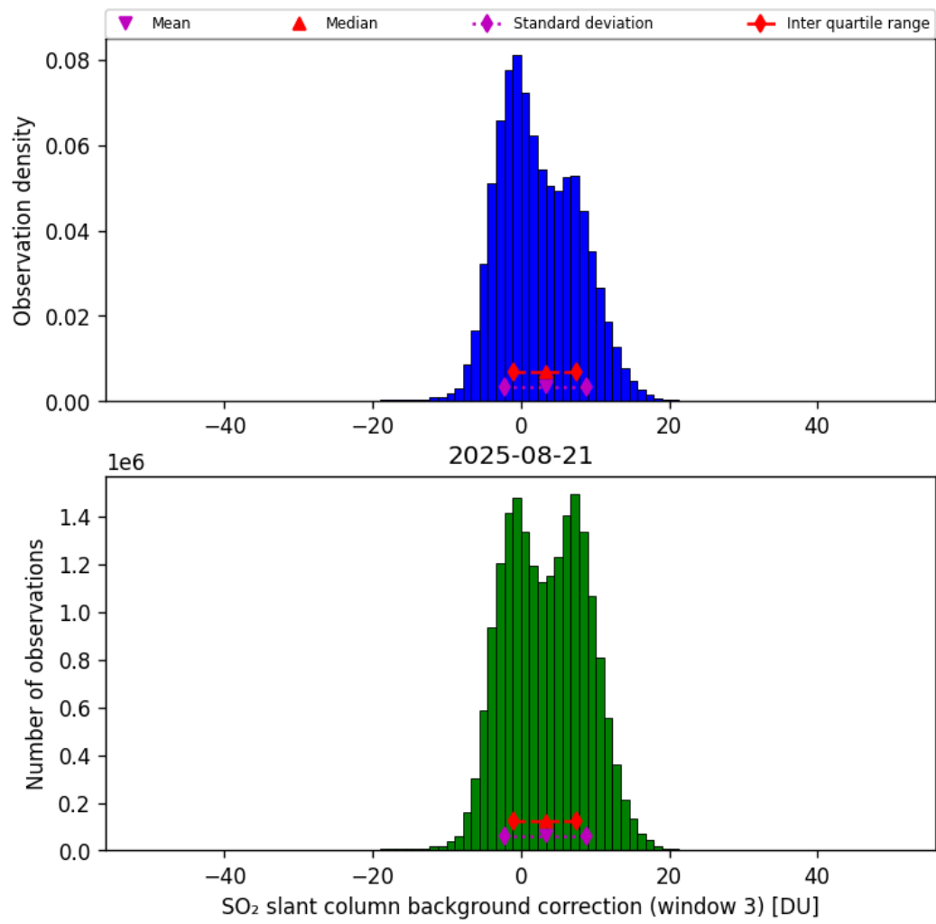
Figure 74: Histogram of “SO 2 slant column background correction (window 3)” for 2025-08-20 to 2025-08-22
