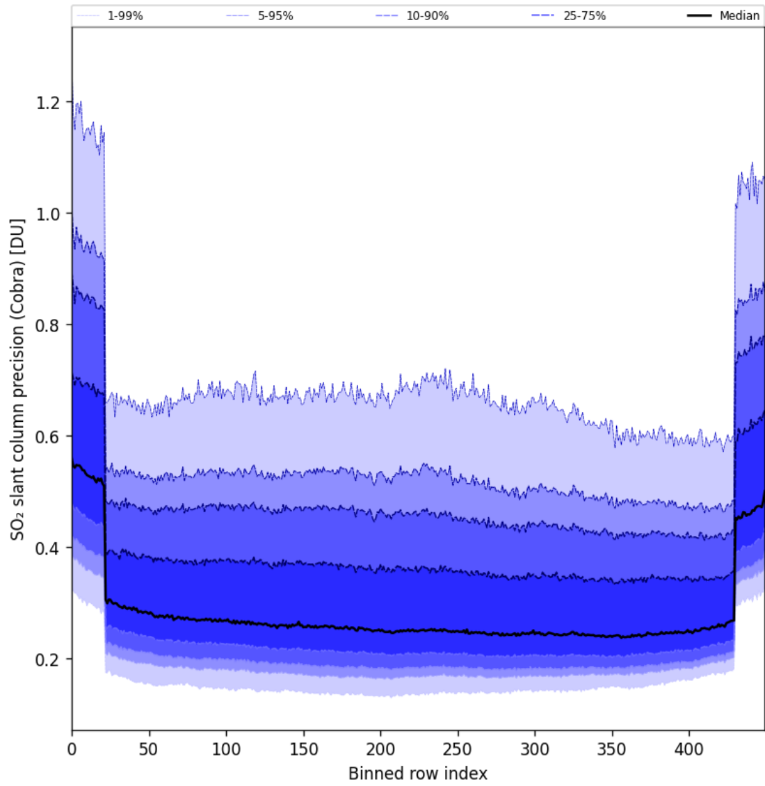
Figure 88: Along track statistics of “SO 2 slant column precision (Cobra)” for 2025-08-20 to 2025-08-22
