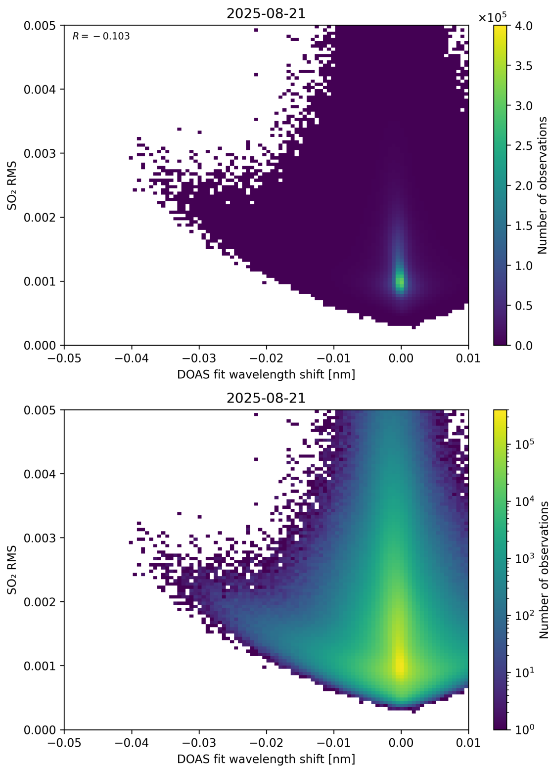
Figure 139: Scatter density plot of “DOAS fit wavelength shift” against “SO 2 RMS” for 2025-08-20 to 2025-08-22.
