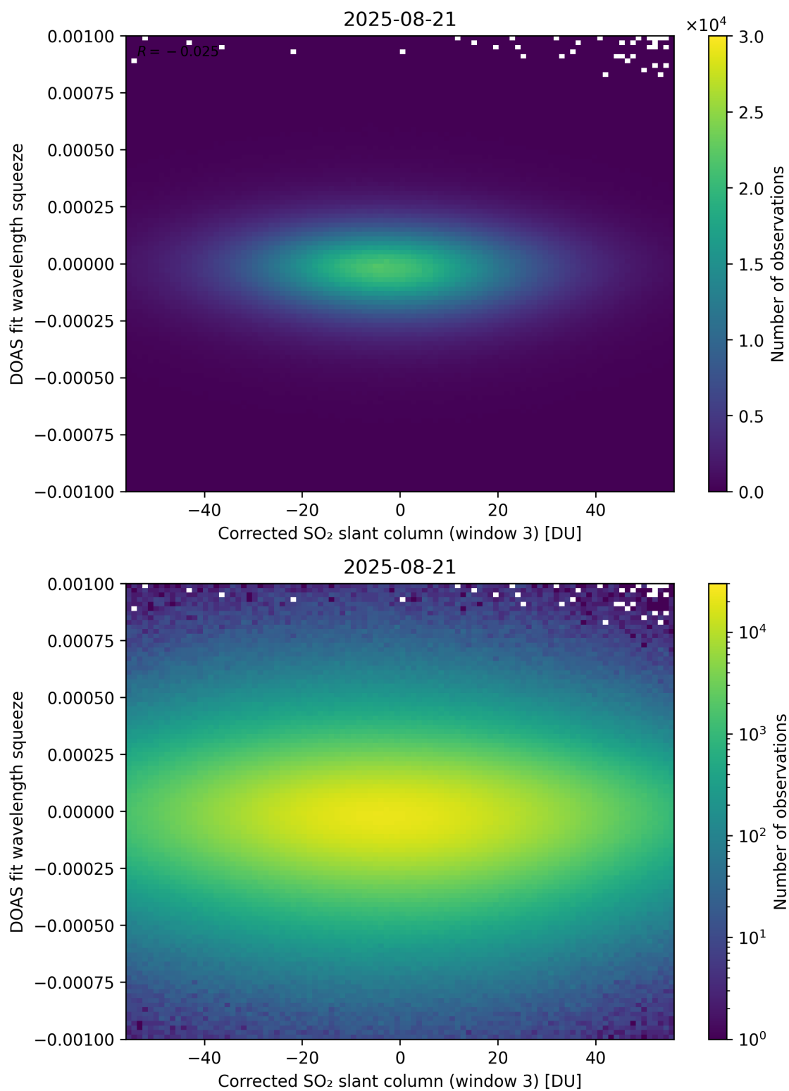
Figure 257: Scatter density plot of “Corrected SO 2 slant column (window 3)” against “DOAS fit wavelength squeeze” for 2025-08-20 to 2025-08-22.
