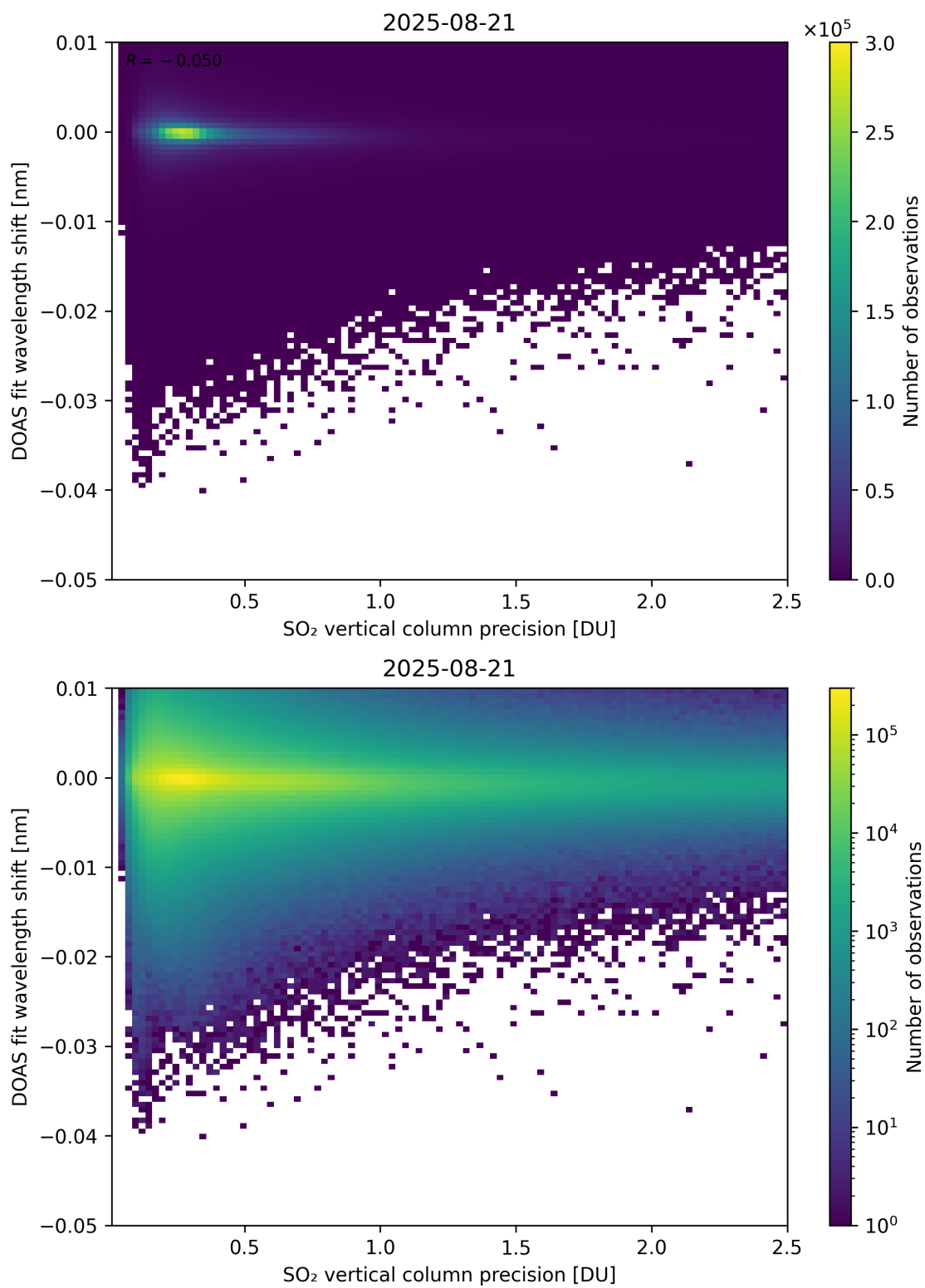
Figure 332: Scatter density plot of “SO 2 vertical column precision” against “DOAS fit wavelength shift” for 2025-08-20 to 2025-08-22.
