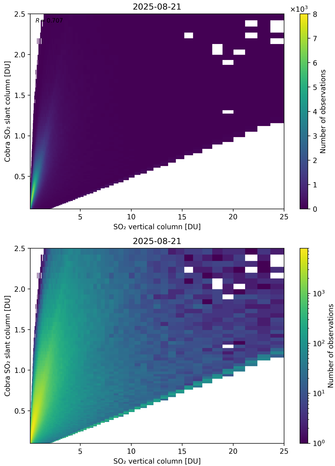
Figure 349: Scatter density plot of “SO 2 vertical column” against “Cobra SO 2 slant column” for 2025-08-20 to 2025-08-22.
