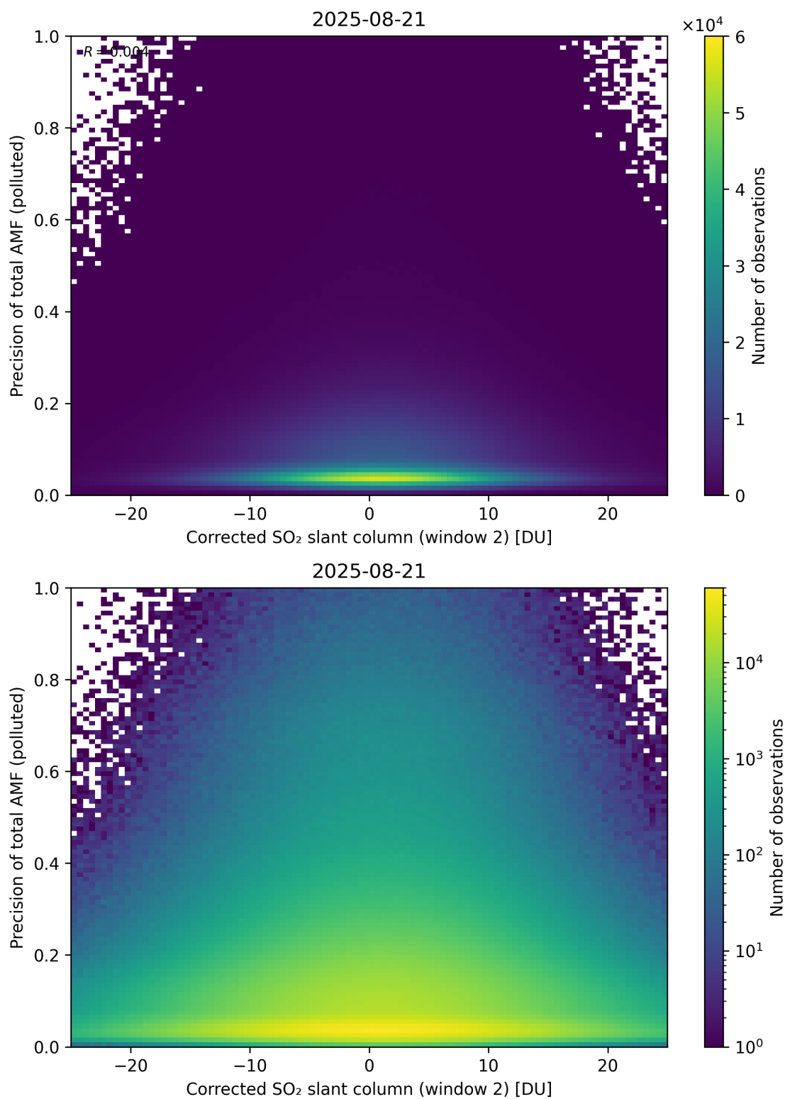
Figure 254: Scatter density plot of “Corrected SO 2 slant column (window 2)” against “Precision of total AMF (polluted)” for 2025-08-20 to 2025-08-22.
