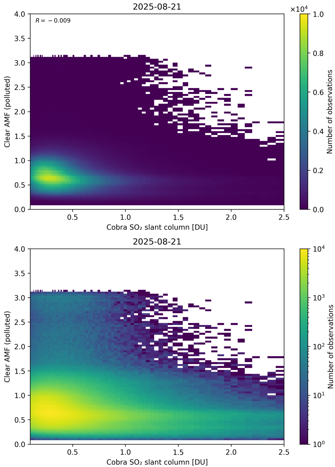
Figure 215: Scatter density plot of “Cobra SO 2 slant column” against “Clear AMF (polluted)” for 2025-08-20 to 2025-08-22.
