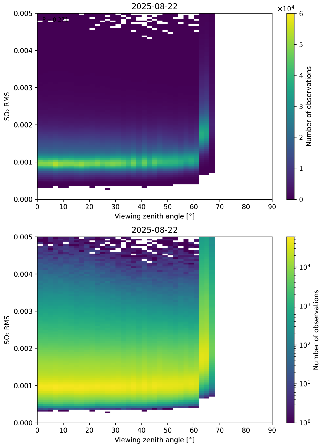
Figure 367: Scatter density plot of “Viewing zenith angle” against “SO 2 RMS” for 2025-08-21 to 2025-08-23.
