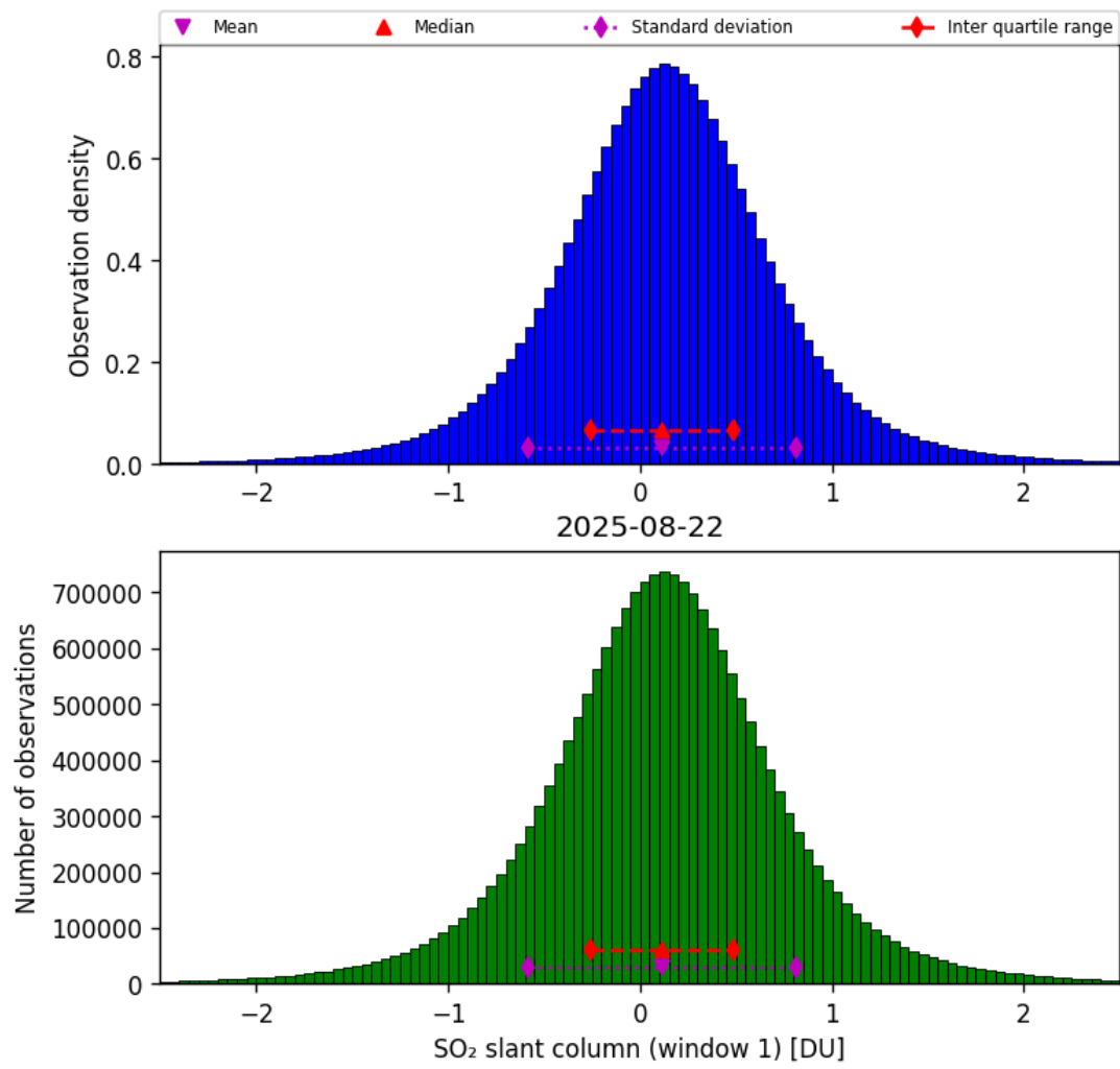
Figure 63: Histogram of “SO 2 slant column (window 1)” for 2025-08-21 to 2025-08-23
