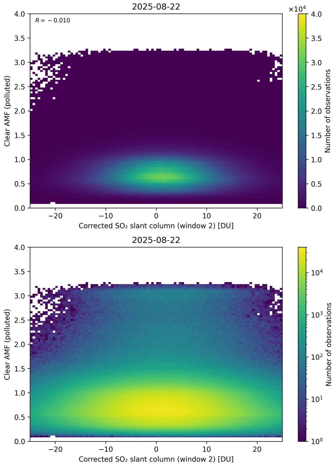
Figure 249: Scatter density plot of “Corrected SO 2 slant column (window 2)” against “Clear AMF (polluted)” for 2025-08-21 to 2025-08-23.
