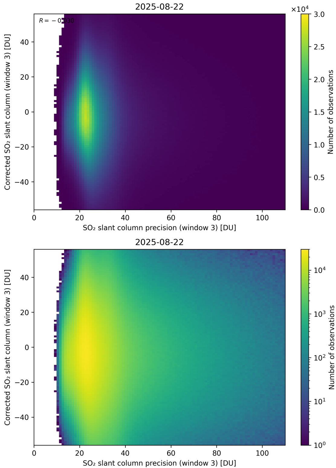
Figure 312: Scatter density plot of “SO 2 slant column precision (window 3)” against “Corrected SO 2 slant column (window 3)” for 2025-08-21 to 2025-08-23.
