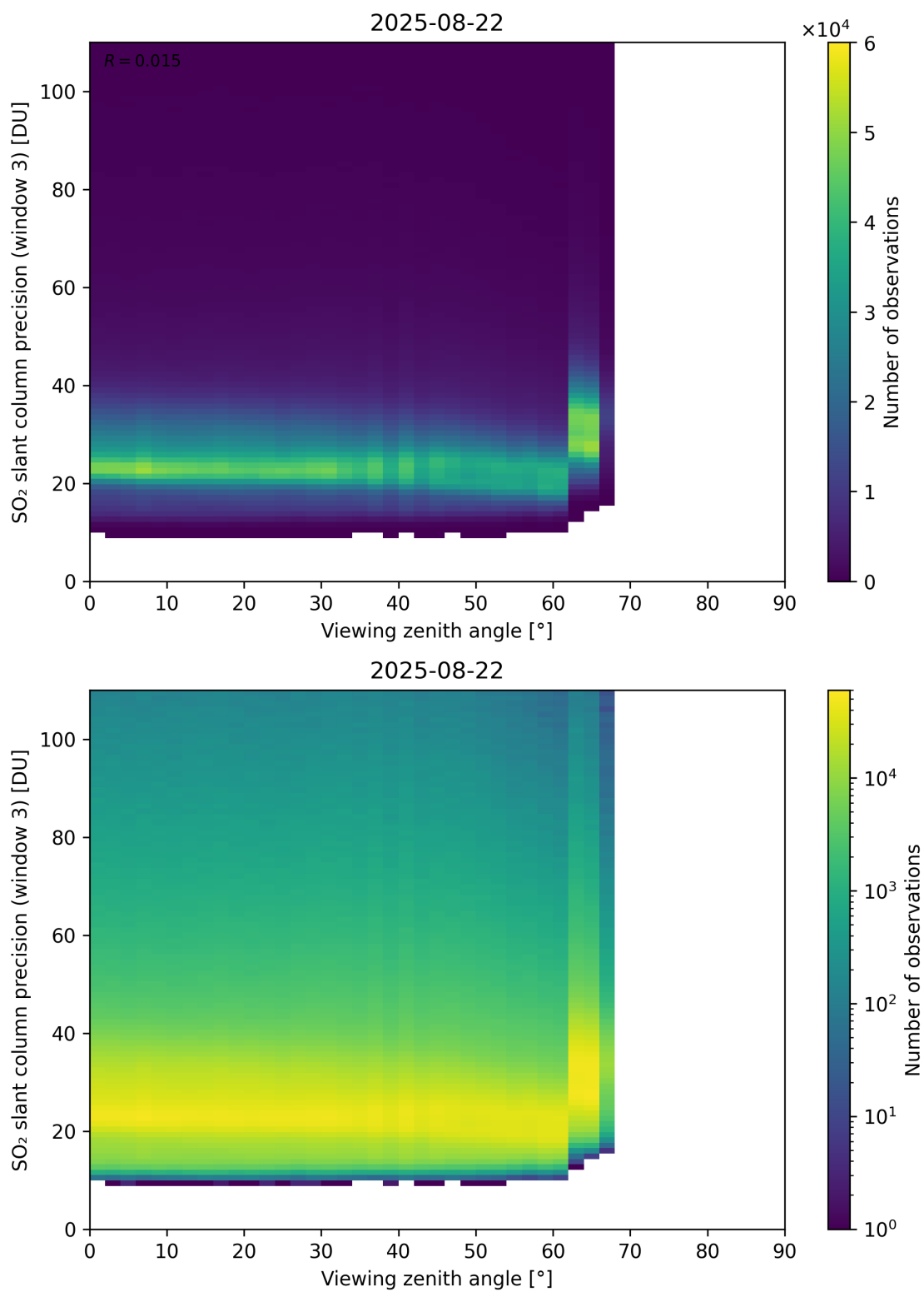
Figure 380: Scatter density plot of “Viewing zenith angle” against “SO 2 slant column precision (window 3)” for 2025-08-21 to 2025-08-23.
