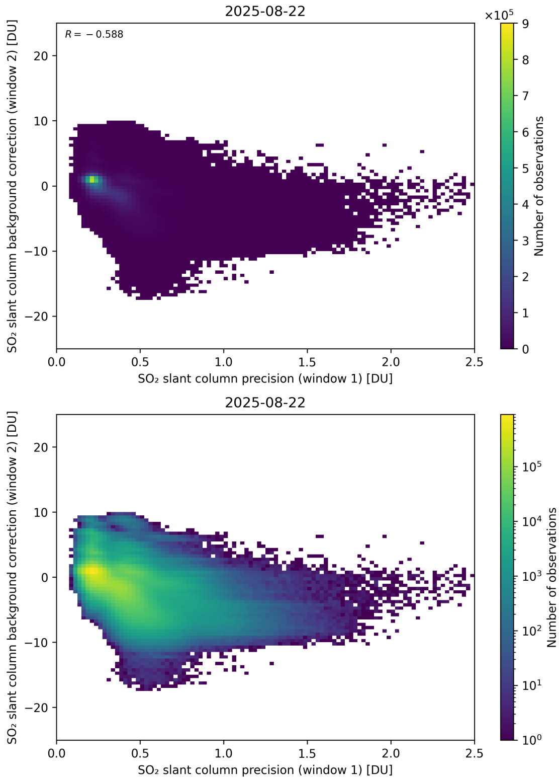
Figure 269: Scatter density plot of “SO 2 slant column precision (window 1)” against “SO 2 slant column background correction (window 2)” for 2025-08-21 to 2025-08-23.
