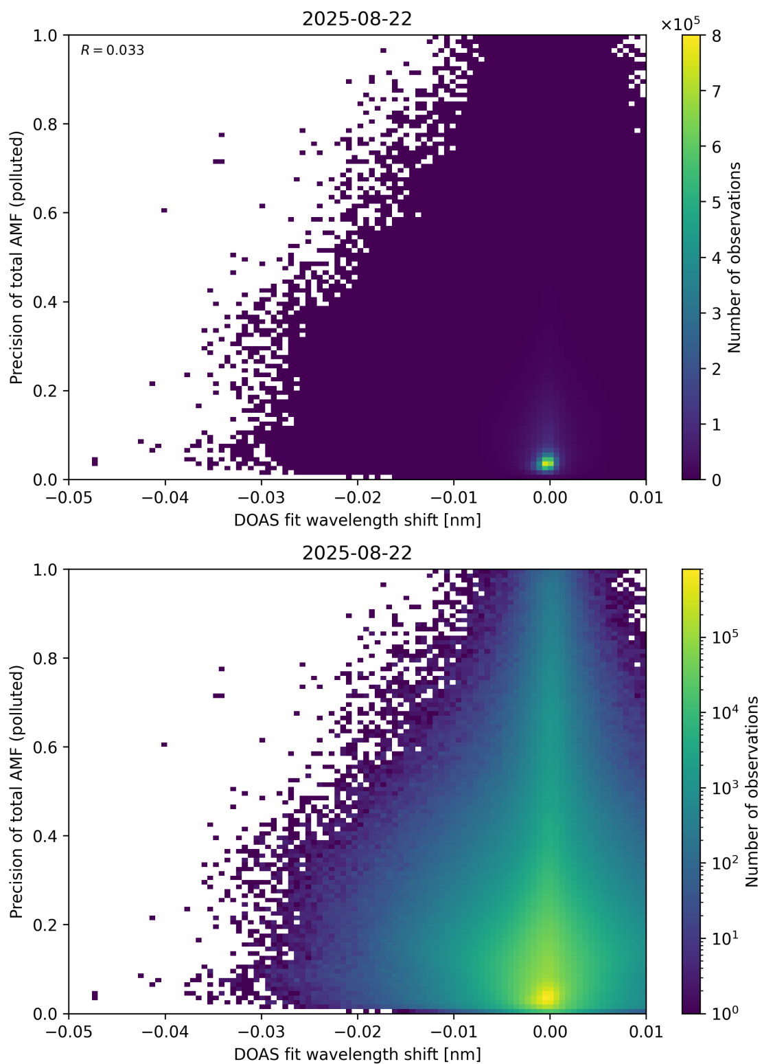
Figure 142: Scatter density plot of “DOAS fit wavelength shift” against “Precision of total AMF (polluted)” for 2025-08-21 to 2025-08-23.
