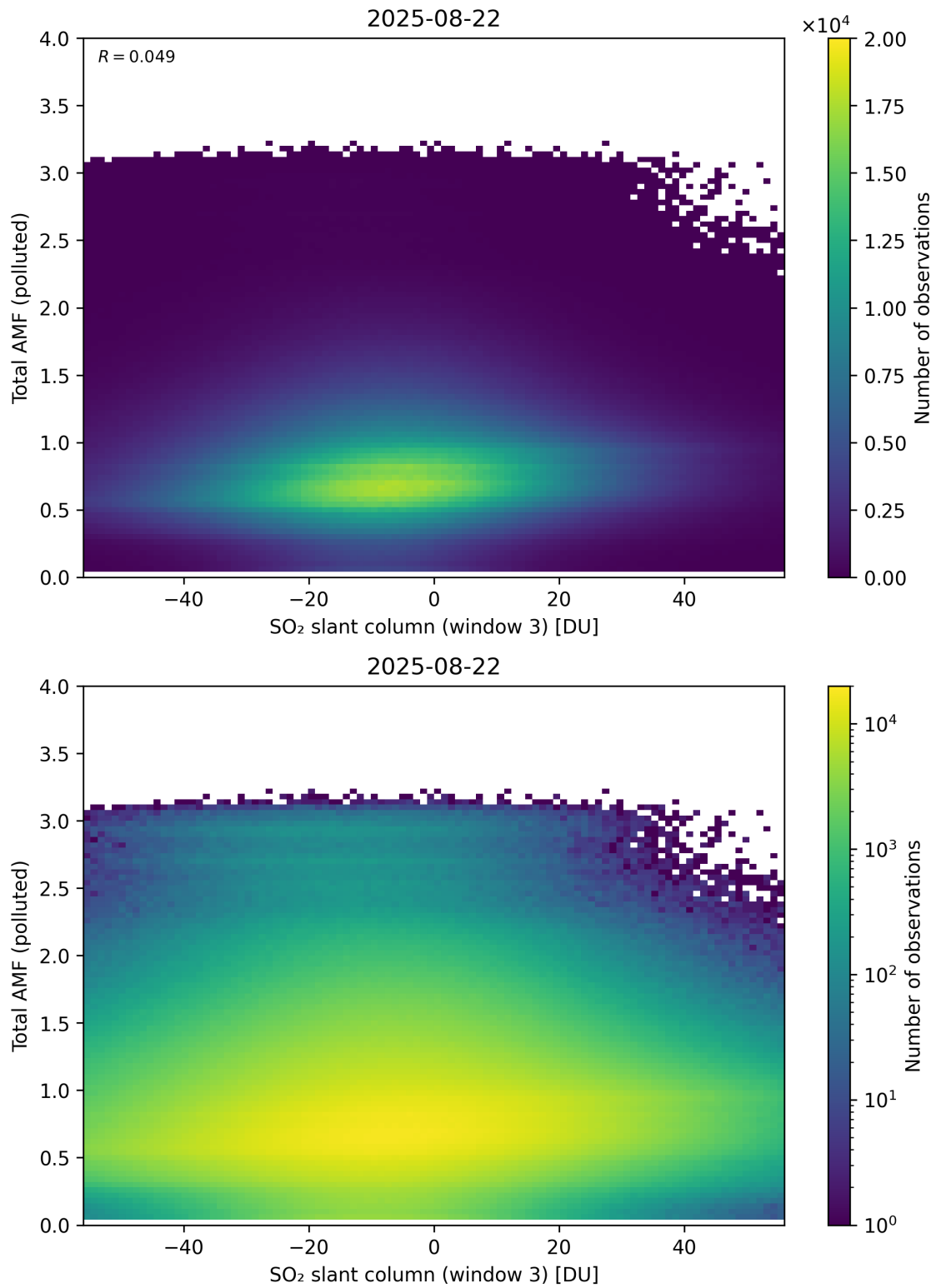
Figure 318: Scatter density plot of “SO 2 slant column (window 3)” against “Total AMF (polluted)” for 2025-08-21 to 2025-08-23.
