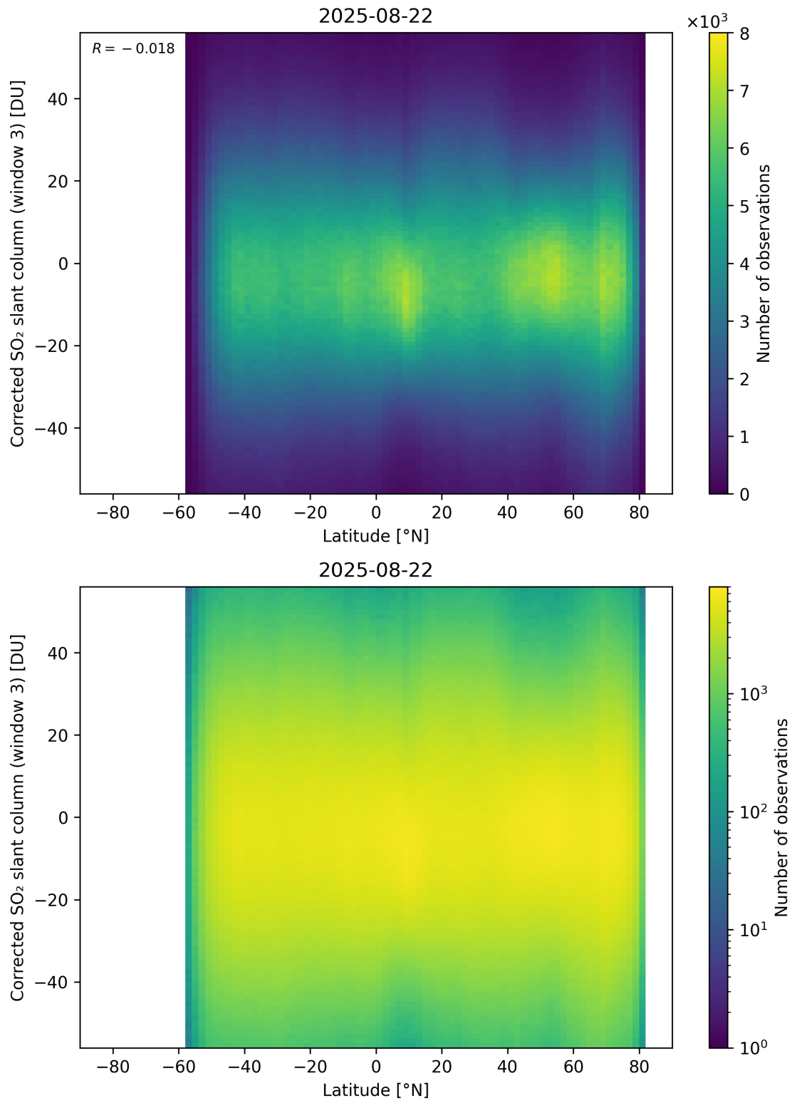
Figure 161: Scatter density plot of “Latitude” against “Corrected SO 2 slant column (window 3)” for 2025-08-21 to 2025-08-23.
