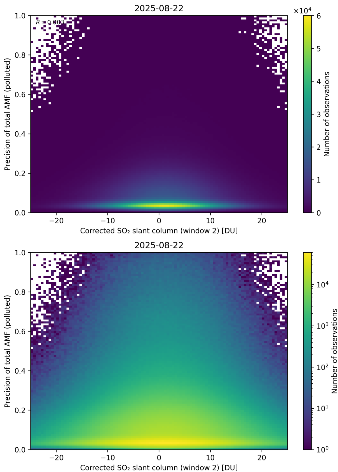
Figure 254: Scatter density plot of “Corrected SO 2 slant column (window 2)” against “Precision of total AMF (polluted)” for 2025-08-21 to 2025-08-23.
