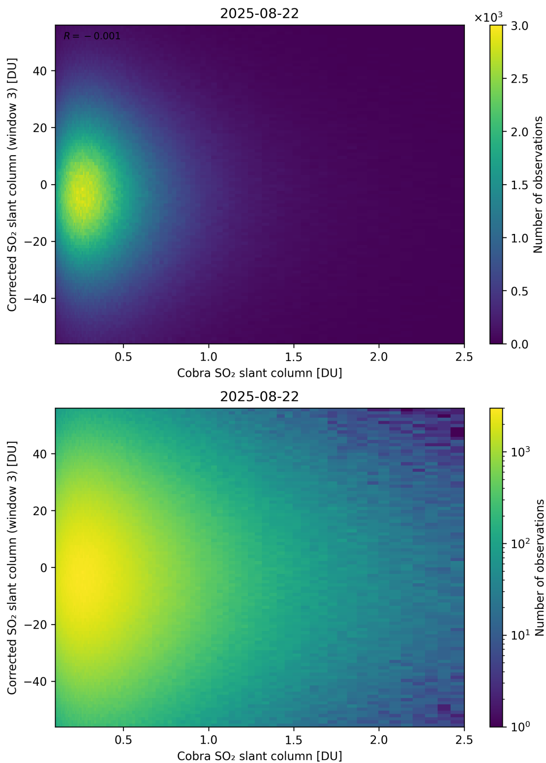
Figure 218: Scatter density plot of “Cobra SO 2 slant column” against “Corrected SO 2 slant column (window 3)” for 2025-08-21 to 2025-08-23.
