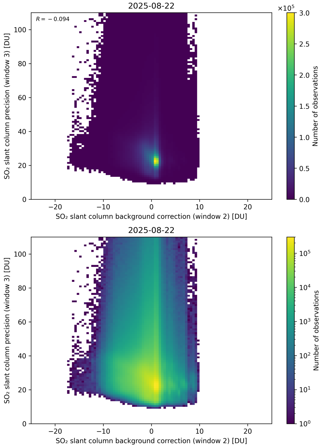
Figure 129: Scatter density plot of “SO 2 slant column background correction (window 2)” against “SO 2 slant column precision (window 3)” for 2025-08-21 to 2025-08-23.
