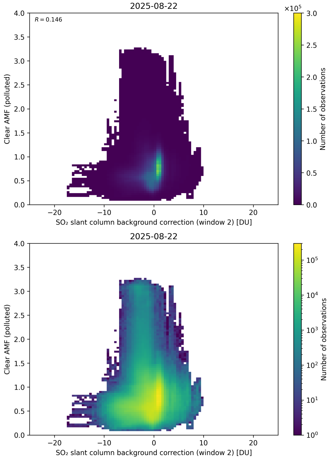
Figure 126: Scatter density plot of “SO 2 slant column background correction (window 2)” against “Clear AMF (polluted)” for 2025-08-21 to 2025-08-23.
