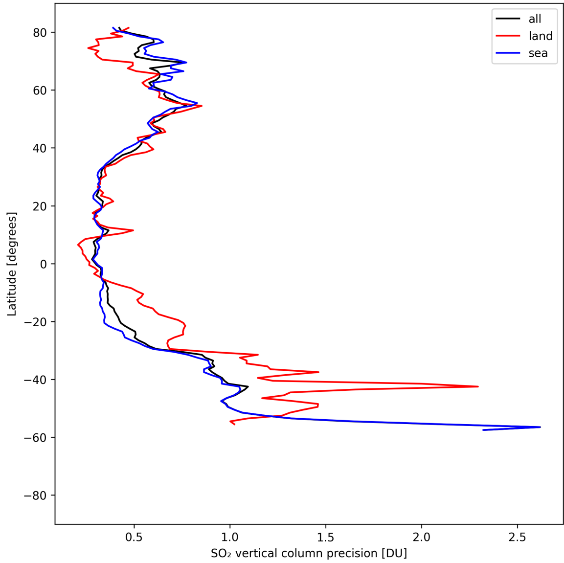
Figure 33: Zonal average of “SO 2 vertical column precision” for 2025-08-21 to 2025-08-23.
