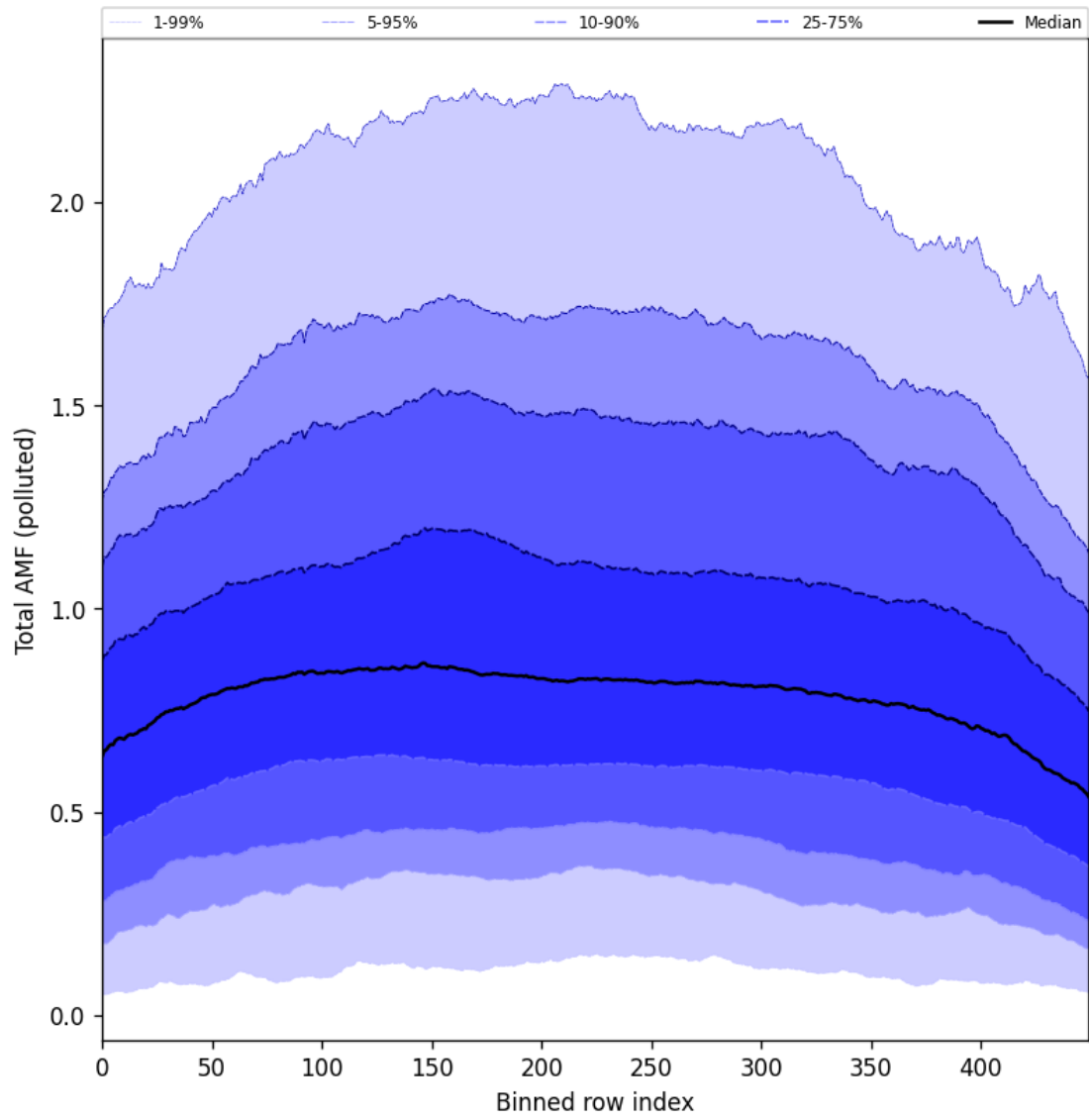
Figure 105: Along track statistics of “Total AMF (polluted)” for 2025-08-21 to 2025-08-23
