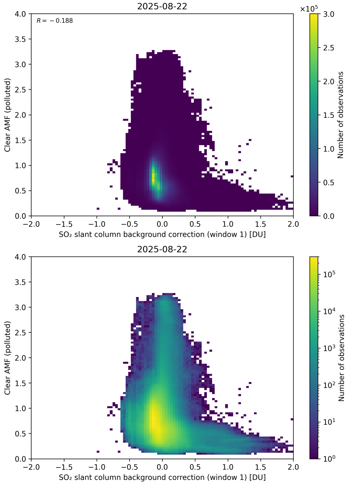
Figure 114: Scatter density plot of “SO 2 slant column background correction (window 1)” against “Clear AMF (polluted)” for 2025-08-21 to 2025-08-23.
