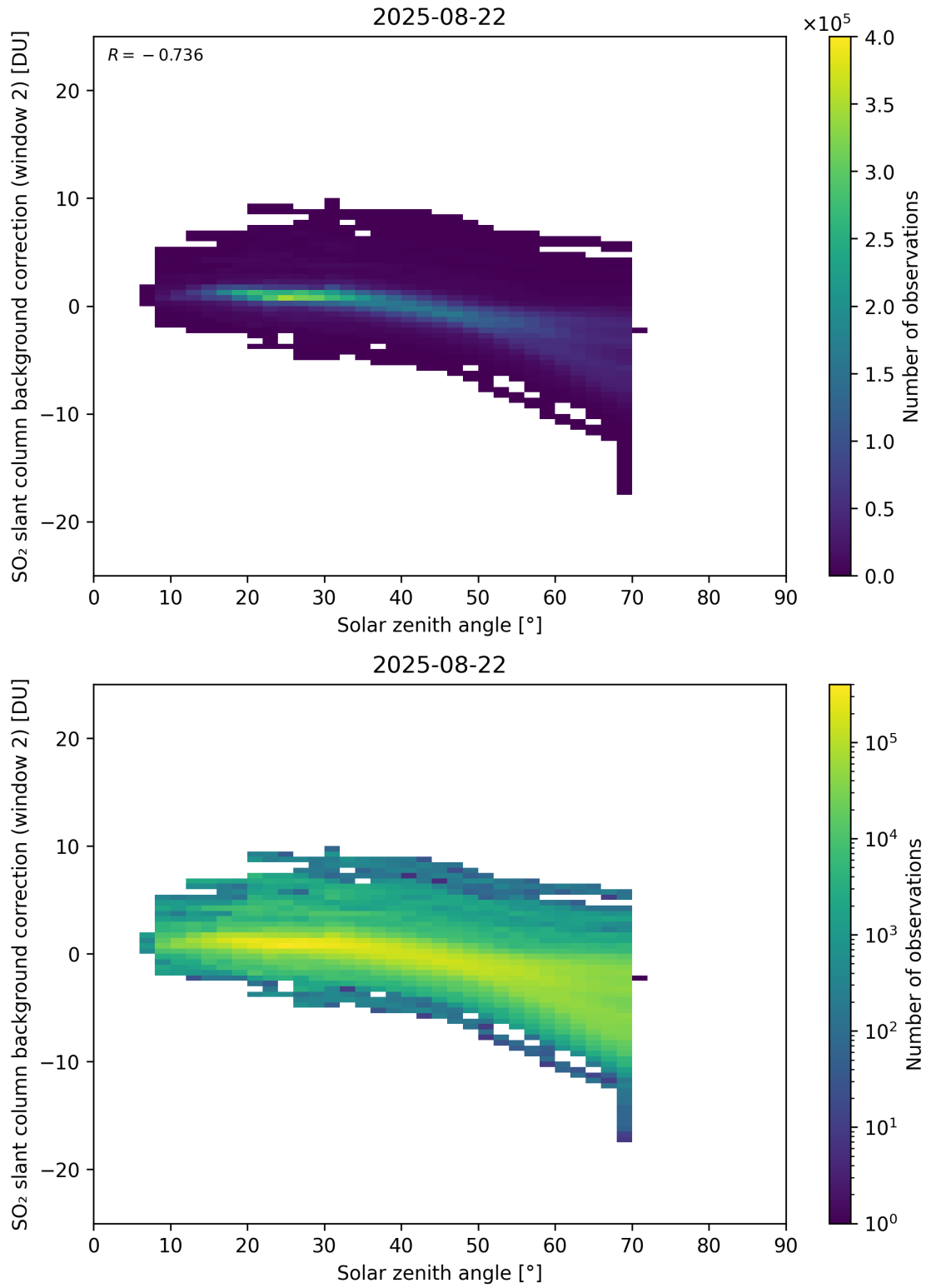
Figure 172: Scatter density plot of “Solar zenith angle” against “SO 2 slant column background correction (window 2)” for 2025-08-21 to 2025-08-23.
