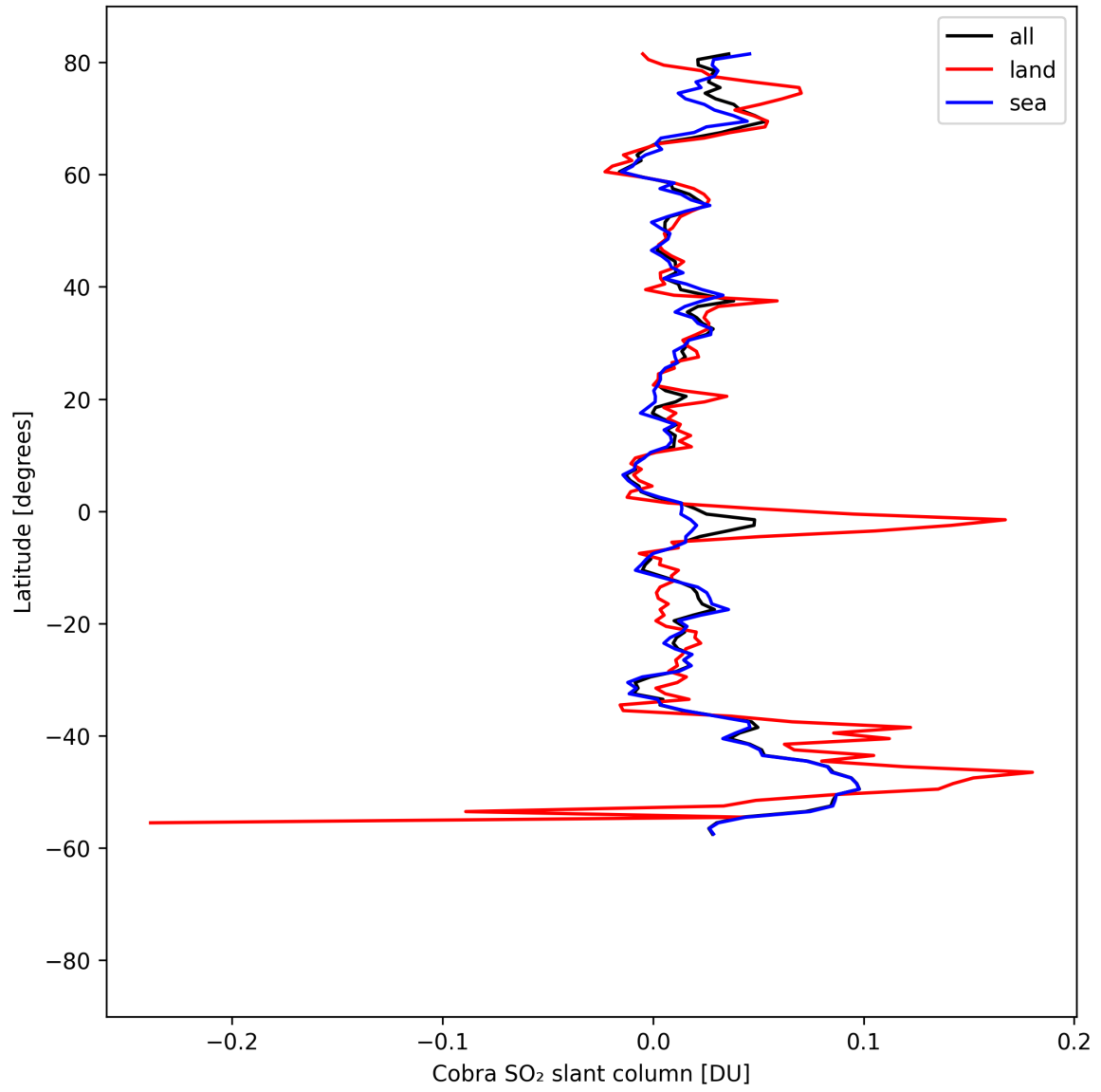
Figure 35: Zonal average of “Cobra SO 2 slant column” for 2025-08-21 to 2025-08-23.
