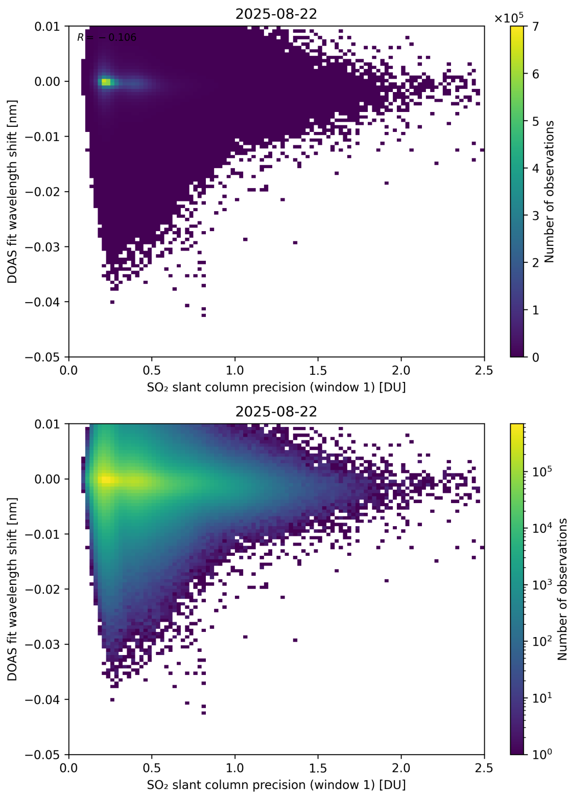
Figure 271: Scatter density plot of “SO 2 slant column precision (window 1)” against “DOAS fit wavelength shift” for 2025-08-21 to 2025-08-23.
