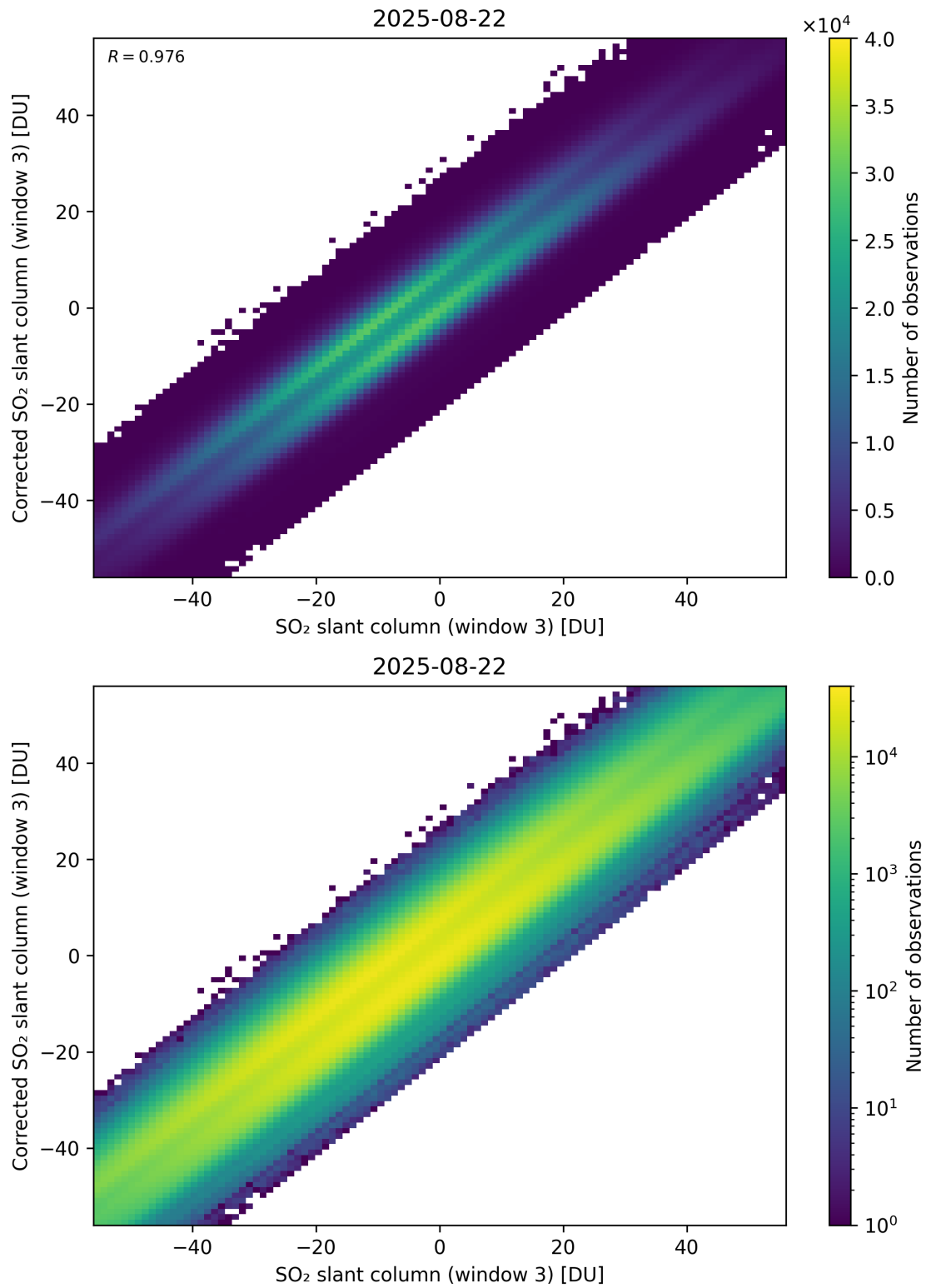
Figure 316: Scatter density plot of “SO 2 slant column (window 3)” against “Corrected SO 2 slant column (window 3)” for 2025-08-21 to 2025-08-23.
