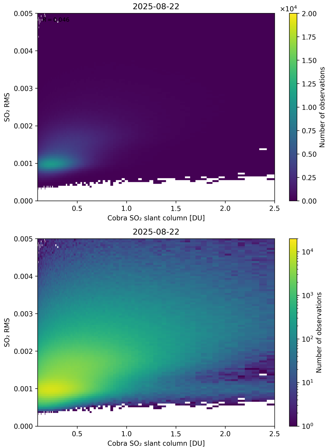
Figure 198: Scatter density plot of “Cobra SO 2 slant column” against “SO 2 RMS” for 2025-08-21 to 2025-08-23.
