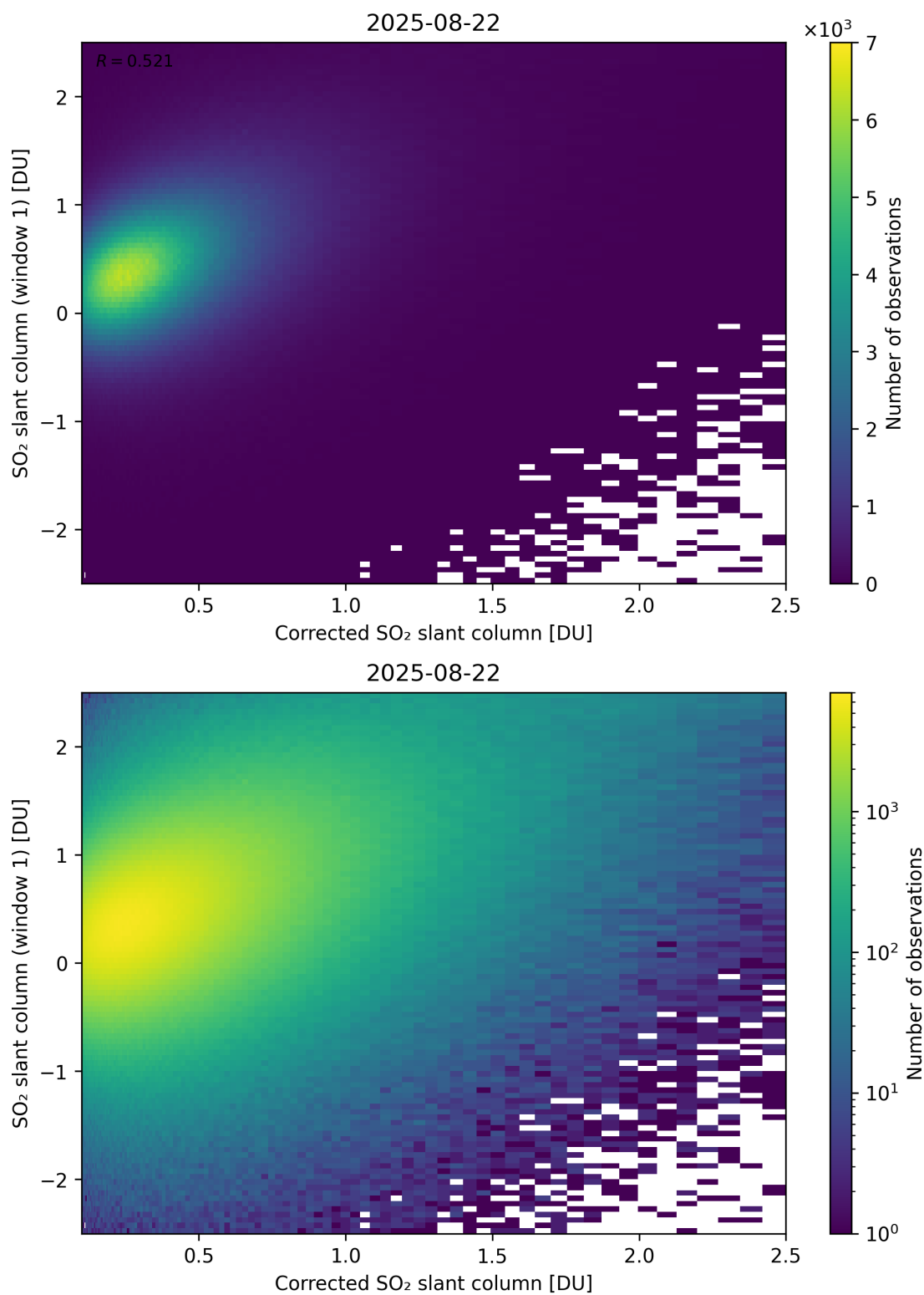
Figure 237: Scatter density plot of “Corrected SO 2 slant column” against “SO 2 slant column (window 1)” for 2025-08-21 to 2025-08-23.
