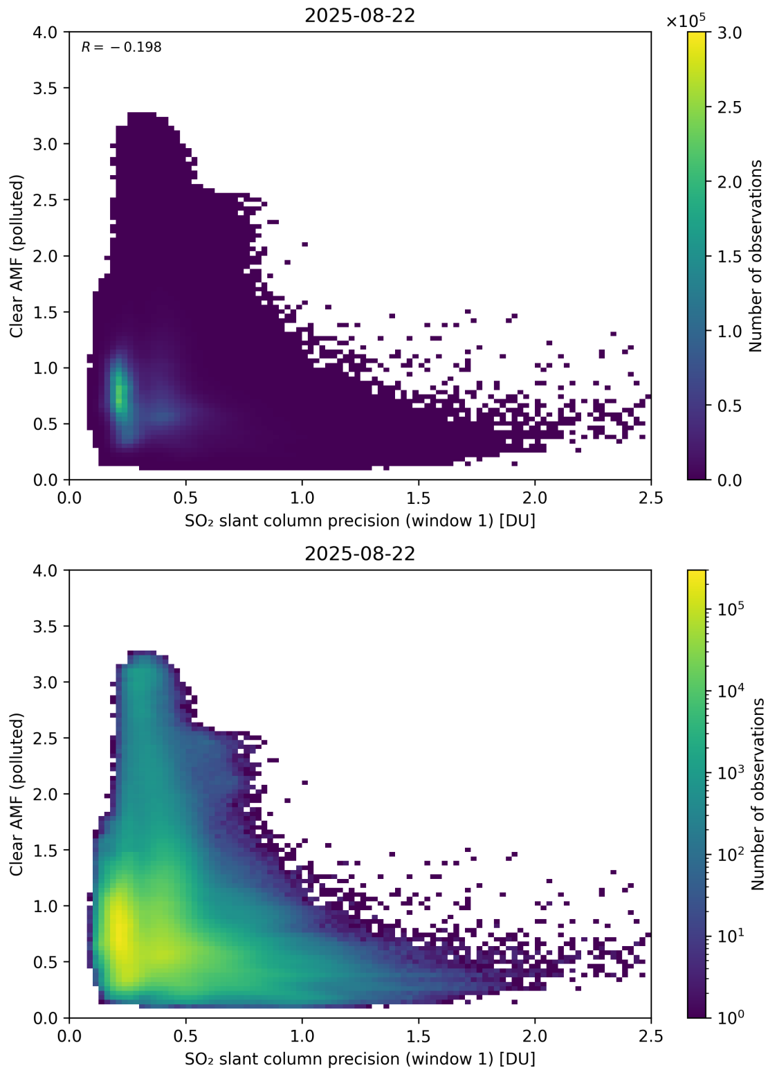
Figure 274: Scatter density plot of “SO 2 slant column precision (window 1)” against “Clear AMF (polluted)” for 2025-08-21 to 2025-08-23.
