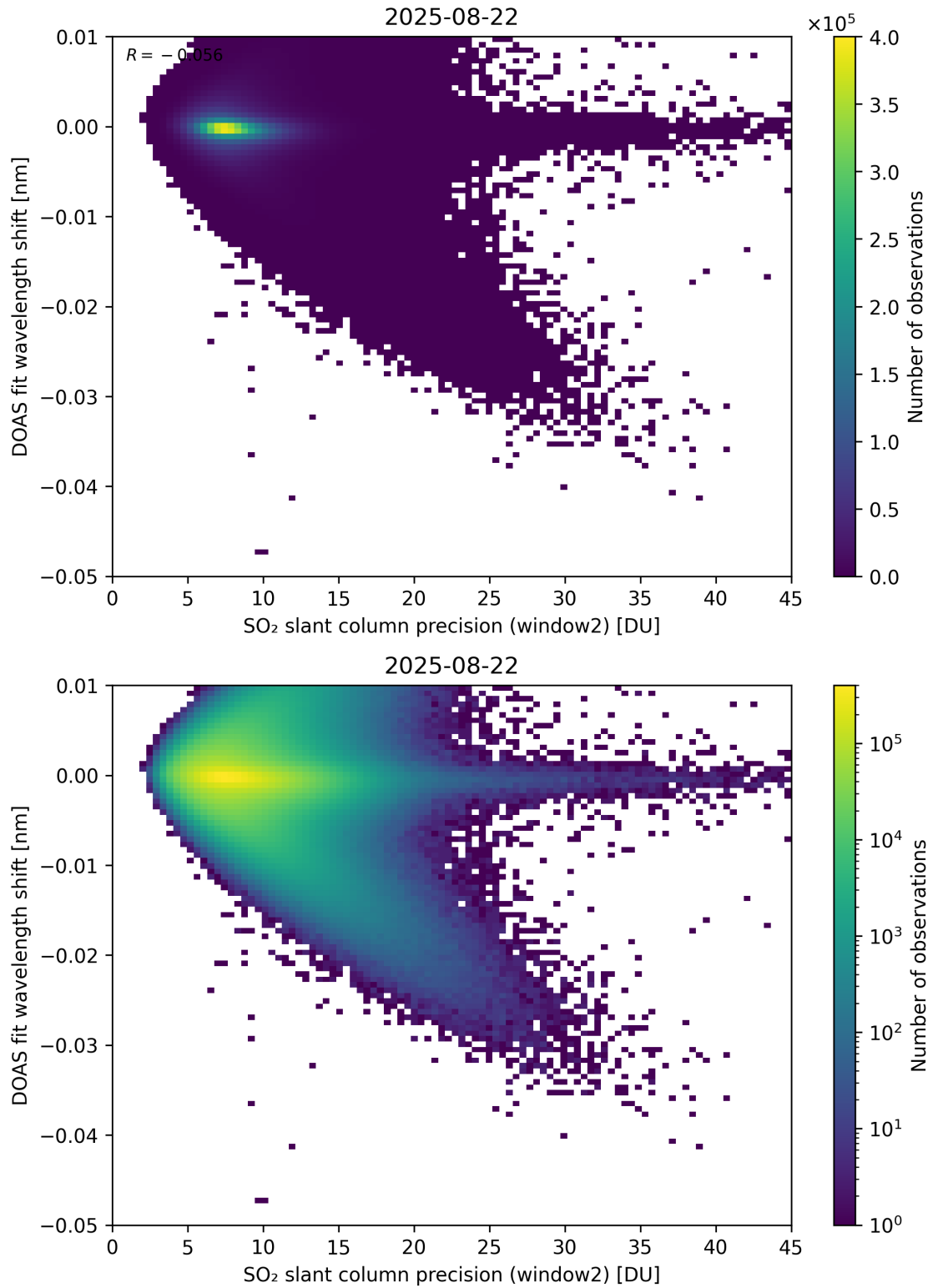
Figure 293: Scatter density plot of “SO 2 slant column precision (window2)” against “DOAS fit wavelength shift” for 2025-08-21 to 2025-08-23.
