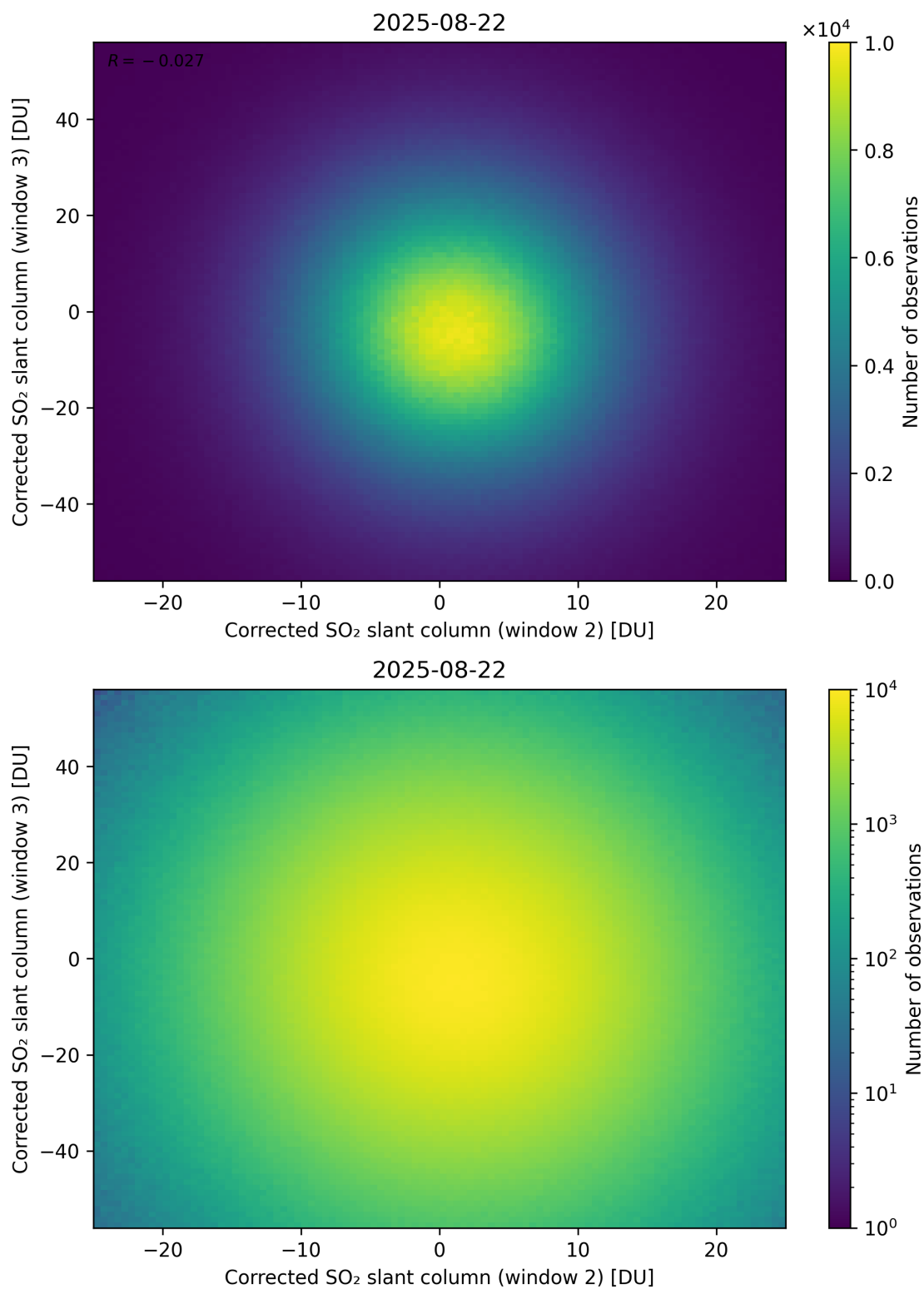
Figure 250: Scatter density plot of “Corrected SO 2 slant column (window 2)” against “Corrected SO 2 slant column (window 3)” for 2025-08-21 to 2025-08-23.
