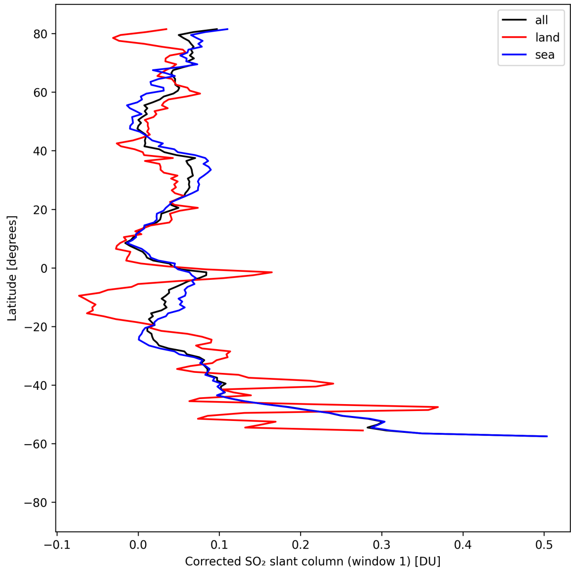
Figure 39: Zonal average of "Corrected SO 2 slant column (window 1)" for 2025-08-21 to 2025-08-23.
