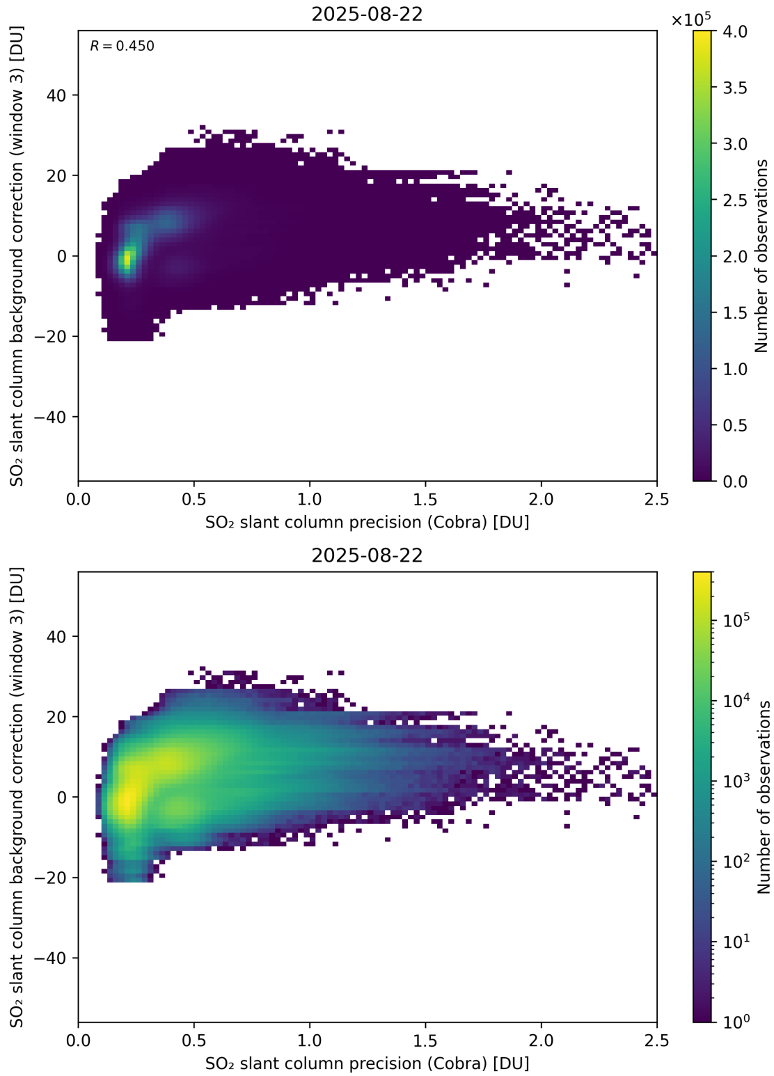
Figure 201: Scatter density plot of “SO 2 slant column precision (Cobra)” against “SO 2 slant column background correction (window 3)” for 2025-08-21 to 2025-08-23.
