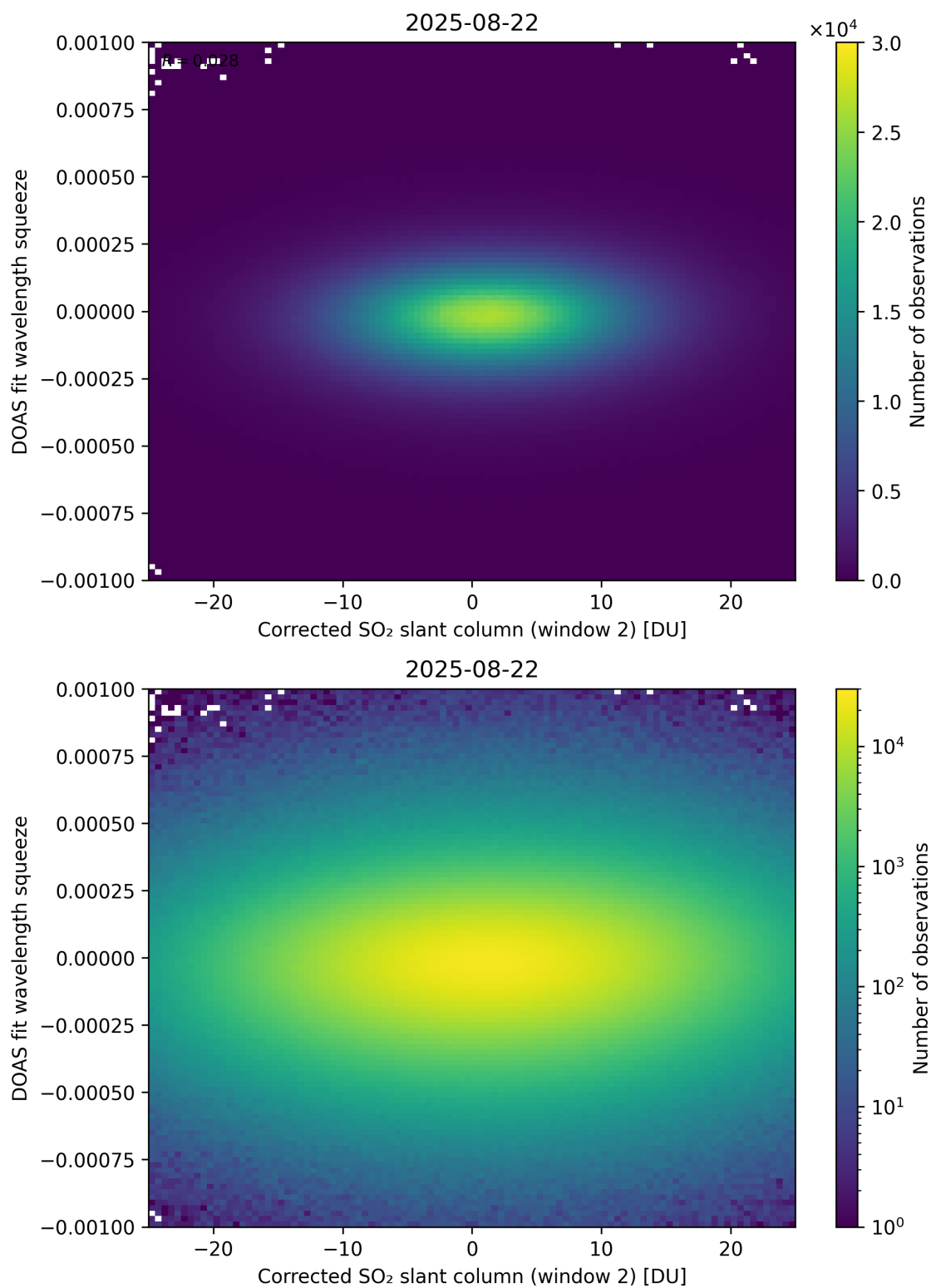
Figure 247: Scatter density plot of “Corrected SO 2 slant column (window 2)” against “DOAS fit wavelength squeeze” for 2025-08-21 to 2025-08-23.
