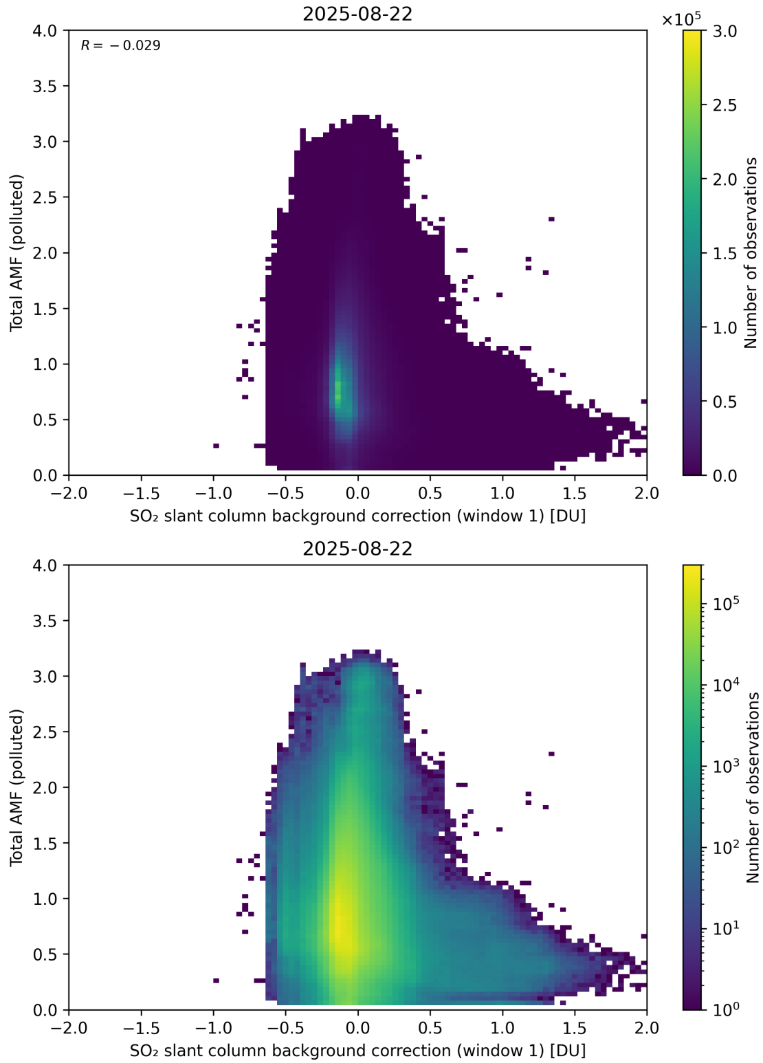
Figure 120: Scatter density plot of “SO 2 slant column background correction (window 1)” against “Total AMF (polluted)” for 2025-08-21 to 2025-08-23.
