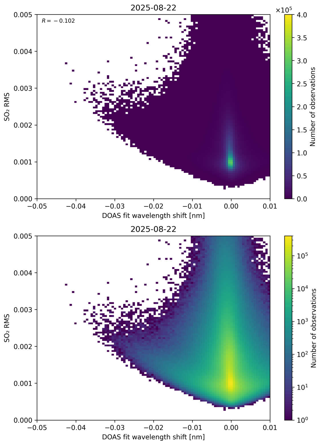
Figure 139: Scatter density plot of “DOAS fit wavelength shift” against “SO 2 RMS” for 2025-08-21 to 2025-08-23.
