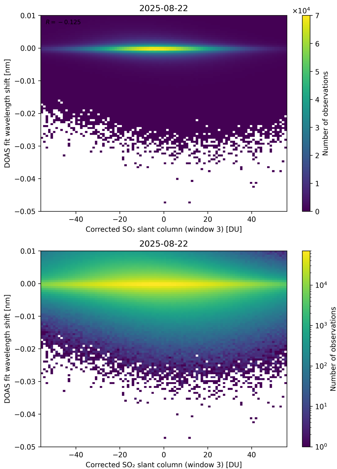
Figure 256: Scatter density plot of “Corrected SO 2 slant column (window 3)” against “DOAS fit wavelength shift” for 2025-08-21 to 2025-08-23.
