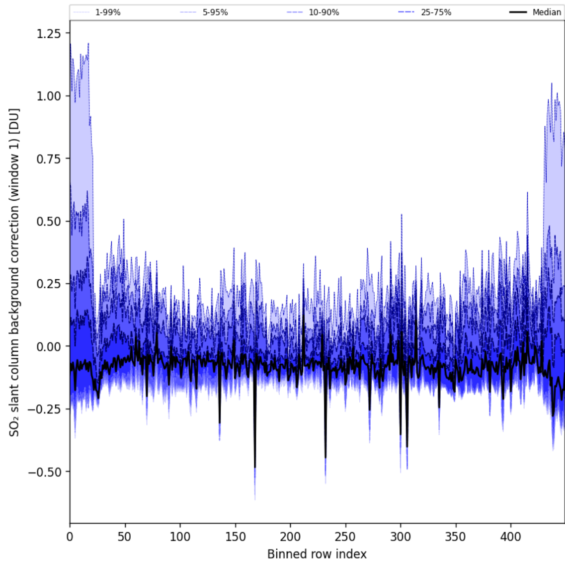
Figure 92: Along track statistics of “SO 2 slant column background correction (window 1)” for 2025-08-21 to 2025-08-23
