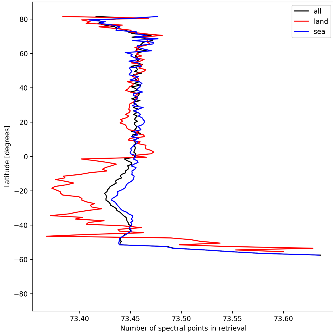
Figure 56: Zonal average of “Number of spectral points in retrieval” for 2025-08-21 to 2025-08-23.
