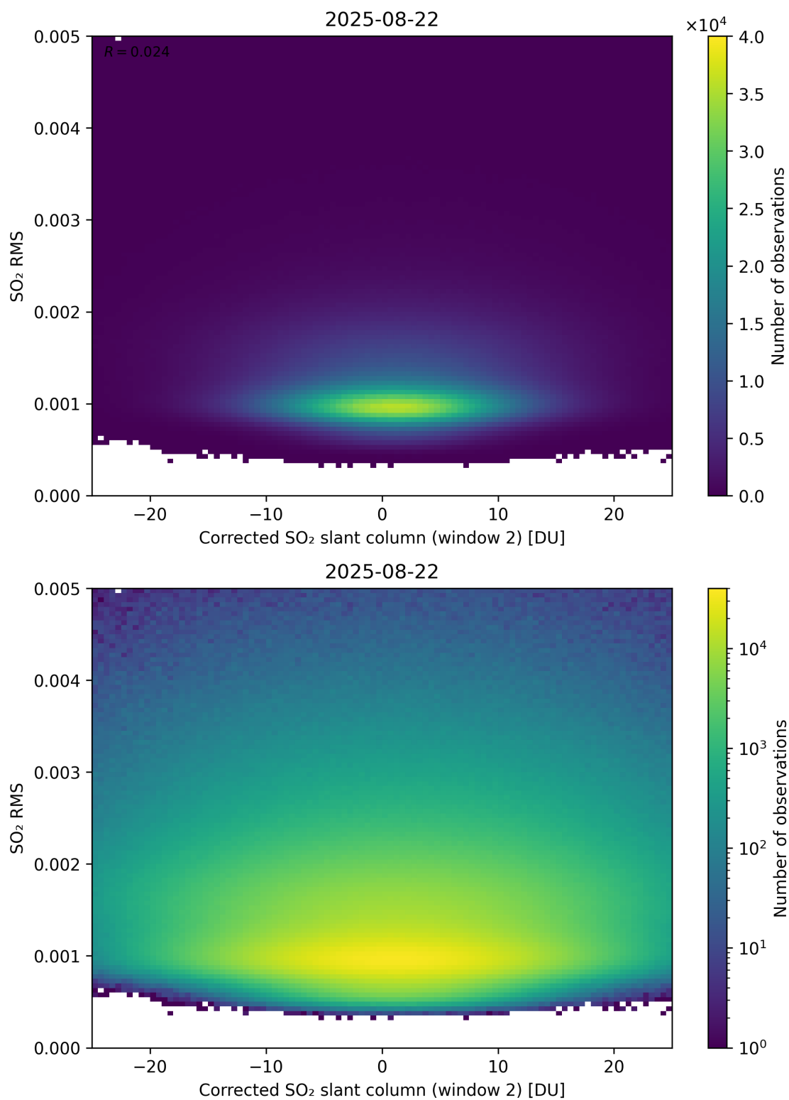
Figure 248: Scatter density plot of “Corrected SO 2 slant column (window 2)” against “SO 2 RMS” for 2025-08-21 to 2025-08-23.
