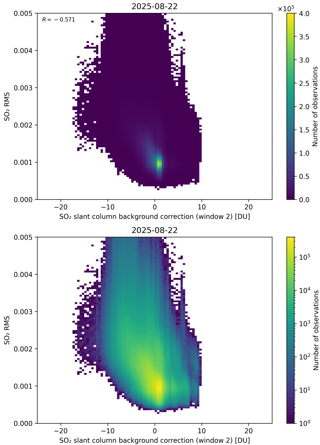
Figure 125: Scatter density plot of “SO 2 slant column background correction (window 2)” against “SO 2 RMS” for 2025-08-21 to 2025-08-23.
