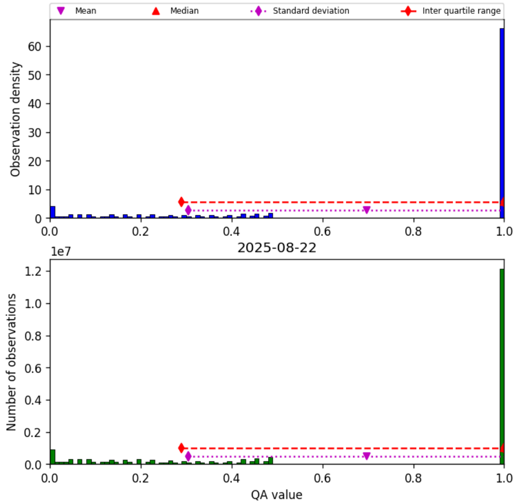
Figure 57: Histogram of “QA value” for 2025-08-21 to 2025-08-23
