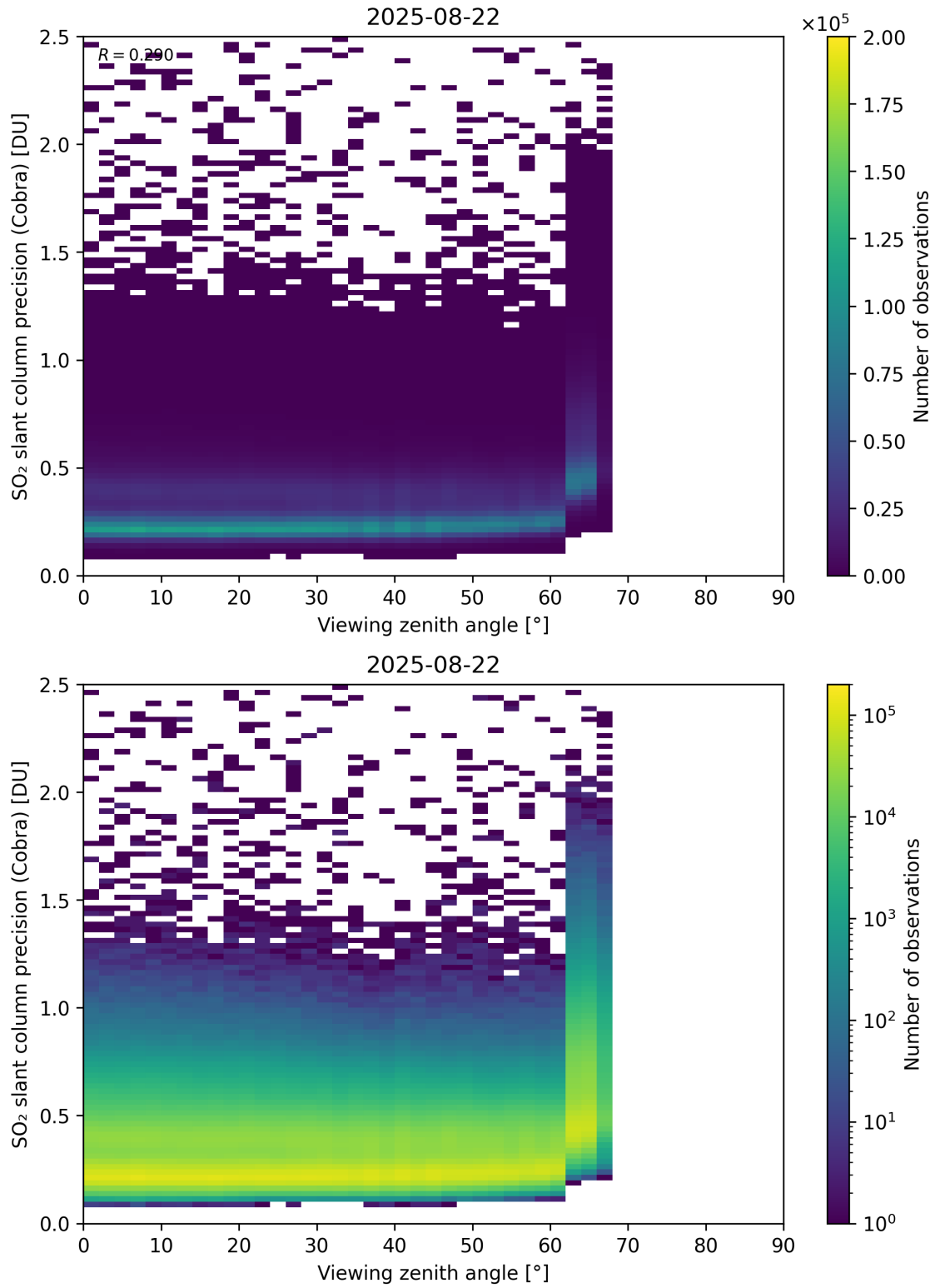
Figure 372: Scatter density plot of “Viewing zenith angle” against “SO 2 slant column precision (Cobra)” for 2025-08-21 to 2025-08-23.
