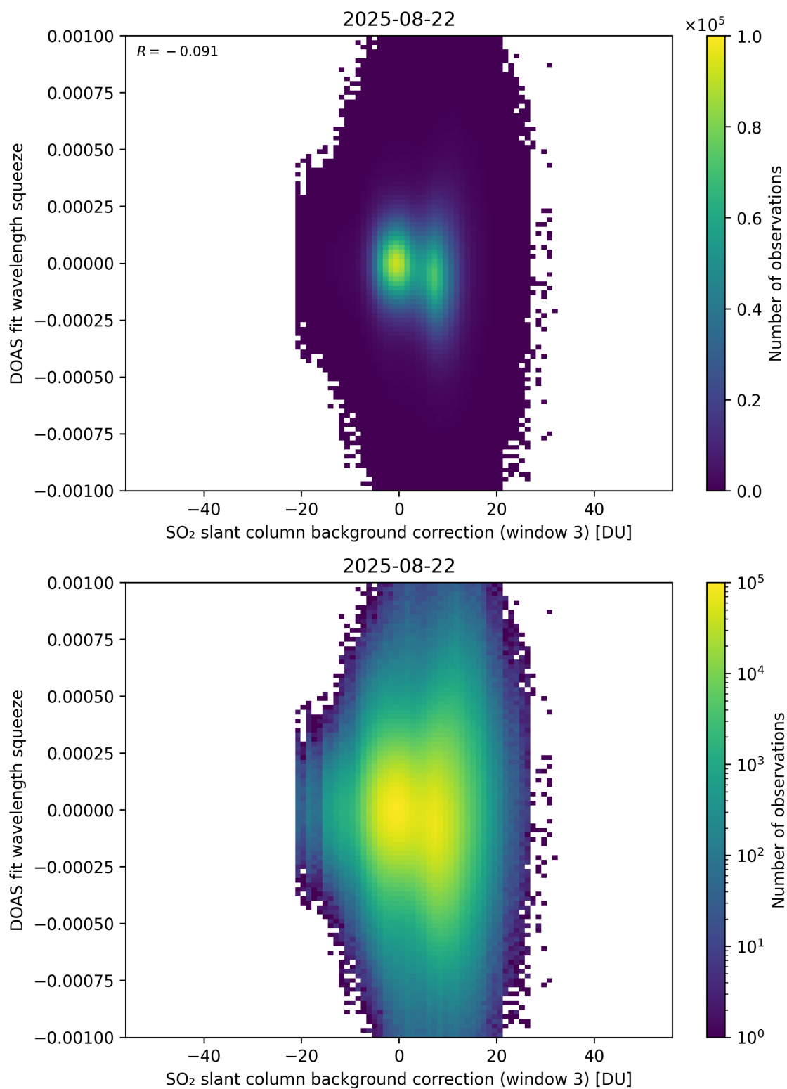
Figure 133: Scatter density plot of “SO 2 slant column background correction (window 3)” against “DOAS fit wavelength squeeze” for 2025-08-21 to 2025-08-23.
