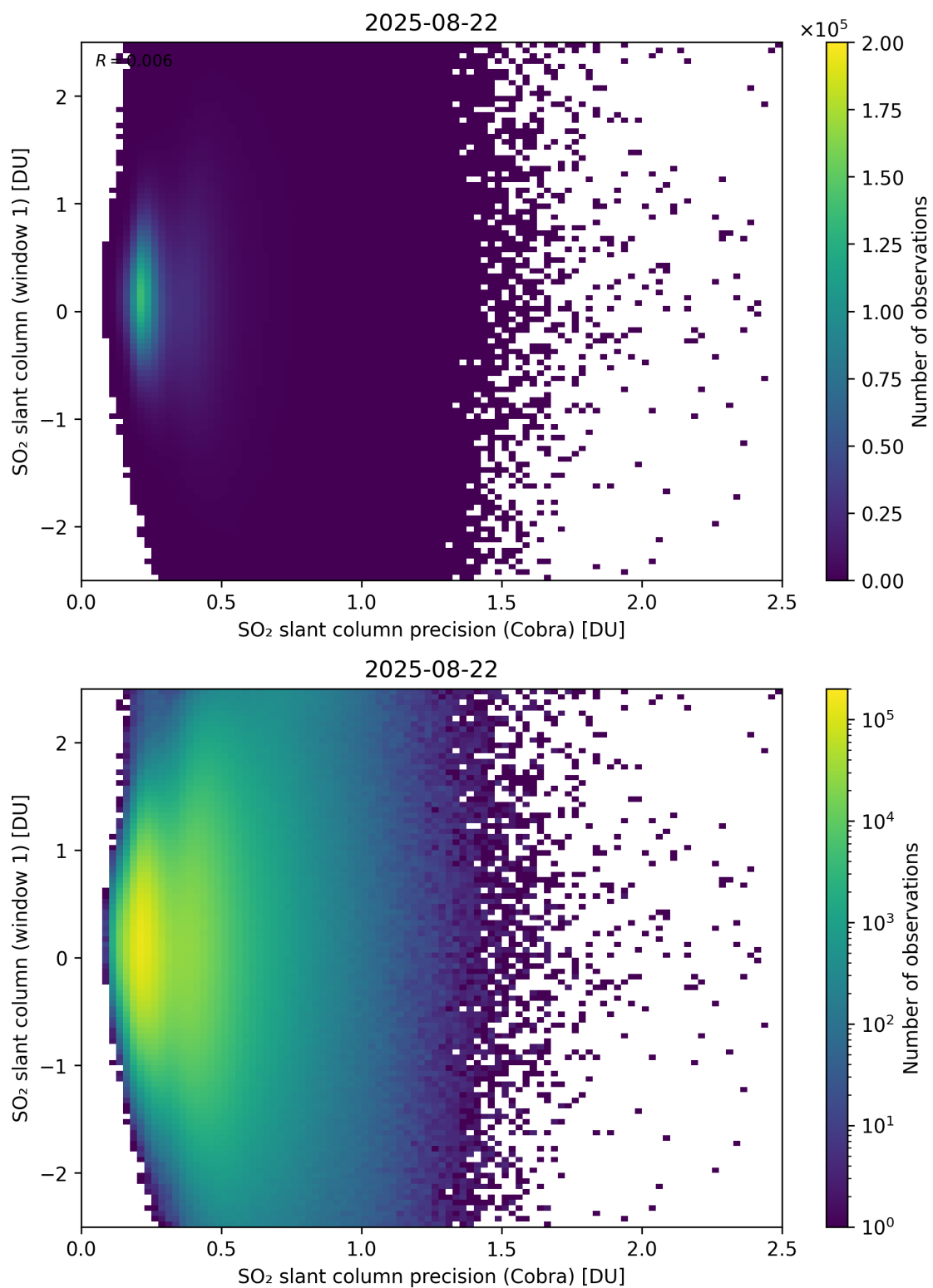
Figure 208: Scatter density plot of “SO 2 slant column precision (Cobra)” against “SO 2 slant column (window 1)” for 2025-08-21 to 2025-08-23.
