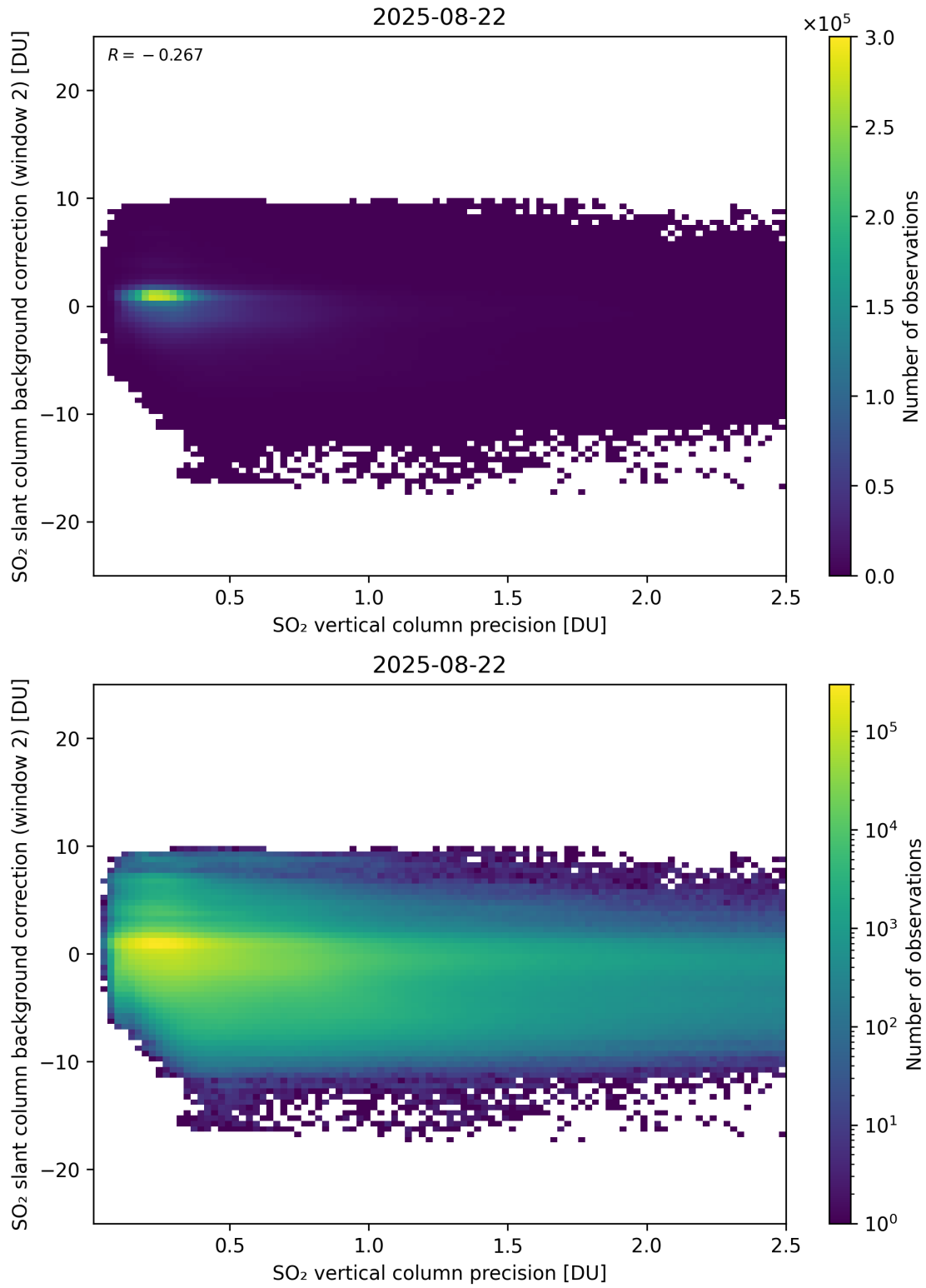
Figure 330: Scatter density plot of “SO 2 vertical column precision” against “SO 2 slant column background correction (window 2)” for 2025-08-21 to 2025-08-23.
