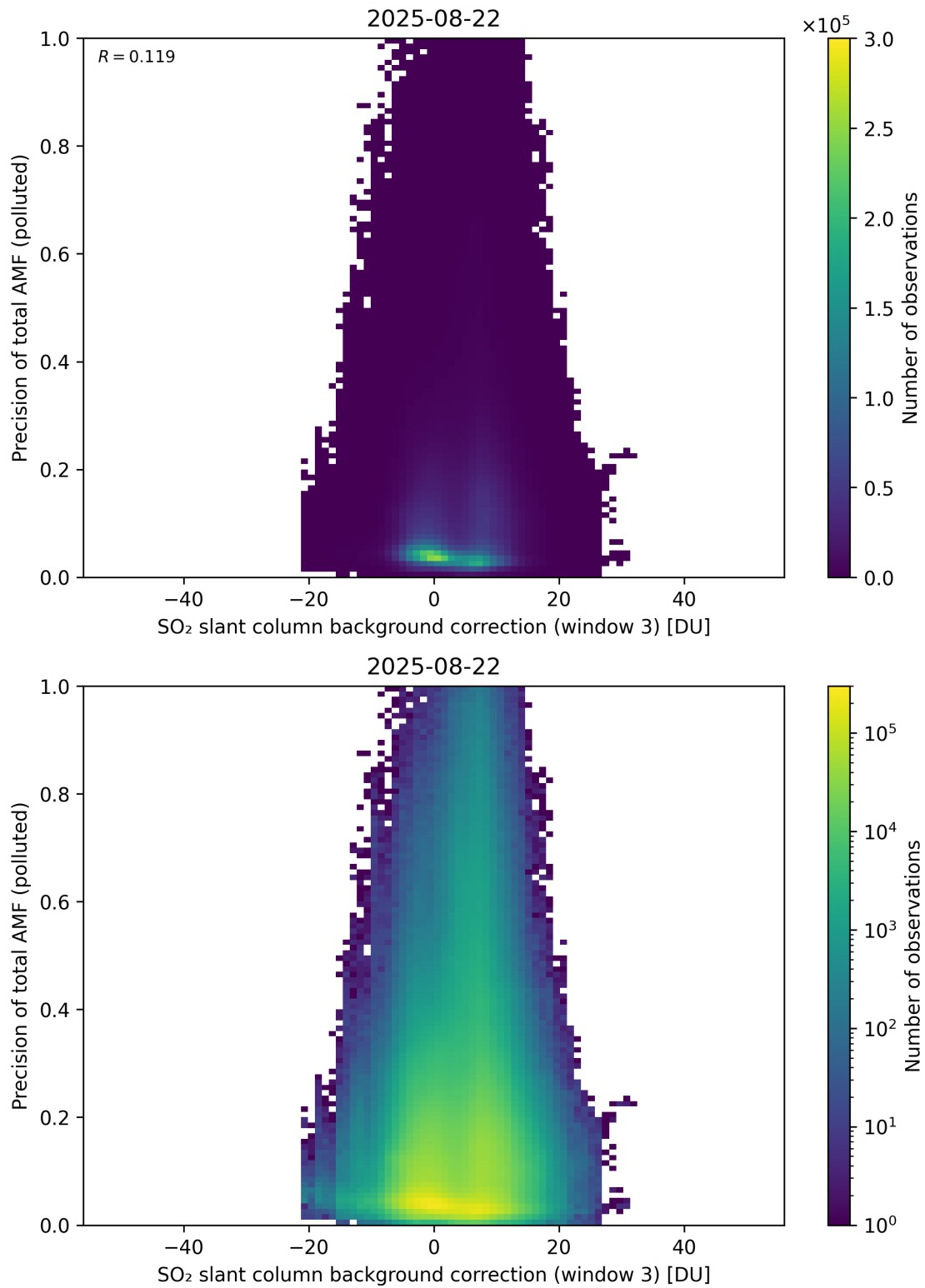
Figure 137: Scatter density plot of “SO 2 slant column background correction (window 3)” against “Precision of total AMF (polluted)” for 2025-08-21 to 2025-08-23.
