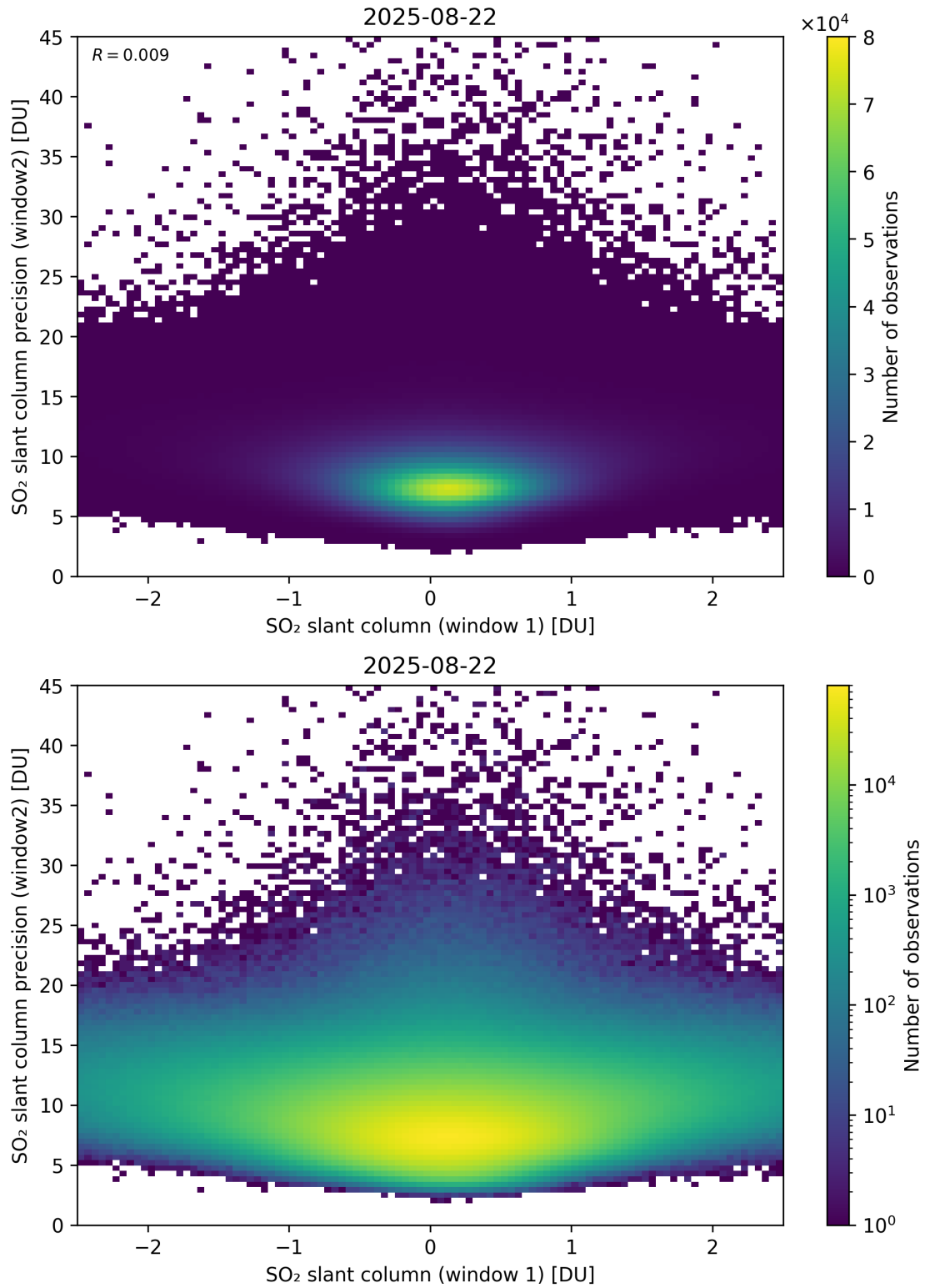
Figure 286: Scatter density plot of “SO 2 slant column (window 1)” against “SO 2 slant column precision (window2)” for 2025-08-21 to 2025-08-23.
