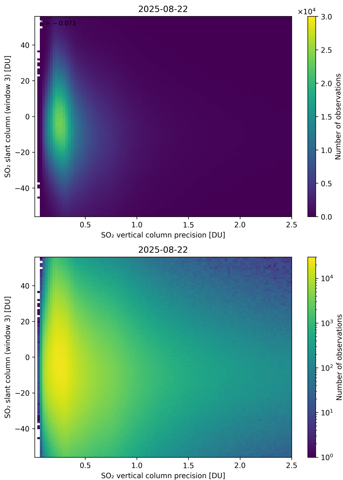
Figure 344: Scatter density plot of “SO 2 vertical column precision” against “SO 2 slant column (window 3)” for 2025-08-21 to 2025-08-23.
