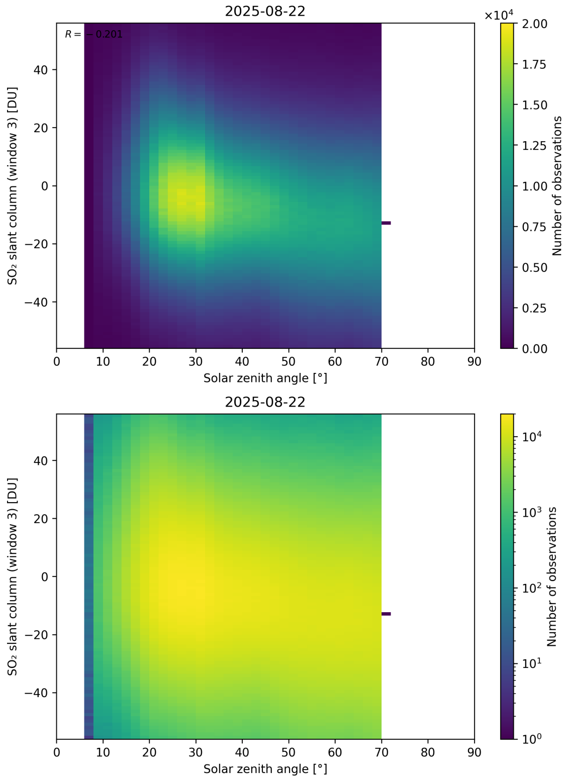
Figure 187: Scatter density plot of “Solar zenith angle” against “SO 2 slant column (window 3)” for 2025-08-21 to 2025-08-23.
