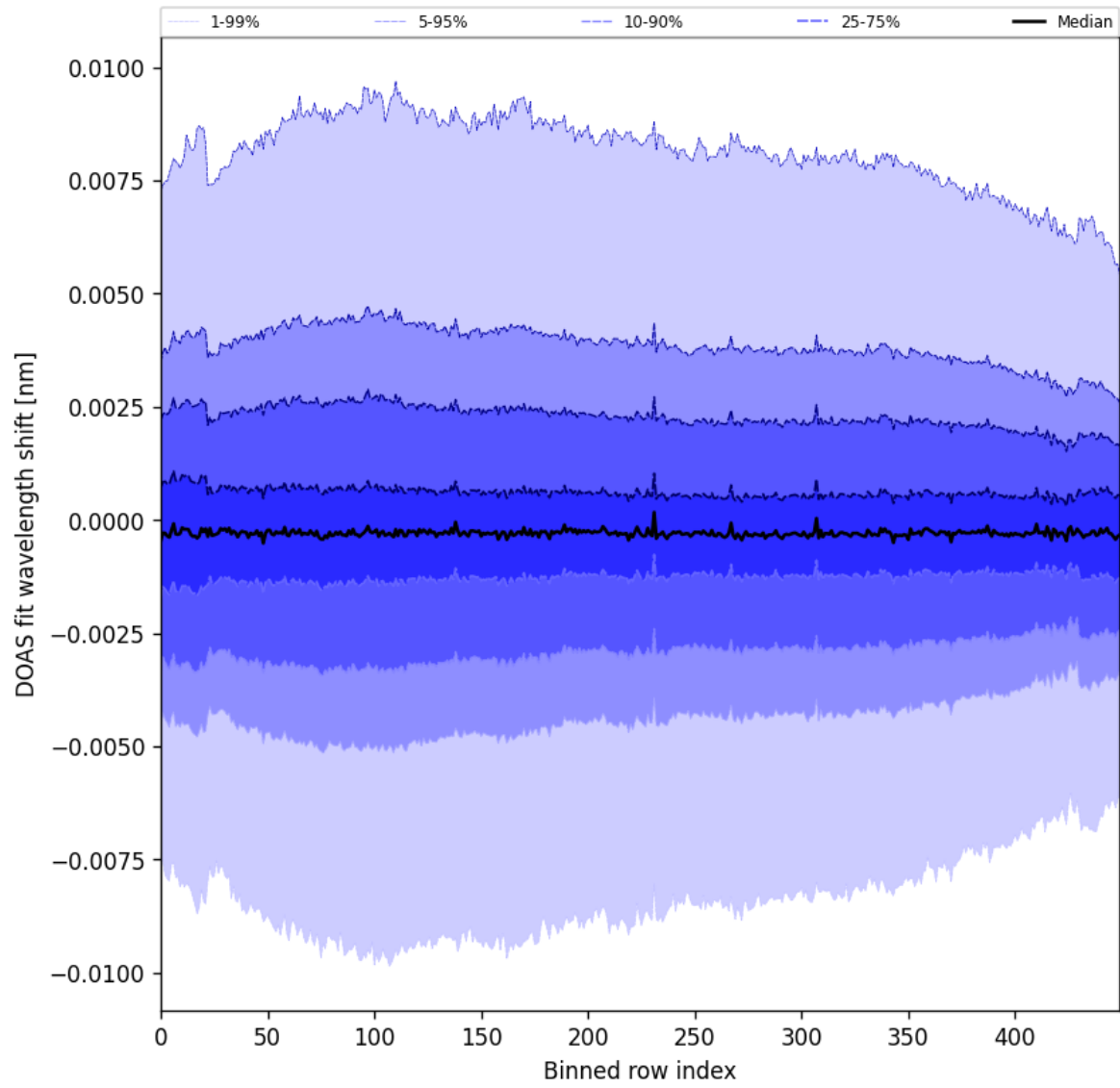
Figure 102: Along track statistics of “DOAS fit wavelength shift” for 2025-08-21 to 2025-08-23
