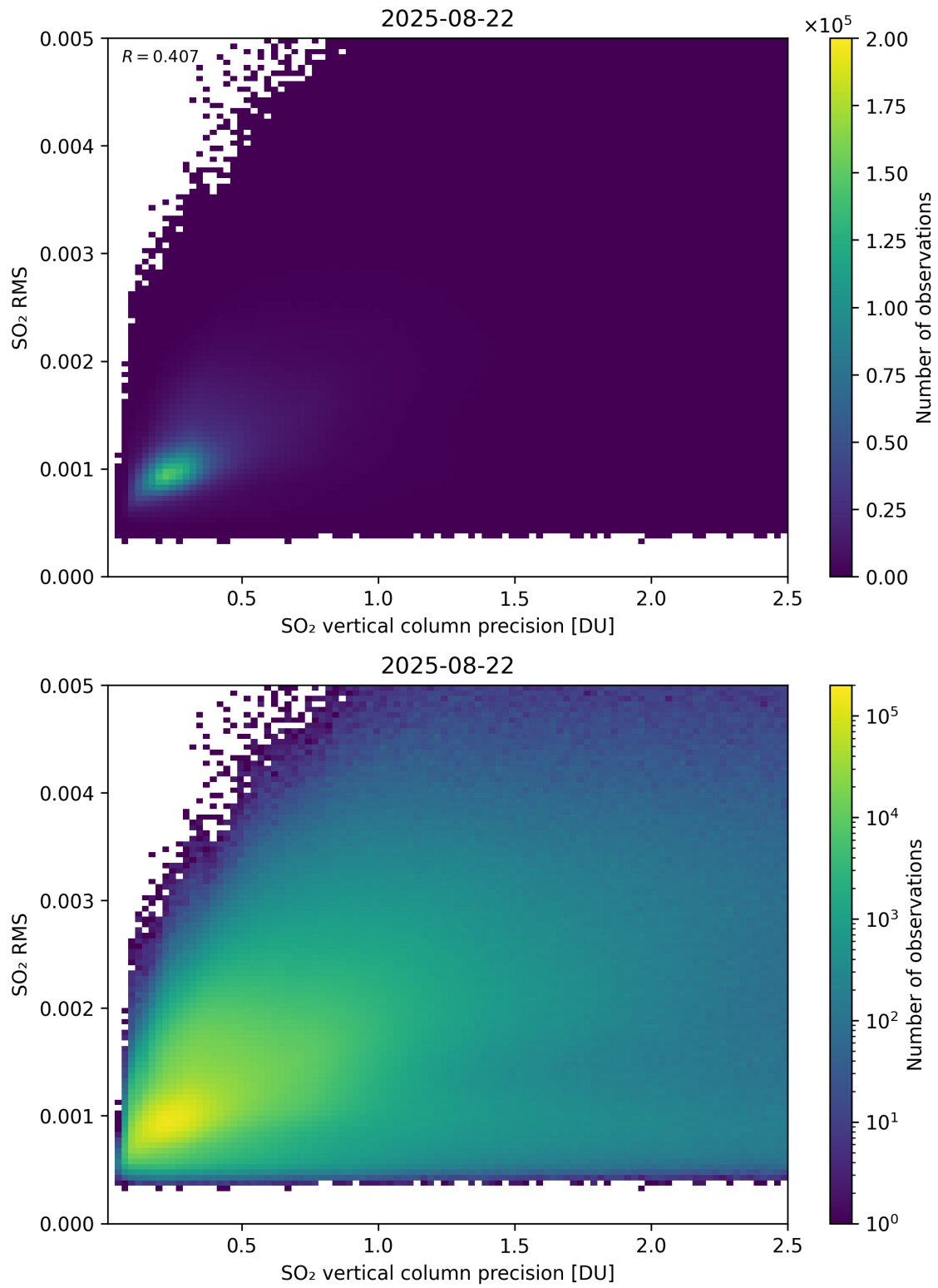
Figure 334: Scatter density plot of “SO 2 vertical column precision” against “SO 2 RMS” for 2025-08-21 to 2025-08-23.
