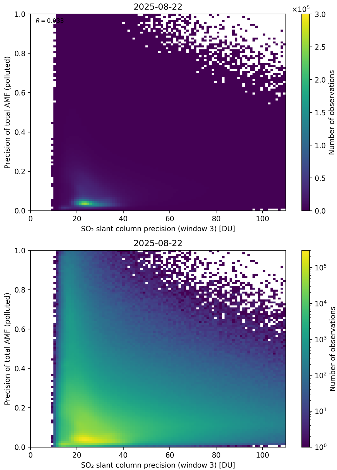
Figure 314: Scatter density plot of “SO 2 slant column precision (window 3)” against “Precision of total AMF (polluted)” for 2025-08-21 to 2025-08-23.
