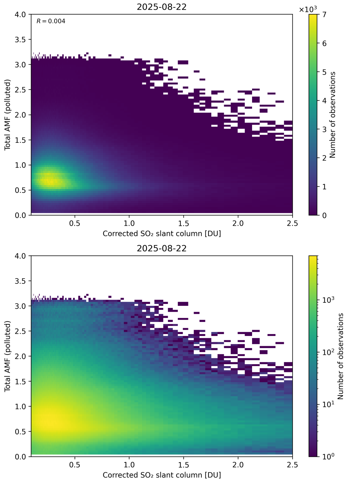
Figure 242: Scatter density plot of “Corrected SO 2 slant column” against “Total AMF (polluted)” for 2025-08-21 to 2025-08-23.
