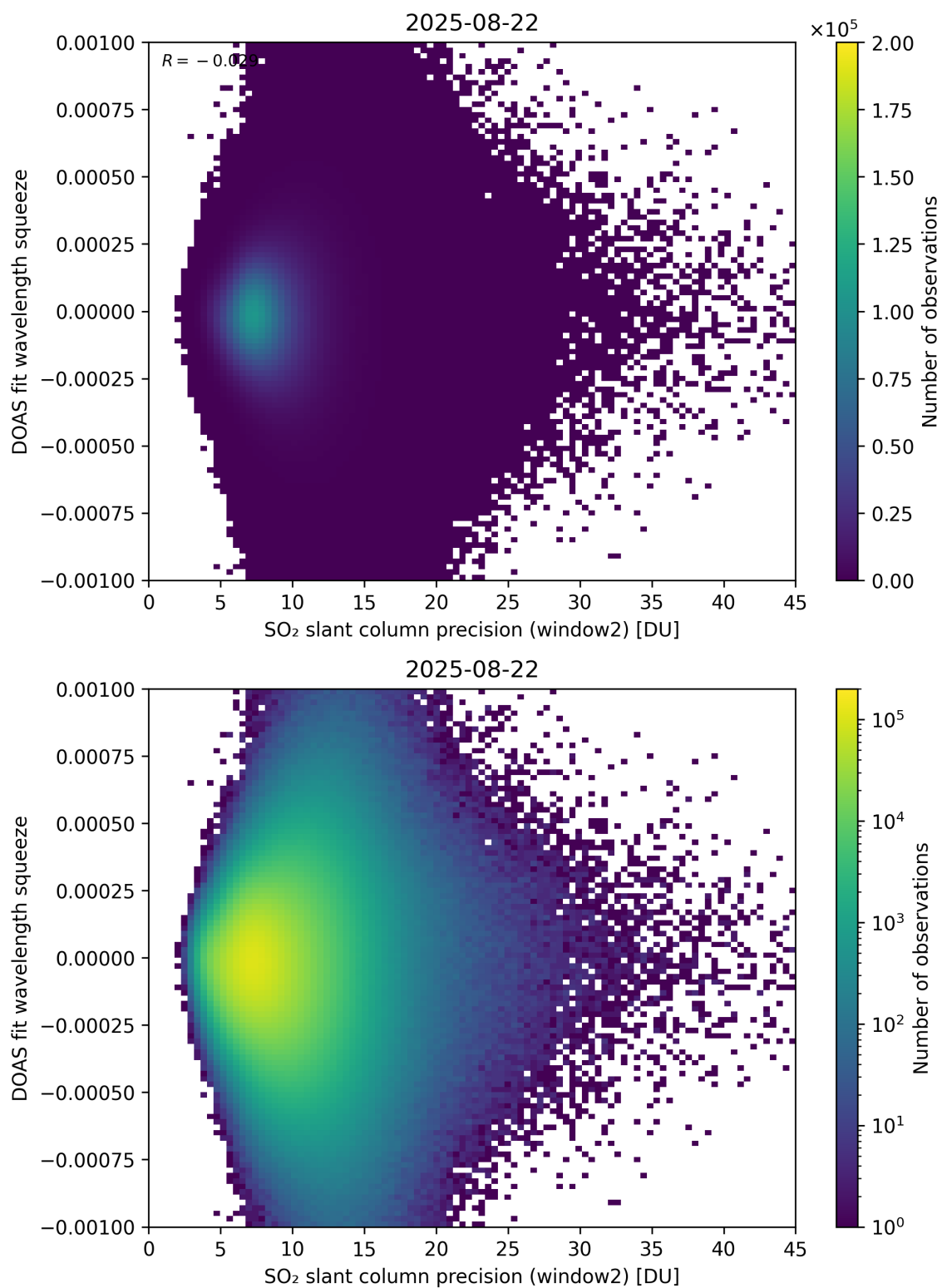
Figure 294: Scatter density plot of “SO 2 slant column precision (window2)” against “DOAS fit wavelength squeeze” for 2025-08-21 to 2025-08-23.
