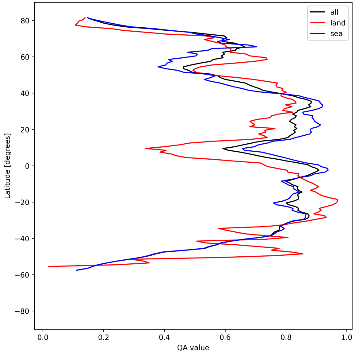
Figure 31: Zonal average of “QA value” for 2025-08-21 to 2025-08-23.
