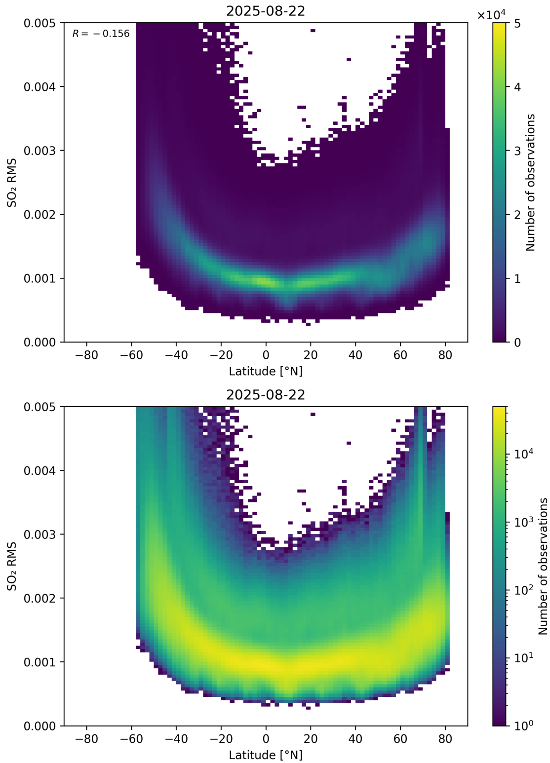
Figure 155: Scatter density plot of “Latitude” against “SO 2 RMS” for 2025-08-21 to 2025-08-23.
