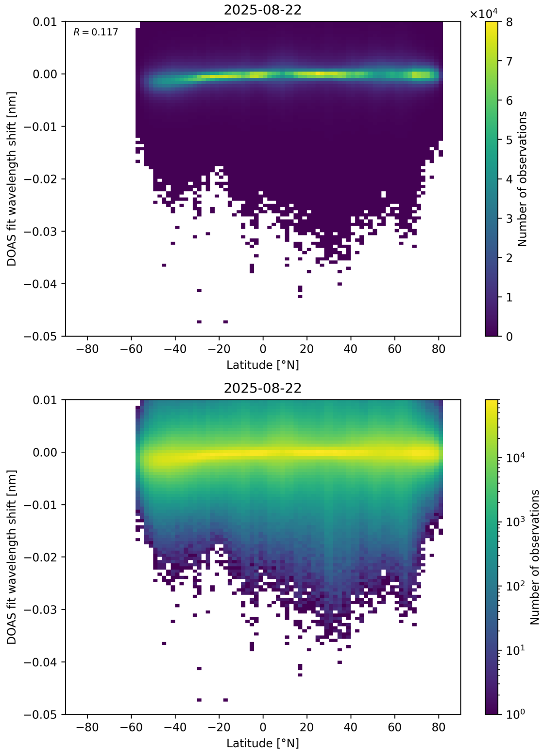
Figure 153: Scatter density plot of “Latitude” against “DOAS fit wavelength shift” for 2025-08-21 to 2025-08-23.
