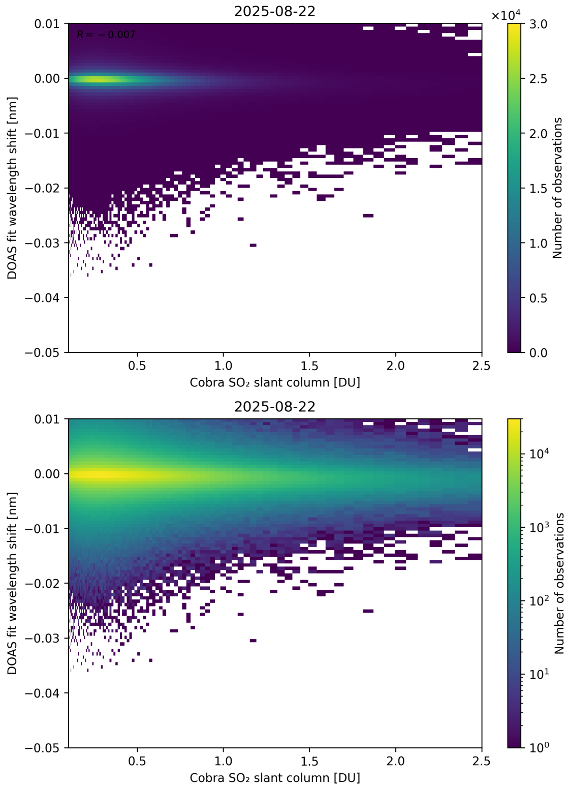
Figure 196: Scatter density plot of “Cobra SO 2 slant column” against “DOAS fit wavelength shift” for 2025-08-21 to 2025-08-23.
