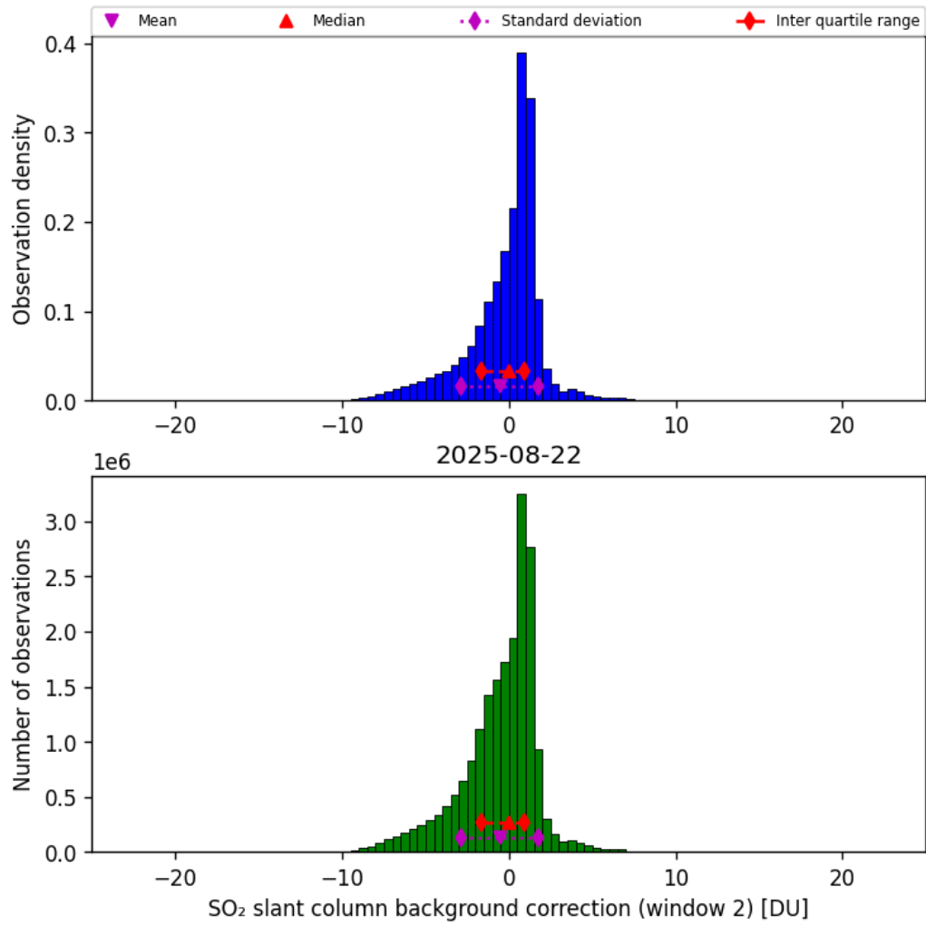
Figure 70: Histogram of “SO 2 slant column background correction (window 2)” for 2025-08-21 to 2025-08-23
