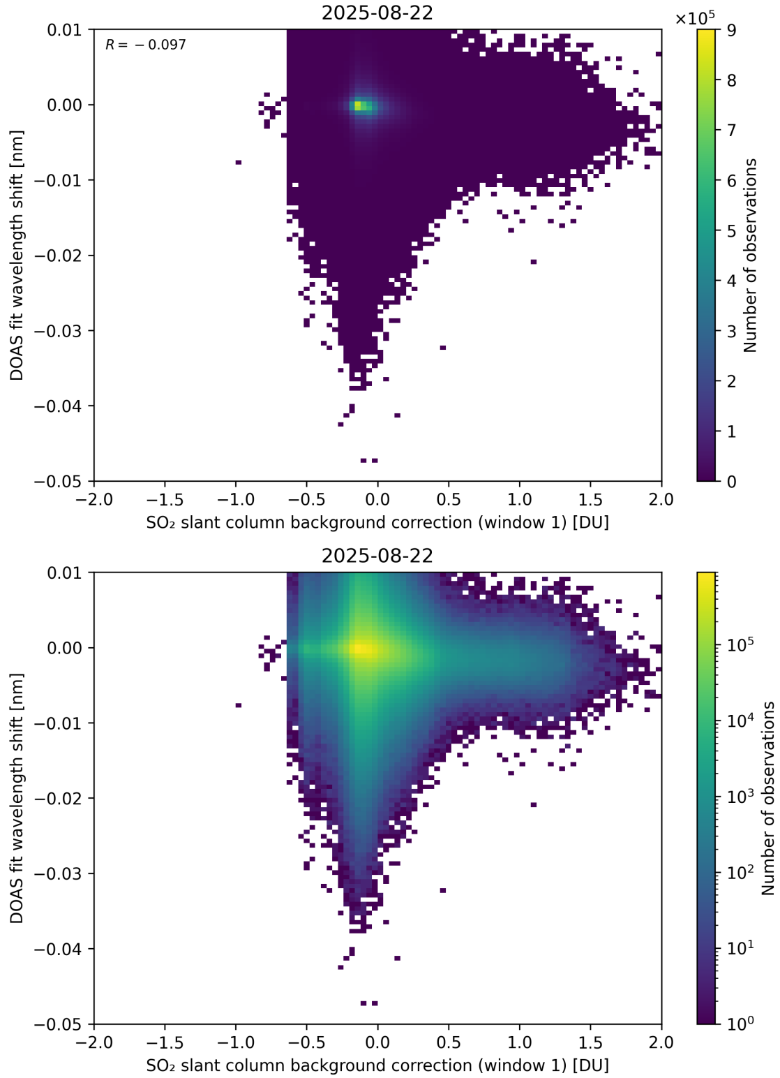
Figure 111: Scatter density plot of “SO 2 slant column background correction (window 1)” against “DOAS fit wavelength shift” for 2025-08-21 to 2025-08-23.
