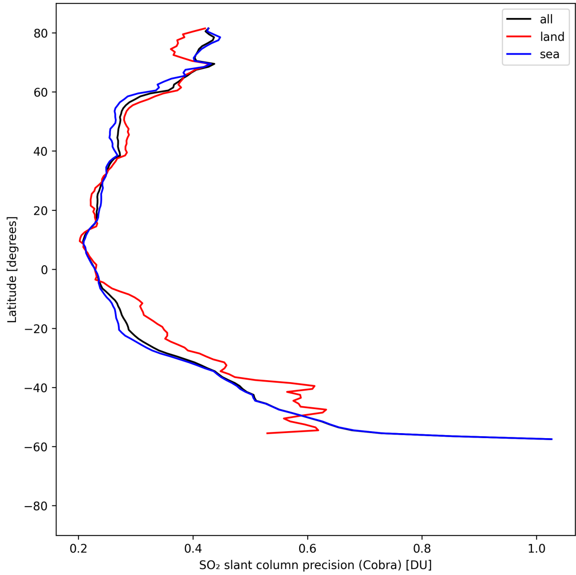
Figure 36: Zonal average of “SO 2 slant column precision (Cobra)” for 2025-08-21 to 2025-08-23.
