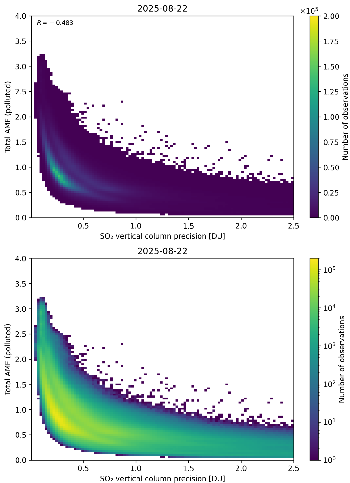
Figure 346: Scatter density plot of “SO 2 vertical column precision” against “Total AMF (polluted)” for 2025-08-21 to 2025-08-23.
