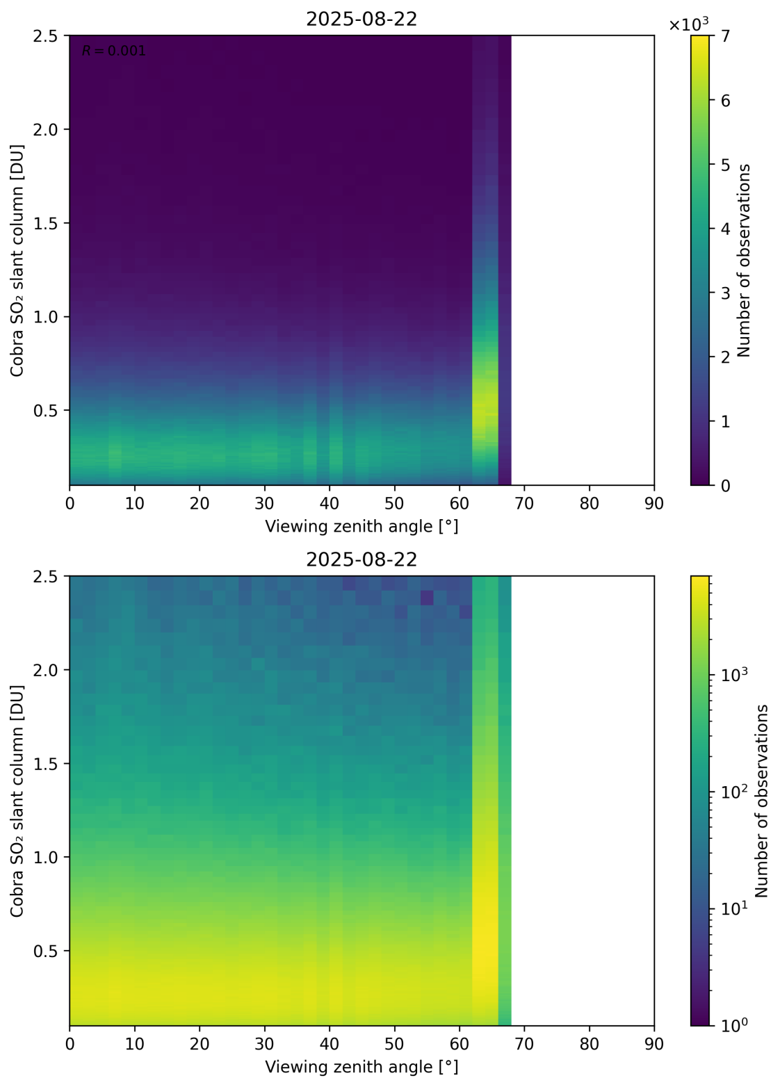
Figure 371: Scatter density plot of “Viewing zenith angle” against “Cobra SO 2 slant column” for 2025-08-21 to 2025-08-23.
