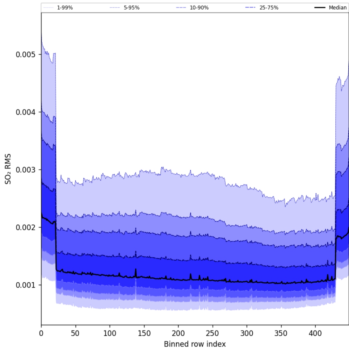
Figure 104: Along track statistics of “SO 2 RMS” for 2025-08-21 to 2025-08-23
