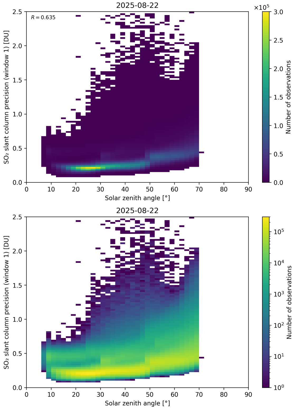
Figure 185: Scatter density plot of “Solar zenith angle” against “SO 2 slant column precision (window 1)” for 2025-08-21 to 2025-08-23.
