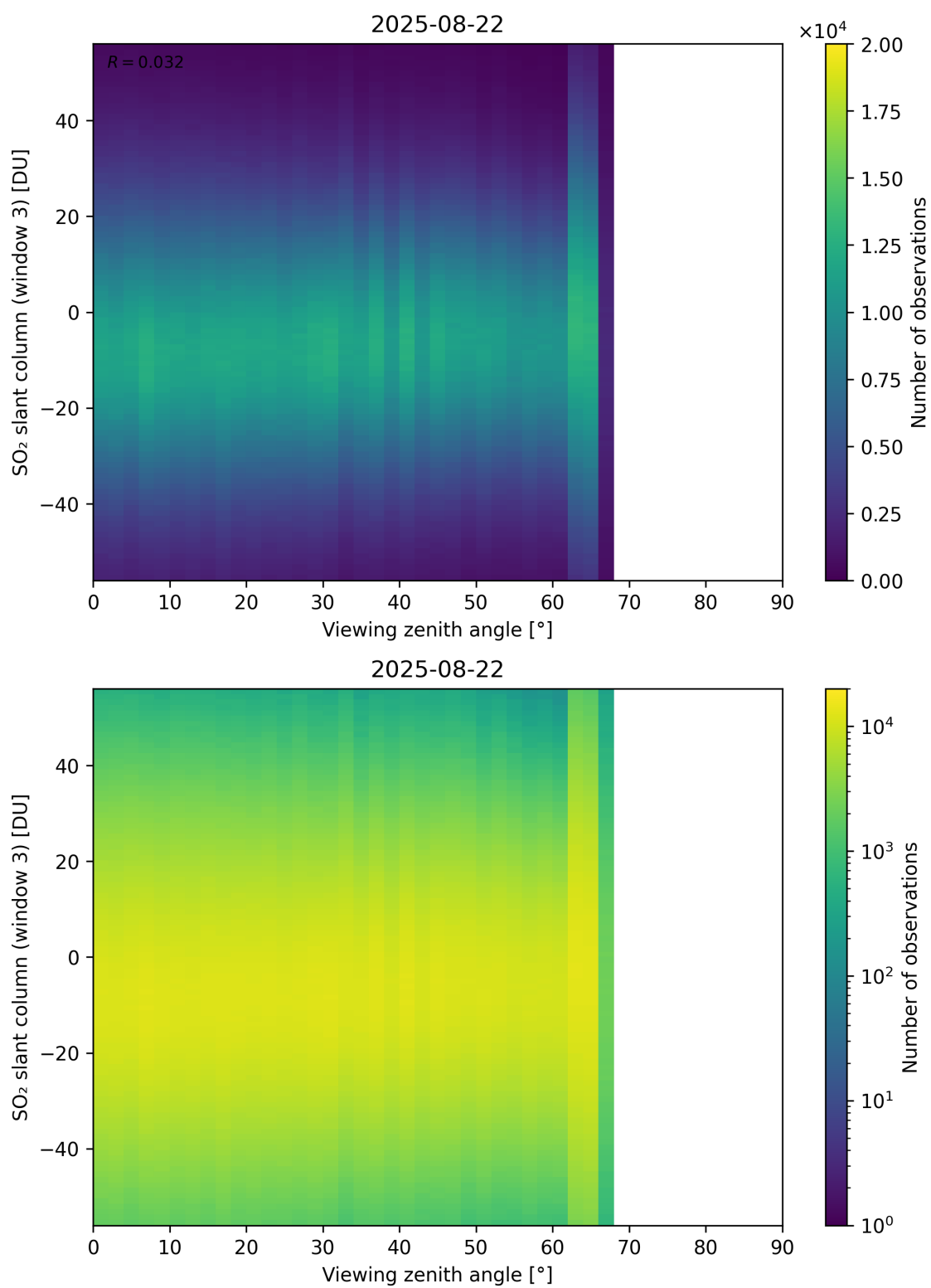
Figure 379: Scatter density plot of “Viewing zenith angle” against “SO 2 slant column (window 3)” for 2025-08-21 to 2025-08-23.
