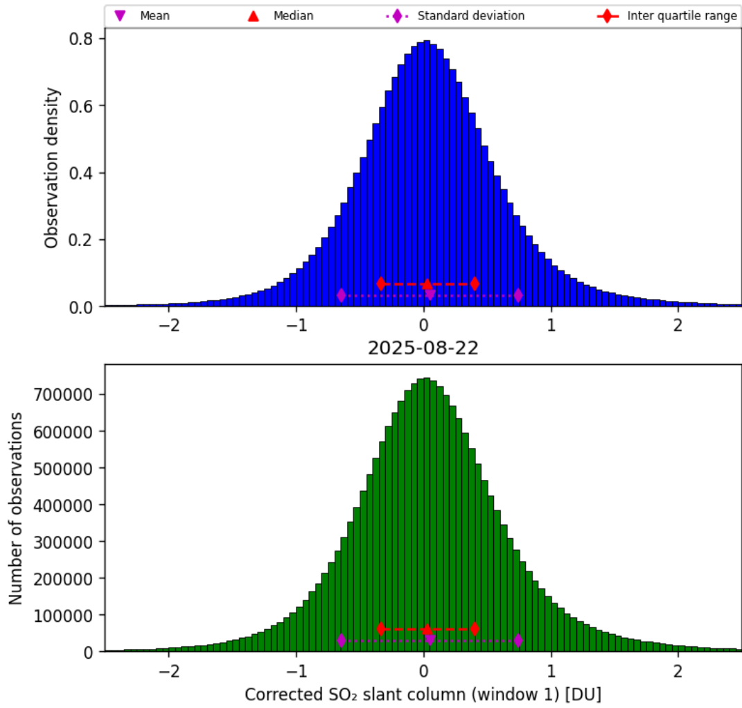
Figure 65: Histogram of “Corrected SO 2 slant column (window 1)” for 2025-08-21 to 2025-08-23
