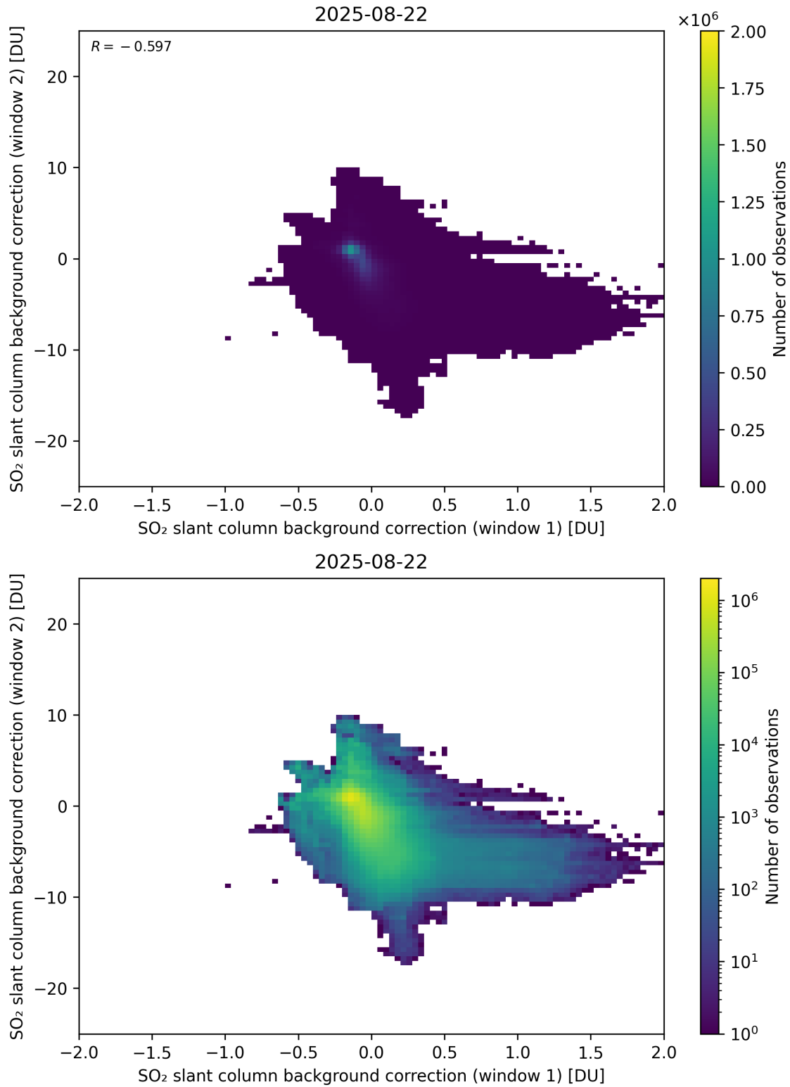
Figure 109: Scatter density plot of “SO 2 slant column background correction (window 1)” against “SO 2 slant column background correction (window 2)” for 2025-08-21 to 2025-08-23.
