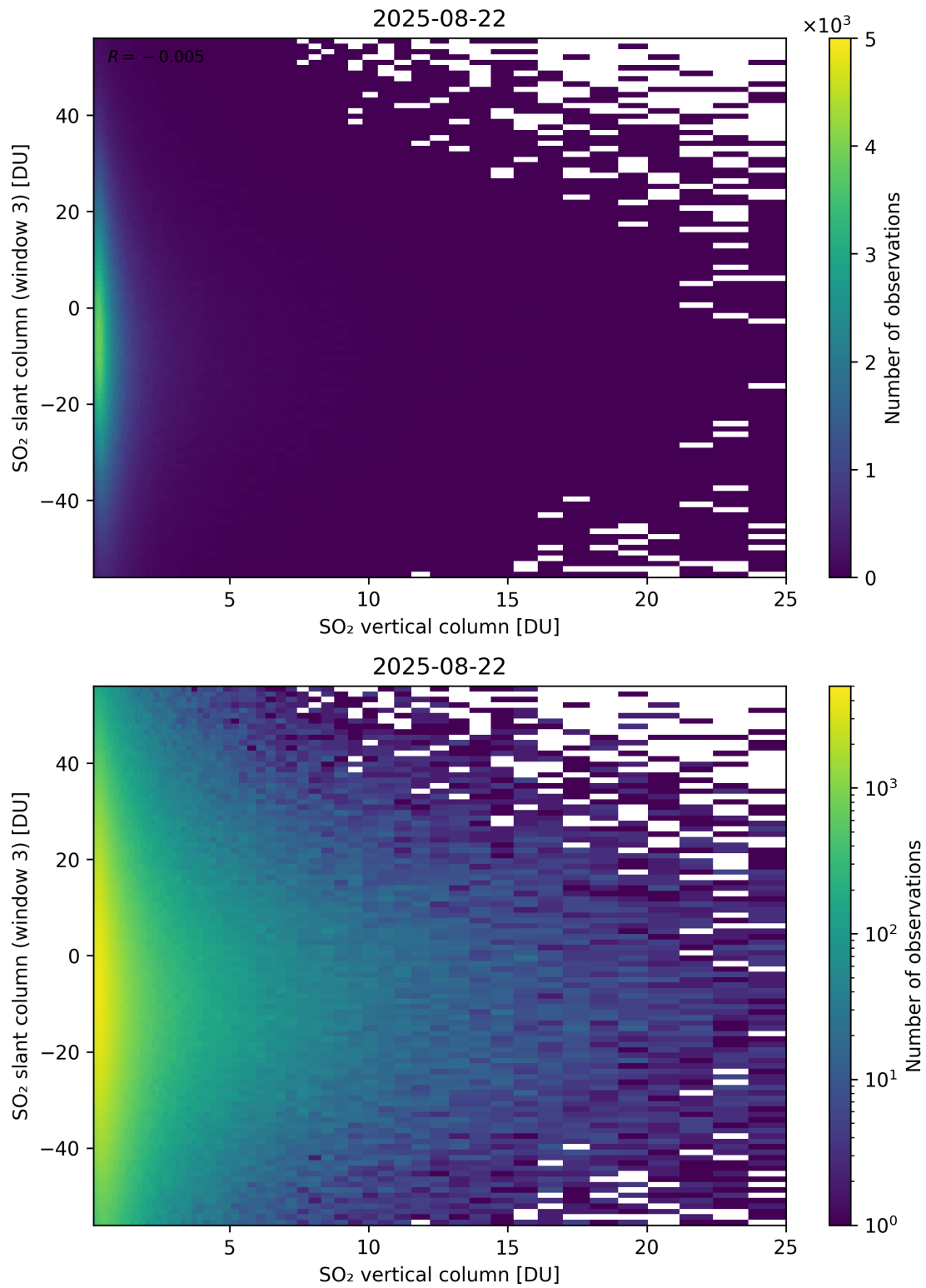
Figure 357: Scatter density plot of “SO 2 vertical column” against “SO 2 slant column (window 3)” for 2025-08-21 to 2025-08-23.
