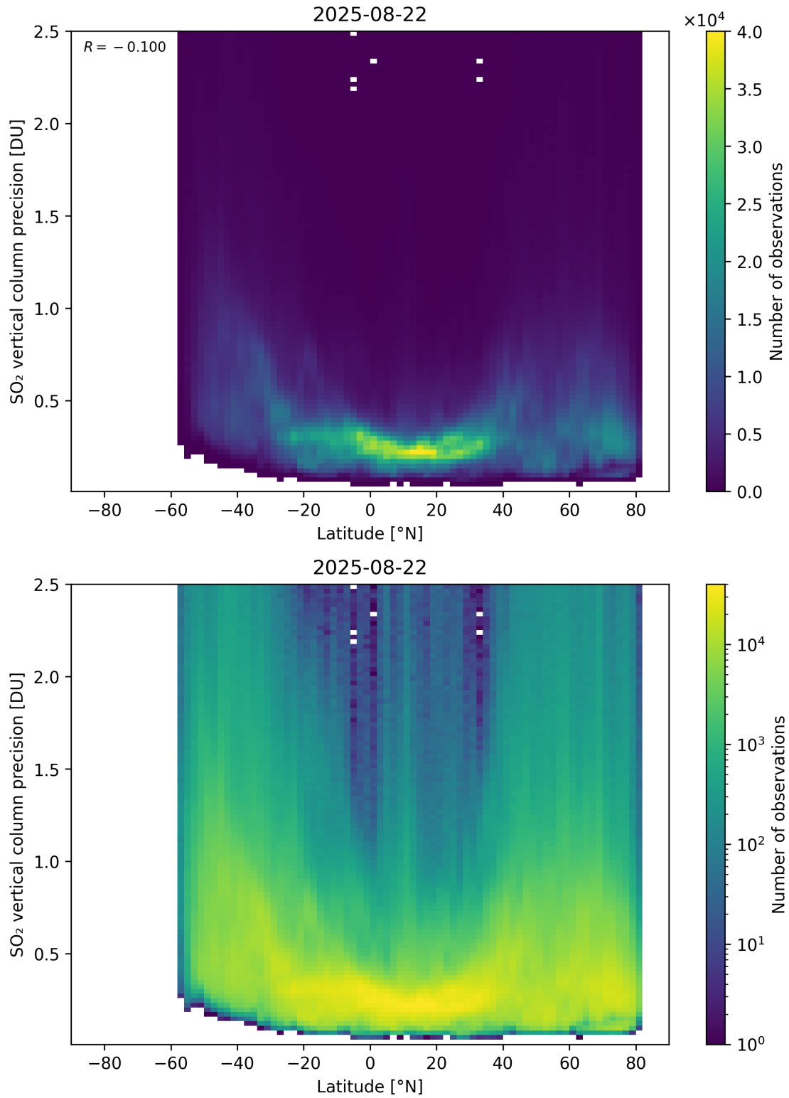
Figure 170: Scatter density plot of “Latitude” against “SO 2 vertical column precision” for 2025-08-21 to 2025-08-23.
