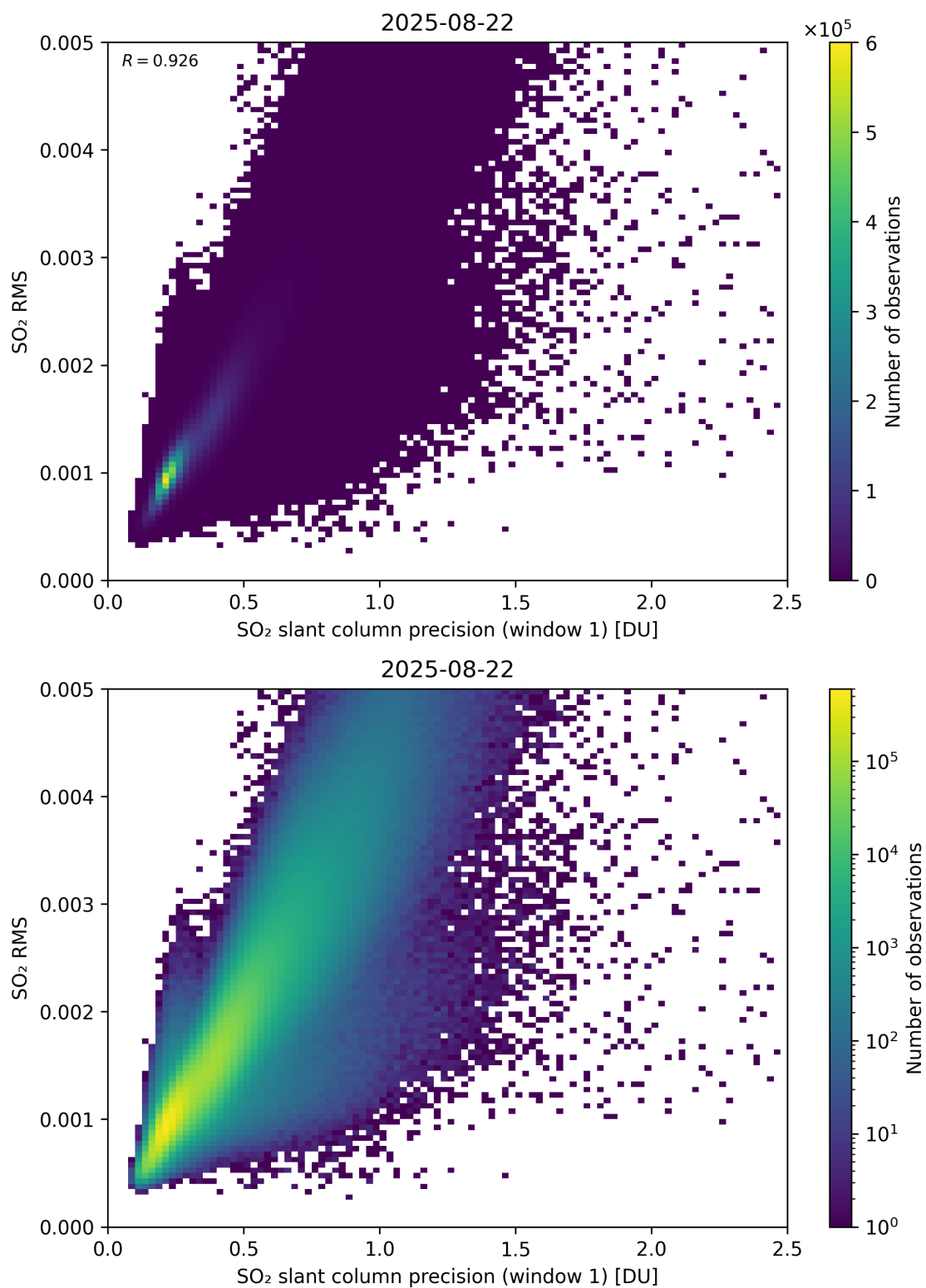
Figure 273: Scatter density plot of “SO 2 slant column precision (window 1)” against “SO 2 RMS” for 2025-08-21 to 2025-08-23.
