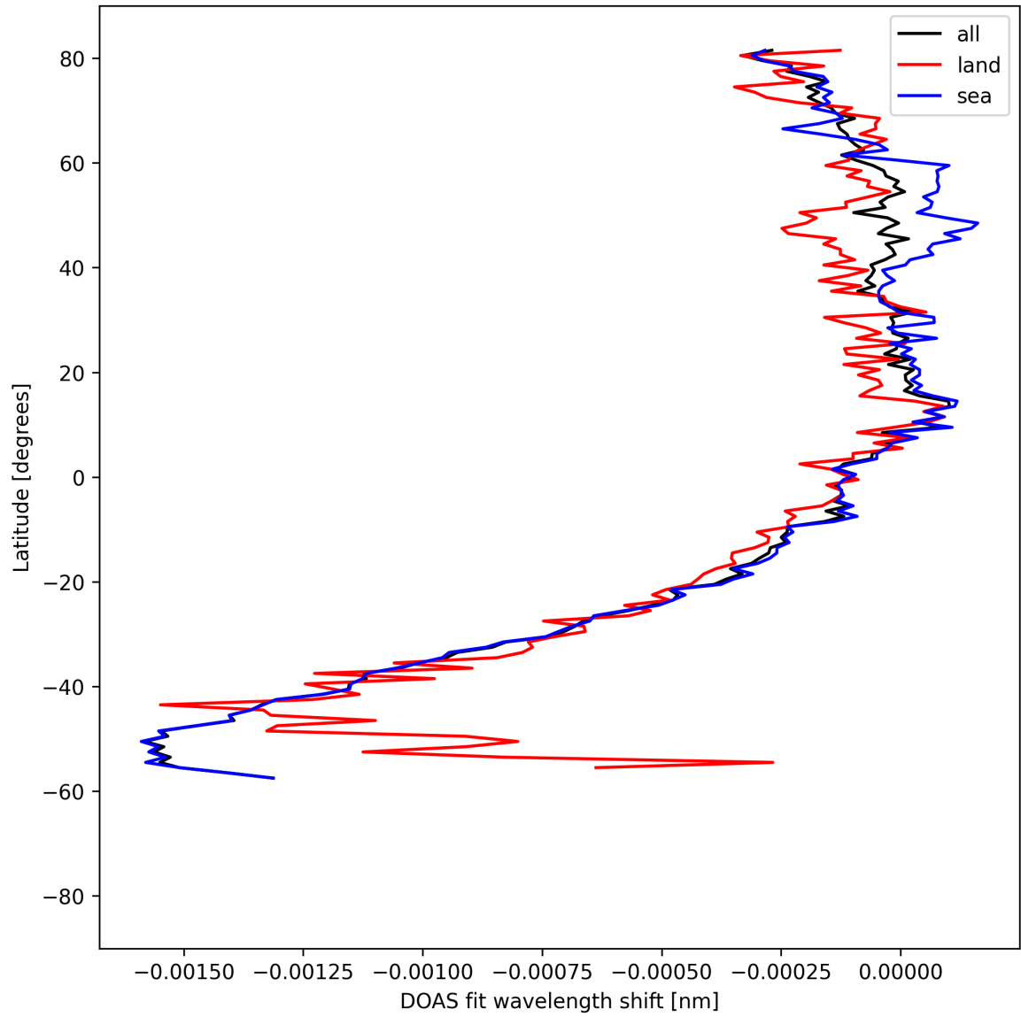
Figure 50: Zonal average of "DOAS fit wavelength shift" for 2025-08-21 to 2025-08-23.
