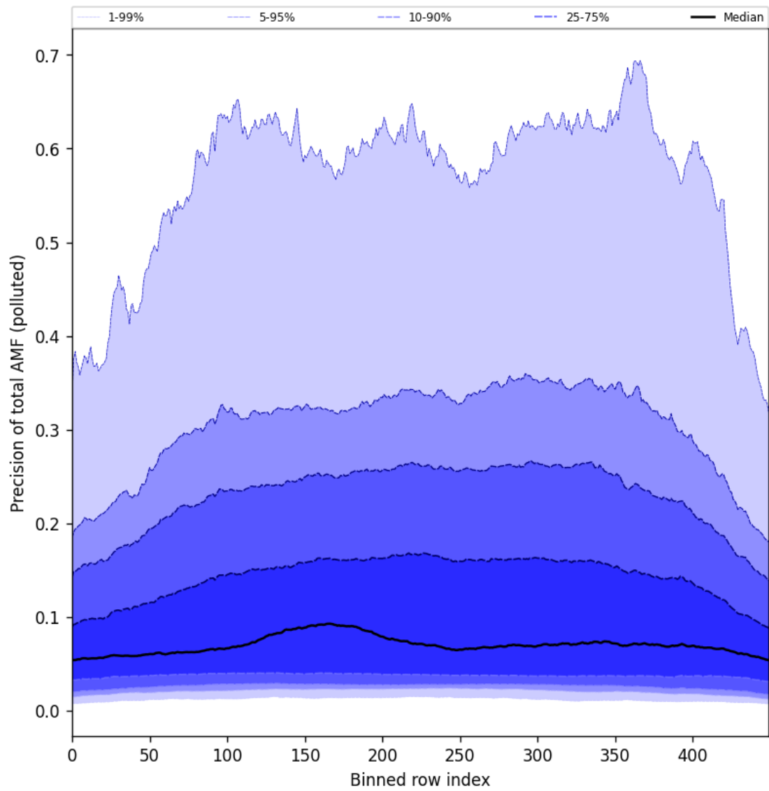
Figure 106: Along track statistics of “Precision of total AMF (polluted)” for 2025-08-21 to 2025-08-23
