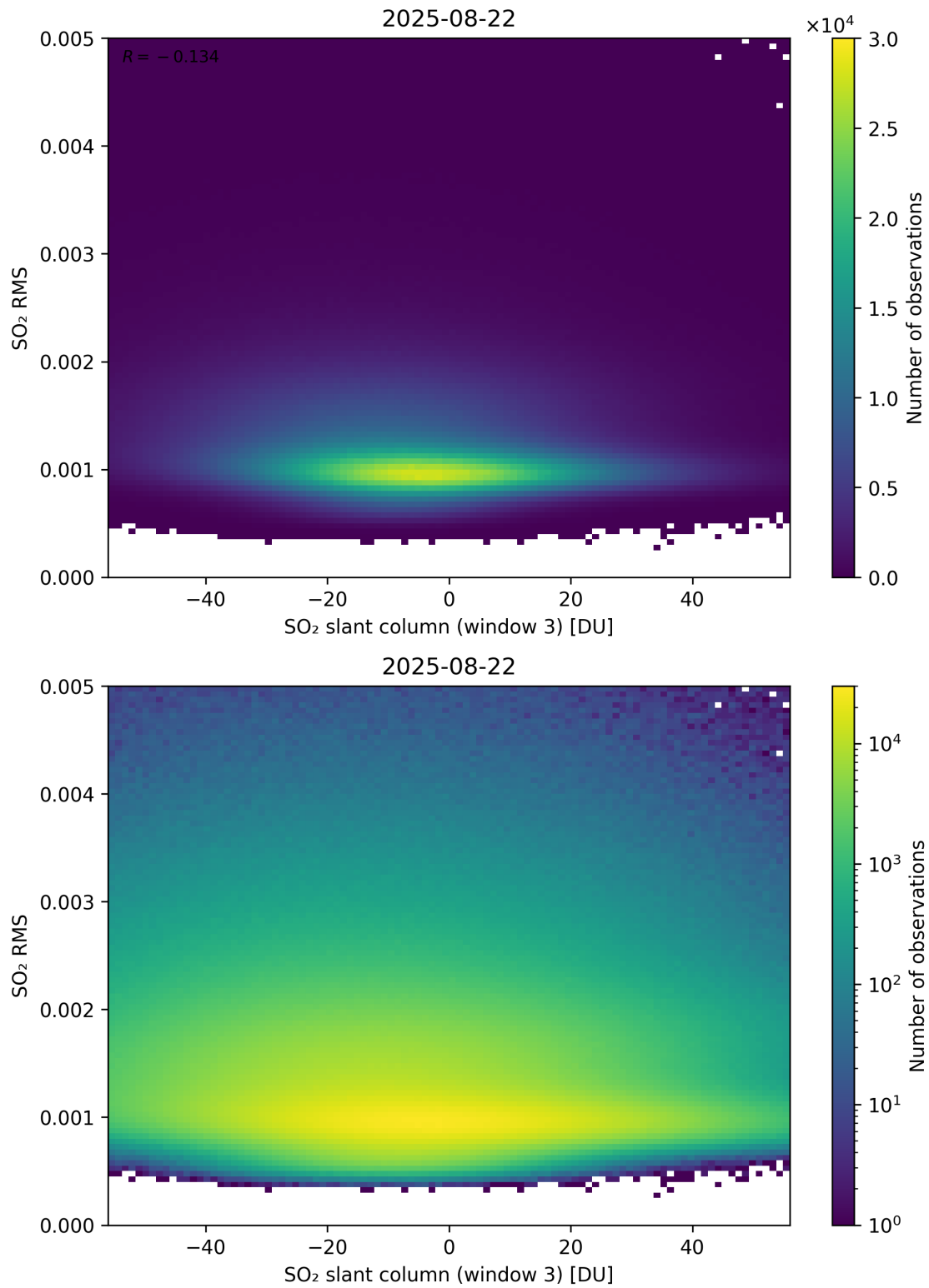
Figure 306: Scatter density plot of “SO 2 slant column (window 3)” against “SO 2 RMS” for 2025-08-21 to 2025-08-23.
