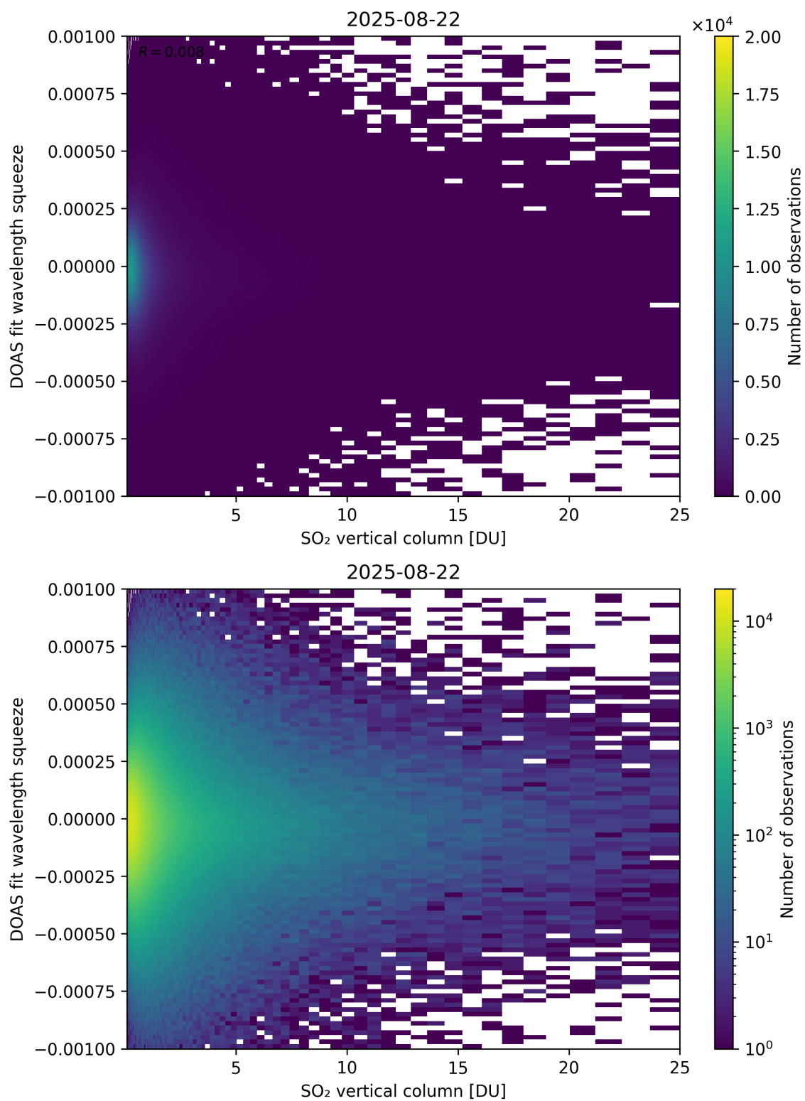
Figure 327: Scatter density plot of “SO 2 vertical column” against “DOAS fit wavelength squeeze” for 2025-08-21 to 2025-08-23.
