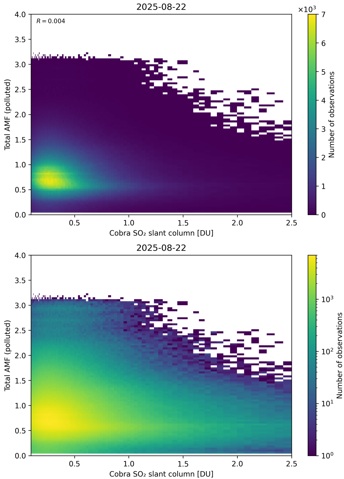
Figure 224: Scatter density plot of “Cobra SO 2 slant column” against “Total AMF (polluted)” for 2025-08-21 to 2025-08-23.
