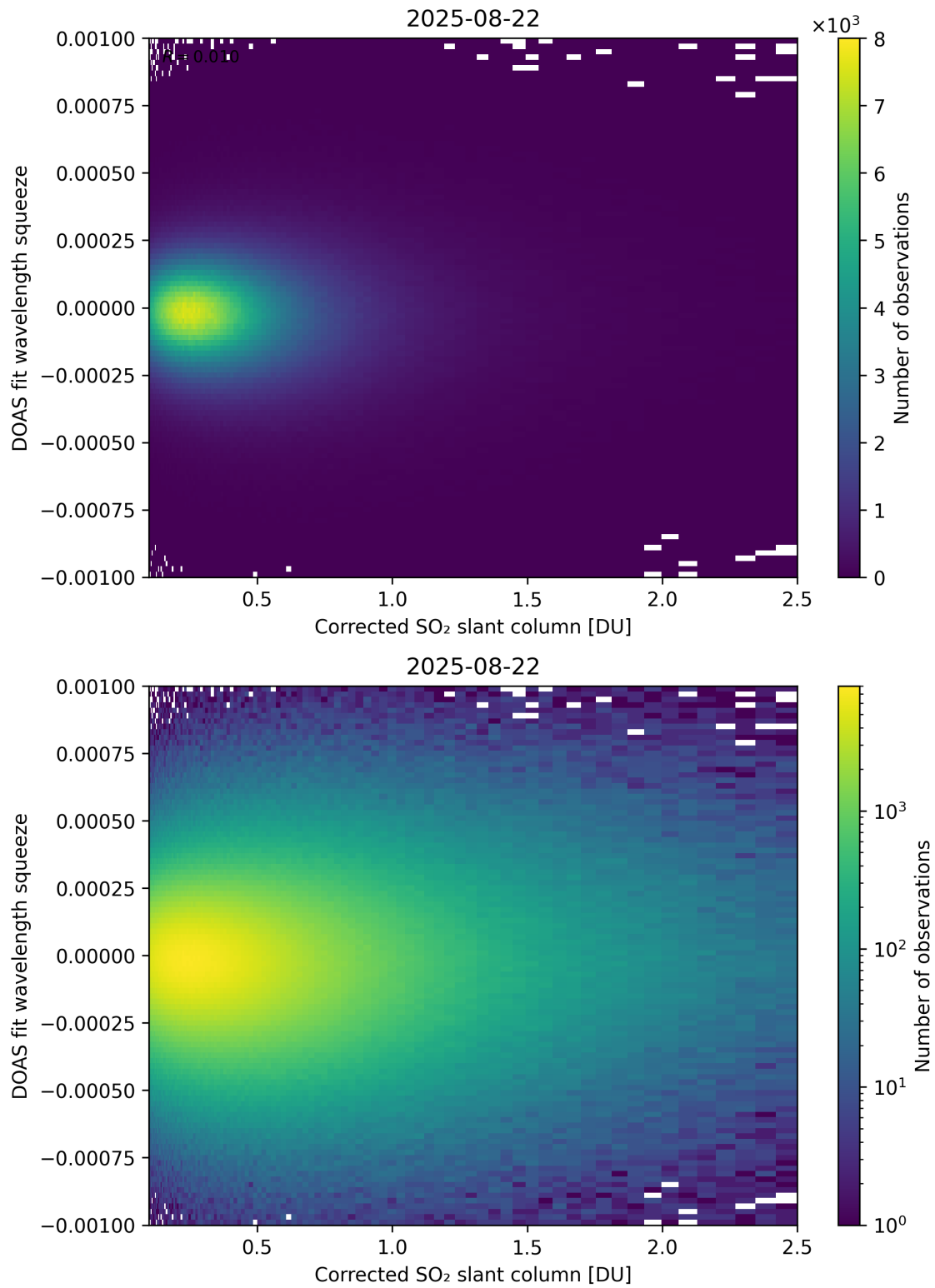
Figure 230: Scatter density plot of "Corrected SO 2 slant column" against "DOAS fit wavelength squeeze" for 2025-08-21 to 2025-08-23.
