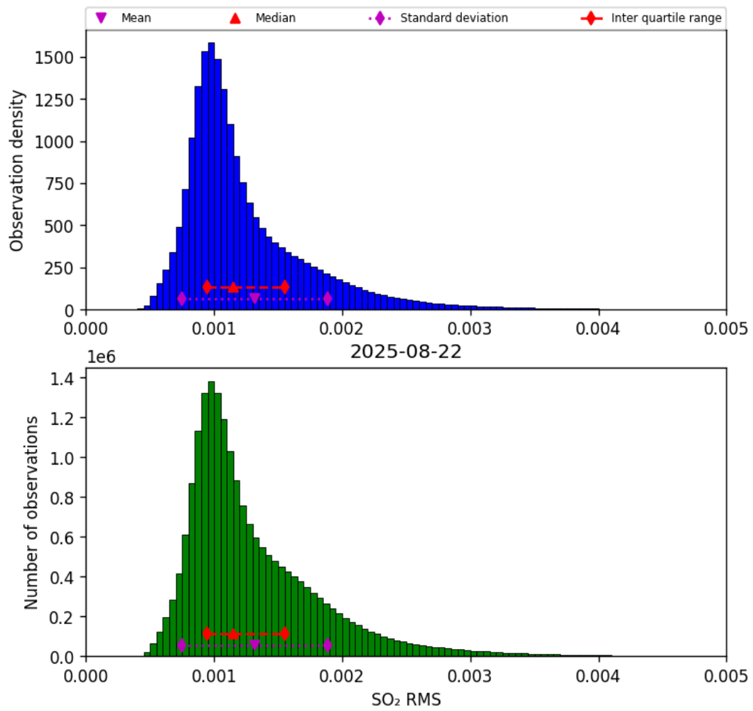
Figure 78: Histogram of “SO 2 RMS” for 2025-08-21 to 2025-08-23
