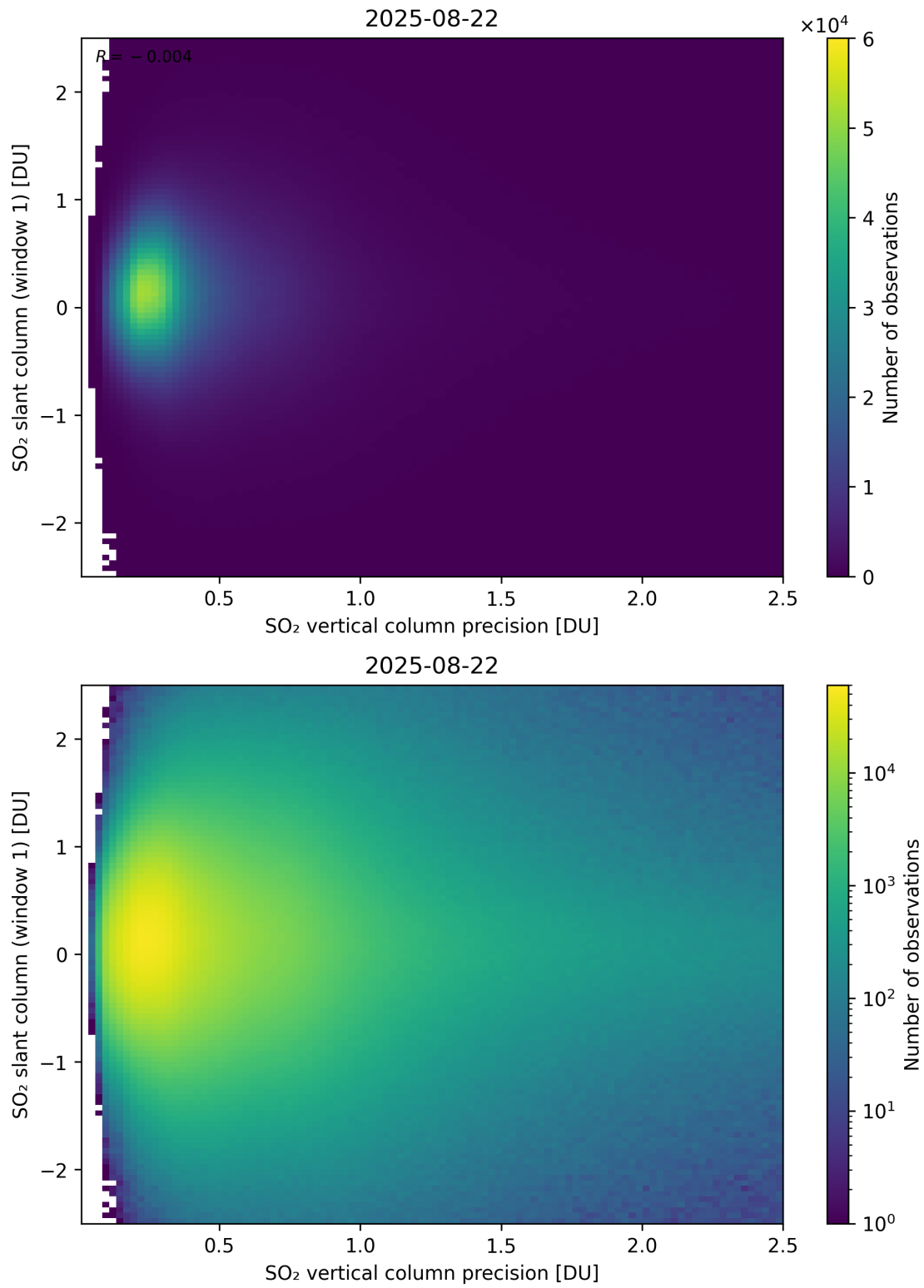
Figure 341: Scatter density plot of “SO 2 vertical column precision” against “SO 2 slant column (window 1)” for 2025-08-21 to 2025-08-23.
