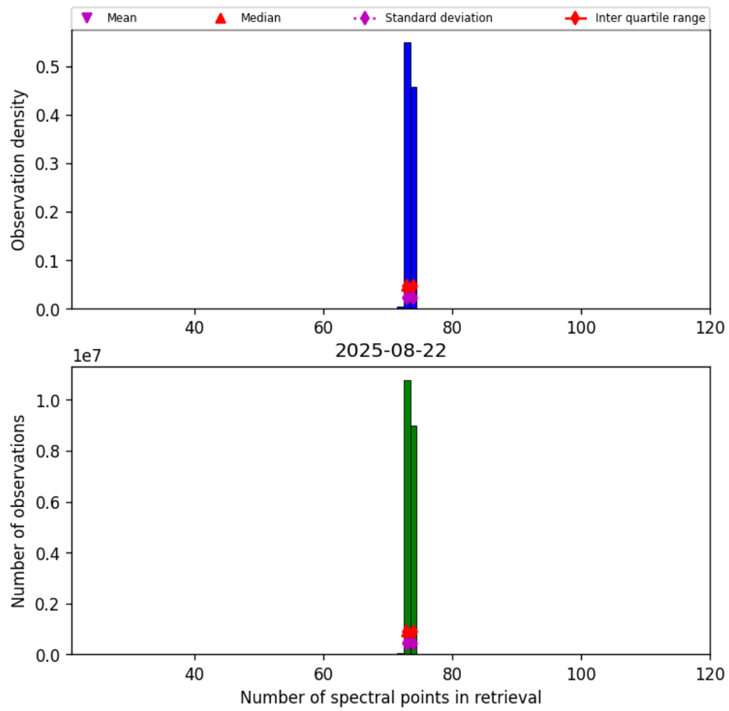
Figure 82: Histogram of “Number of spectral points in retrieval” for 2025-08-21 to 2025-08-23
