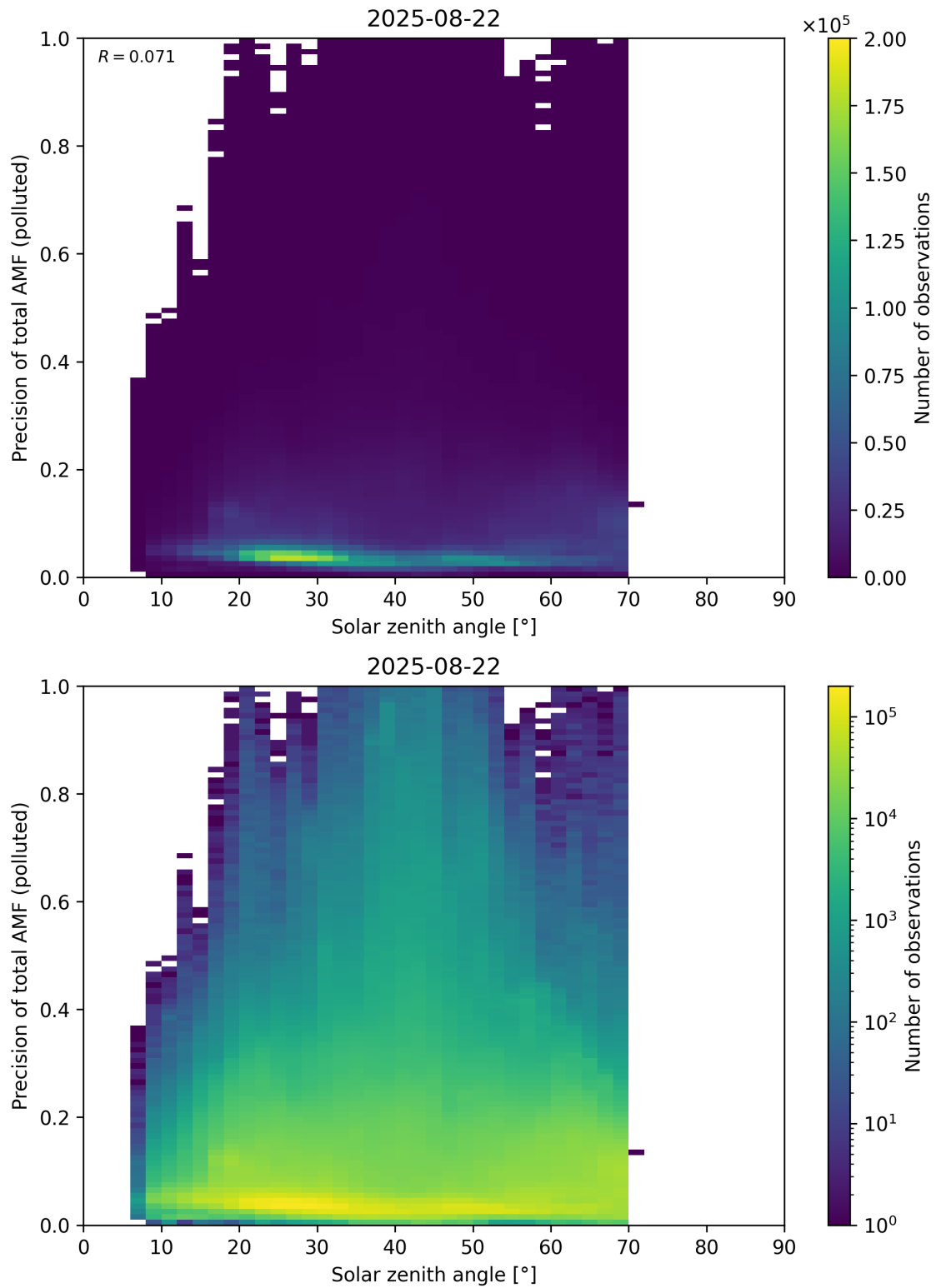
Figure 190: Scatter density plot of “Solar zenith angle” against “Precision of total AMF (polluted)” for 2025-08-21 to 2025-08-23.
