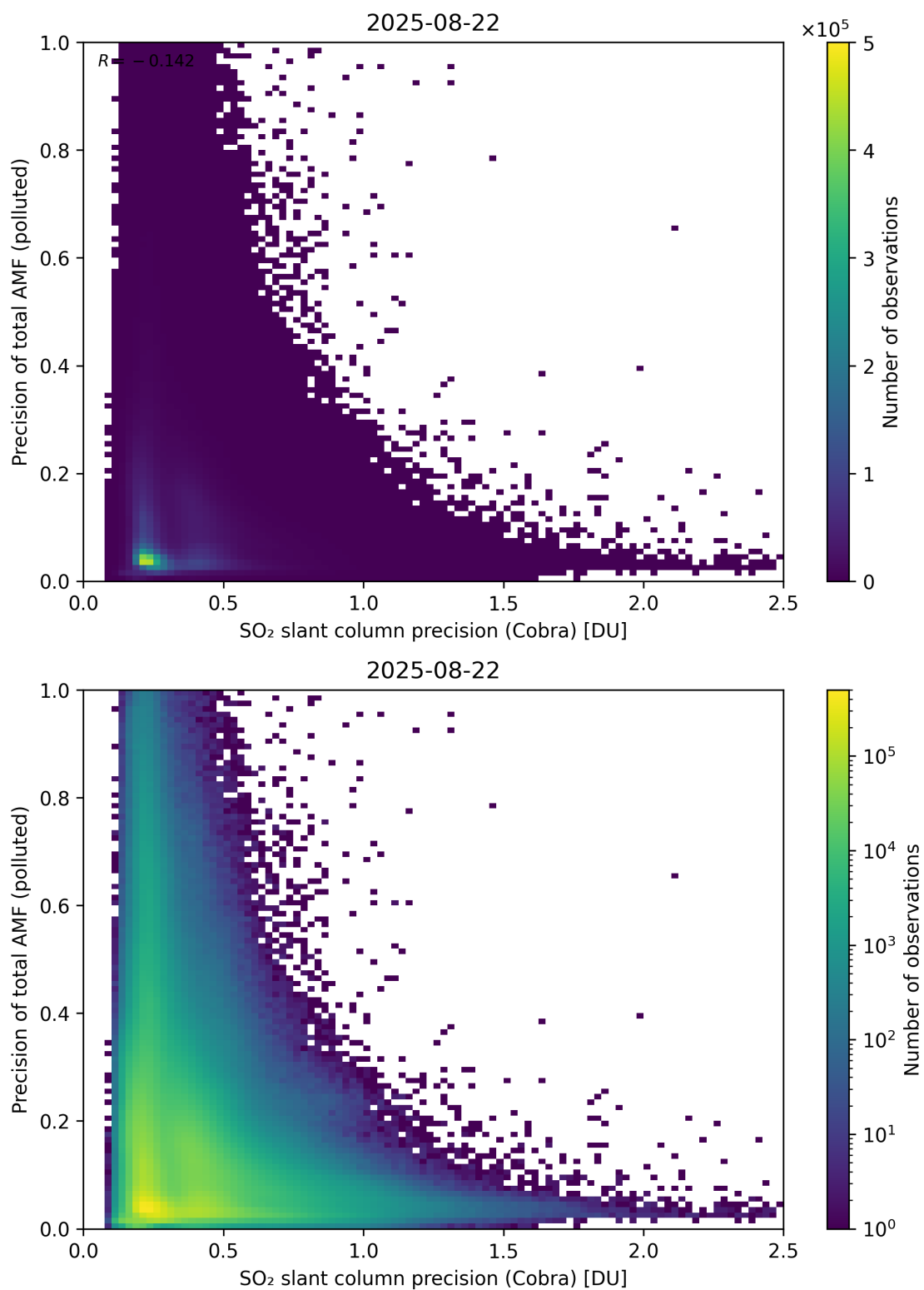
Figure 214: Scatter density plot of “SO 2 slant column precision (Cobra)” against “Precision of total AMF (polluted)” for 2025-08-21 to 2025-08-23.
