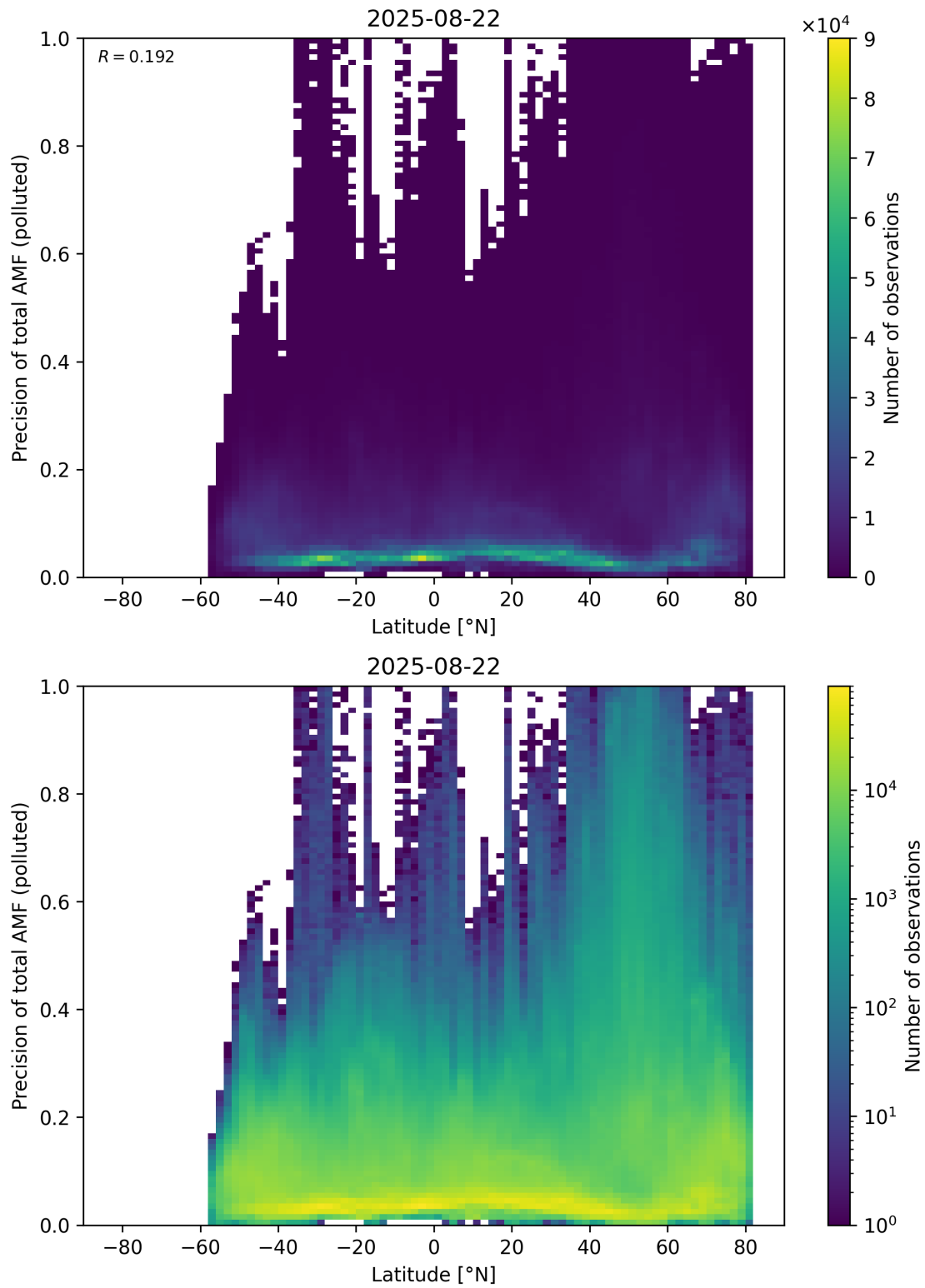
Figure 168: Scatter density plot of “Latitude” against “Precision of total AMF (polluted)” for 2025-08-21 to 2025-08-23.
