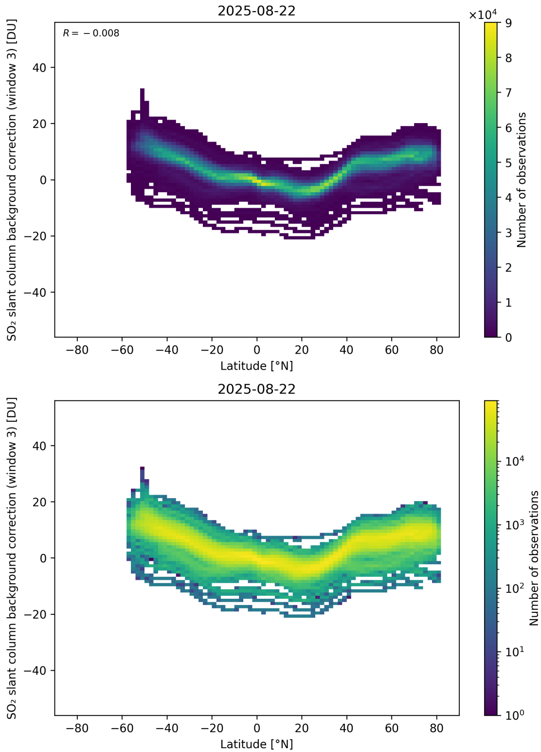
Figure 152: Scatter density plot of “Latitude” against “SO 2 slant column background correction (window 3)” for 2025-08-21 to 2025-08-23.
