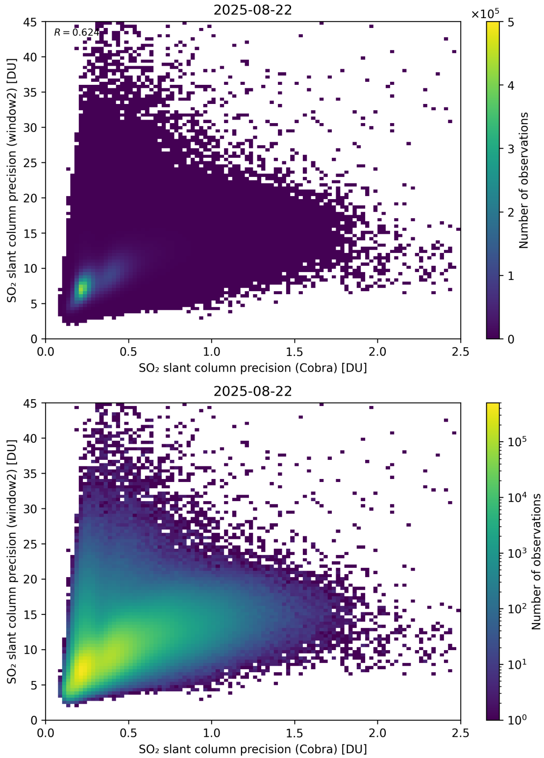
Figure 210: Scatter density plot of “SO 2 slant column precision (Cobra)” against “SO 2 slant column precision (window2)” for 2025-08-21 to 2025-08-23.
