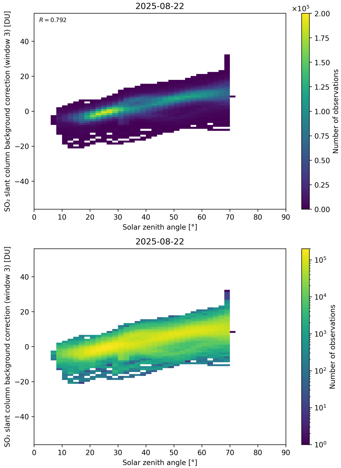
Figure 173: Scatter density plot of “Solar zenith angle” against “SO 2 slant column background correction (window 3)” for 2025-08-21 to 2025-08-23.
