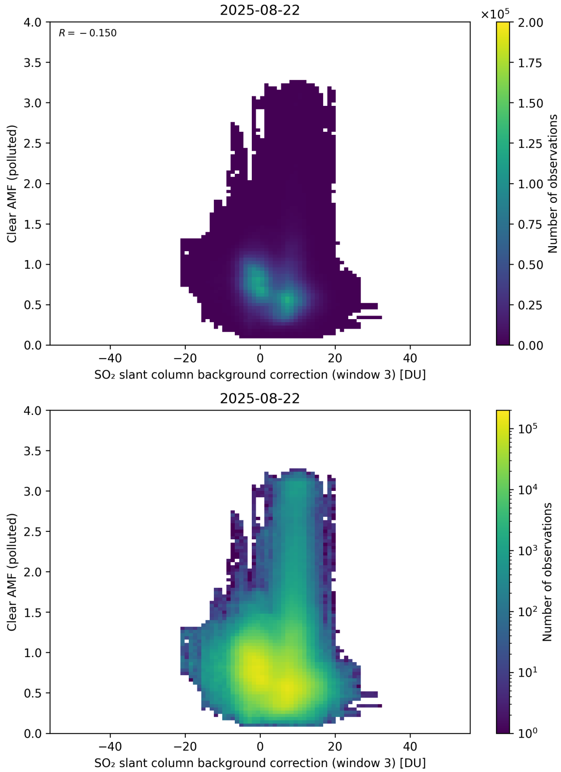
Figure 135: Scatter density plot of “SO 2 slant column background correction (window 3)” against “Clear AMF (polluted)” for 2025-08-21 to 2025-08-23.
