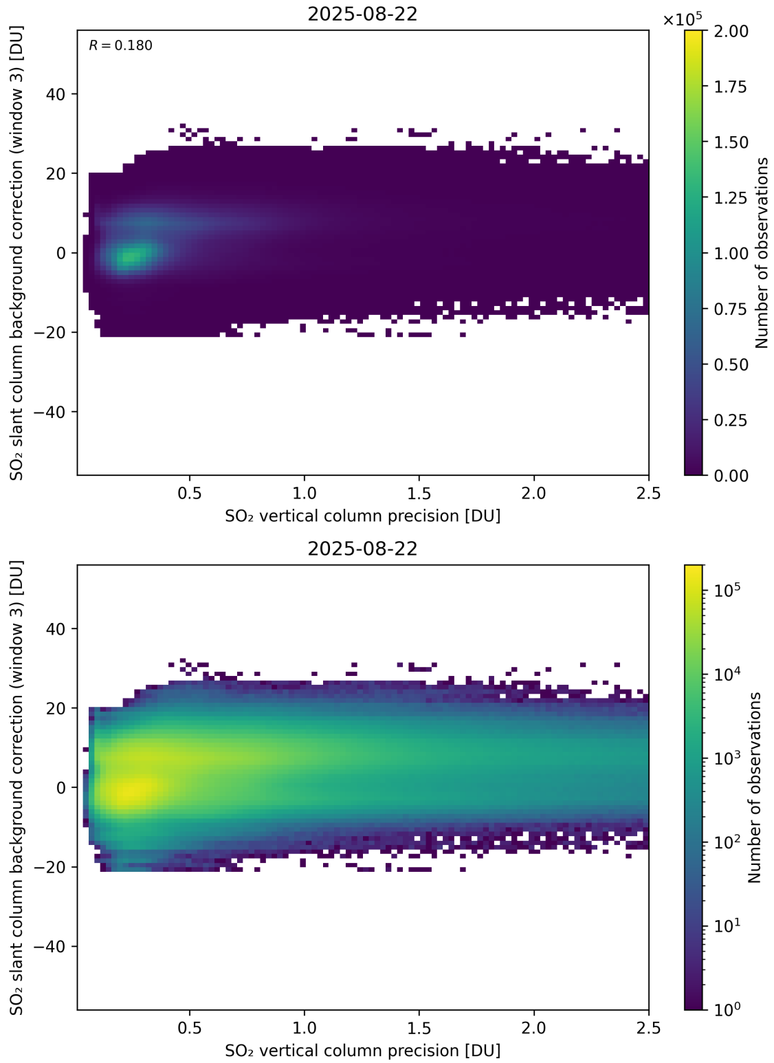
Figure 331: Scatter density plot of “SO 2 vertical column precision” against “SO 2 slant column background correction (window 3)” for 2025-08-21 to 2025-08-23.
