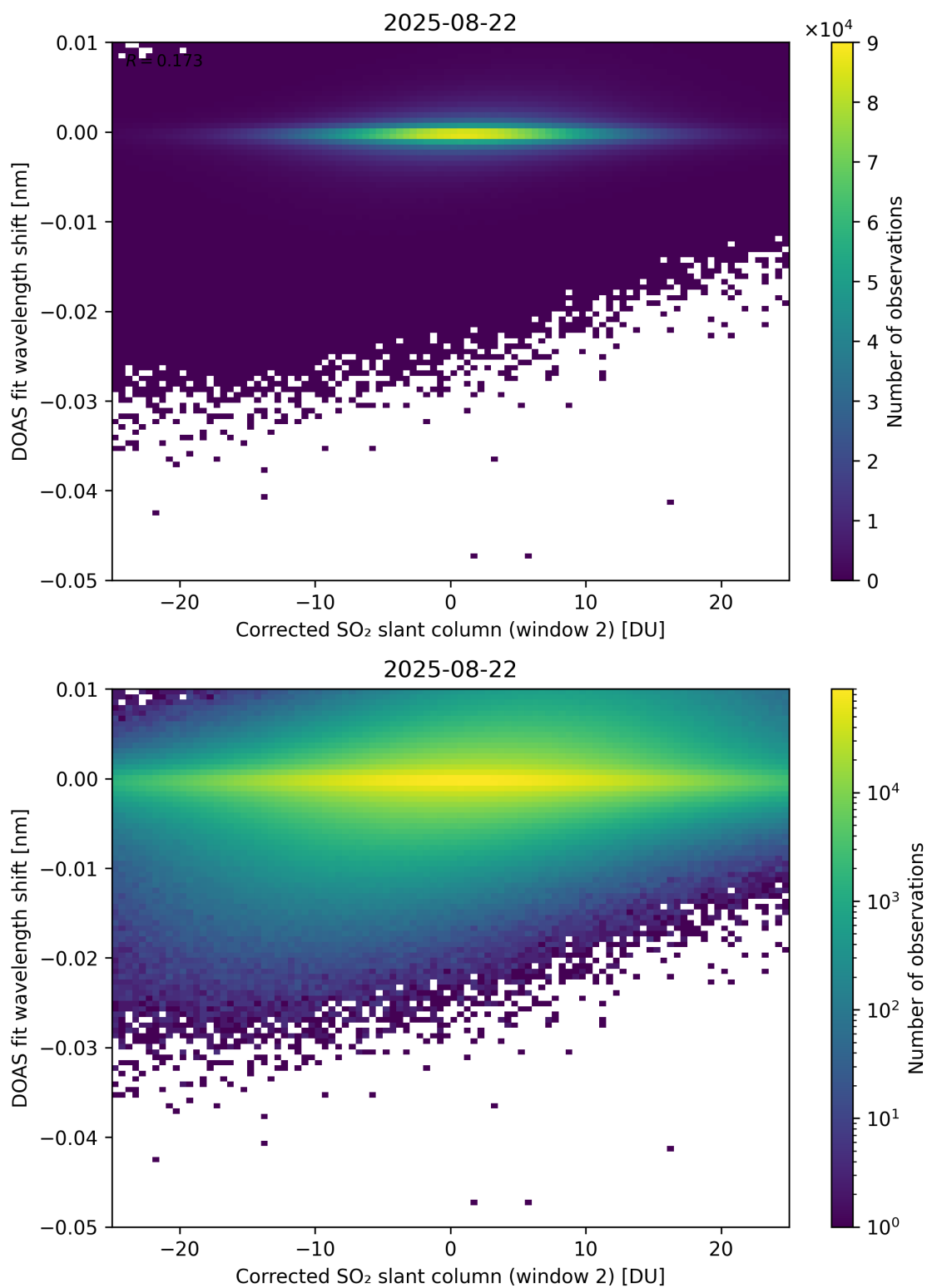
Figure 246: Scatter density plot of “Corrected SO 2 slant column (window 2)” against “DOAS fit wavelength shift” for 2025-08-21 to 2025-08-23.
