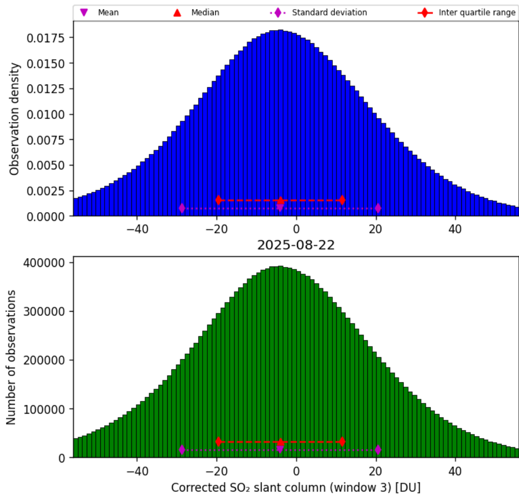
Figure 73: Histogram of “Corrected SO 2 slant column (window 3)” for 2025-08-21 to 2025-08-23
