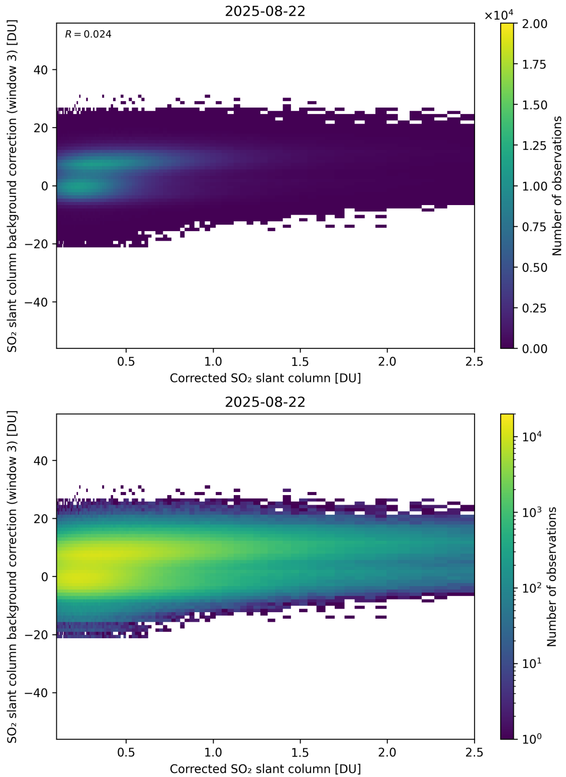
Figure 228: Scatter density plot of “Corrected SO 2 slant column” against “SO 2 slant column background correction (window 3)” for 2025-08-21 to 2025-08-23.
