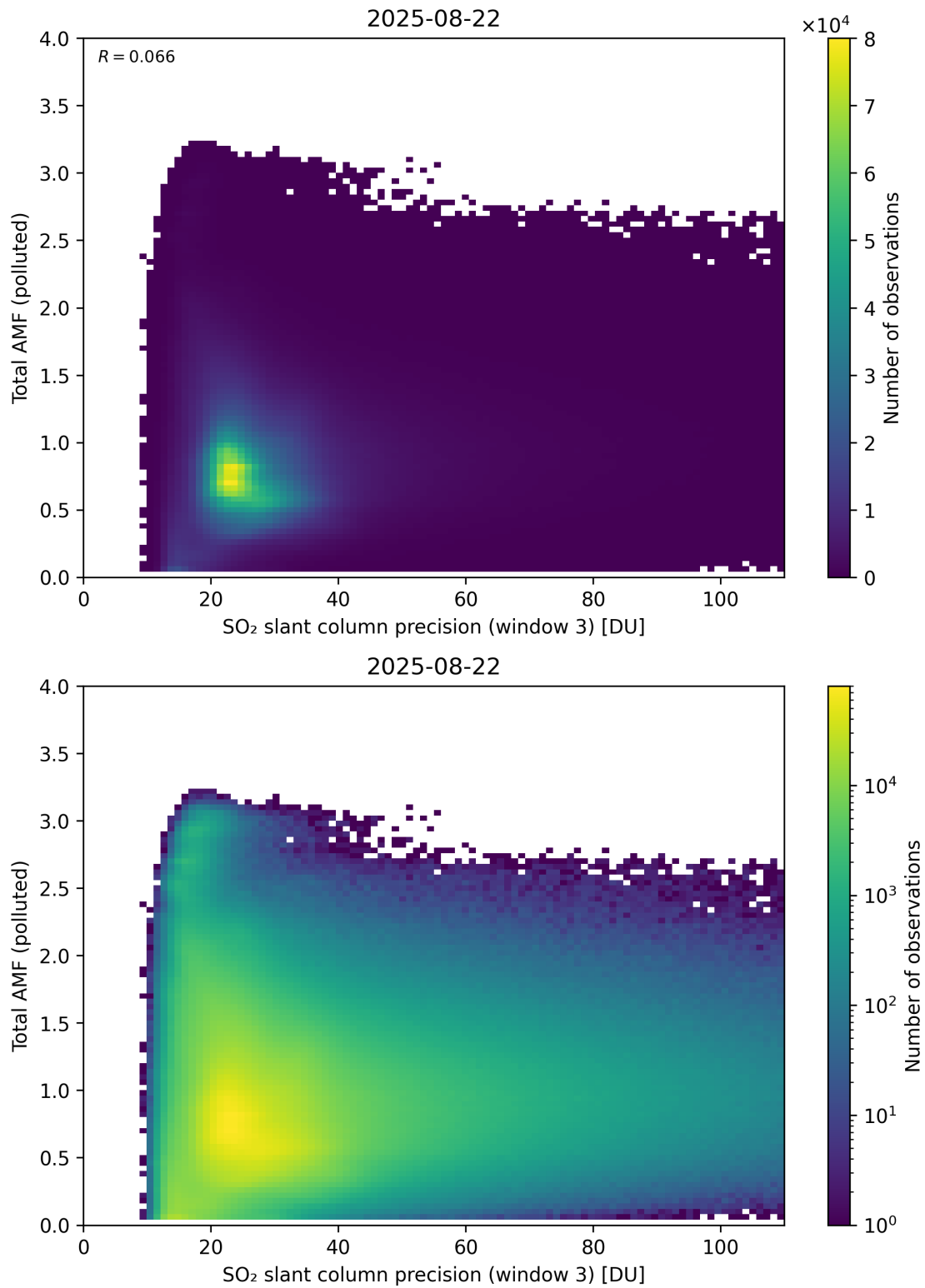
Figure 313: Scatter density plot of “SO 2 slant column precision (window 3)” against “Total AMF (polluted)” for 2025-08-21 to 2025-08-23.
