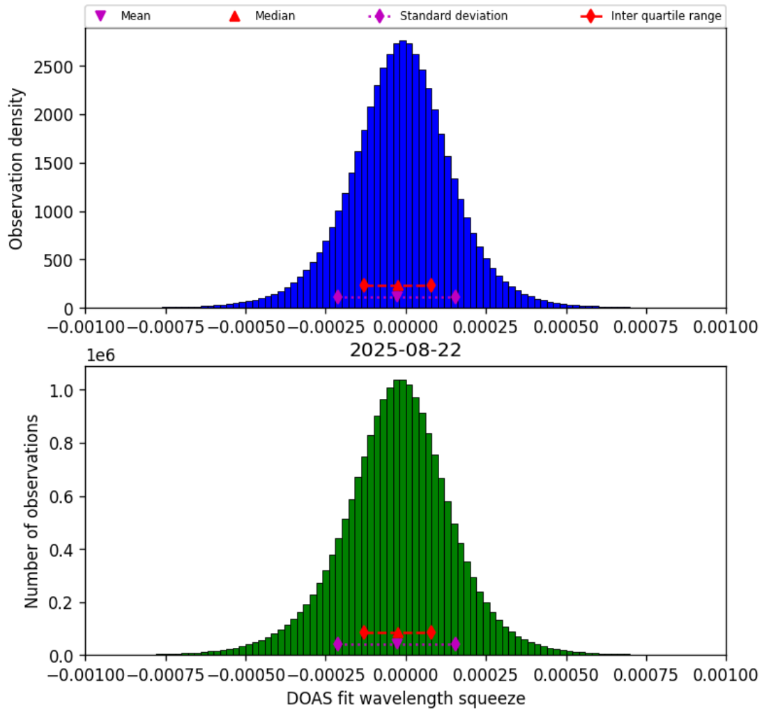
Figure 77: Histogram of “DOAS fit wavelength squeeze” for 2025-08-21 to 2025-08-23
