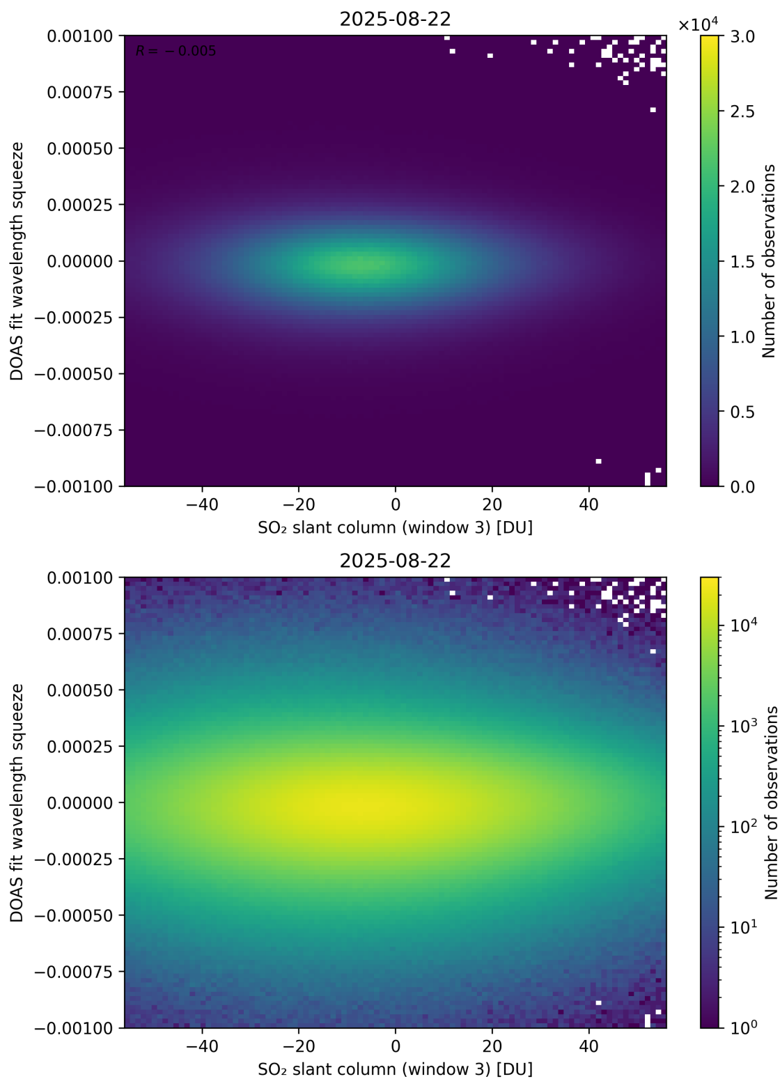
Figure 305: Scatter density plot of “SO 2 slant column (window 3)” against “DOAS fit wavelength squeeze” for 2025-08-21 to 2025-08-23.
