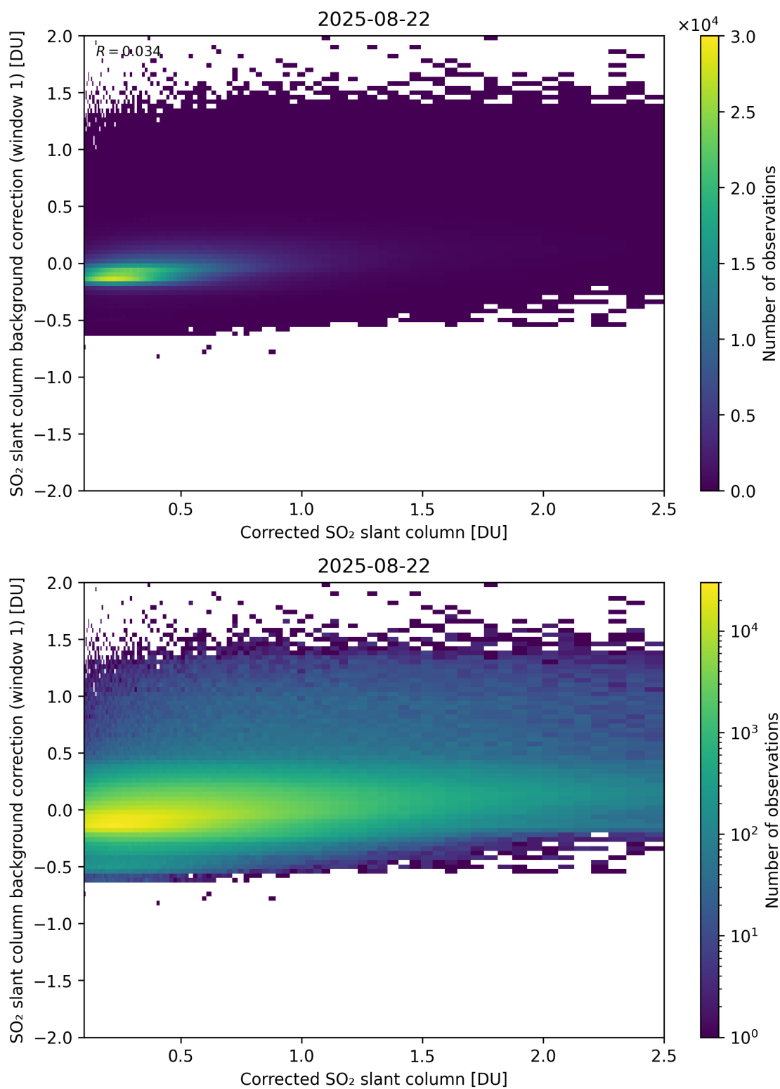
Figure 226: Scatter density plot of “Corrected SO 2 slant column” against “SO 2 slant column background correction (window 1)” for 2025-08-21 to 2025-08-23.
