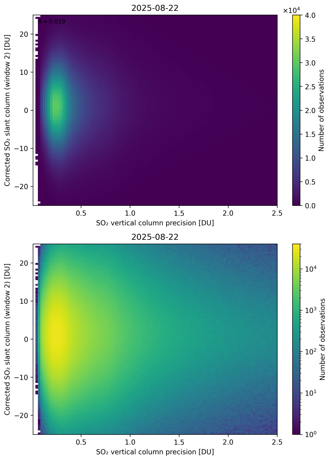
Figure 339: Scatter density plot of “SO 2 vertical column precision” against “Corrected SO 2 slant column (window 2)” for 2025-08-21 to 2025-08-23.
