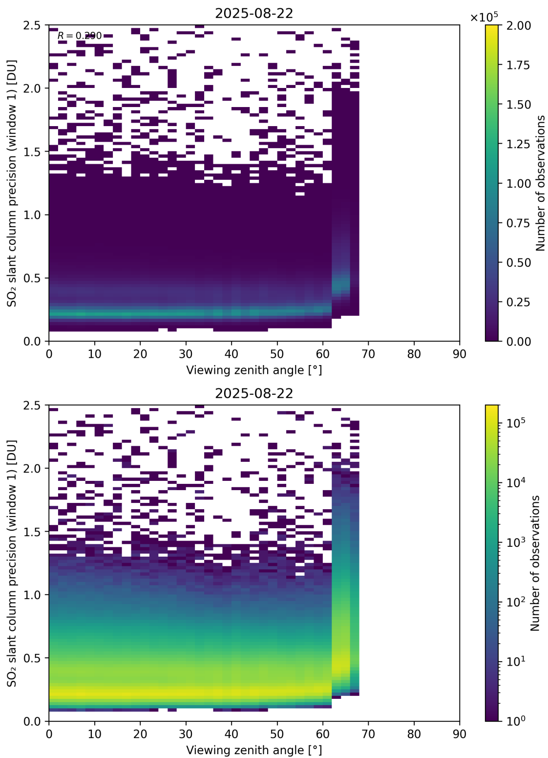
Figure 377: Scatter density plot of “Viewing zenith angle” against “SO 2 slant column precision (window 1)” for 2025-08-21 to 2025-08-23.
