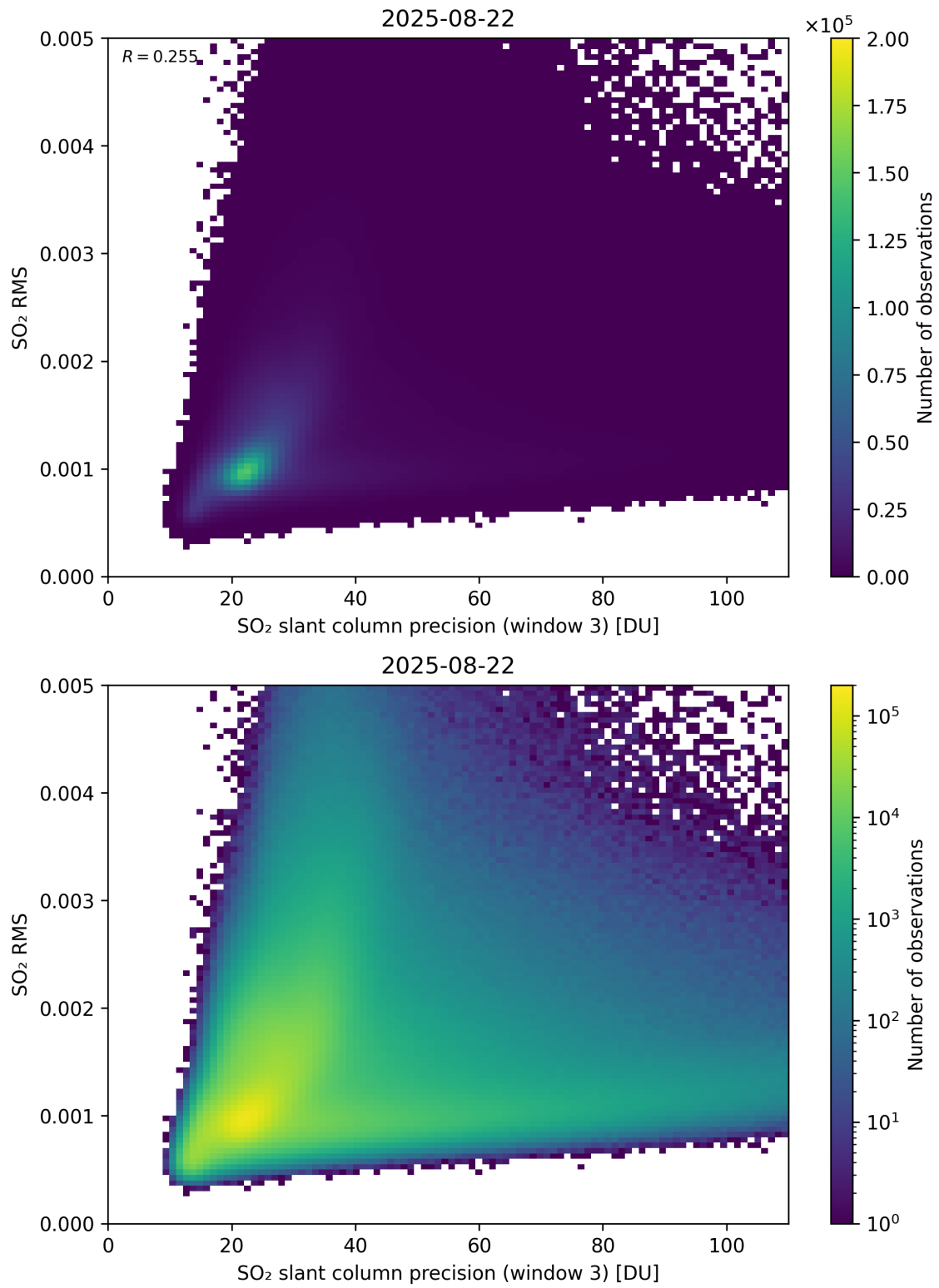
Figure 310: Scatter density plot of “SO 2 slant column precision (window 3)” against “SO 2 RMS” for 2025-08-21 to 2025-08-23.
