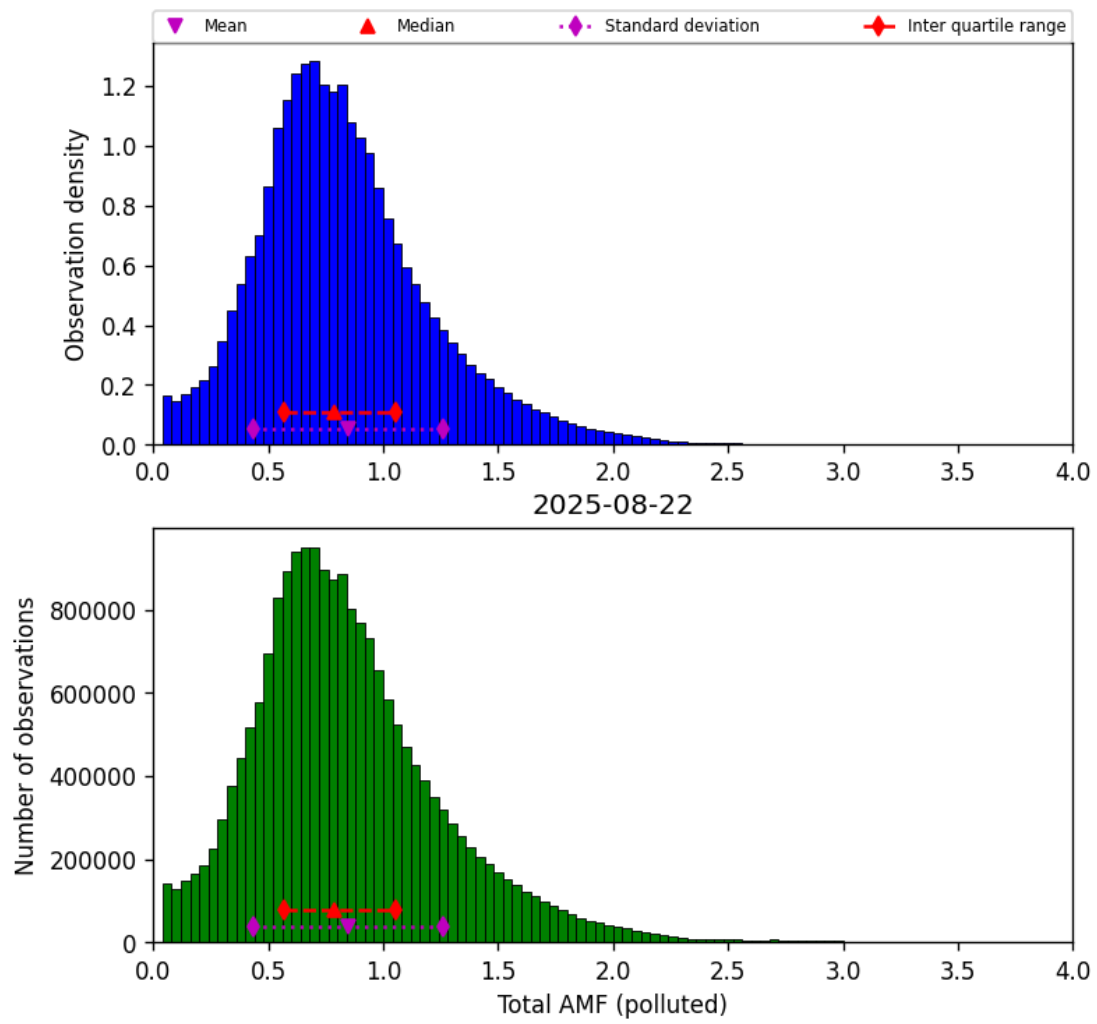
Figure 79: Histogram of “Total AMF (polluted)” for 2025-08-21 to 2025-08-23
