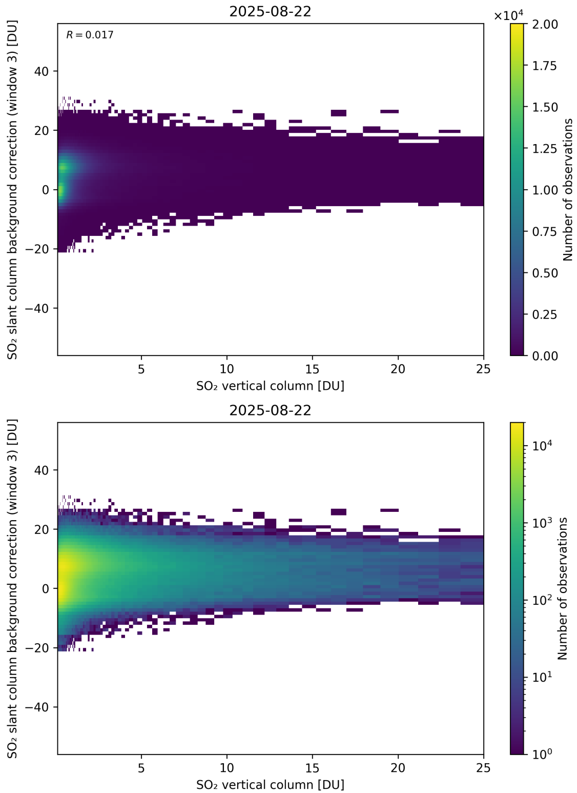
Figure 325: Scatter density plot of “SO 2 vertical column” against “SO 2 slant column background correction (window 3)” for 2025-08-21 to 2025-08-23.
