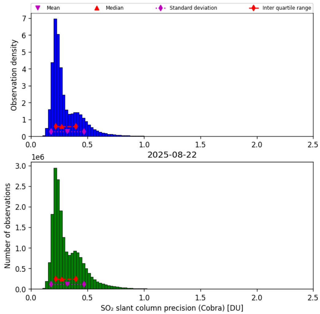
Figure 62: Histogram of “SO 2 slant column precision (Cobra)” for 2025-08-21 to 2025-08-23
