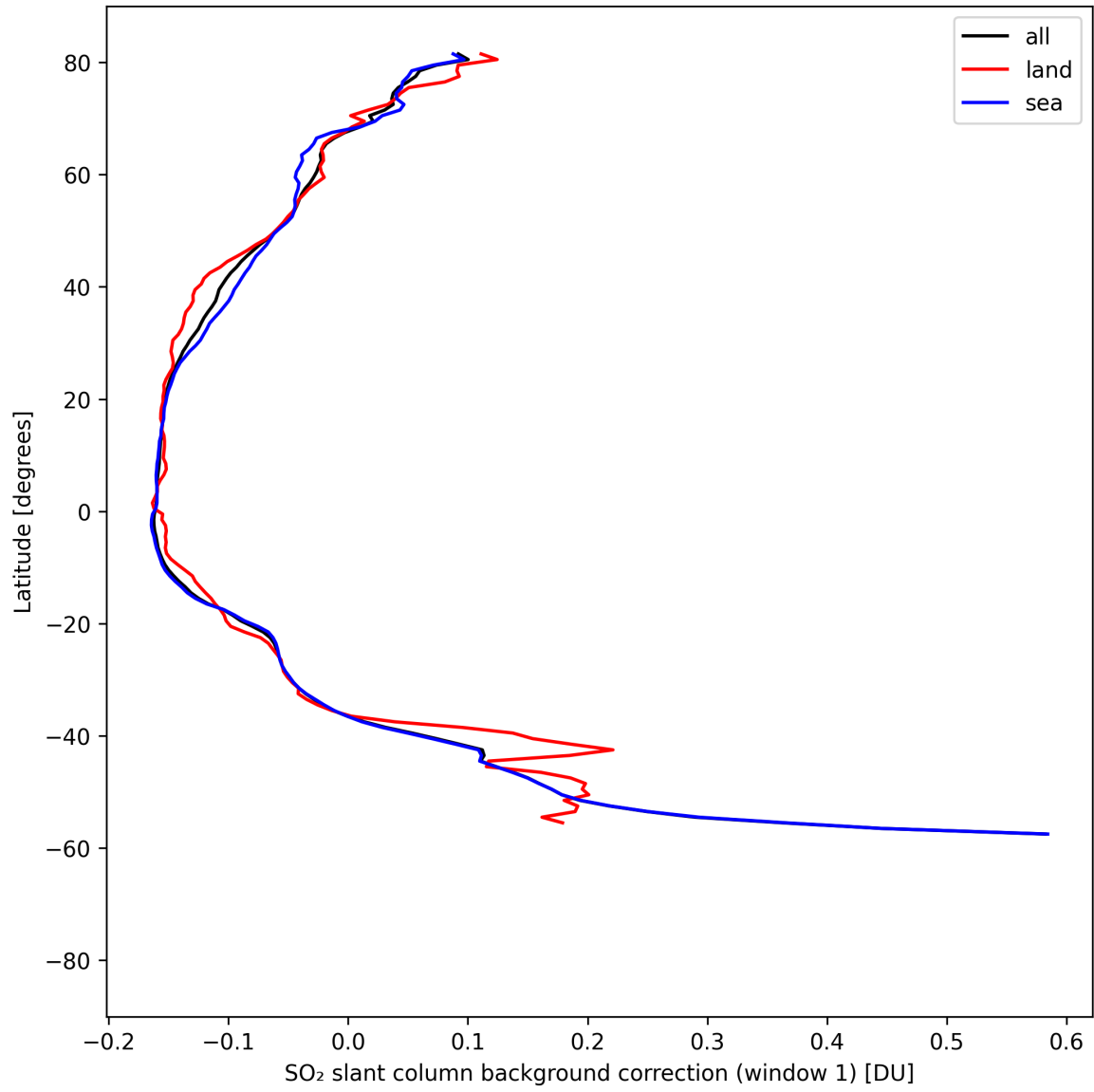
Figure 40: Zonal average of “SO 2 slant column background correction (window 1)” for 2025-08-21 to 2025-08-23.
