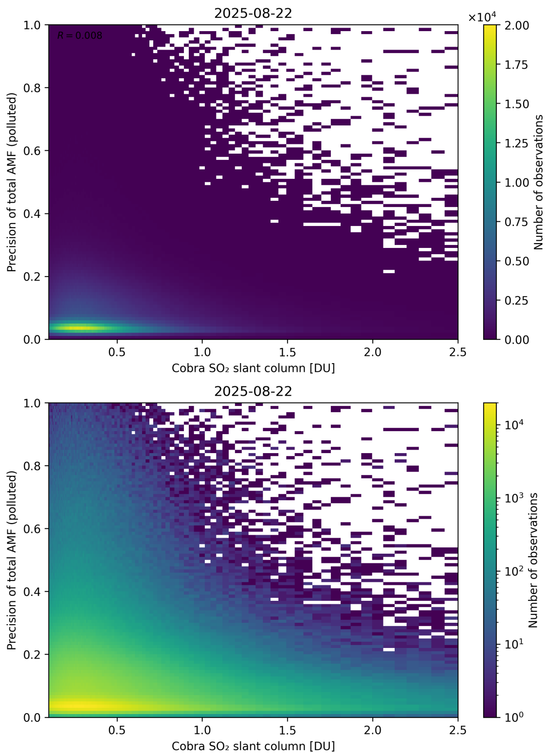
Figure 225: Scatter density plot of “Cobra SO 2 slant column” against “Precision of total AMF (polluted)” for 2025-08-21 to 2025-08-23.
