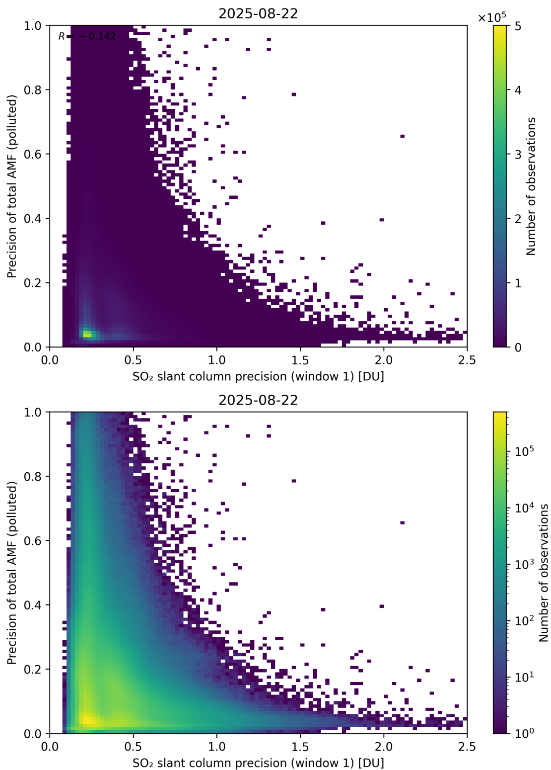
Figure 281: Scatter density plot of “SO 2 slant column precision (window 1)” against “Precision of total AMF (polluted)” for 2025-08-21 to 2025-08-23.
