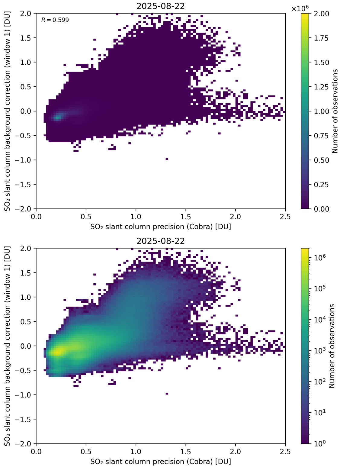
Figure 199: Scatter density plot of “SO 2 slant column precision (Cobra)” against “SO 2 slant column background correction (window 1)” for 2025-08-21 to 2025-08-23.
