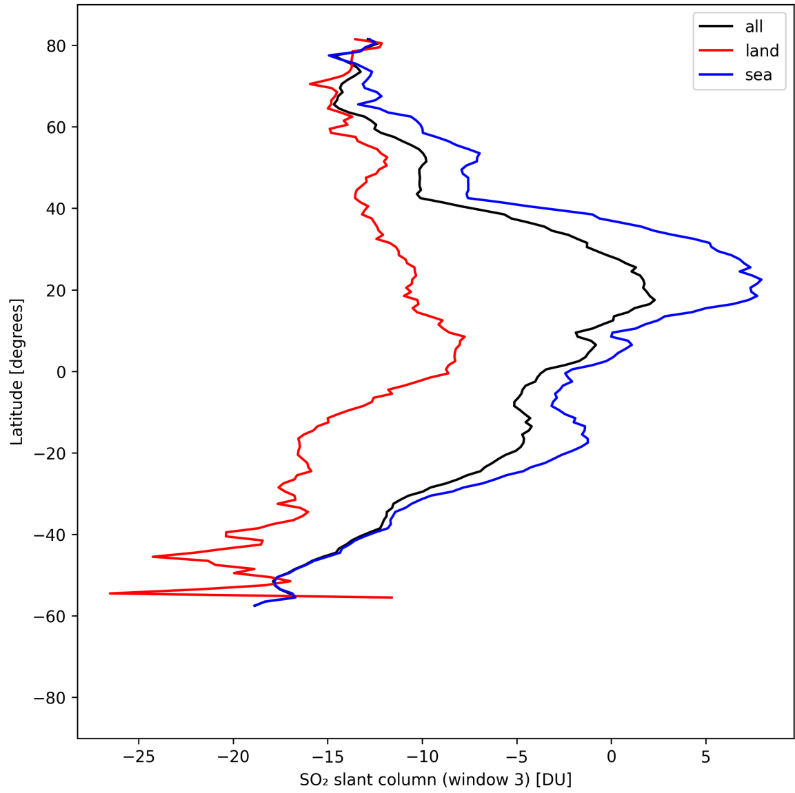
Figure 45: Zonal average of “SO 2 slant column (window 3)” for 2025-08-21 to 2025-08-23.
