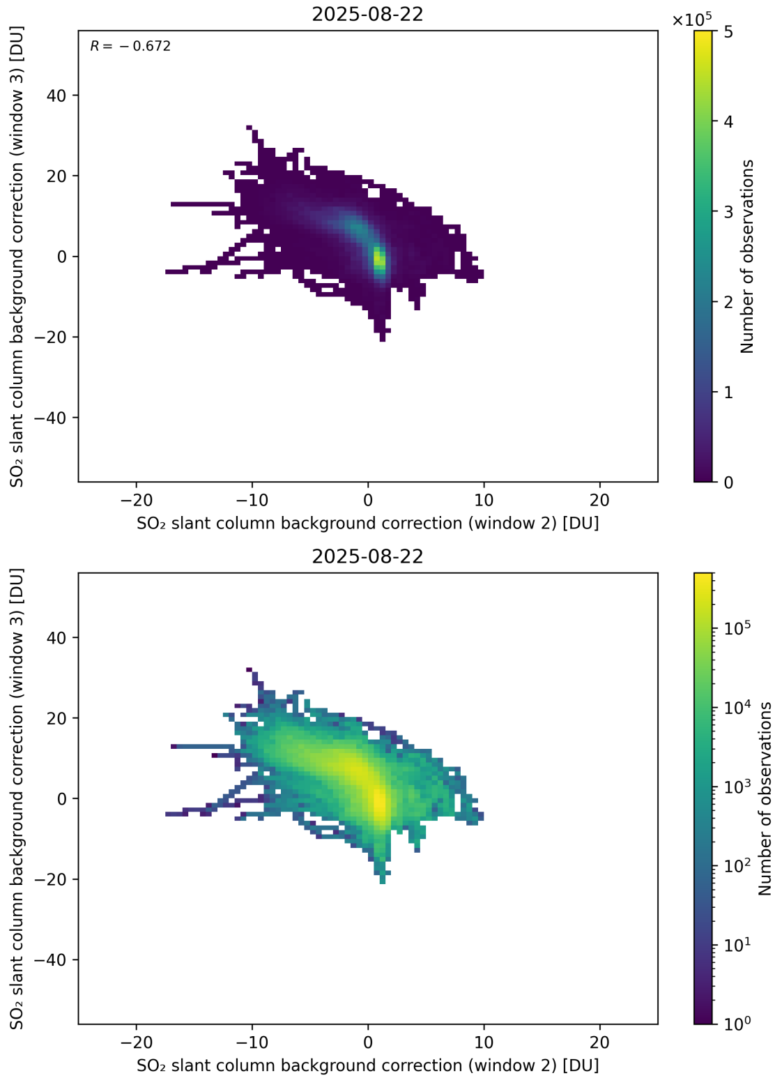
Figure 122: Scatter density plot of “SO 2 slant column background correction (window 2)” against “SO 2 slant column background correction (window 3)” for 2025-08-21 to 2025-08-23.
