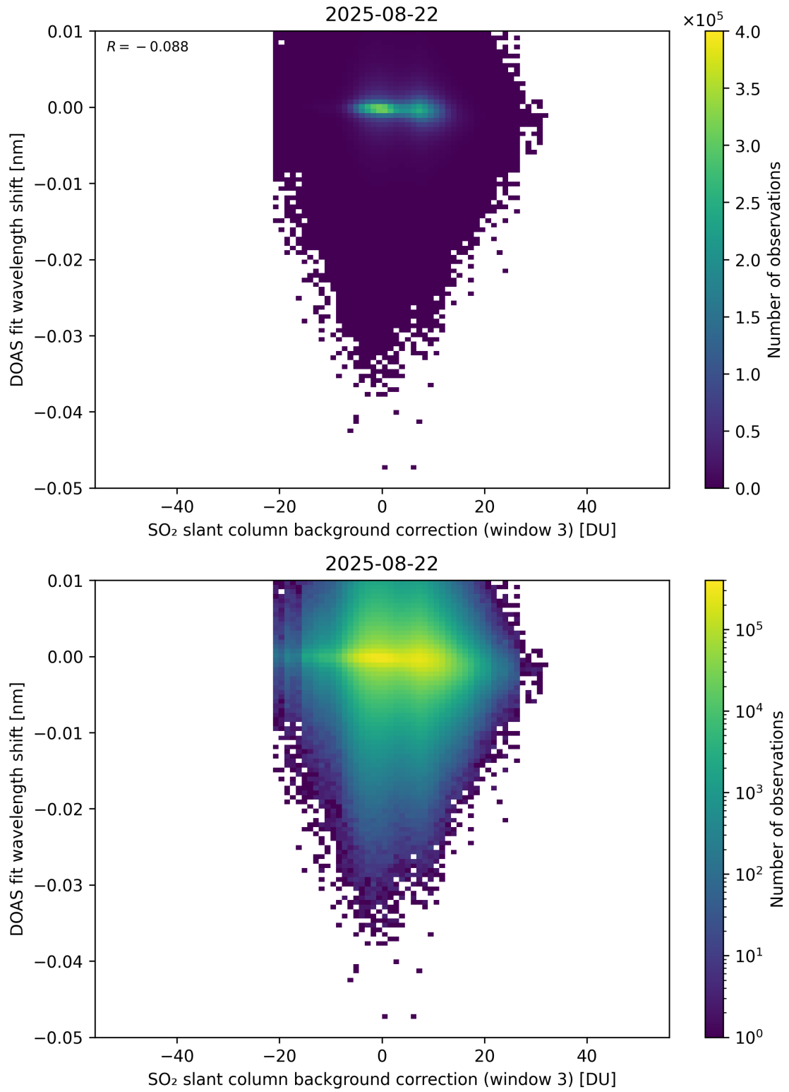
Figure 132: Scatter density plot of “SO 2 slant column background correction (window 3)” against “DOAS fit wavelength shift” for 2025-08-21 to 2025-08-23.
