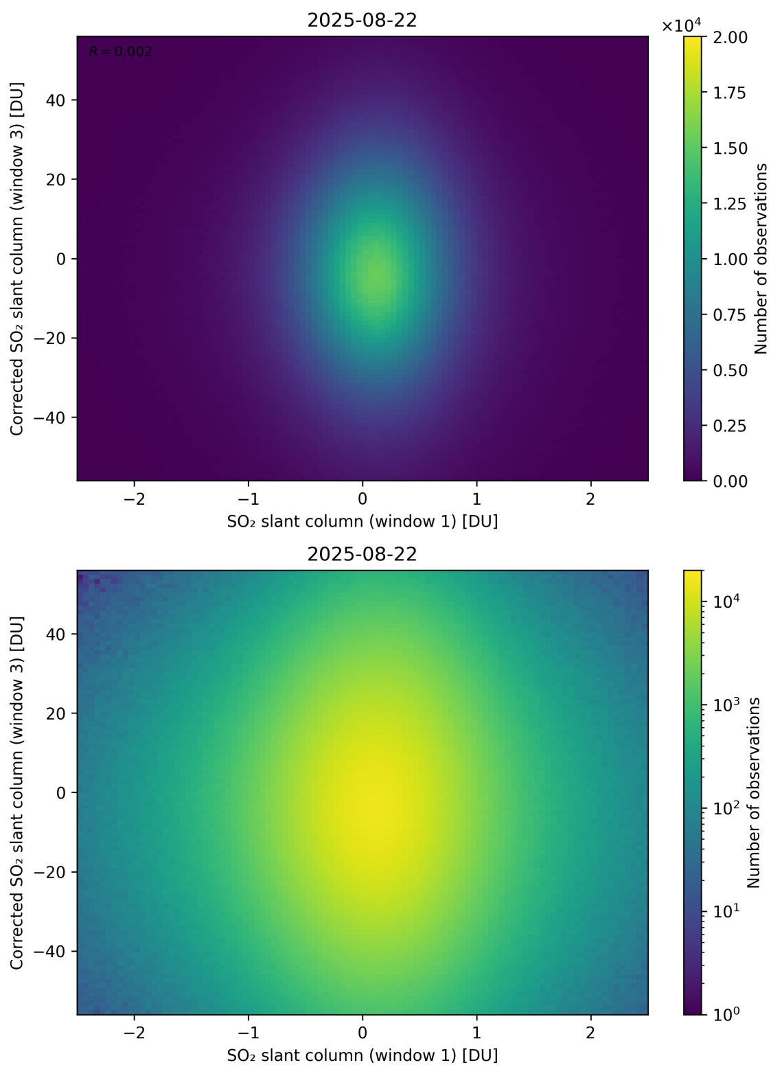
Figure 284: Scatter density plot of “SO 2 slant column (window 1)” against “Corrected SO 2 slant column (window 3)” for 2025-08-21 to 2025-08-23.
