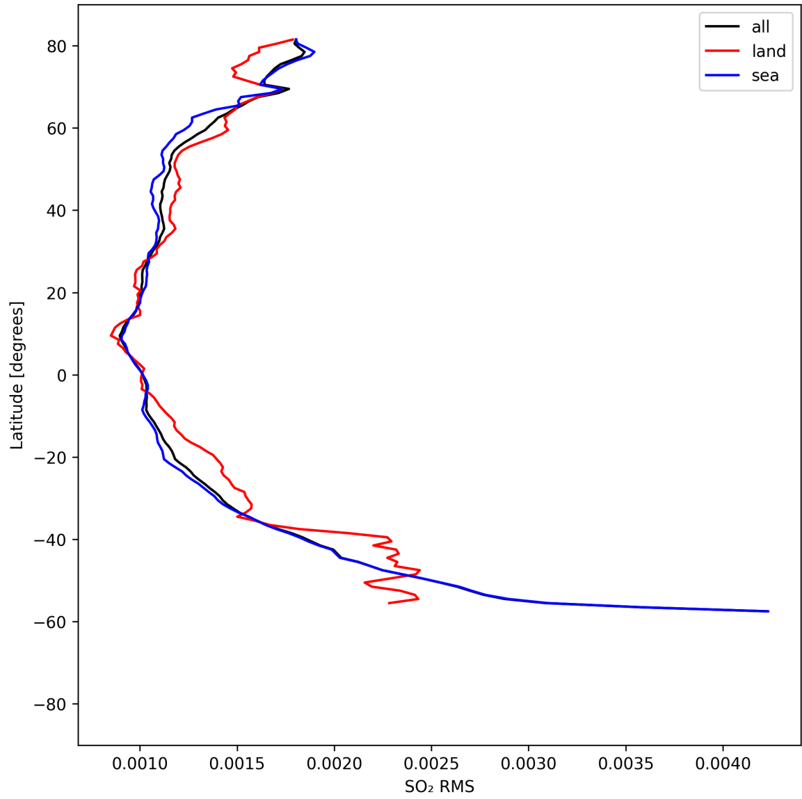
Figure 52: Zonal average of “SO 2 RMS” for 2025-08-21 to 2025-08-23.
