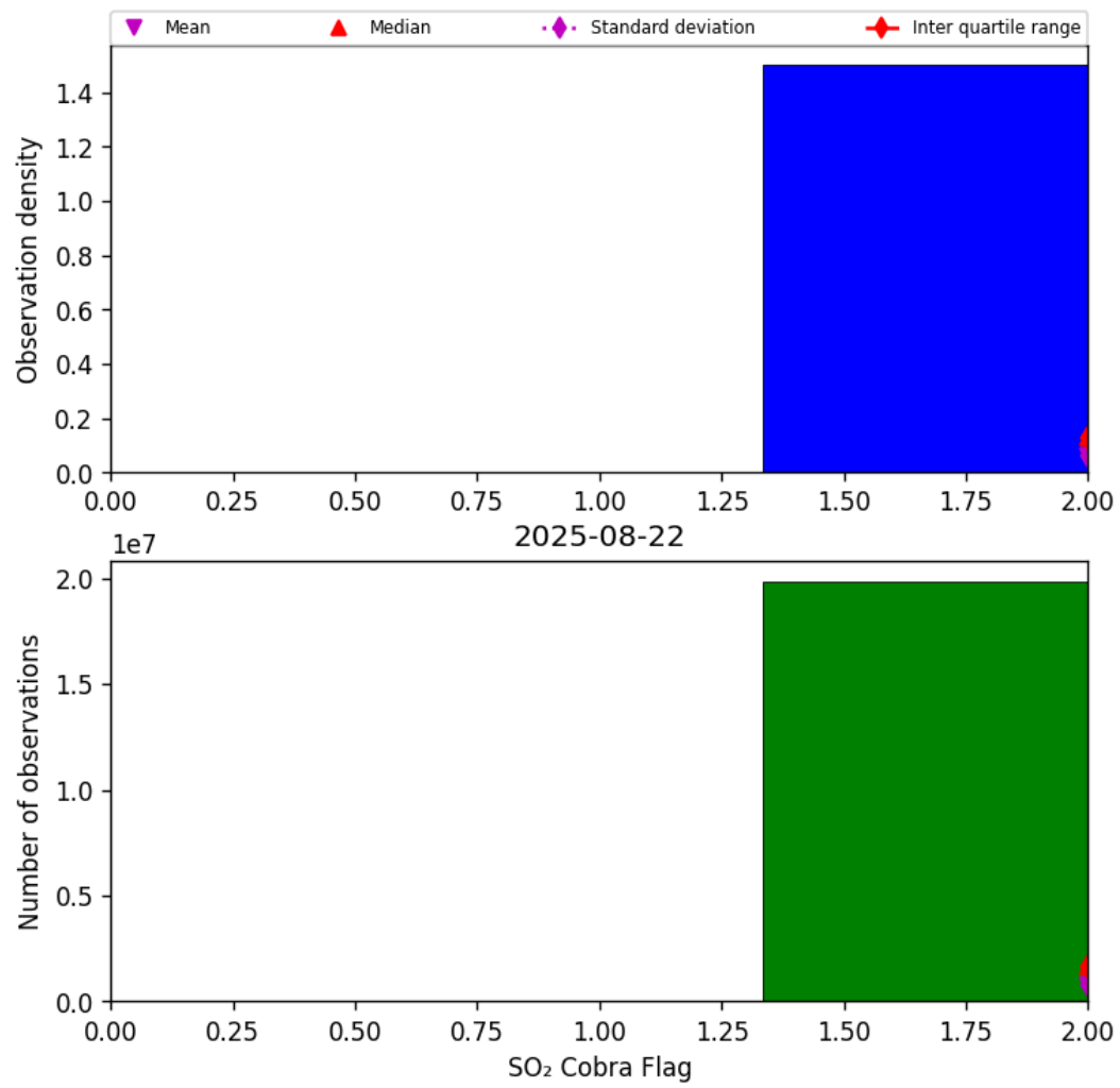
Figure 75: Histogram of “SO 2 Cobra Flag” for 2025-08-21 to 2025-08-23
