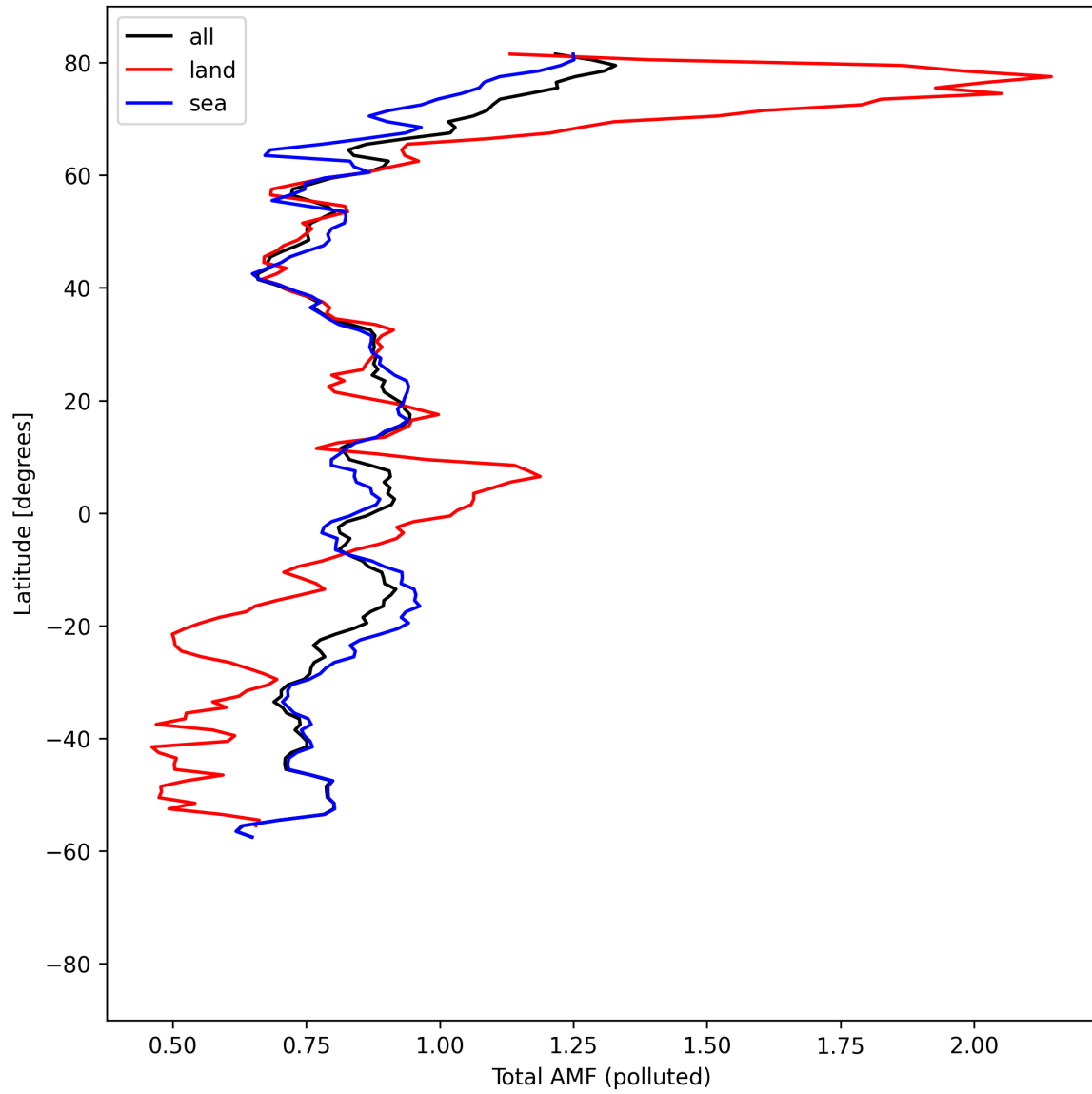
Figure 53: Zonal average of “Total AMF (polluted)” for 2025-08-21 to 2025-08-23.
