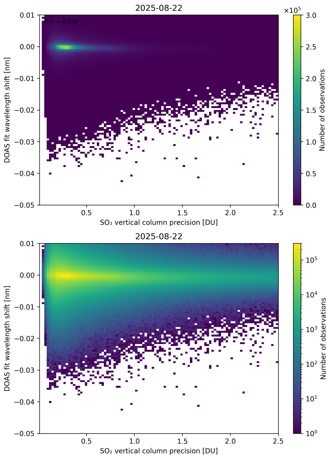
Figure 332: Scatter density plot of “SO 2 vertical column precision” against “DOAS fit wavelength shift” for 2025-08-21 to 2025-08-23.
