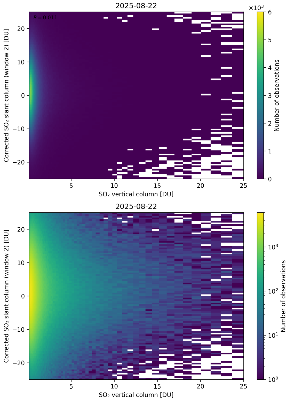
Figure 352: Scatter density plot of “SO 2 vertical column” against “Corrected SO 2 slant column (window 2)” for 2025-08-21 to 2025-08-23.
