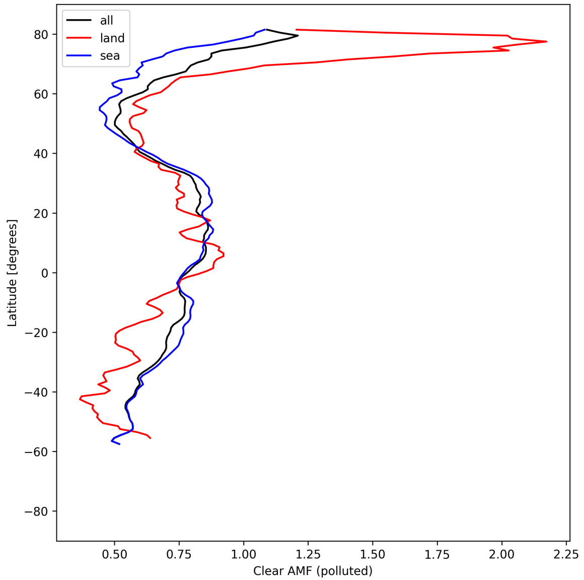
Figure 55: Zonal average of “Clear AMF (polluted)” for 2025-08-21 to 2025-08-23.
