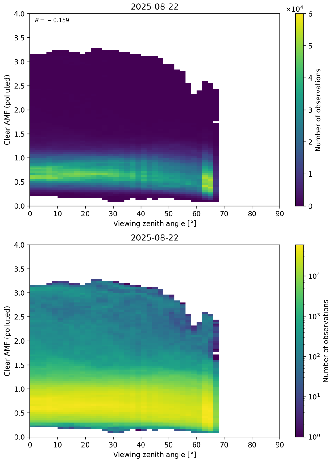
Figure 370: Scatter density plot of “Viewing zenith angle” against “Clear AMF (polluted)” for 2025-08-21 to 2025-08-23.
