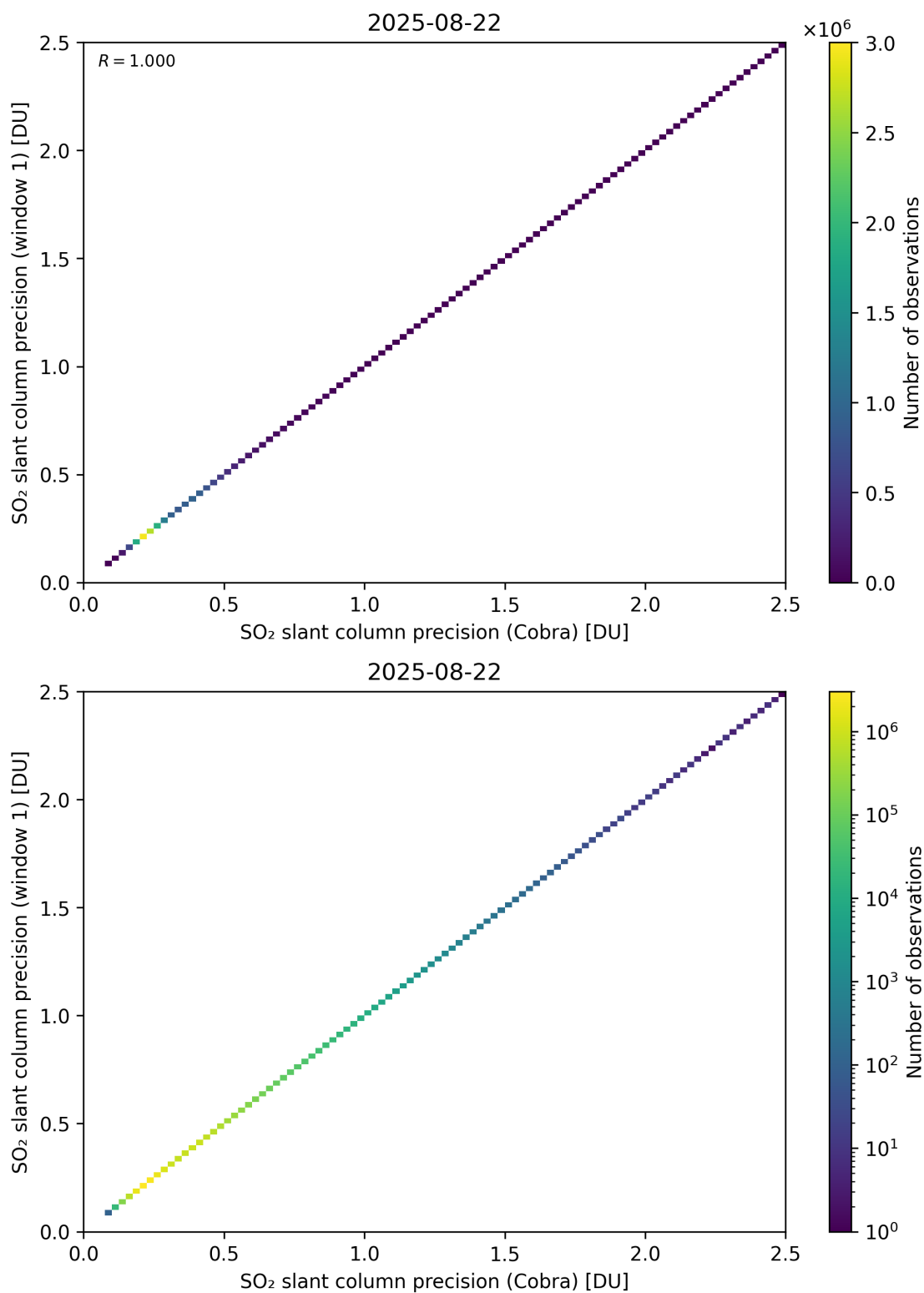
Figure 209: Scatter density plot of “SO 2 slant column precision (Cobra)” against “SO 2 slant column precision (window 1)” for 2025-08-21 to 2025-08-23.
