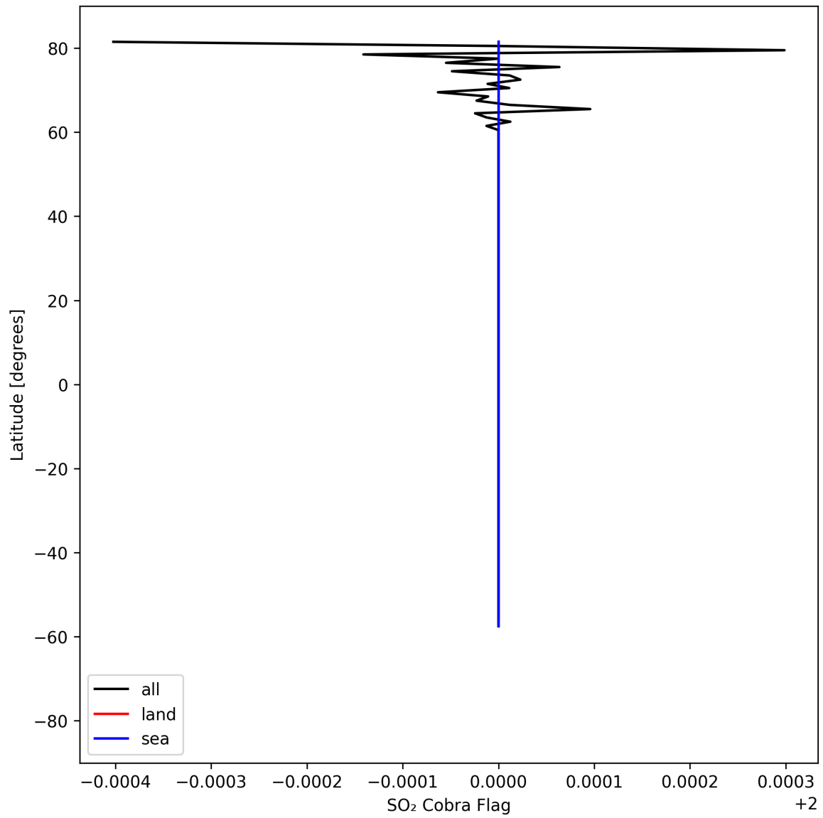
Figure 49: Zonal average of “SO 2 Cobra Flag” for 2025-08-21 to 2025-08-23.
