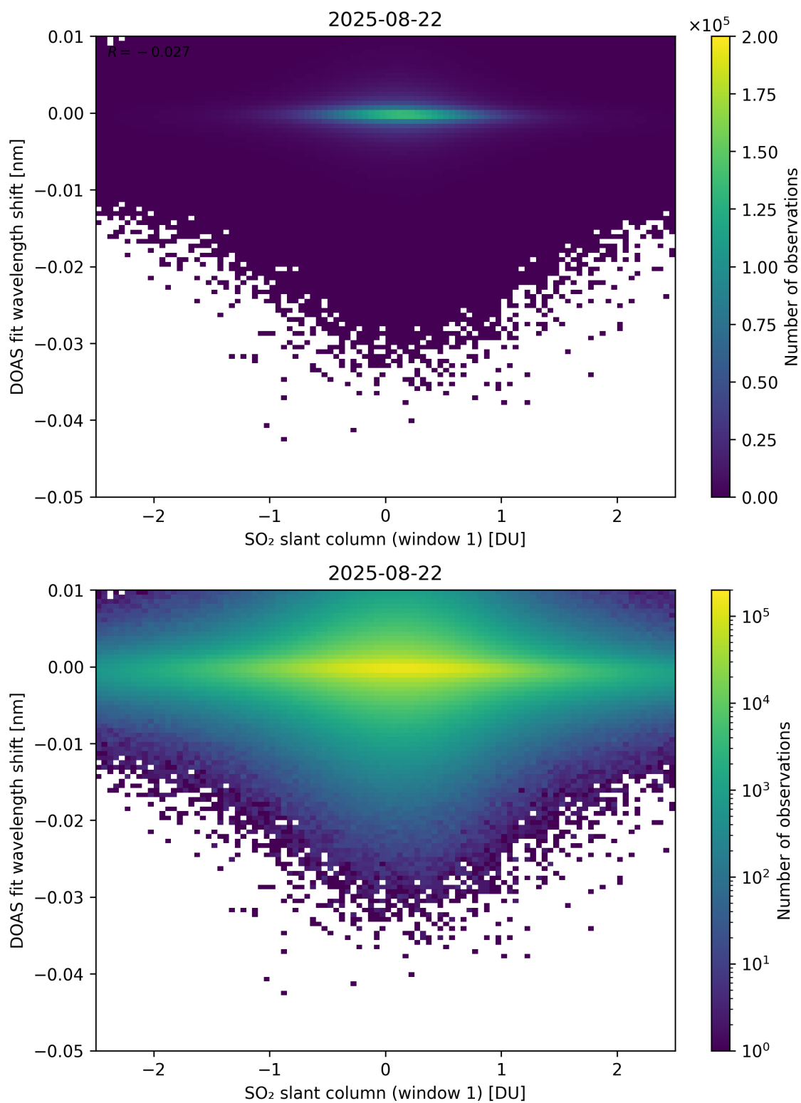
Figure 265: Scatter density plot of “SO 2 slant column (window 1)” against “DOAS fit wavelength shift” for 2025-08-21 to 2025-08-23.
