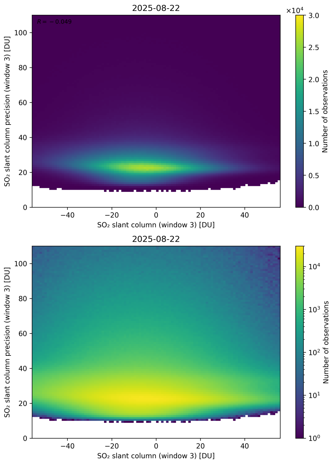
Figure 317: Scatter density plot of “SO 2 slant column (window 3)” against “SO 2 slant column precision (window 3)” for 2025-08-21 to 2025-08-23.
