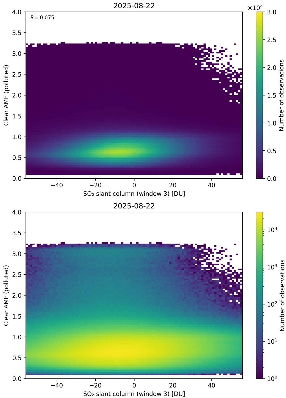
Figure 315: Scatter density plot of “SO 2 slant column (window 3)” against “Clear AMF (polluted)” for 2025-08-21 to 2025-08-23.
