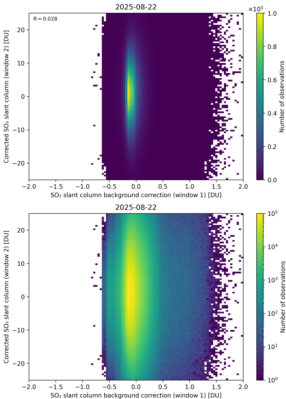
Figure 115: Scatter density plot of “SO 2 slant column background correction (window 1)” against “Corrected SO 2 slant column (window 2)” for 2025-08-21 to 2025-08-23.
