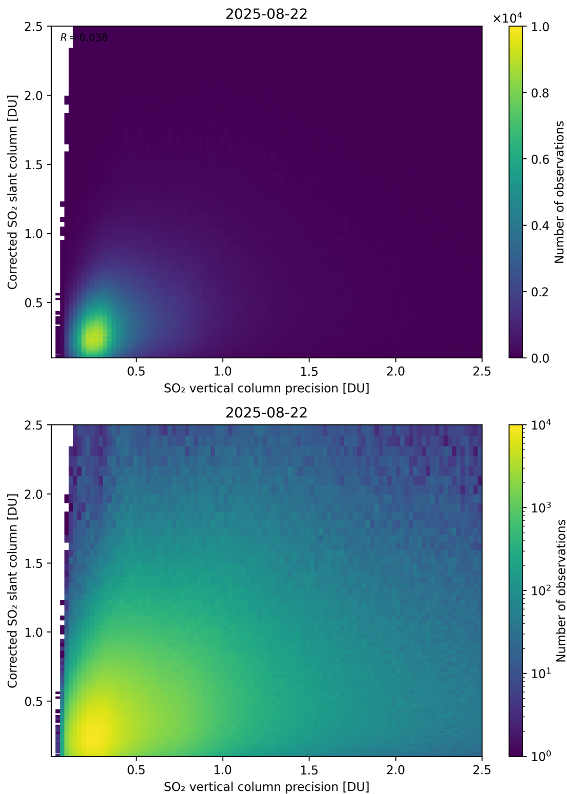
Figure 338: Scatter density plot of “SO 2 vertical column precision” against “Corrected SO 2 slant column” for 2025-08-21 to 2025-08-23.
