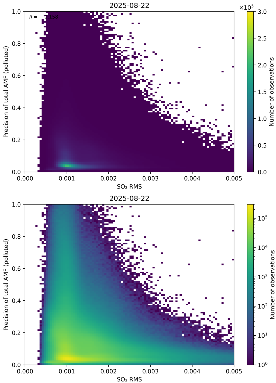
Figure 149: Scatter density plot of “SO 2 RMS” against “Precision of total AMF (polluted)” for 2025-08-21 to 2025-08-23.
