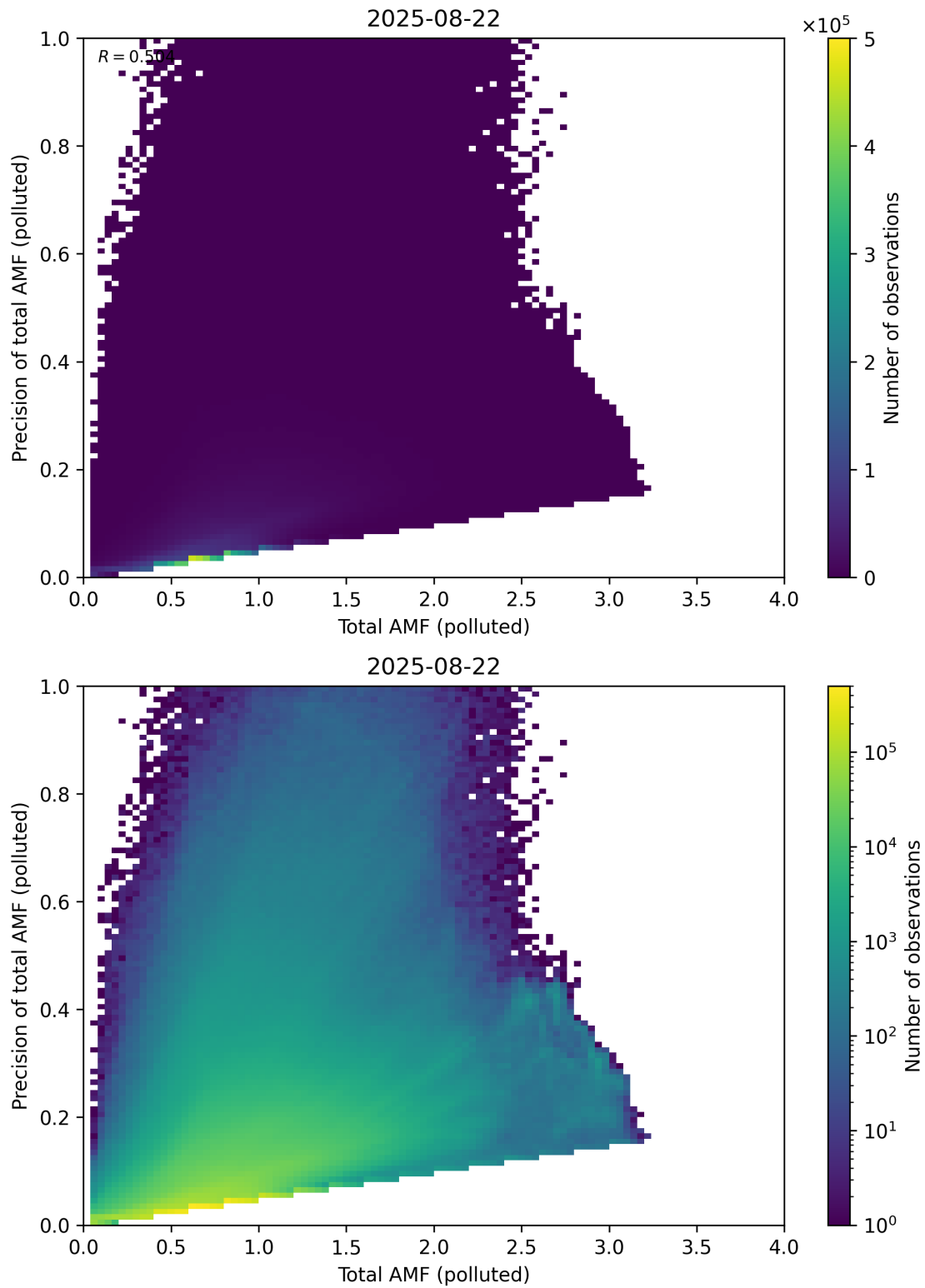
Figure 322: Scatter density plot of “Total AMF (polluted)” against “Precision of total AMF (polluted)” for 2025-08-21 to 2025-08-23.
