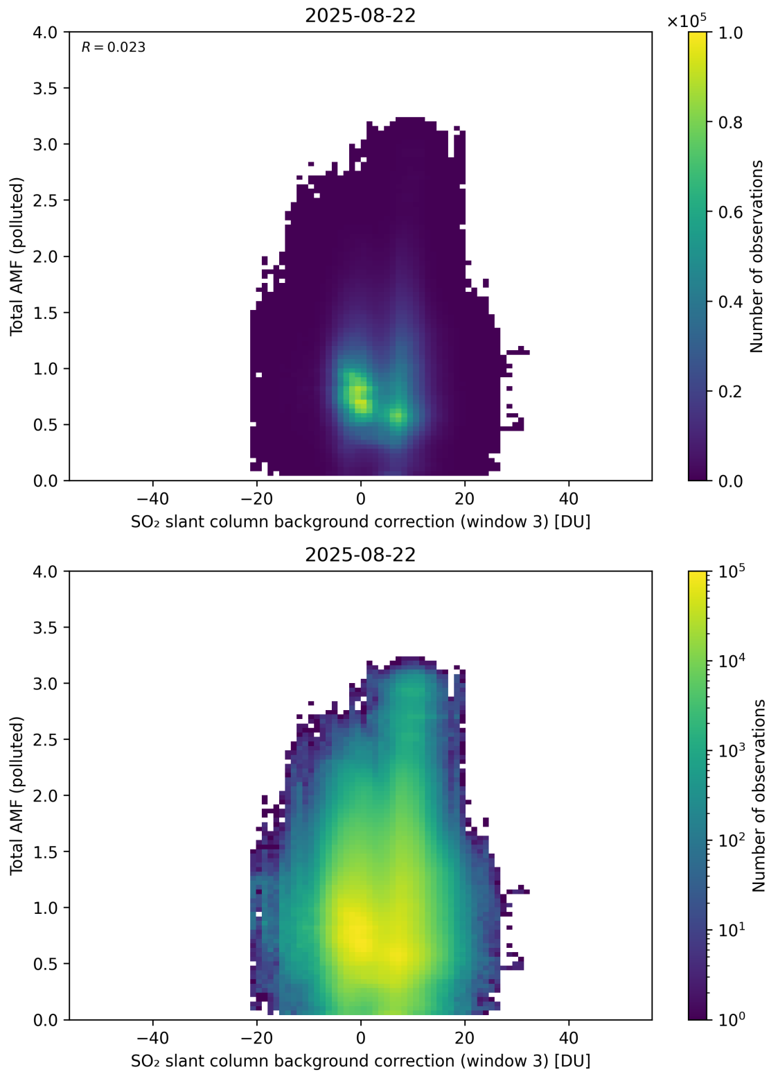
Figure 136: Scatter density plot of “SO 2 slant column background correction (window 3)” against “Total AMF (polluted)” for 2025-08-21 to 2025-08-23.
