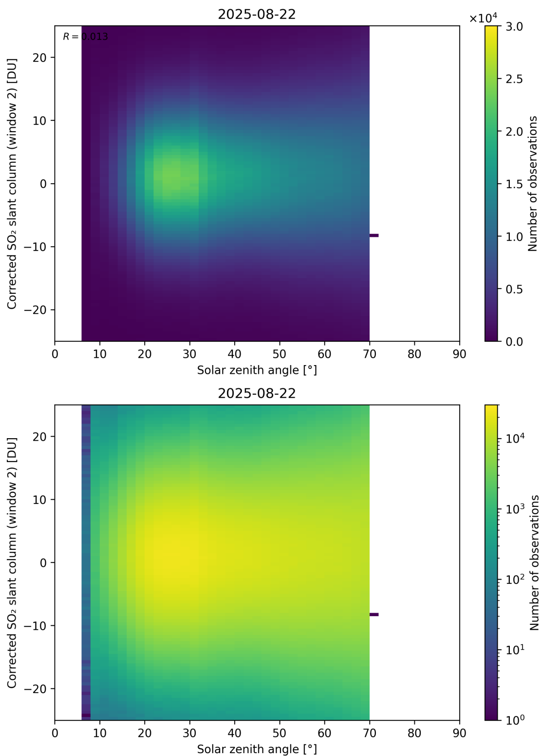
Figure 182: Scatter density plot of “Solar zenith angle” against “Corrected SO 2 slant column (window 2)” for 2025-08-21 to 2025-08-23.
