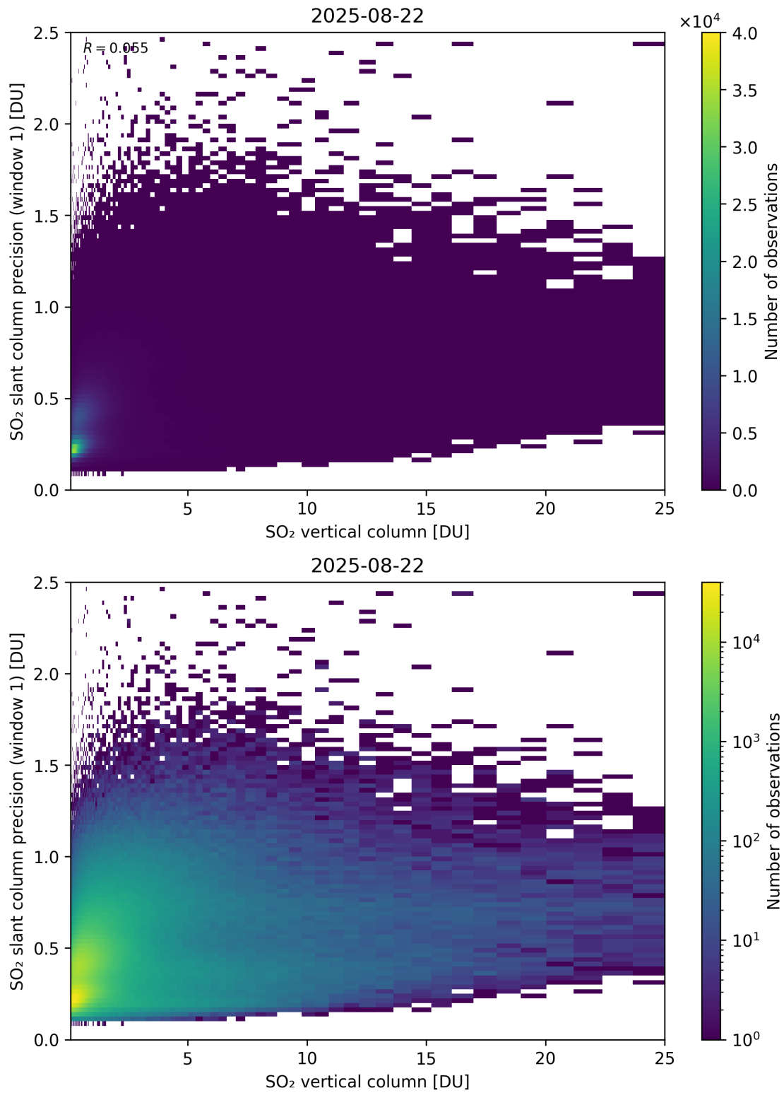
Figure 355: Scatter density plot of “SO 2 vertical column” against “SO 2 slant column precision (window 1)” for 2025-08-21 to 2025-08-23.
