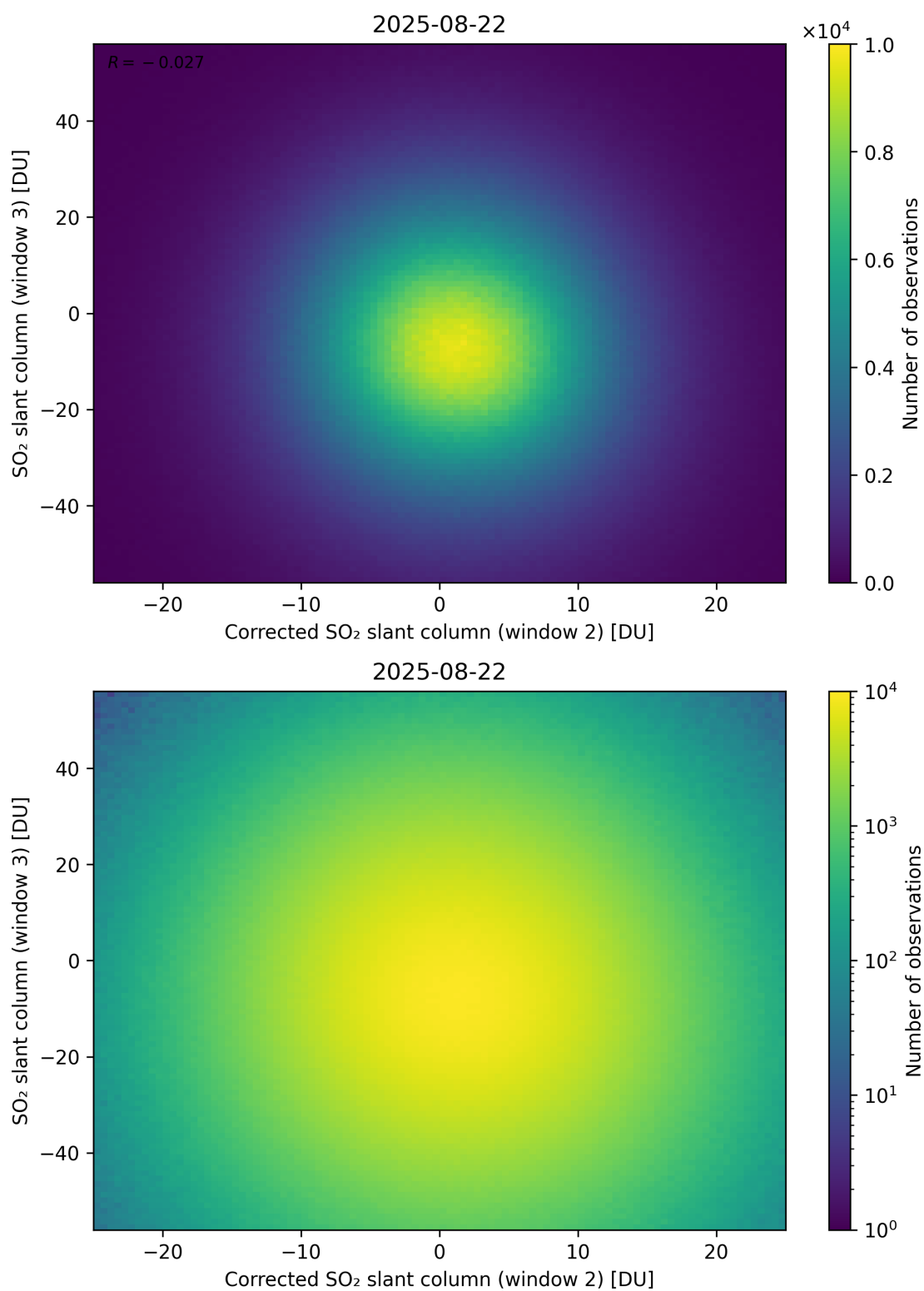
Figure 251: Scatter density plot of “Corrected SO 2 slant column (window 2)” against “SO 2 slant column (window 3)” for 2025-08-21 to 2025-08-23.
