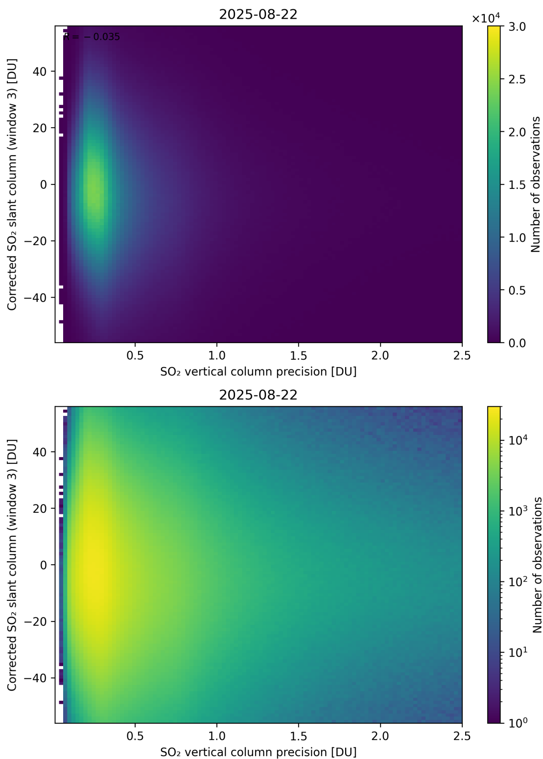
Figure 340: Scatter density plot of “SO 2 vertical column precision” against “Corrected SO 2 slant column (window 3)” for 2025-08-21 to 2025-08-23.
