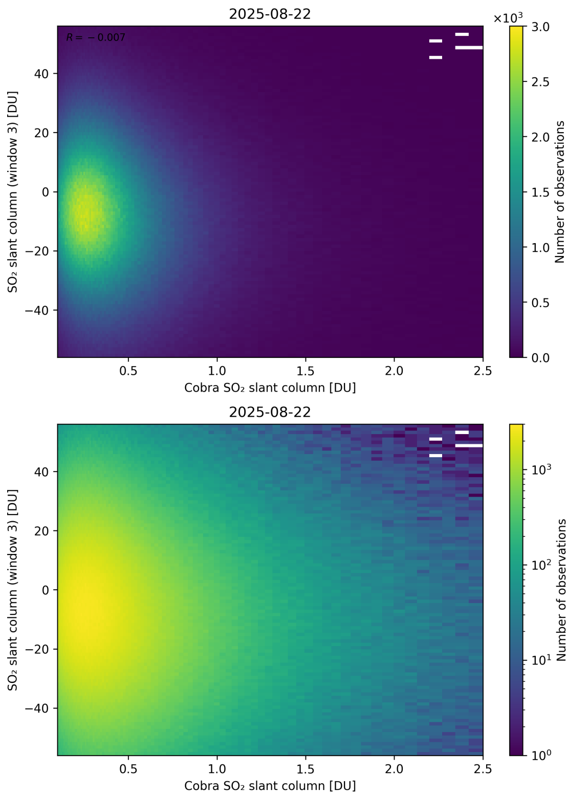
Figure 222: Scatter density plot of “Cobra SO 2 slant column” against “SO 2 slant column (window 3)” for 2025-08-21 to 2025-08-23.
