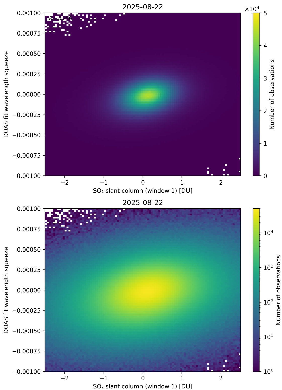
Figure 266: Scatter density plot of “SO 2 slant column (window 1)” against “DOAS fit wavelength squeeze” for 2025-08-21 to 2025-08-23.
