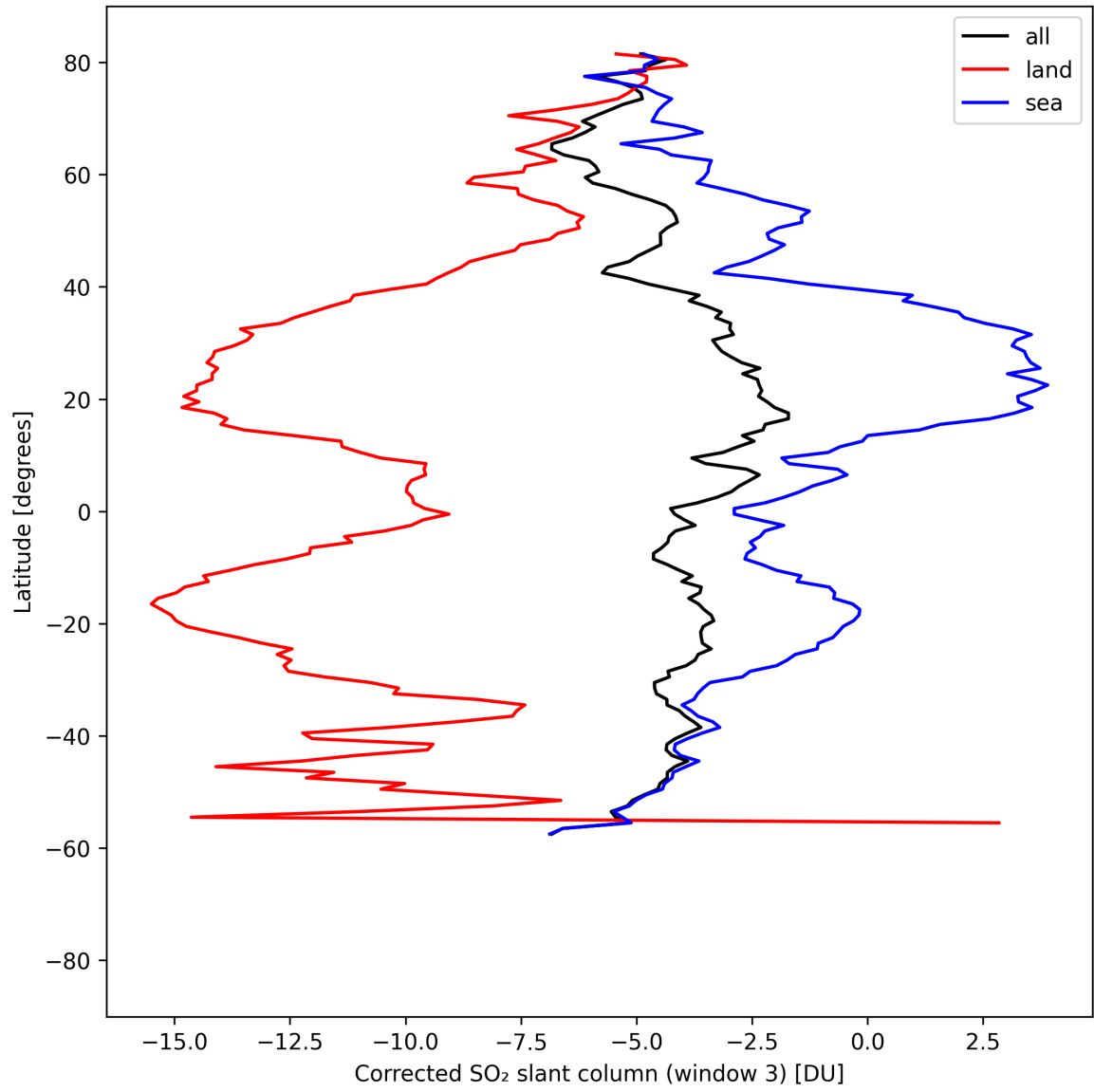
Figure 47: Zonal average of “Corrected SO 2 slant column (window 3)” for 2025-08-21 to 2025-08-23.
