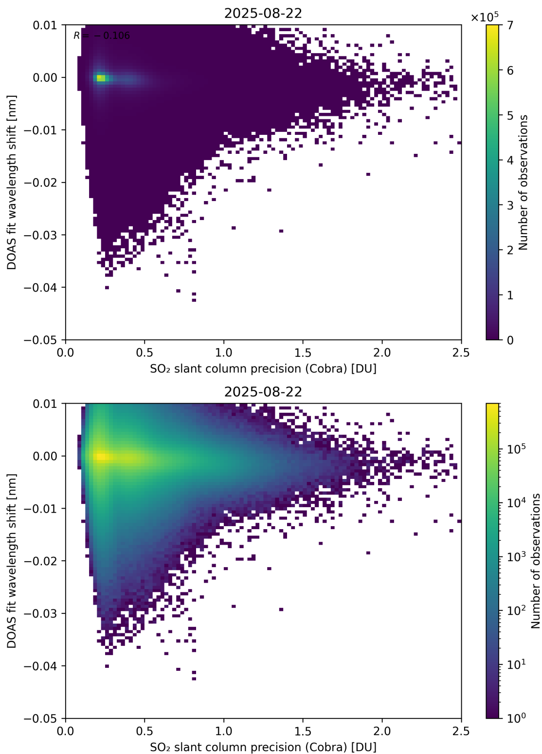
Figure 202: Scatter density plot of “SO 2 slant column precision (Cobra)” against “DOAS fit wavelength shift” for 2025-08-21 to 2025-08-23.
