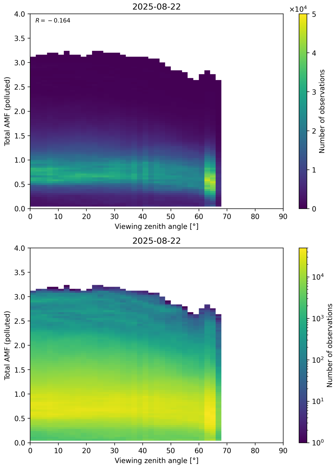
Figure 381: Scatter density plot of “Viewing zenith angle” against “Total AMF (polluted)” for 2025-08-21 to 2025-08-23.
