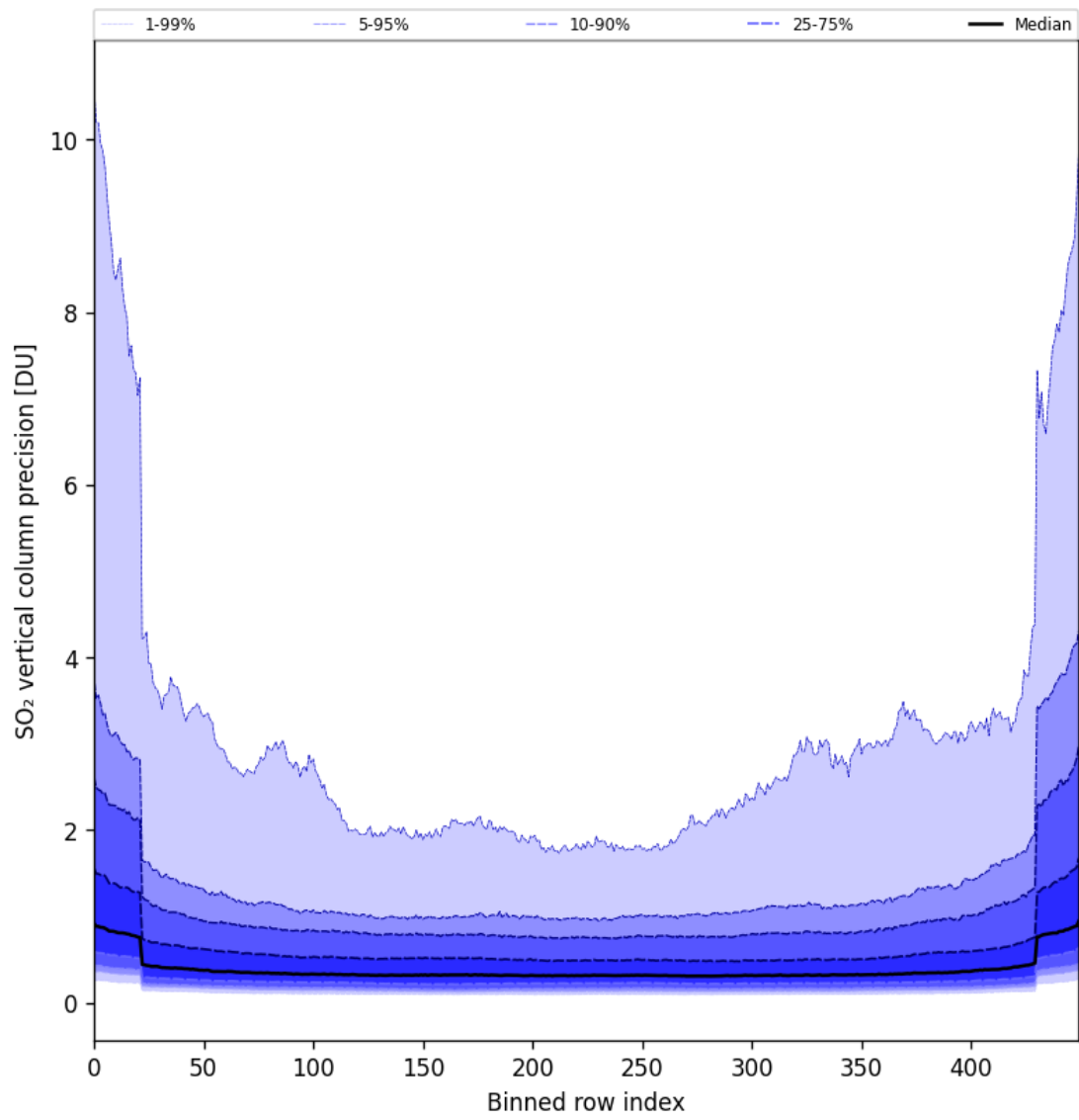
Figure 85: Along track statistics of “SO 2 vertical column precision” for 2025-08-21 to 2025-08-23
