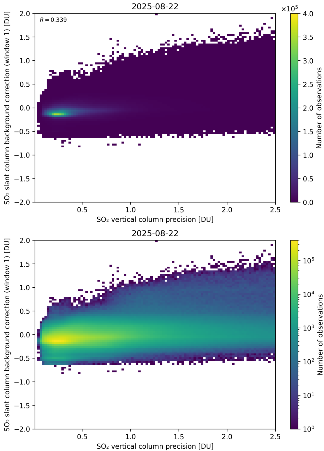
Figure 329: Scatter density plot of “SO 2 vertical column precision” against “SO 2 slant column background correction (window 1)” for 2025-08-21 to 2025-08-23.
