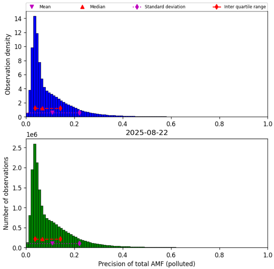
Figure 80: Histogram of “Precision of total AMF (polluted)” for 2025-08-21 to 2025-08-23
