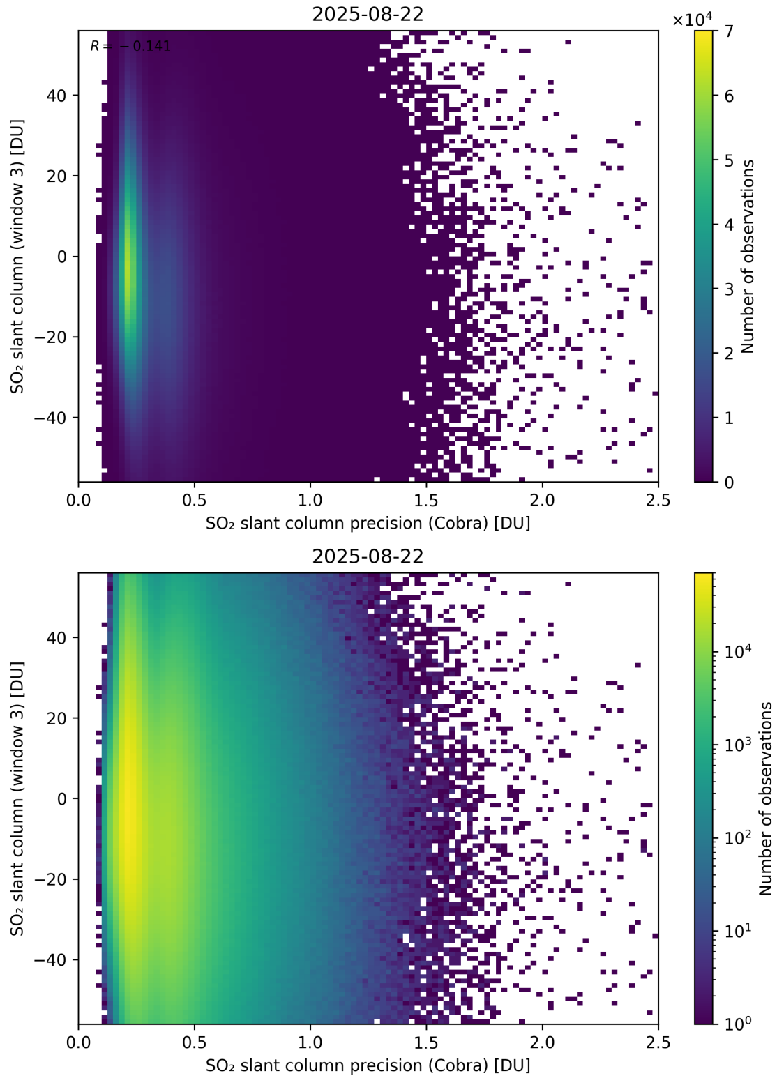
Figure 211: Scatter density plot of “SO 2 slant column precision (Cobra)” against “SO 2 slant column (window 3)” for 2025-08-21 to 2025-08-23.
