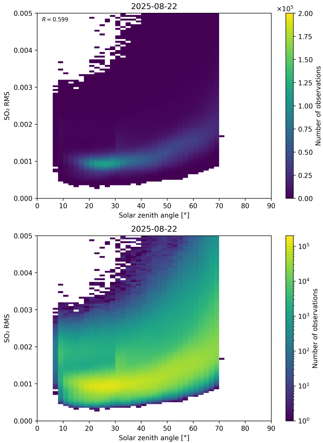
Figure 176: Scatter density plot of “Solar zenith angle” against “SO 2 RMS” for 2025-08-21 to 2025-08-23.
