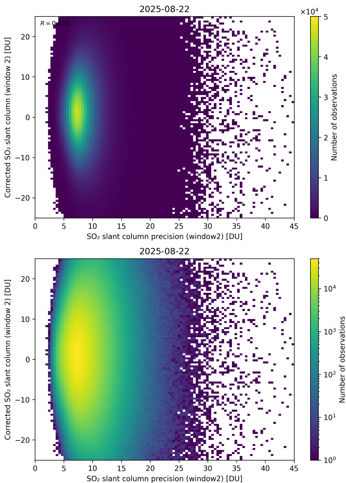
Figure 297: Scatter density plot of “SO 2 slant column precision (window2)” against “Corrected SO 2 slant column (window 2)” for 2025-08-21 to 2025-08-23.
