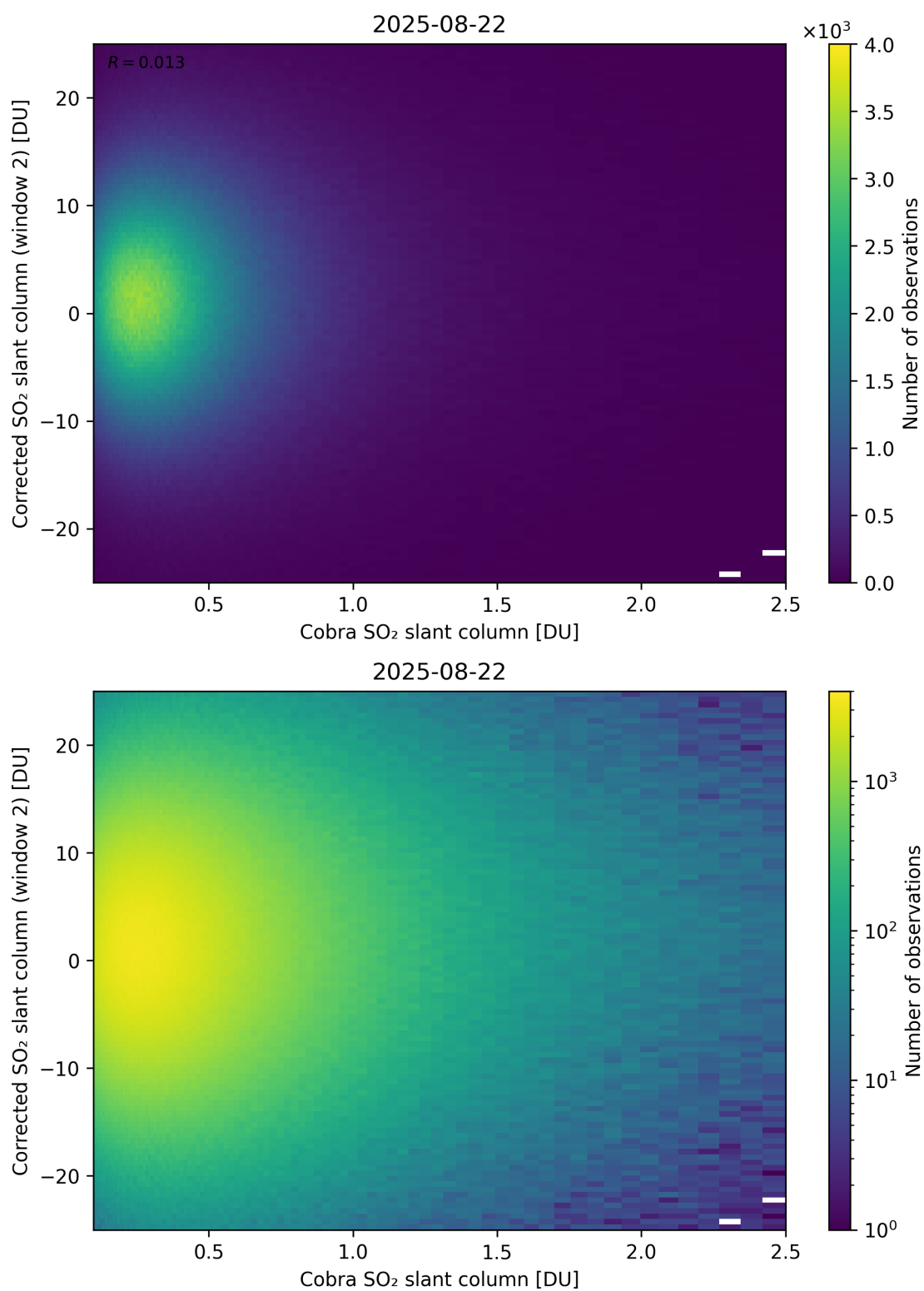
Figure 217: Scatter density plot of “Cobra SO 2 slant column” against “Corrected SO 2 slant column (window 2)” for 2025-08-21 to 2025-08-23.
