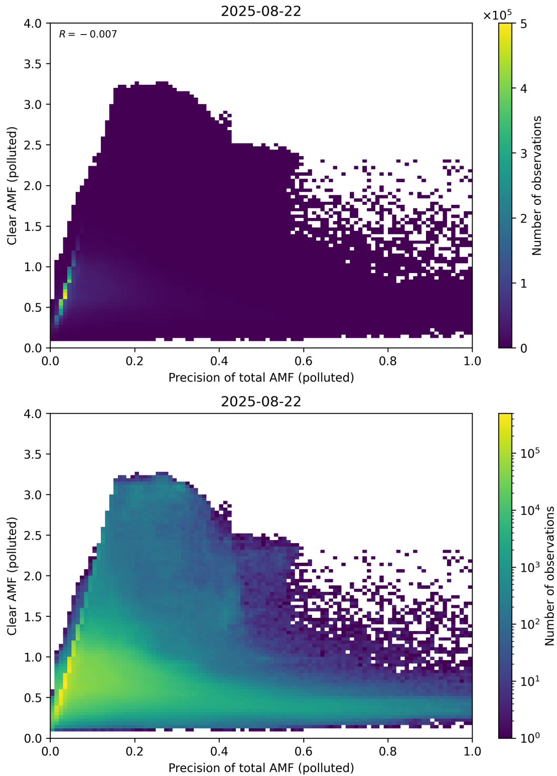
Figure 320: Scatter density plot of “Precision of total AMF (polluted)” against “Clear AMF (polluted)” for 2025-08-21 to 2025-08-23.
