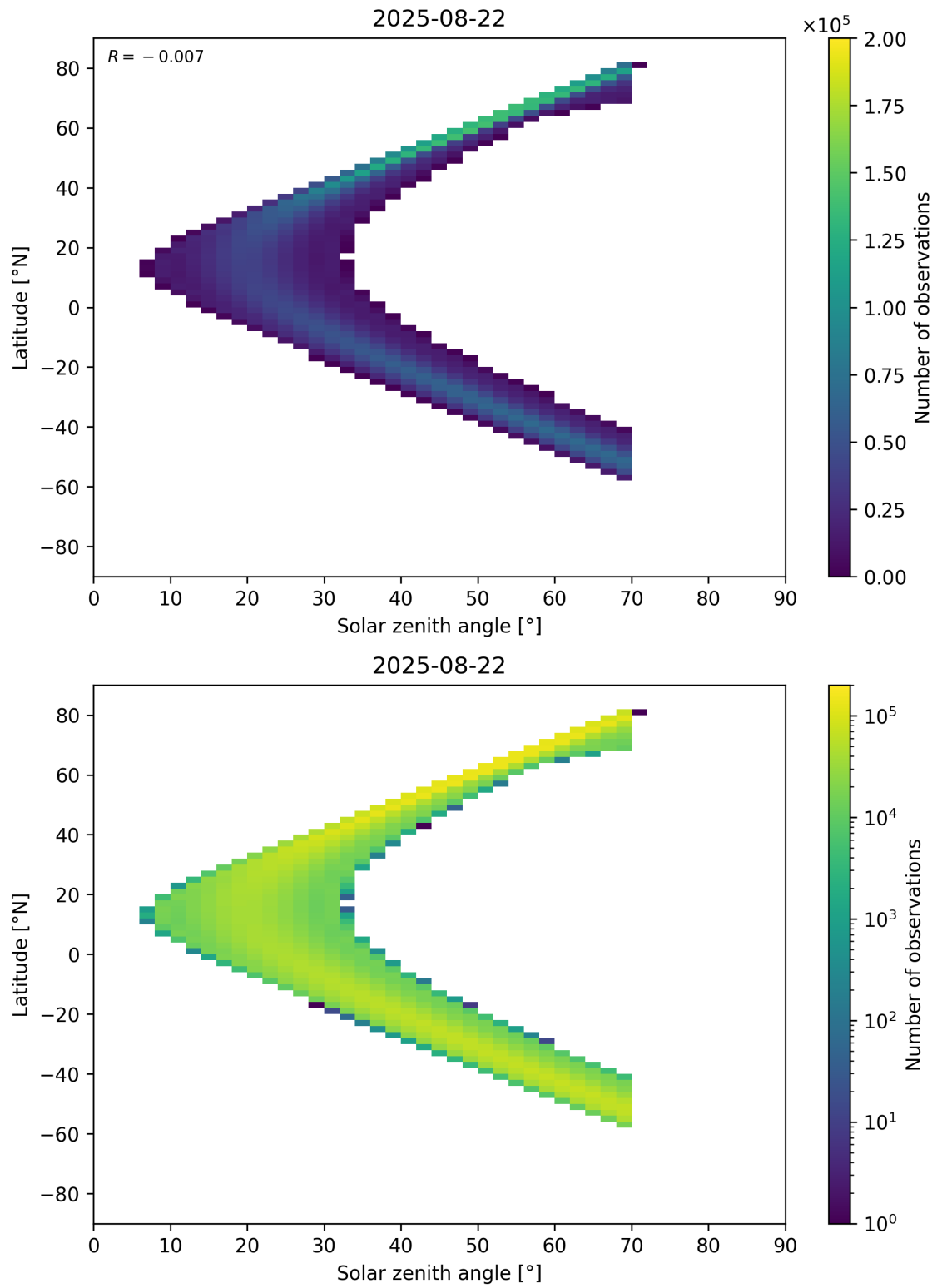
Figure 177: Scatter density plot of “Solar zenith angle” against “Latitude” for 2025-08-21 to 2025-08-23.
