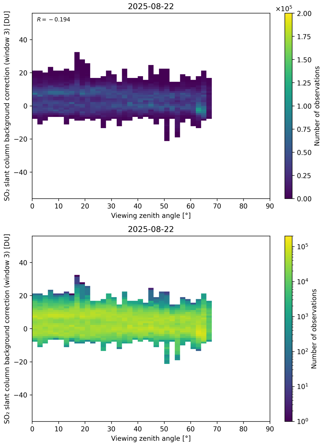
Figure 364: Scatter density plot of “Viewing zenith angle” against “SO 2 slant column background correction (window 3)” for 2025-08-21 to 2025-08-23.
