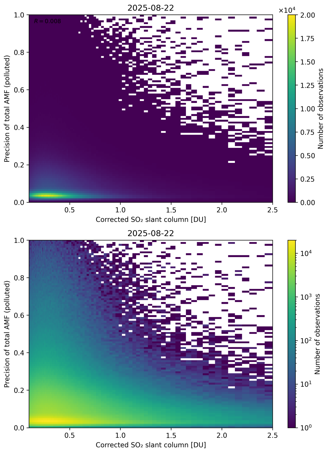
Figure 243: Scatter density plot of “Corrected SO 2 slant column” against “Precision of total AMF (polluted)” for 2025-08-21 to 2025-08-23.
