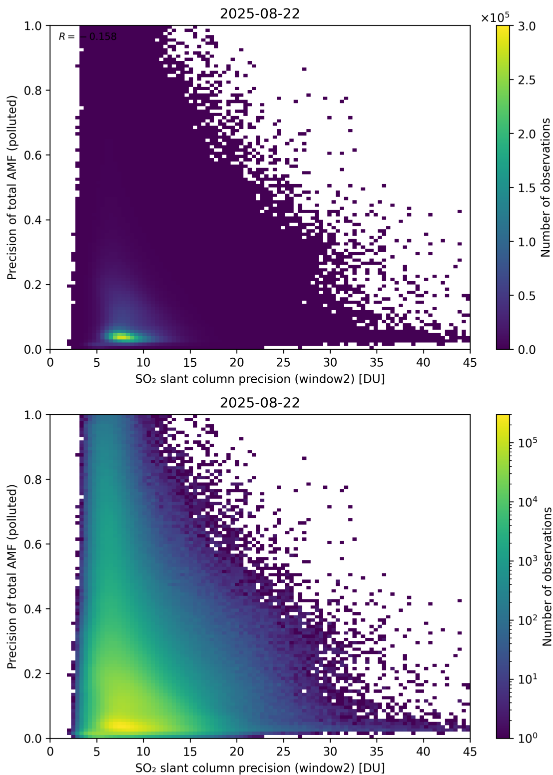
Figure 302: Scatter density plot of “SO 2 slant column precision (window2)” against “Precision of total AMF (polluted)” for 2025-08-21 to 2025-08-23.
