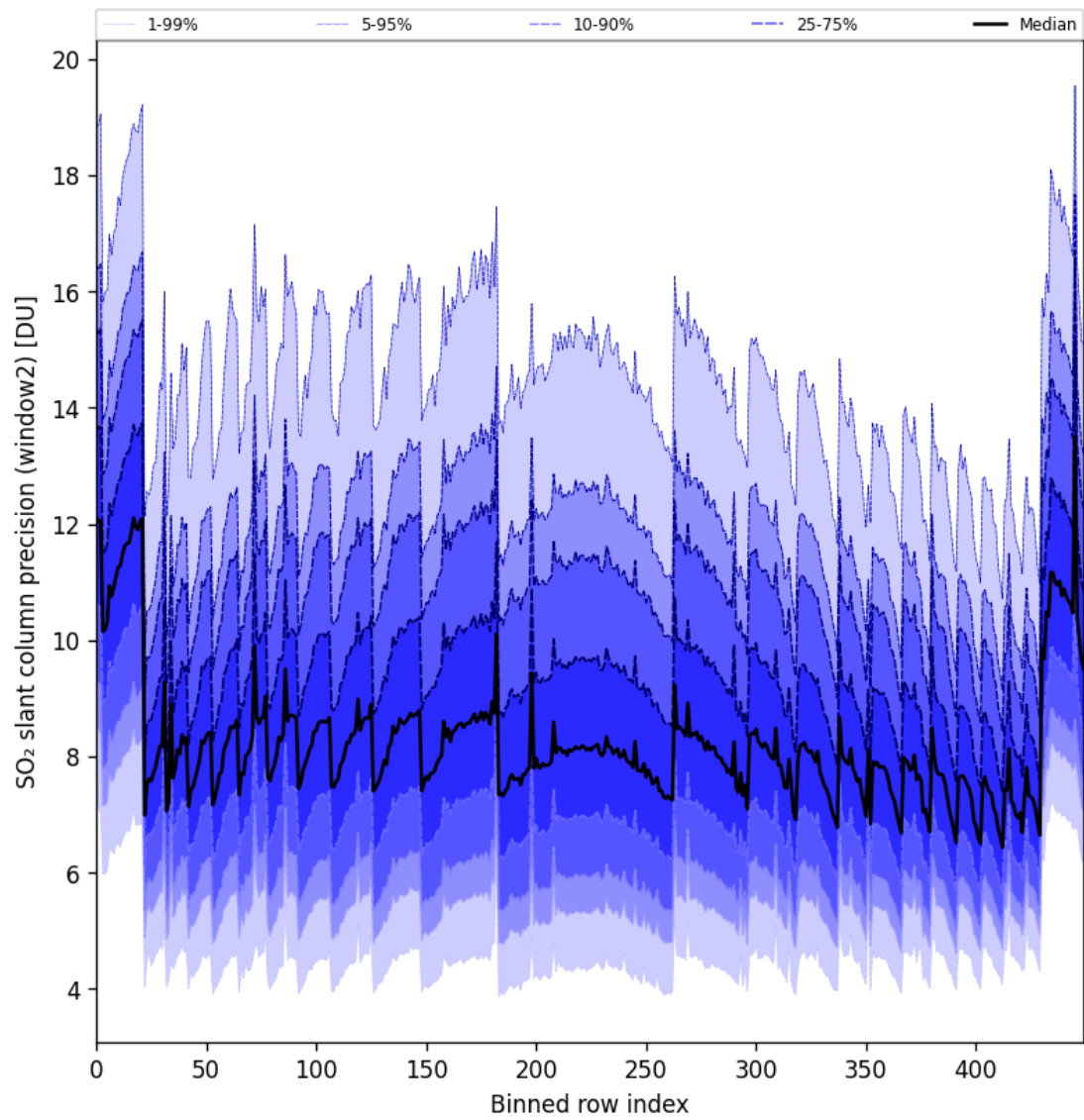
Figure 94: Along track statistics of “SO 2 slant column precision (window2)” for 2025-08-21 to 2025-08-23
