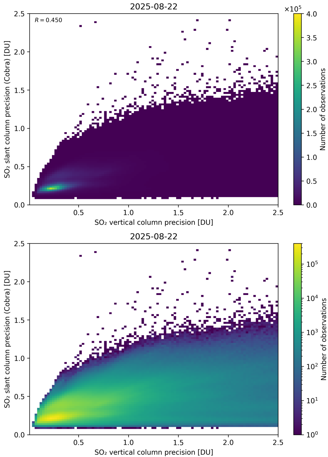
Figure 337: Scatter density plot of “SO 2 vertical column precision” against “SO 2 slant column precision (Cobra)” for 2025-08-21 to 2025-08-23.
