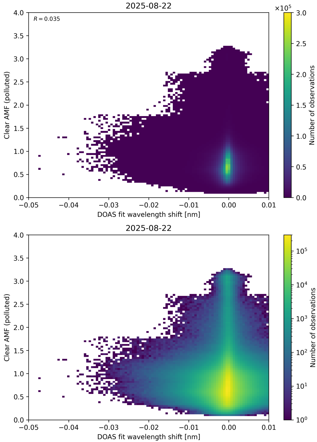
Figure 140: Scatter density plot of “DOAS fit wavelength shift” against “Clear AMF (polluted)” for 2025-08-21 to 2025-08-23.
