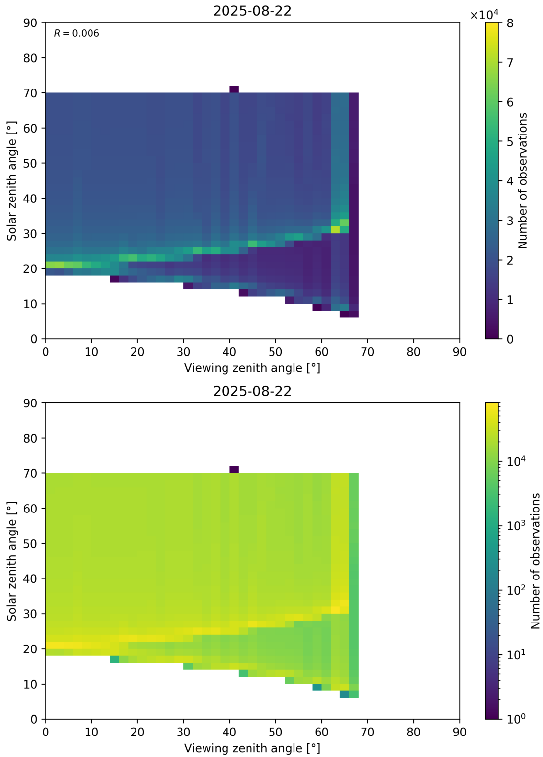
Figure 369: Scatter density plot of “Viewing zenith angle” against “Solar zenith angle” for 2025-08-21 to 2025-08-23.
