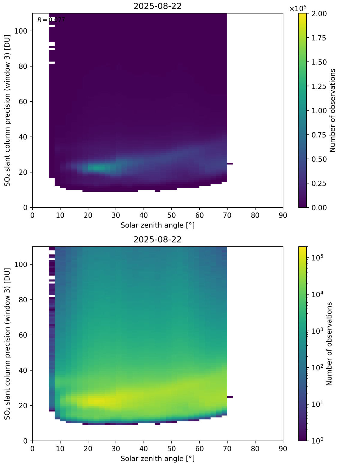
Figure 188: Scatter density plot of “Solar zenith angle” against “SO 2 slant column precision (window 3)” for 2025-08-21 to 2025-08-23.
