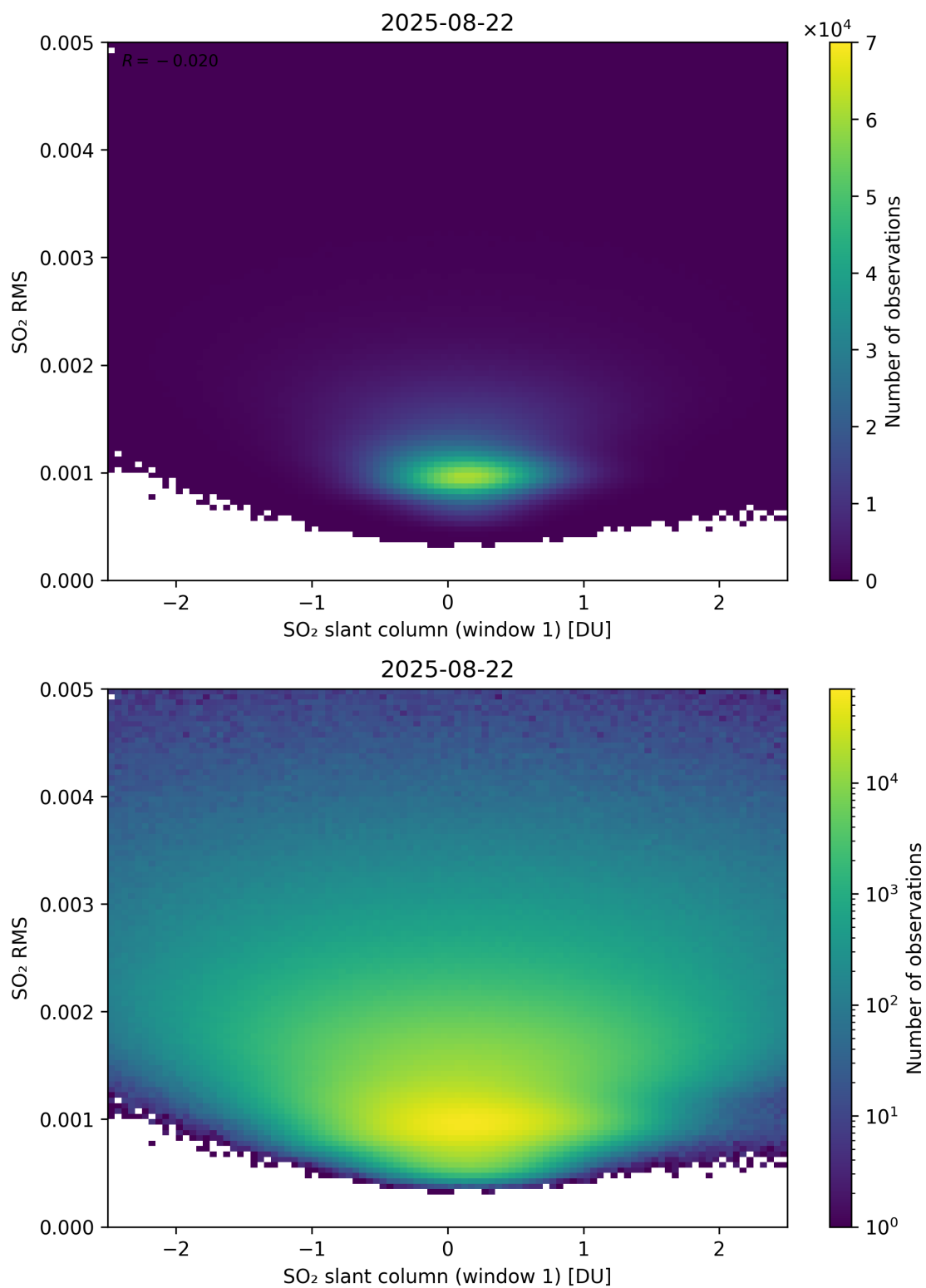
Figure 267: Scatter density plot of “SO 2 slant column (window 1)” against “SO 2 RMS” for 2025-08-21 to 2025-08-23.
