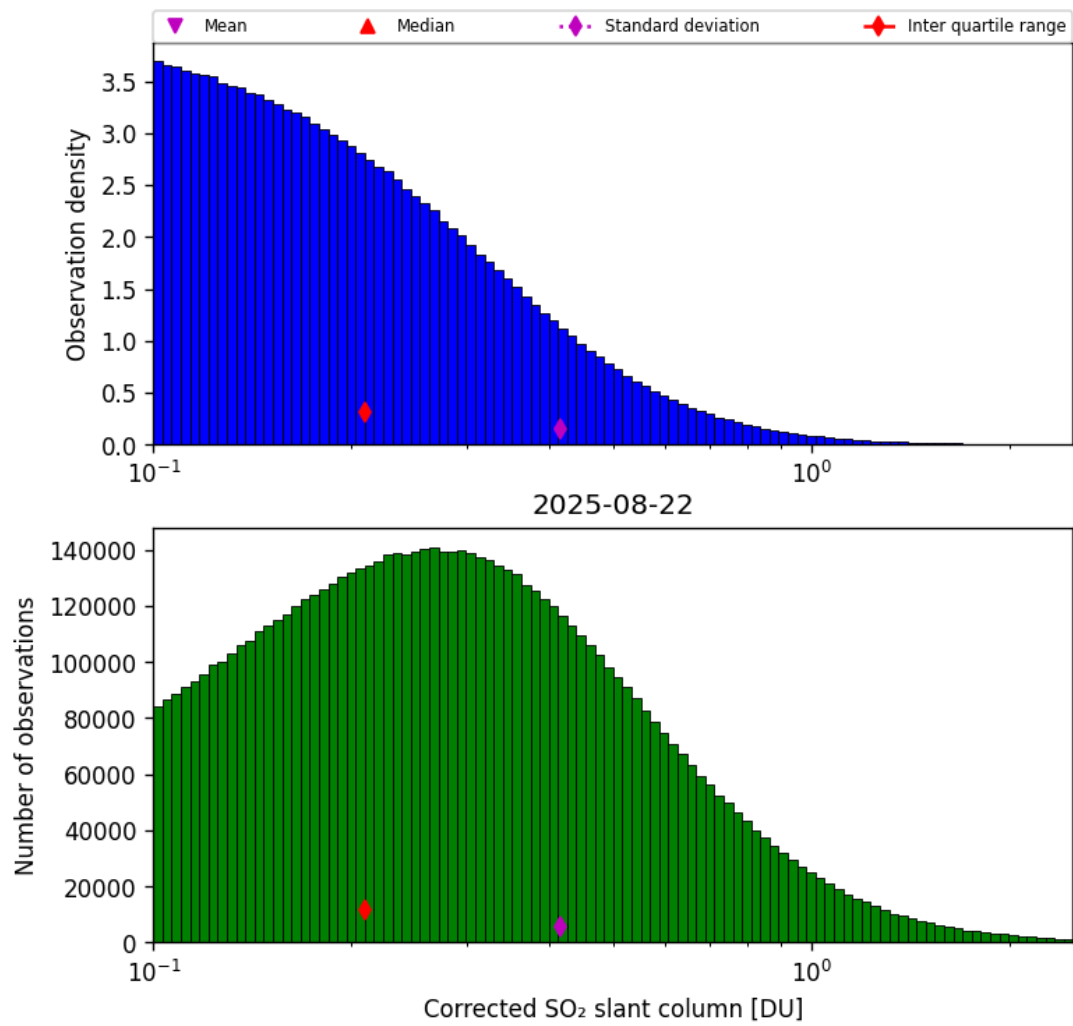
Figure 60: Histogram of “Corrected SO 2 slant column” for 2025-08-21 to 2025-08-23
