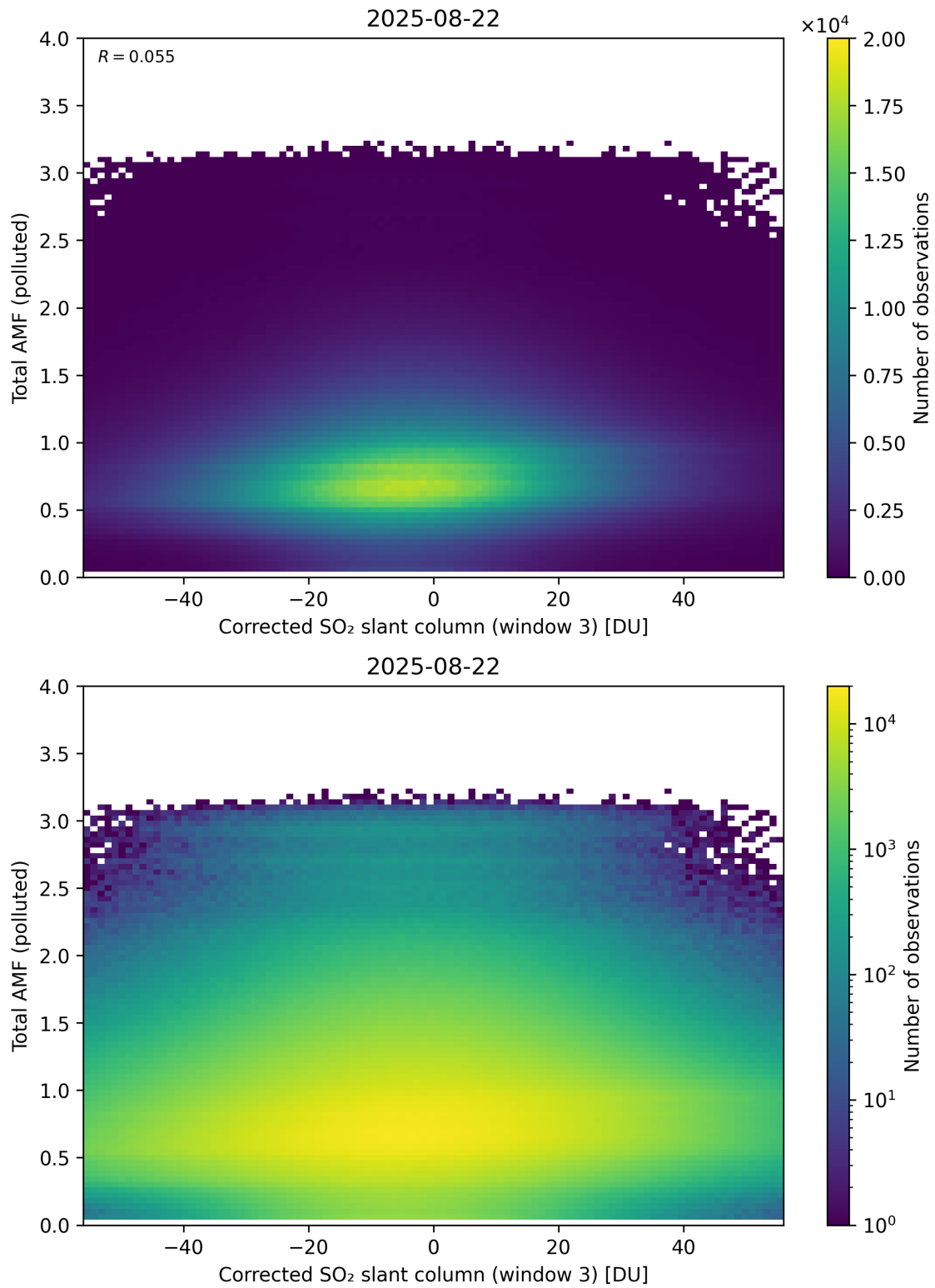
Figure 260: Scatter density plot of “Corrected SO 2 slant column (window 3)” against “Total AMF (polluted)” for 2025-08-21 to 2025-08-23.
