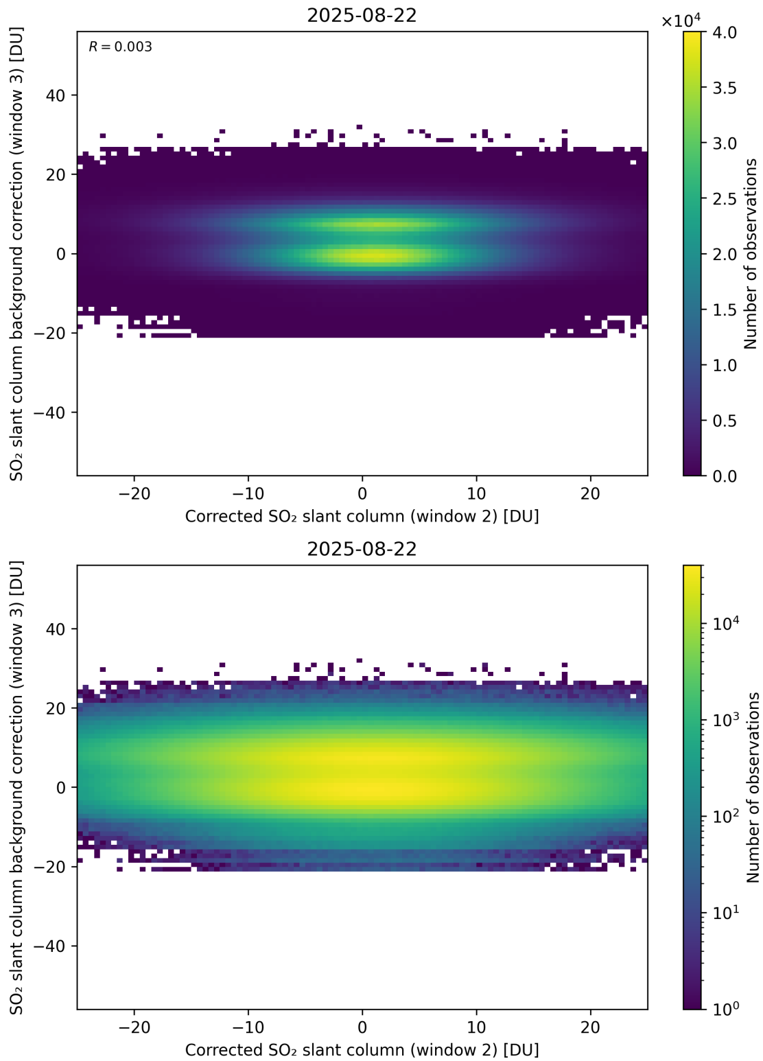
Figure 245: Scatter density plot of “Corrected SO 2 slant column (window 2)” against “SO 2 slant column background correction (window 3)” for 2025-08-21 to 2025-08-23.
