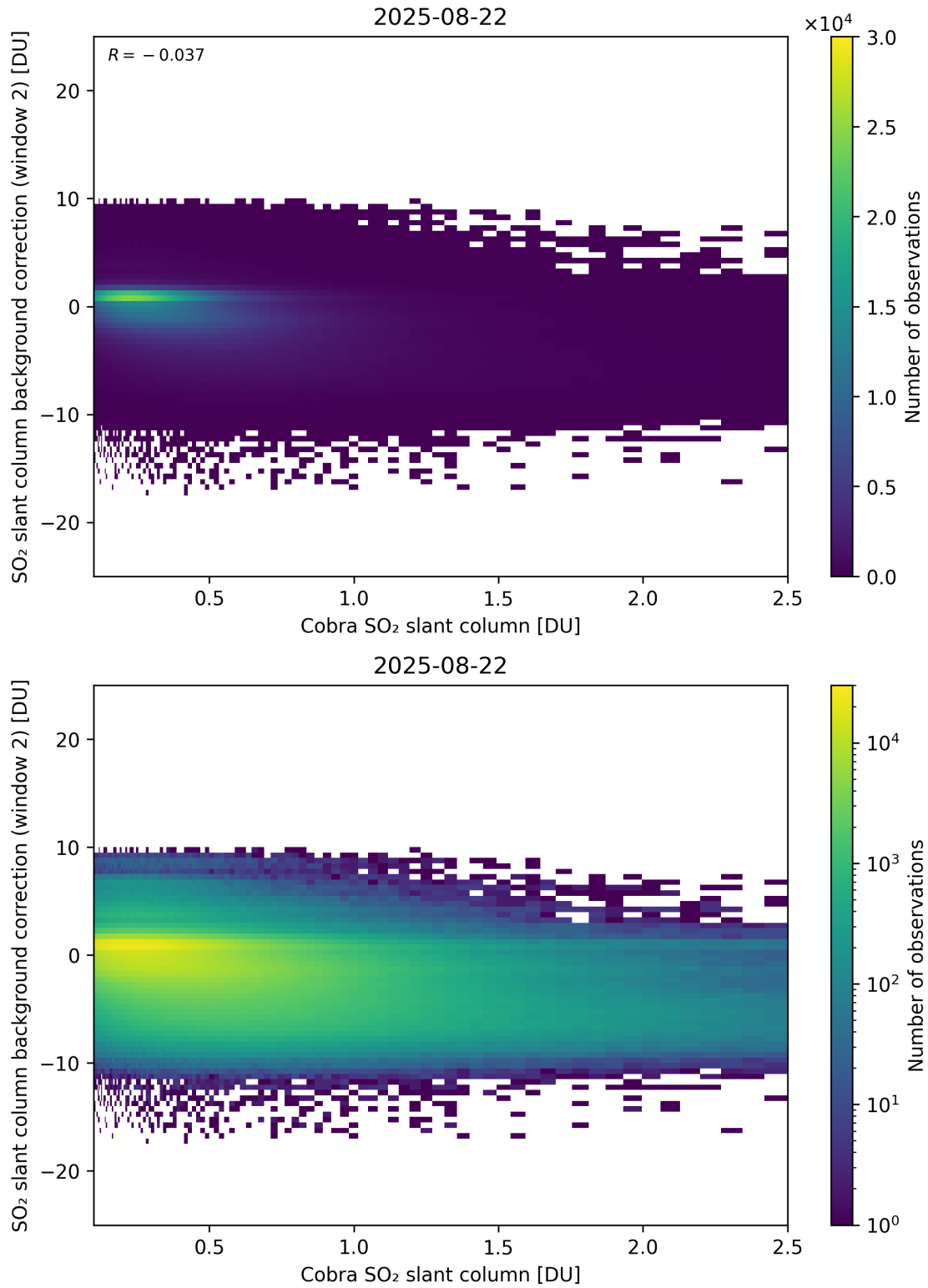
Figure 194: Scatter density plot of “Cobra SO 2 slant column” against “SO 2 slant column background correction (window 2)” for 2025-08-21 to 2025-08-23.
