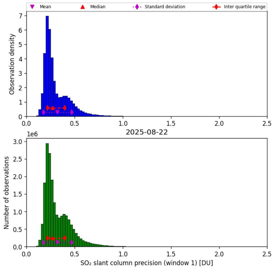
Figure 64: Histogram of “SO 2 slant column precision (window 1)” for 2025-08-21 to 2025-08-23
