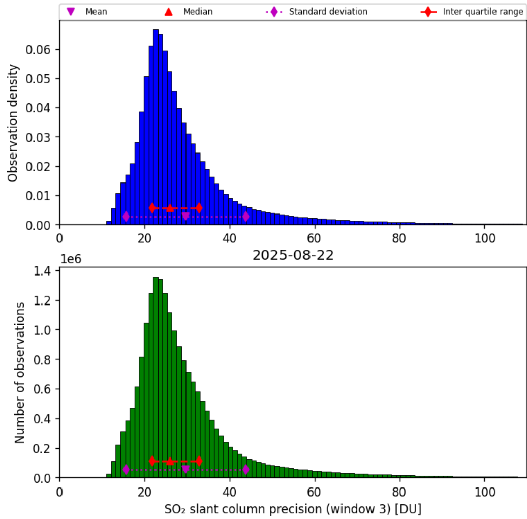
Figure 72: Histogram of “SO 2 slant column precision (window 3)” for 2025-08-21 to 2025-08-23
