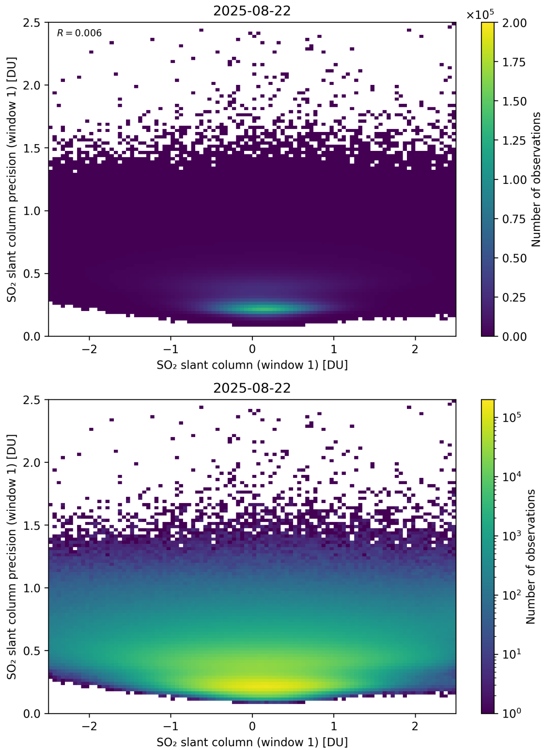
Figure 285: Scatter density plot of “SO 2 slant column (window 1)” against “SO 2 slant column precision (window 1)” for 2025-08-21 to 2025-08-23.
