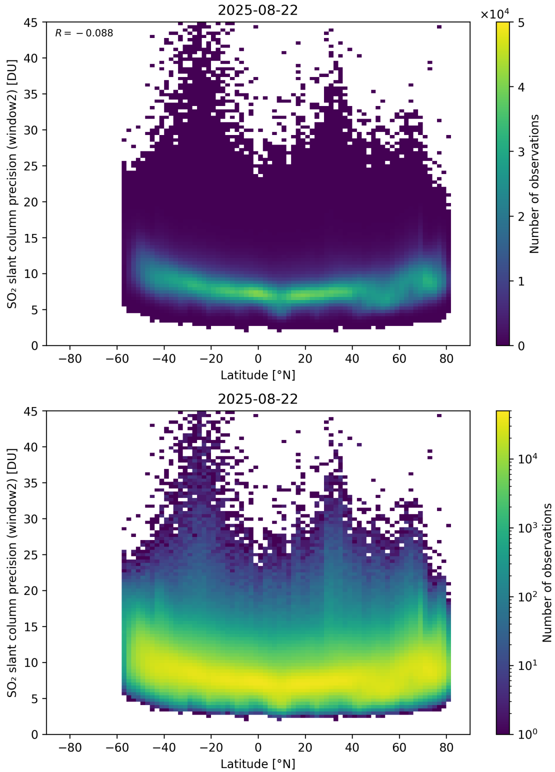
Figure 164: Scatter density plot of “Latitude” against “SO 2 slant column precision (window2)” for 2025-08-21 to 2025-08-23.
