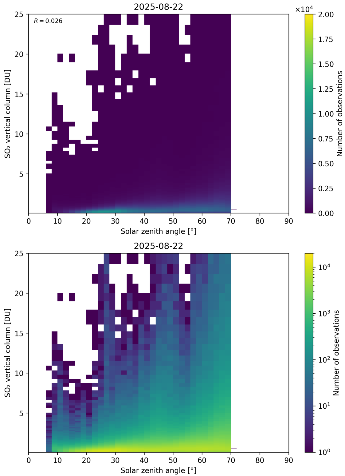
Figure 191: Scatter density plot of “Solar zenith angle” against “SO 2 vertical column” for 2025-08-21 to 2025-08-23.
