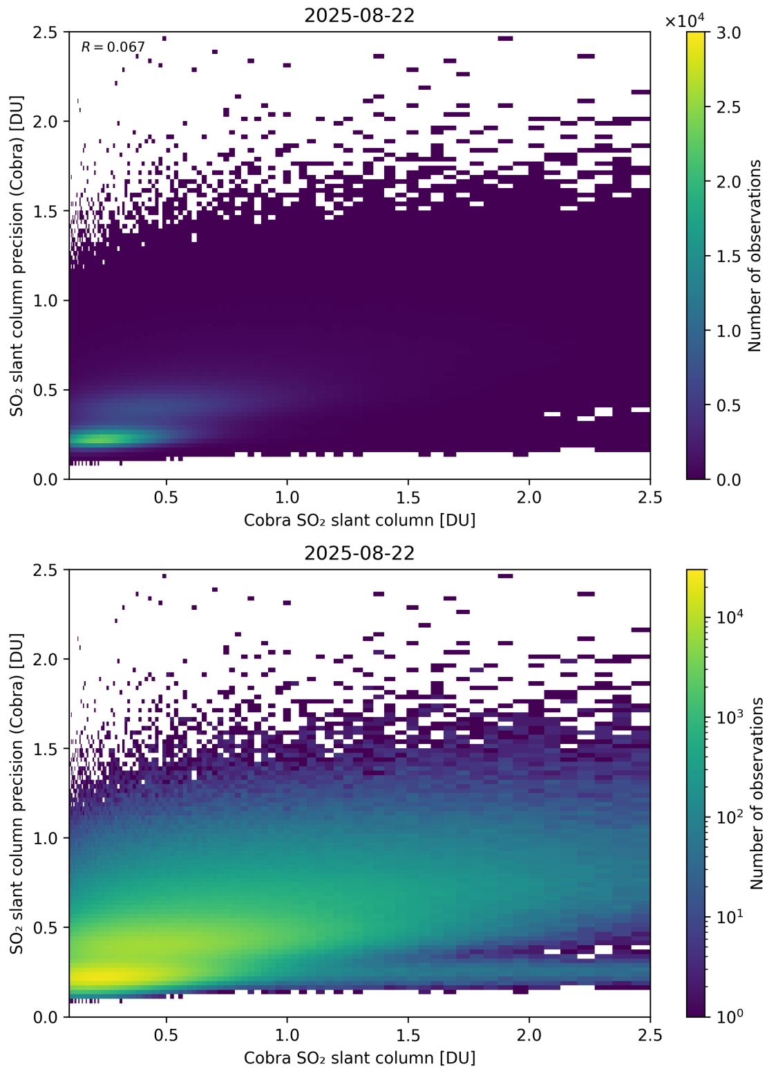
Figure 216: Scatter density plot of “Cobra SO 2 slant column” against “SO 2 slant column precision (Cobra)” for 2025-08-21 to 2025-08-23.
