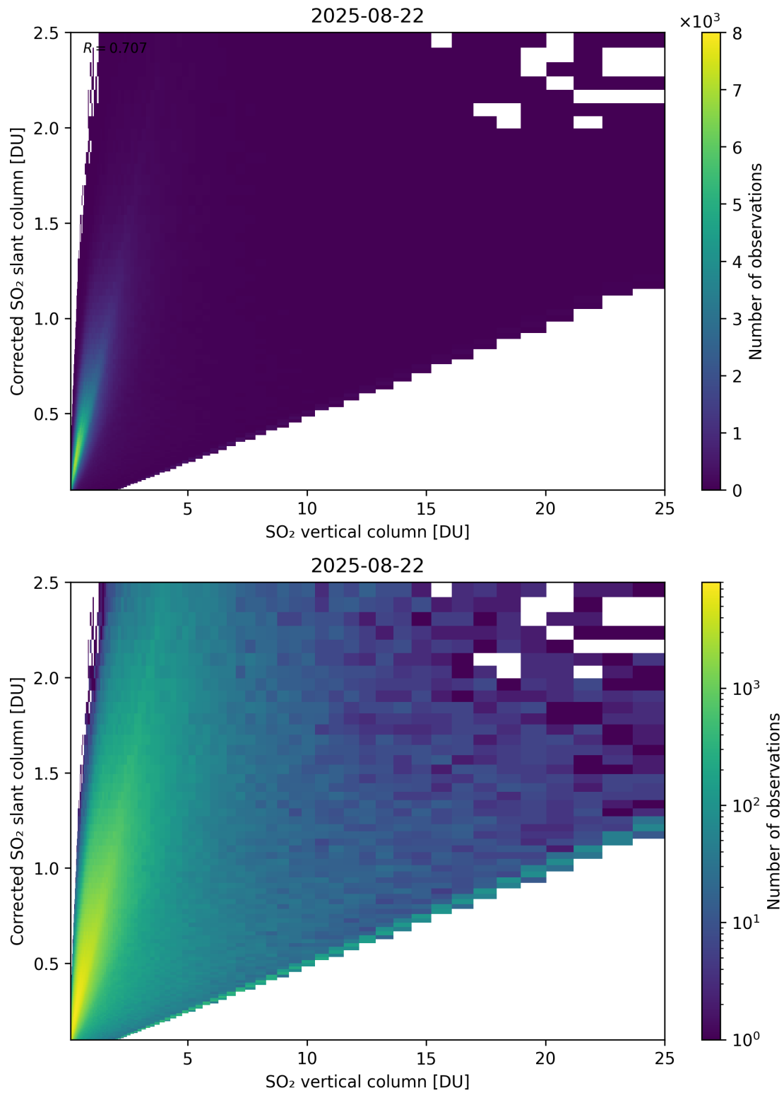
Figure 351: Scatter density plot of “SO 2 vertical column” against “Corrected SO 2 slant column” for 2025-08-21 to 2025-08-23.
