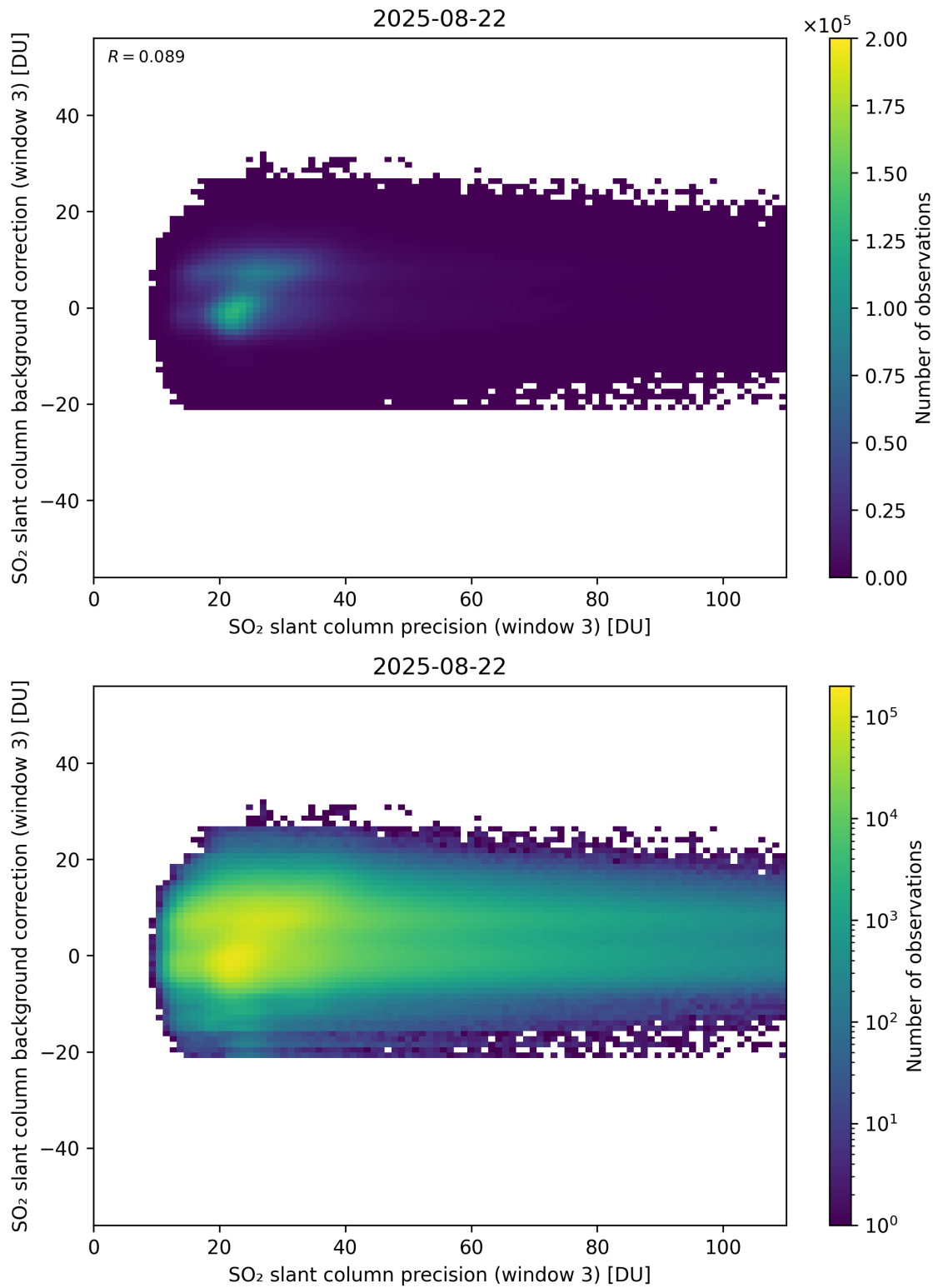
Figure 307: Scatter density plot of “SO 2 slant column precision (window 3)” against “SO 2 slant column background correction (window 3)” for 2025-08-21 to 2025-08-23.
