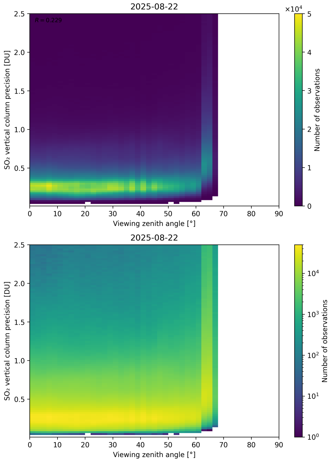
Figure 384: Scatter density plot of “Viewing zenith angle” against “SO 2 vertical column precision” for 2025-08-21 to 2025-08-23.
