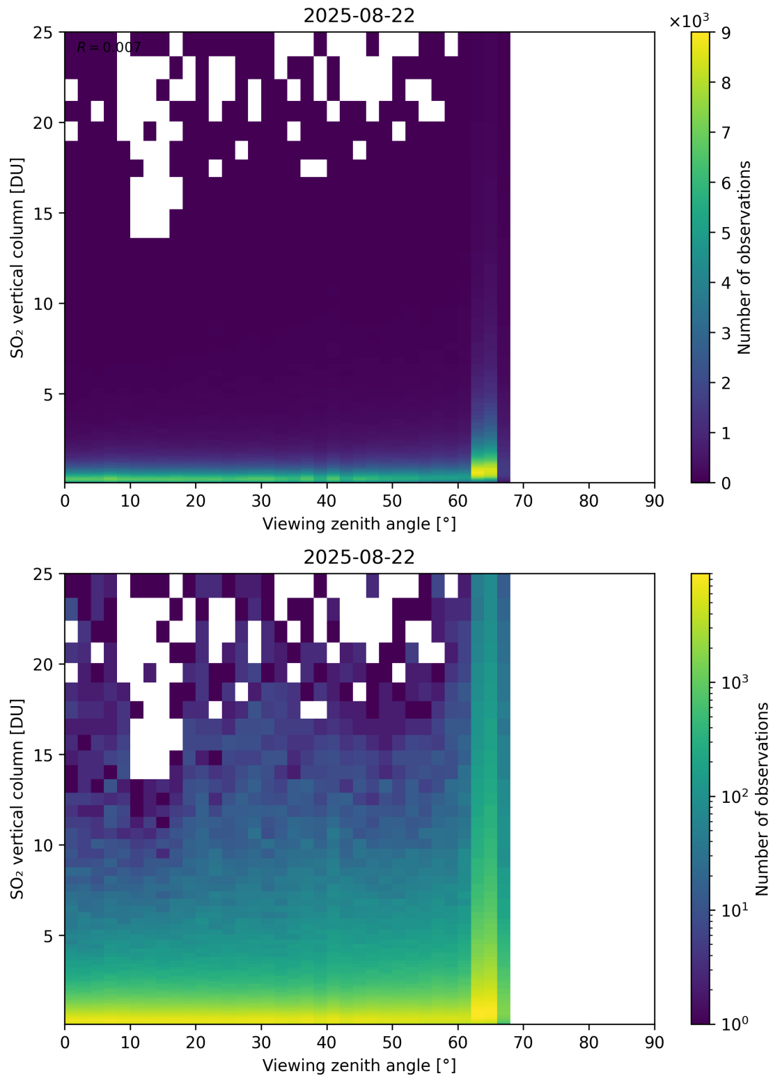
Figure 383: Scatter density plot of “Viewing zenith angle” against “SO 2 vertical column” for 2025-08-21 to 2025-08-23.
