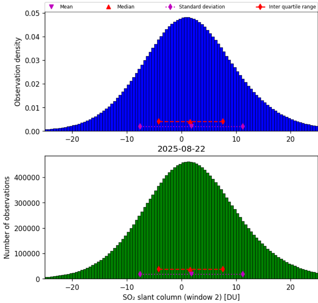
Figure 67: Histogram of “SO 2 slant column (window 2)” for 2025-08-21 to 2025-08-23
