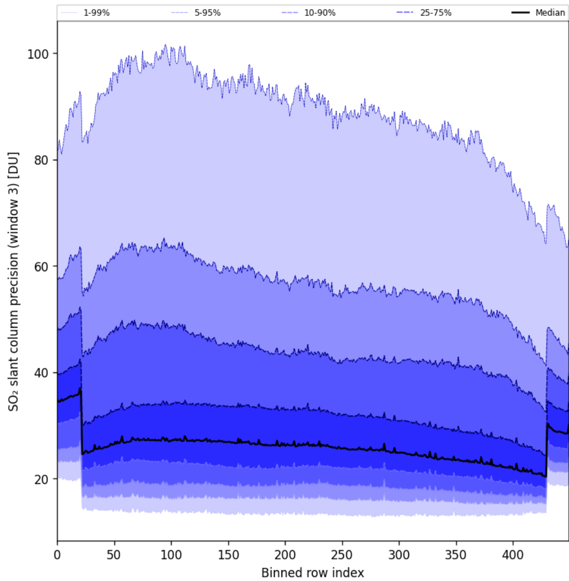
Figure 98: Along track statistics of “SO 2 slant column precision (window 3)” for 2025-08-21 to 2025-08-23
