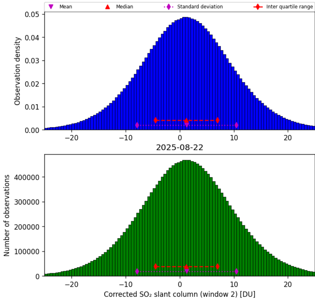
Figure 69: Histogram of “Corrected SO 2 slant column (window 2)” for 2025-08-21 to 2025-08-23
