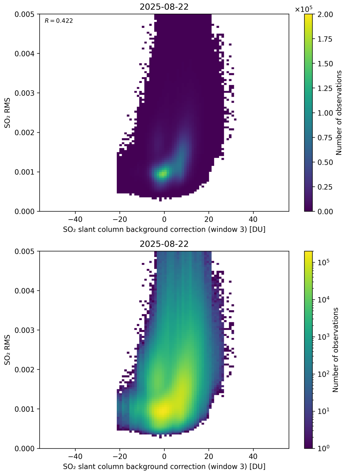
Figure 134: Scatter density plot of “SO 2 slant column background correction (window 3)” against “SO 2 RMS” for 2025-08-21 to 2025-08-23.
