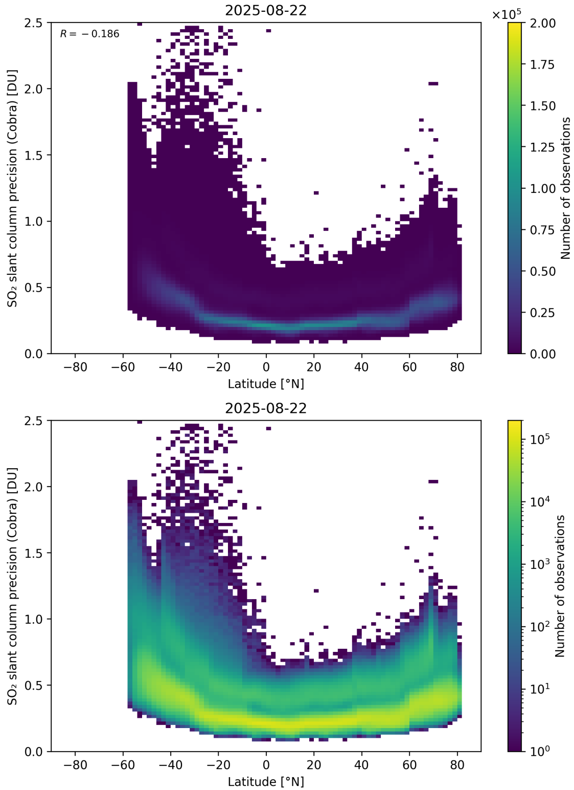
Figure 158: Scatter density plot of “Latitude” against “SO 2 slant column precision (Cobra)” for 2025-08-21 to 2025-08-23.
