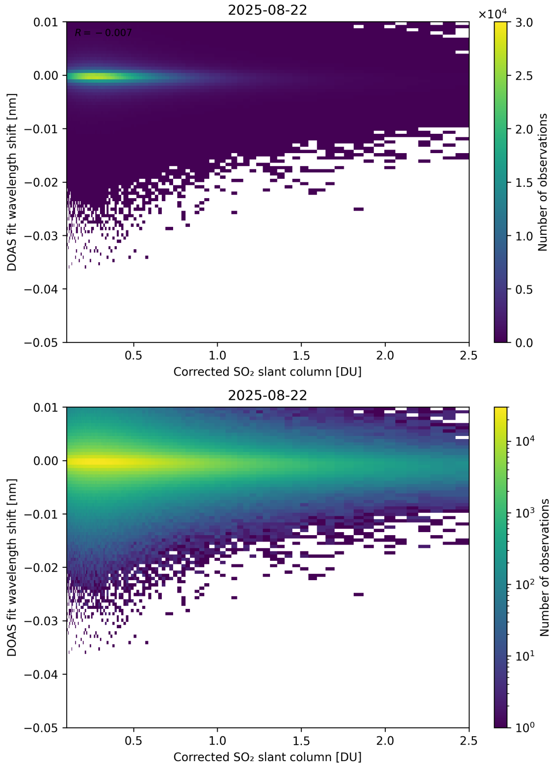
Figure 229: Scatter density plot of “Corrected SO 2 slant column” against “DOAS fit wavelength shift” for 2025-08-21 to 2025-08-23.
