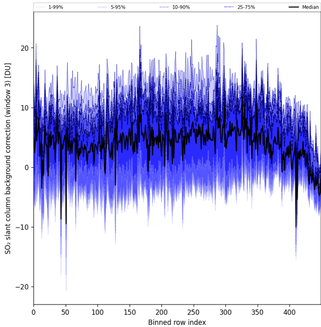
Figure 100: Along track statistics of “SO 2 slant column background correction (window 3)” for 2025-08-21 to 2025-08-23
