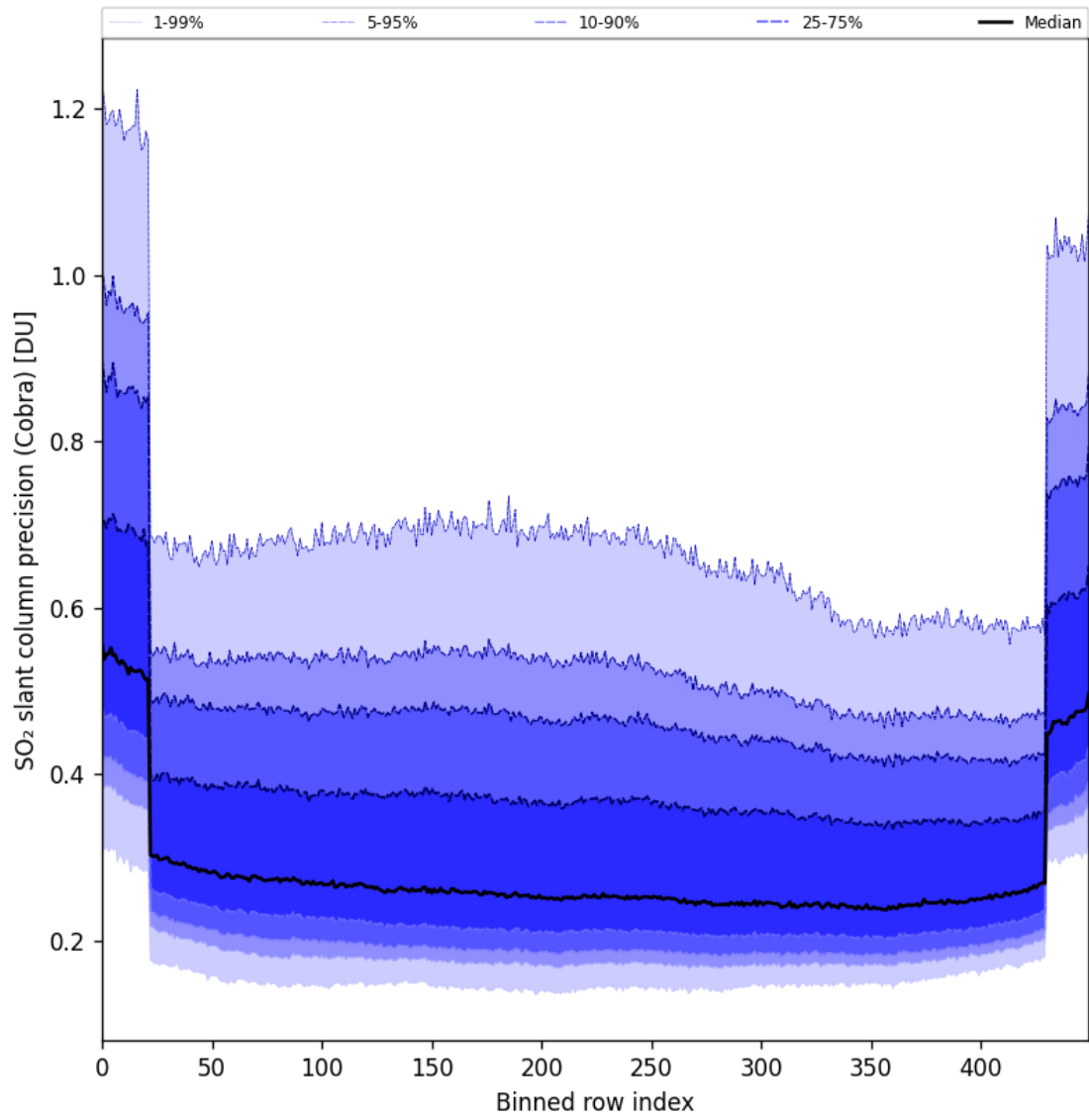
Figure 88: Along track statistics of “SO 2 slant column precision (Cobra)” for 2025-08-21 to 2025-08-23
