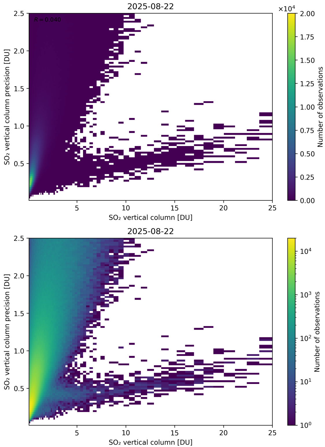
Figure 361: Scatter density plot of “SO 2 vertical column” against “SO 2 vertical column precision” for 2025-08-21 to 2025-08-23.
