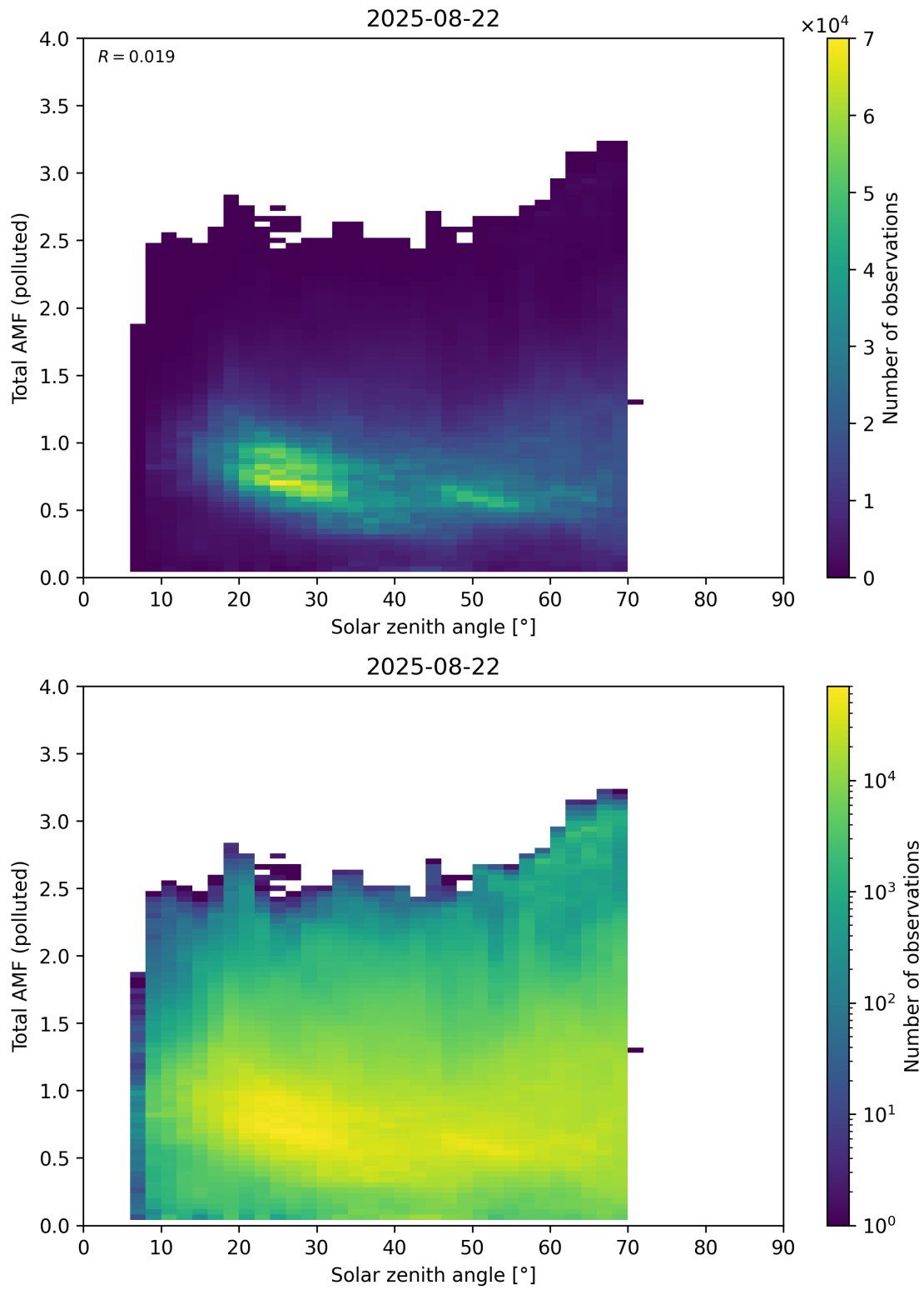
Figure 189: Scatter density plot of “Solar zenith angle” against “Total AMF (polluted)” for 2025-08-21 to 2025-08-23.
