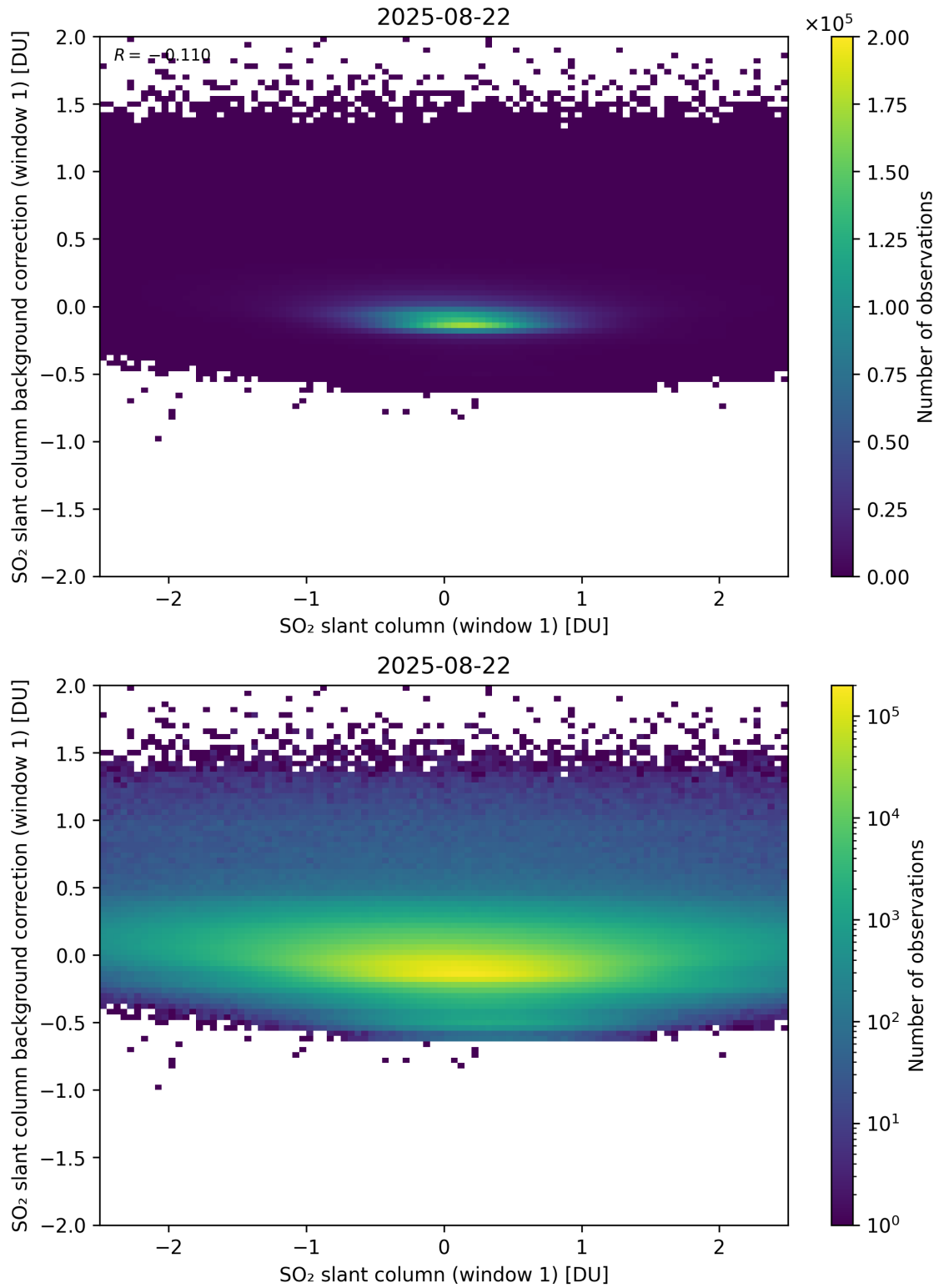
Figure 262: Scatter density plot of “SO 2 slant column (window 1)” against “SO 2 slant column background correction (window 1)” for 2025-08-21 to 2025-08-23.
