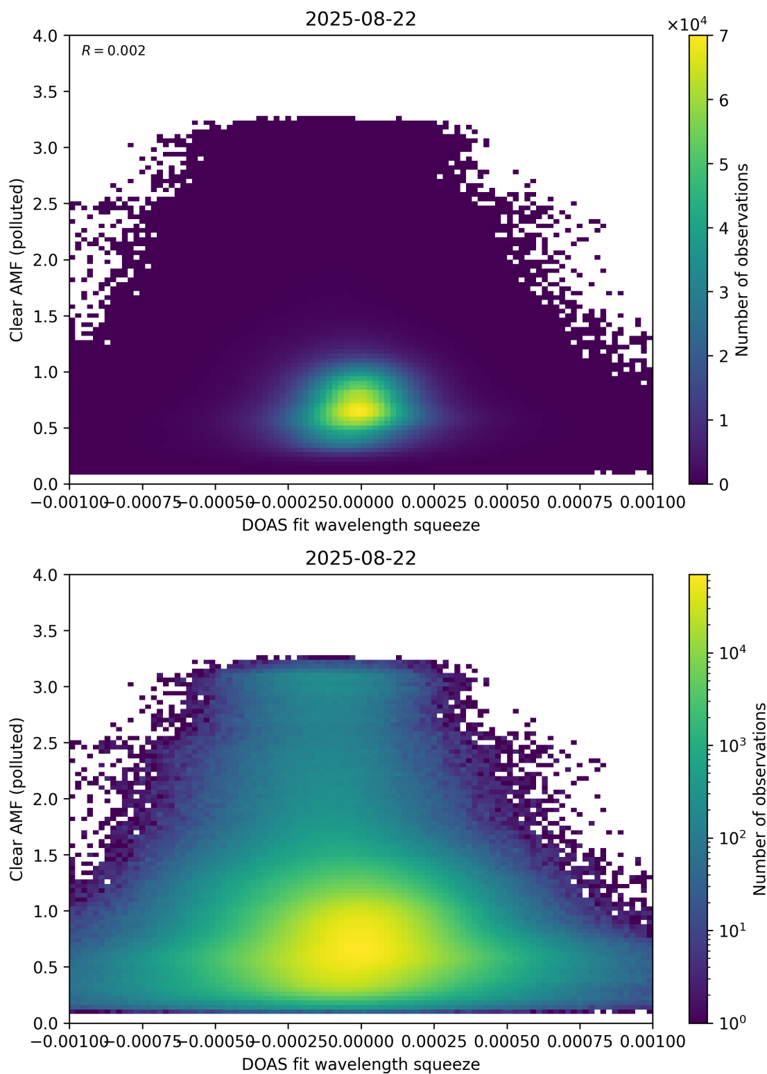
Figure 144: Scatter density plot of “DOAS fit wavelength squeeze” against “Clear AMF (polluted)” for 2025-08-21 to 2025-08-23.
