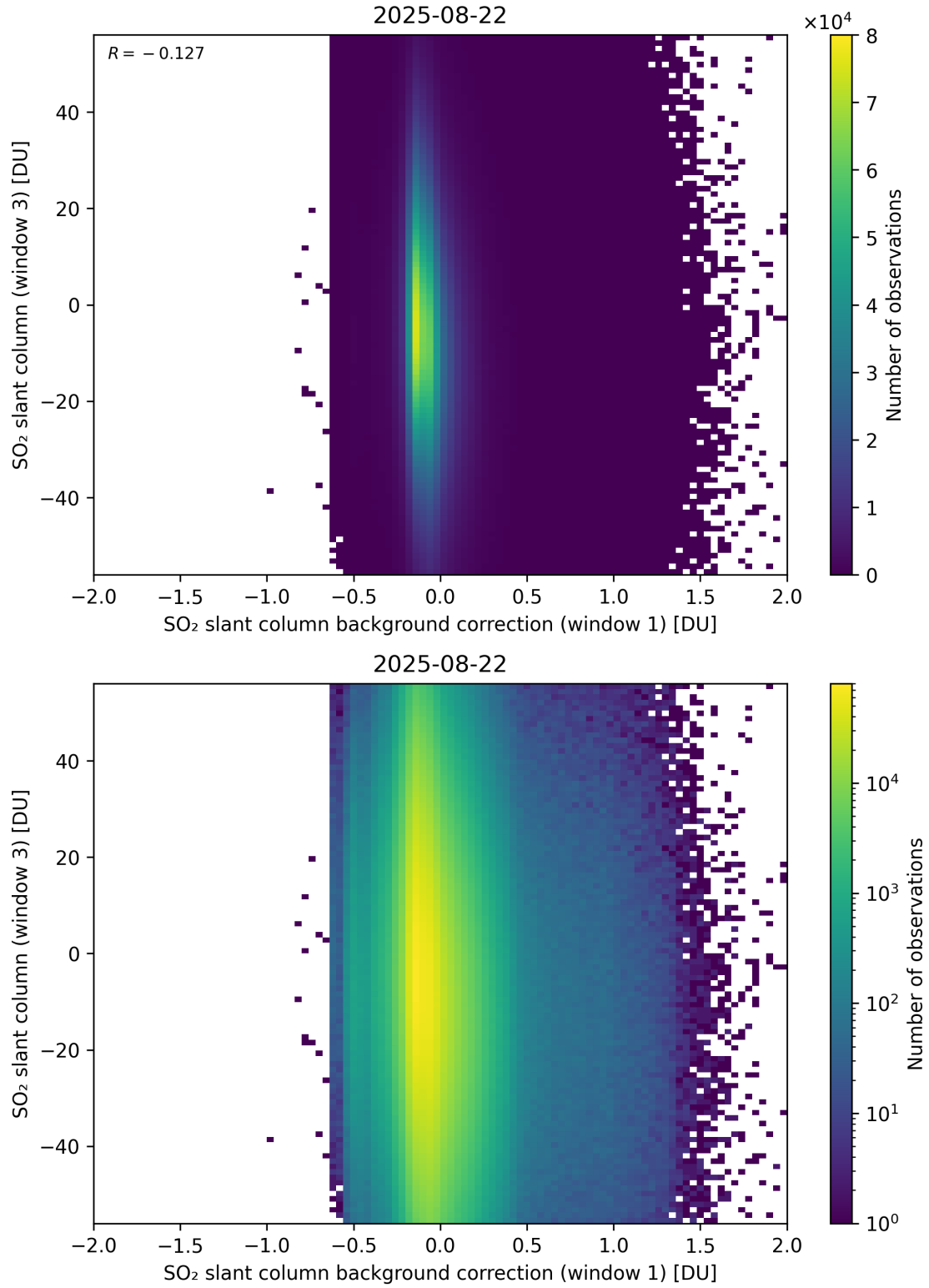
Figure 118: Scatter density plot of “SO 2 slant column background correction (window 1)” against “SO 2 slant column (window 3)” for 2025-08-21 to 2025-08-23.
