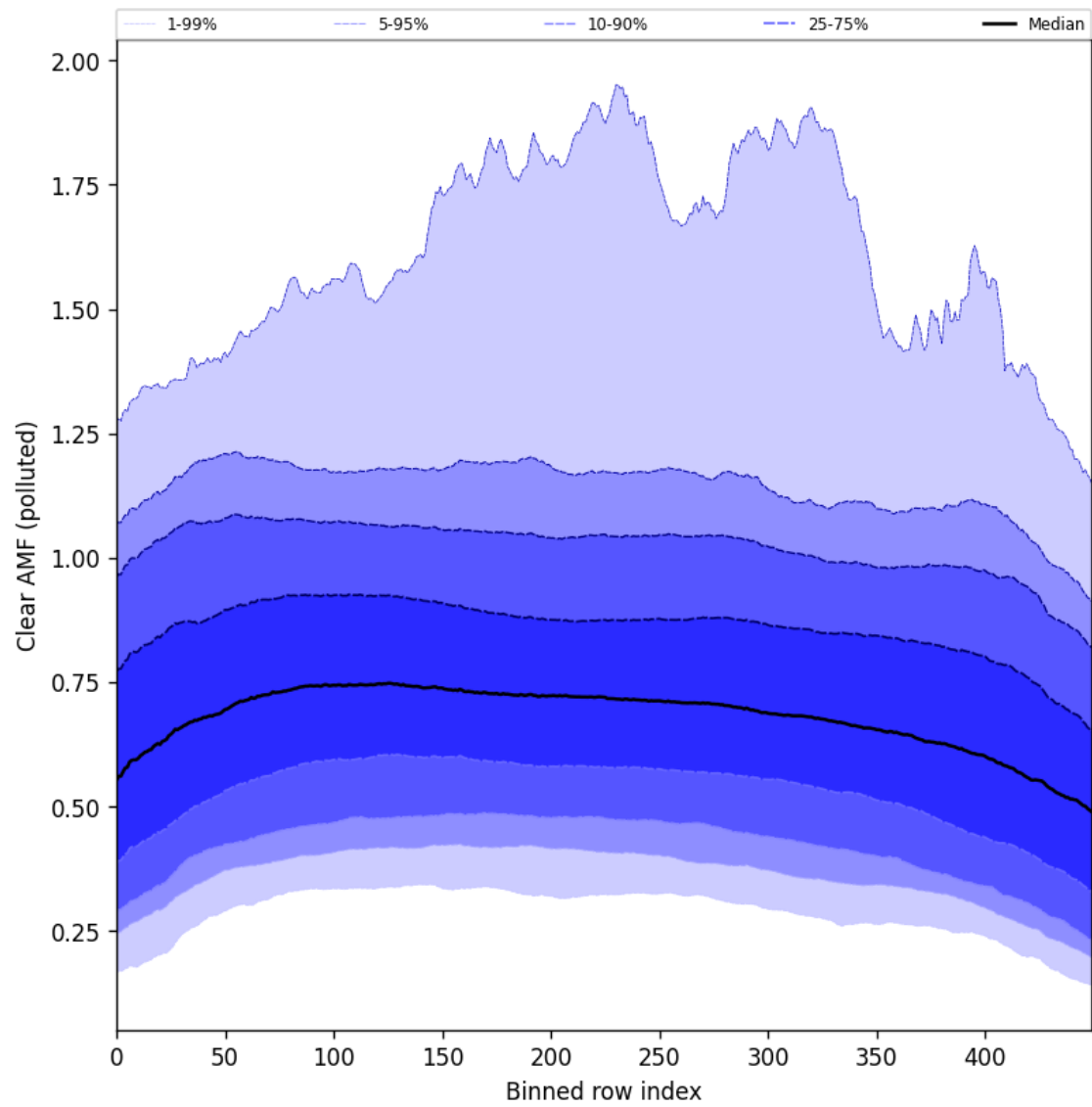
Figure 107: Along track statistics of “Clear AMF (polluted)” for 2025-08-21 to 2025-08-23
