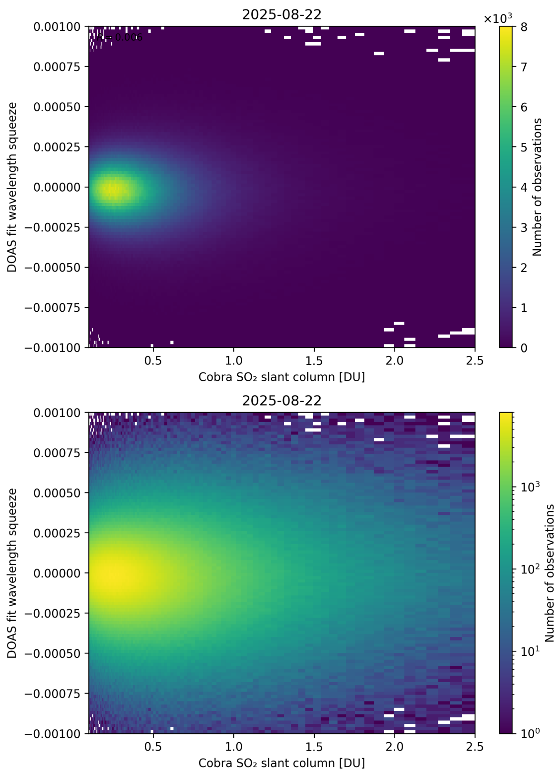
Figure 197: Scatter density plot of “Cobra SO 2 slant column” against “DOAS fit wavelength squeeze” for 2025-08-21 to 2025-08-23.
