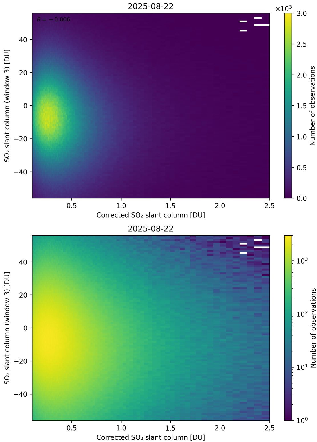
Figure 240: Scatter density plot of “Corrected SO 2 slant column” against “SO 2 slant column (window 3)” for 2025-08-21 to 2025-08-23.
