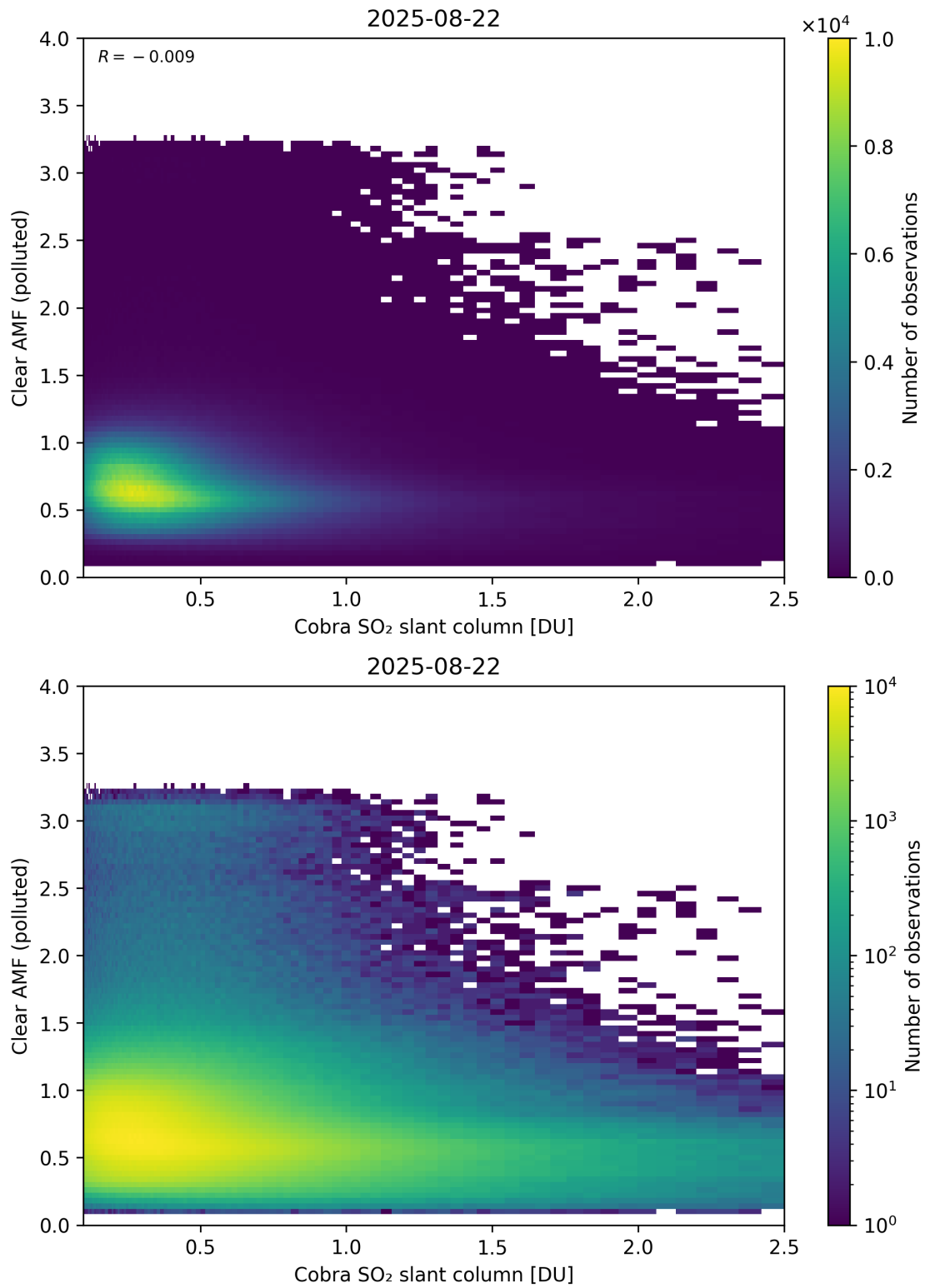
Figure 215: Scatter density plot of “Cobra SO 2 slant column” against “Clear AMF (polluted)” for 2025-08-21 to 2025-08-23.
