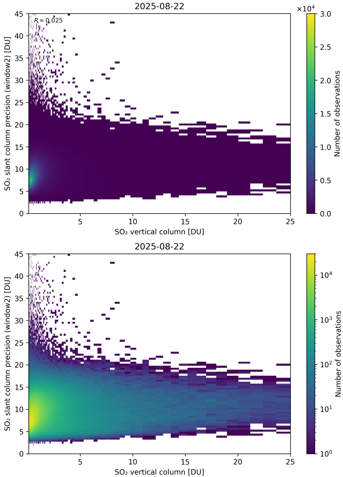
Figure 356: Scatter density plot of “SO 2 vertical column” against “SO 2 slant column precision (window2)” for 2025-08-21 to 2025-08-23.
