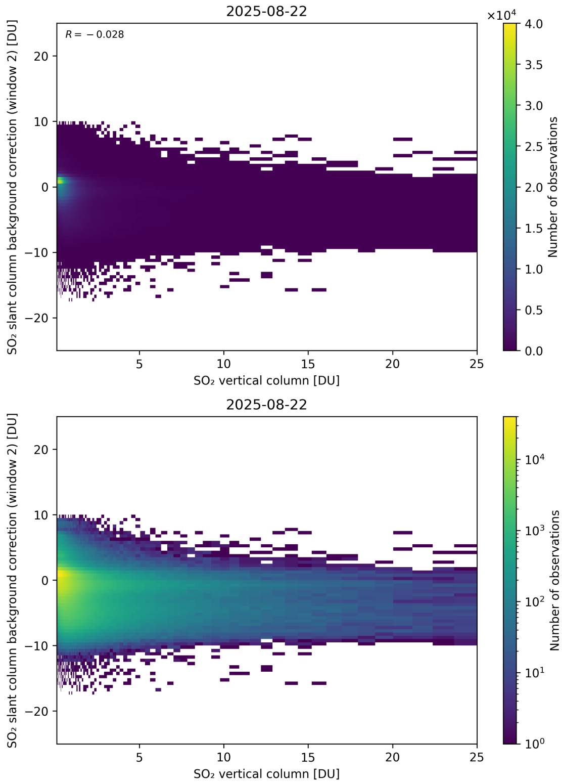
Figure 324: Scatter density plot of “SO 2 vertical column” against “SO 2 slant column background correction (window 2)” for 2025-08-21 to 2025-08-23.
