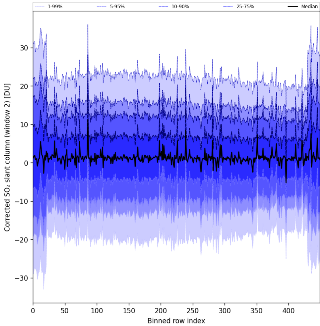
Figure 95: Along track statistics of “Corrected SO 2 slant column (window 2)” for 2025-08-21 to 2025-08-23
