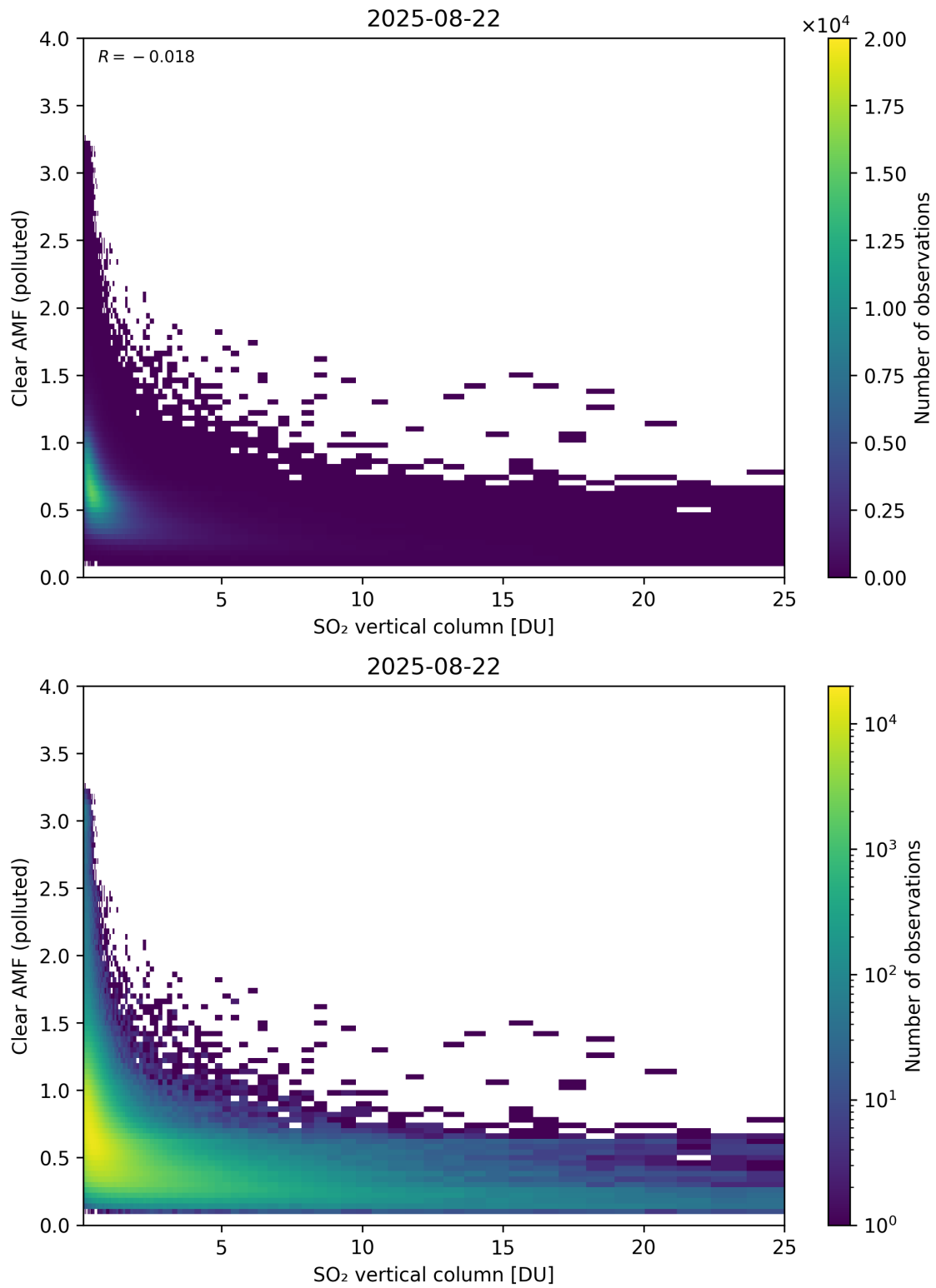
Figure 348: Scatter density plot of “SO 2 vertical column” against “Clear AMF (polluted)” for 2025-08-21 to 2025-08-23.
