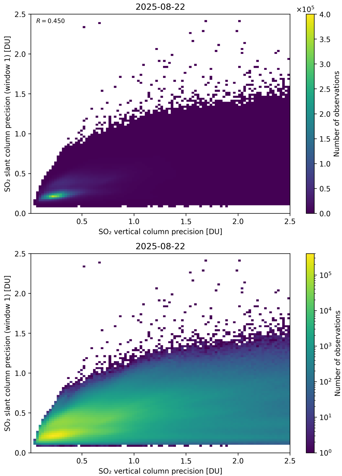
Figure 342: Scatter density plot of “SO 2 vertical column precision” against “SO 2 slant column precision (window 1)” for 2025-08-21 to 2025-08-23.
