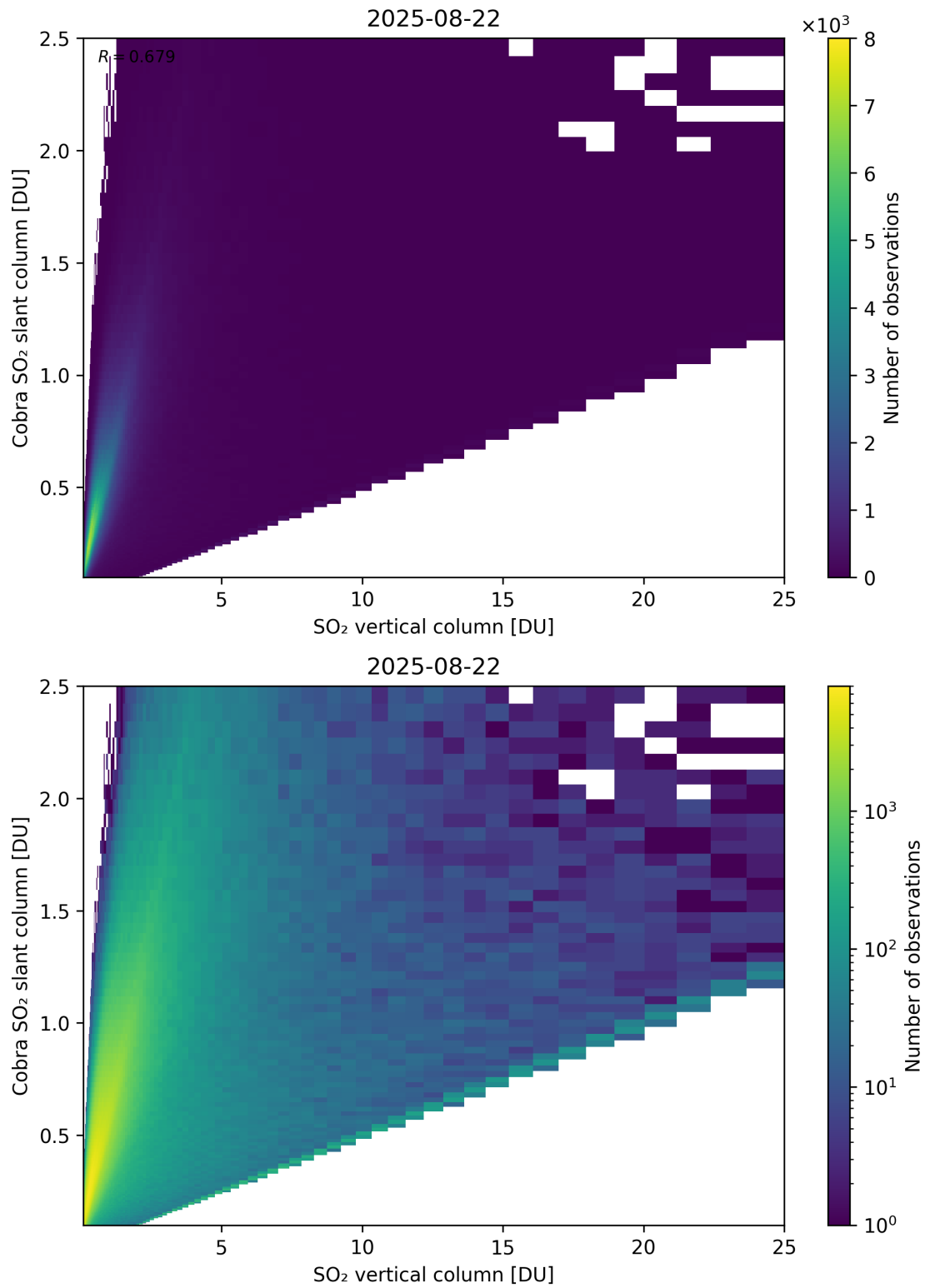
Figure 349: Scatter density plot of “SO 2 vertical column” against “Cobra SO 2 slant column” for 2025-08-21 to 2025-08-23.
