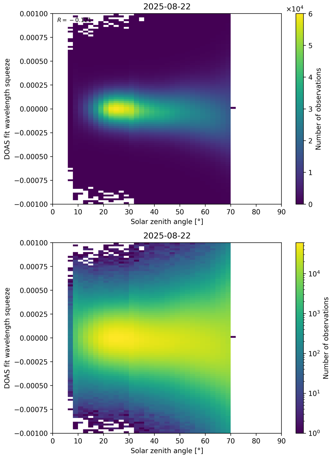
Figure 175: Scatter density plot of “Solar zenith angle” against “DOAS fit wavelength squeeze” for 2025-08-21 to 2025-08-23.
