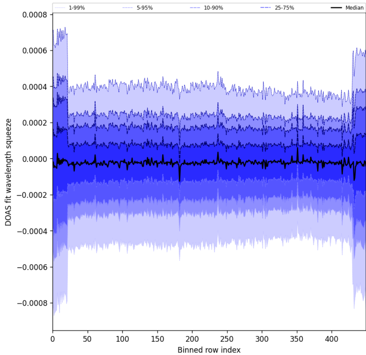
Figure 103: Along track statistics of “DOAS fit wavelength squeeze” for 2025-08-21 to 2025-08-23
