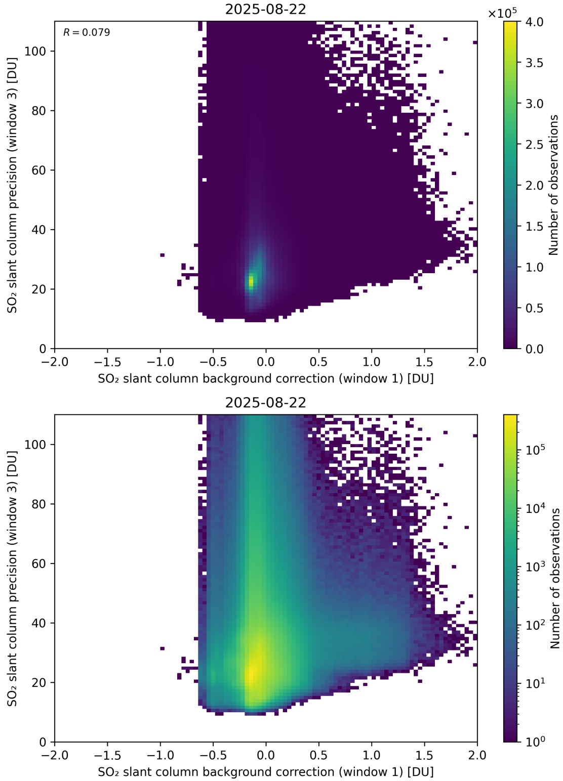
Figure 119: Scatter density plot of “SO 2 slant column background correction (window 1)” against “SO 2 slant column precision (window 3)” for 2025-08-21 to 2025-08-23.
