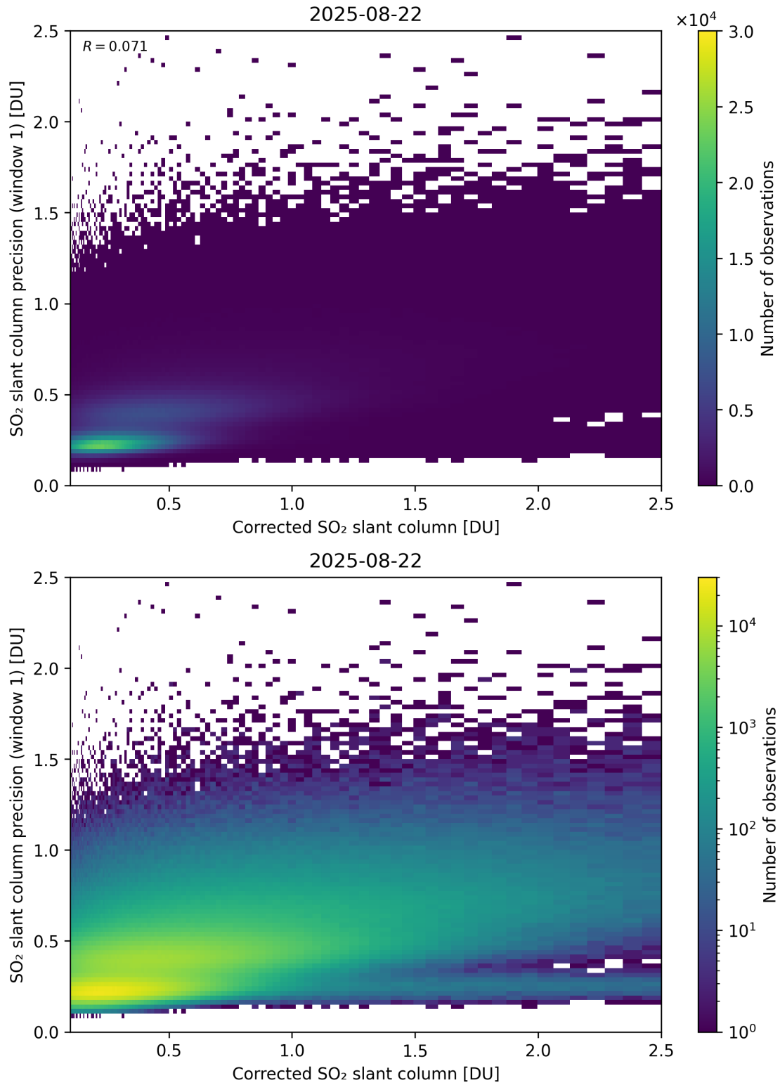
Figure 238: Scatter density plot of “Corrected SO 2 slant column” against “SO 2 slant column precision (window 1)” for 2025-08-21 to 2025-08-23.
