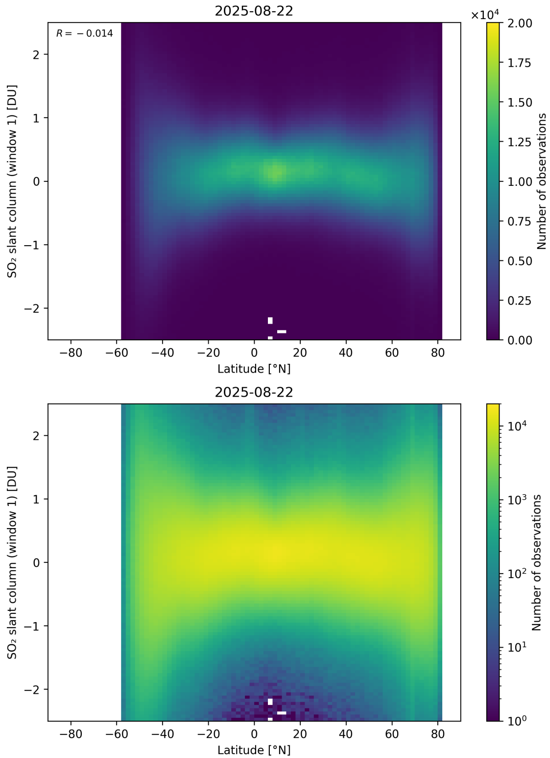
Figure 162: Scatter density plot of “Latitude” against “SO 2 slant column (window 1)” for 2025-08-21 to 2025-08-23.
