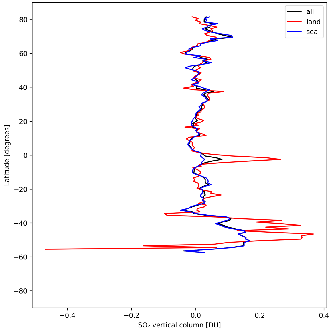
Figure 32: Zonal average of “SO 2 vertical column” for 2025-08-21 to 2025-08-23.
