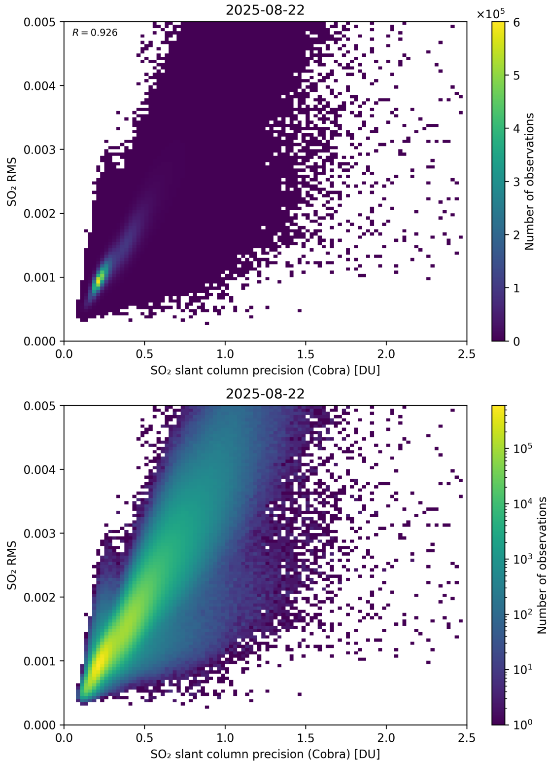
Figure 204: Scatter density plot of “SO 2 slant column precision (Cobra)” against “SO 2 RMS” for 2025-08-21 to 2025-08-23.
