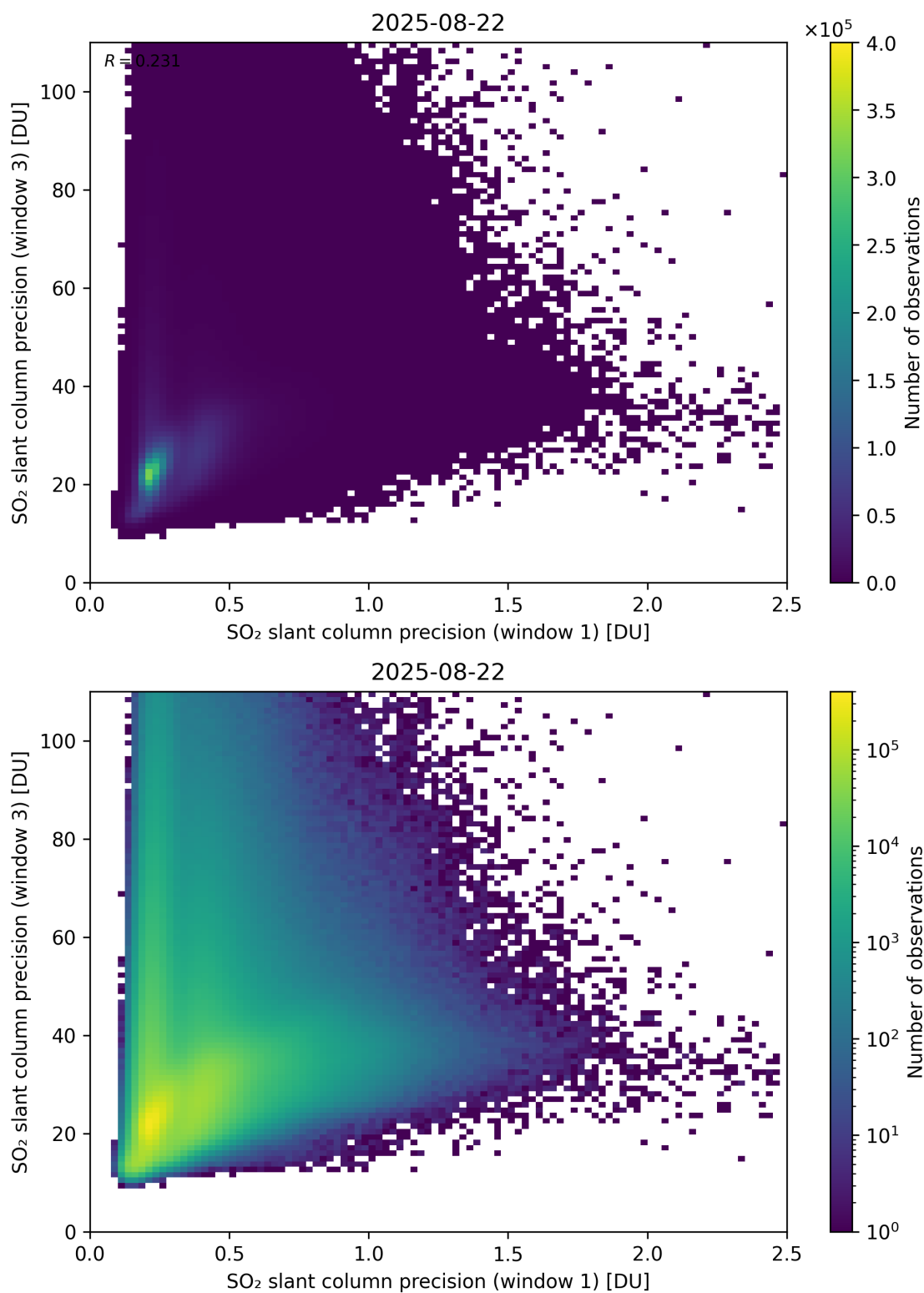
Figure 279: Scatter density plot of “SO 2 slant column precision (window 1)” against “SO 2 slant column precision (window 3)” for 2025-08-21 to 2025-08-23.
