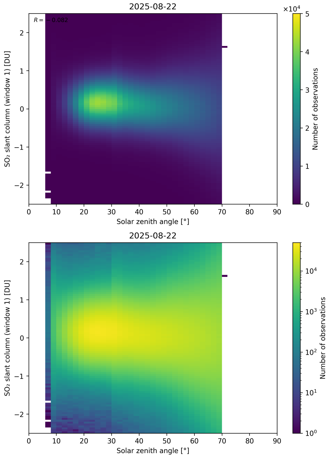
Figure 184: Scatter density plot of “Solar zenith angle” against “SO 2 slant column (window 1)” for 2025-08-21 to 2025-08-23.
