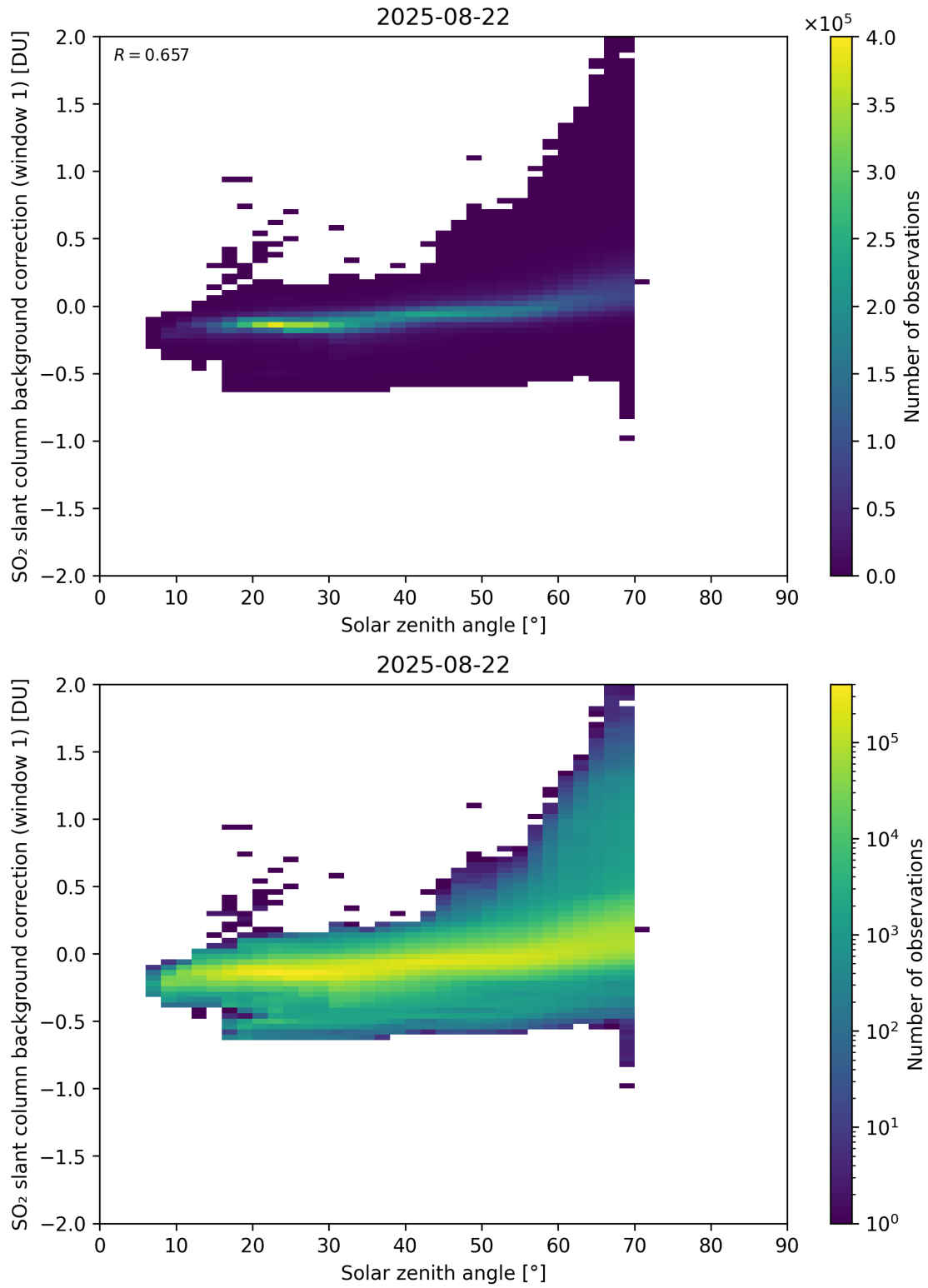
Figure 171: Scatter density plot of “Solar zenith angle” against “SO 2 slant column background correction (window 1)” for 2025-08-21 to 2025-08-23.
