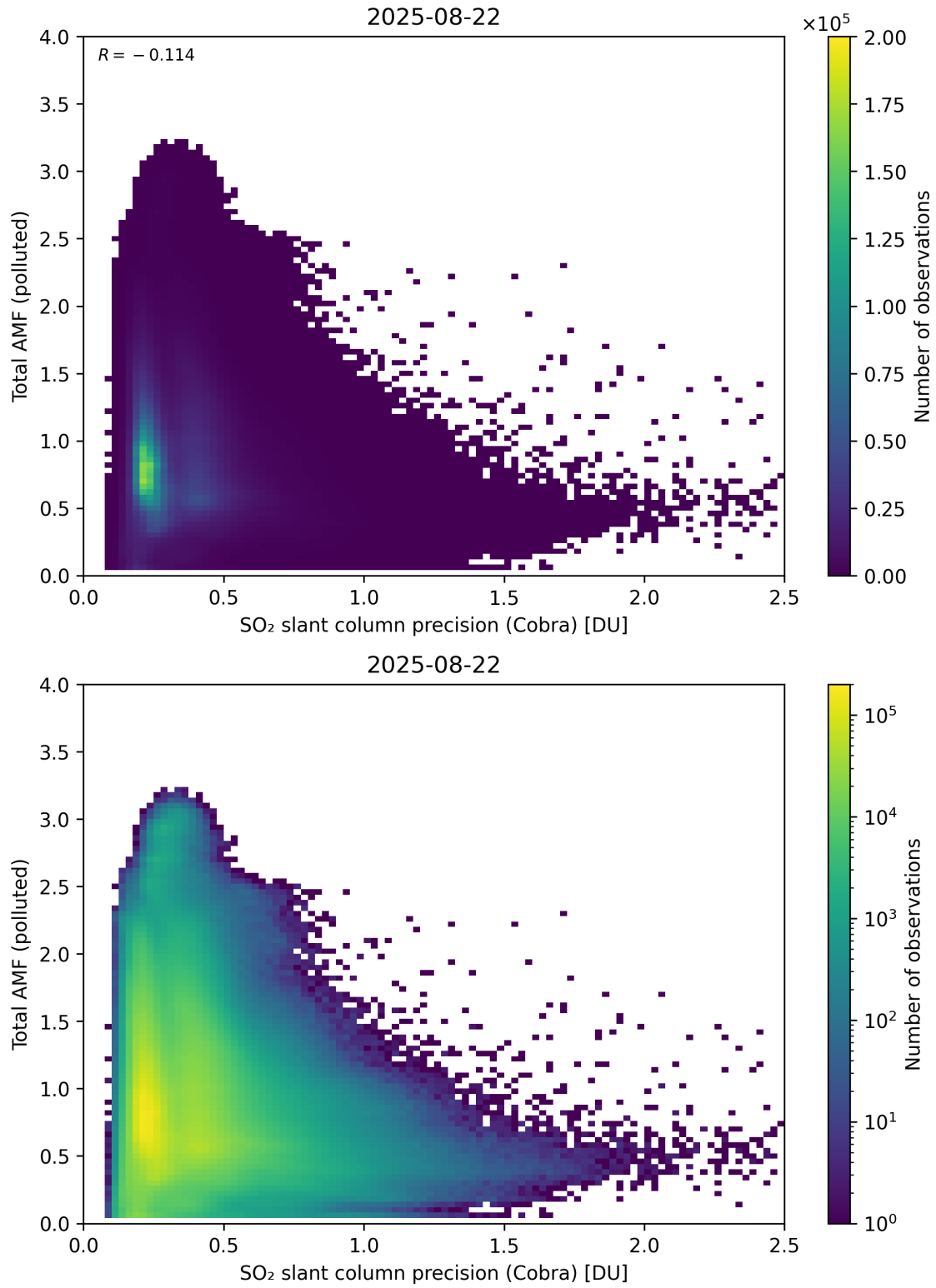
Figure 213: Scatter density plot of “SO 2 slant column precision (Cobra)” against “Total AMF (polluted)” for 2025-08-21 to 2025-08-23.
