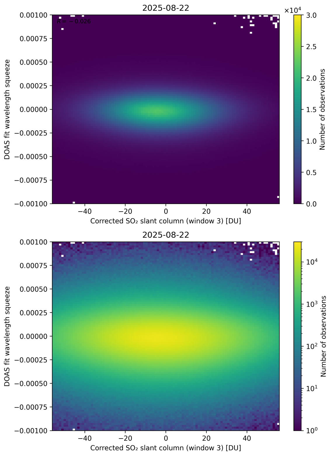
Figure 257: Scatter density plot of “Corrected SO 2 slant column (window 3)” against “DOAS fit wavelength squeeze” for 2025-08-21 to 2025-08-23.
