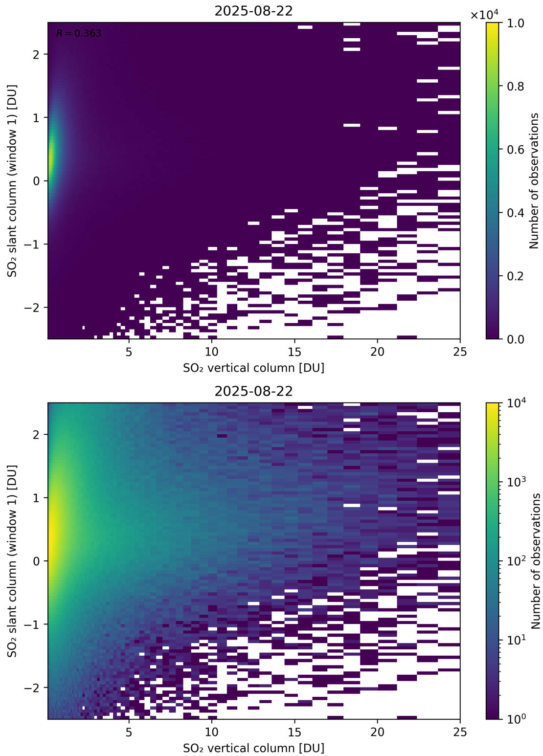
Figure 354: Scatter density plot of “SO 2 vertical column” against “SO 2 slant column (window 1)” for 2025-08-21 to 2025-08-23.
