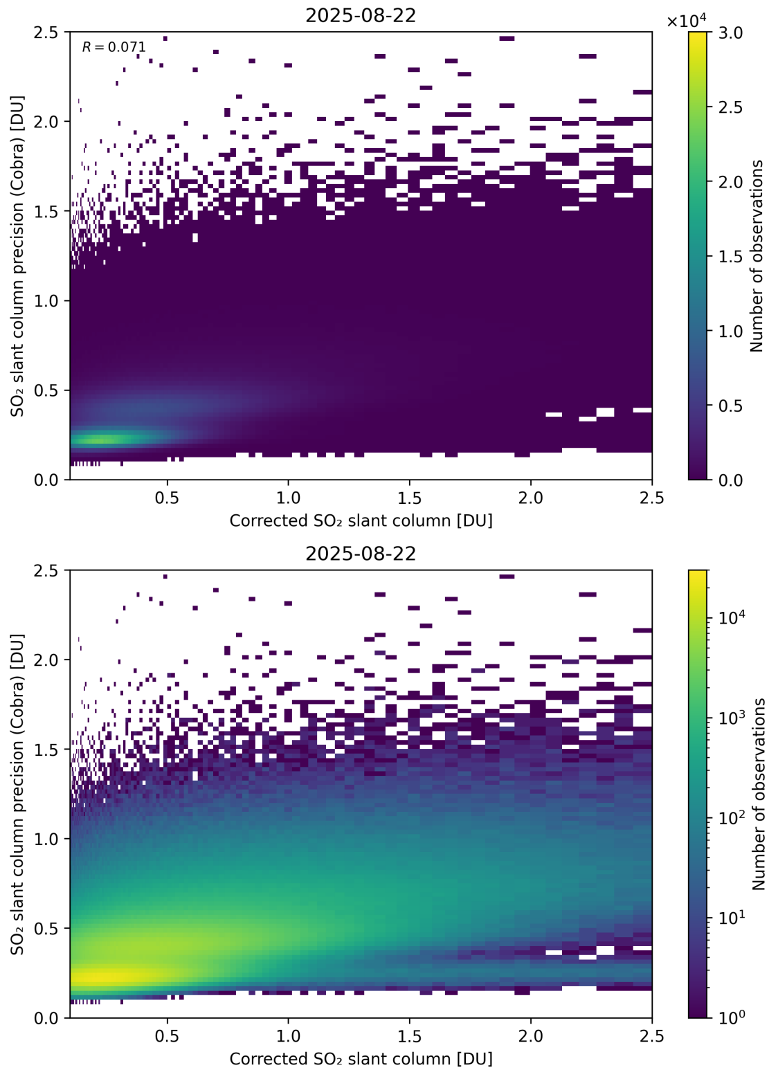
Figure 234: Scatter density plot of “Corrected SO 2 slant column” against “SO 2 slant column precision (Cobra)” for 2025-08-21 to 2025-08-23.
