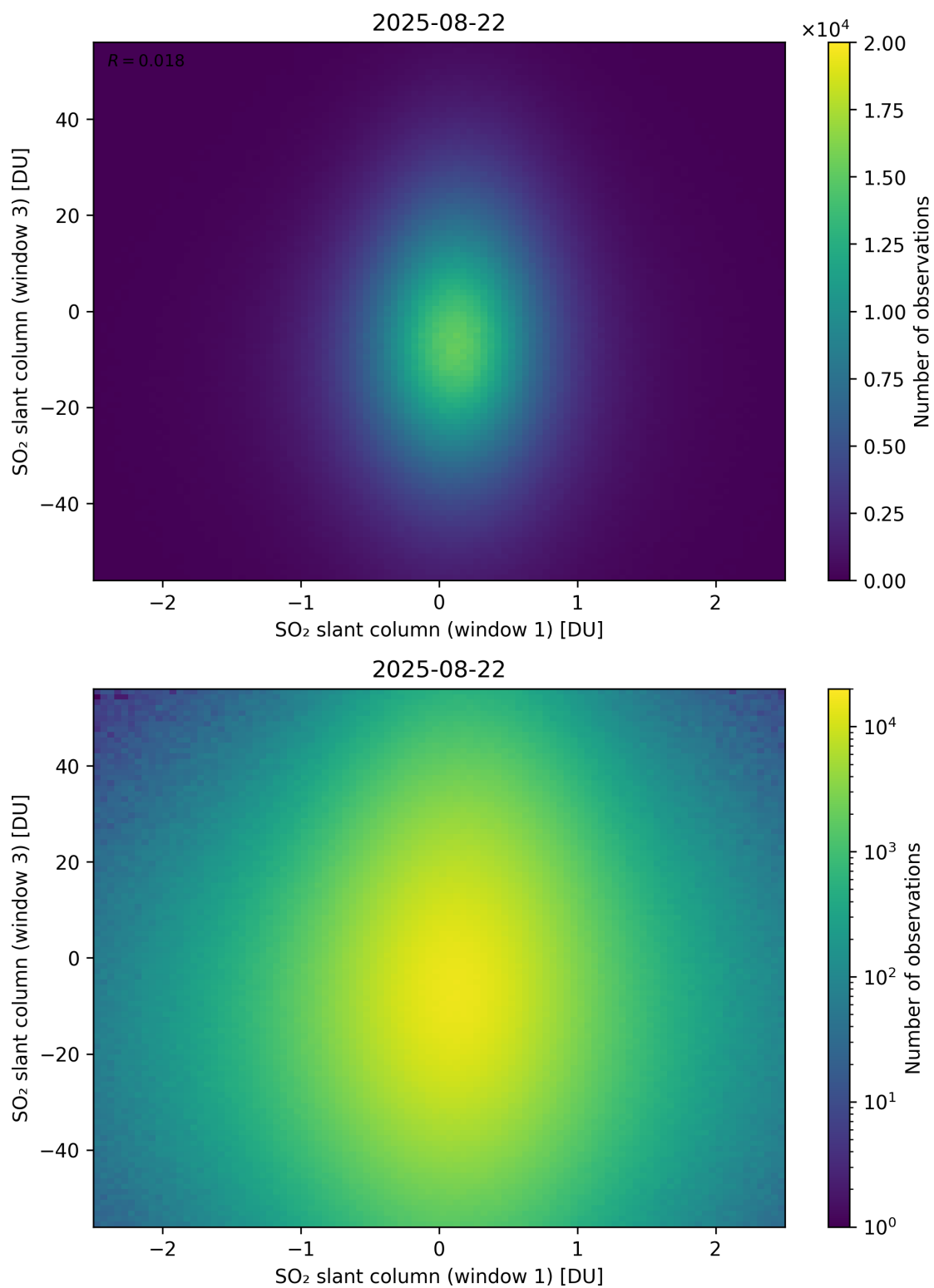
Figure 287: Scatter density plot of “SO 2 slant column (window 1)” against “SO 2 slant column (window 3)” for 2025-08-21 to 2025-08-23.
