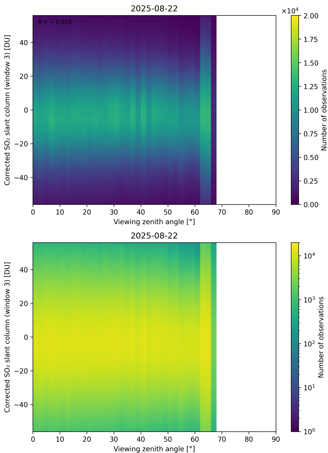
Figure 375: Scatter density plot of “Viewing zenith angle” against “Corrected SO 2 slant column (window 3)” for 2025-08-21 to 2025-08-23.
