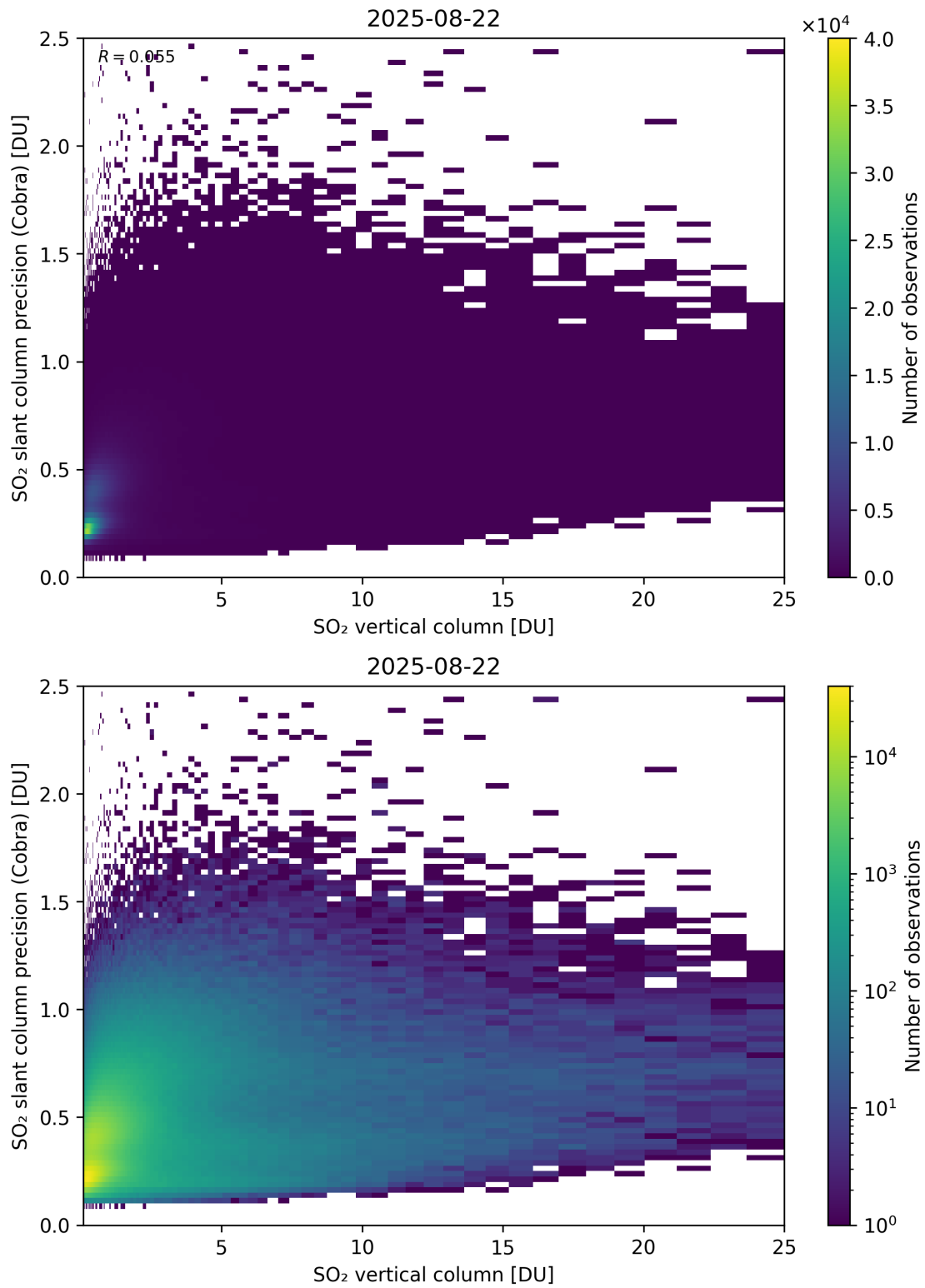
Figure 350: Scatter density plot of “SO 2 vertical column” against “SO 2 slant column precision (Cobra)” for 2025-08-21 to 2025-08-23.
