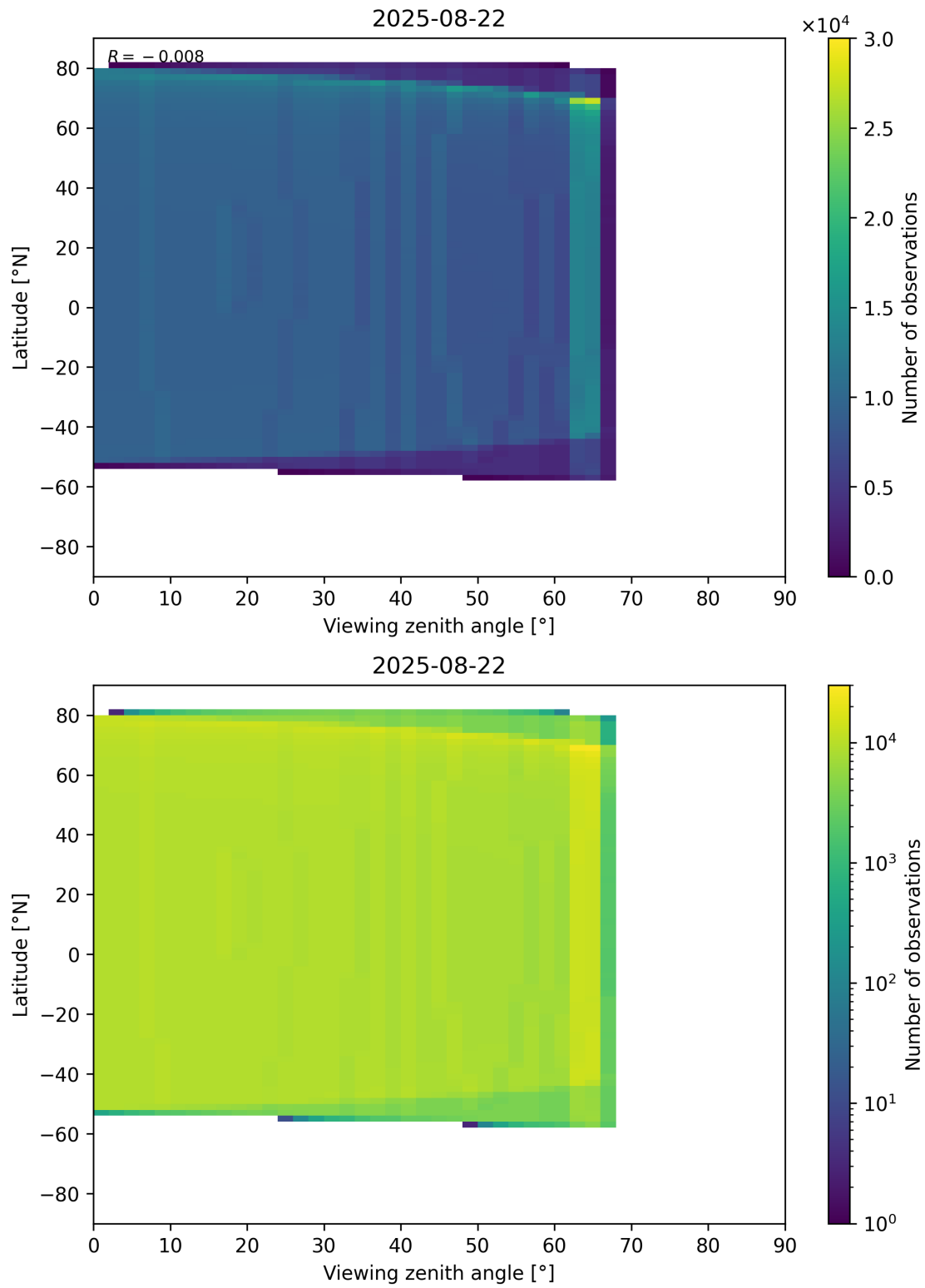
Figure 368: Scatter density plot of “Viewing zenith angle” against “Latitude” for 2025-08-21 to 2025-08-23.
