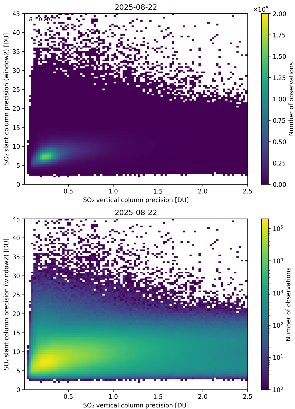
Figure 343: Scatter density plot of “SO 2 vertical column precision” against “SO 2 slant column precision (window2)” for 2025-08-21 to 2025-08-23.
