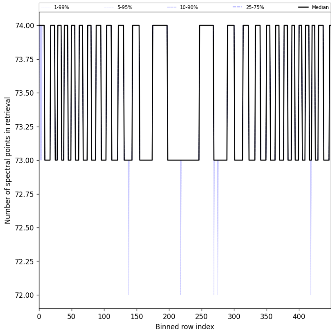
Figure 108: Along track statistics of “Number of spectral points in retrieval” for 2025-08-21 to 2025-08-23
