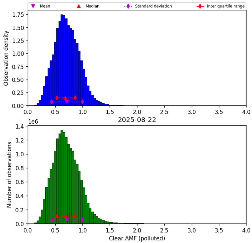
Figure 81: Histogram of “Clear AMF (polluted)” for 2025-08-21 to 2025-08-23
