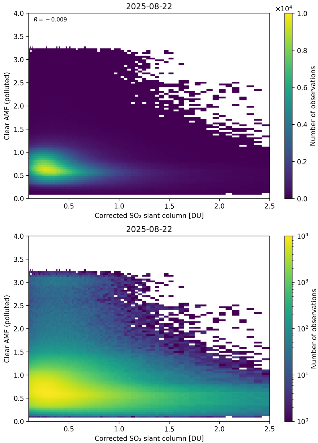
Figure 232: Scatter density plot of “Corrected SO 2 slant column” against “Clear AMF (polluted)” for 2025-08-21 to 2025-08-23.
