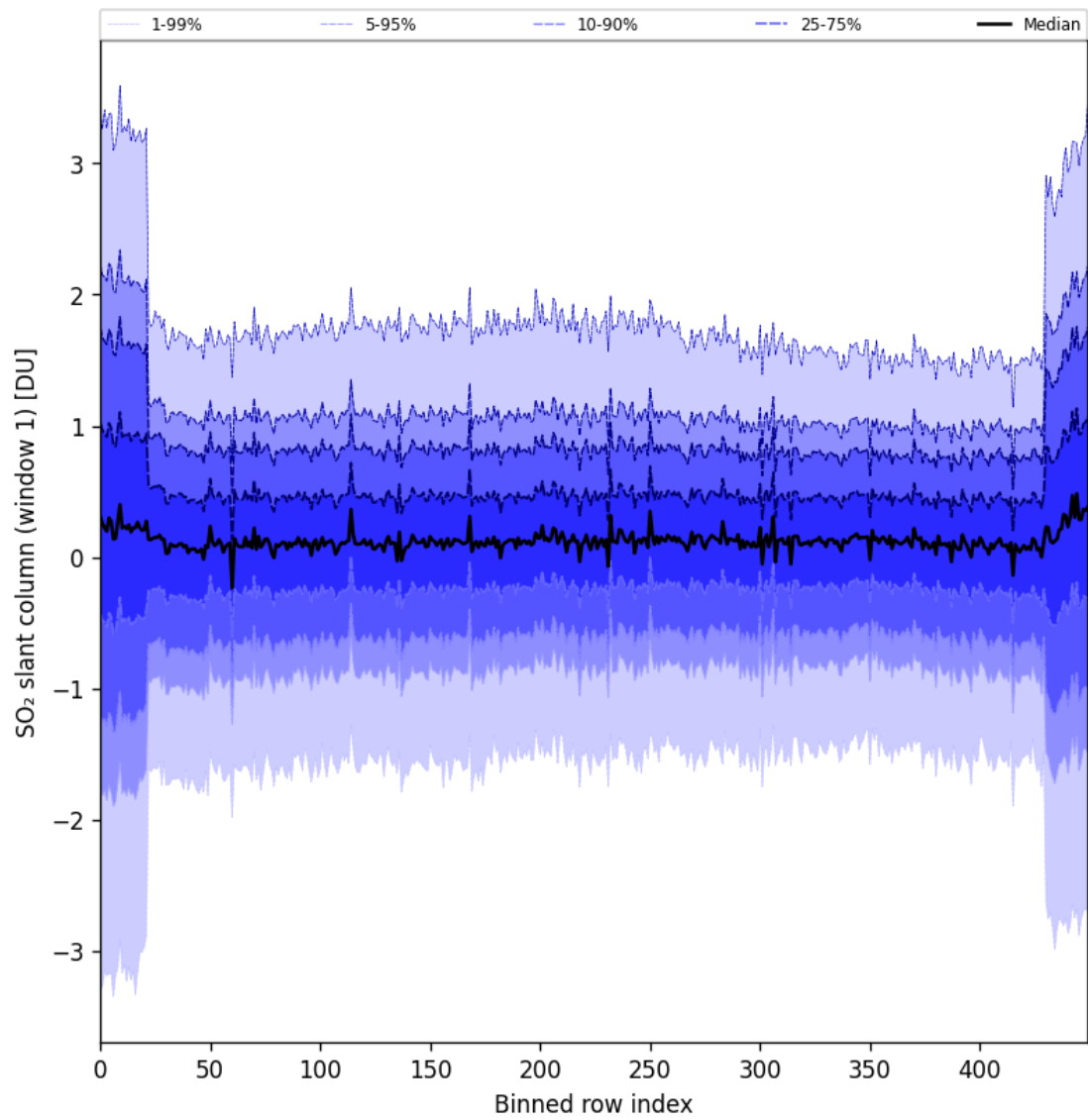
Figure 89: Along track statistics of “SO 2 slant column (window 1)” for 2025-08-21 to 2025-08-23
