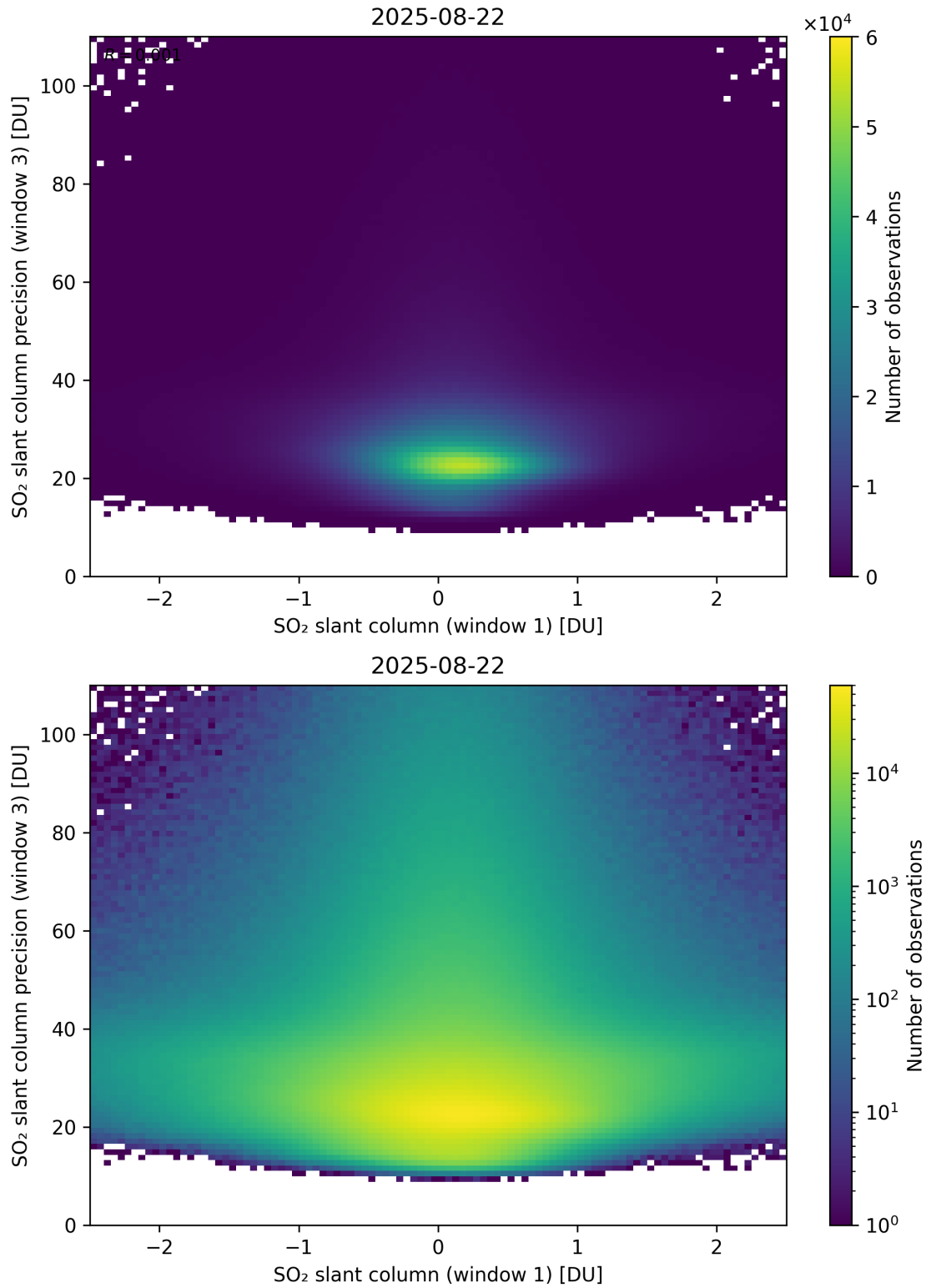
Figure 288: Scatter density plot of “SO 2 slant column (window 1)” against “SO 2 slant column precision (window 3)” for 2025-08-21 to 2025-08-23.
