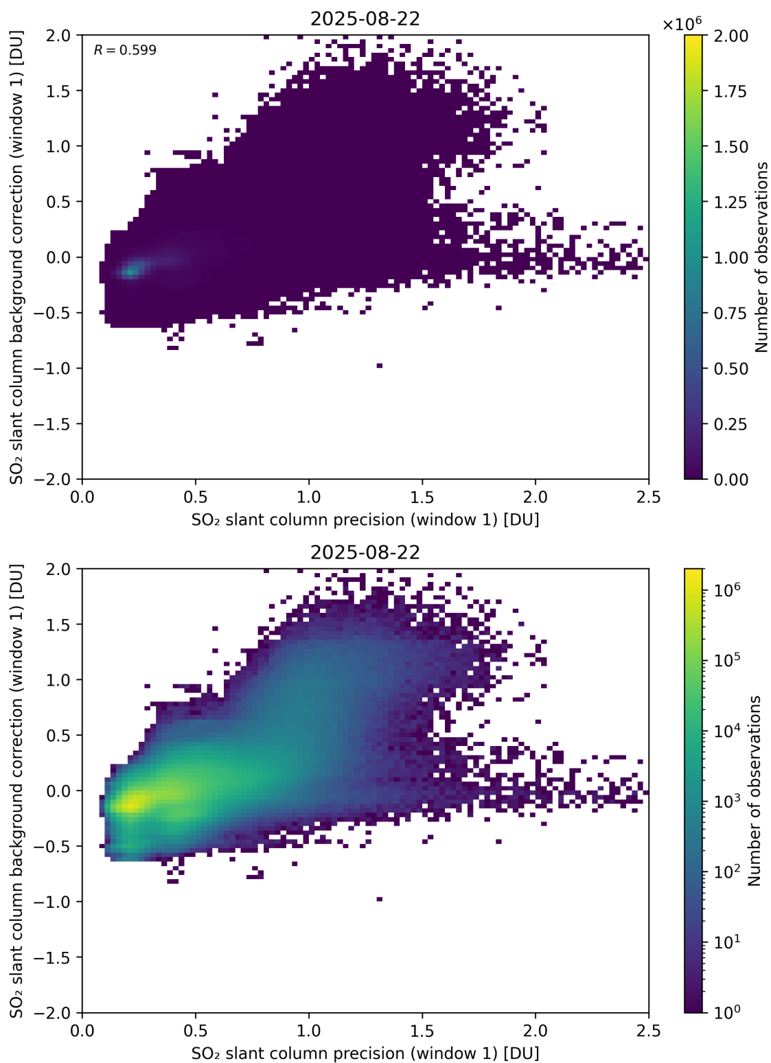
Figure 268: Scatter density plot of “SO 2 slant column precision (window 1)” against “SO 2 slant column background correction (window 1)” for 2025-08-21 to 2025-08-23.
