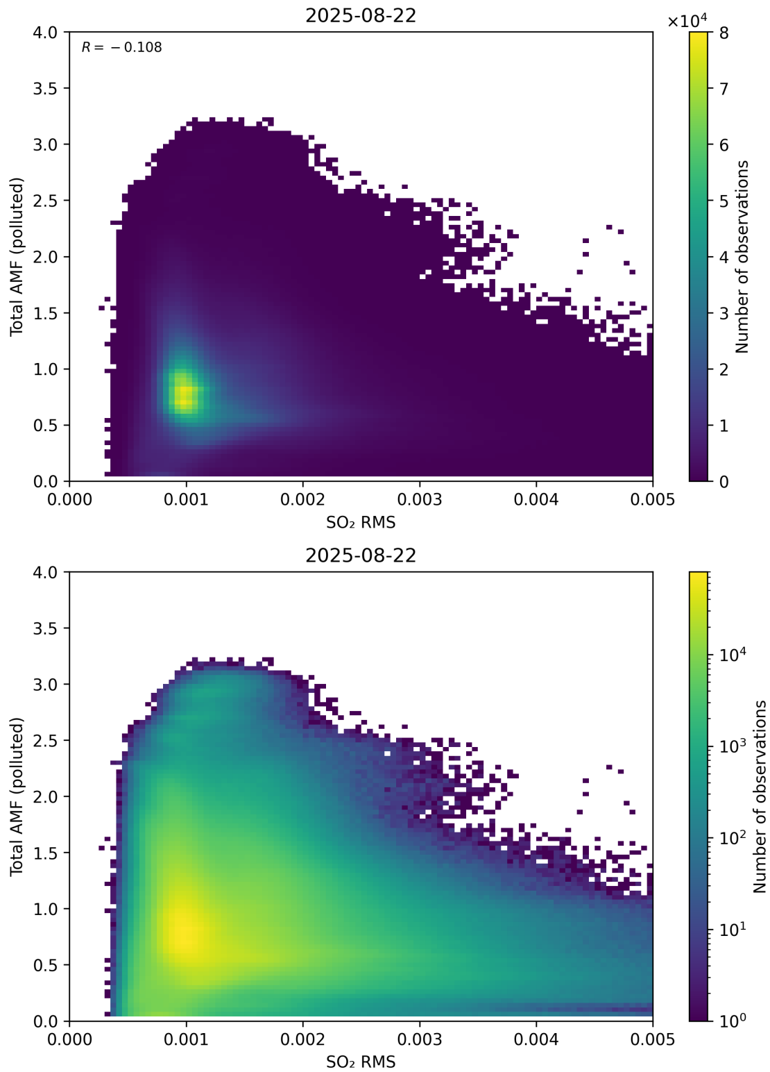
Figure 148: Scatter density plot of “SO 2 RMS” against “Total AMF (polluted)” for 2025-08-21 to 2025-08-23.
