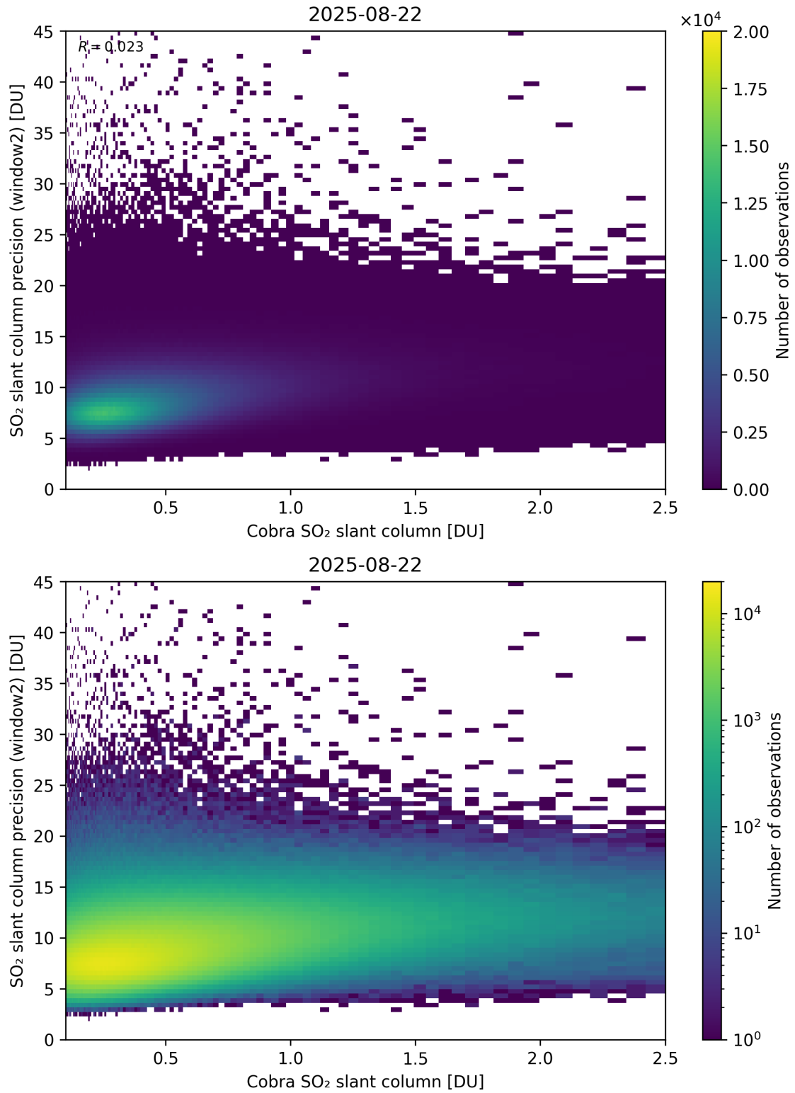
Figure 221: Scatter density plot of “Cobra SO 2 slant column” against “SO 2 slant column precision (window2)” for 2025-08-21 to 2025-08-23.
