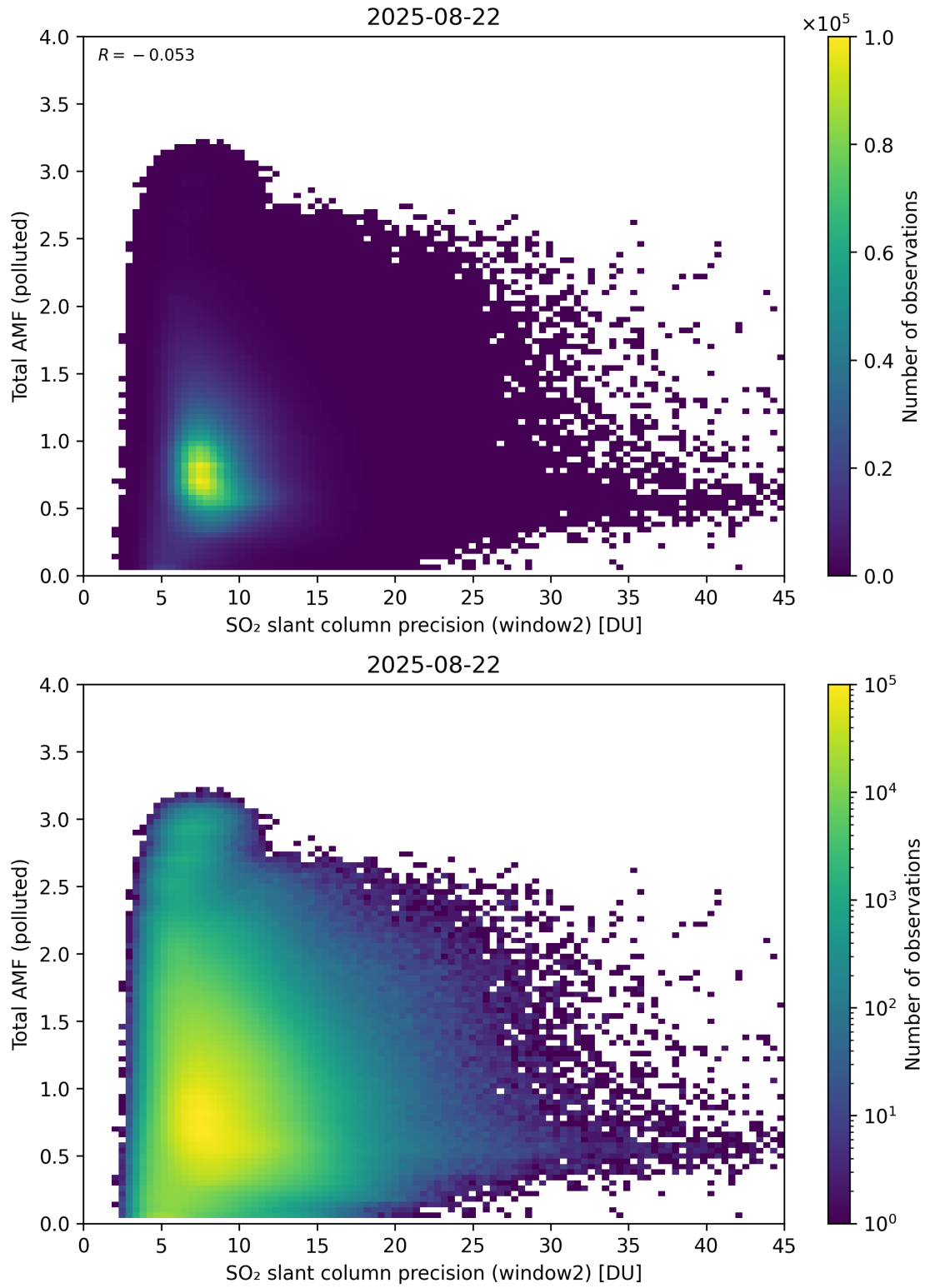
Figure 301: Scatter density plot of “SO 2 slant column precision (window2)” against “Total AMF (polluted)” for 2025-08-21 to 2025-08-23.
