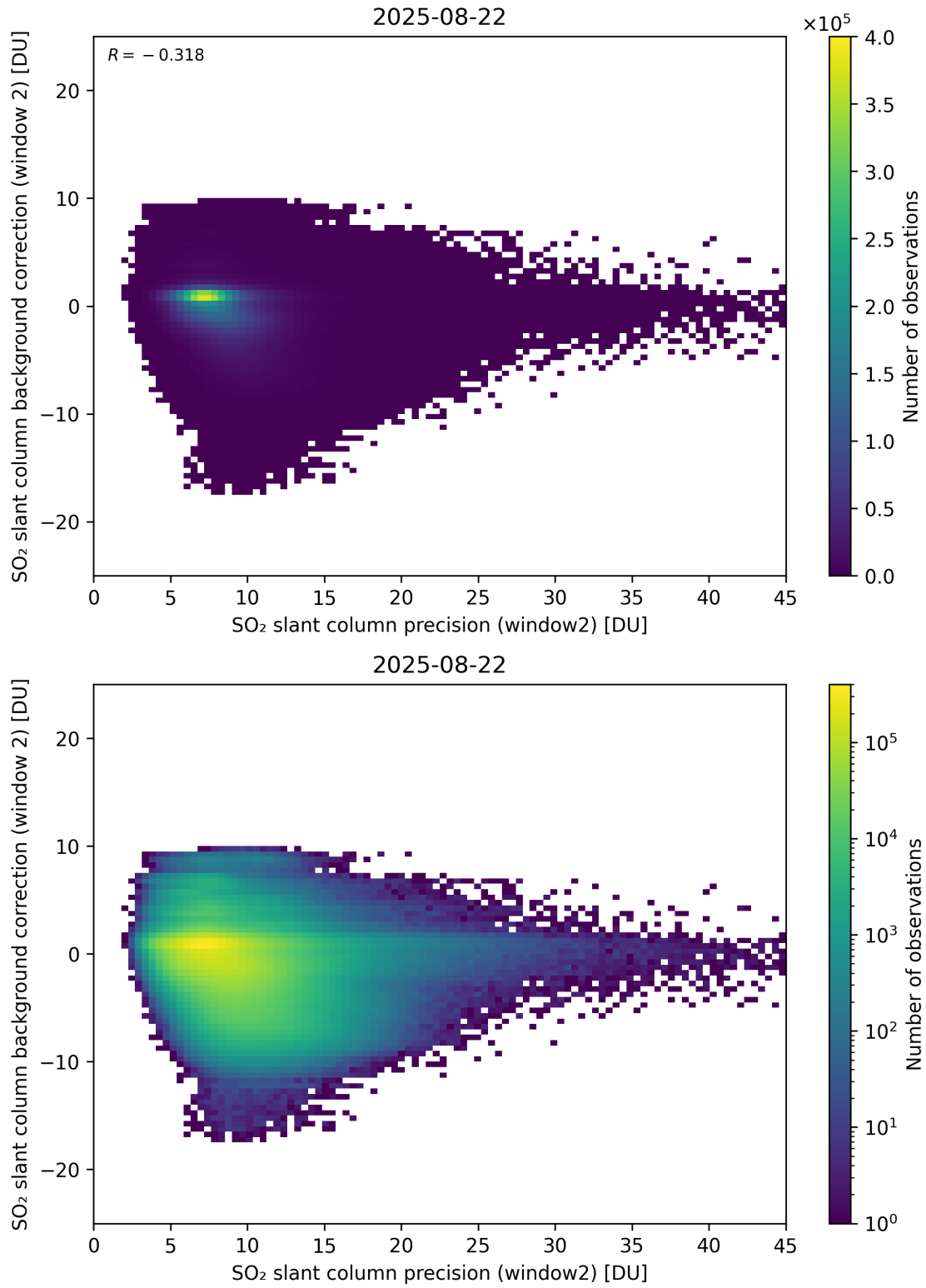
Figure 291: Scatter density plot of “SO 2 slant column precision (window2)” against “SO 2 slant column background correction (window 2)” for 2025-08-21 to 2025-08-23.
