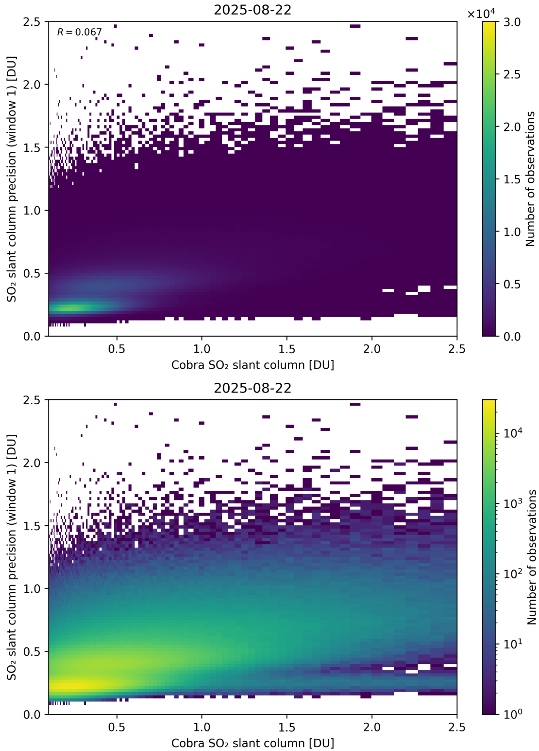
Figure 220: Scatter density plot of “Cobra SO 2 slant column” against “SO 2 slant column precision (window 1)” for 2025-08-21 to 2025-08-23.
