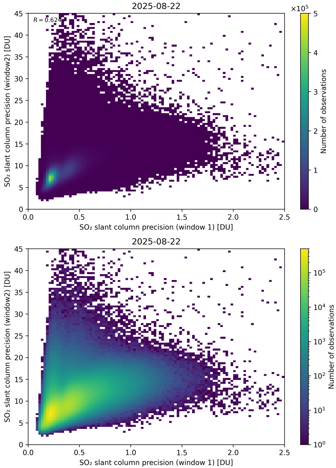
Figure 277: Scatter density plot of “SO 2 slant column precision (window 1)” against “SO 2 slant column precision (window2)” for 2025-08-21 to 2025-08-23.
