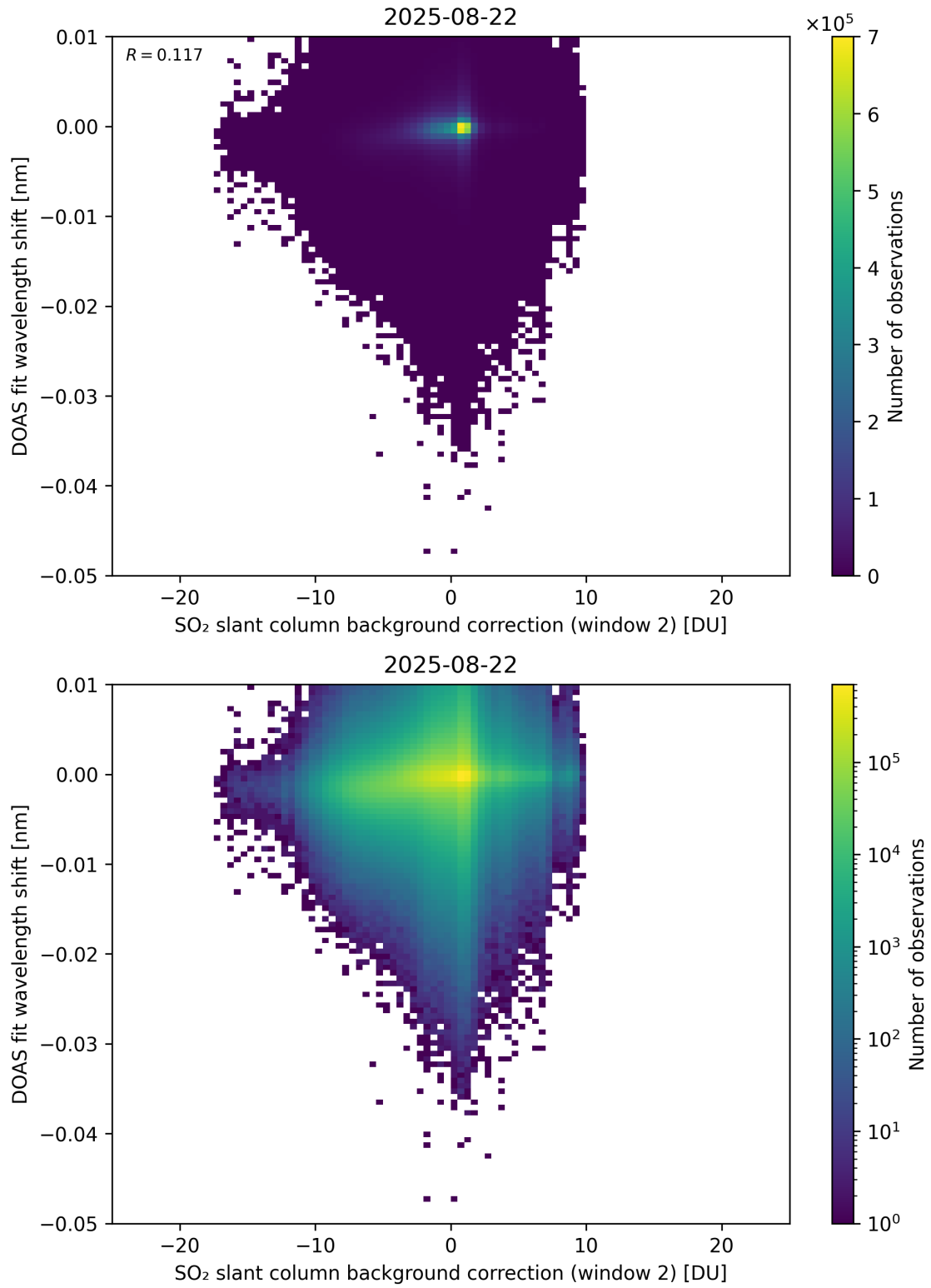
Figure 123: Scatter density plot of “SO 2 slant column background correction (window 2)” against “DOAS fit wavelength shift” for 2025-08-21 to 2025-08-23.
