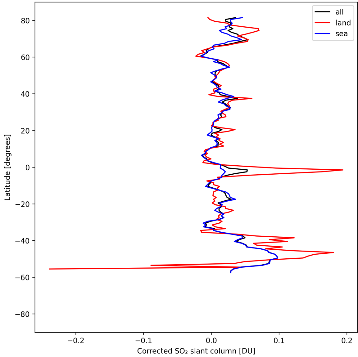
Figure 34: Zonal average of “Corrected SO 2 slant column” for 2025-08-21 to 2025-08-23.
