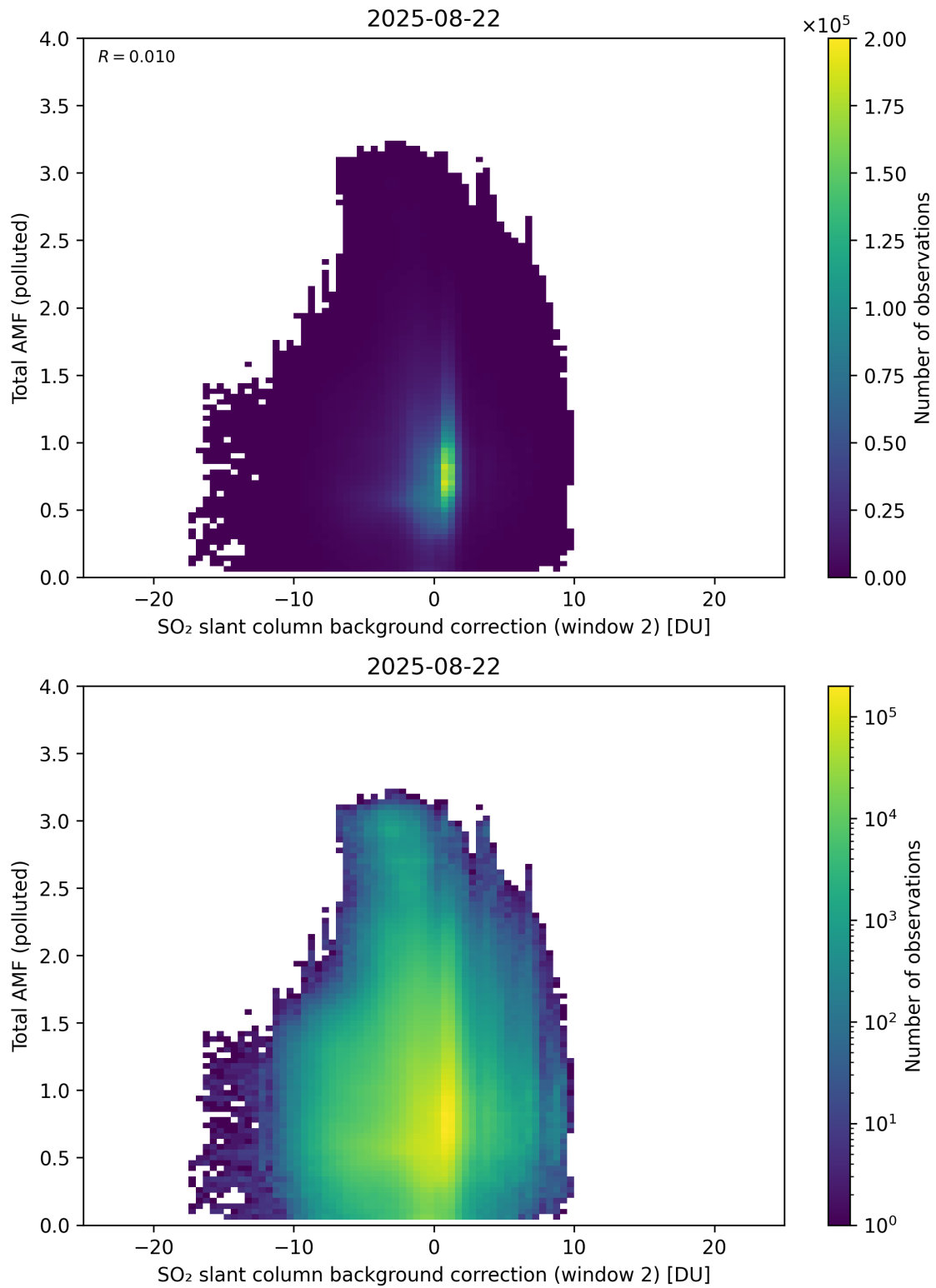
Figure 130: Scatter density plot of “SO 2 slant column background correction (window 2)” against “Total AMF (polluted)” for 2025-08-21 to 2025-08-23.
