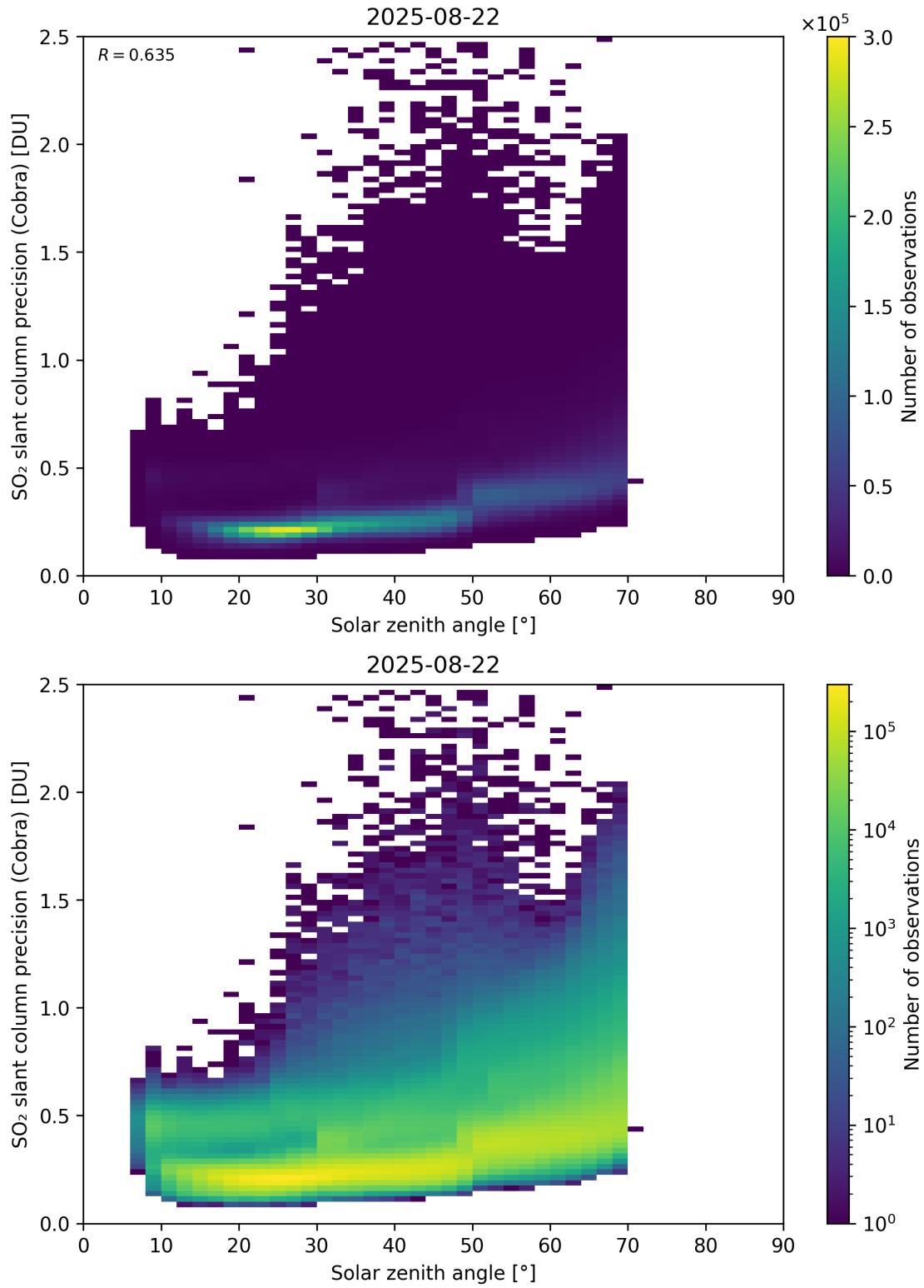
Figure 180: Scatter density plot of “Solar zenith angle” against “SO 2 slant column precision (Cobra)” for 2025-08-21 to 2025-08-23.
