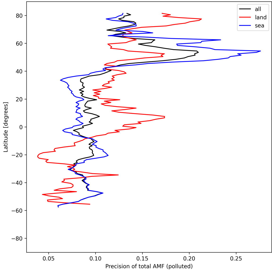
Figure 54: Zonal average of “Precision of total AMF (polluted)” for 2025-08-21 to 2025-08-23.
