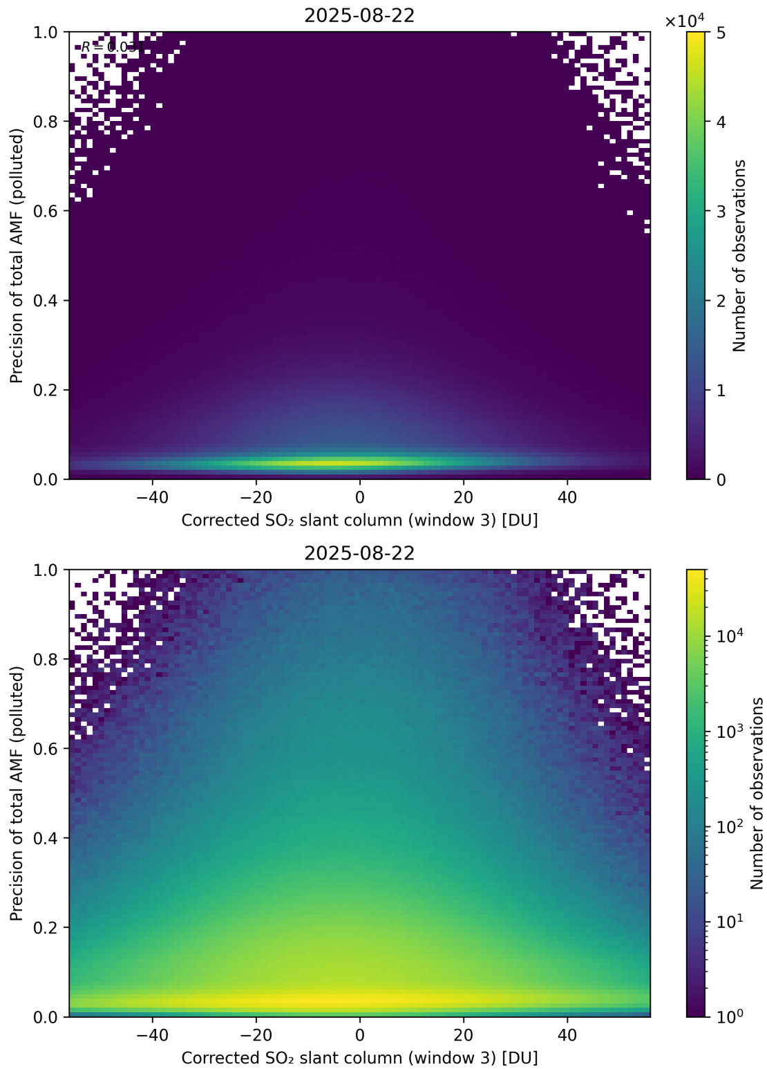
Figure 261: Scatter density plot of “Corrected SO 2 slant column (window 3)” against “Precision of total AMF (polluted)” for 2025-08-21 to 2025-08-23.
