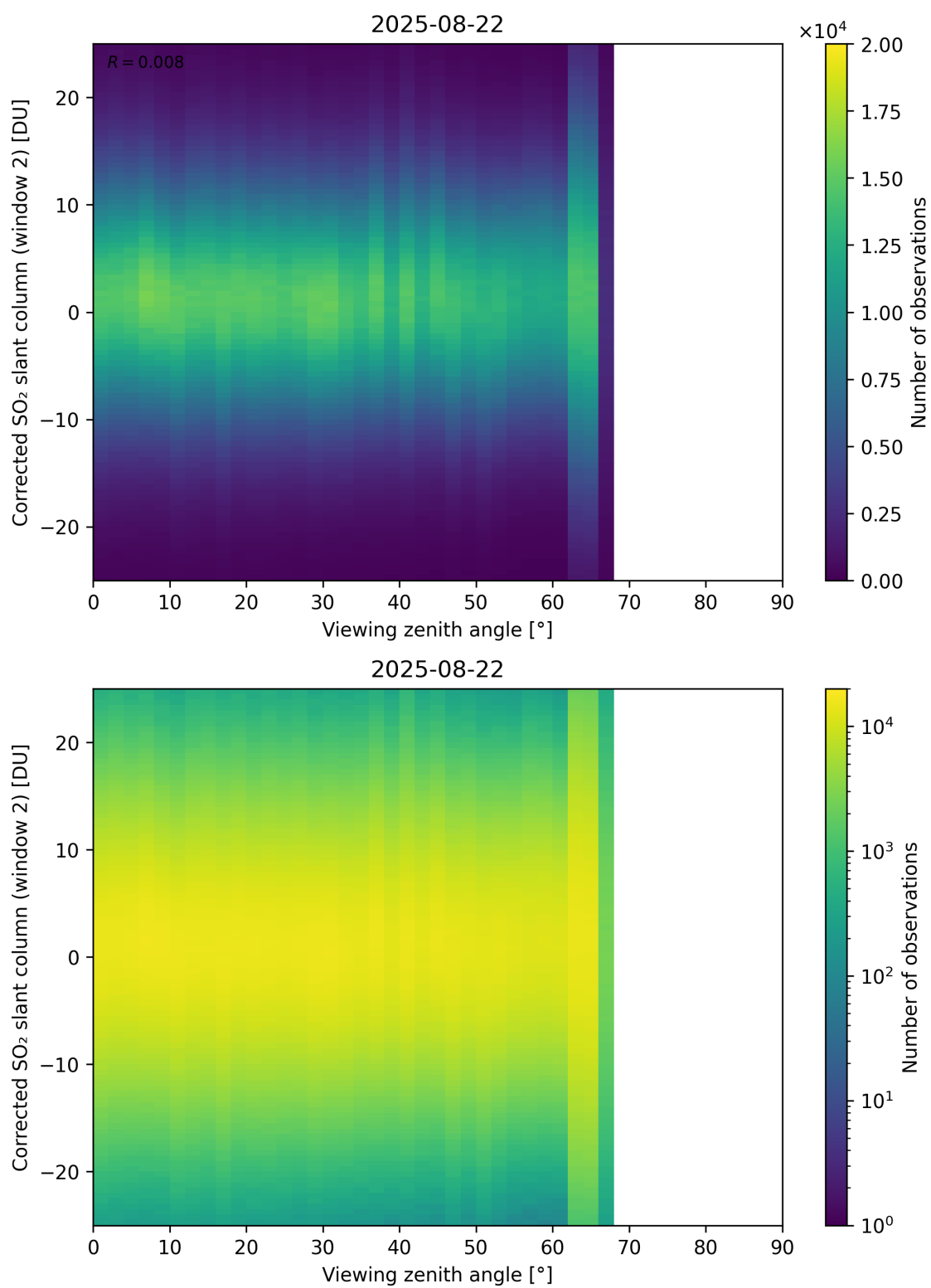
Figure 374: Scatter density plot of “Viewing zenith angle” against “Corrected SO 2 slant column (window 2)” for 2025-08-21 to 2025-08-23.
