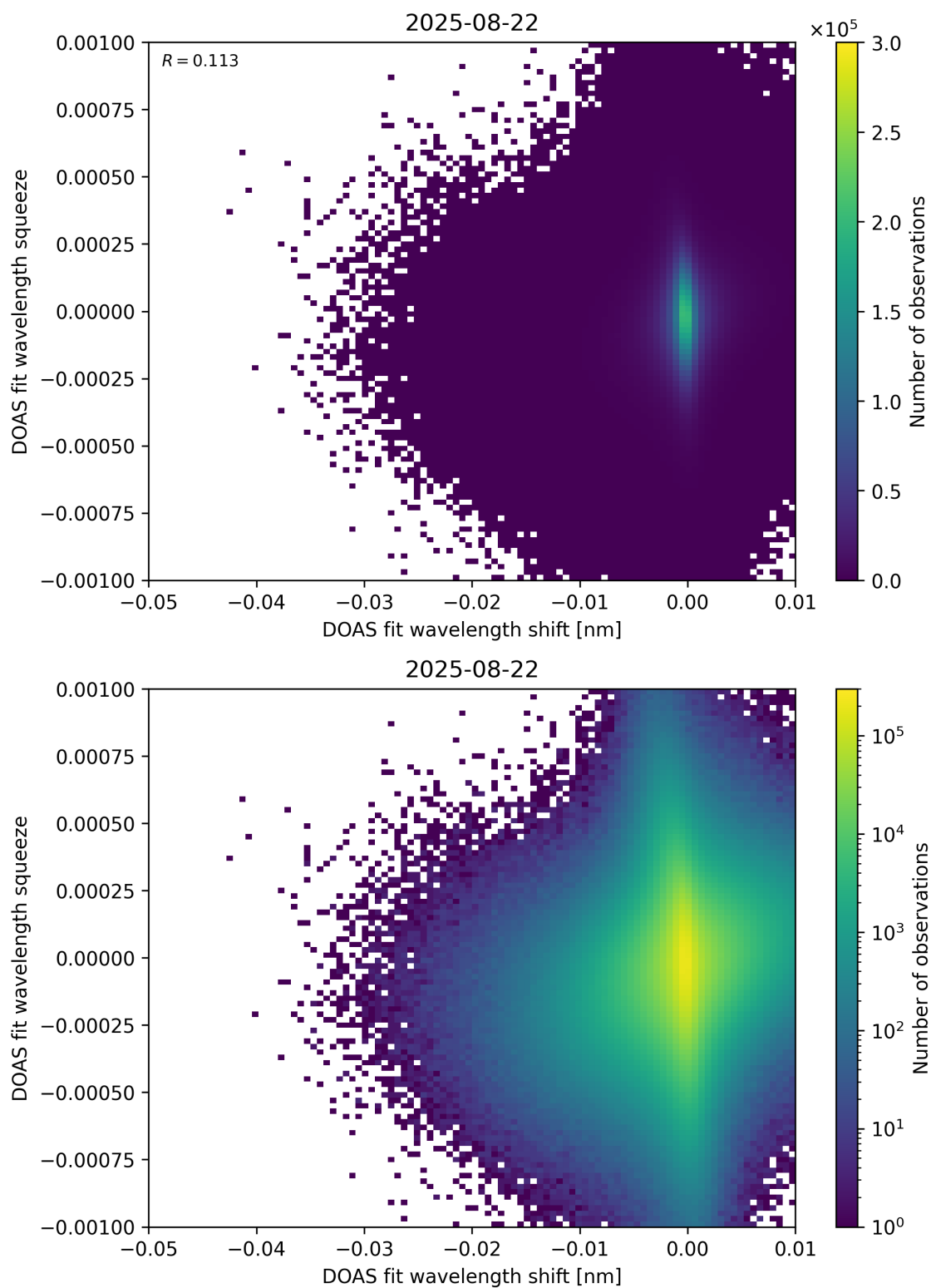
Figure 138: Scatter density plot of “DOAS fit wavelength shift” against “DOAS fit wavelength squeeze” for 2025-08-21 to 2025-08-23.
