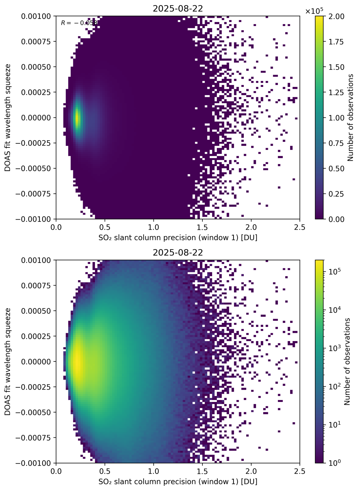
Figure 272: Scatter density plot of “SO 2 slant column precision (window 1)” against “DOAS fit wavelength squeeze” for 2025-08-21 to 2025-08-23.
