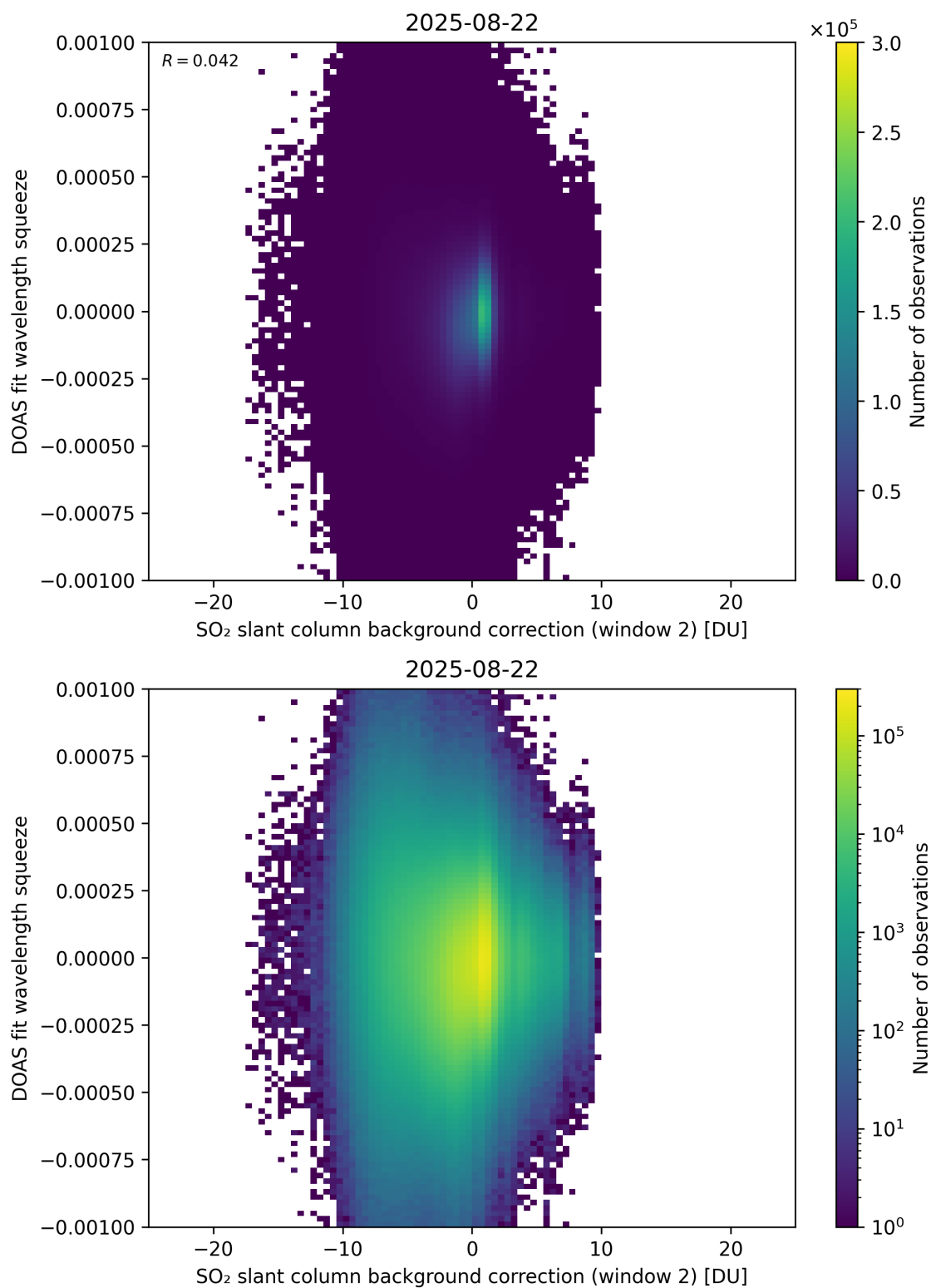
Figure 124: Scatter density plot of “SO 2 slant column background correction (window 2)” against “DOAS fit wavelength squeeze” for 2025-08-21 to 2025-08-23.
