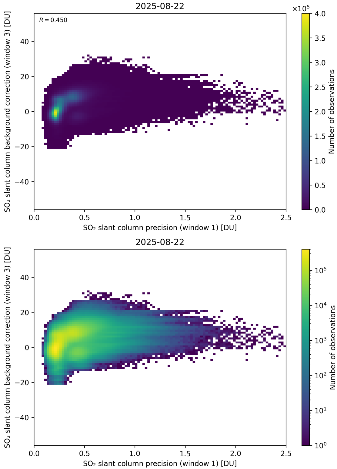
Figure 270: Scatter density plot of “SO 2 slant column precision (window 1)” against “SO 2 slant column background correction (window 3)” for 2025-08-21 to 2025-08-23.
