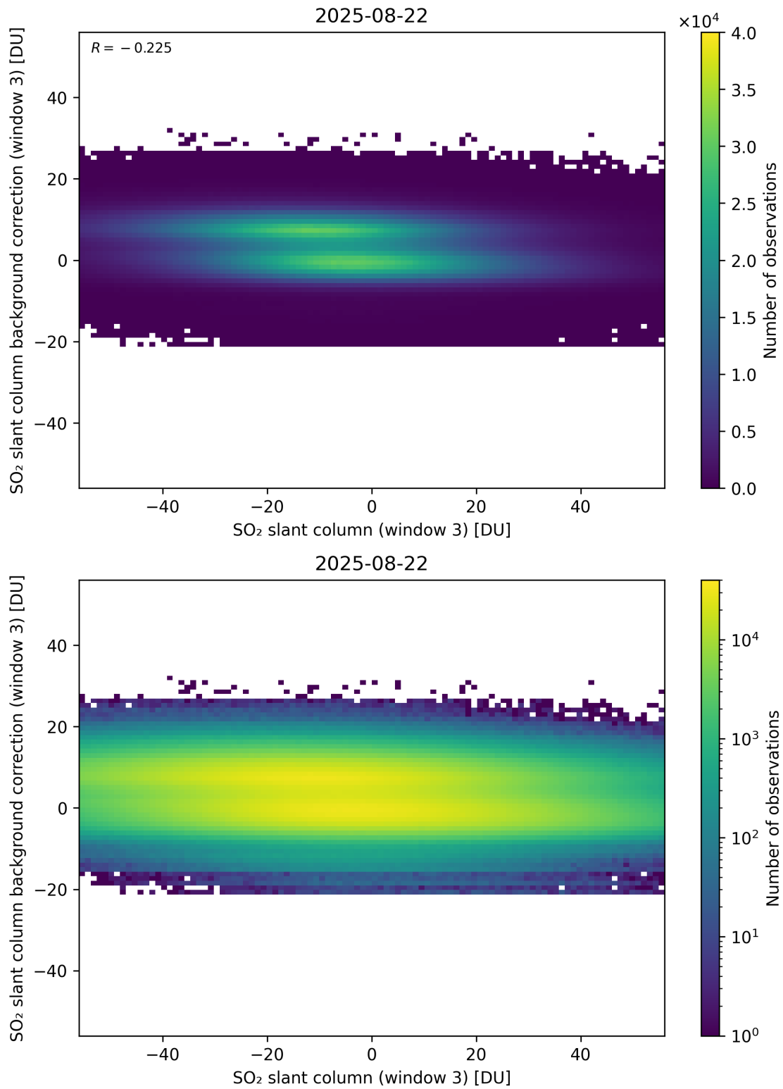
Figure 303: Scatter density plot of “SO 2 slant column (window 3)” against “SO 2 slant column background correction (window 3)” for 2025-08-21 to 2025-08-23.
