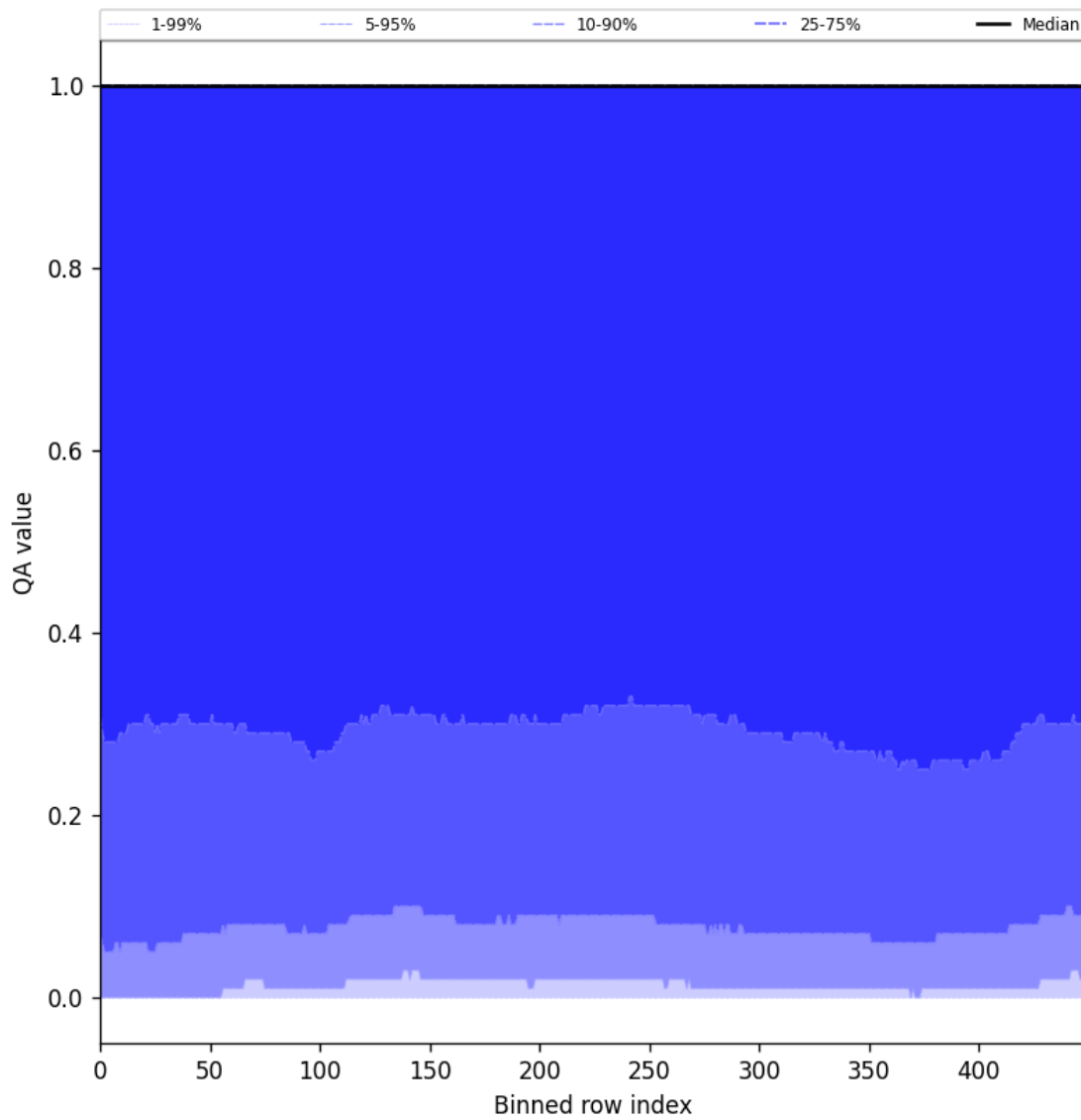
Figure 83: Along track statistics of “QA value” for 2025-08-21 to 2025-08-23
