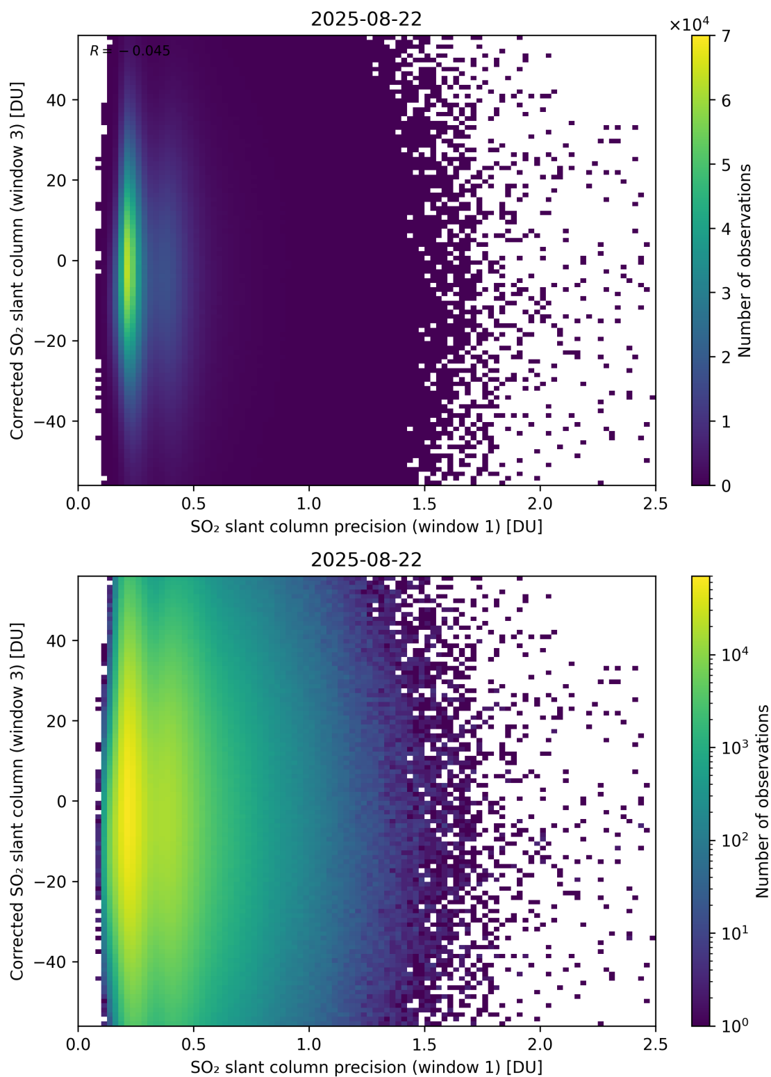
Figure 276: Scatter density plot of “SO 2 slant column precision (window 1)” against “Corrected SO 2 slant column (window 3)” for 2025-08-21 to 2025-08-23.
