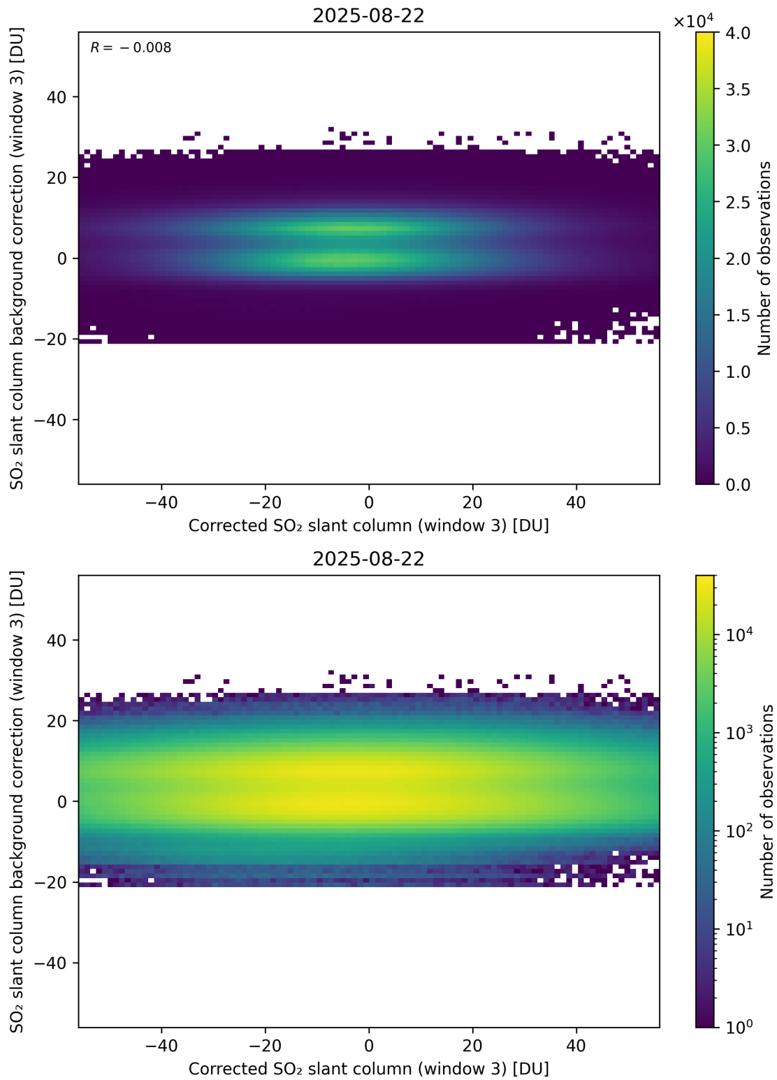
Figure 255: Scatter density plot of “Corrected SO 2 slant column (window 3)” against “SO 2 slant column background correction (window 3)” for 2025-08-21 to 2025-08-23.
