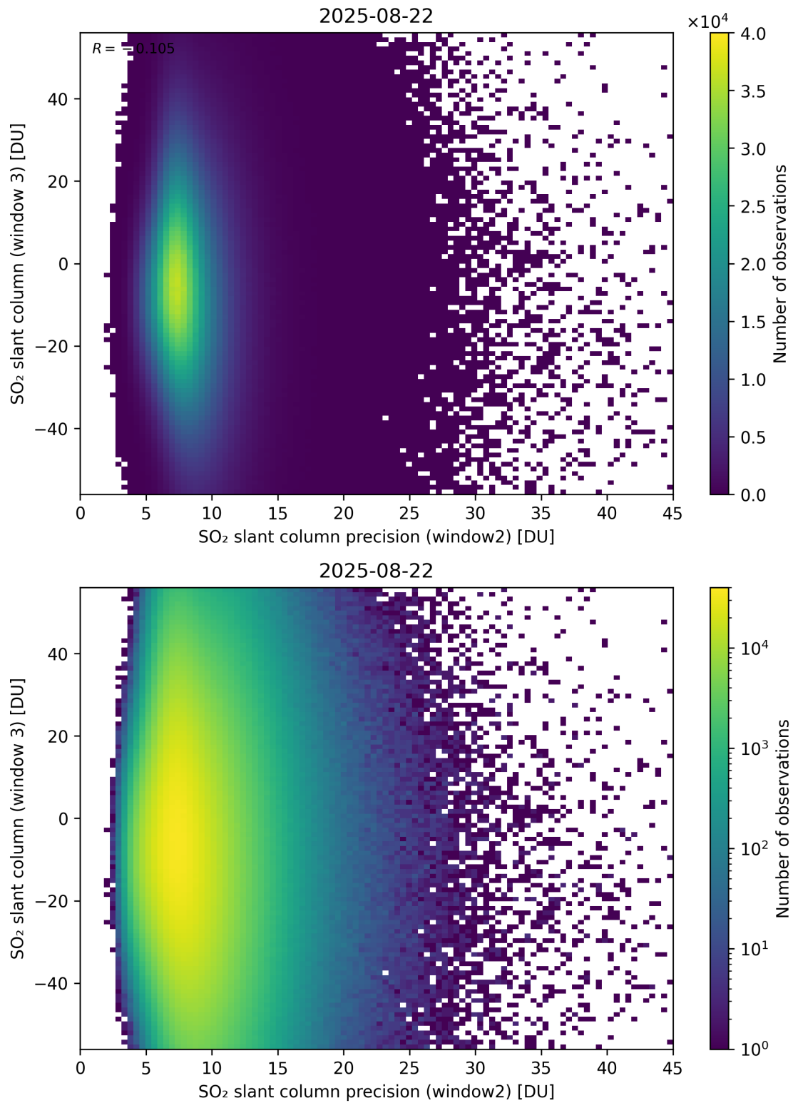
Figure 299: Scatter density plot of “SO 2 slant column precision (window2)” against “SO 2 slant column (window 3)” for 2025-08-21 to 2025-08-23.
