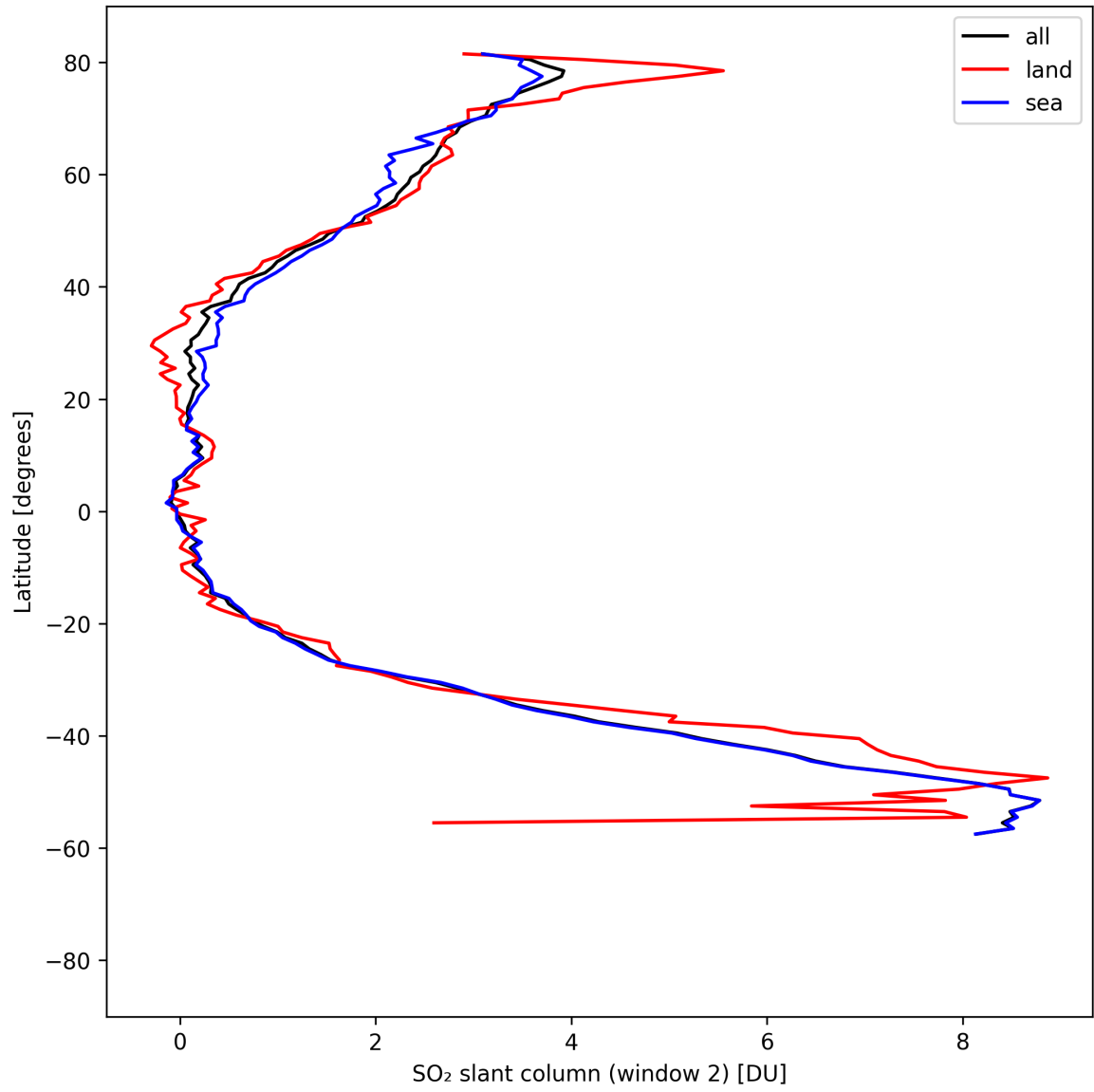
Figure 41: Zonal average of “SO 2 slant column (window 2)” for 2025-08-21 to 2025-08-23.
