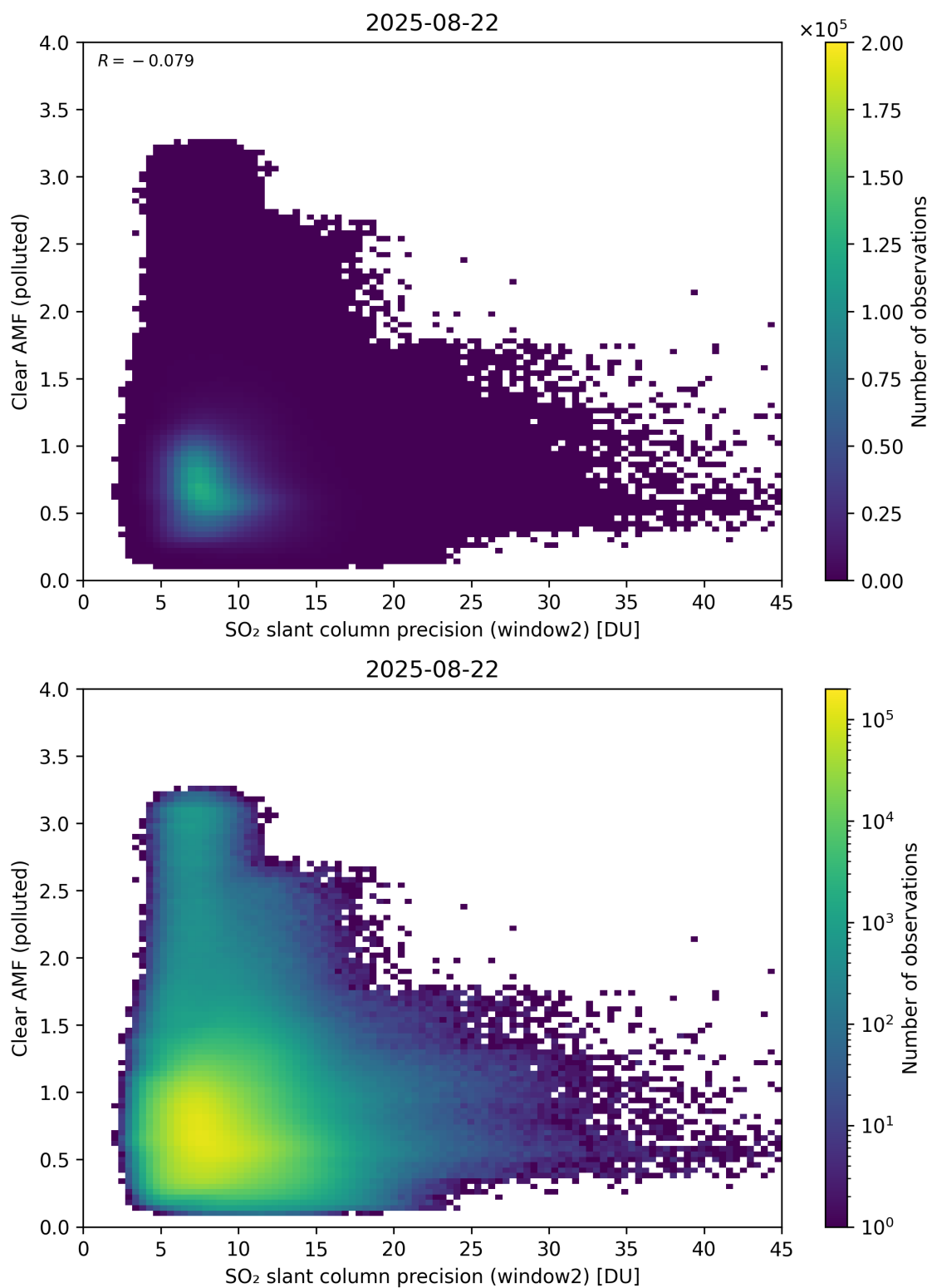
Figure 296: Scatter density plot of “SO 2 slant column precision (window2)” against “Clear AMF (polluted)” for 2025-08-21 to 2025-08-23.
