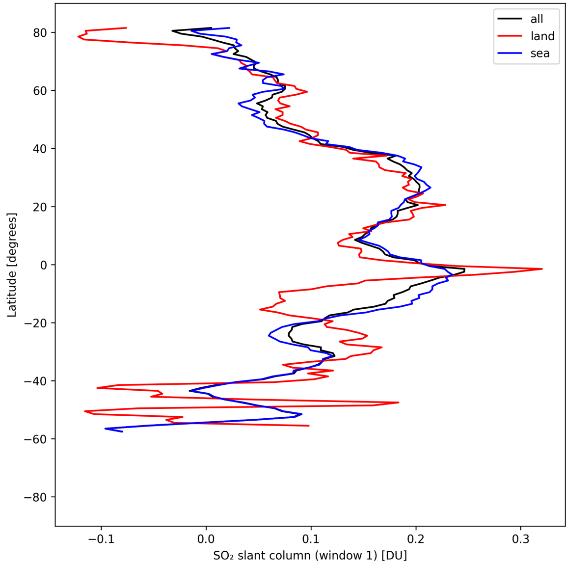
Figure 37: Zonal average of “SO 2 slant column (window 1)” for 2025-08-21 to 2025-08-23.
