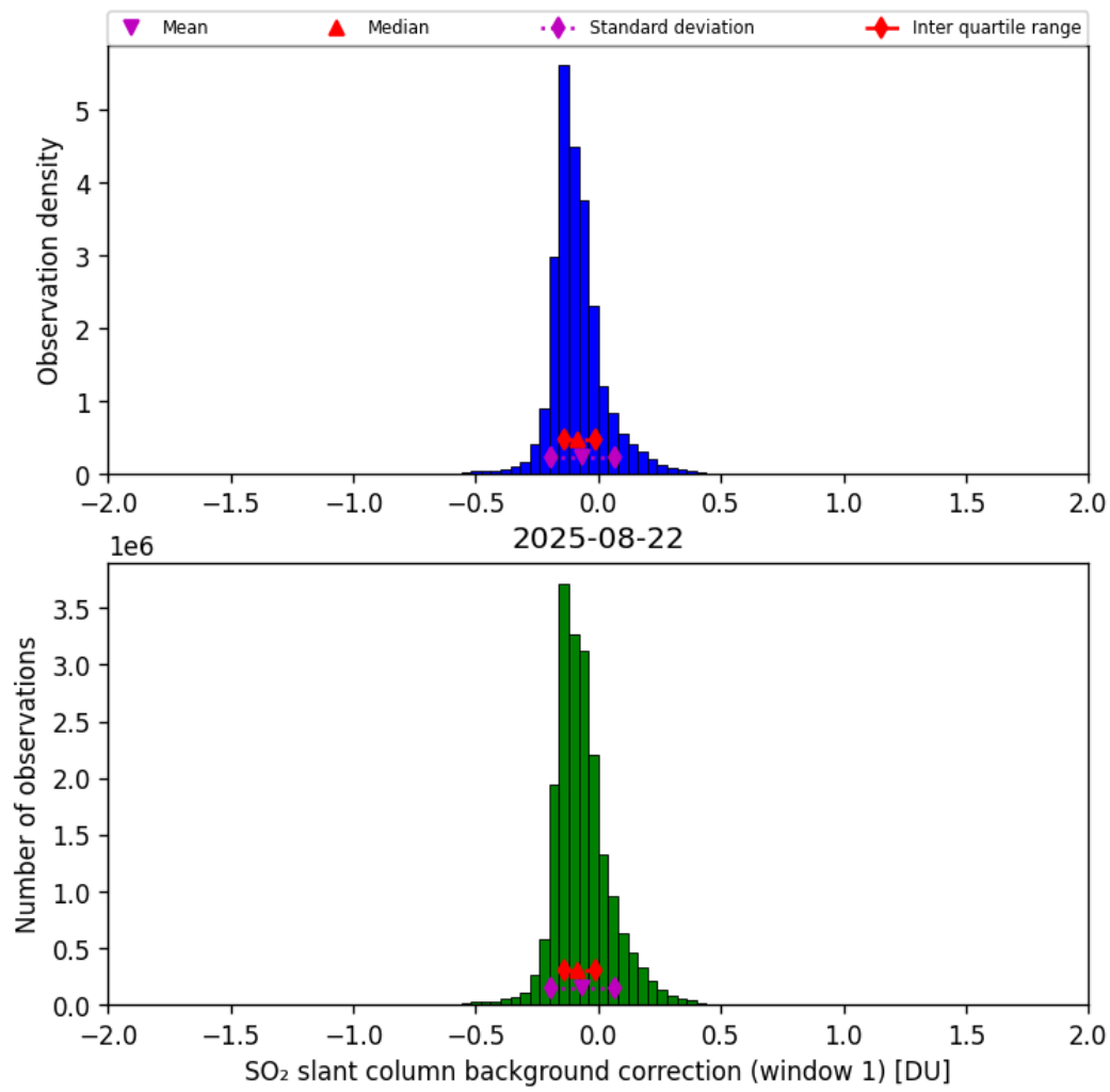
Figure 66: Histogram of “SO 2 slant column background correction (window 1)” for 2025-08-21 to 2025-08-23
