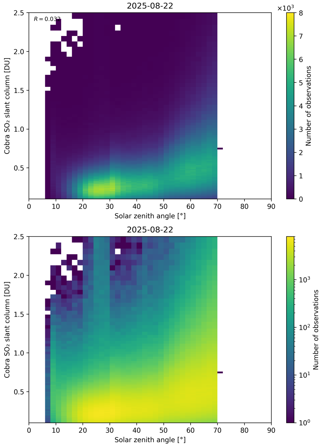
Figure 179: Scatter density plot of “Solar zenith angle” against “Cobra SO 2 slant column” for 2025-08-21 to 2025-08-23.
