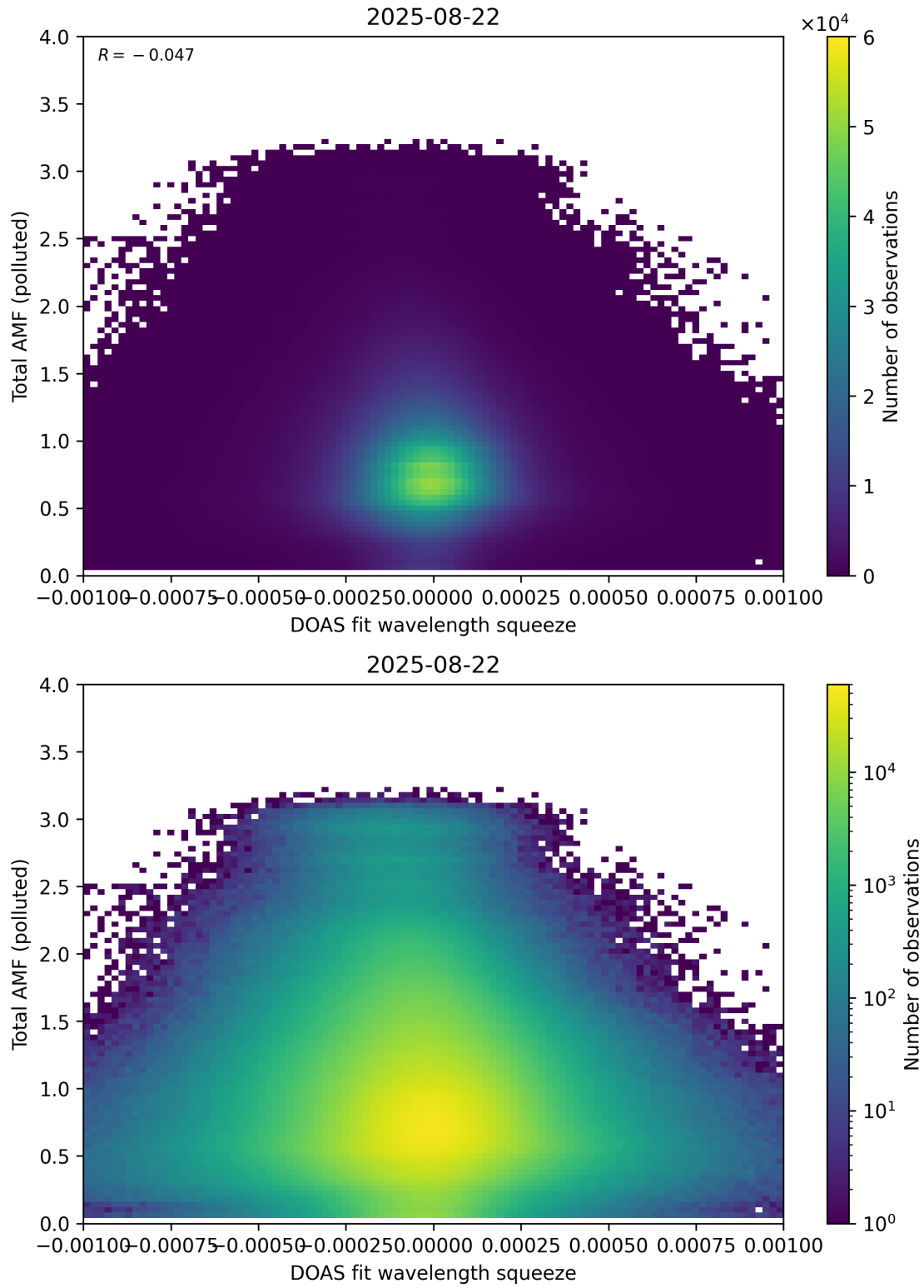
Figure 145: Scatter density plot of “DOAS fit wavelength squeeze” against “Total AMF (polluted)” for 2025-08-21 to 2025-08-23.
