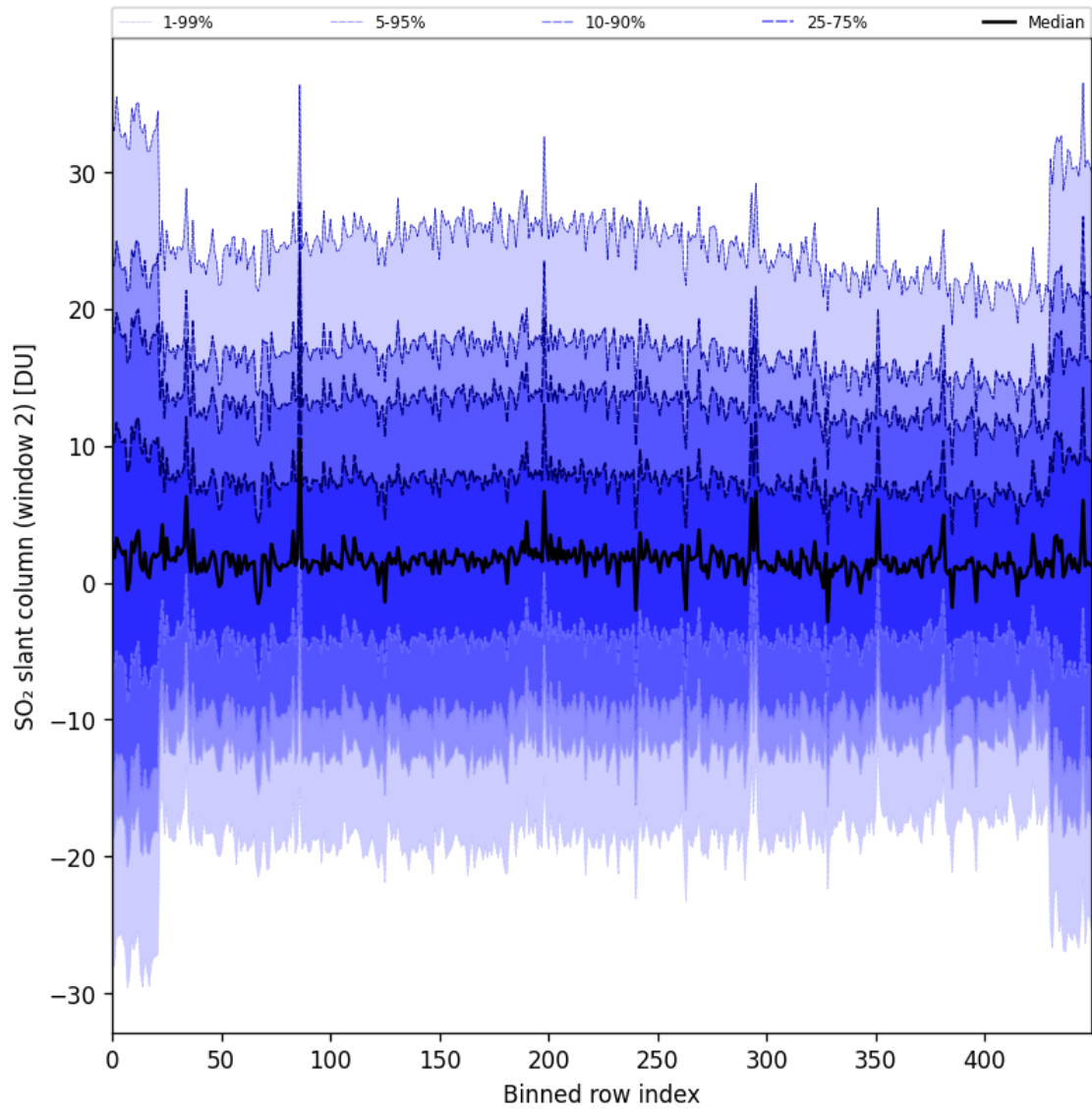
Figure 93: Along track statistics of “SO 2 slant column (window 2)” for 2025-08-21 to 2025-08-23
