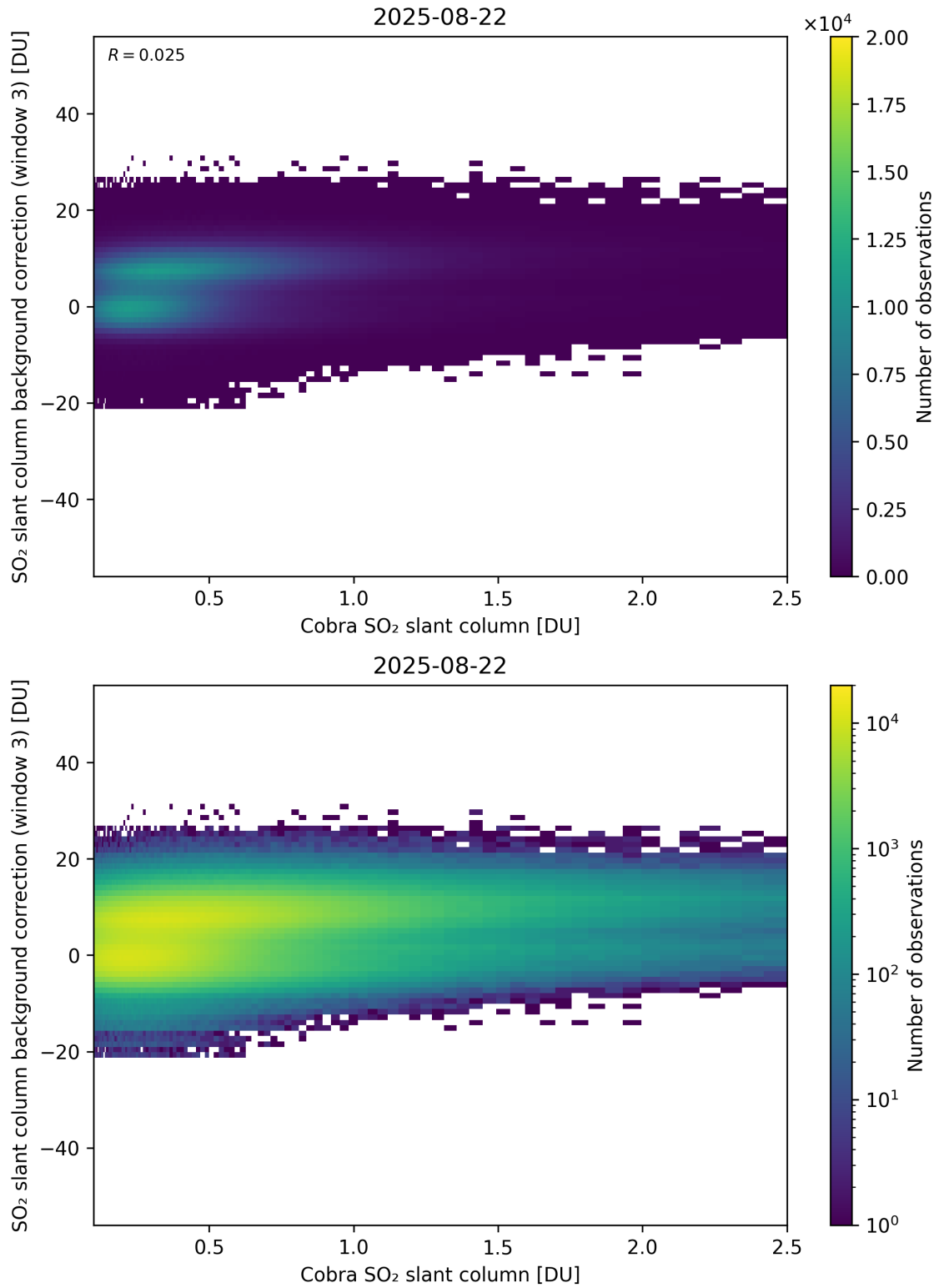
Figure 195: Scatter density plot of “Cobra SO 2 slant column” against “SO 2 slant column background correction (window 3)” for 2025-08-21 to 2025-08-23.
