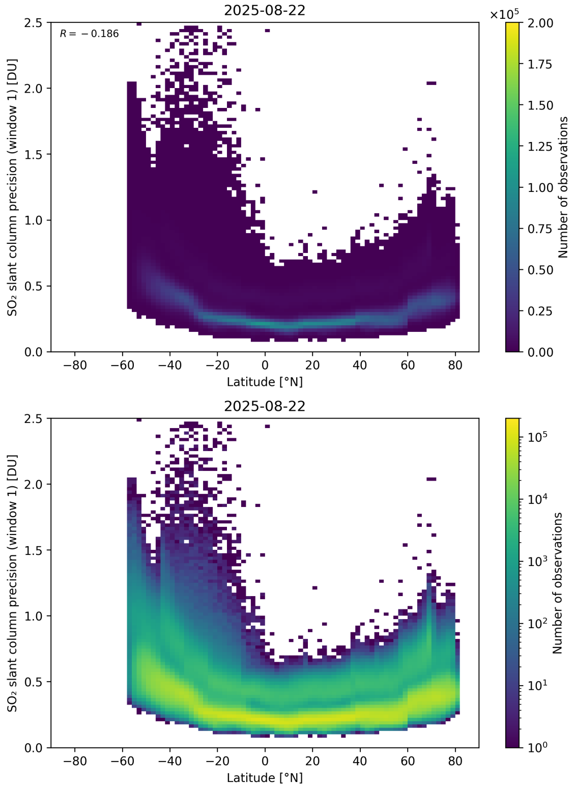
Figure 163: Scatter density plot of “Latitude” against “SO 2 slant column precision (window 1)” for 2025-08-21 to 2025-08-23.
