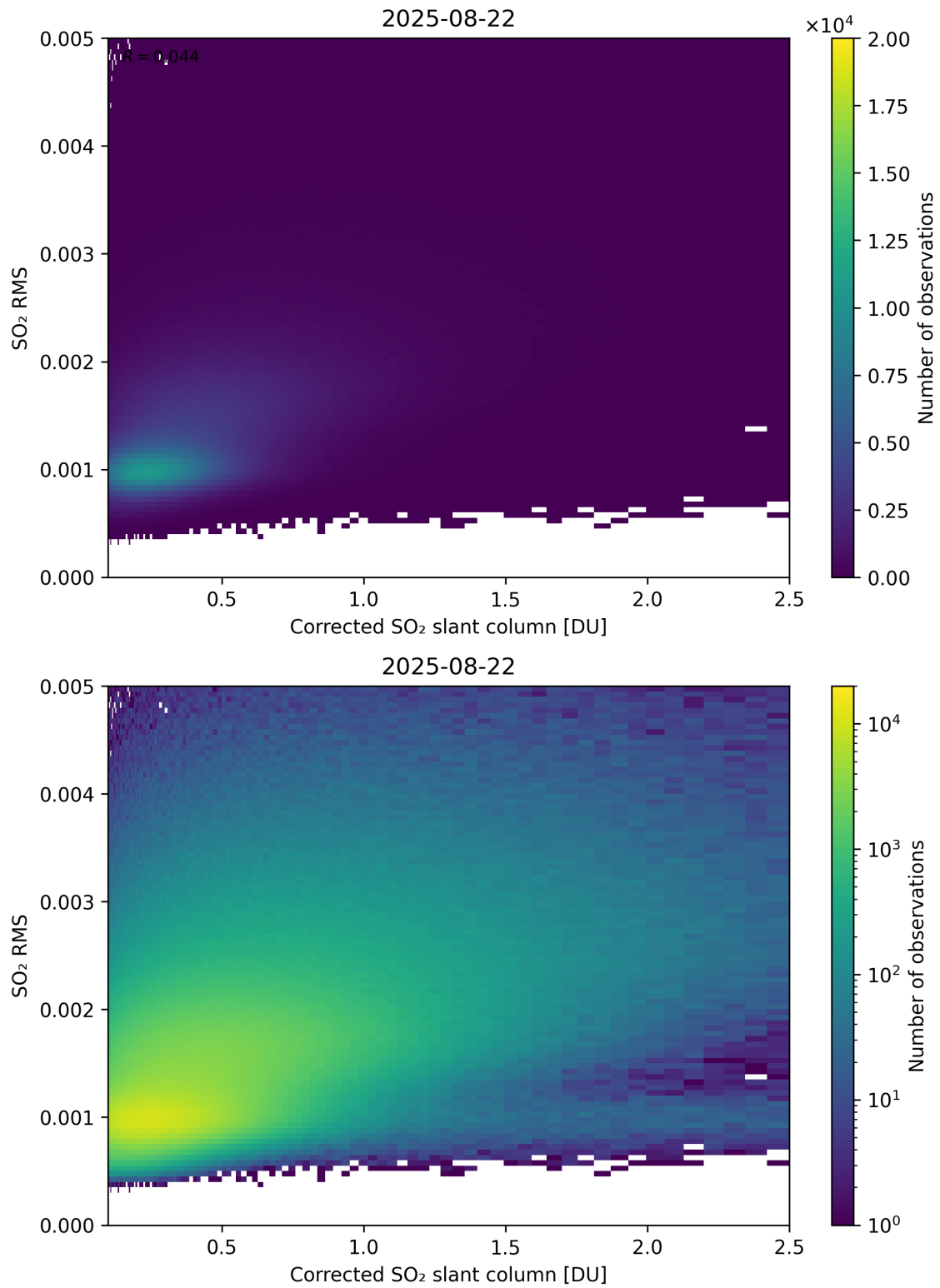
Figure 231: Scatter density plot of “Corrected SO 2 slant column” against “SO 2 RMS” for 2025-08-21 to 2025-08-23.
