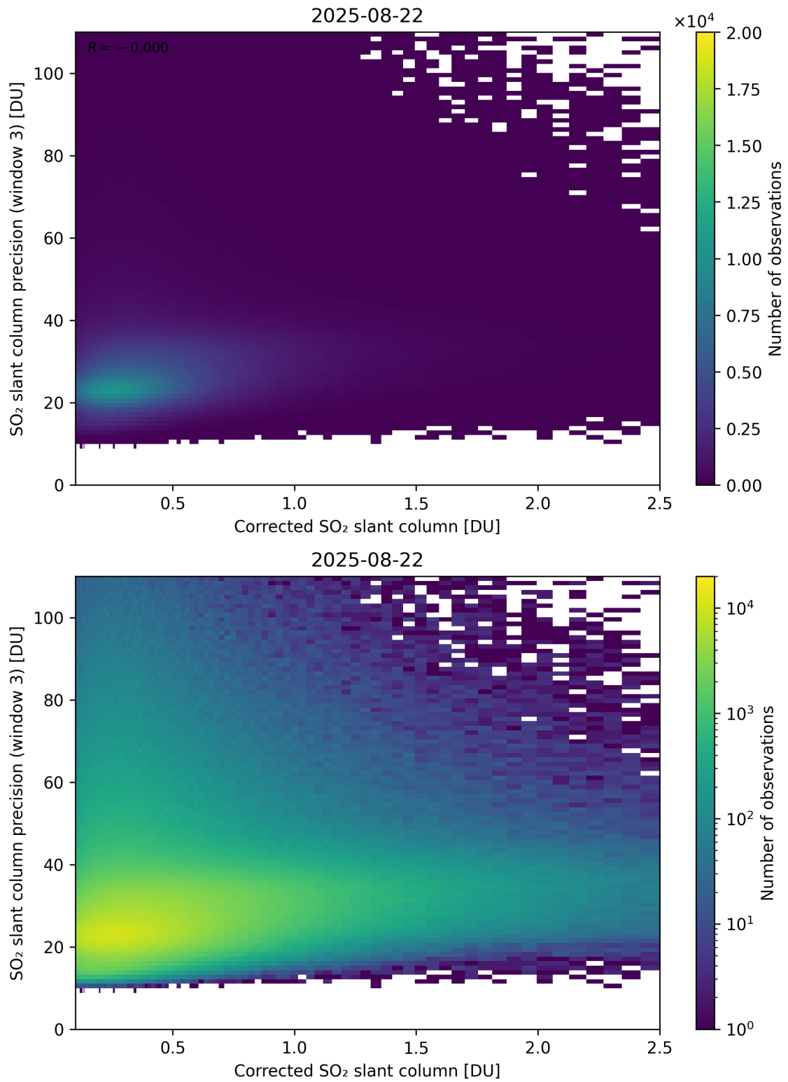
Figure 241: Scatter density plot of “Corrected SO 2 slant column” against “SO 2 slant column precision (window 3)” for 2025-08-21 to 2025-08-23.
