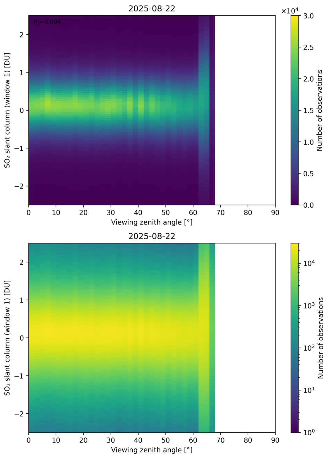
Figure 376: Scatter density plot of “Viewing zenith angle” against “SO 2 slant column (window 1)” for 2025-08-21 to 2025-08-23.
