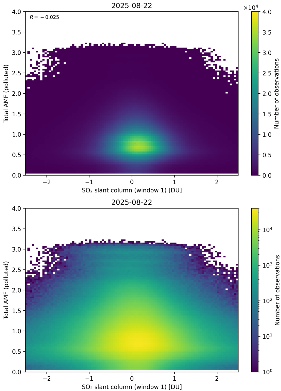
Figure 289: Scatter density plot of “SO 2 slant column (window 1)” against “Total AMF (polluted)” for 2025-08-21 to 2025-08-23.
