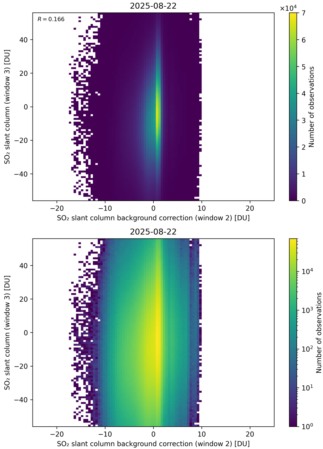
Figure 128: Scatter density plot of “SO 2 slant column background correction (window 2)” against “SO 2 slant column (window 3)” for 2025-08-21 to 2025-08-23.
