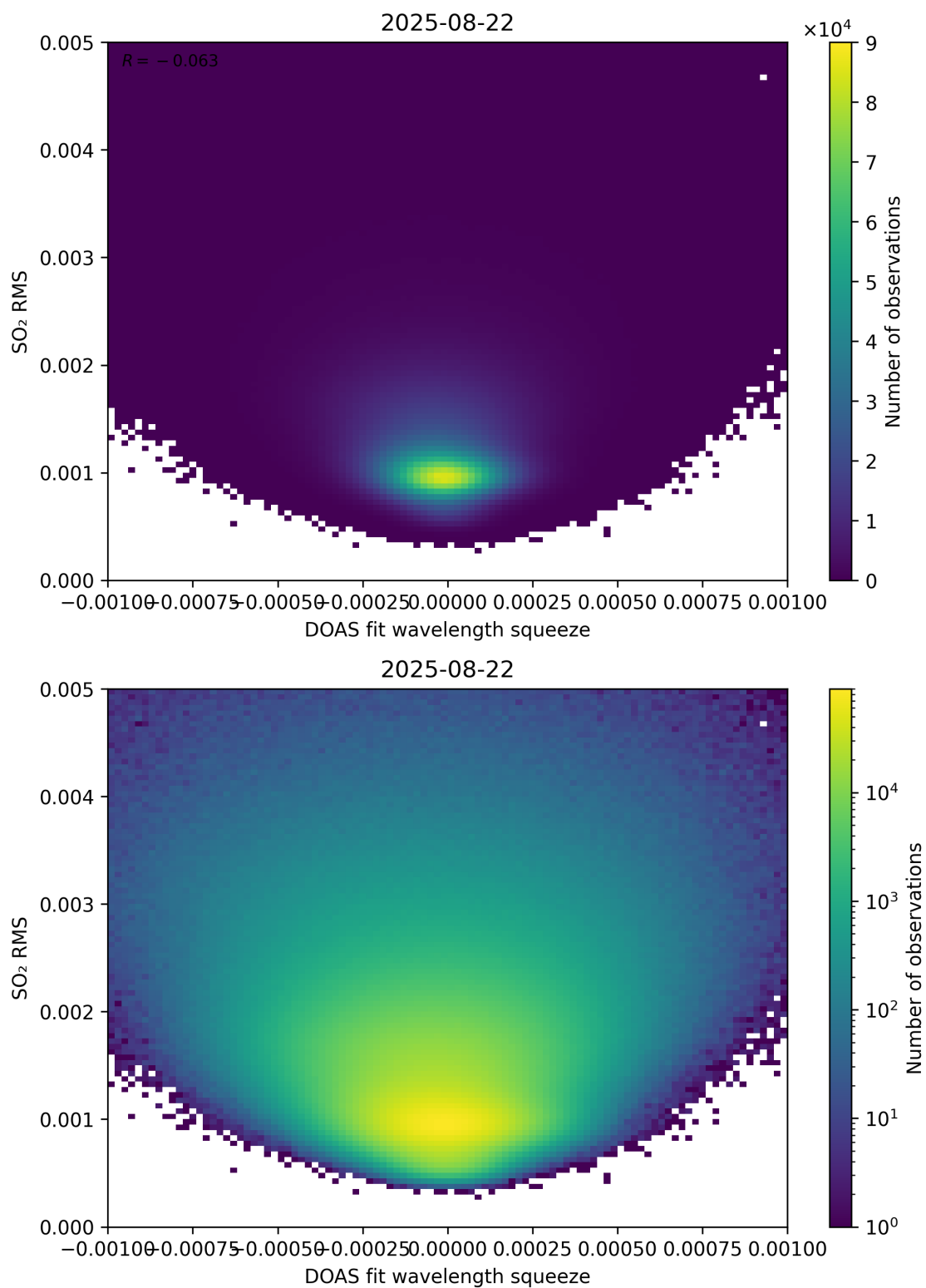
Figure 143: Scatter density plot of “DOAS fit wavelength squeeze” against “SO 2 RMS” for 2025-08-21 to 2025-08-23.
