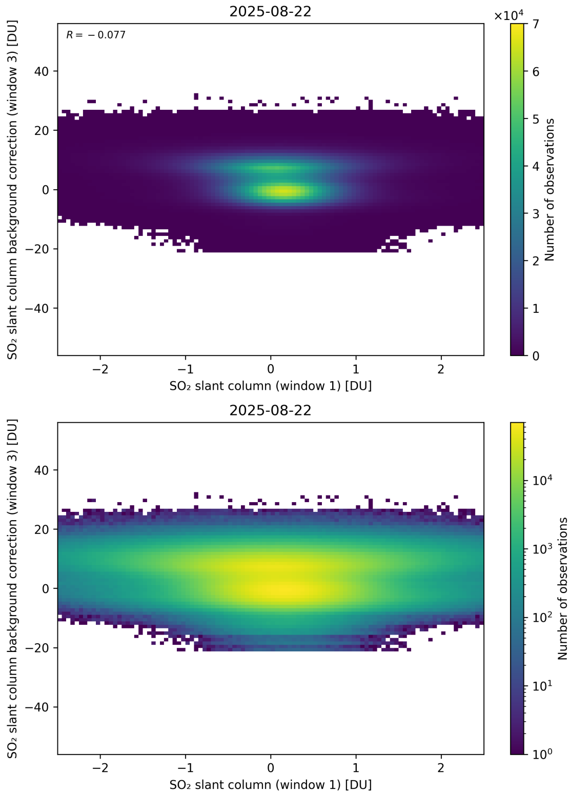
Figure 264: Scatter density plot of “SO 2 slant column (window 1)” against “SO 2 slant column background correction (window 3)” for 2025-08-21 to 2025-08-23.
