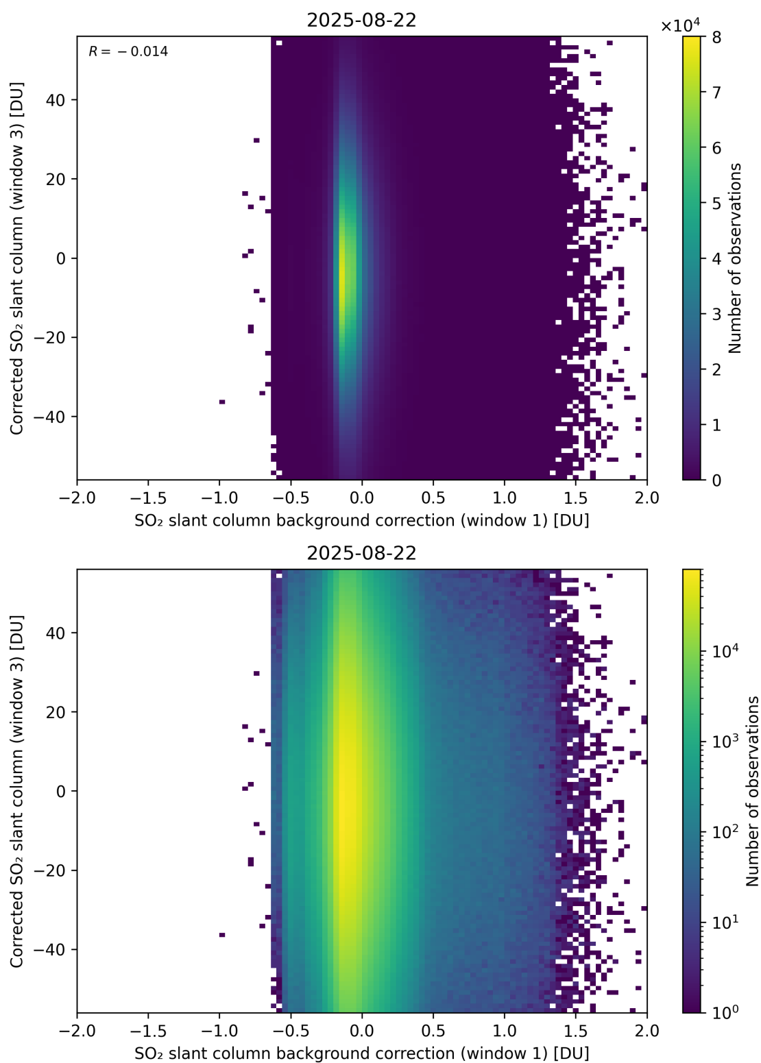
Figure 116: Scatter density plot of “SO 2 slant column background correction (window 1)” against “Corrected SO 2 slant column (window 3)” for 2025-08-21 to 2025-08-23.
