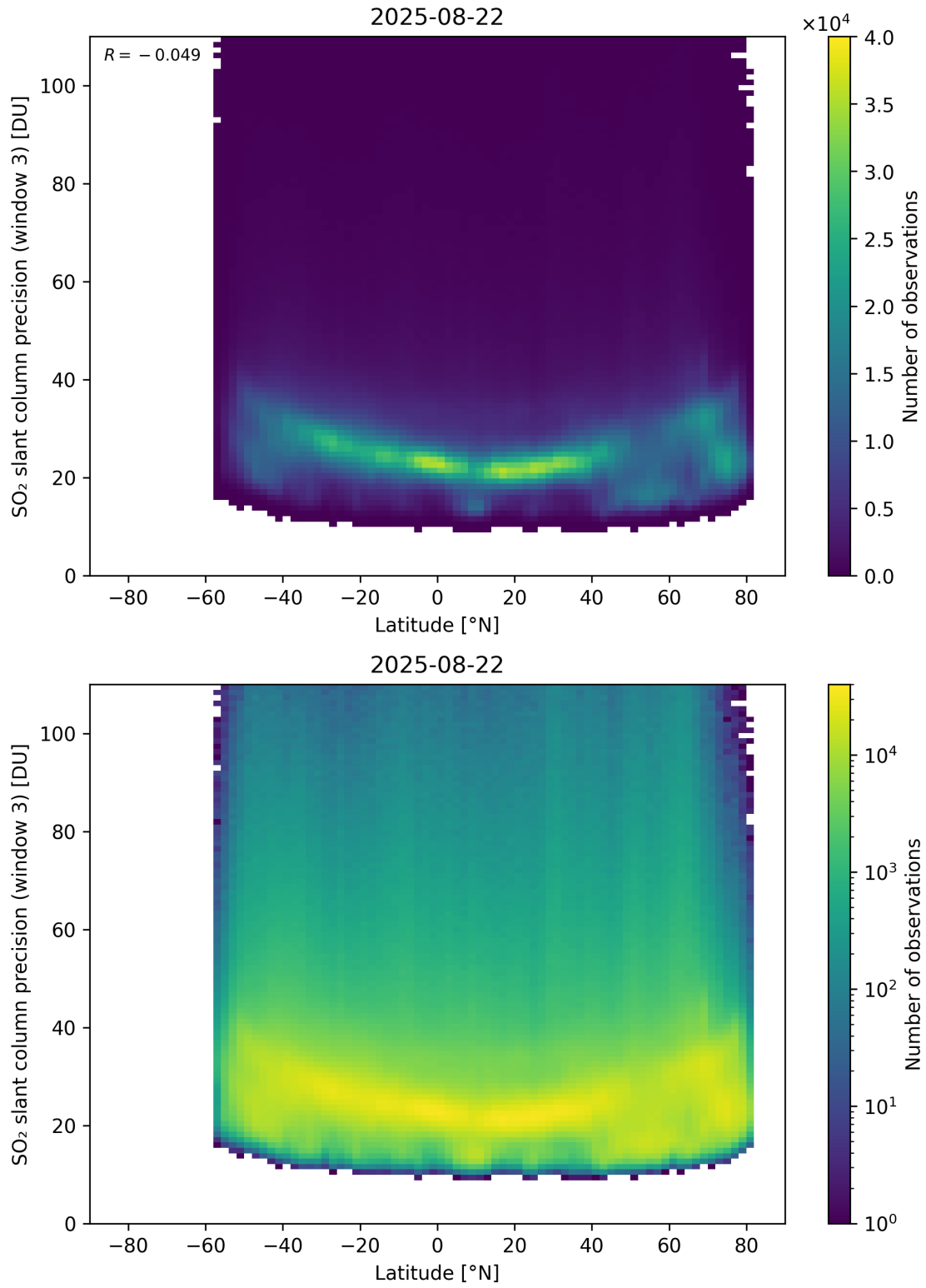
Figure 166: Scatter density plot of “Latitude” against “SO 2 slant column precision (window 3)” for 2025-08-21 to 2025-08-23.
