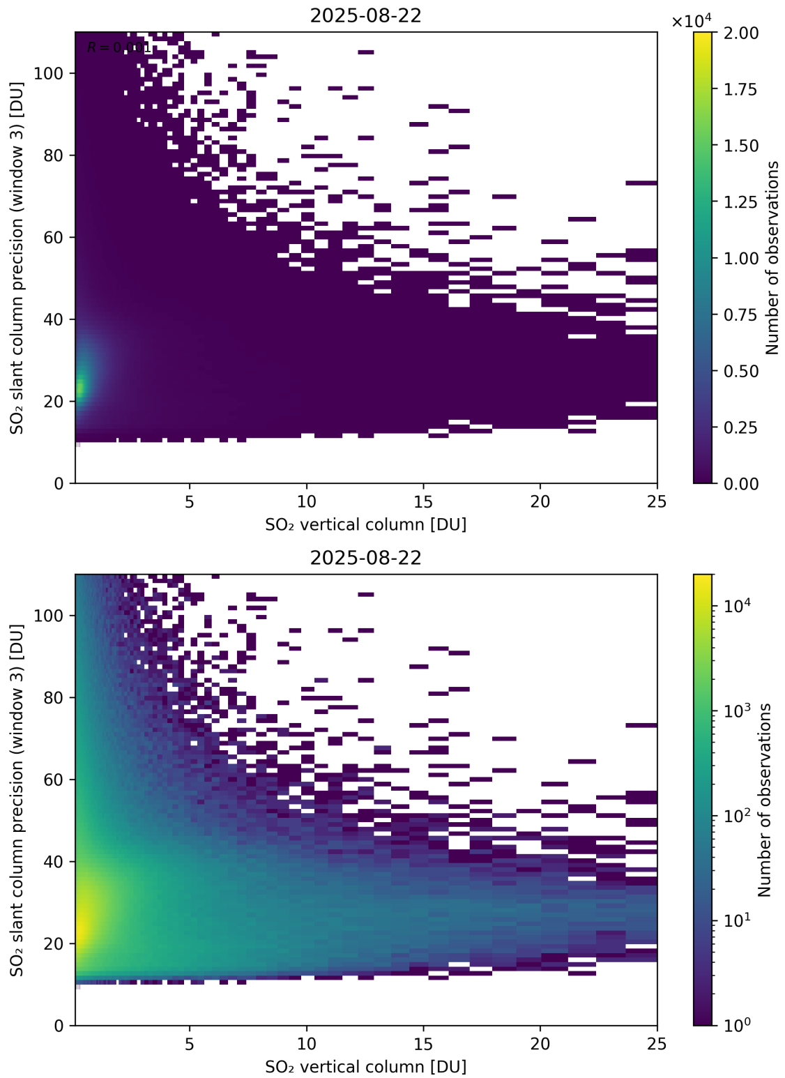
Figure 358: Scatter density plot of “SO 2 vertical column” against “SO 2 slant column precision (window 3)” for 2025-08-21 to 2025-08-23.
