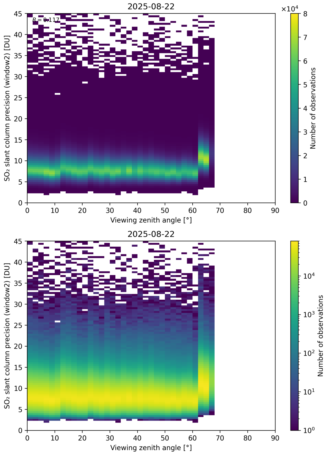
Figure 378: Scatter density plot of “Viewing zenith angle” against “SO 2 slant column precision (window2)” for 2025-08-21 to 2025-08-23.
