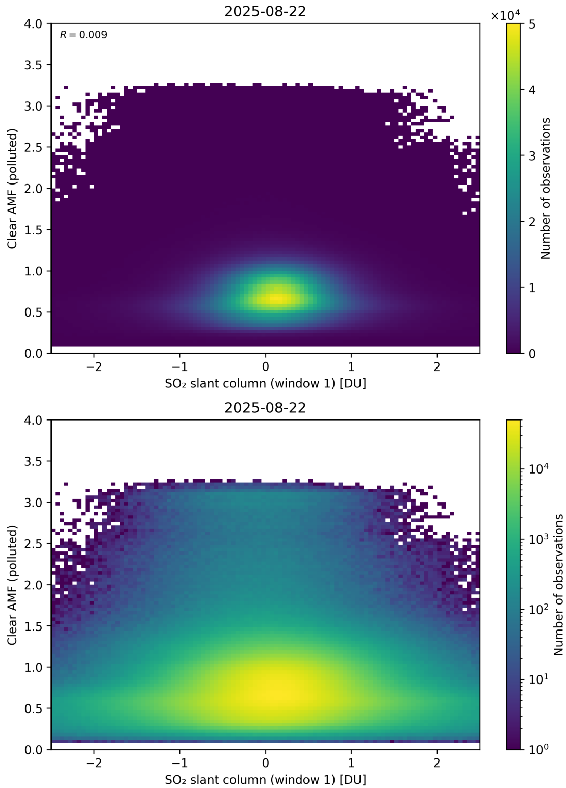
Figure 282: Scatter density plot of “SO 2 slant column (window 1)” against “Clear AMF (polluted)” for 2025-08-21 to 2025-08-23.
