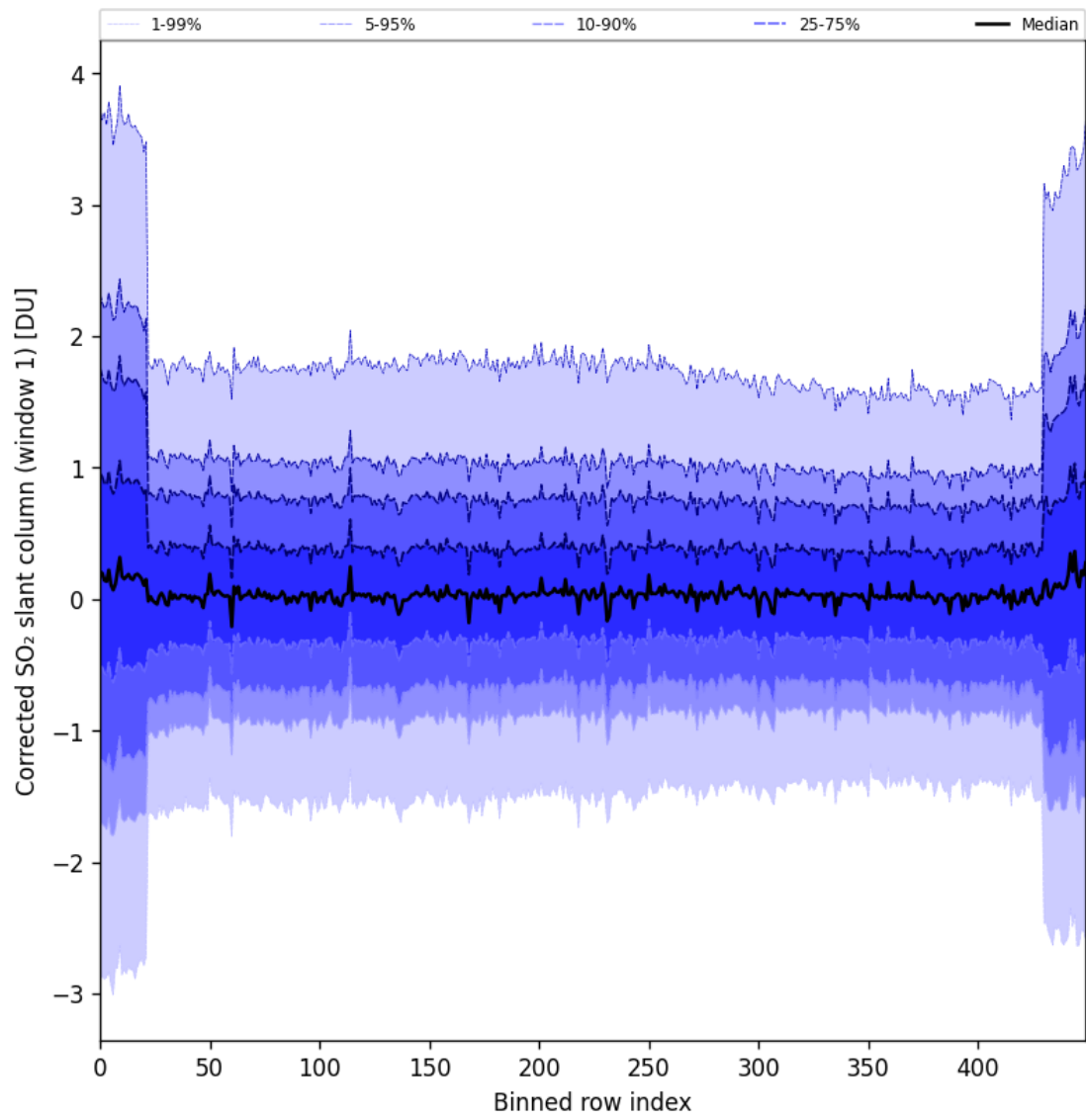
Figure 91: Along track statistics of "Corrected SO 2 slant column (window 1)" for 2025-08-21 to 2025-08-23
