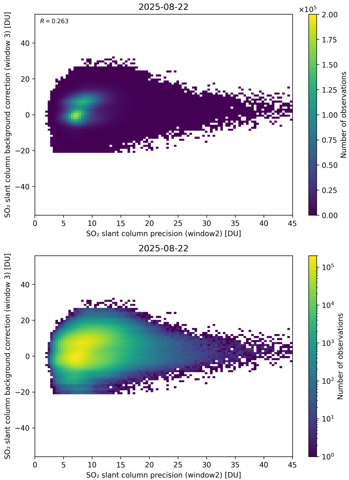
Figure 292: Scatter density plot of “SO 2 slant column precision (window2)” against “SO 2 slant column background correction (window 3)” for 2025-08-21 to 2025-08-23.
