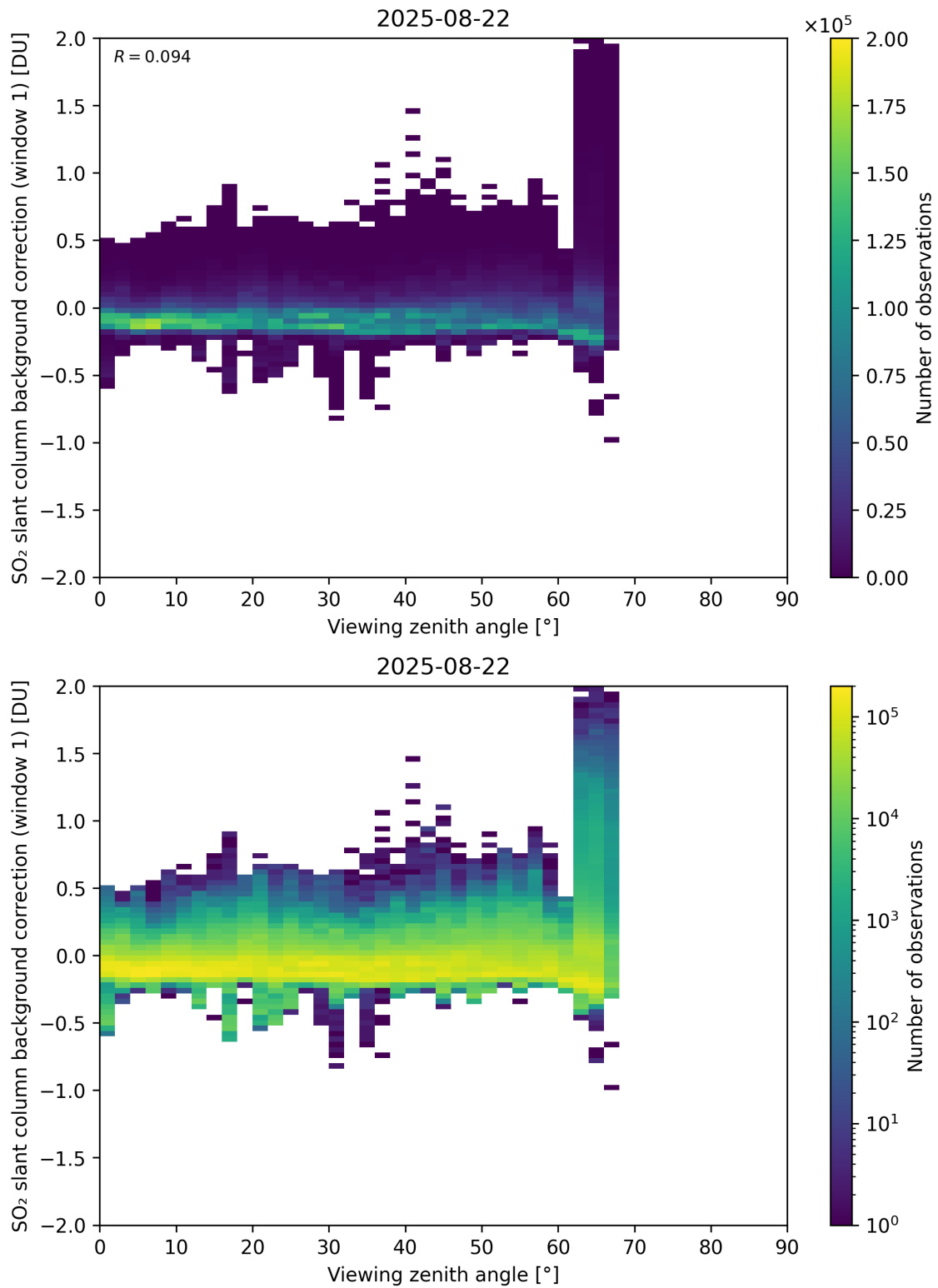
Figure 362: Scatter density plot of “Viewing zenith angle” against “SO 2 slant column background correction (window 1)” for 2025-08-21 to 2025-08-23.
