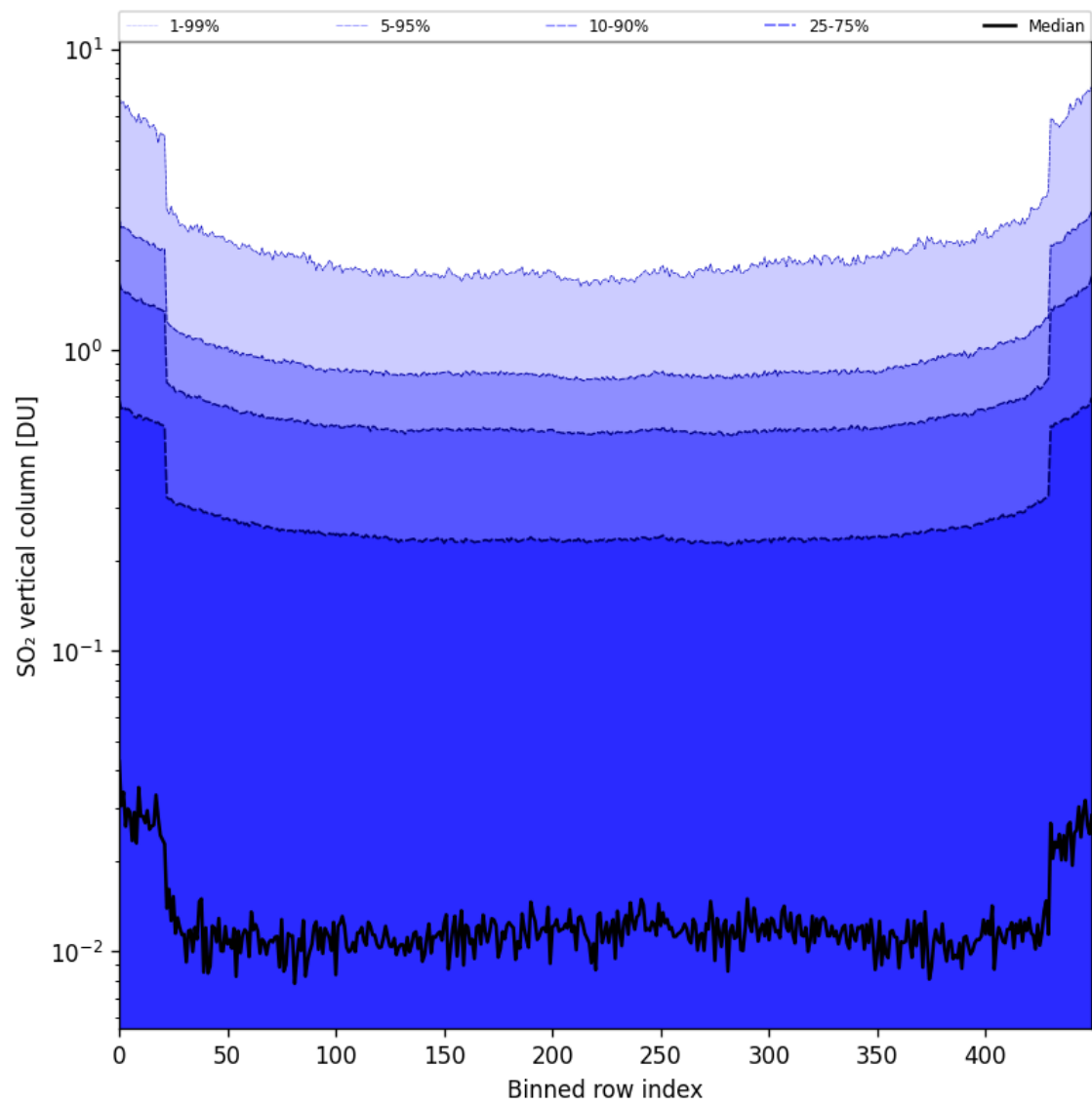
Figure 84: Along track statistics of “SO 2 vertical column” for 2025-08-21 to 2025-08-23
