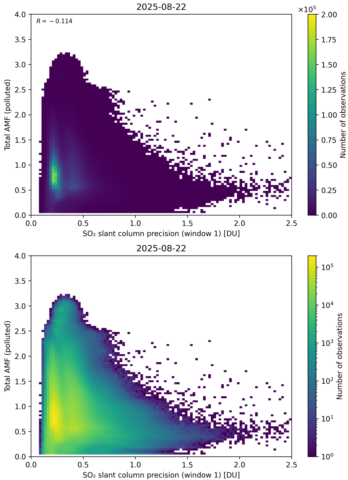
Figure 280: Scatter density plot of “SO 2 slant column precision (window 1)” against “Total AMF (polluted)” for 2025-08-21 to 2025-08-23.
