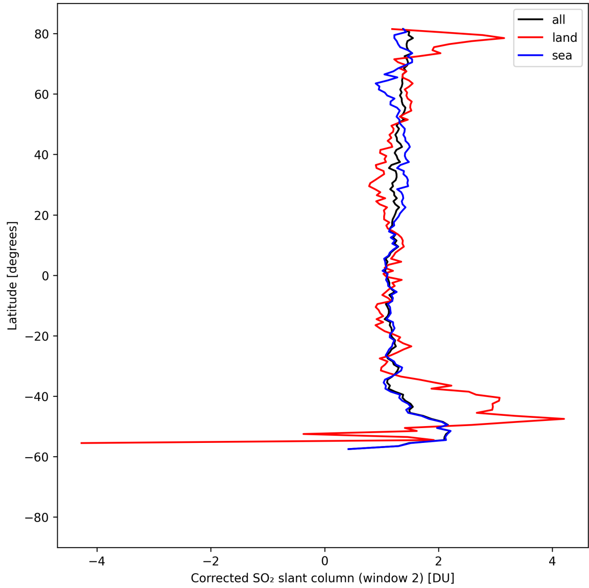
Figure 43: Zonal average of “Corrected SO 2 slant column (window 2)” for 2025-08-21 to 2025-08-23.
