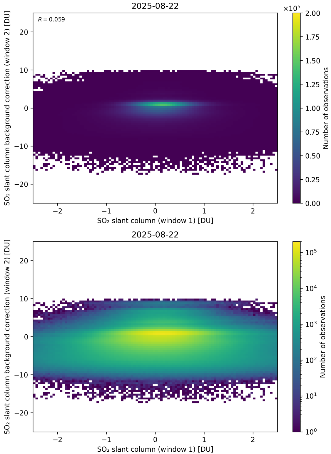
Figure 263: Scatter density plot of “SO 2 slant column (window 1)” against “SO 2 slant column background correction (window 2)” for 2025-08-21 to 2025-08-23.
