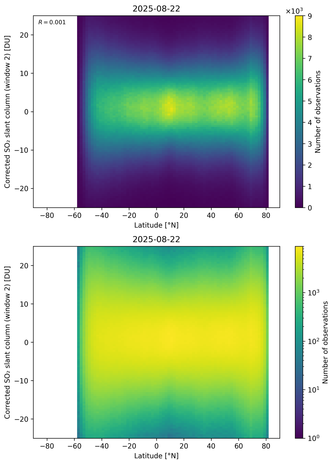
Figure 160: Scatter density plot of “Latitude” against “Corrected SO 2 slant column (window 2)” for 2025-08-21 to 2025-08-23.
