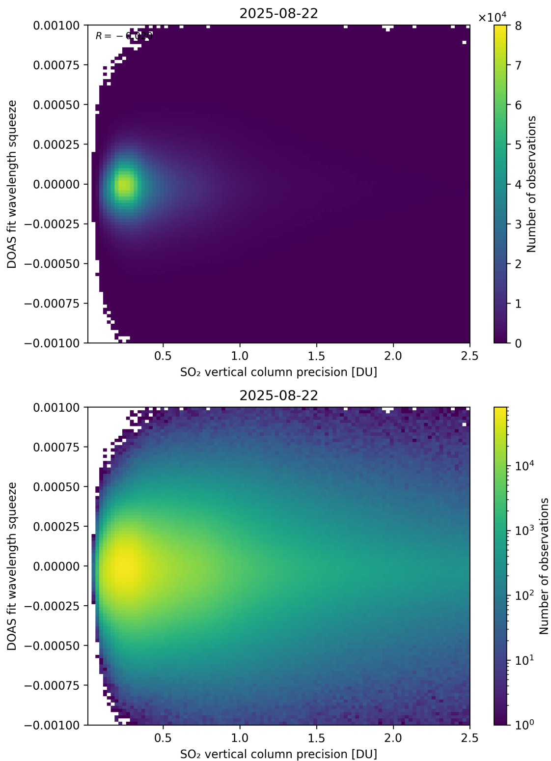
Figure 333: Scatter density plot of “SO 2 vertical column precision” against “DOAS fit wavelength squeeze” for 2025-08-21 to 2025-08-23.
