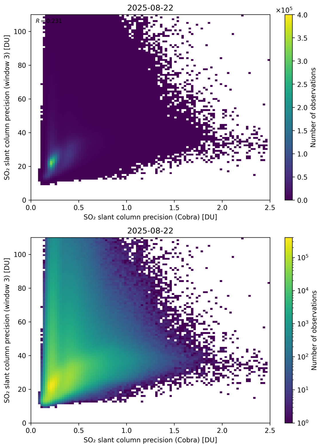
Figure 212: Scatter density plot of “SO 2 slant column precision (Cobra)” against “SO 2 slant column precision (window 3)” for 2025-08-21 to 2025-08-23.
