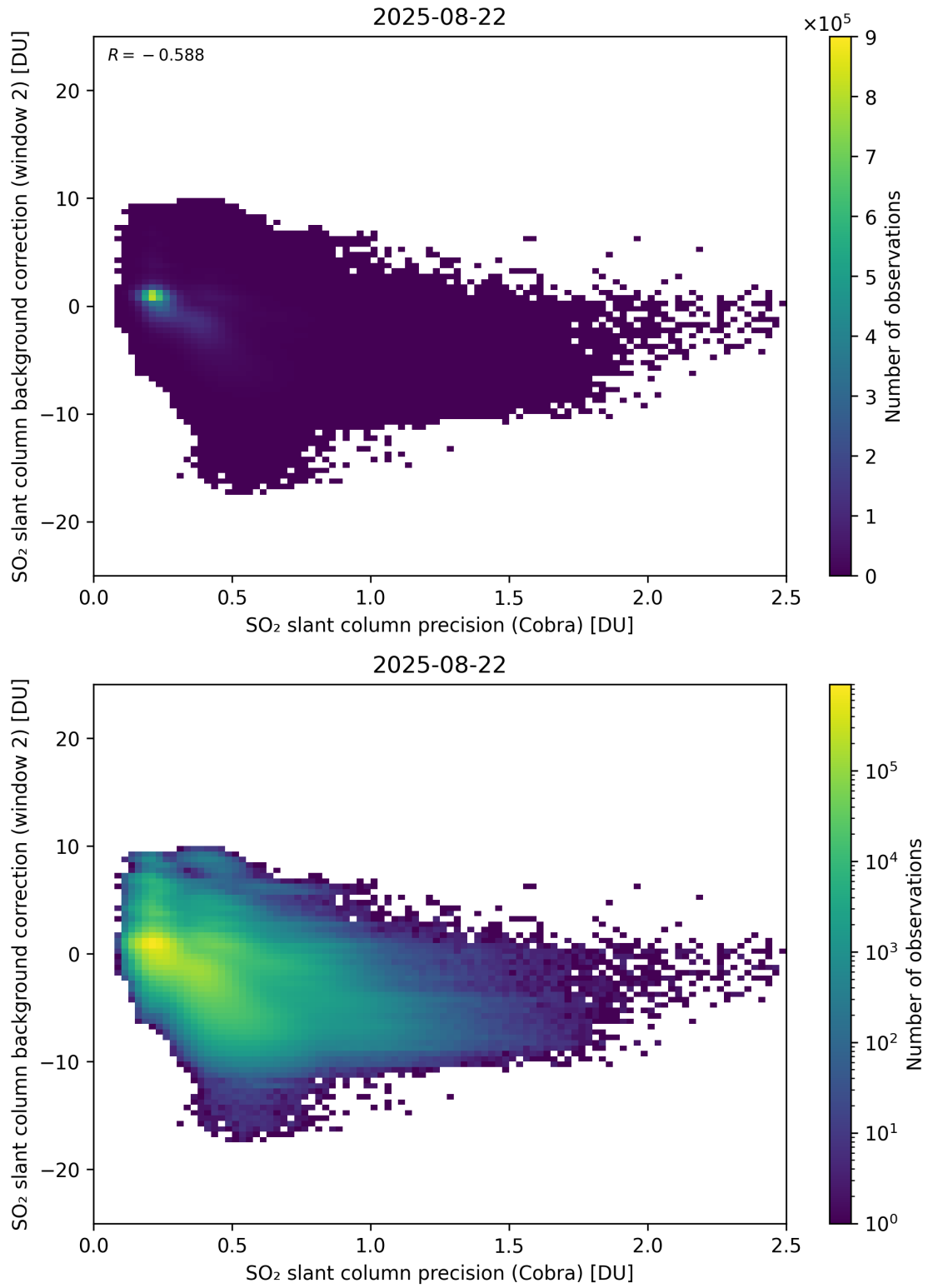
Figure 200: Scatter density plot of “SO 2 slant column precision (Cobra)” against “SO 2 slant column background correction (window 2)” for 2025-08-21 to 2025-08-23.
