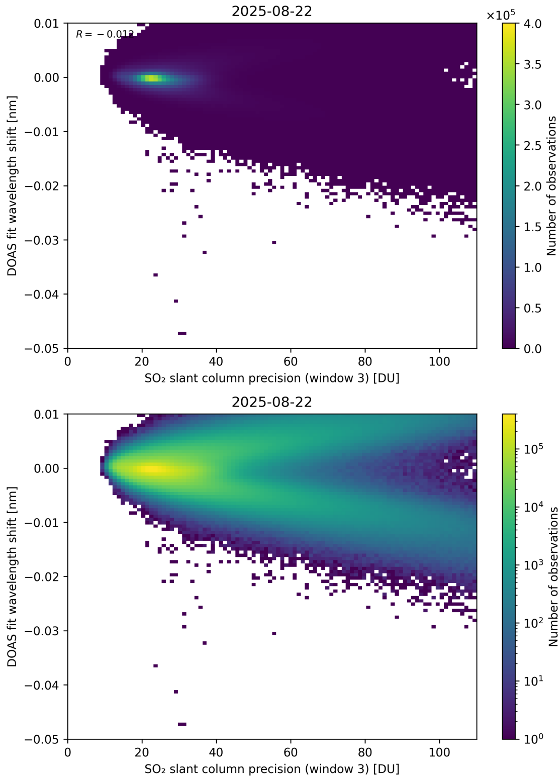
Figure 308: Scatter density plot of “SO 2 slant column precision (window 3)” against “DOAS fit wavelength shift” for 2025-08-21 to 2025-08-23.
