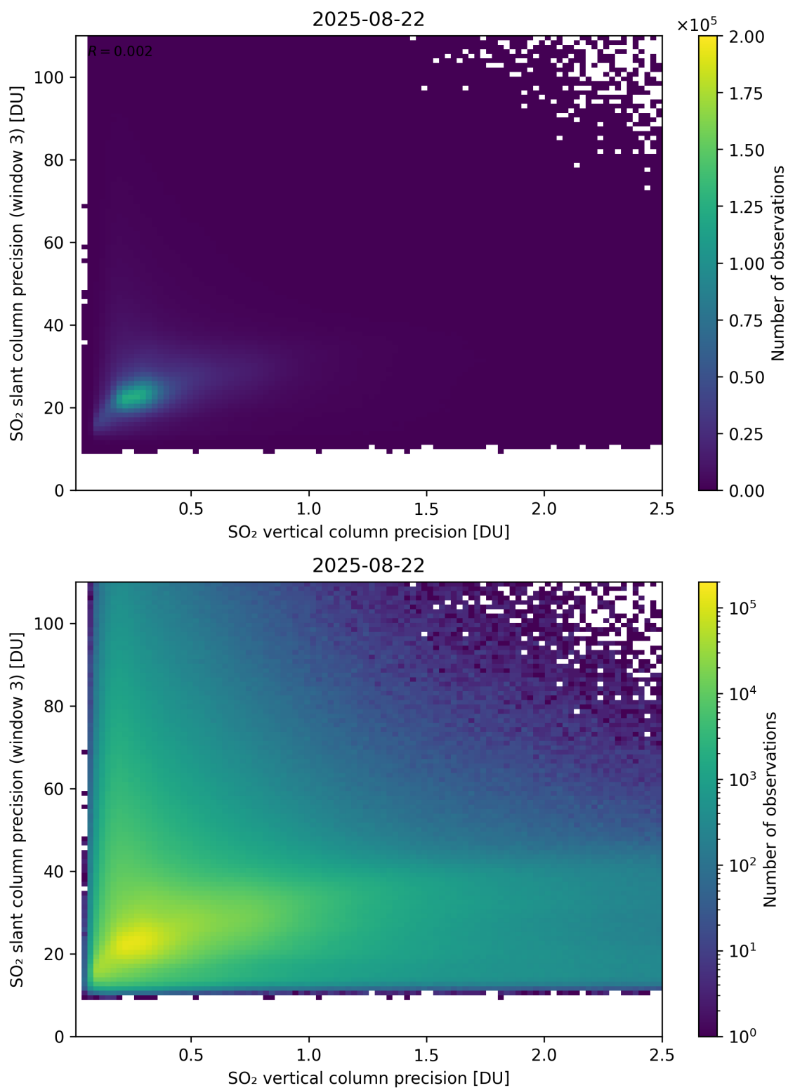
Figure 345: Scatter density plot of “SO 2 vertical column precision” against “SO 2 slant column precision (window 3)” for 2025-08-21 to 2025-08-23.
