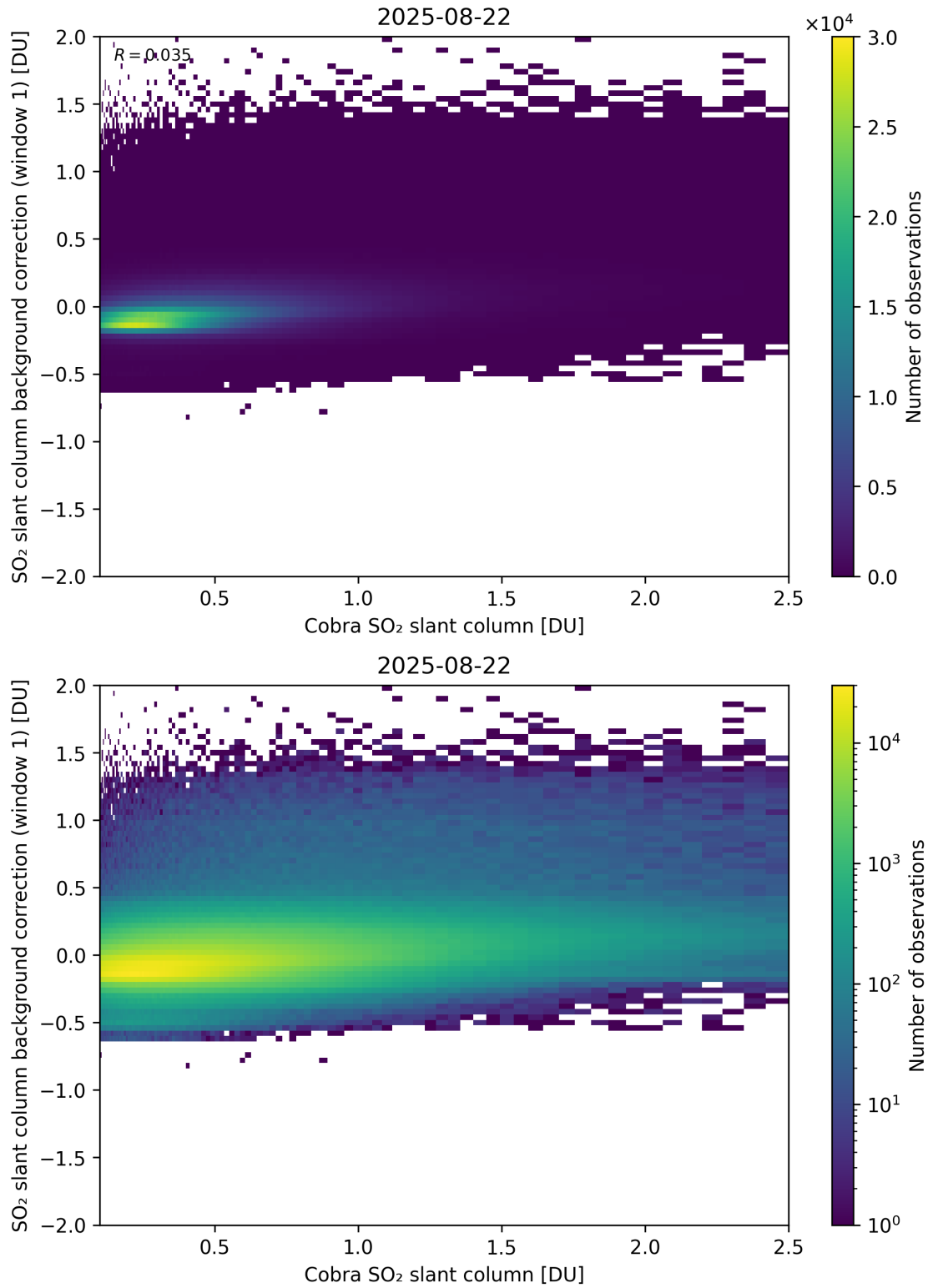
Figure 193: Scatter density plot of “Cobra SO 2 slant column” against “SO 2 slant column background correction (window 1)” for 2025-08-21 to 2025-08-23.
