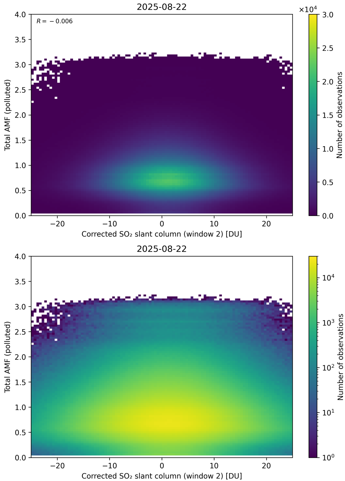
Figure 253: Scatter density plot of “Corrected SO 2 slant column (window 2)” against “Total AMF (polluted)” for 2025-08-21 to 2025-08-23.
