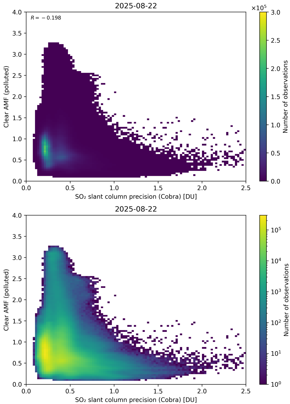
Figure 205: Scatter density plot of “SO 2 slant column precision (Cobra)” against “Clear AMF (polluted)” for 2025-08-21 to 2025-08-23.
