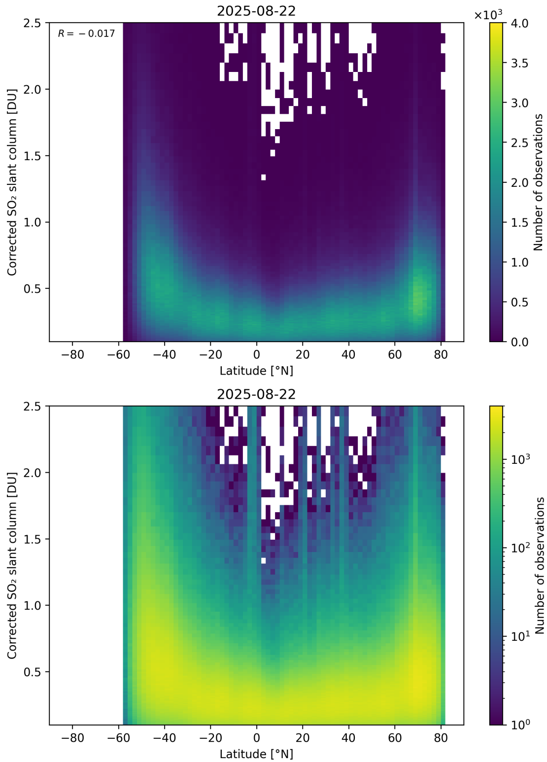
Figure 159: Scatter density plot of “Latitude” against “Corrected SO 2 slant column” for 2025-08-21 to 2025-08-23.
