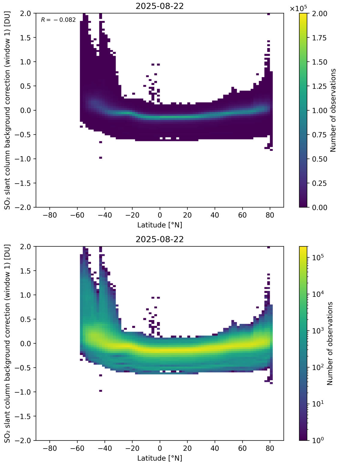
Figure 150: Scatter density plot of “Latitude” against “SO 2 slant column background correction (window 1)” for 2025-08-21 to 2025-08-23.
