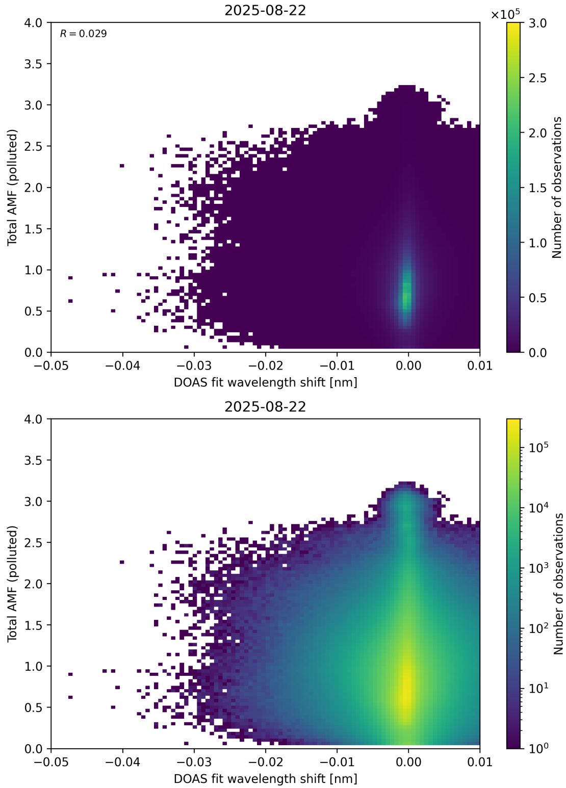
Figure 141: Scatter density plot of “DOAS fit wavelength shift” against “Total AMF (polluted)” for 2025-08-21 to 2025-08-23.
