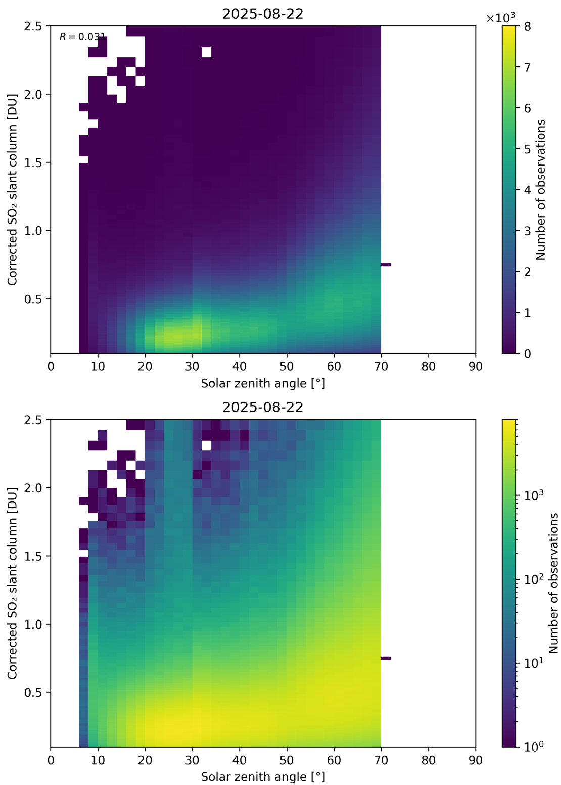
Figure 181: Scatter density plot of “Solar zenith angle” against “Corrected SO 2 slant column” for 2025-08-21 to 2025-08-23.
