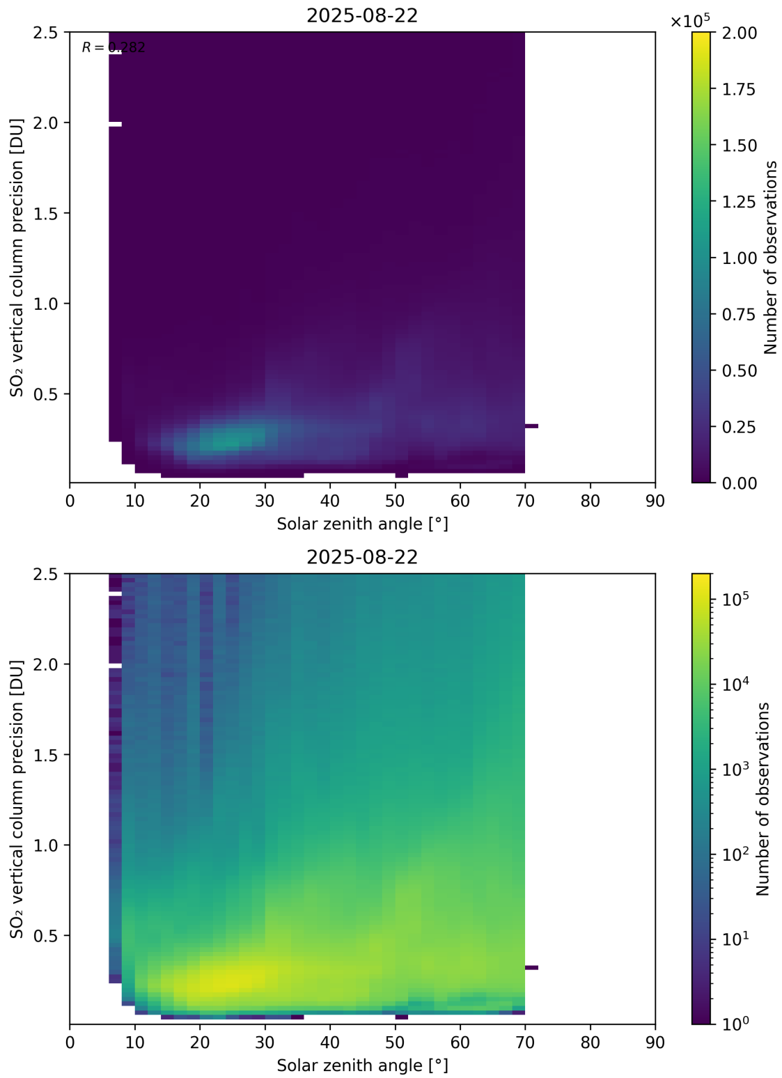
Figure 192: Scatter density plot of “Solar zenith angle” against “SO 2 vertical column precision” for 2025-08-21 to 2025-08-23.
