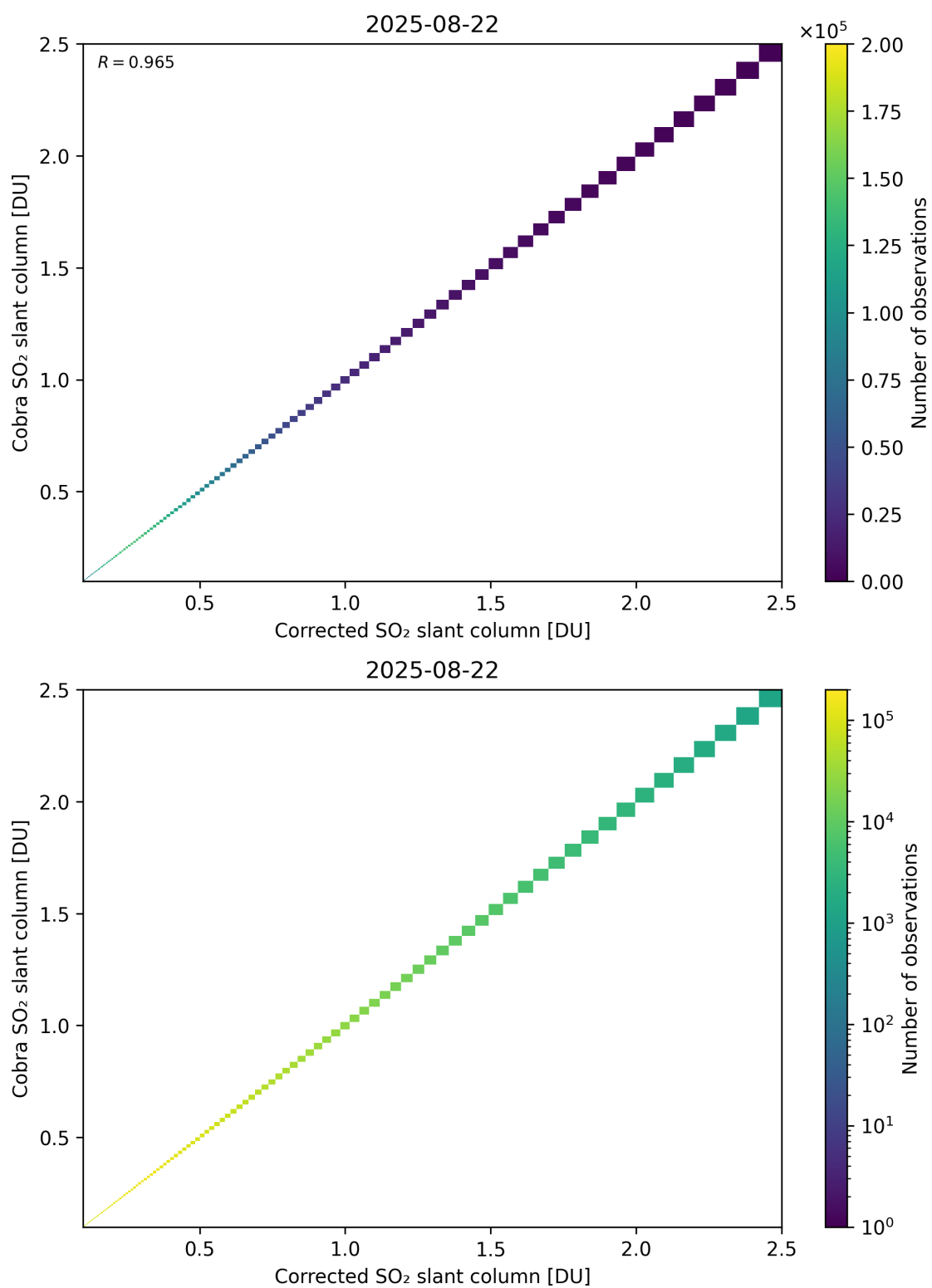
Figure 233: Scatter density plot of “Corrected SO 2 slant column” against “Cobra SO 2 slant column” for 2025-08-21 to 2025-08-23.
