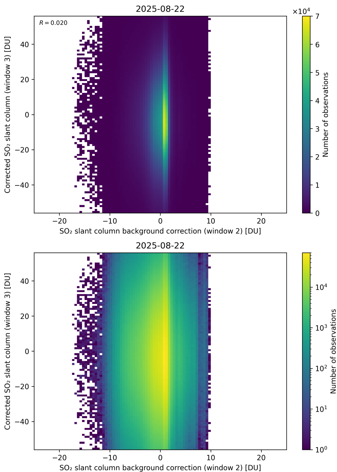
Figure 127: Scatter density plot of “SO 2 slant column background correction (window 2)” against “Corrected SO 2 slant column (window 3)” for 2025-08-21 to 2025-08-23.
