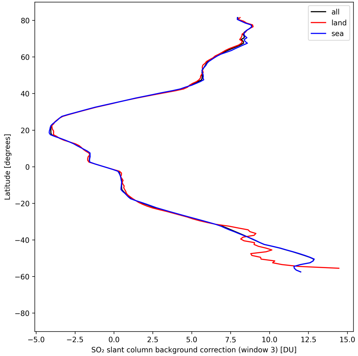
Figure 48: Zonal average of “SO 2 slant column background correction (window 3)” for 2025-08-21 to 2025-08-23.
