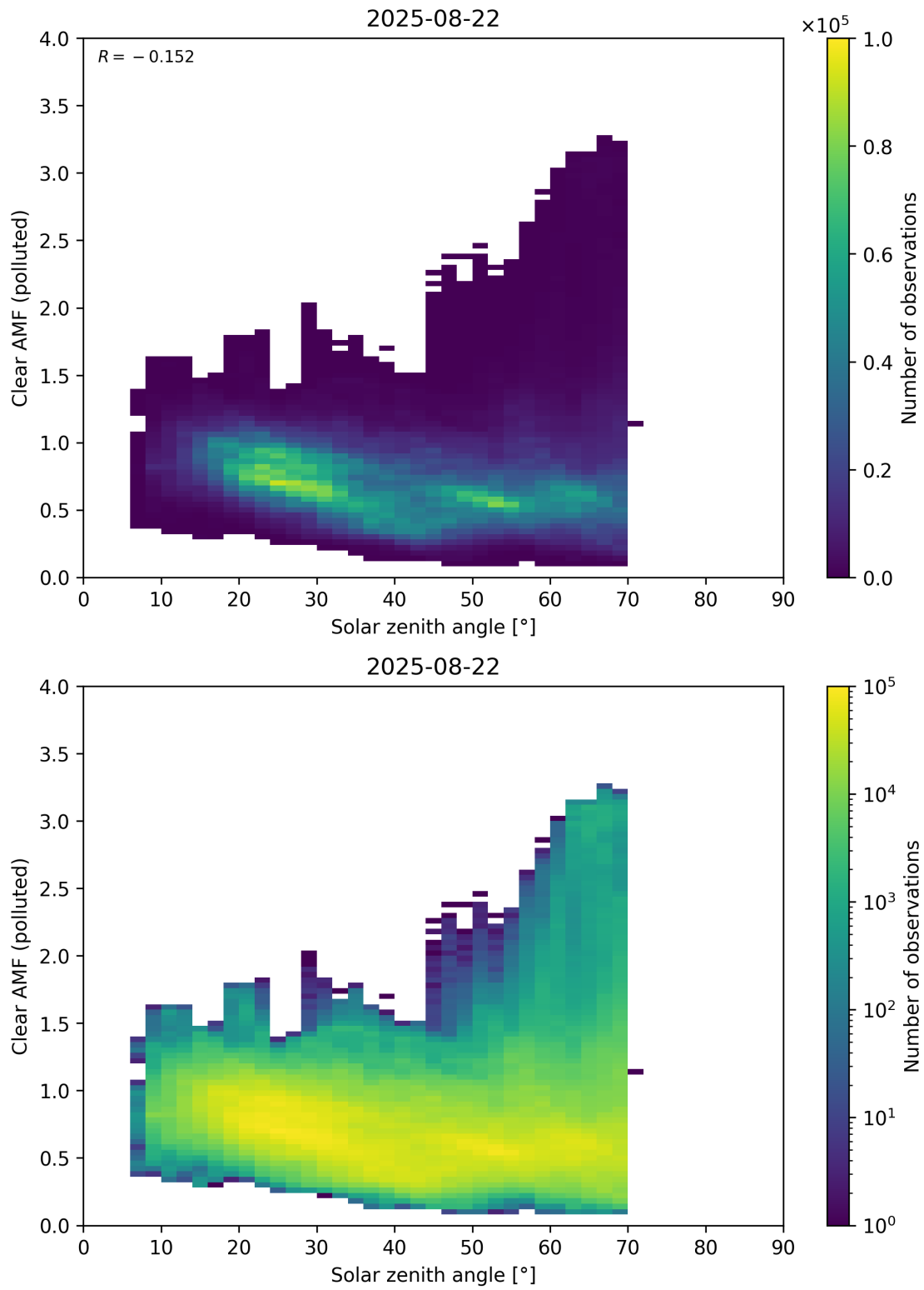
Figure 178: Scatter density plot of “Solar zenith angle” against “Clear AMF (polluted)” for 2025-08-21 to 2025-08-23.
