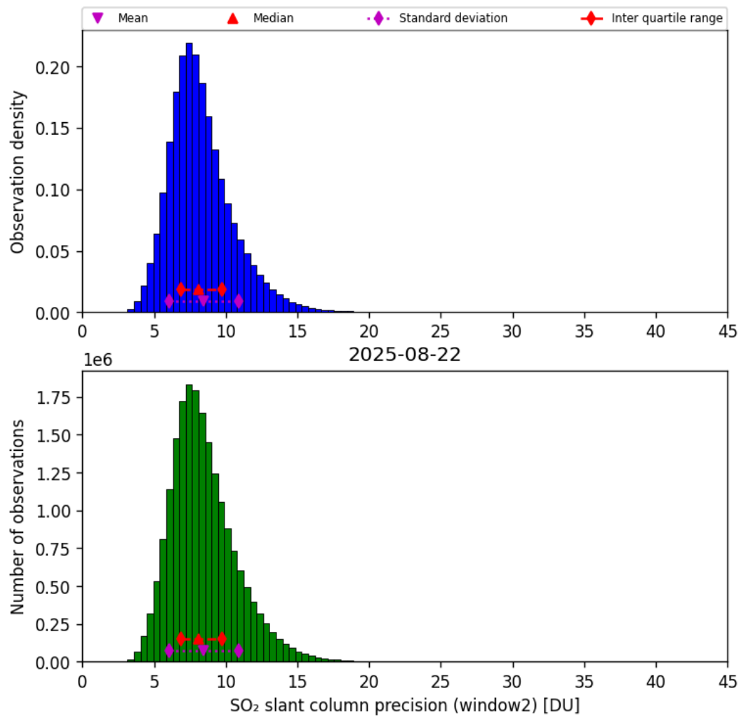
Figure 68: Histogram of “SO 2 slant column precision (window2)” for 2025-08-21 to 2025-08-23
