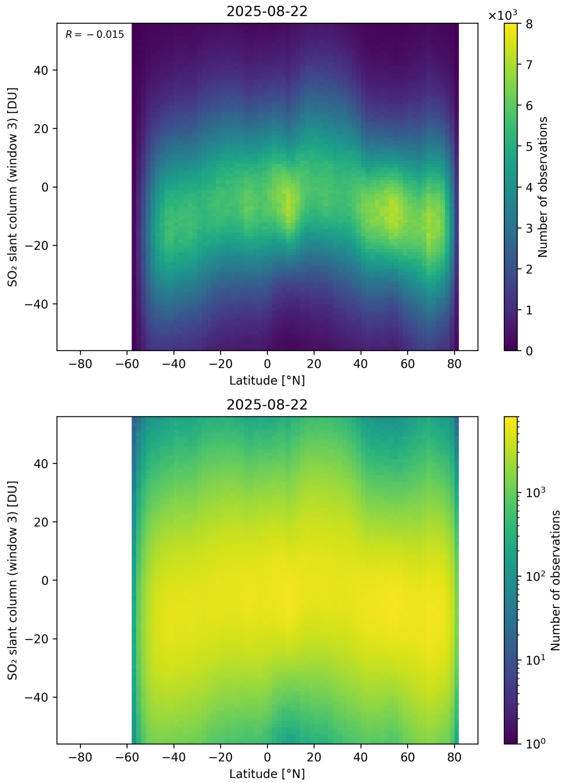
Figure 165: Scatter density plot of “Latitude” against “SO 2 slant column (window 3)” for 2025-08-21 to 2025-08-23.
