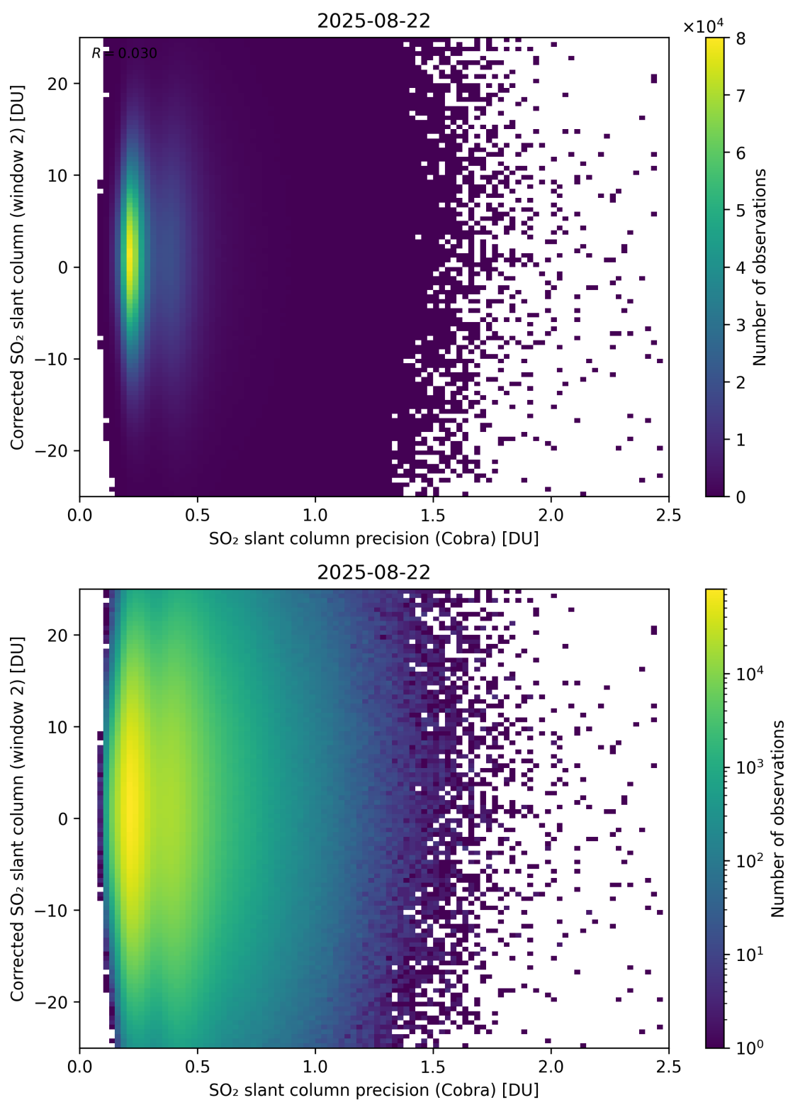
Figure 206: Scatter density plot of “SO 2 slant column precision (Cobra)” against “Corrected SO 2 slant column (window 2)” for 2025-08-21 to 2025-08-23.
