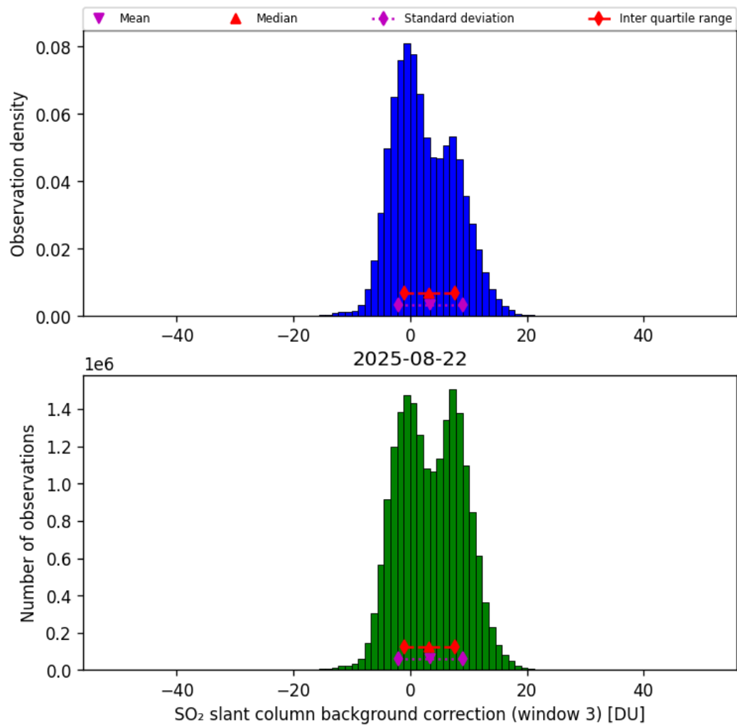
Figure 74: Histogram of “SO 2 slant column background correction (window 3)” for 2025-08-21 to 2025-08-23
