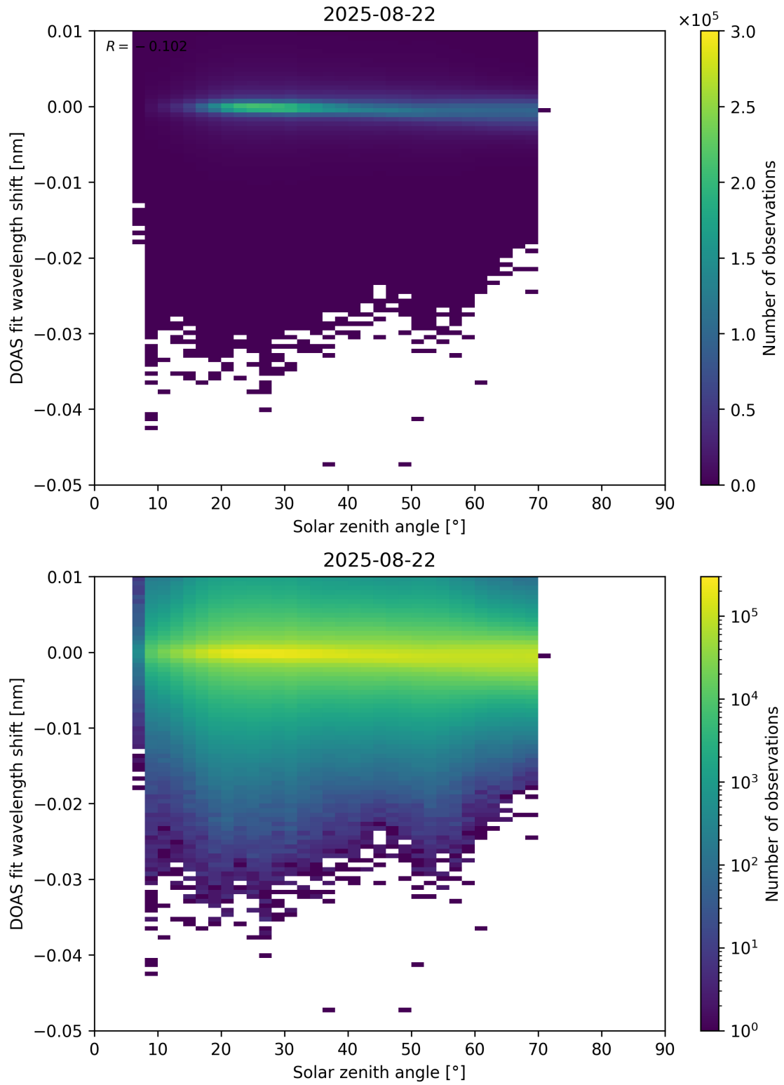
Figure 174: Scatter density plot of “Solar zenith angle” against “DOAS fit wavelength shift” for 2025-08-21 to 2025-08-23.
