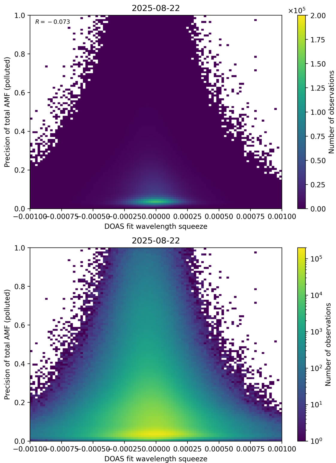
Figure 146: Scatter density plot of “DOAS fit wavelength squeeze” against “Precision of total AMF (polluted)” for 2025-08-21 to 2025-08-23.
