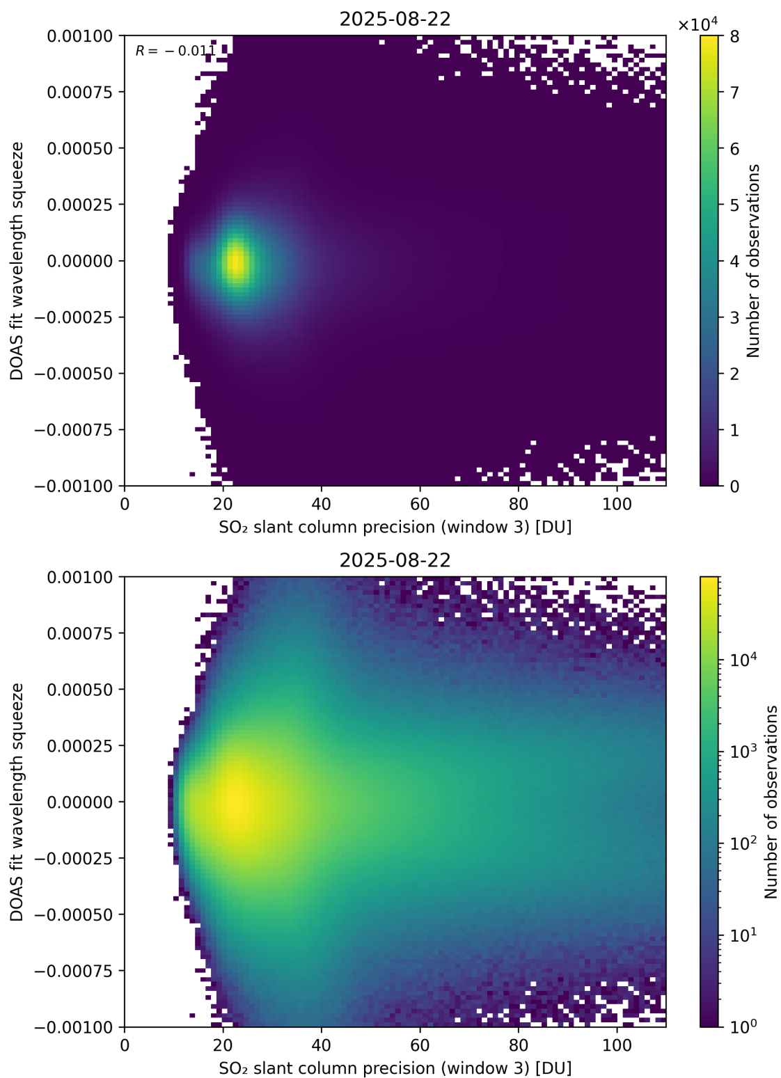
Figure 309: Scatter density plot of “SO 2 slant column precision (window 3)” against “DOAS fit wavelength squeeze” for 2025-08-21 to 2025-08-23.
