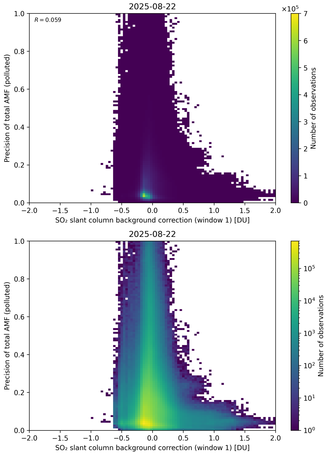
Figure 121: Scatter density plot of “SO 2 slant column background correction (window 1)” against “Precision of total AMF (polluted)” for 2025-08-21 to 2025-08-23.
