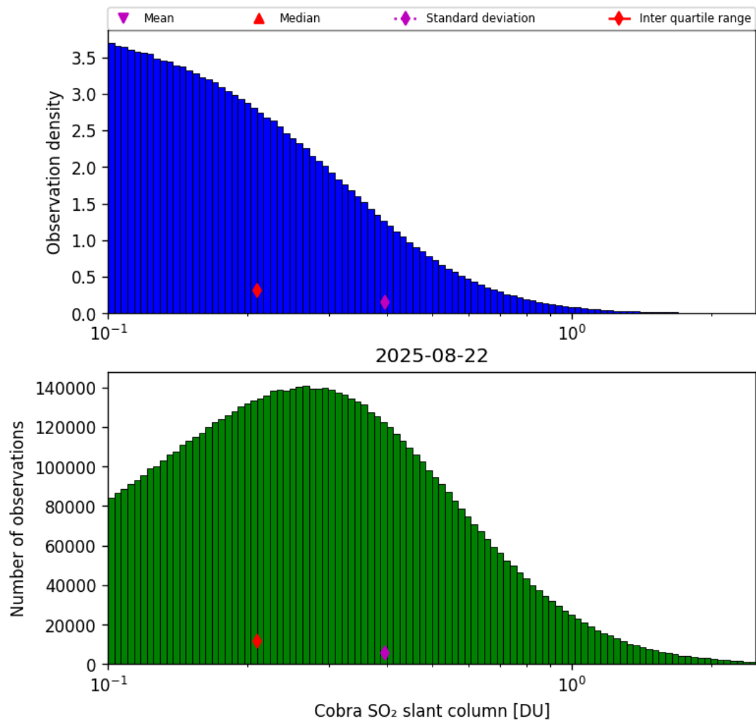
Figure 61: Histogram of “Cobra SO 2 slant column” for 2025-08-21 to 2025-08-23
