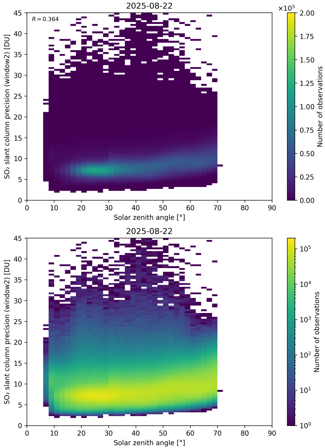
Figure 186: Scatter density plot of “Solar zenith angle” against “SO 2 slant column precision (window2)” for 2025-08-21 to 2025-08-23.
