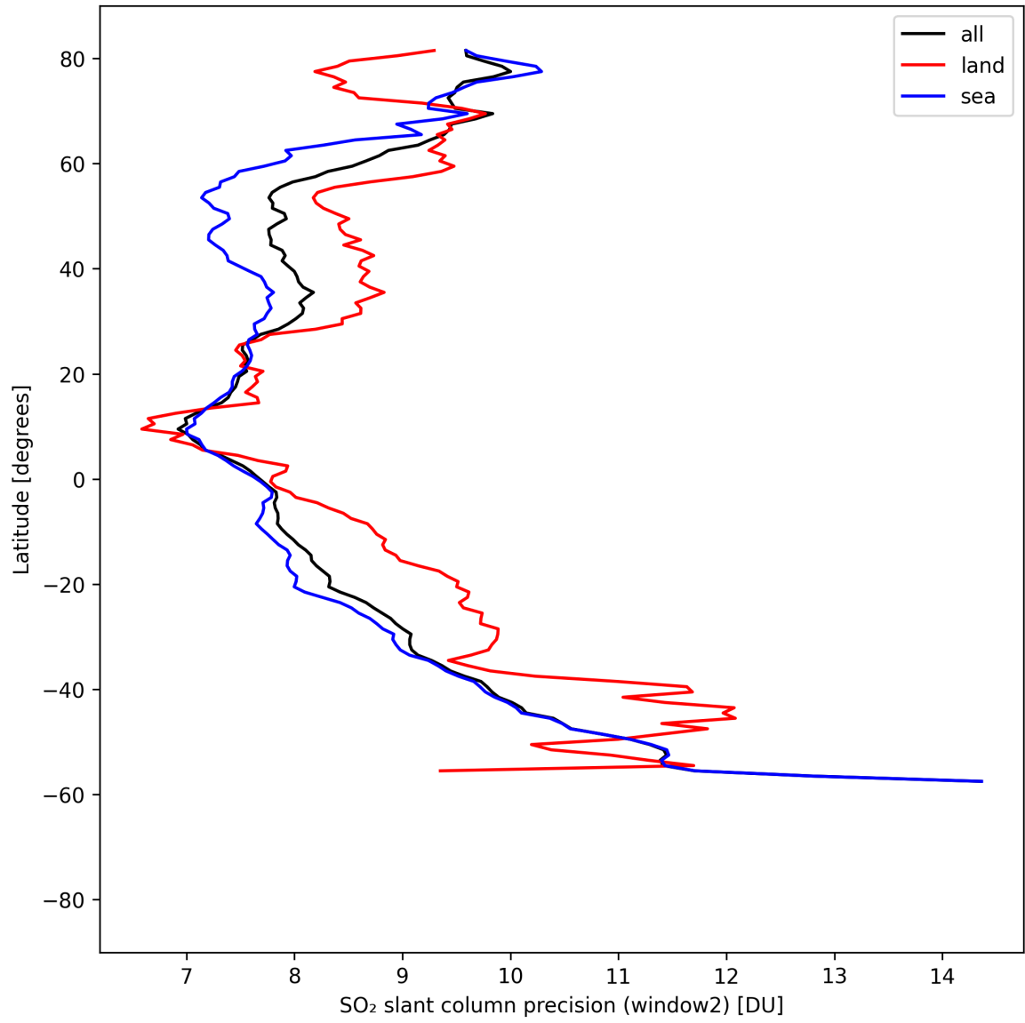
Figure 42: Zonal average of “SO 2 slant column precision (window2)” for 2025-08-21 to 2025-08-23.
