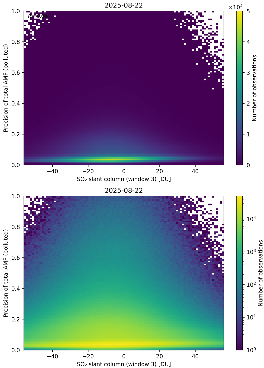
Figure 319: Scatter density plot of “SO 2 slant column (window 3)” against “Precision of total AMF (polluted)” for 2025-08-21 to 2025-08-23.
