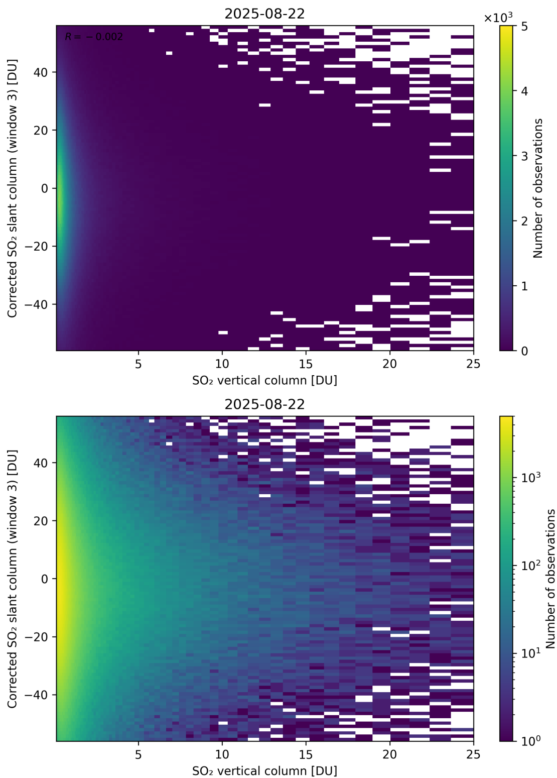
Figure 353: Scatter density plot of “SO 2 vertical column” against “Corrected SO 2 slant column (window 3)” for 2025-08-21 to 2025-08-23.
