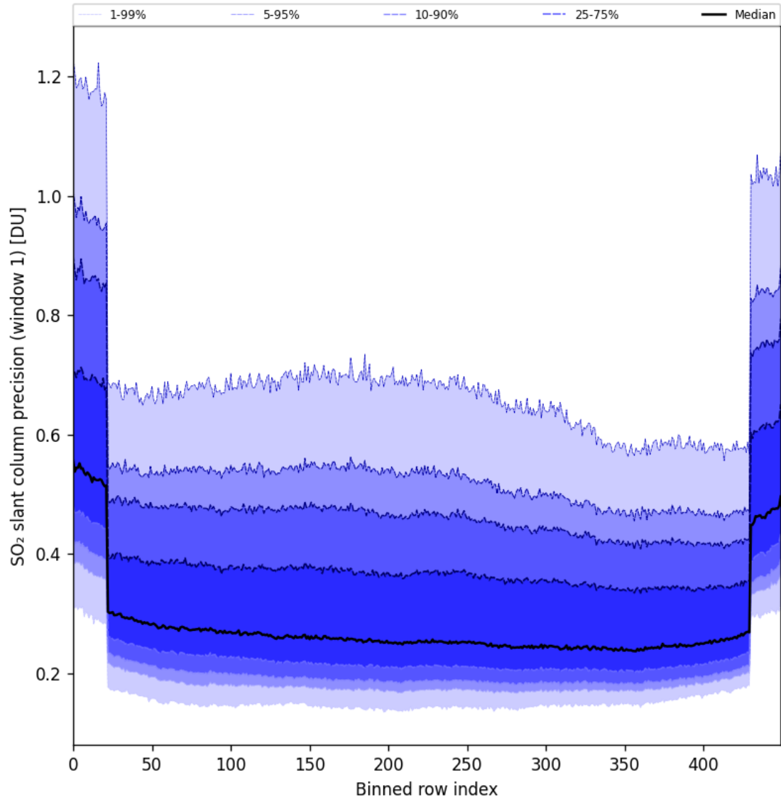
Figure 90: Along track statistics of “SO 2 slant column precision (window 1)” for 2025-08-21 to 2025-08-23
