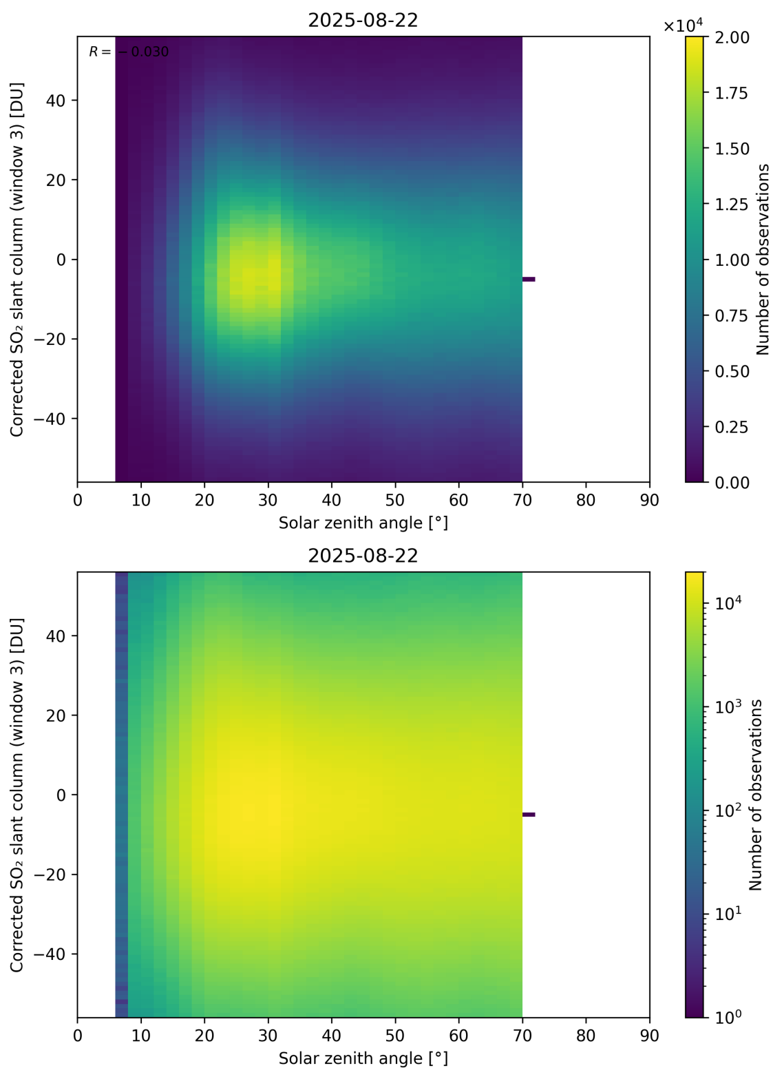
Figure 183: Scatter density plot of “Solar zenith angle” against “Corrected SO 2 slant column (window 3)” for 2025-08-21 to 2025-08-23.
