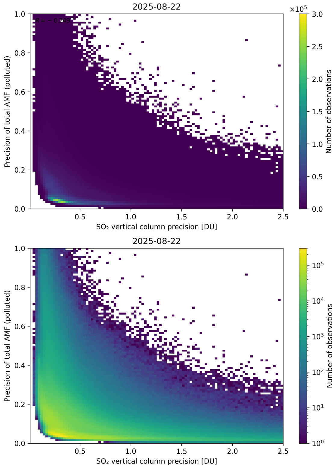
Figure 347: Scatter density plot of “SO 2 vertical column precision” against “Precision of total AMF (polluted)” for 2025-08-21 to 2025-08-23.
