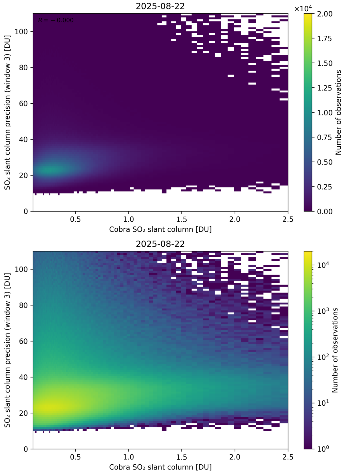
Figure 223: Scatter density plot of “Cobra SO 2 slant column” against “SO 2 slant column precision (window 3)” for 2025-08-21 to 2025-08-23.
