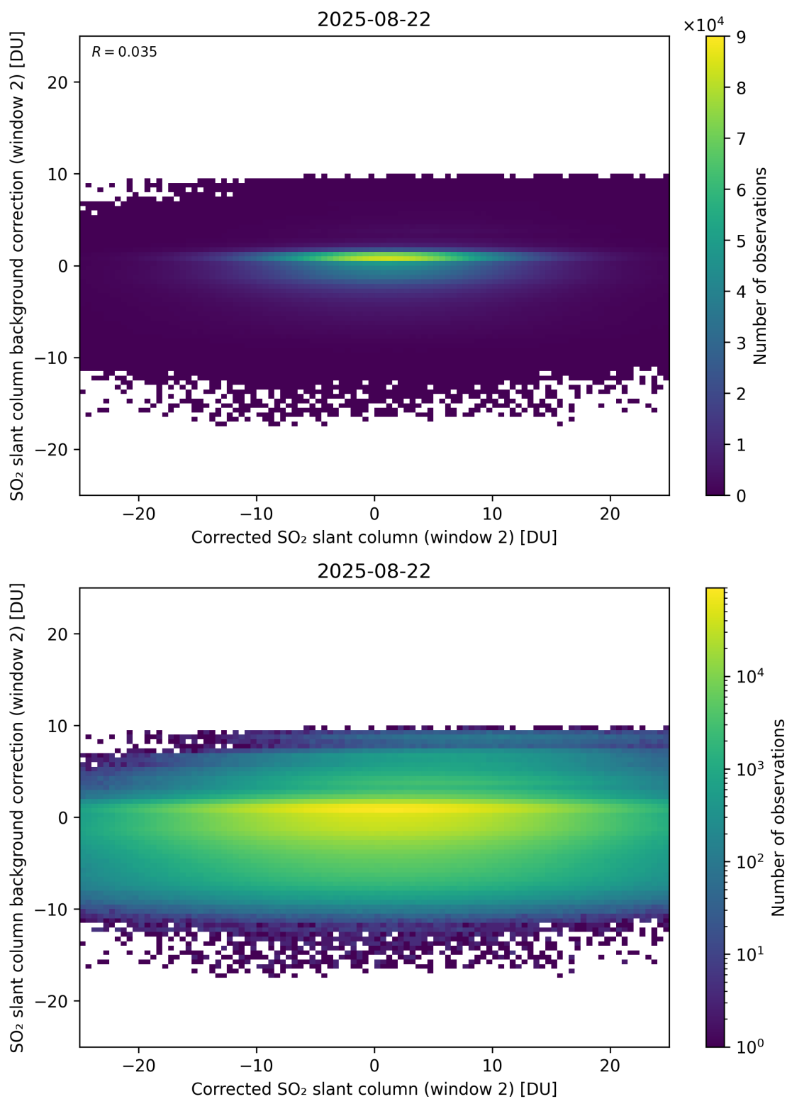
Figure 244: Scatter density plot of “Corrected SO 2 slant column (window 2)” against “SO 2 slant column background correction (window 2)” for 2025-08-21 to 2025-08-23.
