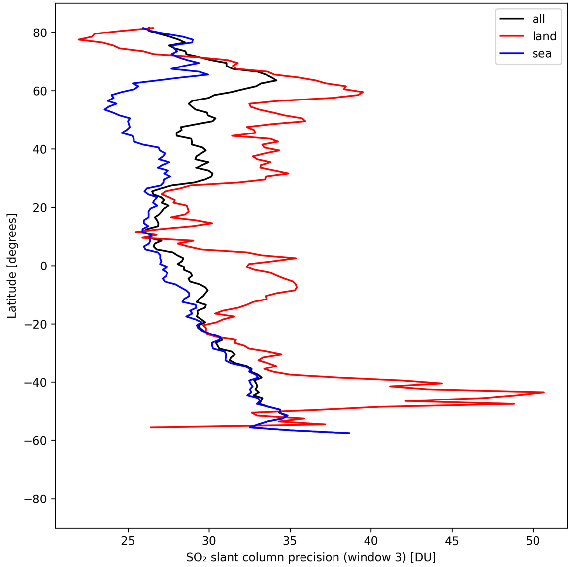
Figure 46: Zonal average of “SO 2 slant column precision (window 3)” for 2025-08-21 to 2025-08-23.
