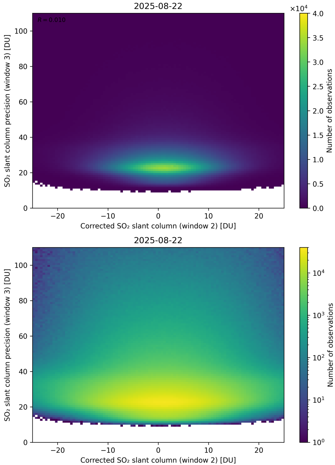
Figure 252: Scatter density plot of “Corrected SO 2 slant column (window 2)” against “SO 2 slant column precision (window 3)” for 2025-08-21 to 2025-08-23.
