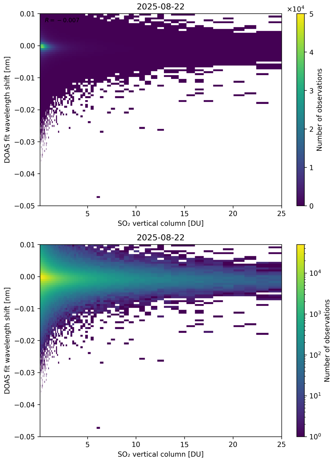
Figure 326: Scatter density plot of “SO 2 vertical column” against “DOAS fit wavelength shift” for 2025-08-21 to 2025-08-23.
