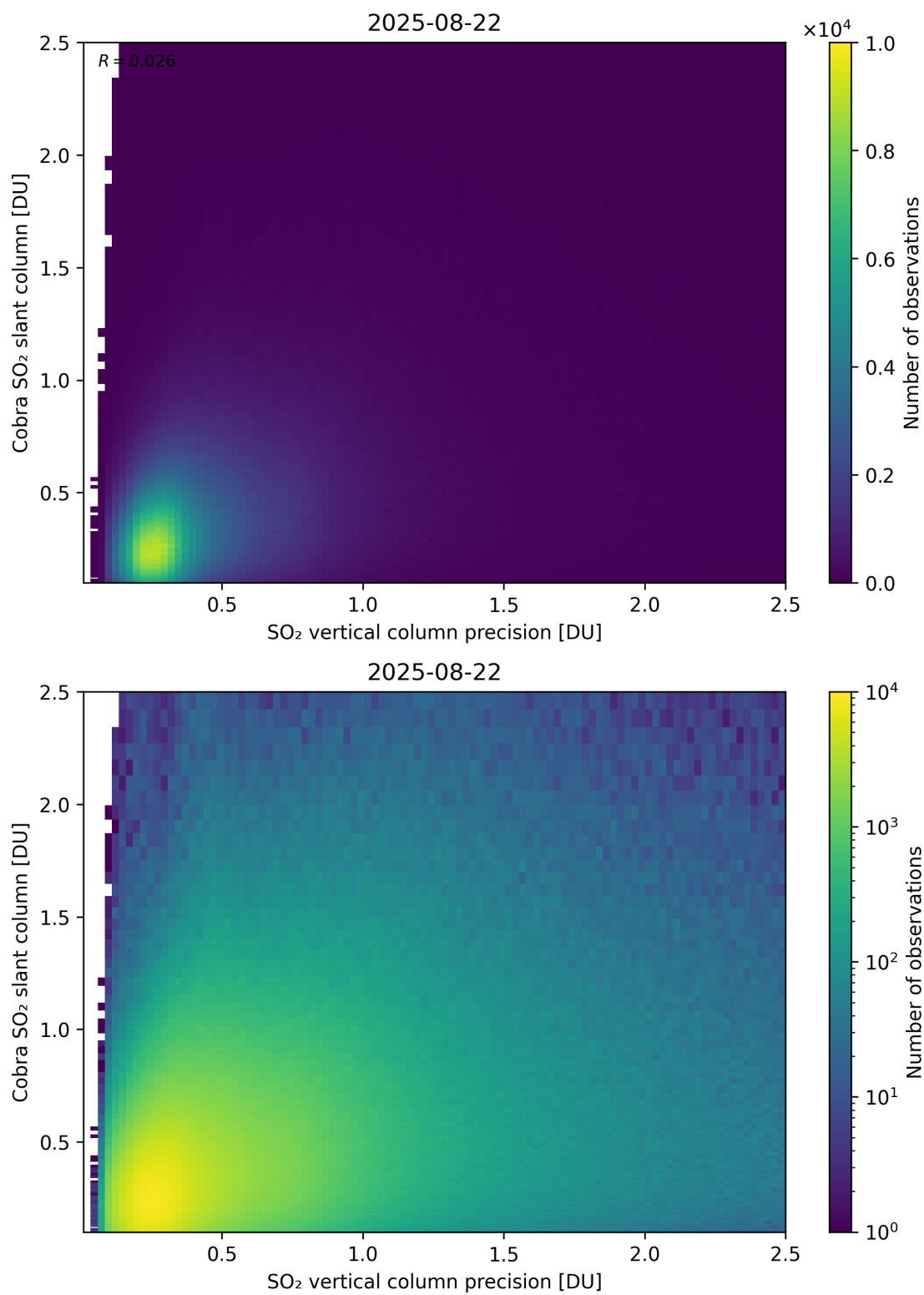
Figure 336: Scatter density plot of “SO 2 vertical column precision” against “Cobra SO 2 slant column” for 2025-08-21 to 2025-08-23.
