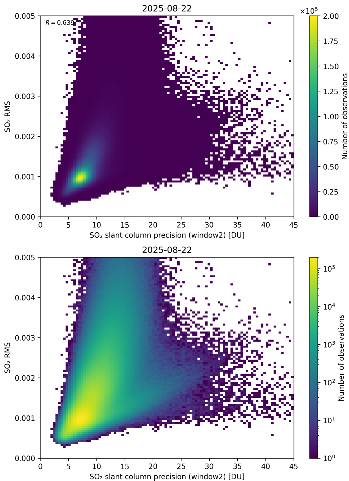
Figure 295: Scatter density plot of “SO 2 slant column precision (window2)” against “SO 2 RMS” for 2025-08-21 to 2025-08-23.
