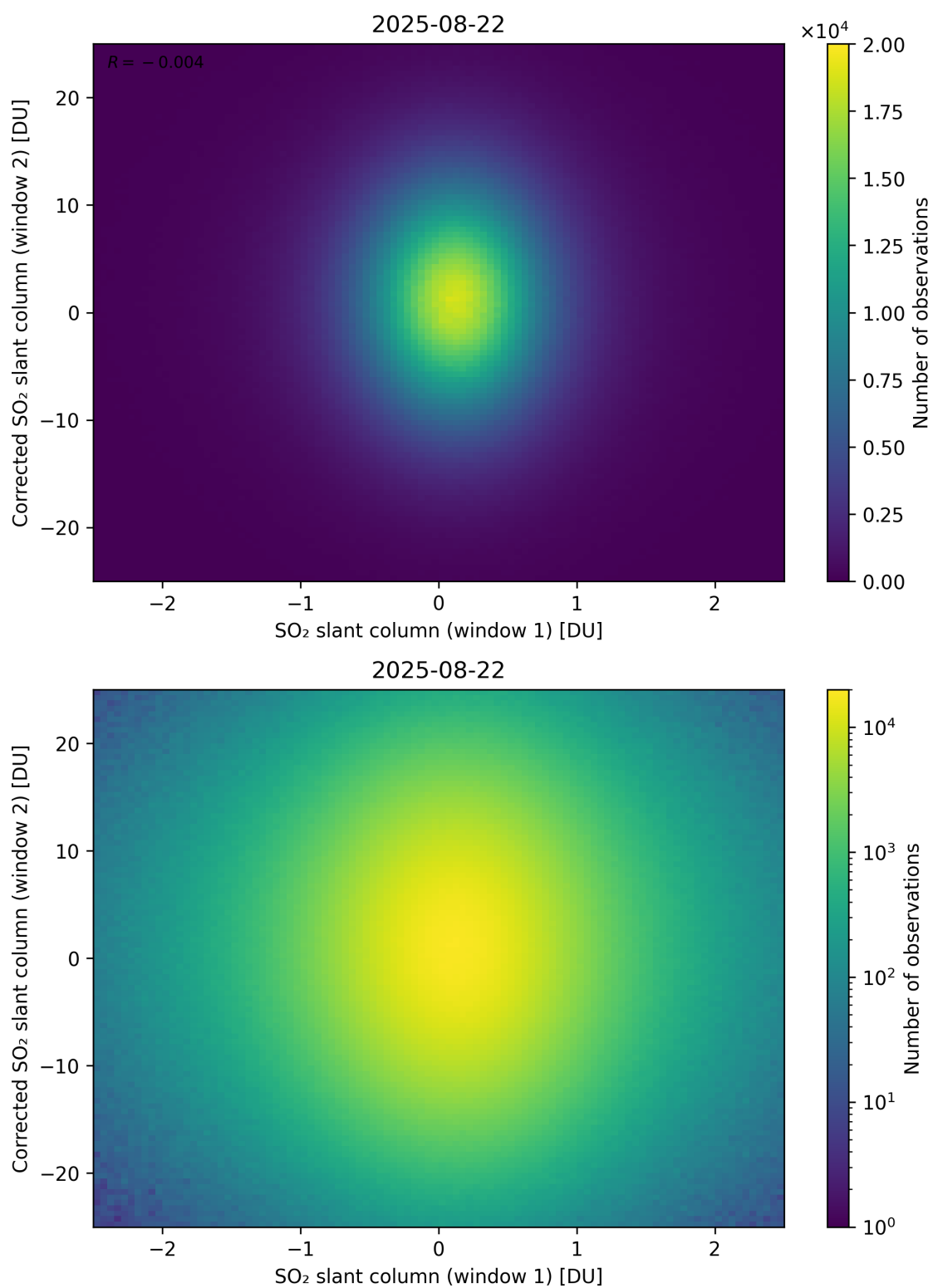
Figure 283: Scatter density plot of “SO 2 slant column (window 1)” against “Corrected SO 2 slant column (window 2)” for 2025-08-21 to 2025-08-23.
