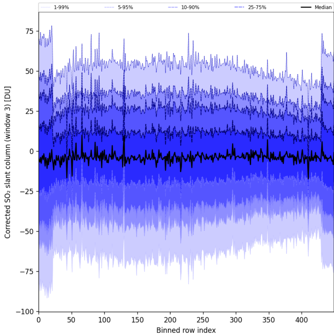
Figure 99: Along track statistics of “Corrected SO 2 slant column (window 3)” for 2025-08-21 to 2025-08-23
