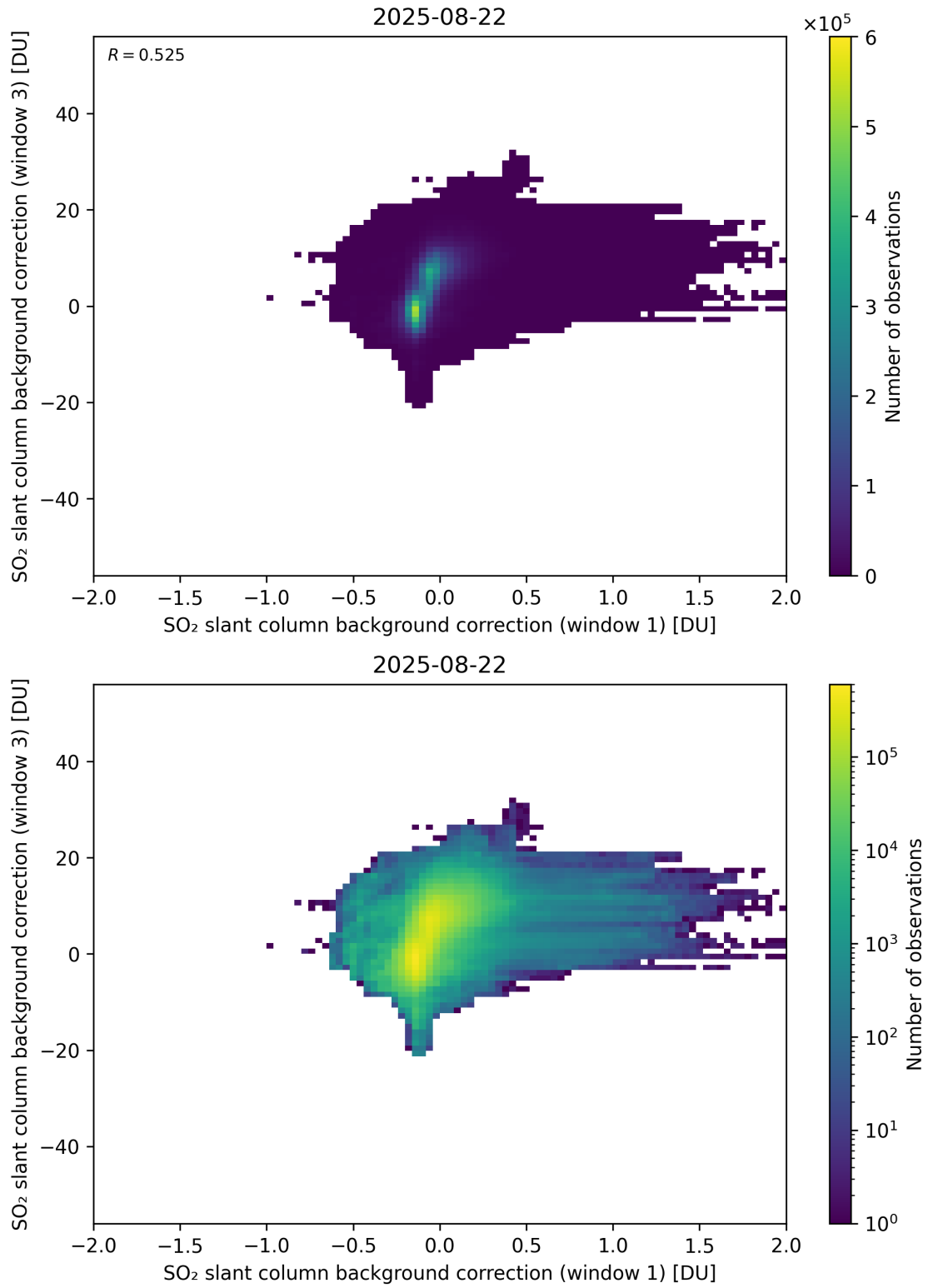
Figure 110: Scatter density plot of “SO 2 slant column background correction (window 1)” against “SO 2 slant column background correction (window 3)” for 2025-08-21 to 2025-08-23.
