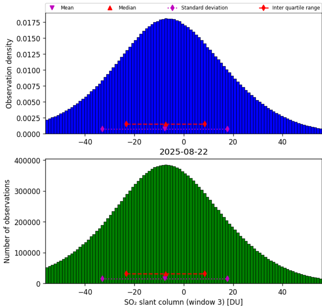
Figure 71: Histogram of “SO 2 slant column (window 3)” for 2025-08-21 to 2025-08-23
