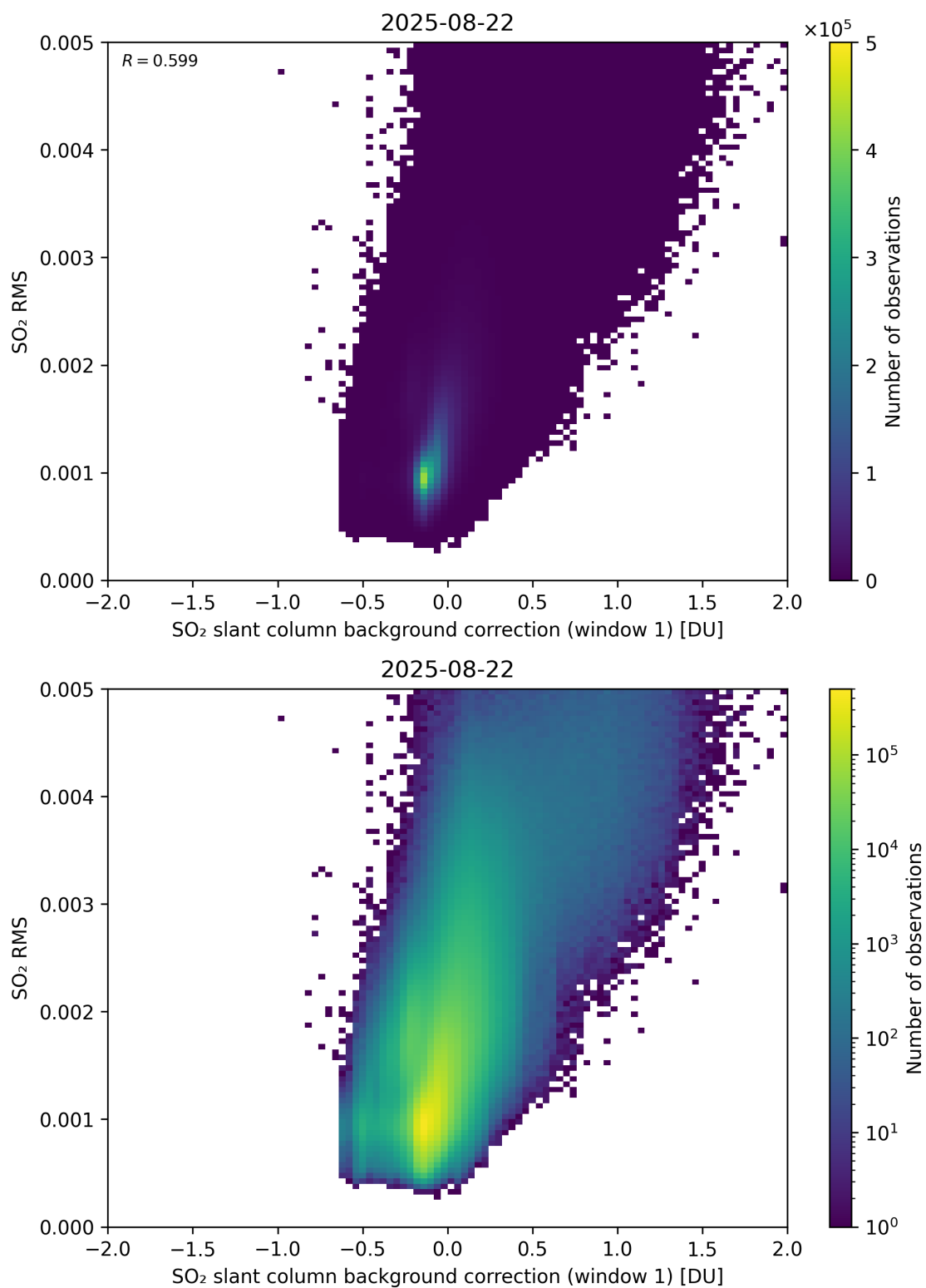
Figure 113: Scatter density plot of “SO 2 slant column background correction (window 1)” against “SO 2 RMS” for 2025-08-21 to 2025-08-23.
