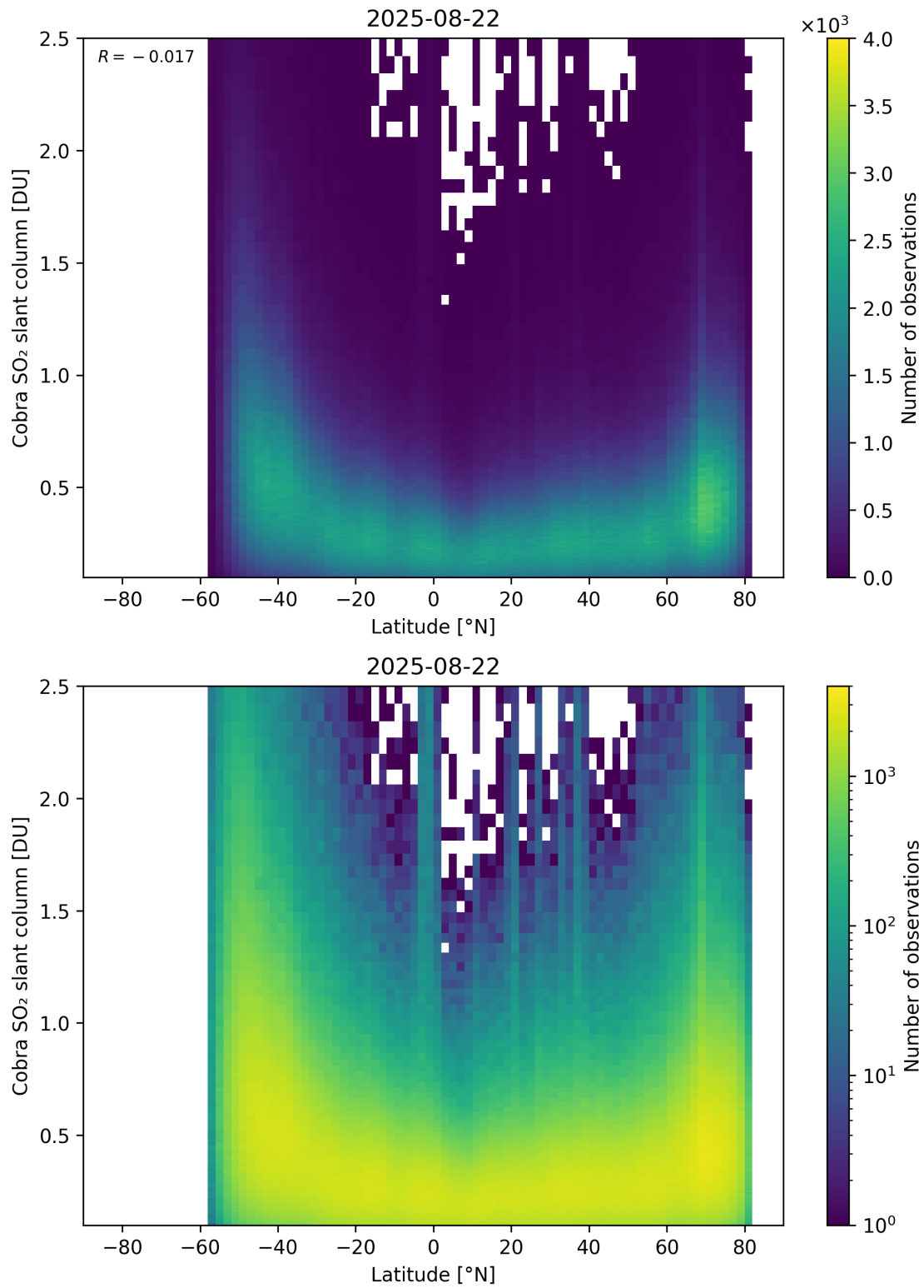
Figure 157: Scatter density plot of “Latitude” against “Cobra SO 2 slant column” for 2025-08-21 to 2025-08-23.
