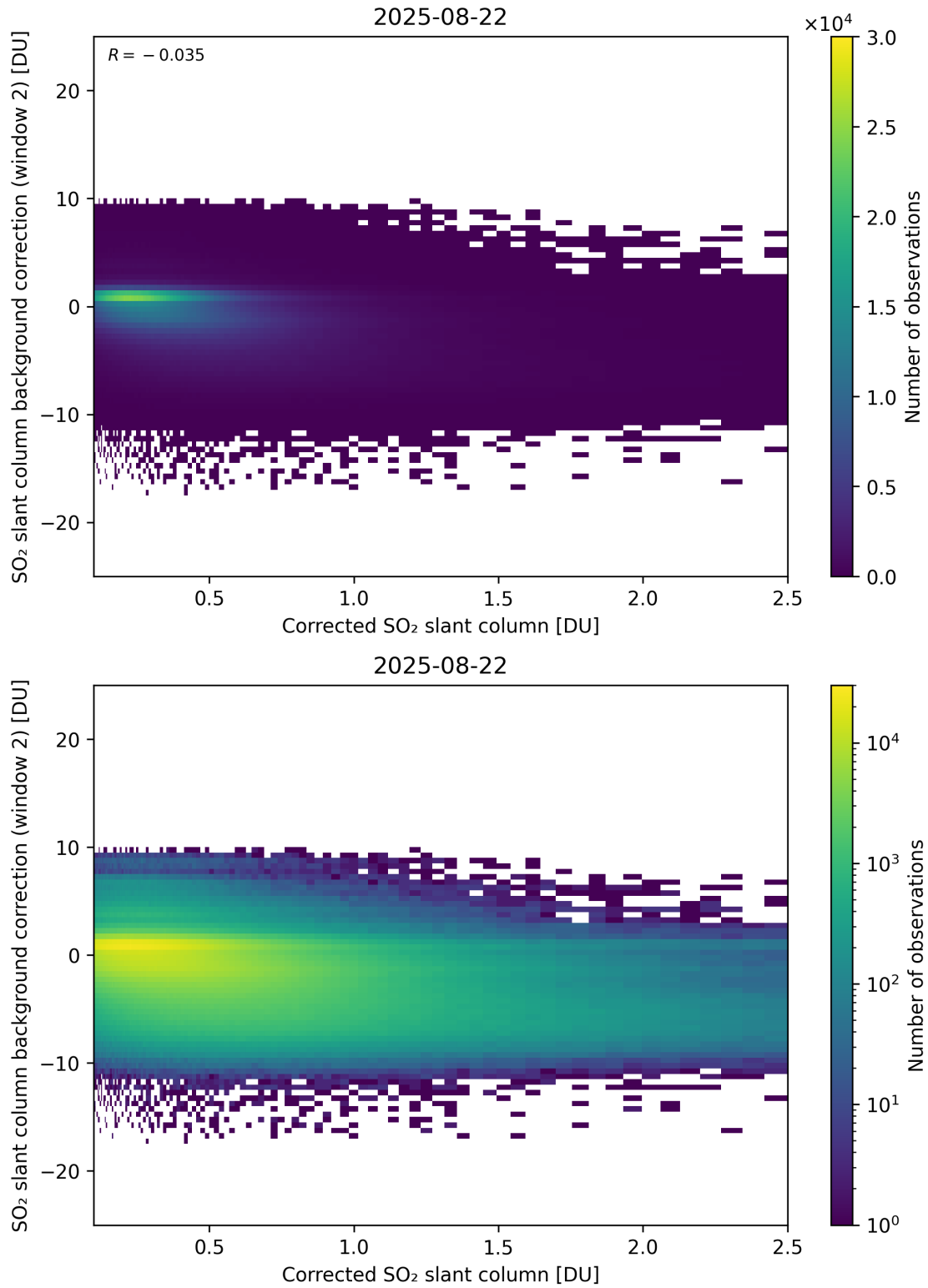
Figure 227: Scatter density plot of “Corrected SO 2 slant column” against “SO 2 slant column background correction (window 2)” for 2025-08-21 to 2025-08-23.
