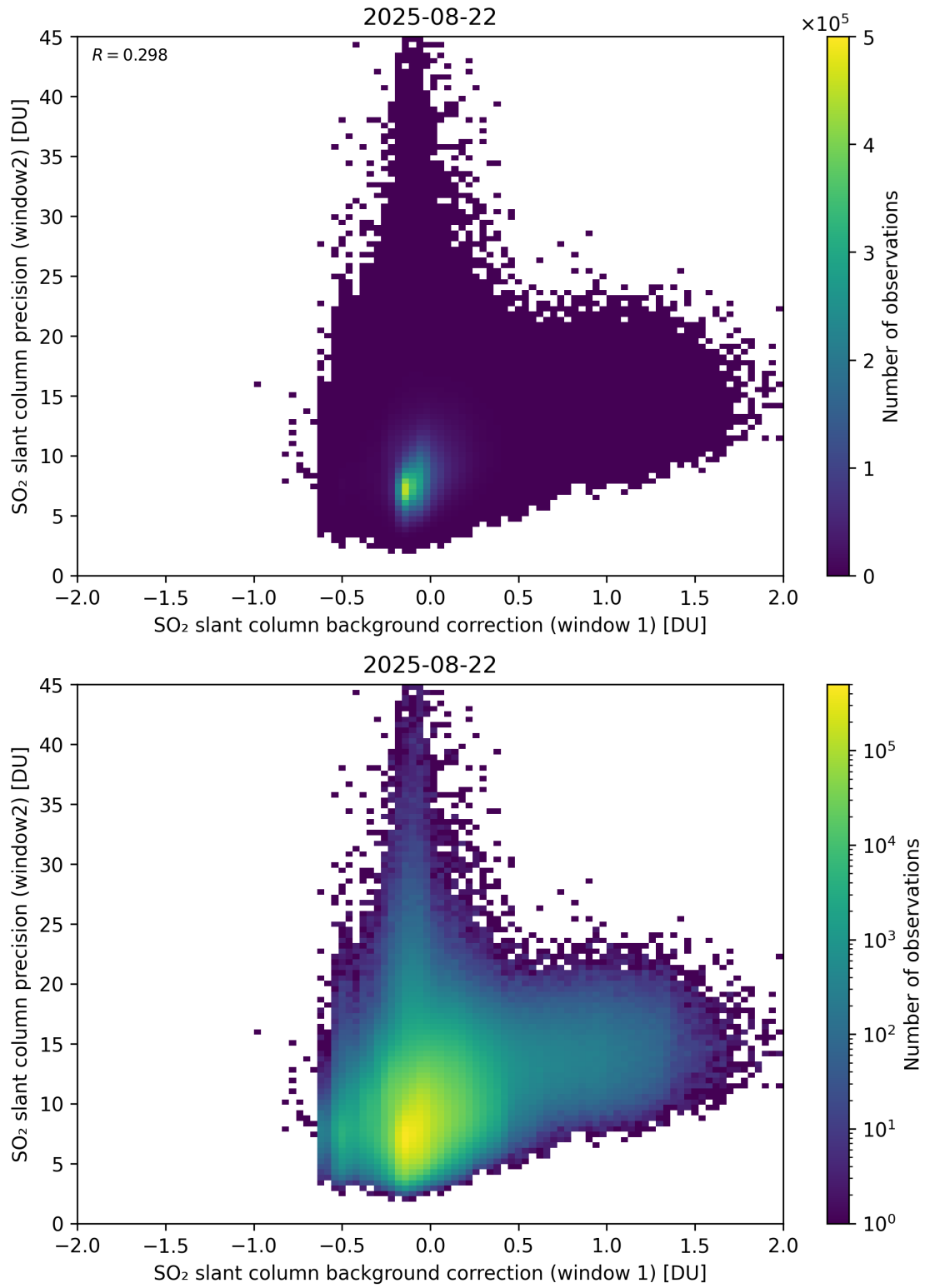
Figure 117: Scatter density plot of “SO 2 slant column background correction (window 1)” against “SO 2 slant column precision (window2)” for 2025-08-21 to 2025-08-23.
