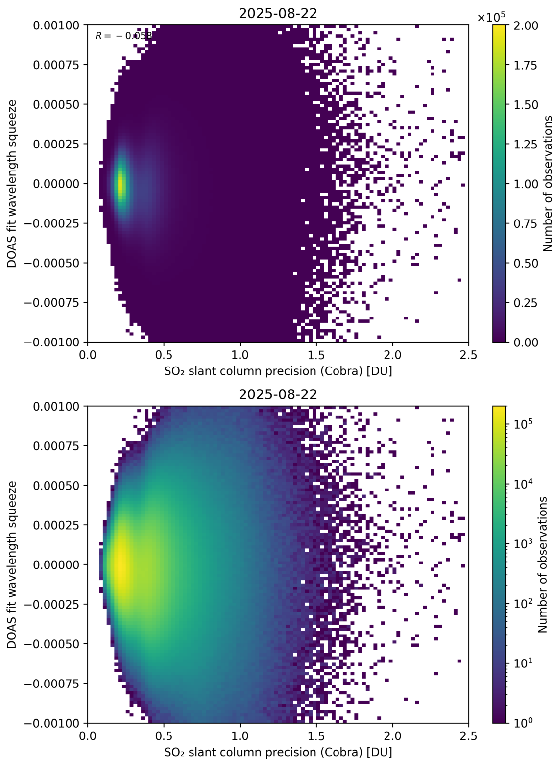
Figure 203: Scatter density plot of “SO 2 slant column precision (Cobra)” against “DOAS fit wavelength squeeze” for 2025-08-21 to 2025-08-23.
