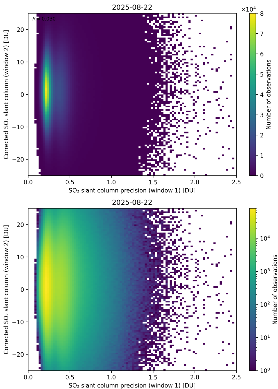
Figure 275: Scatter density plot of “SO 2 slant column precision (window 1)” against “Corrected SO 2 slant column (window 2)” for 2025-08-21 to 2025-08-23.
