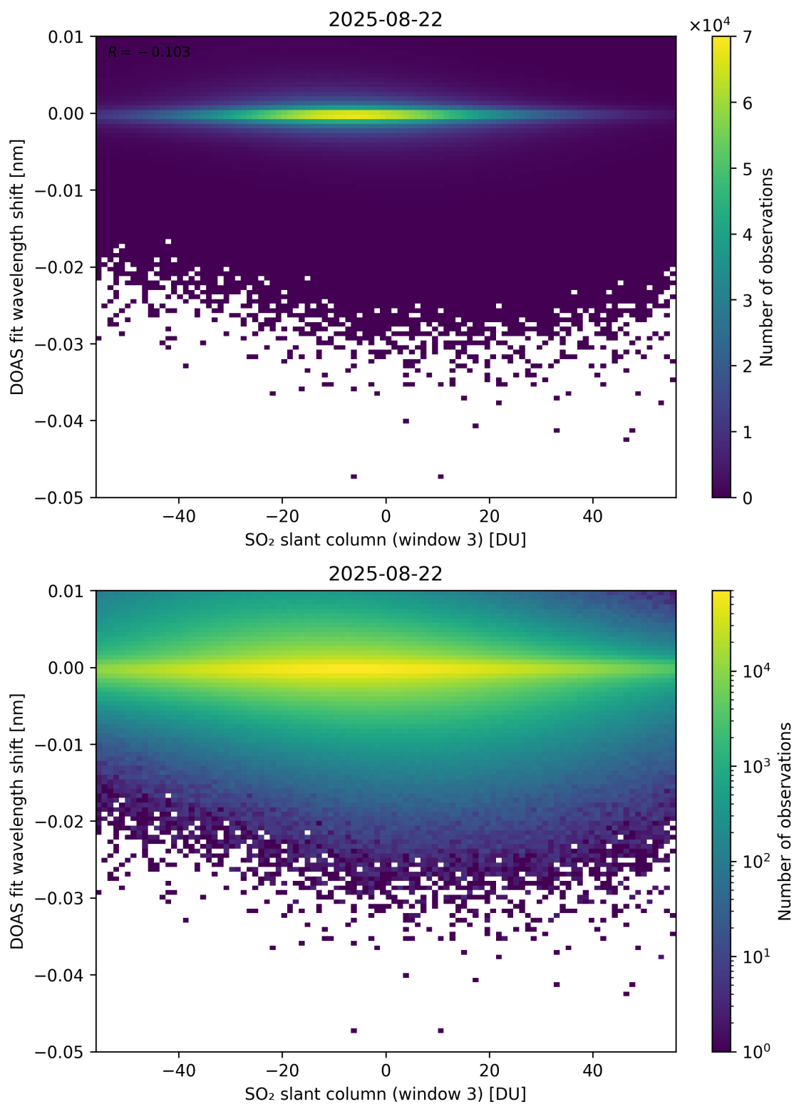
Figure 304: Scatter density plot of “SO 2 slant column (window 3)” against “DOAS fit wavelength shift” for 2025-08-21 to 2025-08-23.
