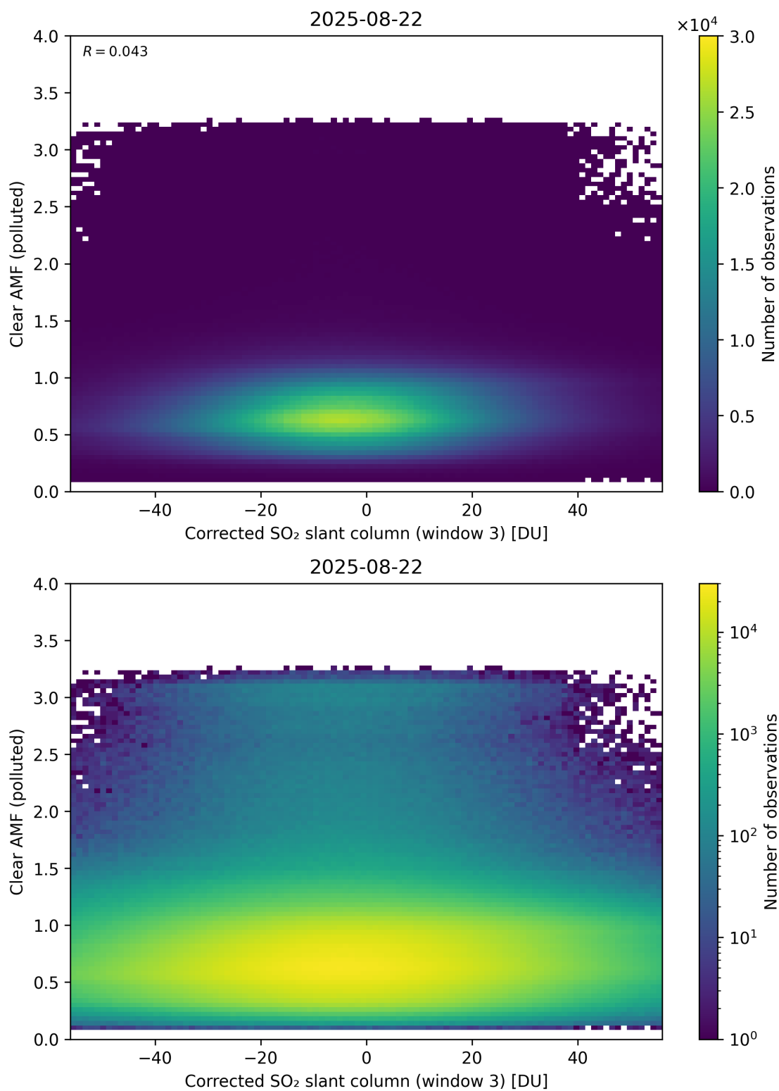
Figure 259: Scatter density plot of “Corrected SO 2 slant column (window 3)” against “Clear AMF (polluted)” for 2025-08-21 to 2025-08-23.
