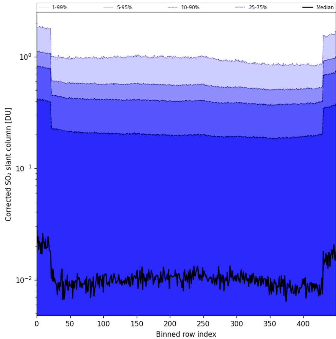
Figure 86: Along track statistics of “Corrected SO 2 slant column” for 2025-08-21 to 2025-08-23
