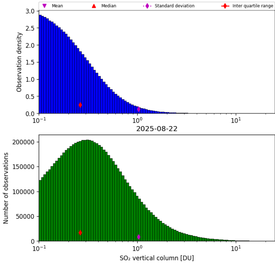
Figure 58: Histogram of “SO 2 vertical column” for 2025-08-21 to 2025-08-23
