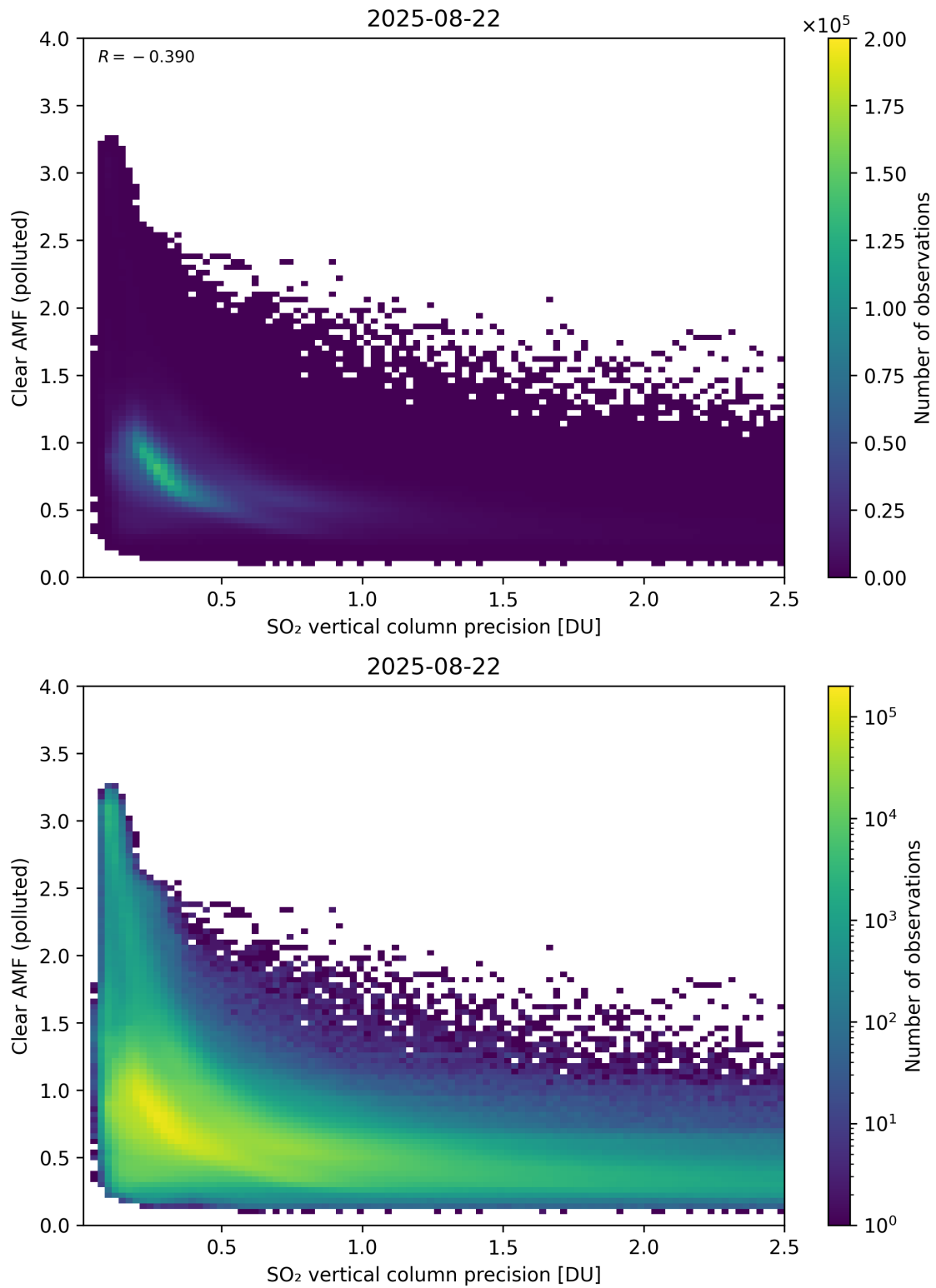
Figure 335: Scatter density plot of “SO 2 vertical column precision” against “Clear AMF (polluted)” for 2025-08-21 to 2025-08-23.
