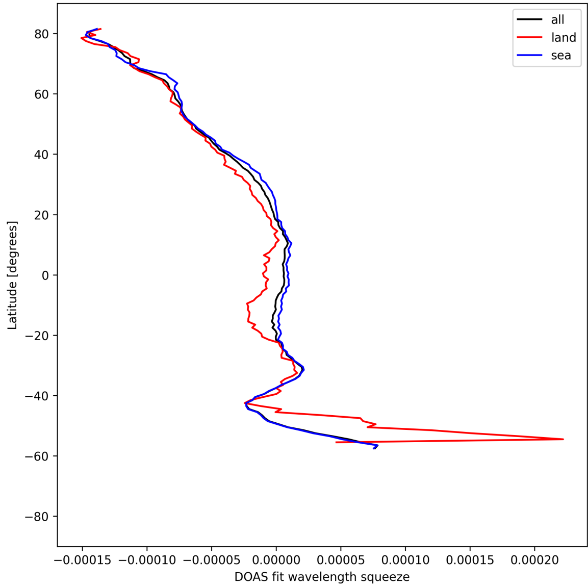
Figure 51: Zonal average of “DOAS fit wavelength squeeze” for 2025-08-21 to 2025-08-23.
