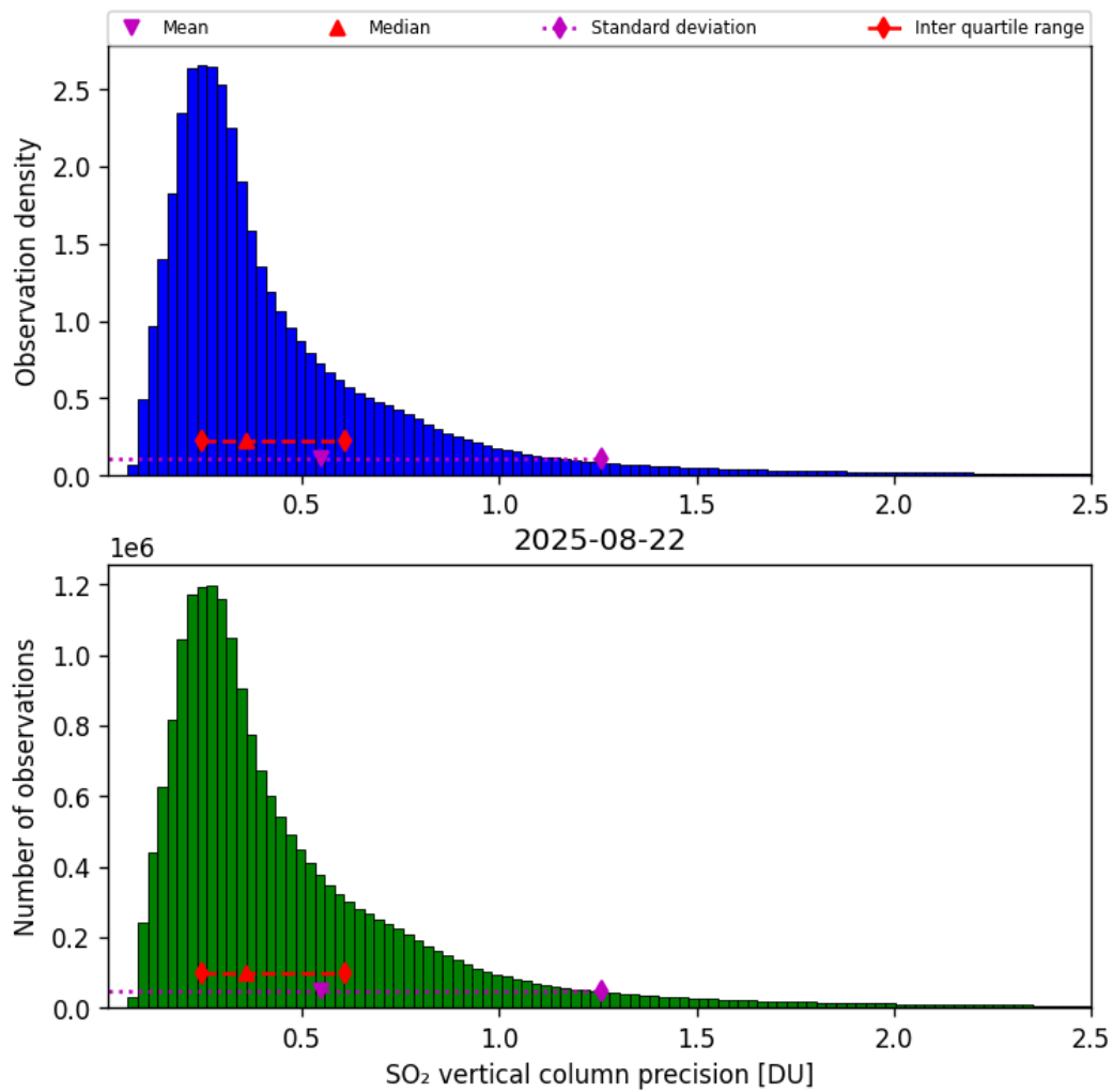
Figure 59: Histogram of “SO 2 vertical column precision” for 2025-08-21 to 2025-08-23
