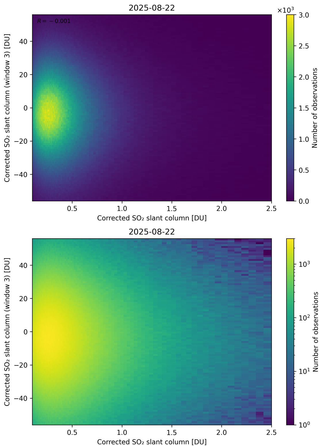
Figure 236: Scatter density plot of “Corrected SO 2 slant column” against “Corrected SO 2 slant column (window 3)” for 2025-08-21 to 2025-08-23.
