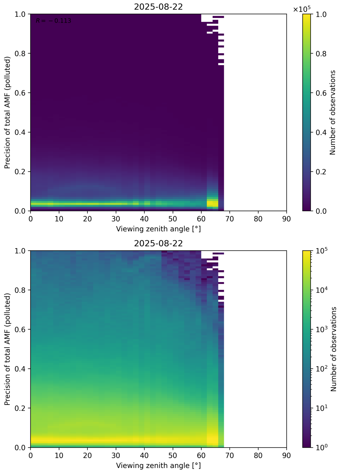
Figure 382: Scatter density plot of “Viewing zenith angle” against “Precision of total AMF (polluted)” for 2025-08-21 to 2025-08-23.
