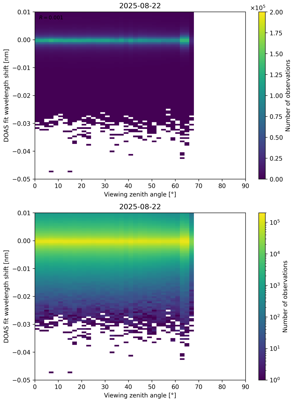
Figure 365: Scatter density plot of “Viewing zenith angle” against “DOAS fit wavelength shift” for 2025-08-21 to 2025-08-23.
