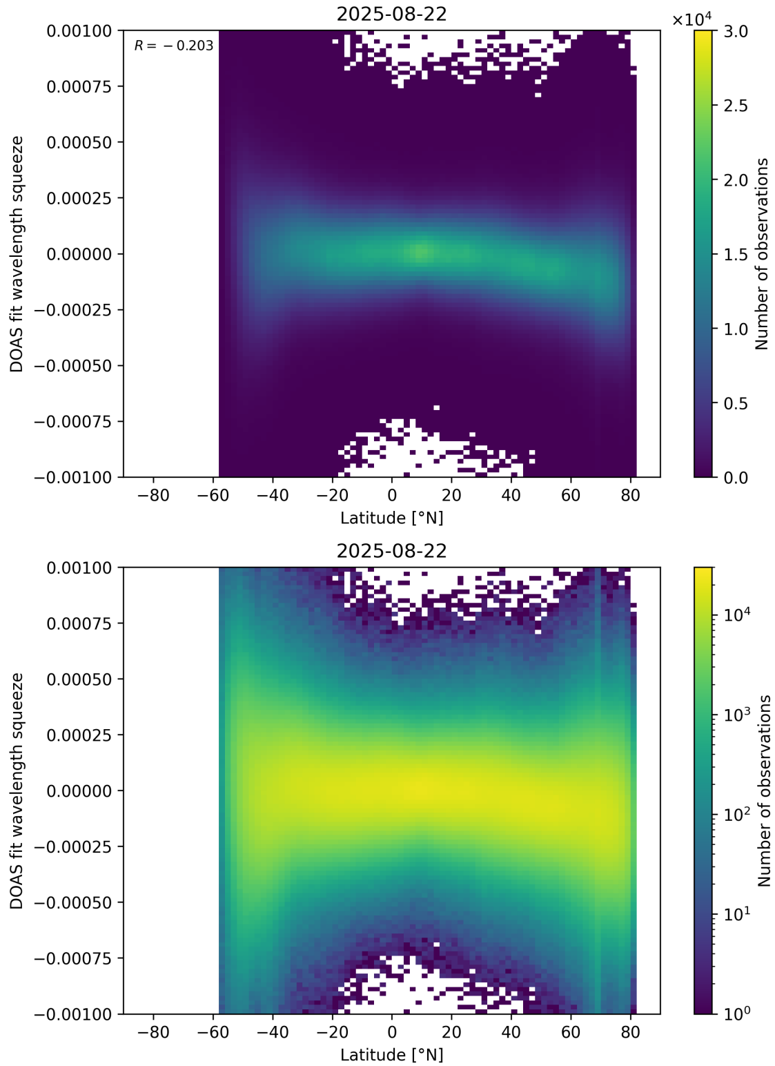
Figure 154: Scatter density plot of “Latitude” against “DOAS fit wavelength squeeze” for 2025-08-21 to 2025-08-23.
