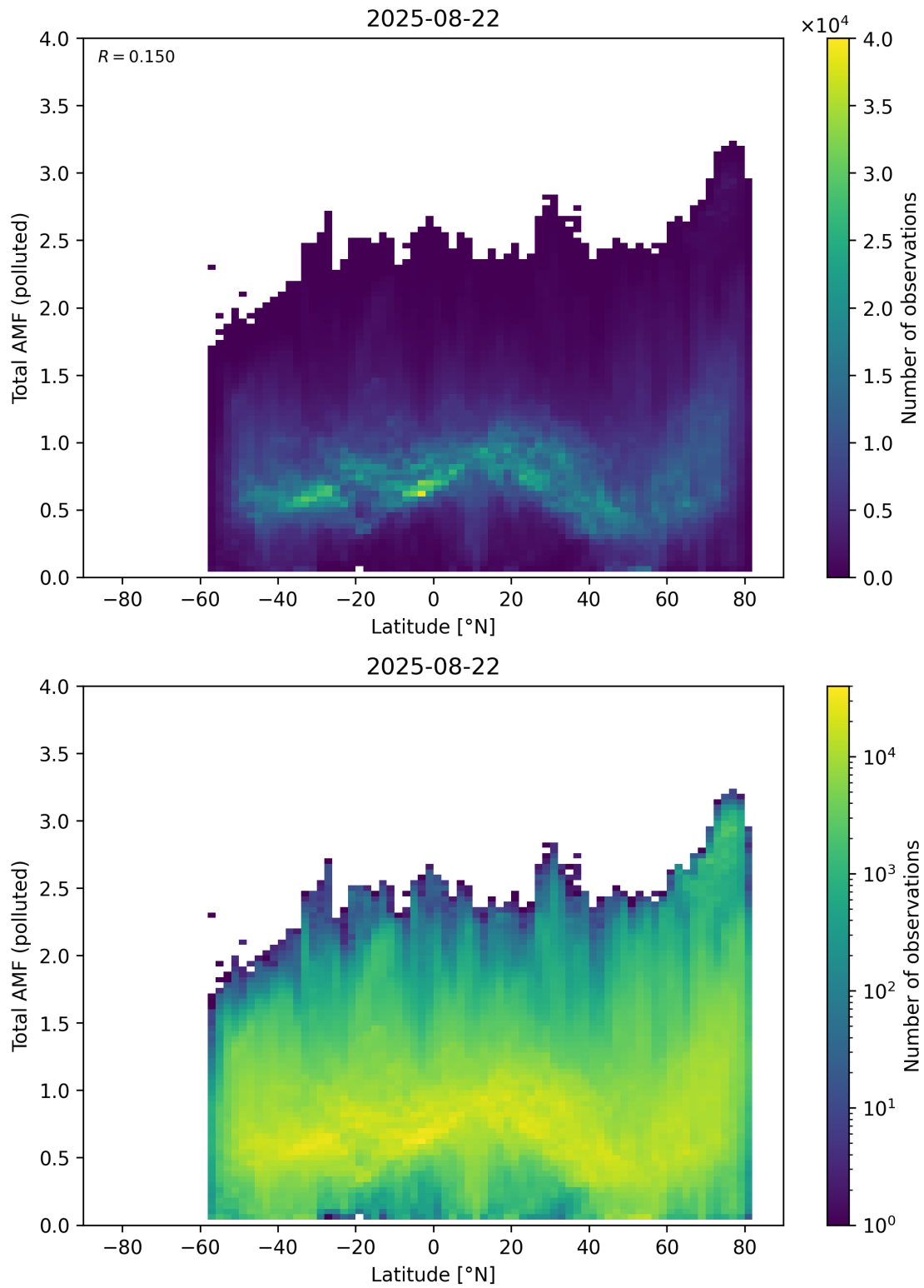
Figure 167: Scatter density plot of “Latitude” against “Total AMF (polluted)” for 2025-08-21 to 2025-08-23.
