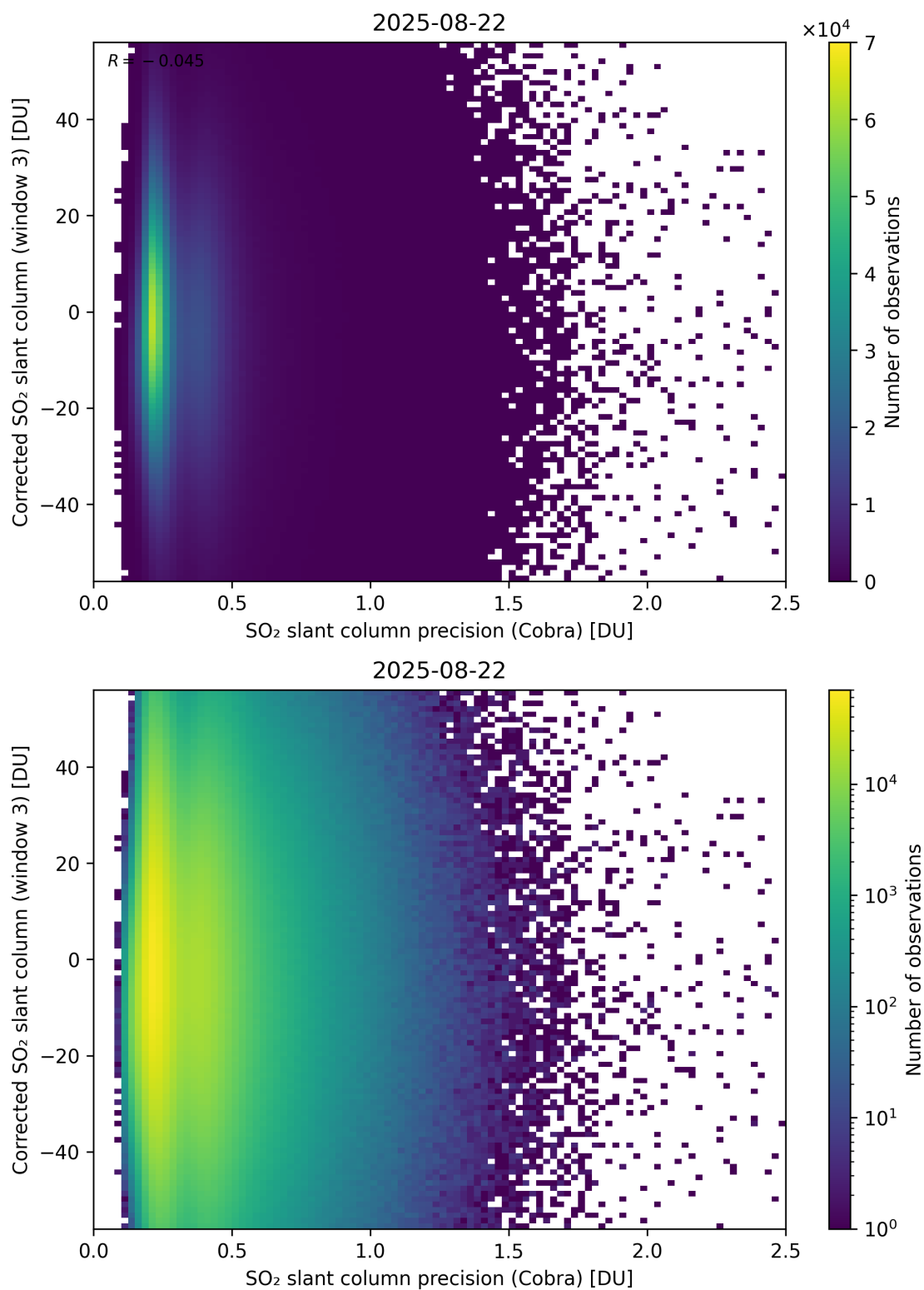
Figure 207: Scatter density plot of “SO 2 slant column precision (Cobra)” against “Corrected SO 2 slant column (window 3)” for 2025-08-21 to 2025-08-23.
