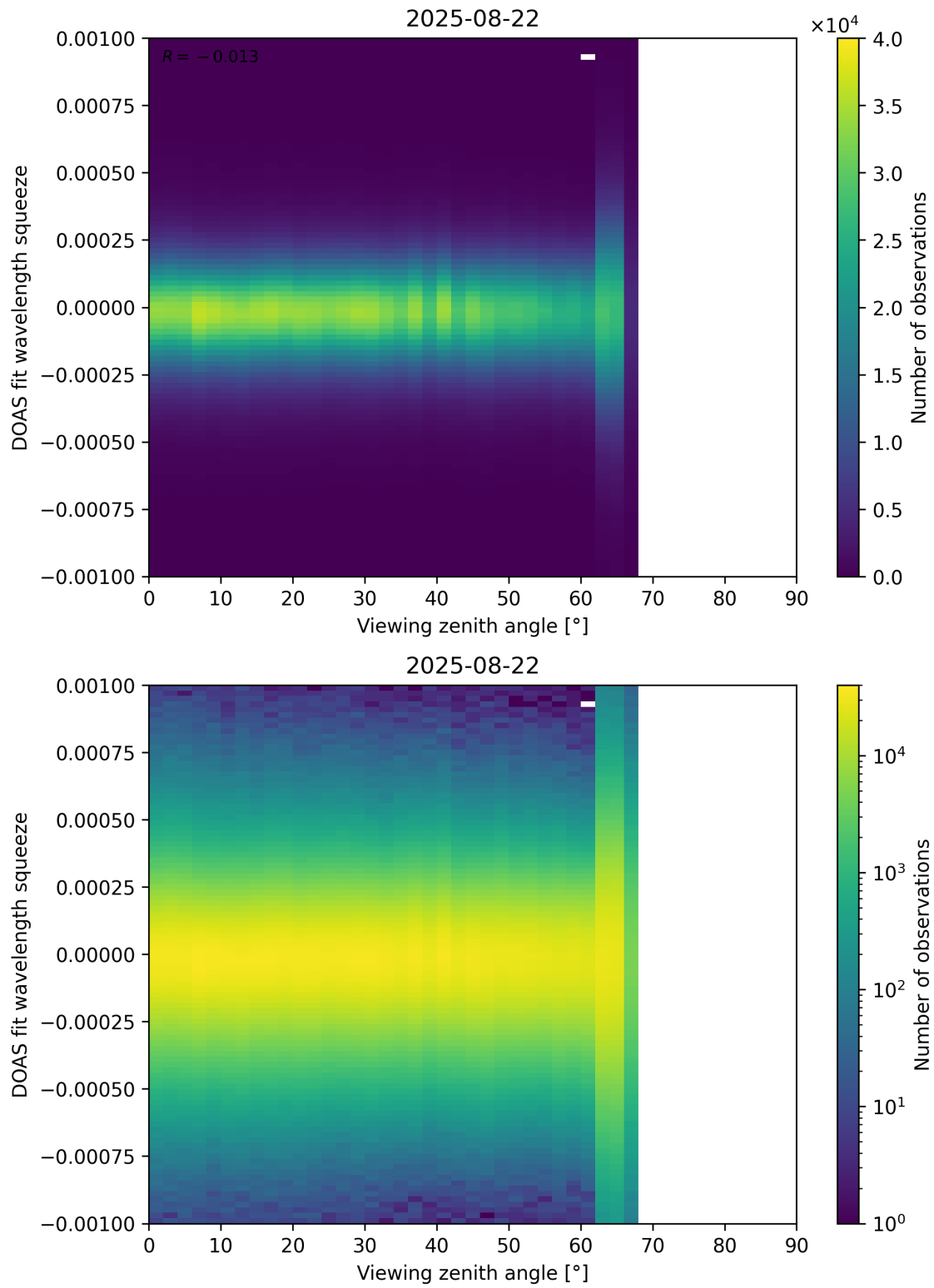
Figure 366: Scatter density plot of “Viewing zenith angle” against “DOAS fit wavelength squeeze” for 2025-08-21 to 2025-08-23.
