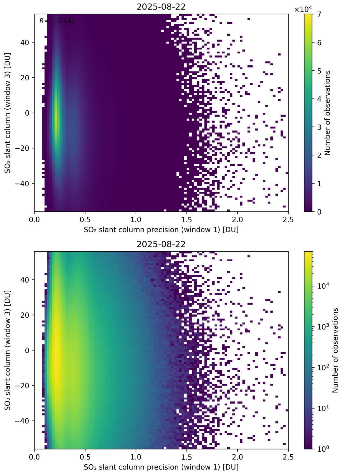
Figure 278: Scatter density plot of “SO 2 slant column precision (window 1)” against “SO 2 slant column (window 3)” for 2025-08-21 to 2025-08-23.
