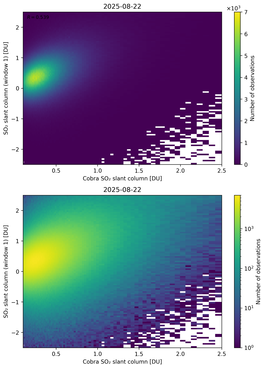
Figure 219: Scatter density plot of “Cobra SO 2 slant column” against “SO 2 slant column (window 1)” for 2025-08-21 to 2025-08-23.
