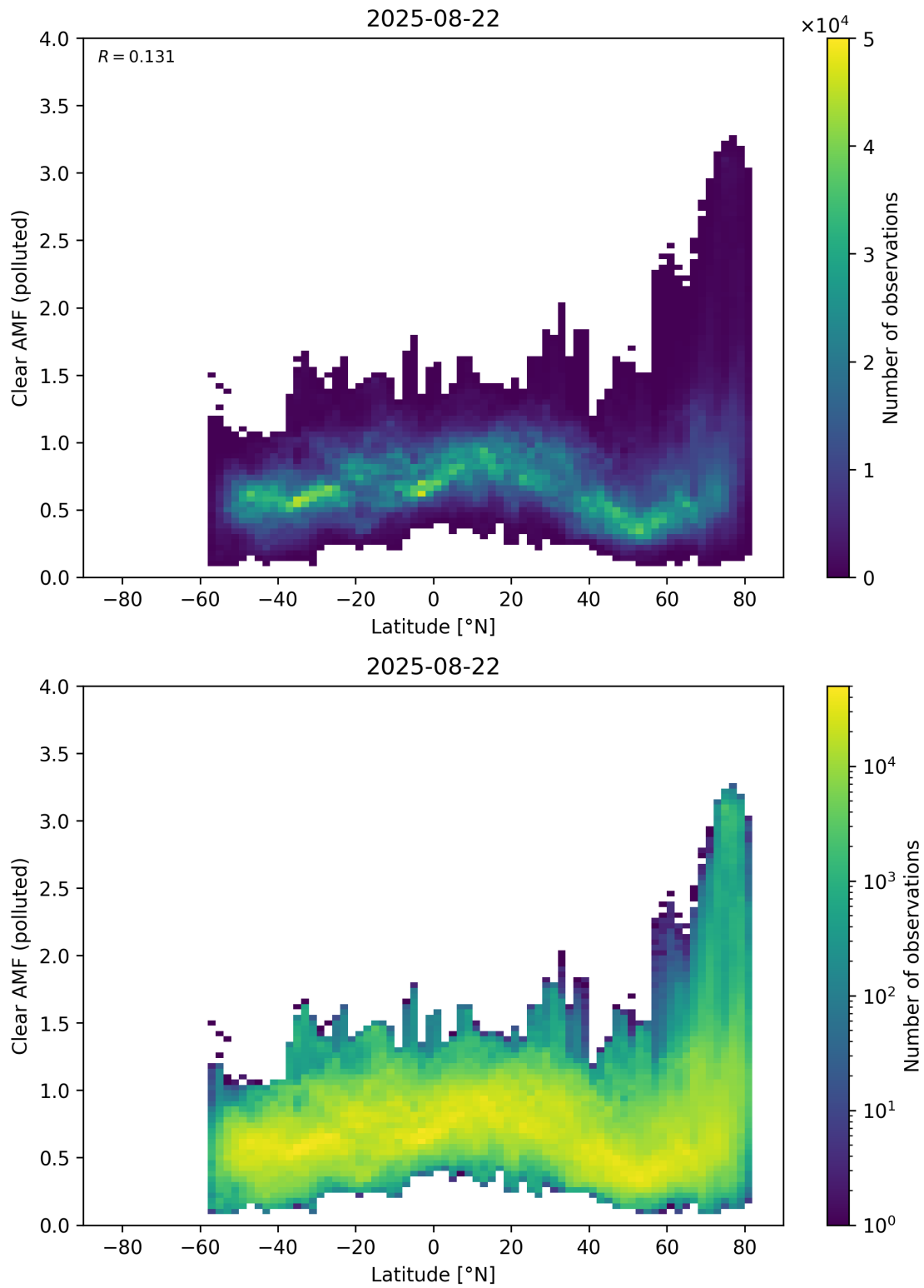
Figure 156: Scatter density plot of “Latitude” against “Clear AMF (polluted)” for 2025-08-21 to 2025-08-23.
