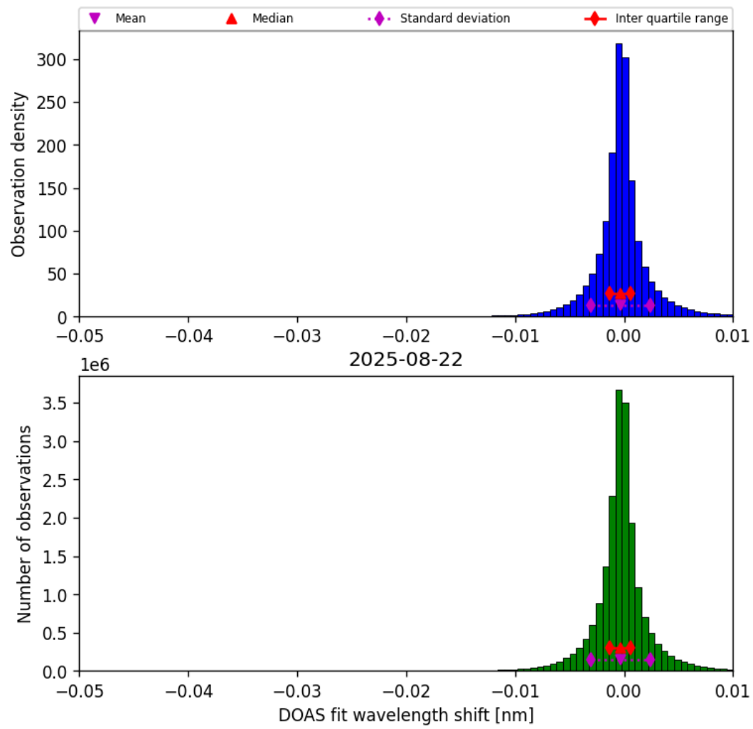
Figure 76: Histogram of “DOAS fit wavelength shift” for 2025-08-21 to 2025-08-23
