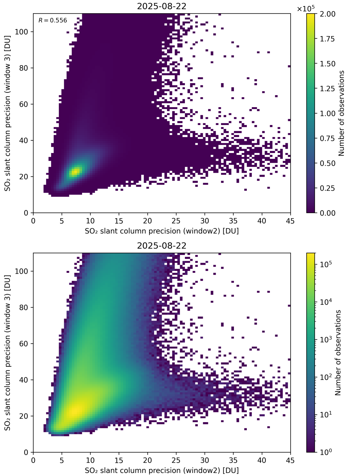
Figure 300: Scatter density plot of “SO 2 slant column precision (window2)” against “SO 2 slant column precision (window 3)” for 2025-08-21 to 2025-08-23.
