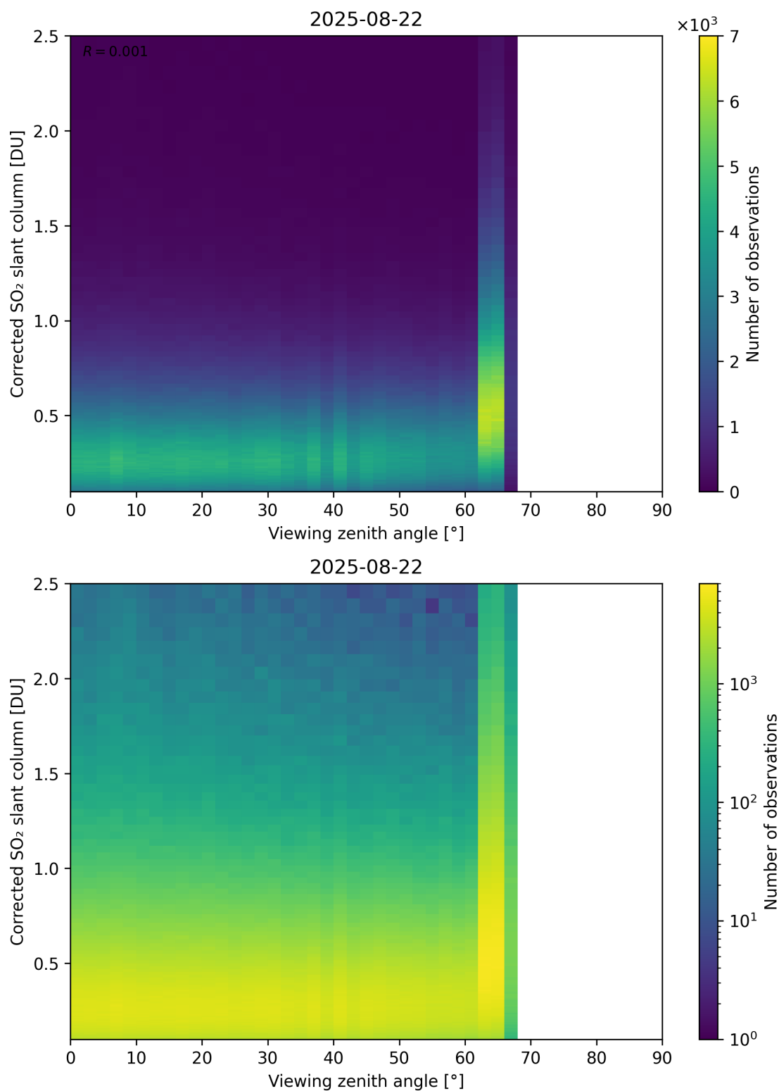
Figure 373: Scatter density plot of “Viewing zenith angle” against “Corrected SO 2 slant column” for 2025-08-21 to 2025-08-23.
