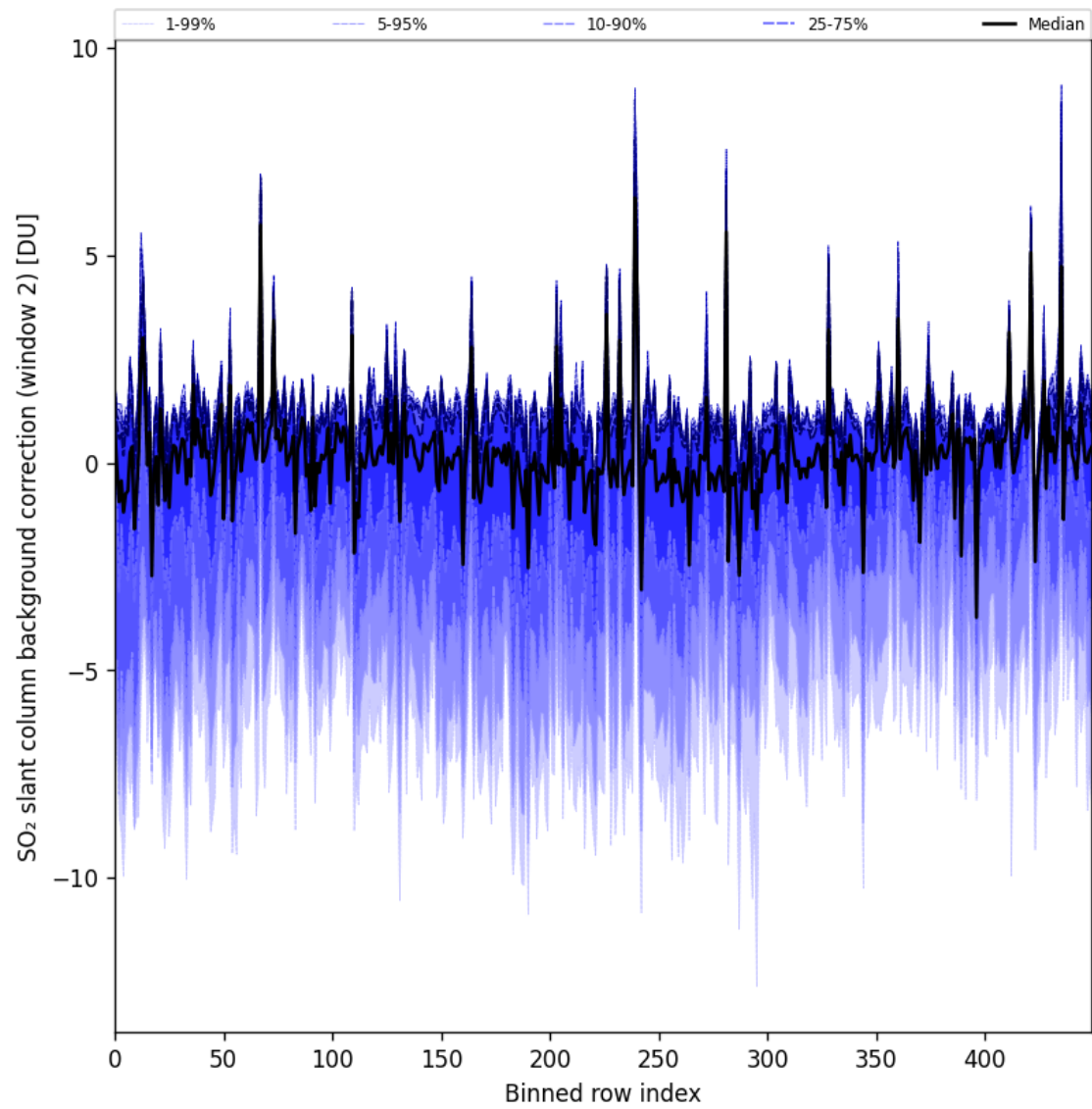
Figure 96: Along track statistics of “SO 2 slant column background correction (window 2)” for 2025-08-21 to 2025-08-23
