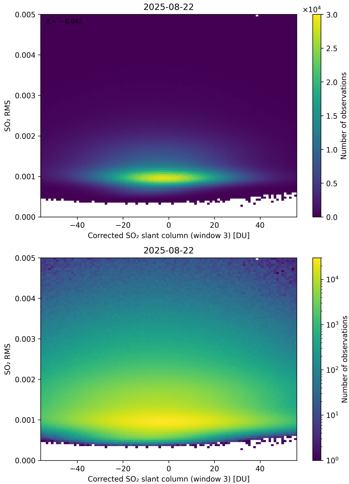
Figure 258: Scatter density plot of “Corrected SO 2 slant column (window 3)” against “SO 2 RMS” for 2025-08-21 to 2025-08-23.
