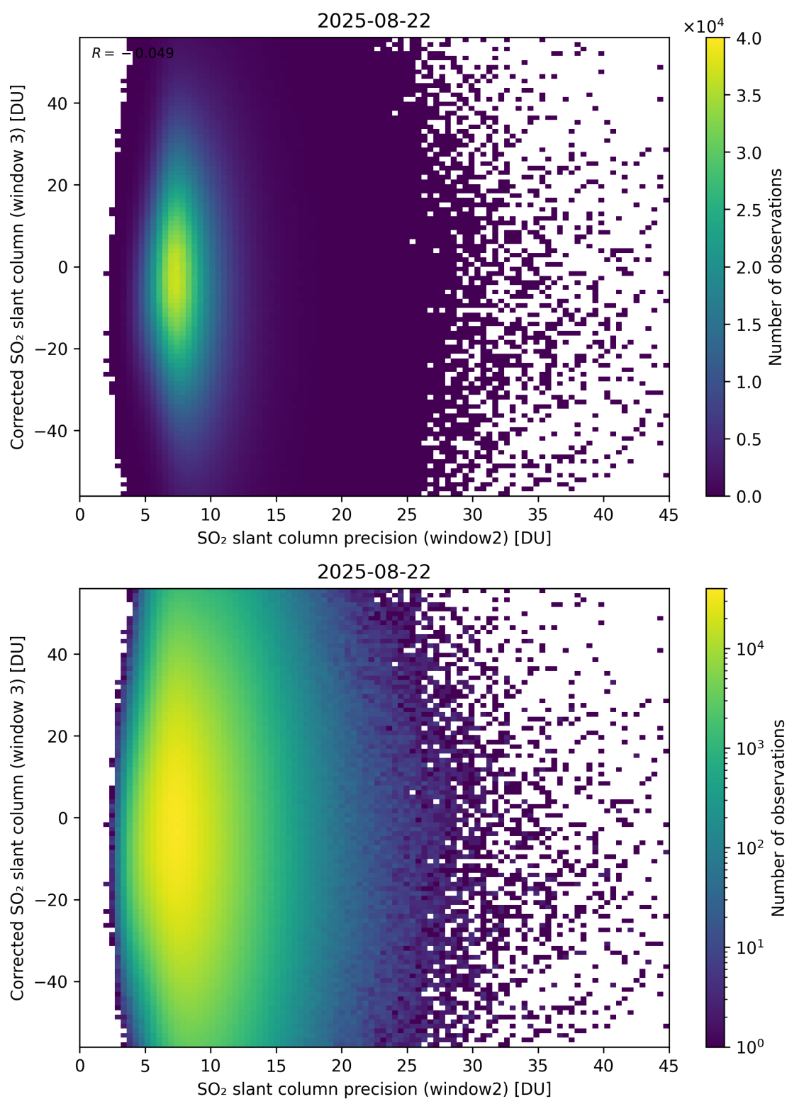
Figure 298: Scatter density plot of “SO 2 slant column precision (window2)” against “Corrected SO 2 slant column (window 3)” for 2025-08-21 to 2025-08-23.
