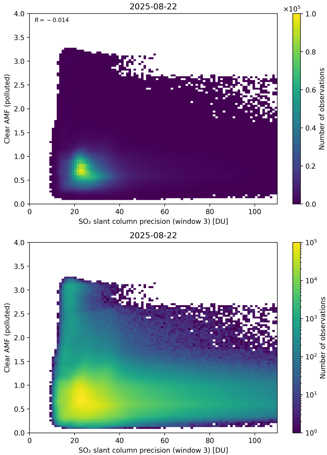
Figure 311: Scatter density plot of “SO 2 slant column precision (window 3)” against “Clear AMF (polluted)” for 2025-08-21 to 2025-08-23.
