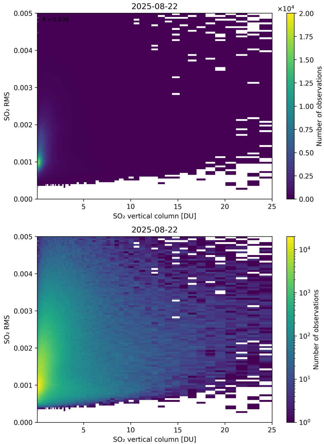
Figure 328: Scatter density plot of “SO 2 vertical column” against “SO 2 RMS” for 2025-08-21 to 2025-08-23.
