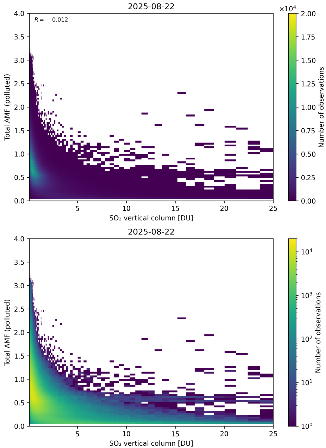
Figure 359: Scatter density plot of “SO 2 vertical column” against “Total AMF (polluted)” for 2025-08-21 to 2025-08-23.
