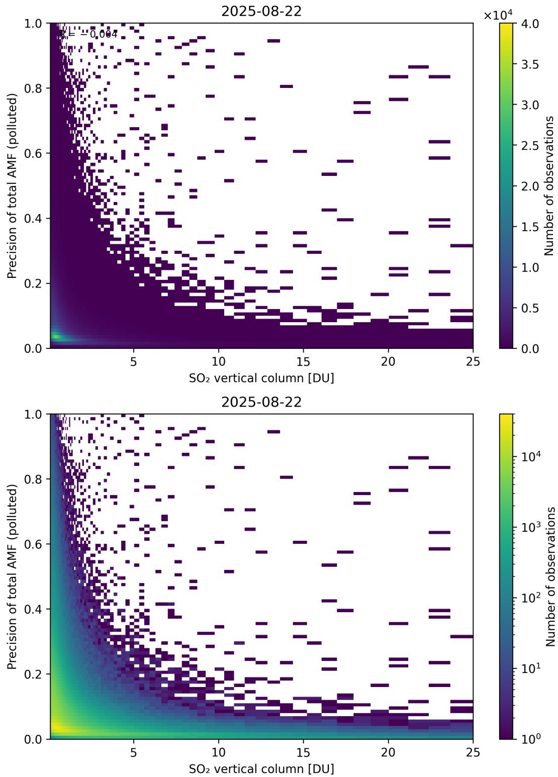
Figure 360: Scatter density plot of “SO 2 vertical column” against “Precision of total AMF (polluted)” for 2025-08-21 to 2025-08-23.
