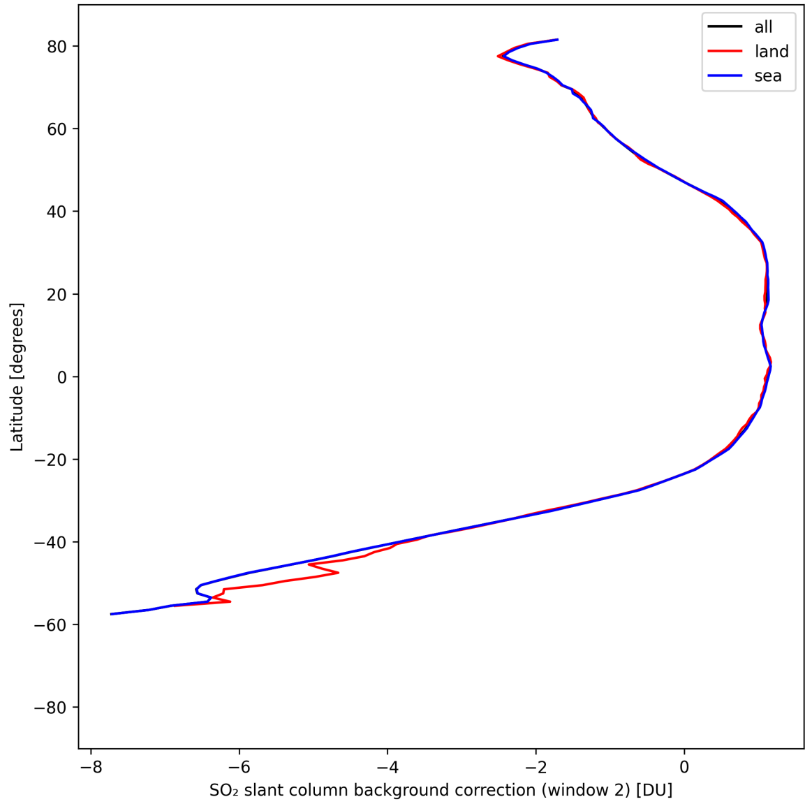
Figure 44: Zonal average of “SO 2 slant column background correction (window 2)” for 2025-08-21 to 2025-08-23.
