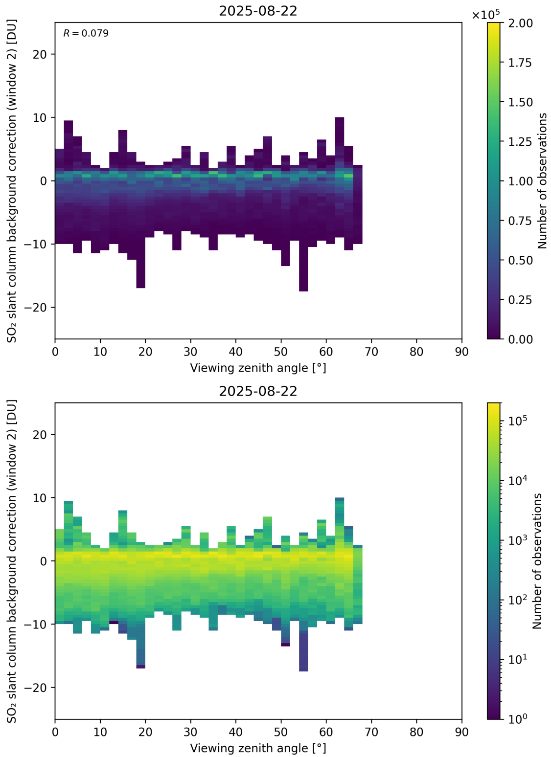
Figure 363: Scatter density plot of “Viewing zenith angle” against “SO 2 slant column background correction (window 2)” for 2025-08-21 to 2025-08-23.
