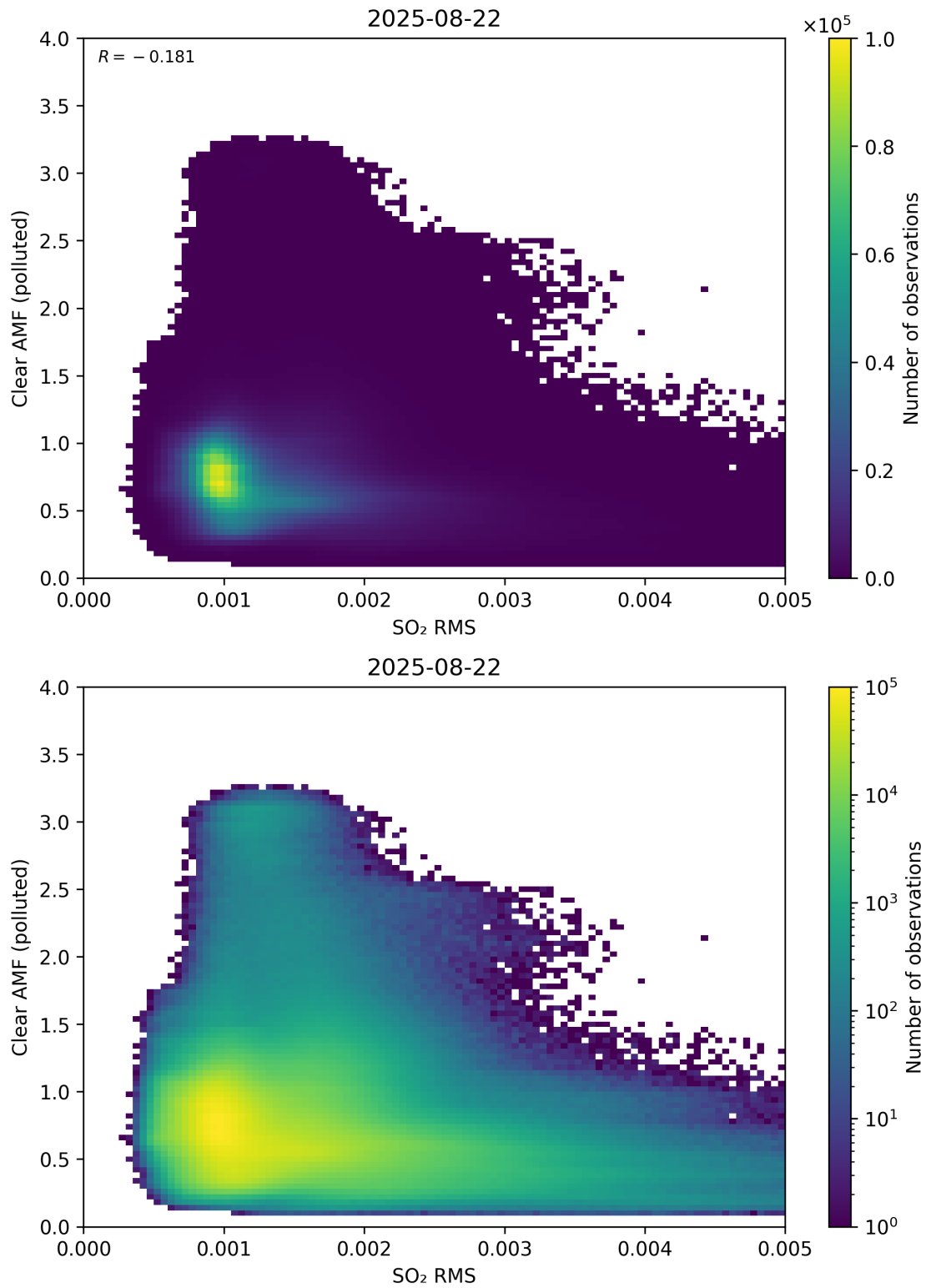
Figure 147: Scatter density plot of “SO 2 RMS” against “Clear AMF (polluted)” for 2025-08-21 to 2025-08-23.
