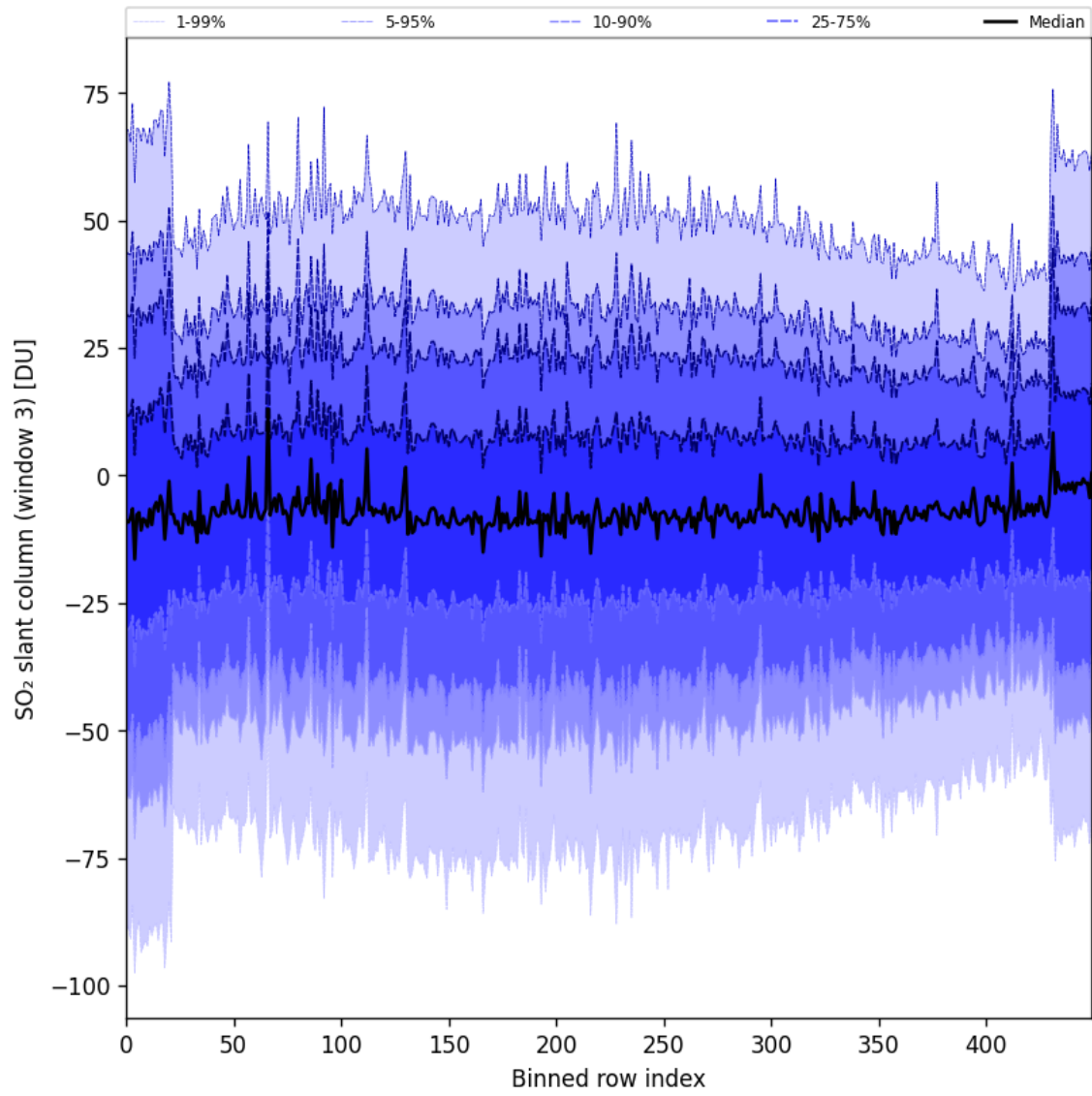
Figure 97: Along track statistics of “SO 2 slant column (window 3)” for 2025-08-21 to 2025-08-23
