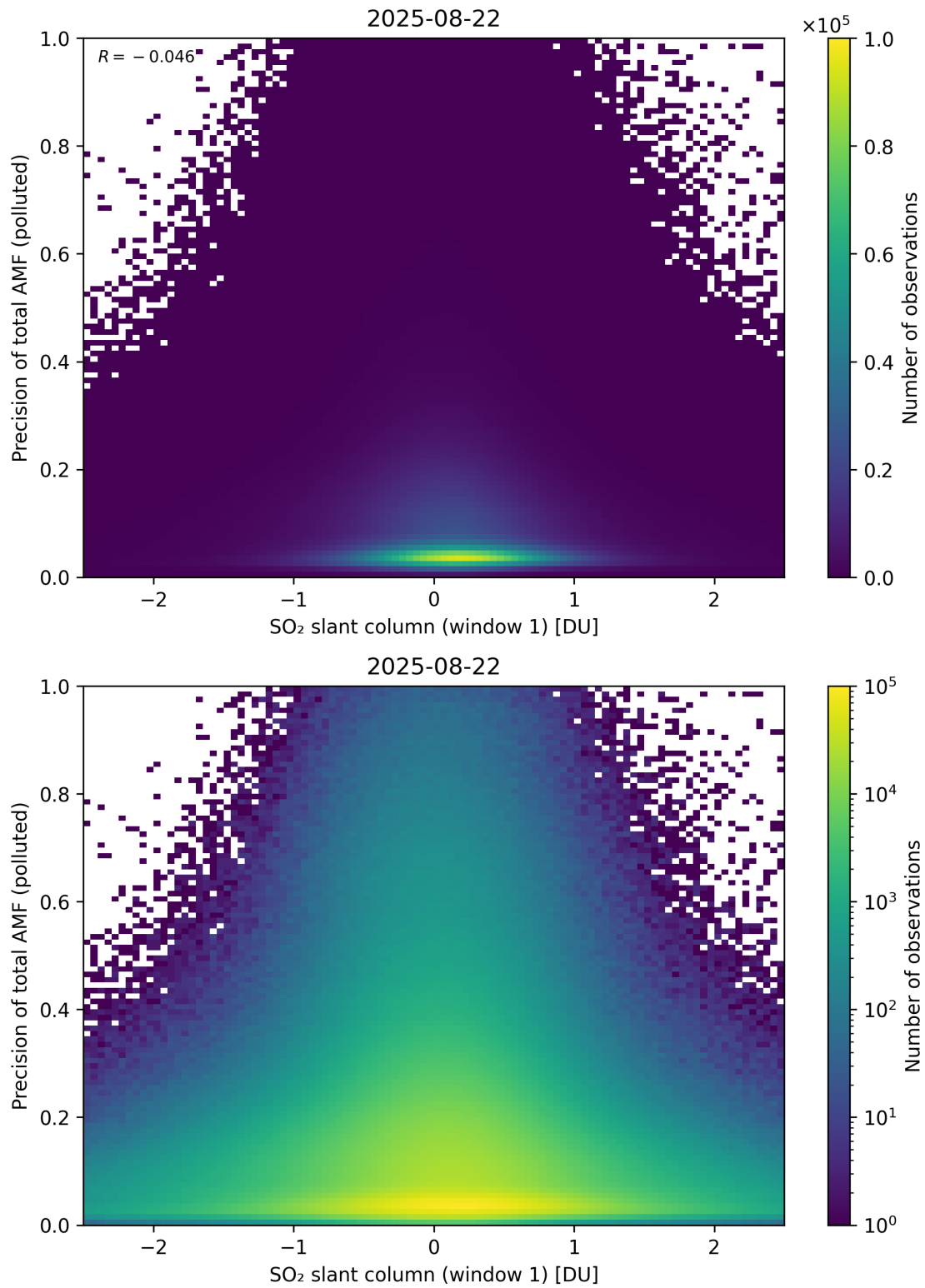
Figure 290: Scatter density plot of “SO 2 slant column (window 1)” against “Precision of total AMF (polluted)” for 2025-08-21 to 2025-08-23.
