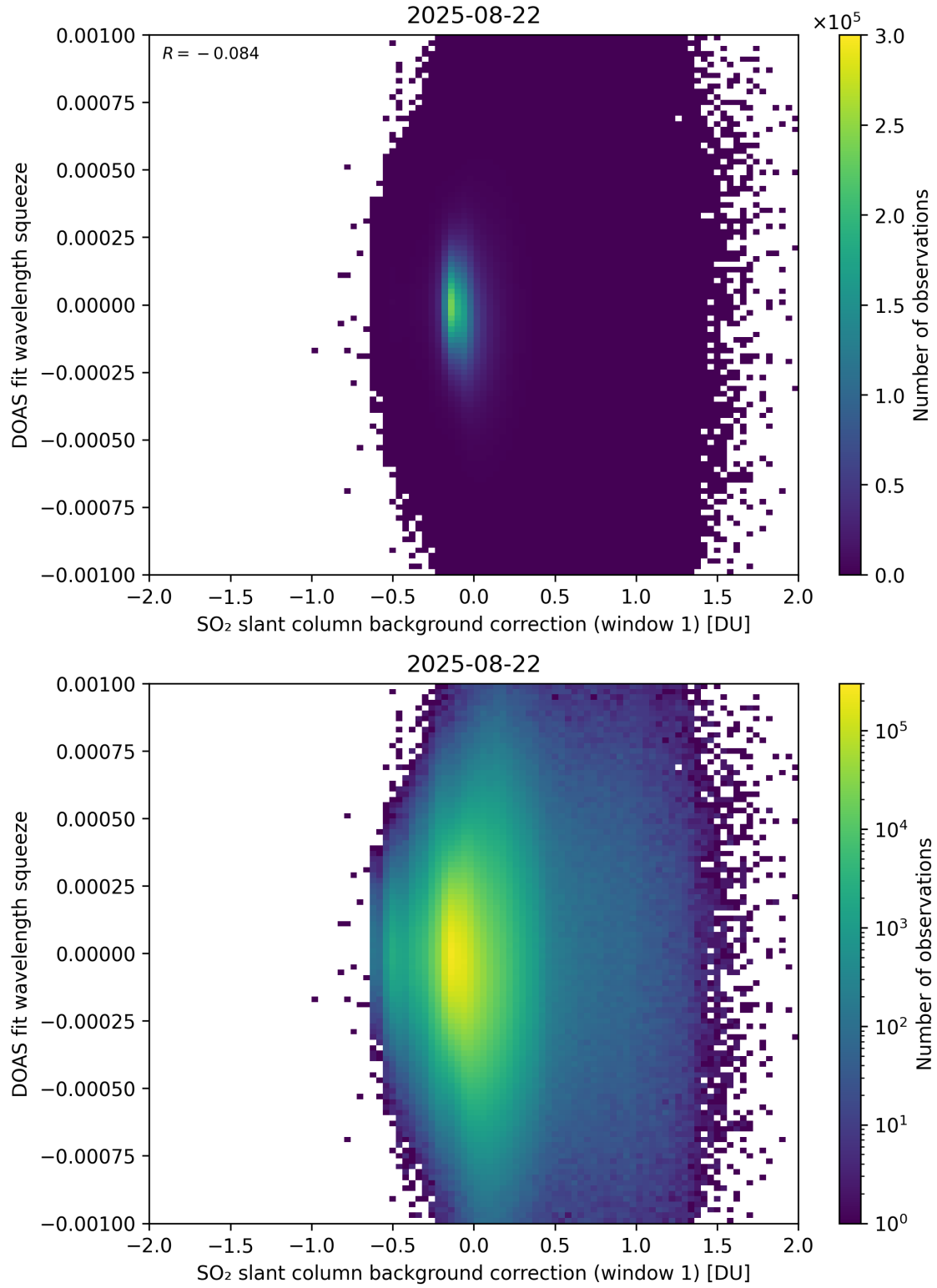
Figure 112: Scatter density plot of “SO 2 slant column background correction (window 1)” against “DOAS fit wavelength squeeze” for 2025-08-21 to 2025-08-23.
