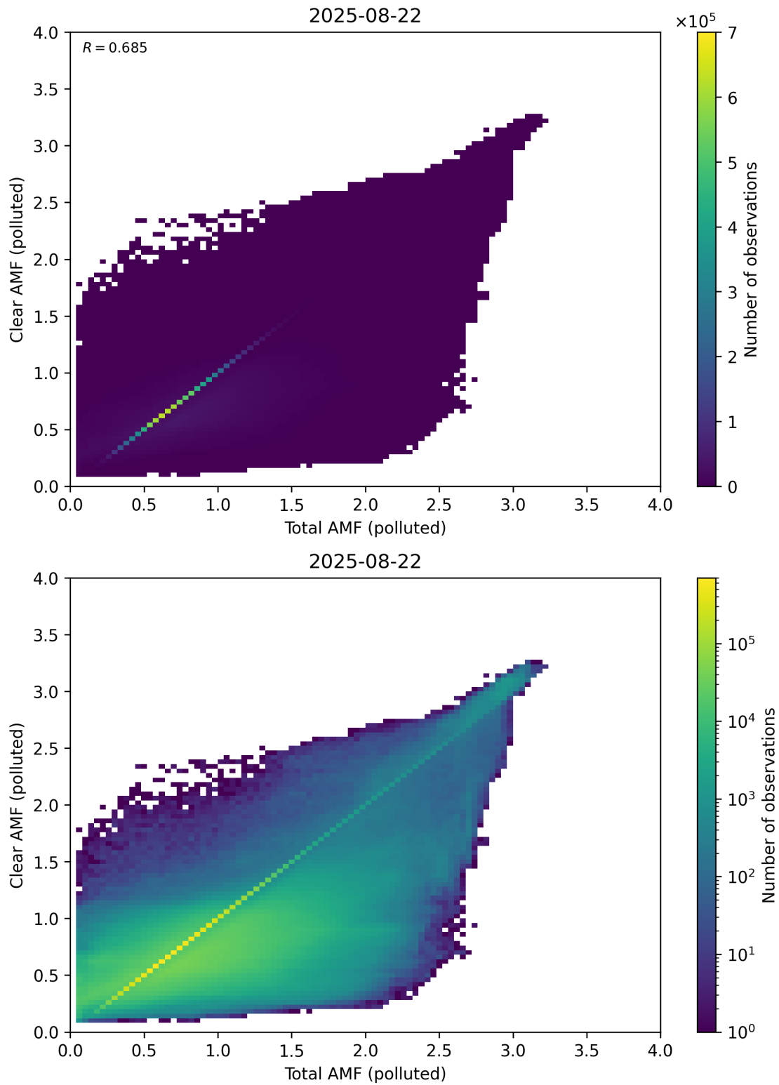
Figure 321: Scatter density plot of “Total AMF (polluted)” against “Clear AMF (polluted)” for 2025-08-21 to 2025-08-23.
