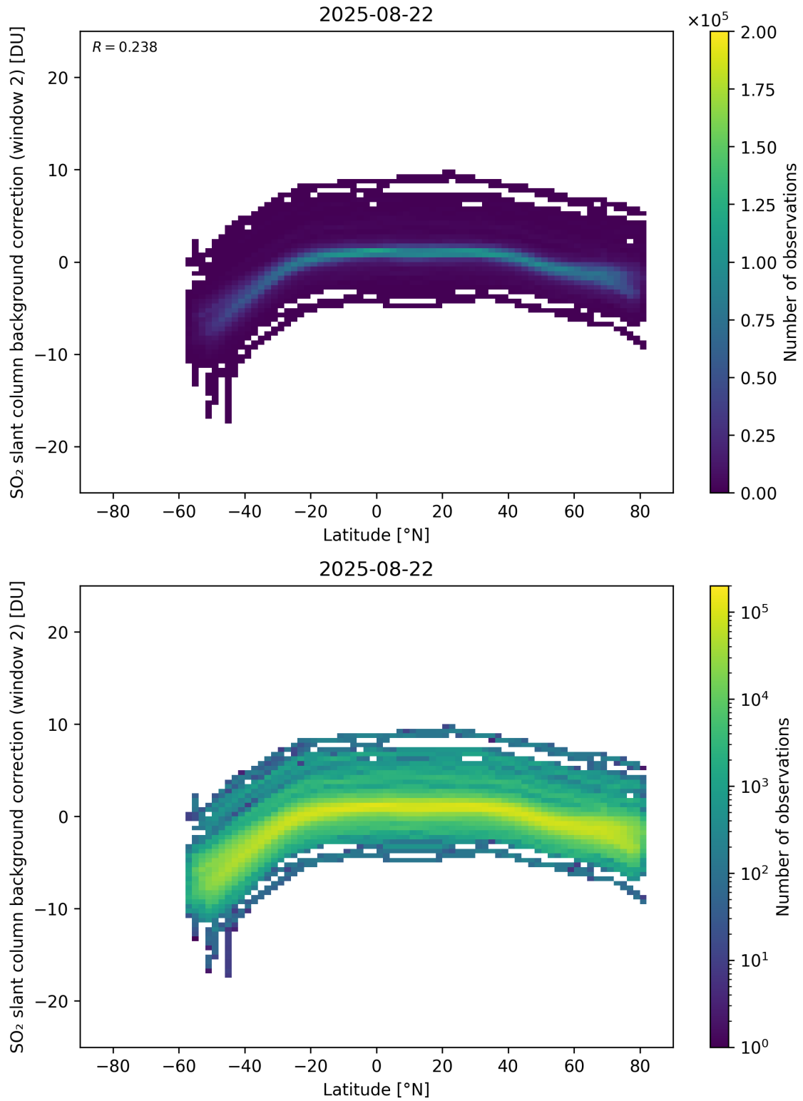
Figure 151: Scatter density plot of “Latitude” against “SO 2 slant column background correction (window 2)” for 2025-08-21 to 2025-08-23.
