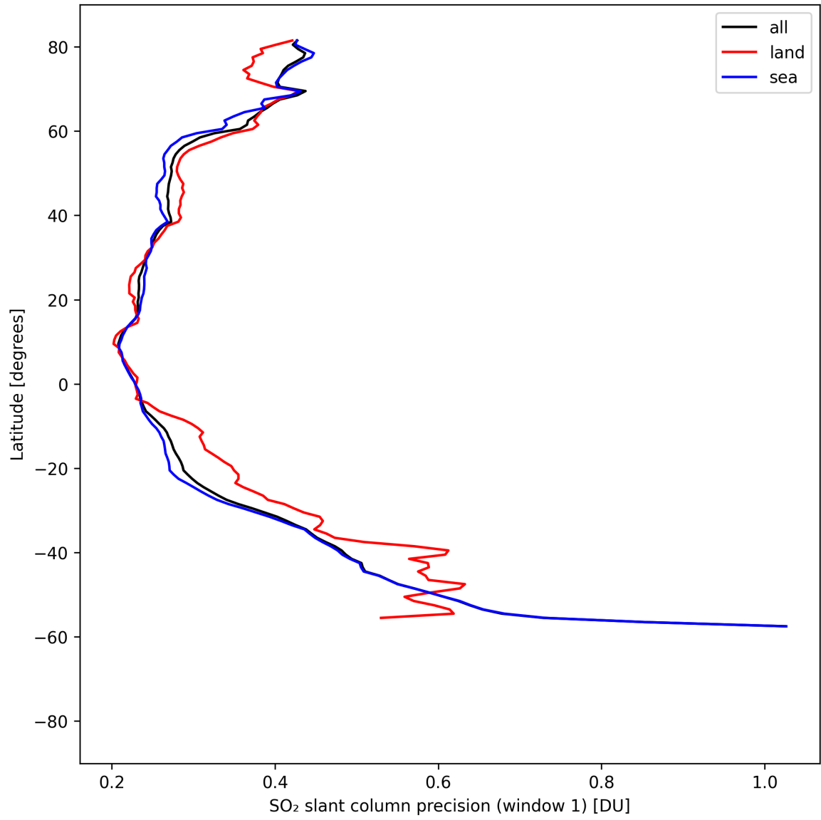
Figure 38: Zonal average of “SO 2 slant column precision (window 1)” for 2025-08-21 to 2025-08-23.
