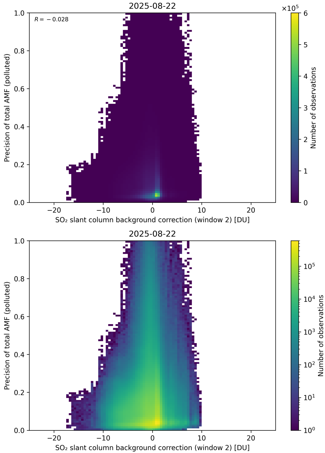
Figure 131: Scatter density plot of “SO 2 slant column background correction (window 2)” against “Precision of total AMF (polluted)” for 2025-08-21 to 2025-08-23.
