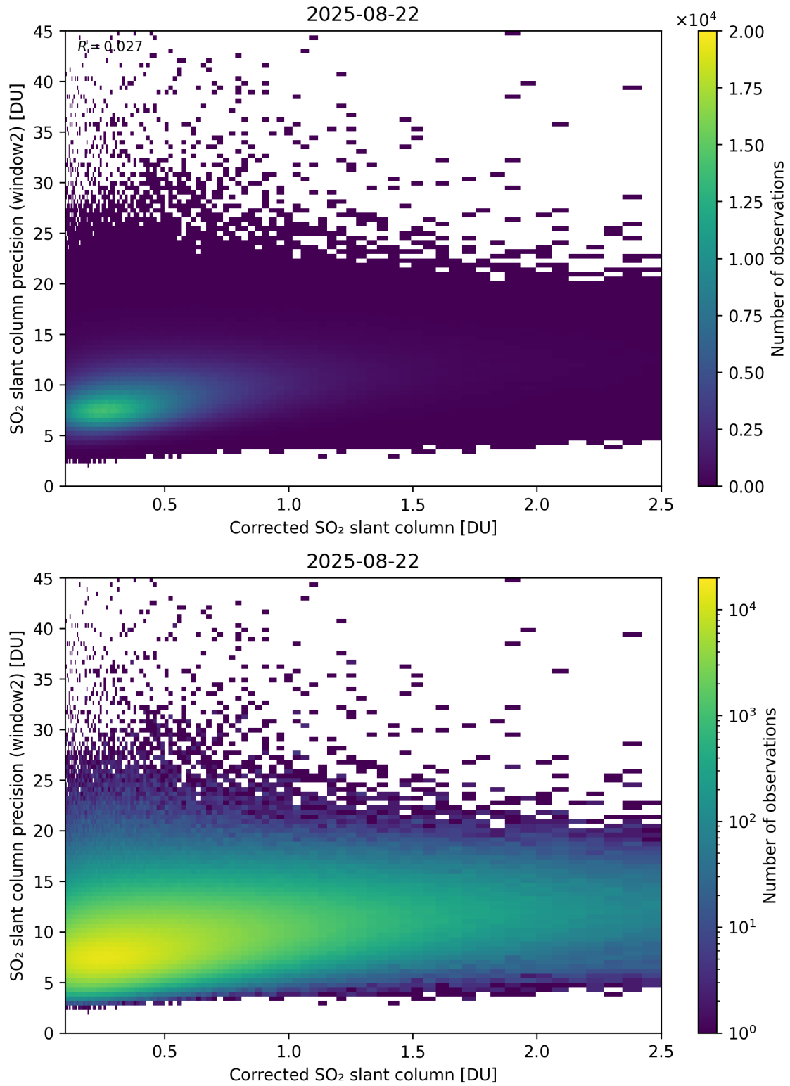
Figure 239: Scatter density plot of “Corrected SO 2 slant column” against “SO 2 slant column precision (window2)” for 2025-08-21 to 2025-08-23.
