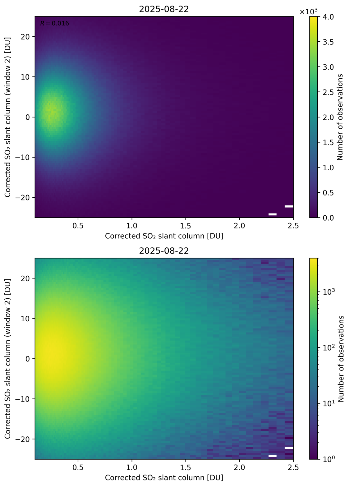
Figure 235: Scatter density plot of “Corrected SO 2 slant column” against “Corrected SO 2 slant column (window 2)” for 2025-08-21 to 2025-08-23.
