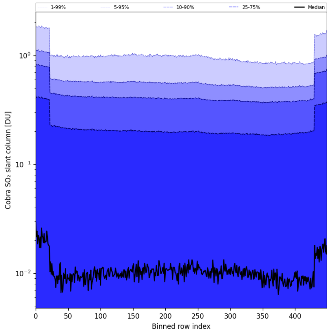
Figure 87: Along track statistics of “Cobra SO 2 slant column” for 2025-08-21 to 2025-08-23
