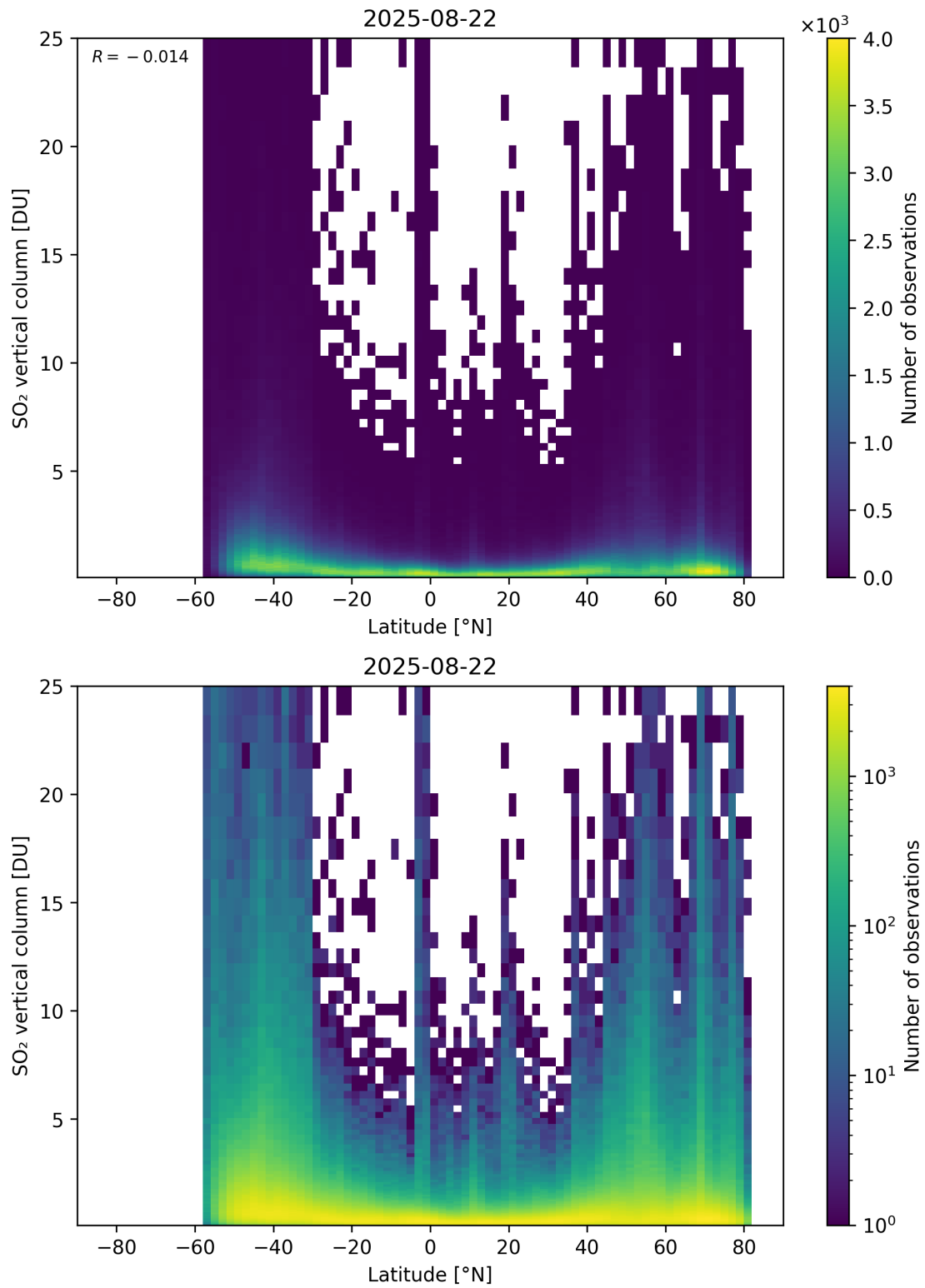
Figure 169: Scatter density plot of “Latitude” against “SO 2 vertical column” for 2025-08-21 to 2025-08-23.
