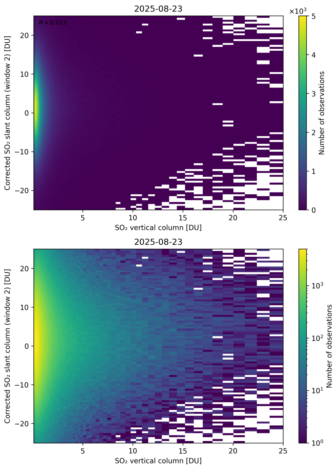
Figure 352: Scatter density plot of “SO 2 vertical column” against “Corrected SO 2 slant column (window 2)” for 2025-08-22 to 2025-08-24.
