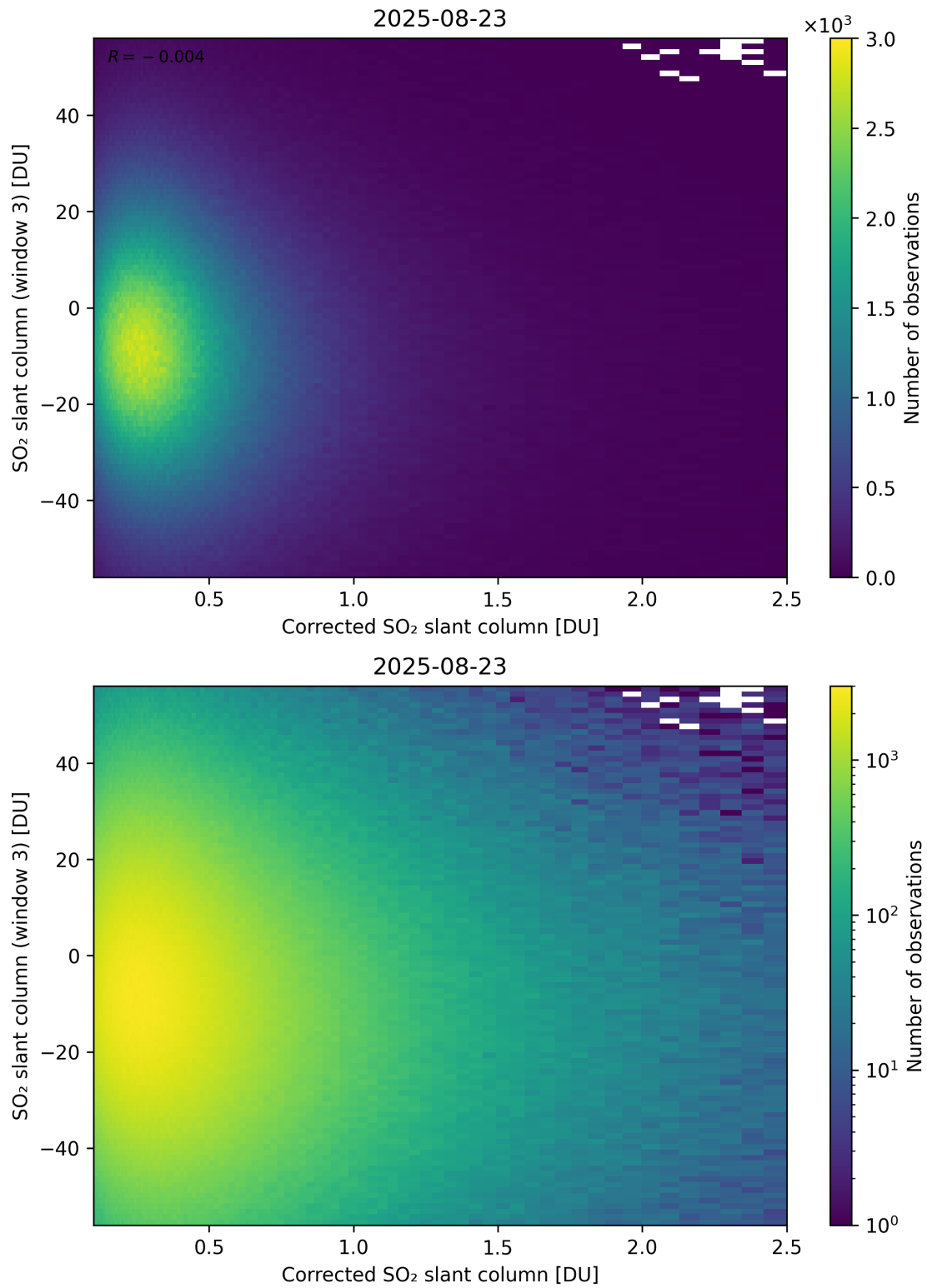
Figure 240: Scatter density plot of “Corrected SO 2 slant column” against “SO 2 slant column (window 3)” for 2025-08-22 to 2025-08-24.
