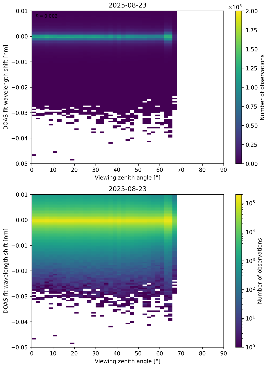
Figure 365: Scatter density plot of “Viewing zenith angle” against “DOAS fit wavelength shift” for 2025-08-22 to 2025-08-24.
