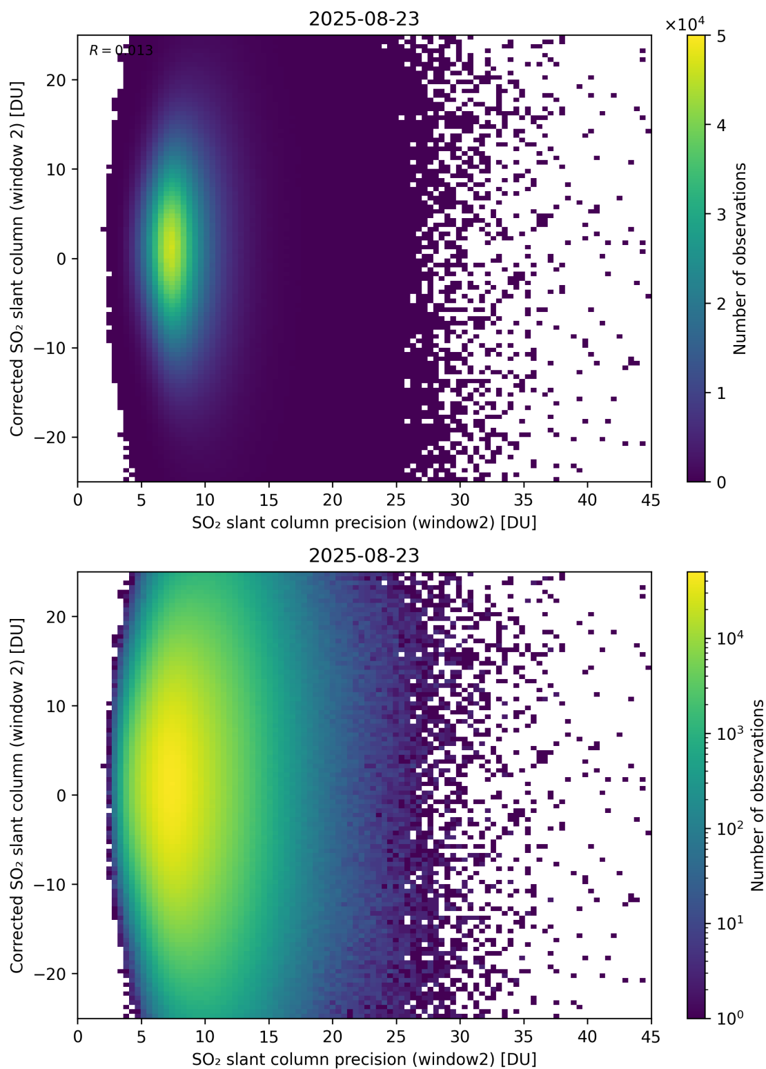
Figure 297: Scatter density plot of “SO 2 slant column precision (window2)” against “Corrected SO 2 slant column (window 2)” for 2025-08-22 to 2025-08-24.
