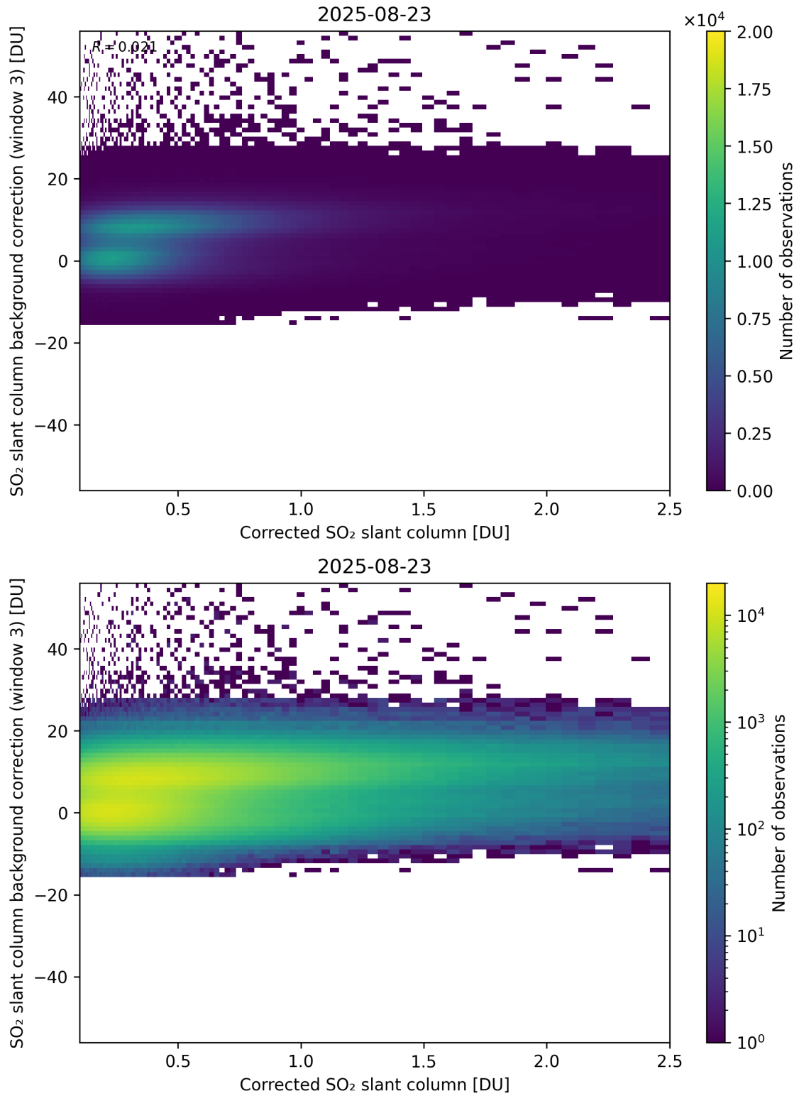
Figure 228: Scatter density plot of “Corrected SO 2 slant column” against “SO 2 slant column background correction (window 3)” for 2025-08-22 to 2025-08-24.
