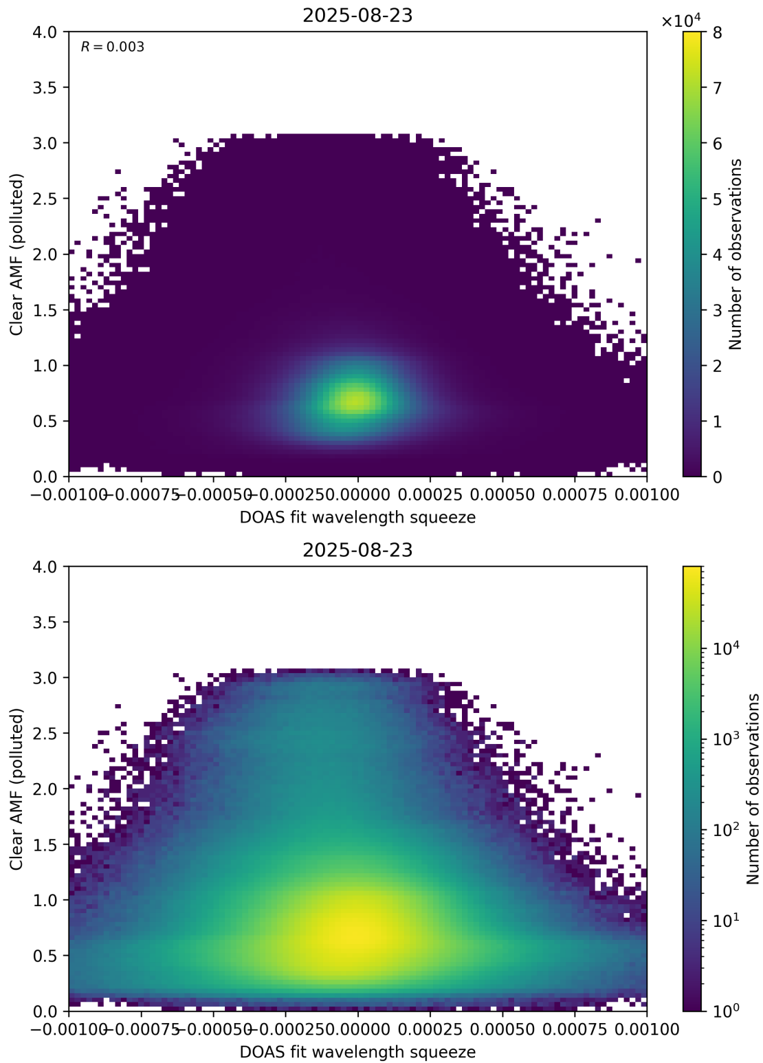
Figure 144: Scatter density plot of “DOAS fit wavelength squeeze” against “Clear AMF (polluted)” for 2025-08-22 to 2025-08-24.
