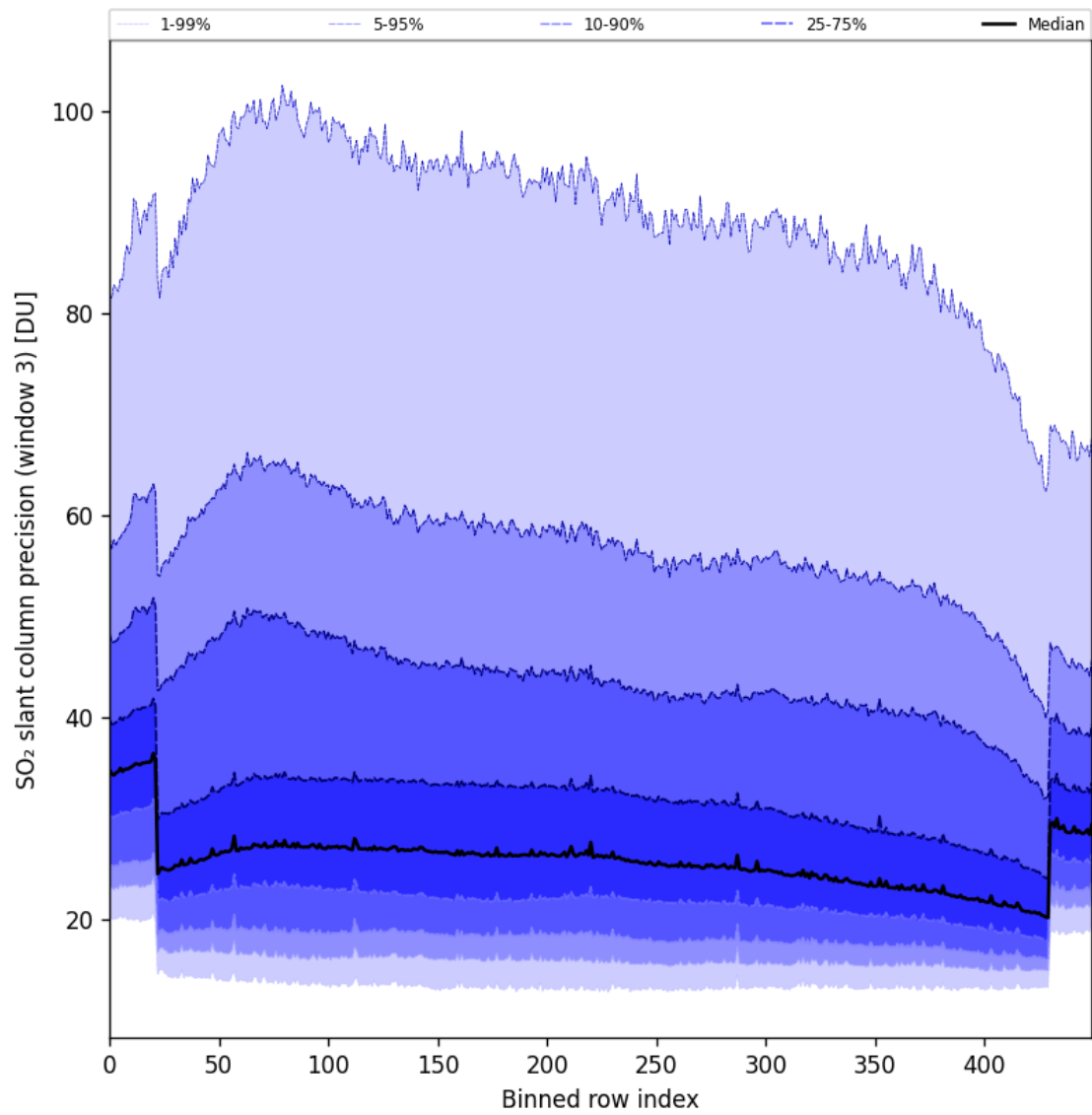
Figure 98: Along track statistics of “SO 2 slant column precision (window 3)” for 2025-08-22 to 2025-08-24
