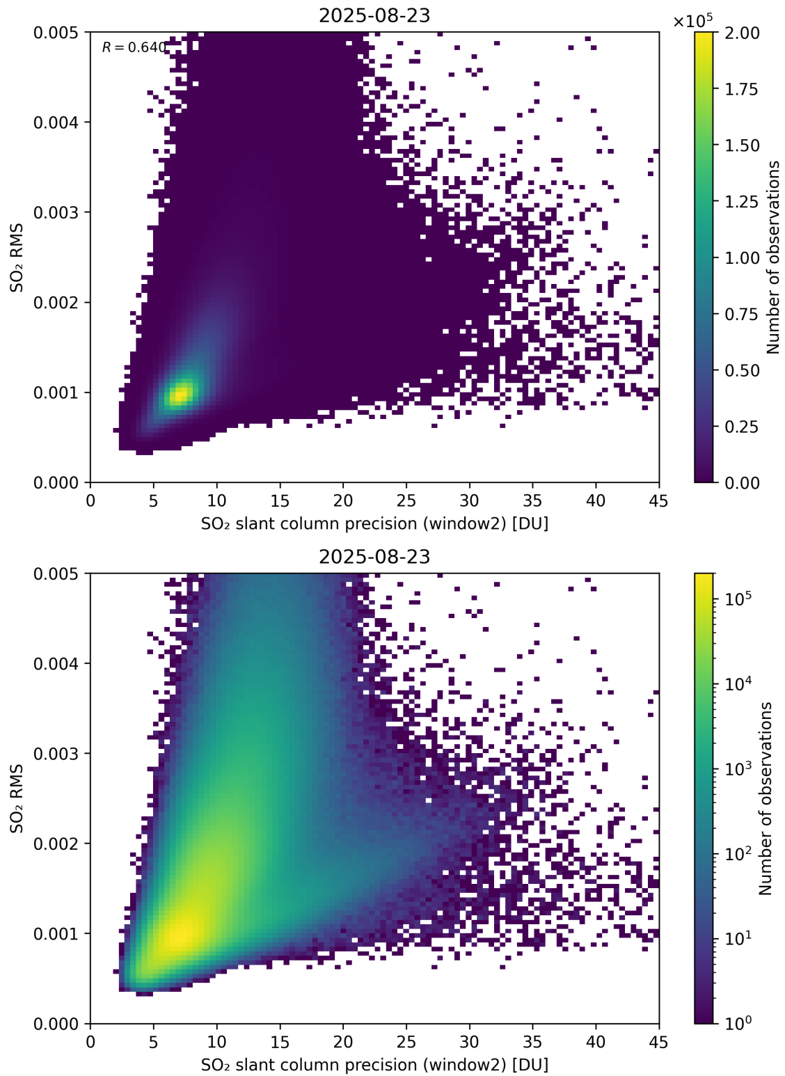
Figure 295: Scatter density plot of “SO 2 slant column precision (window2)” against “SO 2 RMS” for 2025-08-22 to 2025-08-24.
