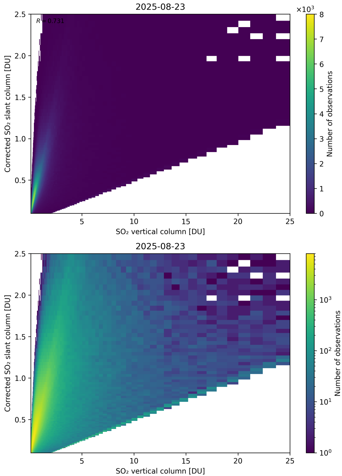
Figure 351: Scatter density plot of “SO 2 vertical column” against “Corrected SO 2 slant column” for 2025-08-22 to 2025-08-24.
