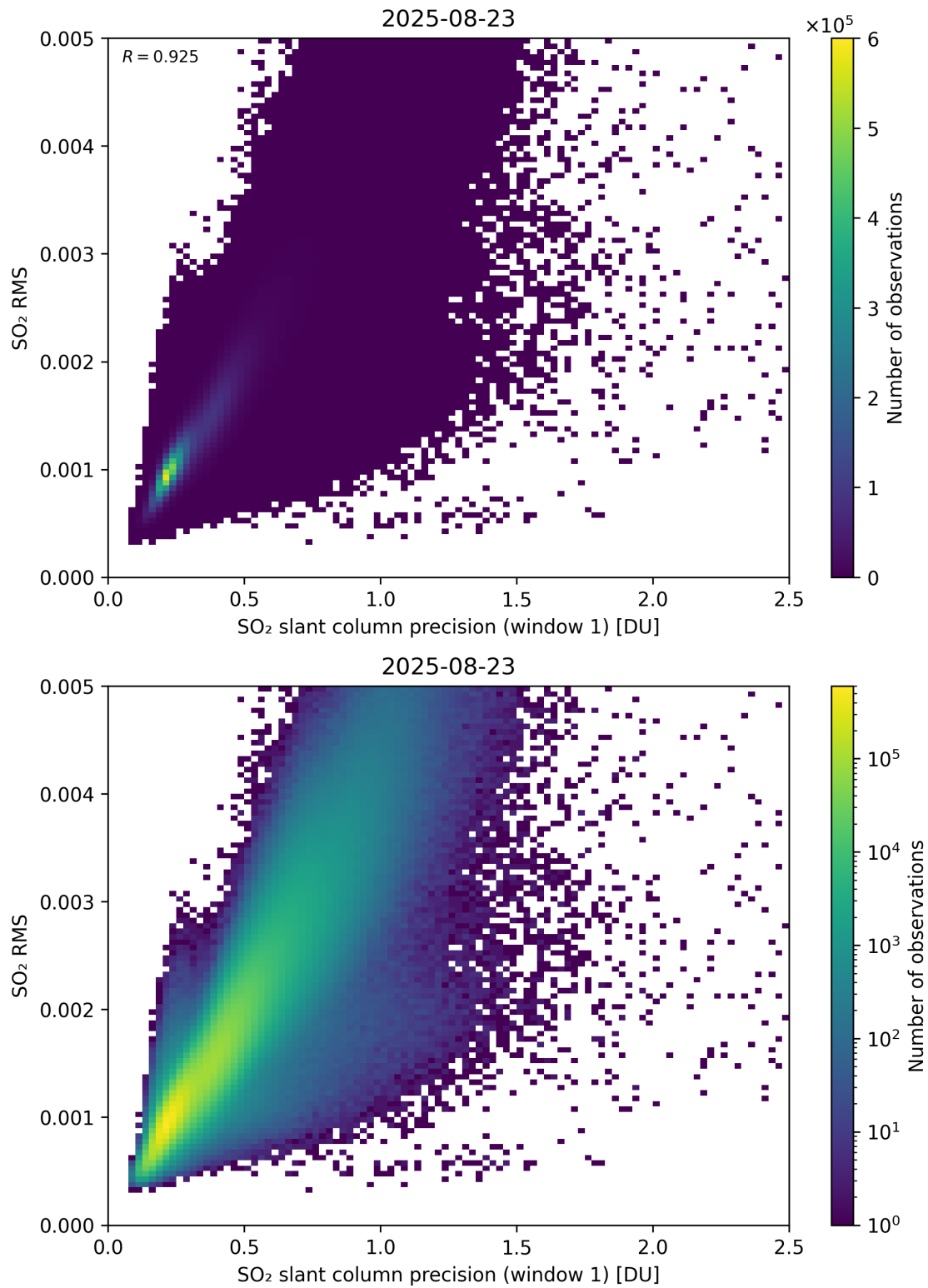
Figure 273: Scatter density plot of “SO 2 slant column precision (window 1)” against “SO 2 RMS” for 2025-08-22 to 2025-08-24.
