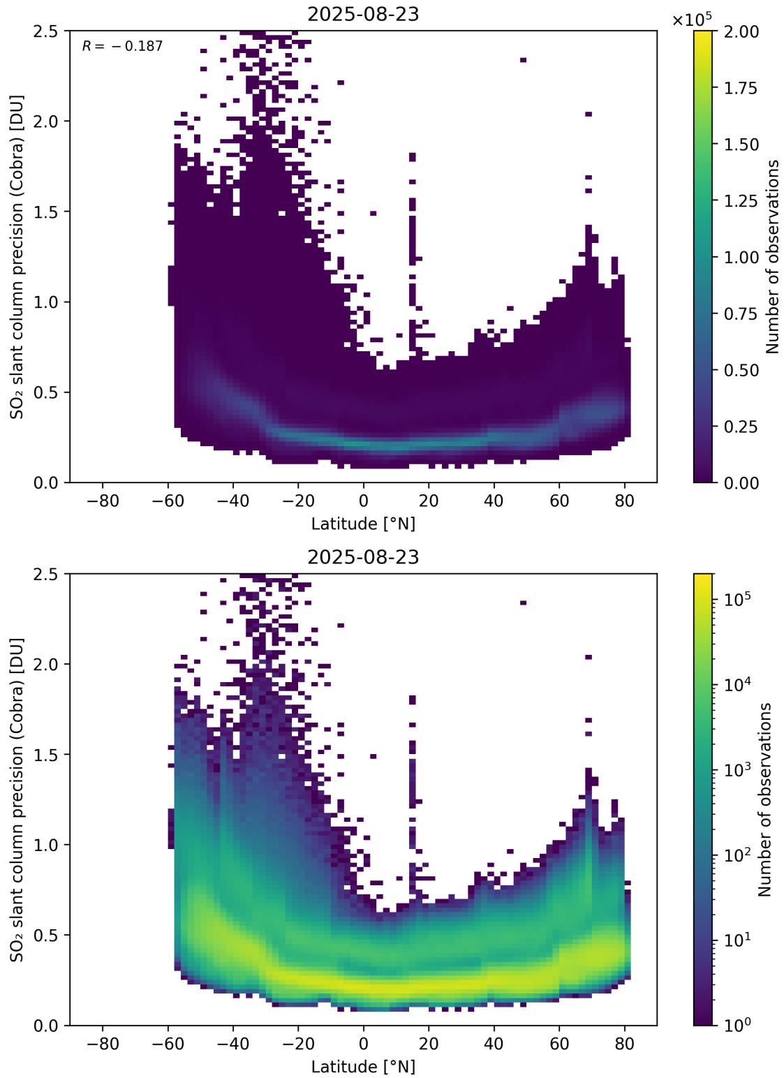
Figure 158: Scatter density plot of “Latitude” against “SO 2 slant column precision (Cobra)” for 2025-08-22 to 2025-08-24.
