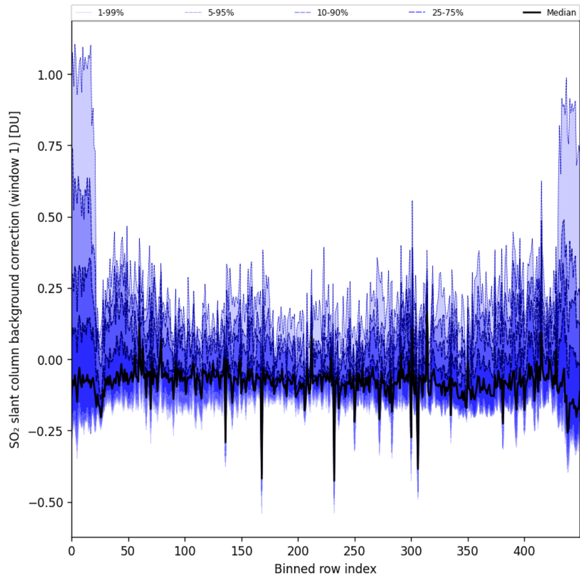
Figure 92: Along track statistics of “SO 2 slant column background correction (window 1)” for 2025-08-22 to 2025-08-24
