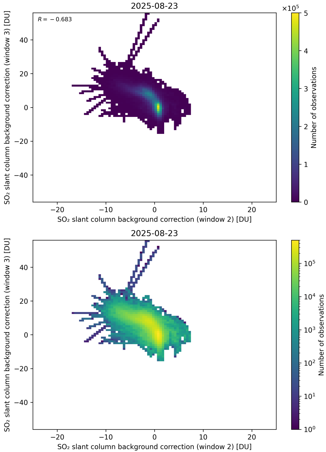
Figure 122: Scatter density plot of “SO 2 slant column background correction (window 2)” against “SO 2 slant column background correction (window 3)” for 2025-08-22 to 2025-08-24.
