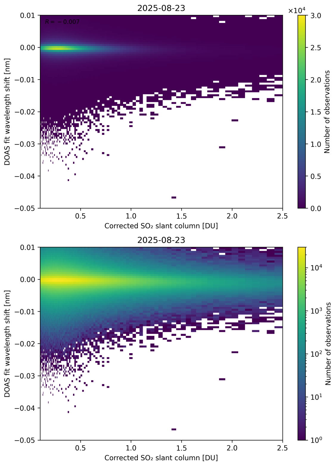
Figure 229: Scatter density plot of “Corrected SO 2 slant column” against “DOAS fit wavelength shift” for 2025-08-22 to 2025-08-24.
