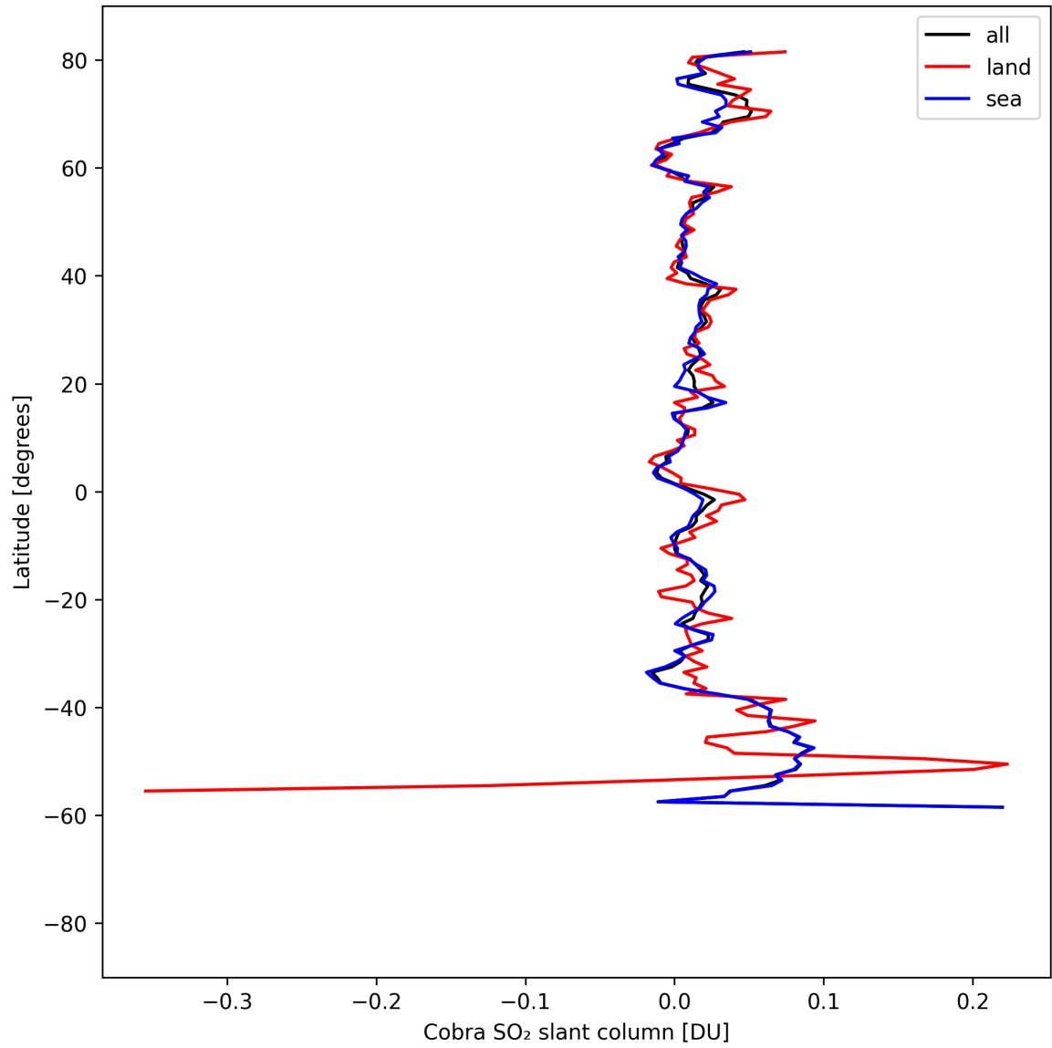
Figure 35: Zonal average of “Cobra SO 2 slant column” for 2025-08-22 to 2025-08-24.
