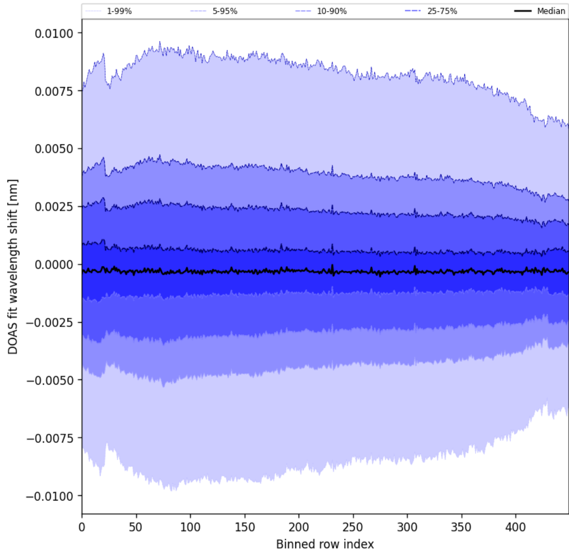
Figure 102: Along track statistics of “DOAS fit wavelength shift” for 2025-08-22 to 2025-08-24
