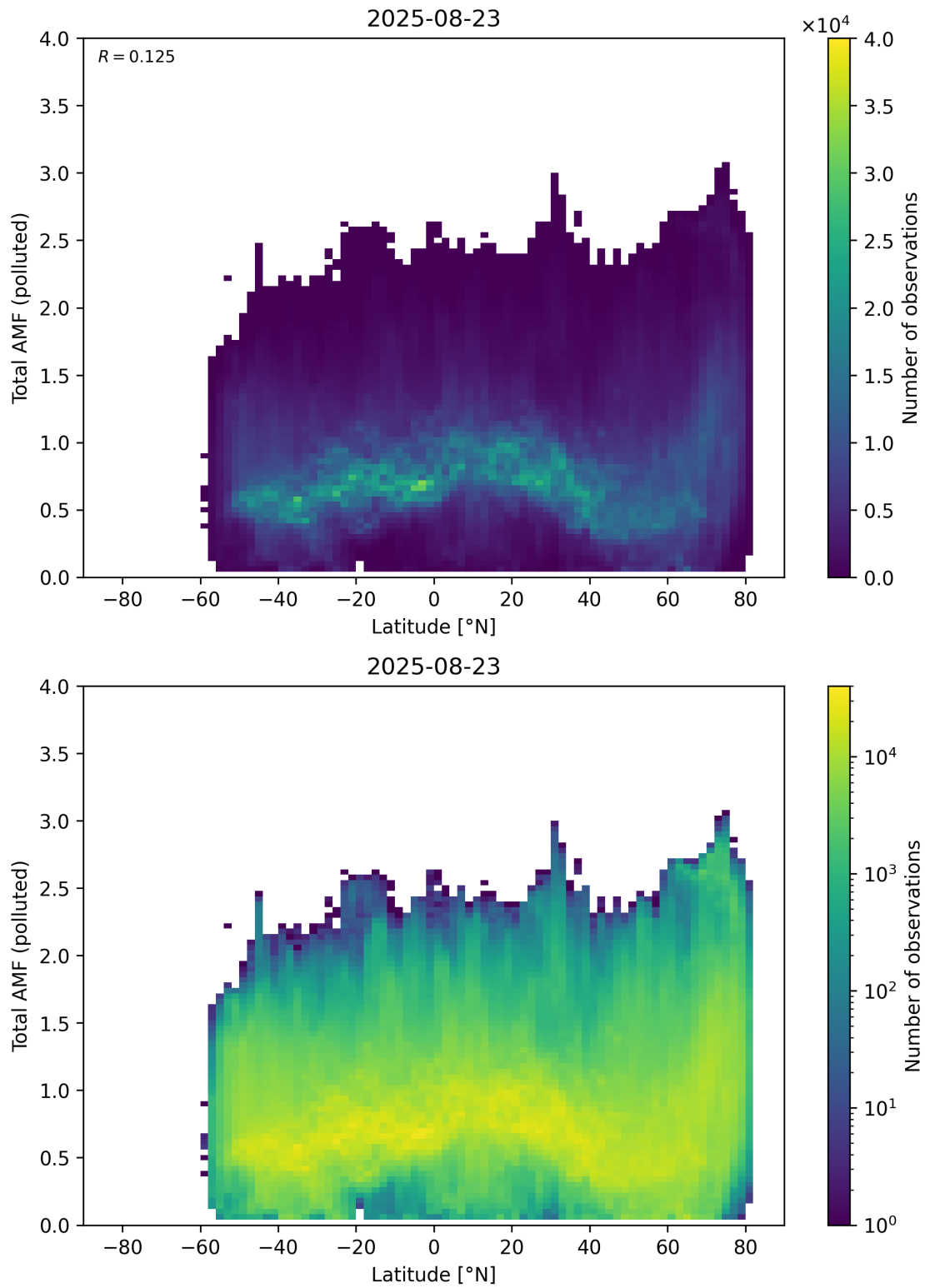
Figure 167: Scatter density plot of “Latitude” against “Total AMF (polluted)” for 2025-08-22 to 2025-08-24.
