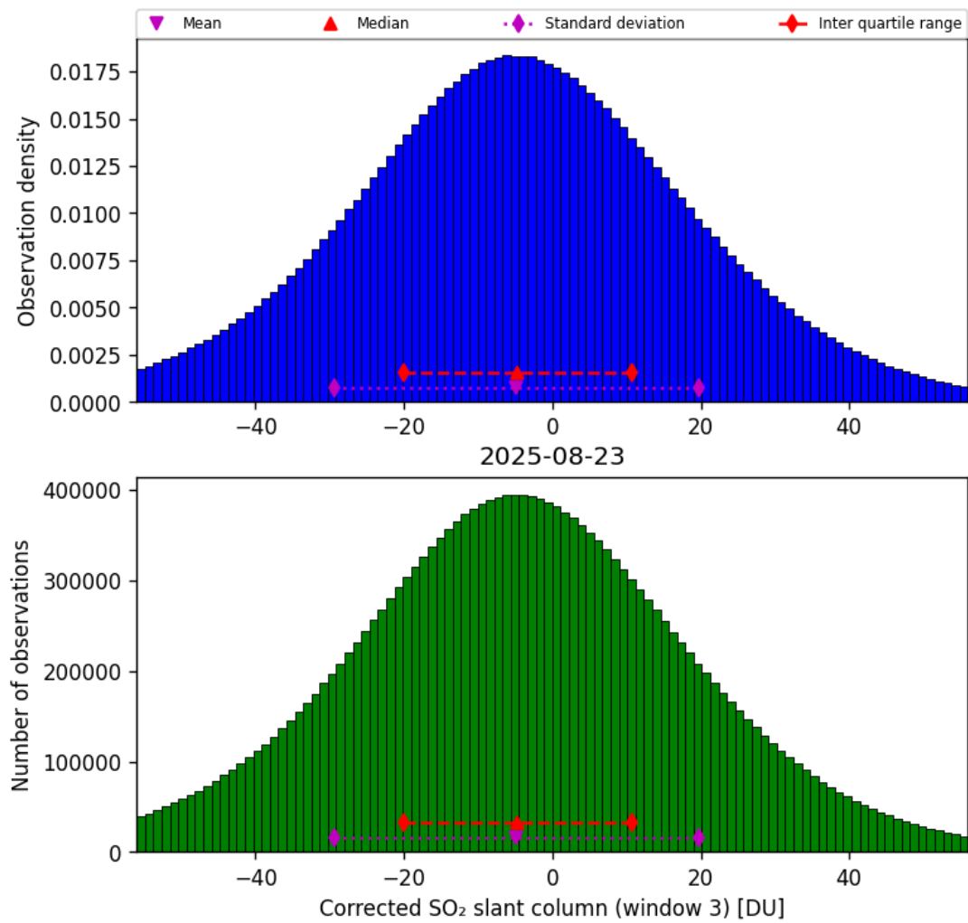
Figure 73: Histogram of “Corrected SO 2 slant column (window 3)” for 2025-08-22 to 2025-08-24
