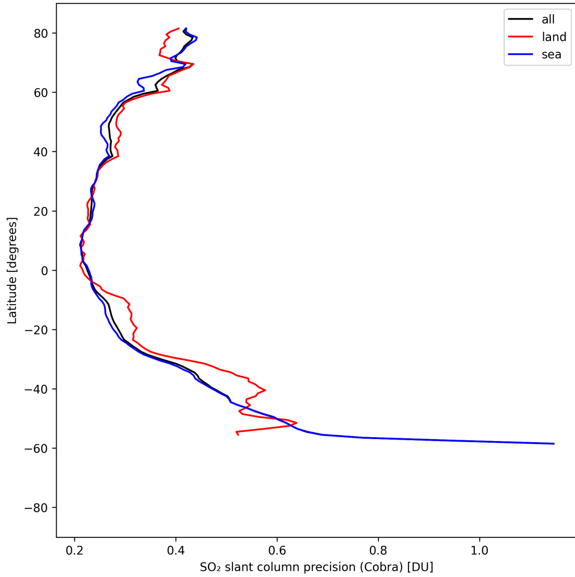
Figure 36: Zonal average of “SO 2 slant column precision (Cobra)” for 2025-08-22 to 2025-08-24.
