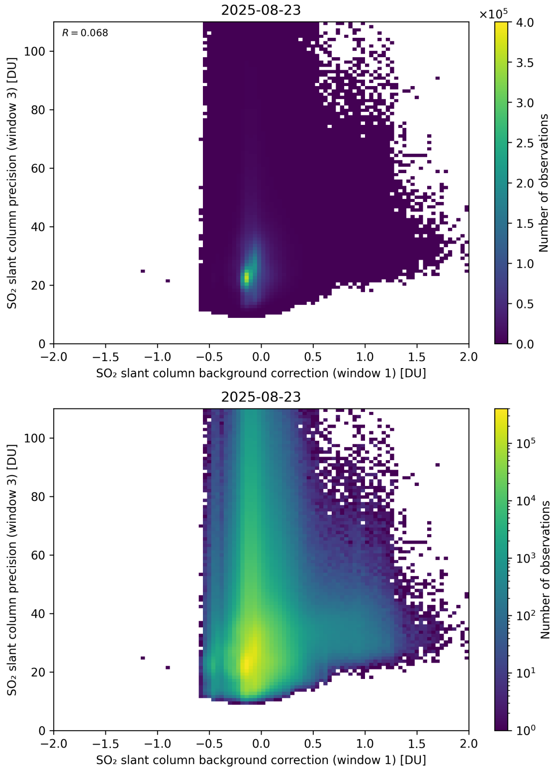
Figure 119: Scatter density plot of “SO 2 slant column background correction (window 1)” against “SO 2 slant column precision (window 3)” for 2025-08-22 to 2025-08-24.
