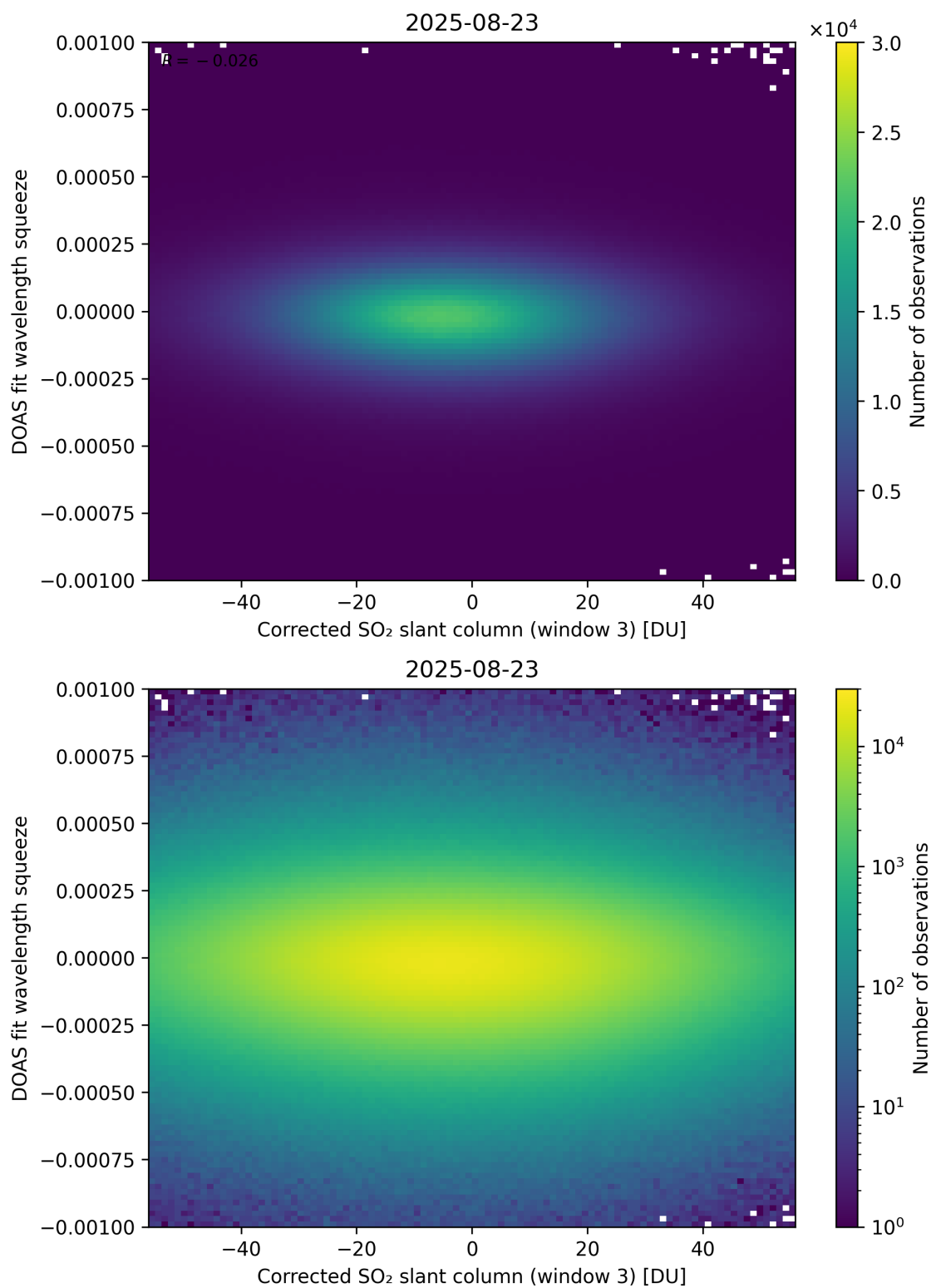
Figure 257: Scatter density plot of “Corrected SO 2 slant column (window 3)” against “DOAS fit wavelength squeeze” for 2025-08-22 to 2025-08-24.
