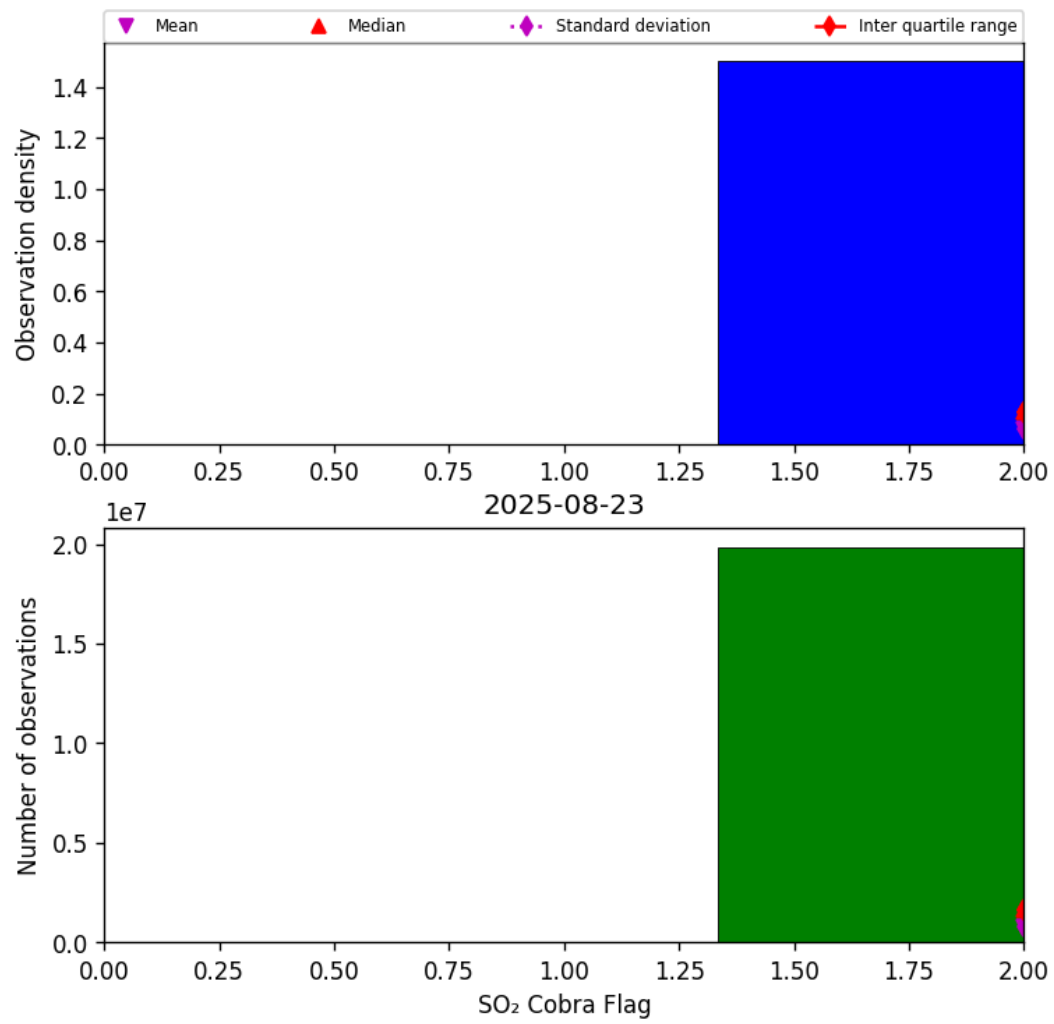
Figure 75: Histogram of “SO 2 Cobra Flag” for 2025-08-22 to 2025-08-24
