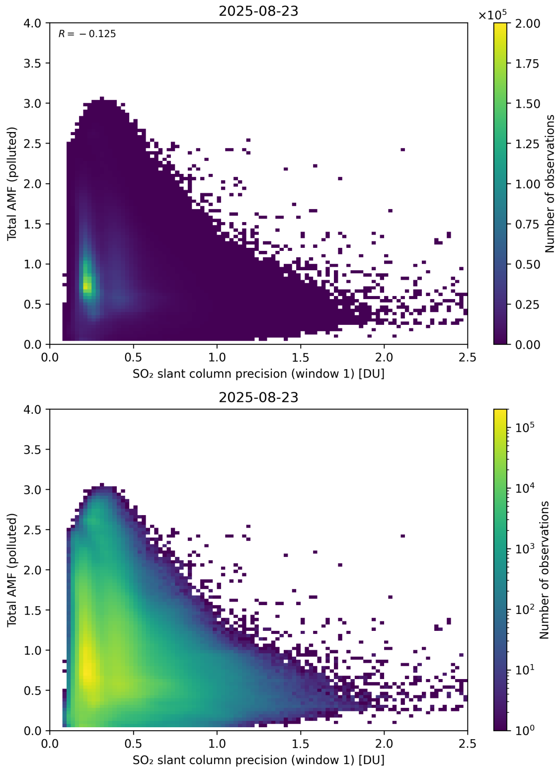
Figure 280: Scatter density plot of “SO 2 slant column precision (window 1)” against “Total AMF (polluted)” for 2025-08-22 to 2025-08-24.
