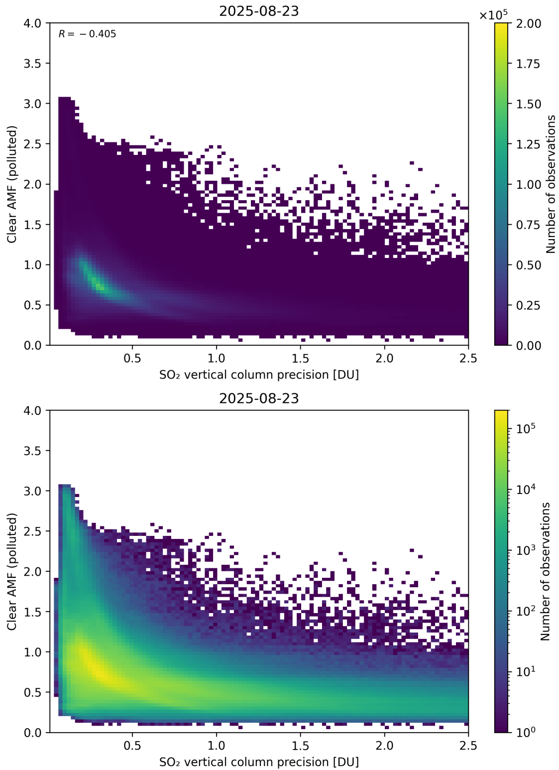
Figure 335: Scatter density plot of “SO 2 vertical column precision” against “Clear AMF (polluted)” for 2025-08-22 to 2025-08-24.
