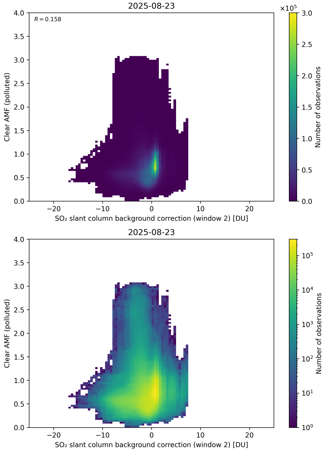
Figure 126: Scatter density plot of “SO 2 slant column background correction (window 2)” against “Clear AMF (polluted)” for 2025-08-22 to 2025-08-24.
