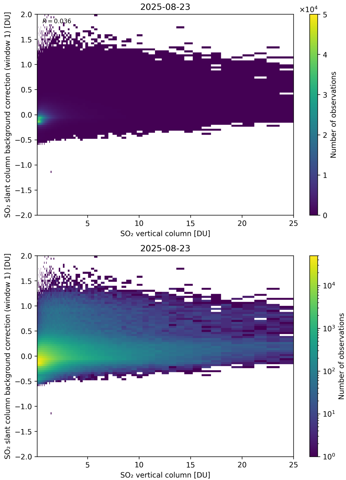
Figure 323: Scatter density plot of “SO 2 vertical column” against “SO 2 slant column background correction (window 1)” for 2025-08-22 to 2025-08-24.
