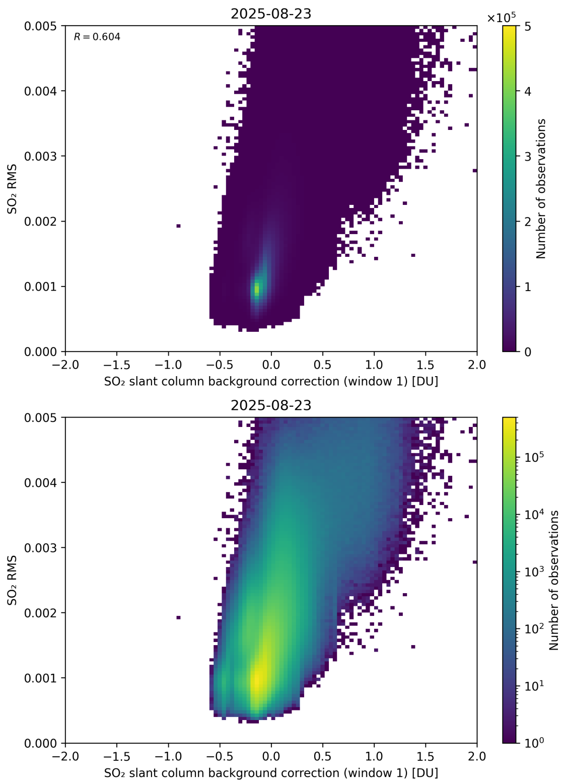
Figure 113: Scatter density plot of “SO 2 slant column background correction (window 1)” against “SO 2 RMS” for 2025-08-22 to 2025-08-24.
