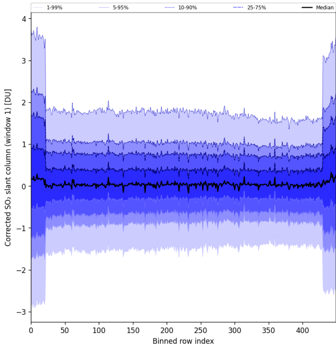
Figure 91: Along track statistics of “Corrected SO 2 slant column (window 1)” for 2025-08-22 to 2025-08-24
