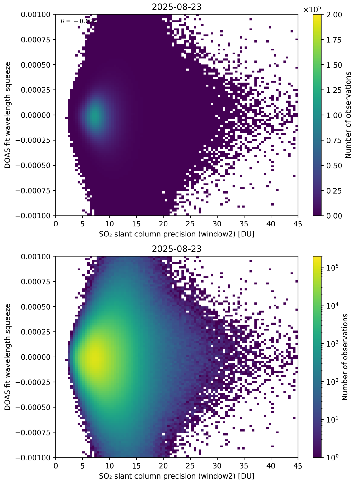
Figure 294: Scatter density plot of “SO 2 slant column precision (window2)” against “DOAS fit wavelength squeeze” for 2025-08-22 to 2025-08-24.
