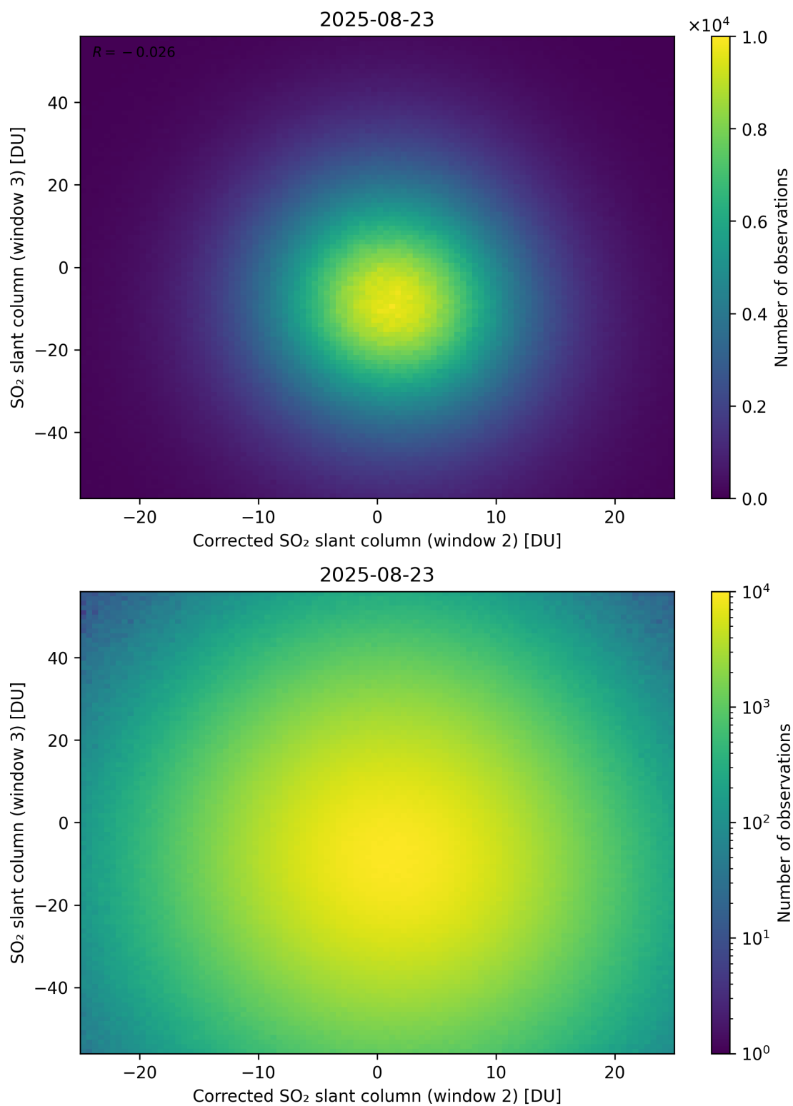
Figure 251: Scatter density plot of “Corrected SO 2 slant column (window 2)” against “SO 2 slant column (window 3)” for 2025-08-22 to 2025-08-24.
