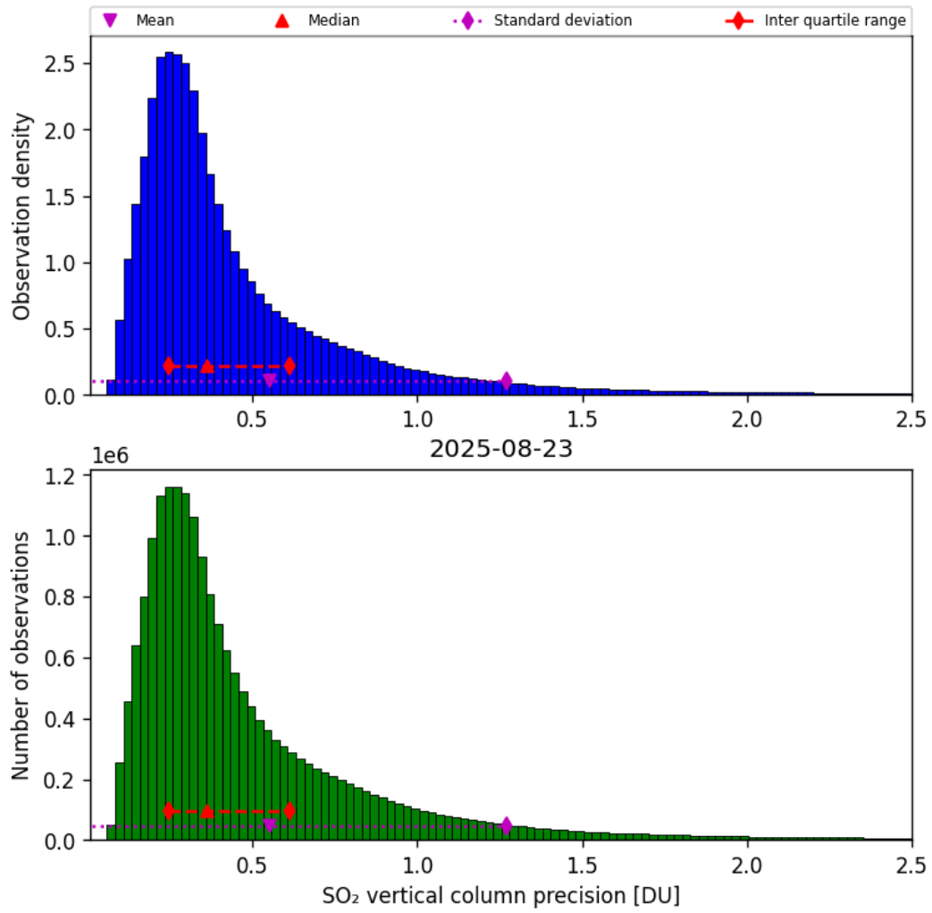
Figure 59: Histogram of “SO 2 vertical column precision” for 2025-08-22 to 2025-08-24
