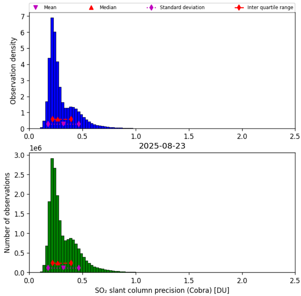
Figure 62: Histogram of “SO 2 slant column precision (Cobra)” for 2025-08-22 to 2025-08-24
