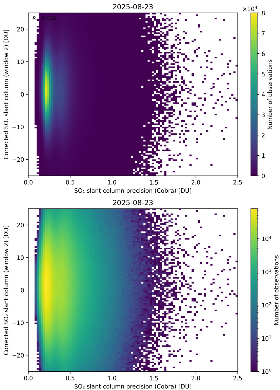
Figure 206: Scatter density plot of “SO 2 slant column precision (Cobra)” against “Corrected SO 2 slant column (window 2)” for 2025-08-22 to 2025-08-24.
