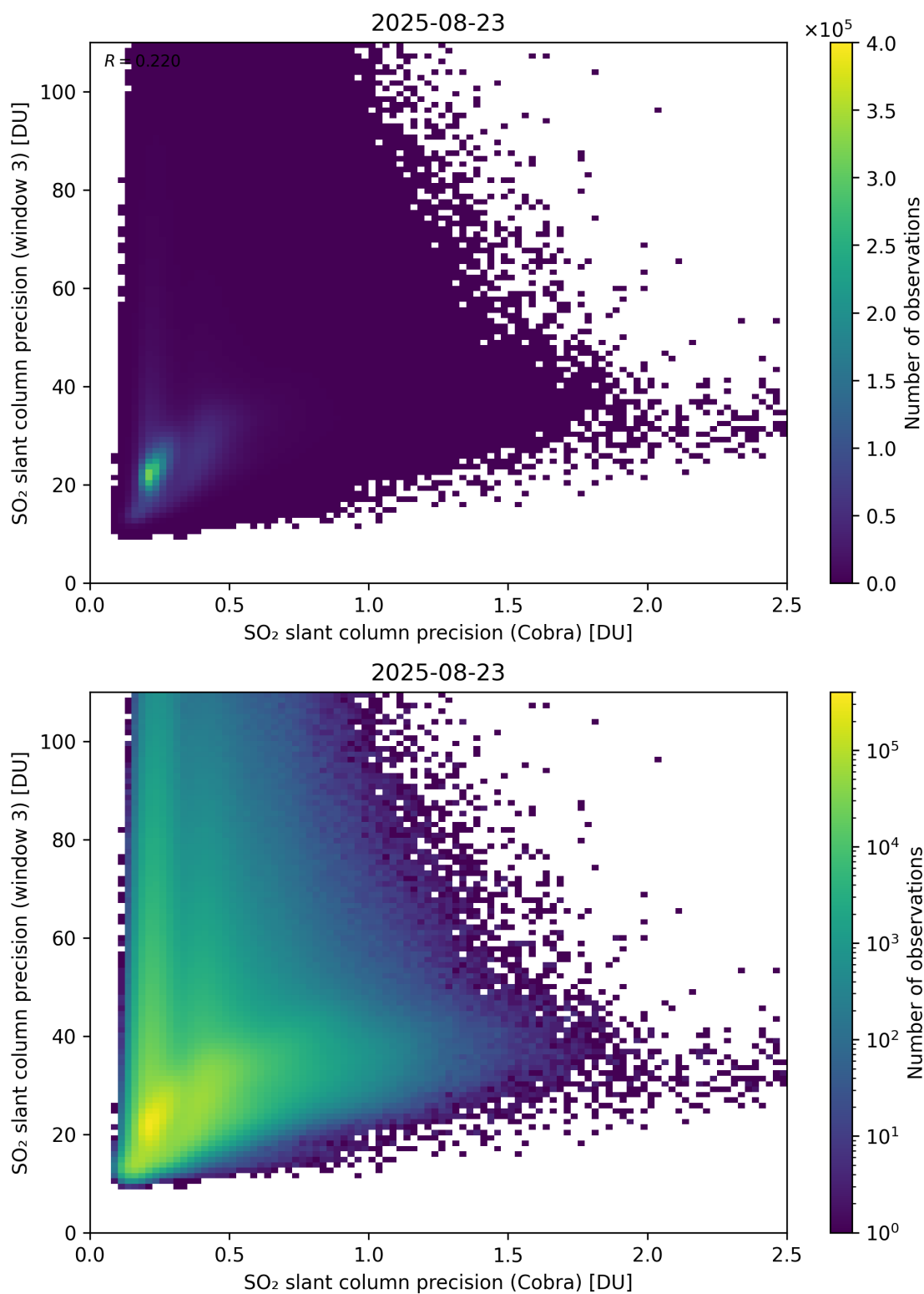
Figure 212: Scatter density plot of “SO 2 slant column precision (Cobra)” against “SO 2 slant column precision (window 3)” for 2025-08-22 to 2025-08-24.
