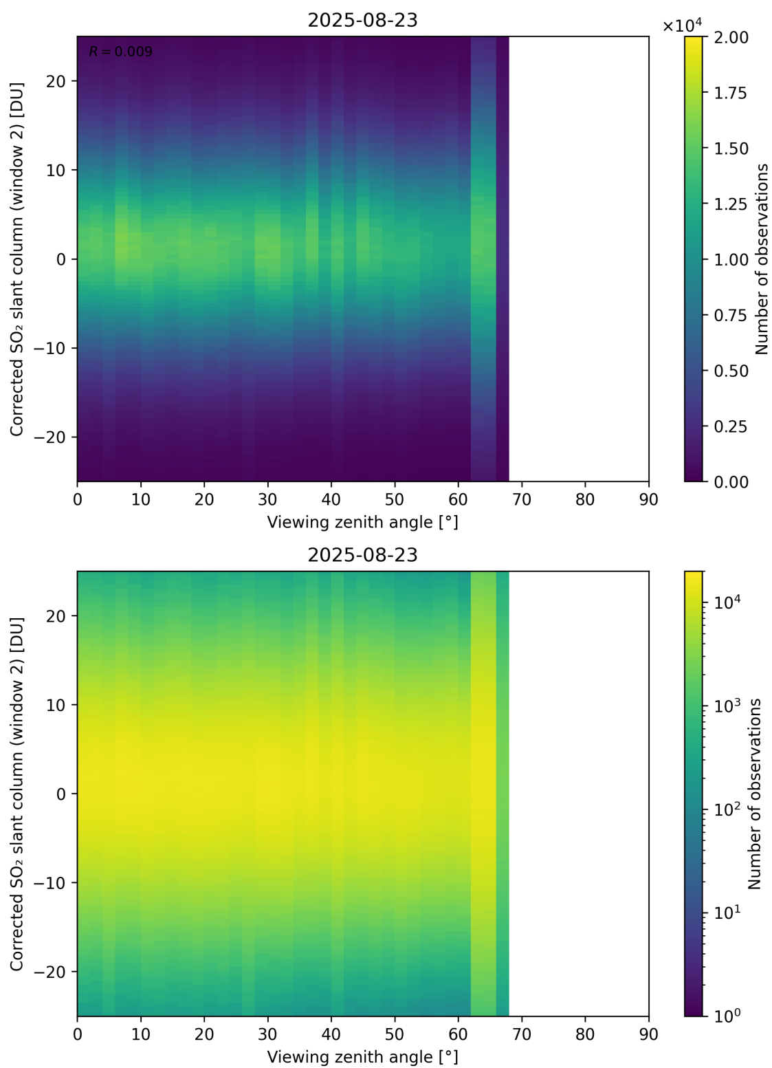
Figure 374: Scatter density plot of “Viewing zenith angle” against “Corrected SO 2 slant column (window 2)” for 2025-08-22 to 2025-08-24.
