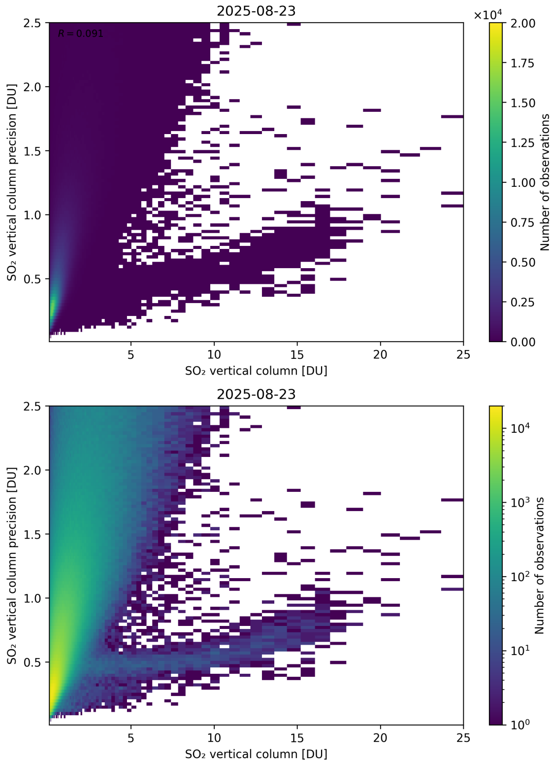
Figure 361: Scatter density plot of “SO 2 vertical column” against “SO 2 vertical column precision” for 2025-08-22 to 2025-08-24.
