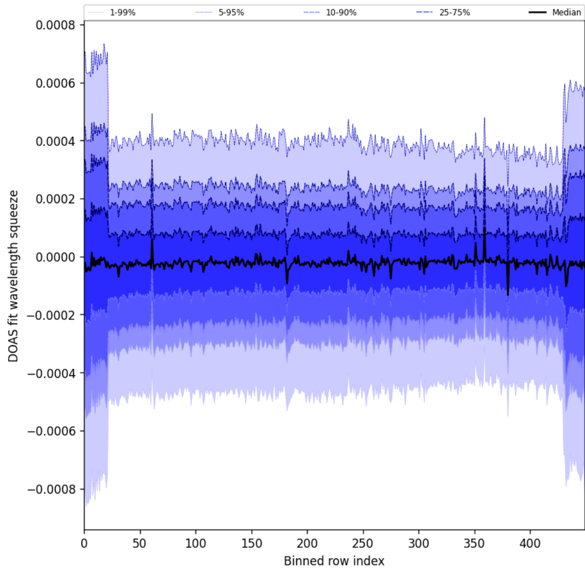
Figure 103: Along track statistics of “DOAS fit wavelength squeeze” for 2025-08-22 to 2025-08-24
