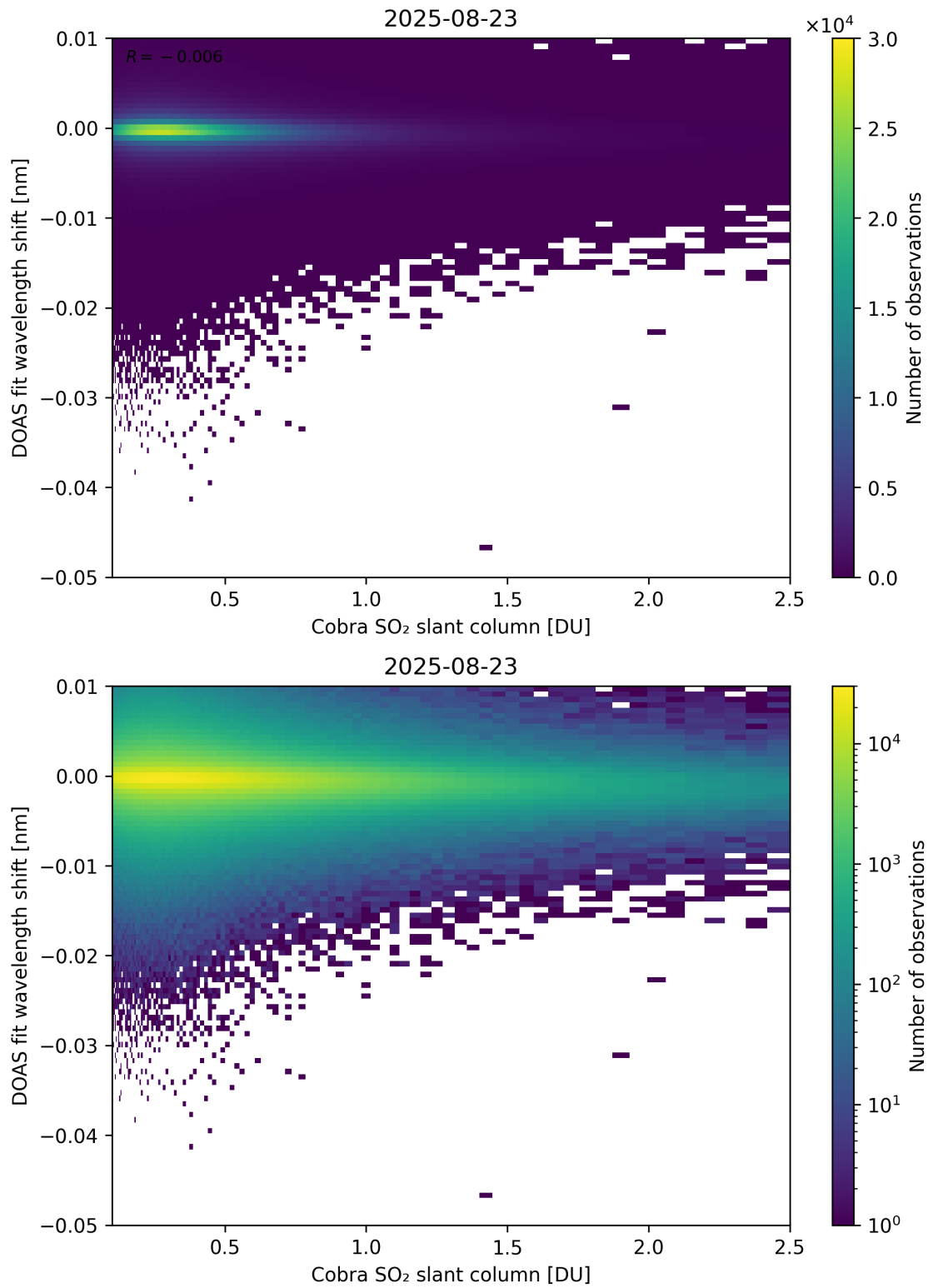
Figure 196: Scatter density plot of “Cobra SO 2 slant column” against “DOAS fit wavelength shift” for 2025-08-22 to 2025-08-24.
