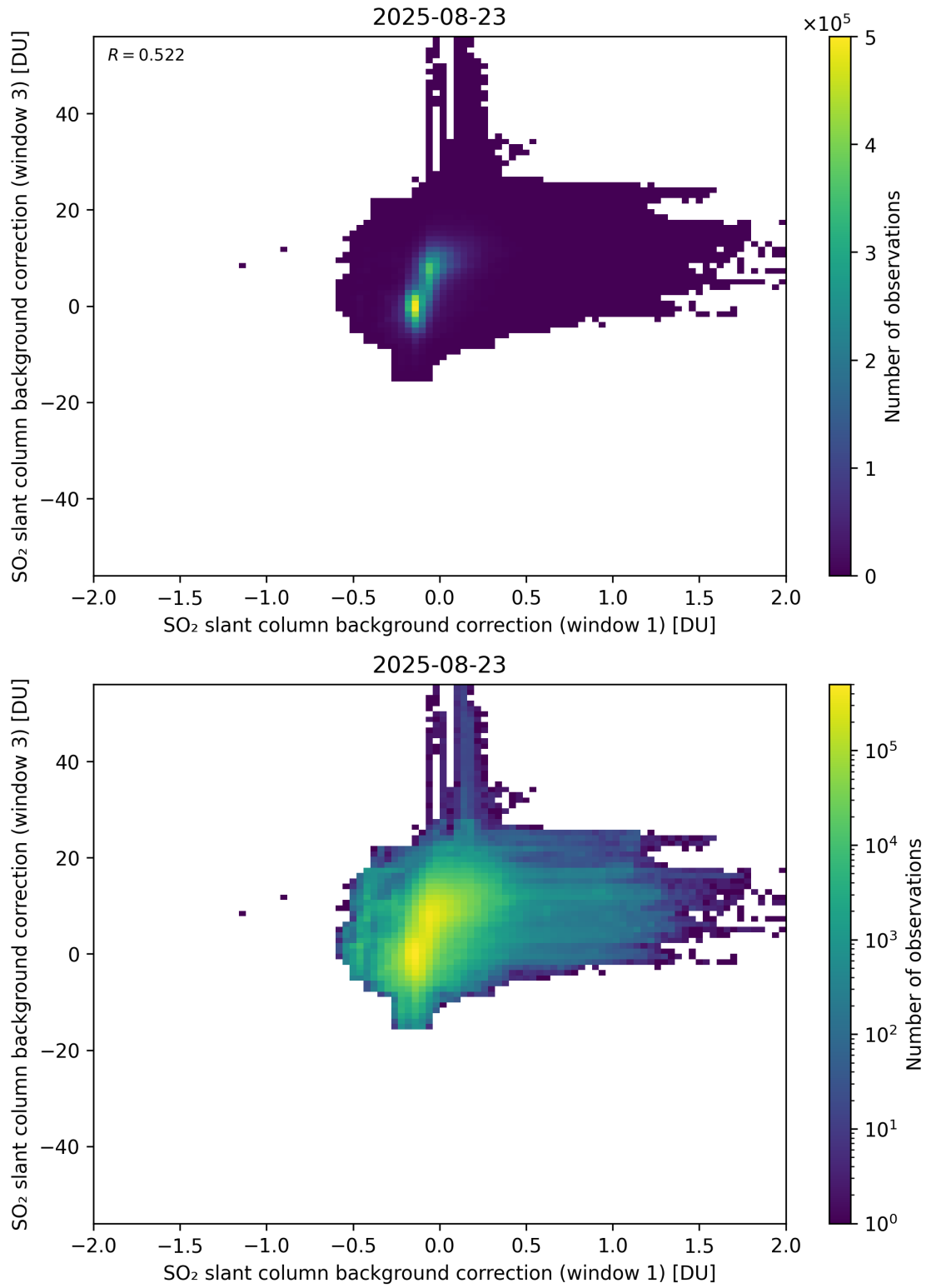
Figure 110: Scatter density plot of “SO 2 slant column background correction (window 1)” against “SO 2 slant column background correction (window 3)” for 2025-08-22 to 2025-08-24.
