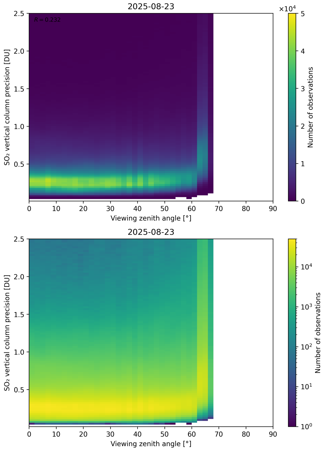
Figure 384: Scatter density plot of “Viewing zenith angle” against “SO 2 vertical column precision” for 2025-08-22 to 2025-08-24.
