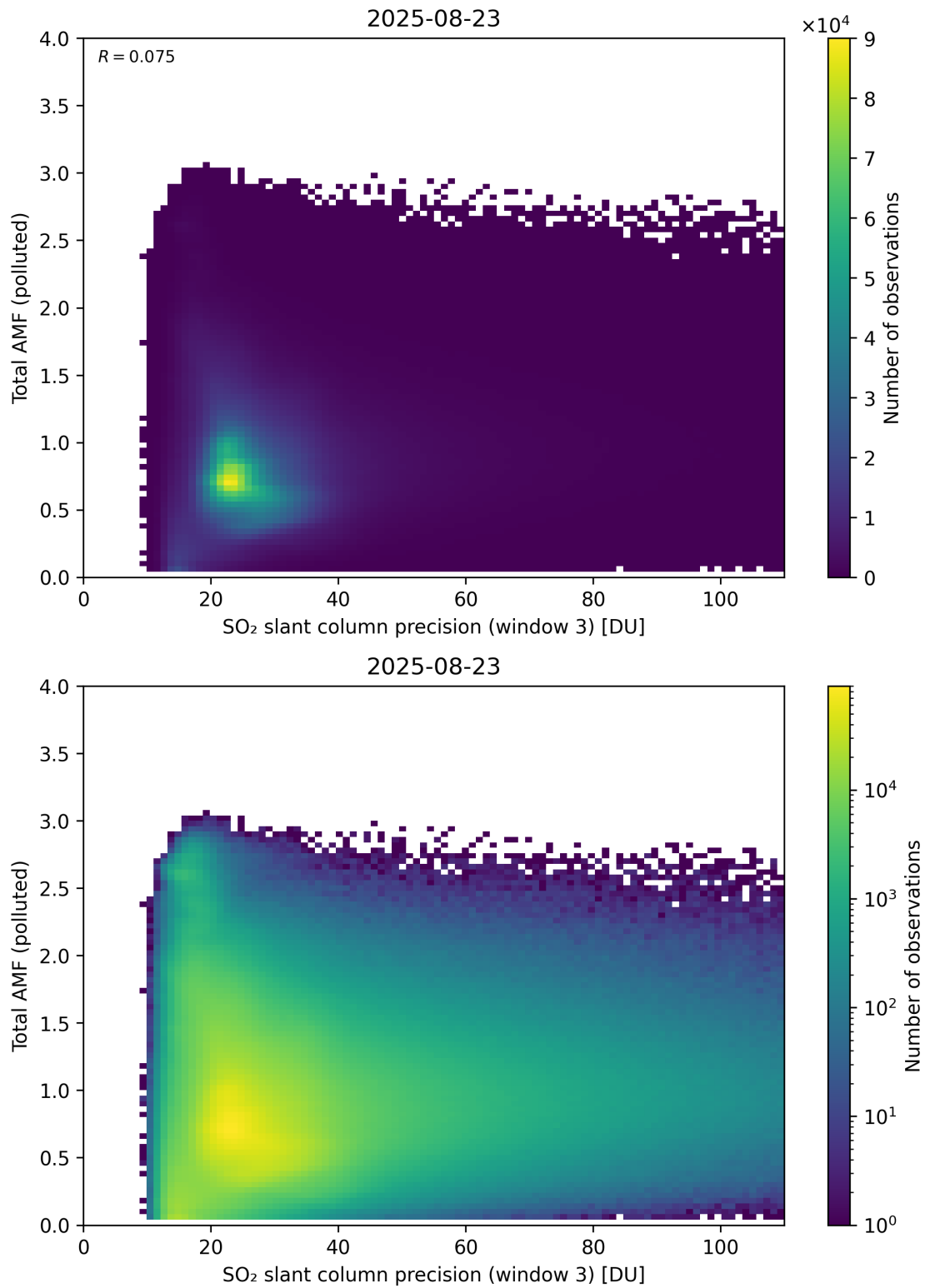
Figure 313: Scatter density plot of “SO 2 slant column precision (window 3)” against “Total AMF (polluted)” for 2025-08-22 to 2025-08-24.
