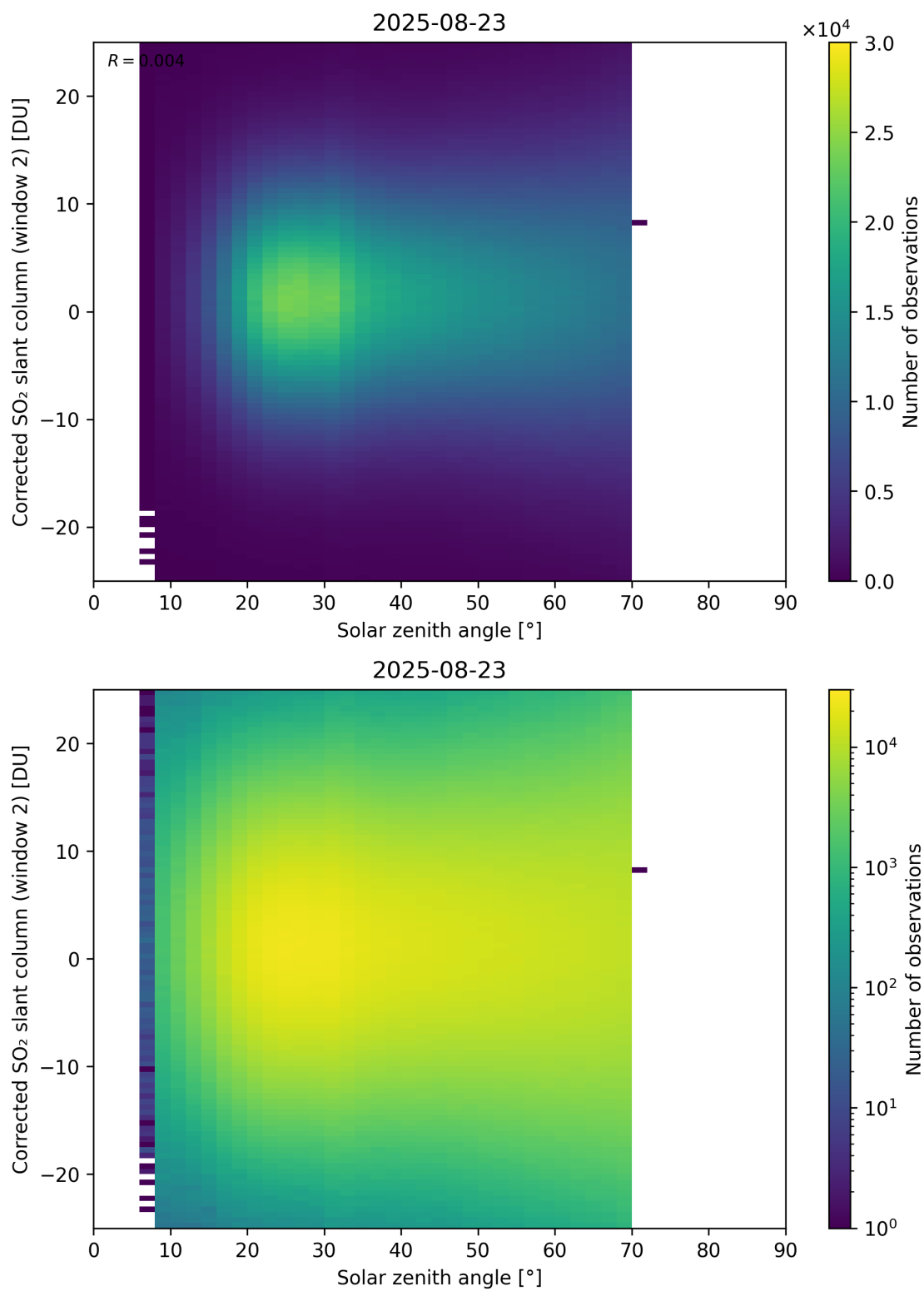
Figure 182: Scatter density plot of “Solar zenith angle” against “Corrected SO 2 slant column (window 2)” for 2025-08-22 to 2025-08-24.
