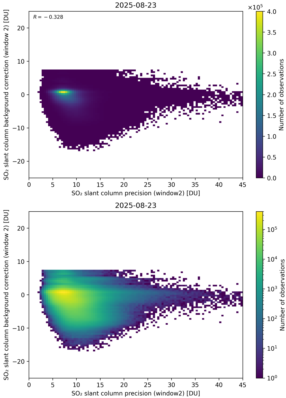
Figure 291: Scatter density plot of “SO 2 slant column precision (window2)” against “SO 2 slant column background correction (window 2)” for 2025-08-22 to 2025-08-24.
