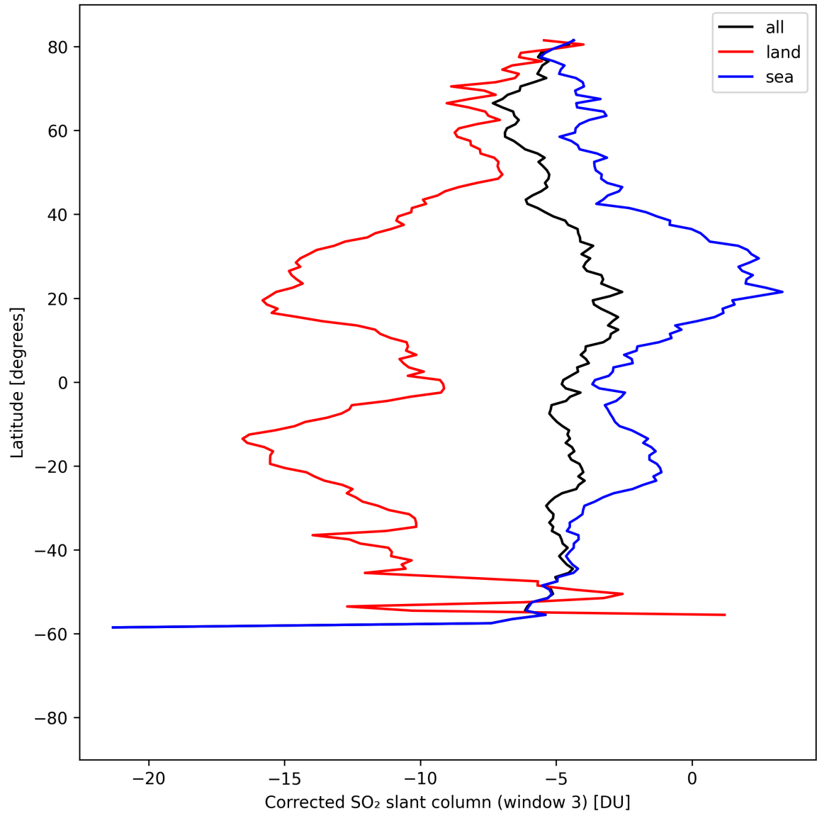
Figure 47: Zonal average of “Corrected SO 2 slant column (window 3)” for 2025-08-22 to 2025-08-24.
