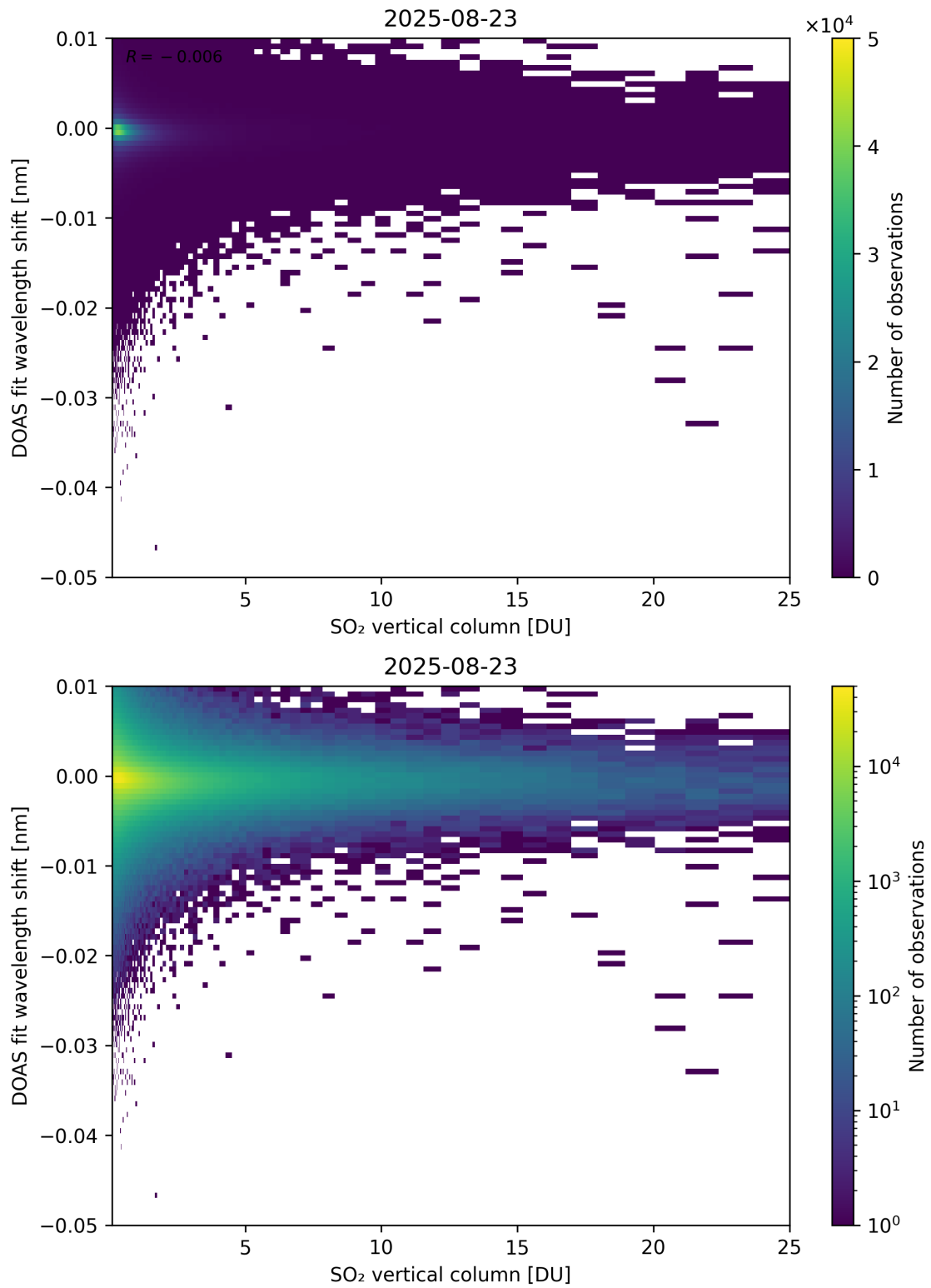
Figure 326: Scatter density plot of “SO 2 vertical column” against “DOAS fit wavelength shift” for 2025-08-22 to 2025-08-24.
