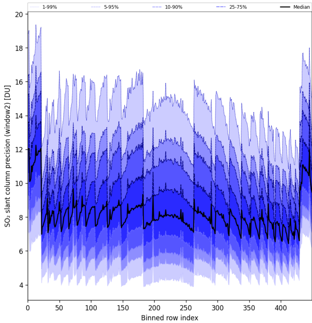
Figure 94: Along track statistics of “SO 2 slant column precision (window2)” for 2025-08-22 to 2025-08-24
