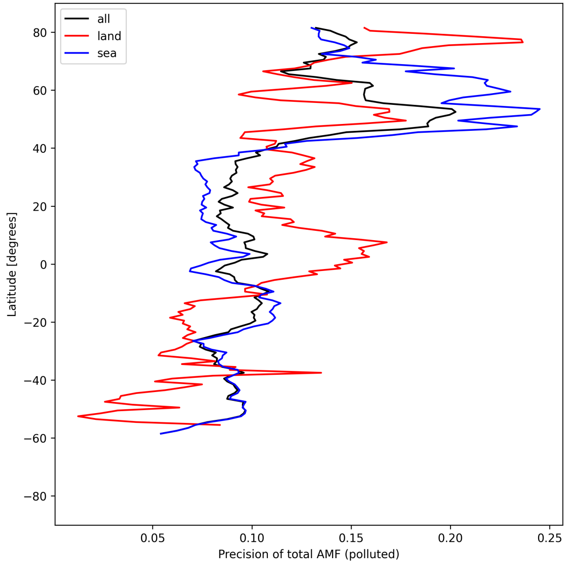
Figure 54: Zonal average of “Precision of total AMF (polluted)” for 2025-08-22 to 2025-08-24.
