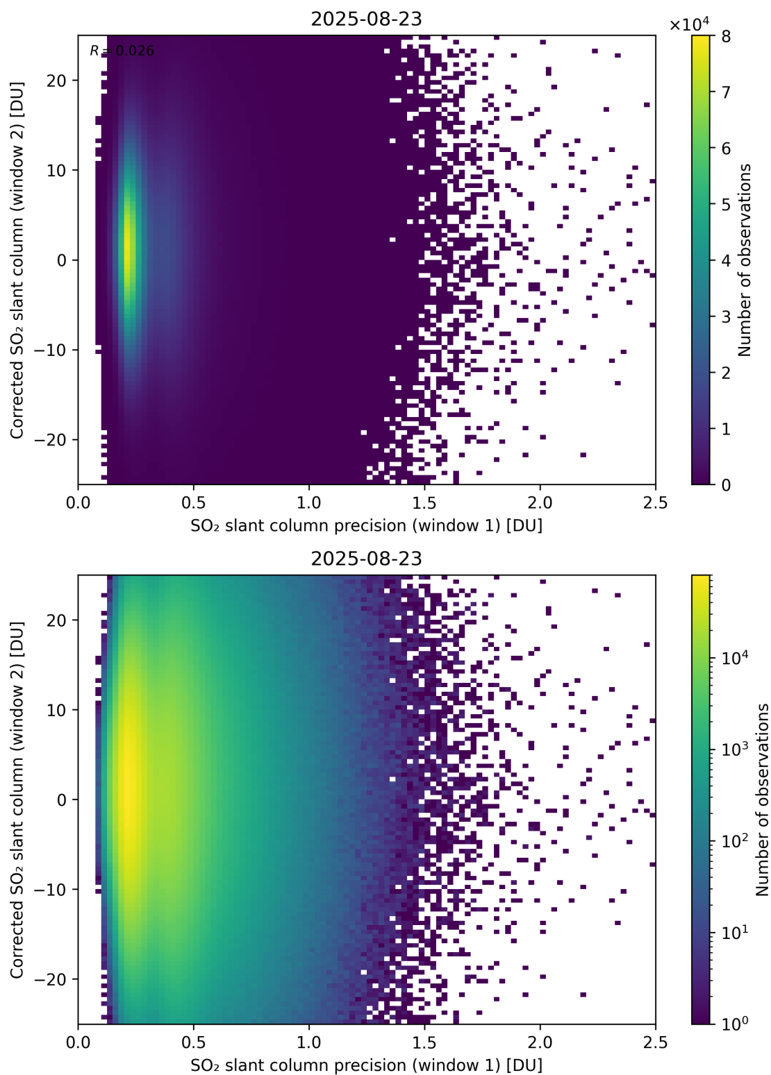
Figure 275: Scatter density plot of “SO 2 slant column precision (window 1)” against “Corrected SO 2 slant column (window 2)” for 2025-08-22 to 2025-08-24.
