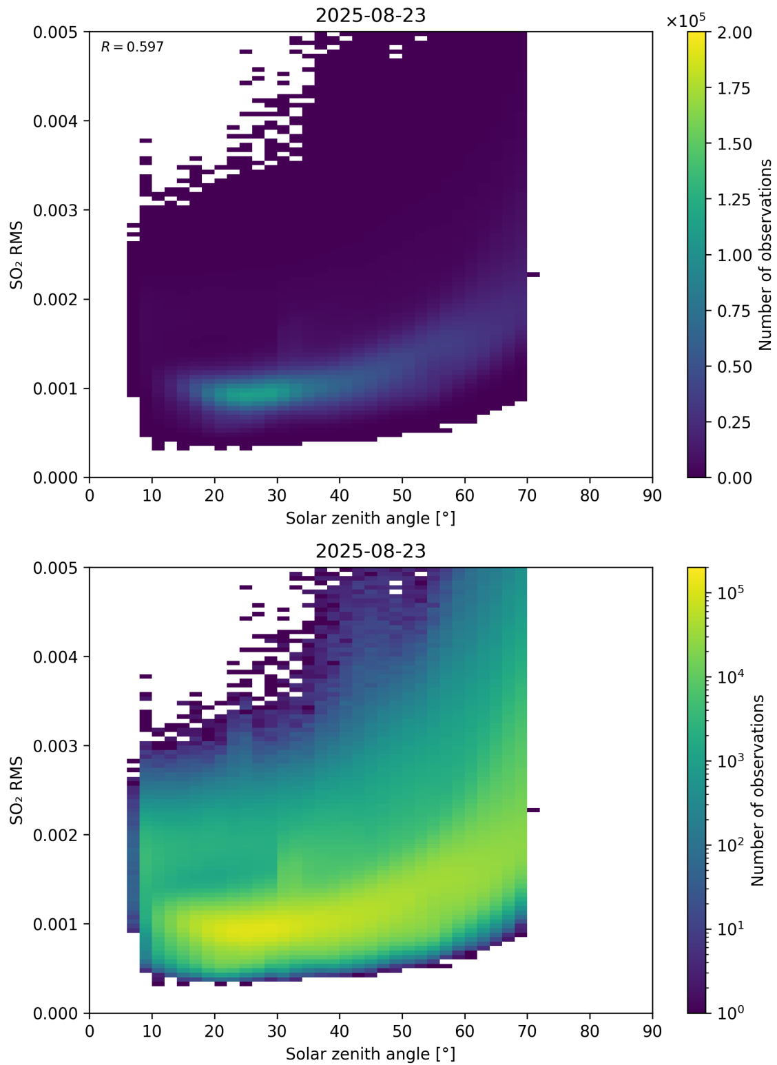
Figure 176: Scatter density plot of “Solar zenith angle” against “SO 2 RMS” for 2025-08-22 to 2025-08-24.
