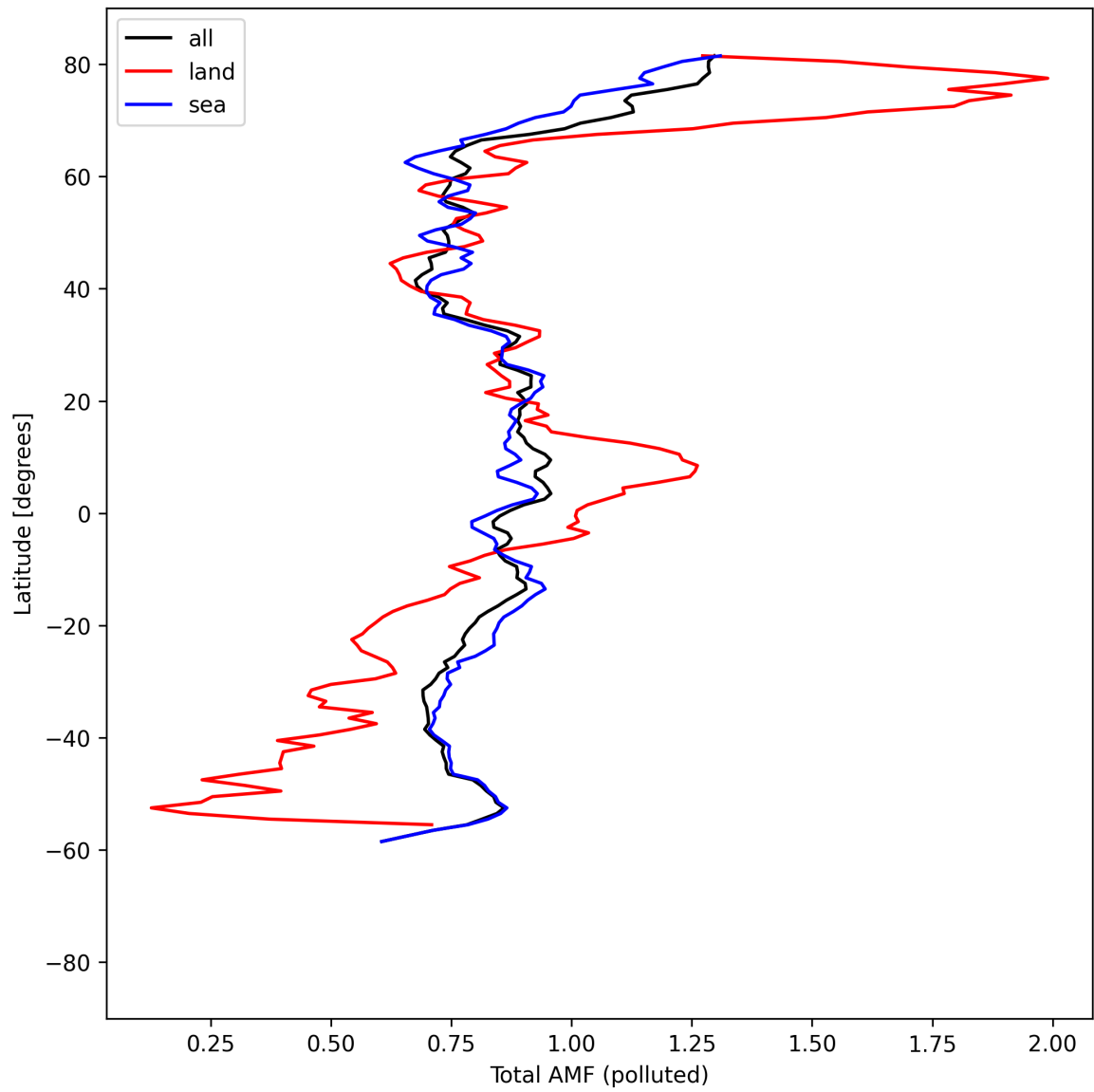
Figure 53: Zonal average of “Total AMF (polluted)” for 2025-08-22 to 2025-08-24.
