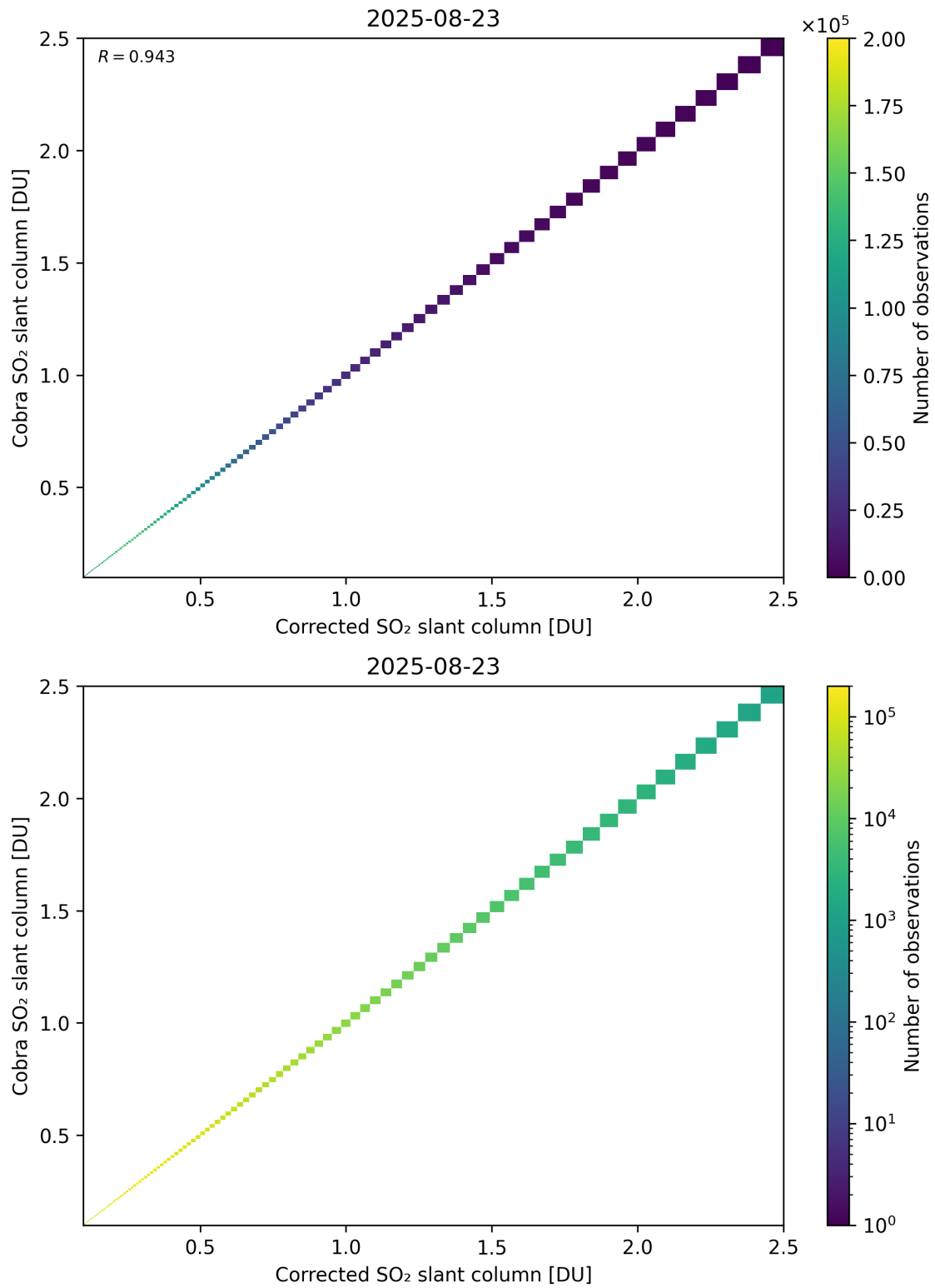
Figure 233: Scatter density plot of “Corrected SO 2 slant column” against “Cobra SO 2 slant column” for 2025-08-22 to 2025-08-24.
