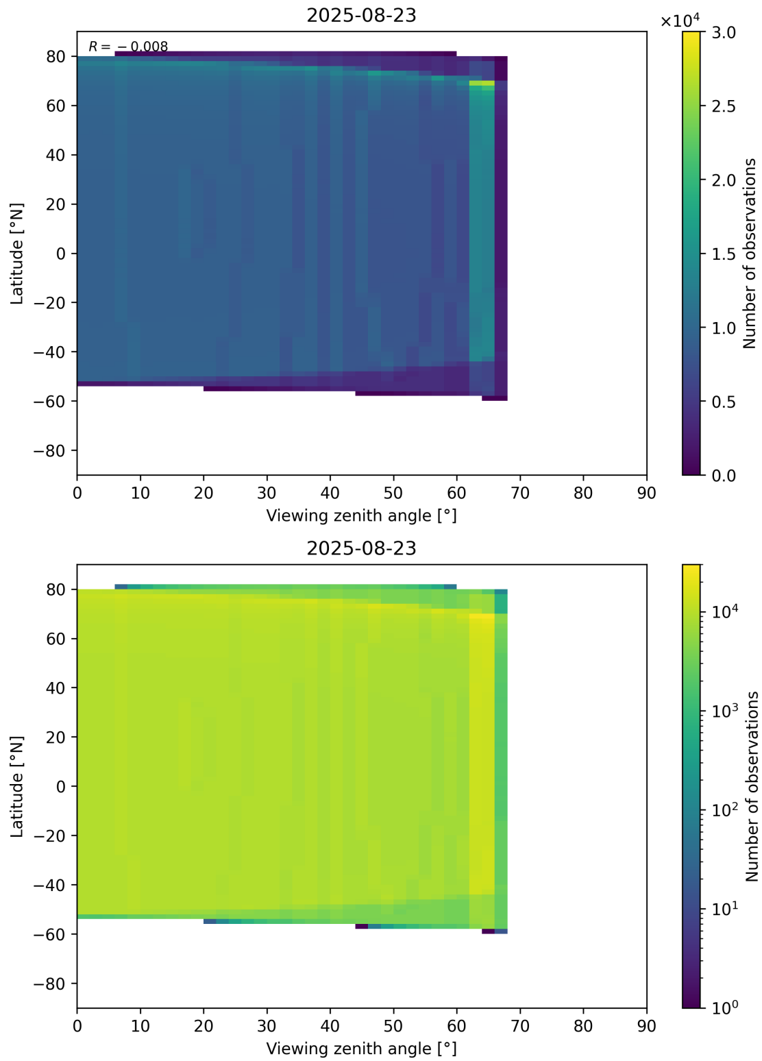
Figure 368: Scatter density plot of “Viewing zenith angle” against “Latitude” for 2025-08-22 to 2025-08-24.
