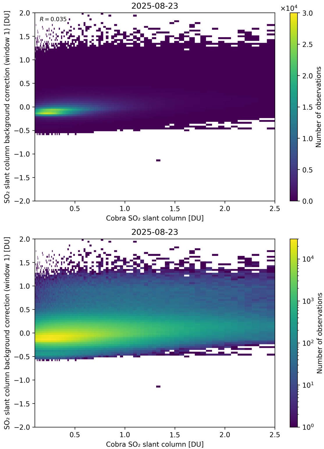
Figure 193: Scatter density plot of “Cobra SO 2 slant column” against “SO 2 slant column background correction (window 1)” for 2025-08-22 to 2025-08-24.
