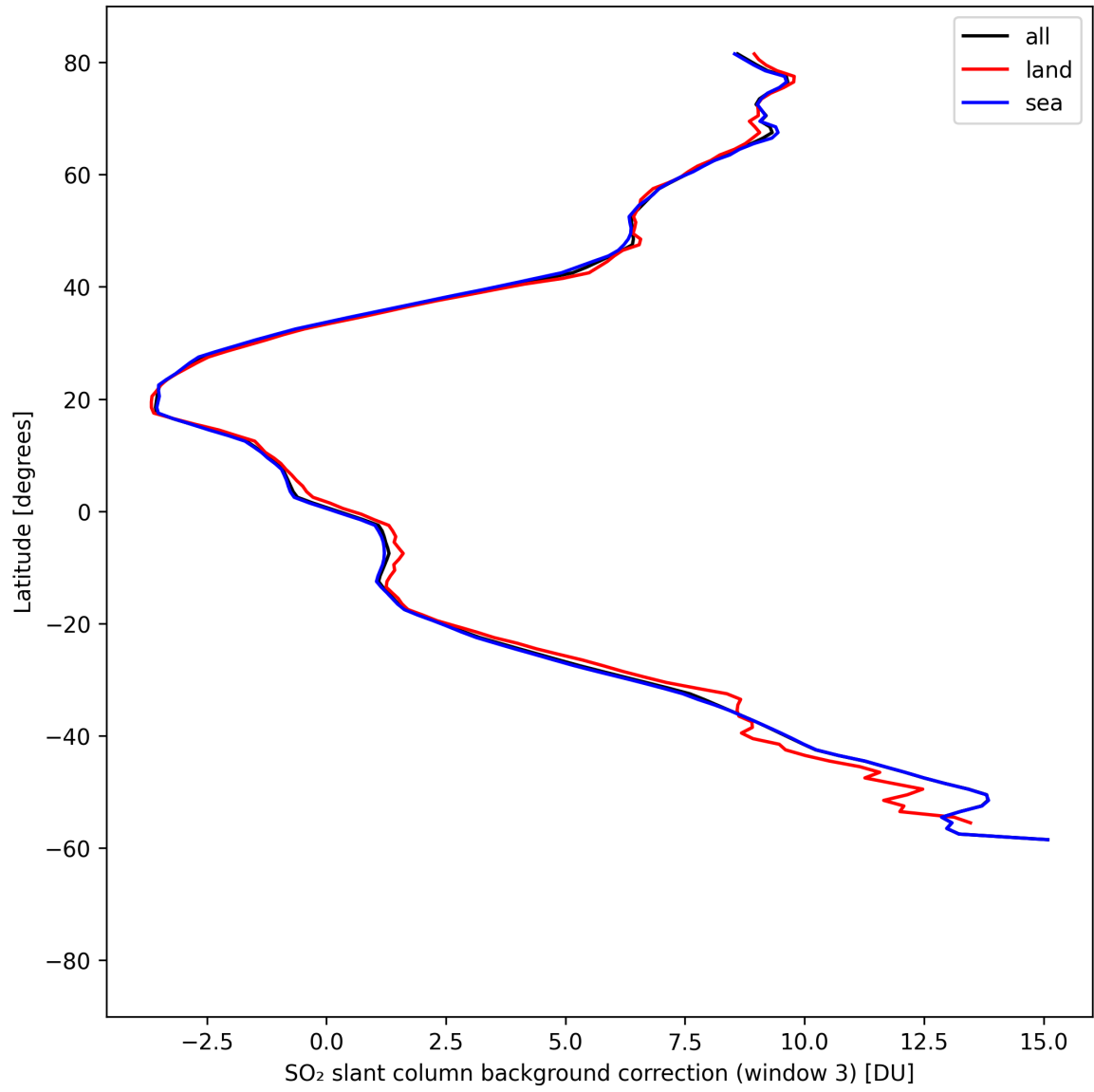
Figure 48: Zonal average of “SO 2 slant column background correction (window 3)” for 2025-08-22 to 2025-08-24.
