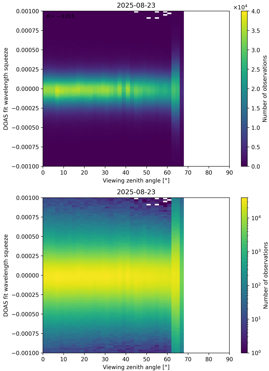
Figure 366: Scatter density plot of “Viewing zenith angle” against “DOAS fit wavelength squeeze” for 2025-08-22 to 2025-08-24.
