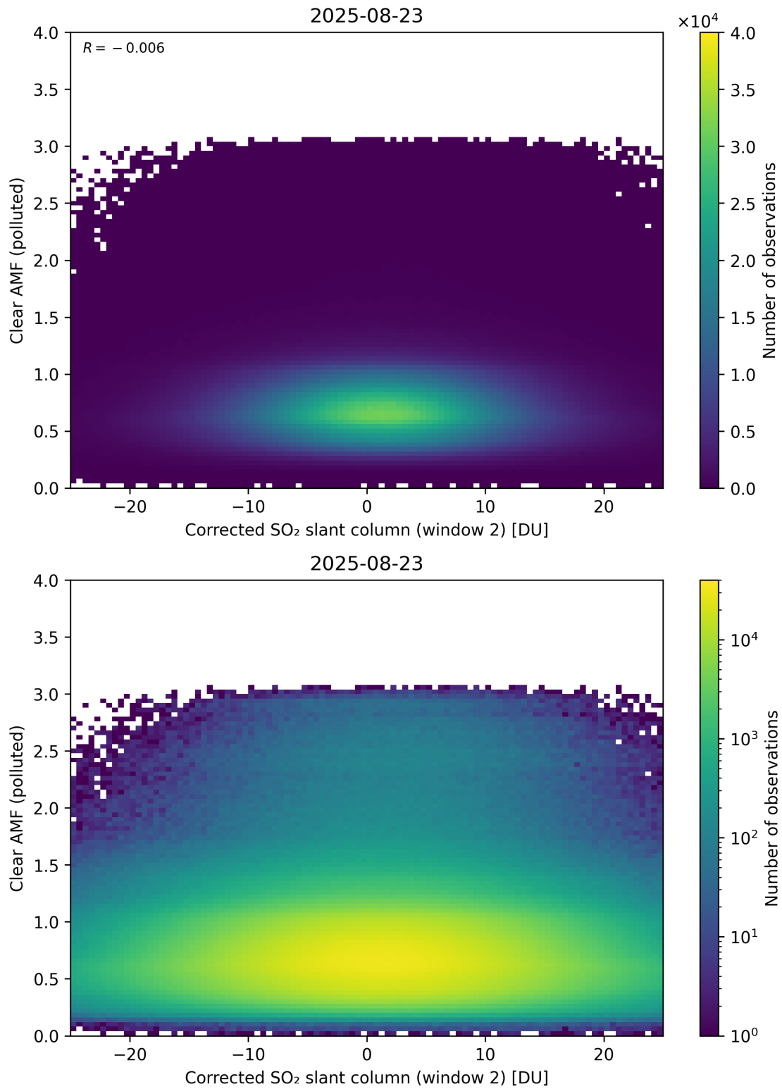
Figure 249: Scatter density plot of “Corrected SO 2 slant column (window 2)” against “Clear AMF (polluted)” for 2025-08-22 to 2025-08-24.
