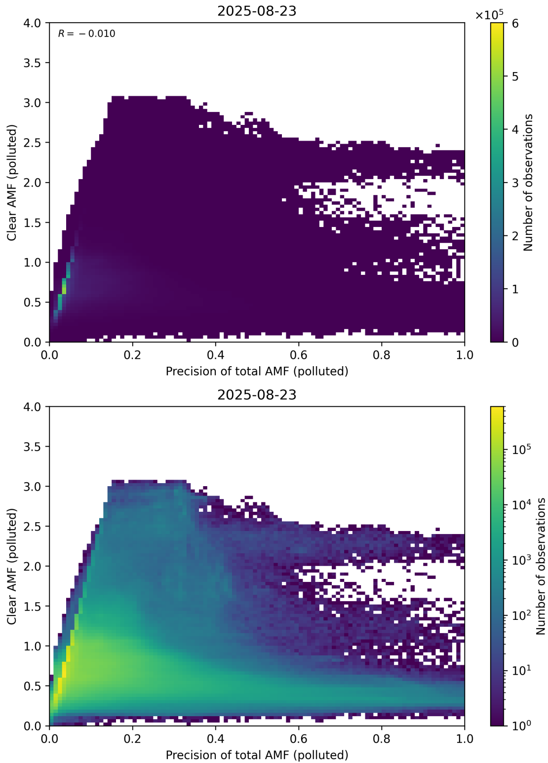
Figure 320: Scatter density plot of “Precision of total AMF (polluted)” against “Clear AMF (polluted)” for 2025-08-22 to 2025-08-24.
