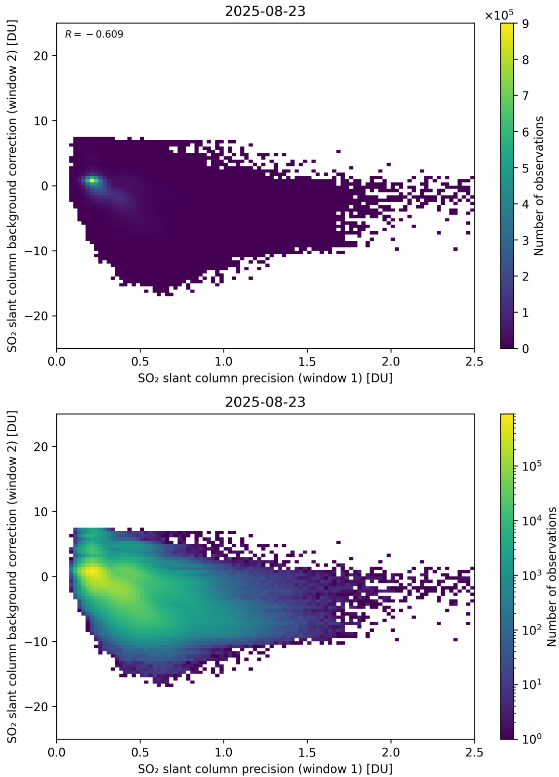
Figure 269: Scatter density plot of “SO 2 slant column precision (window 1)” against “SO 2 slant column background correction (window 2)” for 2025-08-22 to 2025-08-24.
