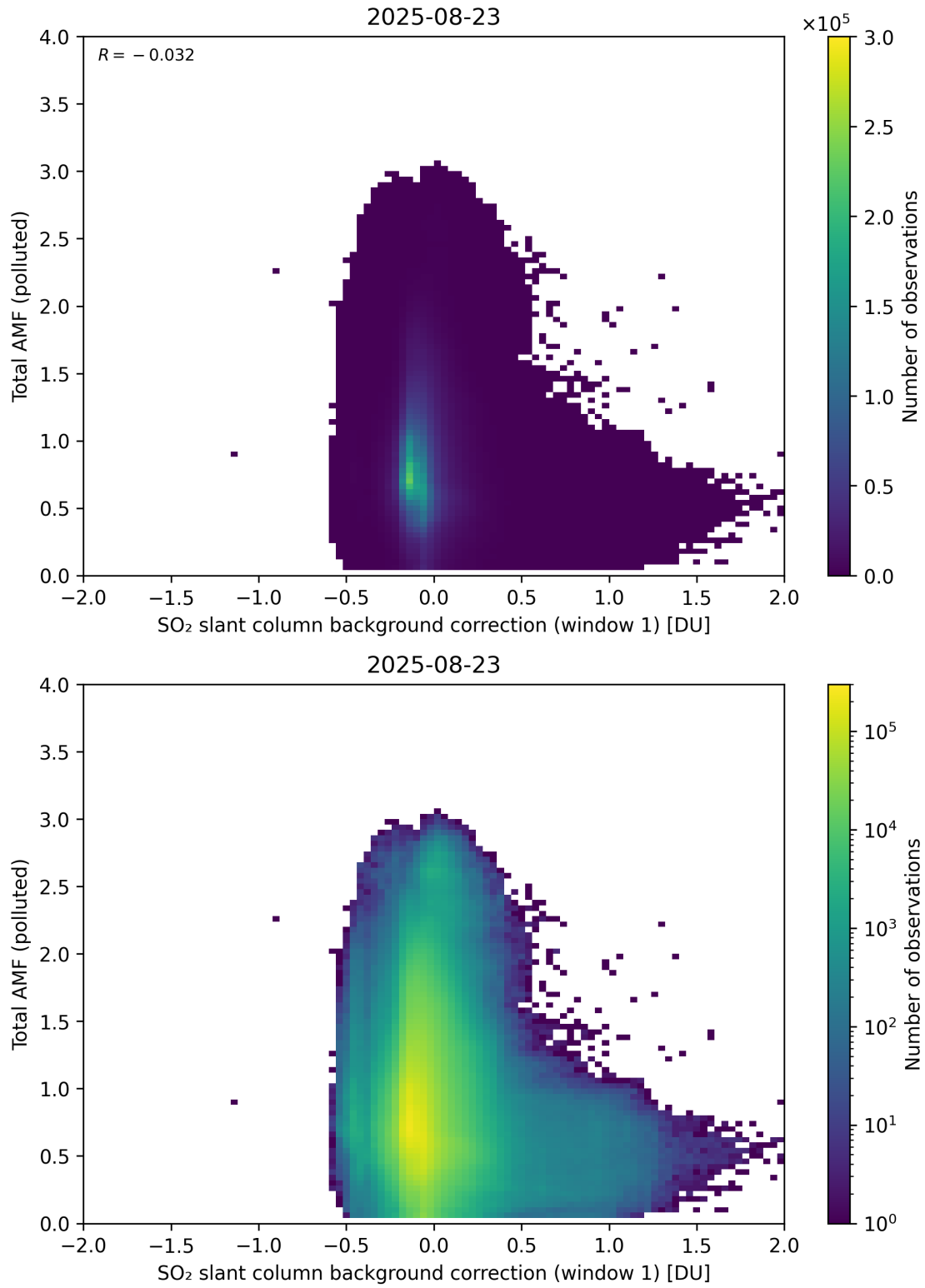
Figure 120: Scatter density plot of “SO 2 slant column background correction (window 1)” against “Total AMF (polluted)” for 2025-08-22 to 2025-08-24.
