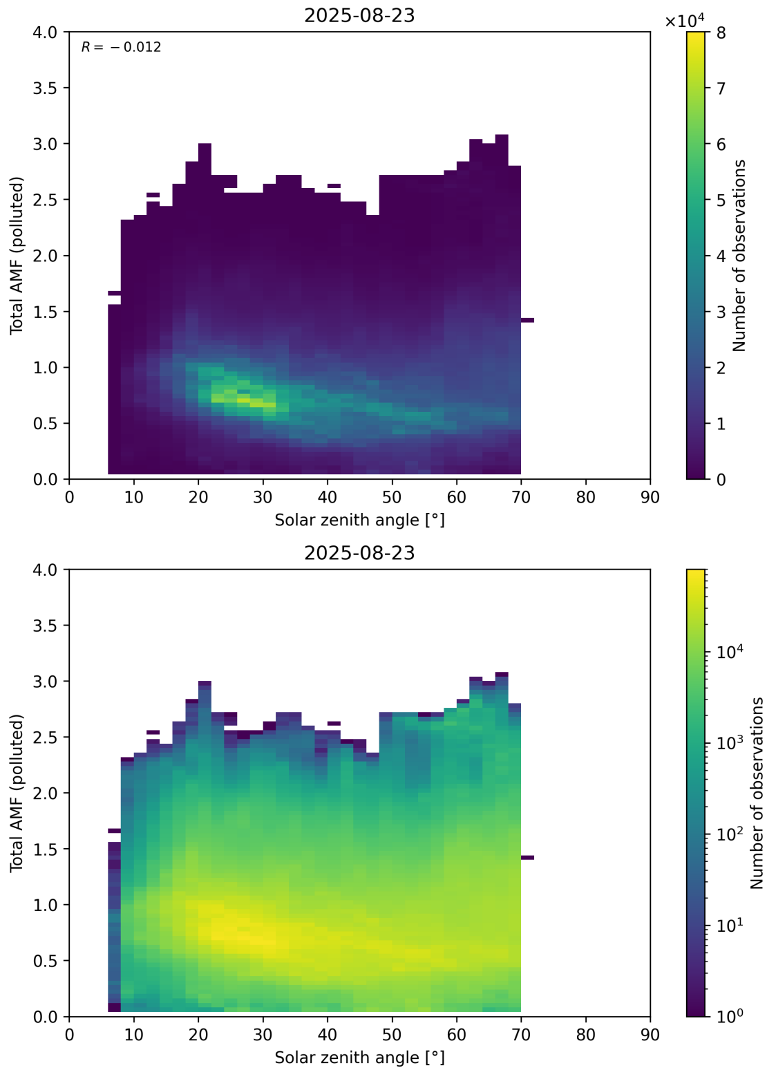
Figure 189: Scatter density plot of “Solar zenith angle” against “Total AMF (polluted)” for 2025-08-22 to 2025-08-24.
