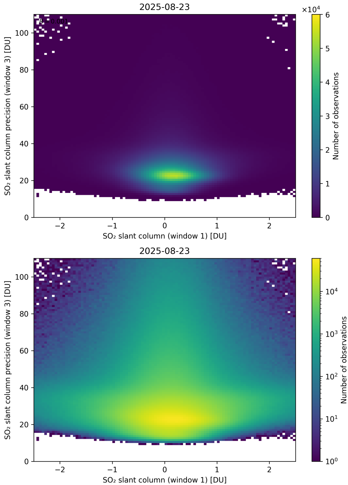
Figure 288: Scatter density plot of “SO 2 slant column (window 1)” against “SO 2 slant column precision (window 3)” for 2025-08-22 to 2025-08-24.
