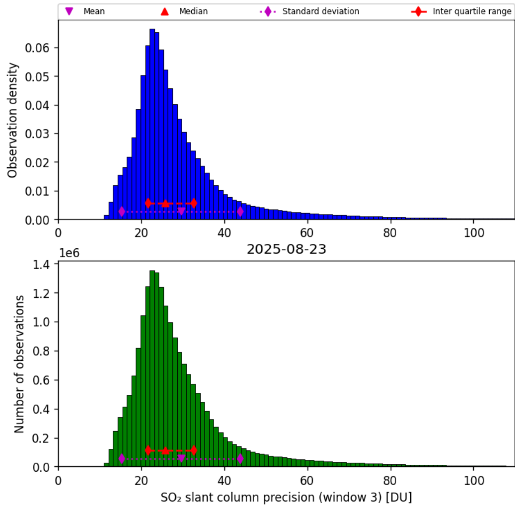
Figure 72: Histogram of “SO 2 slant column precision (window 3)” for 2025-08-22 to 2025-08-24
