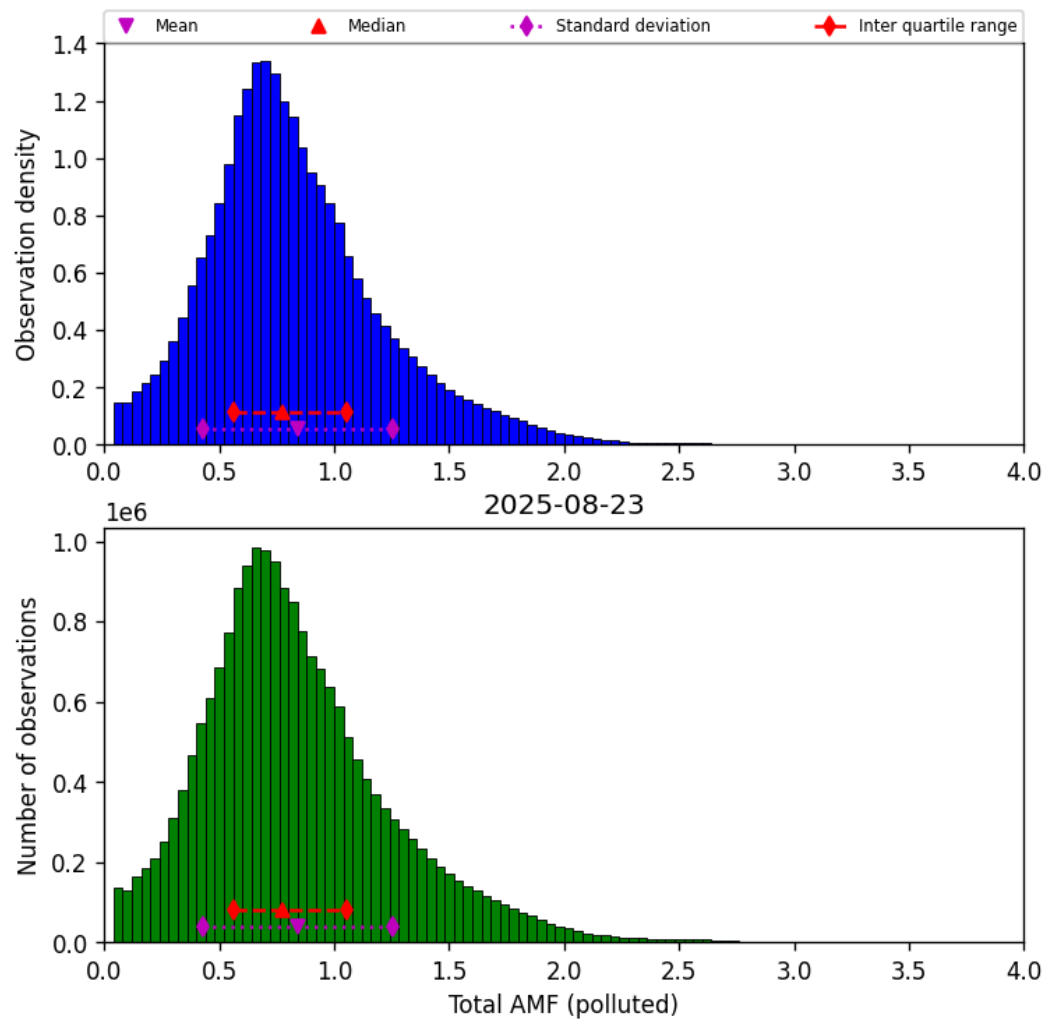
Figure 79: Histogram of “Total AMF (polluted)” for 2025-08-22 to 2025-08-24
