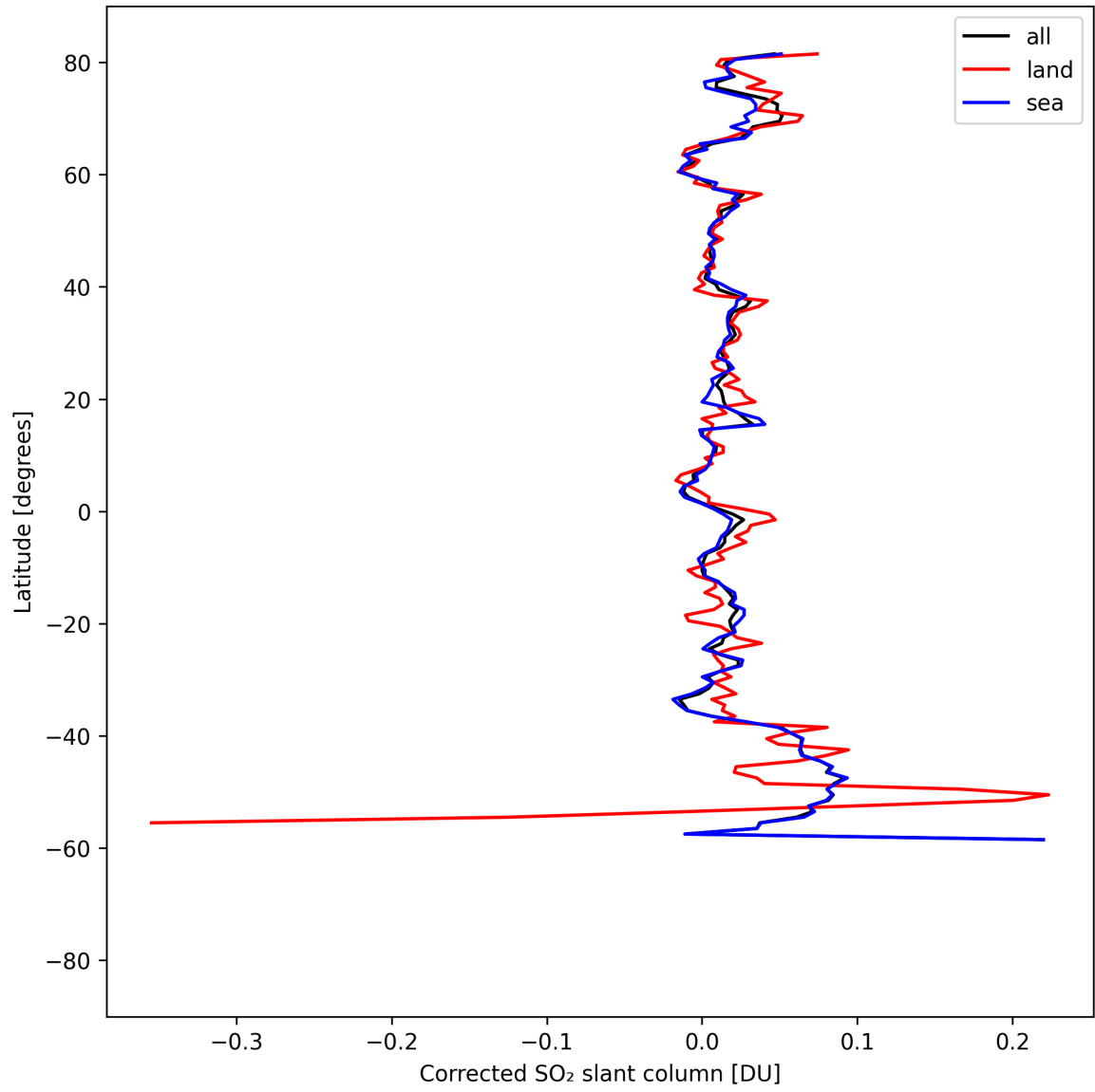
Figure 34: Zonal average of “Corrected SO 2 slant column” for 2025-08-22 to 2025-08-24.
