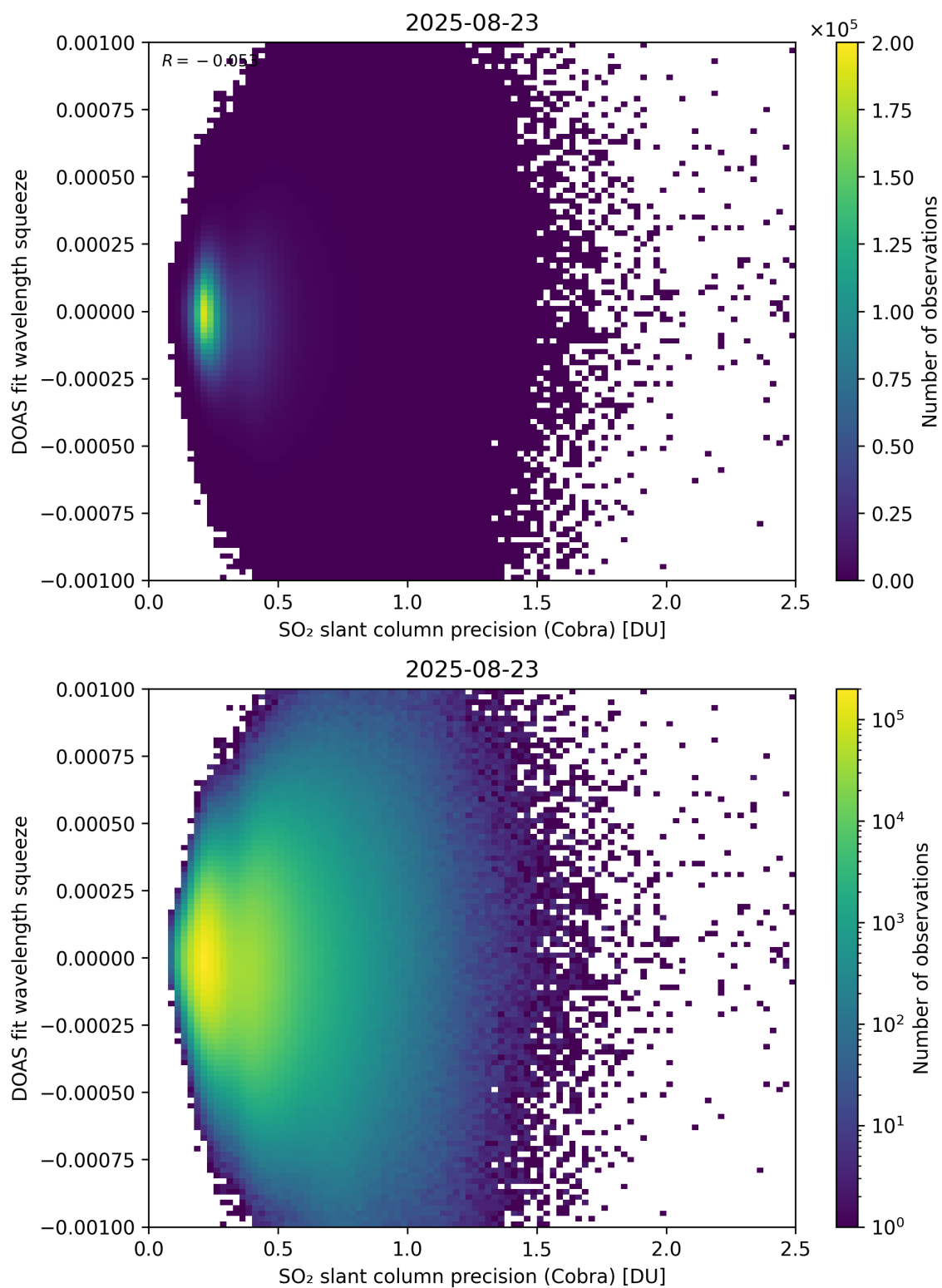
Figure 203: Scatter density plot of “SO 2 slant column precision (Cobra)” against “DOAS fit wavelength squeeze” for 2025-08-22 to 2025-08-24.
