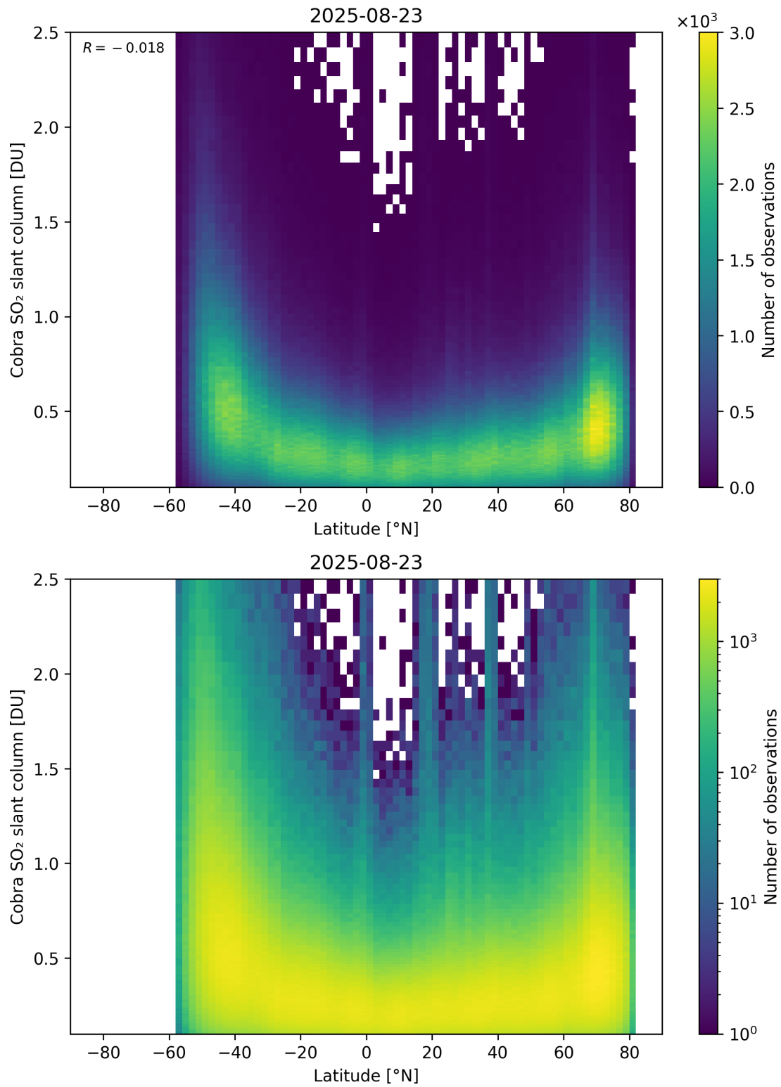
Figure 157: Scatter density plot of “Latitude” against “Cobra SO 2 slant column” for 2025-08-22 to 2025-08-24.
