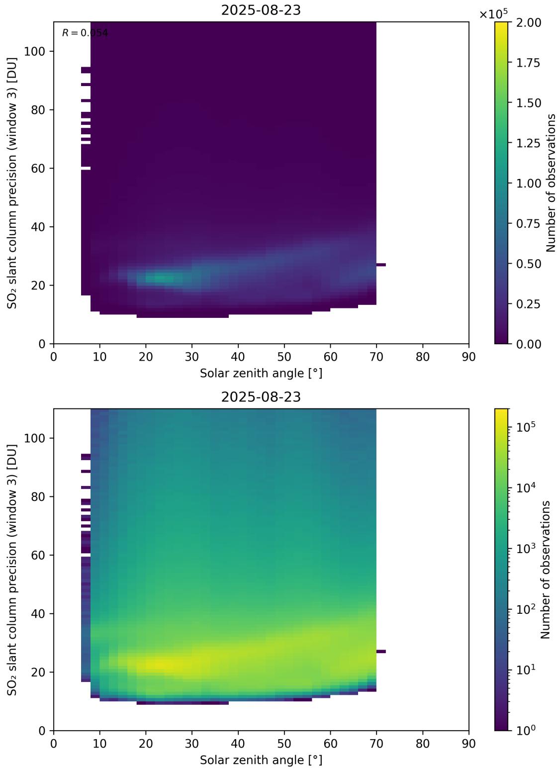
Figure 188: Scatter density plot of “Solar zenith angle” against “SO 2 slant column precision (window 3)” for 2025-08-22 to 2025-08-24.
