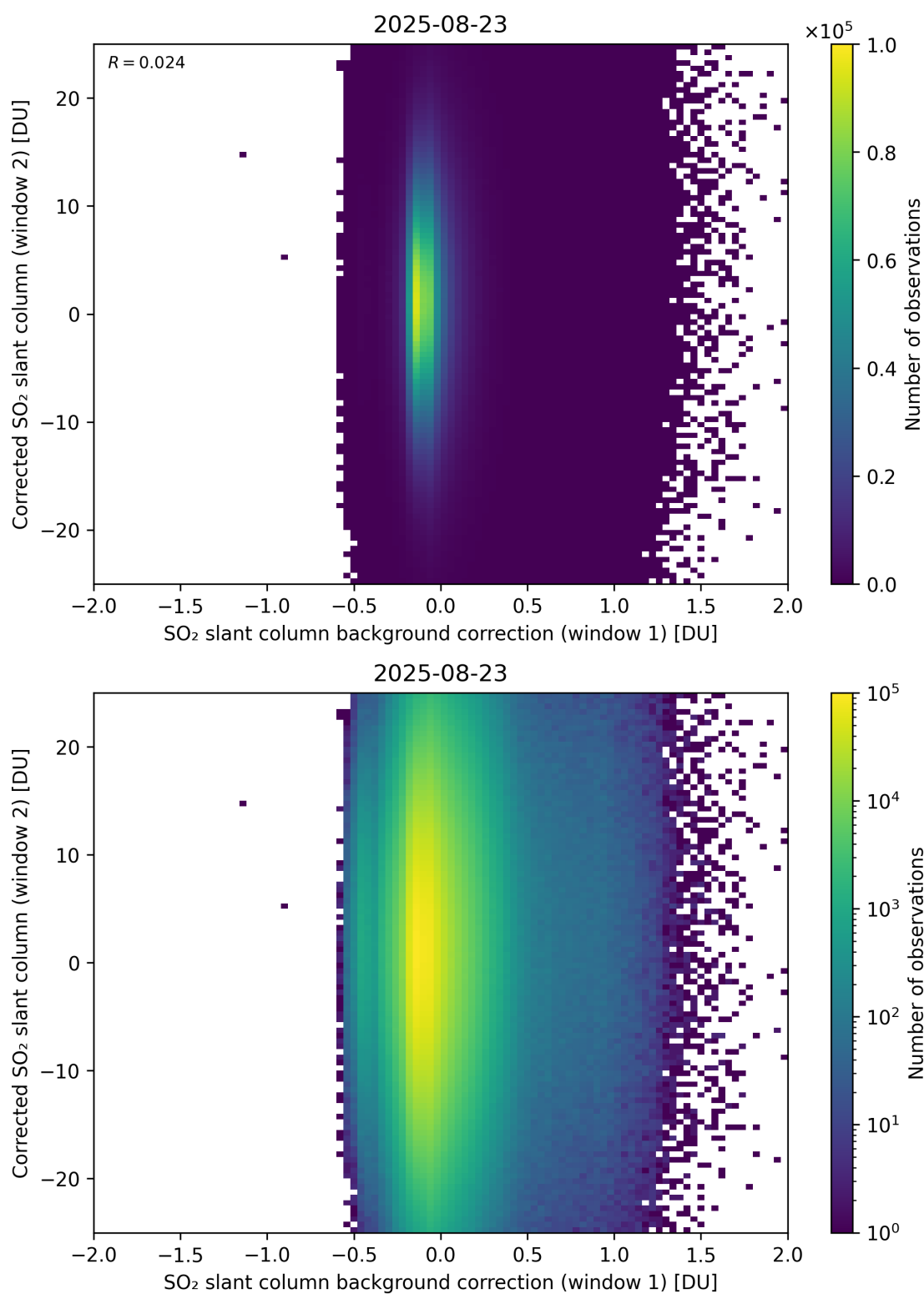
Figure 115: Scatter density plot of “SO 2 slant column background correction (window 1)” against “Corrected SO 2 slant column (window 2)” for 2025-08-22 to 2025-08-24.
