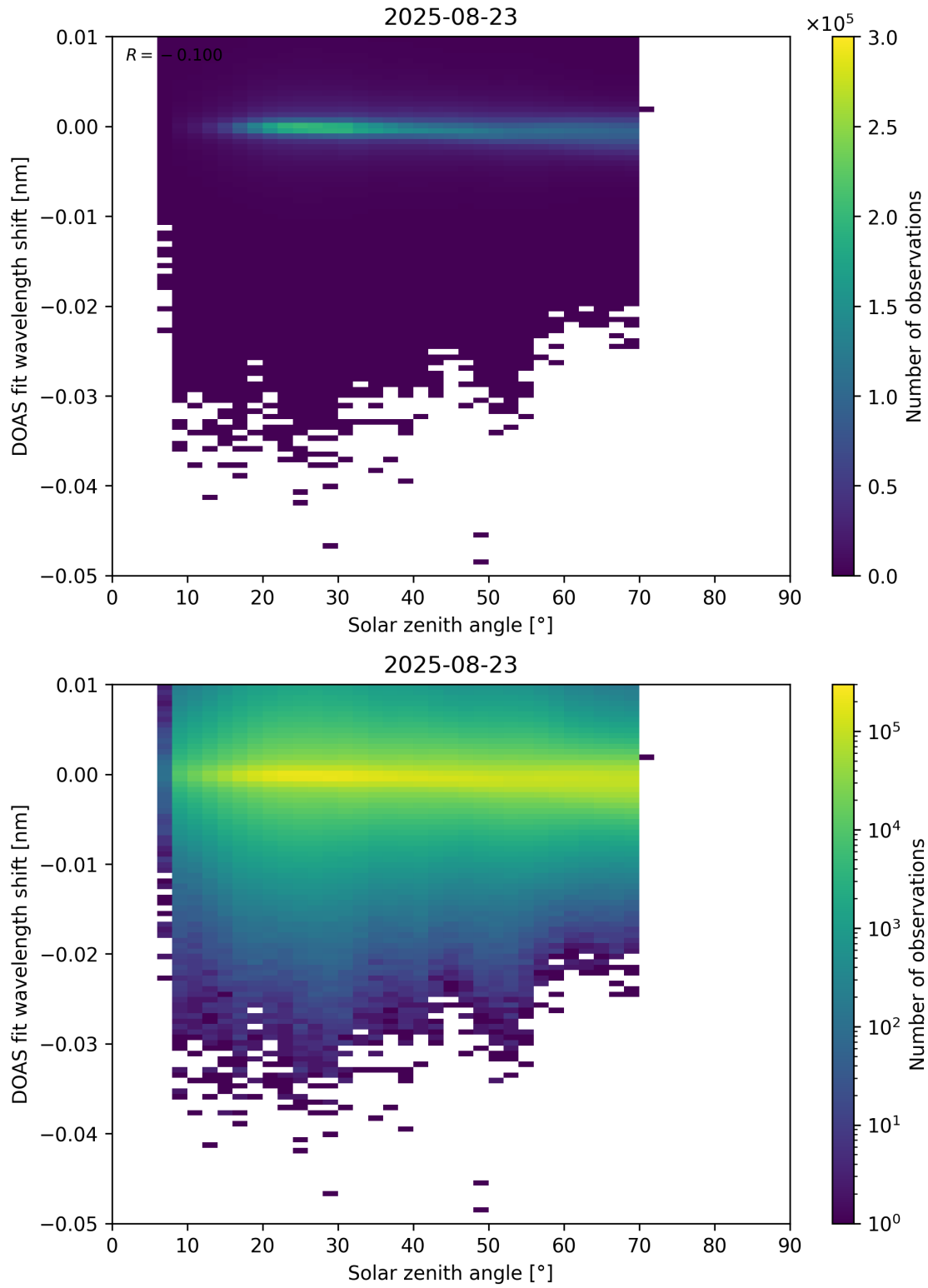
Figure 174: Scatter density plot of “Solar zenith angle” against “DOAS fit wavelength shift” for 2025-08-22 to 2025-08-24.
