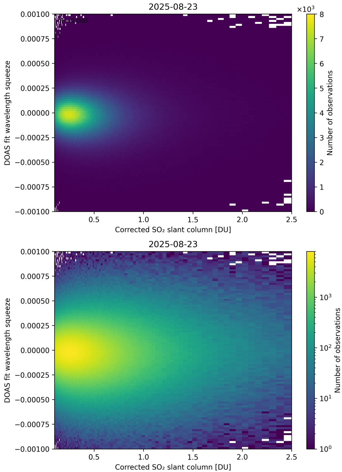
Figure 230: Scatter density plot of "Corrected SO 2 slant column" against "DOAS fit wavelength squeeze" for 2025-08-22 to 2025-08-24.
