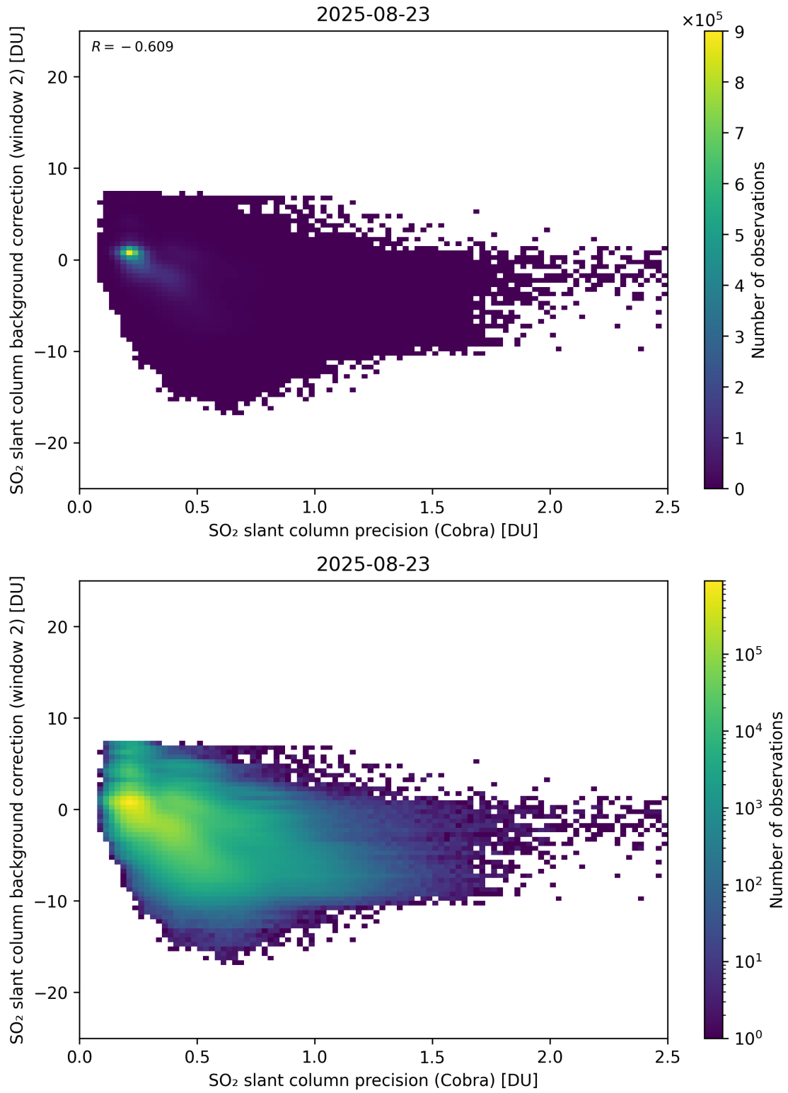
Figure 200: Scatter density plot of “SO 2 slant column precision (Cobra)” against “SO 2 slant column background correction (window 2)” for 2025-08-22 to 2025-08-24.
