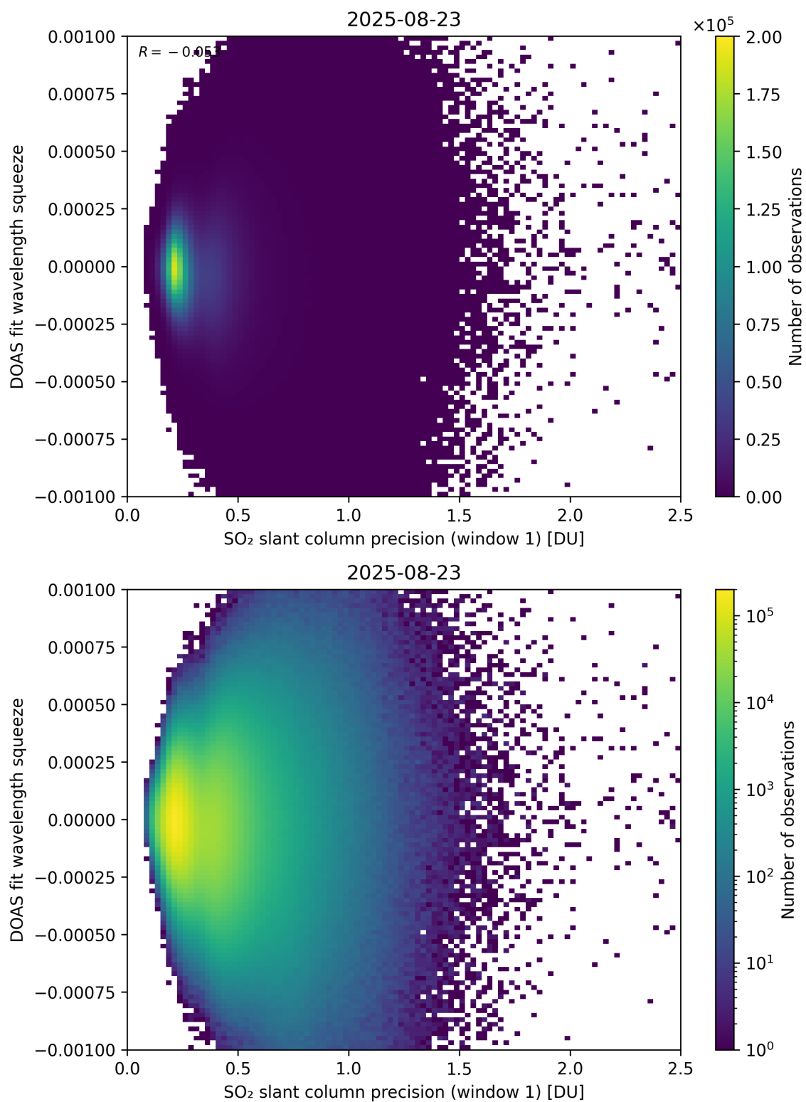
Figure 272: Scatter density plot of “SO 2 slant column precision (window 1)” against “DOAS fit wavelength squeeze” for 2025-08-22 to 2025-08-24.
