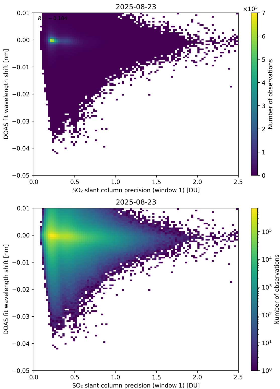
Figure 271: Scatter density plot of “SO 2 slant column precision (window 1)” against “DOAS fit wavelength shift” for 2025-08-22 to 2025-08-24.
