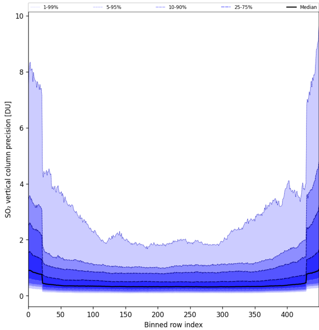
Figure 85: Along track statistics of “SO 2 vertical column precision” for 2025-08-22 to 2025-08-24
