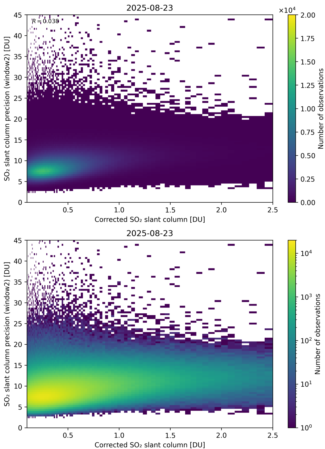
Figure 239: Scatter density plot of “Corrected SO 2 slant column” against “SO 2 slant column precision (window2)” for 2025-08-22 to 2025-08-24.
