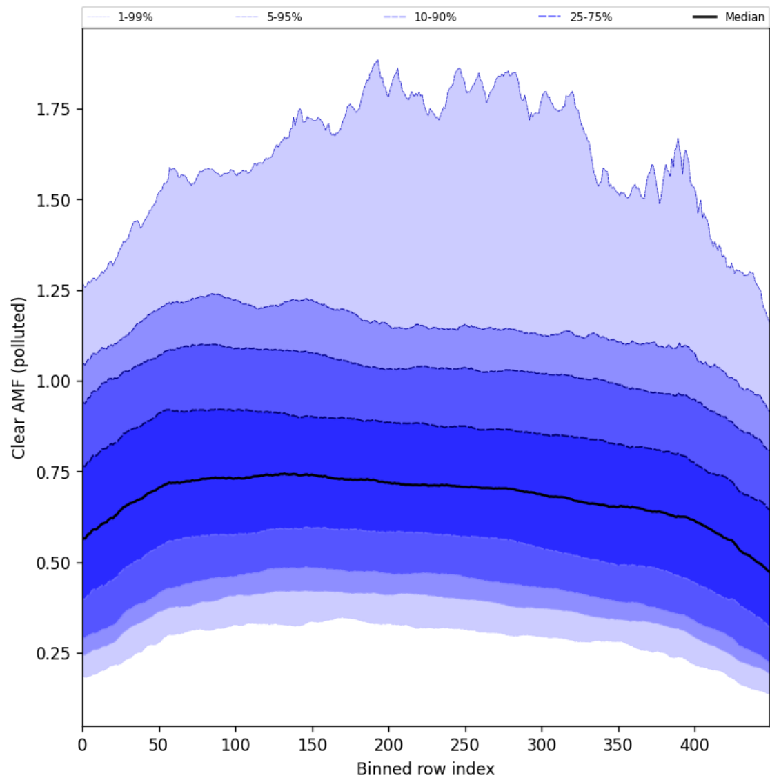
Figure 107: Along track statistics of “Clear AMF (polluted)” for 2025-08-22 to 2025-08-24
