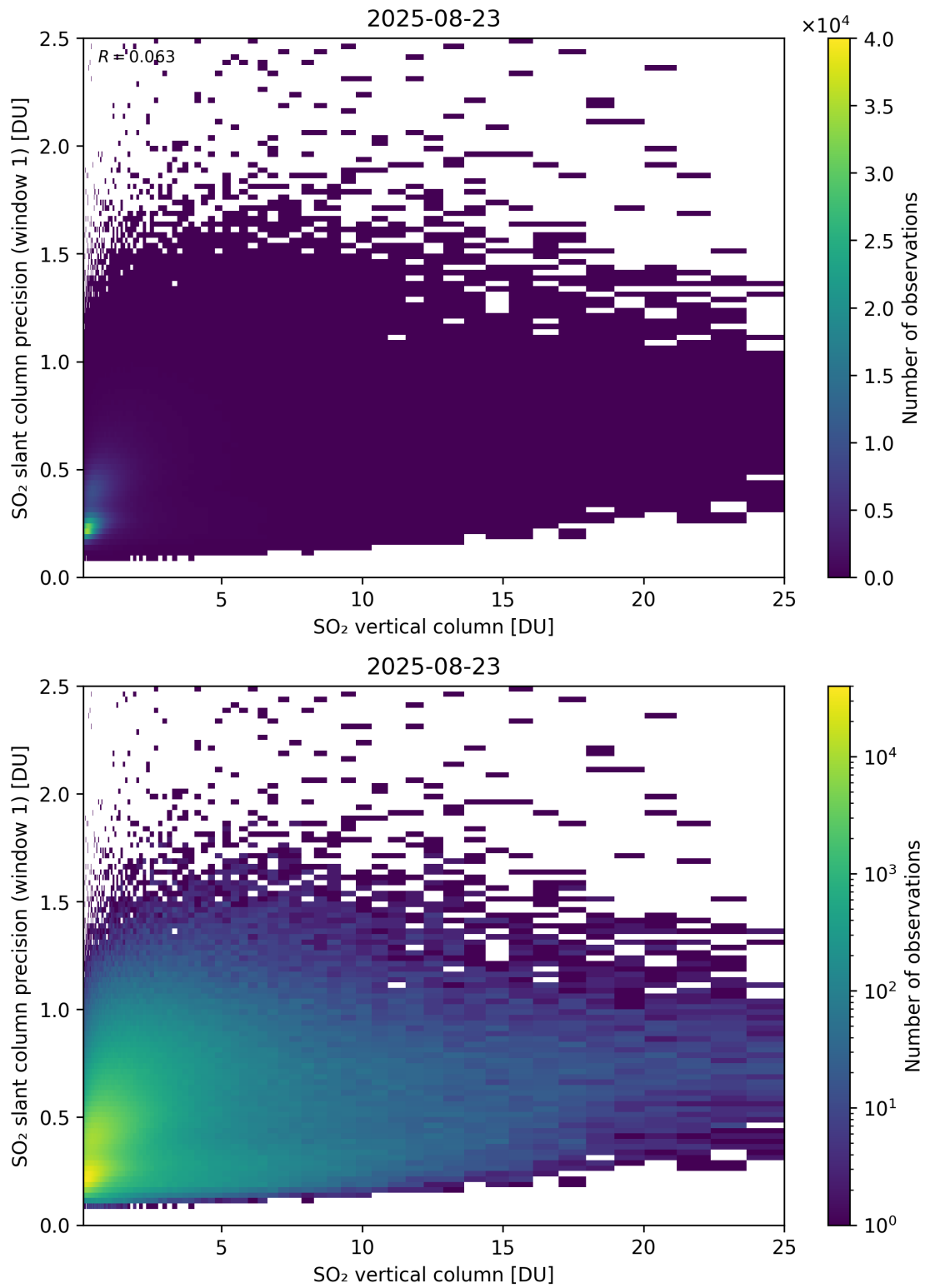
Figure 355: Scatter density plot of “SO 2 vertical column” against “SO 2 slant column precision (window 1)” for 2025-08-22 to 2025-08-24.
