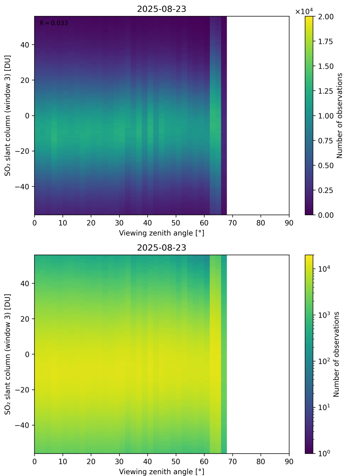
Figure 379: Scatter density plot of “Viewing zenith angle” against “SO 2 slant column (window 3)” for 2025-08-22 to 2025-08-24.
