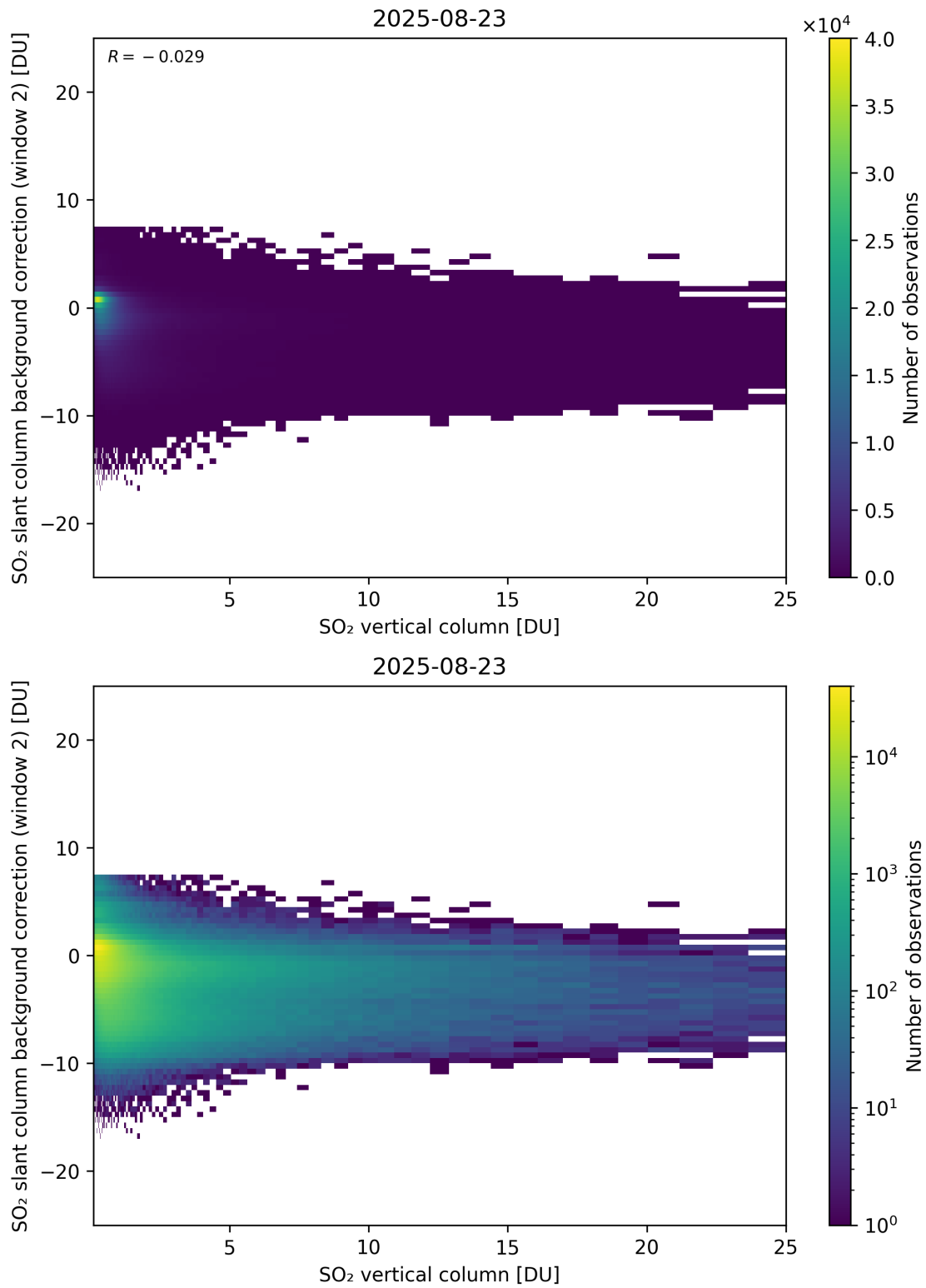
Figure 324: Scatter density plot of “SO 2 vertical column” against “SO 2 slant column background correction (window 2)” for 2025-08-22 to 2025-08-24.
