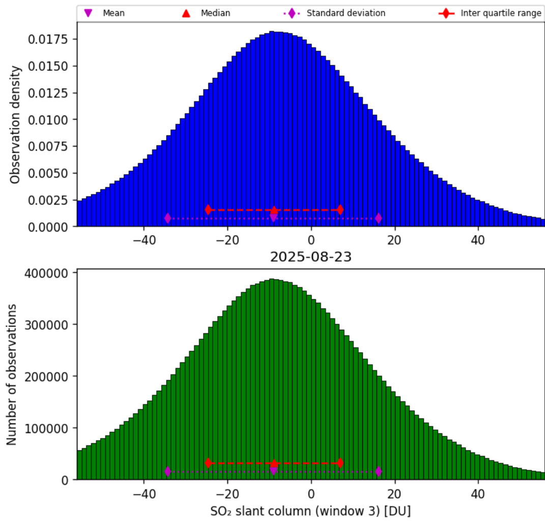
Figure 71: Histogram of “SO 2 slant column (window 3)” for 2025-08-22 to 2025-08-24
