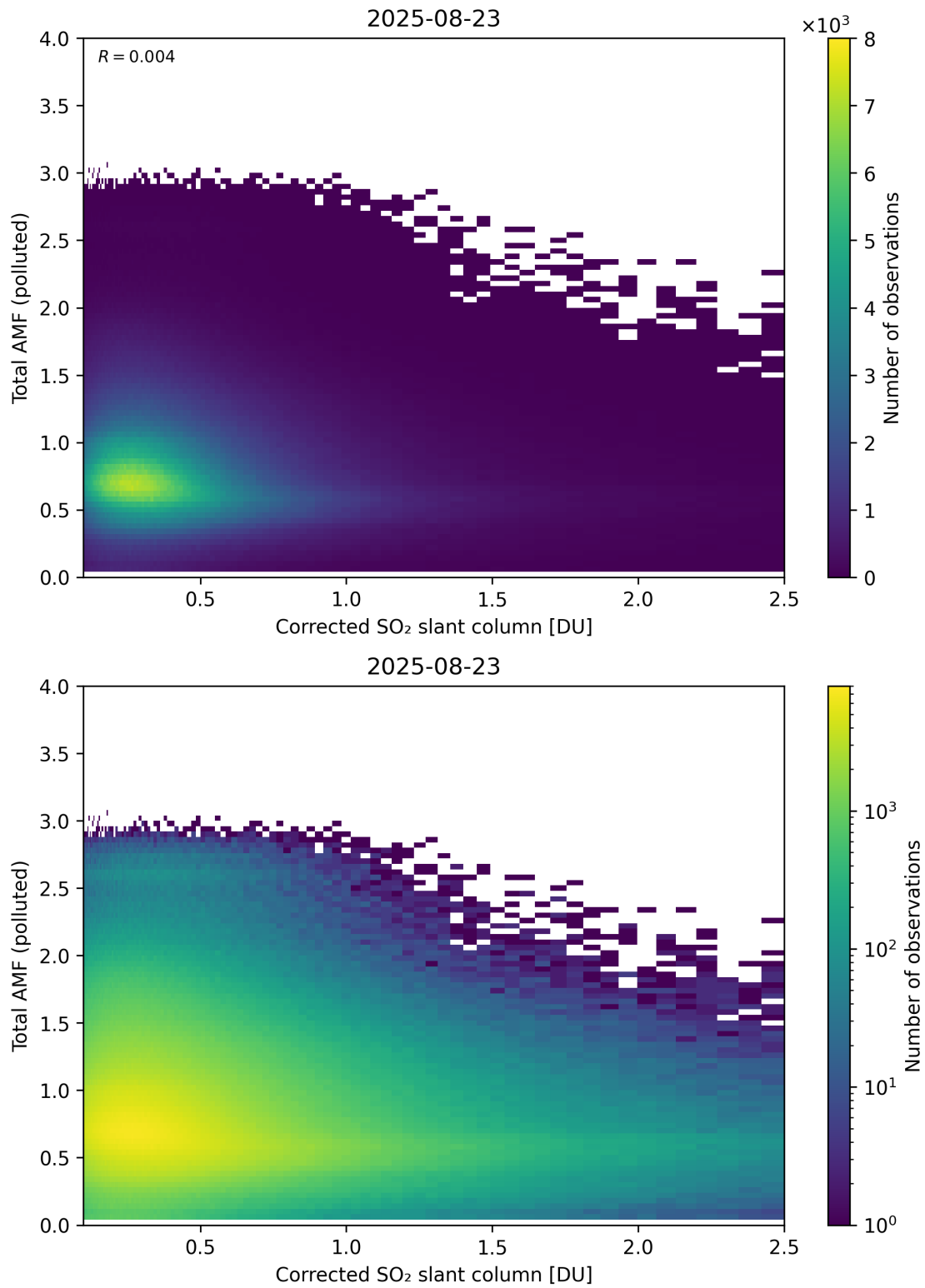
Figure 242: Scatter density plot of “Corrected SO 2 slant column” against “Total AMF (polluted)” for 2025-08-22 to 2025-08-24.
