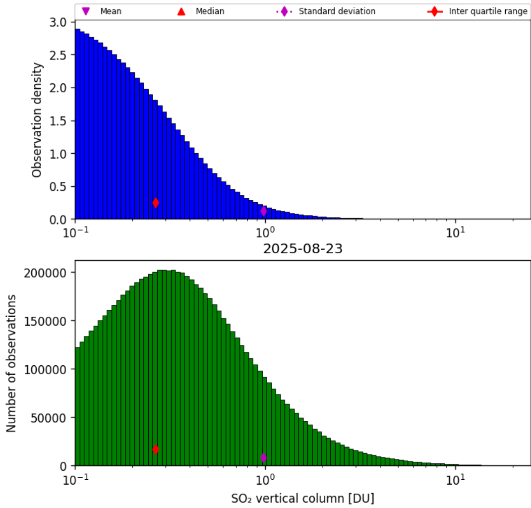
Figure 58: Histogram of “SO 2 vertical column” for 2025-08-22 to 2025-08-24
