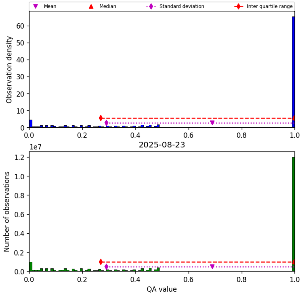
Figure 57: Histogram of “QA value” for 2025-08-22 to 2025-08-24
