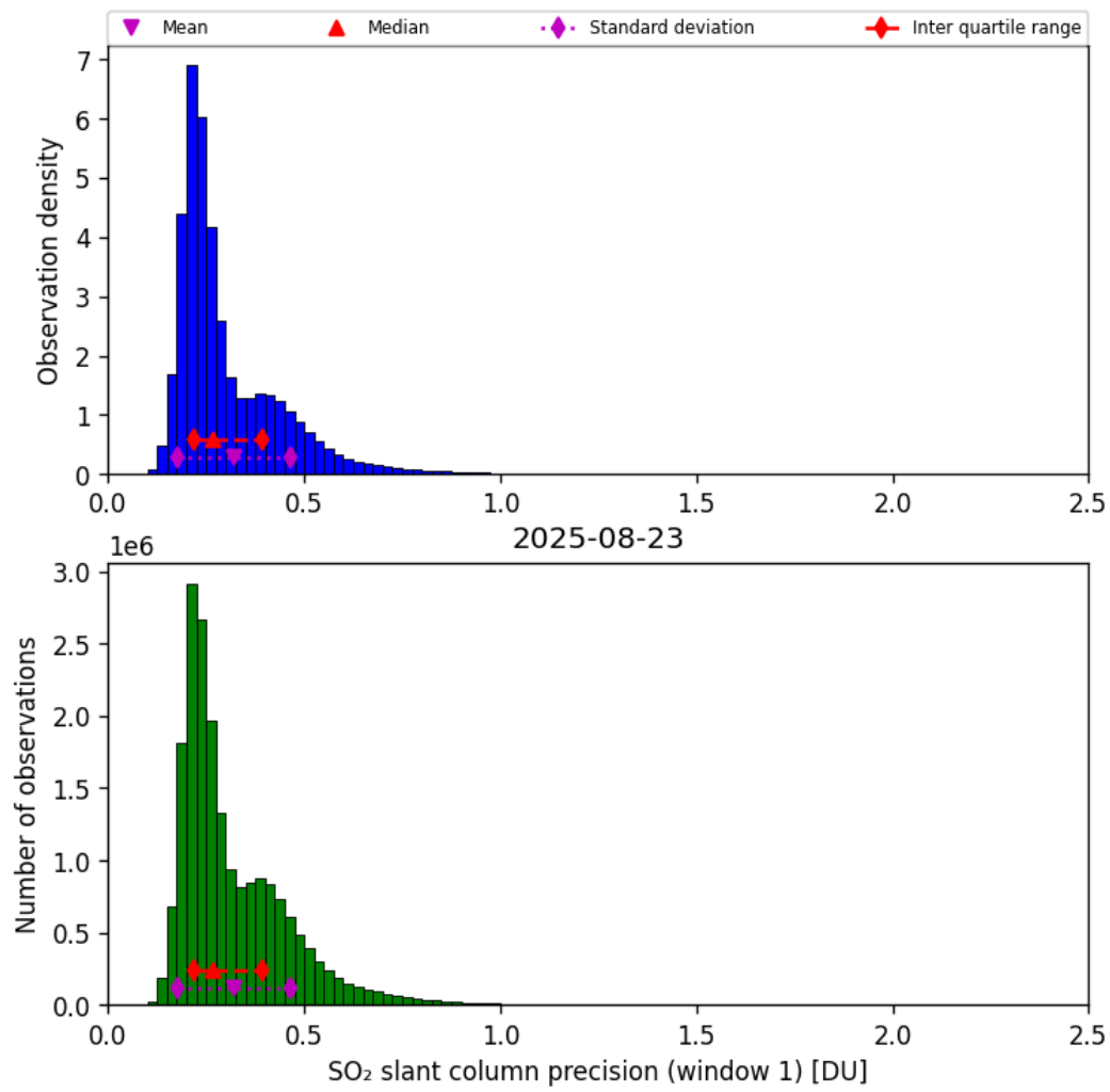
Figure 64: Histogram of “SO 2 slant column precision (window 1)” for 2025-08-22 to 2025-08-24
