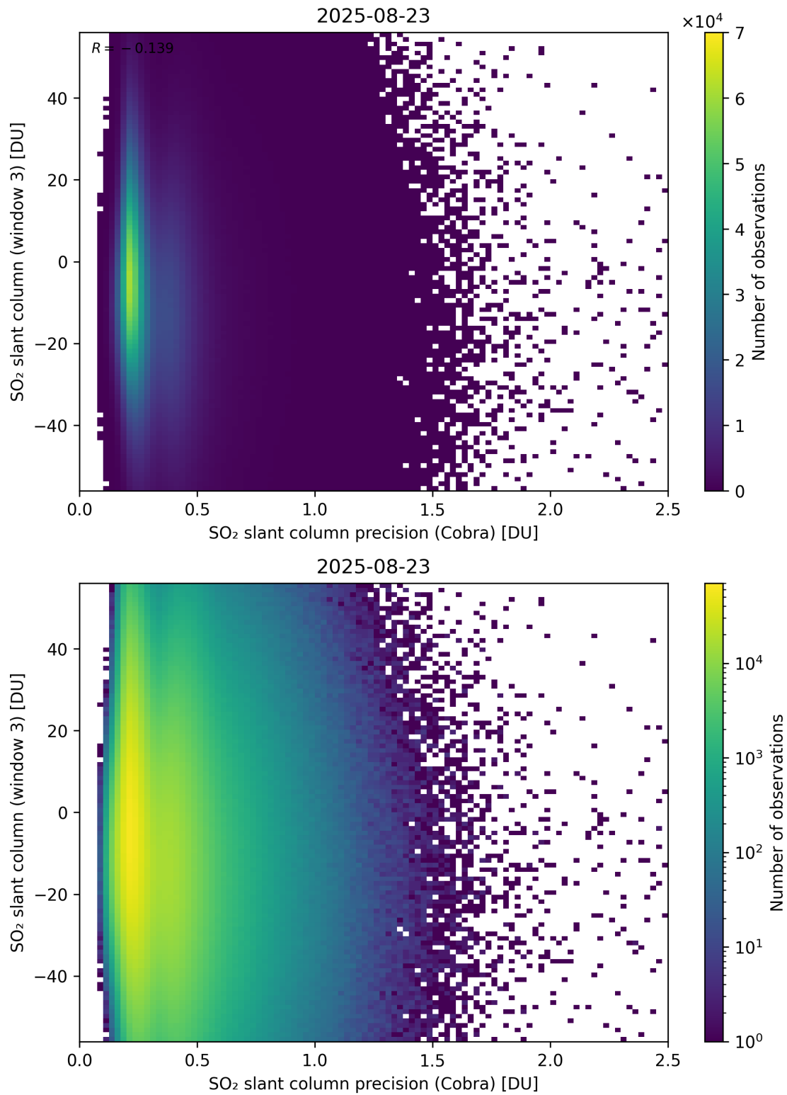
Figure 211: Scatter density plot of “SO 2 slant column precision (Cobra)” against “SO 2 slant column (window 3)” for 2025-08-22 to 2025-08-24.
