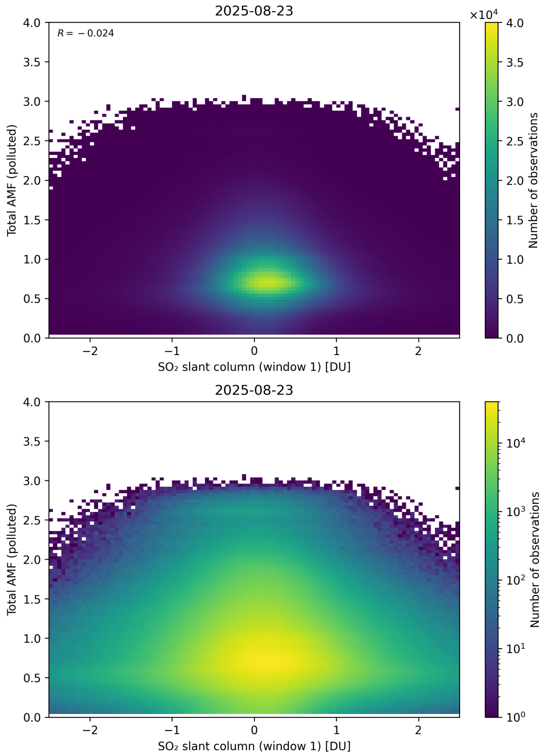
Figure 289: Scatter density plot of “SO 2 slant column (window 1)” against “Total AMF (polluted)” for 2025-08-22 to 2025-08-24.
