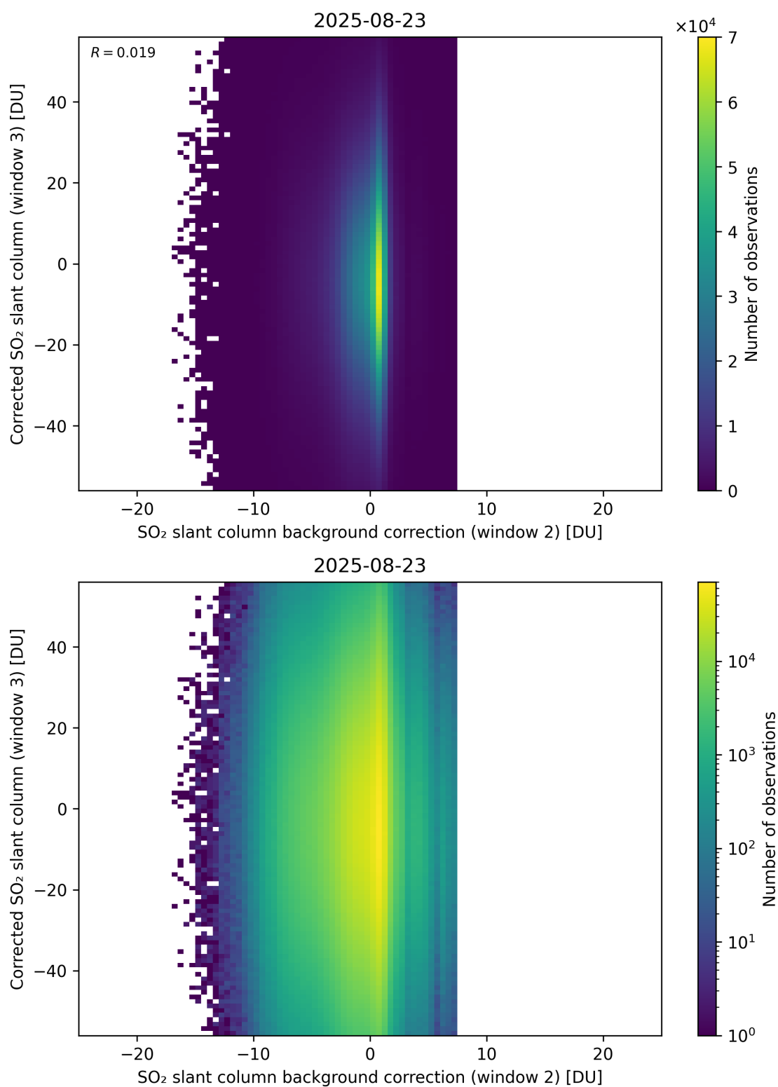
Figure 127: Scatter density plot of “SO 2 slant column background correction (window 2)” against “Corrected SO 2 slant column (window 3)” for 2025-08-22 to 2025-08-24.
