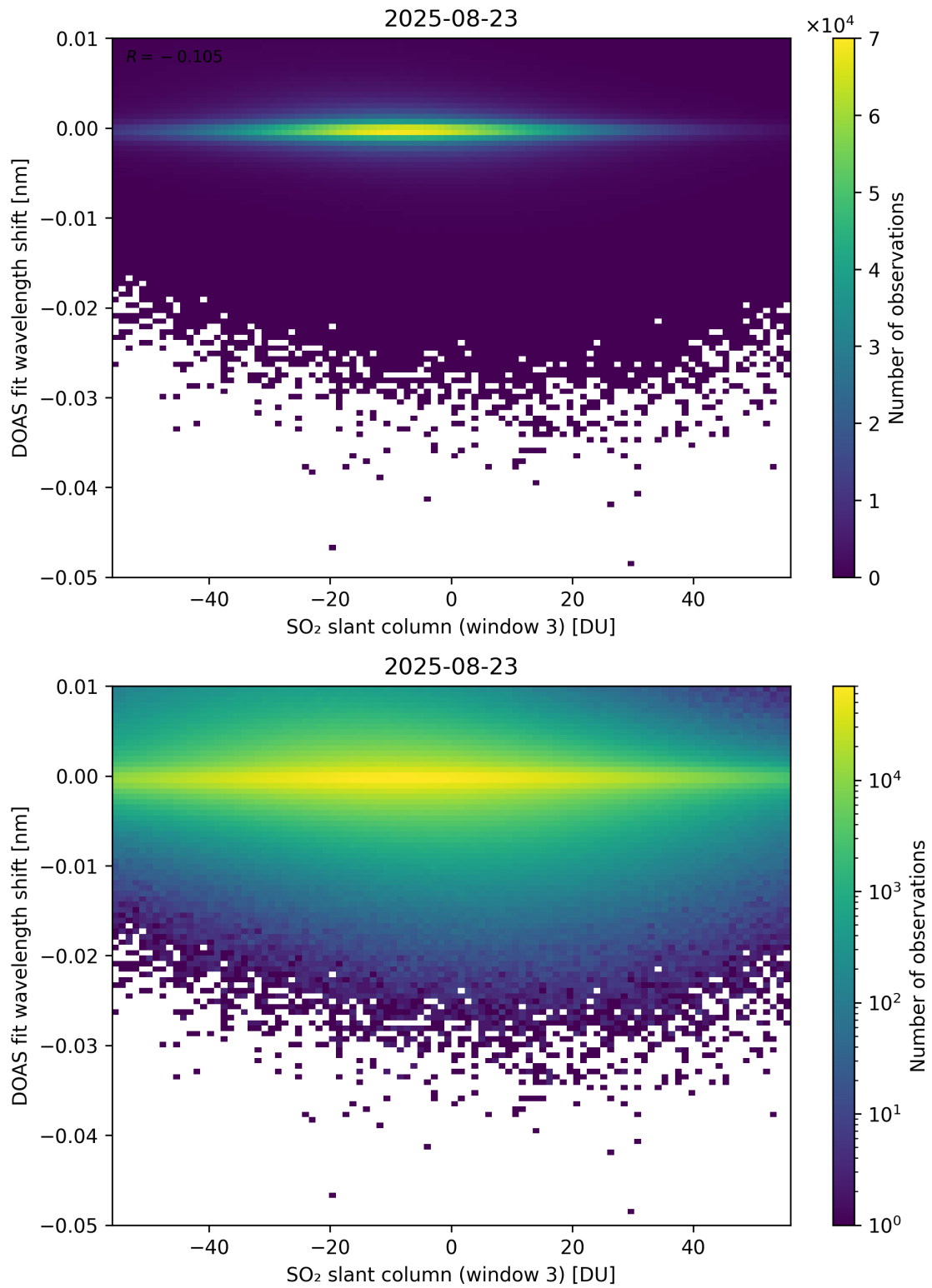
Figure 304: Scatter density plot of “SO 2 slant column (window 3)” against “DOAS fit wavelength shift” for 2025-08-22 to 2025-08-24.
