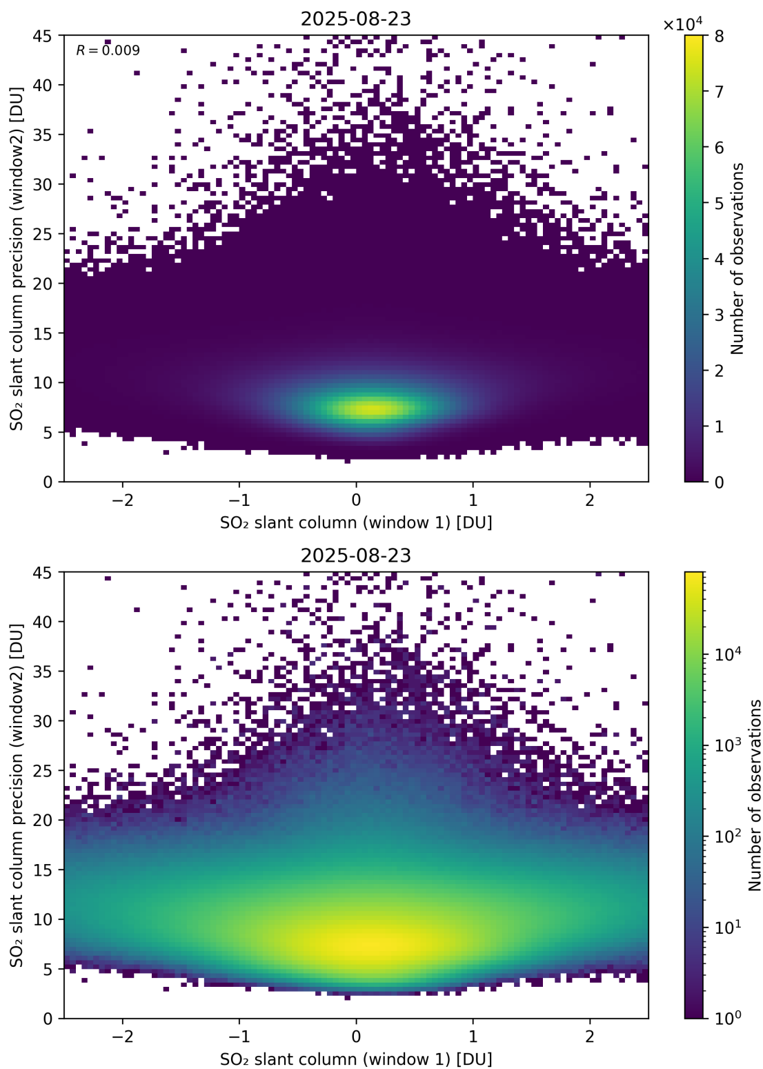
Figure 286: Scatter density plot of “SO 2 slant column (window 1)” against “SO 2 slant column precision (window2)” for 2025-08-22 to 2025-08-24.
