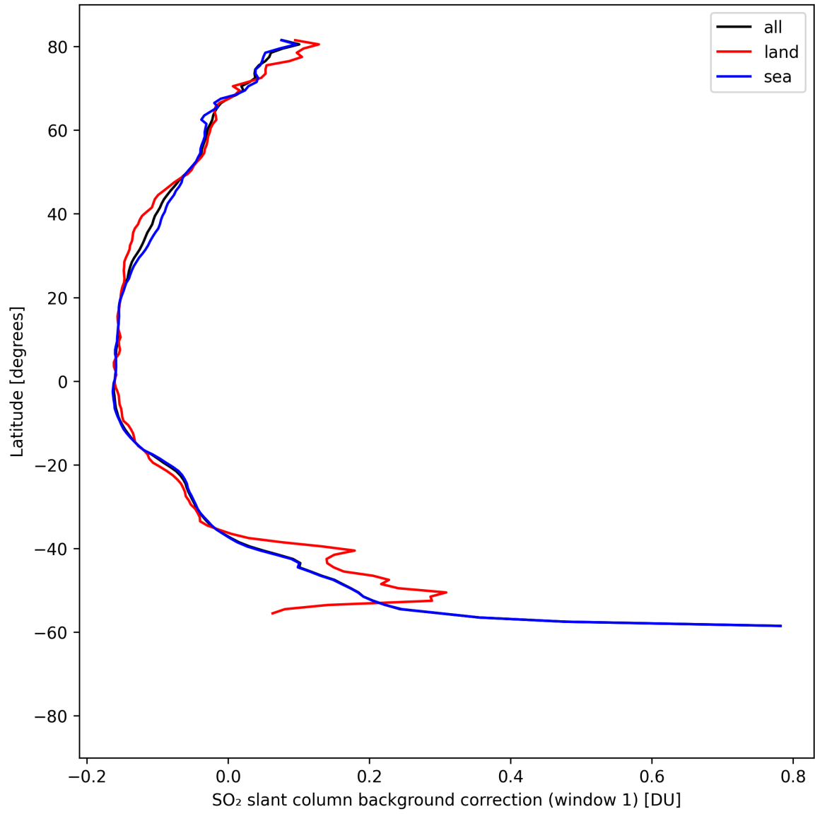
Figure 40: Zonal average of “SO 2 slant column background correction (window 1)” for 2025-08-22 to 2025-08-24.
