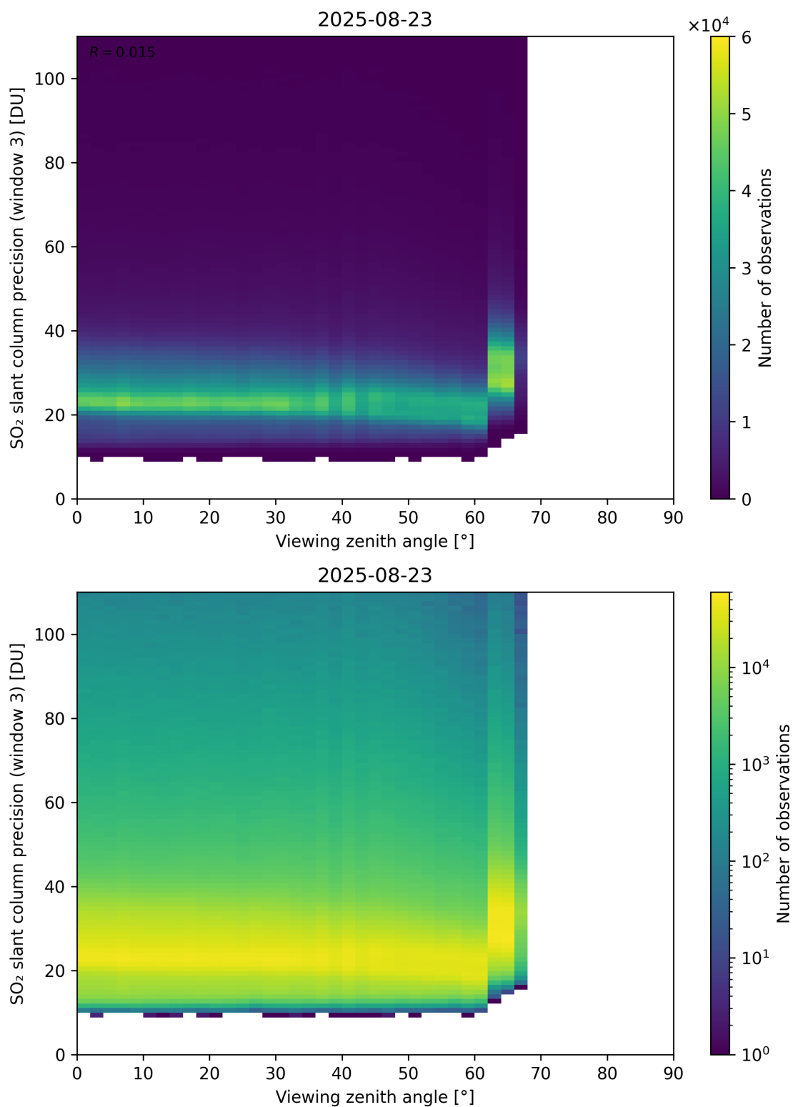
Figure 380: Scatter density plot of “Viewing zenith angle” against “SO 2 slant column precision (window 3)” for 2025-08-22 to 2025-08-24.
