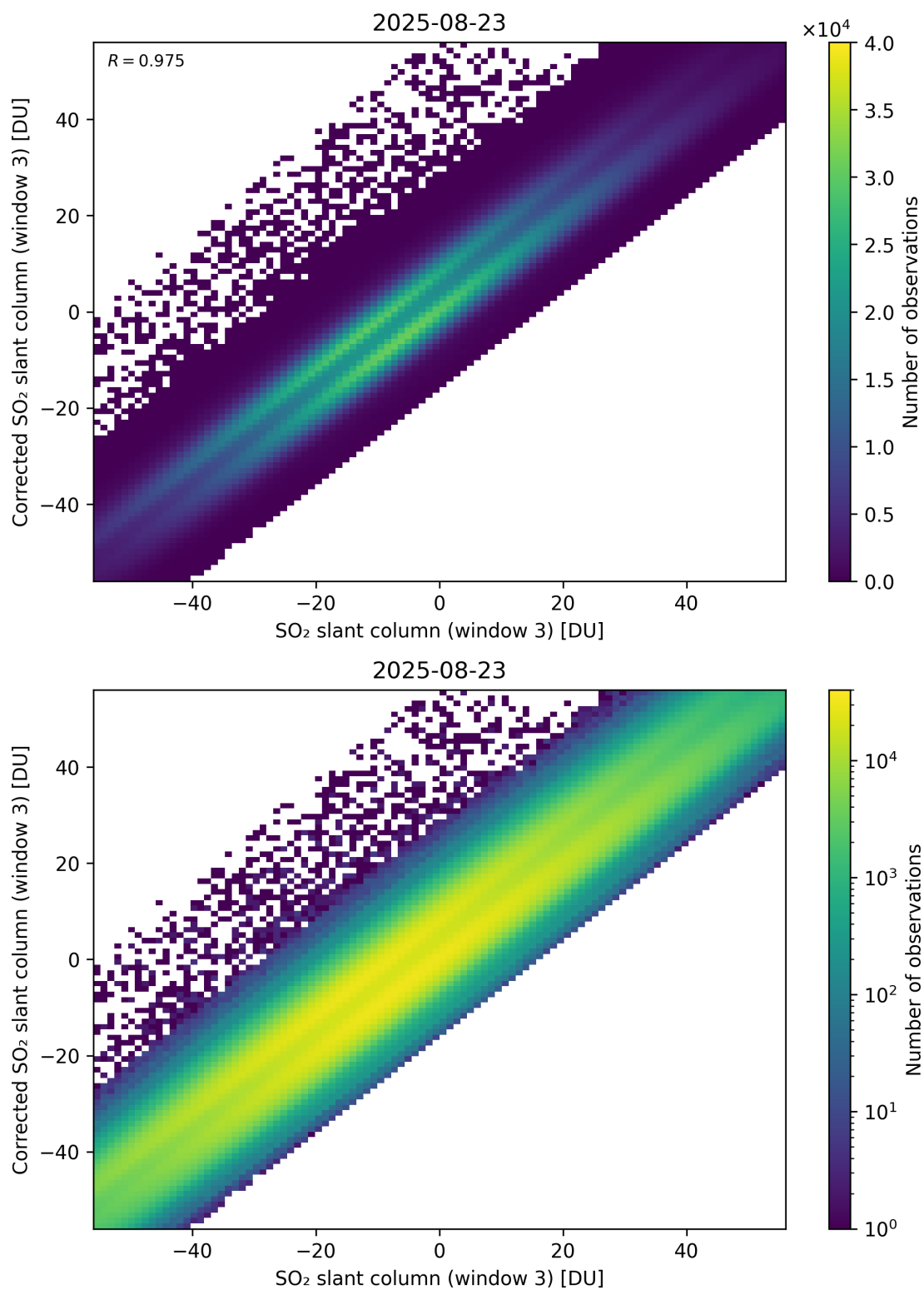
Figure 316: Scatter density plot of “SO 2 slant column (window 3)” against “Corrected SO 2 slant column (window 3)” for 2025-08-22 to 2025-08-24.
