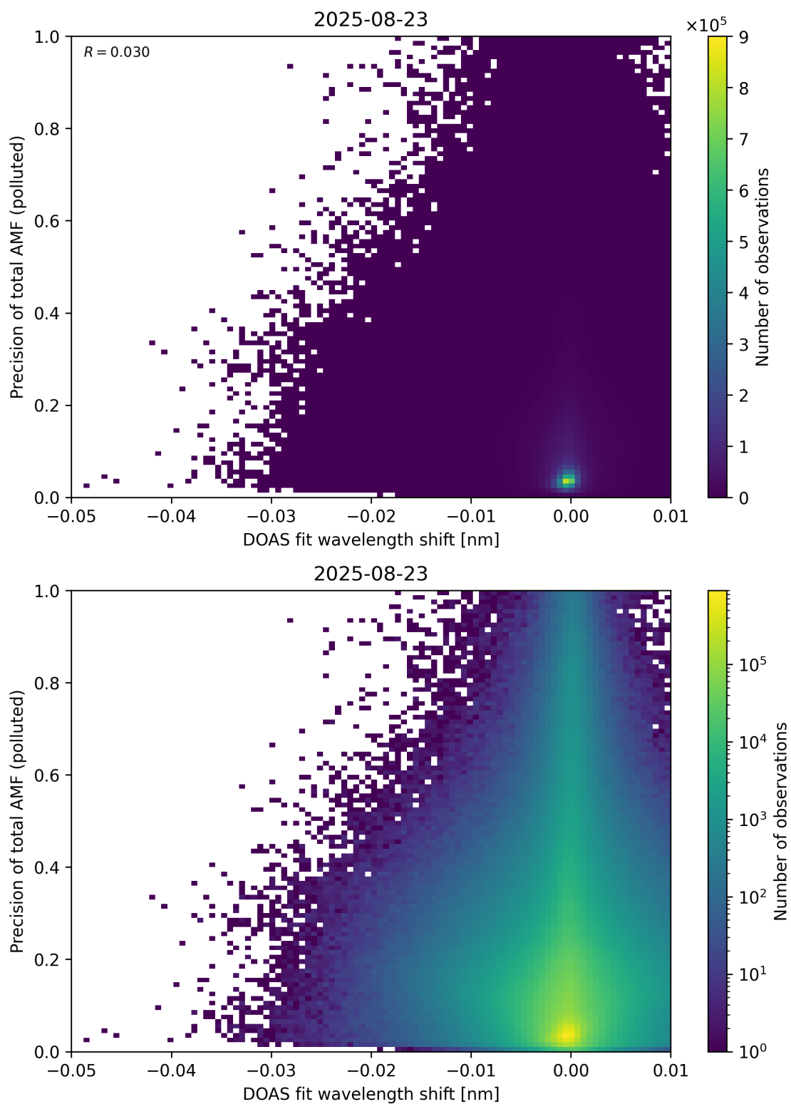
Figure 142: Scatter density plot of “DOAS fit wavelength shift” against “Precision of total AMF (polluted)” for 2025-08-22 to 2025-08-24.
