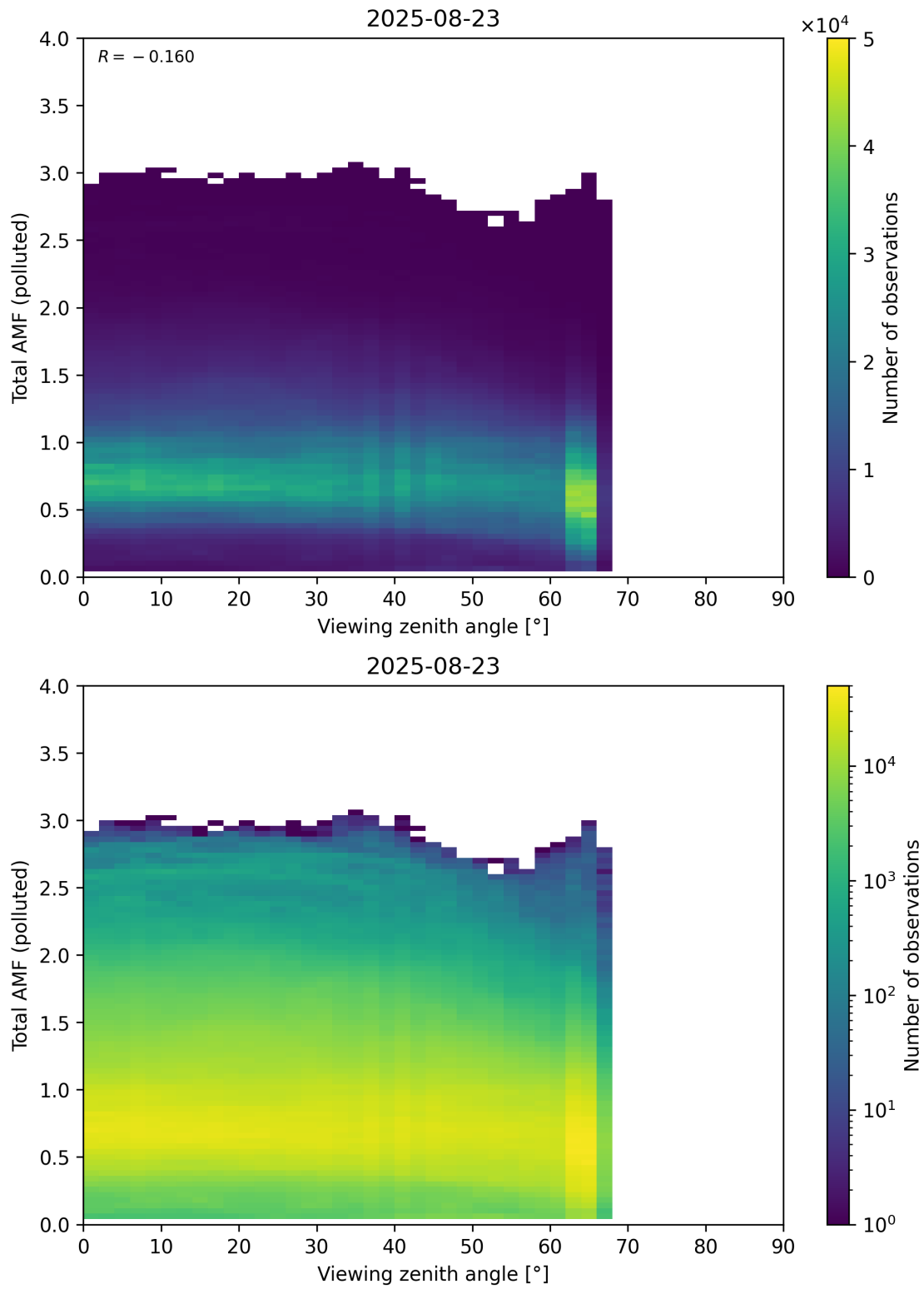
Figure 381: Scatter density plot of “Viewing zenith angle” against “Total AMF (polluted)” for 2025-08-22 to 2025-08-24.
