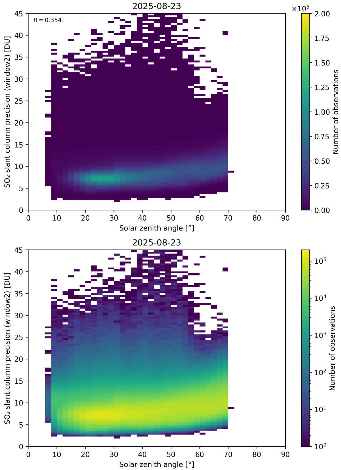
Figure 186: Scatter density plot of “Solar zenith angle” against “SO 2 slant column precision (window2)” for 2025-08-22 to 2025-08-24.
