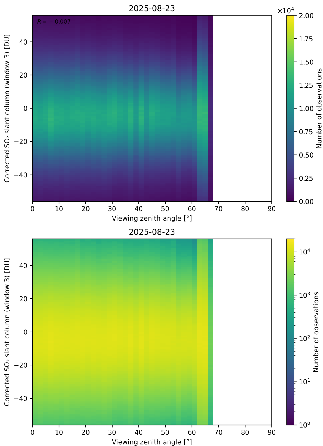
Figure 375: Scatter density plot of “Viewing zenith angle” against “Corrected SO 2 slant column (window 3)” for 2025-08-22 to 2025-08-24.
