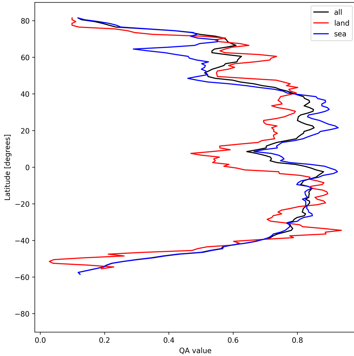
Figure 31: Zonal average of “QA value” for 2025-08-22 to 2025-08-24.
