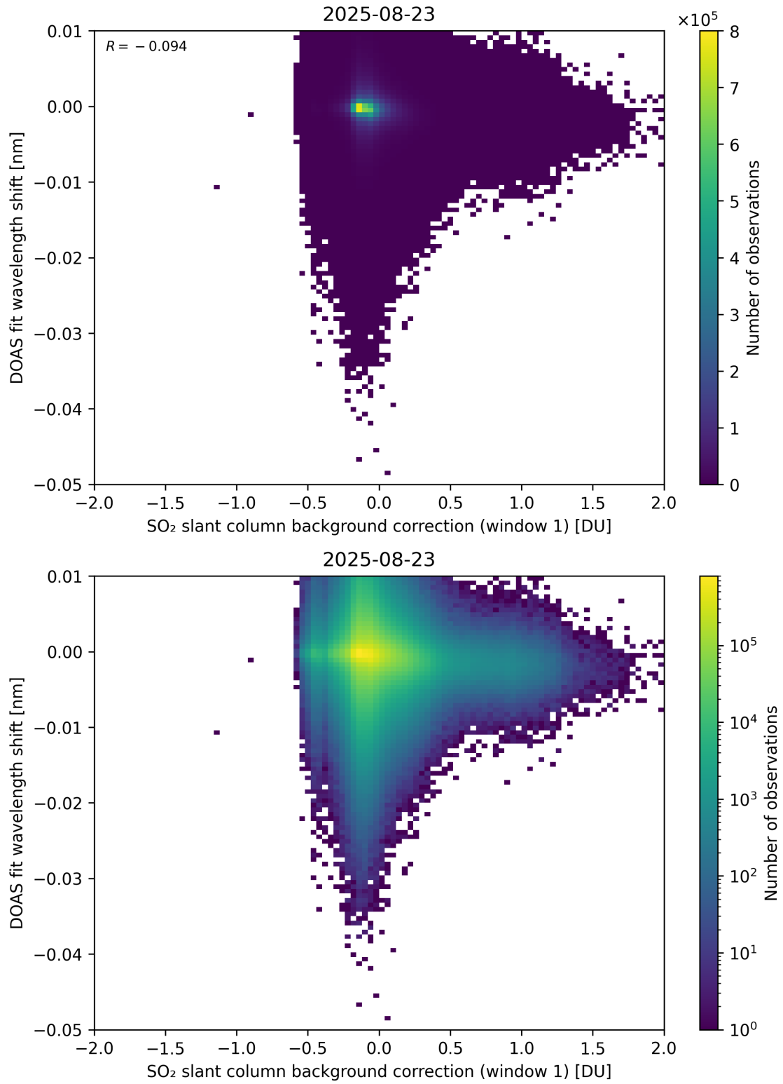
Figure 111: Scatter density plot of “SO 2 slant column background correction (window 1)” against “DOAS fit wavelength shift” for 2025-08-22 to 2025-08-24.
