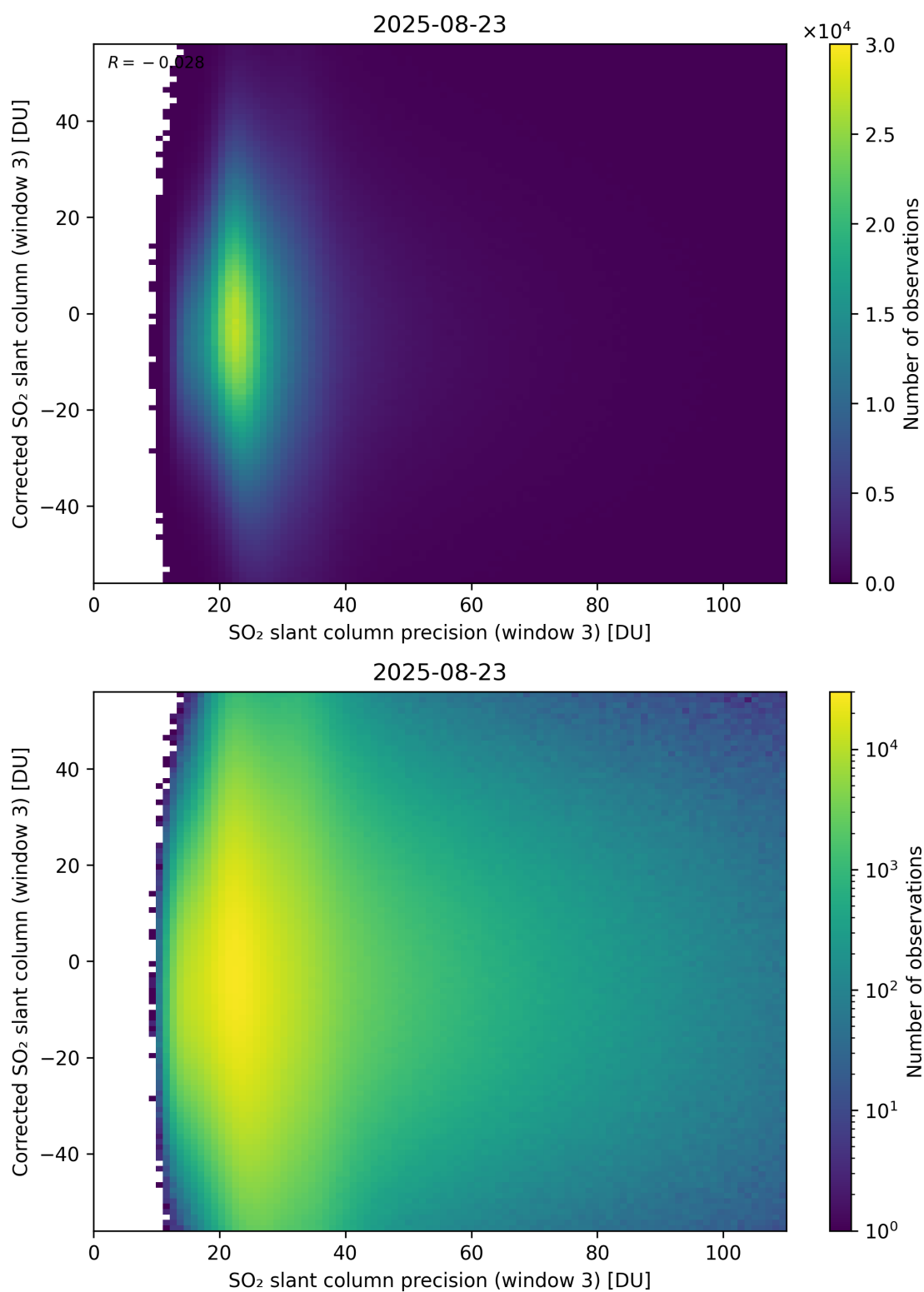
Figure 312: Scatter density plot of “SO 2 slant column precision (window 3)” against “Corrected SO 2 slant column (window 3)” for 2025-08-22 to 2025-08-24.
