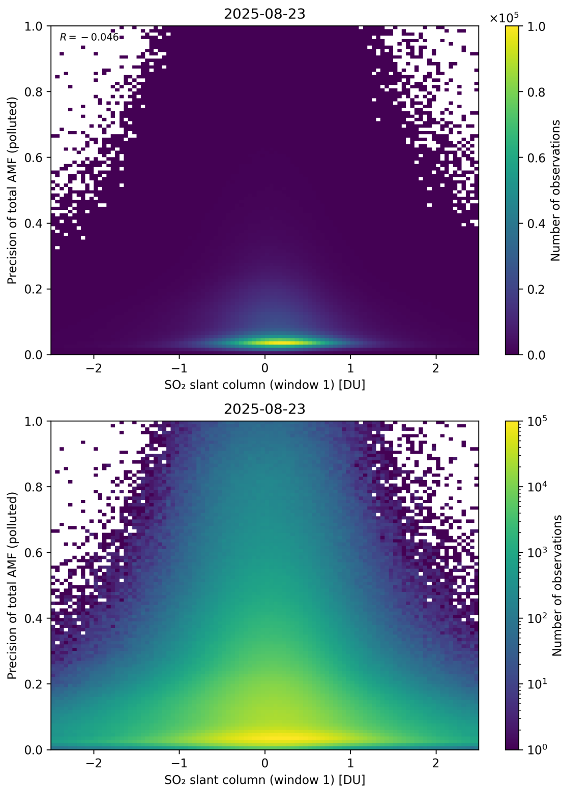
Figure 290: Scatter density plot of “SO 2 slant column (window 1)” against “Precision of total AMF (polluted)” for 2025-08-22 to 2025-08-24.
