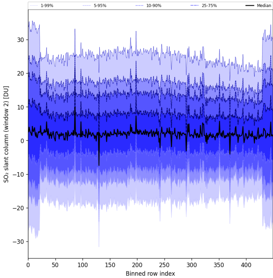
Figure 93: Along track statistics of “SO 2 slant column (window 2)” for 2025-08-22 to 2025-08-24
