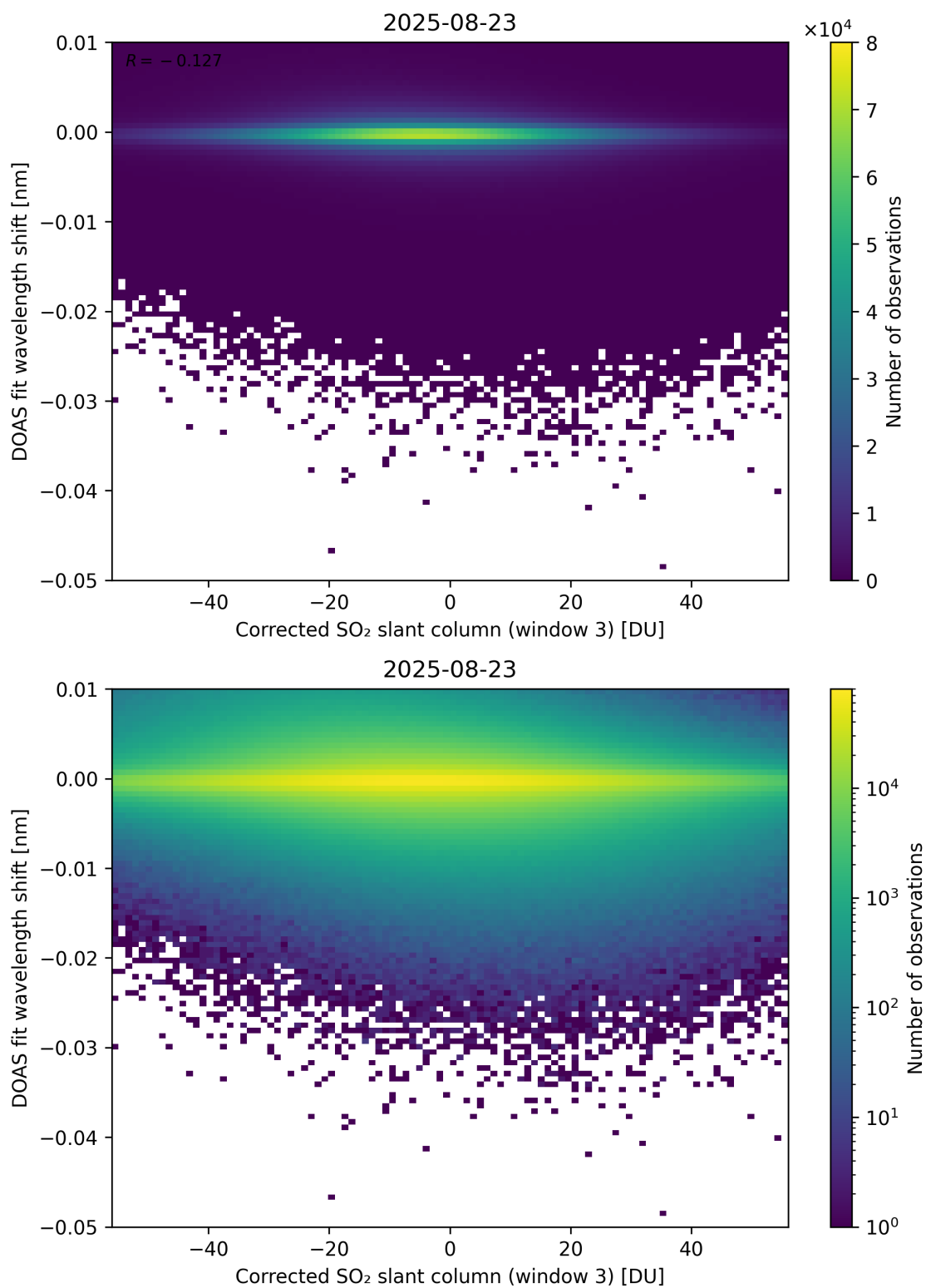
Figure 256: Scatter density plot of “Corrected SO 2 slant column (window 3)” against “DOAS fit wavelength shift” for 2025-08-22 to 2025-08-24.
