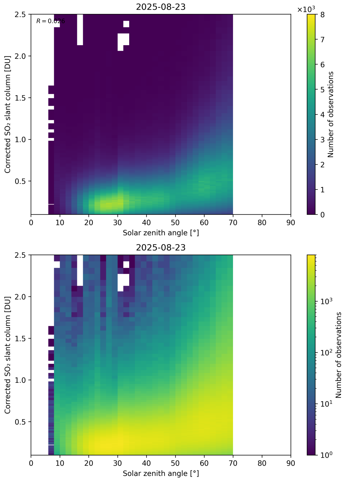
Figure 181: Scatter density plot of “Solar zenith angle” against “Corrected SO 2 slant column” for 2025-08-22 to 2025-08-24.
