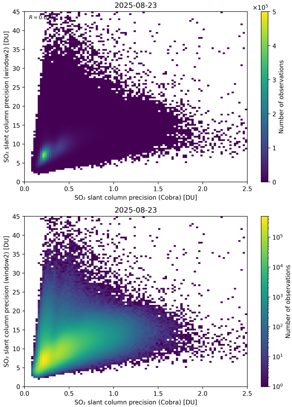
Figure 210: Scatter density plot of “SO 2 slant column precision (Cobra)” against “SO 2 slant column precision (window2)” for 2025-08-22 to 2025-08-24.
