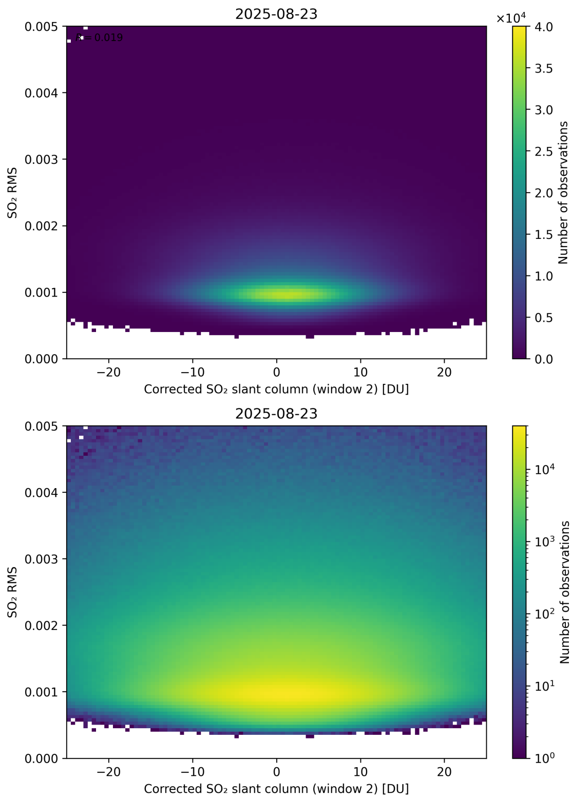
Figure 248: Scatter density plot of “Corrected SO 2 slant column (window 2)” against “SO 2 RMS” for 2025-08-22 to 2025-08-24.
