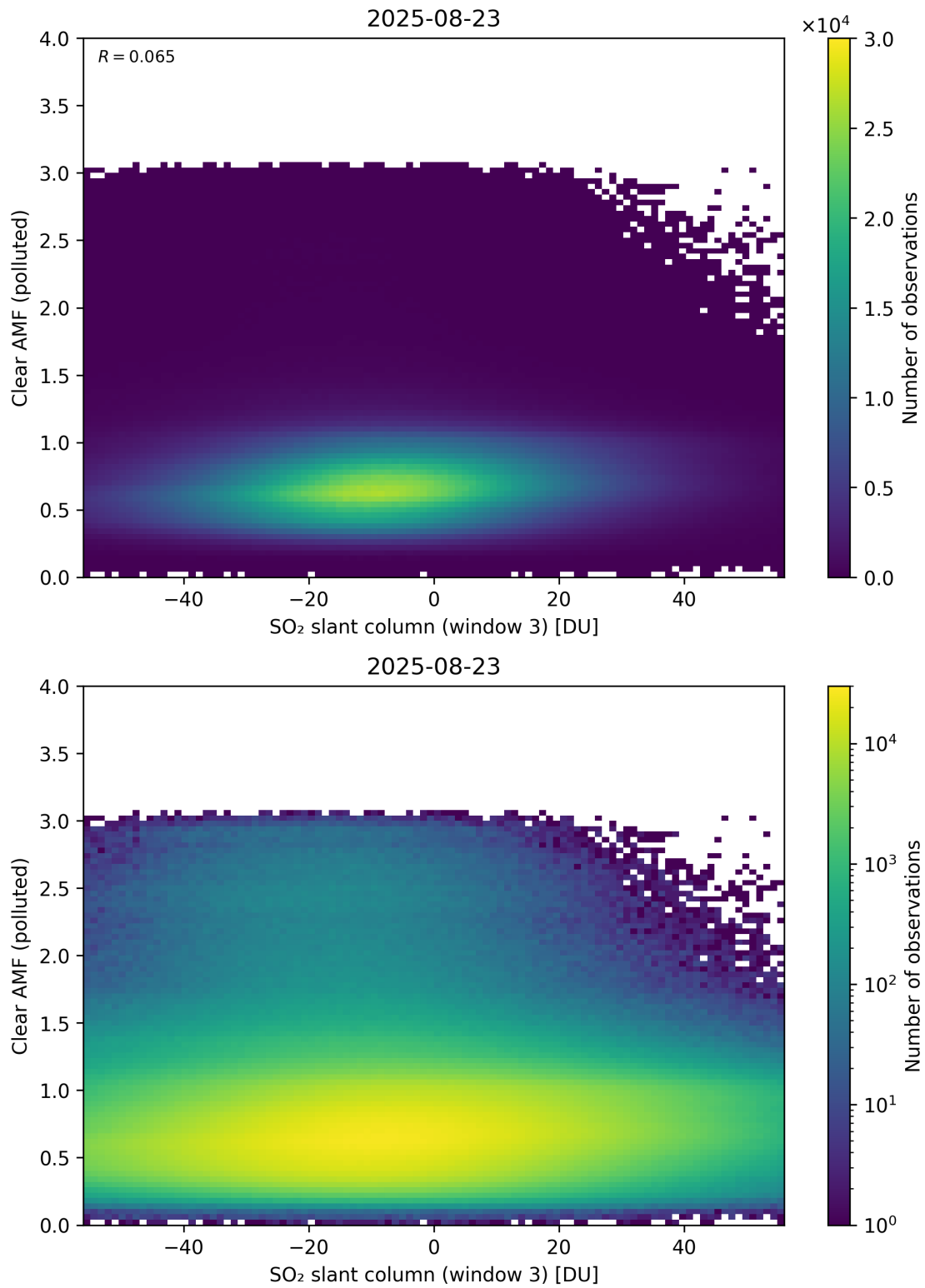
Figure 315: Scatter density plot of “SO 2 slant column (window 3)” against “Clear AMF (polluted)” for 2025-08-22 to 2025-08-24.
