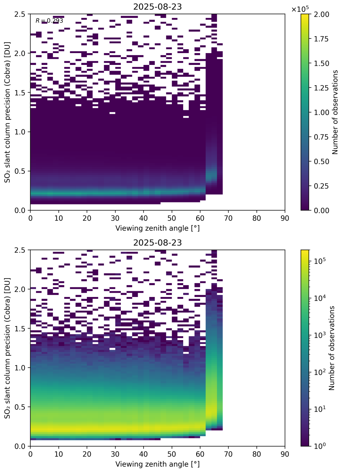
Figure 372: Scatter density plot of “Viewing zenith angle” against “SO 2 slant column precision (Cobra)” for 2025-08-22 to 2025-08-24.
