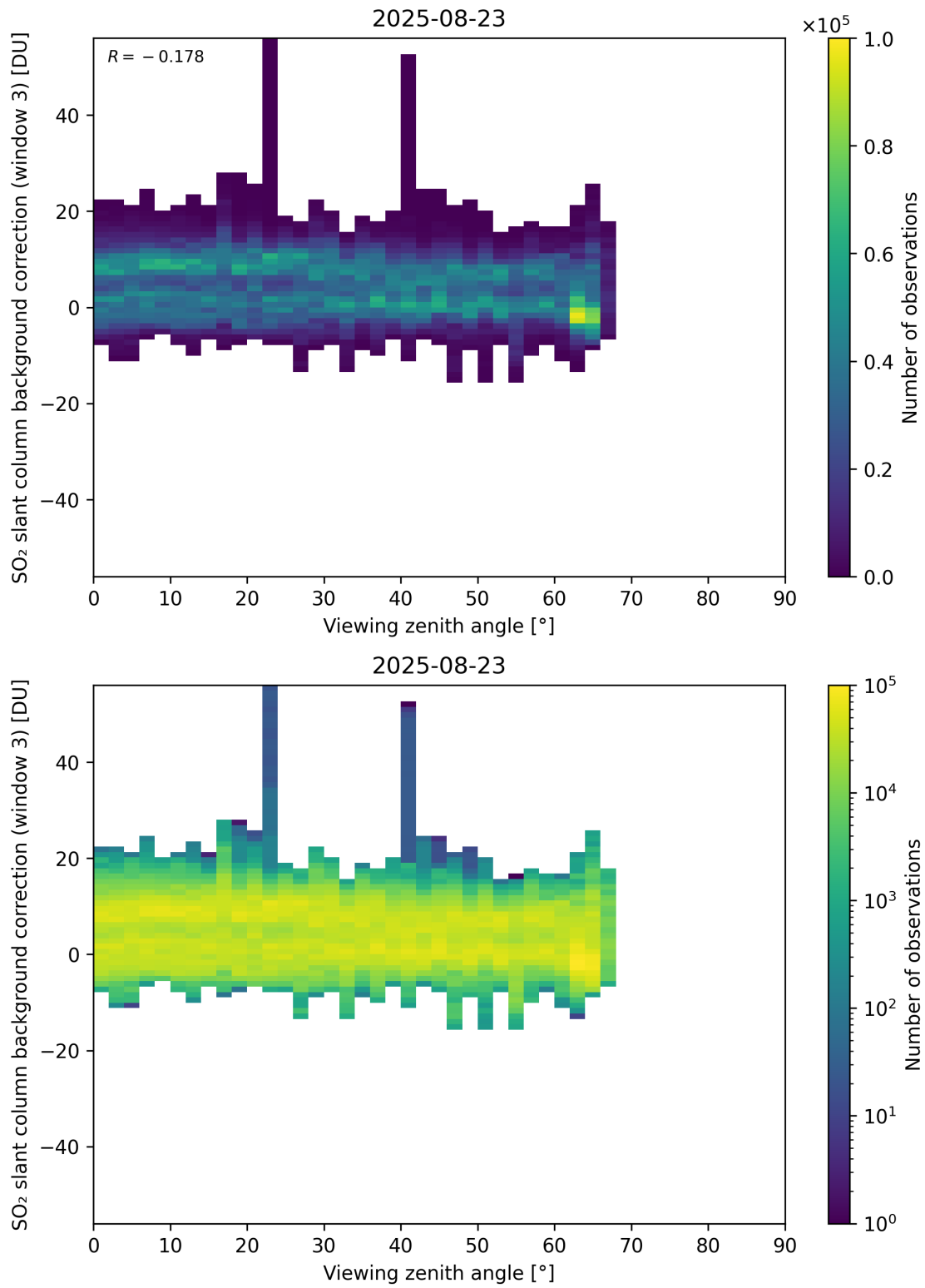
Figure 364: Scatter density plot of “Viewing zenith angle” against “SO 2 slant column background correction (window 3)” for 2025-08-22 to 2025-08-24.
