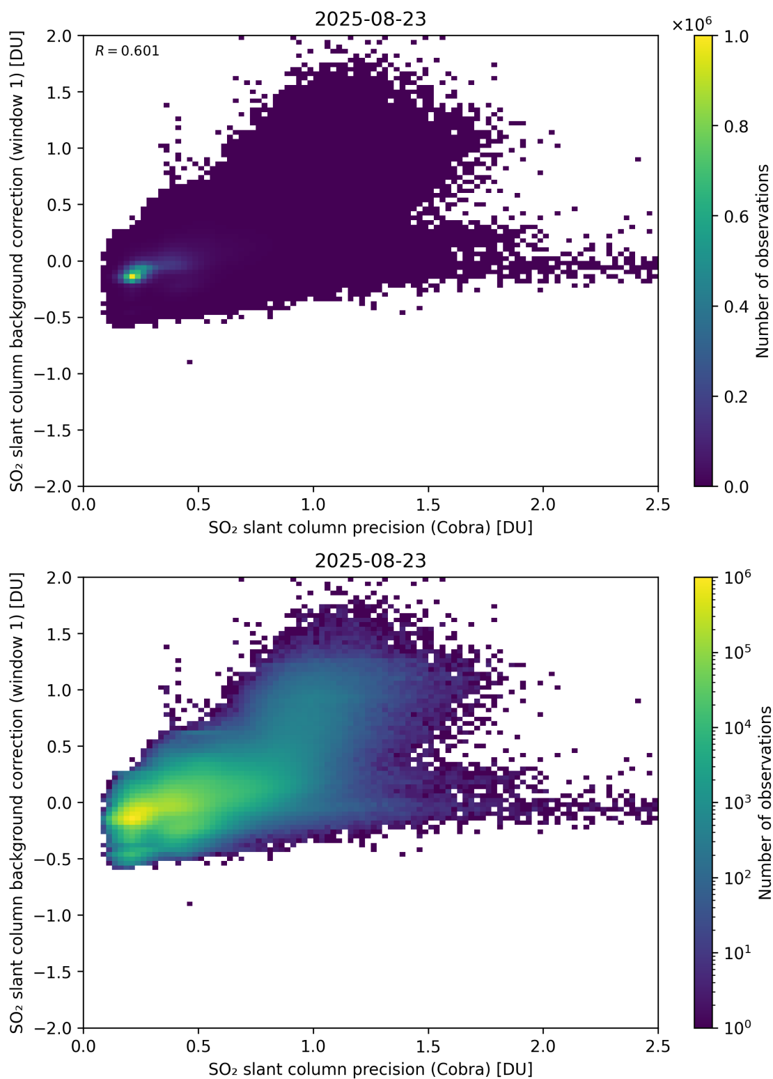
Figure 199: Scatter density plot of “SO 2 slant column precision (Cobra)” against “SO 2 slant column background correction (window 1)” for 2025-08-22 to 2025-08-24.
