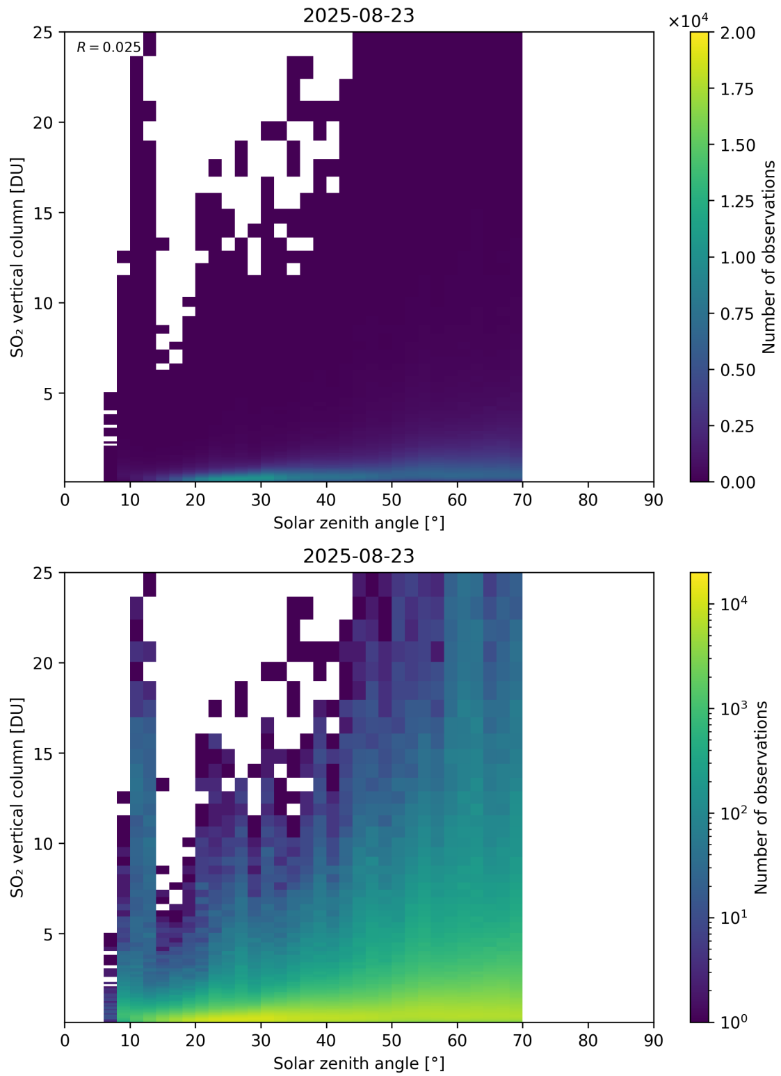
Figure 191: Scatter density plot of “Solar zenith angle” against “SO 2 vertical column” for 2025-08-22 to 2025-08-24.
