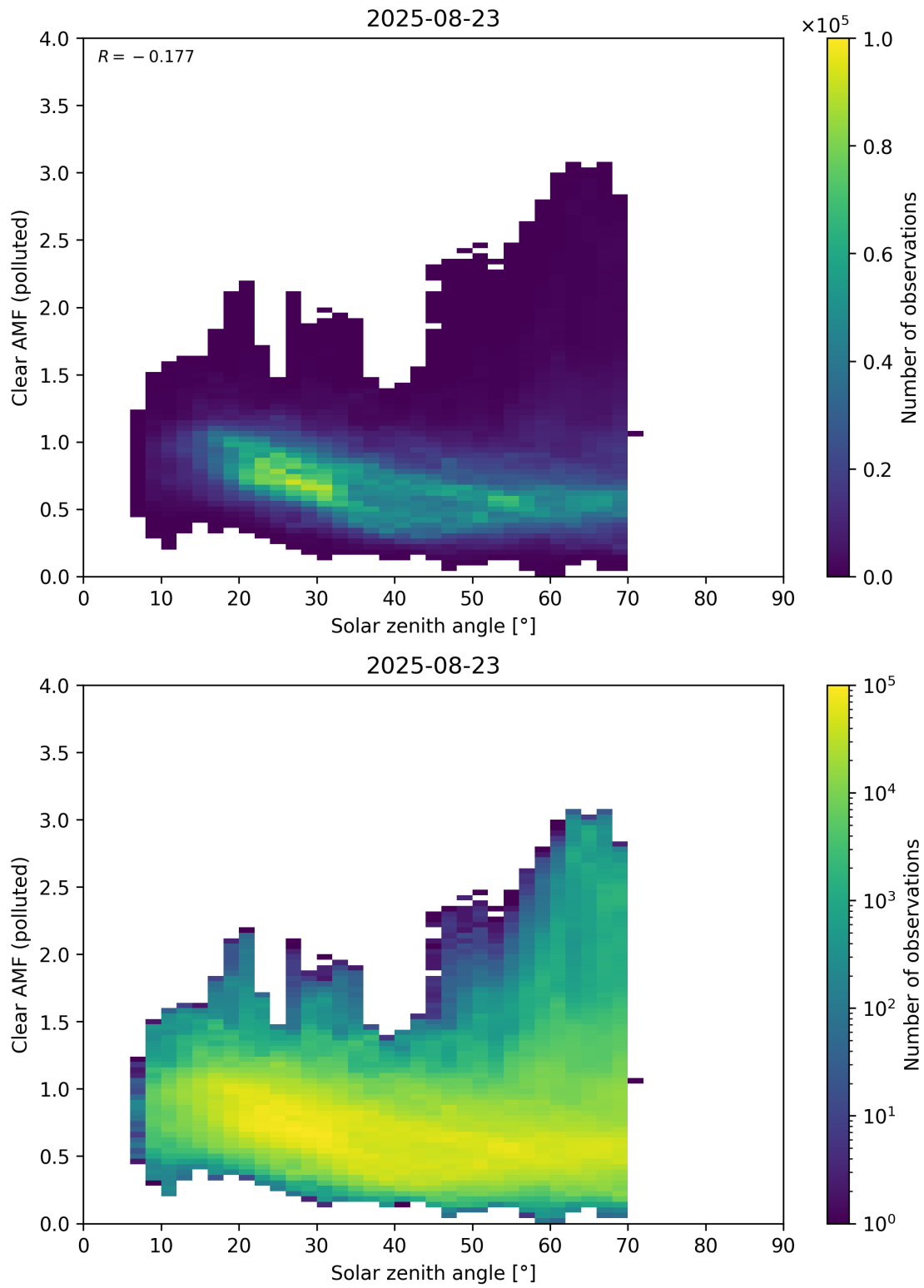
Figure 178: Scatter density plot of “Solar zenith angle” against “Clear AMF (polluted)” for 2025-08-22 to 2025-08-24.
