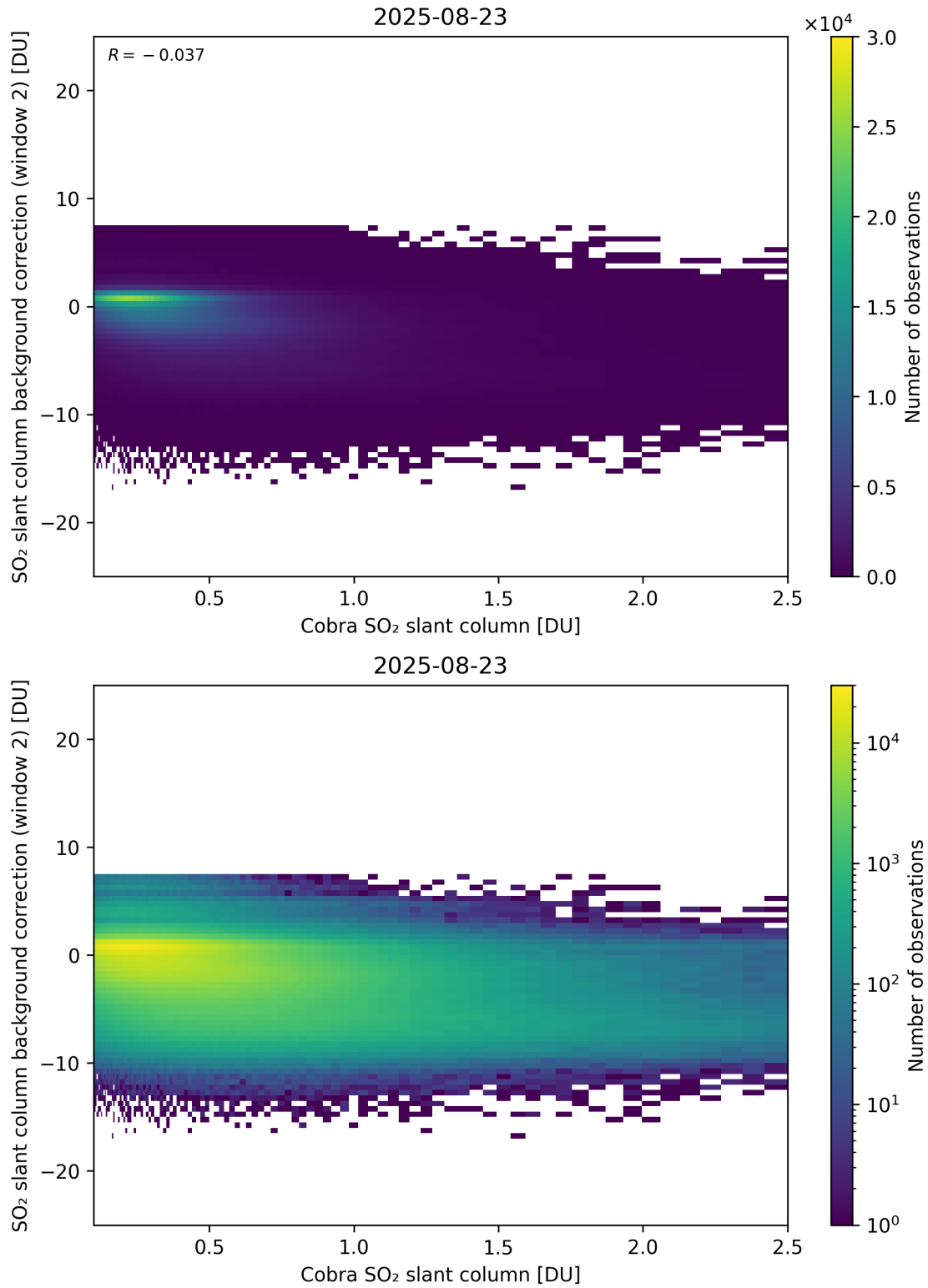
Figure 194: Scatter density plot of “Cobra SO 2 slant column” against “SO 2 slant column background correction (window 2)” for 2025-08-22 to 2025-08-24.
