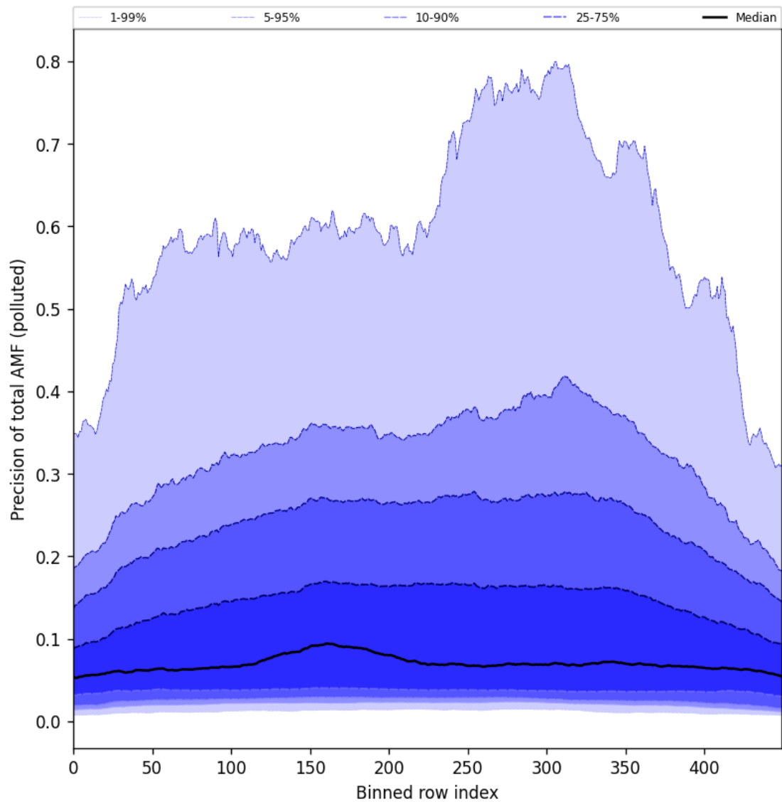
Figure 106: Along track statistics of “Precision of total AMF (polluted)” for 2025-08-22 to 2025-08-24
