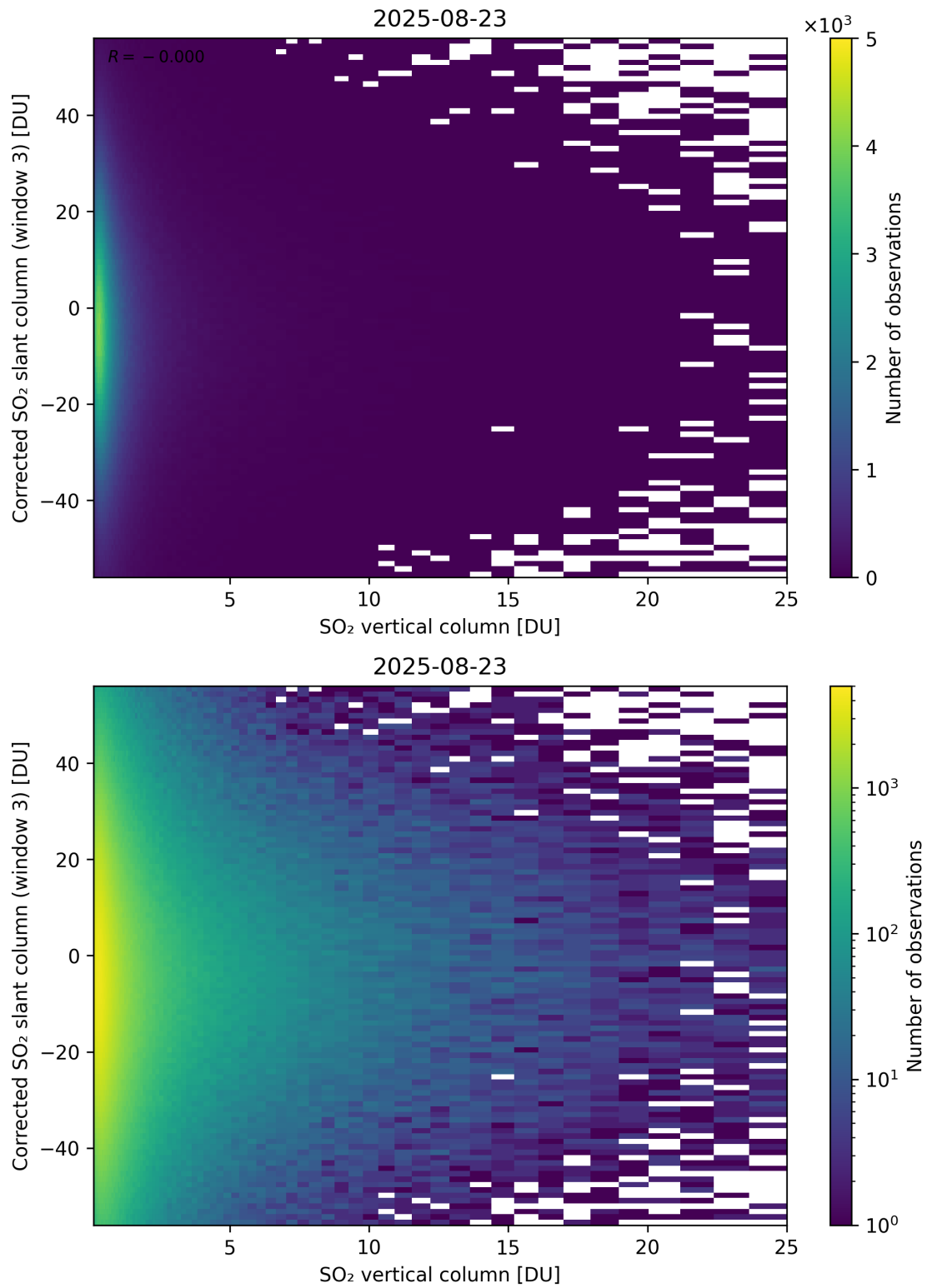
Figure 353: Scatter density plot of “SO 2 vertical column” against “Corrected SO 2 slant column (window 3)” for 2025-08-22 to 2025-08-24.
