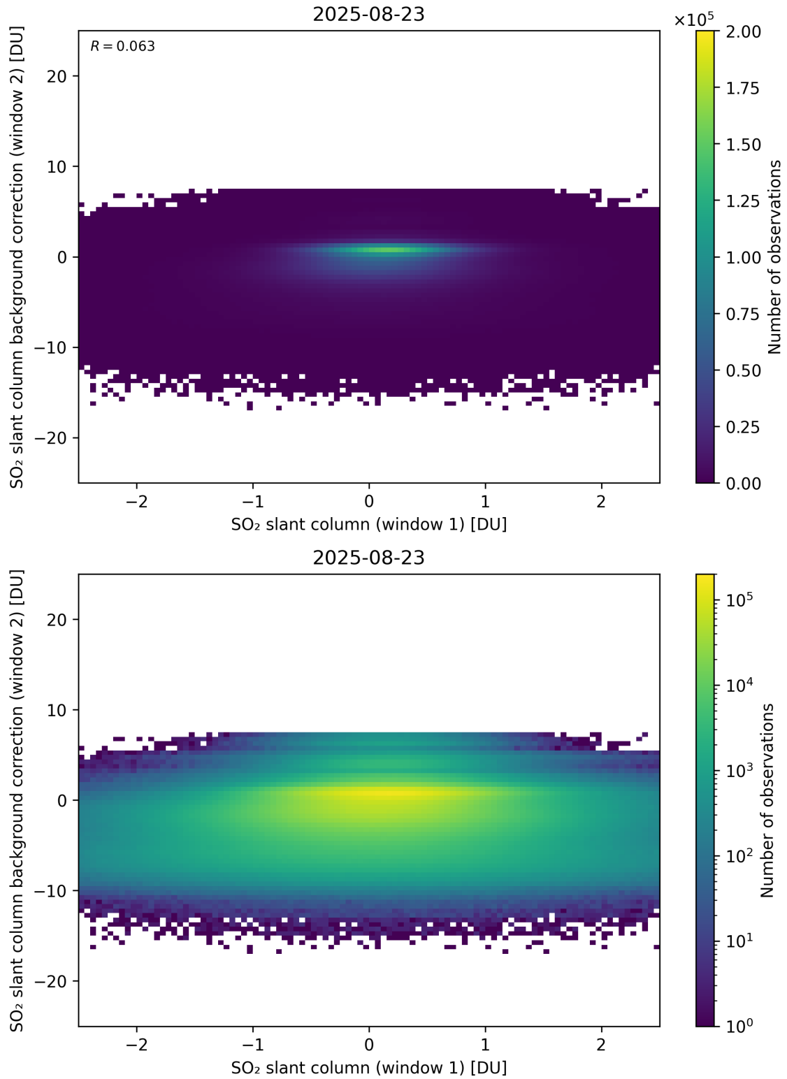
Figure 263: Scatter density plot of “SO 2 slant column (window 1)” against “SO 2 slant column background correction (window 2)” for 2025-08-22 to 2025-08-24.
