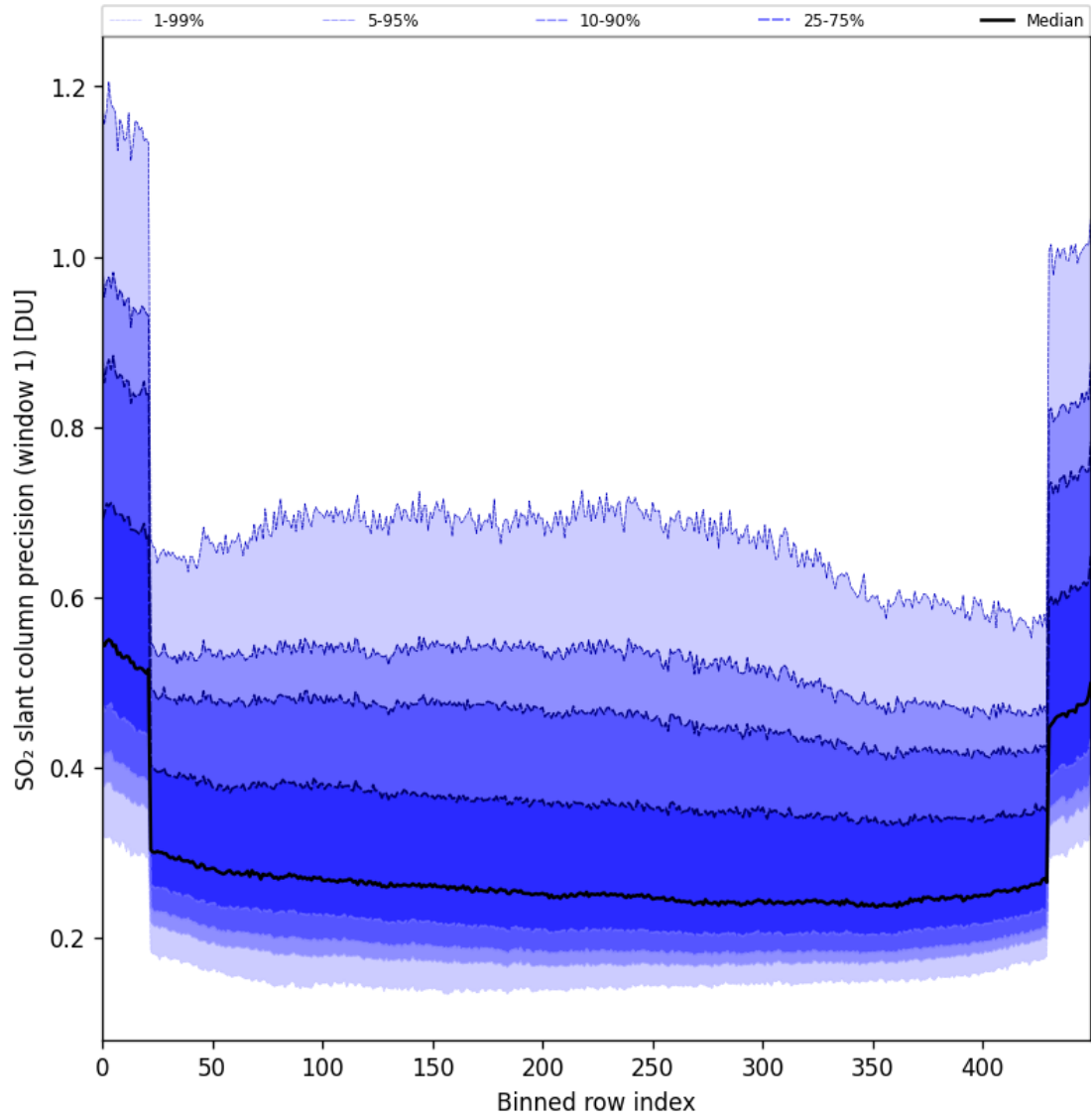
Figure 90: Along track statistics of “SO 2 slant column precision (window 1)” for 2025-08-22 to 2025-08-24
