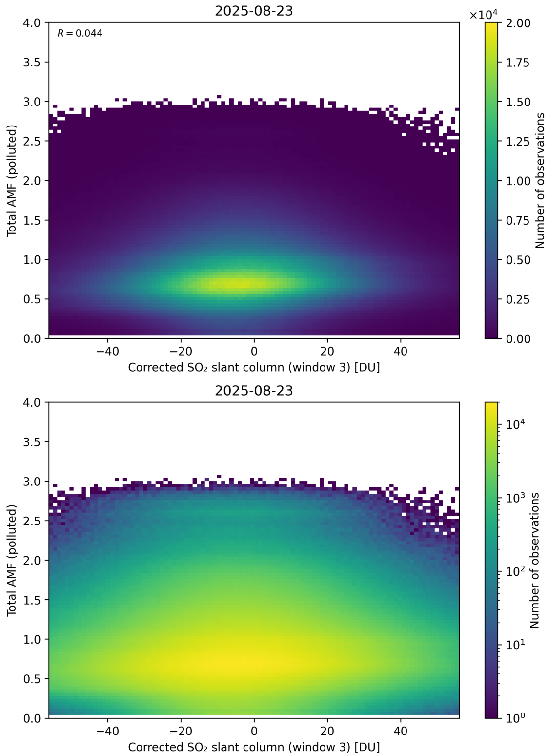
Figure 260: Scatter density plot of “Corrected SO 2 slant column (window 3)” against “Total AMF (polluted)” for 2025-08-22 to 2025-08-24.
