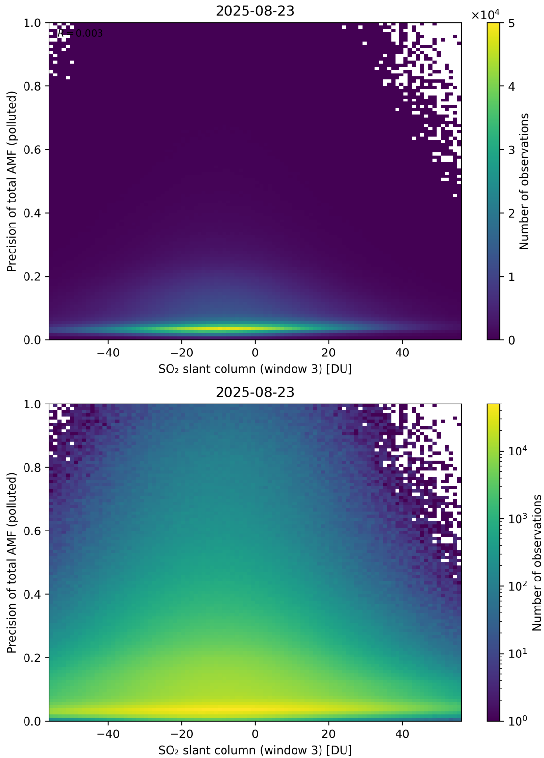
Figure 319: Scatter density plot of “SO 2 slant column (window 3)” against “Precision of total AMF (polluted)” for 2025-08-22 to 2025-08-24.
