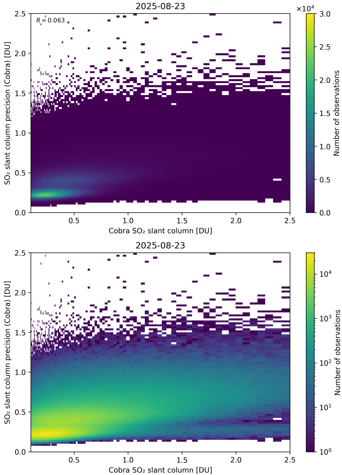
Figure 216: Scatter density plot of “Cobra SO 2 slant column” against “SO 2 slant column precision (Cobra)” for 2025-08-22 to 2025-08-24.
