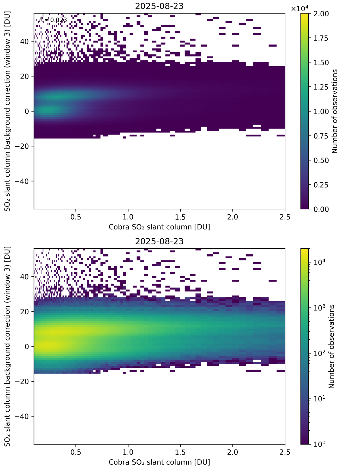
Figure 195: Scatter density plot of “Cobra SO 2 slant column” against “SO 2 slant column background correction (window 3)” for 2025-08-22 to 2025-08-24.
