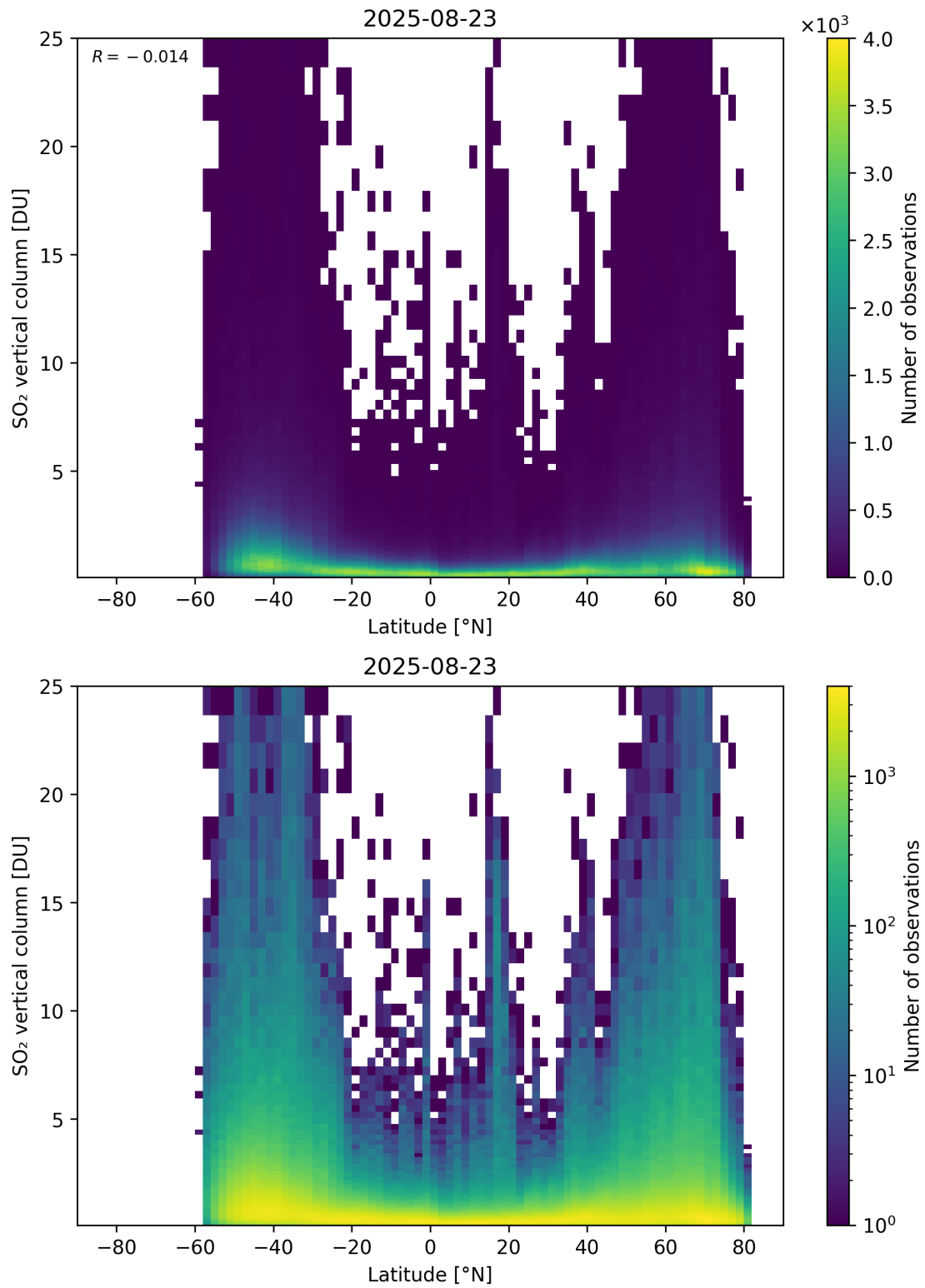
Figure 169: Scatter density plot of “Latitude” against “SO 2 vertical column” for 2025-08-22 to 2025-08-24.
