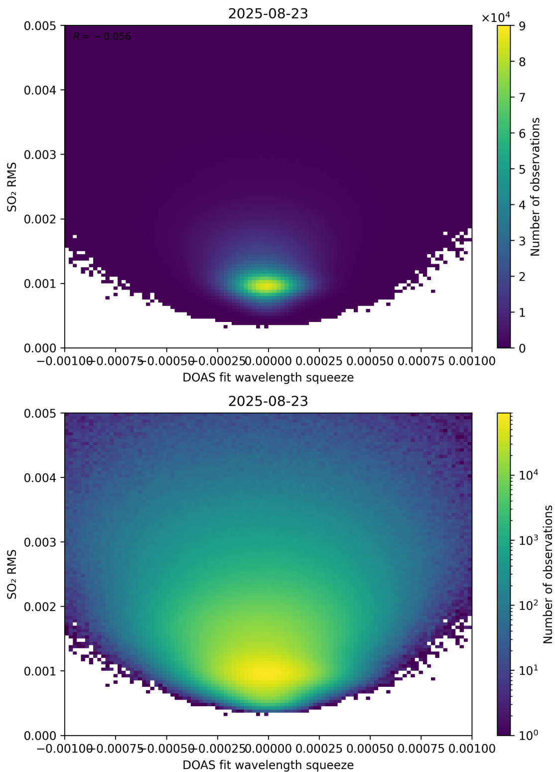
Figure 143: Scatter density plot of “DOAS fit wavelength squeeze” against “SO 2 RMS” for 2025-08-22 to 2025-08-24.
