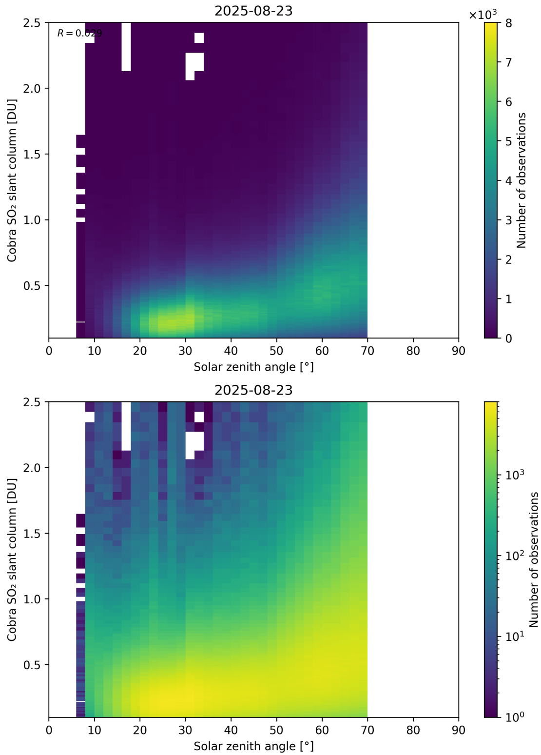
Figure 179: Scatter density plot of “Solar zenith angle” against “Cobra SO 2 slant column” for 2025-08-22 to 2025-08-24.
