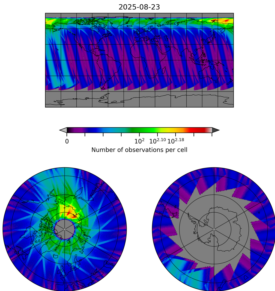
Figure 30: Map of the number of observations for 2025-08-22 to 2025-08-24
