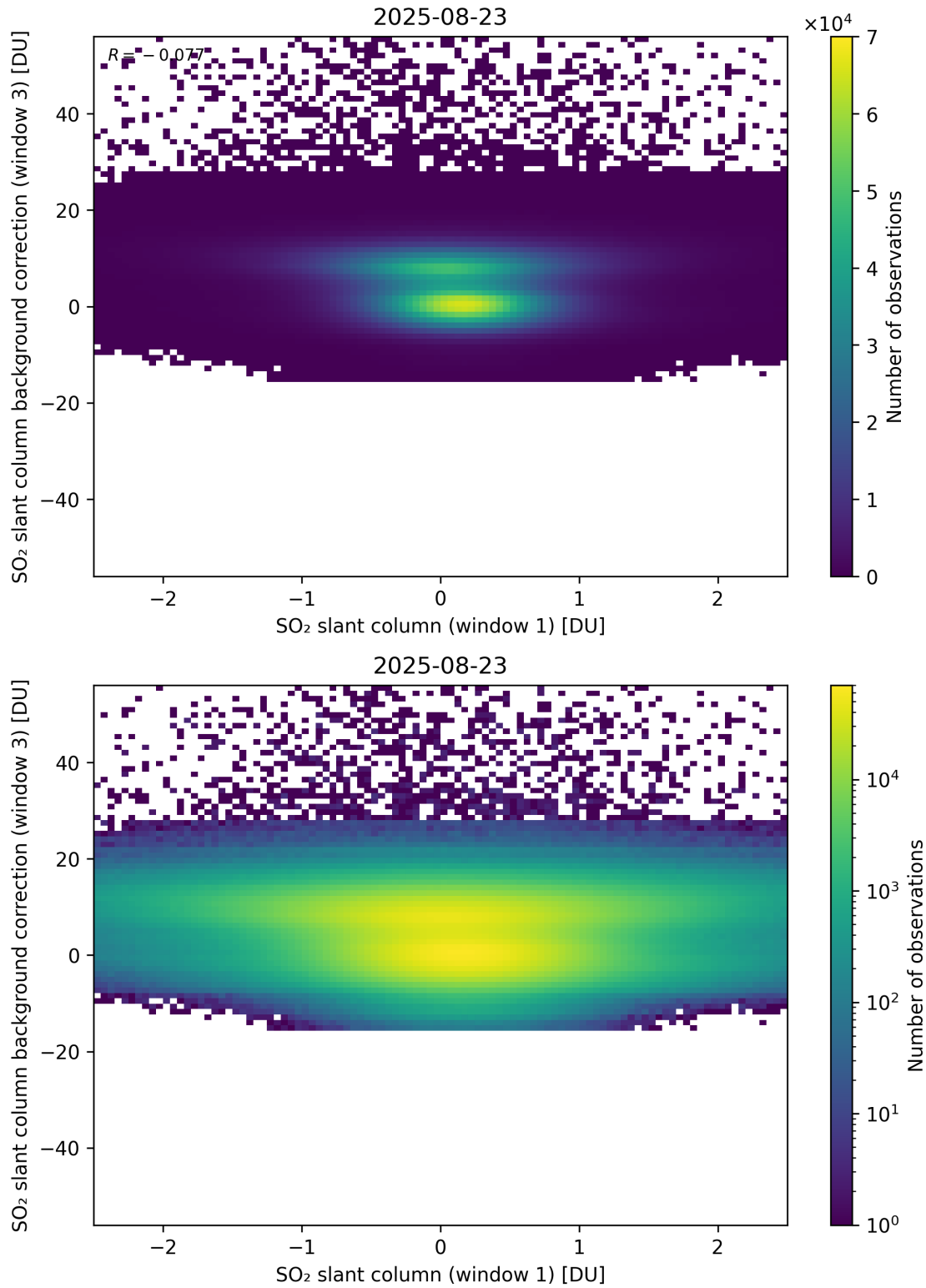
Figure 264: Scatter density plot of “SO 2 slant column (window 1)” against “SO 2 slant column background correction (window 3)” for 2025-08-22 to 2025-08-24.
