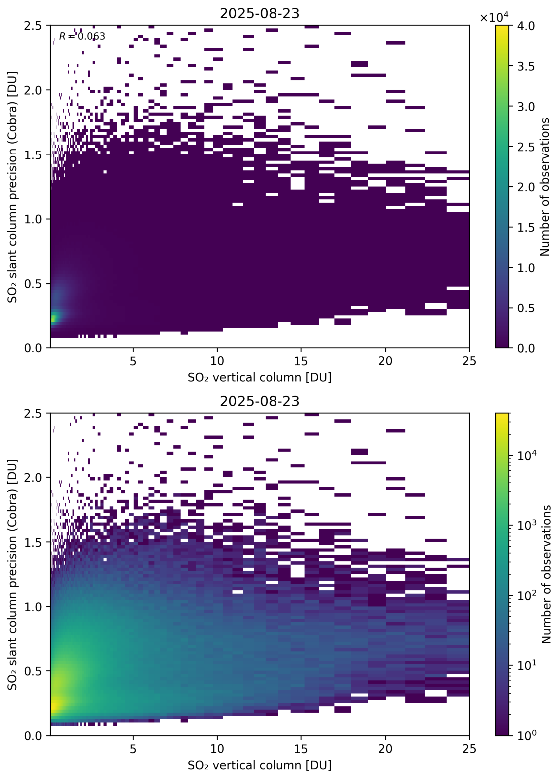
Figure 350: Scatter density plot of “SO 2 vertical column” against “SO 2 slant column precision (Cobra)” for 2025-08-22 to 2025-08-24.
