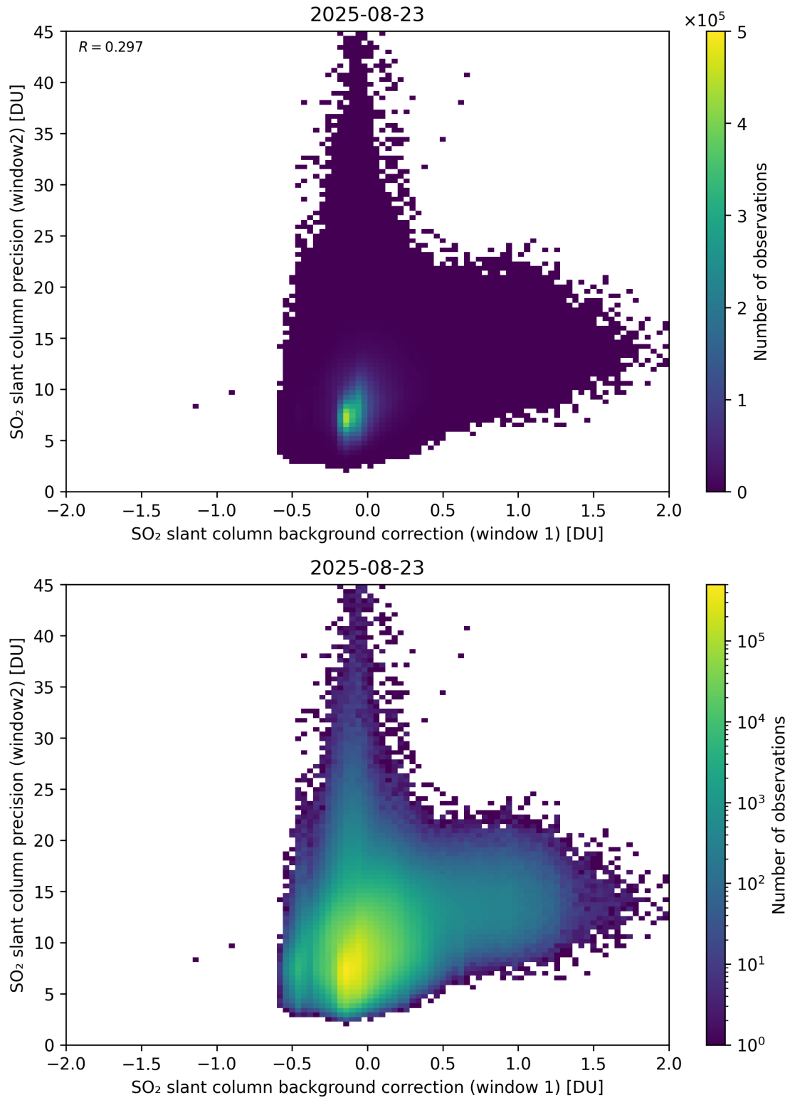
Figure 117: Scatter density plot of “SO 2 slant column background correction (window 1)” against “SO 2 slant column precision (window2)” for 2025-08-22 to 2025-08-24.
