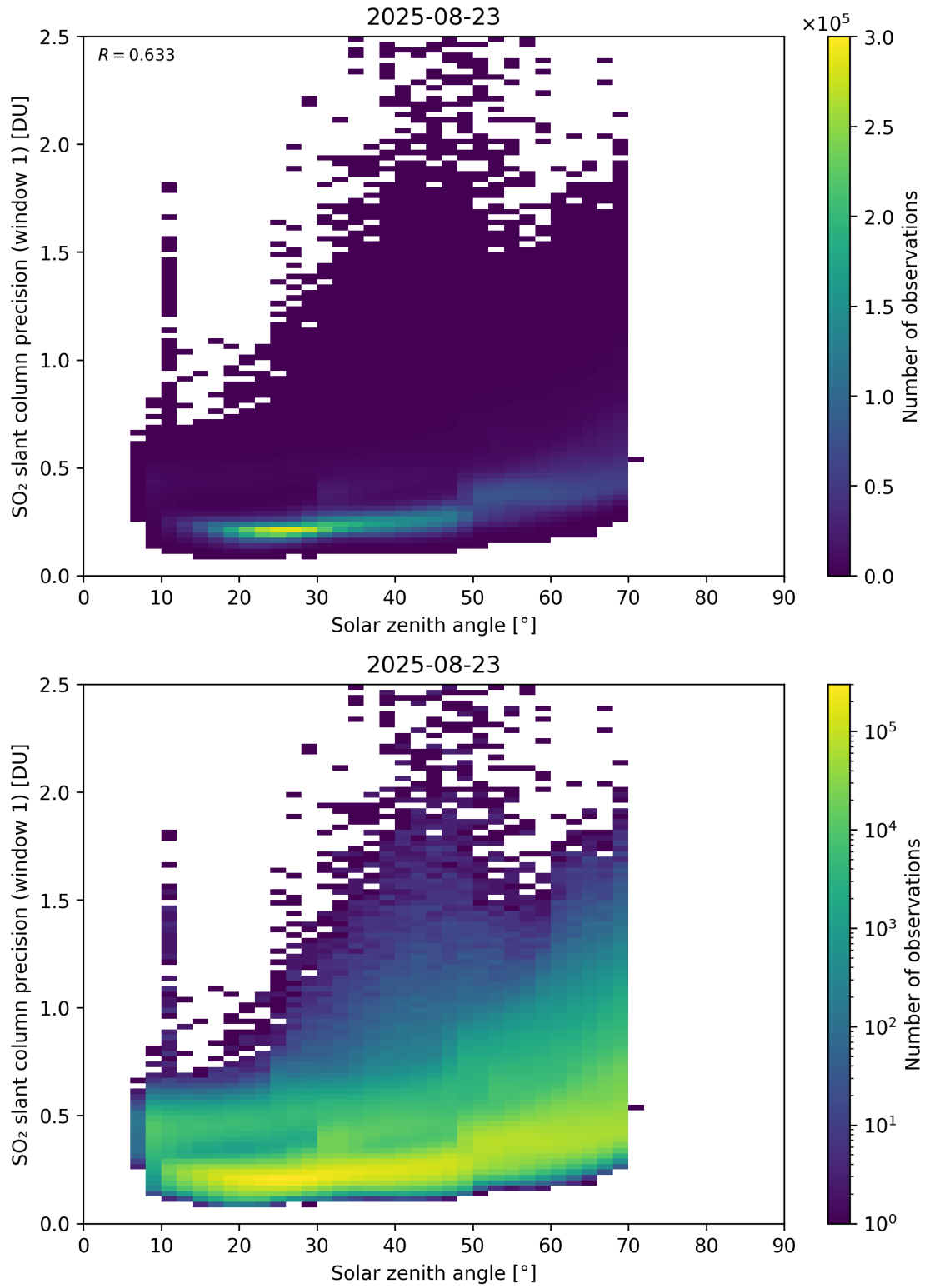
Figure 185: Scatter density plot of “Solar zenith angle” against “SO 2 slant column precision (window 1)” for 2025-08-22 to 2025-08-24.
