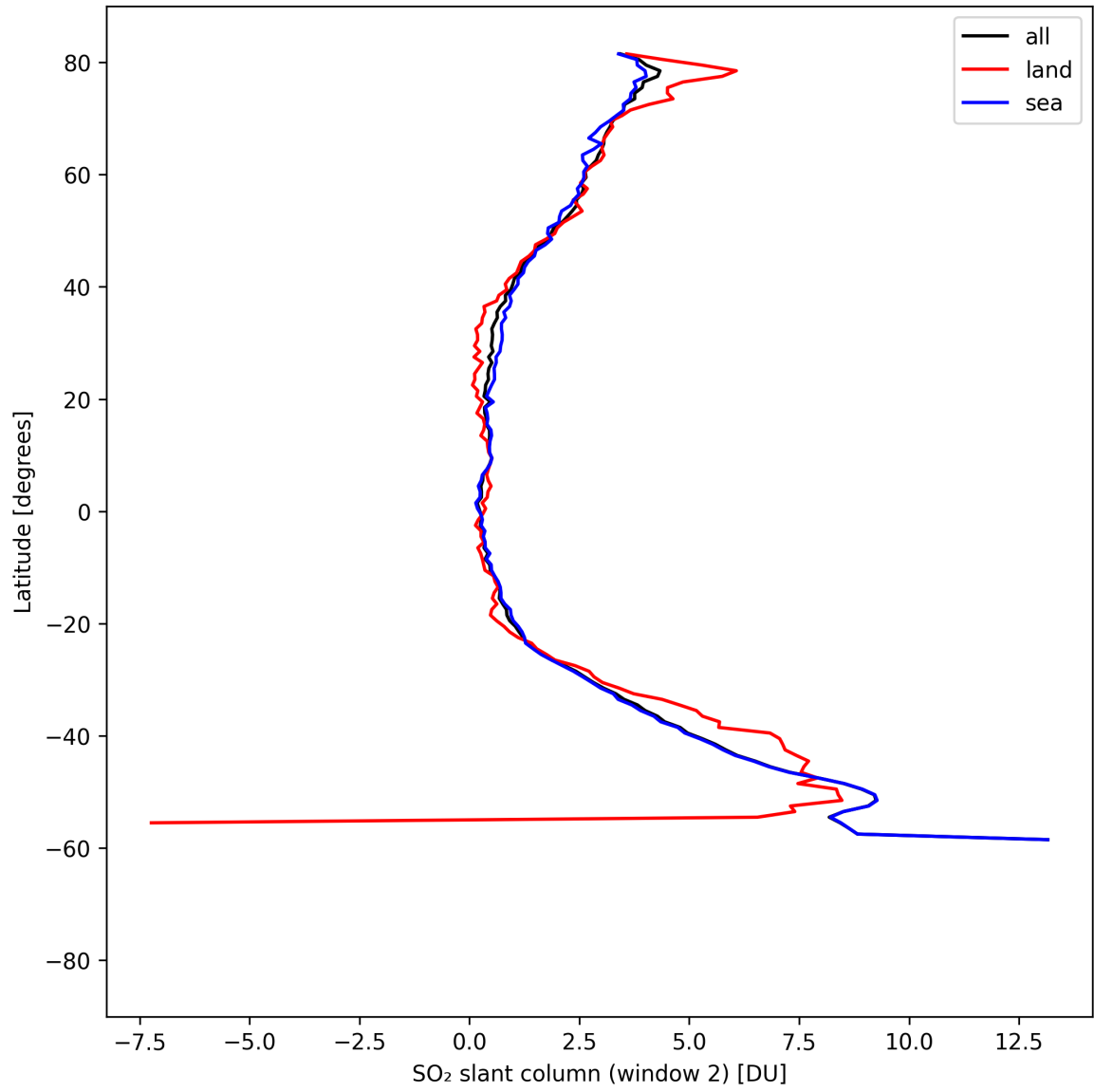
Figure 41: Zonal average of “SO 2 slant column (window 2)” for 2025-08-22 to 2025-08-24.
