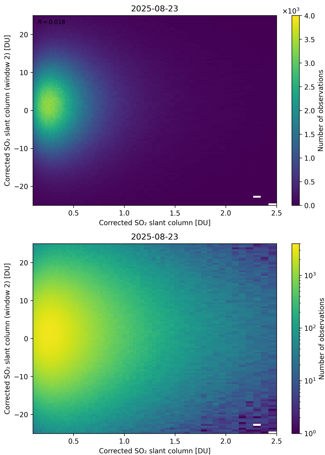
Figure 235: Scatter density plot of “Corrected SO 2 slant column” against “Corrected SO 2 slant column (window 2)” for 2025-08-22 to 2025-08-24.
