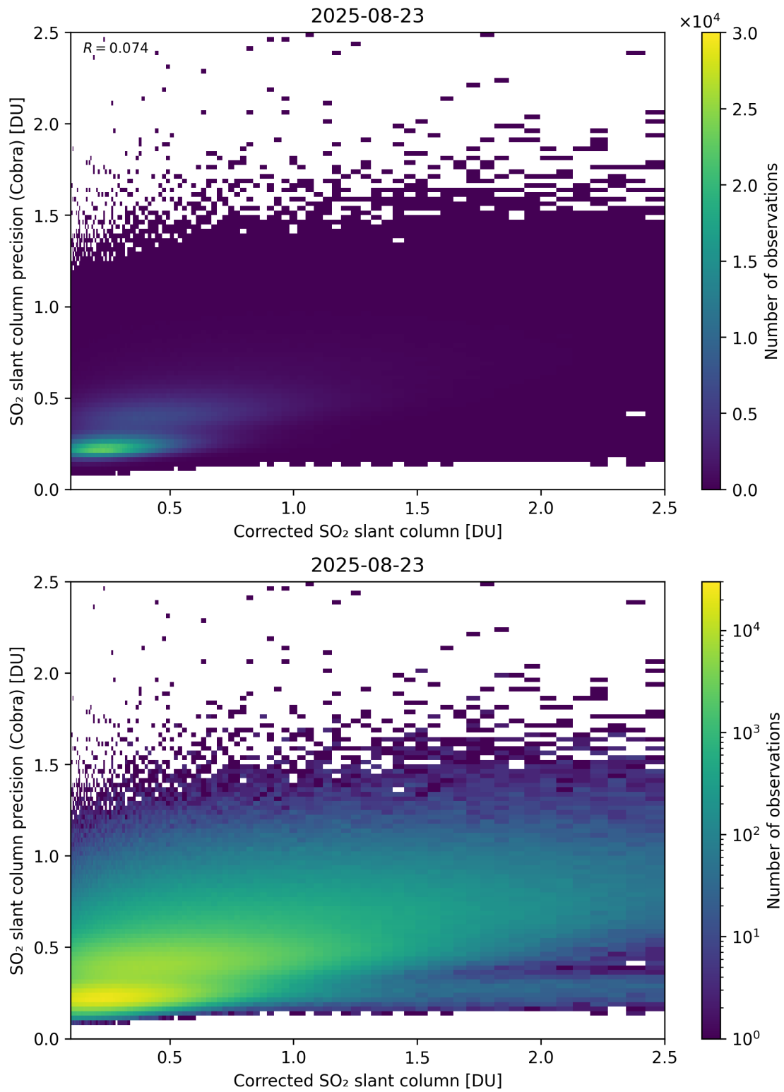
Figure 234: Scatter density plot of “Corrected SO 2 slant column” against “SO 2 slant column precision (Cobra)” for 2025-08-22 to 2025-08-24.
