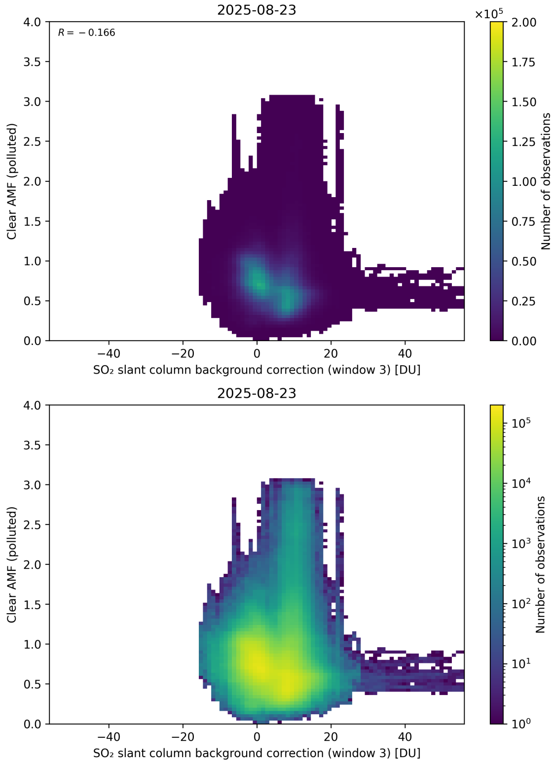
Figure 135: Scatter density plot of “SO 2 slant column background correction (window 3)” against “Clear AMF (polluted)” for 2025-08-22 to 2025-08-24.
