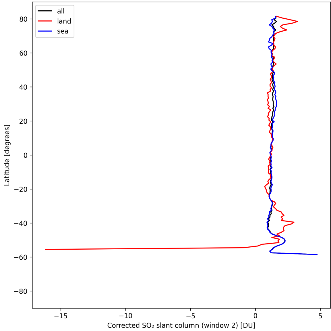
Figure 43: Zonal average of “Corrected SO 2 slant column (window 2)” for 2025-08-22 to 2025-08-24.
