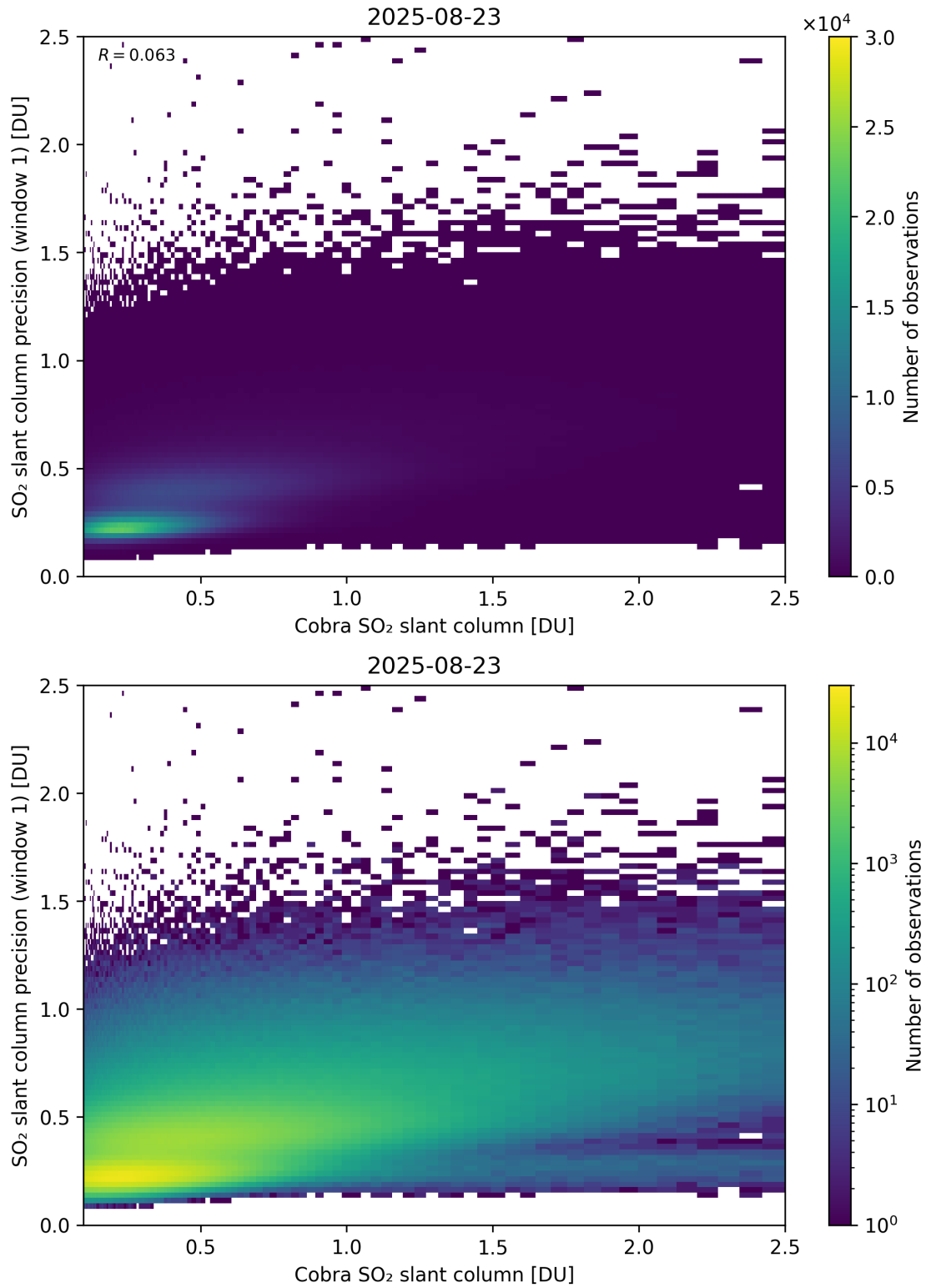
Figure 220: Scatter density plot of “Cobra SO 2 slant column” against “SO 2 slant column precision (window 1)” for 2025-08-22 to 2025-08-24.
