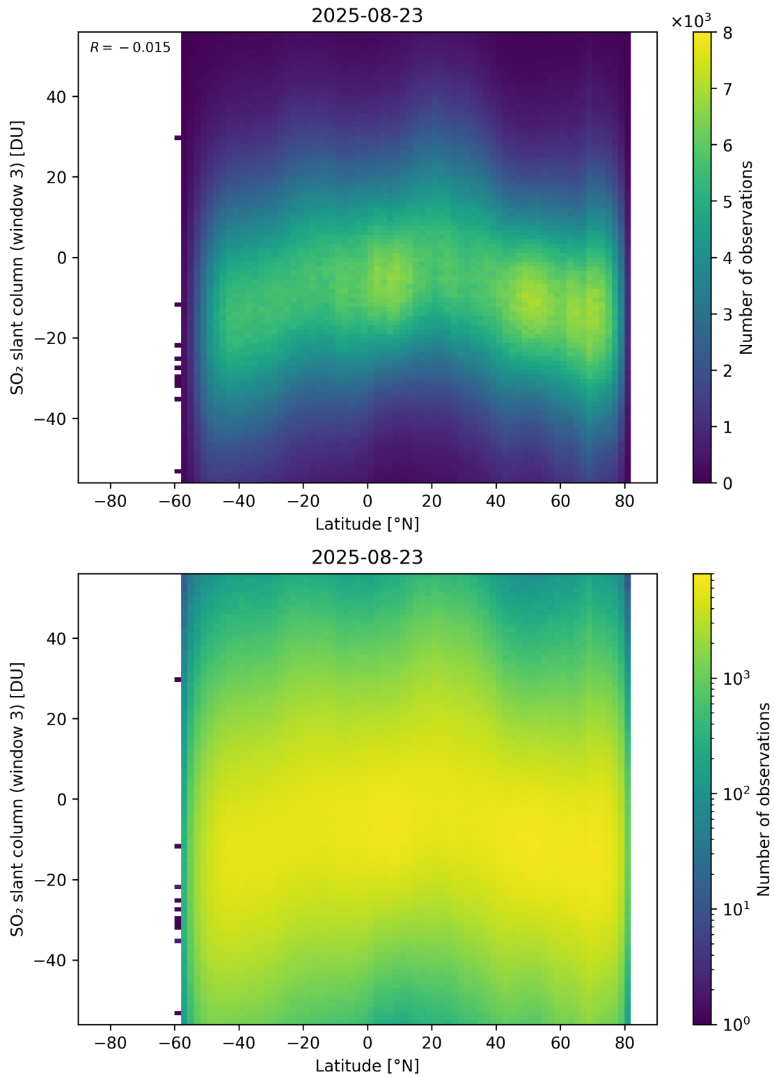
Figure 165: Scatter density plot of “Latitude” against “SO 2 slant column (window 3)” for 2025-08-22 to 2025-08-24.
