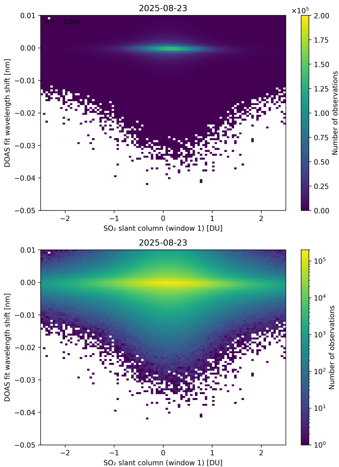
Figure 265: Scatter density plot of “SO 2 slant column (window 1)” against “DOAS fit wavelength shift” for 2025-08-22 to 2025-08-24.
