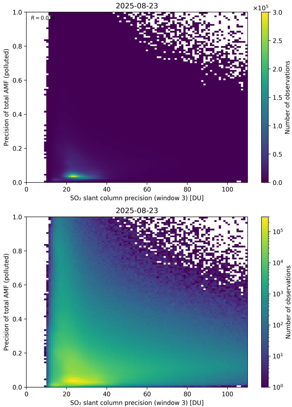
Figure 314: Scatter density plot of “SO 2 slant column precision (window 3)” against “Precision of total AMF (polluted)” for 2025-08-22 to 2025-08-24.
