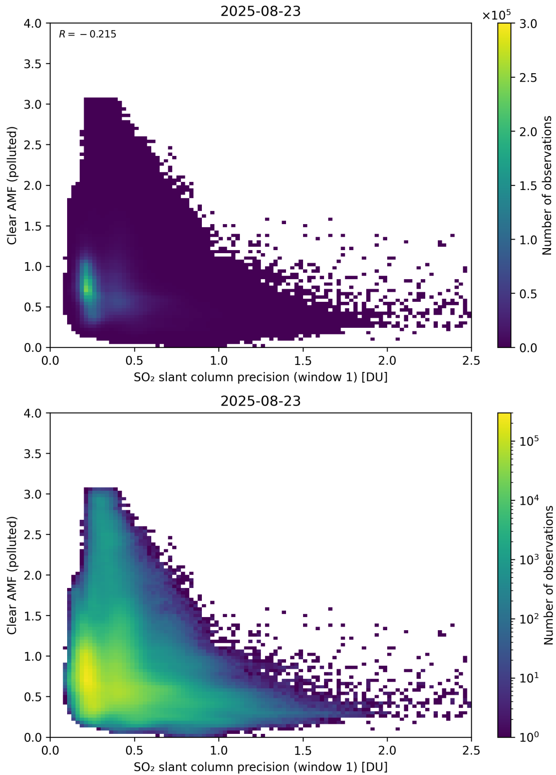
Figure 274: Scatter density plot of “SO 2 slant column precision (window 1)” against “Clear AMF (polluted)” for 2025-08-22 to 2025-08-24.
