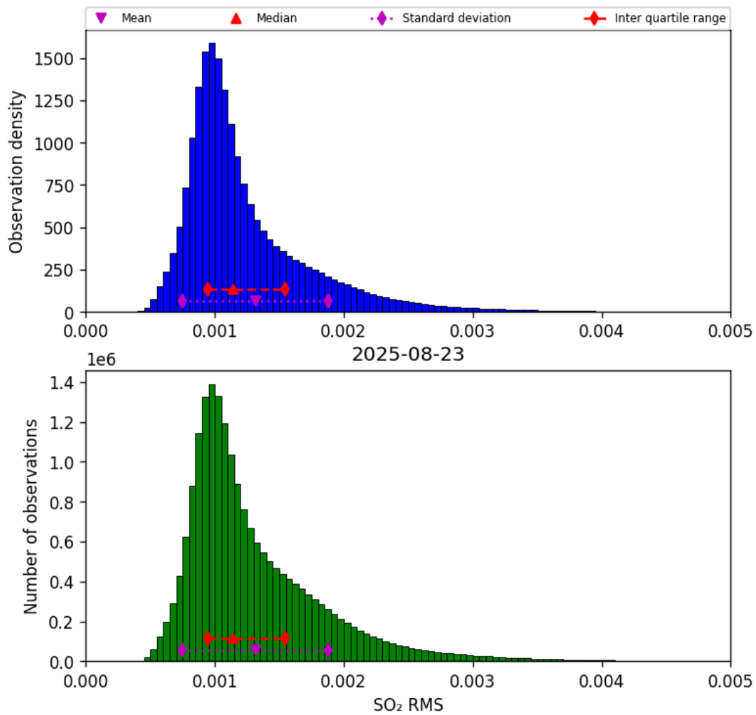
Figure 78: Histogram of “SO 2 RMS” for 2025-08-22 to 2025-08-24
