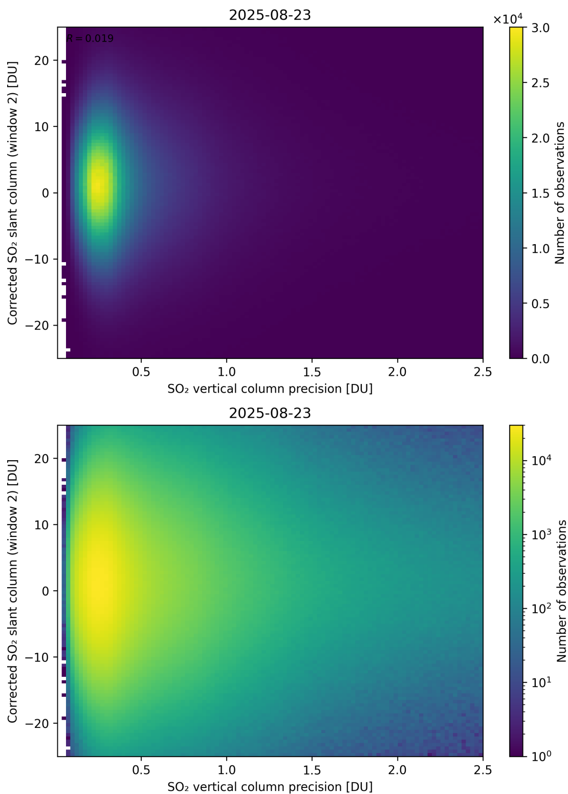
Figure 339: Scatter density plot of “SO 2 vertical column precision” against “Corrected SO 2 slant column (window 2)” for 2025-08-22 to 2025-08-24.
