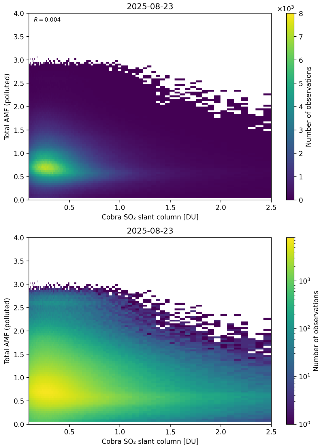
Figure 224: Scatter density plot of “Cobra SO 2 slant column” against “Total AMF (polluted)” for 2025-08-22 to 2025-08-24.
