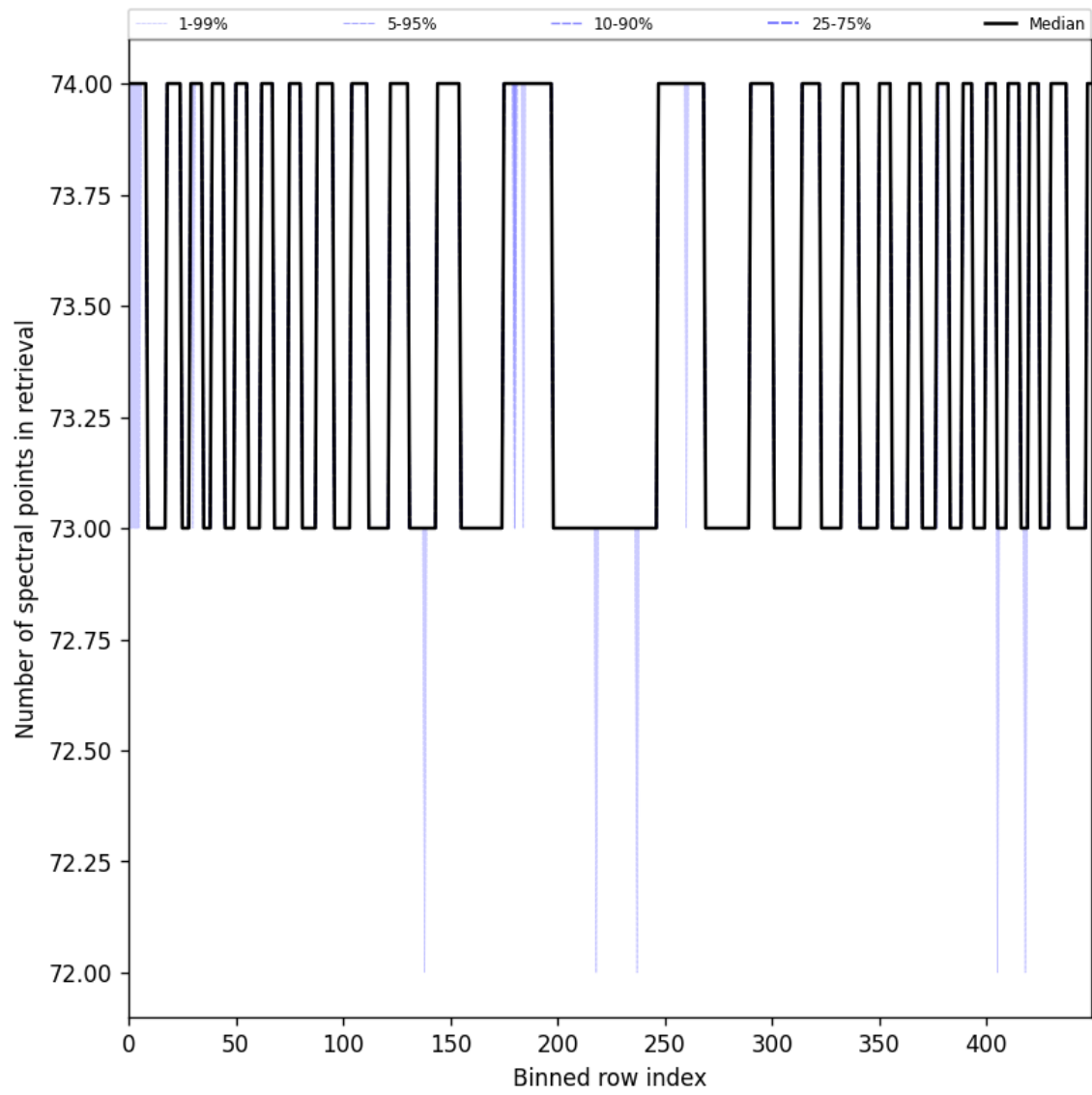
Figure 108: Along track statistics of “Number of spectral points in retrieval” for 2025-08-22 to 2025-08-24
