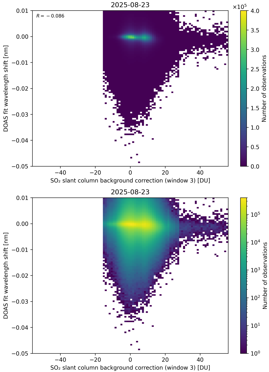
Figure 132: Scatter density plot of “SO 2 slant column background correction (window 3)” against “DOAS fit wavelength shift” for 2025-08-22 to 2025-08-24.
