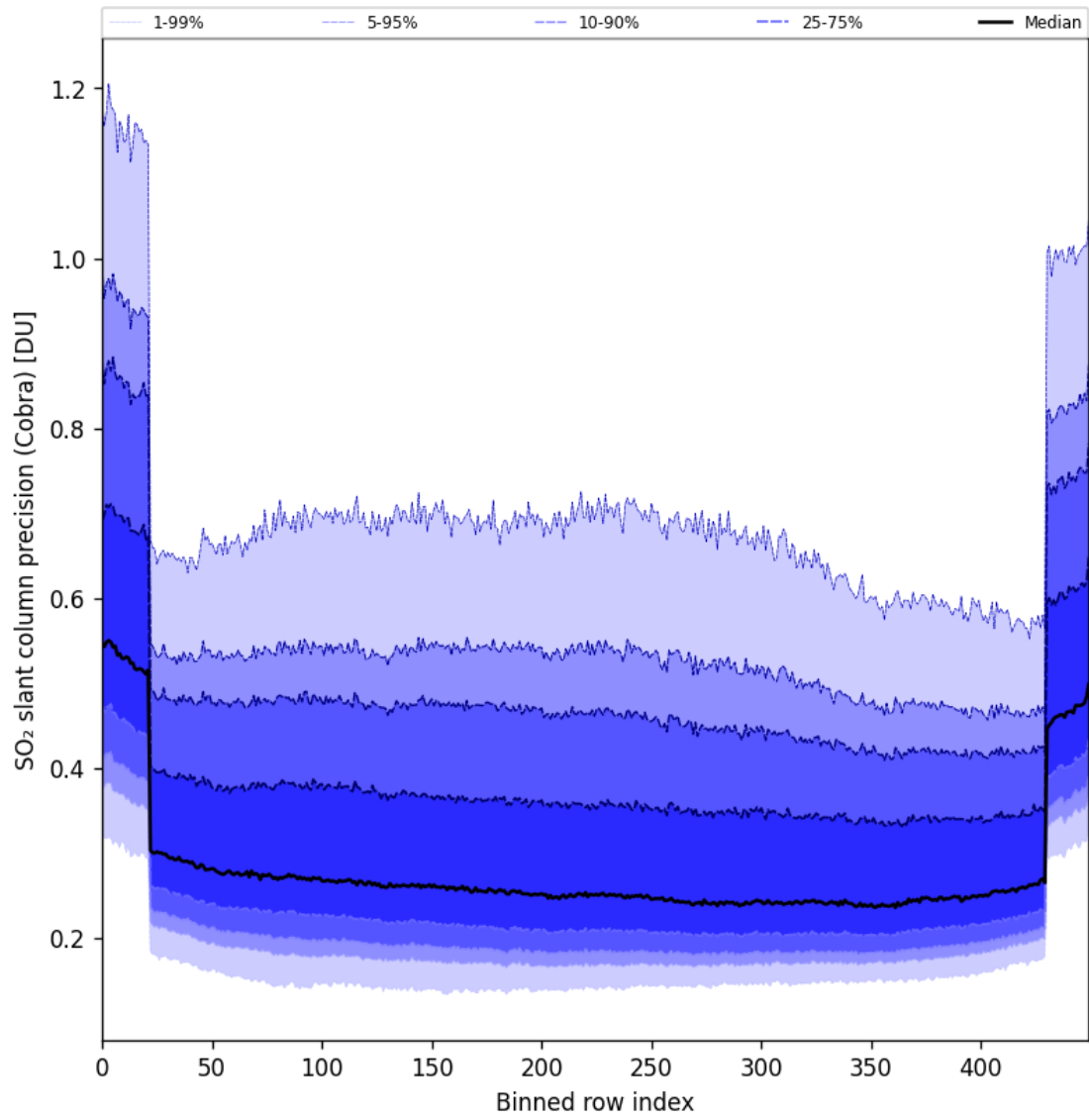
Figure 88: Along track statistics of “SO 2 slant column precision (Cobra)” for 2025-08-22 to 2025-08-24
