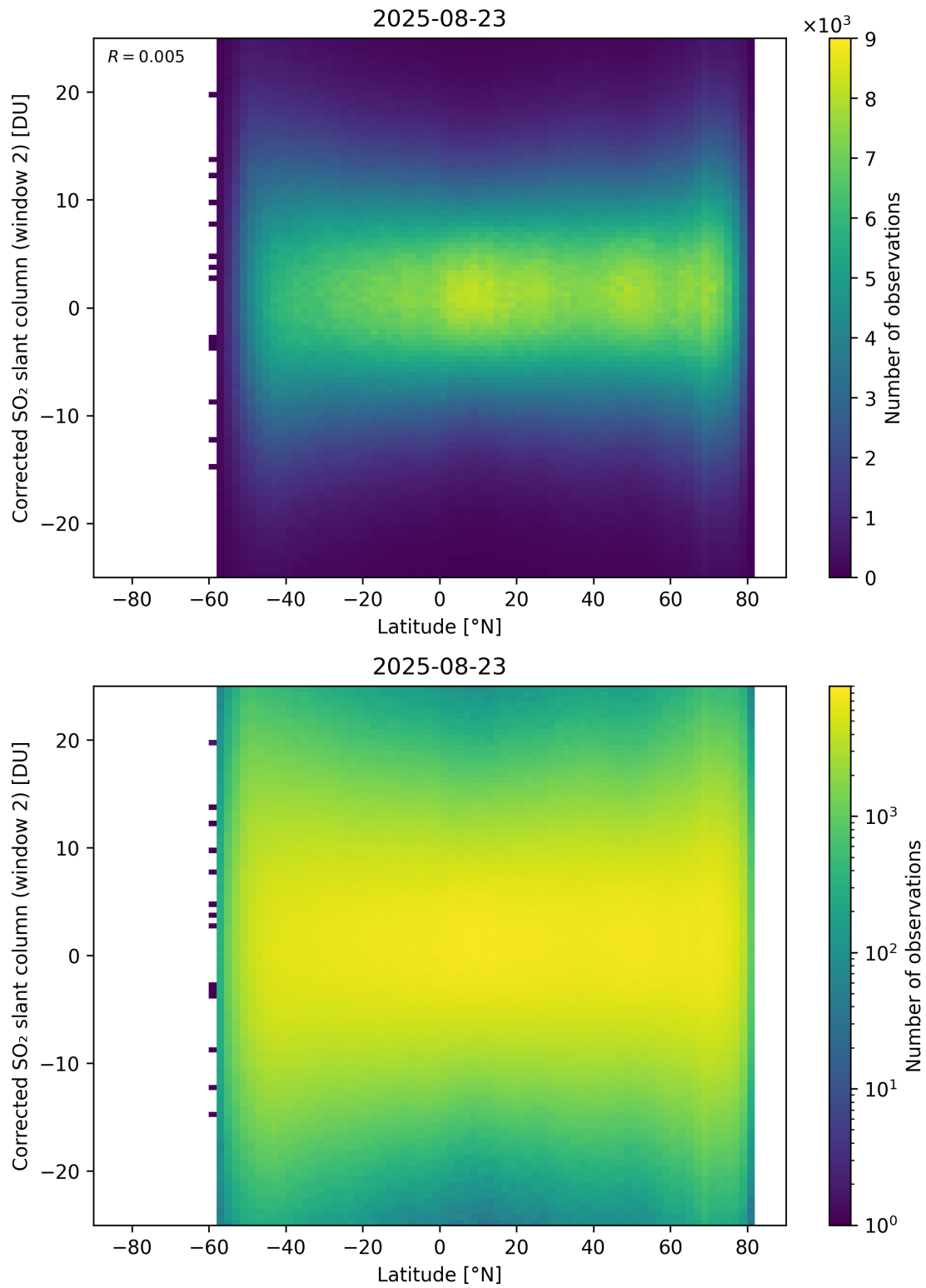
Figure 160: Scatter density plot of “Latitude” against “Corrected SO 2 slant column (window 2)” for 2025-08-22 to 2025-08-24.
