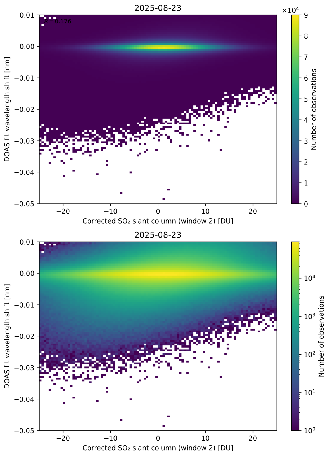
Figure 246: Scatter density plot of “Corrected SO 2 slant column (window 2)” against “DOAS fit wavelength shift” for 2025-08-22 to 2025-08-24.
