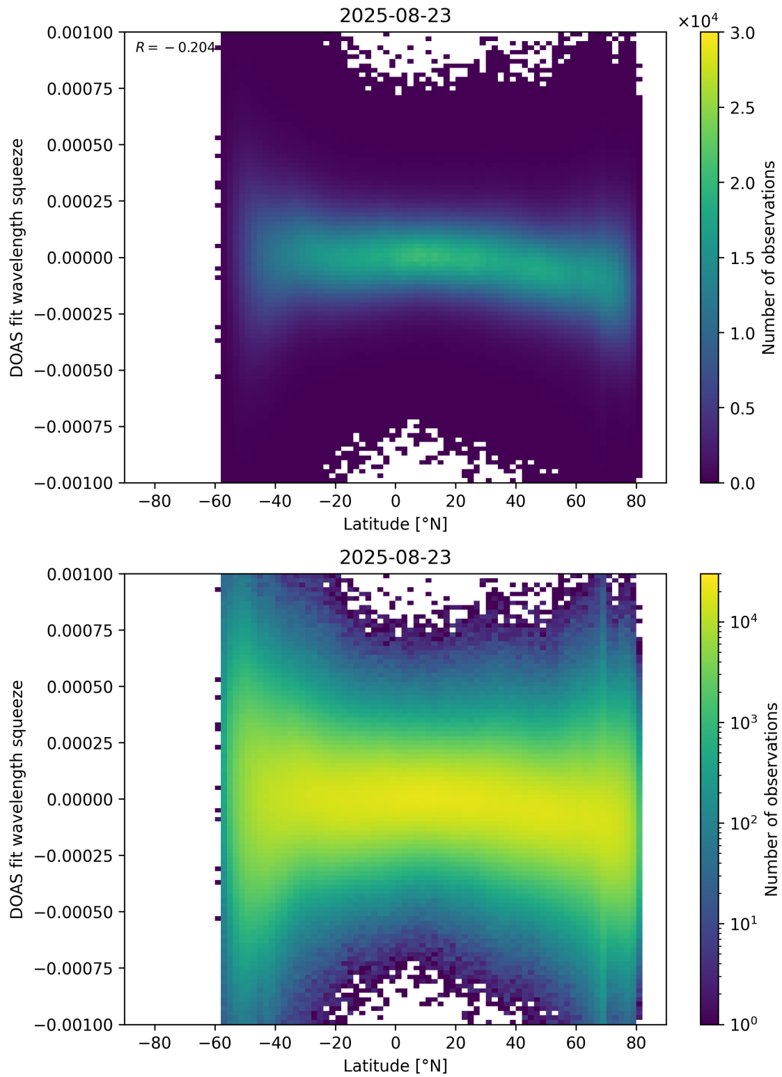
Figure 154: Scatter density plot of “Latitude” against “DOAS fit wavelength squeeze” for 2025-08-22 to 2025-08-24.
