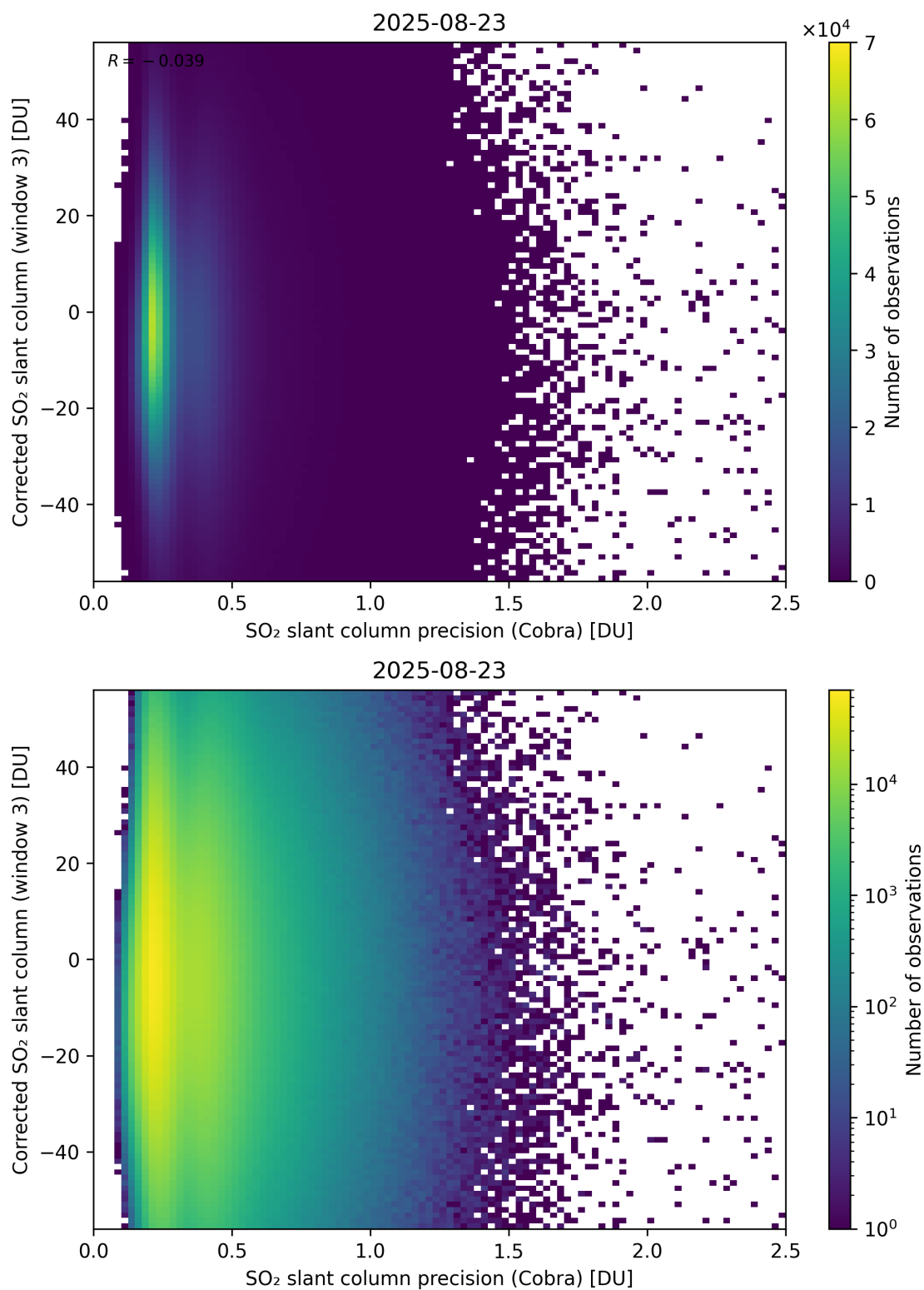
Figure 207: Scatter density plot of “SO 2 slant column precision (Cobra)” against “Corrected SO 2 slant column (window 3)” for 2025-08-22 to 2025-08-24.
