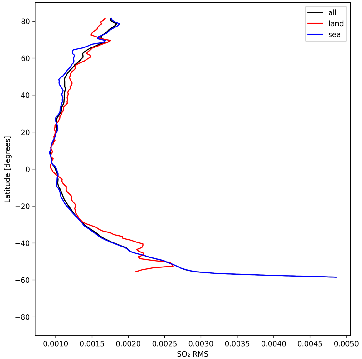
Figure 52: Zonal average of “SO 2 RMS” for 2025-08-22 to 2025-08-24.
