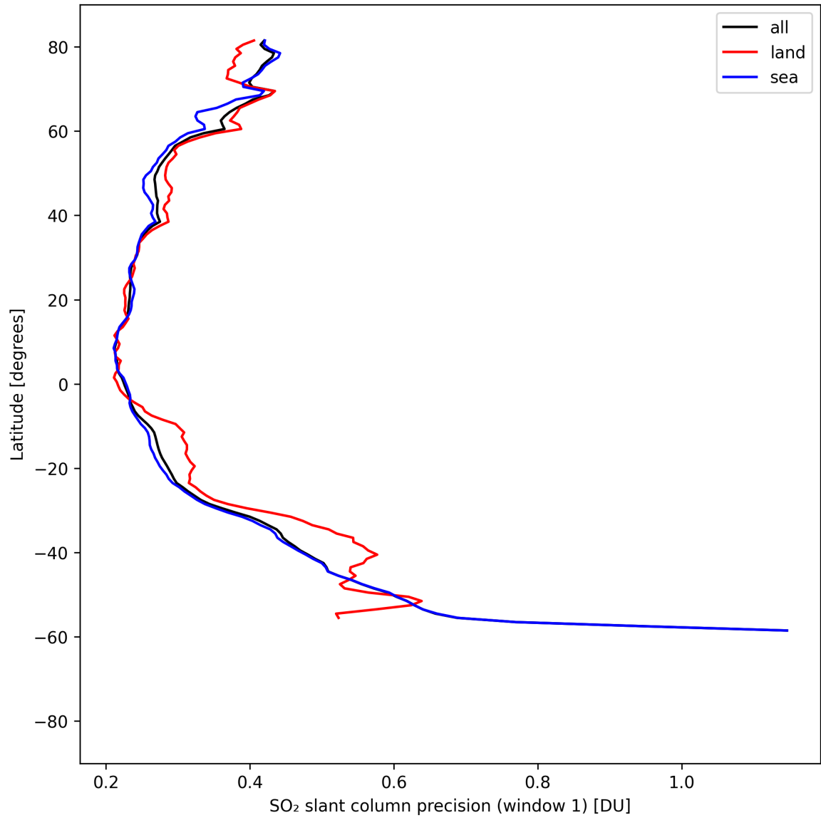
Figure 38: Zonal average of “SO 2 slant column precision (window 1)” for 2025-08-22 to 2025-08-24.
