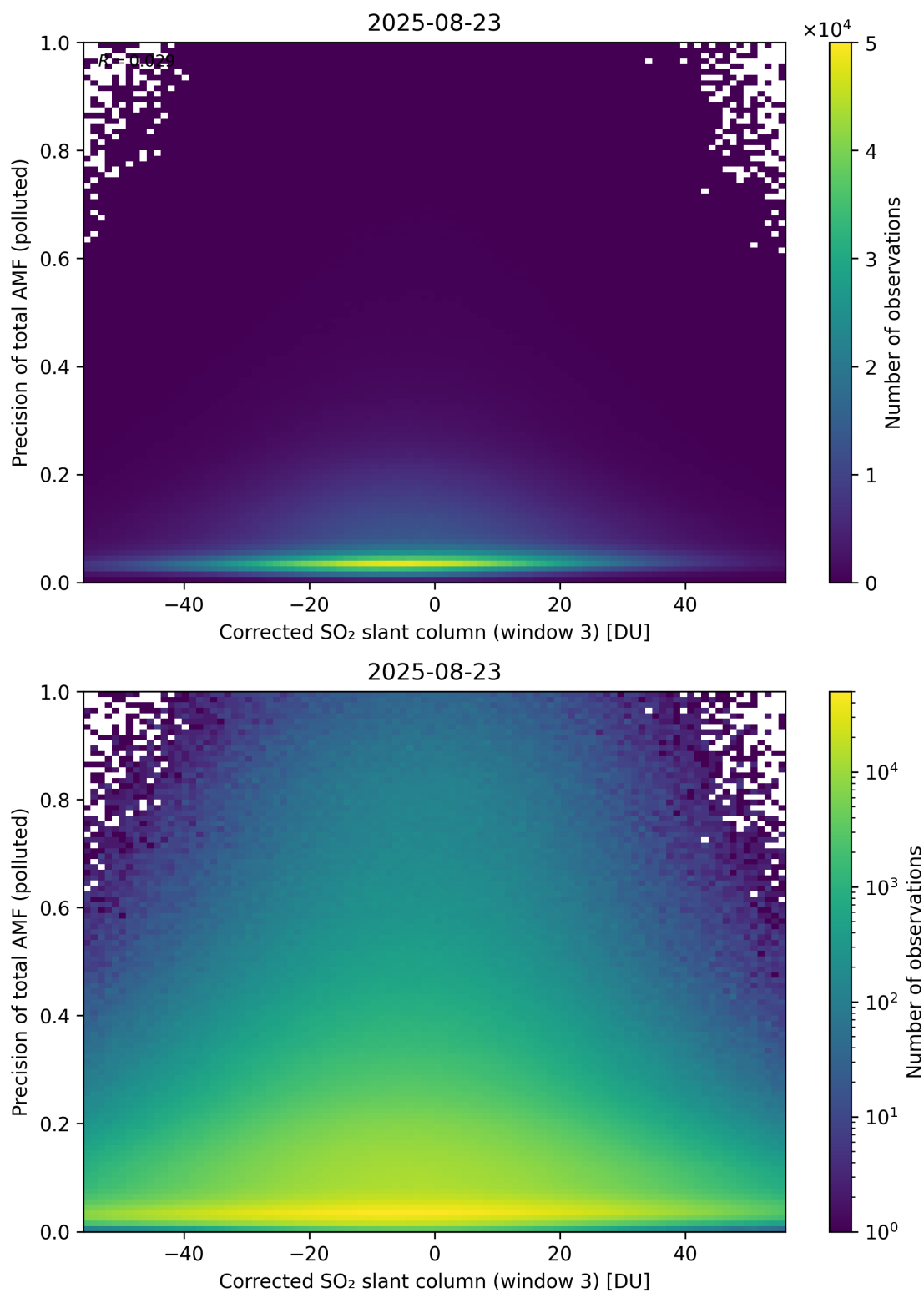
Figure 261: Scatter density plot of “Corrected SO 2 slant column (window 3)” against “Precision of total AMF (polluted)” for 2025-08-22 to 2025-08-24.
