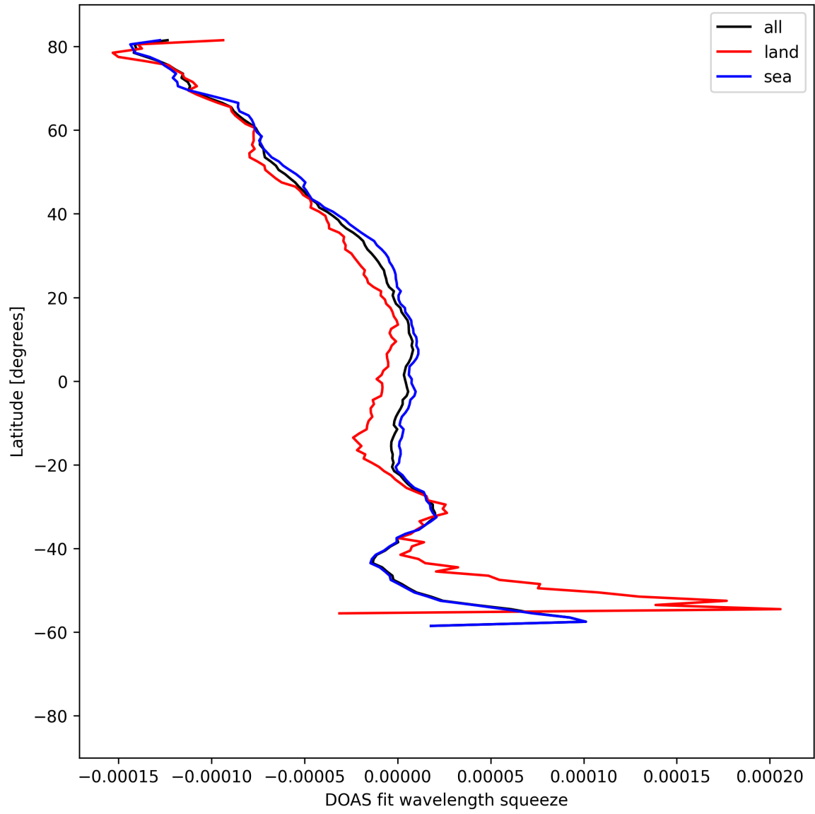
Figure 51: Zonal average of “DOAS fit wavelength squeeze” for 2025-08-22 to 2025-08-24.
