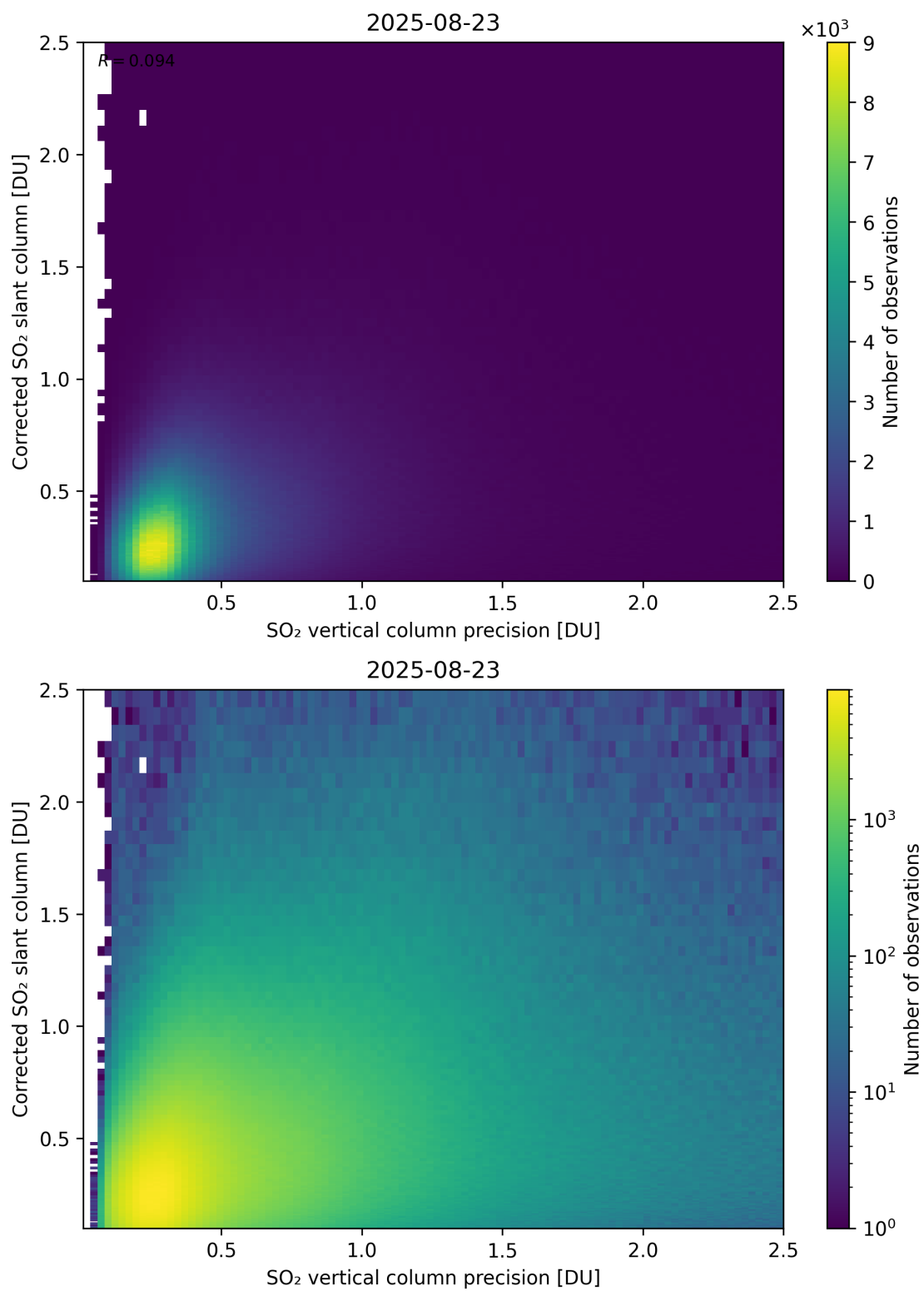
Figure 338: Scatter density plot of “SO 2 vertical column precision” against “Corrected SO 2 slant column” for 2025-08-22 to 2025-08-24.
