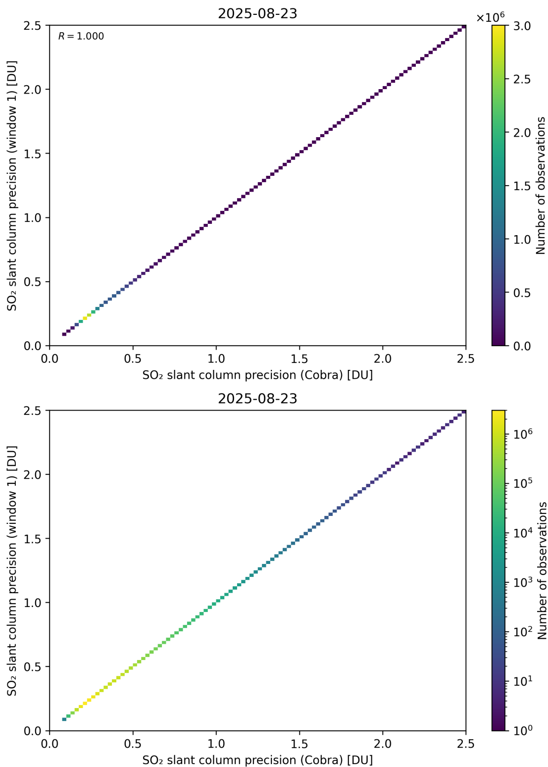
Figure 209: Scatter density plot of “SO 2 slant column precision (Cobra)” against “SO 2 slant column precision (window 1)” for 2025-08-22 to 2025-08-24.
