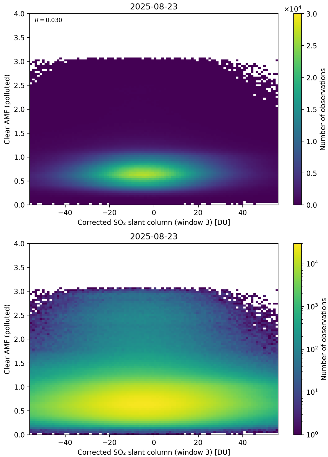
Figure 259: Scatter density plot of “Corrected SO 2 slant column (window 3)” against “Clear AMF (polluted)” for 2025-08-22 to 2025-08-24.
