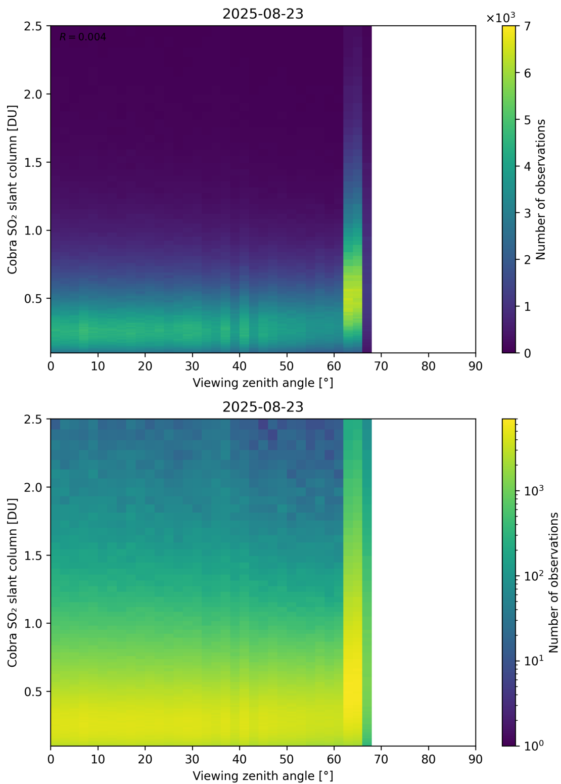
Figure 371: Scatter density plot of “Viewing zenith angle” against “Cobra SO 2 slant column” for 2025-08-22 to 2025-08-24.
