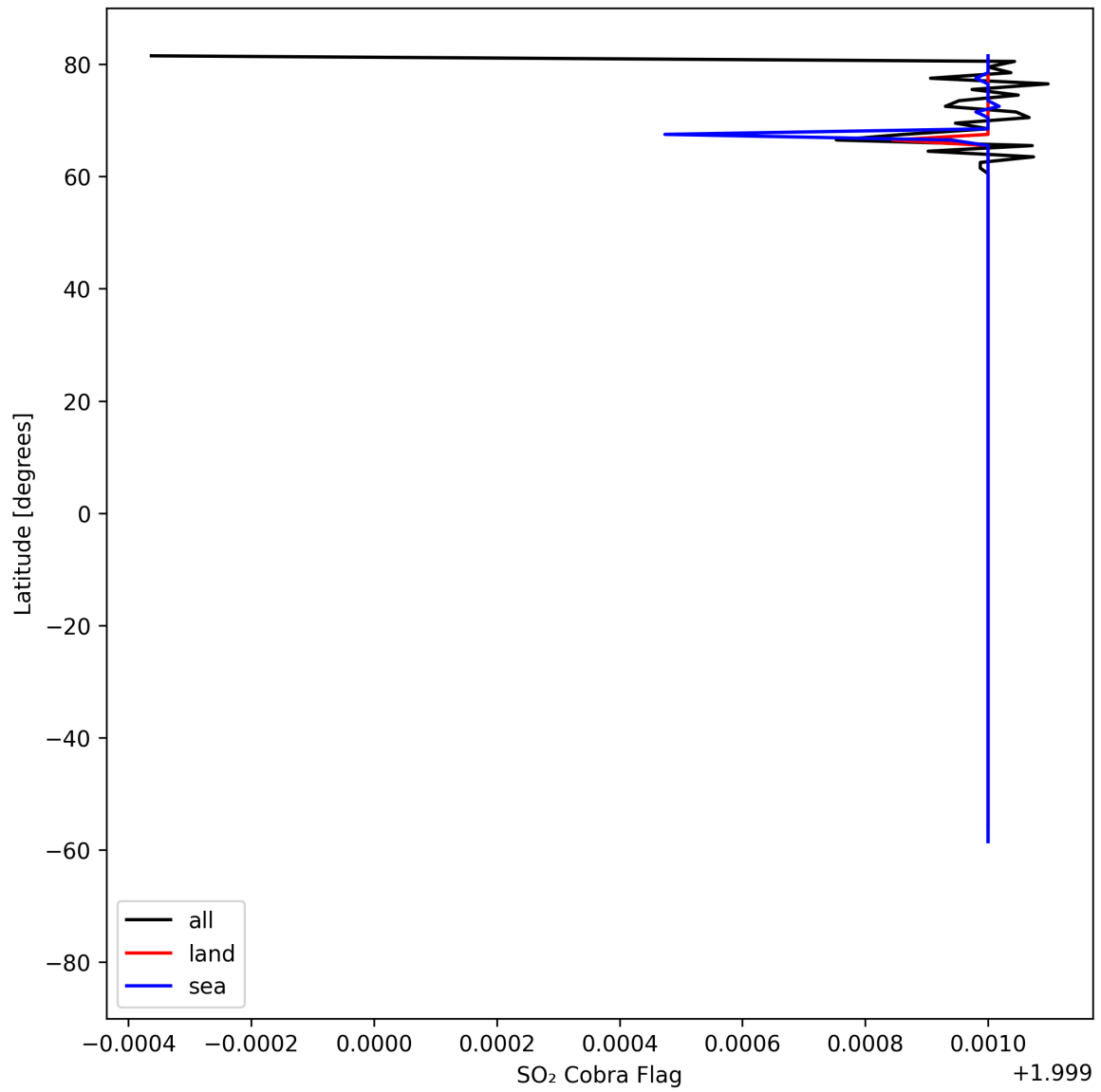
Figure 49: Zonal average of "SO 2 Cobra Flag" for 2025-08-22 to 2025-08-24.
