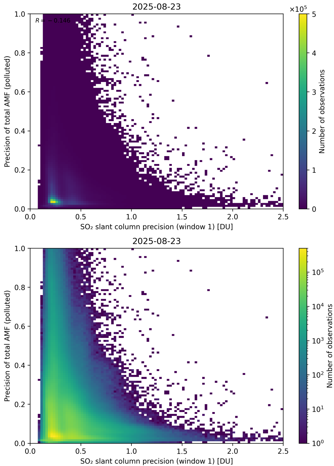
Figure 281: Scatter density plot of “SO 2 slant column precision (window 1)” against “Precision of total AMF (polluted)” for 2025-08-22 to 2025-08-24.
