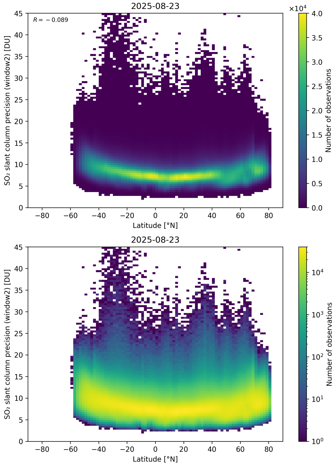
Figure 164: Scatter density plot of “Latitude” against “SO 2 slant column precision (window2)” for 2025-08-22 to 2025-08-24.
