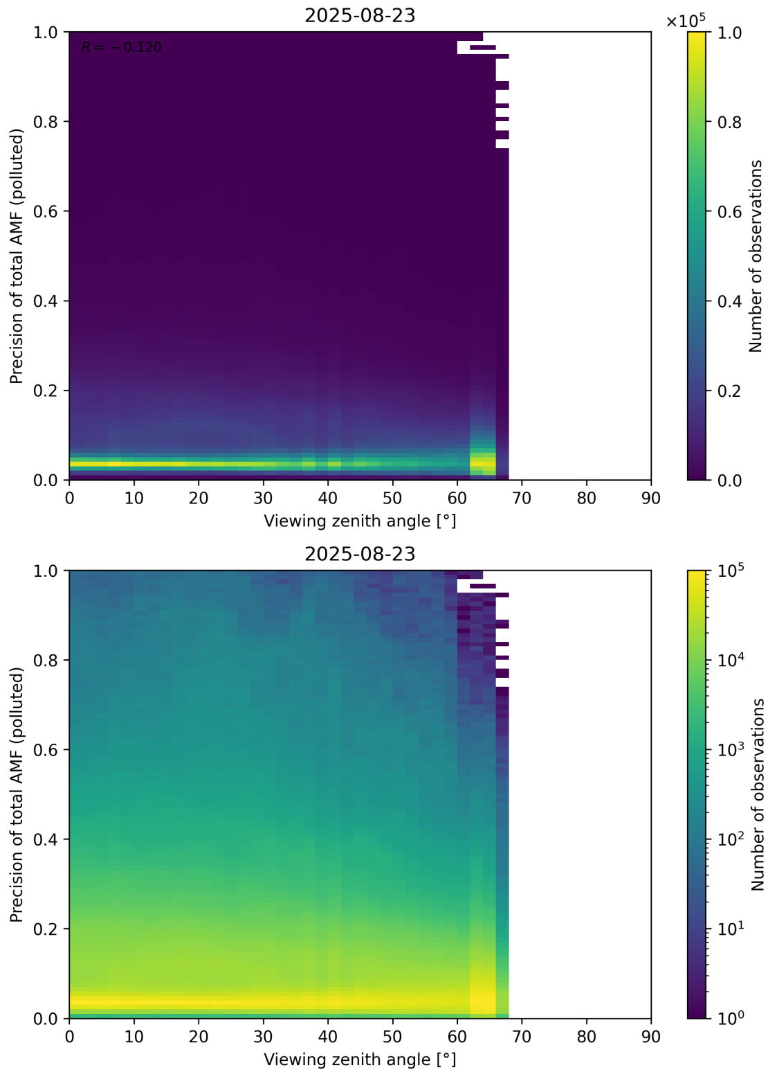
Figure 382: Scatter density plot of “Viewing zenith angle” against “Precision of total AMF (polluted)” for 2025-08-22 to 2025-08-24.
