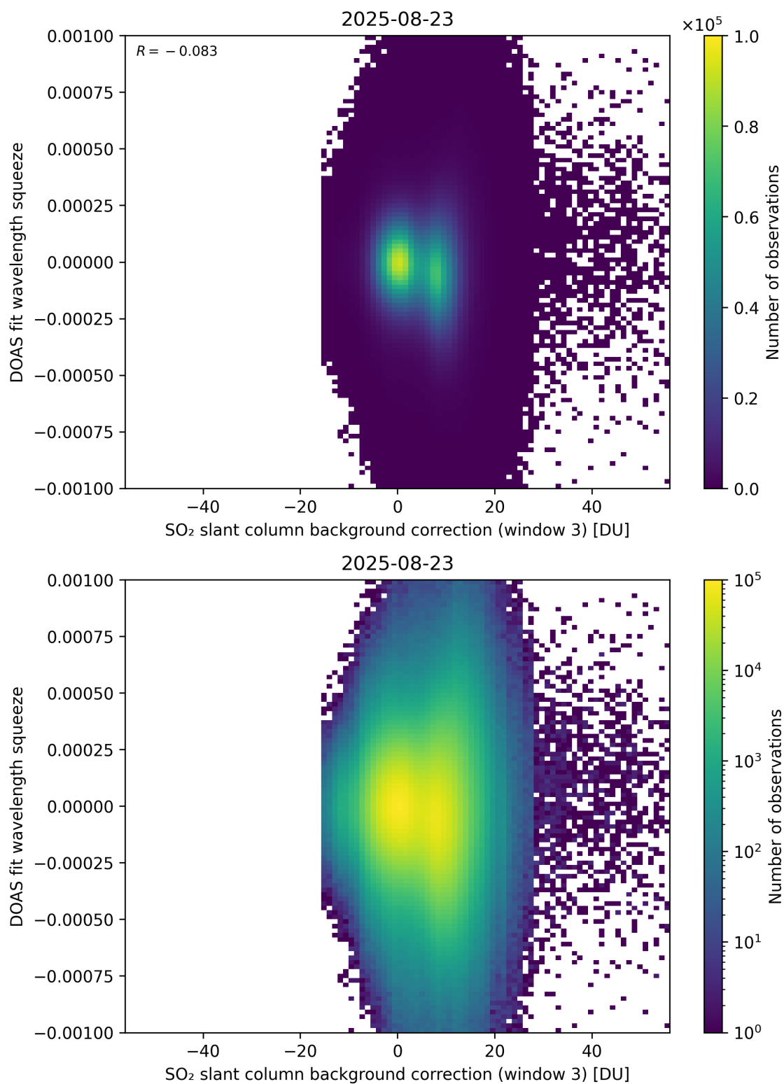
Figure 133: Scatter density plot of “SO 2 slant column background correction (window 3)” against “DOAS fit wavelength squeeze” for 2025-08-22 to 2025-08-24.
