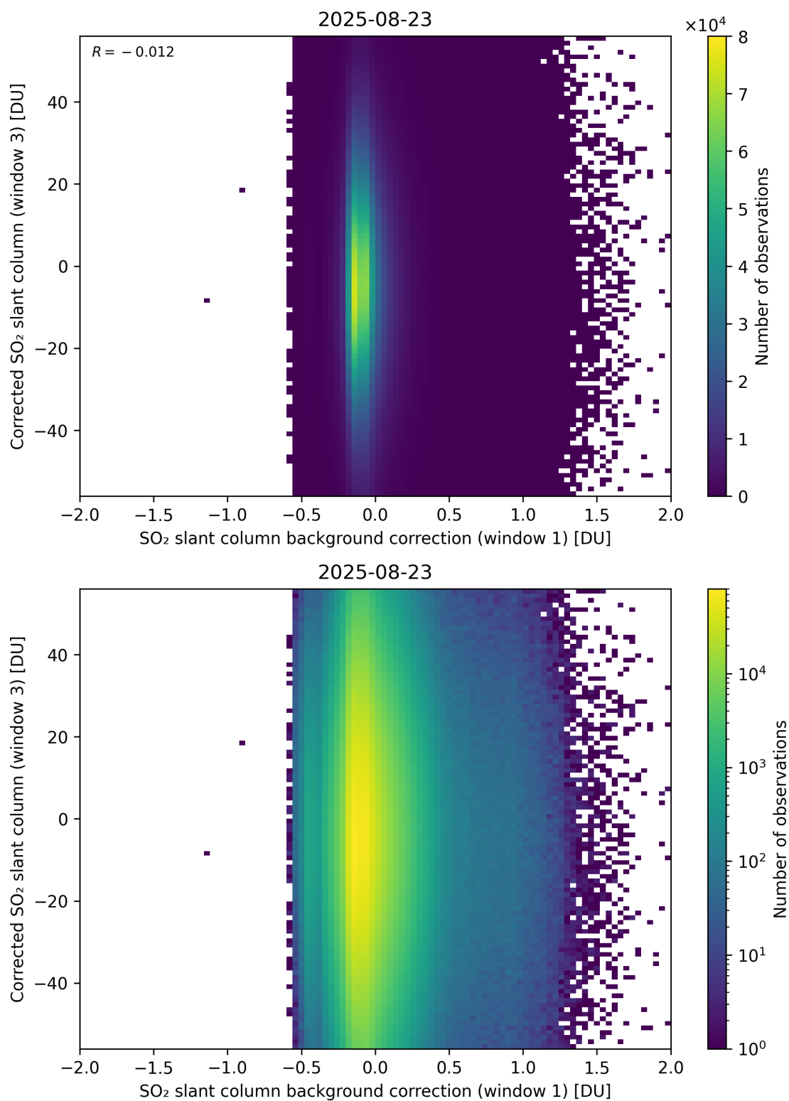
Figure 116: Scatter density plot of “SO 2 slant column background correction (window 1)” against “Corrected SO 2 slant column (window 3)” for 2025-08-22 to 2025-08-24.
