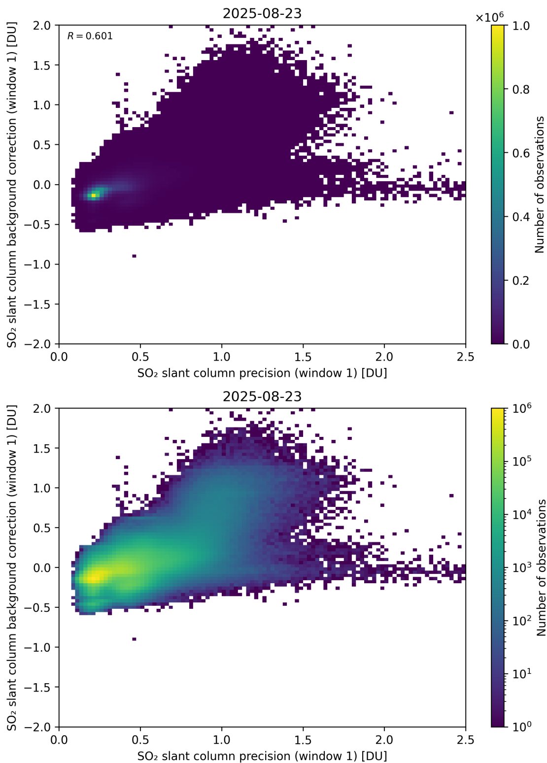
Figure 268: Scatter density plot of “SO 2 slant column precision (window 1)” against “SO 2 slant column background correction (window 1)” for 2025-08-22 to 2025-08-24.
