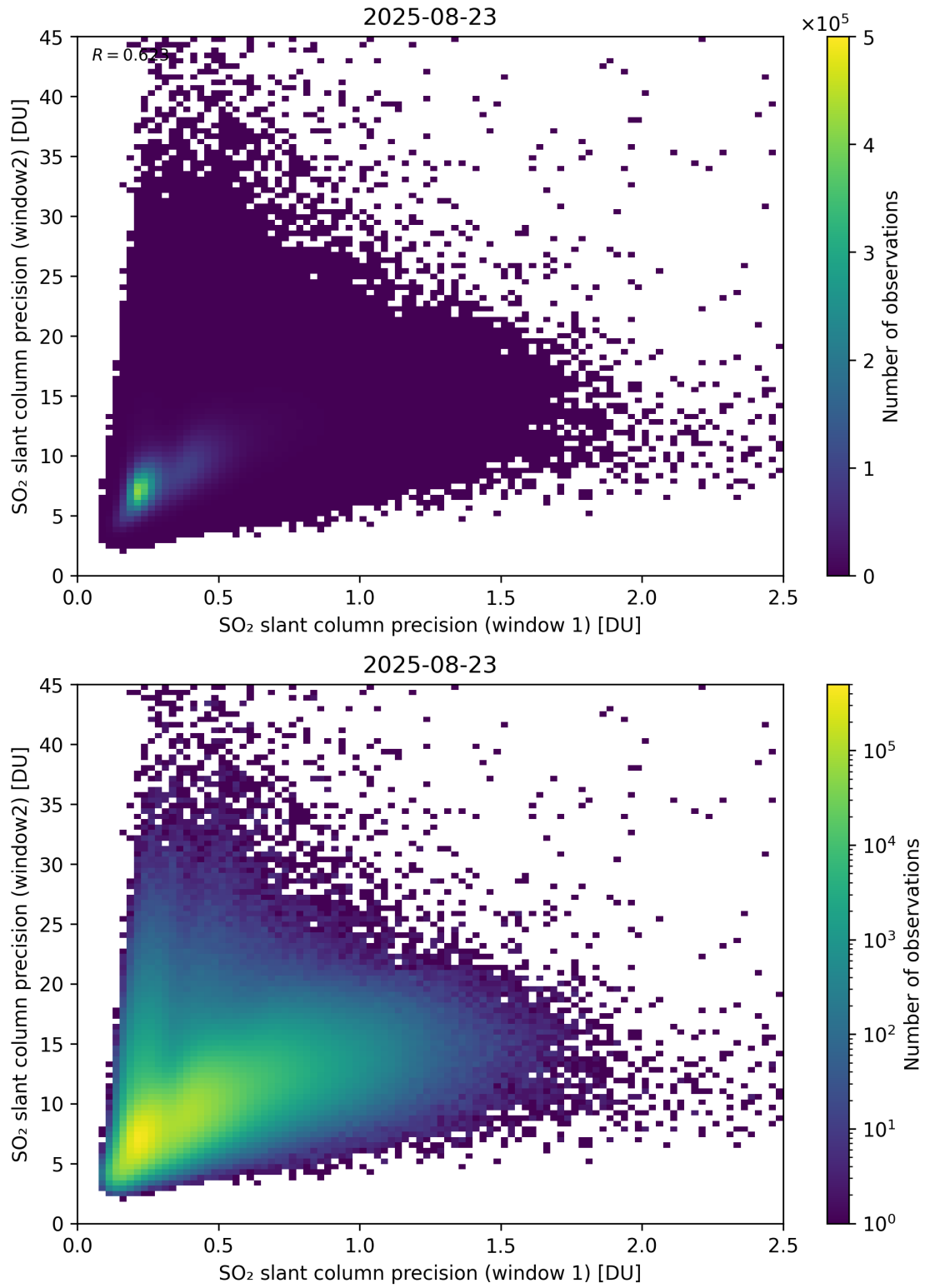
Figure 277: Scatter density plot of “SO 2 slant column precision (window 1)” against “SO 2 slant column precision (window2)” for 2025-08-22 to 2025-08-24.
