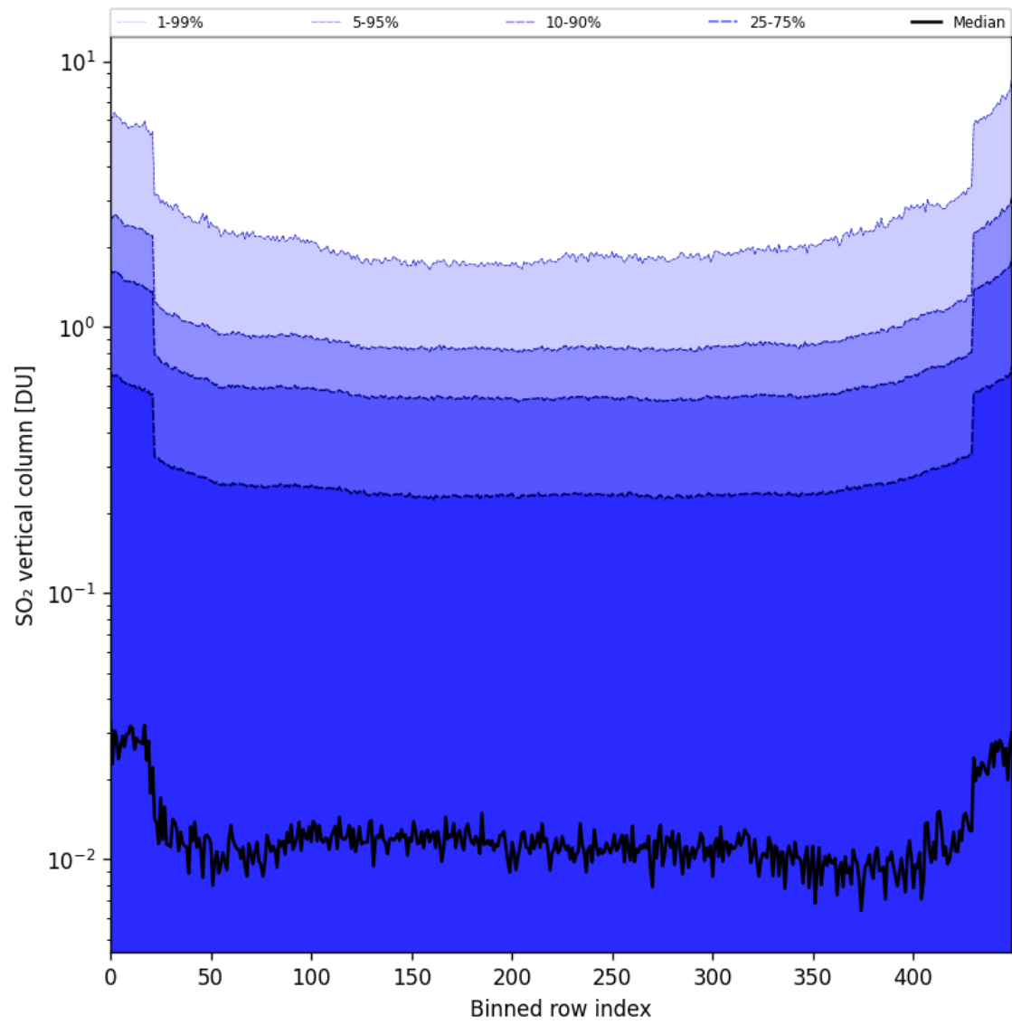
Figure 84: Along track statistics of “SO 2 vertical column” for 2025-08-22 to 2025-08-24
