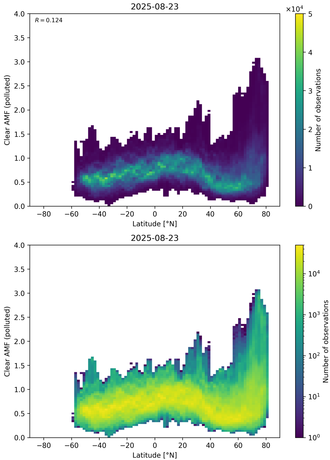
Figure 156: Scatter density plot of “Latitude” against “Clear AMF (polluted)” for 2025-08-22 to 2025-08-24.
