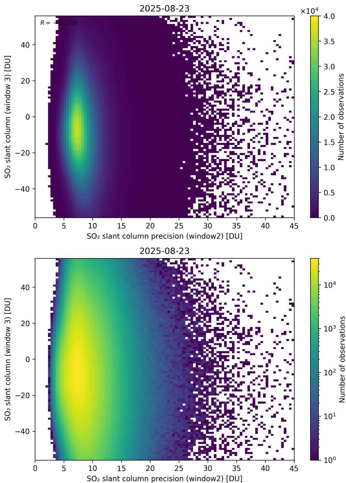
Figure 299: Scatter density plot of “SO 2 slant column precision (window2)” against “SO 2 slant column (window 3)” for 2025-08-22 to 2025-08-24.
