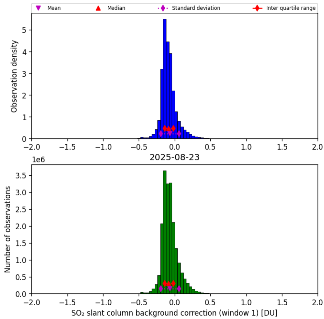
Figure 66: Histogram of “SO 2 slant column background correction (window 1)” for 2025-08-22 to 2025-08-24
