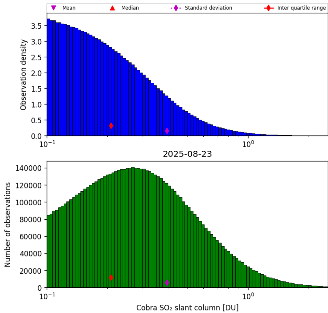
Figure 61: Histogram of “Cobra SO 2 slant column” for 2025-08-22 to 2025-08-24
