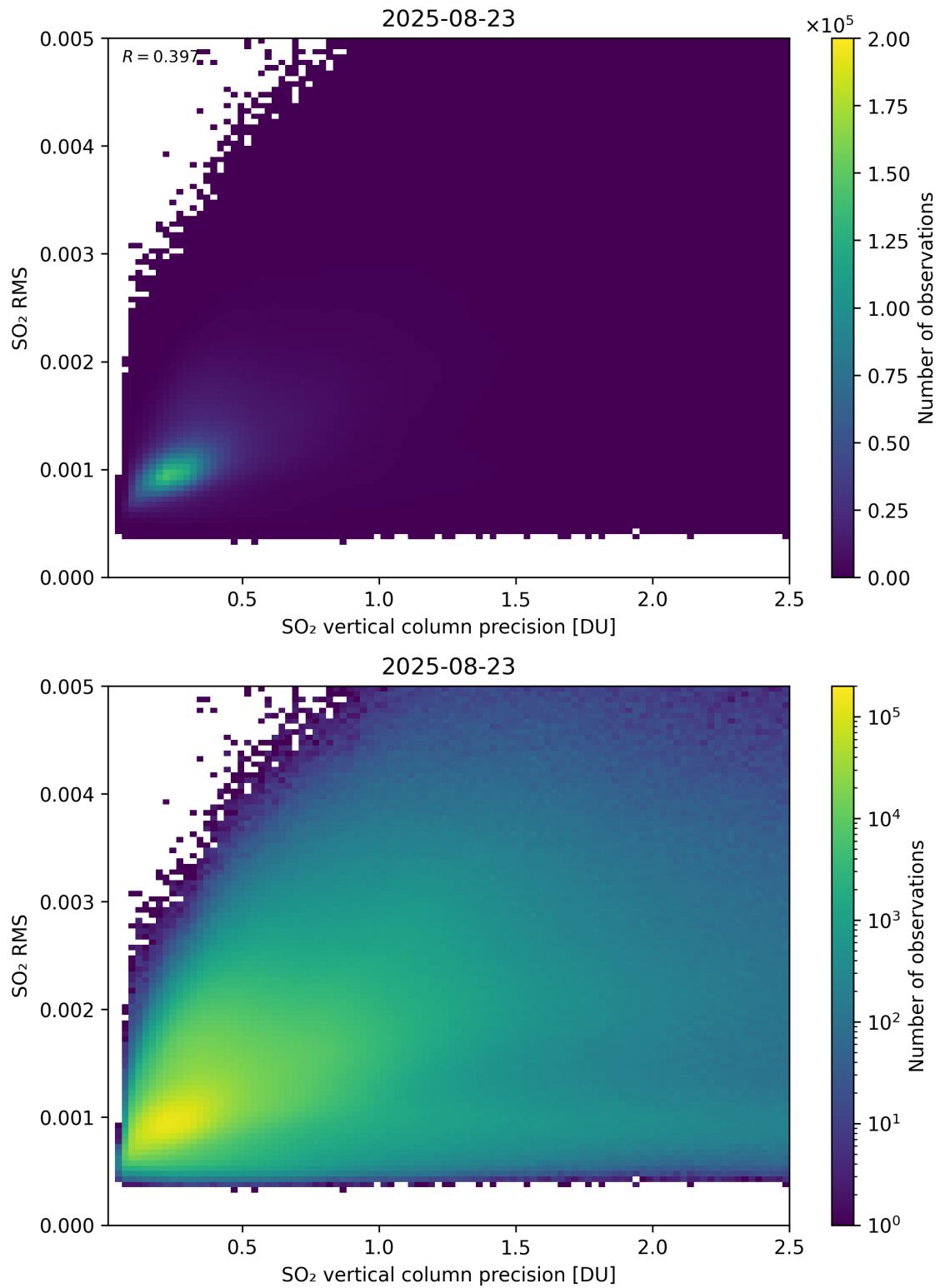
Figure 334: Scatter density plot of “SO 2 vertical column precision” against “SO 2 RMS” for 2025-08-22 to 2025-08-24.
