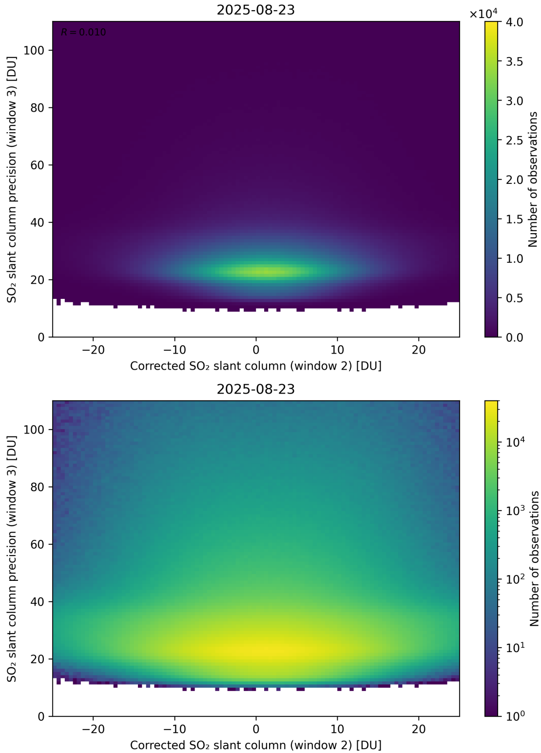
Figure 252: Scatter density plot of “Corrected SO 2 slant column (window 2)” against “SO 2 slant column precision (window 3)” for 2025-08-22 to 2025-08-24.
