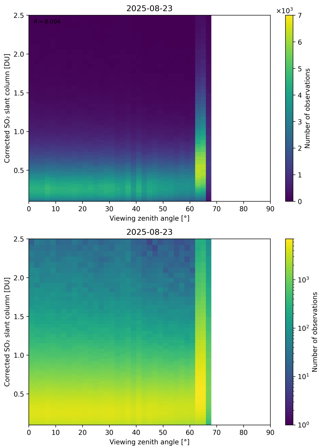
Figure 373: Scatter density plot of “Viewing zenith angle” against “Corrected SO 2 slant column” for 2025-08-22 to 2025-08-24.
