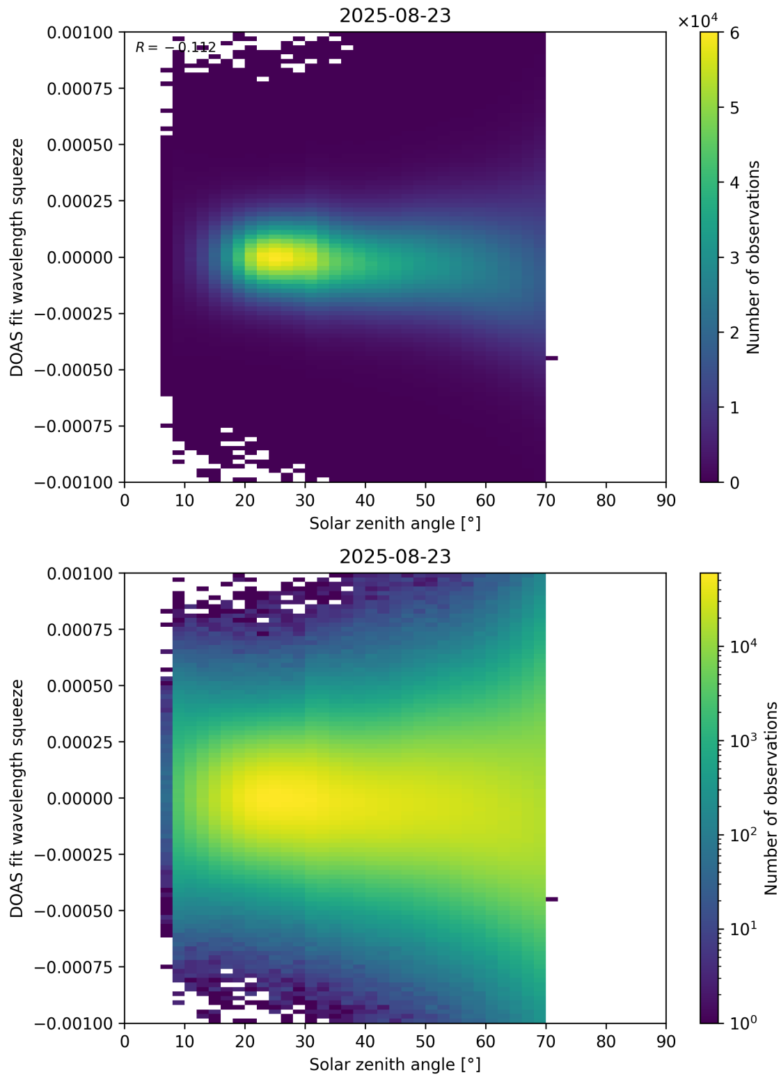
Figure 175: Scatter density plot of “Solar zenith angle” against “DOAS fit wavelength squeeze” for 2025-08-22 to 2025-08-24.
