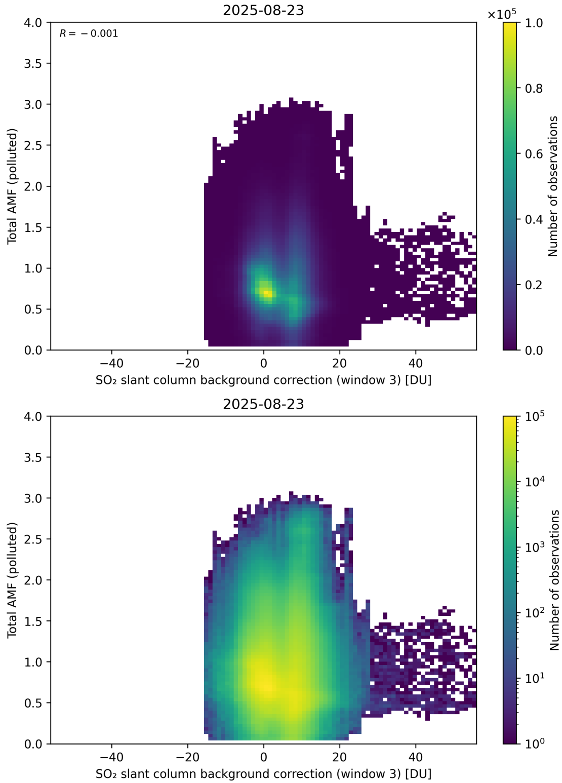
Figure 136: Scatter density plot of “SO 2 slant column background correction (window 3)” against “Total AMF (polluted)” for 2025-08-22 to 2025-08-24.
