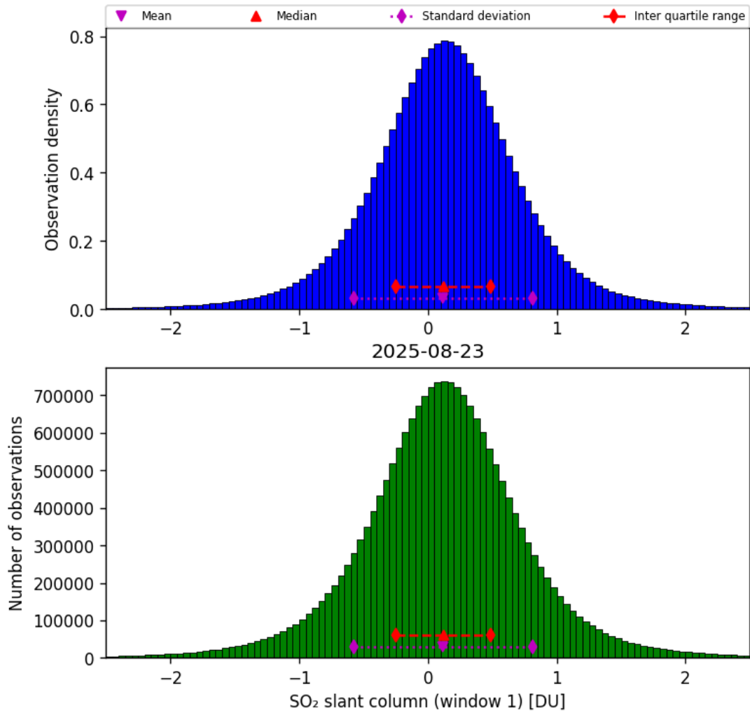
Figure 63: Histogram of “SO 2 slant column (window 1)” for 2025-08-22 to 2025-08-24
