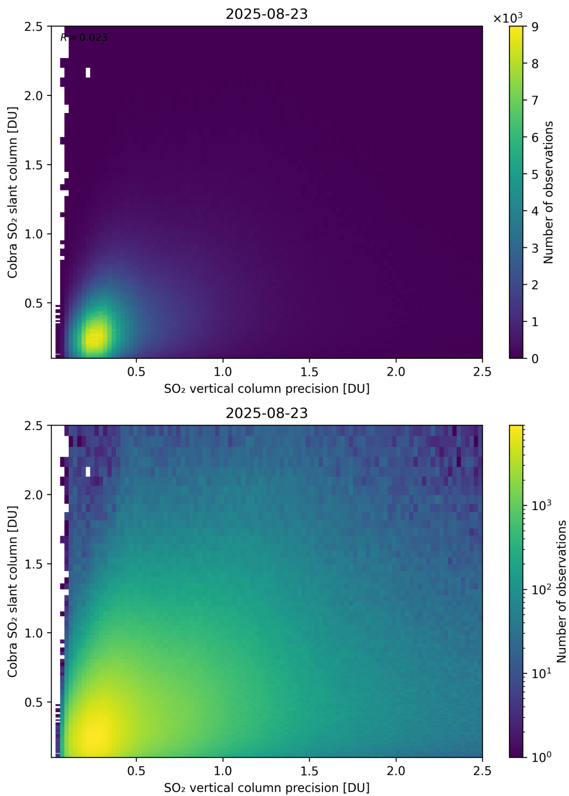
Figure 336: Scatter density plot of “SO 2 vertical column precision” against “Cobra SO 2 slant column” for 2025-08-22 to 2025-08-24.
