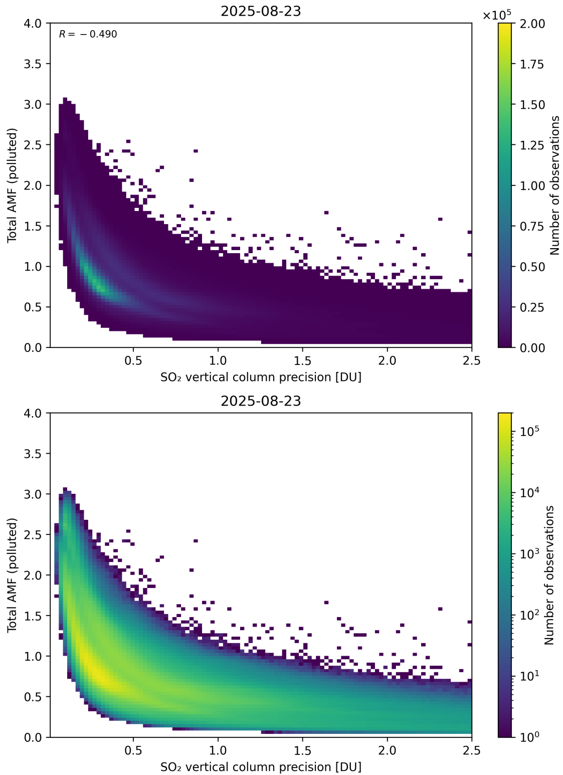
Figure 346: Scatter density plot of “SO 2 vertical column precision” against “Total AMF (polluted)” for 2025-08-22 to 2025-08-24.
