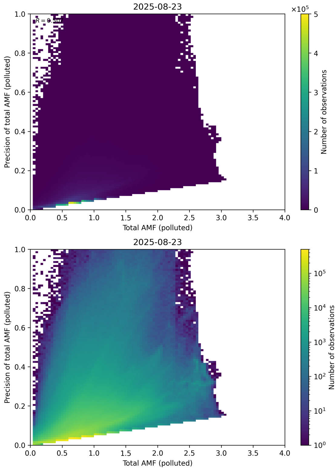
Figure 322: Scatter density plot of “Total AMF (polluted)” against “Precision of total AMF (polluted)” for 2025-08-22 to 2025-08-24.
