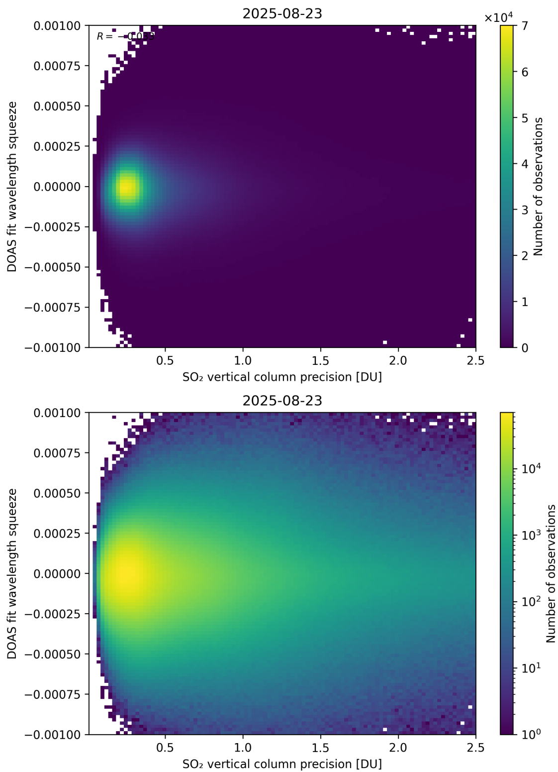
Figure 333: Scatter density plot of “SO 2 vertical column precision” against “DOAS fit wavelength squeeze” for 2025-08-22 to 2025-08-24.
