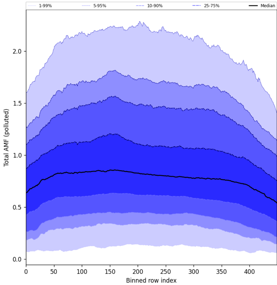
Figure 105: Along track statistics of “Total AMF (polluted)” for 2025-08-22 to 2025-08-24
