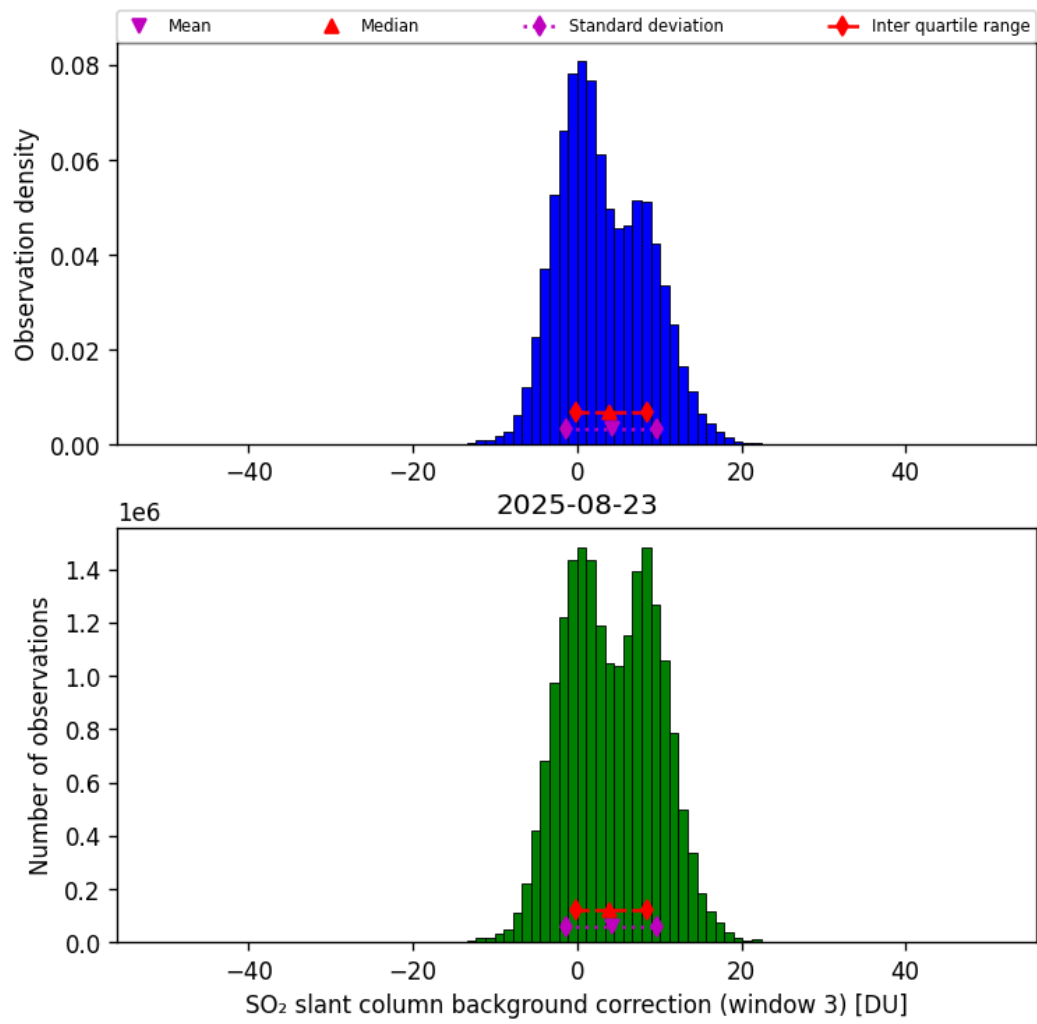
Figure 74: Histogram of “SO 2 slant column background correction (window 3)” for 2025-08-22 to 2025-08-24
