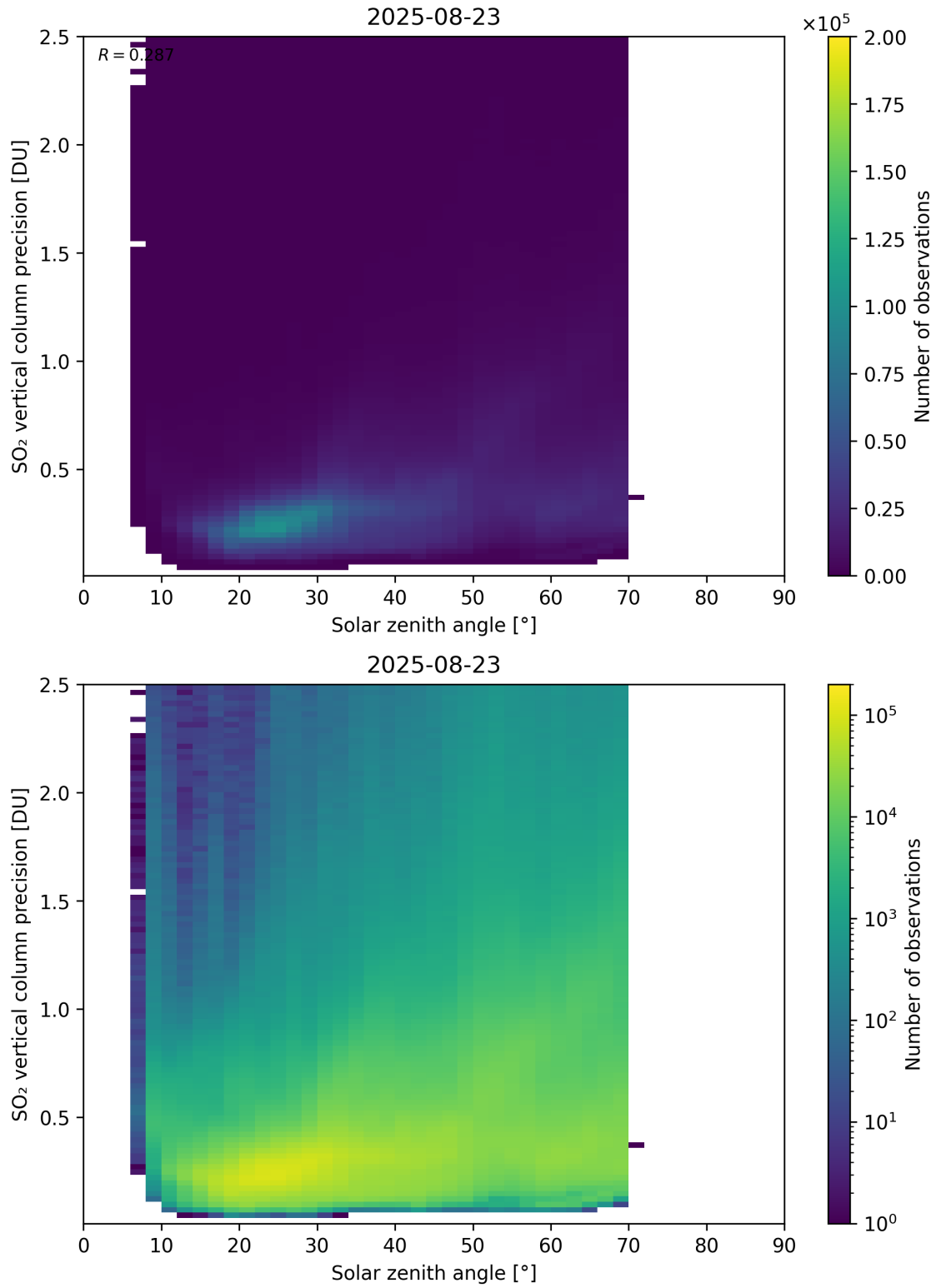
Figure 192: Scatter density plot of “Solar zenith angle” against “SO 2 vertical column precision” for 2025-08-22 to 2025-08-24.
