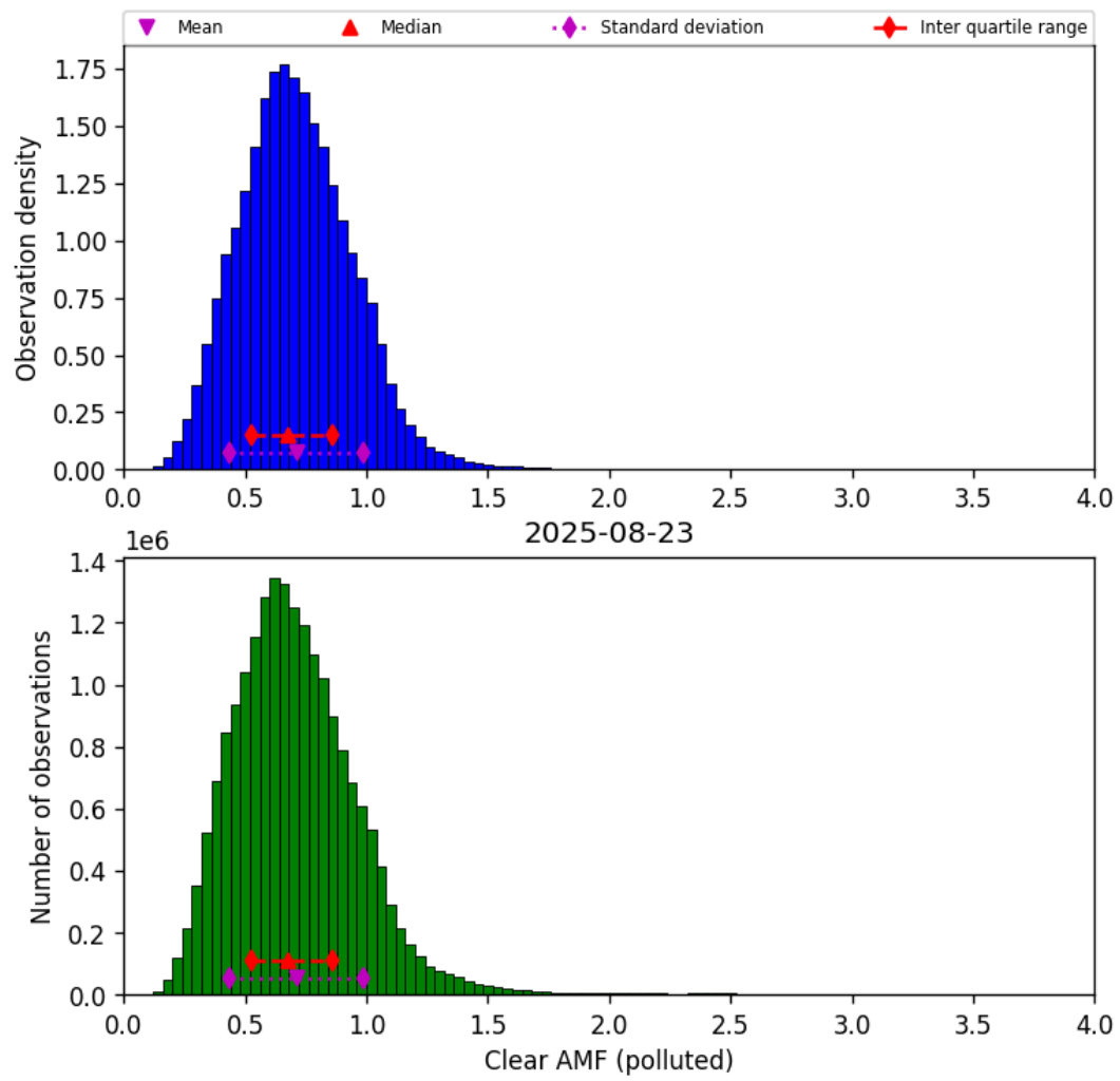
Figure 81: Histogram of “Clear AMF (polluted)” for 2025-08-22 to 2025-08-24
