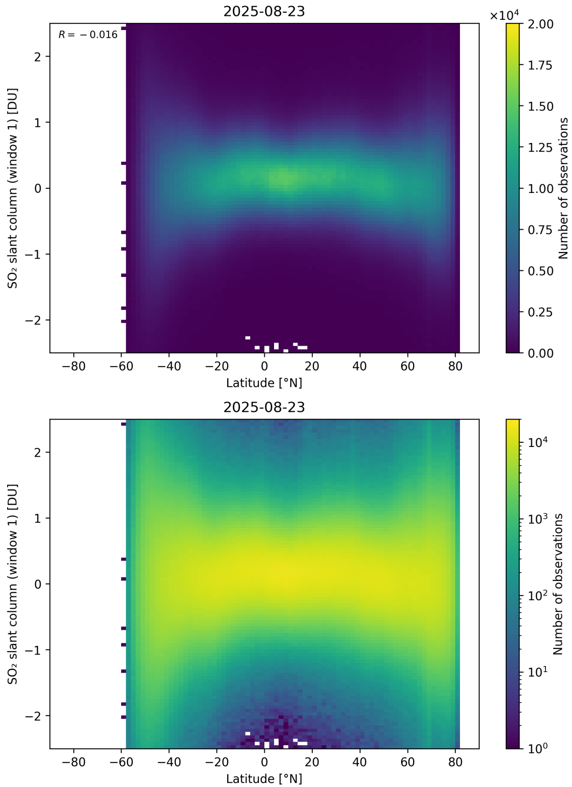
Figure 162: Scatter density plot of “Latitude” against “SO 2 slant column (window 1)” for 2025-08-22 to 2025-08-24.
