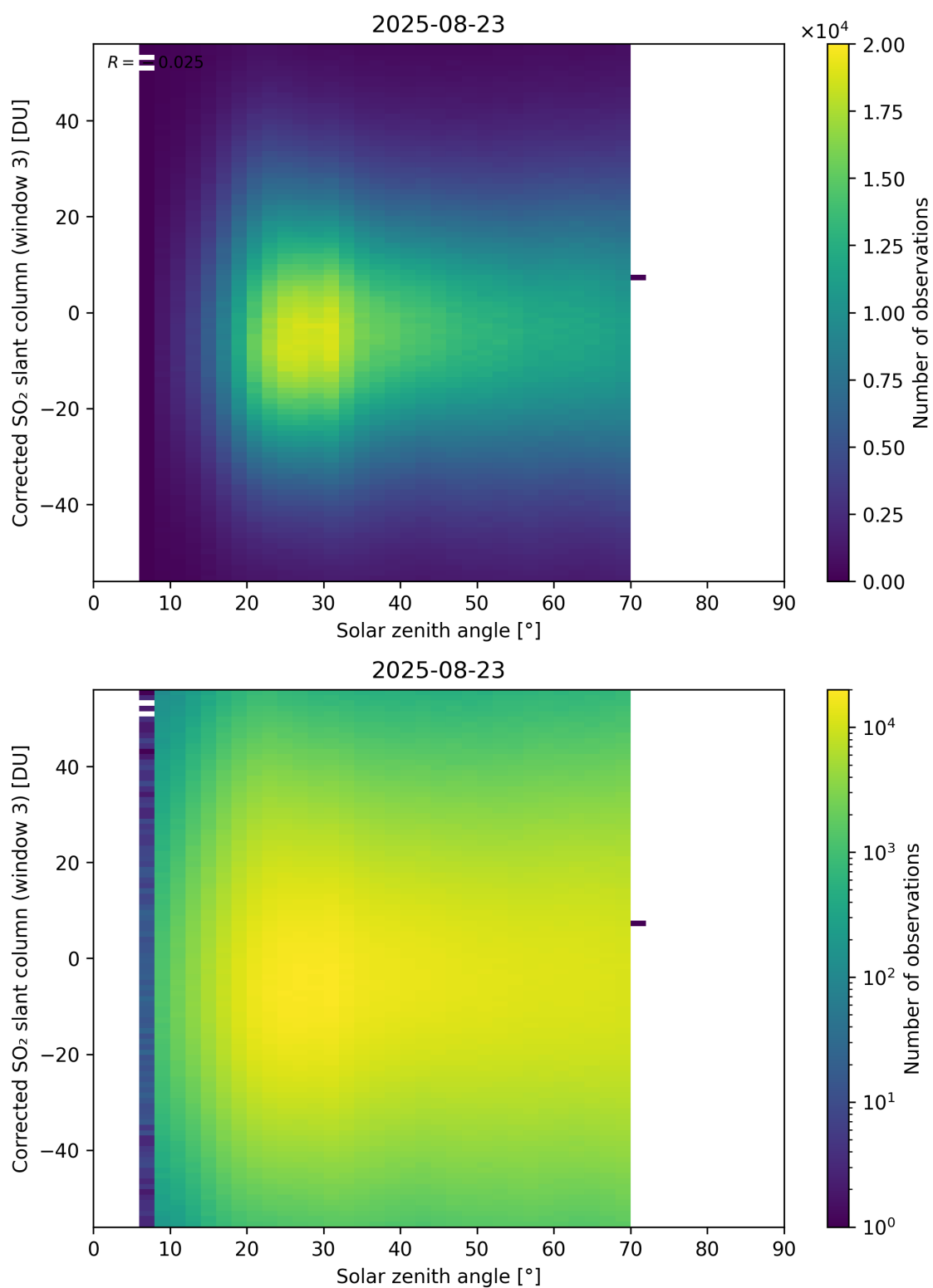
Figure 183: Scatter density plot of “Solar zenith angle” against “Corrected SO 2 slant column (window 3)” for 2025-08-22 to 2025-08-24.
