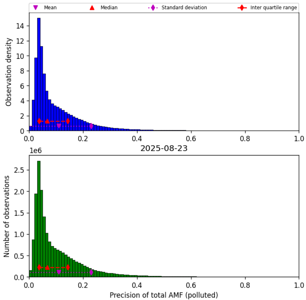
Figure 80: Histogram of “Precision of total AMF (polluted)” for 2025-08-22 to 2025-08-24
