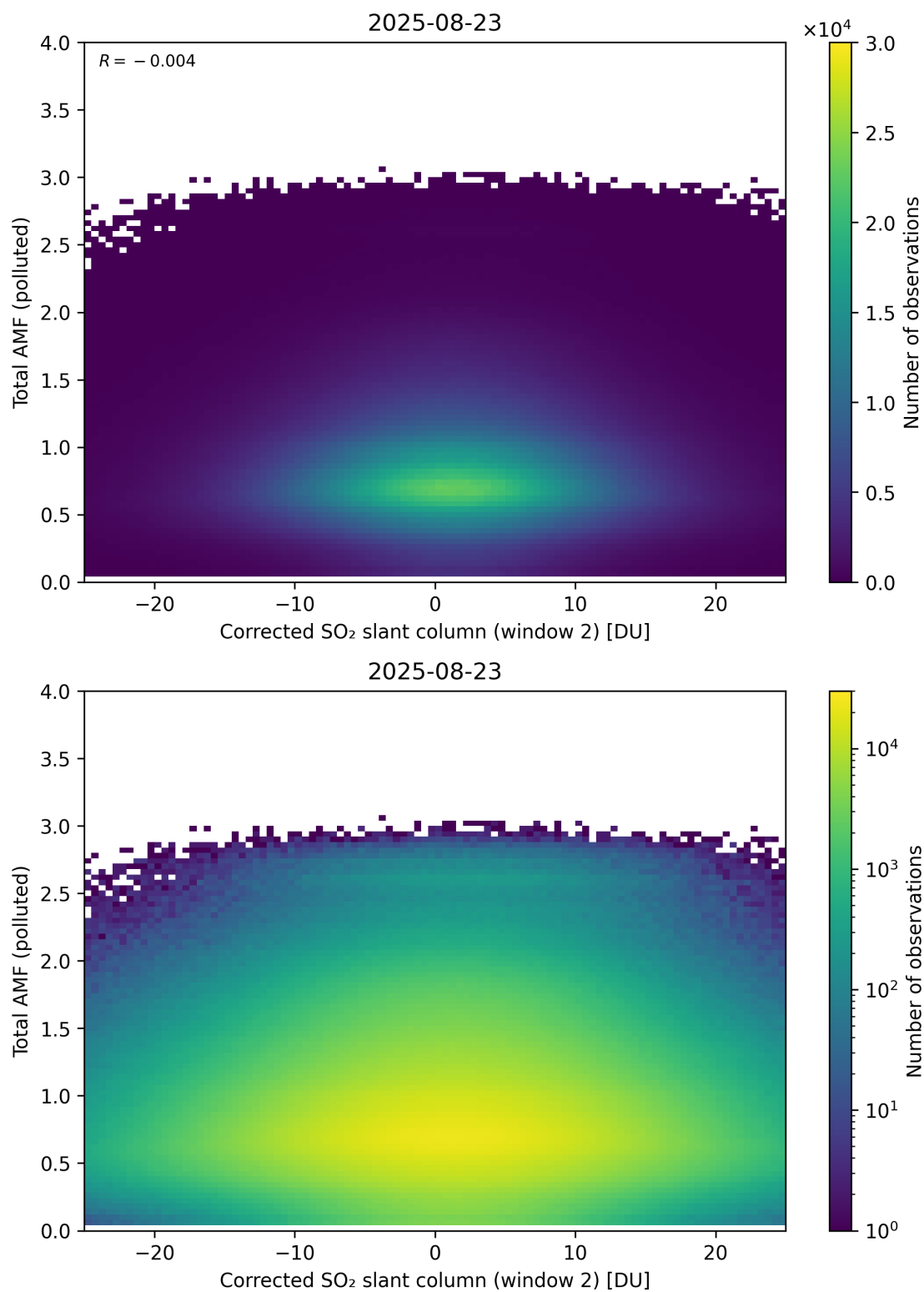
Figure 253: Scatter density plot of “Corrected SO 2 slant column (window 2)” against “Total AMF (polluted)” for 2025-08-22 to 2025-08-24.
