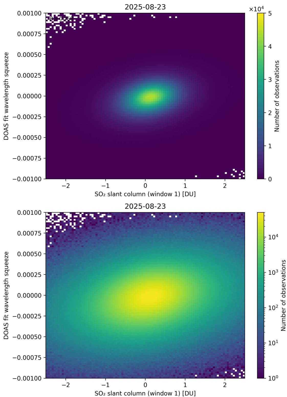
Figure 266: Scatter density plot of “SO 2 slant column (window 1)” against “DOAS fit wavelength squeeze” for 2025-08-22 to 2025-08-24.
