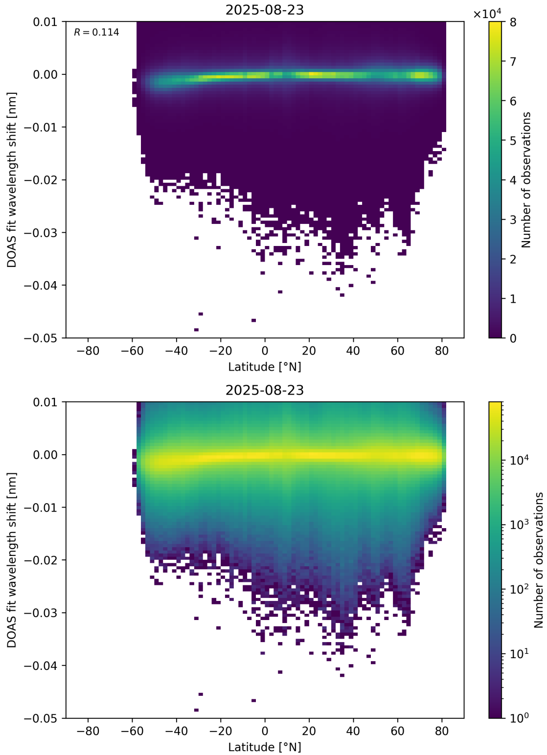
Figure 153: Scatter density plot of “Latitude” against “DOAS fit wavelength shift” for 2025-08-22 to 2025-08-24.
