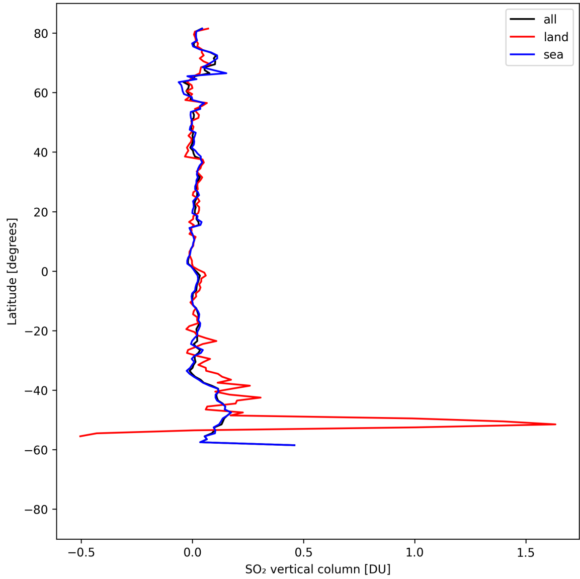
Figure 32: Zonal average of “SO 2 vertical column” for 2025-08-22 to 2025-08-24.
