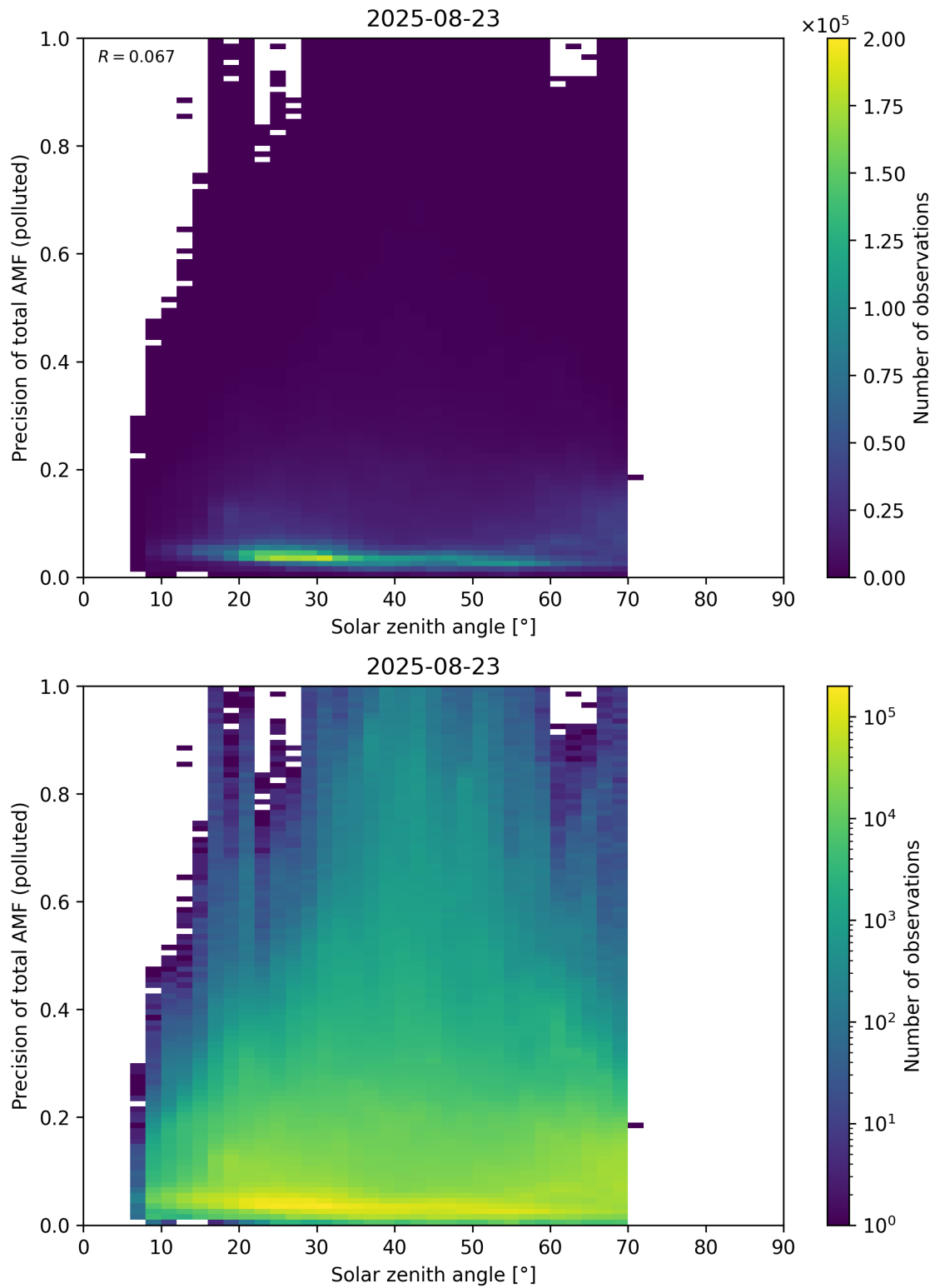
Figure 190: Scatter density plot of “Solar zenith angle” against “Precision of total AMF (polluted)” for 2025-08-22 to 2025-08-24.
