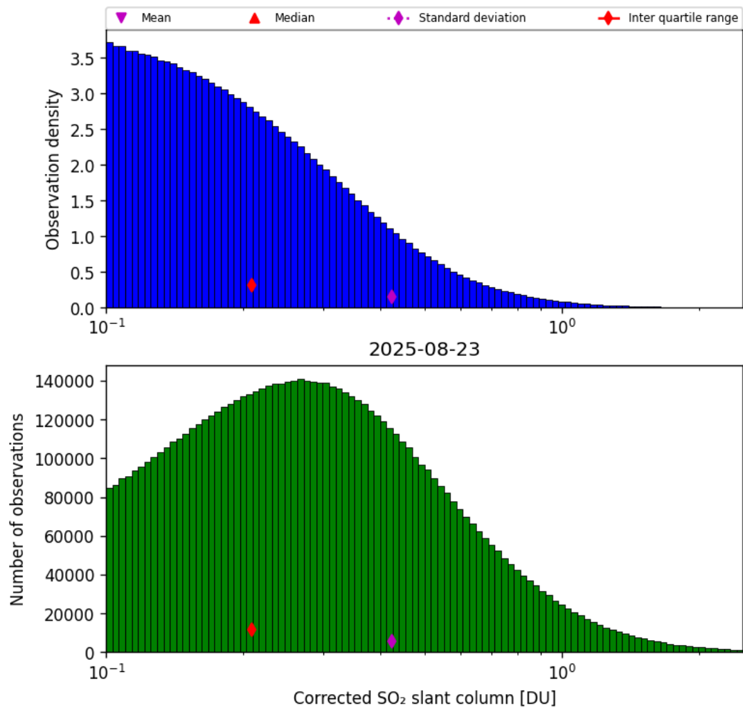
Figure 60: Histogram of "Corrected SO 2 slant column" for 2025-08-22 to 2025-08-24
