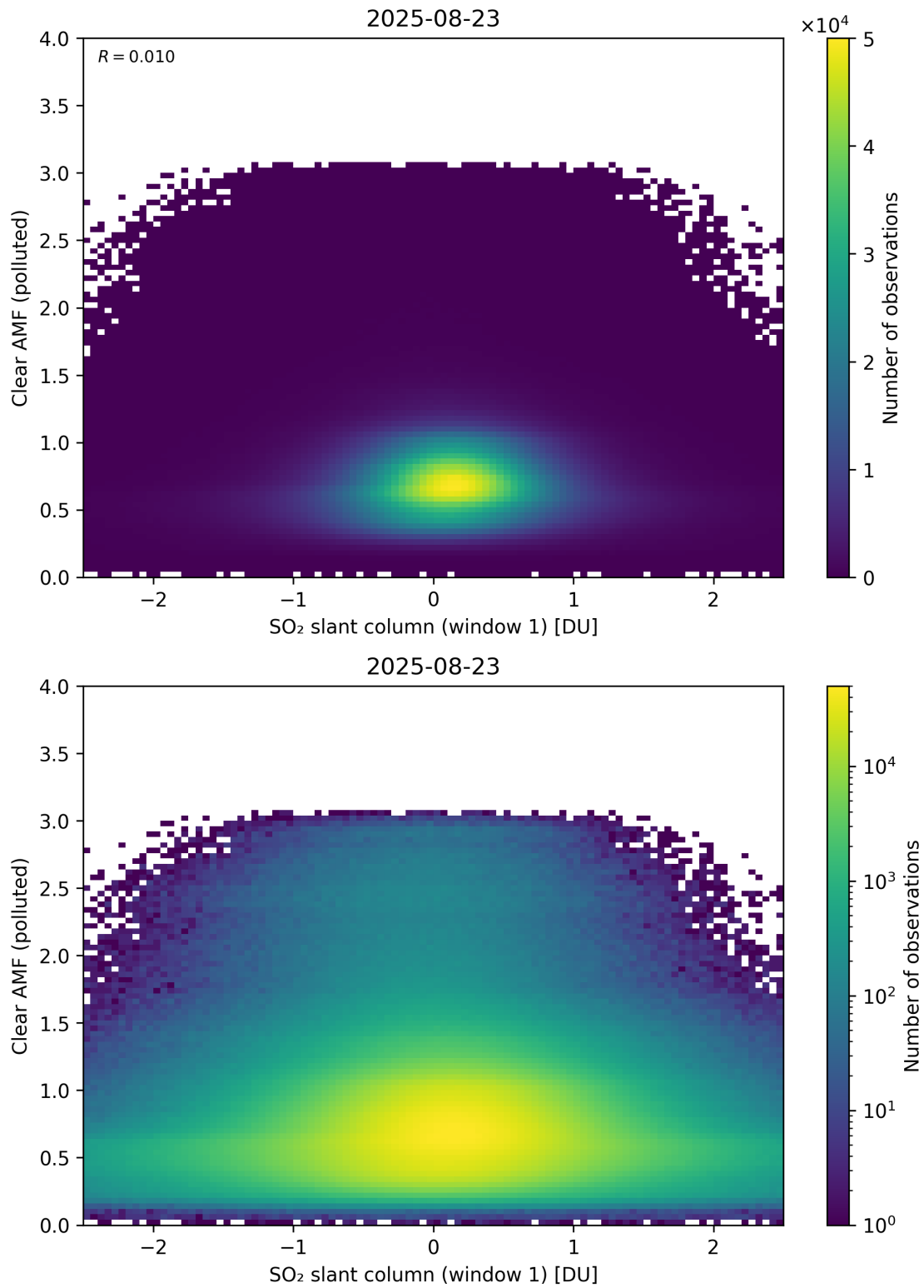
Figure 282: Scatter density plot of “SO 2 slant column (window 1)” against “Clear AMF (polluted)” for 2025-08-22 to 2025-08-24.
