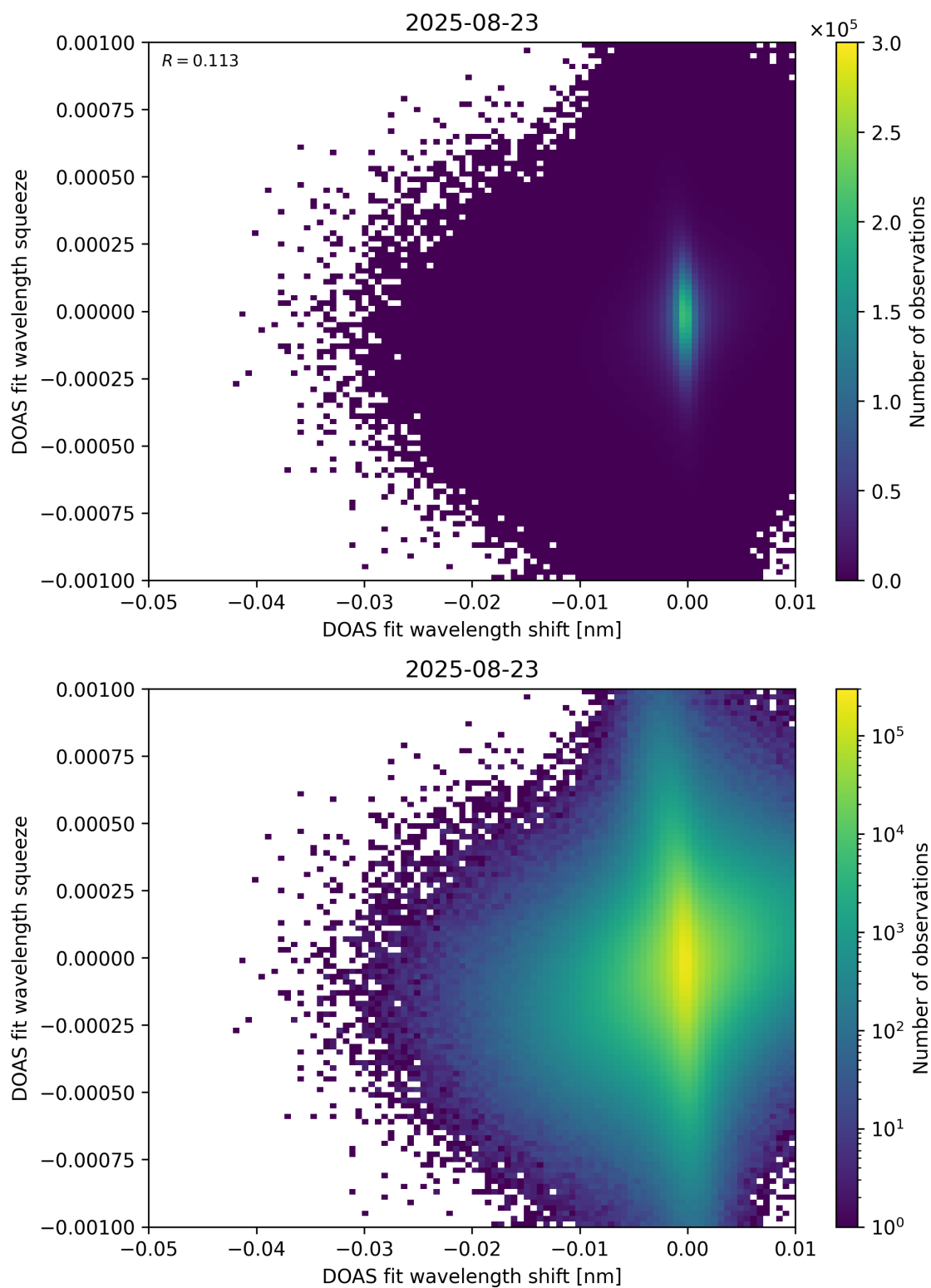
Figure 138: Scatter density plot of “DOAS fit wavelength shift” against “DOAS fit wavelength squeeze” for 2025-08-22 to 2025-08-24.
