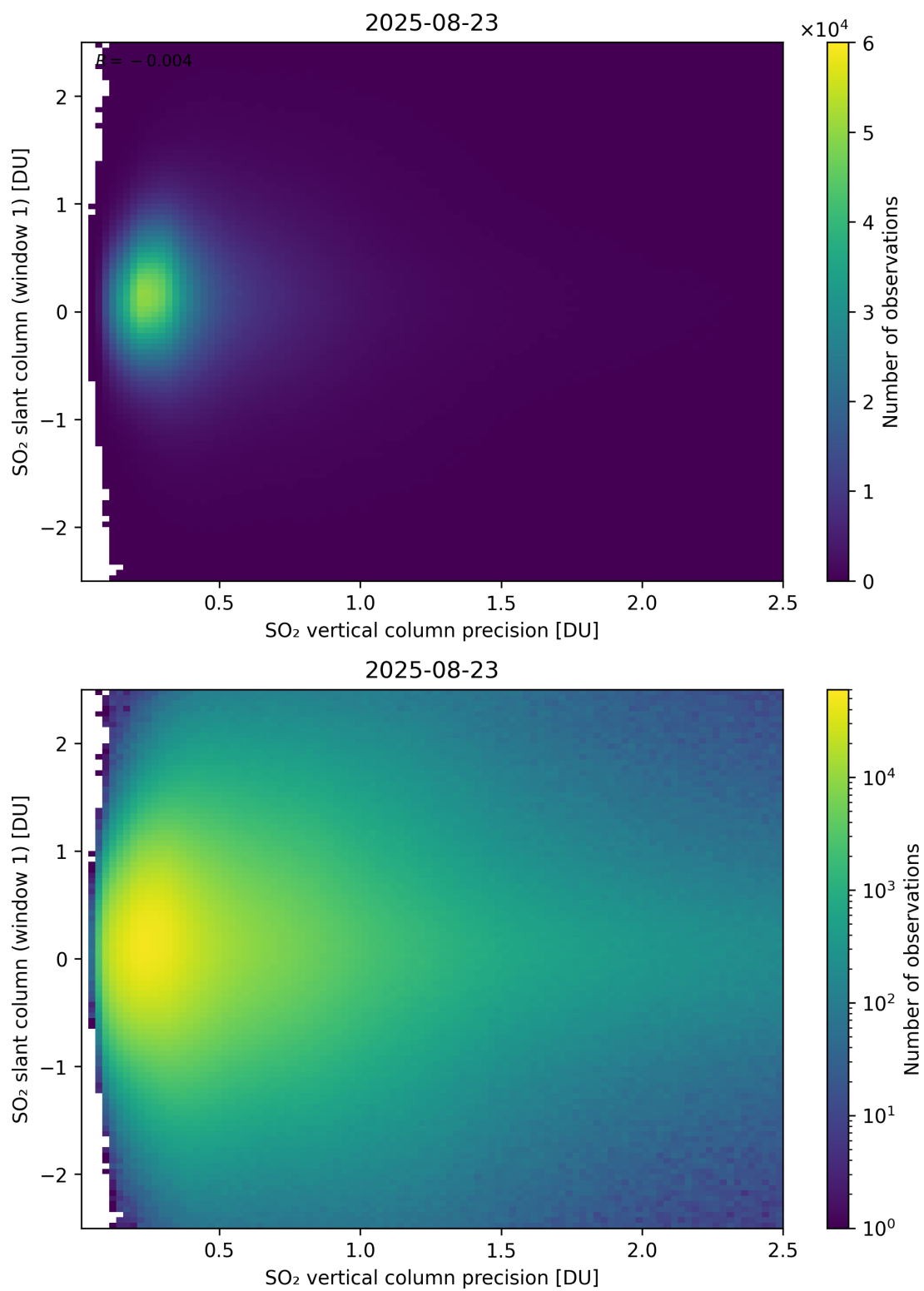
Figure 341: Scatter density plot of “SO 2 vertical column precision” against “SO 2 slant column (window 1)” for 2025-08-22 to 2025-08-24.
