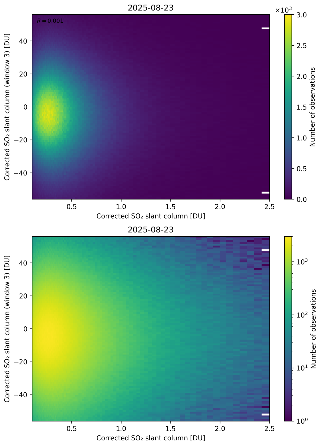
Figure 236: Scatter density plot of “Corrected SO 2 slant column” against “Corrected SO 2 slant column (window 3)” for 2025-08-22 to 2025-08-24.
