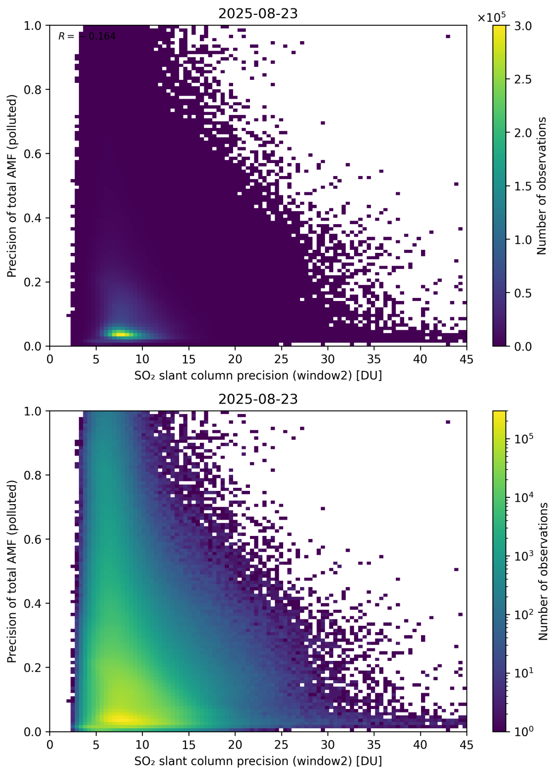
Figure 302: Scatter density plot of “SO 2 slant column precision (window2)” against “Precision of total AMF (polluted)” for 2025-08-22 to 2025-08-24.
