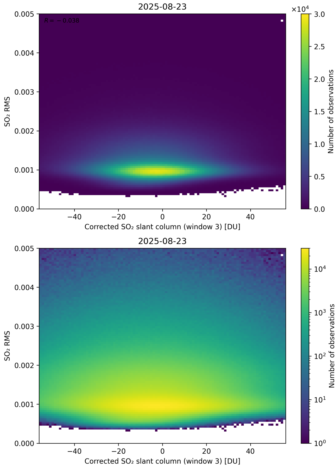
Figure 258: Scatter density plot of “Corrected SO 2 slant column (window 3)” against “SO 2 RMS” for 2025-08-22 to 2025-08-24.
