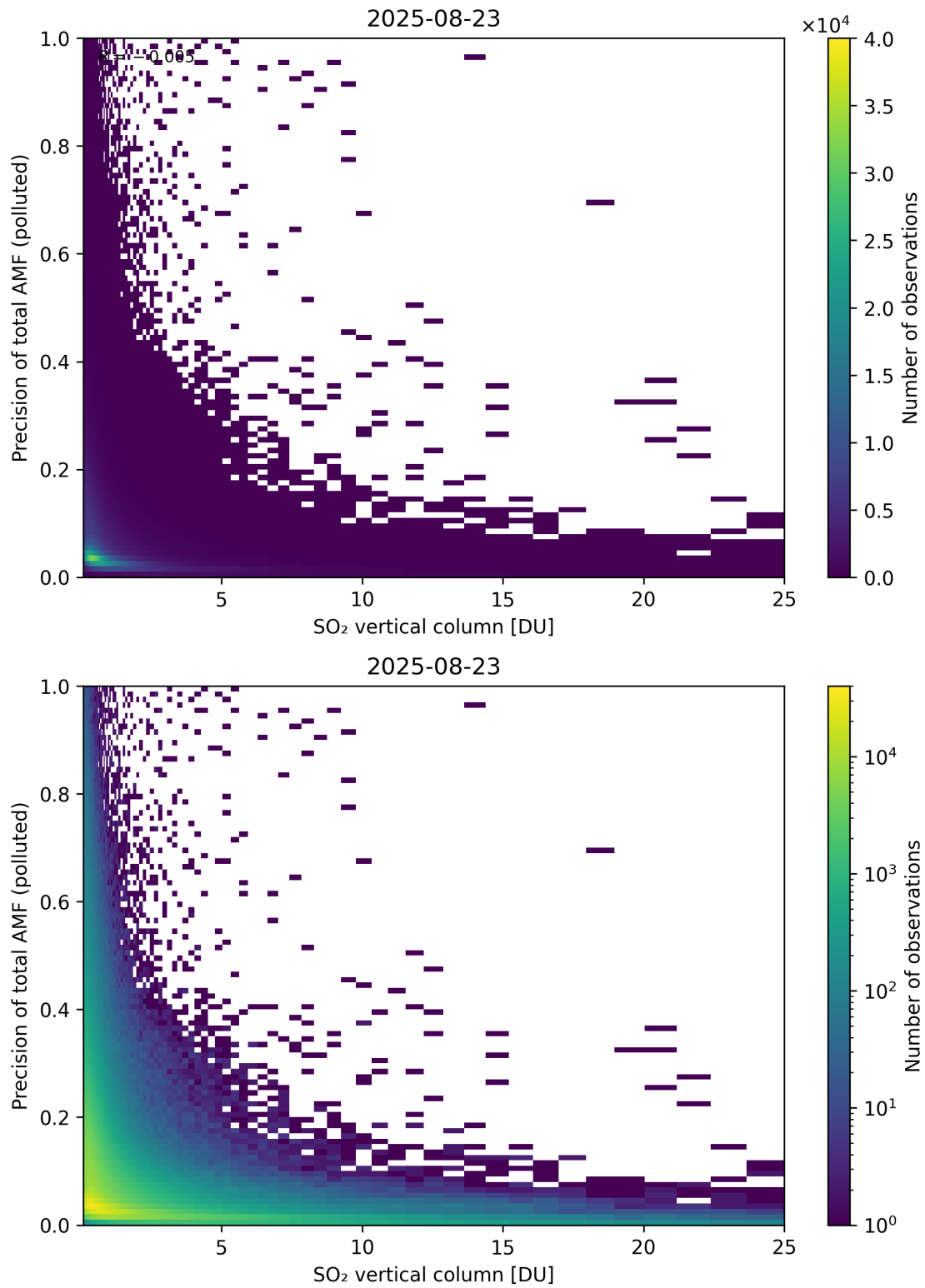
Figure 360: Scatter density plot of “SO 2 vertical column” against “Precision of total AMF (polluted)” for 2025-08-22 to 2025-08-24.
