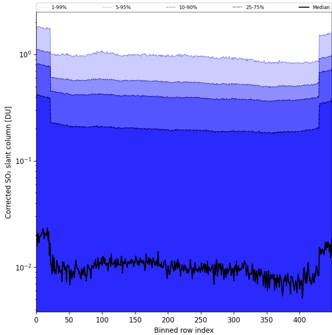
Figure 86: Along track statistics of “Corrected SO 2 slant column” for 2025-08-22 to 2025-08-24
