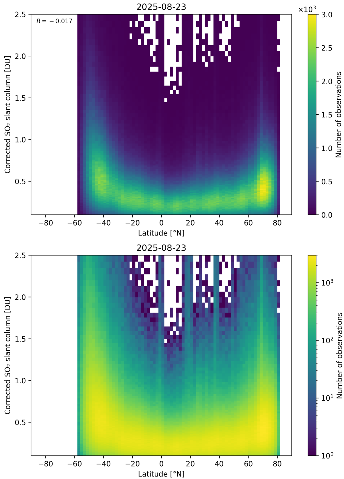
Figure 159: Scatter density plot of “Latitude” against “Corrected SO 2 slant column” for 2025-08-22 to 2025-08-24.
