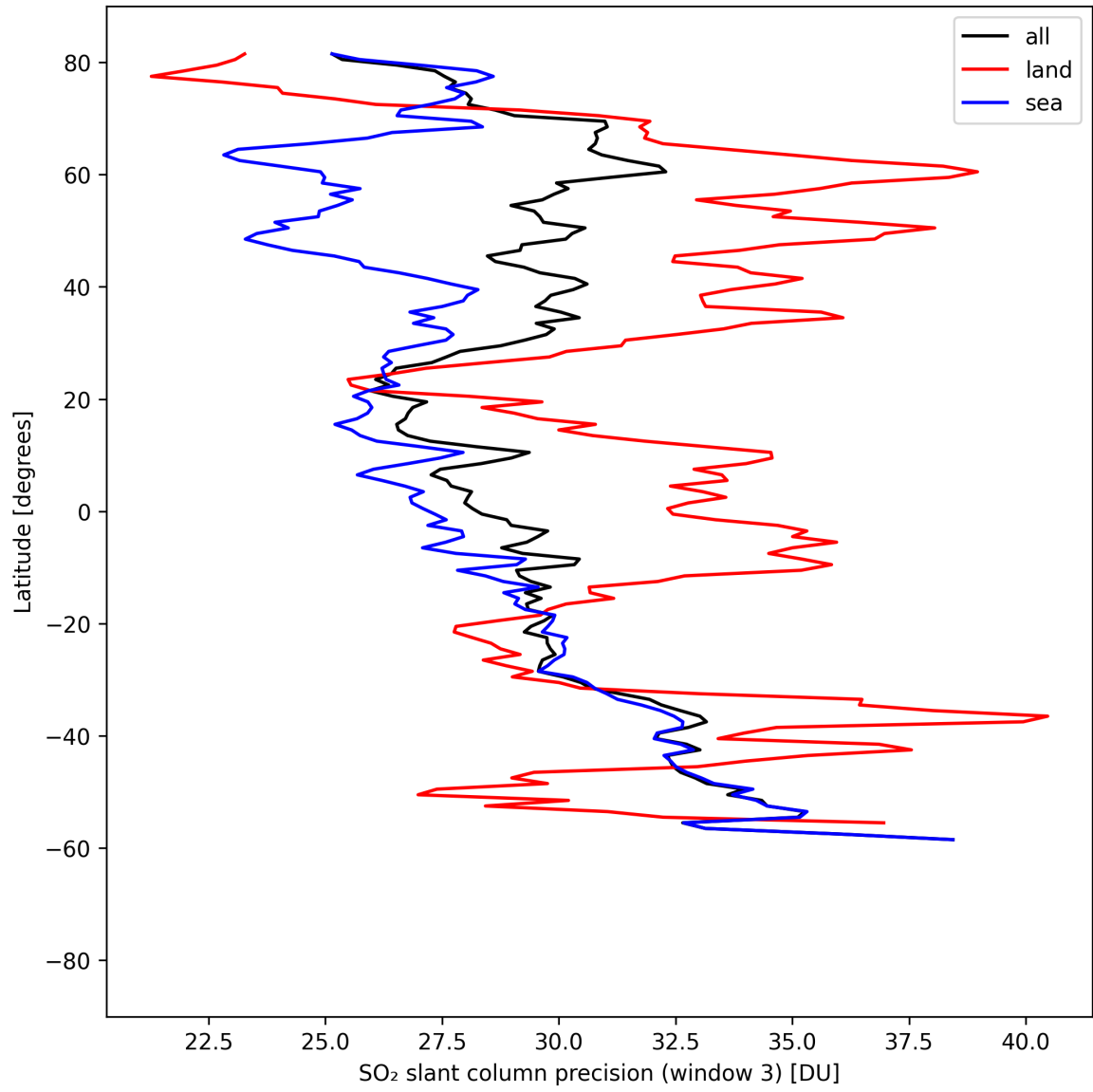
Figure 46: Zonal average of “SO 2 slant column precision (window 3)” for 2025-08-22 to 2025-08-24.
