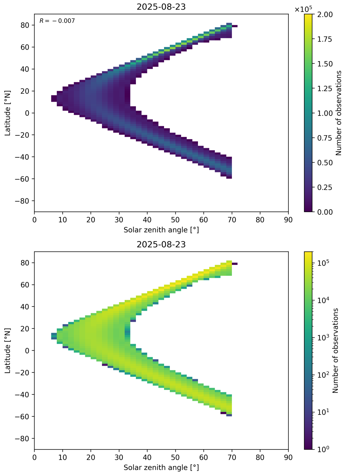
Figure 177: Scatter density plot of “Solar zenith angle” against “Latitude” for 2025-08-22 to 2025-08-24.
