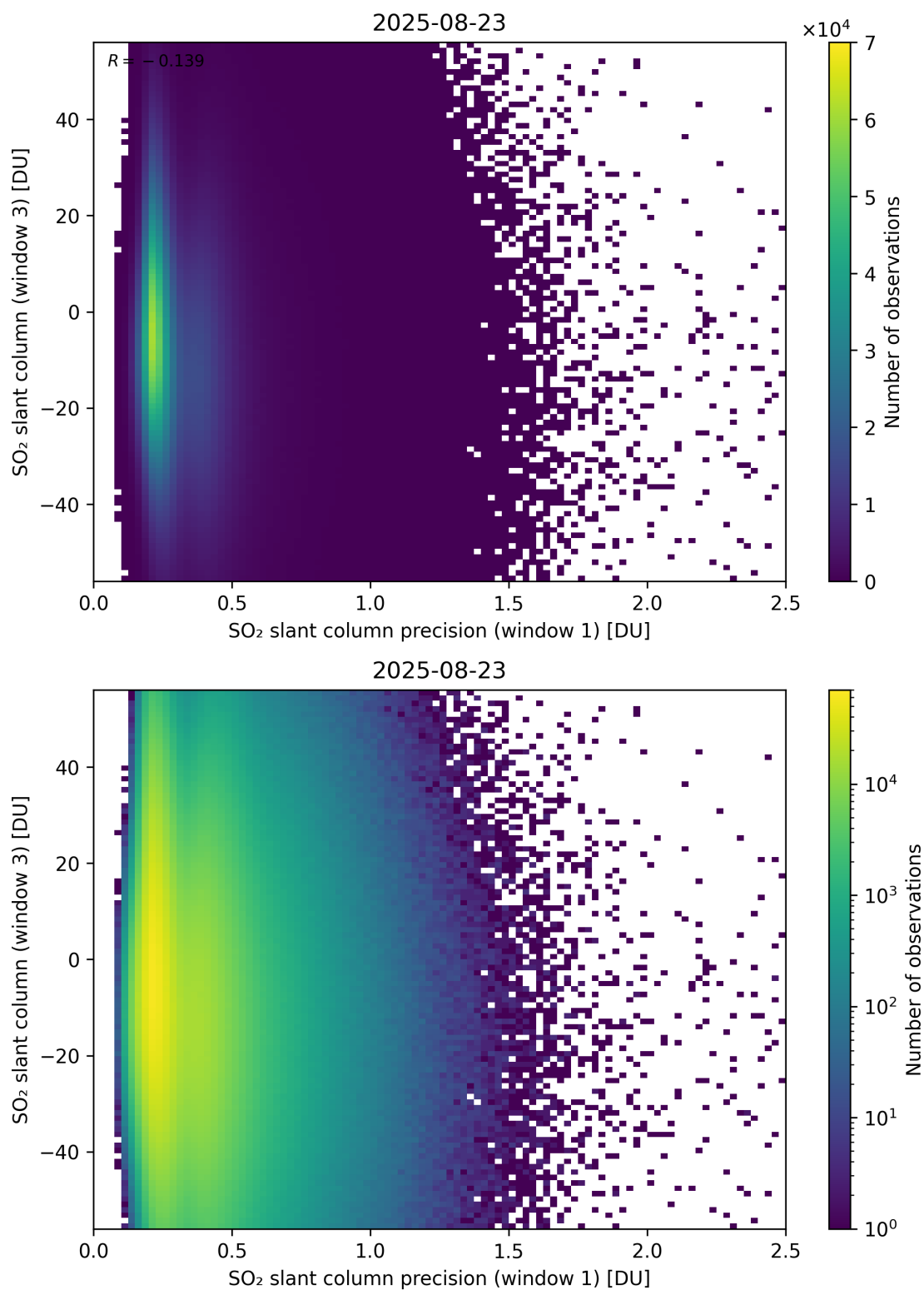
Figure 278: Scatter density plot of “SO 2 slant column precision (window 1)” against “SO 2 slant column (window 3)” for 2025-08-22 to 2025-08-24.
