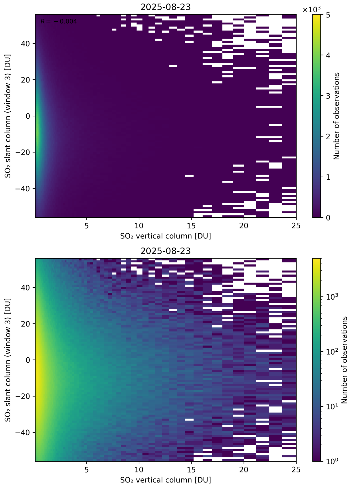
Figure 357: Scatter density plot of “SO 2 vertical column” against “SO 2 slant column (window 3)” for 2025-08-22 to 2025-08-24.
