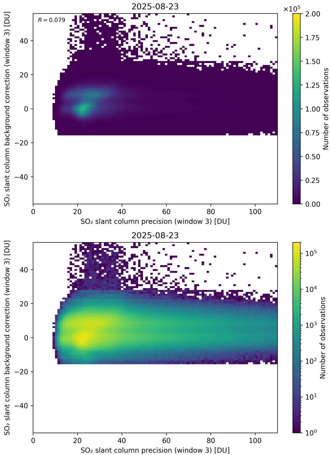
Figure 307: Scatter density plot of “SO 2 slant column precision (window 3)” against “SO 2 slant column background correction (window 3)” for 2025-08-22 to 2025-08-24.
