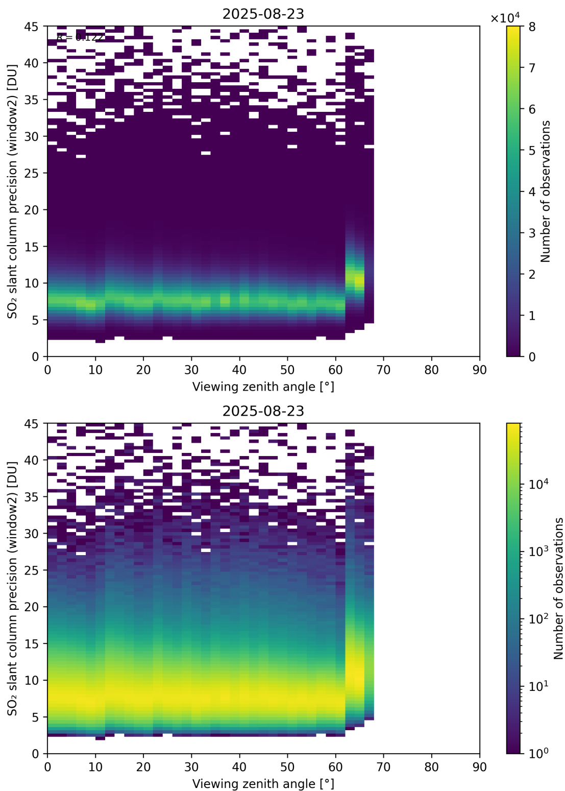
Figure 378: Scatter density plot of “Viewing zenith angle” against “SO 2 slant column precision (window2)” for 2025-08-22 to 2025-08-24.
