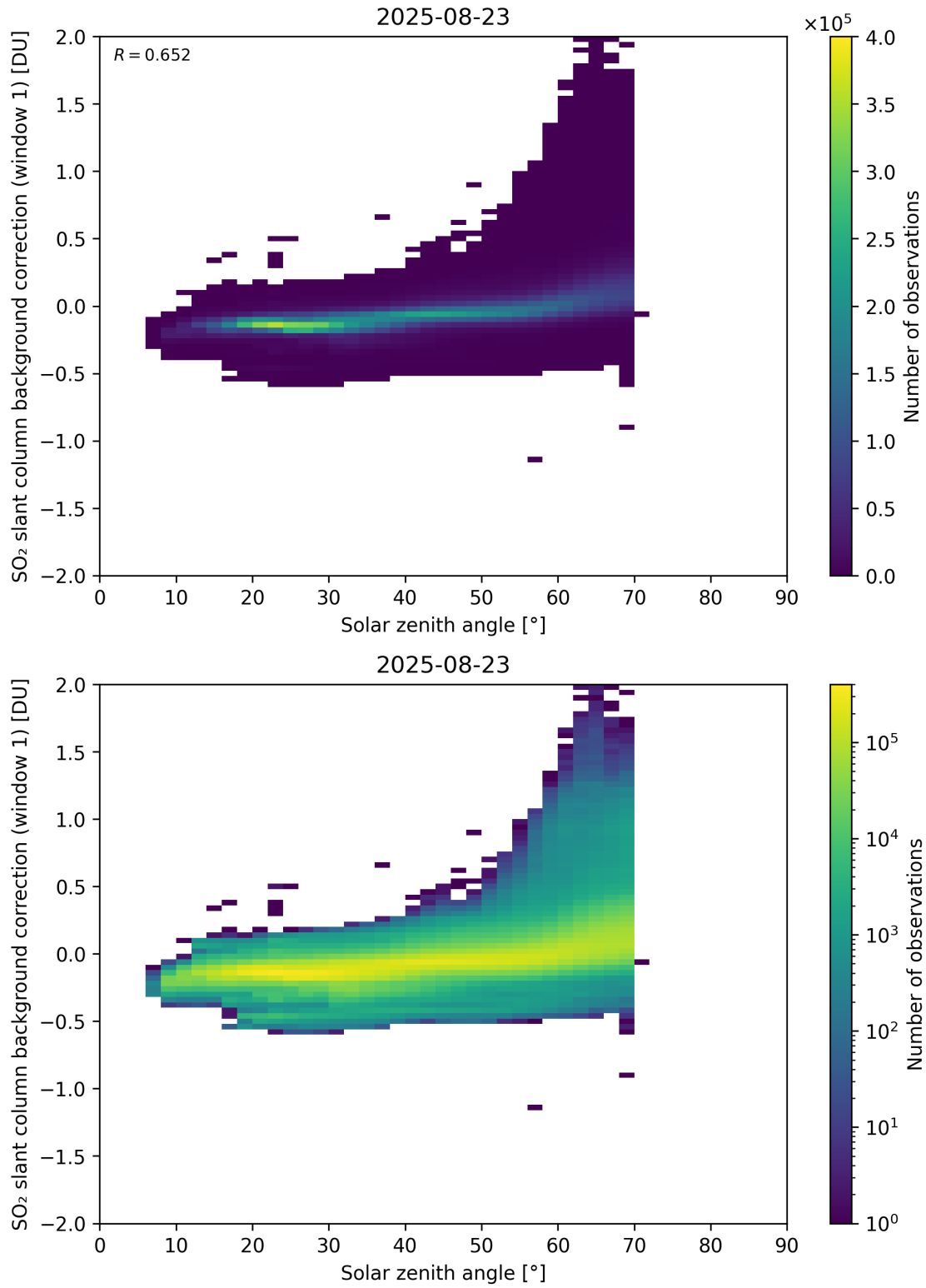
Figure 171: Scatter density plot of “Solar zenith angle” against “SO 2 slant column background correction (window 1)” for 2025-08-22 to 2025-08-24.
