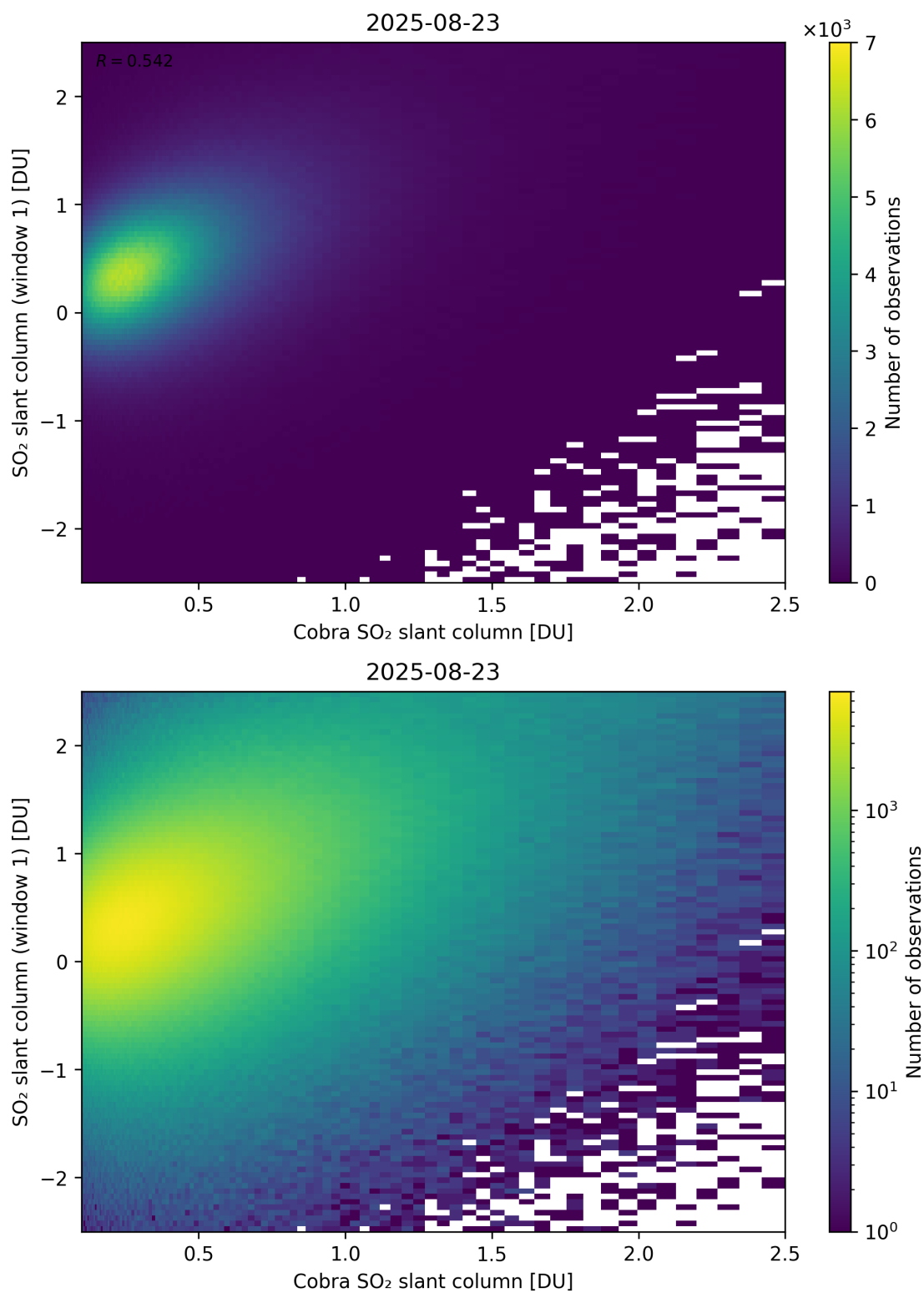
Figure 219: Scatter density plot of “Cobra SO 2 slant column” against “SO 2 slant column (window 1)” for 2025-08-22 to 2025-08-24.
