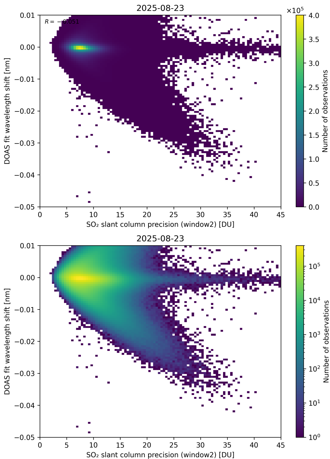
Figure 293: Scatter density plot of “SO 2 slant column precision (window2)” against “DOAS fit wavelength shift” for 2025-08-22 to 2025-08-24.
