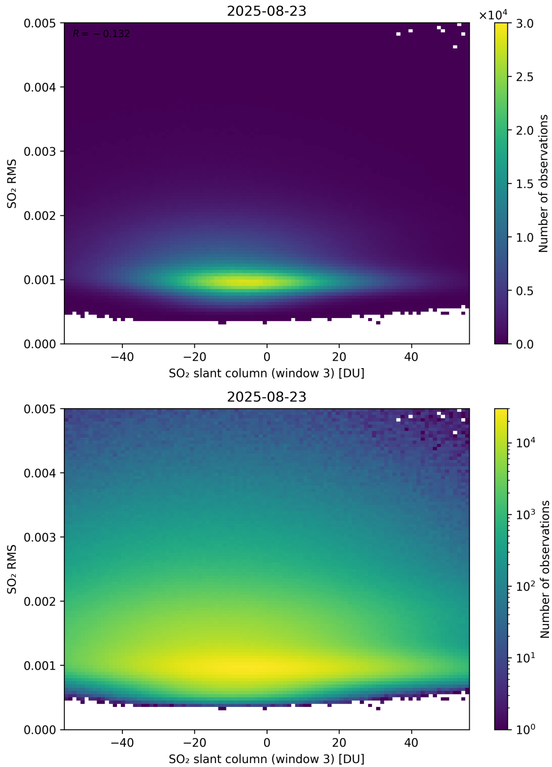
Figure 306: Scatter density plot of “SO 2 slant column (window 3)” against “SO 2 RMS” for 2025-08-22 to 2025-08-24.
