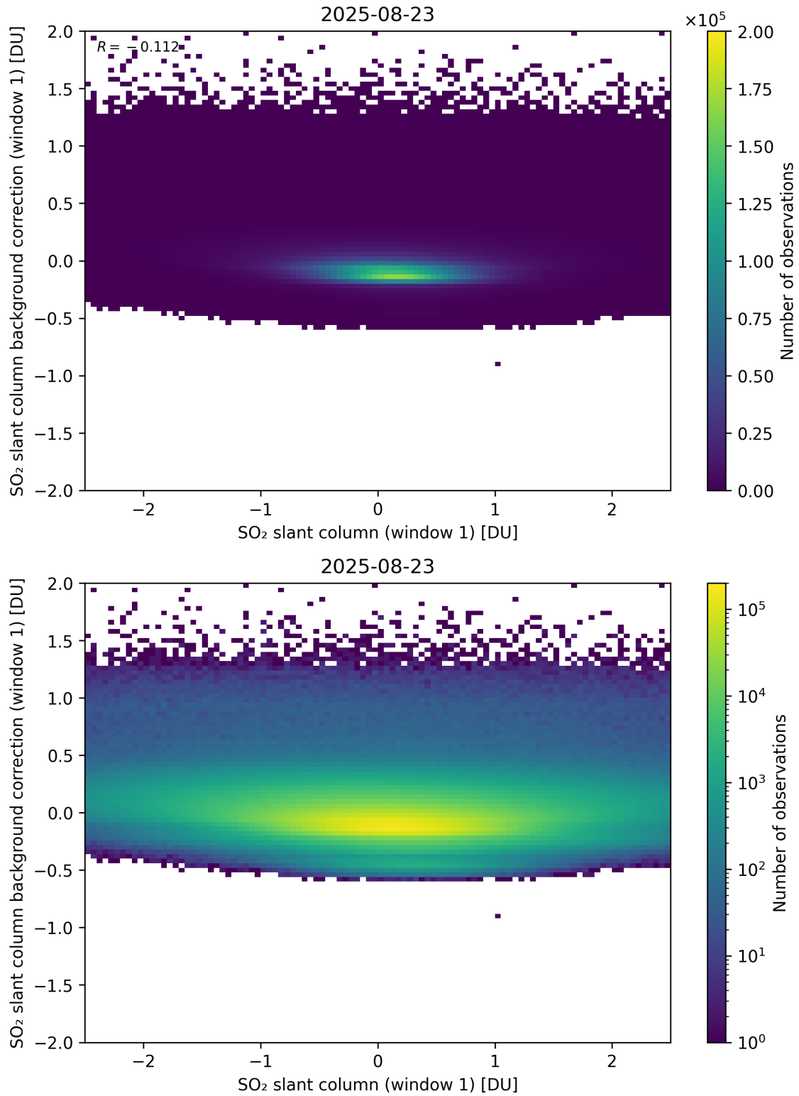
Figure 262: Scatter density plot of “SO 2 slant column (window 1)” against “SO 2 slant column background correction (window 1)” for 2025-08-22 to 2025-08-24.
