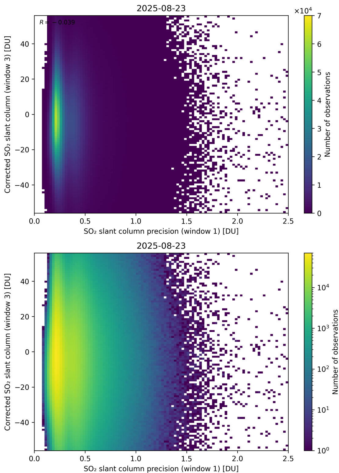
Figure 276: Scatter density plot of “SO 2 slant column precision (window 1)” against “Corrected SO 2 slant column (window 3)” for 2025-08-22 to 2025-08-24.
