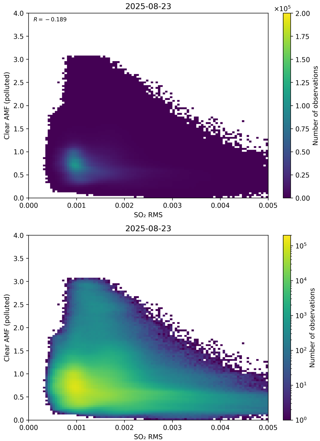
Figure 147: Scatter density plot of “SO 2 RMS” against “Clear AMF (polluted)” for 2025-08-22 to 2025-08-24.
