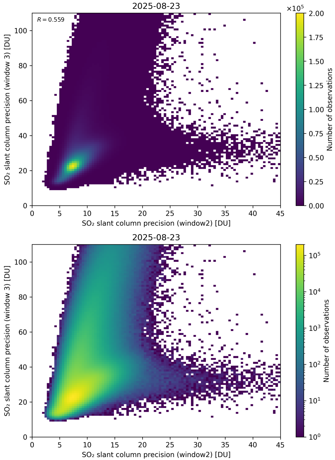
Figure 300: Scatter density plot of “SO 2 slant column precision (window2)” against “SO 2 slant column precision (window 3)” for 2025-08-22 to 2025-08-24.
