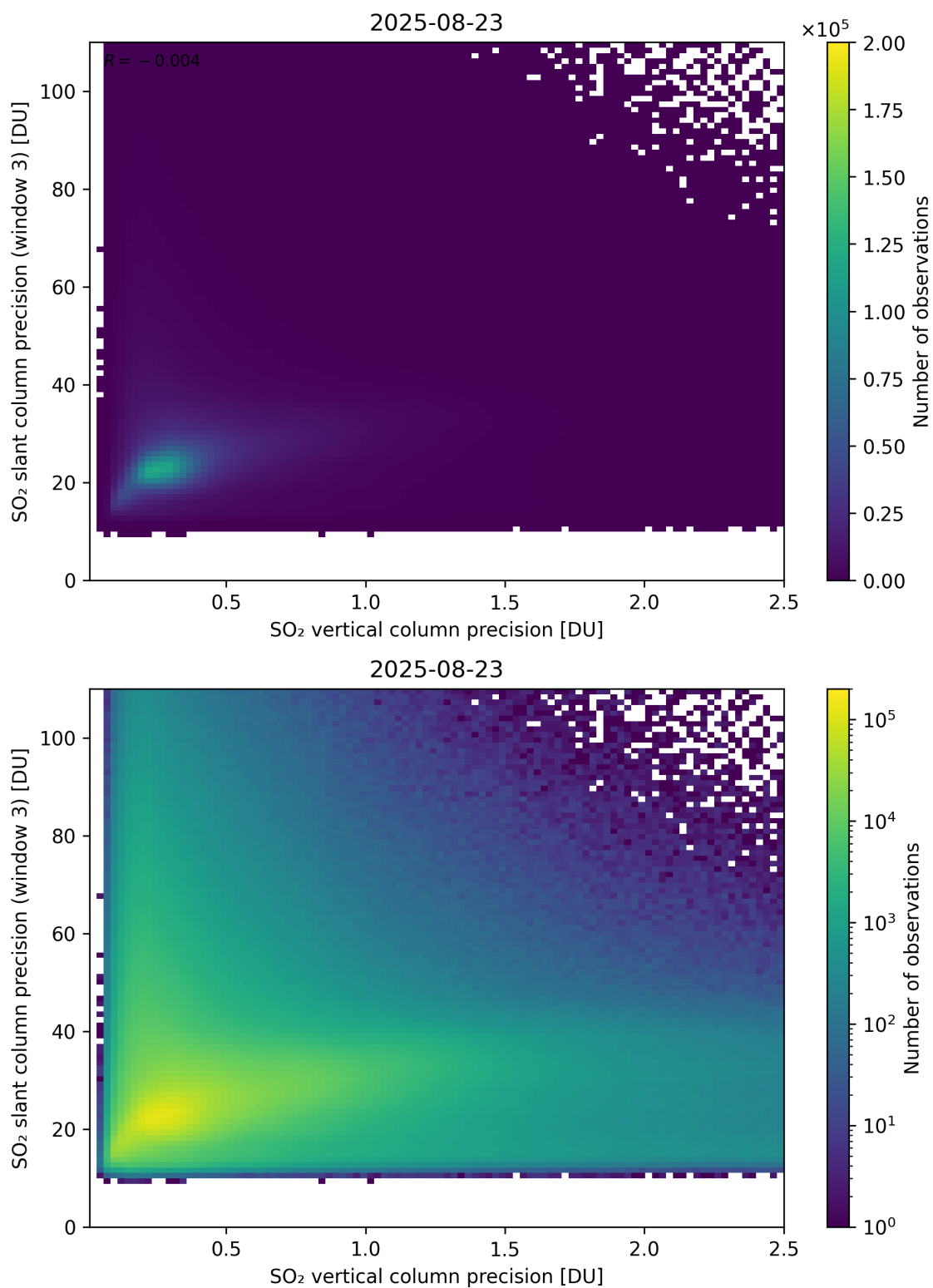
Figure 345: Scatter density plot of “SO 2 vertical column precision” against “SO 2 slant column precision (window 3)” for 2025-08-22 to 2025-08-24.
