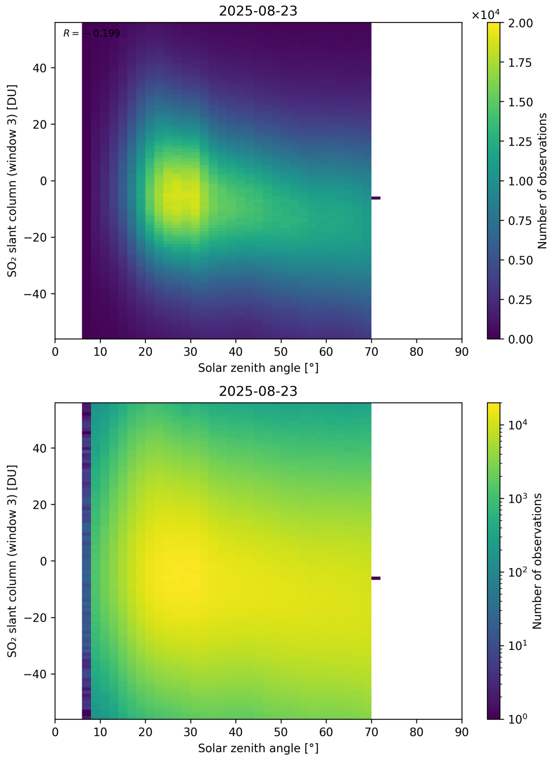
Figure 187: Scatter density plot of “Solar zenith angle” against “SO 2 slant column (window 3)” for 2025-08-22 to 2025-08-24.
