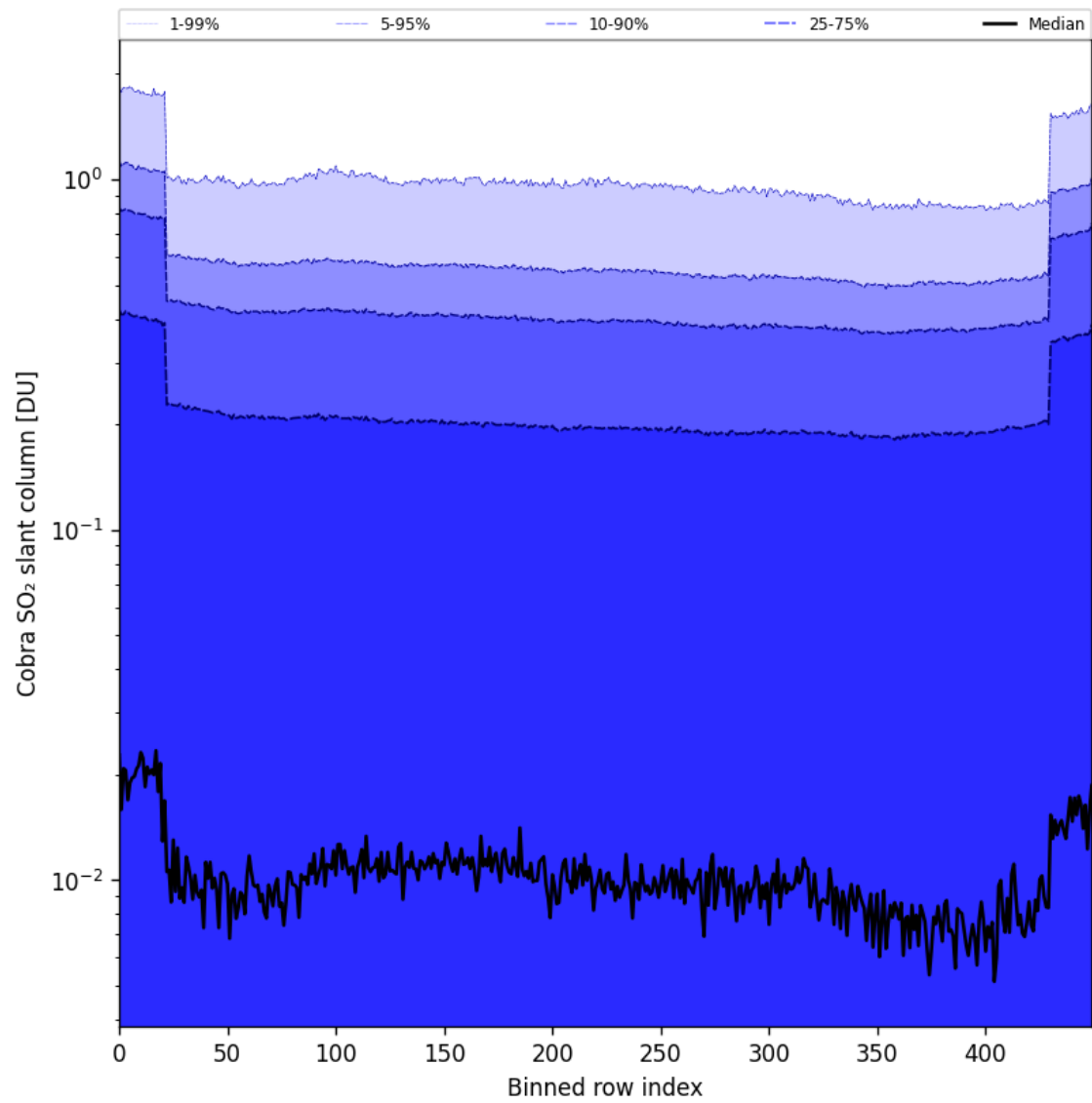
Figure 87: Along track statistics of "Cobra SO 2 slant column" for 2025-08-22 to 2025-08-24
