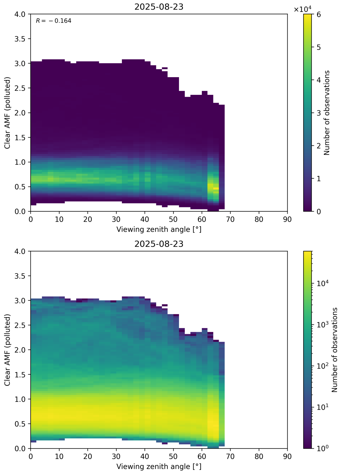
Figure 370: Scatter density plot of “Viewing zenith angle” against “Clear AMF (polluted)” for 2025-08-22 to 2025-08-24.
