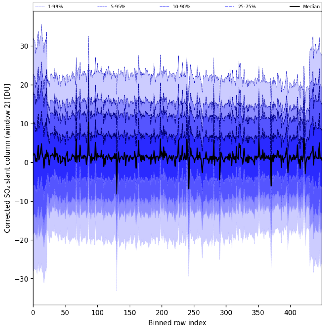
Figure 95: Along track statistics of “Corrected SO 2 slant column (window 2)” for 2025-08-22 to 2025-08-24
