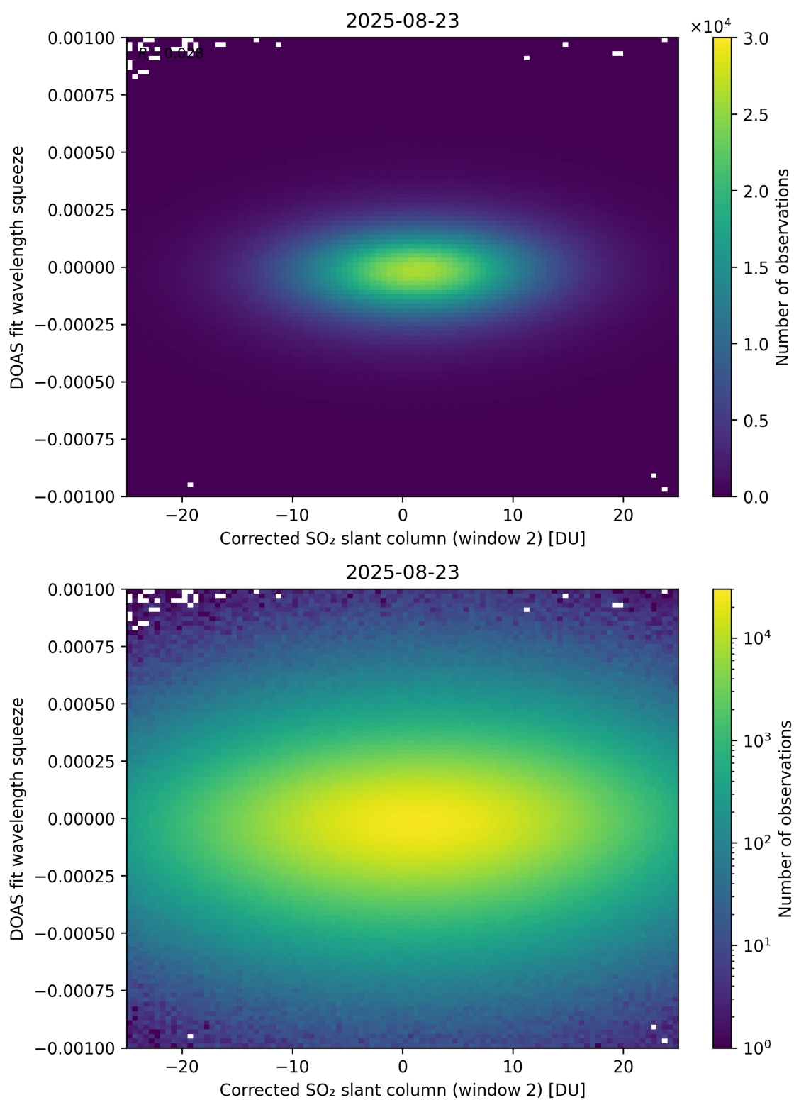
Figure 247: Scatter density plot of “Corrected SO 2 slant column (window 2)” against “DOAS fit wavelength squeeze” for 2025-08-22 to 2025-08-24.
