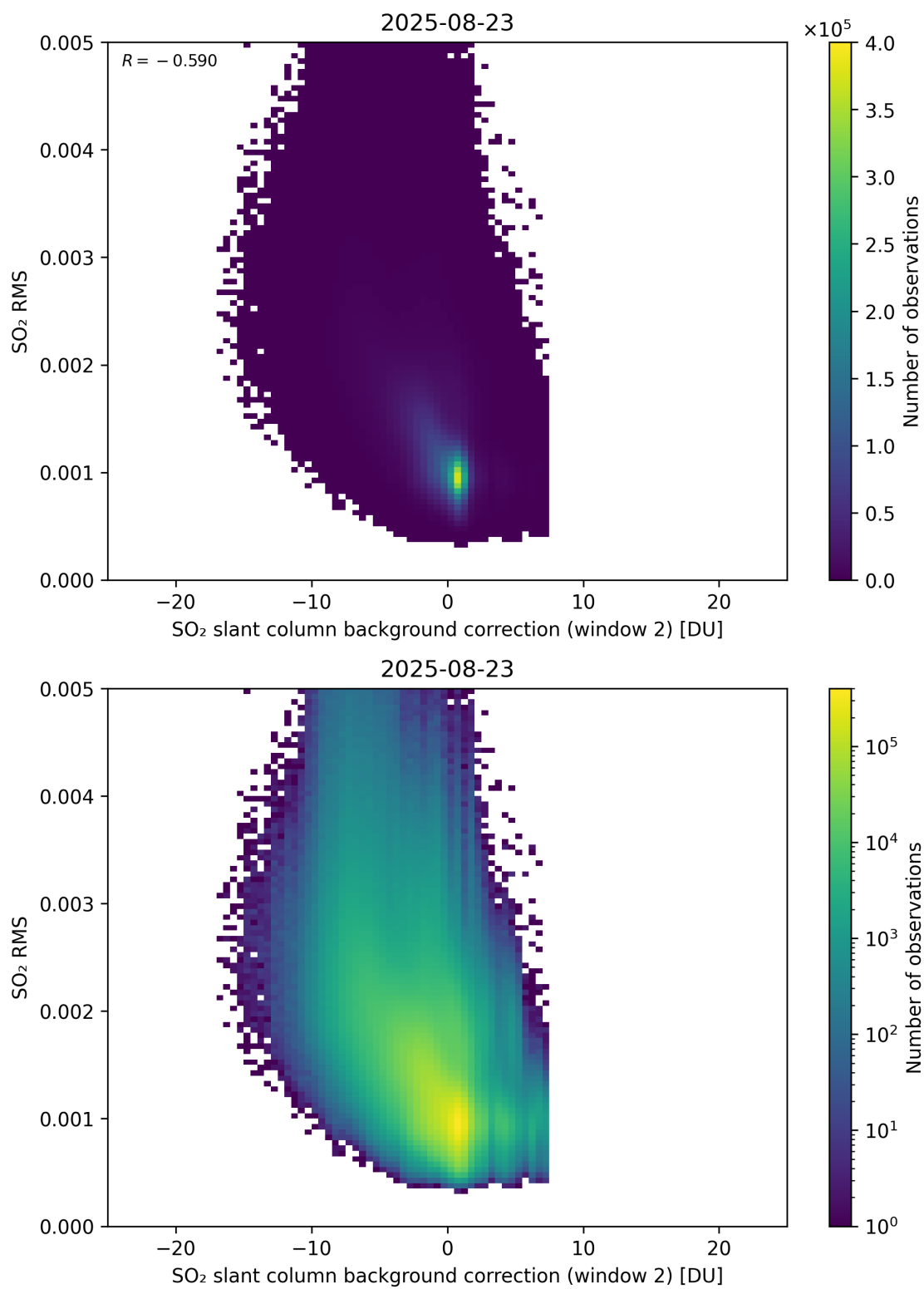
Figure 125: Scatter density plot of “SO 2 slant column background correction (window 2)” against “SO 2 RMS” for 2025-08-22 to 2025-08-24.
