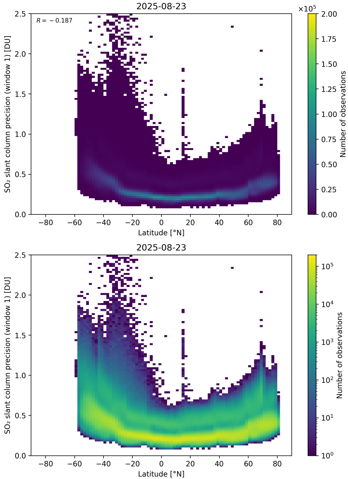
Figure 163: Scatter density plot of “Latitude” against “SO 2 slant column precision (window 1)” for 2025-08-22 to 2025-08-24.
