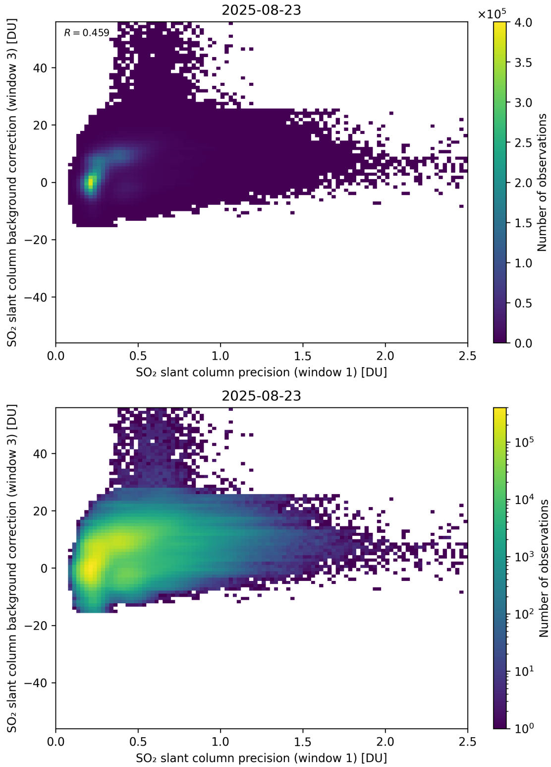
Figure 270: Scatter density plot of “SO 2 slant column precision (window 1)” against “SO 2 slant column background correction (window 3)” for 2025-08-22 to 2025-08-24.
