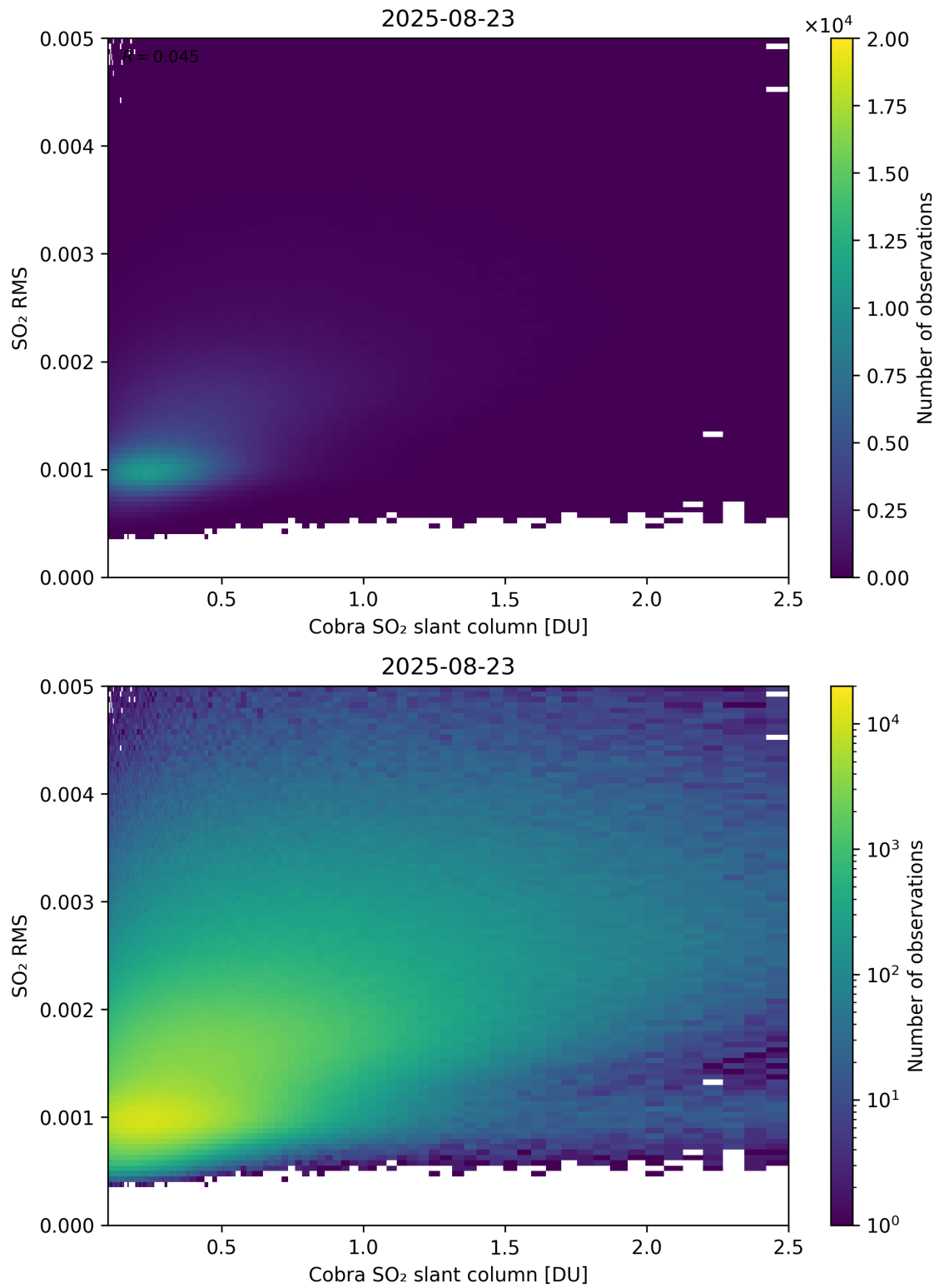
Figure 198: Scatter density plot of “Cobra SO 2 slant column” against “SO 2 RMS” for 2025-08-22 to 2025-08-24.
