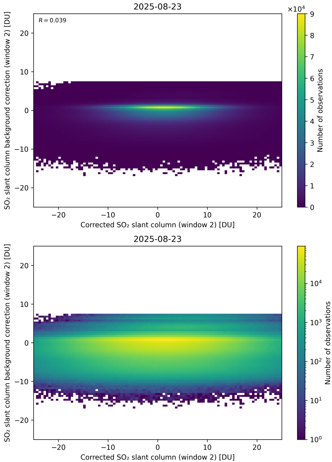
Figure 244: Scatter density plot of “Corrected SO 2 slant column (window 2)” against “SO 2 slant column background correction (window 2)” for 2025-08-22 to 2025-08-24.
