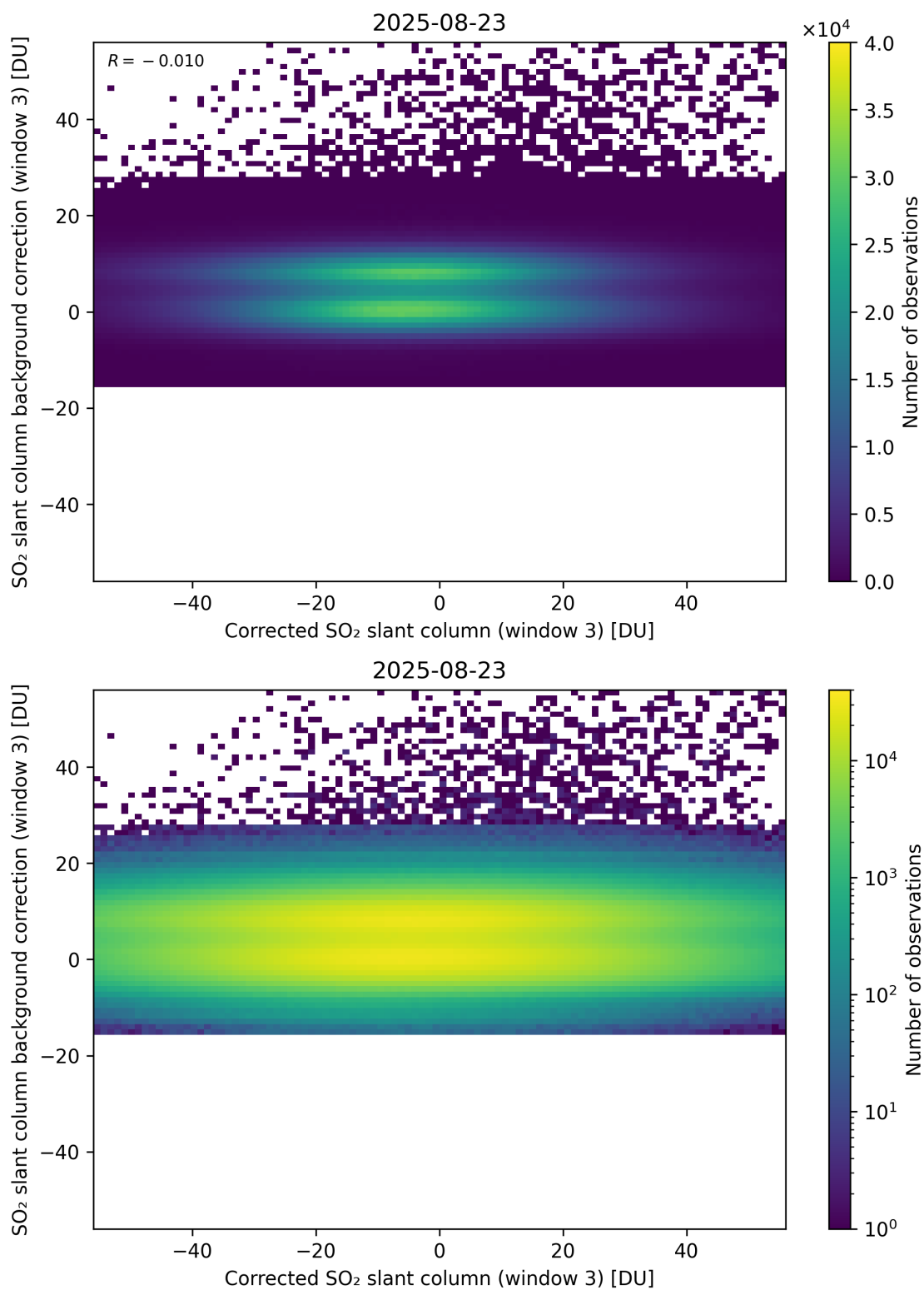
Figure 255: Scatter density plot of “Corrected SO 2 slant column (window 3)” against “SO 2 slant column background correction (window 3)” for 2025-08-22 to 2025-08-24.
