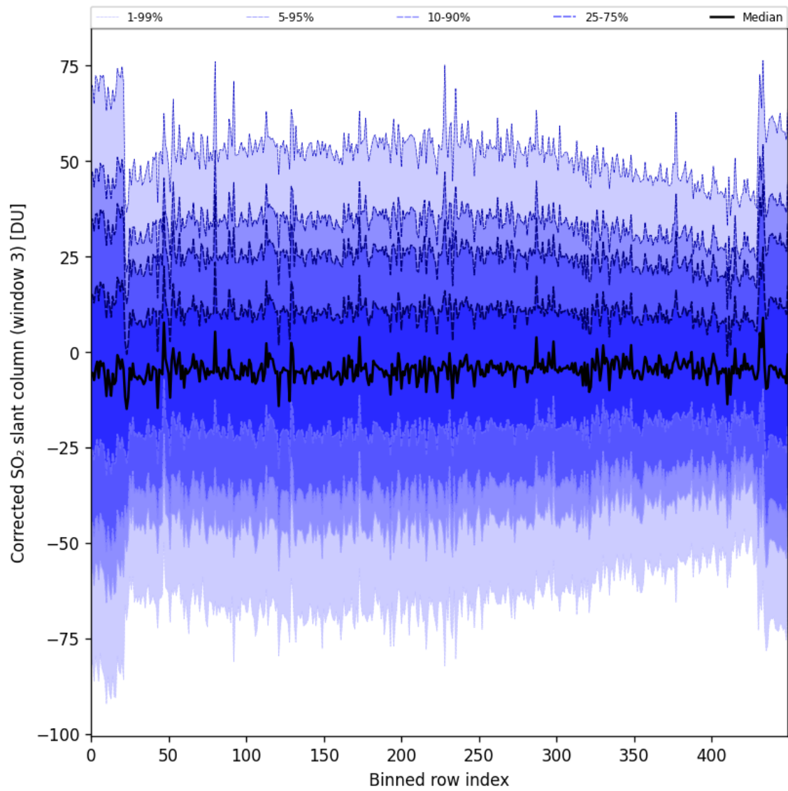
Figure 99: Along track statistics of “Corrected SO 2 slant column (window 3)” for 2025-08-22 to 2025-08-24
