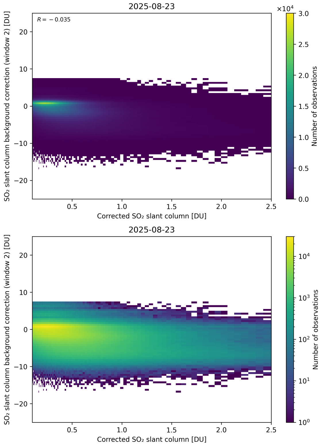
Figure 227: Scatter density plot of “Corrected SO 2 slant column” against “SO 2 slant column background correction (window 2)” for 2025-08-22 to 2025-08-24.
