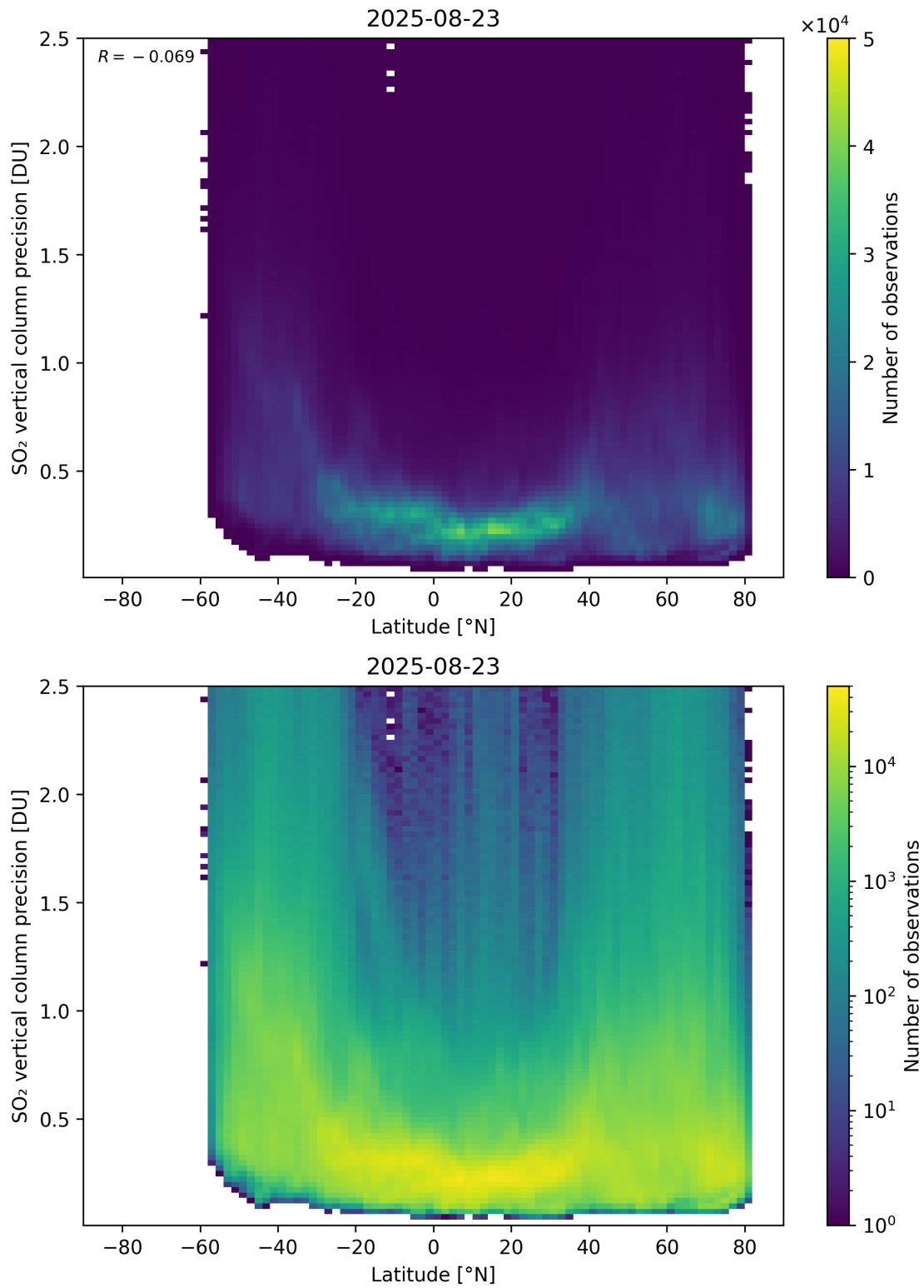
Figure 170: Scatter density plot of “Latitude” against “SO 2 vertical column precision” for 2025-08-22 to 2025-08-24.
