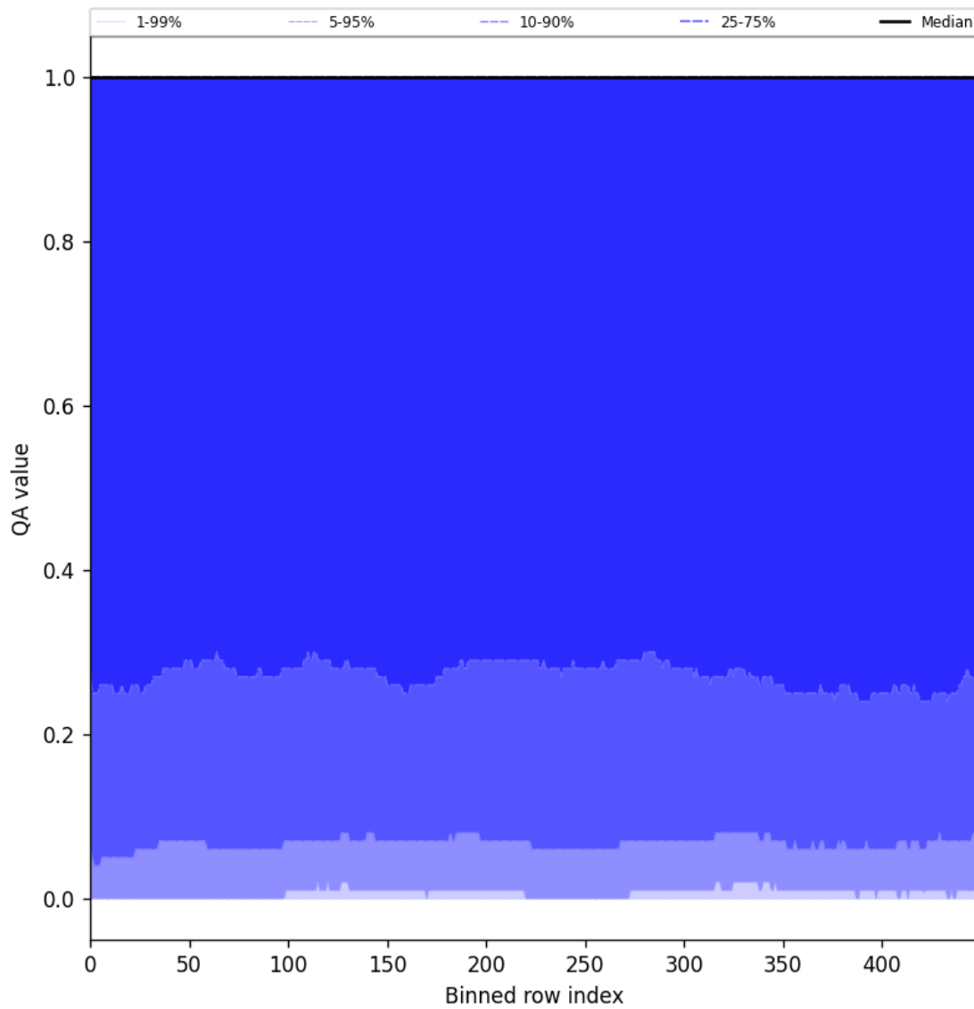
Figure 83: Along track statistics of “QA value” for 2025-08-22 to 2025-08-24
