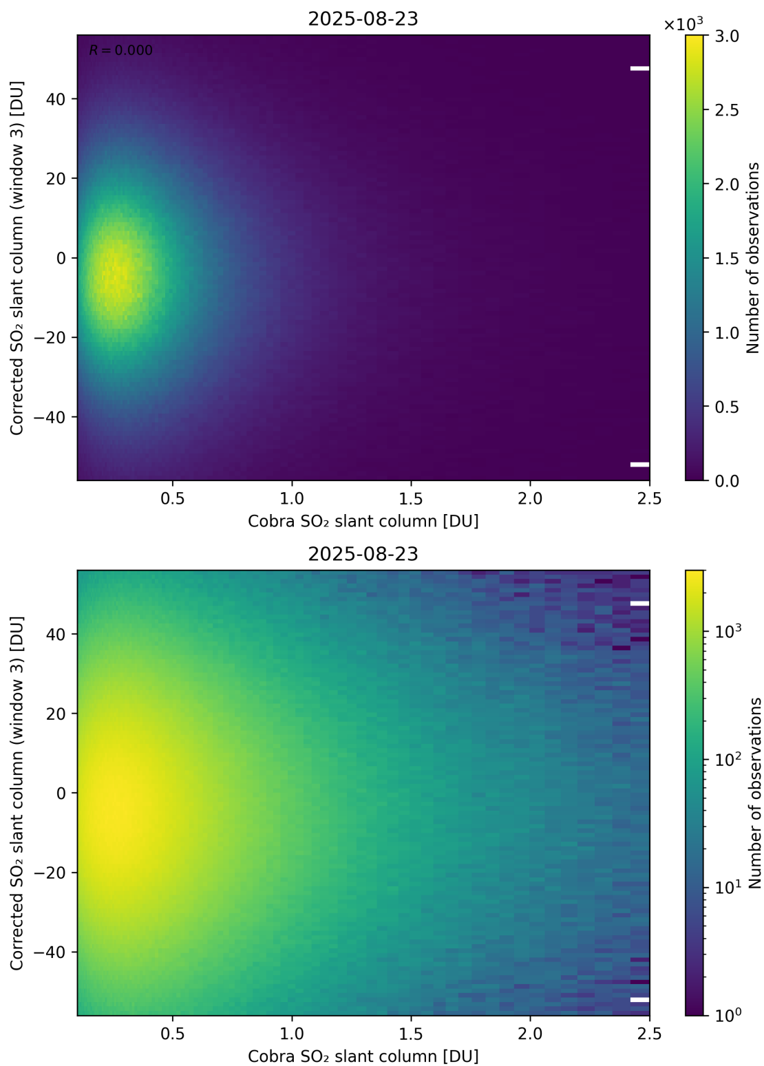
Figure 218: Scatter density plot of “Cobra SO 2 slant column” against “Corrected SO 2 slant column (window 3)” for 2025-08-22 to 2025-08-24.
