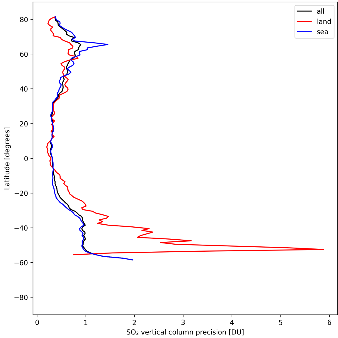
Figure 33: Zonal average of “SO 2 vertical column precision” for 2025-08-22 to 2025-08-24.
