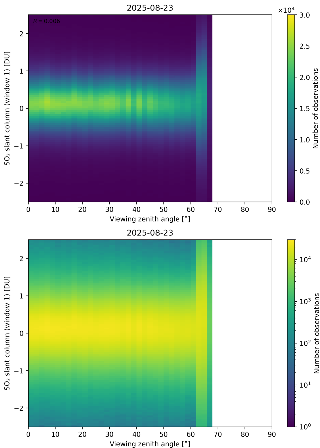
Figure 376: Scatter density plot of “Viewing zenith angle” against “SO 2 slant column (window 1)” for 2025-08-22 to 2025-08-24.
