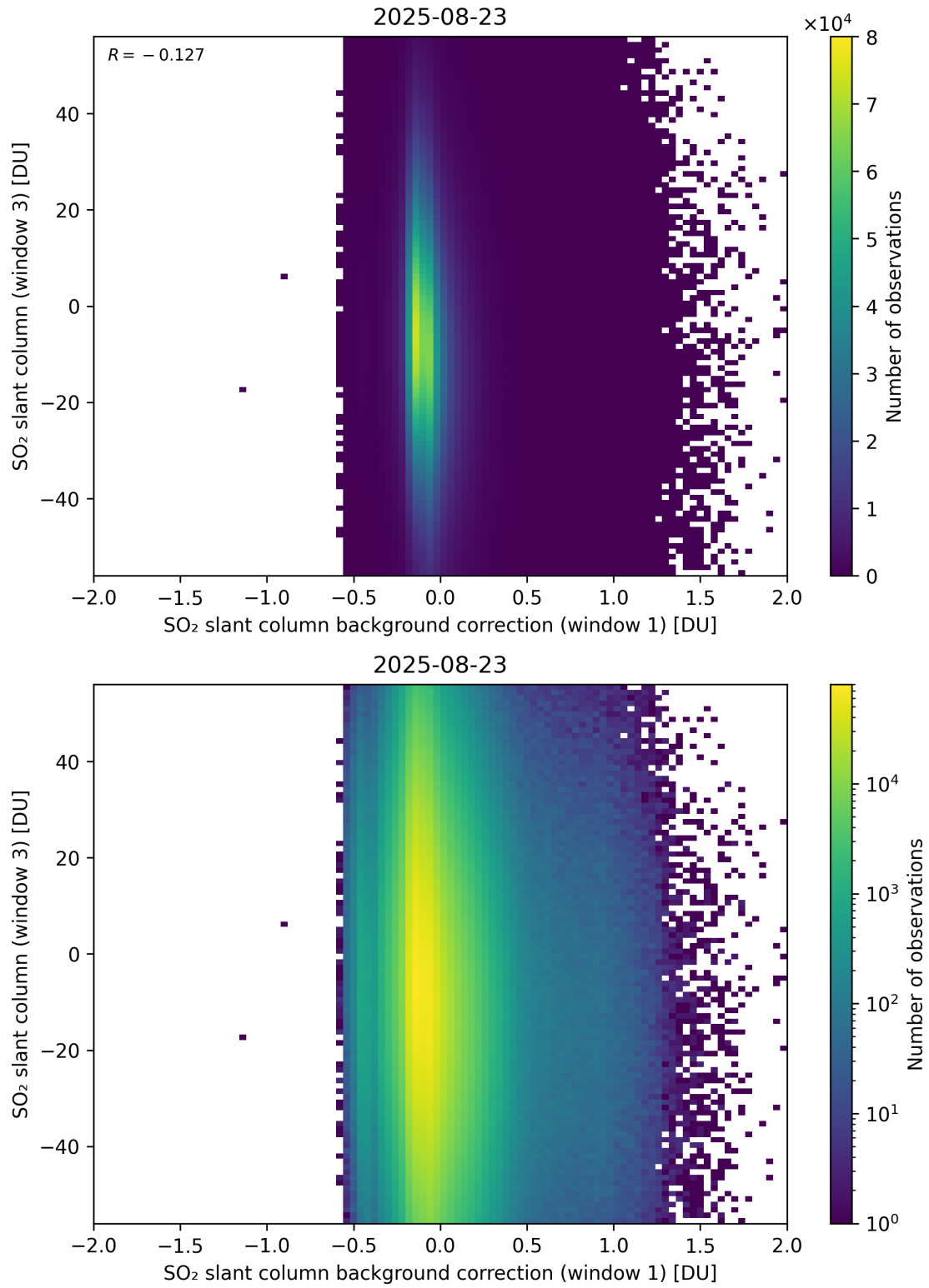
Figure 118: Scatter density plot of “SO 2 slant column background correction (window 1)” against “SO 2 slant column (window 3)” for 2025-08-22 to 2025-08-24.
