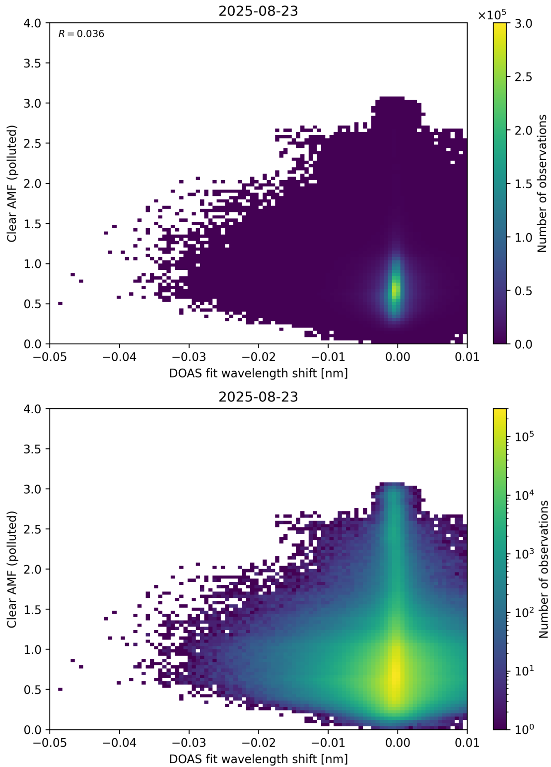
Figure 140: Scatter density plot of “DOAS fit wavelength shift” against “Clear AMF (polluted)” for 2025-08-22 to 2025-08-24.
