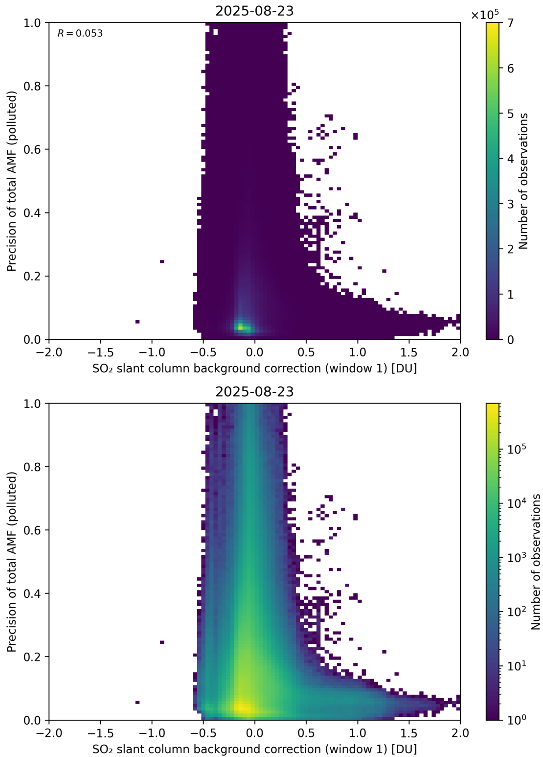
Figure 121: Scatter density plot of “SO 2 slant column background correction (window 1)” against “Precision of total AMF (polluted)” for 2025-08-22 to 2025-08-24.
