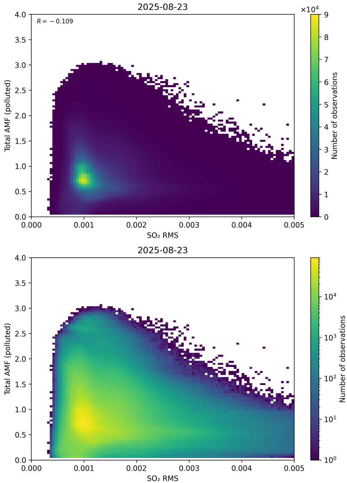
Figure 148: Scatter density plot of “SO 2 RMS” against “Total AMF (polluted)” for 2025-08-22 to 2025-08-24.
