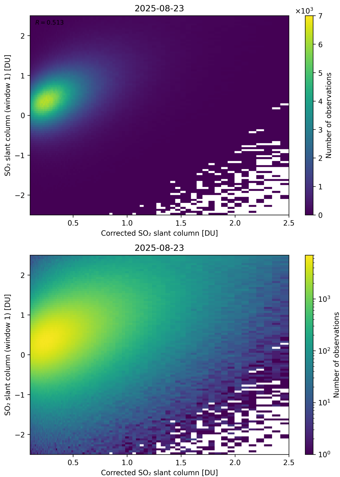
Figure 237: Scatter density plot of “Corrected SO 2 slant column” against “SO 2 slant column (window 1)” for 2025-08-22 to 2025-08-24.
