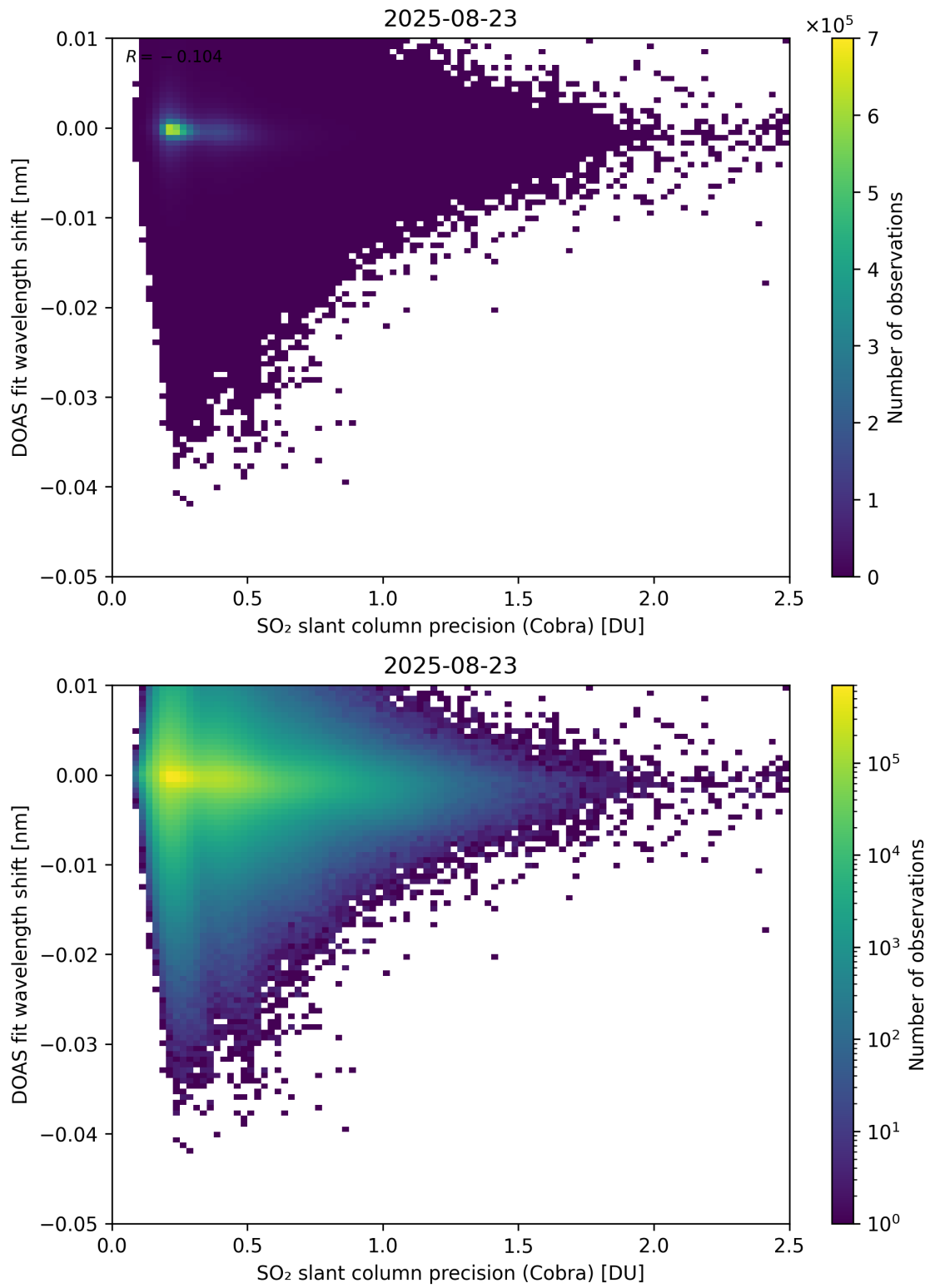
Figure 202: Scatter density plot of “SO 2 slant column precision (Cobra)” against “DOAS fit wavelength shift” for 2025-08-22 to 2025-08-24.
