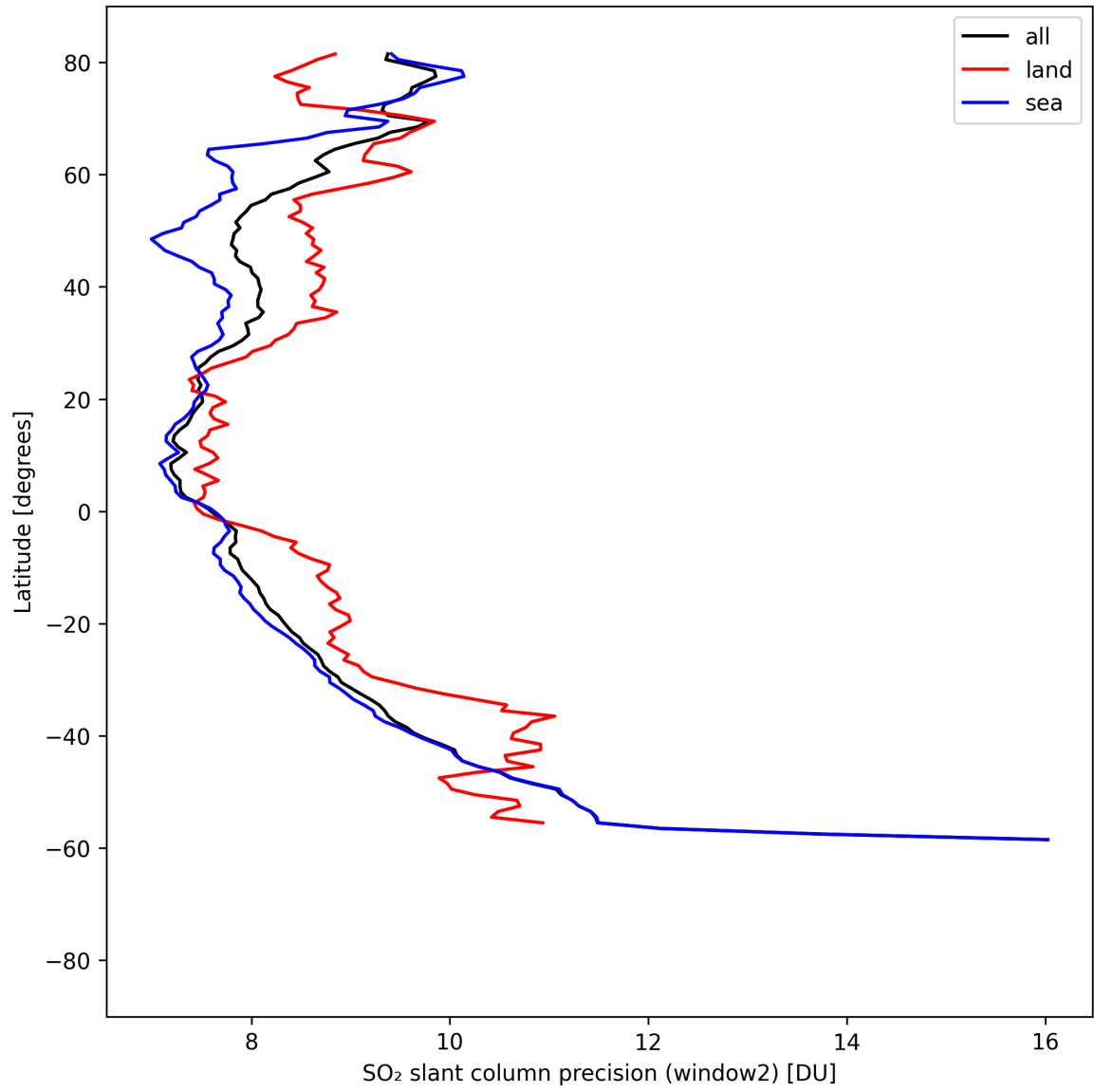
Figure 42: Zonal average of “SO 2 slant column precision (window2)” for 2025-08-22 to 2025-08-24.
