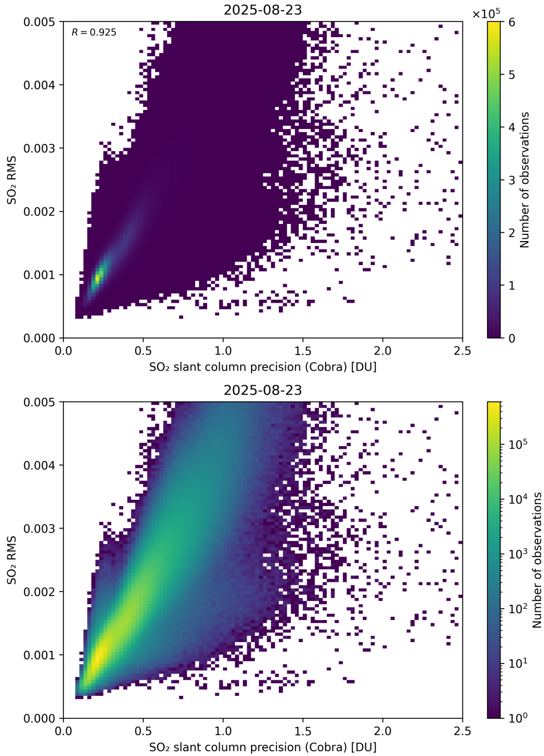
Figure 204: Scatter density plot of “SO 2 slant column precision (Cobra)” against “SO 2 RMS” for 2025-08-22 to 2025-08-24.
