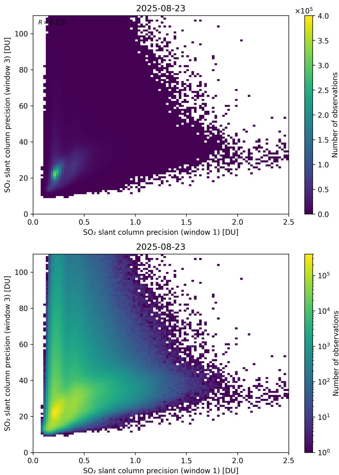
Figure 279: Scatter density plot of “SO 2 slant column precision (window 1)” against “SO 2 slant column precision (window 3)” for 2025-08-22 to 2025-08-24.
