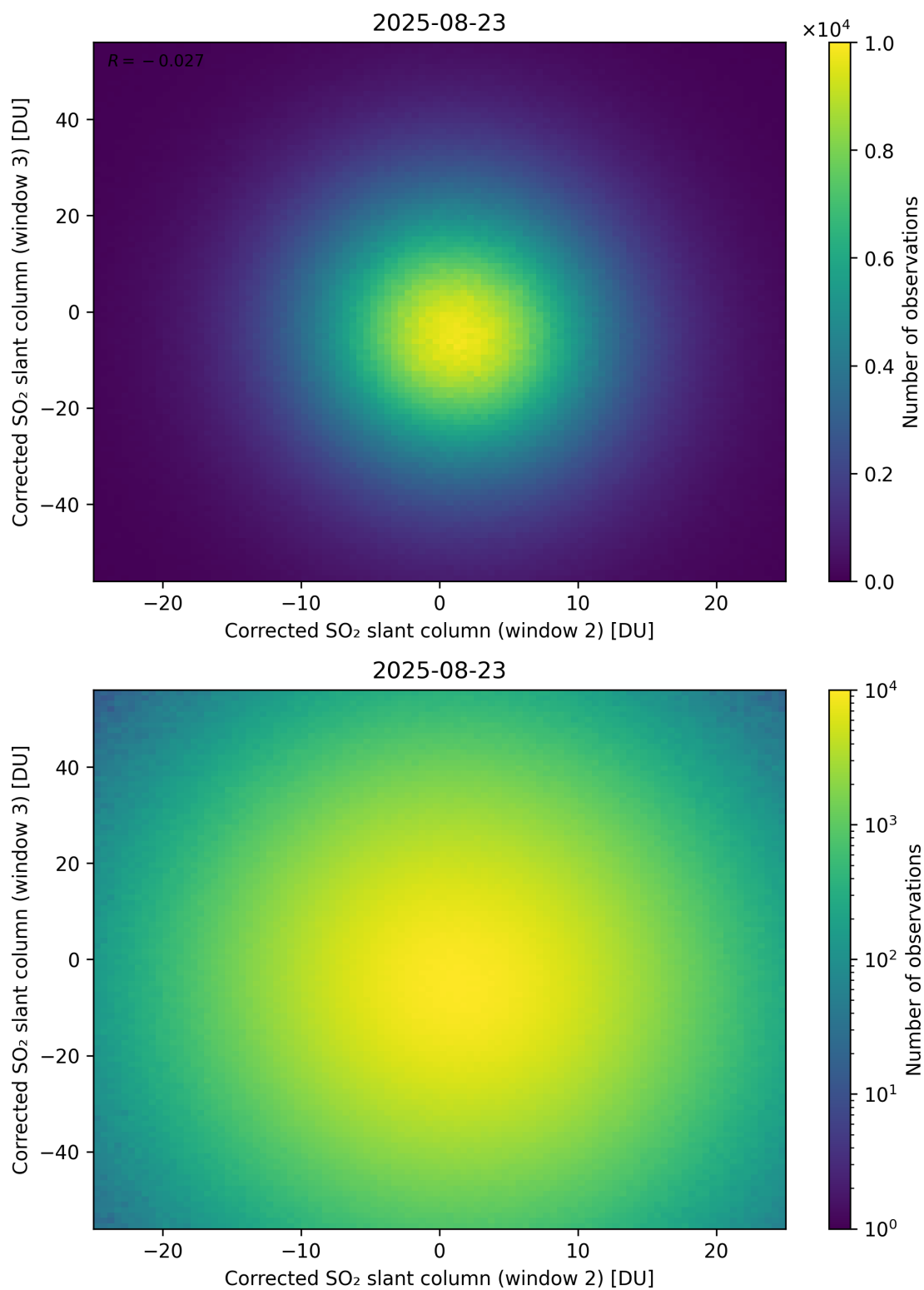
Figure 250: Scatter density plot of “Corrected SO 2 slant column (window 2)” against “Corrected SO 2 slant column (window 3)” for 2025-08-22 to 2025-08-24.
