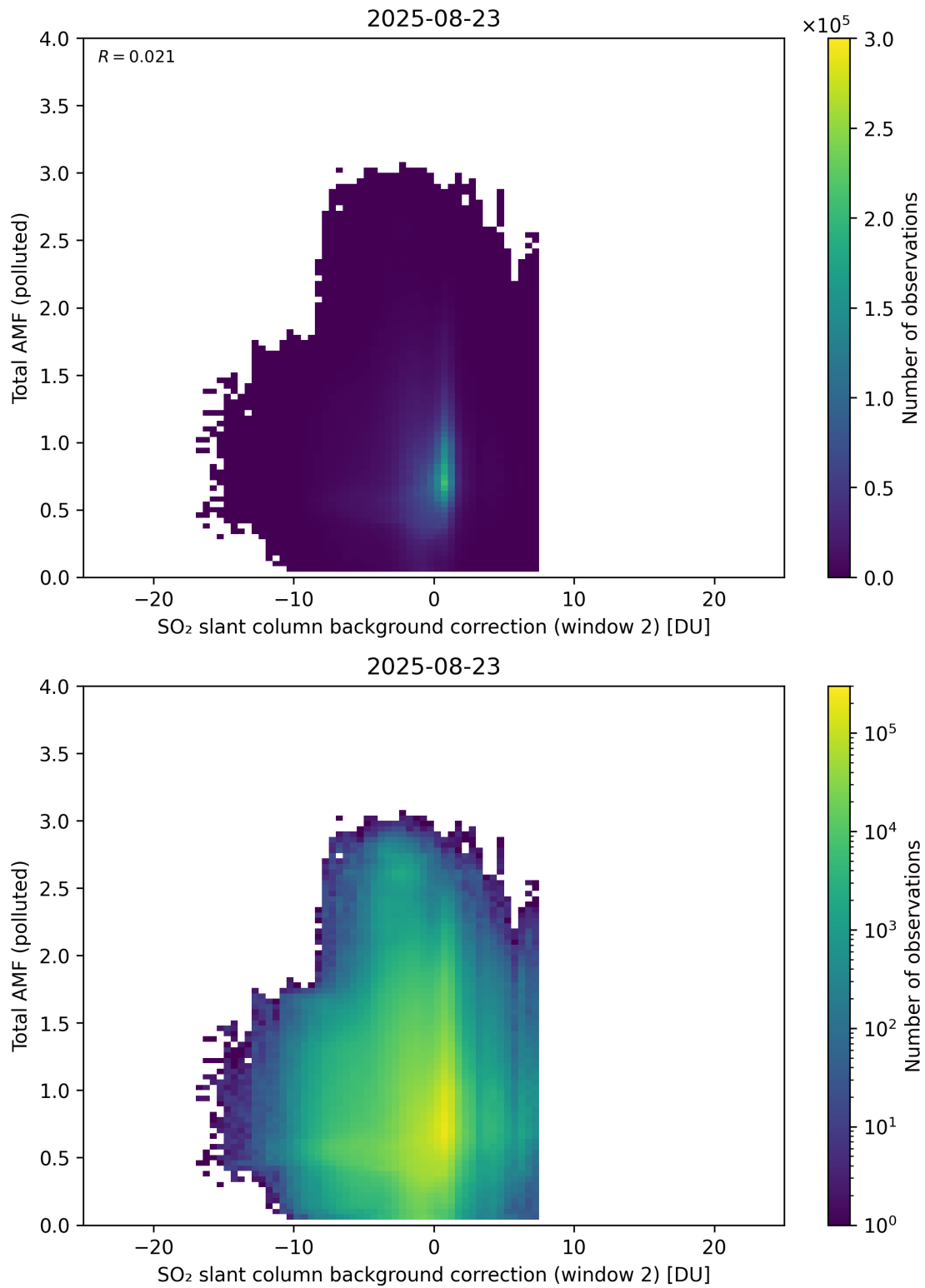
Figure 130: Scatter density plot of “SO 2 slant column background correction (window 2)” against “Total AMF (polluted)” for 2025-08-22 to 2025-08-24.
