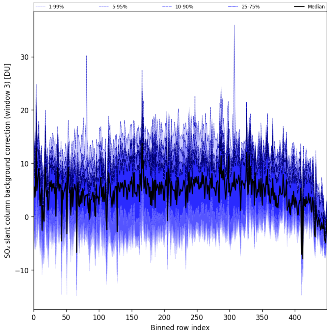
Figure 100: Along track statistics of “SO 2 slant column background correction (window 3)” for 2025-08-22 to 2025-08-24
