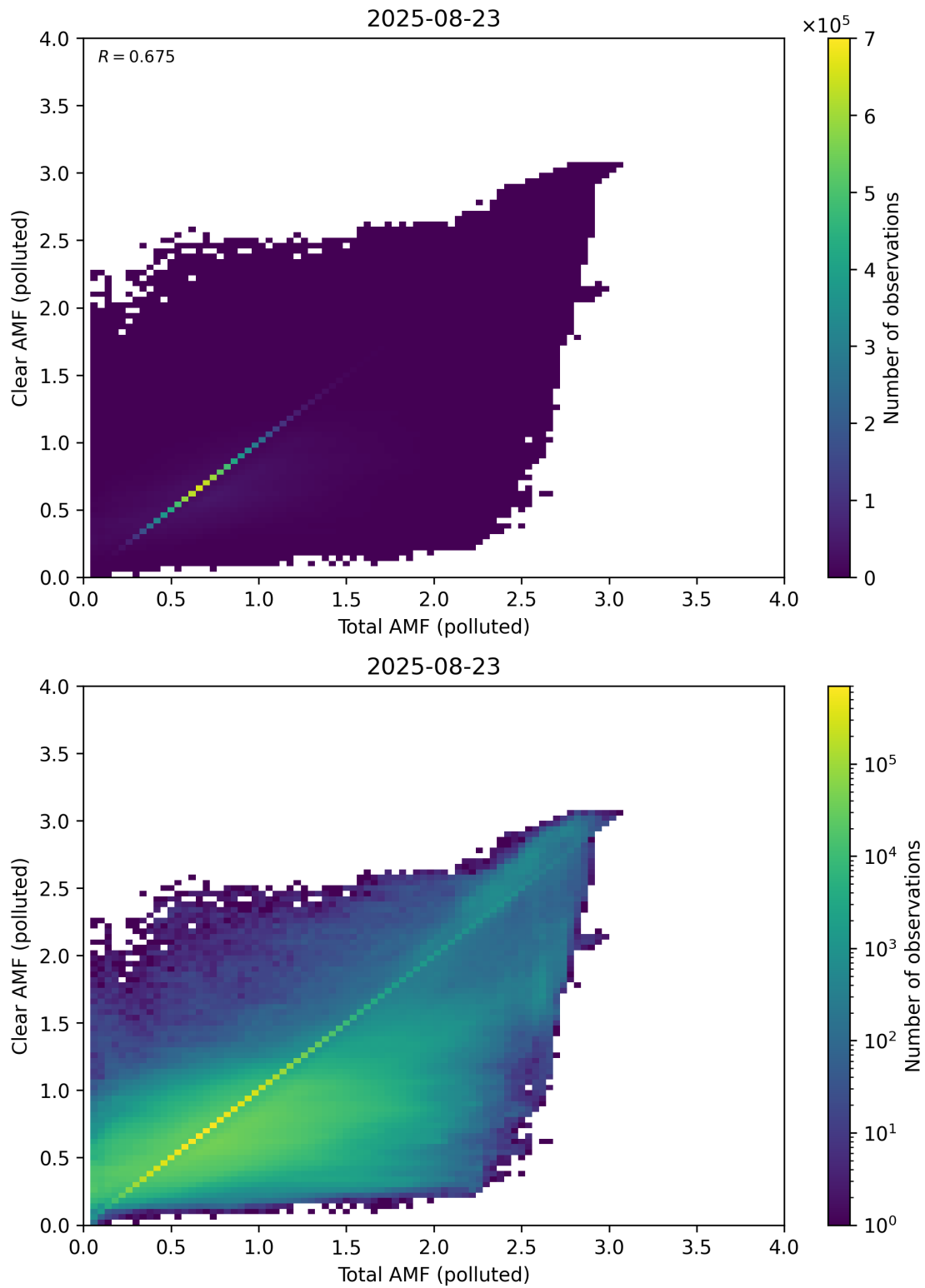
Figure 321: Scatter density plot of “Total AMF (polluted)” against “Clear AMF (polluted)” for 2025-08-22 to 2025-08-24.
