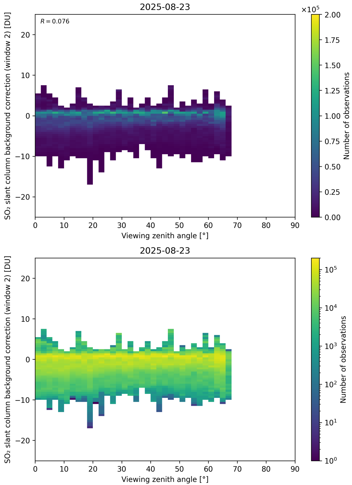
Figure 363: Scatter density plot of “Viewing zenith angle” against “SO 2 slant column background correction (window 2)” for 2025-08-22 to 2025-08-24.
