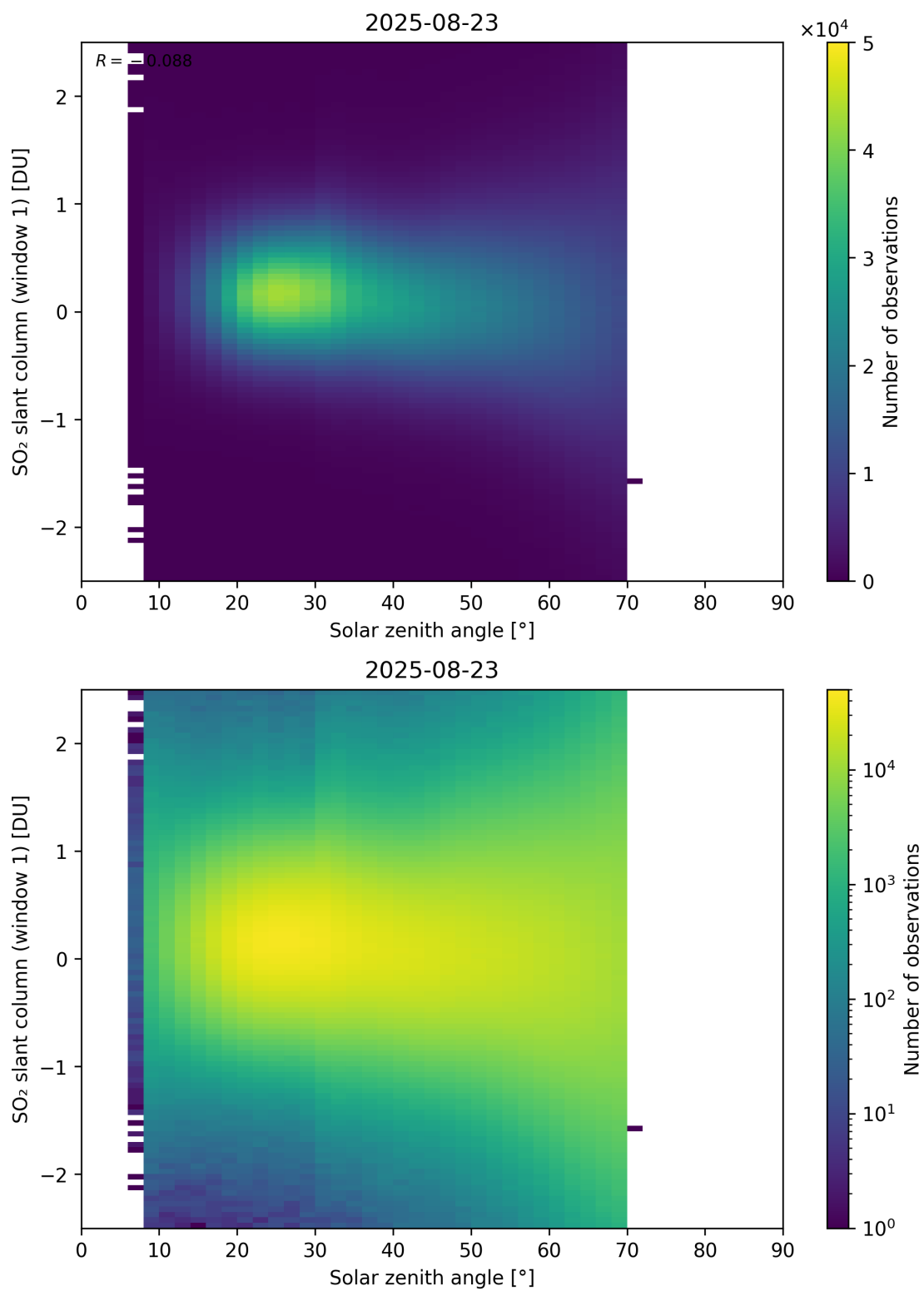
Figure 184: Scatter density plot of “Solar zenith angle” against “SO 2 slant column (window 1)” for 2025-08-22 to 2025-08-24.
