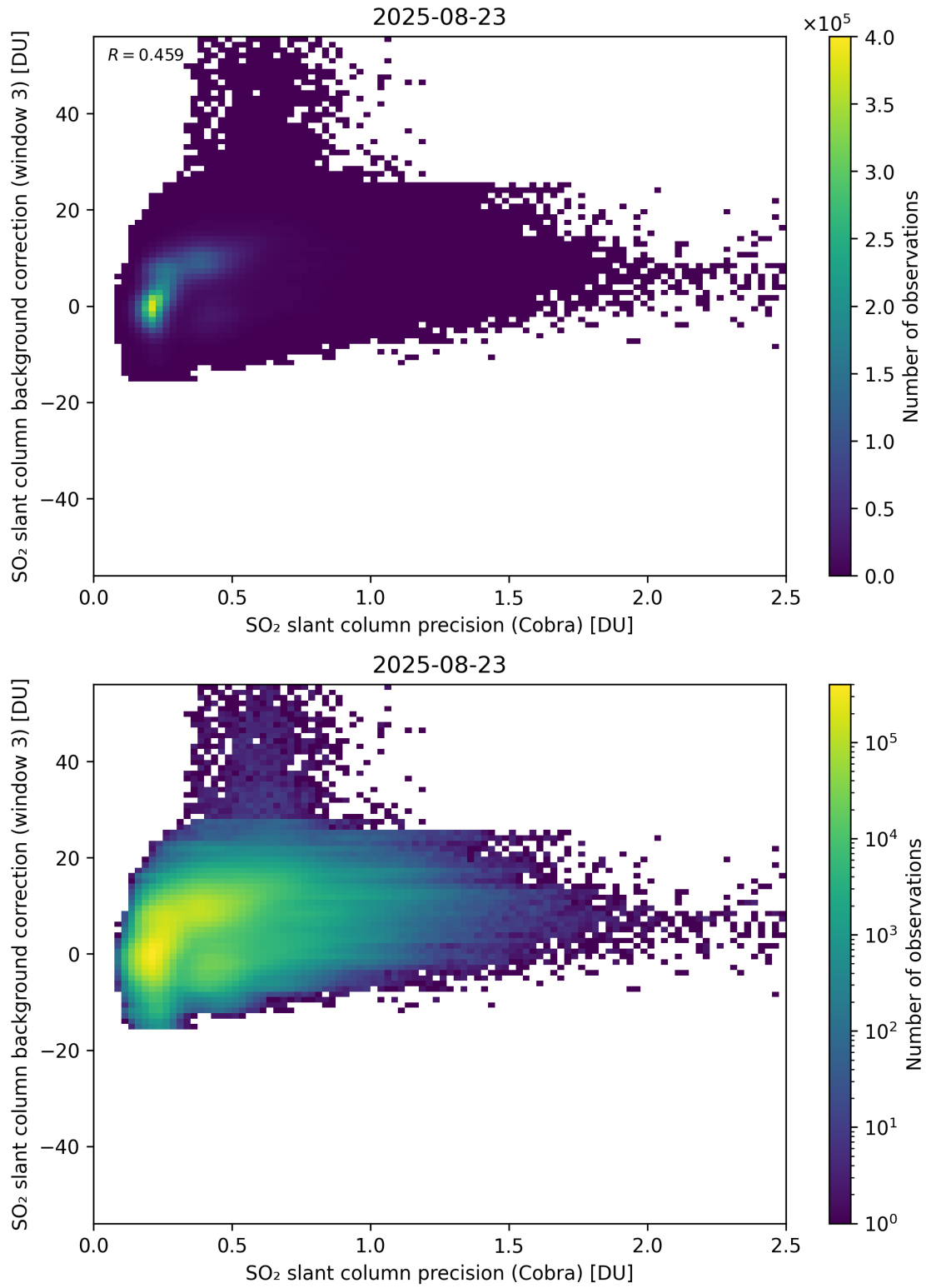
Figure 201: Scatter density plot of “SO 2 slant column precision (Cobra)” against “SO 2 slant column background correction (window 3)” for 2025-08-22 to 2025-08-24.
