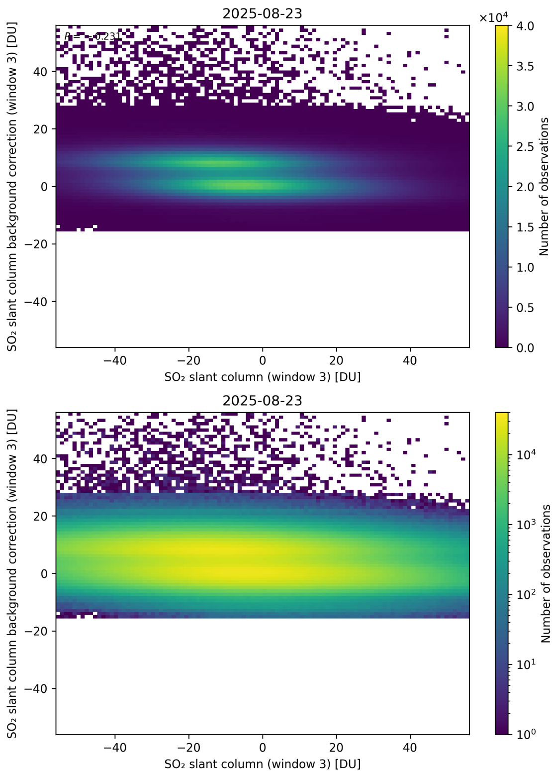
Figure 303: Scatter density plot of “SO 2 slant column (window 3)” against “SO 2 slant column background correction (window 3)” for 2025-08-22 to 2025-08-24.
