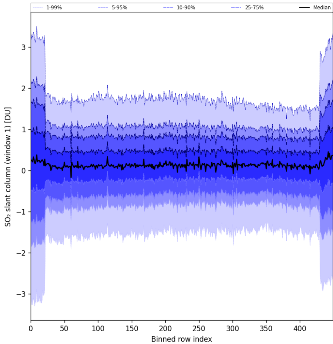
Figure 89: Along track statistics of “SO 2 slant column (window 1)” for 2025-08-22 to 2025-08-24
