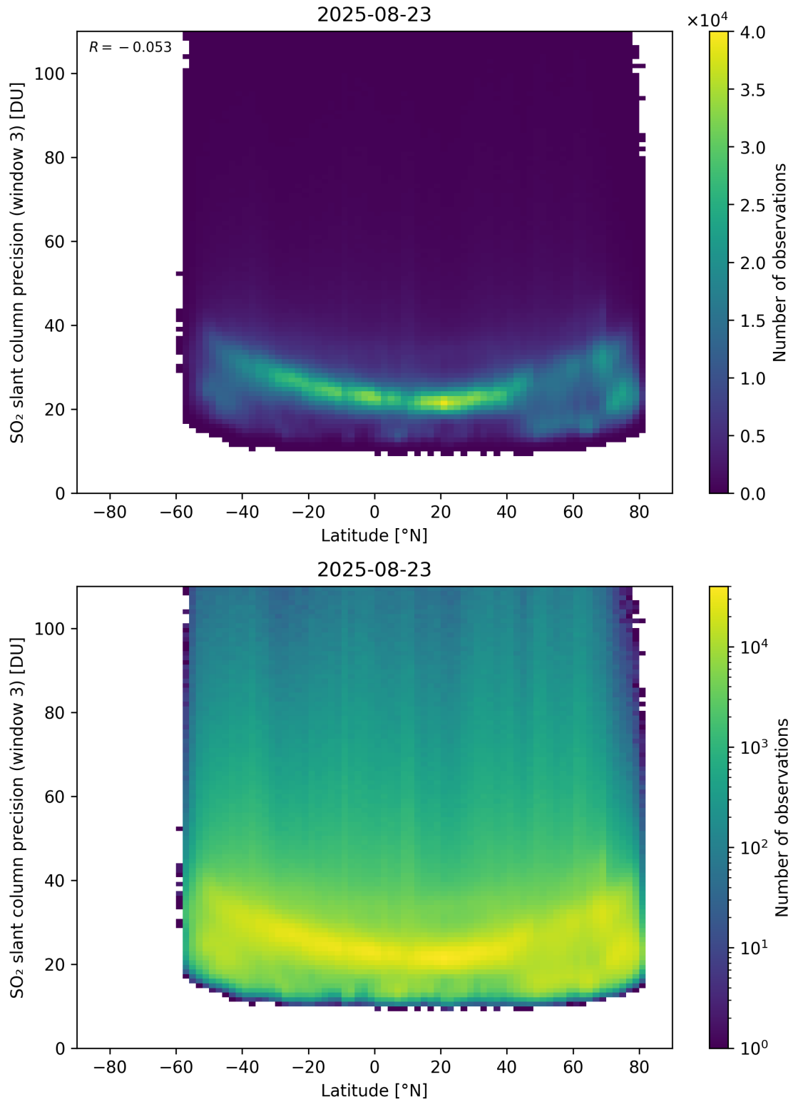
Figure 166: Scatter density plot of “Latitude” against “SO 2 slant column precision (window 3)” for 2025-08-22 to 2025-08-24.
