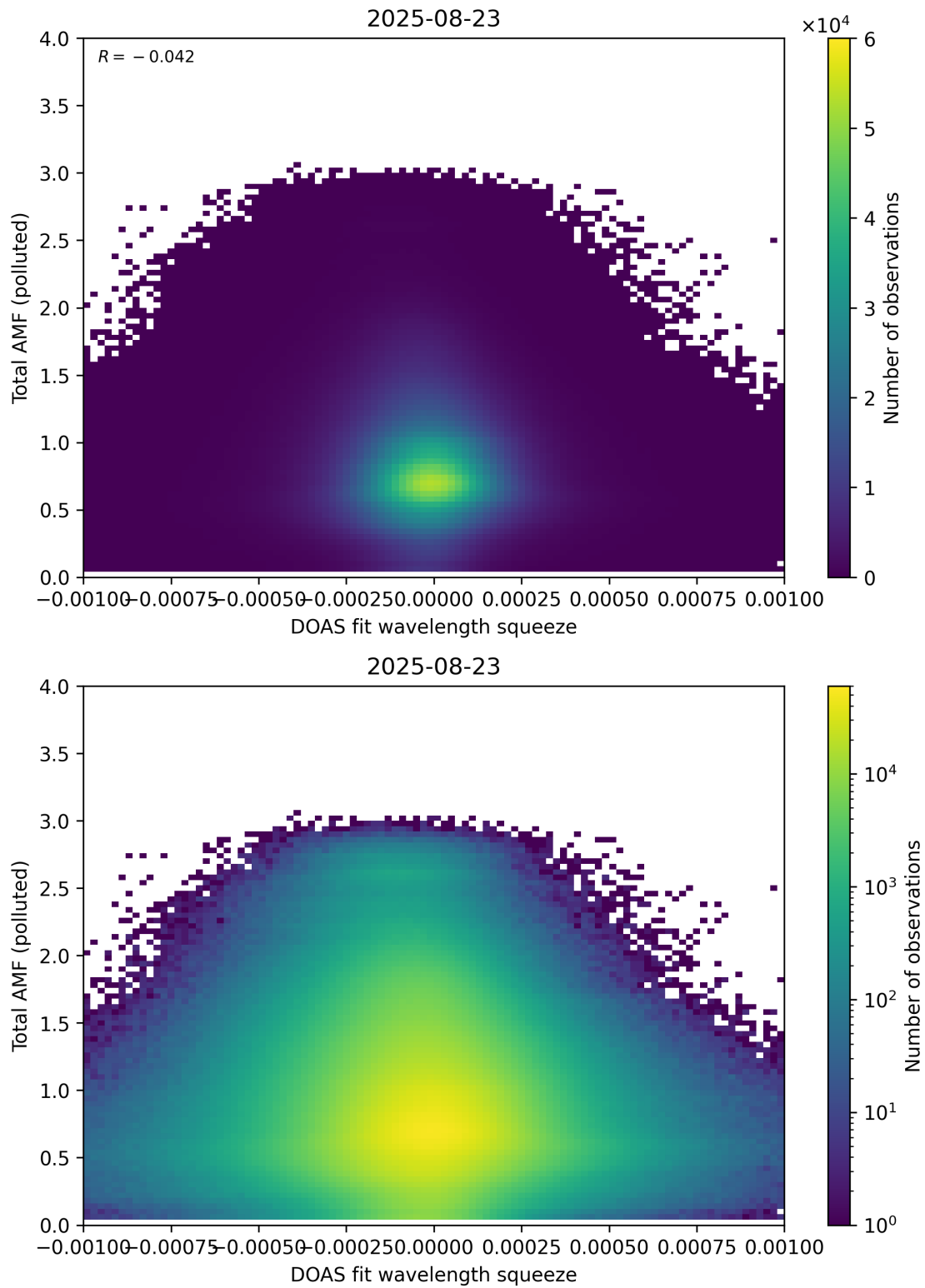
Figure 145: Scatter density plot of “DOAS fit wavelength squeeze” against “Total AMF (polluted)” for 2025-08-22 to 2025-08-24.
