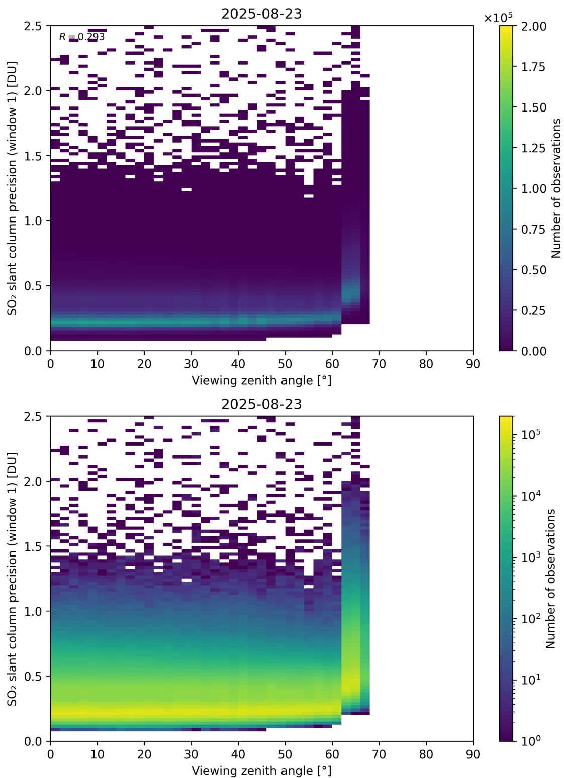
Figure 377: Scatter density plot of “Viewing zenith angle” against “SO 2 slant column precision (window 1)” for 2025-08-22 to 2025-08-24.
