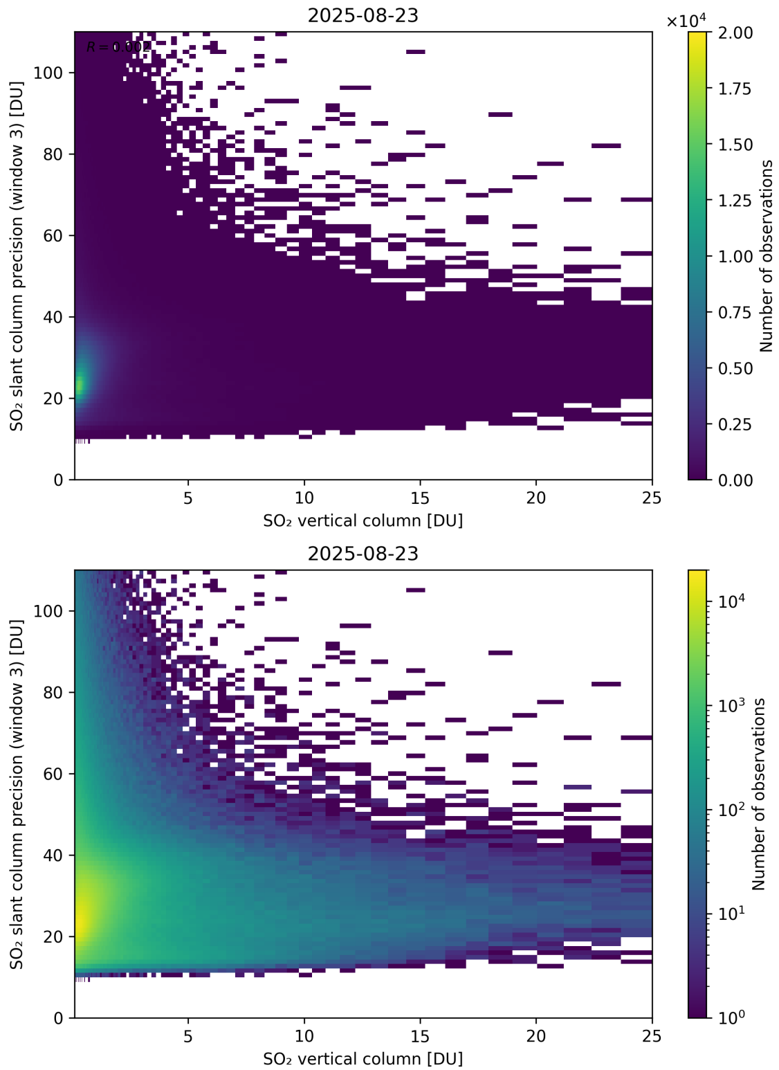
Figure 358: Scatter density plot of “SO 2 vertical column” against “SO 2 slant column precision (window 3)” for 2025-08-22 to 2025-08-24.
