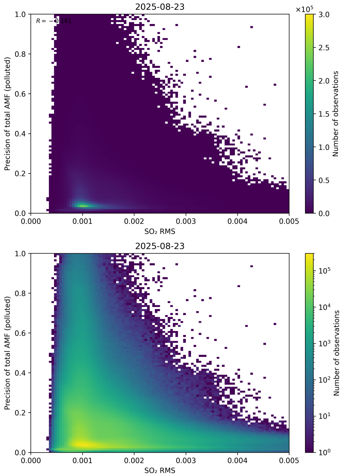
Figure 149: Scatter density plot of “SO 2 RMS” against “Precision of total AMF (polluted)” for 2025-08-22 to 2025-08-24.
