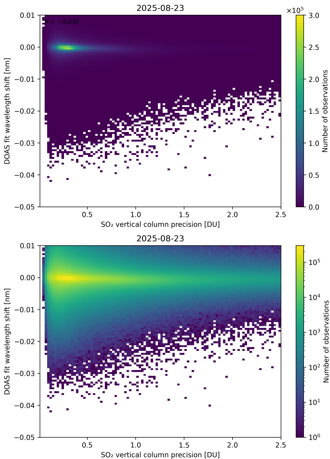
Figure 332: Scatter density plot of “SO 2 vertical column precision” against “DOAS fit wavelength shift” for 2025-08-22 to 2025-08-24.
