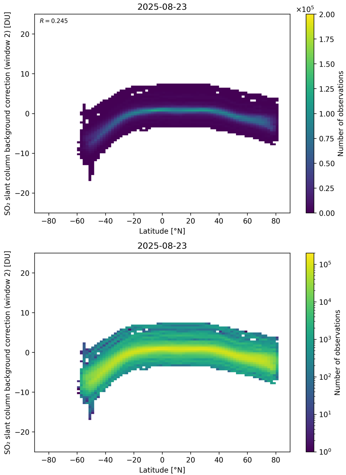
Figure 151: Scatter density plot of “Latitude” against “SO 2 slant column background correction (window 2)” for 2025-08-22 to 2025-08-24.
