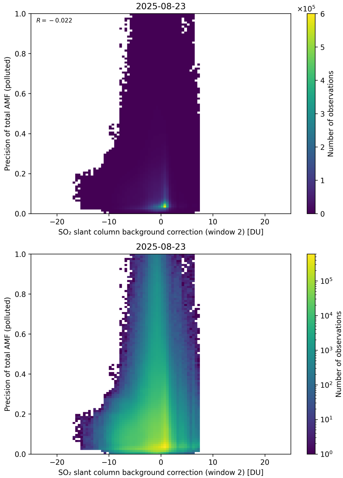
Figure 131: Scatter density plot of “SO 2 slant column background correction (window 2)” against “Precision of total AMF (polluted)” for 2025-08-22 to 2025-08-24.
