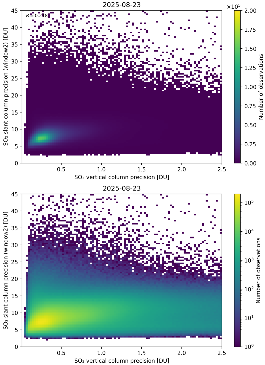
Figure 343: Scatter density plot of “SO 2 vertical column precision” against “SO 2 slant column precision (window2)” for 2025-08-22 to 2025-08-24.
