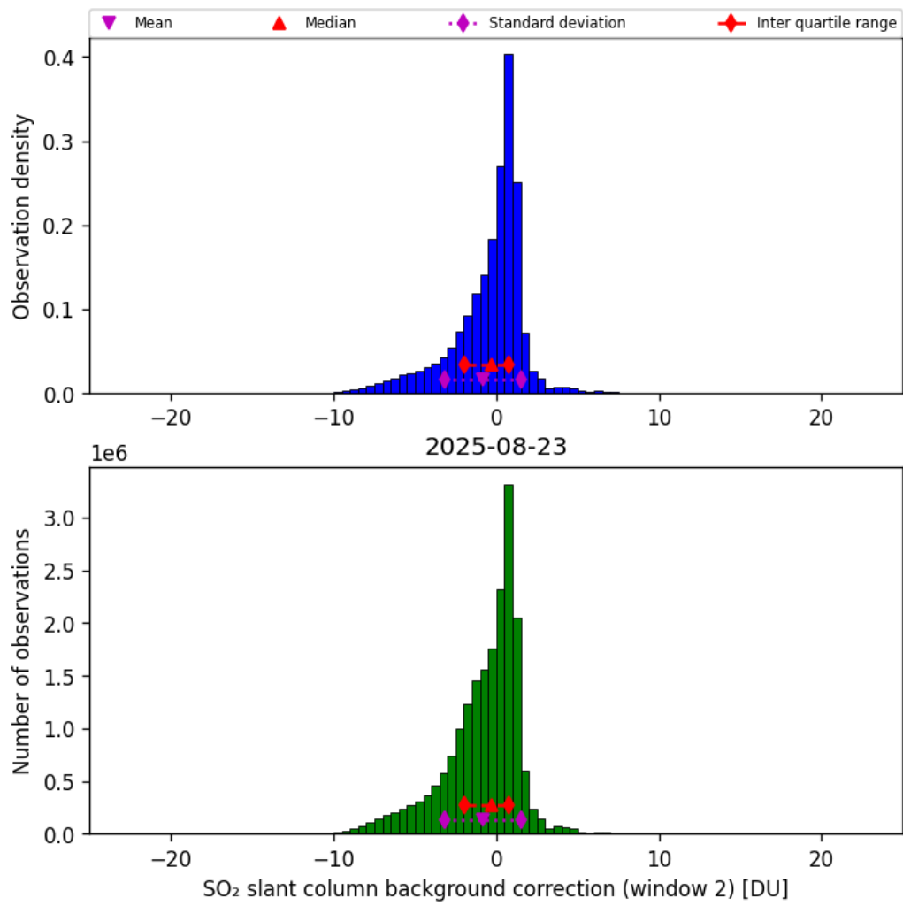
Figure 70: Histogram of “SO 2 slant column background correction (window 2)” for 2025-08-22 to 2025-08-24
