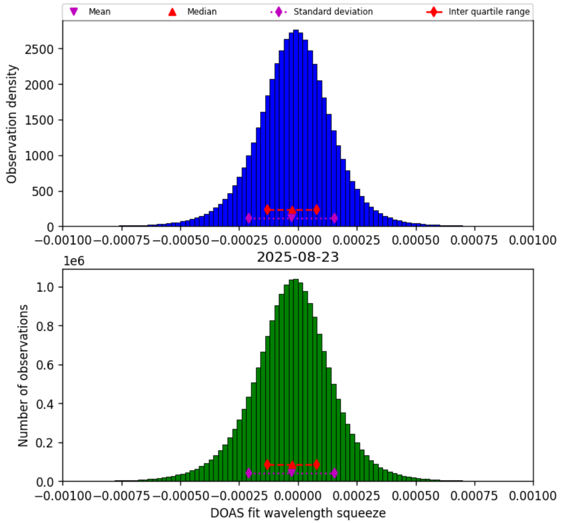
Figure 77: Histogram of “DOAS fit wavelength squeeze” for 2025-08-22 to 2025-08-24
