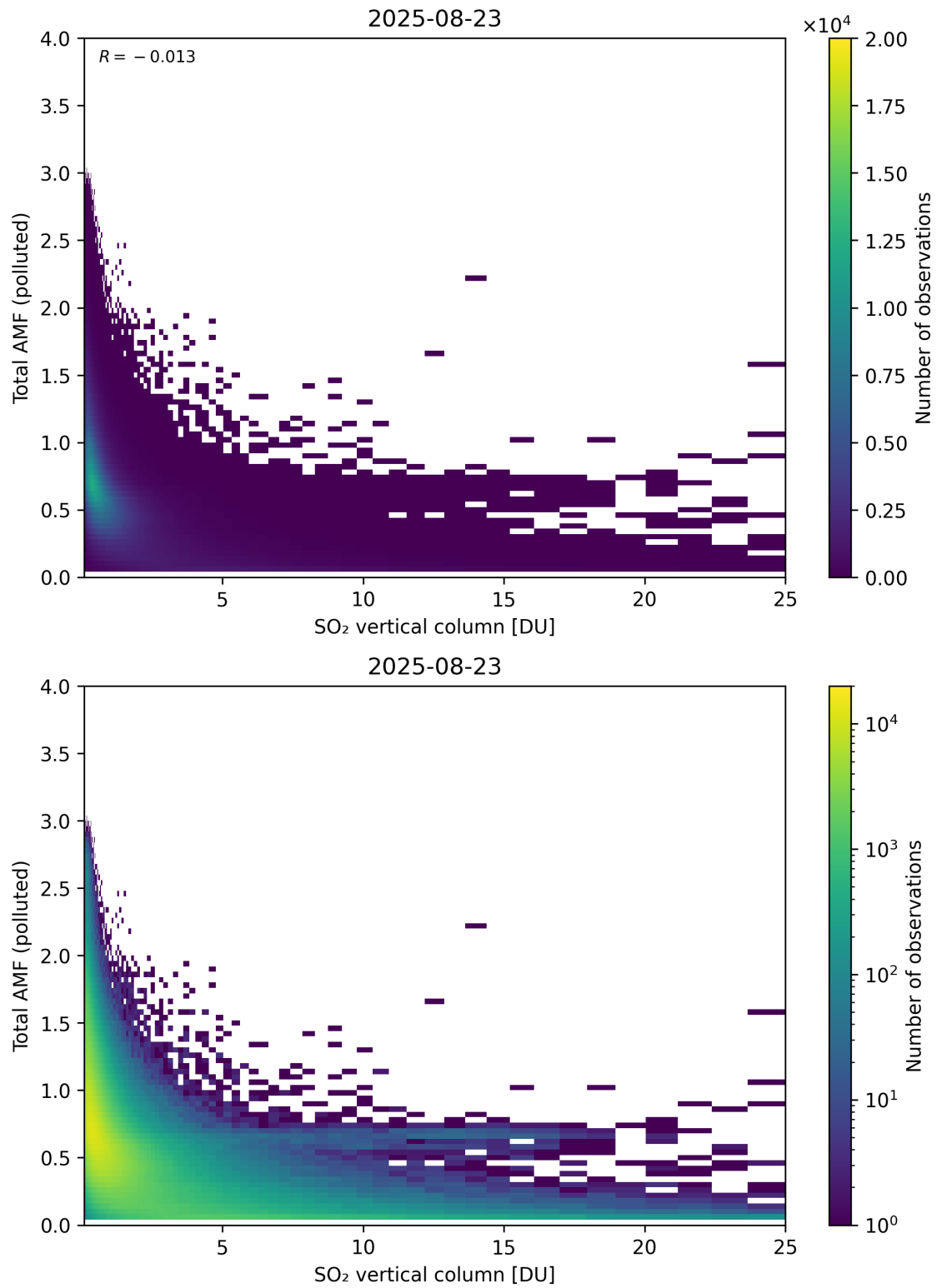
Figure 359: Scatter density plot of “SO 2 vertical column” against “Total AMF (polluted)” for 2025-08-22 to 2025-08-24.
