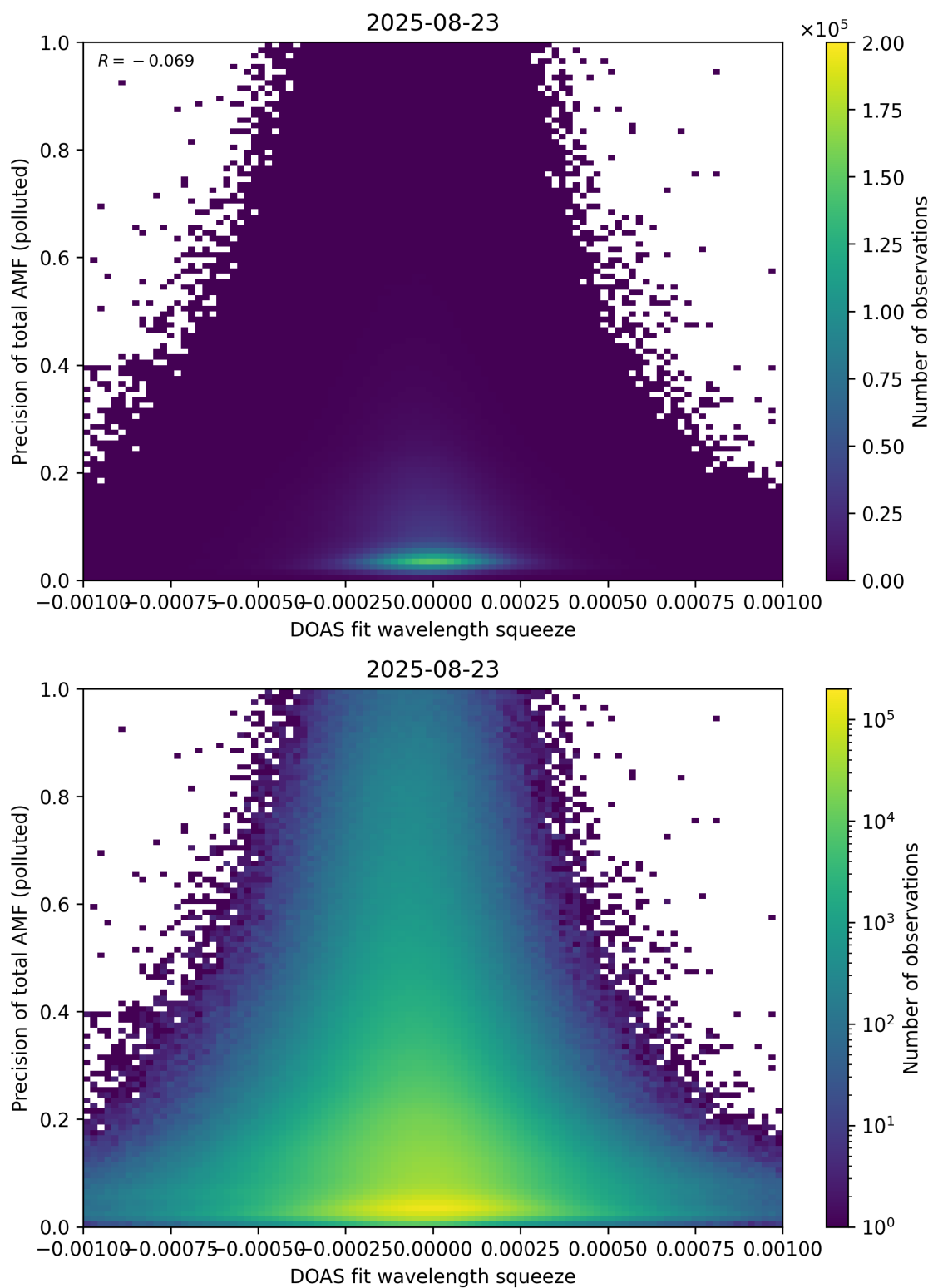
Figure 146: Scatter density plot of “DOAS fit wavelength squeeze” against “Precision of total AMF (polluted)” for 2025-08-22 to 2025-08-24.
