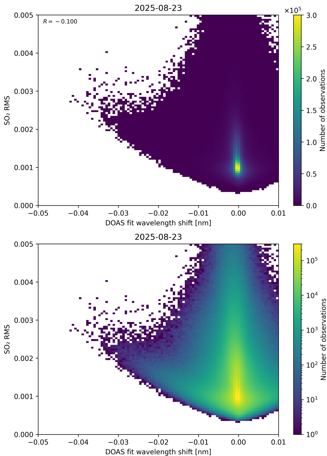
Figure 139: Scatter density plot of “DOAS fit wavelength shift” against “SO 2 RMS” for 2025-08-22 to 2025-08-24.
