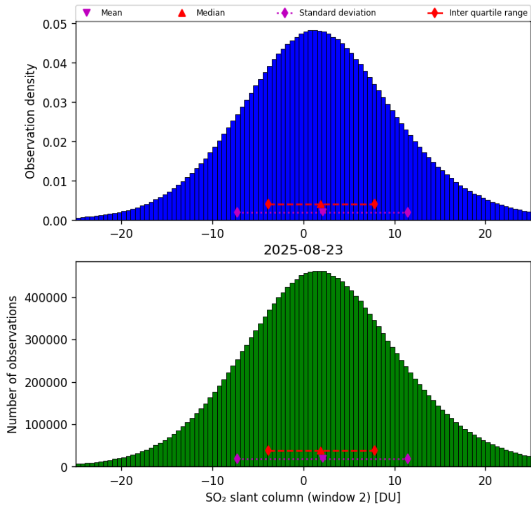
Figure 67: Histogram of “SO 2 slant column (window 2)” for 2025-08-22 to 2025-08-24
