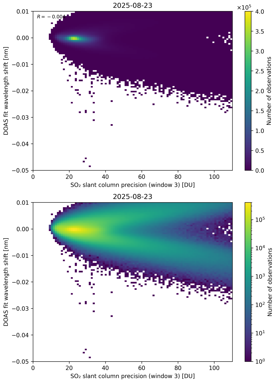
Figure 308: Scatter density plot of “SO 2 slant column precision (window 3)” against “DOAS fit wavelength shift” for 2025-08-22 to 2025-08-24.
