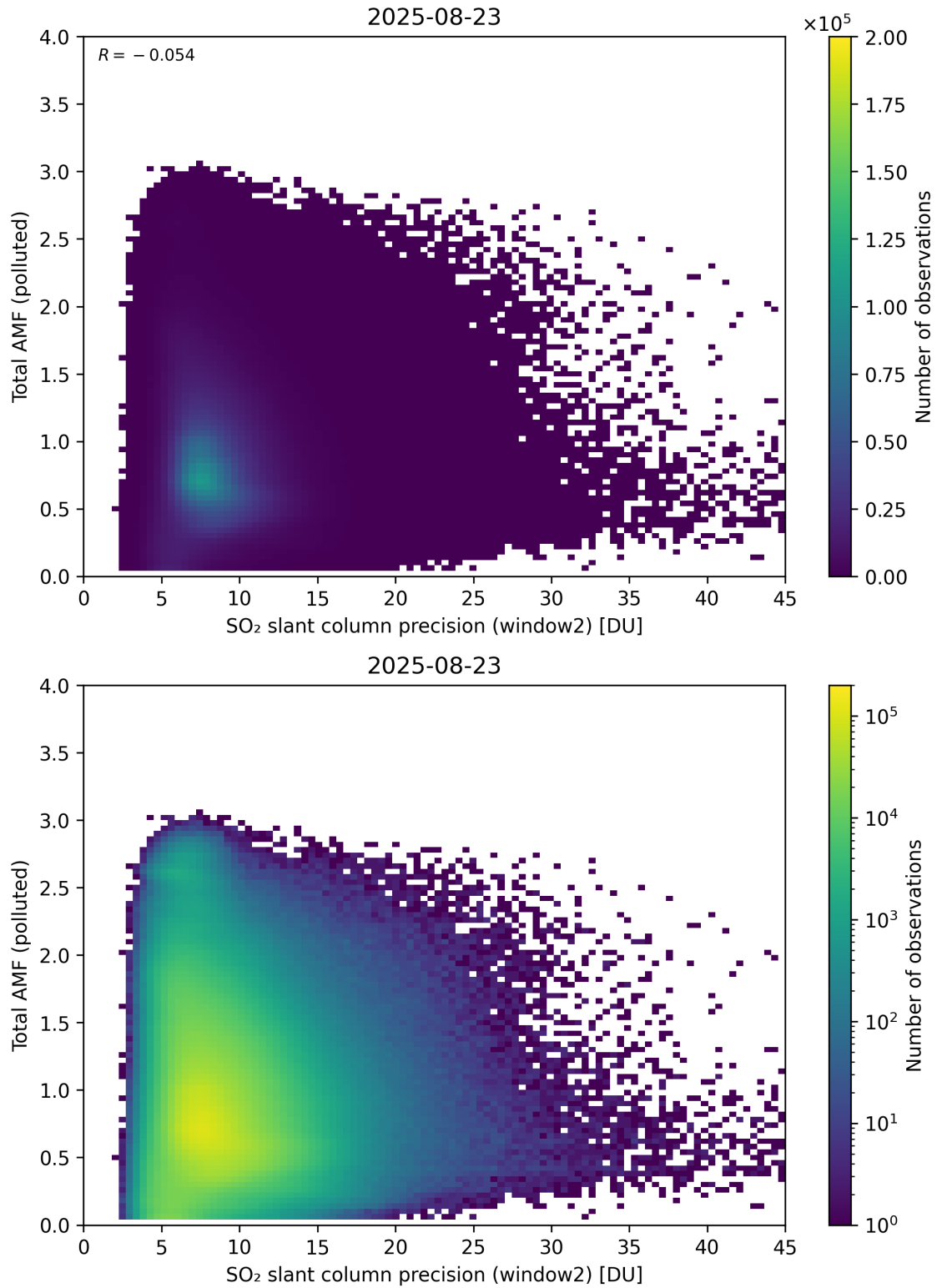
Figure 301: Scatter density plot of “SO 2 slant column precision (window2)” against “Total AMF (polluted)” for 2025-08-22 to 2025-08-24.
