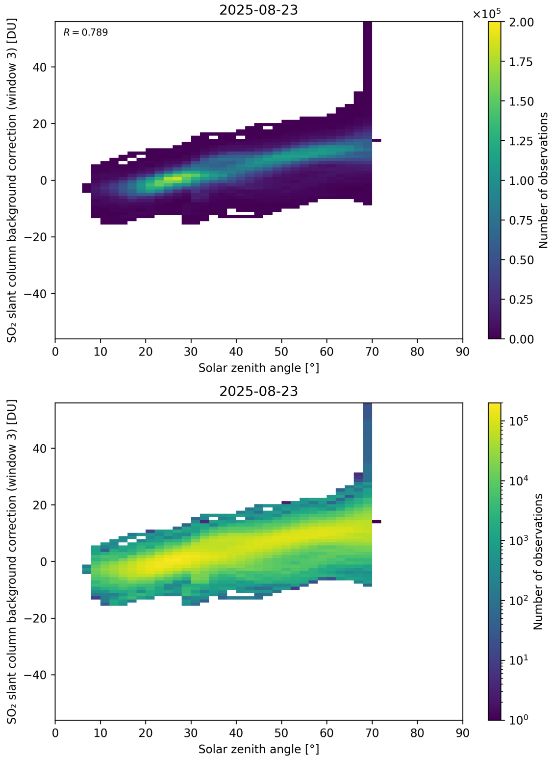
Figure 173: Scatter density plot of “Solar zenith angle” against “SO 2 slant column background correction (window 3)” for 2025-08-22 to 2025-08-24.
