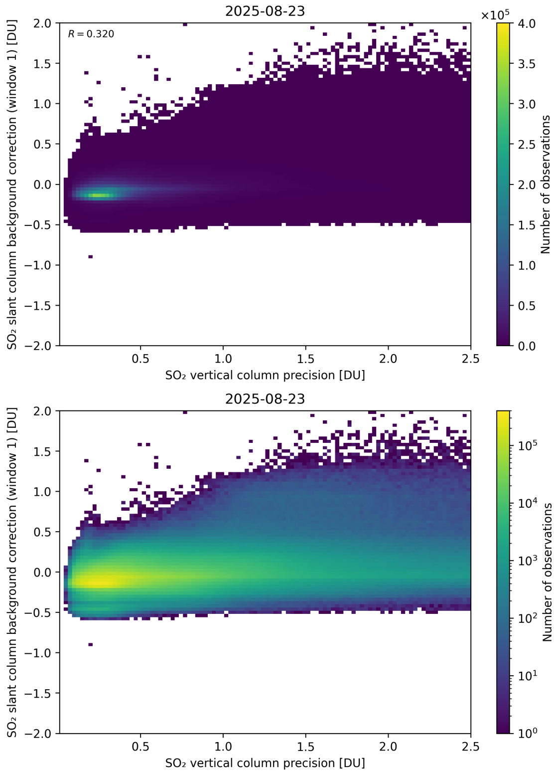
Figure 329: Scatter density plot of “SO 2 vertical column precision” against “SO 2 slant column background correction (window 1)” for 2025-08-22 to 2025-08-24.
