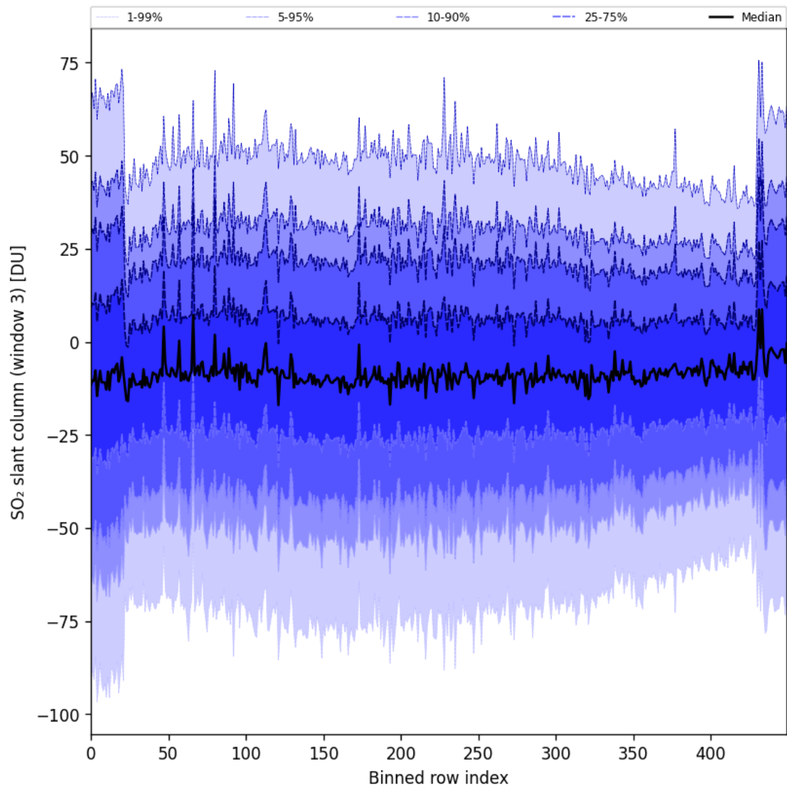
Figure 97: Along track statistics of “SO 2 slant column (window 3)” for 2025-08-22 to 2025-08-24
