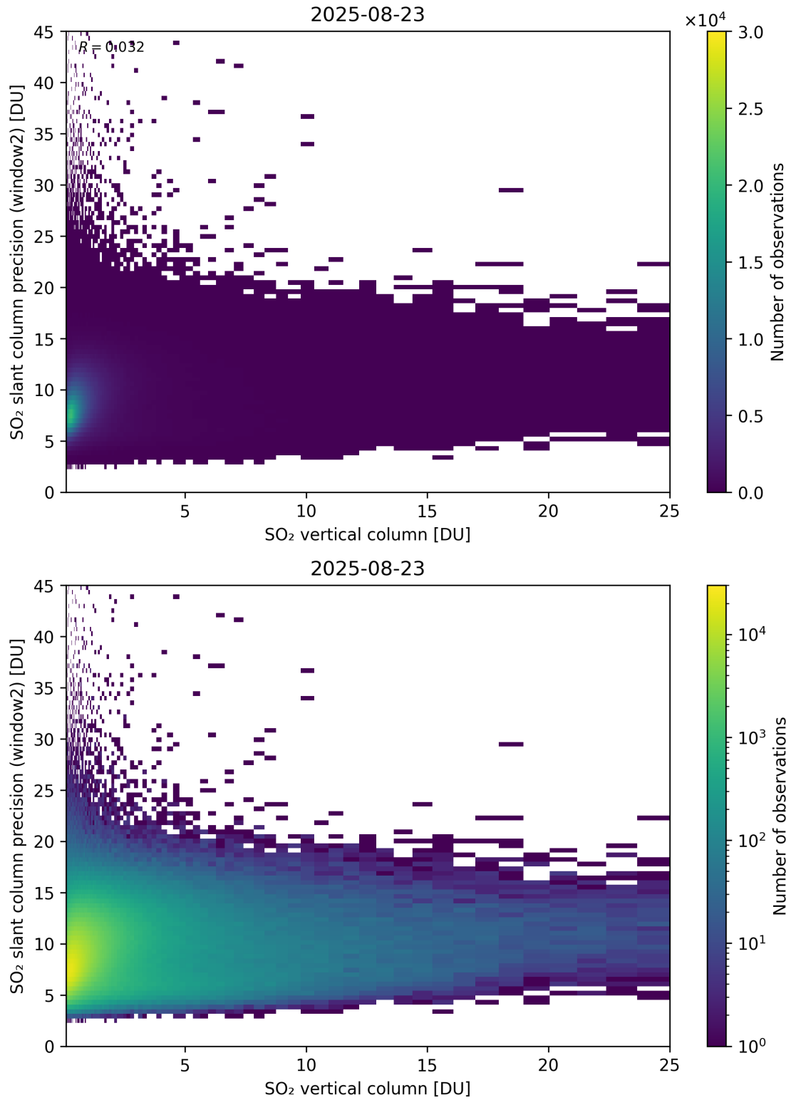
Figure 356: Scatter density plot of “SO 2 vertical column” against “SO 2 slant column precision (window2)” for 2025-08-22 to 2025-08-24.
