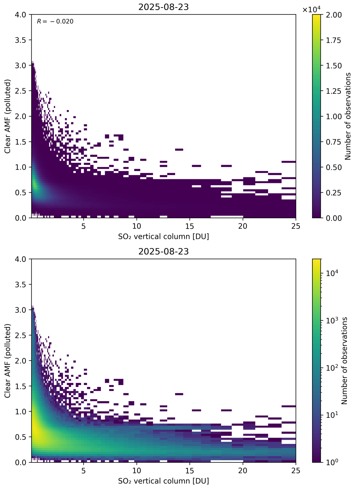
Figure 348: Scatter density plot of “SO 2 vertical column” against “Clear AMF (polluted)” for 2025-08-22 to 2025-08-24.
