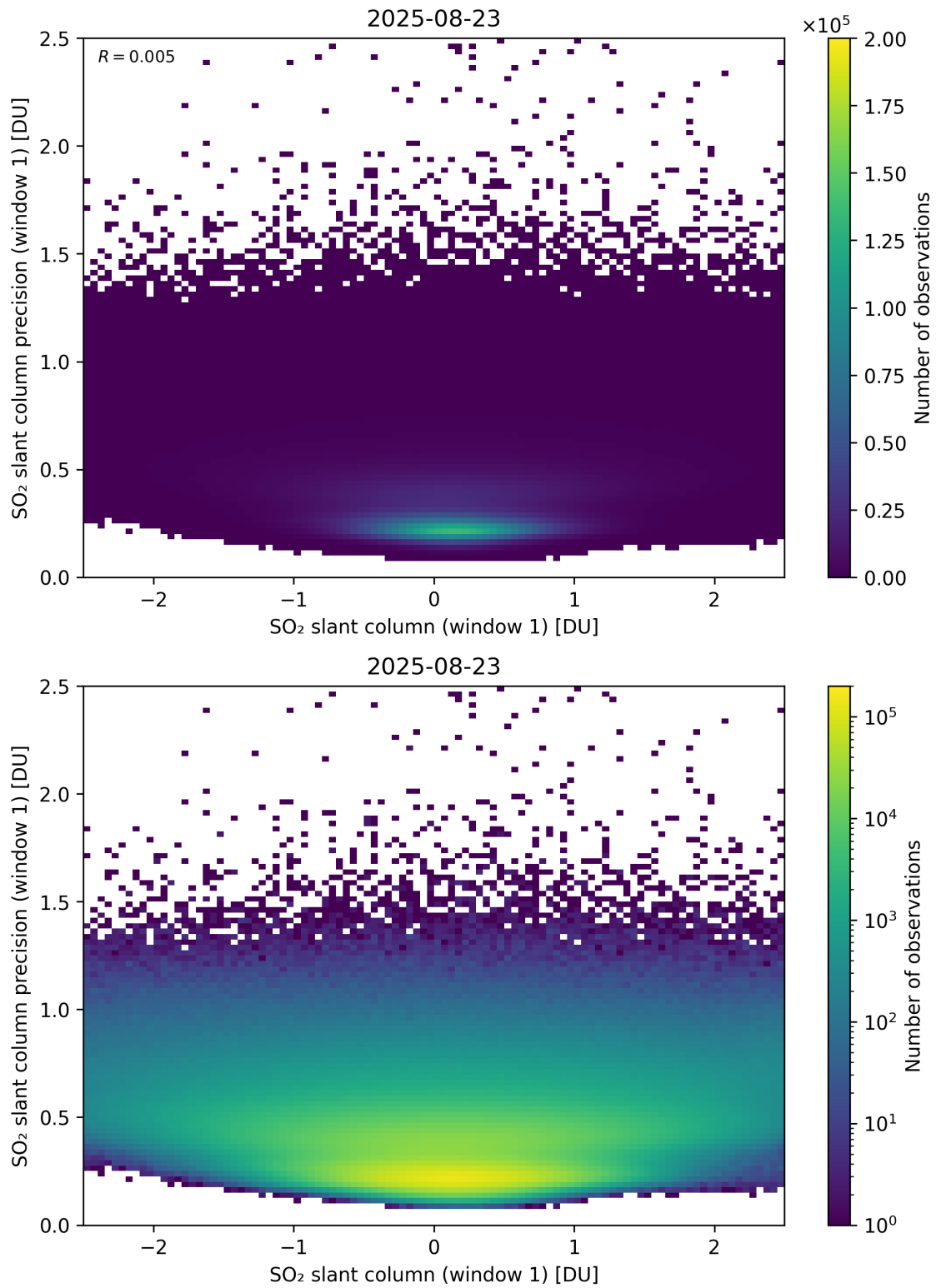
Figure 285: Scatter density plot of “SO 2 slant column (window 1)” against “SO 2 slant column precision (window 1)” for 2025-08-22 to 2025-08-24.
