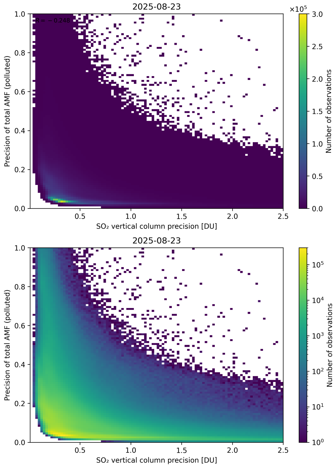
Figure 347: Scatter density plot of “SO 2 vertical column precision” against “Precision of total AMF (polluted)” for 2025-08-22 to 2025-08-24.
