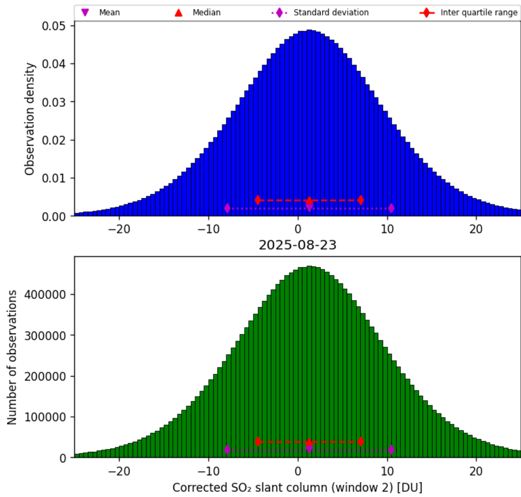
Figure 69: Histogram of “Corrected SO 2 slant column (window 2)” for 2025-08-22 to 2025-08-24
