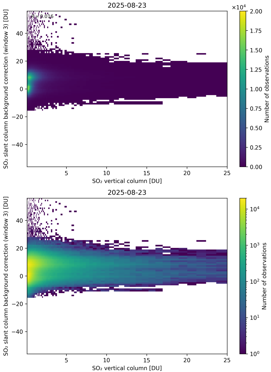
Figure 325: Scatter density plot of “SO 2 vertical column” against “SO 2 slant column background correction (window 3)” for 2025-08-22 to 2025-08-24.
