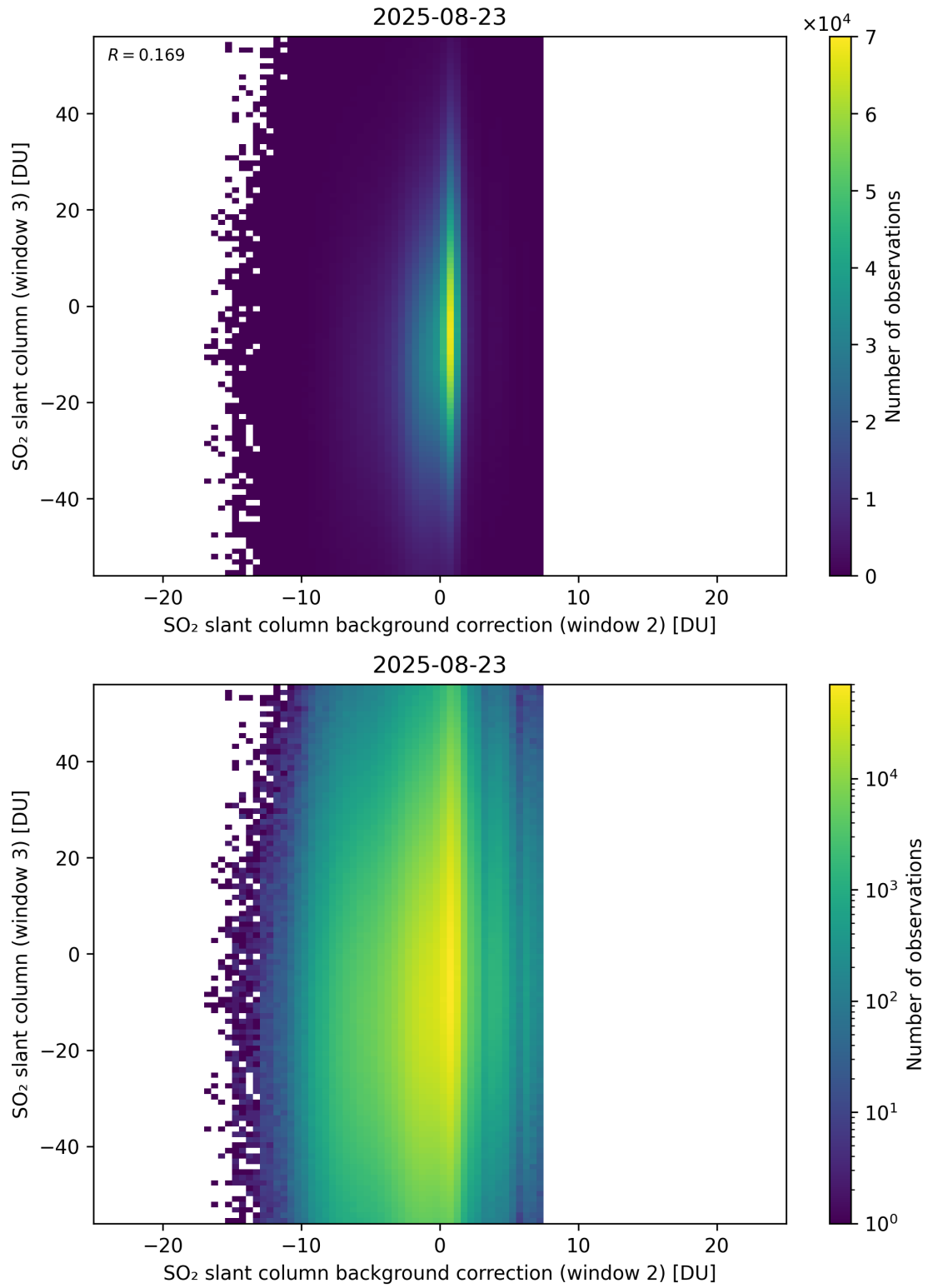
Figure 128: Scatter density plot of “SO 2 slant column background correction (window 2)” against “SO 2 slant column (window 3)” for 2025-08-22 to 2025-08-24.
