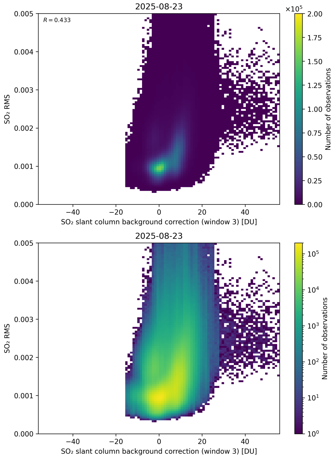
Figure 134: Scatter density plot of “SO 2 slant column background correction (window 3)” against “SO 2 RMS” for 2025-08-22 to 2025-08-24.
