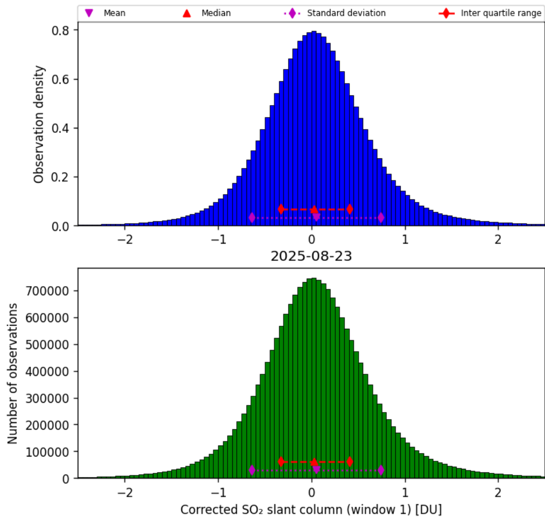
Figure 65: Histogram of “Corrected SO 2 slant column (window 1)” for 2025-08-22 to 2025-08-24
