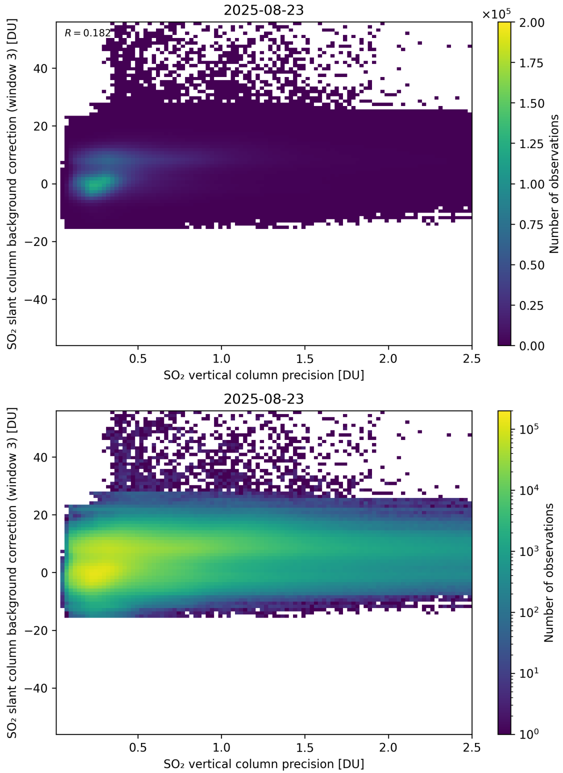
Figure 331: Scatter density plot of “SO 2 vertical column precision” against “SO 2 slant column background correction (window 3)” for 2025-08-22 to 2025-08-24.
