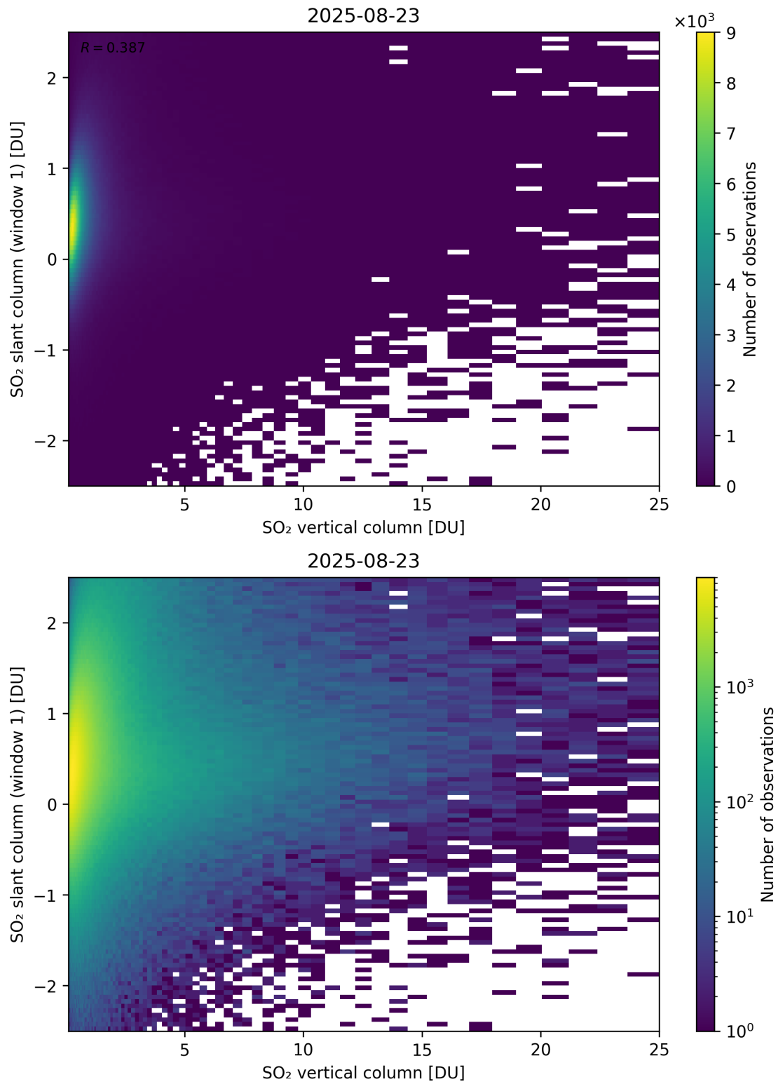
Figure 354: Scatter density plot of “SO 2 vertical column” against “SO 2 slant column (window 1)” for 2025-08-22 to 2025-08-24.
