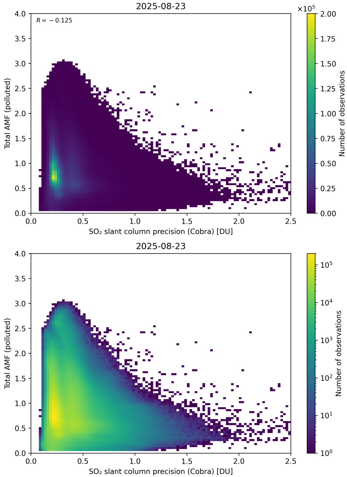
Figure 213: Scatter density plot of “SO 2 slant column precision (Cobra)” against “Total AMF (polluted)” for 2025-08-22 to 2025-08-24.
