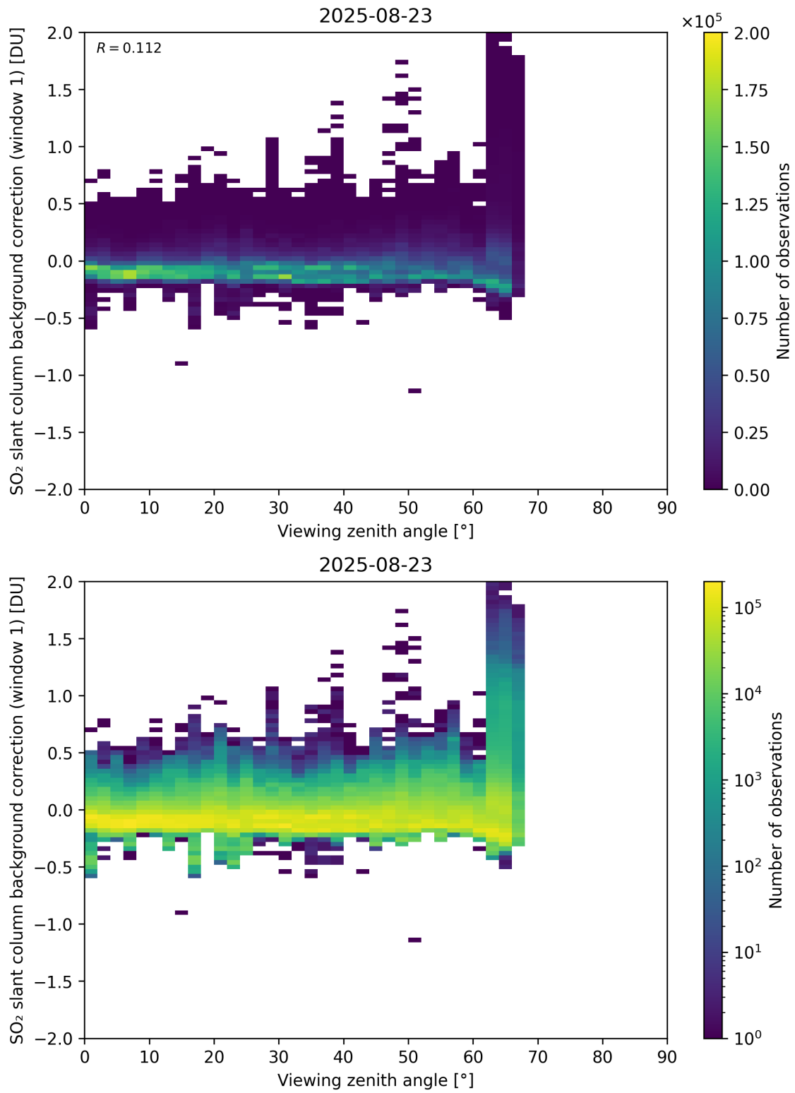
Figure 362: Scatter density plot of “Viewing zenith angle” against “SO 2 slant column background correction (window 1)” for 2025-08-22 to 2025-08-24.
