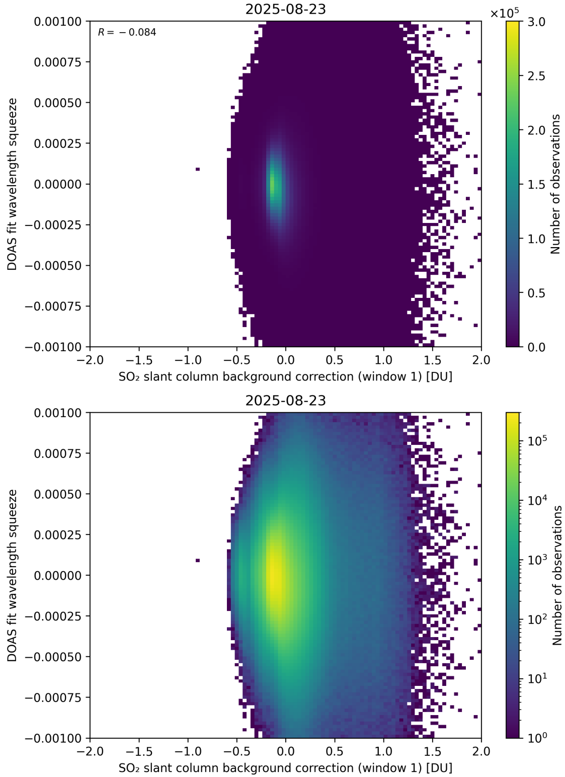
Figure 112: Scatter density plot of “SO 2 slant column background correction (window 1)” against “DOAS fit wavelength squeeze” for 2025-08-22 to 2025-08-24.
