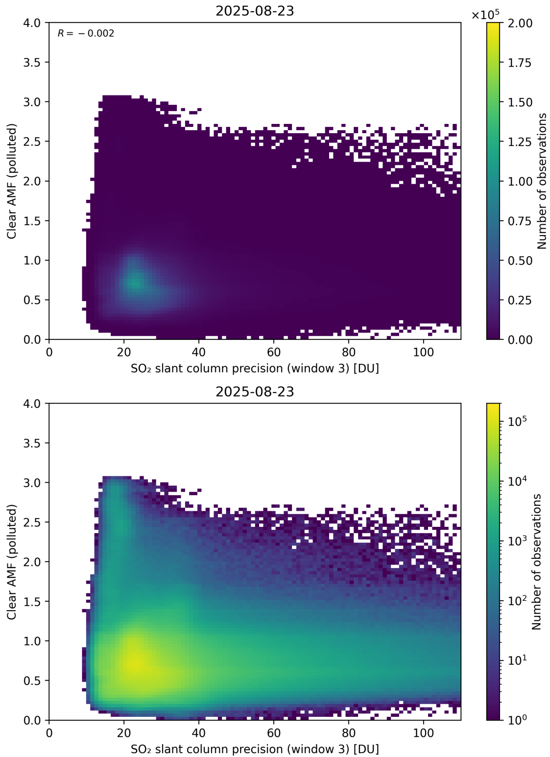
Figure 311: Scatter density plot of “SO 2 slant column precision (window 3)” against “Clear AMF (polluted)” for 2025-08-22 to 2025-08-24.
