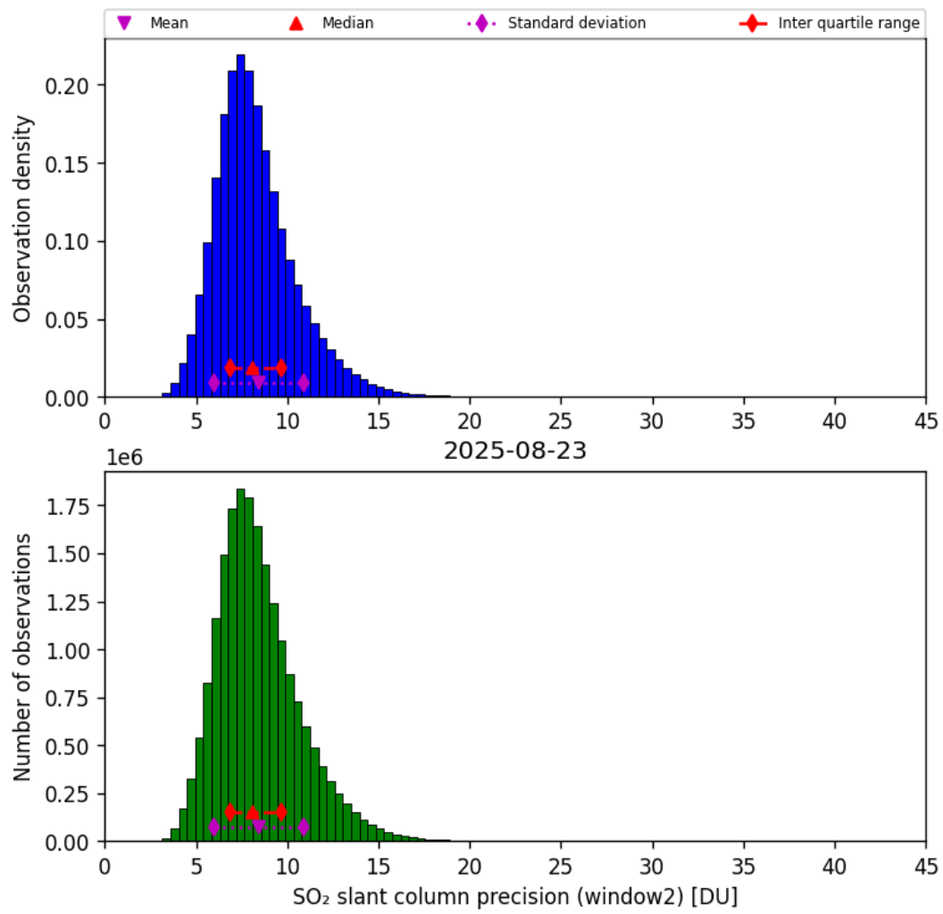
Figure 68: Histogram of “SO 2 slant column precision (window2)” for 2025-08-22 to 2025-08-24
