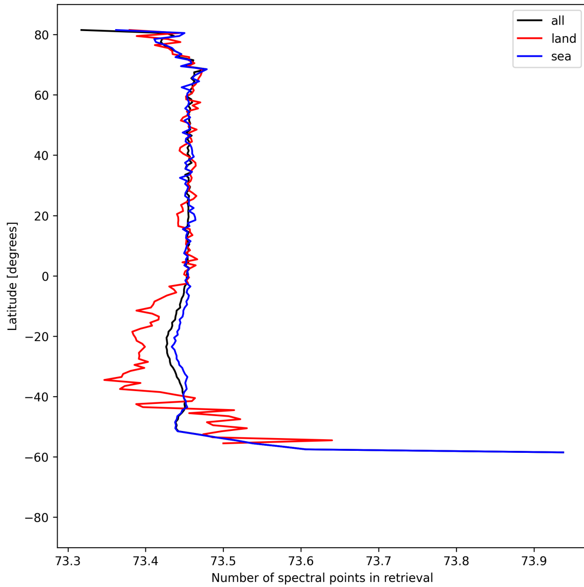
Figure 56: Zonal average of “Number of spectral points in retrieval” for 2025-08-22 to 2025-08-24.
