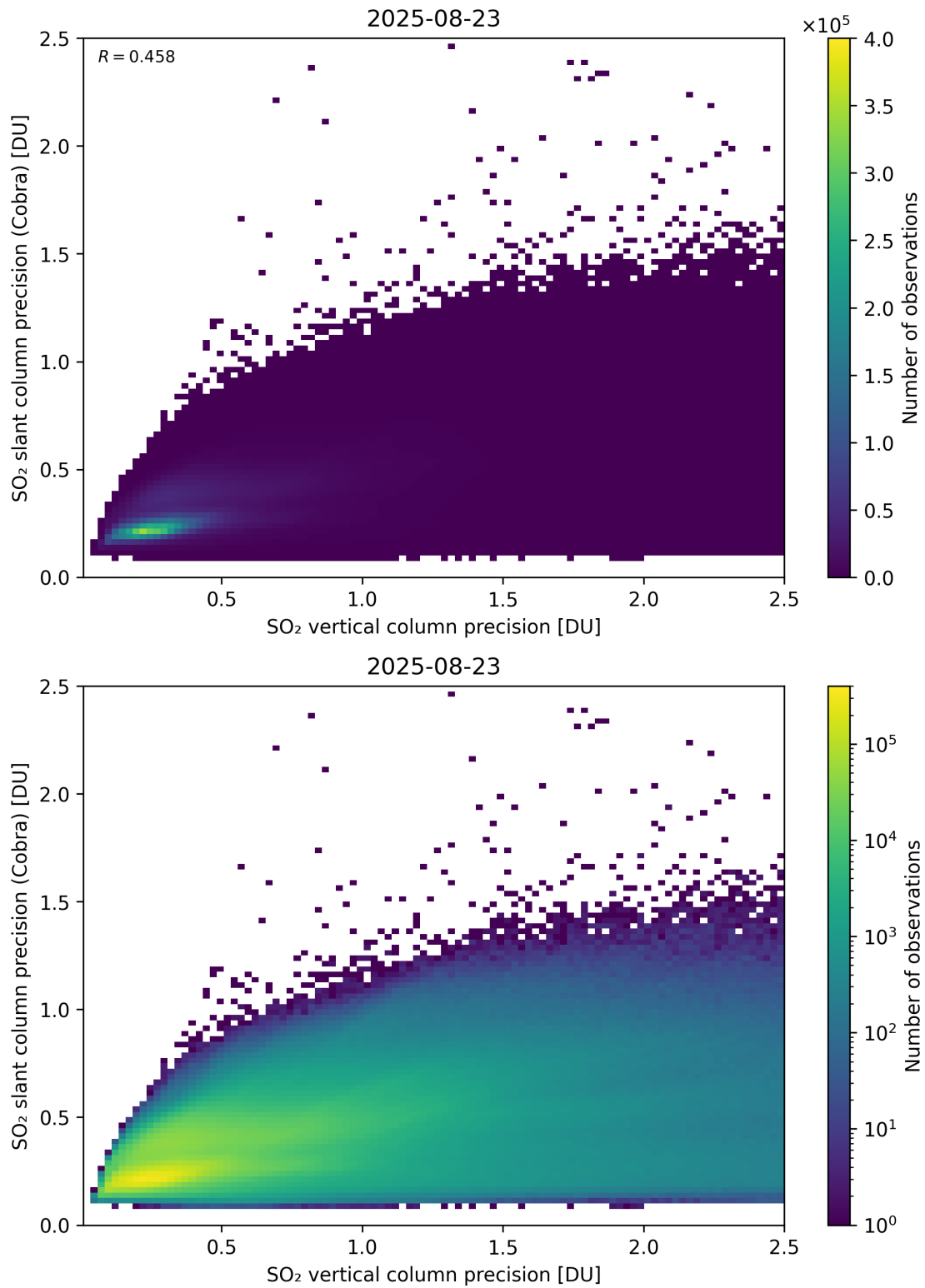
Figure 337: Scatter density plot of “SO 2 vertical column precision” against “SO 2 slant column precision (Cobra)” for 2025-08-22 to 2025-08-24.
