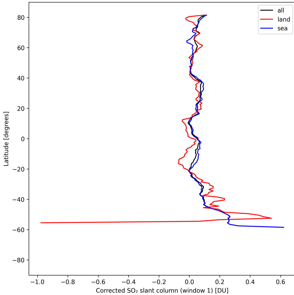
Figure 39: Zonal average of “Corrected SO 2 slant column (window 1)” for 2025-08-22 to 2025-08-24.
