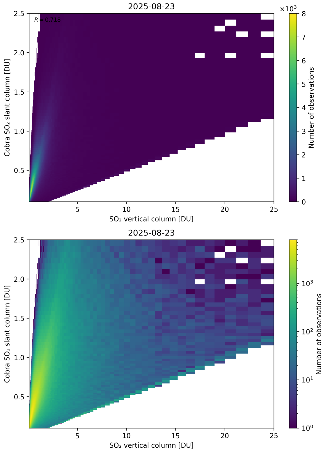
Figure 349: Scatter density plot of “SO 2 vertical column” against “Cobra SO 2 slant column” for 2025-08-22 to 2025-08-24.
