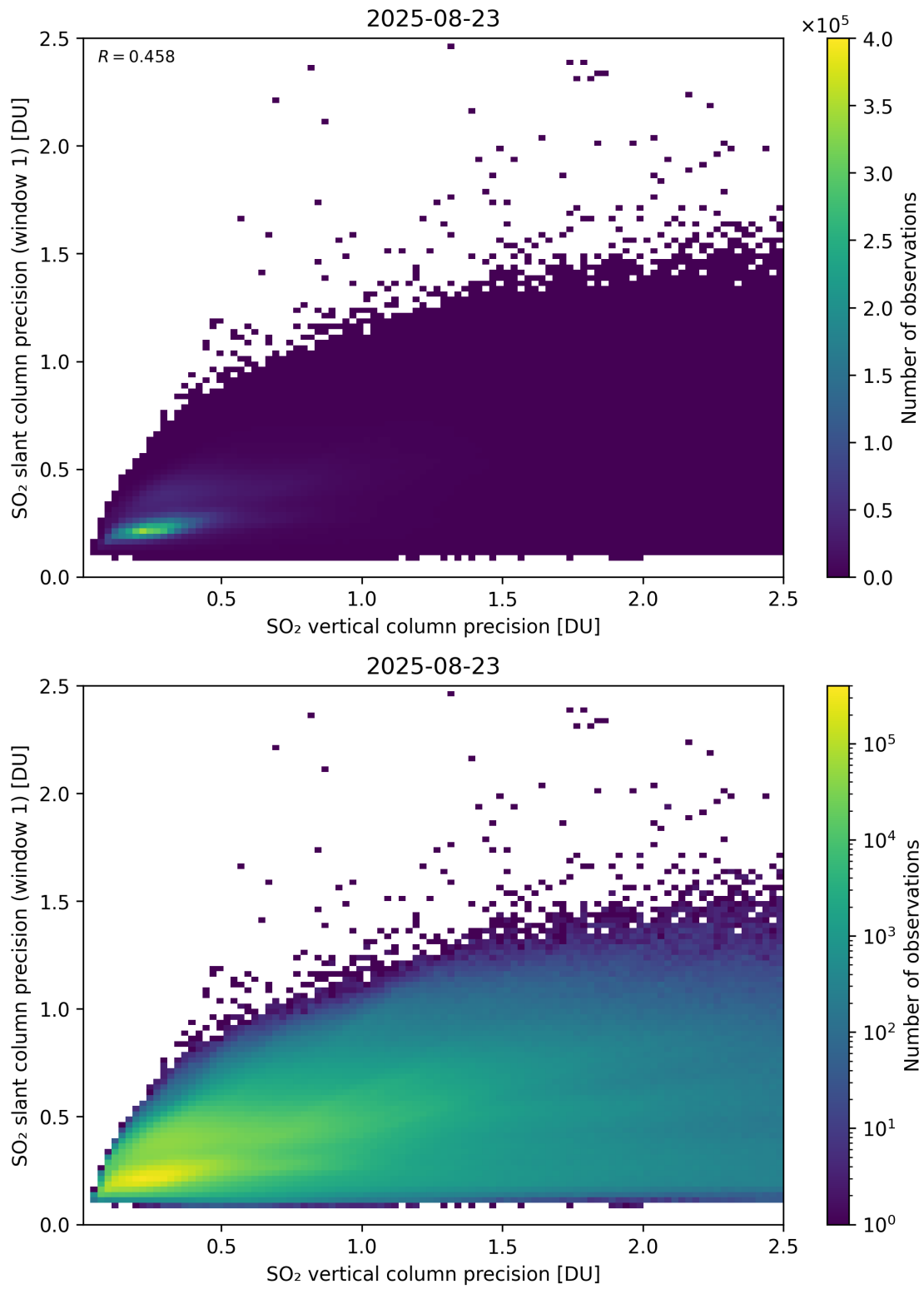
Figure 342: Scatter density plot of “SO 2 vertical column precision” against “SO 2 slant column precision (window 1)” for 2025-08-22 to 2025-08-24.
