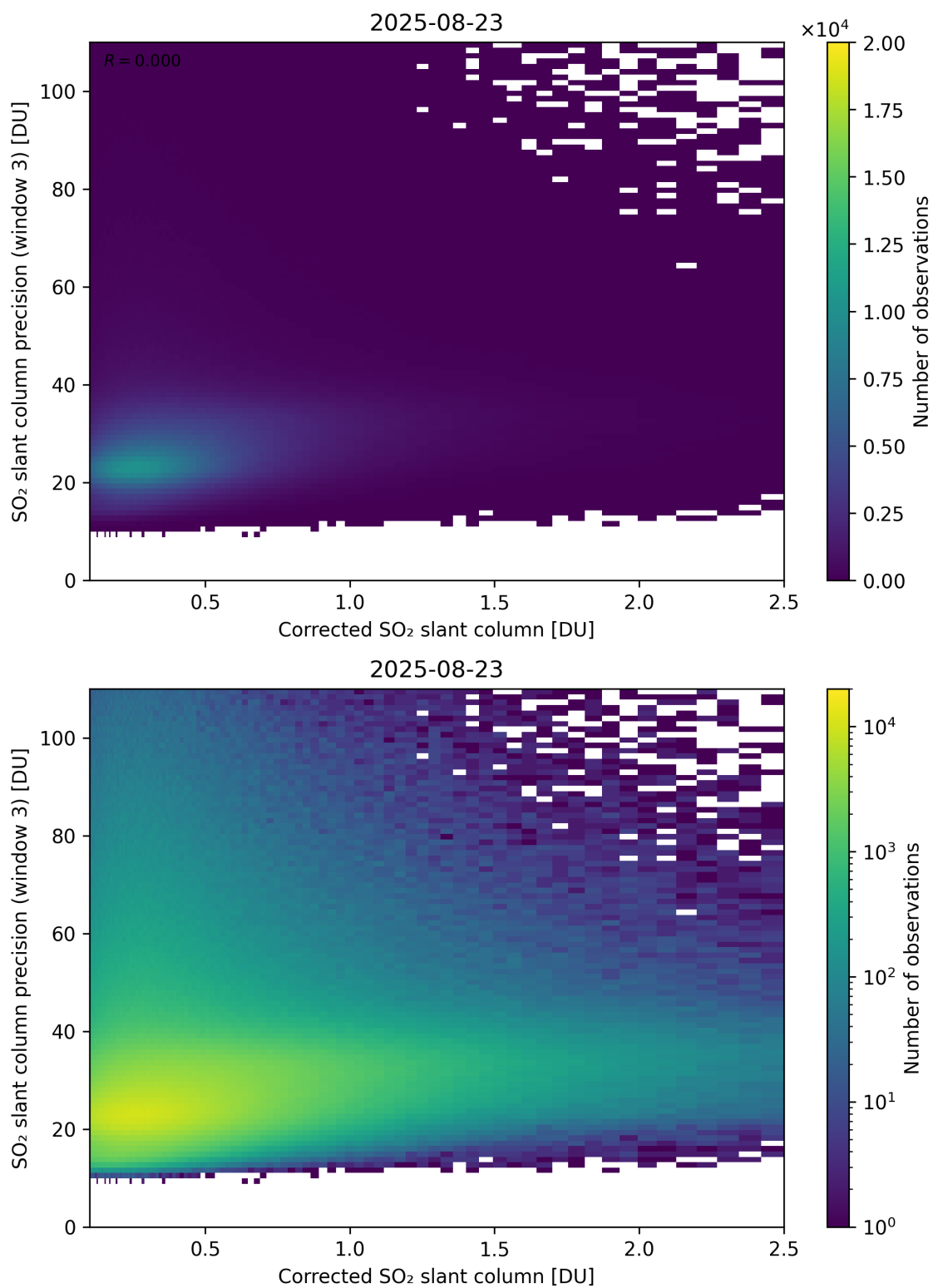
Figure 241: Scatter density plot of “Corrected SO 2 slant column” against “SO 2 slant column precision (window 3)” for 2025-08-22 to 2025-08-24.
