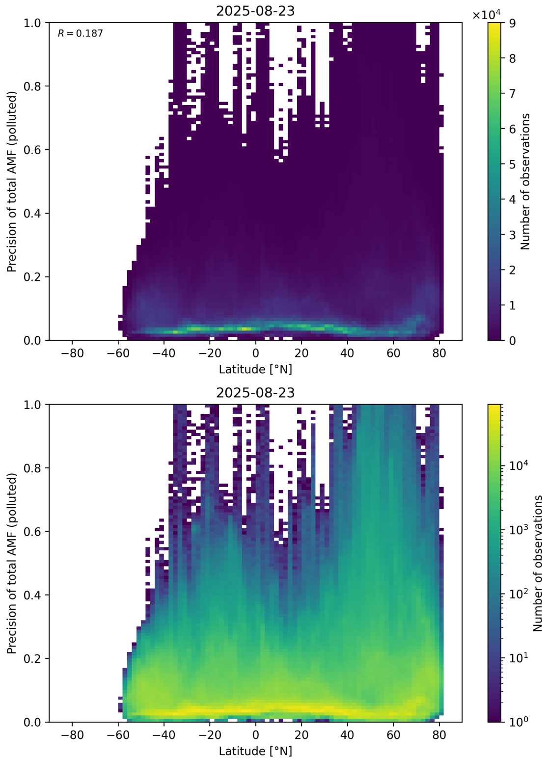
Figure 168: Scatter density plot of “Latitude” against “Precision of total AMF (polluted)” for 2025-08-22 to 2025-08-24.
