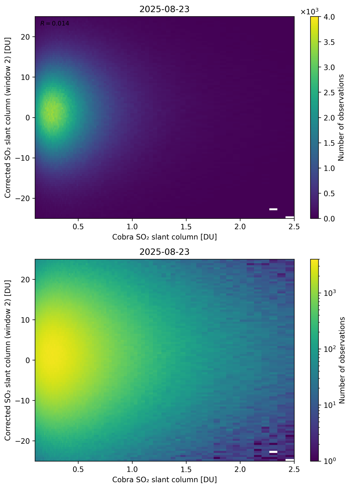
Figure 217: Scatter density plot of “Cobra SO 2 slant column” against “Corrected SO 2 slant column (window 2)” for 2025-08-22 to 2025-08-24.
