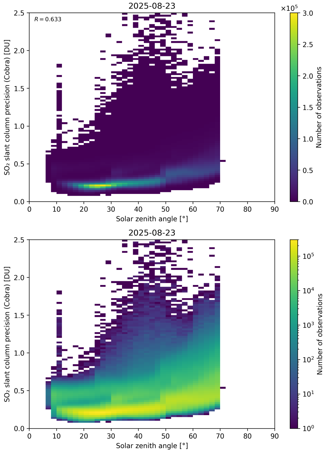
Figure 180: Scatter density plot of “Solar zenith angle” against “SO 2 slant column precision (Cobra)” for 2025-08-22 to 2025-08-24.
