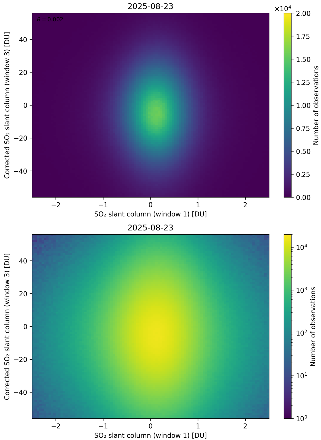
Figure 284: Scatter density plot of “SO 2 slant column (window 1)” against “Corrected SO 2 slant column (window 3)” for 2025-08-22 to 2025-08-24.
