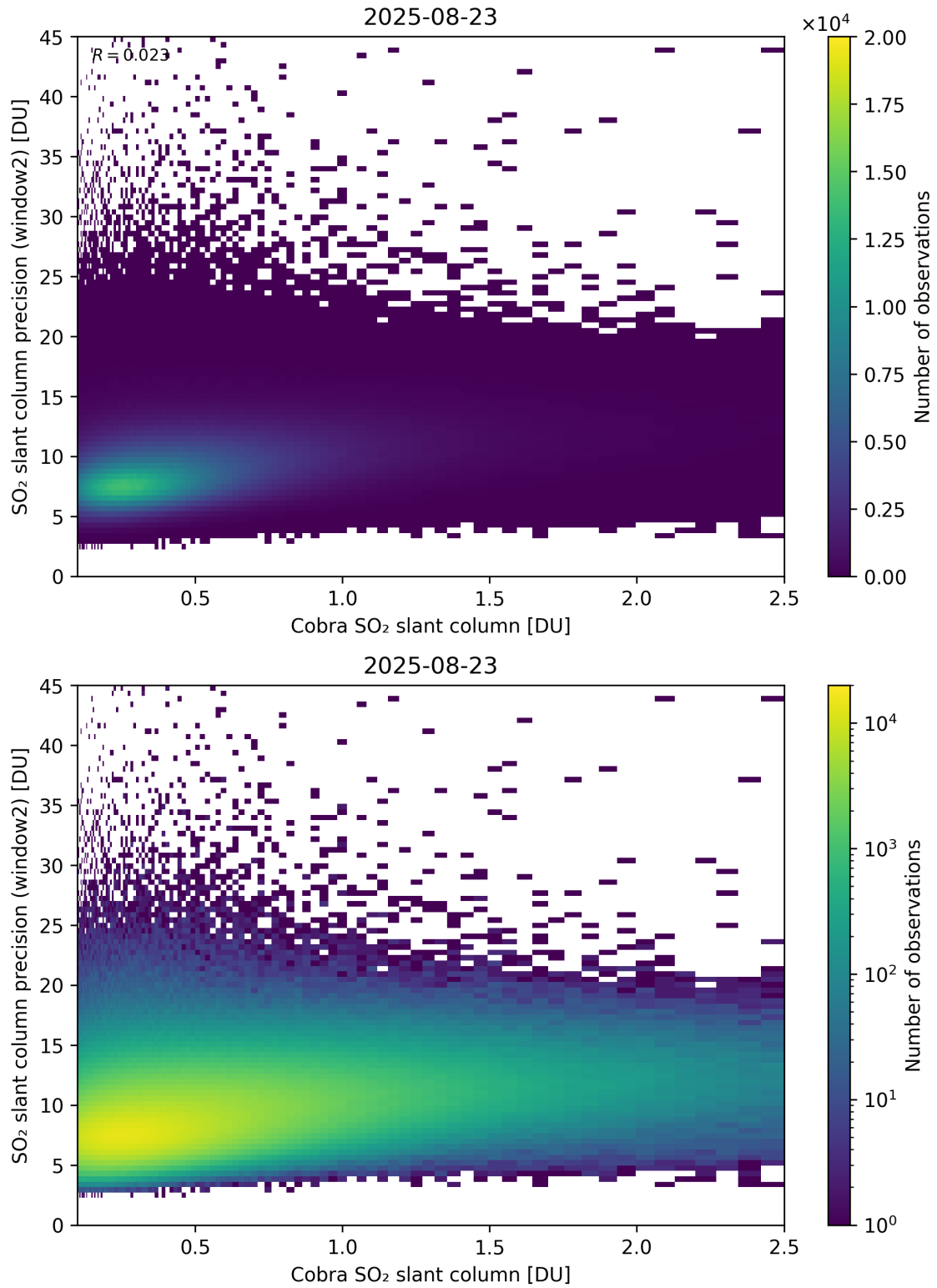
Figure 221: Scatter density plot of “Cobra SO 2 slant column” against “SO 2 slant column precision (window2)” for 2025-08-22 to 2025-08-24.
