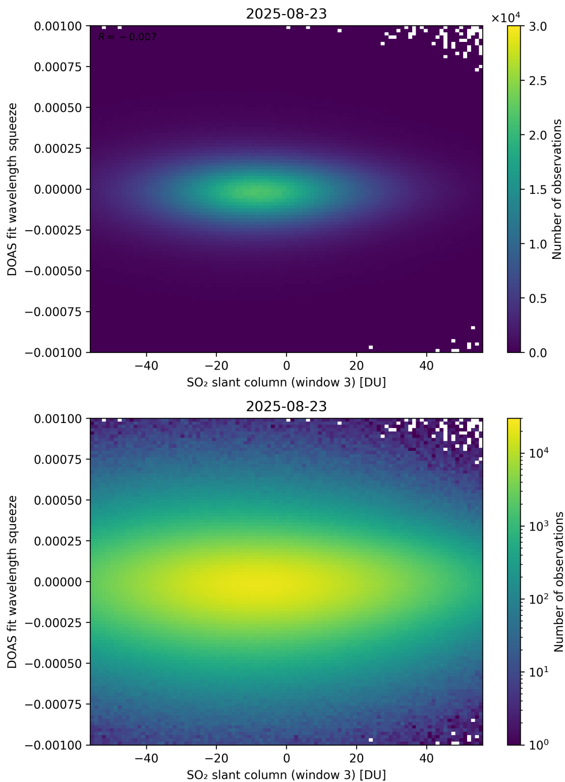
Figure 305: Scatter density plot of “SO 2 slant column (window 3)” against “DOAS fit wavelength squeeze” for 2025-08-22 to 2025-08-24.
