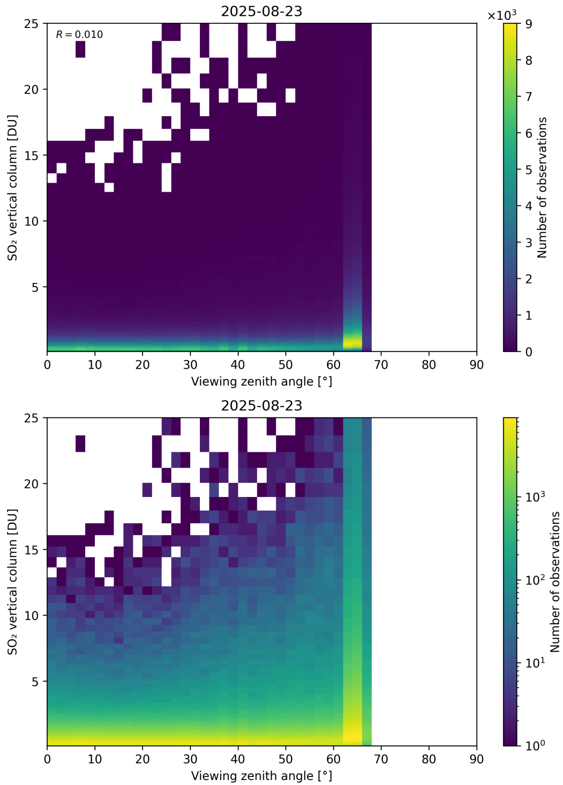
Figure 383: Scatter density plot of “Viewing zenith angle” against “SO 2 vertical column” for 2025-08-22 to 2025-08-24.
