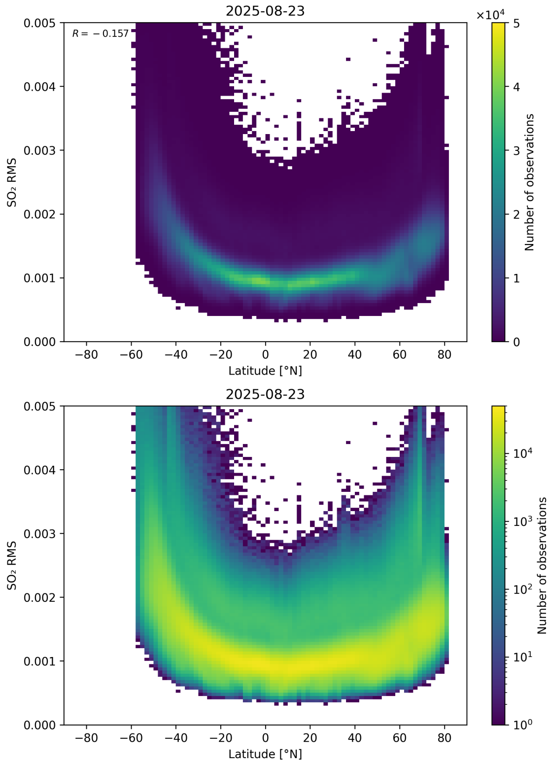
Figure 155: Scatter density plot of “Latitude” against “SO 2 RMS” for 2025-08-22 to 2025-08-24.
