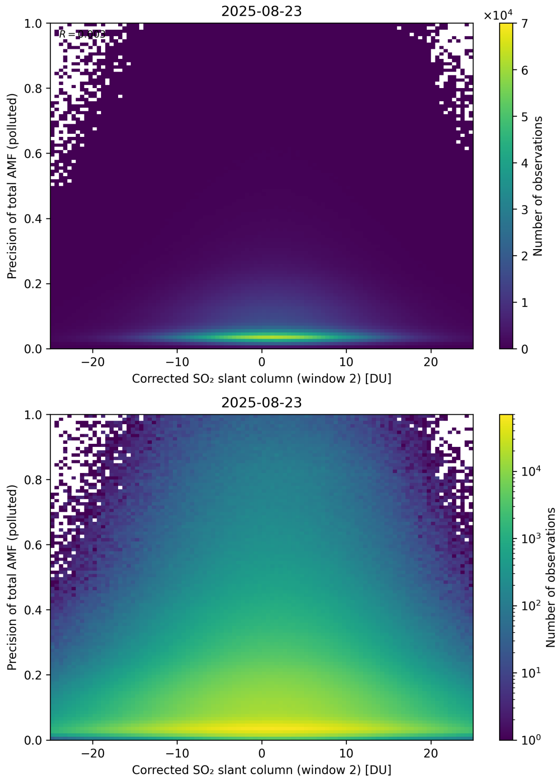
Figure 254: Scatter density plot of “Corrected SO 2 slant column (window 2)” against “Precision of total AMF (polluted)” for 2025-08-22 to 2025-08-24.
