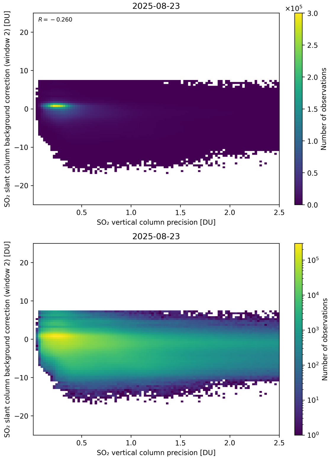
Figure 330: Scatter density plot of “SO 2 vertical column precision” against “SO 2 slant column background correction (window 2)” for 2025-08-22 to 2025-08-24.
