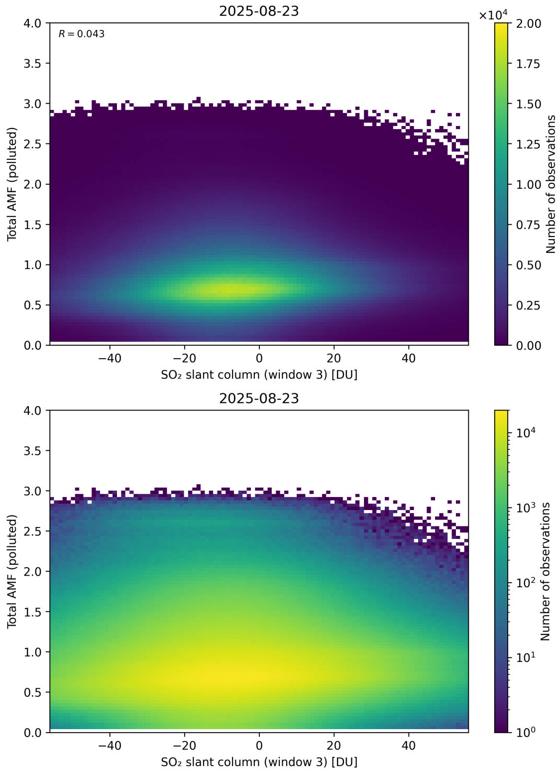
Figure 318: Scatter density plot of “SO 2 slant column (window 3)” against “Total AMF (polluted)” for 2025-08-22 to 2025-08-24.
