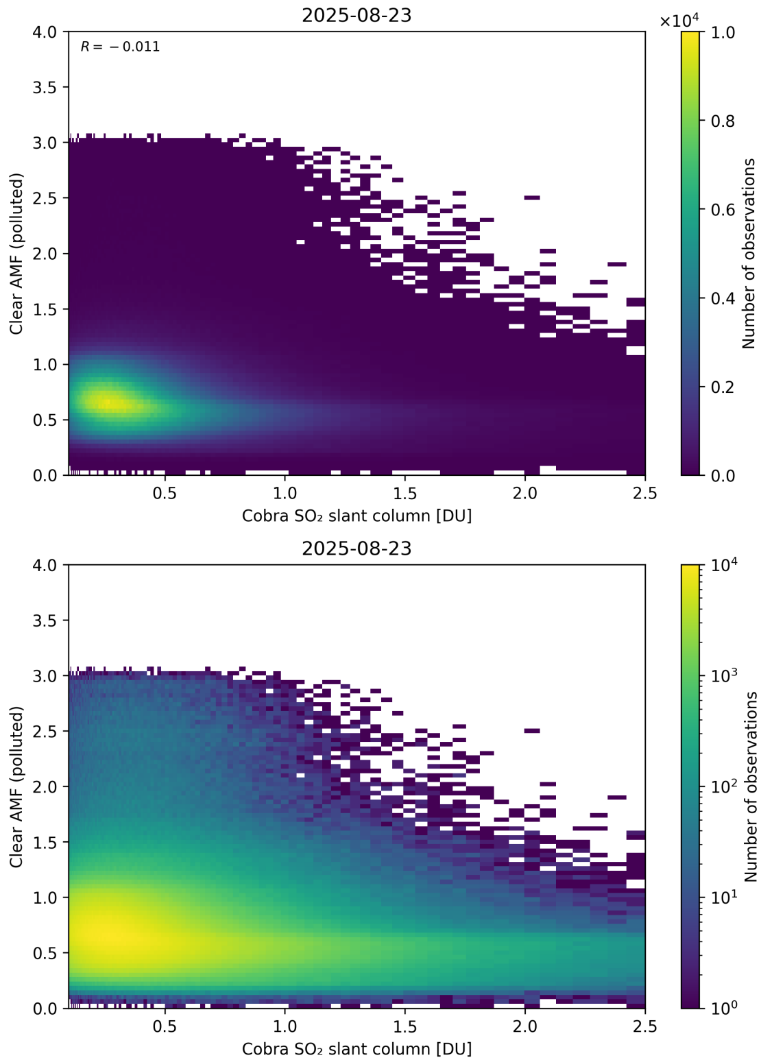
Figure 215: Scatter density plot of “Cobra SO 2 slant column” against “Clear AMF (polluted)” for 2025-08-22 to 2025-08-24.
