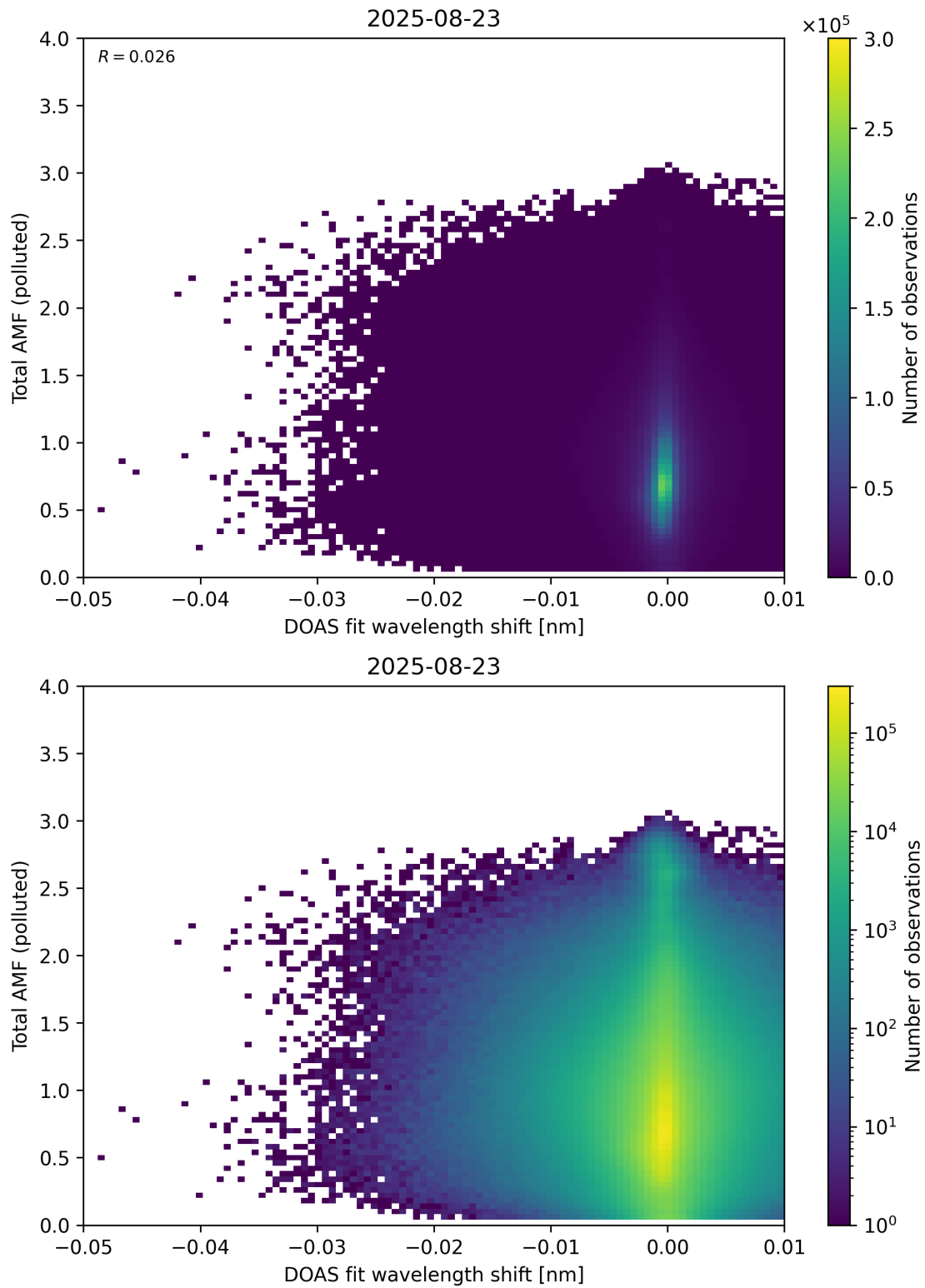
Figure 141: Scatter density plot of “DOAS fit wavelength shift” against “Total AMF (polluted)” for 2025-08-22 to 2025-08-24.
