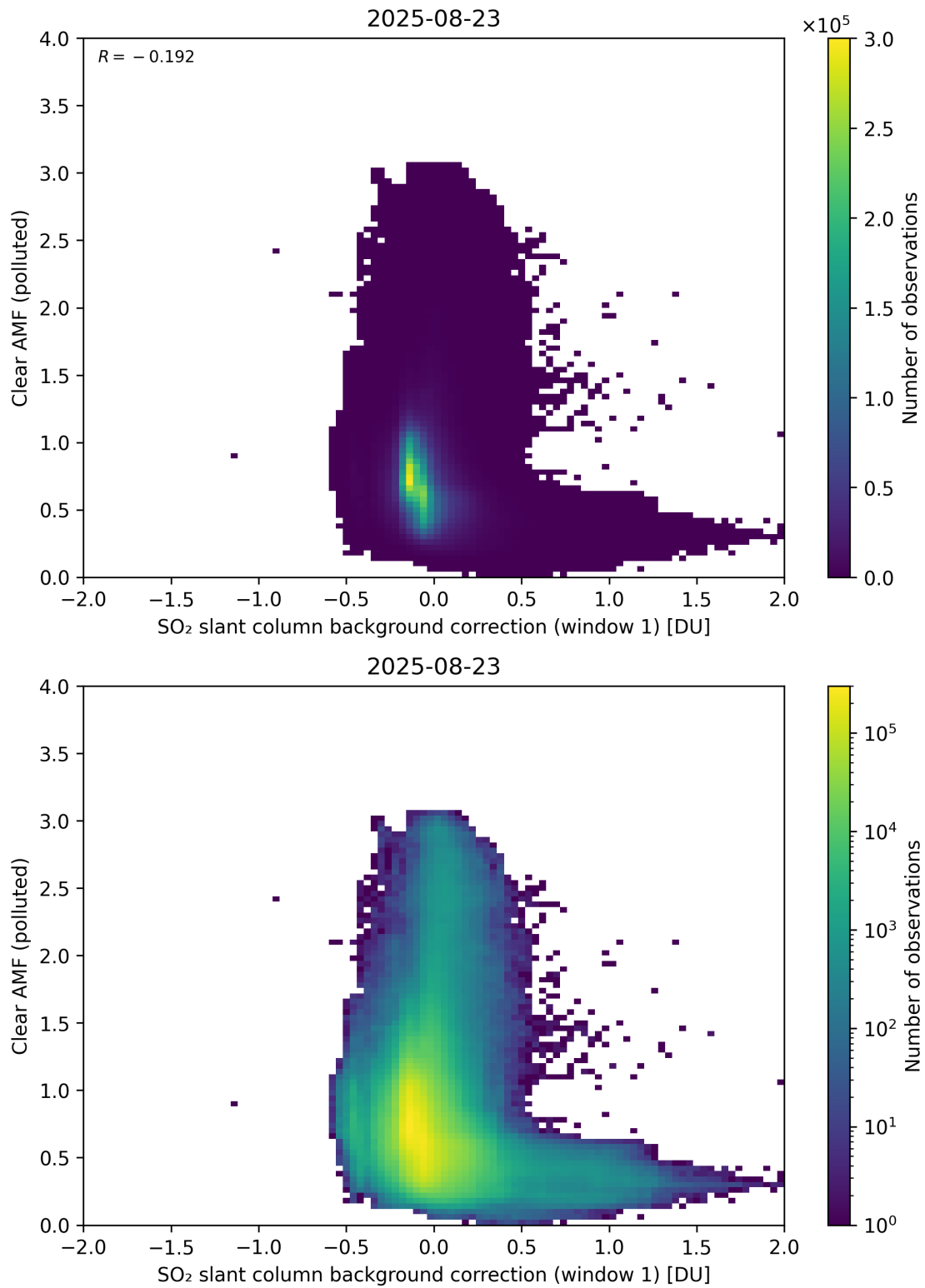
Figure 114: Scatter density plot of “SO 2 slant column background correction (window 1)” against “Clear AMF (polluted)” for 2025-08-22 to 2025-08-24.
