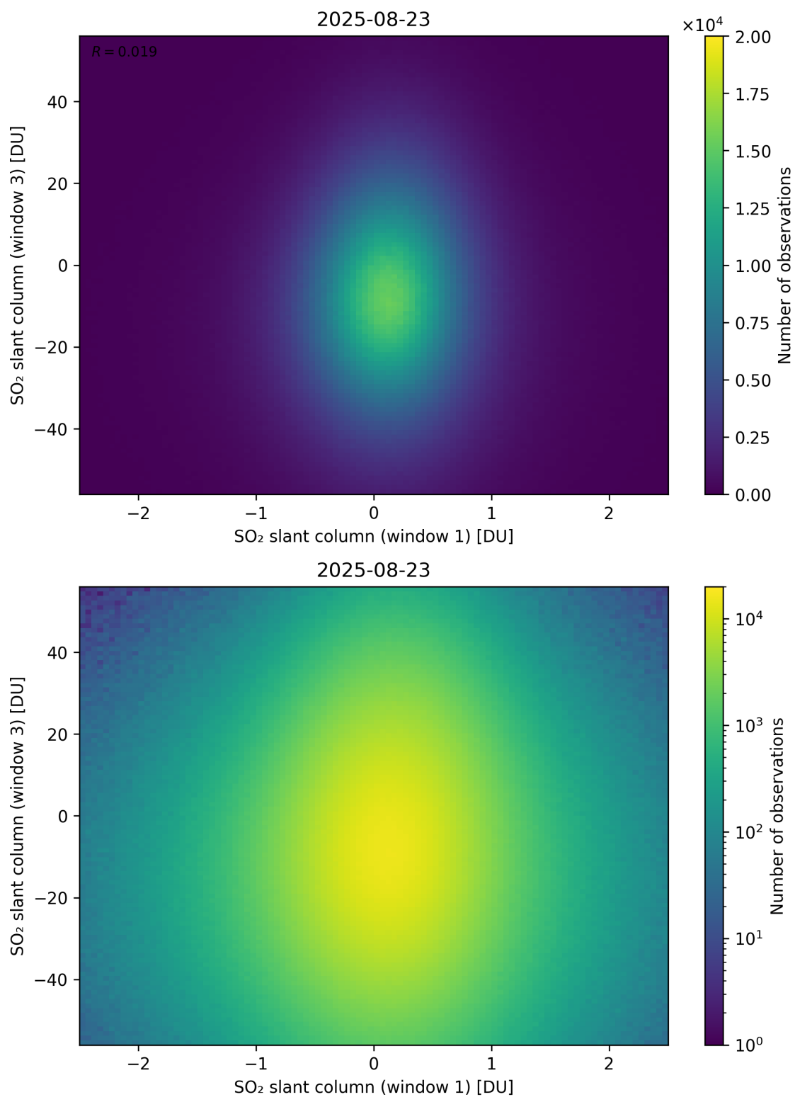
Figure 287: Scatter density plot of “SO 2 slant column (window 1)” against “SO 2 slant column (window 3)” for 2025-08-22 to 2025-08-24.
