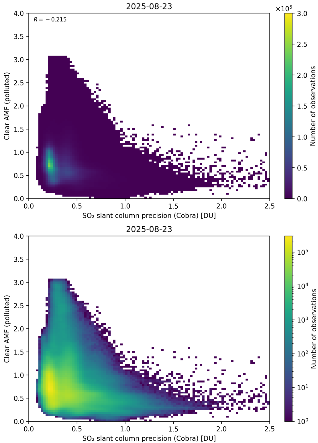
Figure 205: Scatter density plot of “SO 2 slant column precision (Cobra)” against “Clear AMF (polluted)” for 2025-08-22 to 2025-08-24.
