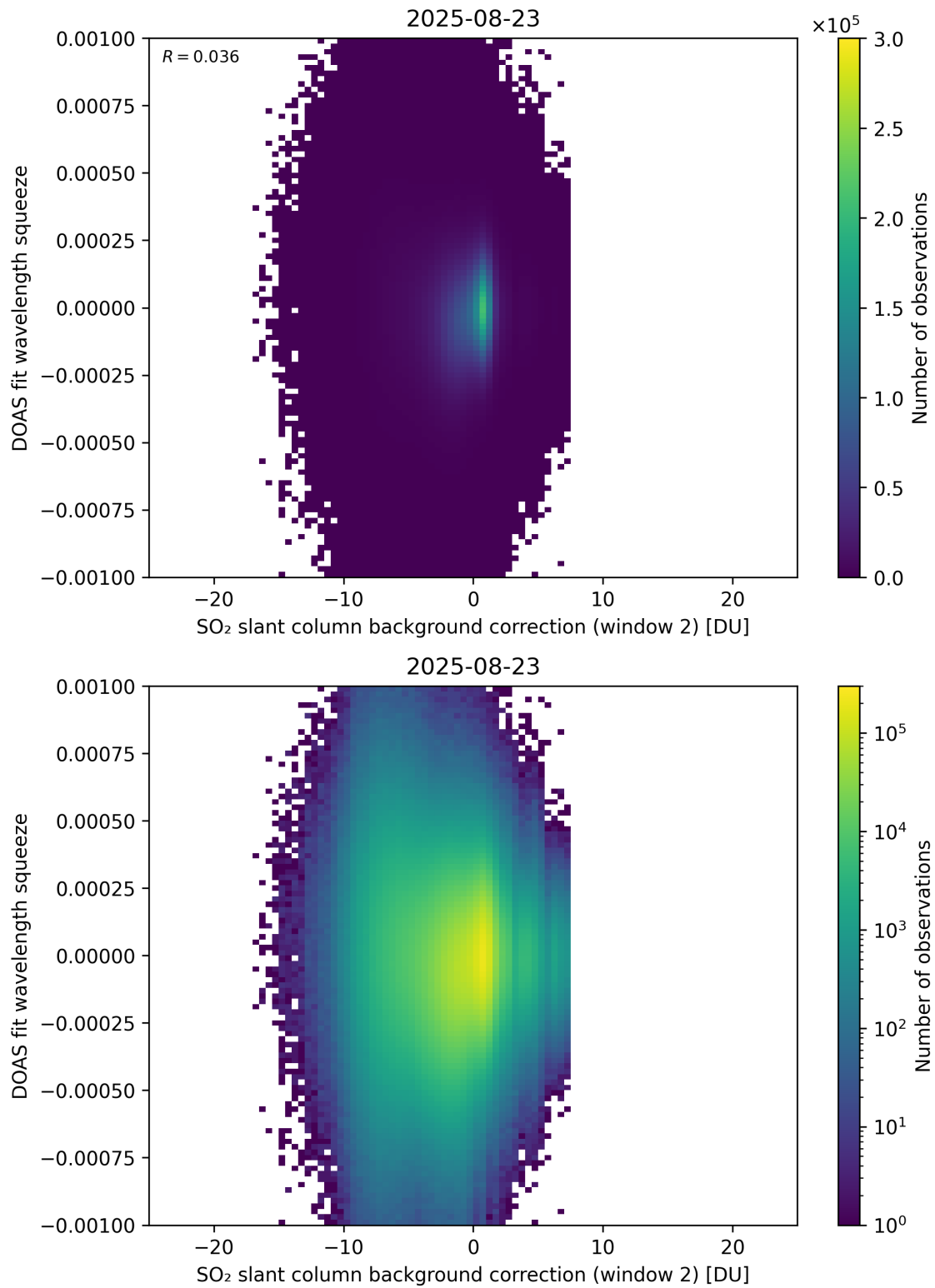
Figure 124: Scatter density plot of “SO 2 slant column background correction (window 2)” against “DOAS fit wavelength squeeze” for 2025-08-22 to 2025-08-24.
