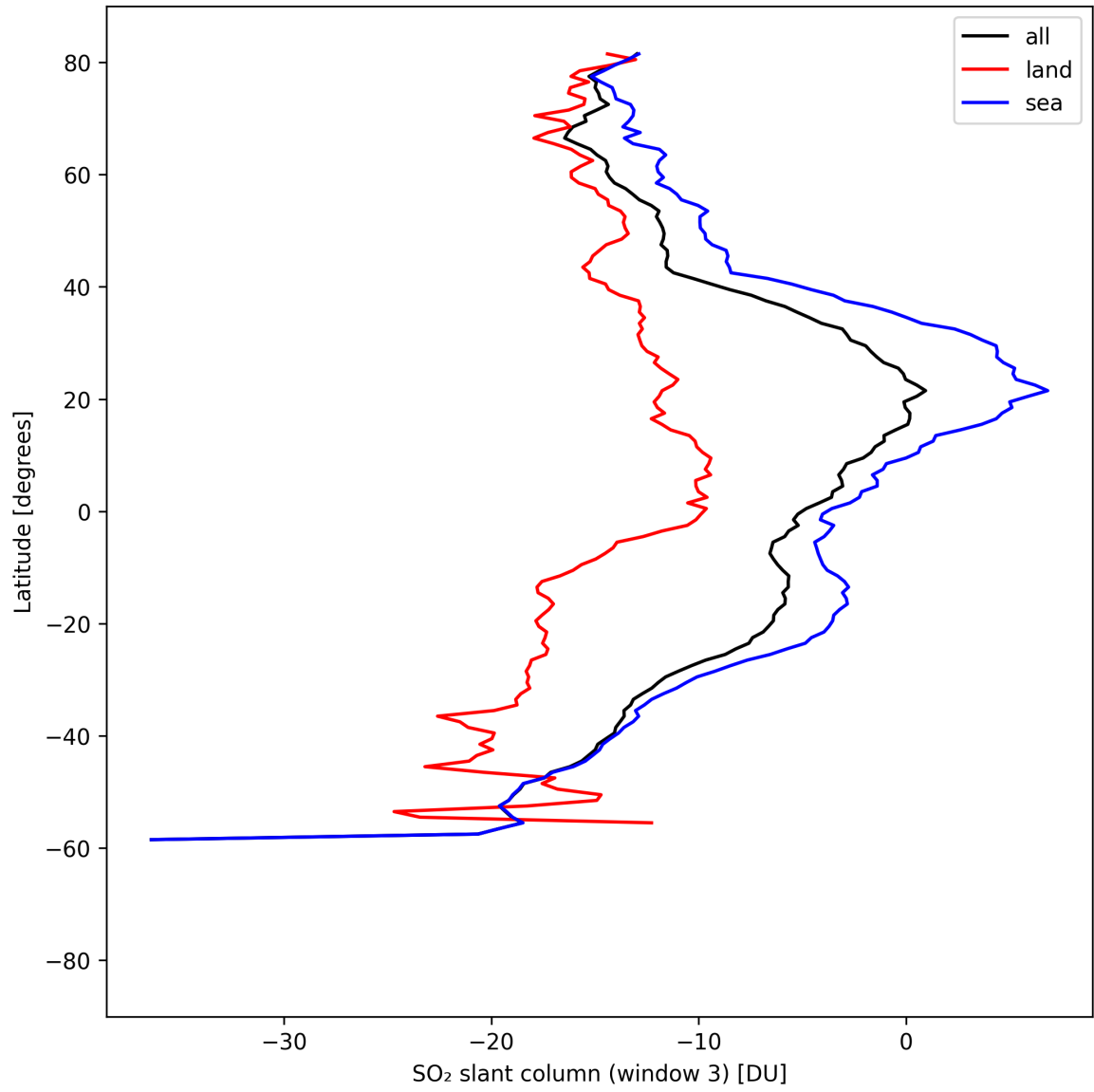
Figure 45: Zonal average of “SO 2 slant column (window 3)” for 2025-08-22 to 2025-08-24.
