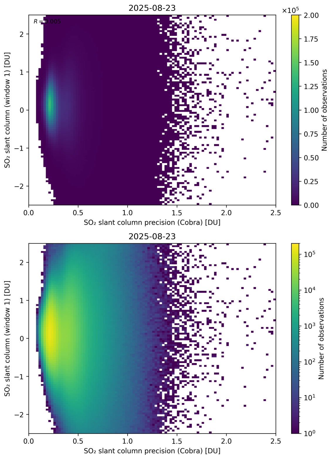
Figure 208: Scatter density plot of “SO 2 slant column precision (Cobra)” against “SO 2 slant column (window 1)” for 2025-08-22 to 2025-08-24.
