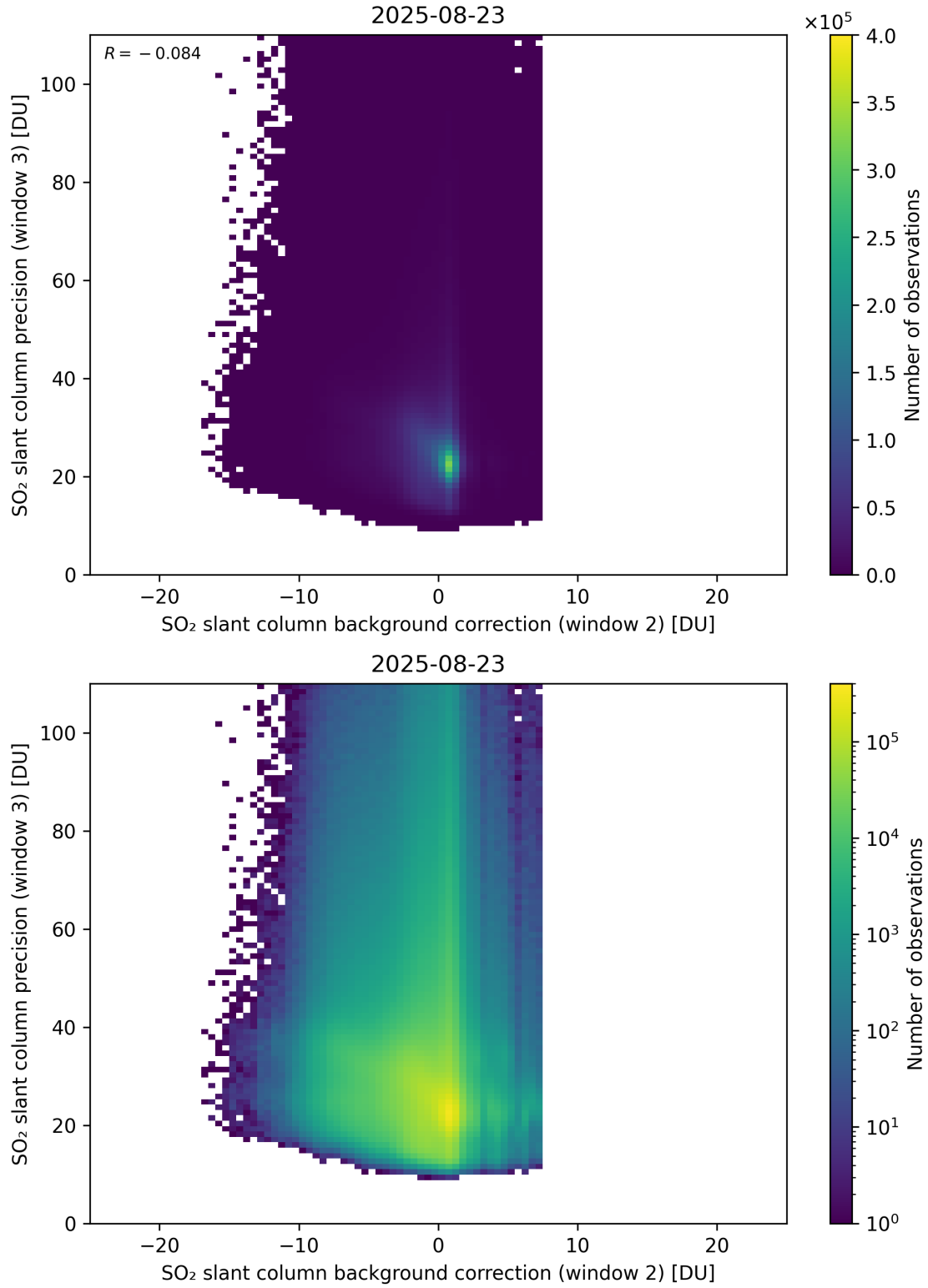
Figure 129: Scatter density plot of “SO 2 slant column background correction (window 2)” against “SO 2 slant column precision (window 3)” for 2025-08-22 to 2025-08-24.
