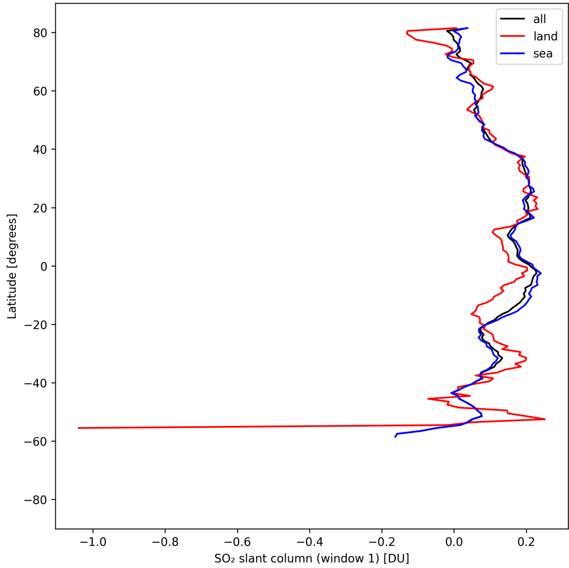
Figure 37: Zonal average of “SO 2 slant column (window 1)” for 2025-08-22 to 2025-08-24.
