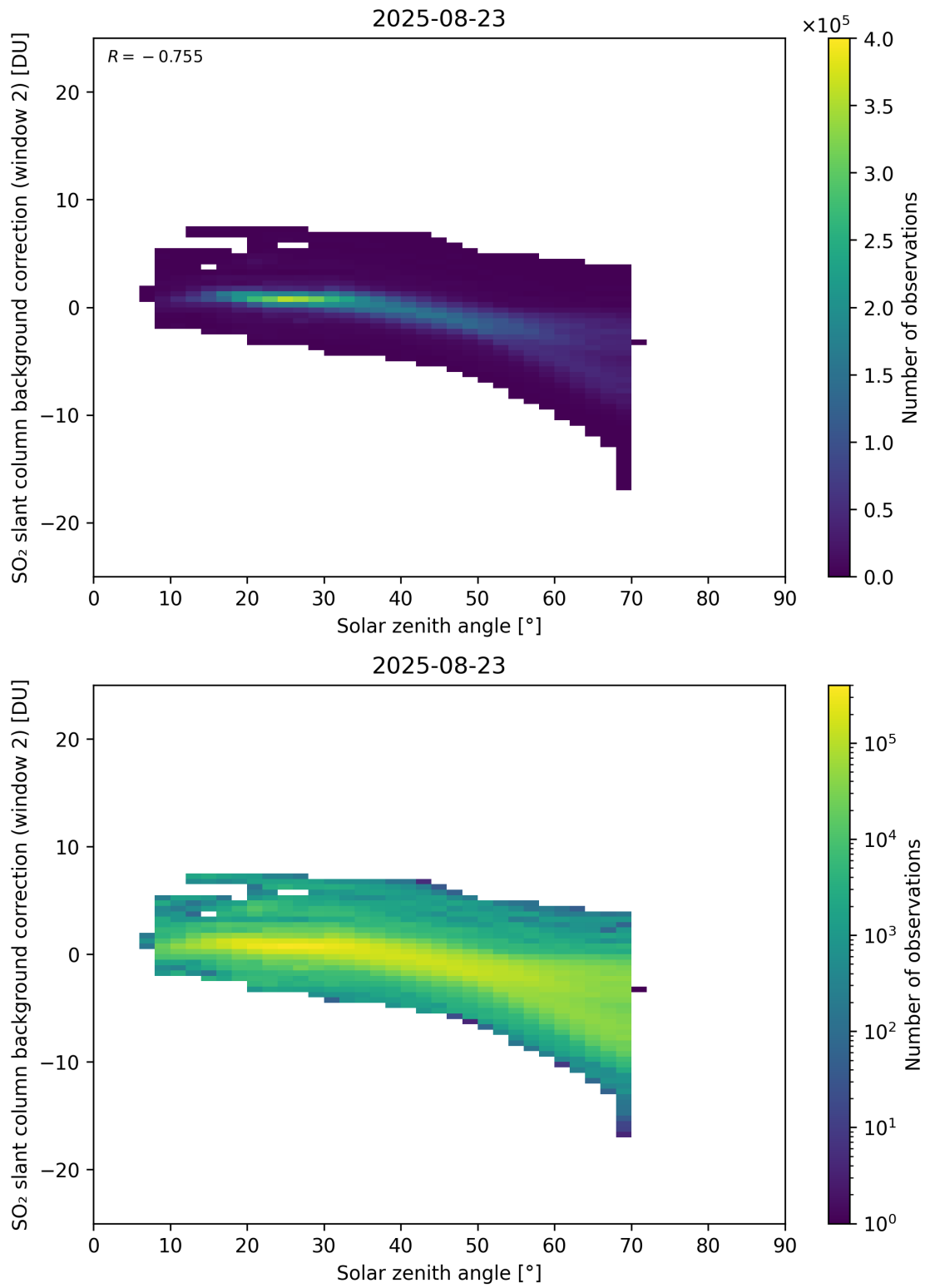
Figure 172: Scatter density plot of “Solar zenith angle” against “SO 2 slant column background correction (window 2)” for 2025-08-22 to 2025-08-24.
