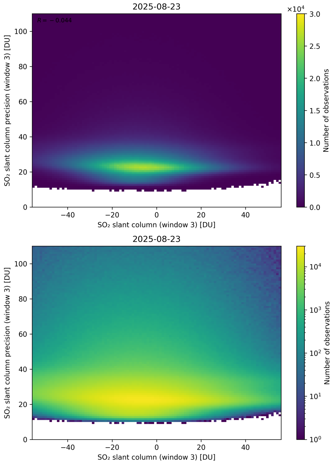
Figure 317: Scatter density plot of “SO 2 slant column (window 3)” against “SO 2 slant column precision (window 3)” for 2025-08-22 to 2025-08-24.
