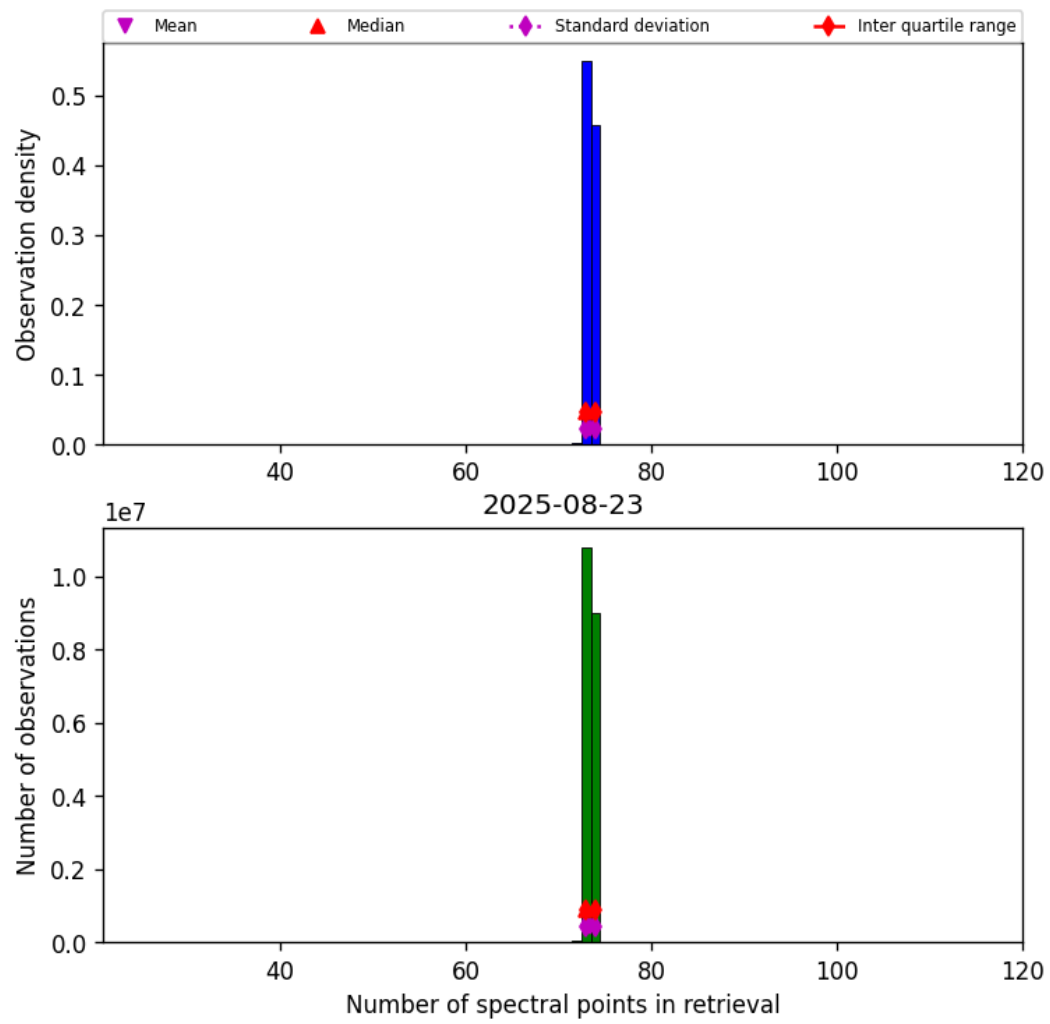
Figure 82: Histogram of “Number of spectral points in retrieval” for 2025-08-22 to 2025-08-24
