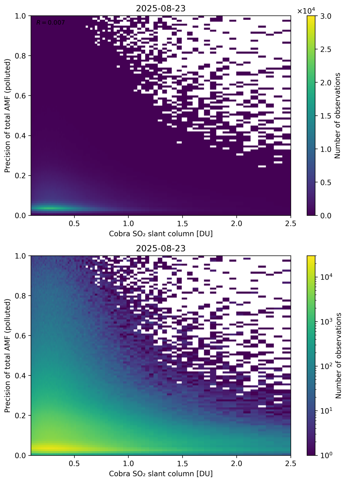
Figure 225: Scatter density plot of “Cobra SO 2 slant column” against “Precision of total AMF (polluted)” for 2025-08-22 to 2025-08-24.
