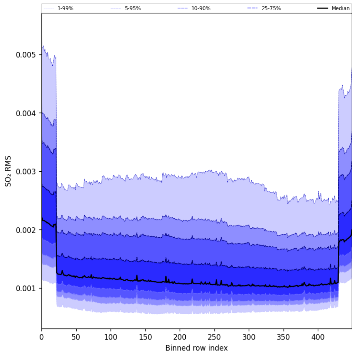
Figure 104: Along track statistics of “SO 2 RMS” for 2025-08-22 to 2025-08-24
