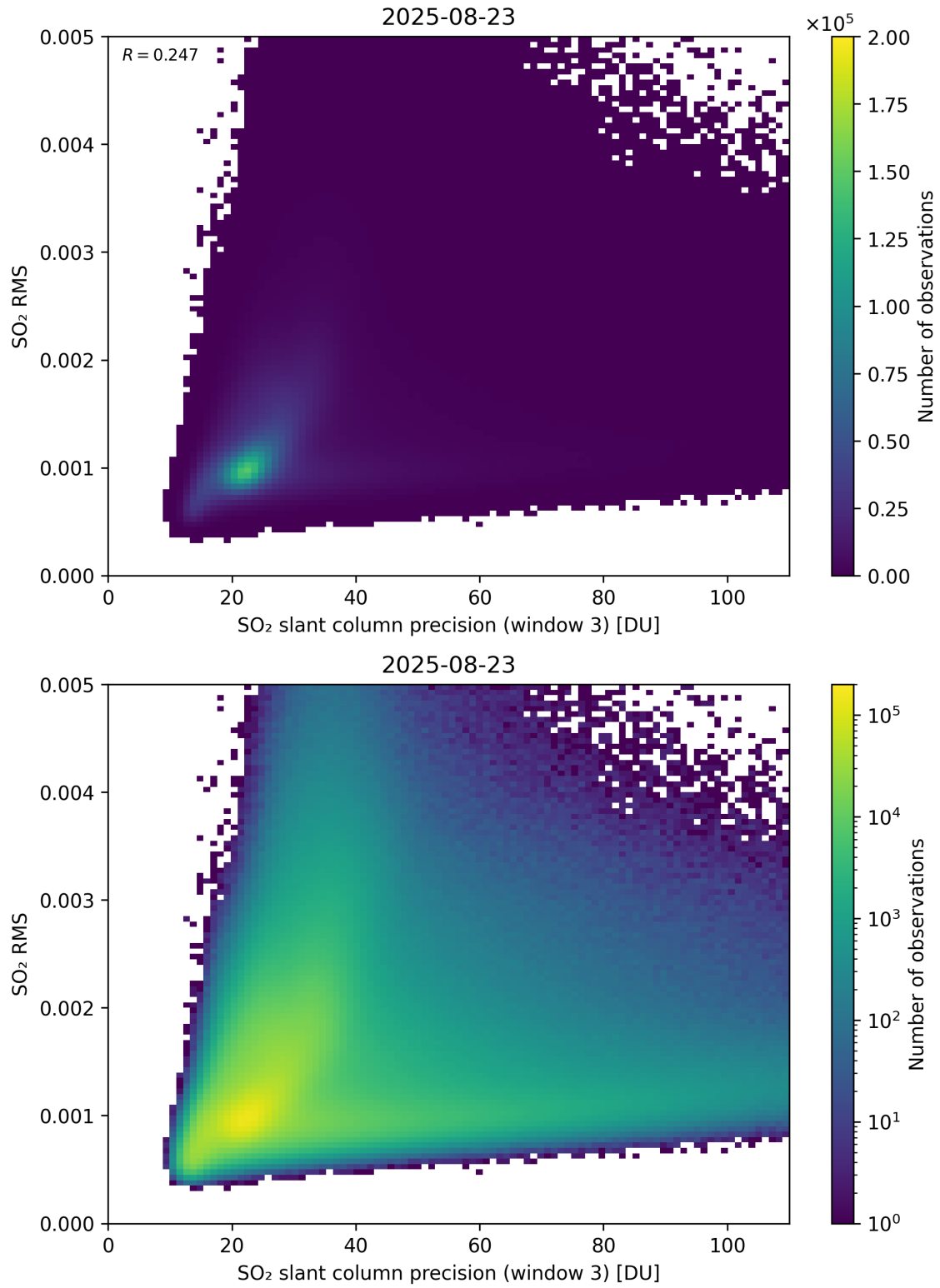
Figure 310: Scatter density plot of “SO 2 slant column precision (window 3)” against “SO 2 RMS” for 2025-08-22 to 2025-08-24.
