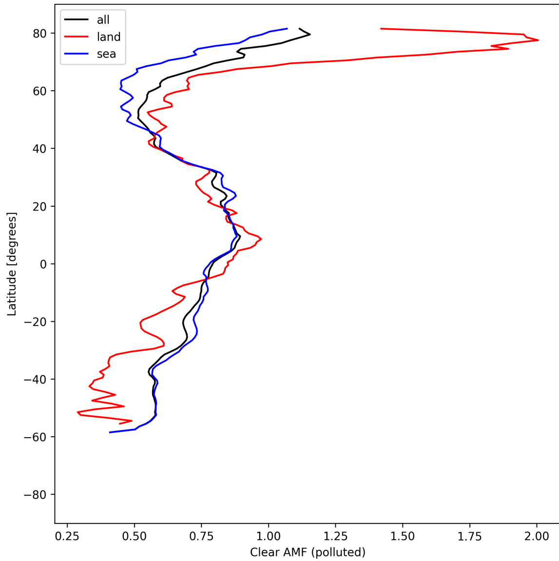
Figure 55: Zonal average of “Clear AMF (polluted)” for 2025-08-22 to 2025-08-24.
