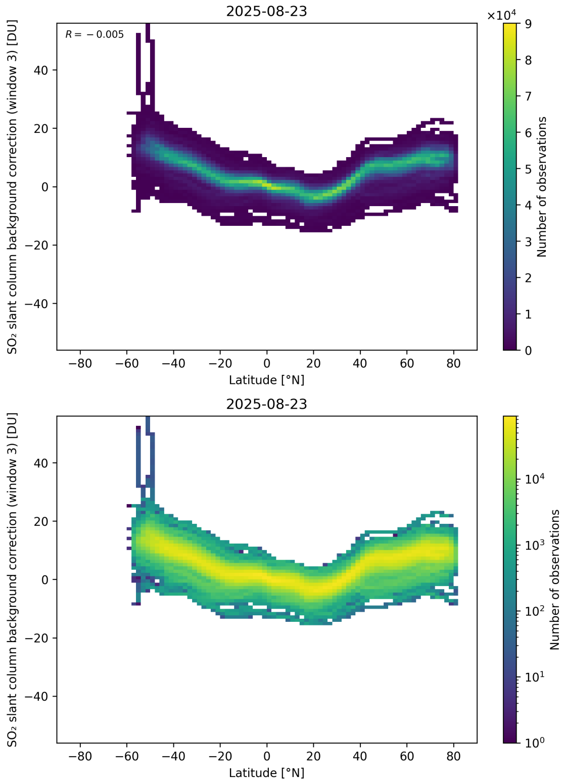
Figure 152: Scatter density plot of “Latitude” against “SO 2 slant column background correction (window 3)” for 2025-08-22 to 2025-08-24.
