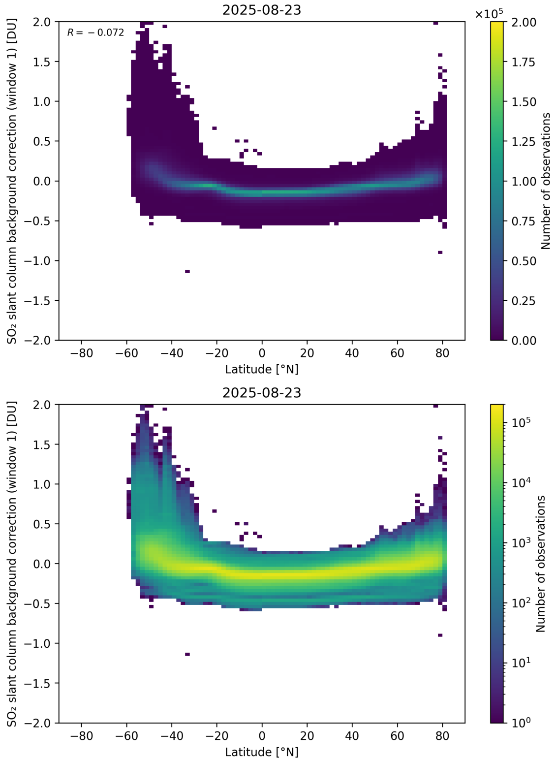
Figure 150: Scatter density plot of “Latitude” against “SO 2 slant column background correction (window 1)” for 2025-08-22 to 2025-08-24.
