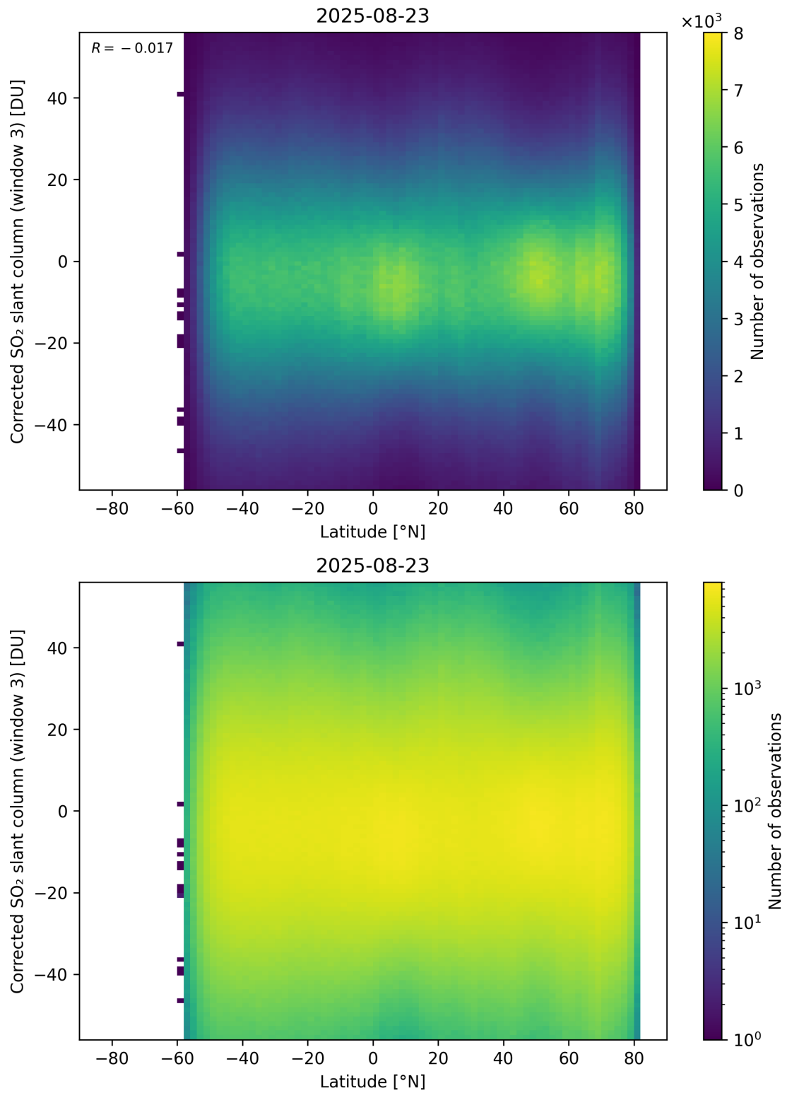
Figure 161: Scatter density plot of “Latitude” against “Corrected SO 2 slant column (window 3)” for 2025-08-22 to 2025-08-24.
