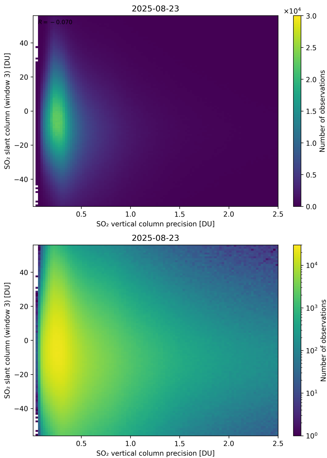
Figure 344: Scatter density plot of “SO 2 vertical column precision” against “SO 2 slant column (window 3)” for 2025-08-22 to 2025-08-24.
