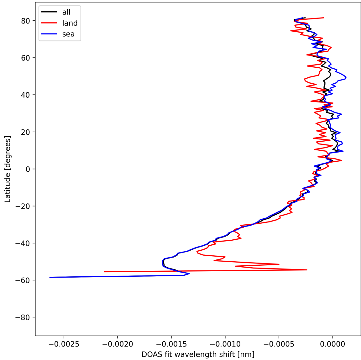
Figure 50: Zonal average of “DOAS fit wavelength shift” for 2025-08-22 to 2025-08-24.
