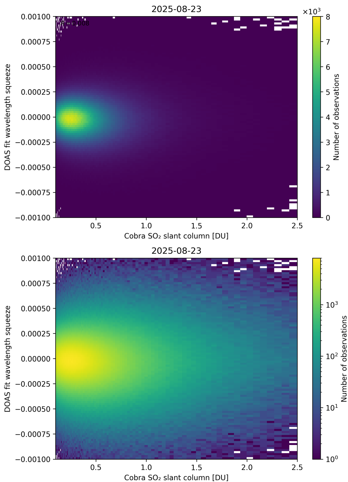
Figure 197: Scatter density plot of “Cobra SO 2 slant column” against “DOAS fit wavelength squeeze” for 2025-08-22 to 2025-08-24.
