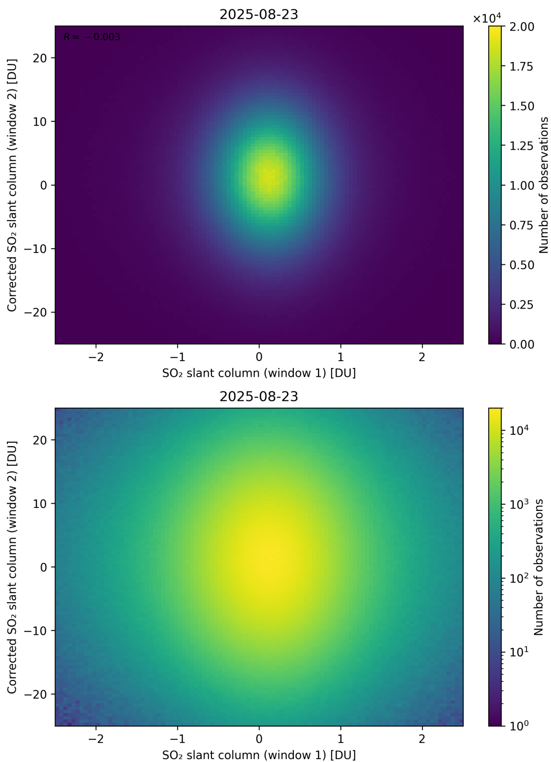
Figure 283: Scatter density plot of “SO 2 slant column (window 1)” against “Corrected SO 2 slant column (window 2)” for 2025-08-22 to 2025-08-24.
