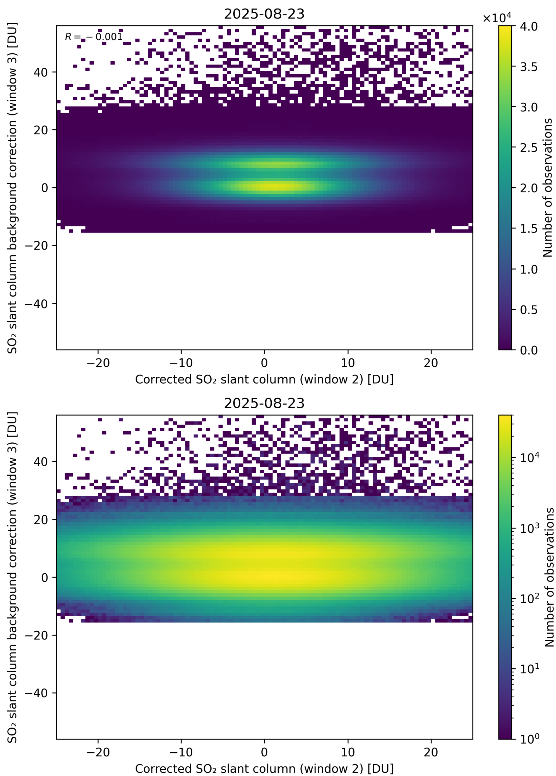
Figure 245: Scatter density plot of “Corrected SO 2 slant column (window 2)” against “SO 2 slant column background correction (window 3)” for 2025-08-22 to 2025-08-24.
