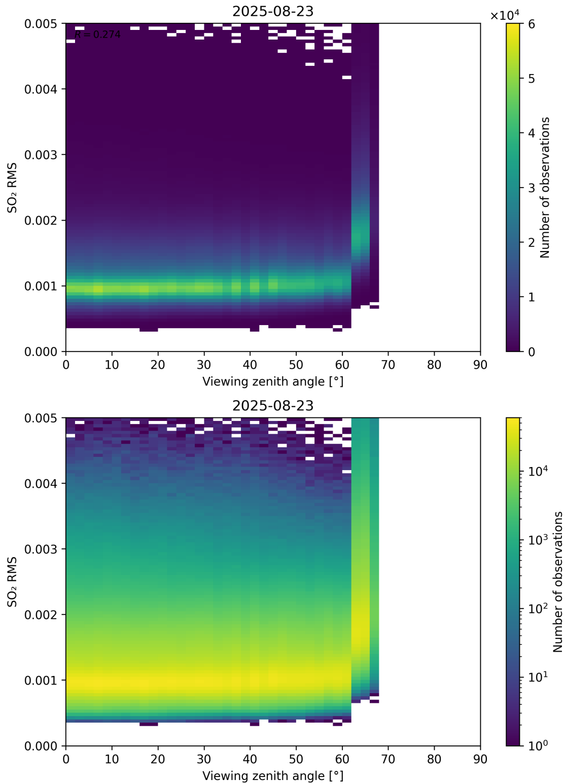
Figure 367: Scatter density plot of “Viewing zenith angle” against “SO 2 RMS” for 2025-08-22 to 2025-08-24.
