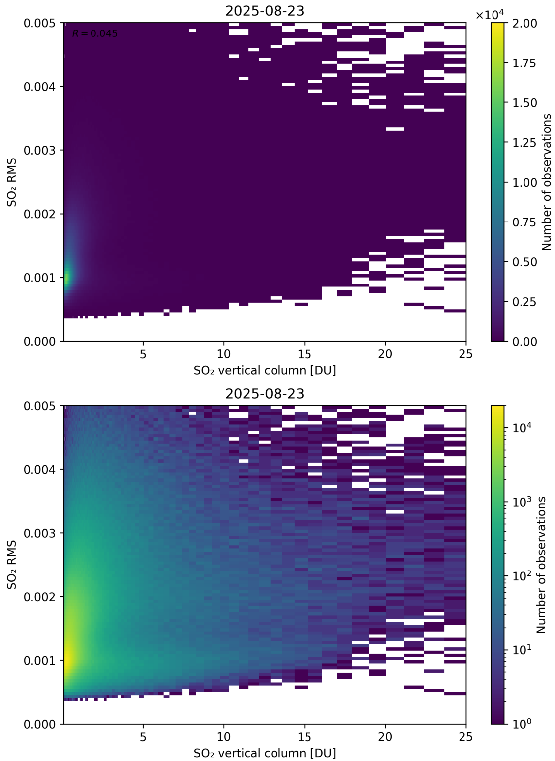
Figure 328: Scatter density plot of “SO 2 vertical column” against “SO 2 RMS” for 2025-08-22 to 2025-08-24.
