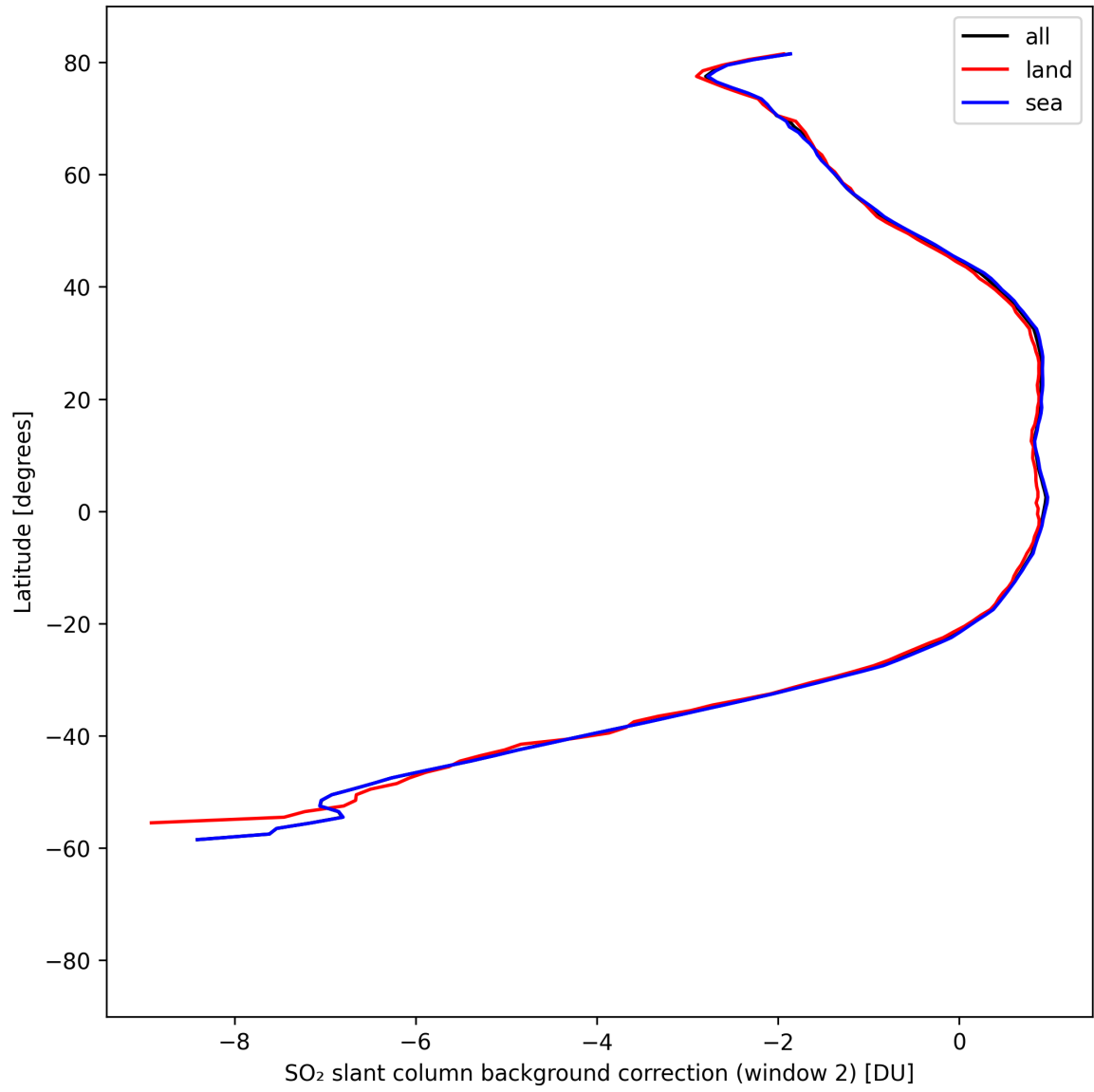
Figure 44: Zonal average of “SO 2 slant column background correction (window 2)” for 2025-08-22 to 2025-08-24.
