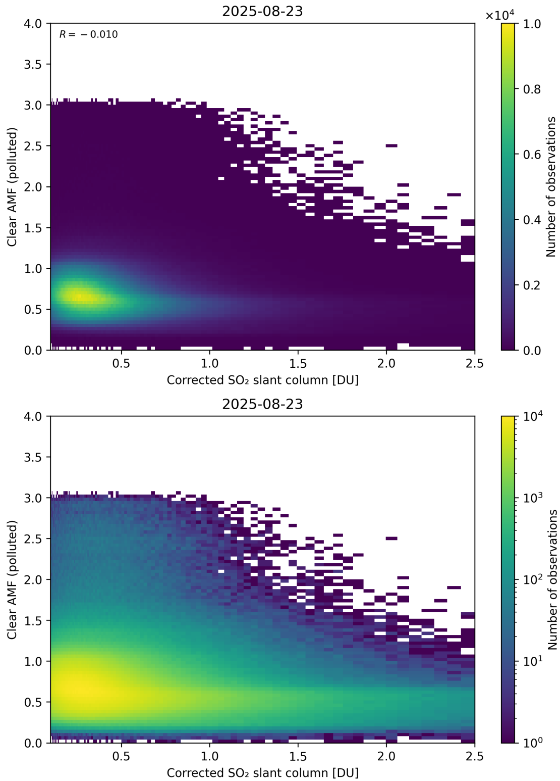
Figure 232: Scatter density plot of “Corrected SO 2 slant column” against “Clear AMF (polluted)” for 2025-08-22 to 2025-08-24.
