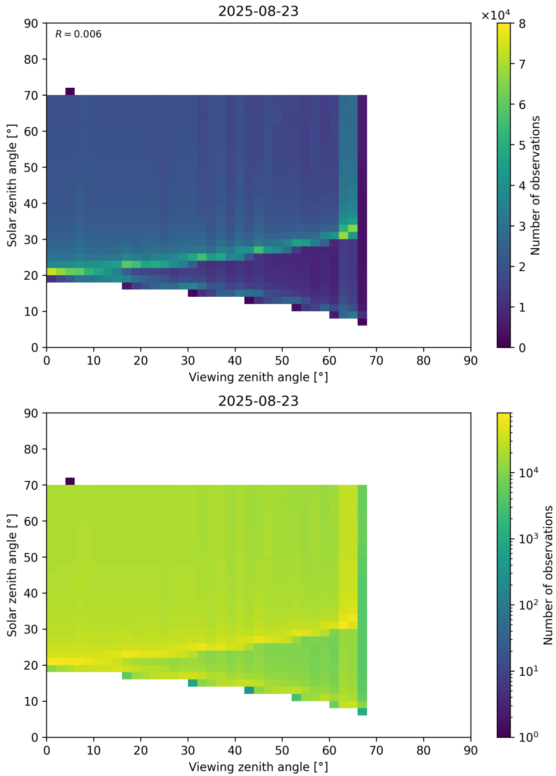
Figure 369: Scatter density plot of “Viewing zenith angle” against “Solar zenith angle” for 2025-08-22 to 2025-08-24.
