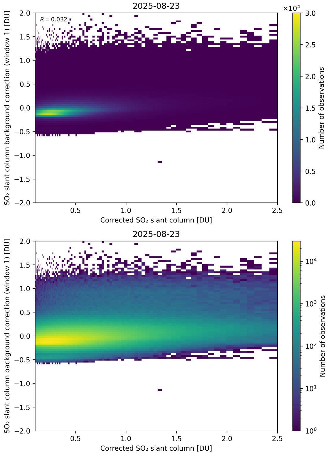
Figure 226: Scatter density plot of “Corrected SO 2 slant column” against “SO 2 slant column background correction (window 1)” for 2025-08-22 to 2025-08-24.
