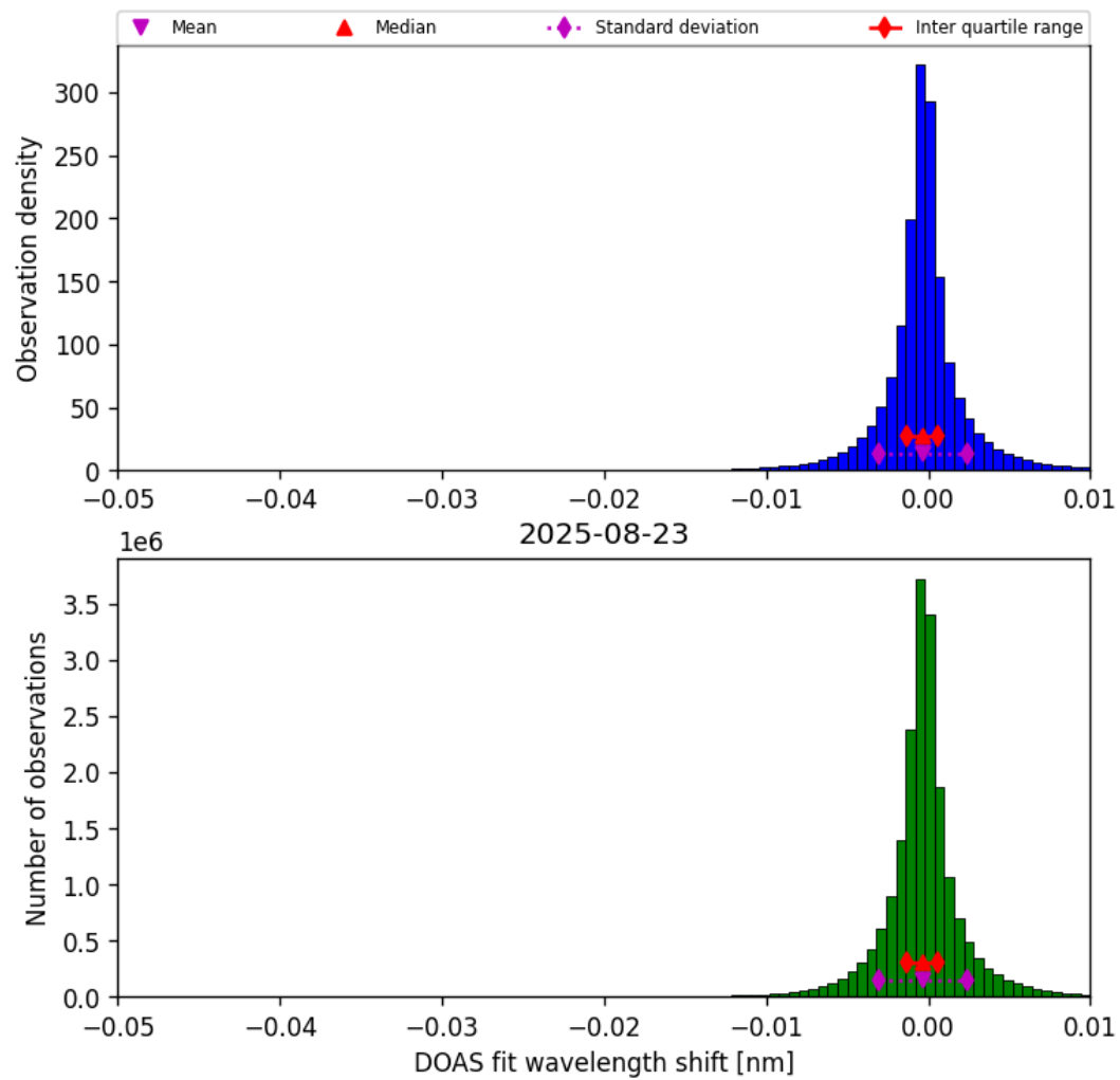
Figure 76: Histogram of “DOAS fit wavelength shift” for 2025-08-22 to 2025-08-24
