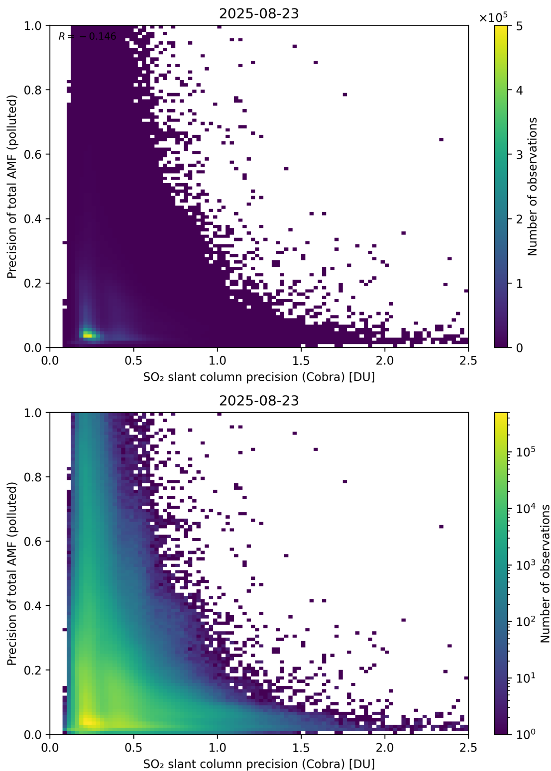
Figure 214: Scatter density plot of “SO 2 slant column precision (Cobra)” against “Precision of total AMF (polluted)” for 2025-08-22 to 2025-08-24.
