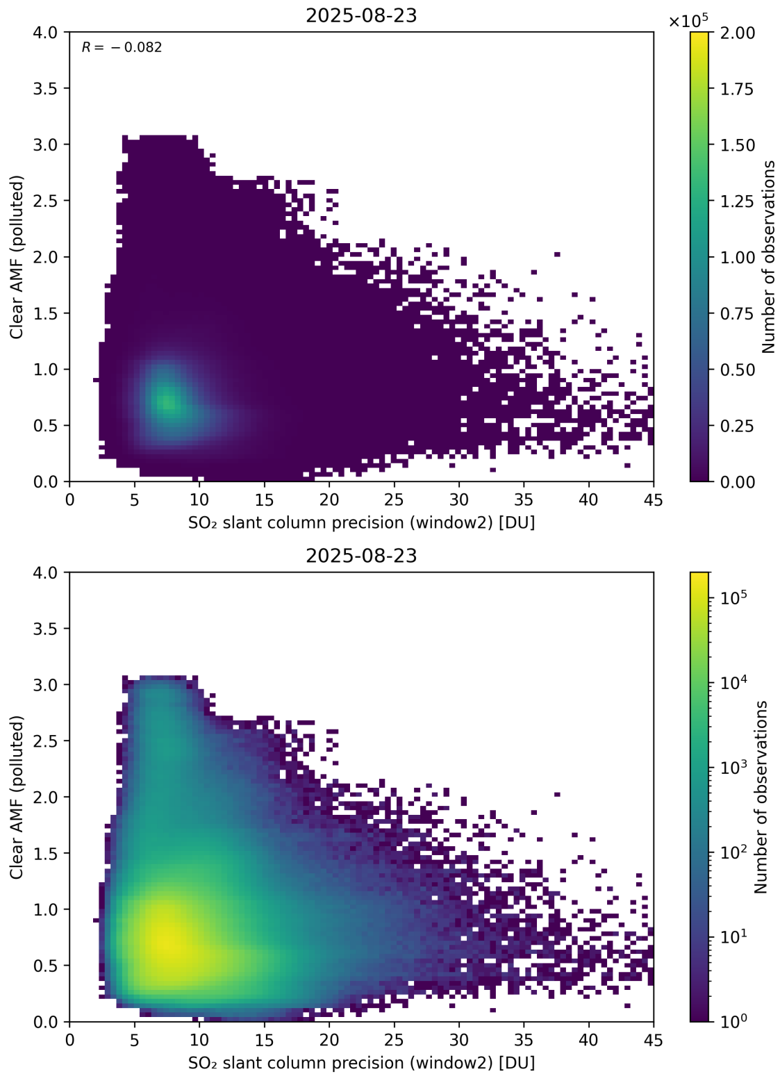
Figure 296: Scatter density plot of “SO 2 slant column precision (window2)” against “Clear AMF (polluted)” for 2025-08-22 to 2025-08-24.
