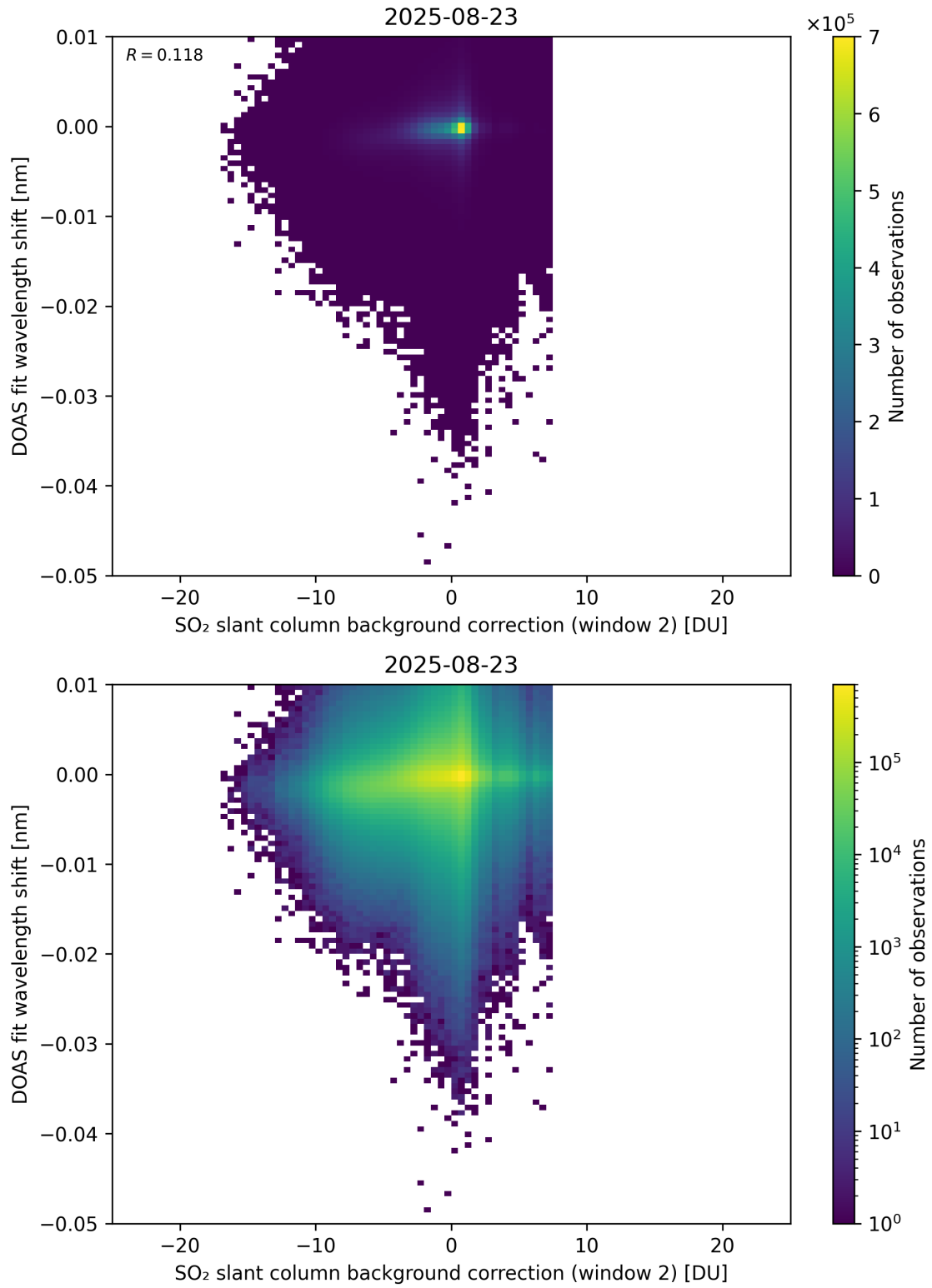
Figure 123: Scatter density plot of “SO 2 slant column background correction (window 2)” against “DOAS fit wavelength shift” for 2025-08-22 to 2025-08-24.
