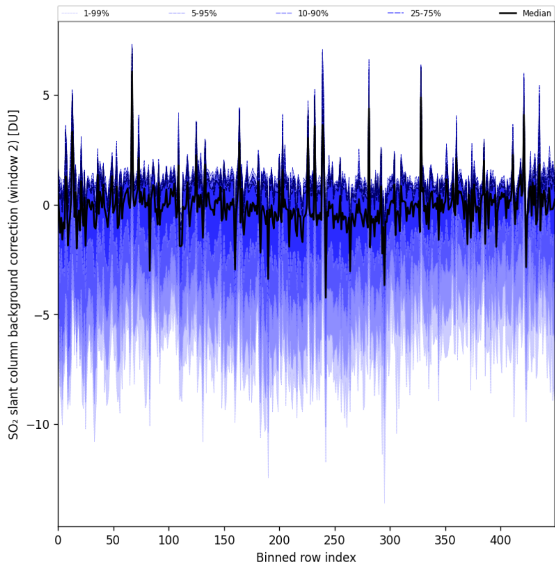
Figure 96: Along track statistics of “SO 2 slant column background correction (window 2)” for 2025-08-22 to 2025-08-24
