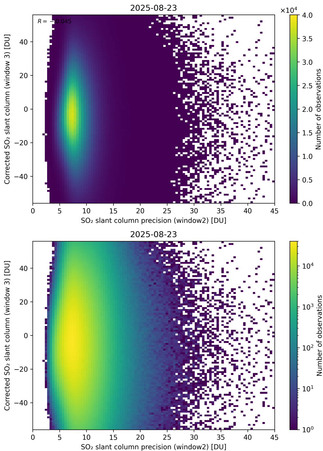
Figure 298: Scatter density plot of “SO 2 slant column precision (window2)” against “Corrected SO 2 slant column (window 3)” for 2025-08-22 to 2025-08-24.
