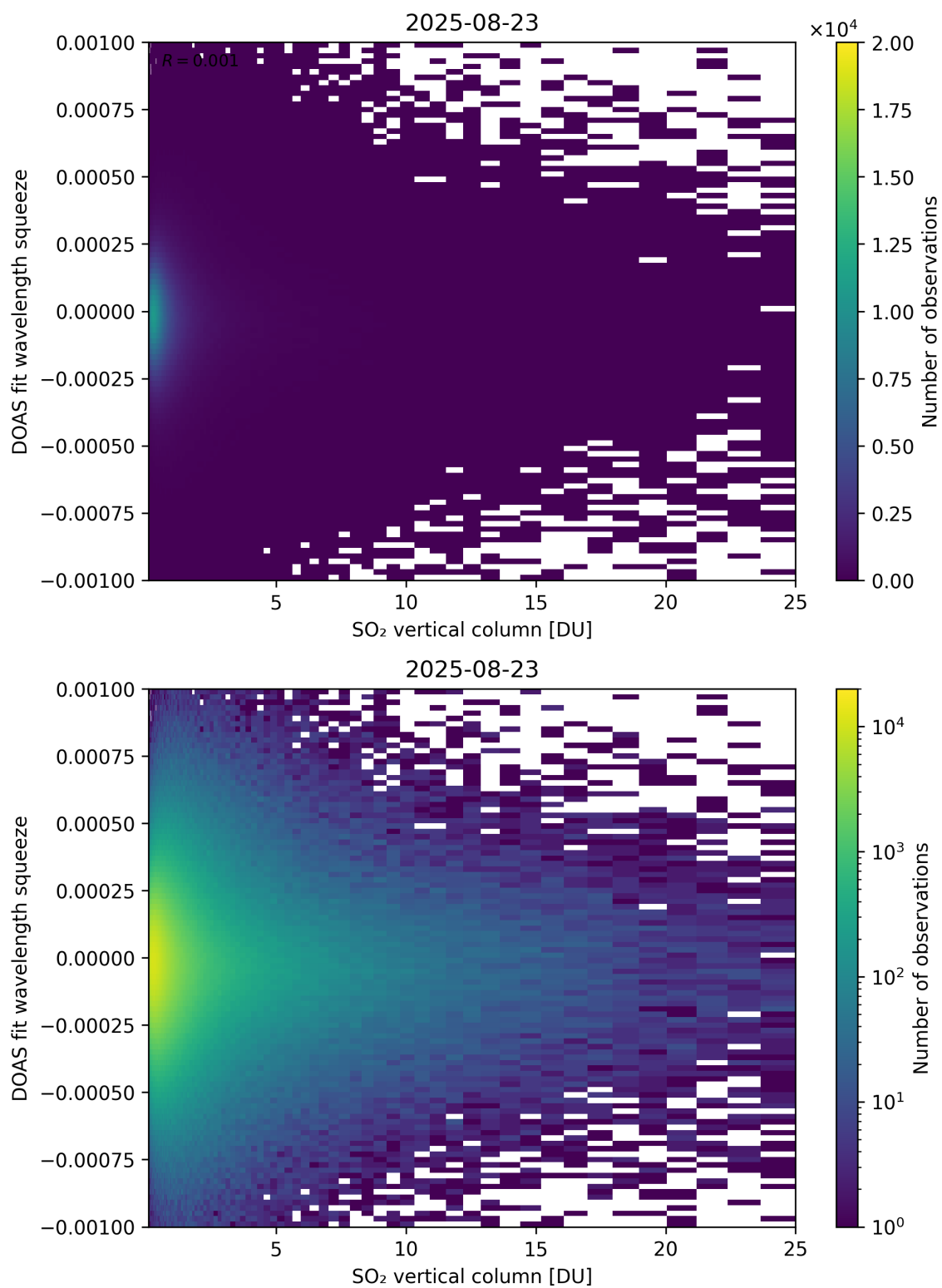
Figure 327: Scatter density plot of “SO 2 vertical column” against “DOAS fit wavelength squeeze” for 2025-08-22 to 2025-08-24.
