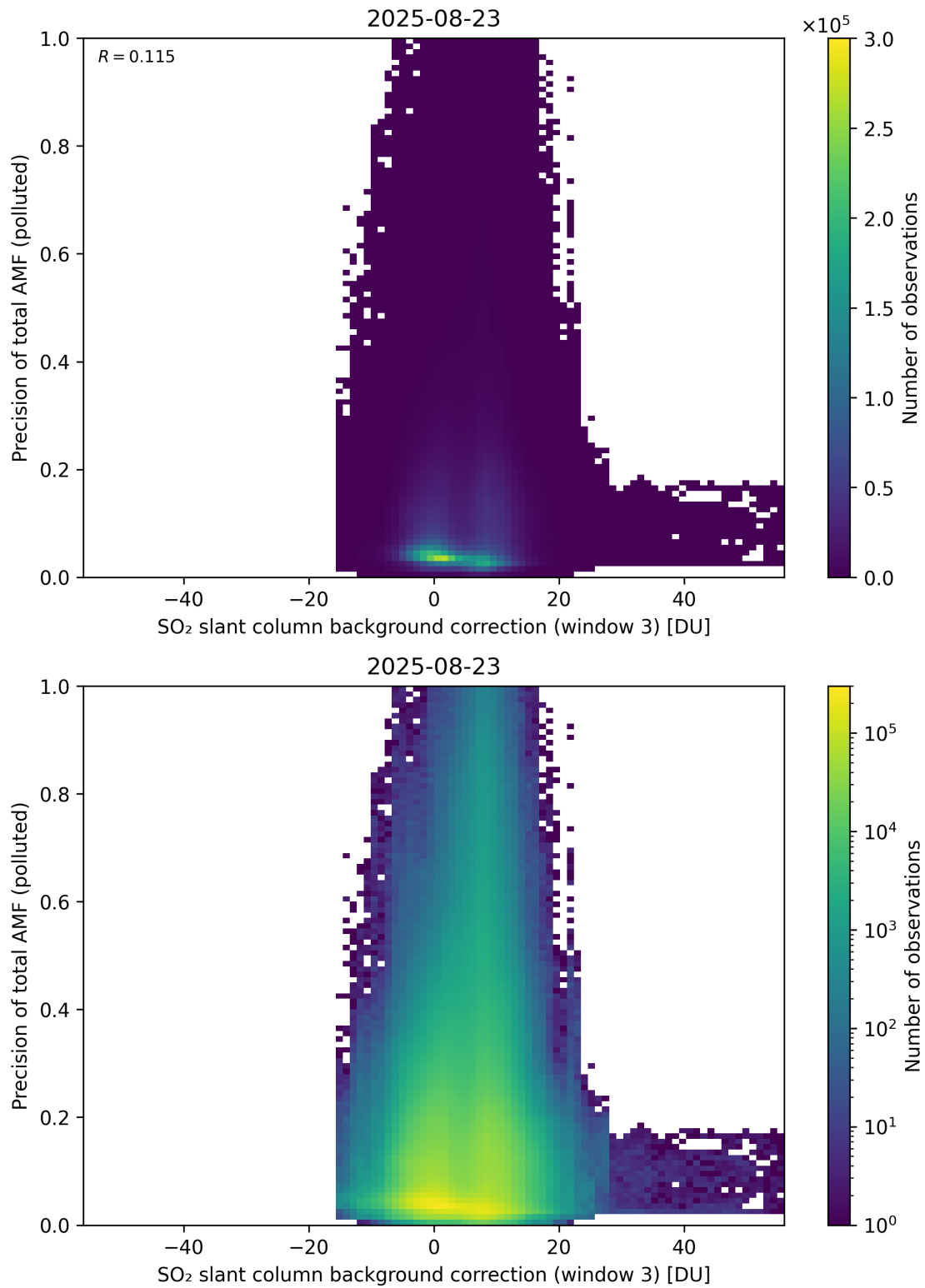
Figure 137: Scatter density plot of “SO 2 slant column background correction (window 3)” against “Precision of total AMF (polluted)” for 2025-08-22 to 2025-08-24.
