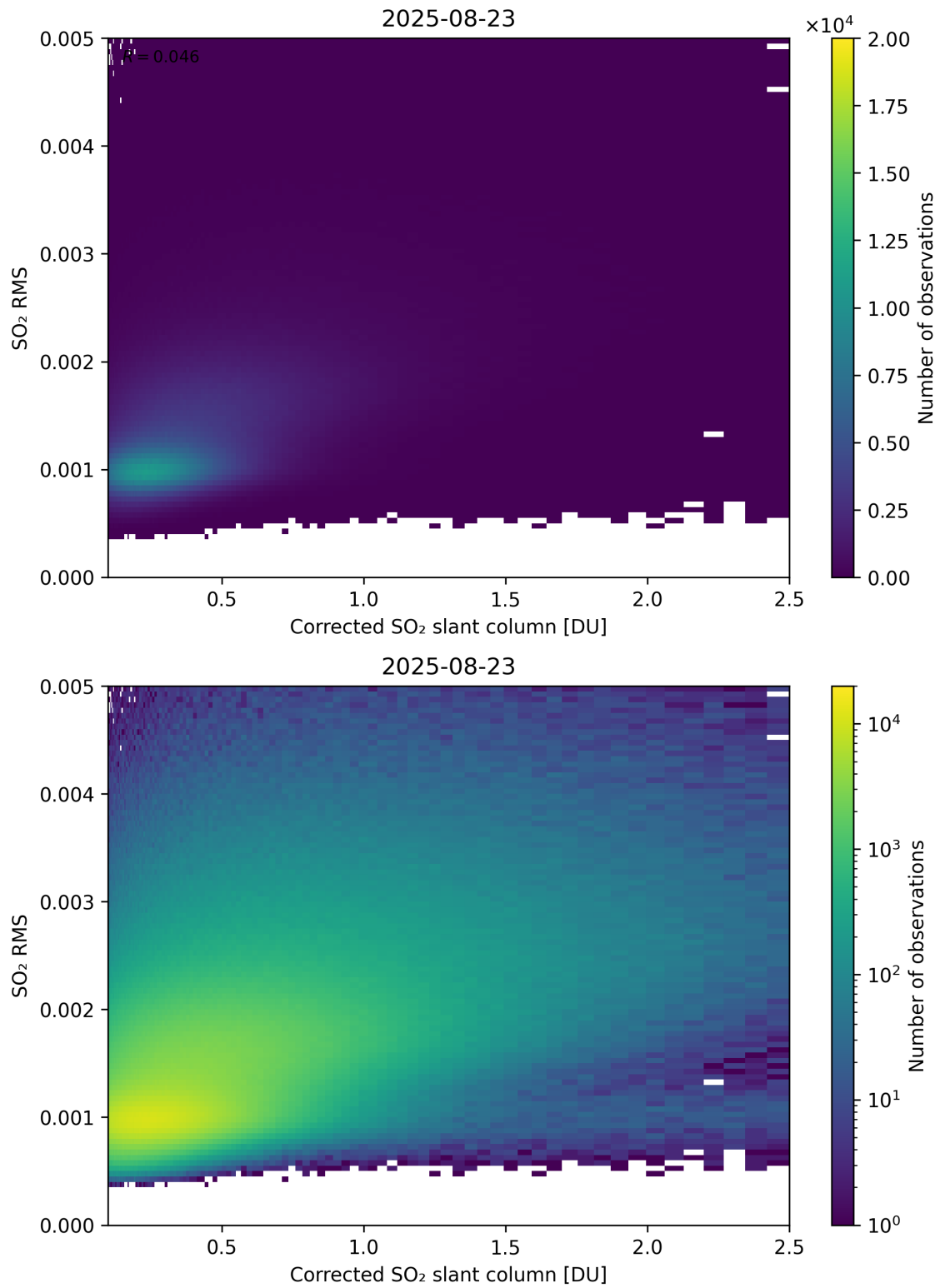
Figure 231: Scatter density plot of “Corrected SO 2 slant column” against “SO 2 RMS” for 2025-08-22 to 2025-08-24.
