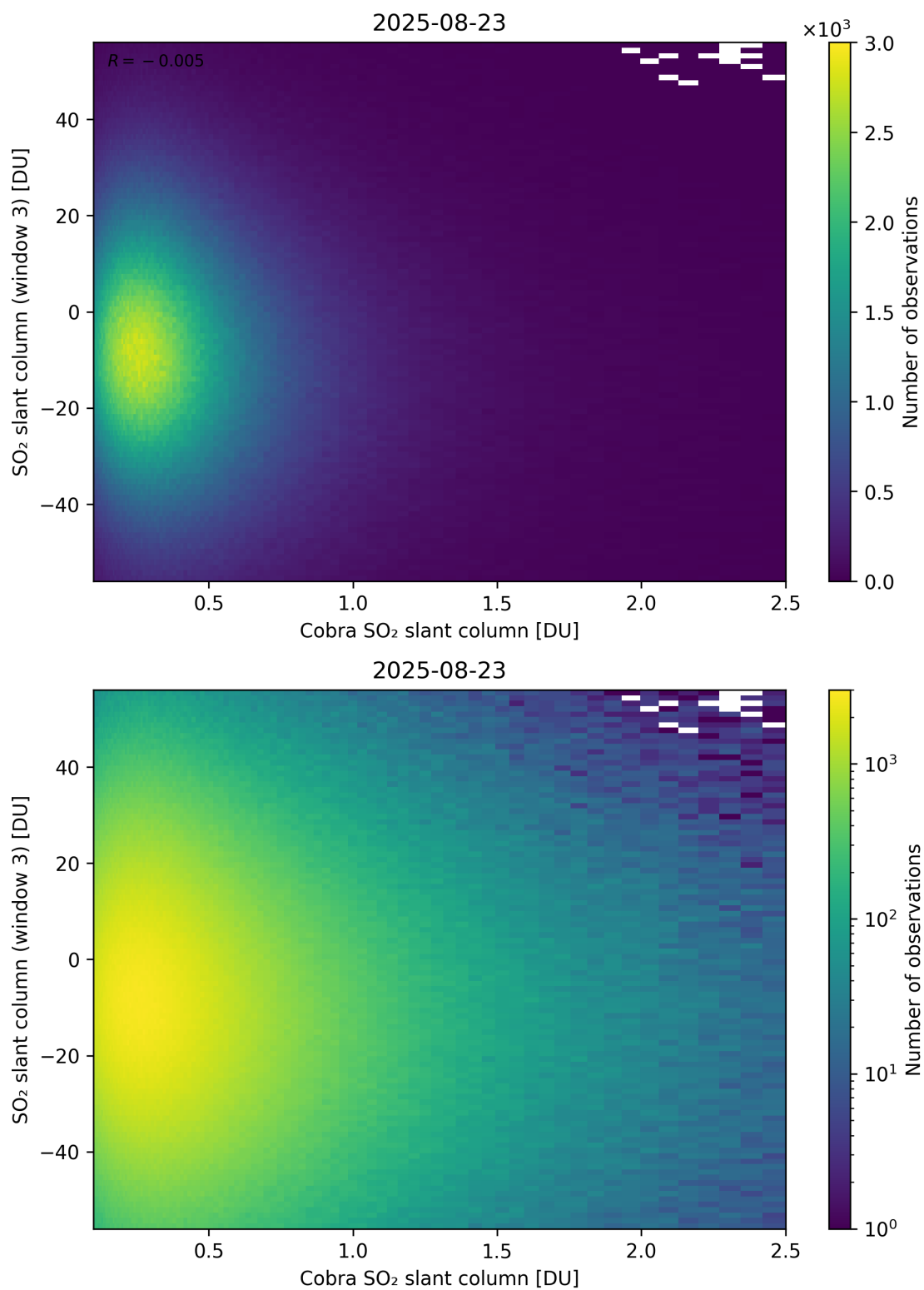
Figure 222: Scatter density plot of “Cobra SO 2 slant column” against “SO 2 slant column (window 3)” for 2025-08-22 to 2025-08-24.
