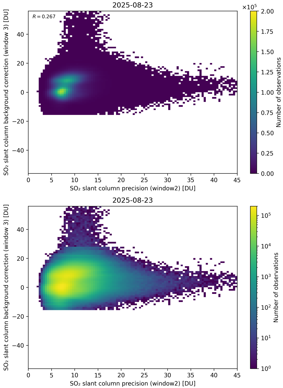
Figure 292: Scatter density plot of “SO 2 slant column precision (window2)” against “SO 2 slant column background correction (window 3)” for 2025-08-22 to 2025-08-24.
