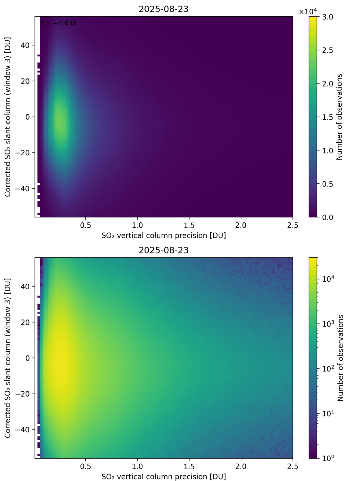
Figure 340: Scatter density plot of “SO 2 vertical column precision” against “Corrected SO 2 slant column (window 3)” for 2025-08-22 to 2025-08-24.
