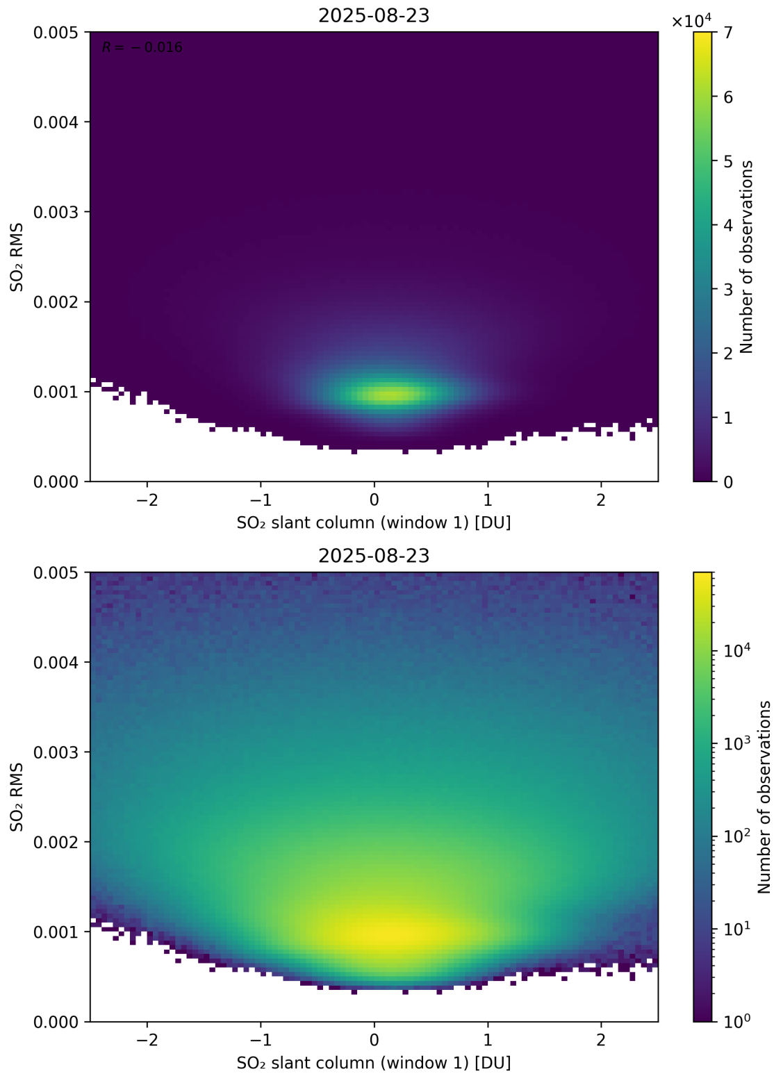
Figure 267: Scatter density plot of “SO 2 slant column (window 1)” against “SO 2 RMS” for 2025-08-22 to 2025-08-24.
