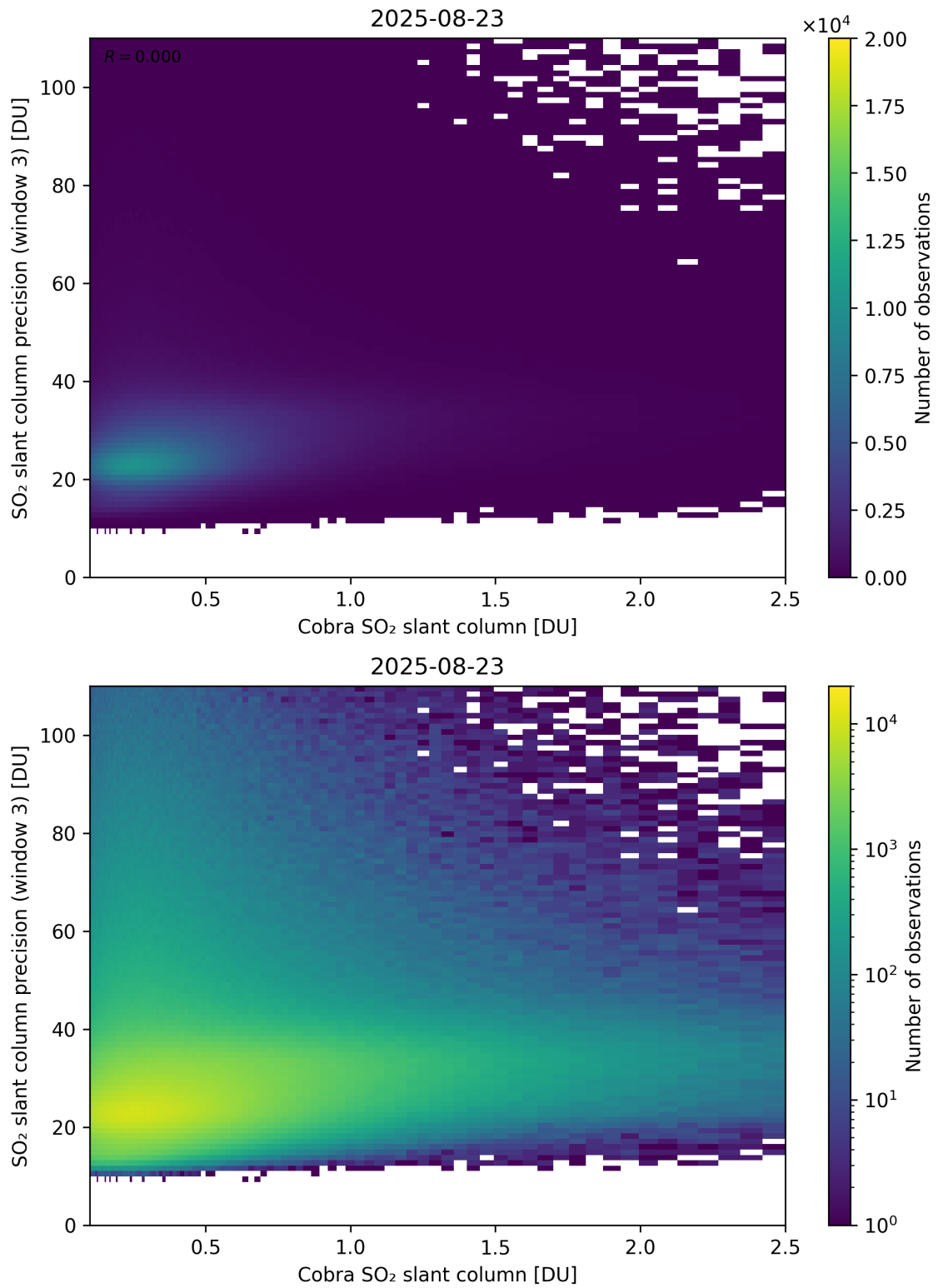
Figure 223: Scatter density plot of “Cobra SO 2 slant column” against “SO 2 slant column precision (window 3)” for 2025-08-22 to 2025-08-24.
