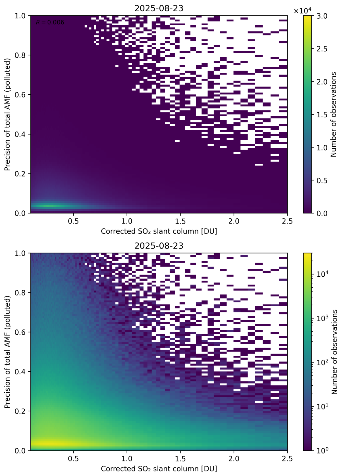
Figure 243: Scatter density plot of “Corrected SO 2 slant column” against “Precision of total AMF (polluted)” for 2025-08-22 to 2025-08-24.
