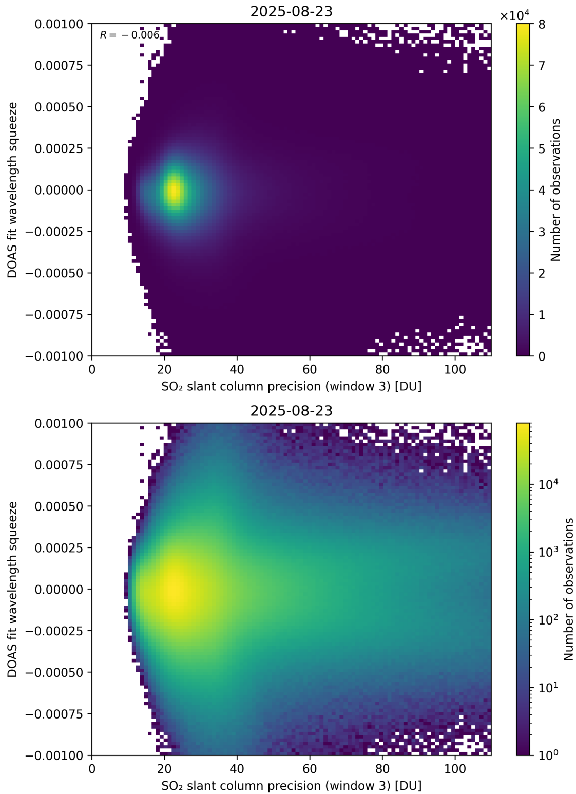
Figure 309: Scatter density plot of “SO 2 slant column precision (window 3)” against “DOAS fit wavelength squeeze” for 2025-08-22 to 2025-08-24.
