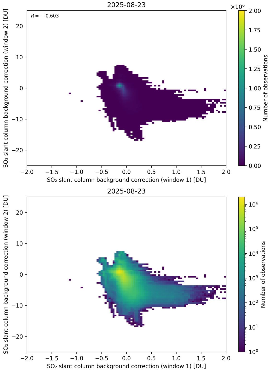
Figure 109: Scatter density plot of “SO 2 slant column background correction (window 1)” against “SO 2 slant column background correction (window 2)” for 2025-08-22 to 2025-08-24.
