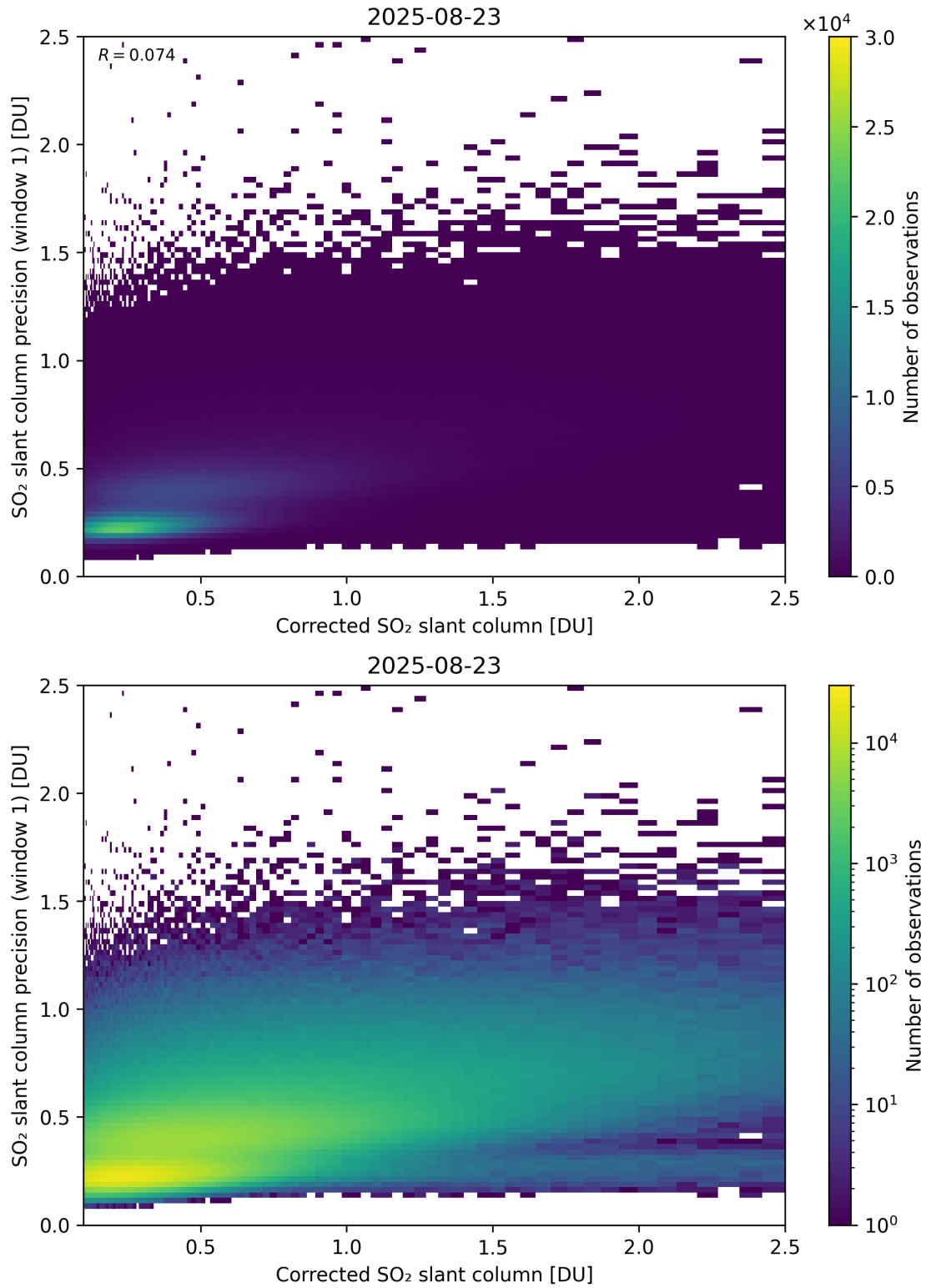
Figure 238: Scatter density plot of “Corrected SO 2 slant column” against “SO 2 slant column precision (window 1)” for 2025-08-22 to 2025-08-24.
