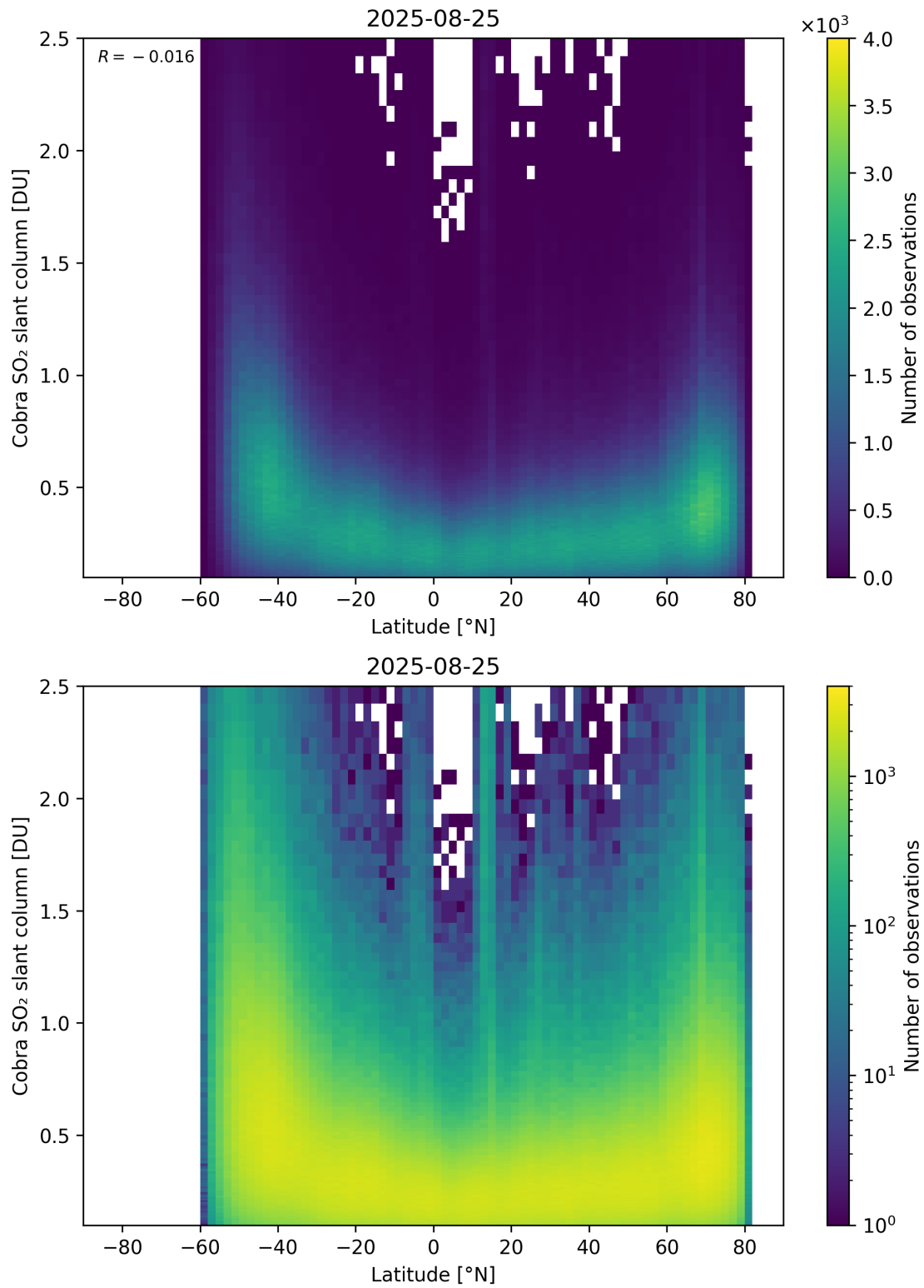
Figure 157: Scatter density plot of “Latitude” against “Cobra SO 2 slant column” for 2025-08-25 to 2025-08-26.
