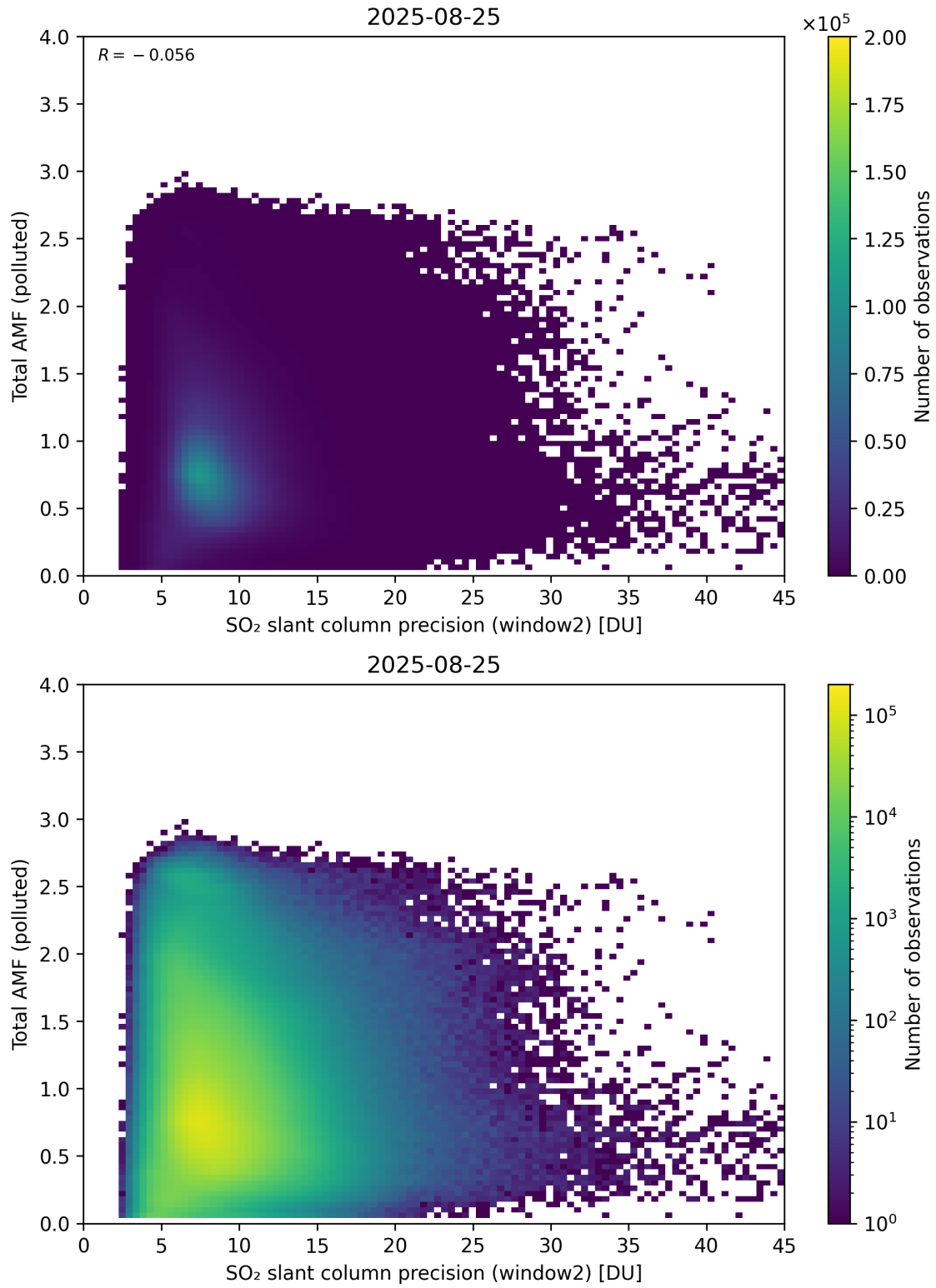
Figure 301: Scatter density plot of “SO 2 slant column precision (window2)” against “Total AMF (polluted)” for 2025-08-25 to 2025-08-26.
