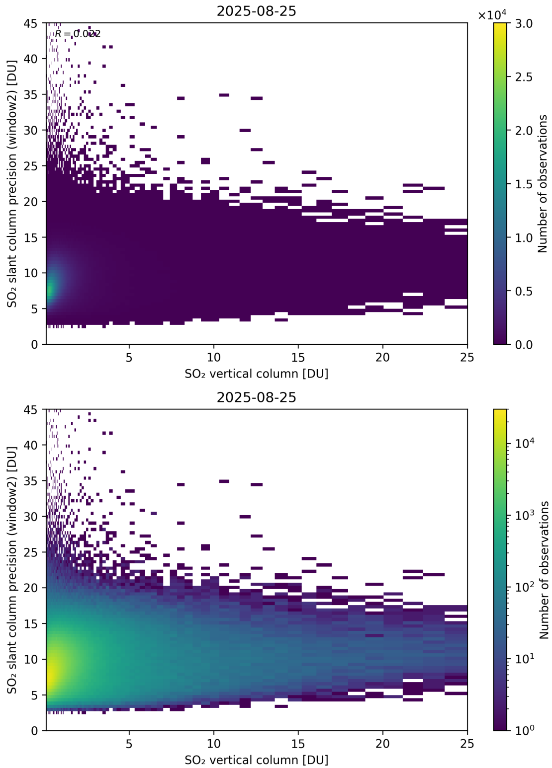
Figure 356: Scatter density plot of “SO 2 vertical column” against “SO 2 slant column precision (window2)” for 2025-08-25 to 2025-08-26.
