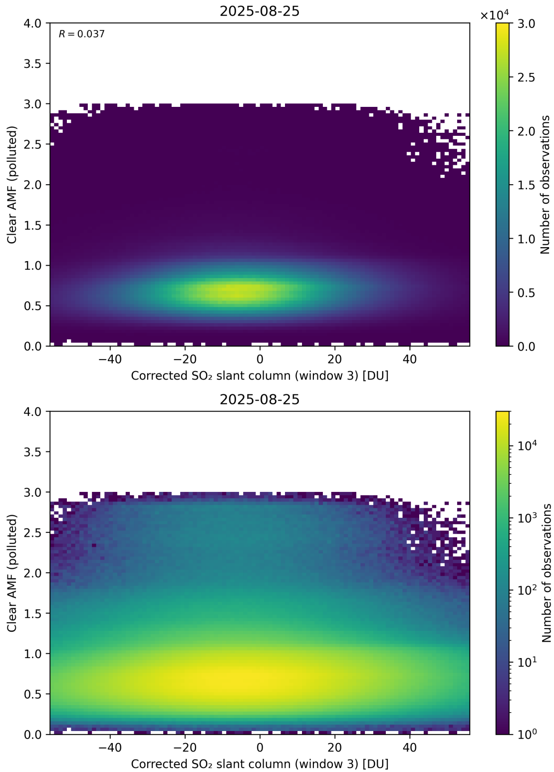
Figure 259: Scatter density plot of “Corrected SO 2 slant column (window 3)” against “Clear AMF (polluted)” for 2025-08-25 to 2025-08-26.
