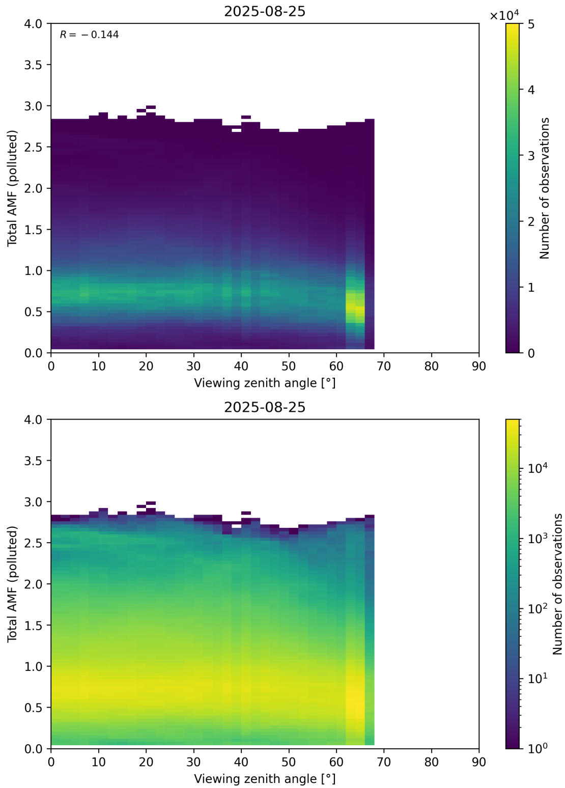
Figure 381: Scatter density plot of “Viewing zenith angle” against “Total AMF (polluted)” for 2025-08-25 to 2025-08-26.
