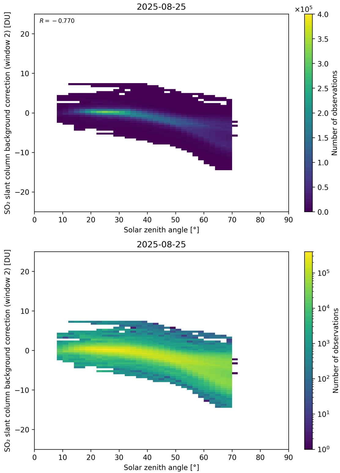
Figure 172: Scatter density plot of “Solar zenith angle” against “SO 2 slant column background correction (window 2)” for 2025-08-25 to 2025-08-26.
