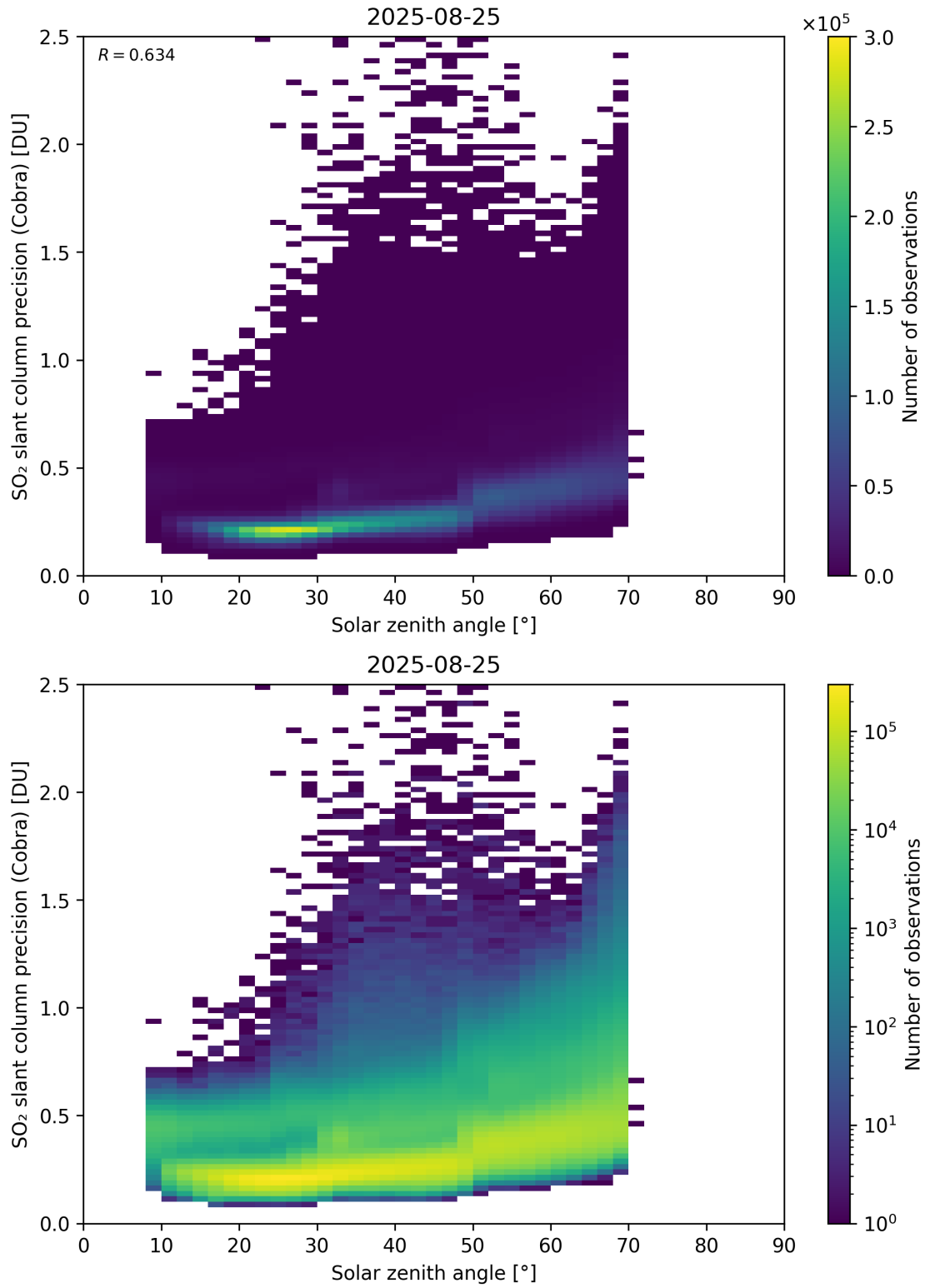
Figure 180: Scatter density plot of “Solar zenith angle” against “SO 2 slant column precision (Cobra)” for 2025-08-25 to 2025-08-26.
