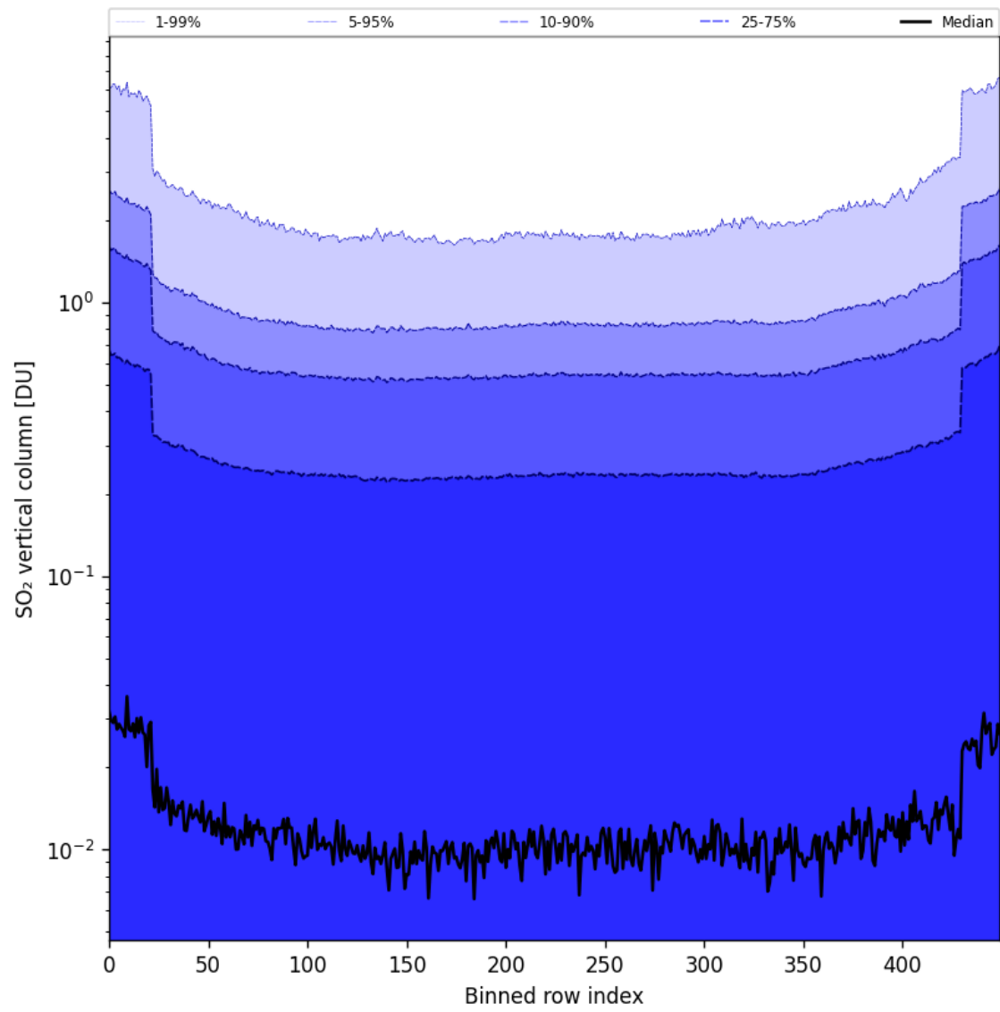
Figure 84: Along track statistics of “SO 2 vertical column” for 2025-08-25 to 2025-08-26
