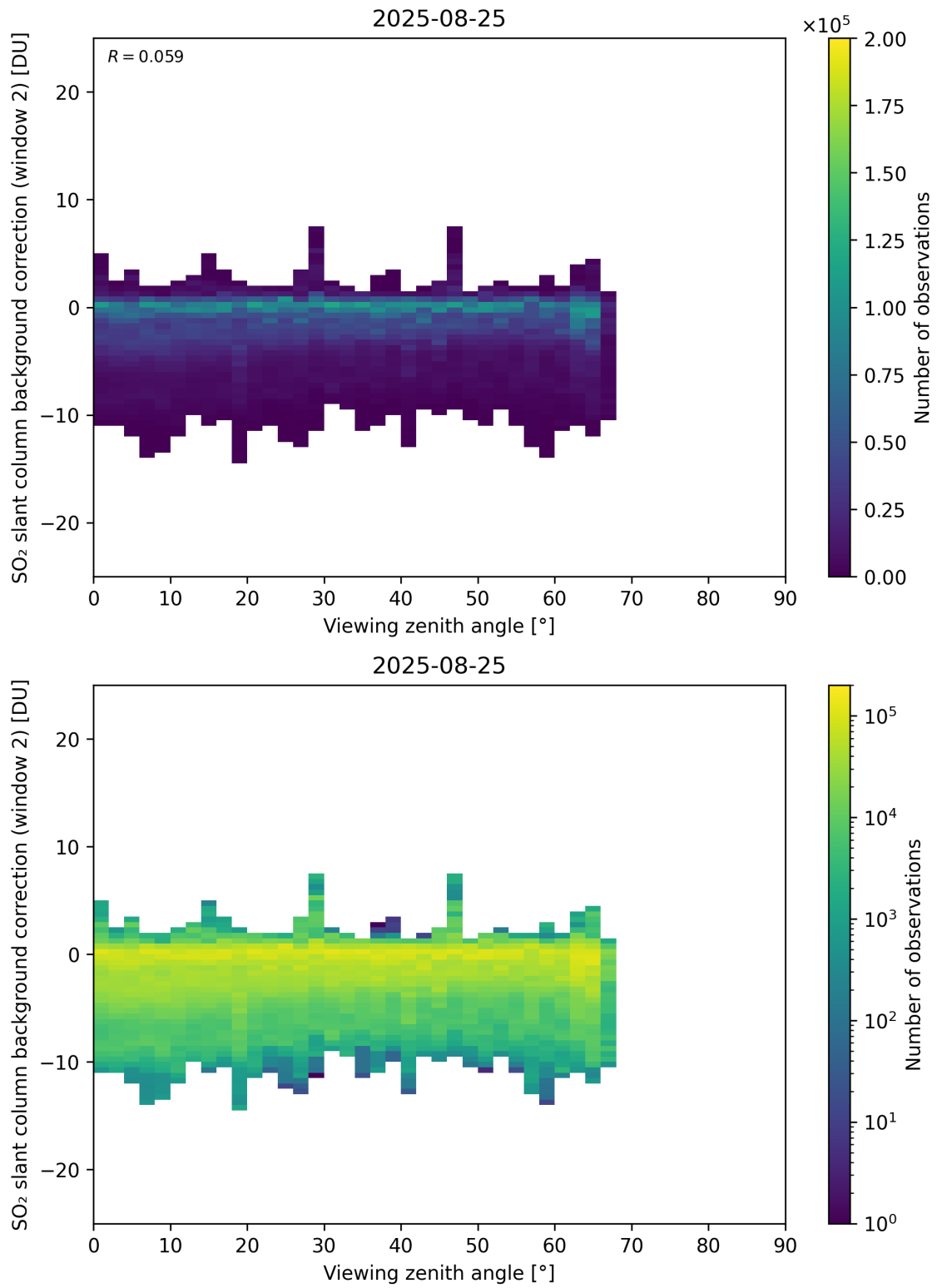
Figure 363: Scatter density plot of “Viewing zenith angle” against “SO 2 slant column background correction (window 2)” for 2025-08-25 to 2025-08-26.
