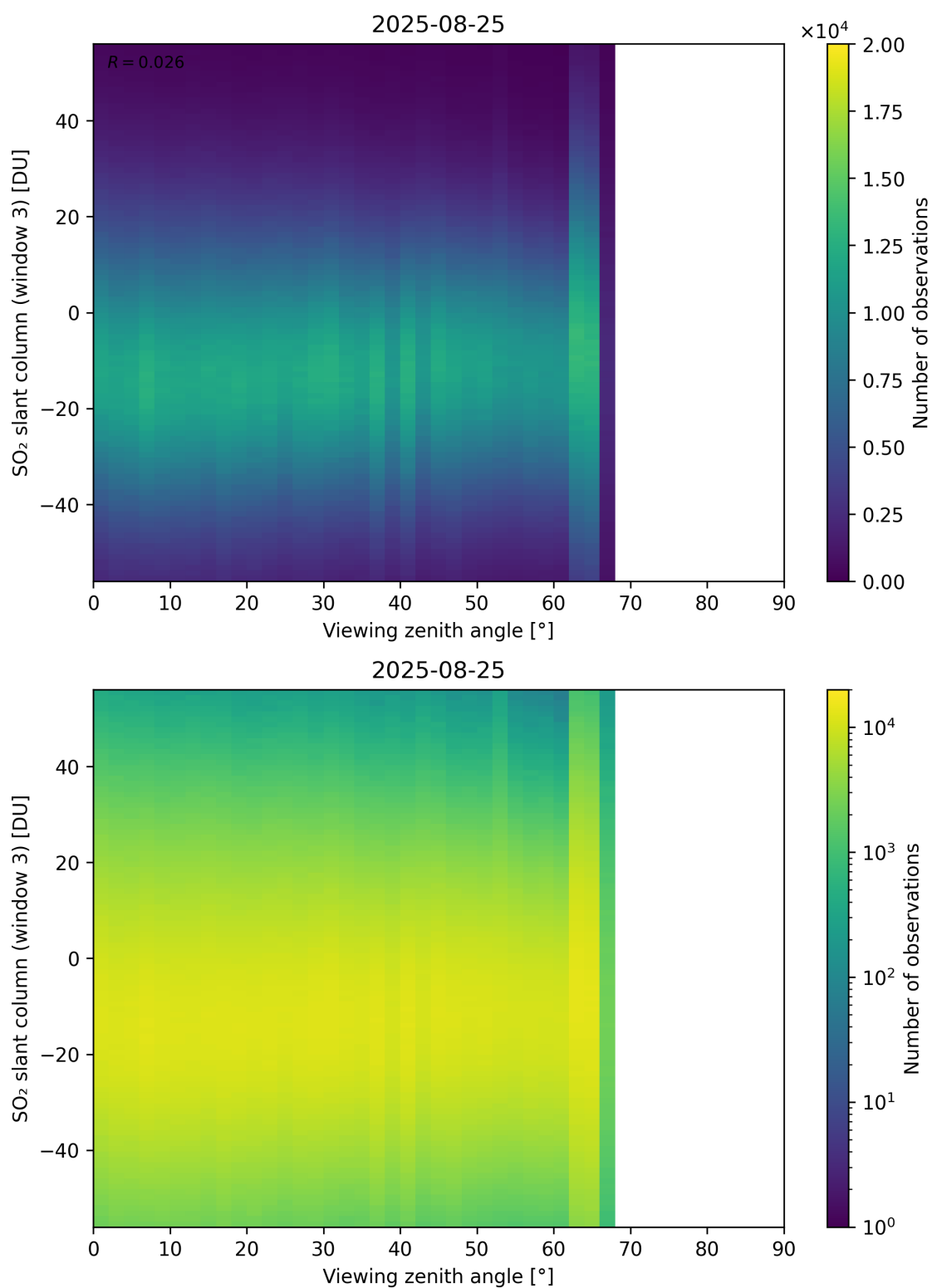
Figure 379: Scatter density plot of “Viewing zenith angle” against “SO 2 slant column (window 3)” for 2025-08-25 to 2025-08-26.
