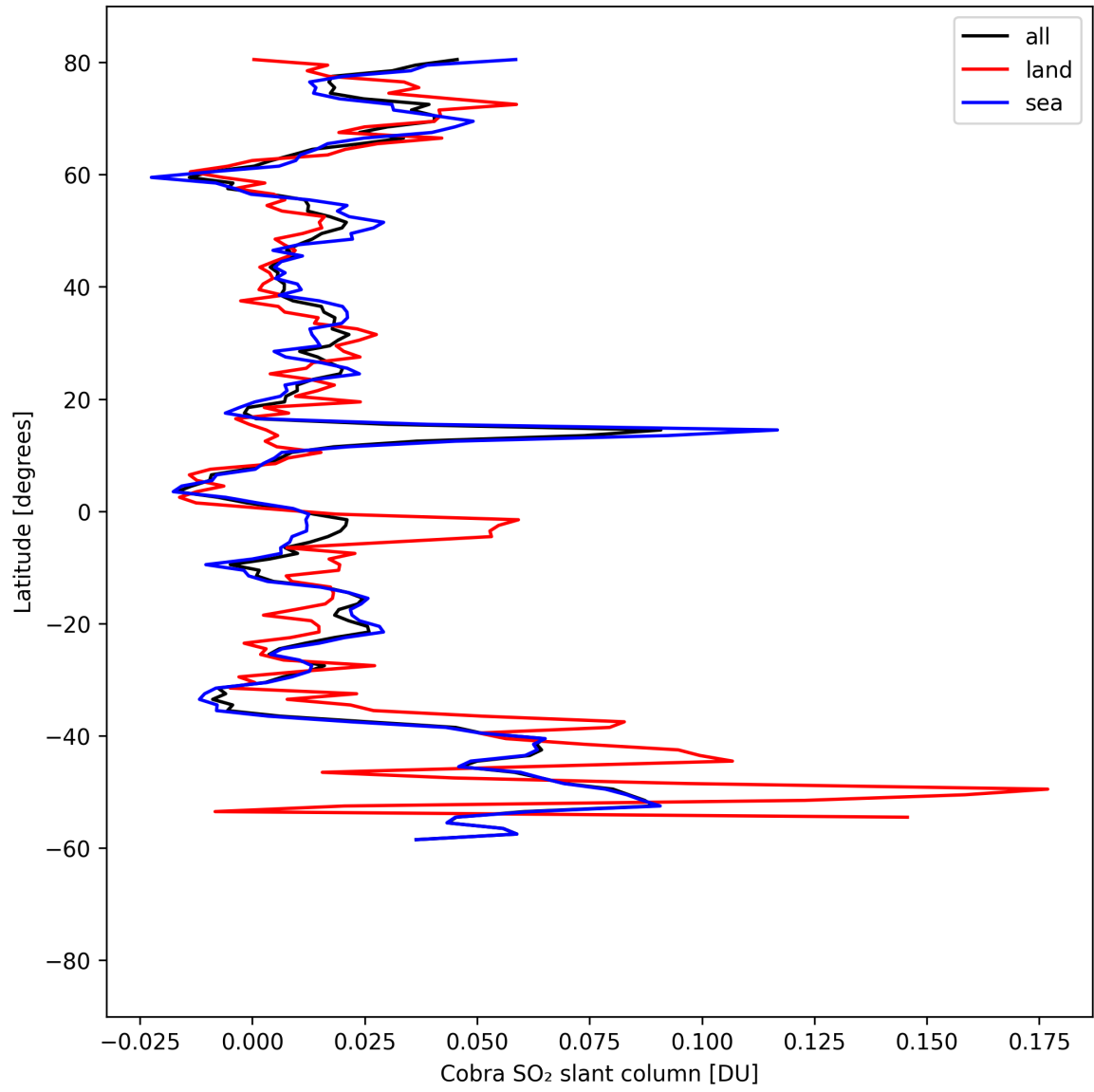
Figure 35: Zonal average of “Cobra SO 2 slant column” for 2025-08-25 to 2025-08-26.
