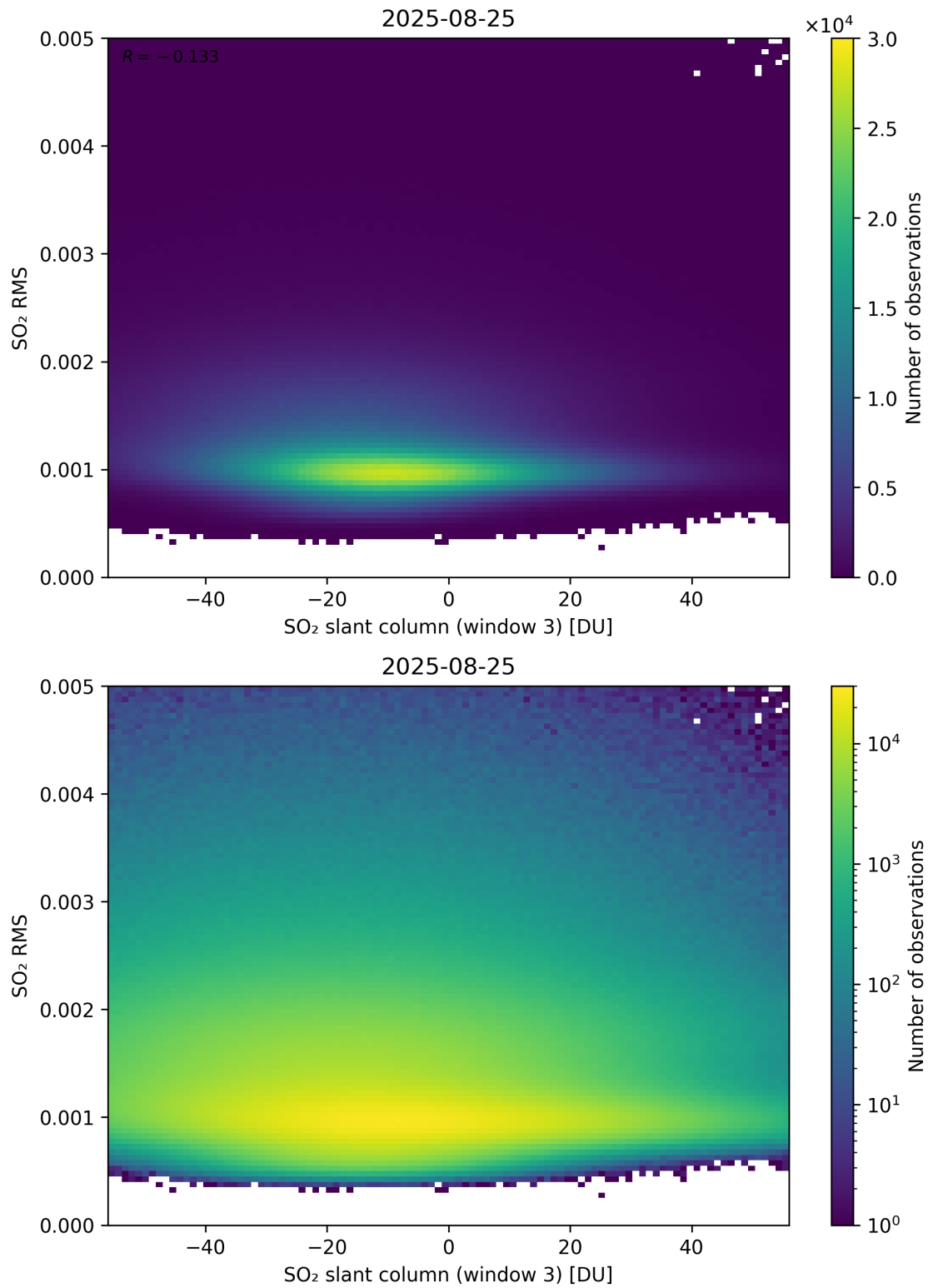
Figure 306: Scatter density plot of “SO 2 slant column (window 3)” against “SO 2 RMS” for 2025-08-25 to 2025-08-26.
