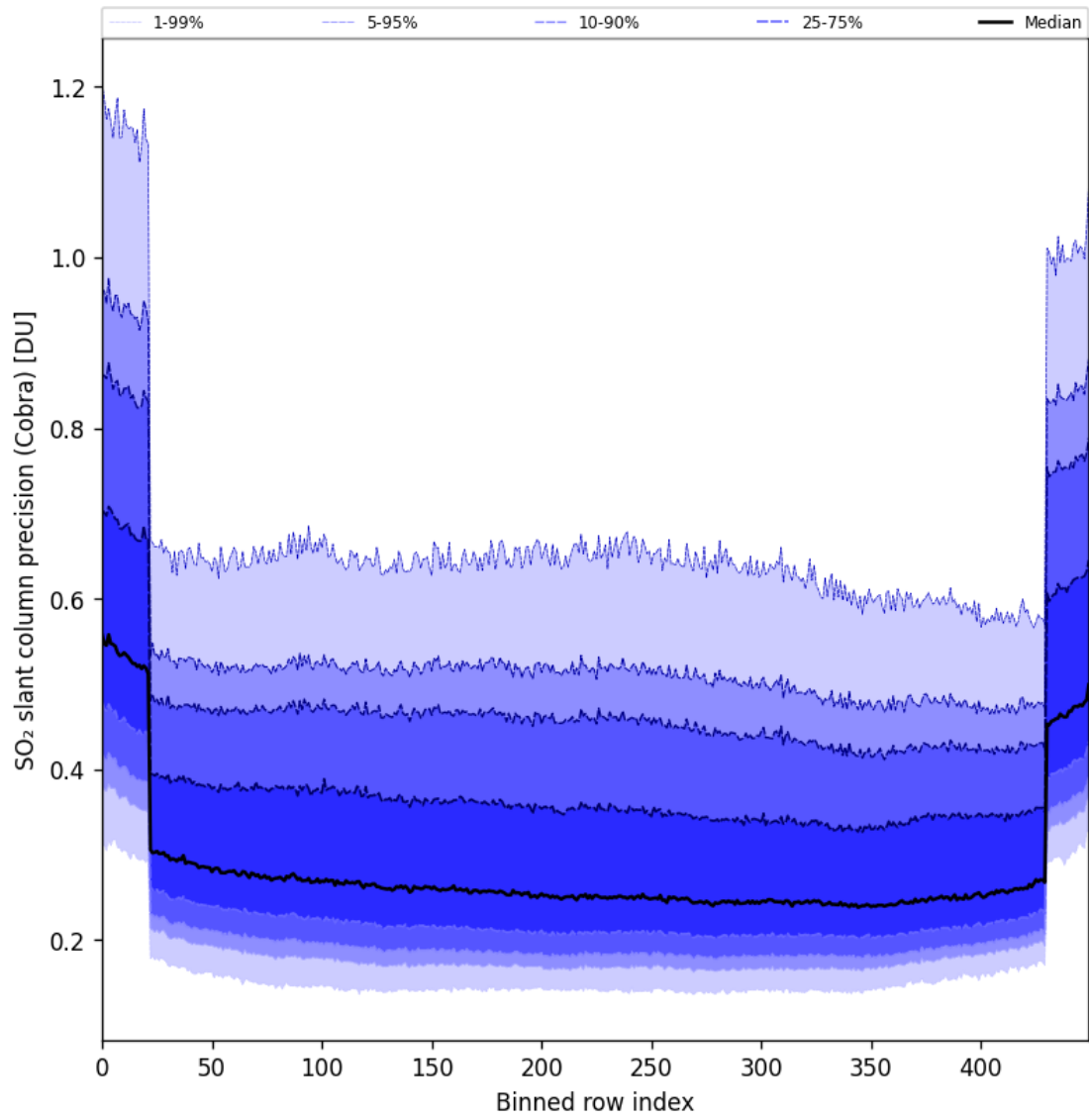
Figure 88: Along track statistics of “SO 2 slant column precision (Cobra)” for 2025-08-25 to 2025-08-26
