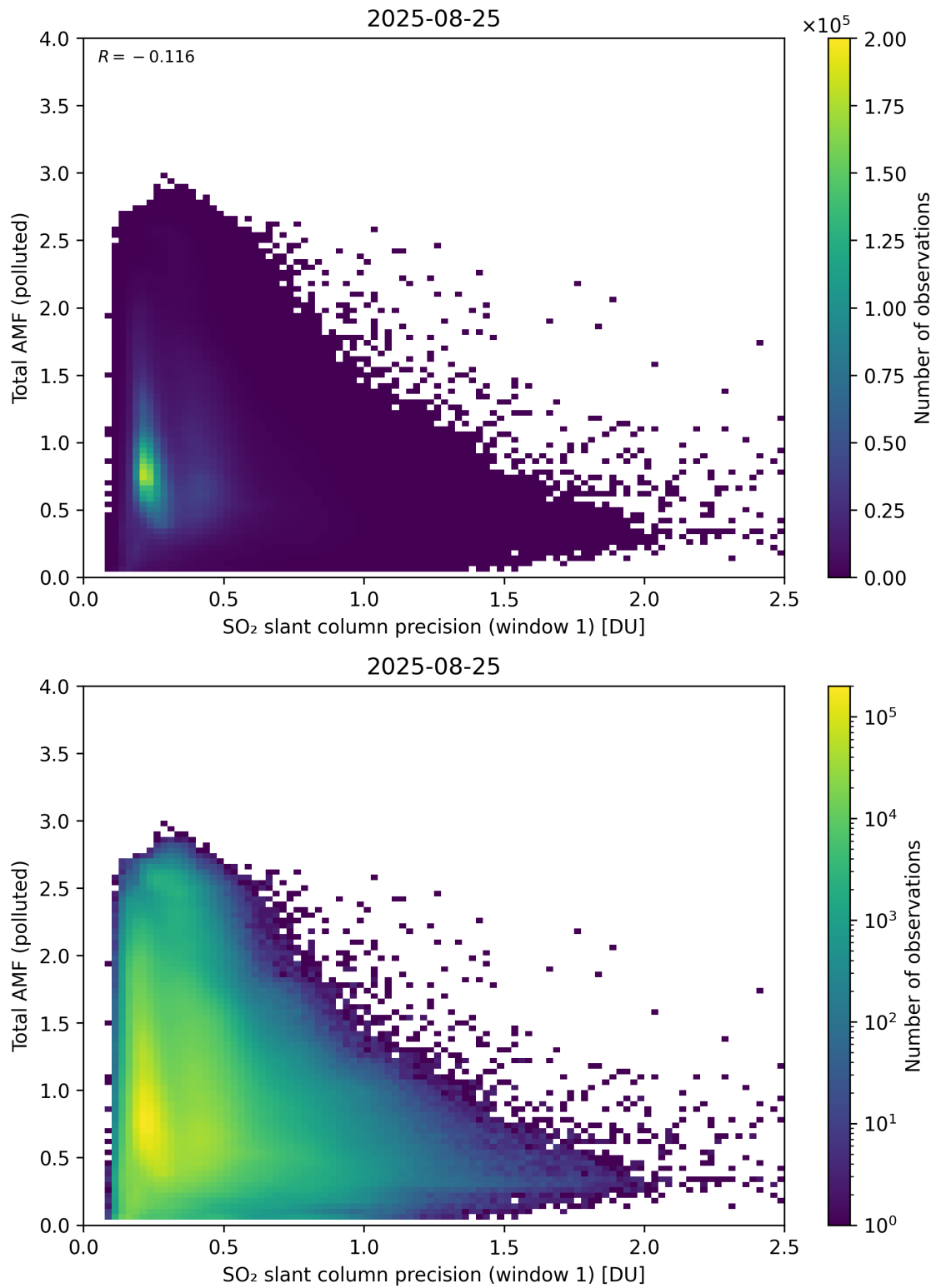
Figure 280: Scatter density plot of “SO 2 slant column precision (window 1)” against “Total AMF (polluted)” for 2025-08-25 to 2025-08-26.
