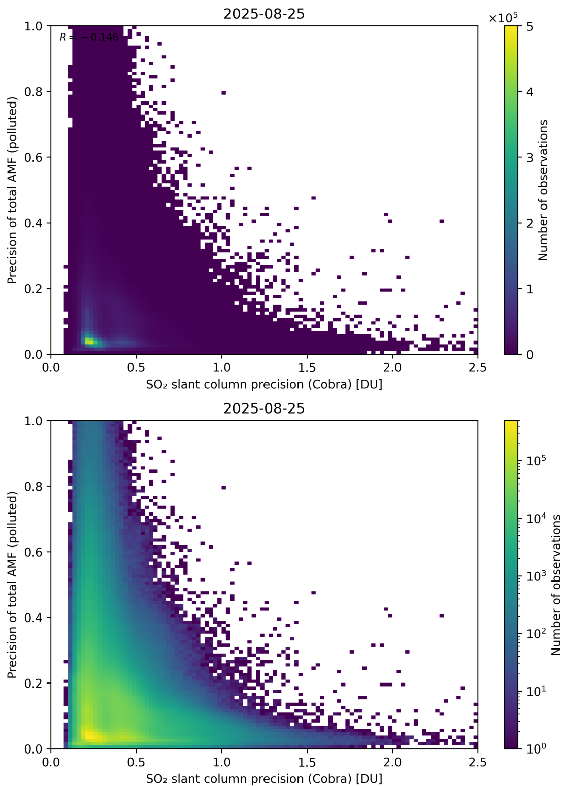
Figure 214: Scatter density plot of “SO 2 slant column precision (Cobra)” against “Precision of total AMF (polluted)” for 2025-08-25 to 2025-08-26.
