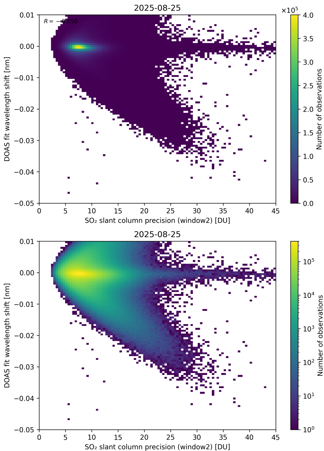
Figure 293: Scatter density plot of “SO 2 slant column precision (window2)” against “DOAS fit wavelength shift” for 2025-08-25 to 2025-08-26.
