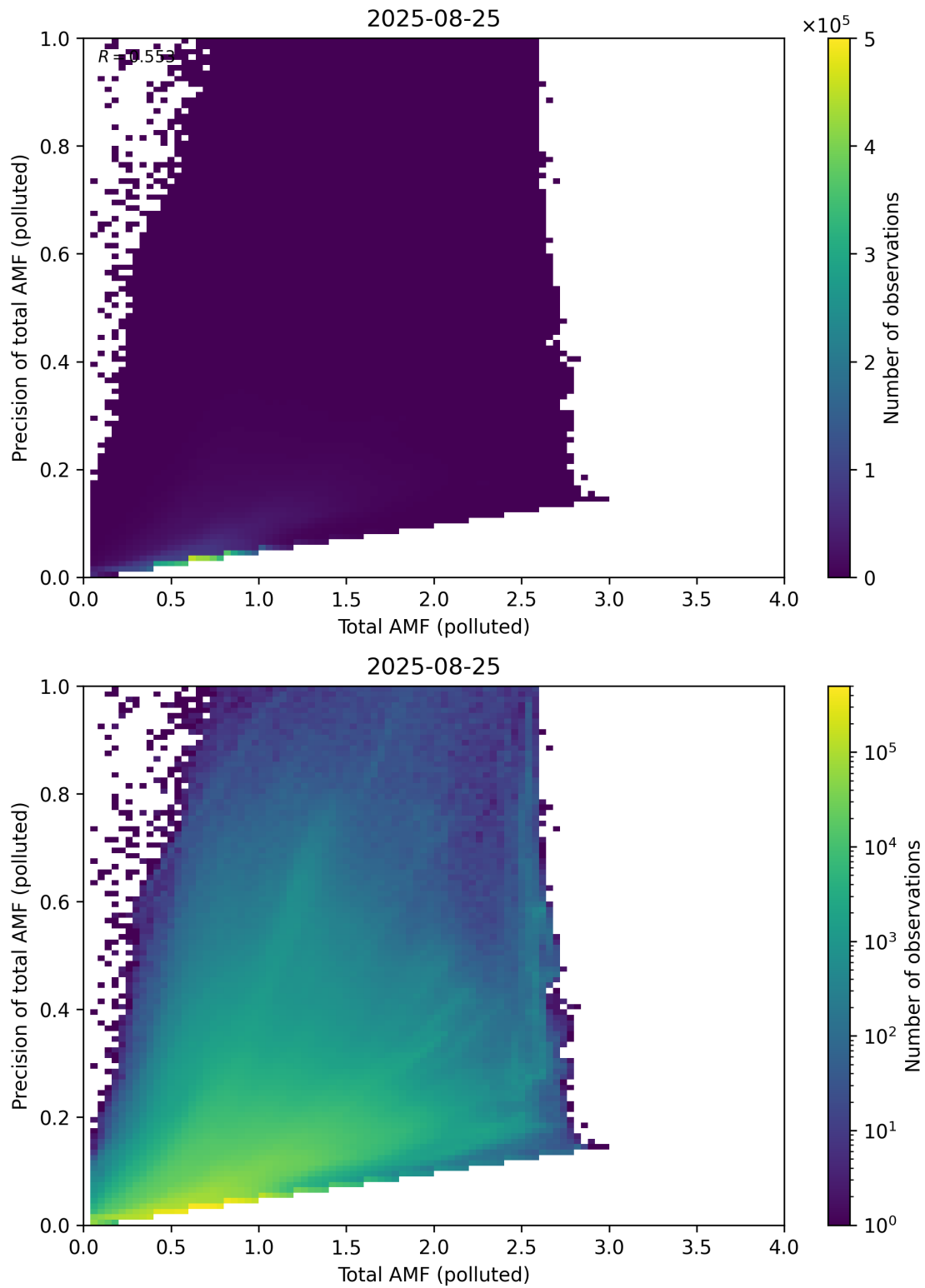
Figure 322: Scatter density plot of “Total AMF (polluted)” against “Precision of total AMF (polluted)” for 2025-08-25 to 2025-08-26.
