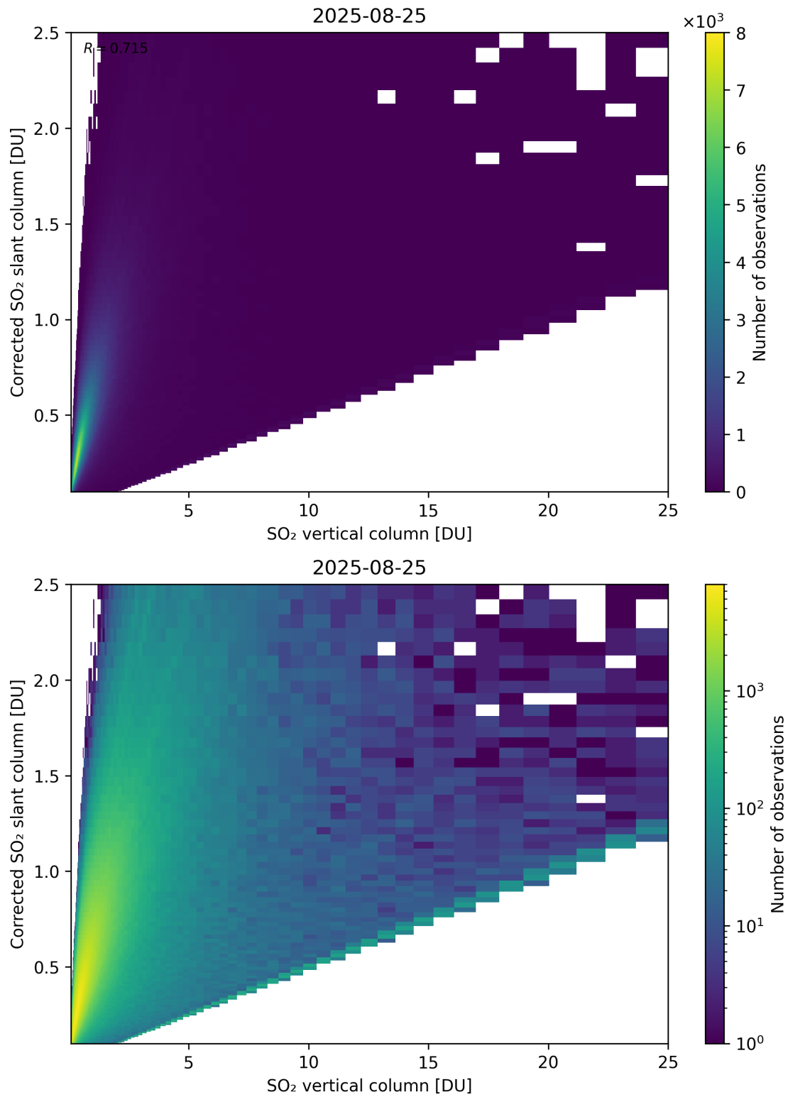
Figure 351: Scatter density plot of “SO 2 vertical column” against “Corrected SO 2 slant column” for 2025-08-25 to 2025-08-26.
