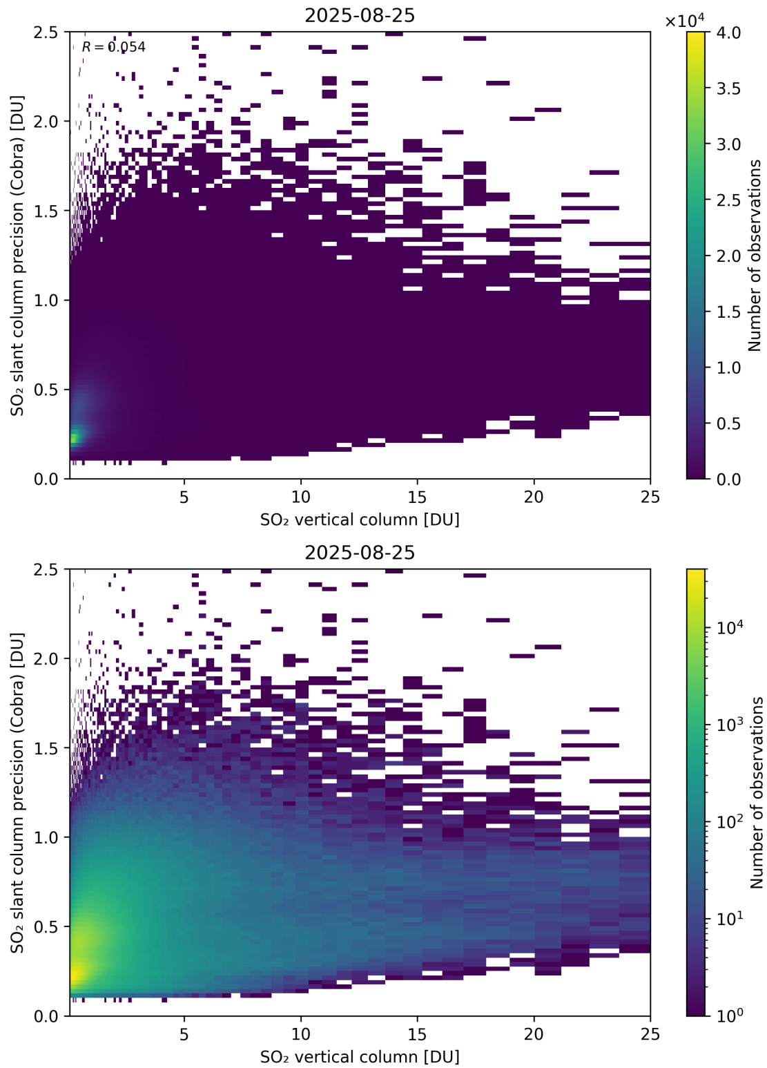
Figure 350: Scatter density plot of “SO 2 vertical column” against “SO 2 slant column precision (Cobra)” for 2025-08-25 to 2025-08-26.
