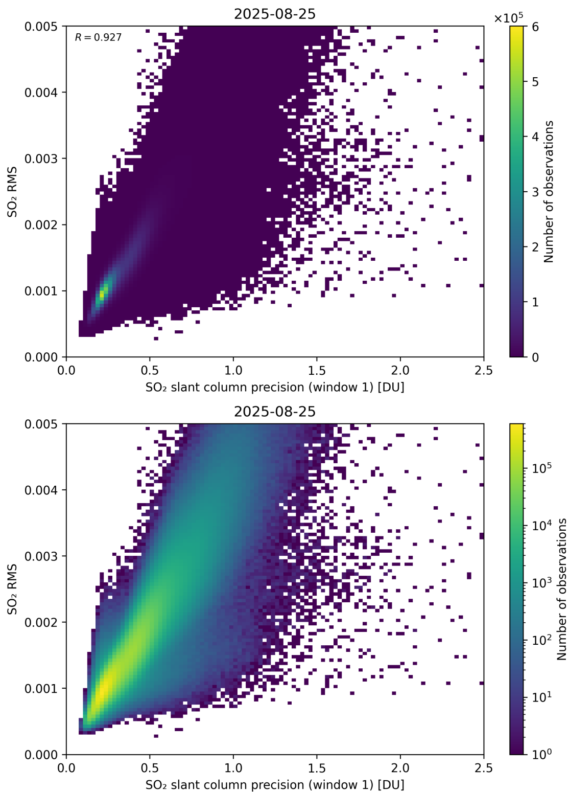
Figure 273: Scatter density plot of “SO 2 slant column precision (window 1)” against “SO 2 RMS” for 2025-08-25 to 2025-08-26.
