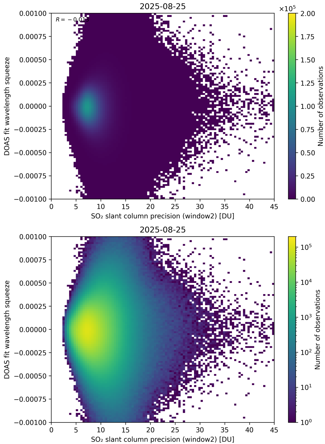
Figure 294: Scatter density plot of “SO 2 slant column precision (window2)” against “DOAS fit wavelength squeeze” for 2025-08-25 to 2025-08-26.
