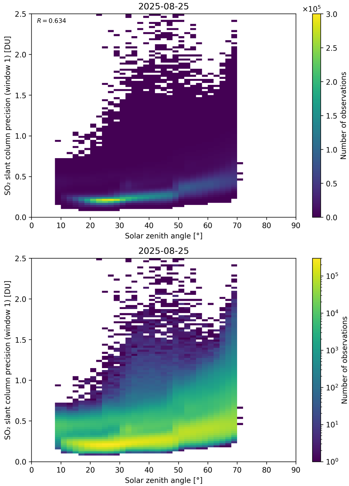
Figure 185: Scatter density plot of “Solar zenith angle” against “SO 2 slant column precision (window 1)” for 2025-08-25 to 2025-08-26.
