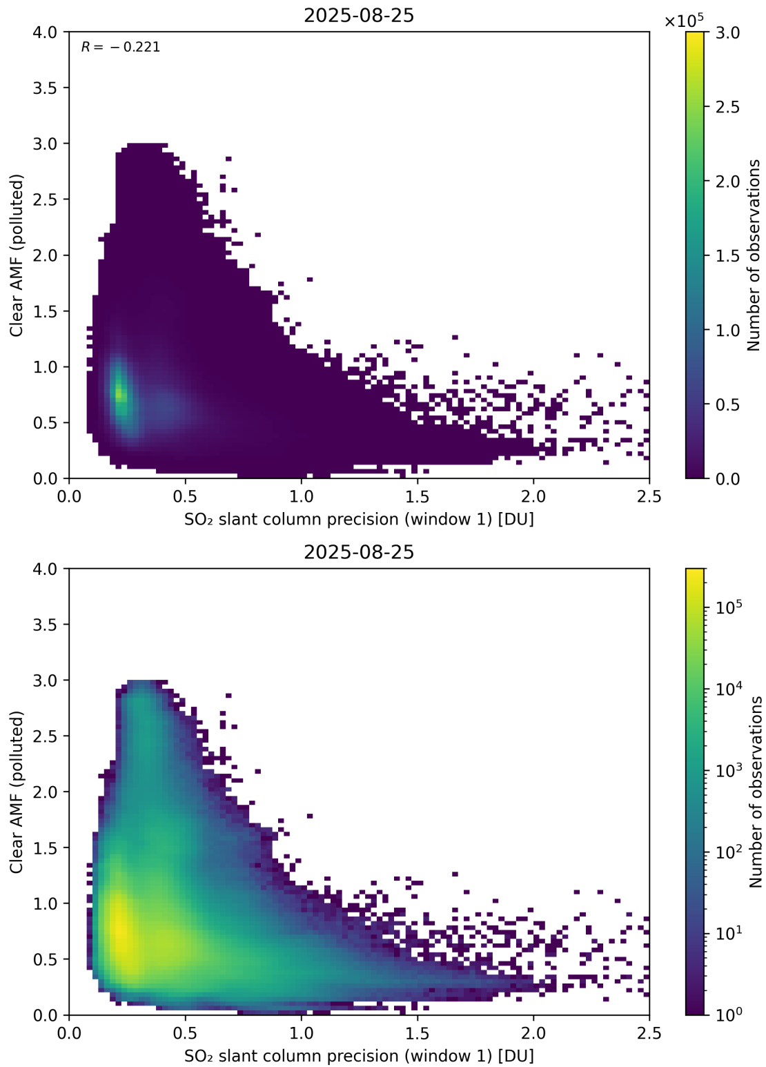
Figure 274: Scatter density plot of “SO 2 slant column precision (window 1)” against “Clear AMF (polluted)” for 2025-08-25 to 2025-08-26.
