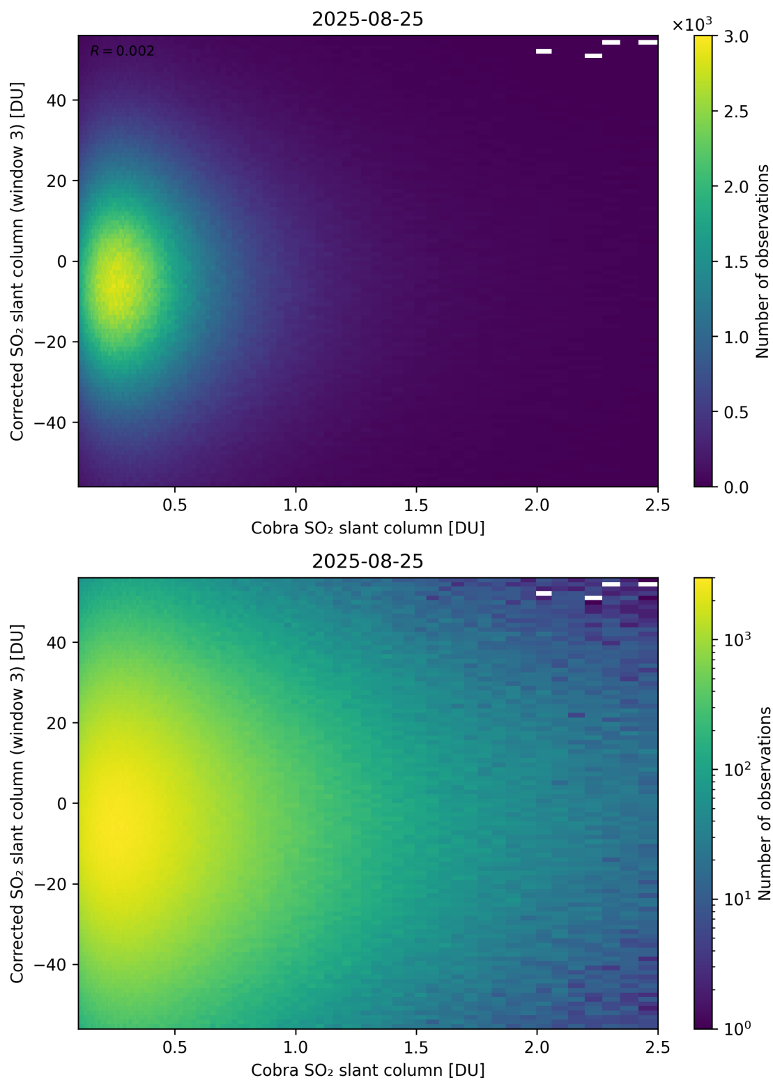
Figure 218: Scatter density plot of “Cobra SO 2 slant column” against “Corrected SO 2 slant column (window 3)” for 2025-08-25 to 2025-08-26.
