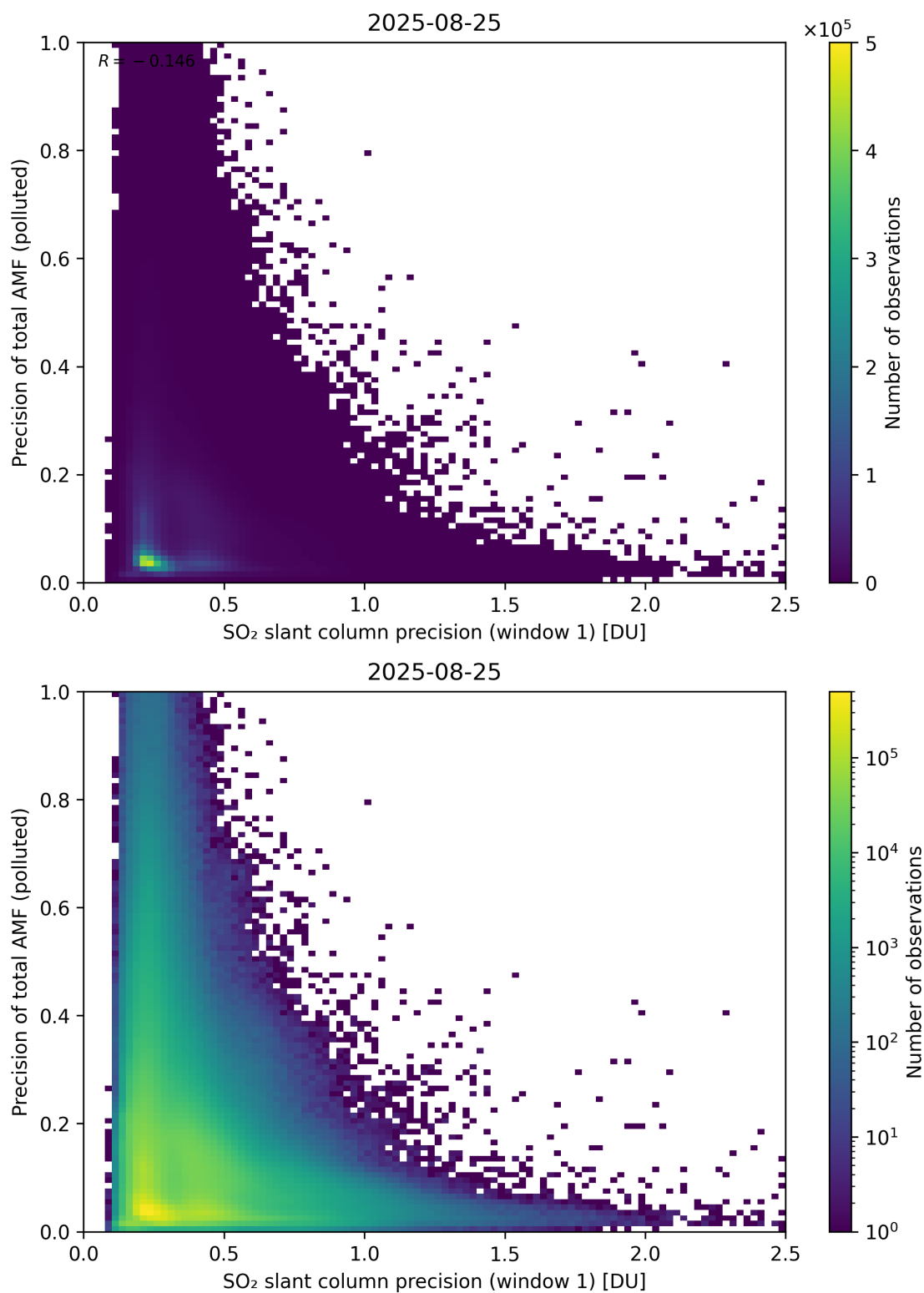
Figure 281: Scatter density plot of “SO 2 slant column precision (window 1)” against “Precision of total AMF (polluted)” for 2025-08-25 to 2025-08-26.
