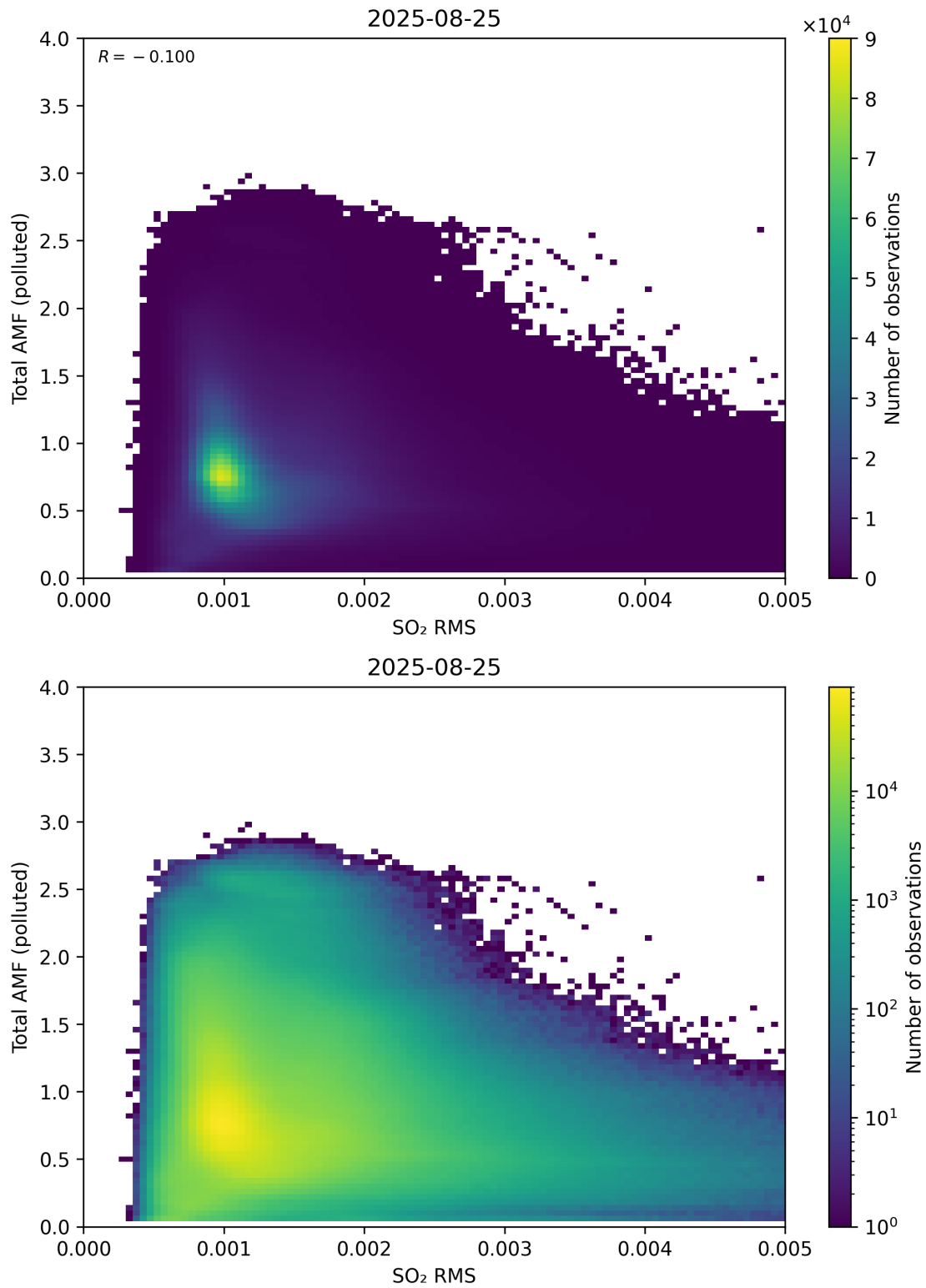
Figure 148: Scatter density plot of “SO 2 RMS” against “Total AMF (polluted)” for 2025-08-25 to 2025-08-26.
