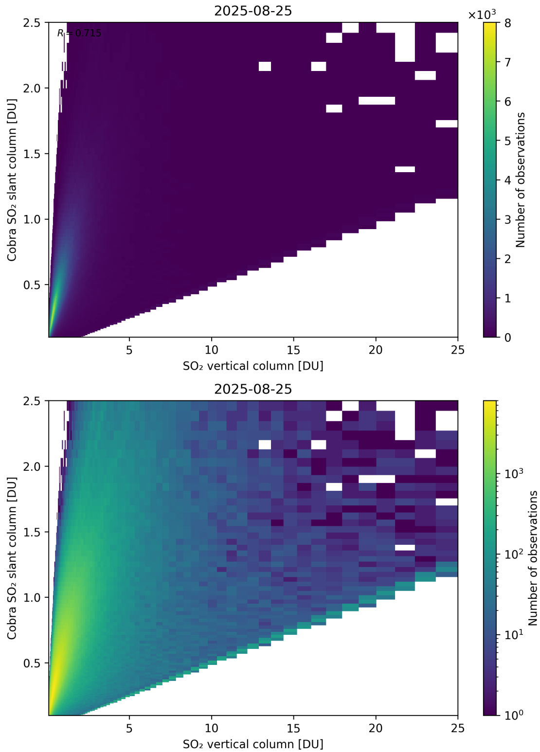
Figure 349: Scatter density plot of “SO 2 vertical column” against “Cobra SO 2 slant column” for 2025-08-25 to 2025-08-26.
