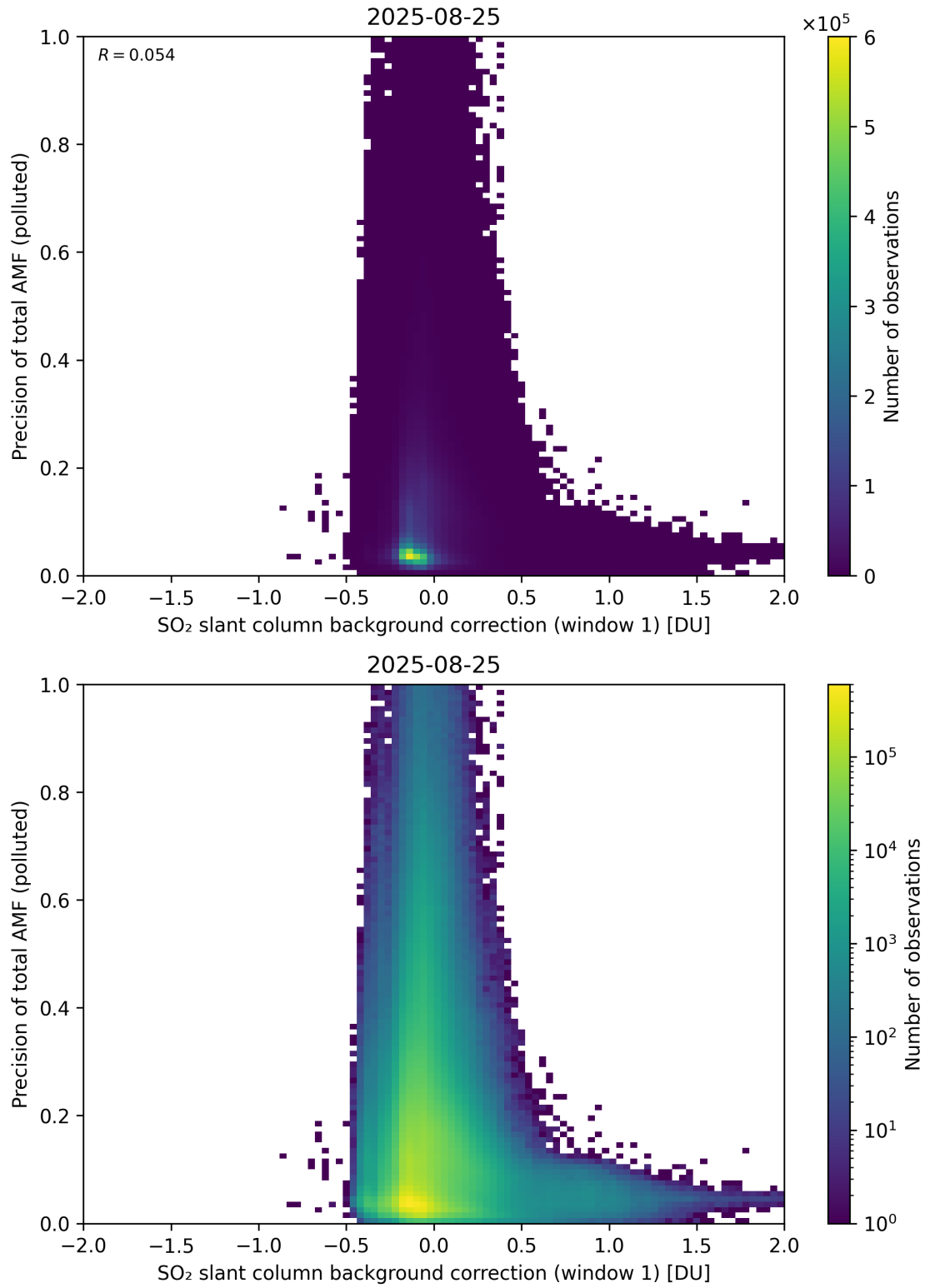
Figure 121: Scatter density plot of “SO 2 slant column background correction (window 1)” against “Precision of total AMF (polluted)” for 2025-08-25 to 2025-08-26.
