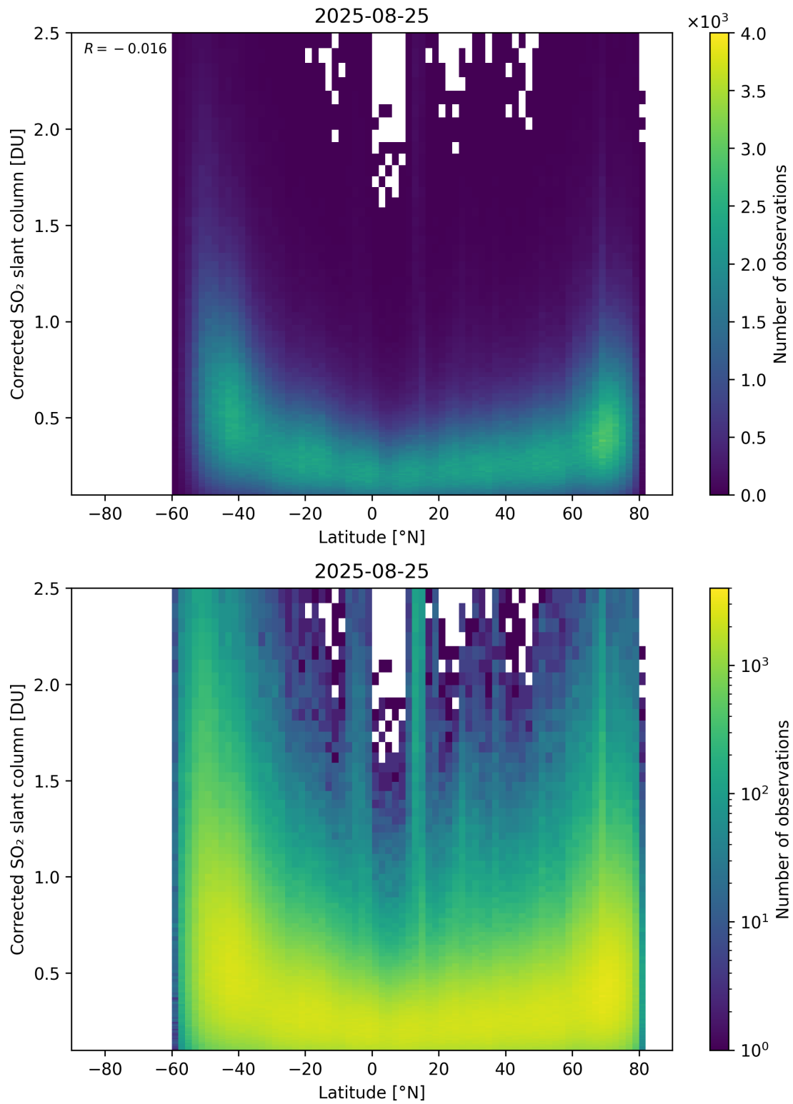
Figure 159: Scatter density plot of “Latitude” against “Corrected SO 2 slant column” for 2025-08-25 to 2025-08-26.
