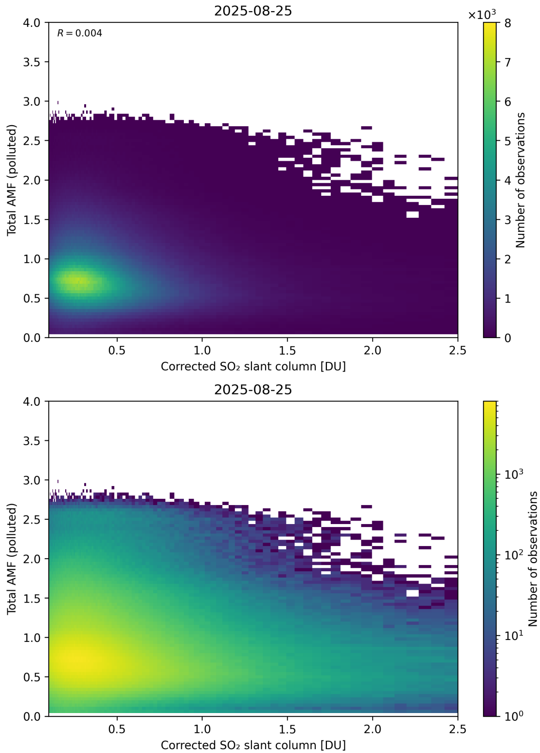
Figure 242: Scatter density plot of “Corrected SO 2 slant column” against “Total AMF (polluted)” for 2025-08-25 to 2025-08-26.
