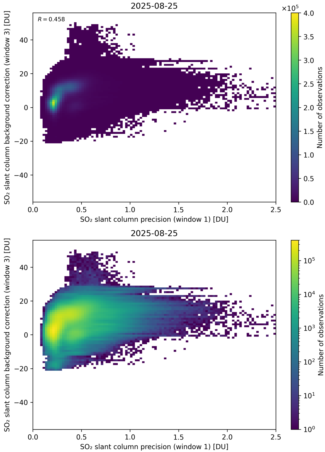
Figure 270: Scatter density plot of “SO 2 slant column precision (window 1)” against “SO 2 slant column background correction (window 3)” for 2025-08-25 to 2025-08-26.
