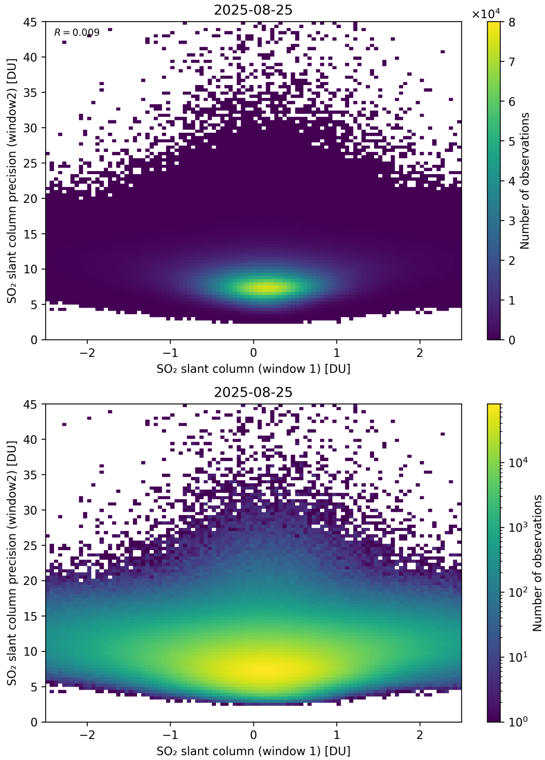
Figure 286: Scatter density plot of “SO 2 slant column (window 1)” against “SO 2 slant column precision (window2)” for 2025-08-25 to 2025-08-26.
