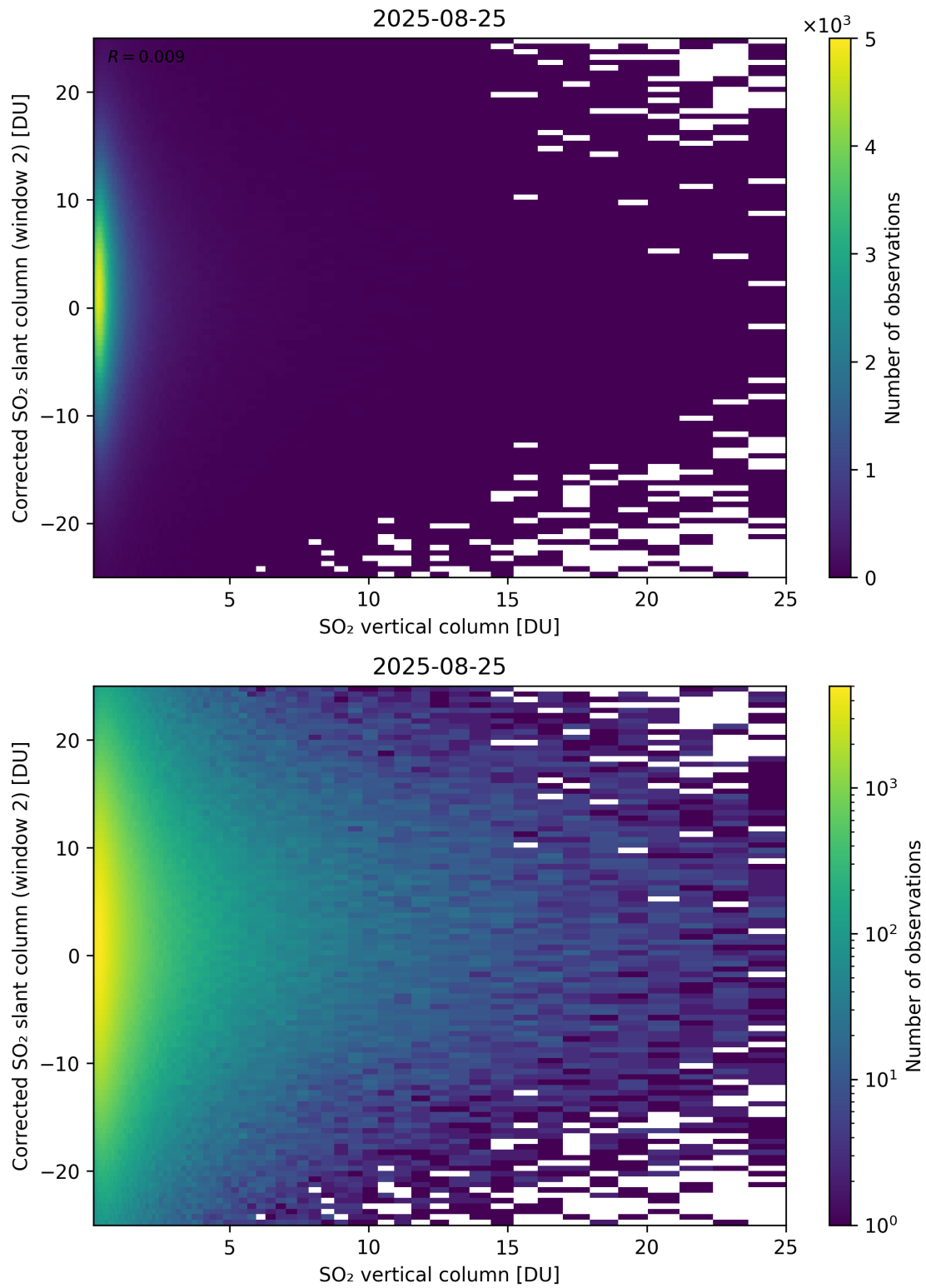
Figure 352: Scatter density plot of “SO 2 vertical column” against “Corrected SO 2 slant column (window 2)” for 2025-08-25 to 2025-08-26.
