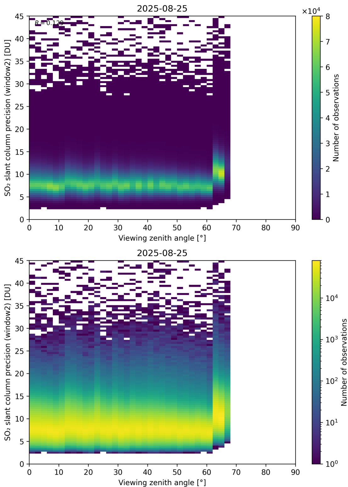
Figure 378: Scatter density plot of “Viewing zenith angle” against “SO 2 slant column precision (window2)” for 2025-08-25 to 2025-08-26.
