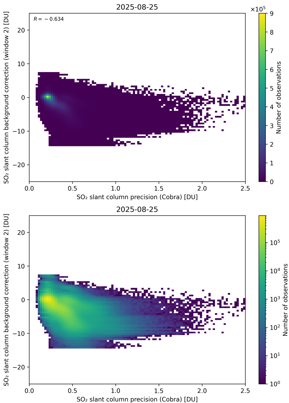
Figure 200: Scatter density plot of “SO 2 slant column precision (Cobra)” against “SO 2 slant column background correction (window 2)” for 2025-08-25 to 2025-08-26.
