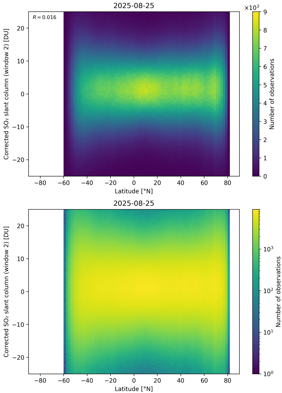
Figure 160: Scatter density plot of “Latitude” against “Corrected SO 2 slant column (window 2)” for 2025-08-25 to 2025-08-26.
