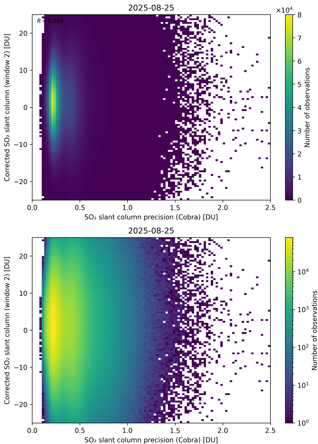
Figure 206: Scatter density plot of “SO 2 slant column precision (Cobra)” against “Corrected SO 2 slant column (window 2)” for 2025-08-25 to 2025-08-26.
