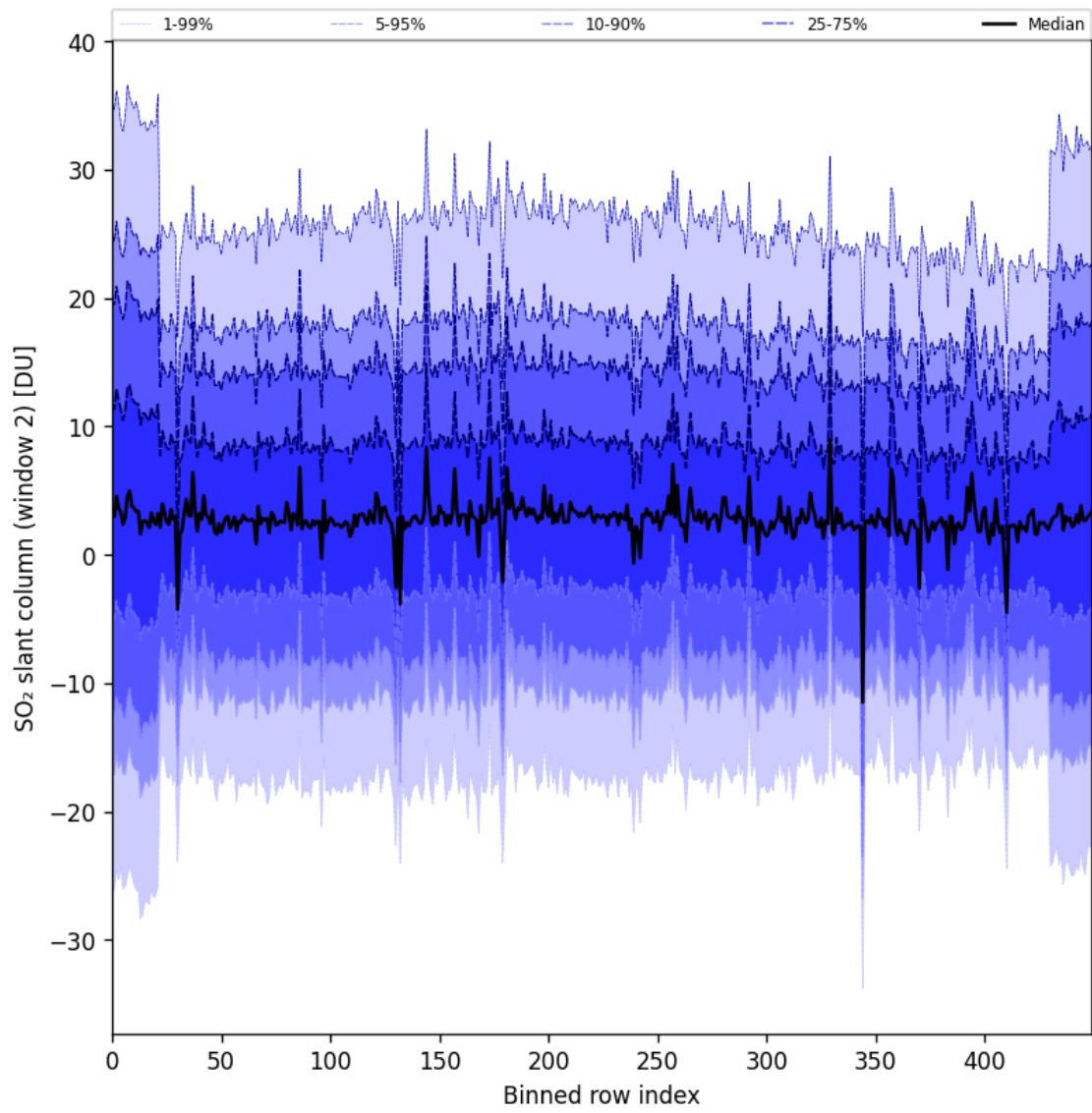
Figure 93: Along track statistics of “SO 2 slant column (window 2)” for 2025-08-25 to 2025-08-26
