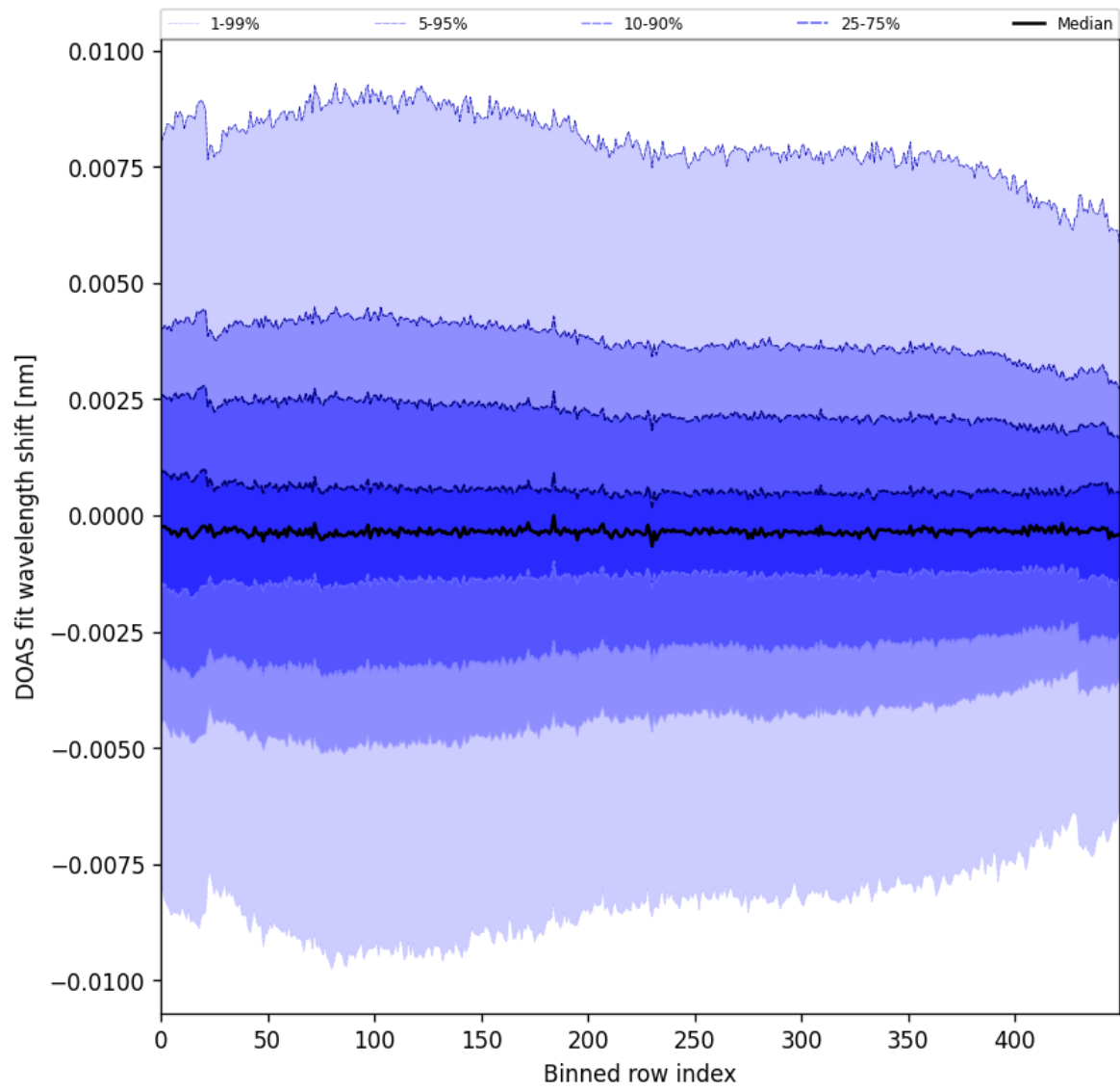
Figure 102: Along track statistics of “DOAS fit wavelength shift” for 2025-08-25 to 2025-08-26
