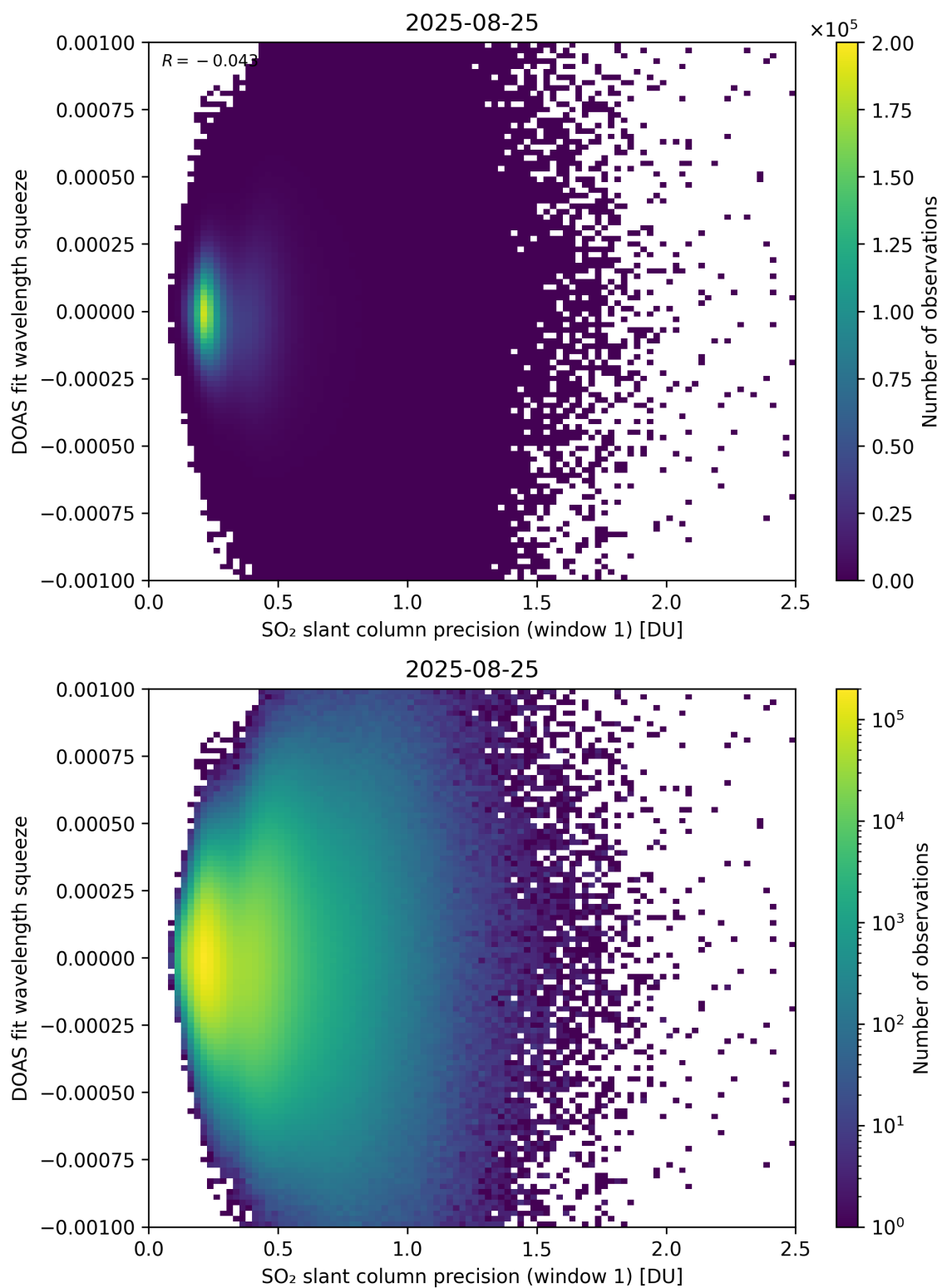
Figure 272: Scatter density plot of “SO 2 slant column precision (window 1)” against “DOAS fit wavelength squeeze” for 2025-08-25 to 2025-08-26.
