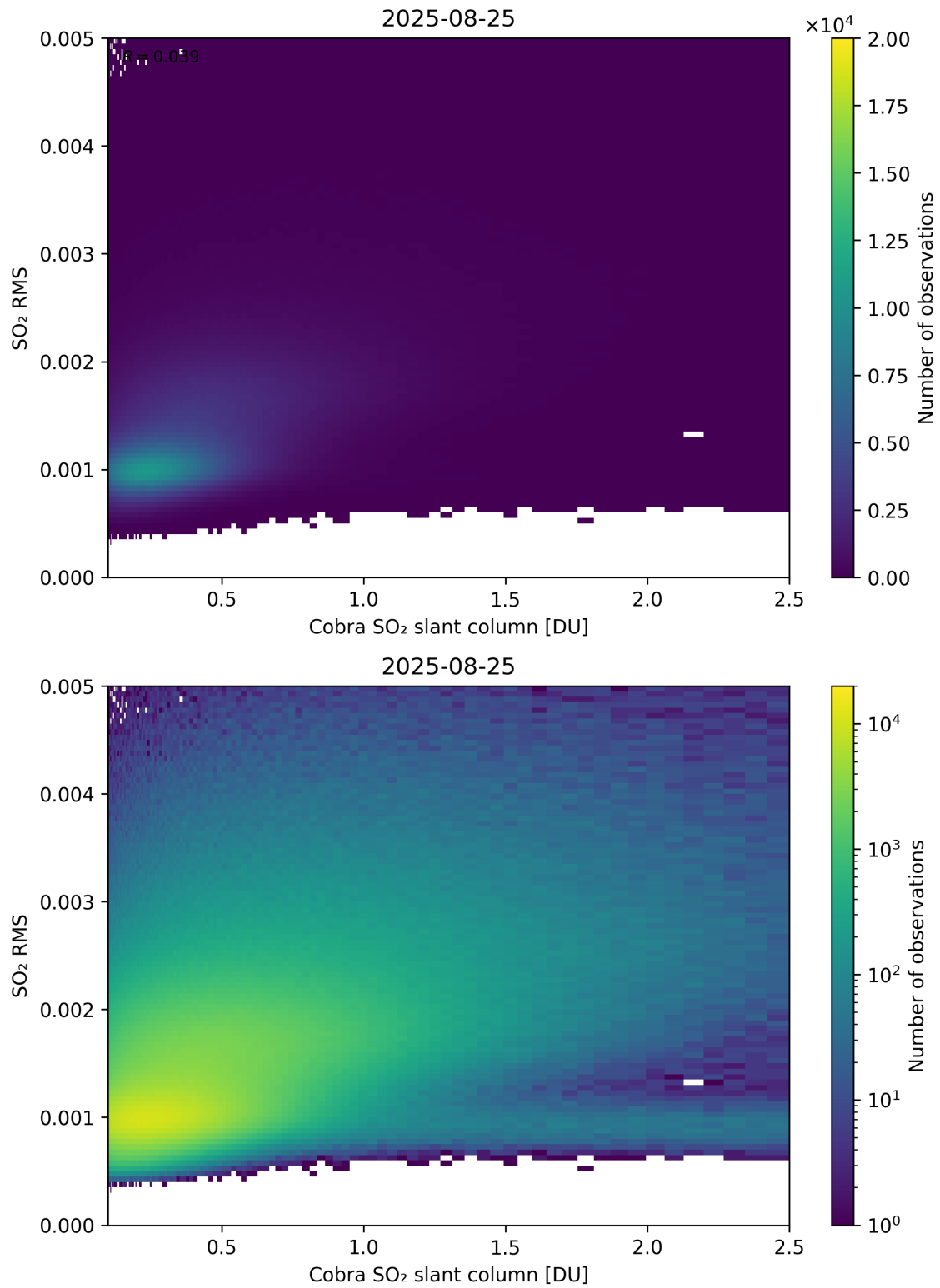
Figure 198: Scatter density plot of “Cobra SO 2 slant column” against “SO 2 RMS” for 2025-08-25 to 2025-08-26.
