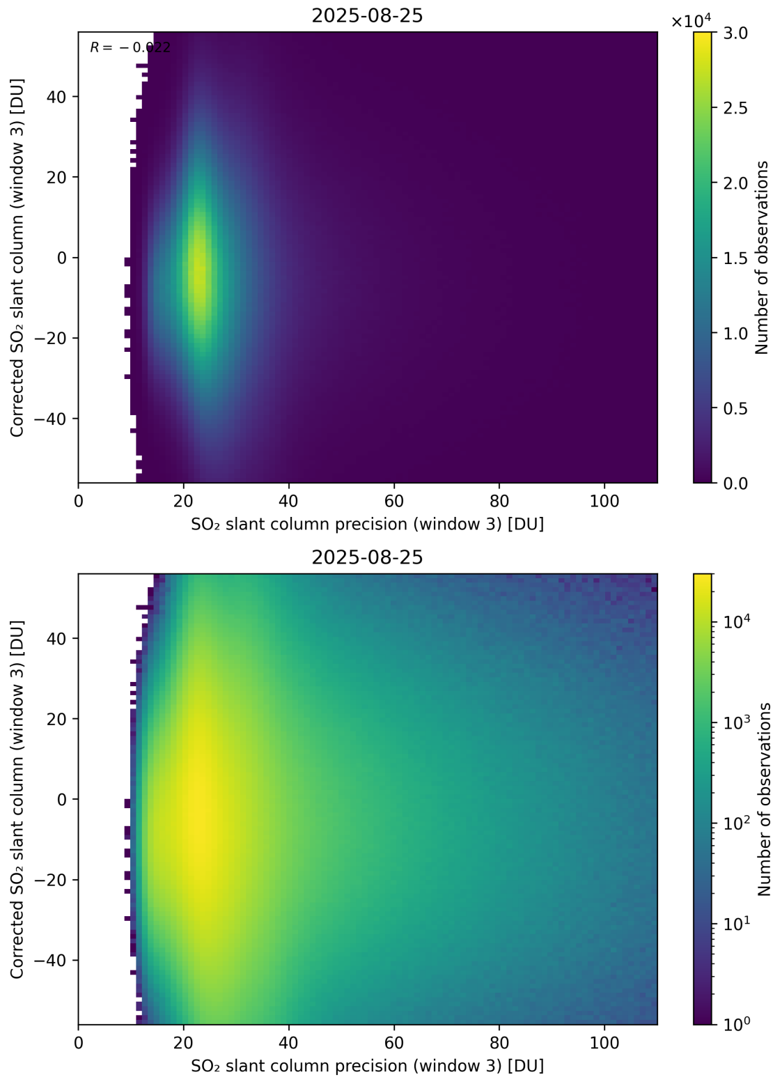
Figure 312: Scatter density plot of “SO 2 slant column precision (window 3)” against “Corrected SO 2 slant column (window 3)” for 2025-08-25 to 2025-08-26.
