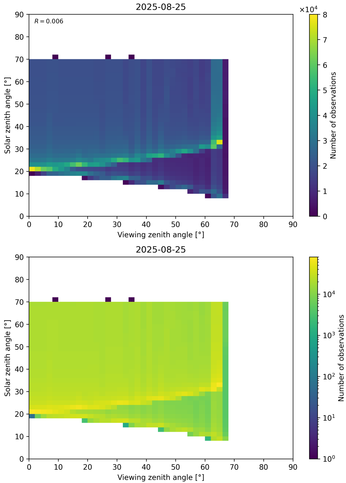
Figure 369: Scatter density plot of “Viewing zenith angle” against “Solar zenith angle” for 2025-08-25 to 2025-08-26.
