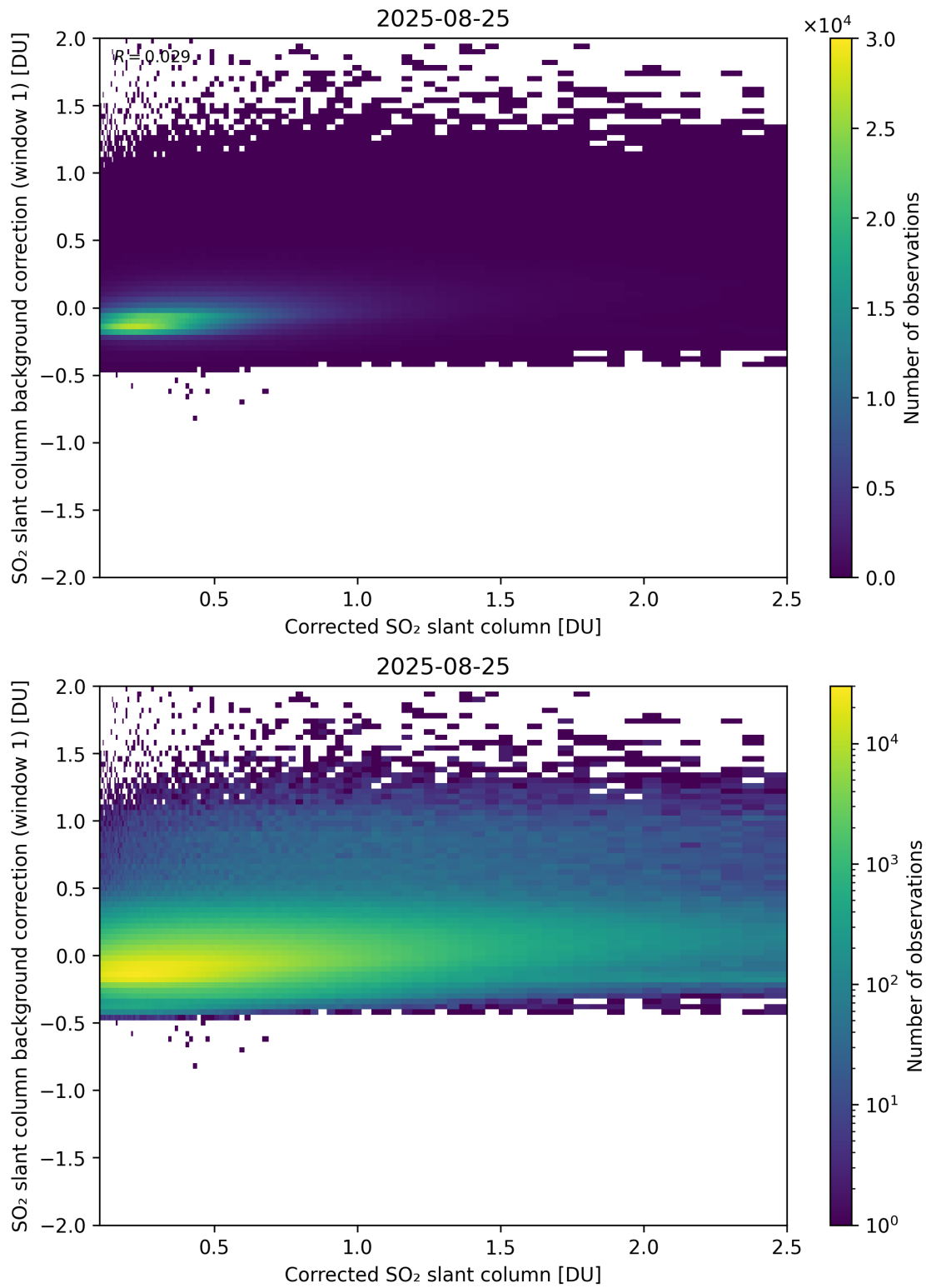
Figure 226: Scatter density plot of “Corrected SO 2 slant column” against “SO 2 slant column background correction (window 1)” for 2025-08-25 to 2025-08-26.
