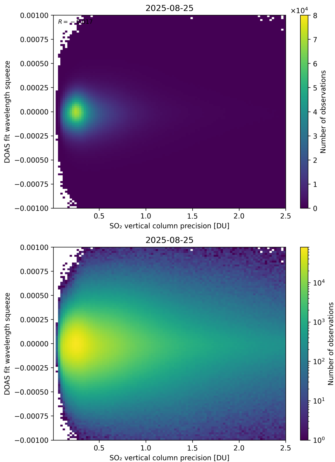
Figure 333: Scatter density plot of “SO 2 vertical column precision” against “DOAS fit wavelength squeeze” for 2025-08-25 to 2025-08-26.
