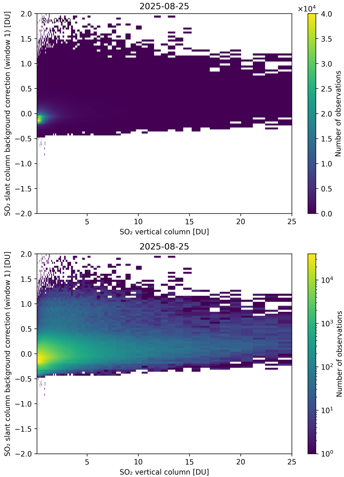
Figure 323: Scatter density plot of “SO 2 vertical column” against “SO 2 slant column background correction (window 1)” for 2025-08-25 to 2025-08-26.
