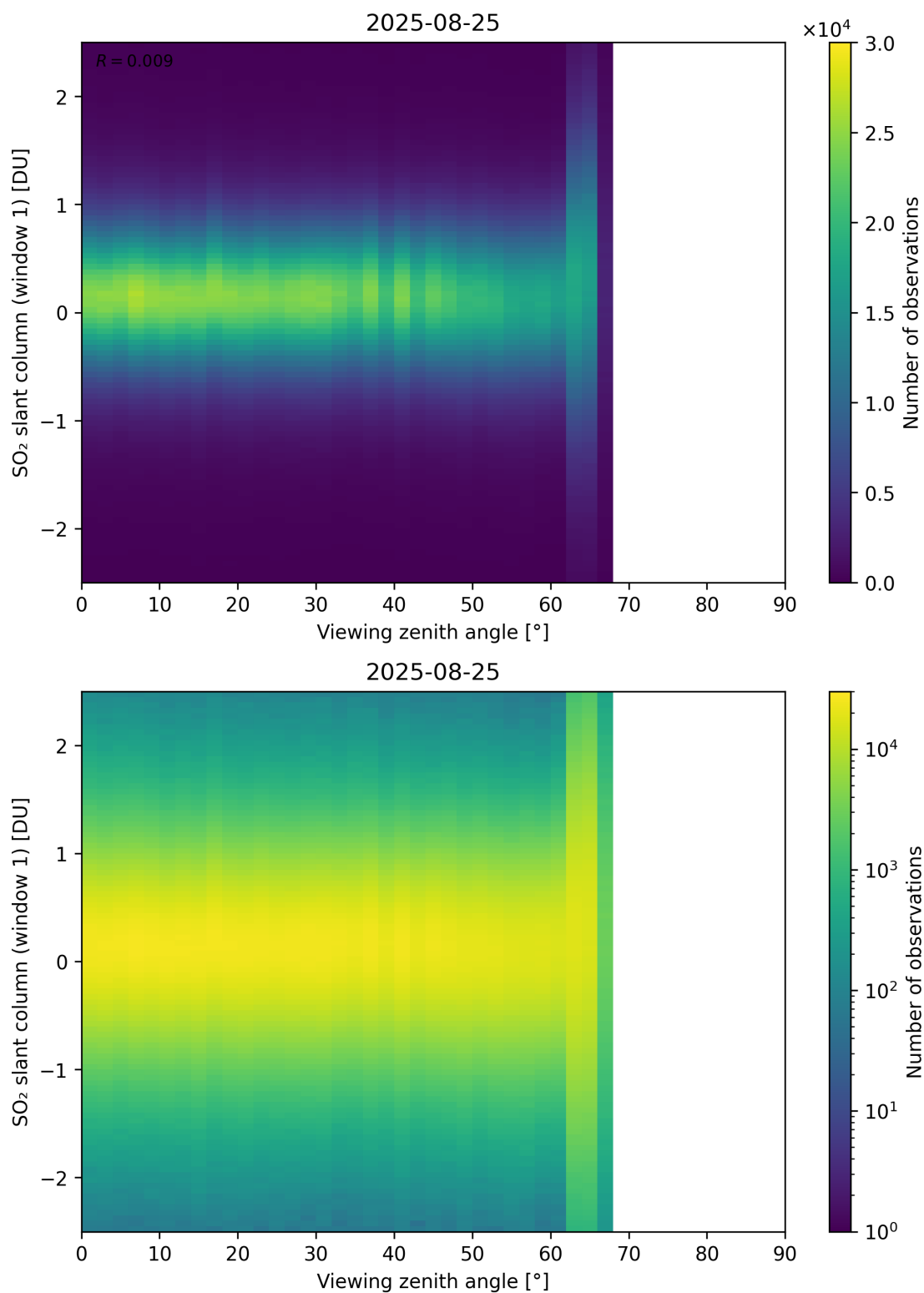
Figure 376: Scatter density plot of “Viewing zenith angle” against “SO 2 slant column (window 1)” for 2025-08-25 to 2025-08-26.
