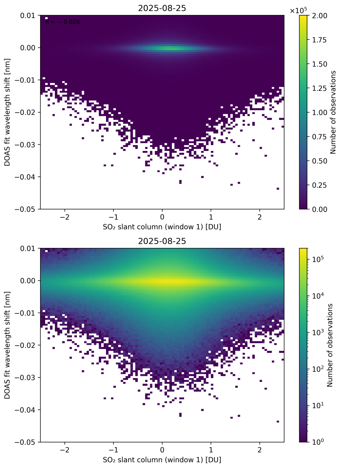
Figure 265: Scatter density plot of “SO 2 slant column (window 1)” against “DOAS fit wavelength shift” for 2025-08-25 to 2025-08-26.
