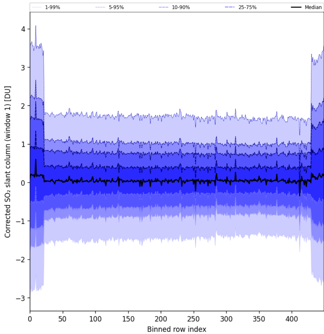
Figure 91: Along track statistics of “Corrected SO 2 slant column (window 1)” for 2025-08-25 to 2025-08-26
