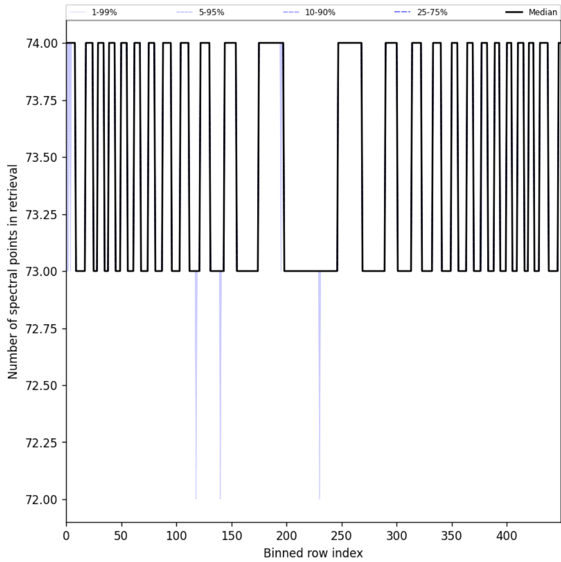
Figure 108: Along track statistics of “Number of spectral points in retrieval” for 2025-08-25 to 2025-08-26
