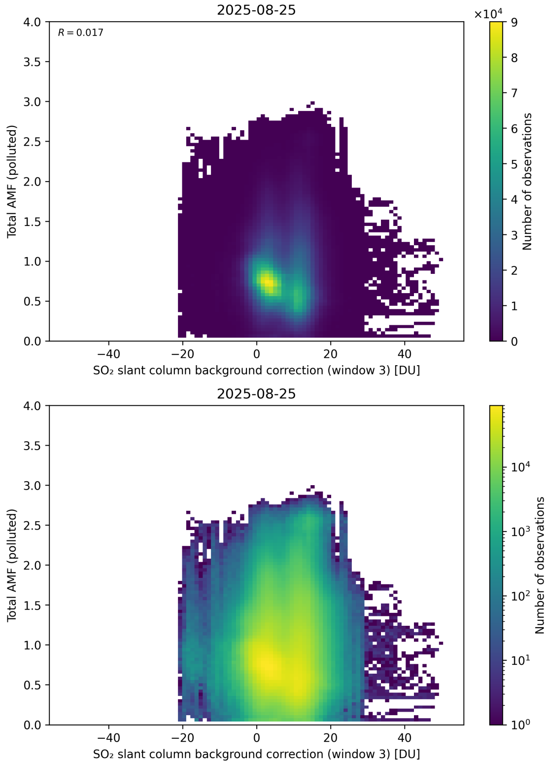
Figure 136: Scatter density plot of “SO 2 slant column background correction (window 3)” against “Total AMF (polluted)” for 2025-08-25 to 2025-08-26.
