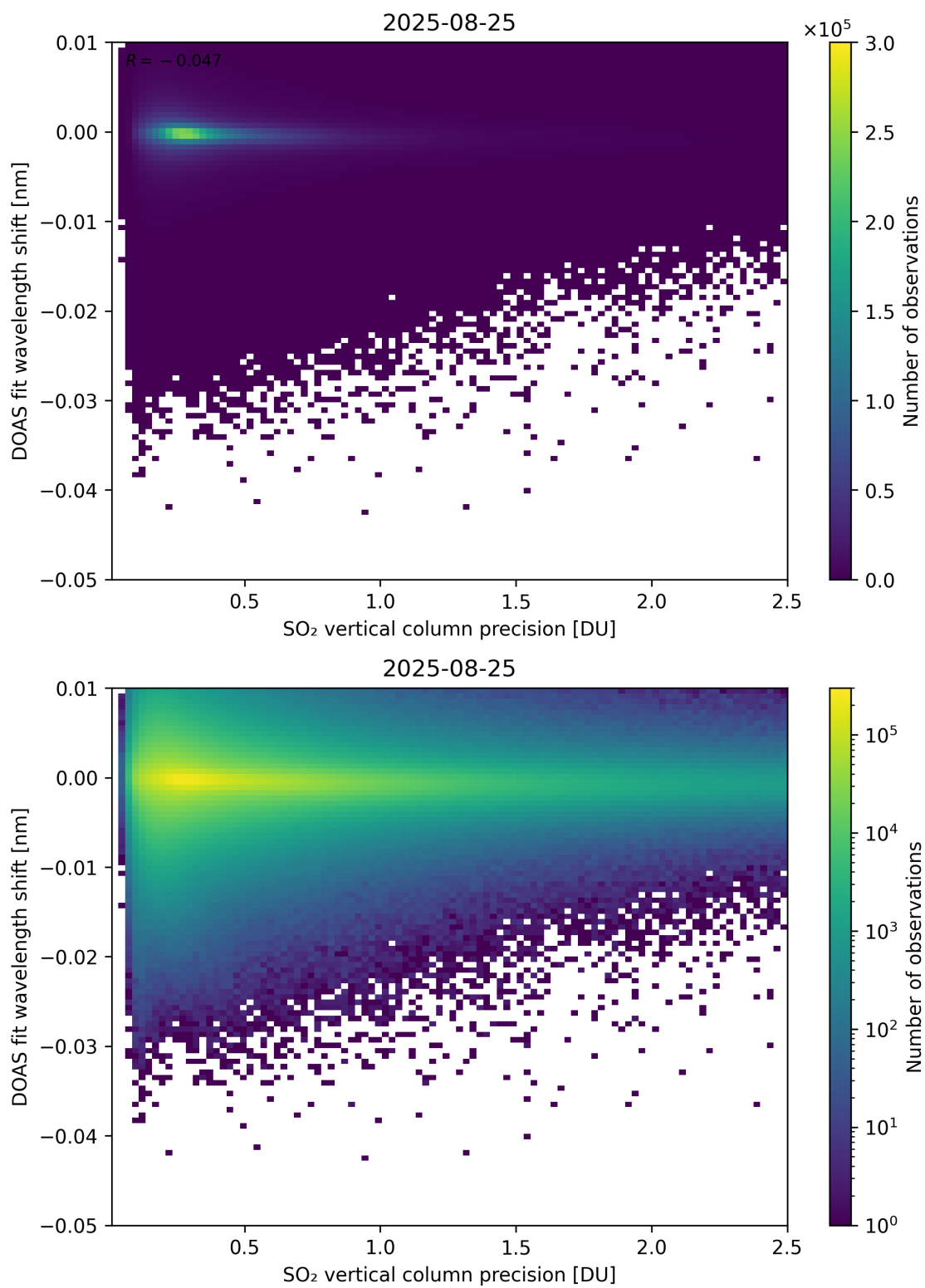
Figure 332: Scatter density plot of “SO 2 vertical column precision” against “DOAS fit wavelength shift” for 2025-08-25 to 2025-08-26.
