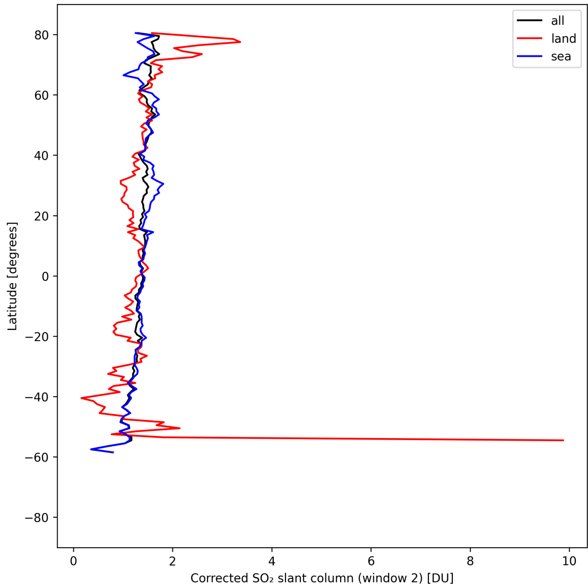
Figure 43: Zonal average of “Corrected SO 2 slant column (window 2)” for 2025-08-25 to 2025-08-26.
