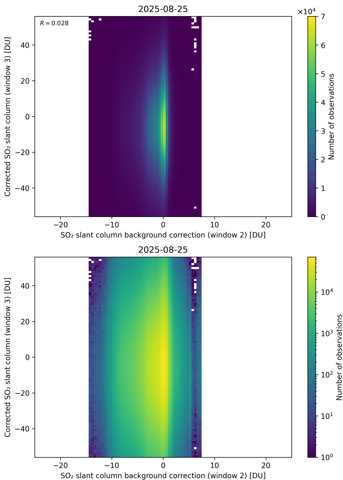
Figure 127: Scatter density plot of “SO 2 slant column background correction (window 2)” against “Corrected SO 2 slant column (window 3)” for 2025-08-25 to 2025-08-26.
