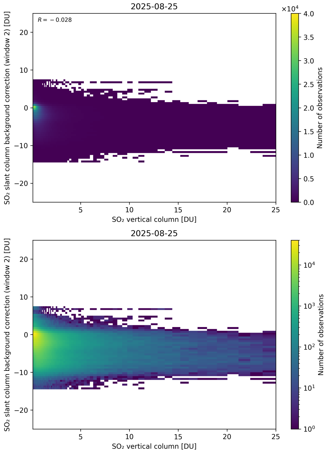
Figure 324: Scatter density plot of “SO 2 vertical column” against “SO 2 slant column background correction (window 2)” for 2025-08-25 to 2025-08-26.
