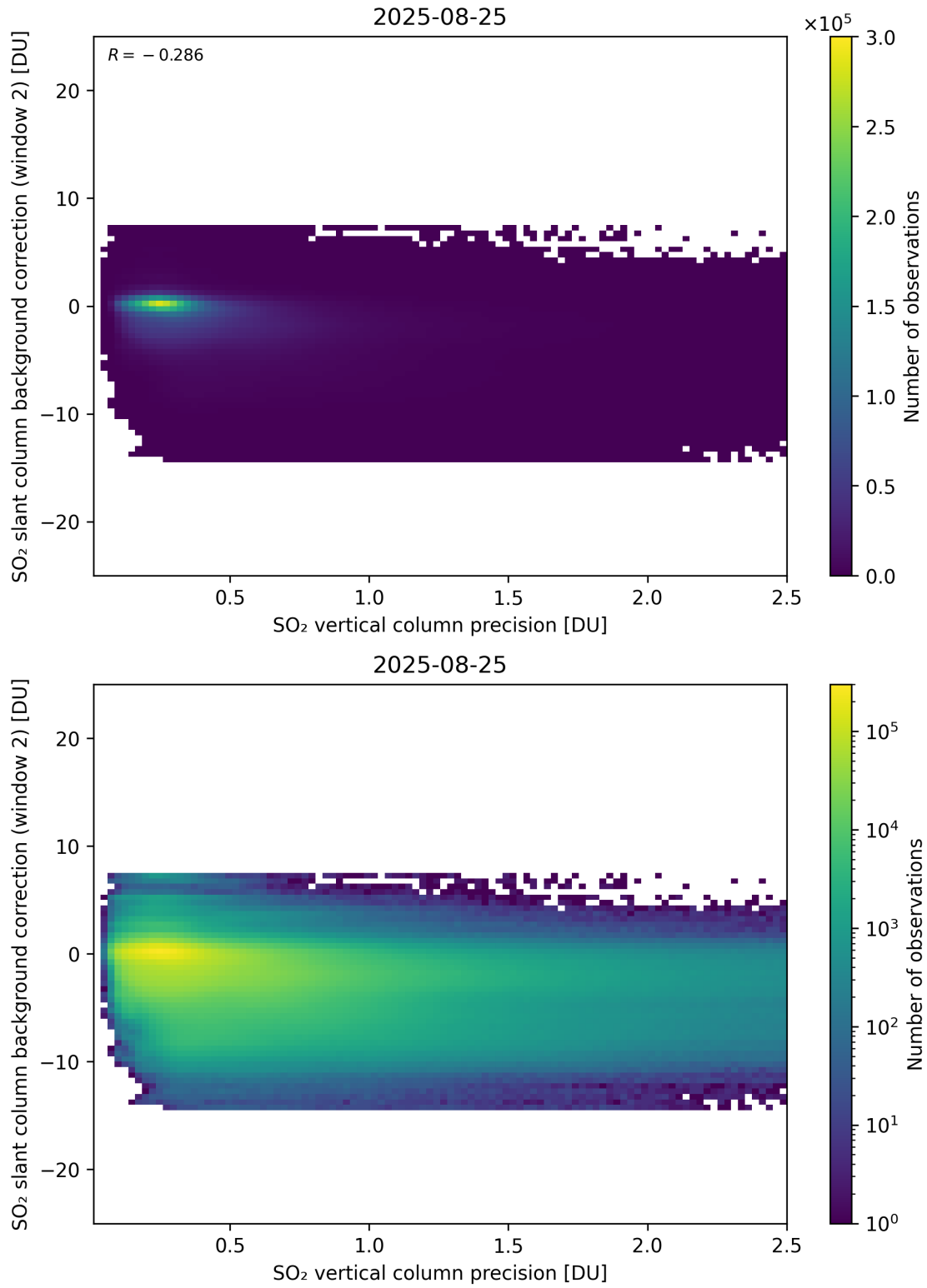
Figure 330: Scatter density plot of “SO 2 vertical column precision” against “SO 2 slant column background correction (window 2)” for 2025-08-25 to 2025-08-26.
