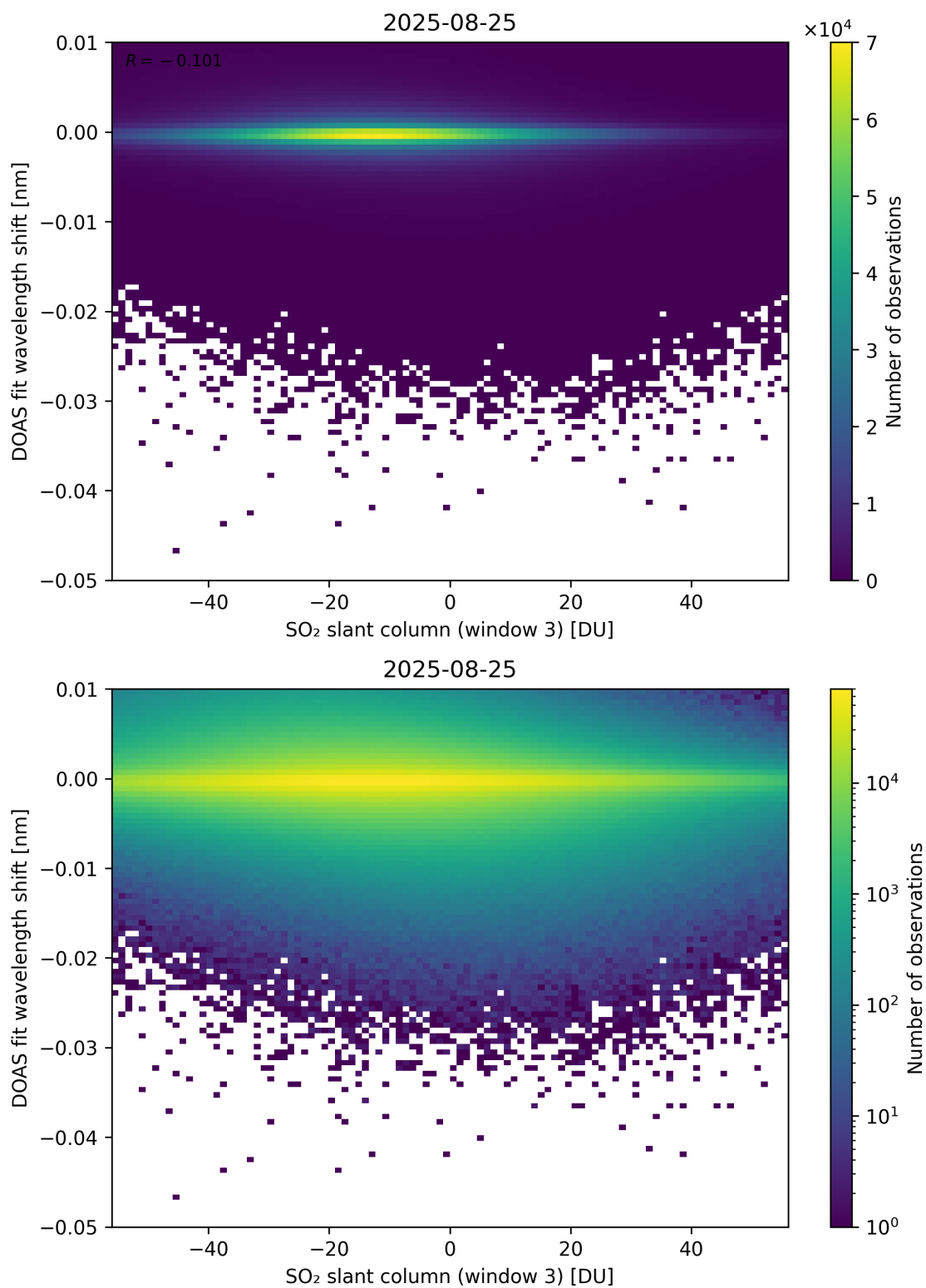
Figure 304: Scatter density plot of “SO 2 slant column (window 3)” against “DOAS fit wavelength shift” for 2025-08-25 to 2025-08-26.
