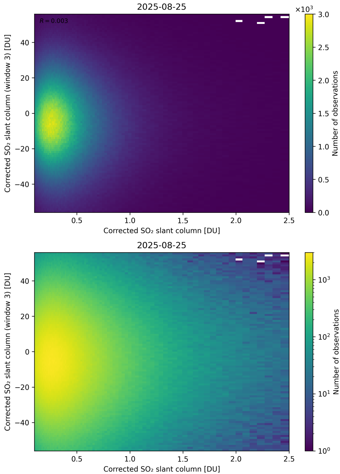
Figure 236: Scatter density plot of “Corrected SO 2 slant column” against “Corrected SO 2 slant column (window 3)” for 2025-08-25 to 2025-08-26.
