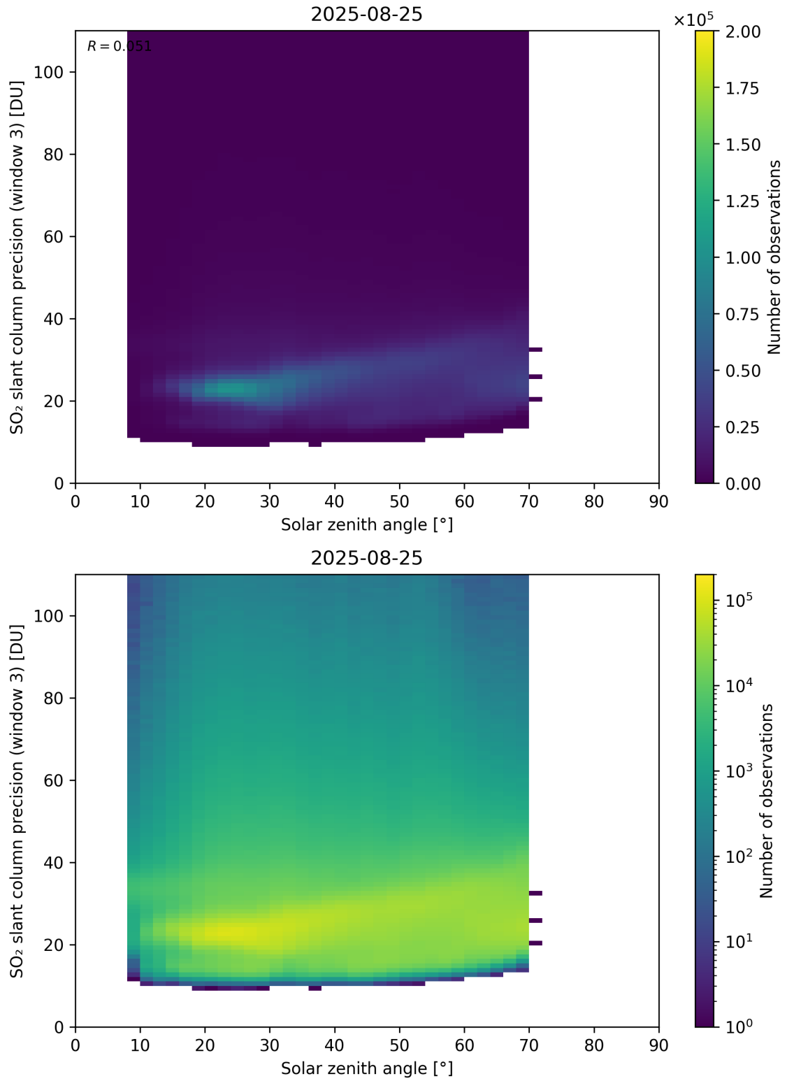
Figure 188: Scatter density plot of “Solar zenith angle” against “SO 2 slant column precision (window 3)” for 2025-08-25 to 2025-08-26.
