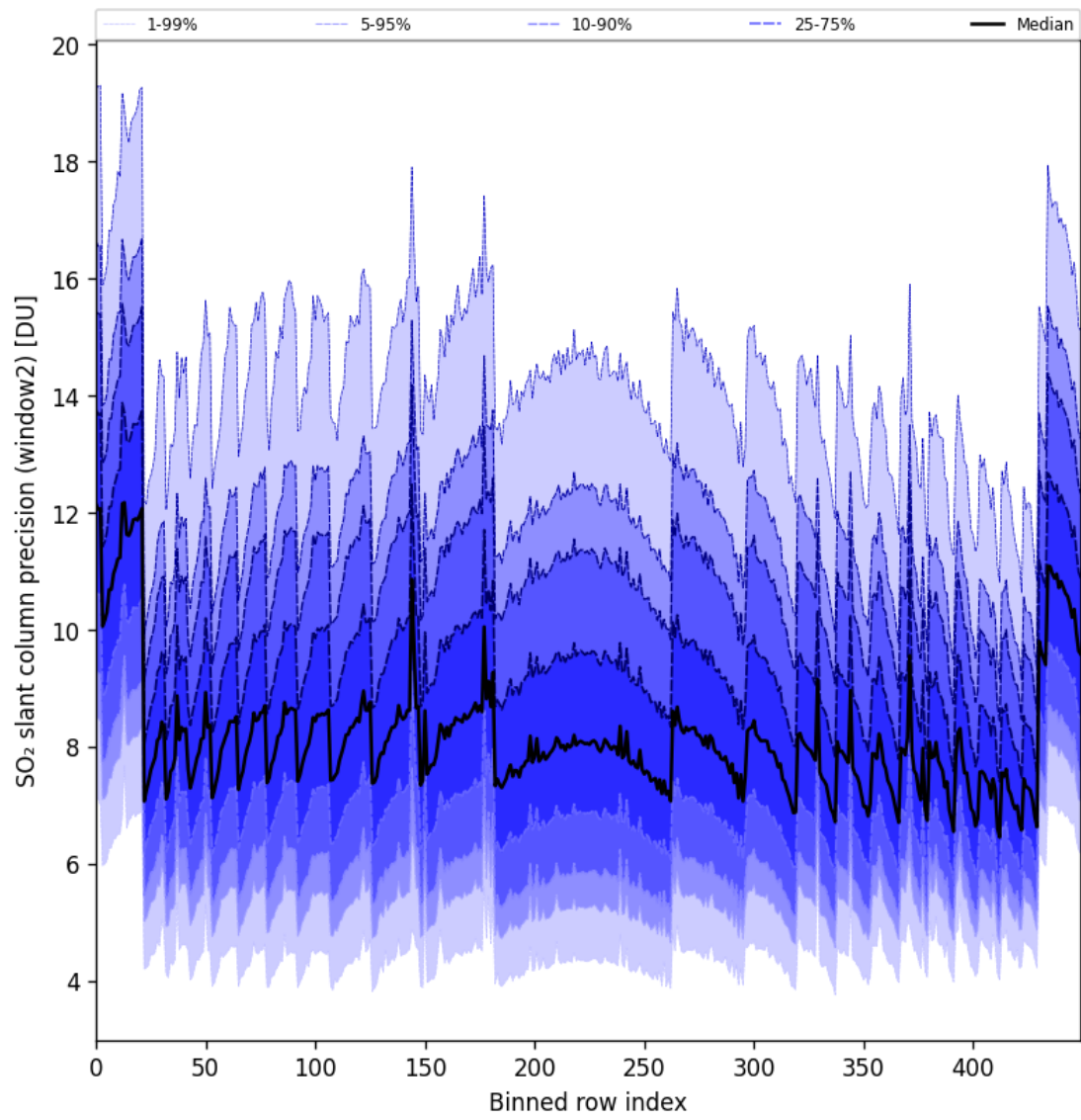
Figure 94: Along track statistics of “SO 2 slant column precision (window2)” for 2025-08-25 to 2025-08-26
