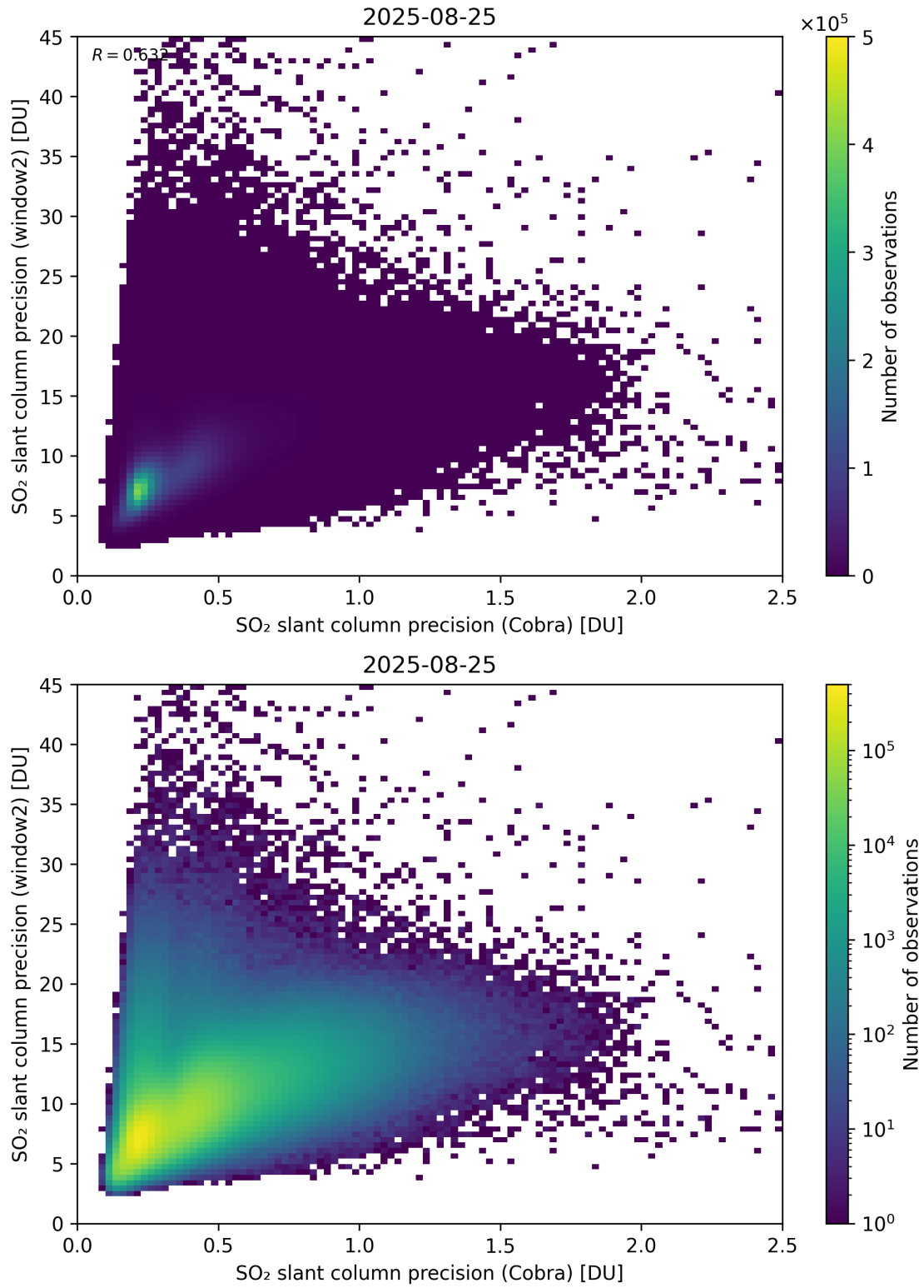
Figure 210: Scatter density plot of “SO 2 slant column precision (Cobra)” against “SO 2 slant column precision (window2)” for 2025-08-25 to 2025-08-26.
