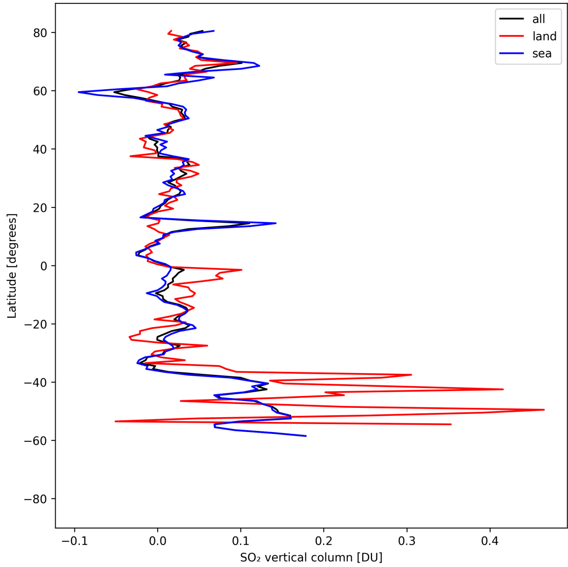
Figure 32: Zonal average of “SO 2 vertical column” for 2025-08-25 to 2025-08-26.
