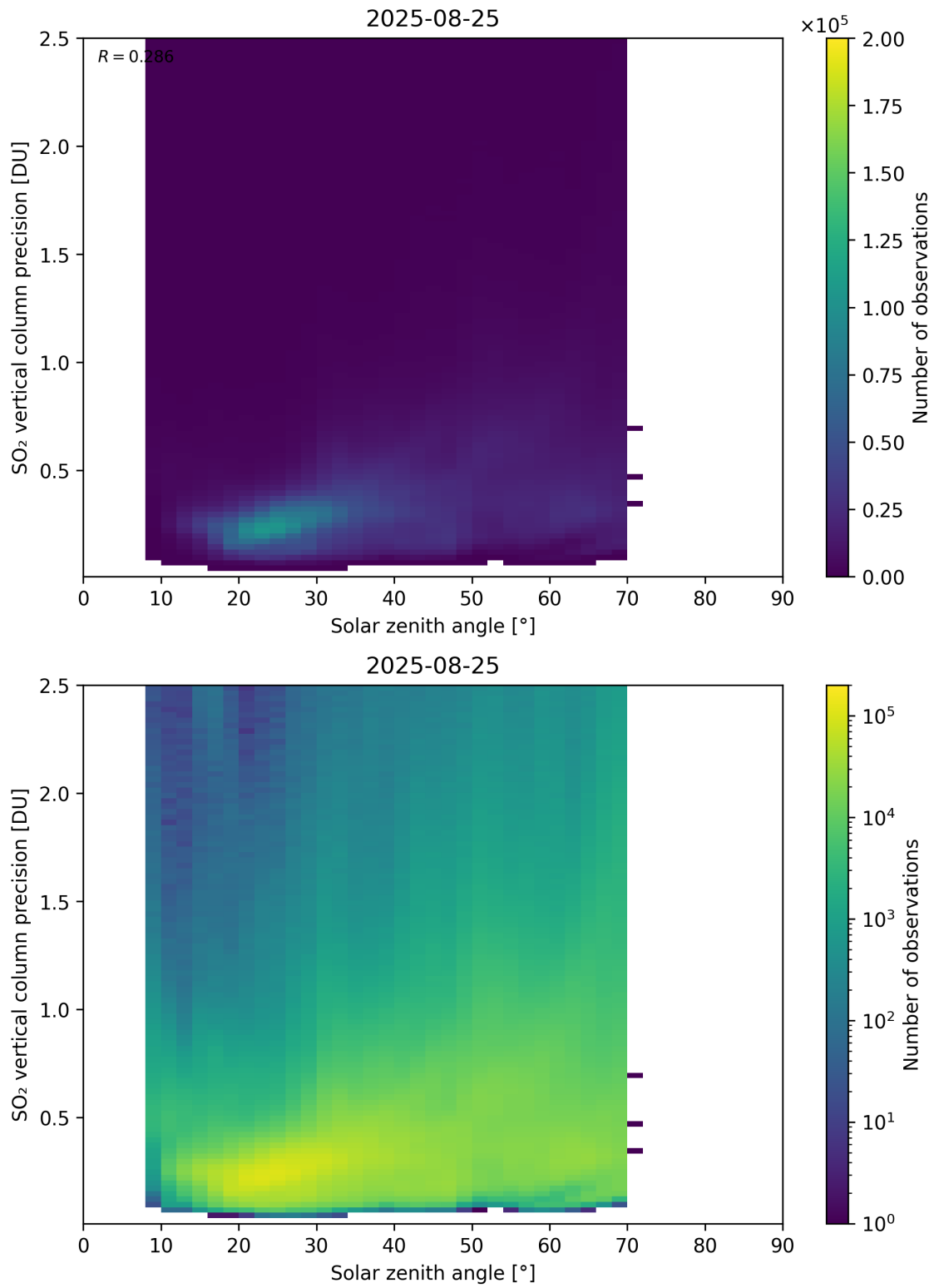
Figure 192: Scatter density plot of “Solar zenith angle” against “SO 2 vertical column precision” for 2025-08-25 to 2025-08-26.
