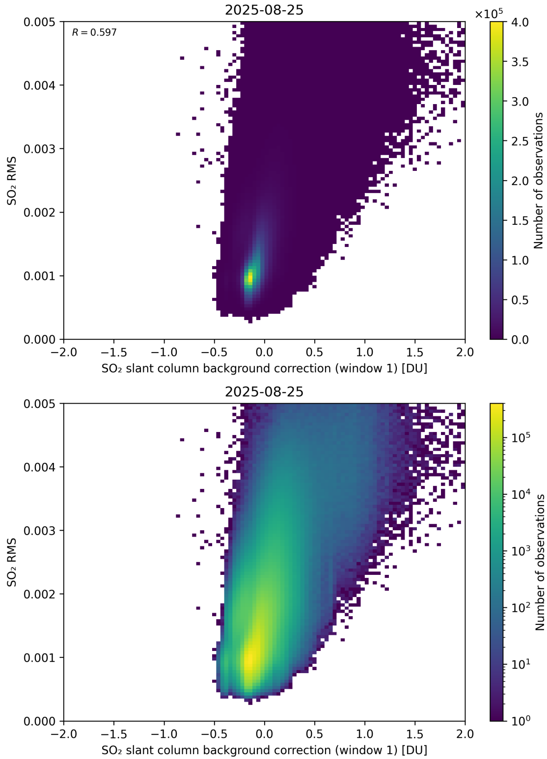
Figure 113: Scatter density plot of “SO 2 slant column background correction (window 1)” against “SO 2 RMS” for 2025-08-25 to 2025-08-26.
