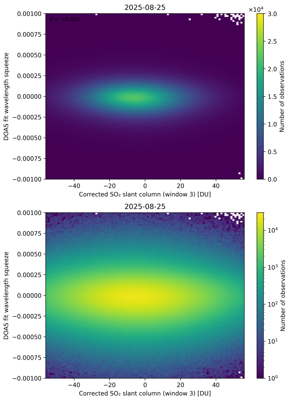
Figure 257: Scatter density plot of “Corrected SO 2 slant column (window 3)” against “DOAS fit wavelength squeeze” for 2025-08-25 to 2025-08-26.
