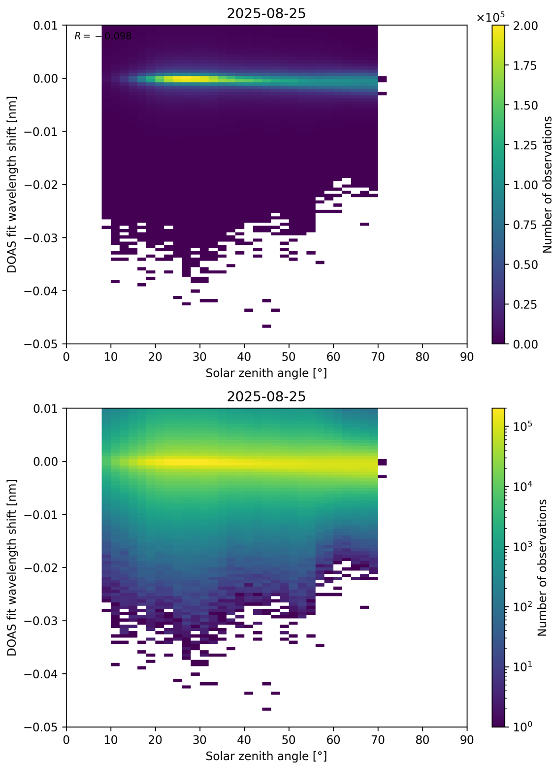
Figure 174: Scatter density plot of “Solar zenith angle” against “DOAS fit wavelength shift” for 2025-08-25 to 2025-08-26.
