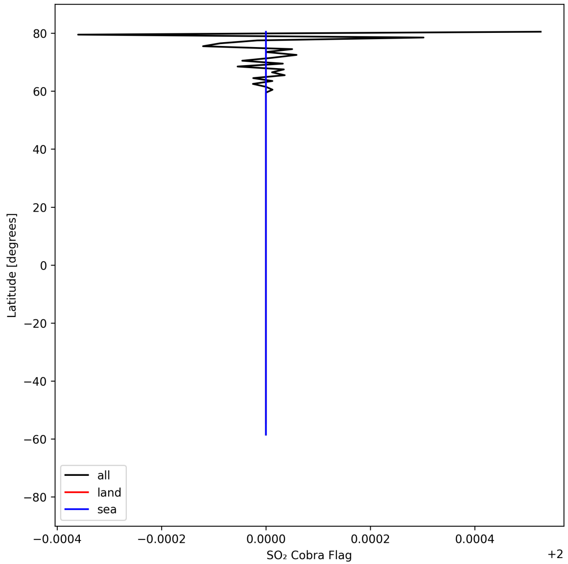
Figure 49: Zonal average of "SO 2 Cobra Flag" for 2025-08-25 to 2025-08-26.
