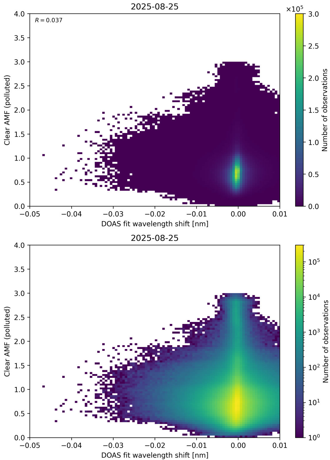
Figure 140: Scatter density plot of “DOAS fit wavelength shift” against “Clear AMF (polluted)” for 2025-08-25 to 2025-08-26.
