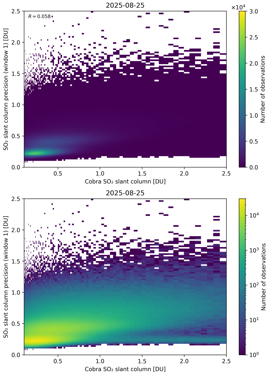
Figure 220: Scatter density plot of “Cobra SO 2 slant column” against “SO 2 slant column precision (window 1)” for 2025-08-25 to 2025-08-26.
