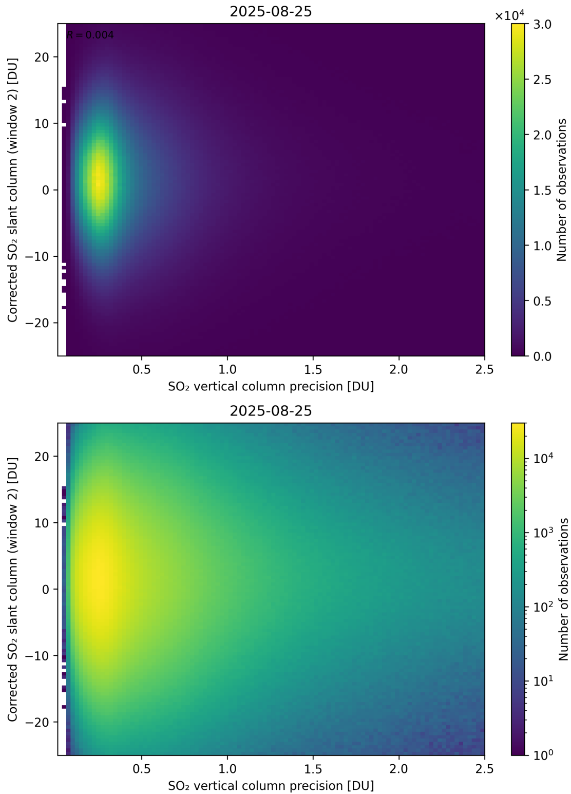
Figure 339: Scatter density plot of “SO 2 vertical column precision” against “Corrected SO 2 slant column (window 2)” for 2025-08-25 to 2025-08-26.
