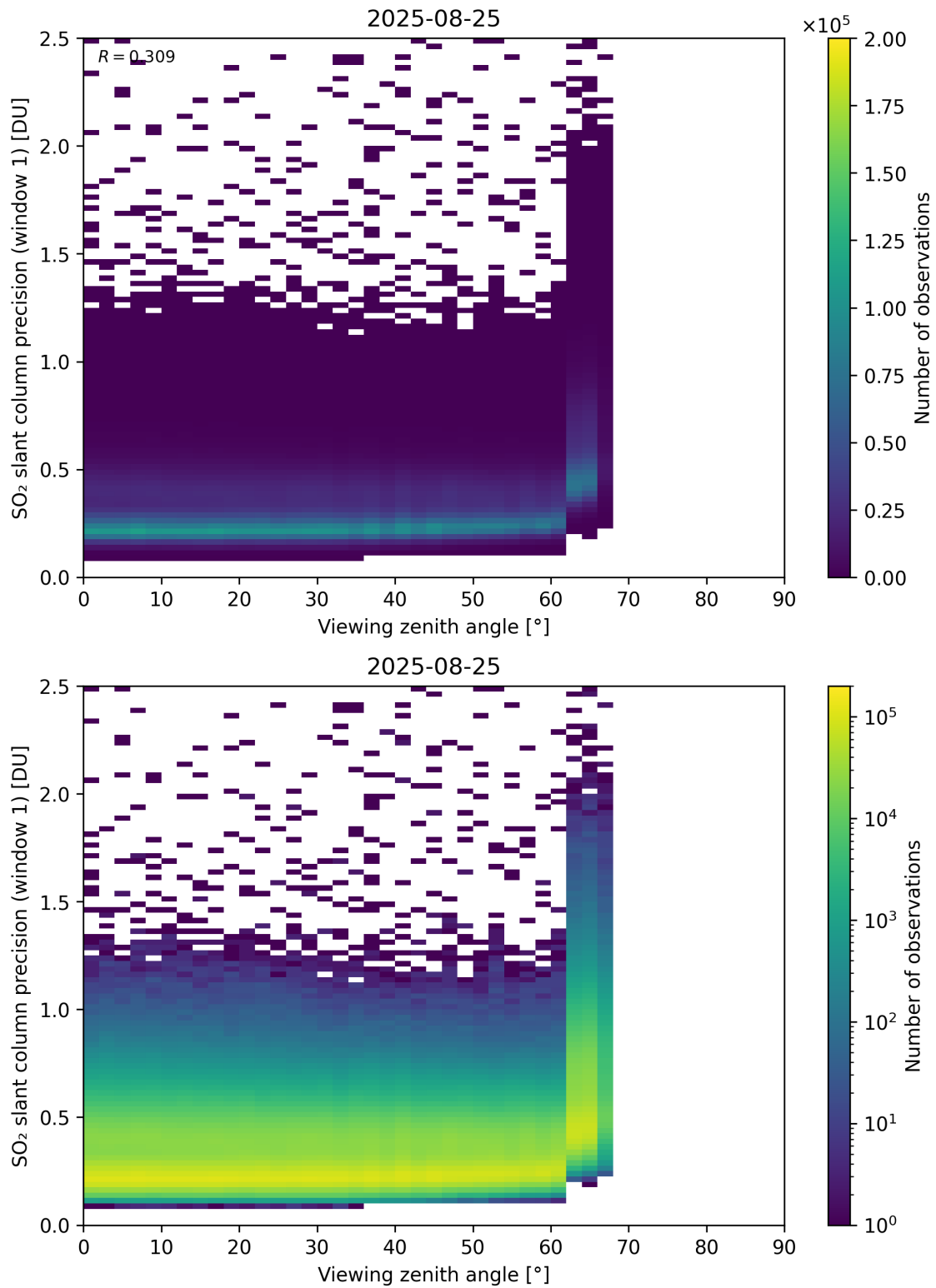
Figure 377: Scatter density plot of “Viewing zenith angle” against “SO 2 slant column precision (window 1)” for 2025-08-25 to 2025-08-26.
