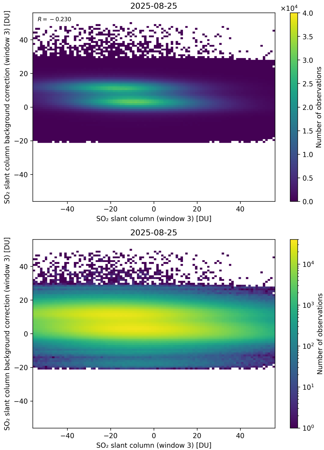
Figure 303: Scatter density plot of “SO 2 slant column (window 3)” against “SO 2 slant column background correction (window 3)” for 2025-08-25 to 2025-08-26.
