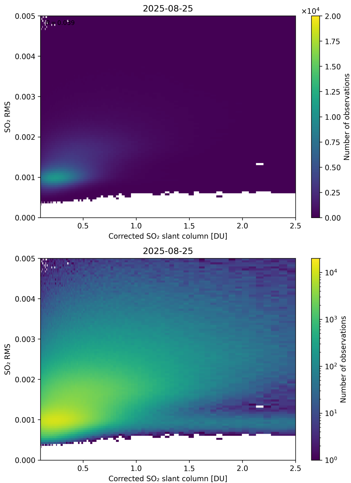
Figure 231: Scatter density plot of “Corrected SO 2 slant column” against “SO 2 RMS” for 2025-08-25 to 2025-08-26.
