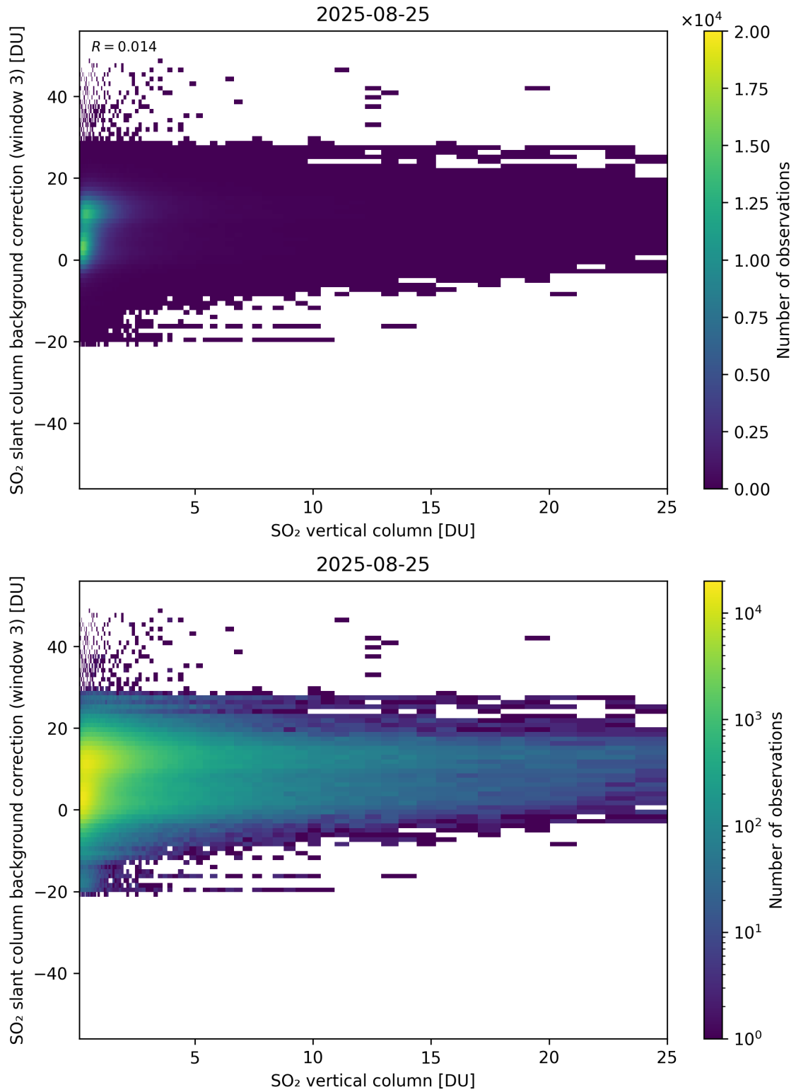
Figure 325: Scatter density plot of “SO 2 vertical column” against “SO 2 slant column background correction (window 3)” for 2025-08-25 to 2025-08-26.
