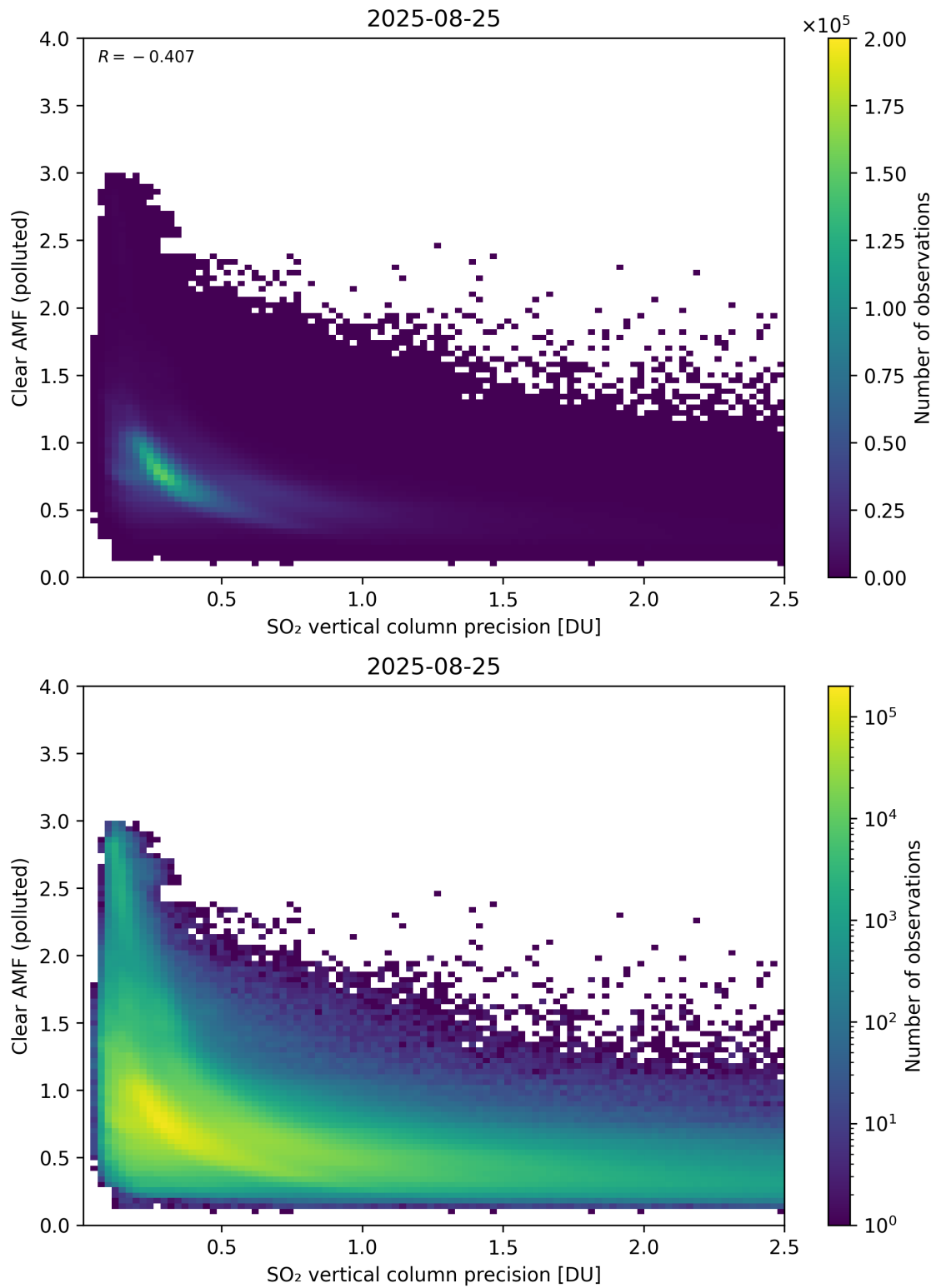
Figure 335: Scatter density plot of “SO 2 vertical column precision” against “Clear AMF (polluted)” for 2025-08-25 to 2025-08-26.
