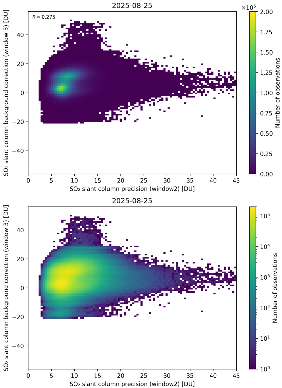
Figure 292: Scatter density plot of “SO 2 slant column precision (window2)” against “SO 2 slant column background correction (window 3)” for 2025-08-25 to 2025-08-26.
