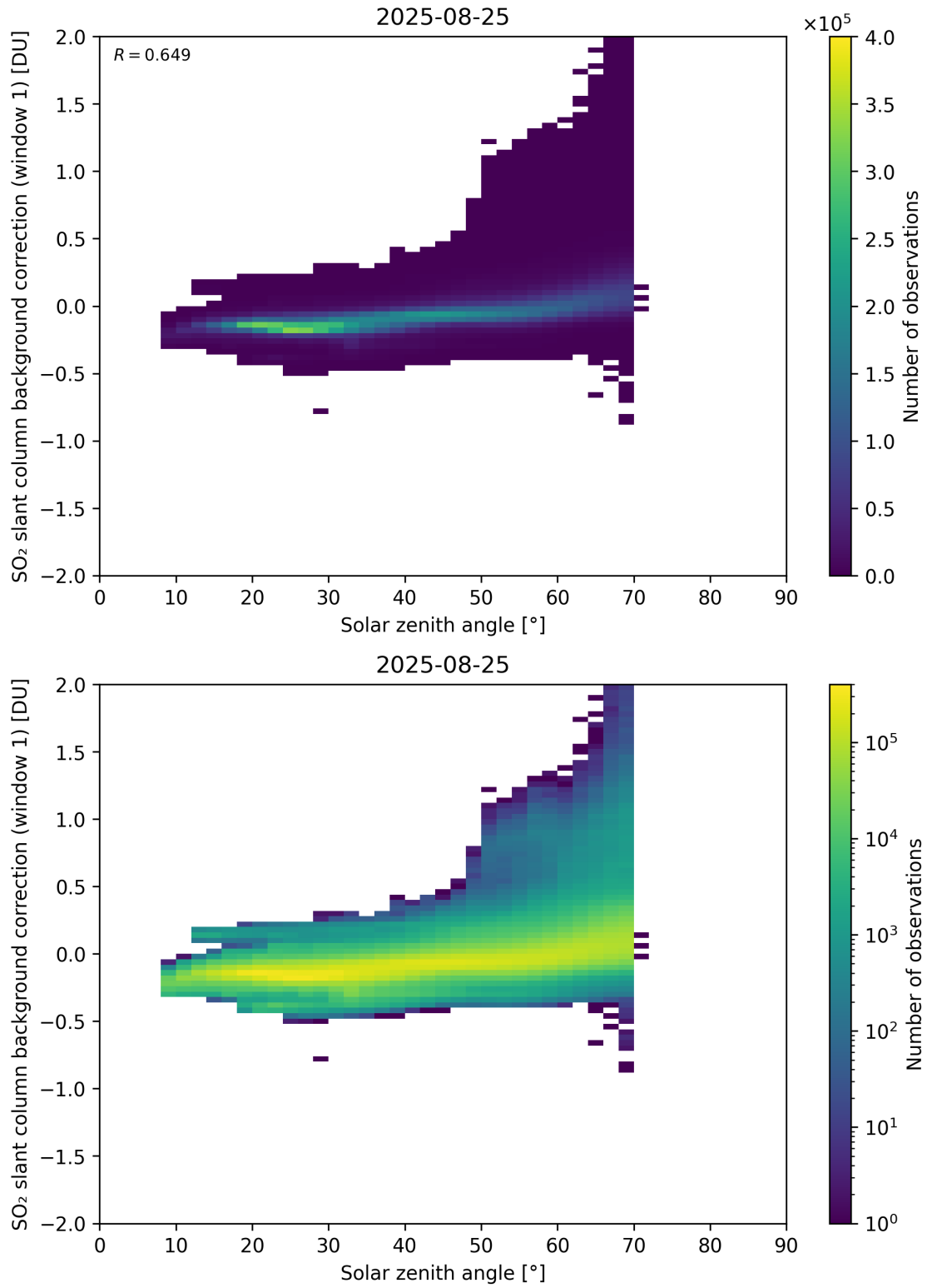
Figure 171: Scatter density plot of “Solar zenith angle” against “SO 2 slant column background correction (window 1)” for 2025-08-25 to 2025-08-26.
