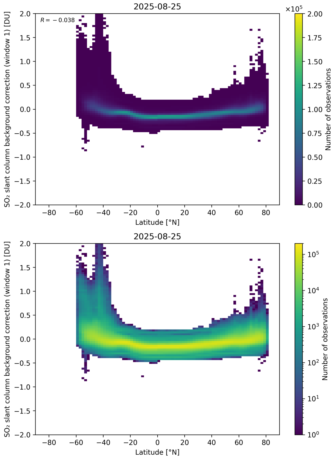
Figure 150: Scatter density plot of “Latitude” against “SO 2 slant column background correction (window 1)” for 2025-08-25 to 2025-08-26.
