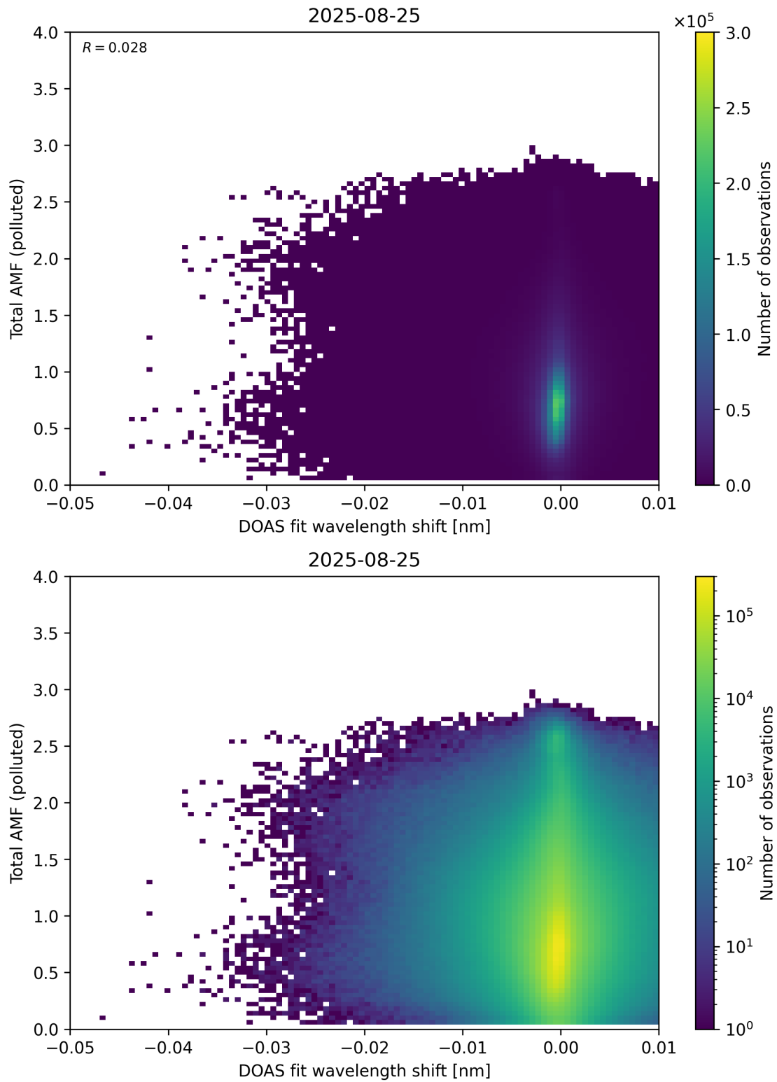
Figure 141: Scatter density plot of “DOAS fit wavelength shift” against “Total AMF (polluted)” for 2025-08-25 to 2025-08-26.
