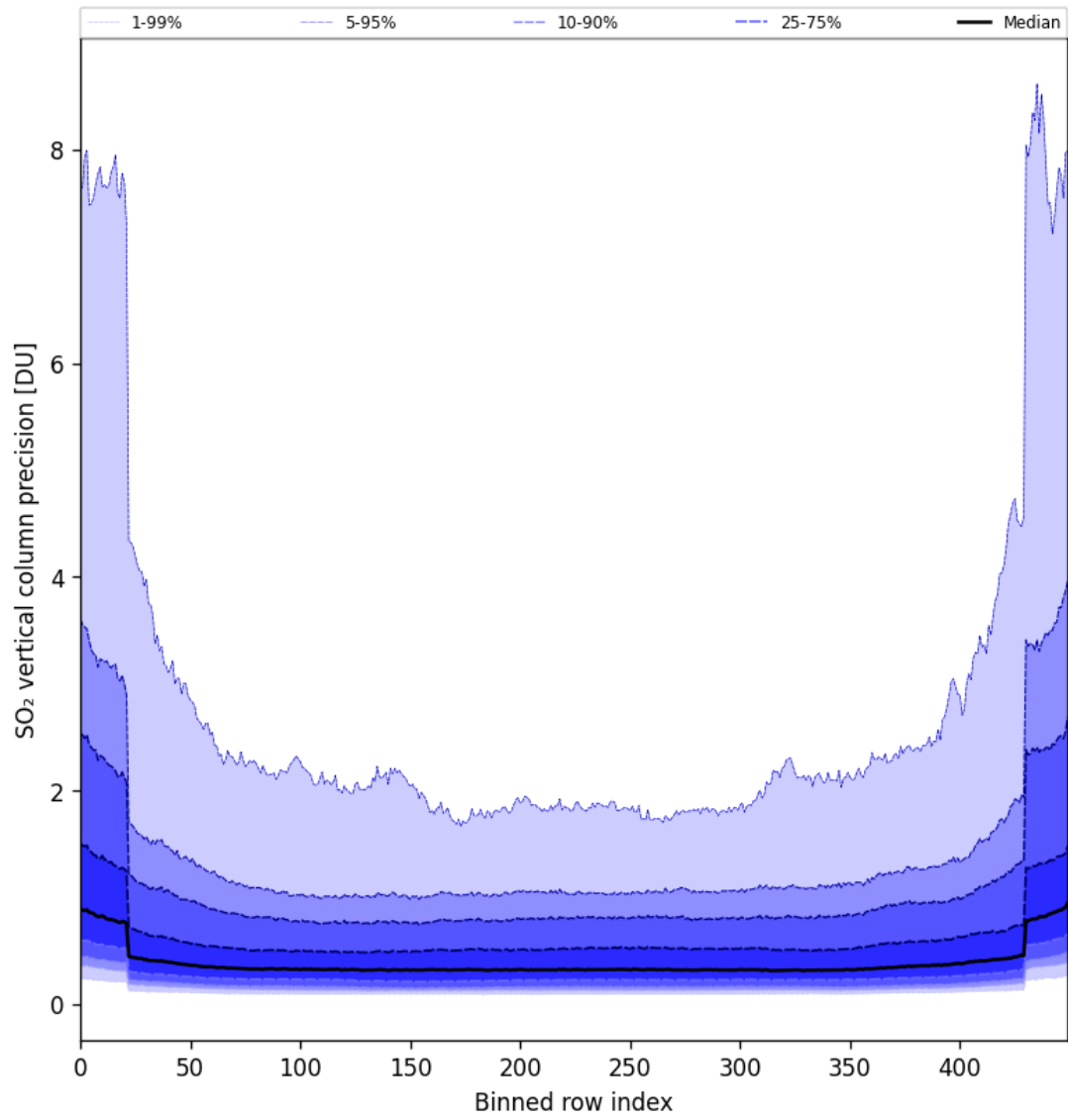
Figure 85: Along track statistics of “SO 2 vertical column precision” for 2025-08-25 to 2025-08-26
