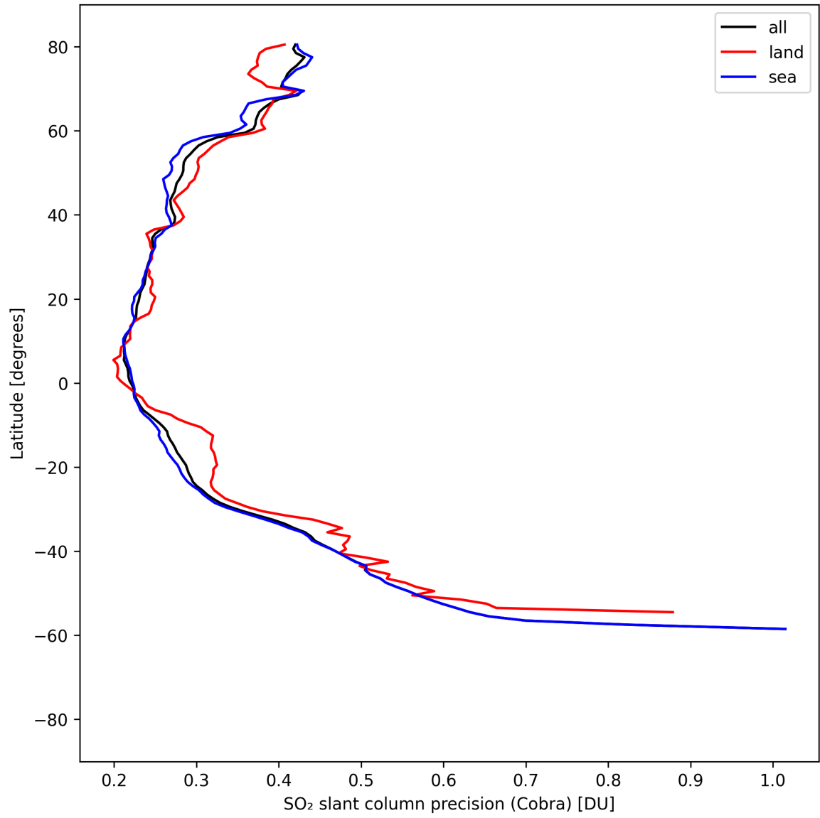
Figure 36: Zonal average of “SO 2 slant column precision (Cobra)” for 2025-08-25 to 2025-08-26.
