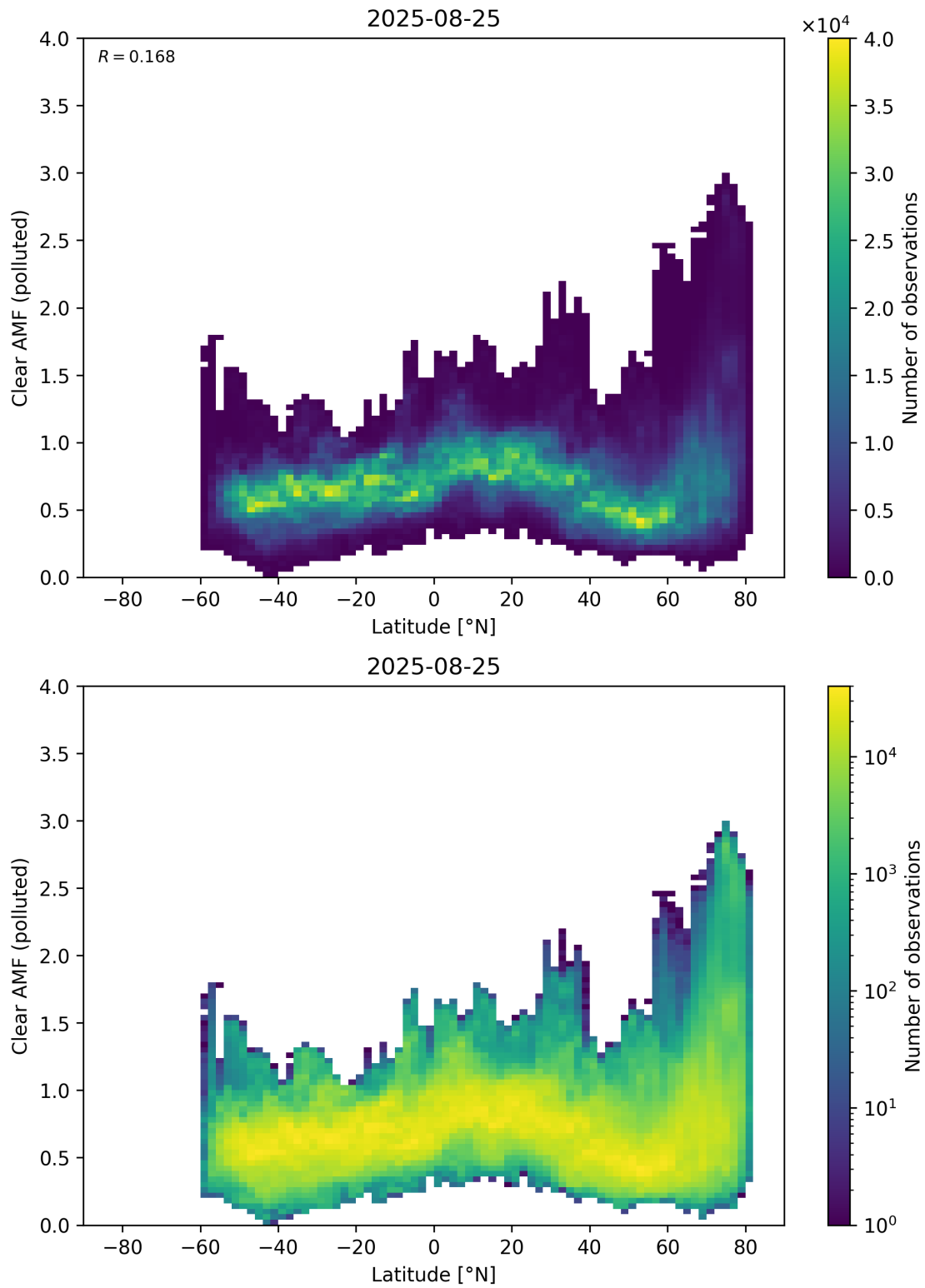
Figure 156: Scatter density plot of “Latitude” against “Clear AMF (polluted)” for 2025-08-25 to 2025-08-26.
