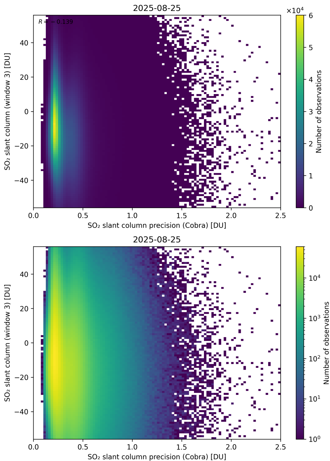
Figure 211: Scatter density plot of “SO 2 slant column precision (Cobra)” against “SO 2 slant column (window 3)” for 2025-08-25 to 2025-08-26.
