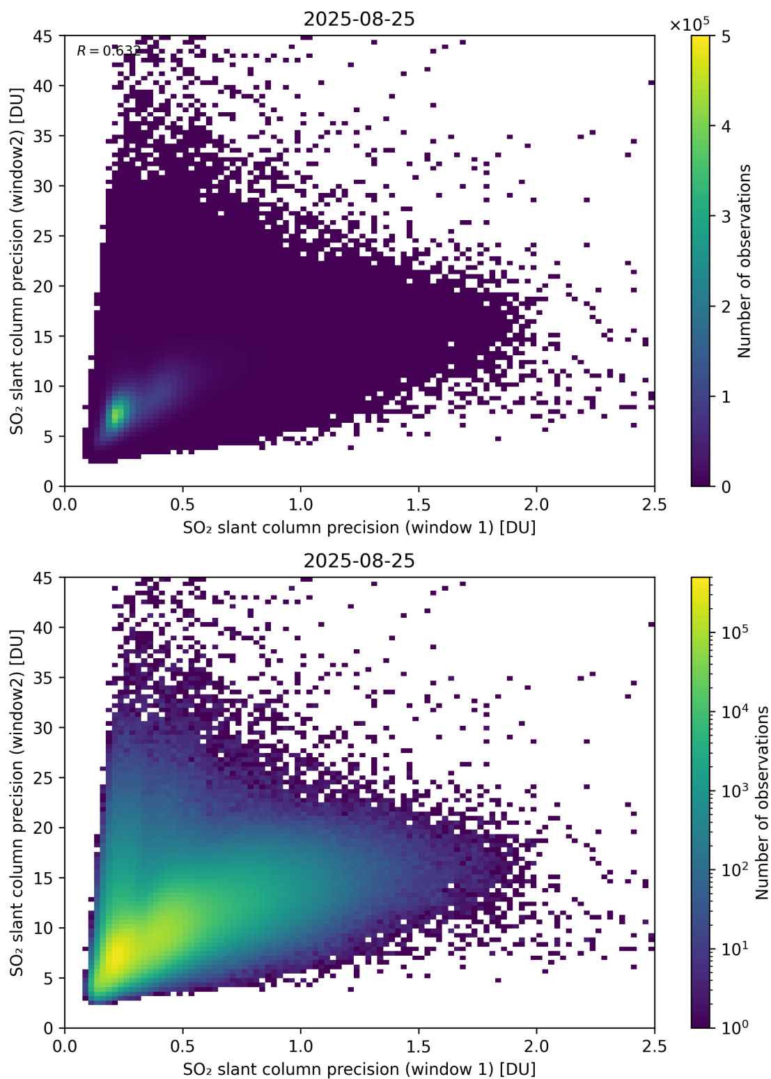
Figure 277: Scatter density plot of “SO 2 slant column precision (window 1)” against “SO 2 slant column precision (window2)” for 2025-08-25 to 2025-08-26.
