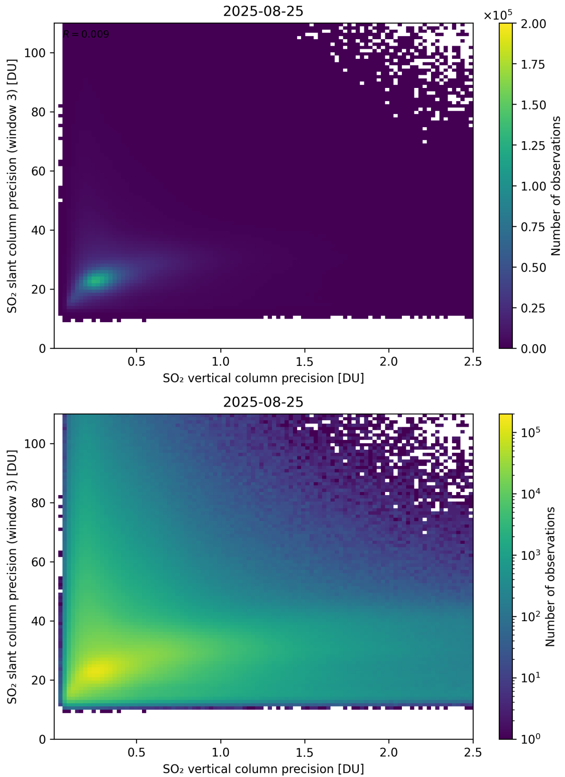
Figure 345: Scatter density plot of “SO 2 vertical column precision” against “SO 2 slant column precision (window 3)” for 2025-08-25 to 2025-08-26.
