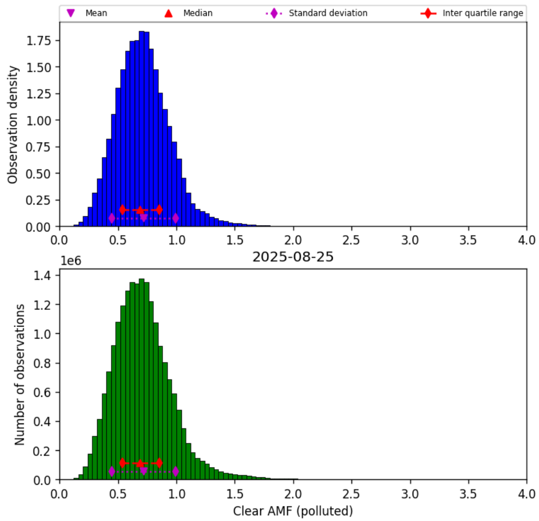
Figure 81: Histogram of “Clear AMF (polluted)” for 2025-08-25 to 2025-08-26
