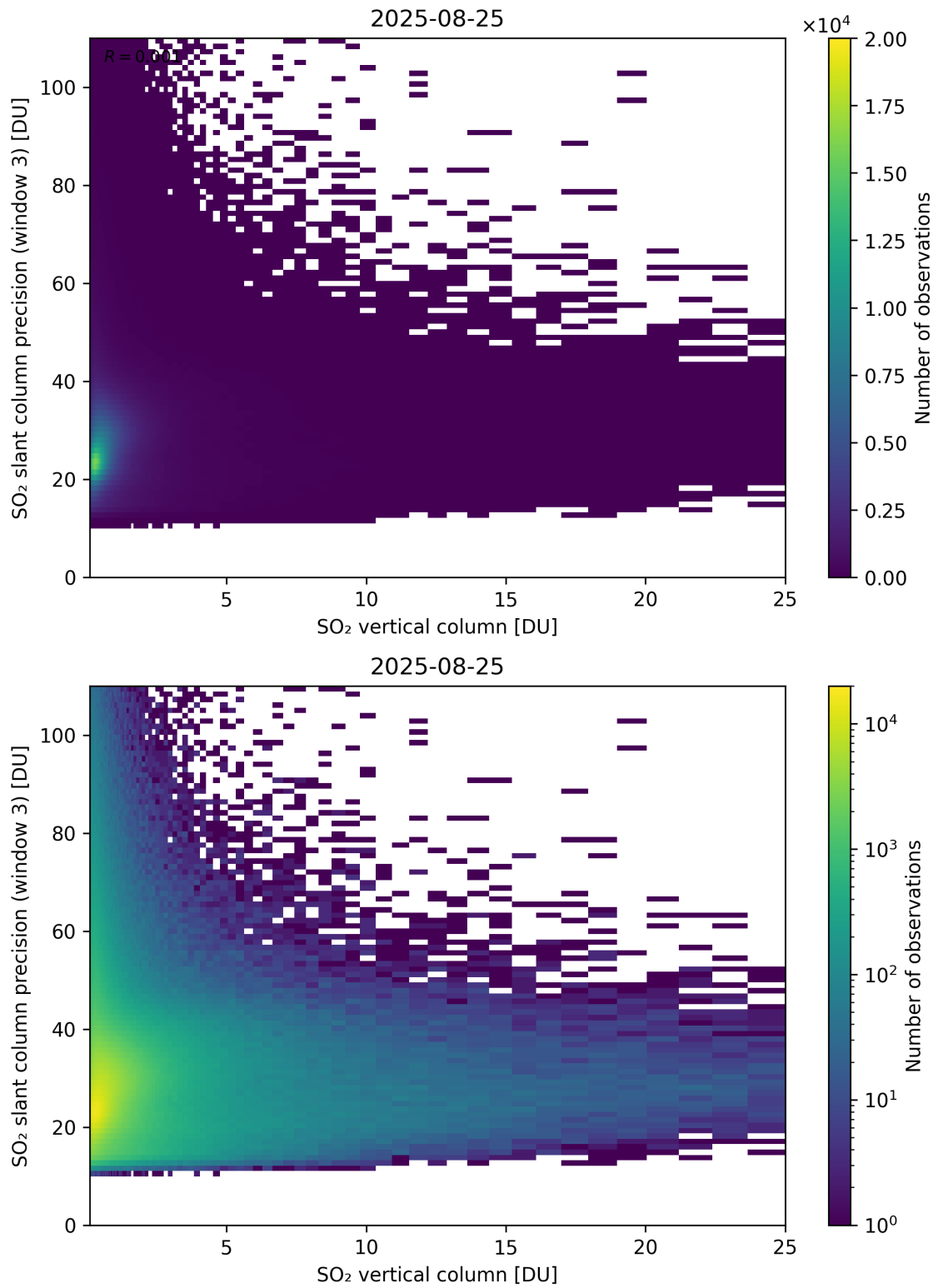
Figure 358: Scatter density plot of “SO 2 vertical column” against “SO 2 slant column precision (window 3)” for 2025-08-25 to 2025-08-26.
