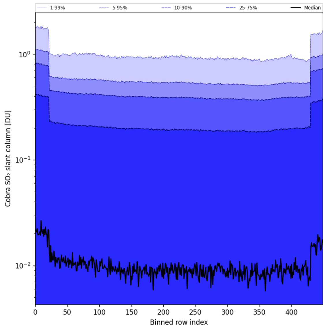
Figure 87: Along track statistics of “Cobra SO 2 slant column” for 2025-08-25 to 2025-08-26
