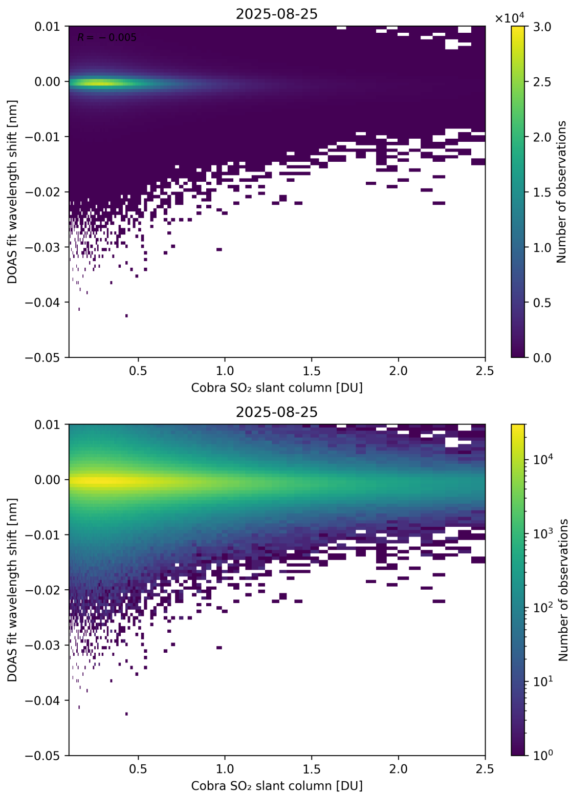
Figure 196: Scatter density plot of “Cobra SO 2 slant column” against “DOAS fit wavelength shift” for 2025-08-25 to 2025-08-26.
