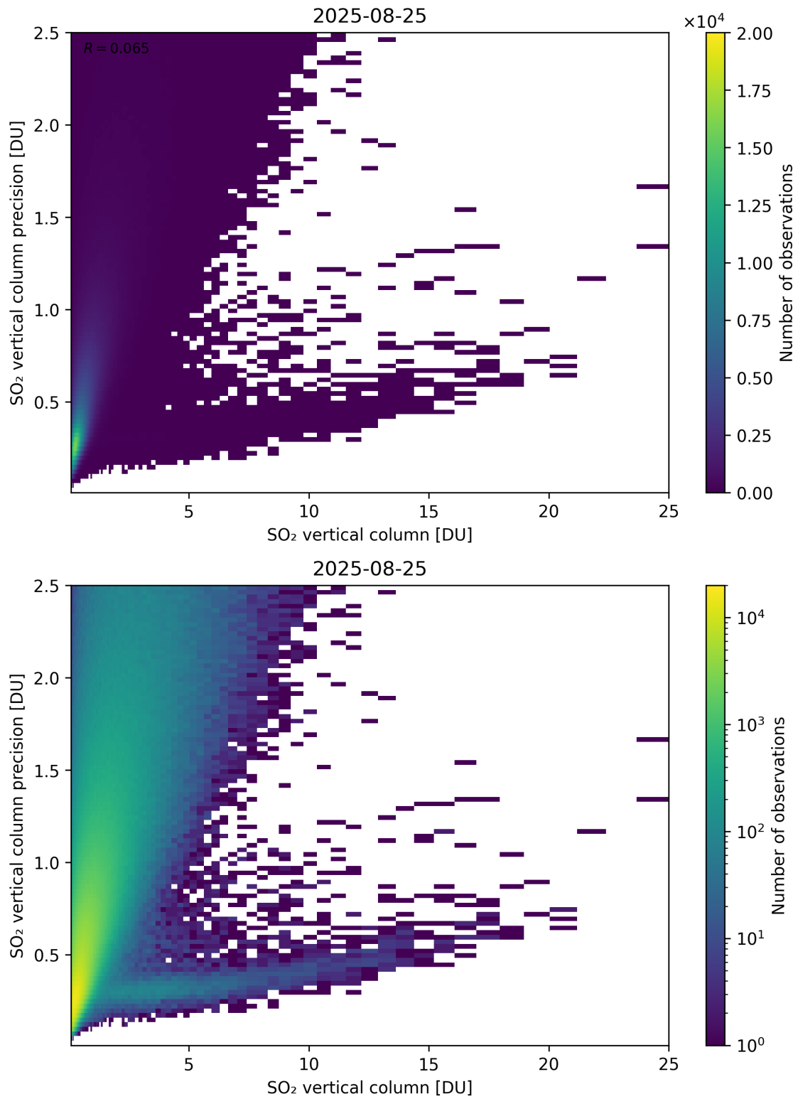
Figure 361: Scatter density plot of “SO 2 vertical column” against “SO 2 vertical column precision” for 2025-08-25 to 2025-08-26.
