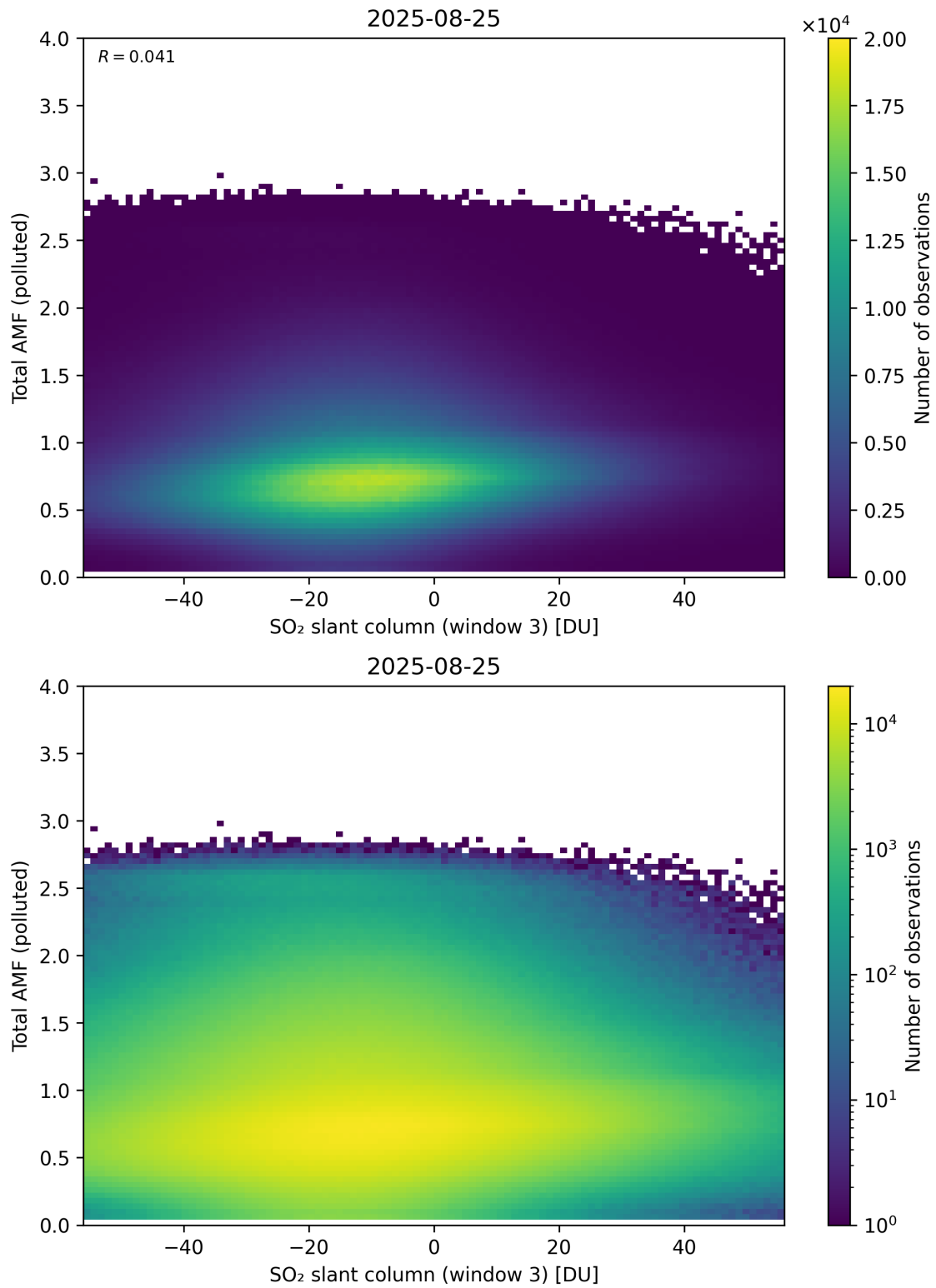
Figure 318: Scatter density plot of “SO 2 slant column (window 3)” against “Total AMF (polluted)” for 2025-08-25 to 2025-08-26.
