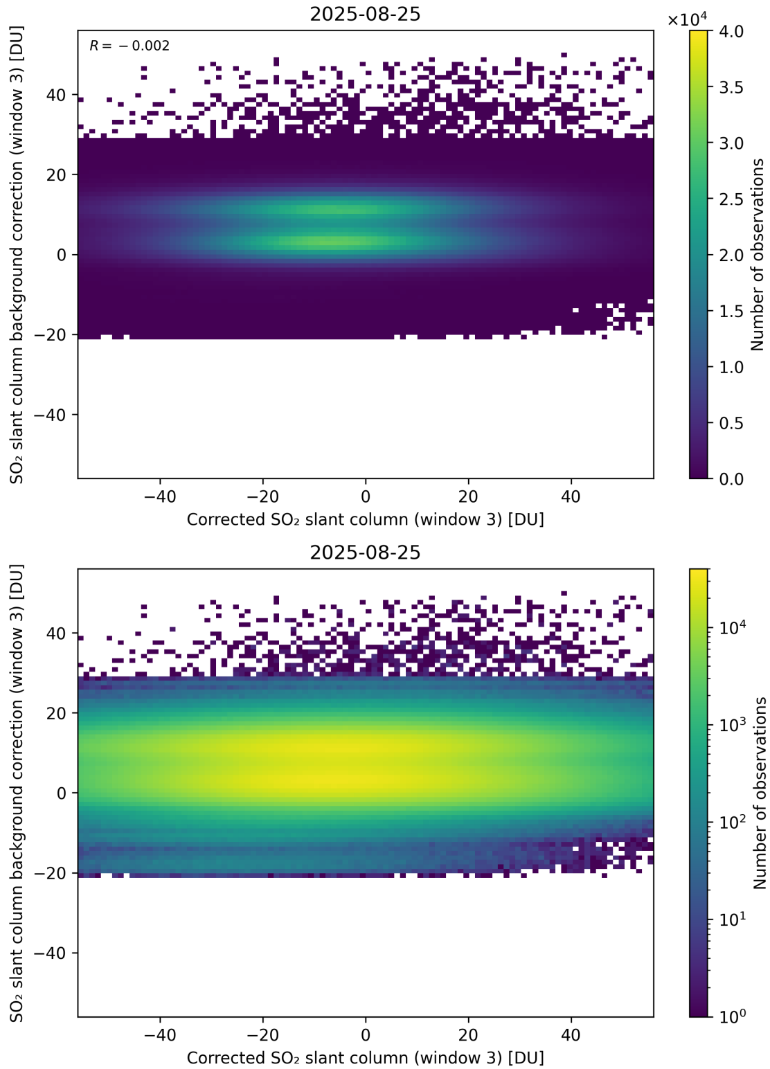
Figure 255: Scatter density plot of “Corrected SO 2 slant column (window 3)” against “SO 2 slant column background correction (window 3)” for 2025-08-25 to 2025-08-26.
