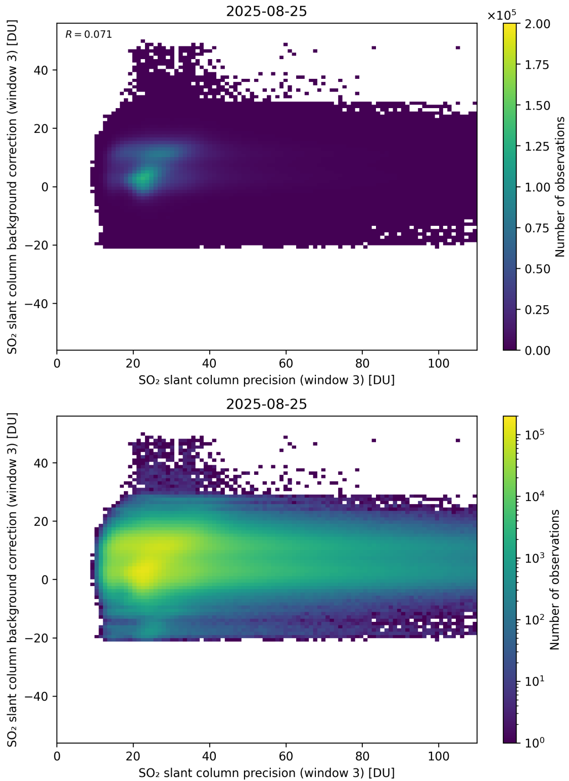
Figure 307: Scatter density plot of “SO 2 slant column precision (window 3)” against “SO 2 slant column background correction (window 3)” for 2025-08-25 to 2025-08-26.
