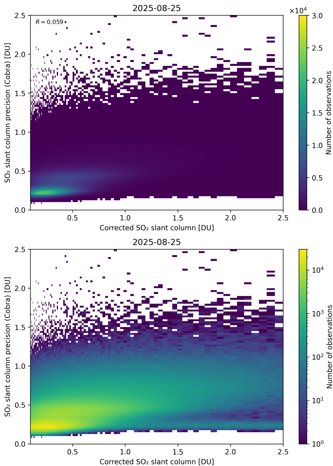
Figure 234: Scatter density plot of “Corrected SO 2 slant column” against “SO 2 slant column precision (Cobra)” for 2025-08-25 to 2025-08-26.
