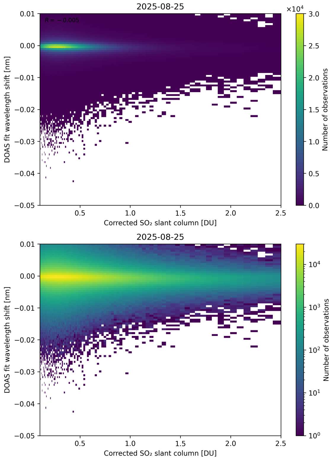
Figure 229: Scatter density plot of “Corrected SO 2 slant column” against “DOAS fit wavelength shift” for 2025-08-25 to 2025-08-26.
