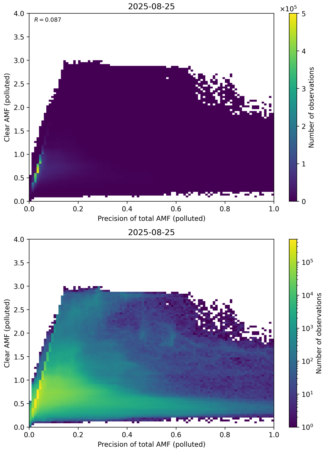
Figure 320: Scatter density plot of “Precision of total AMF (polluted)” against “Clear AMF (polluted)” for 2025-08-25 to 2025-08-26.
