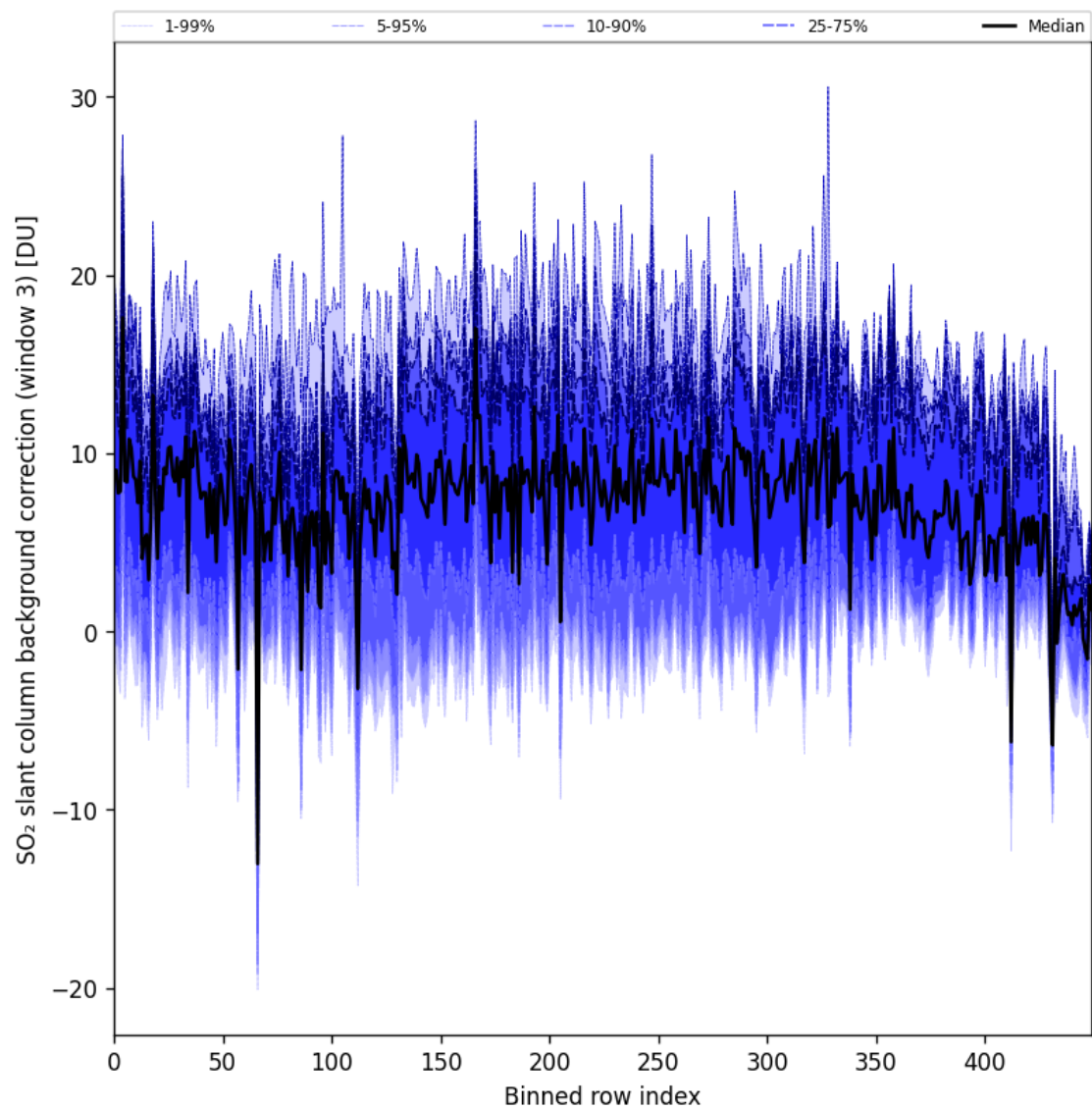
Figure 100: Along track statistics of “SO 2 slant column background correction (window 3)” for 2025-08-25 to 2025-08-26
