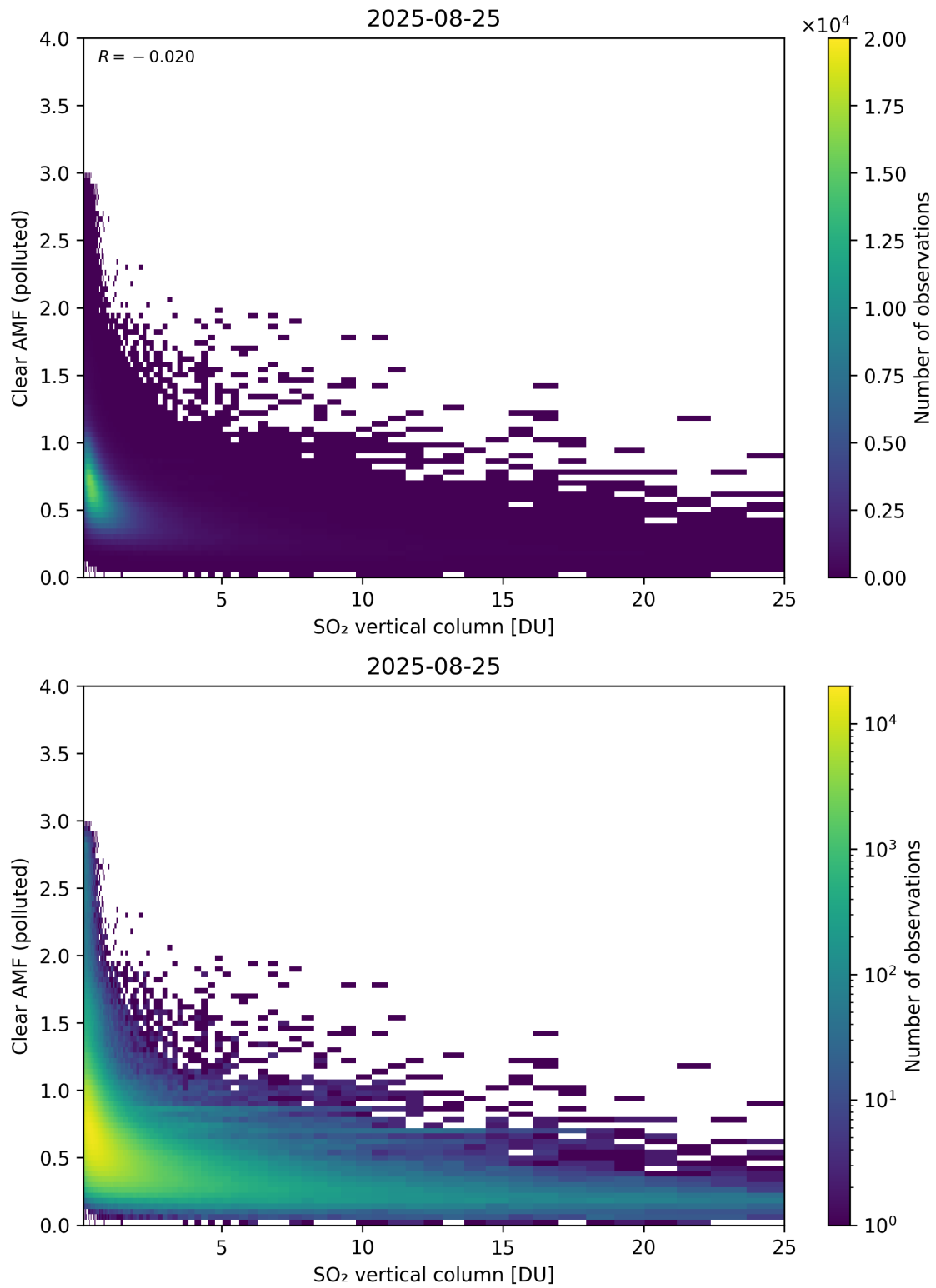
Figure 348: Scatter density plot of “SO 2 vertical column” against “Clear AMF (polluted)” for 2025-08-25 to 2025-08-26.
