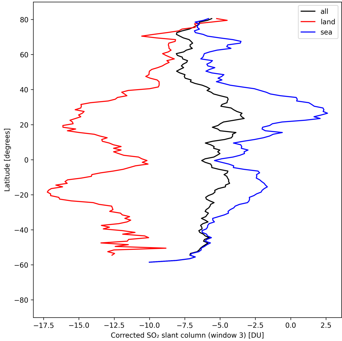
Figure 47: Zonal average of “Corrected SO 2 slant column (window 3)” for 2025-08-25 to 2025-08-26.
