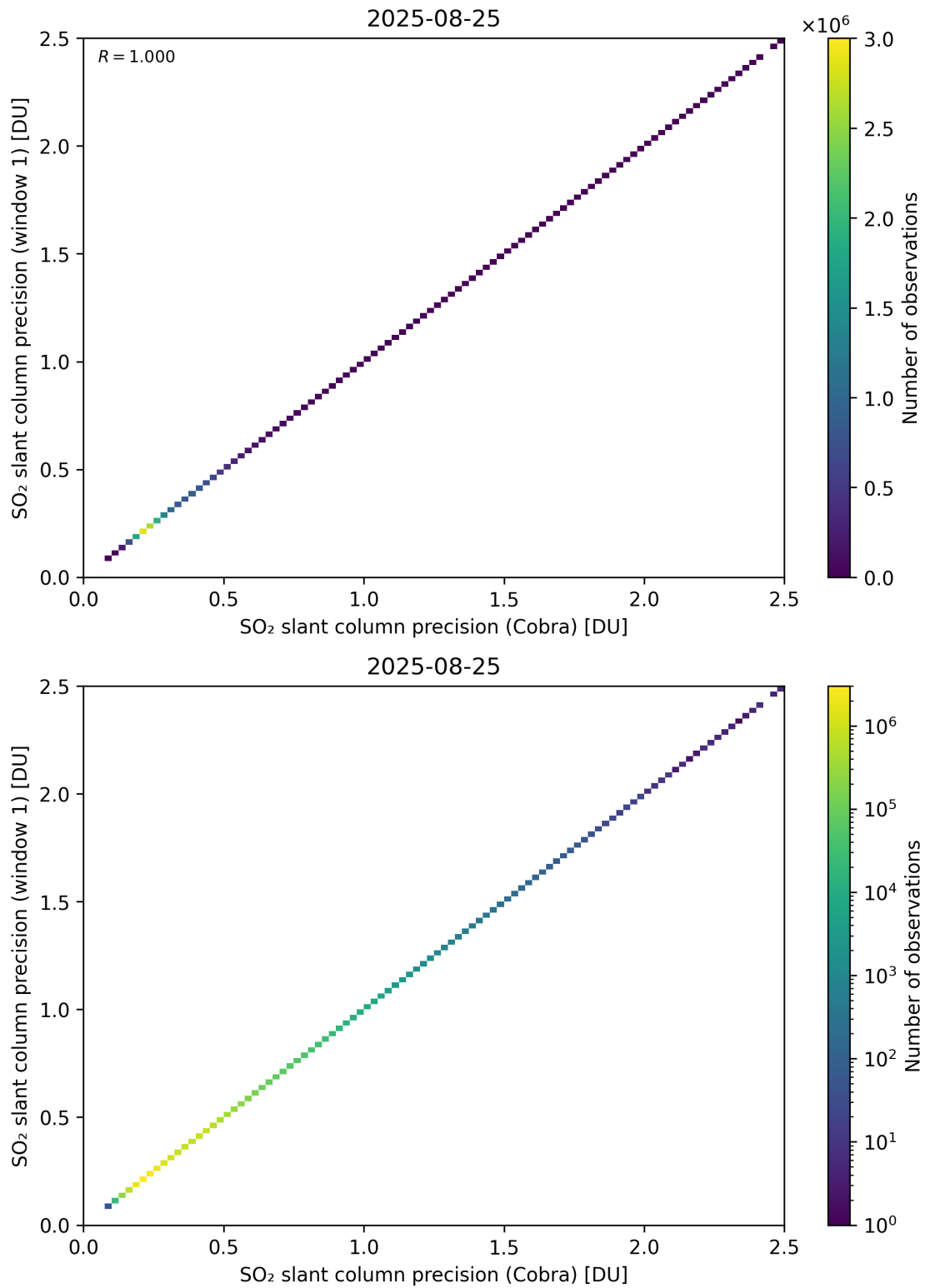
Figure 209: Scatter density plot of “SO 2 slant column precision (Cobra)” against “SO 2 slant column precision (window 1)” for 2025-08-25 to 2025-08-26.
