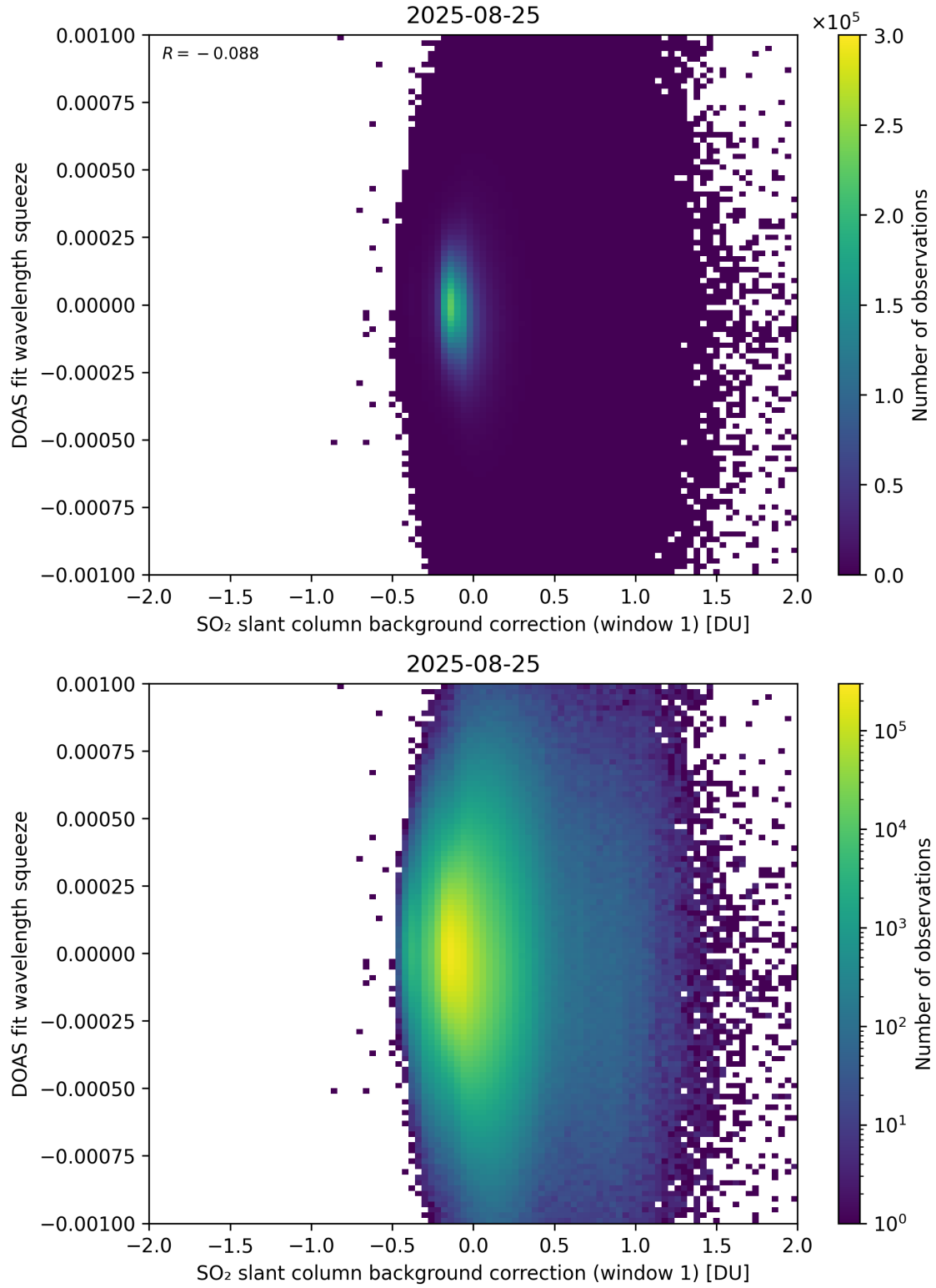
Figure 112: Scatter density plot of “SO 2 slant column background correction (window 1)” against “DOAS fit wavelength squeeze” for 2025-08-25 to 2025-08-26.
