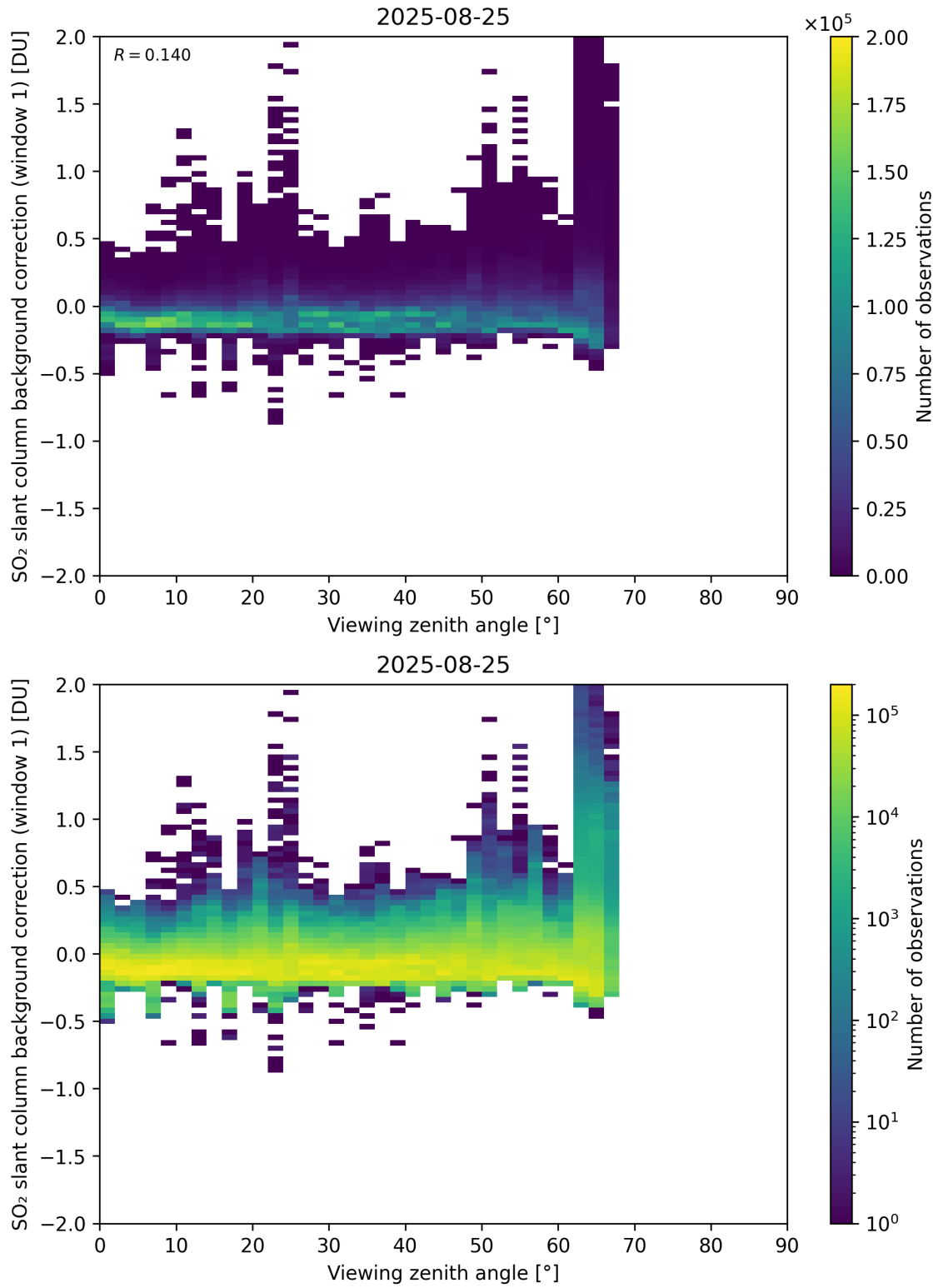
Figure 362: Scatter density plot of “Viewing zenith angle” against “SO 2 slant column background correction (window 1)” for 2025-08-25 to 2025-08-26.
