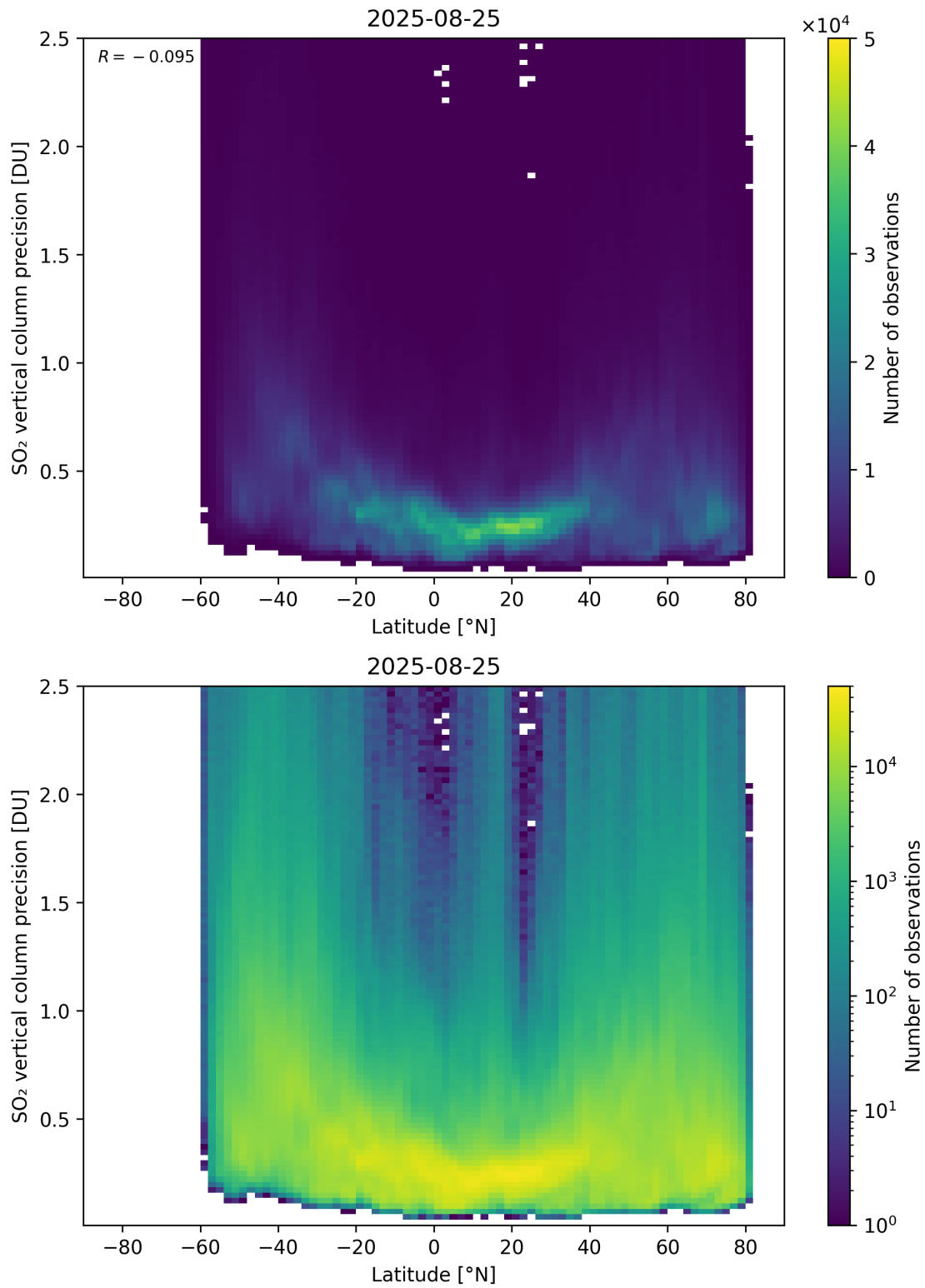
Figure 170: Scatter density plot of “Latitude” against “SO 2 vertical column precision” for 2025-08-25 to 2025-08-26.
