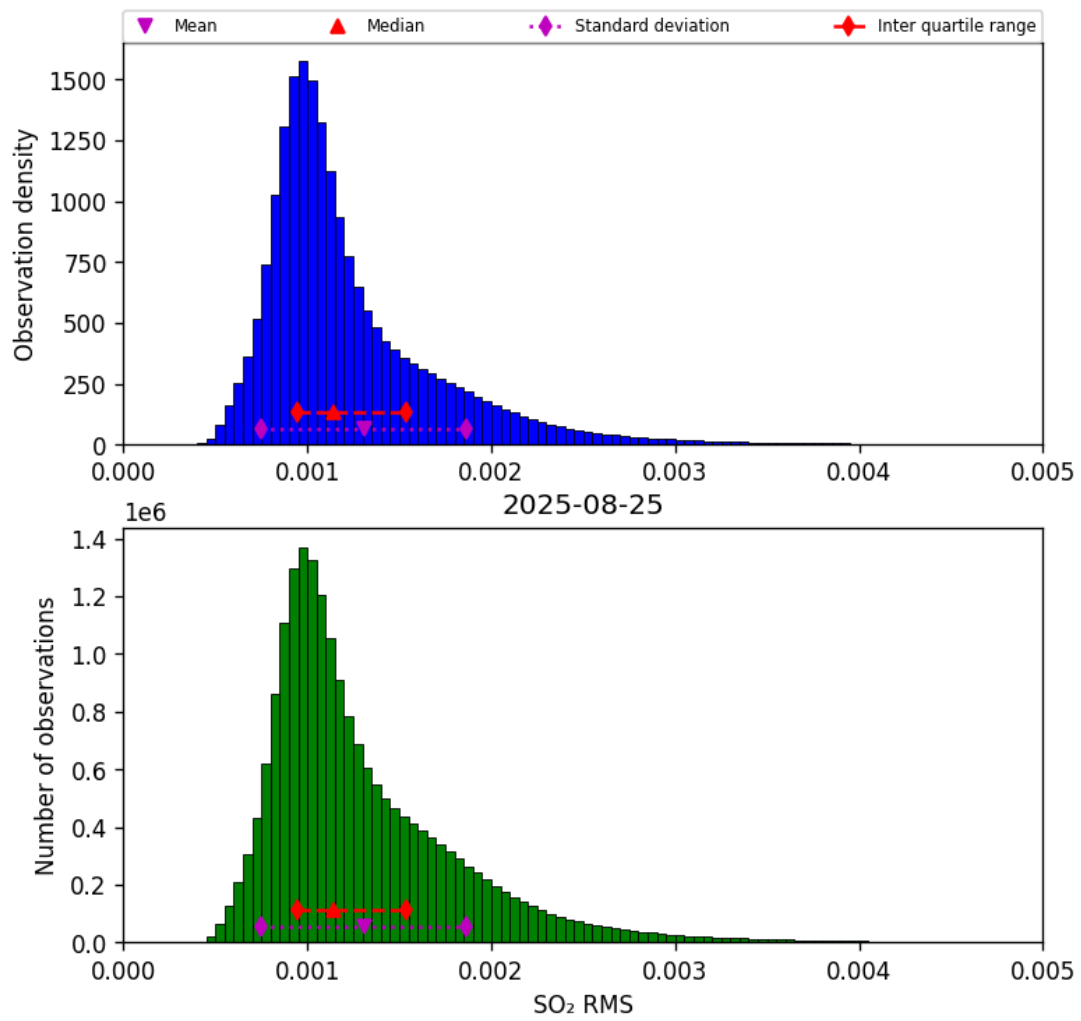
Figure 78: Histogram of "SO 2 RMS" for 2025-08-25 to 2025-08-26
