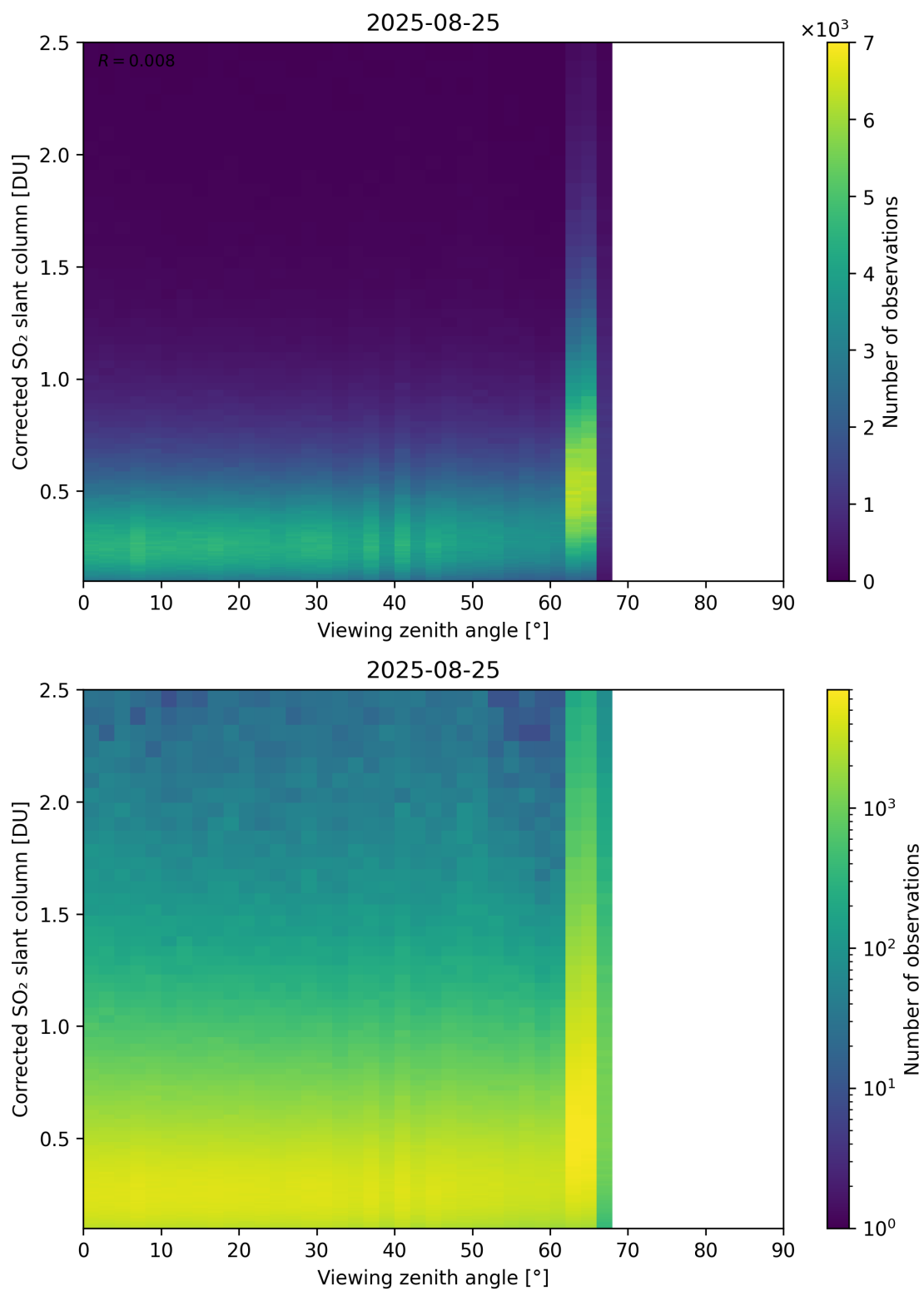
Figure 373: Scatter density plot of “Viewing zenith angle” against “Corrected SO 2 slant column” for 2025-08-25 to 2025-08-26.
