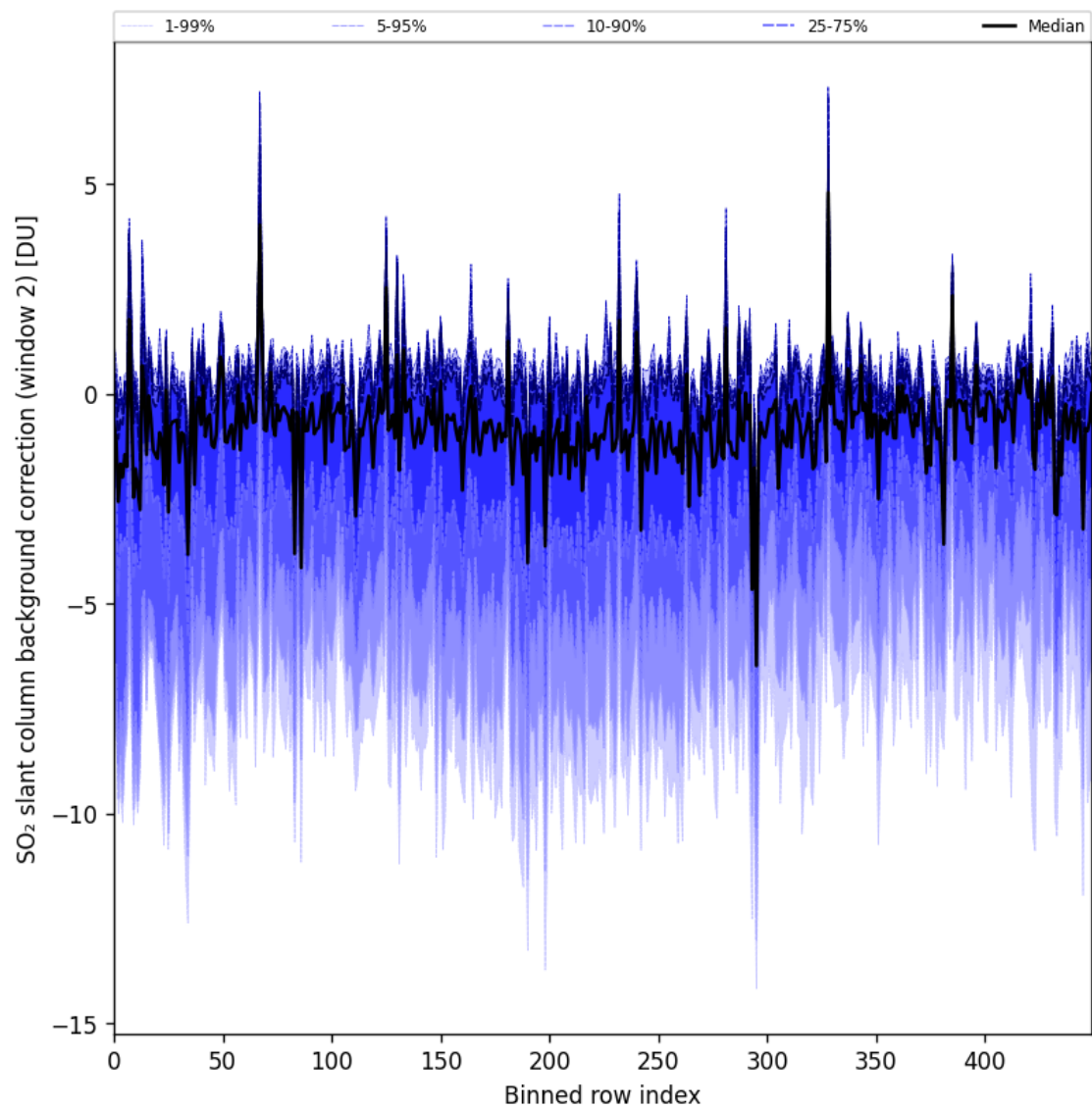
Figure 96: Along track statistics of “SO 2 slant column background correction (window 2)” for 2025-08-25 to 2025-08-26
