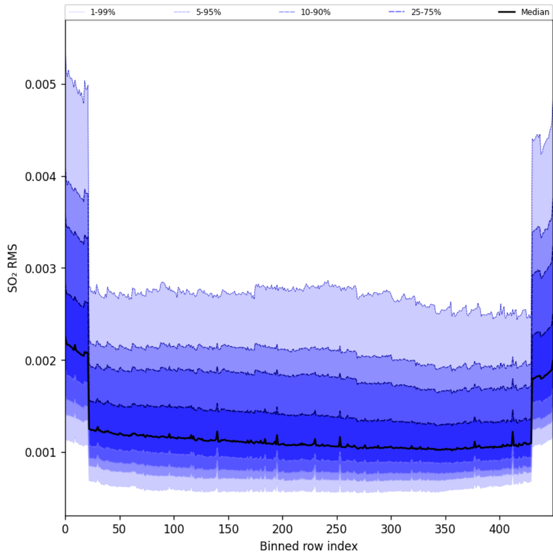
Figure 104: Along track statistics of “SO 2 RMS” for 2025-08-25 to 2025-08-26
