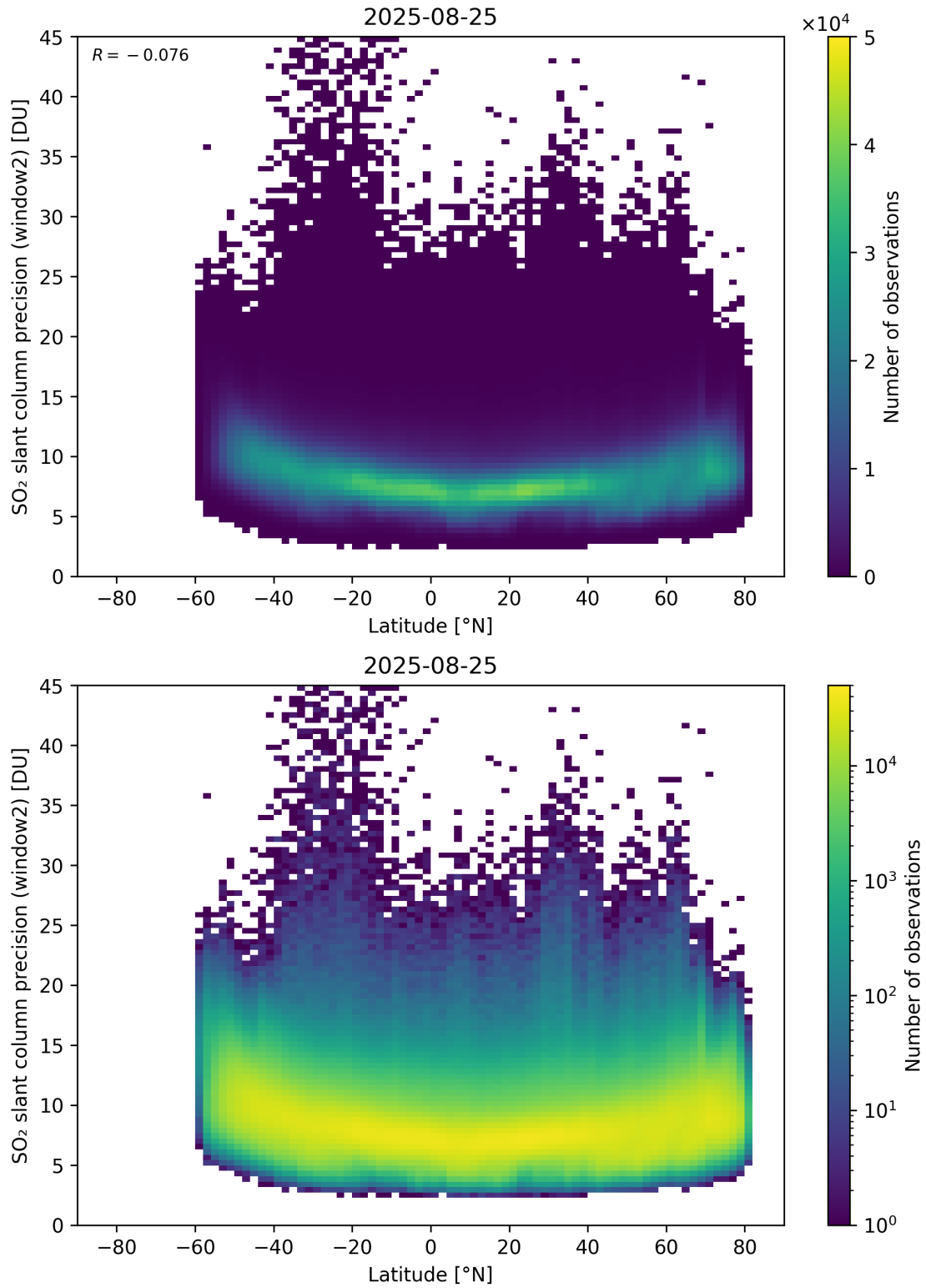
Figure 164: Scatter density plot of “Latitude” against “SO 2 slant column precision (window2)” for 2025-08-25 to 2025-08-26.
