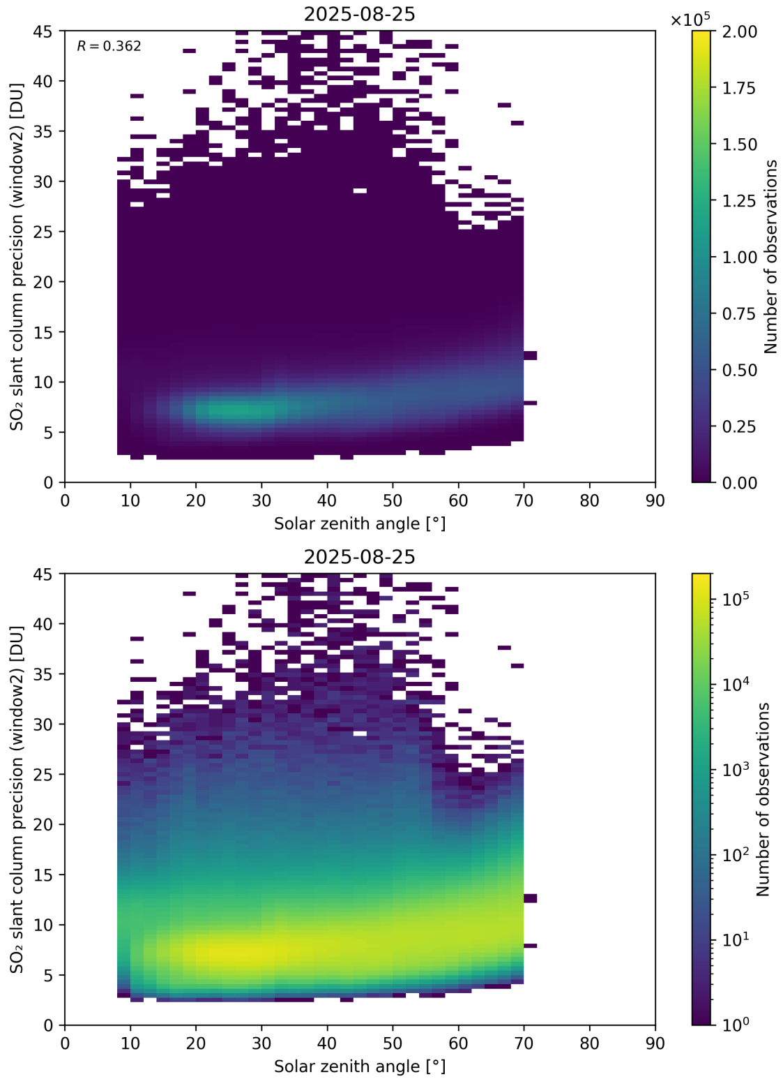
Figure 186: Scatter density plot of “Solar zenith angle” against “SO 2 slant column precision (window2)” for 2025-08-25 to 2025-08-26.
