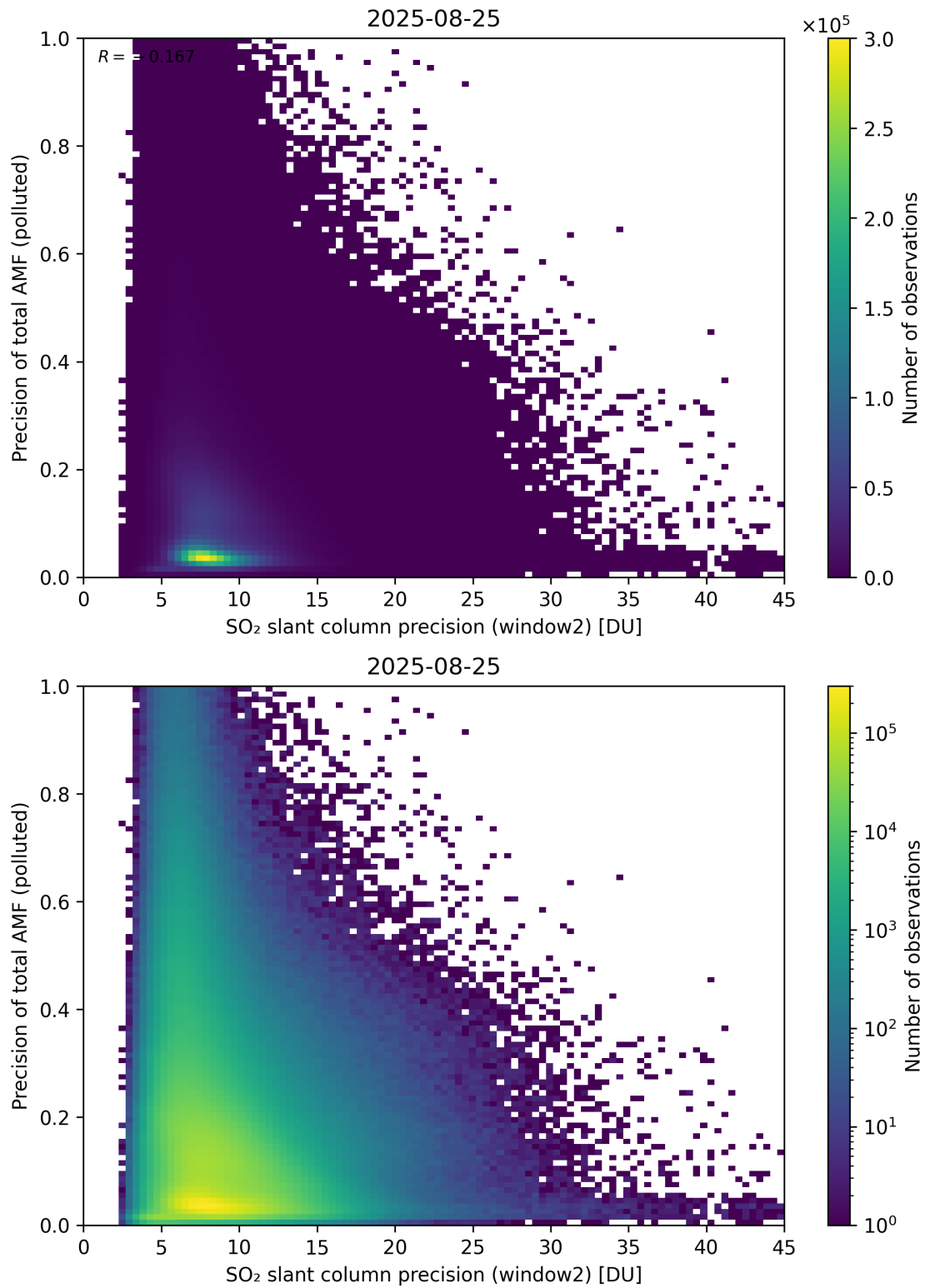
Figure 302: Scatter density plot of “SO 2 slant column precision (window2)” against “Precision of total AMF (polluted)” for 2025-08-25 to 2025-08-26.
