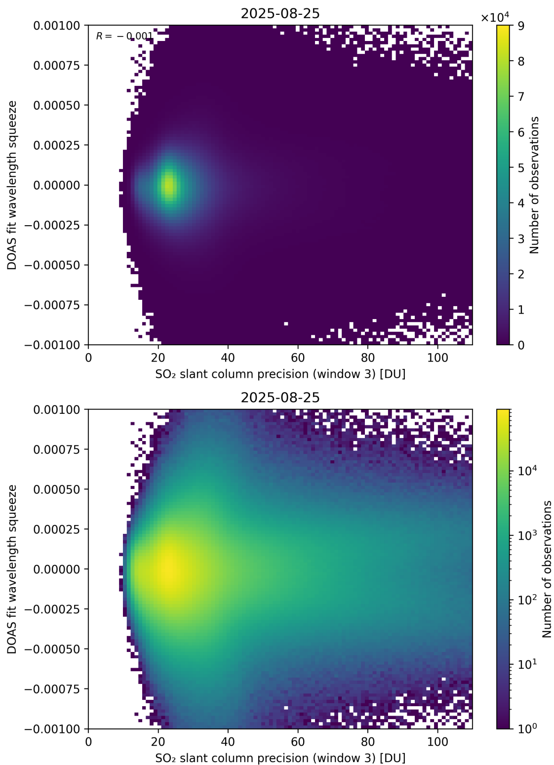
Figure 309: Scatter density plot of “SO 2 slant column precision (window 3)” against “DOAS fit wavelength squeeze” for 2025-08-25 to 2025-08-26.
