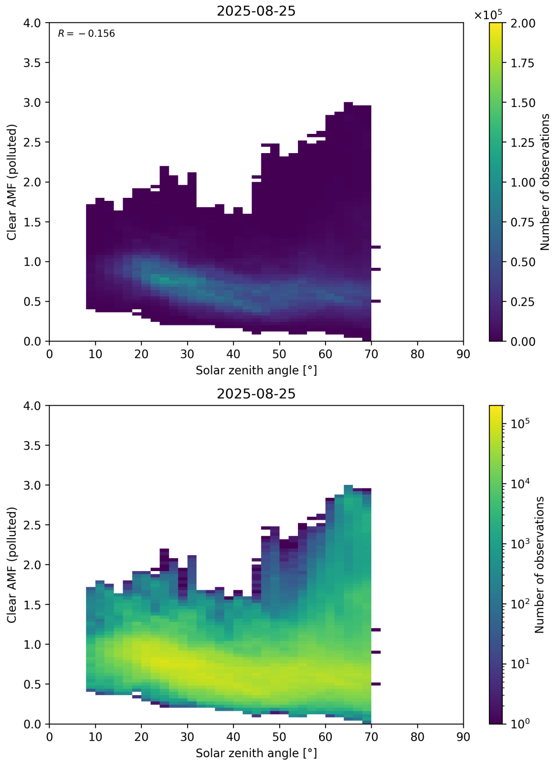
Figure 178: Scatter density plot of “Solar zenith angle” against “Clear AMF (polluted)” for 2025-08-25 to 2025-08-26.
