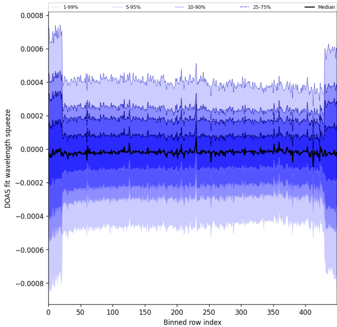
Figure 103: Along track statistics of “DOAS fit wavelength squeeze” for 2025-08-25 to 2025-08-26
