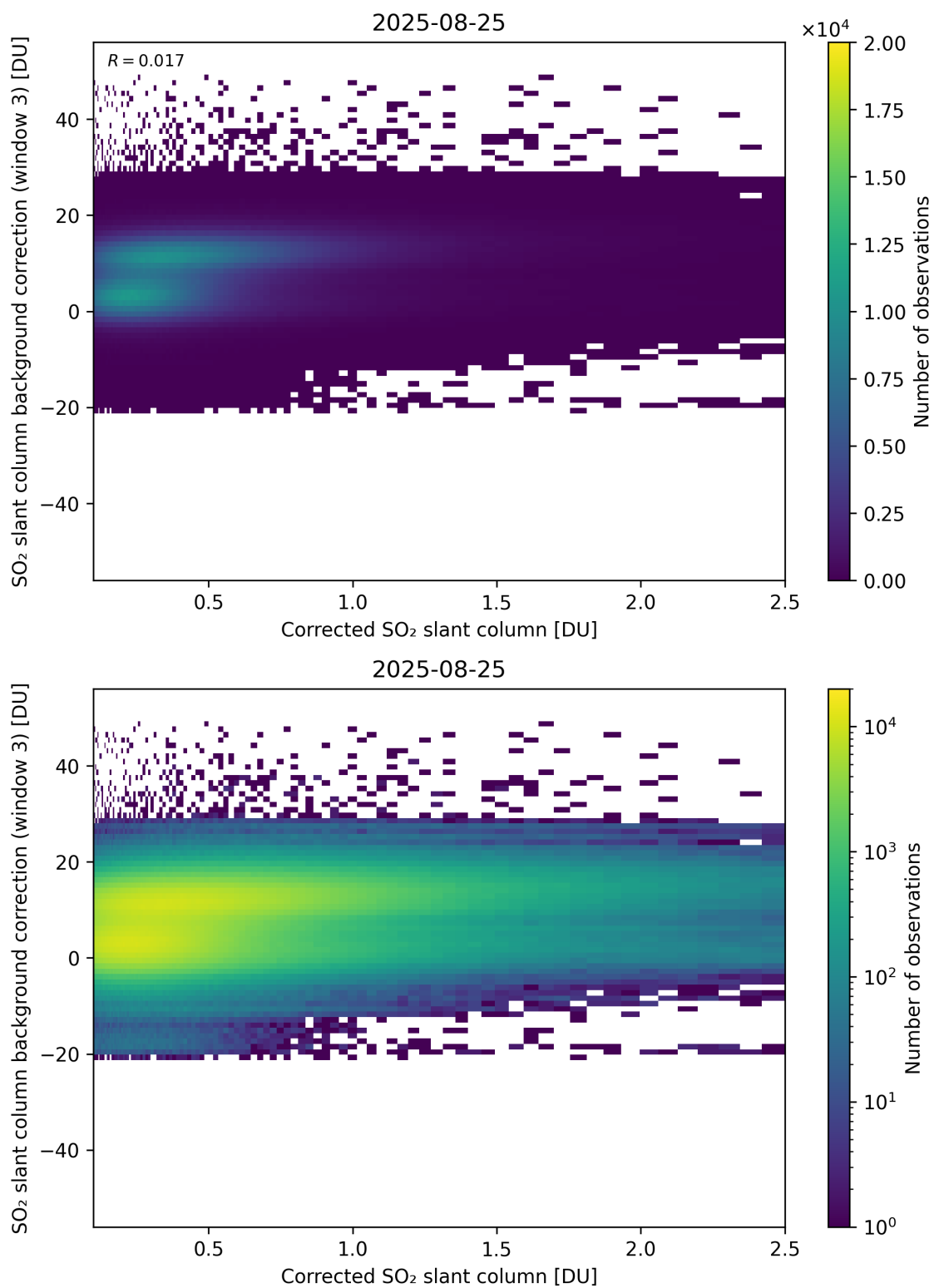
Figure 228: Scatter density plot of “Corrected SO 2 slant column” against “SO 2 slant column background correction (window 3)” for 2025-08-25 to 2025-08-26.
