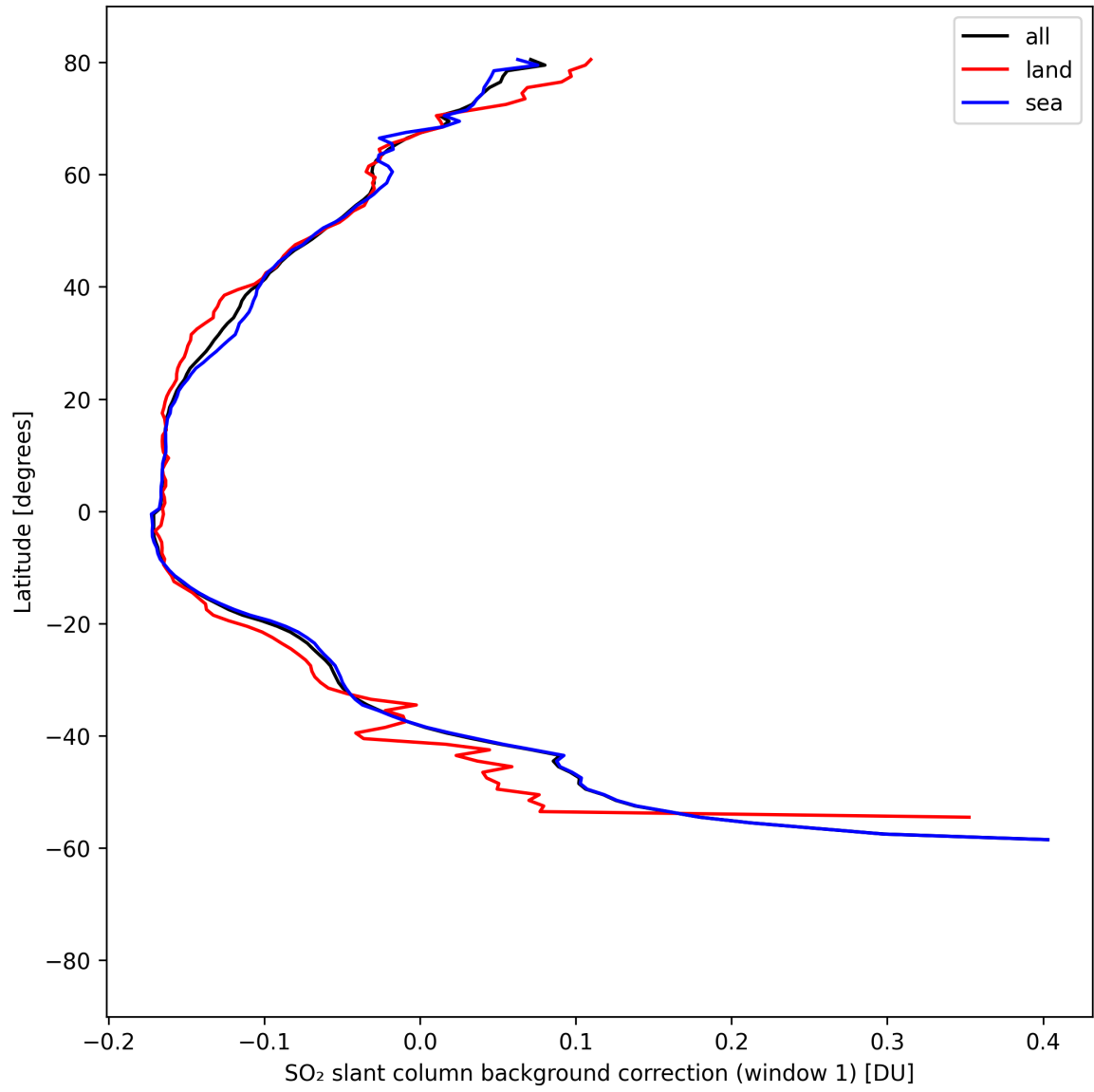
Figure 40: Zonal average of “SO 2 slant column background correction (window 1)” for 2025-08-25 to 2025-08-26.
