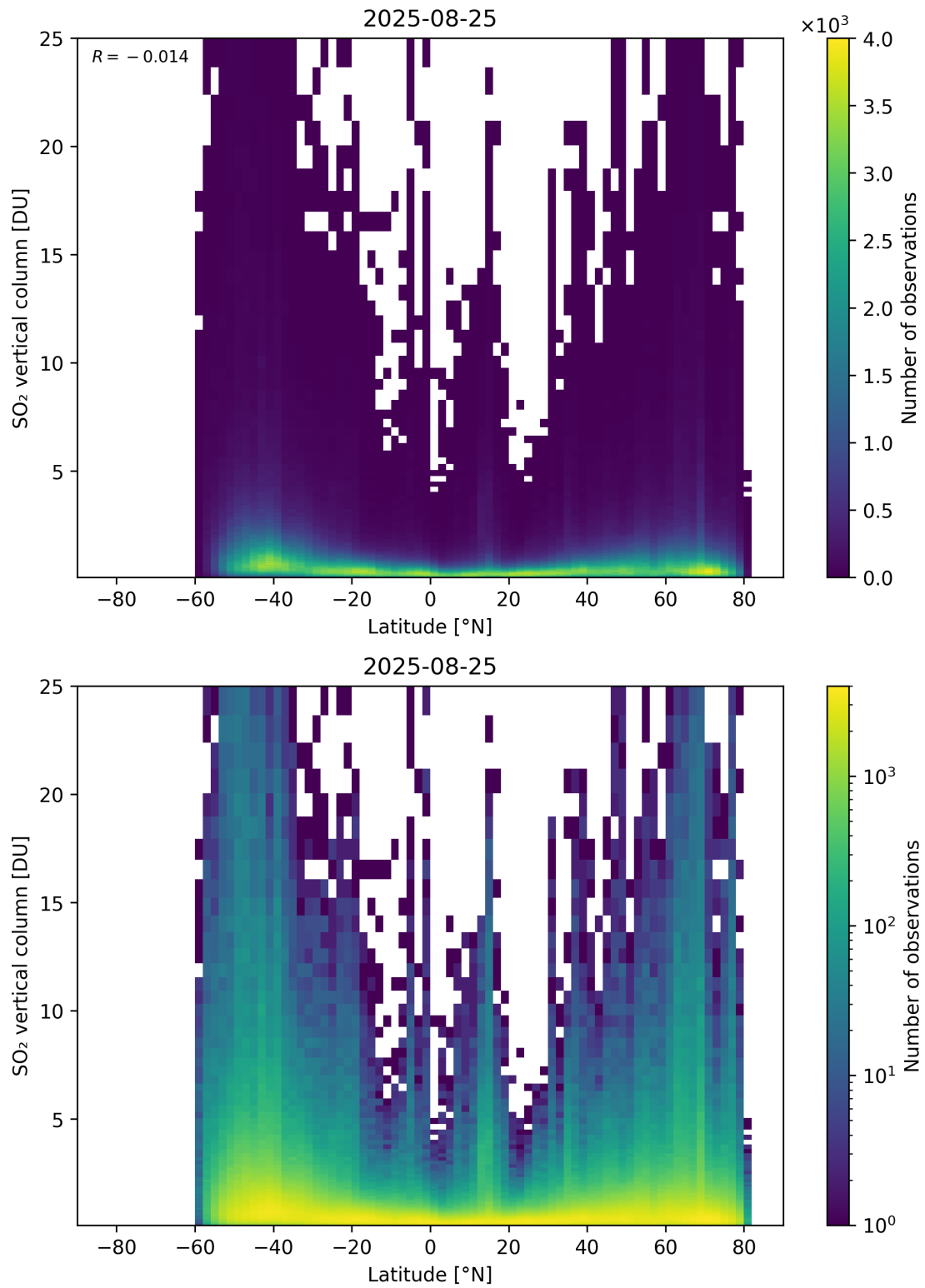
Figure 169: Scatter density plot of “Latitude” against “SO 2 vertical column” for 2025-08-25 to 2025-08-26.
