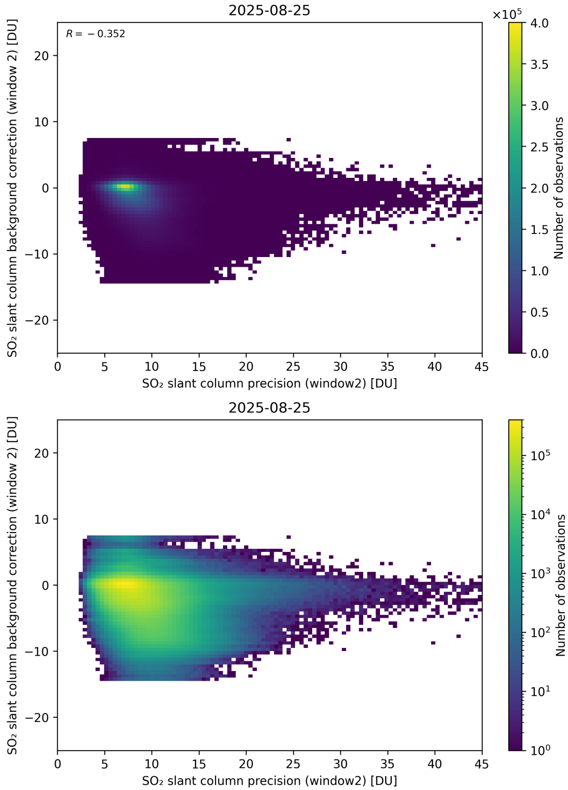
Figure 291: Scatter density plot of “SO 2 slant column precision (window2)” against “SO 2 slant column background correction (window 2)” for 2025-08-25 to 2025-08-26.
