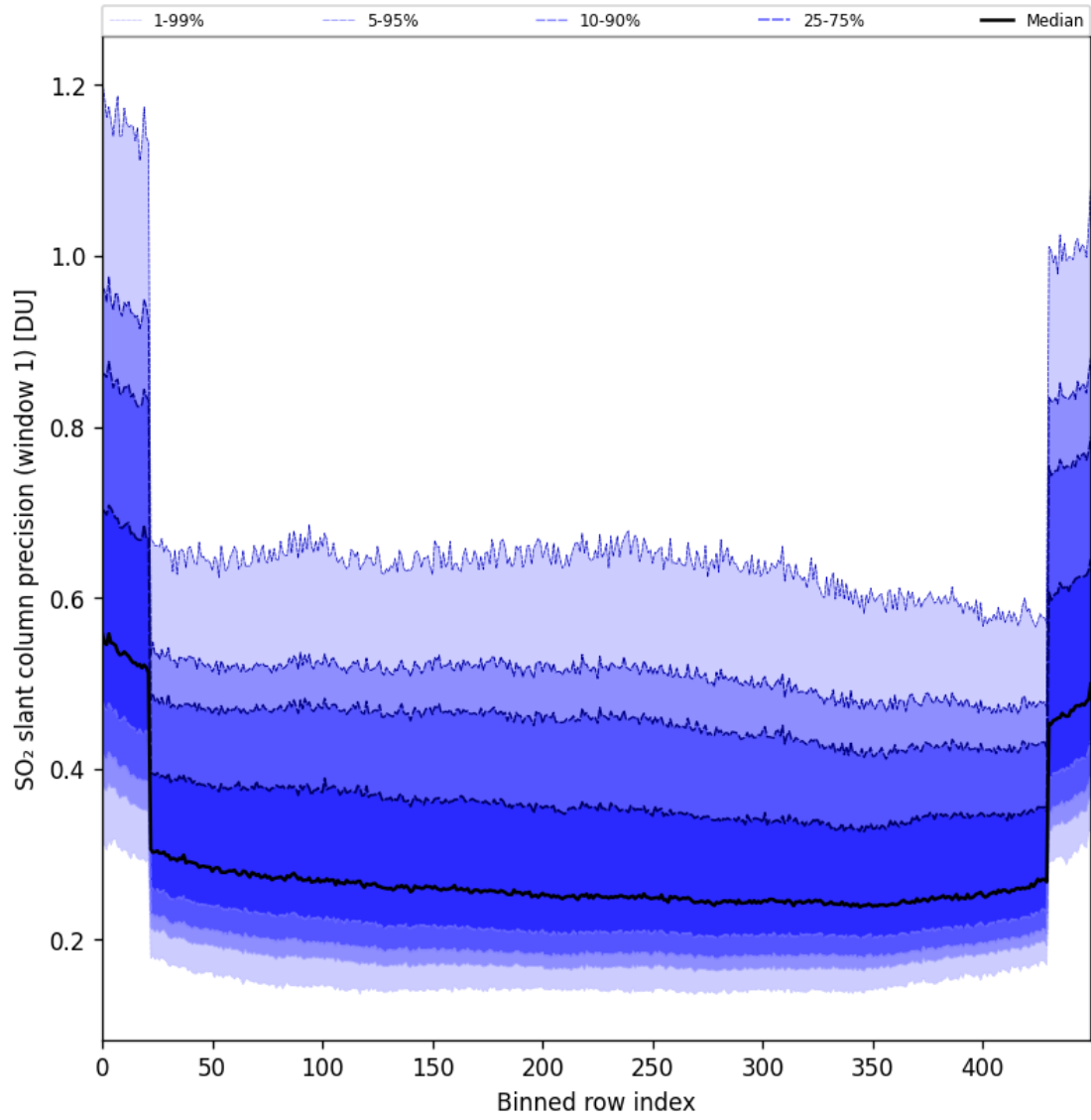
Figure 90: Along track statistics of “SO 2 slant column precision (window 1)” for 2025-08-25 to 2025-08-26
