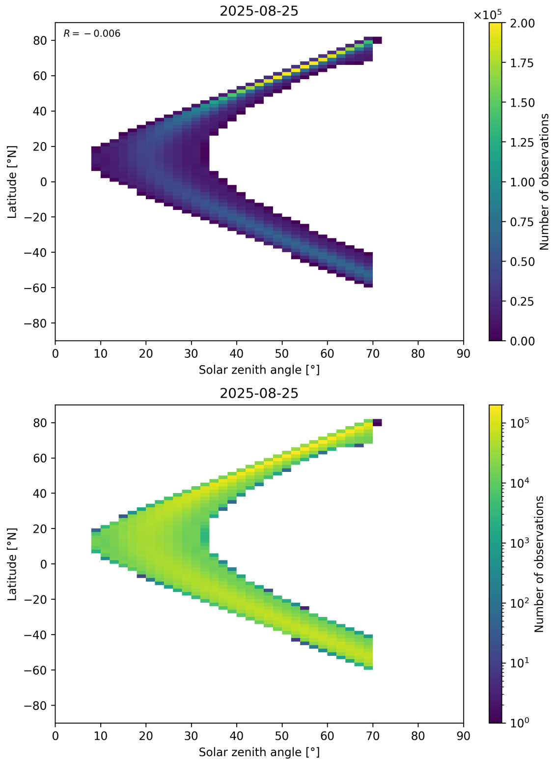
Figure 177: Scatter density plot of “Solar zenith angle” against “Latitude” for 2025-08-25 to 2025-08-26.
