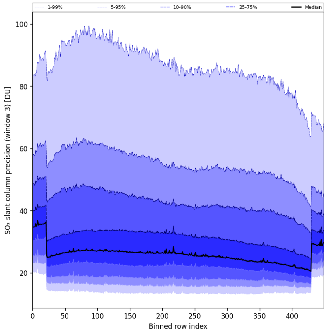
Figure 98: Along track statistics of “SO 2 slant column precision (window 3)” for 2025-08-25 to 2025-08-26
