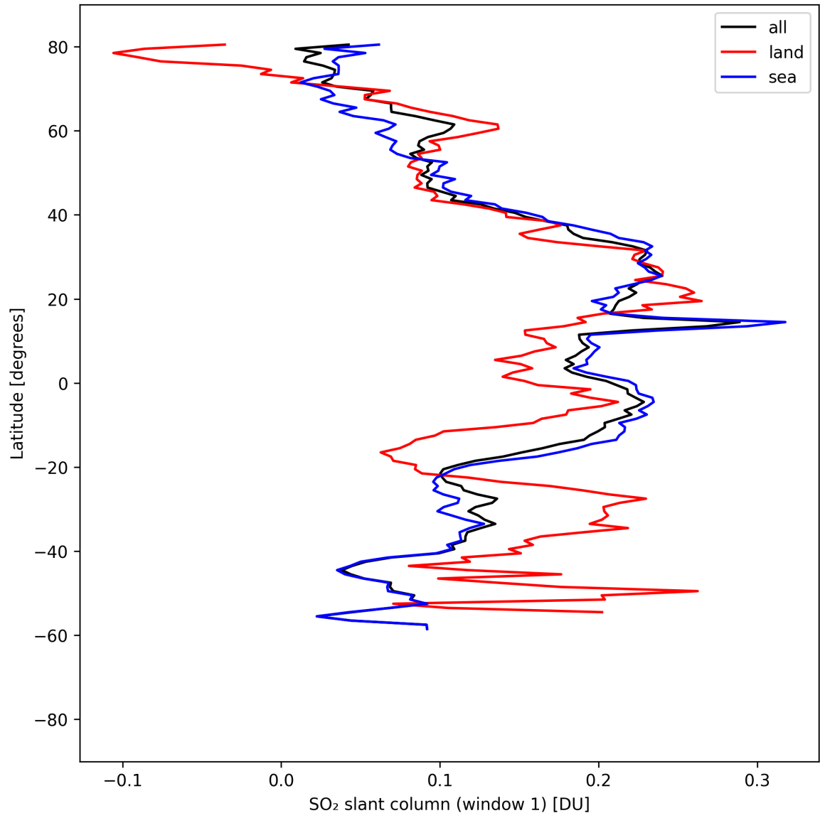
Figure 37: Zonal average of “SO 2 slant column (window 1)” for 2025-08-25 to 2025-08-26.
