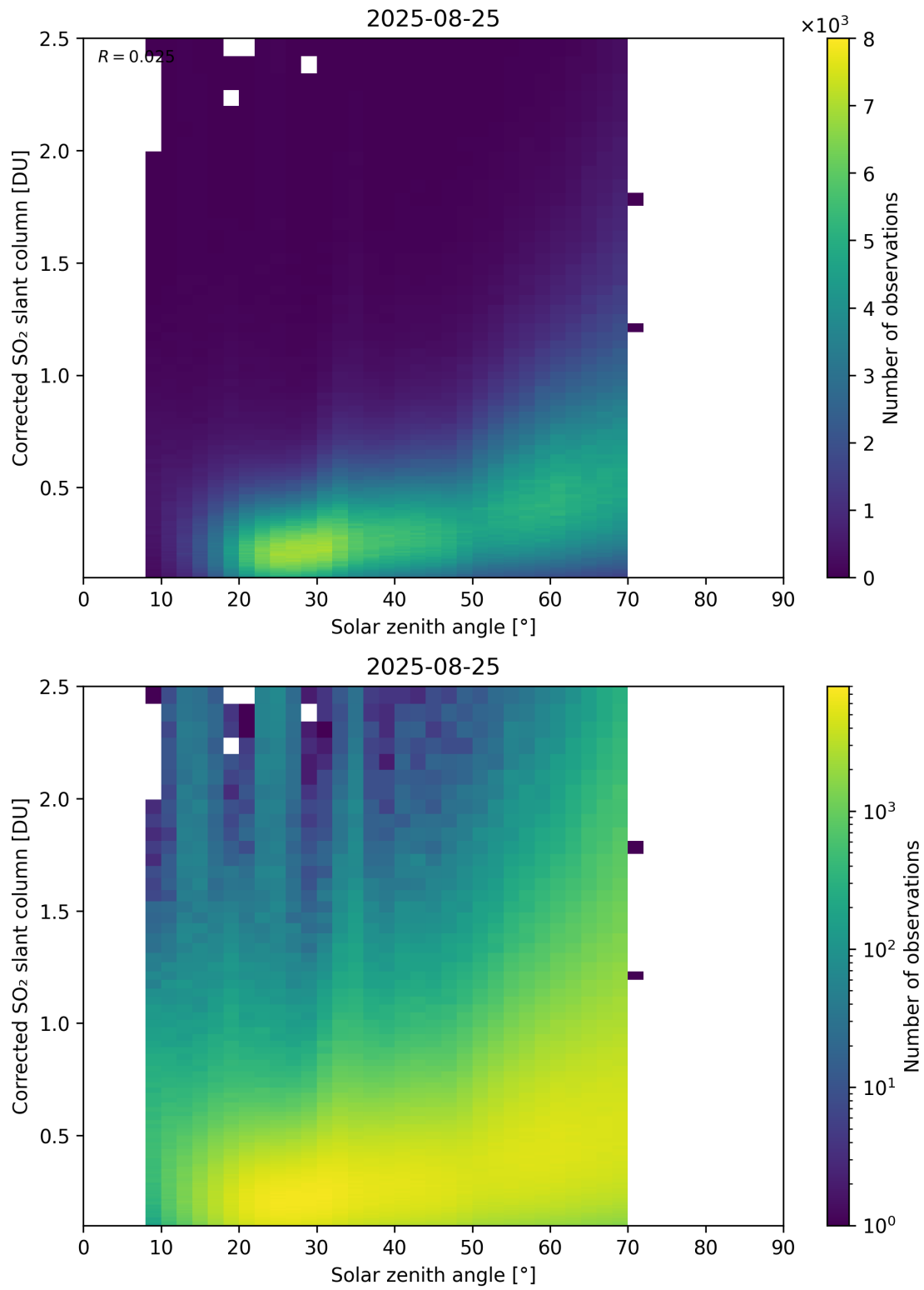
Figure 181: Scatter density plot of “Solar zenith angle” against “Corrected SO 2 slant column” for 2025-08-25 to 2025-08-26.
