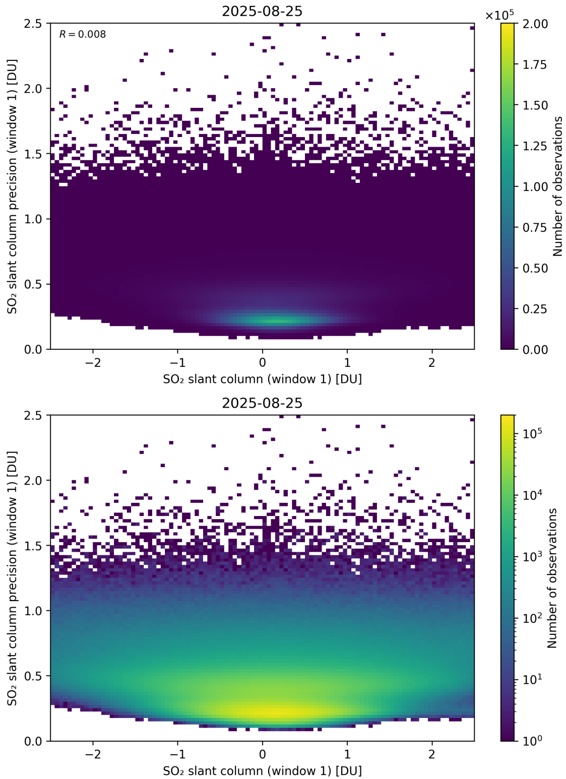
Figure 285: Scatter density plot of “SO 2 slant column (window 1)” against “SO 2 slant column precision (window 1)” for 2025-08-25 to 2025-08-26.
