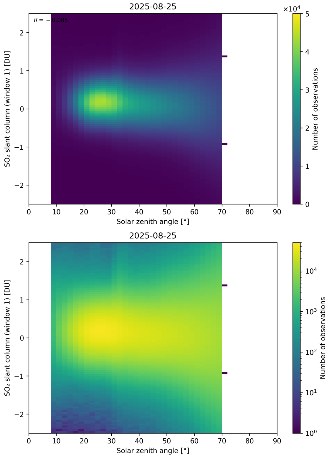
Figure 184: Scatter density plot of “Solar zenith angle” against “SO 2 slant column (window 1)” for 2025-08-25 to 2025-08-26.
