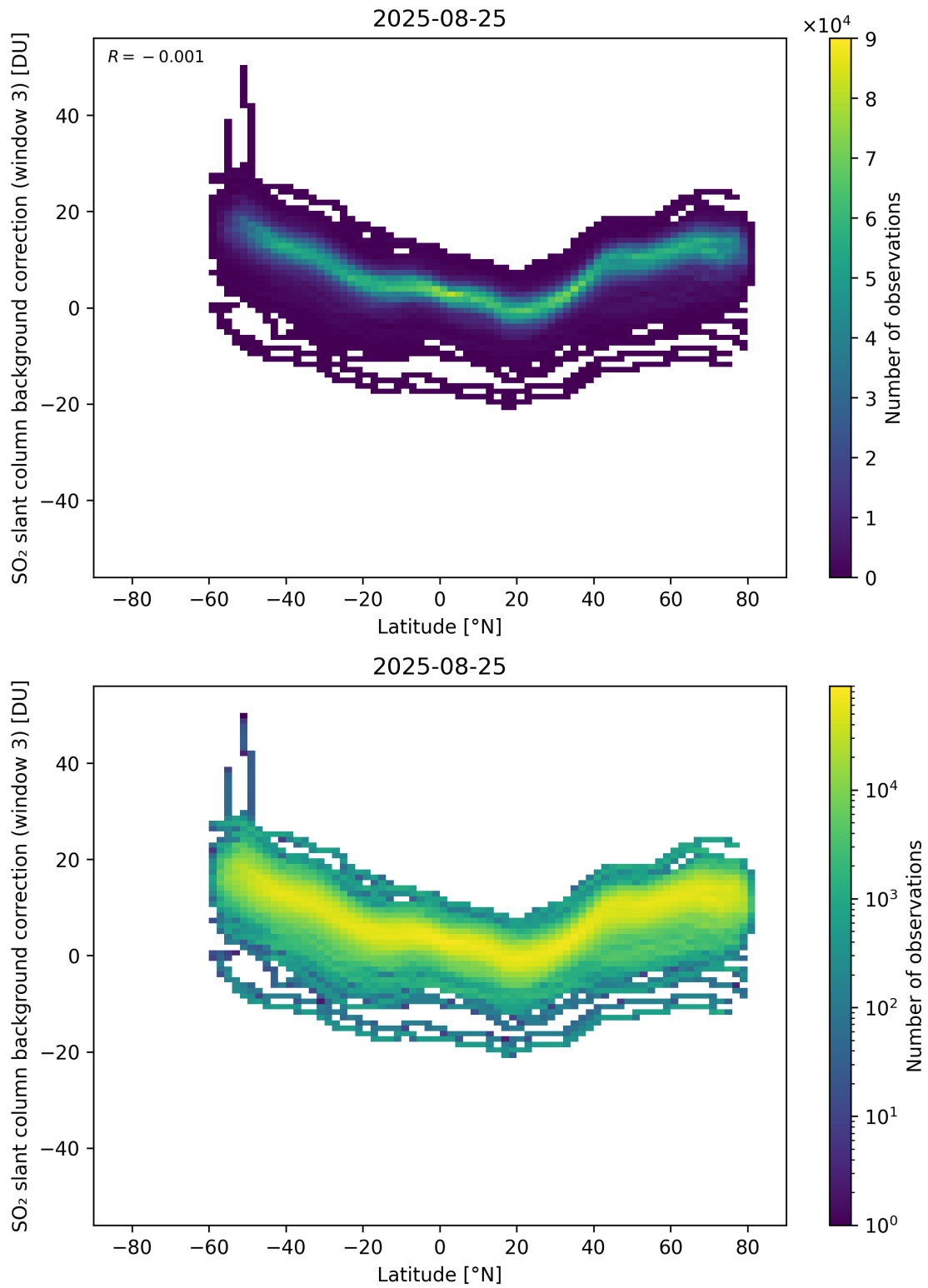
Figure 152: Scatter density plot of “Latitude” against “SO 2 slant column background correction (window 3)” for 2025-08-25 to 2025-08-26.
