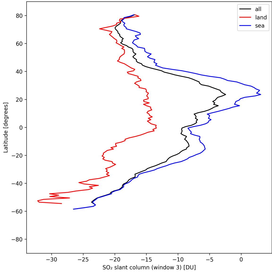
Figure 45: Zonal average of “SO 2 slant column (window 3)” for 2025-08-25 to 2025-08-26.
