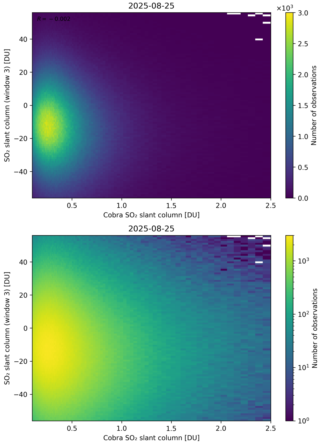
Figure 222: Scatter density plot of “Cobra SO 2 slant column” against “SO 2 slant column (window 3)” for 2025-08-25 to 2025-08-26.
