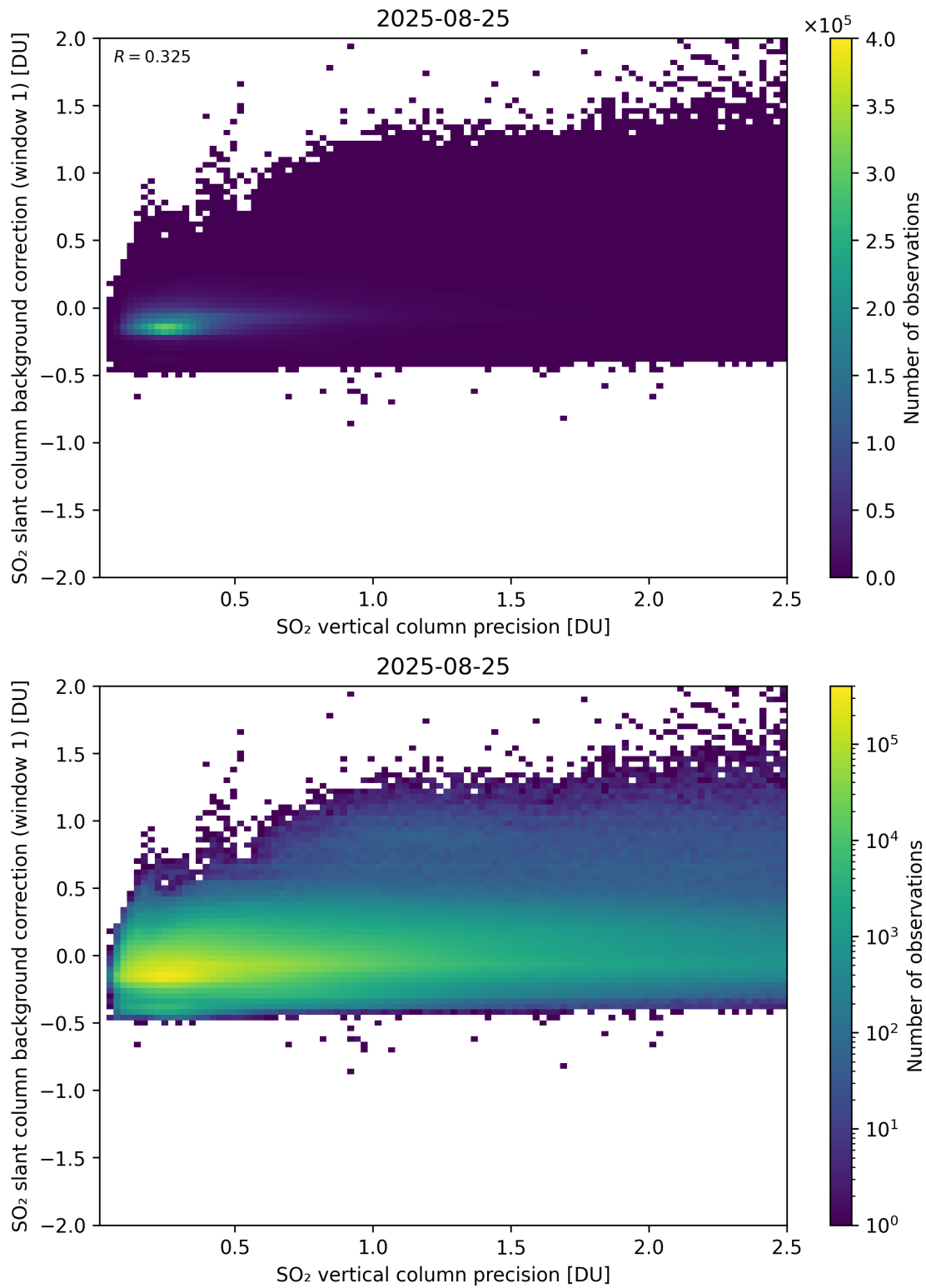
Figure 329: Scatter density plot of “SO 2 vertical column precision” against “SO 2 slant column background correction (window 1)” for 2025-08-25 to 2025-08-26.
