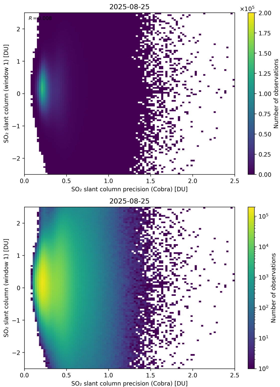
Figure 208: Scatter density plot of “SO 2 slant column precision (Cobra)” against “SO 2 slant column (window 1)” for 2025-08-25 to 2025-08-26.
