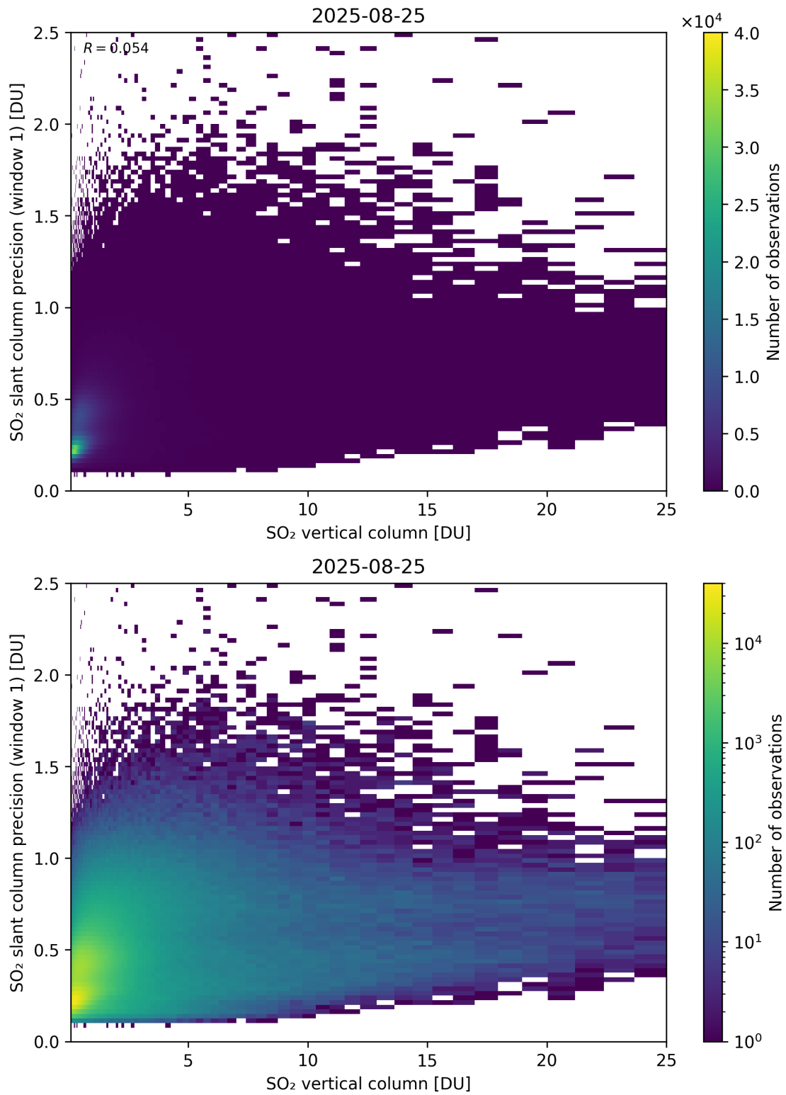
Figure 355: Scatter density plot of “SO 2 vertical column” against “SO 2 slant column precision (window 1)” for 2025-08-25 to 2025-08-26.
