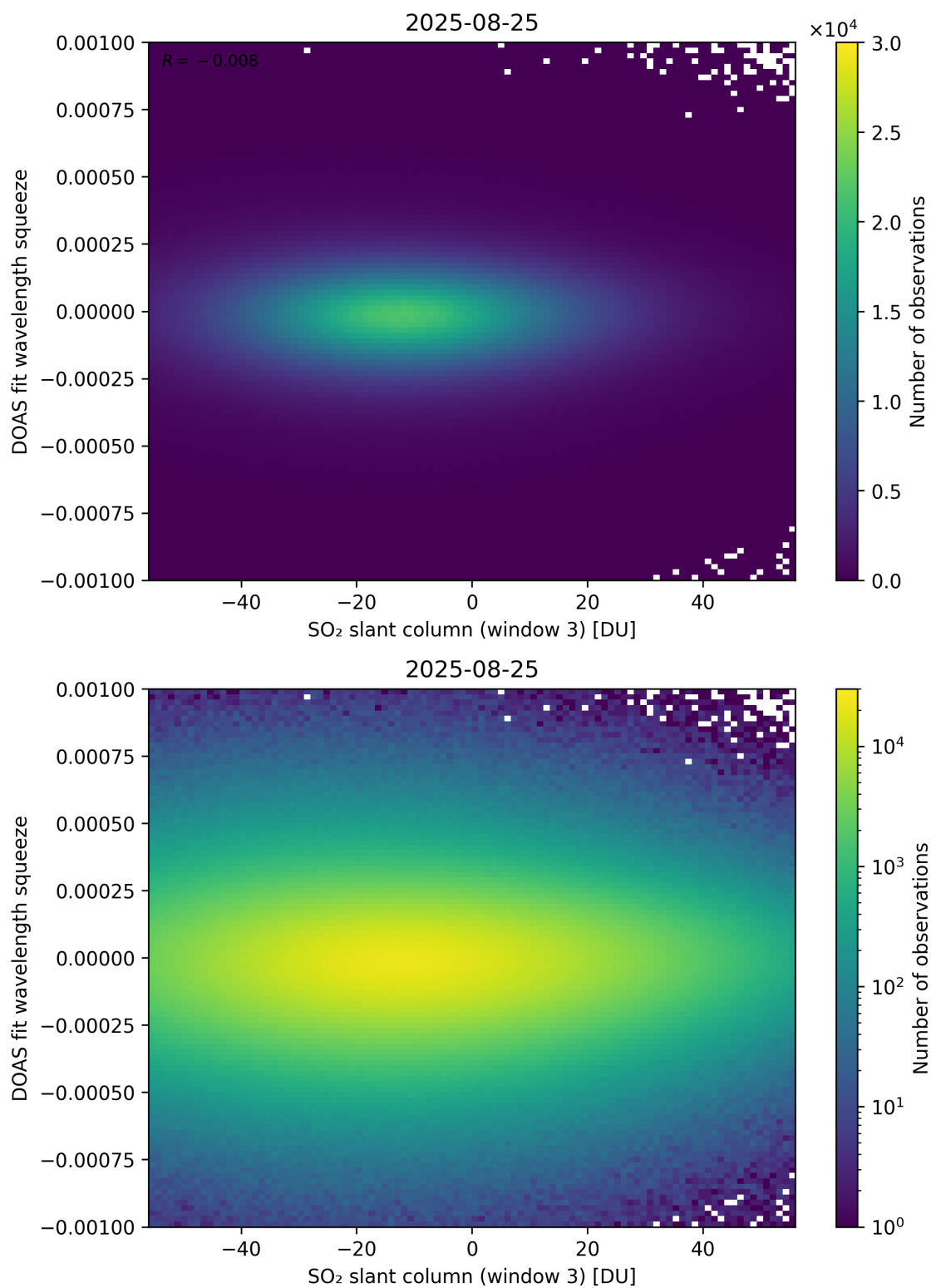
Figure 305: Scatter density plot of “SO 2 slant column (window 3)” against “DOAS fit wavelength squeeze” for 2025-08-25 to 2025-08-26.
