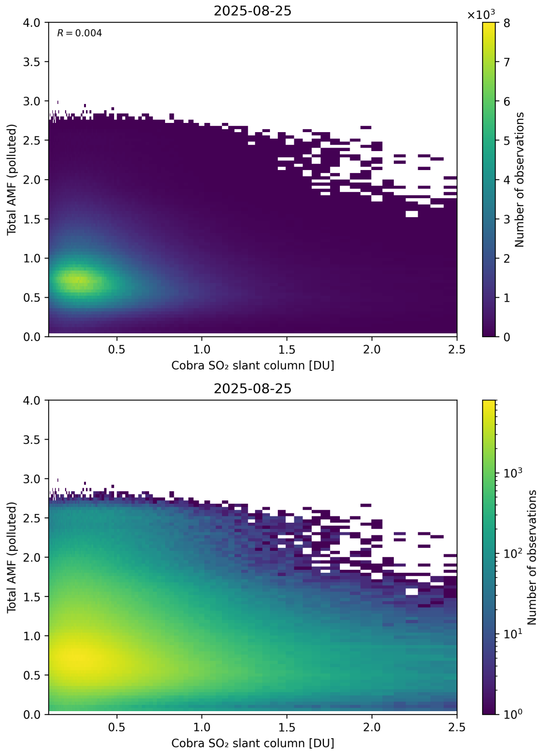
Figure 224: Scatter density plot of “Cobra SO 2 slant column” against “Total AMF (polluted)” for 2025-08-25 to 2025-08-26.
