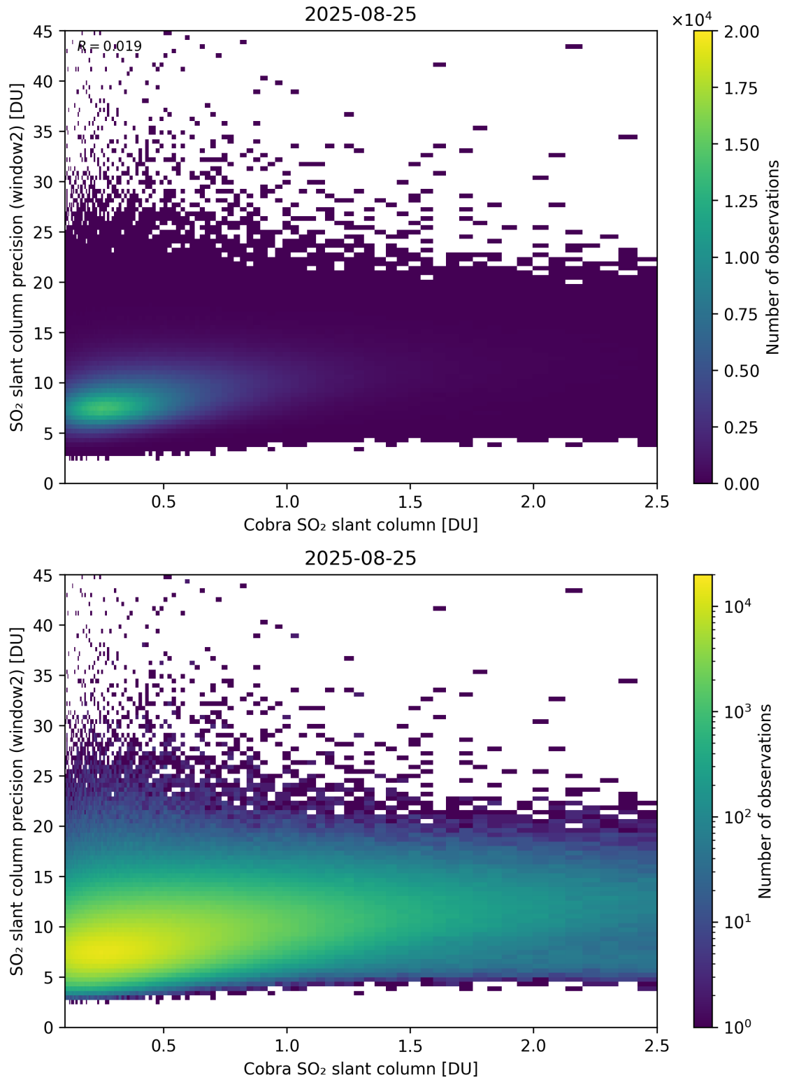
Figure 221: Scatter density plot of “Cobra SO 2 slant column” against “SO 2 slant column precision (window2)” for 2025-08-25 to 2025-08-26.
