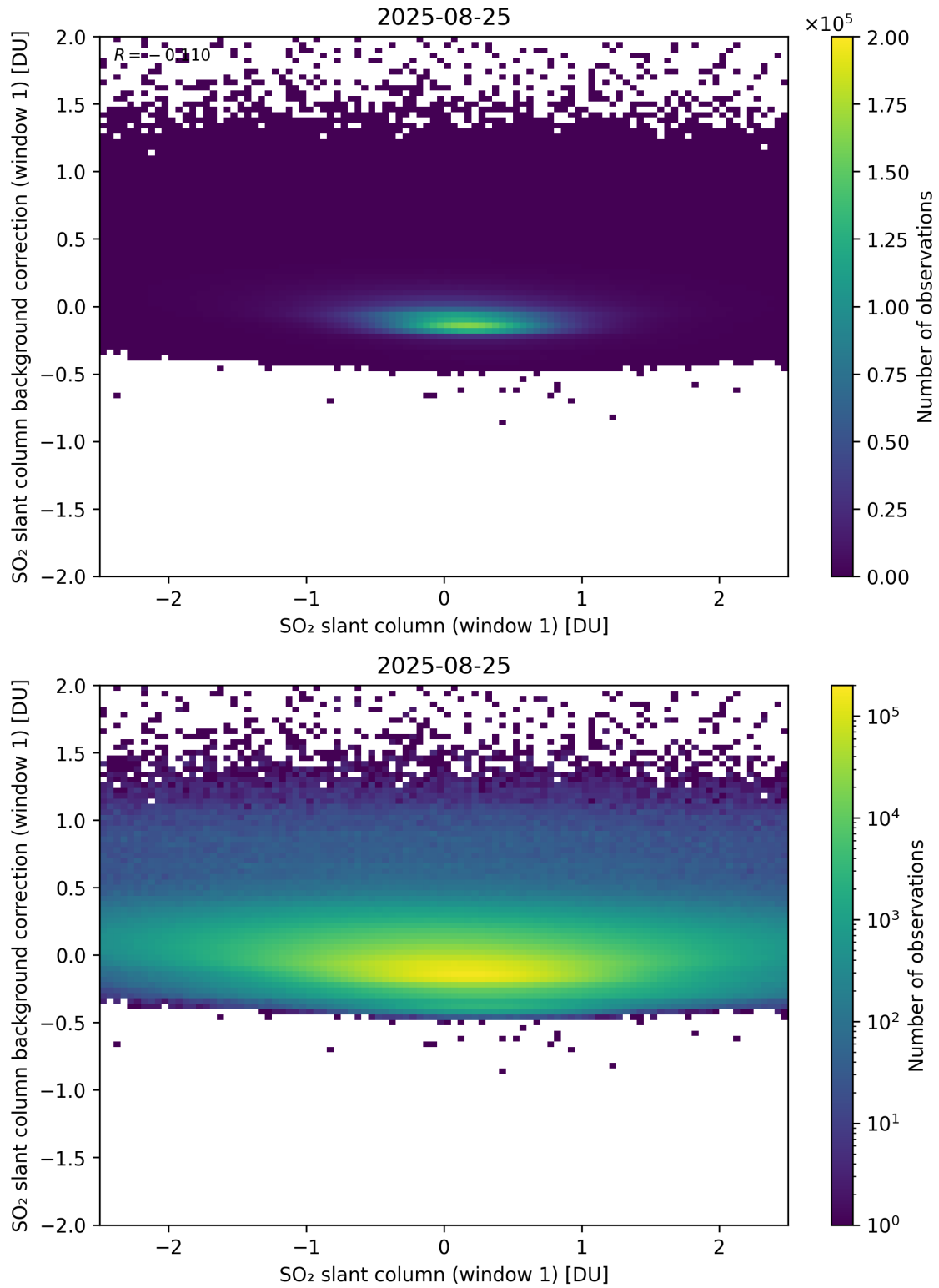
Figure 262: Scatter density plot of “SO 2 slant column (window 1)” against “SO 2 slant column background correction (window 1)” for 2025-08-25 to 2025-08-26.
