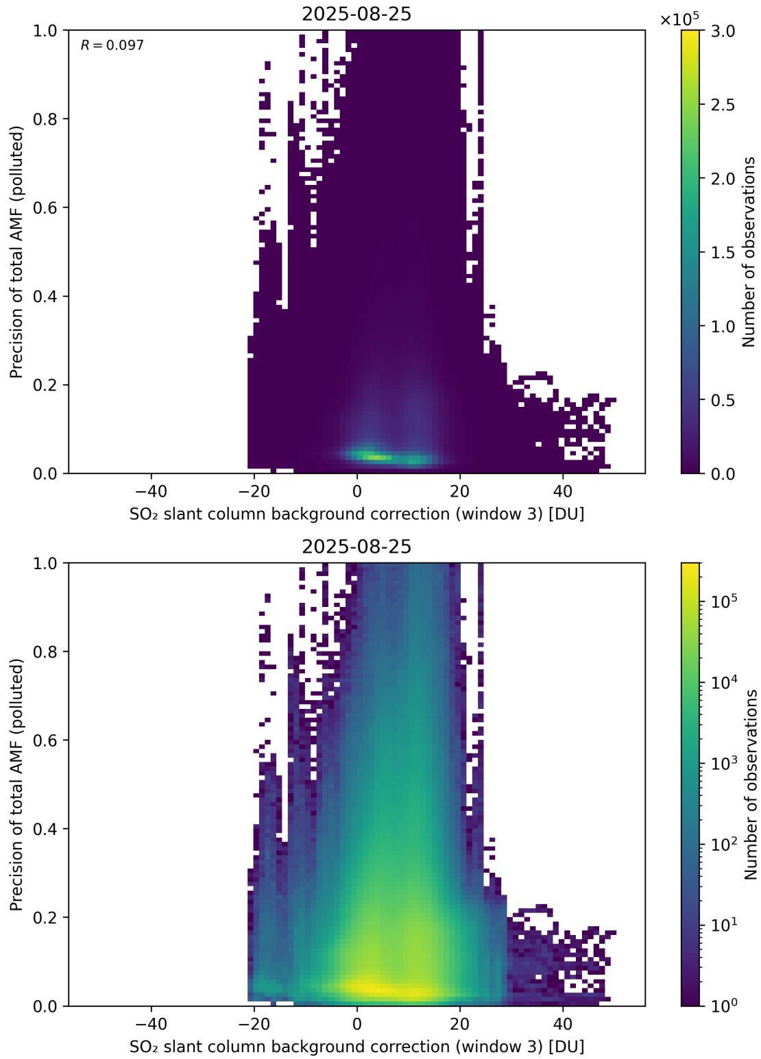
Figure 137: Scatter density plot of “SO 2 slant column background correction (window 3)” against “Precision of total AMF (polluted)” for 2025-08-25 to 2025-08-26.
