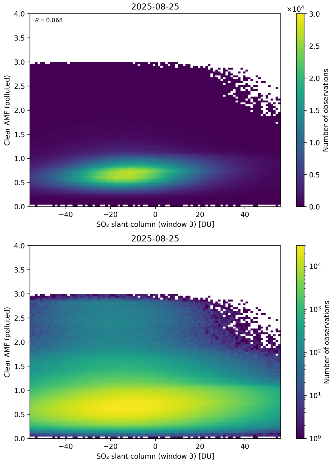
Figure 315: Scatter density plot of “SO 2 slant column (window 3)” against “Clear AMF (polluted)” for 2025-08-25 to 2025-08-26.
