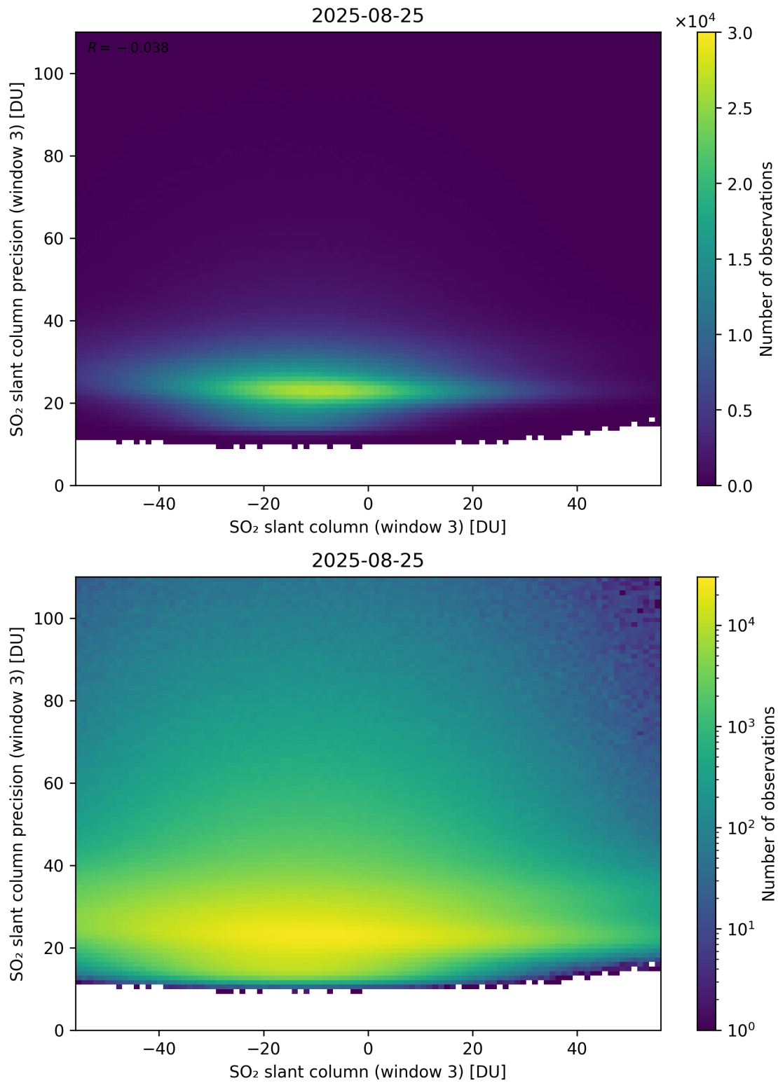
Figure 317: Scatter density plot of “SO 2 slant column (window 3)” against “SO 2 slant column precision (window 3)” for 2025-08-25 to 2025-08-26.
