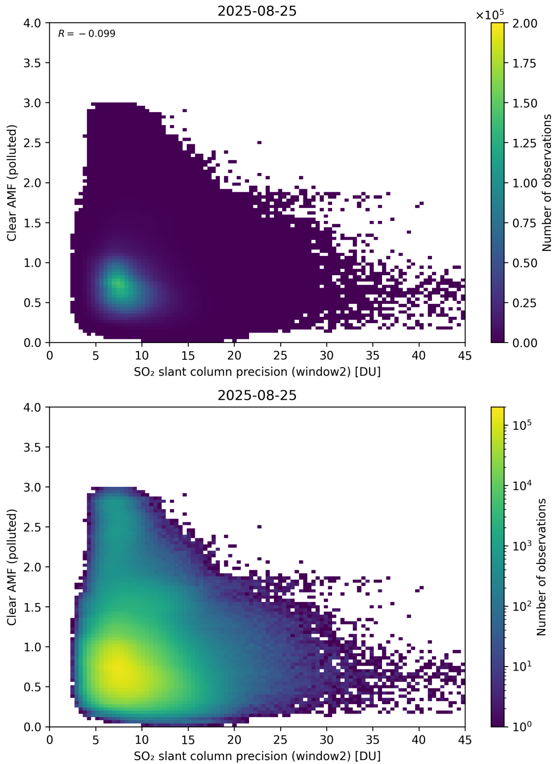
Figure 296: Scatter density plot of “SO 2 slant column precision (window2)” against “Clear AMF (polluted)” for 2025-08-25 to 2025-08-26.
