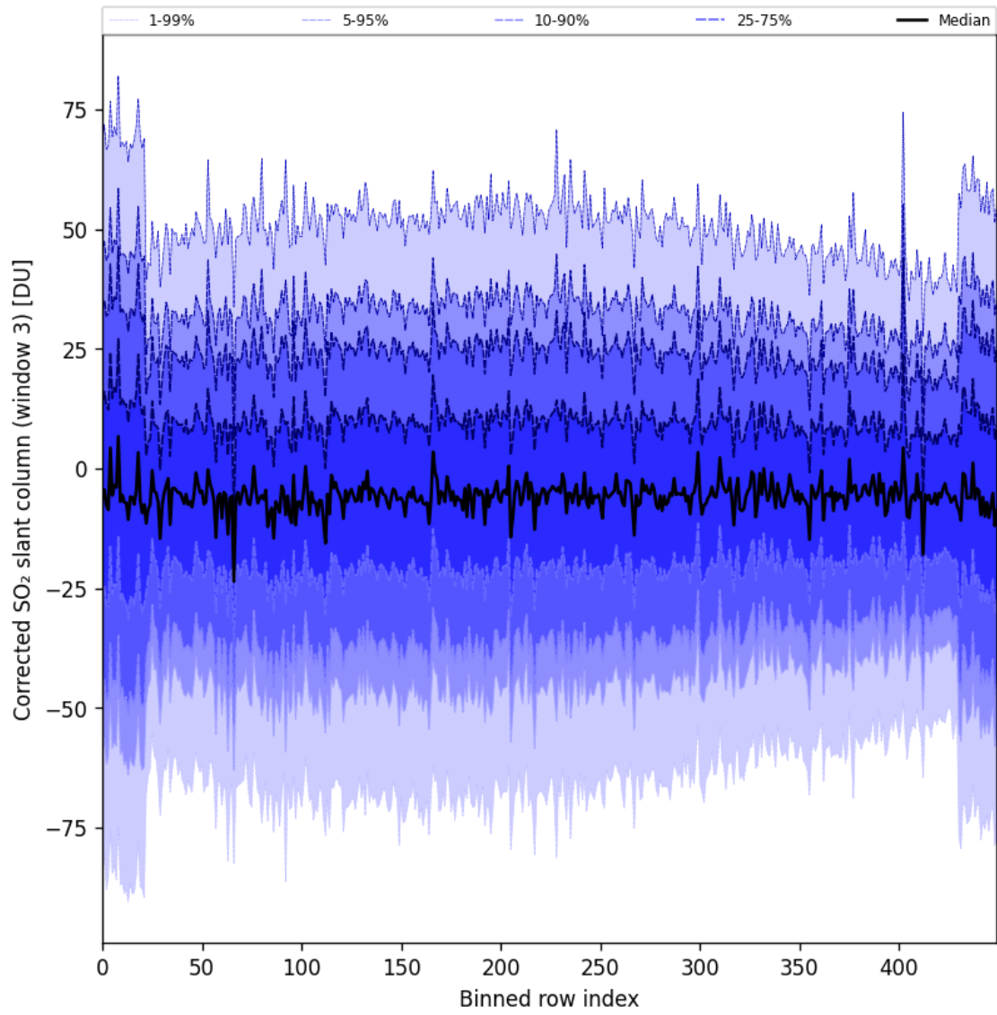
Figure 99: Along track statistics of “Corrected SO 2 slant column (window 3)” for 2025-08-25 to 2025-08-26
