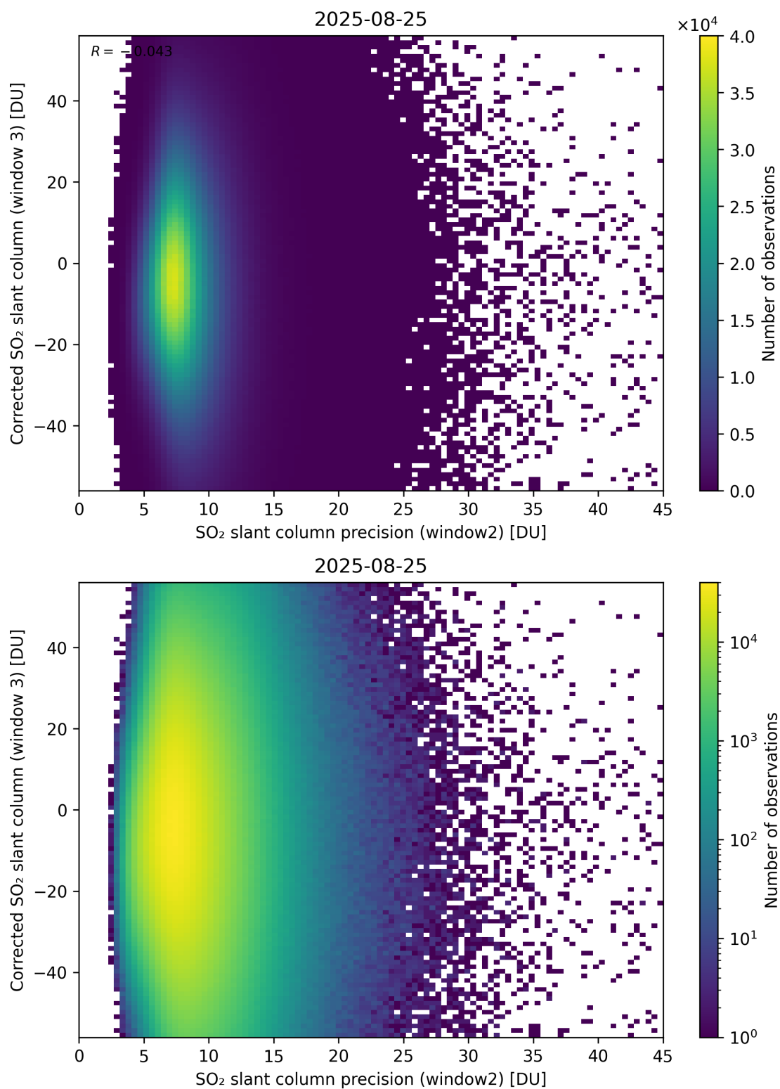
Figure 298: Scatter density plot of “SO 2 slant column precision (window2)” against “Corrected SO 2 slant column (window 3)” for 2025-08-25 to 2025-08-26.
