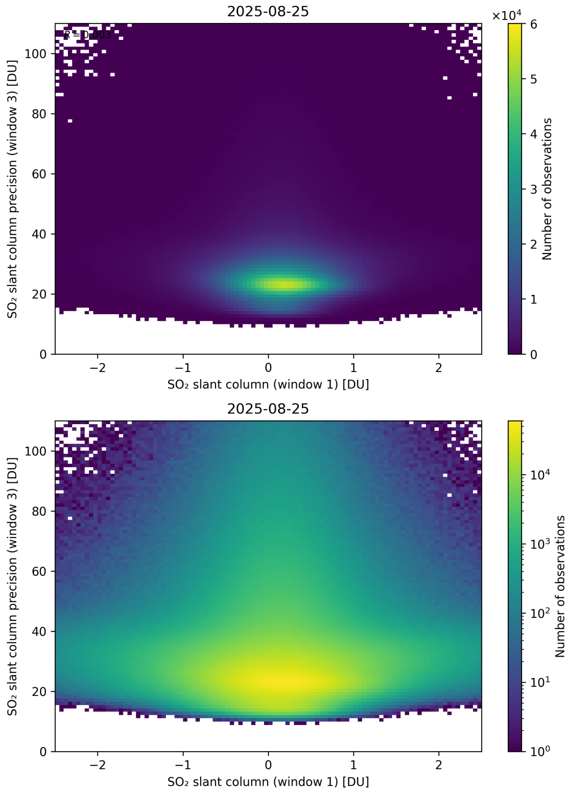
Figure 288: Scatter density plot of “SO 2 slant column (window 1)” against “SO 2 slant column precision (window 3)” for 2025-08-25 to 2025-08-26.
