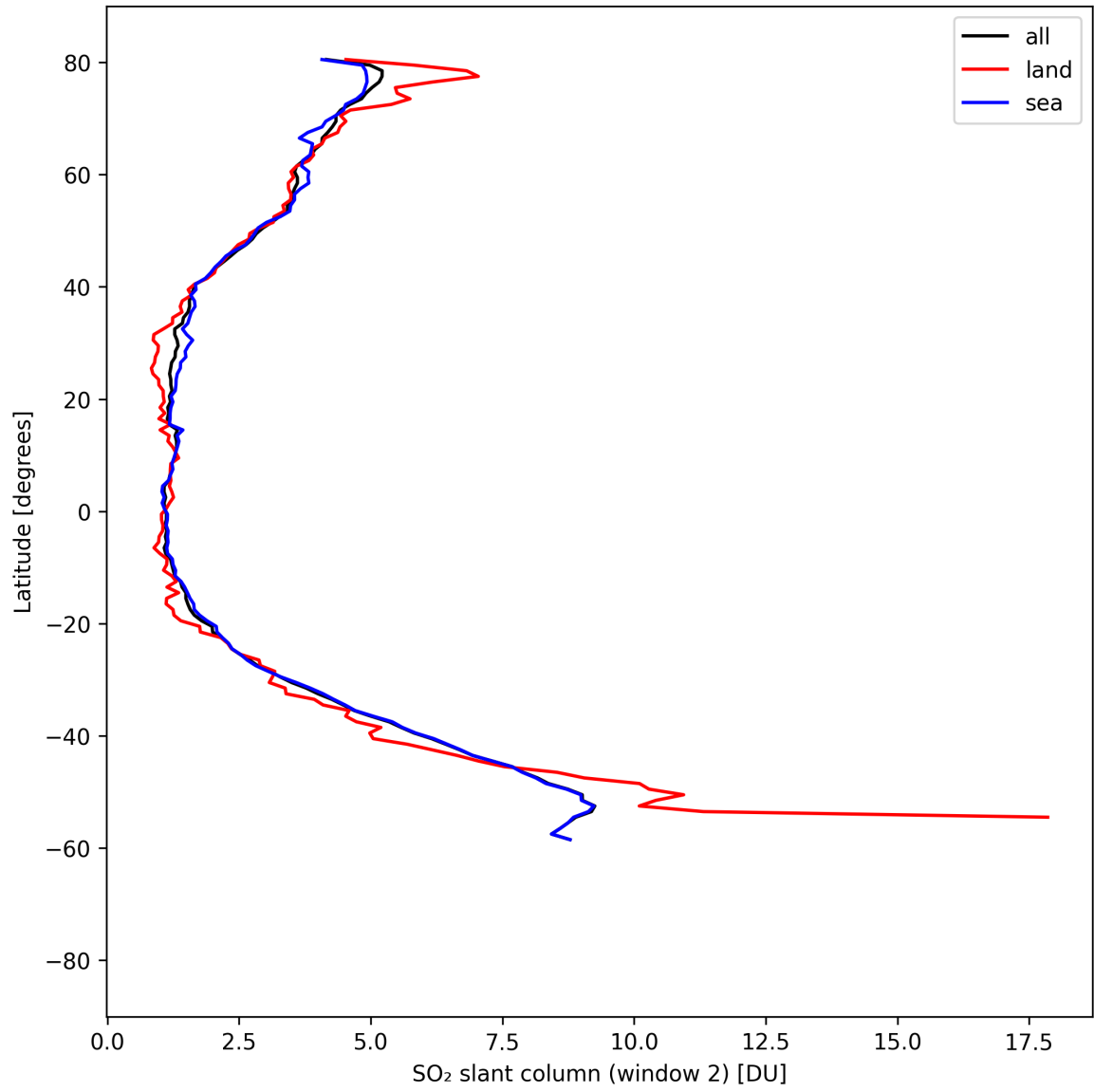
Figure 41: Zonal average of “SO 2 slant column (window 2)” for 2025-08-25 to 2025-08-26.
