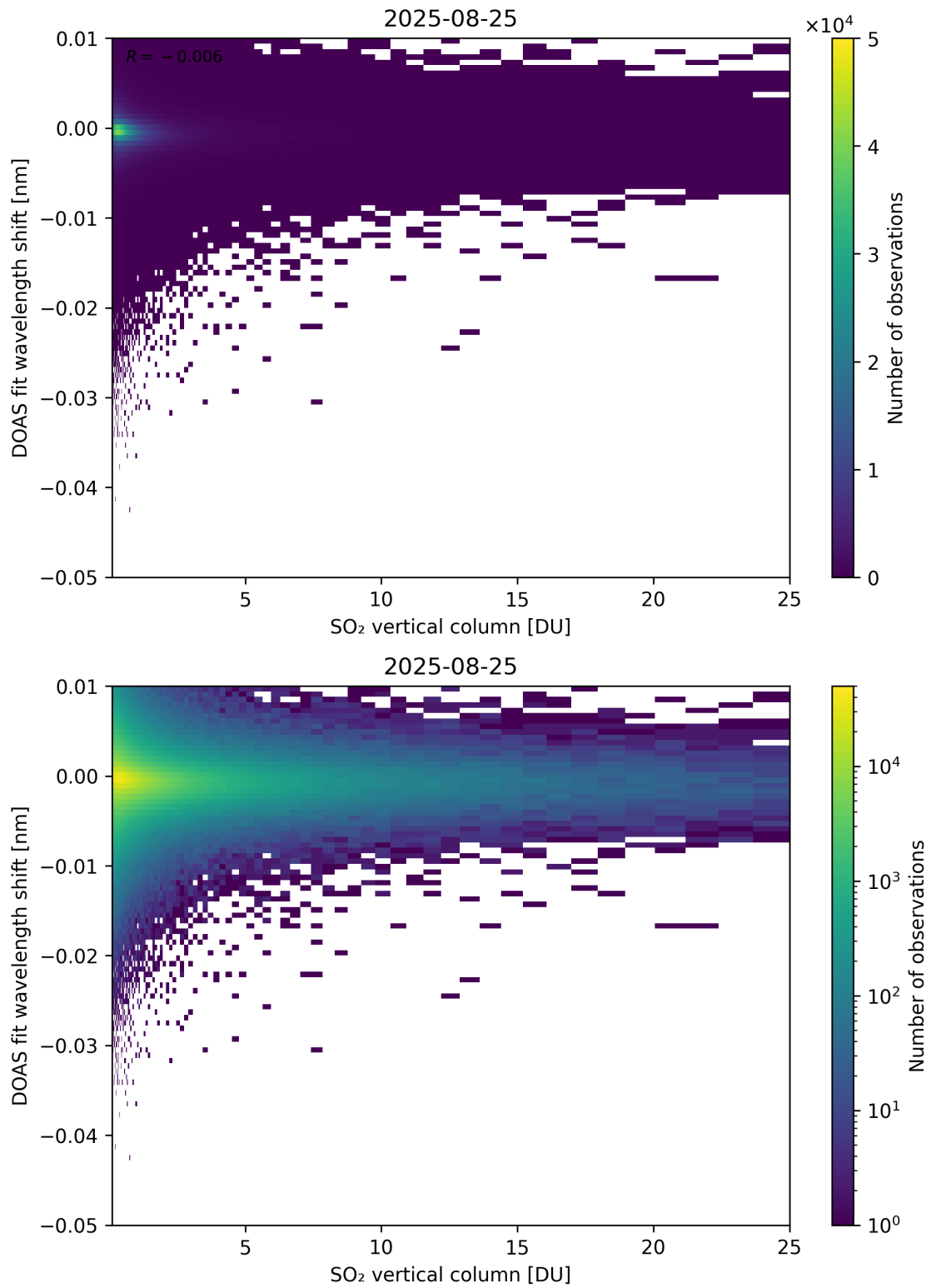
Figure 326: Scatter density plot of “SO 2 vertical column” against “DOAS fit wavelength shift” for 2025-08-25 to 2025-08-26.
