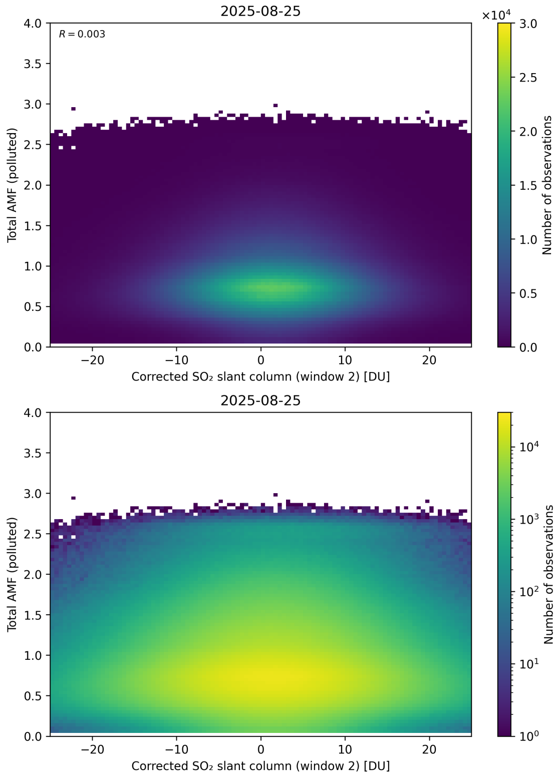
Figure 253: Scatter density plot of “Corrected SO 2 slant column (window 2)” against “Total AMF (polluted)” for 2025-08-25 to 2025-08-26.
