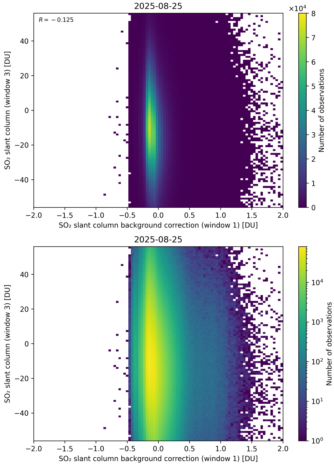
Figure 118: Scatter density plot of “SO 2 slant column background correction (window 1)” against “SO 2 slant column (window 3)” for 2025-08-25 to 2025-08-26.
