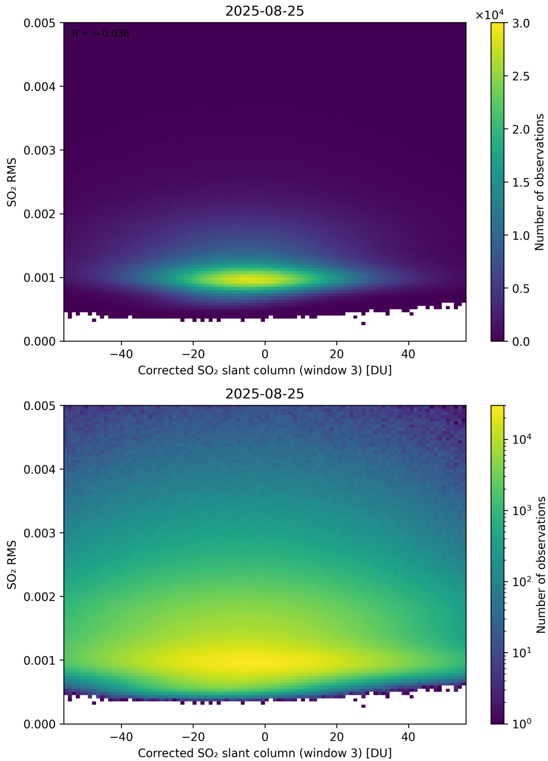
Figure 258: Scatter density plot of “Corrected SO 2 slant column (window 3)” against “SO 2 RMS” for 2025-08-25 to 2025-08-26.
