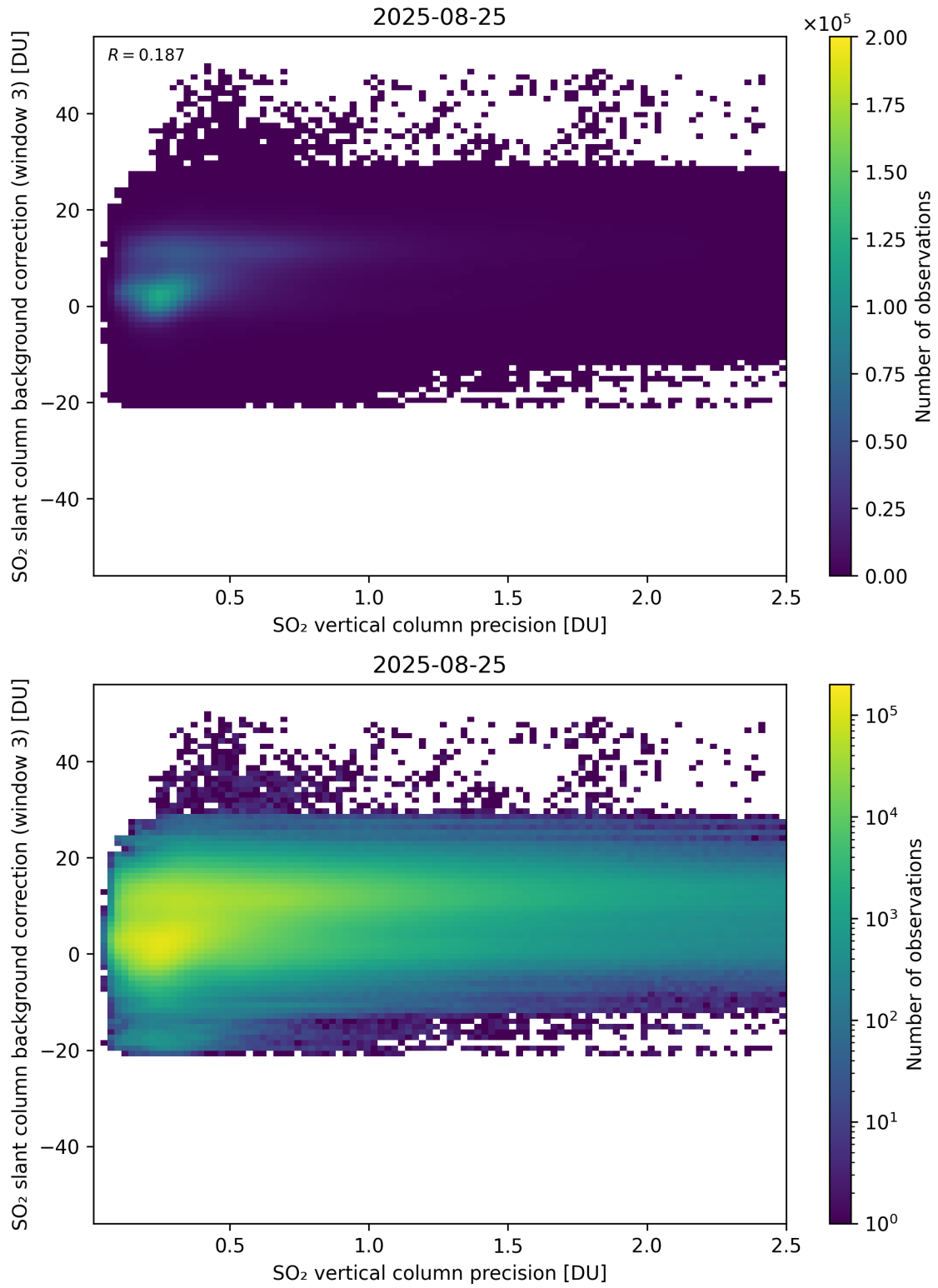
Figure 331: Scatter density plot of “SO 2 vertical column precision” against “SO 2 slant column background correction (window 3)” for 2025-08-25 to 2025-08-26.
