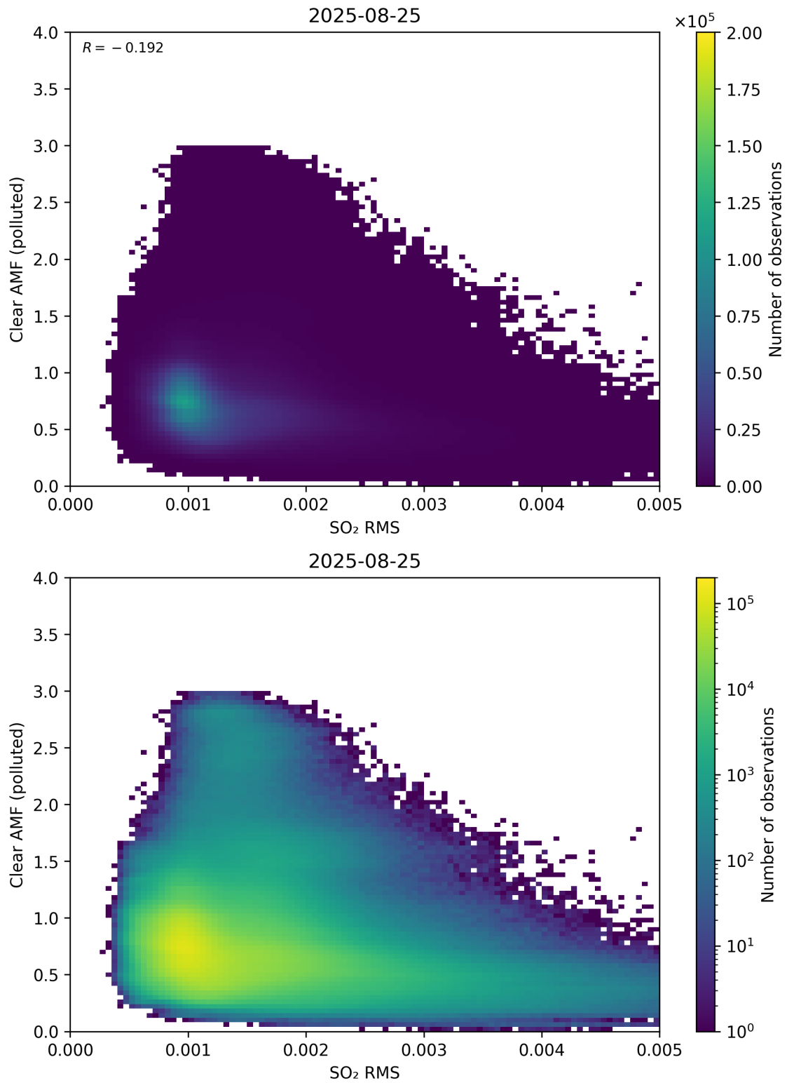
Figure 147: Scatter density plot of “SO 2 RMS” against “Clear AMF (polluted)” for 2025-08-25 to 2025-08-26.
