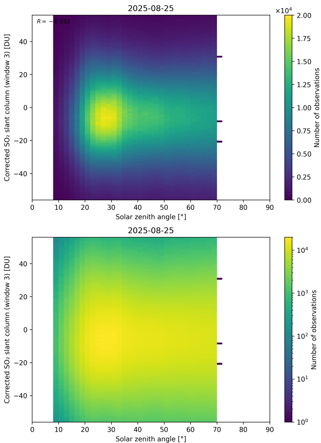
Figure 183: Scatter density plot of “Solar zenith angle” against “Corrected SO 2 slant column (window 3)” for 2025-08-25 to 2025-08-26.
