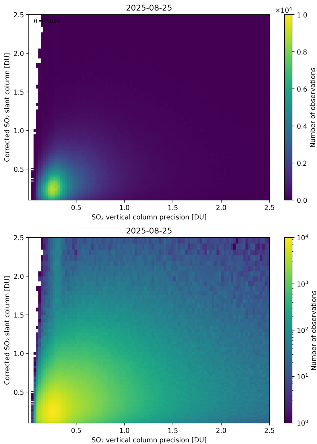
Figure 338: Scatter density plot of “SO 2 vertical column precision” against “Corrected SO 2 slant column” for 2025-08-25 to 2025-08-26.
