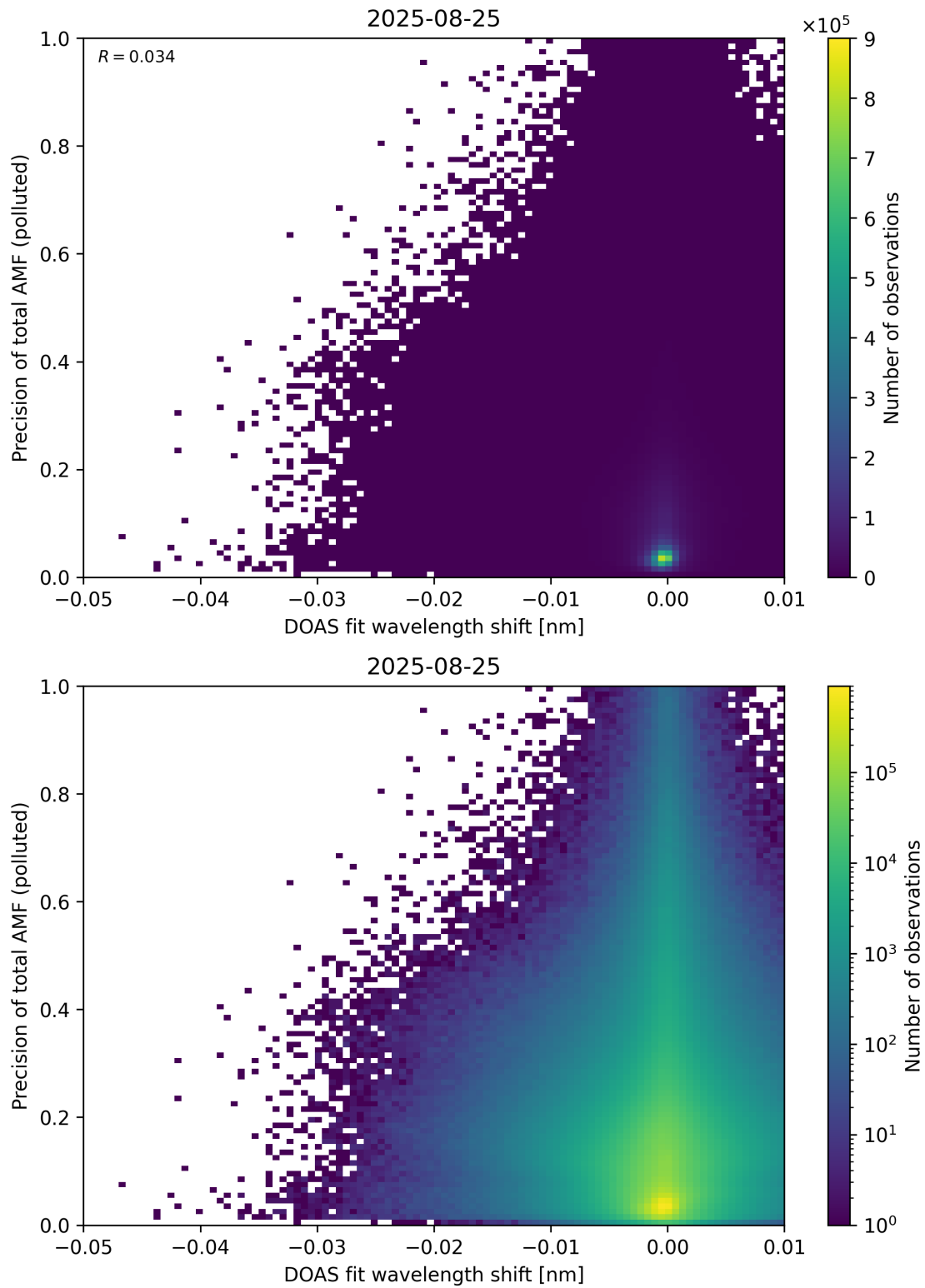
Figure 142: Scatter density plot of “DOAS fit wavelength shift” against “Precision of total AMF (polluted)” for 2025-08-25 to 2025-08-26.
