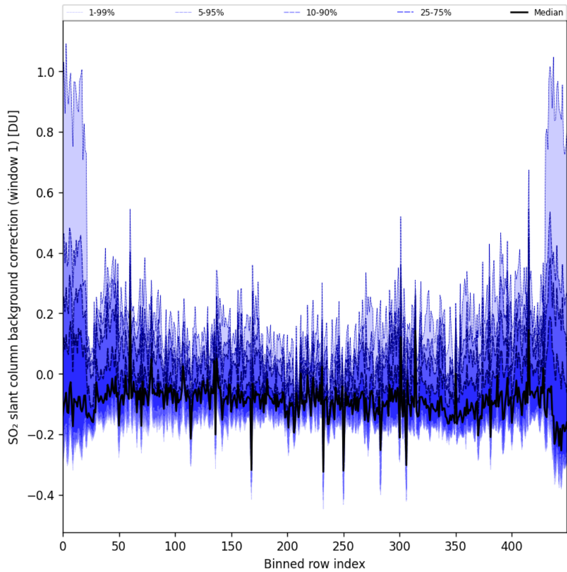
Figure 92: Along track statistics of “SO 2 slant column background correction (window 1)” for 2025-08-25 to 2025-08-26
