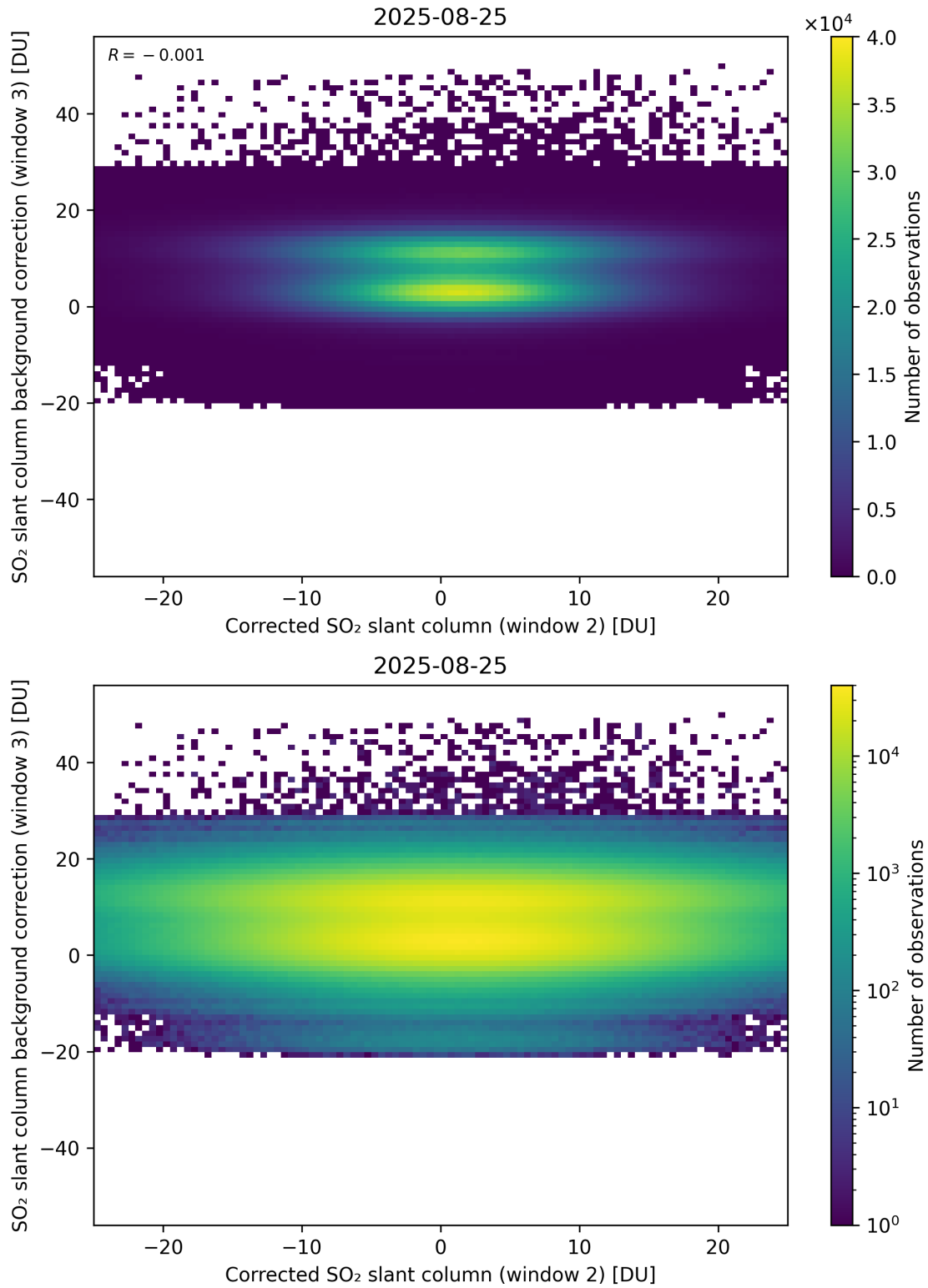
Figure 245: Scatter density plot of “Corrected SO 2 slant column (window 2)” against “SO 2 slant column background correction (window 3)” for 2025-08-25 to 2025-08-26.
