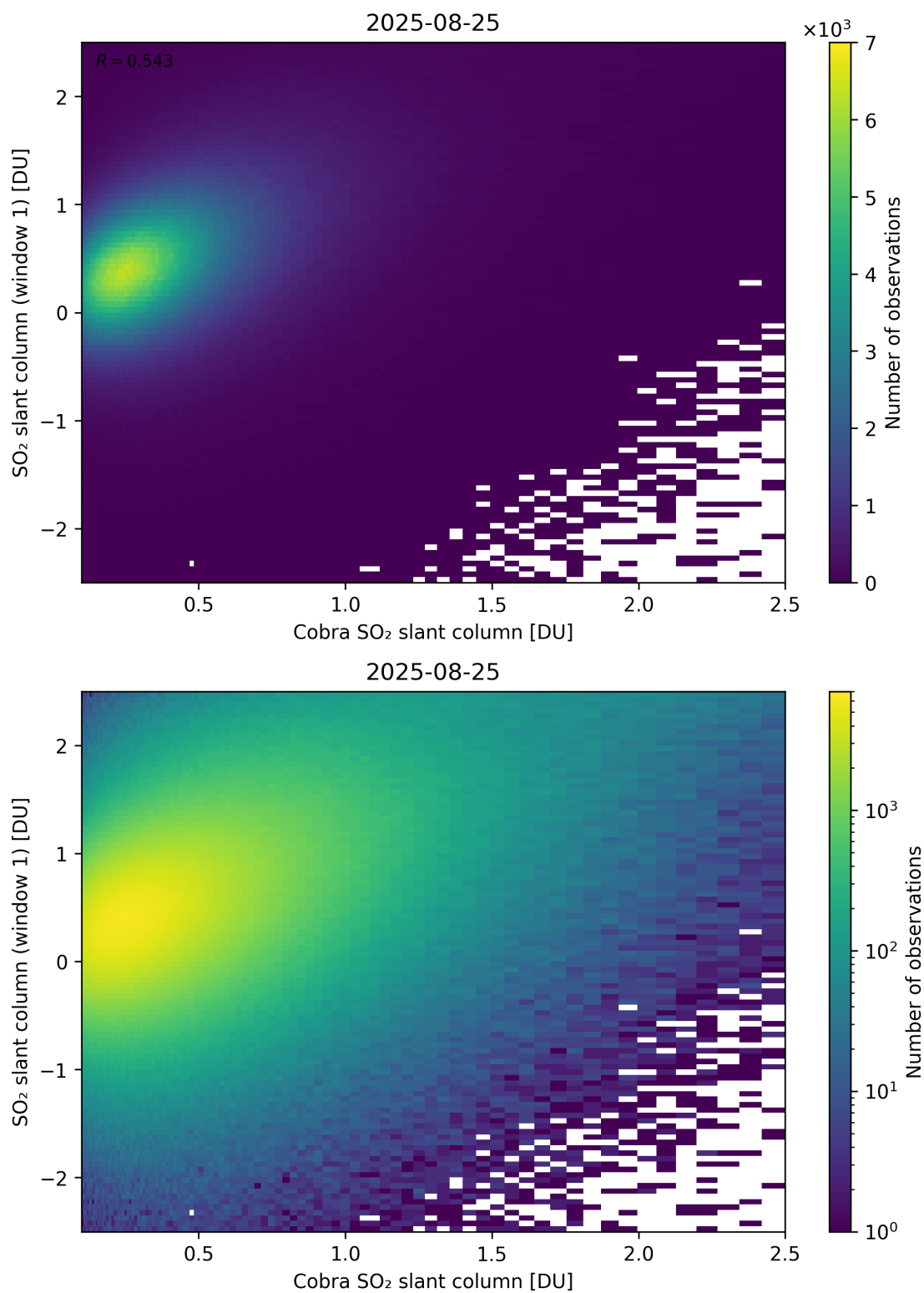
Figure 219: Scatter density plot of “Cobra SO 2 slant column” against “SO 2 slant column (window 1)” for 2025-08-25 to 2025-08-26.
