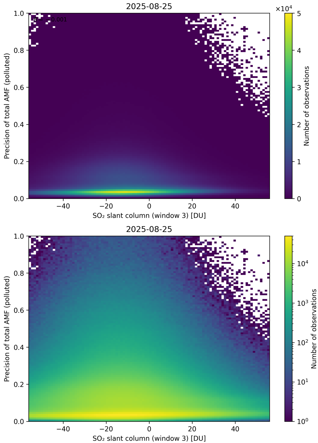
Figure 319: Scatter density plot of “SO 2 slant column (window 3)” against “Precision of total AMF (polluted)” for 2025-08-25 to 2025-08-26.
