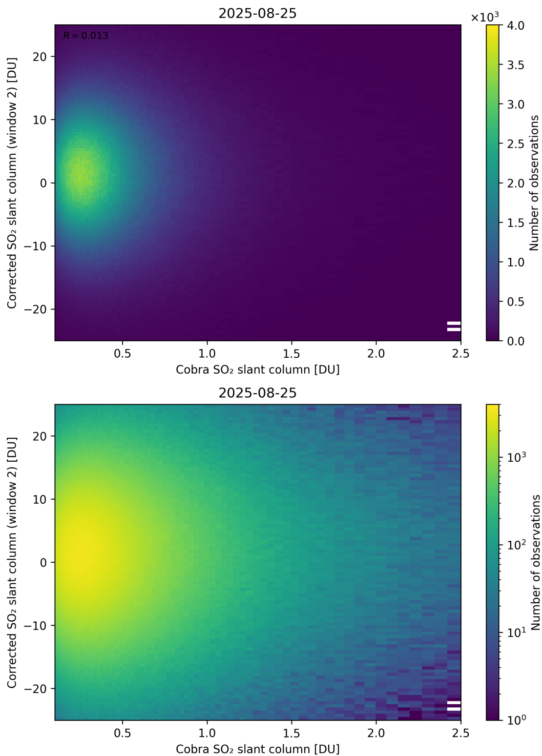
Figure 217: Scatter density plot of “Cobra SO 2 slant column” against “Corrected SO 2 slant column (window 2)” for 2025-08-25 to 2025-08-26.
