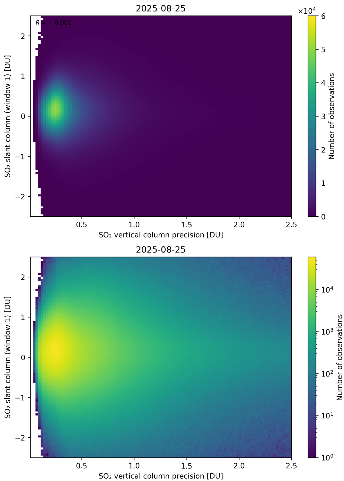
Figure 341: Scatter density plot of “SO 2 vertical column precision” against “SO 2 slant column (window 1)” for 2025-08-25 to 2025-08-26.
