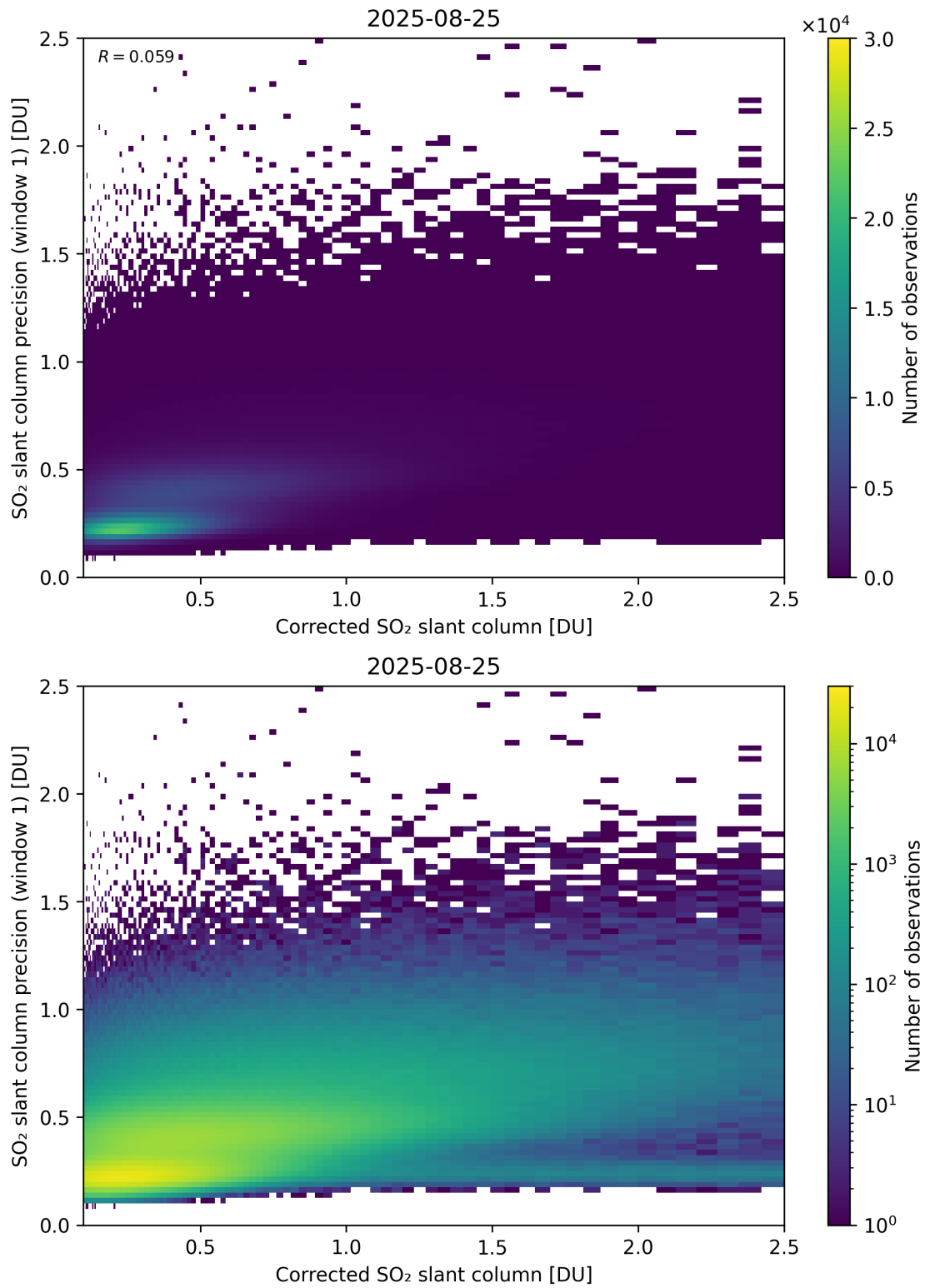
Figure 238: Scatter density plot of “Corrected SO 2 slant column” against “SO 2 slant column precision (window 1)” for 2025-08-25 to 2025-08-26.
