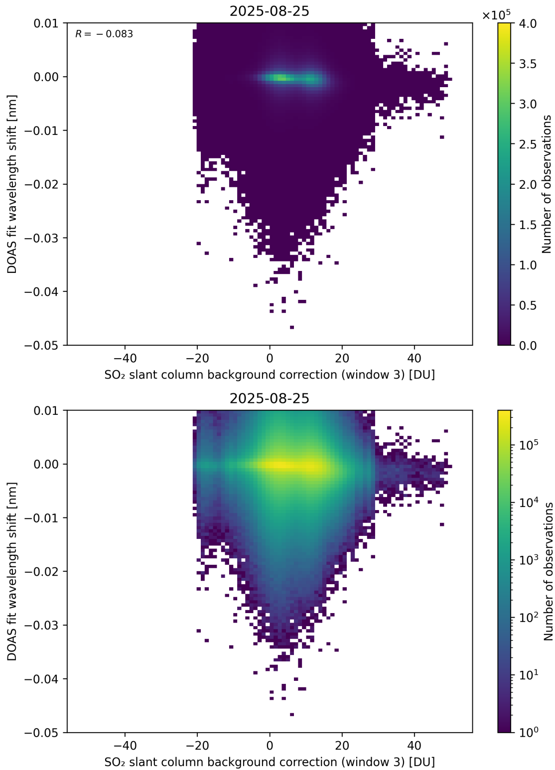
Figure 132: Scatter density plot of “SO 2 slant column background correction (window 3)” against “DOAS fit wavelength shift” for 2025-08-25 to 2025-08-26.
