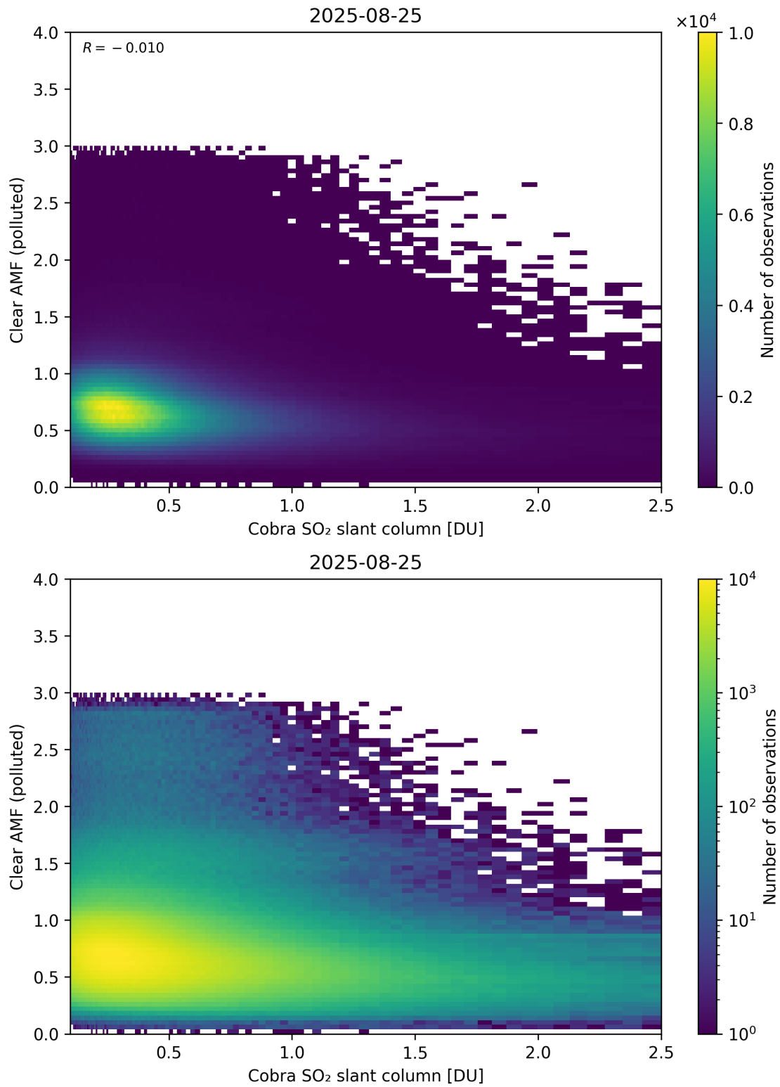
Figure 215: Scatter density plot of “Cobra SO 2 slant column” against “Clear AMF (polluted)” for 2025-08-25 to 2025-08-26.
