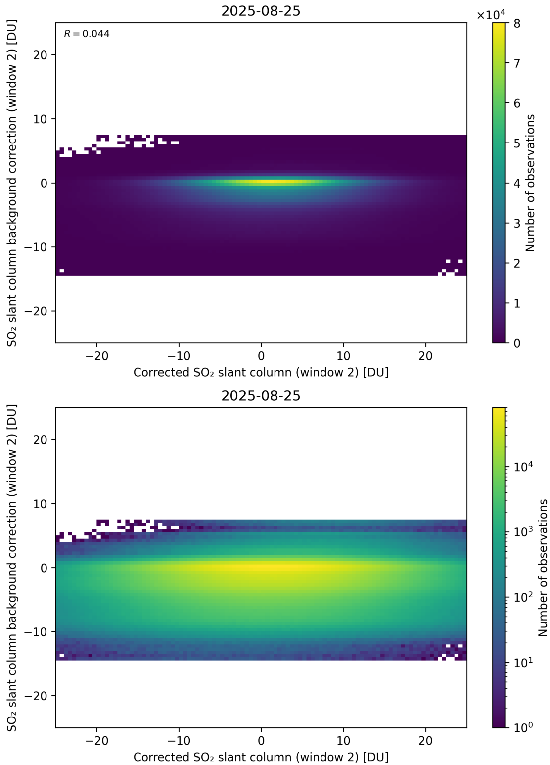
Figure 244: Scatter density plot of “Corrected SO 2 slant column (window 2)” against “SO 2 slant column background correction (window 2)” for 2025-08-25 to 2025-08-26.
