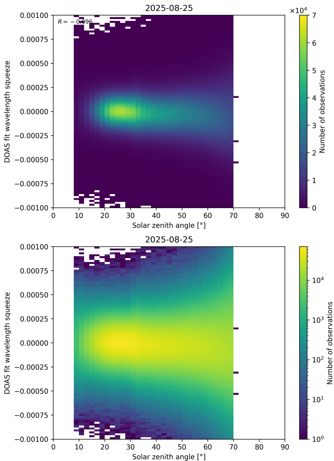
Figure 175: Scatter density plot of “Solar zenith angle” against “DOAS fit wavelength squeeze” for 2025-08-25 to 2025-08-26.
