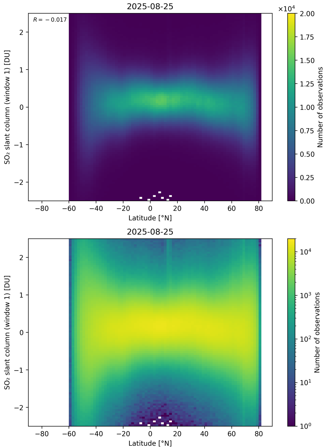
Figure 162: Scatter density plot of “Latitude” against “SO 2 slant column (window 1)” for 2025-08-25 to 2025-08-26.
