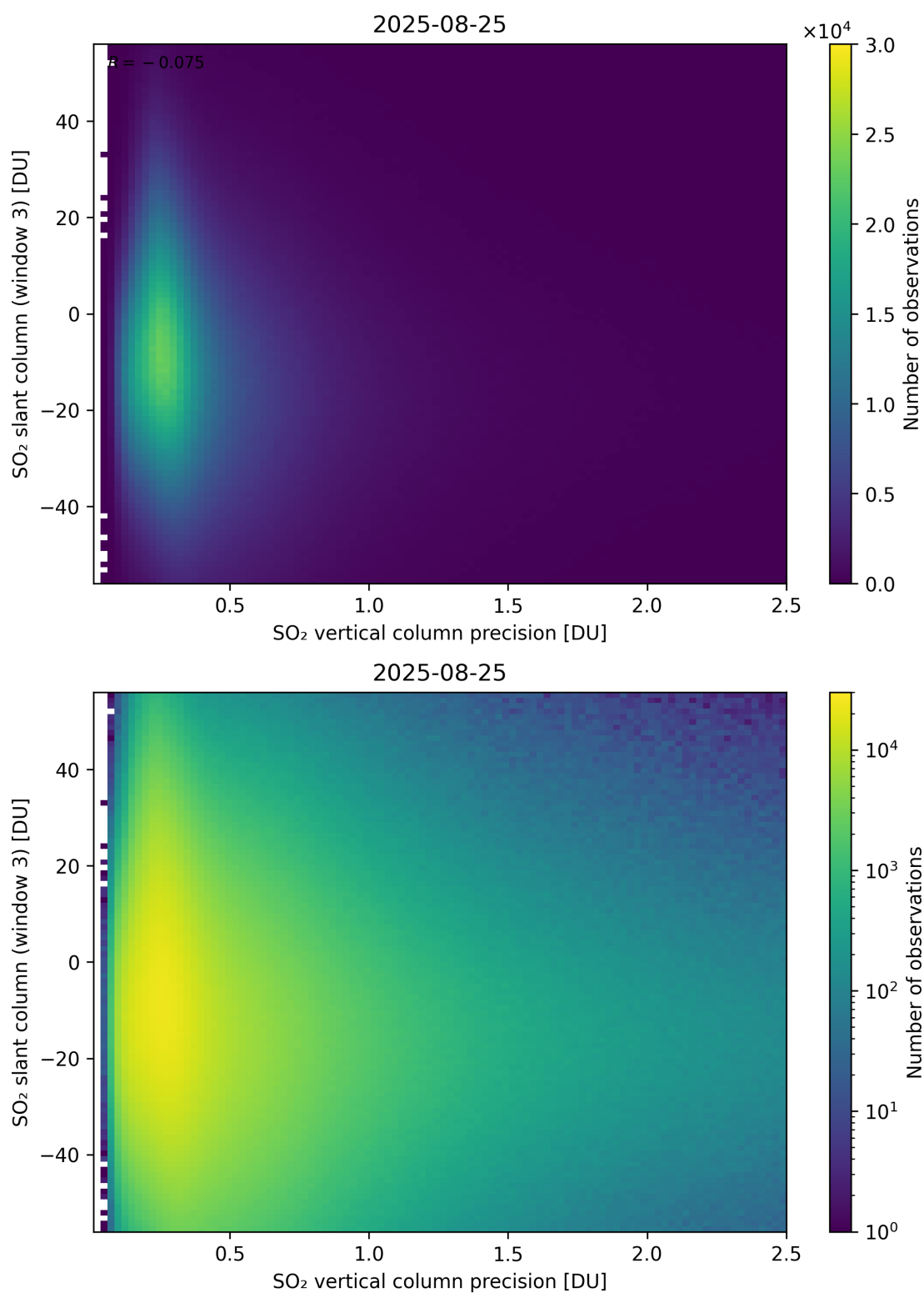
Figure 344: Scatter density plot of “SO 2 vertical column precision” against “SO 2 slant column (window 3)” for 2025-08-25 to 2025-08-26.
