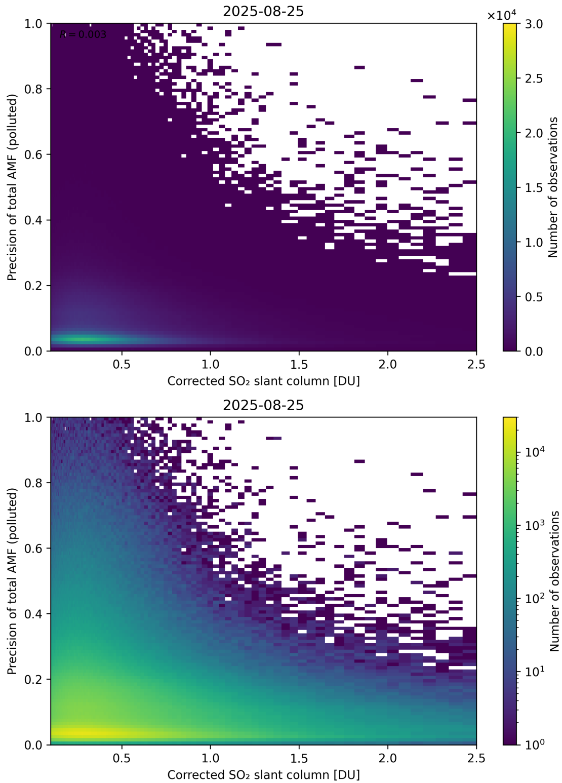
Figure 243: Scatter density plot of “Corrected SO 2 slant column” against “Precision of total AMF (polluted)” for 2025-08-25 to 2025-08-26.
