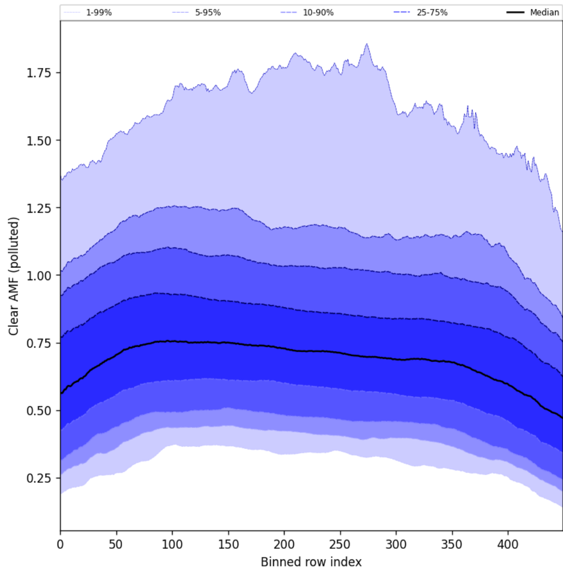
Figure 107: Along track statistics of “Clear AMF (polluted)” for 2025-08-25 to 2025-08-26
