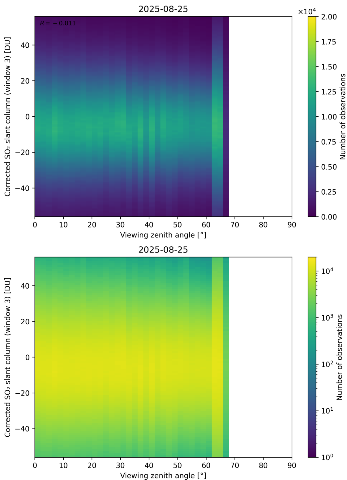
Figure 375: Scatter density plot of “Viewing zenith angle” against “Corrected SO 2 slant column (window 3)” for 2025-08-25 to 2025-08-26.
