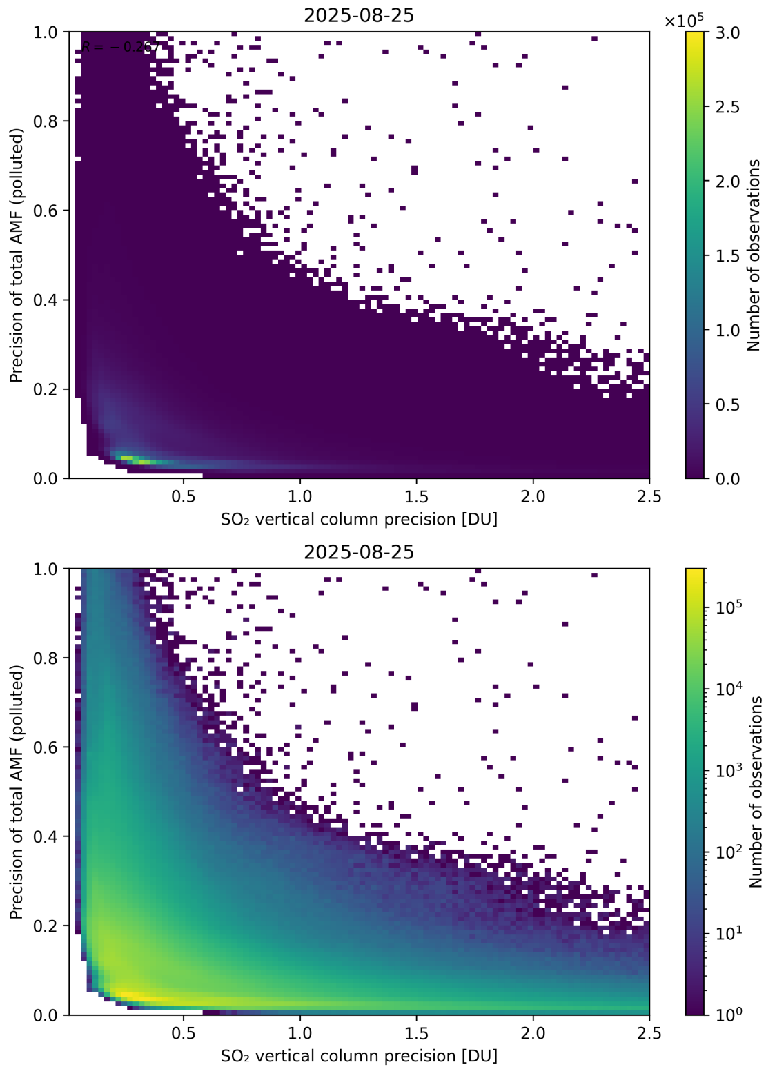
Figure 347: Scatter density plot of “SO 2 vertical column precision” against “Precision of total AMF (polluted)” for 2025-08-25 to 2025-08-26.
