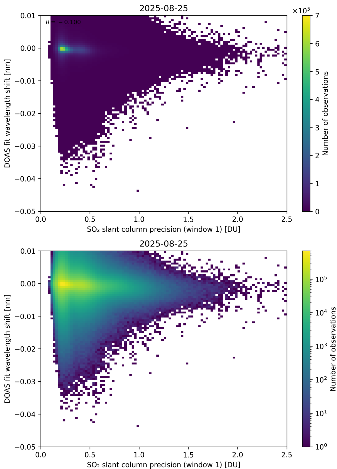
Figure 271: Scatter density plot of “SO 2 slant column precision (window 1)” against “DOAS fit wavelength shift” for 2025-08-25 to 2025-08-26.
