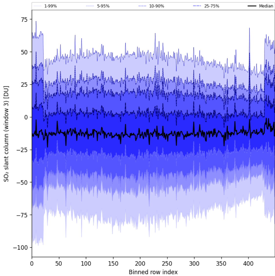
Figure 97: Along track statistics of “SO 2 slant column (window 3)” for 2025-08-25 to 2025-08-26
