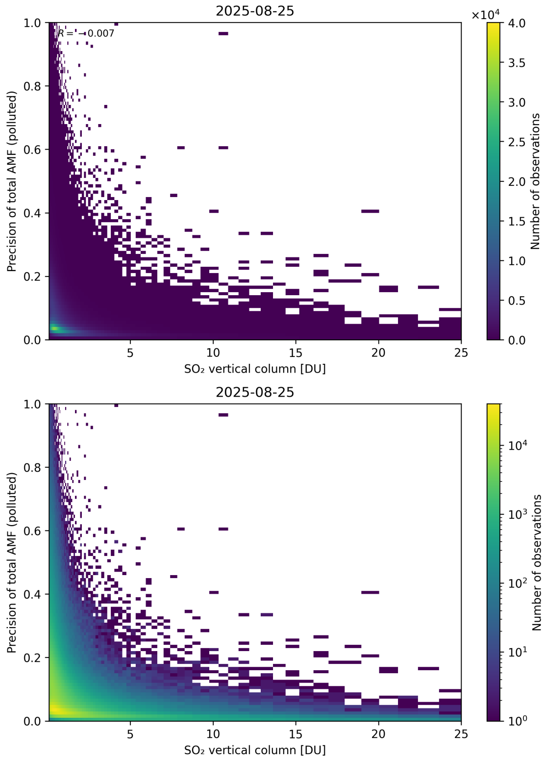
Figure 360: Scatter density plot of “SO 2 vertical column” against “Precision of total AMF (polluted)” for 2025-08-25 to 2025-08-26.
