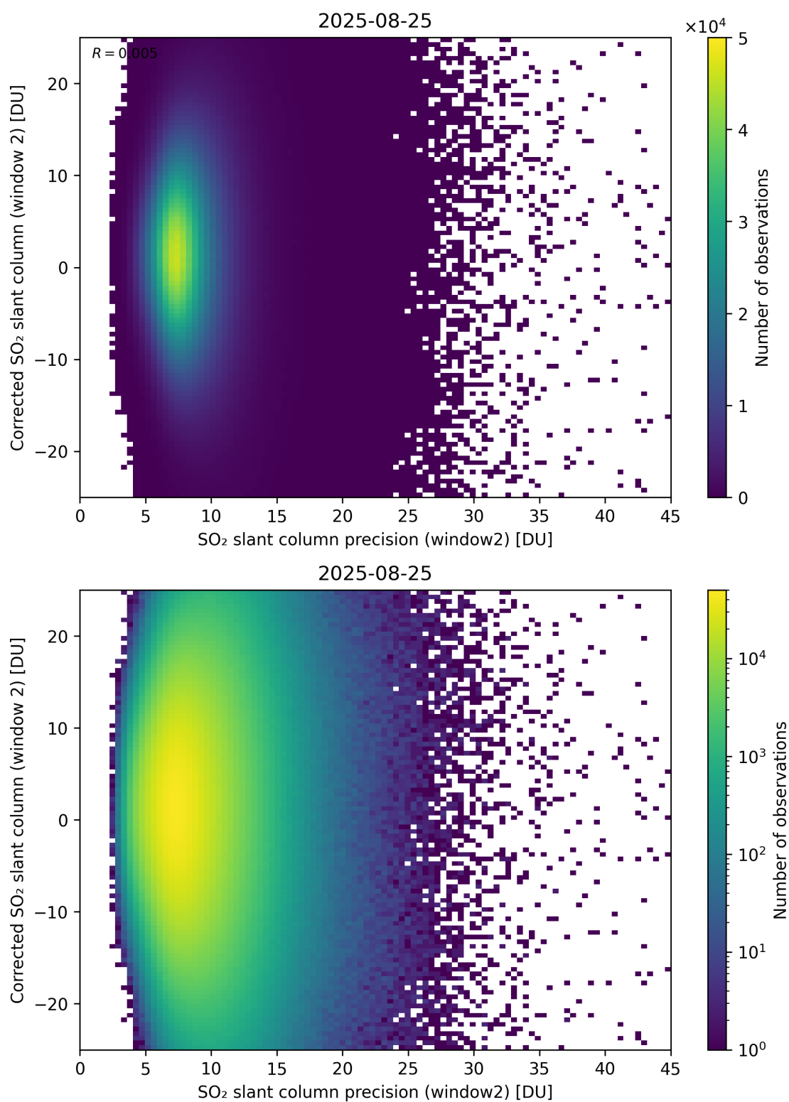
Figure 297: Scatter density plot of “SO 2 slant column precision (window2)” against “Corrected SO 2 slant column (window 2)” for 2025-08-25 to 2025-08-26.
