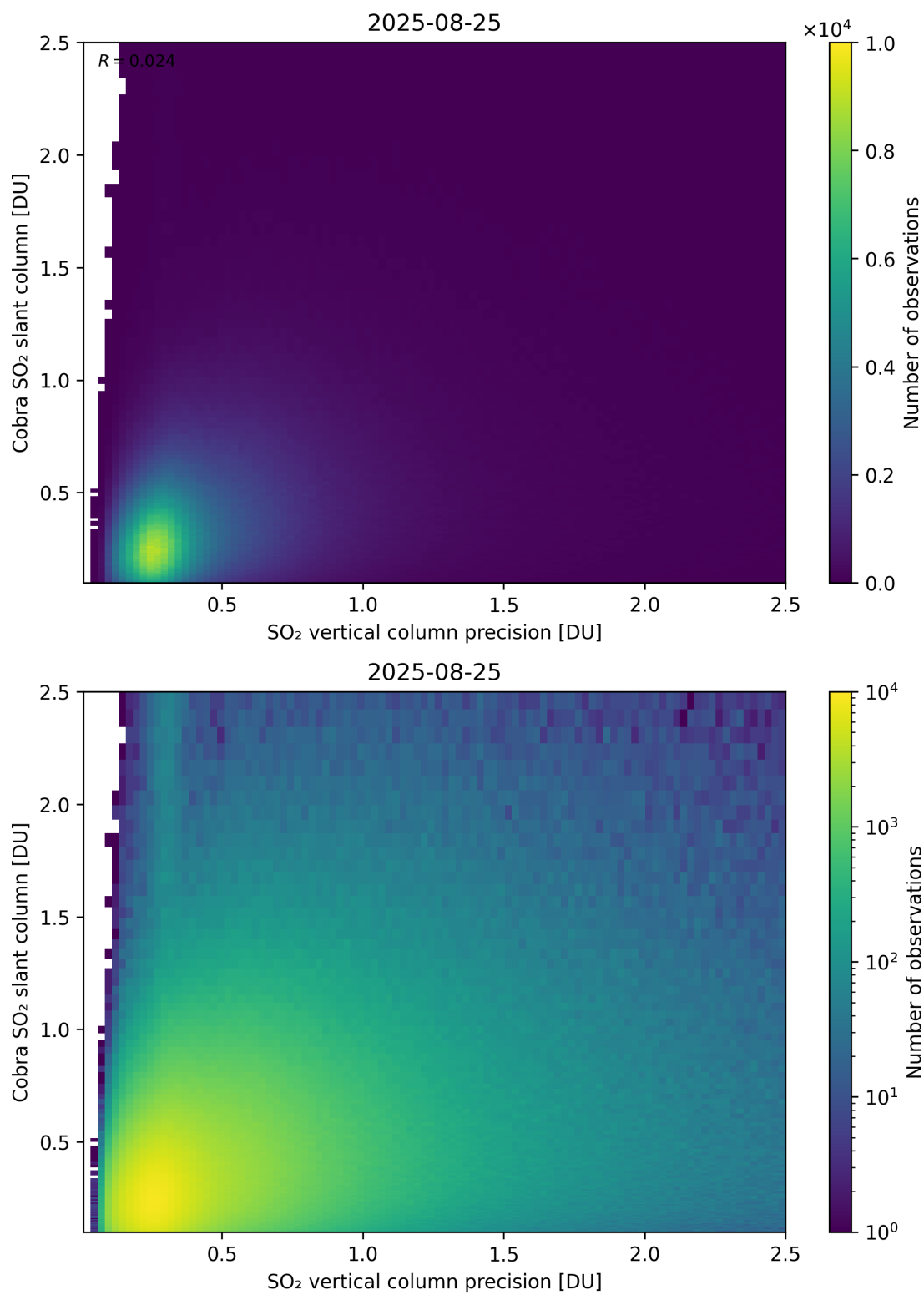
Figure 336: Scatter density plot of “SO 2 vertical column precision” against “Cobra SO 2 slant column” for 2025-08-25 to 2025-08-26.
