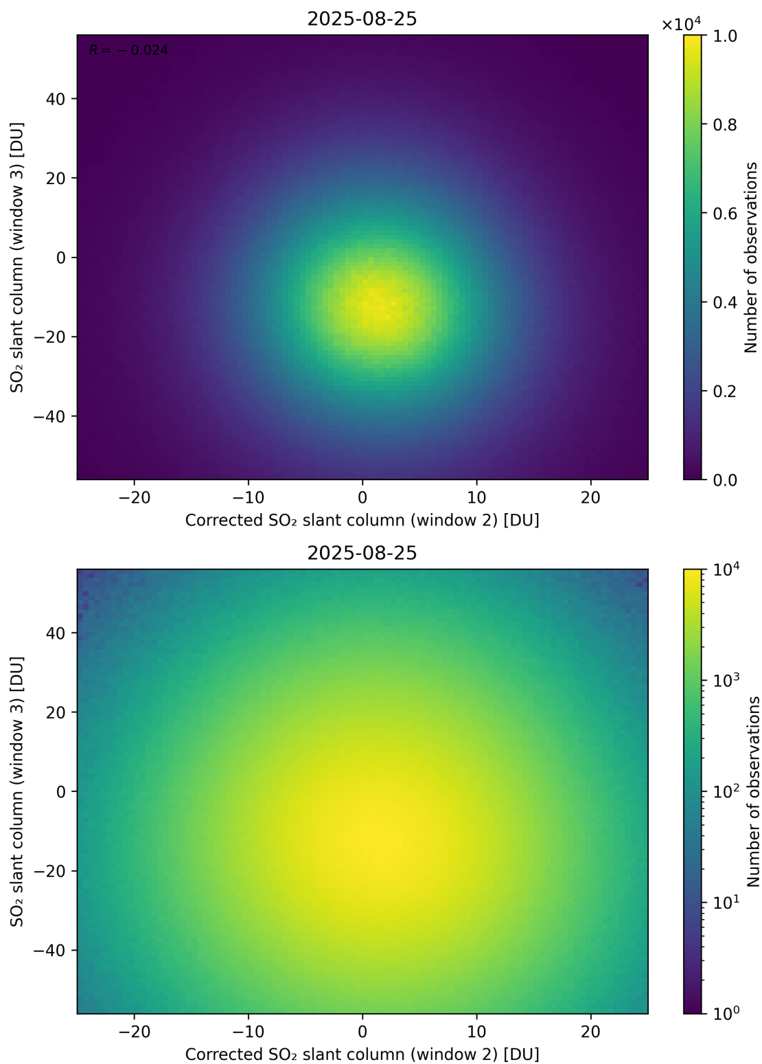
Figure 251: Scatter density plot of “Corrected SO 2 slant column (window 2)” against “SO 2 slant column (window 3)” for 2025-08-25 to 2025-08-26.
