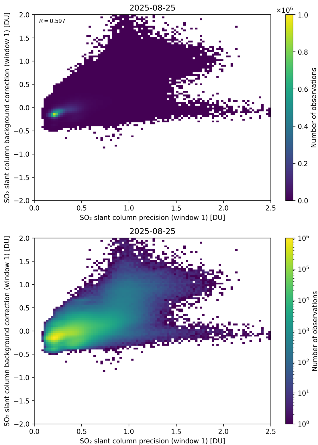
Figure 268: Scatter density plot of “SO 2 slant column precision (window 1)” against “SO 2 slant column background correction (window 1)” for 2025-08-25 to 2025-08-26.
