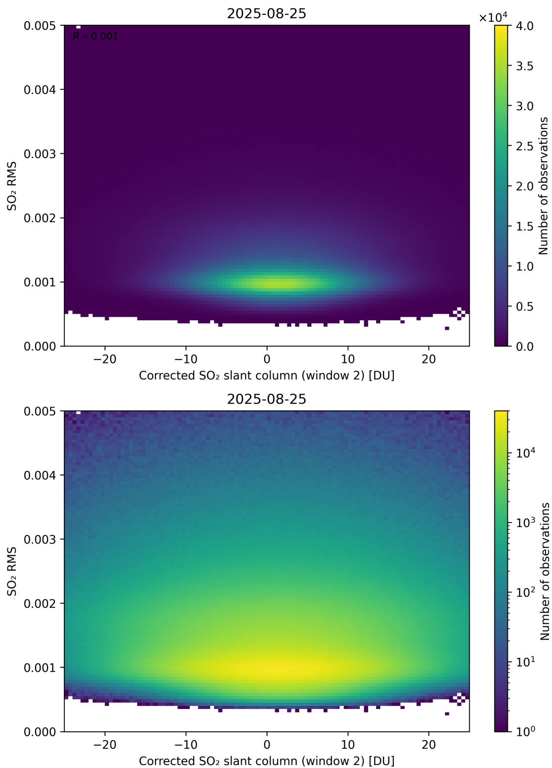
Figure 248: Scatter density plot of “Corrected SO 2 slant column (window 2)” against “SO 2 RMS” for 2025-08-25 to 2025-08-26.
