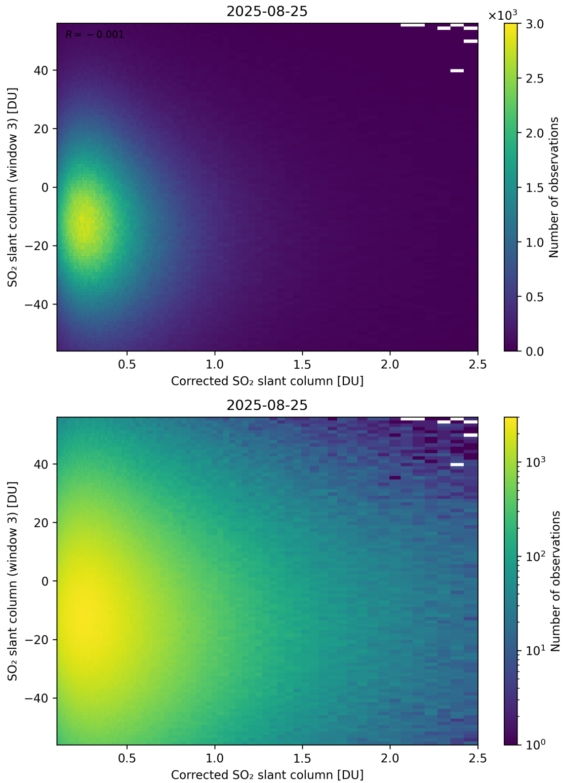
Figure 240: Scatter density plot of “Corrected SO 2 slant column” against “SO 2 slant column (window 3)” for 2025-08-25 to 2025-08-26.
