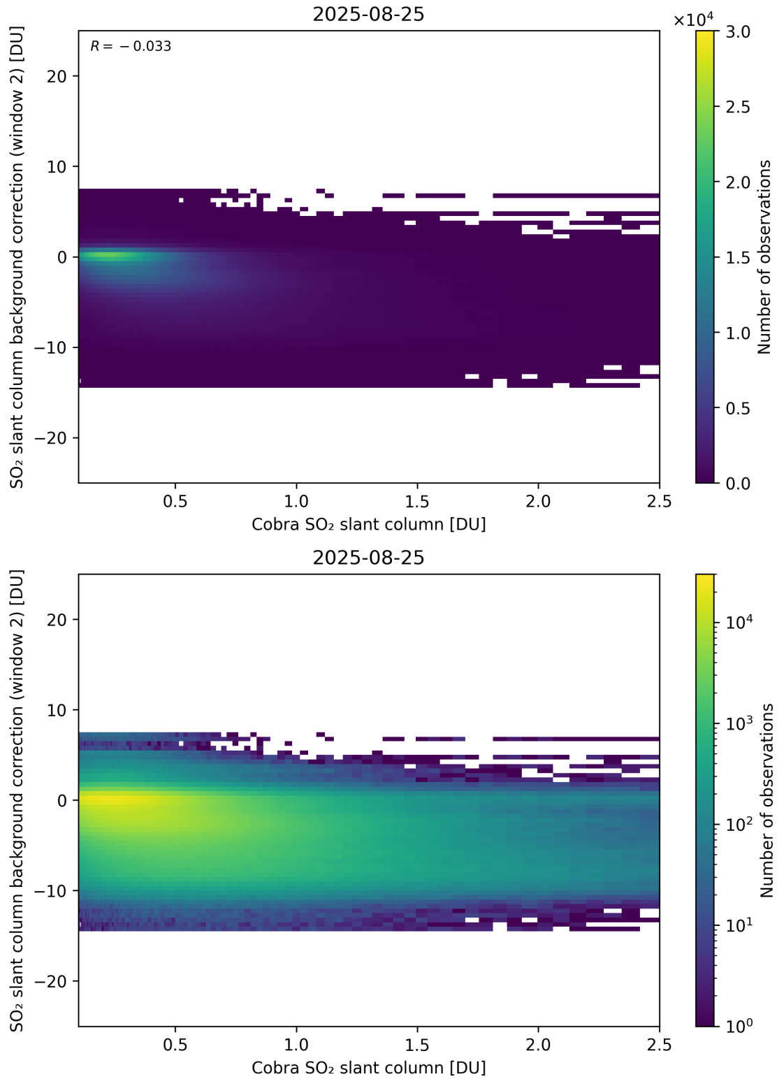
Figure 194: Scatter density plot of “Cobra SO 2 slant column” against “SO 2 slant column background correction (window 2)” for 2025-08-25 to 2025-08-26.
