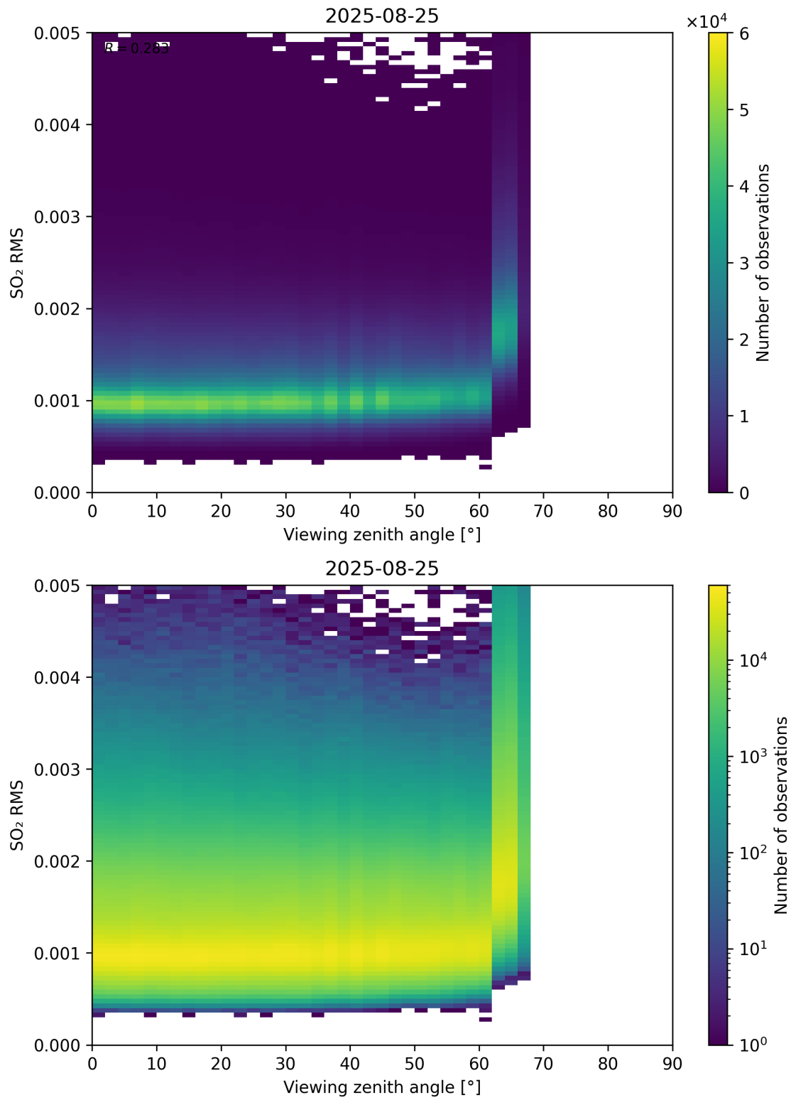
Figure 367: Scatter density plot of “Viewing zenith angle” against “SO 2 RMS” for 2025-08-25 to 2025-08-26.
