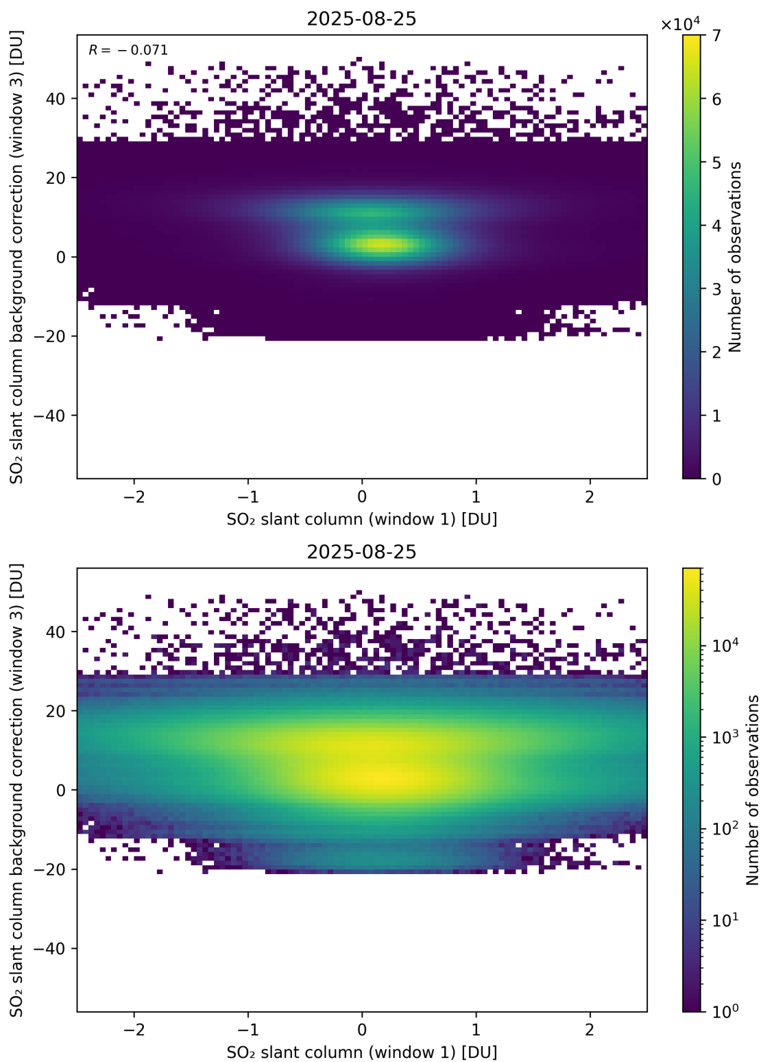
Figure 264: Scatter density plot of “SO 2 slant column (window 1)” against “SO 2 slant column background correction (window 3)” for 2025-08-25 to 2025-08-26.
