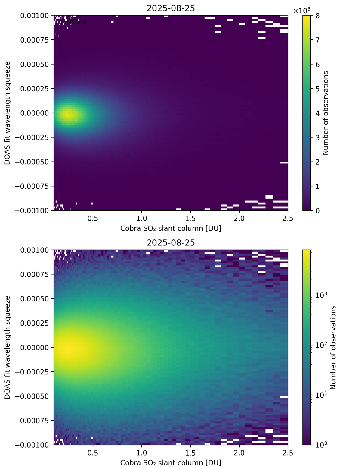
Figure 197: Scatter density plot of “Cobra SO 2 slant column” against “DOAS fit wavelength squeeze” for 2025-08-25 to 2025-08-26.
