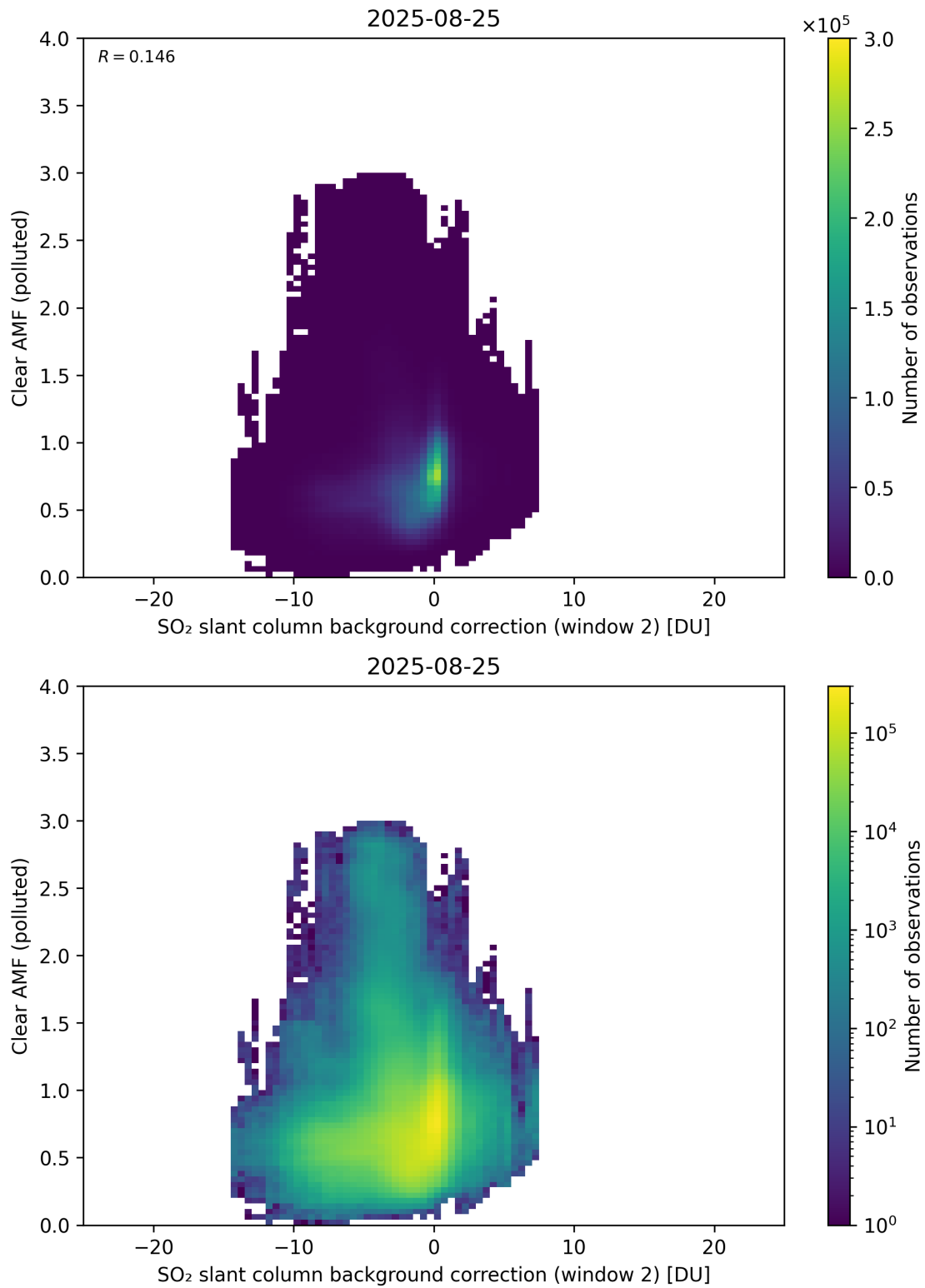
Figure 126: Scatter density plot of “SO 2 slant column background correction (window 2)” against “Clear AMF (polluted)” for 2025-08-25 to 2025-08-26.
