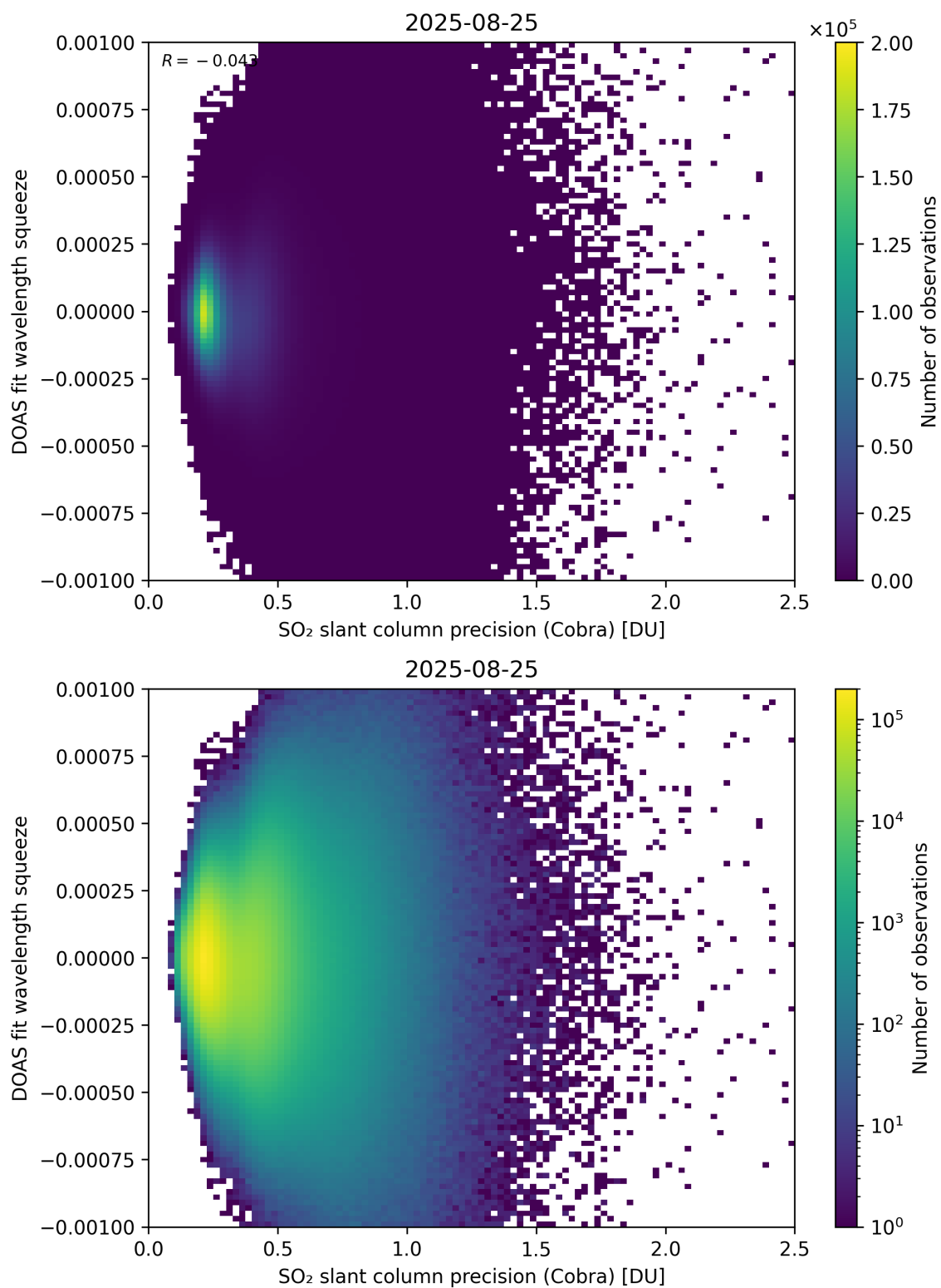
Figure 203: Scatter density plot of “SO 2 slant column precision (Cobra)” against “DOAS fit wavelength squeeze” for 2025-08-25 to 2025-08-26.
