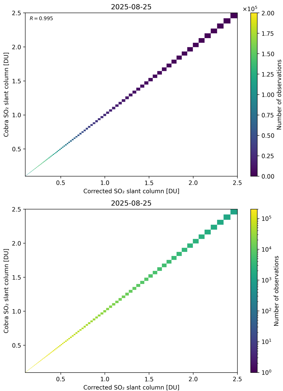
Figure 233: Scatter density plot of “Corrected SO 2 slant column” against “Cobra SO 2 slant column” for 2025-08-25 to 2025-08-26.
