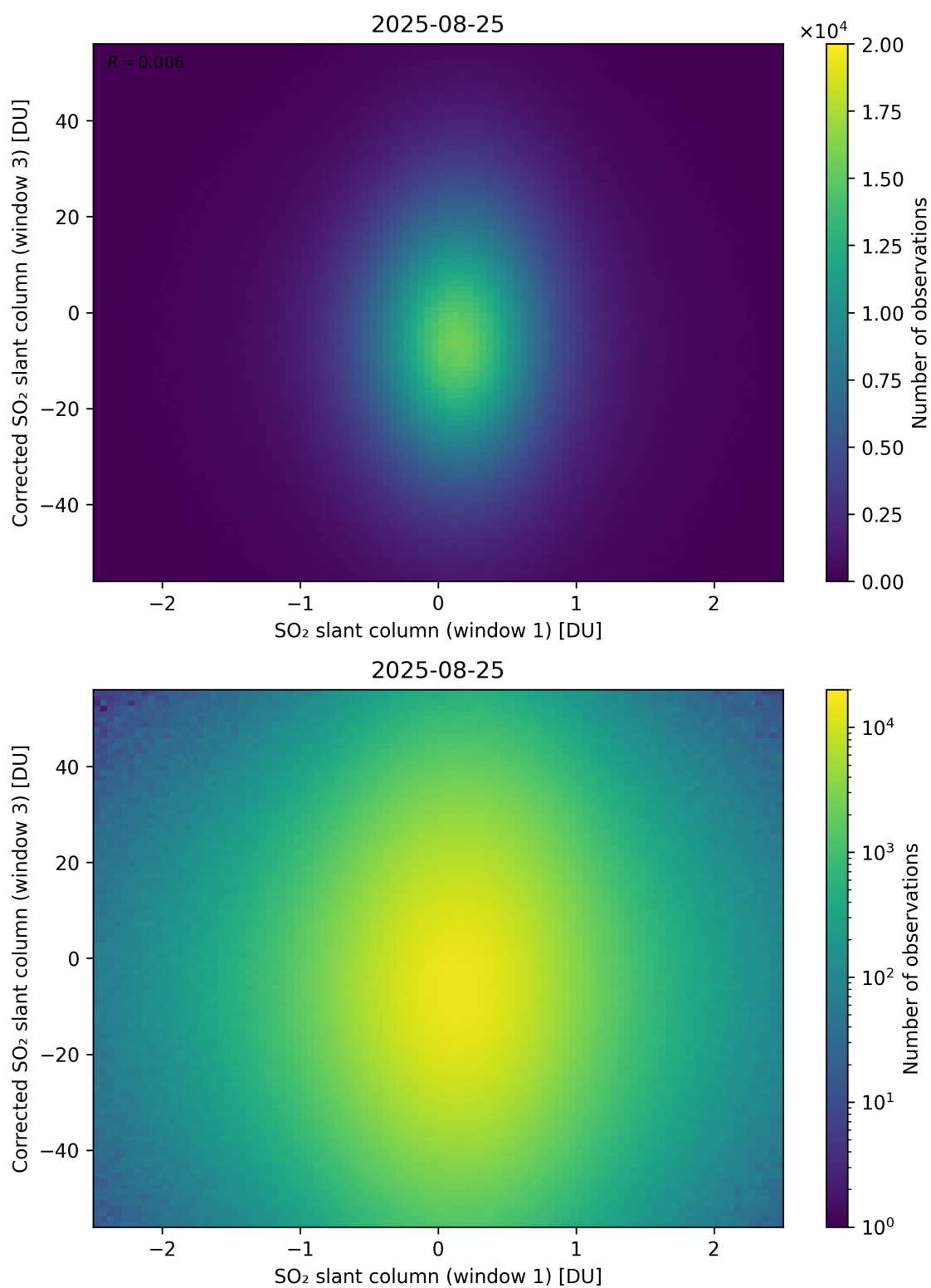
Figure 284: Scatter density plot of “SO 2 slant column (window 1)” against “Corrected SO 2 slant column (window 3)” for 2025-08-25 to 2025-08-26.
