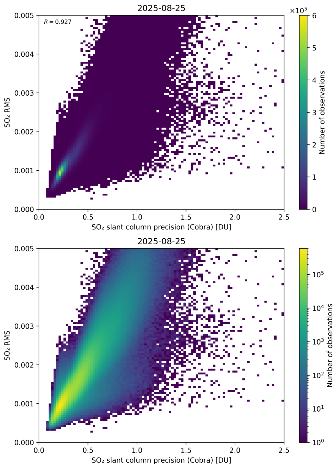
Figure 204: Scatter density plot of “SO 2 slant column precision (Cobra)” against “SO 2 RMS” for 2025-08-25 to 2025-08-26.
