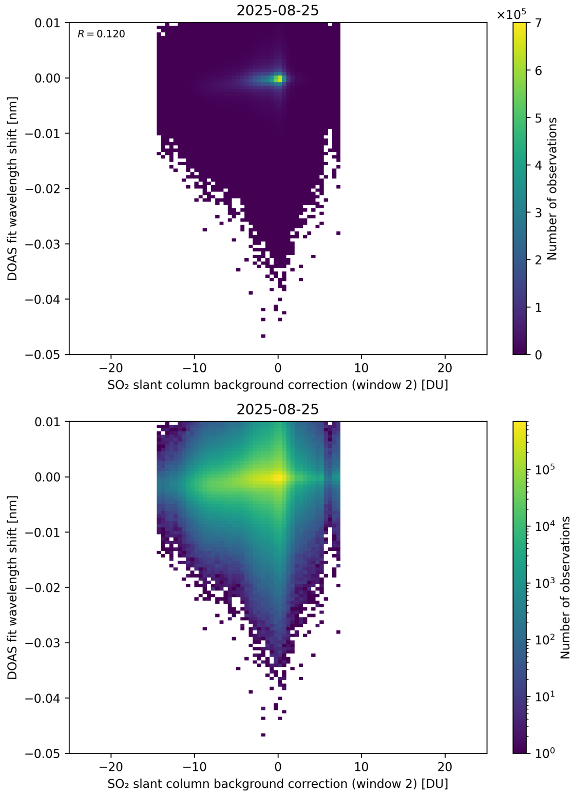
Figure 123: Scatter density plot of “SO 2 slant column background correction (window 2)” against “DOAS fit wavelength shift” for 2025-08-25 to 2025-08-26.
