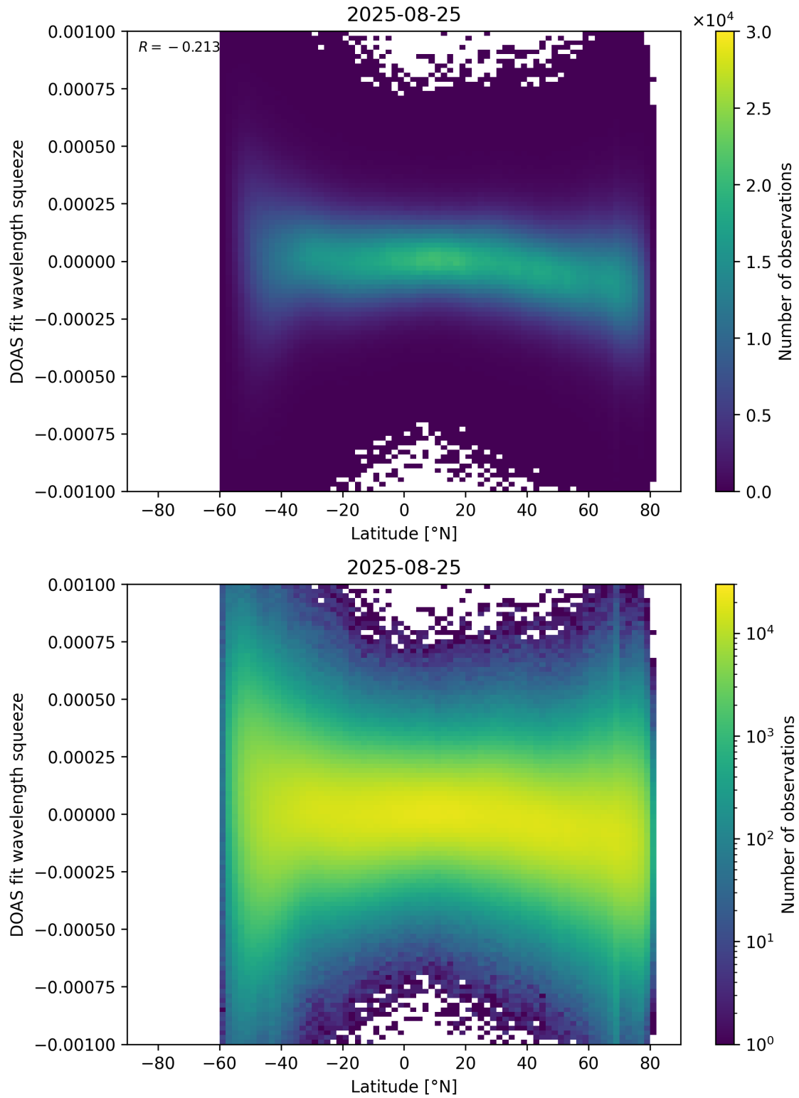
Figure 154: Scatter density plot of “Latitude” against “DOAS fit wavelength squeeze” for 2025-08-25 to 2025-08-26.
