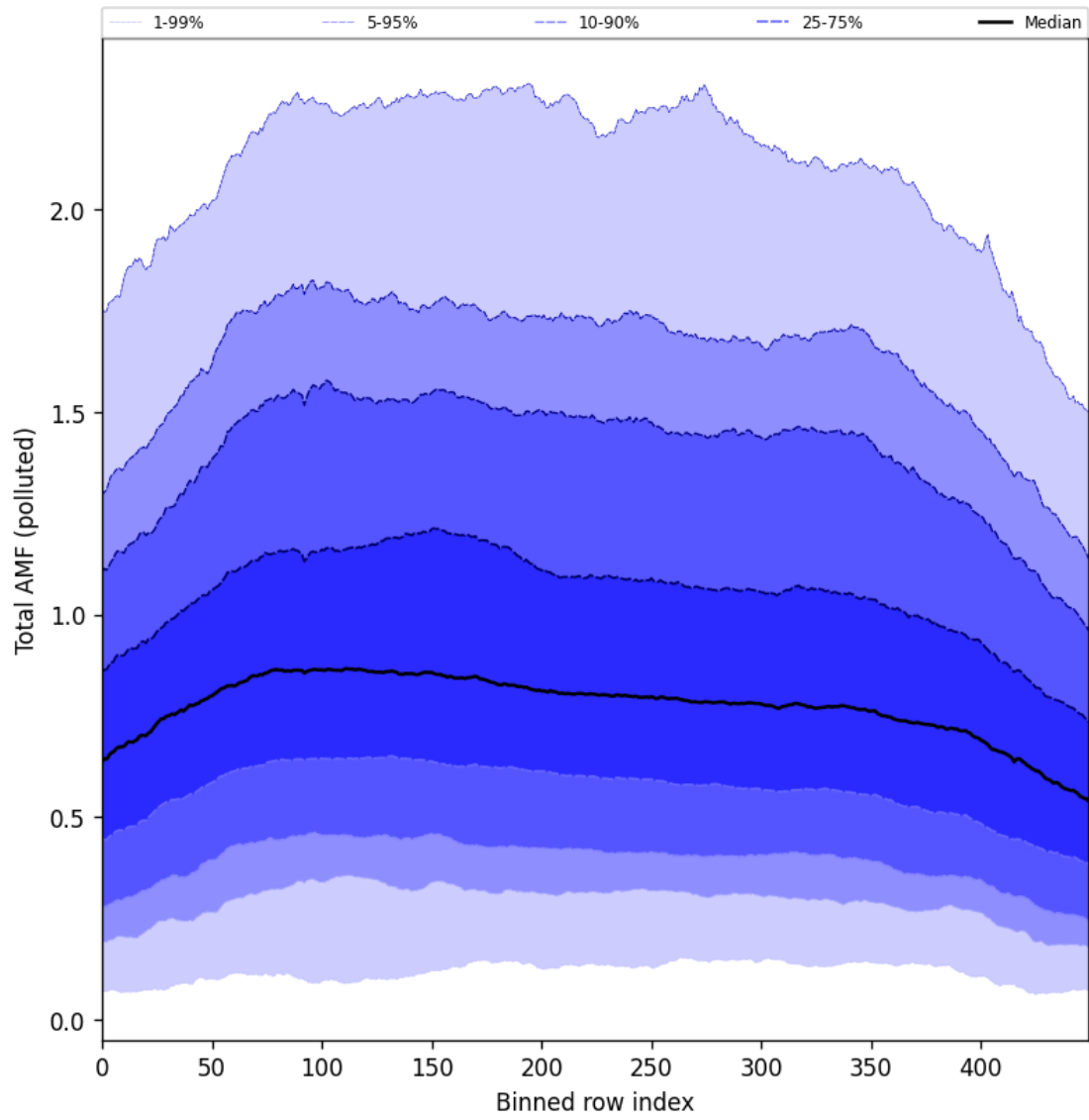
Figure 105: Along track statistics of “Total AMF (polluted)” for 2025-08-25 to 2025-08-26
