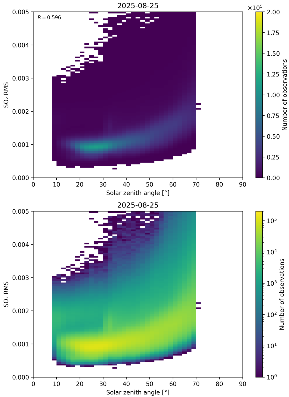
Figure 176: Scatter density plot of “Solar zenith angle” against “SO 2 RMS” for 2025-08-25 to 2025-08-26.
