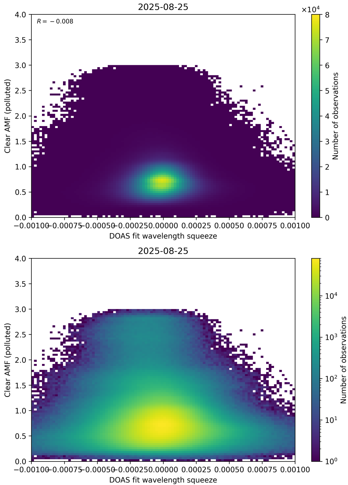
Figure 144: Scatter density plot of “DOAS fit wavelength squeeze” against “Clear AMF (polluted)” for 2025-08-25 to 2025-08-26.
