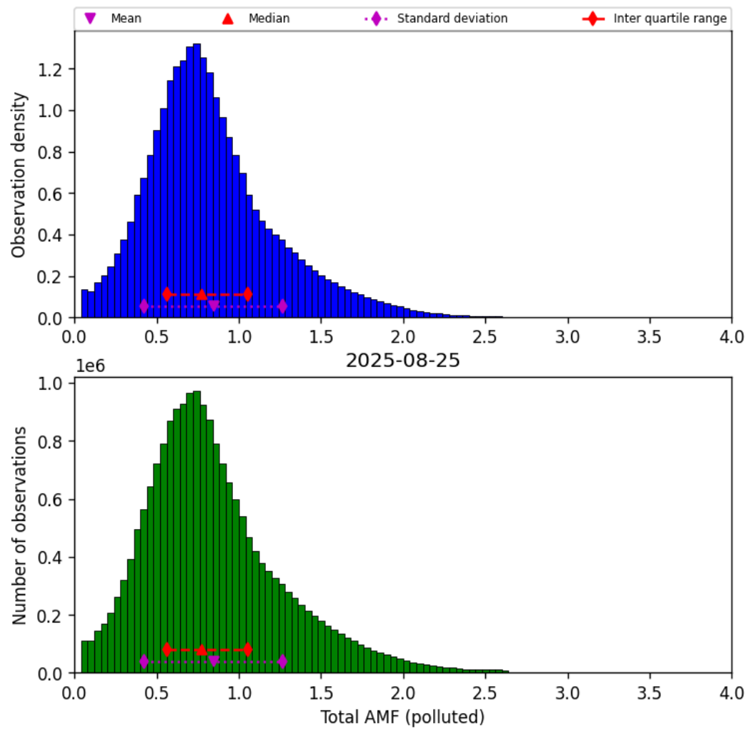
Figure 79: Histogram of “Total AMF (polluted)” for 2025-08-25 to 2025-08-26
