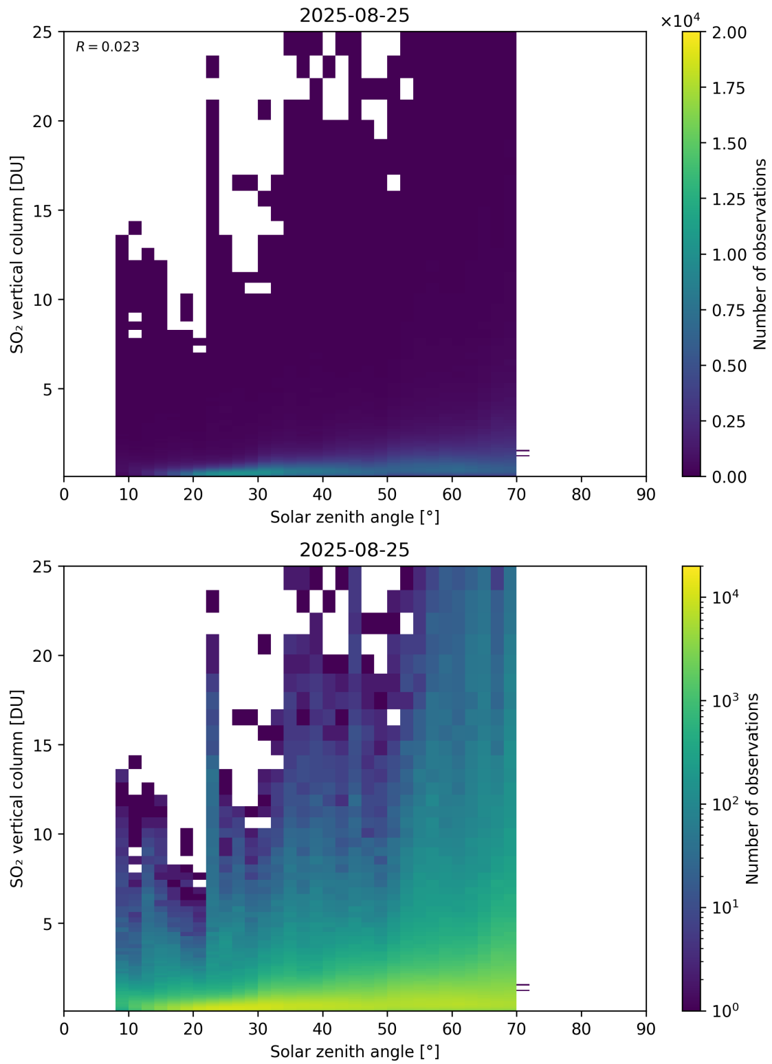
Figure 191: Scatter density plot of “Solar zenith angle” against “SO 2 vertical column” for 2025-08-25 to 2025-08-26.
