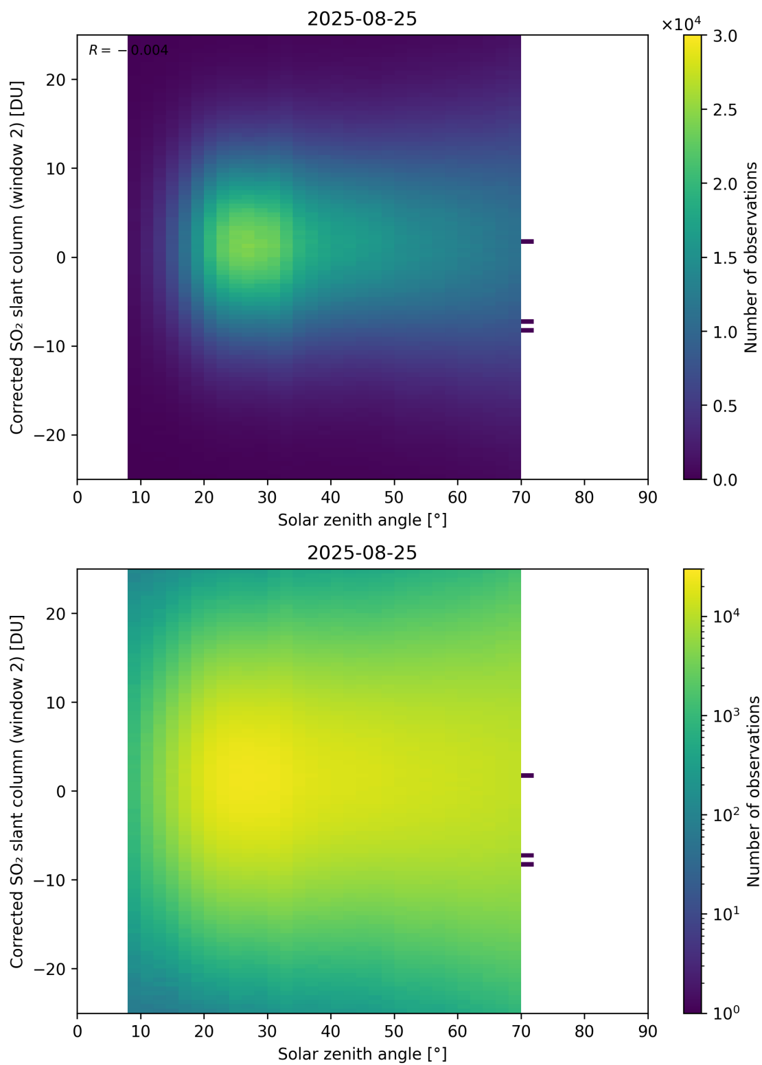
Figure 182: Scatter density plot of “Solar zenith angle” against “Corrected SO 2 slant column (window 2)” for 2025-08-25 to 2025-08-26.
