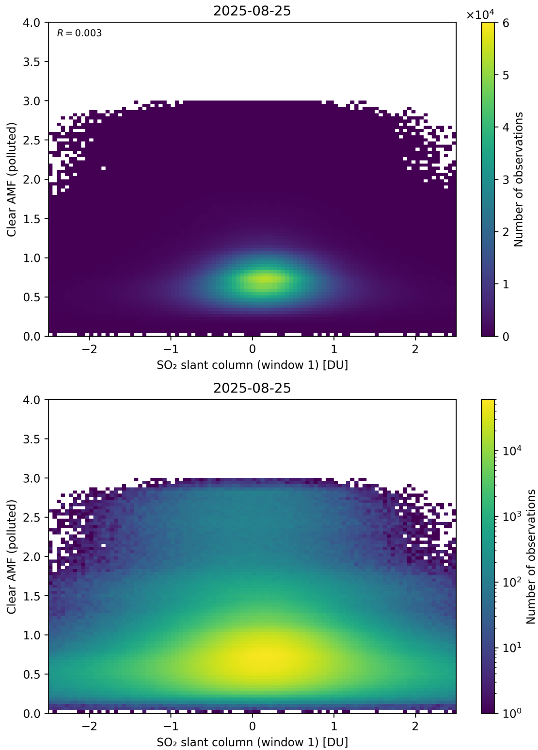
Figure 282: Scatter density plot of “SO 2 slant column (window 1)” against “Clear AMF (polluted)” for 2025-08-25 to 2025-08-26.
