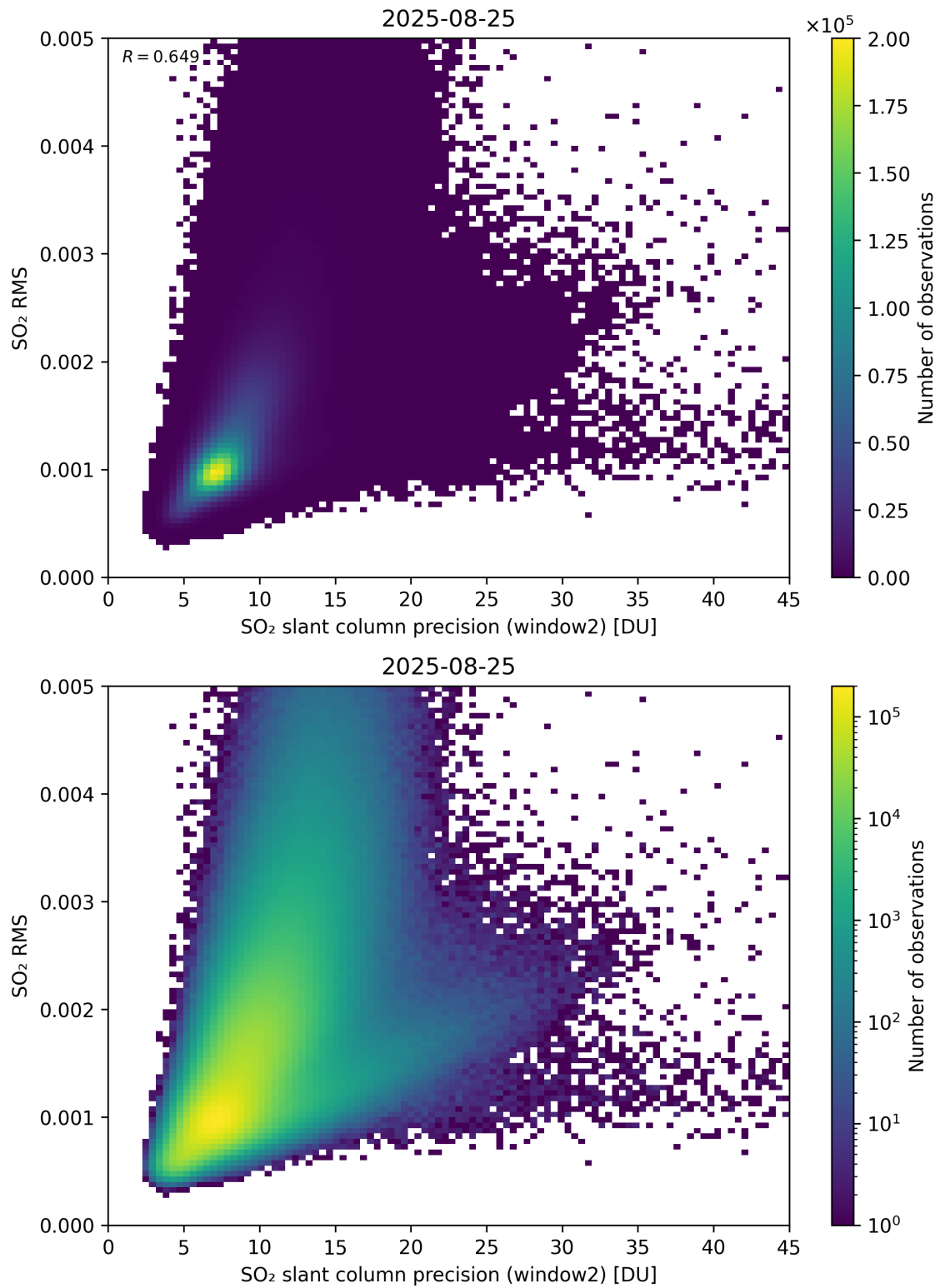
Figure 295: Scatter density plot of “SO 2 slant column precision (window2)” against “SO 2 RMS” for 2025-08-25 to 2025-08-26.
