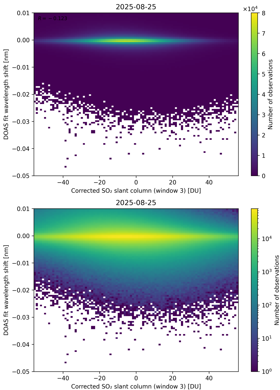
Figure 256: Scatter density plot of “Corrected SO 2 slant column (window 3)” against “DOAS fit wavelength shift” for 2025-08-25 to 2025-08-26.
