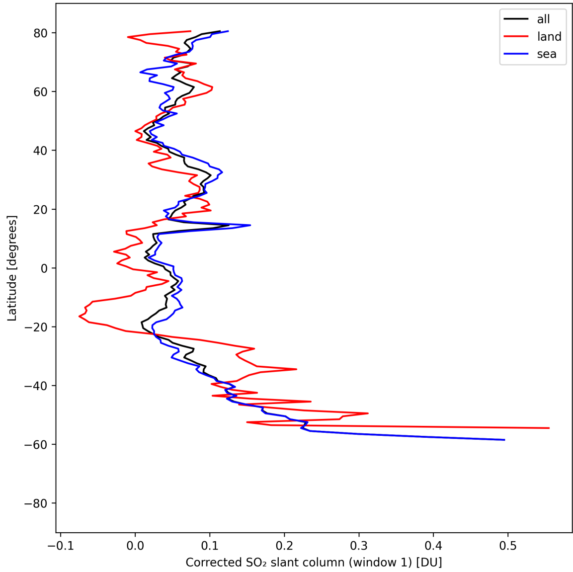
Figure 39: Zonal average of “Corrected SO 2 slant column (window 1)” for 2025-08-25 to 2025-08-26.
