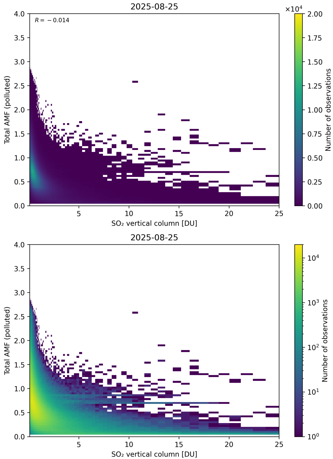
Figure 359: Scatter density plot of “SO 2 vertical column” against “Total AMF (polluted)” for 2025-08-25 to 2025-08-26.
