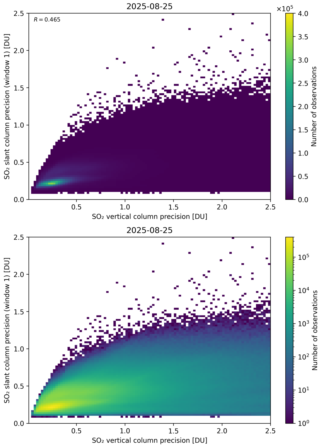
Figure 342: Scatter density plot of “SO 2 vertical column precision” against “SO 2 slant column precision (window 1)” for 2025-08-25 to 2025-08-26.
