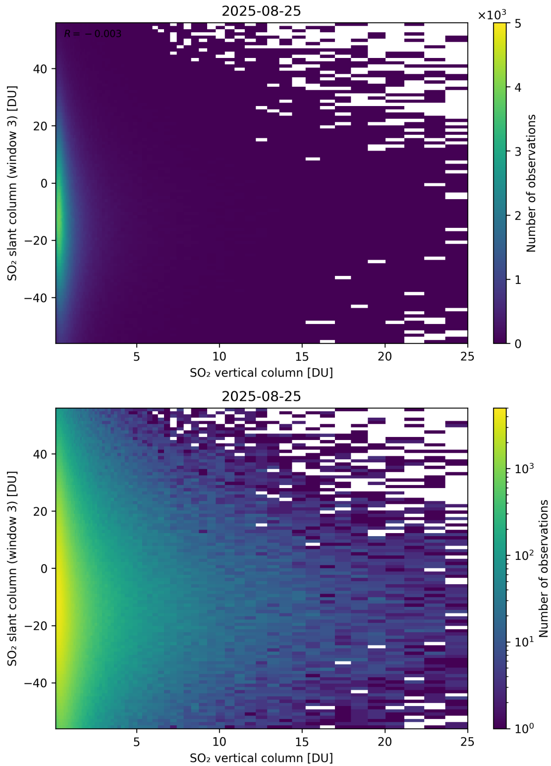
Figure 357: Scatter density plot of “SO 2 vertical column” against “SO 2 slant column (window 3)” for 2025-08-25 to 2025-08-26.
