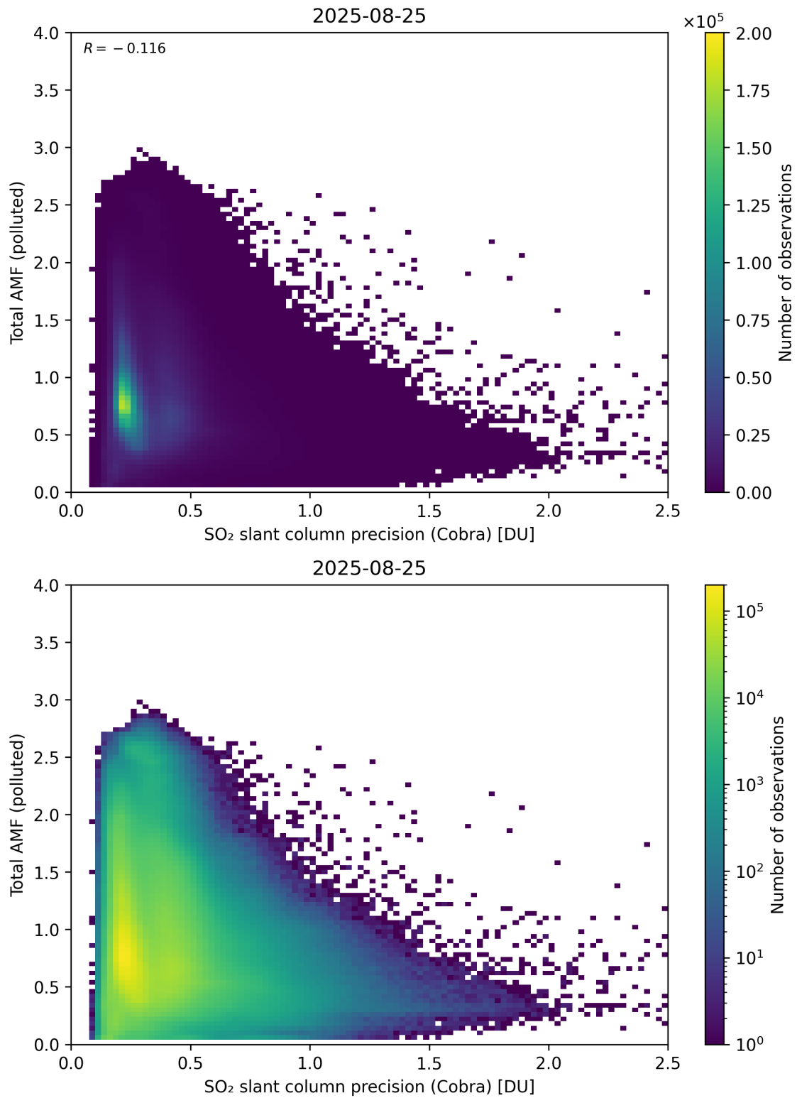
Figure 213: Scatter density plot of “SO 2 slant column precision (Cobra)” against “Total AMF (polluted)” for 2025-08-25 to 2025-08-26.
