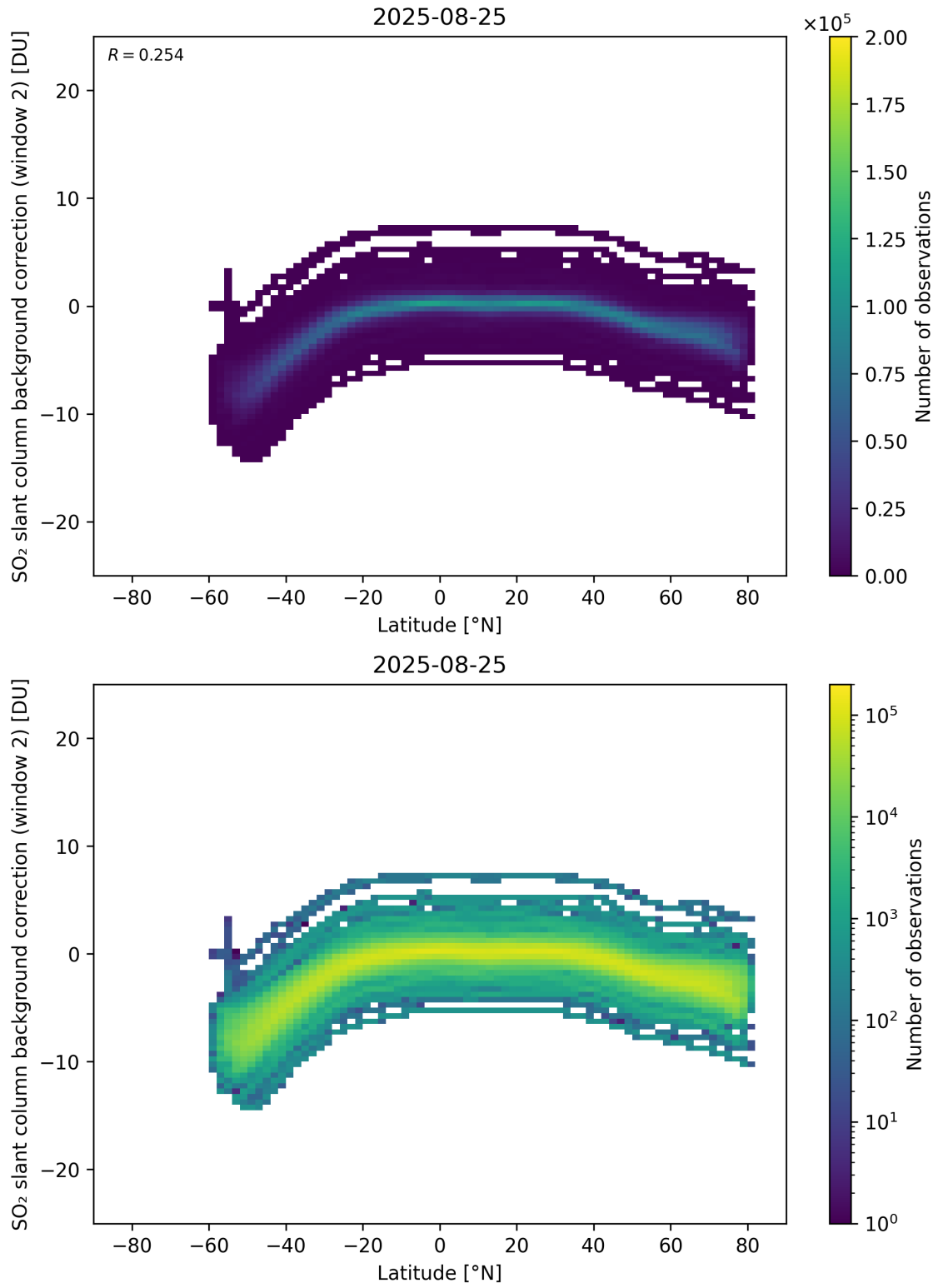
Figure 151: Scatter density plot of “Latitude” against “SO 2 slant column background correction (window 2)” for 2025-08-25 to 2025-08-26.
