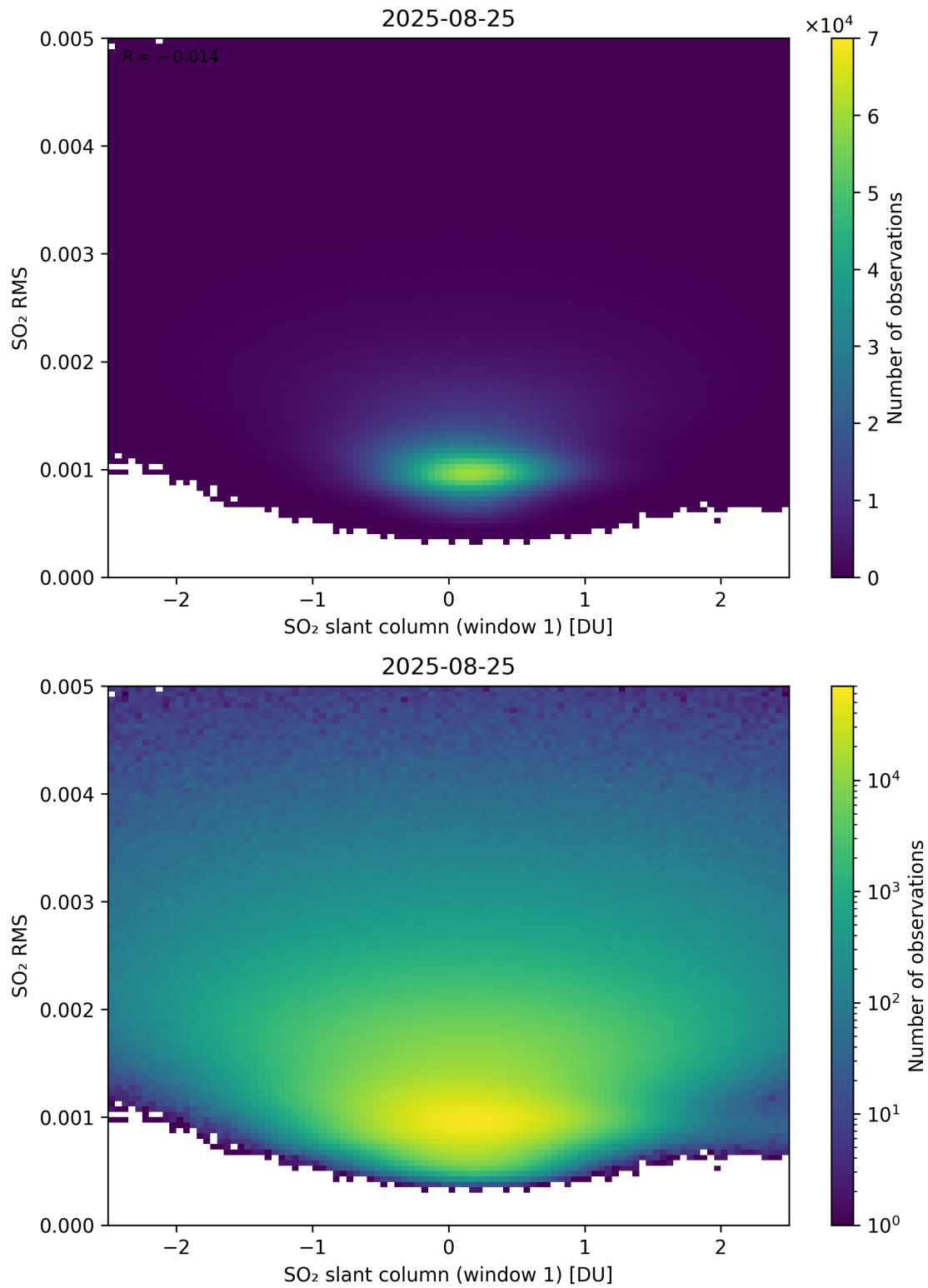
Figure 267: Scatter density plot of “SO 2 slant column (window 1)” against “SO 2 RMS” for 2025-08-25 to 2025-08-26.
