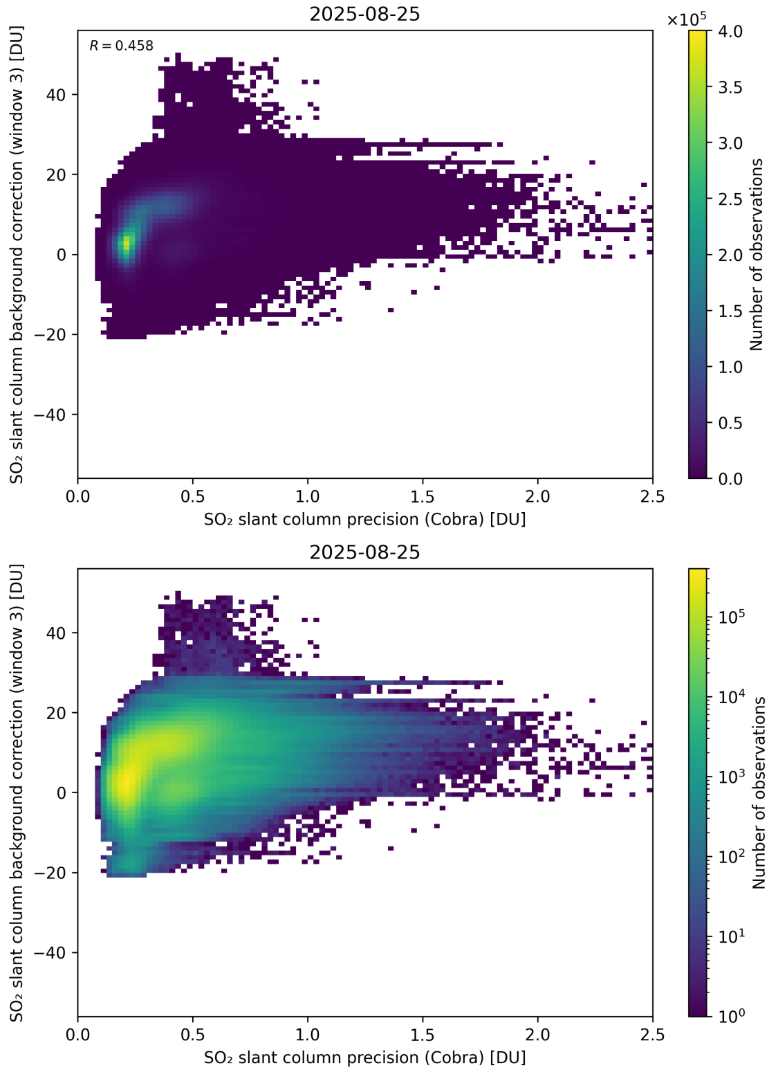
Figure 201: Scatter density plot of “SO 2 slant column precision (Cobra)” against “SO 2 slant column background correction (window 3)” for 2025-08-25 to 2025-08-26.
