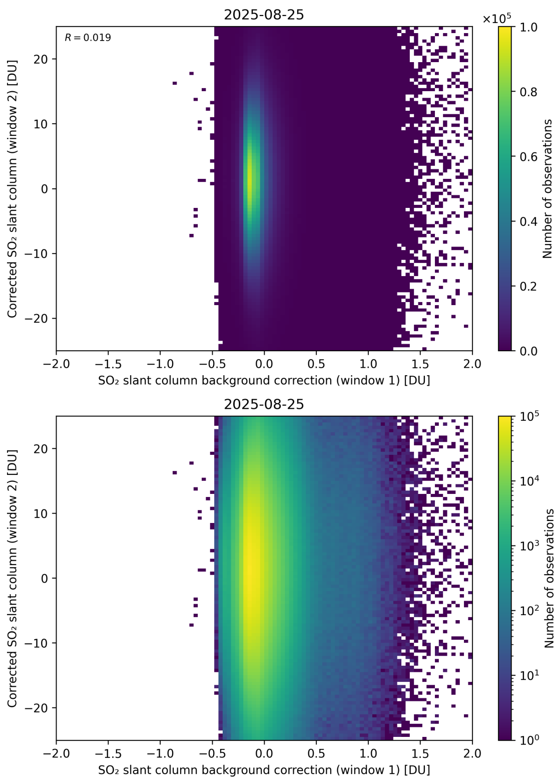
Figure 115: Scatter density plot of “SO 2 slant column background correction (window 1)” against “Corrected SO 2 slant column (window 2)” for 2025-08-25 to 2025-08-26.
