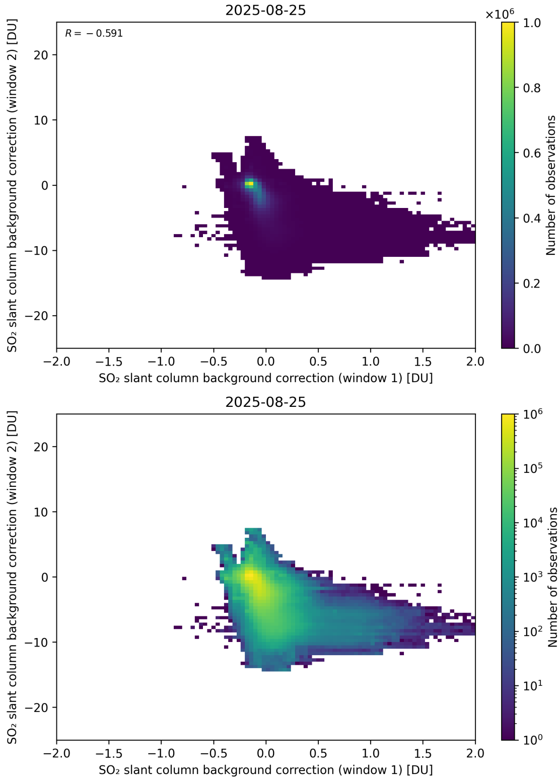
Figure 109: Scatter density plot of “SO 2 slant column background correction (window 1)” against “SO 2 slant column background correction (window 2)” for 2025-08-25 to 2025-08-26.
