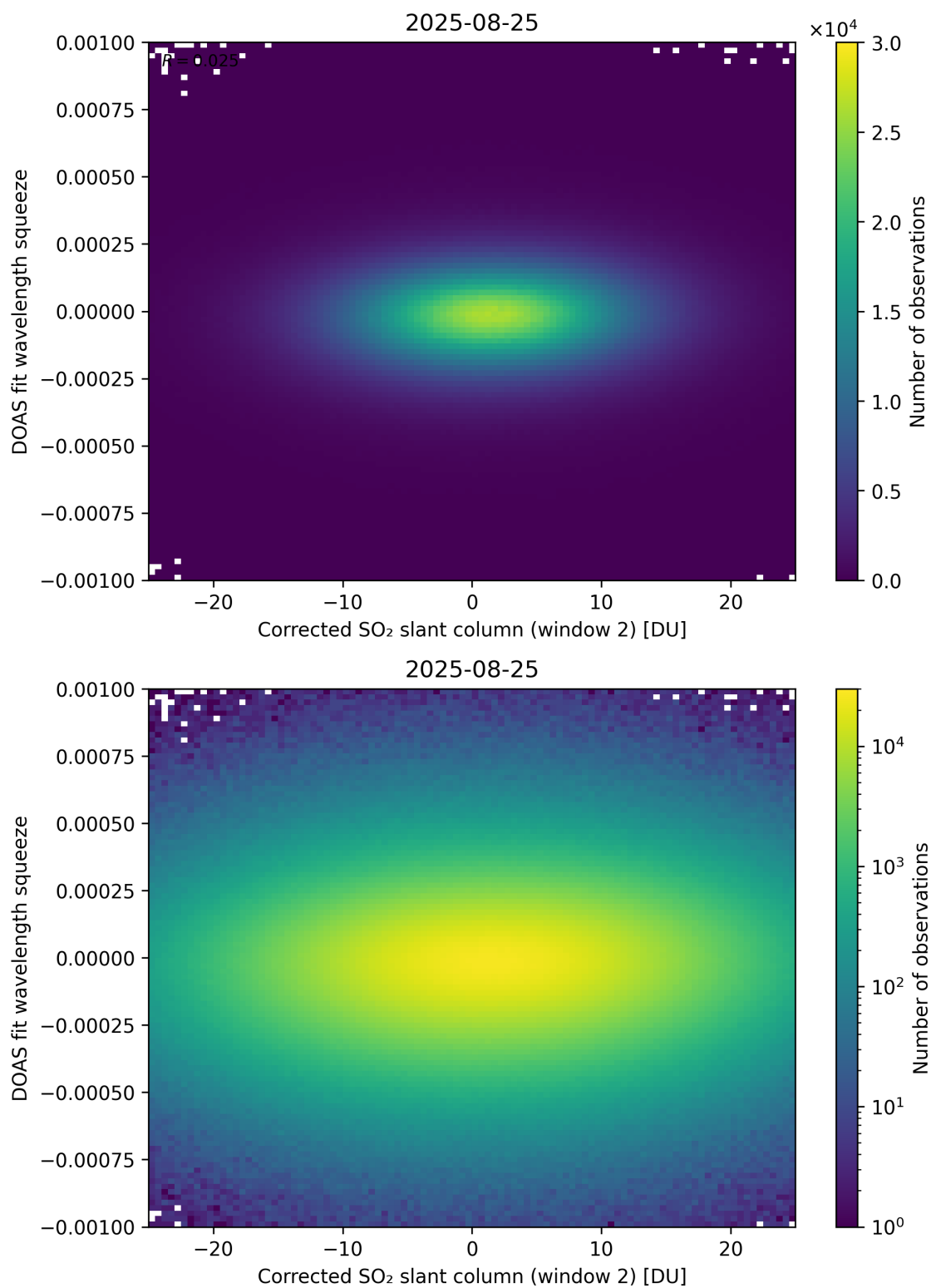
Figure 247: Scatter density plot of “Corrected SO 2 slant column (window 2)” against “DOAS fit wavelength squeeze” for 2025-08-25 to 2025-08-26.
