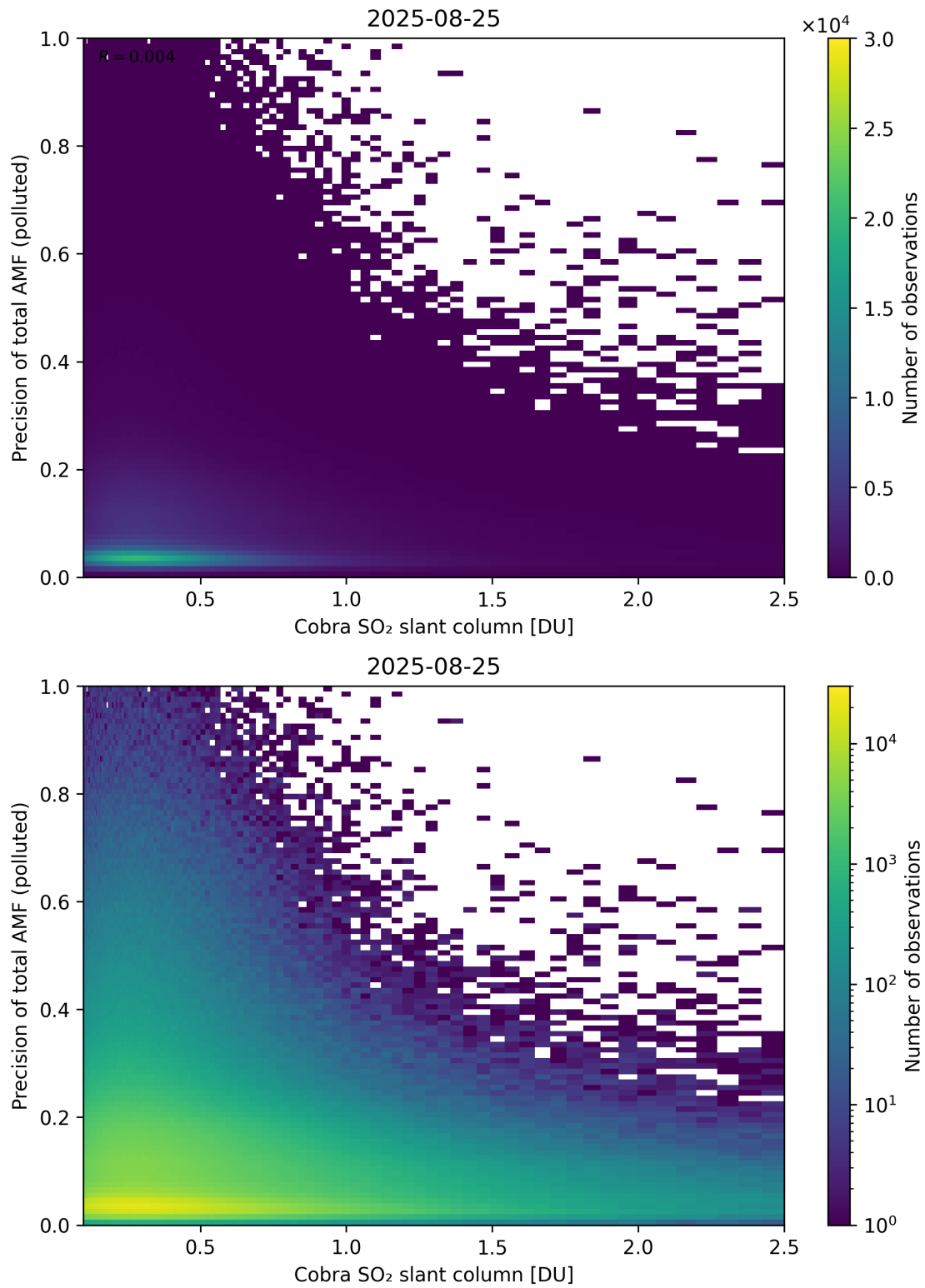
Figure 225: Scatter density plot of “Cobra SO 2 slant column” against “Precision of total AMF (polluted)” for 2025-08-25 to 2025-08-26.
