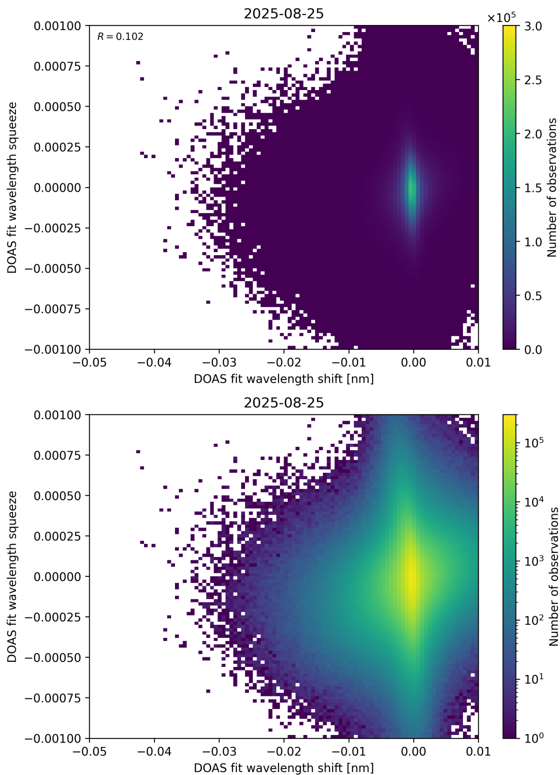
Figure 138: Scatter density plot of “DOAS fit wavelength shift” against “DOAS fit wavelength squeeze” for 2025-08-25 to 2025-08-26.
