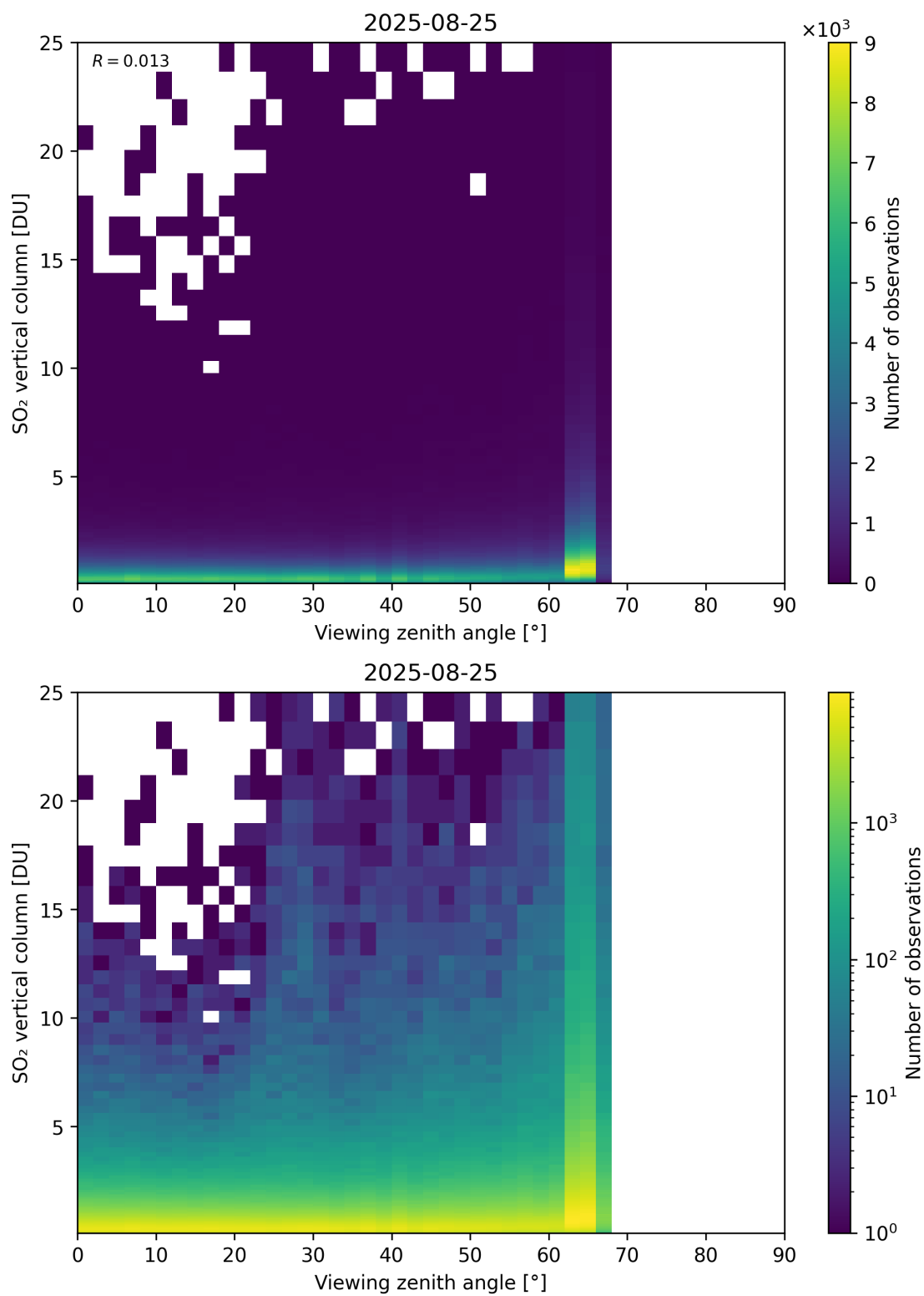
Figure 383: Scatter density plot of “Viewing zenith angle” against “SO 2 vertical column” for 2025-08-25 to 2025-08-26.
