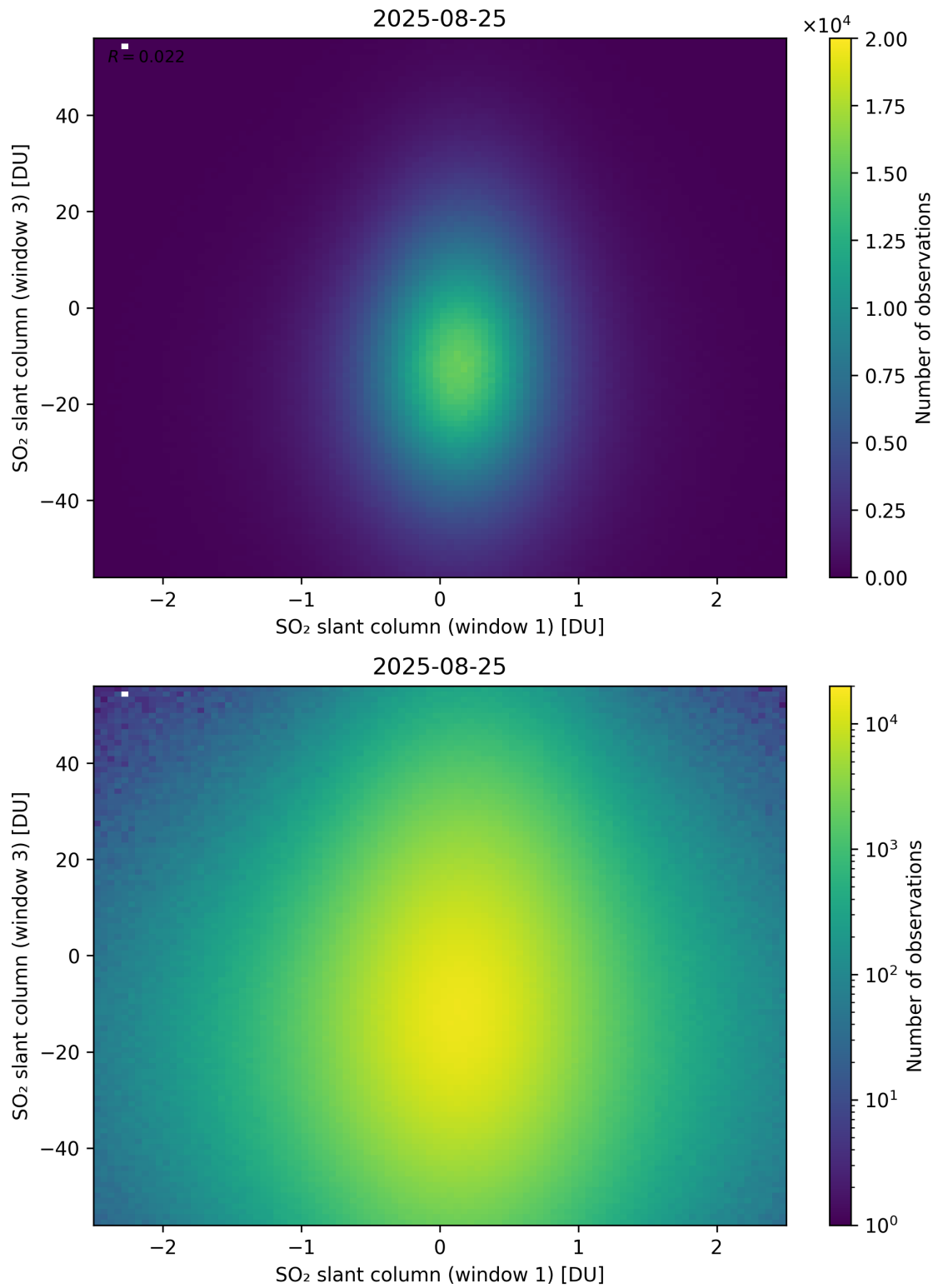
Figure 287: Scatter density plot of “SO 2 slant column (window 1)” against “SO 2 slant column (window 3)” for 2025-08-25 to 2025-08-26.
