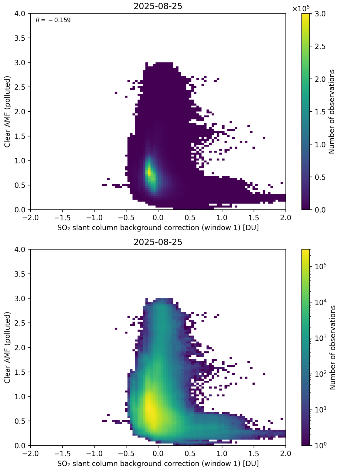
Figure 114: Scatter density plot of “SO 2 slant column background correction (window 1)” against “Clear AMF (polluted)” for 2025-08-25 to 2025-08-26.
