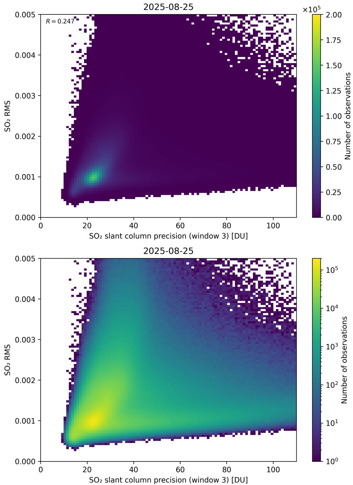
Figure 310: Scatter density plot of “SO 2 slant column precision (window 3)” against “SO 2 RMS” for 2025-08-25 to 2025-08-26.
