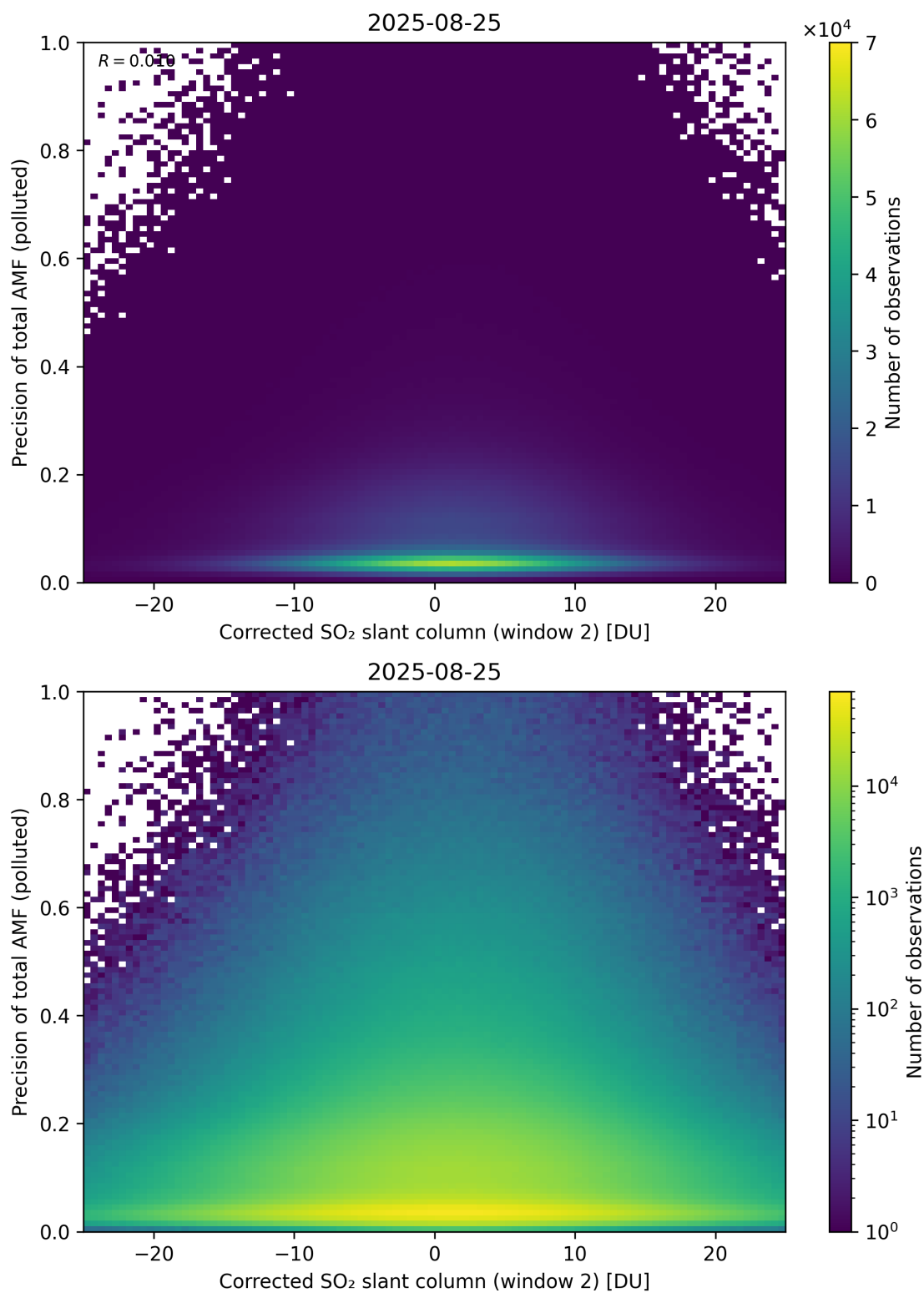
Figure 254: Scatter density plot of “Corrected SO 2 slant column (window 2)” against “Precision of total AMF (polluted)” for 2025-08-25 to 2025-08-26.
