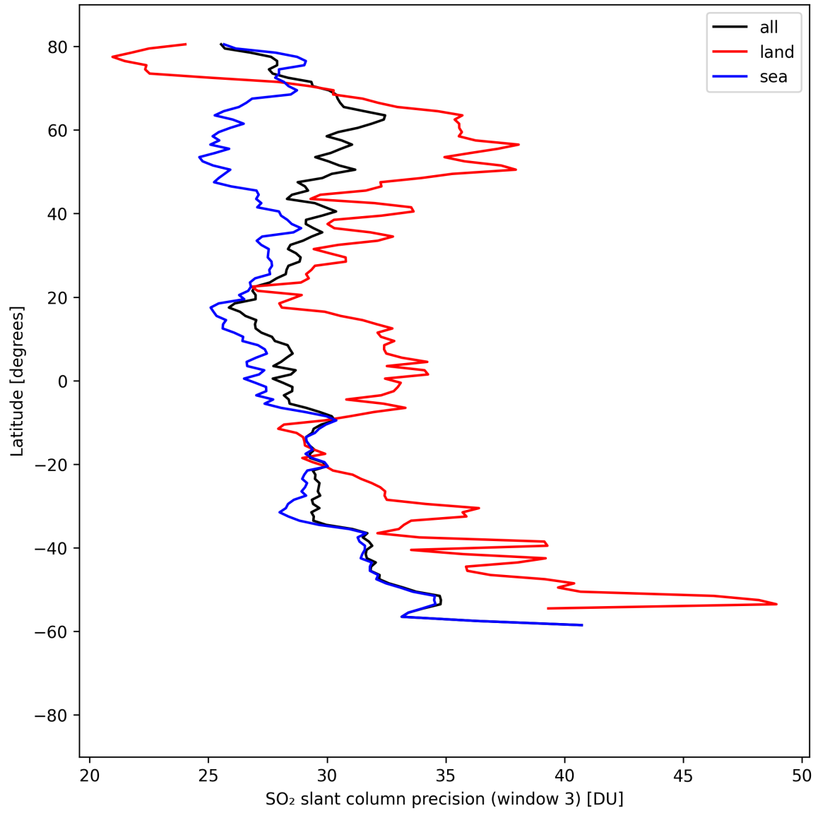
Figure 46: Zonal average of “SO 2 slant column precision (window 3)” for 2025-08-25 to 2025-08-26.
