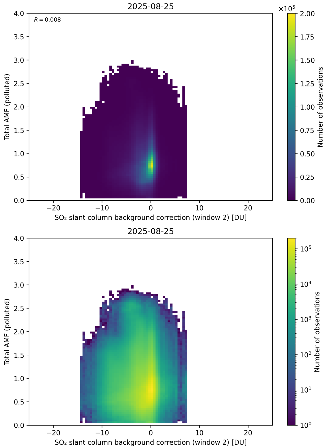
Figure 130: Scatter density plot of “SO 2 slant column background correction (window 2)” against “Total AMF (polluted)” for 2025-08-25 to 2025-08-26.
