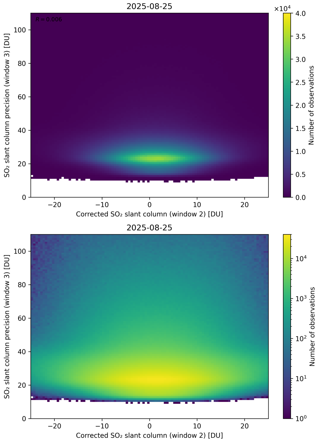
Figure 252: Scatter density plot of “Corrected SO 2 slant column (window 2)” against “SO 2 slant column precision (window 3)” for 2025-08-25 to 2025-08-26.
