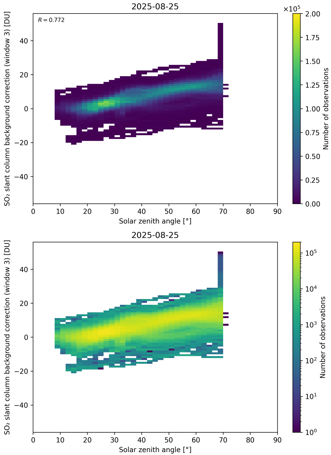
Figure 173: Scatter density plot of “Solar zenith angle” against “SO 2 slant column background correction (window 3)” for 2025-08-25 to 2025-08-26.
