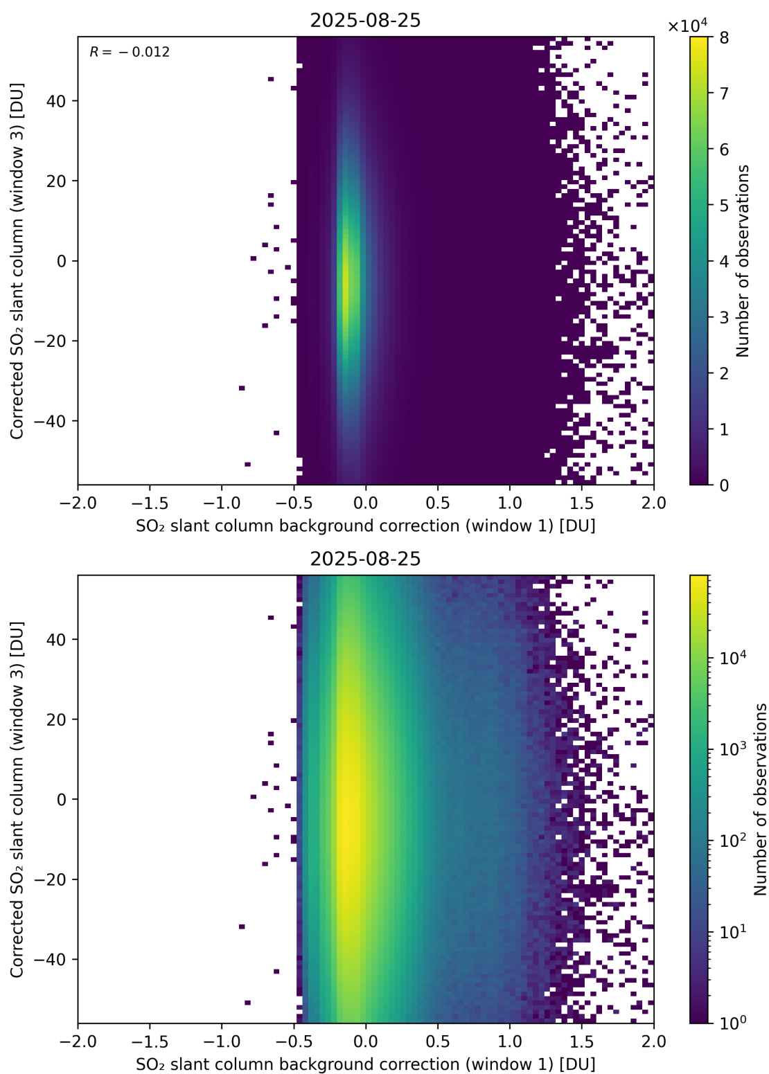
Figure 116: Scatter density plot of “SO 2 slant column background correction (window 1)” against “Corrected SO 2 slant column (window 3)” for 2025-08-25 to 2025-08-26.
