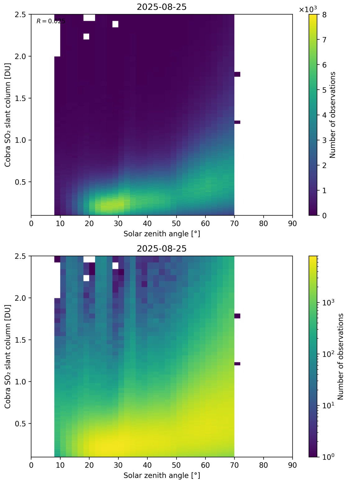
Figure 179: Scatter density plot of “Solar zenith angle” against “Cobra SO 2 slant column” for 2025-08-25 to 2025-08-26.
