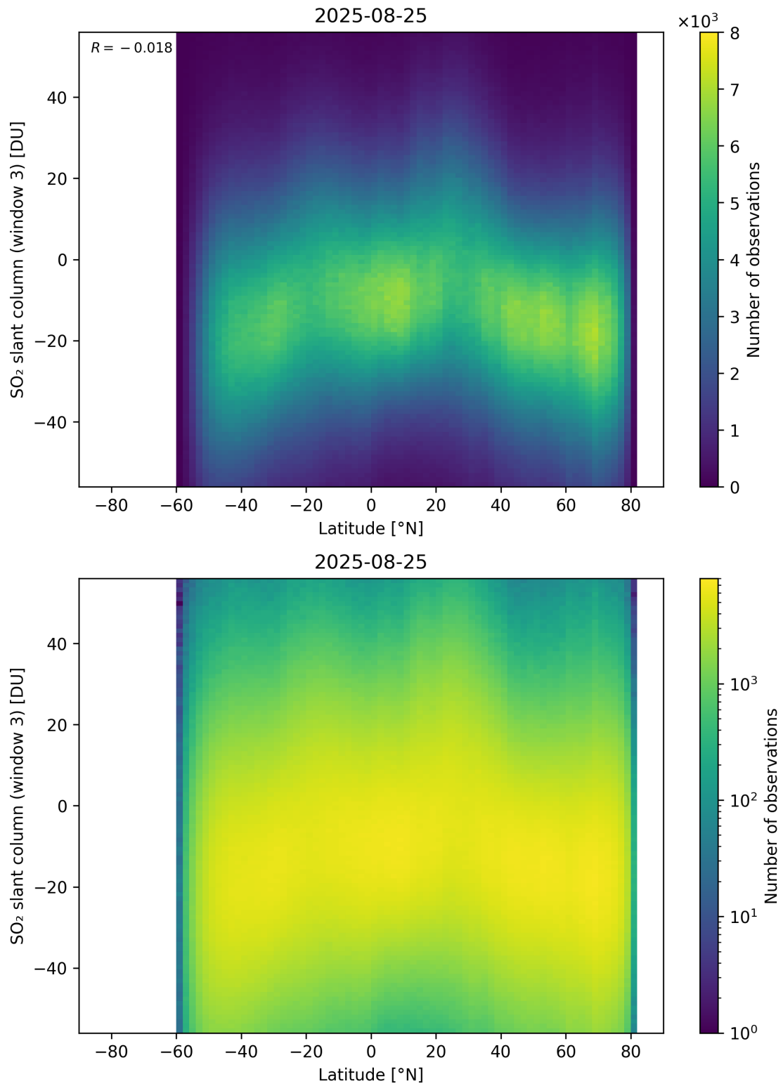
Figure 165: Scatter density plot of “Latitude” against “SO 2 slant column (window 3)” for 2025-08-25 to 2025-08-26.
