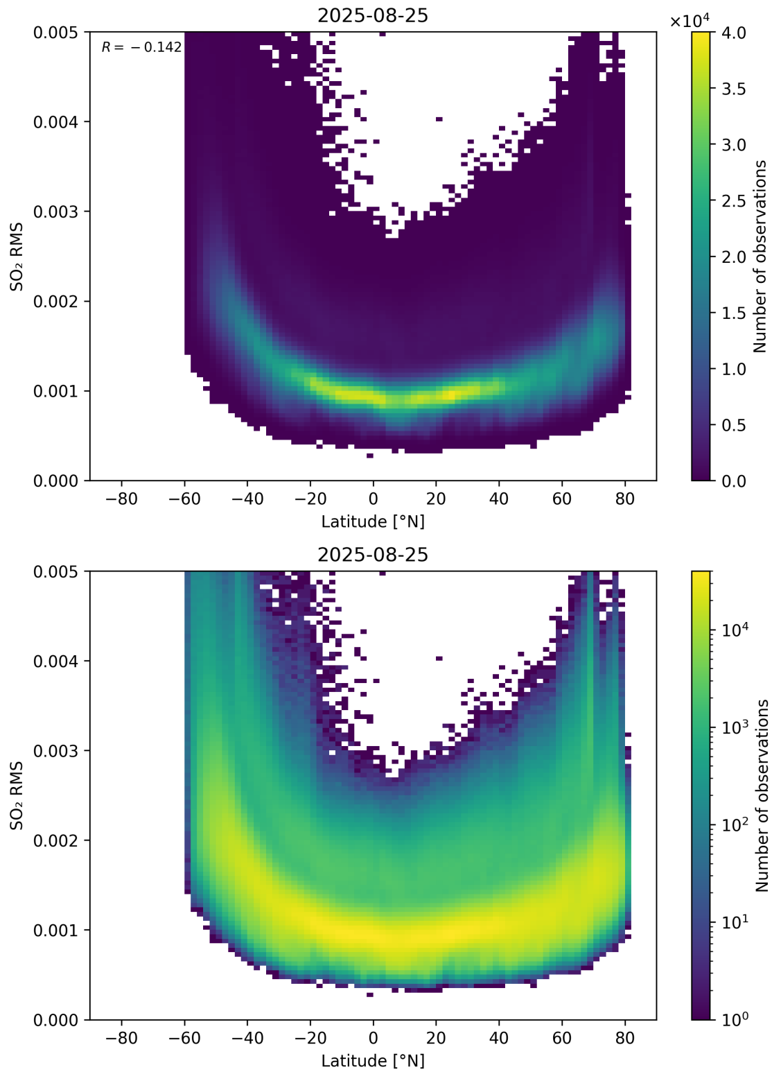
Figure 155: Scatter density plot of “Latitude” against “SO 2 RMS” for 2025-08-25 to 2025-08-26.
