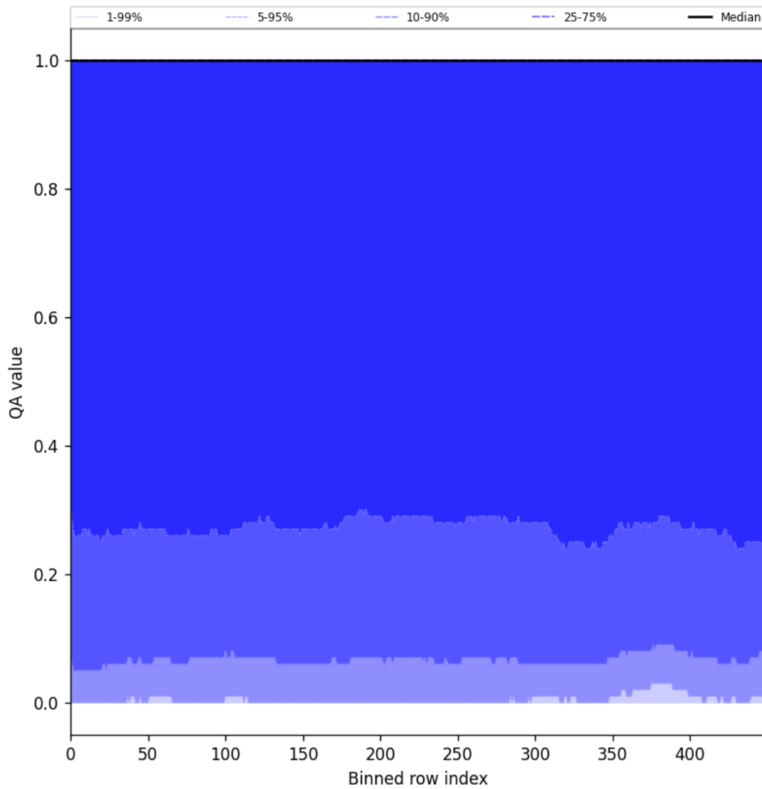
Figure 83: Along track statistics of “QA value” for 2025-08-25 to 2025-08-26
