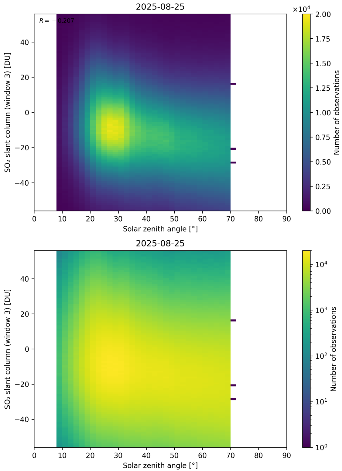
Figure 187: Scatter density plot of “Solar zenith angle” against “SO 2 slant column (window 3)” for 2025-08-25 to 2025-08-26.
