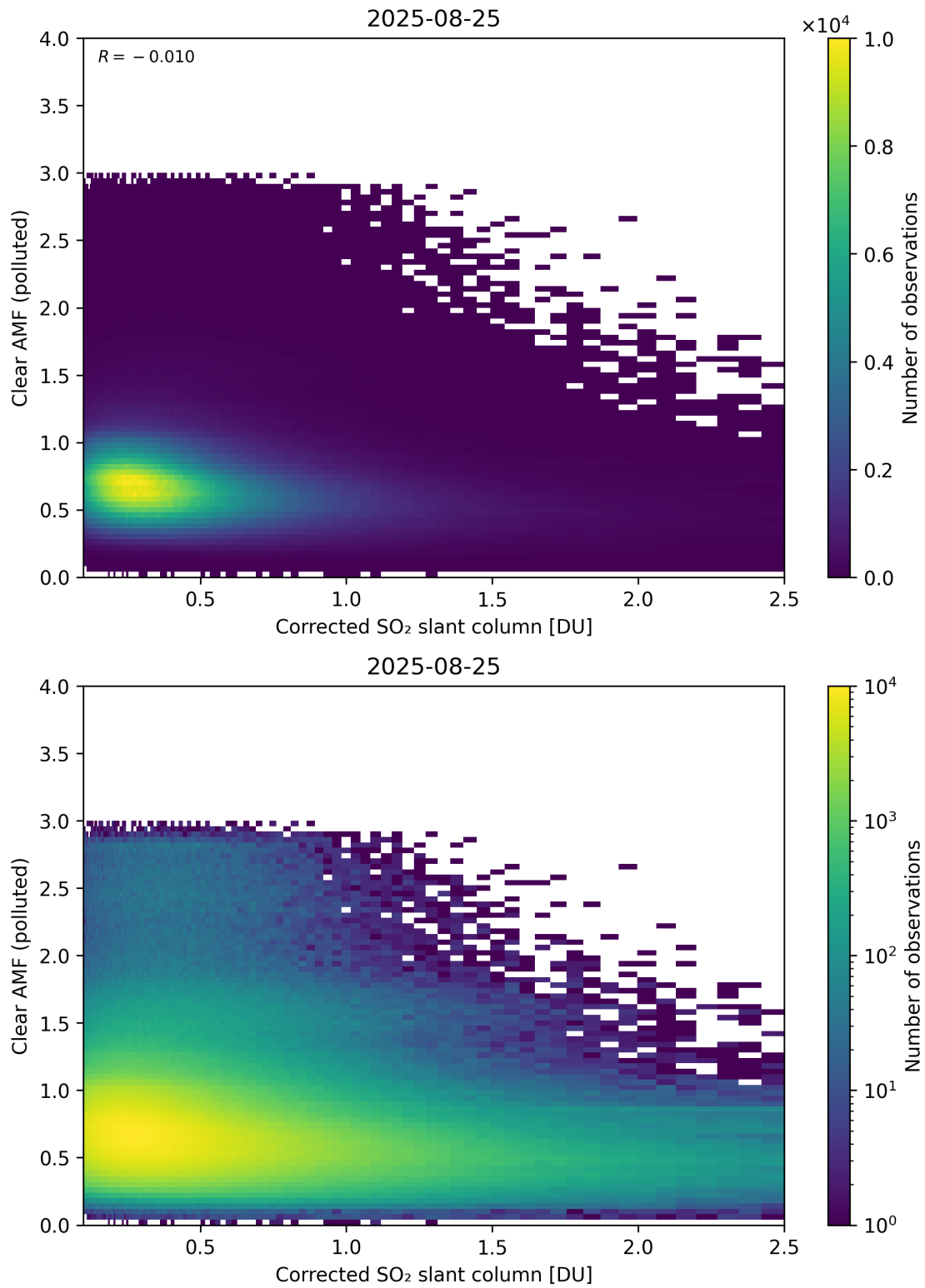
Figure 232: Scatter density plot of “Corrected SO 2 slant column” against “Clear AMF (polluted)” for 2025-08-25 to 2025-08-26.
