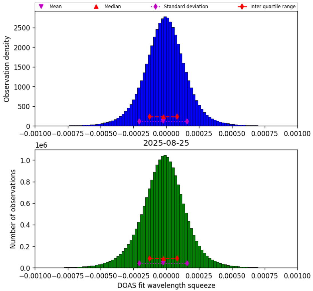
Figure 77: Histogram of “DOAS fit wavelength squeeze” for 2025-08-25 to 2025-08-26
