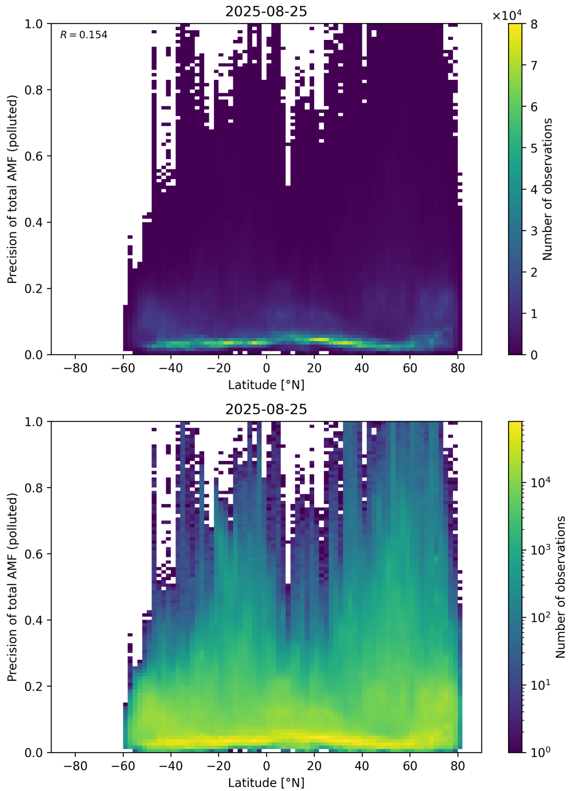
Figure 168: Scatter density plot of “Latitude” against “Precision of total AMF (polluted)” for 2025-08-25 to 2025-08-26.
