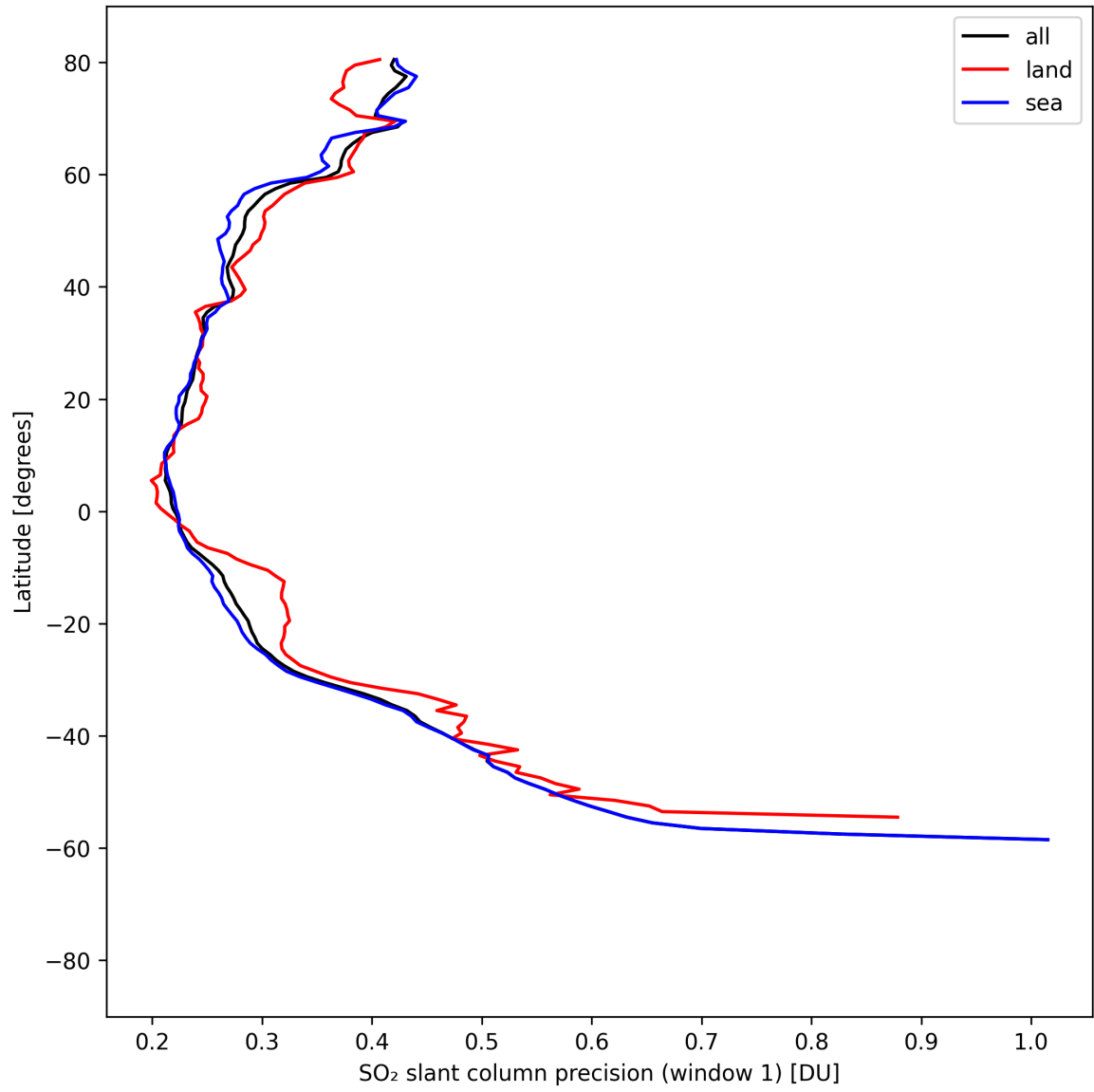
Figure 38: Zonal average of “SO 2 slant column precision (window 1)” for 2025-08-25 to 2025-08-26.
