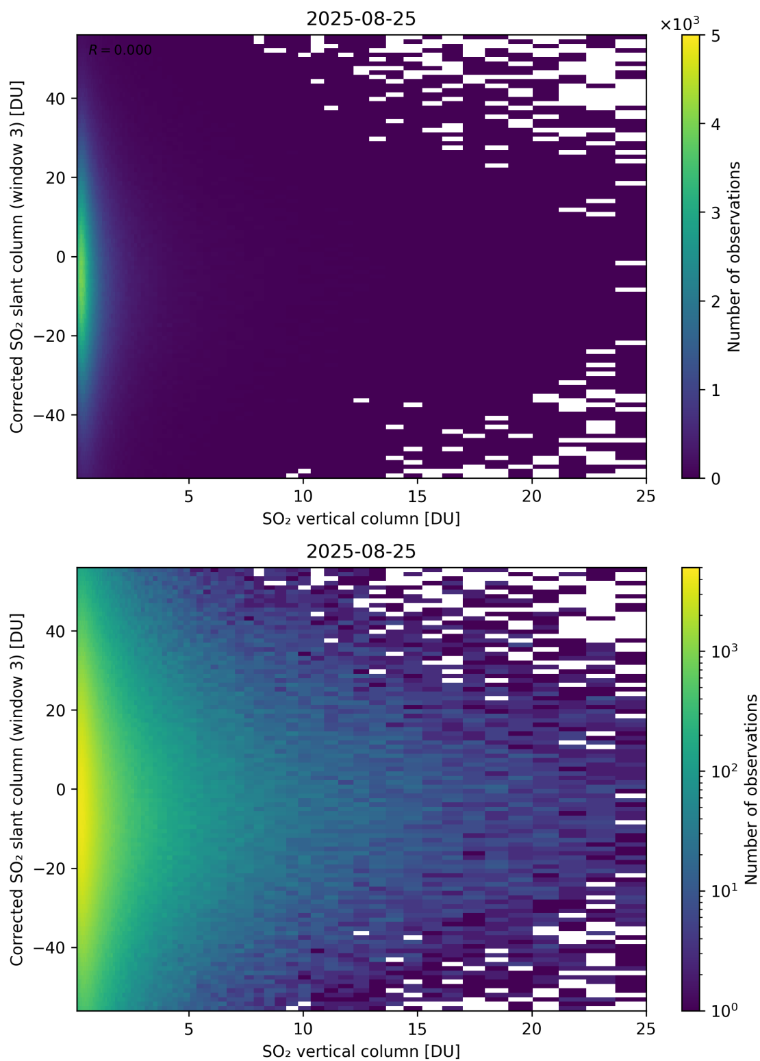
Figure 353: Scatter density plot of “SO 2 vertical column” against “Corrected SO 2 slant column (window 3)” for 2025-08-25 to 2025-08-26.
