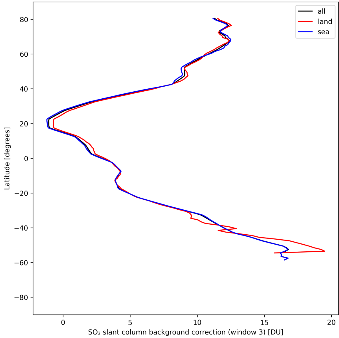
Figure 48: Zonal average of “SO 2 slant column background correction (window 3)” for 2025-08-25 to 2025-08-26.
