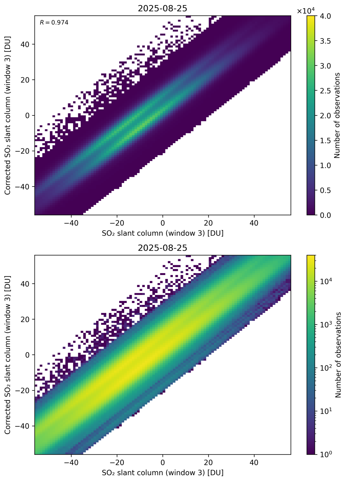
Figure 316: Scatter density plot of “SO 2 slant column (window 3)” against “Corrected SO 2 slant column (window 3)” for 2025-08-25 to 2025-08-26.
