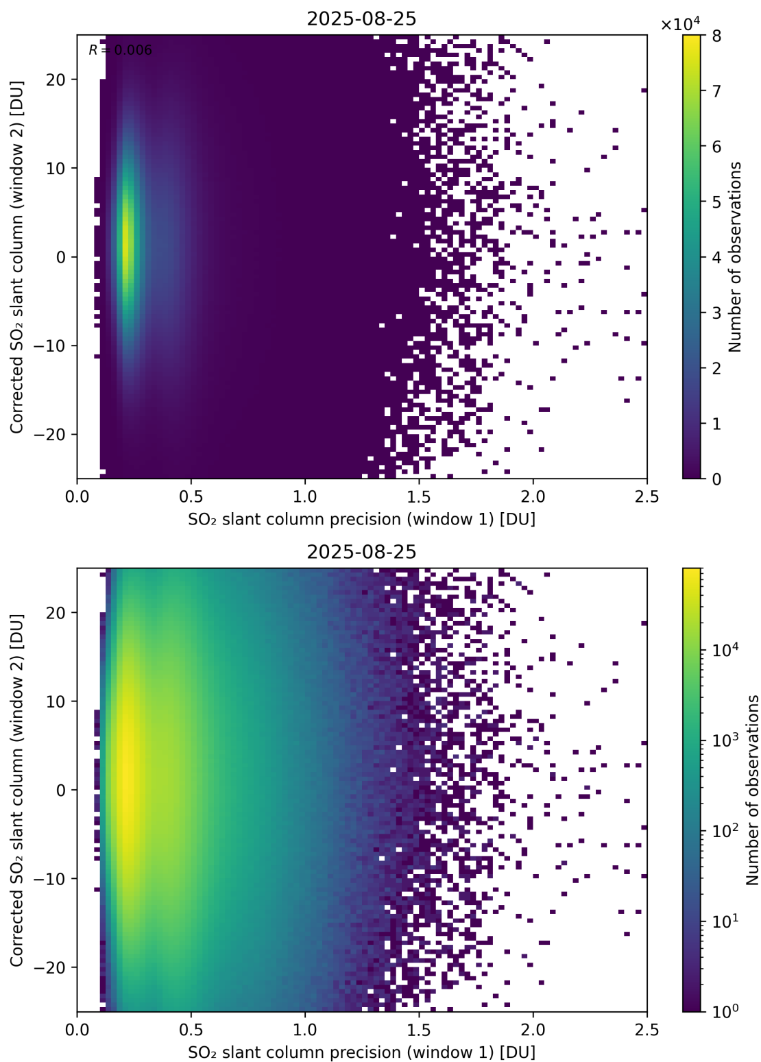
Figure 275: Scatter density plot of “SO 2 slant column precision (window 1)” against “Corrected SO 2 slant column (window 2)” for 2025-08-25 to 2025-08-26.
