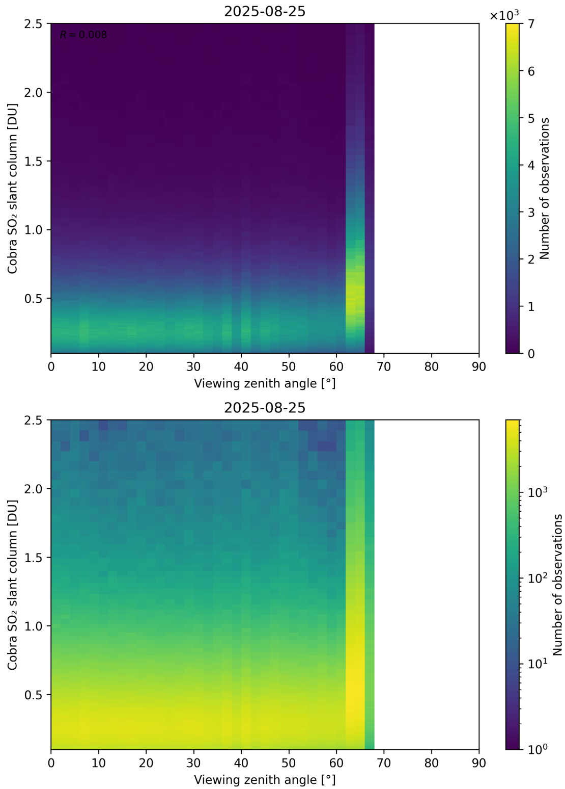
Figure 371: Scatter density plot of “Viewing zenith angle” against “Cobra SO 2 slant column” for 2025-08-25 to 2025-08-26.
