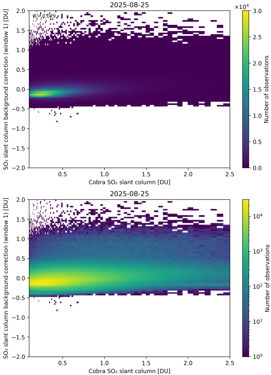
Figure 193: Scatter density plot of “Cobra SO 2 slant column” against “SO 2 slant column background correction (window 1)” for 2025-08-25 to 2025-08-26.
