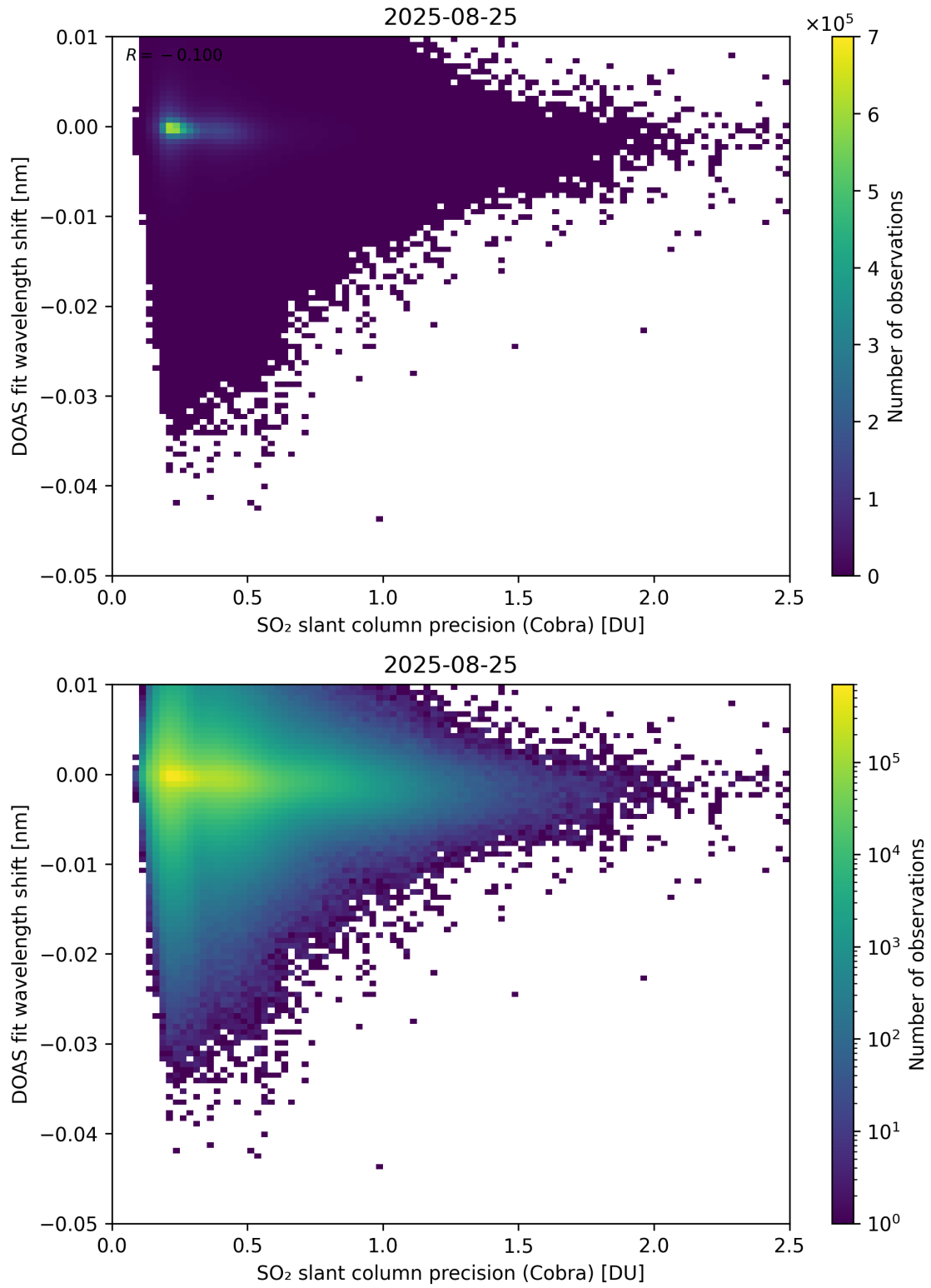
Figure 202: Scatter density plot of “SO 2 slant column precision (Cobra)” against “DOAS fit wavelength shift” for 2025-08-25 to 2025-08-26.
