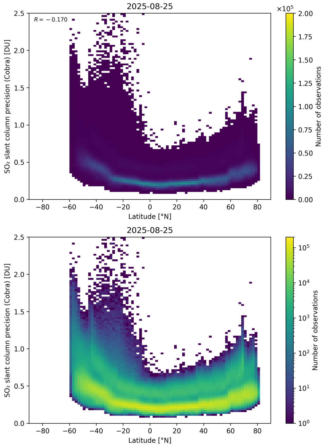
Figure 158: Scatter density plot of “Latitude” against “SO 2 slant column precision (Cobra)” for 2025-08-25 to 2025-08-26.
