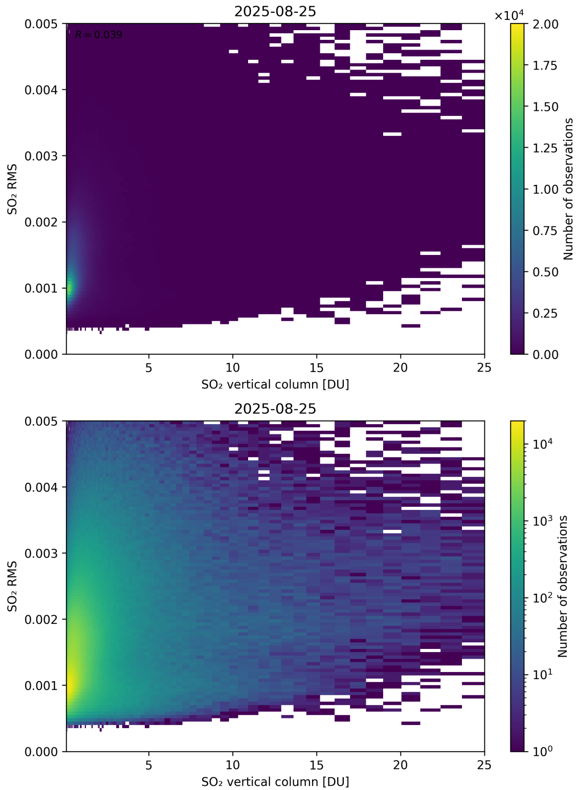
Figure 328: Scatter density plot of “SO 2 vertical column” against “SO 2 RMS” for 2025-08-25 to 2025-08-26.
