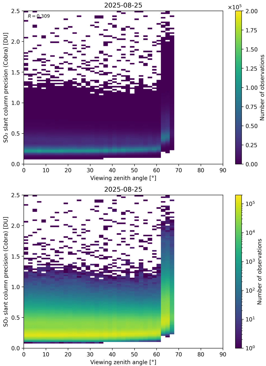
Figure 372: Scatter density plot of “Viewing zenith angle” against “SO 2 slant column precision (Cobra)” for 2025-08-25 to 2025-08-26.
