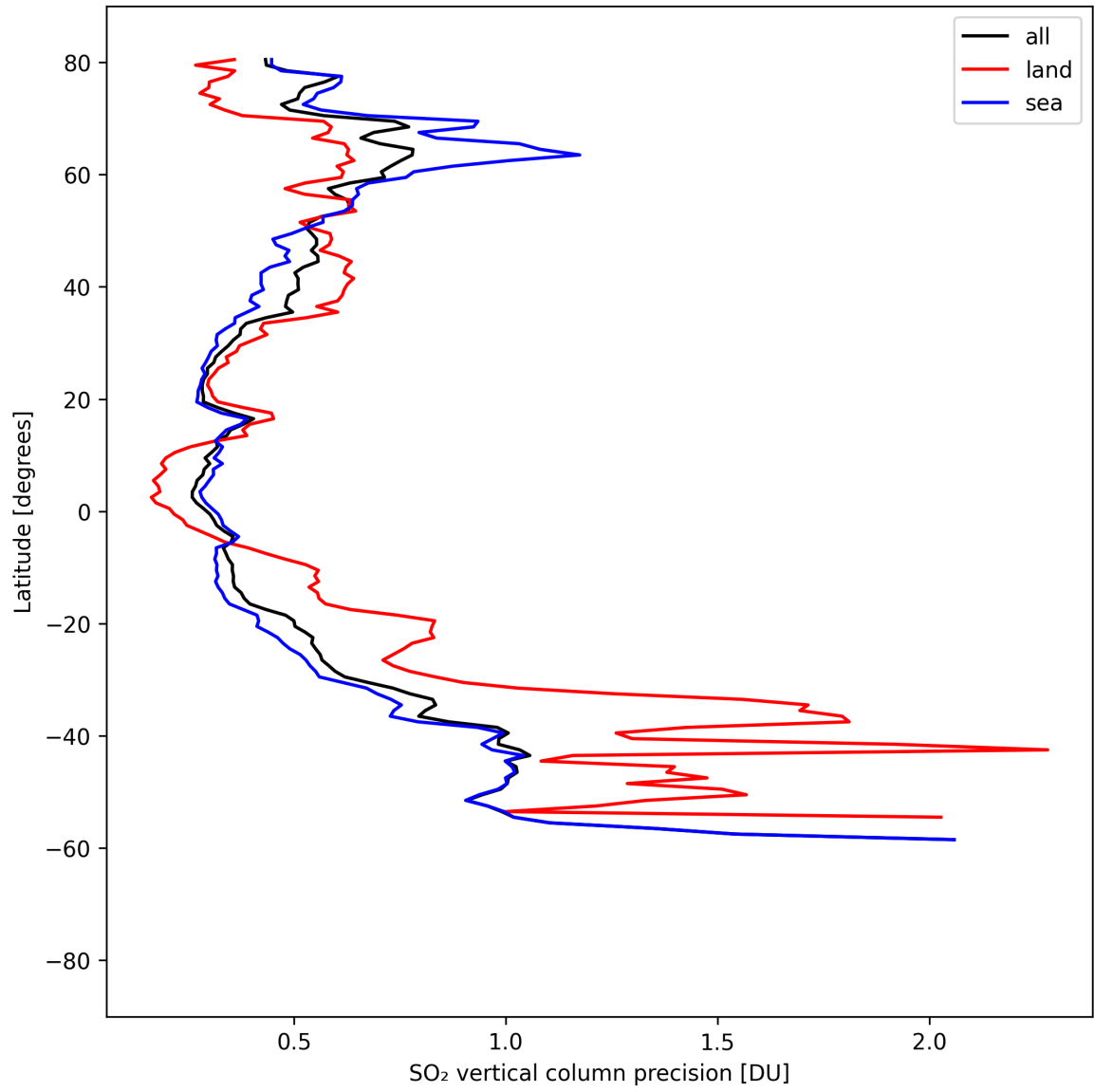
Figure 33: Zonal average of “SO 2 vertical column precision” for 2025-08-25 to 2025-08-26.
