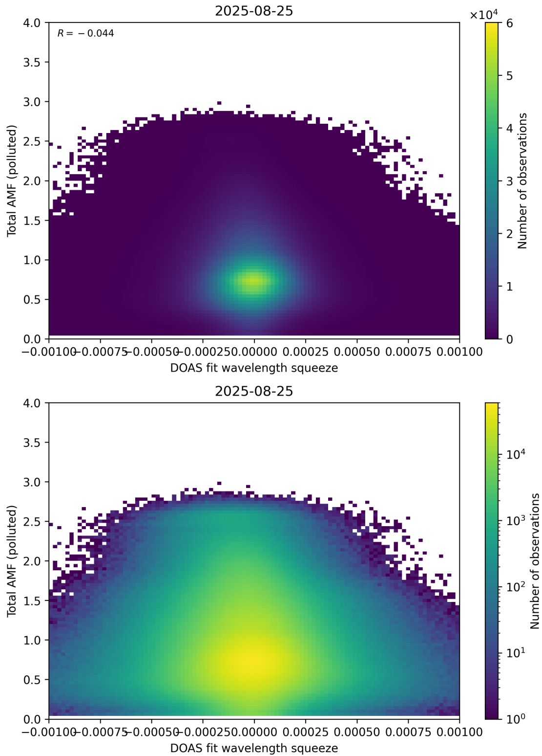
Figure 145: Scatter density plot of “DOAS fit wavelength squeeze” against “Total AMF (polluted)” for 2025-08-25 to 2025-08-26.
