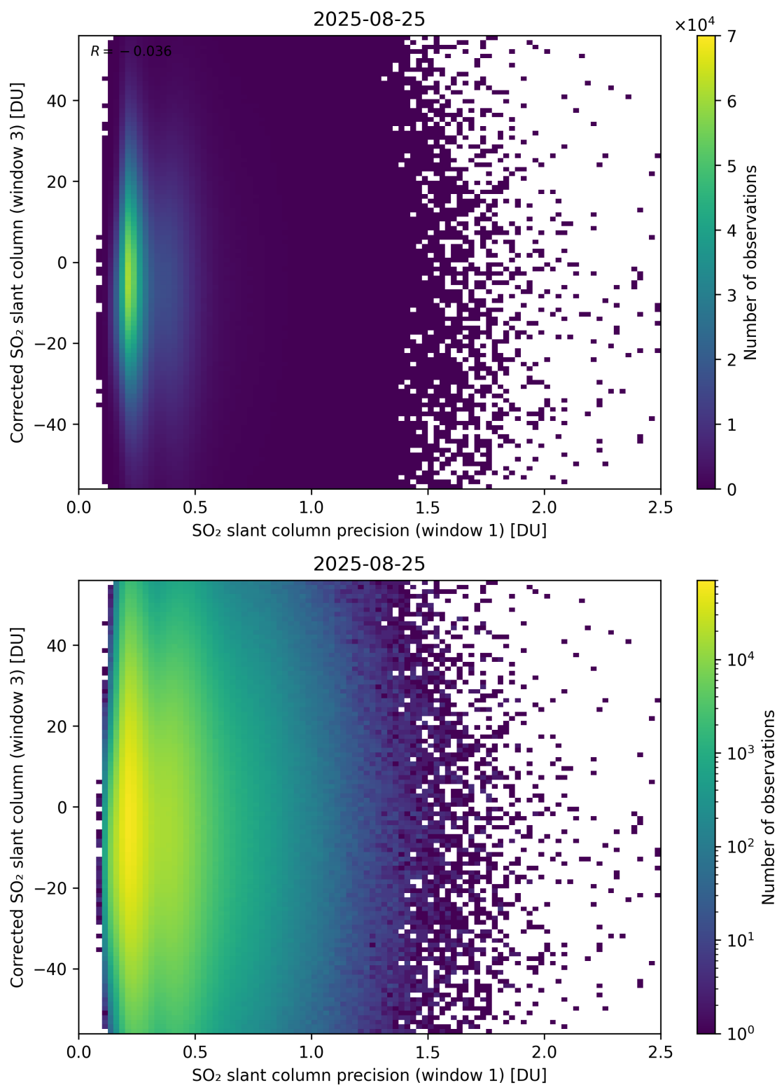
Figure 276: Scatter density plot of “SO 2 slant column precision (window 1)” against “Corrected SO 2 slant column (window 3)” for 2025-08-25 to 2025-08-26.
