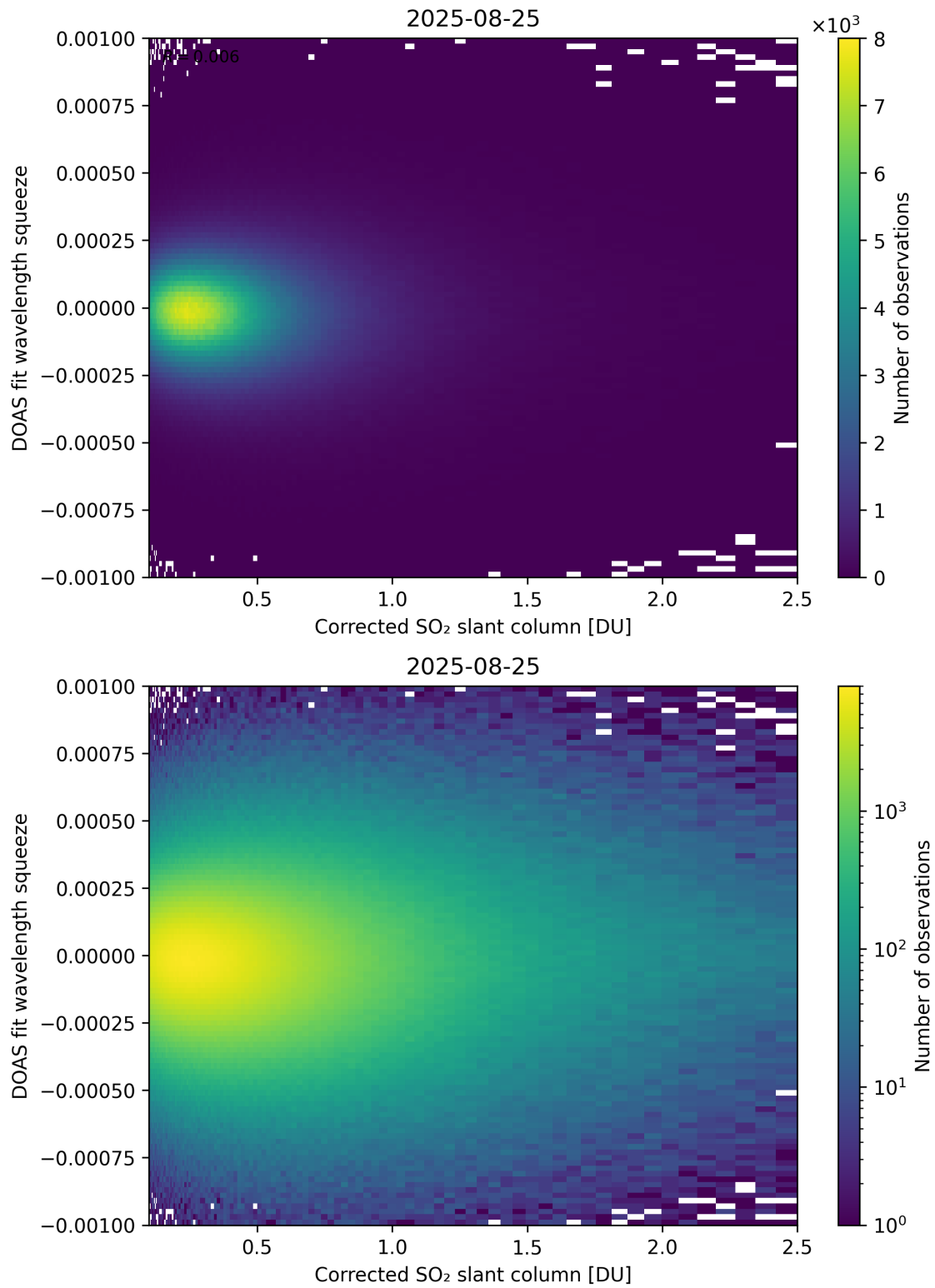
Figure 230: Scatter density plot of “Corrected SO 2 slant column” against “DOAS fit wavelength squeeze” for 2025-08-25 to 2025-08-26.
