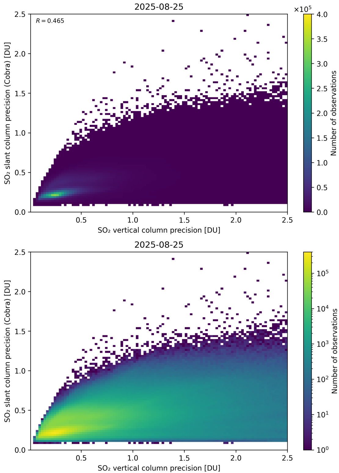
Figure 337: Scatter density plot of “SO 2 vertical column precision” against “SO 2 slant column precision (Cobra)” for 2025-08-25 to 2025-08-26.
