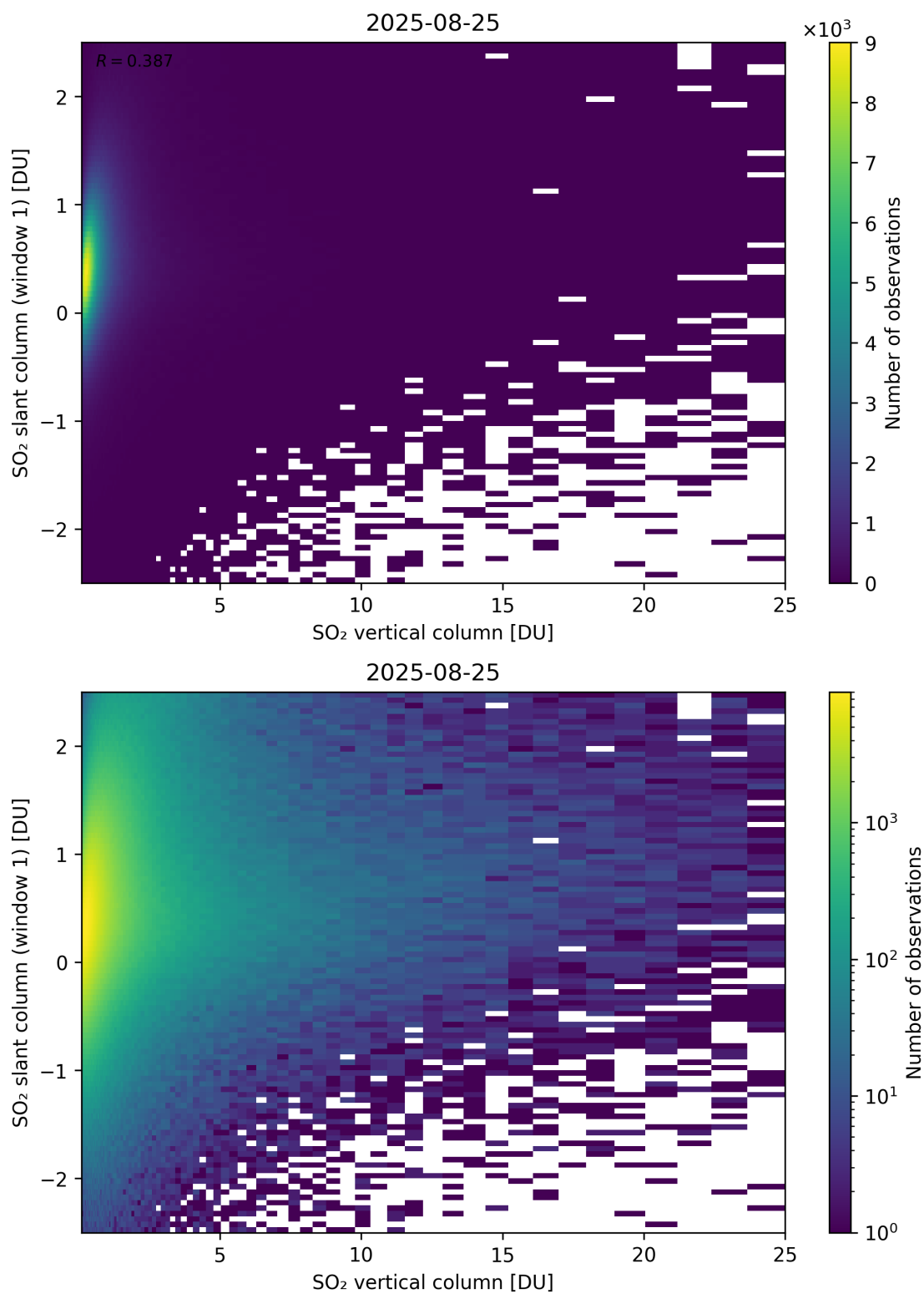
Figure 354: Scatter density plot of “SO 2 vertical column” against “SO 2 slant column (window 1)” for 2025-08-25 to 2025-08-26.
