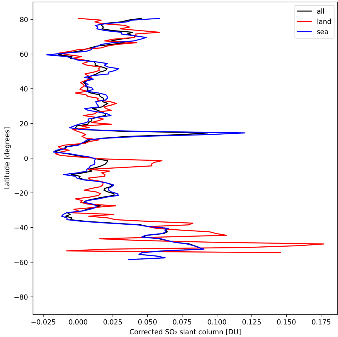
Figure 34: Zonal average of “Corrected SO 2 slant column” for 2025-08-25 to 2025-08-26.
