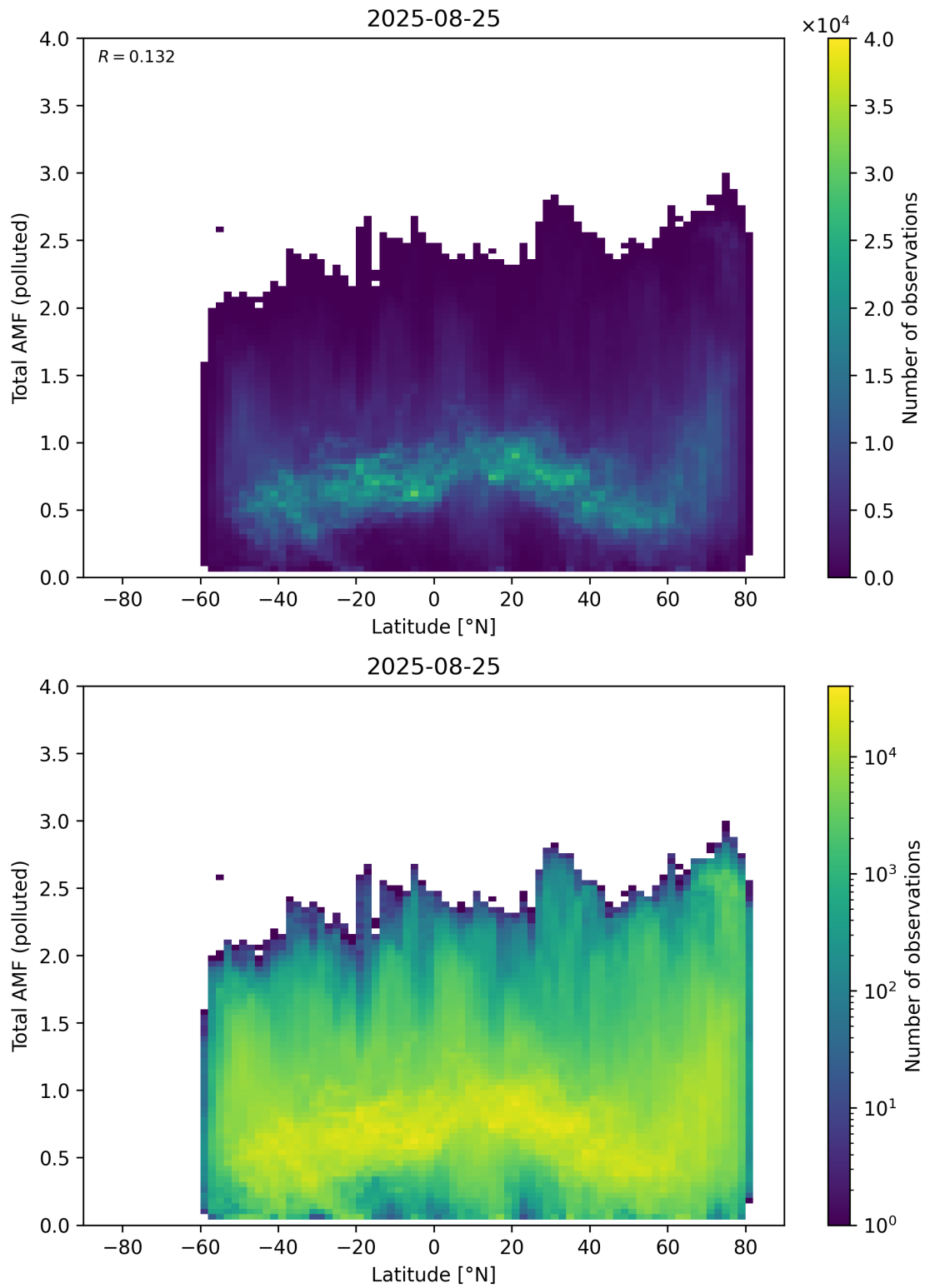
Figure 167: Scatter density plot of “Latitude” against “Total AMF (polluted)” for 2025-08-25 to 2025-08-26.
