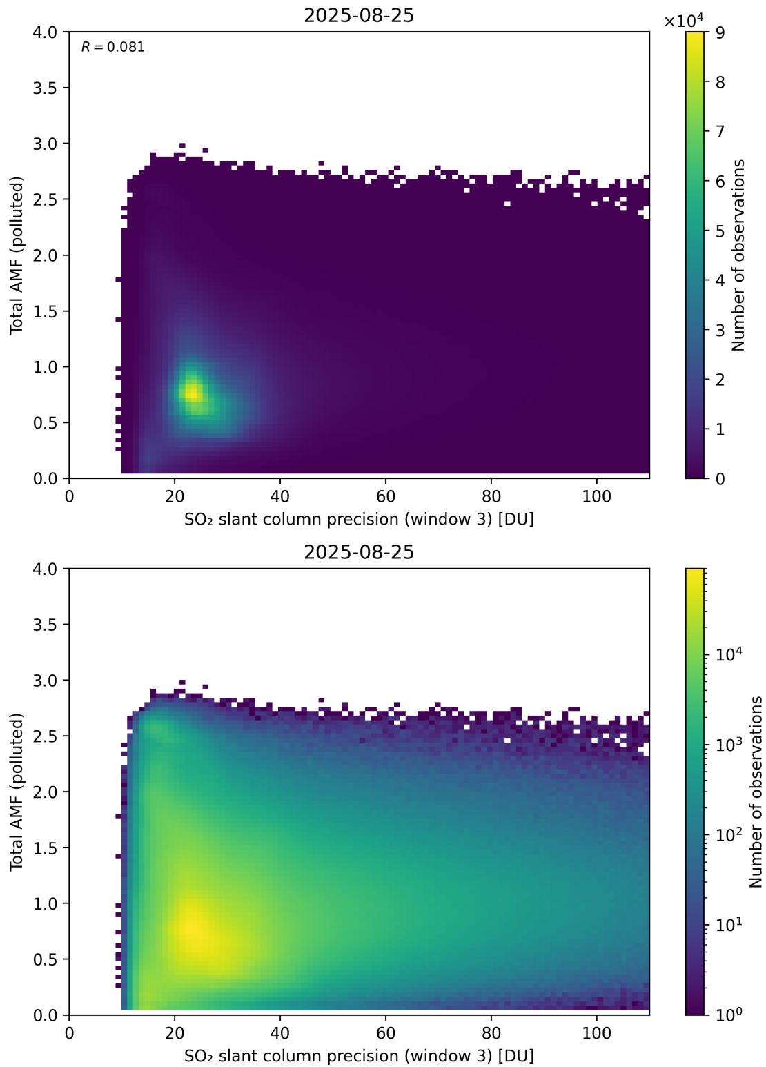
Figure 313: Scatter density plot of “SO 2 slant column precision (window 3)” against “Total AMF (polluted)” for 2025-08-25 to 2025-08-26.
