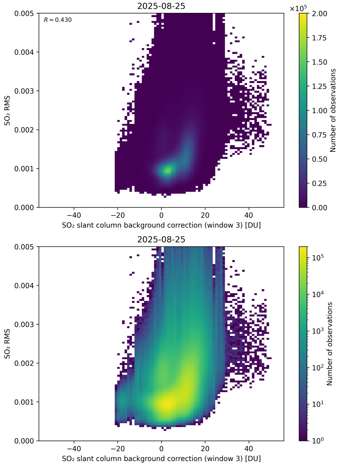
Figure 134: Scatter density plot of “SO 2 slant column background correction (window 3)” against “SO 2 RMS” for 2025-08-25 to 2025-08-26.
