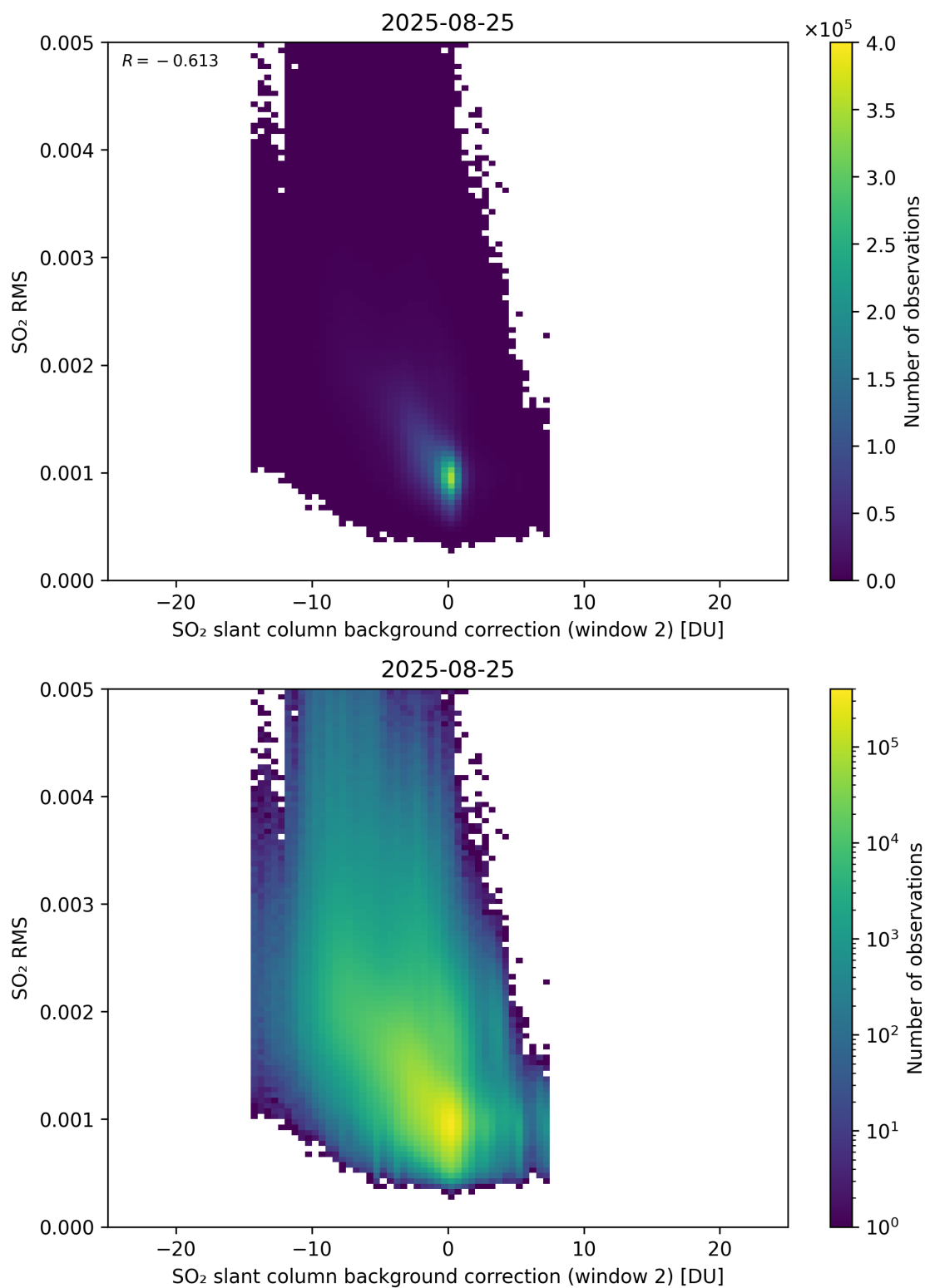
Figure 125: Scatter density plot of “SO 2 slant column background correction (window 2)” against “SO 2 RMS” for 2025-08-25 to 2025-08-26.
