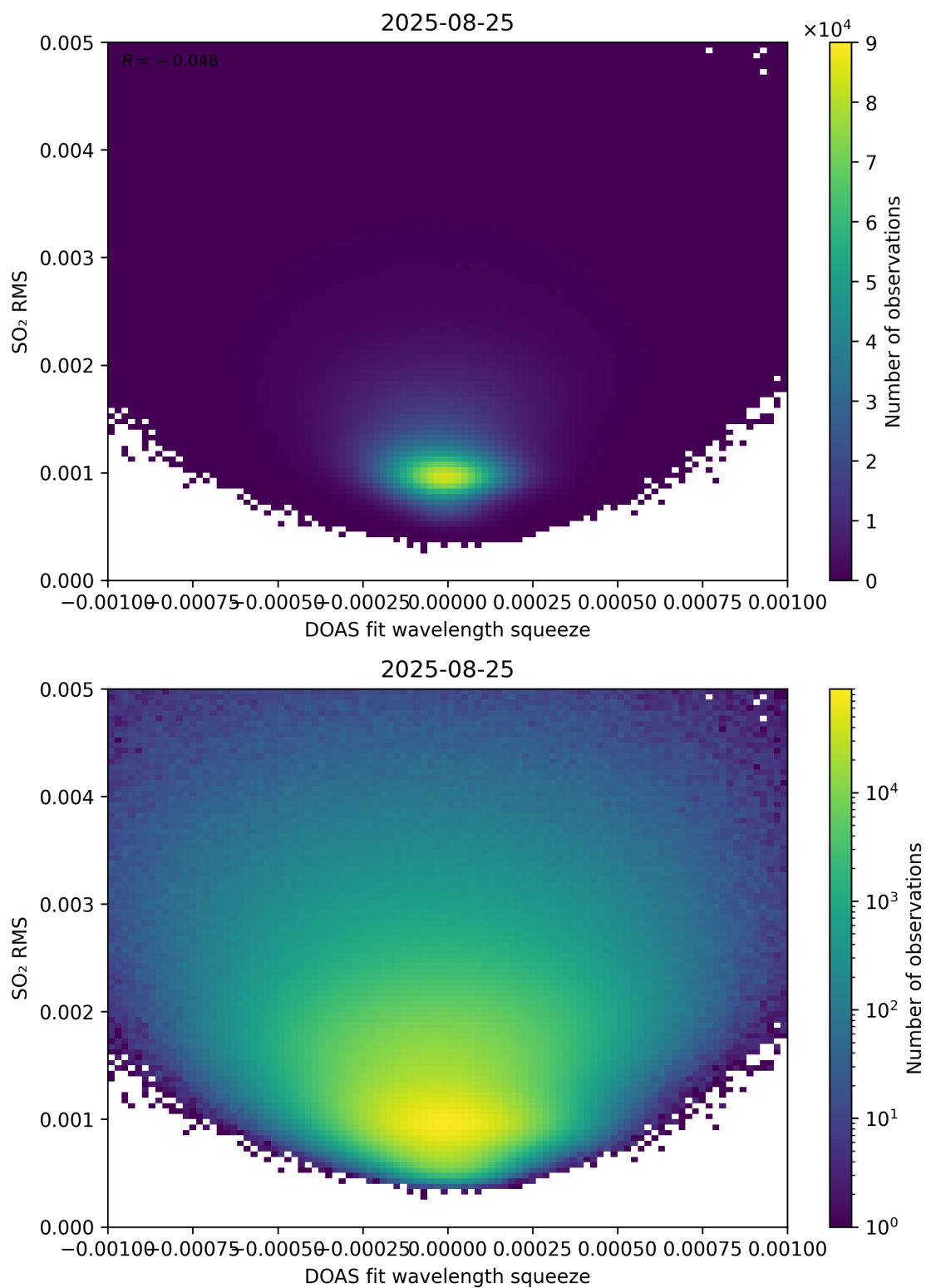
Figure 143: Scatter density plot of “DOAS fit wavelength squeeze” against “SO 2 RMS” for 2025-08-25 to 2025-08-26.
