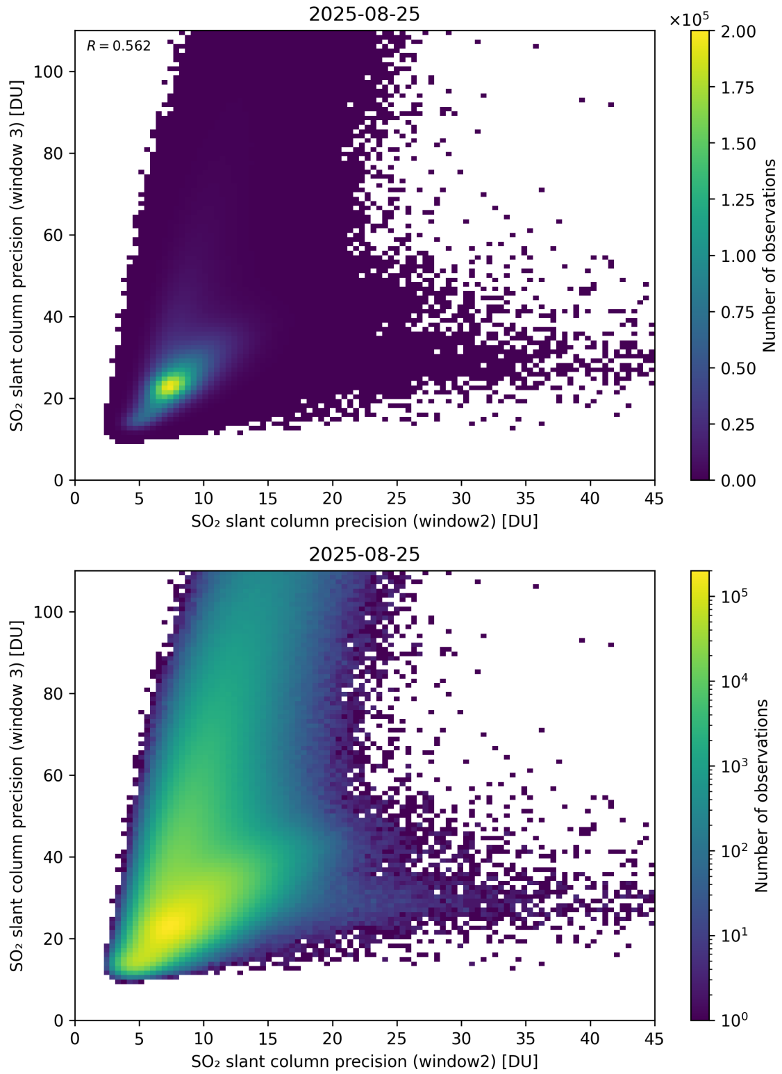
Figure 300: Scatter density plot of “SO 2 slant column precision (window2)” against “SO 2 slant column precision (window 3)” for 2025-08-25 to 2025-08-26.
