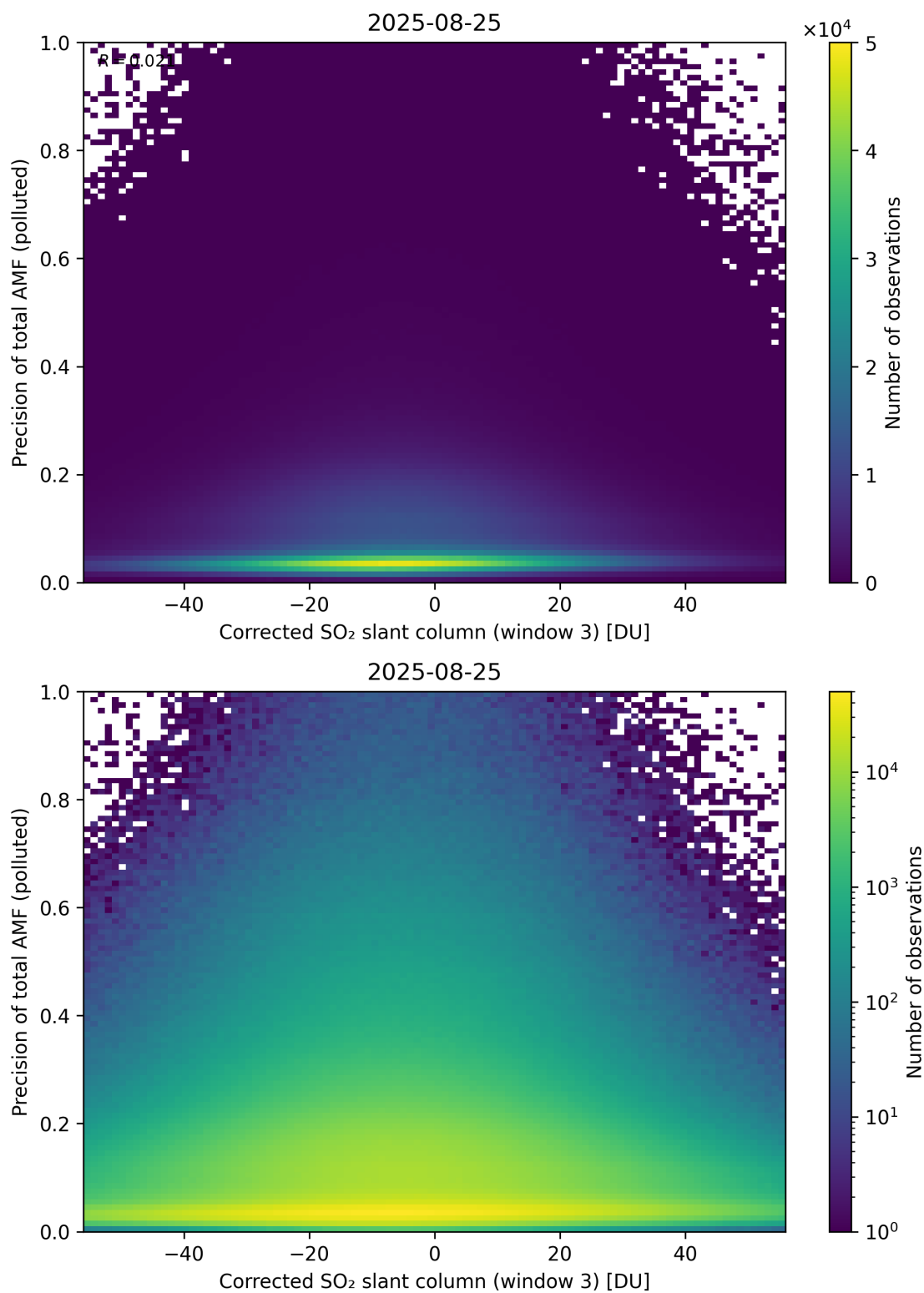
Figure 261: Scatter density plot of “Corrected SO 2 slant column (window 3)” against “Precision of total AMF (polluted)” for 2025-08-25 to 2025-08-26.
