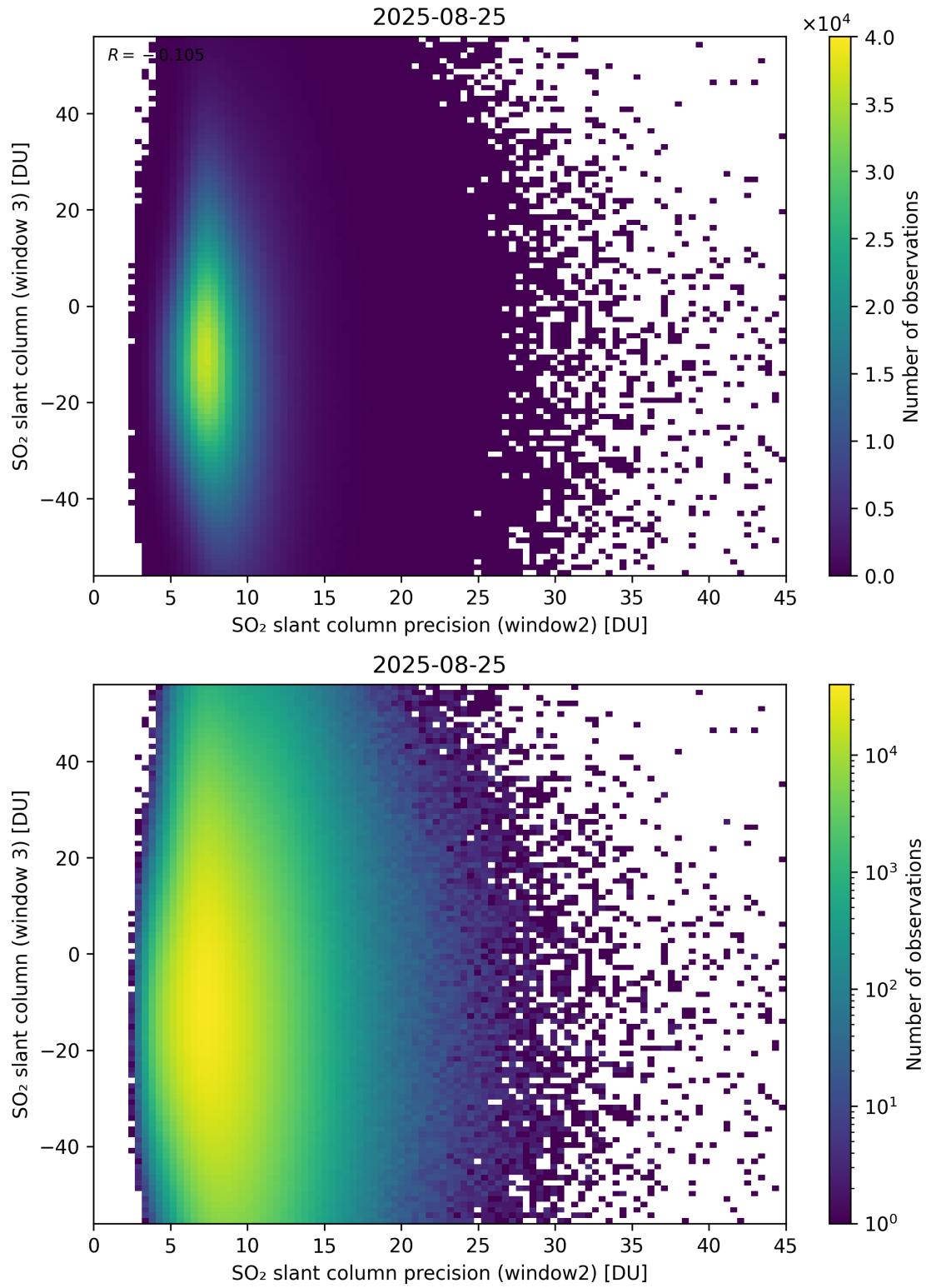
Figure 299: Scatter density plot of “SO 2 slant column precision (window2)” against “SO 2 slant column (window 3)” for 2025-08-25 to 2025-08-26.
