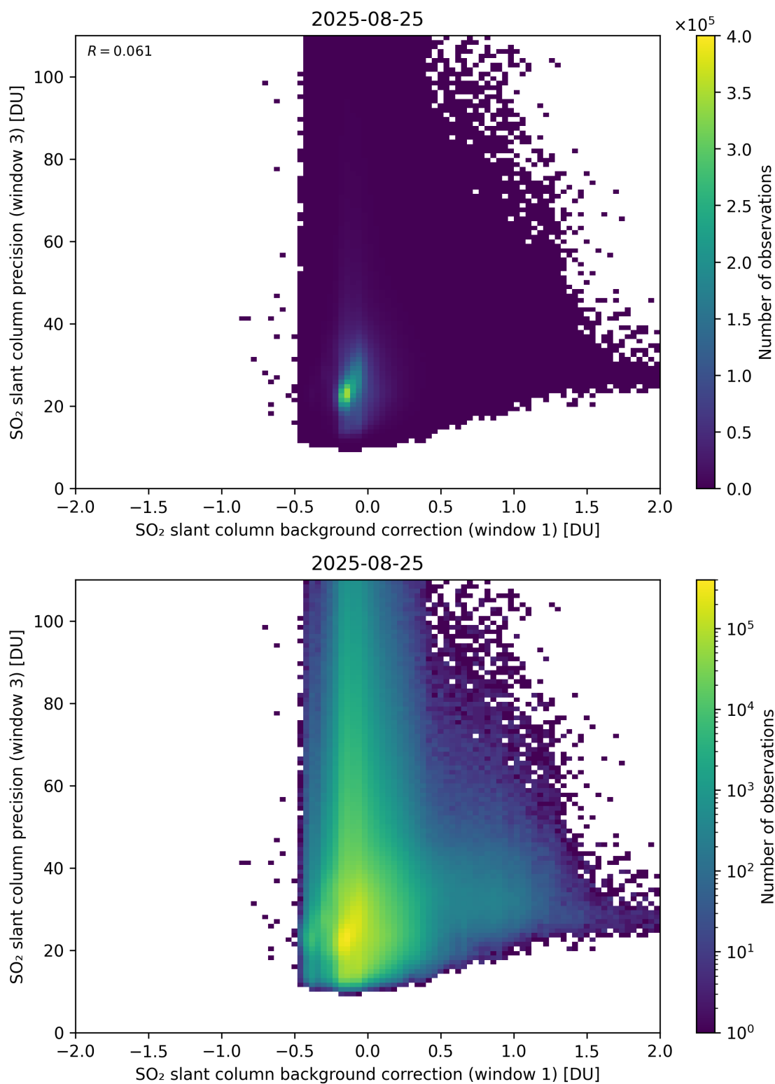
Figure 119: Scatter density plot of “SO 2 slant column background correction (window 1)” against “SO 2 slant column precision (window 3)” for 2025-08-25 to 2025-08-26.
