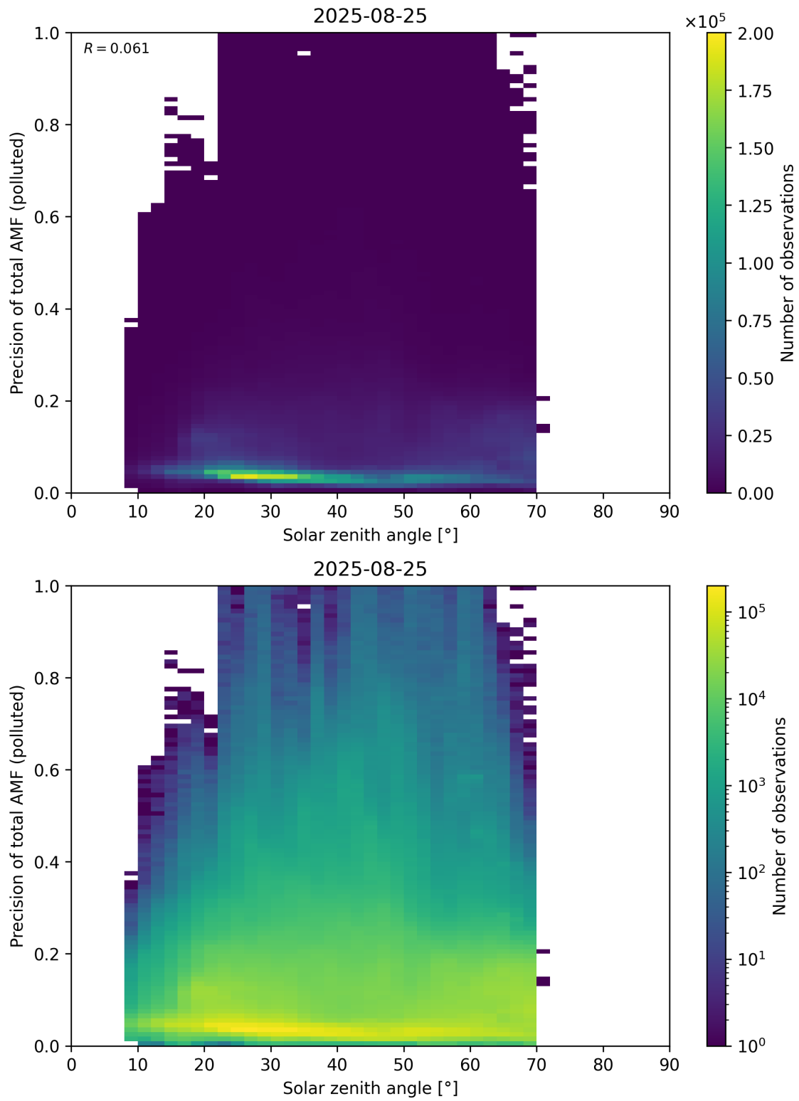
Figure 190: Scatter density plot of “Solar zenith angle” against “Precision of total AMF (polluted)” for 2025-08-25 to 2025-08-26.
