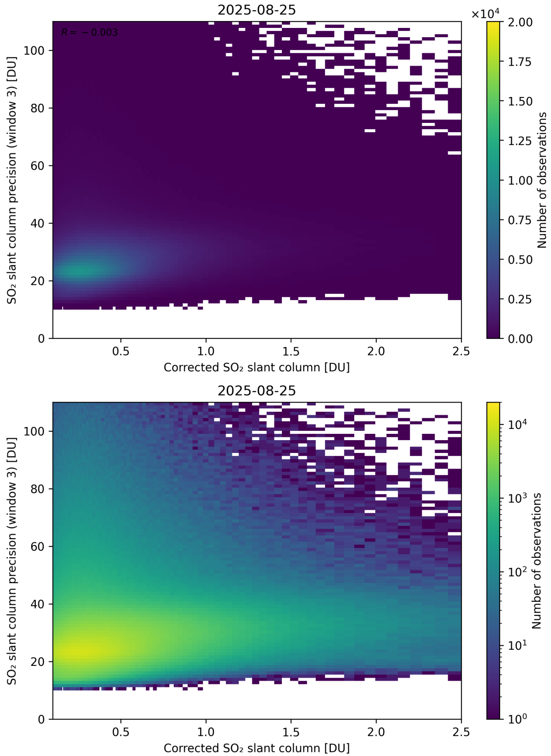
Figure 241: Scatter density plot of “Corrected SO 2 slant column” against “SO 2 slant column precision (window 3)” for 2025-08-25 to 2025-08-26.
