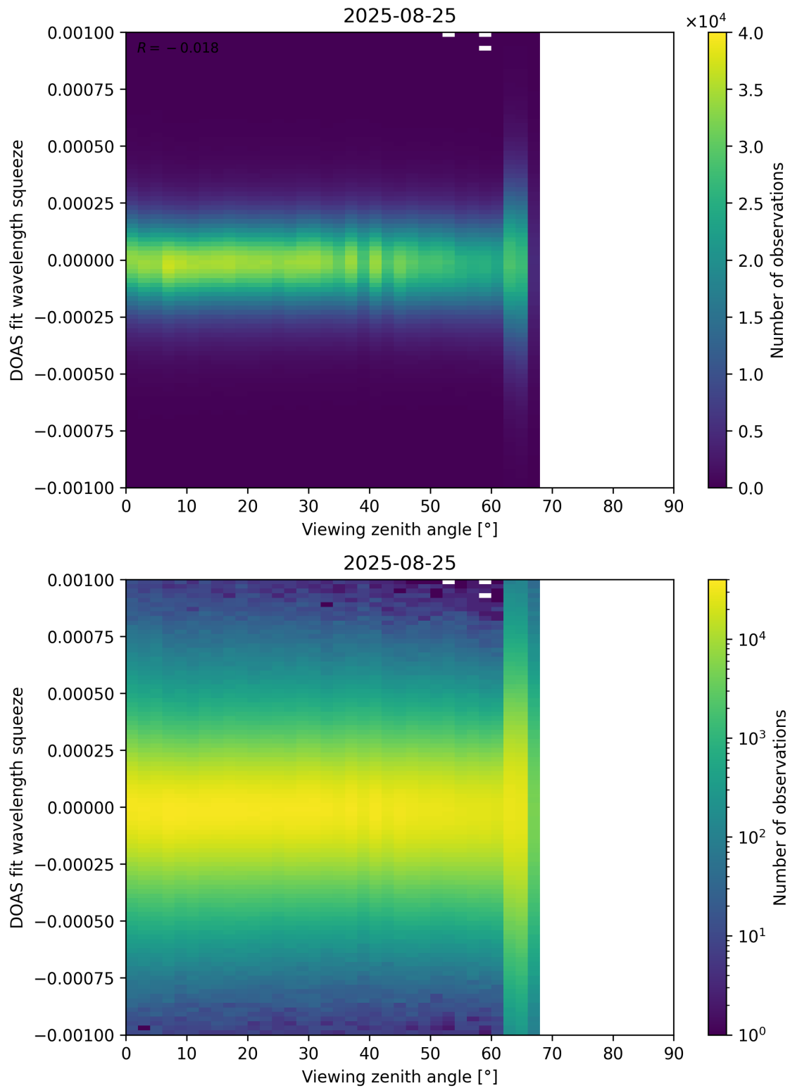
Figure 366: Scatter density plot of “Viewing zenith angle” against “DOAS fit wavelength squeeze” for 2025-08-25 to 2025-08-26.
