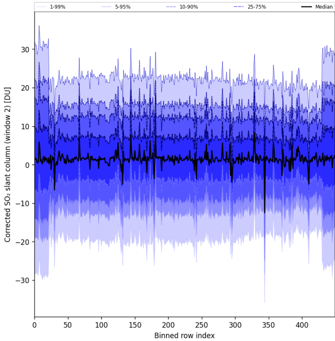
Figure 95: Along track statistics of "Corrected SO 2 slant column (window 2)" for 2025-08-25 to 2025-08-26
