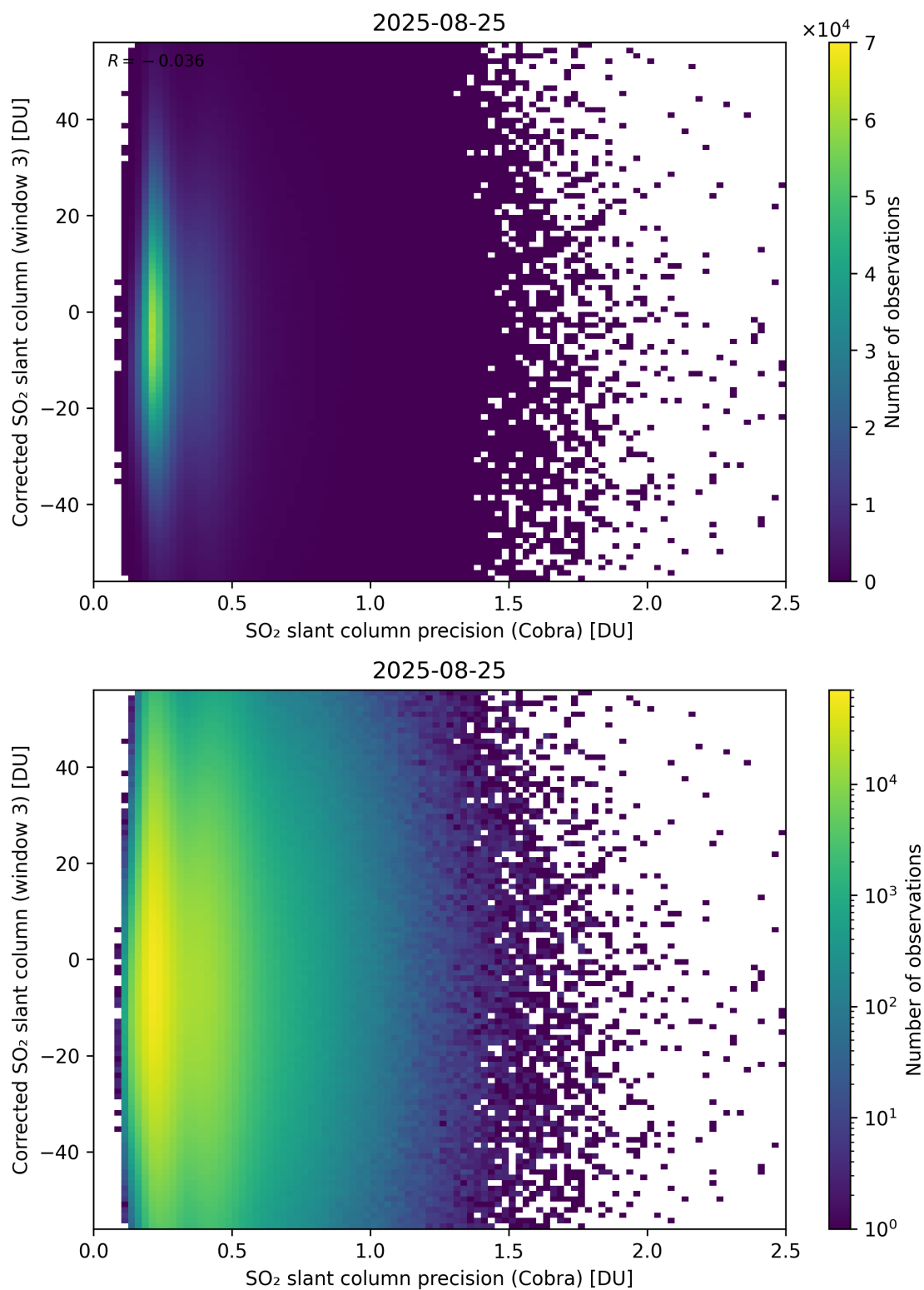
Figure 207: Scatter density plot of “SO 2 slant column precision (Cobra)” against “Corrected SO 2 slant column (window 3)” for 2025-08-25 to 2025-08-26.
