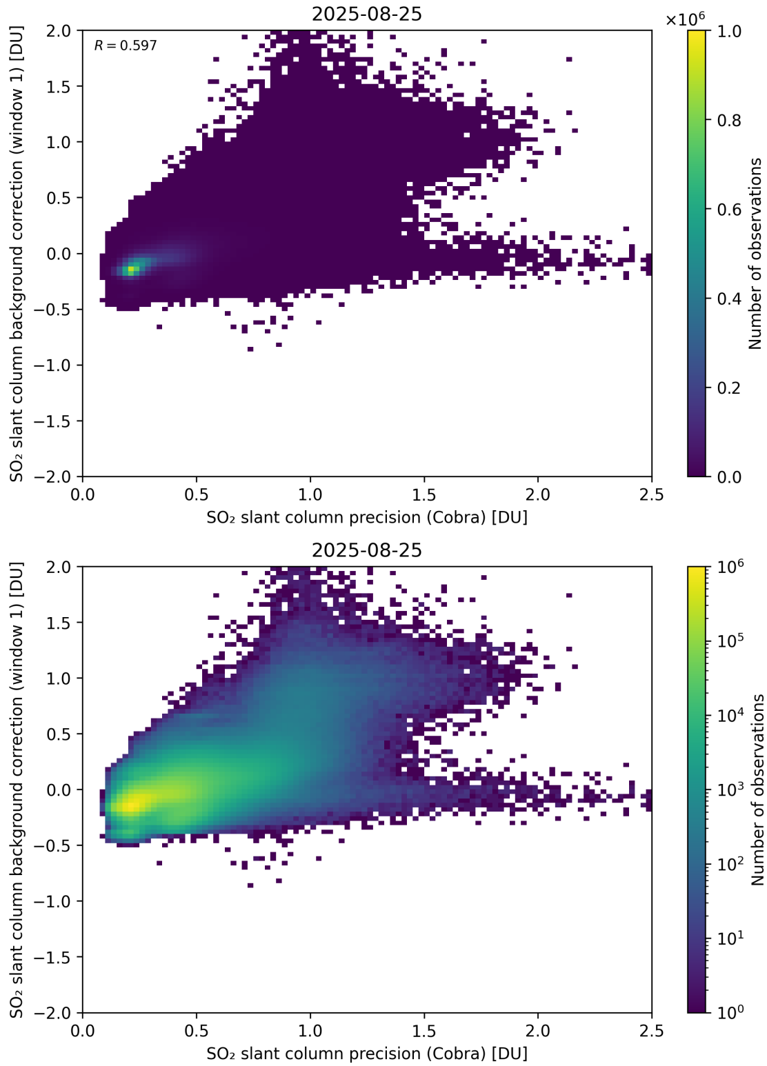
Figure 199: Scatter density plot of “SO 2 slant column precision (Cobra)” against “SO 2 slant column background correction (window 1)” for 2025-08-25 to 2025-08-26.
