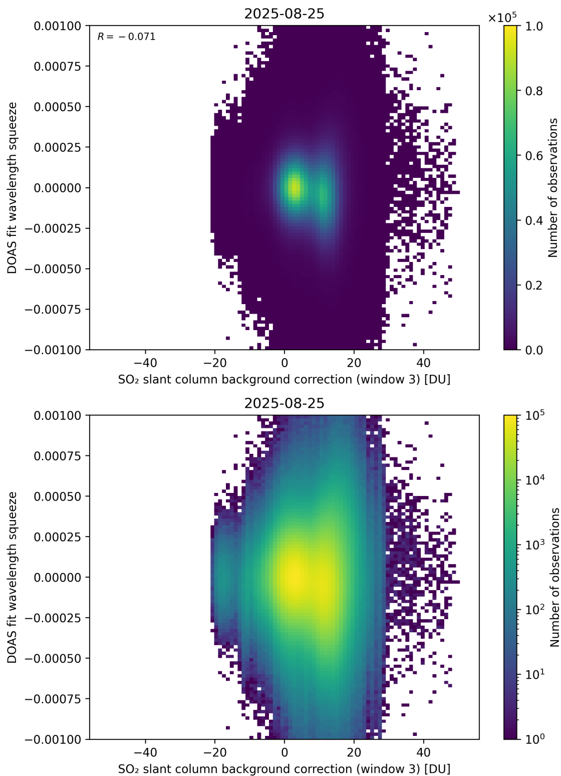
Figure 133: Scatter density plot of “SO 2 slant column background correction (window 3)” against “DOAS fit wavelength squeeze” for 2025-08-25 to 2025-08-26.
