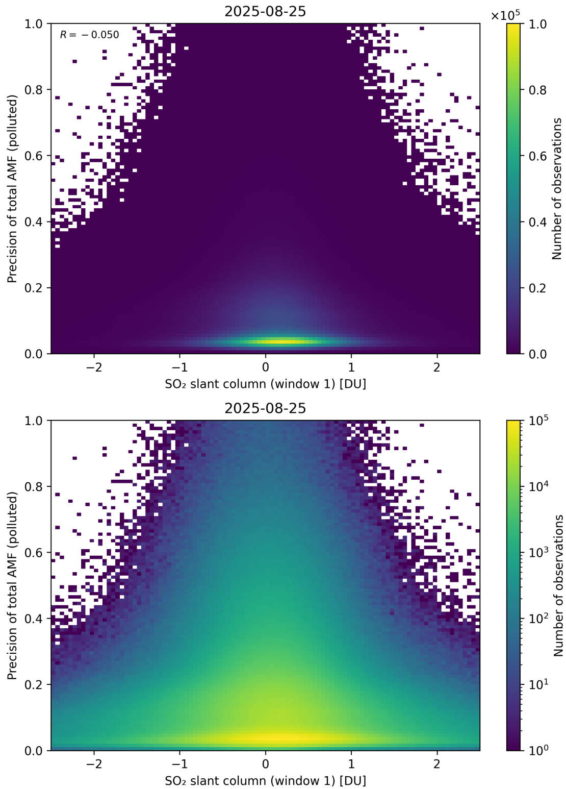
Figure 290: Scatter density plot of “SO 2 slant column (window 1)” against “Precision of total AMF (polluted)” for 2025-08-25 to 2025-08-26.
