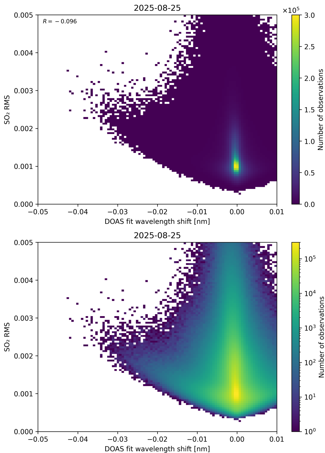
Figure 139: Scatter density plot of “DOAS fit wavelength shift” against “SO 2 RMS” for 2025-08-25 to 2025-08-26.
