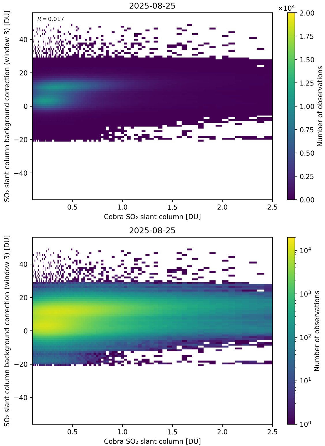
Figure 195: Scatter density plot of “Cobra SO 2 slant column” against “SO 2 slant column background correction (window 3)” for 2025-08-25 to 2025-08-26.
