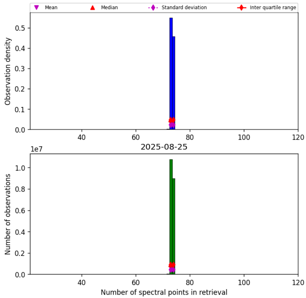
Figure 82: Histogram of “Number of spectral points in retrieval” for 2025-08-25 to 2025-08-26
