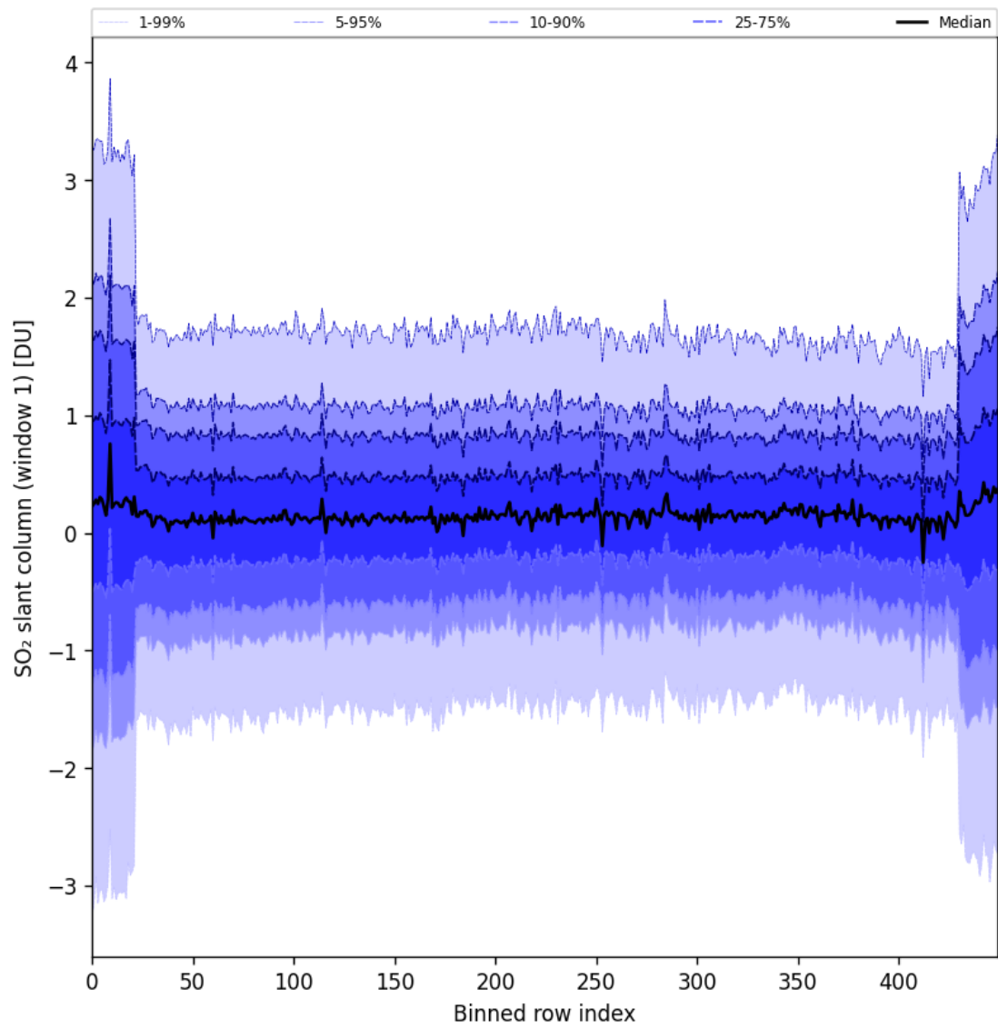
Figure 89: Along track statistics of “SO 2 slant column (window 1)” for 2025-08-25 to 2025-08-26
