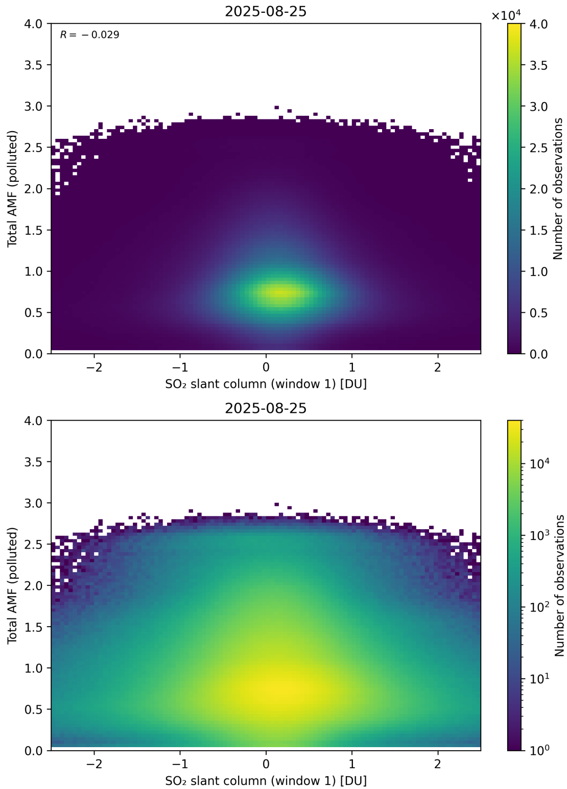
Figure 289: Scatter density plot of “SO 2 slant column (window 1)” against “Total AMF (polluted)” for 2025-08-25 to 2025-08-26.
