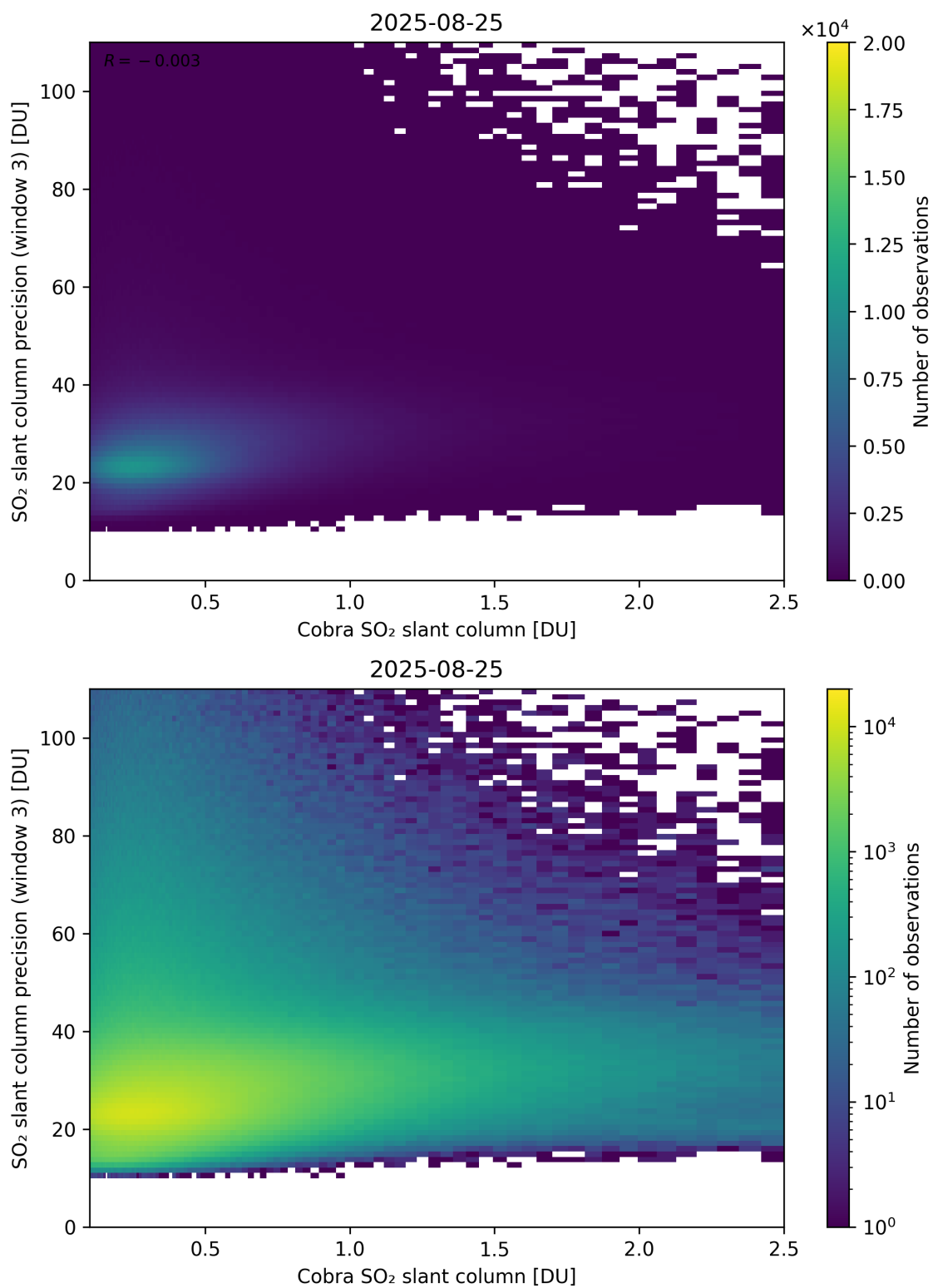
Figure 223: Scatter density plot of “Cobra SO 2 slant column” against “SO 2 slant column precision (window 3)” for 2025-08-25 to 2025-08-26.
