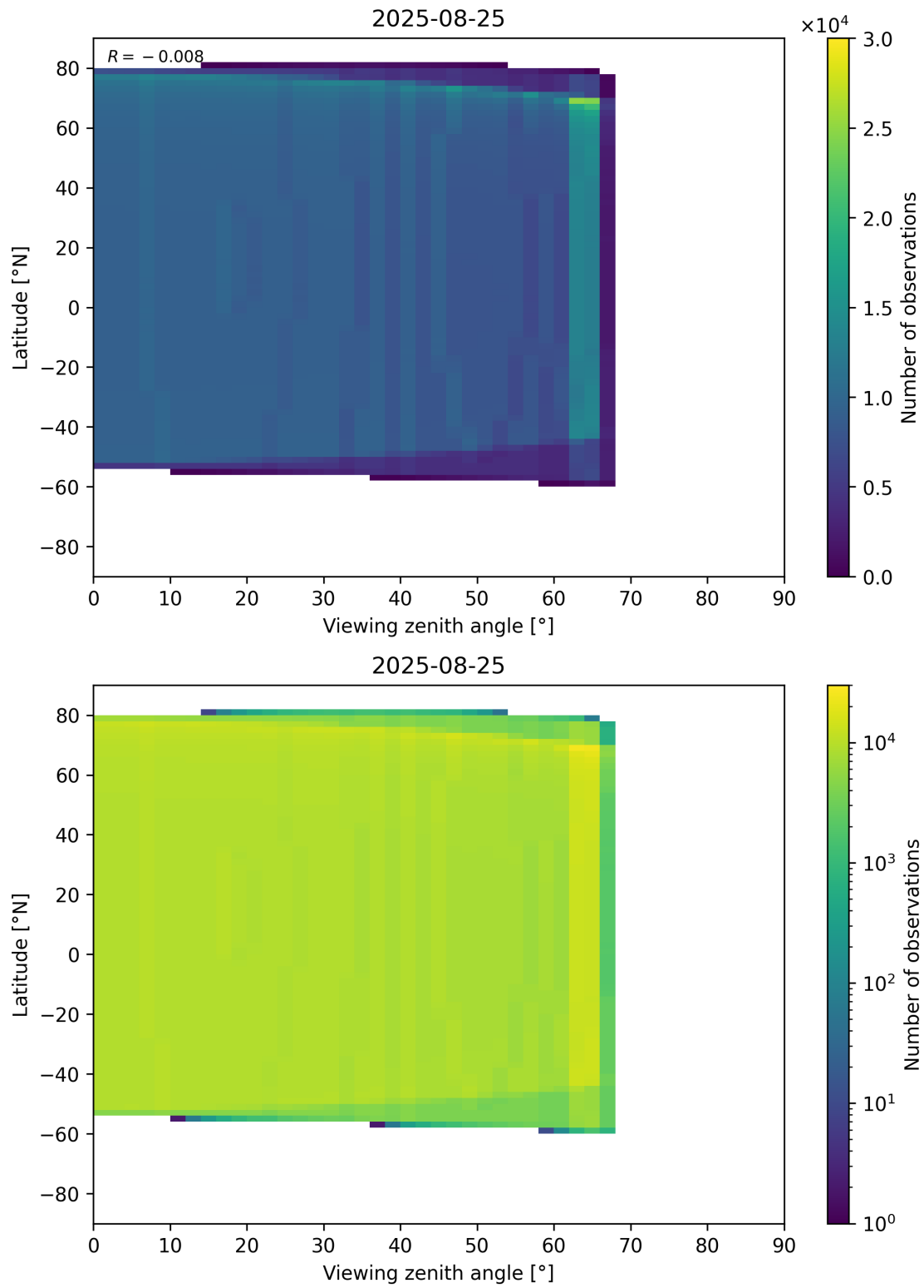
Figure 368: Scatter density plot of “Viewing zenith angle” against “Latitude” for 2025-08-25 to 2025-08-26.
