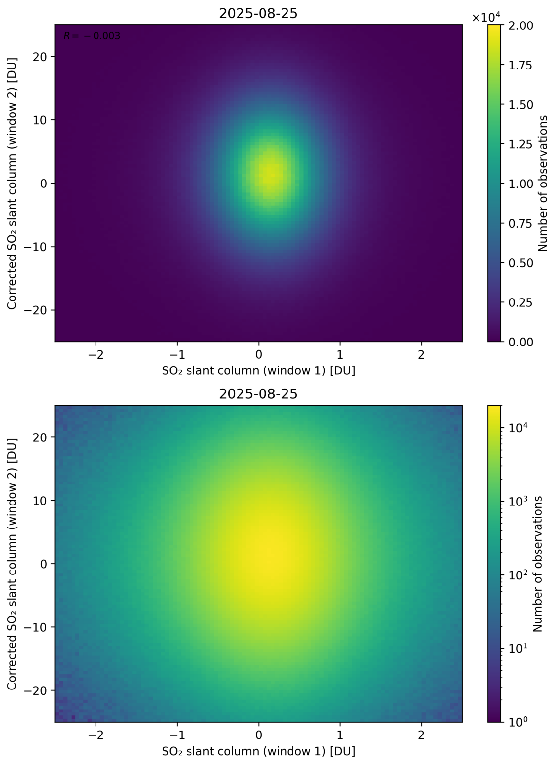
Figure 283: Scatter density plot of “SO 2 slant column (window 1)” against “Corrected SO 2 slant column (window 2)” for 2025-08-25 to 2025-08-26.
