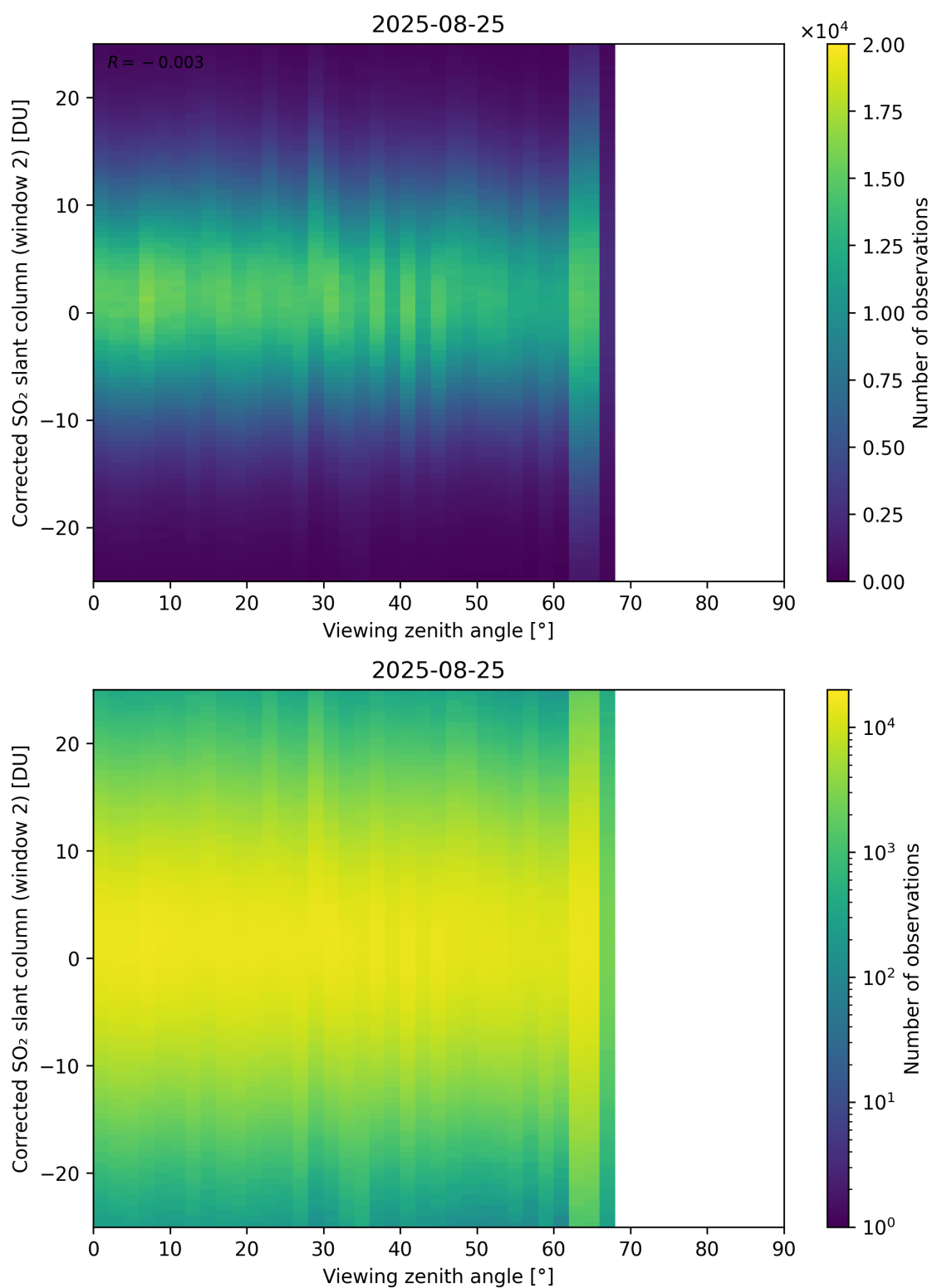
Figure 374: Scatter density plot of “Viewing zenith angle” against “Corrected SO 2 slant column (window 2)” for 2025-08-25 to 2025-08-26.
