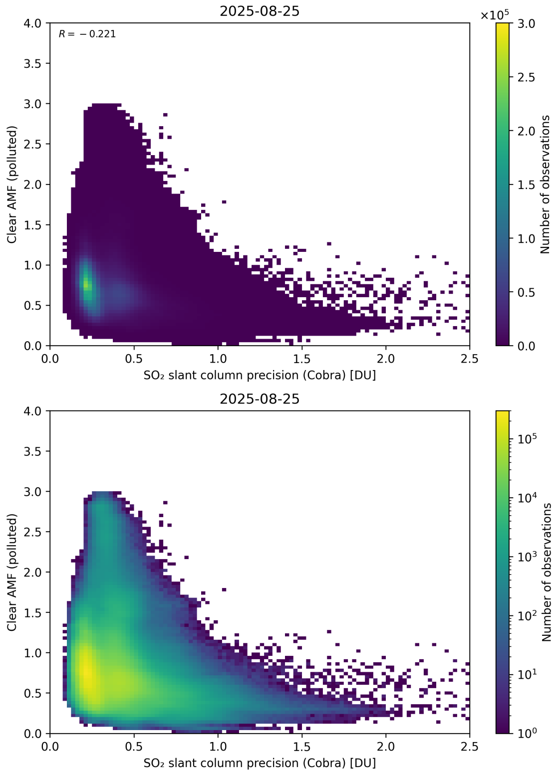
Figure 205: Scatter density plot of “SO 2 slant column precision (Cobra)” against “Clear AMF (polluted)” for 2025-08-25 to 2025-08-26.
