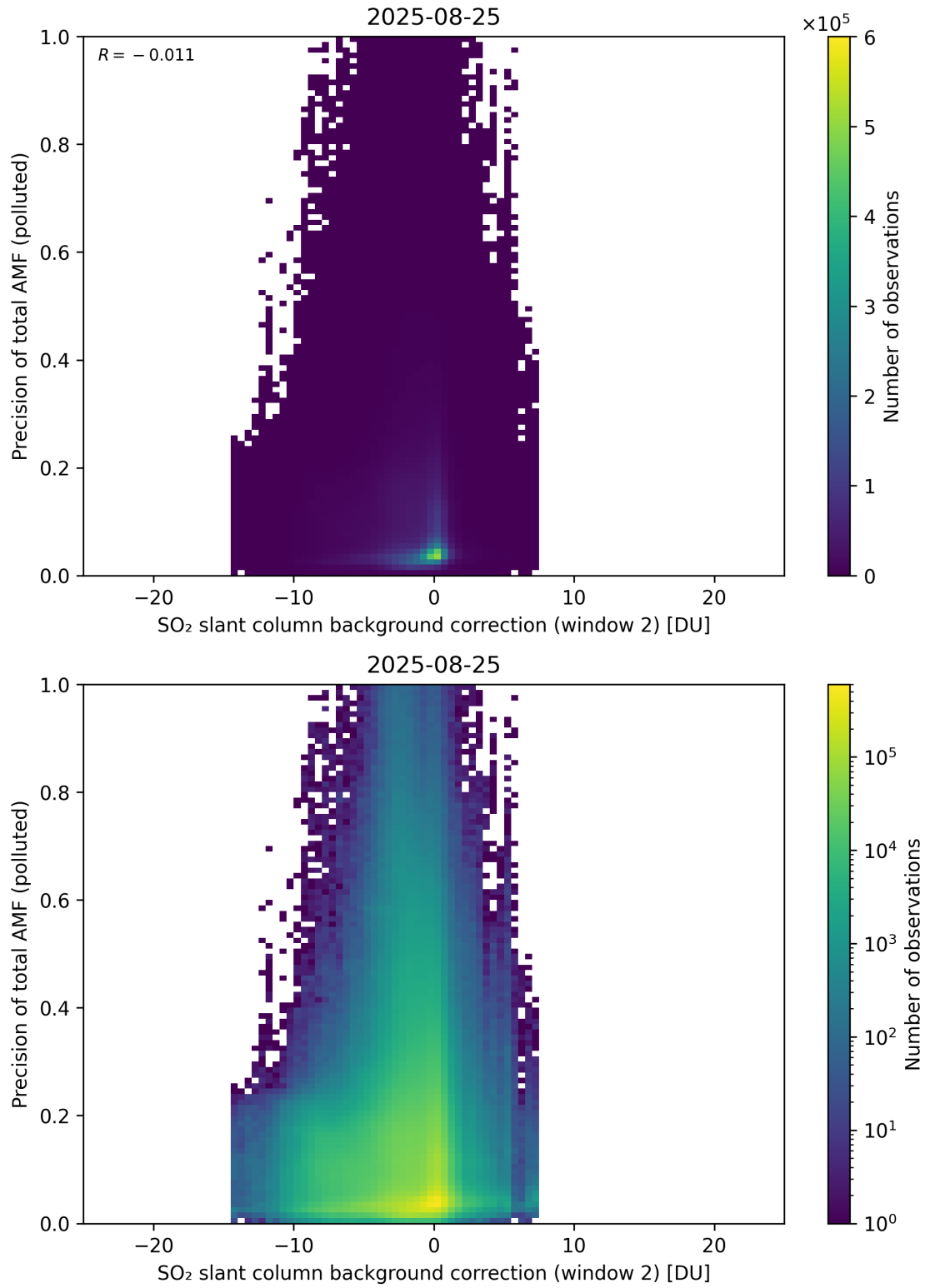
Figure 131: Scatter density plot of “SO 2 slant column background correction (window 2)” against “Precision of total AMF (polluted)” for 2025-08-25 to 2025-08-26.
