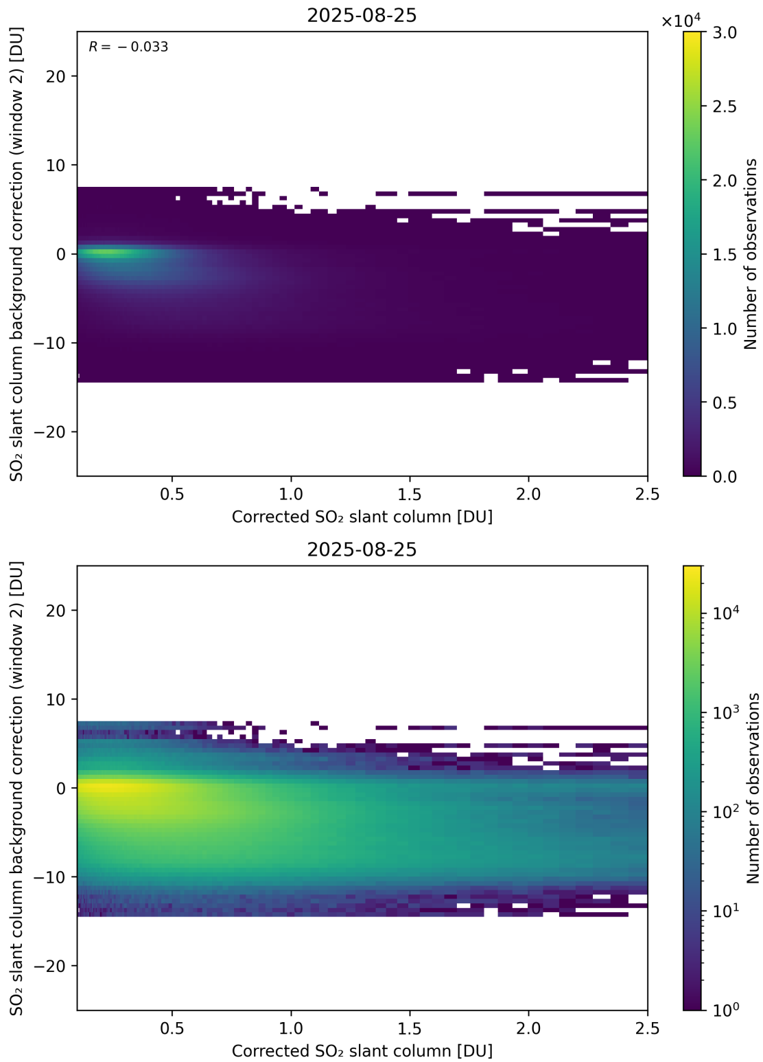
Figure 227: Scatter density plot of “Corrected SO 2 slant column” against “SO 2 slant column background correction (window 2)” for 2025-08-25 to 2025-08-26.
