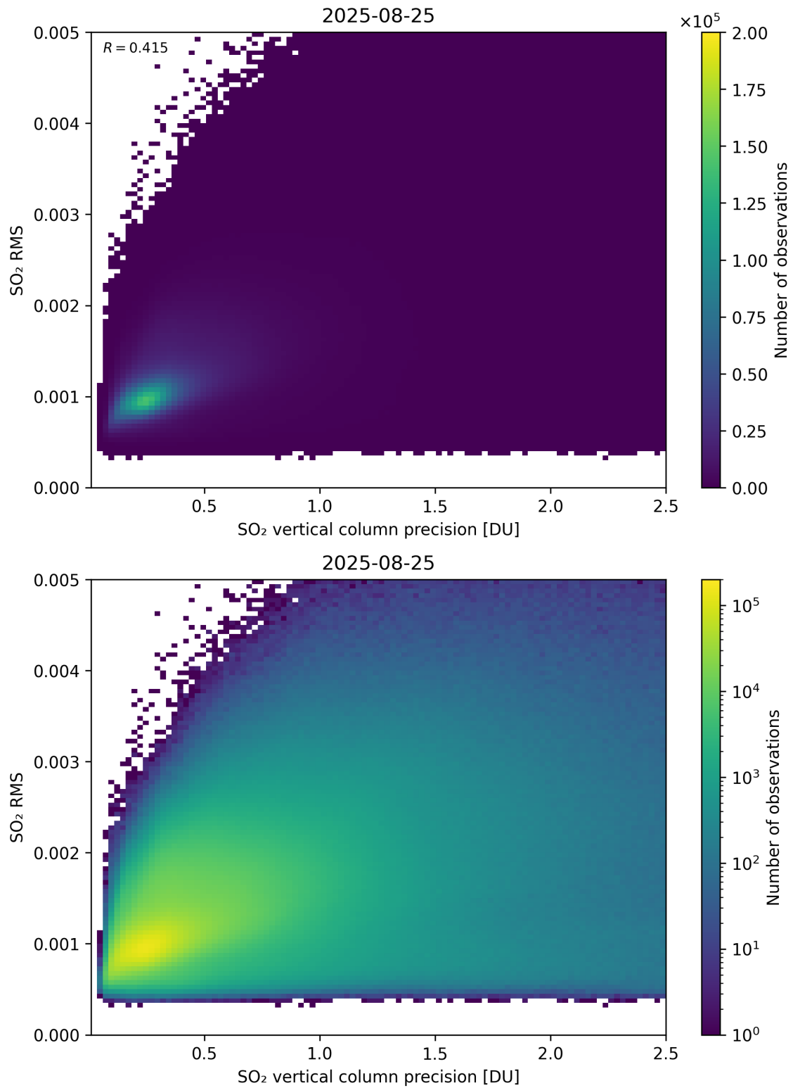
Figure 334: Scatter density plot of “SO 2 vertical column precision” against “SO 2 RMS” for 2025-08-25 to 2025-08-26.
