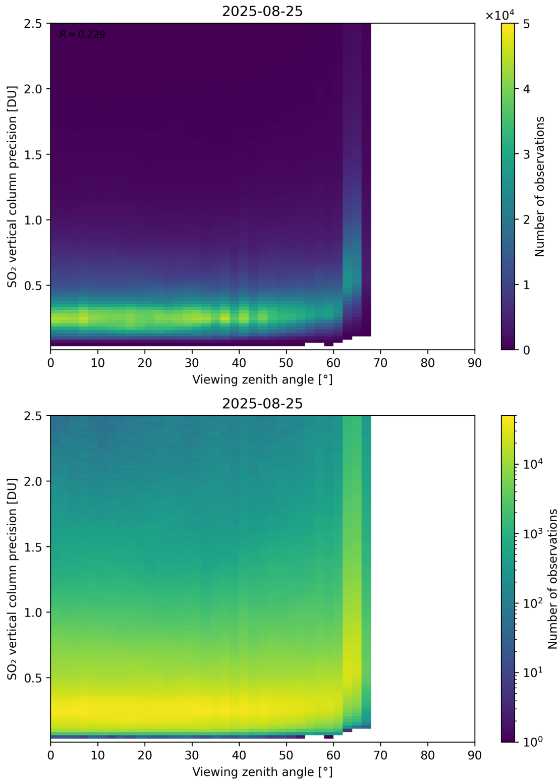
Figure 384: Scatter density plot of “Viewing zenith angle” against “SO 2 vertical column precision” for 2025-08-25 to 2025-08-26.
