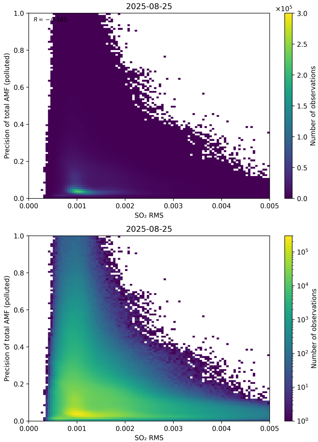
Figure 149: Scatter density plot of “SO 2 RMS” against “Precision of total AMF (polluted)” for 2025-08-25 to 2025-08-26.
