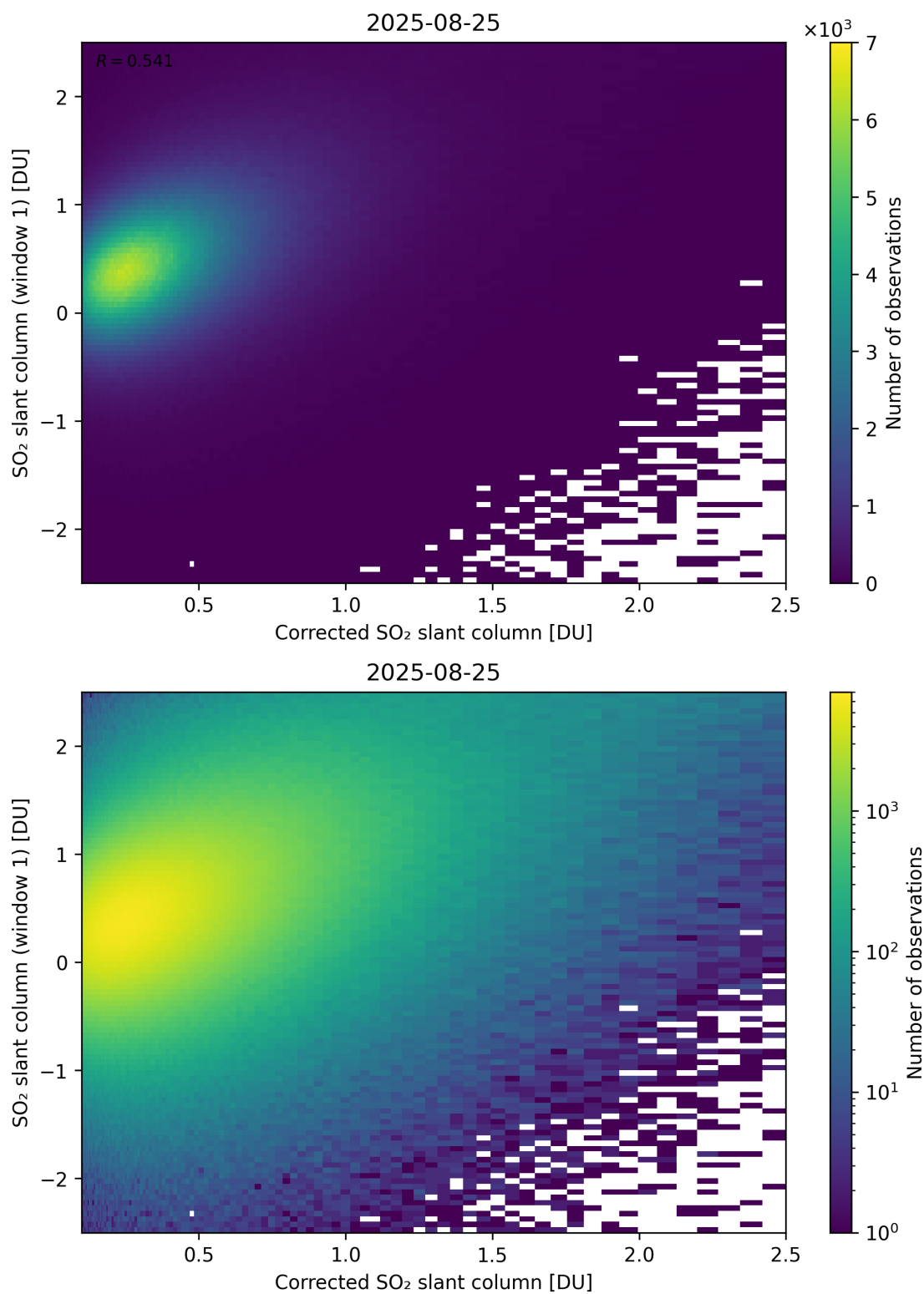
Figure 237: Scatter density plot of “Corrected SO 2 slant column” against “SO 2 slant column (window 1)” for 2025-08-25 to 2025-08-26.
