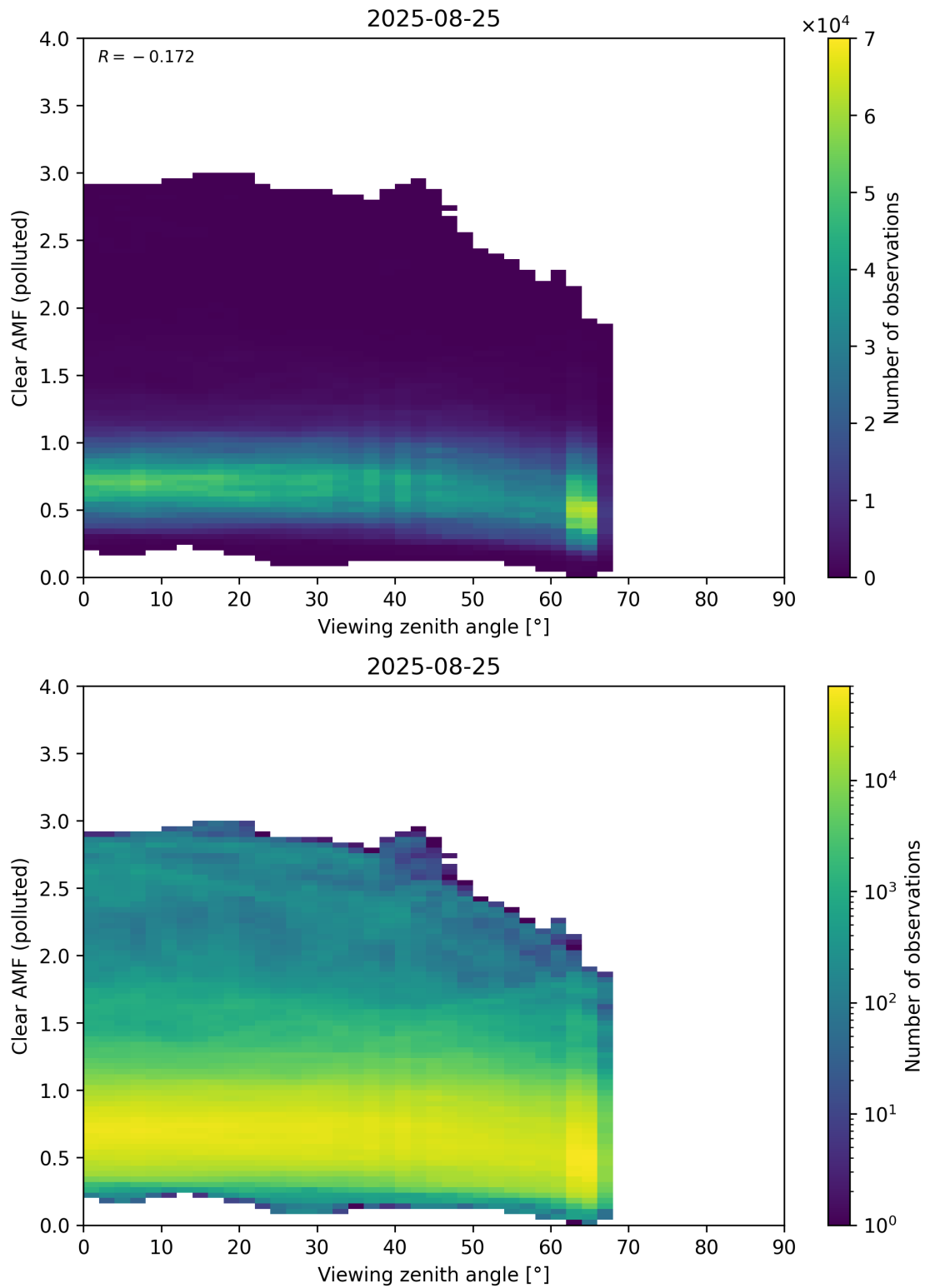
Figure 370: Scatter density plot of “Viewing zenith angle” against “Clear AMF (polluted)” for 2025-08-25 to 2025-08-26.
