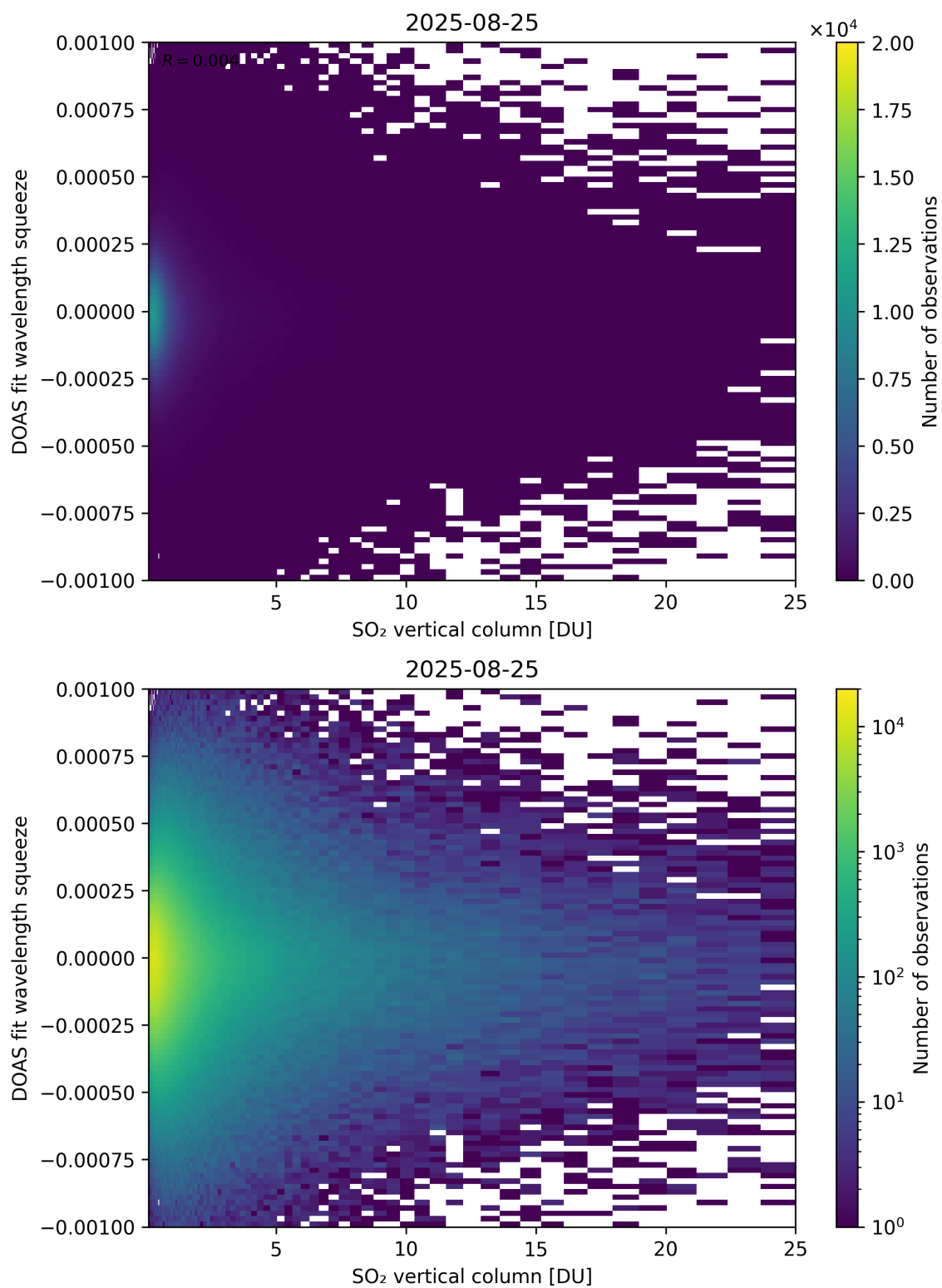
Figure 327: Scatter density plot of “SO 2 vertical column” against “DOAS fit wavelength squeeze” for 2025-08-25 to 2025-08-26.
