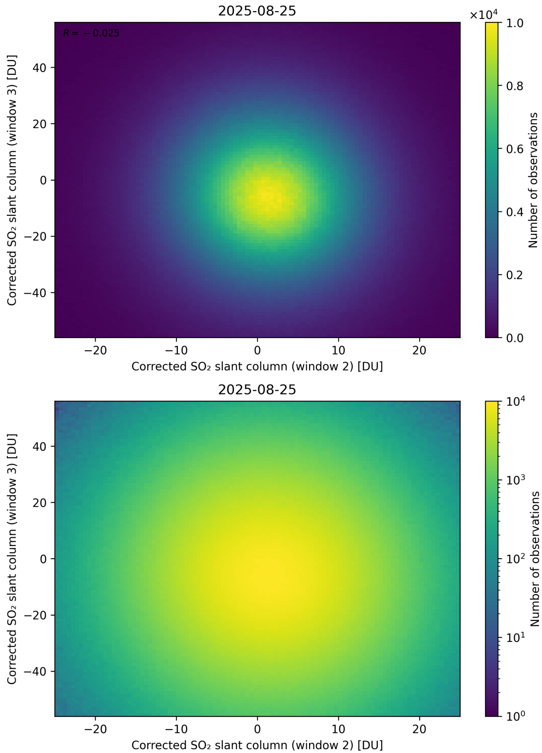
Figure 250: Scatter density plot of “Corrected SO 2 slant column (window 2)” against “Corrected SO 2 slant column (window 3)” for 2025-08-25 to 2025-08-26.
