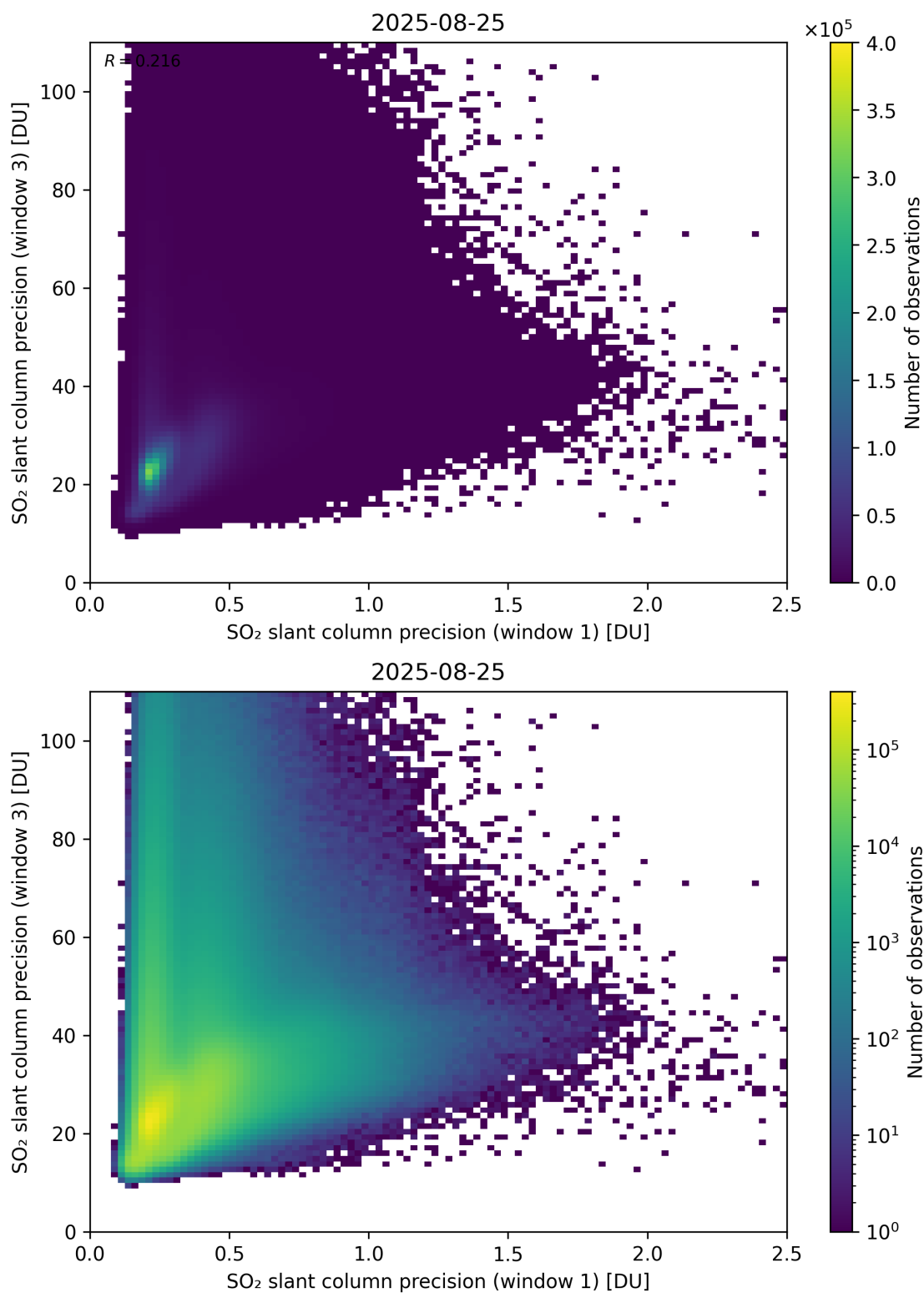
Figure 279: Scatter density plot of “SO 2 slant column precision (window 1)” against “SO 2 slant column precision (window 3)” for 2025-08-25 to 2025-08-26.
