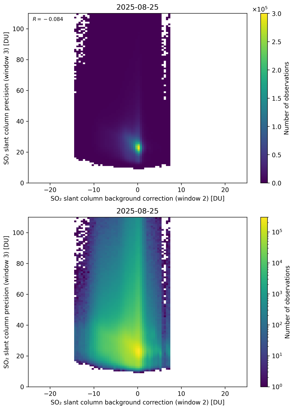
Figure 129: Scatter density plot of “SO 2 slant column background correction (window 2)” against “SO 2 slant column precision (window 3)” for 2025-08-25 to 2025-08-26.
