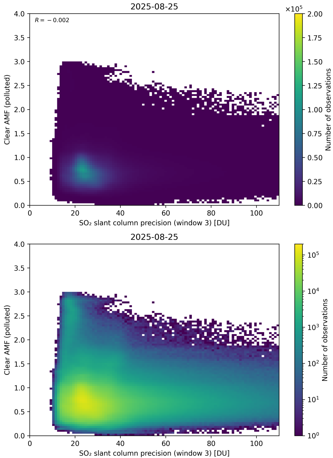
Figure 311: Scatter density plot of “SO 2 slant column precision (window 3)” against “Clear AMF (polluted)” for 2025-08-25 to 2025-08-26.
