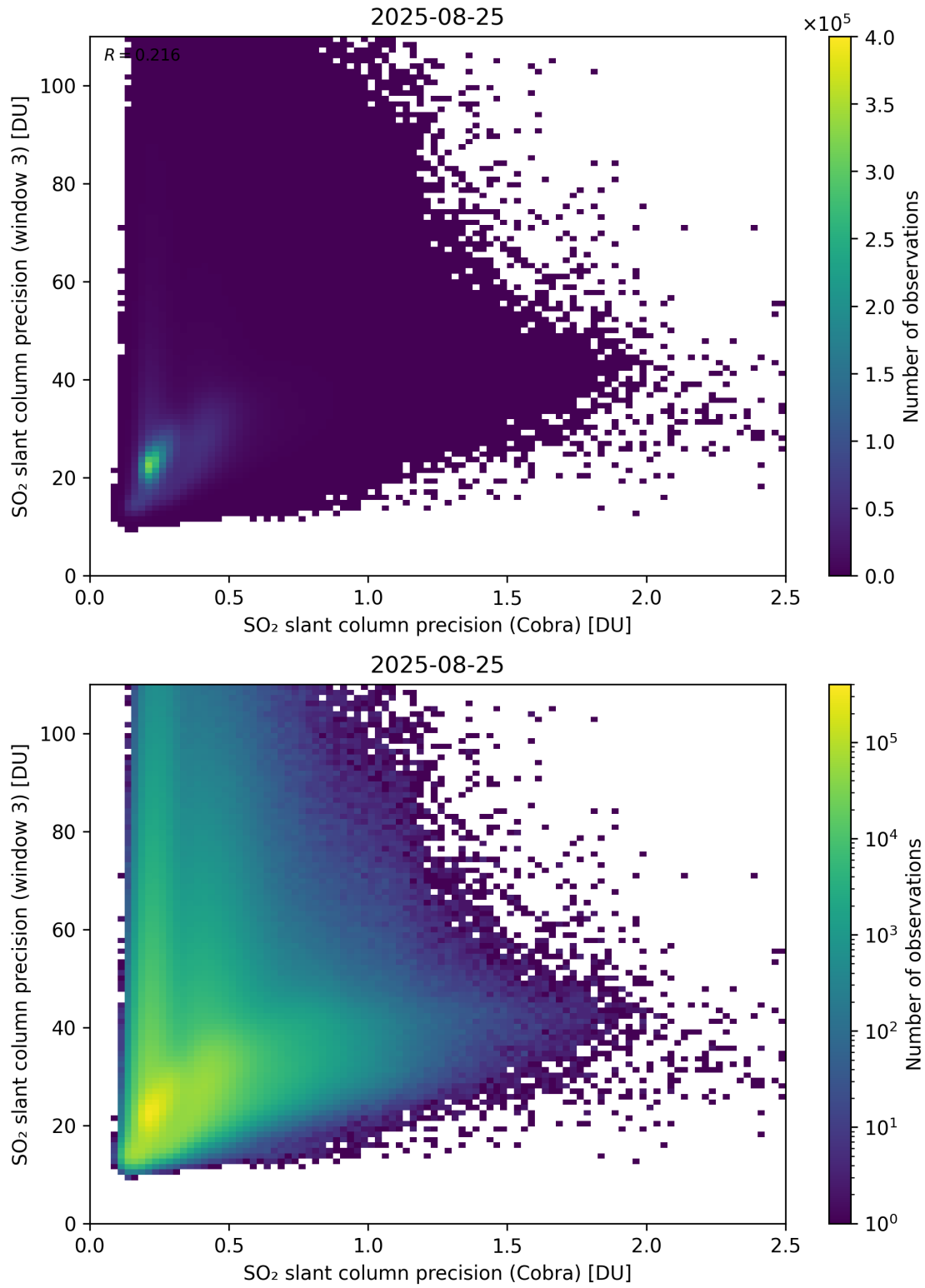
Figure 212: Scatter density plot of “SO 2 slant column precision (Cobra)” against “SO 2 slant column precision (window 3)” for 2025-08-25 to 2025-08-26.
