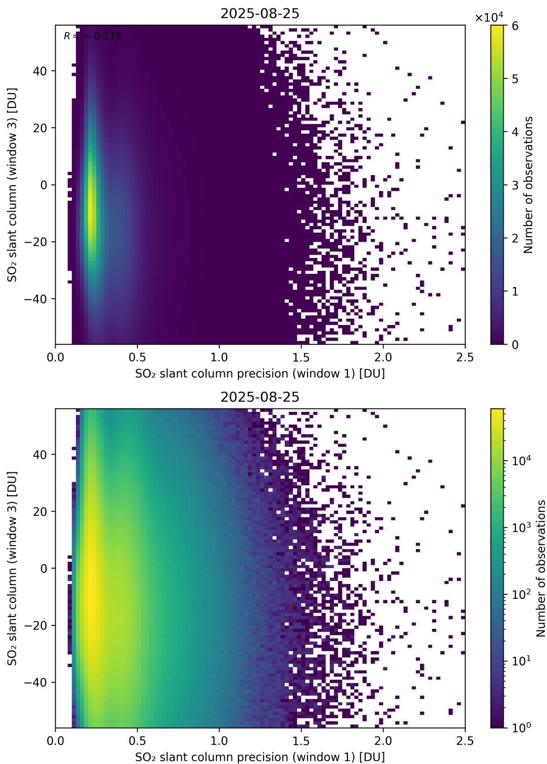
Figure 278: Scatter density plot of “SO 2 slant column precision (window 1)” against “SO 2 slant column (window 3)” for 2025-08-25 to 2025-08-26.
