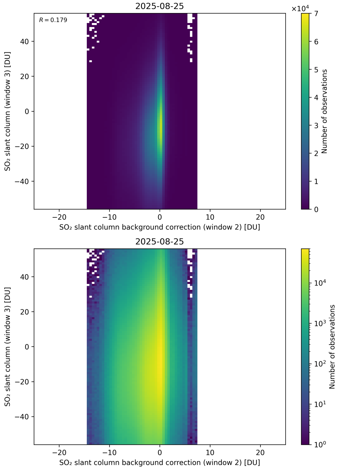
Figure 128: Scatter density plot of “SO 2 slant column background correction (window 2)” against “SO 2 slant column (window 3)” for 2025-08-25 to 2025-08-26.
