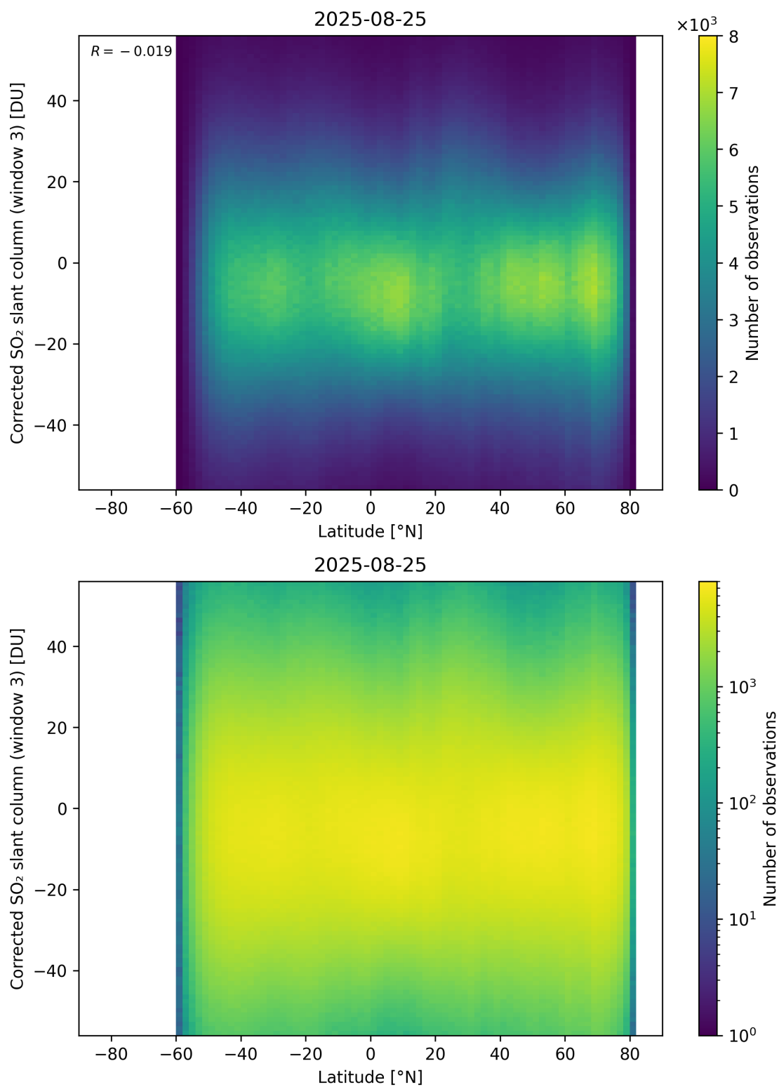
Figure 161: Scatter density plot of “Latitude” against “Corrected SO 2 slant column (window 3)” for 2025-08-25 to 2025-08-26.
