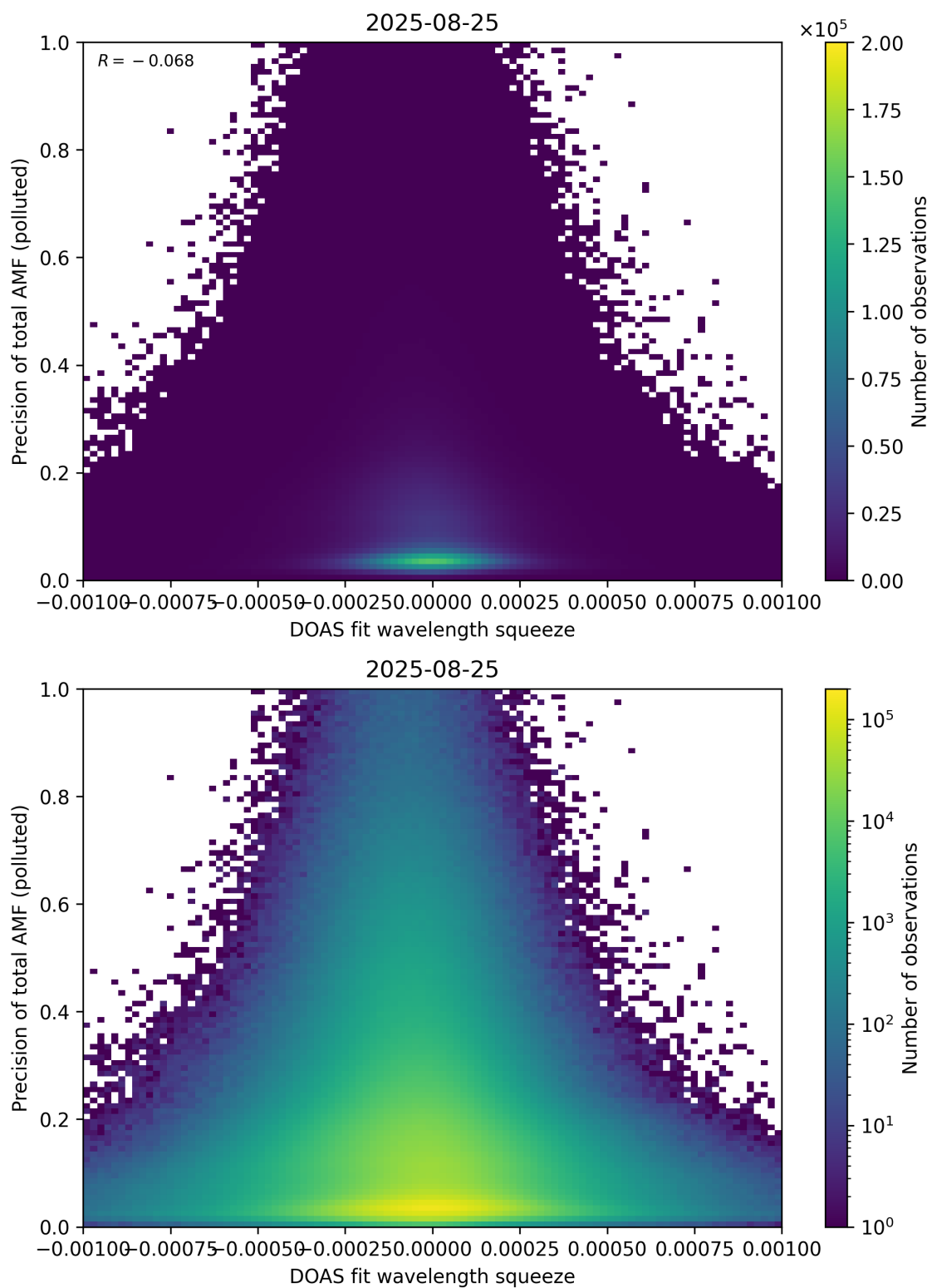
Figure 146: Scatter density plot of “DOAS fit wavelength squeeze” against “Precision of total AMF (polluted)” for 2025-08-25 to 2025-08-26.
