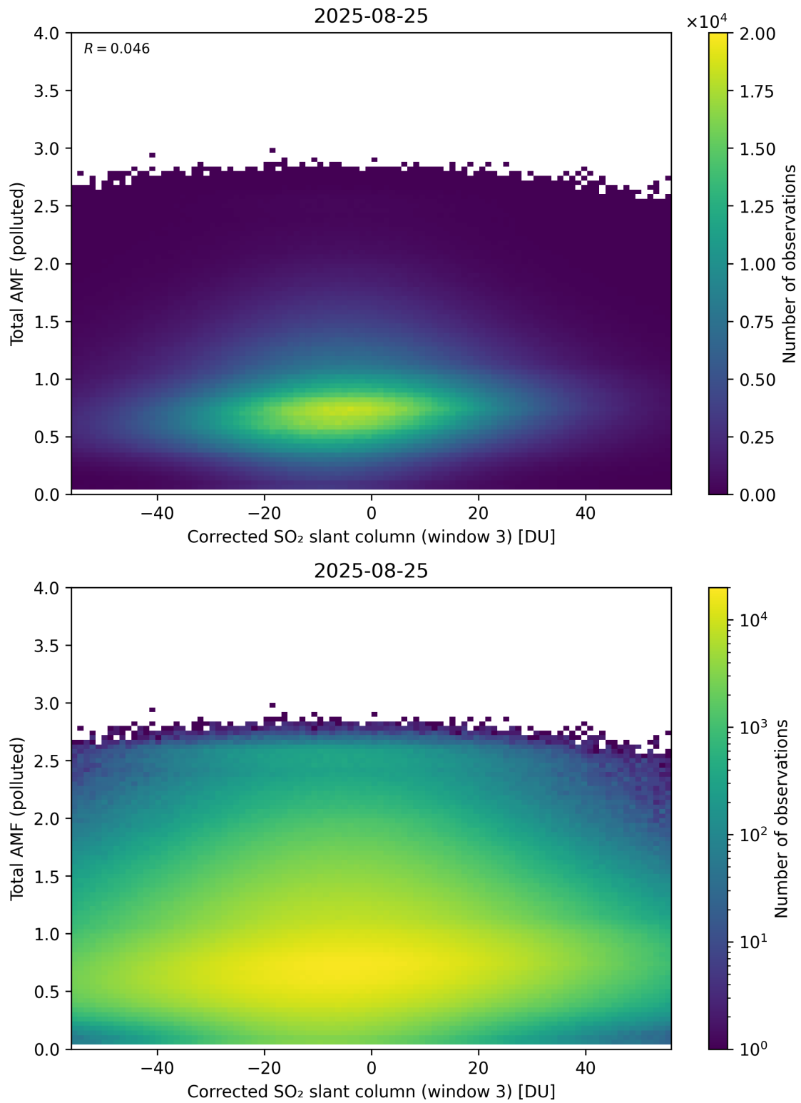
Figure 260: Scatter density plot of “Corrected SO 2 slant column (window 3)” against “Total AMF (polluted)” for 2025-08-25 to 2025-08-26.
