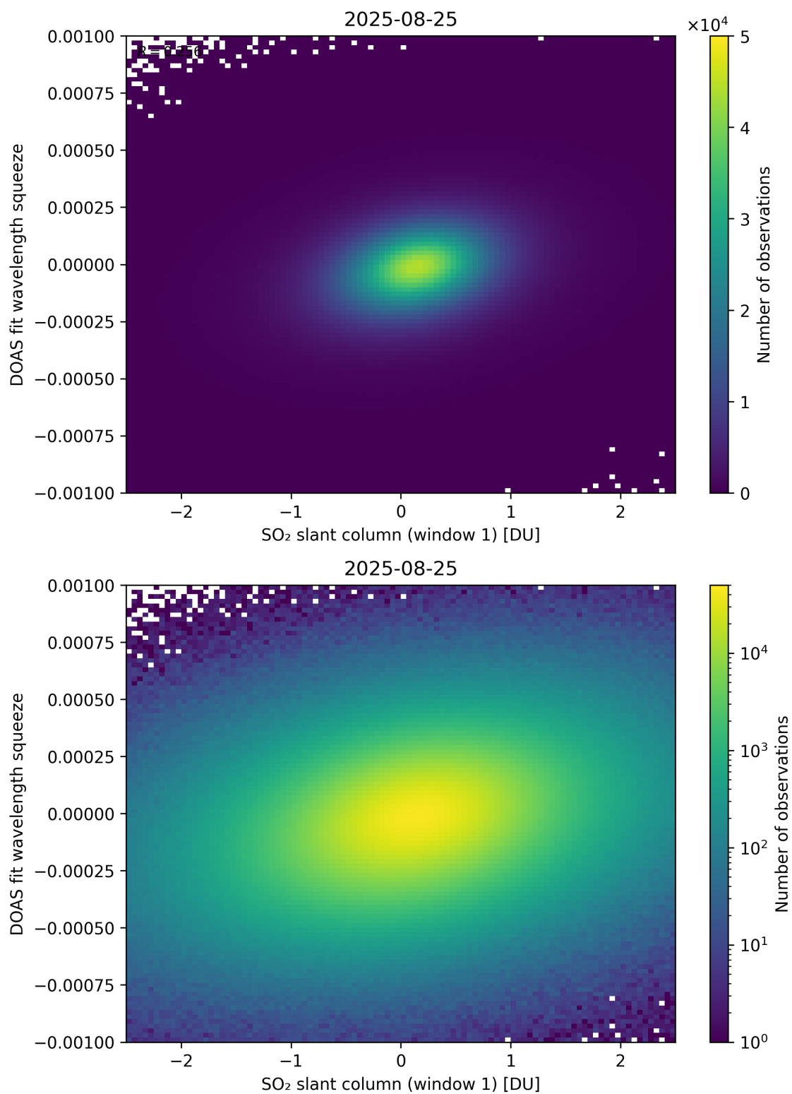
Figure 266: Scatter density plot of “SO 2 slant column (window 1)” against “DOAS fit wavelength squeeze” for 2025-08-25 to 2025-08-26.
