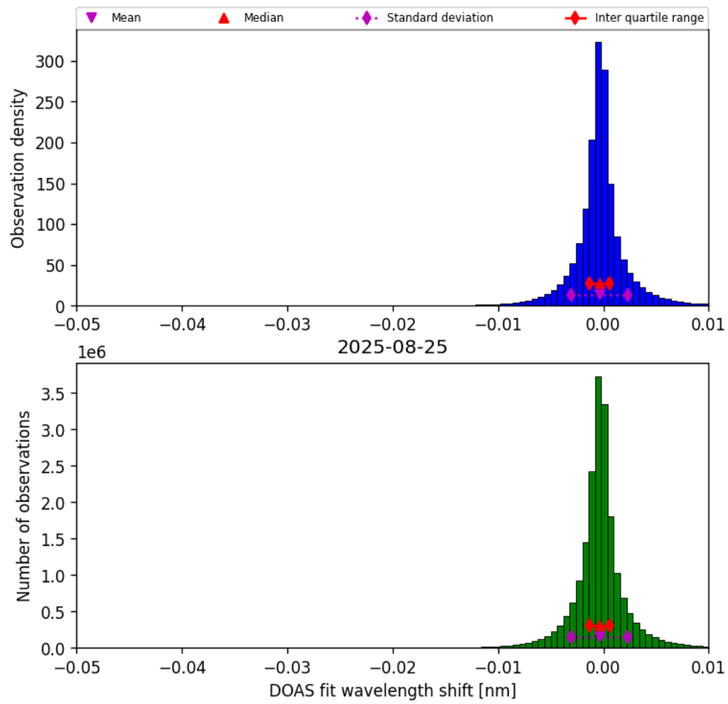
Figure 76: Histogram of “DOAS fit wavelength shift” for 2025-08-25 to 2025-08-26
