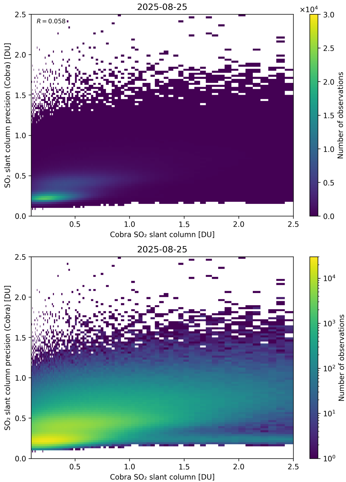
Figure 216: Scatter density plot of “Cobra SO 2 slant column” against “SO 2 slant column precision (Cobra)” for 2025-08-25 to 2025-08-26.
