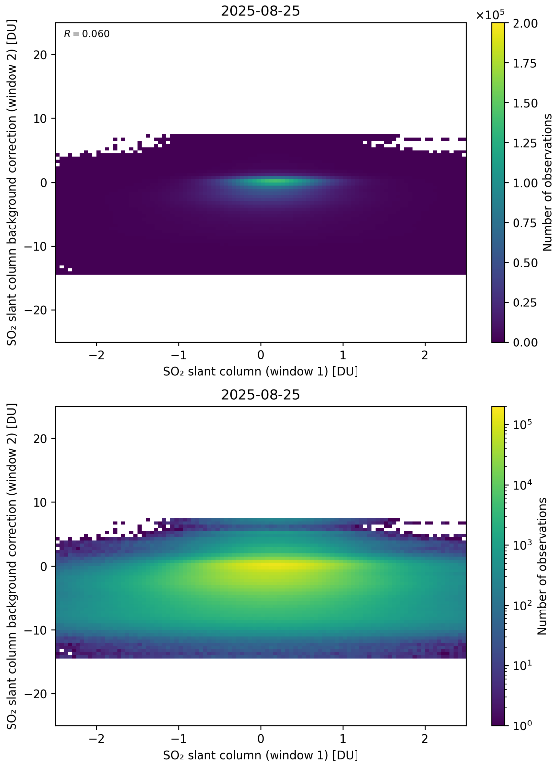
Figure 263: Scatter density plot of “SO 2 slant column (window 1)” against “SO 2 slant column background correction (window 2)” for 2025-08-25 to 2025-08-26.
