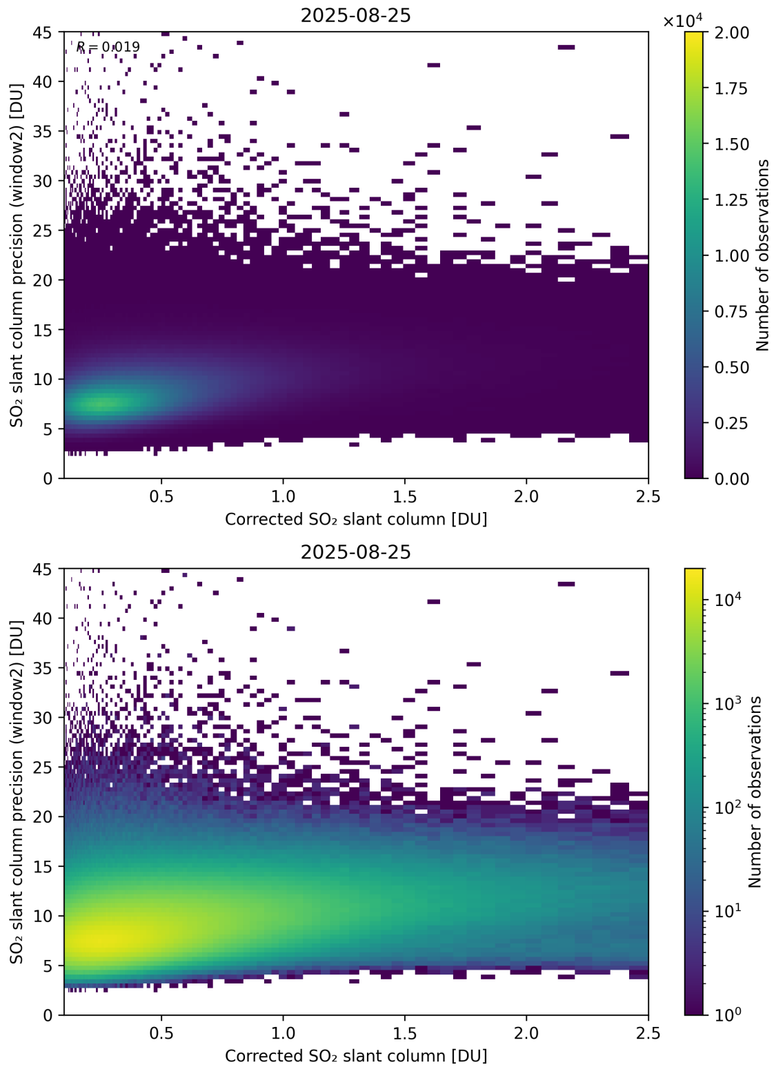
Figure 239: Scatter density plot of “Corrected SO 2 slant column” against “SO 2 slant column precision (window2)” for 2025-08-25 to 2025-08-26.
