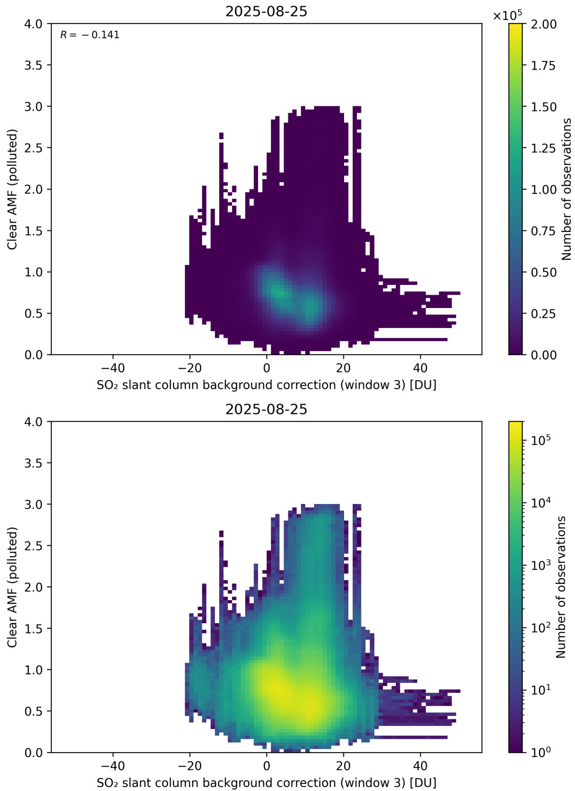
Figure 135: Scatter density plot of “SO 2 slant column background correction (window 3)” against “Clear AMF (polluted)” for 2025-08-25 to 2025-08-26.
