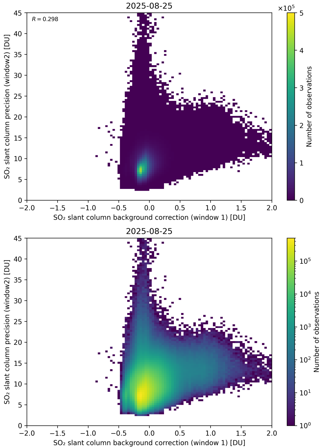
Figure 117: Scatter density plot of “SO 2 slant column background correction (window 1)” against “SO 2 slant column precision (window2)” for 2025-08-25 to 2025-08-26.
