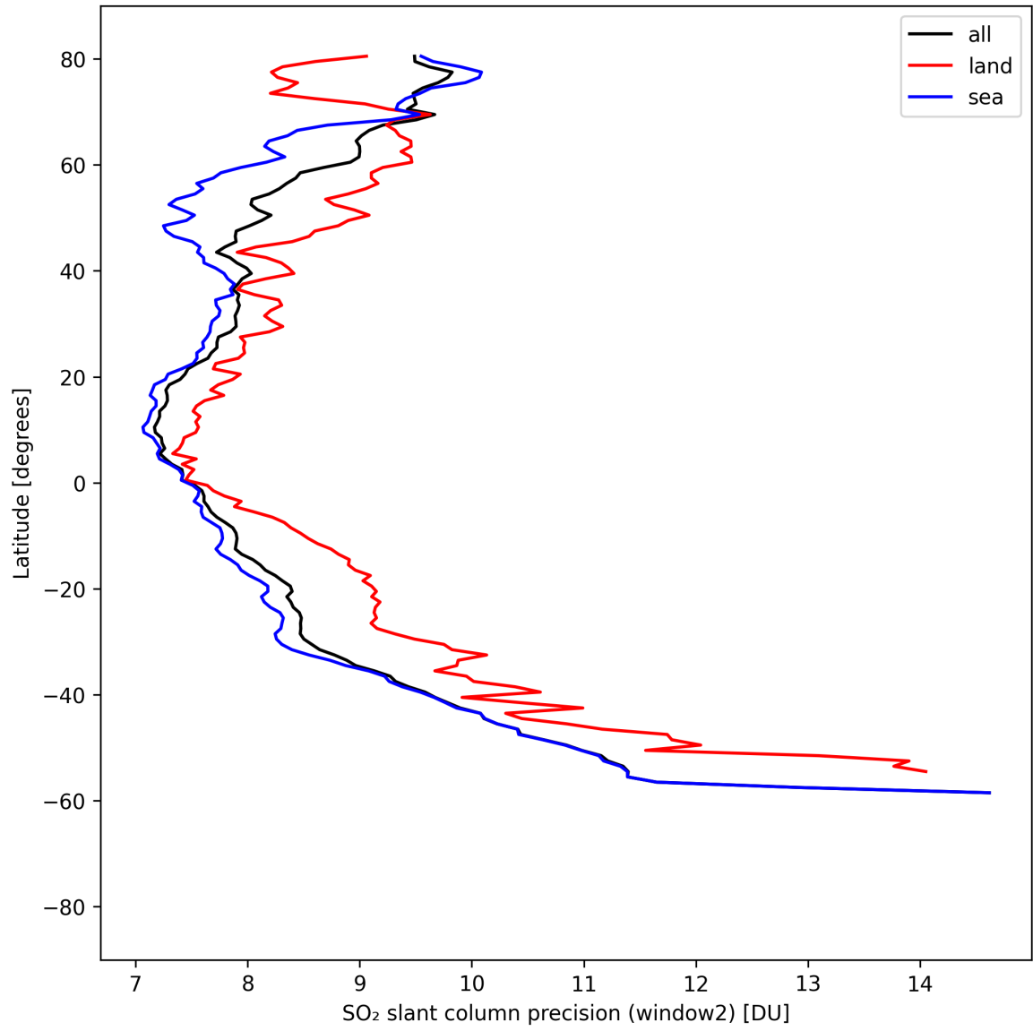
Figure 42: Zonal average of “SO 2 slant column precision (window2)” for 2025-08-25 to 2025-08-26.
