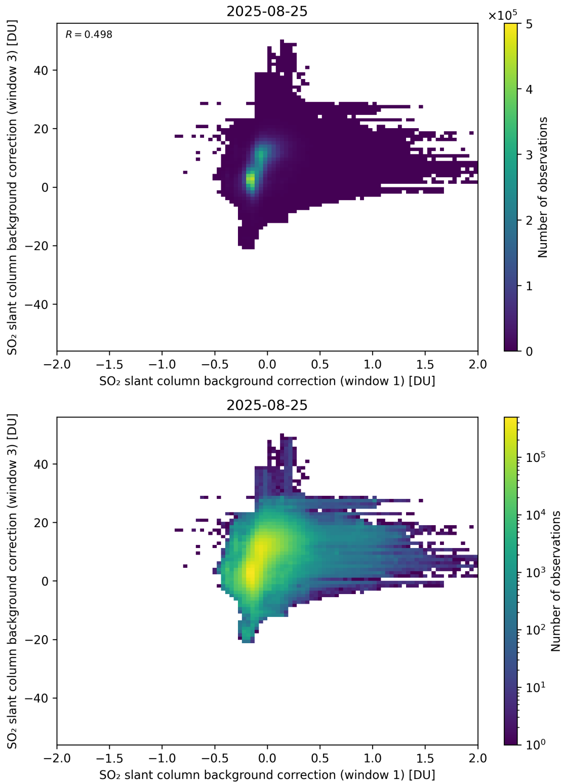
Figure 110: Scatter density plot of “SO 2 slant column background correction (window 1)” against “SO 2 slant column background correction (window 3)” for 2025-08-25 to 2025-08-26.
