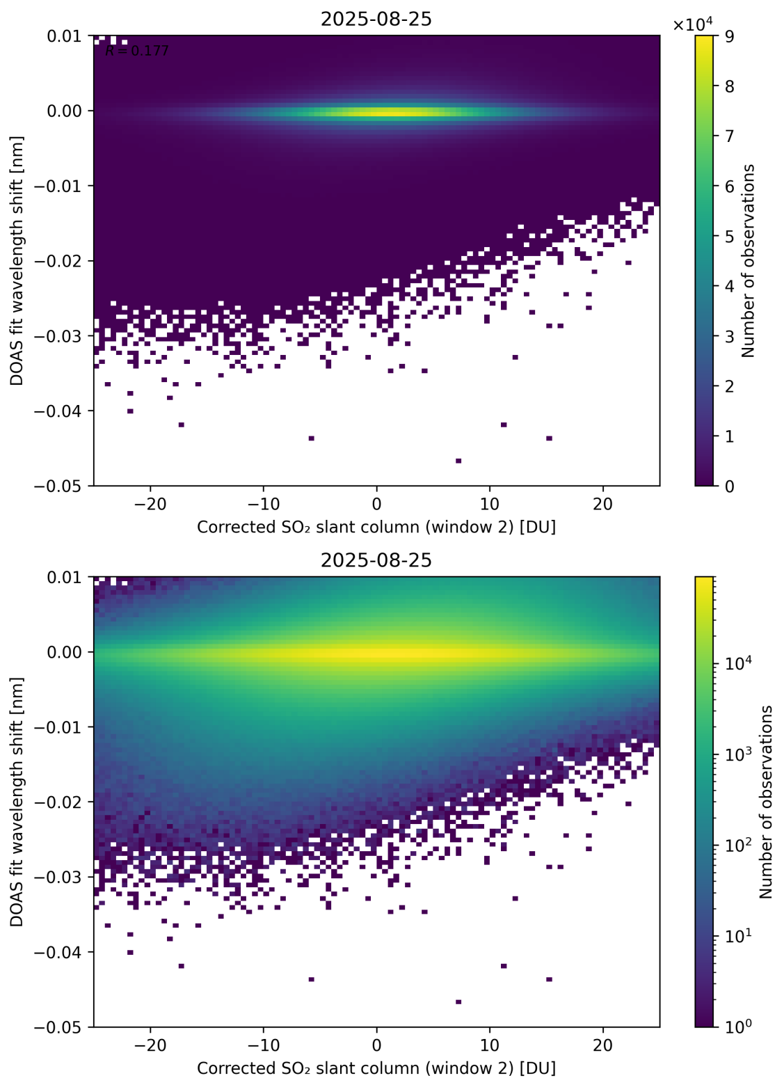
Figure 246: Scatter density plot of “Corrected SO 2 slant column (window 2)” against “DOAS fit wavelength shift” for 2025-08-25 to 2025-08-26.
