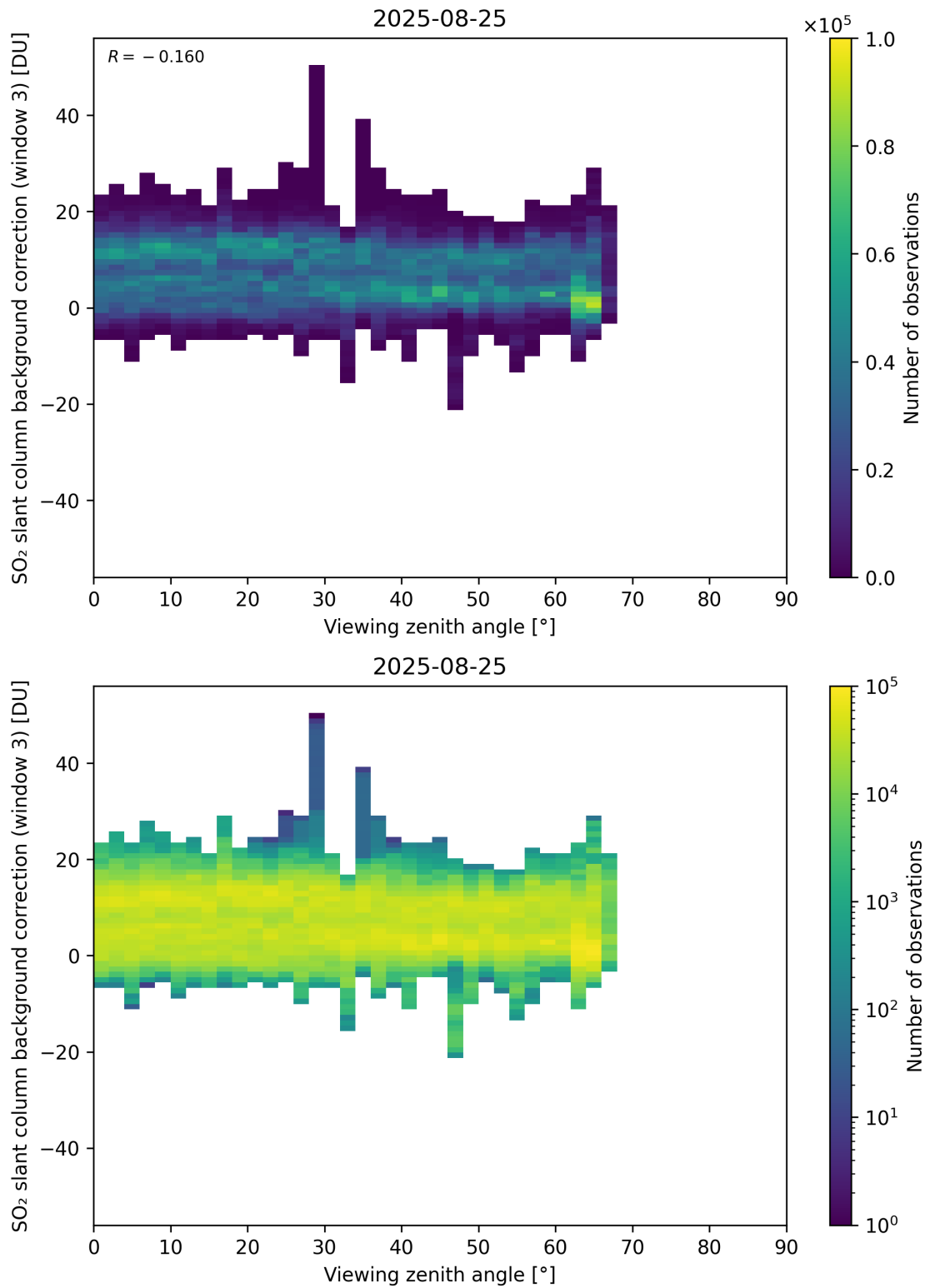
Figure 364: Scatter density plot of “Viewing zenith angle” against “SO 2 slant column background correction (window 3)” for 2025-08-25 to 2025-08-26.
