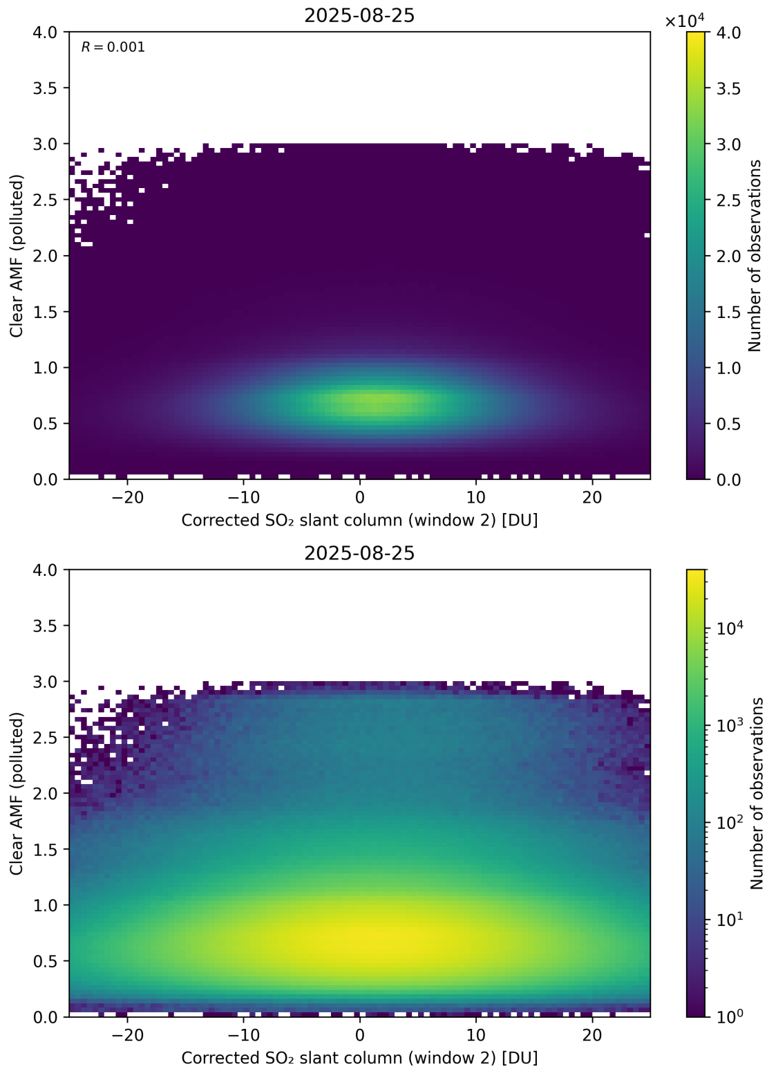
Figure 249: Scatter density plot of “Corrected SO 2 slant column (window 2)” against “Clear AMF (polluted)” for 2025-08-25 to 2025-08-26.
