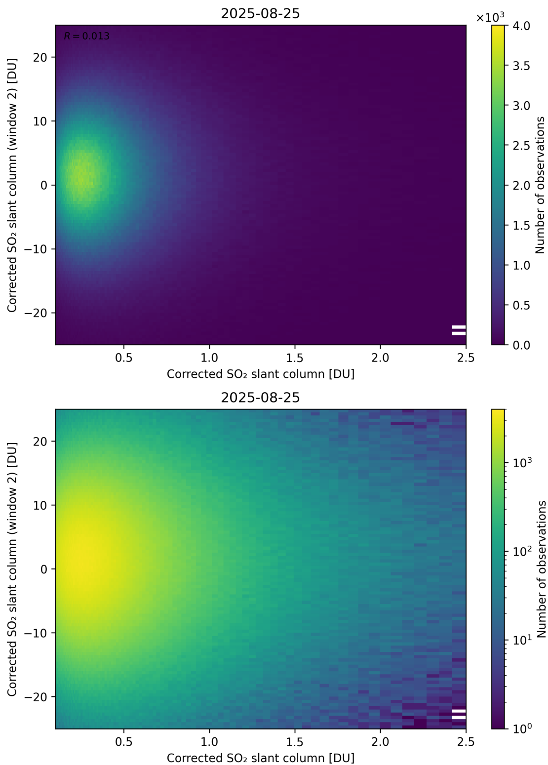
Figure 235: Scatter density plot of “Corrected SO 2 slant column” against “Corrected SO 2 slant column (window 2)” for 2025-08-25 to 2025-08-26.
