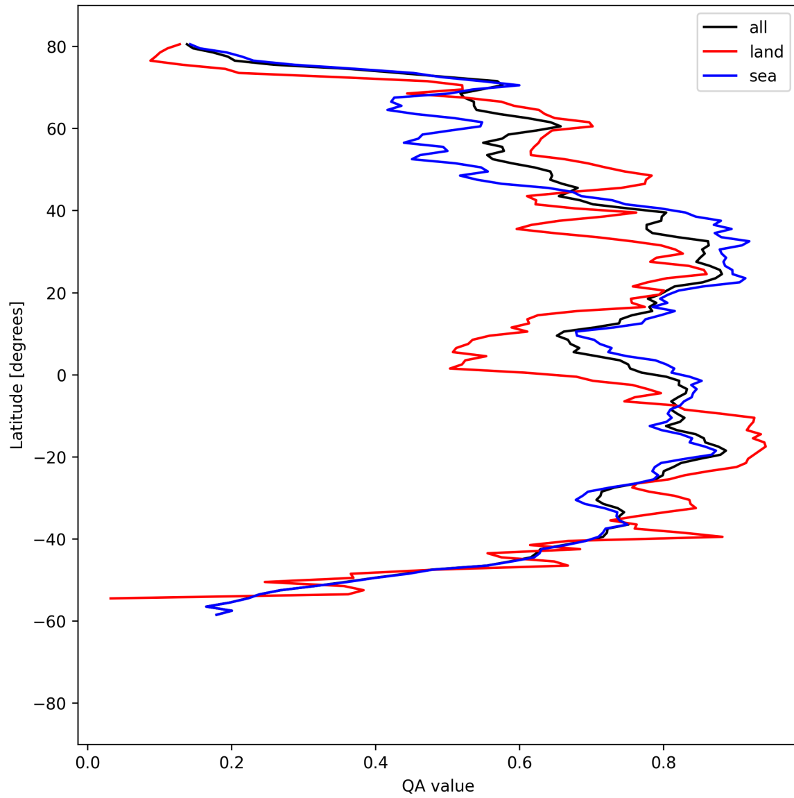
Figure 31: Zonal average of “QA value” for 2025-08-25 to 2025-08-26.
