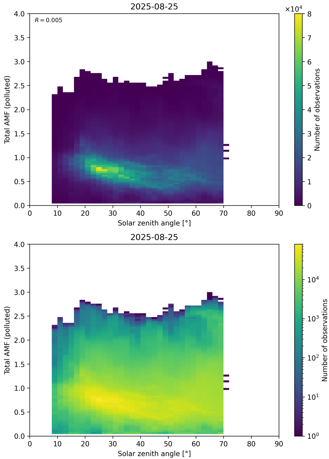
Figure 189: Scatter density plot of “Solar zenith angle” against “Total AMF (polluted)” for 2025-08-25 to 2025-08-26.
