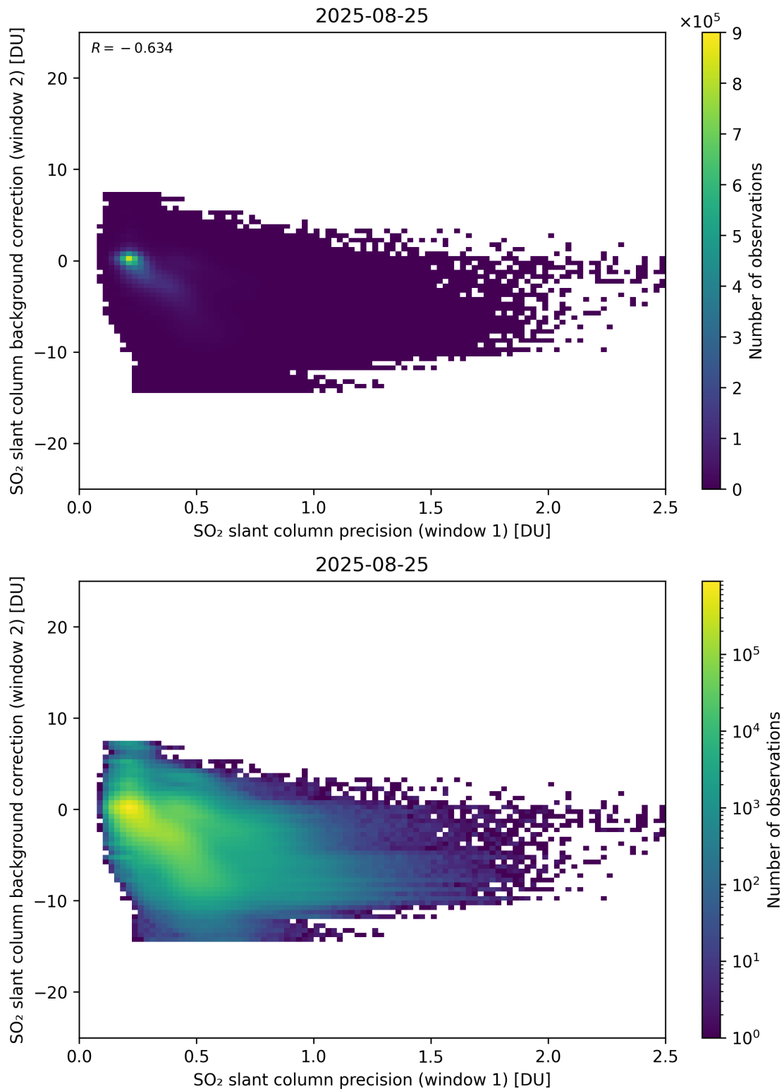
Figure 269: Scatter density plot of “SO 2 slant column precision (window 1)” against “SO 2 slant column background correction (window 2)” for 2025-08-25 to 2025-08-26.
