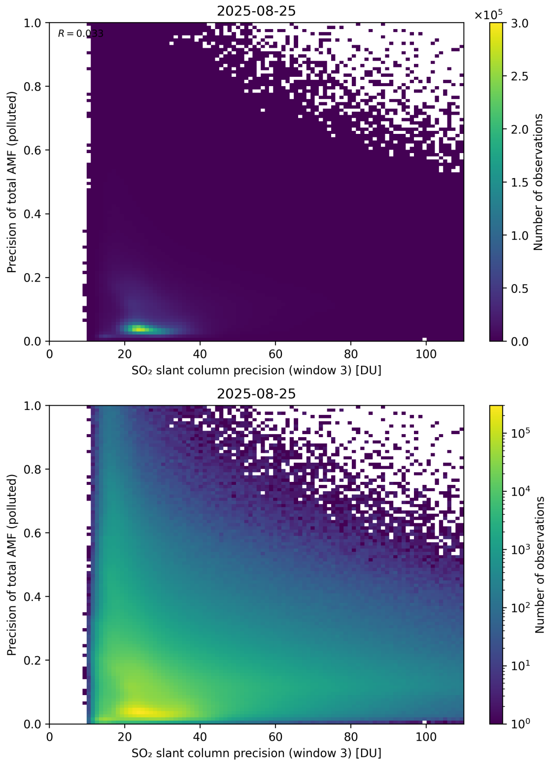
Figure 314: Scatter density plot of “SO 2 slant column precision (window 3)” against “Precision of total AMF (polluted)” for 2025-08-25 to 2025-08-26.
