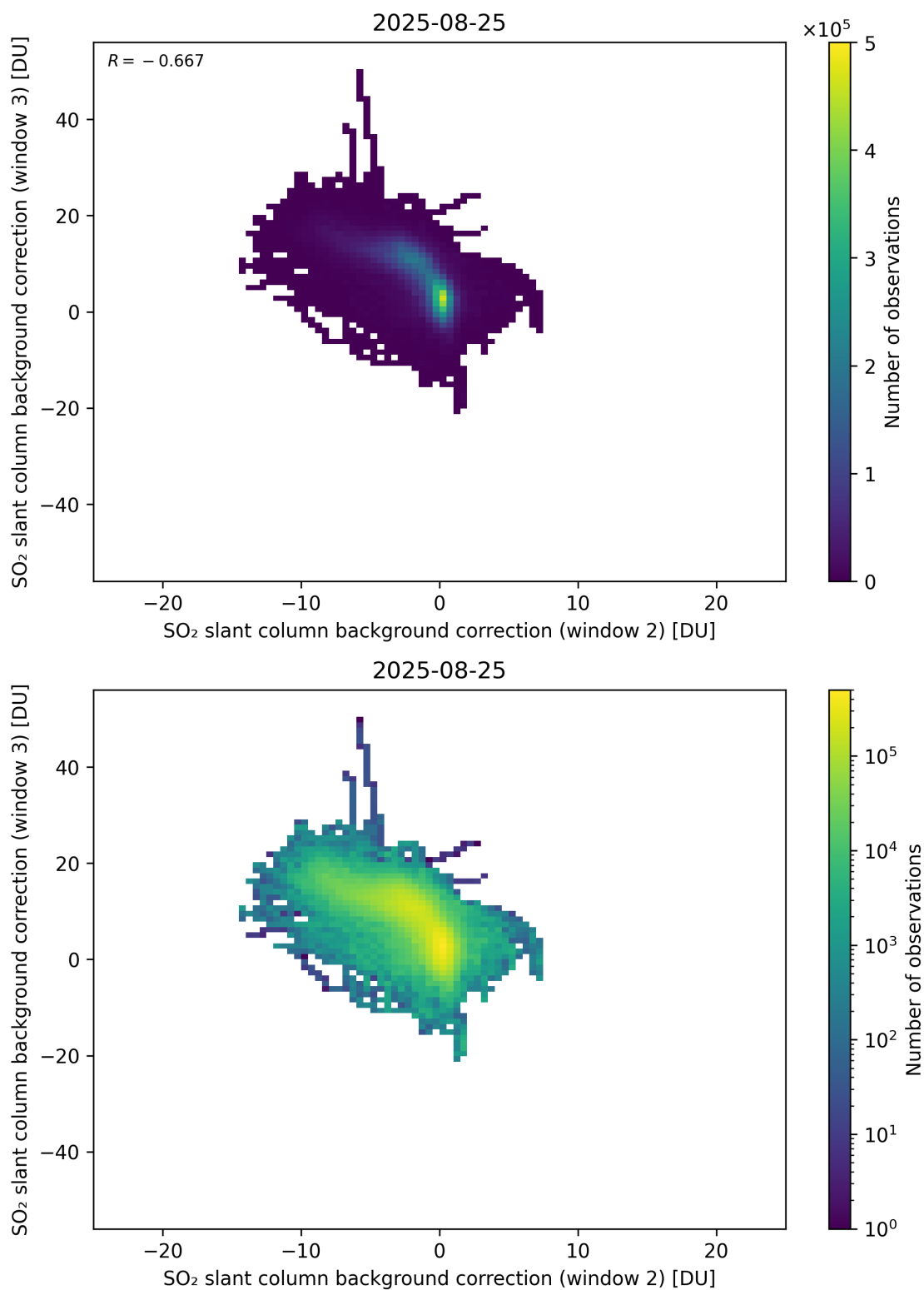
Figure 122: Scatter density plot of “SO 2 slant column background correction (window 2)” against “SO 2 slant column background correction (window 3)” for 2025-08-25 to 2025-08-26.
