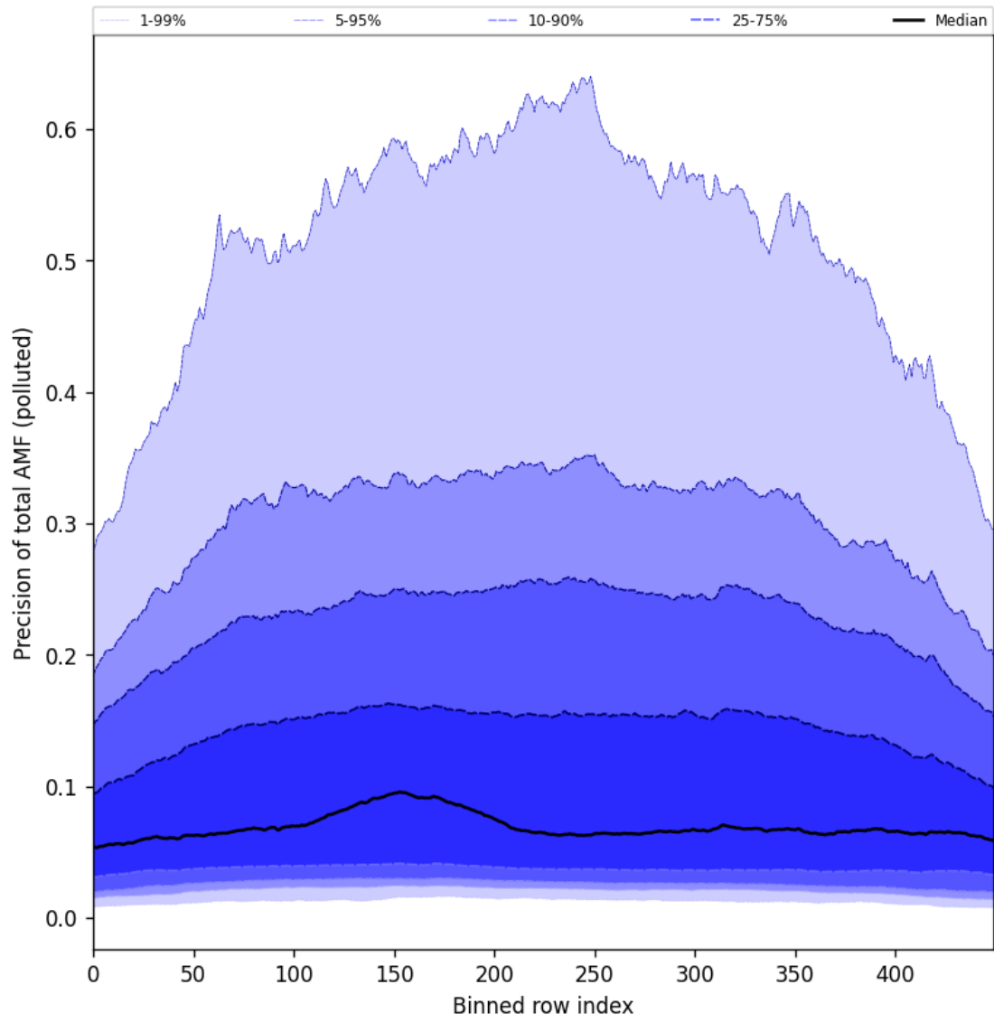
Figure 106: Along track statistics of “Precision of total AMF (polluted)” for 2025-08-25 to 2025-08-26
