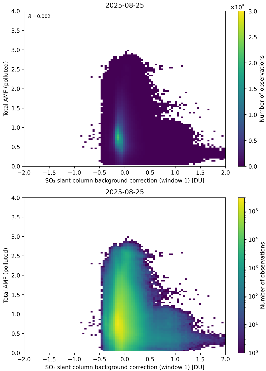
Figure 120: Scatter density plot of “SO 2 slant column background correction (window 1)” against “Total AMF (polluted)” for 2025-08-25 to 2025-08-26.
