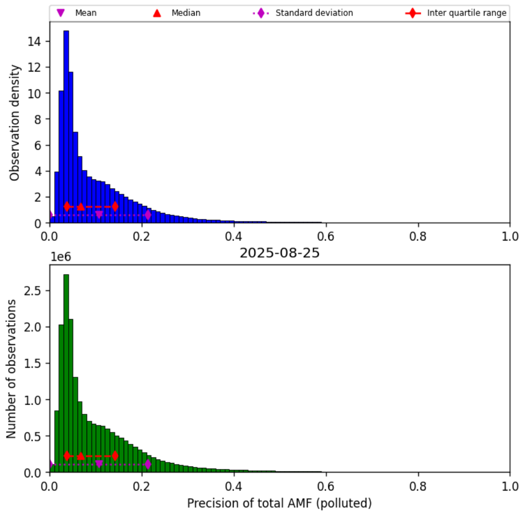
Figure 80: Histogram of “Precision of total AMF (polluted)” for 2025-08-25 to 2025-08-26
