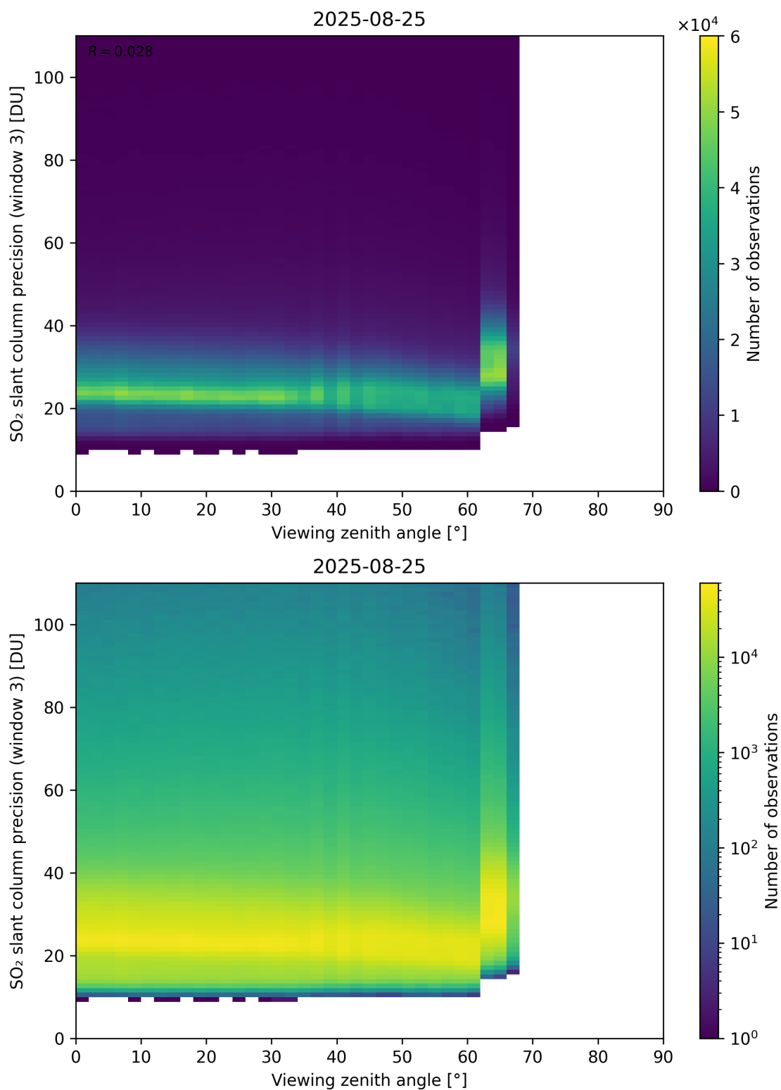
Figure 380: Scatter density plot of “Viewing zenith angle” against “SO 2 slant column precision (window 3)” for 2025-08-25 to 2025-08-26.
