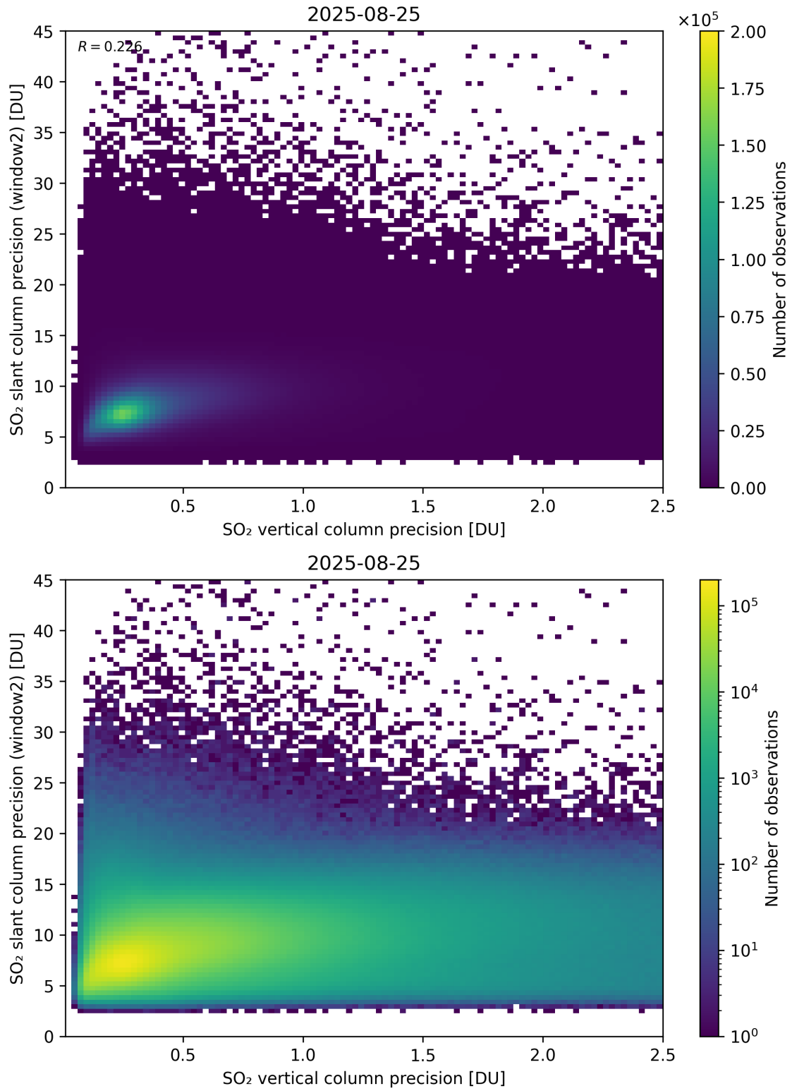
Figure 343: Scatter density plot of “SO 2 vertical column precision” against “SO 2 slant column precision (window2)” for 2025-08-25 to 2025-08-26.
