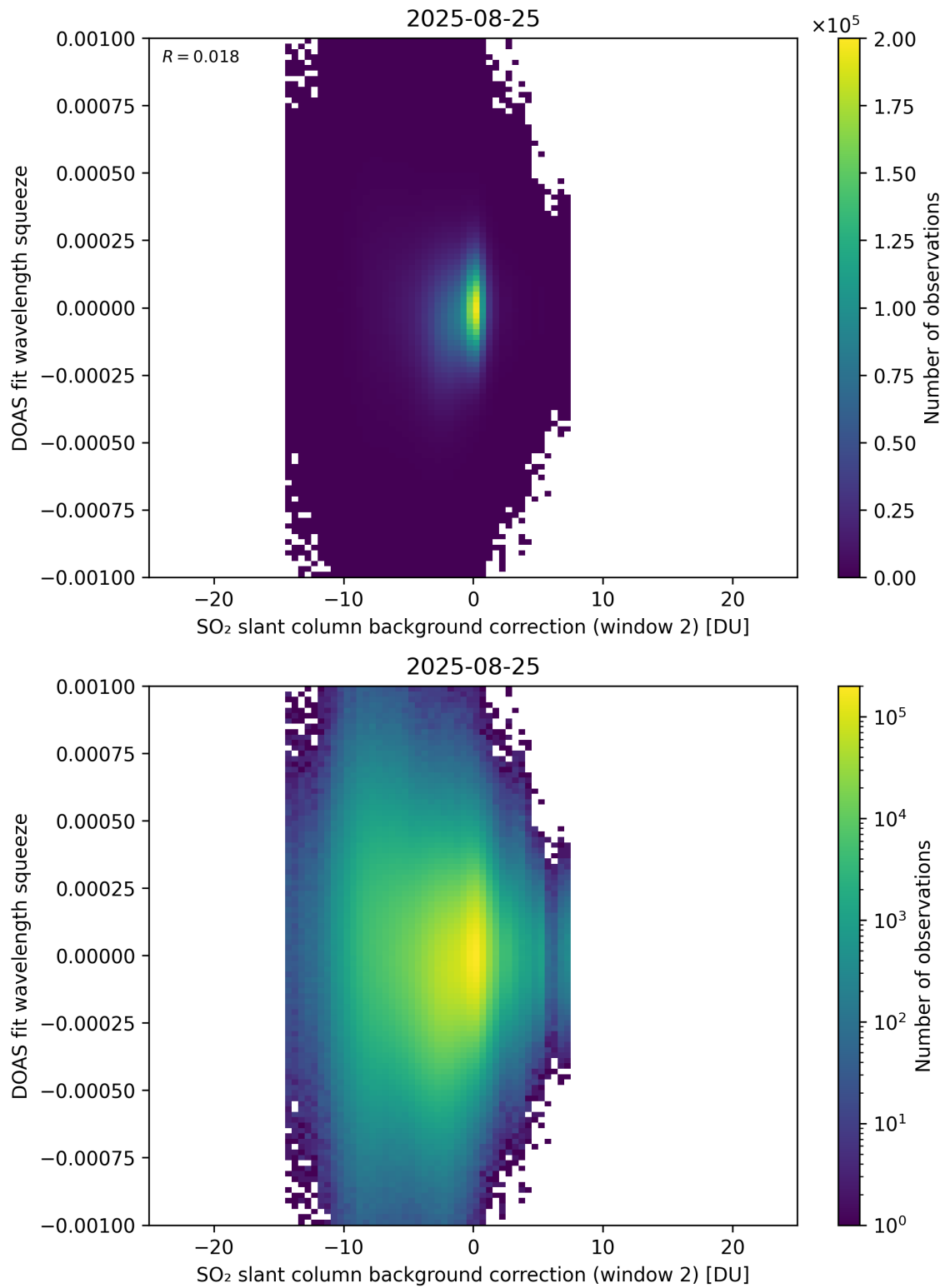
Figure 124: Scatter density plot of “SO 2 slant column background correction (window 2)” against “DOAS fit wavelength squeeze” for 2025-08-25 to 2025-08-26.
