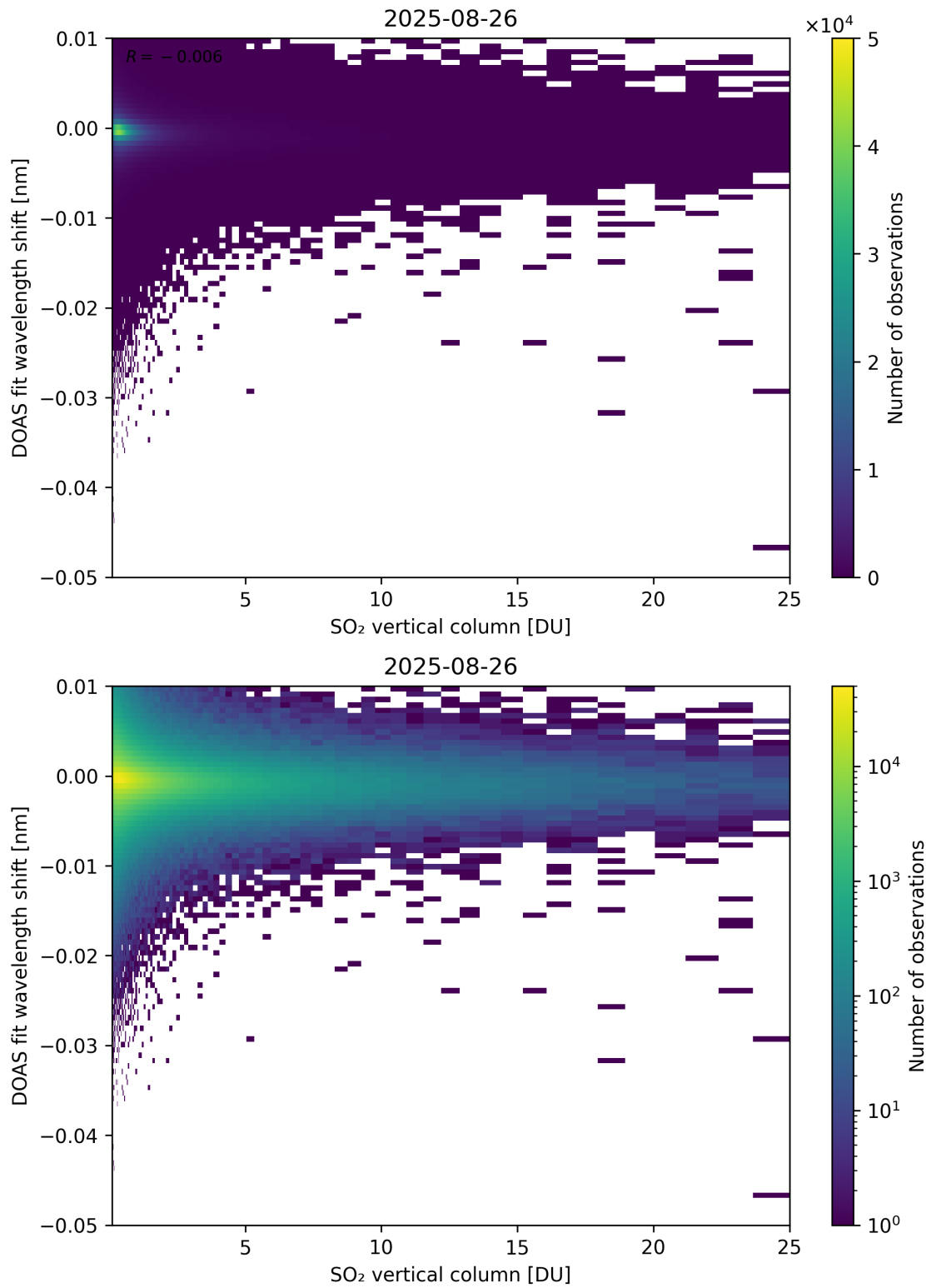
Figure 326: Scatter density plot of “SO 2 vertical column” against “DOAS fit wavelength shift” for 2025-08-25 to 2025-08-27.
