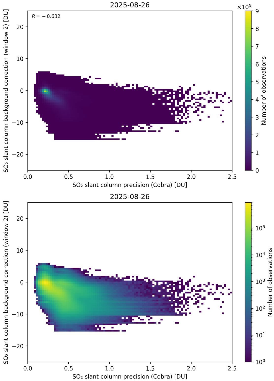
Figure 200: Scatter density plot of “SO 2 slant column precision (Cobra)” against “SO 2 slant column background correction (window 2)” for 2025-08-25 to 2025-08-27.
