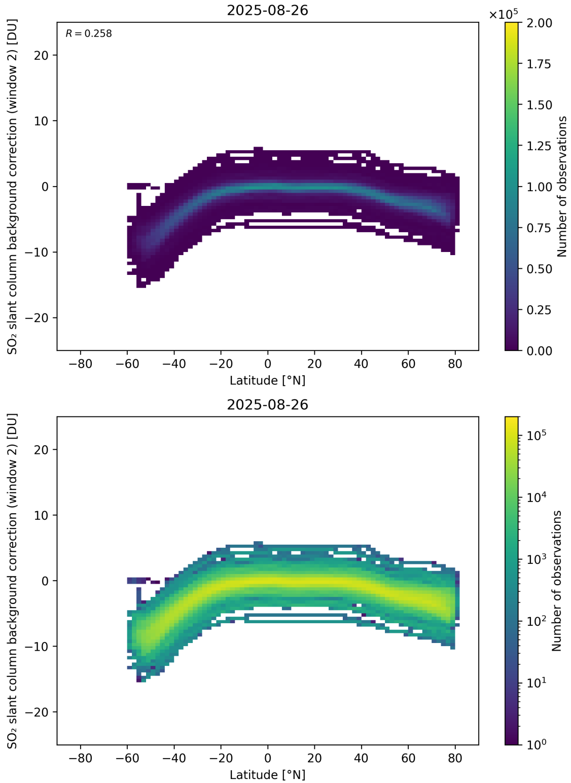
Figure 151: Scatter density plot of “Latitude” against “SO 2 slant column background correction (window 2)” for 2025-08-25 to 2025-08-27.
