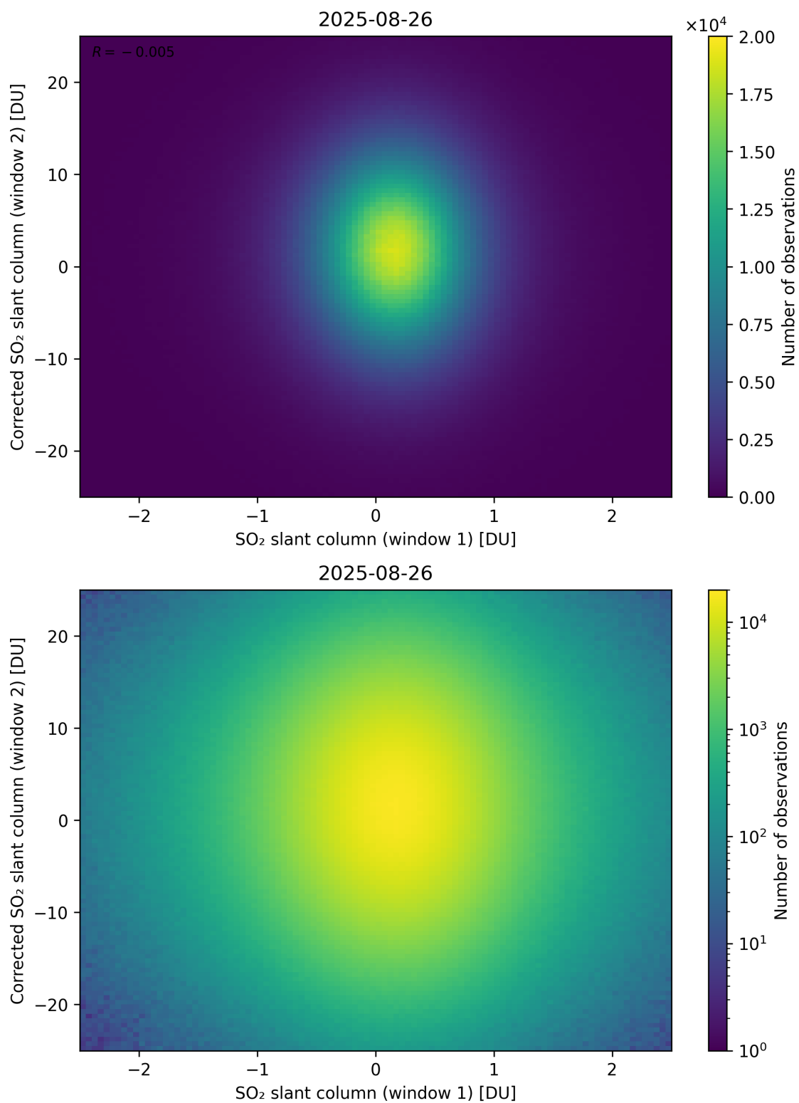
Figure 283: Scatter density plot of “SO 2 slant column (window 1)” against “Corrected SO 2 slant column (window 2)” for 2025-08-25 to 2025-08-27.
