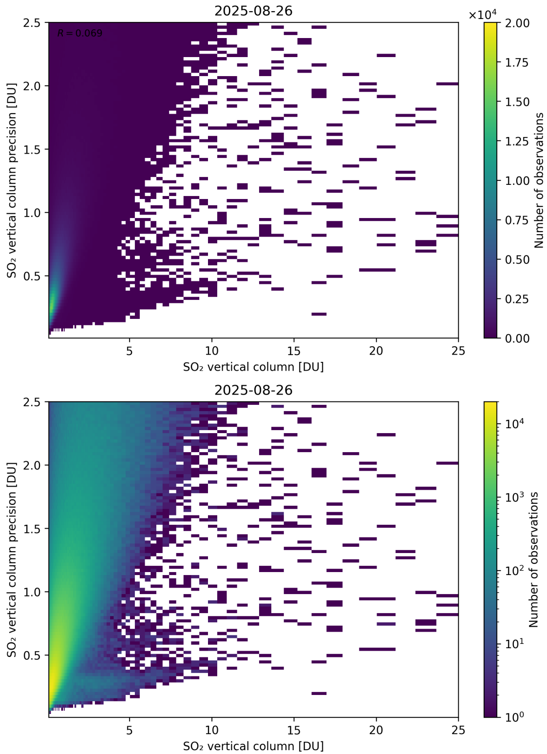
Figure 361: Scatter density plot of “SO 2 vertical column” against “SO 2 vertical column precision” for 2025-08-25 to 2025-08-27.
