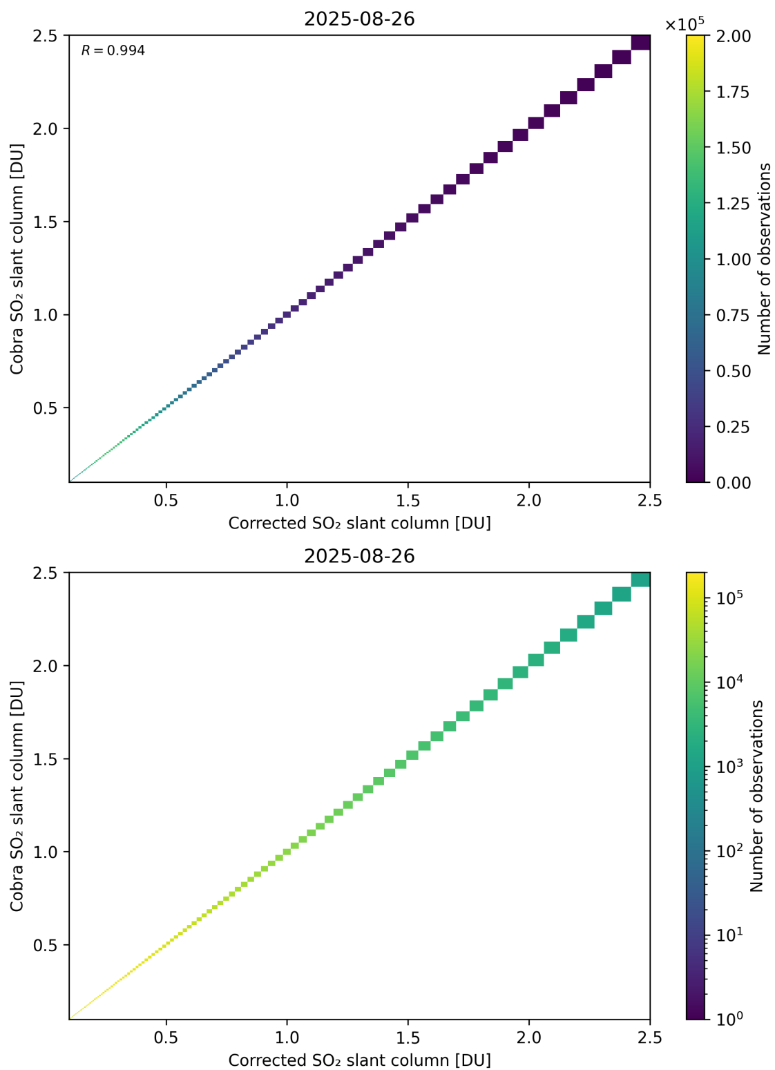
Figure 233: Scatter density plot of “Corrected SO 2 slant column” against “Cobra SO 2 slant column” for 2025-08-25 to 2025-08-27.
