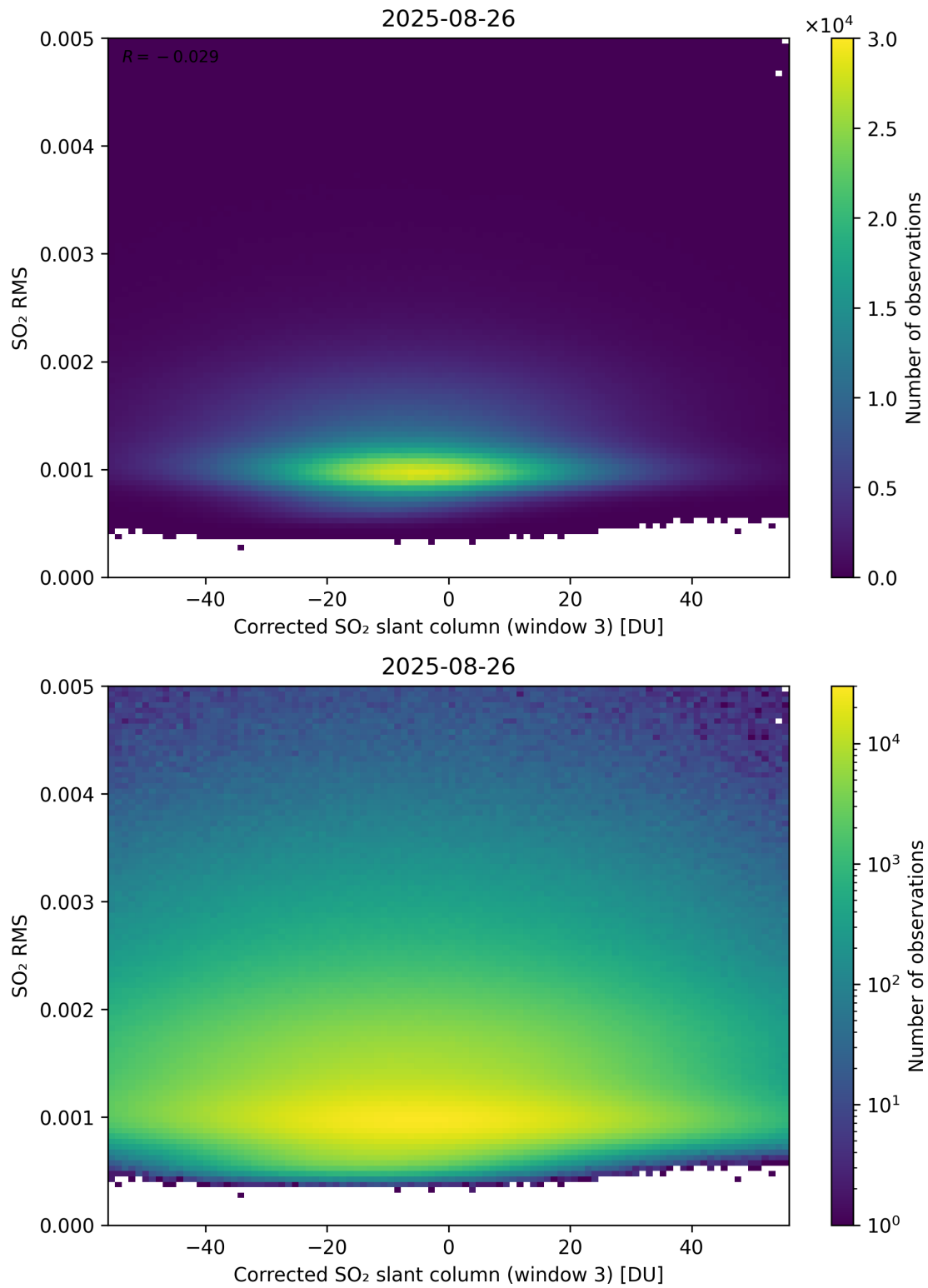
Figure 258: Scatter density plot of “Corrected SO 2 slant column (window 3)” against “SO 2 RMS” for 2025-08-25 to 2025-08-27.
