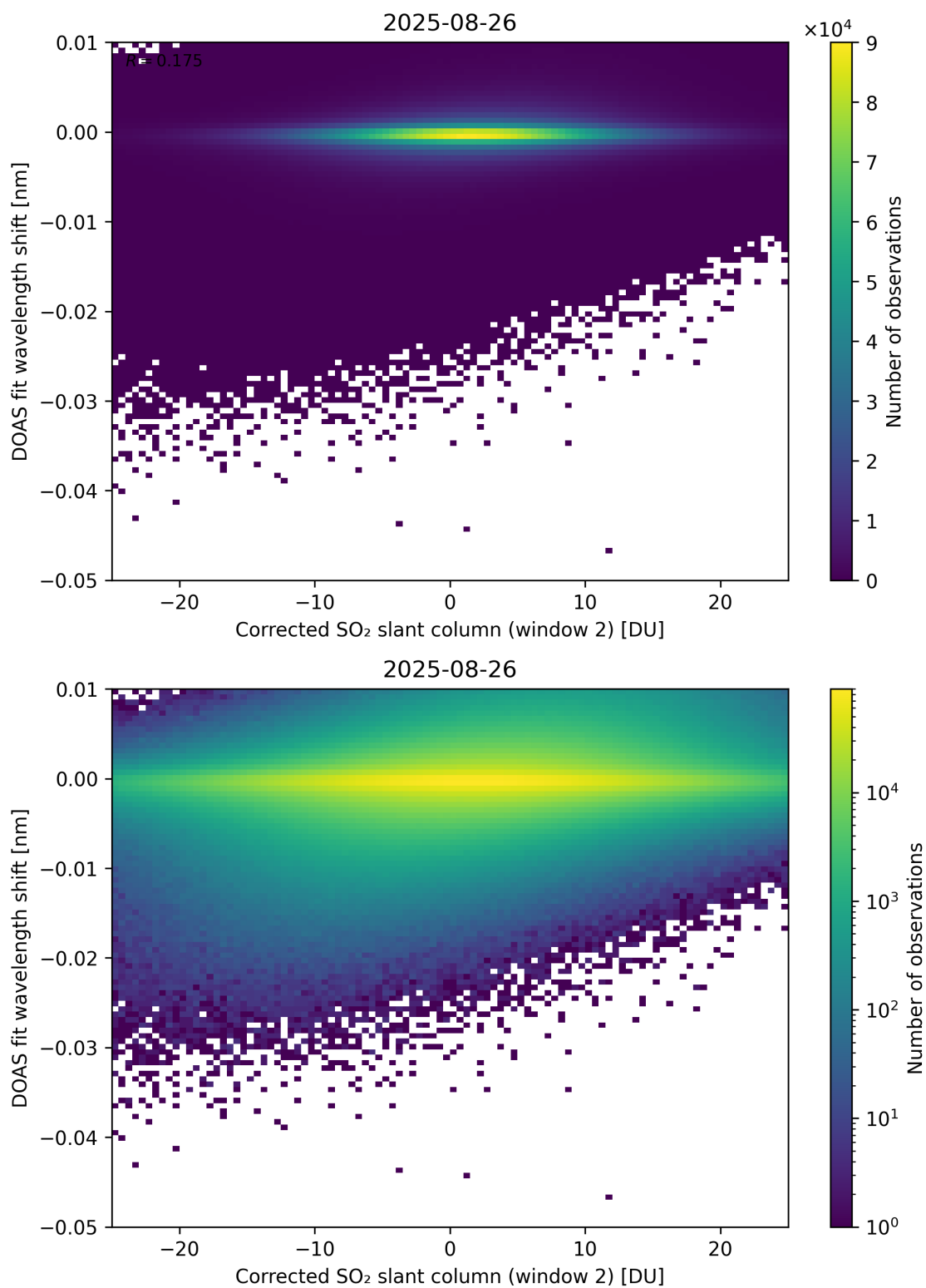
Figure 246: Scatter density plot of “Corrected SO 2 slant column (window 2)” against “DOAS fit wavelength shift” for 2025-08-25 to 2025-08-27.
