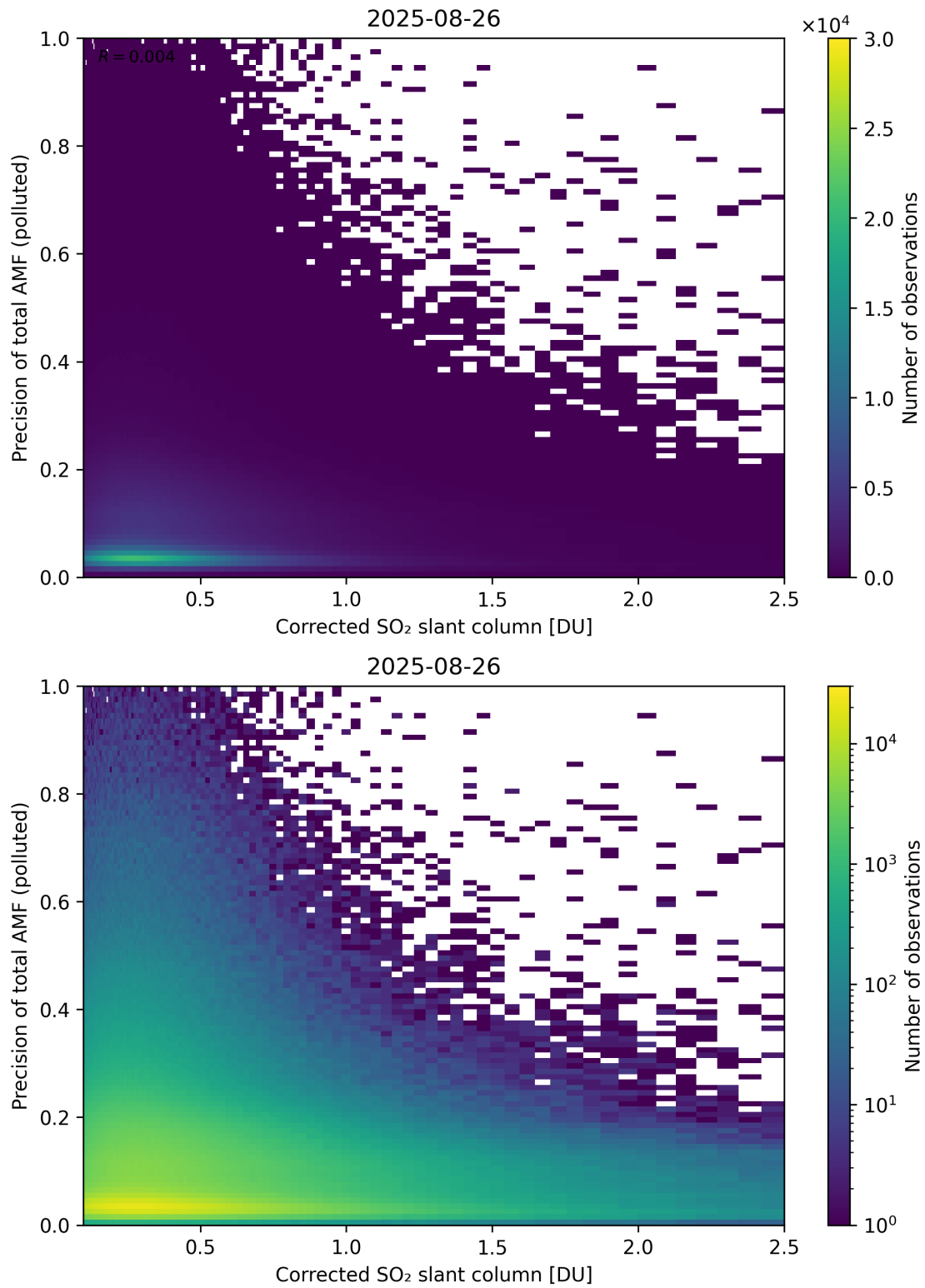
Figure 243: Scatter density plot of “Corrected SO 2 slant column” against “Precision of total AMF (polluted)” for 2025-08-25 to 2025-08-27.
