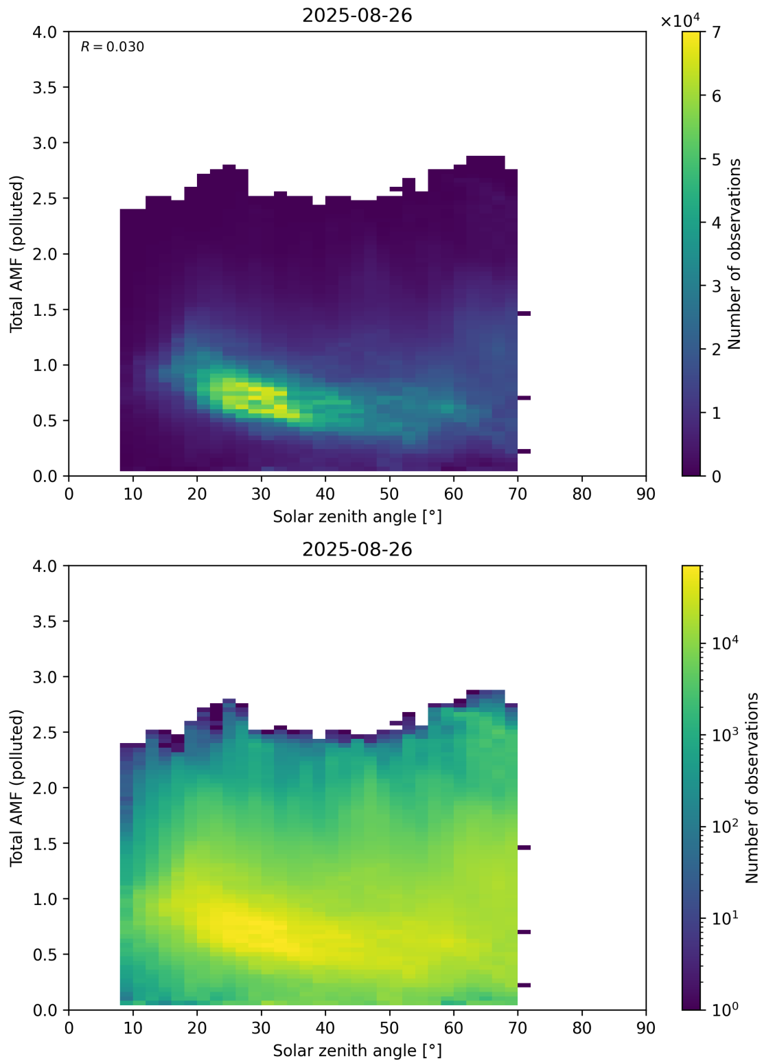
Figure 189: Scatter density plot of “Solar zenith angle” against “Total AMF (polluted)” for 2025-08-25 to 2025-08-27.
