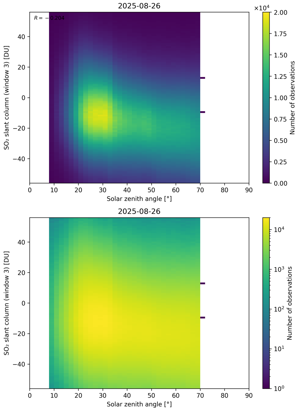
Figure 187: Scatter density plot of “Solar zenith angle” against “SO 2 slant column (window 3)” for 2025-08-25 to 2025-08-27.
