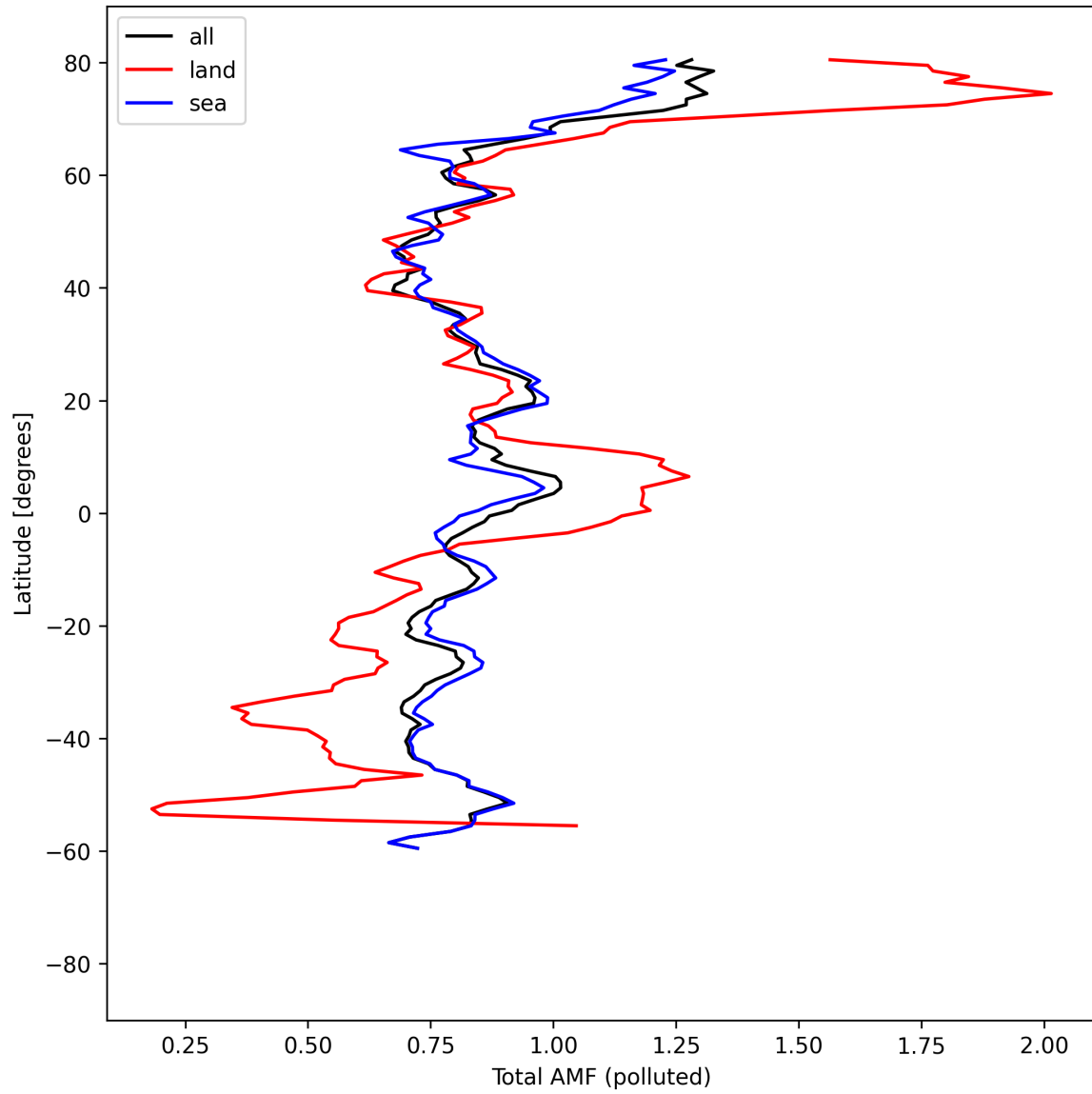
Figure 53: Zonal average of “Total AMF (polluted)” for 2025-08-25 to 2025-08-27.
