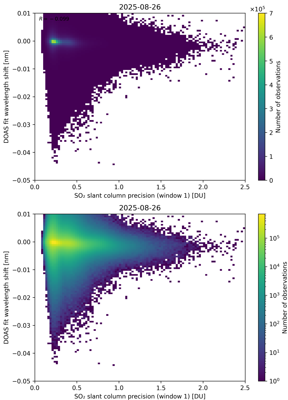
Figure 271: Scatter density plot of “SO 2 slant column precision (window 1)” against “DOAS fit wavelength shift” for 2025-08-25 to 2025-08-27.
