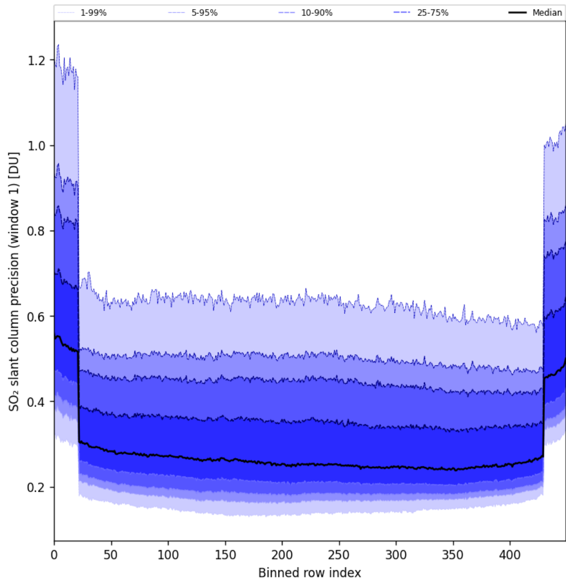
Figure 90: Along track statistics of "SO 2 slant column precision (window 1)" for 2025-08-25 to 2025-08-27
