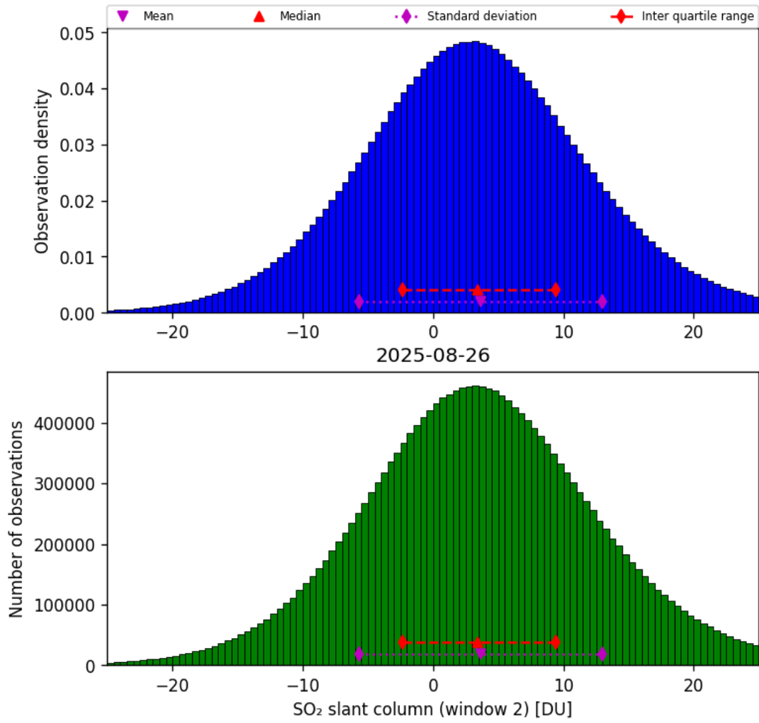
Figure 67: Histogram of “SO 2 slant column (window 2)” for 2025-08-25 to 2025-08-27
