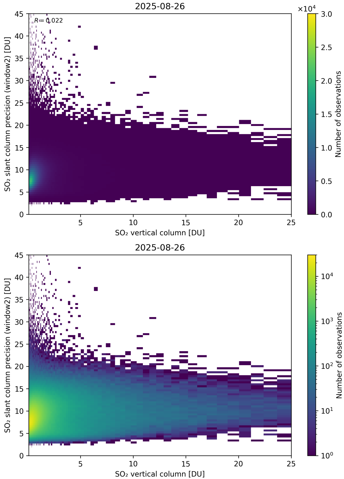
Figure 356: Scatter density plot of “SO 2 vertical column” against “SO 2 slant column precision (window2)” for 2025-08-25 to 2025-08-27.
