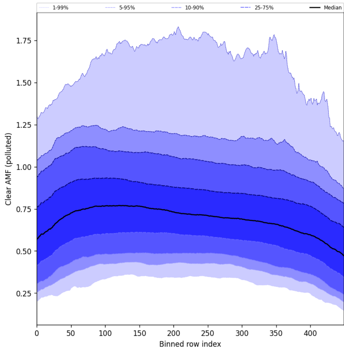
Figure 107: Along track statistics of “Clear AMF (polluted)” for 2025-08-25 to 2025-08-27
