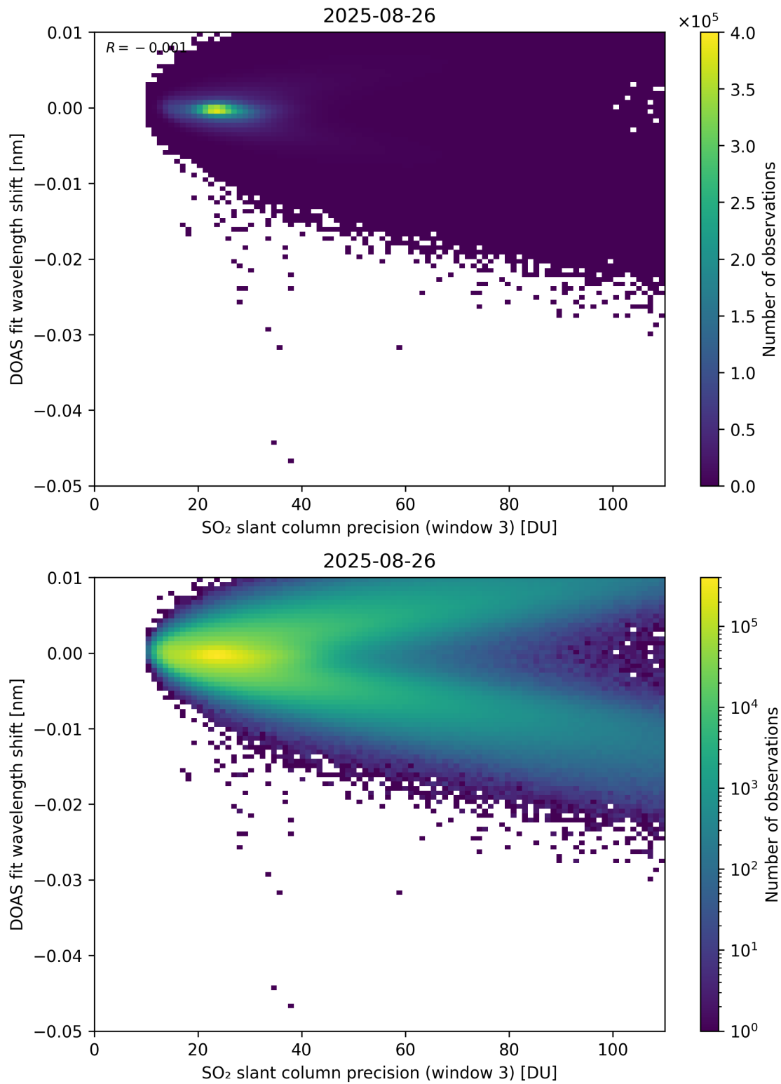
Figure 308: Scatter density plot of “SO 2 slant column precision (window 3)” against “DOAS fit wavelength shift” for 2025-08-25 to 2025-08-27.
