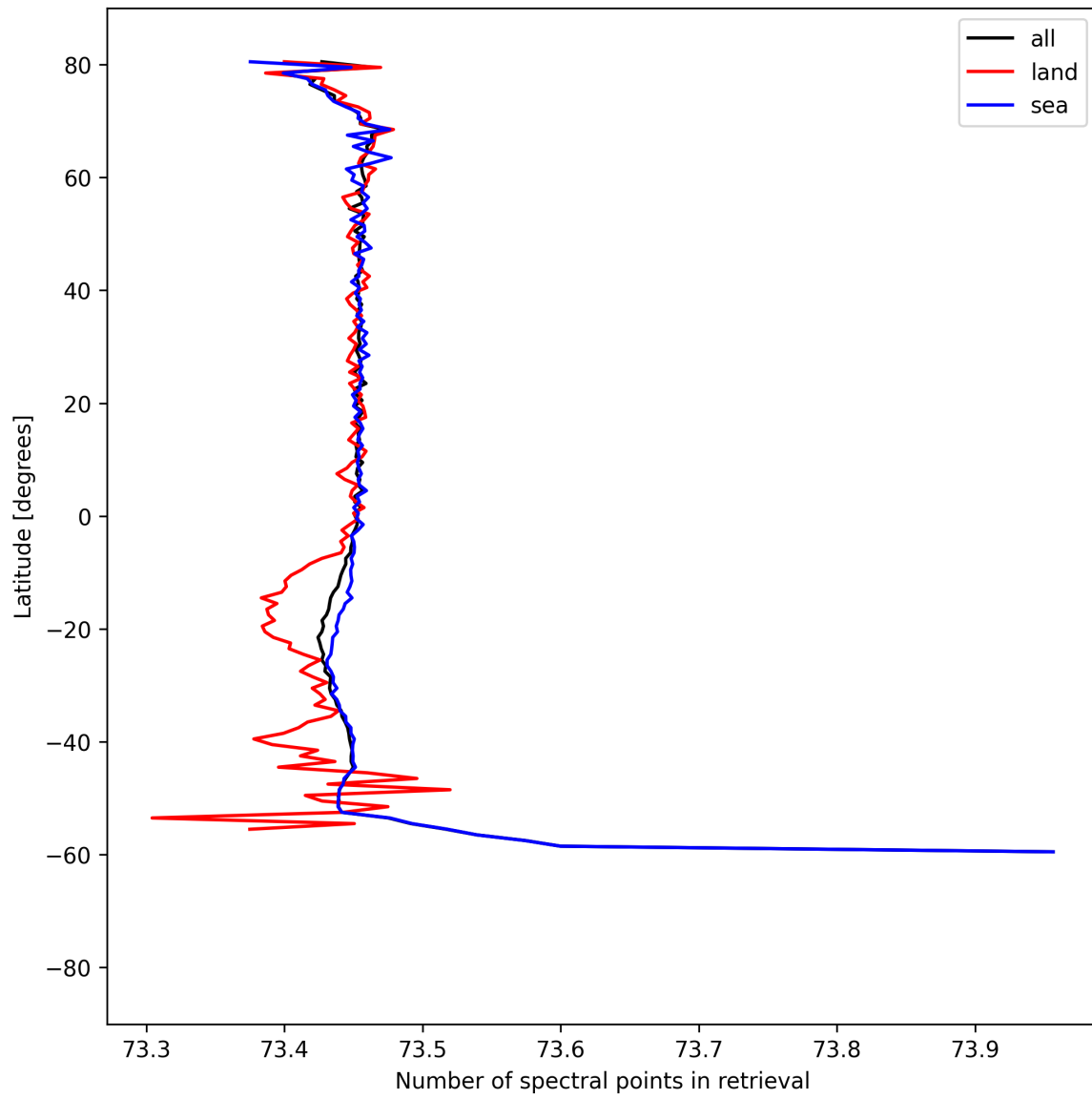
Figure 56: Zonal average of “Number of spectral points in retrieval” for 2025-08-25 to 2025-08-27.
