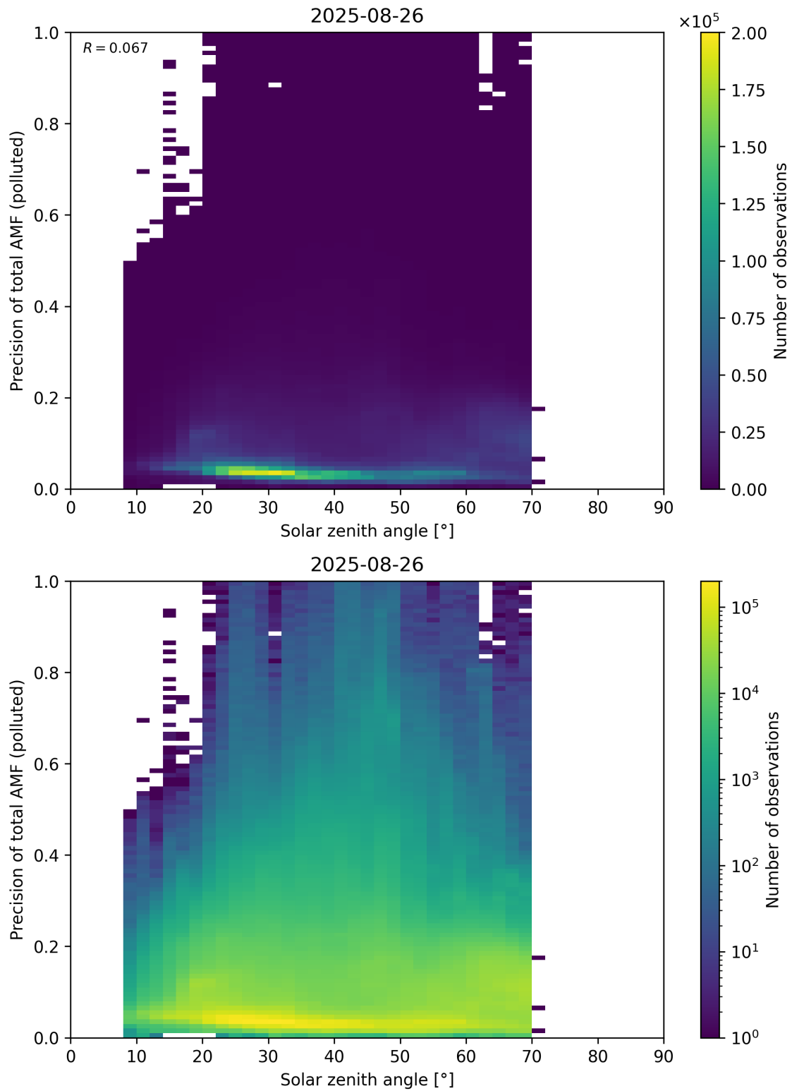
Figure 190: Scatter density plot of “Solar zenith angle” against “Precision of total AMF (polluted)” for 2025-08-25 to 2025-08-27.
