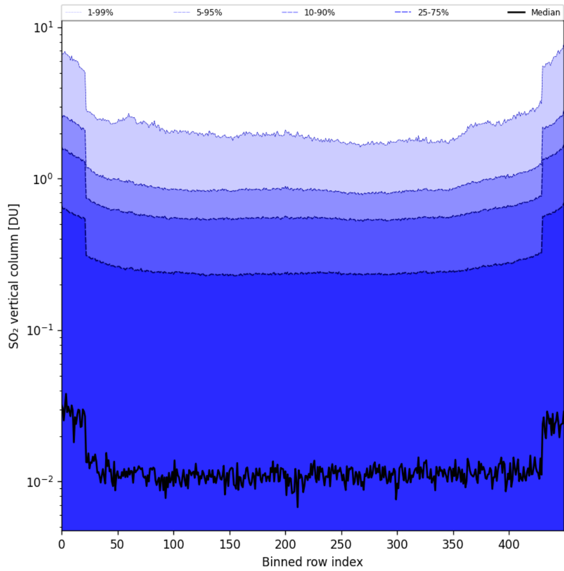
Figure 84: Along track statistics of “SO 2 vertical column” for 2025-08-25 to 2025-08-27
