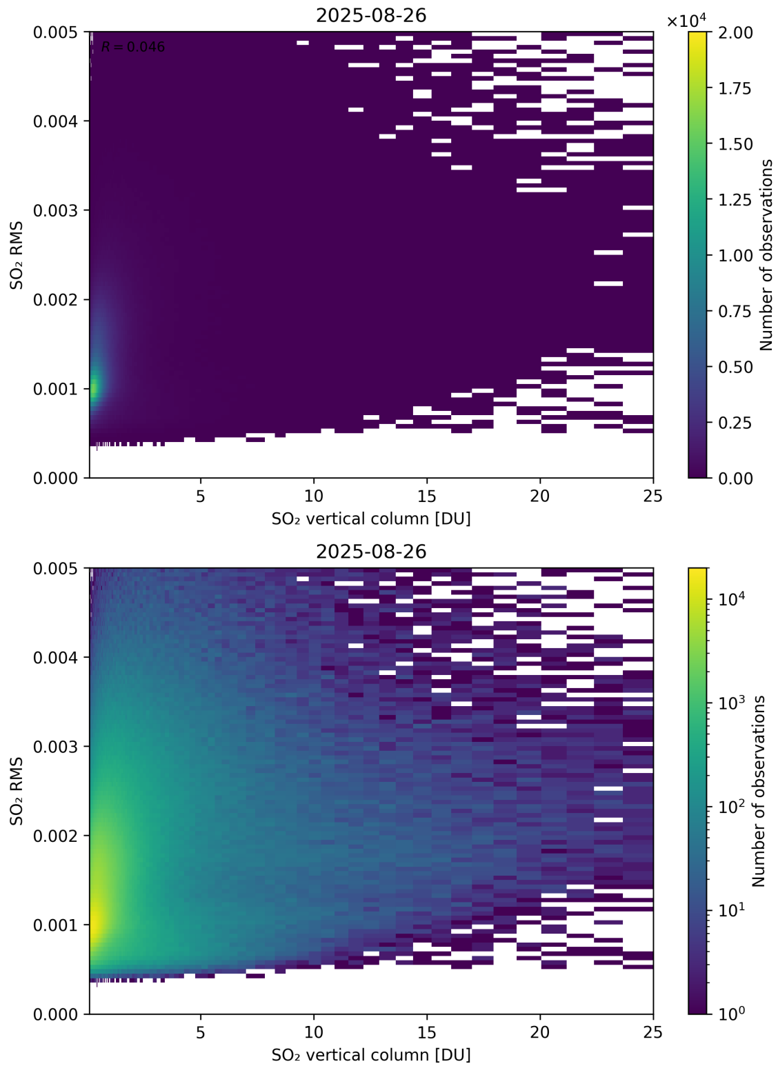
Figure 328: Scatter density plot of “SO 2 vertical column” against “SO 2 RMS” for 2025-08-25 to 2025-08-27.
