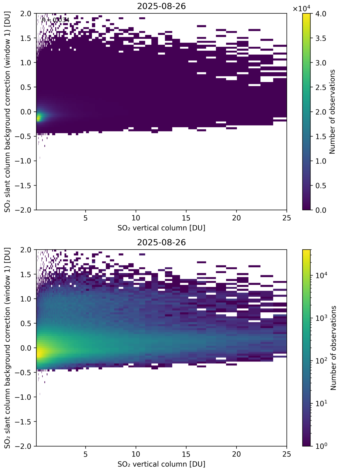
Figure 323: Scatter density plot of “SO 2 vertical column” against “SO 2 slant column background correction (window 1)” for 2025-08-25 to 2025-08-27.
