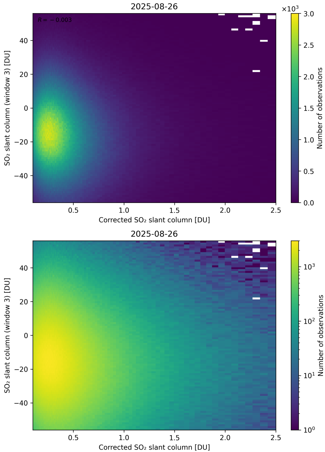
Figure 240: Scatter density plot of “Corrected SO 2 slant column” against “SO 2 slant column (window 3)” for 2025-08-25 to 2025-08-27.
