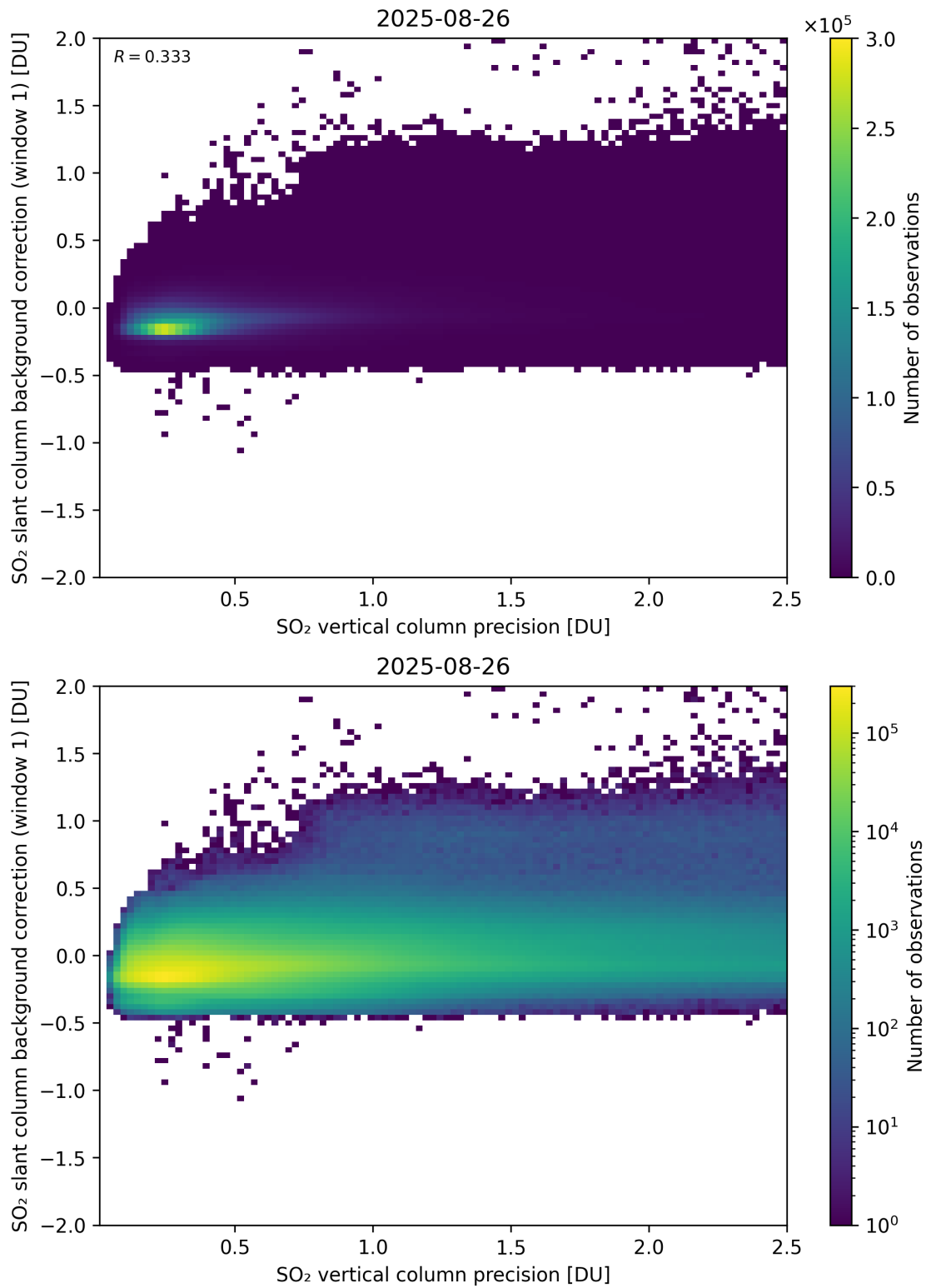
Figure 329: Scatter density plot of “SO 2 vertical column precision” against “SO 2 slant column background correction (window 1)” for 2025-08-25 to 2025-08-27.
