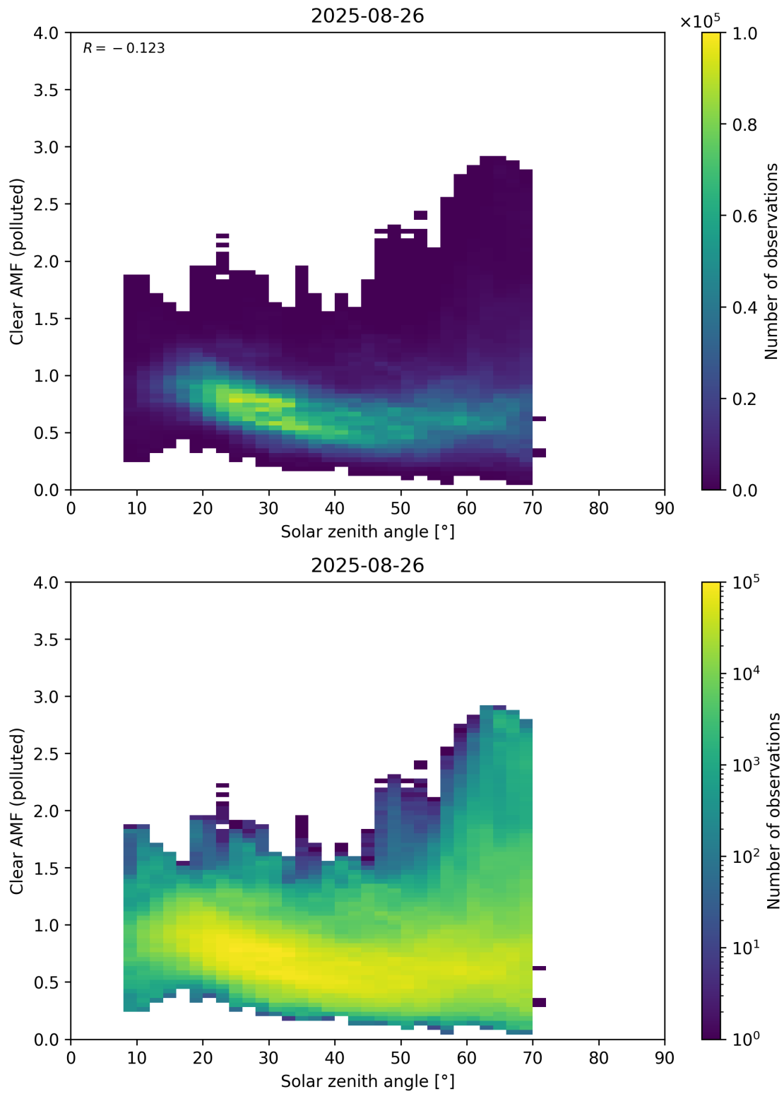
Figure 178: Scatter density plot of “Solar zenith angle” against “Clear AMF (polluted)” for 2025-08-25 to 2025-08-27.
