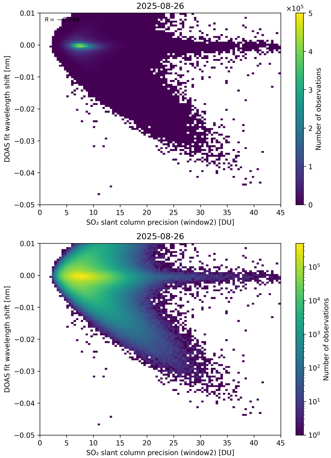
Figure 293: Scatter density plot of “SO 2 slant column precision (window2)” against “DOAS fit wavelength shift” for 2025-08-25 to 2025-08-27.
