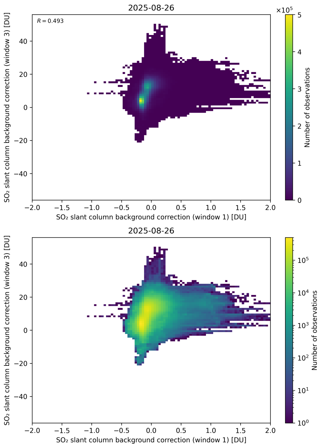
Figure 110: Scatter density plot of “SO 2 slant column background correction (window 1)” against “SO 2 slant column background correction (window 3)” for 2025-08-25 to 2025-08-27.
