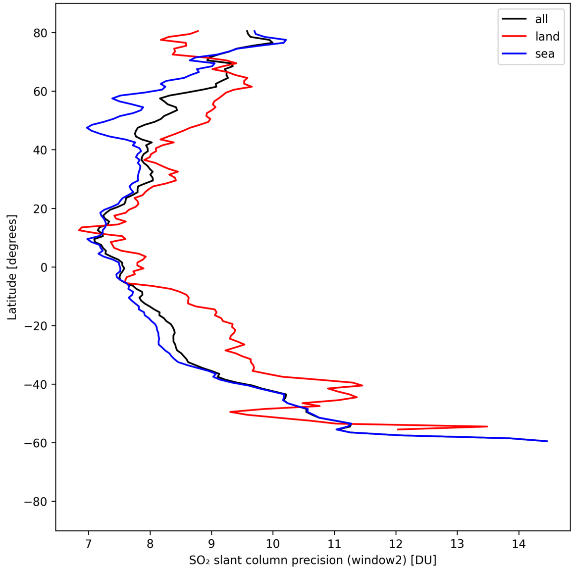
Figure 42: Zonal average of “SO 2 slant column precision (window2)” for 2025-08-25 to 2025-08-27.
