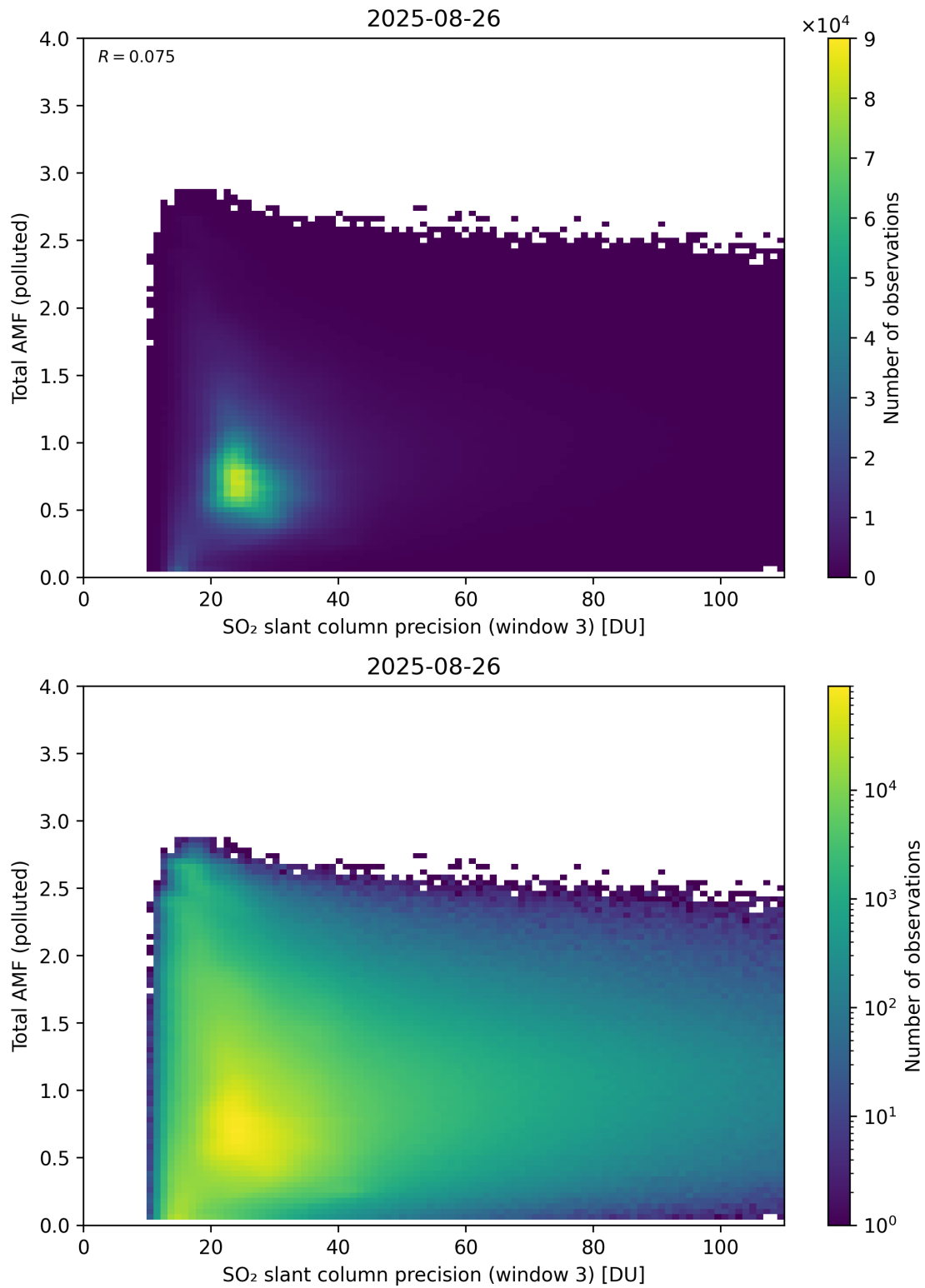
Figure 313: Scatter density plot of “SO 2 slant column precision (window 3)” against “Total AMF (polluted)” for 2025-08-25 to 2025-08-27.
