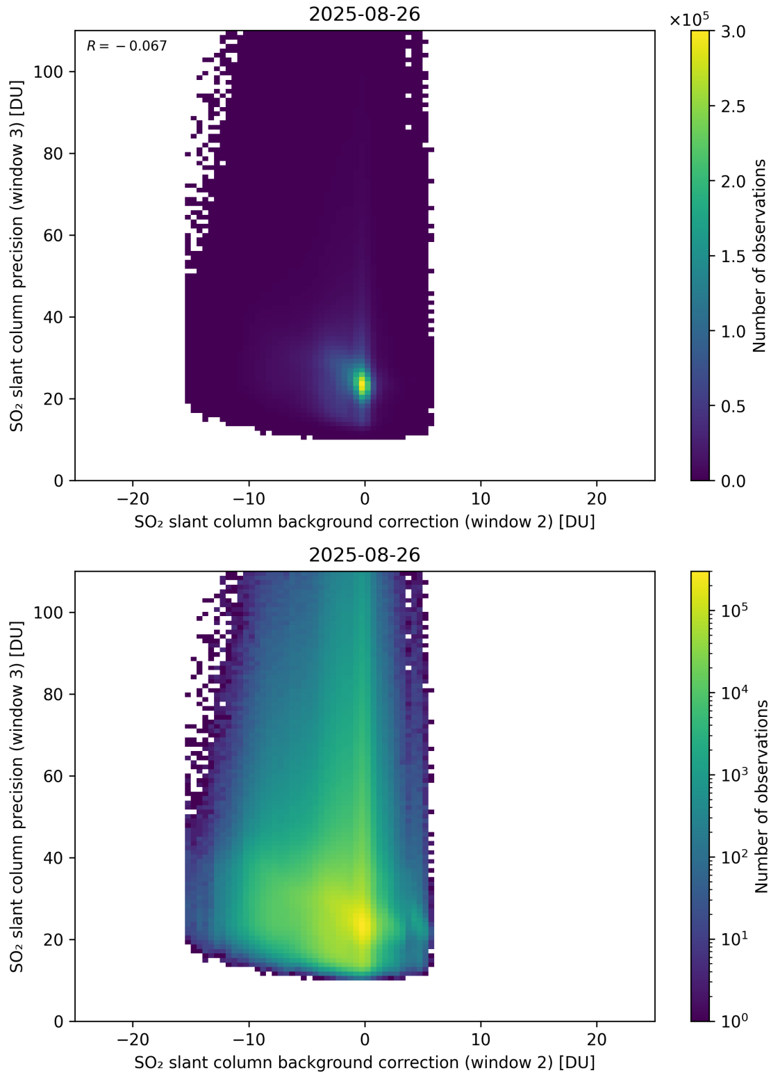
Figure 129: Scatter density plot of “SO 2 slant column background correction (window 2)” against “SO 2 slant column precision (window 3)” for 2025-08-25 to 2025-08-27.
