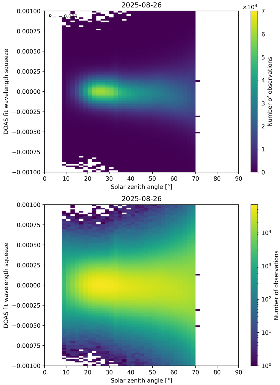
Figure 175: Scatter density plot of “Solar zenith angle” against “DOAS fit wavelength squeeze” for 2025-08-25 to 2025-08-27.
