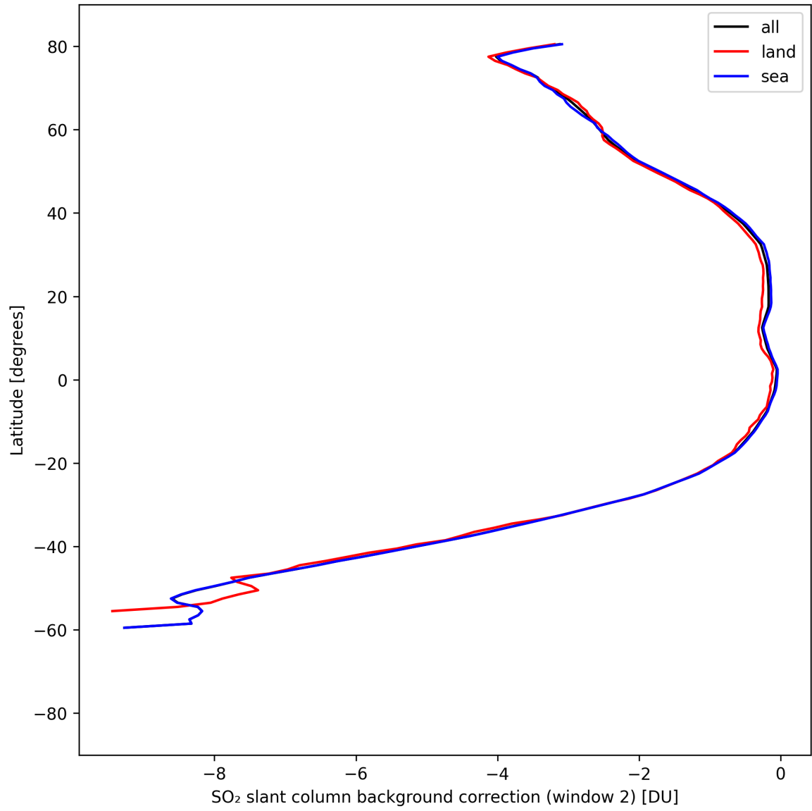
Figure 44: Zonal average of “SO 2 slant column background correction (window 2)” for 2025-08-25 to 2025-08-27.
