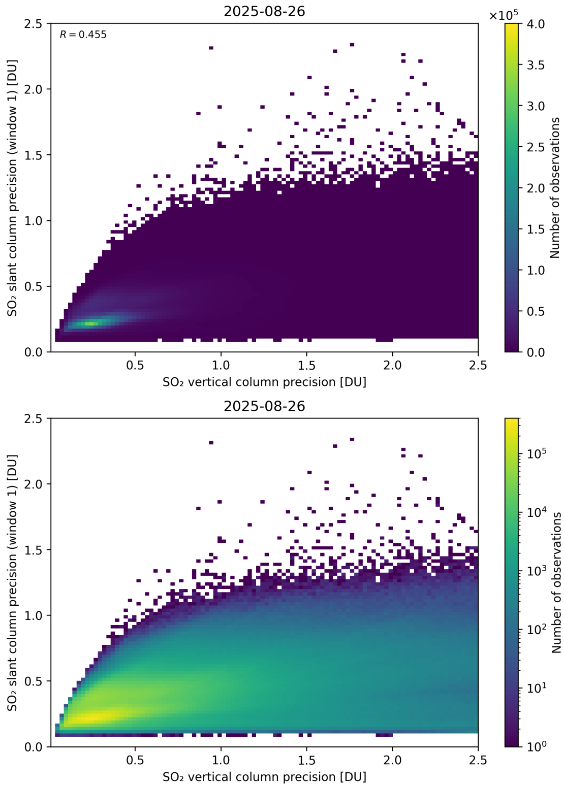
Figure 342: Scatter density plot of “SO 2 vertical column precision” against “SO 2 slant column precision (window 1)” for 2025-08-25 to 2025-08-27.
