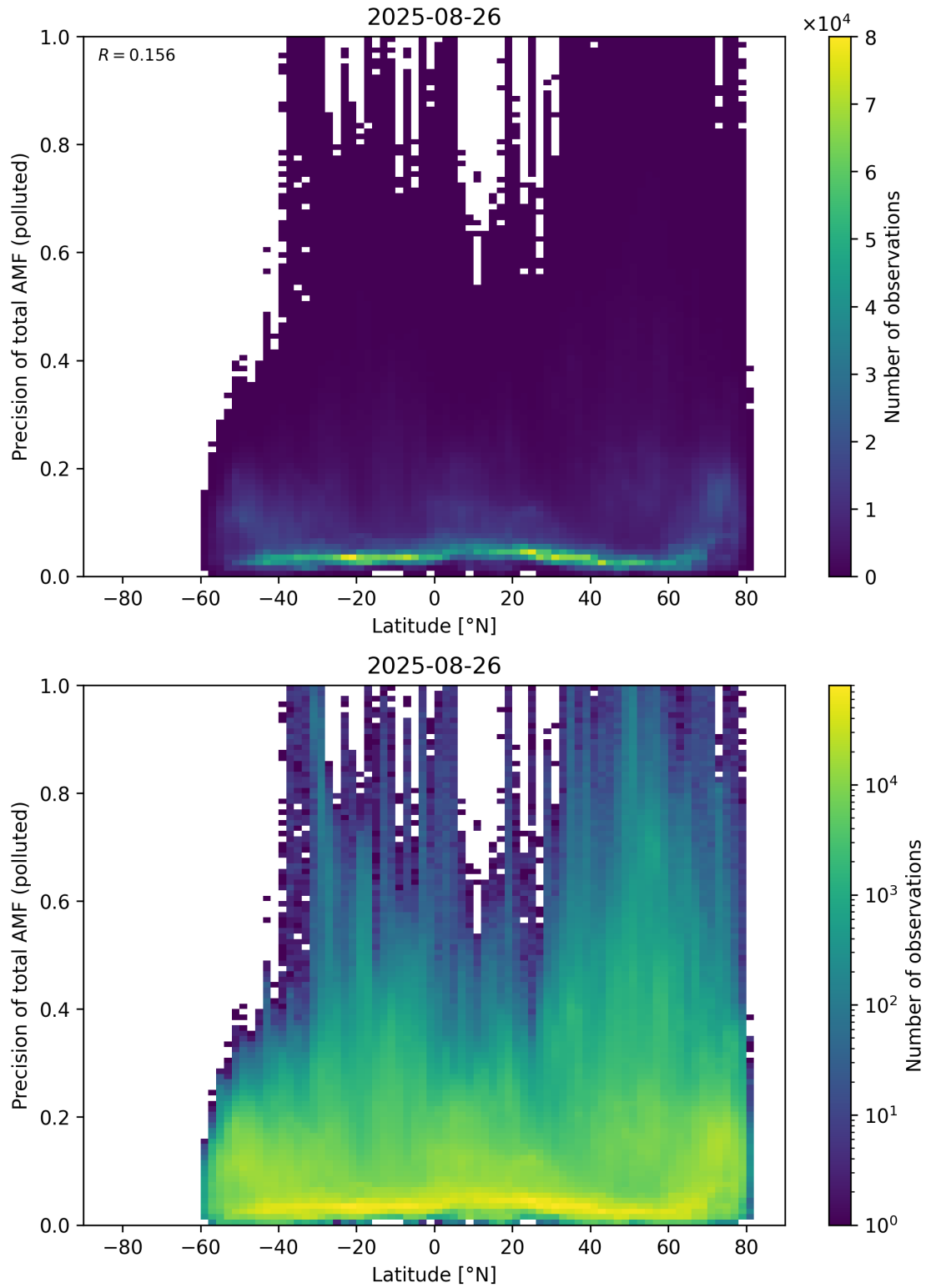
Figure 168: Scatter density plot of “Latitude” against “Precision of total AMF (polluted)” for 2025-08-25 to 2025-08-27.
