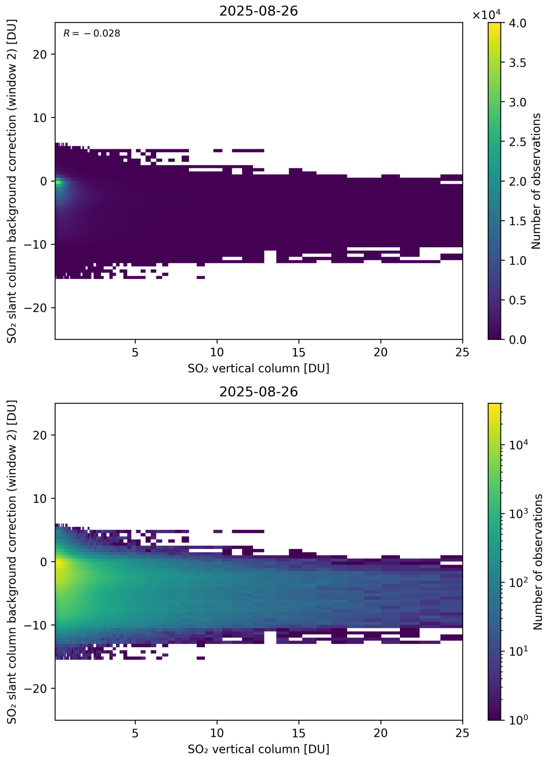
Figure 324: Scatter density plot of “SO 2 vertical column” against “SO 2 slant column background correction (window 2)” for 2025-08-25 to 2025-08-27.
