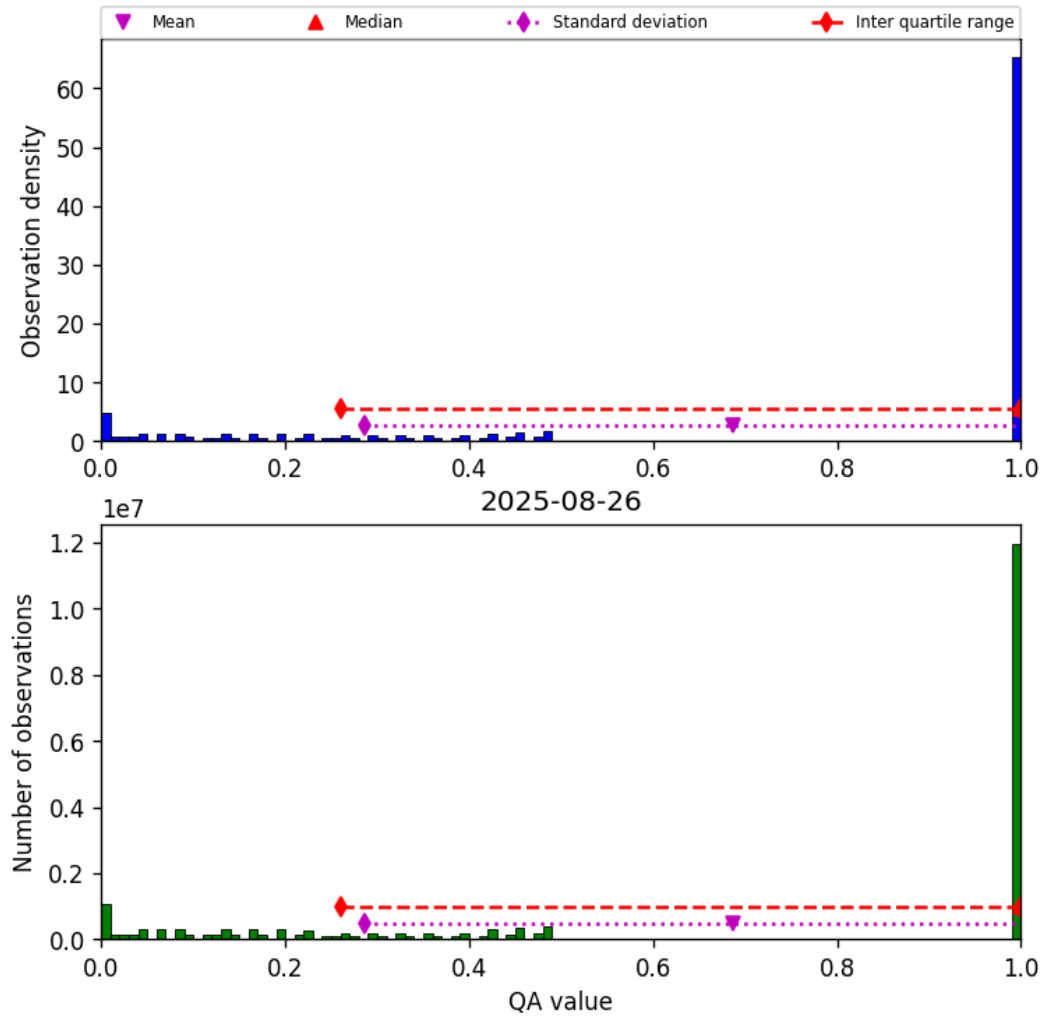
Figure 57: Histogram of “QA value” for 2025-08-25 to 2025-08-27
