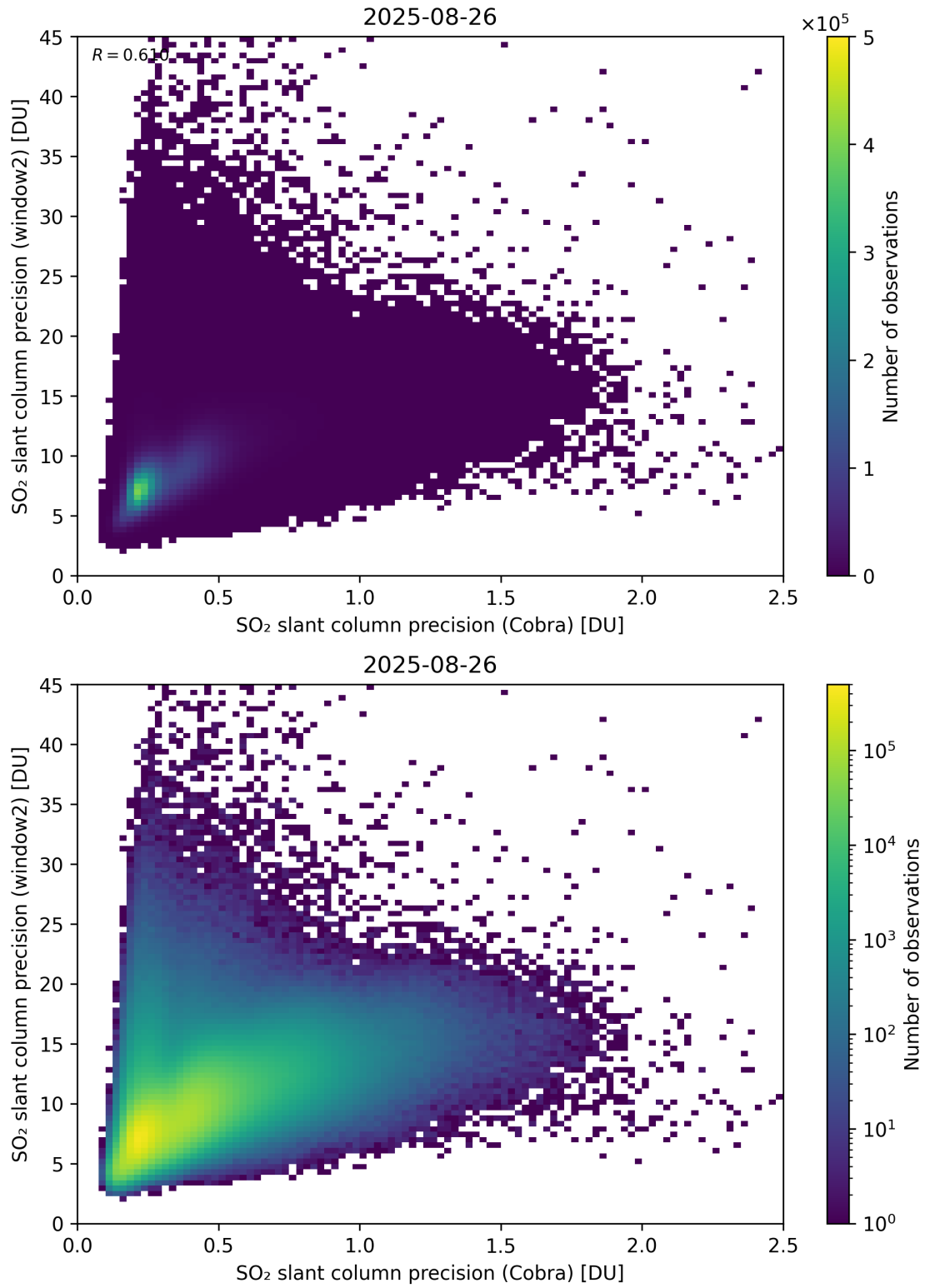
Figure 210: Scatter density plot of “SO 2 slant column precision (Cobra)” against “SO 2 slant column precision (window2)” for 2025-08-25 to 2025-08-27.
