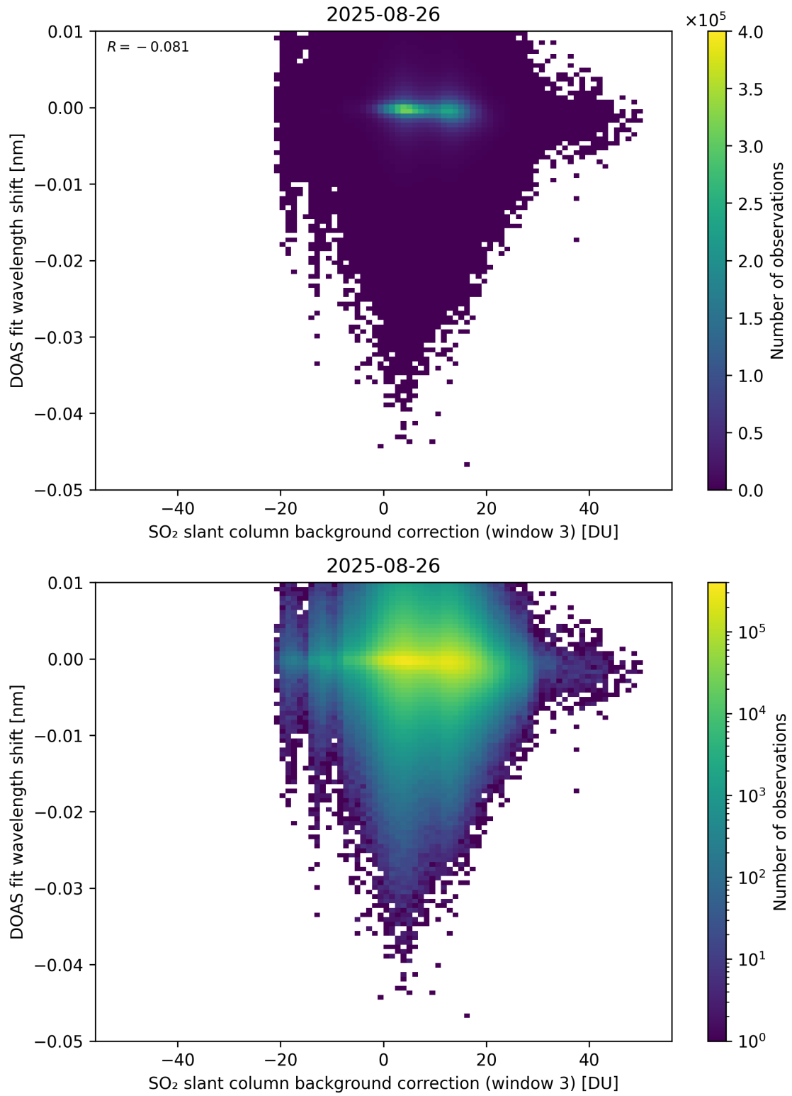
Figure 132: Scatter density plot of “SO 2 slant column background correction (window 3)” against “DOAS fit wavelength shift” for 2025-08-25 to 2025-08-27.
