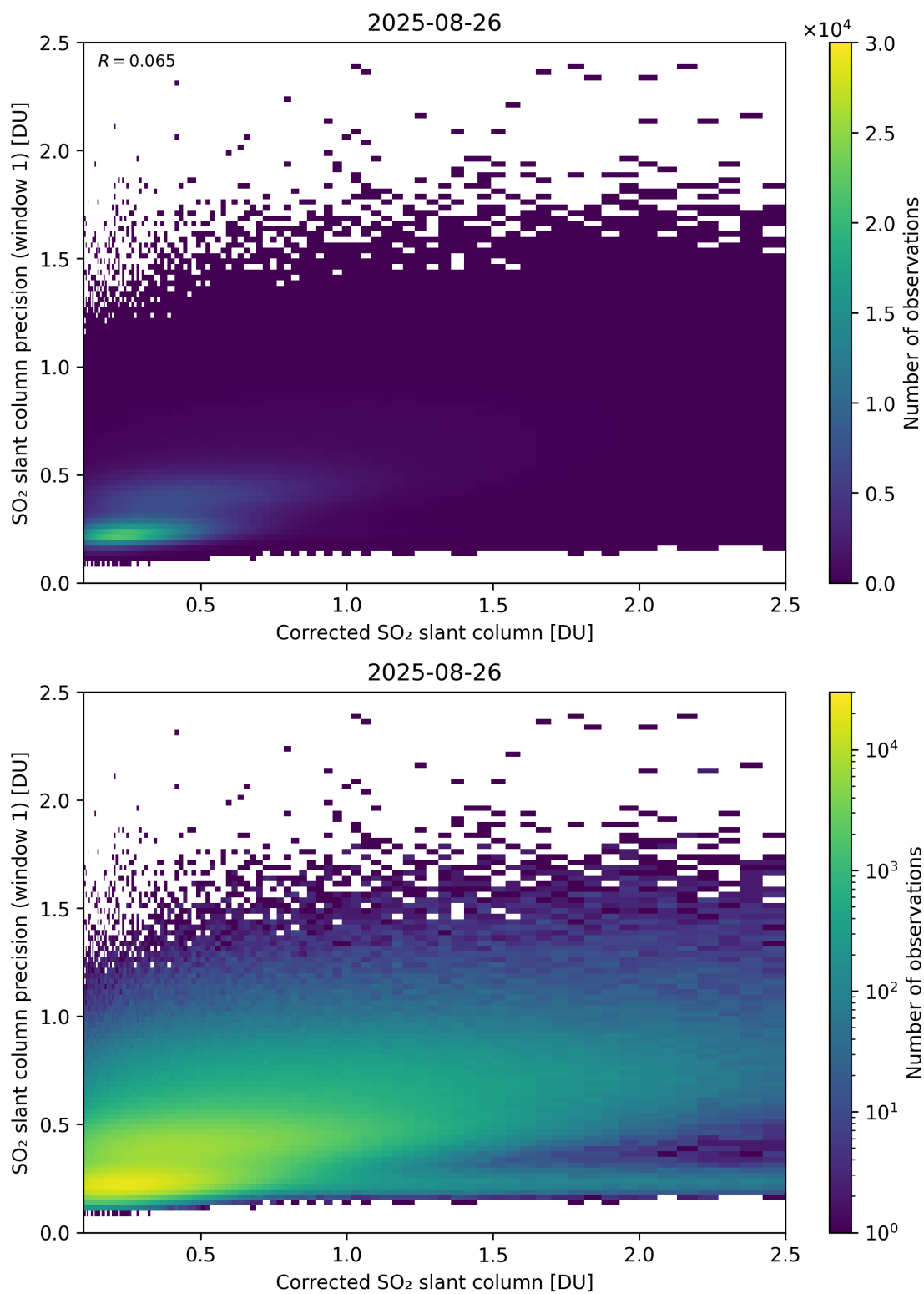
Figure 238: Scatter density plot of “Corrected SO 2 slant column” against “SO 2 slant column precision (window 1)” for 2025-08-25 to 2025-08-27.
