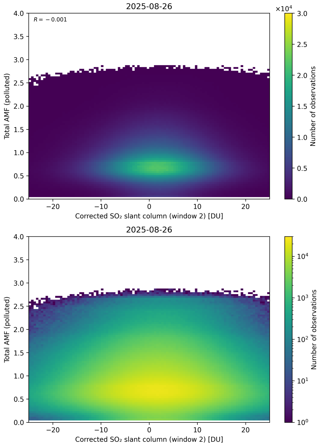
Figure 253: Scatter density plot of “Corrected SO 2 slant column (window 2)” against “Total AMF (polluted)” for 2025-08-25 to 2025-08-27.
