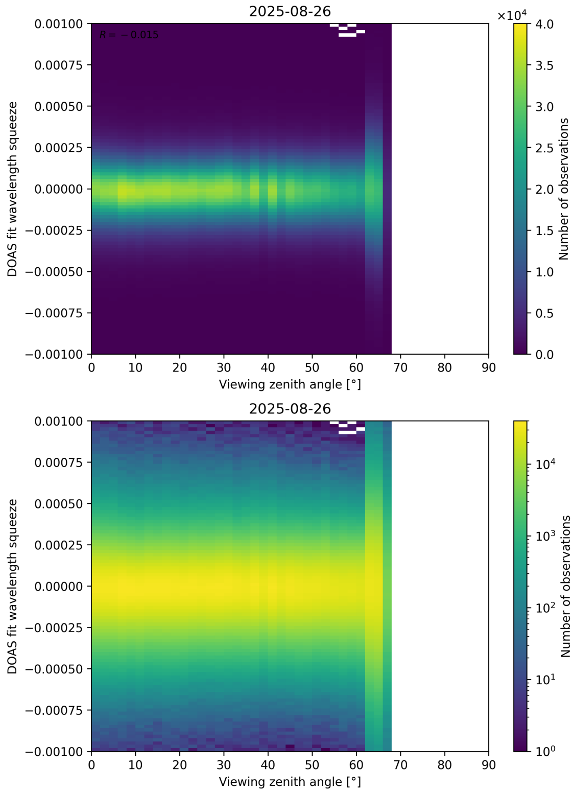
Figure 366: Scatter density plot of “Viewing zenith angle” against “DOAS fit wavelength squeeze” for 2025-08-25 to 2025-08-27.
