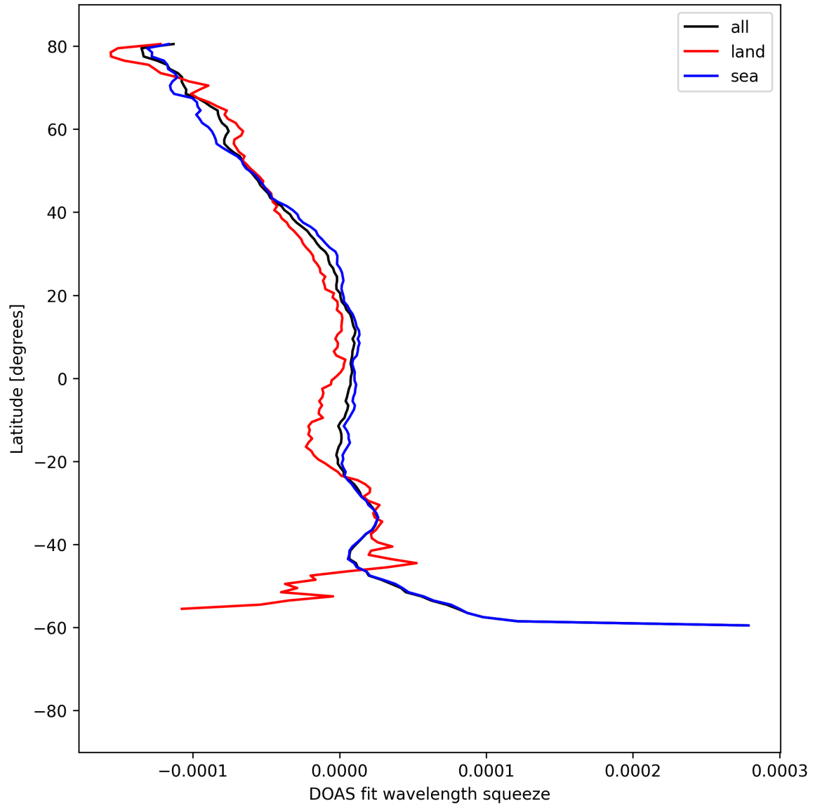
Figure 51: Zonal average of “DOAS fit wavelength squeeze” for 2025-08-25 to 2025-08-27.
