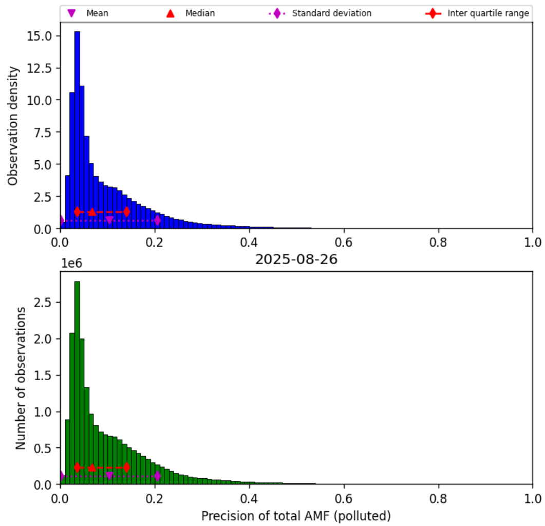
Figure 80: Histogram of “Precision of total AMF (polluted)” for 2025-08-25 to 2025-08-27
