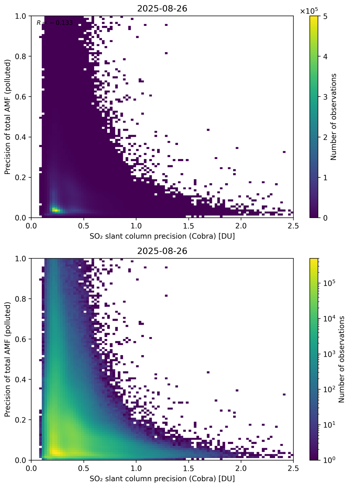
Figure 214: Scatter density plot of “SO 2 slant column precision (Cobra)” against “Precision of total AMF (polluted)” for 2025-08-25 to 2025-08-27.
