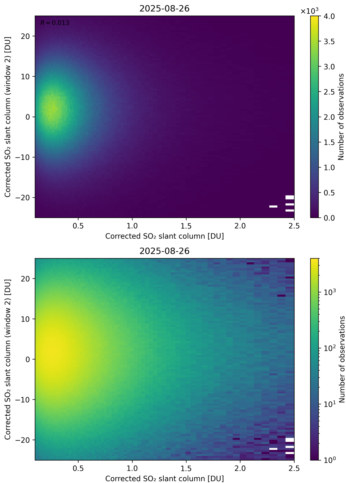
Figure 235: Scatter density plot of “Corrected SO 2 slant column” against “Corrected SO 2 slant column (window 2)” for 2025-08-25 to 2025-08-27.
