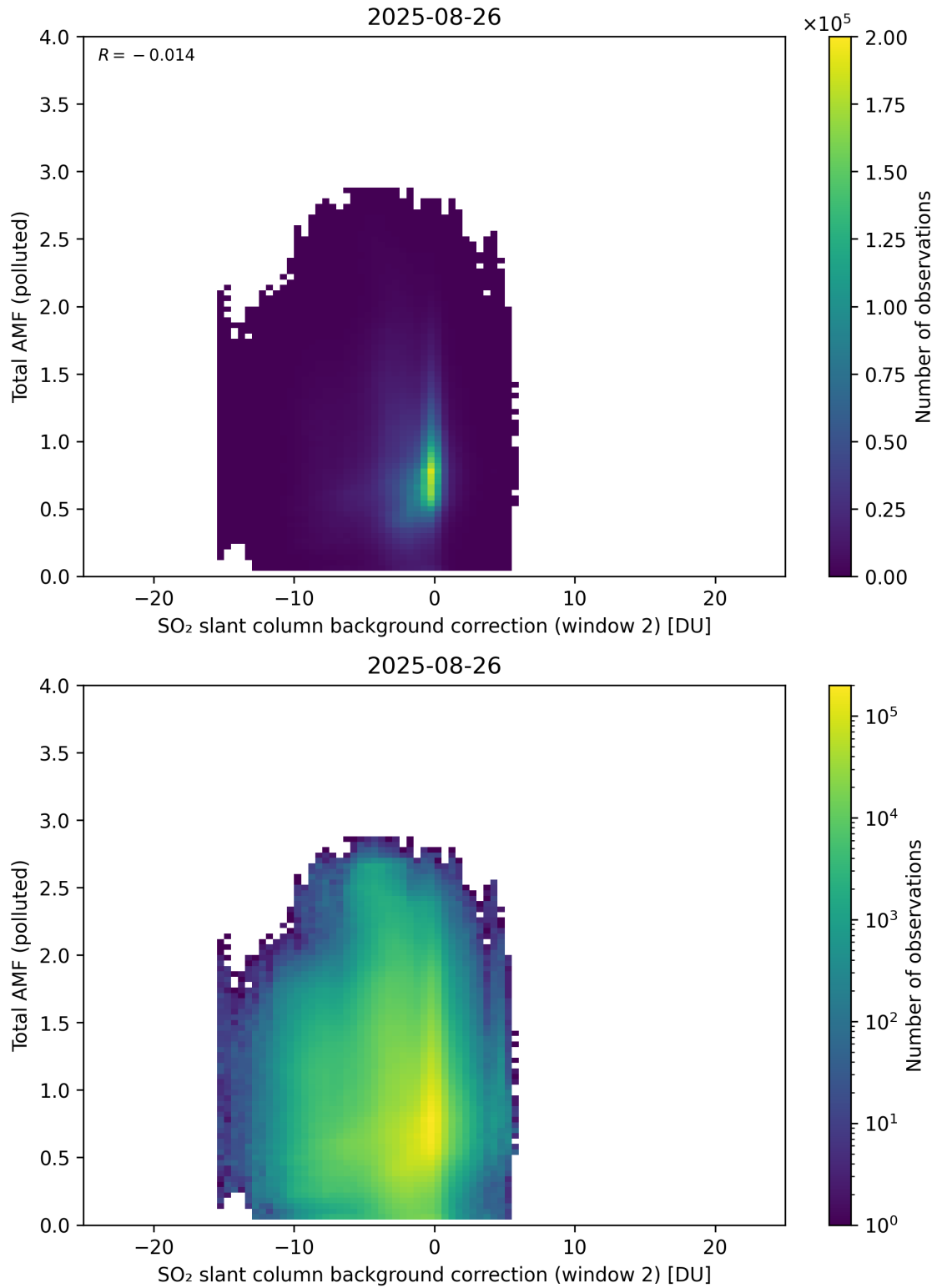
Figure 130: Scatter density plot of “SO 2 slant column background correction (window 2)” against “Total AMF (polluted)” for 2025-08-25 to 2025-08-27.
