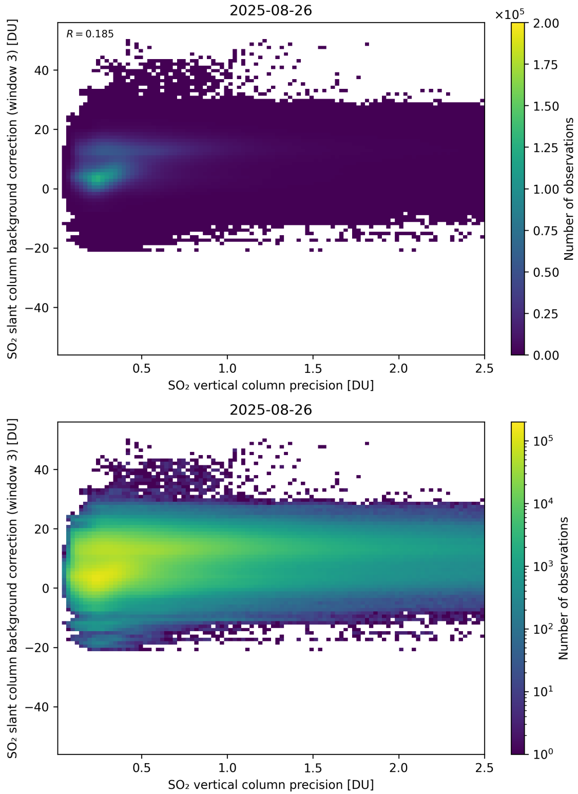
Figure 331: Scatter density plot of “SO 2 vertical column precision” against “SO 2 slant column background correction (window 3)” for 2025-08-25 to 2025-08-27.
