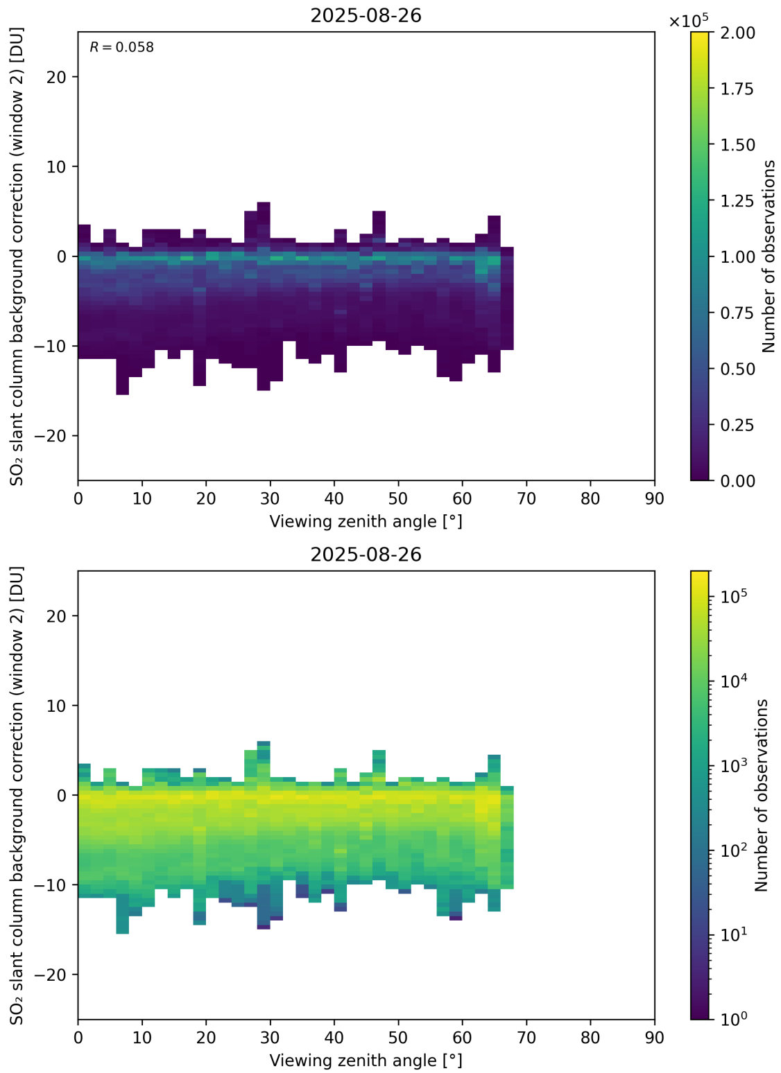
Figure 363: Scatter density plot of “Viewing zenith angle” against “SO 2 slant column background correction (window 2)” for 2025-08-25 to 2025-08-27.
