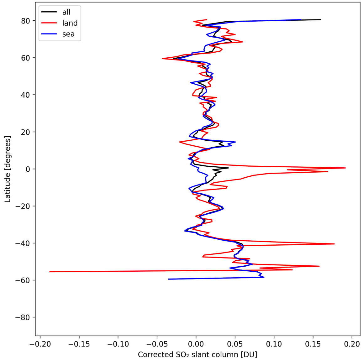
Figure 34: Zonal average of “Corrected SO 2 slant column” for 2025-08-25 to 2025-08-27.
