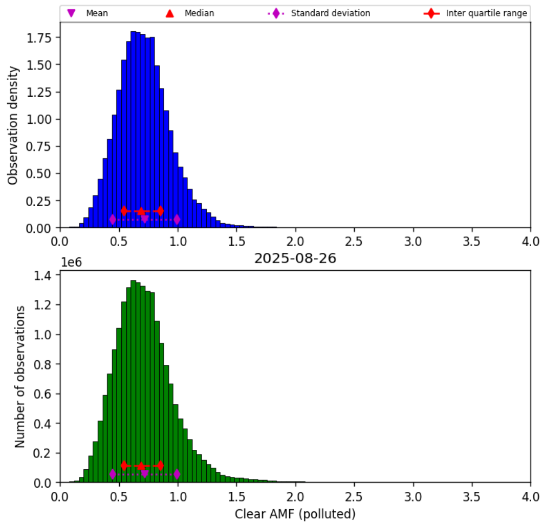
Figure 81: Histogram of “Clear AMF (polluted)” for 2025-08-25 to 2025-08-27
