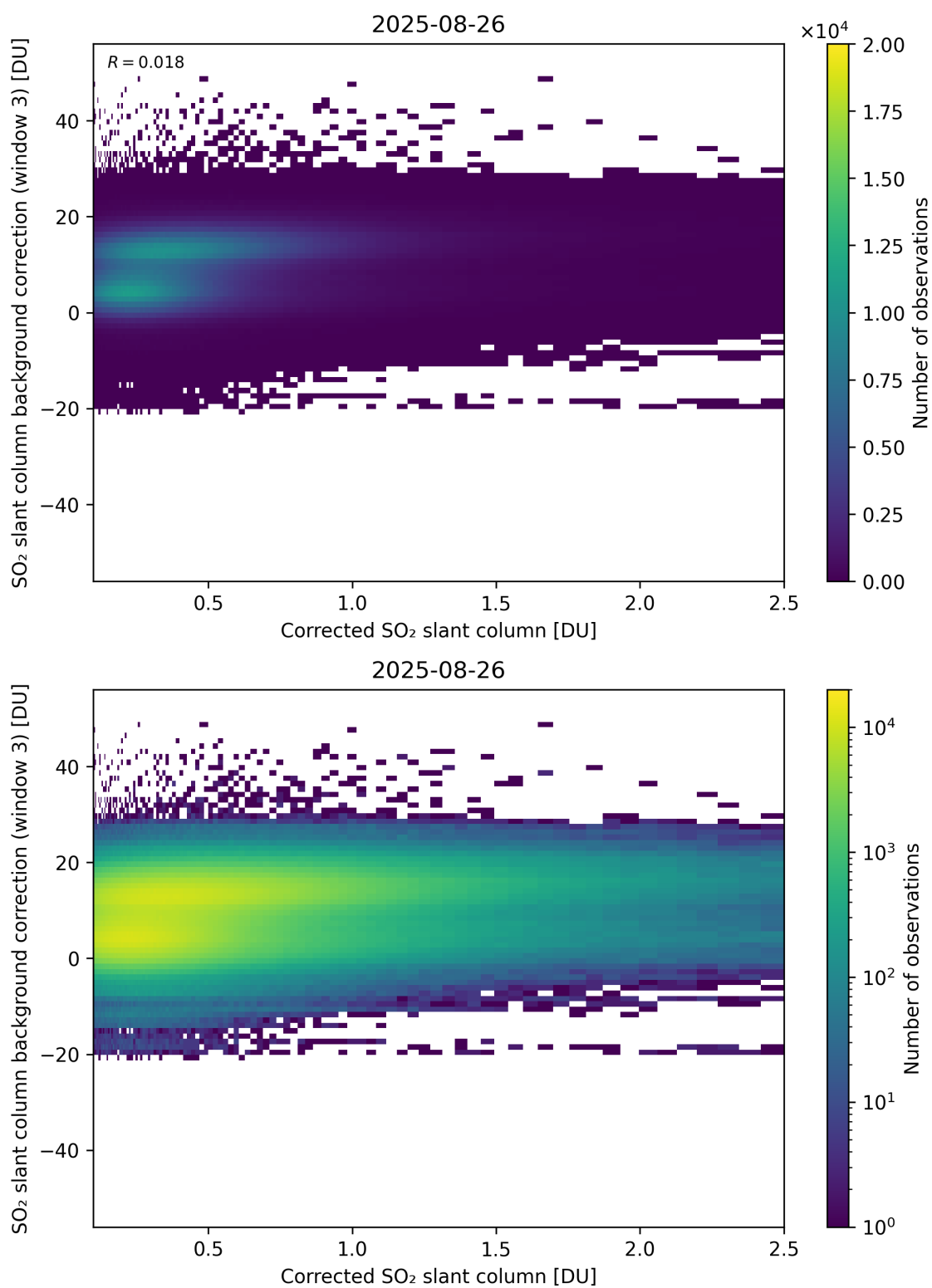
Figure 228: Scatter density plot of “Corrected SO 2 slant column” against “SO 2 slant column background correction (window 3)” for 2025-08-25 to 2025-08-27.
