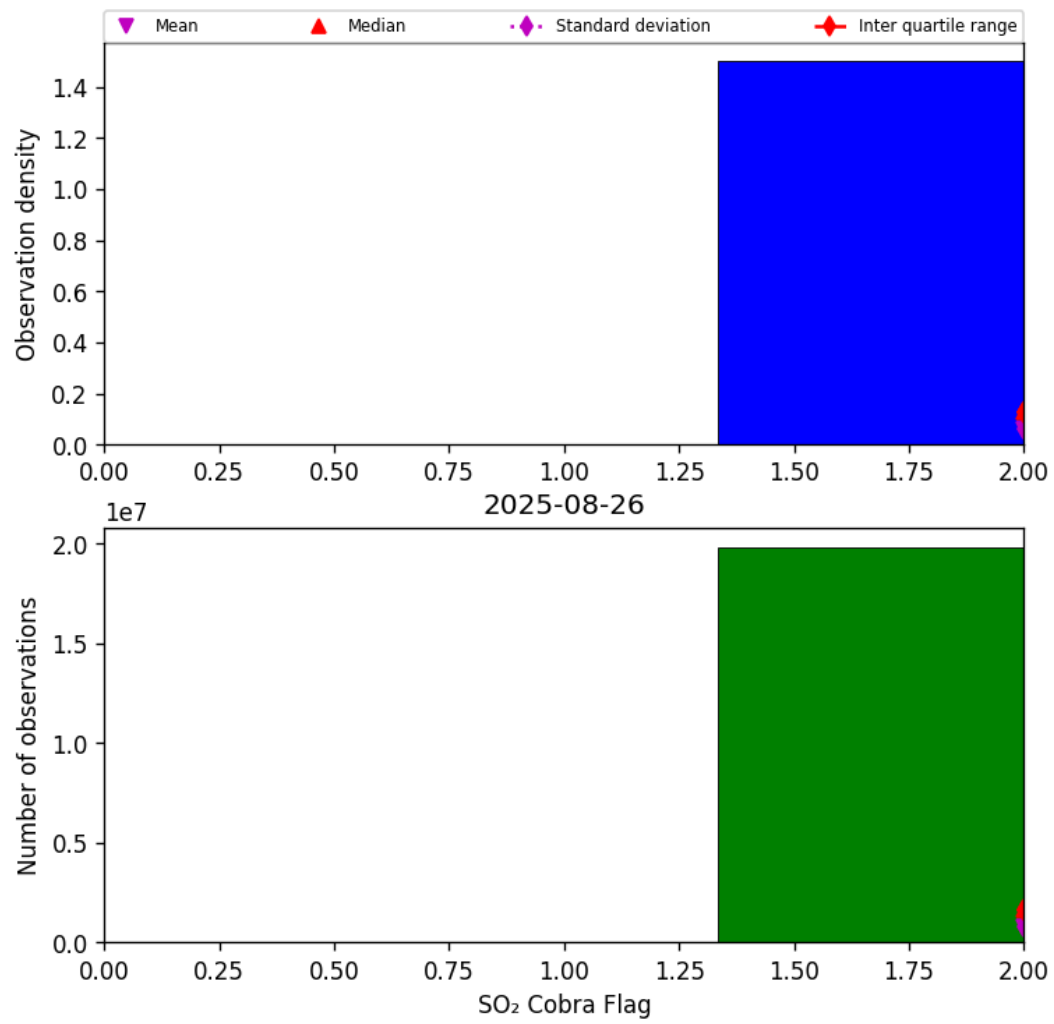
Figure 75: Histogram of “SO 2 Cobra Flag” for 2025-08-25 to 2025-08-27
