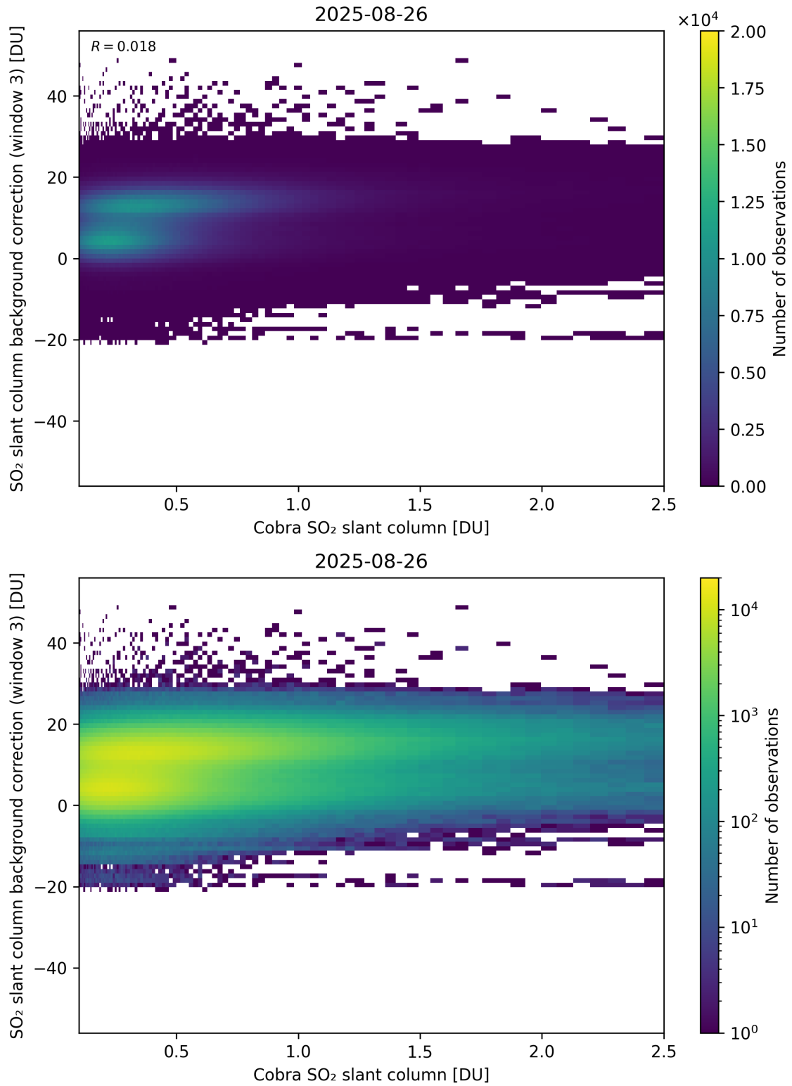
Figure 195: Scatter density plot of “Cobra SO 2 slant column” against “SO 2 slant column background correction (window 3)” for 2025-08-25 to 2025-08-27.
