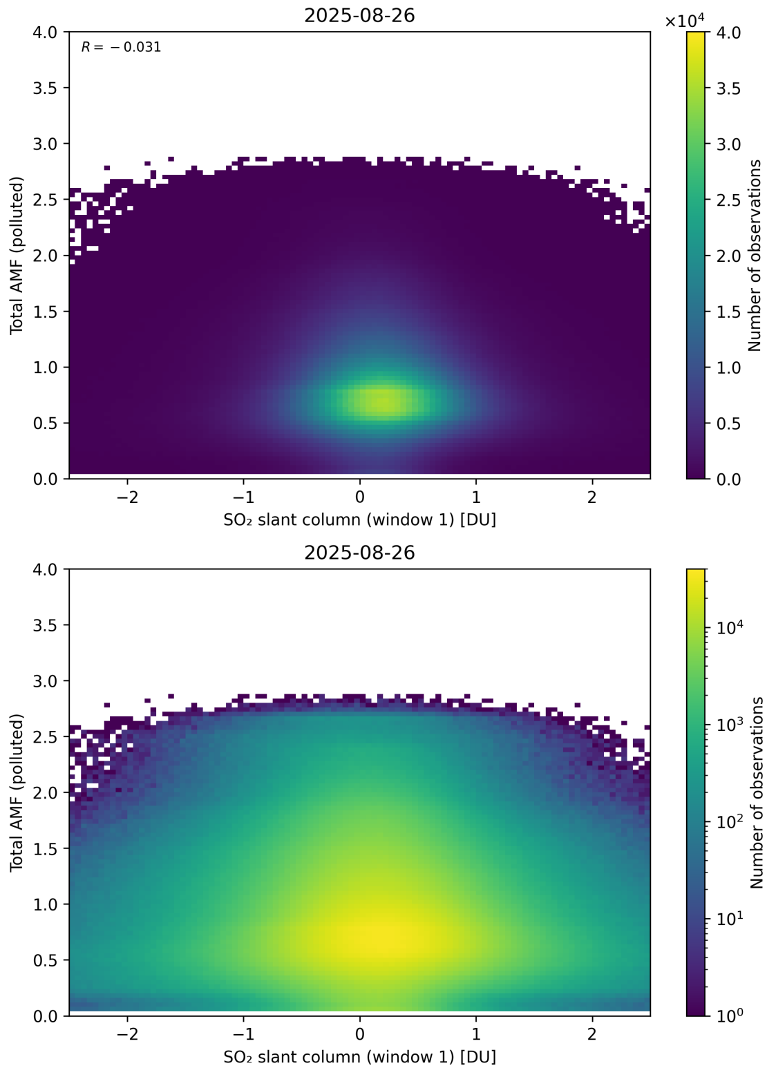
Figure 289: Scatter density plot of “SO 2 slant column (window 1)” against “Total AMF (polluted)” for 2025-08-25 to 2025-08-27.
