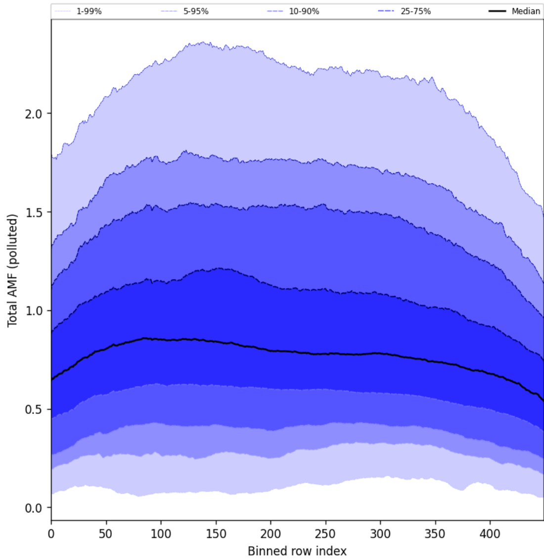
Figure 105: Along track statistics of “Total AMF (polluted)” for 2025-08-25 to 2025-08-27
