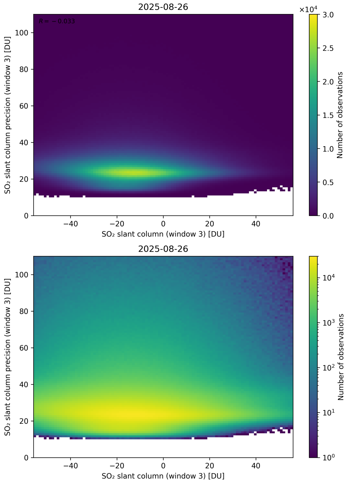
Figure 317: Scatter density plot of “SO 2 slant column (window 3)” against “SO 2 slant column precision (window 3)” for 2025-08-25 to 2025-08-27.
