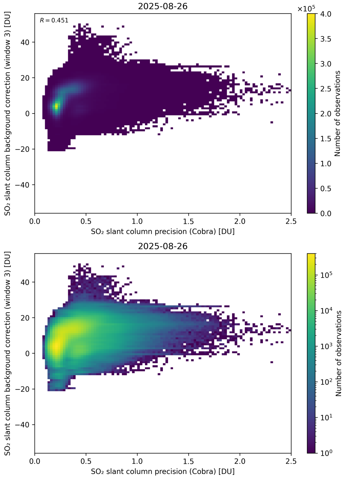
Figure 201: Scatter density plot of “SO 2 slant column precision (Cobra)” against “SO 2 slant column background correction (window 3)” for 2025-08-25 to 2025-08-27.
