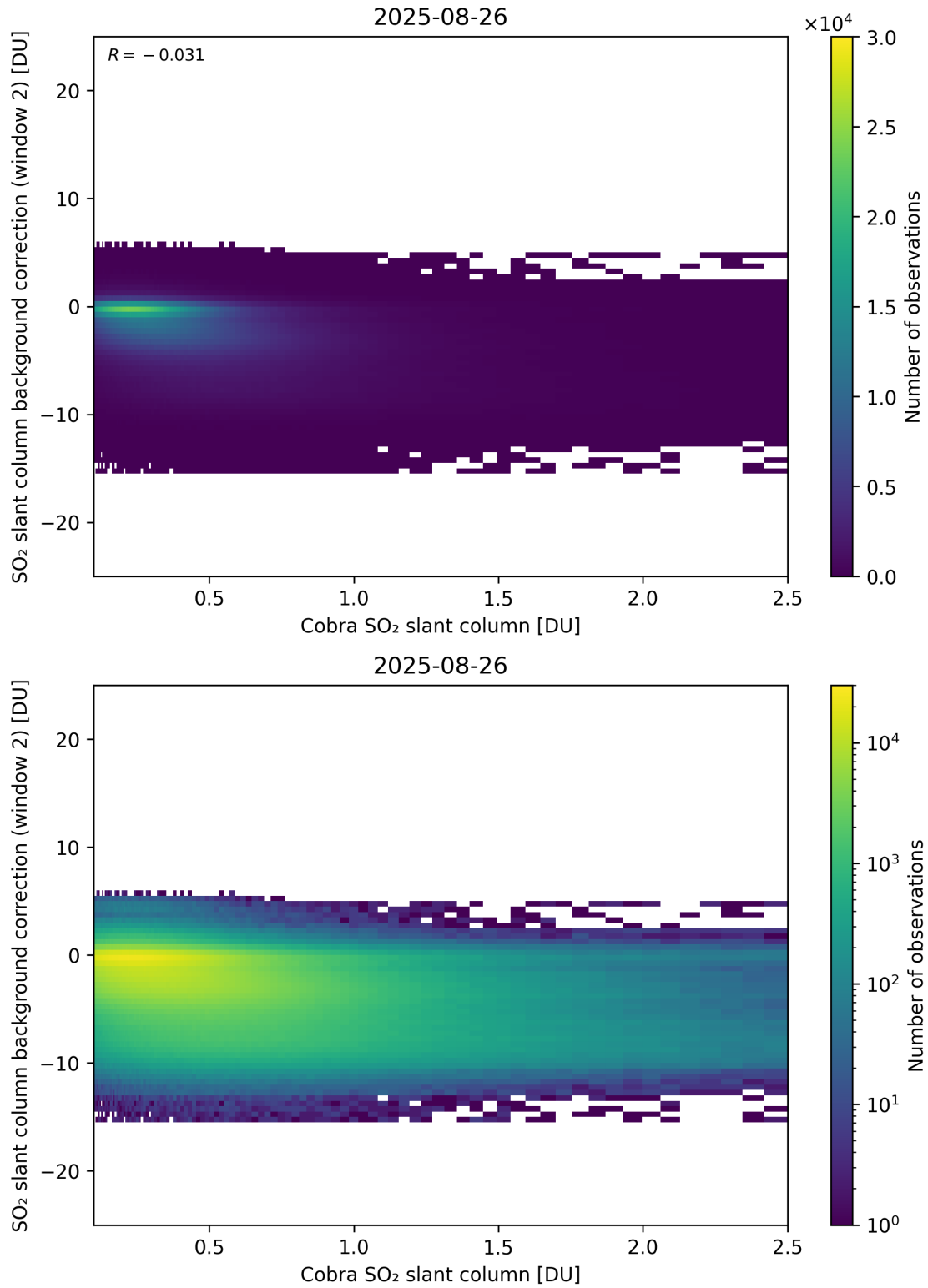
Figure 194: Scatter density plot of “Cobra SO 2 slant column” against “SO 2 slant column background correction (window 2)” for 2025-08-25 to 2025-08-27.
