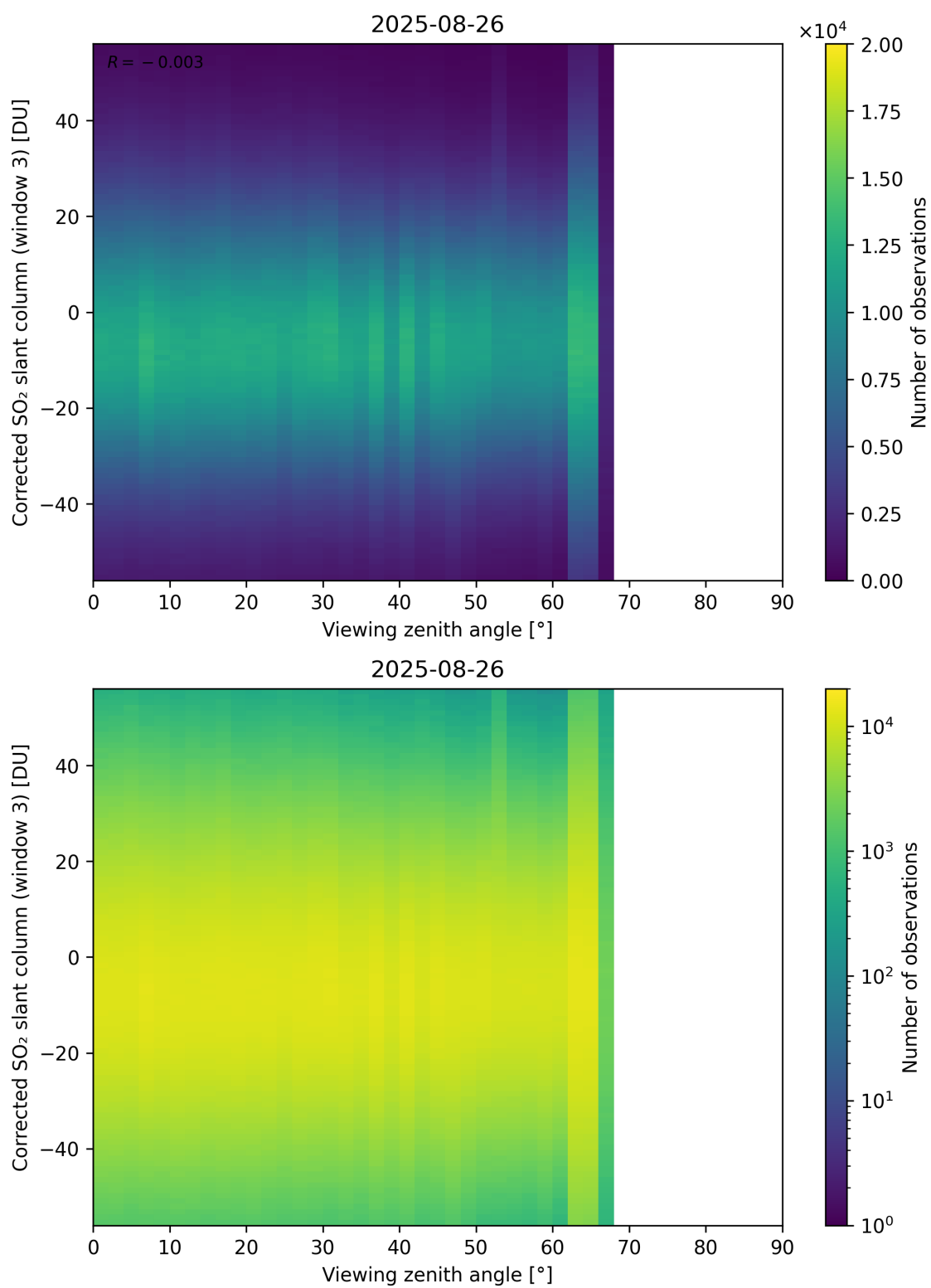
Figure 375: Scatter density plot of “Viewing zenith angle” against “Corrected SO 2 slant column (window 3)” for 2025-08-25 to 2025-08-27.
