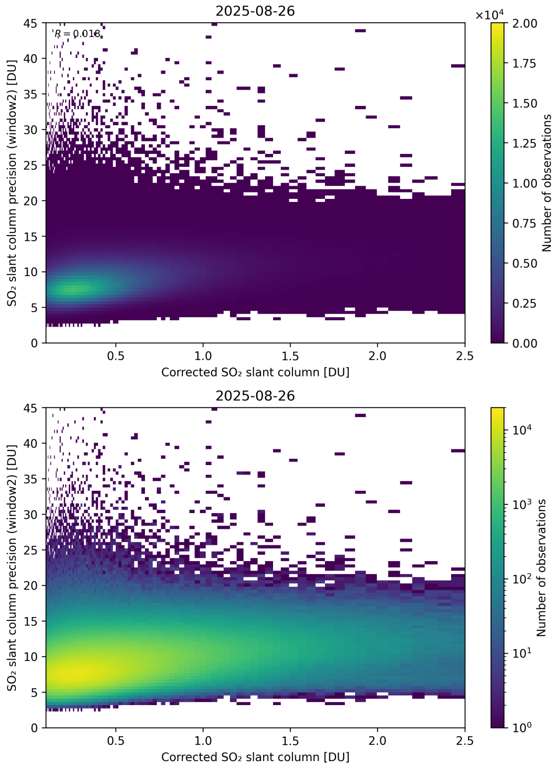
Figure 239: Scatter density plot of “Corrected SO 2 slant column” against “SO 2 slant column precision (window2)” for 2025-08-25 to 2025-08-27.
