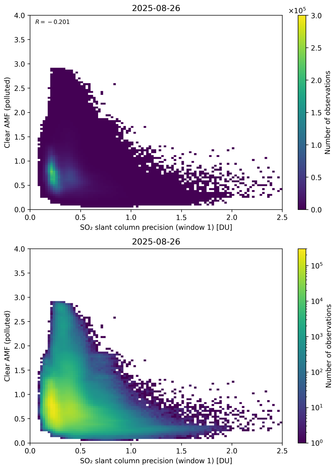
Figure 274: Scatter density plot of “SO 2 slant column precision (window 1)” against “Clear AMF (polluted)” for 2025-08-25 to 2025-08-27.
