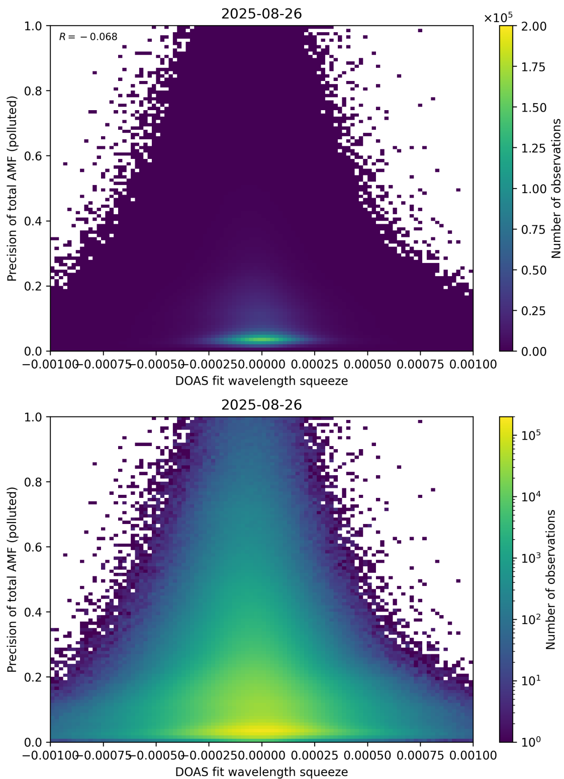
Figure 146: Scatter density plot of “DOAS fit wavelength squeeze” against “Precision of total AMF (polluted)” for 2025-08-25 to 2025-08-27.
