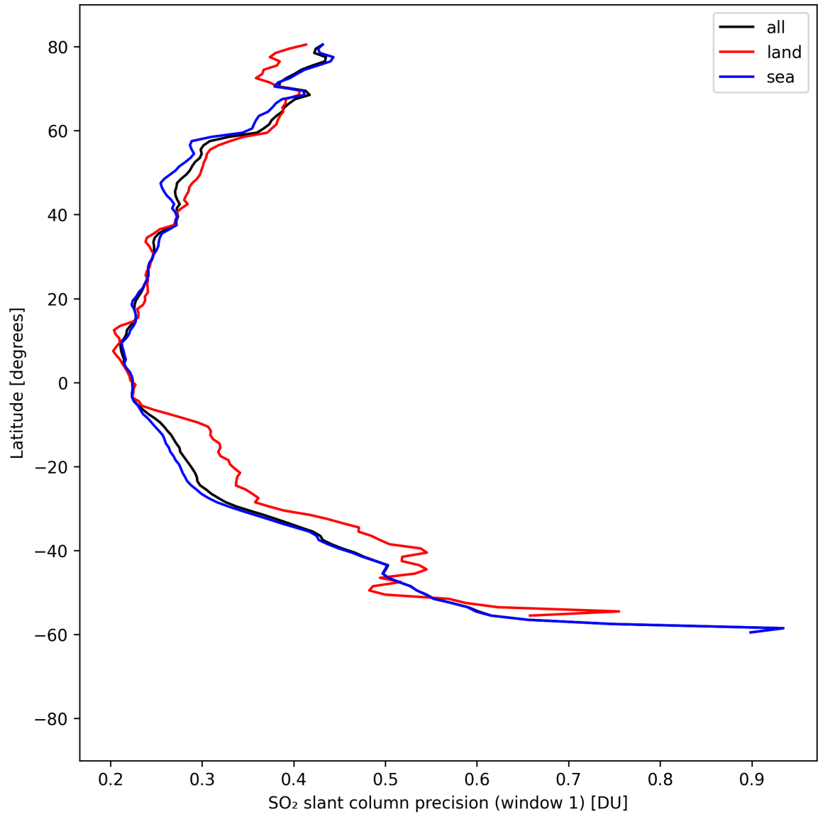
Figure 38: Zonal average of “SO 2 slant column precision (window 1)” for 2025-08-25 to 2025-08-27.
