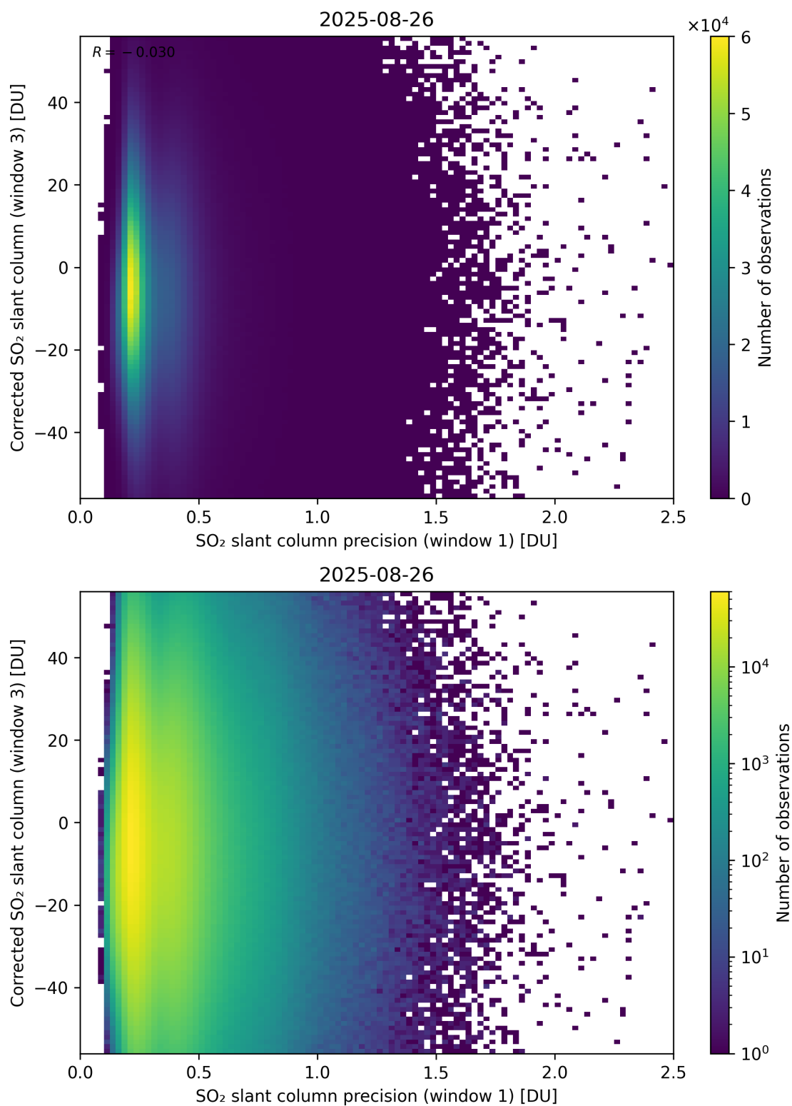
Figure 276: Scatter density plot of “SO 2 slant column precision (window 1)” against “Corrected SO 2 slant column (window 3)” for 2025-08-25 to 2025-08-27.
