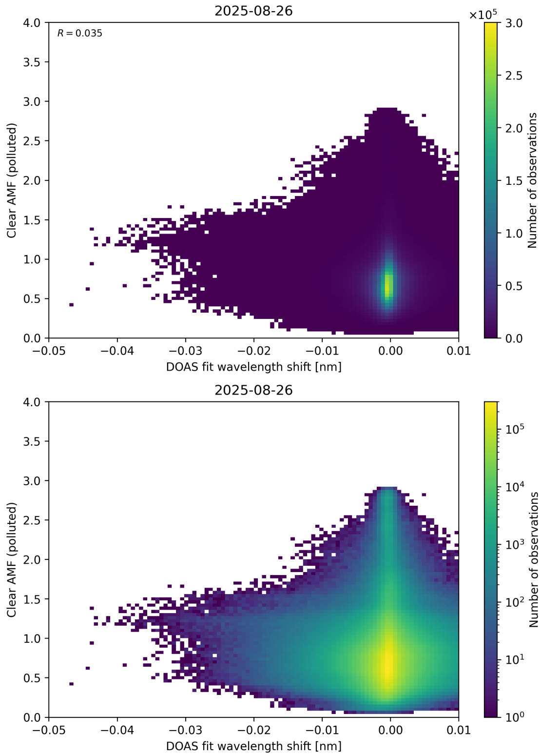
Figure 140: Scatter density plot of “DOAS fit wavelength shift” against “Clear AMF (polluted)” for 2025-08-25 to 2025-08-27.
