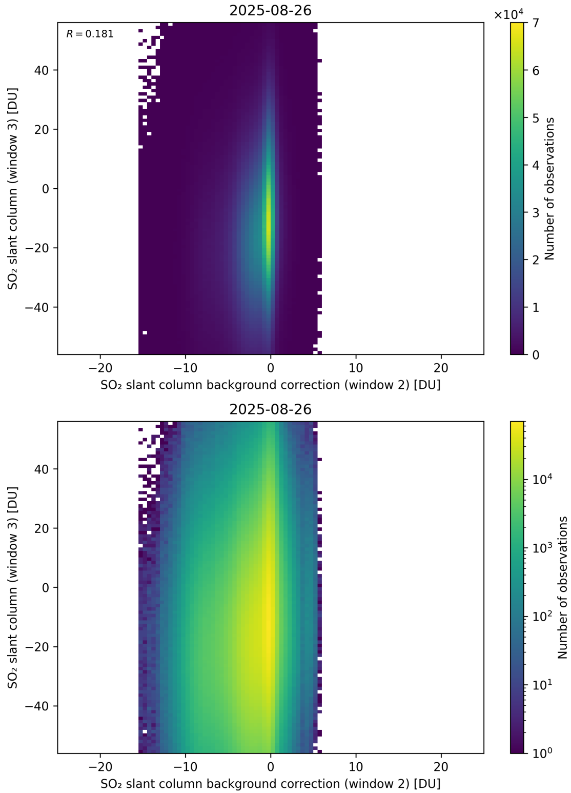
Figure 128: Scatter density plot of “SO 2 slant column background correction (window 2)” against “SO 2 slant column (window 3)” for 2025-08-25 to 2025-08-27.
