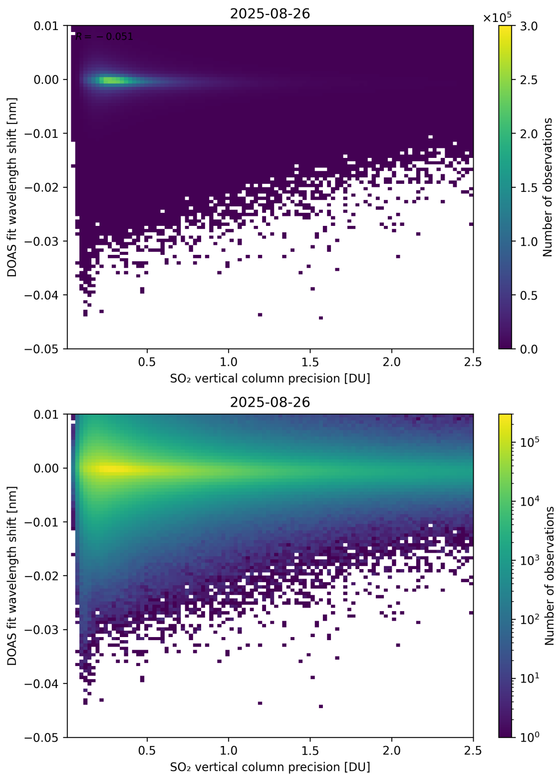
Figure 332: Scatter density plot of “SO 2 vertical column precision” against “DOAS fit wavelength shift” for 2025-08-25 to 2025-08-27.
