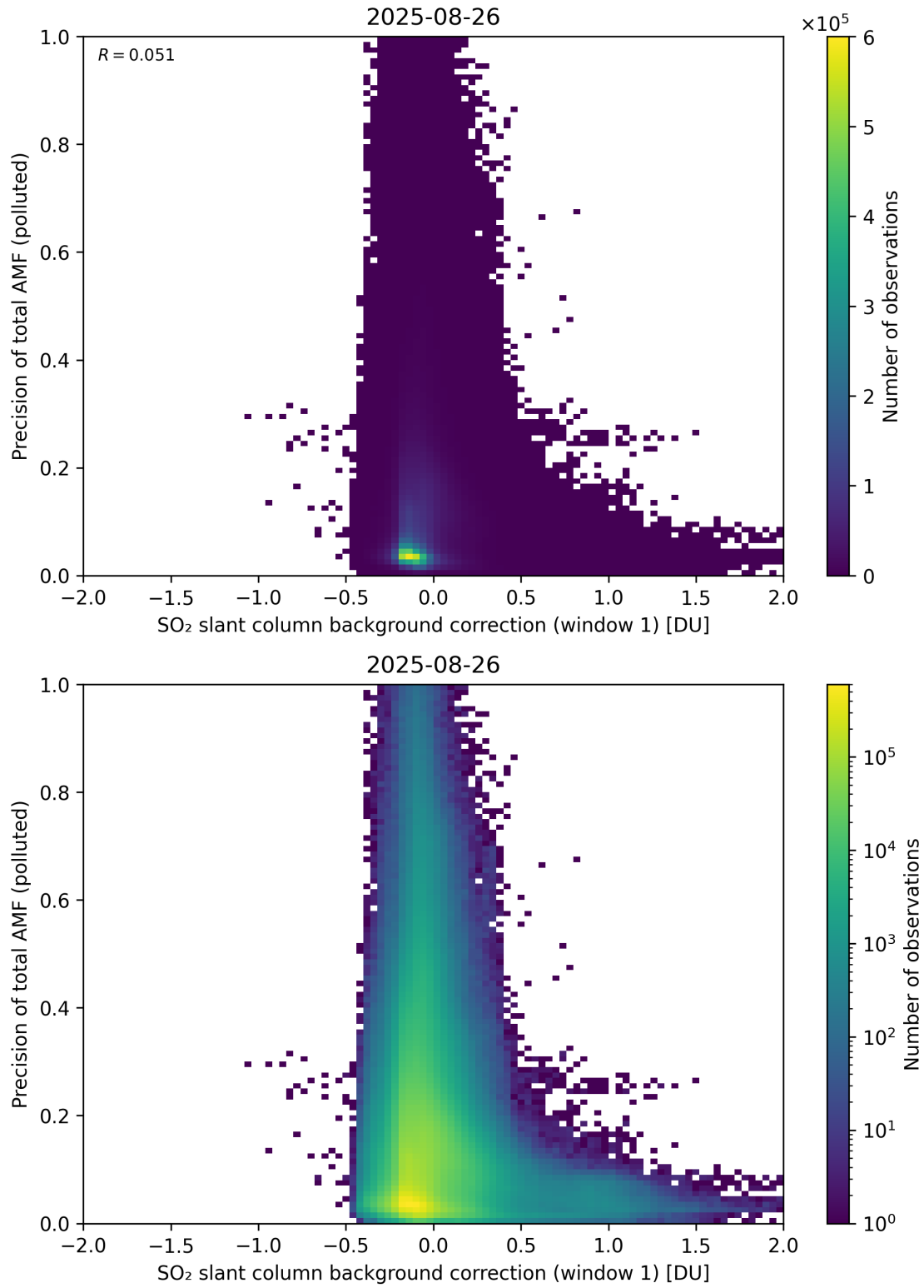
Figure 121: Scatter density plot of “SO 2 slant column background correction (window 1)” against “Precision of total AMF (polluted)” for 2025-08-25 to 2025-08-27.
