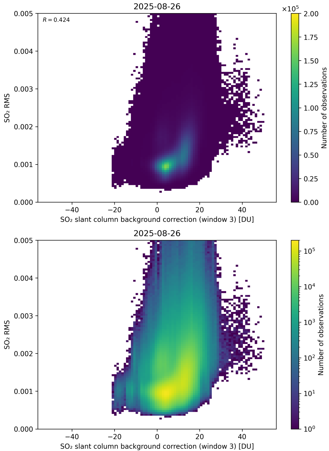
Figure 134: Scatter density plot of “SO 2 slant column background correction (window 3)” against “SO 2 RMS” for 2025-08-25 to 2025-08-27.
