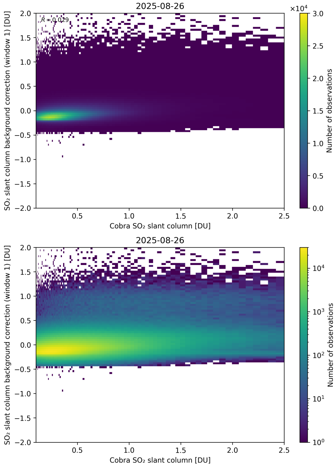
Figure 193: Scatter density plot of “Cobra SO 2 slant column” against “SO 2 slant column background correction (window 1)” for 2025-08-25 to 2025-08-27.
