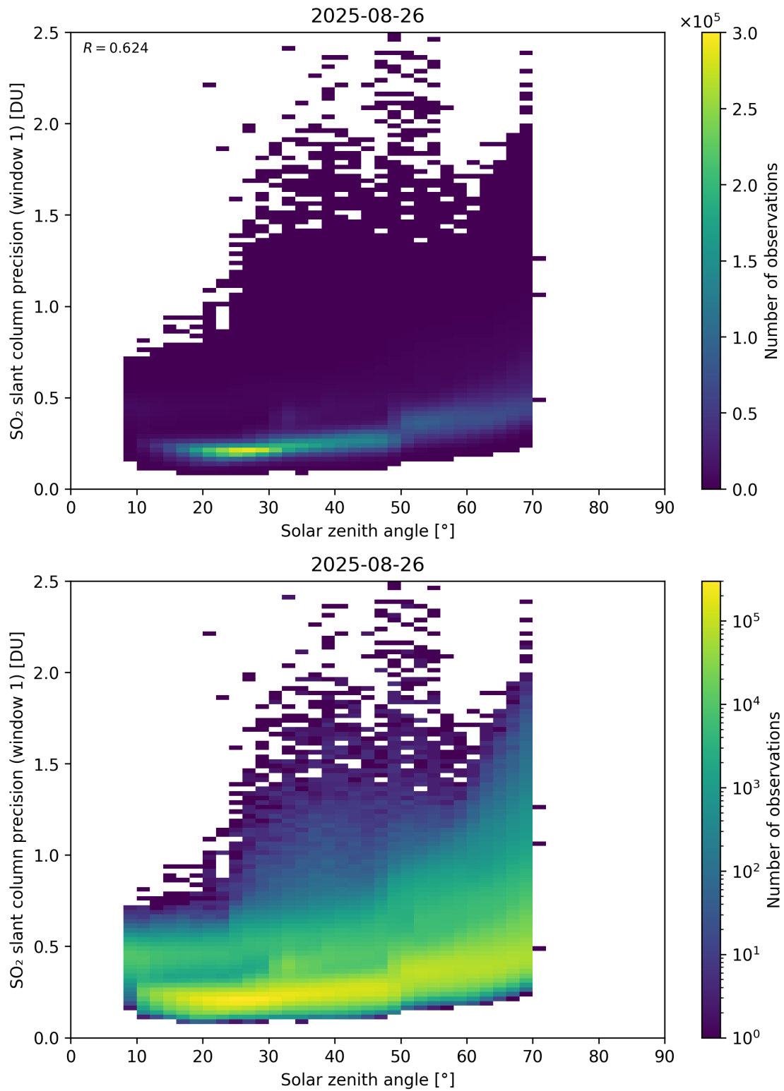
Figure 185: Scatter density plot of “Solar zenith angle” against “SO 2 slant column precision (window 1)” for 2025-08-25 to 2025-08-27.
