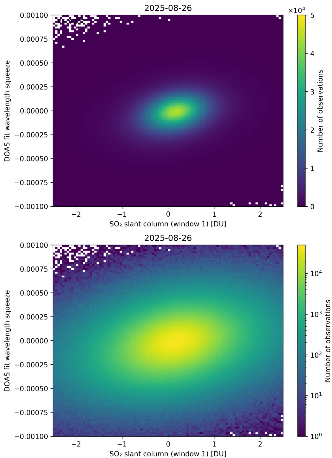
Figure 266: Scatter density plot of “SO 2 slant column (window 1)” against “DOAS fit wavelength squeeze” for 2025-08-25 to 2025-08-27.
