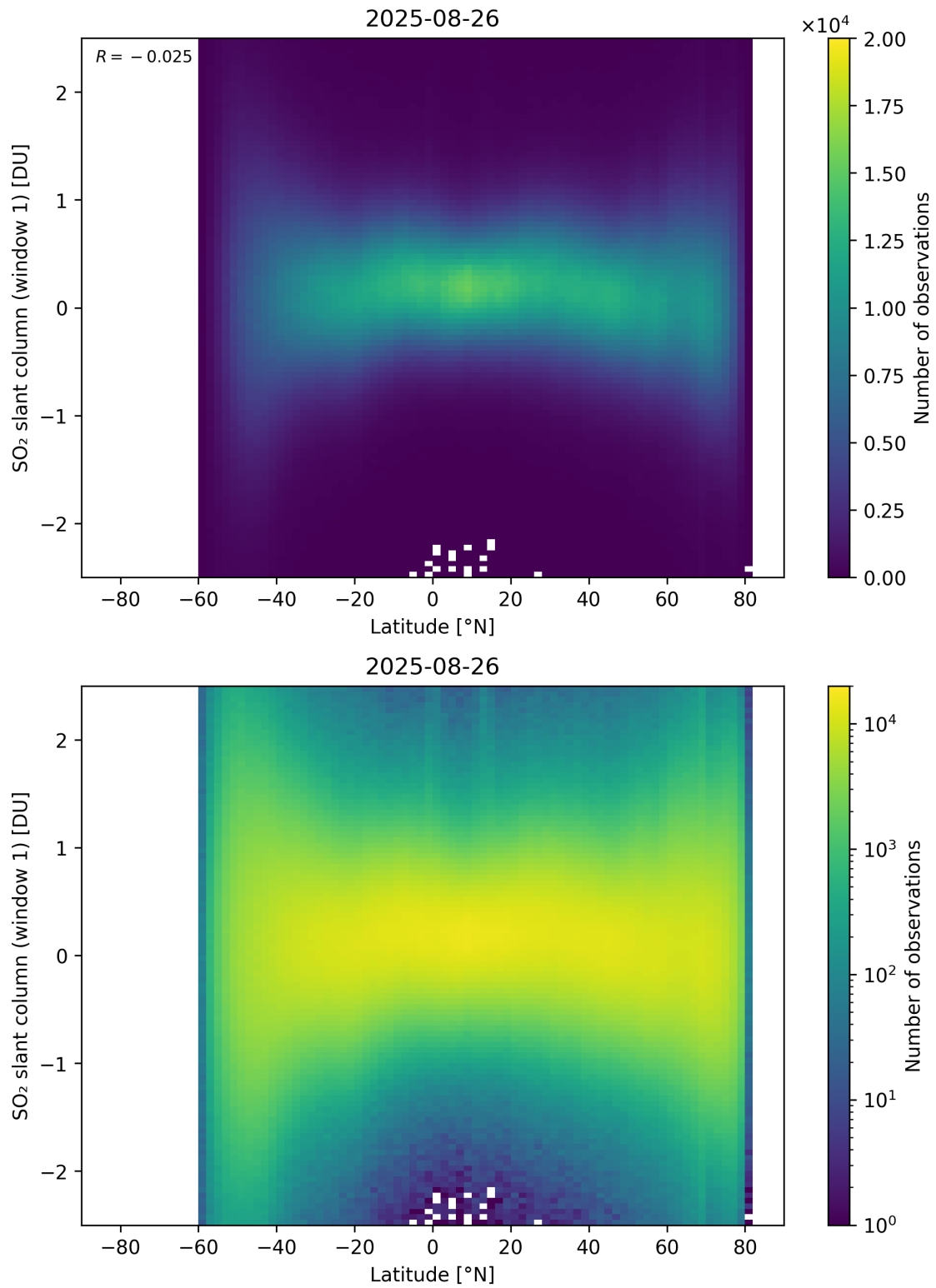
Figure 162: Scatter density plot of “Latitude” against “SO 2 slant column (window 1)” for 2025-08-25 to 2025-08-27.
