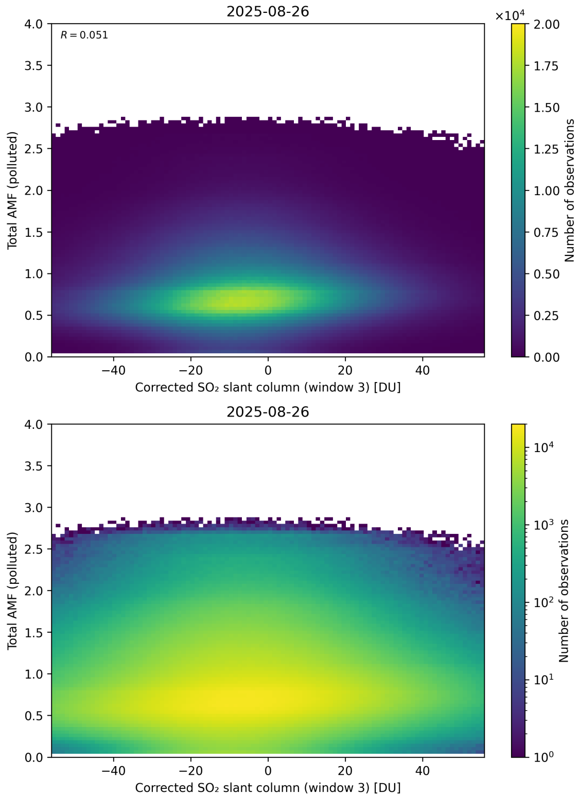
Figure 260: Scatter density plot of “Corrected SO 2 slant column (window 3)” against “Total AMF (polluted)” for 2025-08-25 to 2025-08-27.
