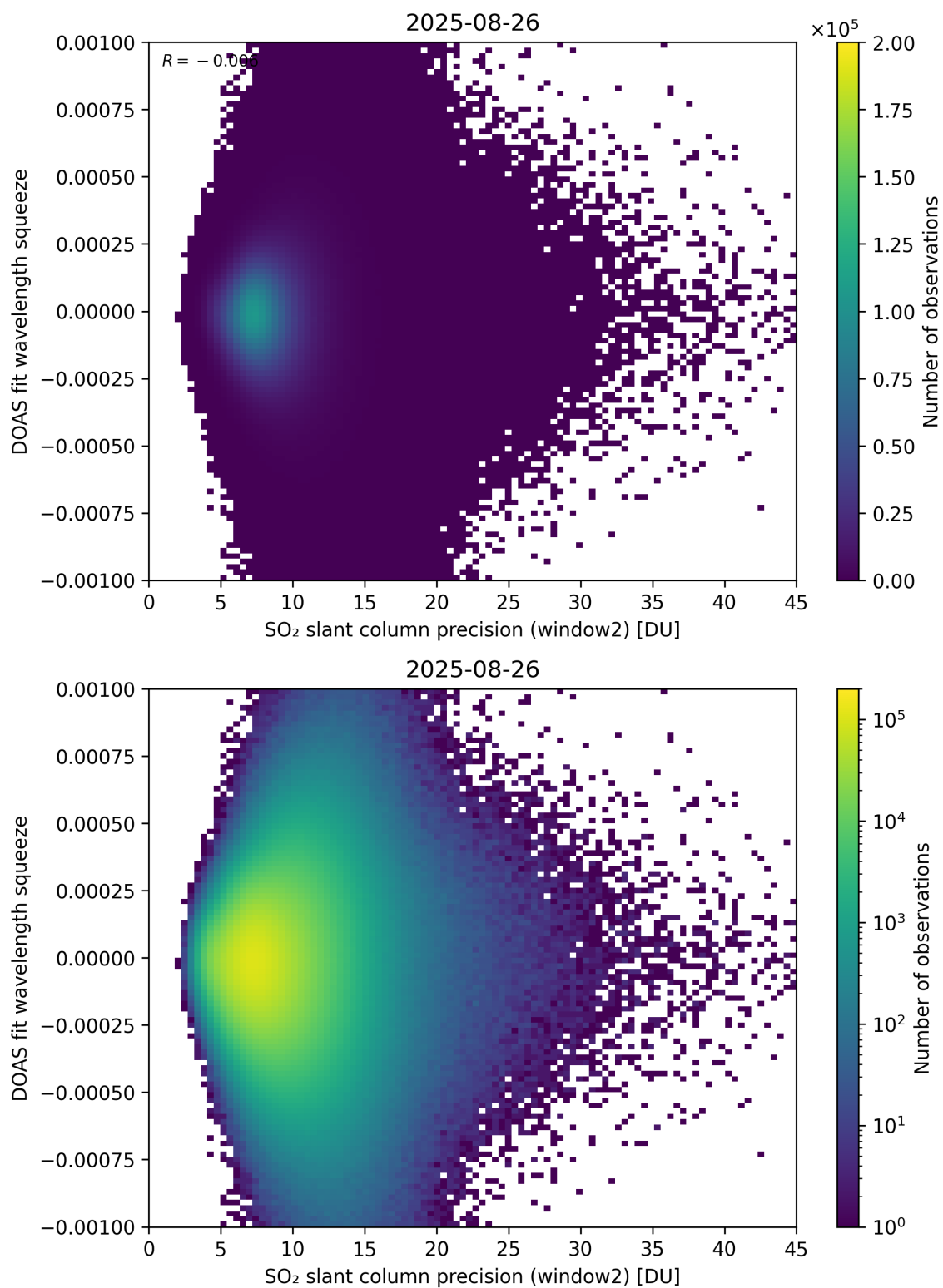
Figure 294: Scatter density plot of “SO 2 slant column precision (window2)” against “DOAS fit wavelength squeeze” for 2025-08-25 to 2025-08-27.
