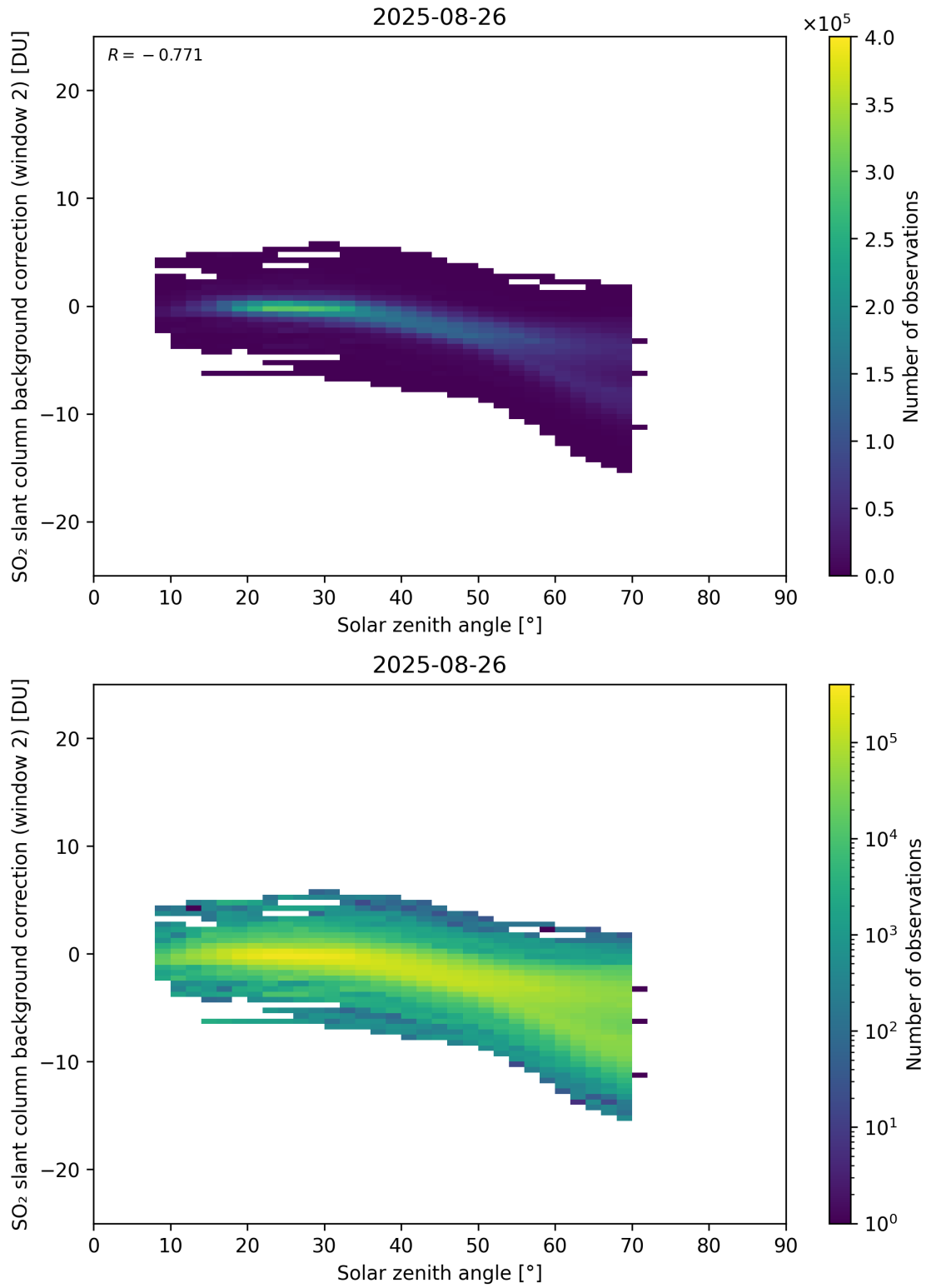
Figure 172: Scatter density plot of “Solar zenith angle” against “SO 2 slant column background correction (window 2)” for 2025-08-25 to 2025-08-27.
