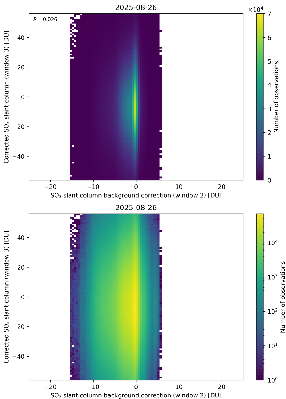
Figure 127: Scatter density plot of “SO 2 slant column background correction (window 2)” against “Corrected SO 2 slant column (window 3)” for 2025-08-25 to 2025-08-27.
