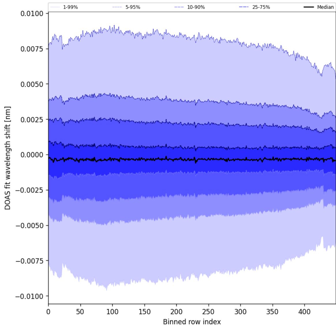
Figure 102: Along track statistics of “DOAS fit wavelength shift” for 2025-08-25 to 2025-08-27
