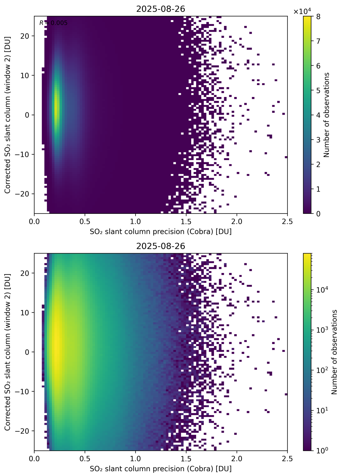
Figure 206: Scatter density plot of “SO 2 slant column precision (Cobra)” against “Corrected SO 2 slant column (window 2)” for 2025-08-25 to 2025-08-27.
