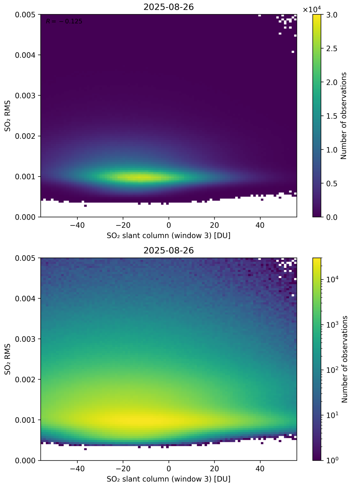
Figure 306: Scatter density plot of “SO 2 slant column (window 3)” against “SO 2 RMS” for 2025-08-25 to 2025-08-27.
