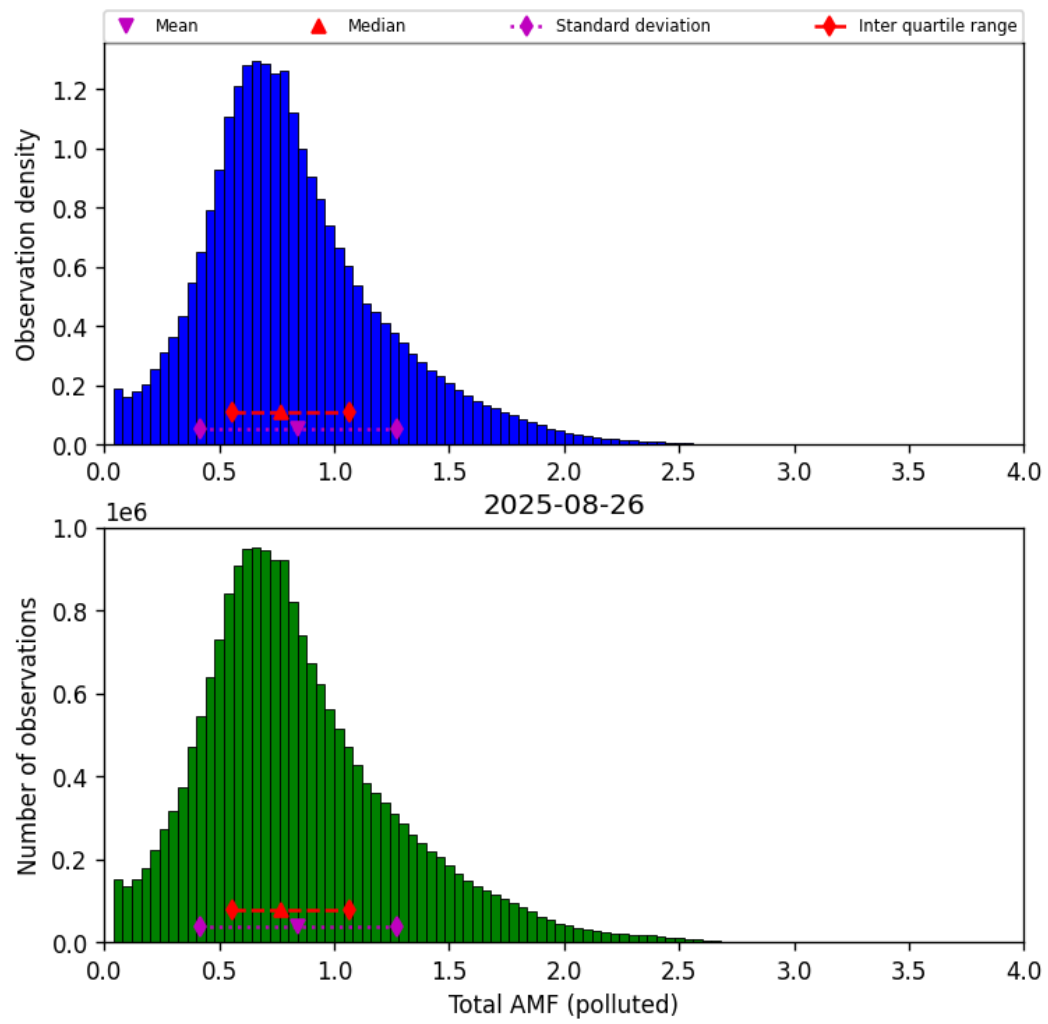
Figure 79: Histogram of “Total AMF (polluted)” for 2025-08-25 to 2025-08-27
