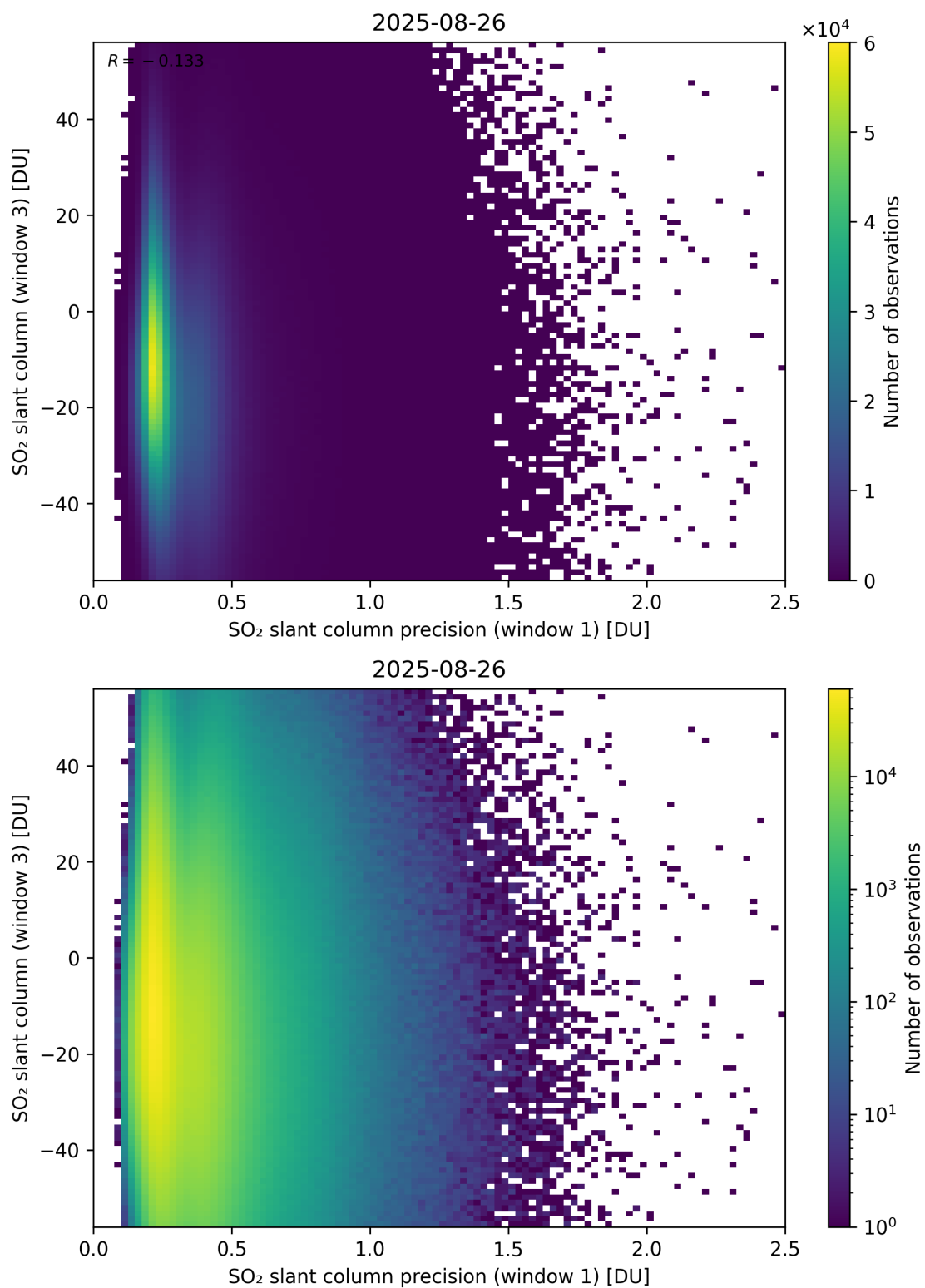
Figure 278: Scatter density plot of “SO 2 slant column precision (window 1)” against “SO 2 slant column (window 3)” for 2025-08-25 to 2025-08-27.
