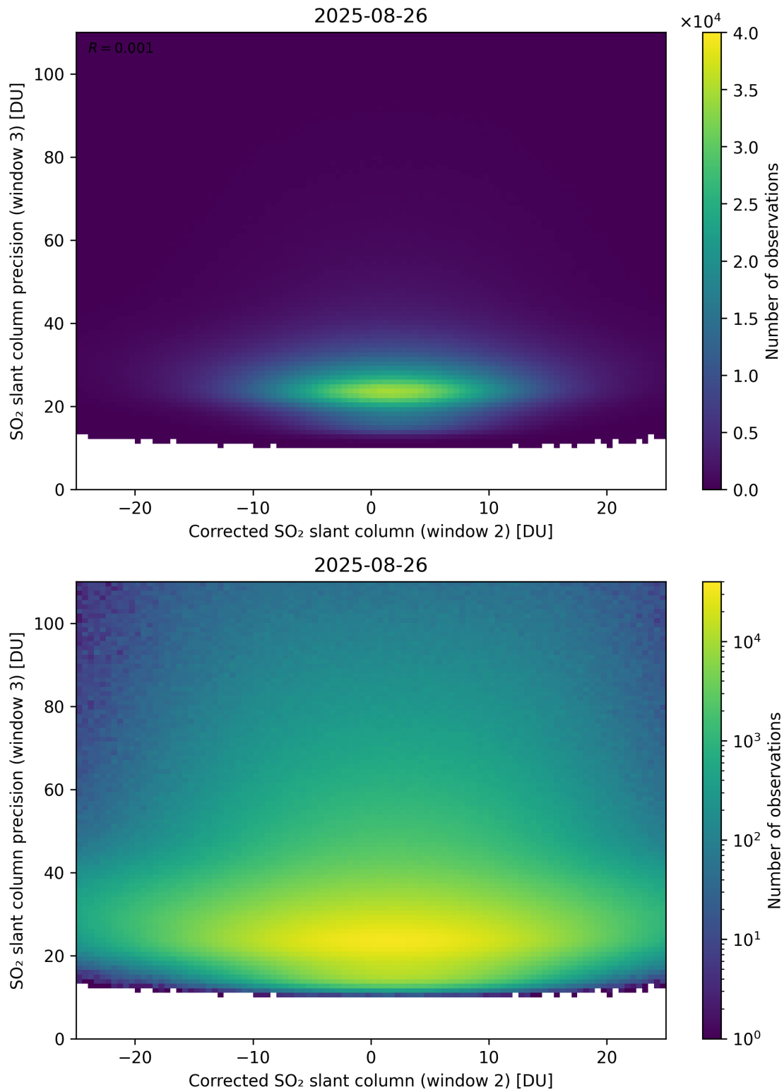
Figure 252: Scatter density plot of “Corrected SO 2 slant column (window 2)” against “SO 2 slant column precision (window 3)” for 2025-08-25 to 2025-08-27.
