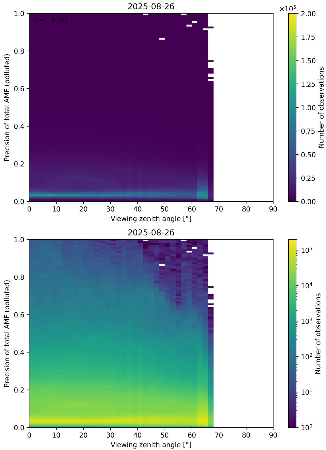
Figure 382: Scatter density plot of “Viewing zenith angle” against “Precision of total AMF (polluted)” for 2025-08-25 to 2025-08-27.
