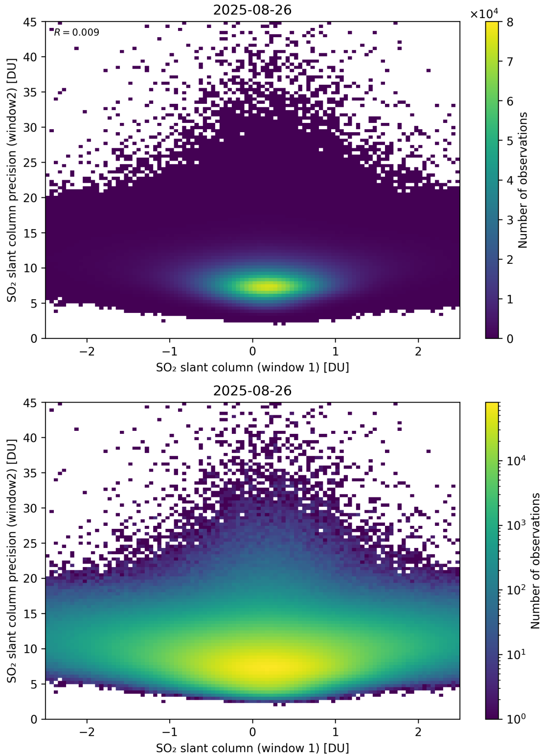
Figure 286: Scatter density plot of “SO 2 slant column (window 1)” against “SO 2 slant column precision (window2)” for 2025-08-25 to 2025-08-27.
