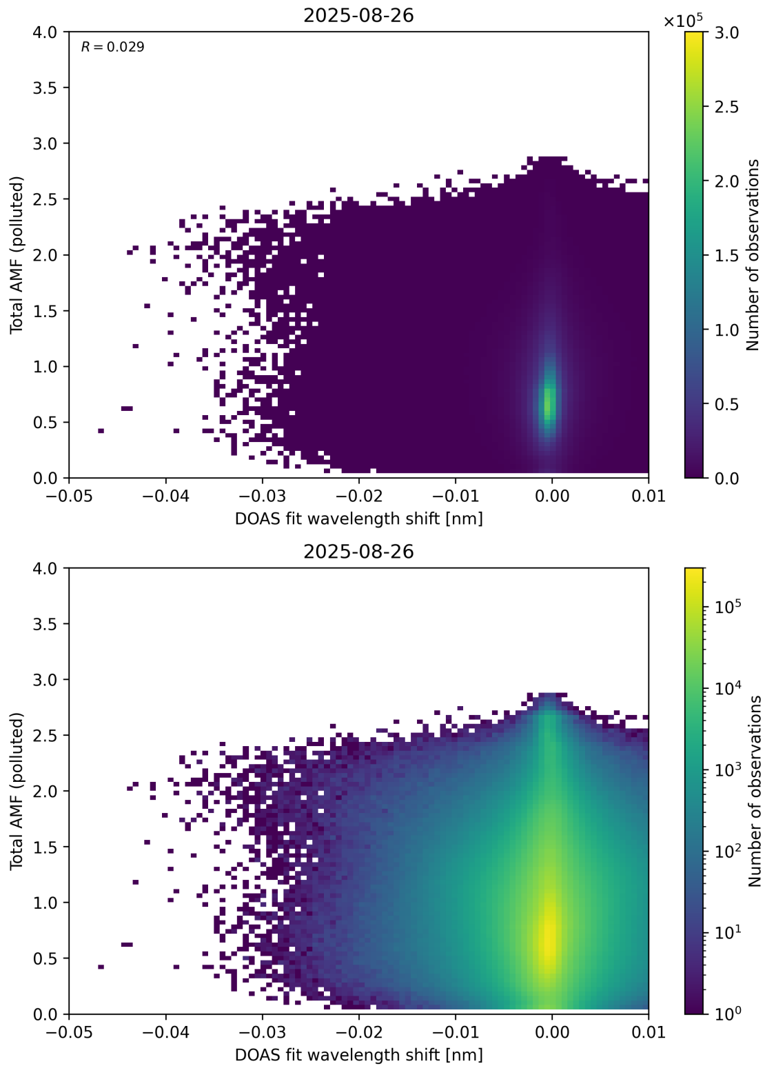
Figure 141: Scatter density plot of “DOAS fit wavelength shift” against “Total AMF (polluted)” for 2025-08-25 to 2025-08-27.
