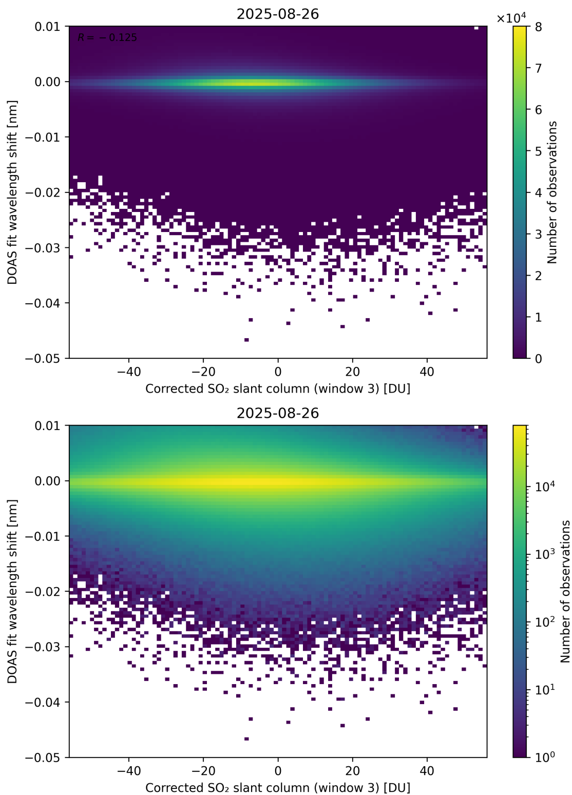
Figure 256: Scatter density plot of “Corrected SO 2 slant column (window 3)” against “DOAS fit wavelength shift” for 2025-08-25 to 2025-08-27.
