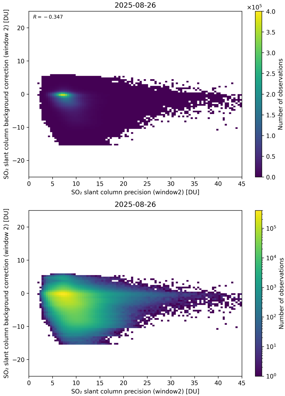
Figure 291: Scatter density plot of “SO 2 slant column precision (window2)” against “SO 2 slant column background correction (window 2)” for 2025-08-25 to 2025-08-27.
