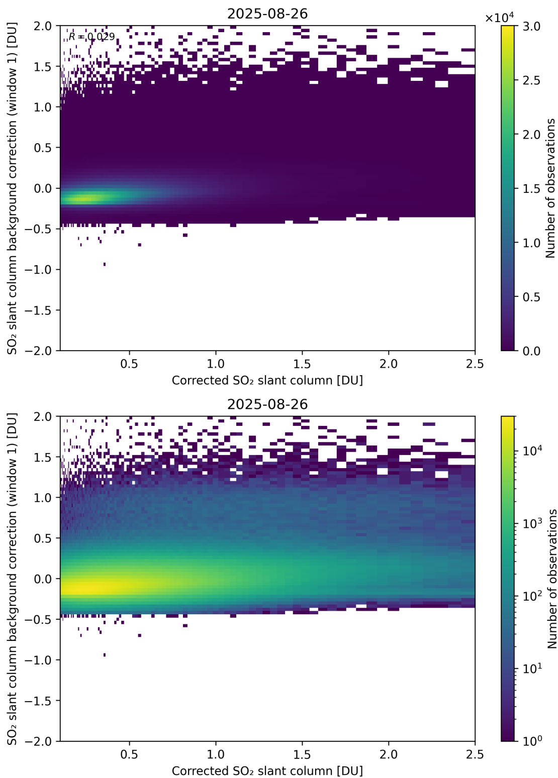
Figure 226: Scatter density plot of “Corrected SO 2 slant column” against “SO 2 slant column background correction (window 1)” for 2025-08-25 to 2025-08-27.
