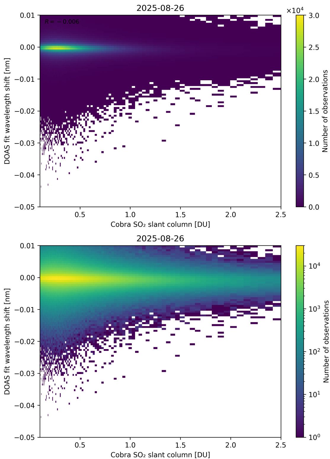
Figure 196: Scatter density plot of “Cobra SO 2 slant column” against “DOAS fit wavelength shift” for 2025-08-25 to 2025-08-27.
