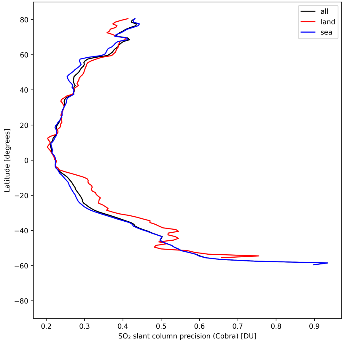
Figure 36: Zonal average of “SO 2 slant column precision (Cobra)” for 2025-08-25 to 2025-08-27.
