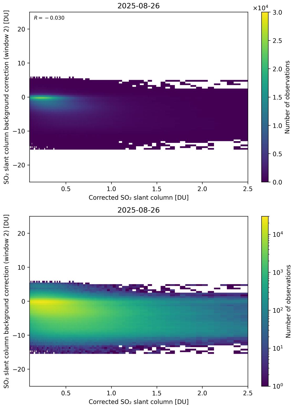
Figure 227: Scatter density plot of “Corrected SO 2 slant column” against “SO 2 slant column background correction (window 2)” for 2025-08-25 to 2025-08-27.
