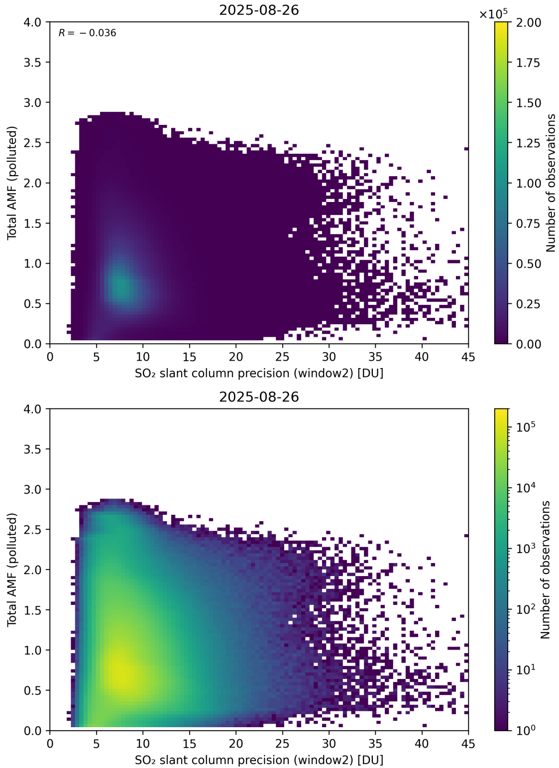
Figure 301: Scatter density plot of “SO 2 slant column precision (window2)” against “Total AMF (polluted)” for 2025-08-25 to 2025-08-27.
