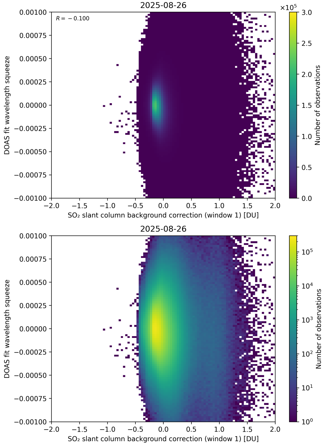
Figure 112: Scatter density plot of “SO 2 slant column background correction (window 1)” against “DOAS fit wavelength squeeze” for 2025-08-25 to 2025-08-27.
