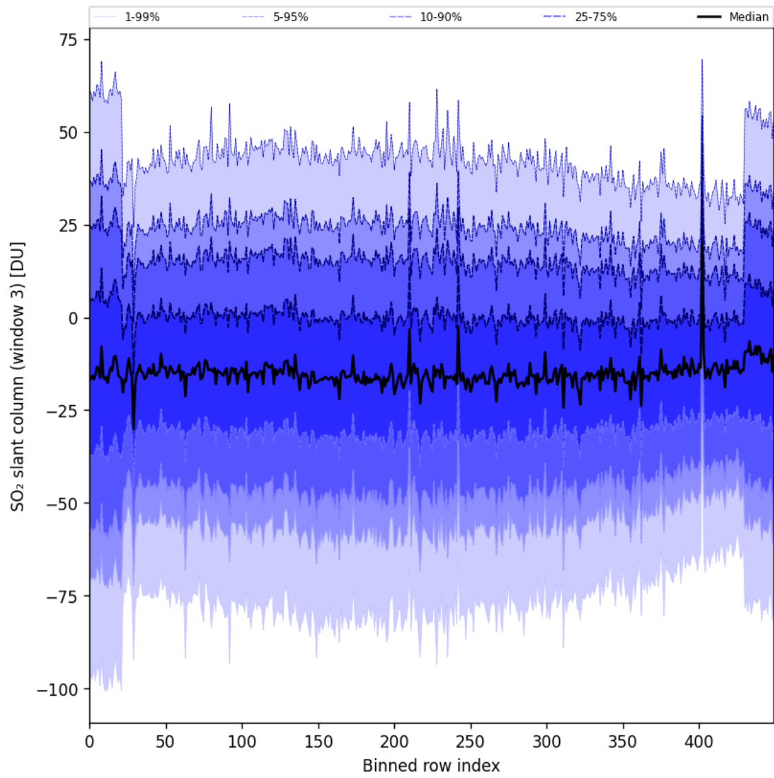
Figure 97: Along track statistics of “SO 2 slant column (window 3)” for 2025-08-25 to 2025-08-27
