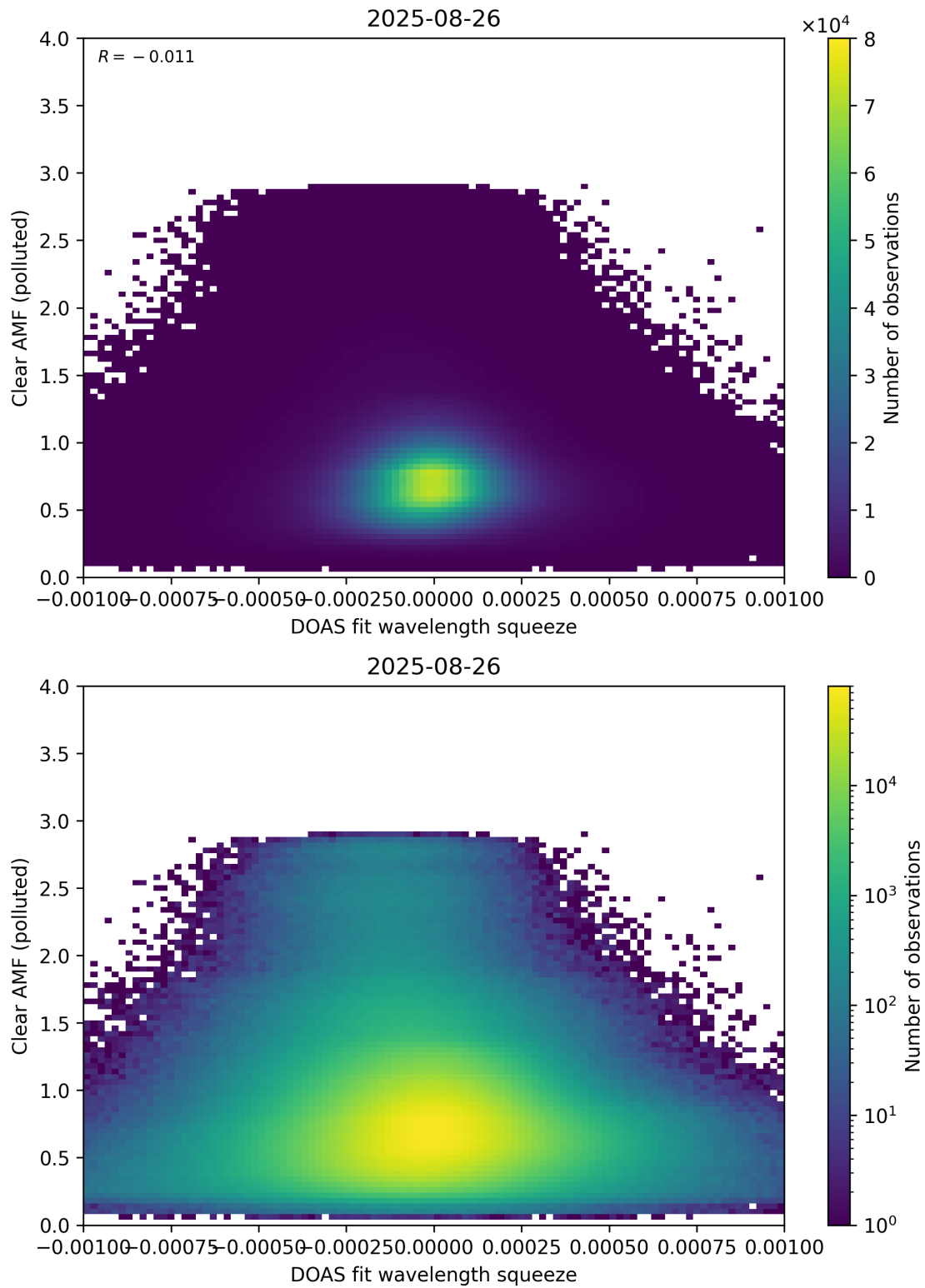
Figure 144: Scatter density plot of “DOAS fit wavelength squeeze” against “Clear AMF (polluted)” for 2025-08-25 to 2025-08-27.
