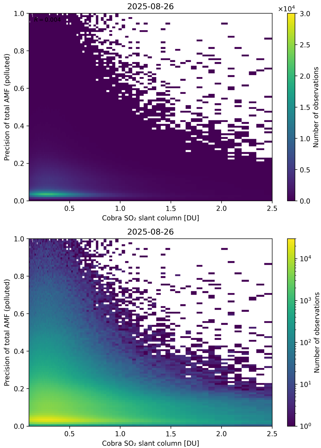
Figure 225: Scatter density plot of “Cobra SO 2 slant column” against “Precision of total AMF (polluted)” for 2025-08-25 to 2025-08-27.
