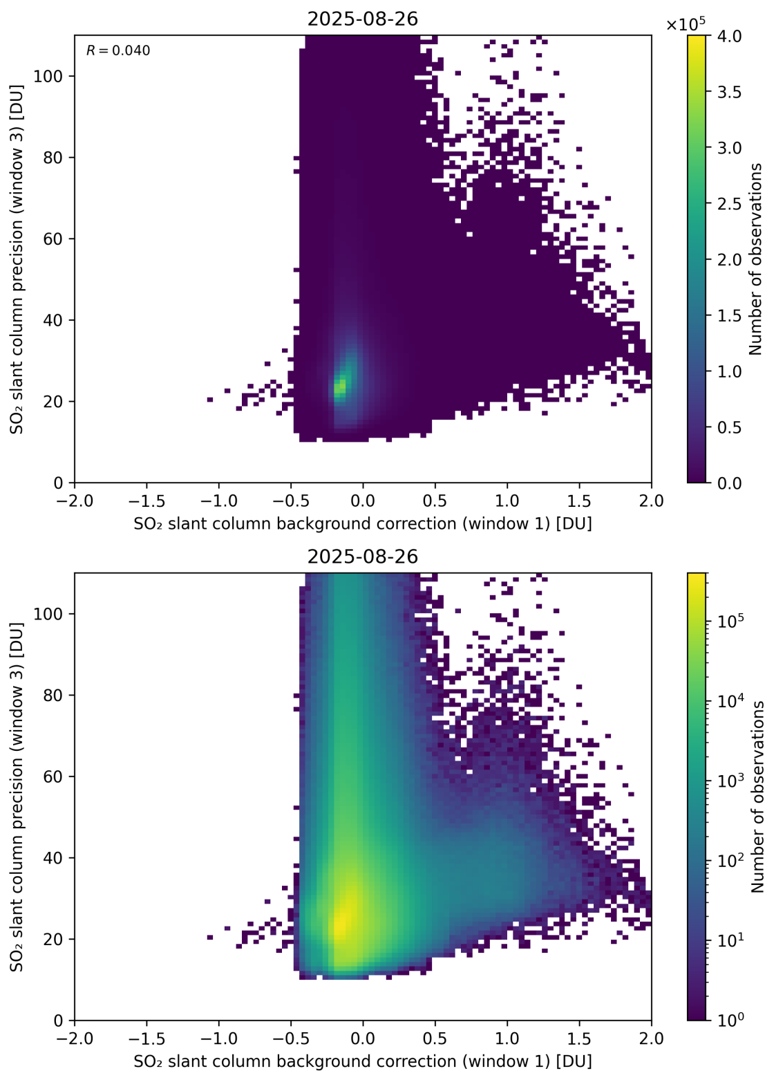
Figure 119: Scatter density plot of “SO 2 slant column background correction (window 1)” against “SO 2 slant column precision (window 3)” for 2025-08-25 to 2025-08-27.
