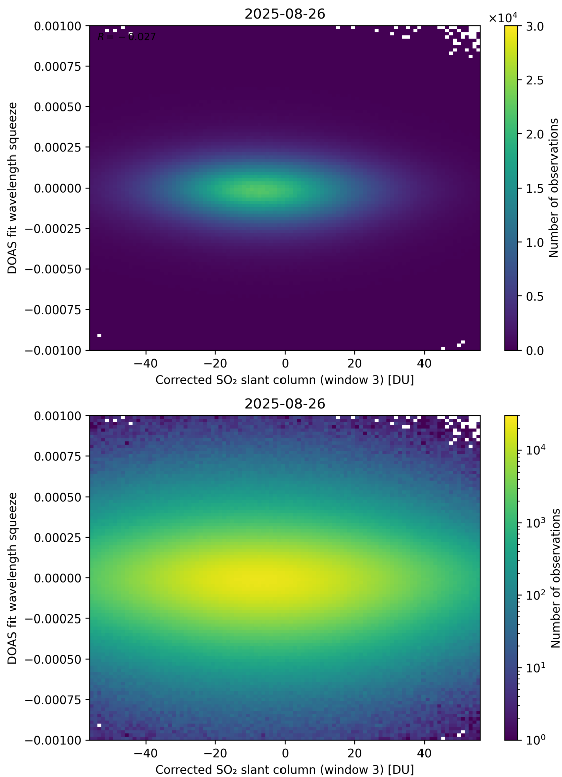
Figure 257: Scatter density plot of “Corrected SO 2 slant column (window 3)” against “DOAS fit wavelength squeeze” for 2025-08-25 to 2025-08-27.
