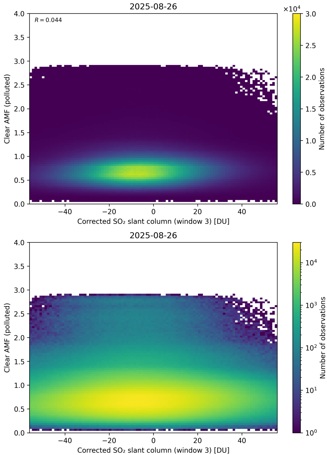
Figure 259: Scatter density plot of “Corrected SO 2 slant column (window 3)” against “Clear AMF (polluted)” for 2025-08-25 to 2025-08-27.
