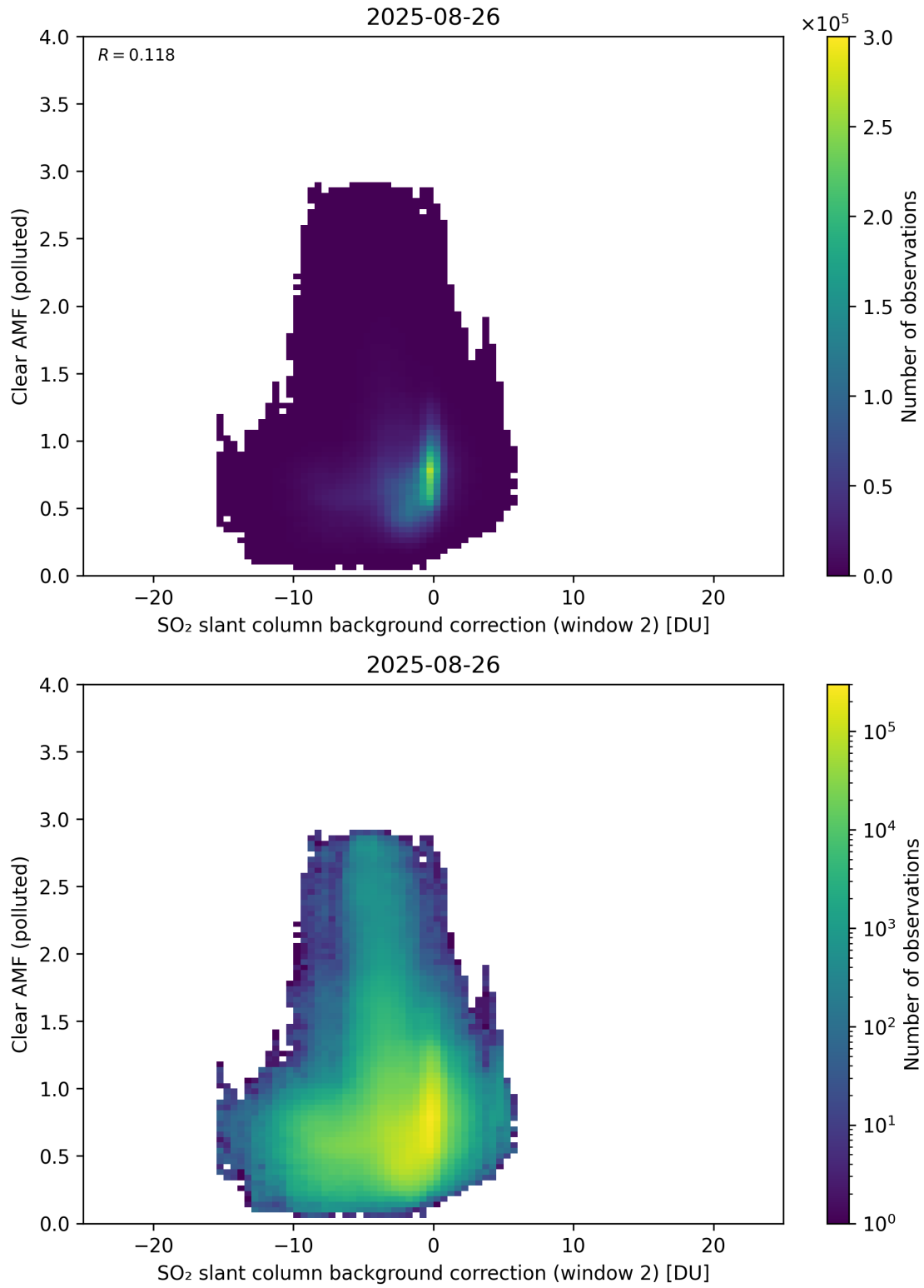
Figure 126: Scatter density plot of “SO 2 slant column background correction (window 2)” against “Clear AMF (polluted)” for 2025-08-25 to 2025-08-27.
