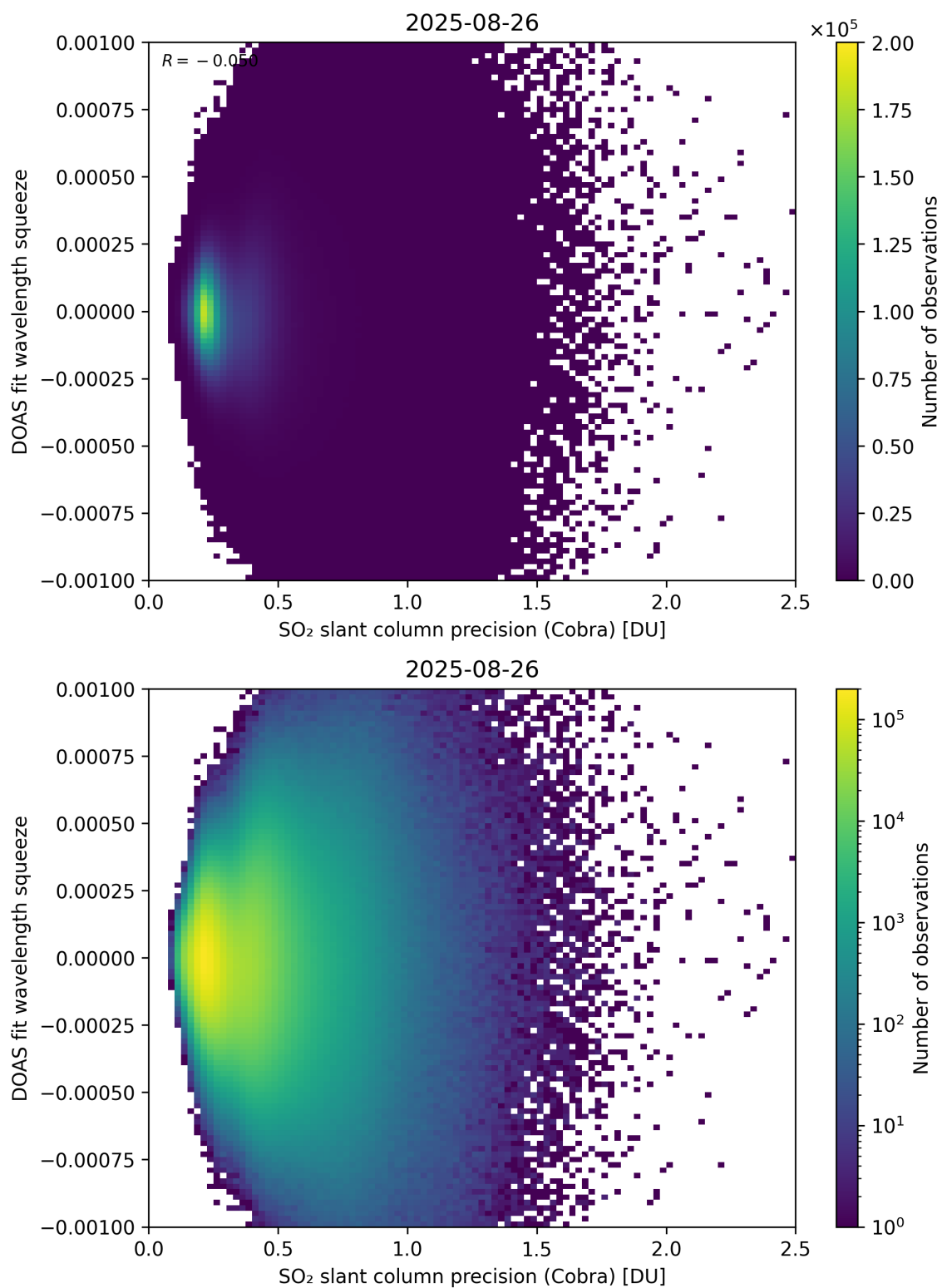
Figure 203: Scatter density plot of “SO 2 slant column precision (Cobra)” against “DOAS fit wavelength squeeze” for 2025-08-25 to 2025-08-27.
