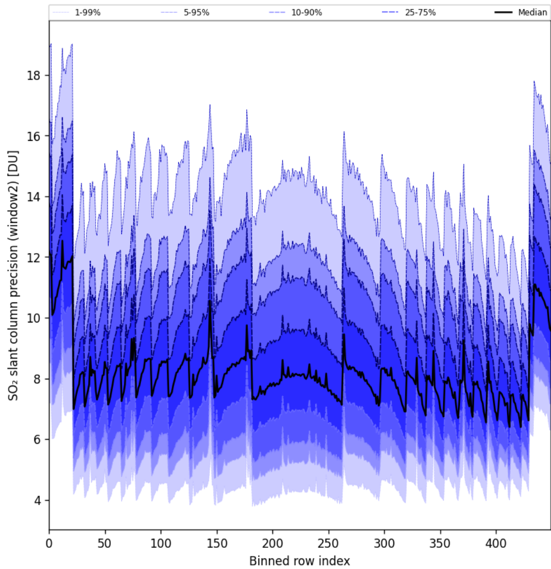
Figure 94: Along track statistics of “SO 2 slant column precision (window2)” for 2025-08-25 to 2025-08-27
