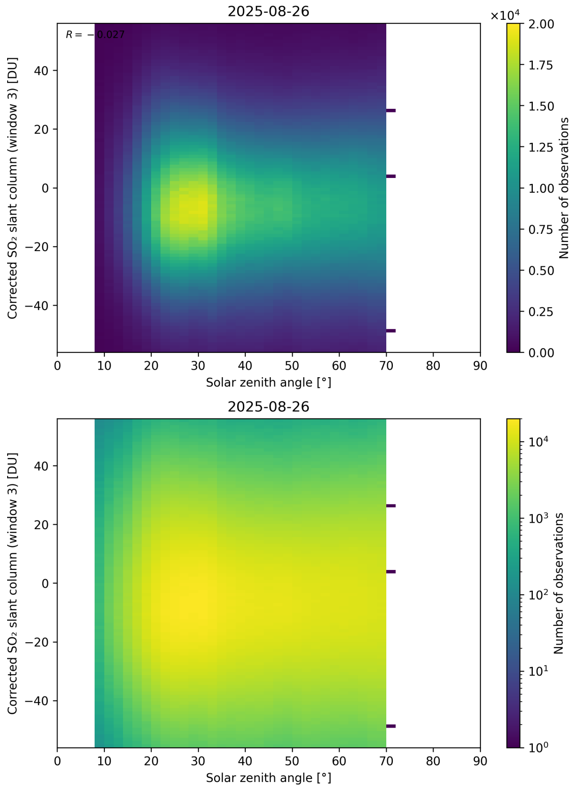
Figure 183: Scatter density plot of “Solar zenith angle” against “Corrected SO 2 slant column (window 3)” for 2025-08-25 to 2025-08-27.
