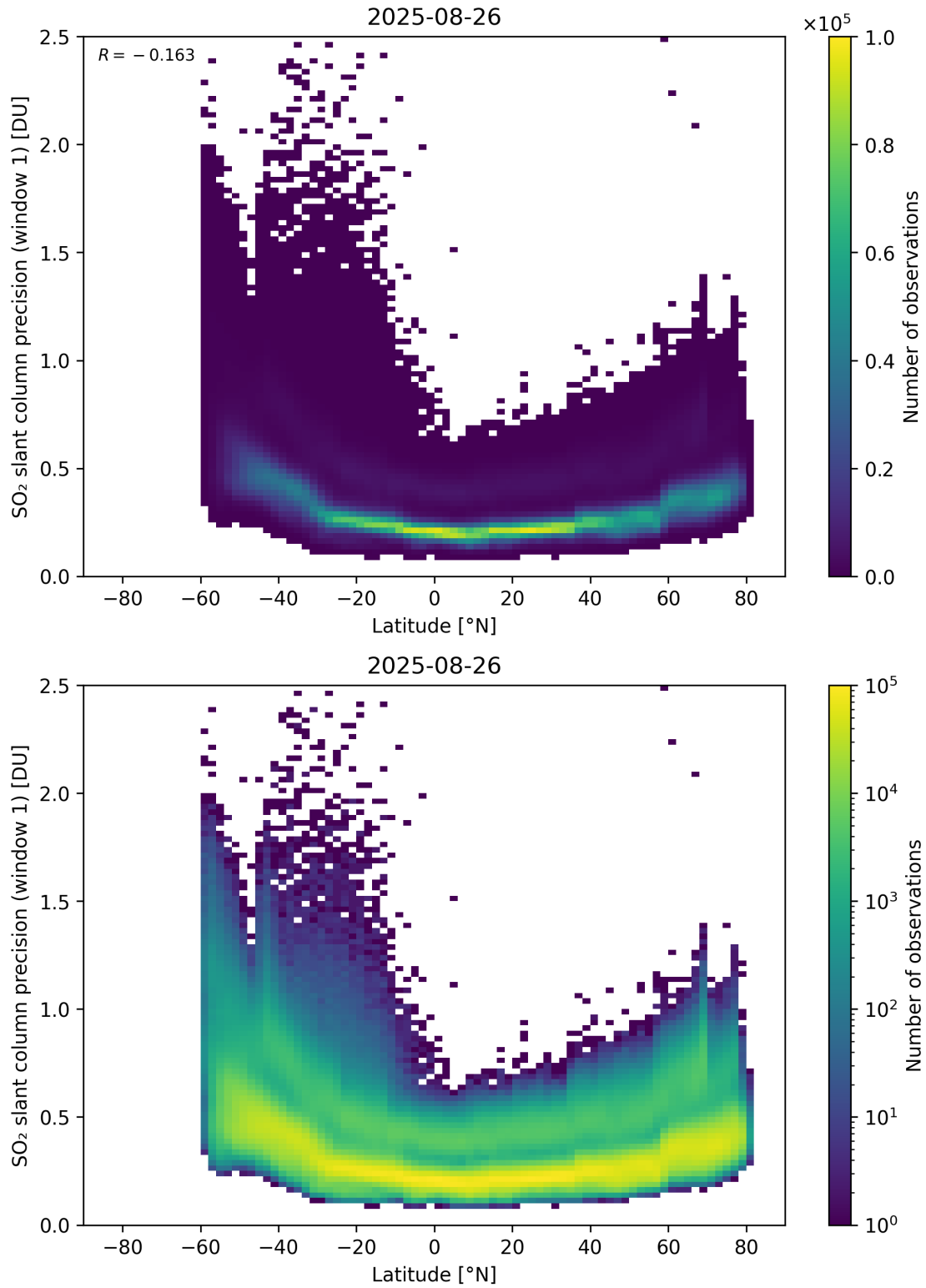
Figure 163: Scatter density plot of “Latitude” against “SO 2 slant column precision (window 1)” for 2025-08-25 to 2025-08-27.
