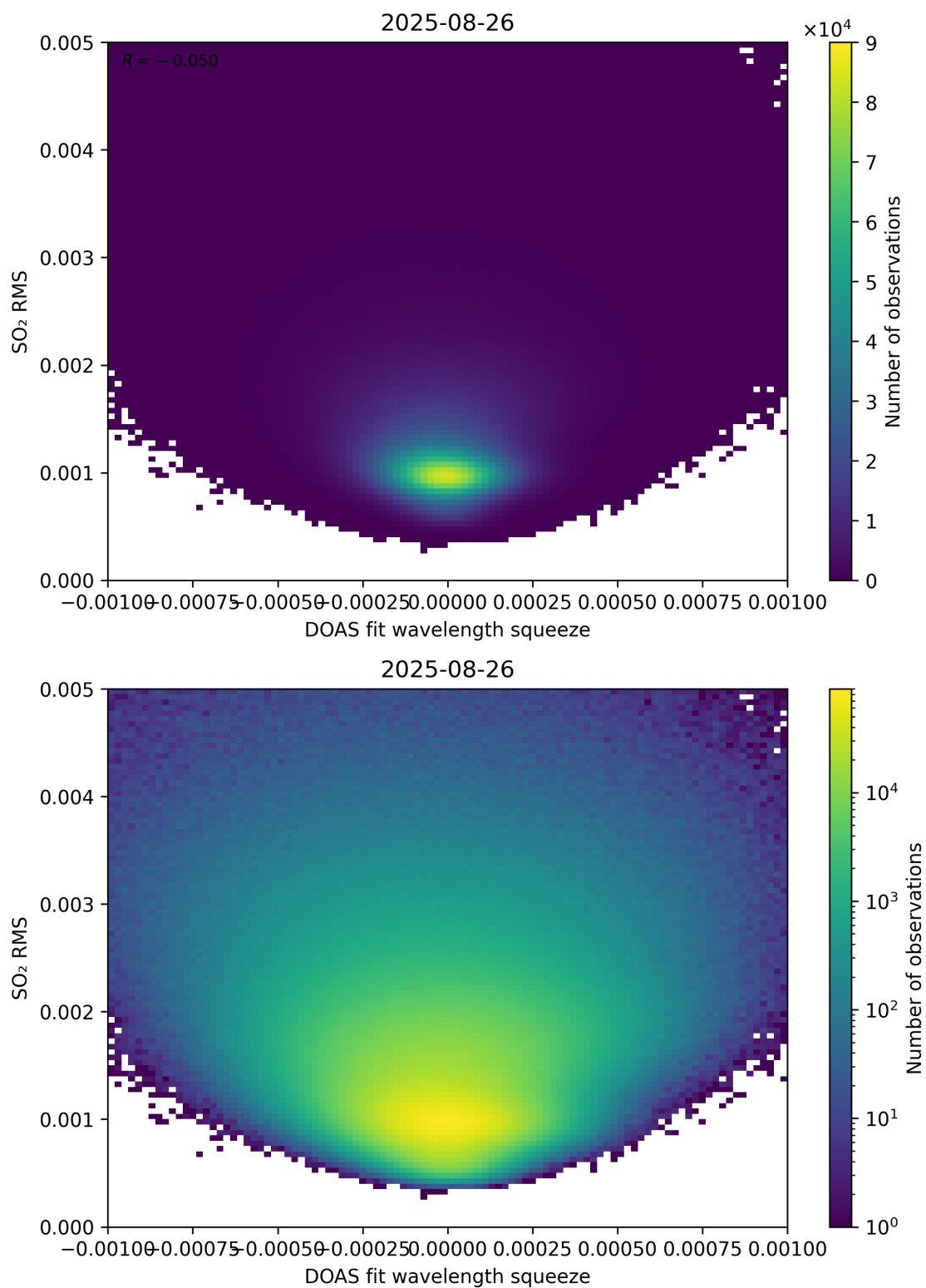
Figure 143: Scatter density plot of “DOAS fit wavelength squeeze” against “SO 2 RMS” for 2025-08-25 to 2025-08-27.
