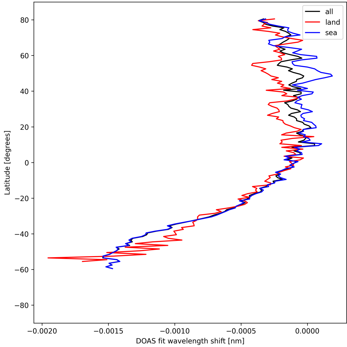
Figure 50: Zonal average of “DOAS fit wavelength shift” for 2025-08-25 to 2025-08-27.
