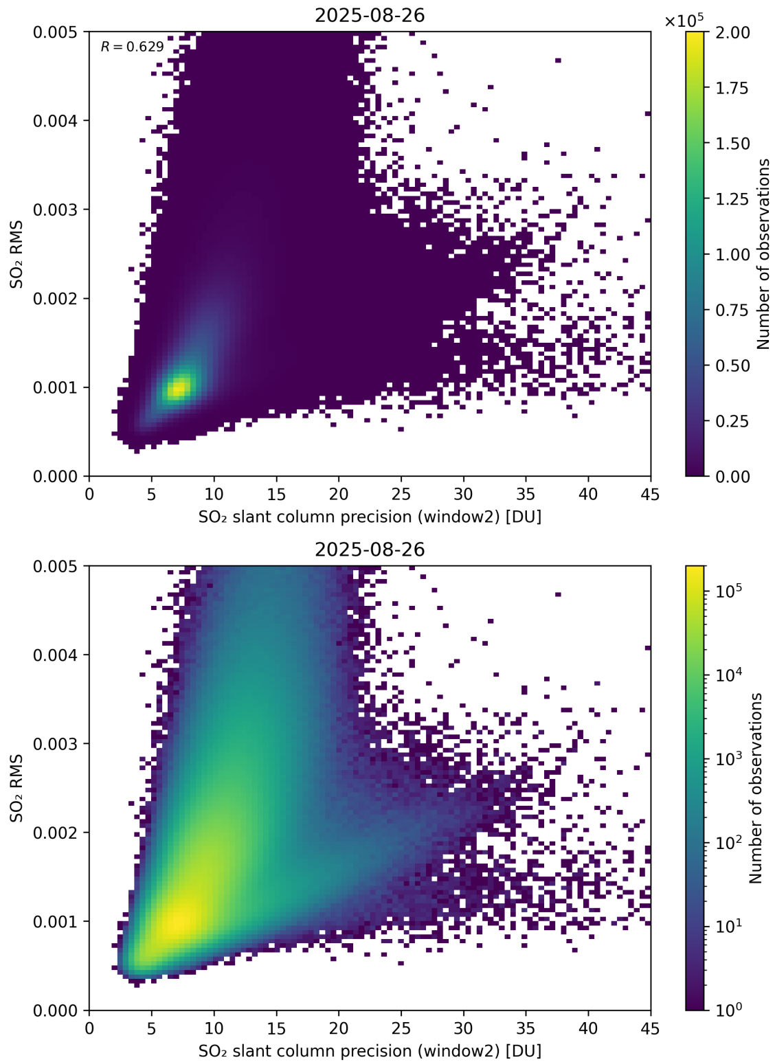
Figure 295: Scatter density plot of “SO 2 slant column precision (window2)” against “SO 2 RMS” for 2025-08-25 to 2025-08-27.
