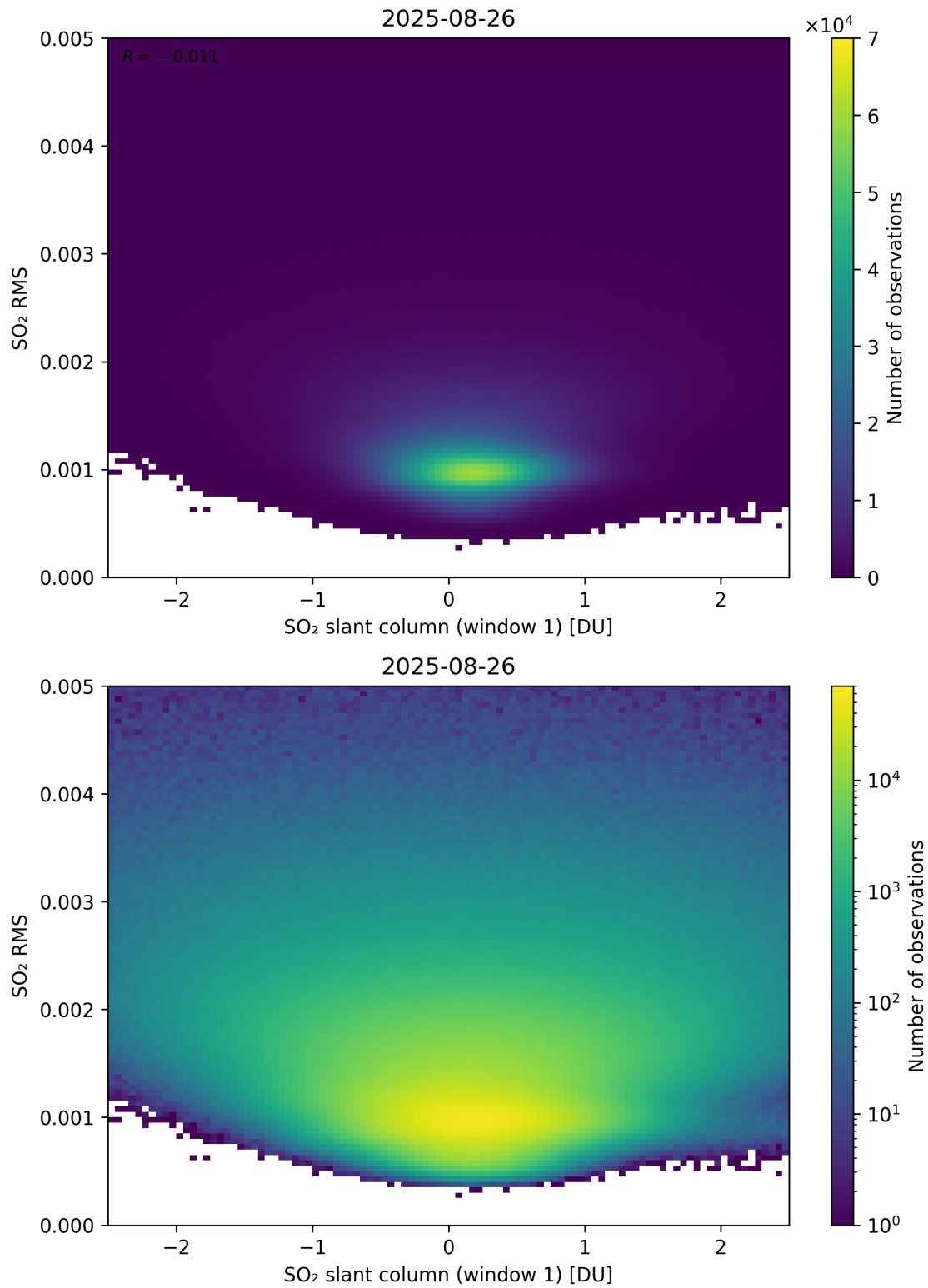
Figure 267: Scatter density plot of “SO 2 slant column (window 1)” against “SO 2 RMS” for 2025-08-25 to 2025-08-27.
