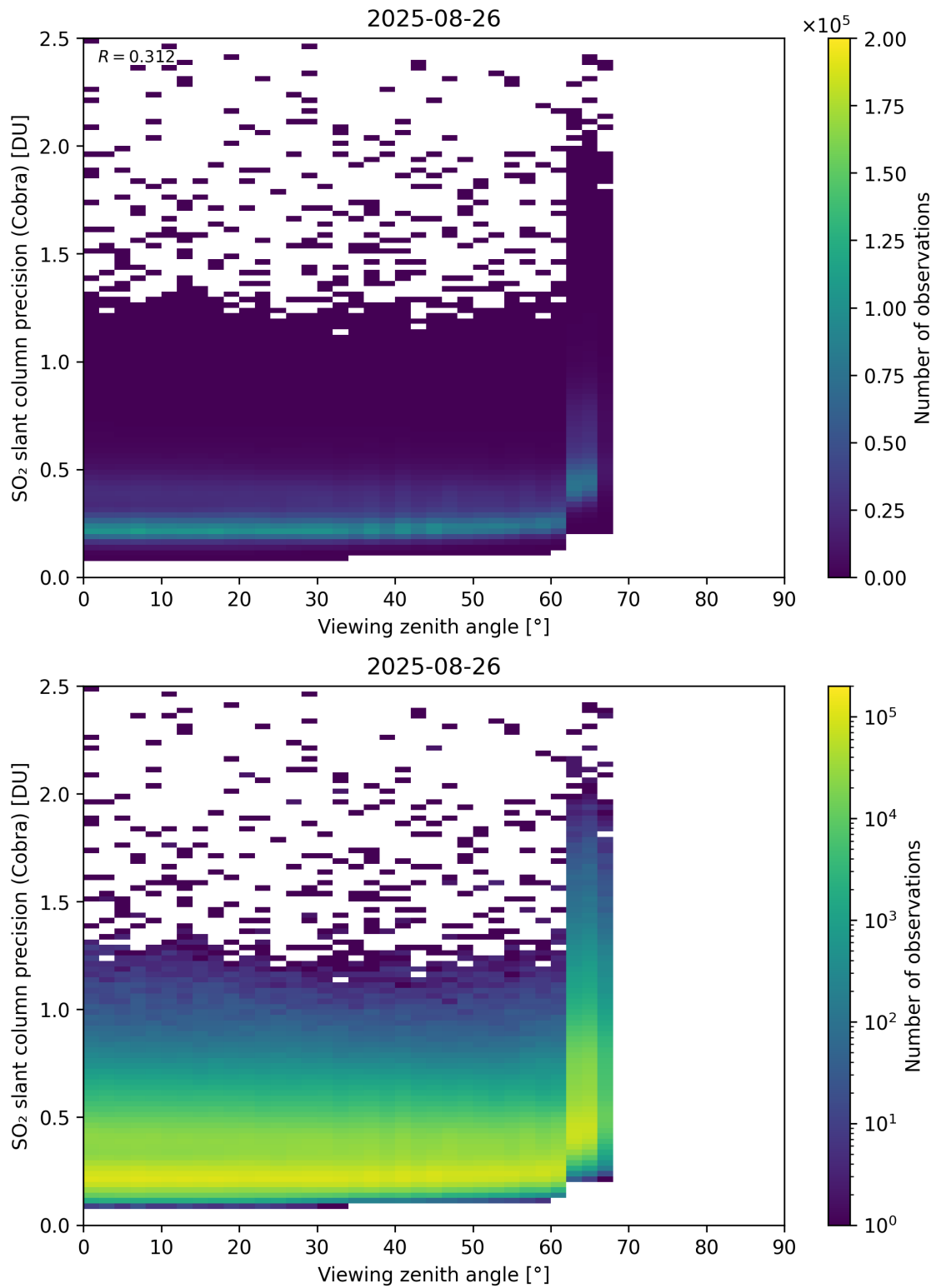
Figure 372: Scatter density plot of “Viewing zenith angle” against “SO 2 slant column precision (Cobra)” for 2025-08-25 to 2025-08-27.
