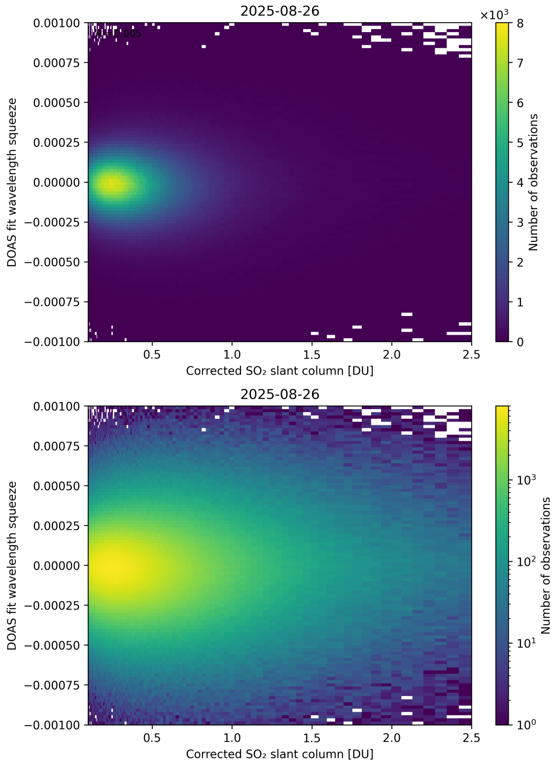
Figure 230: Scatter density plot of “Corrected SO 2 slant column” against “DOAS fit wavelength squeeze” for 2025-08-25 to 2025-08-27.
