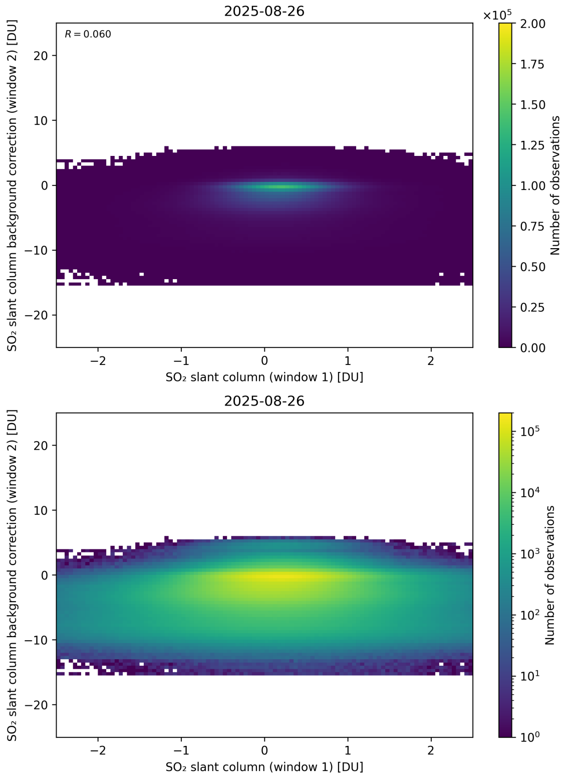
Figure 263: Scatter density plot of “SO 2 slant column (window 1)” against “SO 2 slant column background correction (window 2)” for 2025-08-25 to 2025-08-27.
