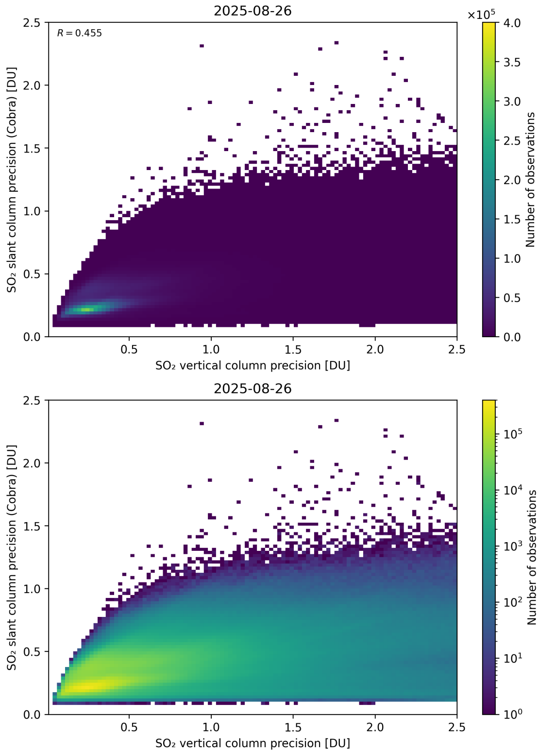
Figure 337: Scatter density plot of “SO 2 vertical column precision” against “SO 2 slant column precision (Cobra)” for 2025-08-25 to 2025-08-27.
