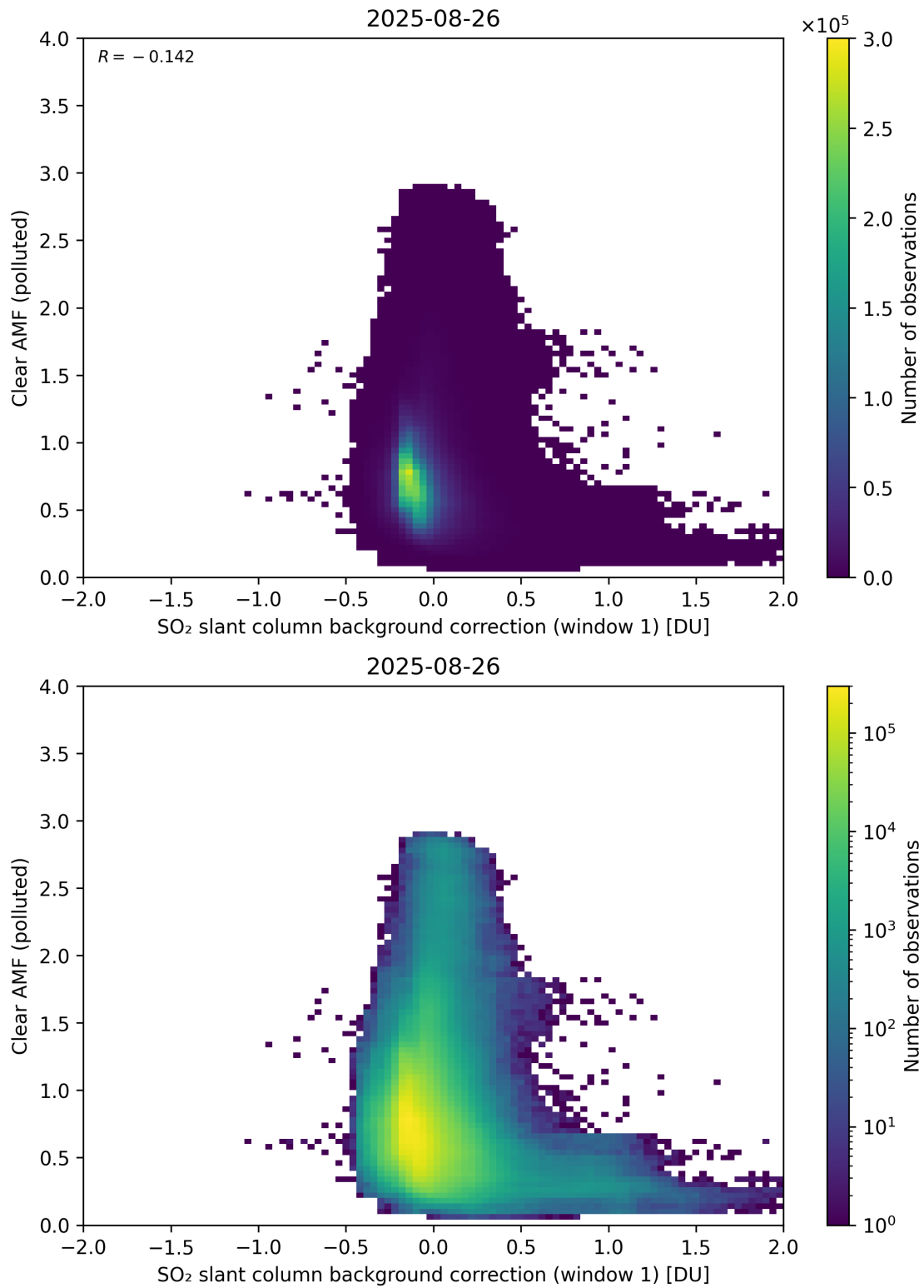
Figure 114: Scatter density plot of “SO 2 slant column background correction (window 1)” against “Clear AMF (polluted)” for 2025-08-25 to 2025-08-27.
