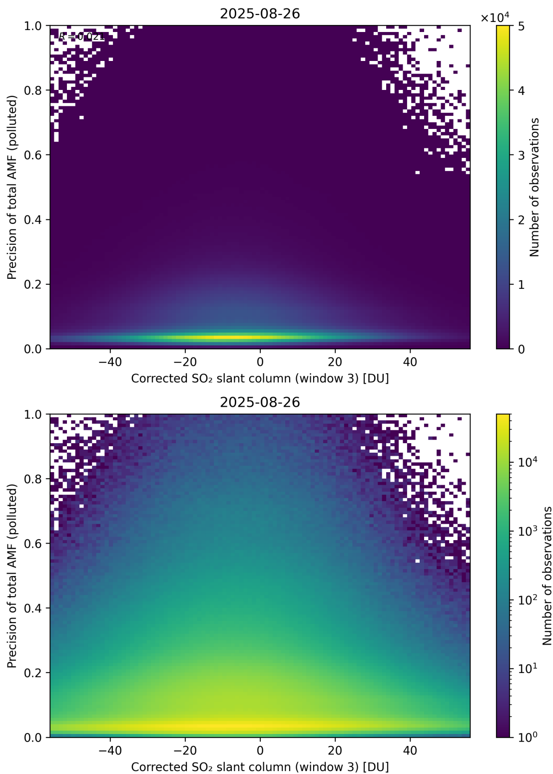
Figure 261: Scatter density plot of “Corrected SO 2 slant column (window 3)” against “Precision of total AMF (polluted)” for 2025-08-25 to 2025-08-27.
