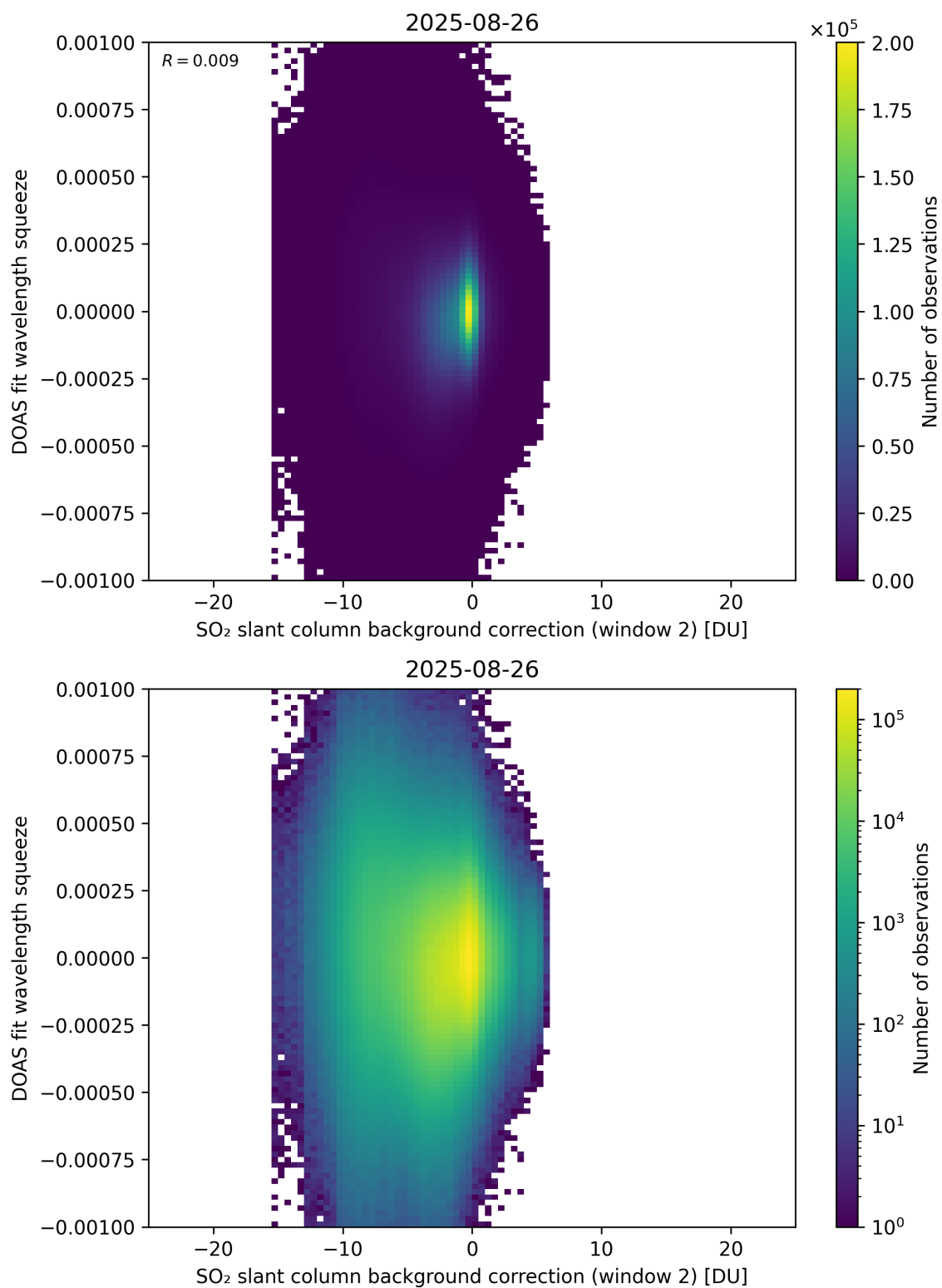
Figure 124: Scatter density plot of “SO 2 slant column background correction (window 2)” against “DOAS fit wavelength squeeze” for 2025-08-25 to 2025-08-27.
