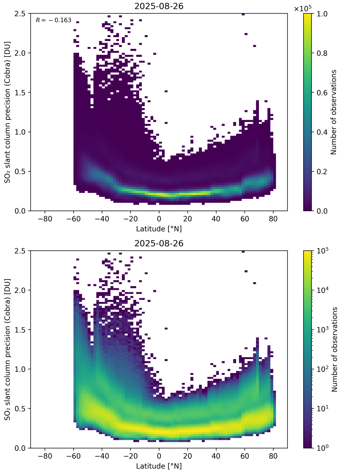
Figure 158: Scatter density plot of “Latitude” against “SO 2 slant column precision (Cobra)” for 2025-08-25 to 2025-08-27.
