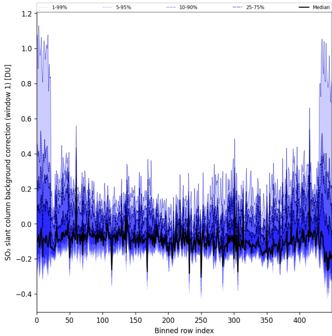
Figure 92: Along track statistics of “SO 2 slant column background correction (window 1)” for 2025-08-25 to 2025-08-27
