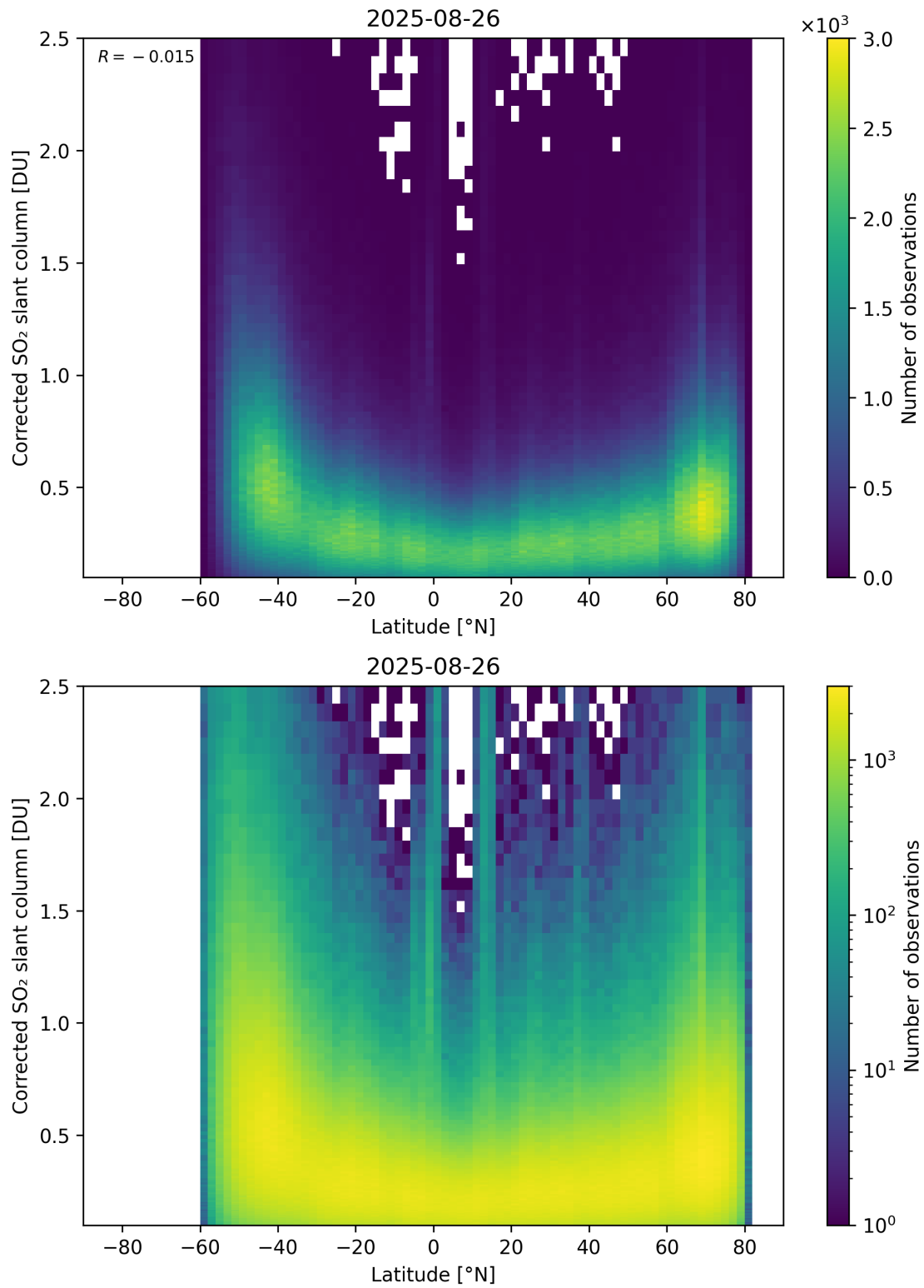
Figure 159: Scatter density plot of “Latitude” against “Corrected SO 2 slant column” for 2025-08-25 to 2025-08-27.
