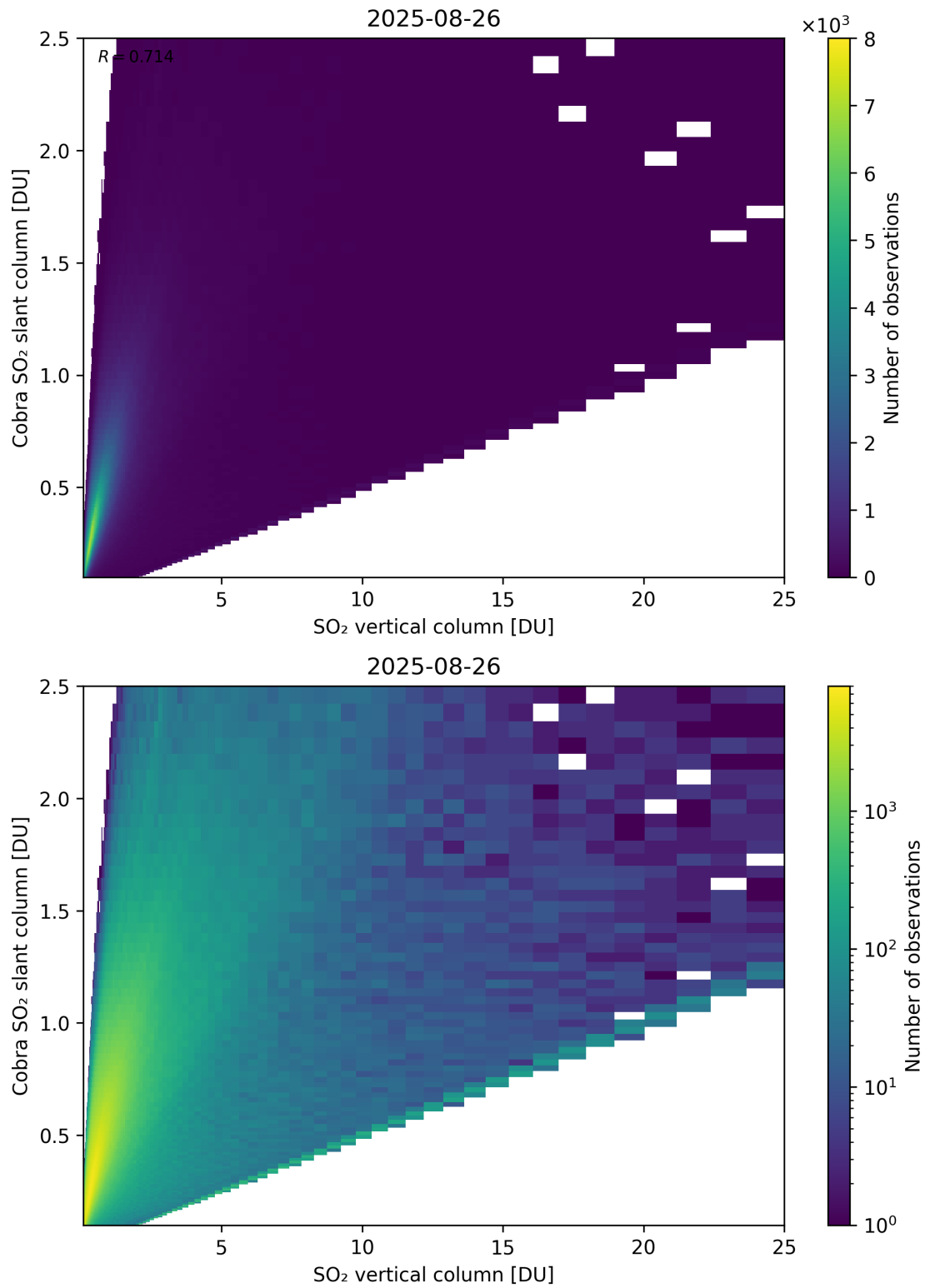
Figure 349: Scatter density plot of “SO 2 vertical column” against “Cobra SO 2 slant column” for 2025-08-25 to 2025-08-27.
