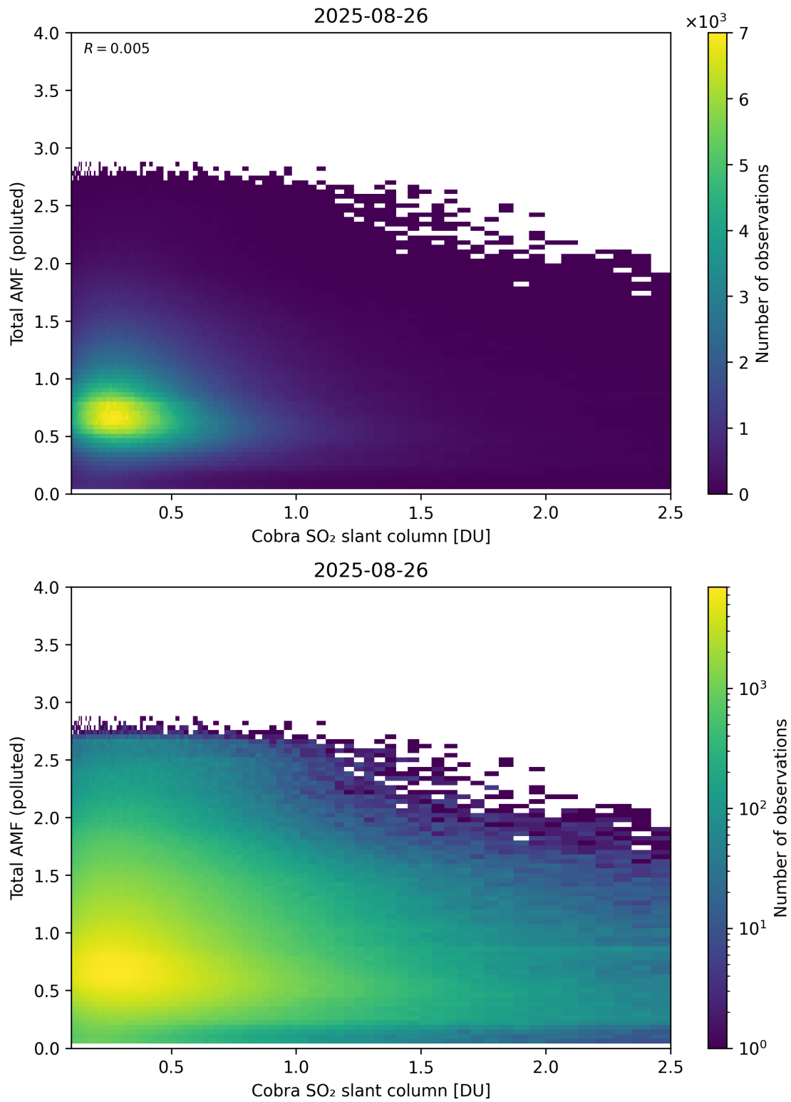
Figure 224: Scatter density plot of “Cobra SO 2 slant column” against “Total AMF (polluted)” for 2025-08-25 to 2025-08-27.
