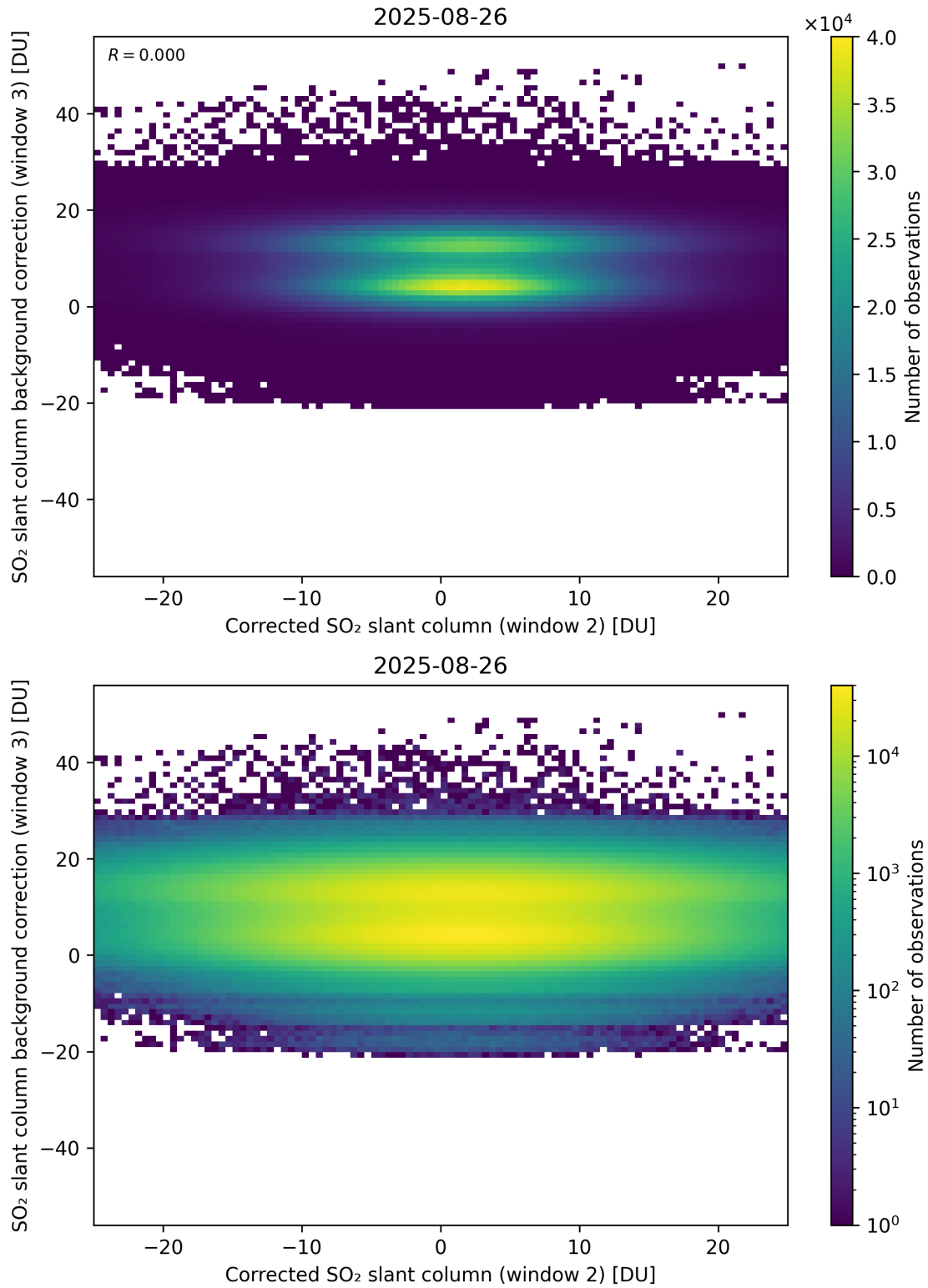
Figure 245: Scatter density plot of “Corrected SO 2 slant column (window 2)” against “SO 2 slant column background correction (window 3)” for 2025-08-25 to 2025-08-27.
