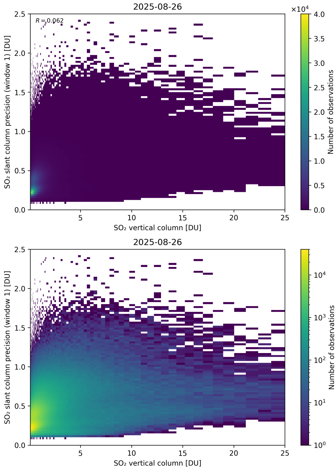
Figure 355: Scatter density plot of “SO 2 vertical column” against “SO 2 slant column precision (window 1)” for 2025-08-25 to 2025-08-27.
