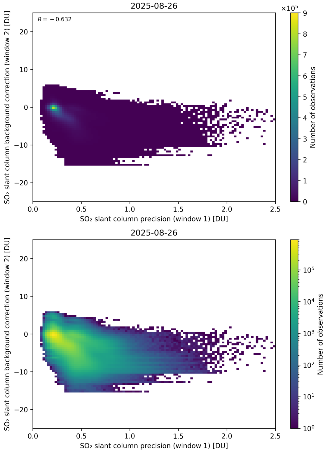
Figure 269: Scatter density plot of “SO 2 slant column precision (window 1)” against “SO 2 slant column background correction (window 2)” for 2025-08-25 to 2025-08-27.
