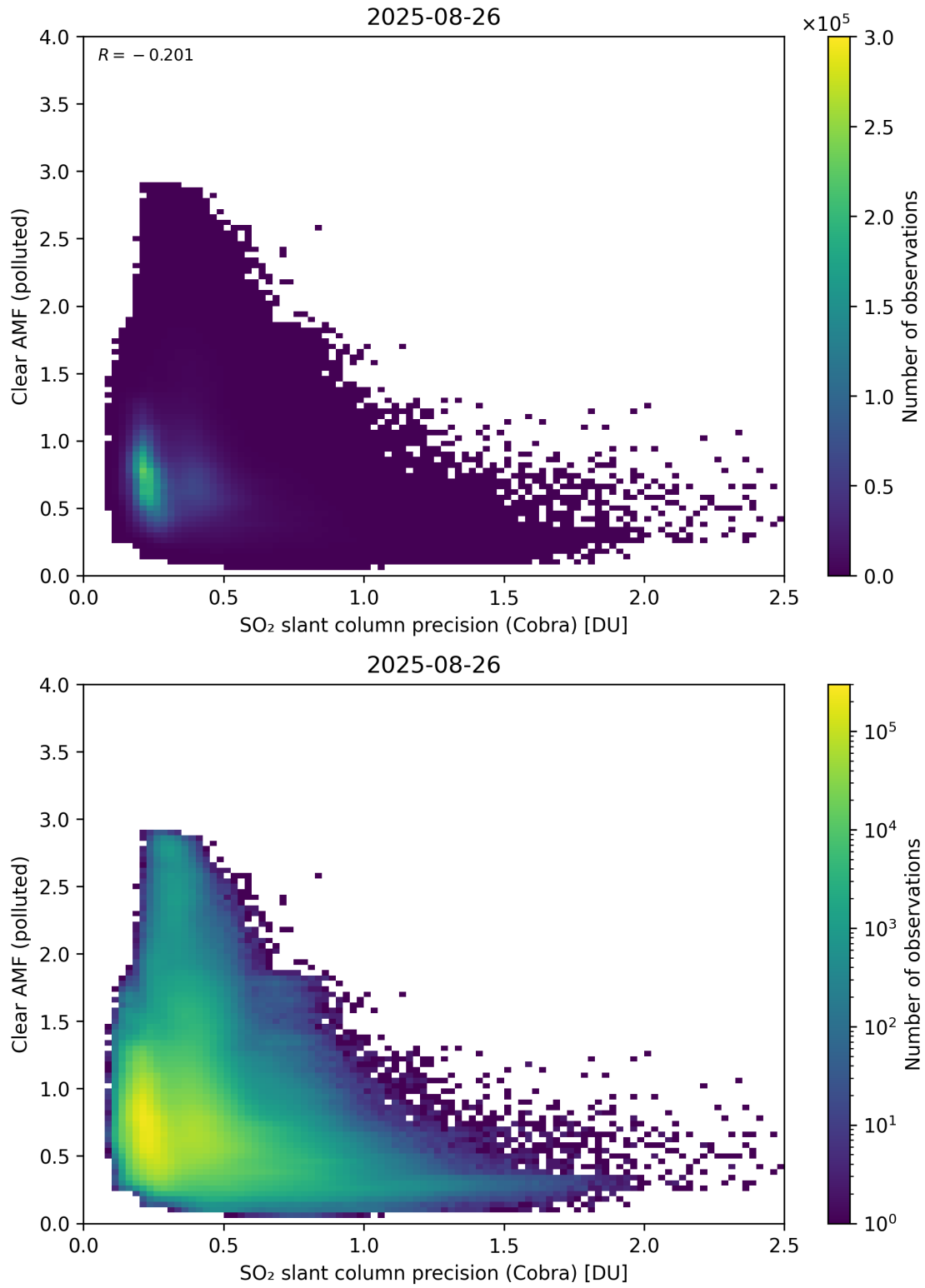
Figure 205: Scatter density plot of “SO 2 slant column precision (Cobra)” against “Clear AMF (polluted)” for 2025-08-25 to 2025-08-27.
