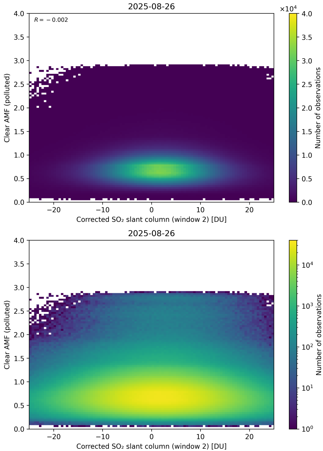
Figure 249: Scatter density plot of “Corrected SO 2 slant column (window 2)” against “Clear AMF (polluted)” for 2025-08-25 to 2025-08-27.
