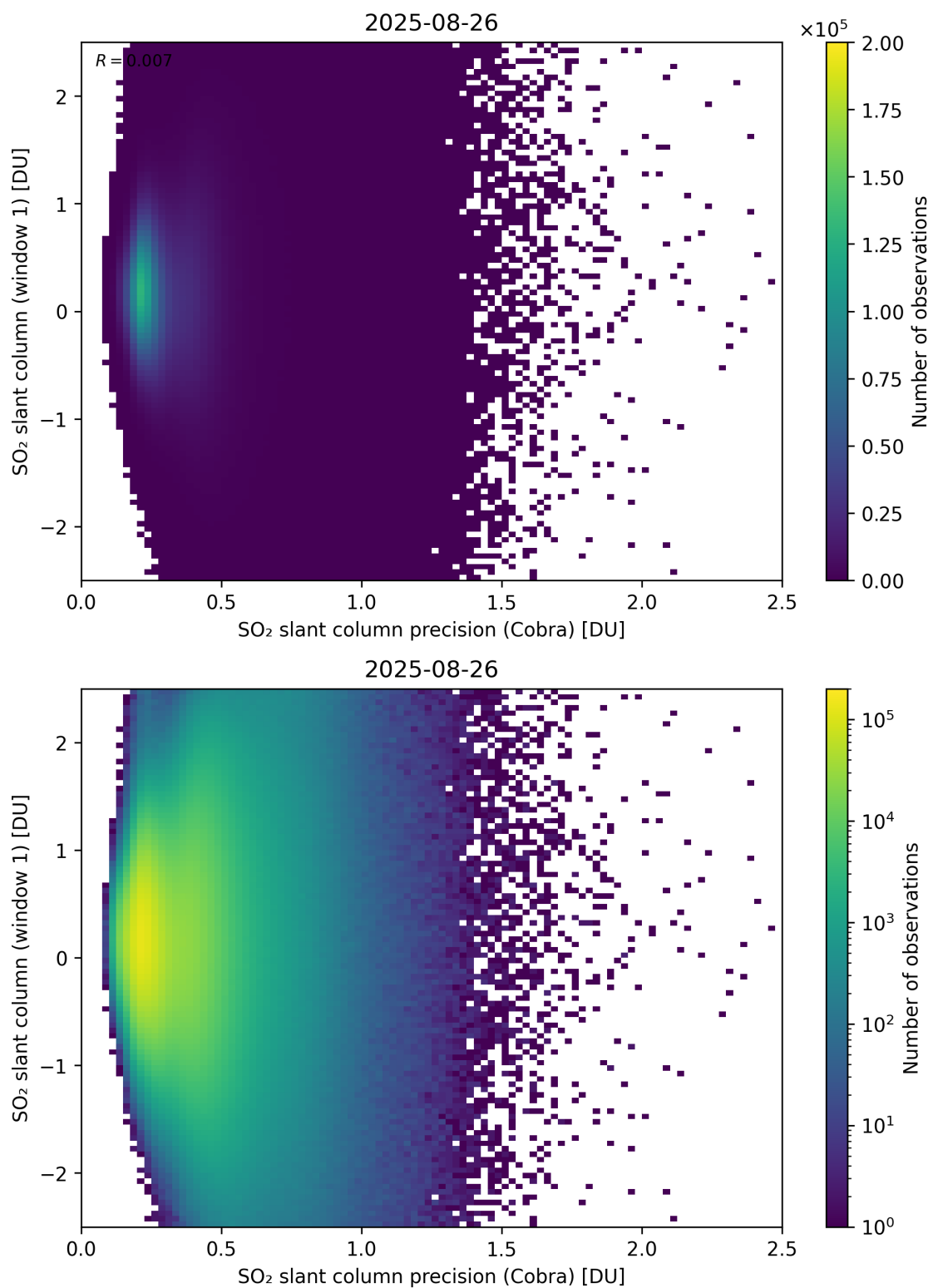
Figure 208: Scatter density plot of “SO 2 slant column precision (Cobra)” against “SO 2 slant column (window 1)” for 2025-08-25 to 2025-08-27.
