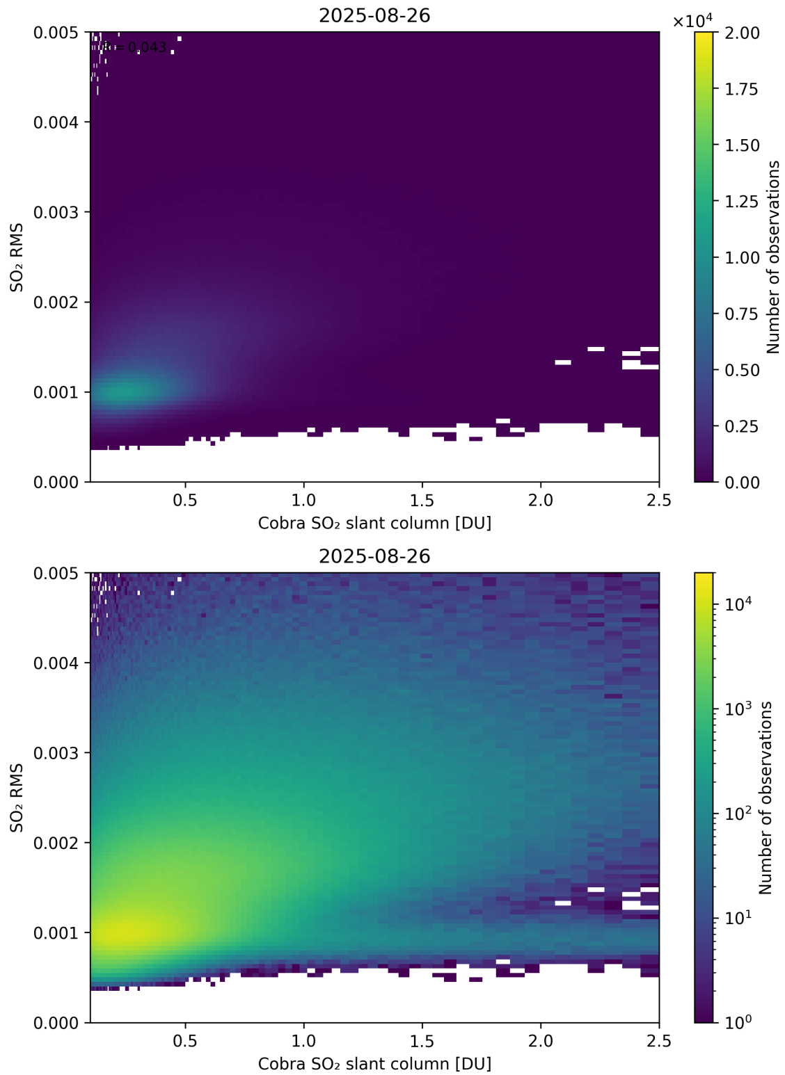
Figure 198: Scatter density plot of “Cobra SO 2 slant column” against “SO 2 RMS” for 2025-08-25 to 2025-08-27.
