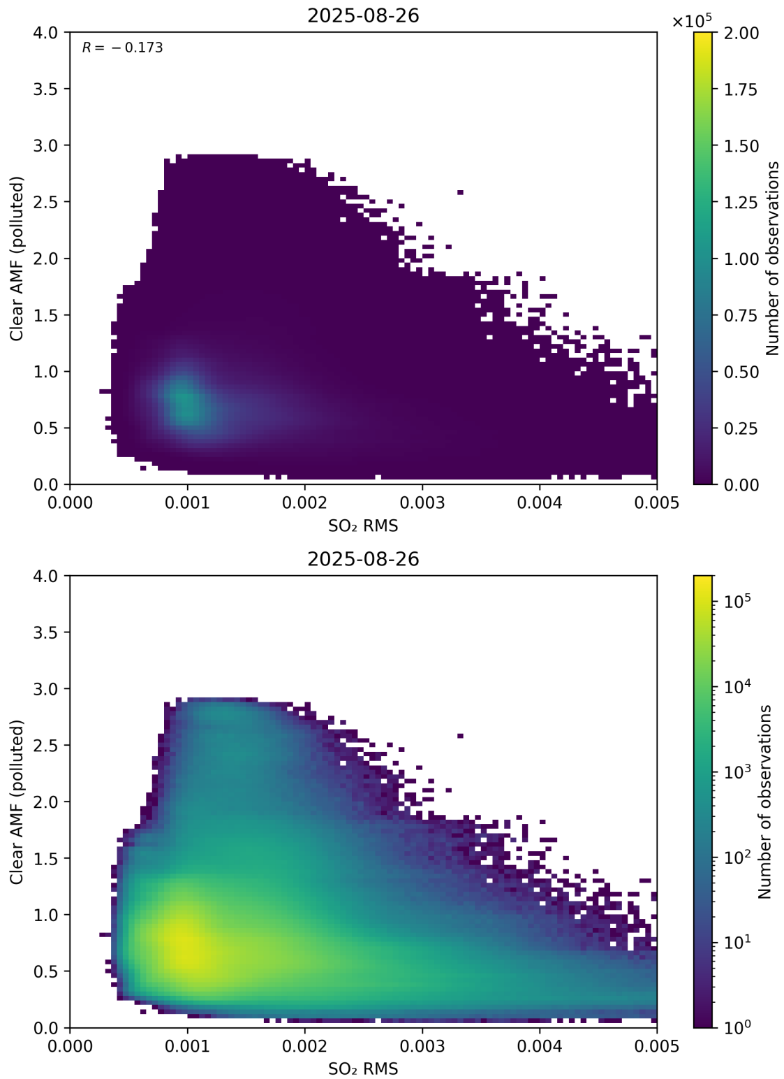
Figure 147: Scatter density plot of “SO 2 RMS” against “Clear AMF (polluted)” for 2025-08-25 to 2025-08-27.
