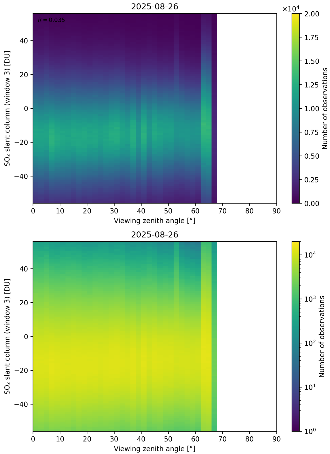
Figure 379: Scatter density plot of “Viewing zenith angle” against “SO 2 slant column (window 3)” for 2025-08-25 to 2025-08-27.
