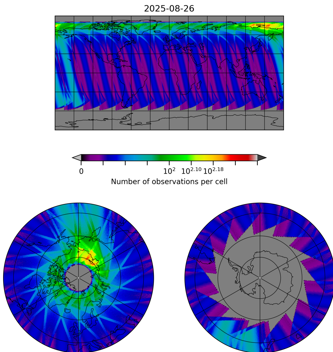
Figure 30: Map of the number of observations for 2025-08-25 to 2025-08-27
