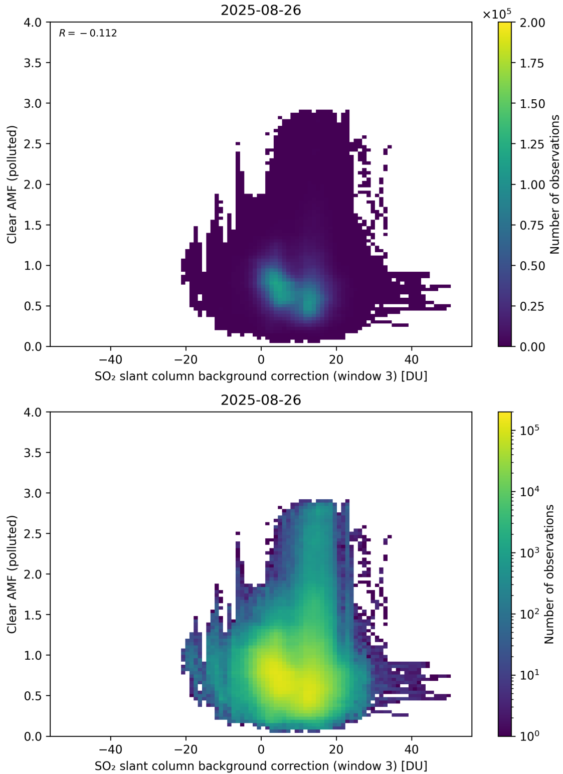
Figure 135: Scatter density plot of “SO 2 slant column background correction (window 3)” against “Clear AMF (polluted)” for 2025-08-25 to 2025-08-27.
