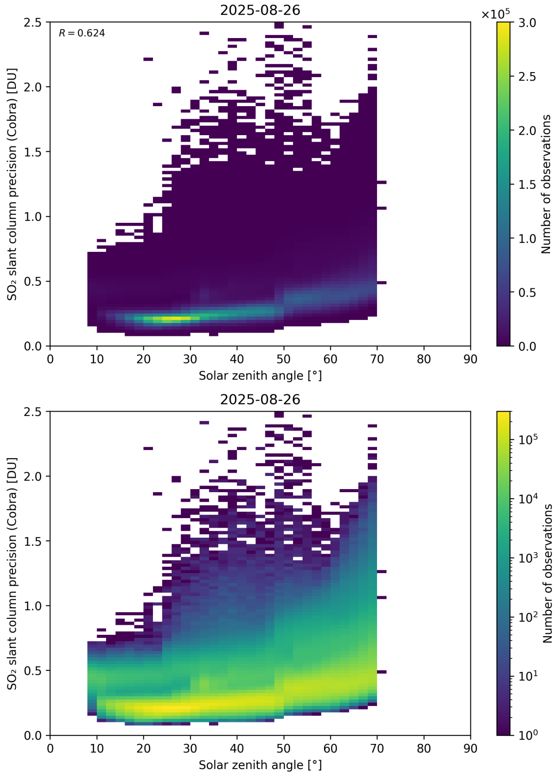
Figure 180: Scatter density plot of “Solar zenith angle” against “SO 2 slant column precision (Cobra)” for 2025-08-25 to 2025-08-27.
