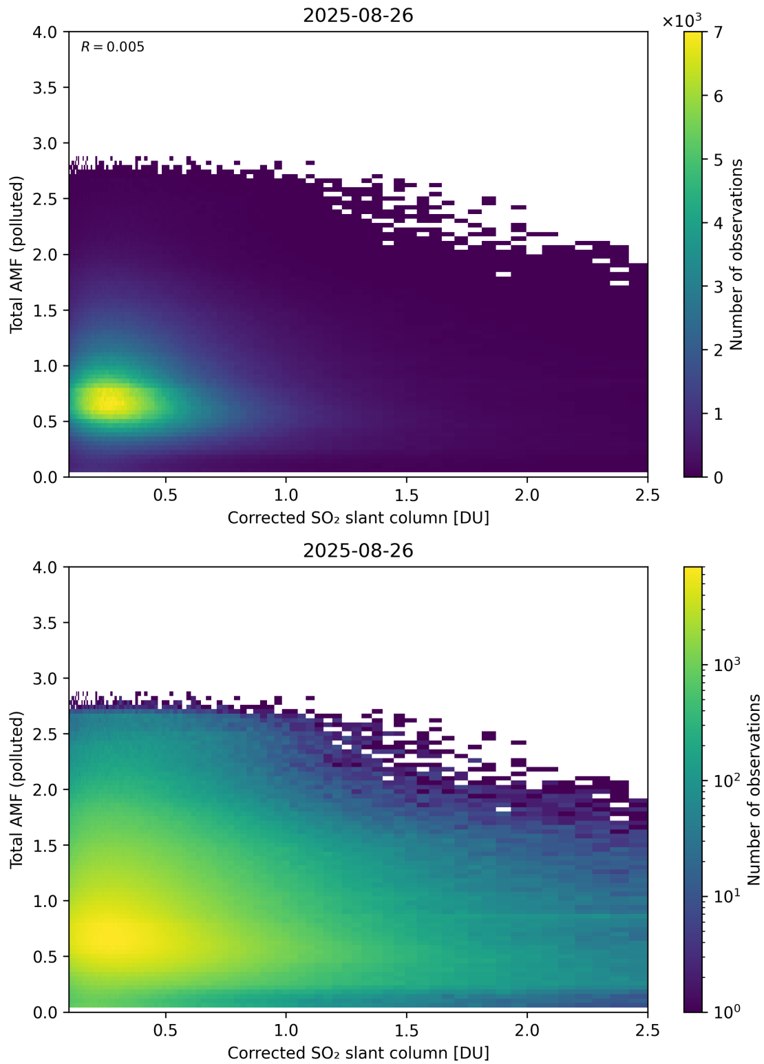
Figure 242: Scatter density plot of “Corrected SO 2 slant column” against “Total AMF (polluted)” for 2025-08-25 to 2025-08-27.
