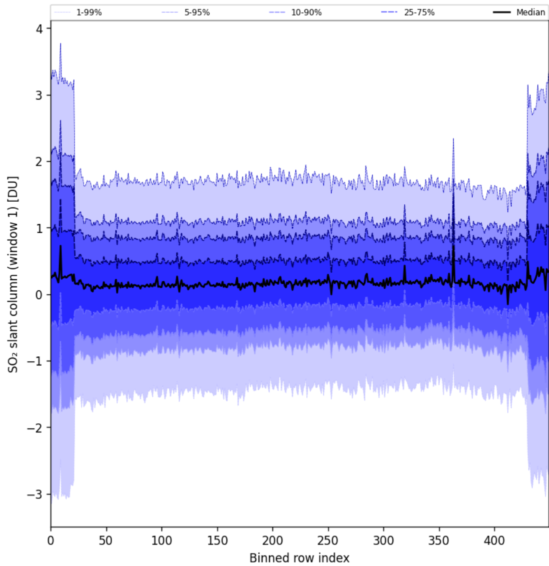
Figure 89: Along track statistics of “SO 2 slant column (window 1)” for 2025-08-25 to 2025-08-27
