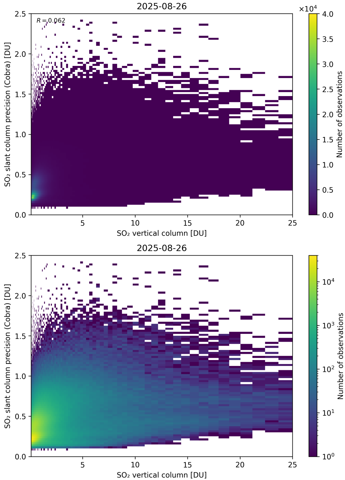
Figure 350: Scatter density plot of “SO 2 vertical column” against “SO 2 slant column precision (Cobra)” for 2025-08-25 to 2025-08-27.
