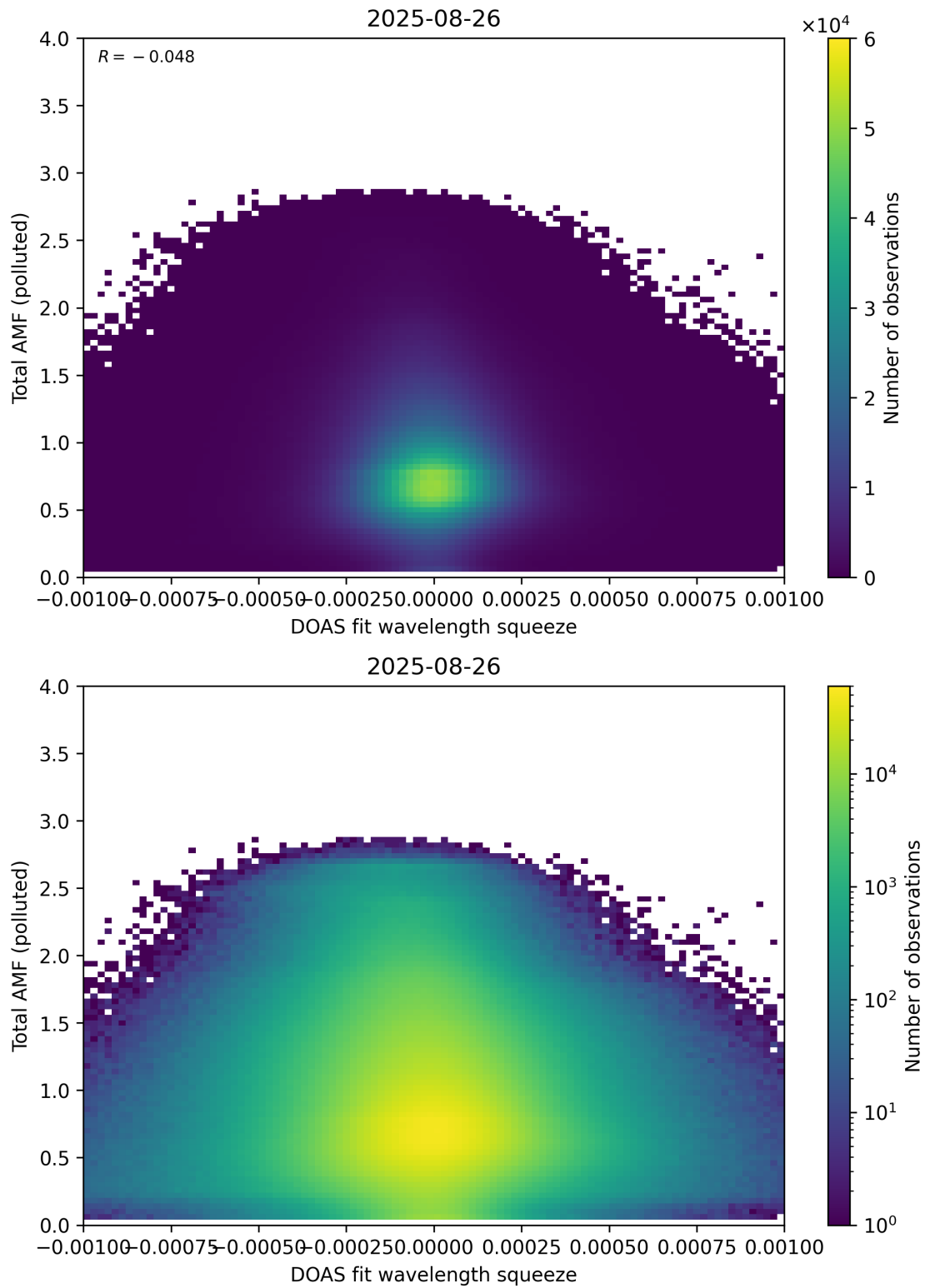
Figure 145: Scatter density plot of “DOAS fit wavelength squeeze” against “Total AMF (polluted)” for 2025-08-25 to 2025-08-27.
