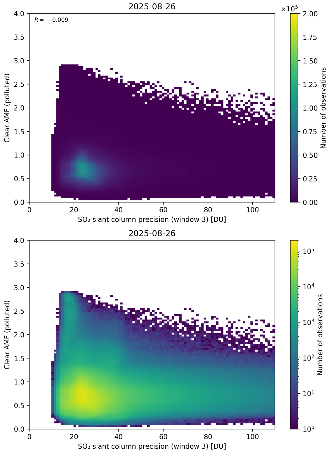
Figure 311: Scatter density plot of “SO 2 slant column precision (window 3)” against “Clear AMF (polluted)” for 2025-08-25 to 2025-08-27.
