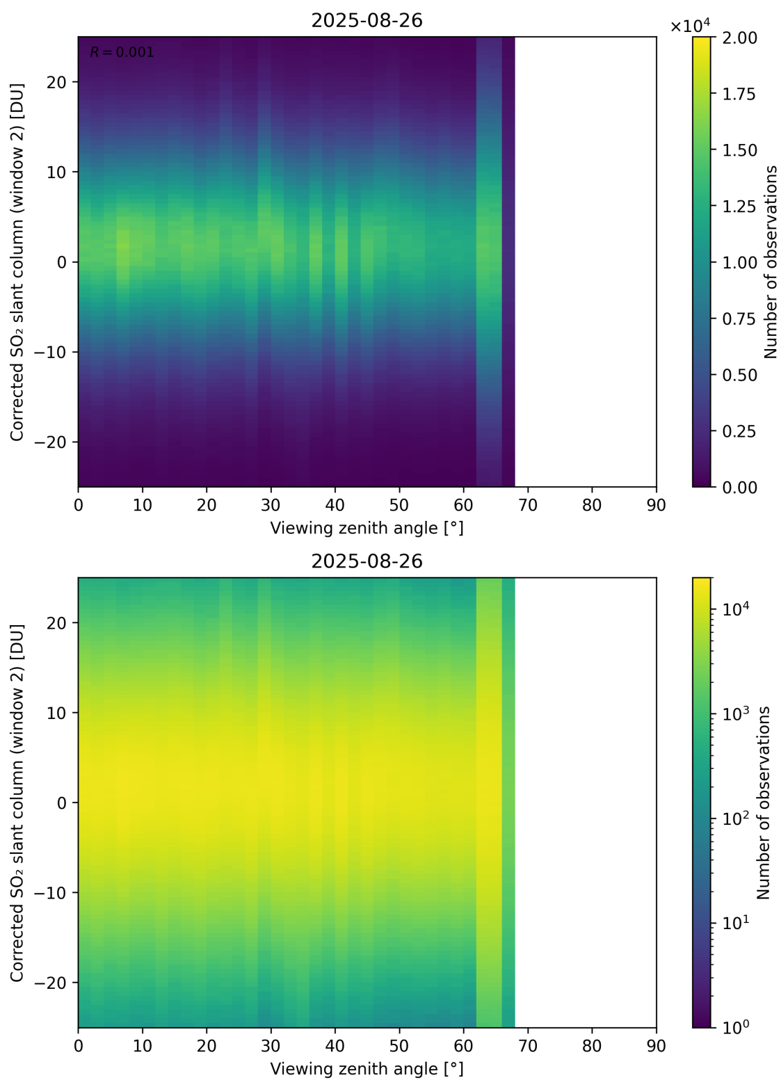
Figure 374: Scatter density plot of “Viewing zenith angle” against “Corrected SO 2 slant column (window 2)” for 2025-08-25 to 2025-08-27.
