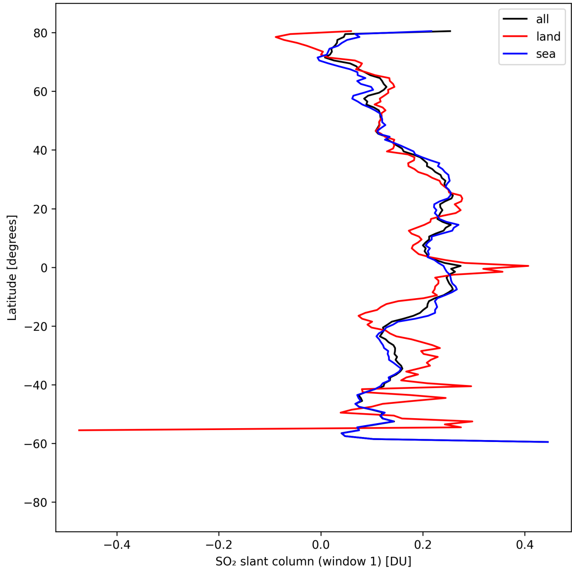
Figure 37: Zonal average of “SO 2 slant column (window 1)” for 2025-08-25 to 2025-08-27.
