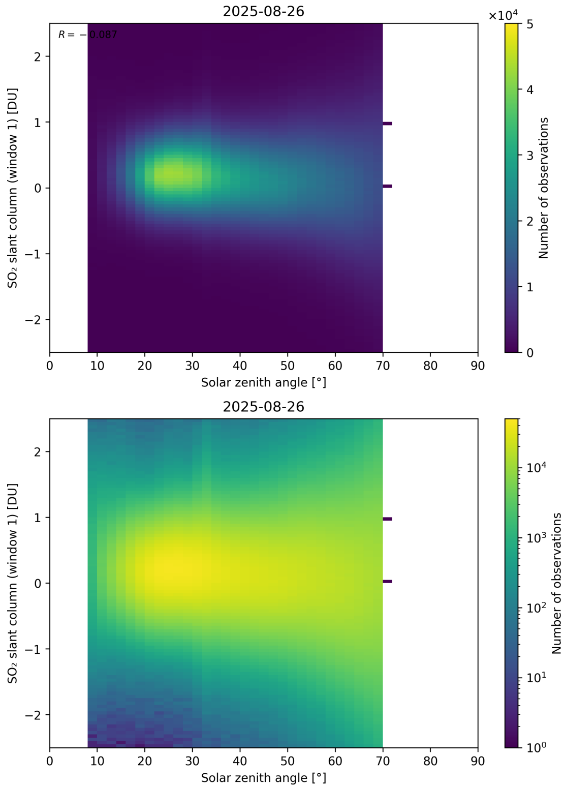
Figure 184: Scatter density plot of “Solar zenith angle” against “SO 2 slant column (window 1)” for 2025-08-25 to 2025-08-27.
