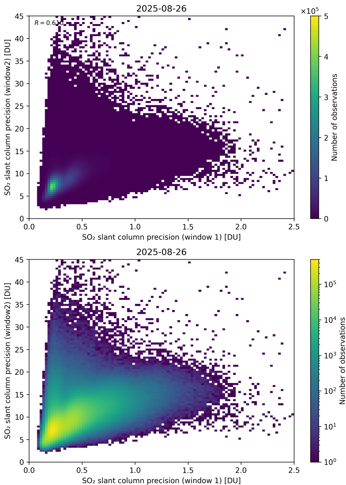
Figure 277: Scatter density plot of “SO 2 slant column precision (window 1)” against “SO 2 slant column precision (window2)” for 2025-08-25 to 2025-08-27.
