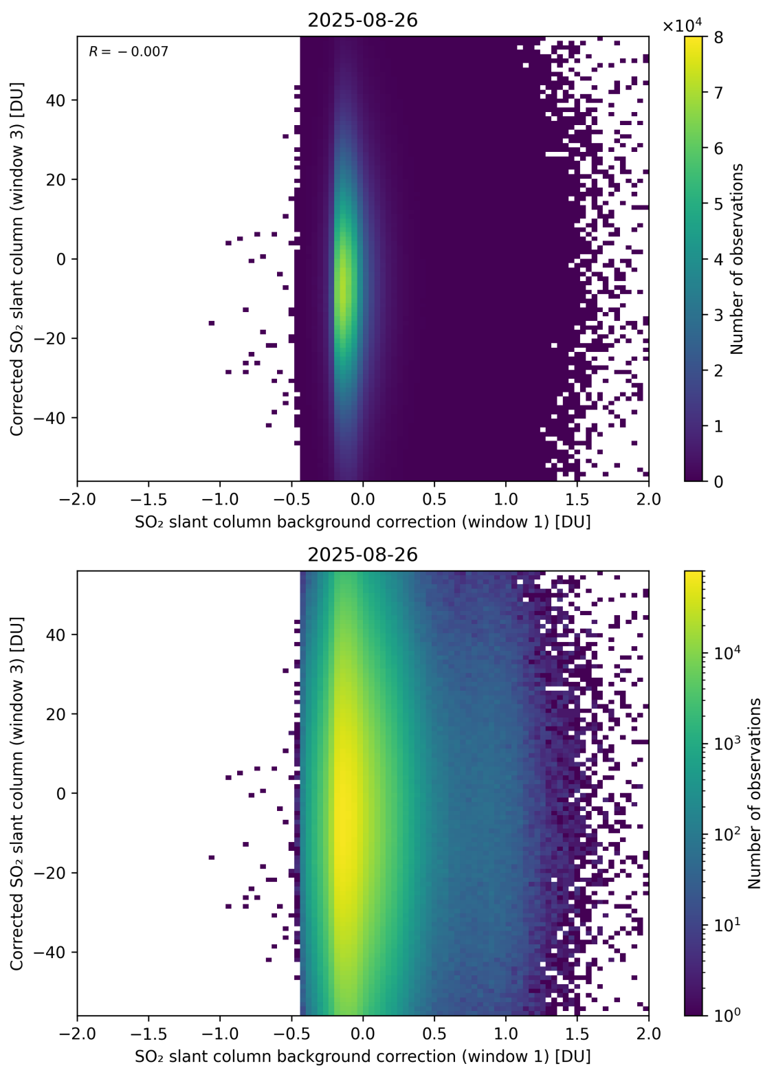
Figure 116: Scatter density plot of “SO 2 slant column background correction (window 1)” against “Corrected SO 2 slant column (window 3)” for 2025-08-25 to 2025-08-27.
