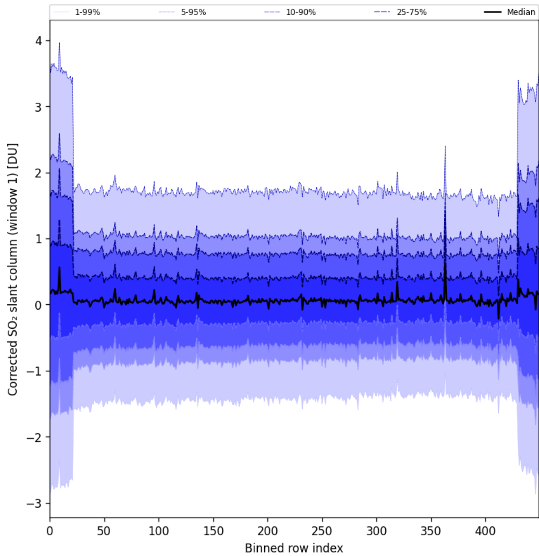
Figure 91: Along track statistics of “Corrected SO 2 slant column (window 1)” for 2025-08-25 to 2025-08-27
