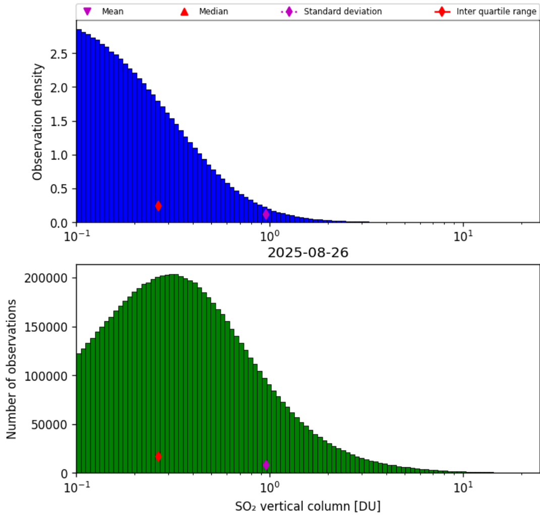
Figure 58: Histogram of “SO 2 vertical column” for 2025-08-25 to 2025-08-27
