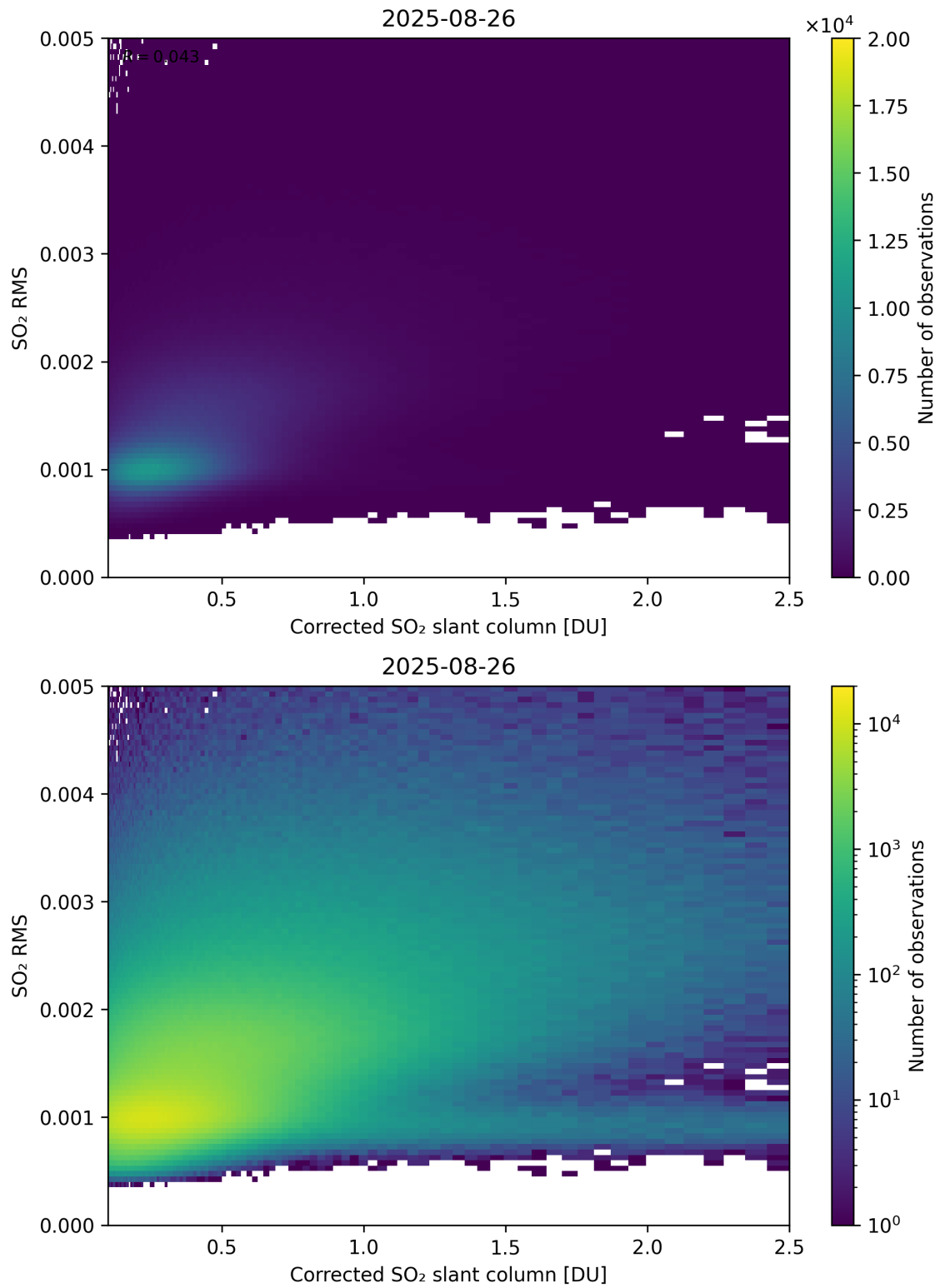
Figure 231: Scatter density plot of “Corrected SO 2 slant column” against “SO 2 RMS” for 2025-08-25 to 2025-08-27.
