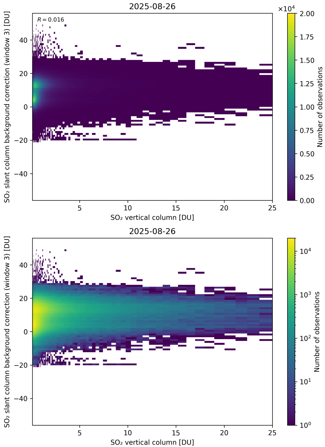
Figure 325: Scatter density plot of “SO 2 vertical column” against “SO 2 slant column background correction (window 3)” for 2025-08-25 to 2025-08-27.
