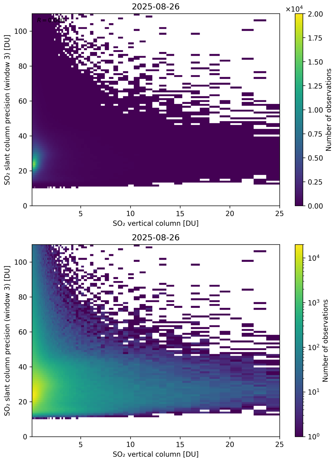
Figure 358: Scatter density plot of “SO 2 vertical column” against “SO 2 slant column precision (window 3)” for 2025-08-25 to 2025-08-27.
