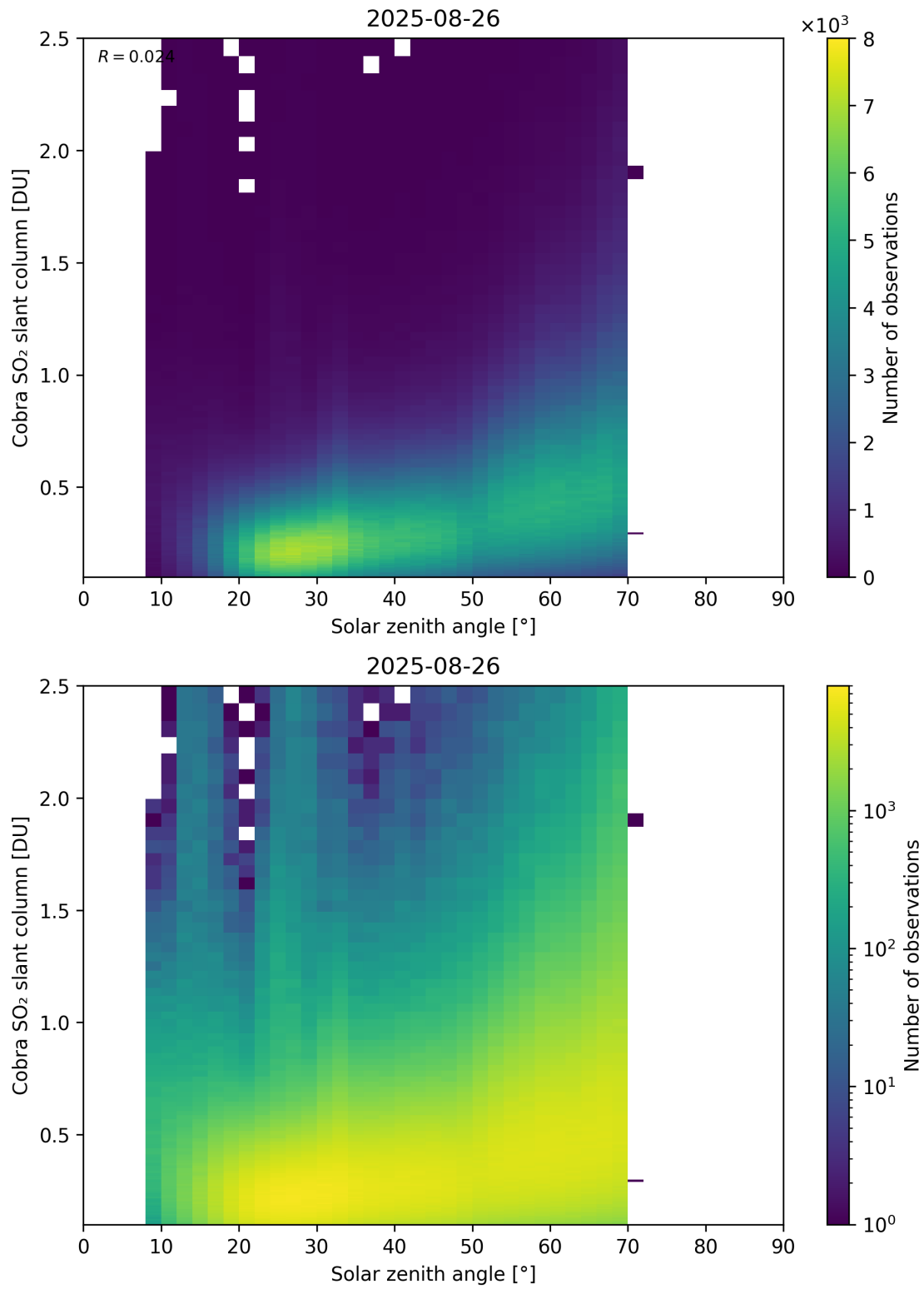
Figure 179: Scatter density plot of “Solar zenith angle” against “Cobra SO 2 slant column” for 2025-08-25 to 2025-08-27.
