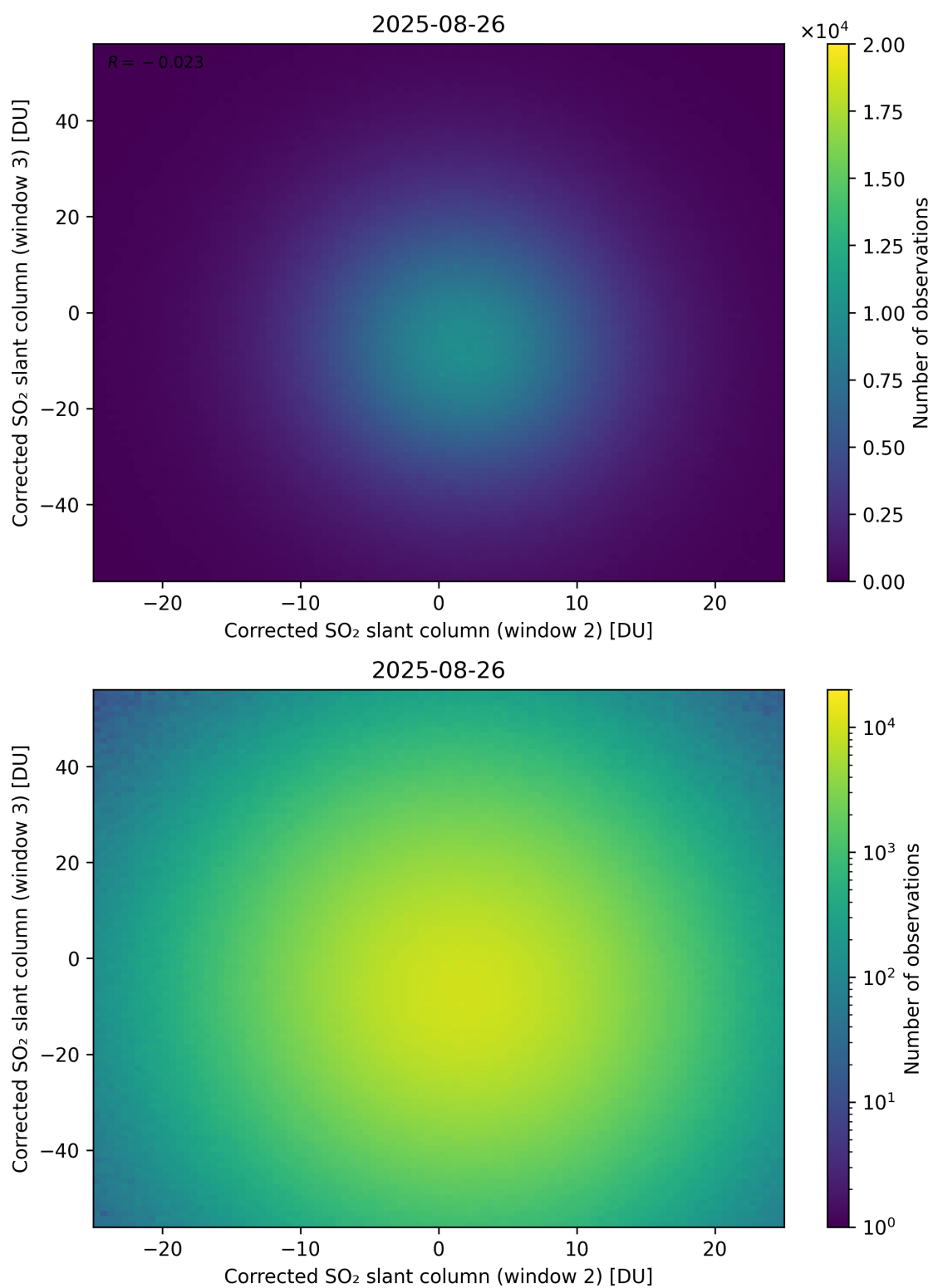
Figure 250: Scatter density plot of “Corrected SO 2 slant column (window 2)” against “Corrected SO 2 slant column (window 3)” for 2025-08-25 to 2025-08-27.
