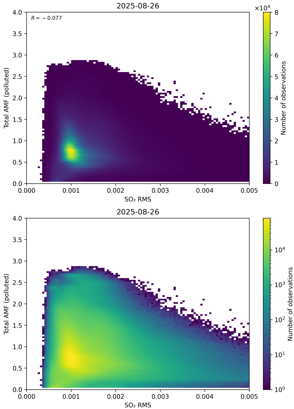
Figure 148: Scatter density plot of “SO 2 RMS” against “Total AMF (polluted)” for 2025-08-25 to 2025-08-27.
