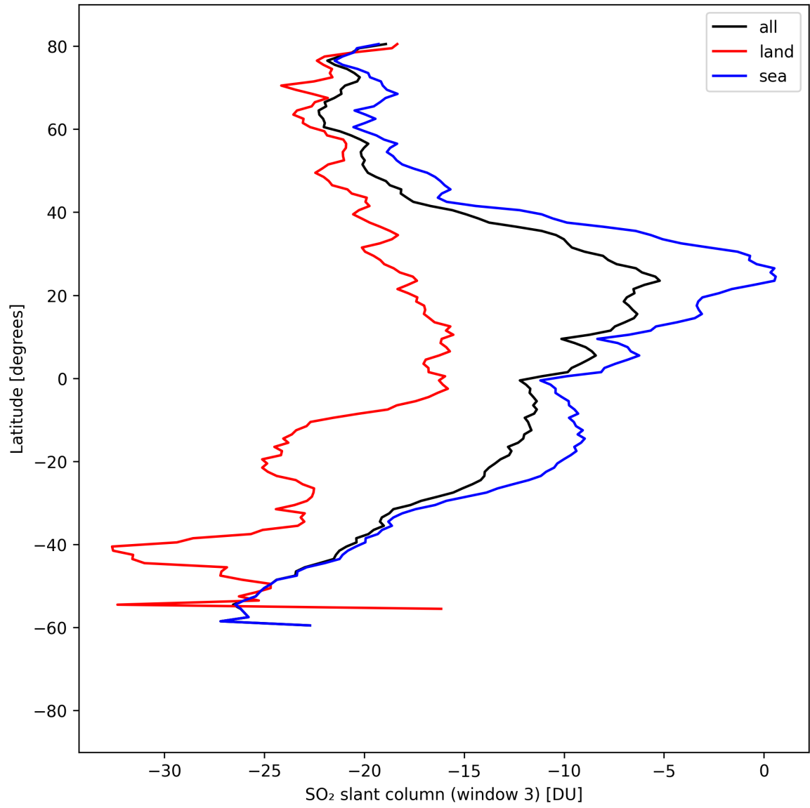
Figure 45: Zonal average of “SO 2 slant column (window 3)” for 2025-08-25 to 2025-08-27.
