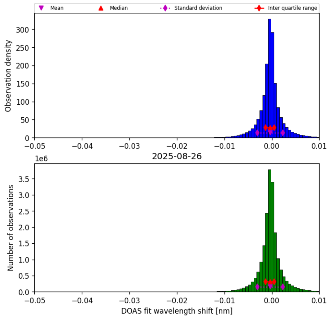
Figure 76: Histogram of “DOAS fit wavelength shift” for 2025-08-25 to 2025-08-27
