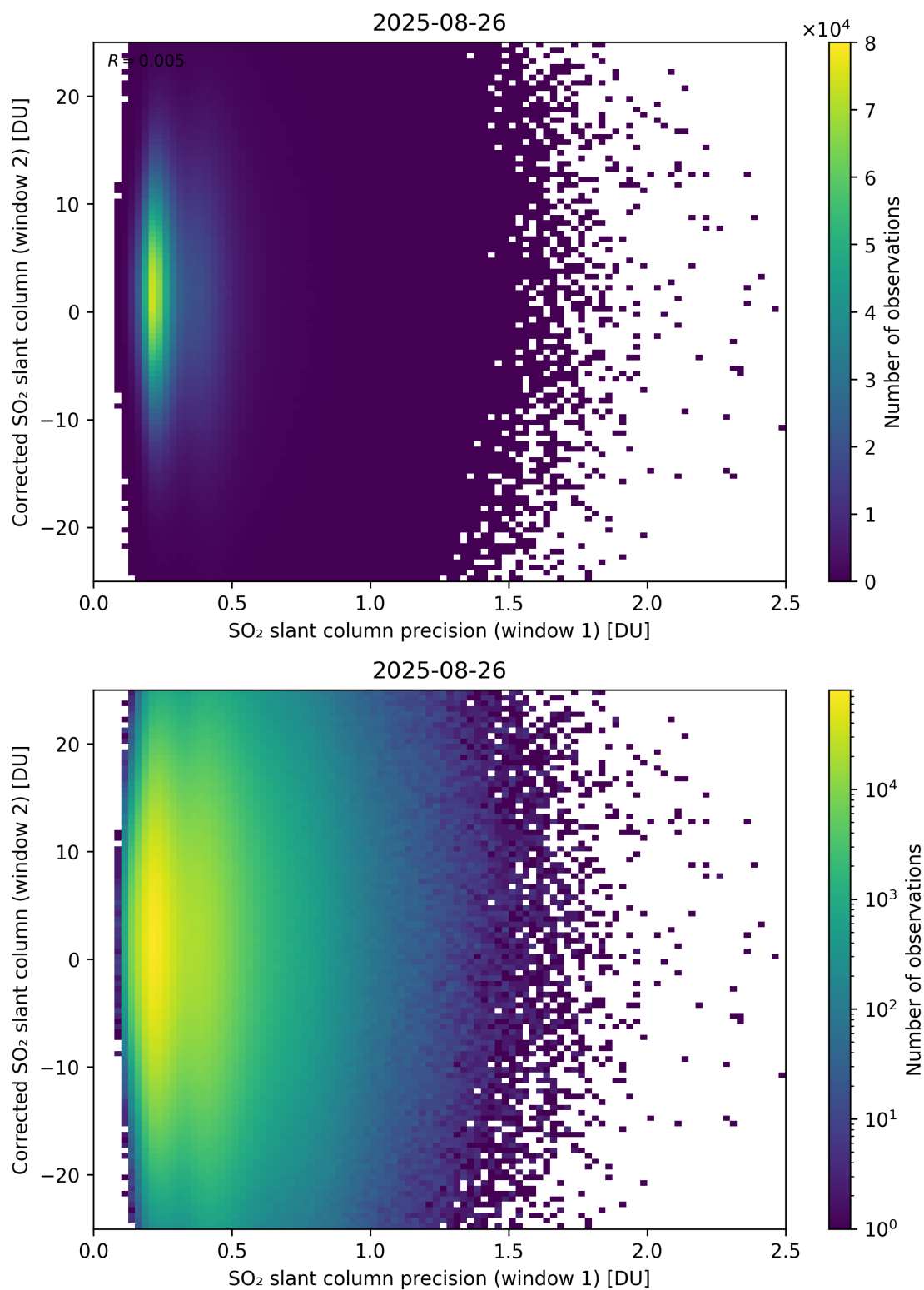
Figure 275: Scatter density plot of “SO 2 slant column precision (window 1)” against “Corrected SO 2 slant column (window 2)” for 2025-08-25 to 2025-08-27.
