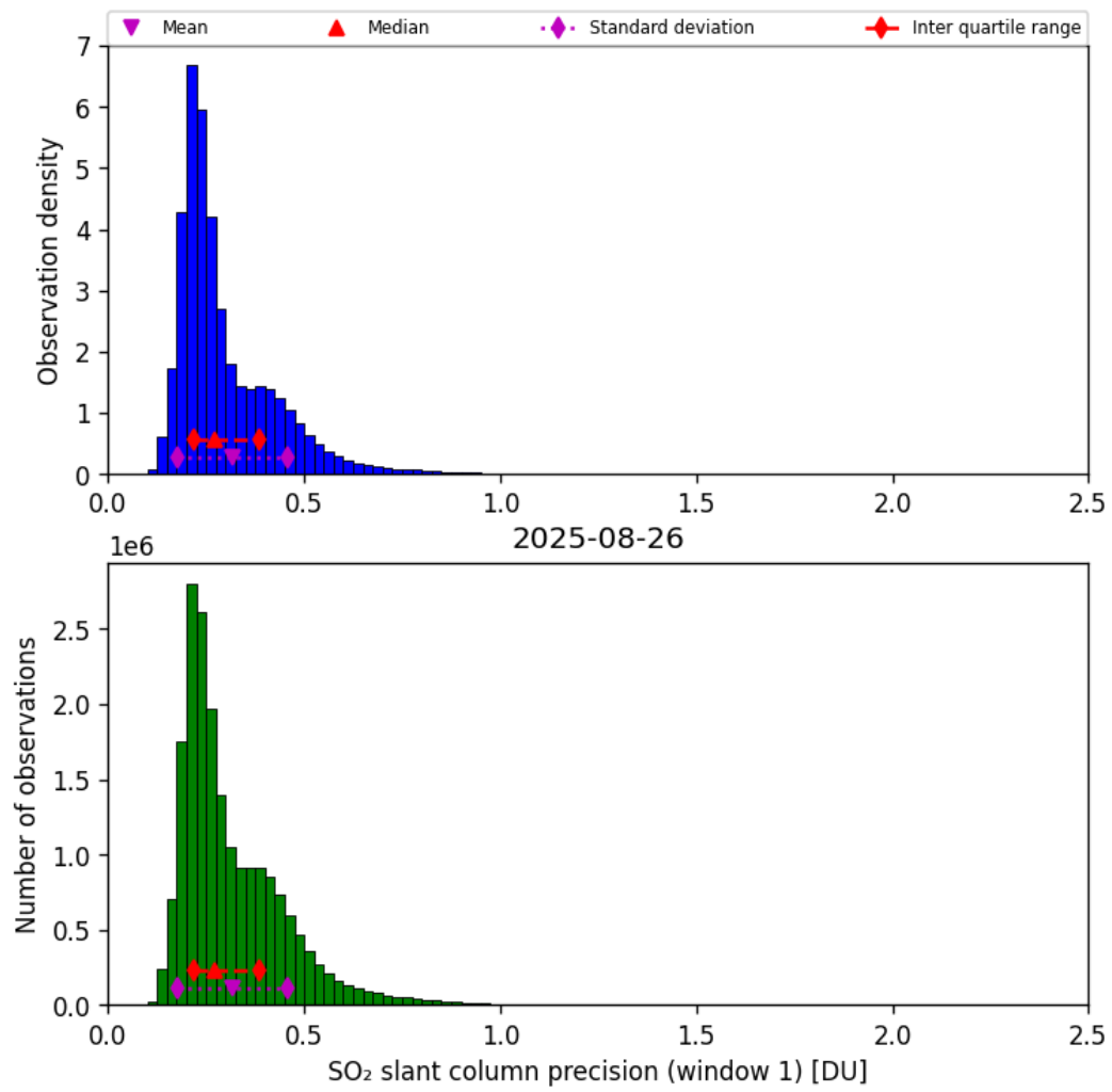
Figure 64: Histogram of “SO 2 slant column precision (window 1)” for 2025-08-25 to 2025-08-27
