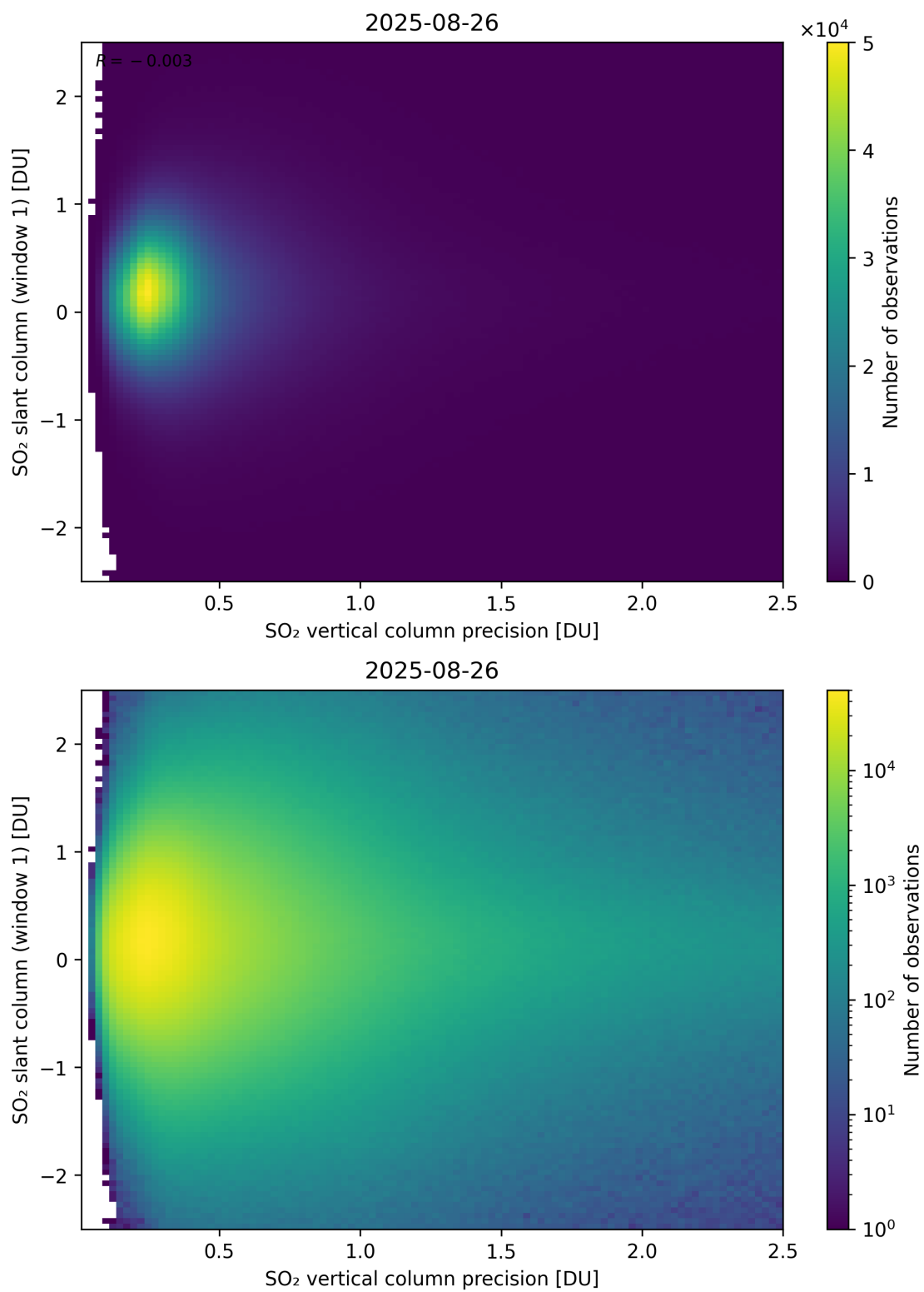
Figure 341: Scatter density plot of “SO 2 vertical column precision” against “SO 2 slant column (window 1)” for 2025-08-25 to 2025-08-27.
