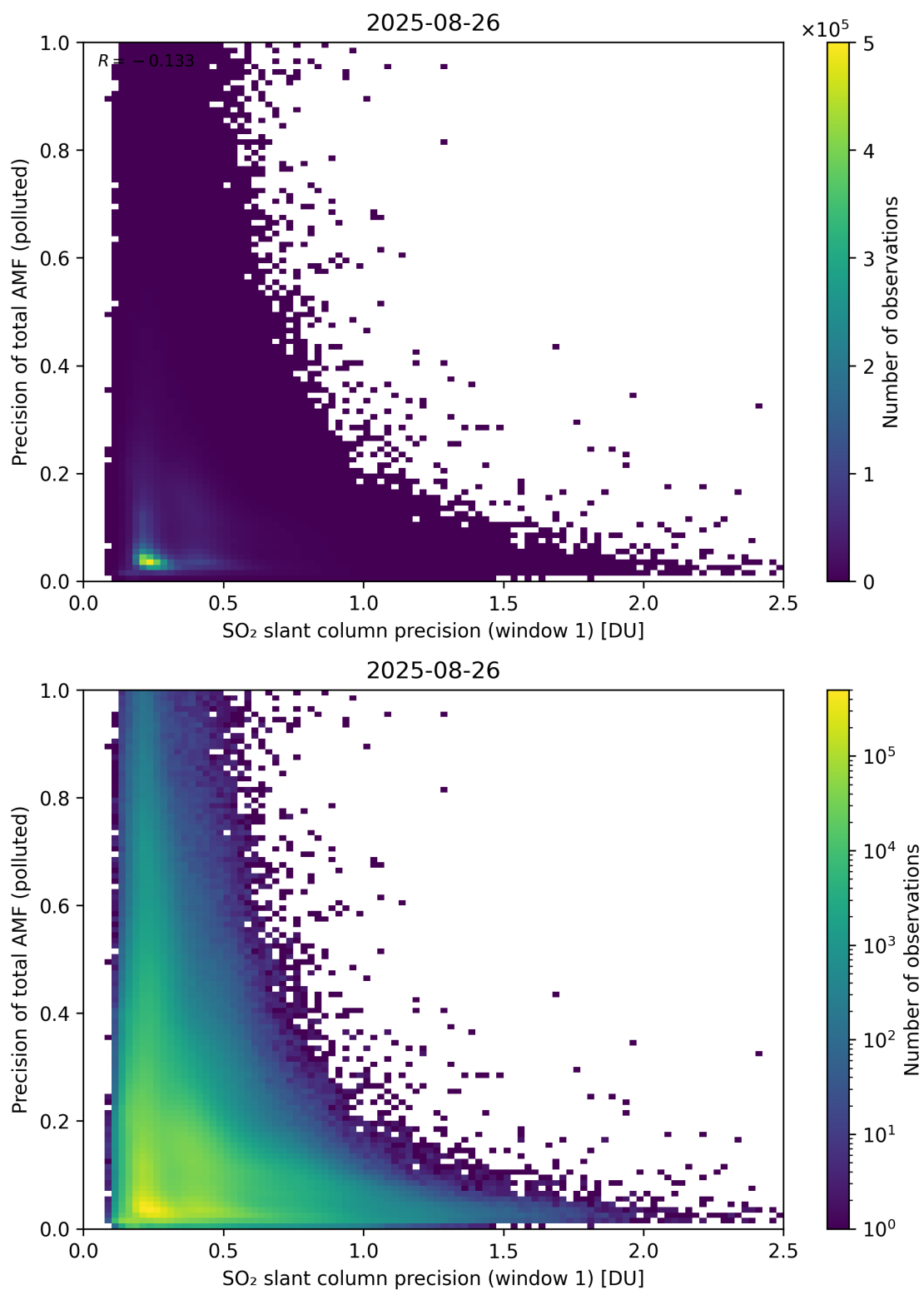
Figure 281: Scatter density plot of “SO 2 slant column precision (window 1)” against “Precision of total AMF (polluted)” for 2025-08-25 to 2025-08-27.
