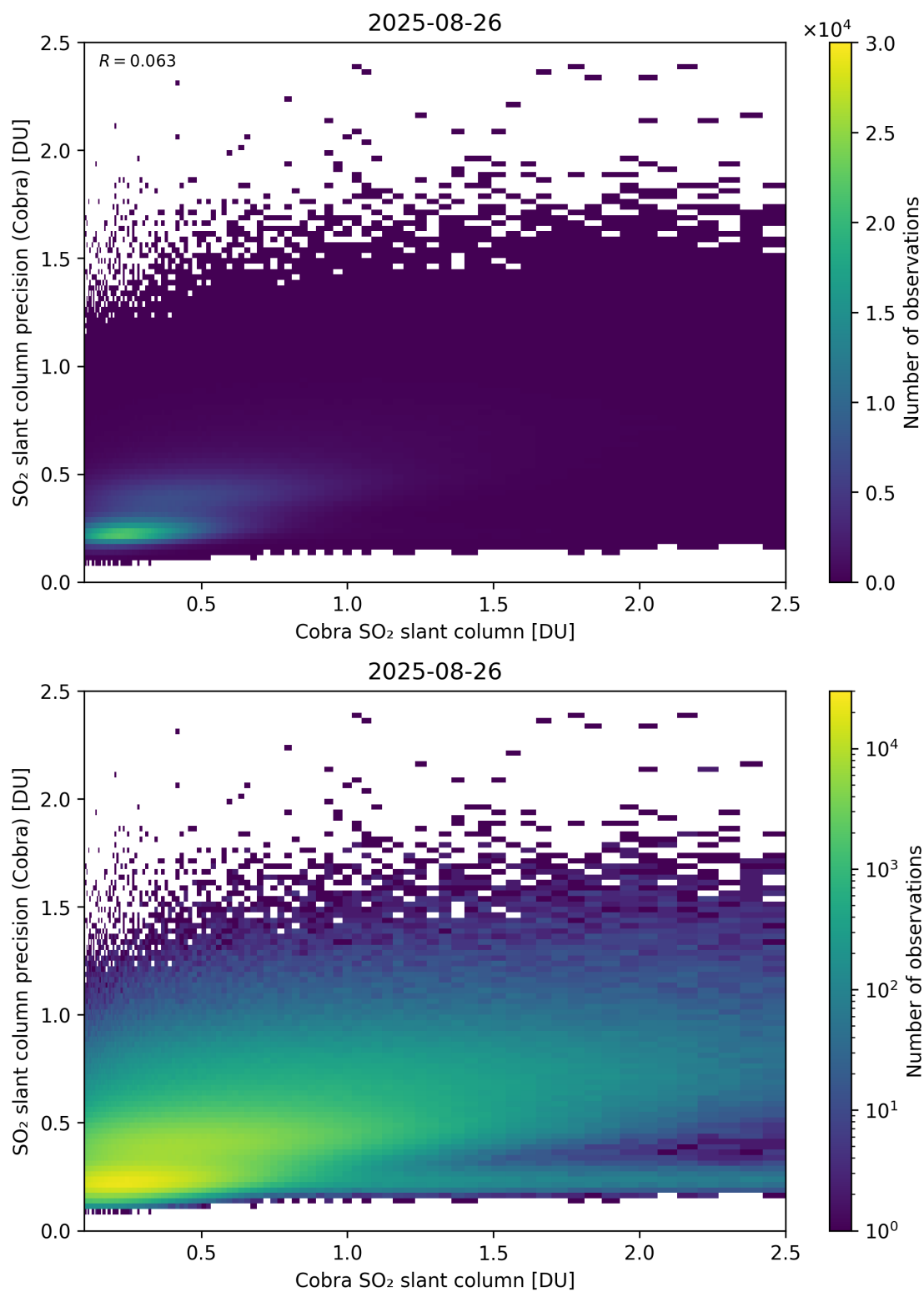
Figure 216: Scatter density plot of “Cobra SO 2 slant column” against “SO 2 slant column precision (Cobra)” for 2025-08-25 to 2025-08-27.
