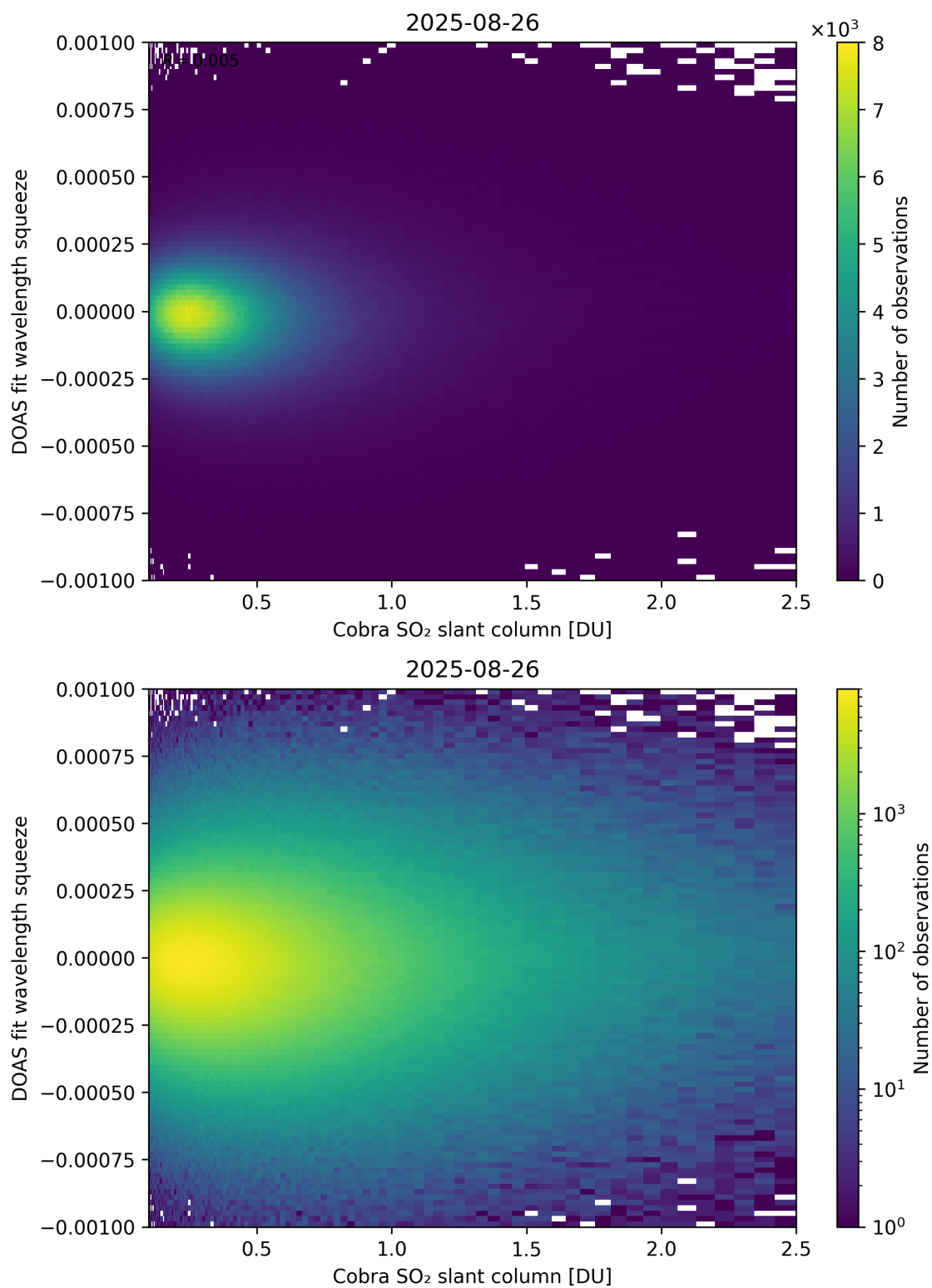
Figure 197: Scatter density plot of “Cobra SO 2 slant column” against “DOAS fit wavelength squeeze” for 2025-08-25 to 2025-08-27.
