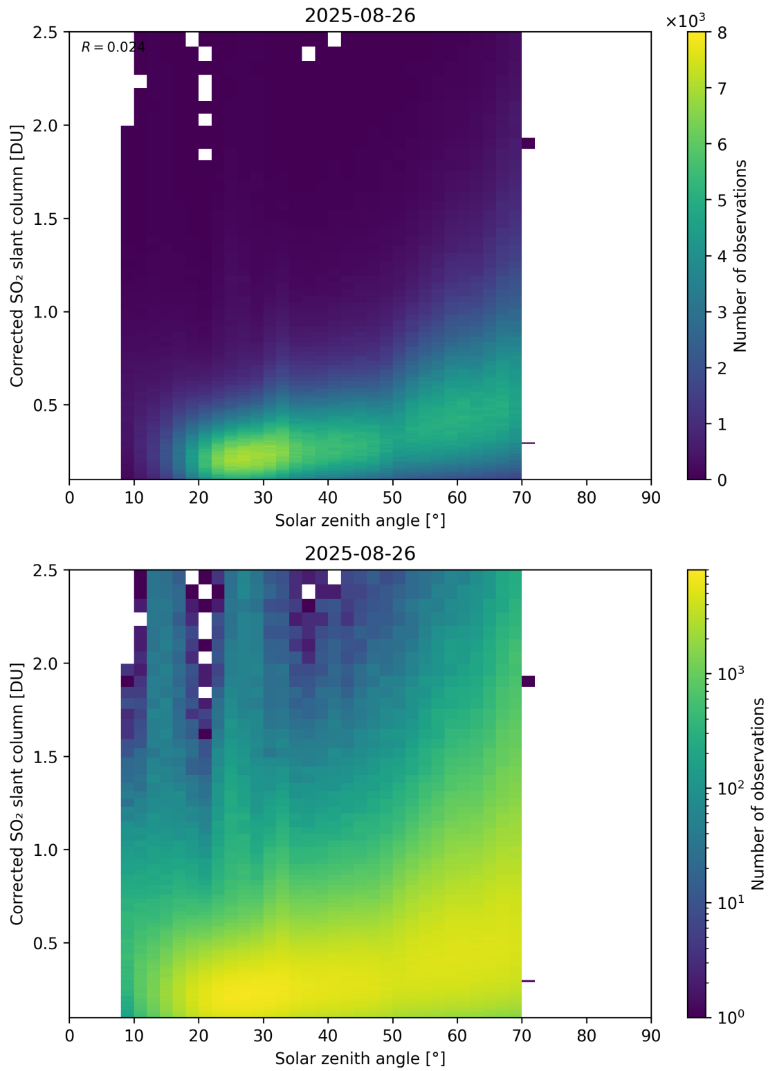
Figure 181: Scatter density plot of “Solar zenith angle” against “Corrected SO 2 slant column” for 2025-08-25 to 2025-08-27.
