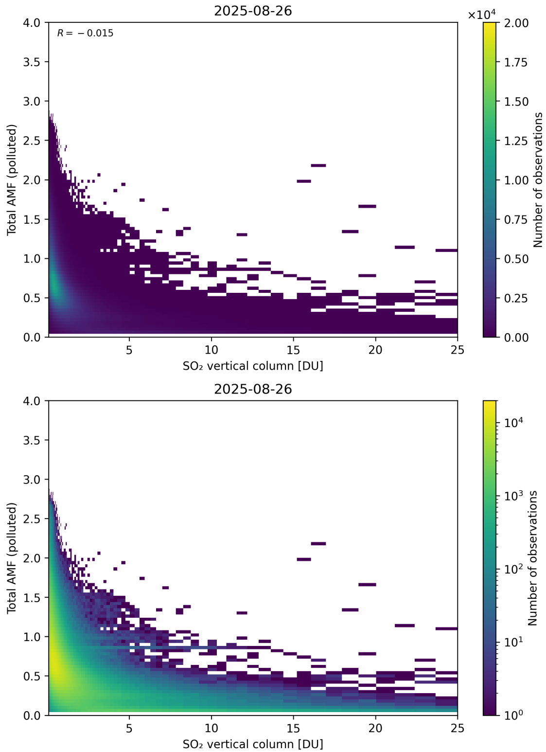
Figure 359: Scatter density plot of “SO 2 vertical column” against “Total AMF (polluted)” for 2025-08-25 to 2025-08-27.
