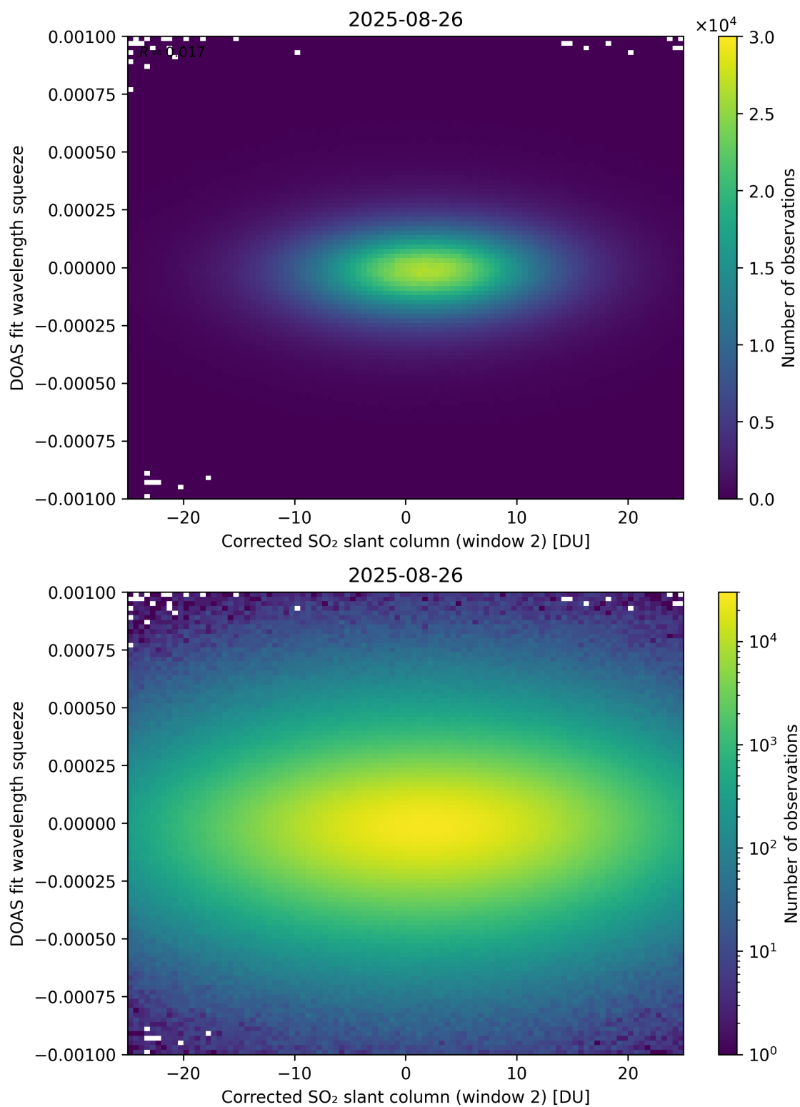
Figure 247: Scatter density plot of “Corrected SO 2 slant column (window 2)” against “DOAS fit wavelength squeeze” for 2025-08-25 to 2025-08-27.
