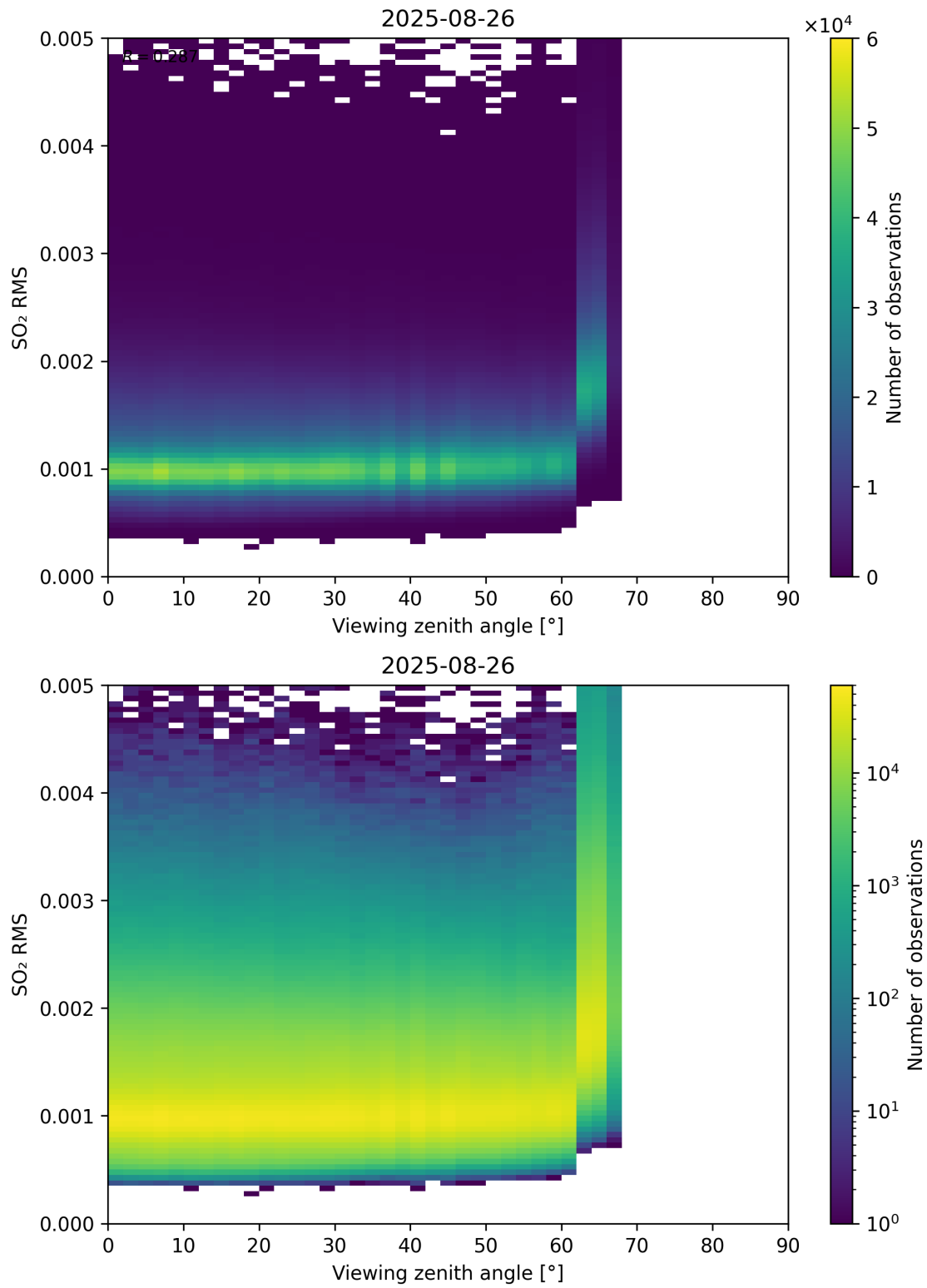
Figure 367: Scatter density plot of “Viewing zenith angle” against “SO 2 RMS” for 2025-08-25 to 2025-08-27.
