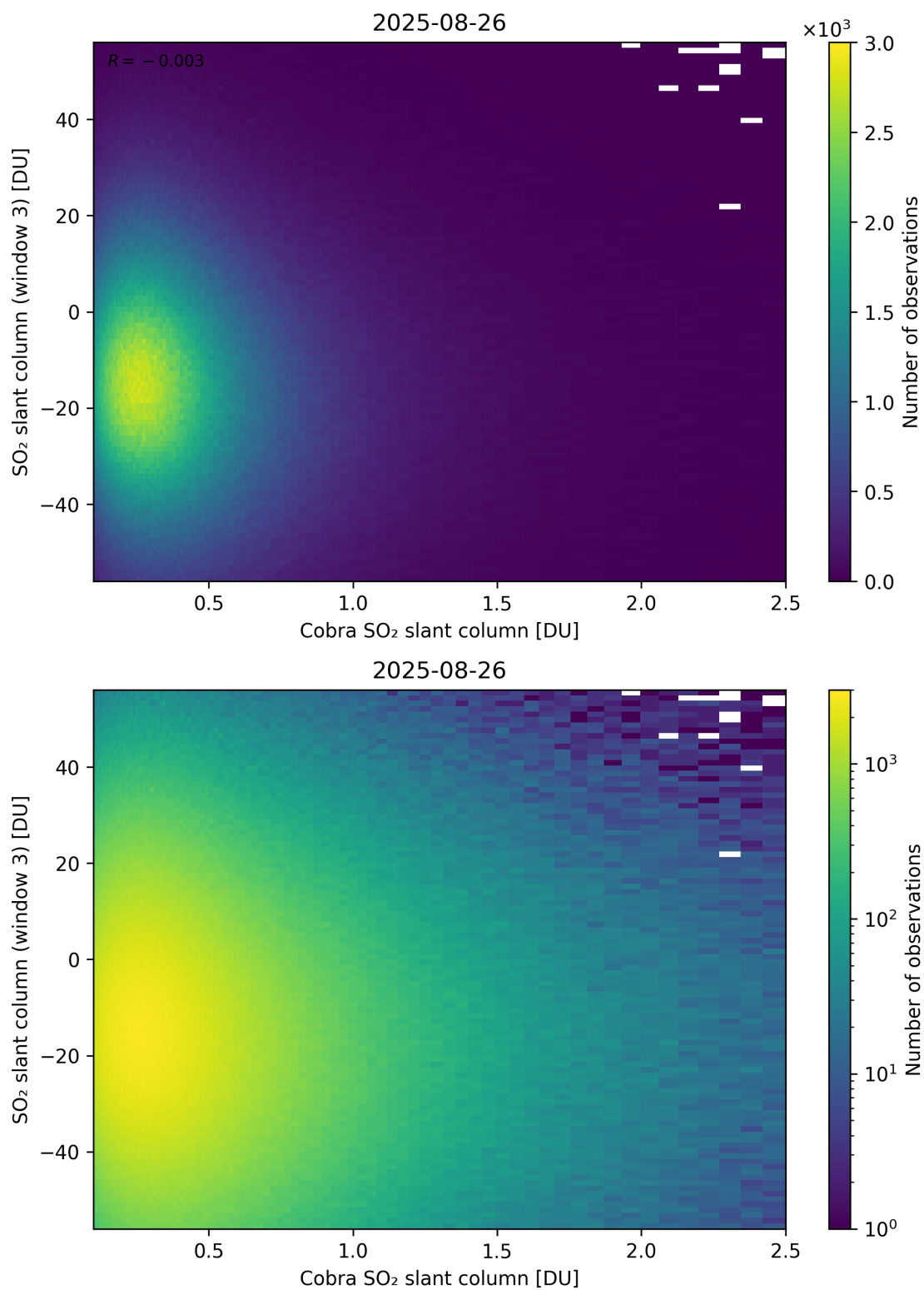
Figure 222: Scatter density plot of “Cobra SO 2 slant column” against “SO 2 slant column (window 3)” for 2025-08-25 to 2025-08-27.
