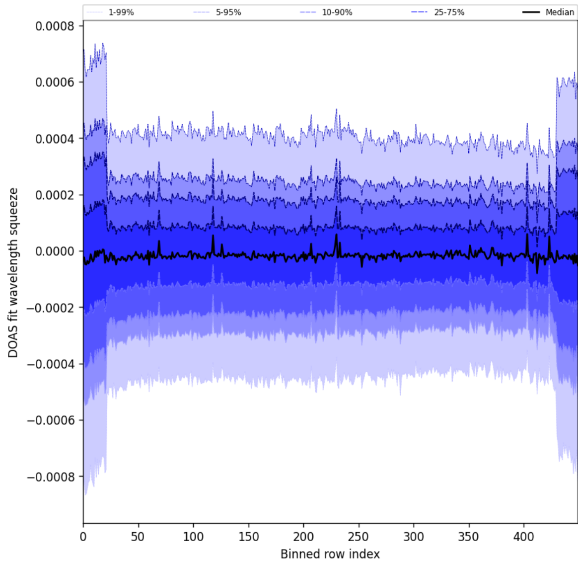
Figure 103: Along track statistics of “DOAS fit wavelength squeeze” for 2025-08-25 to 2025-08-27
