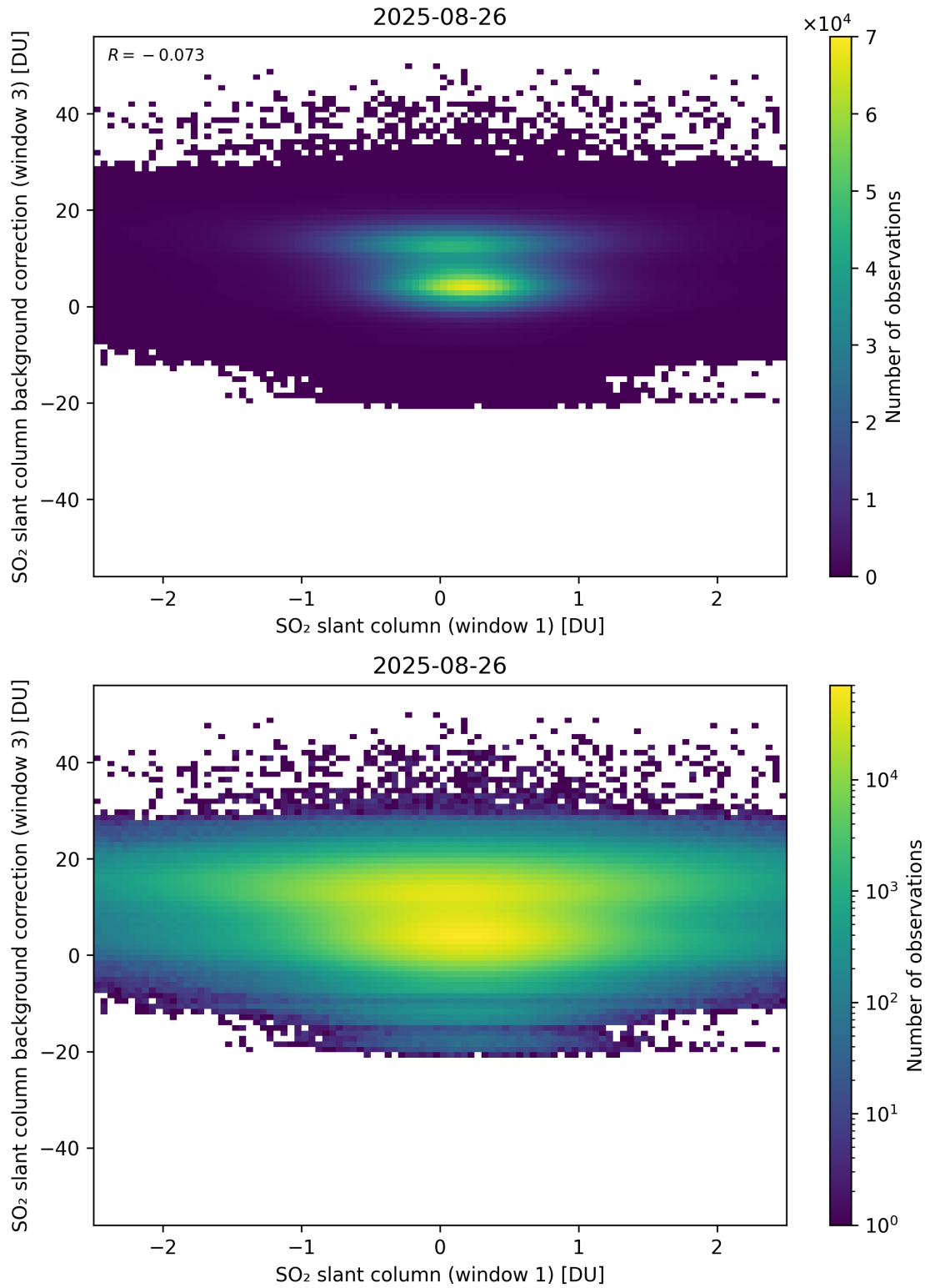
Figure 264: Scatter density plot of “SO 2 slant column (window 1)” against “SO 2 slant column background correction (window 3)” for 2025-08-25 to 2025-08-27.
