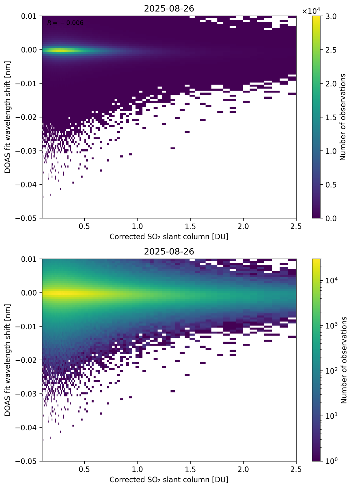
Figure 229: Scatter density plot of “Corrected SO 2 slant column” against “DOAS fit wavelength shift” for 2025-08-25 to 2025-08-27.
