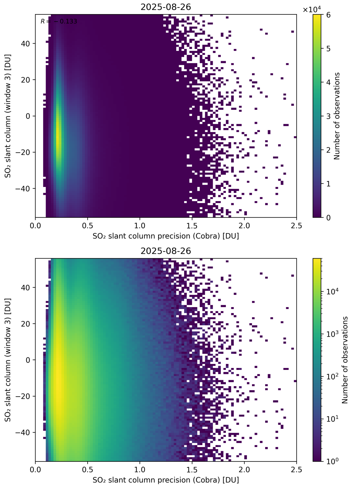
Figure 211: Scatter density plot of “SO 2 slant column precision (Cobra)” against “SO 2 slant column (window 3)” for 2025-08-25 to 2025-08-27.
