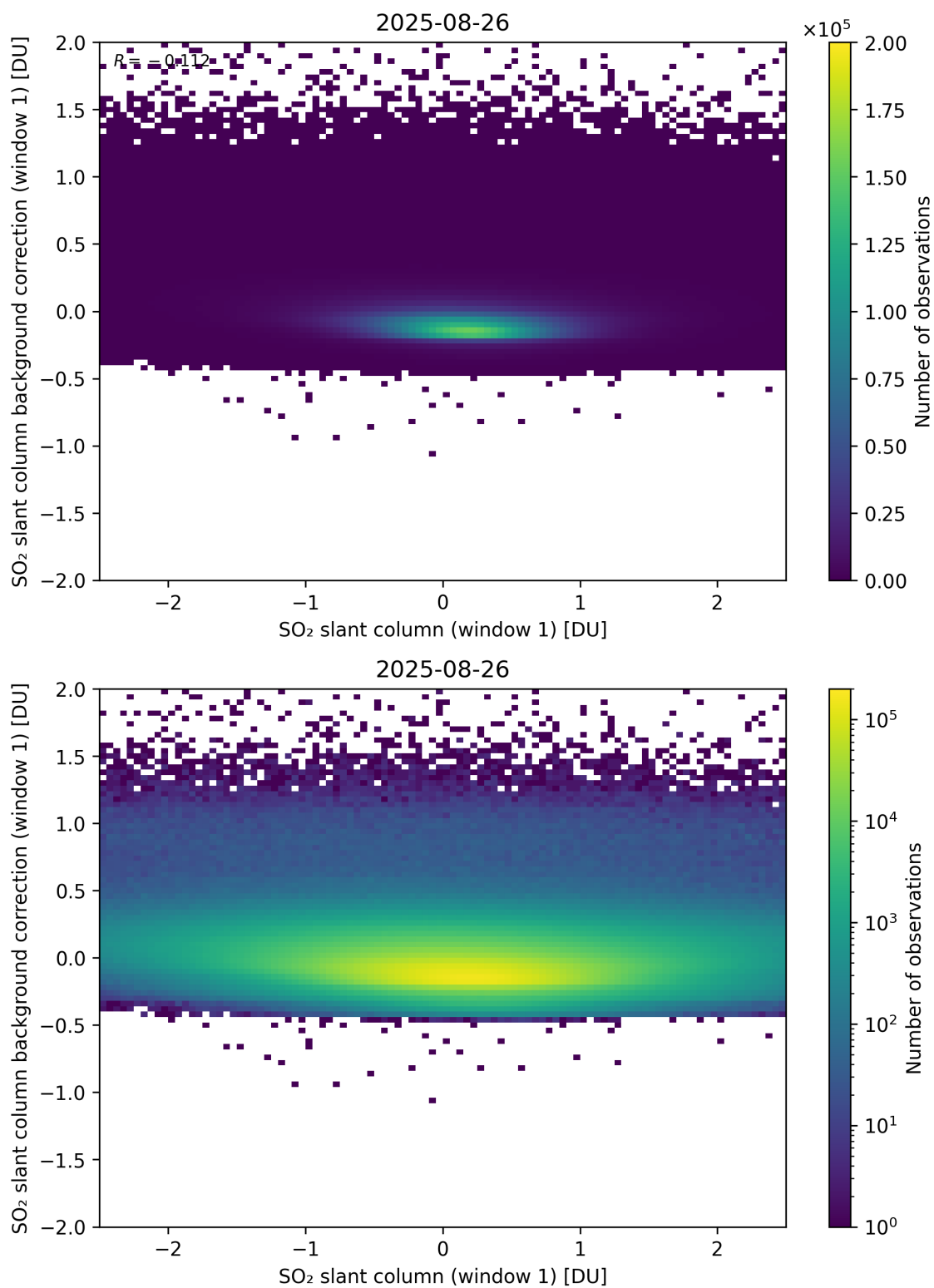
Figure 262: Scatter density plot of “SO 2 slant column (window 1)” against “SO 2 slant column background correction (window 1)” for 2025-08-25 to 2025-08-27.
