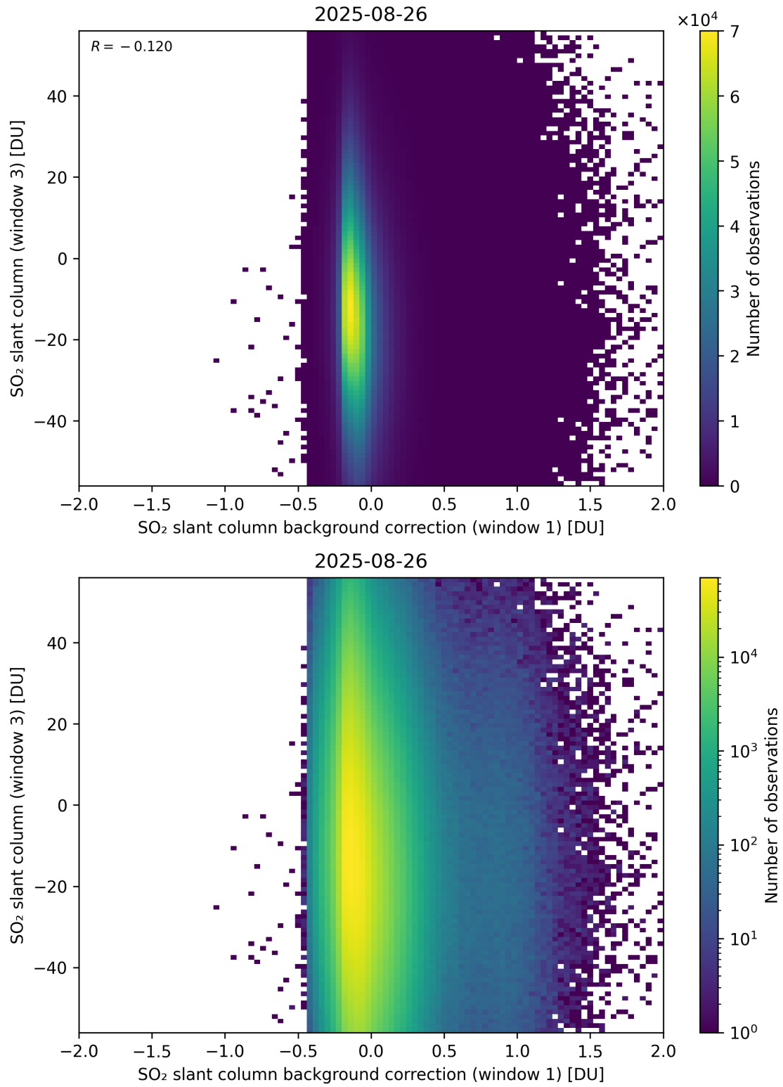
Figure 118: Scatter density plot of “SO 2 slant column background correction (window 1)” against “SO 2 slant column (window 3)” for 2025-08-25 to 2025-08-27.
