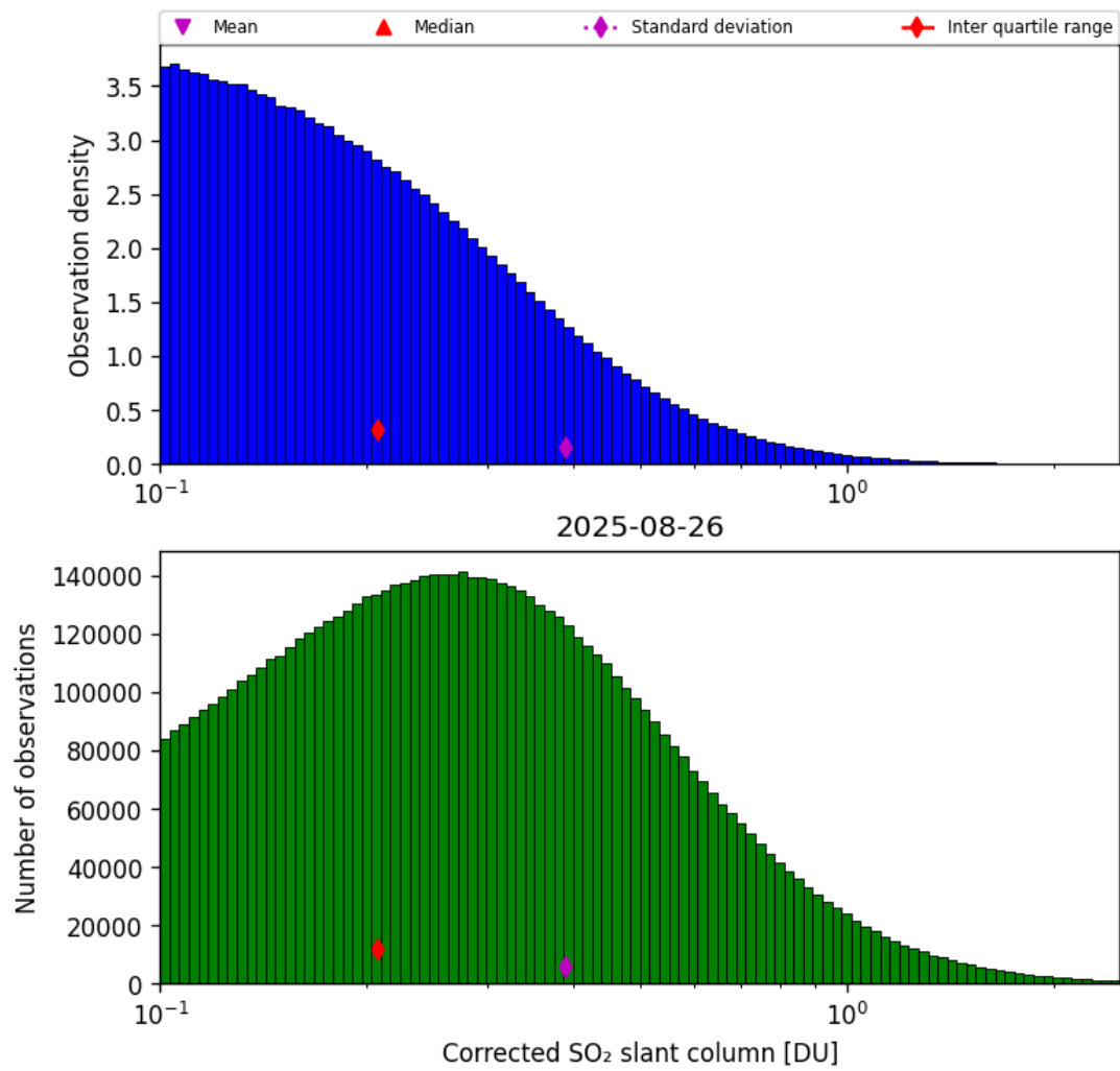
Figure 60: Histogram of "Corrected SO 2 slant column" for 2025-08-25 to 2025-08-27
