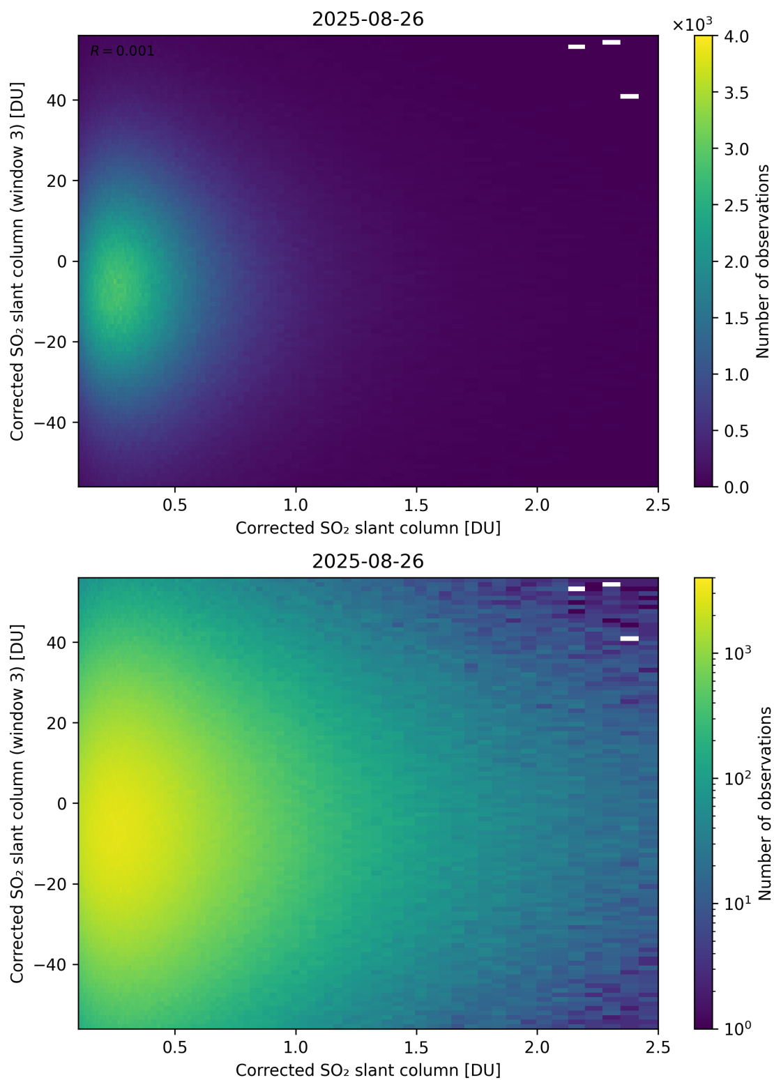
Figure 236: Scatter density plot of “Corrected SO 2 slant column” against “Corrected SO 2 slant column (window 3)” for 2025-08-25 to 2025-08-27.
