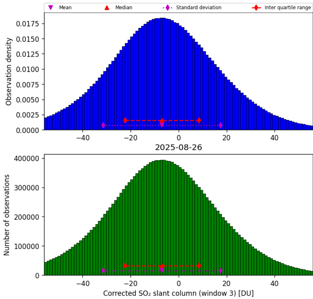
Figure 73: Histogram of “Corrected SO 2 slant column (window 3)” for 2025-08-25 to 2025-08-27
