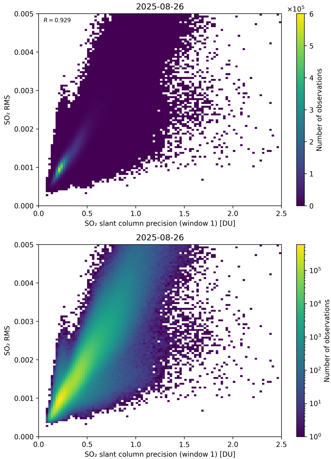
Figure 273: Scatter density plot of “SO 2 slant column precision (window 1)” against “SO 2 RMS” for 2025-08-25 to 2025-08-27.
