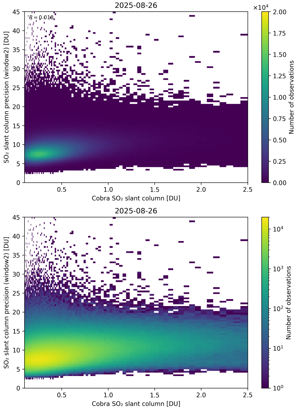
Figure 221: Scatter density plot of “Cobra SO 2 slant column” against “SO 2 slant column precision (window2)” for 2025-08-25 to 2025-08-27.
