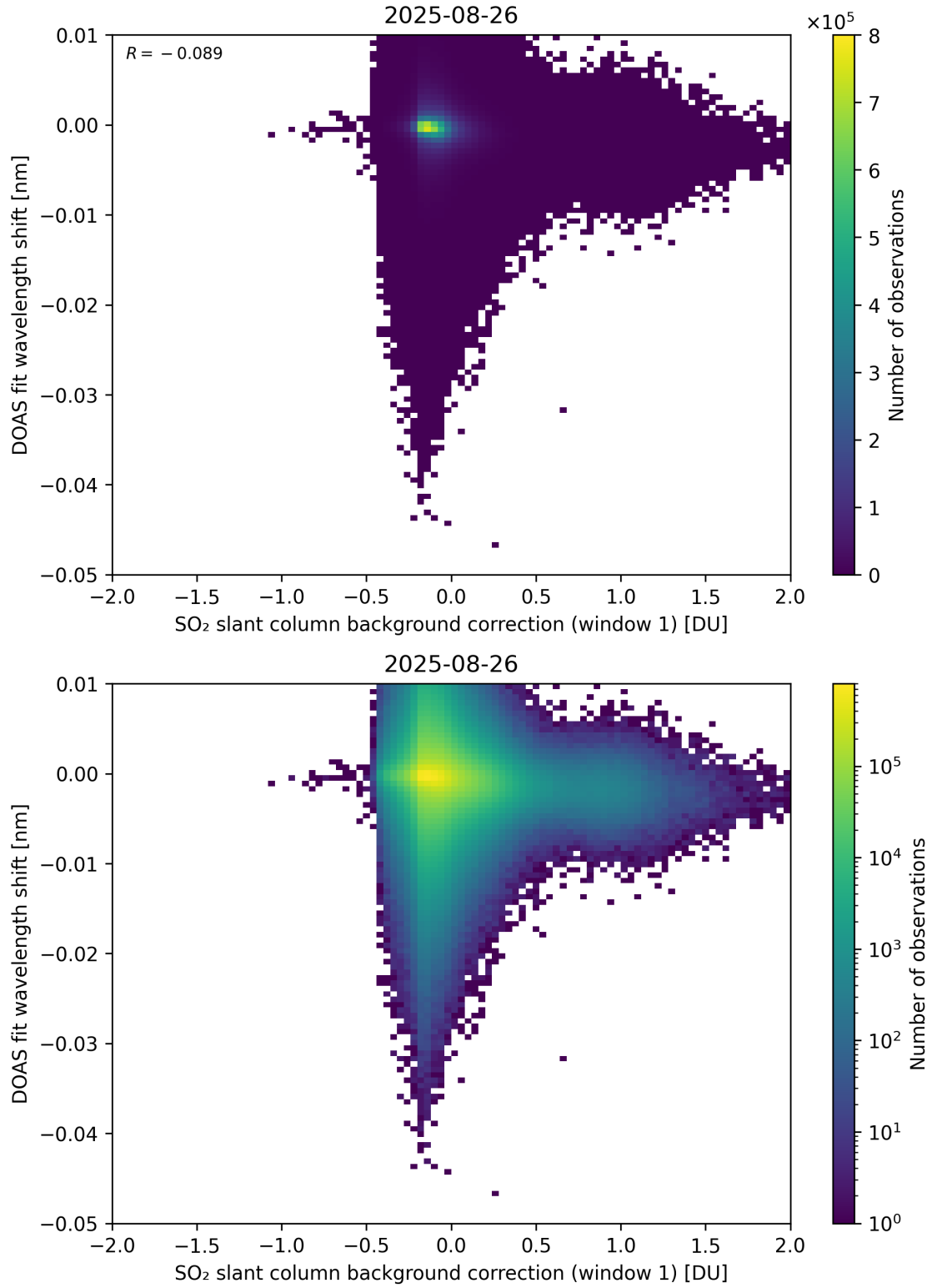
Figure 111: Scatter density plot of “SO 2 slant column background correction (window 1)” against “DOAS fit wavelength shift” for 2025-08-25 to 2025-08-27.
