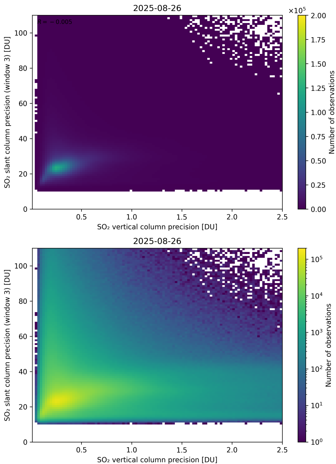
Figure 345: Scatter density plot of “SO 2 vertical column precision” against “SO 2 slant column precision (window 3)” for 2025-08-25 to 2025-08-27.
