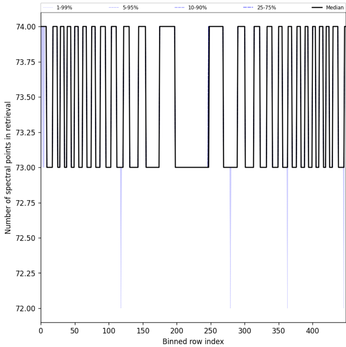
Figure 108: Along track statistics of “Number of spectral points in retrieval” for 2025-08-25 to 2025-08-27
