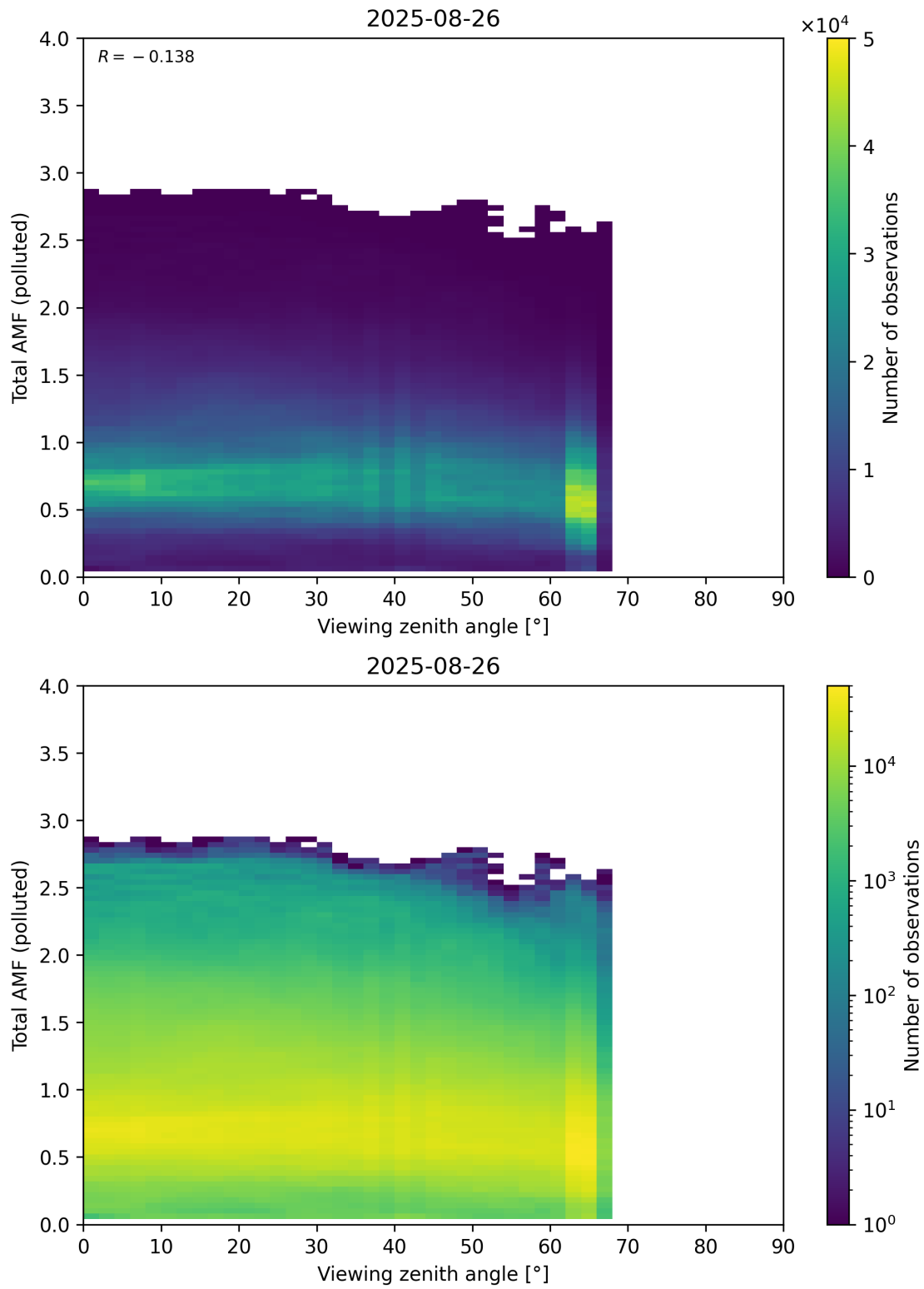
Figure 381: Scatter density plot of “Viewing zenith angle” against “Total AMF (polluted)” for 2025-08-25 to 2025-08-27.
