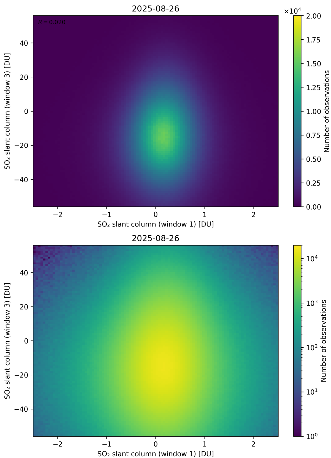
Figure 287: Scatter density plot of “SO 2 slant column (window 1)” against “SO 2 slant column (window 3)” for 2025-08-25 to 2025-08-27.
