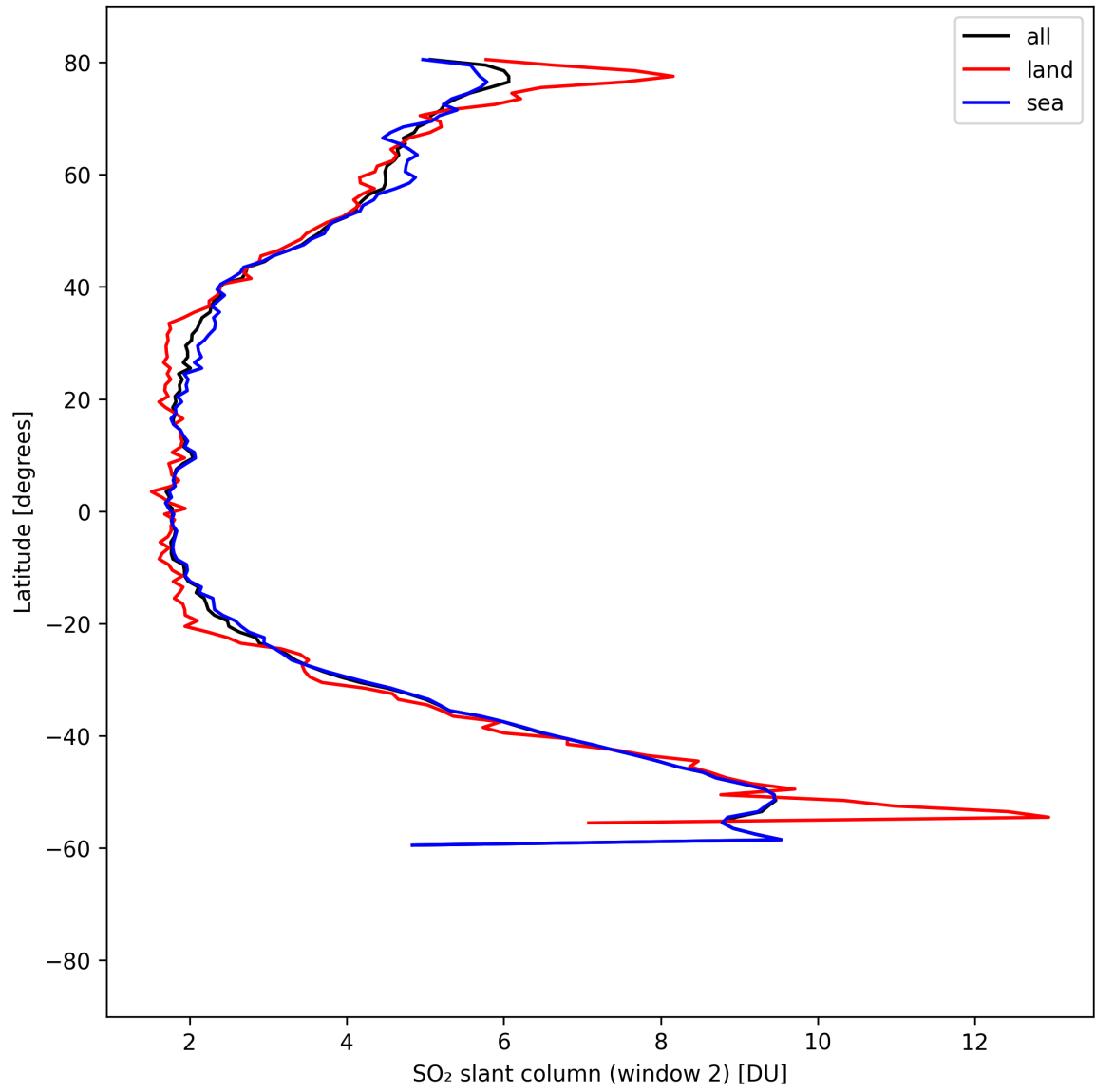
Figure 41: Zonal average of “SO 2 slant column (window 2)” for 2025-08-25 to 2025-08-27.
