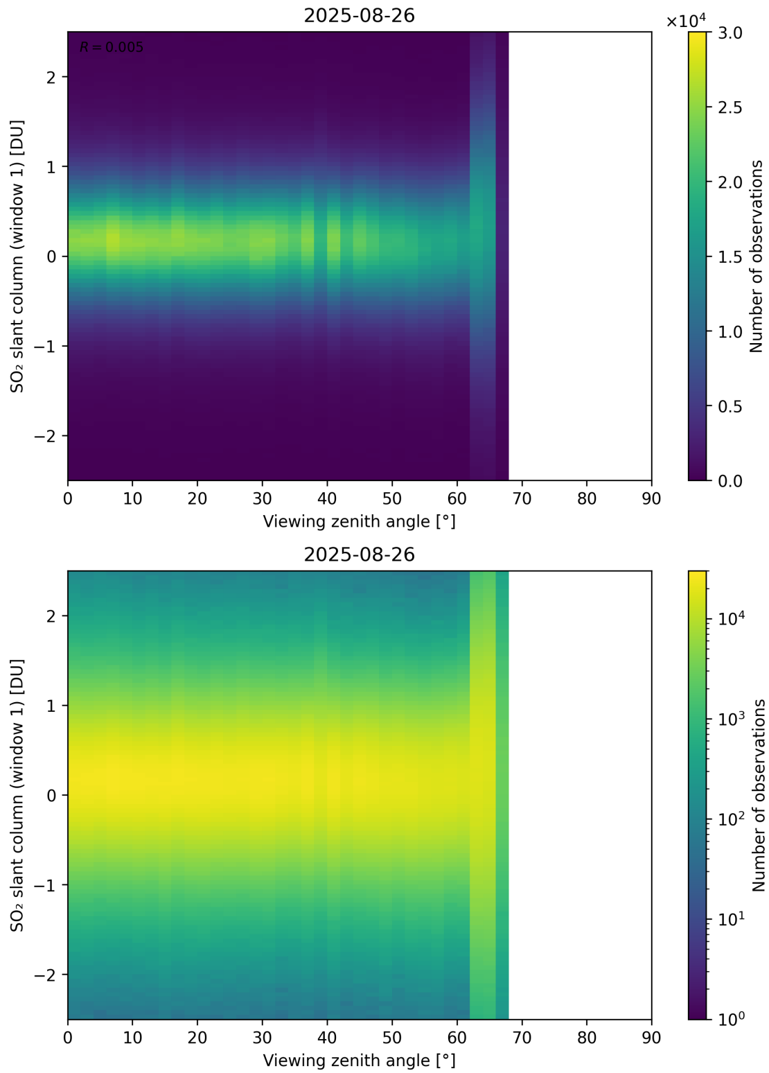
Figure 376: Scatter density plot of “Viewing zenith angle” against “SO 2 slant column (window 1)” for 2025-08-25 to 2025-08-27.
