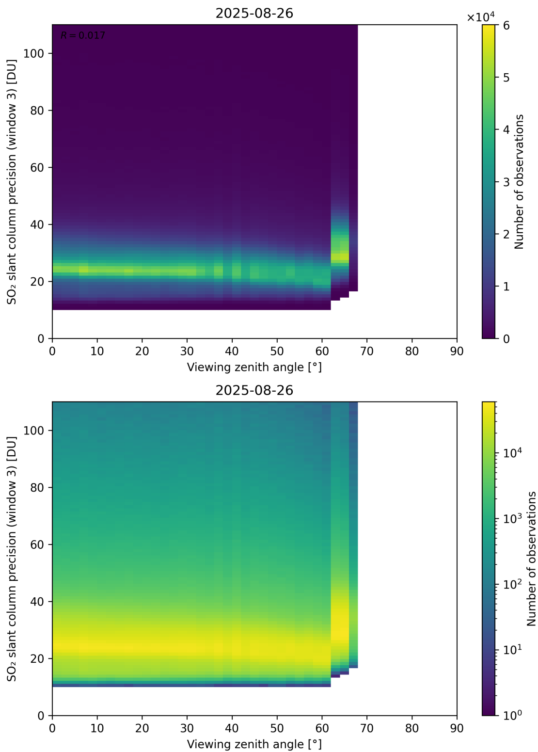
Figure 380: Scatter density plot of “Viewing zenith angle” against “SO 2 slant column precision (window 3)” for 2025-08-25 to 2025-08-27.
