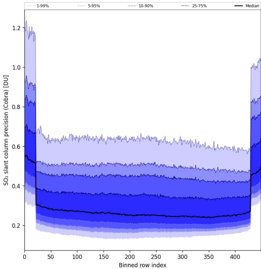
Figure 88: Along track statistics of “SO 2 slant column precision (Cobra)” for 2025-08-25 to 2025-08-27
