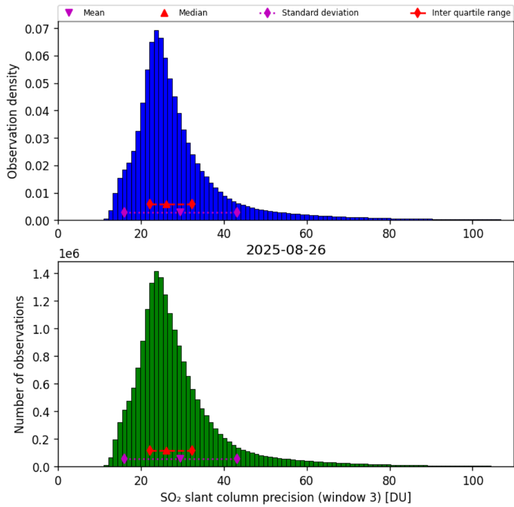
Figure 72: Histogram of “SO 2 slant column precision (window 3)” for 2025-08-25 to 2025-08-27
