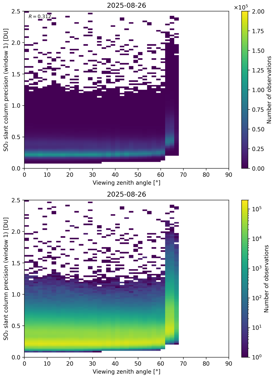
Figure 377: Scatter density plot of “Viewing zenith angle” against “SO 2 slant column precision (window 1)” for 2025-08-25 to 2025-08-27.
