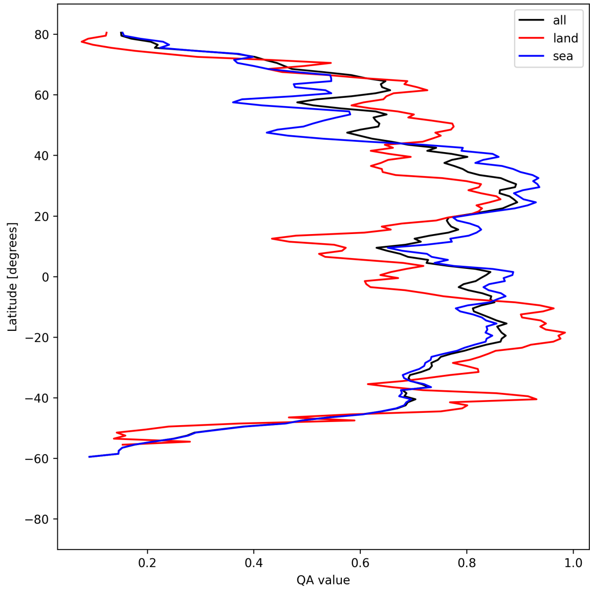
Figure 31: Zonal average of “QA value” for 2025-08-25 to 2025-08-27.
