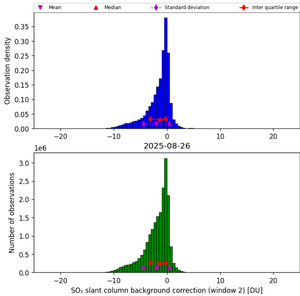
Figure 70: Histogram of “SO 2 slant column background correction (window 2)” for 2025-08-25 to 2025-08-27
