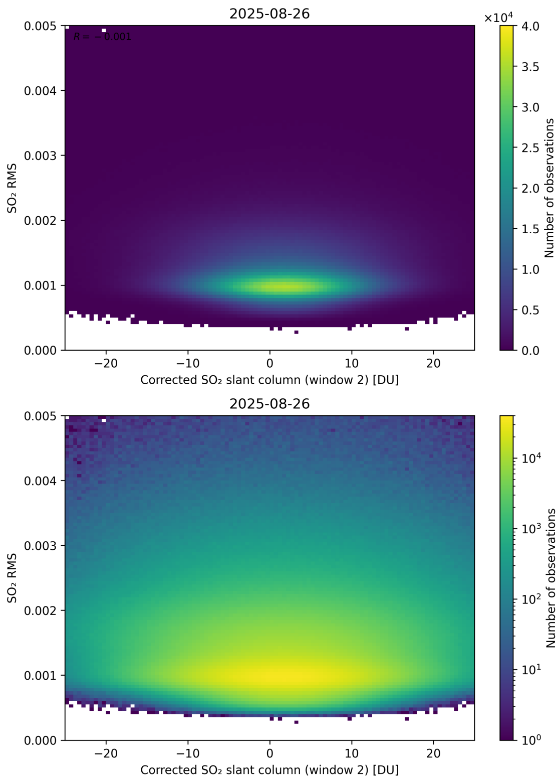
Figure 248: Scatter density plot of “Corrected SO 2 slant column (window 2)” against “SO 2 RMS” for 2025-08-25 to 2025-08-27.
