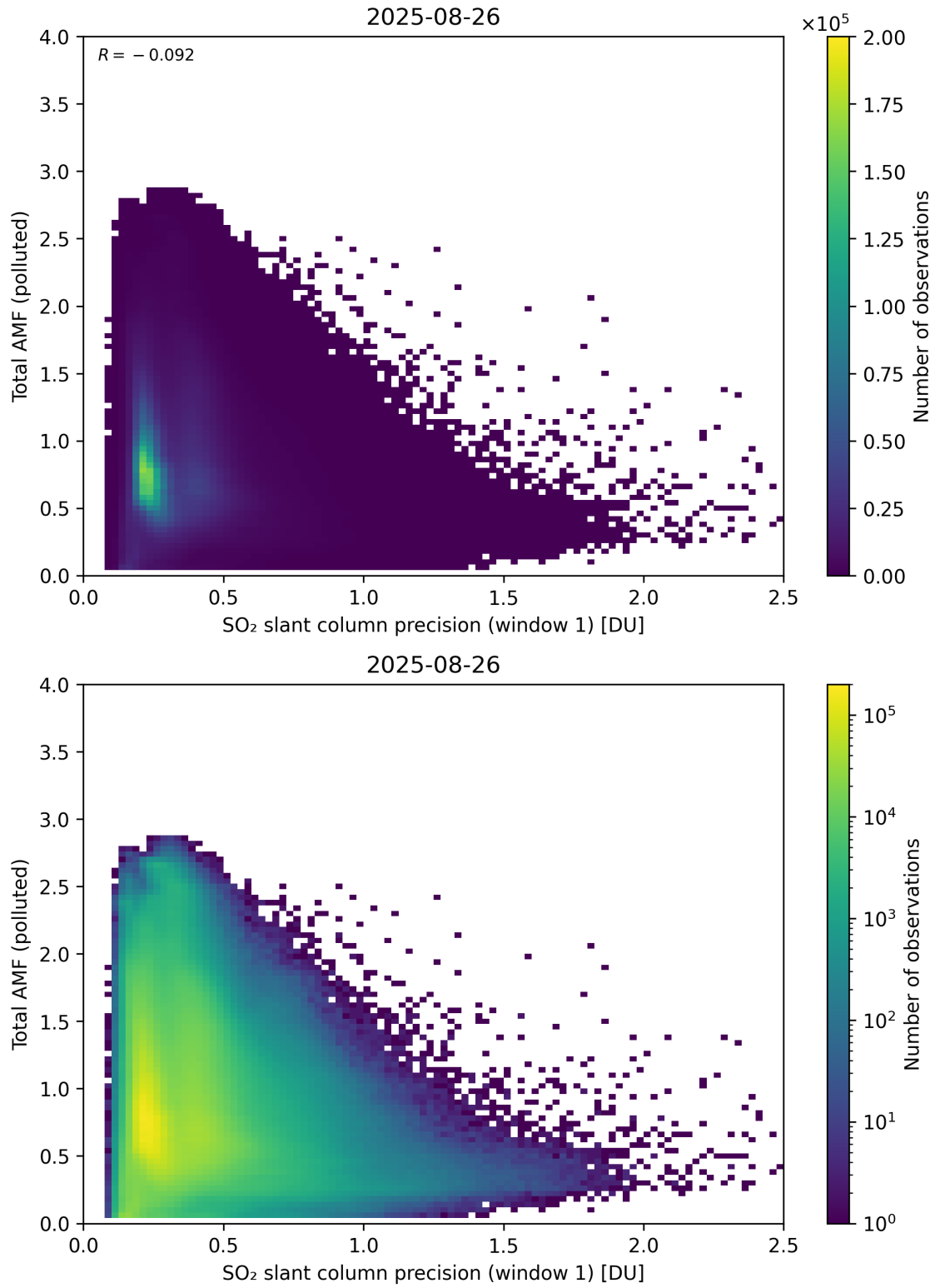
Figure 280: Scatter density plot of “SO 2 slant column precision (window 1)” against “Total AMF (polluted)” for 2025-08-25 to 2025-08-27.
