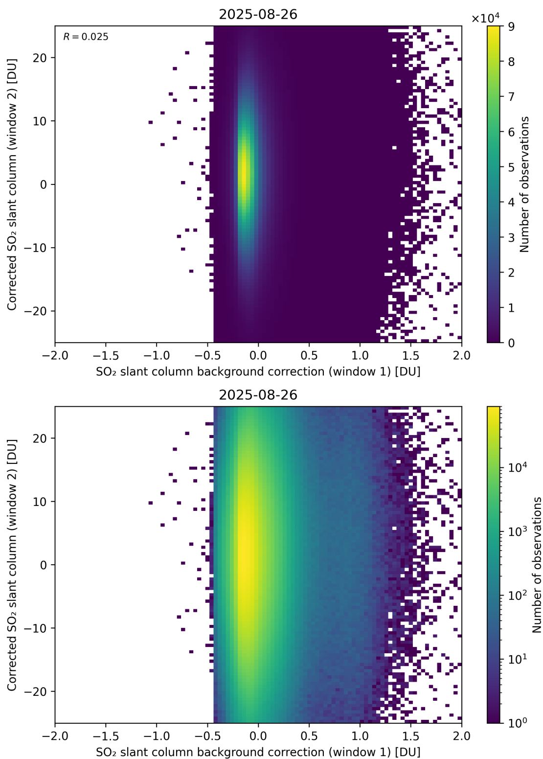
Figure 115: Scatter density plot of “SO 2 slant column background correction (window 1)” against “Corrected SO 2 slant column (window 2)” for 2025-08-25 to 2025-08-27.
