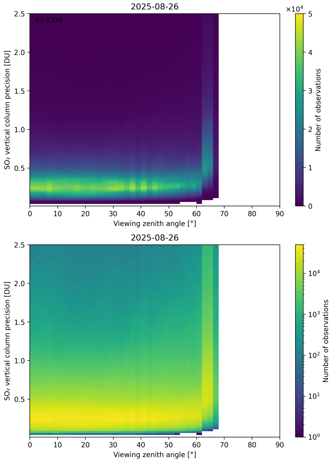
Figure 384: Scatter density plot of “Viewing zenith angle” against “SO 2 vertical column precision” for 2025-08-25 to 2025-08-27.
