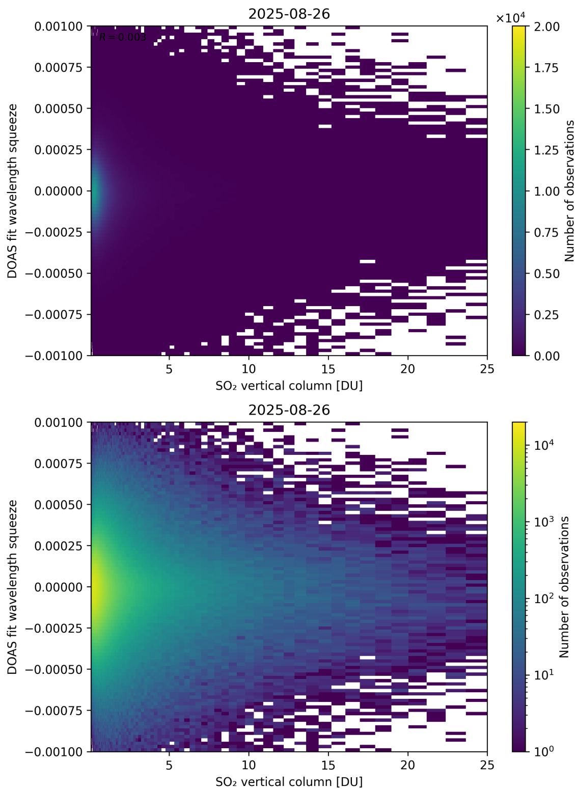
Figure 327: Scatter density plot of “SO 2 vertical column” against “DOAS fit wavelength squeeze” for 2025-08-25 to 2025-08-27.
