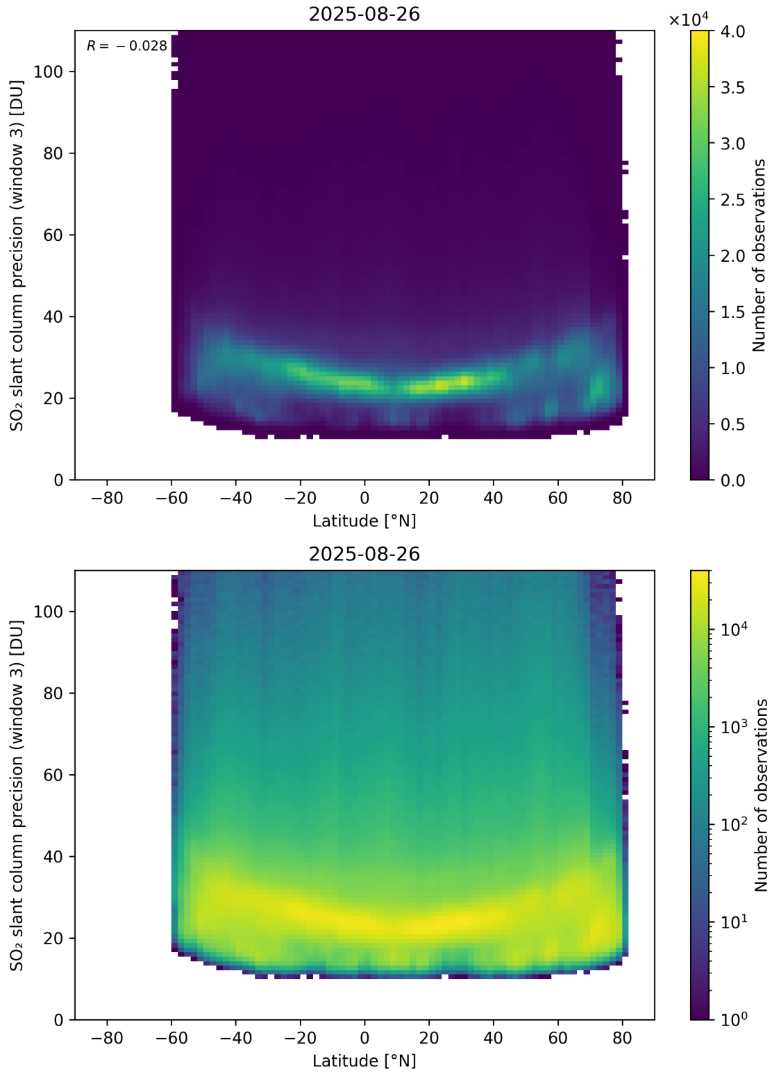
Figure 166: Scatter density plot of “Latitude” against “SO 2 slant column precision (window 3)” for 2025-08-25 to 2025-08-27.
