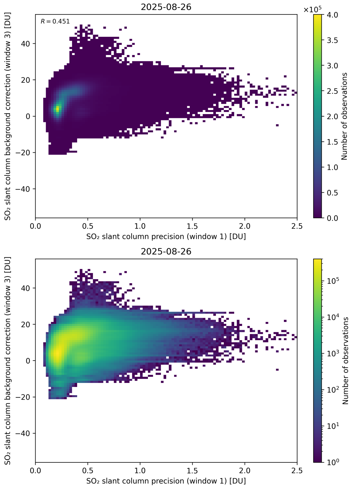
Figure 270: Scatter density plot of “SO 2 slant column precision (window 1)” against “SO 2 slant column background correction (window 3)” for 2025-08-25 to 2025-08-27.
