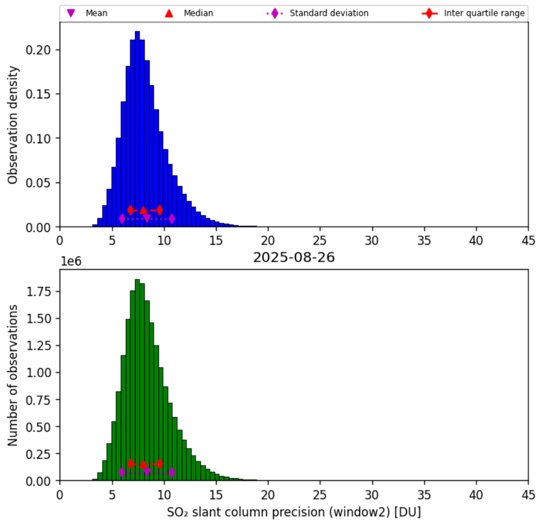
Figure 68: Histogram of “SO 2 slant column precision (window2)” for 2025-08-25 to 2025-08-27
