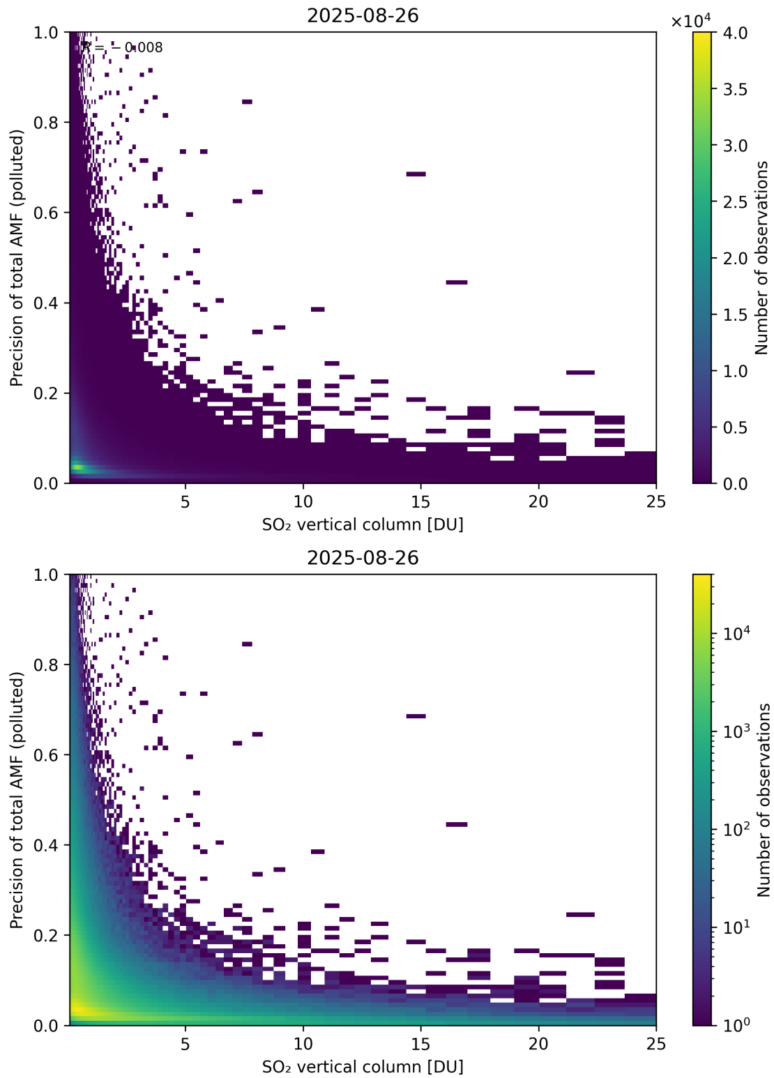
Figure 360: Scatter density plot of “SO 2 vertical column” against “Precision of total AMF (polluted)” for 2025-08-25 to 2025-08-27.
