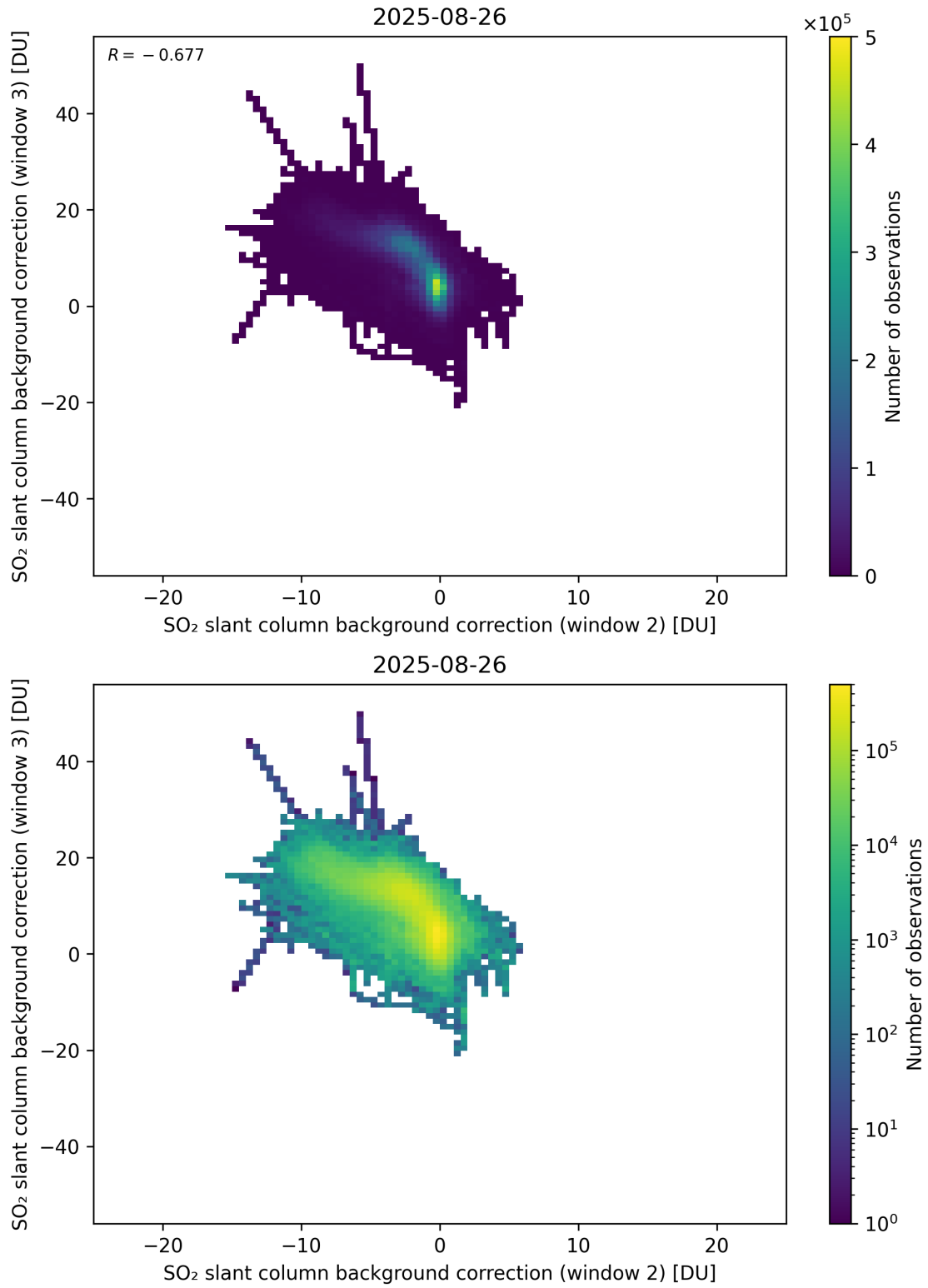
Figure 122: Scatter density plot of “SO 2 slant column background correction (window 2)” against “SO 2 slant column background correction (window 3)” for 2025-08-25 to 2025-08-27.
