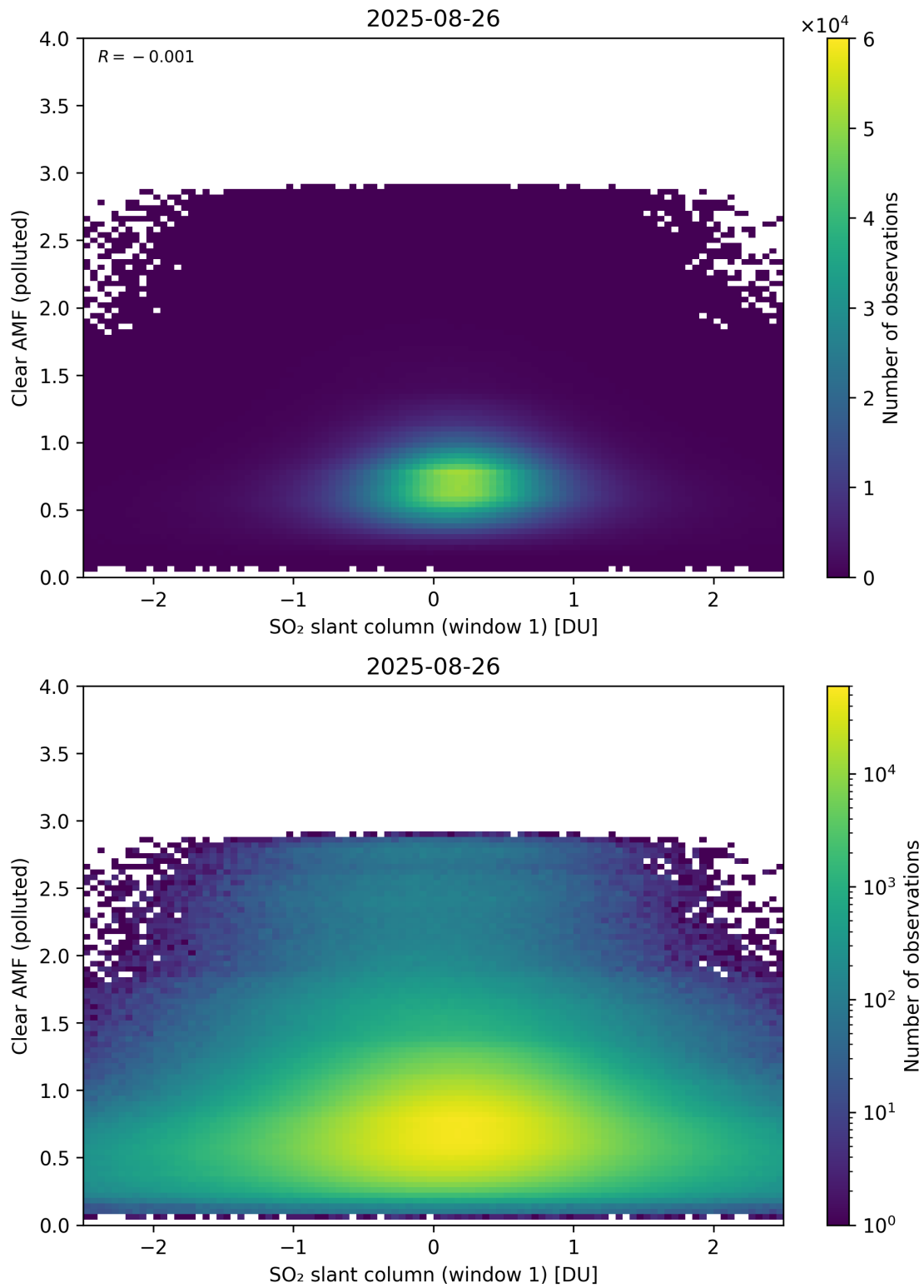
Figure 282: Scatter density plot of “SO 2 slant column (window 1)” against “Clear AMF (polluted)” for 2025-08-25 to 2025-08-27.
