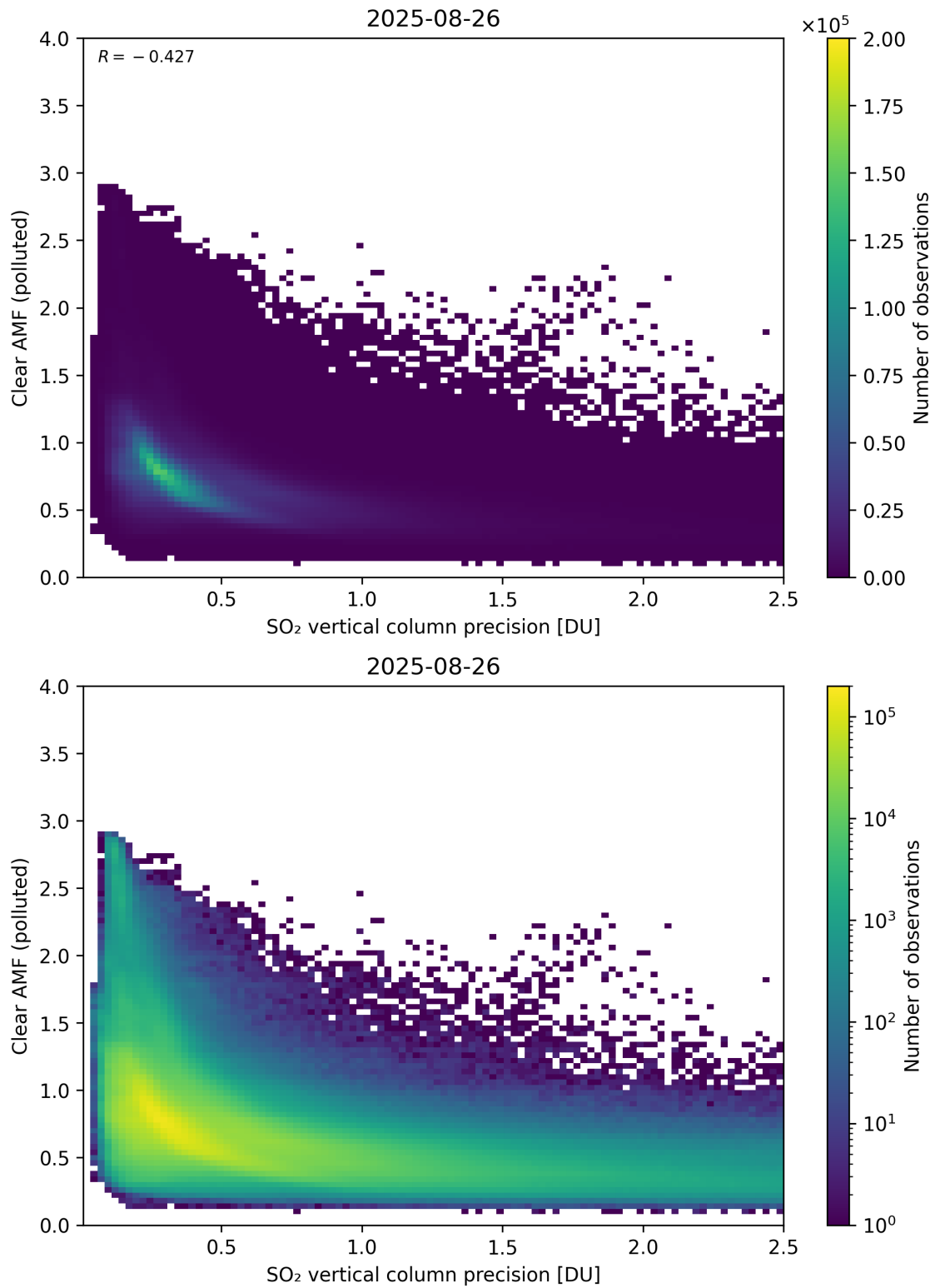
Figure 335: Scatter density plot of “SO 2 vertical column precision” against “Clear AMF (polluted)” for 2025-08-25 to 2025-08-27.
