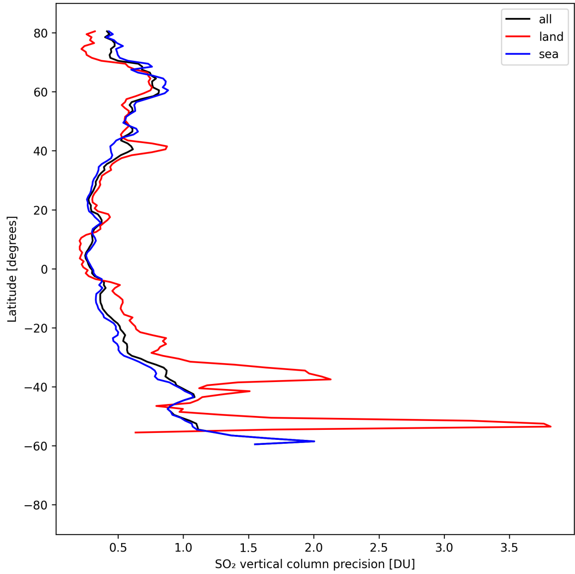
Figure 33: Zonal average of “SO 2 vertical column precision” for 2025-08-25 to 2025-08-27.
