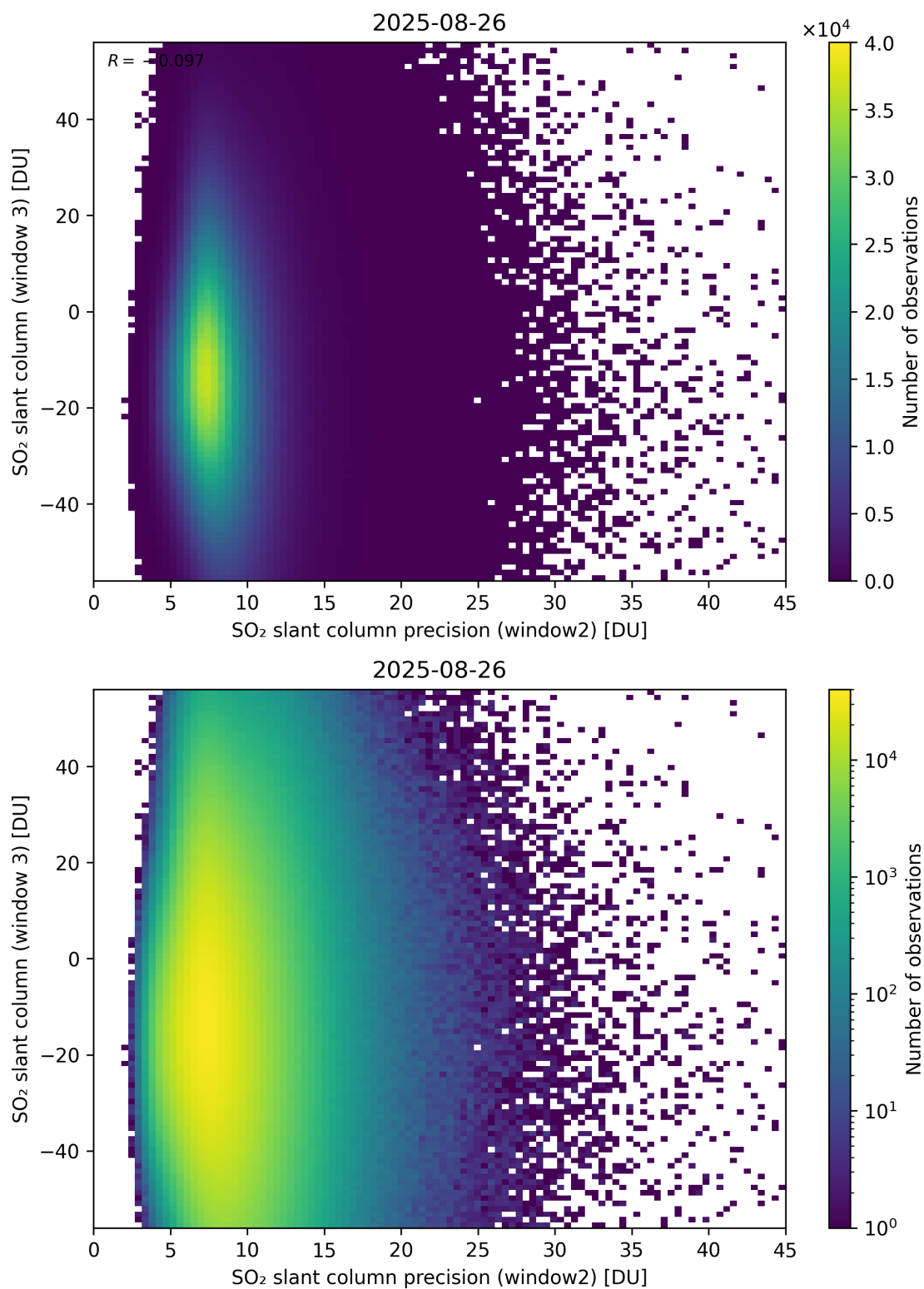
Figure 299: Scatter density plot of “SO 2 slant column precision (window2)” against “SO 2 slant column (window 3)” for 2025-08-25 to 2025-08-27.
