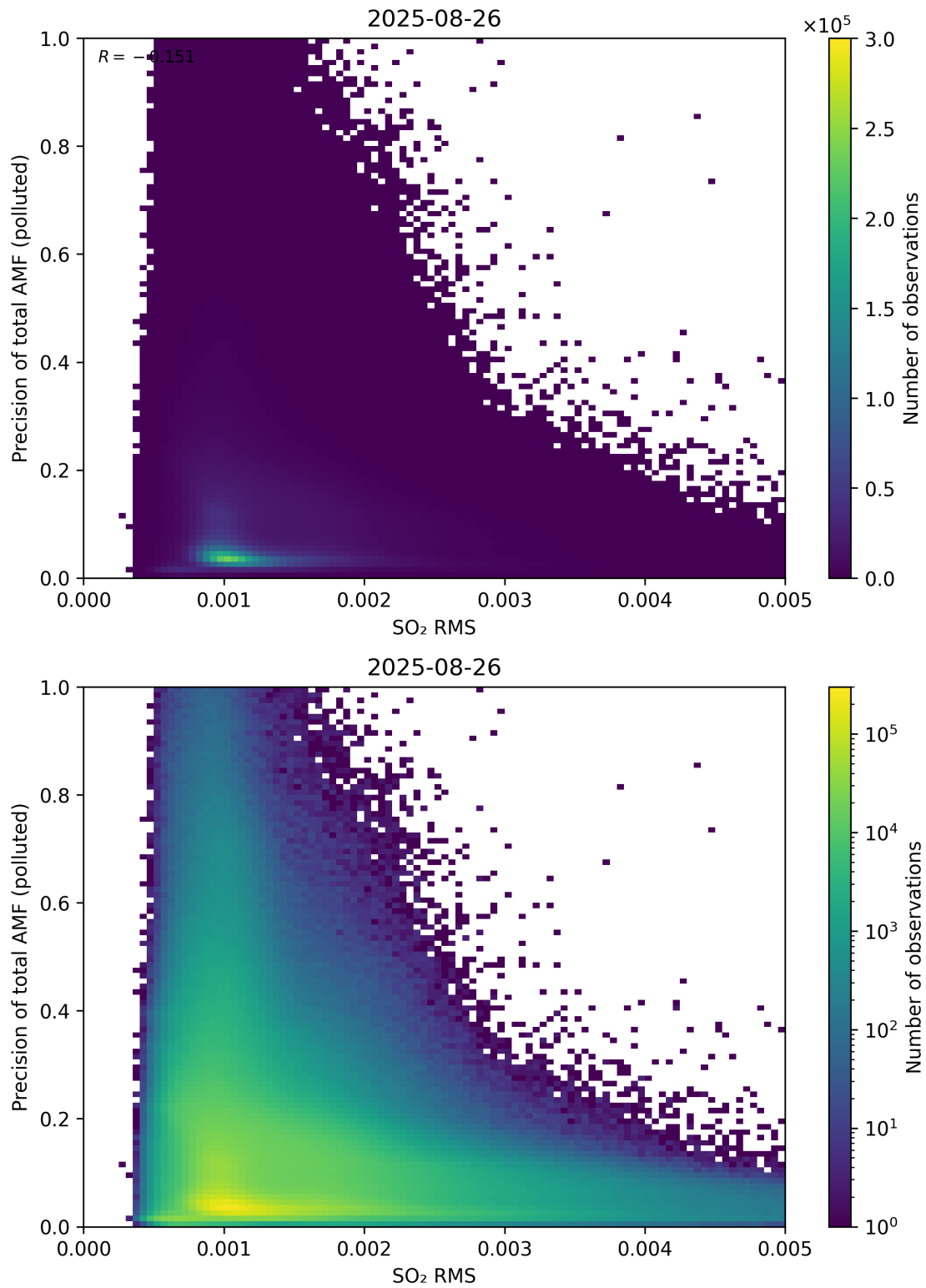
Figure 149: Scatter density plot of “SO 2 RMS” against “Precision of total AMF (polluted)” for 2025-08-25 to 2025-08-27.
