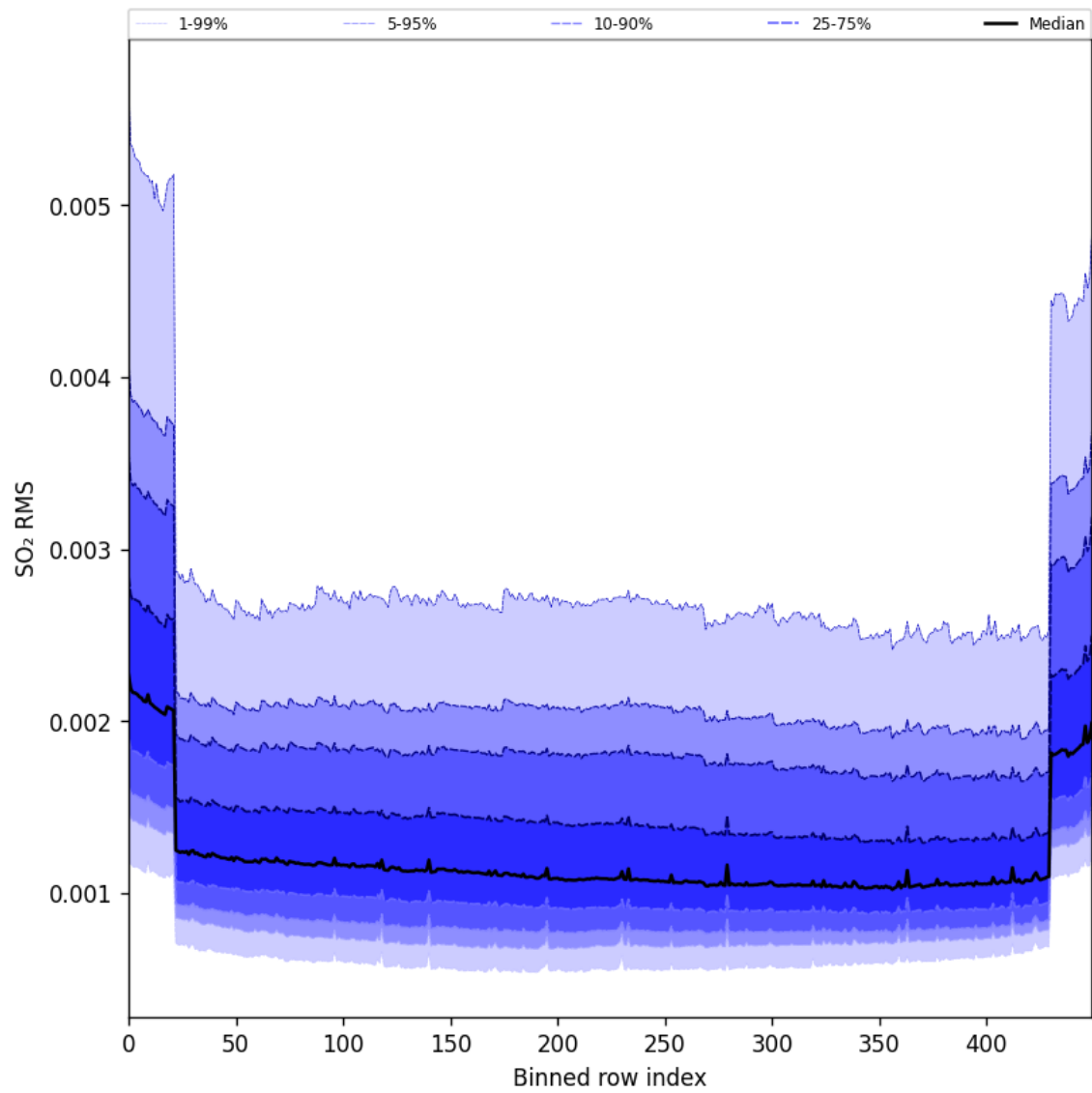
Figure 104: Along track statistics of “SO 2 RMS” for 2025-08-25 to 2025-08-27
