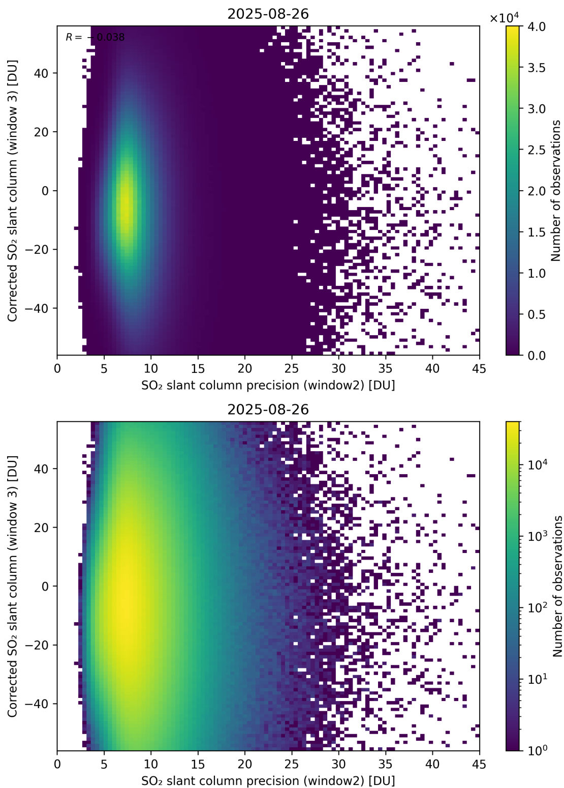
Figure 298: Scatter density plot of “SO 2 slant column precision (window2)” against “Corrected SO 2 slant column (window 3)” for 2025-08-25 to 2025-08-27.
