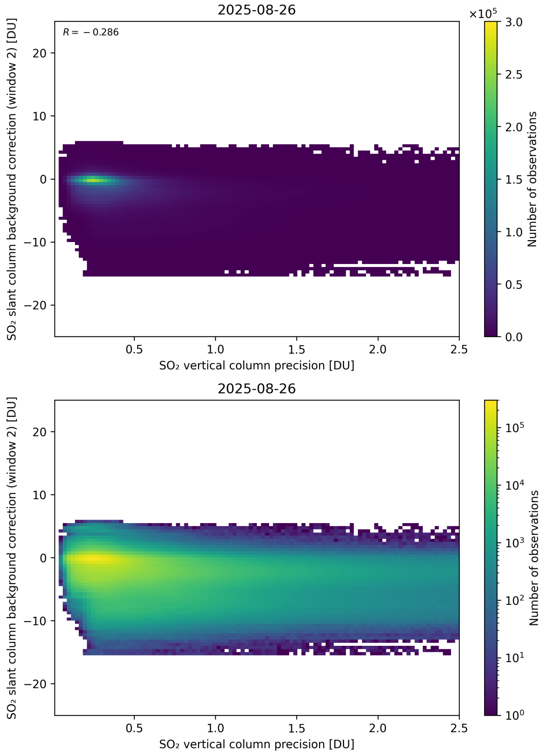
Figure 330: Scatter density plot of “SO 2 vertical column precision” against “SO 2 slant column background correction (window 2)” for 2025-08-25 to 2025-08-27.
