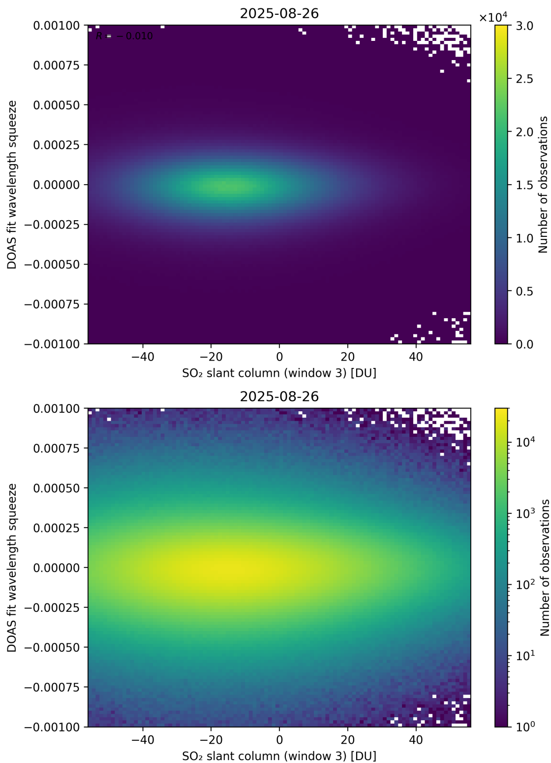
Figure 305: Scatter density plot of “SO 2 slant column (window 3)” against “DOAS fit wavelength squeeze” for 2025-08-25 to 2025-08-27.
