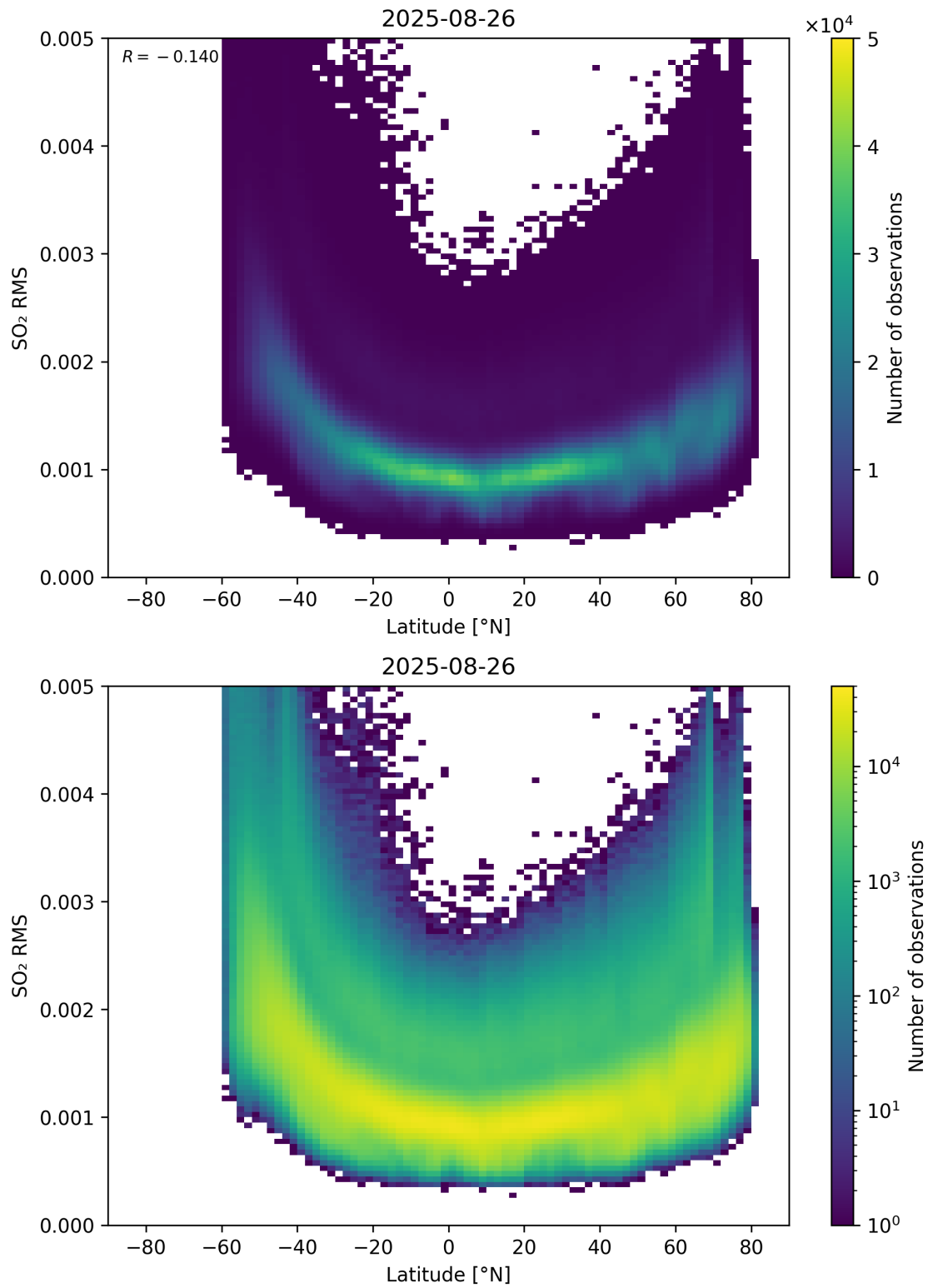
Figure 155: Scatter density plot of “Latitude” against “SO 2 RMS” for 2025-08-25 to 2025-08-27.
