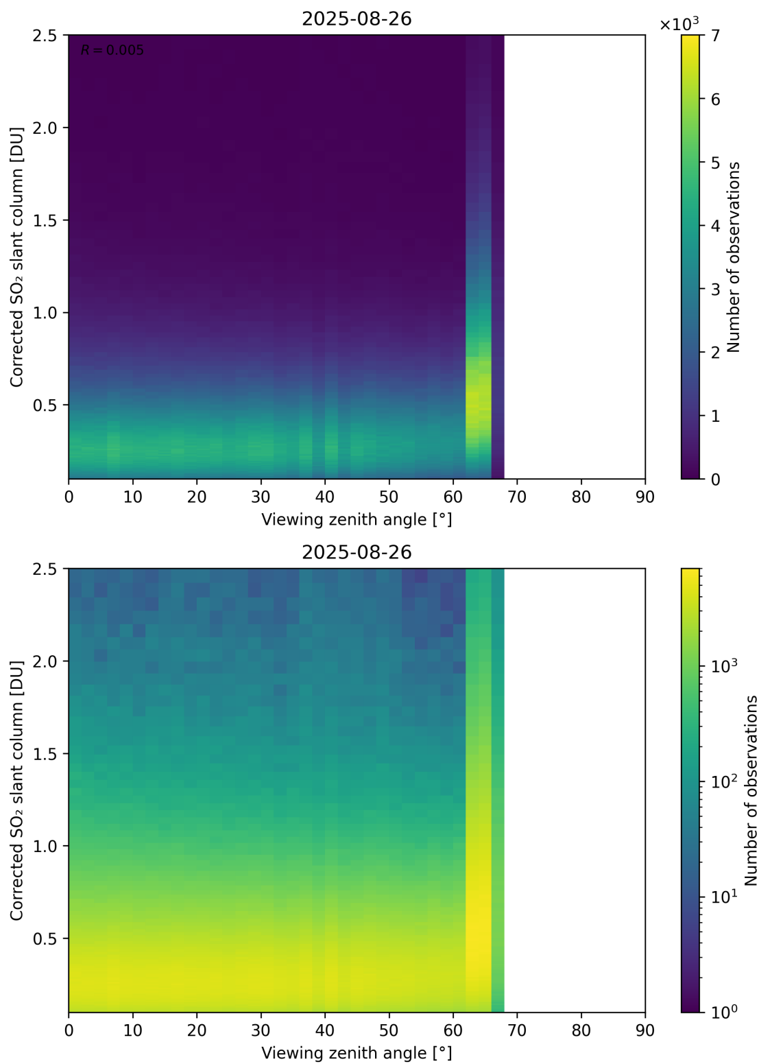
Figure 373: Scatter density plot of “Viewing zenith angle” against “Corrected SO 2 slant column” for 2025-08-25 to 2025-08-27.
