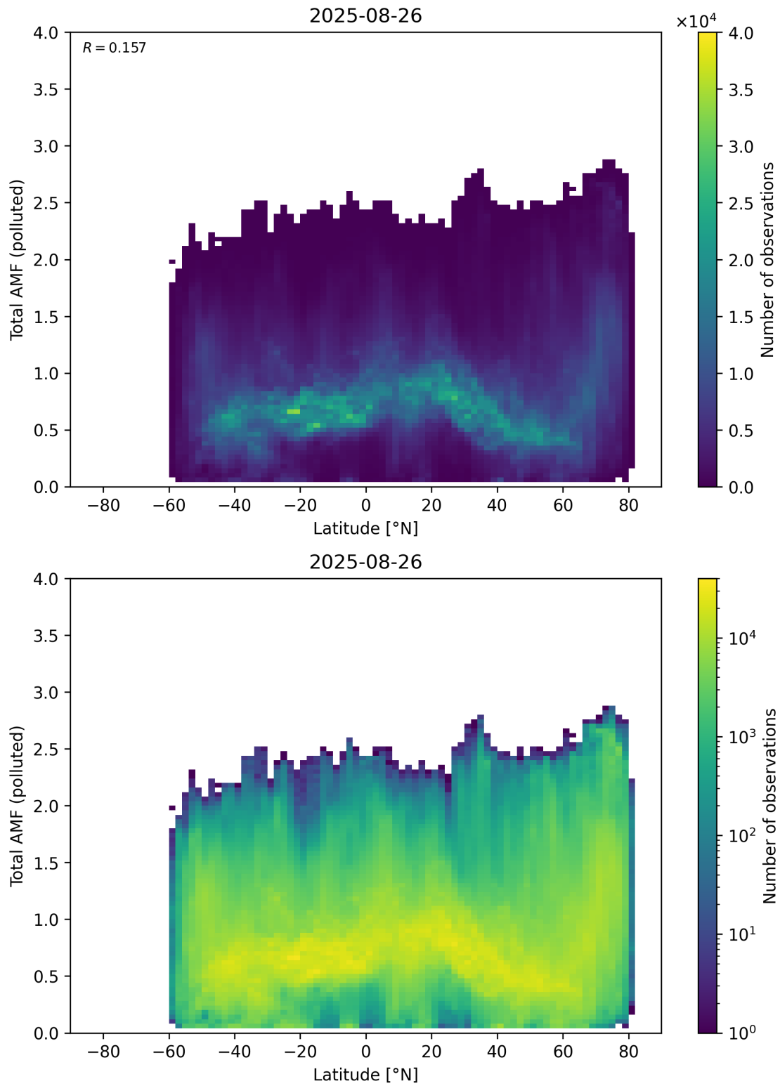
Figure 167: Scatter density plot of “Latitude” against “Total AMF (polluted)” for 2025-08-25 to 2025-08-27.
