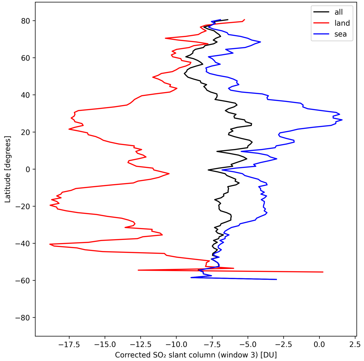
Figure 47: Zonal average of “Corrected SO 2 slant column (window 3)” for 2025-08-25 to 2025-08-27.
