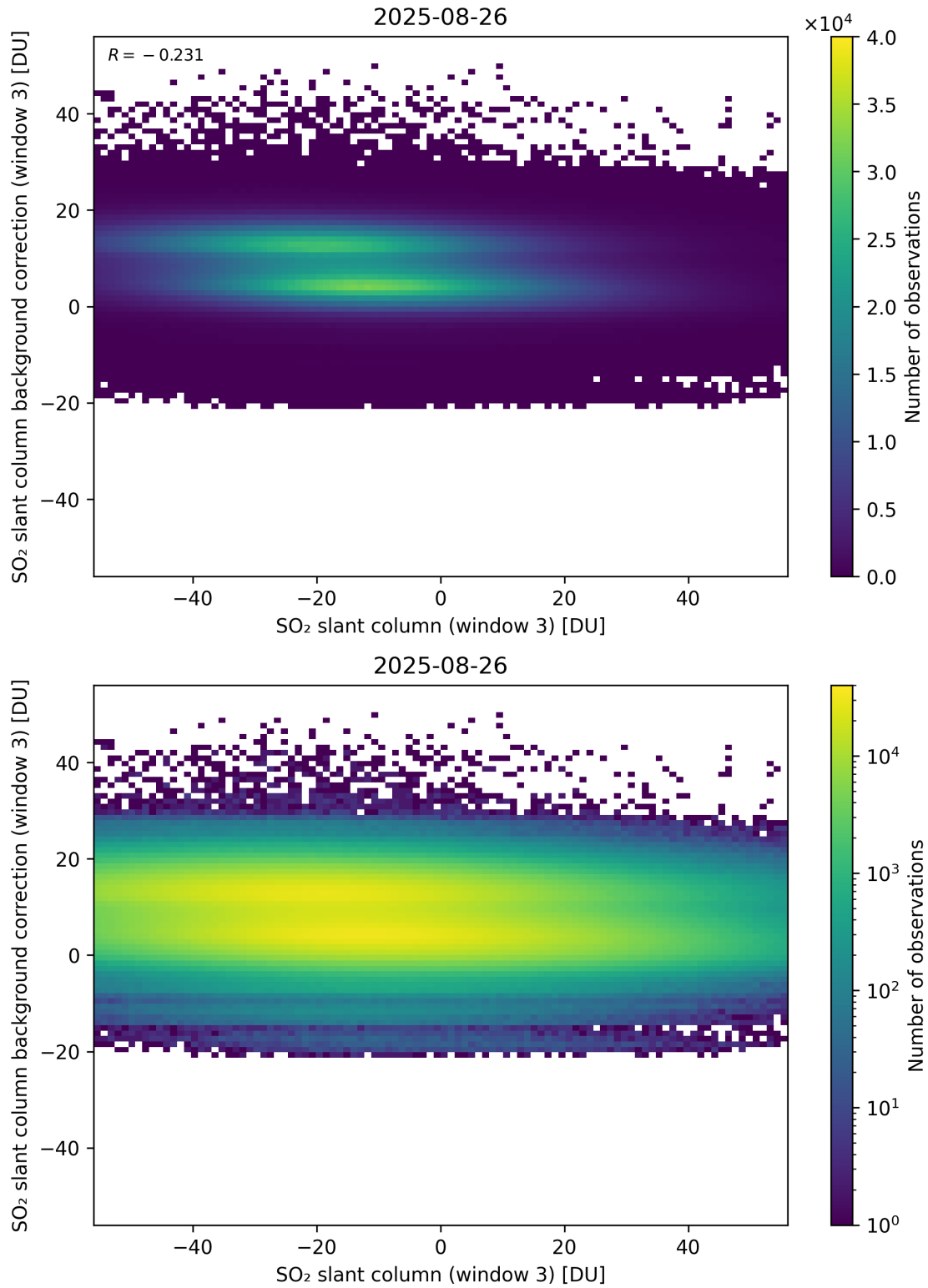
Figure 303: Scatter density plot of “SO 2 slant column (window 3)” against “SO 2 slant column background correction (window 3)” for 2025-08-25 to 2025-08-27.
