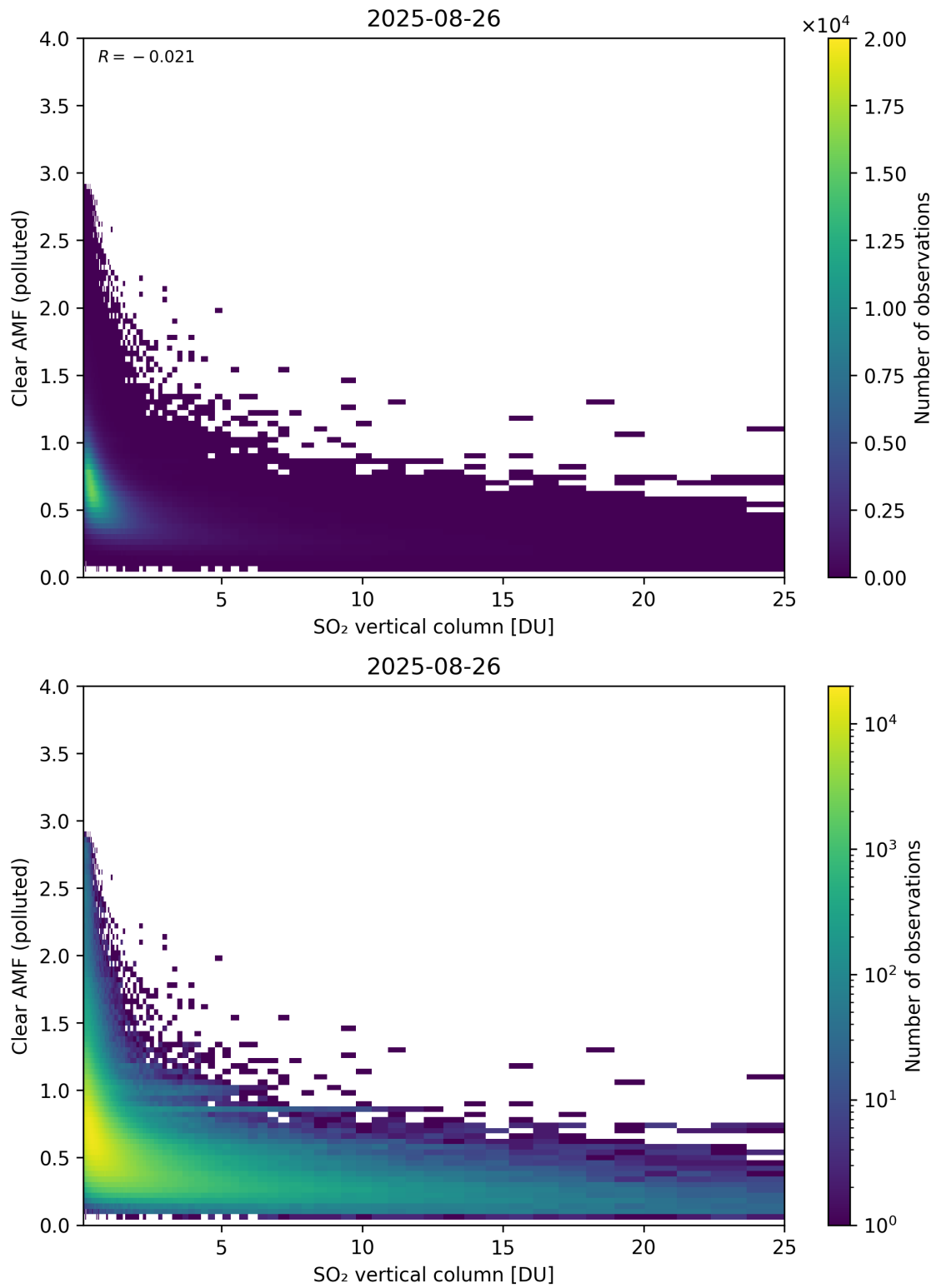
Figure 348: Scatter density plot of “SO 2 vertical column” against “Clear AMF (polluted)” for 2025-08-25 to 2025-08-27.
