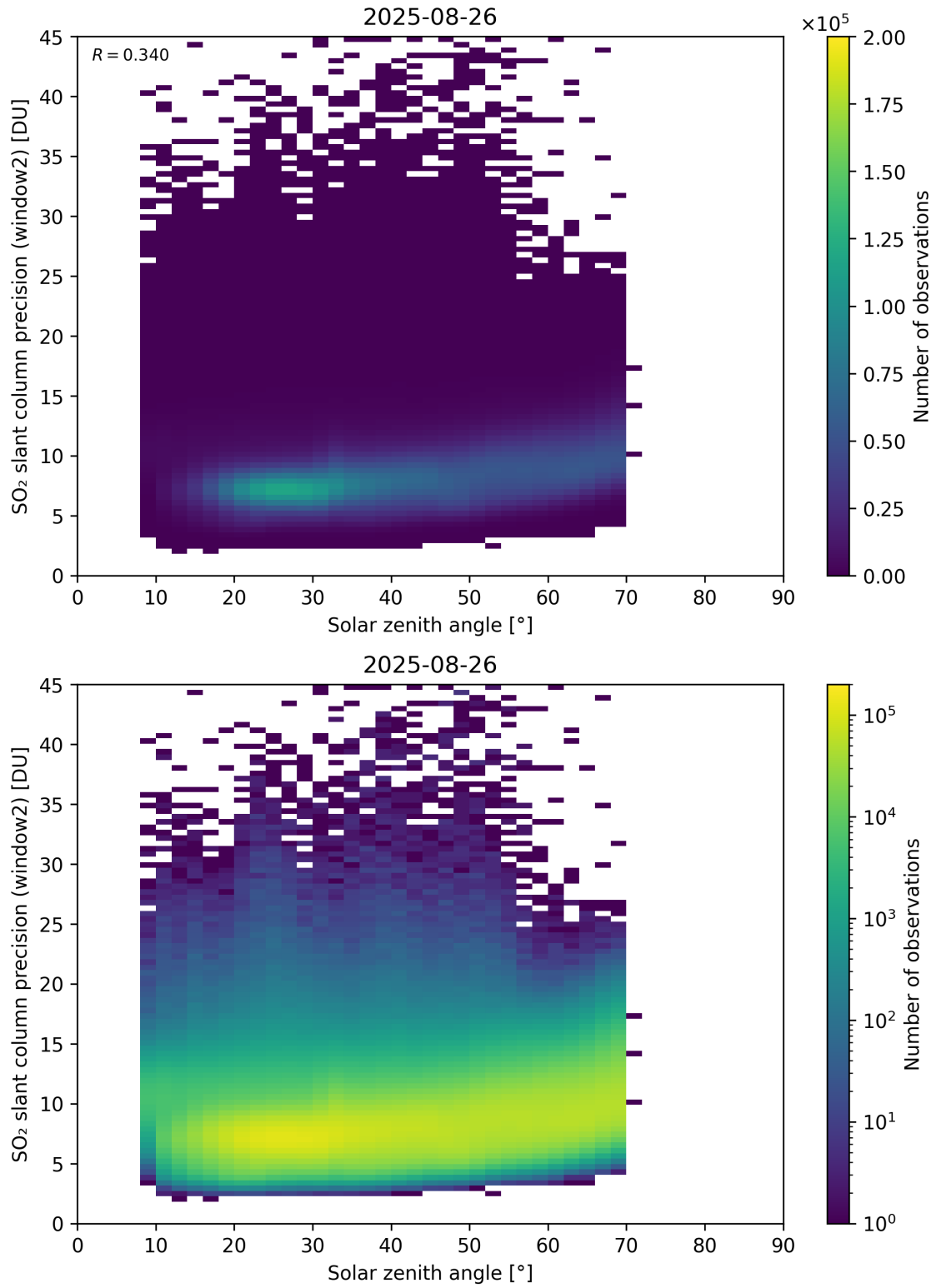
Figure 186: Scatter density plot of “Solar zenith angle” against “SO 2 slant column precision (window2)” for 2025-08-25 to 2025-08-27.
