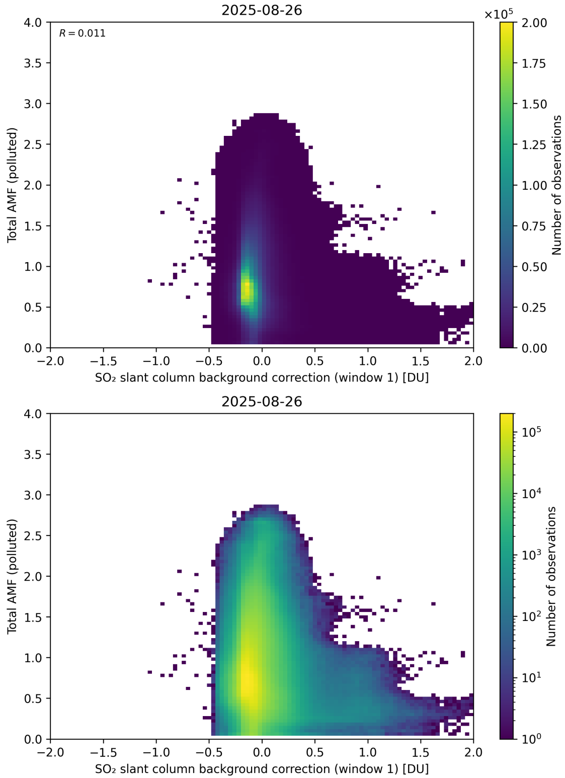
Figure 120: Scatter density plot of “SO 2 slant column background correction (window 1)” against “Total AMF (polluted)” for 2025-08-25 to 2025-08-27.
