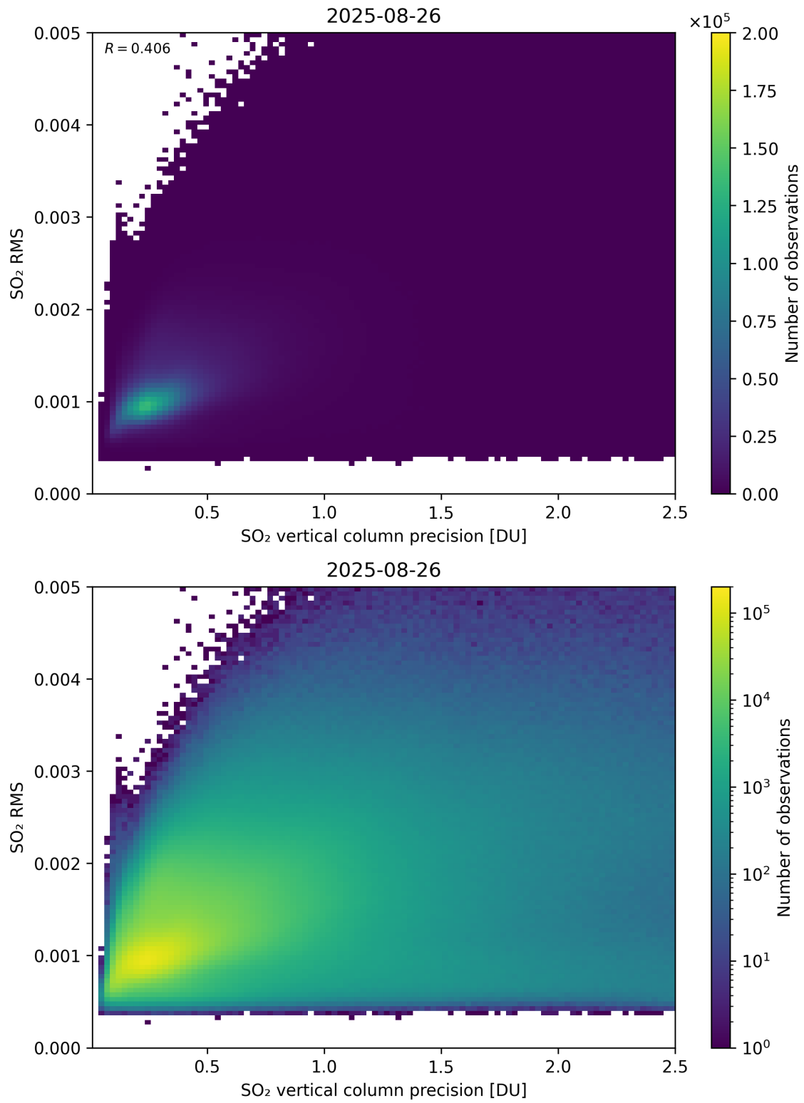
Figure 334: Scatter density plot of “SO 2 vertical column precision” against “SO 2 RMS” for 2025-08-25 to 2025-08-27.
