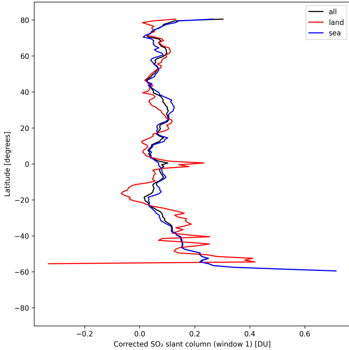
Figure 39: Zonal average of “Corrected SO 2 slant column (window 1)” for 2025-08-25 to 2025-08-27.
