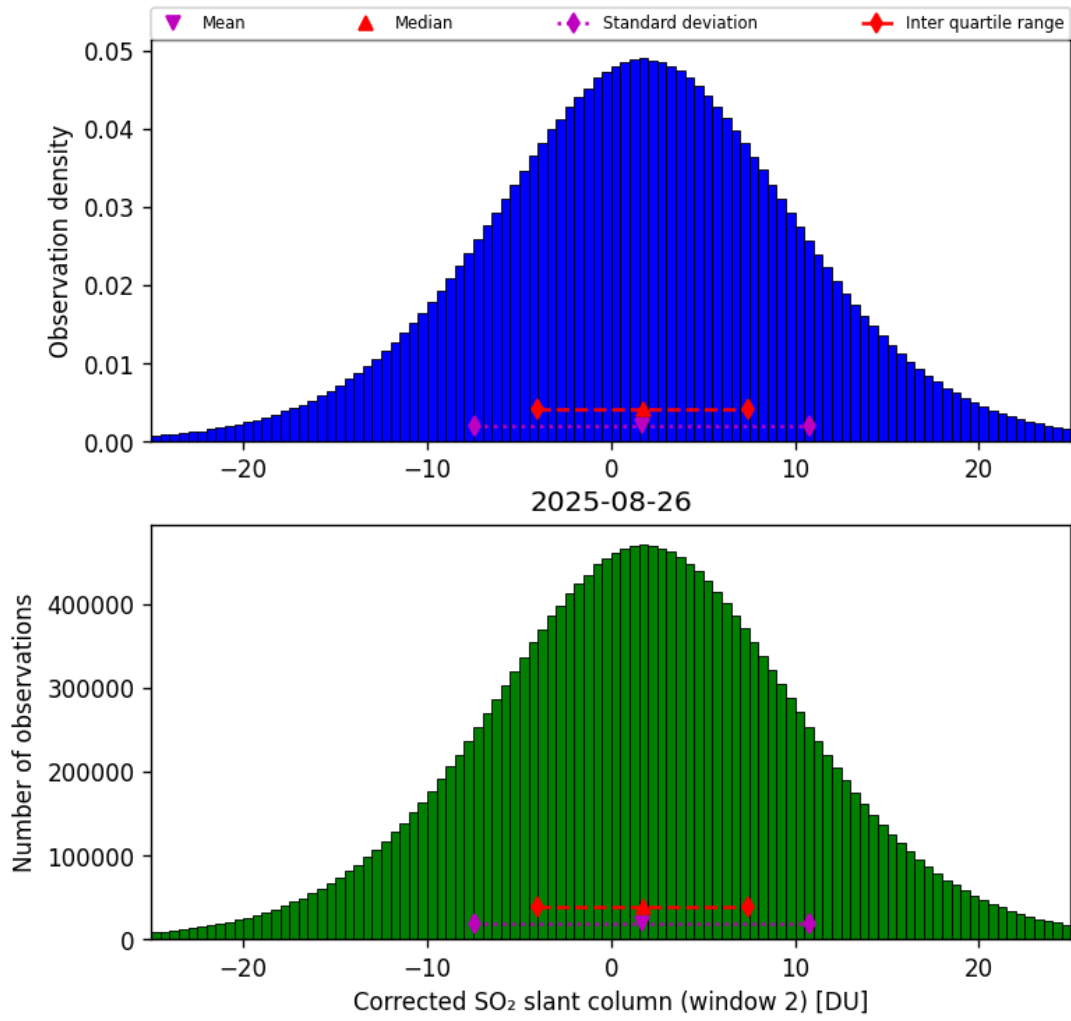
Figure 69: Histogram of “Corrected SO 2 slant column (window 2)” for 2025-08-25 to 2025-08-27
