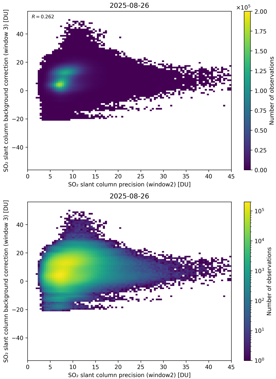
Figure 292: Scatter density plot of “SO 2 slant column precision (window2)” against “SO 2 slant column background correction (window 3)” for 2025-08-25 to 2025-08-27.
