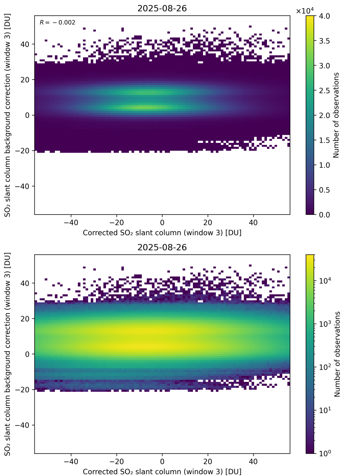
Figure 255: Scatter density plot of “Corrected SO 2 slant column (window 3)” against “SO 2 slant column background correction (window 3)” for 2025-08-25 to 2025-08-27.
