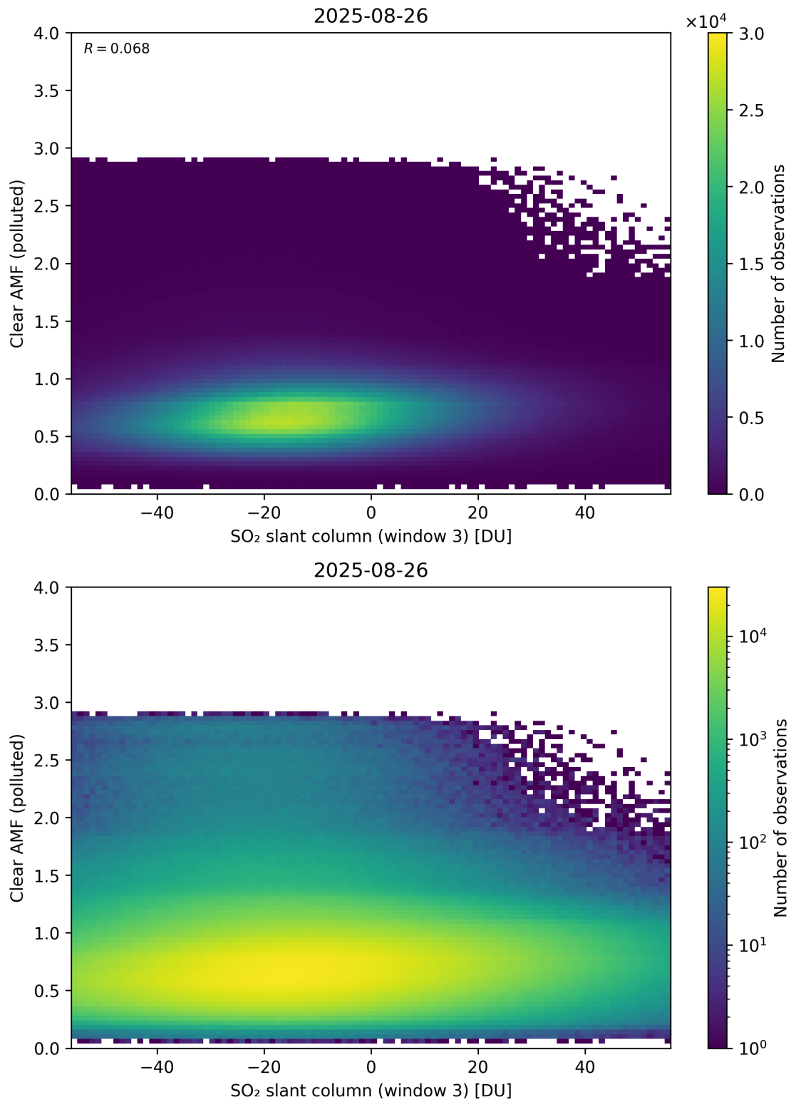
Figure 315: Scatter density plot of “SO 2 slant column (window 3)” against “Clear AMF (polluted)” for 2025-08-25 to 2025-08-27.
