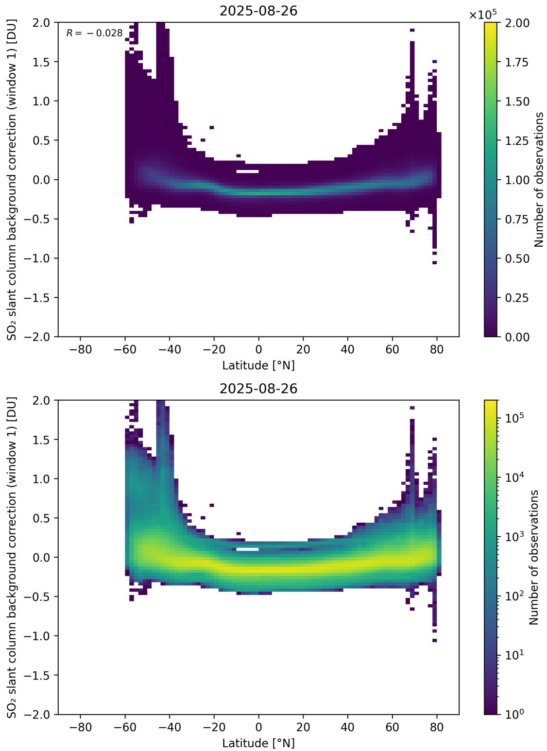
Figure 150: Scatter density plot of “Latitude” against “SO 2 slant column background correction (window 1)” for 2025-08-25 to 2025-08-27.
