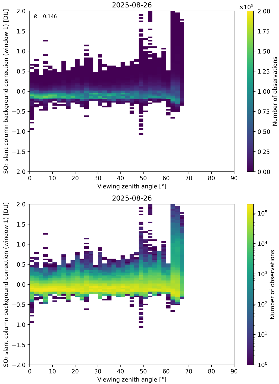
Figure 362: Scatter density plot of “Viewing zenith angle” against “SO 2 slant column background correction (window 1)” for 2025-08-25 to 2025-08-27.
