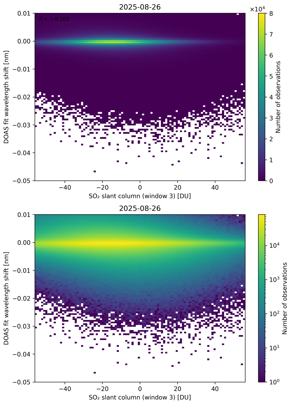
Figure 304: Scatter density plot of “SO 2 slant column (window 3)” against “DOAS fit wavelength shift” for 2025-08-25 to 2025-08-27.
