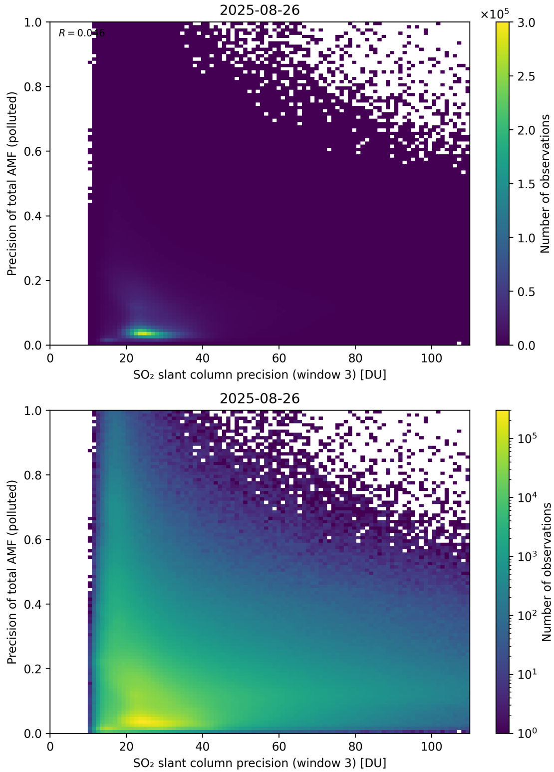
Figure 314: Scatter density plot of “SO 2 slant column precision (window 3)” against “Precision of total AMF (polluted)” for 2025-08-25 to 2025-08-27.
