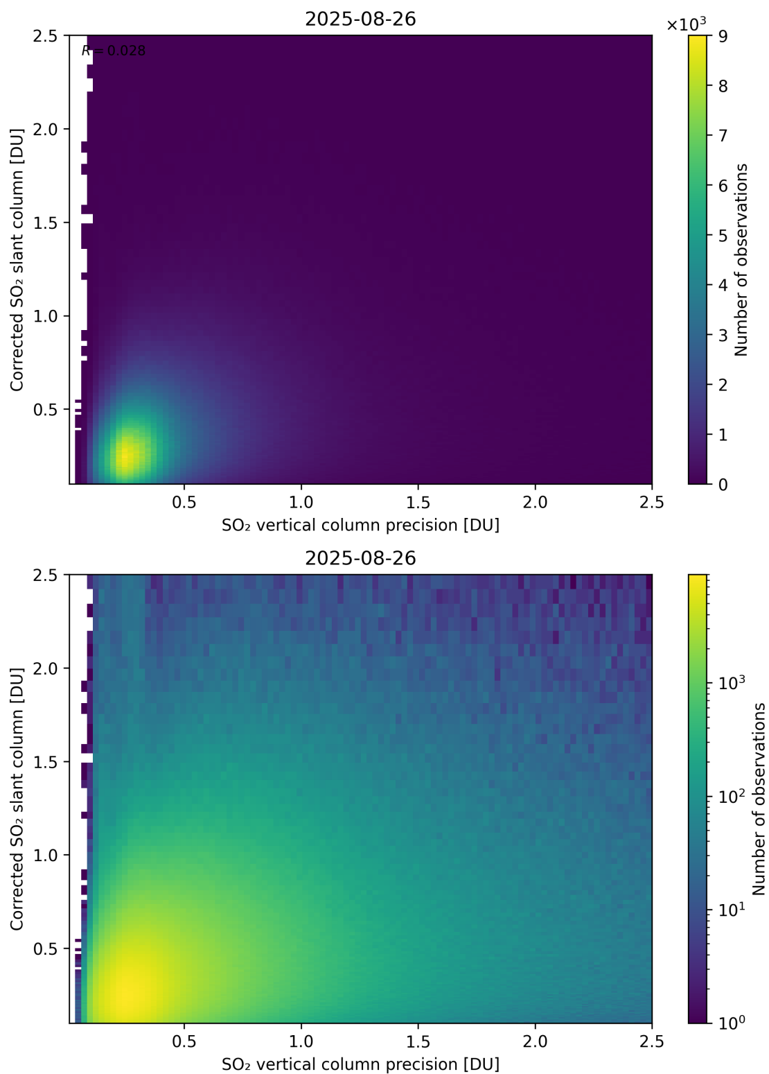
Figure 338: Scatter density plot of “SO 2 vertical column precision” against “Corrected SO 2 slant column” for 2025-08-25 to 2025-08-27.
