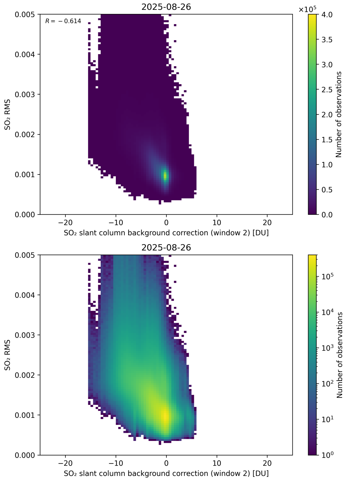
Figure 125: Scatter density plot of “SO 2 slant column background correction (window 2)” against “SO 2 RMS” for 2025-08-25 to 2025-08-27.
