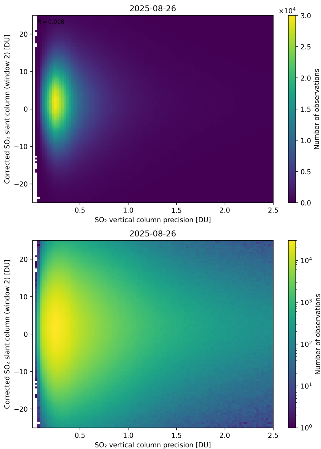
Figure 339: Scatter density plot of “SO 2 vertical column precision” against “Corrected SO 2 slant column (window 2)” for 2025-08-25 to 2025-08-27.
