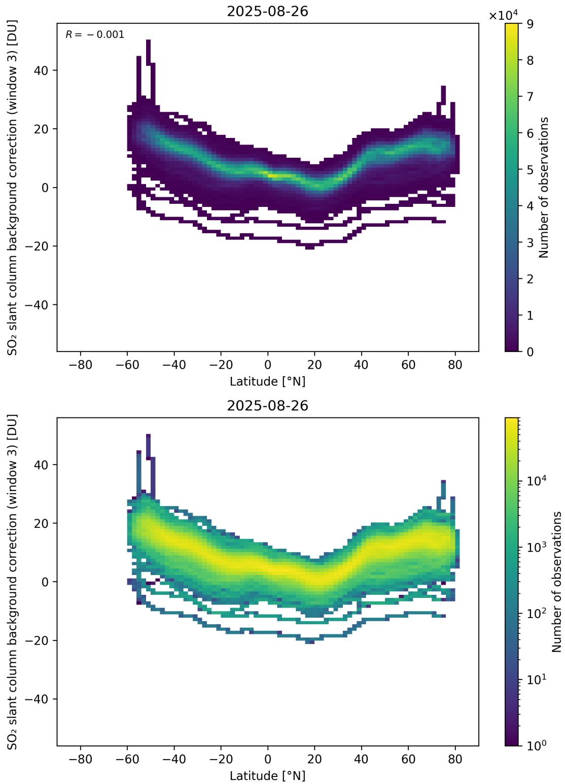
Figure 152: Scatter density plot of “Latitude” against “SO 2 slant column background correction (window 3)” for 2025-08-25 to 2025-08-27.
