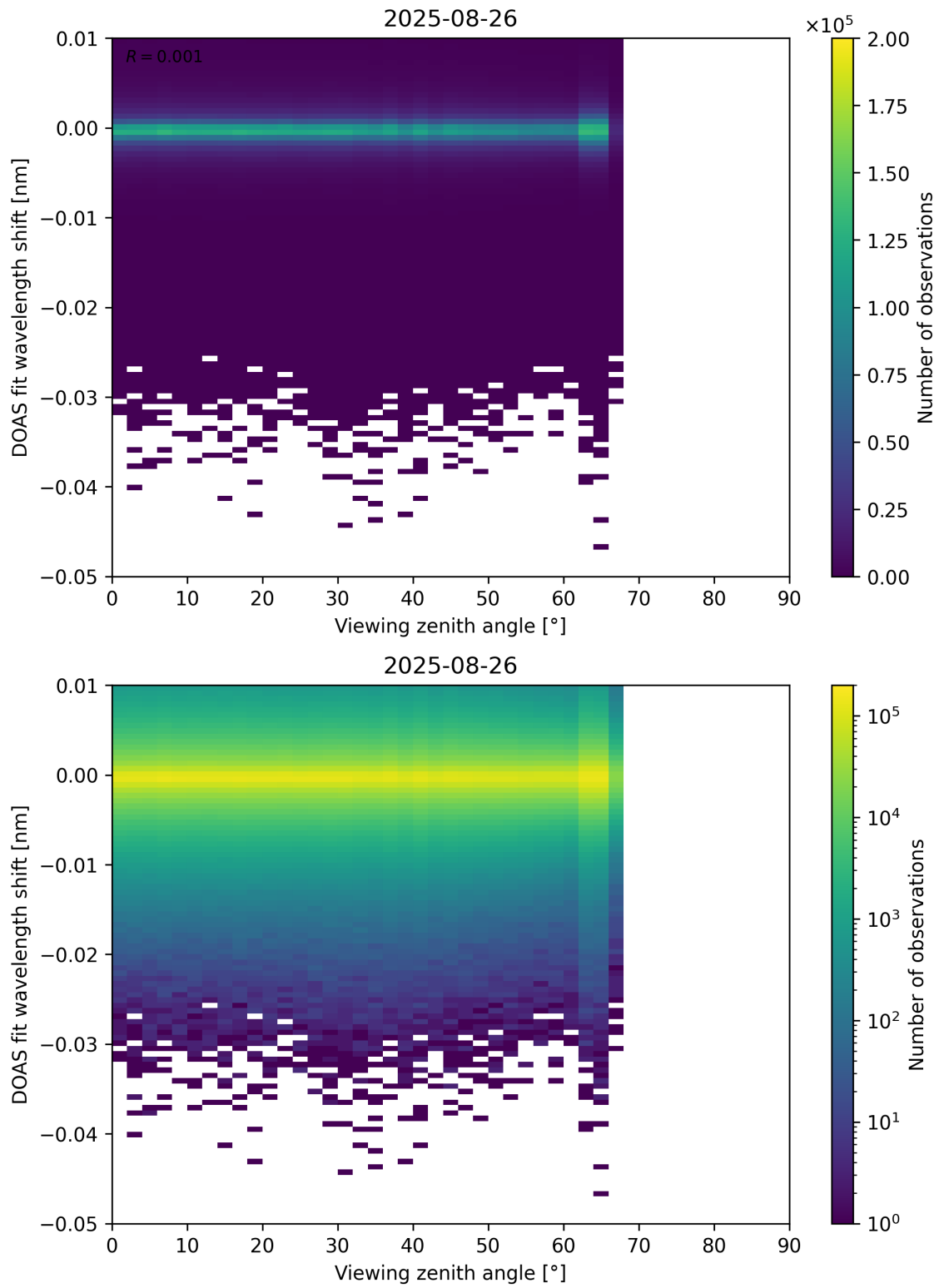
Figure 365: Scatter density plot of “Viewing zenith angle” against “DOAS fit wavelength shift” for 2025-08-25 to 2025-08-27.
