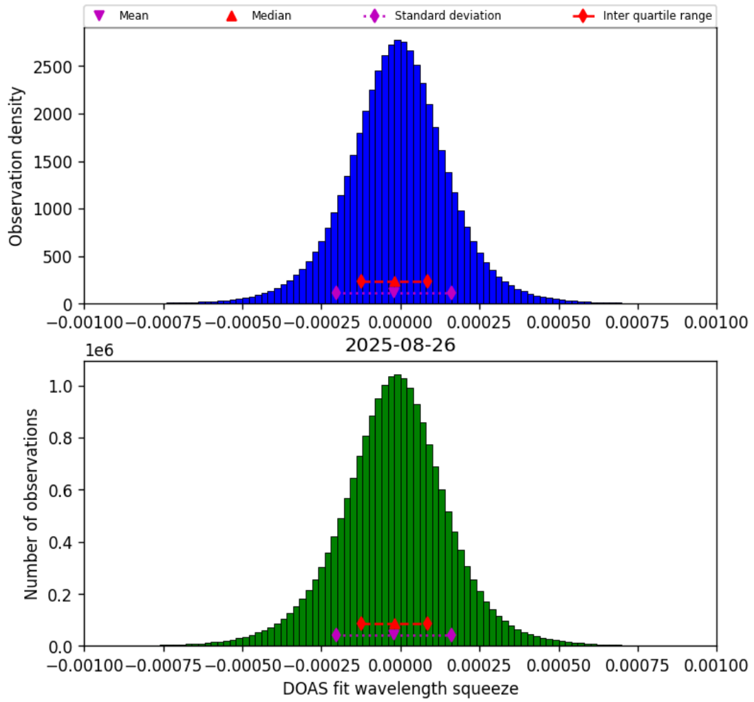
Figure 77: Histogram of “DOAS fit wavelength squeeze” for 2025-08-25 to 2025-08-27
