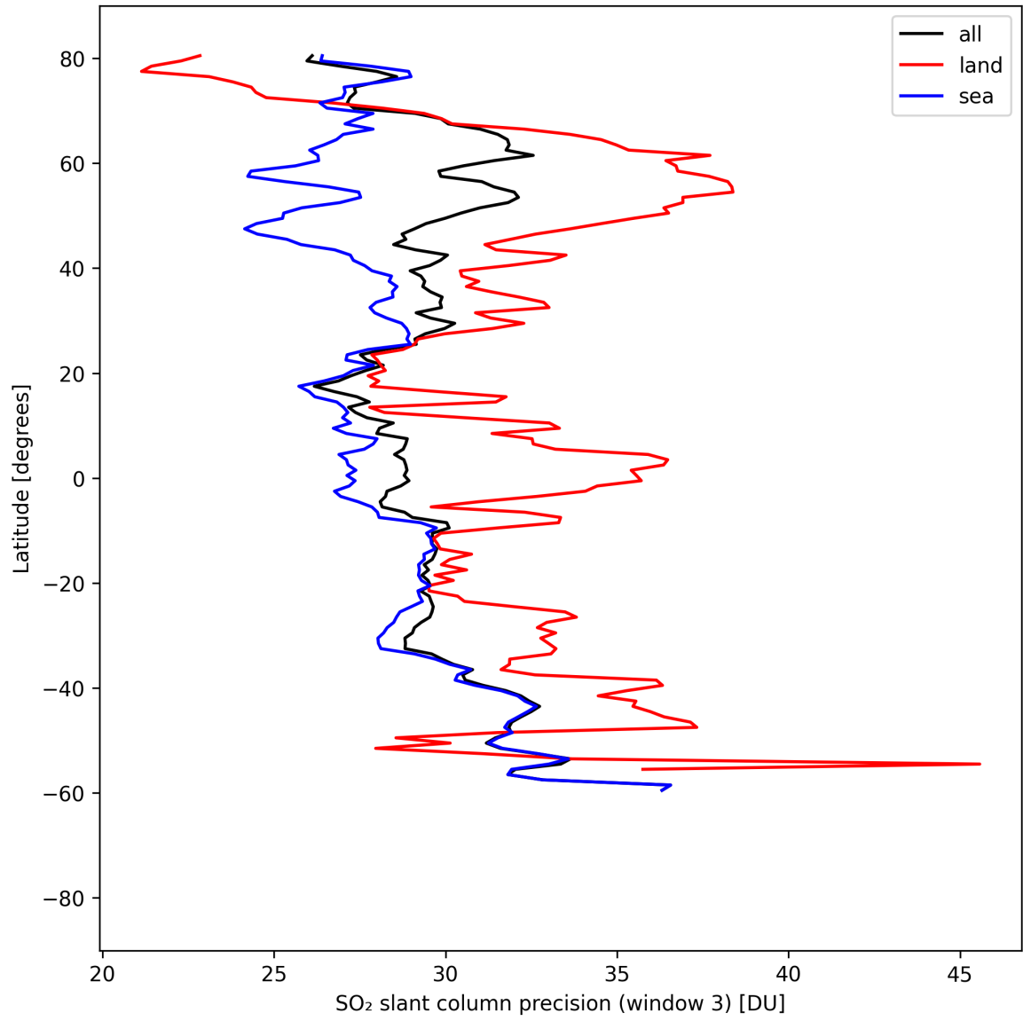
Figure 46: Zonal average of “SO 2 slant column precision (window 3)” for 2025-08-25 to 2025-08-27.
