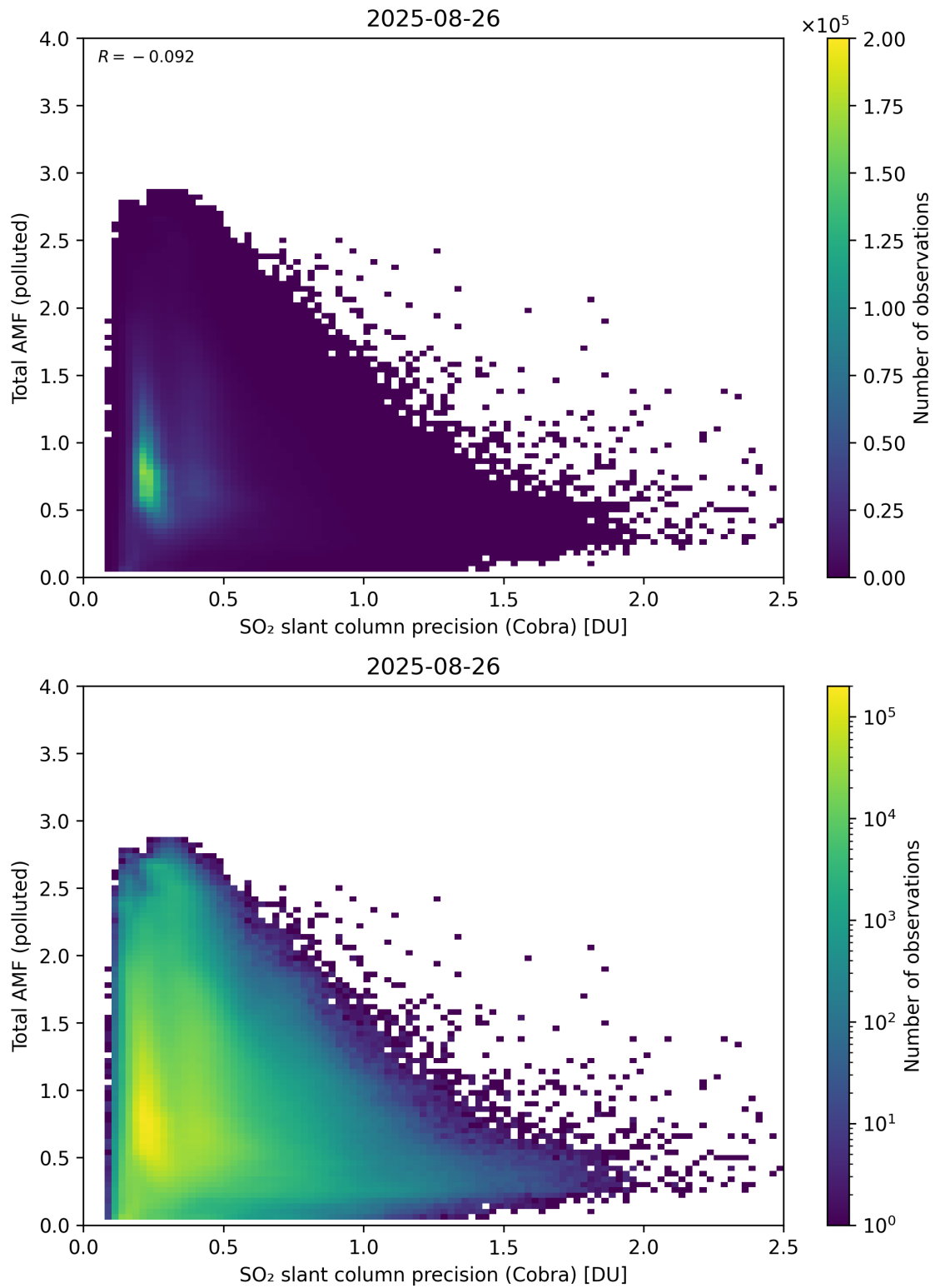
Figure 213: Scatter density plot of “SO 2 slant column precision (Cobra)” against “Total AMF (polluted)” for 2025-08-25 to 2025-08-27.
