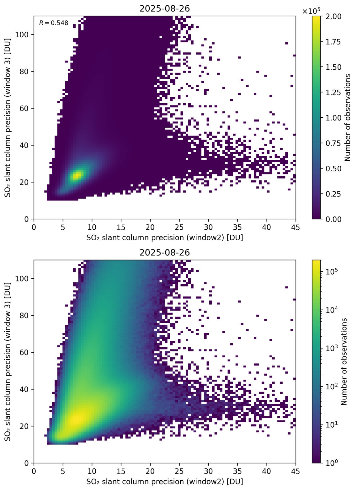
Figure 300: Scatter density plot of “SO 2 slant column precision (window2)” against “SO 2 slant column precision (window 3)” for 2025-08-25 to 2025-08-27.
