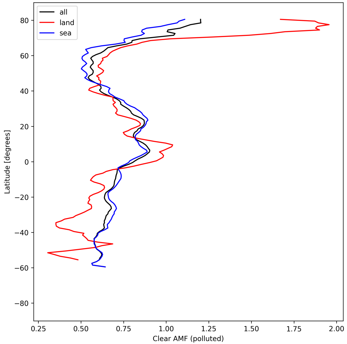
Figure 55: Zonal average of “Clear AMF (polluted)” for 2025-08-25 to 2025-08-27.
