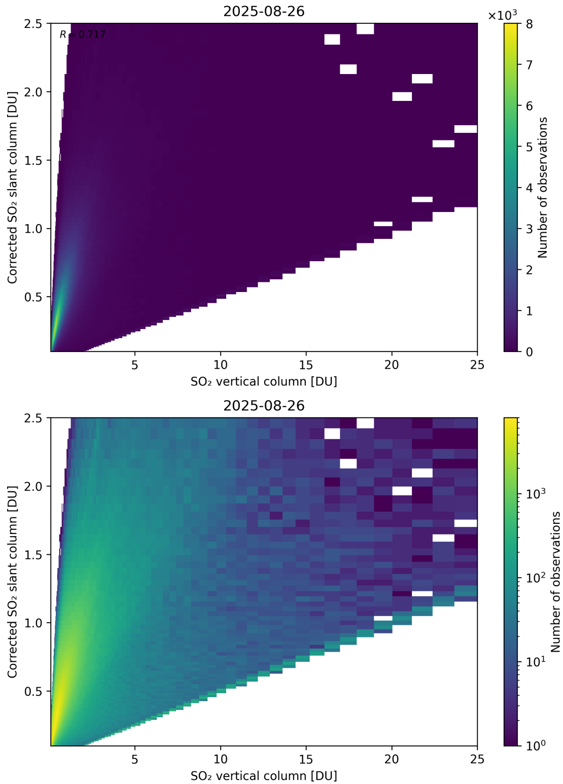
Figure 351: Scatter density plot of “SO 2 vertical column” against “Corrected SO 2 slant column” for 2025-08-25 to 2025-08-27.
