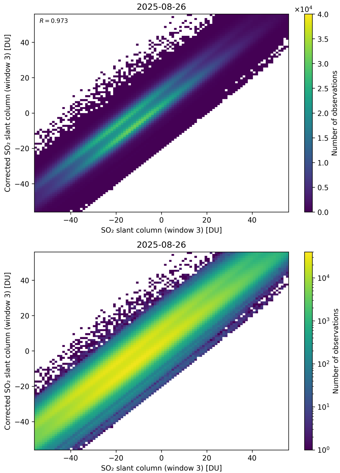
Figure 316: Scatter density plot of “SO 2 slant column (window 3)” against “Corrected SO 2 slant column (window 3)” for 2025-08-25 to 2025-08-27.
