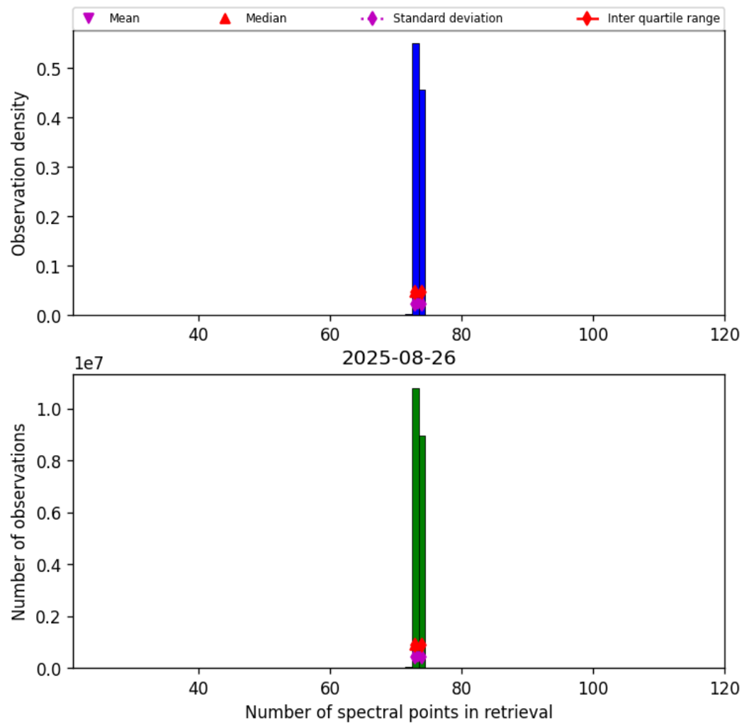
Figure 82: Histogram of “Number of spectral points in retrieval” for 2025-08-25 to 2025-08-27
