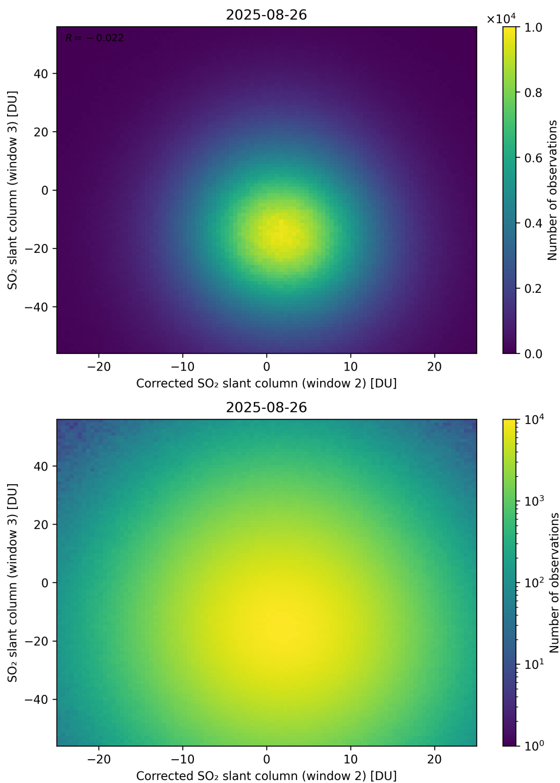
Figure 251: Scatter density plot of “Corrected SO 2 slant column (window 2)” against “SO 2 slant column (window 3)” for 2025-08-25 to 2025-08-27.
