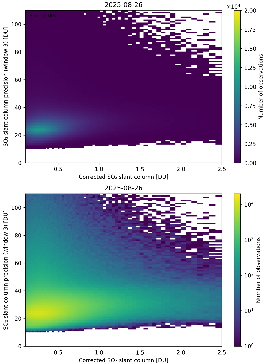
Figure 241: Scatter density plot of “Corrected SO 2 slant column” against “SO 2 slant column precision (window 3)” for 2025-08-25 to 2025-08-27.
