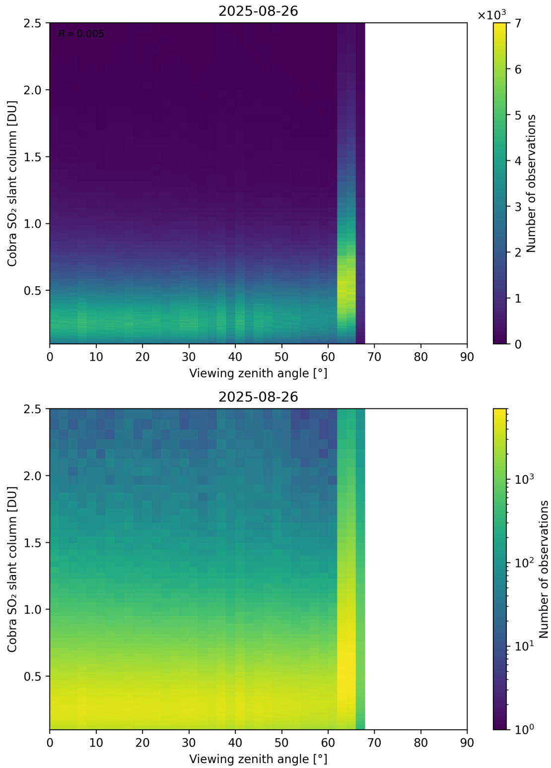
Figure 371: Scatter density plot of “Viewing zenith angle” against “Cobra SO 2 slant column” for 2025-08-25 to 2025-08-27.
