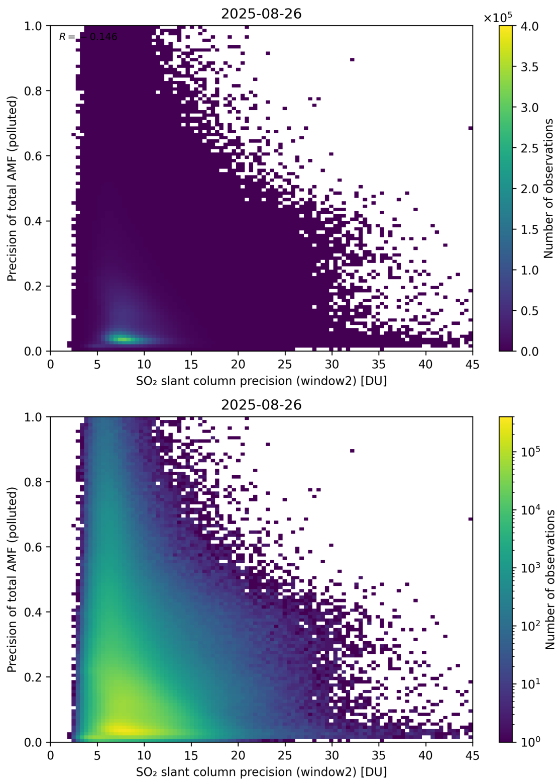
Figure 302: Scatter density plot of “SO 2 slant column precision (window2)” against “Precision of total AMF (polluted)” for 2025-08-25 to 2025-08-27.
