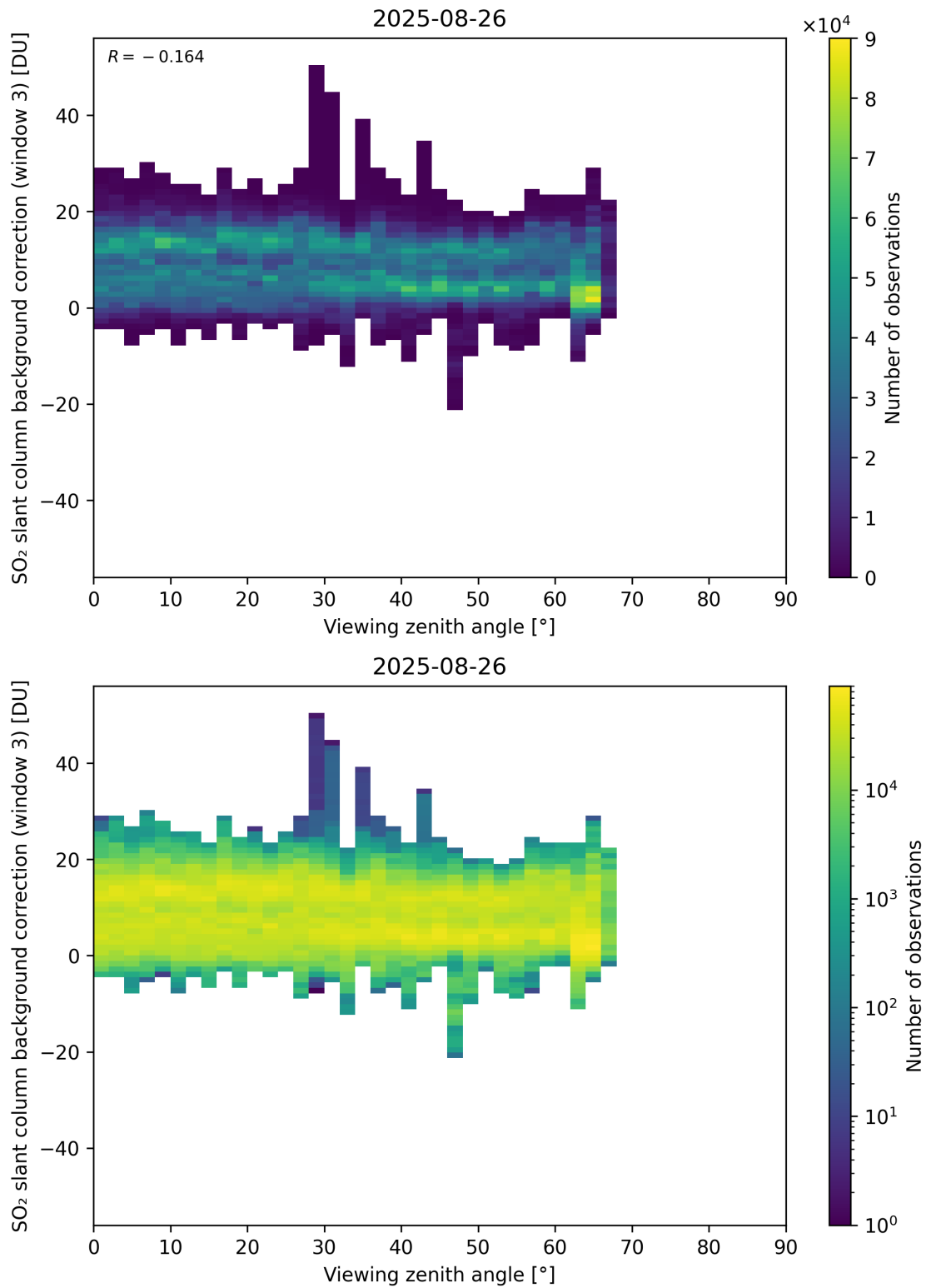
Figure 364: Scatter density plot of “Viewing zenith angle” against “SO 2 slant column background correction (window 3)” for 2025-08-25 to 2025-08-27.
