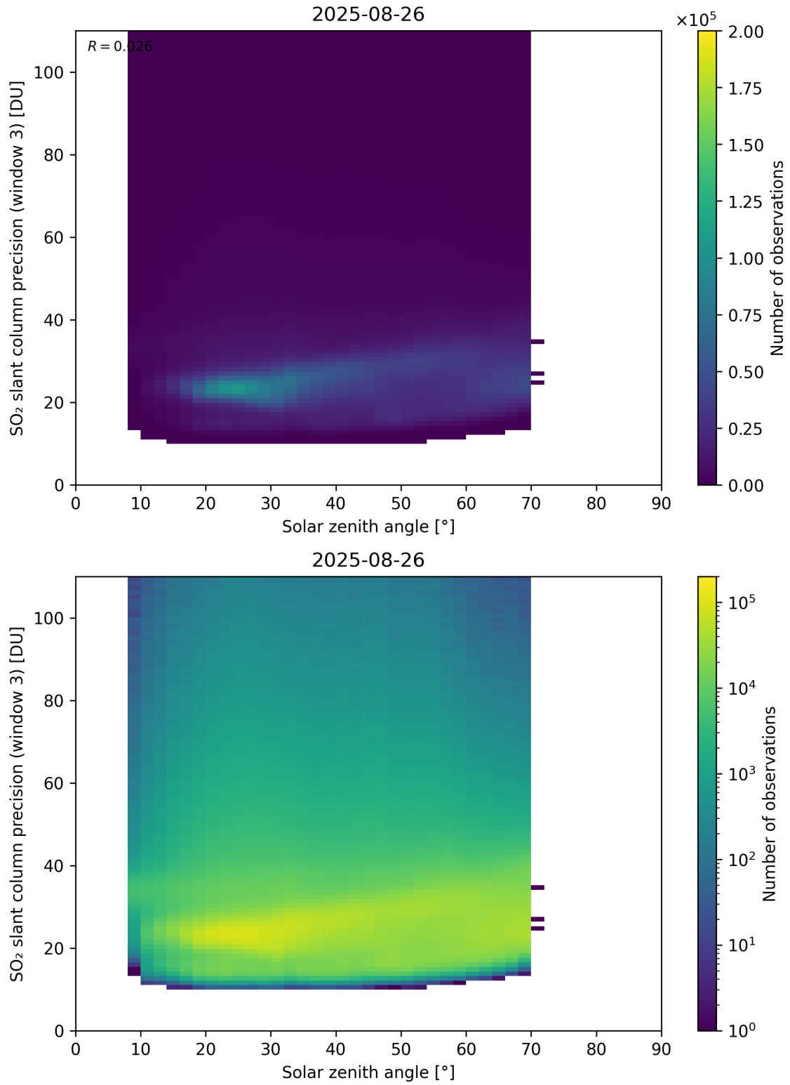
Figure 188: Scatter density plot of “Solar zenith angle” against “SO 2 slant column precision (window 3)” for 2025-08-25 to 2025-08-27.
