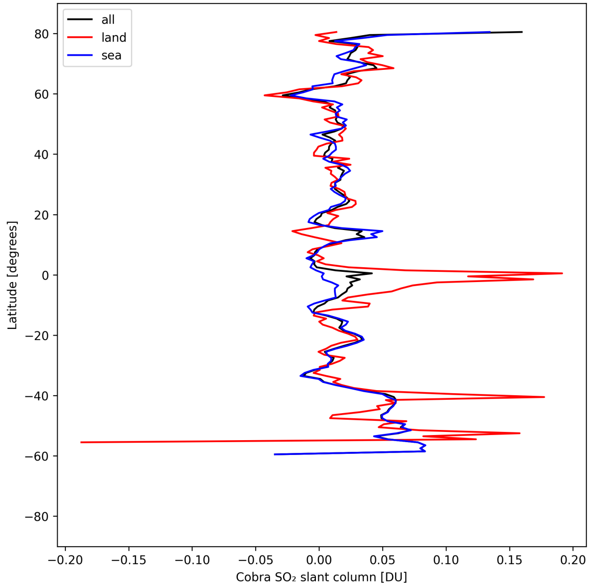
Figure 35: Zonal average of “Cobra SO 2 slant column” for 2025-08-25 to 2025-08-27.
