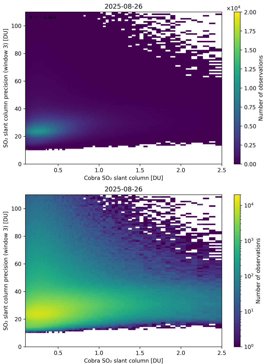
Figure 223: Scatter density plot of “Cobra SO 2 slant column” against “SO 2 slant column precision (window 3)” for 2025-08-25 to 2025-08-27.
