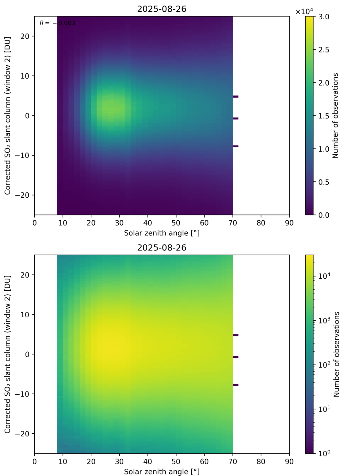
Figure 182: Scatter density plot of “Solar zenith angle” against “Corrected SO 2 slant column (window 2)” for 2025-08-25 to 2025-08-27.
