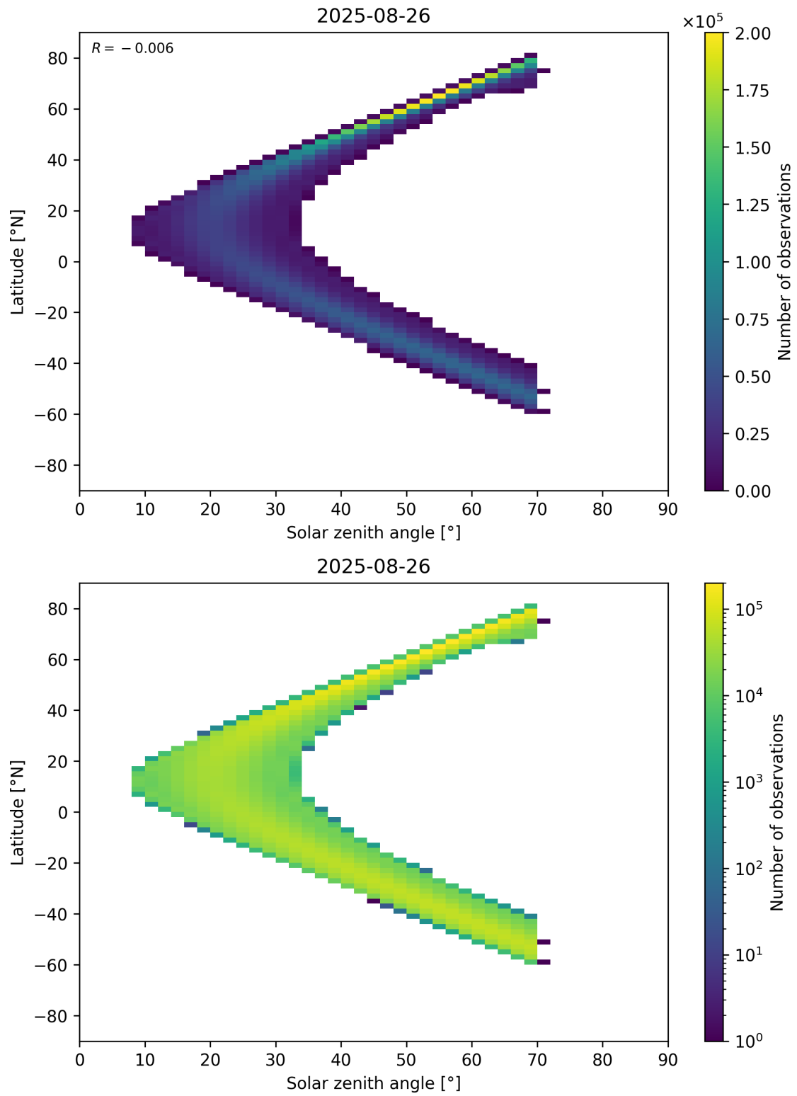
Figure 177: Scatter density plot of “Solar zenith angle” against “Latitude” for 2025-08-25 to 2025-08-27.
