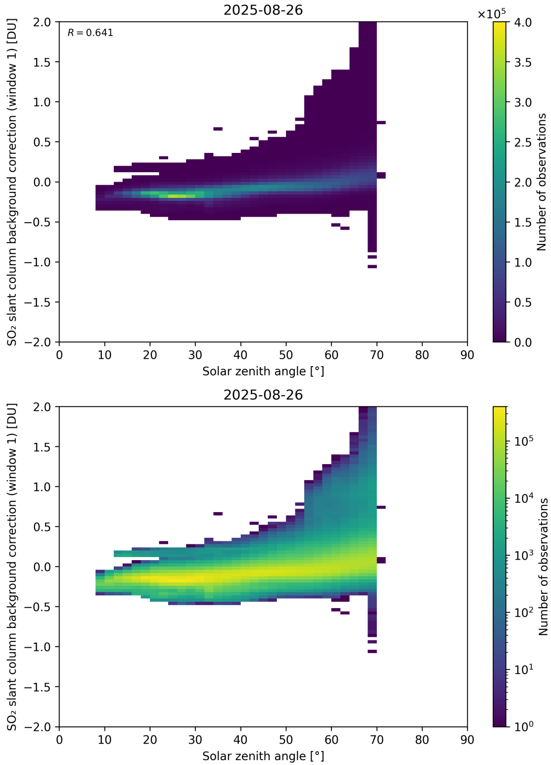
Figure 171: Scatter density plot of “Solar zenith angle” against “SO 2 slant column background correction (window 1)” for 2025-08-25 to 2025-08-27.
