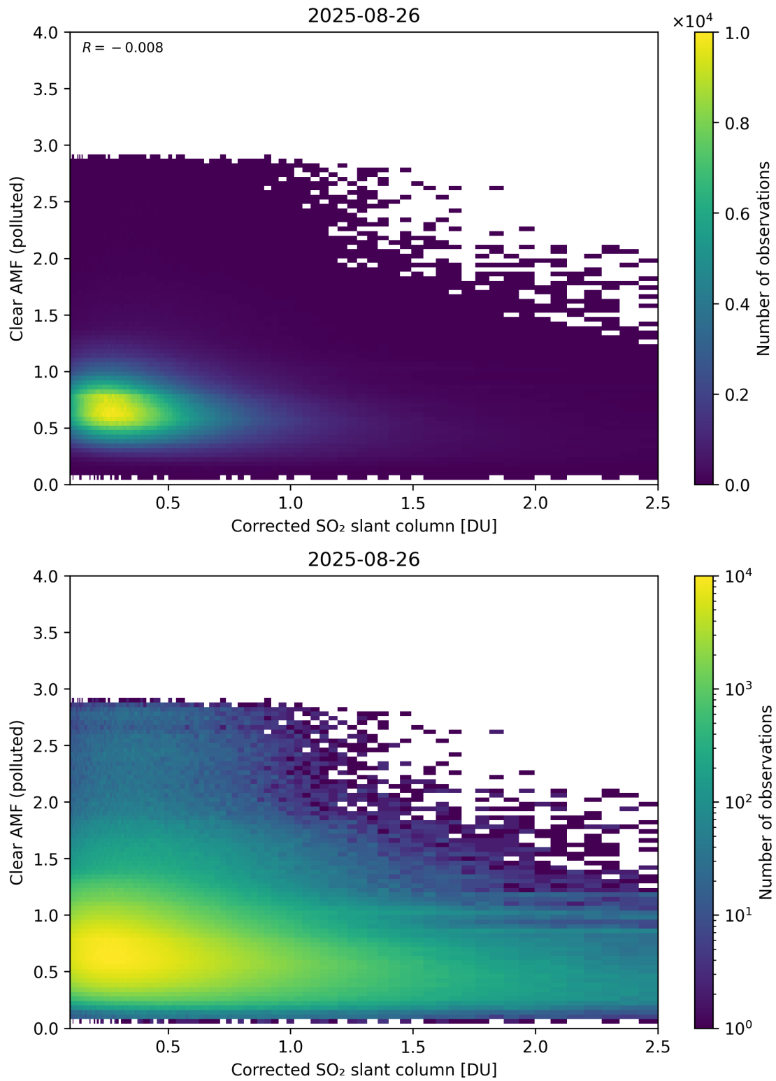
Figure 232: Scatter density plot of “Corrected SO 2 slant column” against “Clear AMF (polluted)” for 2025-08-25 to 2025-08-27.
