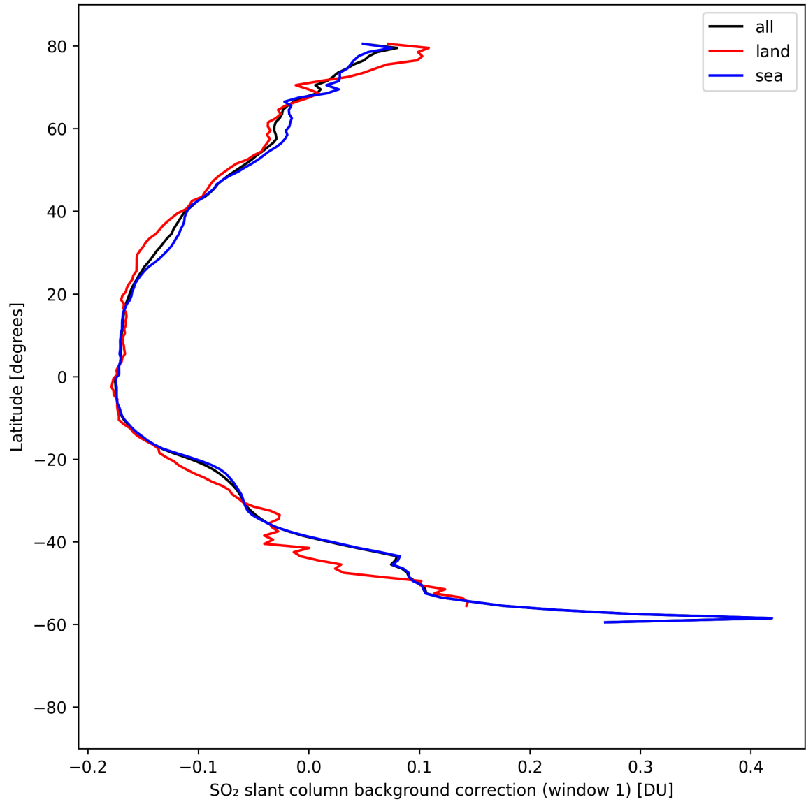
Figure 40: Zonal average of "SO 2 slant column background correction (window 1)" for 2025-08-25 to 2025-08-27.
