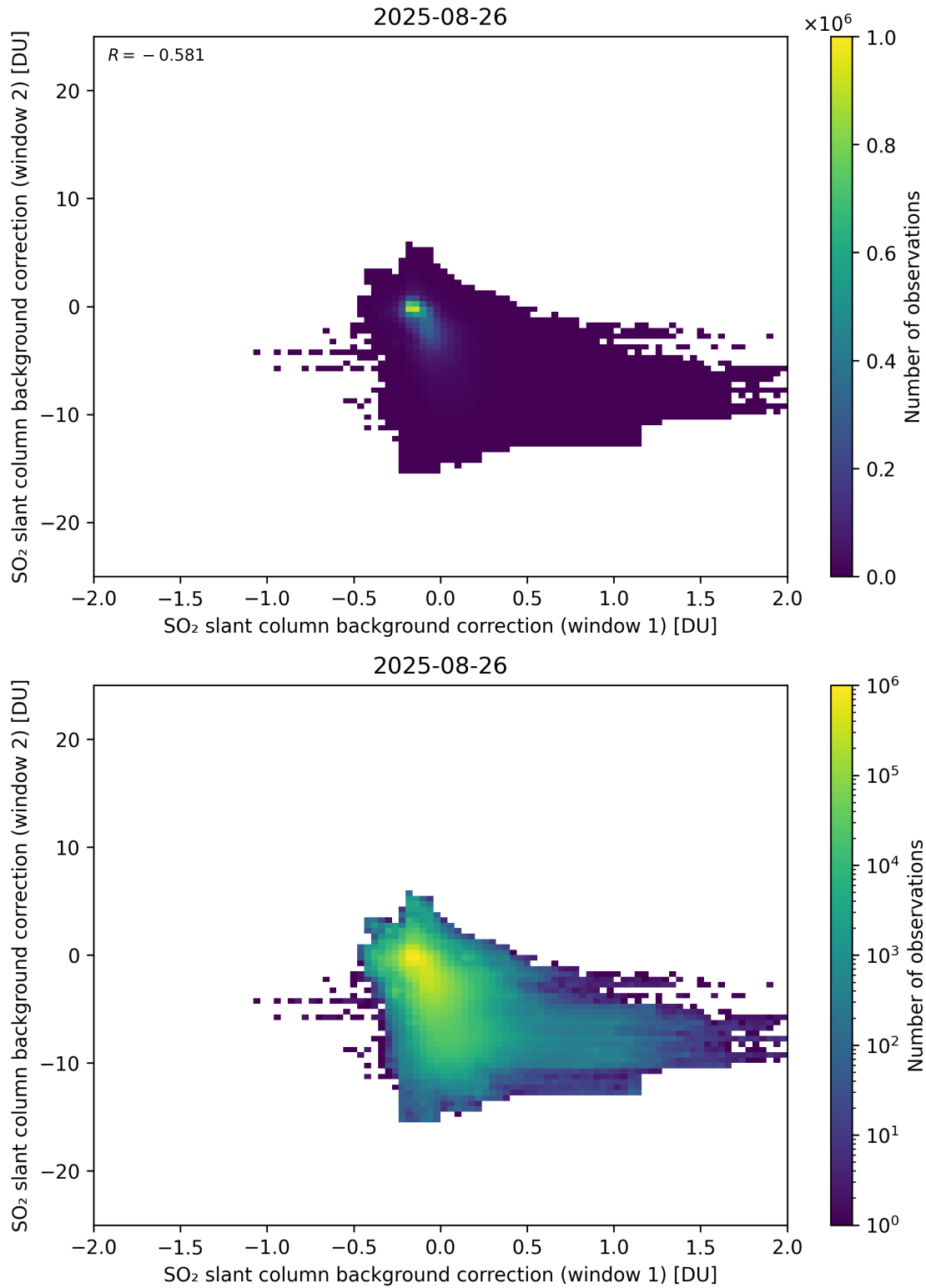
Figure 109: Scatter density plot of “SO 2 slant column background correction (window 1)” against “SO 2 slant column background correction (window 2)” for 2025-08-25 to 2025-08-27.
