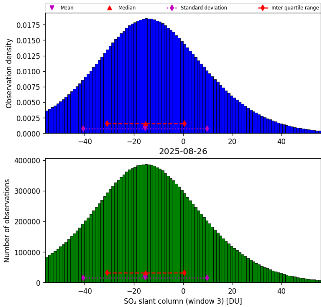
Figure 71: Histogram of “SO 2 slant column (window 3)” for 2025-08-25 to 2025-08-27
