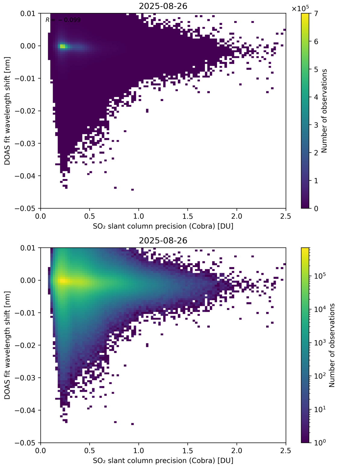
Figure 202: Scatter density plot of “SO 2 slant column precision (Cobra)” against “DOAS fit wavelength shift” for 2025-08-25 to 2025-08-27.
