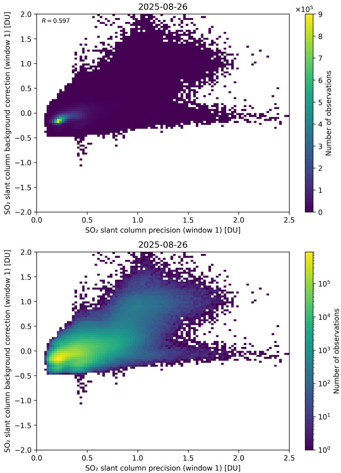
Figure 268: Scatter density plot of “SO 2 slant column precision (window 1)” against “SO 2 slant column background correction (window 1)” for 2025-08-25 to 2025-08-27.
