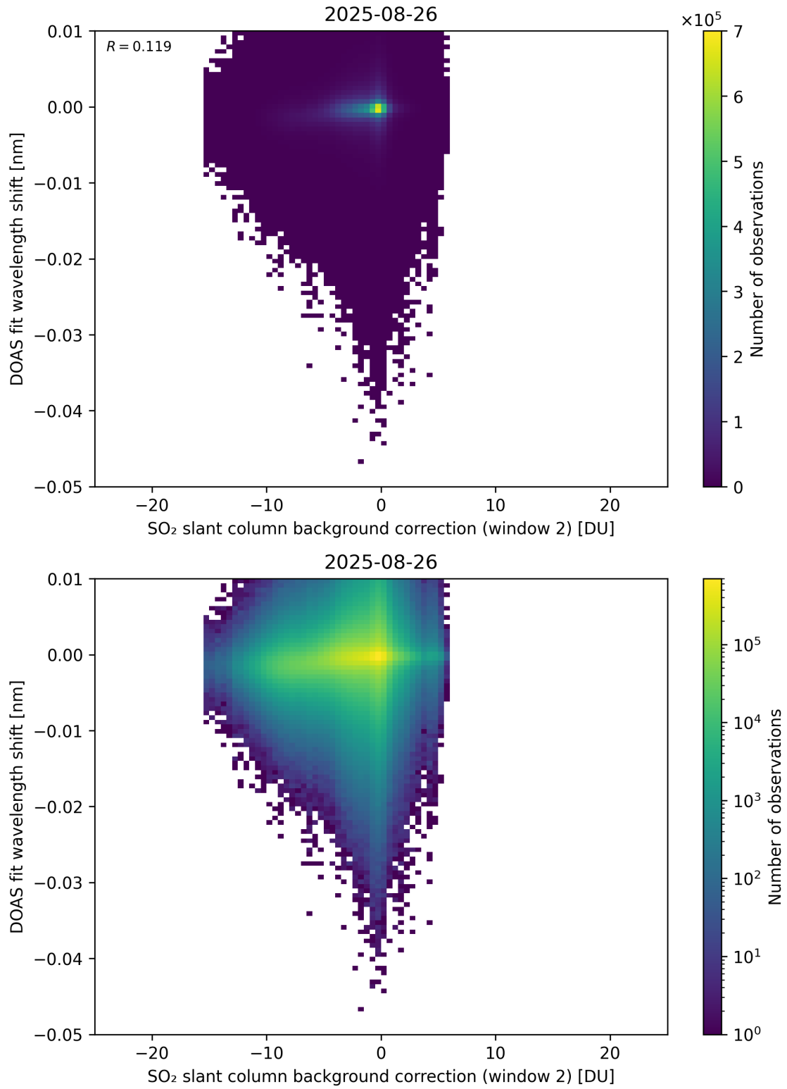
Figure 123: Scatter density plot of “SO 2 slant column background correction (window 2)” against “DOAS fit wavelength shift” for 2025-08-25 to 2025-08-27.
