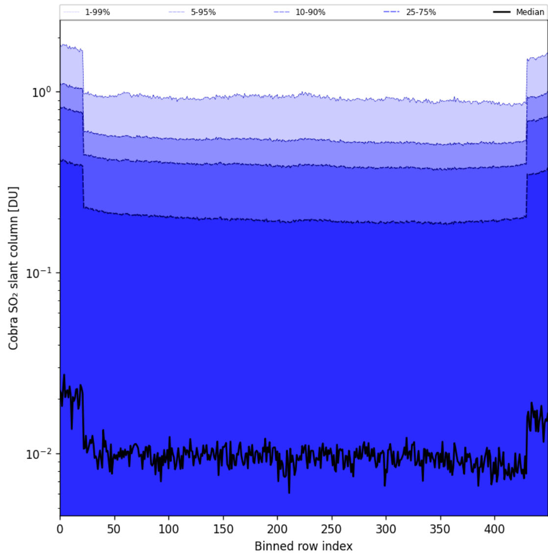
Figure 87: Along track statistics of "Cobra SO 2 slant column" for 2025-08-25 to 2025-08-27
