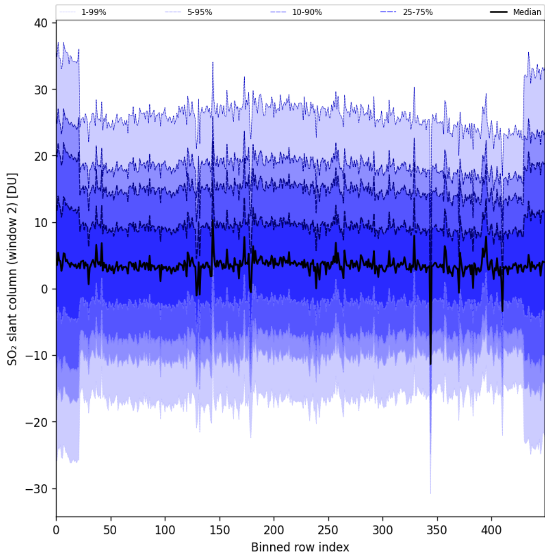
Figure 93: Along track statistics of “SO 2 slant column (window 2)” for 2025-08-25 to 2025-08-27
