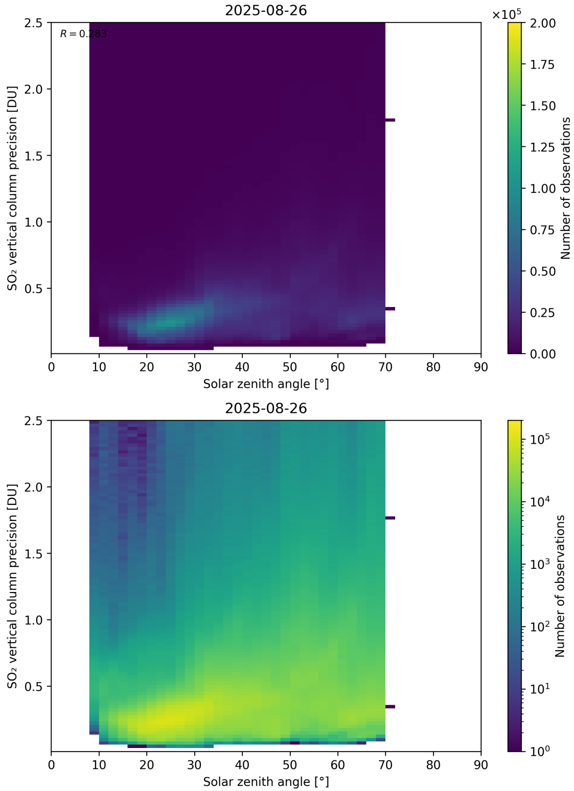
Figure 192: Scatter density plot of “Solar zenith angle” against “SO 2 vertical column precision” for 2025-08-25 to 2025-08-27.
