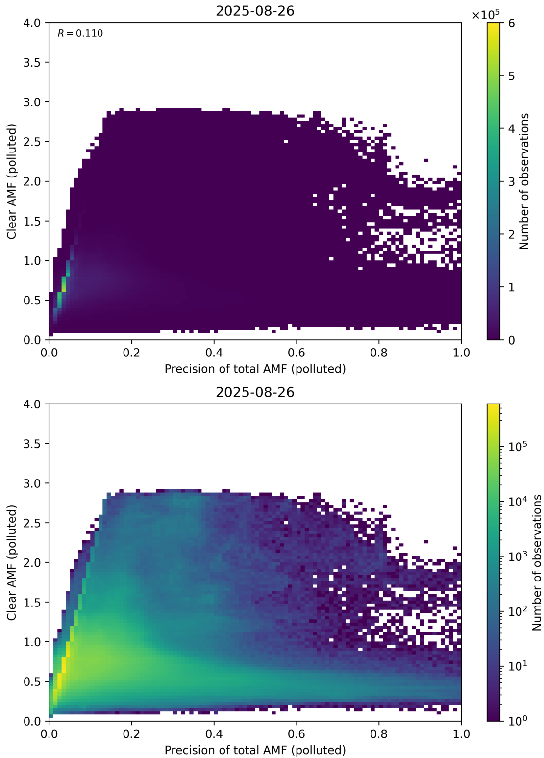
Figure 320: Scatter density plot of “Precision of total AMF (polluted)” against “Clear AMF (polluted)” for 2025-08-25 to 2025-08-27.
