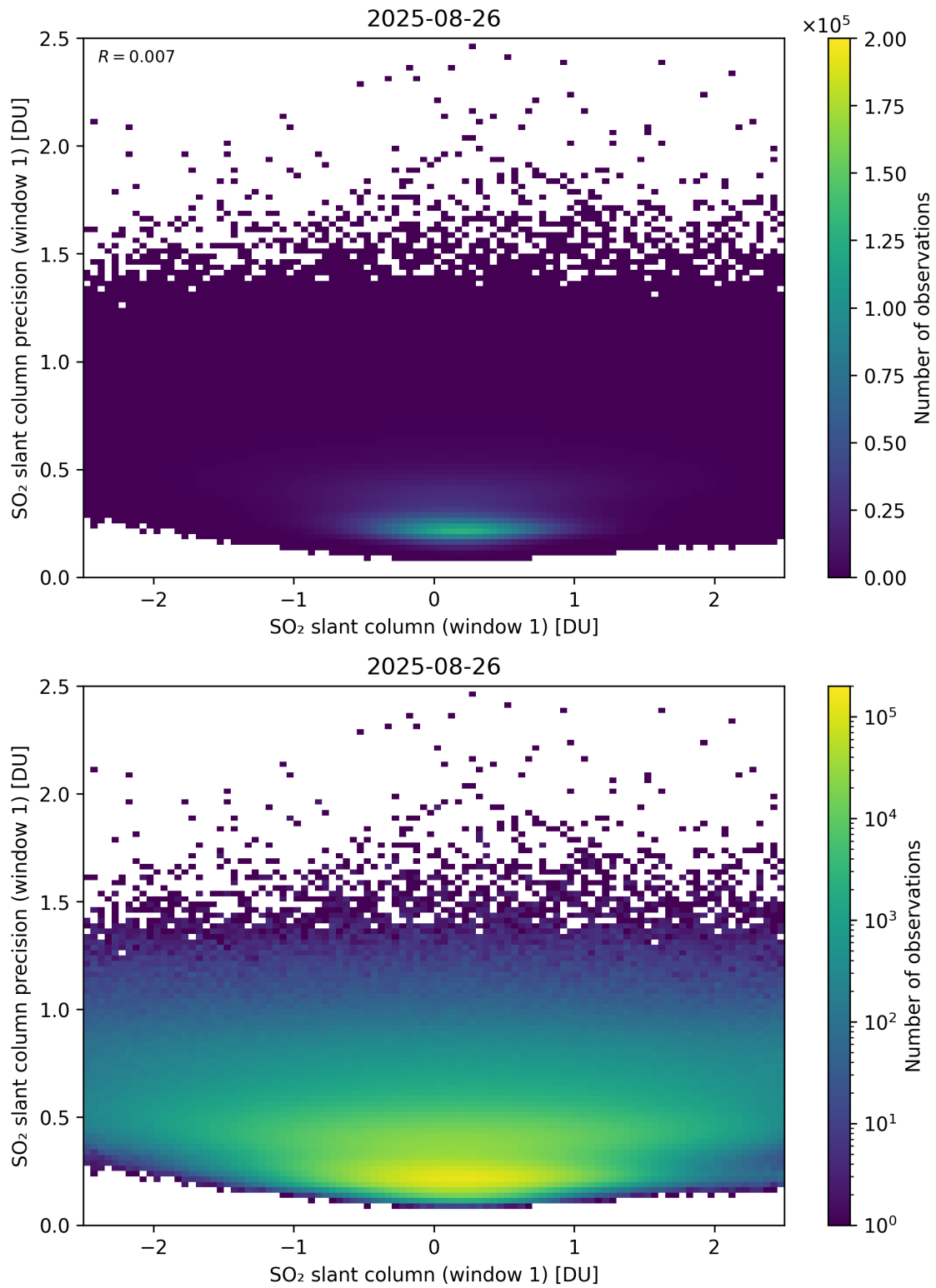
Figure 285: Scatter density plot of “SO 2 slant column (window 1)” against “SO 2 slant column precision (window 1)” for 2025-08-25 to 2025-08-27.
