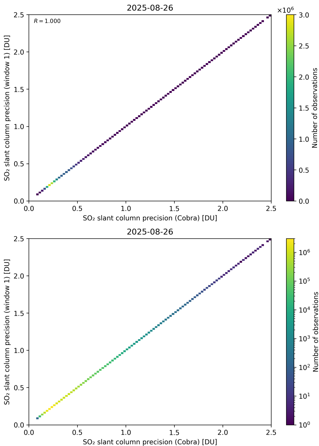
Figure 209: Scatter density plot of “SO 2 slant column precision (Cobra)” against “SO 2 slant column precision (window 1)” for 2025-08-25 to 2025-08-27.
