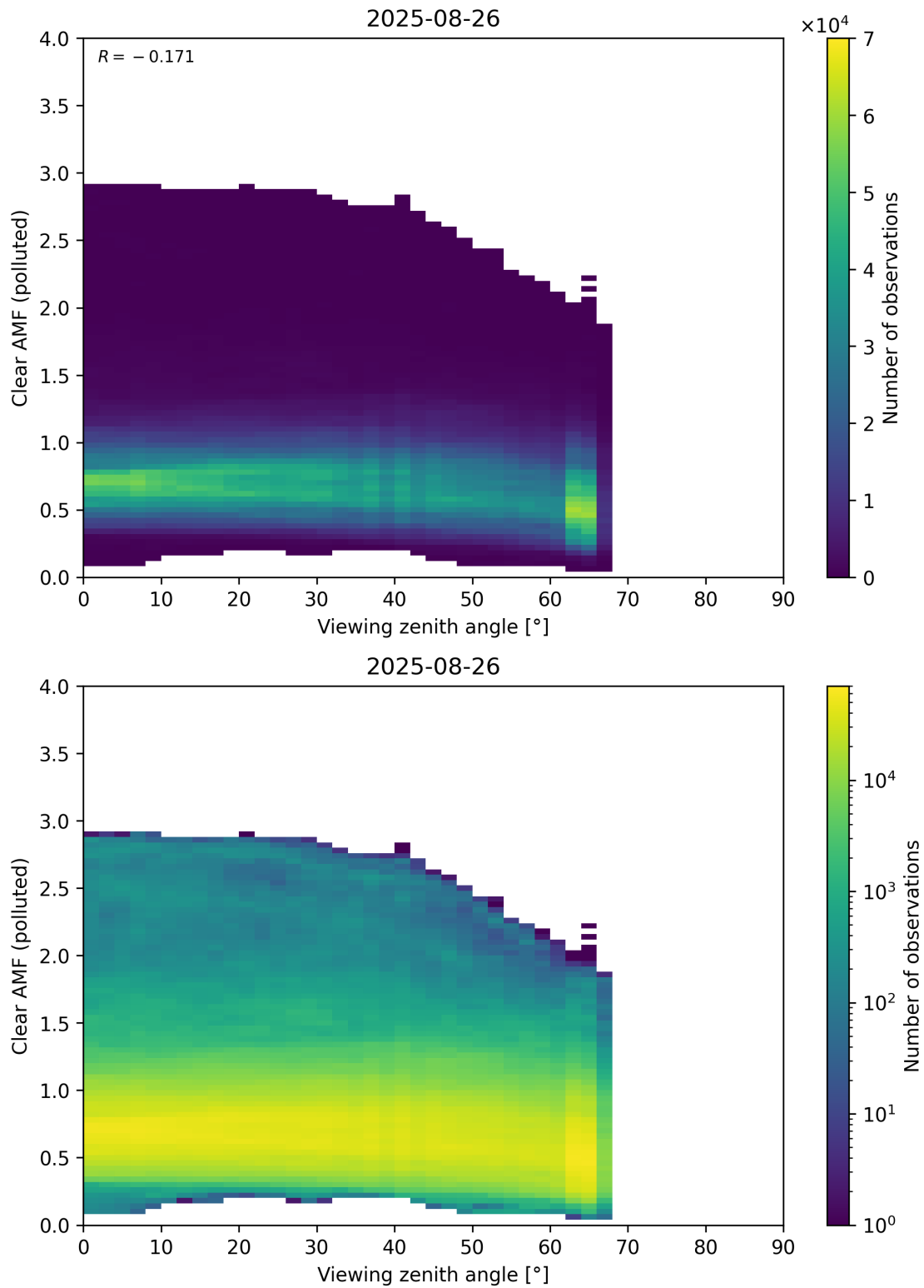
Figure 370: Scatter density plot of “Viewing zenith angle” against “Clear AMF (polluted)” for 2025-08-25 to 2025-08-27.
