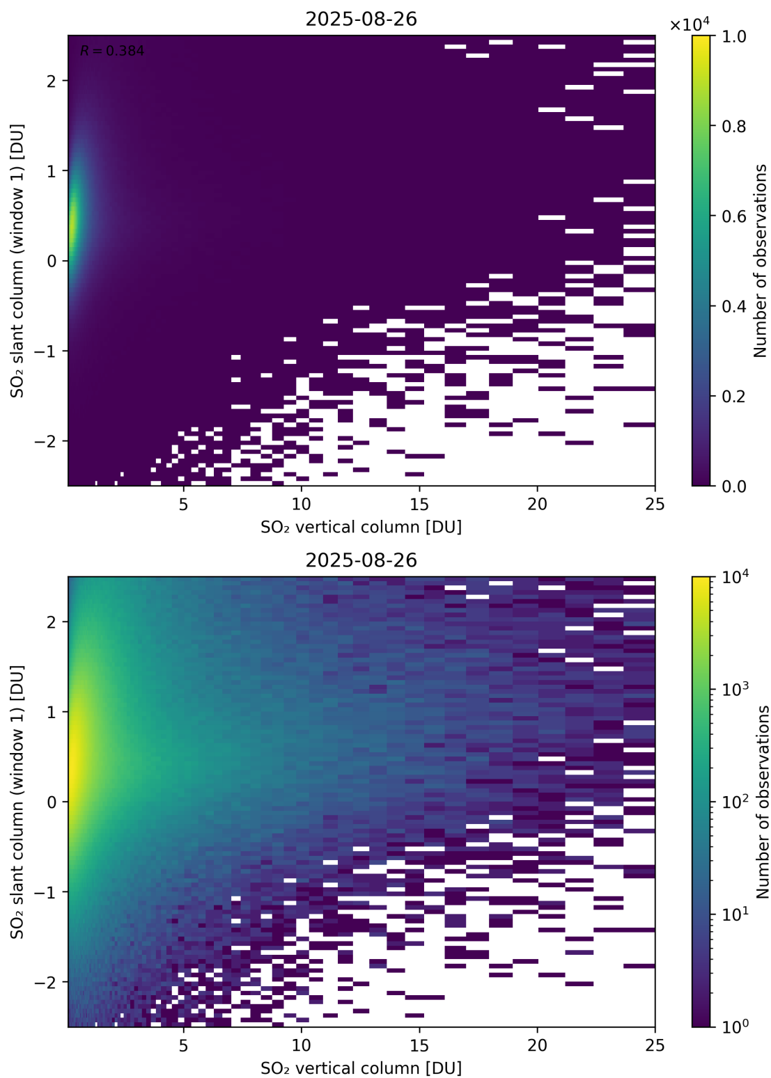
Figure 354: Scatter density plot of “SO 2 vertical column” against “SO 2 slant column (window 1)” for 2025-08-25 to 2025-08-27.
