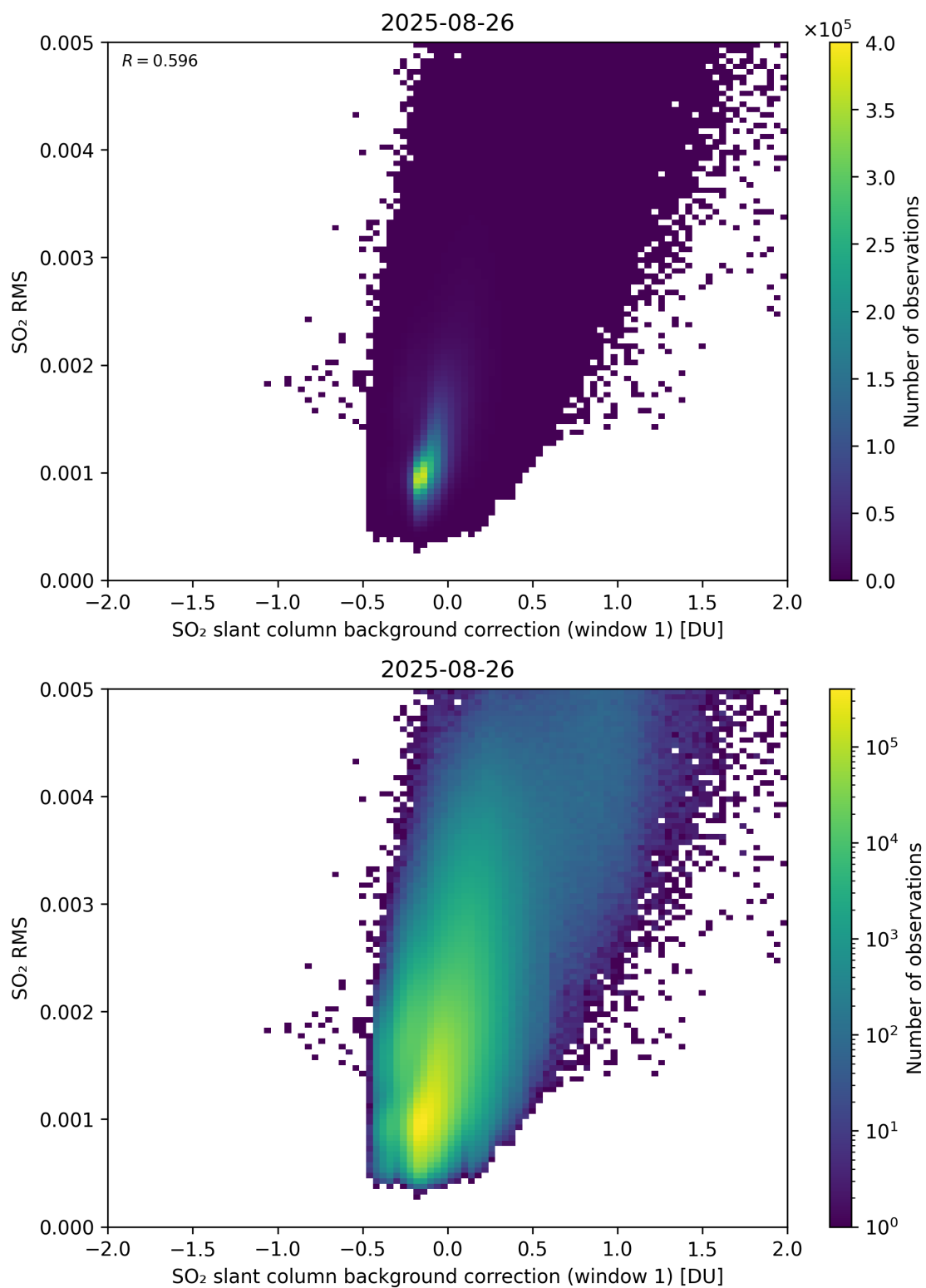
Figure 113: Scatter density plot of “SO 2 slant column background correction (window 1)” against “SO 2 RMS” for 2025-08-25 to 2025-08-27.
