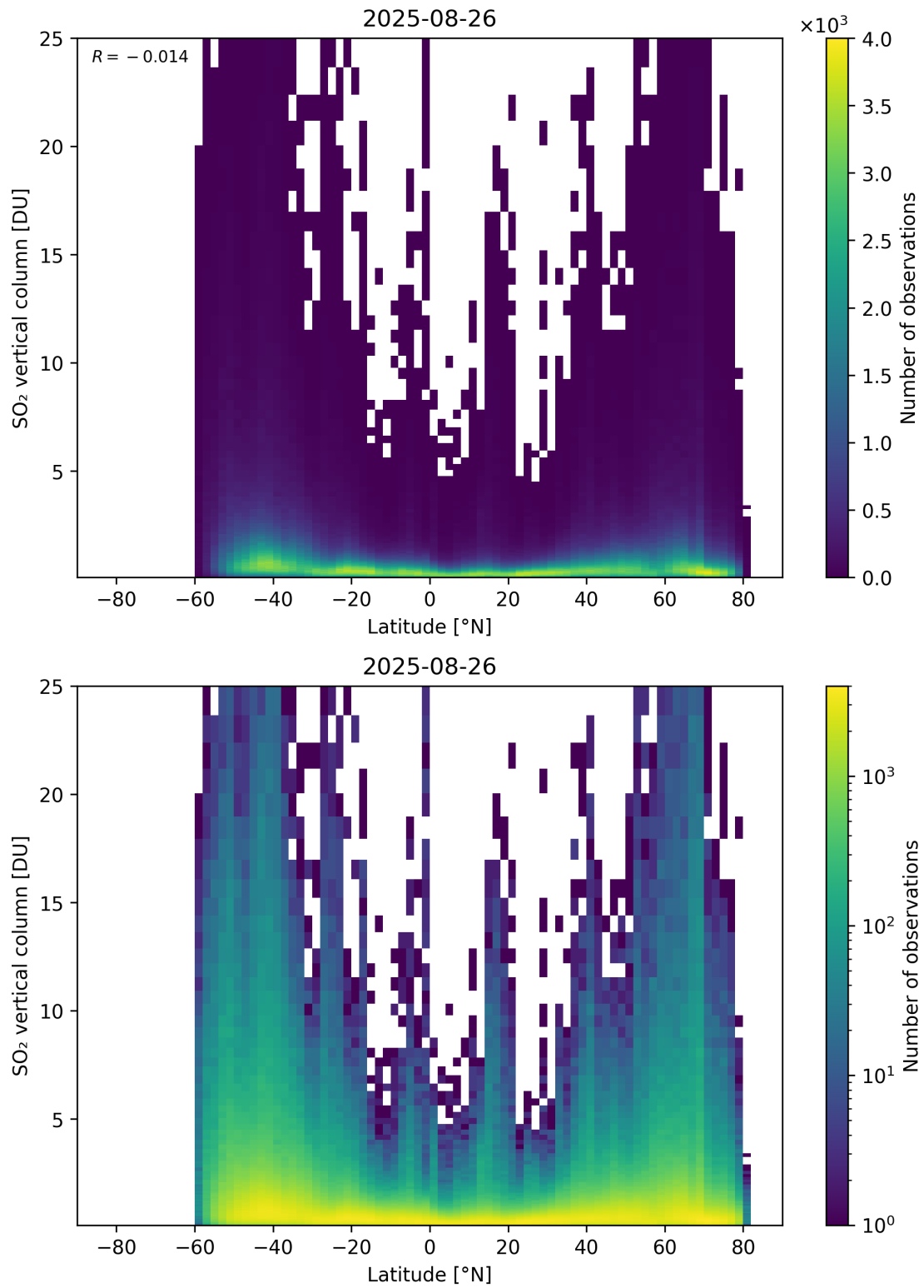
Figure 169: Scatter density plot of “Latitude” against “SO 2 vertical column” for 2025-08-25 to 2025-08-27.
