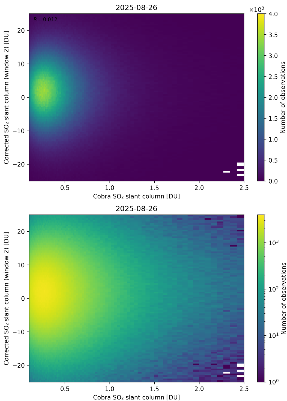
Figure 217: Scatter density plot of “Cobra SO 2 slant column” against “Corrected SO 2 slant column (window 2)” for 2025-08-25 to 2025-08-27.
