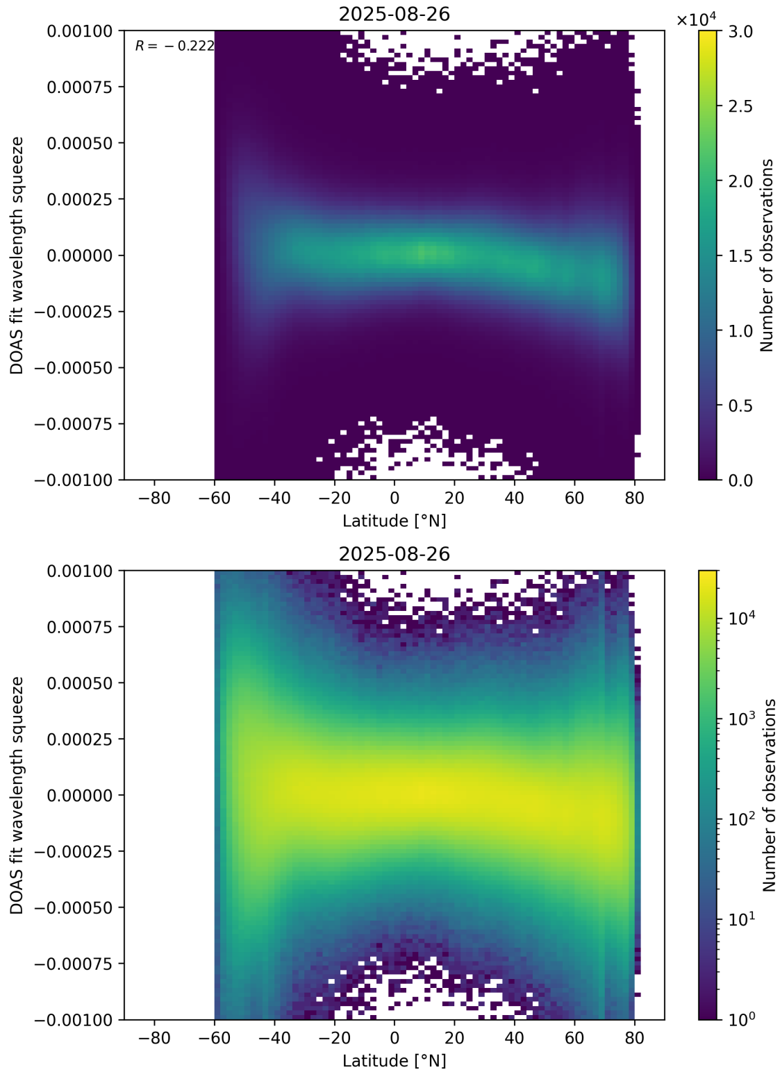
Figure 154: Scatter density plot of “Latitude” against “DOAS fit wavelength squeeze” for 2025-08-25 to 2025-08-27.
