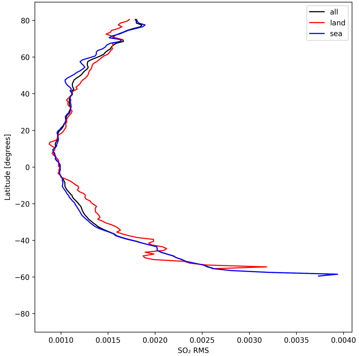
Figure 52: Zonal average of “SO 2 RMS” for 2025-08-25 to 2025-08-27.
