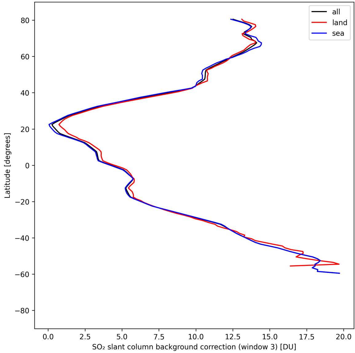
Figure 48: Zonal average of “SO 2 slant column background correction (window 3)” for 2025-08-25 to 2025-08-27.
