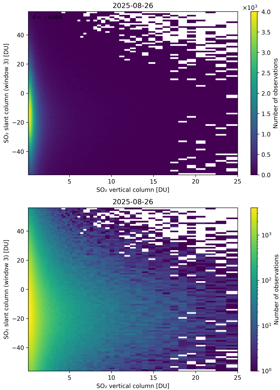
Figure 357: Scatter density plot of “SO 2 vertical column” against “SO 2 slant column (window 3)” for 2025-08-25 to 2025-08-27.
