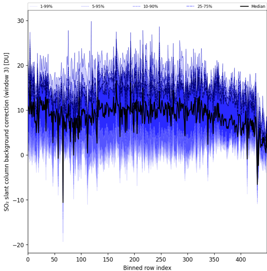
Figure 100: Along track statistics of “SO 2 slant column background correction (window 3)” for 2025-08-25 to 2025-08-27
