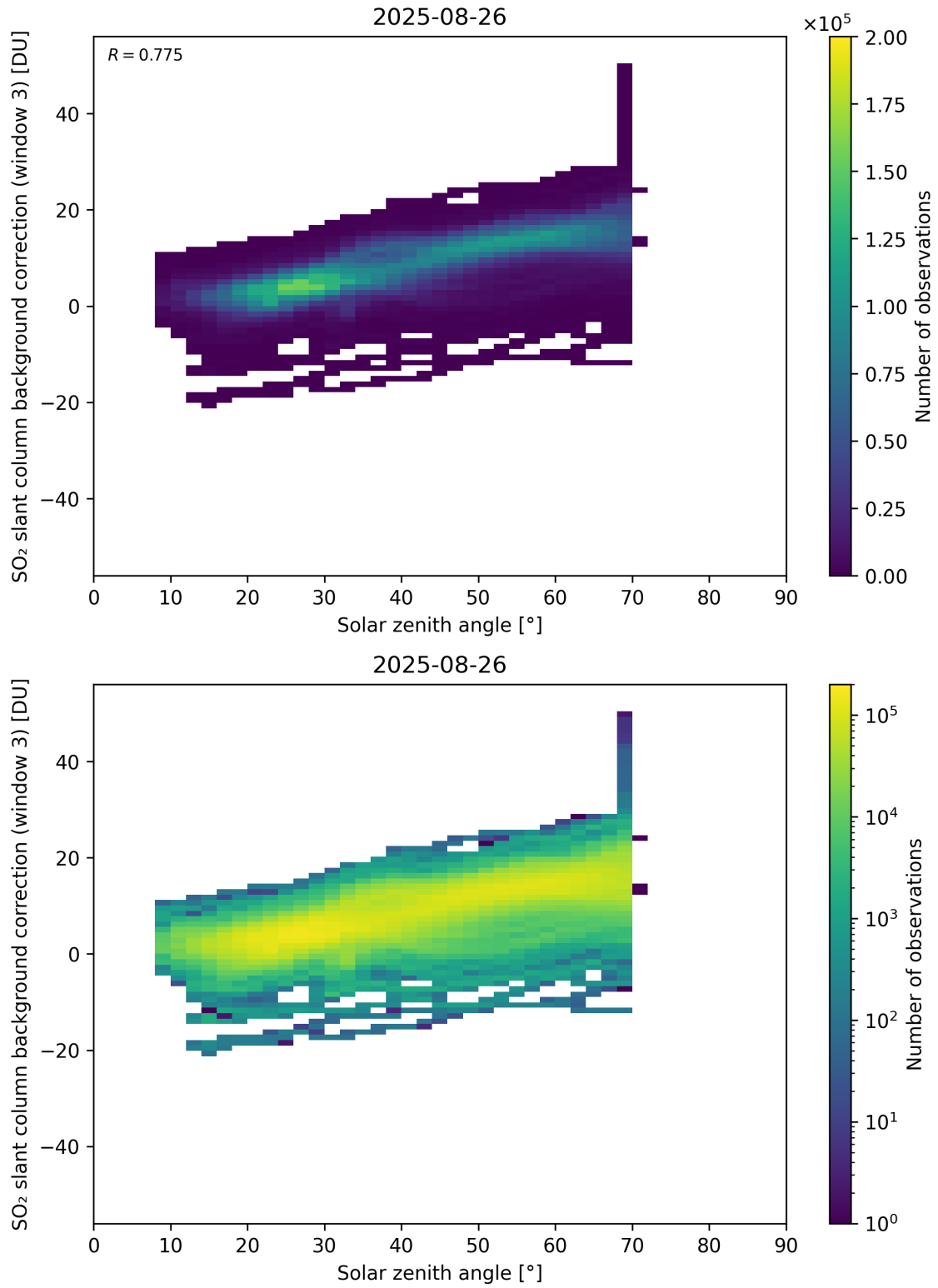
Figure 173: Scatter density plot of “Solar zenith angle” against “SO 2 slant column background correction (window 3)” for 2025-08-25 to 2025-08-27.
