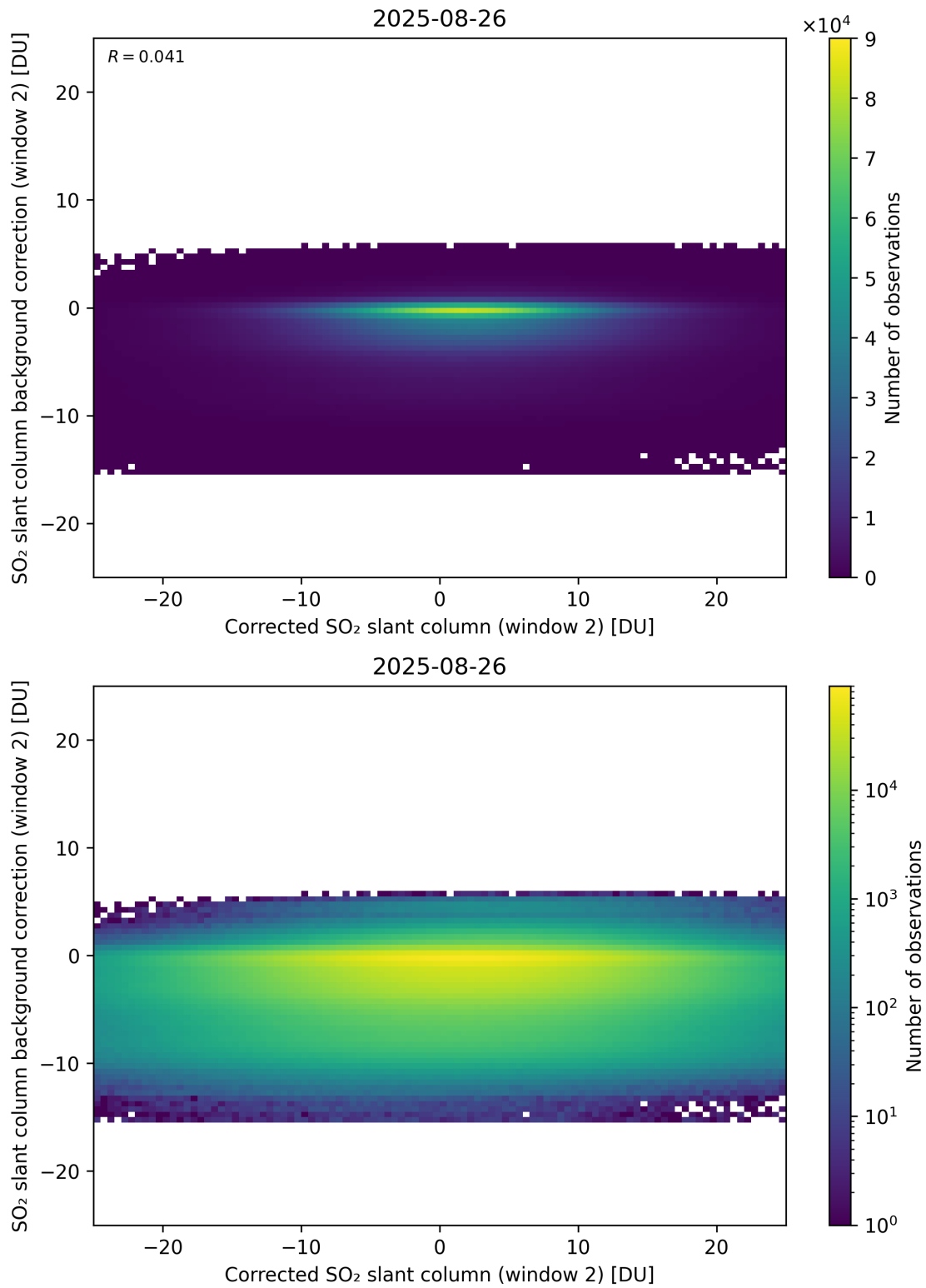
Figure 244: Scatter density plot of “Corrected SO 2 slant column (window 2)” against “SO 2 slant column background correction (window 2)” for 2025-08-25 to 2025-08-27.
