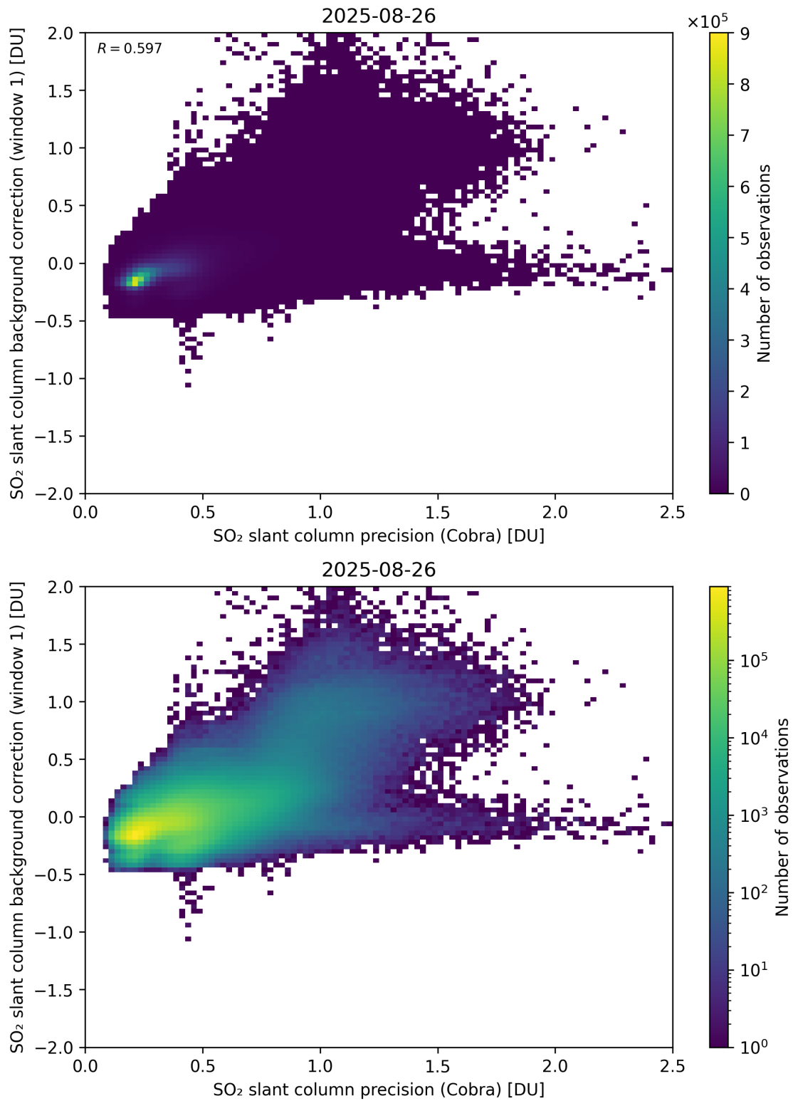
Figure 199: Scatter density plot of “SO 2 slant column precision (Cobra)” against “SO 2 slant column background correction (window 1)” for 2025-08-25 to 2025-08-27.
