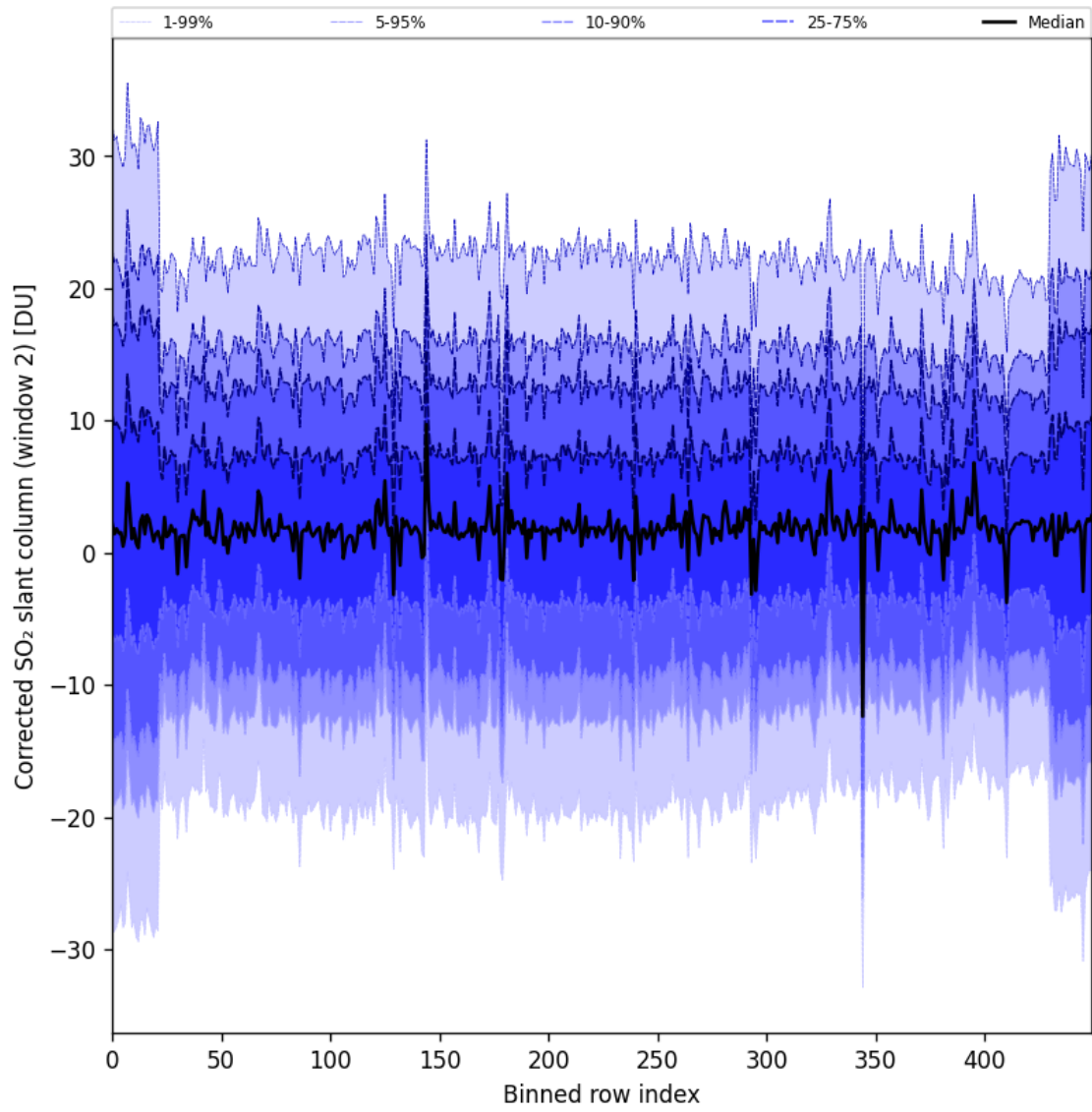
Figure 95: Along track statistics of “Corrected SO 2 slant column (window 2)” for 2025-08-25 to 2025-08-27
