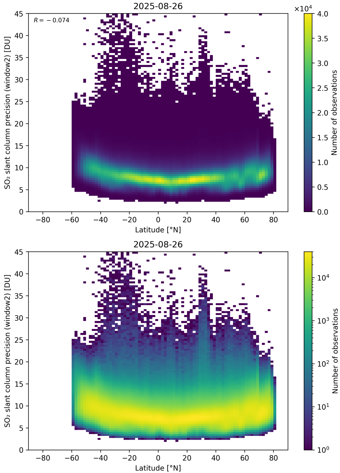
Figure 164: Scatter density plot of “Latitude” against “SO 2 slant column precision (window2)” for 2025-08-25 to 2025-08-27.
