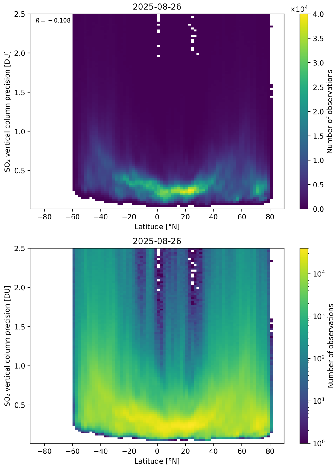
Figure 170: Scatter density plot of “Latitude” against “SO 2 vertical column precision” for 2025-08-25 to 2025-08-27.
