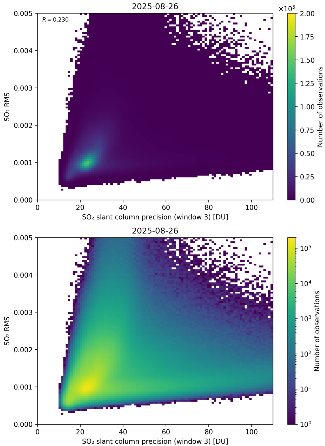
Figure 310: Scatter density plot of “SO 2 slant column precision (window 3)” against “SO 2 RMS” for 2025-08-25 to 2025-08-27.
