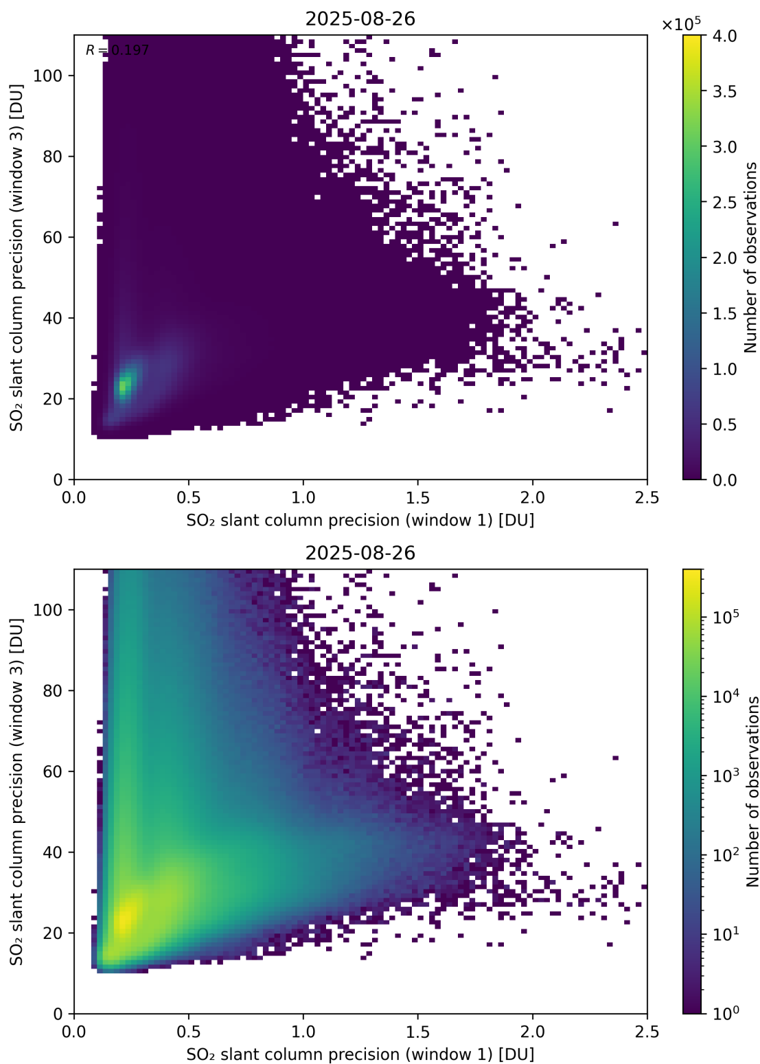
Figure 279: Scatter density plot of “SO 2 slant column precision (window 1)” against “SO 2 slant column precision (window 3)” for 2025-08-25 to 2025-08-27.
