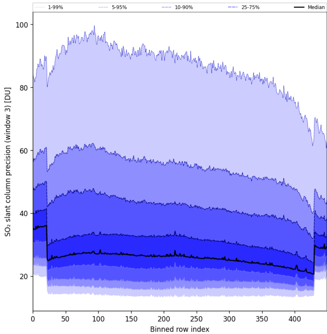
Figure 98: Along track statistics of “SO 2 slant column precision (window 3)” for 2025-08-25 to 2025-08-27
