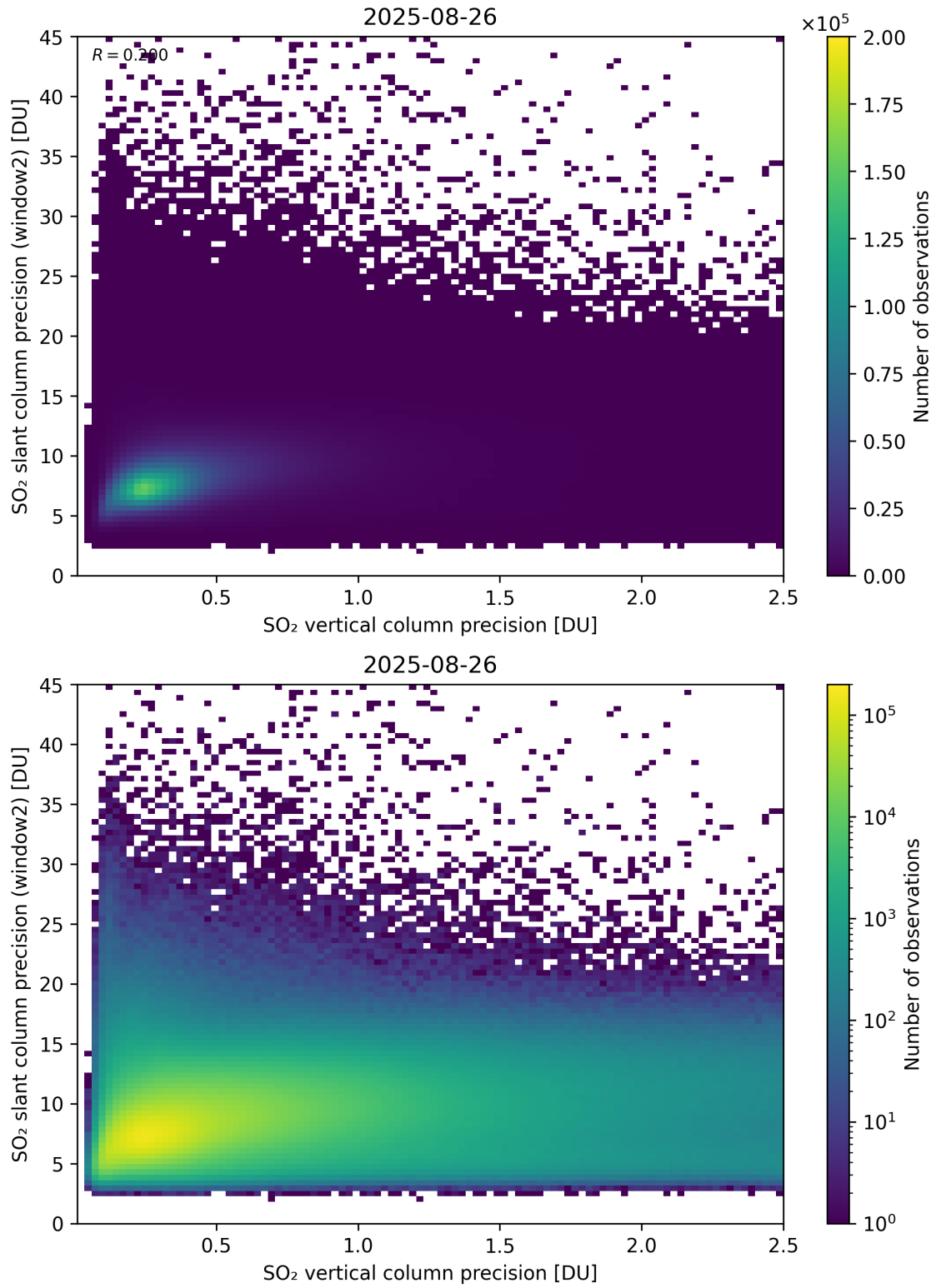
Figure 343: Scatter density plot of “SO 2 vertical column precision” against “SO 2 slant column precision (window2)” for 2025-08-25 to 2025-08-27.
