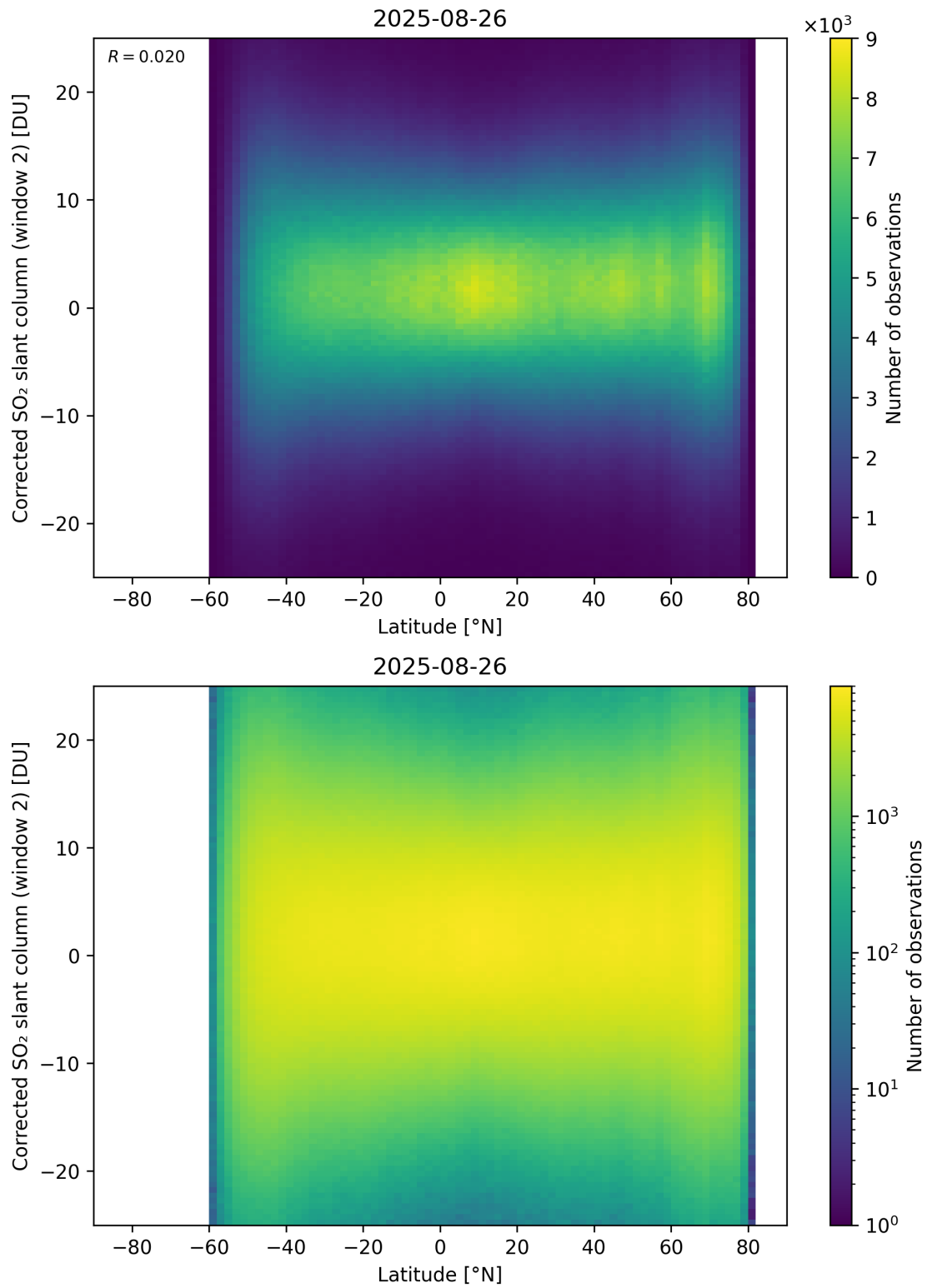
Figure 160: Scatter density plot of “Latitude” against “Corrected SO 2 slant column (window 2)” for 2025-08-25 to 2025-08-27.
