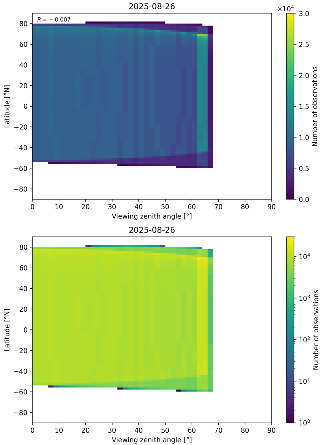
Figure 368: Scatter density plot of “Viewing zenith angle” against “Latitude” for 2025-08-25 to 2025-08-27.
