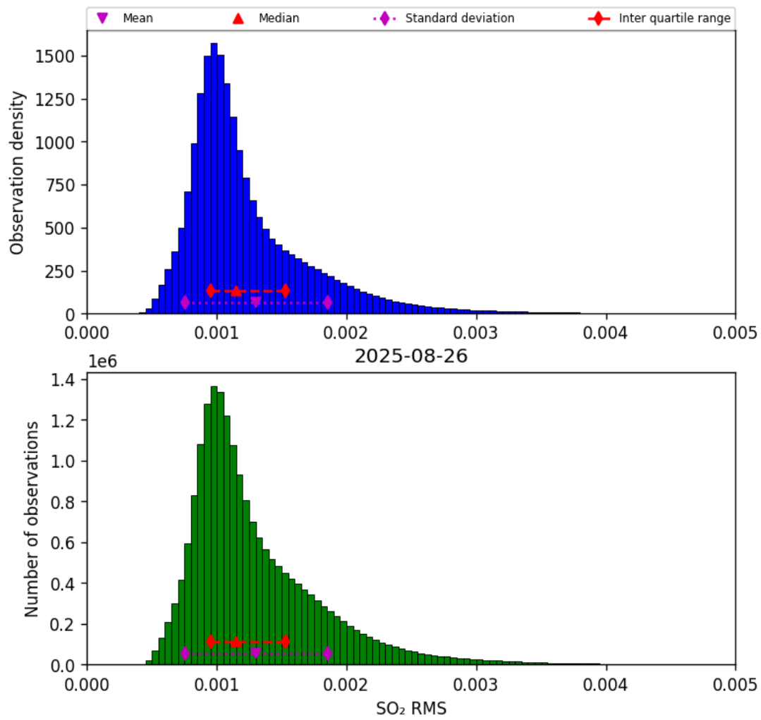
Figure 78: Histogram of “SO 2 RMS” for 2025-08-25 to 2025-08-27
