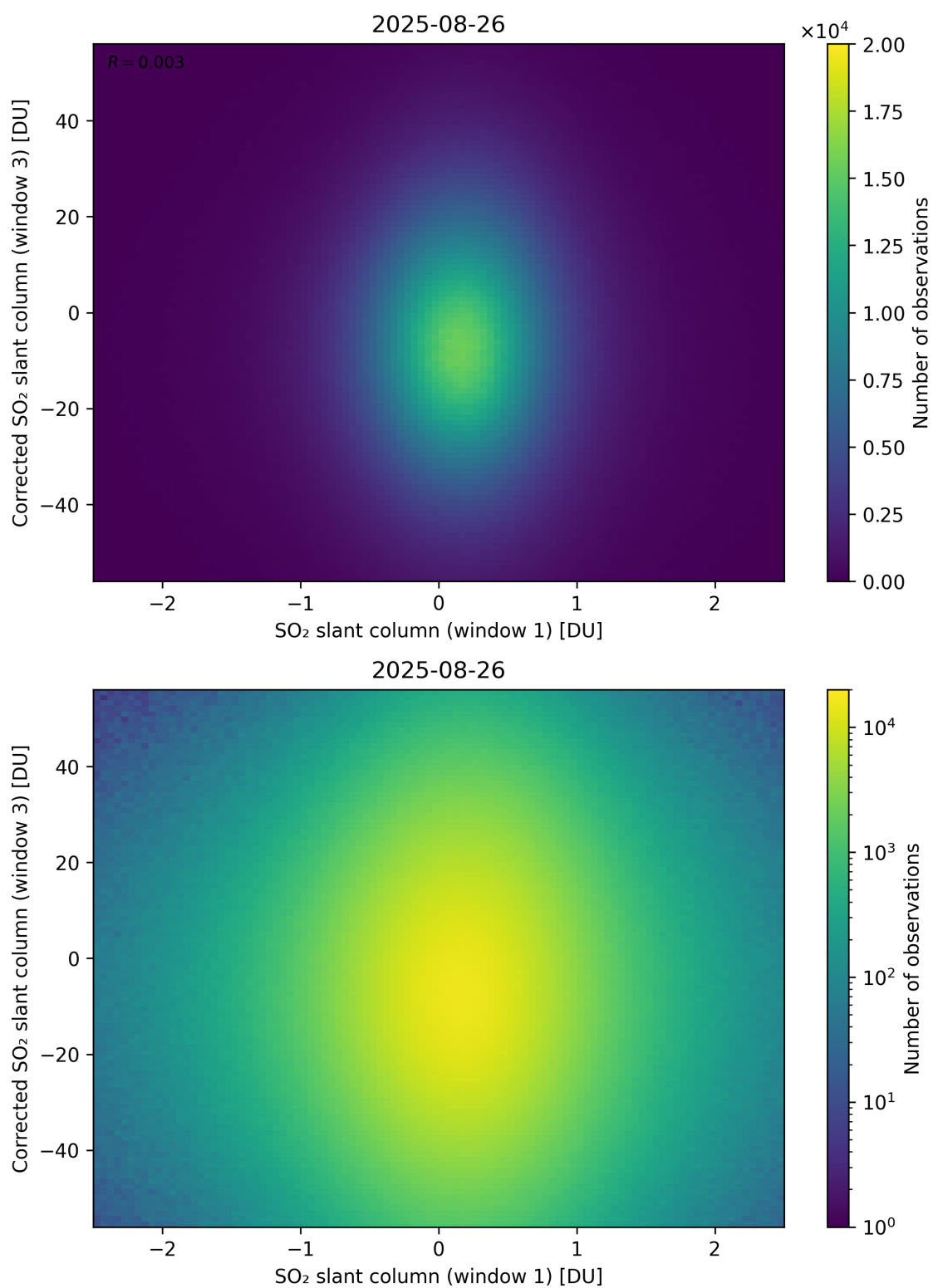
Figure 284: Scatter density plot of “SO 2 slant column (window 1)” against “Corrected SO 2 slant column (window 3)” for 2025-08-25 to 2025-08-27.
