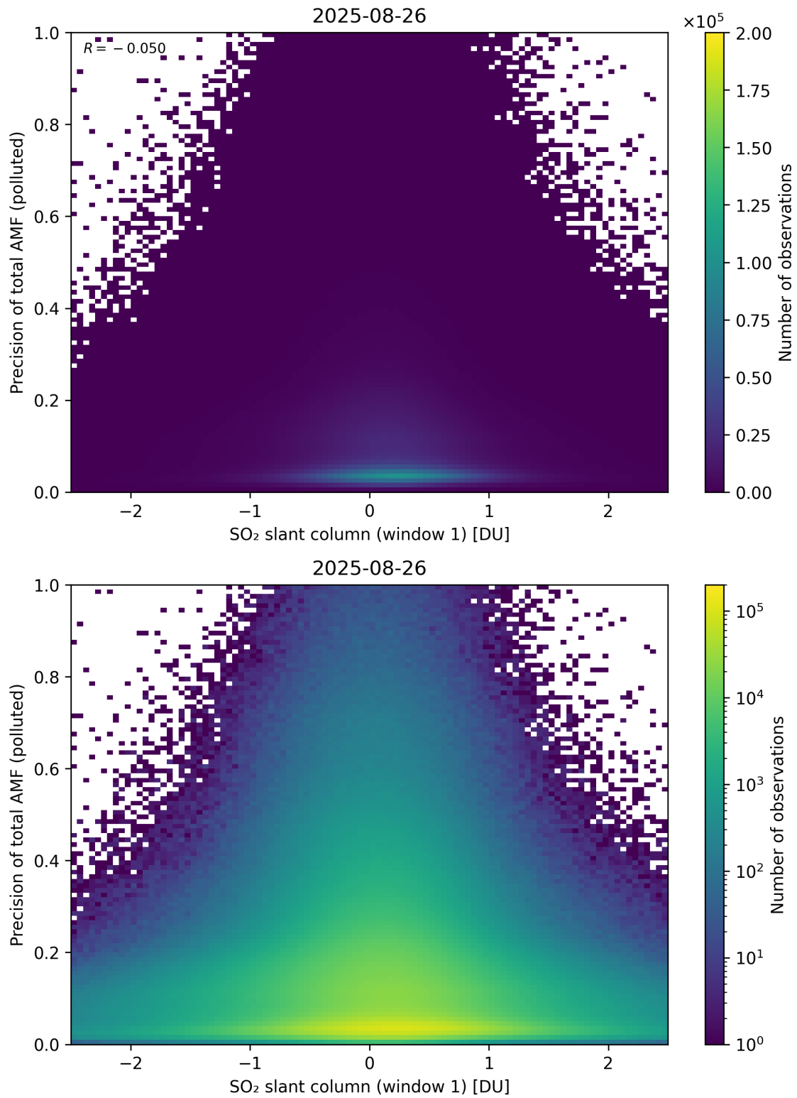
Figure 290: Scatter density plot of “SO 2 slant column (window 1)” against “Precision of total AMF (polluted)” for 2025-08-25 to 2025-08-27.
