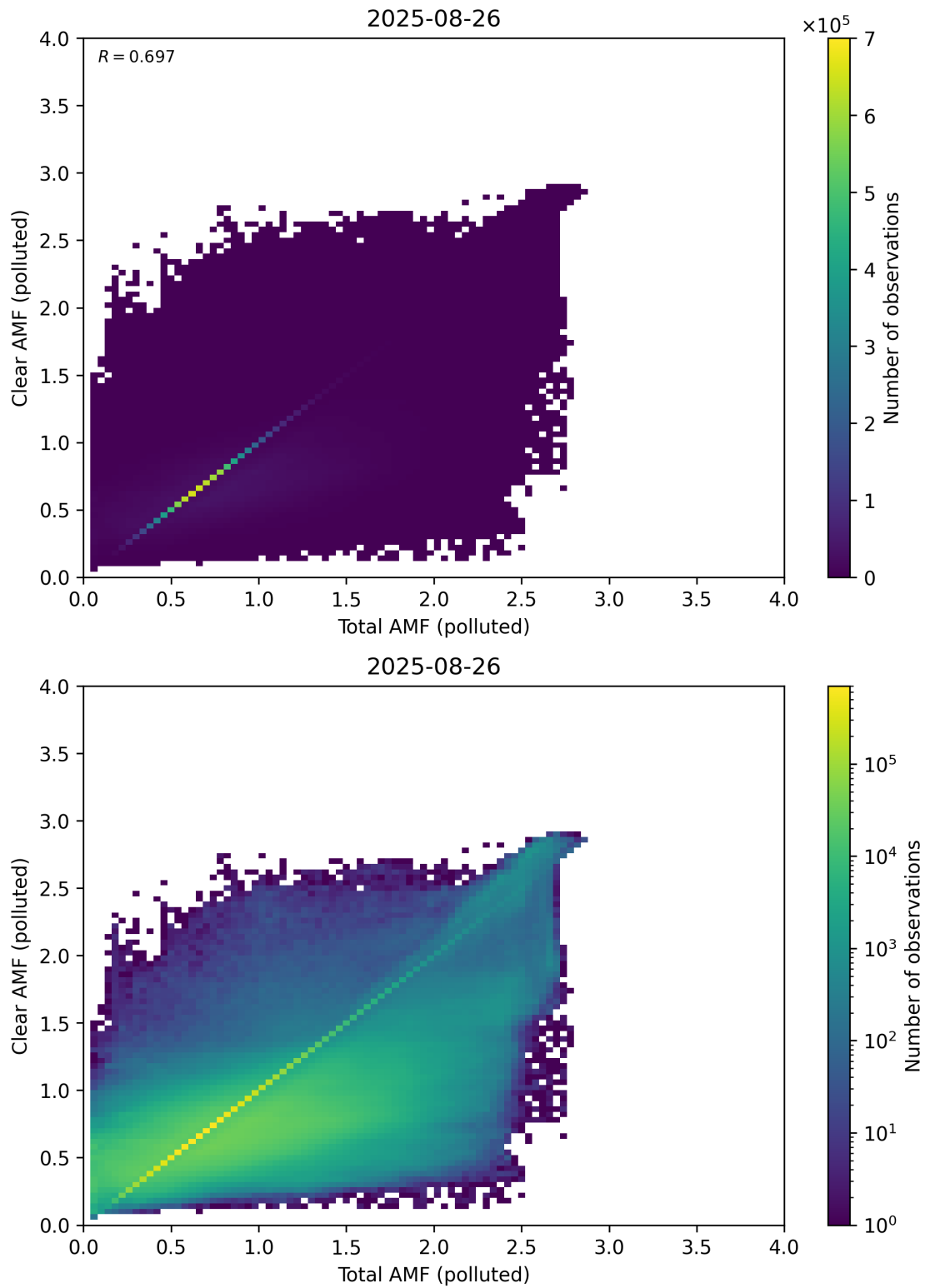
Figure 321: Scatter density plot of “Total AMF (polluted)” against “Clear AMF (polluted)” for 2025-08-25 to 2025-08-27.
