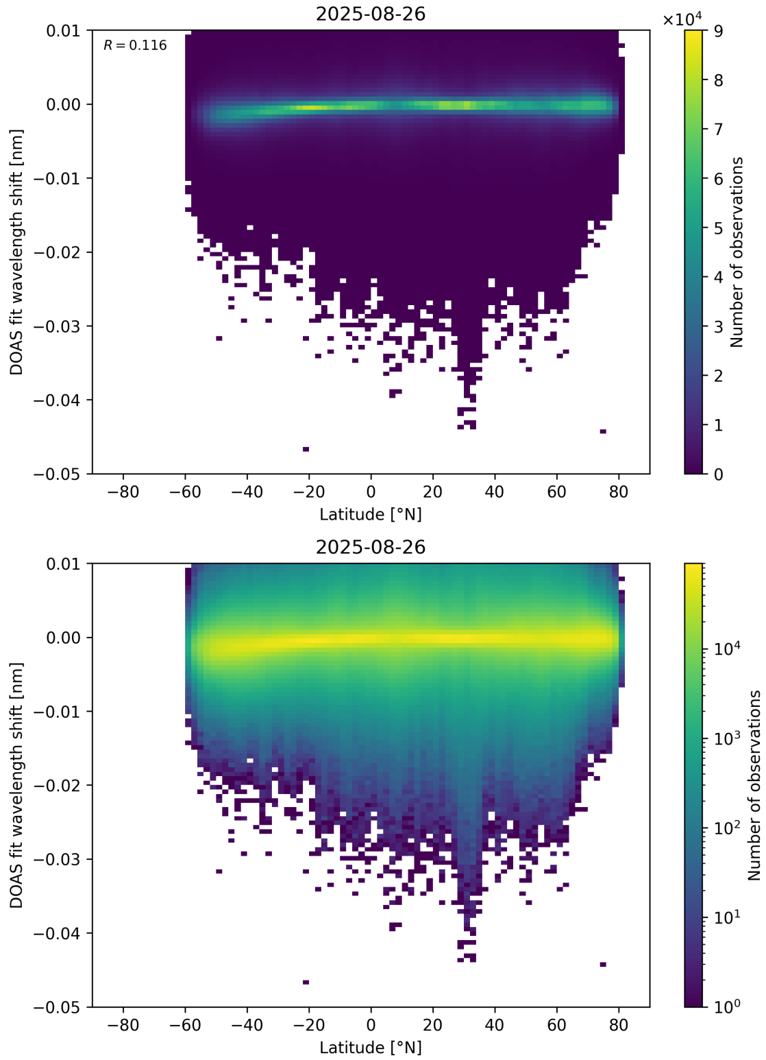
Figure 153: Scatter density plot of “Latitude” against “DOAS fit wavelength shift” for 2025-08-25 to 2025-08-27.
