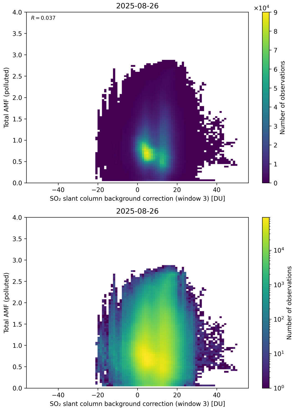
Figure 136: Scatter density plot of “SO 2 slant column background correction (window 3)” against “Total AMF (polluted)” for 2025-08-25 to 2025-08-27.
