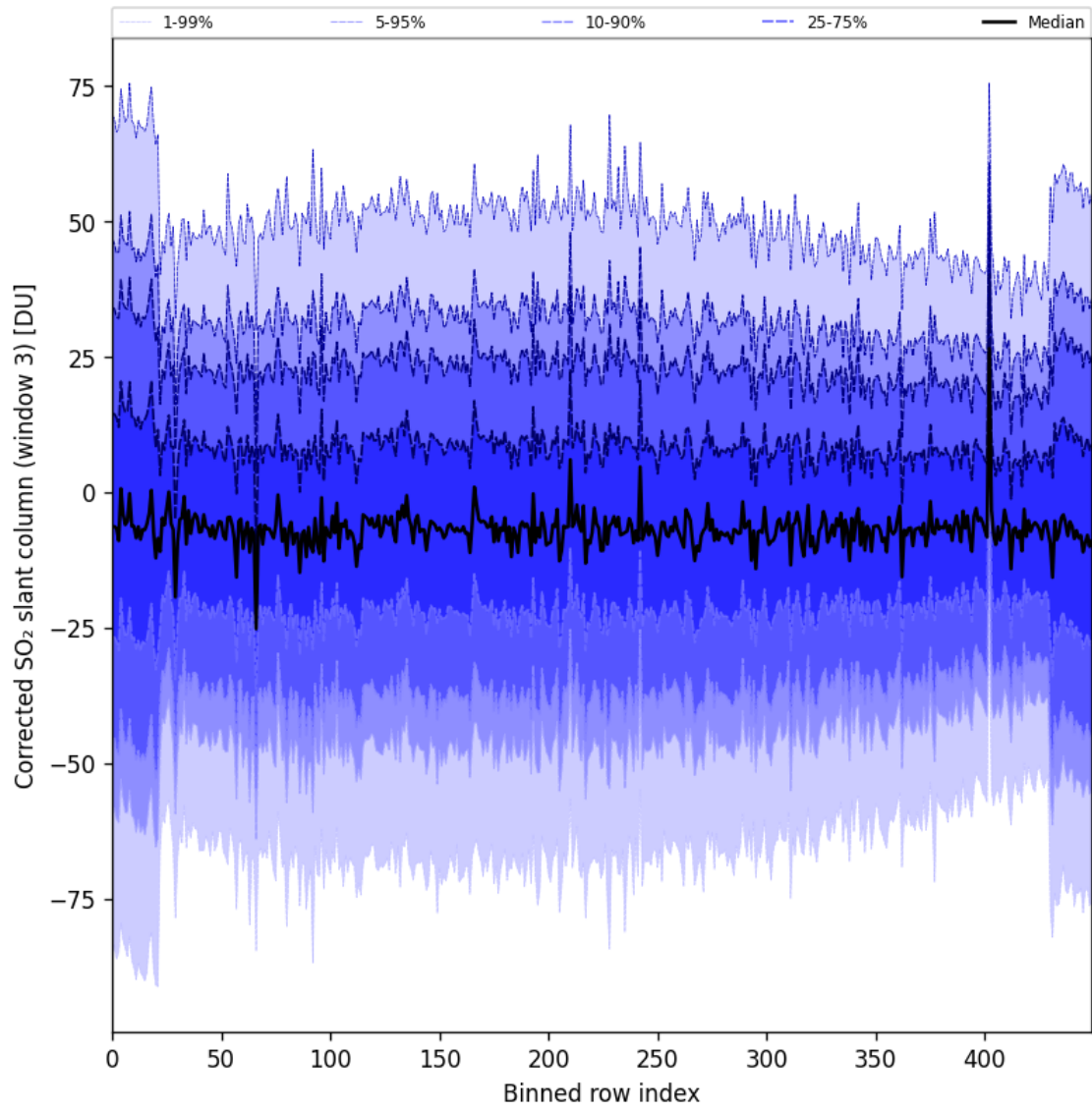
Figure 99: Along track statistics of “Corrected SO 2 slant column (window 3)” for 2025-08-25 to 2025-08-27
