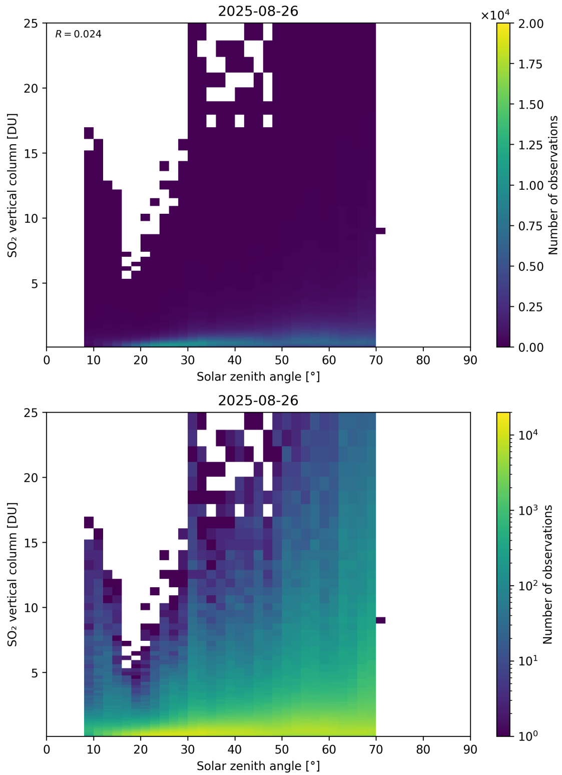
Figure 191: Scatter density plot of “Solar zenith angle” against “SO 2 vertical column” for 2025-08-25 to 2025-08-27.
