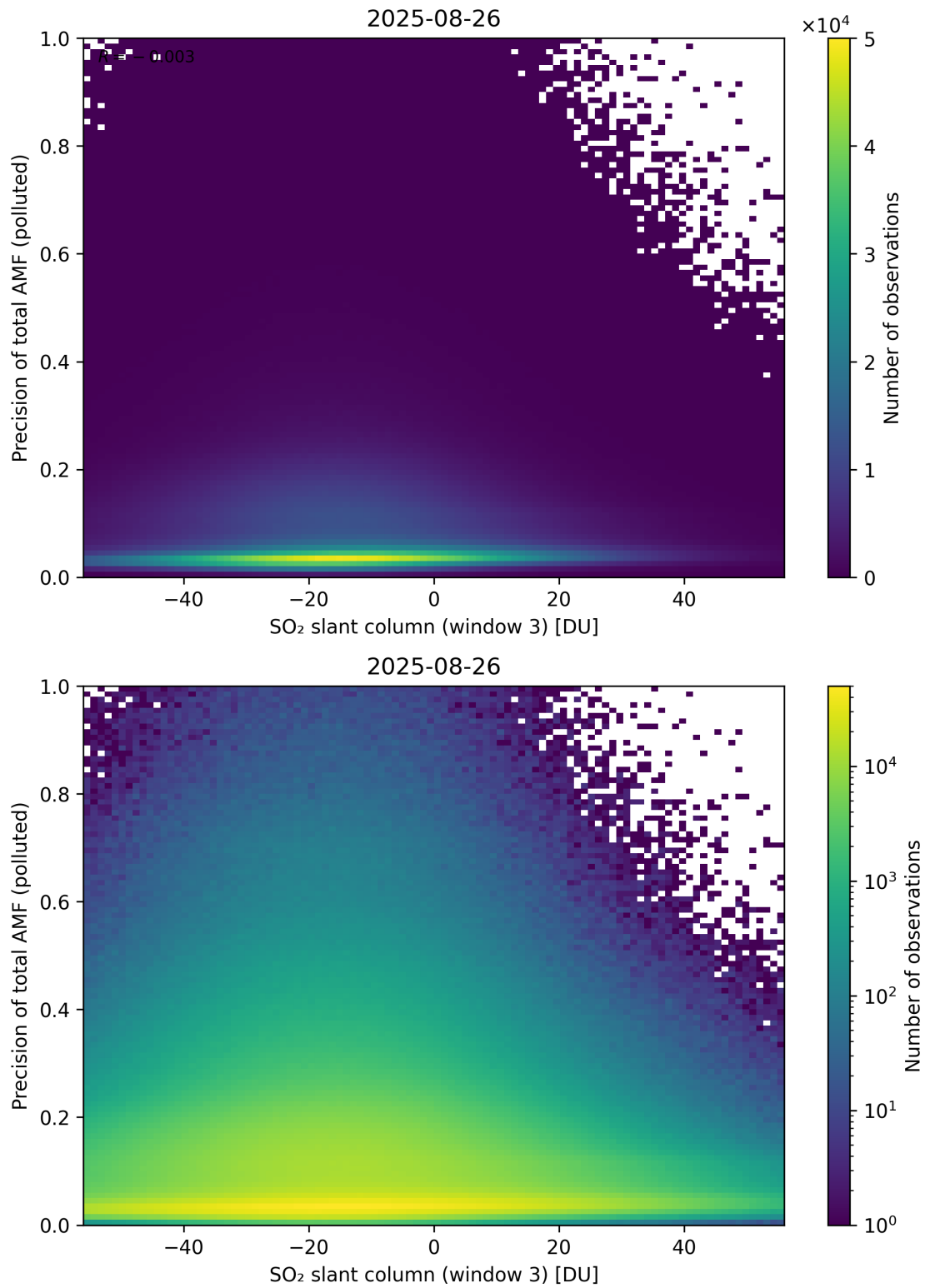
Figure 319: Scatter density plot of “SO 2 slant column (window 3)” against “Precision of total AMF (polluted)” for 2025-08-25 to 2025-08-27.
