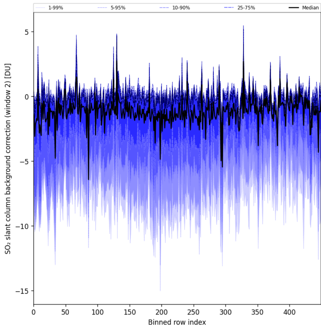
Figure 96: Along track statistics of “SO 2 slant column background correction (window 2)” for 2025-08-25 to 2025-08-27
