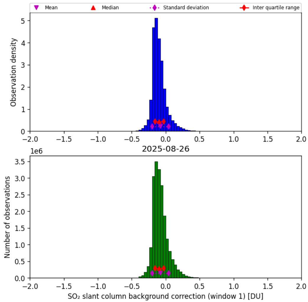
Figure 66: Histogram of “SO 2 slant column background correction (window 1)” for 2025-08-25 to 2025-08-27
