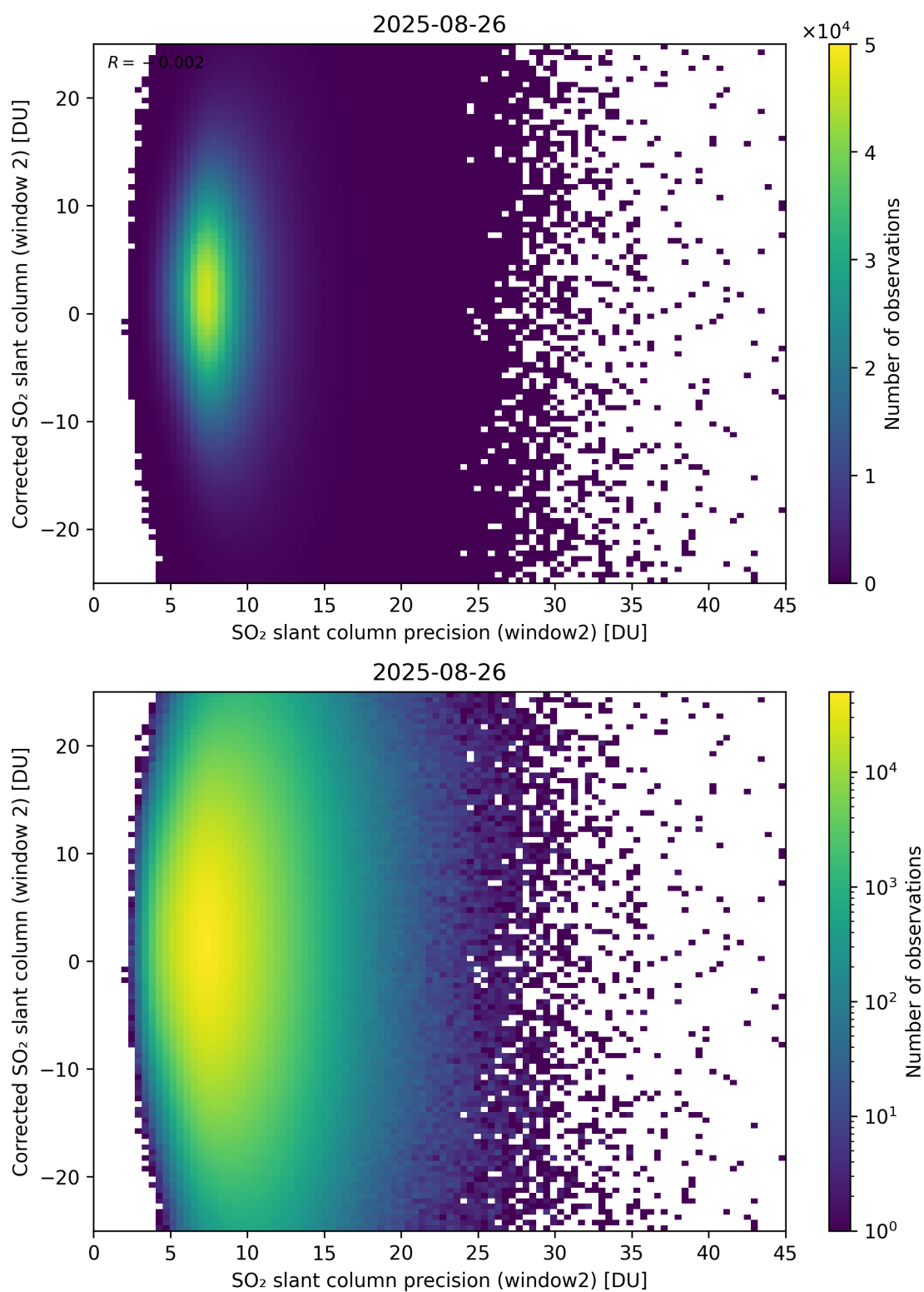
Figure 297: Scatter density plot of “SO 2 slant column precision (window2)” against “Corrected SO 2 slant column (window 2)” for 2025-08-25 to 2025-08-27.
