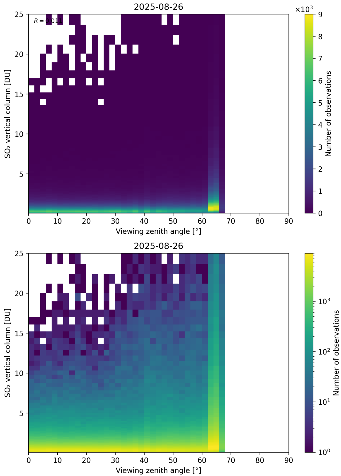
Figure 383: Scatter density plot of “Viewing zenith angle” against “SO 2 vertical column” for 2025-08-25 to 2025-08-27.
