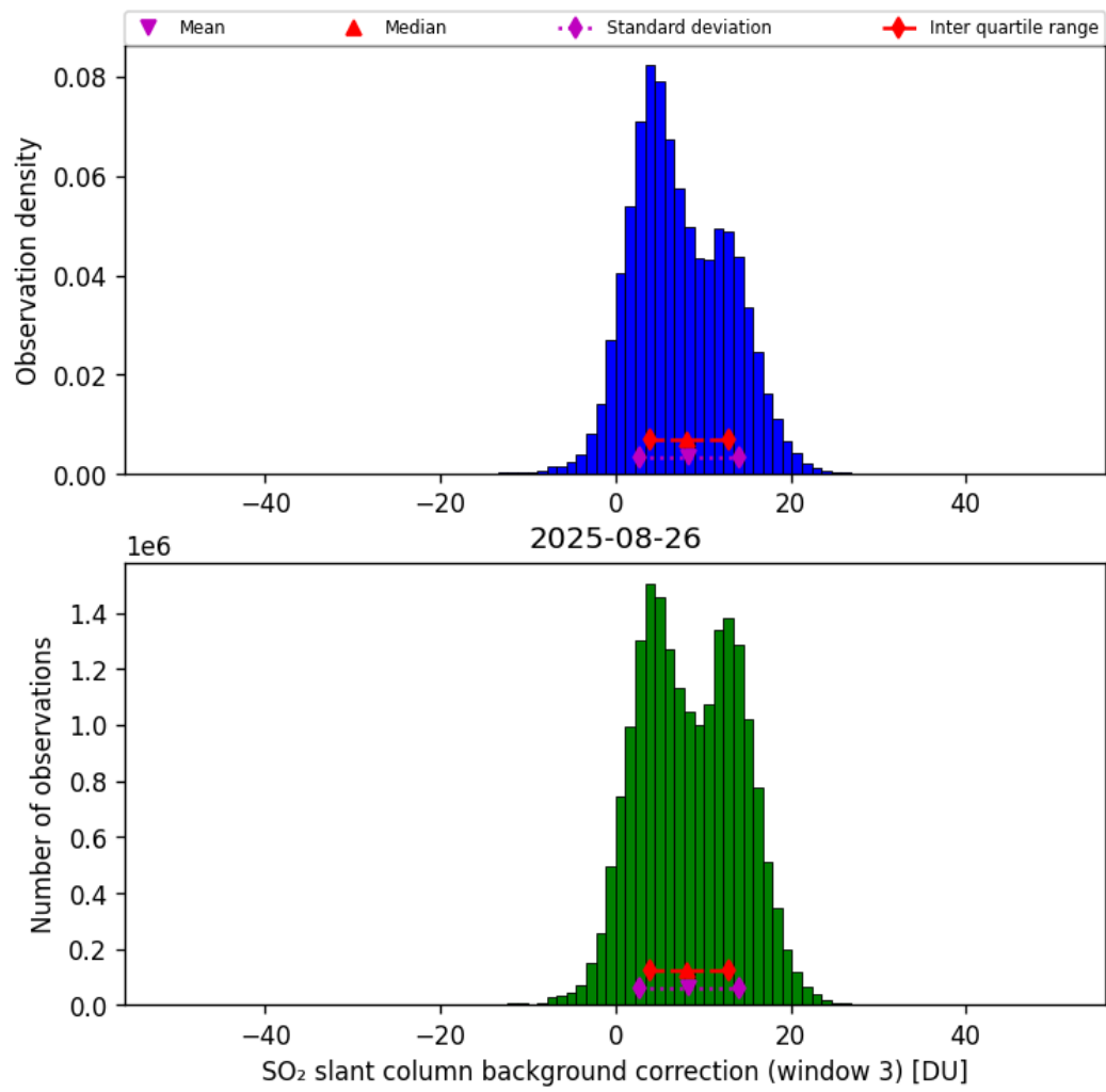
Figure 74: Histogram of “SO 2 slant column background correction (window 3)” for 2025-08-25 to 2025-08-27
