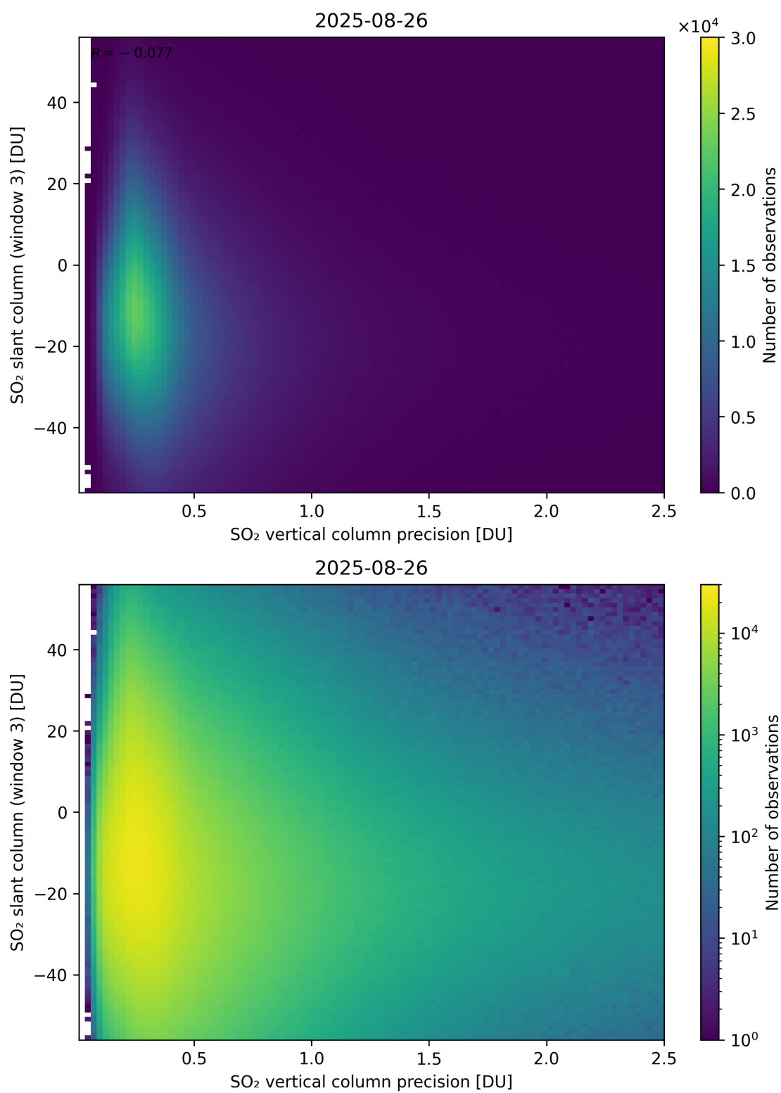
Figure 344: Scatter density plot of “SO 2 vertical column precision” against “SO 2 slant column (window 3)” for 2025-08-25 to 2025-08-27.
