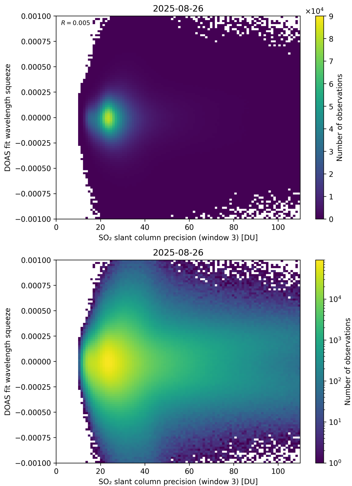
Figure 309: Scatter density plot of “SO 2 slant column precision (window 3)” against “DOAS fit wavelength squeeze” for 2025-08-25 to 2025-08-27.
