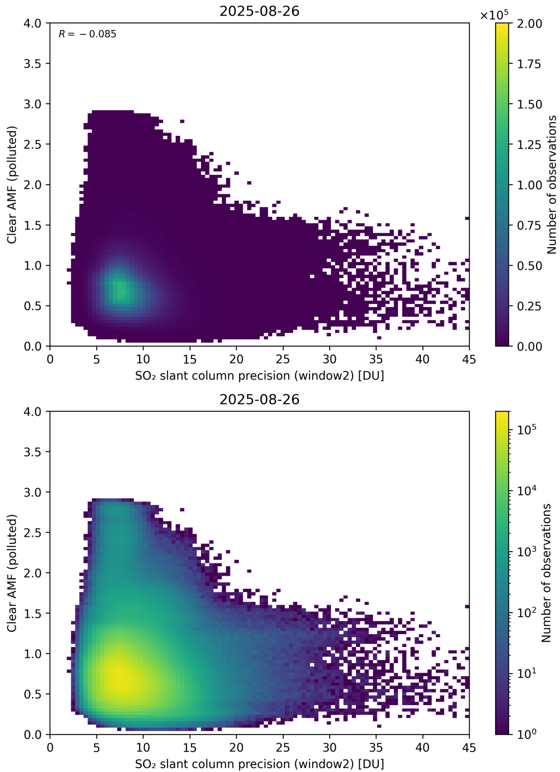
Figure 296: Scatter density plot of “SO 2 slant column precision (window2)” against “Clear AMF (polluted)” for 2025-08-25 to 2025-08-27.
