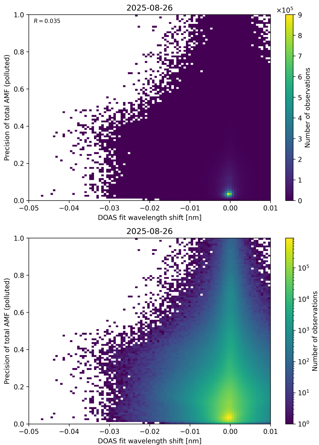
Figure 142: Scatter density plot of “DOAS fit wavelength shift” against “Precision of total AMF (polluted)” for 2025-08-25 to 2025-08-27.
