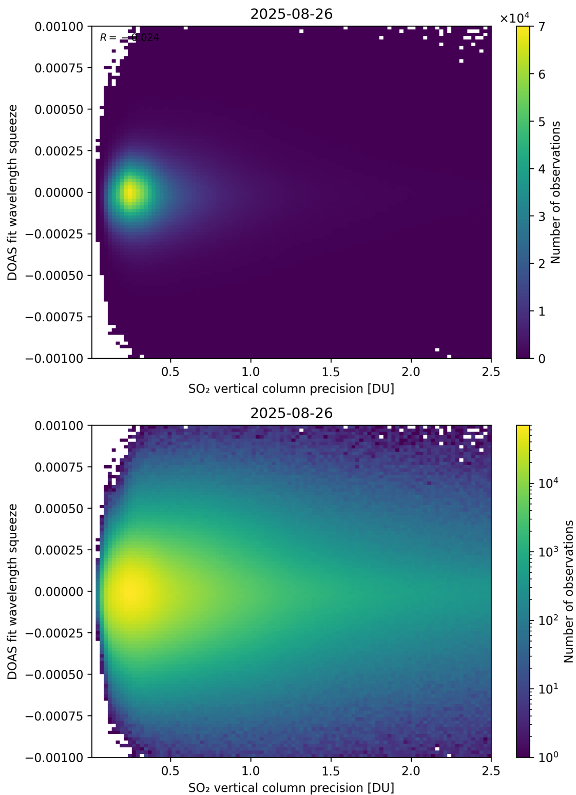
Figure 333: Scatter density plot of “SO 2 vertical column precision” against “DOAS fit wavelength squeeze” for 2025-08-25 to 2025-08-27.
