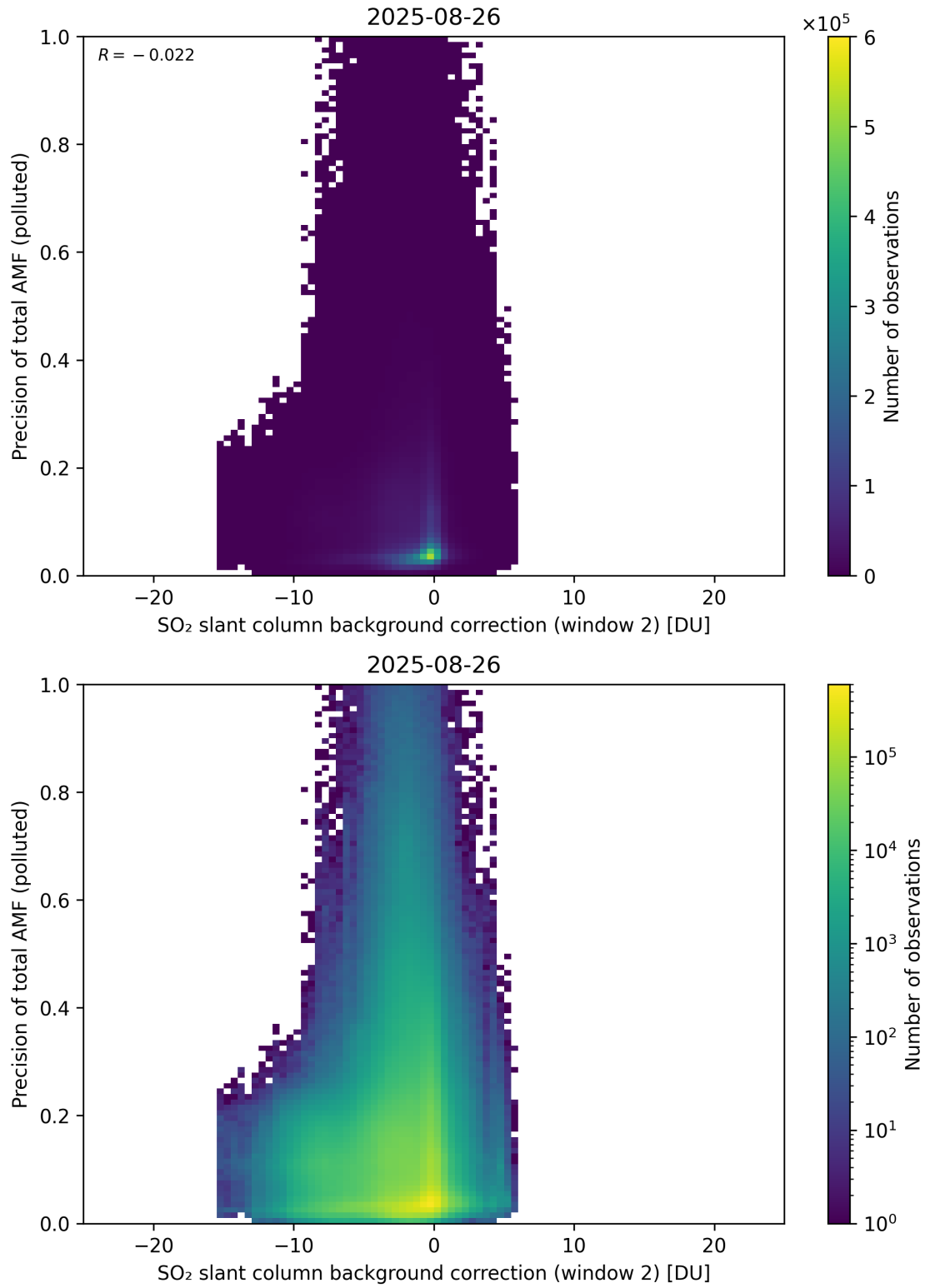
Figure 131: Scatter density plot of “SO 2 slant column background correction (window 2)” against “Precision of total AMF (polluted)” for 2025-08-25 to 2025-08-27.
