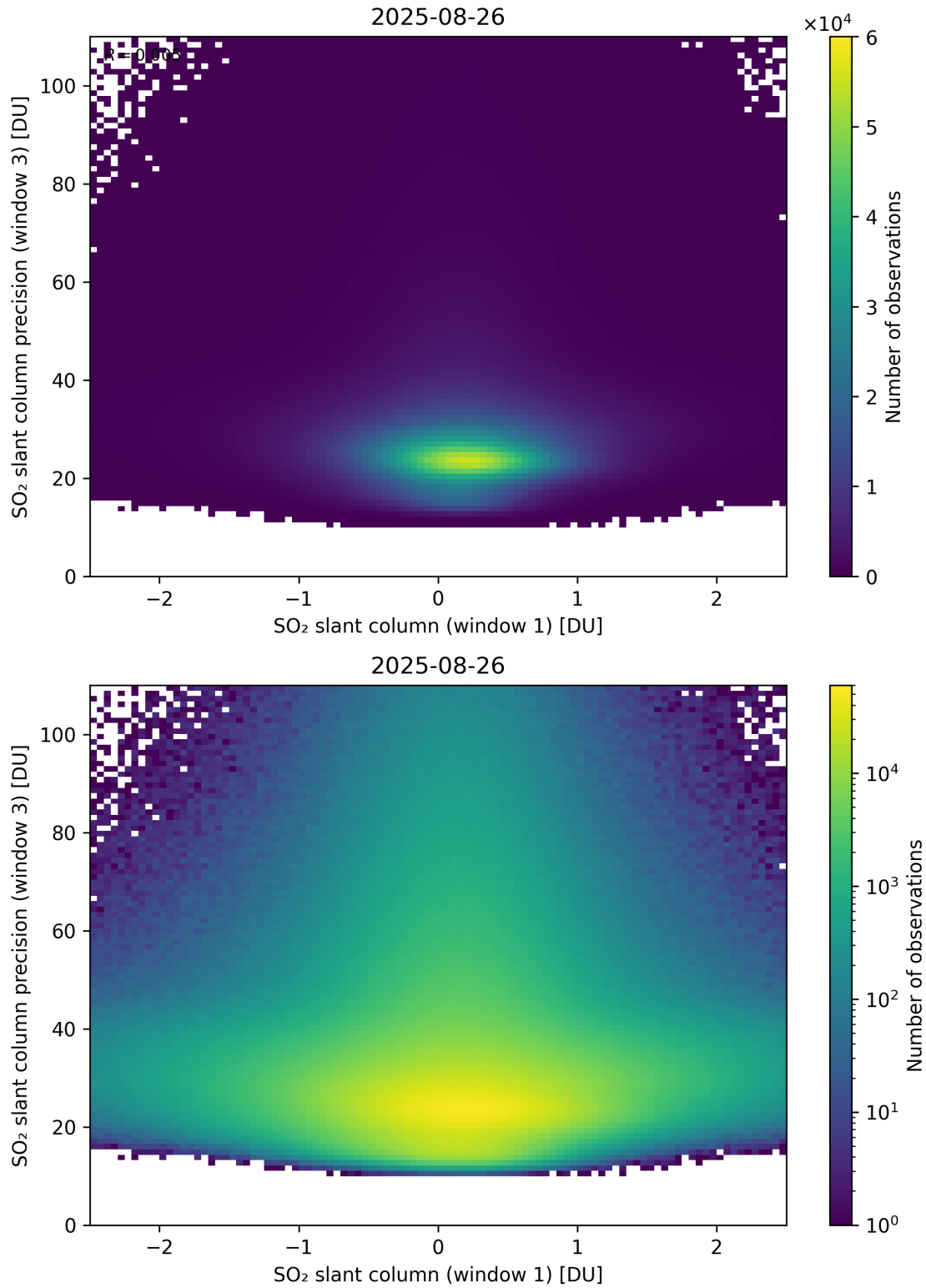
Figure 288: Scatter density plot of “SO 2 slant column (window 1)” against “SO 2 slant column precision (window 3)” for 2025-08-25 to 2025-08-27.
