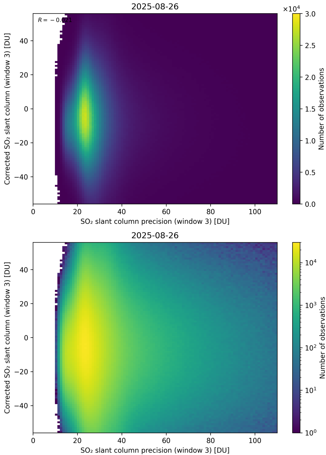
Figure 312: Scatter density plot of “SO 2 slant column precision (window 3)” against “Corrected SO 2 slant column (window 3)” for 2025-08-25 to 2025-08-27.
