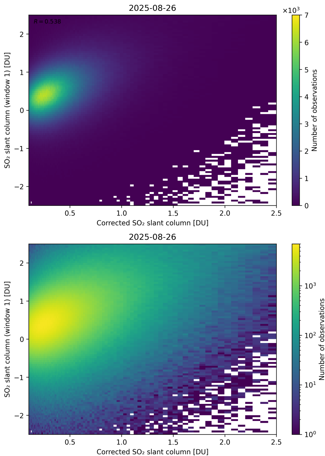
Figure 237: Scatter density plot of “Corrected SO 2 slant column” against “SO 2 slant column (window 1)” for 2025-08-25 to 2025-08-27.
