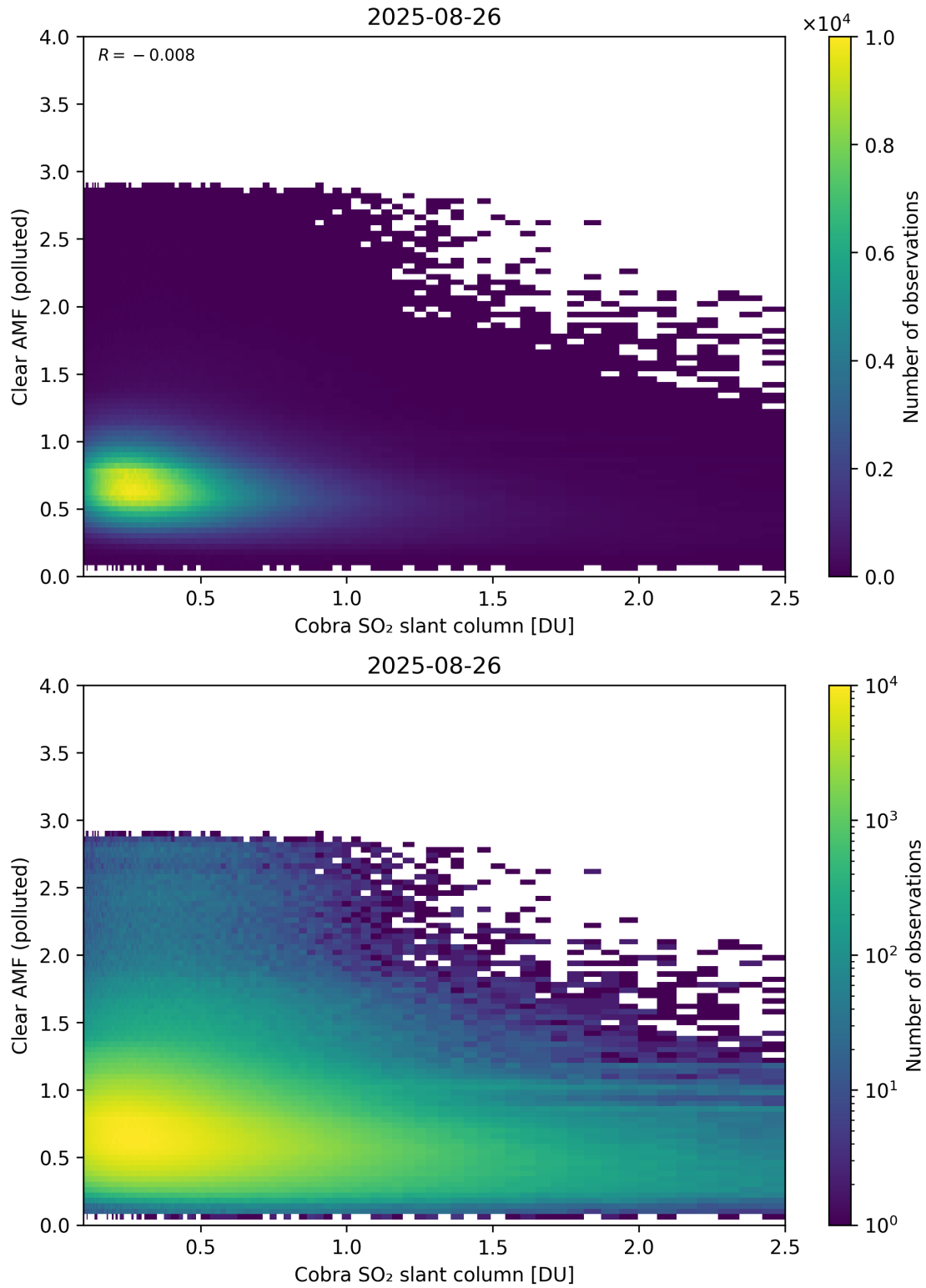
Figure 215: Scatter density plot of “Cobra SO 2 slant column” against “Clear AMF (polluted)” for 2025-08-25 to 2025-08-27.
