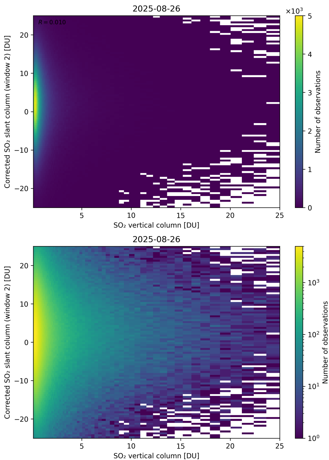
Figure 352: Scatter density plot of “SO 2 vertical column” against “Corrected SO 2 slant column (window 2)” for 2025-08-25 to 2025-08-27.
