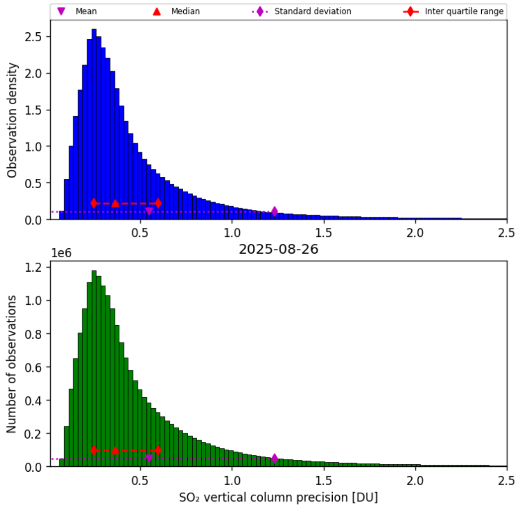
Figure 59: Histogram of “SO 2 vertical column precision” for 2025-08-25 to 2025-08-27
