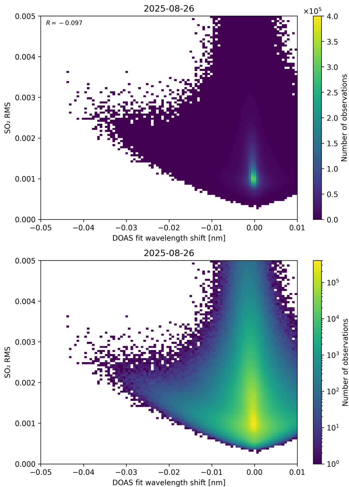
Figure 139: Scatter density plot of “DOAS fit wavelength shift” against “SO 2 RMS” for 2025-08-25 to 2025-08-27.
