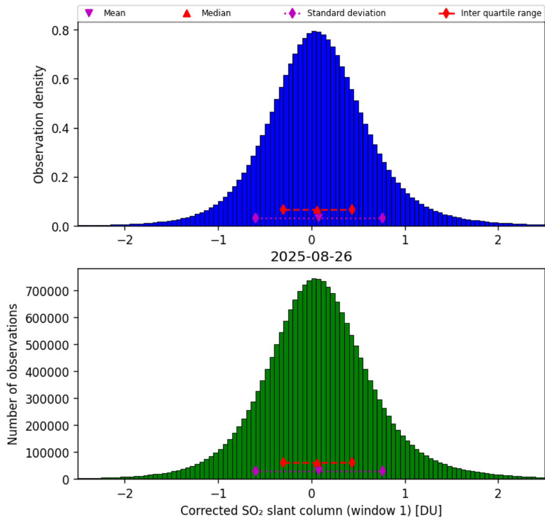
Figure 65: Histogram of “Corrected SO 2 slant column (window 1)” for 2025-08-25 to 2025-08-27
