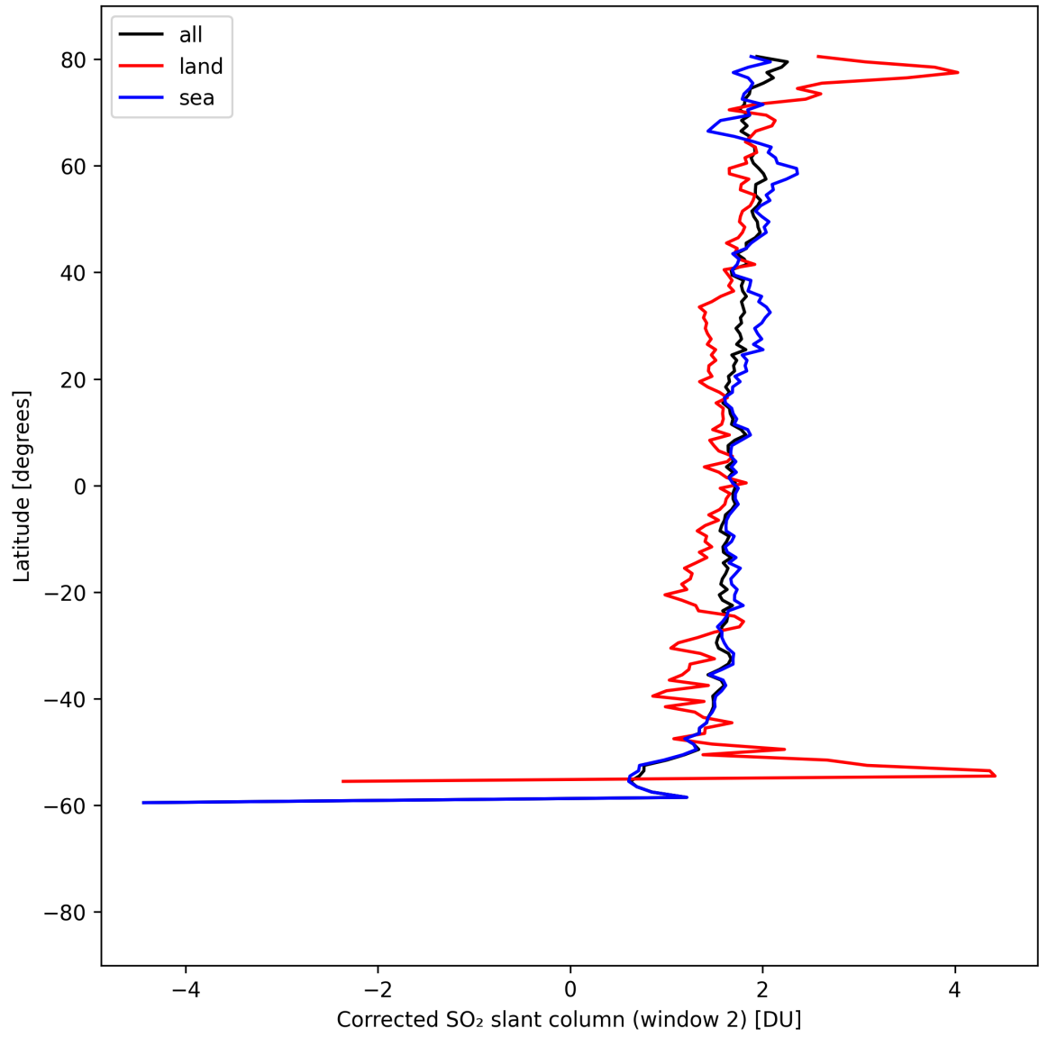
Figure 43: Zonal average of “Corrected SO 2 slant column (window 2)” for 2025-08-25 to 2025-08-27.
