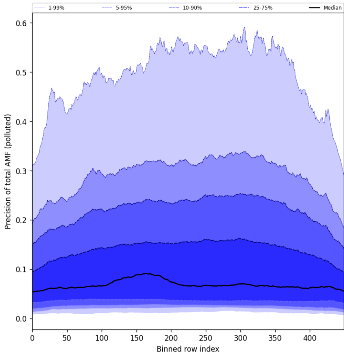
Figure 106: Along track statistics of “Precision of total AMF (polluted)” for 2025-08-25 to 2025-08-27
