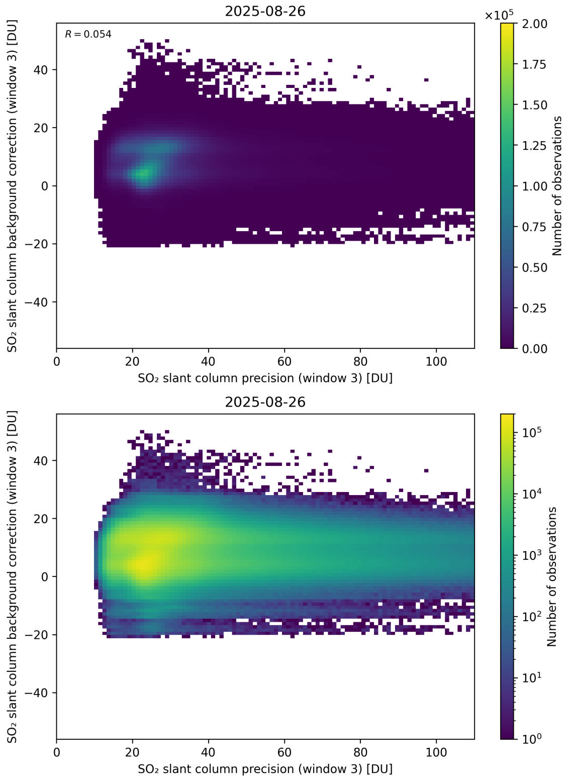
Figure 307: Scatter density plot of “SO 2 slant column precision (window 3)” against “SO 2 slant column background correction (window 3)” for 2025-08-25 to 2025-08-27.
