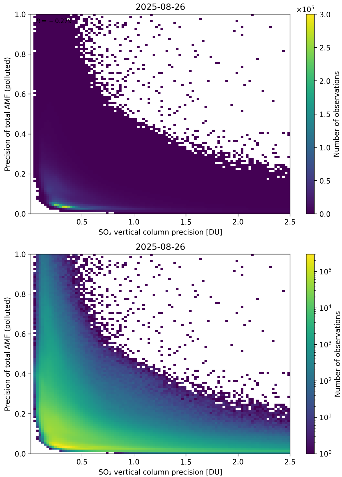
Figure 347: Scatter density plot of “SO 2 vertical column precision” against “Precision of total AMF (polluted)” for 2025-08-25 to 2025-08-27.
