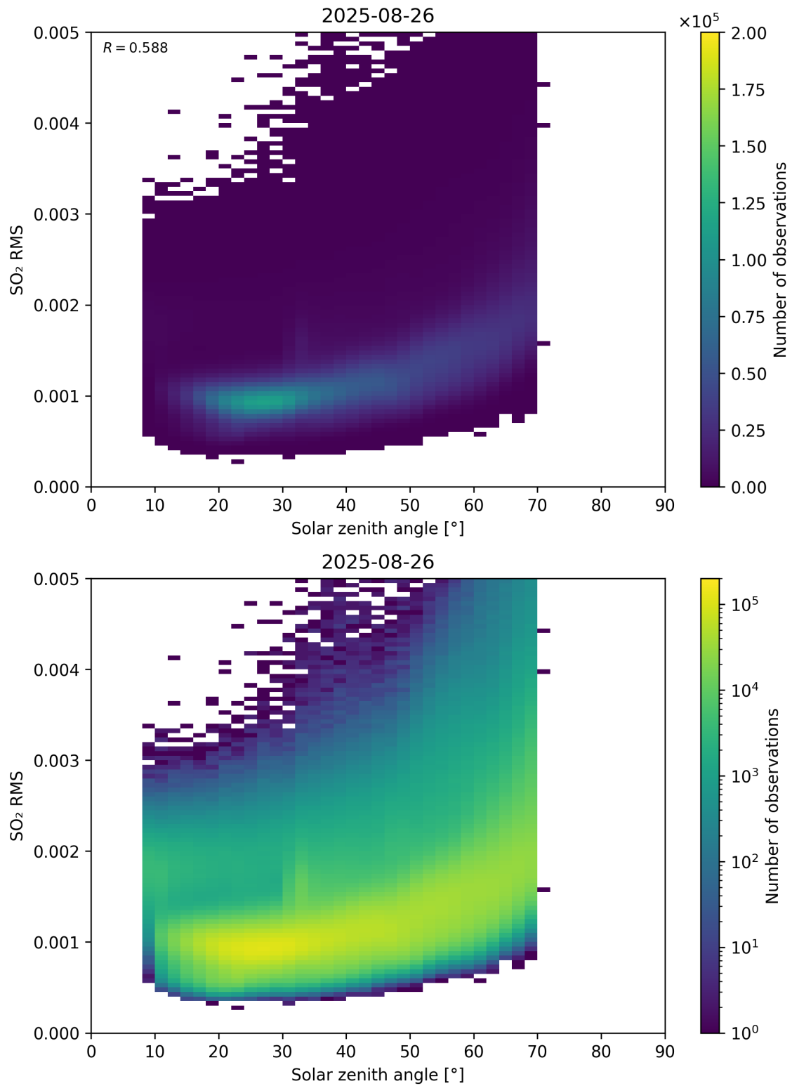
Figure 176: Scatter density plot of “Solar zenith angle” against “SO 2 RMS” for 2025-08-25 to 2025-08-27.
