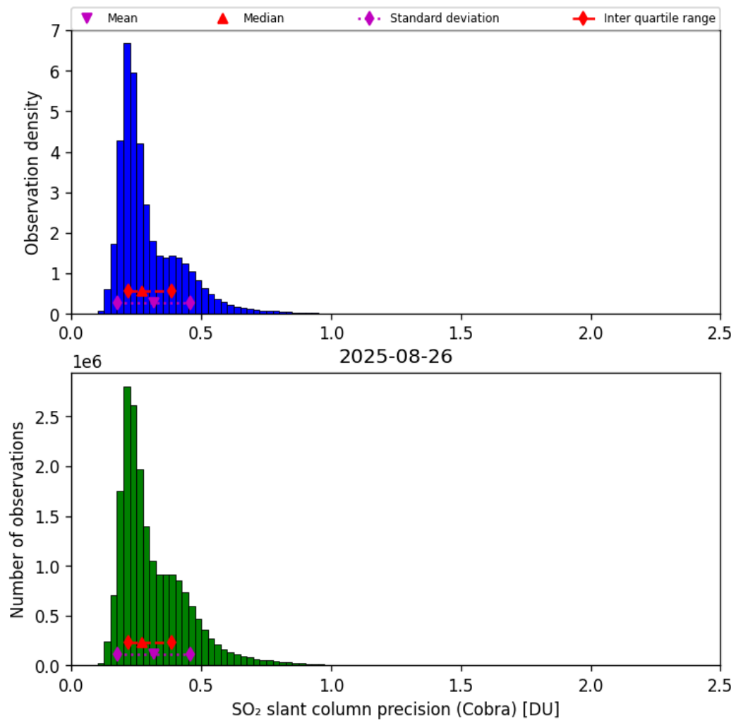
Figure 62: Histogram of “SO 2 slant column precision (Cobra)” for 2025-08-25 to 2025-08-27
