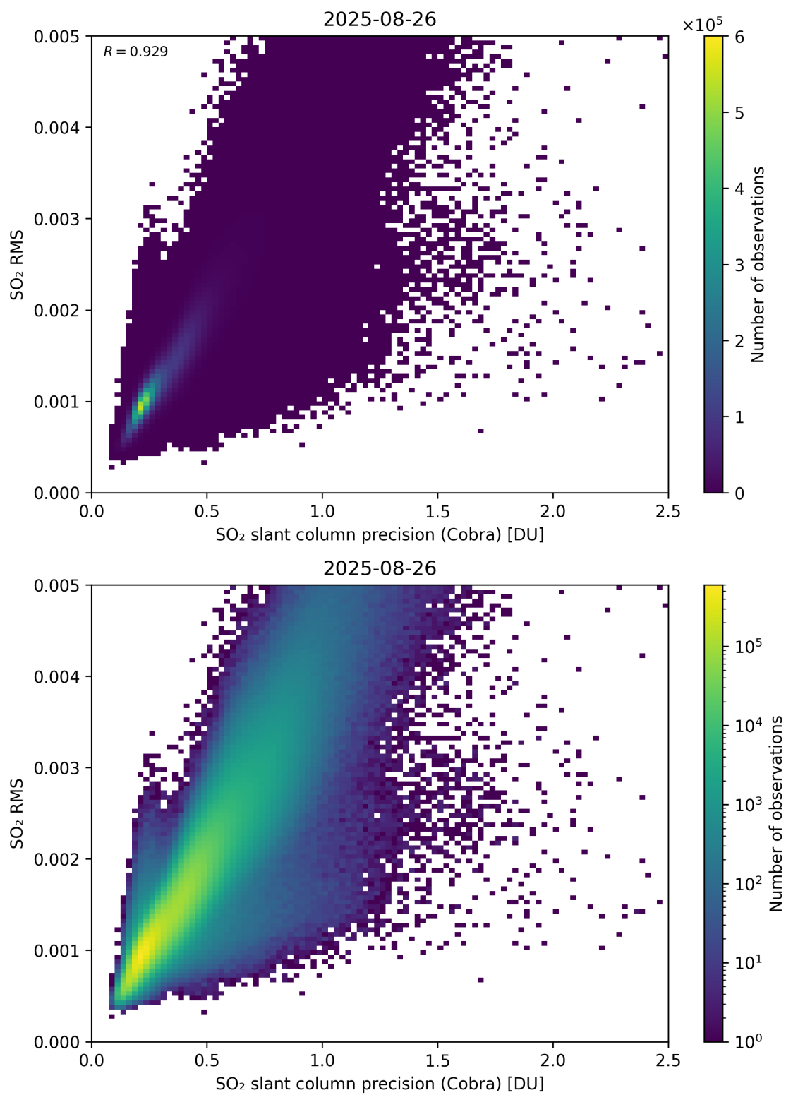
Figure 204: Scatter density plot of “SO 2 slant column precision (Cobra)” against “SO 2 RMS” for 2025-08-25 to 2025-08-27.
