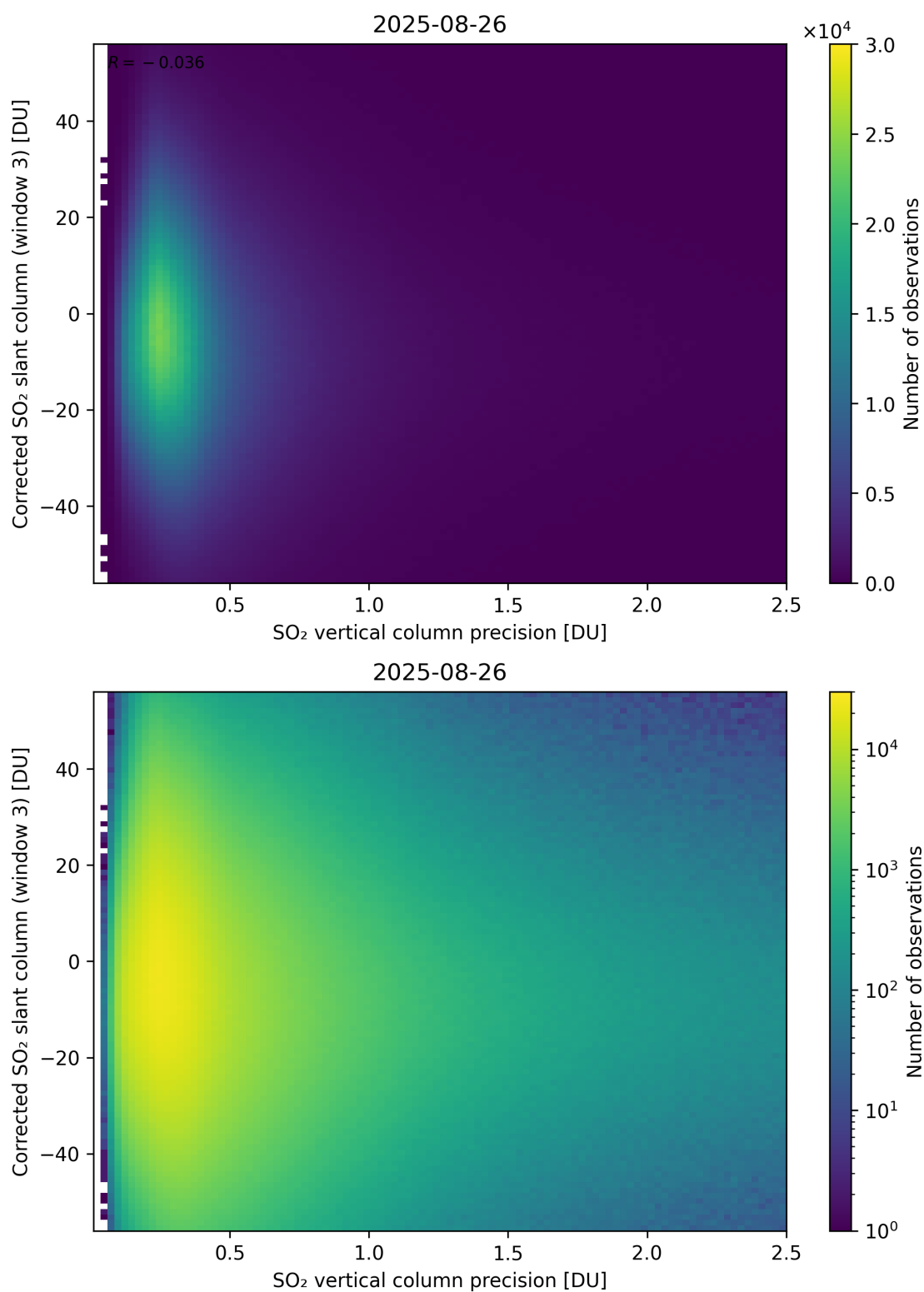
Figure 340: Scatter density plot of “SO 2 vertical column precision” against “Corrected SO 2 slant column (window 3)” for 2025-08-25 to 2025-08-27.
