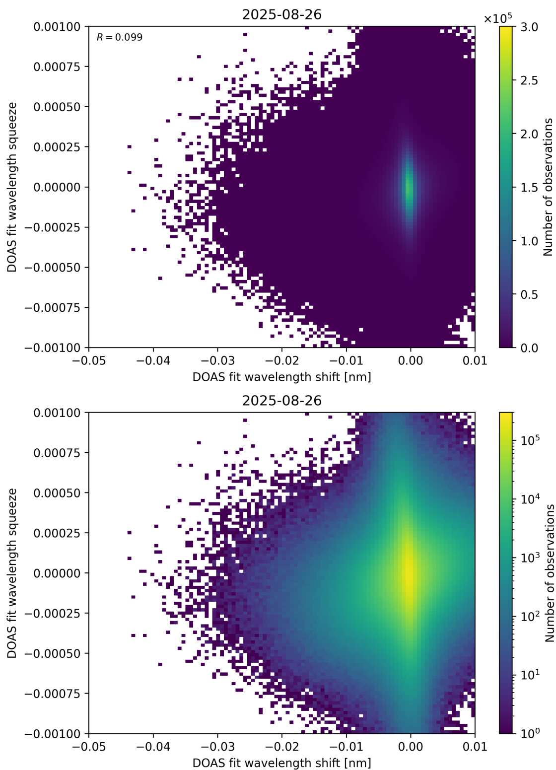
Figure 138: Scatter density plot of “DOAS fit wavelength shift” against “DOAS fit wavelength squeeze” for 2025-08-25 to 2025-08-27.
