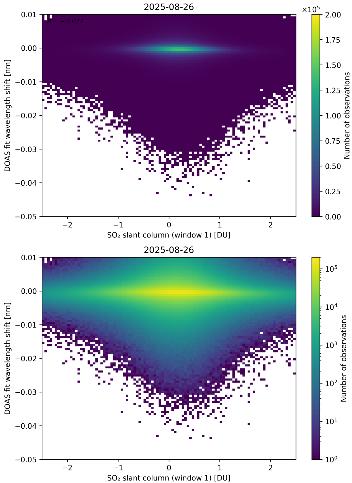
Figure 265: Scatter density plot of “SO 2 slant column (window 1)” against “DOAS fit wavelength shift” for 2025-08-25 to 2025-08-27.
