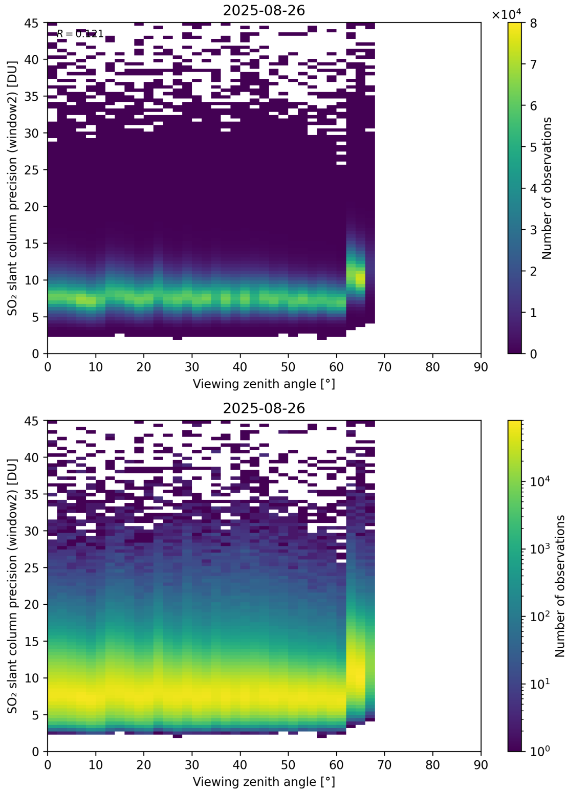
Figure 378: Scatter density plot of “Viewing zenith angle” against “SO 2 slant column precision (window2)” for 2025-08-25 to 2025-08-27.
