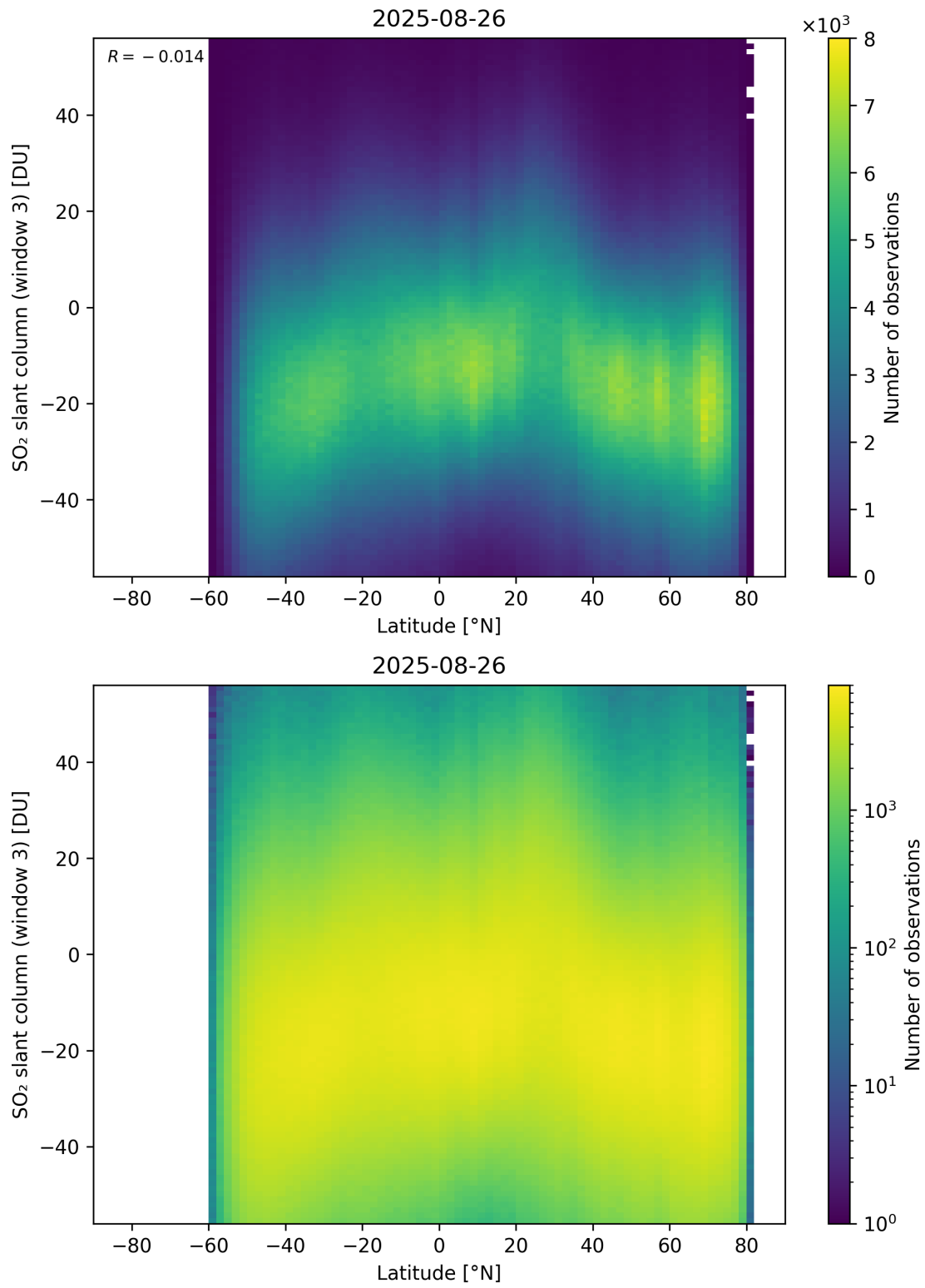
Figure 165: Scatter density plot of “Latitude” against “SO 2 slant column (window 3)” for 2025-08-25 to 2025-08-27.
