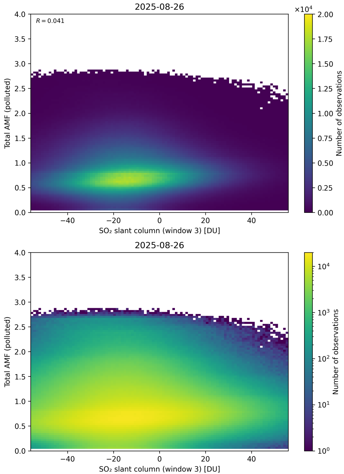
Figure 318: Scatter density plot of “SO 2 slant column (window 3)” against “Total AMF (polluted)” for 2025-08-25 to 2025-08-27.
