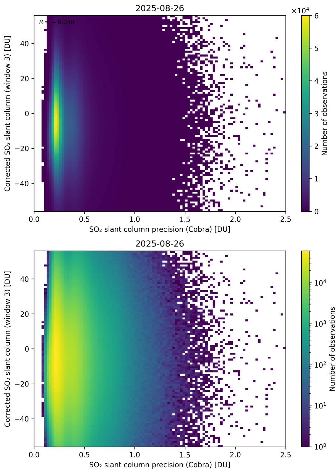
Figure 207: Scatter density plot of “SO 2 slant column precision (Cobra)” against “Corrected SO 2 slant column (window 3)” for 2025-08-25 to 2025-08-27.
