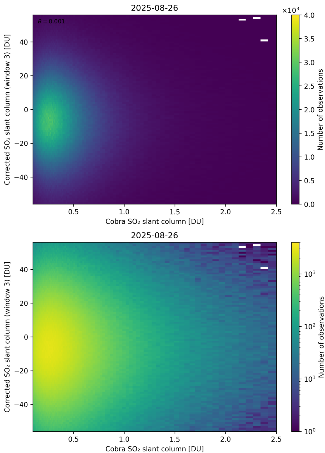
Figure 218: Scatter density plot of “Cobra SO 2 slant column” against “Corrected SO 2 slant column (window 3)” for 2025-08-25 to 2025-08-27.
