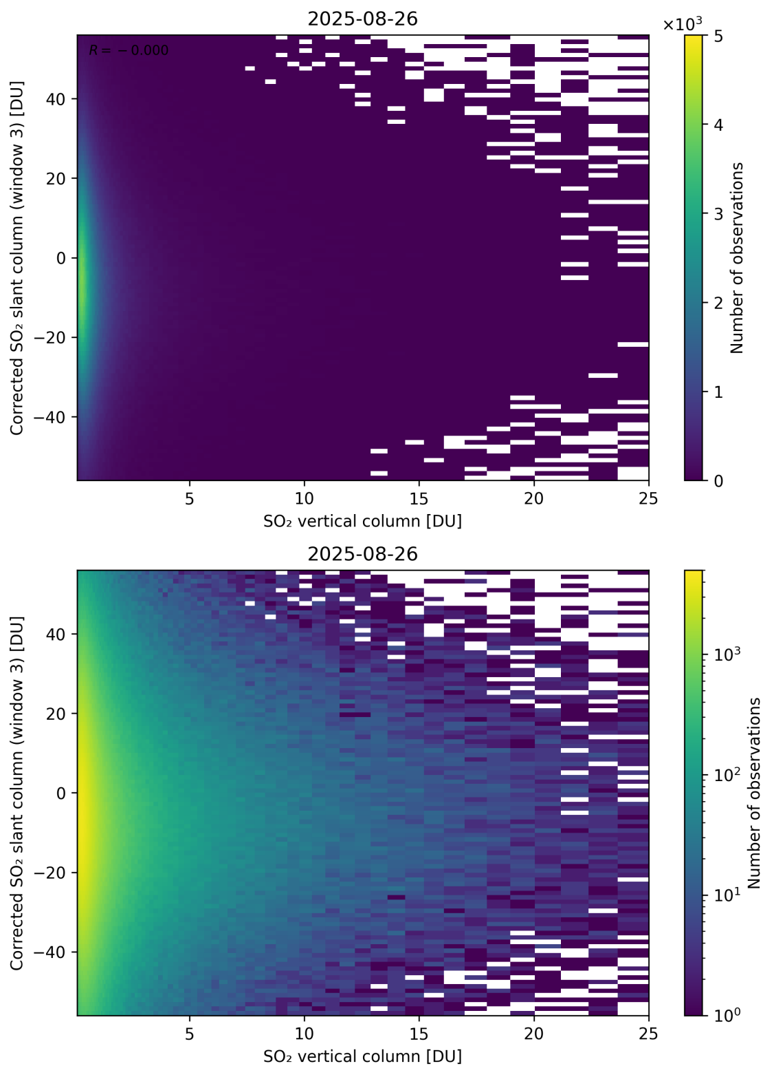
Figure 353: Scatter density plot of “SO 2 vertical column” against “Corrected SO 2 slant column (window 3)” for 2025-08-25 to 2025-08-27.
