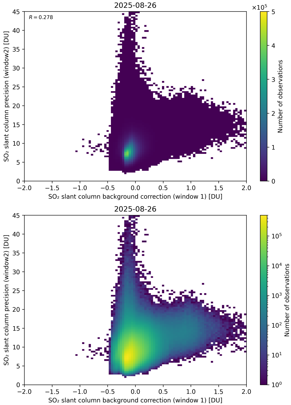
Figure 117: Scatter density plot of “SO 2 slant column background correction (window 1)” against “SO 2 slant column precision (window2)” for 2025-08-25 to 2025-08-27.
