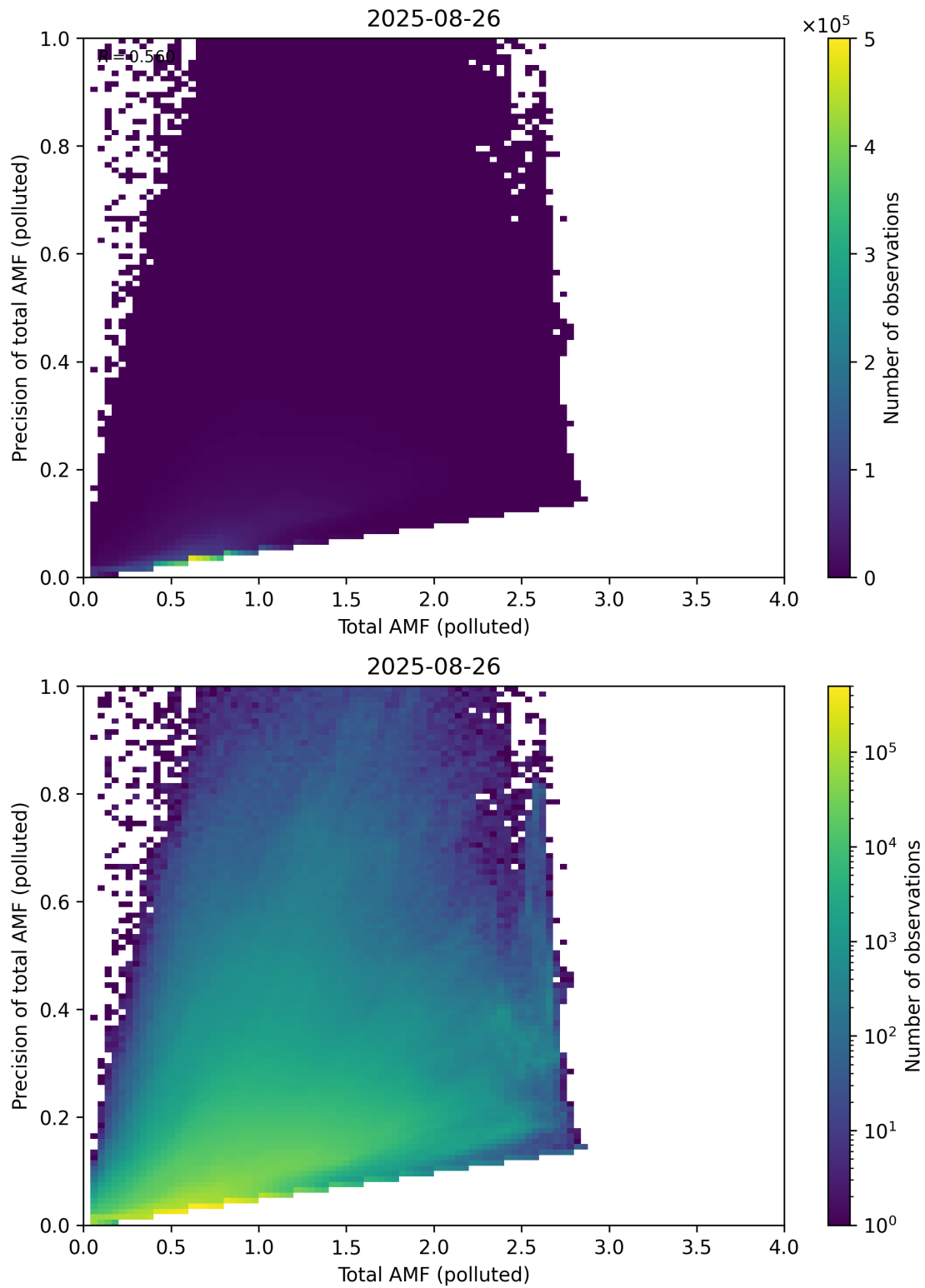
Figure 322: Scatter density plot of “Total AMF (polluted)” against “Precision of total AMF (polluted)” for 2025-08-25 to 2025-08-27.
