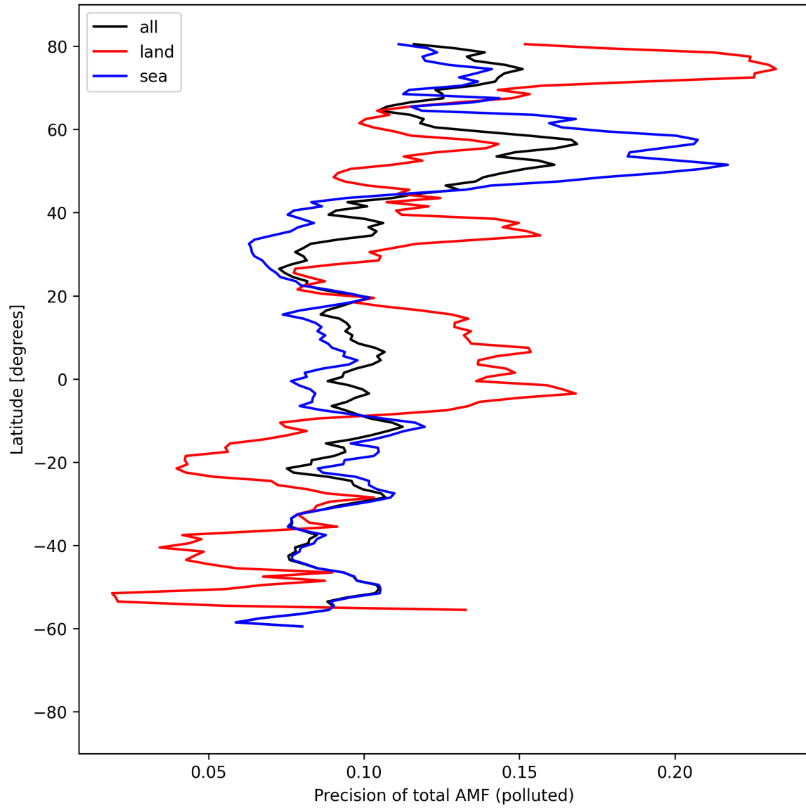
Figure 54: Zonal average of “Precision of total AMF (polluted)” for 2025-08-25 to 2025-08-27.
