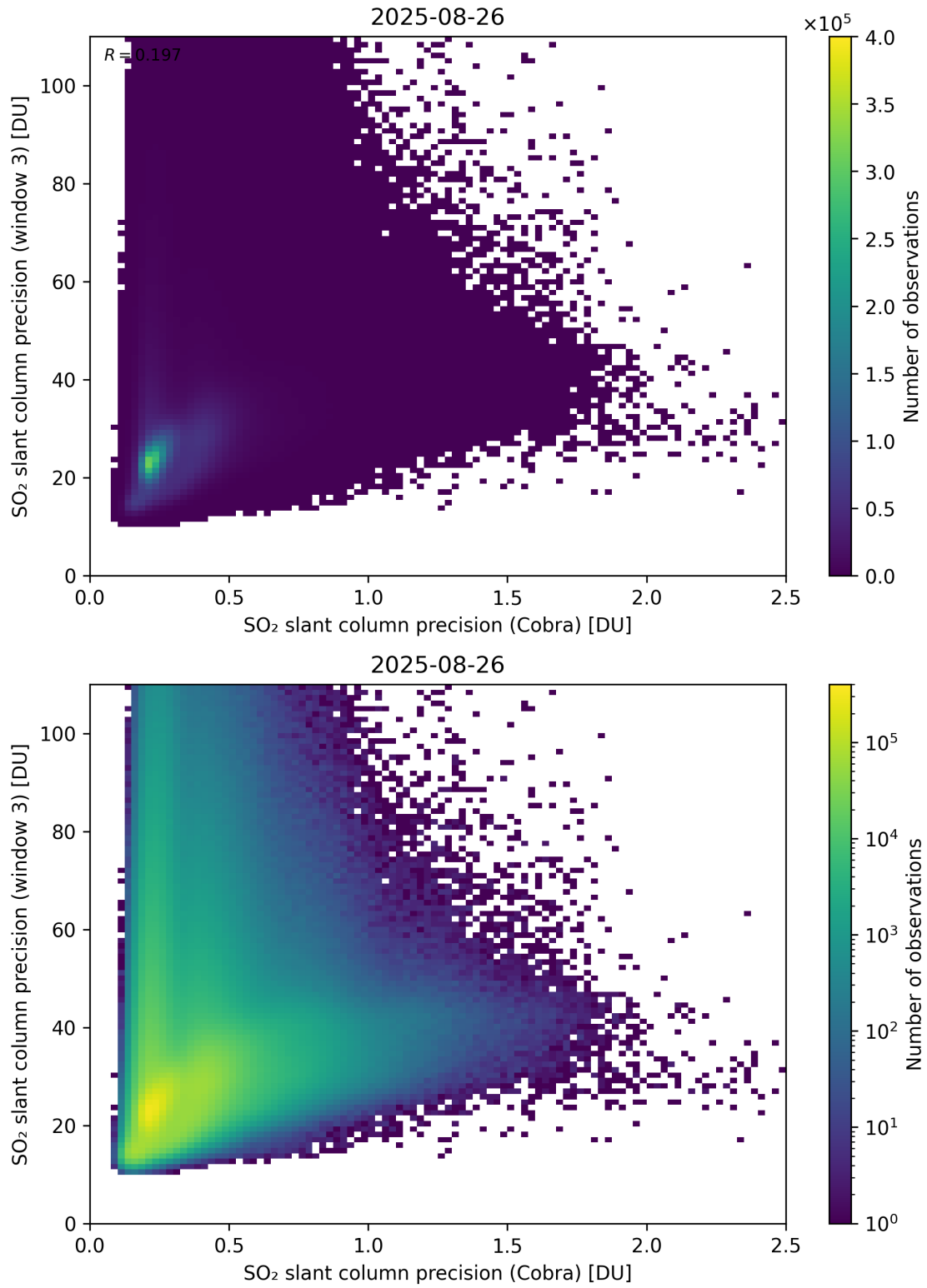
Figure 212: Scatter density plot of “SO 2 slant column precision (Cobra)” against “SO 2 slant column precision (window 3)” for 2025-08-25 to 2025-08-27.
