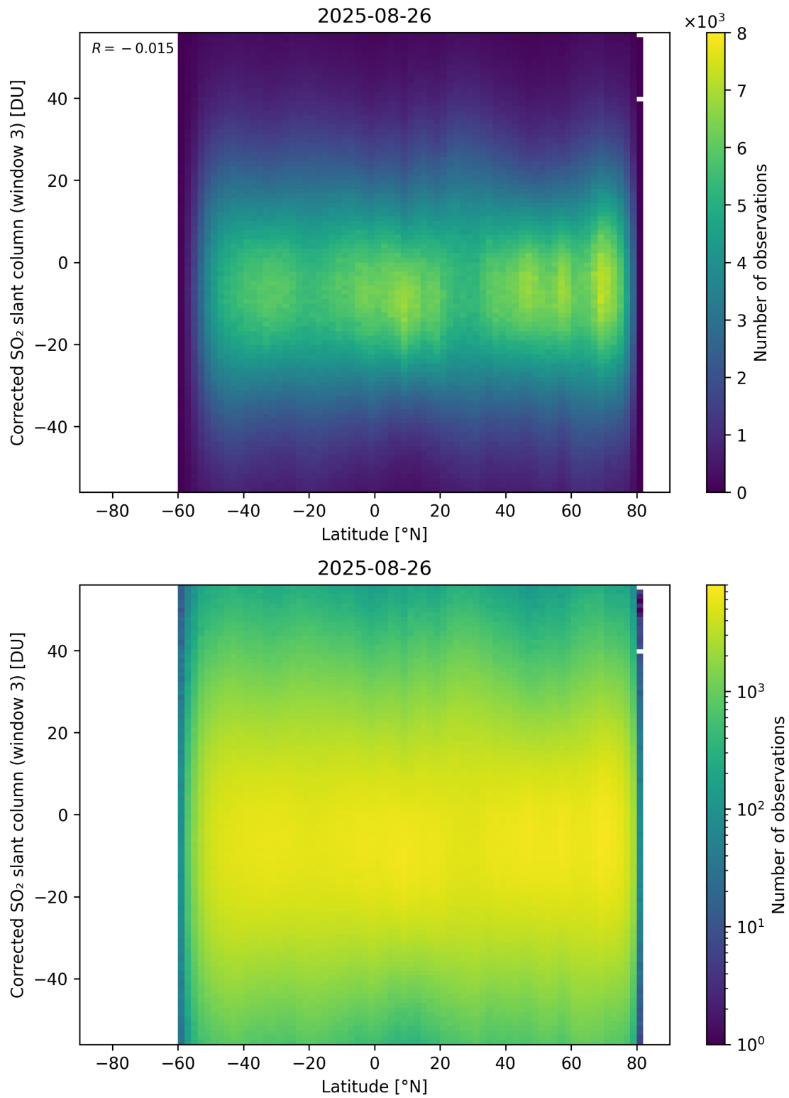
Figure 161: Scatter density plot of “Latitude” against “Corrected SO 2 slant column (window 3)” for 2025-08-25 to 2025-08-27.
