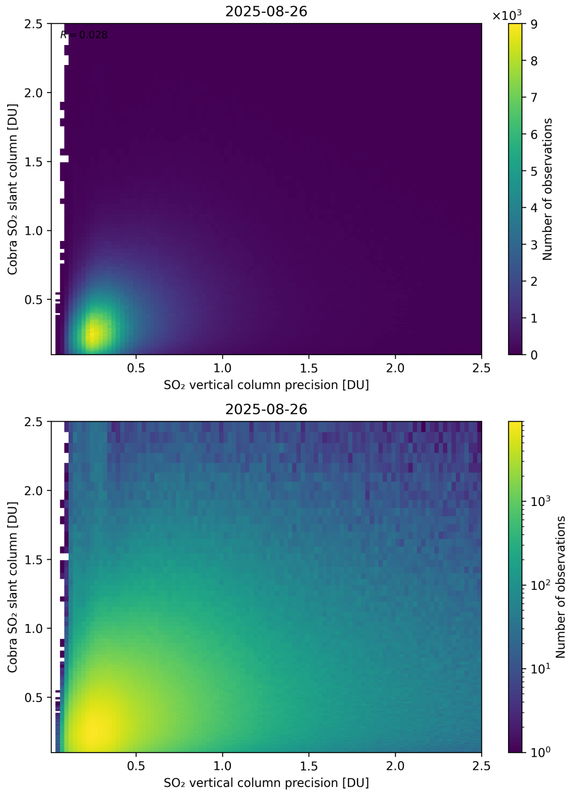
Figure 336: Scatter density plot of “SO 2 vertical column precision” against “Cobra SO 2 slant column” for 2025-08-25 to 2025-08-27.
