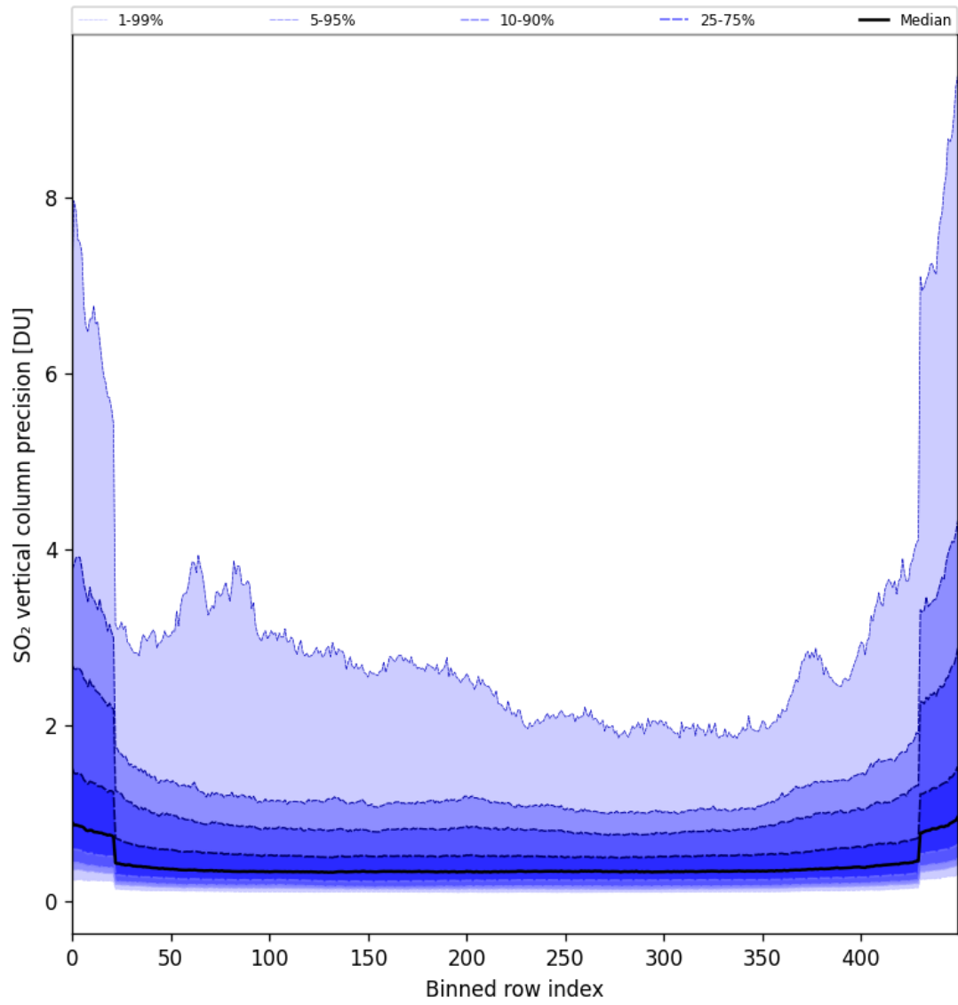
Figure 85: Along track statistics of “SO 2 vertical column precision” for 2025-08-25 to 2025-08-27
