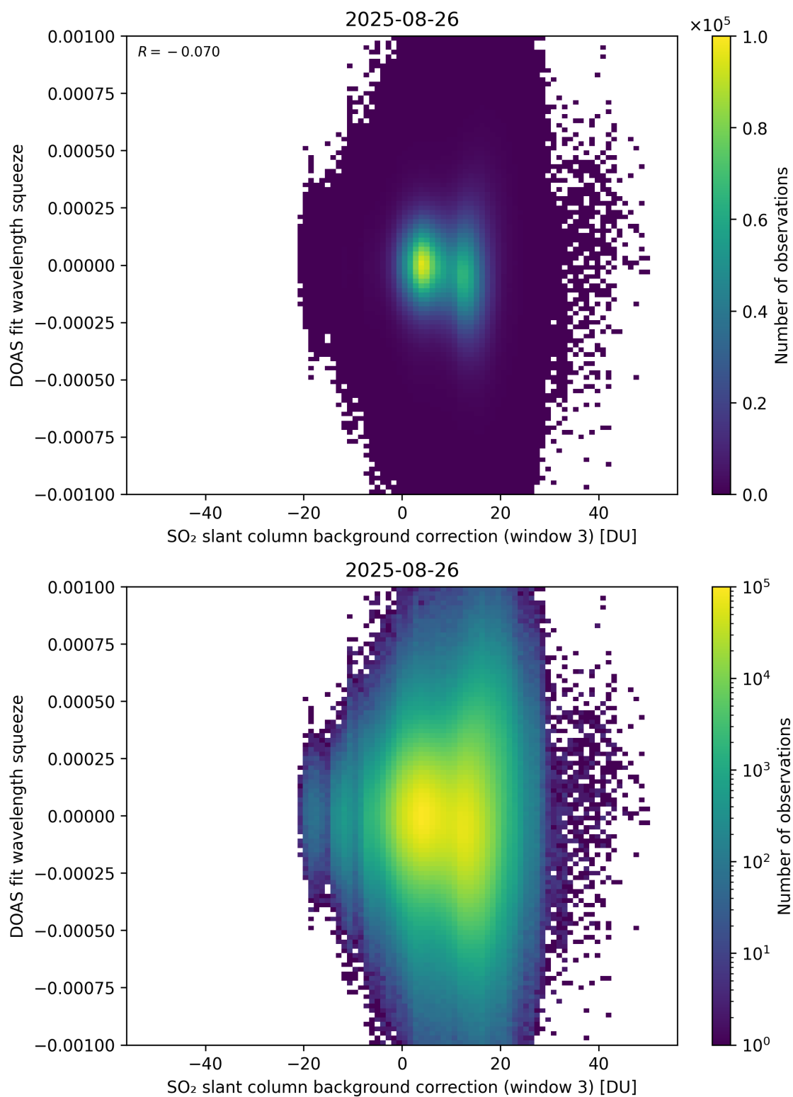
Figure 133: Scatter density plot of “SO 2 slant column background correction (window 3)” against “DOAS fit wavelength squeeze” for 2025-08-25 to 2025-08-27.
