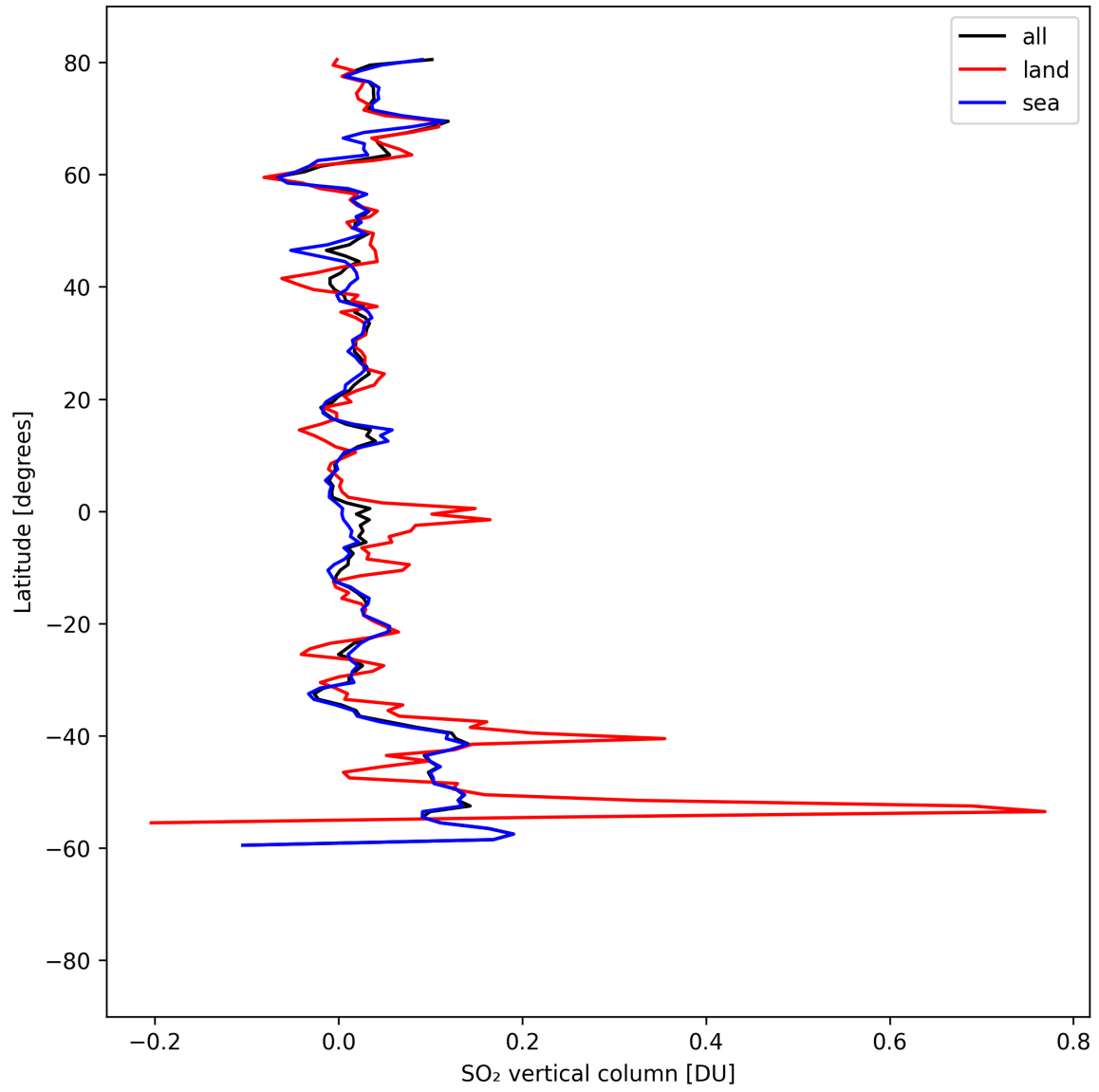
Figure 32: Zonal average of “SO 2 vertical column” for 2025-08-25 to 2025-08-27.
