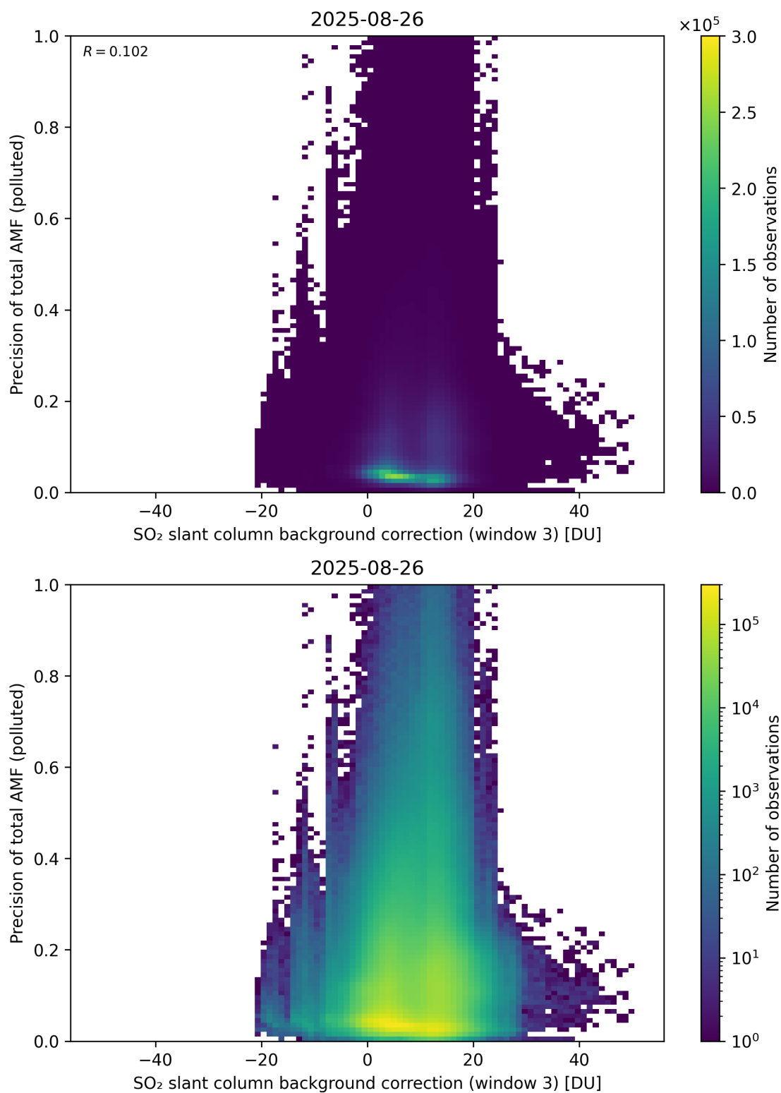
Figure 137: Scatter density plot of “SO 2 slant column background correction (window 3)” against “Precision of total AMF (polluted)” for 2025-08-25 to 2025-08-27.
