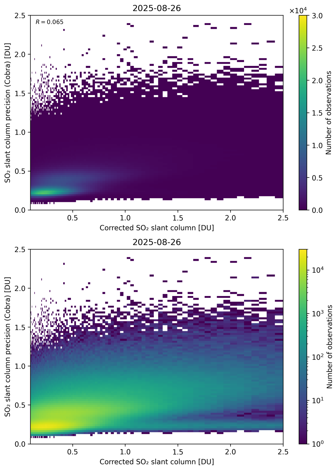
Figure 234: Scatter density plot of “Corrected SO 2 slant column” against “SO 2 slant column precision (Cobra)” for 2025-08-25 to 2025-08-27.
