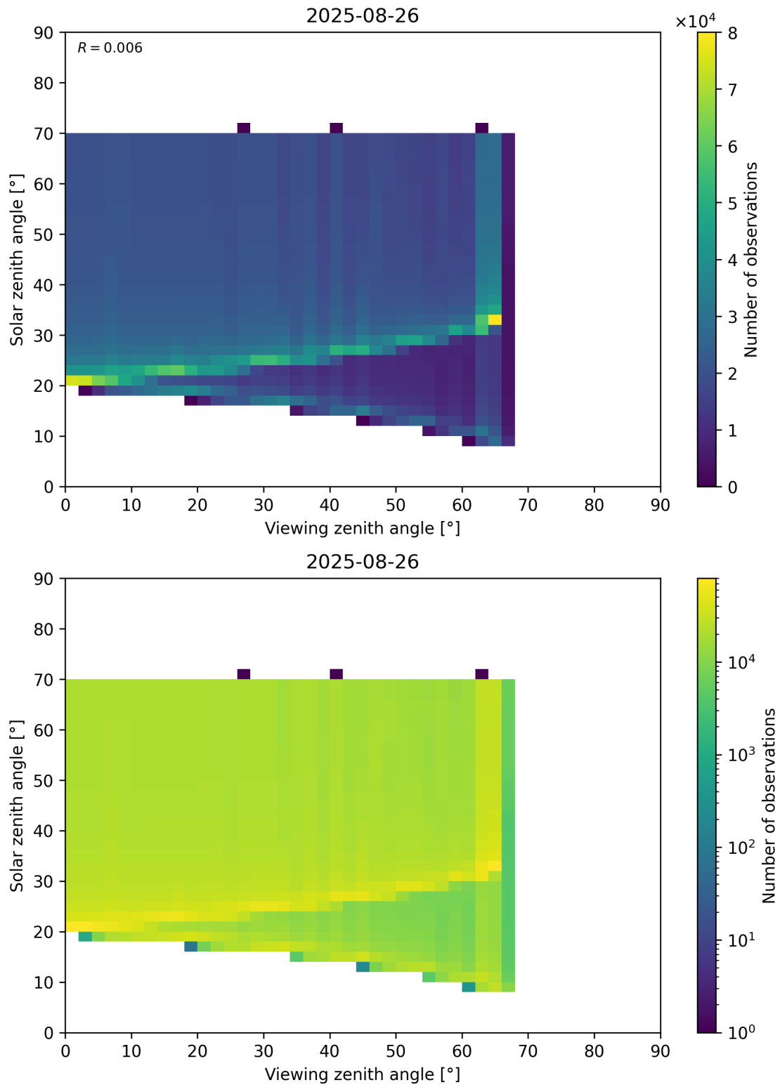
Figure 369: Scatter density plot of “Viewing zenith angle” against “Solar zenith angle” for 2025-08-25 to 2025-08-27.
