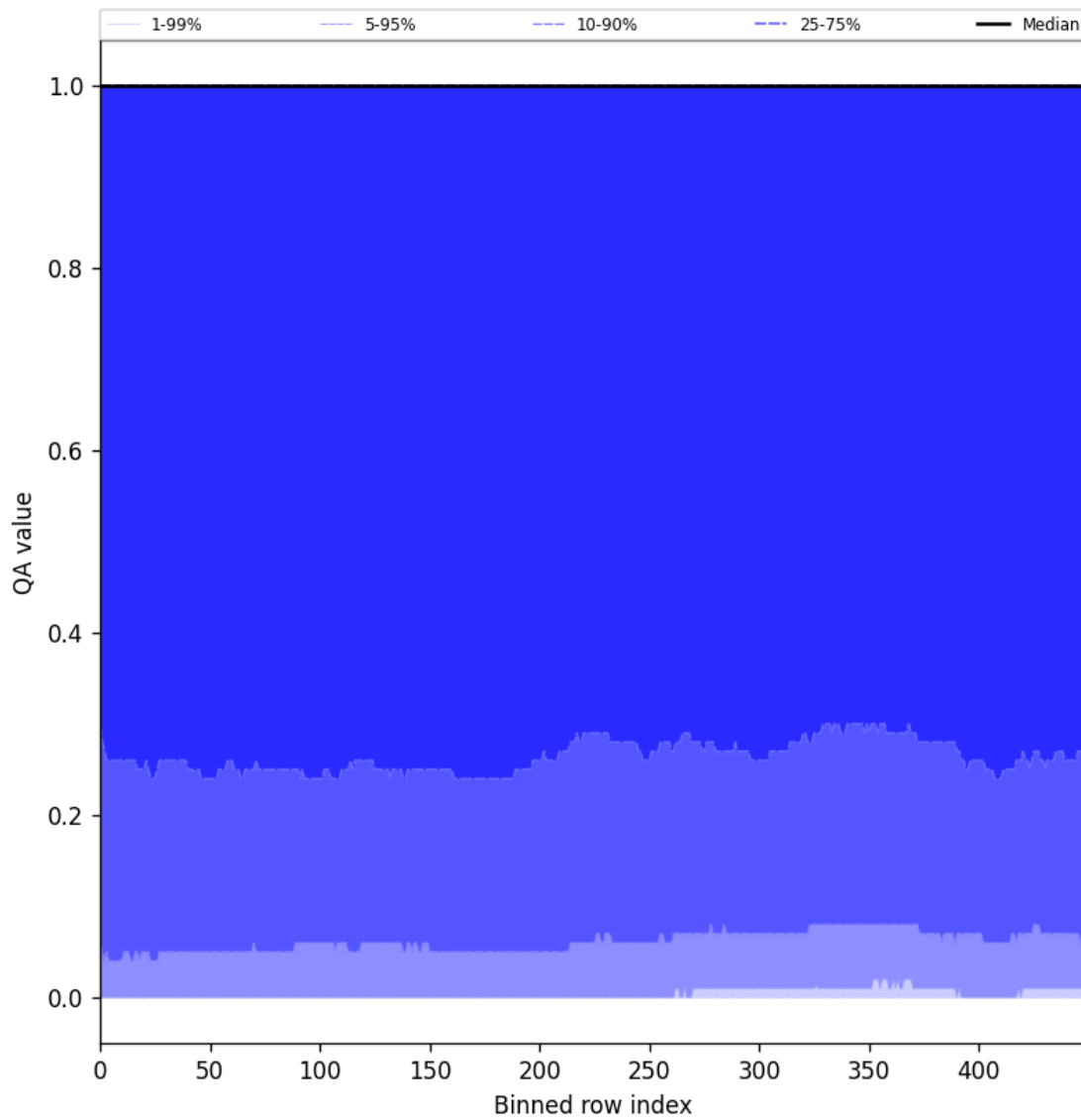
Figure 83: Along track statistics of “QA value” for 2025-08-25 to 2025-08-27
