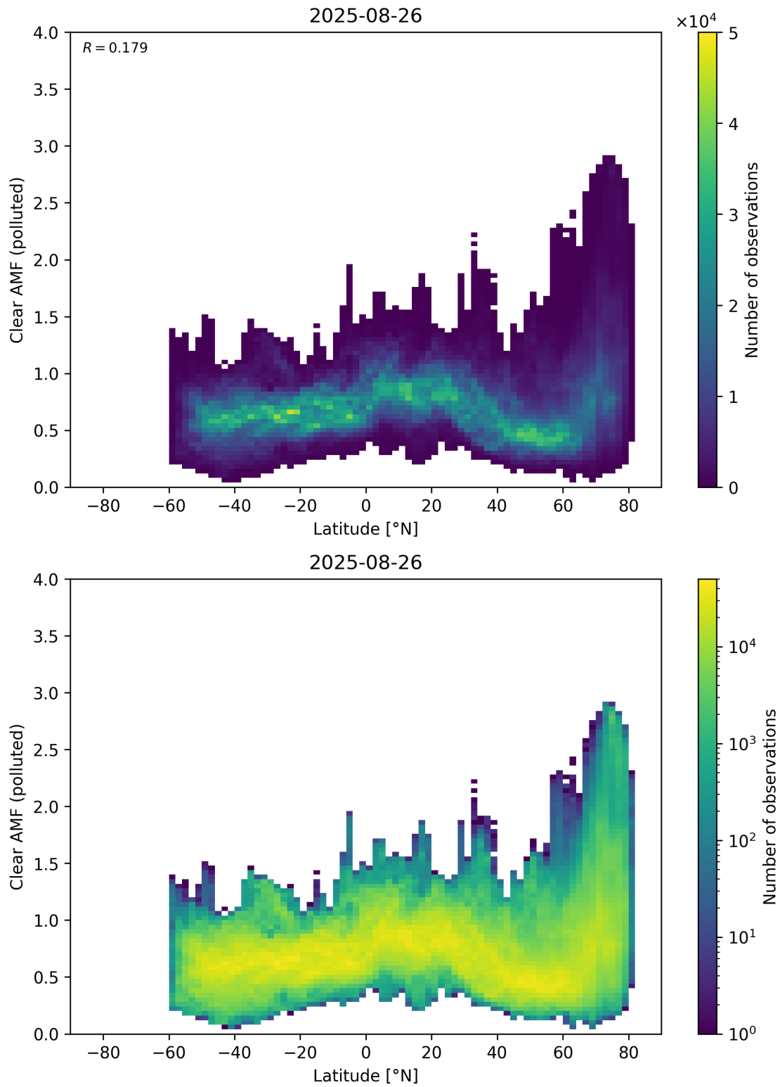
Figure 156: Scatter density plot of “Latitude” against “Clear AMF (polluted)” for 2025-08-25 to 2025-08-27.
