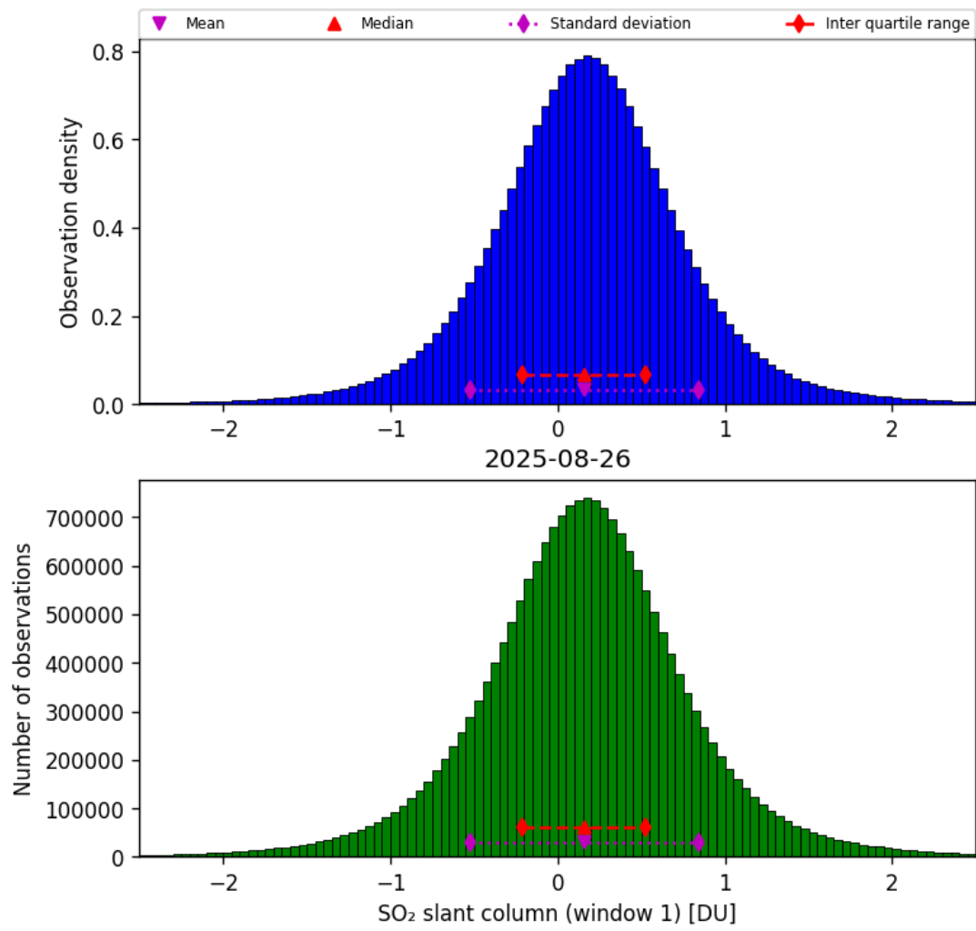
Figure 63: Histogram of “SO 2 slant column (window 1)” for 2025-08-25 to 2025-08-27
