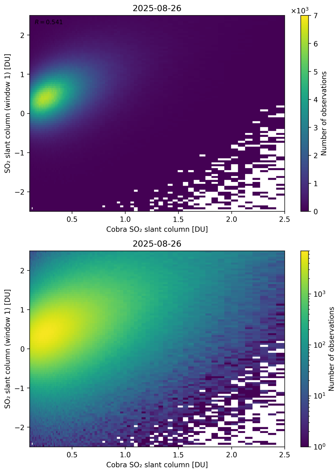
Figure 219: Scatter density plot of “Cobra SO 2 slant column” against “SO 2 slant column (window 1)” for 2025-08-25 to 2025-08-27.
