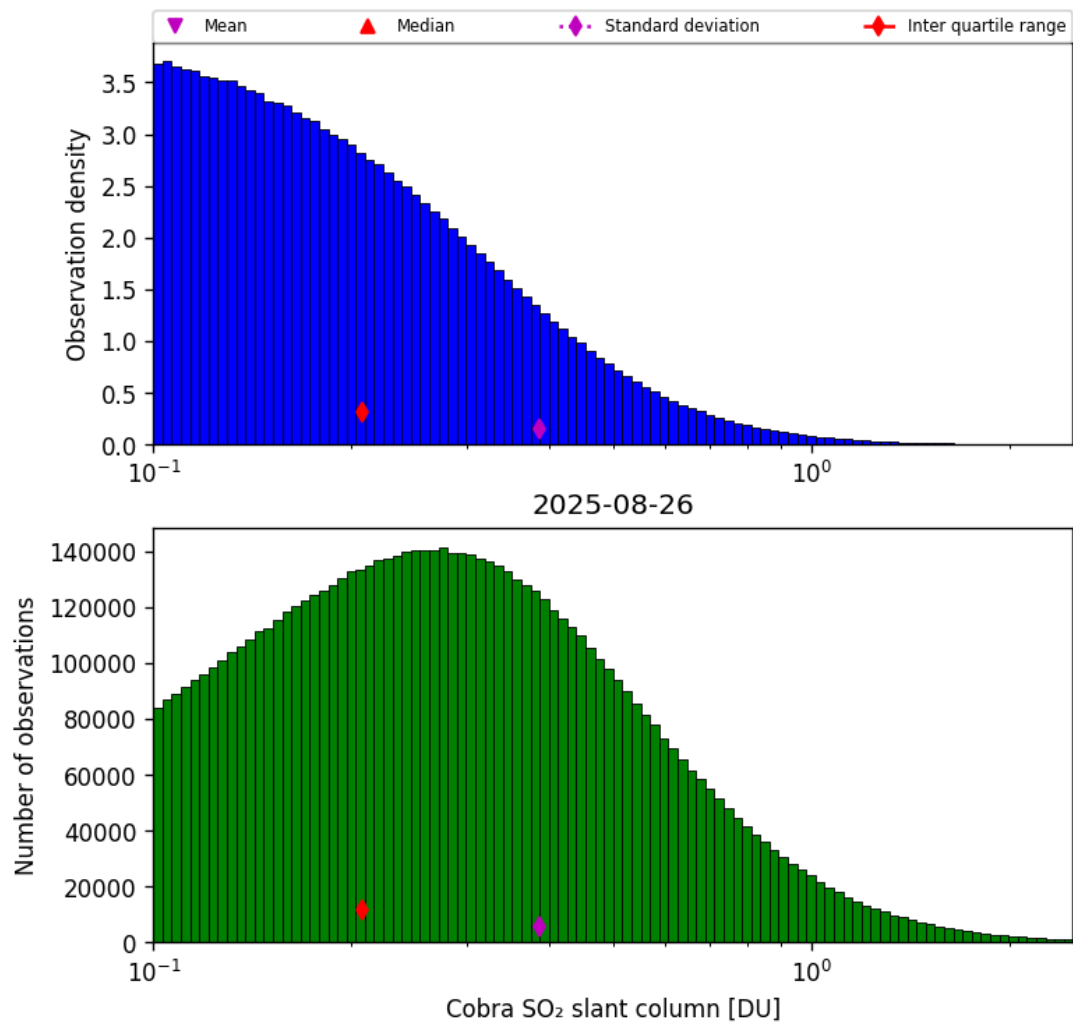
Figure 61: Histogram of “Cobra SO 2 slant column” for 2025-08-25 to 2025-08-27
