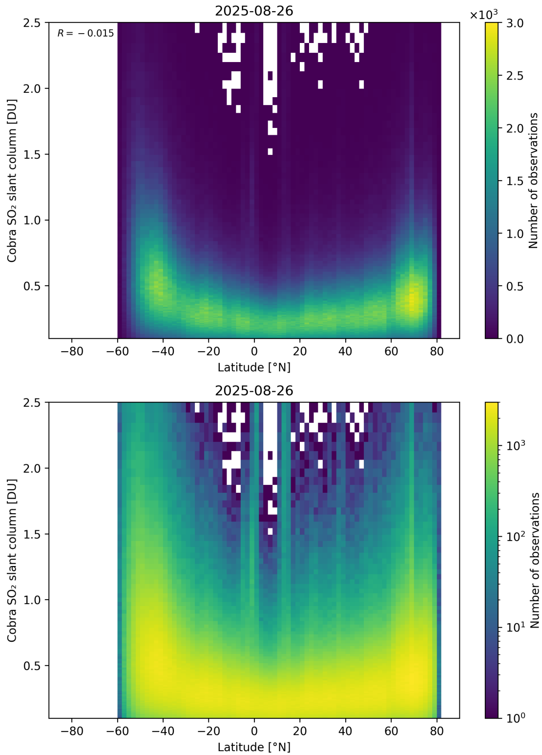
Figure 157: Scatter density plot of “Latitude” against “Cobra SO 2 slant column” for 2025-08-25 to 2025-08-27.
