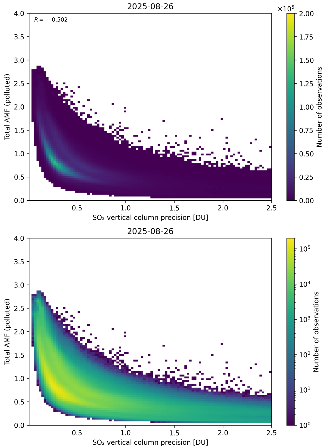
Figure 346: Scatter density plot of “SO 2 vertical column precision” against “Total AMF (polluted)” for 2025-08-25 to 2025-08-27.
