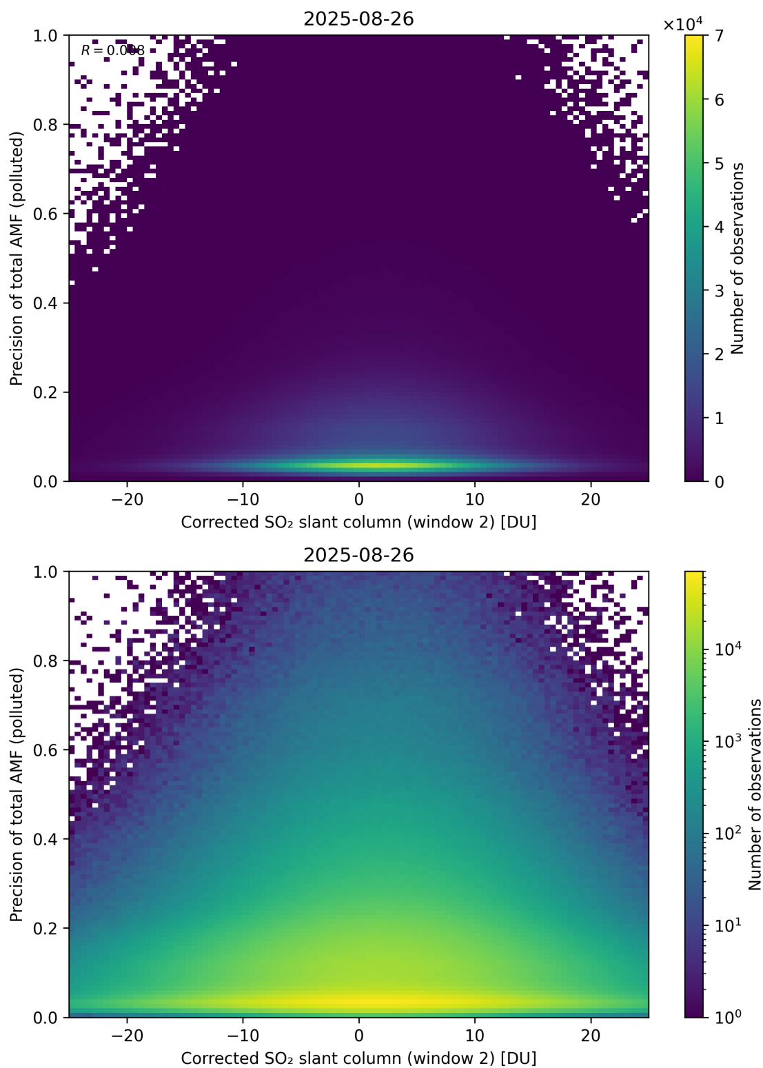
Figure 254: Scatter density plot of “Corrected SO 2 slant column (window 2)” against “Precision of total AMF (polluted)” for 2025-08-25 to 2025-08-27.
