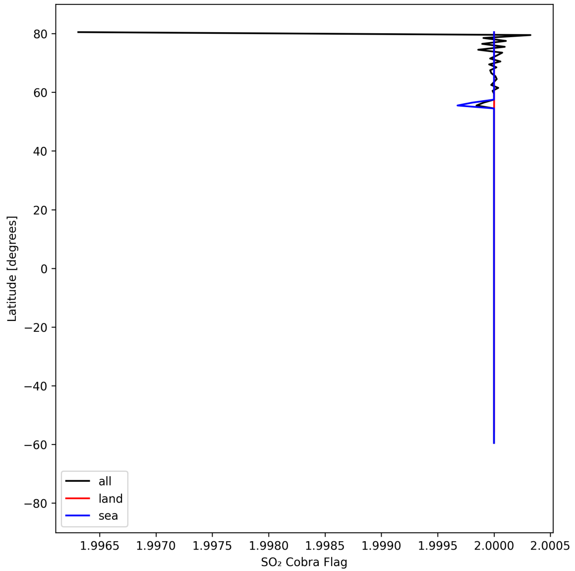
Figure 49: Zonal average of “SO 2 Cobra Flag” for 2025-08-25 to 2025-08-27.
