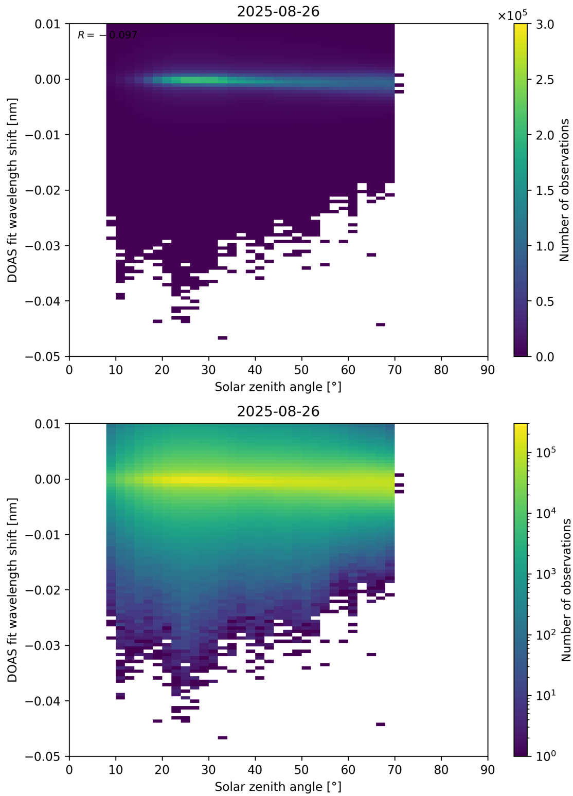
Figure 174: Scatter density plot of “Solar zenith angle” against “DOAS fit wavelength shift” for 2025-08-25 to 2025-08-27.
