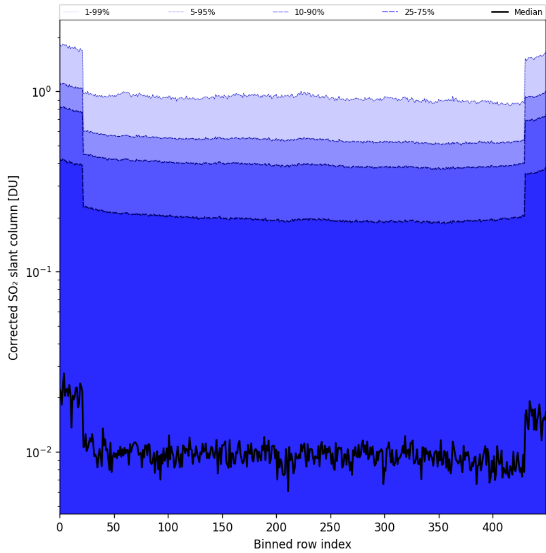
Figure 86: Along track statistics of “Corrected SO 2 slant column” for 2025-08-25 to 2025-08-27
