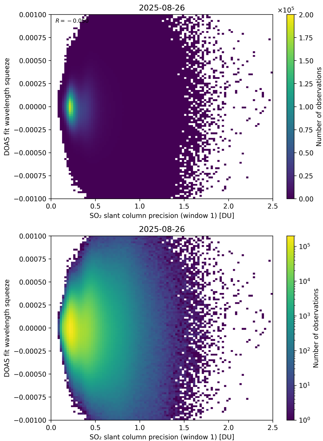
Figure 272: Scatter density plot of “SO 2 slant column precision (window 1)” against “DOAS fit wavelength squeeze” for 2025-08-25 to 2025-08-27.
