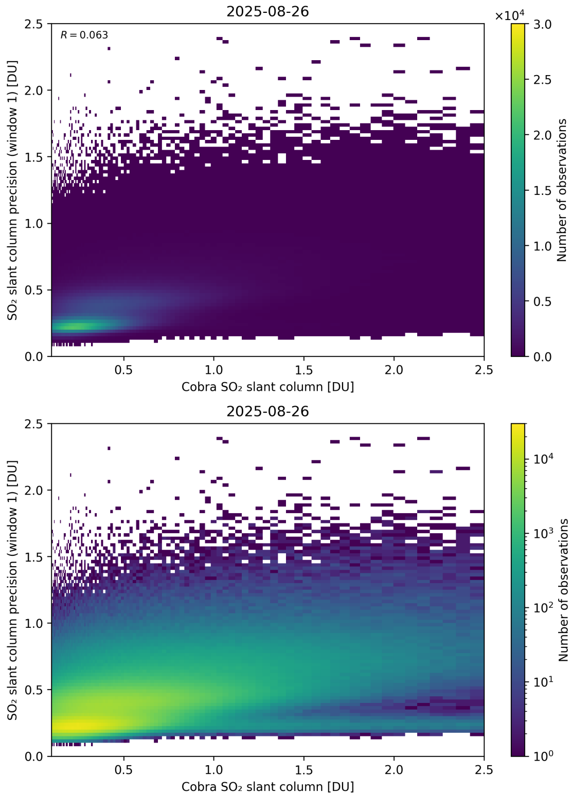
Figure 220: Scatter density plot of “Cobra SO 2 slant column” against “SO 2 slant column precision (window 1)” for 2025-08-25 to 2025-08-27.
