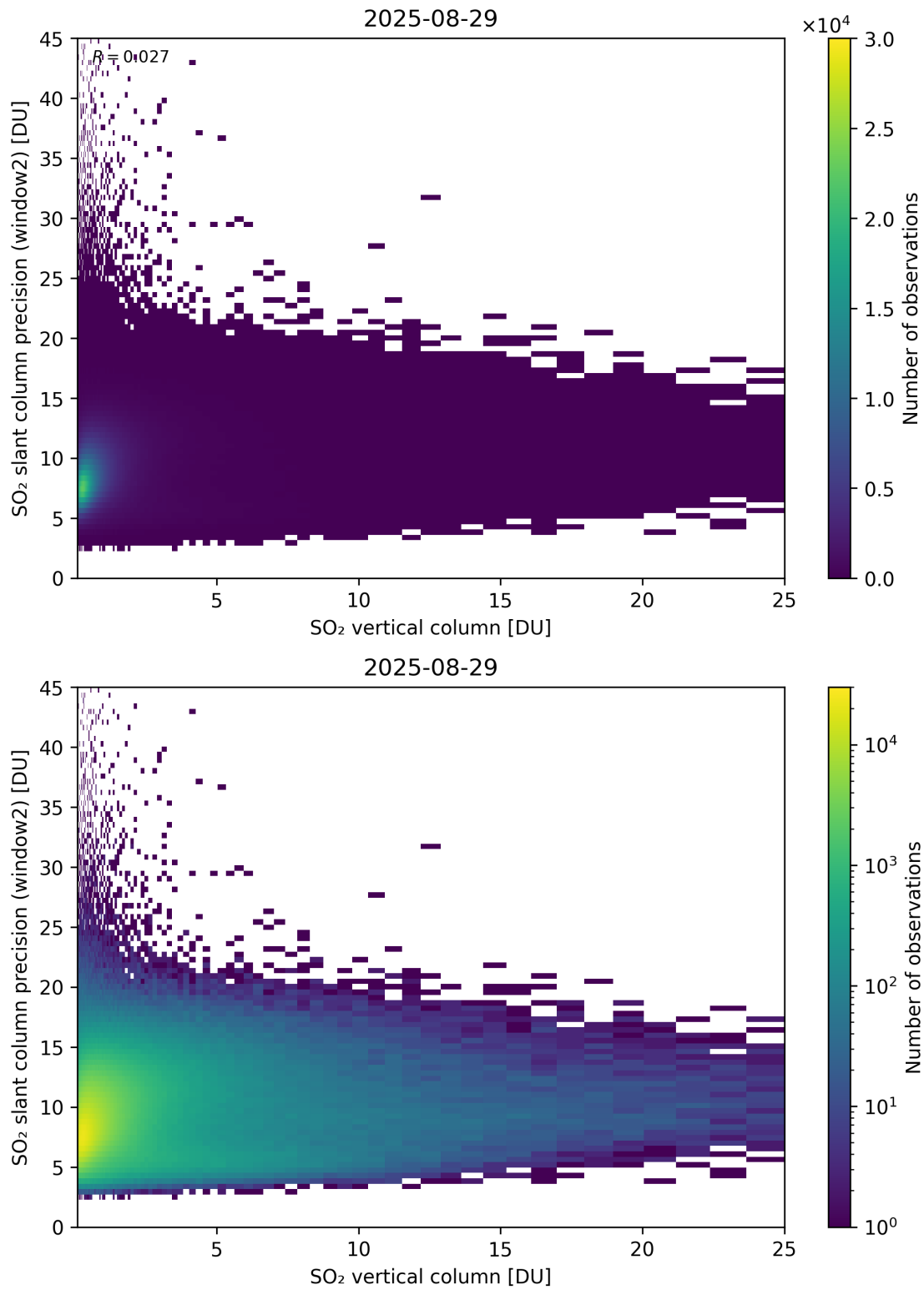
Figure 356: Scatter density plot of “SO 2 vertical column” against “SO 2 slant column precision (window2)” for 2025-08-28 to 2025-08-30.
