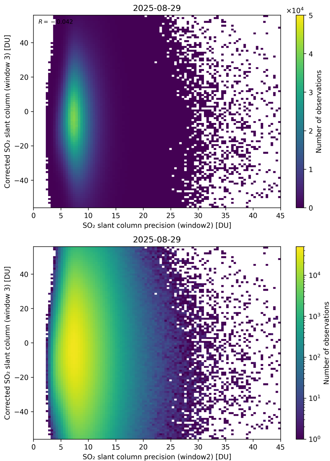
Figure 298: Scatter density plot of “SO 2 slant column precision (window2)” against “Corrected SO 2 slant column (window 3)” for 2025-08-28 to 2025-08-30.
