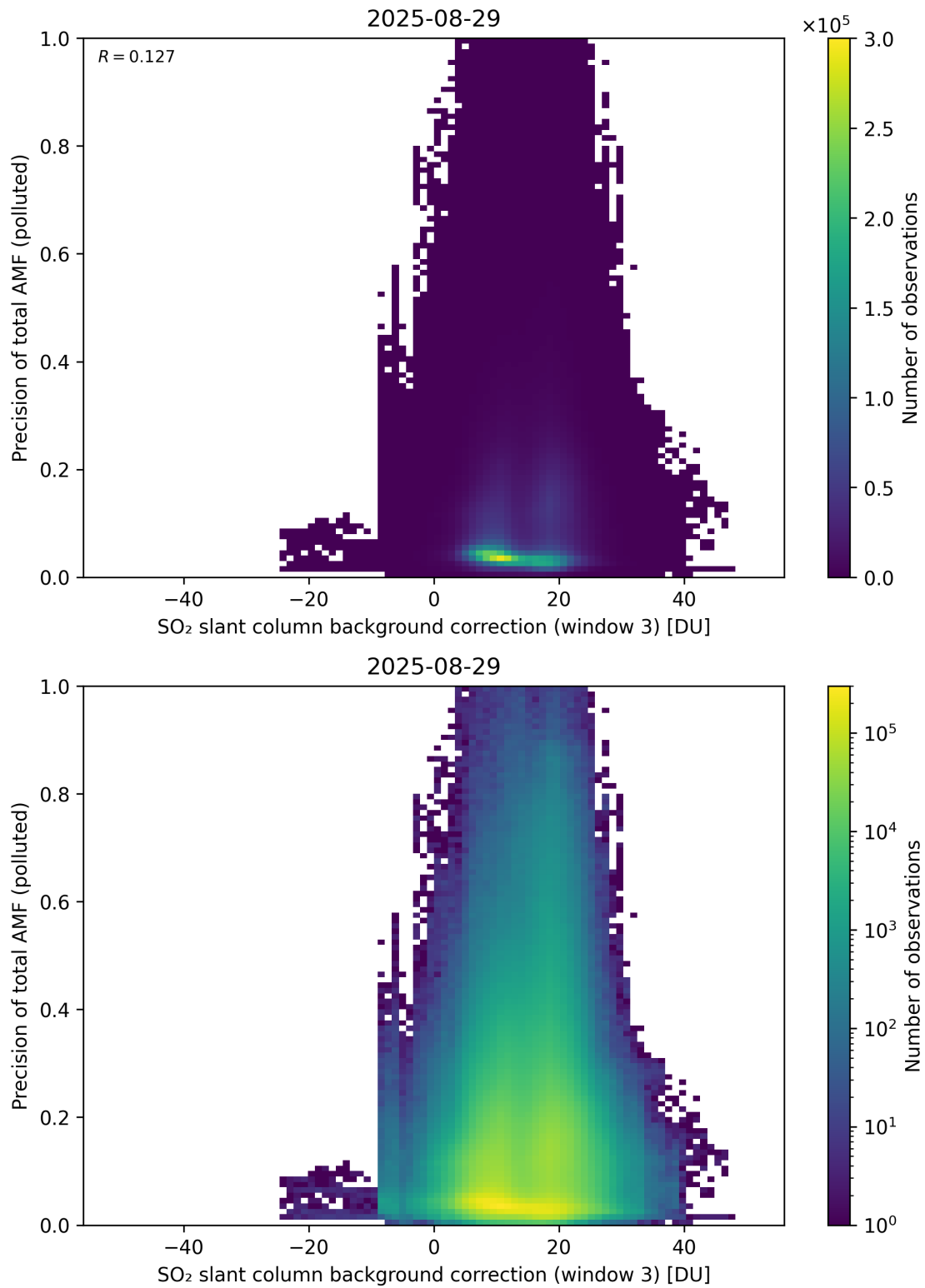
Figure 137: Scatter density plot of “SO 2 slant column background correction (window 3)” against “Precision of total AMF (polluted)” for 2025-08-28 to 2025-08-30.
