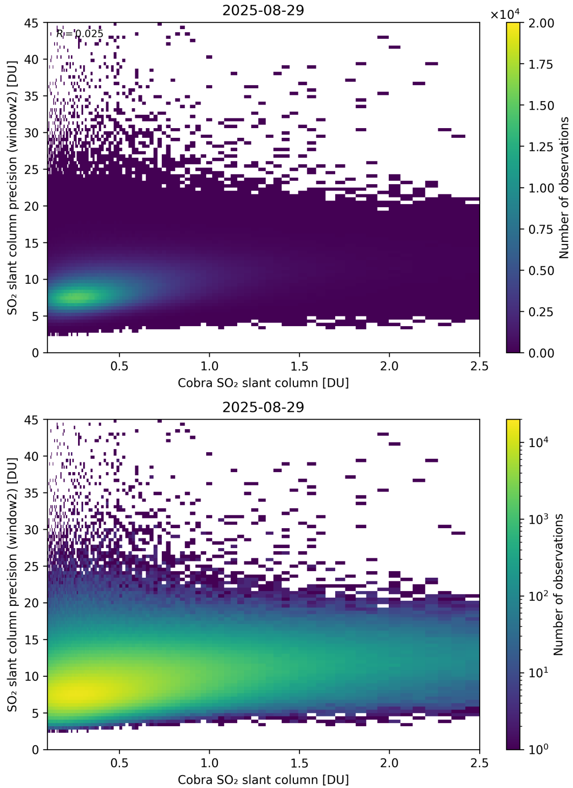
Figure 221: Scatter density plot of “Cobra SO 2 slant column” against “SO 2 slant column precision (window2)” for 2025-08-28 to 2025-08-30.
