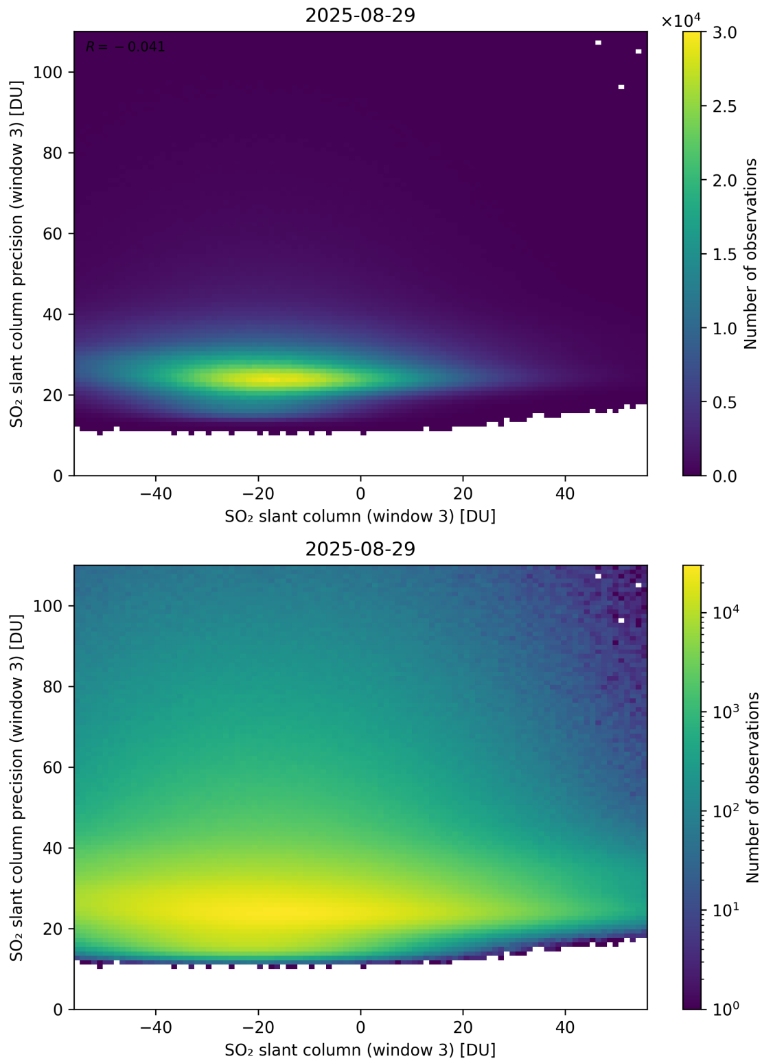
Figure 317: Scatter density plot of “SO 2 slant column (window 3)” against “SO 2 slant column precision (window 3)” for 2025-08-28 to 2025-08-30.
