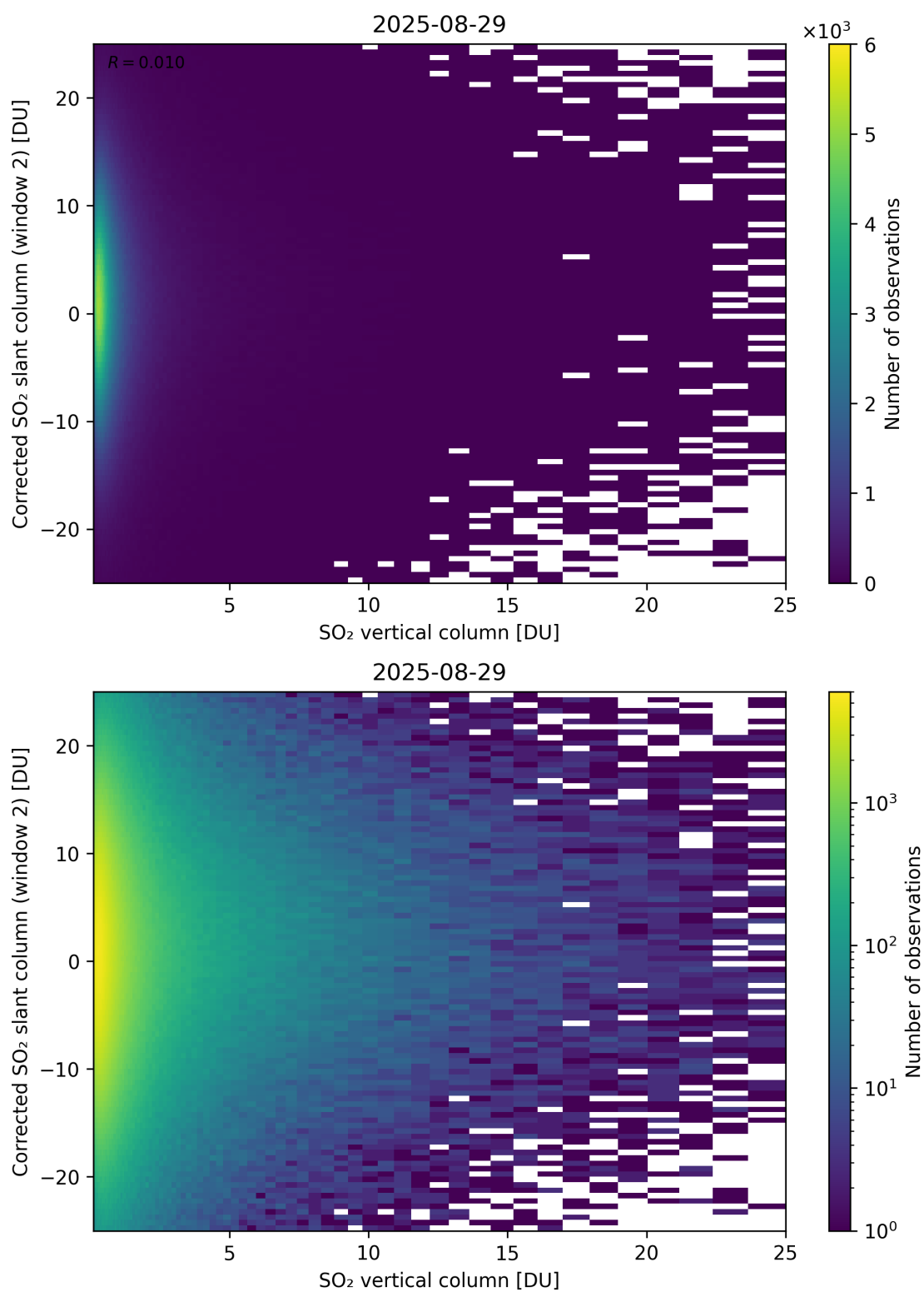
Figure 352: Scatter density plot of “SO 2 vertical column” against “Corrected SO 2 slant column (window 2)” for 2025-08-28 to 2025-08-30.
