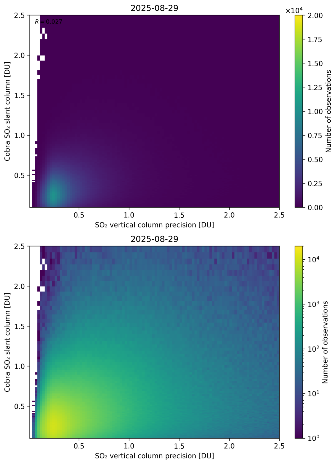
Figure 336: Scatter density plot of “SO 2 vertical column precision” against “Cobra SO 2 slant column” for 2025-08-28 to 2025-08-30.
