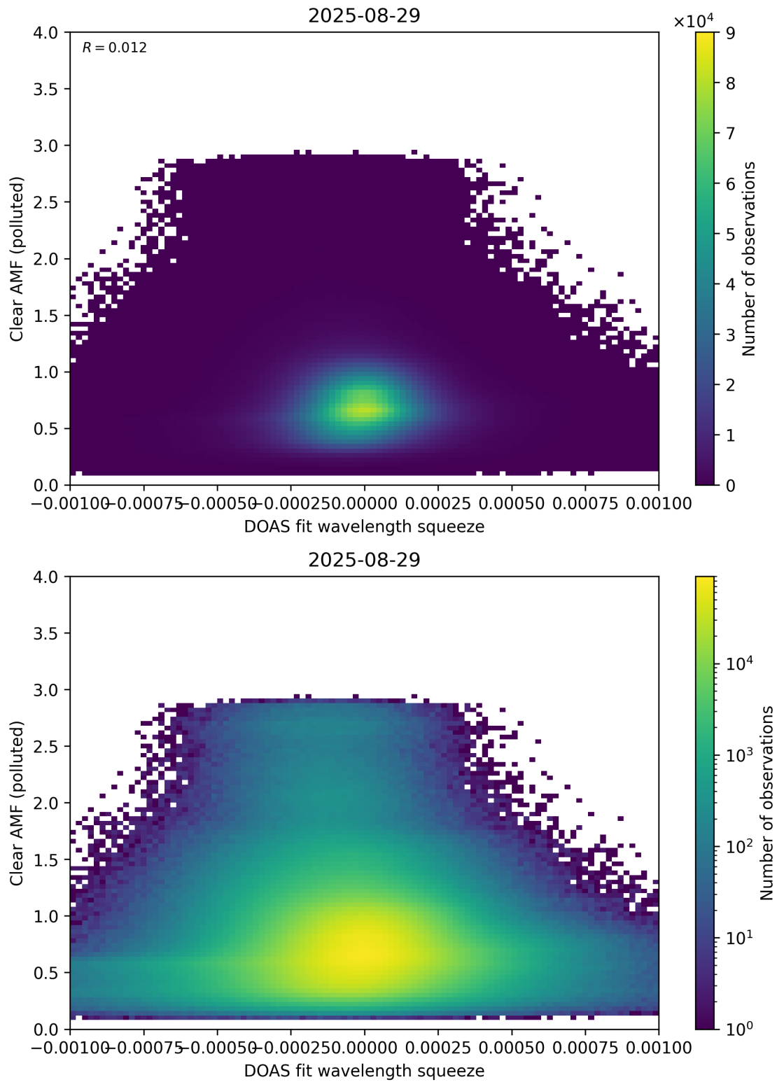
Figure 144: Scatter density plot of “DOAS fit wavelength squeeze” against “Clear AMF (polluted)” for 2025-08-28 to 2025-08-30.
