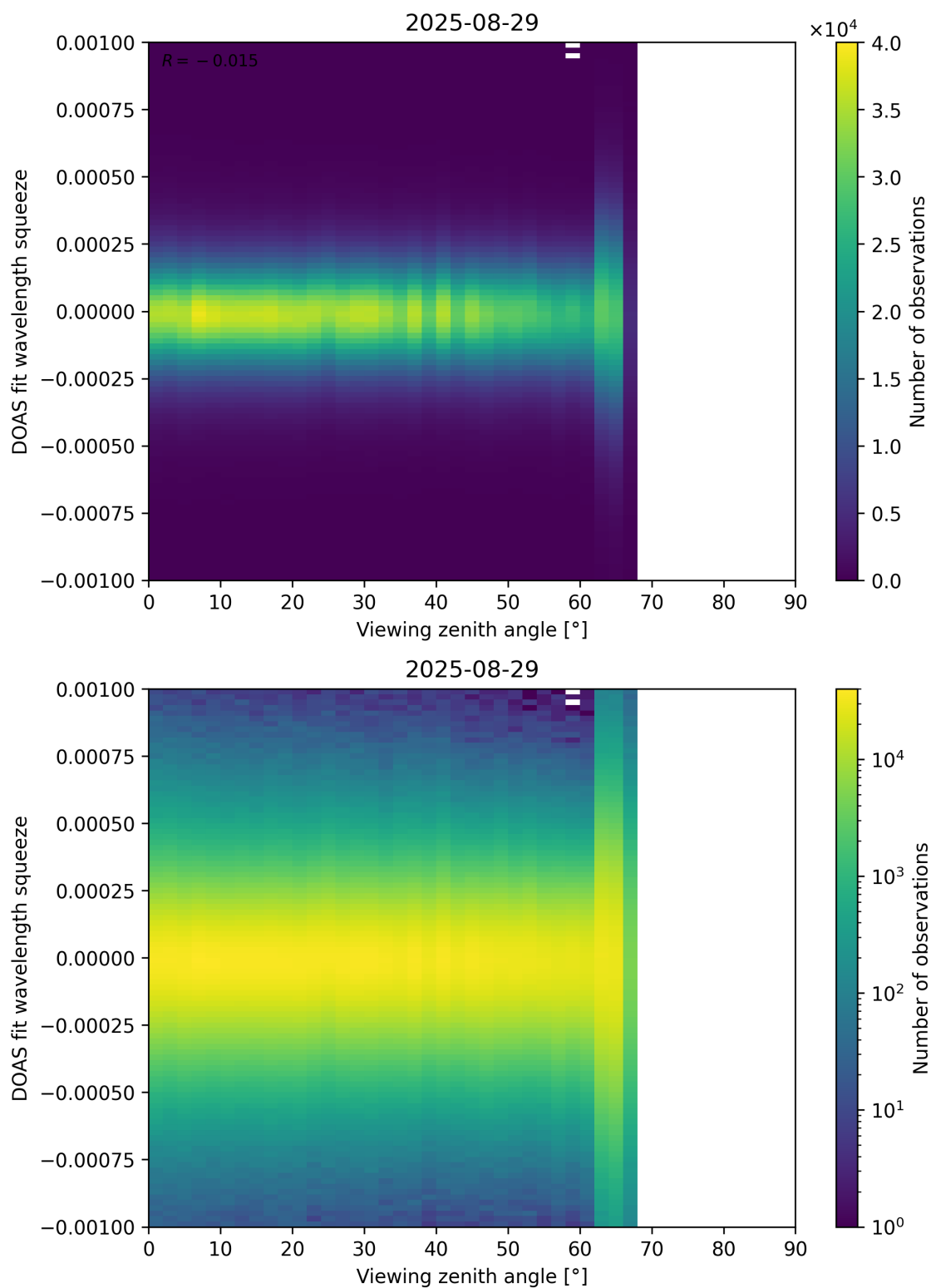
Figure 366: Scatter density plot of “Viewing zenith angle” against “DOAS fit wavelength squeeze” for 2025-08-28 to 2025-08-30.
