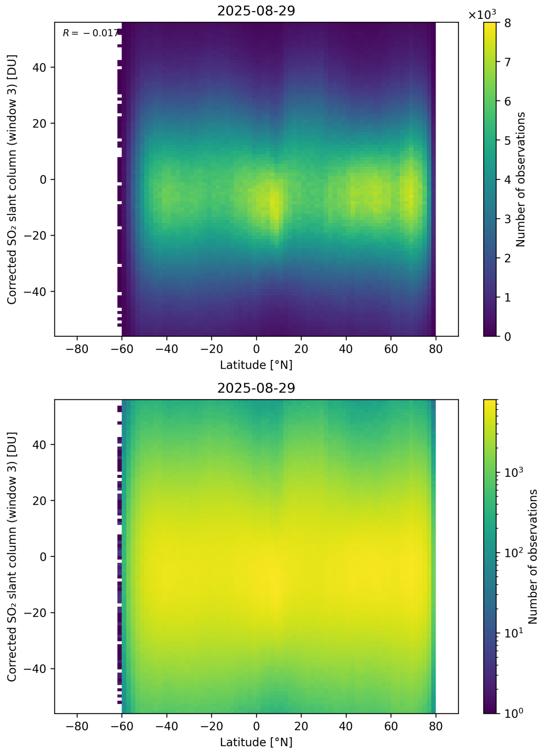
Figure 161: Scatter density plot of “Latitude” against “Corrected SO 2 slant column (window 3)” for 2025-08-28 to 2025-08-30.
