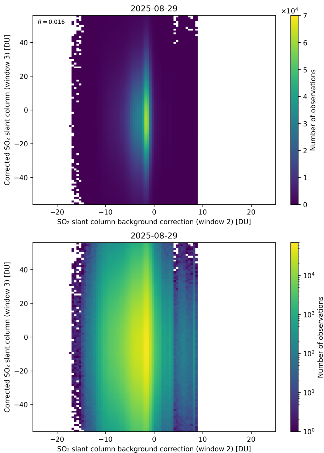
Figure 127: Scatter density plot of “SO 2 slant column background correction (window 2)” against “Corrected SO 2 slant column (window 3)” for 2025-08-28 to 2025-08-30.
