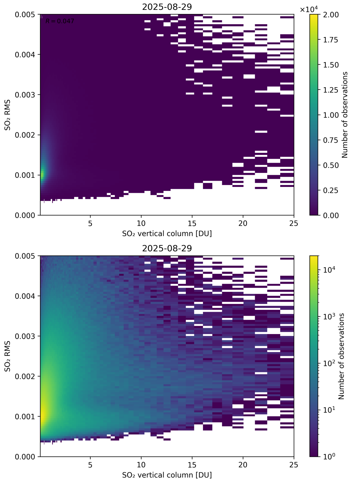
Figure 328: Scatter density plot of “SO 2 vertical column” against “SO 2 RMS” for 2025-08-28 to 2025-08-30.
