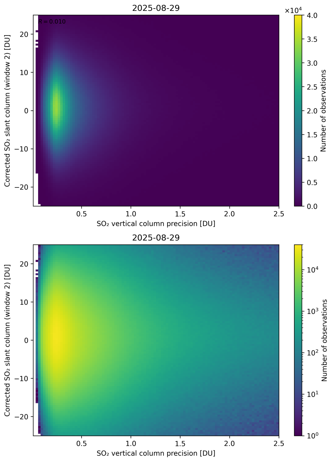
Figure 339: Scatter density plot of “SO 2 vertical column precision” against “Corrected SO 2 slant column (window 2)” for 2025-08-28 to 2025-08-30.
