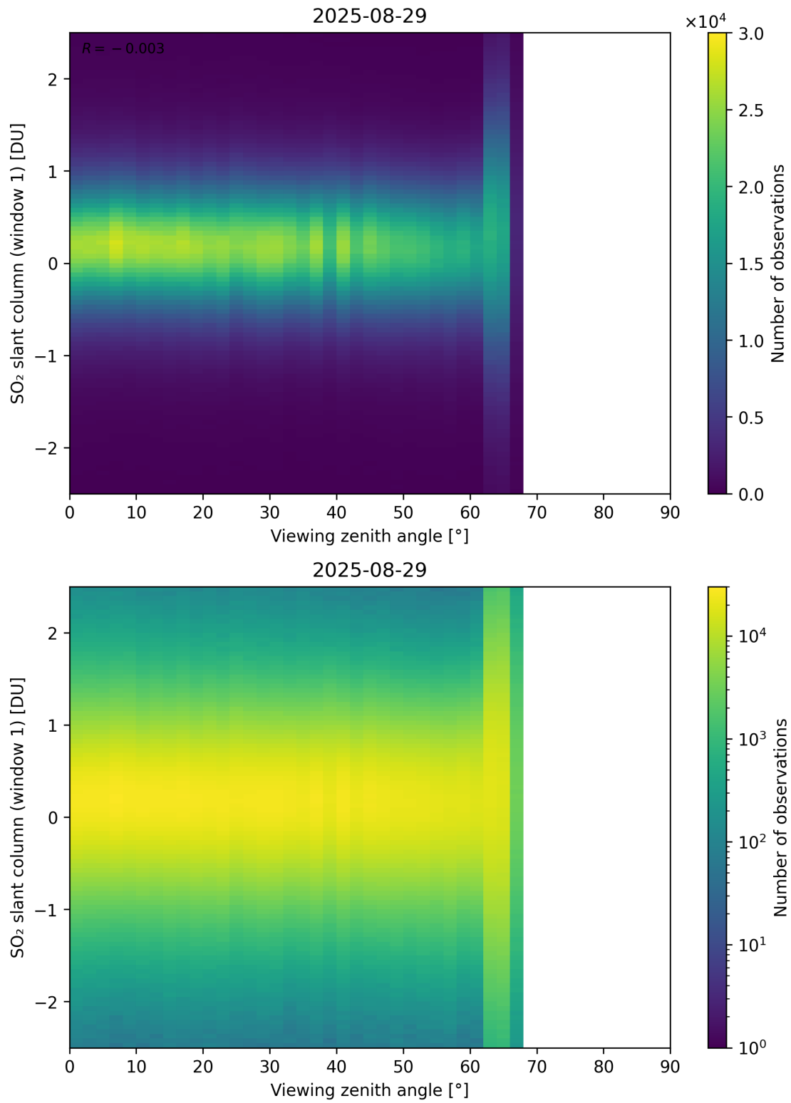
Figure 376: Scatter density plot of “Viewing zenith angle” against “SO 2 slant column (window 1)” for 2025-08-28 to 2025-08-30.
