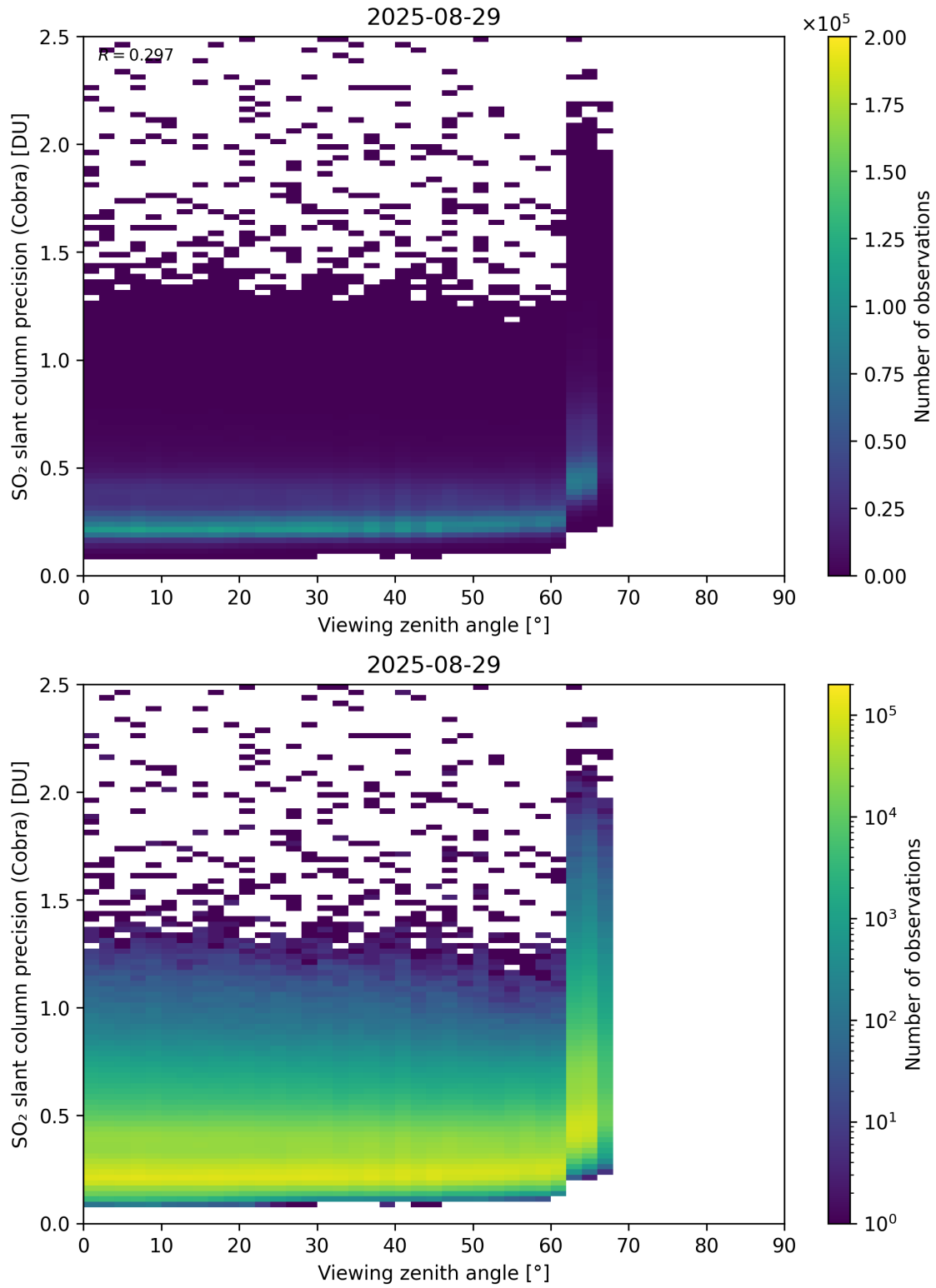
Figure 372: Scatter density plot of “Viewing zenith angle” against “SO 2 slant column precision (Cobra)” for 2025-08-28 to 2025-08-30.
