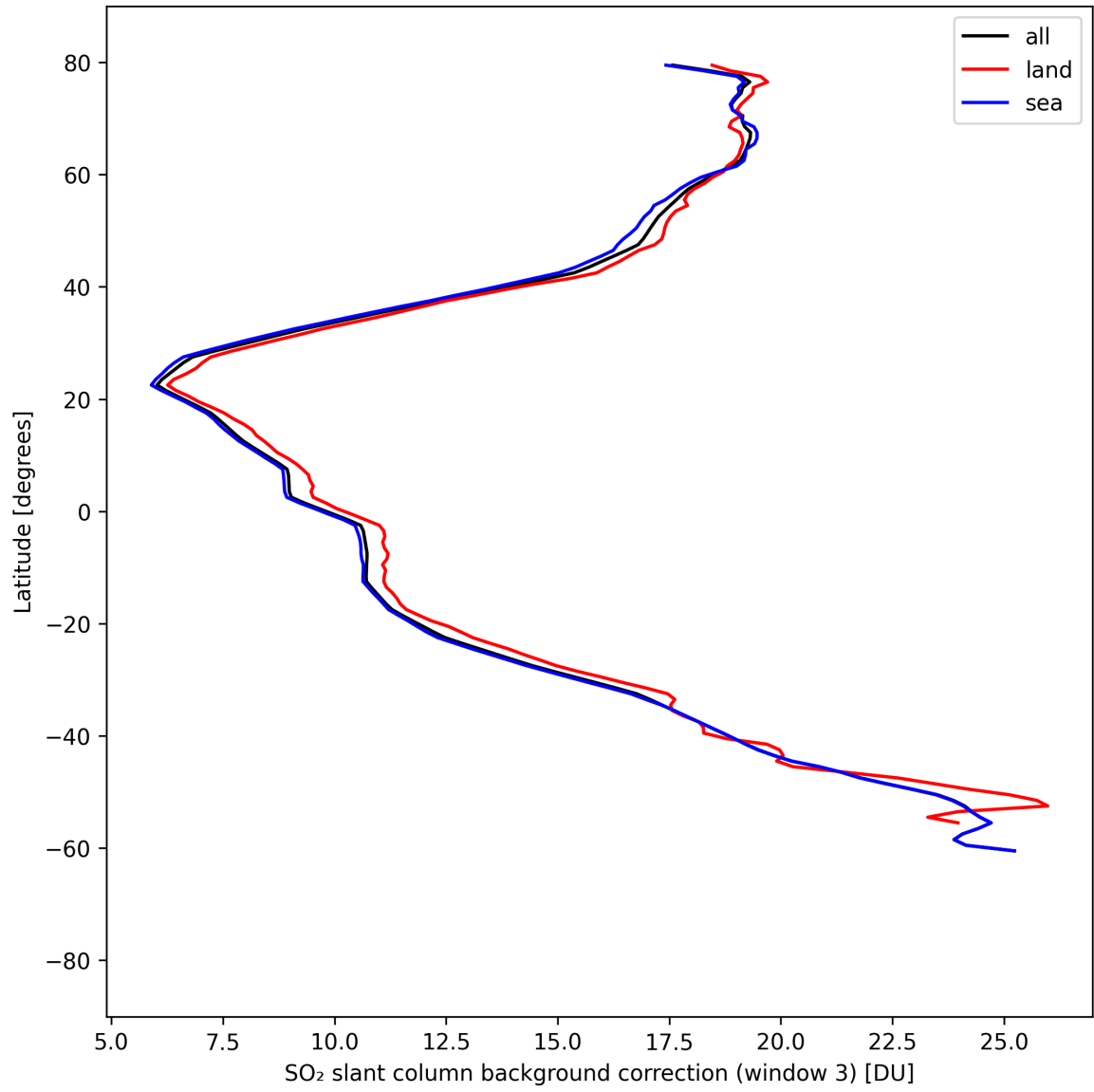
Figure 48: Zonal average of “SO 2 slant column background correction (window 3)” for 2025-08-28 to 2025-08-30.
