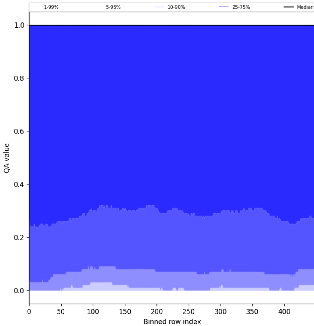
Figure 83: Along track statistics of “QA value” for 2025-08-28 to 2025-08-30
