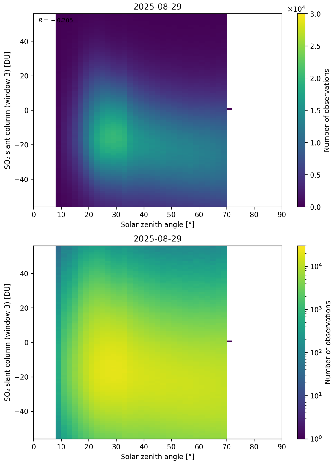
Figure 187: Scatter density plot of “Solar zenith angle” against “SO 2 slant column (window 3)” for 2025-08-28 to 2025-08-30.
