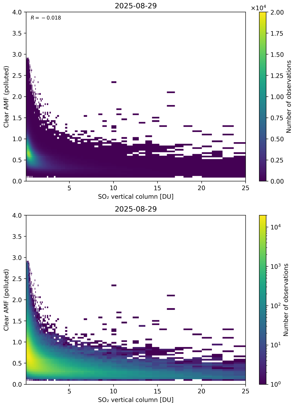
Figure 348: Scatter density plot of “SO 2 vertical column” against “Clear AMF (polluted)” for 2025-08-28 to 2025-08-30.
