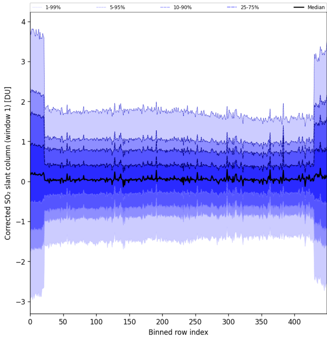
Figure 91: Along track statistics of “Corrected SO 2 slant column (window 1)” for 2025-08-28 to 2025-08-30
