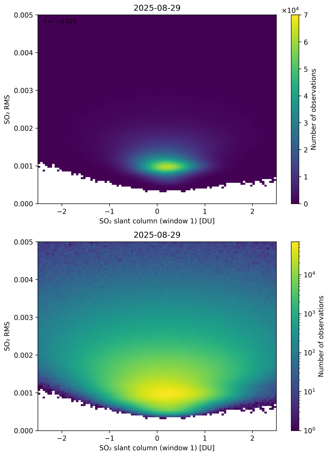
Figure 267: Scatter density plot of “SO 2 slant column (window 1)” against “SO 2 RMS” for 2025-08-28 to 2025-08-30.
