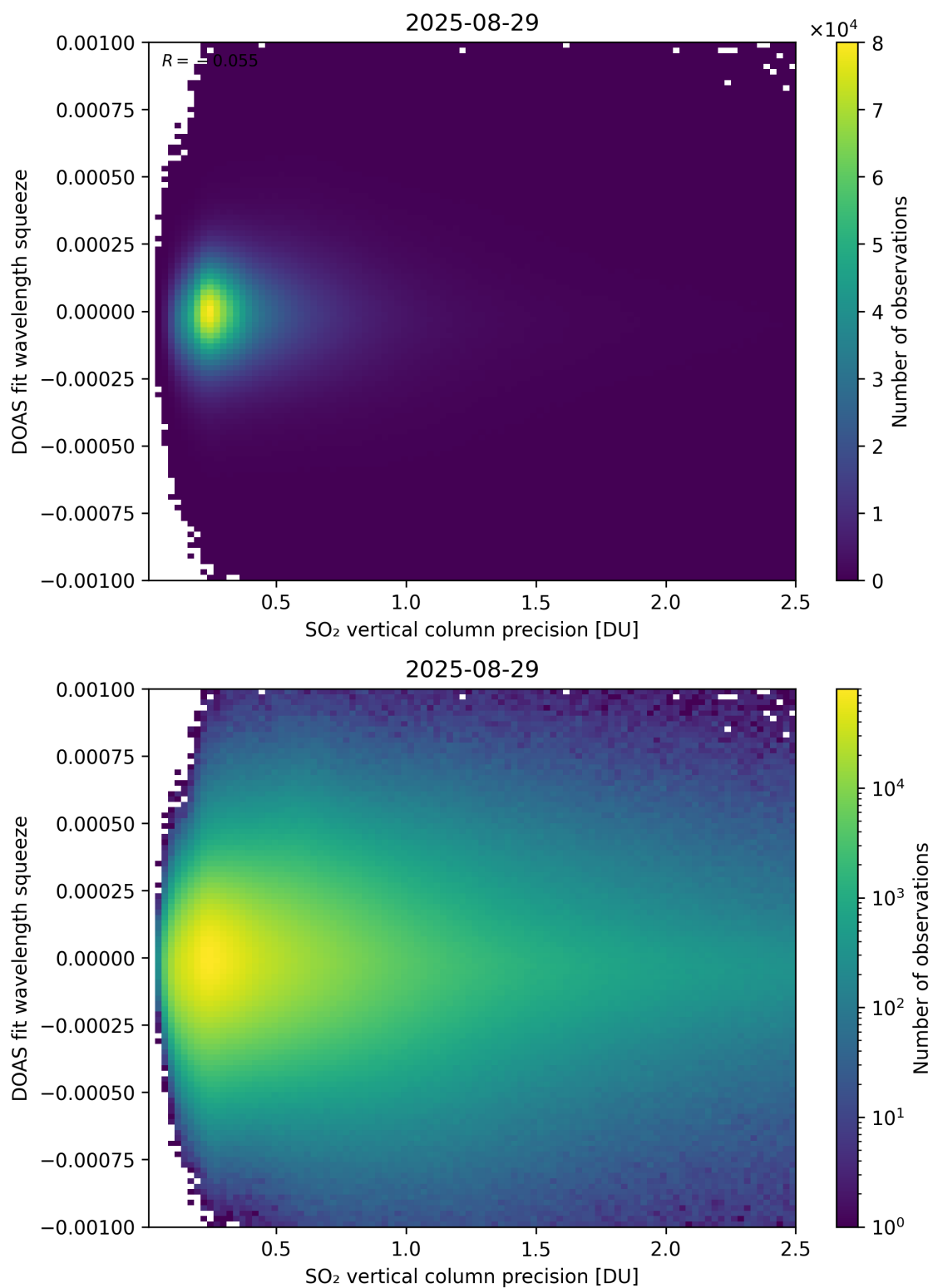
Figure 333: Scatter density plot of “SO 2 vertical column precision” against “DOAS fit wavelength squeeze” for 2025-08-28 to 2025-08-30.
