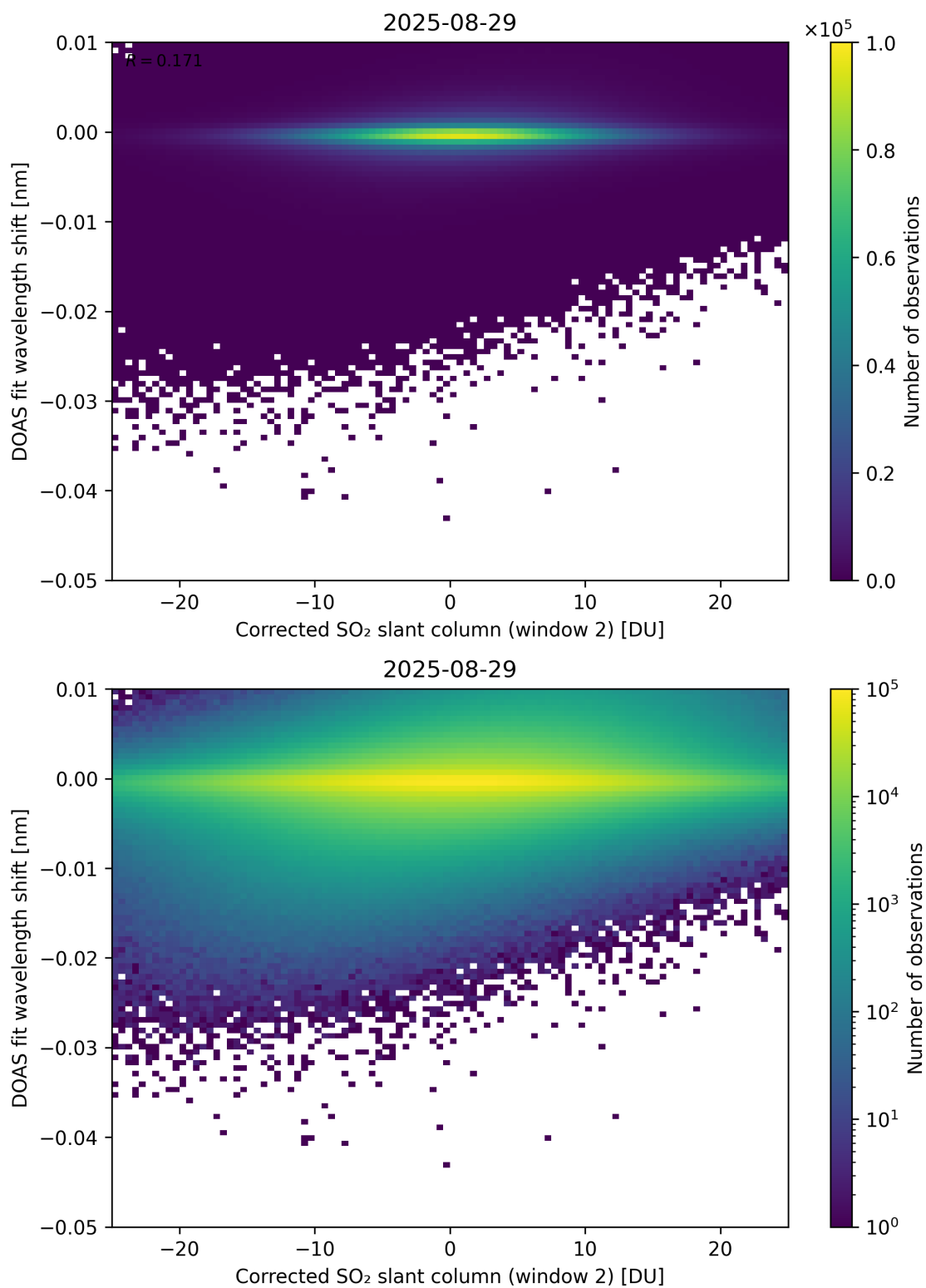
Figure 246: Scatter density plot of “Corrected SO 2 slant column (window 2)” against “DOAS fit wavelength shift” for 2025-08-28 to 2025-08-30.
