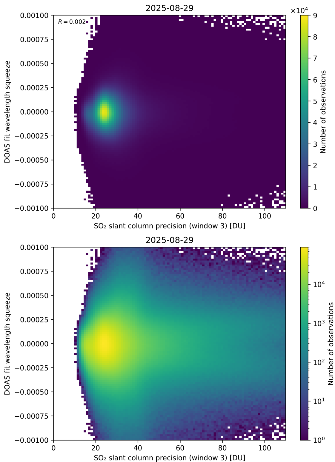
Figure 309: Scatter density plot of “SO 2 slant column precision (window 3)” against “DOAS fit wavelength squeeze” for 2025-08-28 to 2025-08-30.
