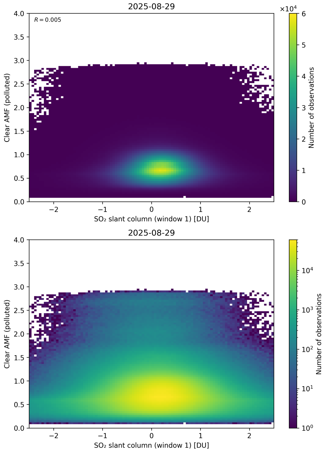
Figure 282: Scatter density plot of “SO 2 slant column (window 1)” against “Clear AMF (polluted)” for 2025-08-28 to 2025-08-30.
