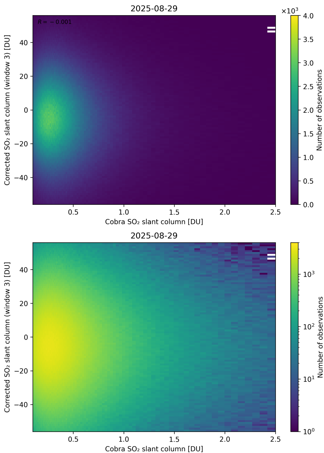
Figure 218: Scatter density plot of “Cobra SO 2 slant column” against “Corrected SO 2 slant column (window 3)” for 2025-08-28 to 2025-08-30.
