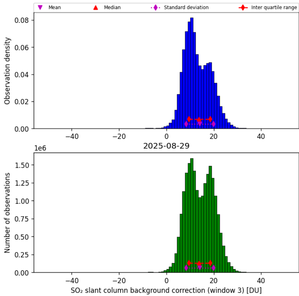
Figure 74: Histogram of “SO 2 slant column background correction (window 3)” for 2025-08-28 to 2025-08-30
