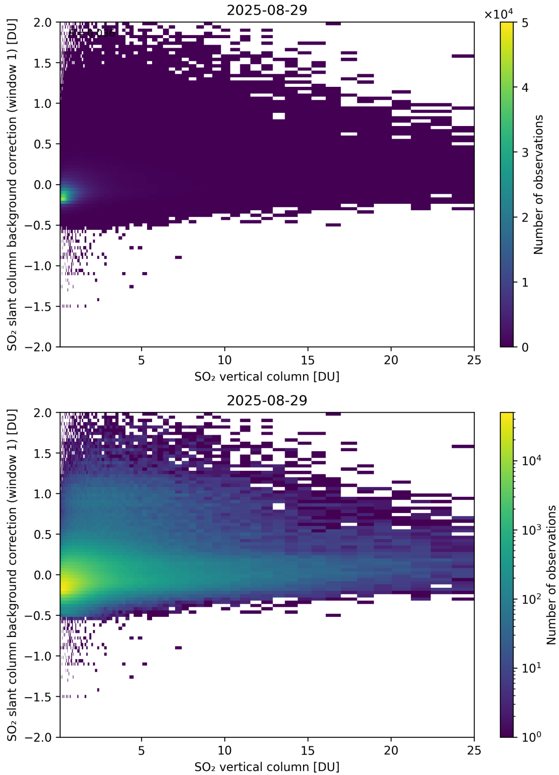
Figure 323: Scatter density plot of “SO 2 vertical column” against “SO 2 slant column background correction (window 1)” for 2025-08-28 to 2025-08-30.
