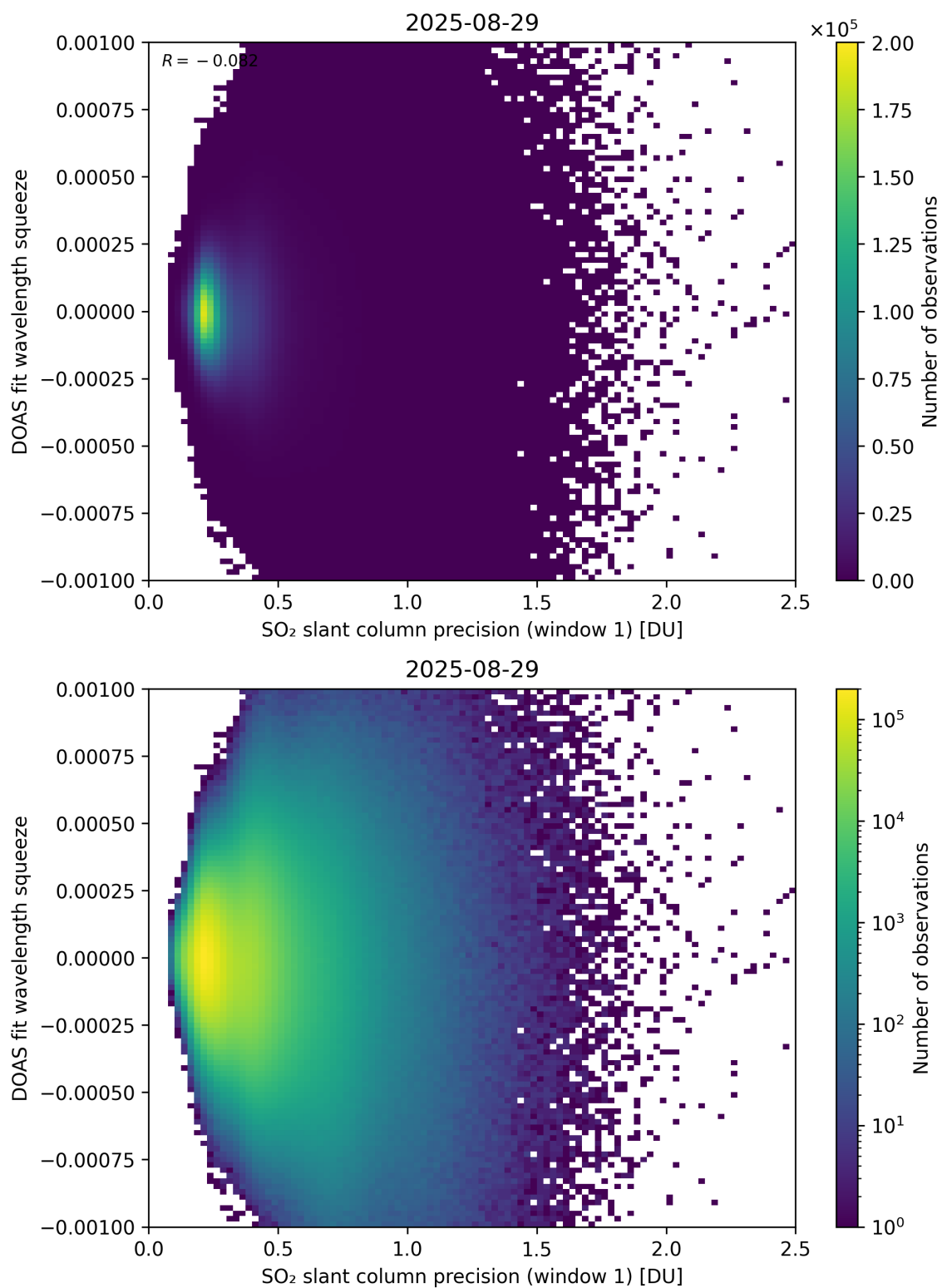
Figure 272: Scatter density plot of “SO 2 slant column precision (window 1)” against “DOAS fit wavelength squeeze” for 2025-08-28 to 2025-08-30.
