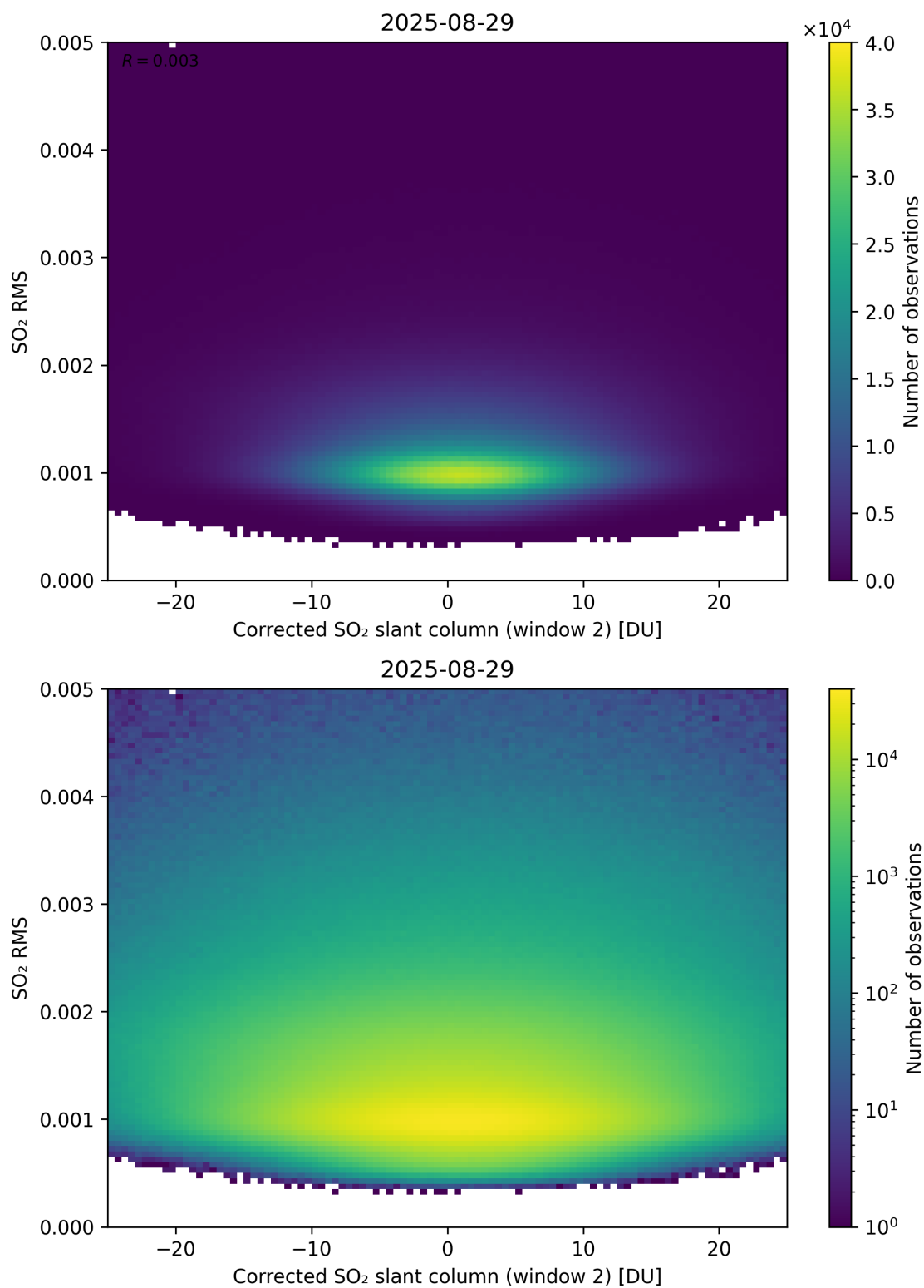
Figure 248: Scatter density plot of “Corrected SO 2 slant column (window 2)” against “SO 2 RMS” for 2025-08-28 to 2025-08-30.
