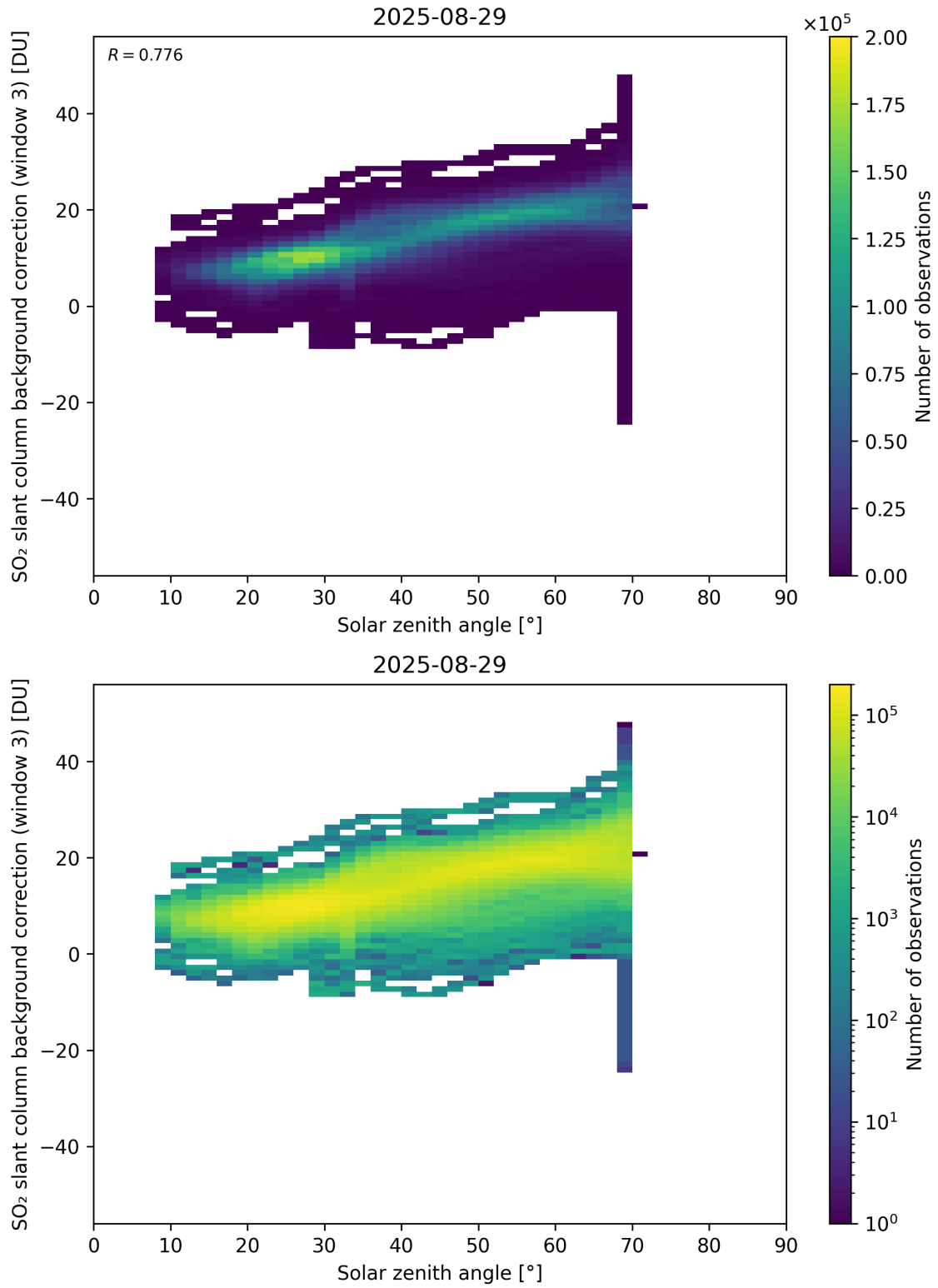
Figure 173: Scatter density plot of “Solar zenith angle” against “SO 2 slant column background correction (window 3)” for 2025-08-28 to 2025-08-30.
