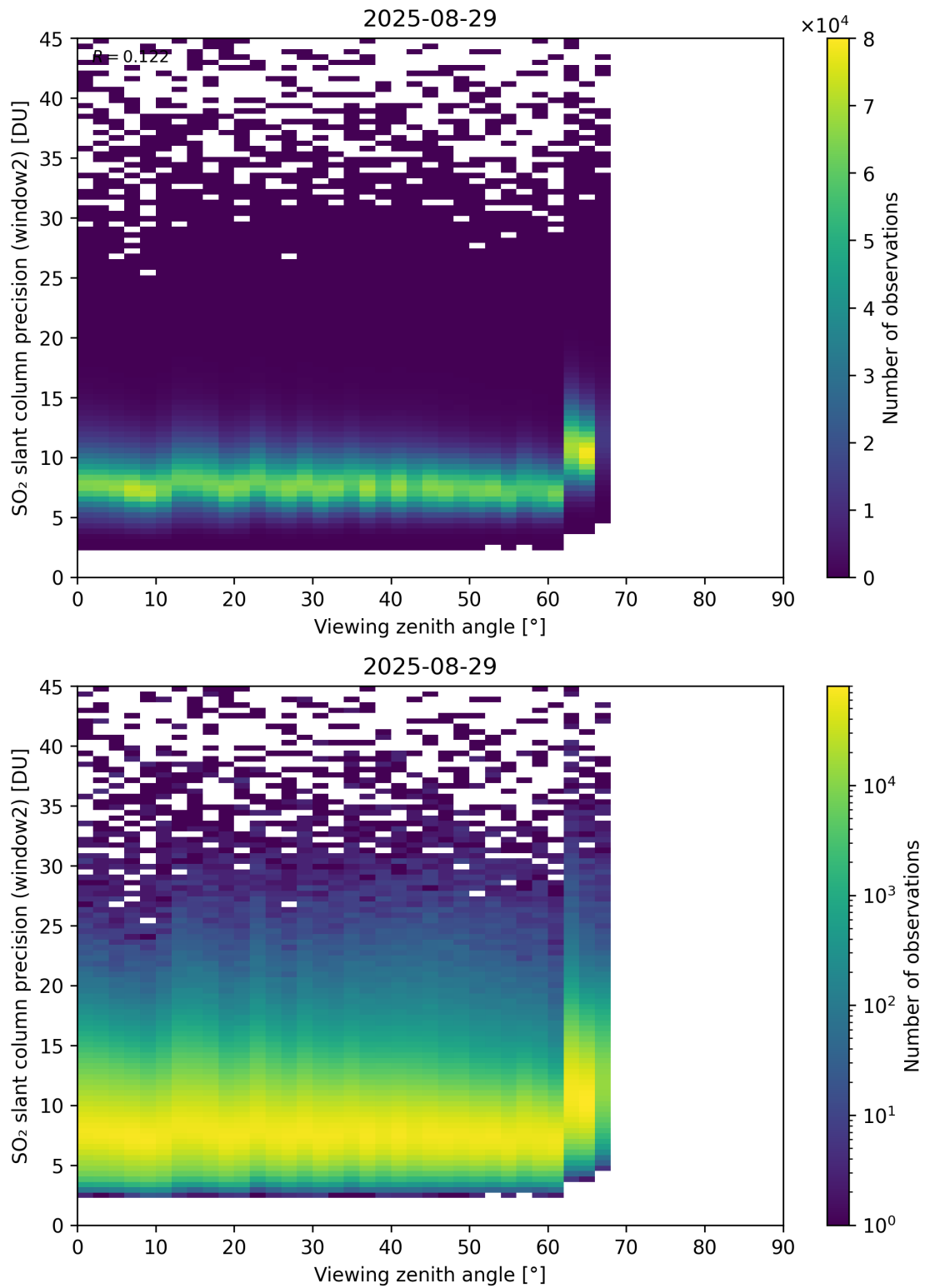
Figure 378: Scatter density plot of “Viewing zenith angle” against “SO 2 slant column precision (window2)” for 2025-08-28 to 2025-08-30.
