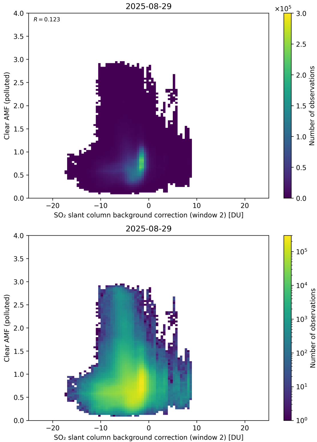
Figure 126: Scatter density plot of “SO 2 slant column background correction (window 2)” against “Clear AMF (polluted)” for 2025-08-28 to 2025-08-30.
