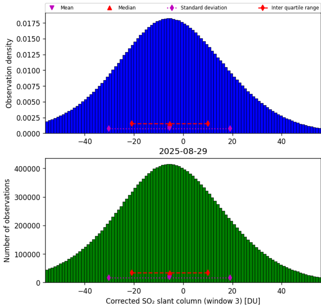
Figure 73: Histogram of “Corrected SO 2 slant column (window 3)” for 2025-08-28 to 2025-08-30
