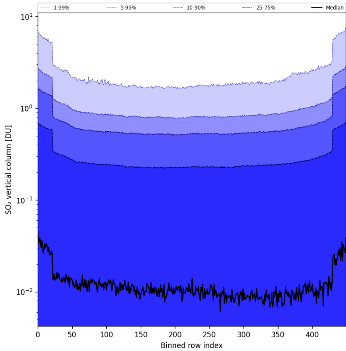
Figure 84: Along track statistics of “SO 2 vertical column” for 2025-08-28 to 2025-08-30
