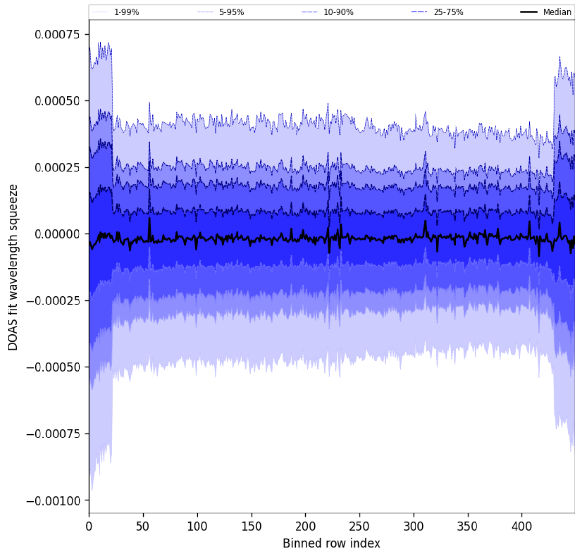
Figure 103: Along track statistics of “DOAS fit wavelength squeeze” for 2025-08-28 to 2025-08-30
