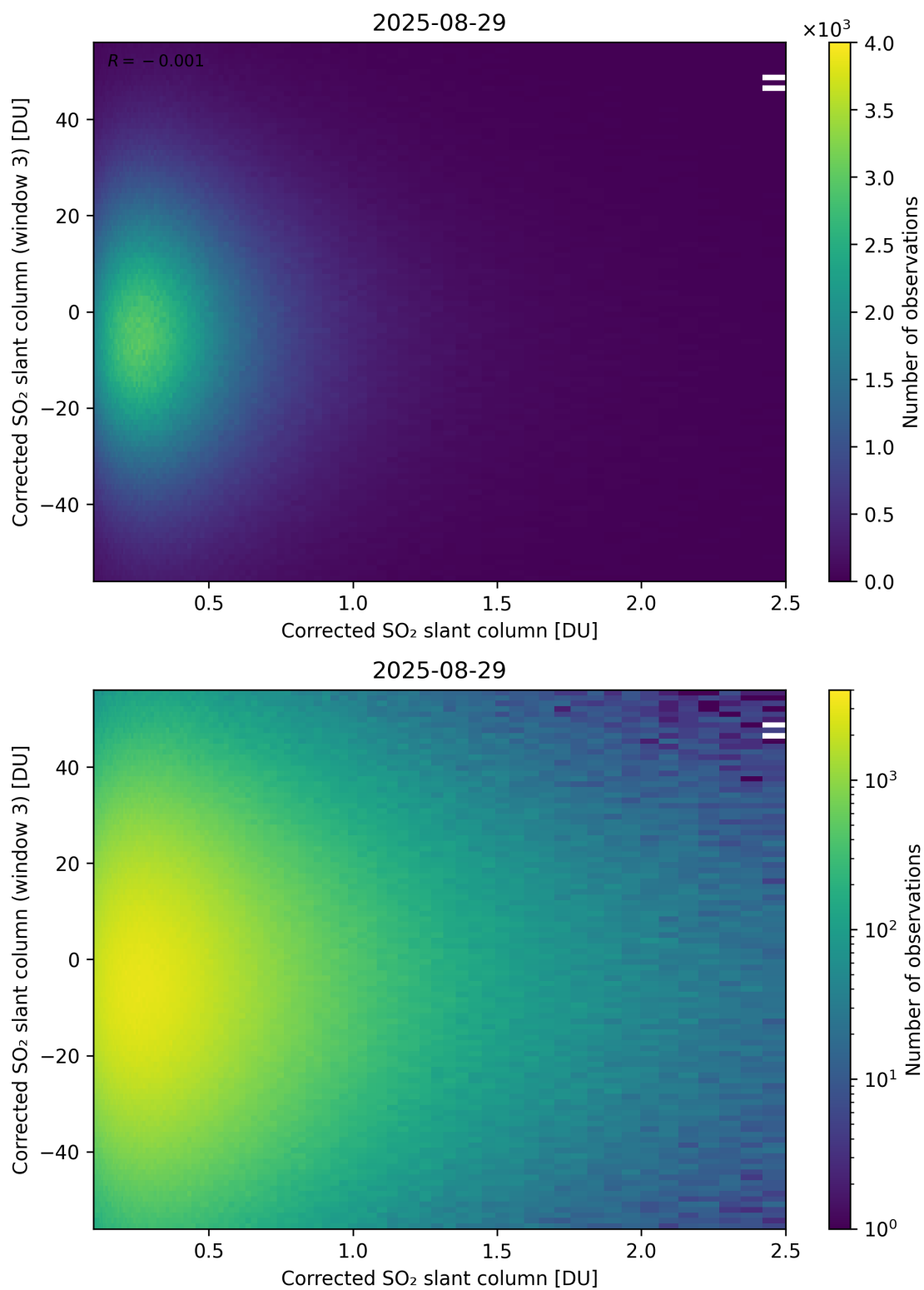
Figure 236: Scatter density plot of “Corrected SO 2 slant column” against “Corrected SO 2 slant column (window 3)” for 2025-08-28 to 2025-08-30.
