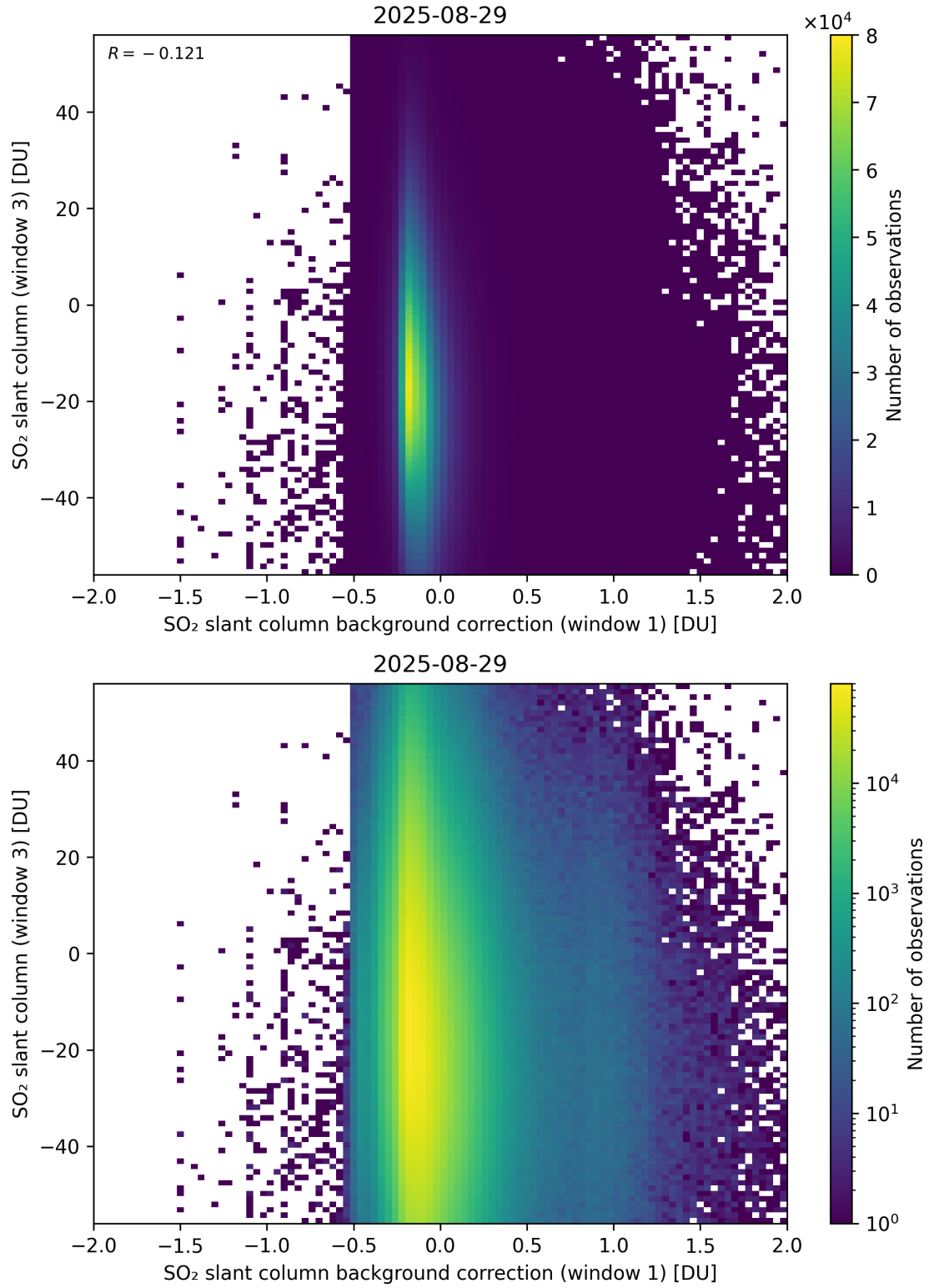
Figure 118: Scatter density plot of “SO 2 slant column background correction (window 1)” against “SO 2 slant column (window 3)” for 2025-08-28 to 2025-08-30.
