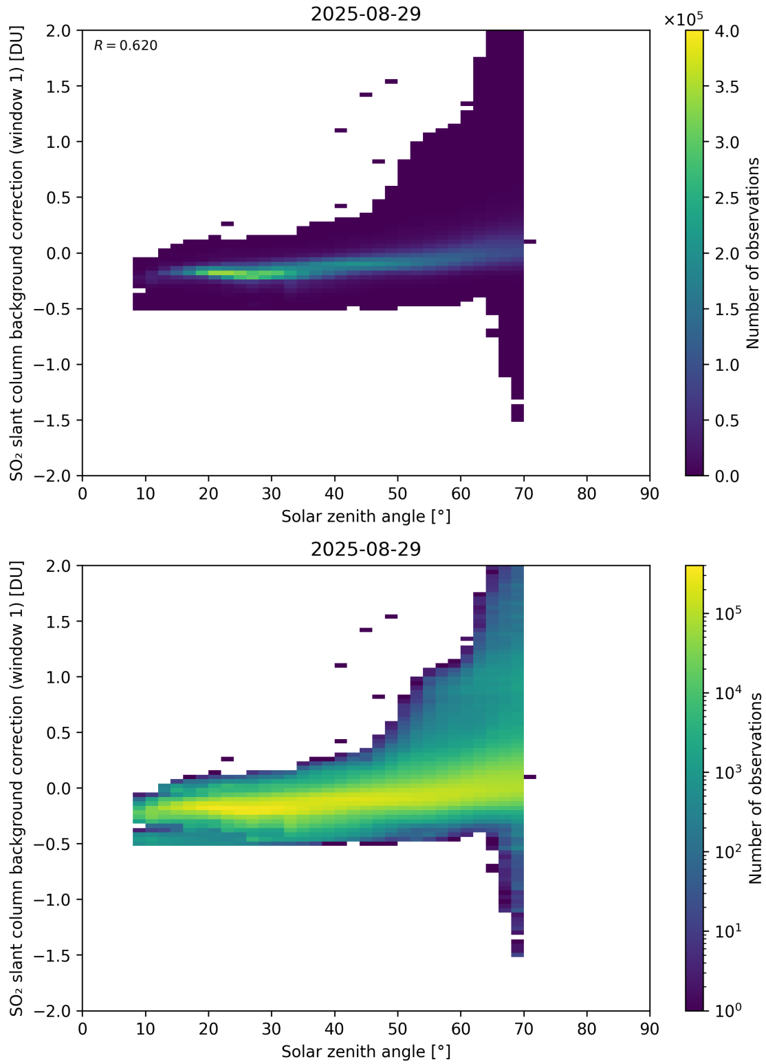
Figure 171: Scatter density plot of “Solar zenith angle” against “SO 2 slant column background correction (window 1)” for 2025-08-28 to 2025-08-30.
