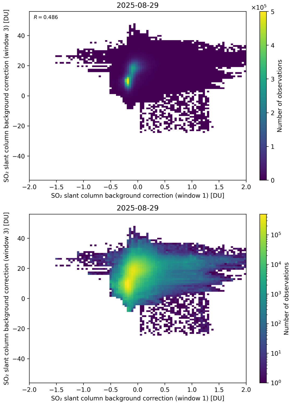
Figure 110: Scatter density plot of “SO 2 slant column background correction (window 1)” against “SO 2 slant column background correction (window 3)” for 2025-08-28 to 2025-08-30.
