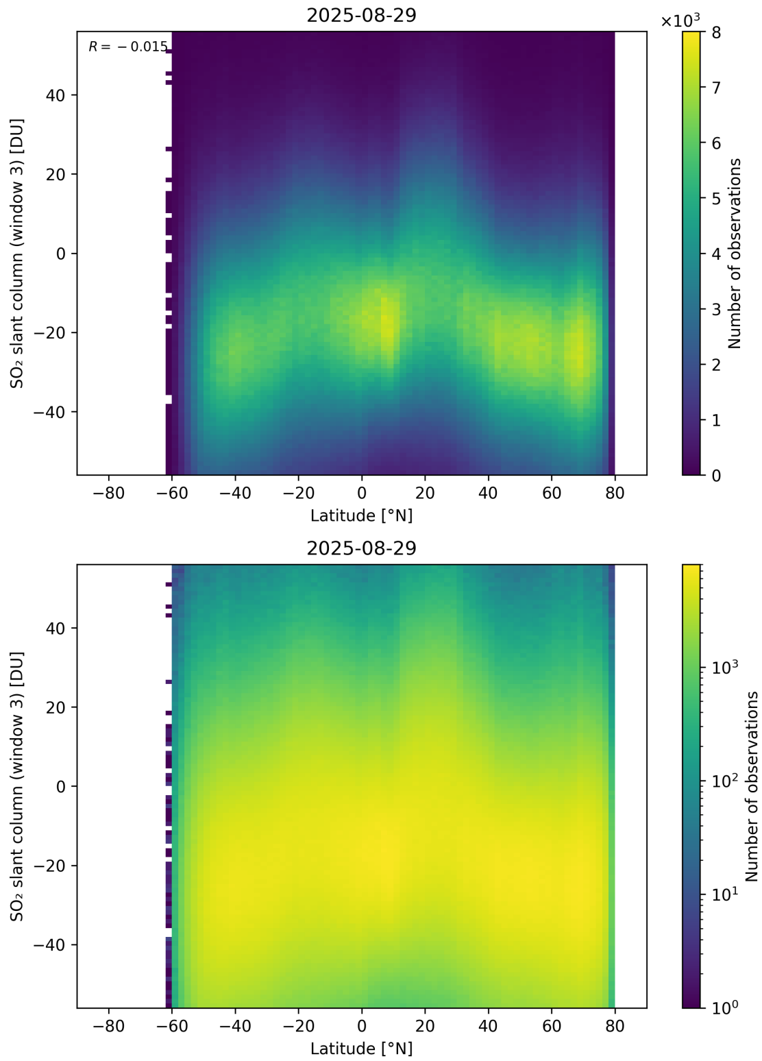
Figure 165: Scatter density plot of “Latitude” against “SO 2 slant column (window 3)” for 2025-08-28 to 2025-08-30.
