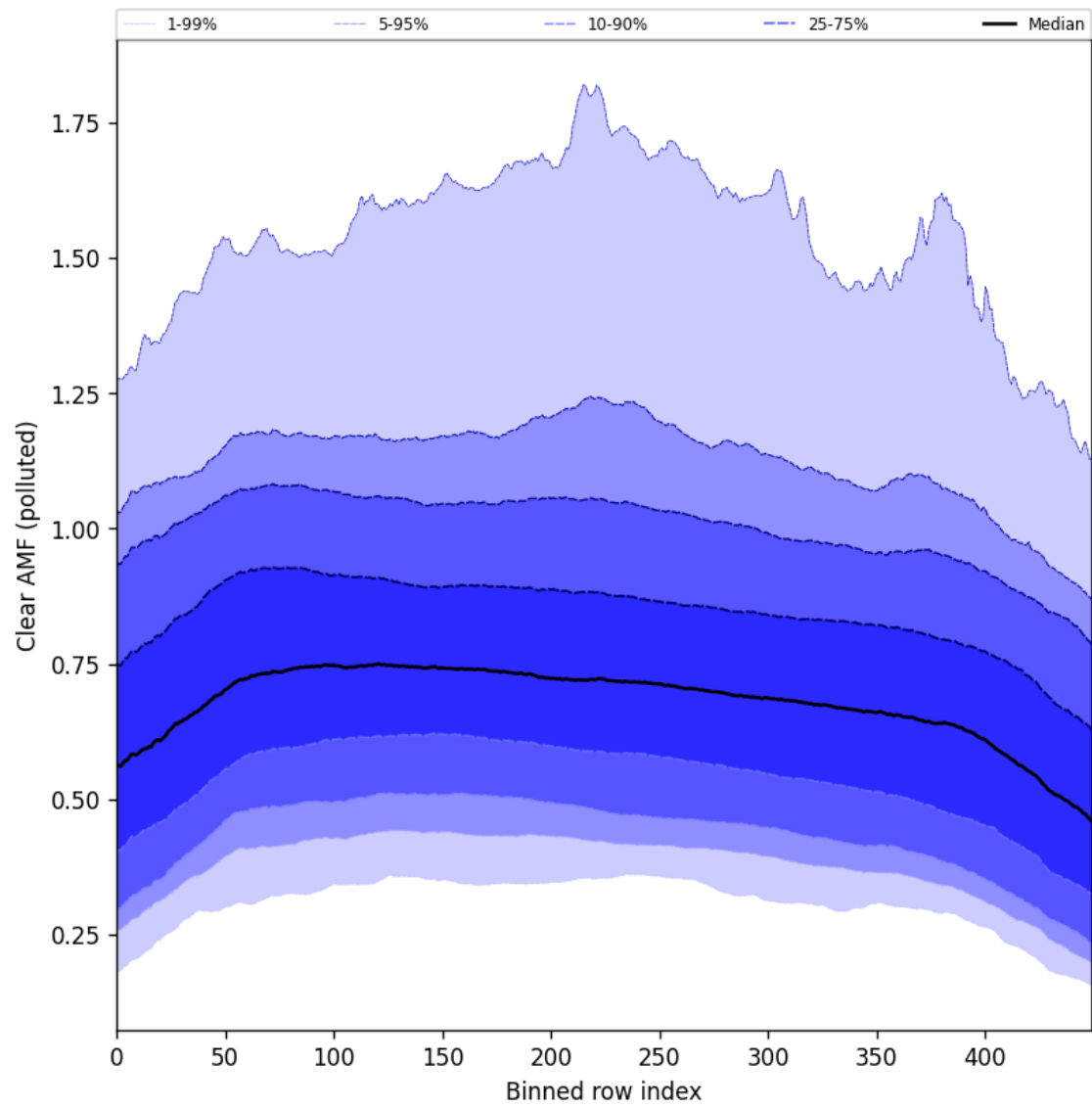
Figure 107: Along track statistics of “Clear AMF (polluted)” for 2025-08-28 to 2025-08-30
