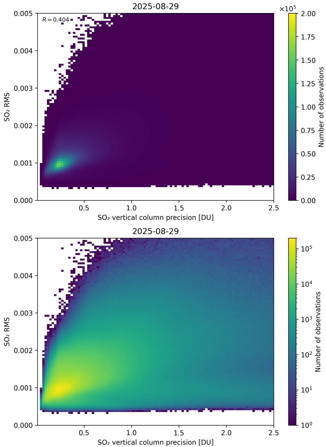
Figure 334: Scatter density plot of “SO 2 vertical column precision” against “SO 2 RMS” for 2025-08-28 to 2025-08-30.
