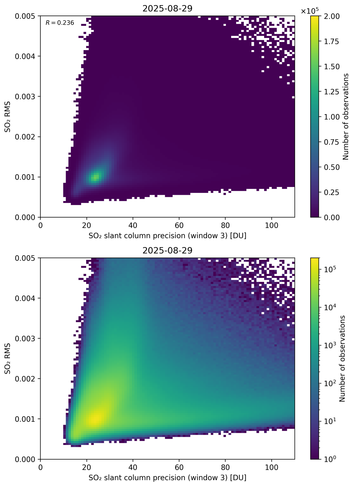
Figure 310: Scatter density plot of “SO 2 slant column precision (window 3)” against “SO 2 RMS” for 2025-08-28 to 2025-08-30.
