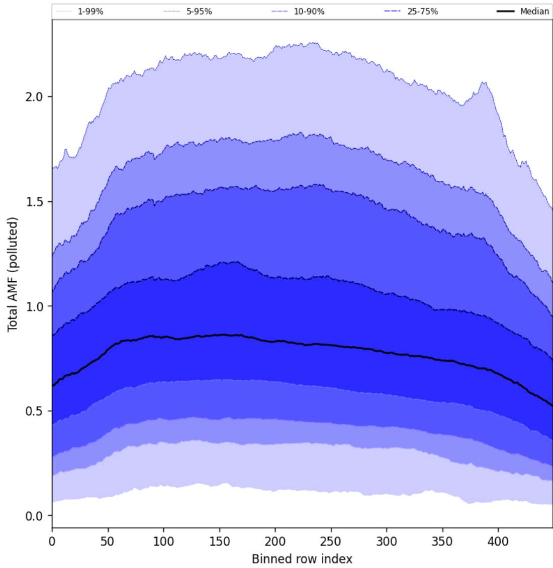
Figure 105: Along track statistics of “Total AMF (polluted)” for 2025-08-28 to 2025-08-30
