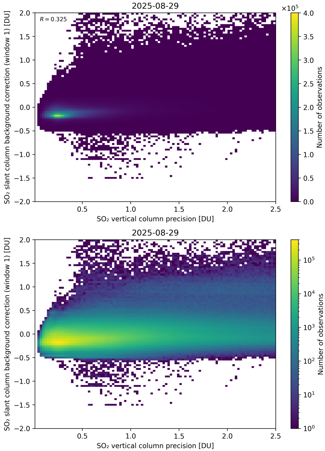
Figure 329: Scatter density plot of “SO 2 vertical column precision” against “SO 2 slant column background correction (window 1)” for 2025-08-28 to 2025-08-30.
