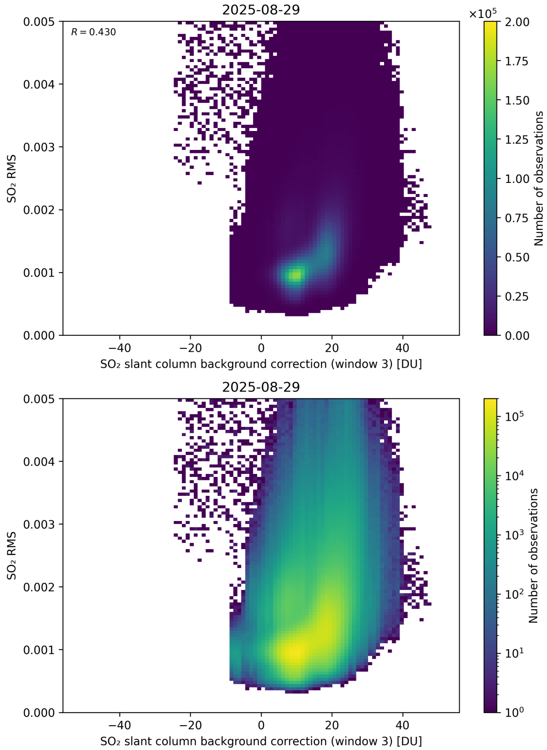
Figure 134: Scatter density plot of “SO 2 slant column background correction (window 3)” against “SO 2 RMS” for 2025-08-28 to 2025-08-30.
