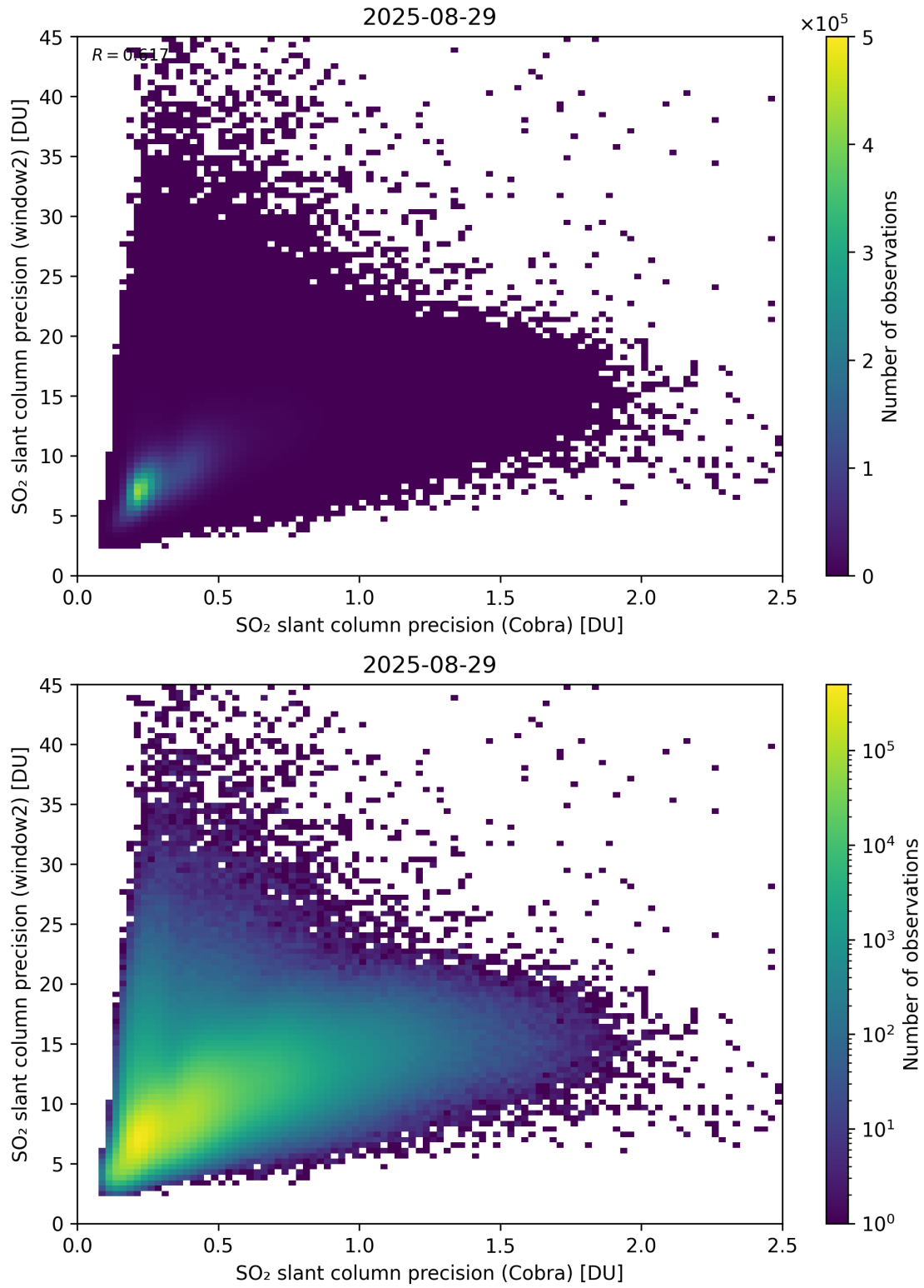
Figure 210: Scatter density plot of “SO 2 slant column precision (Cobra)” against “SO 2 slant column precision (window2)” for 2025-08-28 to 2025-08-30.
