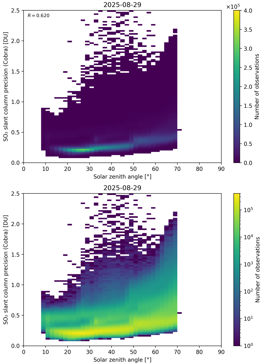
Figure 180: Scatter density plot of “Solar zenith angle” against “SO 2 slant column precision (Cobra)” for 2025-08-28 to 2025-08-30.
