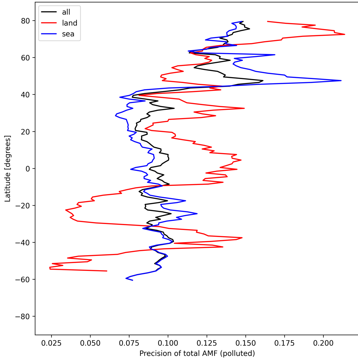
Figure 54: Zonal average of “Precision of total AMF (polluted)” for 2025-08-28 to 2025-08-30.
