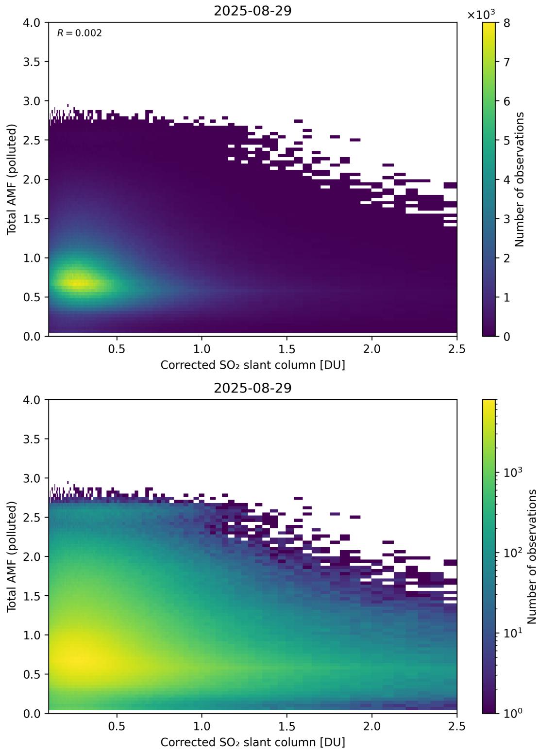
Figure 242: Scatter density plot of “Corrected SO 2 slant column” against “Total AMF (polluted)” for 2025-08-28 to 2025-08-30.
