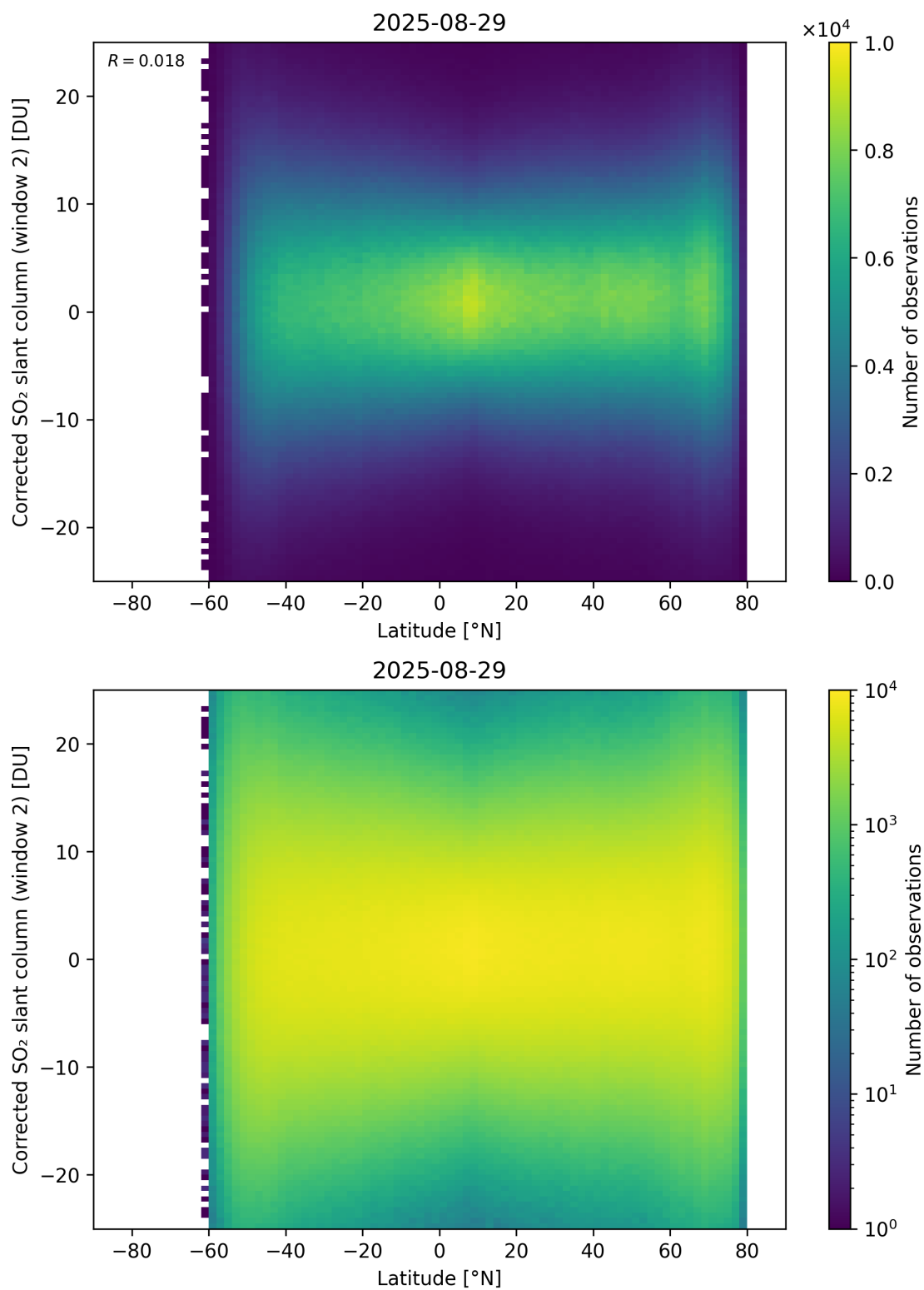
Figure 160: Scatter density plot of “Latitude” against “Corrected SO 2 slant column (window 2)” for 2025-08-28 to 2025-08-30.
