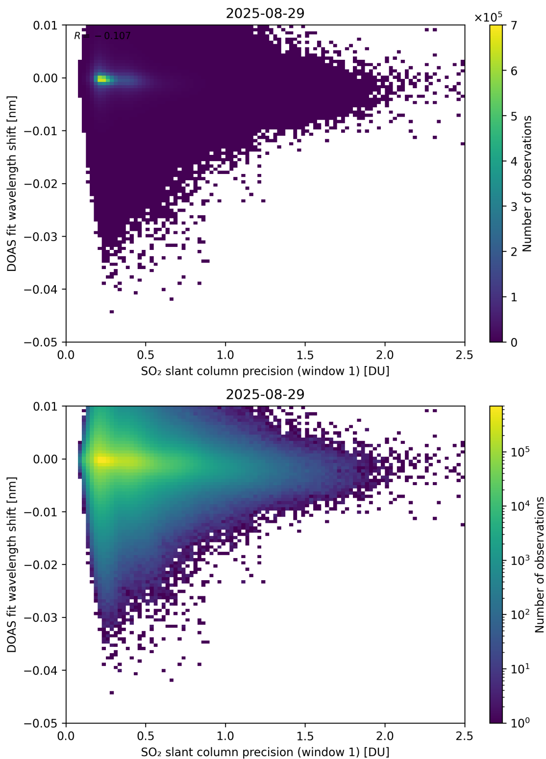
Figure 271: Scatter density plot of “SO 2 slant column precision (window 1)” against “DOAS fit wavelength shift” for 2025-08-28 to 2025-08-30.
