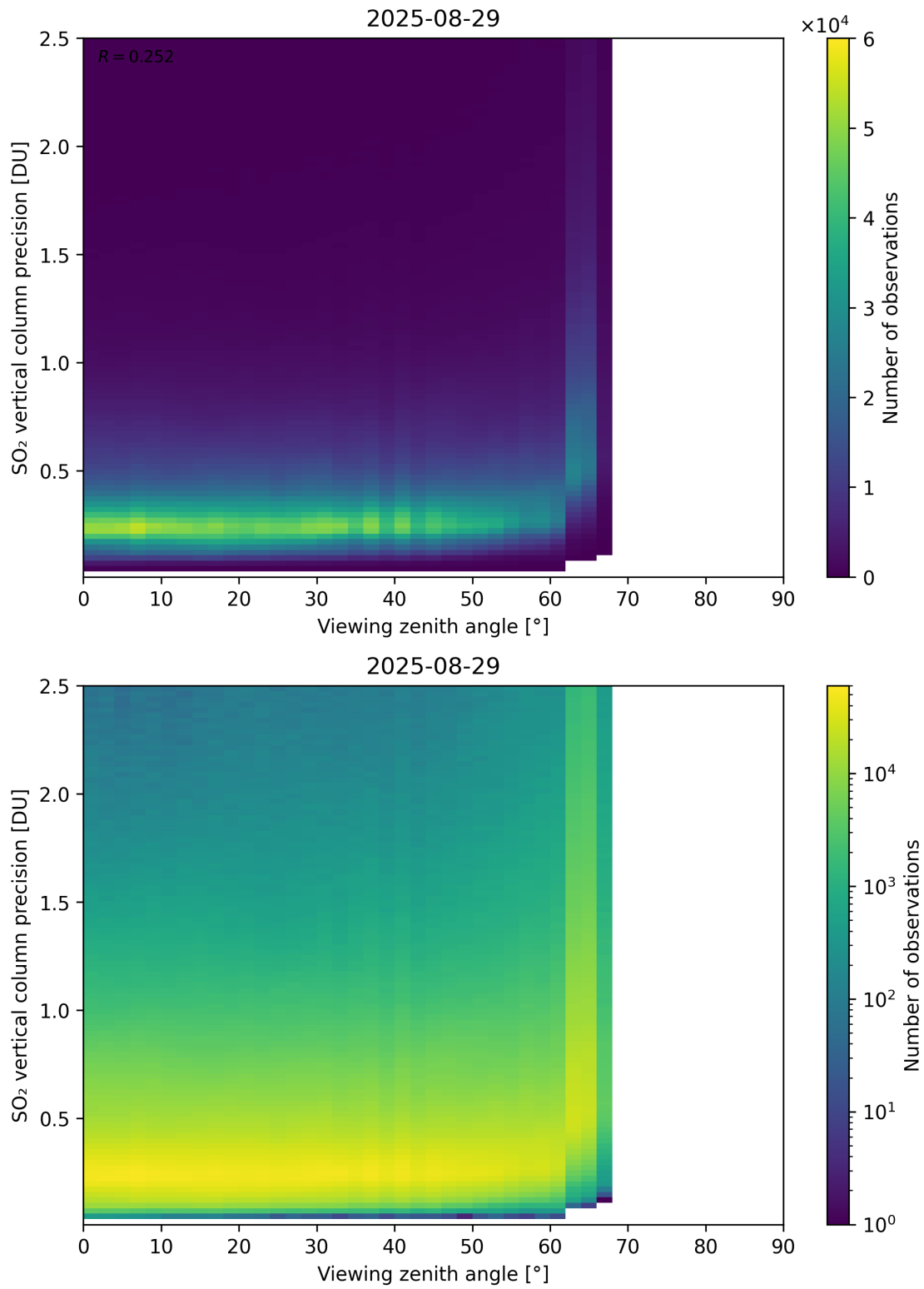
Figure 384: Scatter density plot of “Viewing zenith angle” against “SO 2 vertical column precision” for 2025-08-28 to 2025-08-30.
