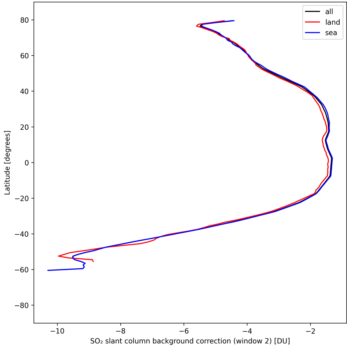
Figure 44: Zonal average of “SO 2 slant column background correction (window 2)” for 2025-08-28 to 2025-08-30.
