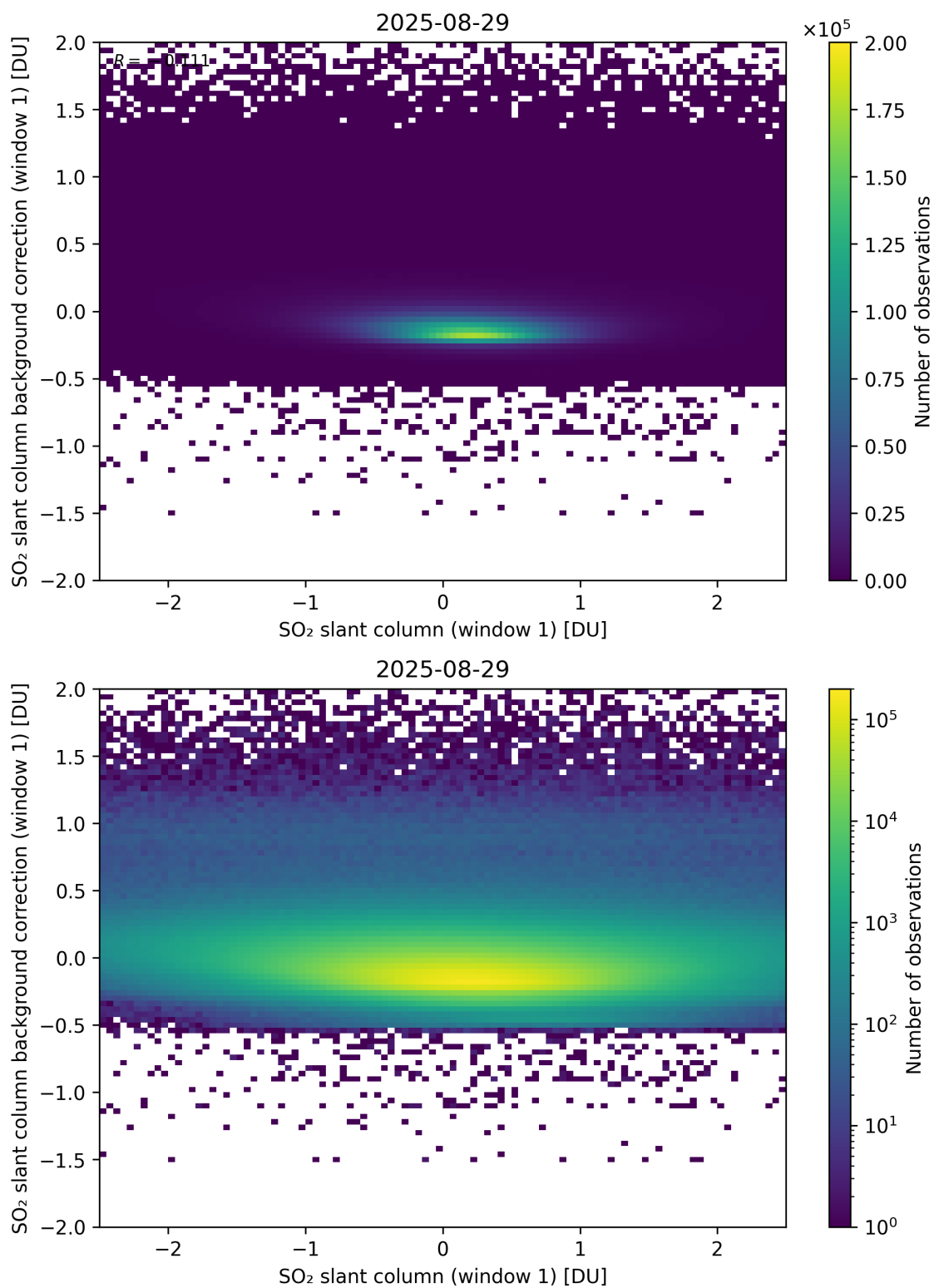
Figure 262: Scatter density plot of “SO 2 slant column (window 1)” against “SO 2 slant column background correction (window 1)” for 2025-08-28 to 2025-08-30.
