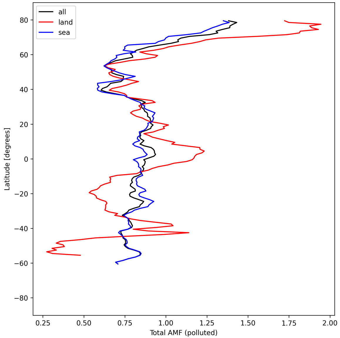
Figure 53: Zonal average of “Total AMF (polluted)” for 2025-08-28 to 2025-08-30.
