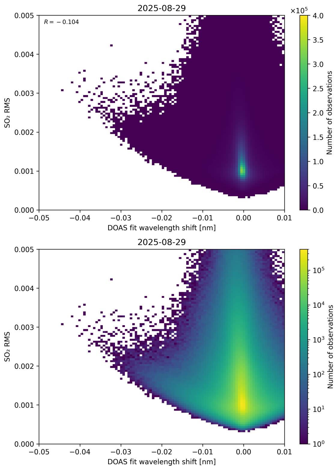
Figure 139: Scatter density plot of “DOAS fit wavelength shift” against “SO 2 RMS” for 2025-08-28 to 2025-08-30.
