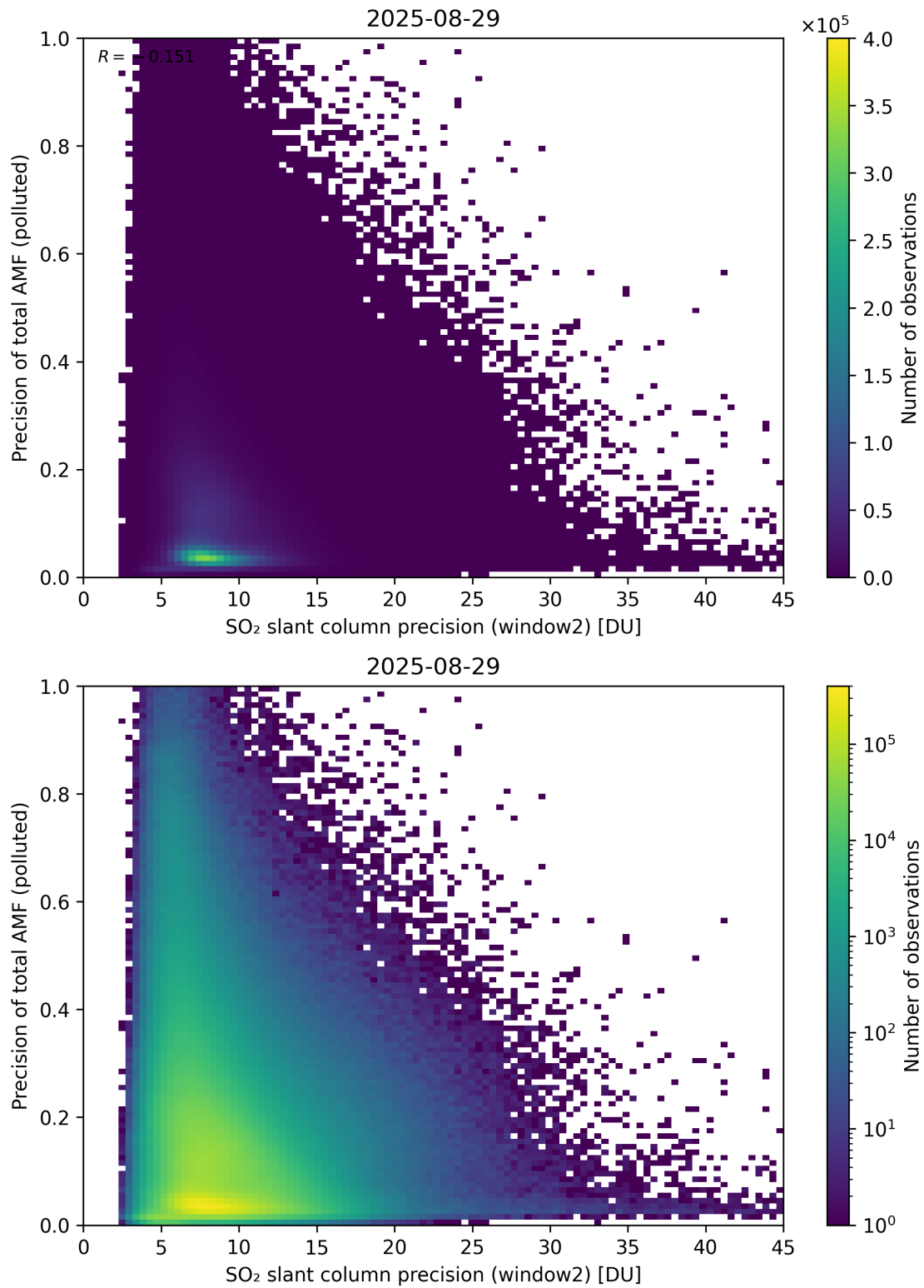
Figure 302: Scatter density plot of “SO 2 slant column precision (window2)” against “Precision of total AMF (polluted)” for 2025-08-28 to 2025-08-30.
