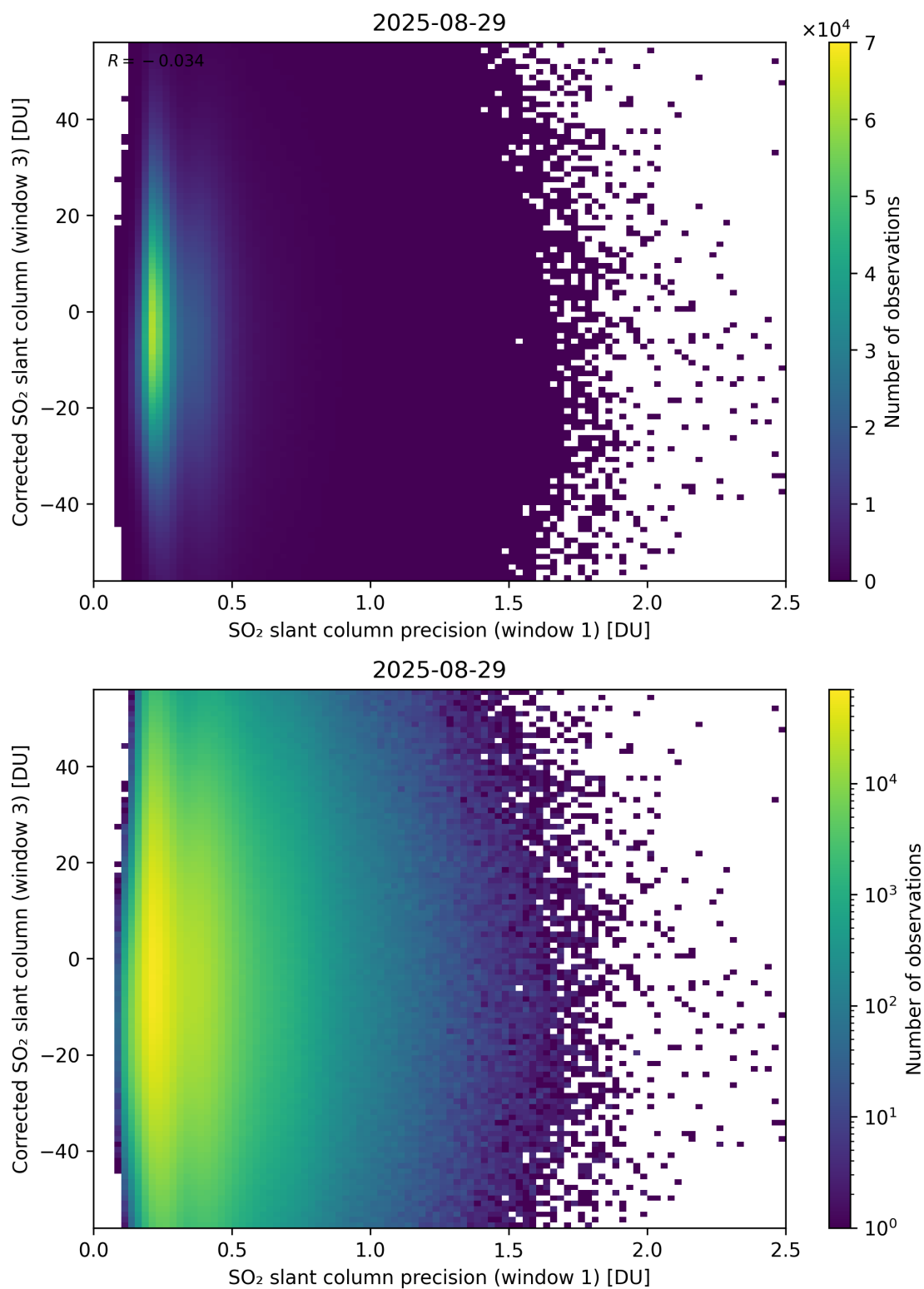
Figure 276: Scatter density plot of “SO 2 slant column precision (window 1)” against “Corrected SO 2 slant column (window 3)” for 2025-08-28 to 2025-08-30.
