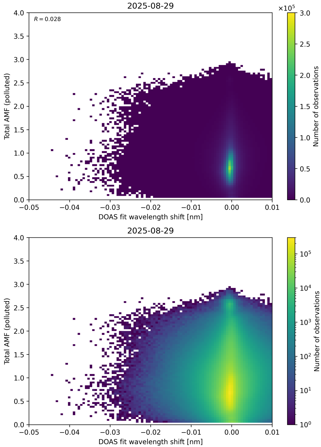
Figure 141: Scatter density plot of “DOAS fit wavelength shift” against “Total AMF (polluted)” for 2025-08-28 to 2025-08-30.
