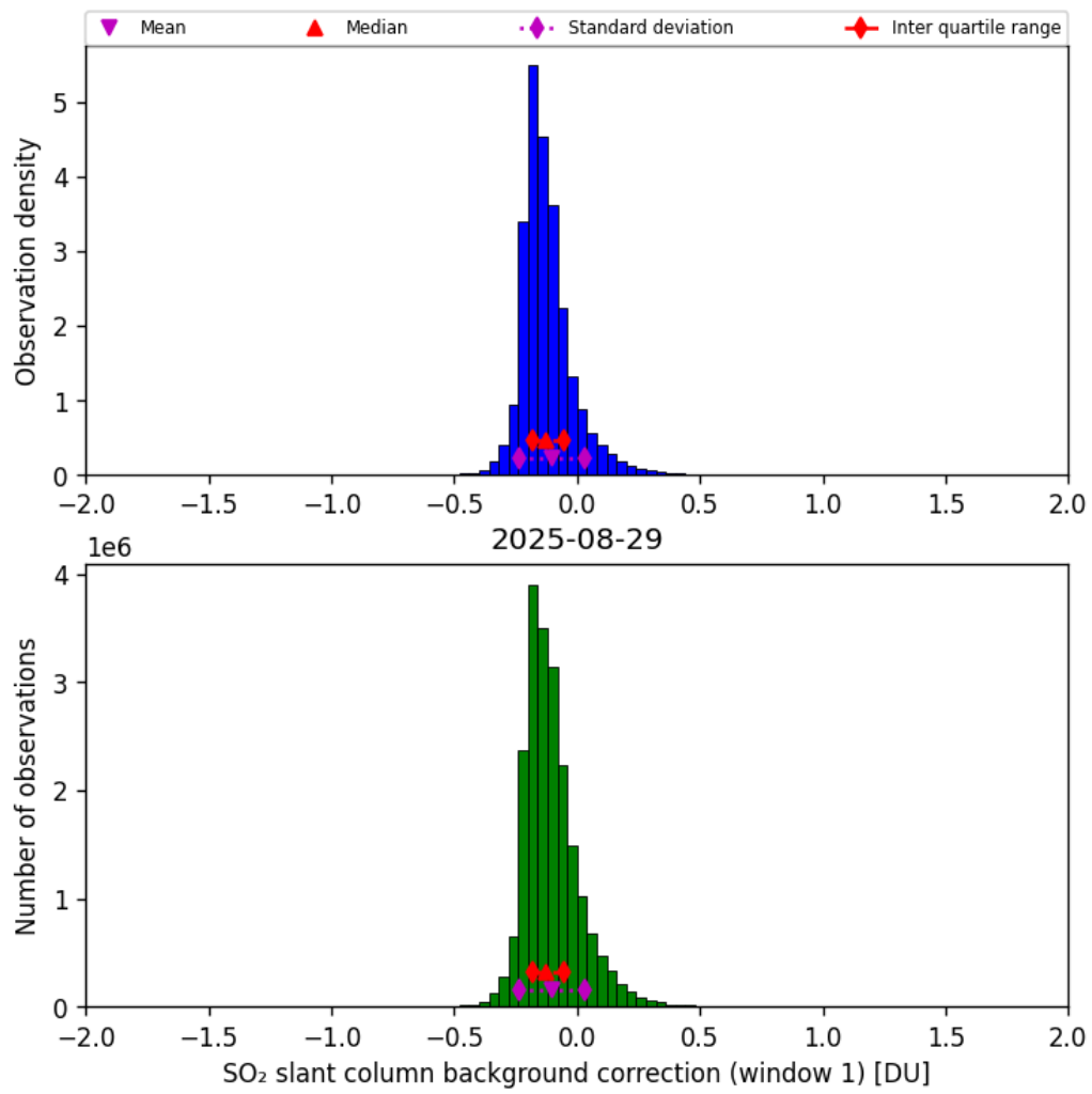
Figure 66: Histogram of “SO 2 slant column background correction (window 1)” for 2025-08-28 to 2025-08-30
