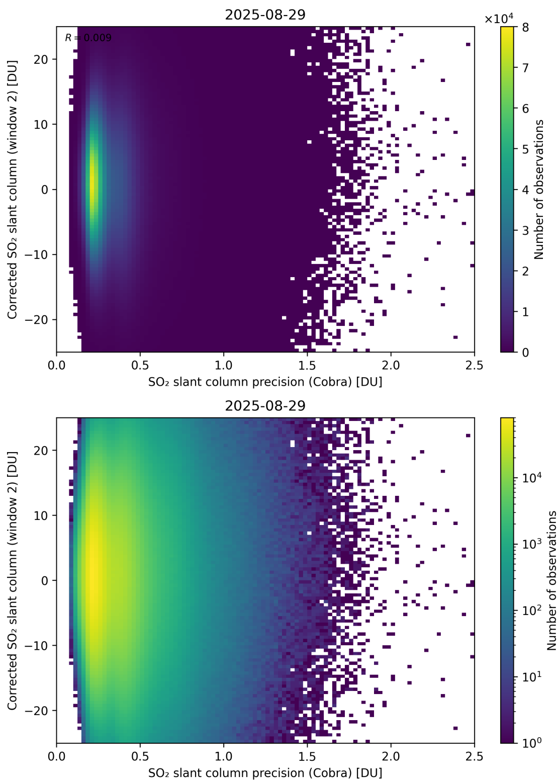
Figure 206: Scatter density plot of “SO 2 slant column precision (Cobra)” against “Corrected SO 2 slant column (window 2)” for 2025-08-28 to 2025-08-30.
