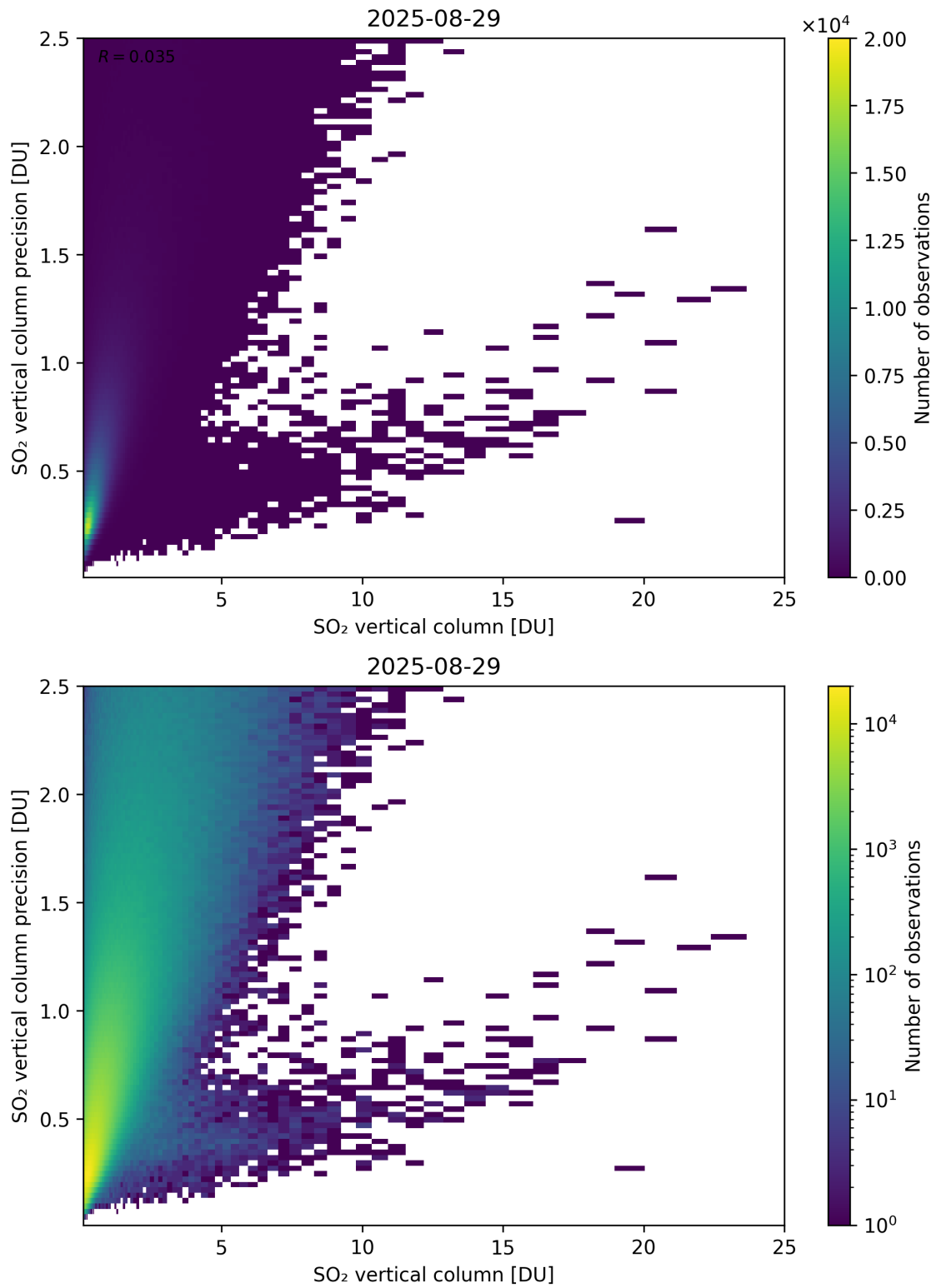
Figure 361: Scatter density plot of “SO 2 vertical column” against “SO 2 vertical column precision” for 2025-08-28 to 2025-08-30.
