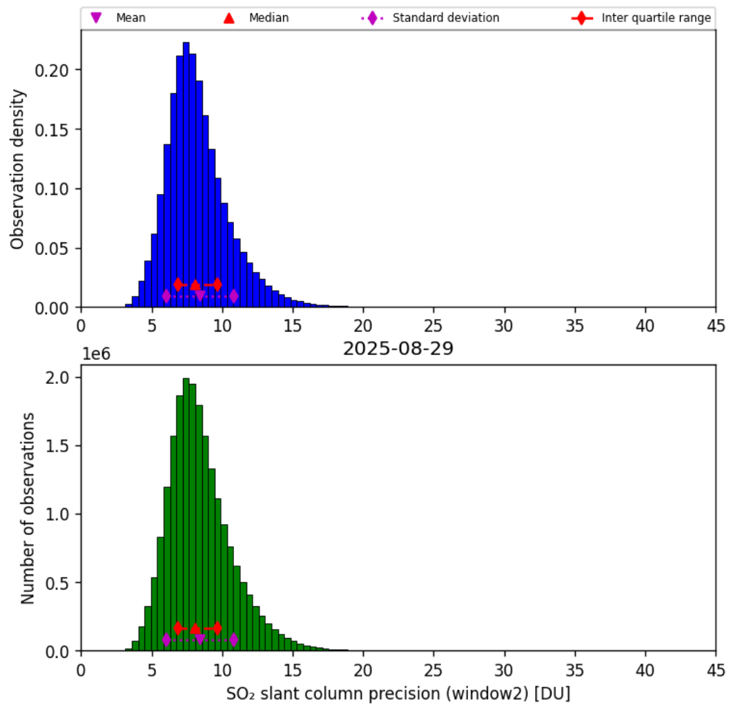
Figure 68: Histogram of “SO 2 slant column precision (window2)” for 2025-08-28 to 2025-08-30
