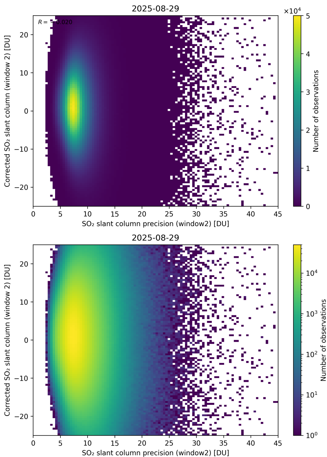
Figure 297: Scatter density plot of “SO 2 slant column precision (window2)” against “Corrected SO 2 slant column (window 2)” for 2025-08-28 to 2025-08-30.
