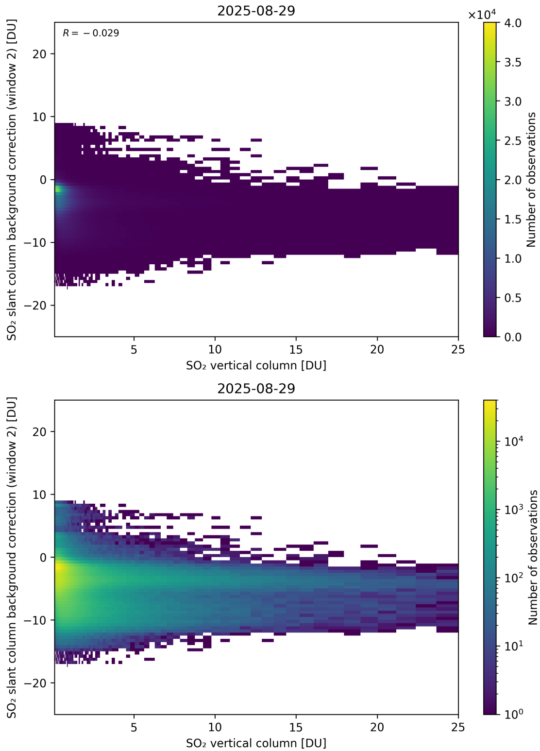
Figure 324: Scatter density plot of “SO 2 vertical column” against “SO 2 slant column background correction (window 2)” for 2025-08-28 to 2025-08-30.
