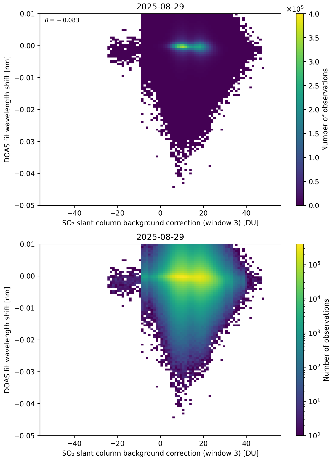
Figure 132: Scatter density plot of “SO 2 slant column background correction (window 3)” against “DOAS fit wavelength shift” for 2025-08-28 to 2025-08-30.
