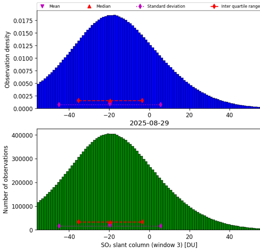
Figure 71: Histogram of “SO 2 slant column (window 3)” for 2025-08-28 to 2025-08-30
