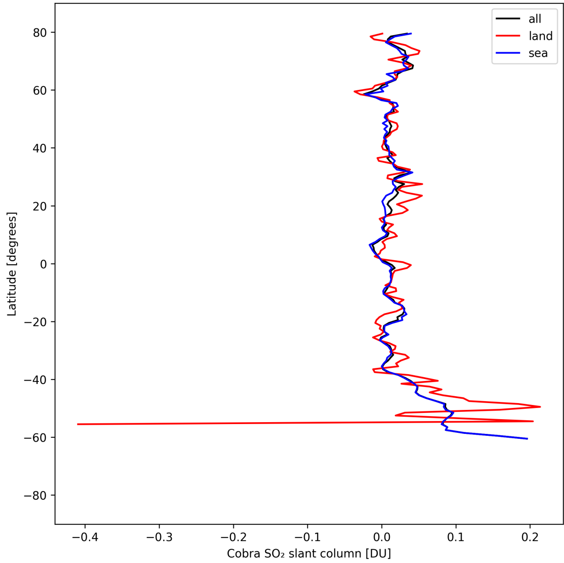
Figure 35: Zonal average of “Cobra SO 2 slant column” for 2025-08-28 to 2025-08-30.
