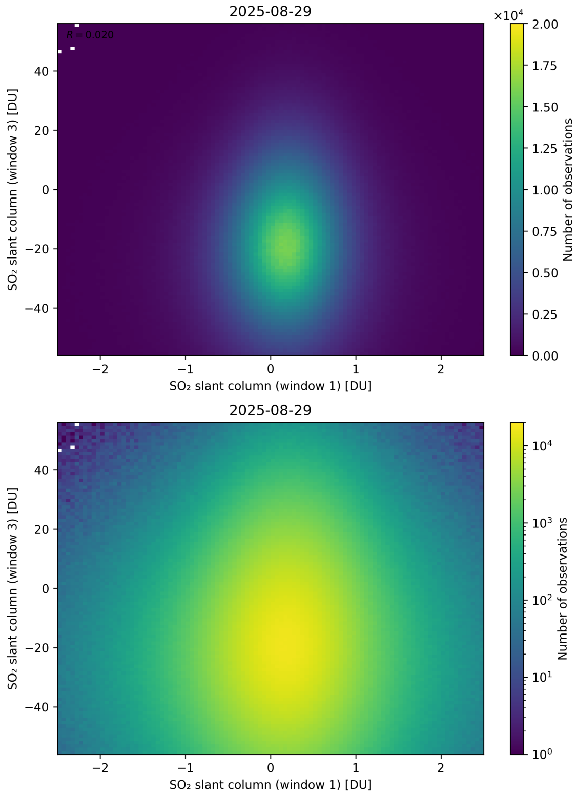
Figure 287: Scatter density plot of “SO 2 slant column (window 1)” against “SO 2 slant column (window 3)” for 2025-08-28 to 2025-08-30.
