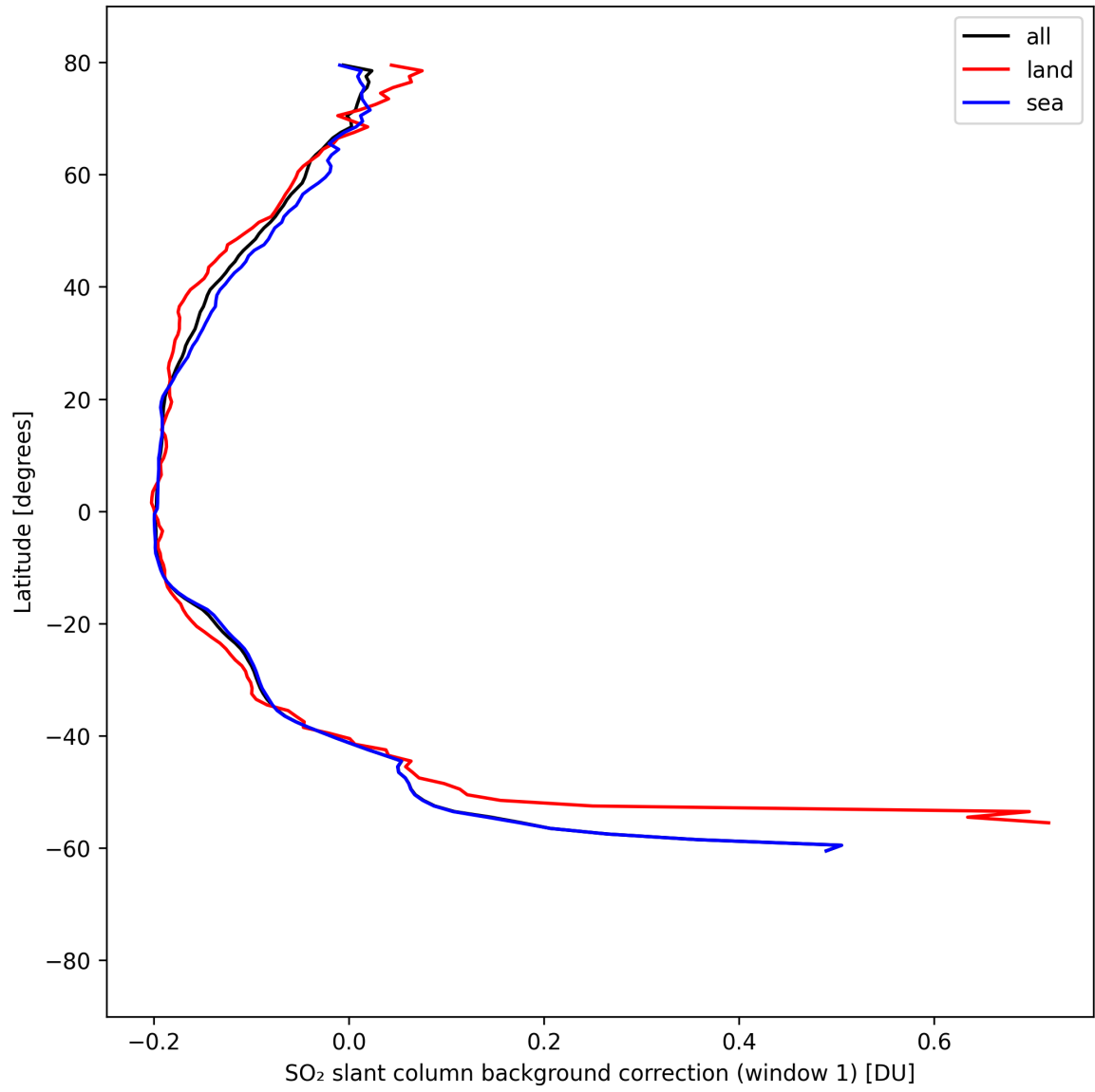
Figure 40: Zonal average of “SO 2 slant column background correction (window 1)” for 2025-08-28 to 2025-08-30.
