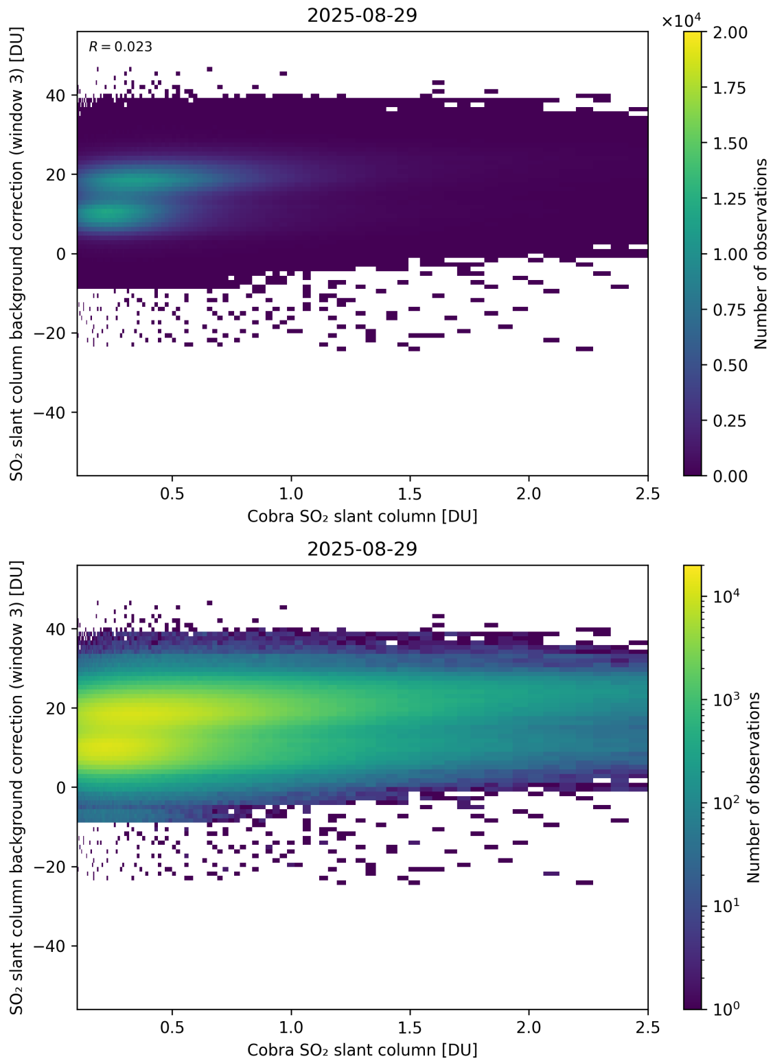
Figure 195: Scatter density plot of “Cobra SO 2 slant column” against “SO 2 slant column background correction (window 3)” for 2025-08-28 to 2025-08-30.
