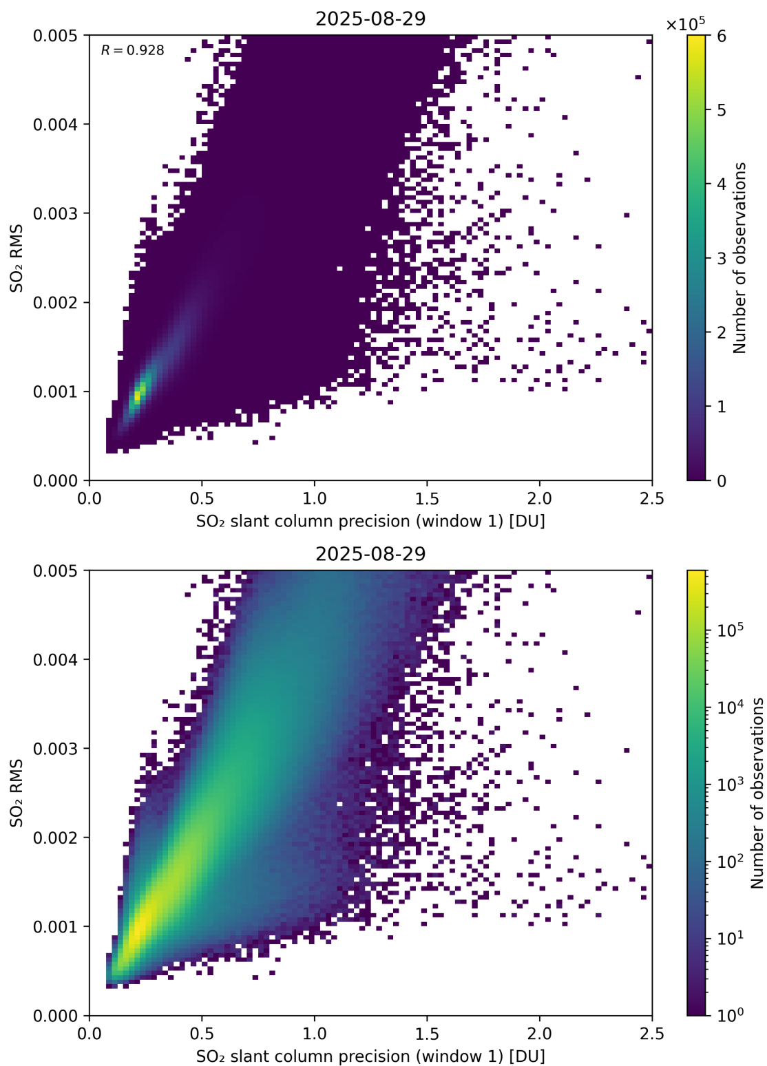
Figure 273: Scatter density plot of “SO 2 slant column precision (window 1)” against “SO 2 RMS” for 2025-08-28 to 2025-08-30.
