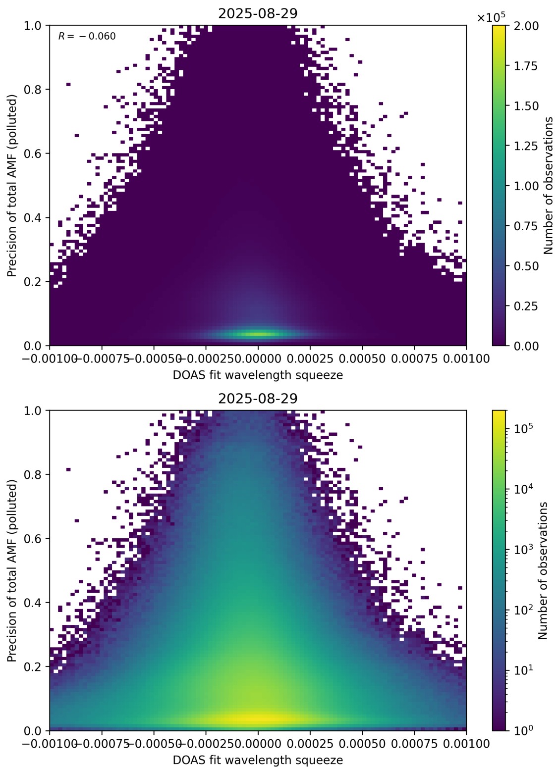
Figure 146: Scatter density plot of “DOAS fit wavelength squeeze” against “Precision of total AMF (polluted)” for 2025-08-28 to 2025-08-30.
