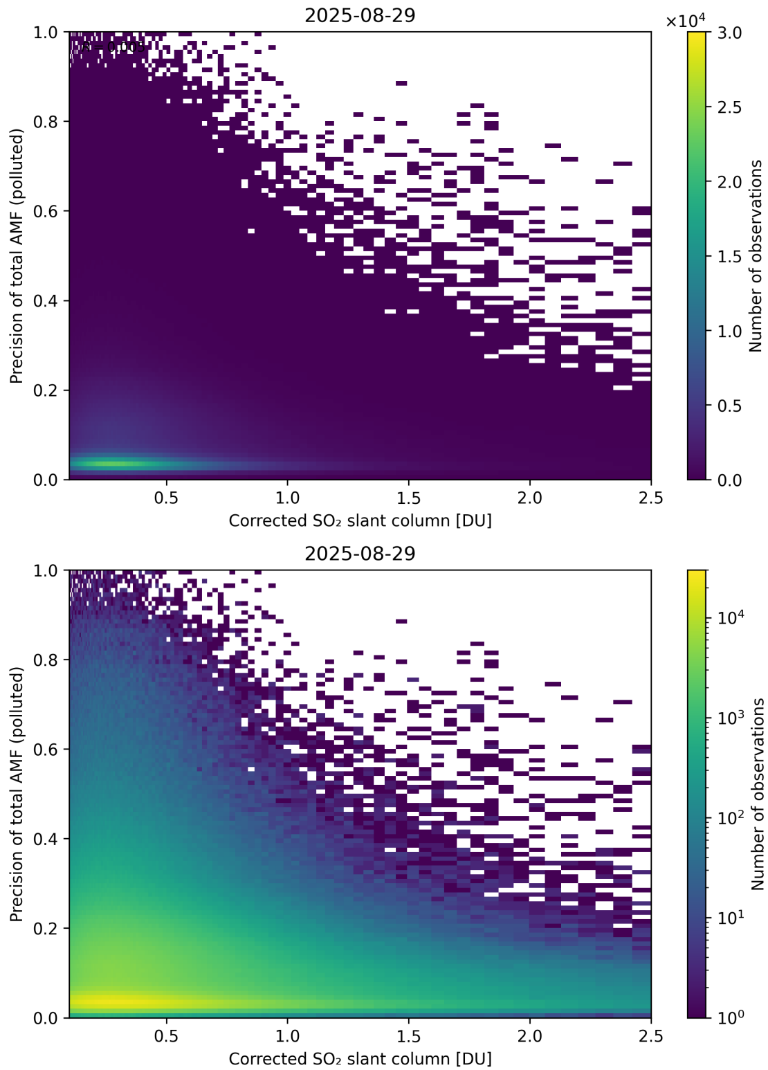
Figure 243: Scatter density plot of “Corrected SO 2 slant column” against “Precision of total AMF (polluted)” for 2025-08-28 to 2025-08-30.
