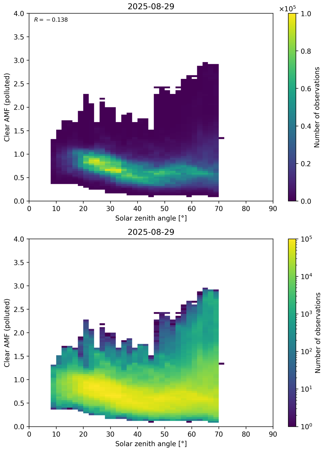
Figure 178: Scatter density plot of “Solar zenith angle” against “Clear AMF (polluted)” for 2025-08-28 to 2025-08-30.
