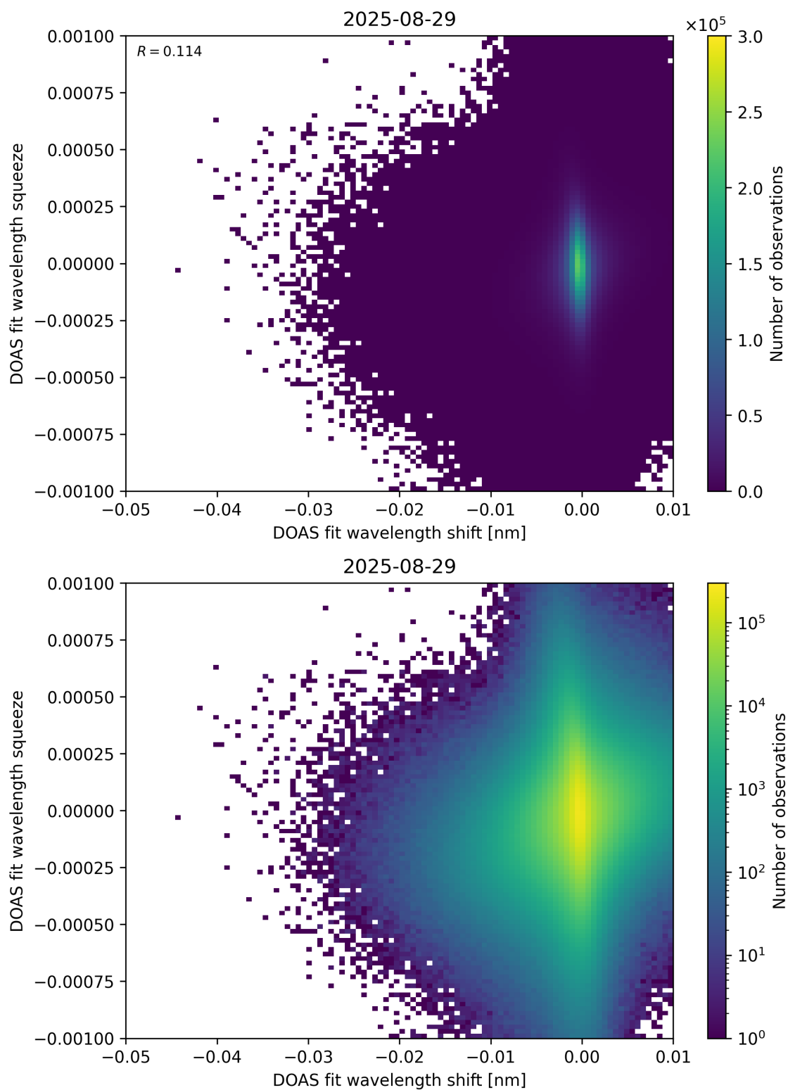
Figure 138: Scatter density plot of “DOAS fit wavelength shift” against “DOAS fit wavelength squeeze” for 2025-08-28 to 2025-08-30.
