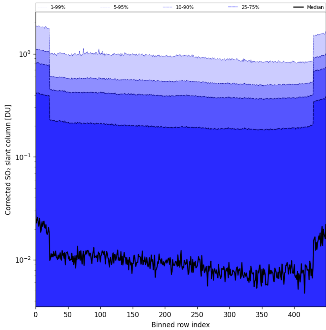
Figure 86: Along track statistics of “Corrected SO 2 slant column” for 2025-08-28 to 2025-08-30
