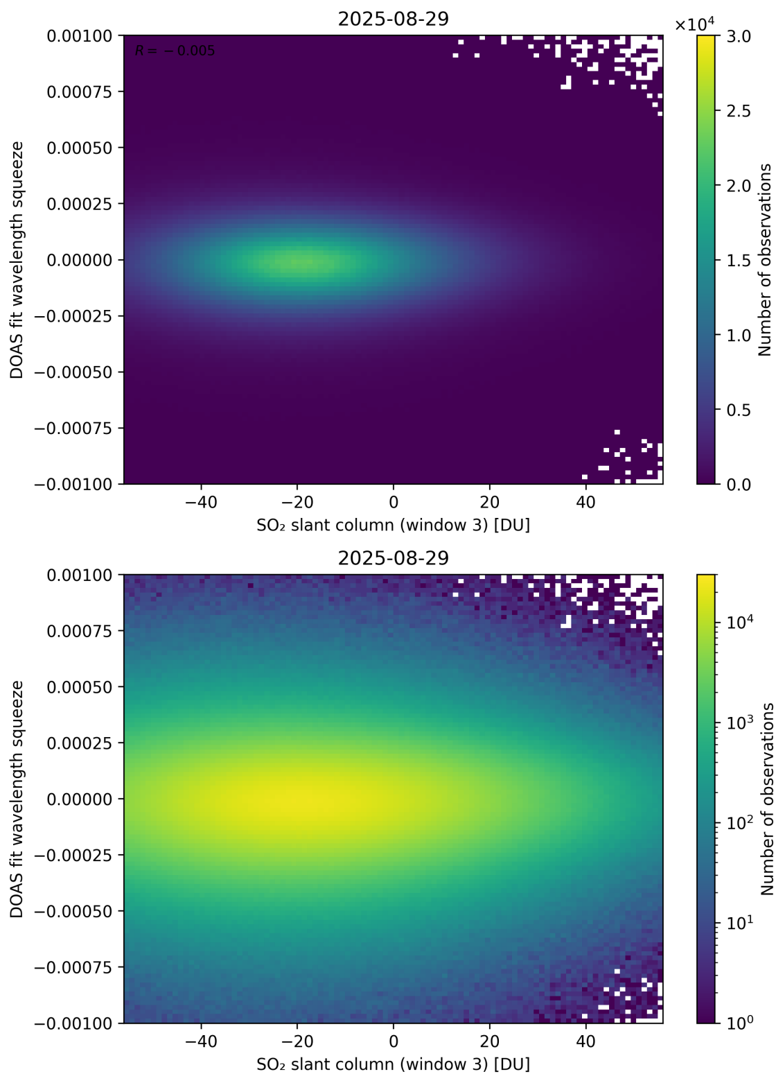
Figure 305: Scatter density plot of “SO 2 slant column (window 3)” against “DOAS fit wavelength squeeze” for 2025-08-28 to 2025-08-30.
