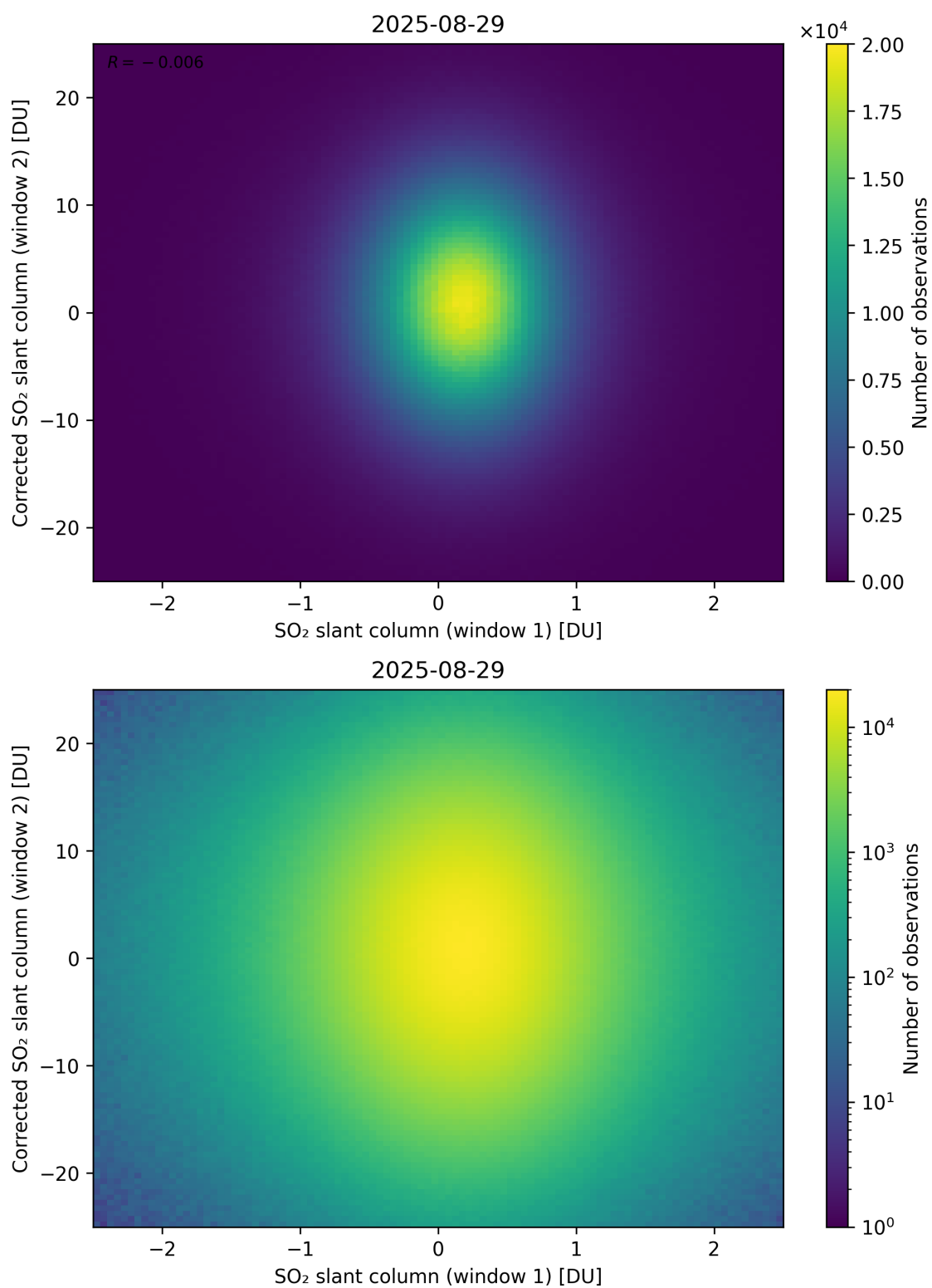
Figure 283: Scatter density plot of “SO 2 slant column (window 1)” against “Corrected SO 2 slant column (window 2)” for 2025-08-28 to 2025-08-30.
