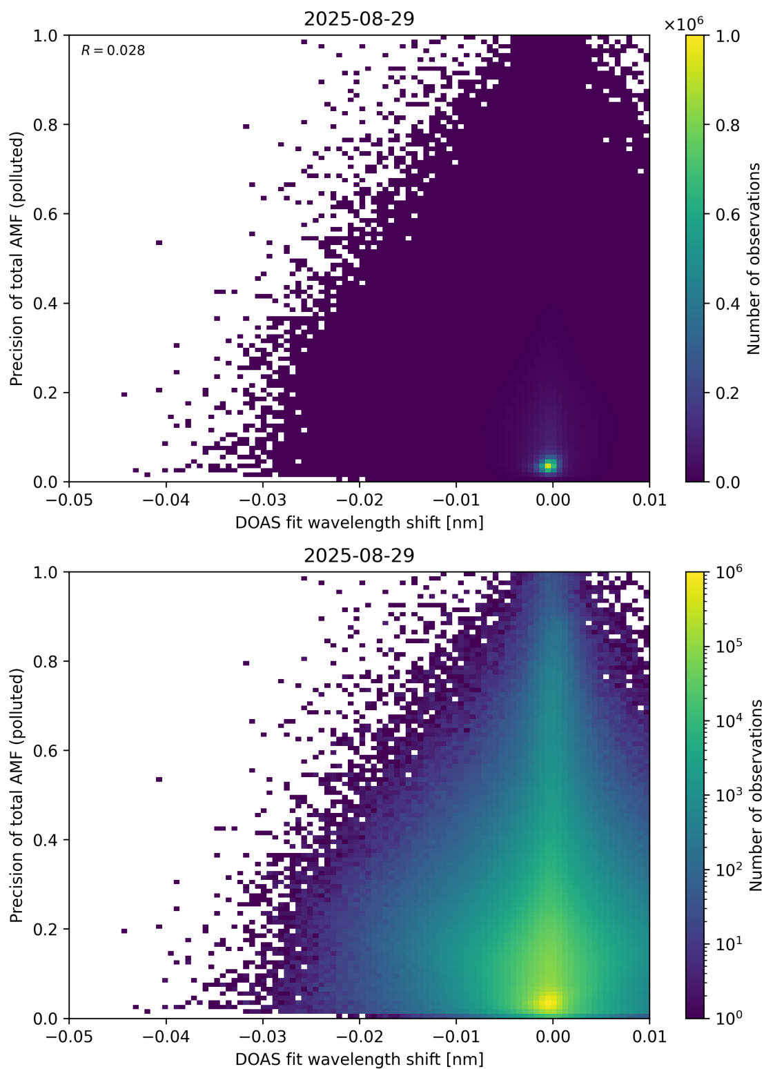
Figure 142: Scatter density plot of “DOAS fit wavelength shift” against “Precision of total AMF (polluted)” for 2025-08-28 to 2025-08-30.
