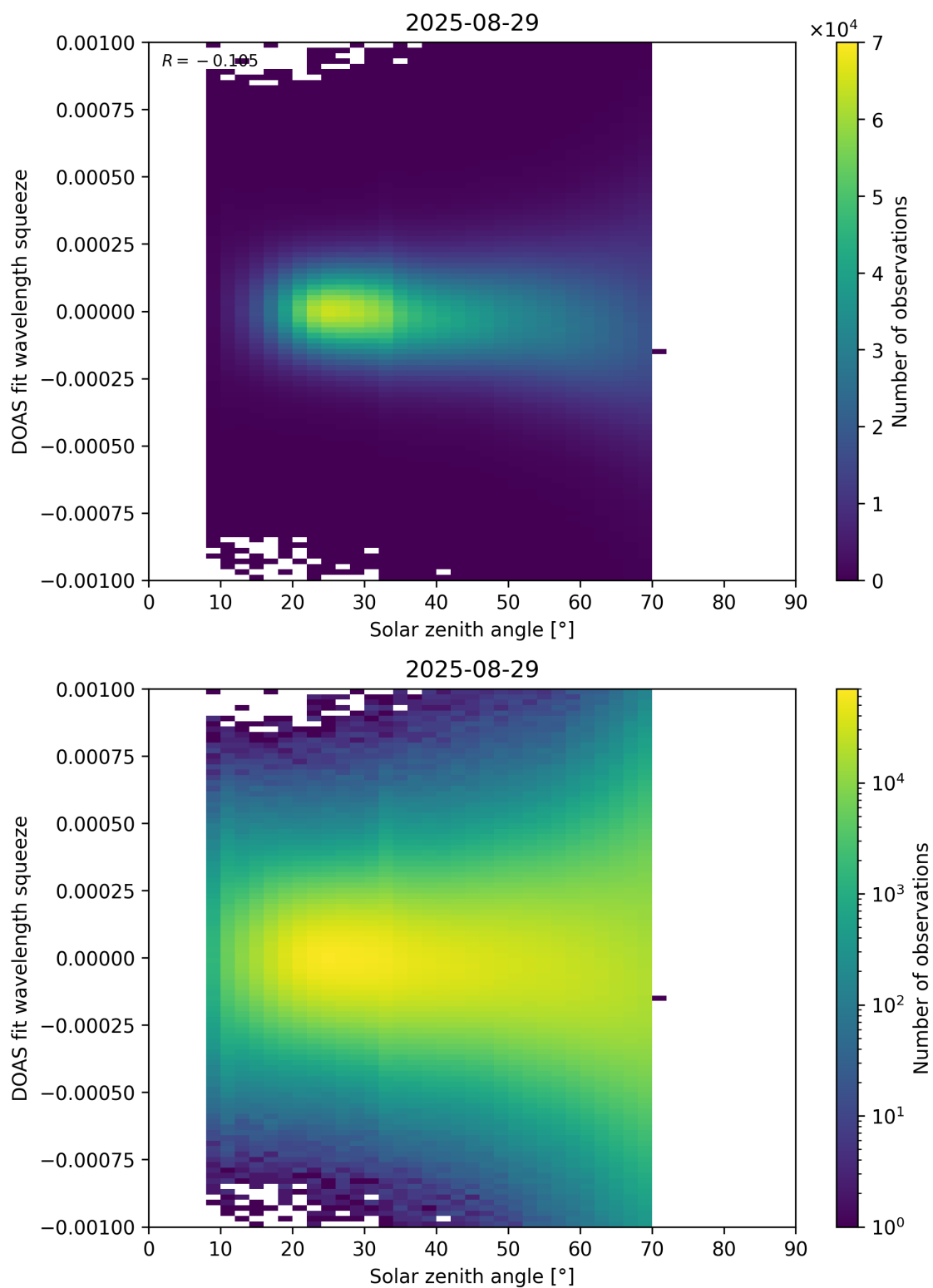
Figure 175: Scatter density plot of “Solar zenith angle” against “DOAS fit wavelength squeeze” for 2025-08-28 to 2025-08-30.
