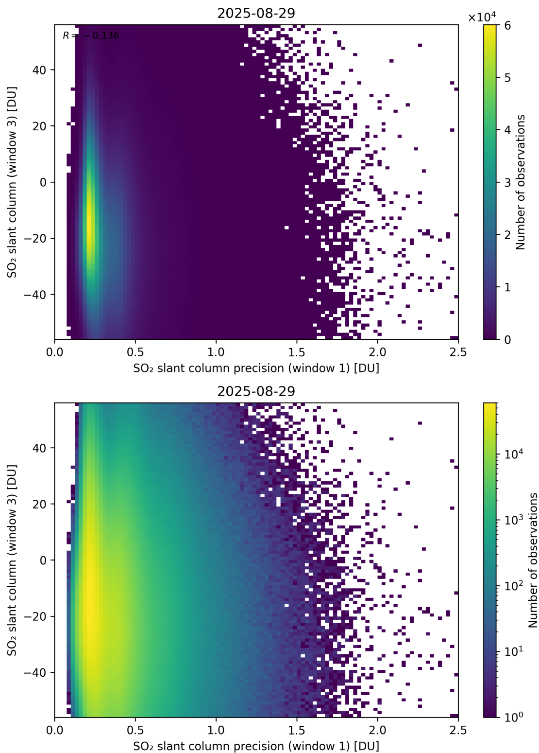
Figure 278: Scatter density plot of “SO 2 slant column precision (window 1)” against “SO 2 slant column (window 3)” for 2025-08-28 to 2025-08-30.
