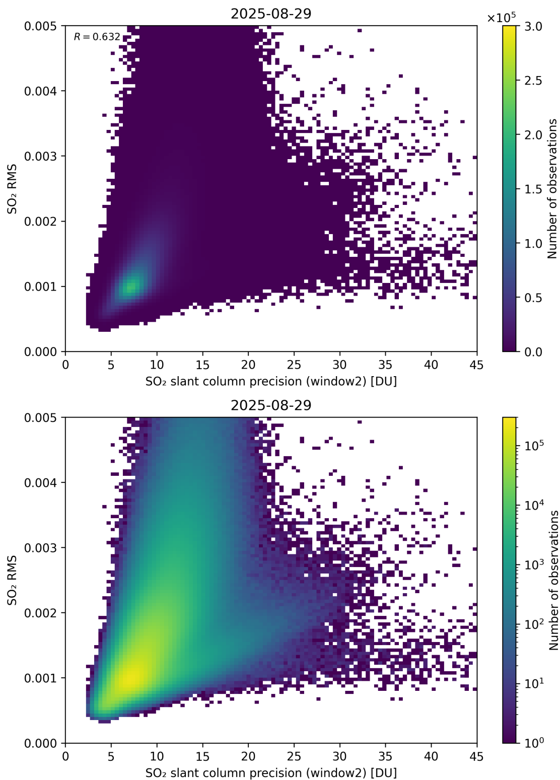
Figure 295: Scatter density plot of “SO 2 slant column precision (window2)” against “SO 2 RMS” for 2025-08-28 to 2025-08-30.
