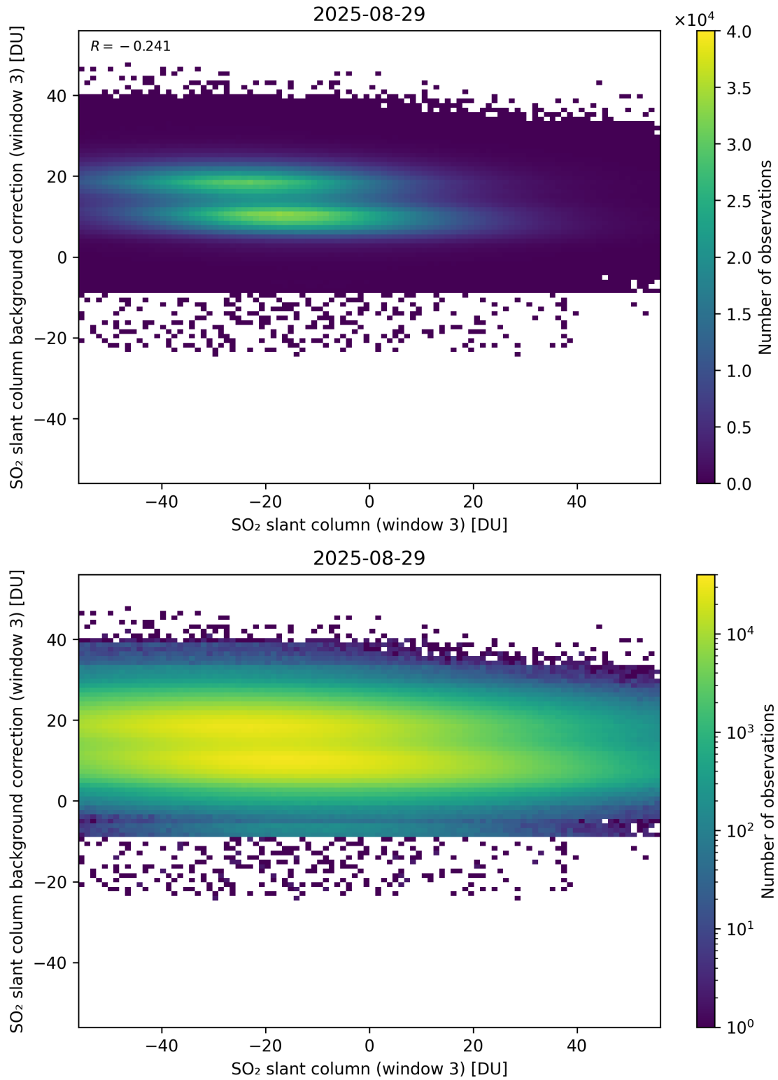
Figure 303: Scatter density plot of “SO 2 slant column (window 3)” against “SO 2 slant column background correction (window 3)” for 2025-08-28 to 2025-08-30.
