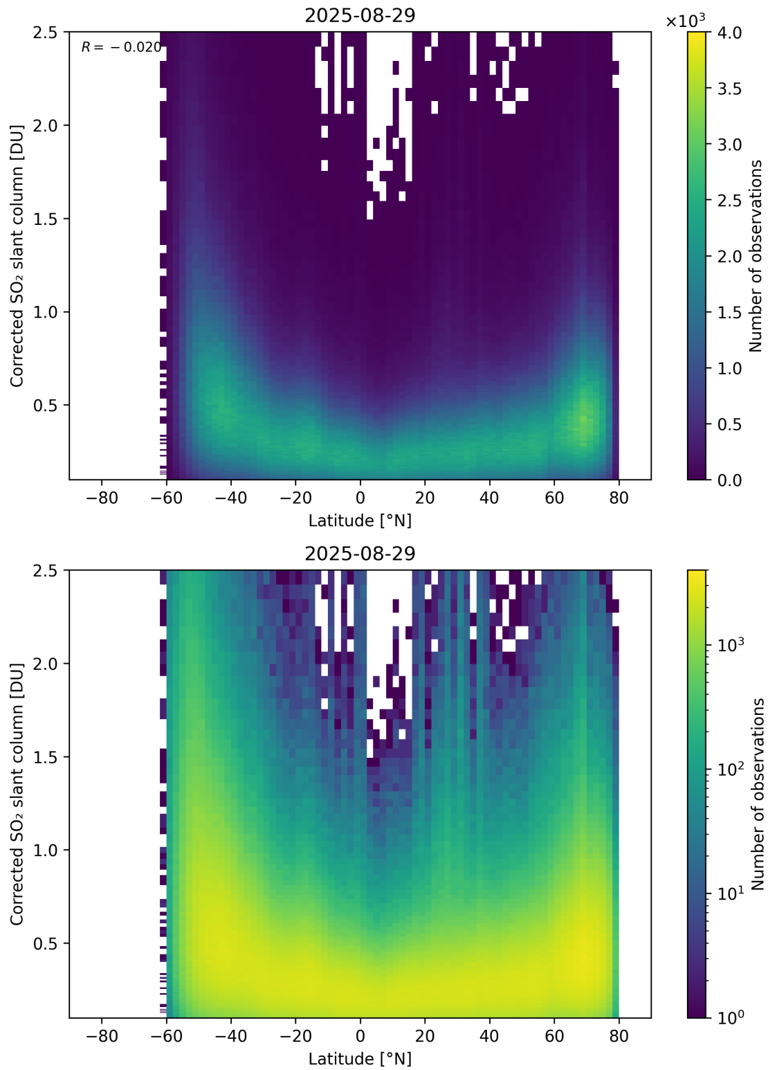
Figure 159: Scatter density plot of “Latitude” against “Corrected SO 2 slant column” for 2025-08-28 to 2025-08-30.
