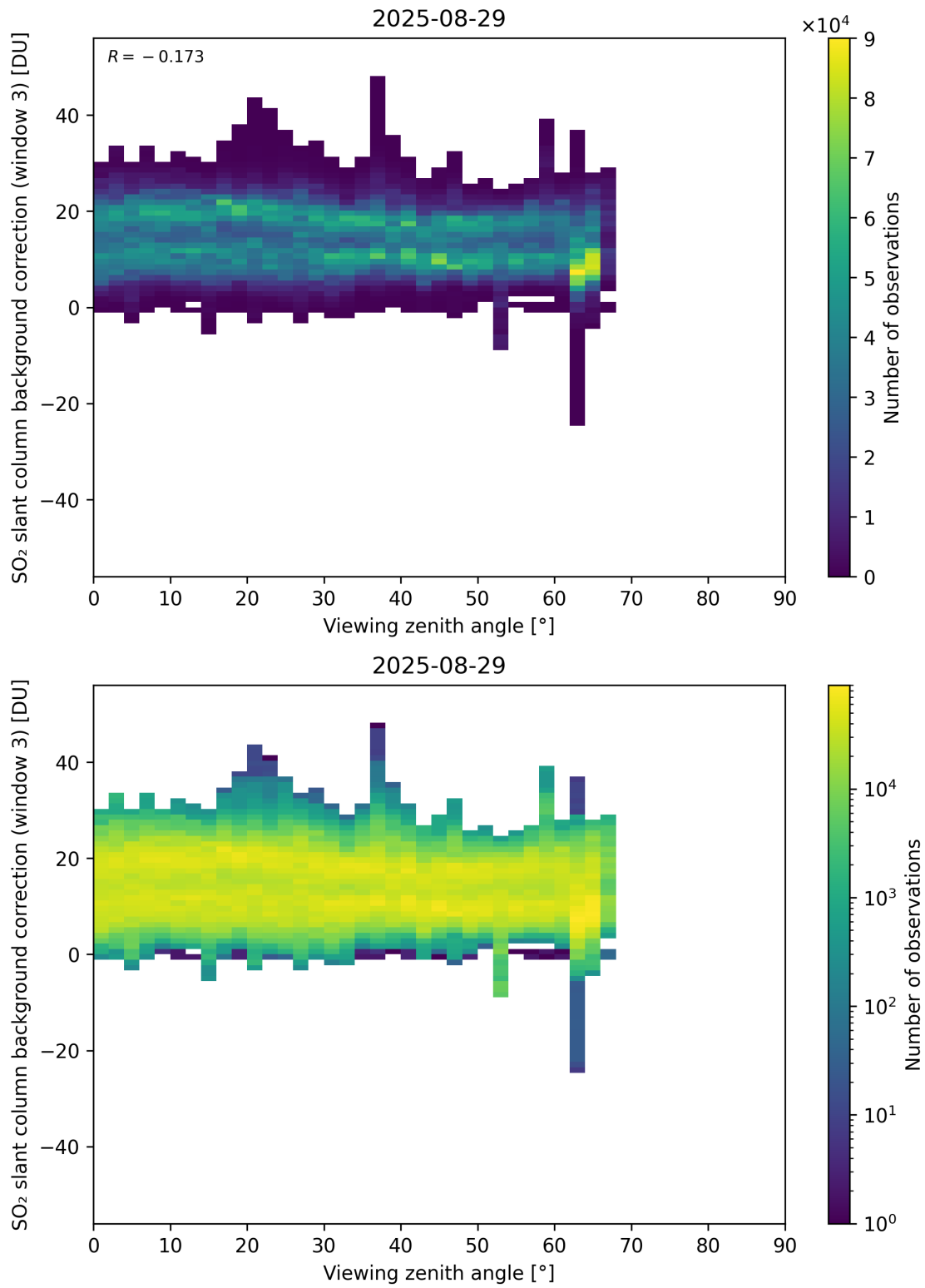
Figure 364: Scatter density plot of “Viewing zenith angle” against “SO 2 slant column background correction (window 3)” for 2025-08-28 to 2025-08-30.
