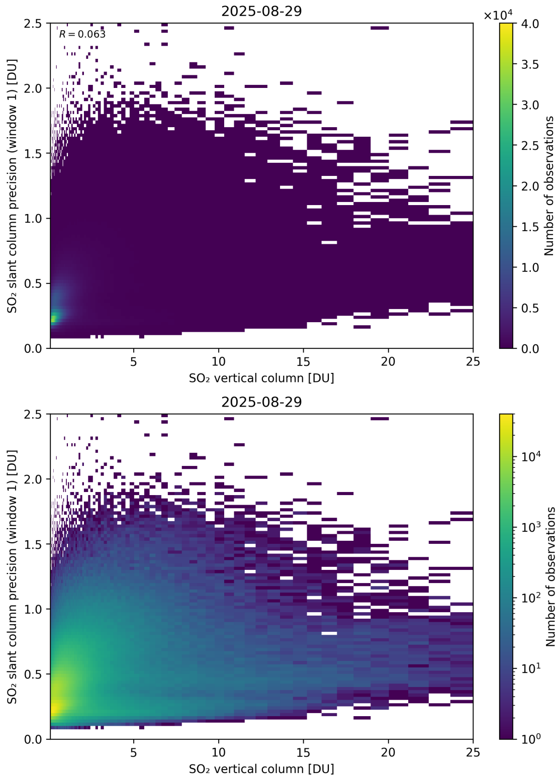
Figure 355: Scatter density plot of “SO 2 vertical column” against “SO 2 slant column precision (window 1)” for 2025-08-28 to 2025-08-30.
