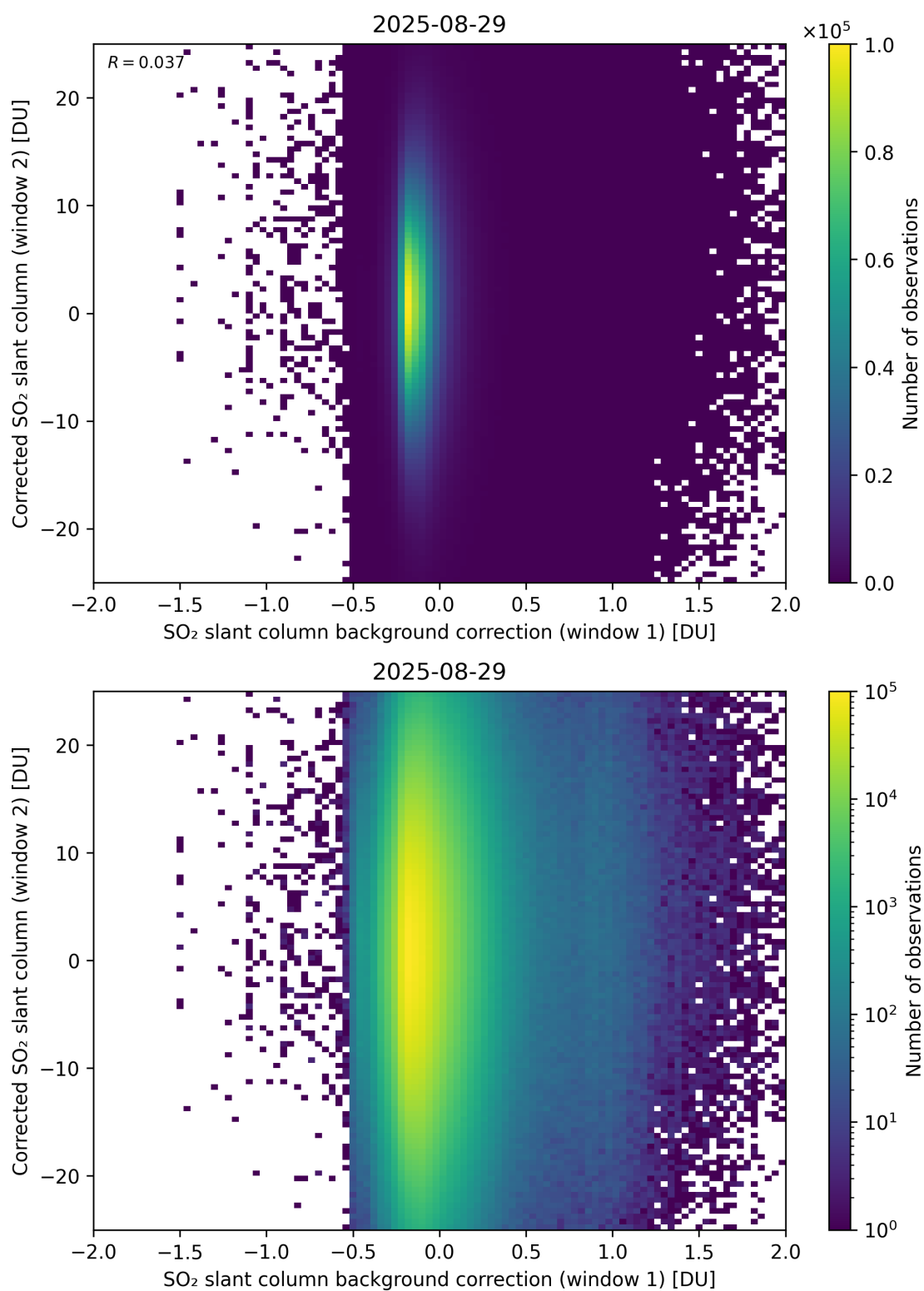
Figure 115: Scatter density plot of “SO 2 slant column background correction (window 1)” against “Corrected SO 2 slant column (window 2)” for 2025-08-28 to 2025-08-30.
