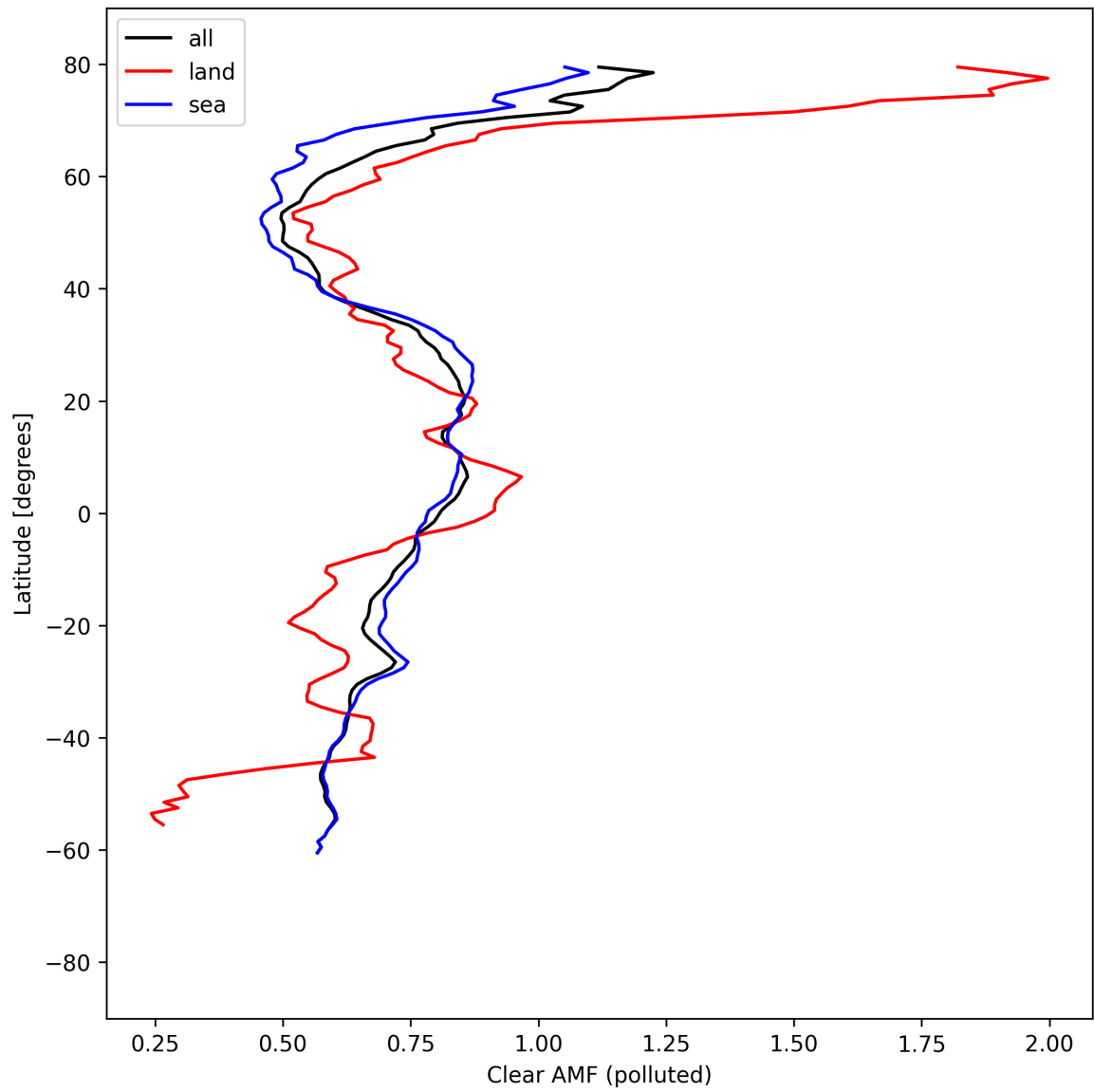
Figure 55: Zonal average of “Clear AMF (polluted)” for 2025-08-28 to 2025-08-30.
