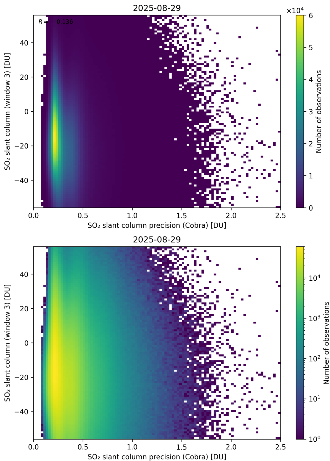
Figure 211: Scatter density plot of “SO 2 slant column precision (Cobra)” against “SO 2 slant column (window 3)” for 2025-08-28 to 2025-08-30.
