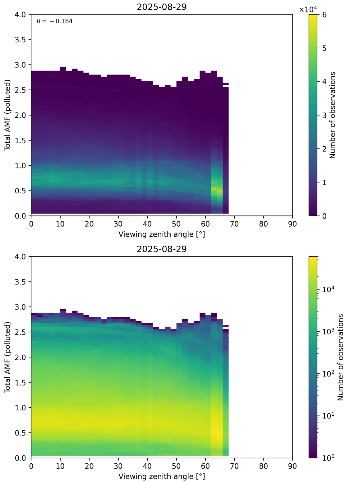
Figure 381: Scatter density plot of “Viewing zenith angle” against “Total AMF (polluted)” for 2025-08-28 to 2025-08-30.
