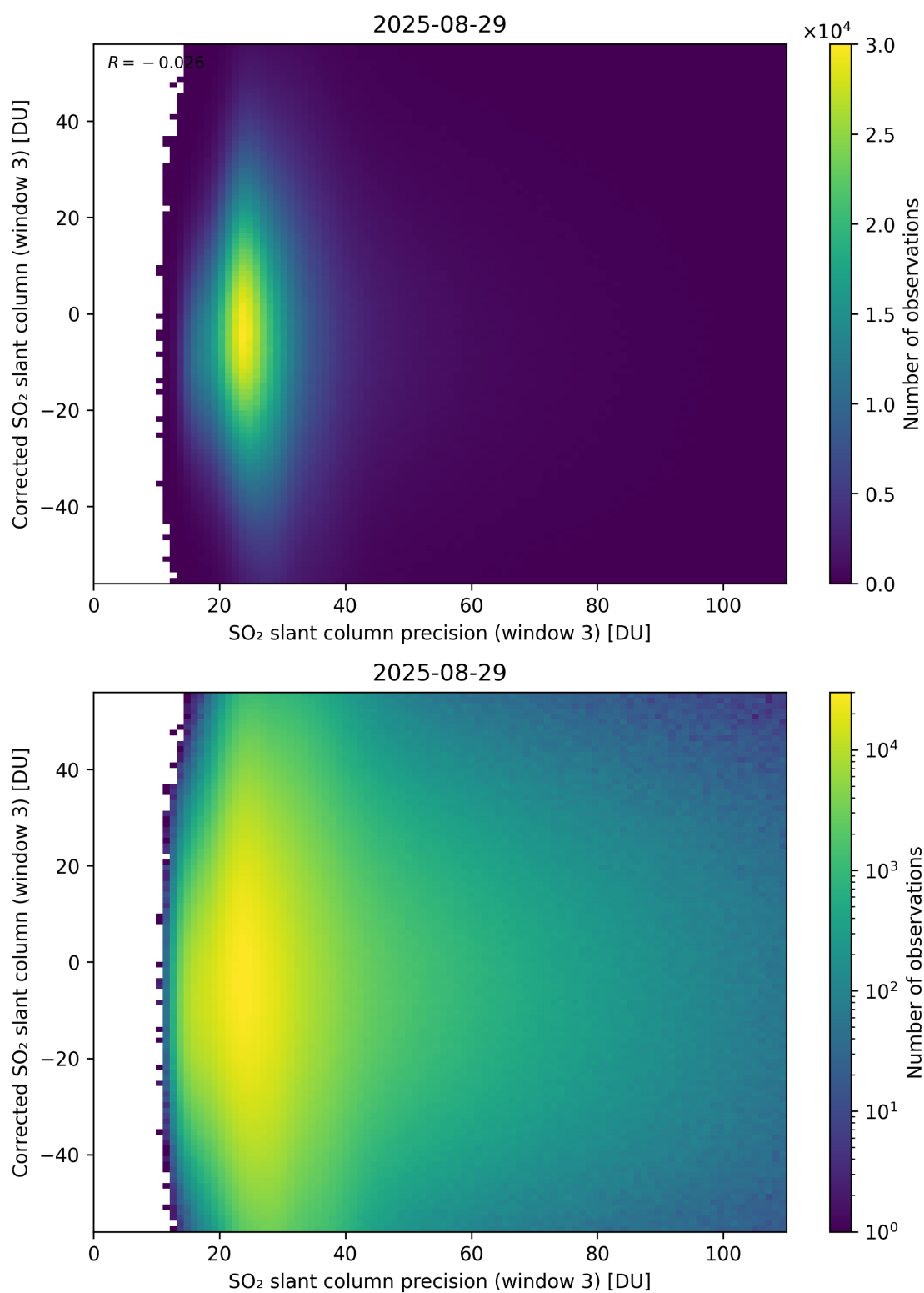
Figure 312: Scatter density plot of “SO 2 slant column precision (window 3)” against “Corrected SO 2 slant column (window 3)” for 2025-08-28 to 2025-08-30.
