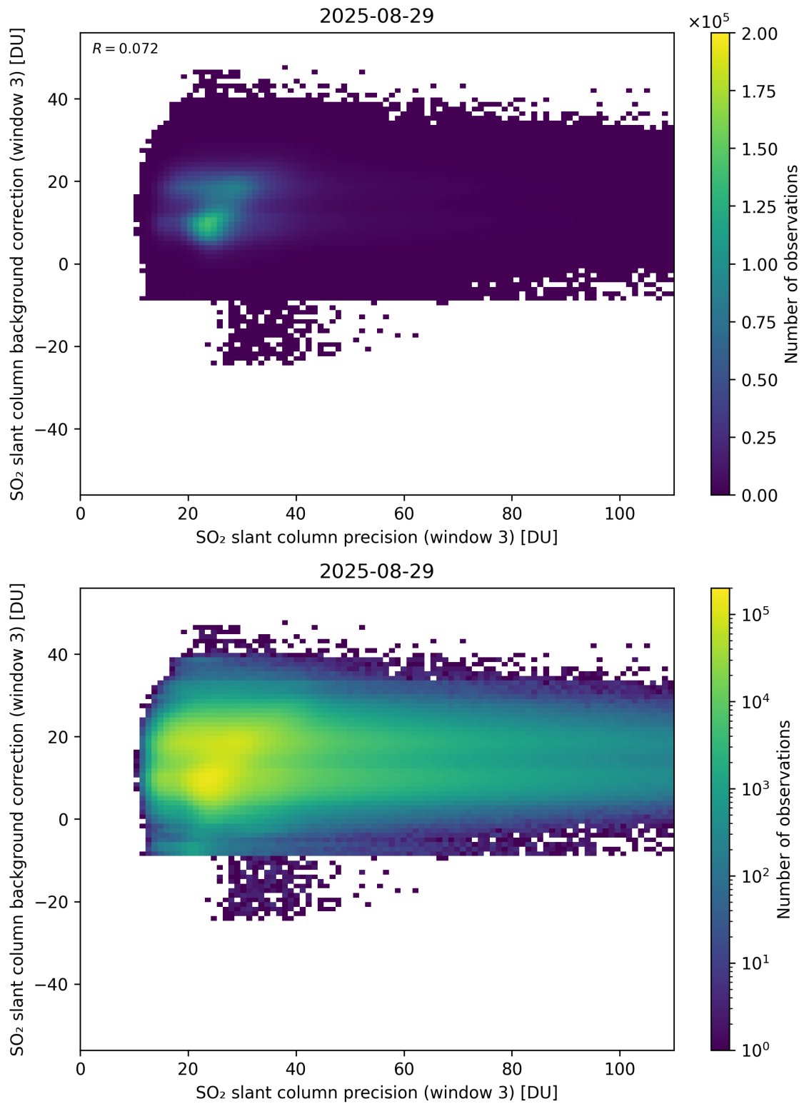
Figure 307: Scatter density plot of “SO 2 slant column precision (window 3)” against “SO 2 slant column background correction (window 3)” for 2025-08-28 to 2025-08-30.
