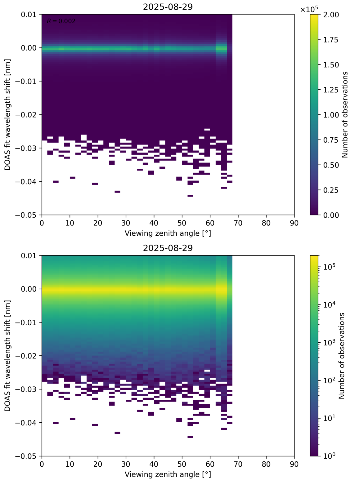
Figure 365: Scatter density plot of “Viewing zenith angle” against “DOAS fit wavelength shift” for 2025-08-28 to 2025-08-30.
