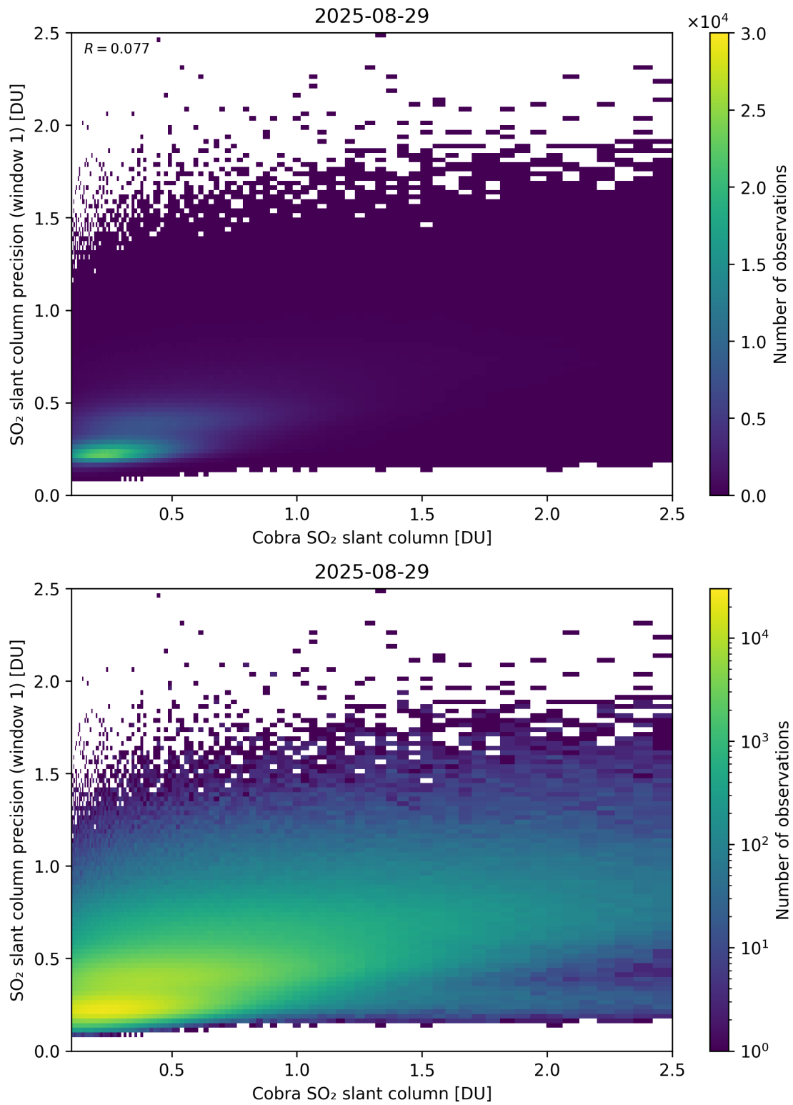
Figure 220: Scatter density plot of “Cobra SO 2 slant column” against “SO 2 slant column precision (window 1)” for 2025-08-28 to 2025-08-30.
