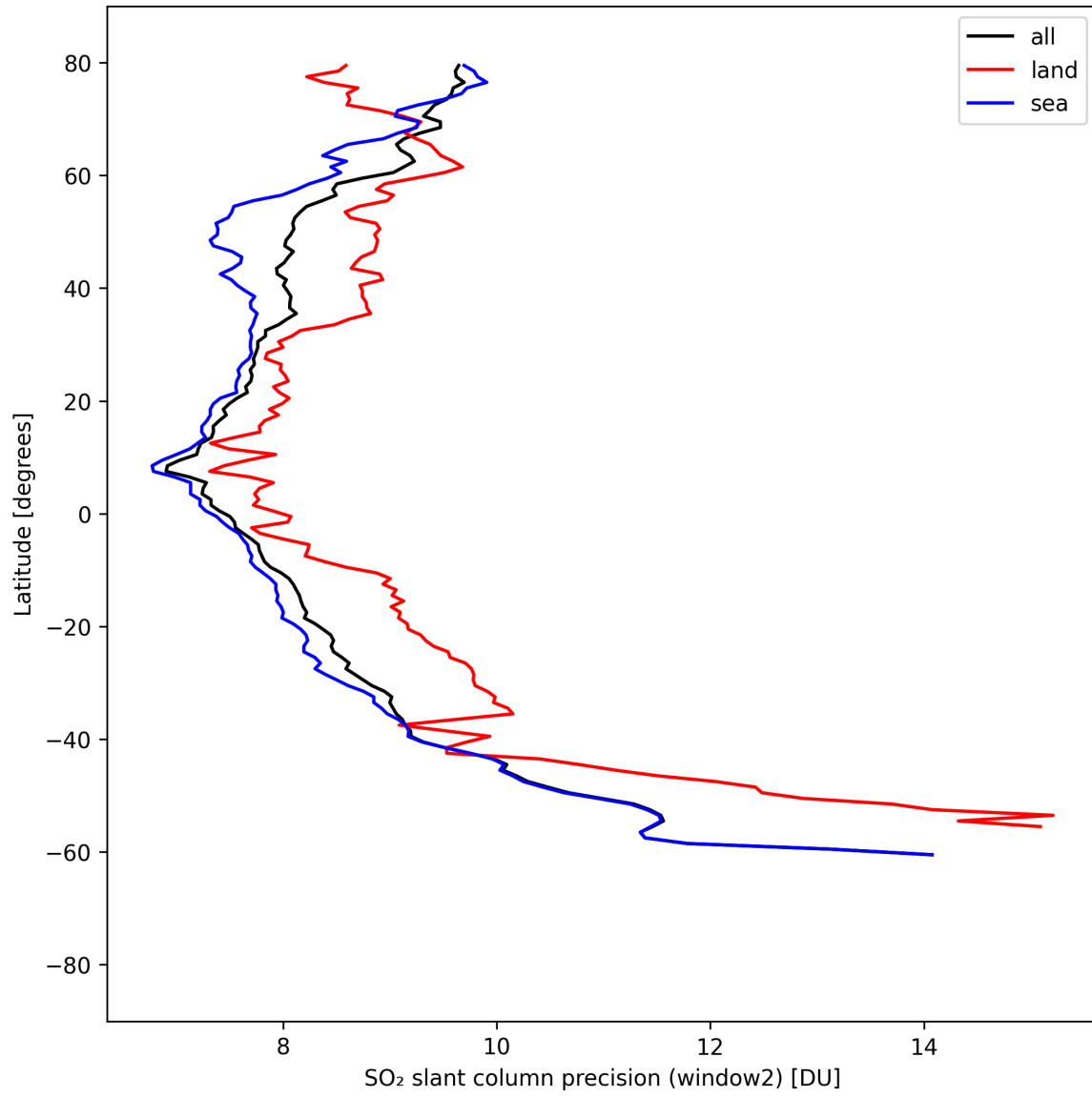
Figure 42: Zonal average of “SO 2 slant column precision (window2)” for 2025-08-28 to 2025-08-30.
