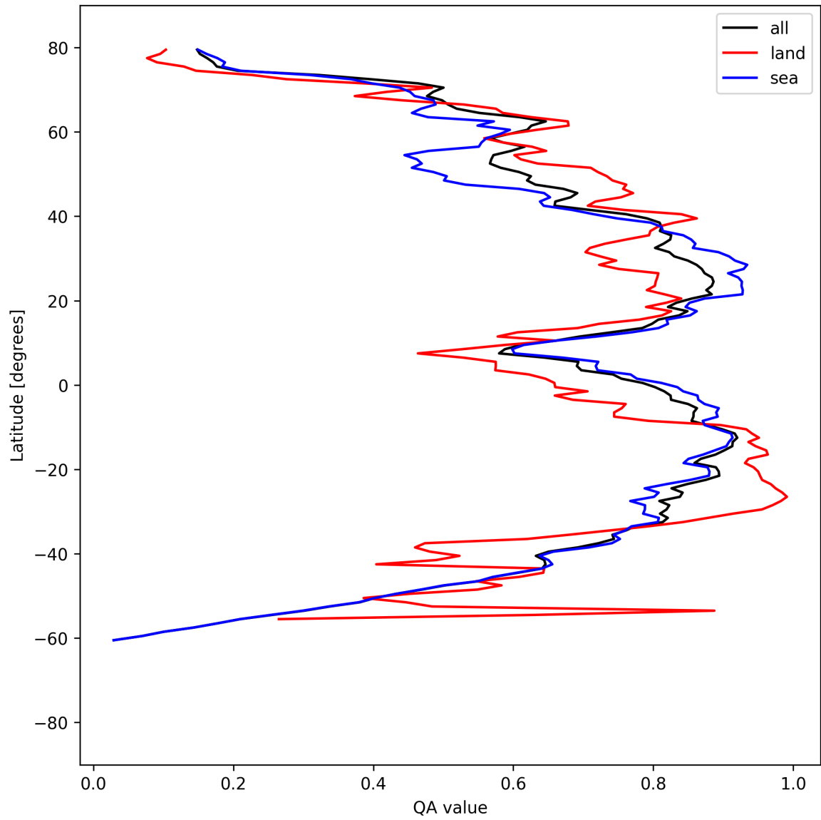
Figure 31: Zonal average of “QA value” for 2025-08-28 to 2025-08-30.
