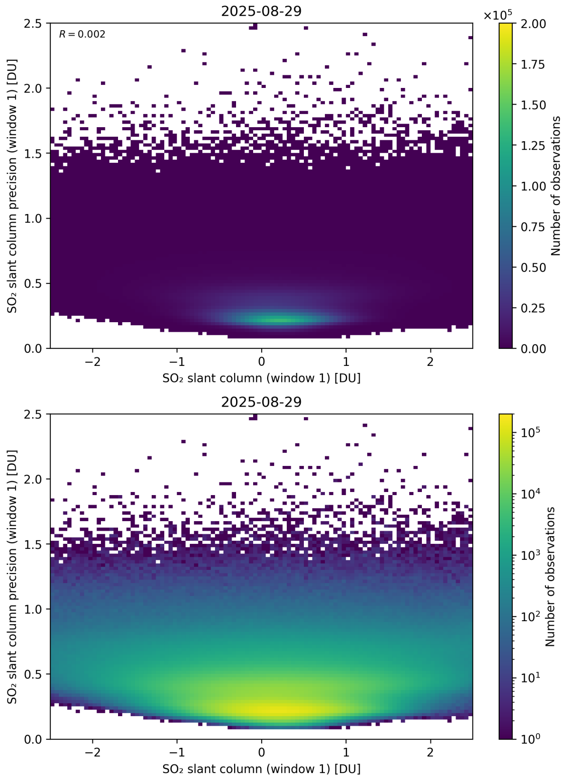
Figure 285: Scatter density plot of “SO 2 slant column (window 1)” against “SO 2 slant column precision (window 1)” for 2025-08-28 to 2025-08-30.
