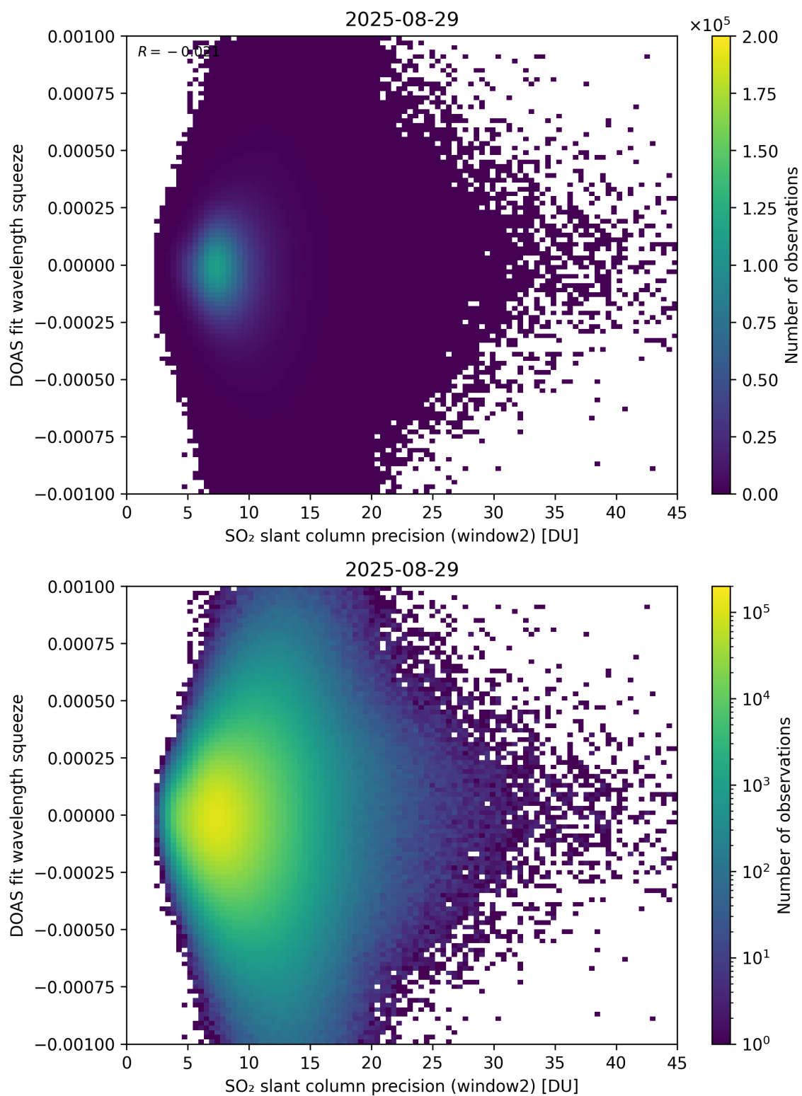
Figure 294: Scatter density plot of “SO 2 slant column precision (window2)” against “DOAS fit wavelength squeeze” for 2025-08-28 to 2025-08-30.
