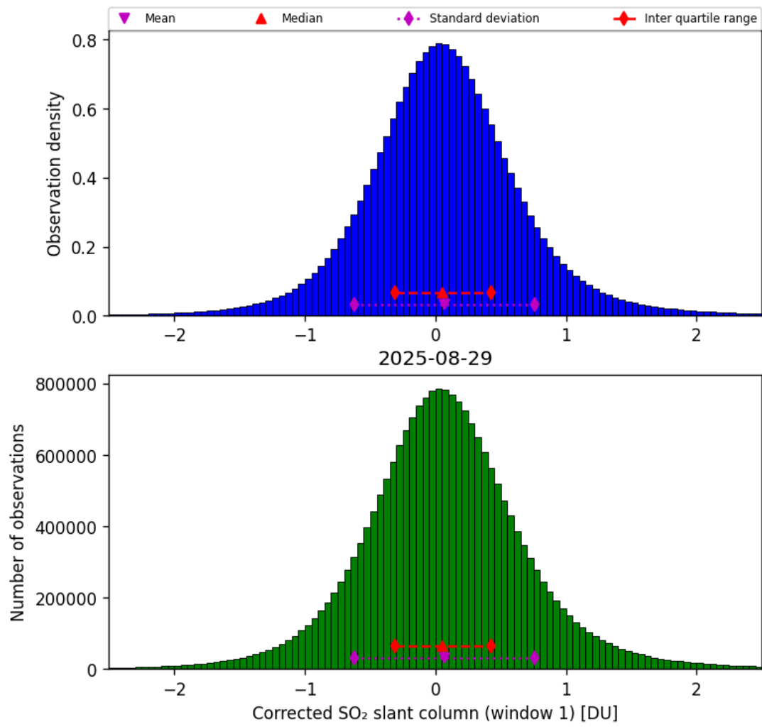
Figure 65: Histogram of “Corrected SO 2 slant column (window 1)” for 2025-08-28 to 2025-08-30
