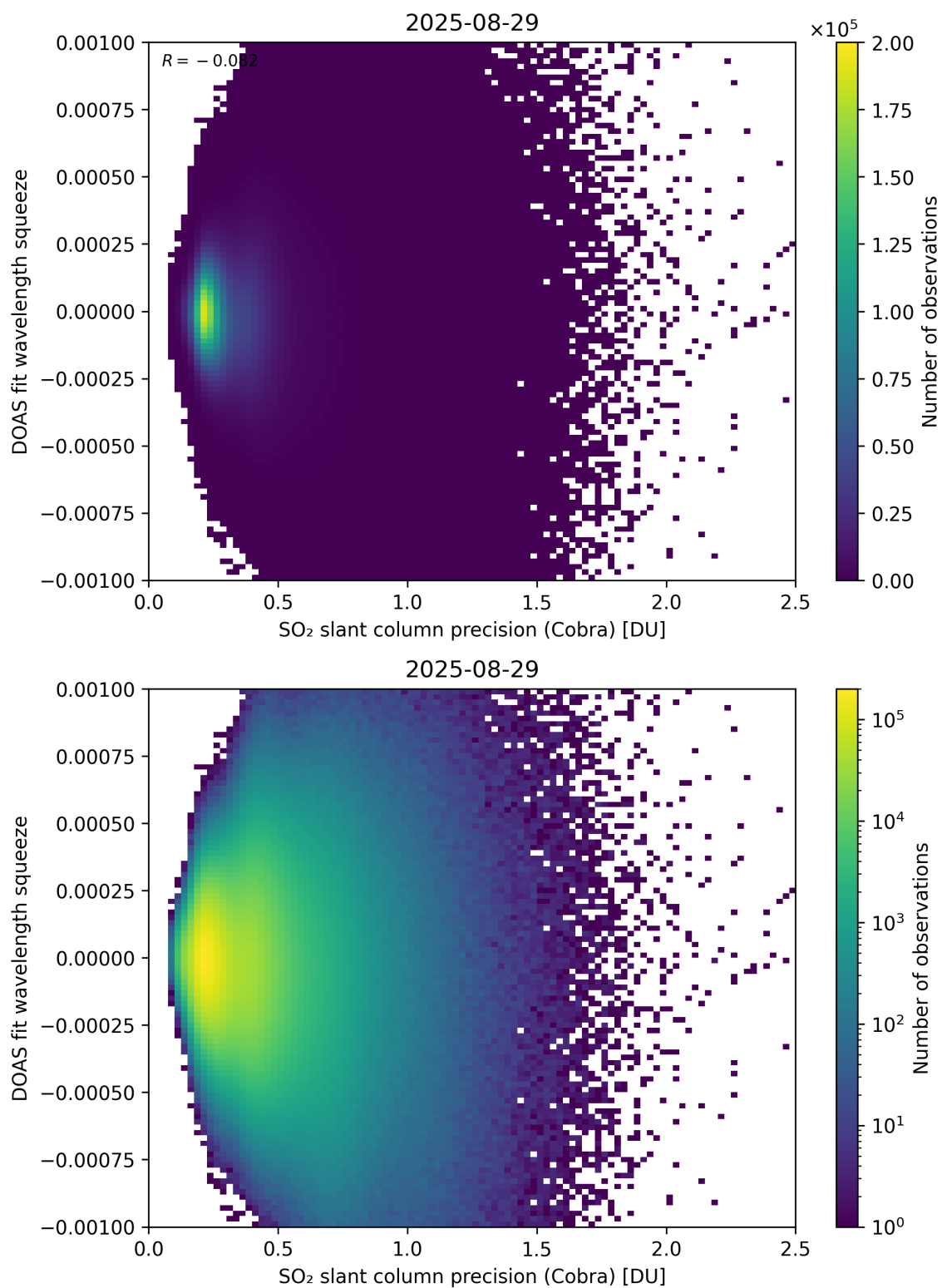
Figure 203: Scatter density plot of “SO 2 slant column precision (Cobra)” against “DOAS fit wavelength squeeze” for 2025-08-28 to 2025-08-30.
