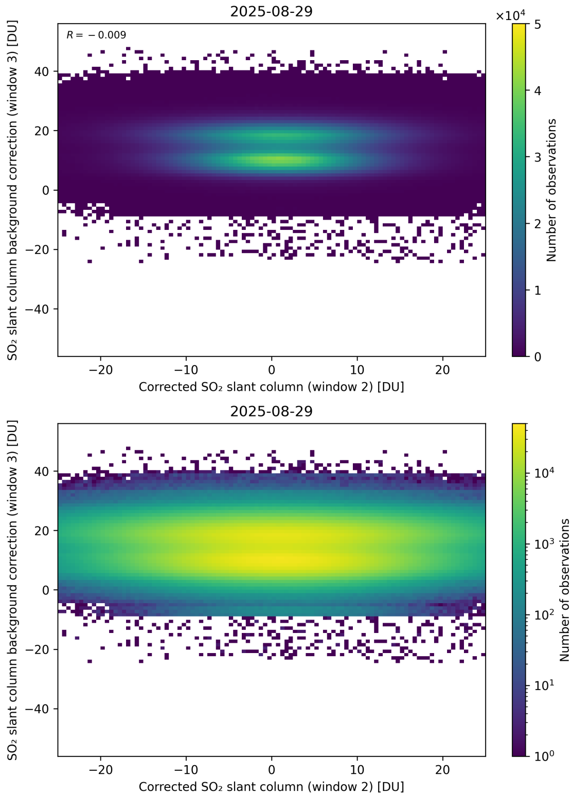
Figure 245: Scatter density plot of “Corrected SO 2 slant column (window 2)” against “SO 2 slant column background correction (window 3)” for 2025-08-28 to 2025-08-30.
