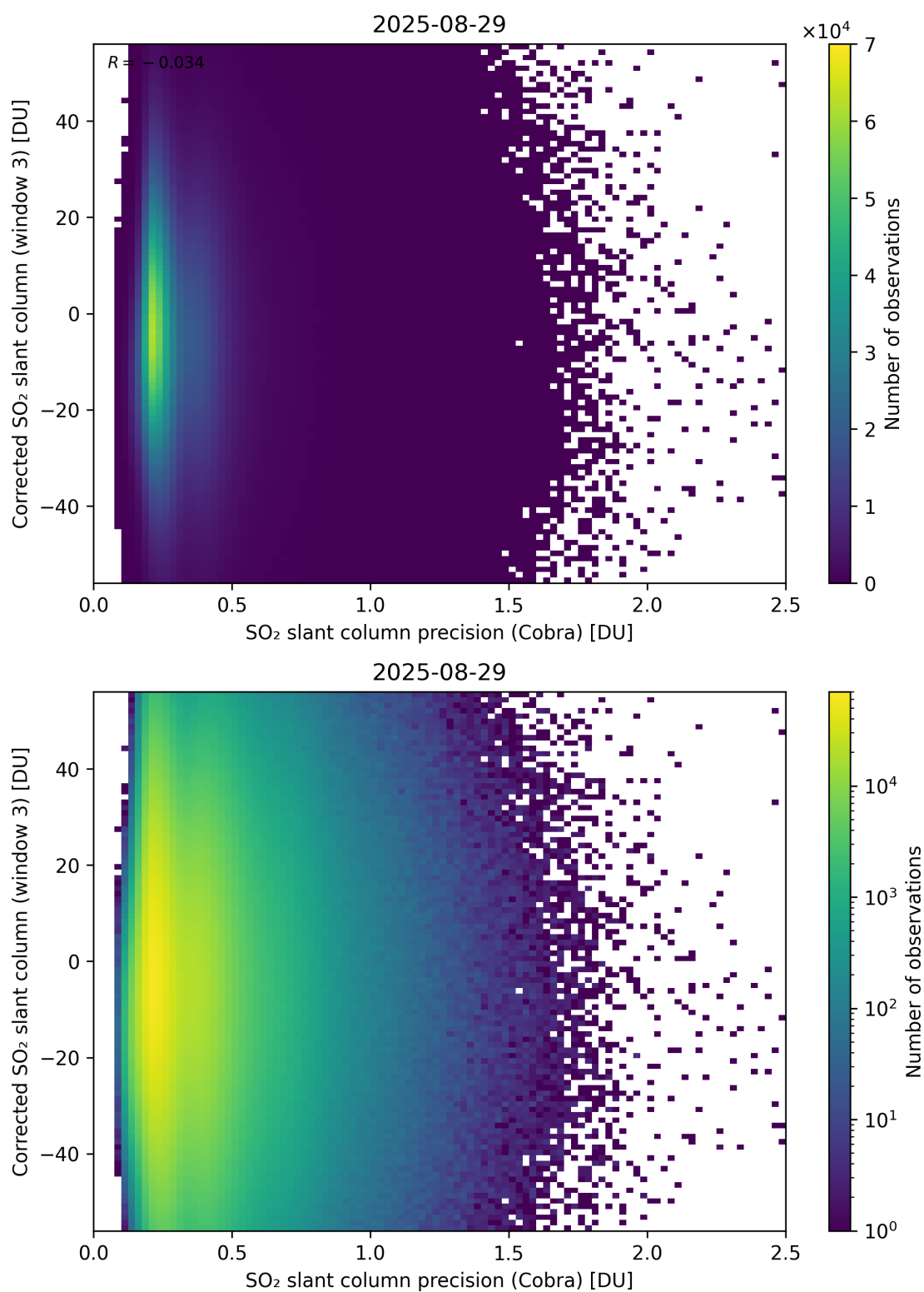
Figure 207: Scatter density plot of “SO 2 slant column precision (Cobra)” against “Corrected SO 2 slant column (window 3)” for 2025-08-28 to 2025-08-30.
