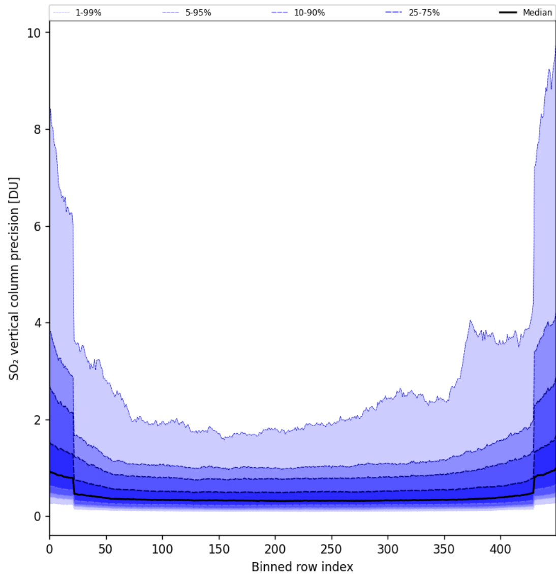
Figure 85: Along track statistics of “SO 2 vertical column precision” for 2025-08-28 to 2025-08-30
