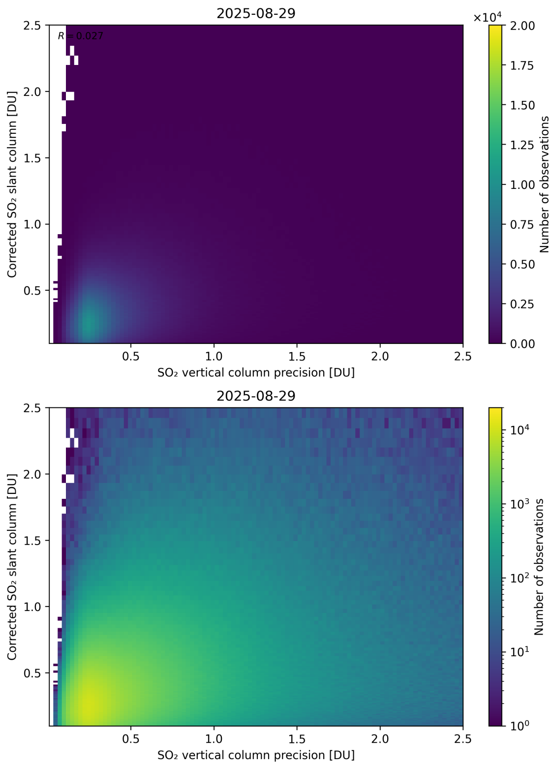
Figure 338: Scatter density plot of “SO 2 vertical column precision” against “Corrected SO 2 slant column” for 2025-08-28 to 2025-08-30.
