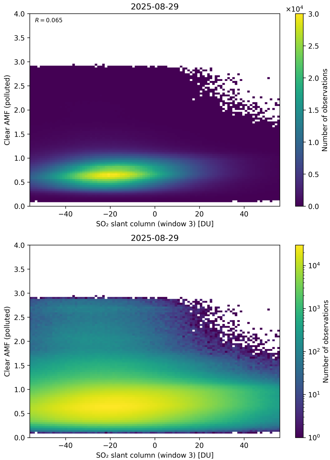
Figure 315: Scatter density plot of “SO 2 slant column (window 3)” against “Clear AMF (polluted)” for 2025-08-28 to 2025-08-30.
