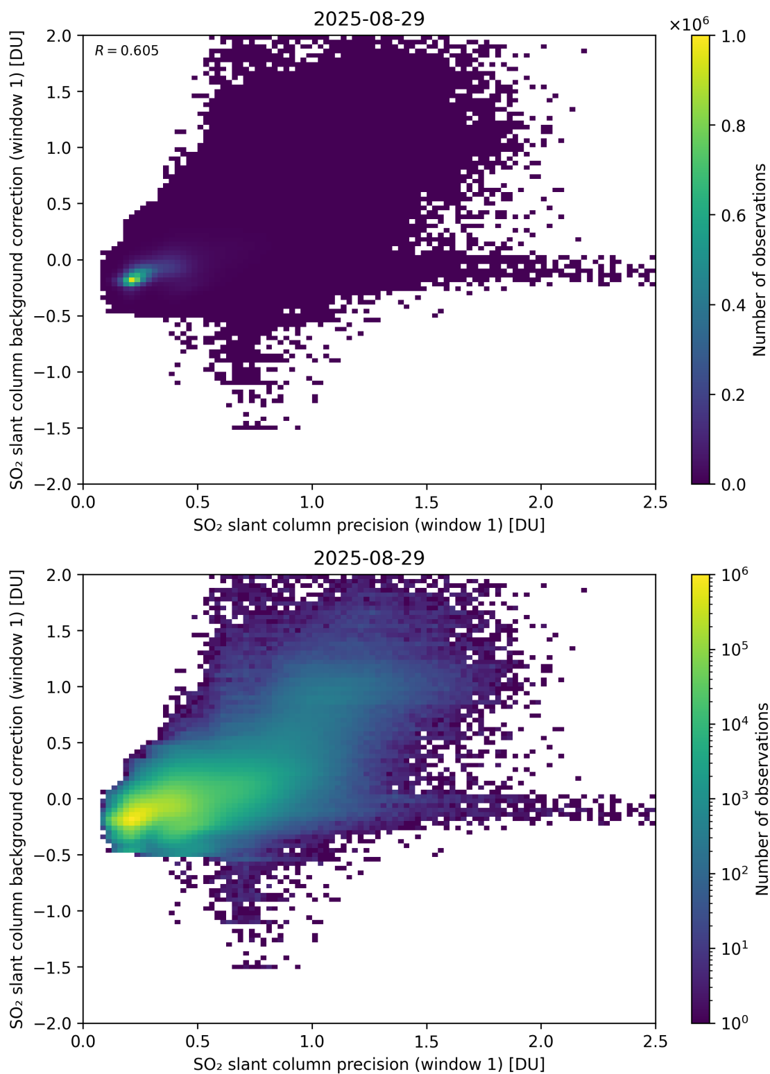
Figure 268: Scatter density plot of “SO 2 slant column precision (window 1)” against “SO 2 slant column background correction (window 1)” for 2025-08-28 to 2025-08-30.
