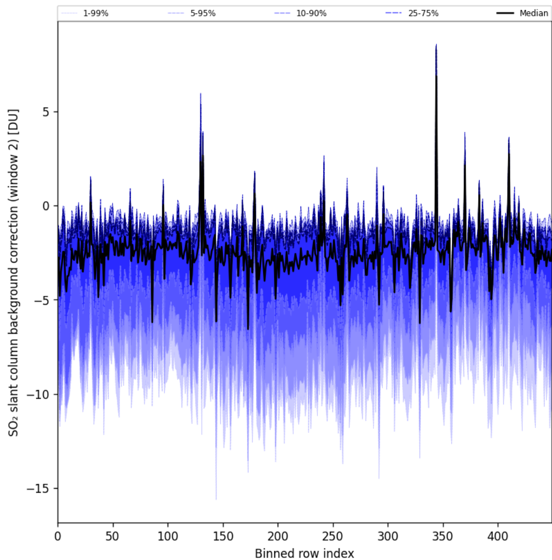
Figure 96: Along track statistics of “SO 2 slant column background correction (window 2)” for 2025-08-28 to 2025-08-30
