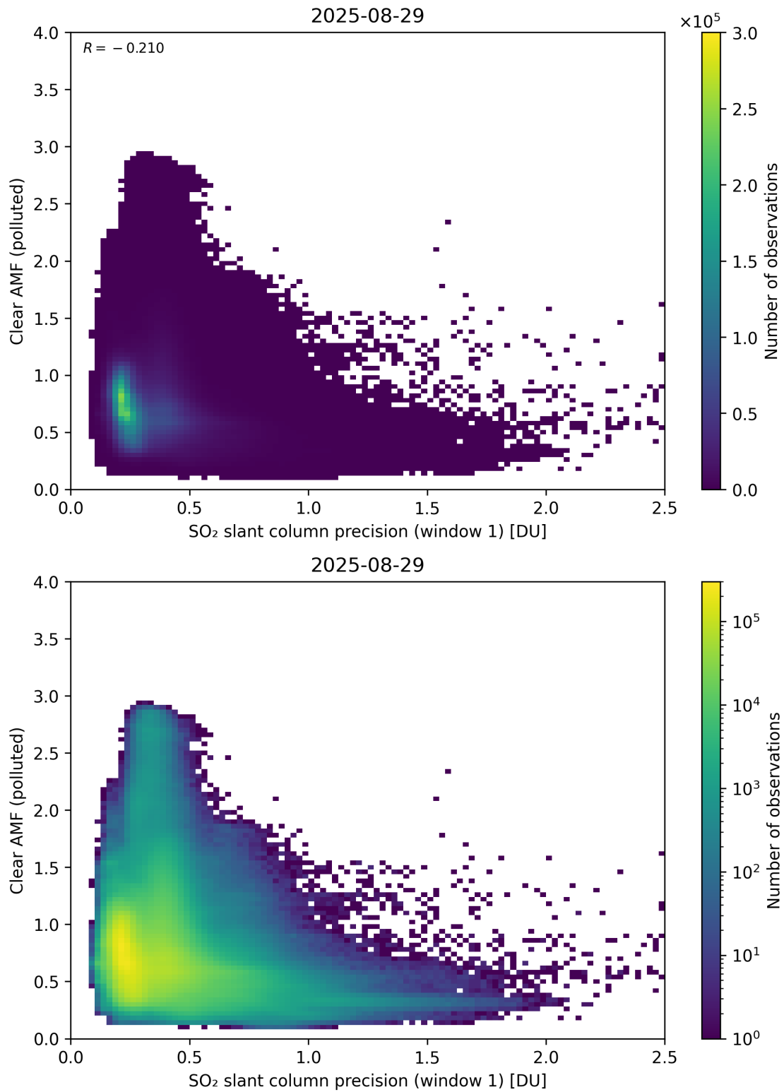
Figure 274: Scatter density plot of “SO 2 slant column precision (window 1)” against “Clear AMF (polluted)” for 2025-08-28 to 2025-08-30.
