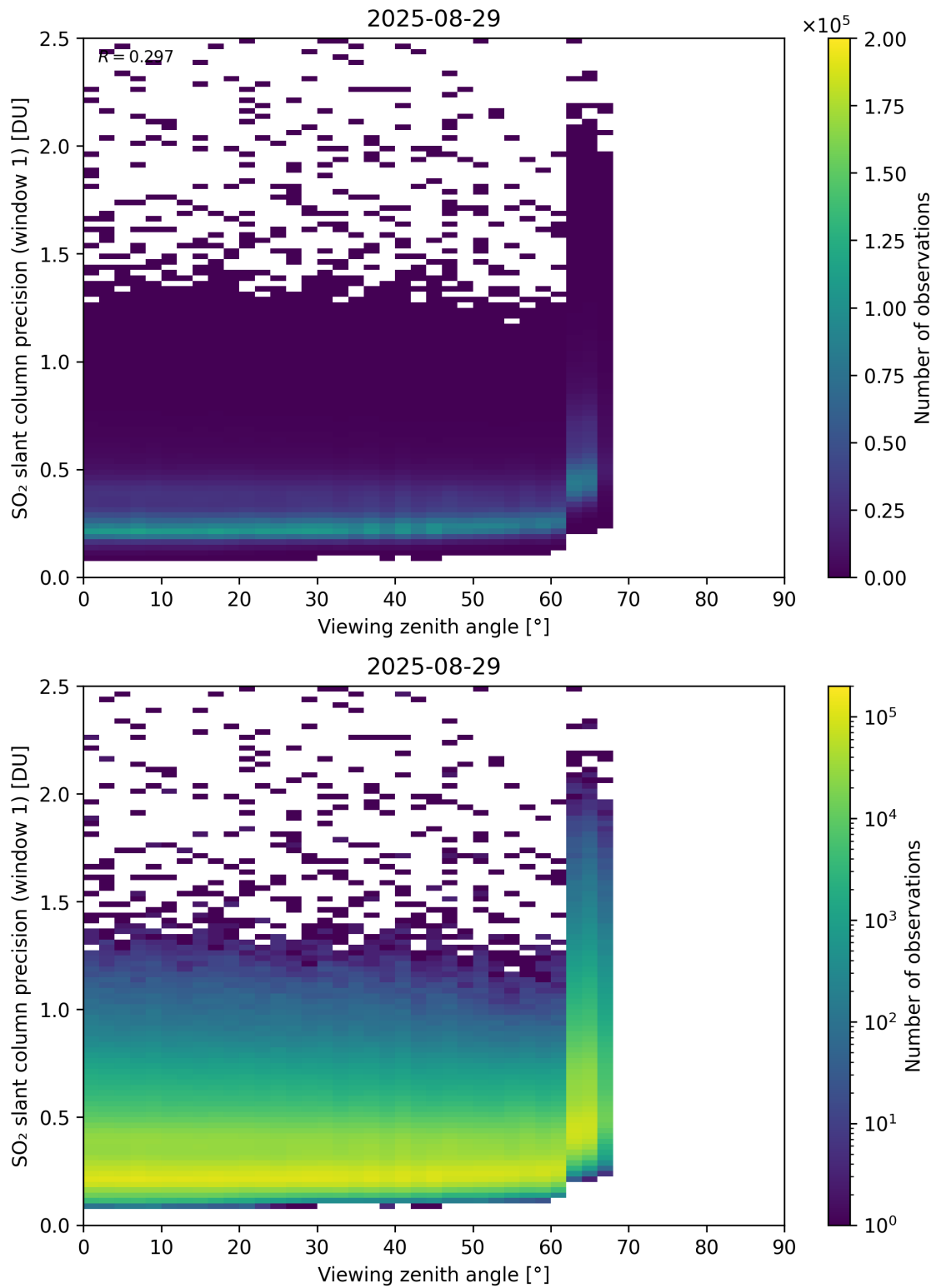
Figure 377: Scatter density plot of “Viewing zenith angle” against “SO 2 slant column precision (window 1)” for 2025-08-28 to 2025-08-30.
