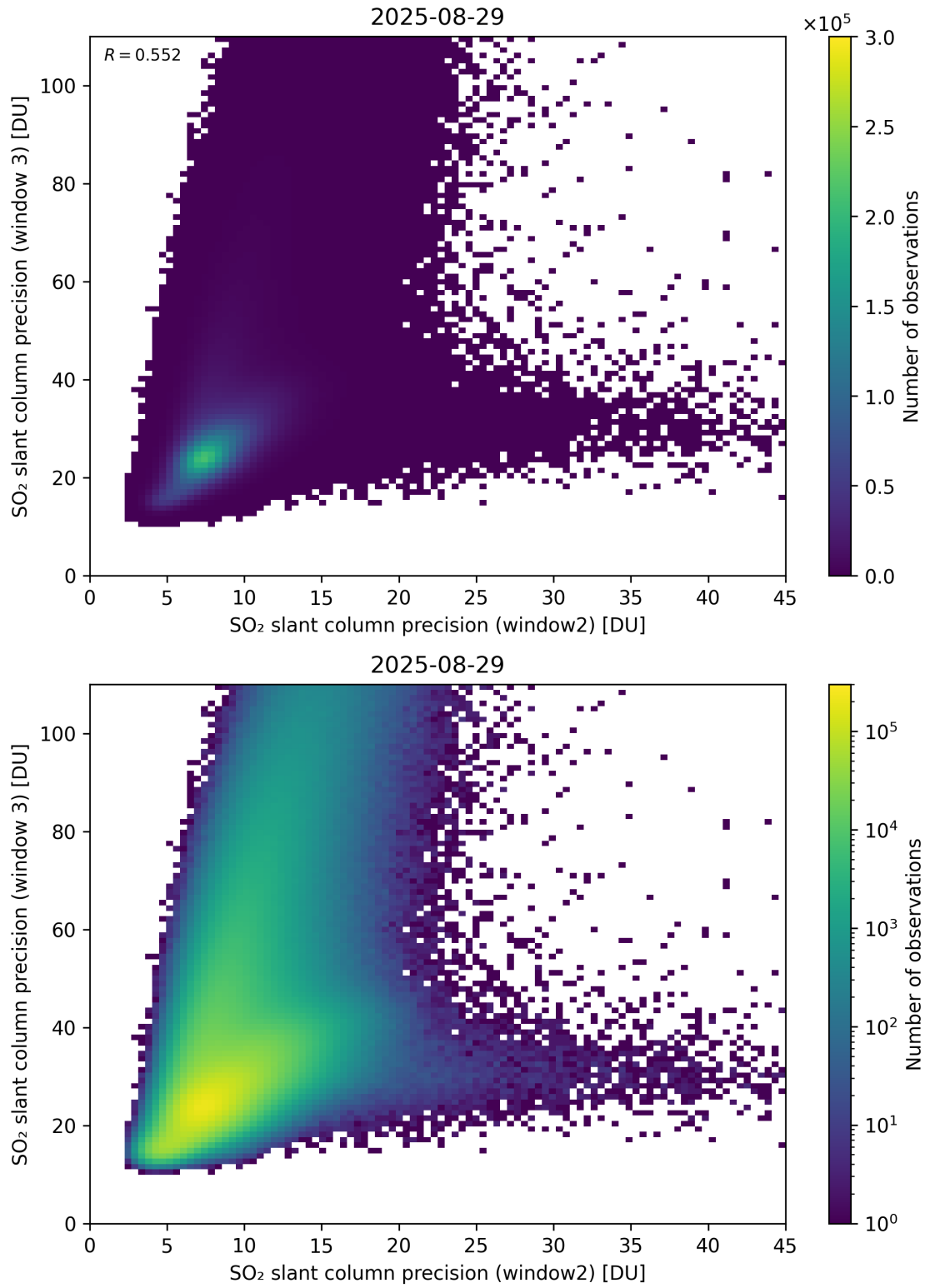
Figure 300: Scatter density plot of “SO 2 slant column precision (window2)” against “SO 2 slant column precision (window 3)” for 2025-08-28 to 2025-08-30.
