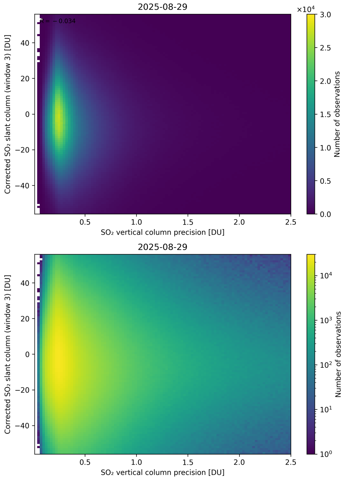
Figure 340: Scatter density plot of “SO 2 vertical column precision” against “Corrected SO 2 slant column (window 3)” for 2025-08-28 to 2025-08-30.
