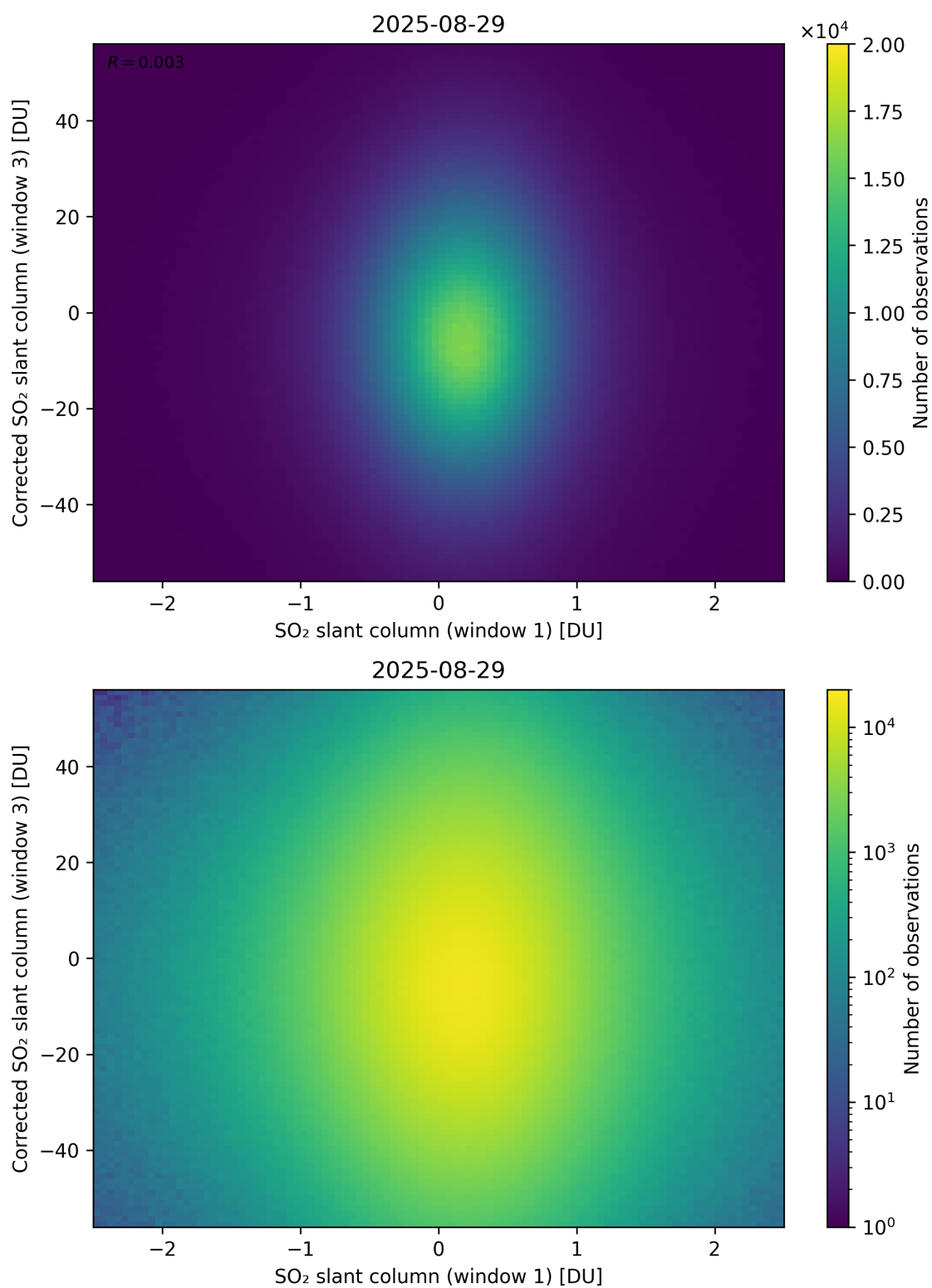
Figure 284: Scatter density plot of “SO 2 slant column (window 1)” against “Corrected SO 2 slant column (window 3)” for 2025-08-28 to 2025-08-30.
