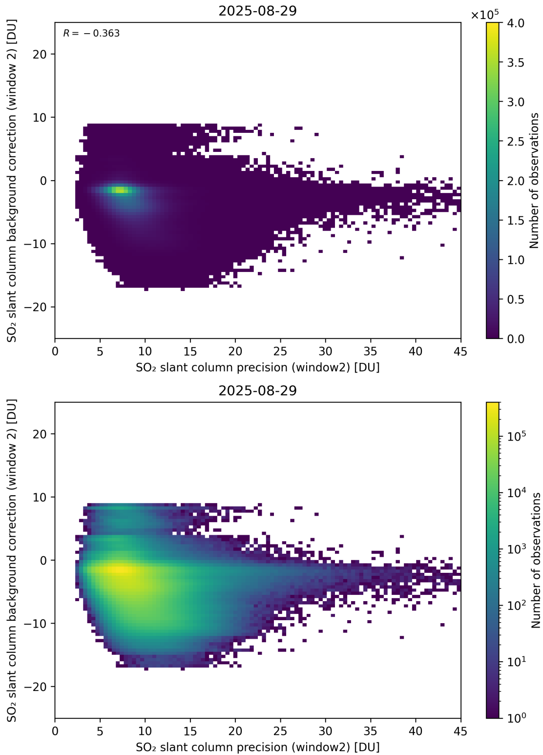
Figure 291: Scatter density plot of “SO 2 slant column precision (window2)” against “SO 2 slant column background correction (window 2)” for 2025-08-28 to 2025-08-30.
