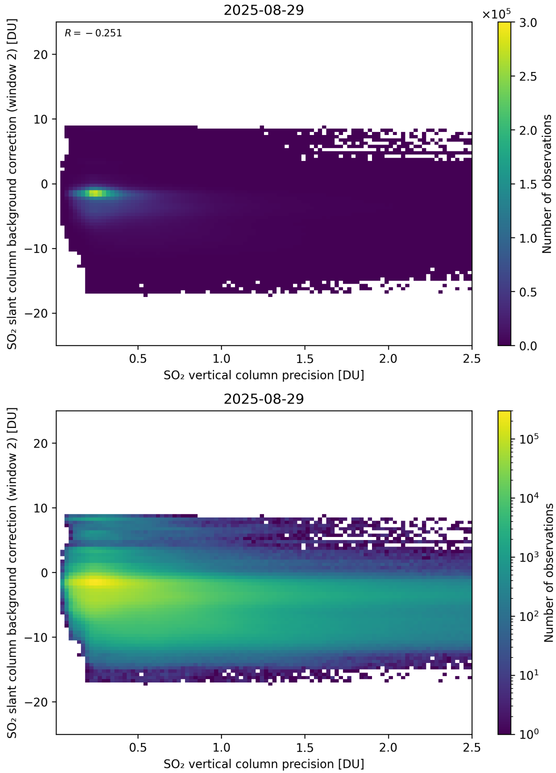
Figure 330: Scatter density plot of “SO 2 vertical column precision” against “SO 2 slant column background correction (window 2)” for 2025-08-28 to 2025-08-30.
