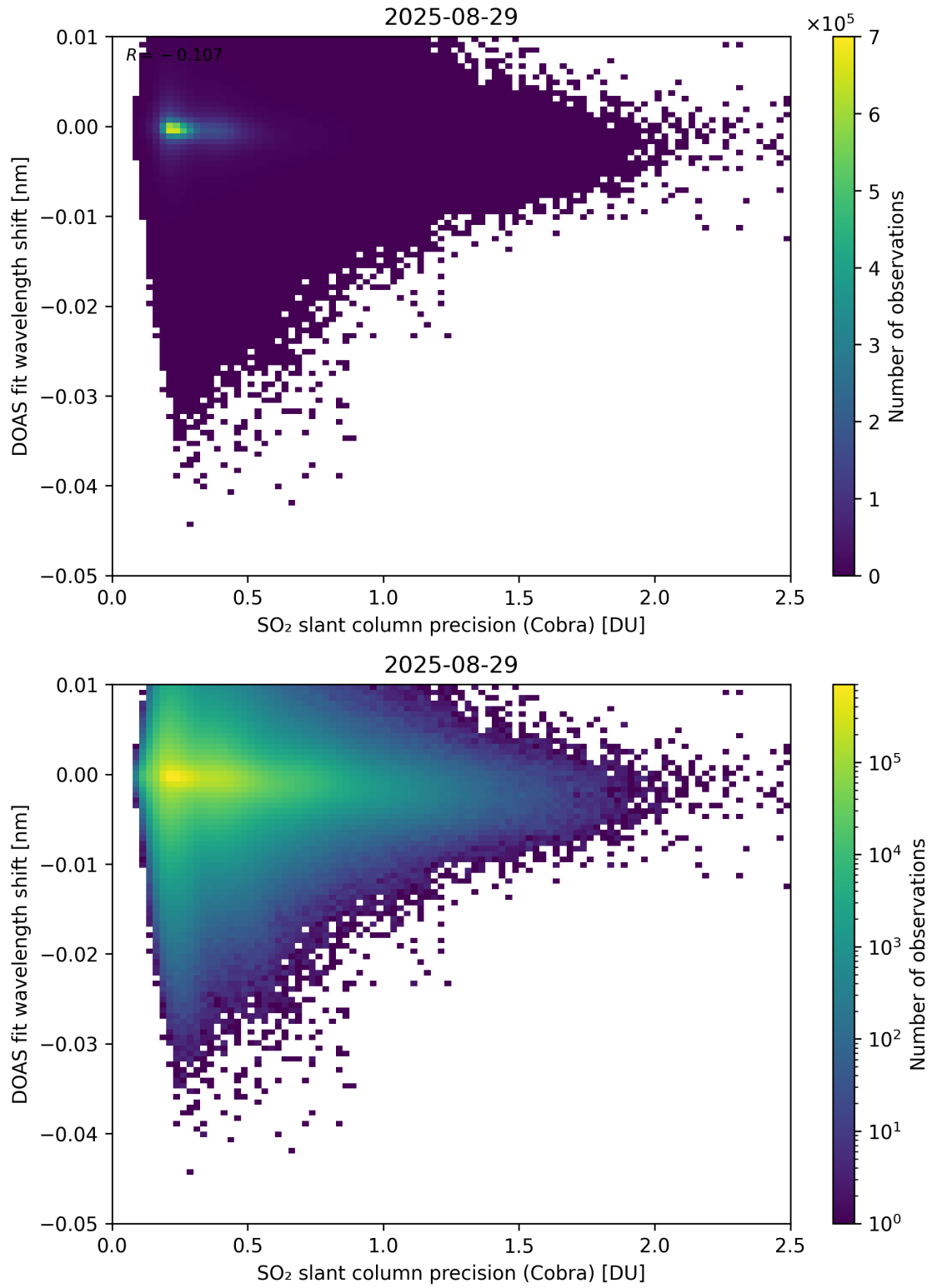
Figure 202: Scatter density plot of “SO 2 slant column precision (Cobra)” against “DOAS fit wavelength shift” for 2025-08-28 to 2025-08-30.
