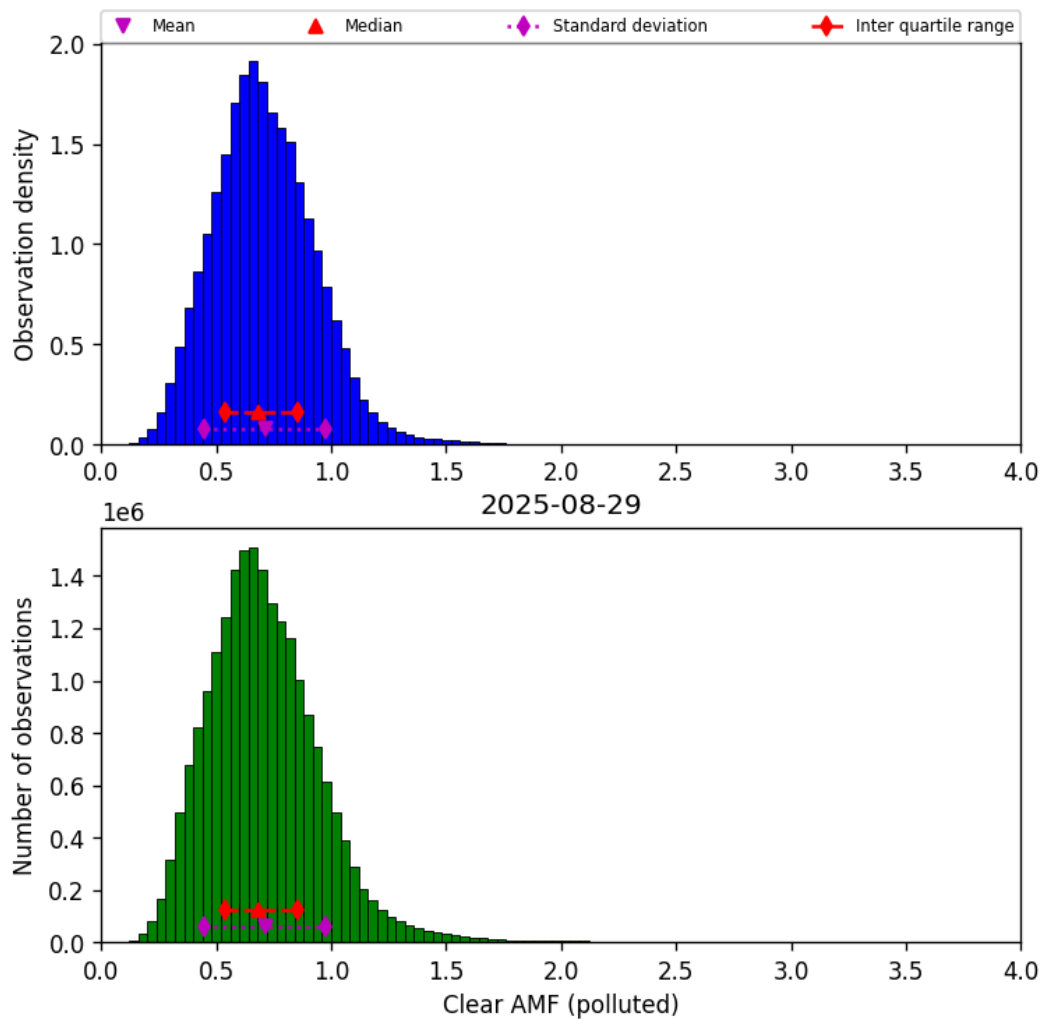
Figure 81: Histogram of “Clear AMF (polluted)” for 2025-08-28 to 2025-08-30
