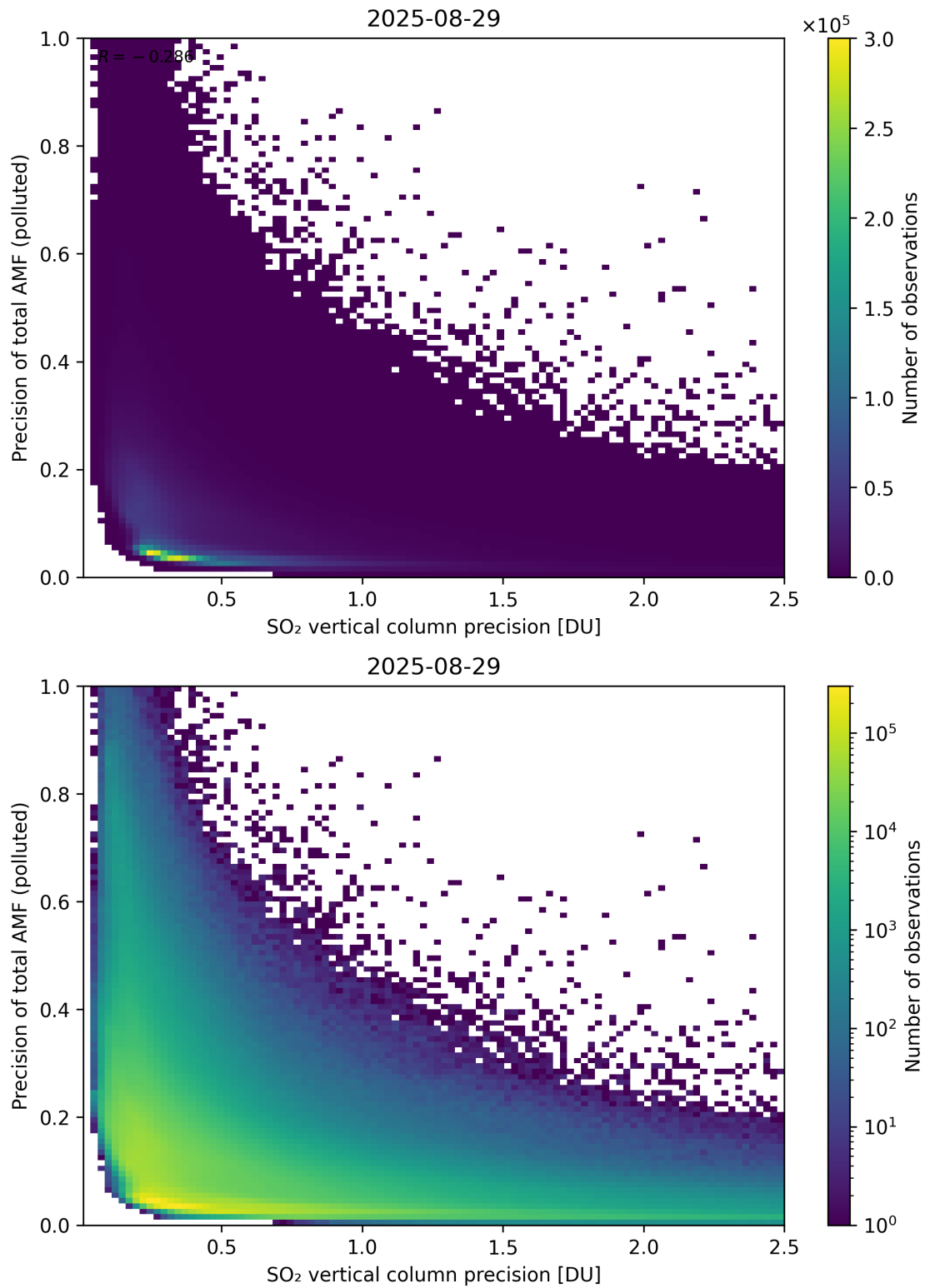
Figure 347: Scatter density plot of “SO 2 vertical column precision” against “Precision of total AMF (polluted)” for 2025-08-28 to 2025-08-30.
