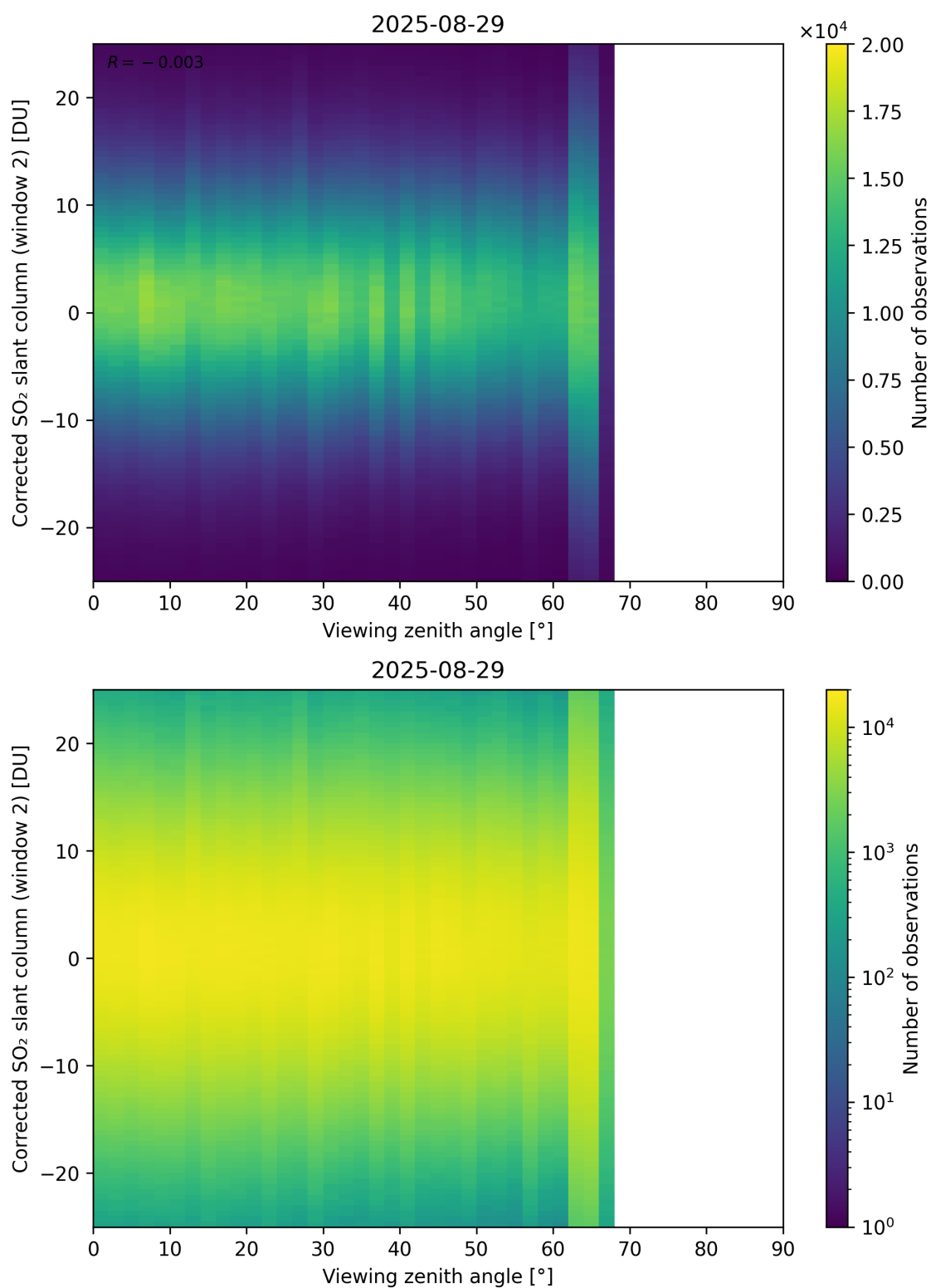
Figure 374: Scatter density plot of “Viewing zenith angle” against “Corrected SO 2 slant column (window 2)” for 2025-08-28 to 2025-08-30.
