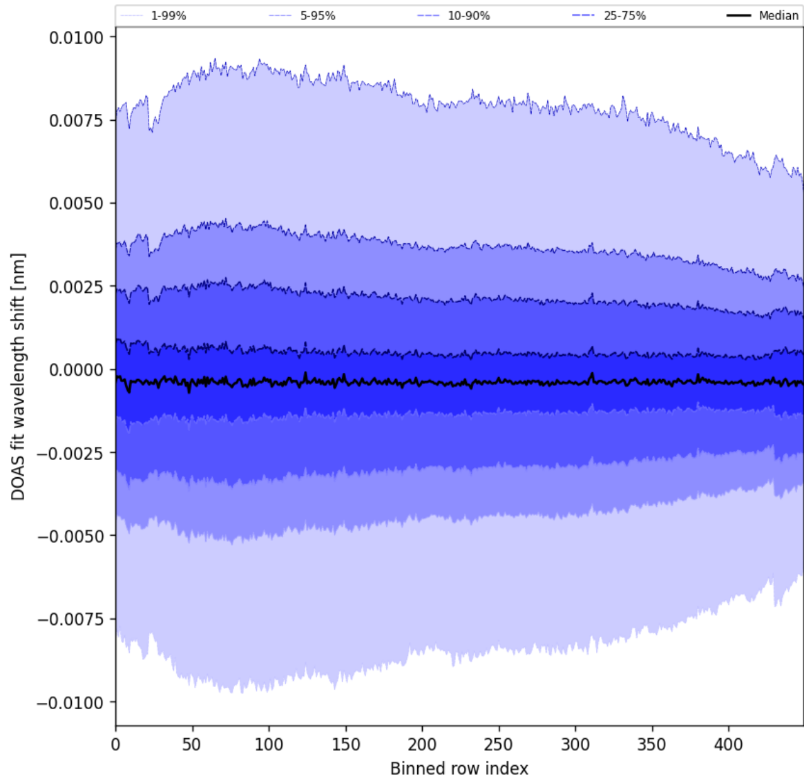
Figure 102: Along track statistics of “DOAS fit wavelength shift” for 2025-08-28 to 2025-08-30
