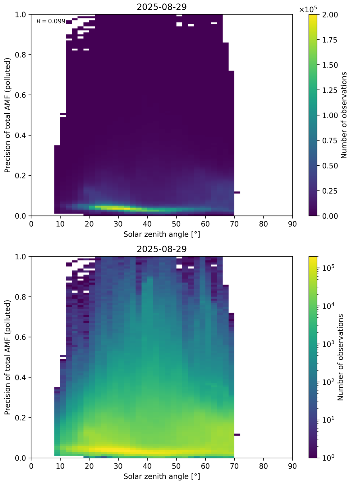
Figure 190: Scatter density plot of “Solar zenith angle” against “Precision of total AMF (polluted)” for 2025-08-28 to 2025-08-30.
