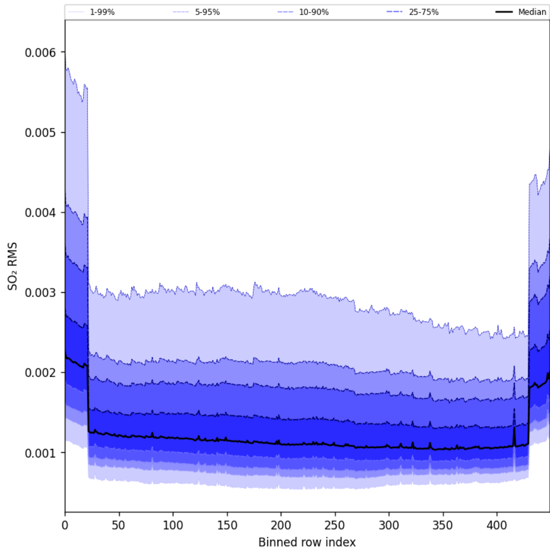
Figure 104: Along track statistics of “SO 2 RMS” for 2025-08-28 to 2025-08-30
