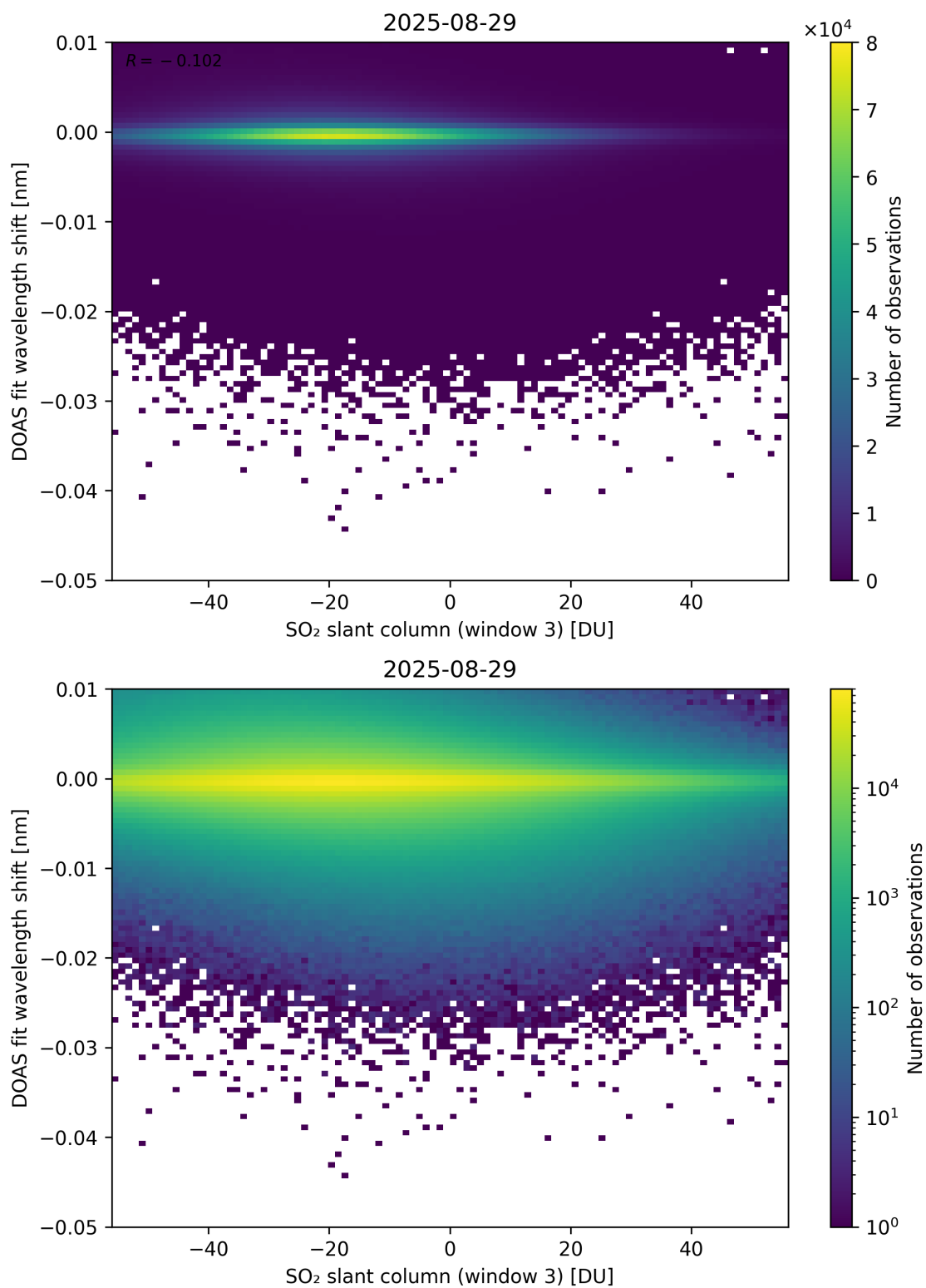
Figure 304: Scatter density plot of “SO 2 slant column (window 3)” against “DOAS fit wavelength shift” for 2025-08-28 to 2025-08-30.
