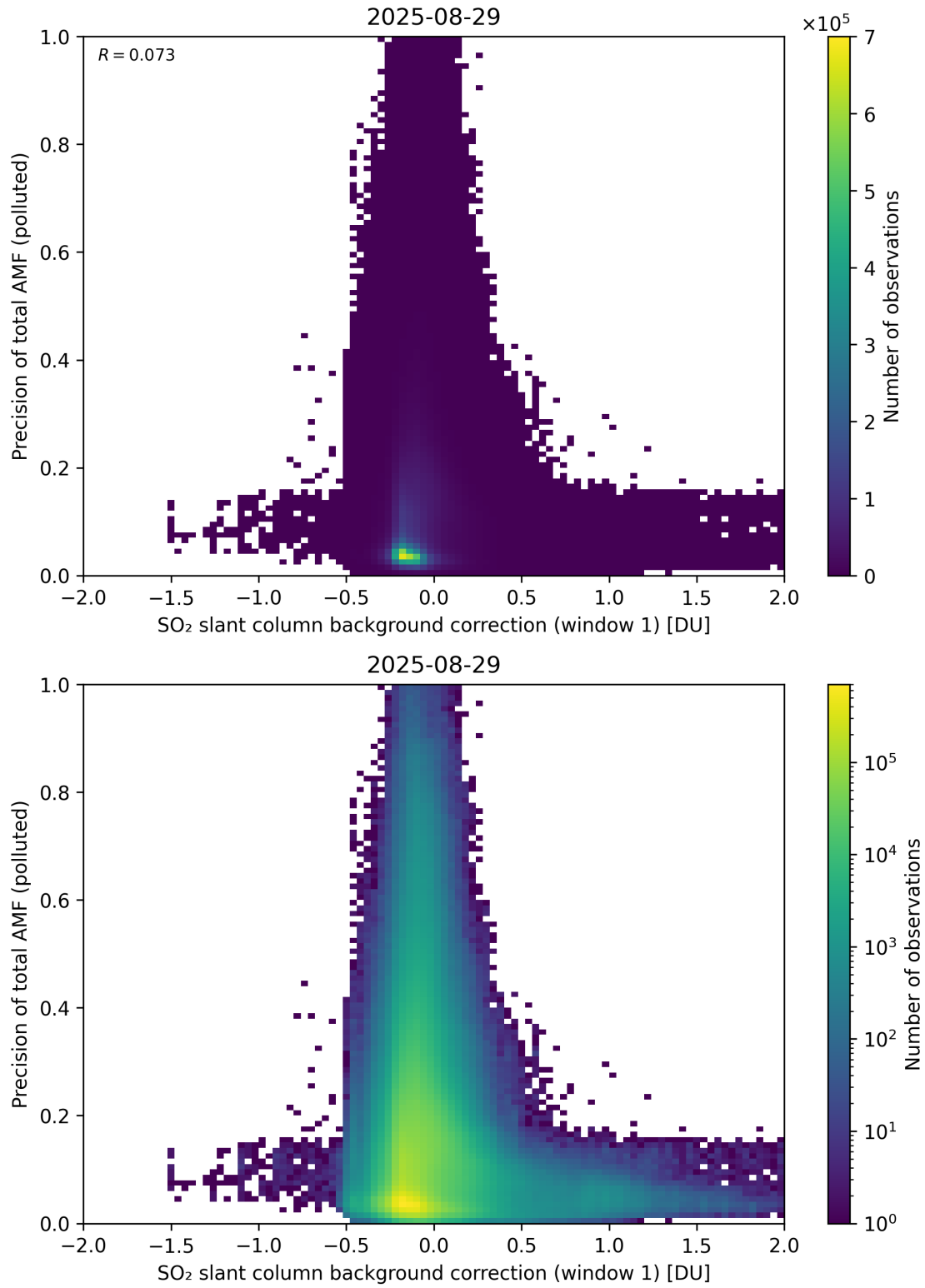
Figure 121: Scatter density plot of “SO 2 slant column background correction (window 1)” against “Precision of total AMF (polluted)” for 2025-08-28 to 2025-08-30.
