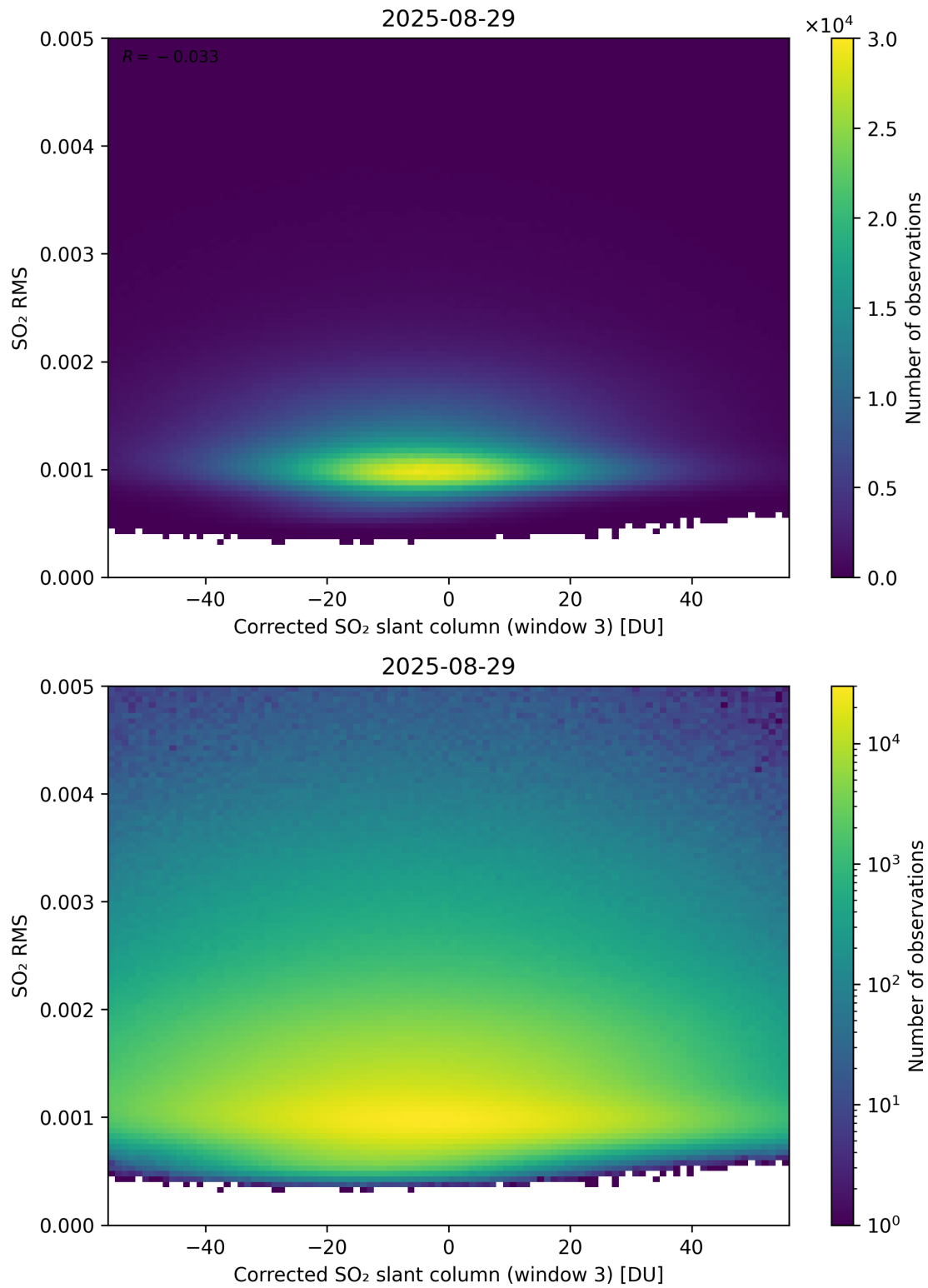
Figure 258: Scatter density plot of “Corrected SO 2 slant column (window 3)” against “SO 2 RMS” for 2025-08-28 to 2025-08-30.
