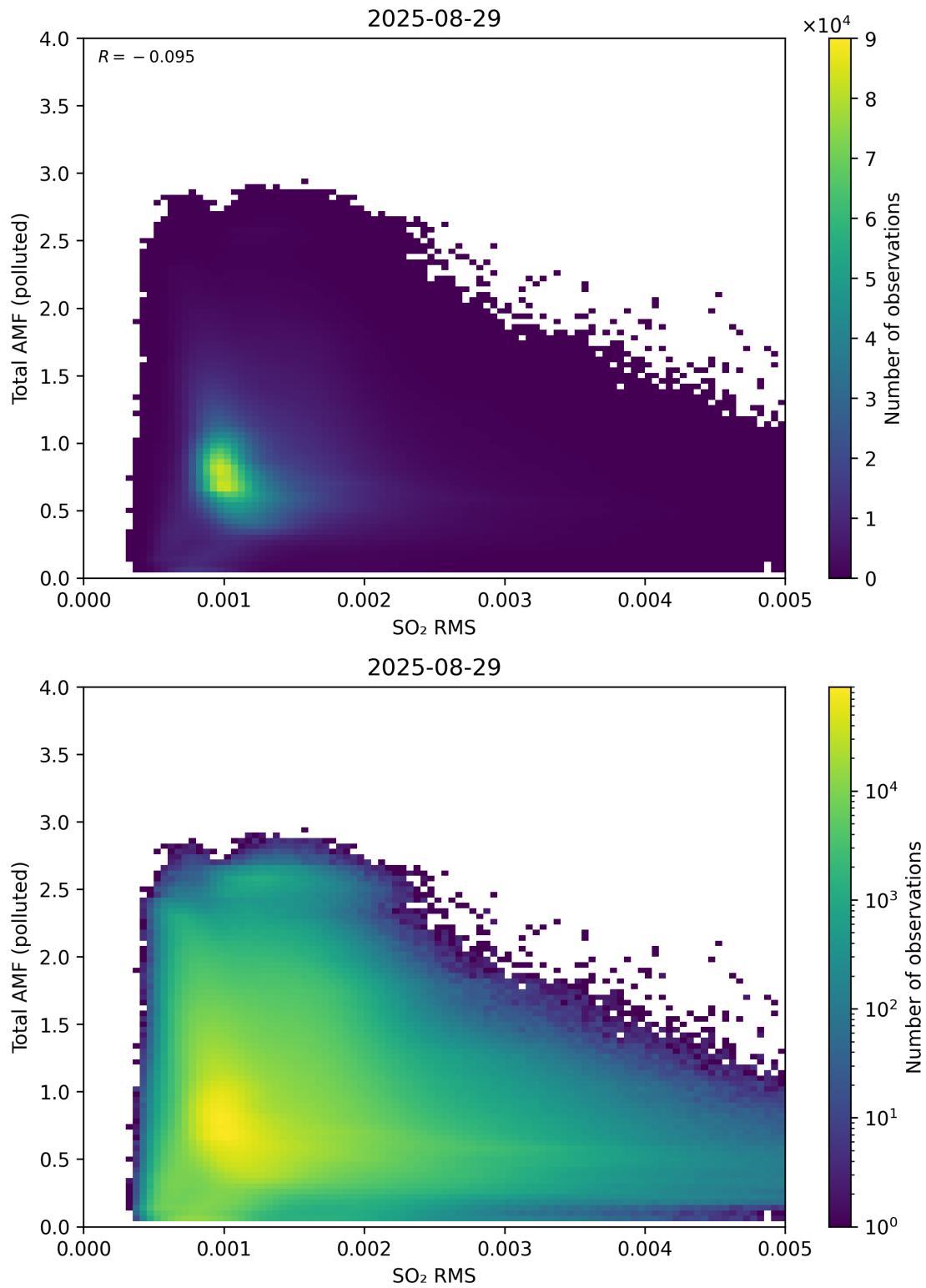
Figure 148: Scatter density plot of “SO 2 RMS” against “Total AMF (polluted)” for 2025-08-28 to 2025-08-30.
