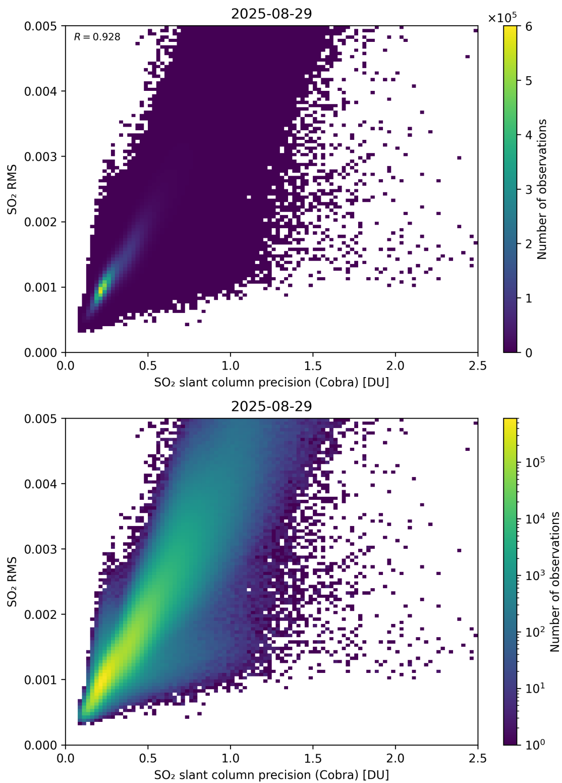
Figure 204: Scatter density plot of “SO 2 slant column precision (Cobra)” against “SO 2 RMS” for 2025-08-28 to 2025-08-30.
