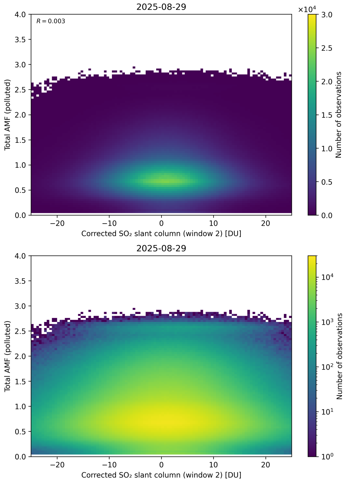
Figure 253: Scatter density plot of “Corrected SO 2 slant column (window 2)” against “Total AMF (polluted)” for 2025-08-28 to 2025-08-30.
