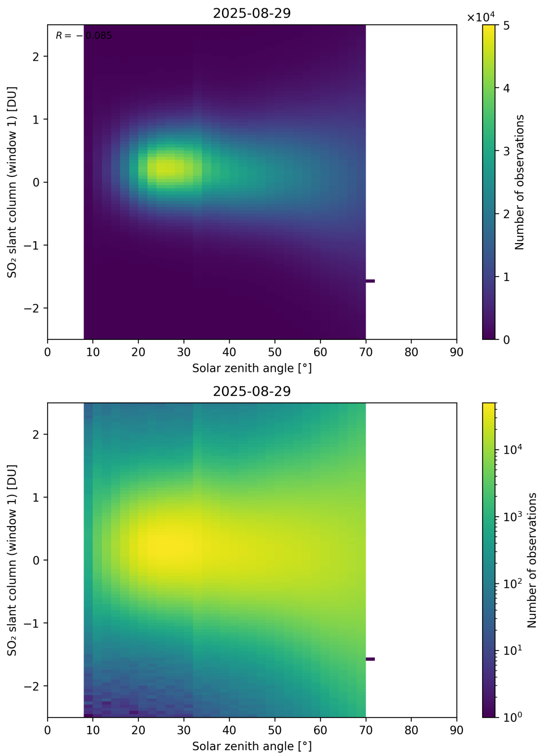
Figure 184: Scatter density plot of “Solar zenith angle” against “SO 2 slant column (window 1)” for 2025-08-28 to 2025-08-30.
