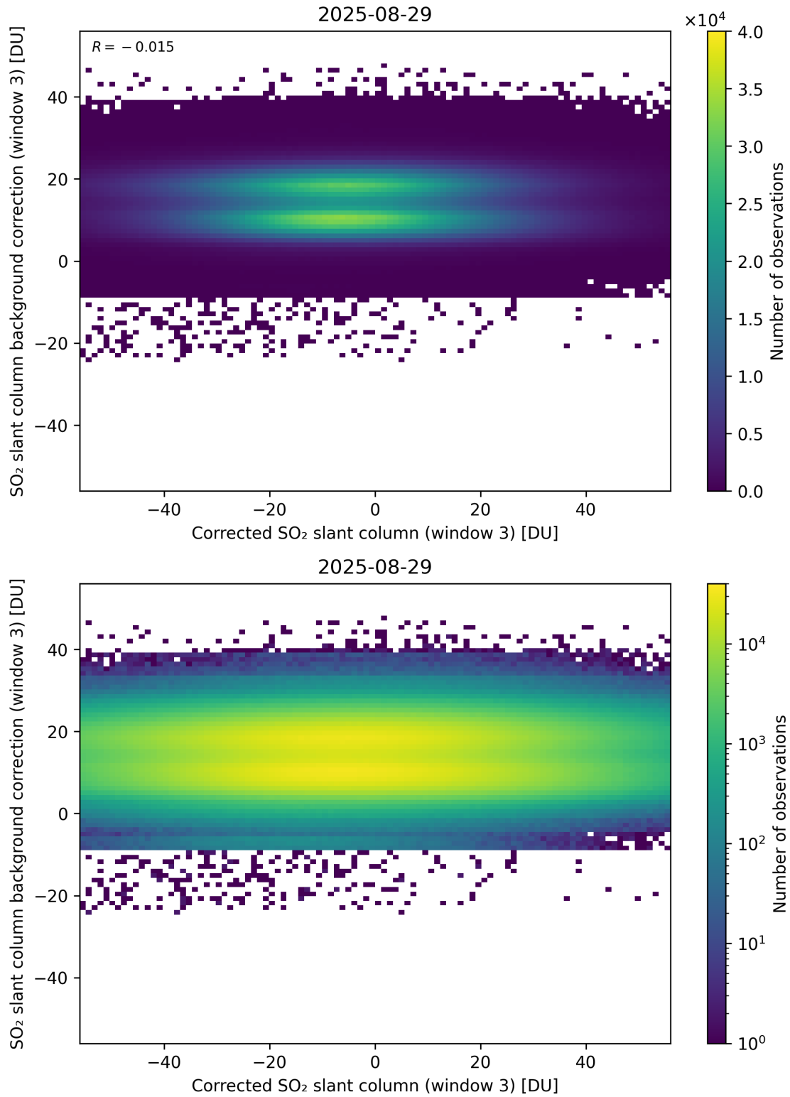
Figure 255: Scatter density plot of “Corrected SO 2 slant column (window 3)” against “SO 2 slant column background correction (window 3)” for 2025-08-28 to 2025-08-30.
