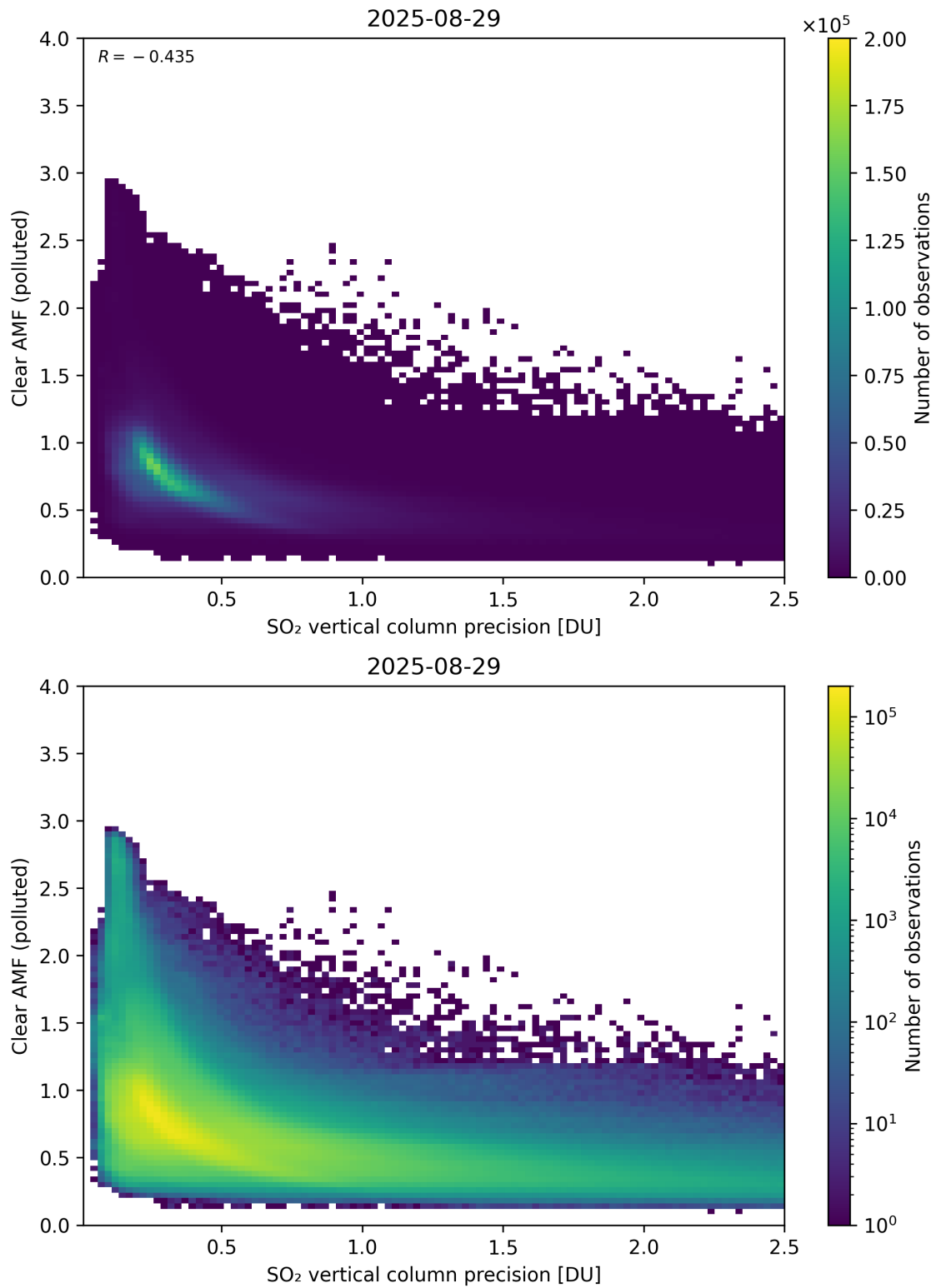
Figure 335: Scatter density plot of “SO 2 vertical column precision” against “Clear AMF (polluted)” for 2025-08-28 to 2025-08-30.
