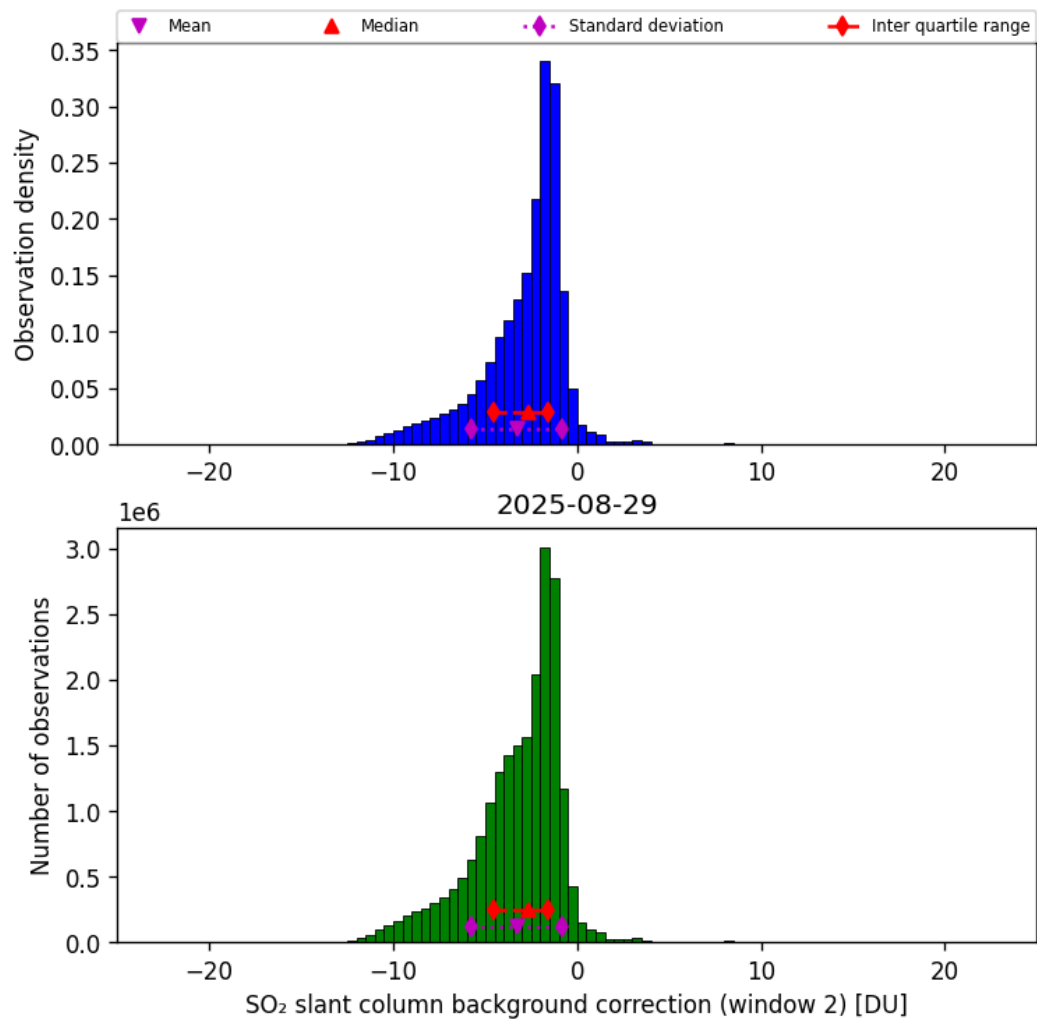
Figure 70: Histogram of “SO 2 slant column background correction (window 2)” for 2025-08-28 to 2025-08-30
