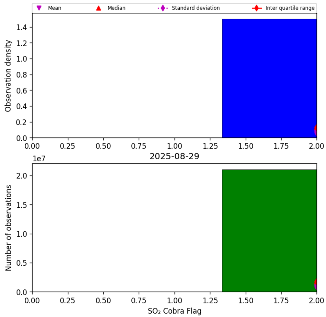
Figure 75: Histogram of “SO 2 Cobra Flag” for 2025-08-28 to 2025-08-30
