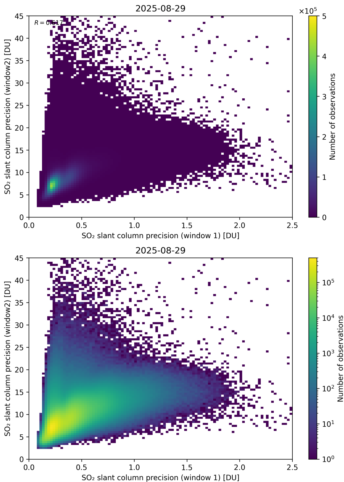
Figure 277: Scatter density plot of “SO 2 slant column precision (window 1)” against “SO 2 slant column precision (window2)” for 2025-08-28 to 2025-08-30.
