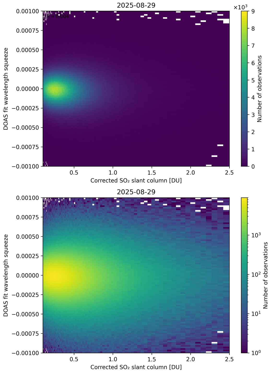
Figure 230: Scatter density plot of “Corrected SO 2 slant column” against “DOAS fit wavelength squeeze” for 2025-08-28 to 2025-08-30.
