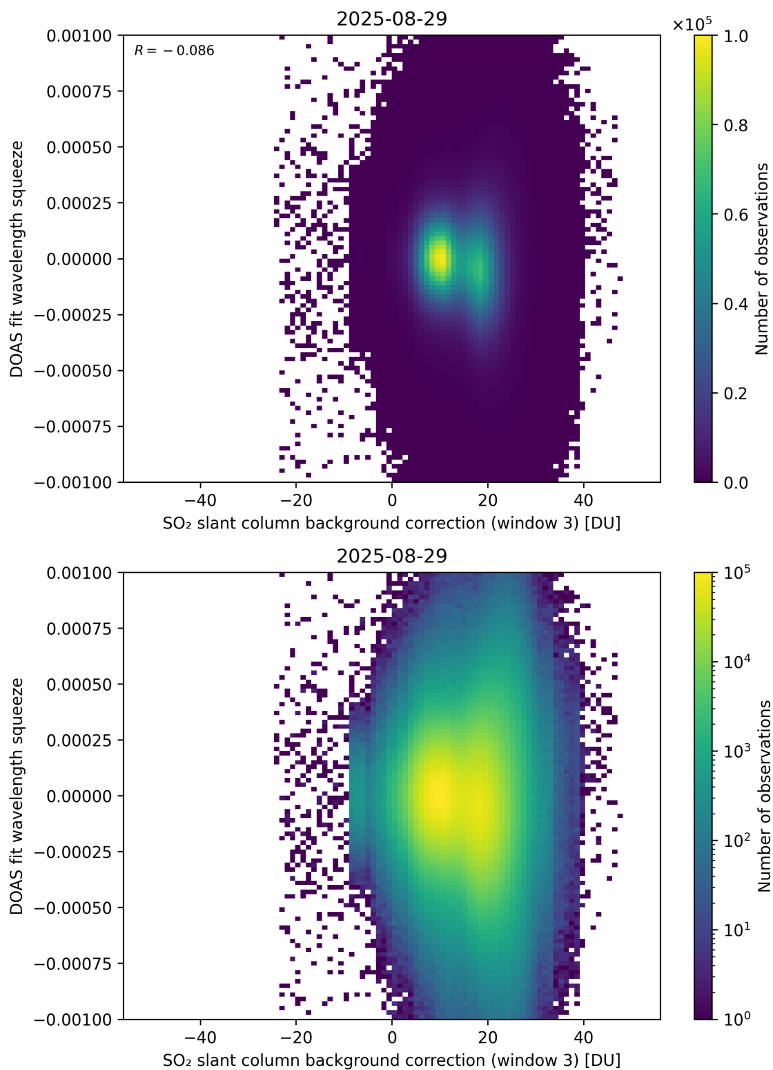
Figure 133: Scatter density plot of “SO 2 slant column background correction (window 3)” against “DOAS fit wavelength squeeze” for 2025-08-28 to 2025-08-30.
