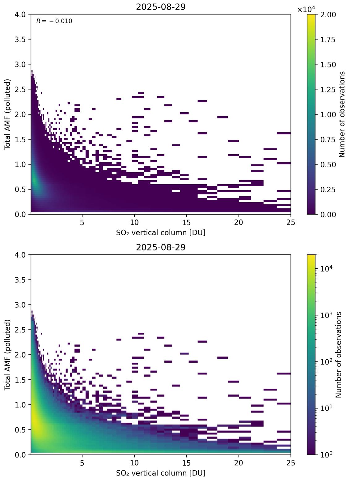
Figure 359: Scatter density plot of “SO 2 vertical column” against “Total AMF (polluted)” for 2025-08-28 to 2025-08-30.
