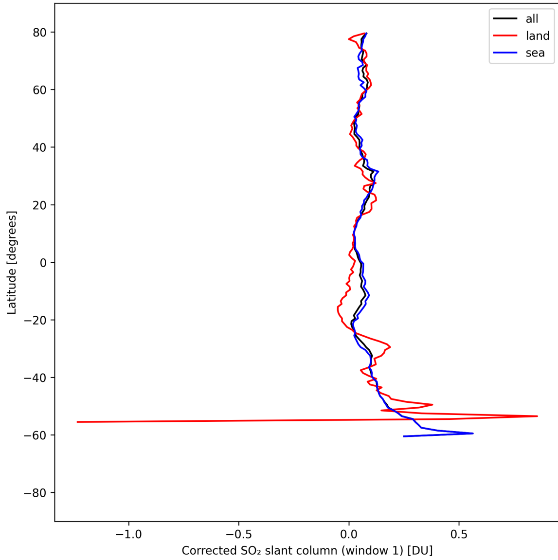
Figure 39: Zonal average of “Corrected SO 2 slant column (window 1)” for 2025-08-28 to 2025-08-30.
