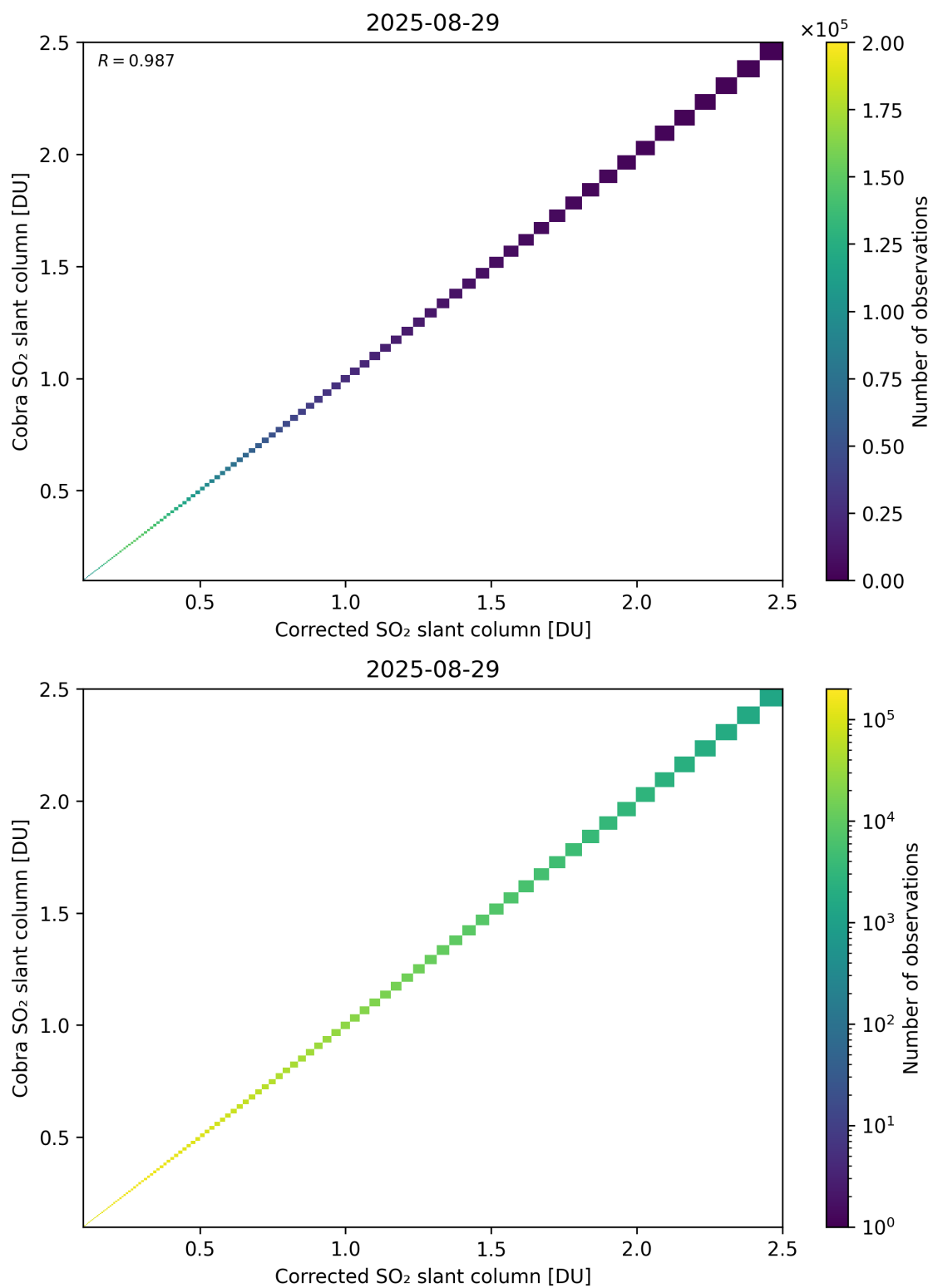
Figure 233: Scatter density plot of “Corrected SO 2 slant column” against “Cobra SO 2 slant column” for 2025-08-28 to 2025-08-30.
