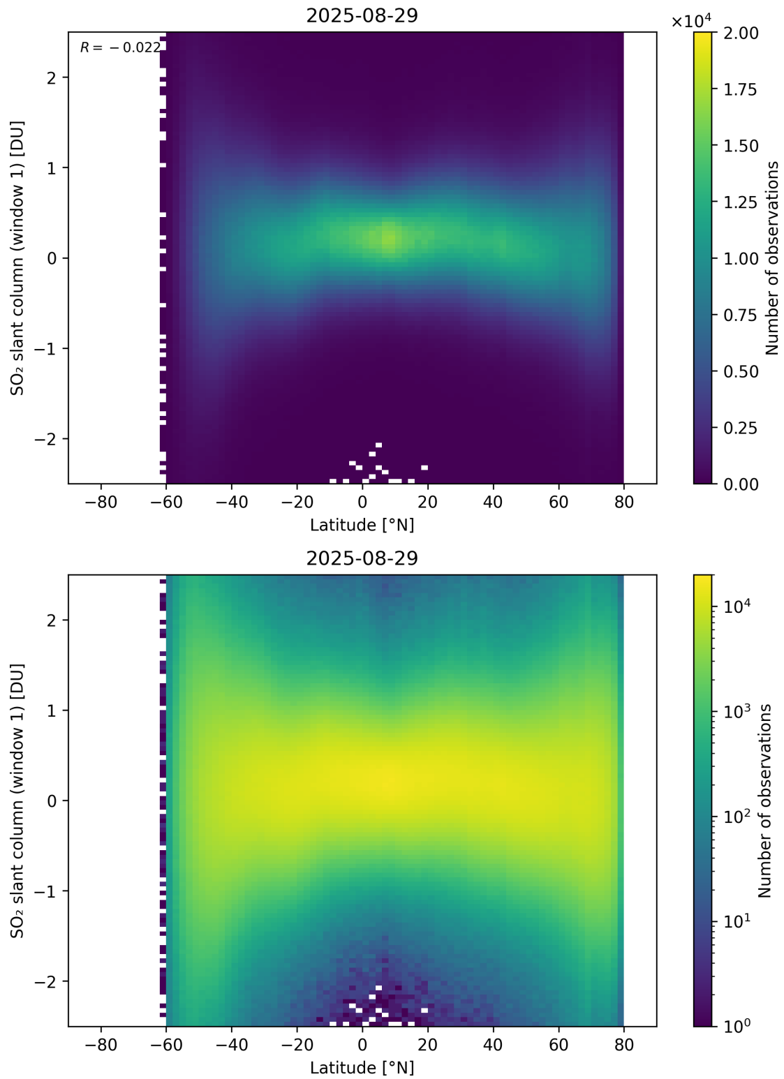
Figure 162: Scatter density plot of “Latitude” against “SO 2 slant column (window 1)” for 2025-08-28 to 2025-08-30.
