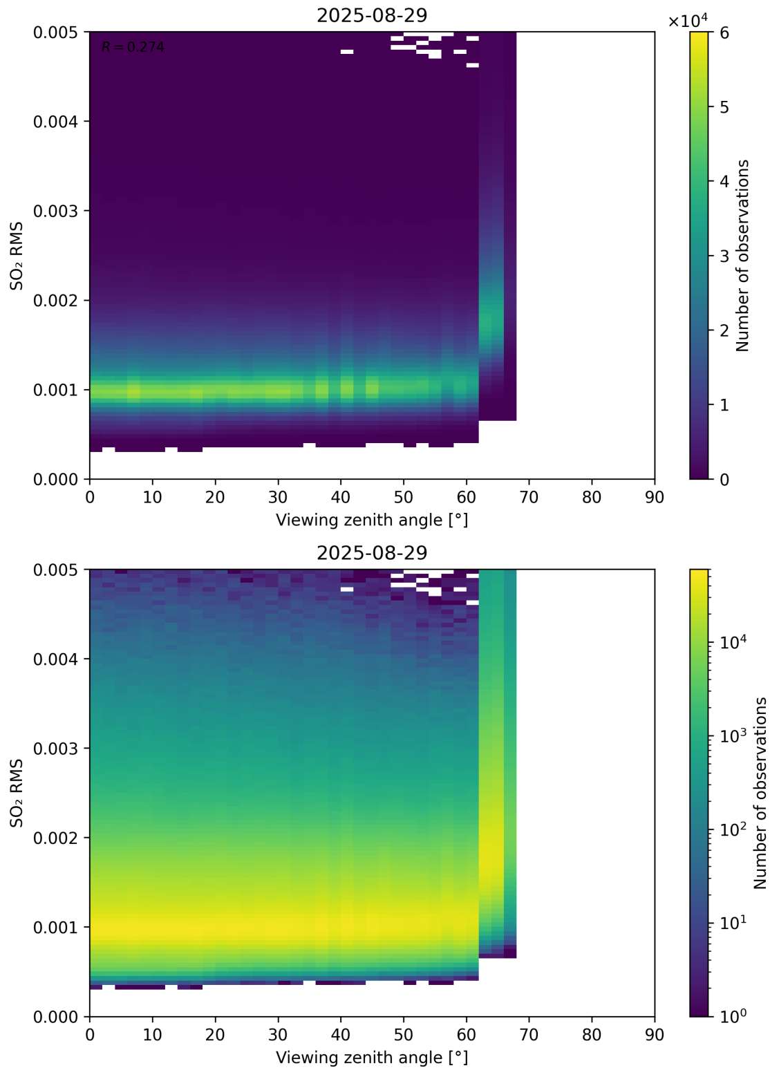
Figure 367: Scatter density plot of “Viewing zenith angle” against “SO 2 RMS” for 2025-08-28 to 2025-08-30.
