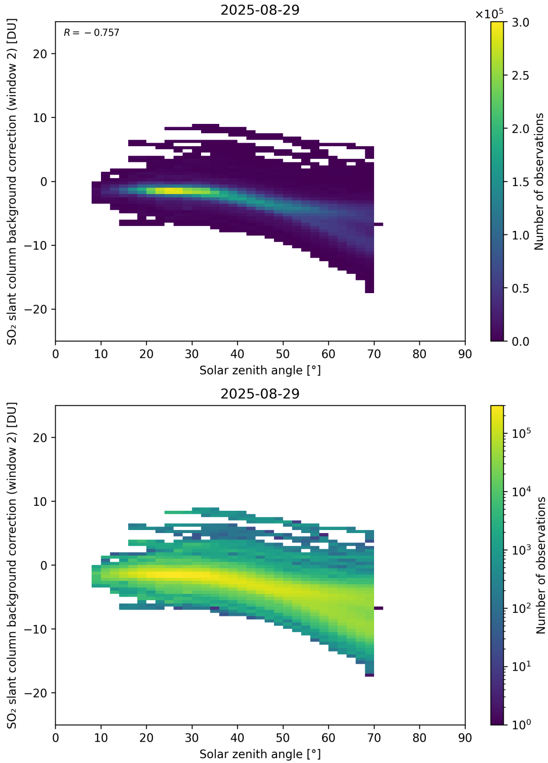
Figure 172: Scatter density plot of “Solar zenith angle” against “SO 2 slant column background correction (window 2)” for 2025-08-28 to 2025-08-30.
