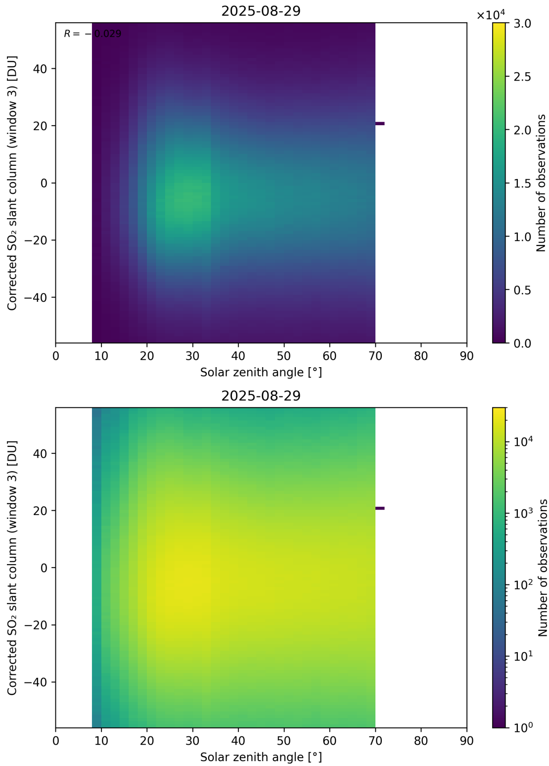
Figure 183: Scatter density plot of “Solar zenith angle” against “Corrected SO 2 slant column (window 3)” for 2025-08-28 to 2025-08-30.
