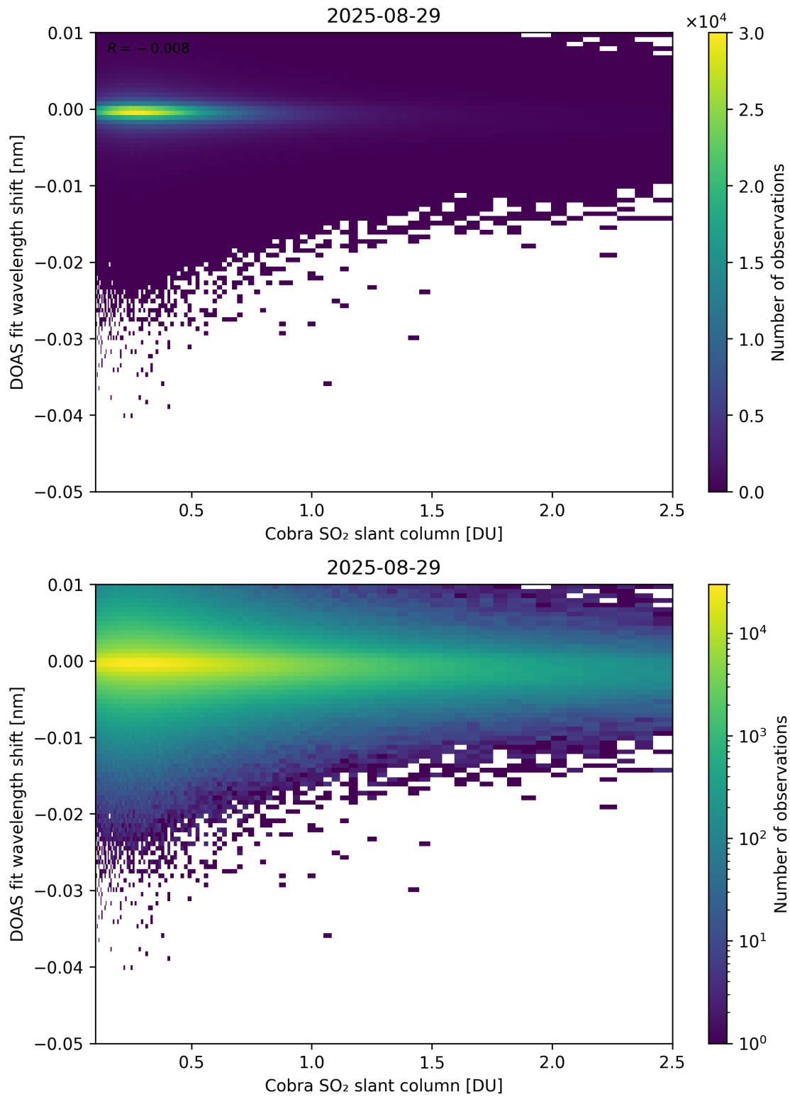
Figure 196: Scatter density plot of “Cobra SO 2 slant column” against “DOAS fit wavelength shift” for 2025-08-28 to 2025-08-30.
