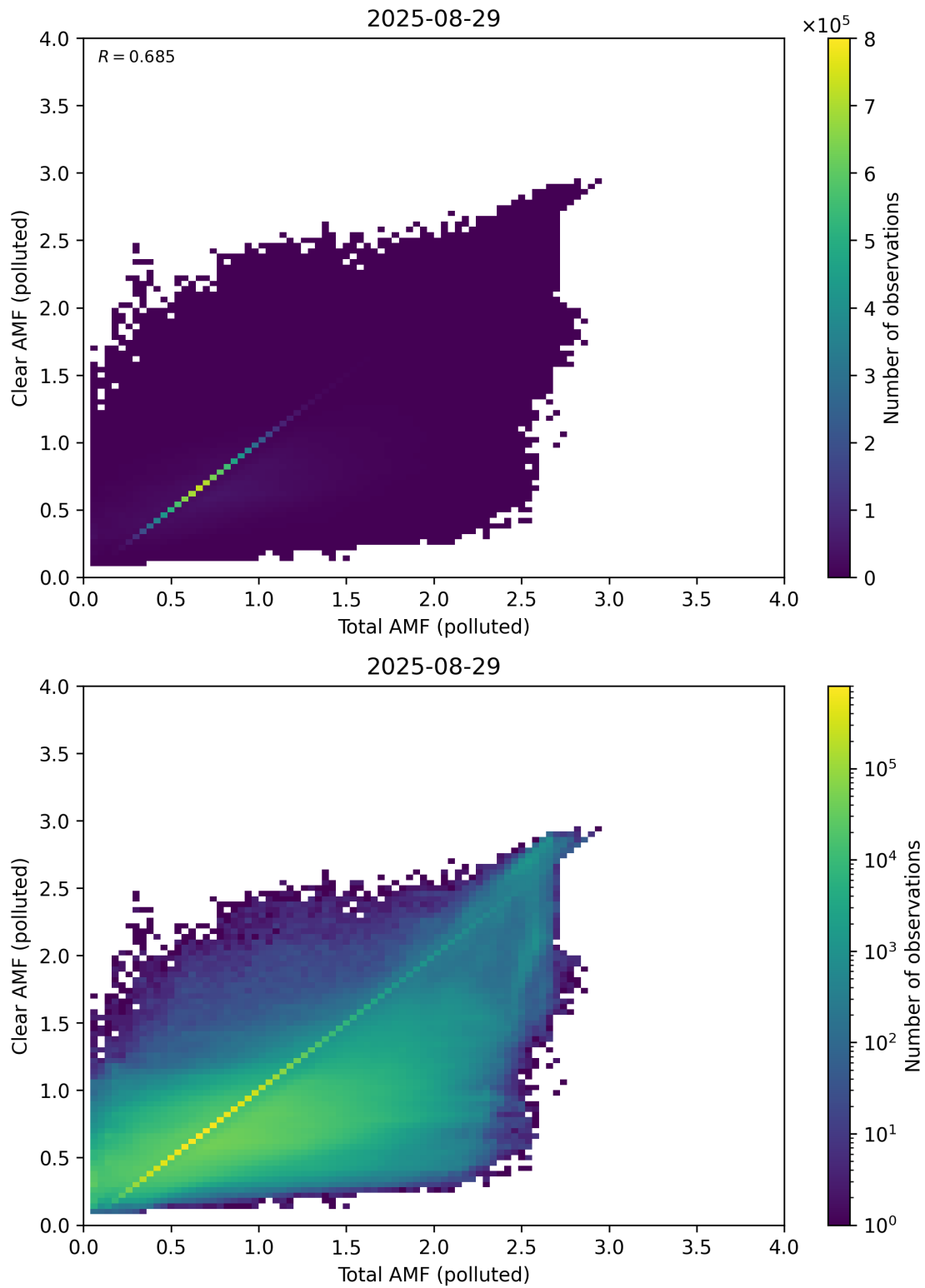
Figure 321: Scatter density plot of “Total AMF (polluted)” against “Clear AMF (polluted)” for 2025-08-28 to 2025-08-30.
