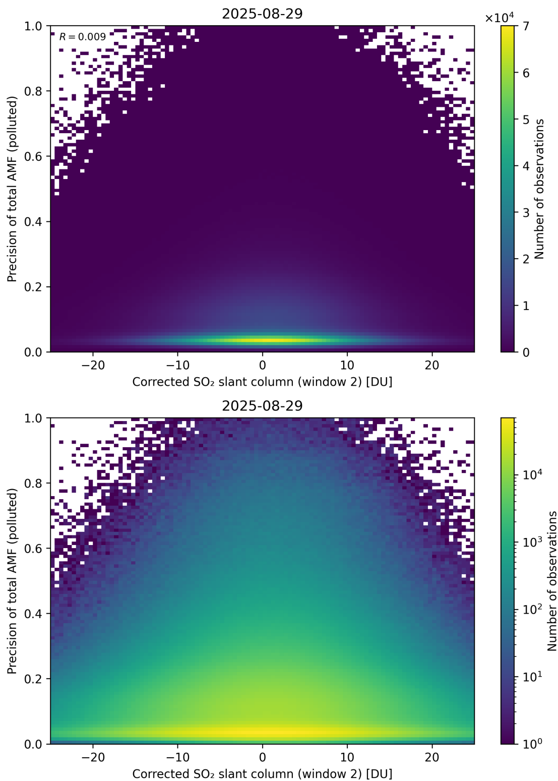
Figure 254: Scatter density plot of “Corrected SO 2 slant column (window 2)” against “Precision of total AMF (polluted)” for 2025-08-28 to 2025-08-30.
