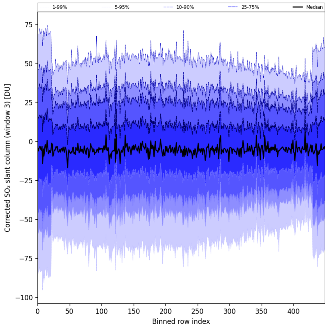
Figure 99: Along track statistics of “Corrected SO 2 slant column (window 3)” for 2025-08-28 to 2025-08-30
