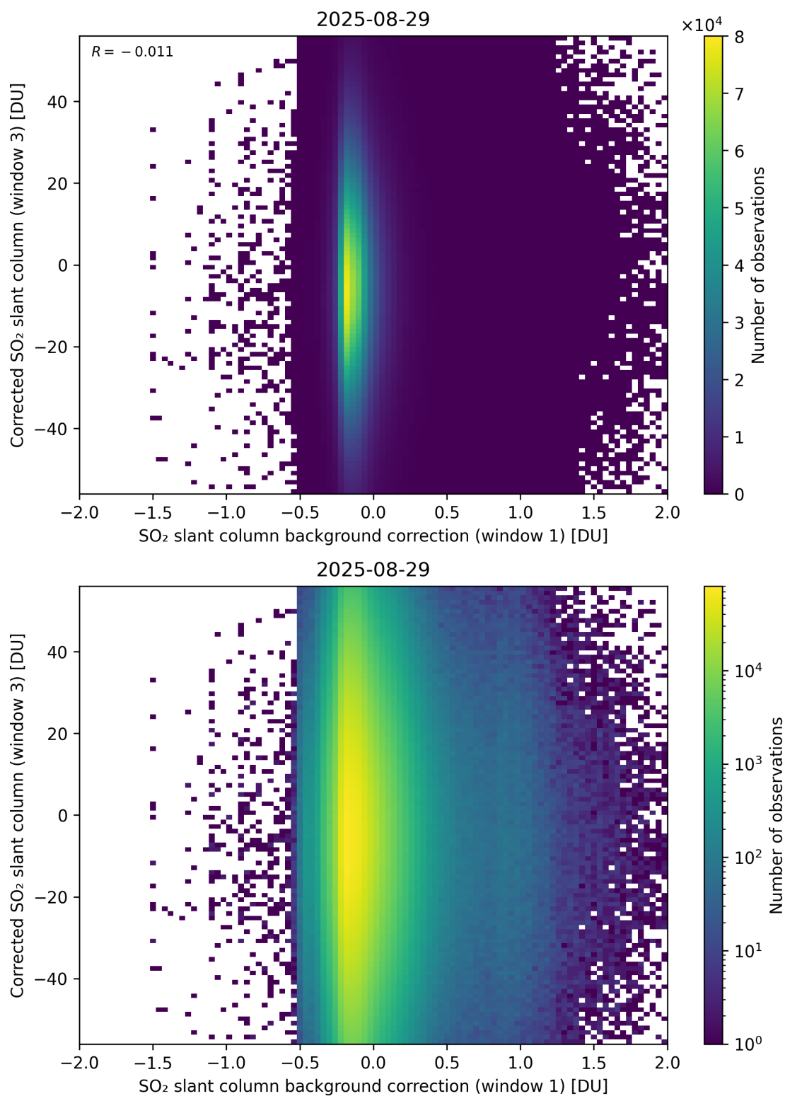
Figure 116: Scatter density plot of “SO 2 slant column background correction (window 1)” against “Corrected SO 2 slant column (window 3)” for 2025-08-28 to 2025-08-30.
