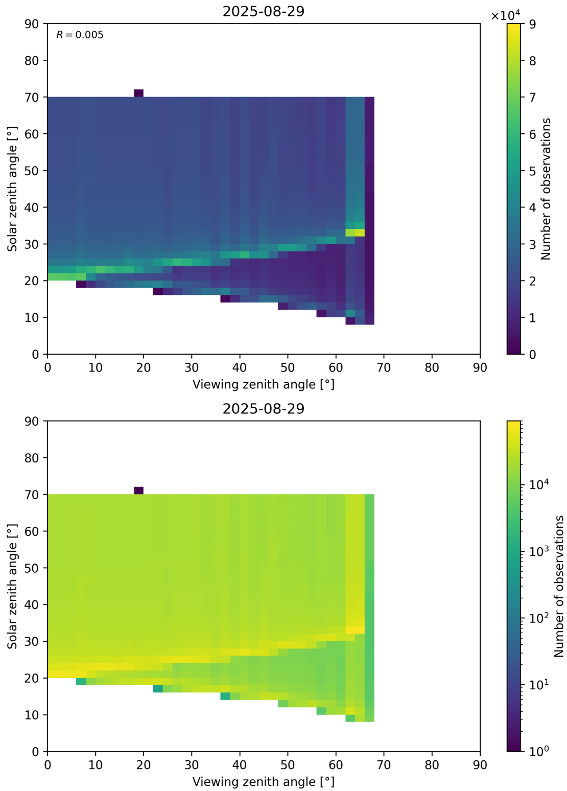
Figure 369: Scatter density plot of “Viewing zenith angle” against “Solar zenith angle” for 2025-08-28 to 2025-08-30.
