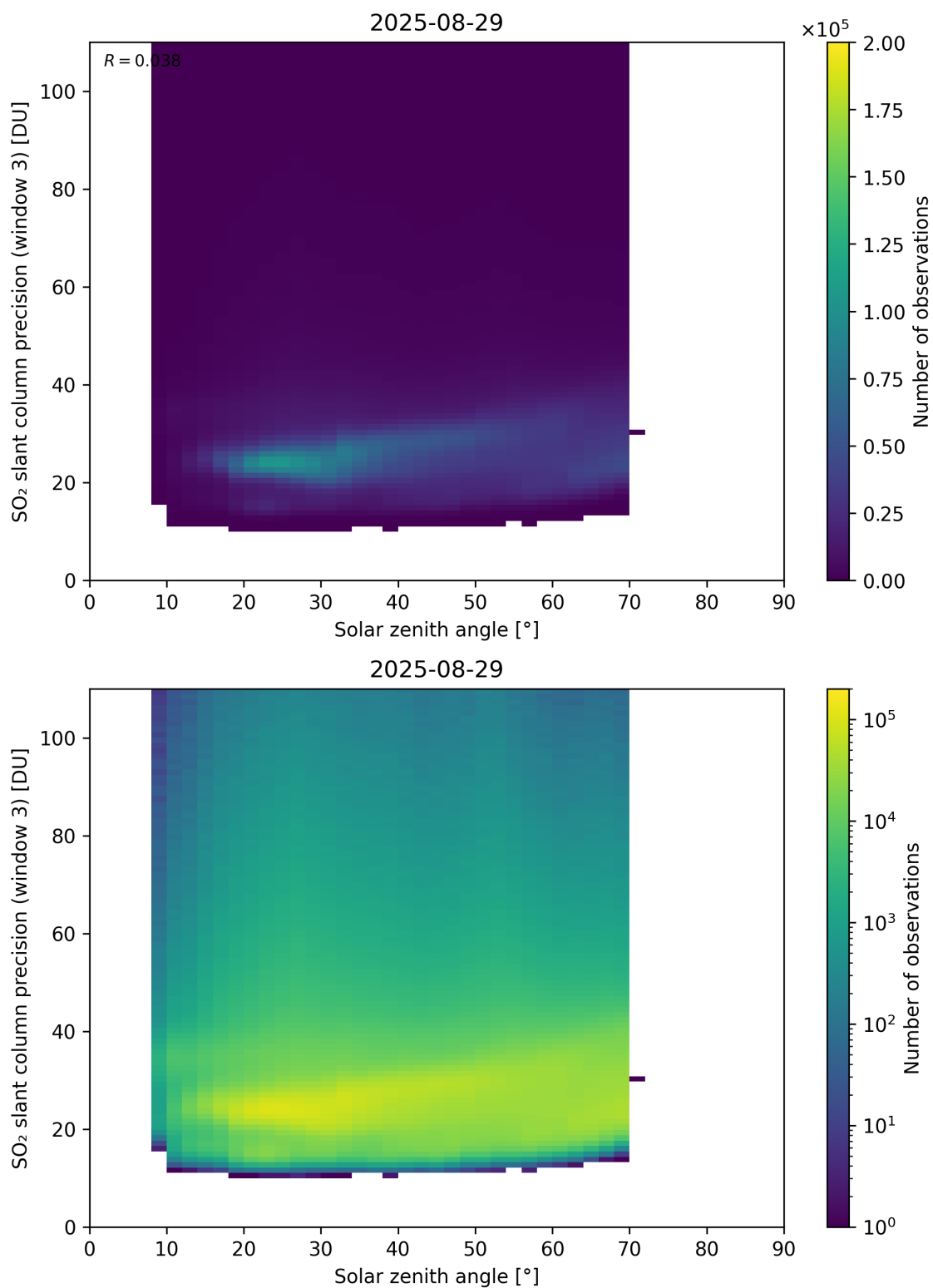
Figure 188: Scatter density plot of “Solar zenith angle” against “SO 2 slant column precision (window 3)” for 2025-08-28 to 2025-08-30.
