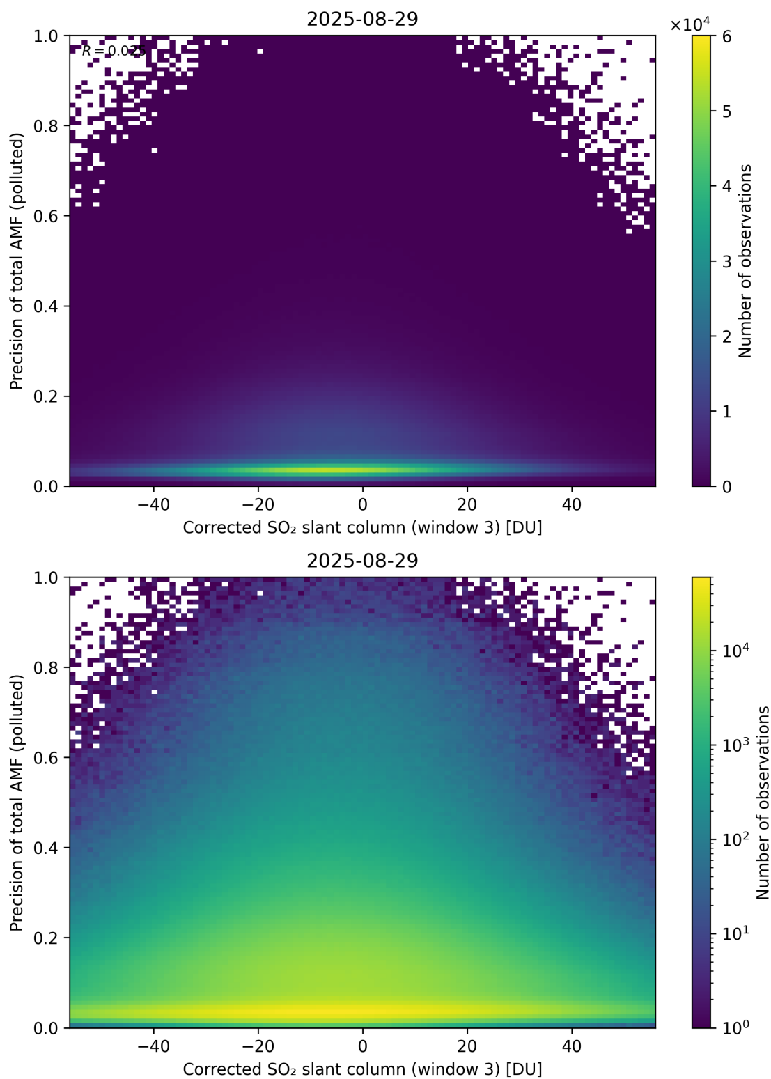
Figure 261: Scatter density plot of “Corrected SO 2 slant column (window 3)” against “Precision of total AMF (polluted)” for 2025-08-28 to 2025-08-30.
