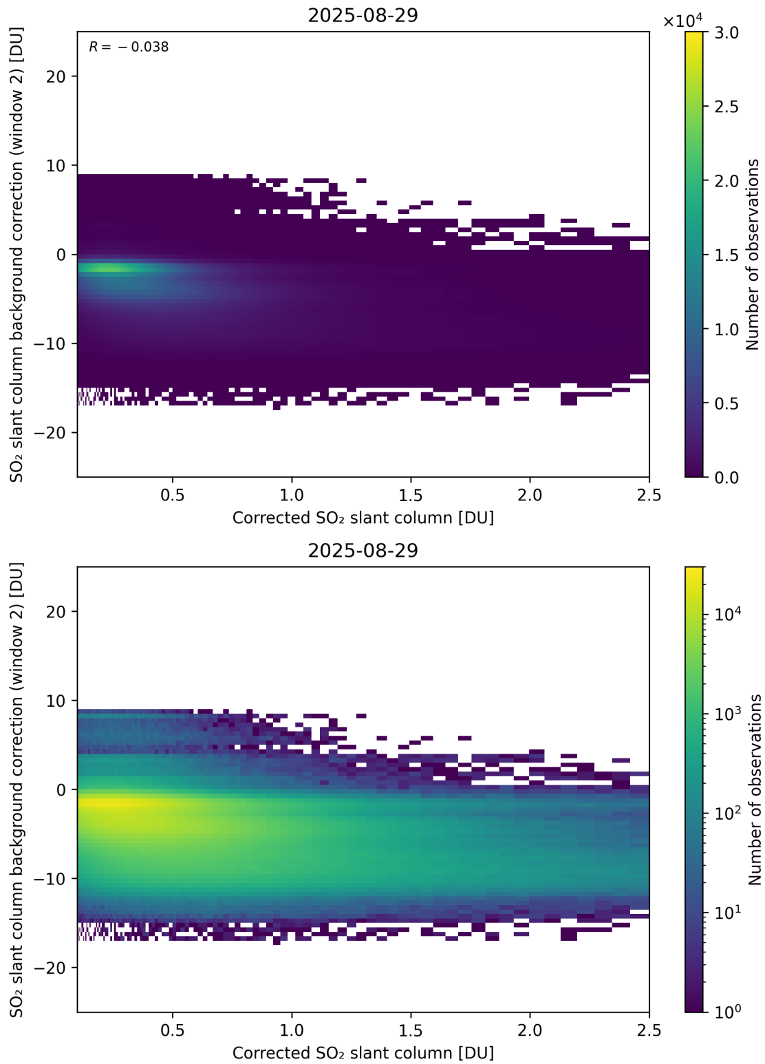
Figure 227: Scatter density plot of “Corrected SO 2 slant column” against “SO 2 slant column background correction (window 2)” for 2025-08-28 to 2025-08-30.
