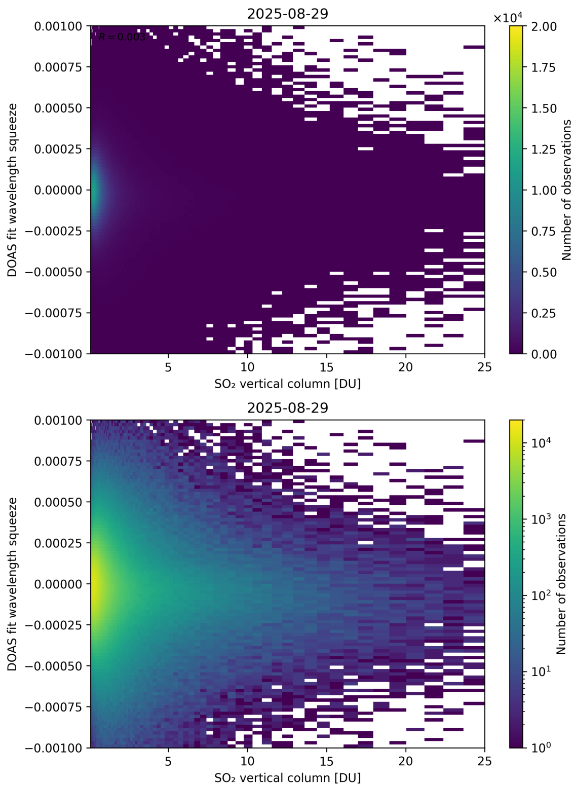
Figure 327: Scatter density plot of “SO 2 vertical column” against “DOAS fit wavelength squeeze” for 2025-08-28 to 2025-08-30.
