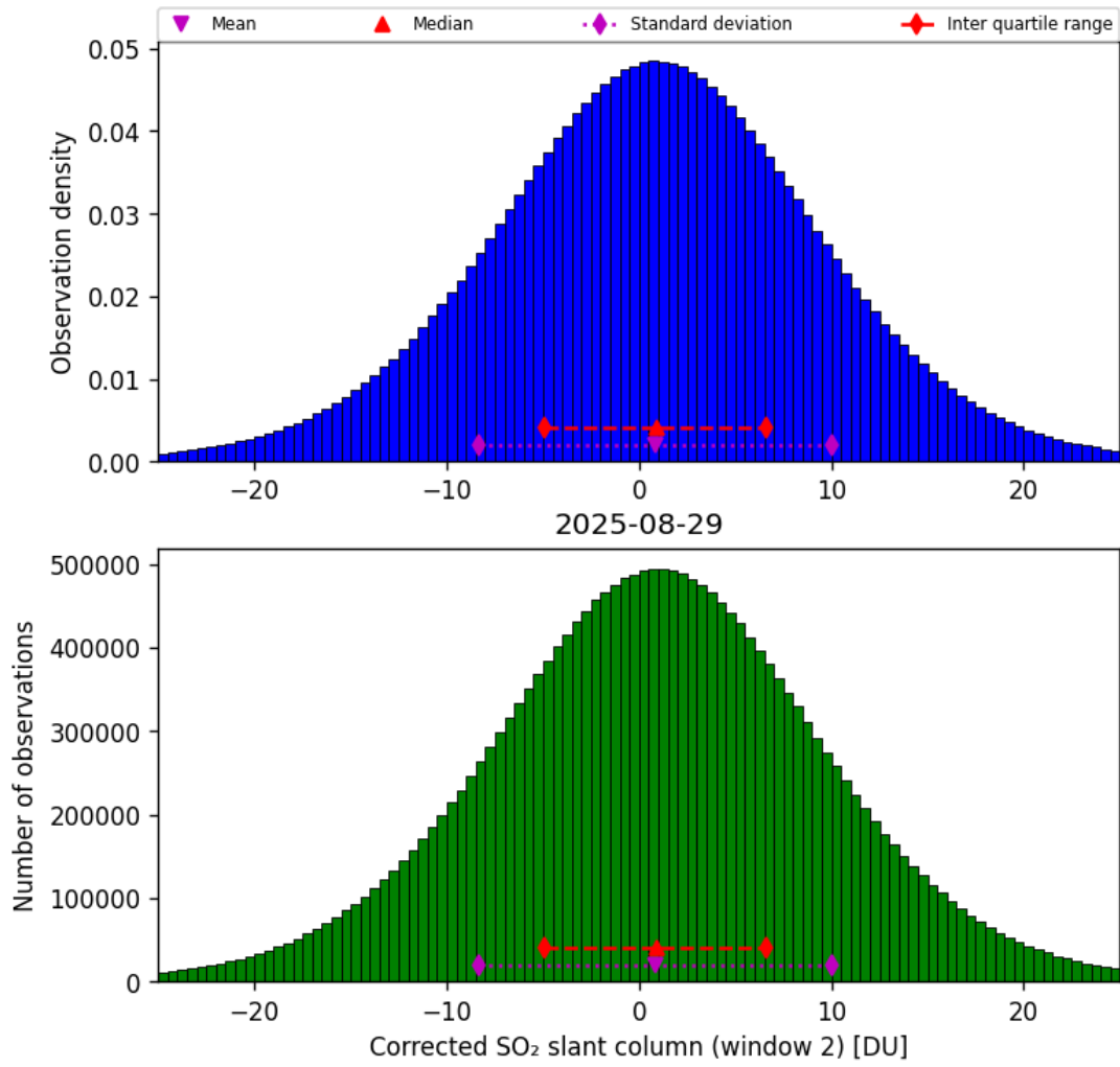
Figure 69: Histogram of “Corrected SO 2 slant column (window 2)” for 2025-08-28 to 2025-08-30
