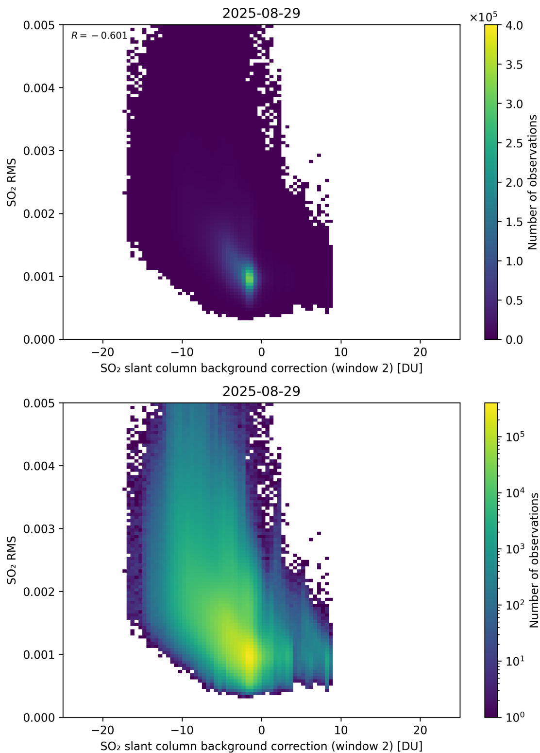
Figure 125: Scatter density plot of “SO 2 slant column background correction (window 2)” against “SO 2 RMS” for 2025-08-28 to 2025-08-30.
