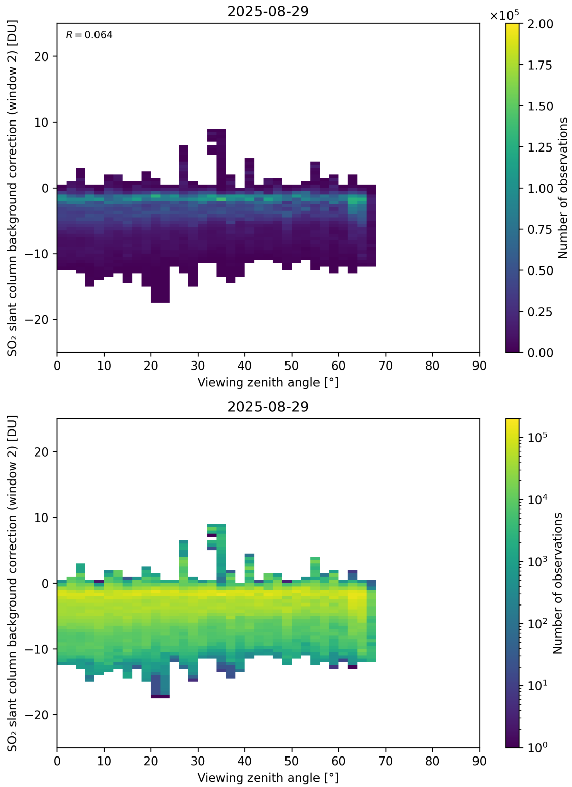
Figure 363: Scatter density plot of “Viewing zenith angle” against “SO 2 slant column background correction (window 2)” for 2025-08-28 to 2025-08-30.
