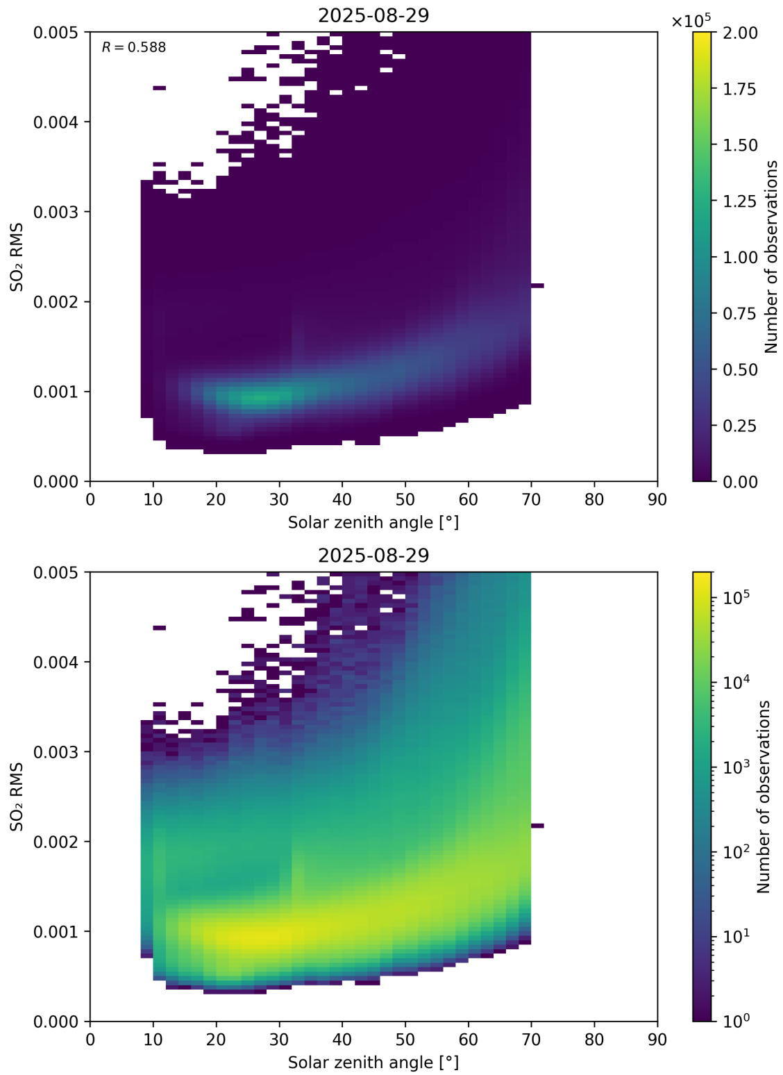
Figure 176: Scatter density plot of “Solar zenith angle” against “SO 2 RMS” for 2025-08-28 to 2025-08-30.
