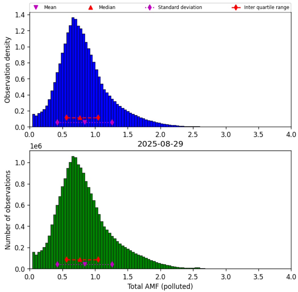
Figure 79: Histogram of “Total AMF (polluted)” for 2025-08-28 to 2025-08-30
