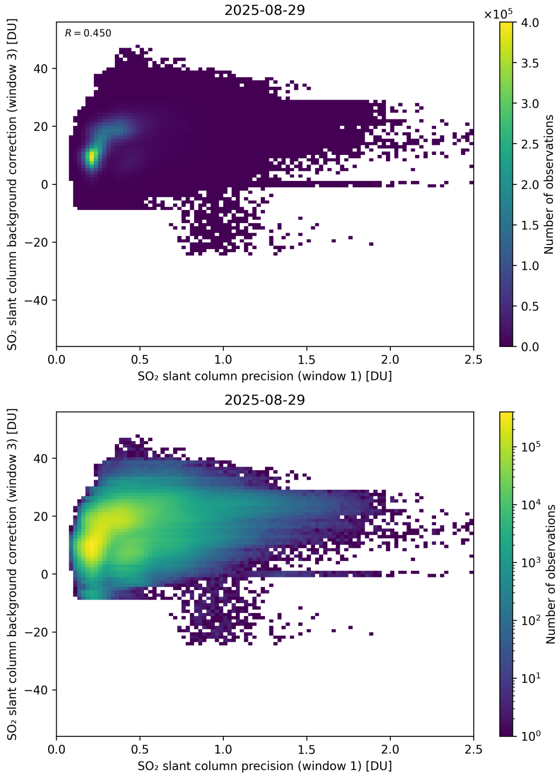
Figure 270: Scatter density plot of “SO 2 slant column precision (window 1)” against “SO 2 slant column background correction (window 3)” for 2025-08-28 to 2025-08-30.
