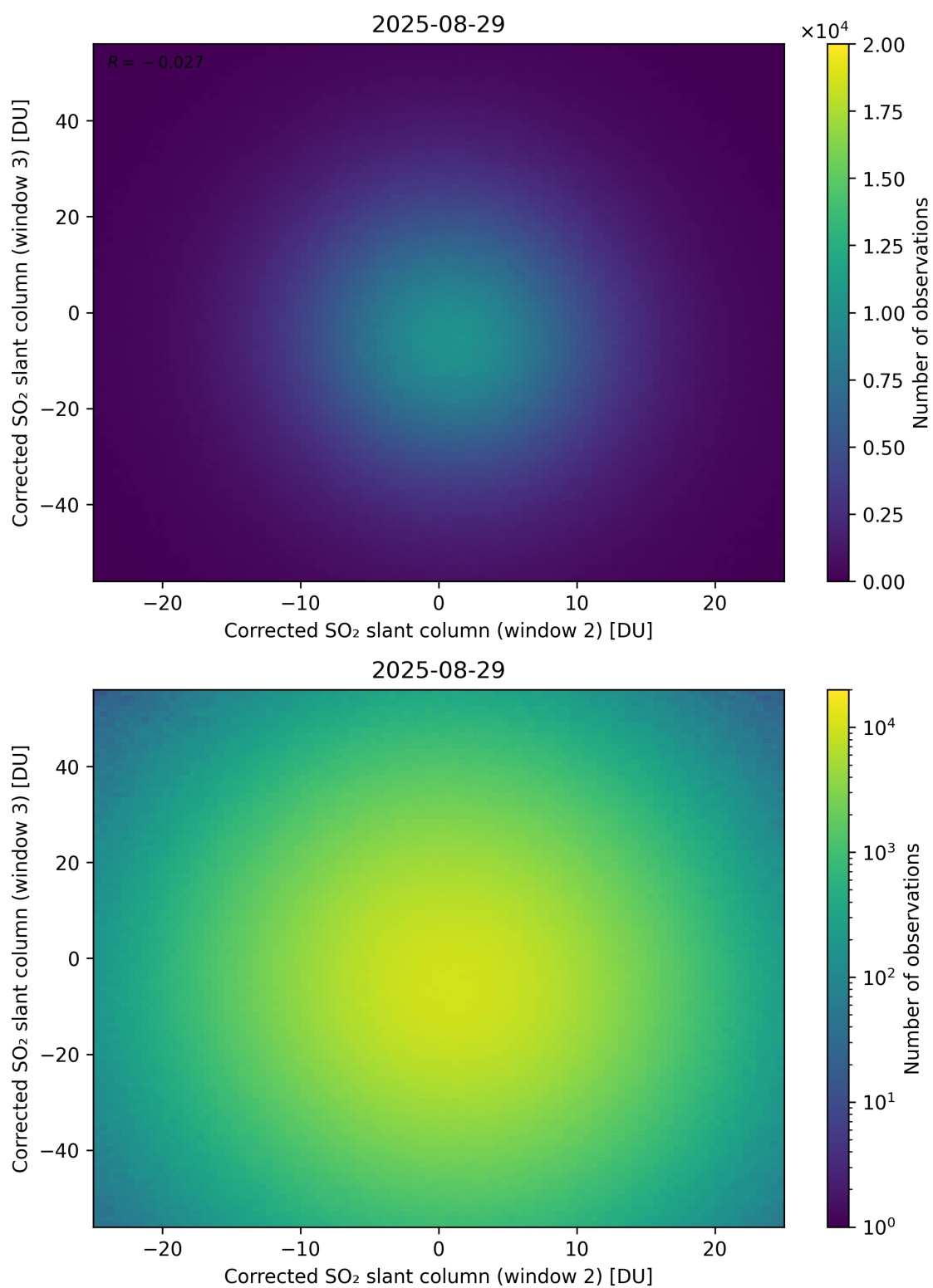
Figure 250: Scatter density plot of “Corrected SO 2 slant column (window 2)” against “Corrected SO 2 slant column (window 3)” for 2025-08-28 to 2025-08-30.
