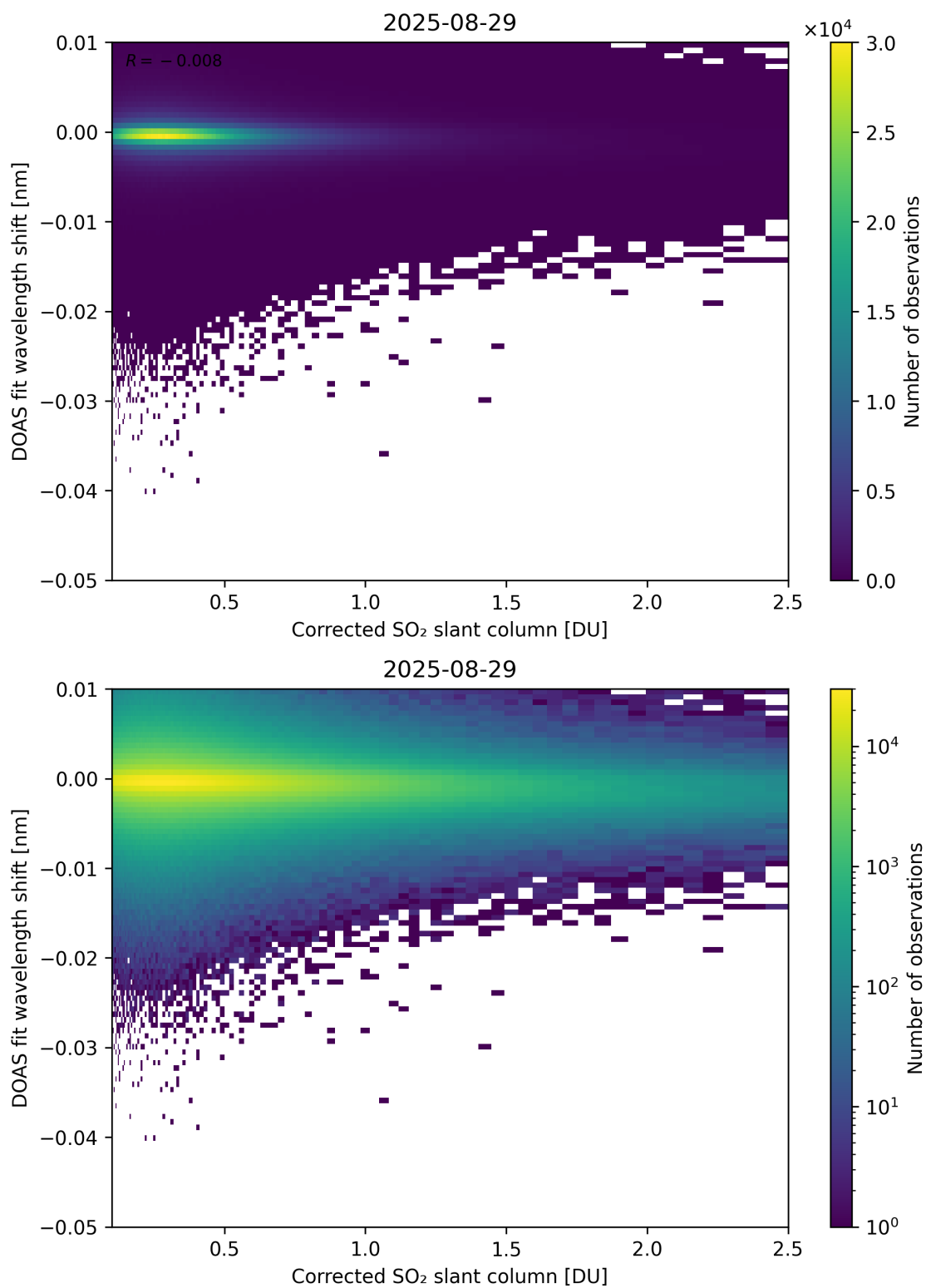
Figure 229: Scatter density plot of “Corrected SO 2 slant column” against “DOAS fit wavelength shift” for 2025-08-28 to 2025-08-30.
