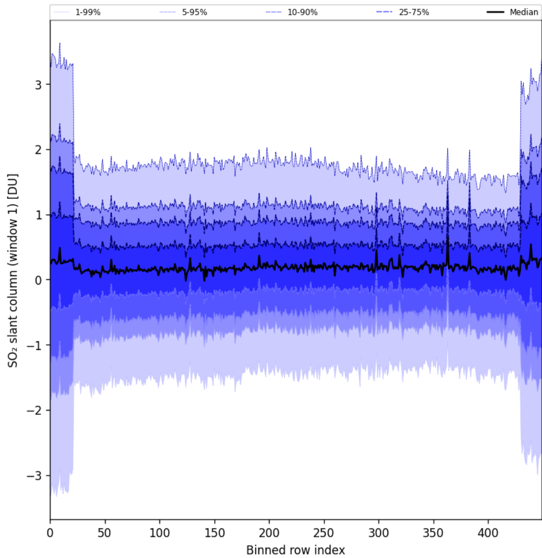
Figure 89: Along track statistics of “SO 2 slant column (window 1)” for 2025-08-28 to 2025-08-30
