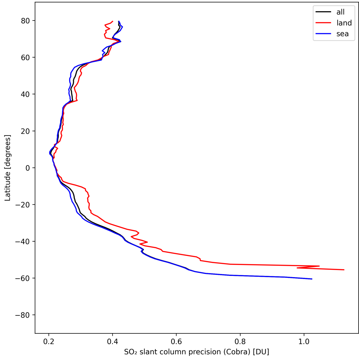
Figure 36: Zonal average of “SO 2 slant column precision (Cobra)” for 2025-08-28 to 2025-08-30.
