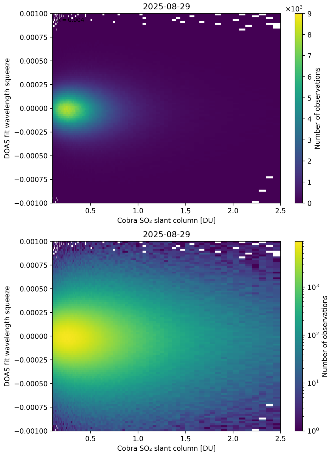
Figure 197: Scatter density plot of “Cobra SO 2 slant column” against “DOAS fit wavelength squeeze” for 2025-08-28 to 2025-08-30.
