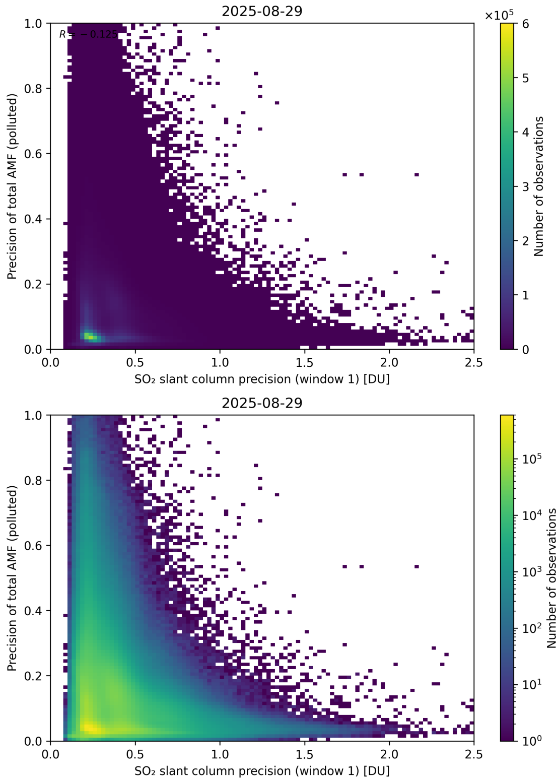
Figure 281: Scatter density plot of “SO 2 slant column precision (window 1)” against “Precision of total AMF (polluted)” for 2025-08-28 to 2025-08-30.
