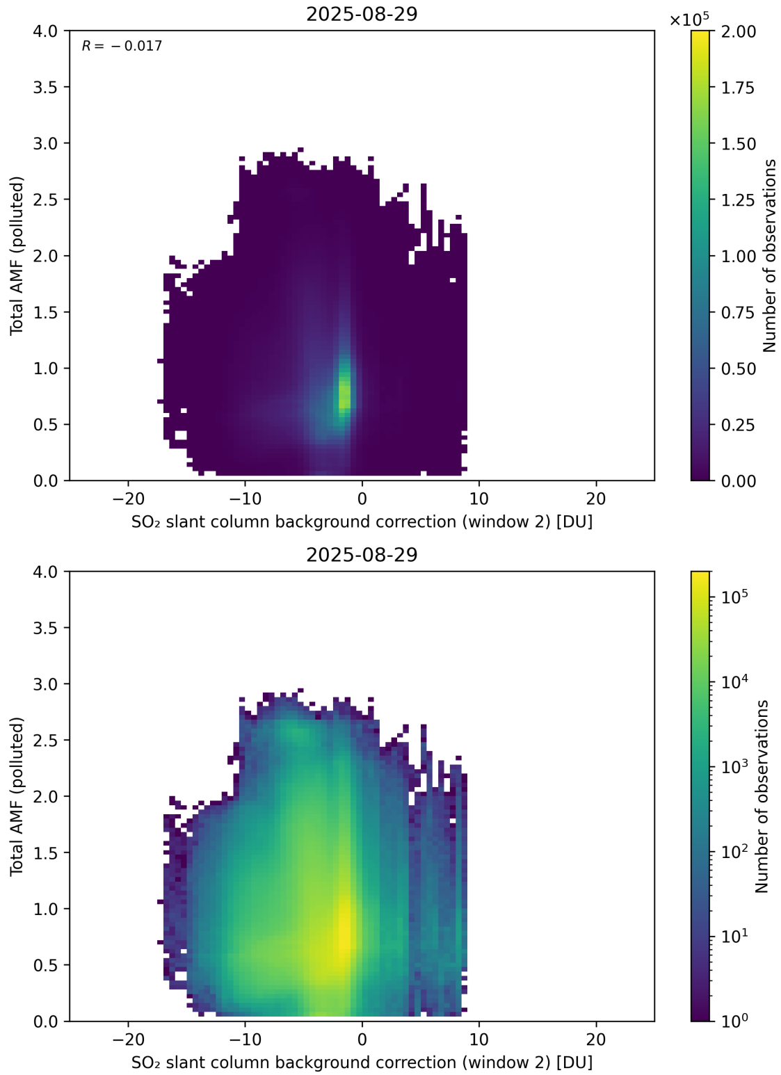
Figure 130: Scatter density plot of “SO 2 slant column background correction (window 2)” against “Total AMF (polluted)” for 2025-08-28 to 2025-08-30.
