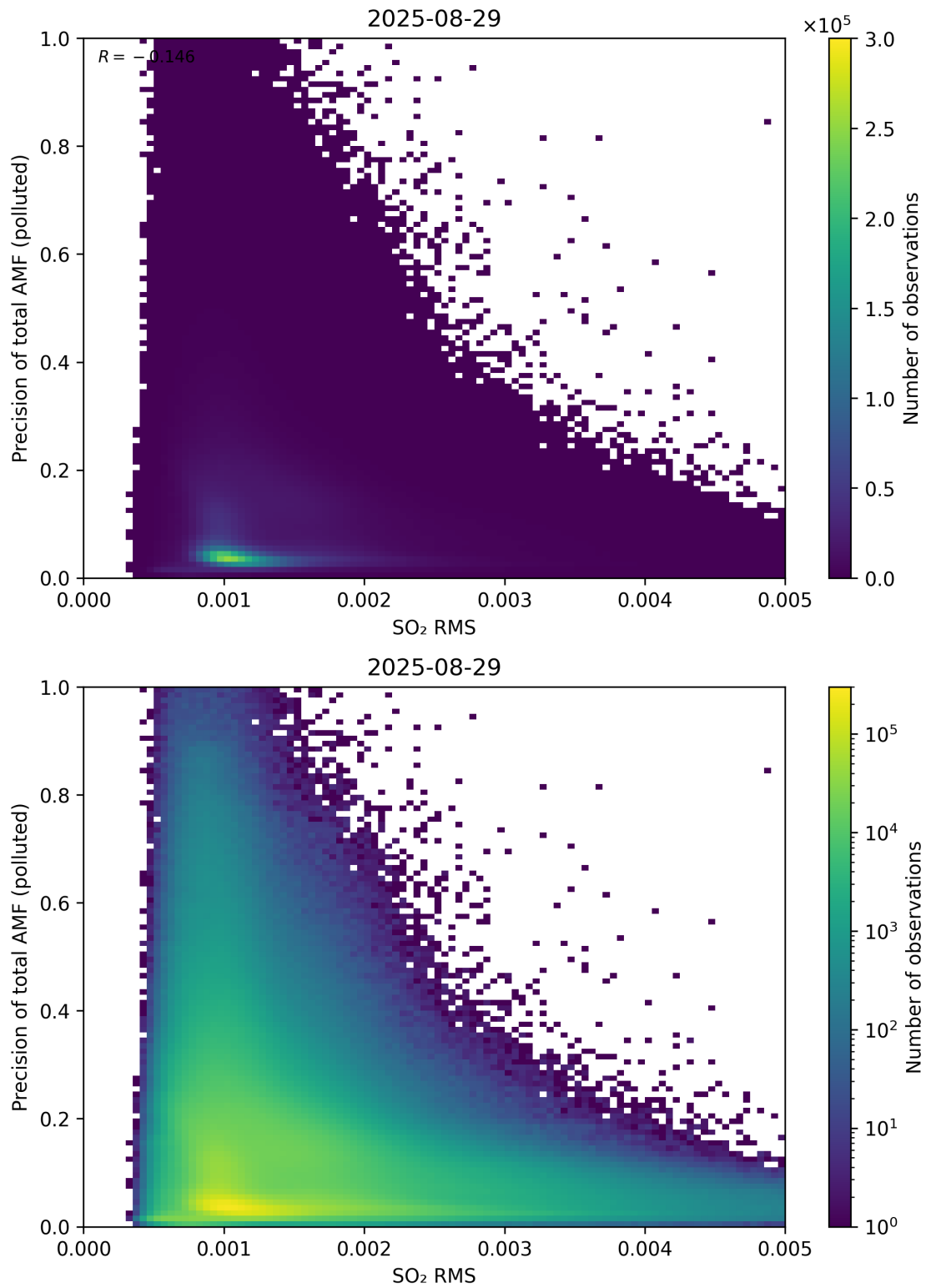
Figure 149: Scatter density plot of “SO 2 RMS” against “Precision of total AMF (polluted)” for 2025-08-28 to 2025-08-30.
