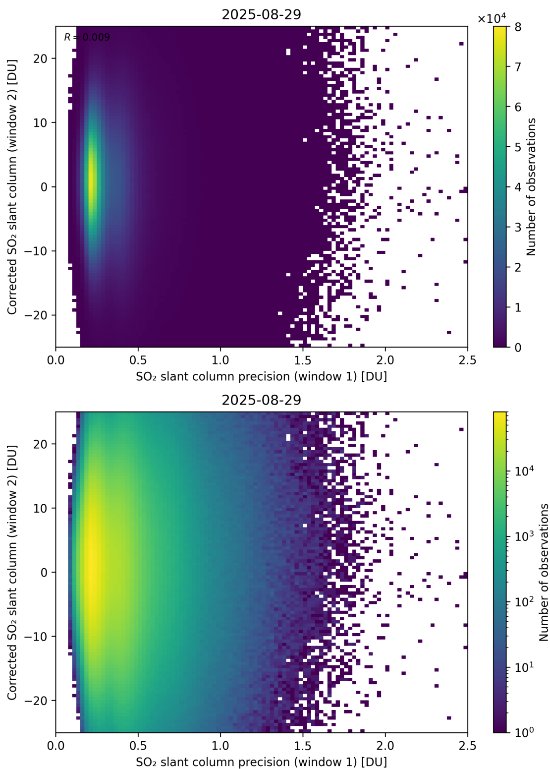
Figure 275: Scatter density plot of “SO 2 slant column precision (window 1)” against “Corrected SO 2 slant column (window 2)” for 2025-08-28 to 2025-08-30.
