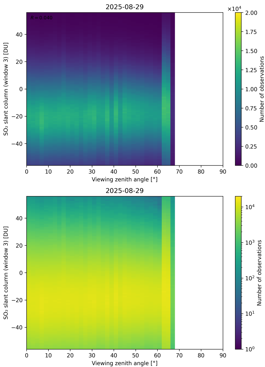
Figure 379: Scatter density plot of “Viewing zenith angle” against “SO 2 slant column (window 3)” for 2025-08-28 to 2025-08-30.
