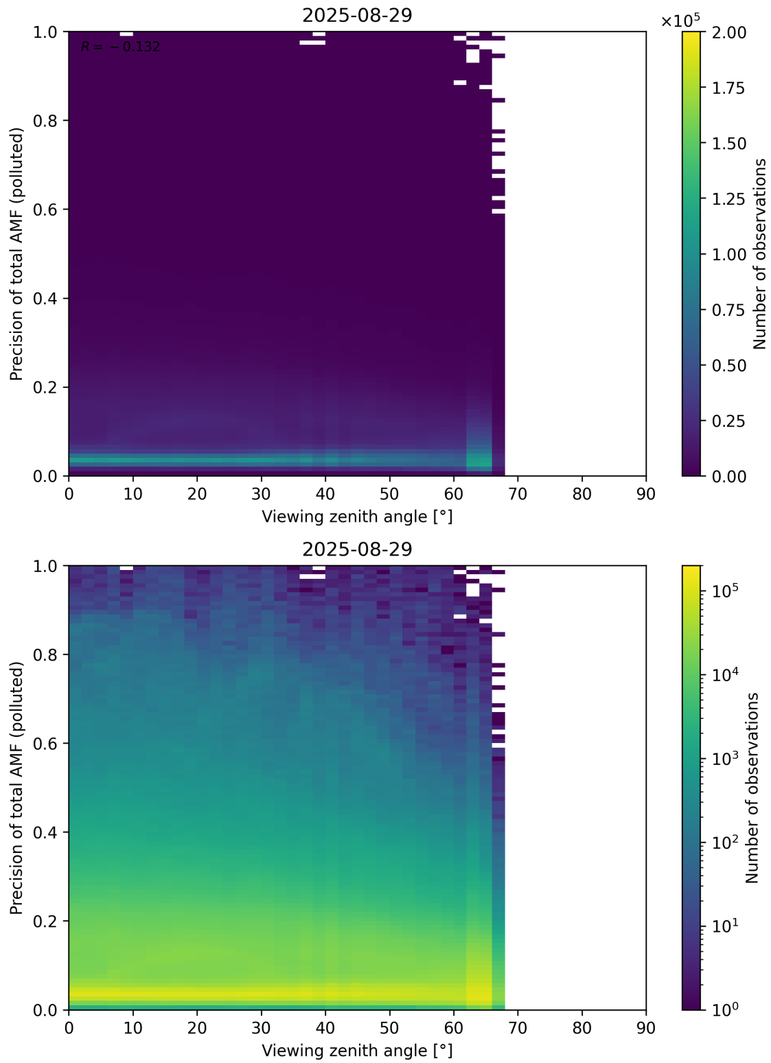
Figure 382: Scatter density plot of “Viewing zenith angle” against “Precision of total AMF (polluted)” for 2025-08-28 to 2025-08-30.
