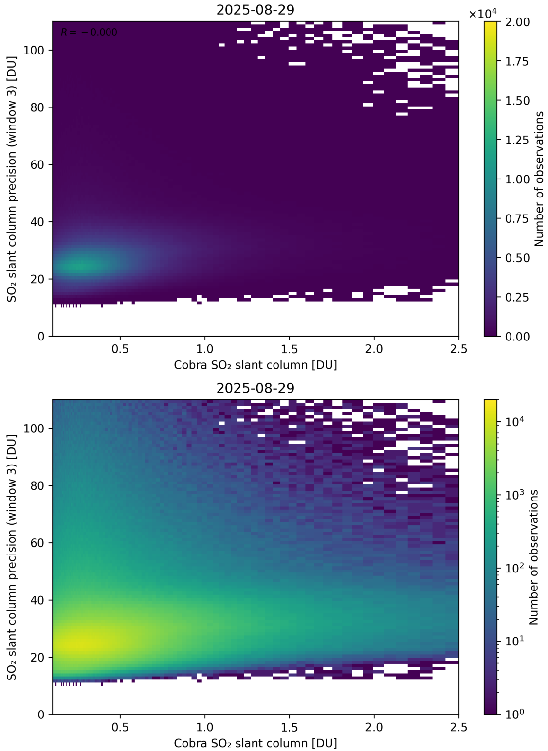
Figure 223: Scatter density plot of “Cobra SO 2 slant column” against “SO 2 slant column precision (window 3)” for 2025-08-28 to 2025-08-30.
