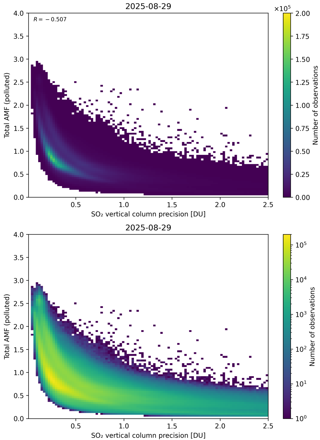
Figure 346: Scatter density plot of “SO 2 vertical column precision” against “Total AMF (polluted)” for 2025-08-28 to 2025-08-30.
