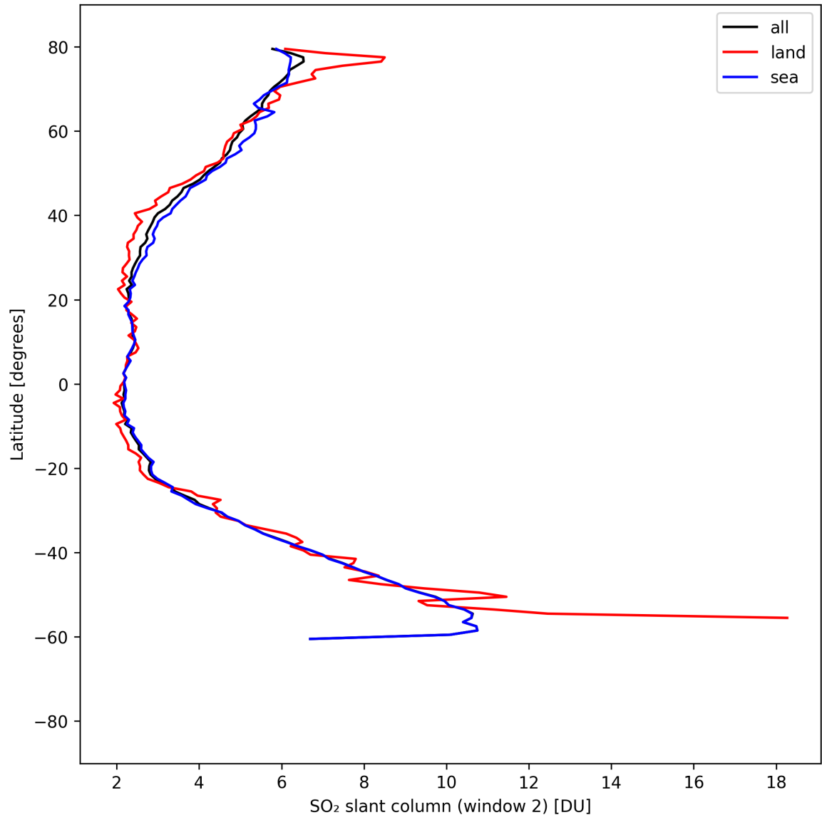
Figure 41: Zonal average of “SO 2 slant column (window 2)” for 2025-08-28 to 2025-08-30.
