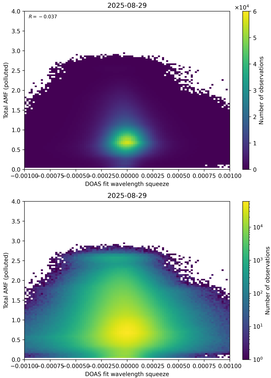
Figure 145: Scatter density plot of “DOAS fit wavelength squeeze” against “Total AMF (polluted)” for 2025-08-28 to 2025-08-30.
