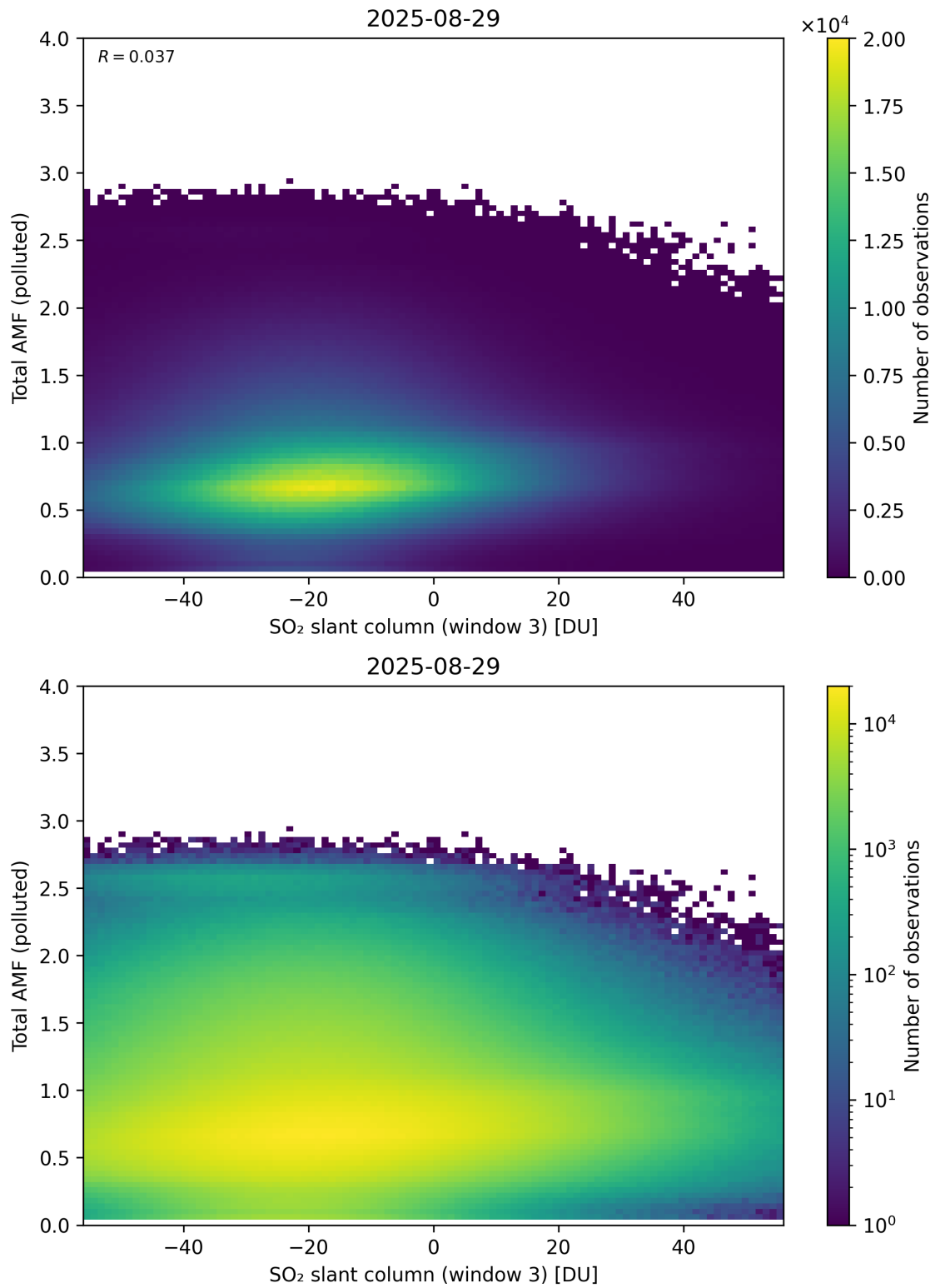
Figure 318: Scatter density plot of “SO 2 slant column (window 3)” against “Total AMF (polluted)” for 2025-08-28 to 2025-08-30.
