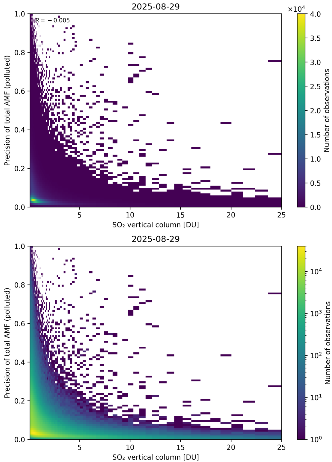
Figure 360: Scatter density plot of “SO 2 vertical column” against “Precision of total AMF (polluted)” for 2025-08-28 to 2025-08-30.
