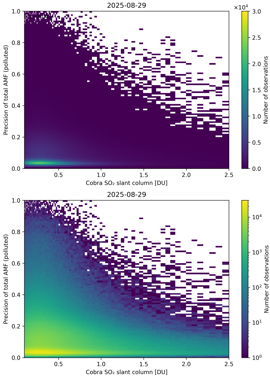
Figure 225: Scatter density plot of “Cobra SO 2 slant column” against “Precision of total AMF (polluted)” for 2025-08-28 to 2025-08-30.
