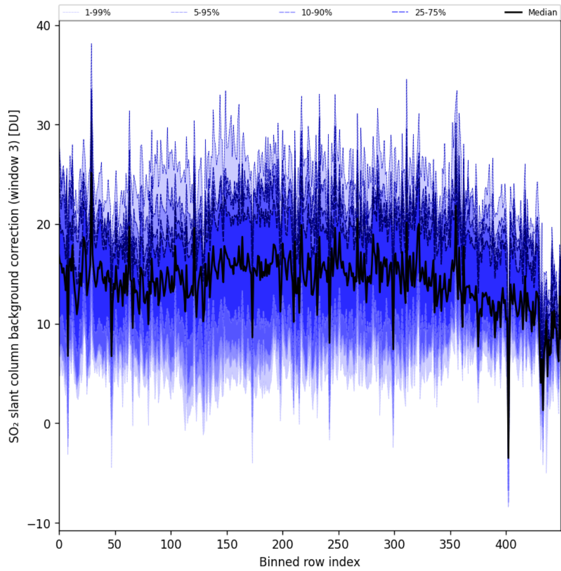
Figure 100: Along track statistics of “SO 2 slant column background correction (window 3)” for 2025-08-28 to 2025-08-30
