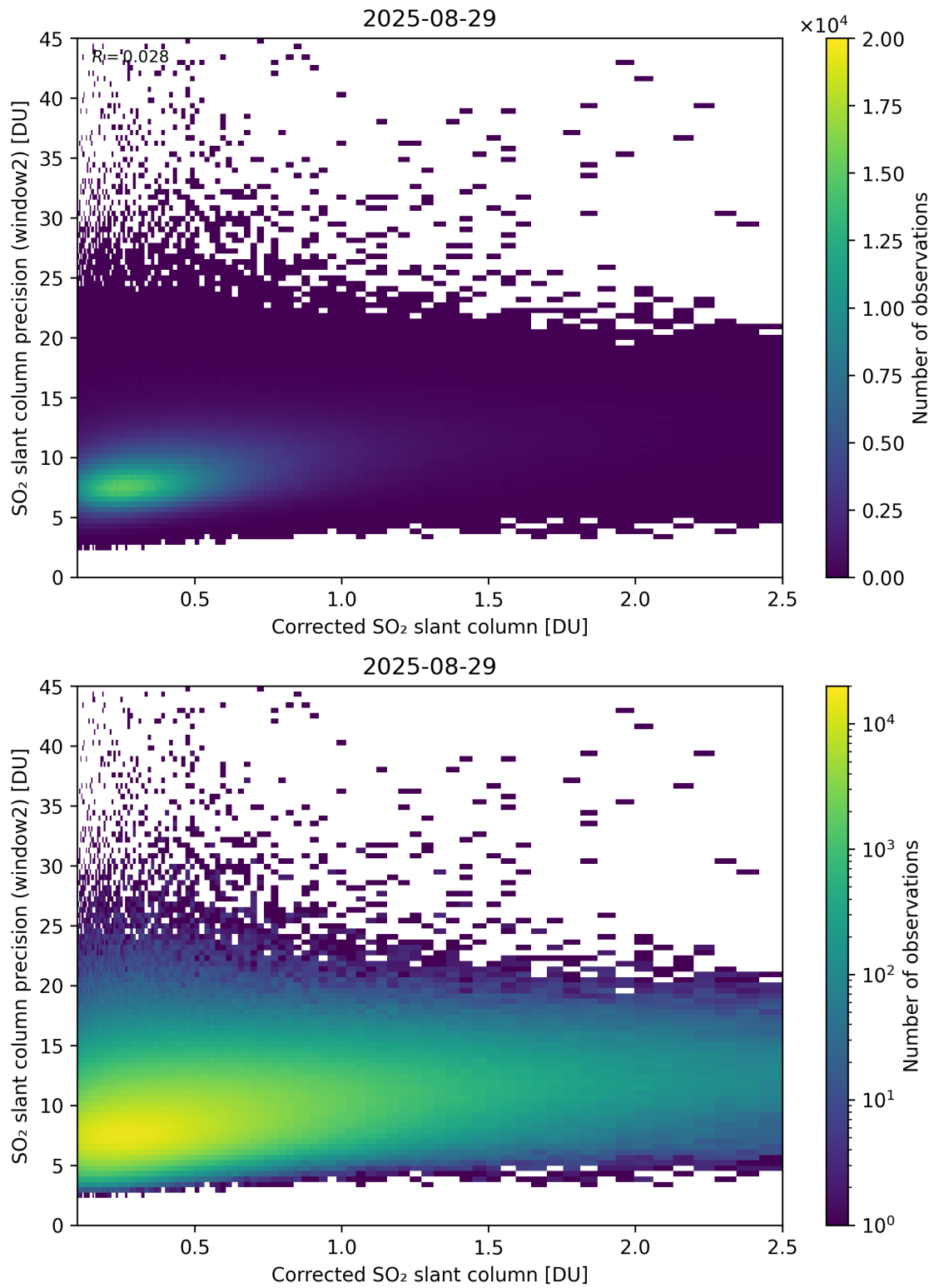
Figure 239: Scatter density plot of “Corrected SO 2 slant column” against “SO 2 slant column precision (window2)” for 2025-08-28 to 2025-08-30.
