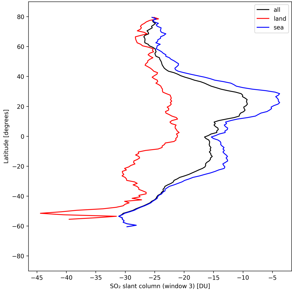
Figure 45: Zonal average of “SO 2 slant column (window 3)” for 2025-08-28 to 2025-08-30.
