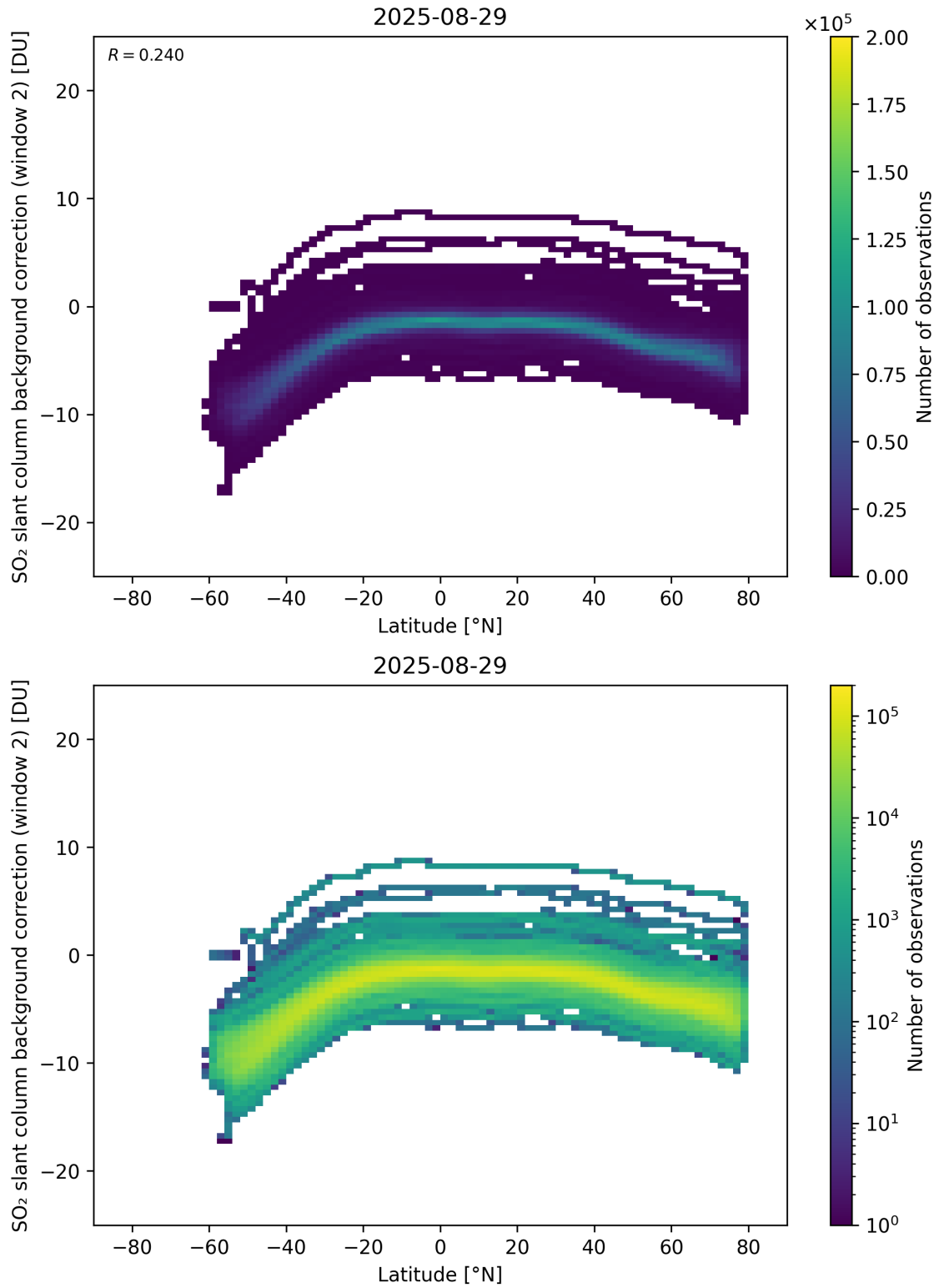
Figure 151: Scatter density plot of “Latitude” against “SO 2 slant column background correction (window 2)” for 2025-08-28 to 2025-08-30.
