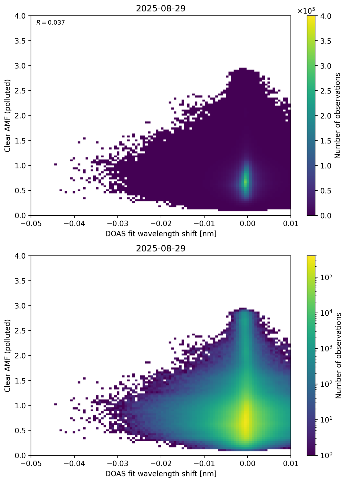
Figure 140: Scatter density plot of “DOAS fit wavelength shift” against “Clear AMF (polluted)” for 2025-08-28 to 2025-08-30.
