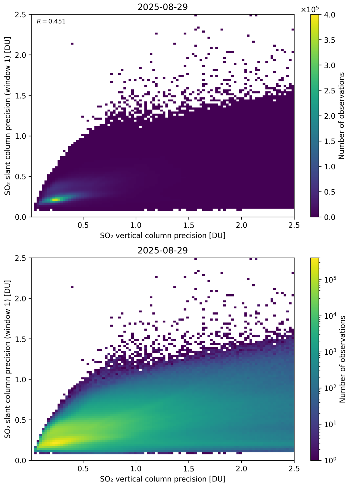
Figure 342: Scatter density plot of “SO 2 vertical column precision” against “SO 2 slant column precision (window 1)” for 2025-08-28 to 2025-08-30.
