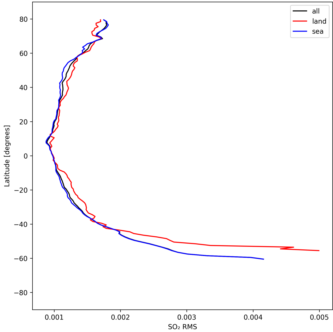
Figure 52: Zonal average of “SO 2 RMS” for 2025-08-28 to 2025-08-30.
