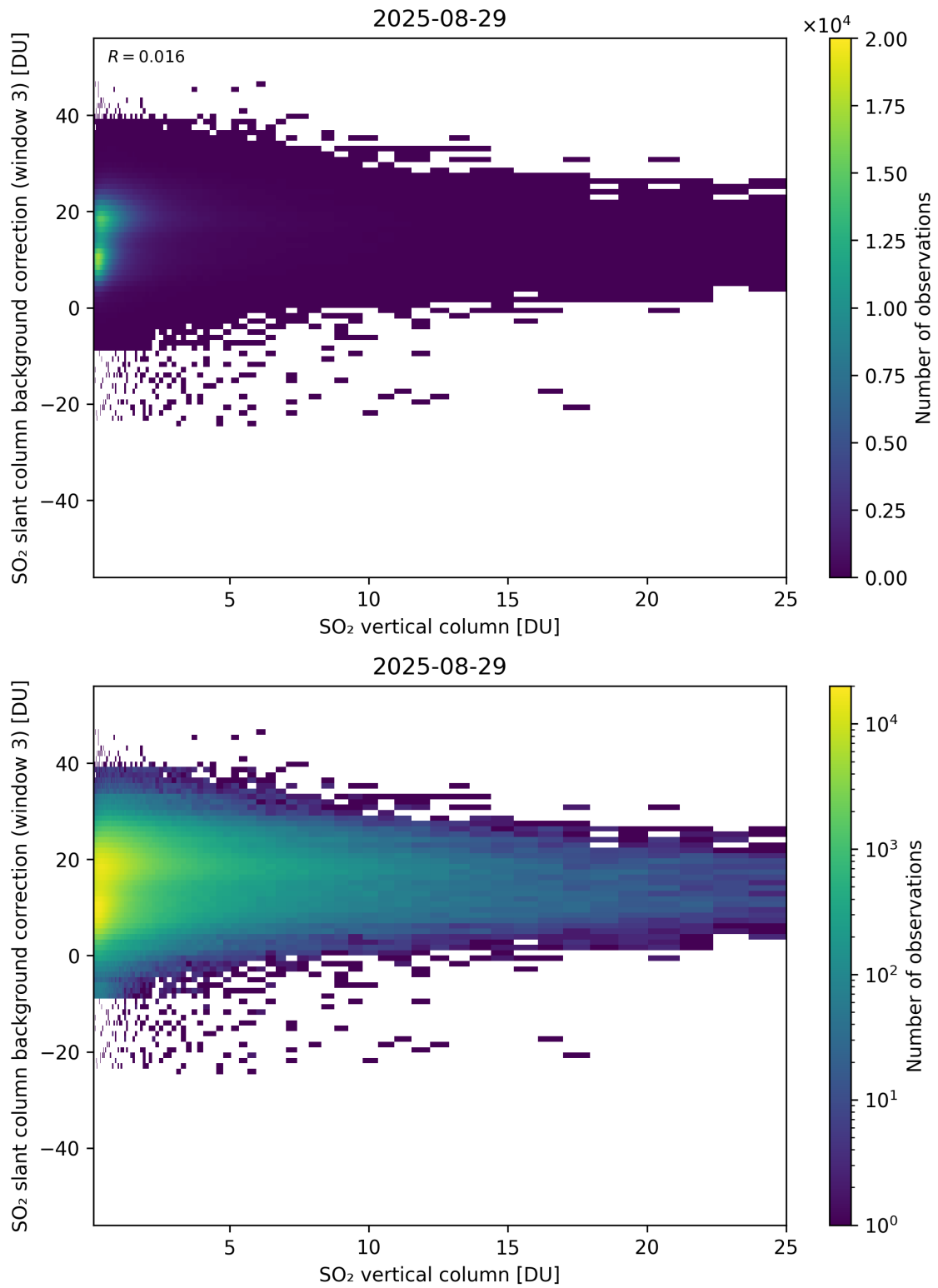
Figure 325: Scatter density plot of “SO 2 vertical column” against “SO 2 slant column background correction (window 3)” for 2025-08-28 to 2025-08-30.
