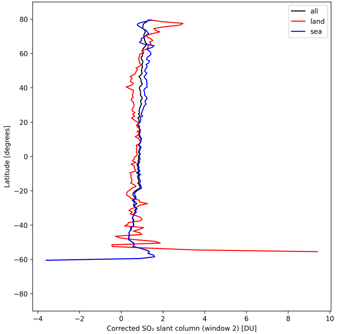
Figure 43: Zonal average of “Corrected SO 2 slant column (window 2)” for 2025-08-28 to 2025-08-30.
