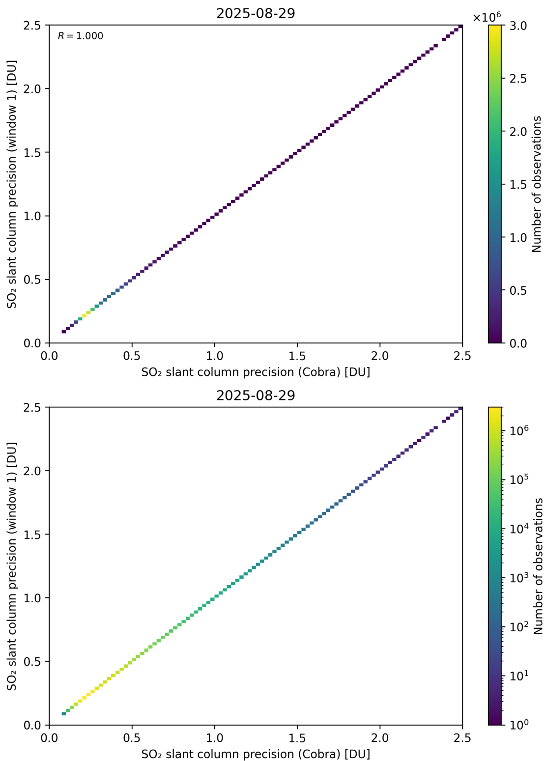
Figure 209: Scatter density plot of “SO 2 slant column precision (Cobra)” against “SO 2 slant column precision (window 1)” for 2025-08-28 to 2025-08-30.
