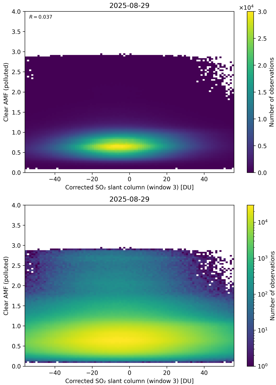
Figure 259: Scatter density plot of “Corrected SO 2 slant column (window 3)” against “Clear AMF (polluted)” for 2025-08-28 to 2025-08-30.
