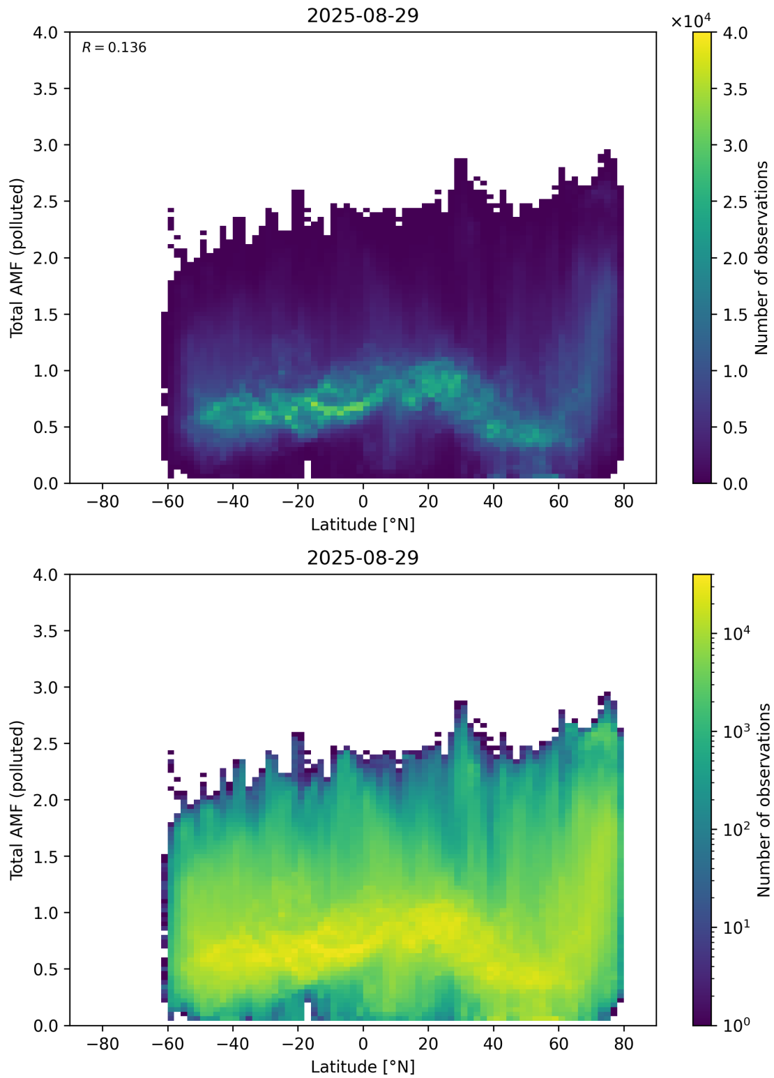
Figure 167: Scatter density plot of “Latitude” against “Total AMF (polluted)” for 2025-08-28 to 2025-08-30.
