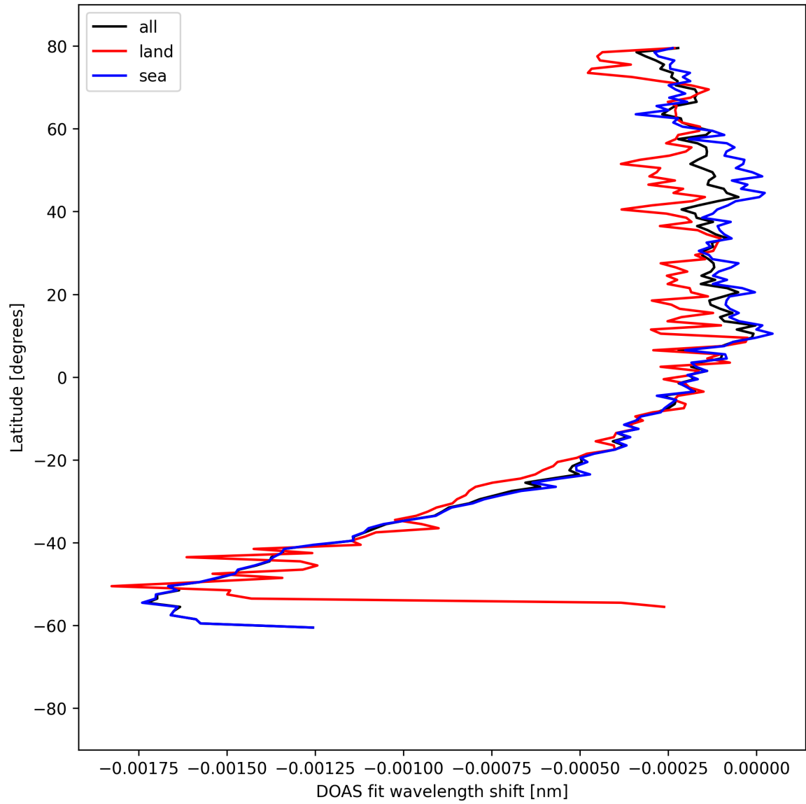
Figure 50: Zonal average of “DOAS fit wavelength shift” for 2025-08-28 to 2025-08-30.
