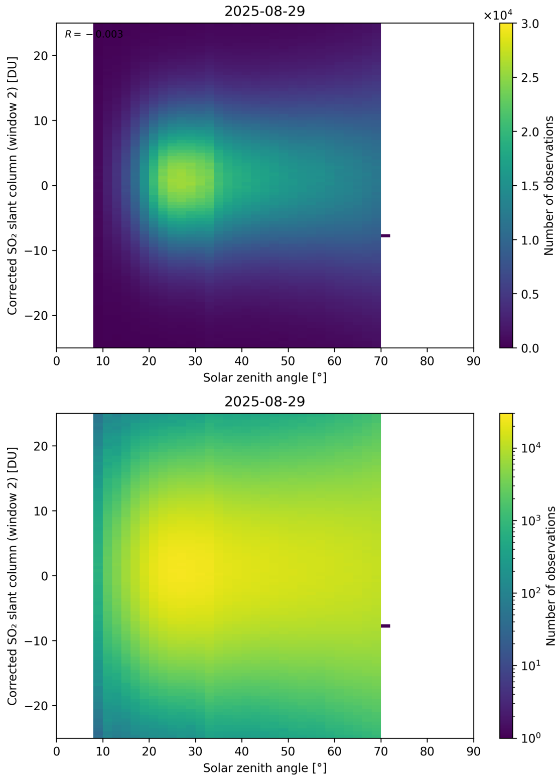
Figure 182: Scatter density plot of “Solar zenith angle” against “Corrected SO 2 slant column (window 2)” for 2025-08-28 to 2025-08-30.
