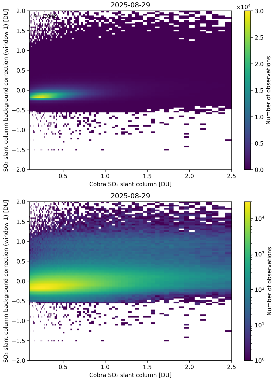
Figure 193: Scatter density plot of “Cobra SO 2 slant column” against “SO 2 slant column background correction (window 1)” for 2025-08-28 to 2025-08-30.
