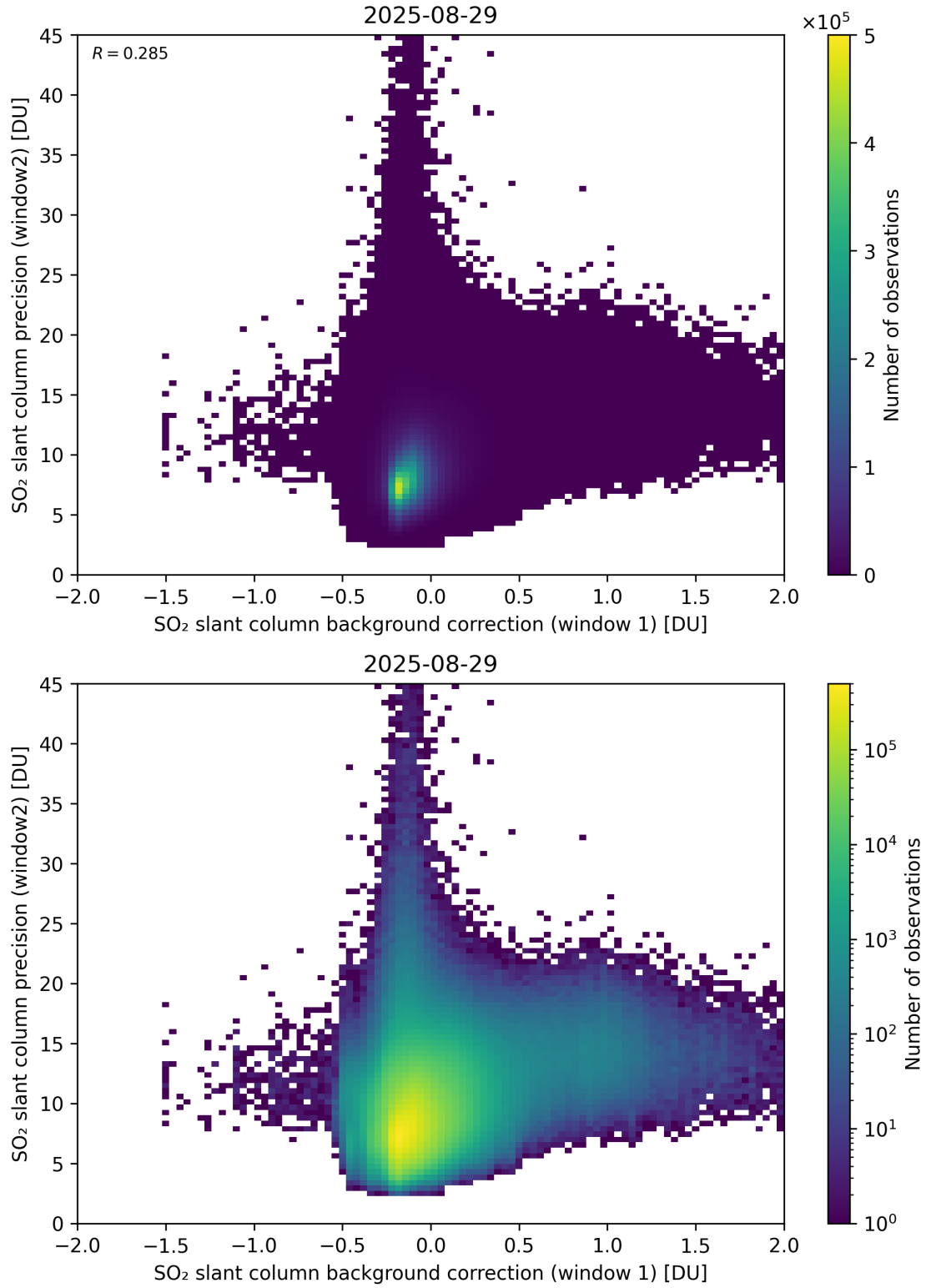
Figure 117: Scatter density plot of “SO 2 slant column background correction (window 1)” against “SO 2 slant column precision (window2)” for 2025-08-28 to 2025-08-30.
