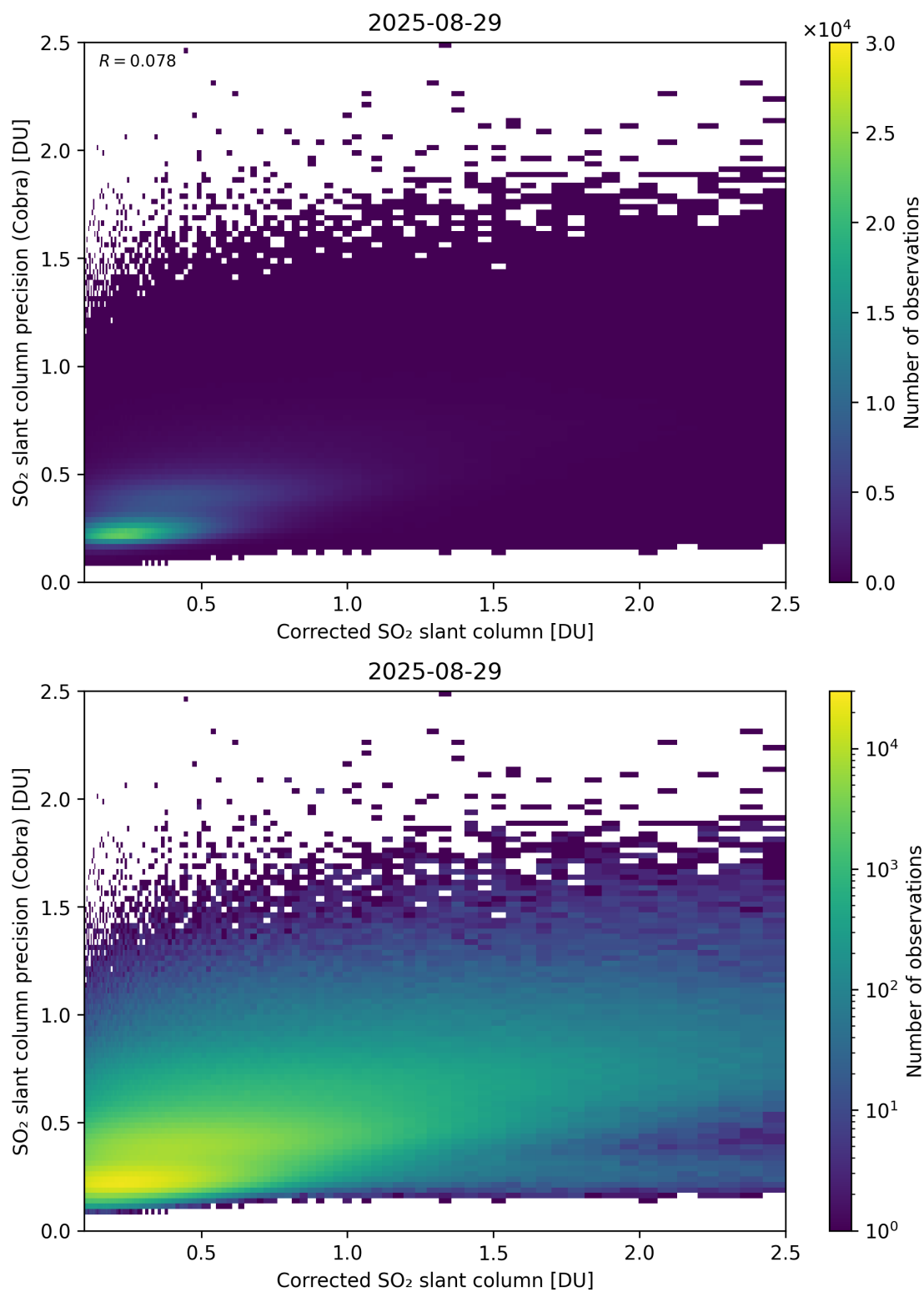
Figure 234: Scatter density plot of “Corrected SO 2 slant column” against “SO 2 slant column precision (Cobra)” for 2025-08-28 to 2025-08-30.
