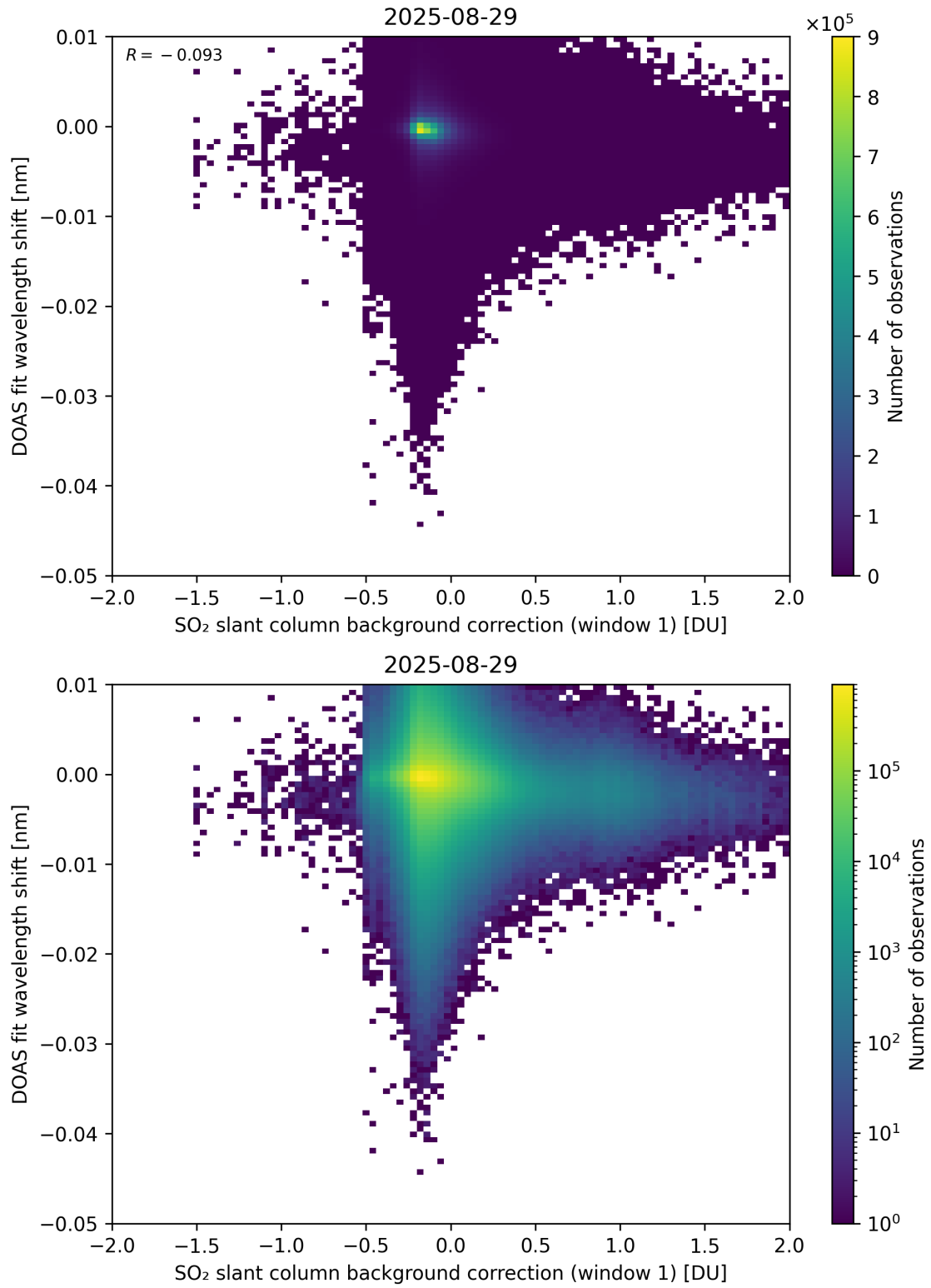
Figure 111: Scatter density plot of “SO 2 slant column background correction (window 1)” against “DOAS fit wavelength shift” for 2025-08-28 to 2025-08-30.
