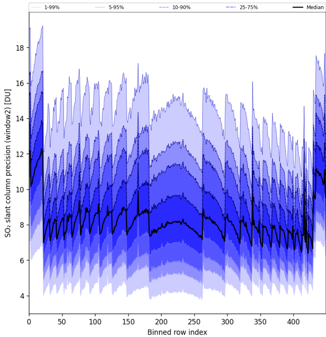
Figure 94: Along track statistics of “SO 2 slant column precision (window2)” for 2025-08-28 to 2025-08-30
