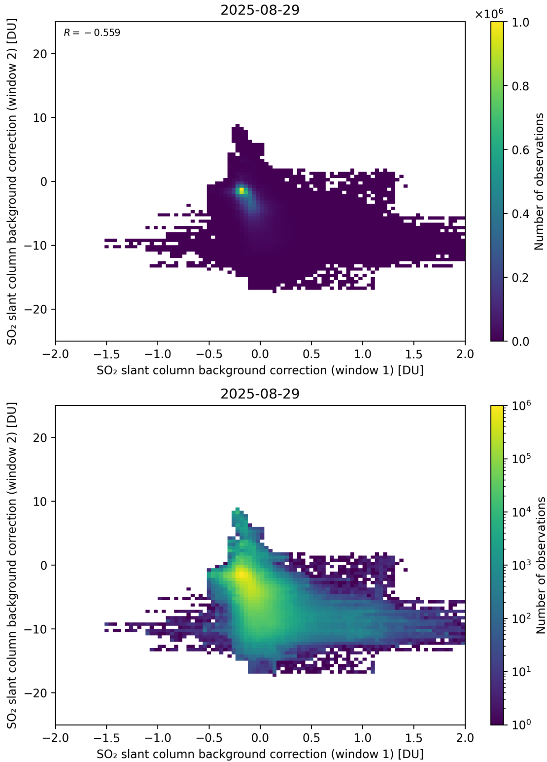
Figure 109: Scatter density plot of “SO 2 slant column background correction (window 1)” against “SO 2 slant column background correction (window 2)” for 2025-08-28 to 2025-08-30.
