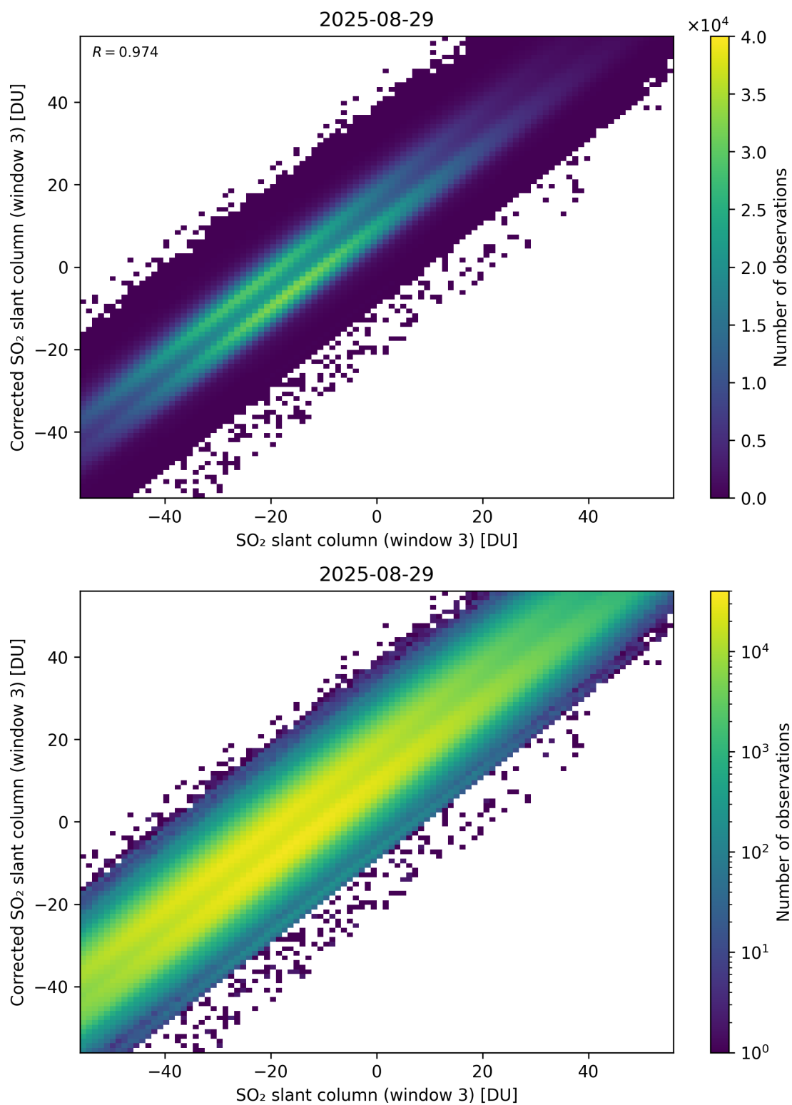
Figure 316: Scatter density plot of “SO 2 slant column (window 3)” against “Corrected SO 2 slant column (window 3)” for 2025-08-28 to 2025-08-30.
