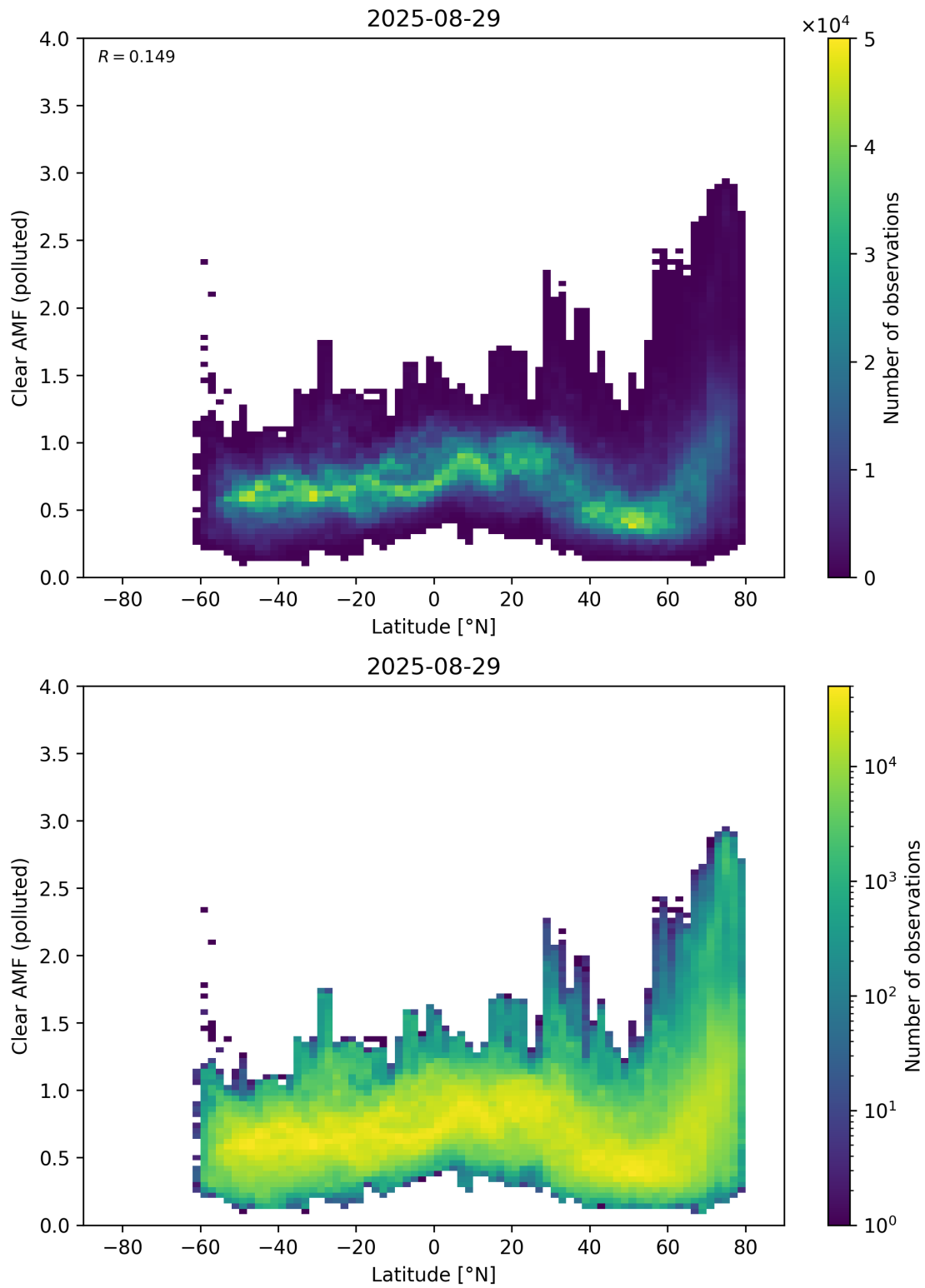
Figure 156: Scatter density plot of “Latitude” against “Clear AMF (polluted)” for 2025-08-28 to 2025-08-30.
