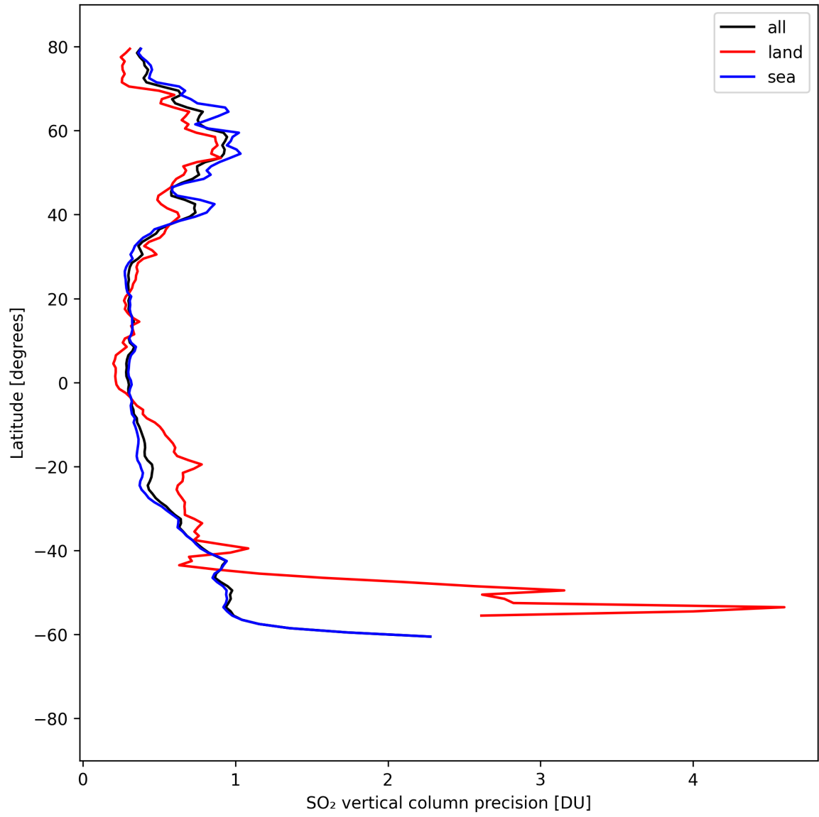
Figure 33: Zonal average of “SO 2 vertical column precision” for 2025-08-28 to 2025-08-30.
