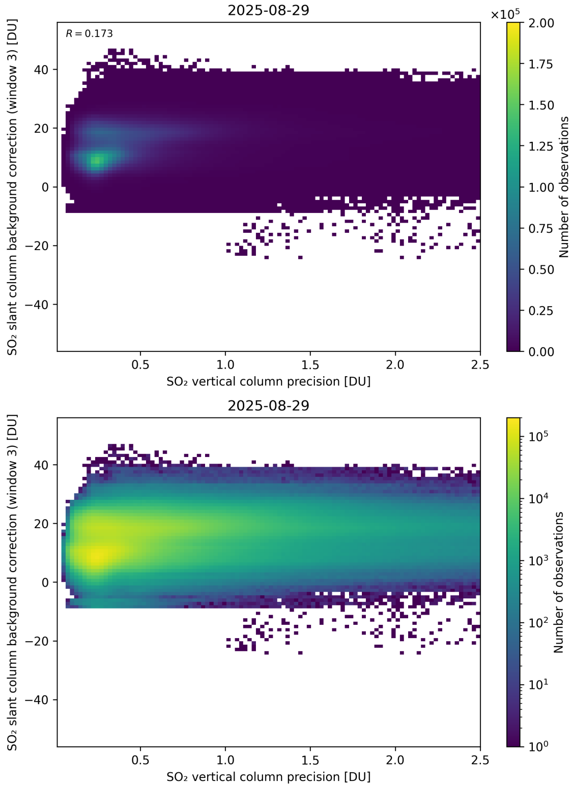
Figure 331: Scatter density plot of “SO 2 vertical column precision” against “SO 2 slant column background correction (window 3)” for 2025-08-28 to 2025-08-30.
