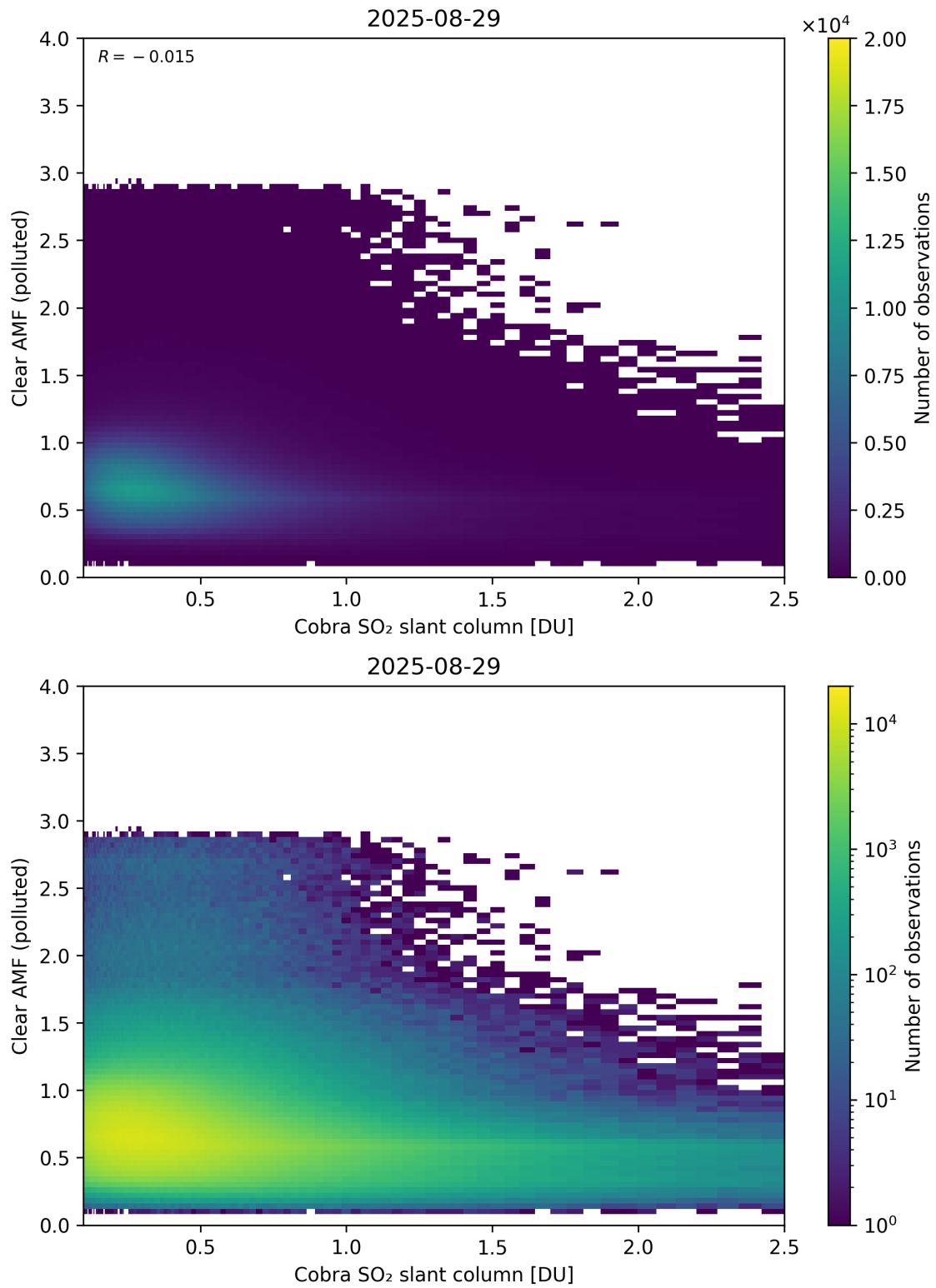
Figure 215: Scatter density plot of “Cobra SO 2 slant column” against “Clear AMF (polluted)” for 2025-08-28 to 2025-08-30.
