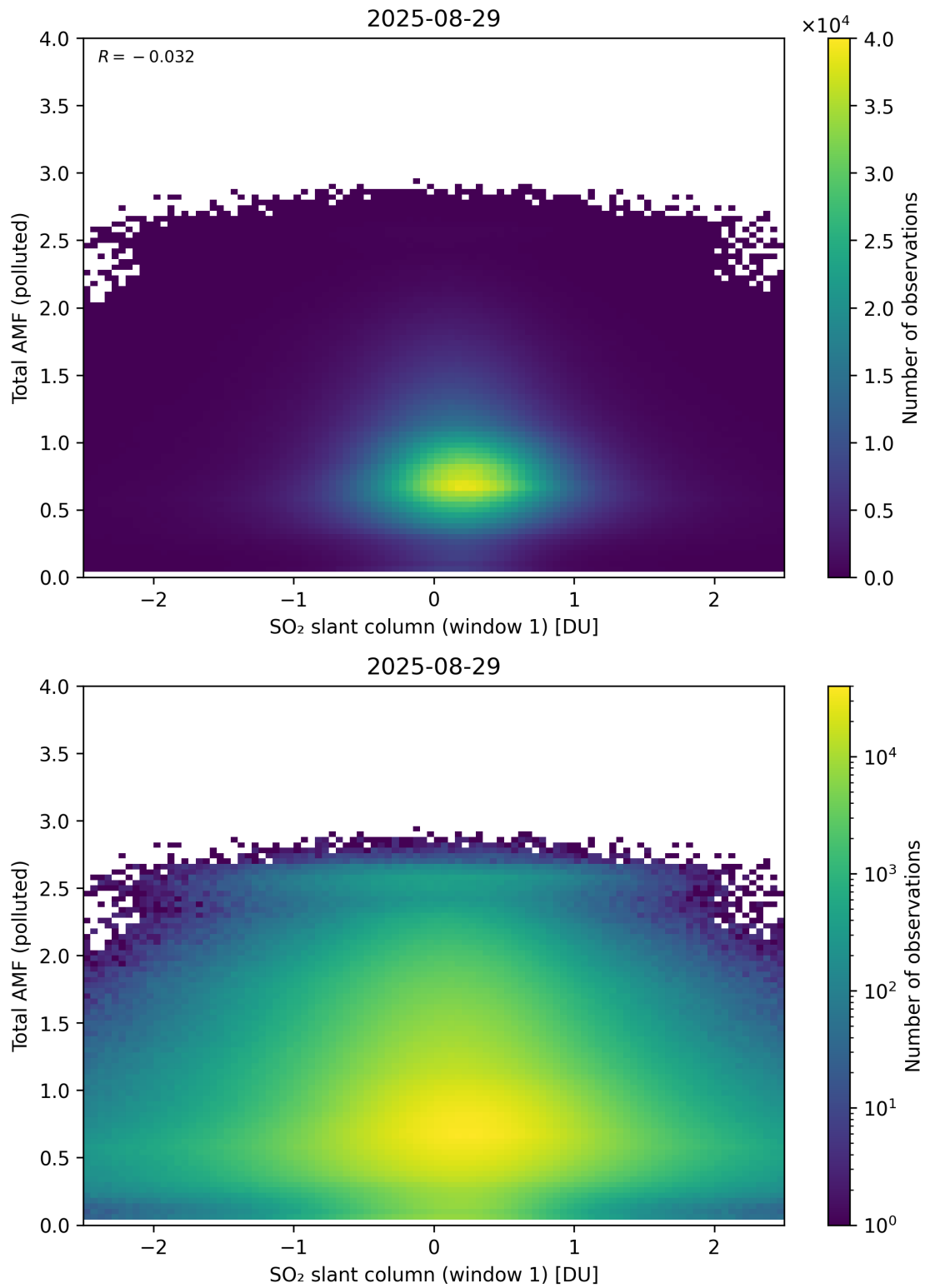
Figure 289: Scatter density plot of “SO 2 slant column (window 1)” against “Total AMF (polluted)” for 2025-08-28 to 2025-08-30.
