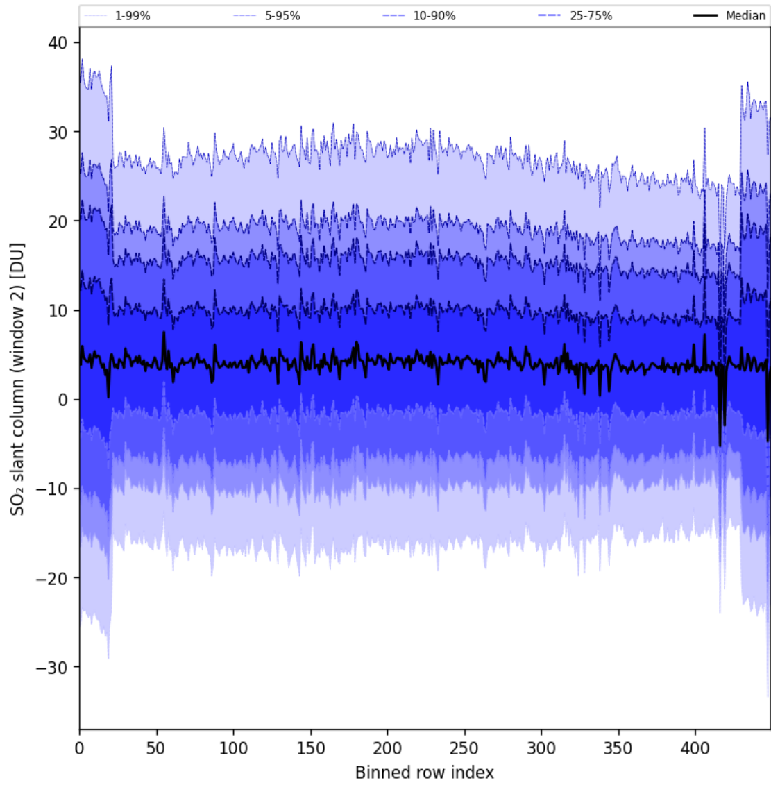
Figure 93: Along track statistics of “SO 2 slant column (window 2)” for 2025-08-28 to 2025-08-30
