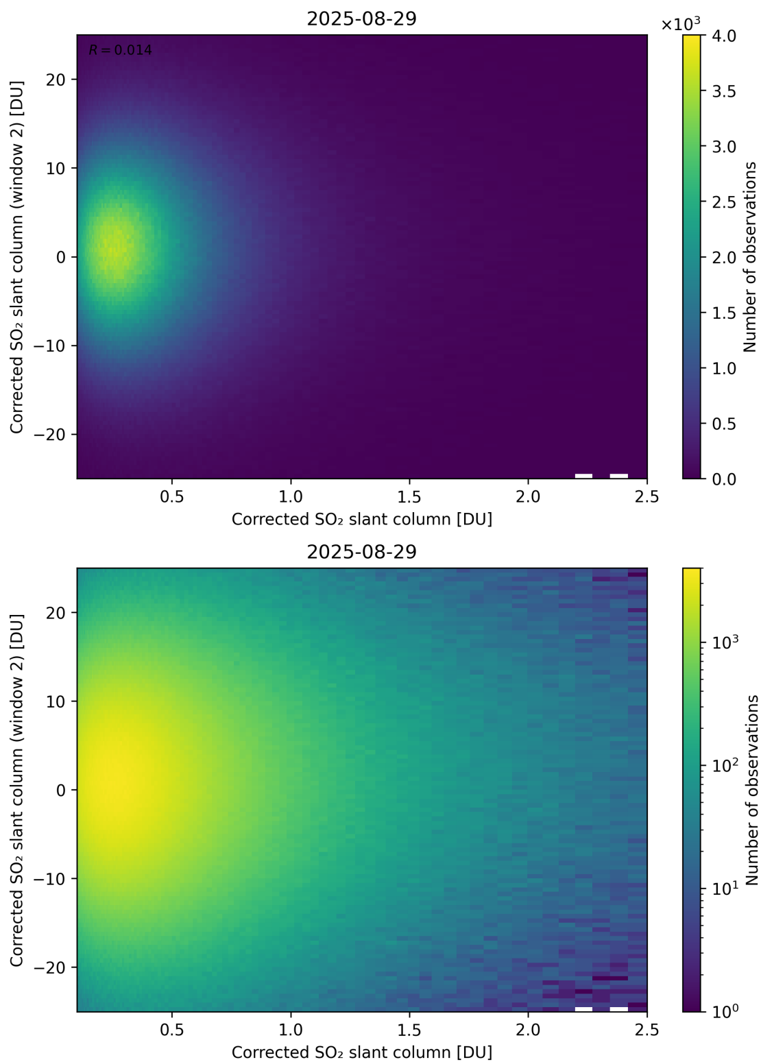
Figure 235: Scatter density plot of “Corrected SO 2 slant column” against “Corrected SO 2 slant column (window 2)” for 2025-08-28 to 2025-08-30.
