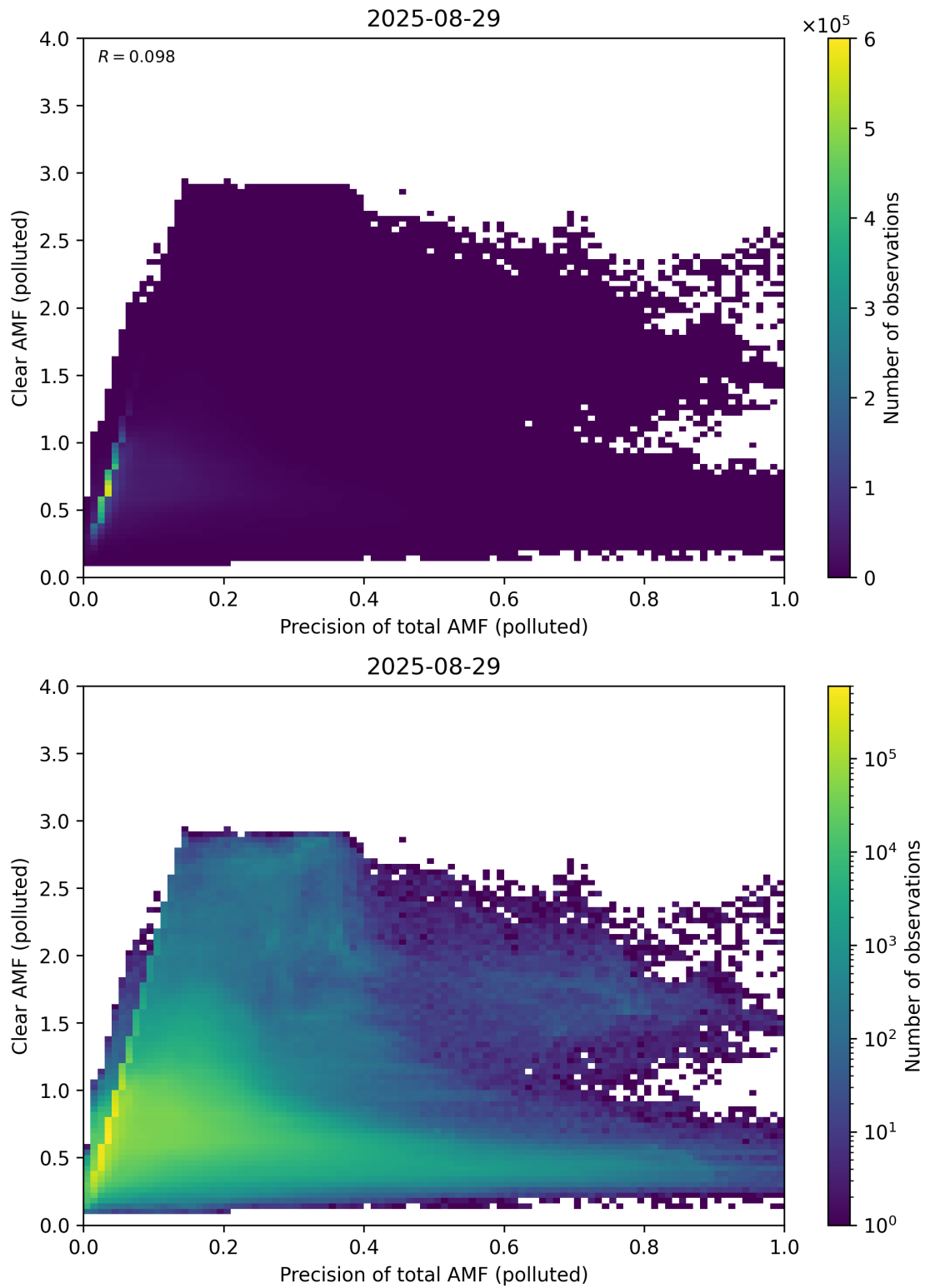
Figure 320: Scatter density plot of “Precision of total AMF (polluted)” against “Clear AMF (polluted)” for 2025-08-28 to 2025-08-30.
