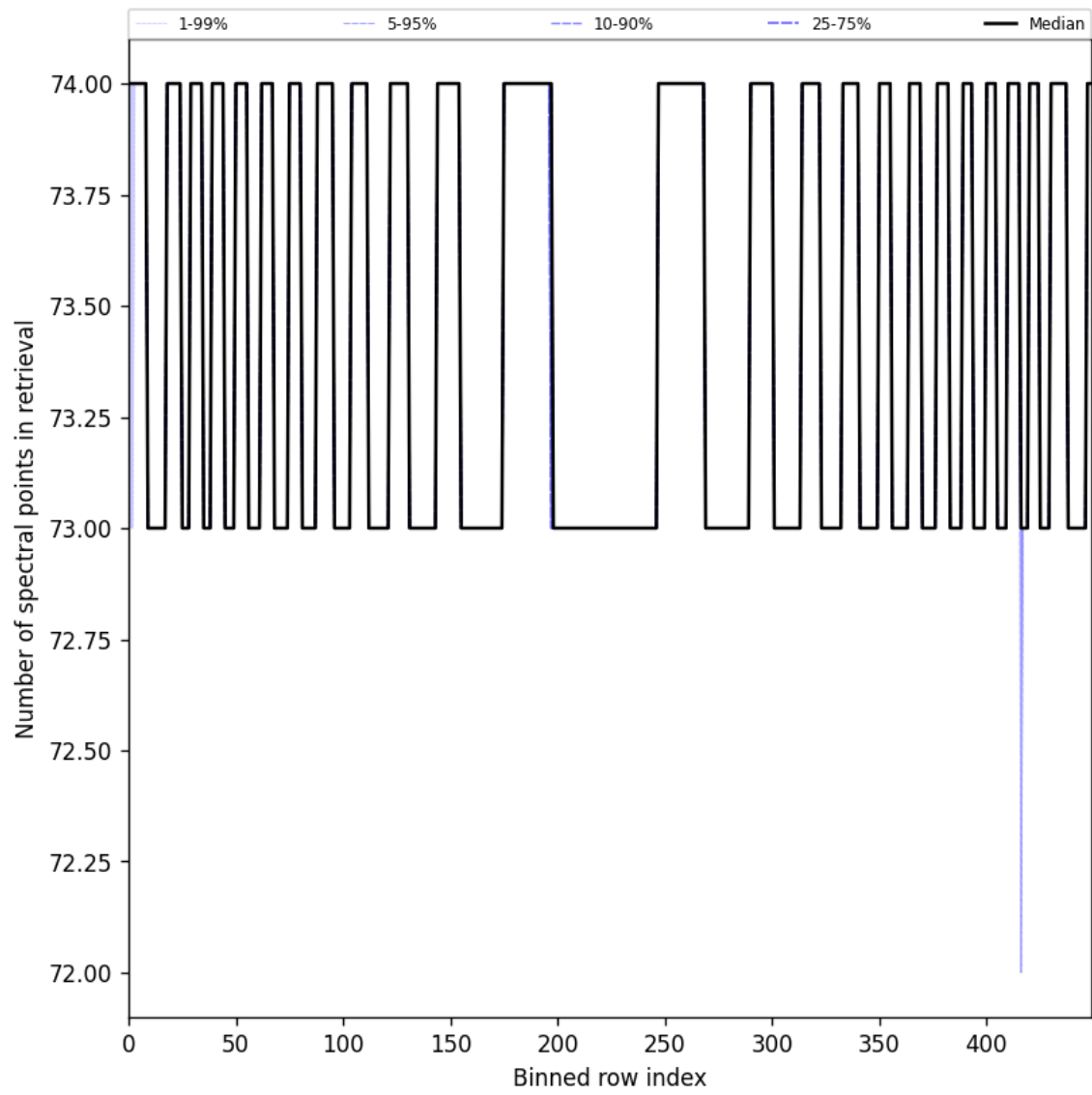
Figure 108: Along track statistics of “Number of spectral points in retrieval” for 2025-08-28 to 2025-08-30
