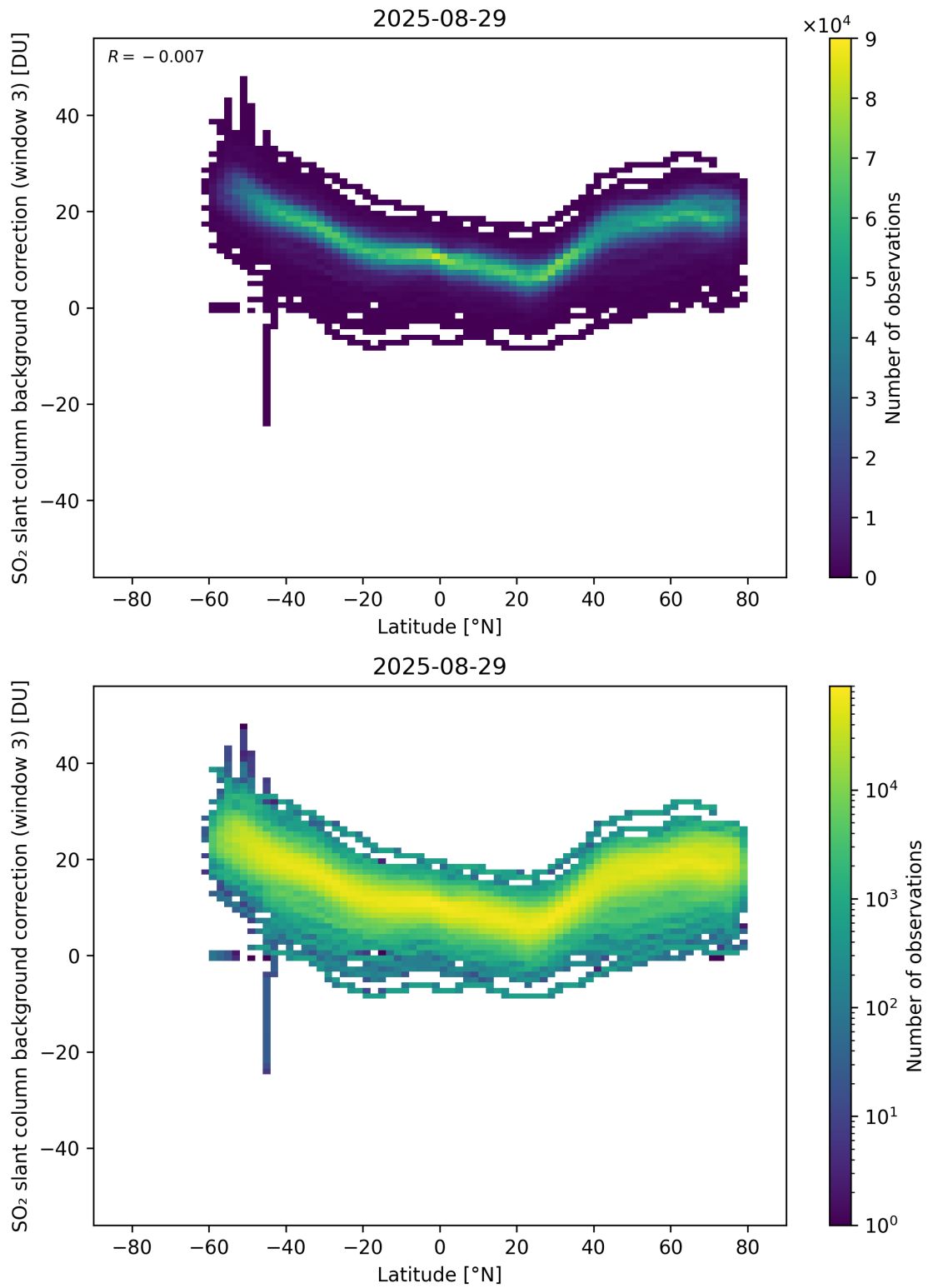
Figure 152: Scatter density plot of “Latitude” against “SO 2 slant column background correction (window 3)” for 2025-08-28 to 2025-08-30.
