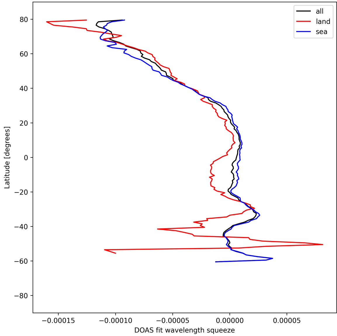
Figure 51: Zonal average of “DOAS fit wavelength squeeze” for 2025-08-28 to 2025-08-30.
