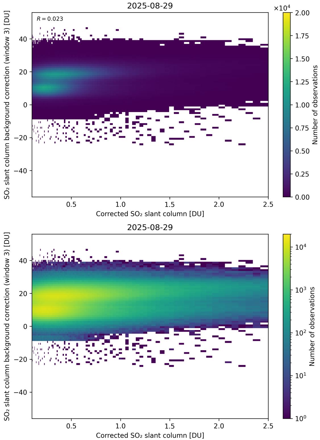
Figure 228: Scatter density plot of “Corrected SO 2 slant column” against “SO 2 slant column background correction (window 3)” for 2025-08-28 to 2025-08-30.
