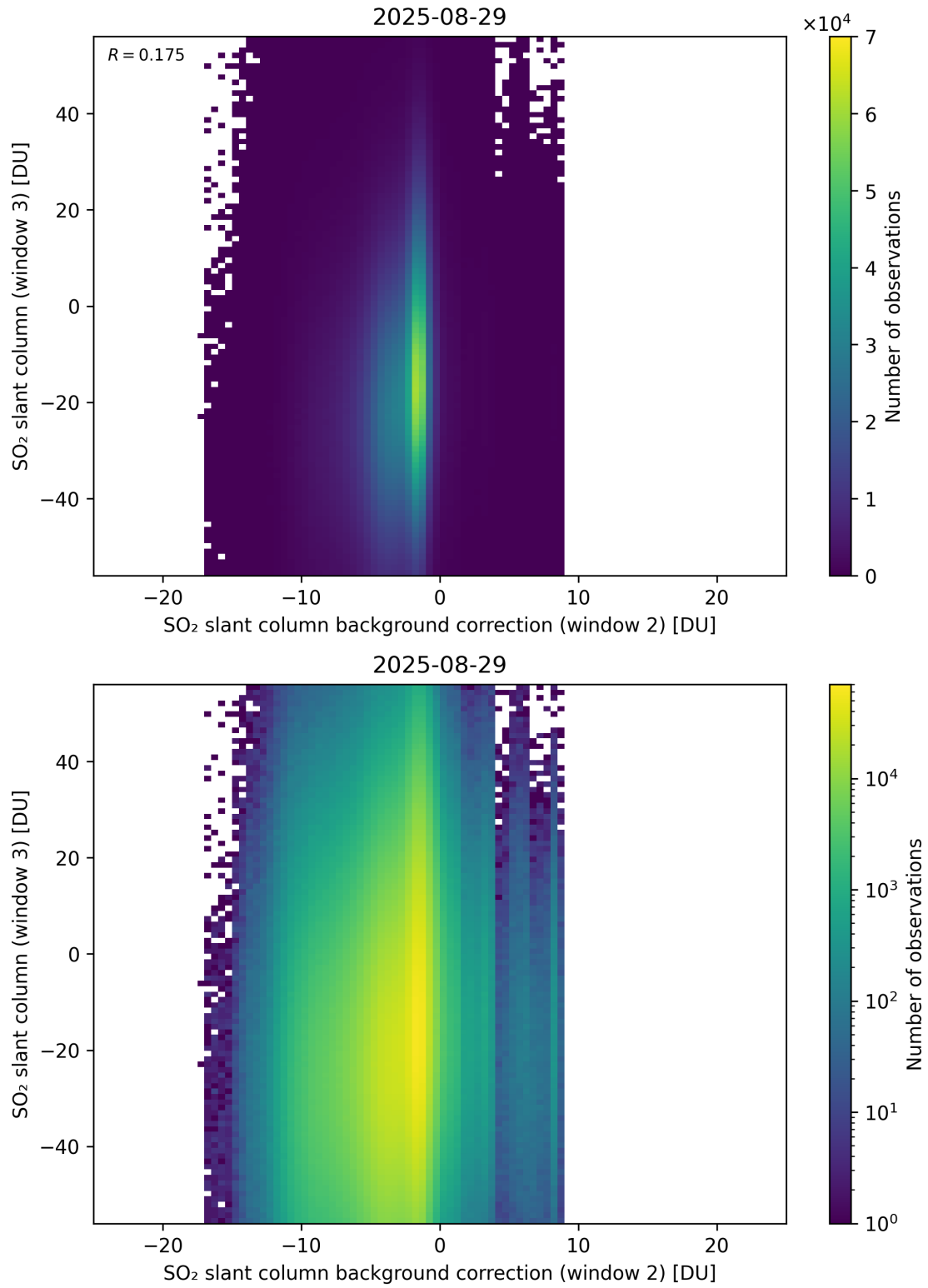
Figure 128: Scatter density plot of “SO 2 slant column background correction (window 2)” against “SO 2 slant column (window 3)” for 2025-08-28 to 2025-08-30.
