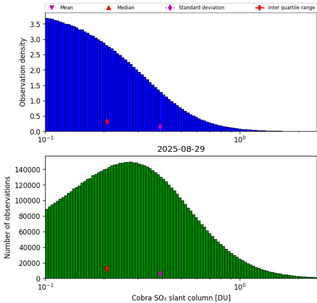
Figure 61: Histogram of “Cobra SO 2 slant column” for 2025-08-28 to 2025-08-30
