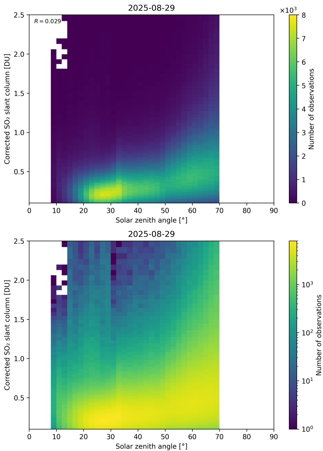
Figure 181: Scatter density plot of “Solar zenith angle” against “Corrected SO 2 slant column” for 2025-08-28 to 2025-08-30.
