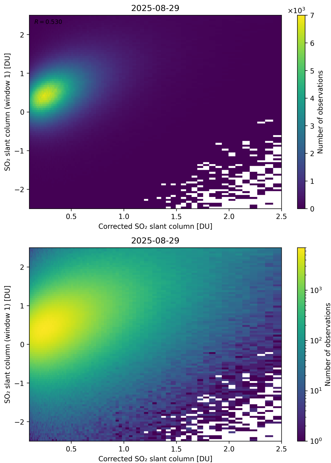
Figure 237: Scatter density plot of “Corrected SO 2 slant column” against “SO 2 slant column (window 1)” for 2025-08-28 to 2025-08-30.
