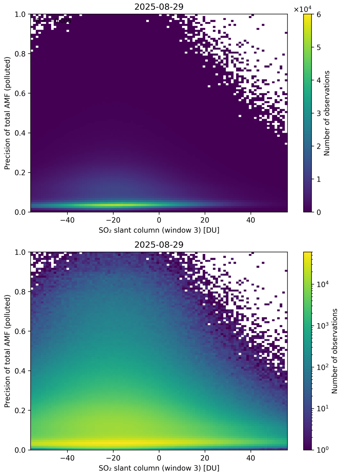
Figure 319: Scatter density plot of “SO 2 slant column (window 3)” against “Precision of total AMF (polluted)” for 2025-08-28 to 2025-08-30.
