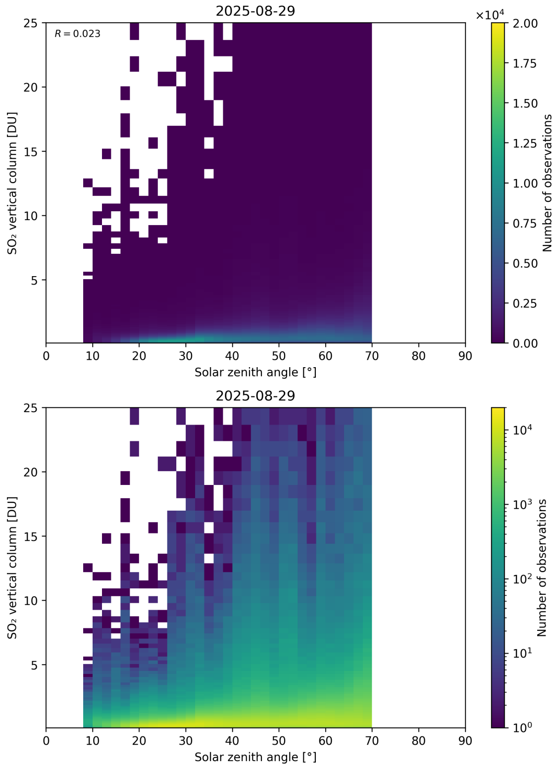
Figure 191: Scatter density plot of “Solar zenith angle” against “SO 2 vertical column” for 2025-08-28 to 2025-08-30.
