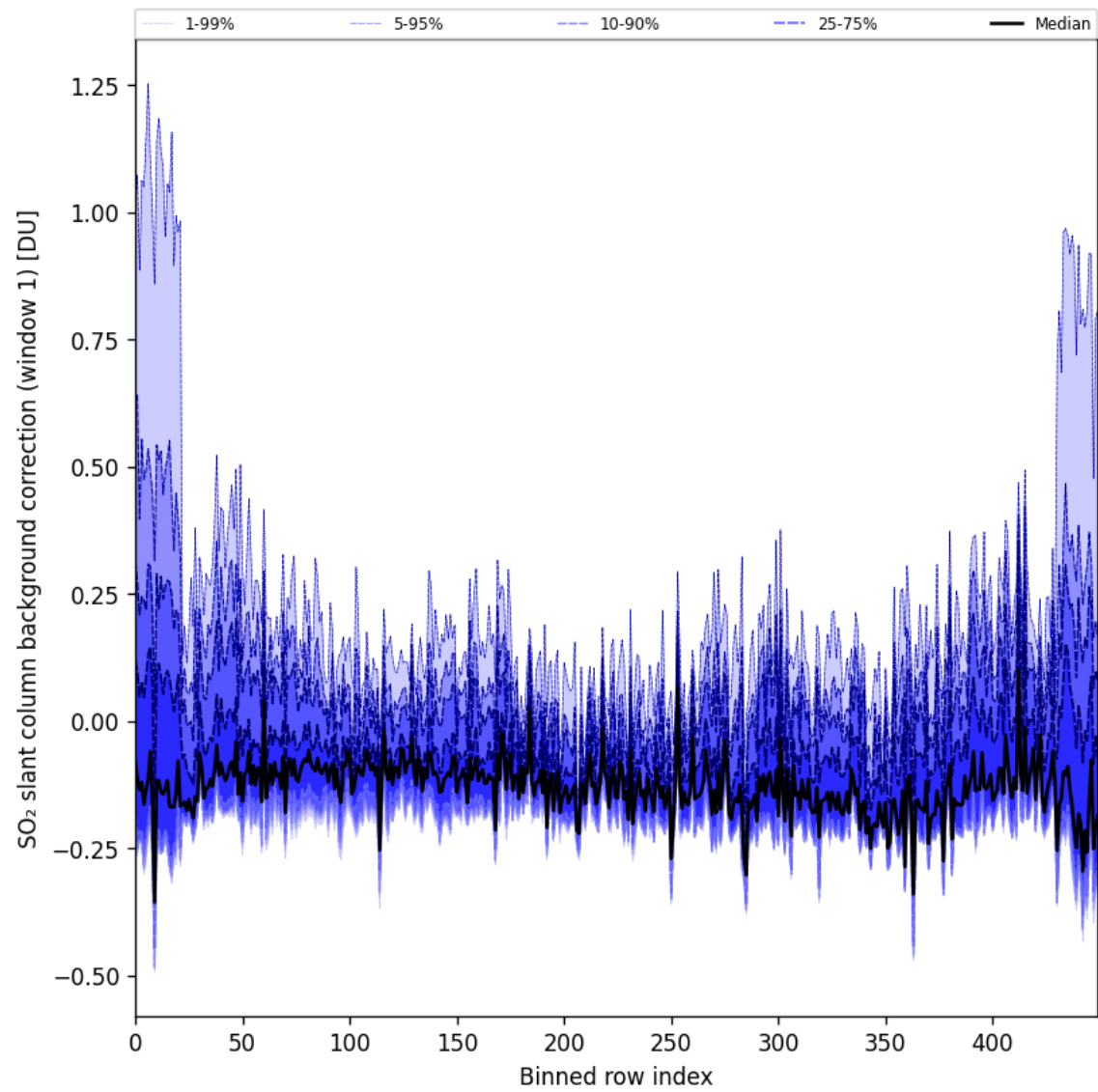
Figure 92: Along track statistics of “SO 2 slant column background correction (window 1)” for 2025-08-28 to 2025-08-30
