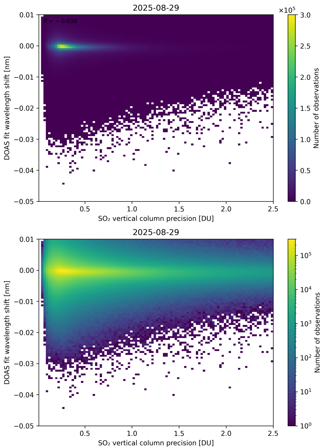
Figure 332: Scatter density plot of “SO 2 vertical column precision” against “DOAS fit wavelength shift” for 2025-08-28 to 2025-08-30.
