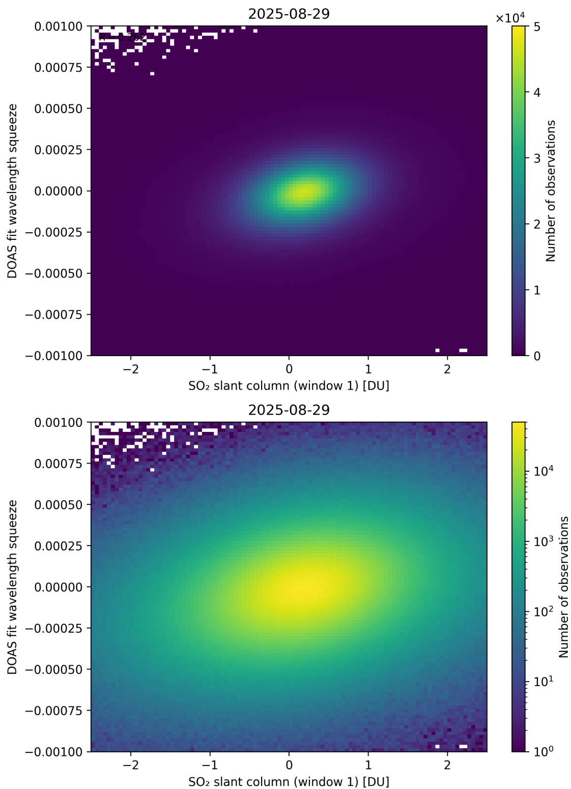
Figure 266: Scatter density plot of “SO 2 slant column (window 1)” against “DOAS fit wavelength squeeze” for 2025-08-28 to 2025-08-30.
