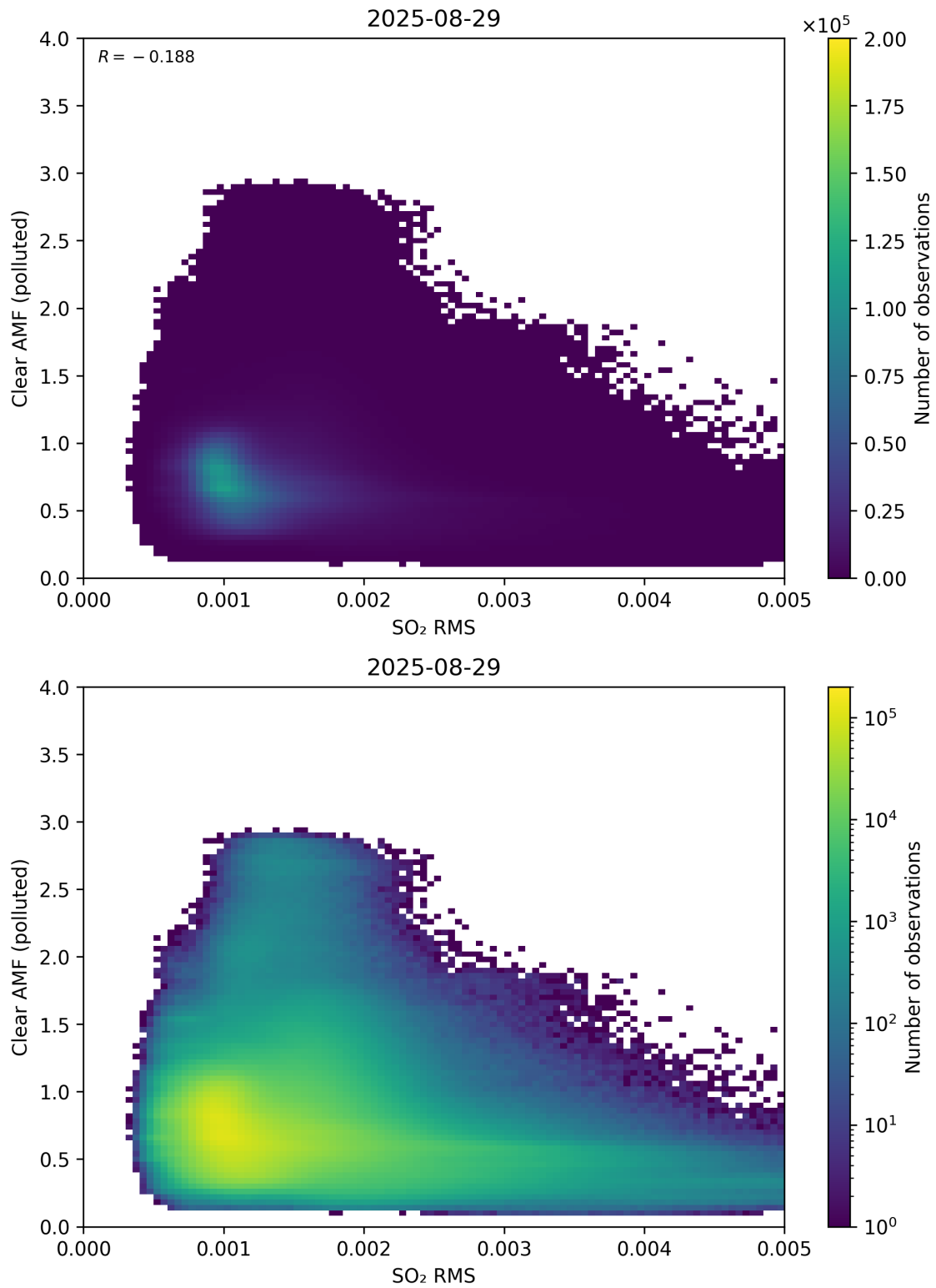
Figure 147: Scatter density plot of “SO 2 RMS” against “Clear AMF (polluted)” for 2025-08-28 to 2025-08-30.
