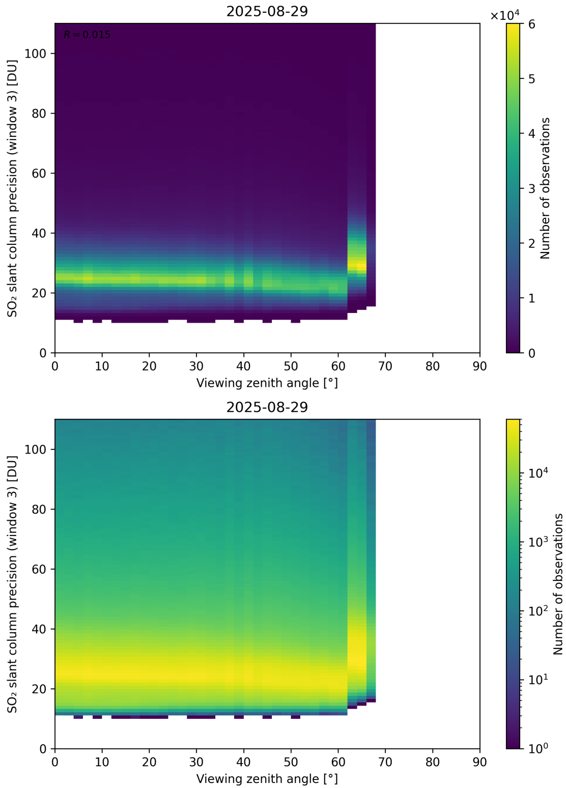
Figure 380: Scatter density plot of “Viewing zenith angle” against “SO 2 slant column precision (window 3)” for 2025-08-28 to 2025-08-30.
