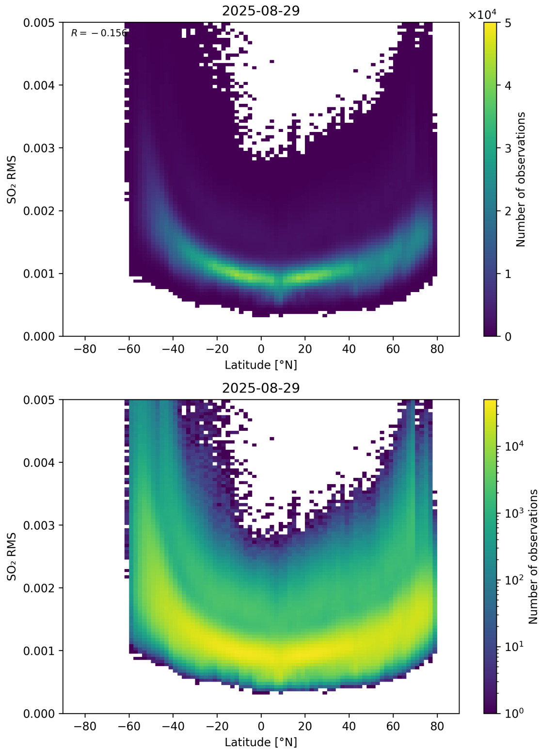
Figure 155: Scatter density plot of “Latitude” against “SO 2 RMS” for 2025-08-28 to 2025-08-30.
