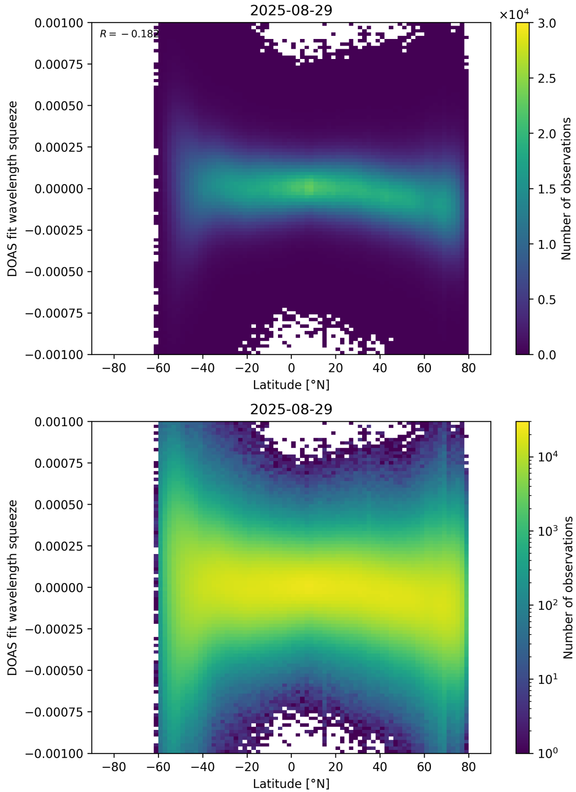
Figure 154: Scatter density plot of “Latitude” against “DOAS fit wavelength squeeze” for 2025-08-28 to 2025-08-30.
