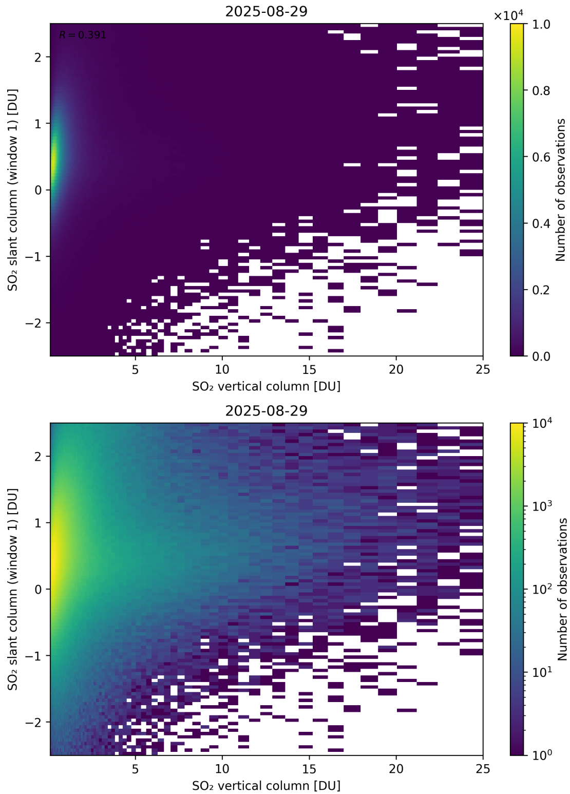
Figure 354: Scatter density plot of “SO 2 vertical column” against “SO 2 slant column (window 1)” for 2025-08-28 to 2025-08-30.
