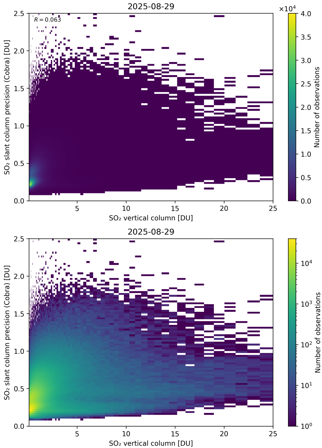
Figure 350: Scatter density plot of “SO 2 vertical column” against “SO 2 slant column precision (Cobra)” for 2025-08-28 to 2025-08-30.
