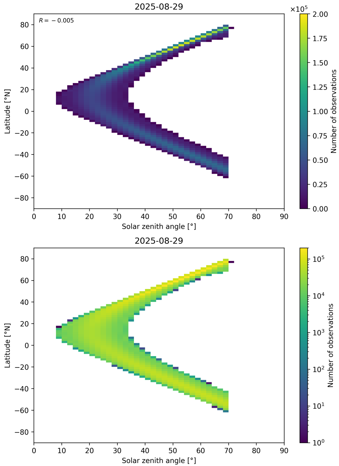
Figure 177: Scatter density plot of “Solar zenith angle” against “Latitude” for 2025-08-28 to 2025-08-30.
