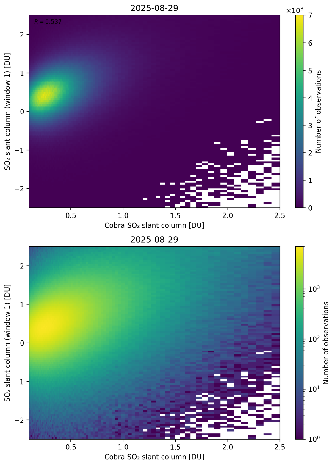
Figure 219: Scatter density plot of “Cobra SO 2 slant column” against “SO 2 slant column (window 1)” for 2025-08-28 to 2025-08-30.
