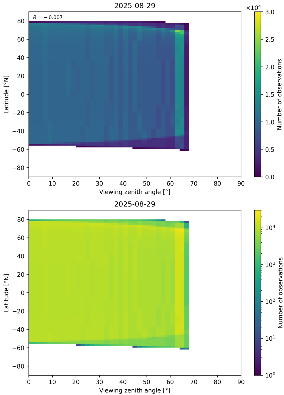
Figure 368: Scatter density plot of “Viewing zenith angle” against “Latitude” for 2025-08-28 to 2025-08-30.
