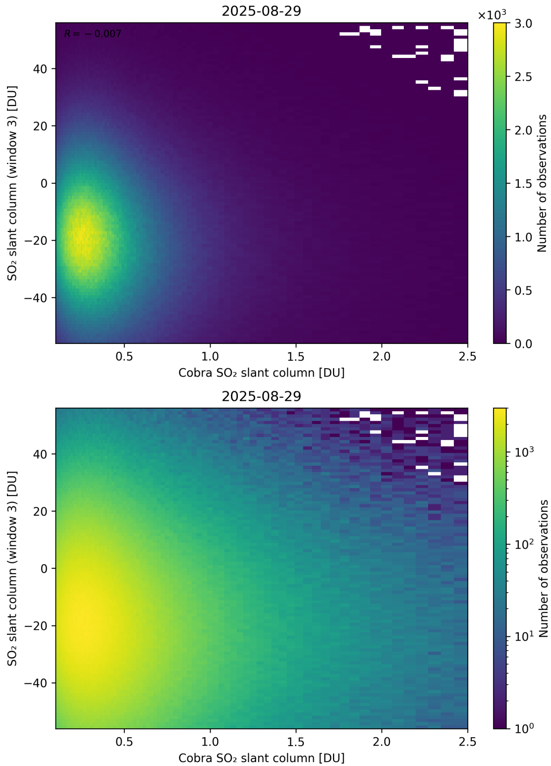
Figure 222: Scatter density plot of “Cobra SO 2 slant column” against “SO 2 slant column (window 3)” for 2025-08-28 to 2025-08-30.
