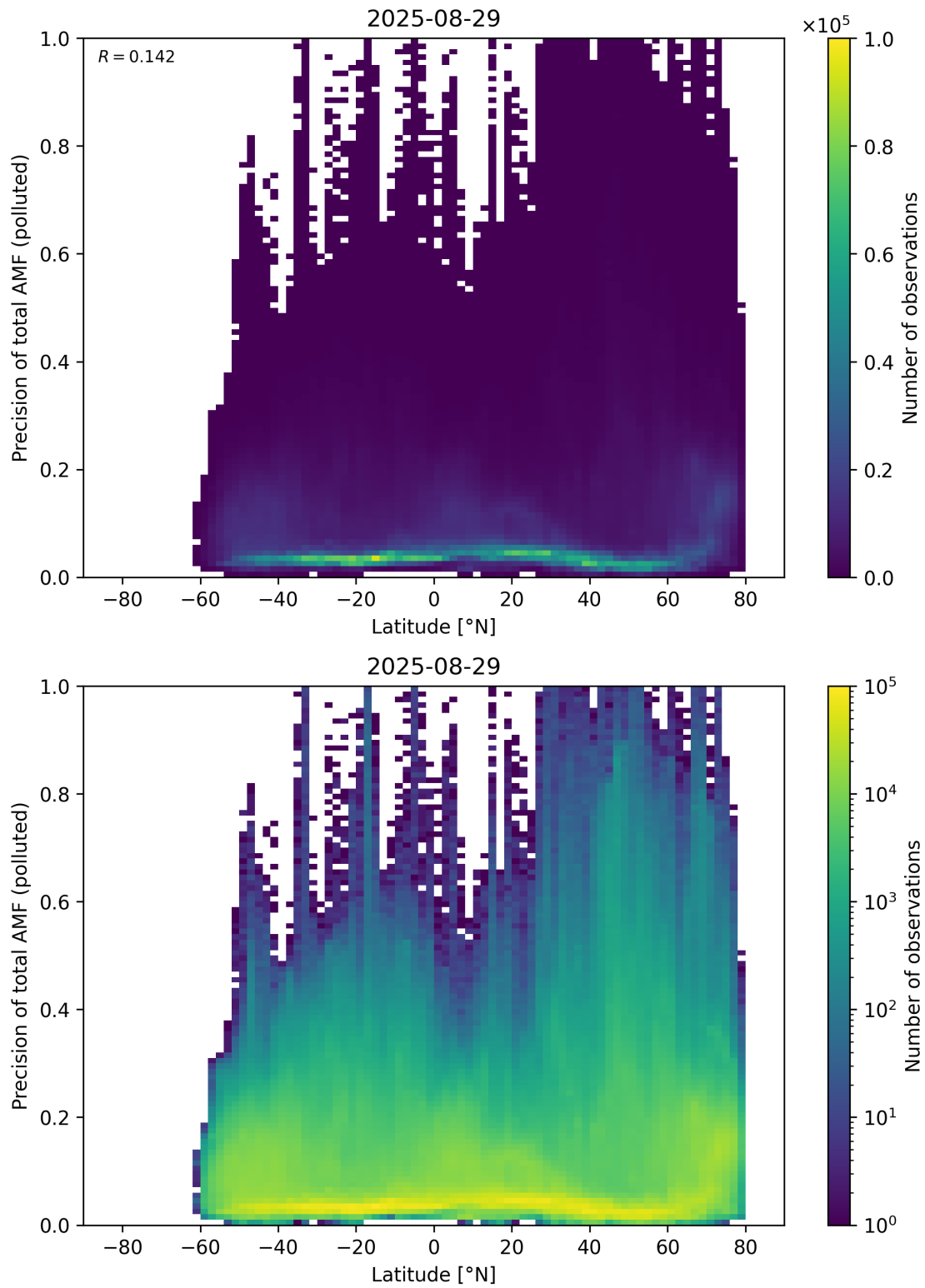
Figure 168: Scatter density plot of “Latitude” against “Precision of total AMF (polluted)” for 2025-08-28 to 2025-08-30.
