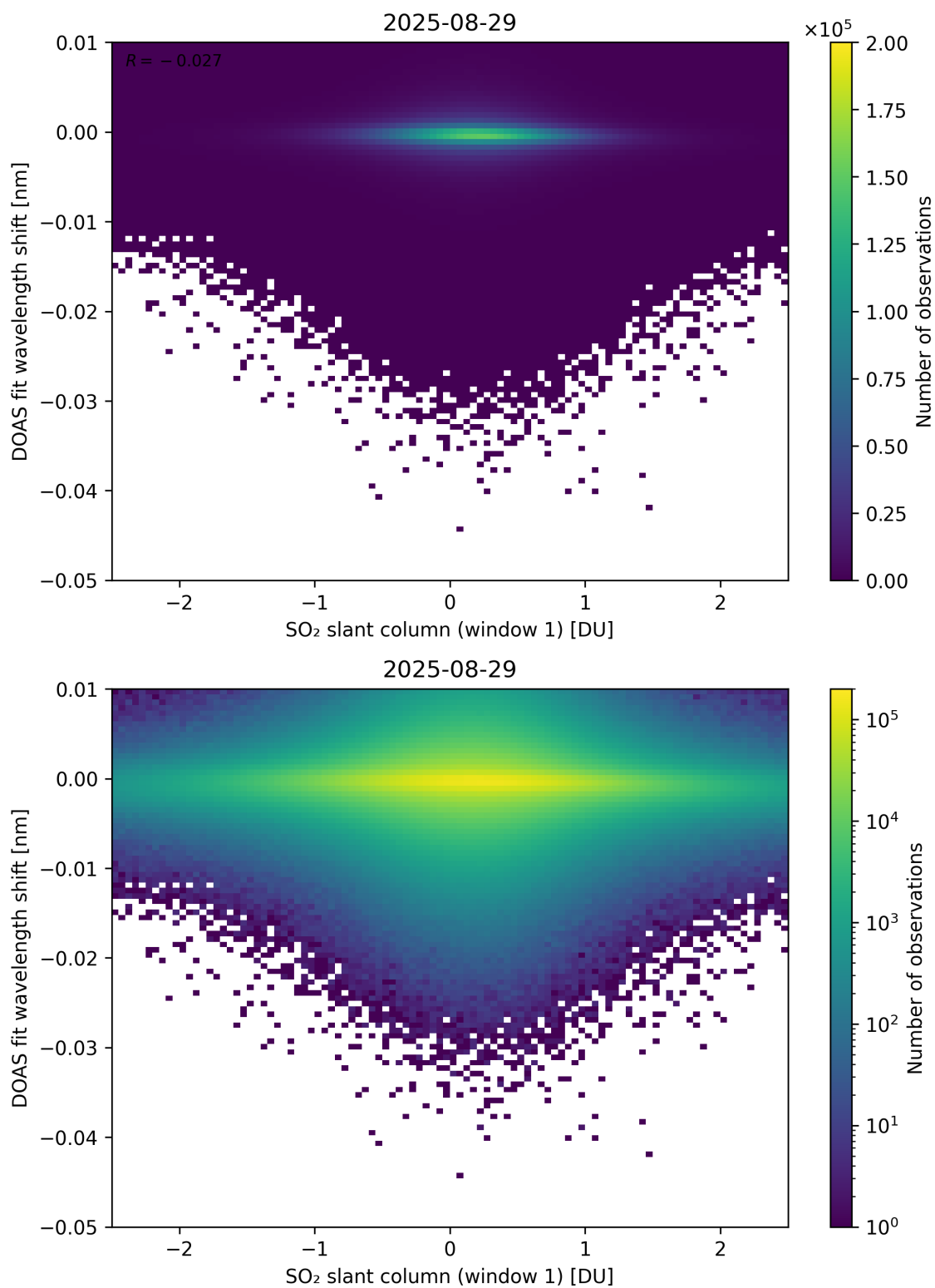
Figure 265: Scatter density plot of “SO 2 slant column (window 1)” against “DOAS fit wavelength shift” for 2025-08-28 to 2025-08-30.
