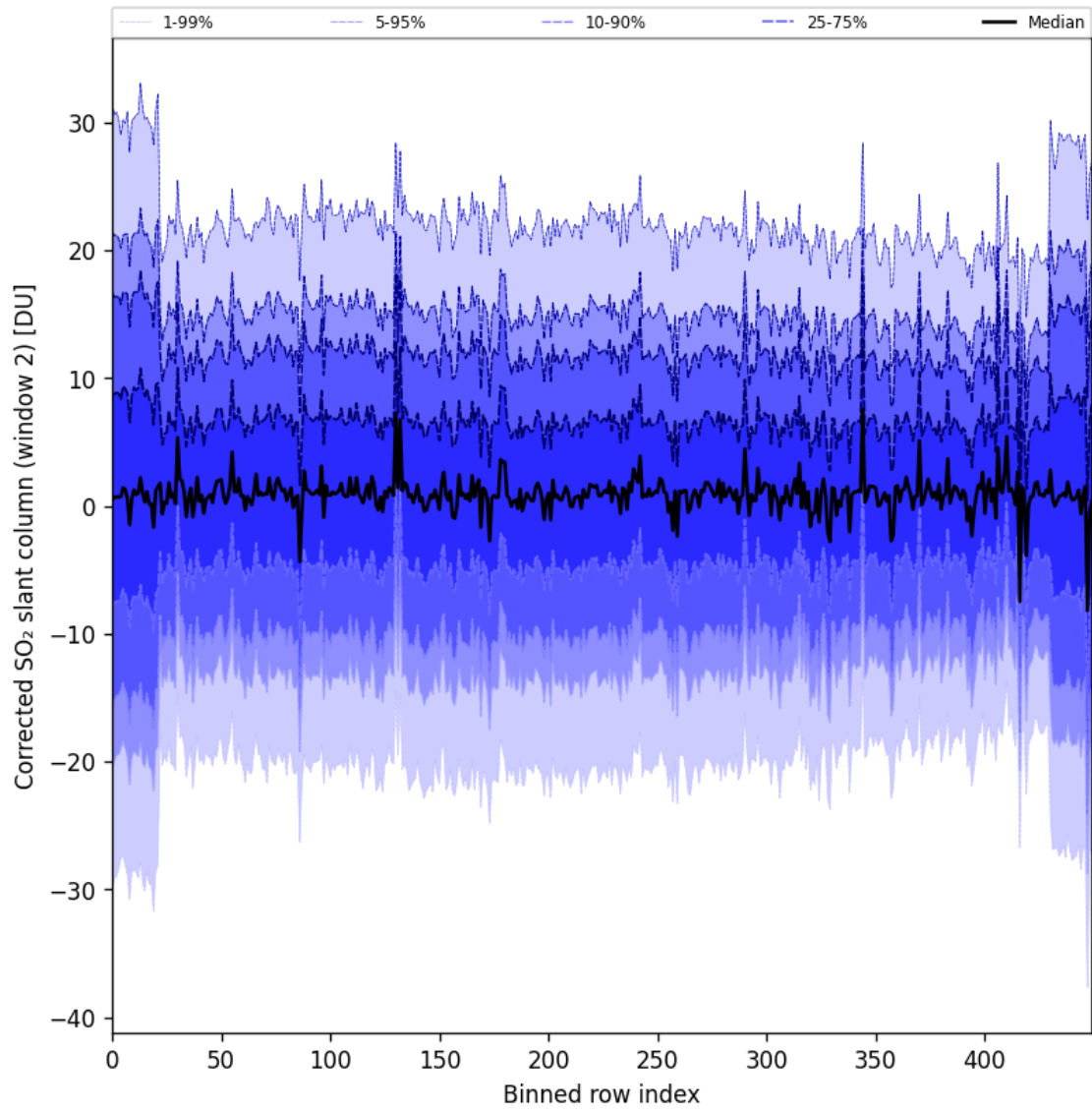
Figure 95: Along track statistics of “Corrected SO 2 slant column (window 2)” for 2025-08-28 to 2025-08-30
