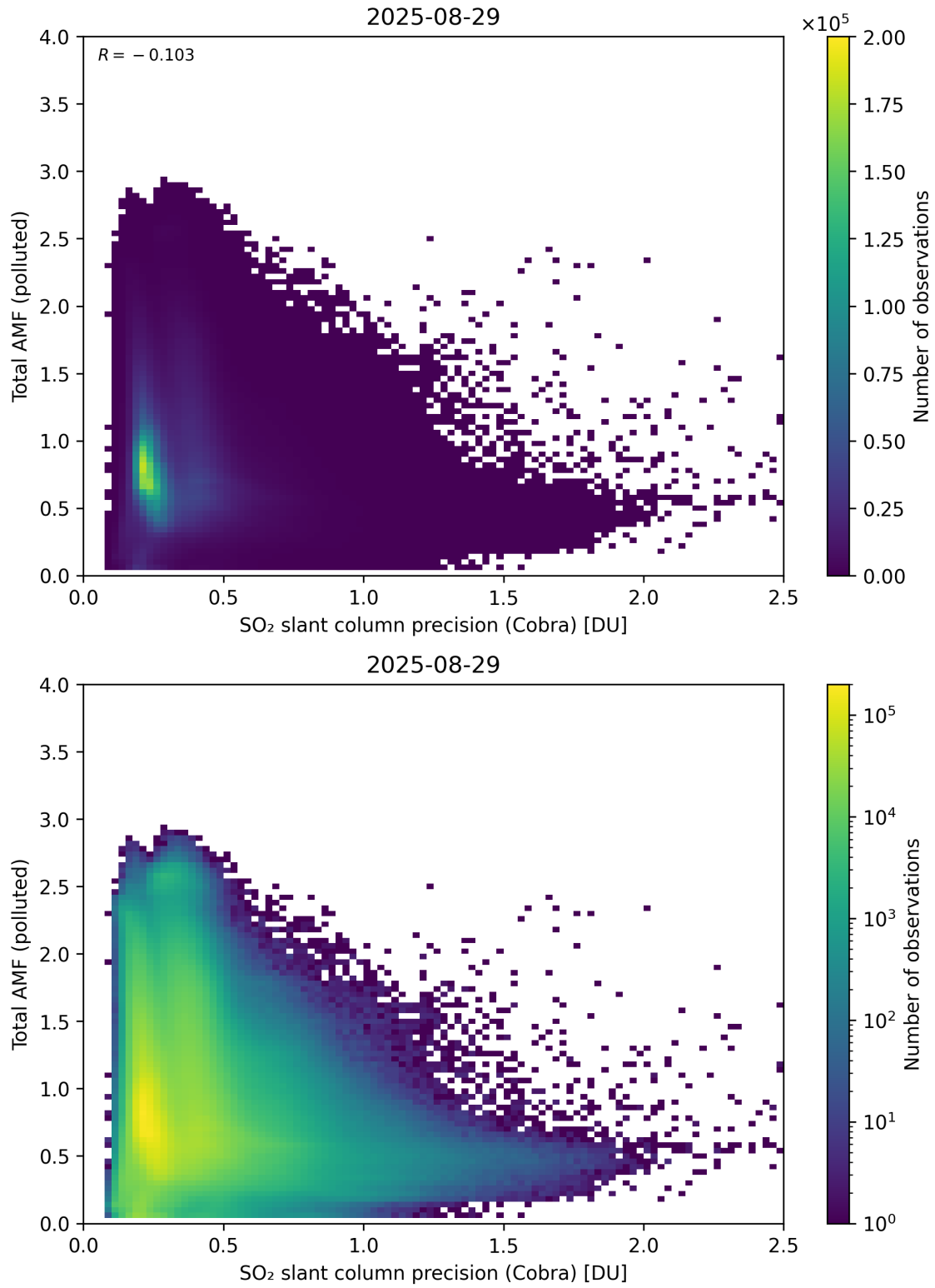
Figure 213: Scatter density plot of “SO 2 slant column precision (Cobra)” against “Total AMF (polluted)” for 2025-08-28 to 2025-08-30.
