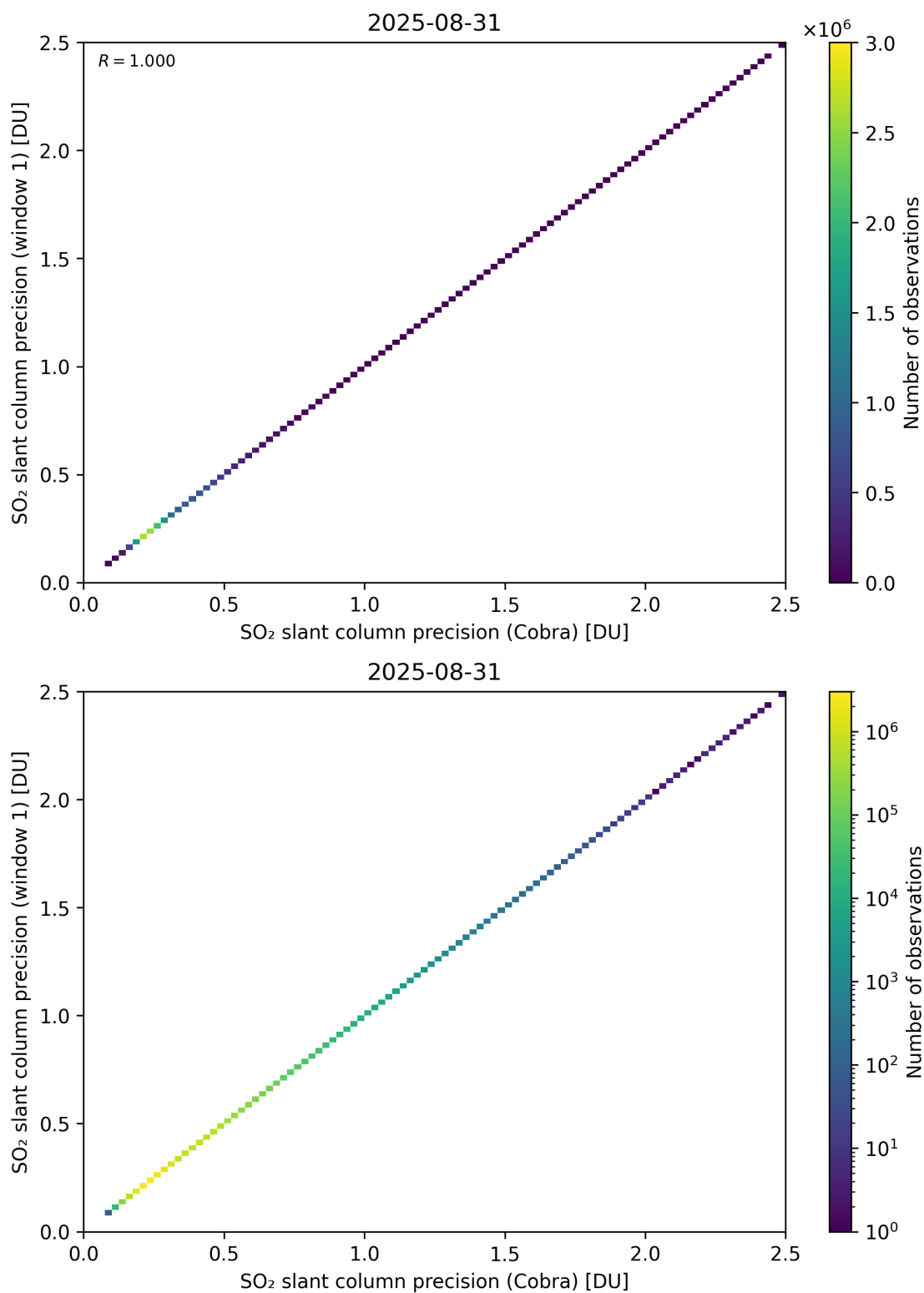
Figure 209: Scatter density plot of “SO 2 slant column precision (Cobra)” against “SO 2 slant column precision (window 1)” for 2025-08-30 to 2025-09-01.
