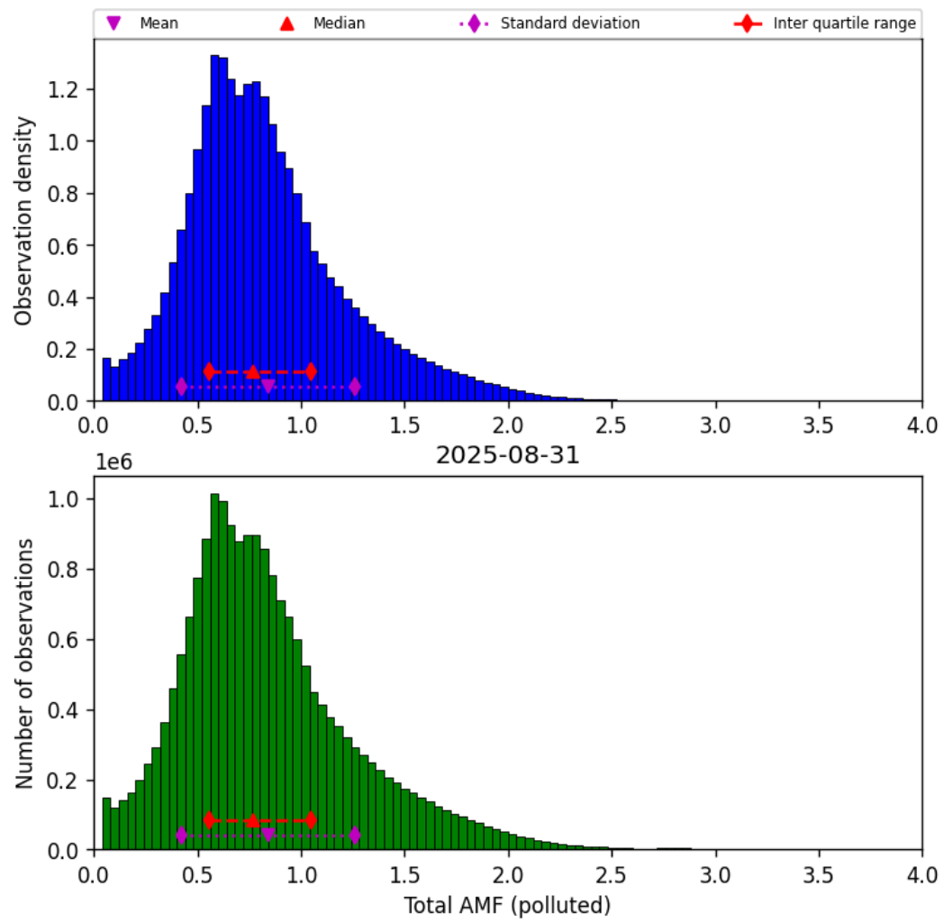
Figure 79: Histogram of “Total AMF (polluted)” for 2025-08-30 to 2025-09-01
