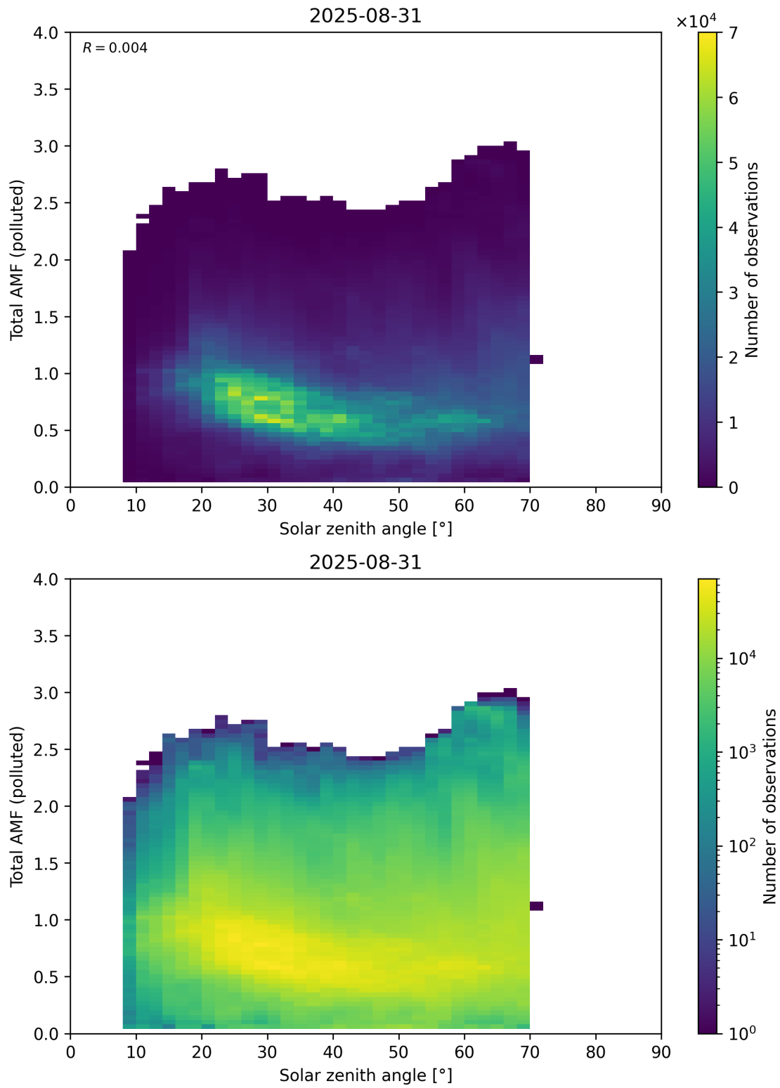
Figure 189: Scatter density plot of “Solar zenith angle” against “Total AMF (polluted)” for 2025-08-30 to 2025-09-01.
