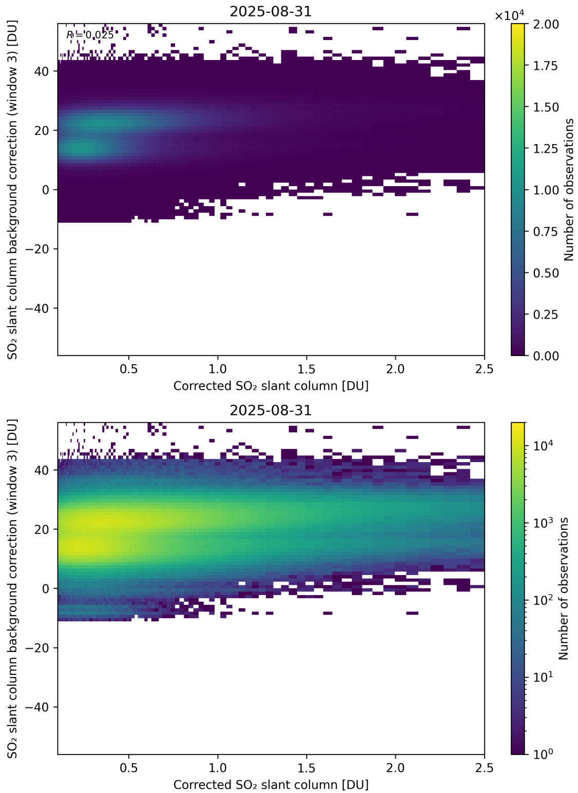
Figure 228: Scatter density plot of “Corrected SO 2 slant column” against “SO 2 slant column background correction (window 3)” for 2025-08-30 to 2025-09-01.
