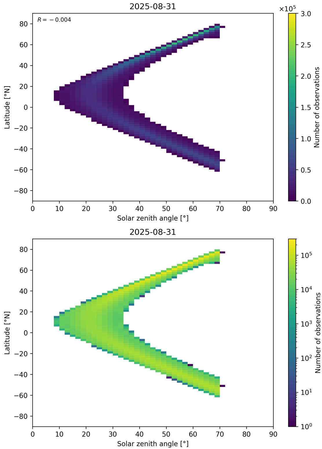
Figure 177: Scatter density plot of “Solar zenith angle” against “Latitude” for 2025-08-30 to 2025-09-01.
