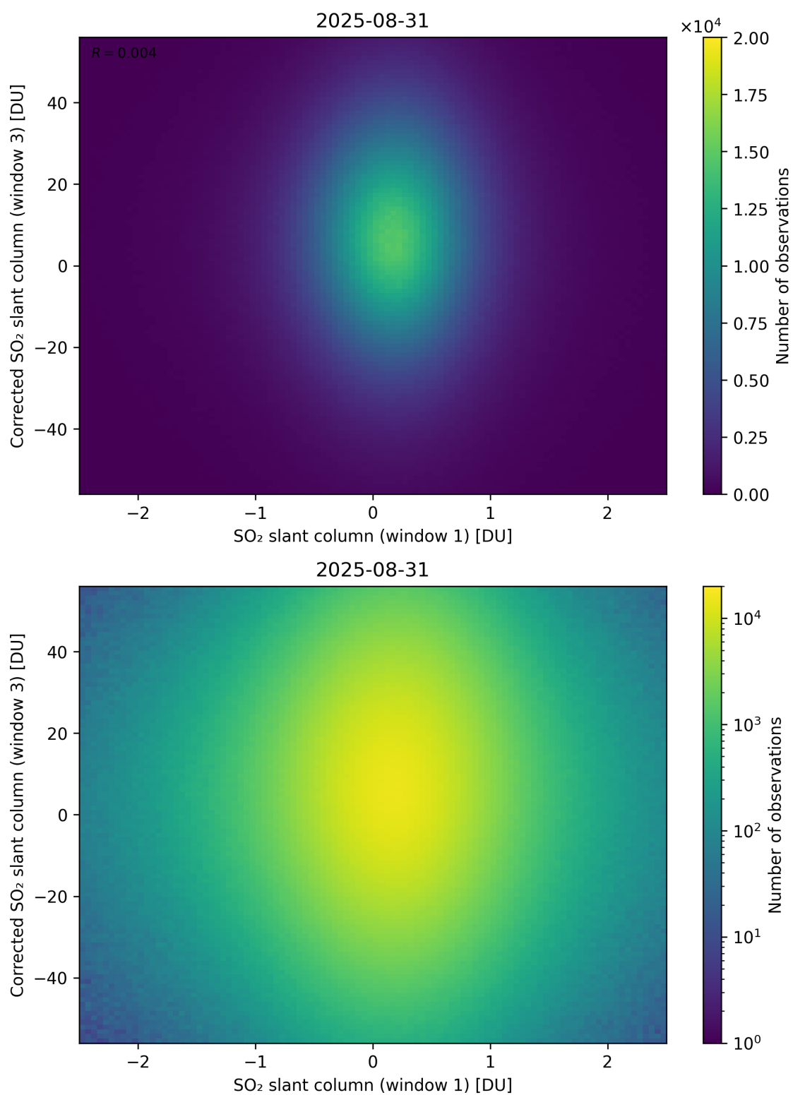
Figure 284: Scatter density plot of “SO 2 slant column (window 1)” against “Corrected SO 2 slant column (window 3)” for 2025-08-30 to 2025-09-01.
