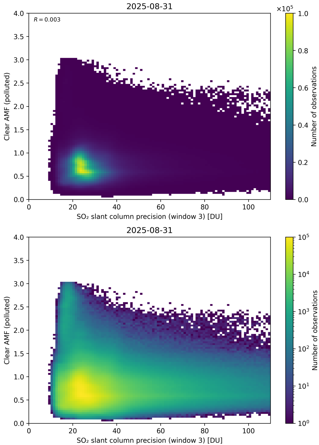
Figure 311: Scatter density plot of “SO 2 slant column precision (window 3)” against “Clear AMF (polluted)” for 2025-08-30 to 2025-09-01.
