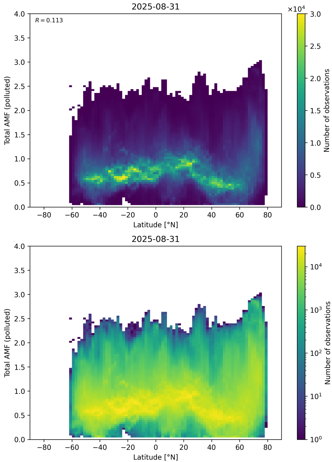
Figure 167: Scatter density plot of “Latitude” against “Total AMF (polluted)” for 2025-08-30 to 2025-09-01.
