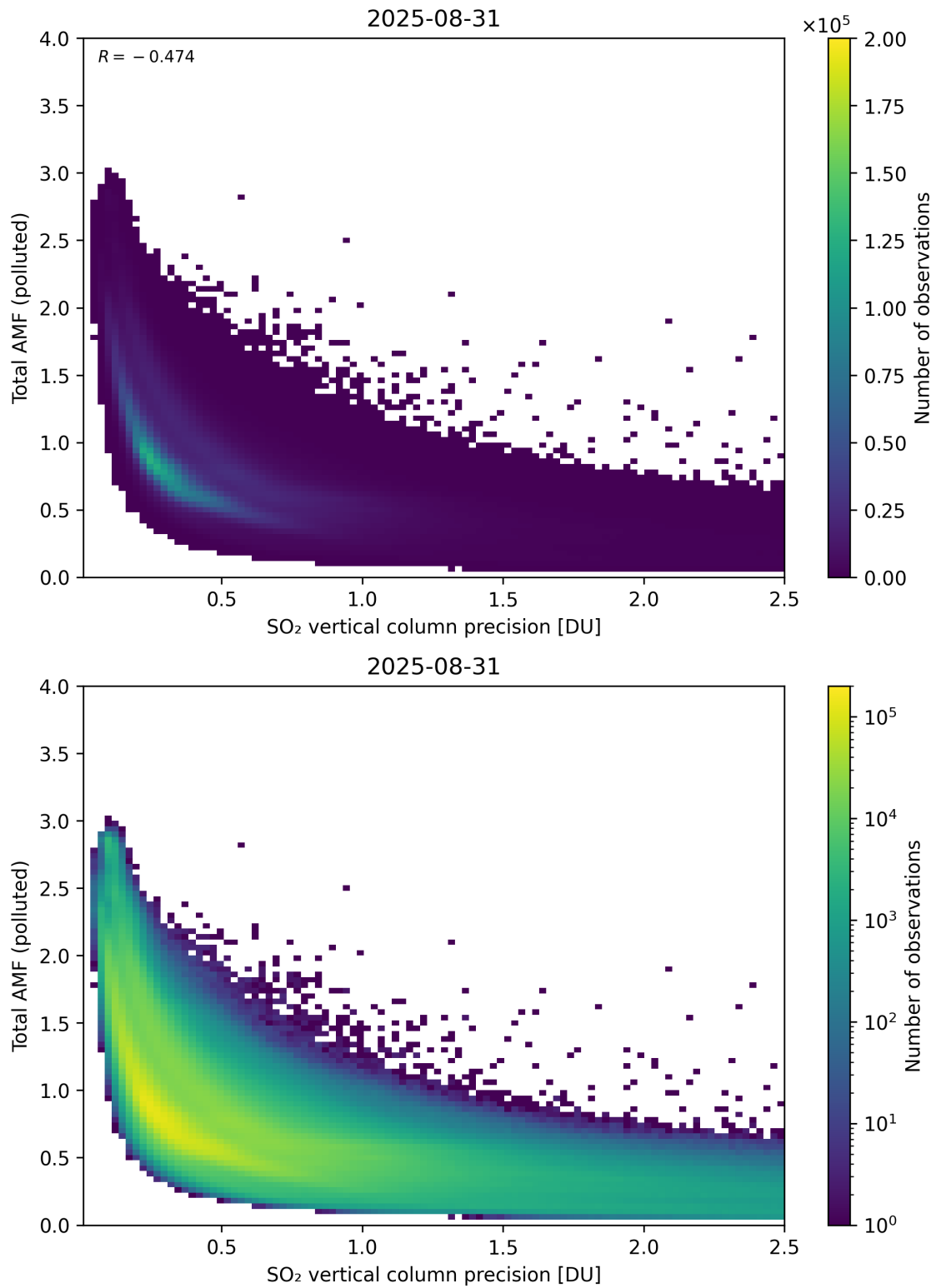
Figure 346: Scatter density plot of “SO 2 vertical column precision” against “Total AMF (polluted)” for 2025-08-30 to 2025-09-01.
