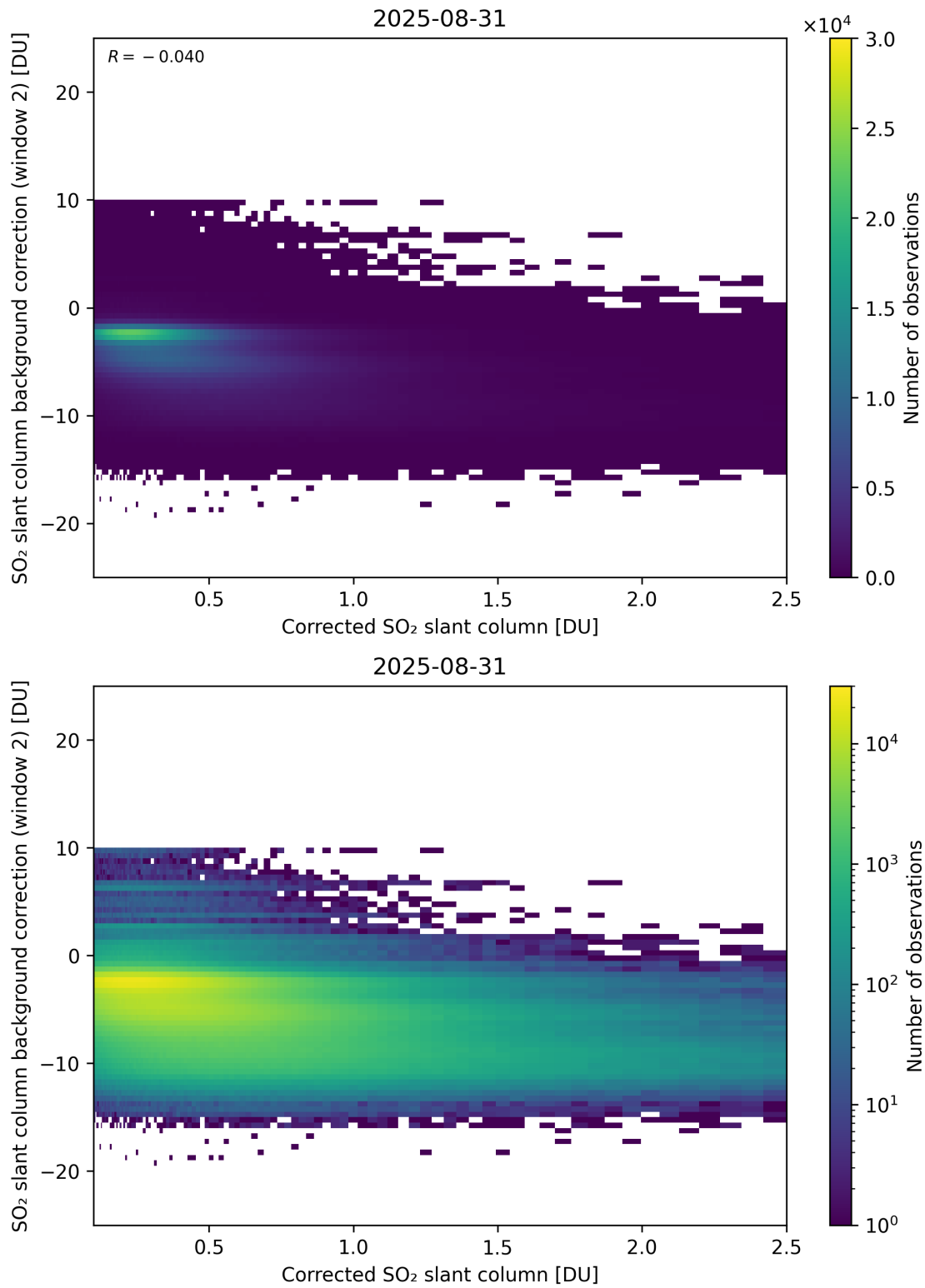
Figure 227: Scatter density plot of “Corrected SO 2 slant column” against “SO 2 slant column background correction (window 2)” for 2025-08-30 to 2025-09-01.
