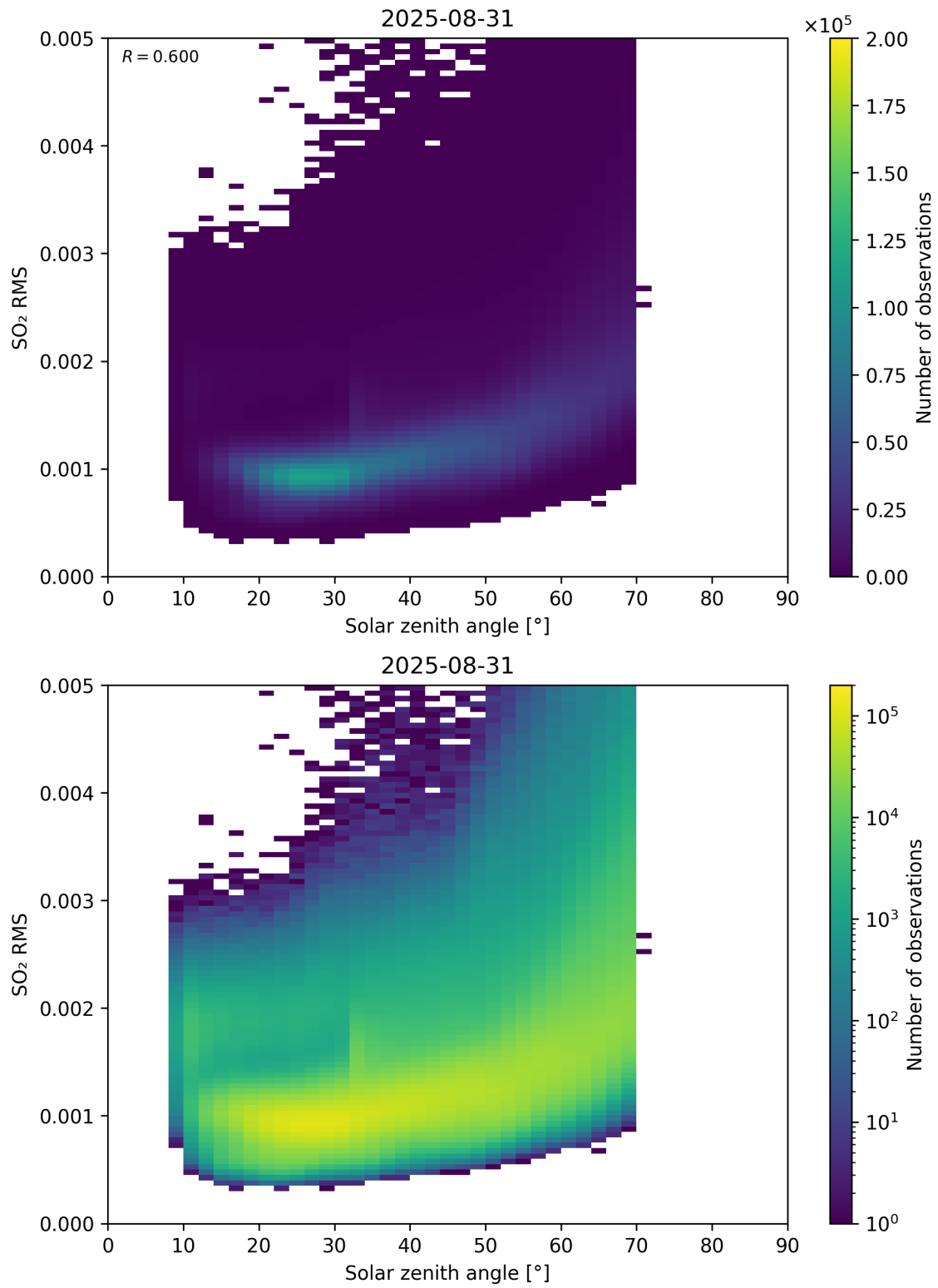
Figure 176: Scatter density plot of “Solar zenith angle” against “SO 2 RMS” for 2025-08-30 to 2025-09-01.
