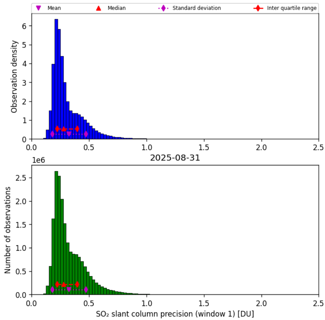
Figure 64: Histogram of “SO 2 slant column precision (window 1)” for 2025-08-30 to 2025-09-01
