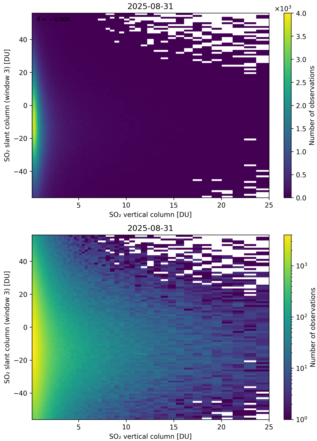
Figure 357: Scatter density plot of “SO 2 vertical column” against “SO 2 slant column (window 3)” for 2025-08-30 to 2025-09-01.
