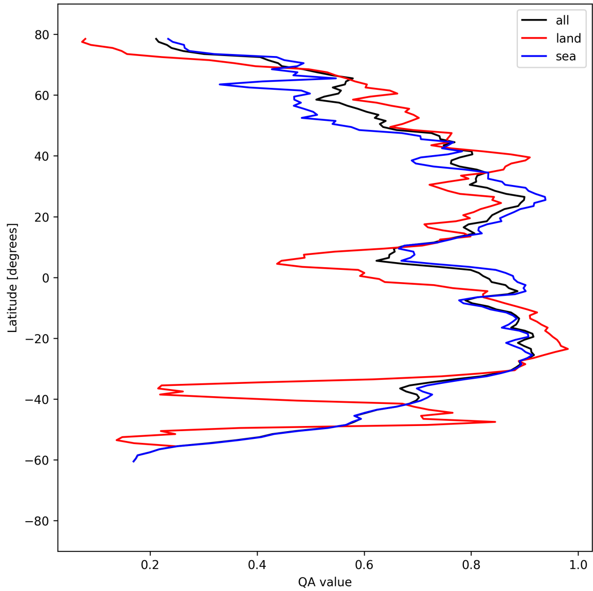
Figure 31: Zonal average of “QA value” for 2025-08-30 to 2025-09-01.
