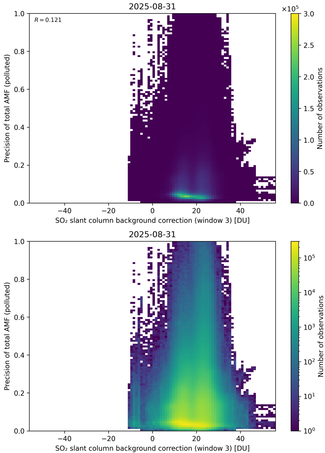
Figure 137: Scatter density plot of “SO 2 slant column background correction (window 3)” against “Precision of total AMF (polluted)” for 2025-08-30 to 2025-09-01.
