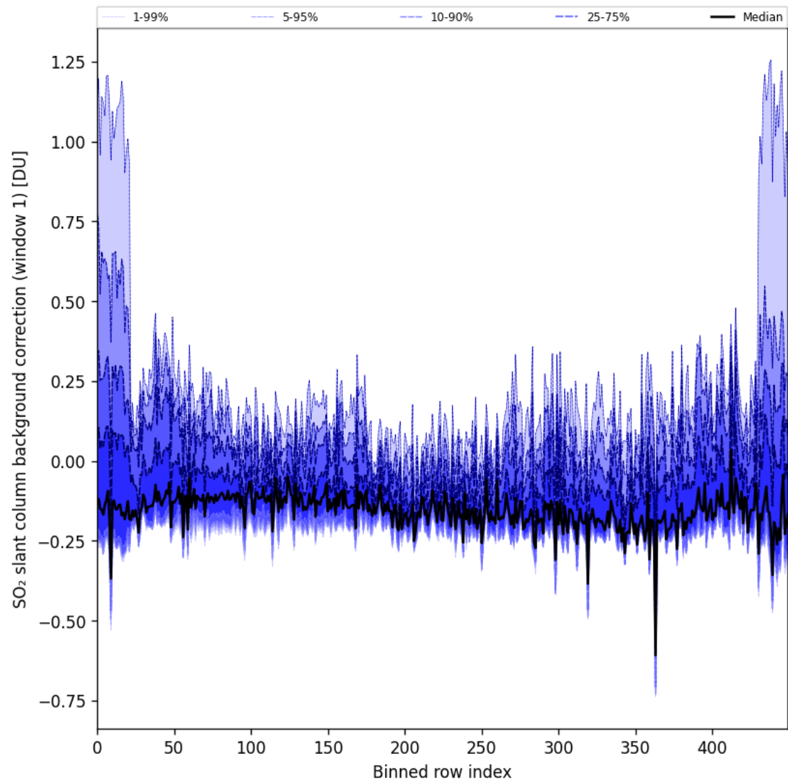
Figure 92: Along track statistics of “SO 2 slant column background correction (window 1)” for 2025-08-30 to 2025-09-01
