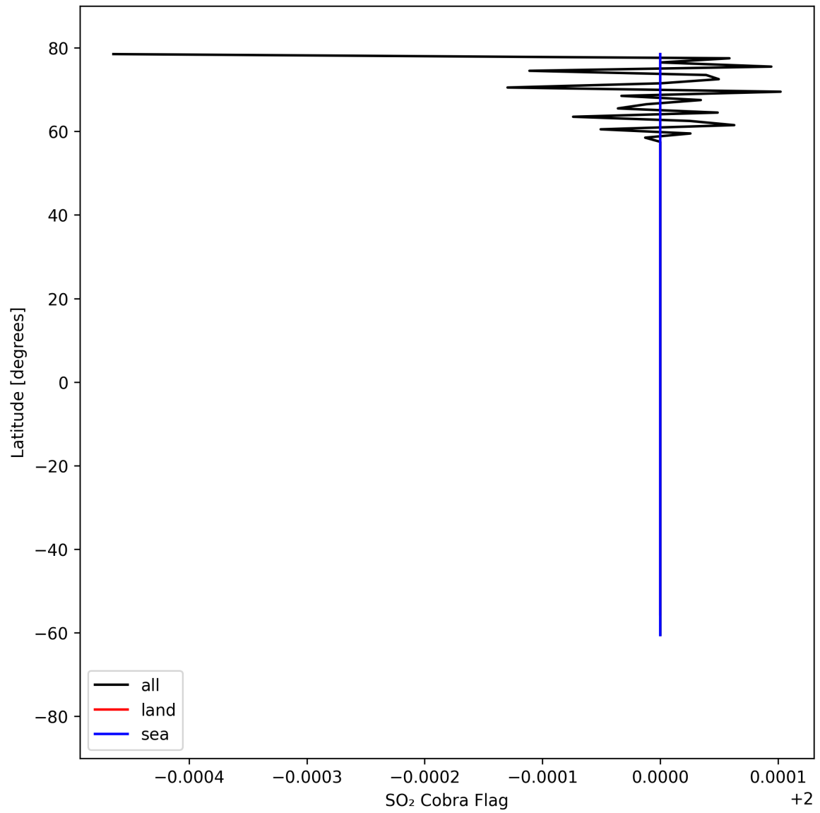
Figure 49: Zonal average of “SO 2 Cobra Flag” for 2025-08-30 to 2025-09-01.
