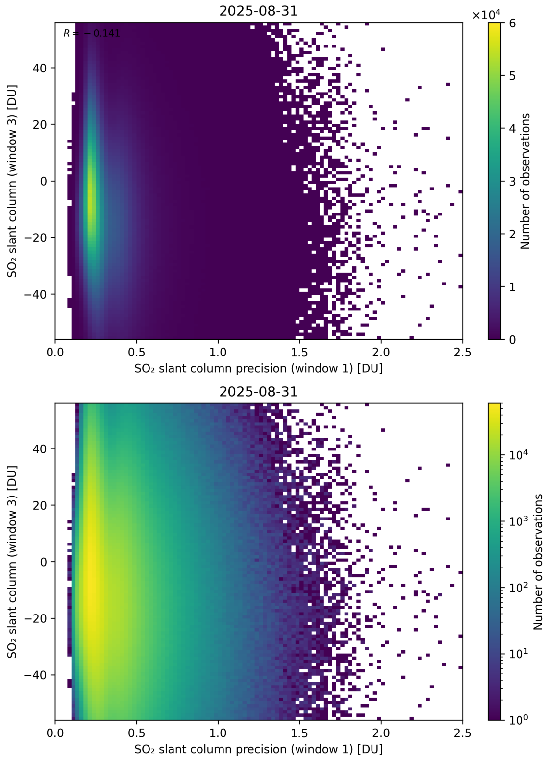
Figure 278: Scatter density plot of “SO 2 slant column precision (window 1)” against “SO 2 slant column (window 3)” for 2025-08-30 to 2025-09-01.
