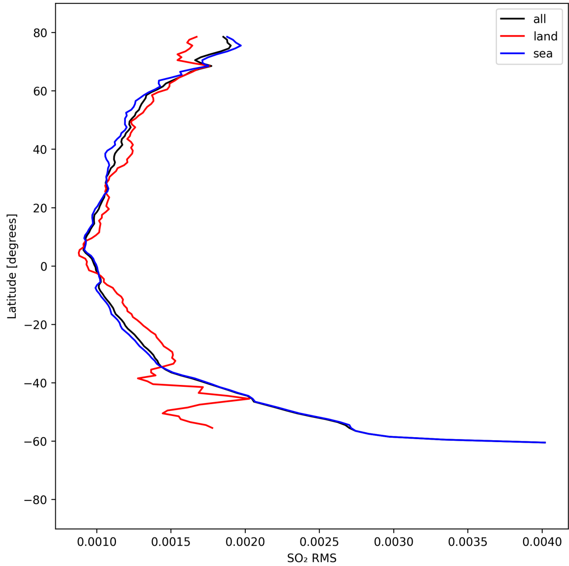
Figure 52: Zonal average of “SO 2 RMS” for 2025-08-30 to 2025-09-01.
