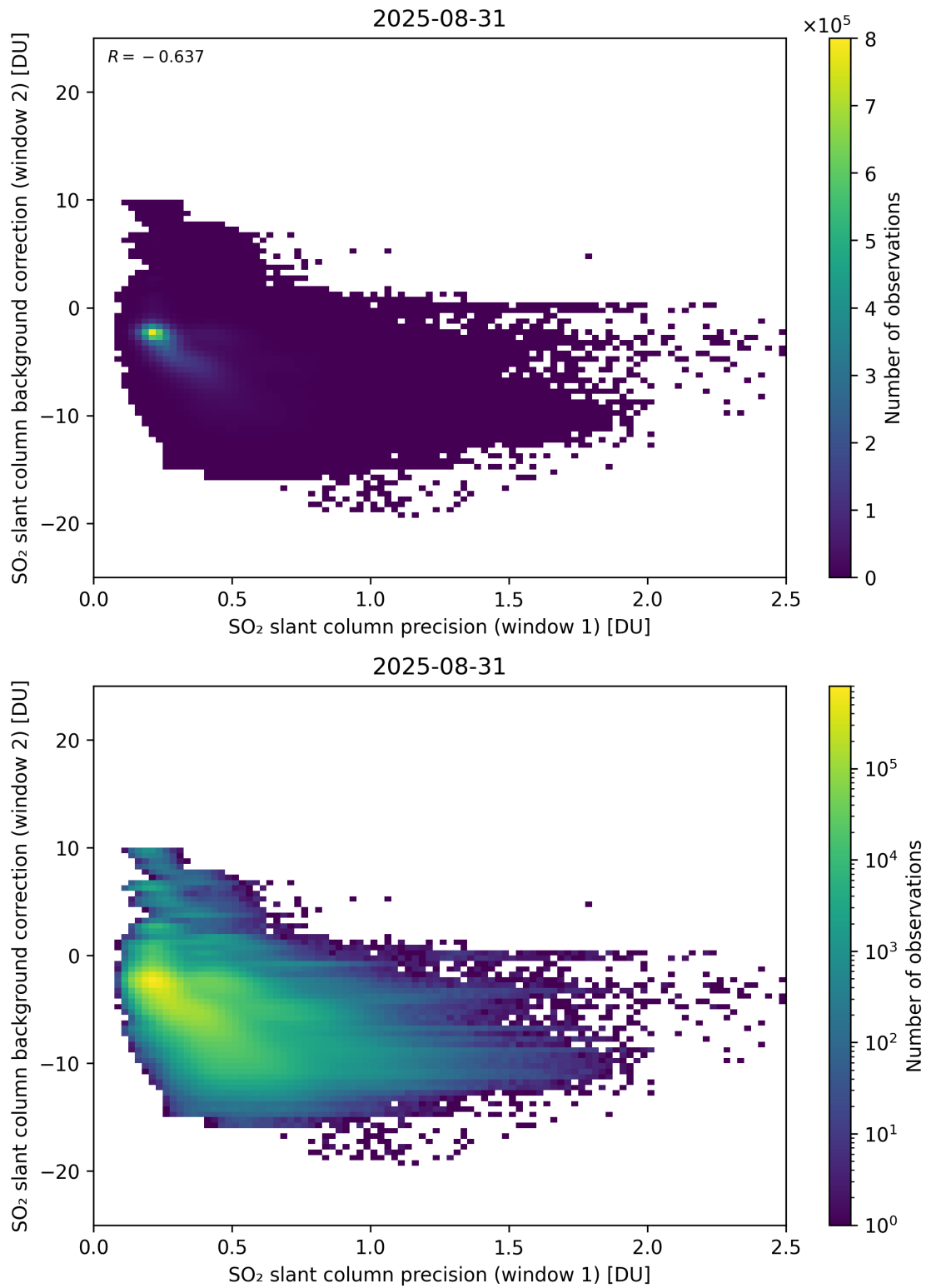
Figure 269: Scatter density plot of “SO 2 slant column precision (window 1)” against “SO 2 slant column background correction (window 2)” for 2025-08-30 to 2025-09-01.
