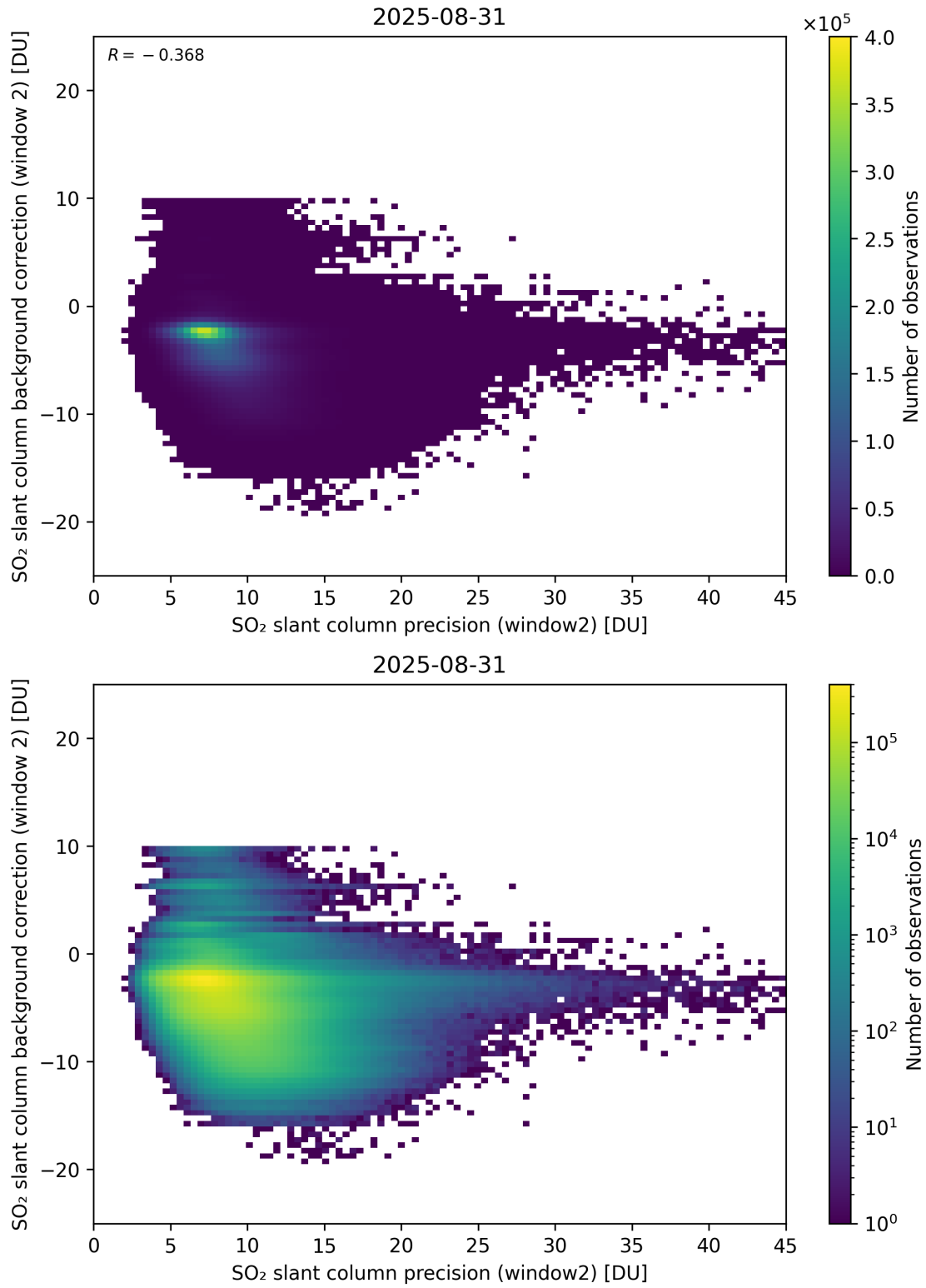
Figure 291: Scatter density plot of “SO 2 slant column precision (window2)” against “SO 2 slant column background correction (window 2)” for 2025-08-30 to 2025-09-01.
