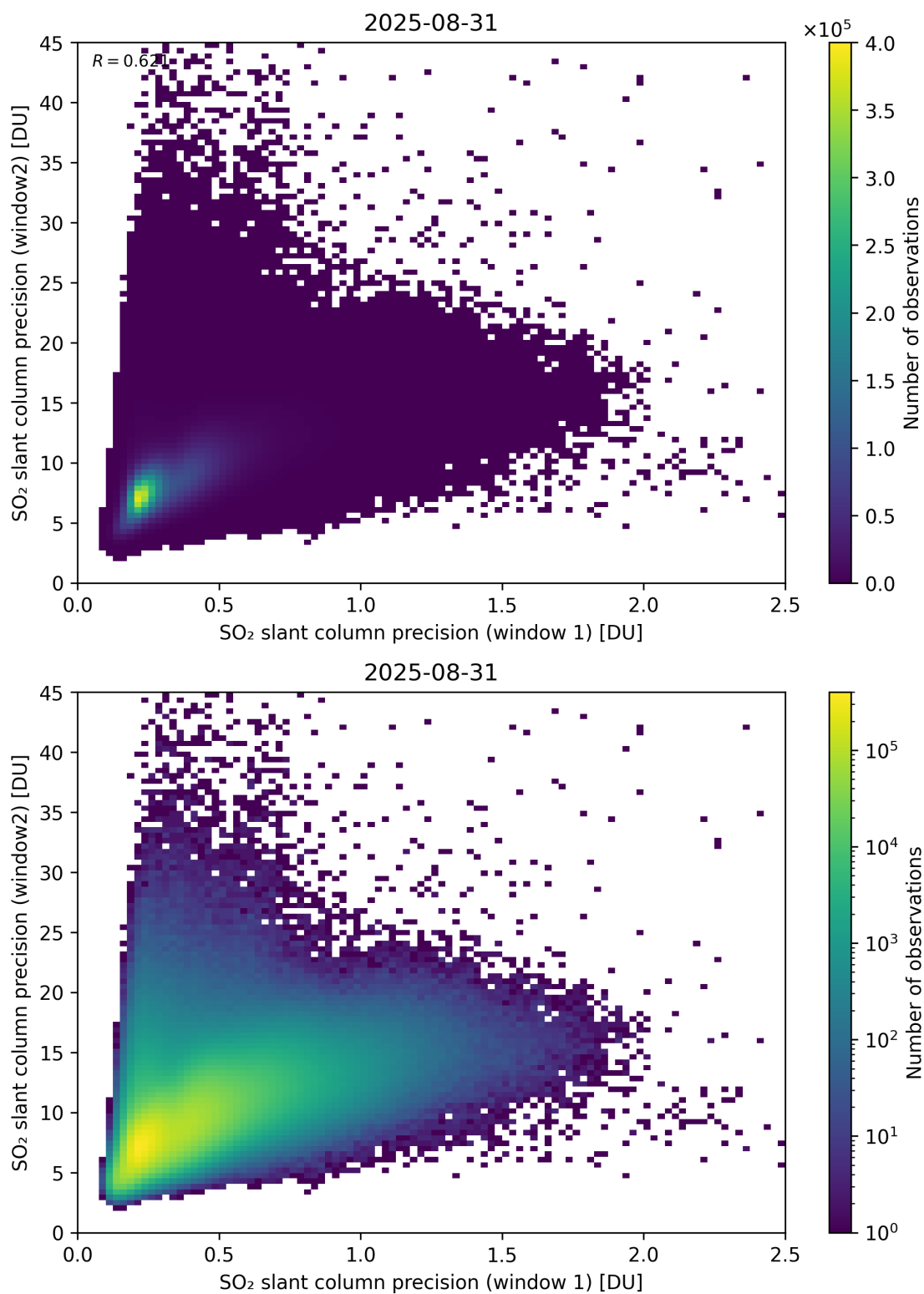
Figure 277: Scatter density plot of “SO 2 slant column precision (window 1)” against “SO 2 slant column precision (window2)” for 2025-08-30 to 2025-09-01.
