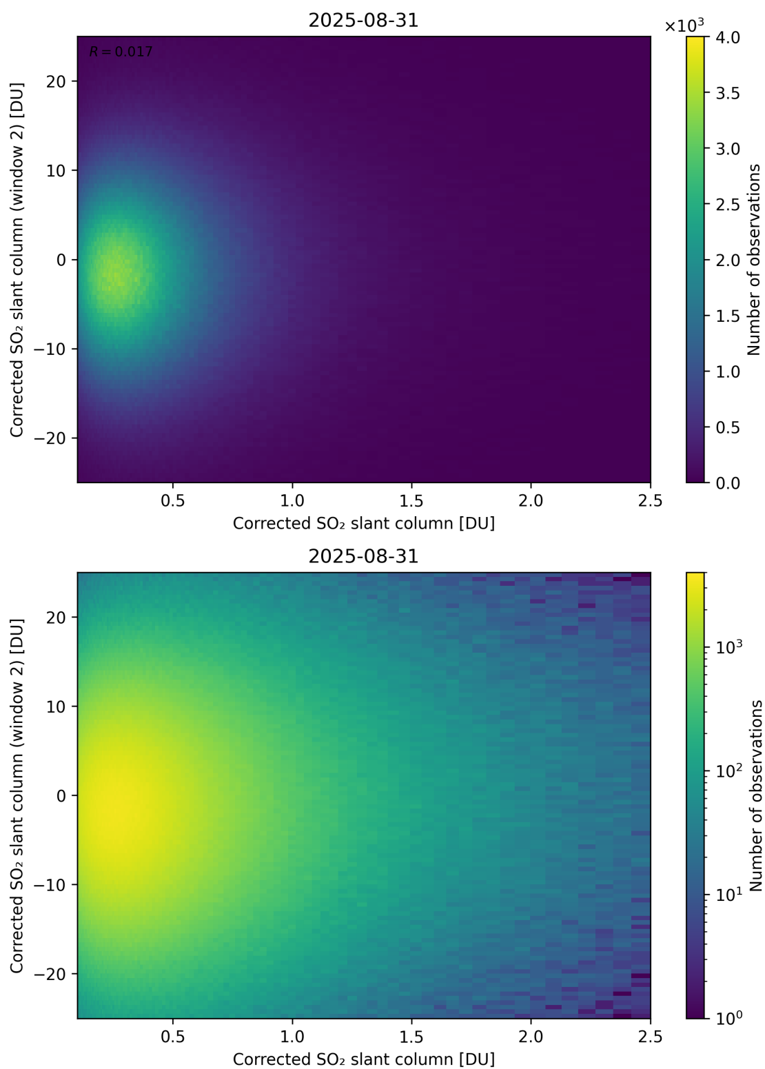
Figure 235: Scatter density plot of “Corrected SO 2 slant column” against “Corrected SO 2 slant column (window 2)” for 2025-08-30 to 2025-09-01.
