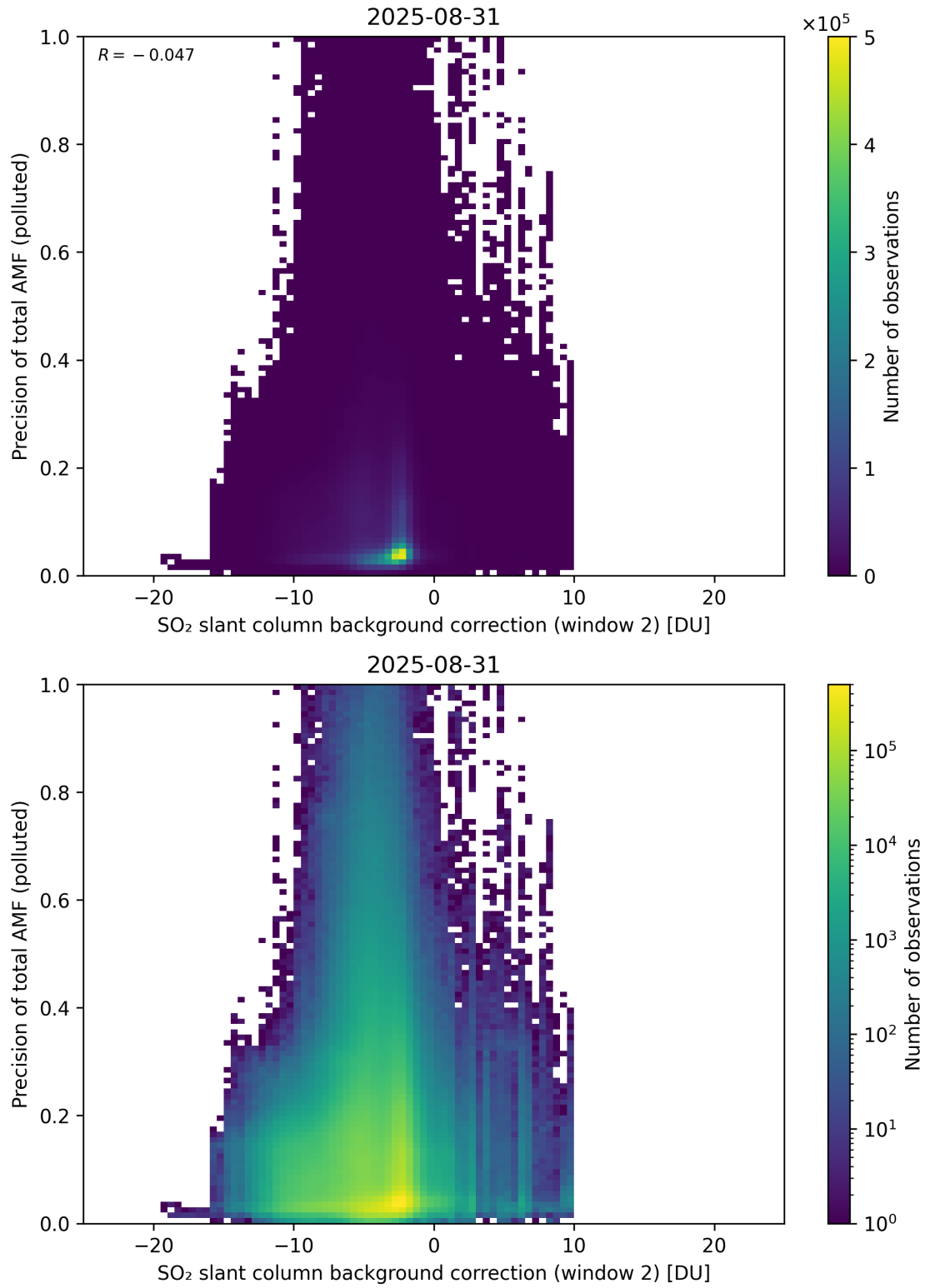
Figure 131: Scatter density plot of “SO 2 slant column background correction (window 2)” against “Precision of total AMF (polluted)” for 2025-08-30 to 2025-09-01.
