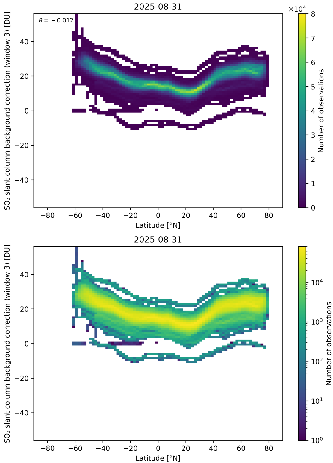
Figure 152: Scatter density plot of “Latitude” against “SO 2 slant column background correction (window 3)” for 2025-08-30 to 2025-09-01.
