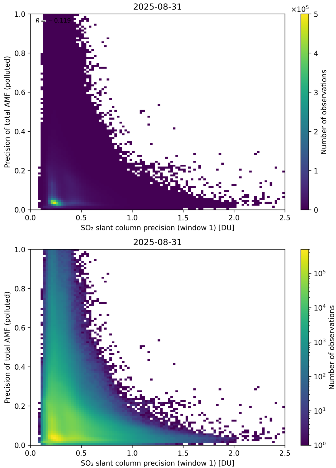
Figure 281: Scatter density plot of “SO 2 slant column precision (window 1)” against “Precision of total AMF (polluted)” for 2025-08-30 to 2025-09-01.
