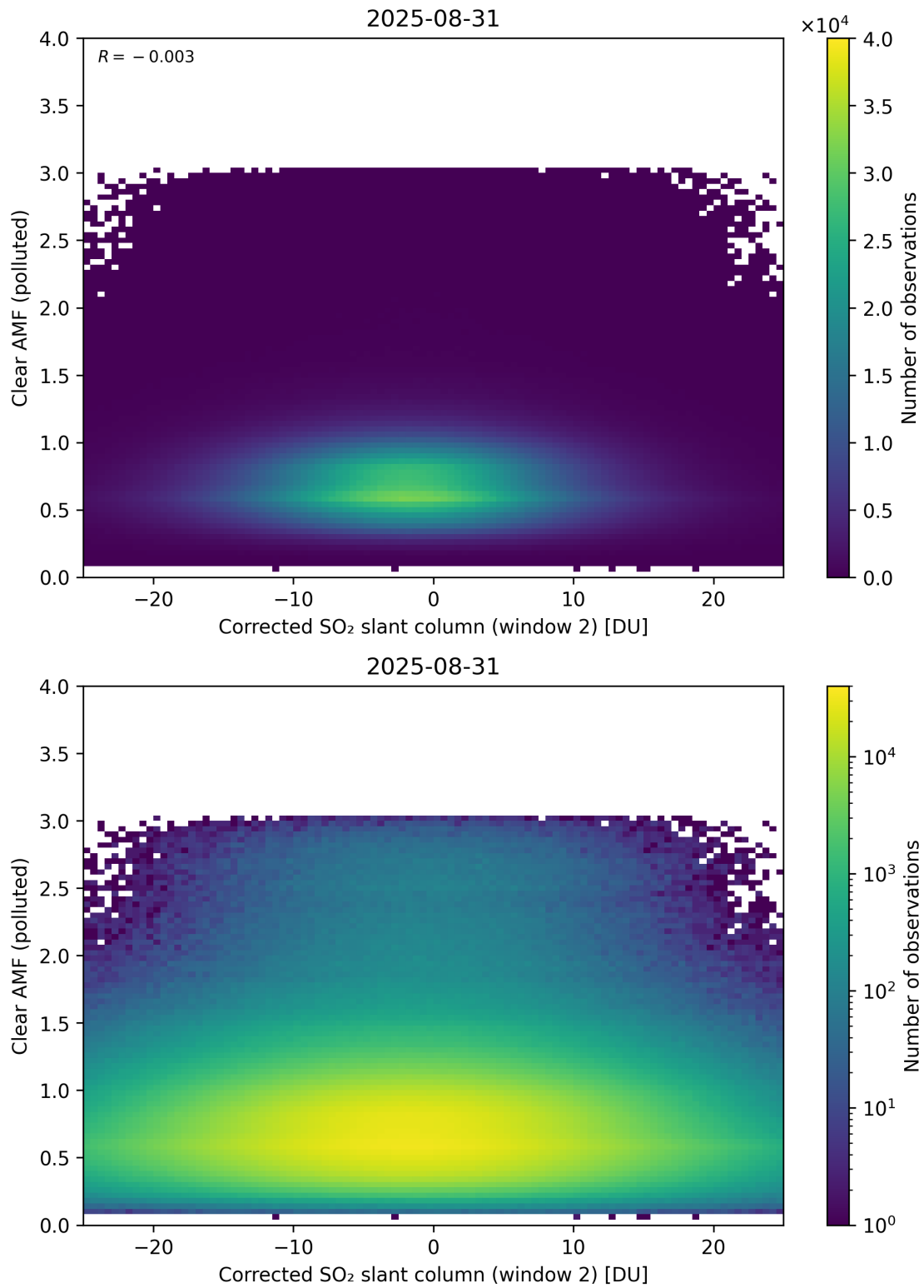
Figure 249: Scatter density plot of “Corrected SO 2 slant column (window 2)” against “Clear AMF (polluted)” for 2025-08-30 to 2025-09-01.
