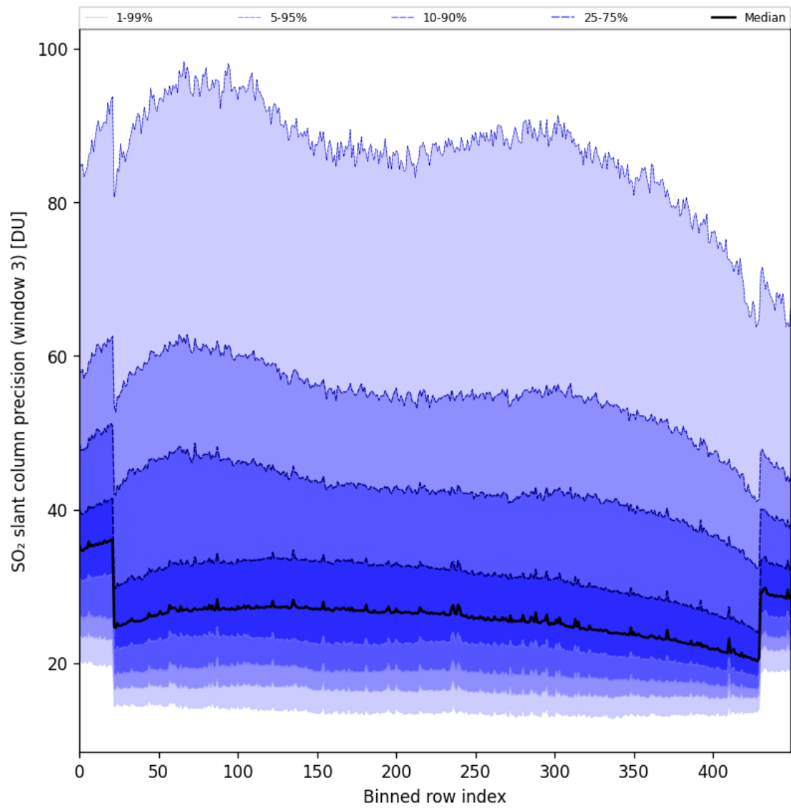
Figure 98: Along track statistics of “SO 2 slant column precision (window 3)” for 2025-08-30 to 2025-09-01
