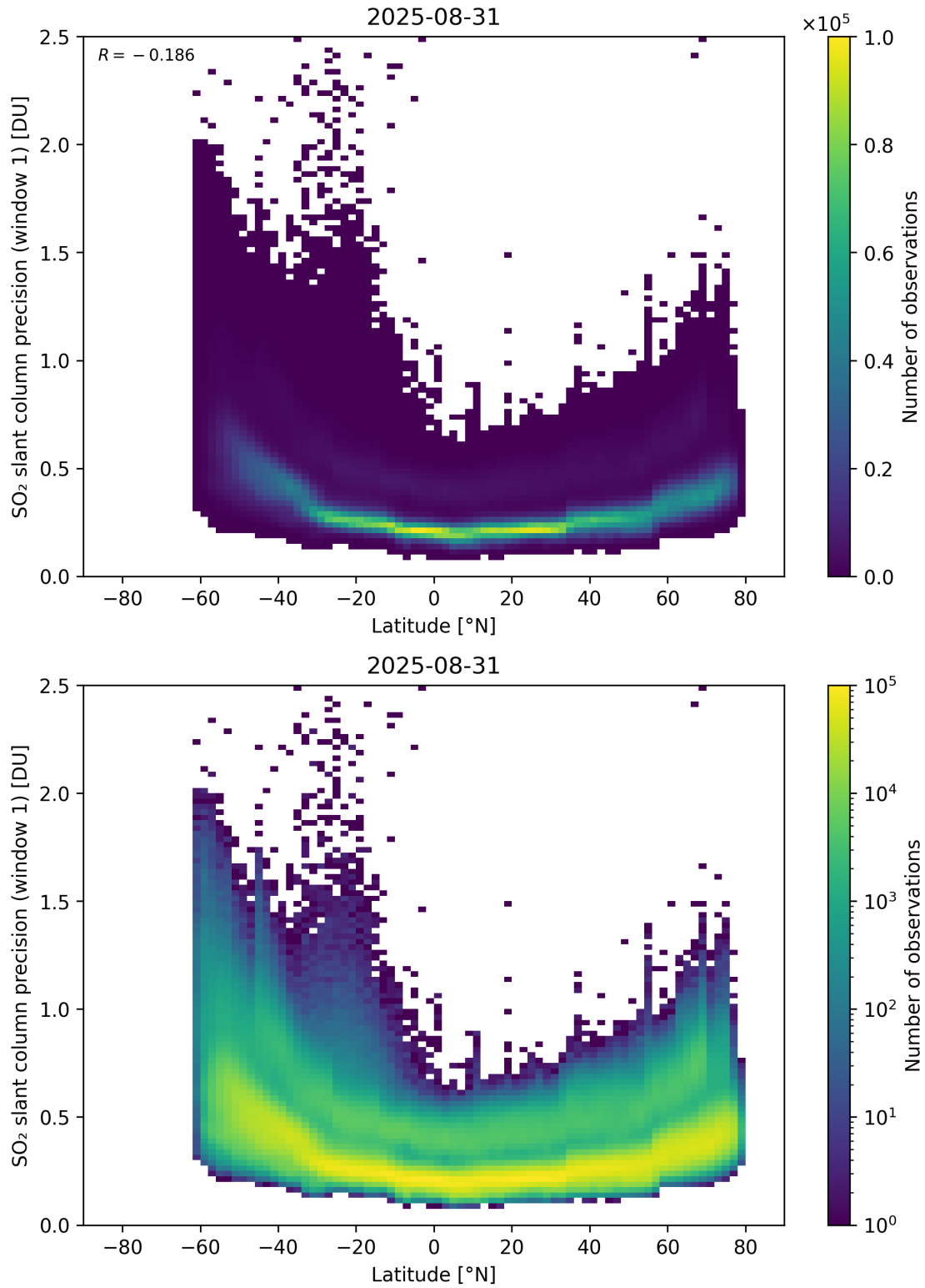
Figure 163: Scatter density plot of “Latitude” against “SO 2 slant column precision (window 1)” for 2025-08-30 to 2025-09-01.
