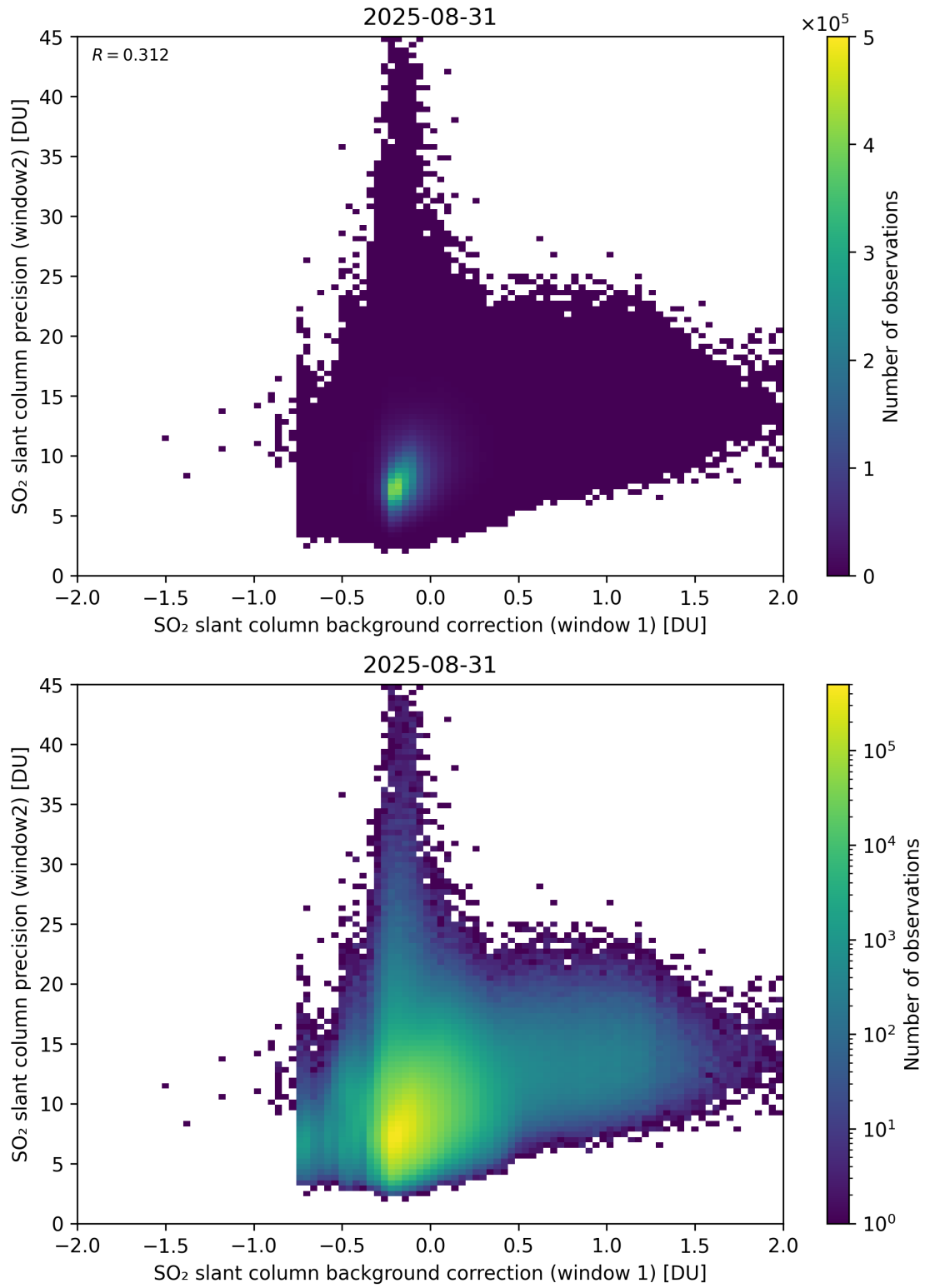
Figure 117: Scatter density plot of “SO 2 slant column background correction (window 1)” against “SO 2 slant column precision (window2)” for 2025-08-30 to 2025-09-01.
