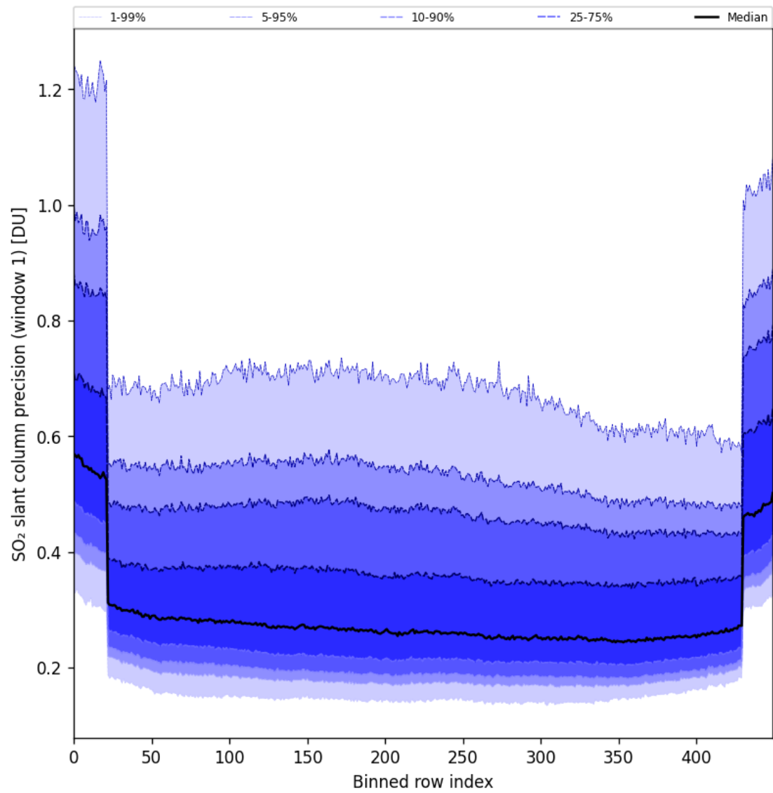
Figure 90: Along track statistics of “SO 2 slant column precision (window 1)” for 2025-08-30 to 2025-09-01
