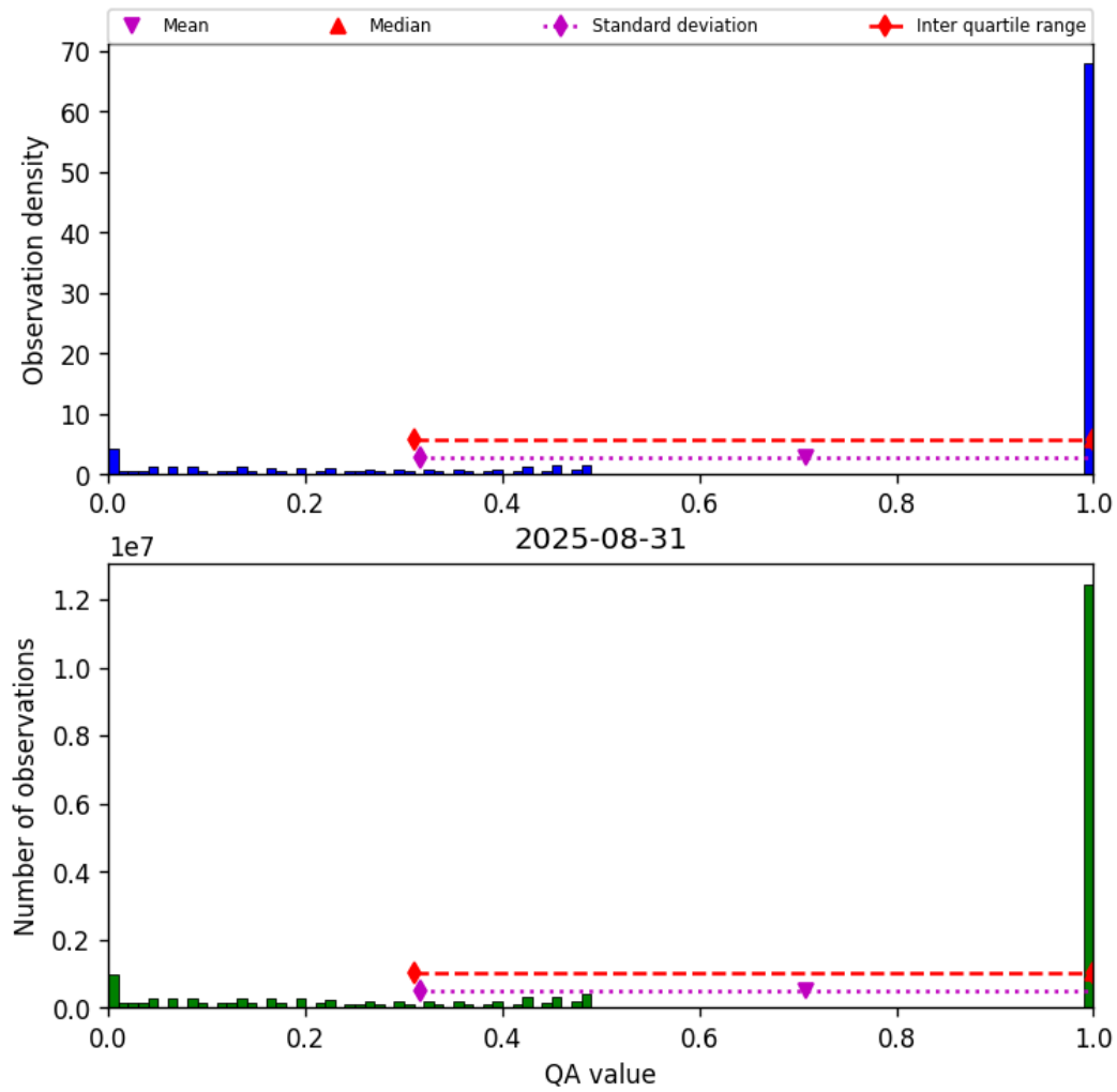
Figure 57: Histogram of “QA value” for 2025-08-30 to 2025-09-01
