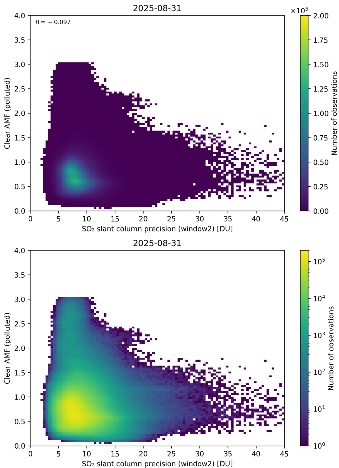
Figure 296: Scatter density plot of “SO 2 slant column precision (window2)” against “Clear AMF (polluted)” for 2025-08-30 to 2025-09-01.
