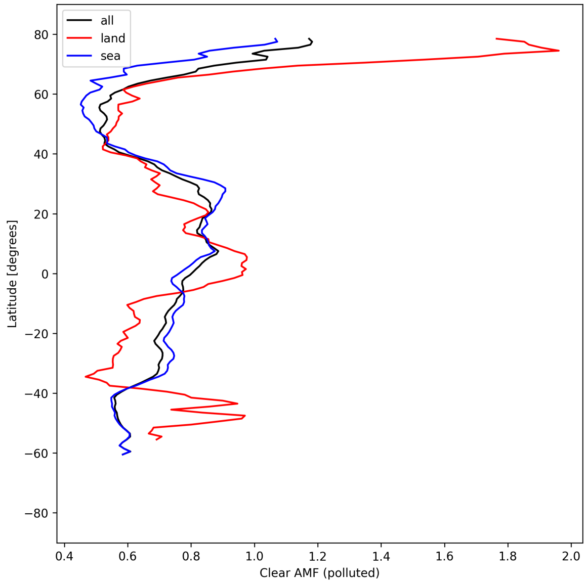
Figure 55: Zonal average of “Clear AMF (polluted)” for 2025-08-30 to 2025-09-01.
