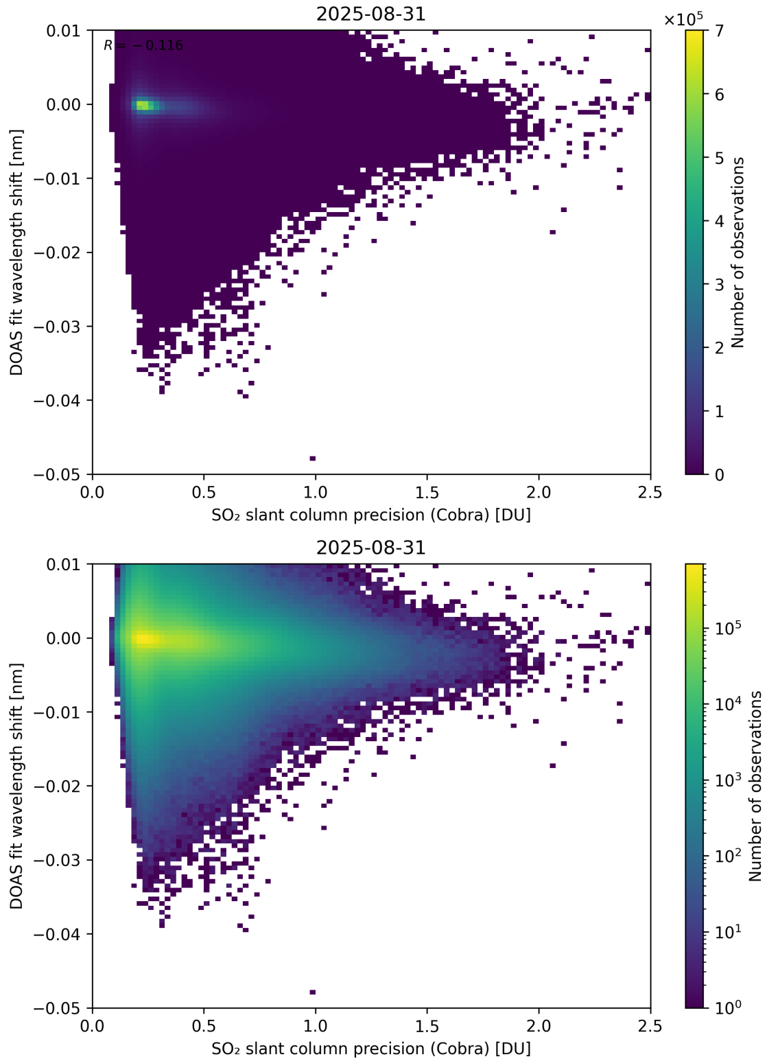
Figure 202: Scatter density plot of “SO 2 slant column precision (Cobra)” against “DOAS fit wavelength shift” for 2025-08-30 to 2025-09-01.
