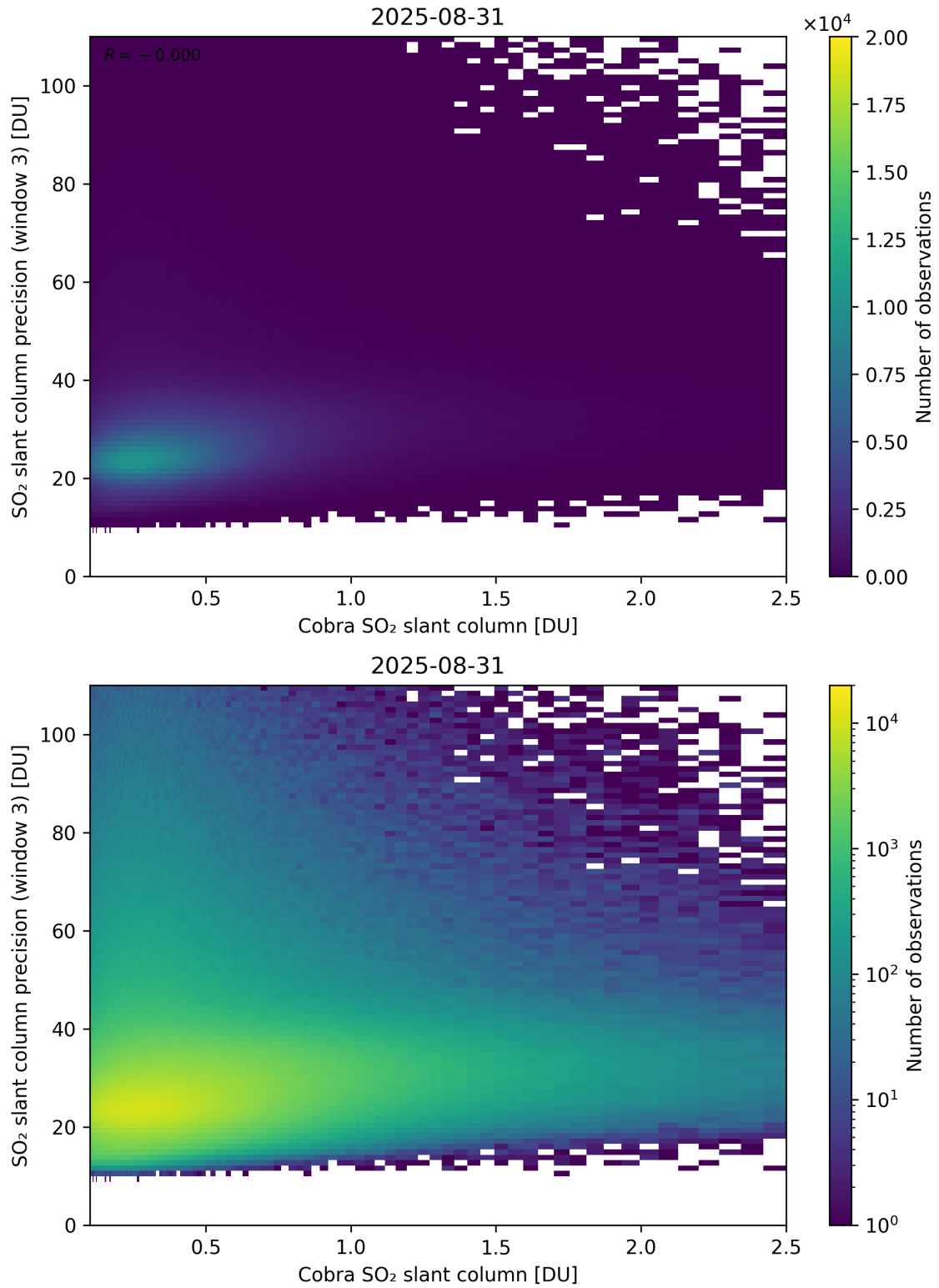
Figure 223: Scatter density plot of “Cobra SO 2 slant column” against “SO 2 slant column precision (window 3)” for 2025-08-30 to 2025-09-01.
