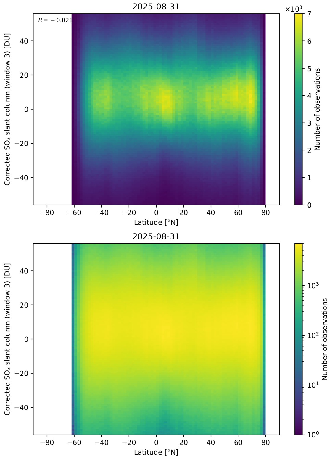
Figure 161: Scatter density plot of “Latitude” against “Corrected SO 2 slant column (window 3)” for 2025-08-30 to 2025-09-01.
