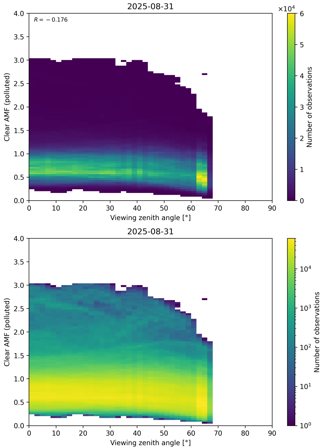
Figure 370: Scatter density plot of “Viewing zenith angle” against “Clear AMF (polluted)” for 2025-08-30 to 2025-09-01.
