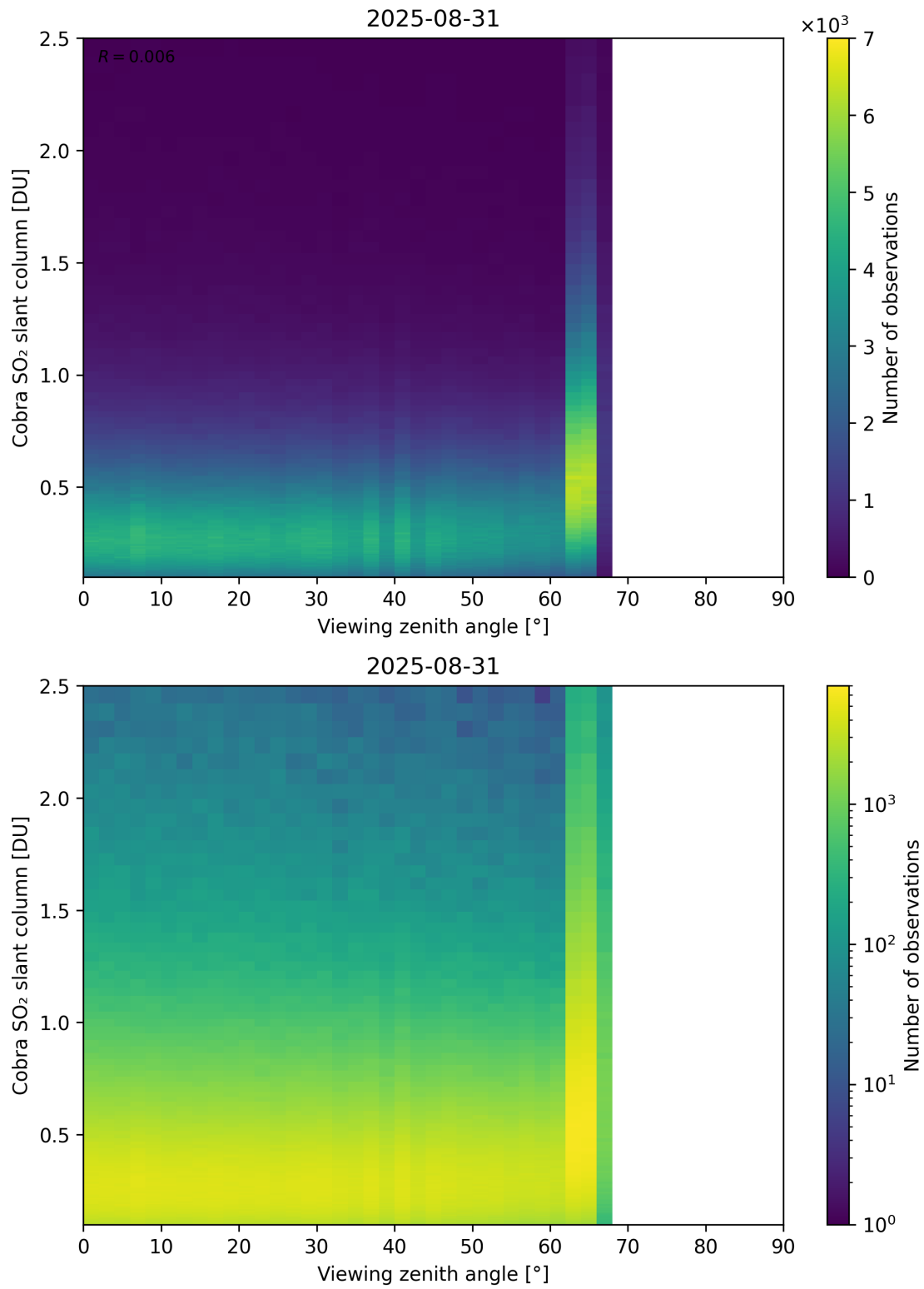
Figure 371: Scatter density plot of “Viewing zenith angle” against “Cobra SO 2 slant column” for 2025-08-30 to 2025-09-01.
