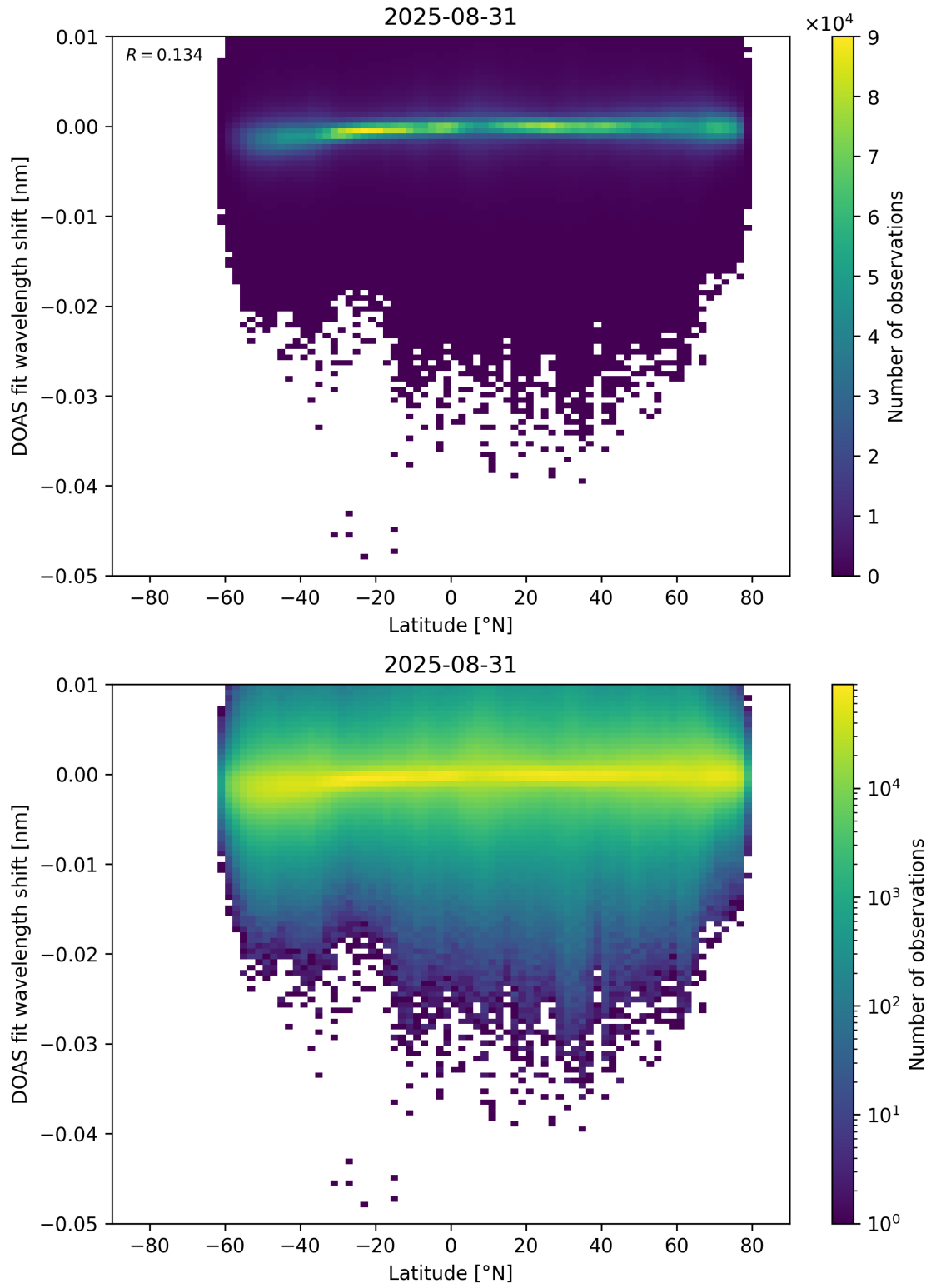
Figure 153: Scatter density plot of “Latitude” against “DOAS fit wavelength shift” for 2025-08-30 to 2025-09-01.
