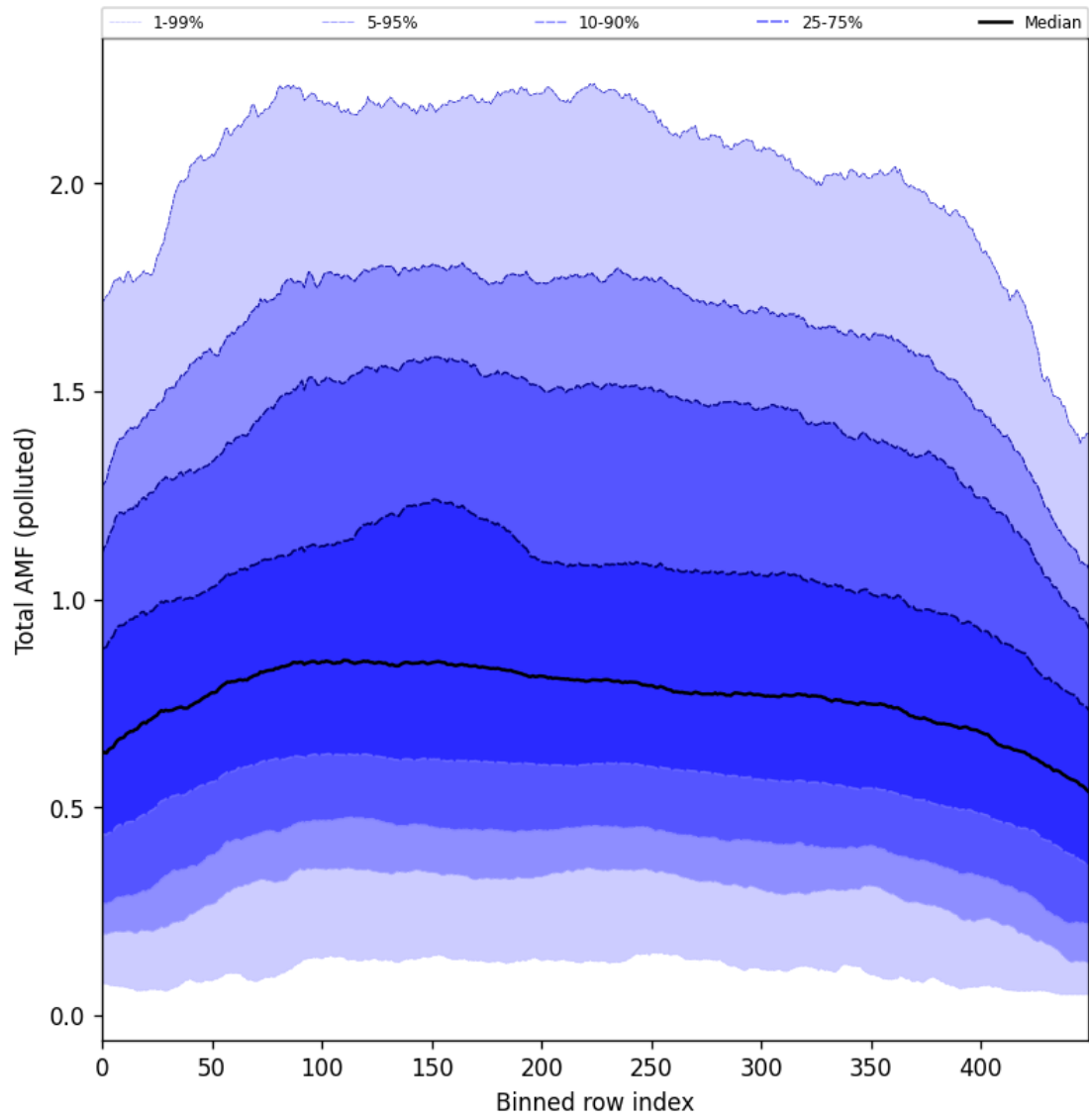
Figure 105: Along track statistics of “Total AMF (polluted)” for 2025-08-30 to 2025-09-01
