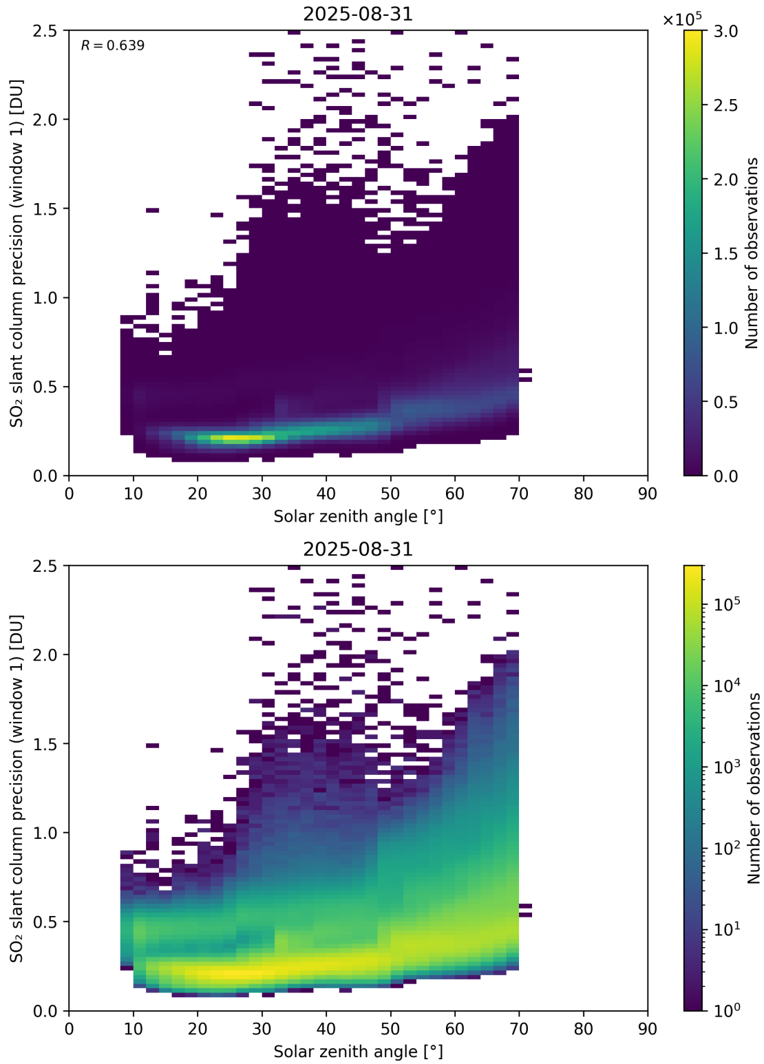
Figure 185: Scatter density plot of “Solar zenith angle” against “SO 2 slant column precision (window 1)” for 2025-08-30 to 2025-09-01.
