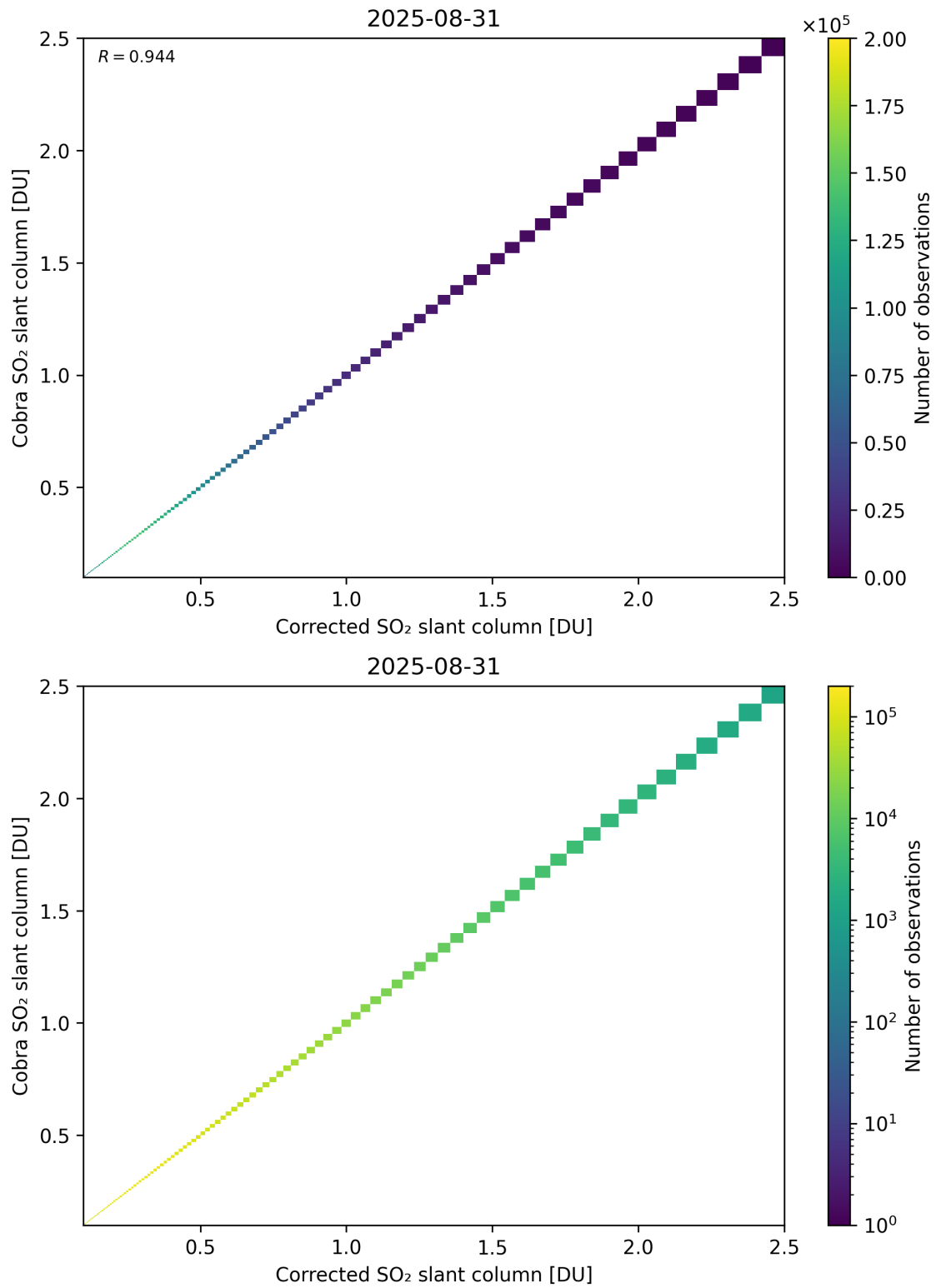
Figure 233: Scatter density plot of “Corrected SO 2 slant column” against “Cobra SO 2 slant column” for 2025-08-30 to 2025-09-01.
