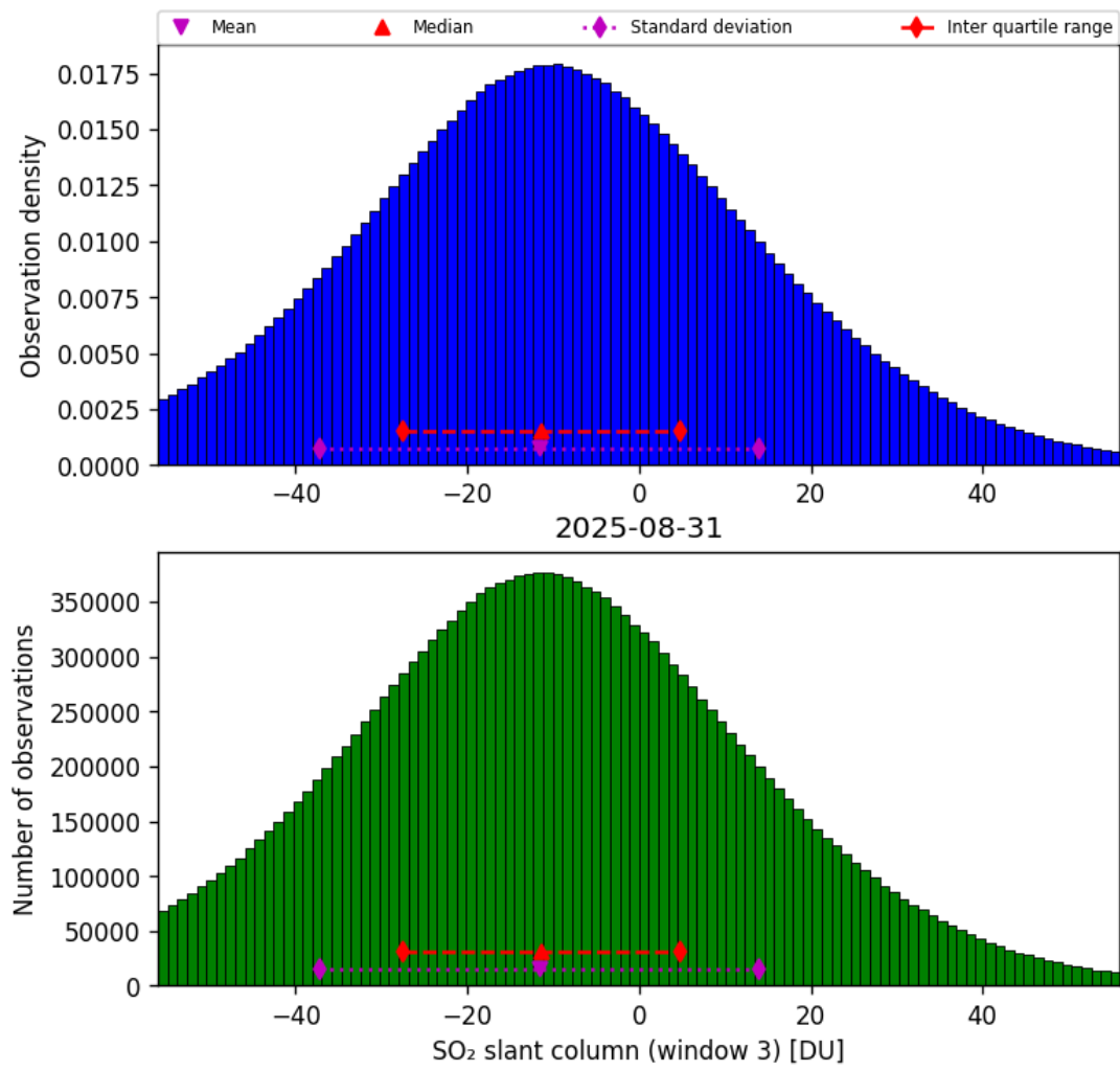
Figure 71: Histogram of “SO 2 slant column (window 3)” for 2025-08-30 to 2025-09-01
