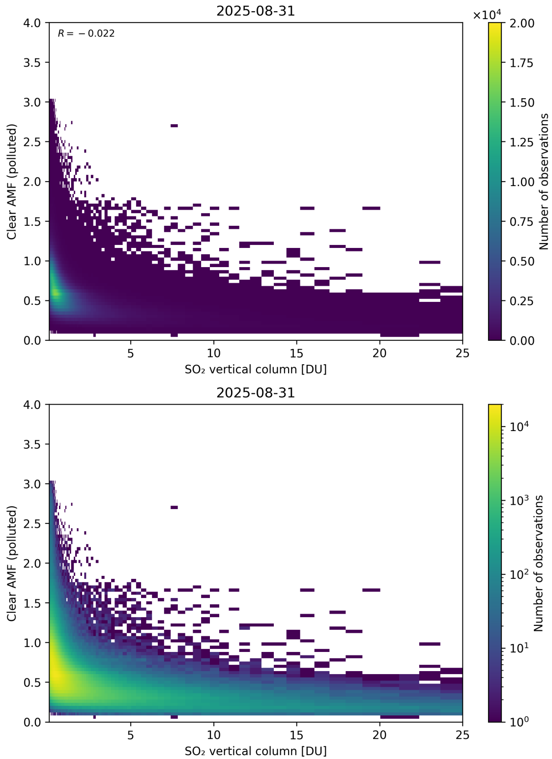
Figure 348: Scatter density plot of “SO 2 vertical column” against “Clear AMF (polluted)” for 2025-08-30 to 2025-09-01.
