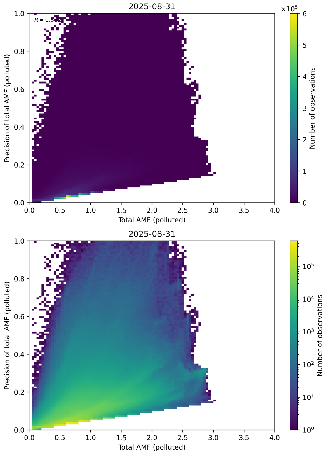
Figure 322: Scatter density plot of “Total AMF (polluted)” against “Precision of total AMF (polluted)” for 2025-08-30 to 2025-09-01.
