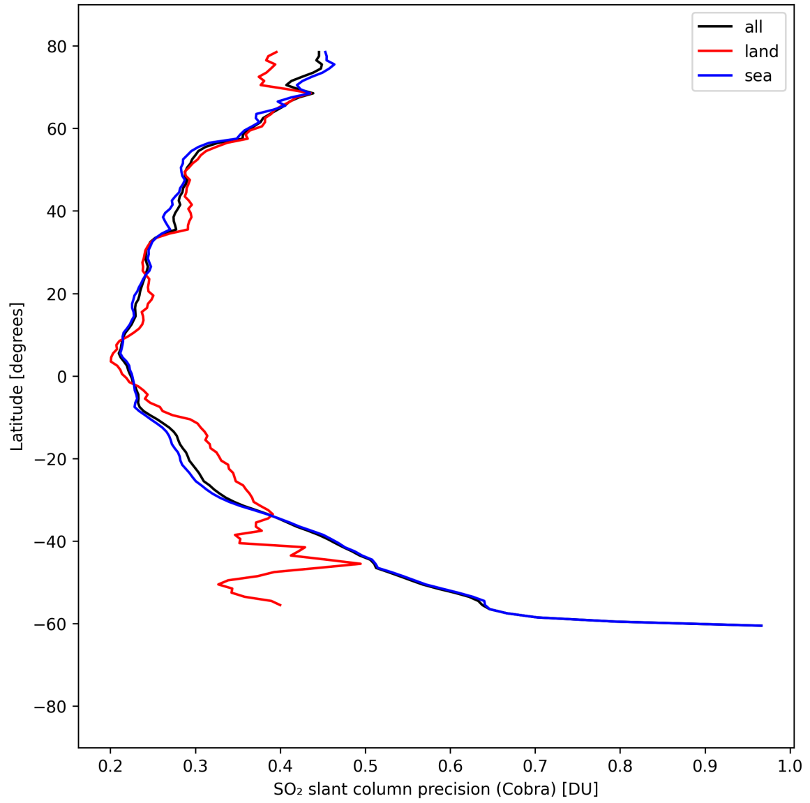
Figure 36: Zonal average of “SO 2 slant column precision (Cobra)” for 2025-08-30 to 2025-09-01.
