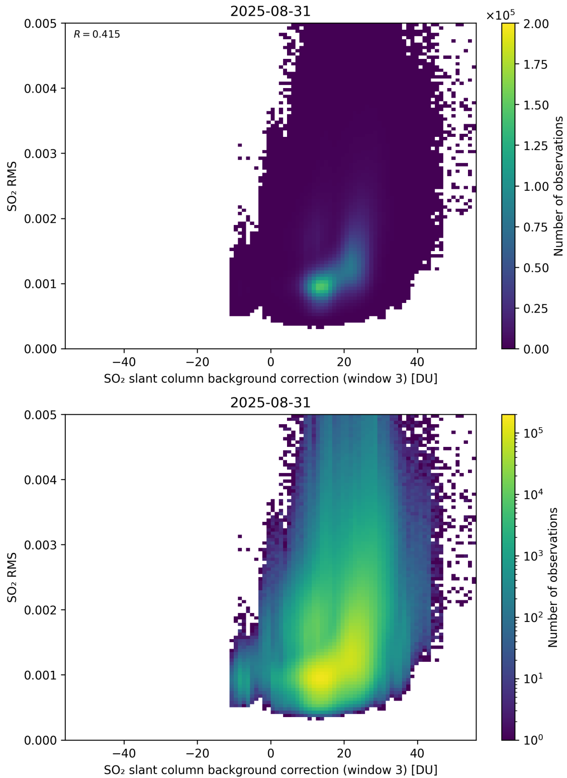
Figure 134: Scatter density plot of “SO 2 slant column background correction (window 3)” against “SO 2 RMS” for 2025-08-30 to 2025-09-01.
