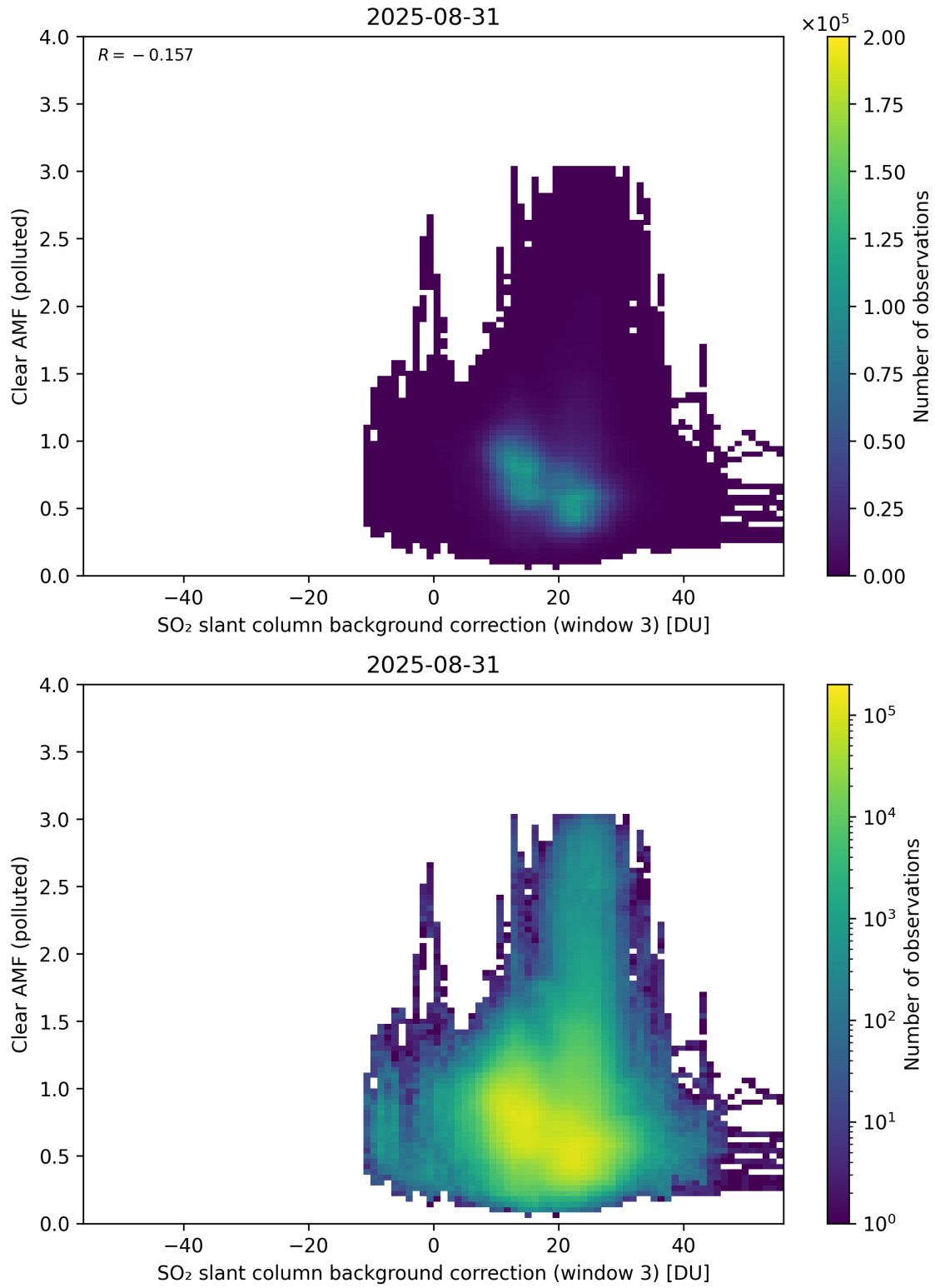
Figure 135: Scatter density plot of “SO 2 slant column background correction (window 3)” against “Clear AMF (polluted)” for 2025-08-30 to 2025-09-01.
