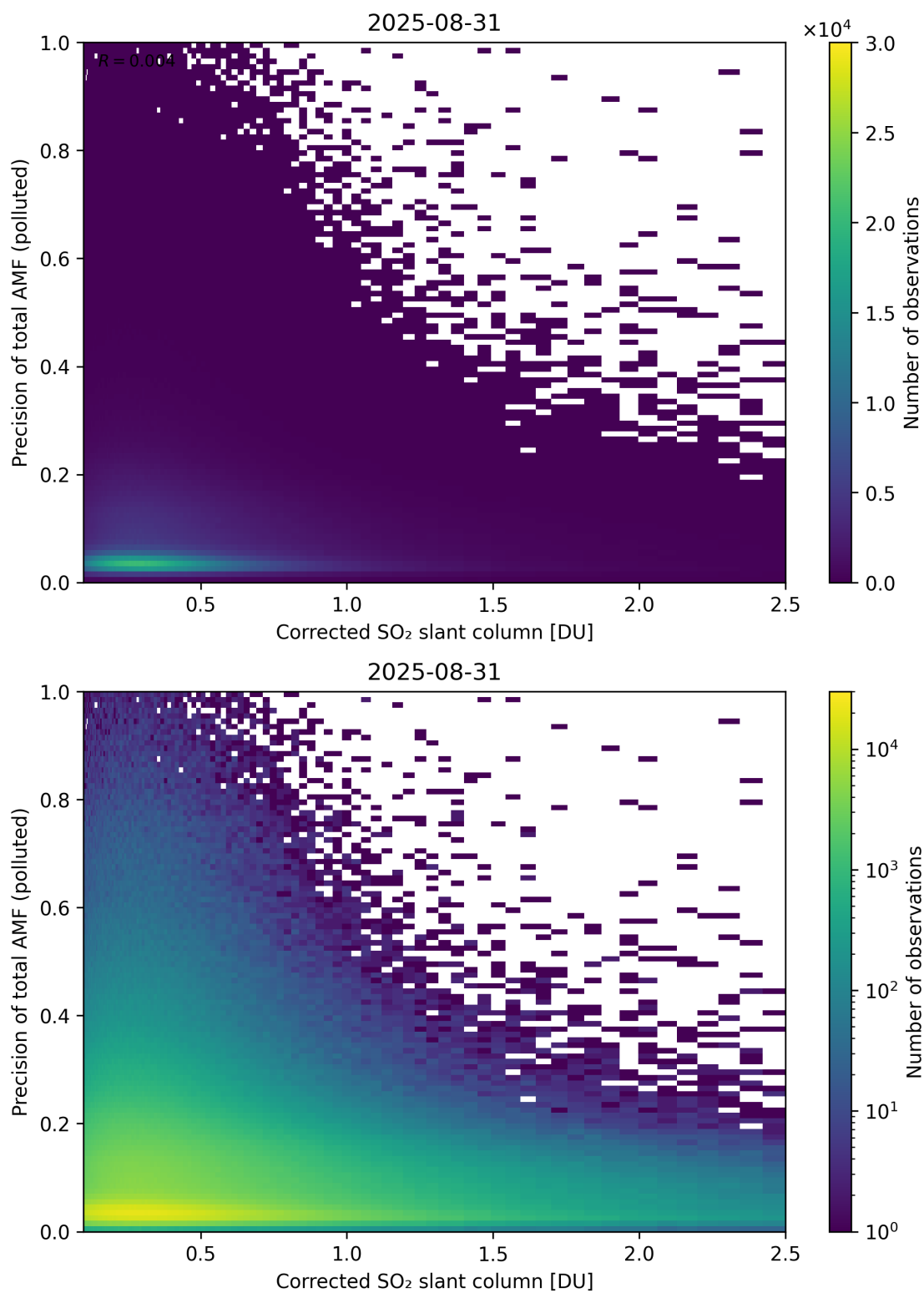
Figure 243: Scatter density plot of “Corrected SO 2 slant column” against “Precision of total AMF (polluted)” for 2025-08-30 to 2025-09-01.
