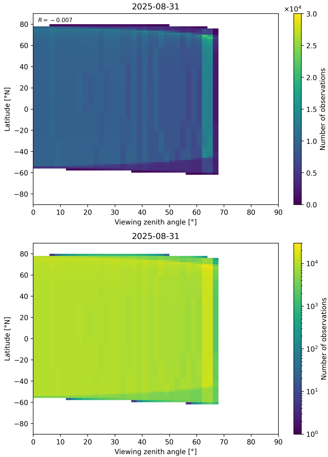
Figure 368: Scatter density plot of “Viewing zenith angle” against “Latitude” for 2025-08-30 to 2025-09-01.
