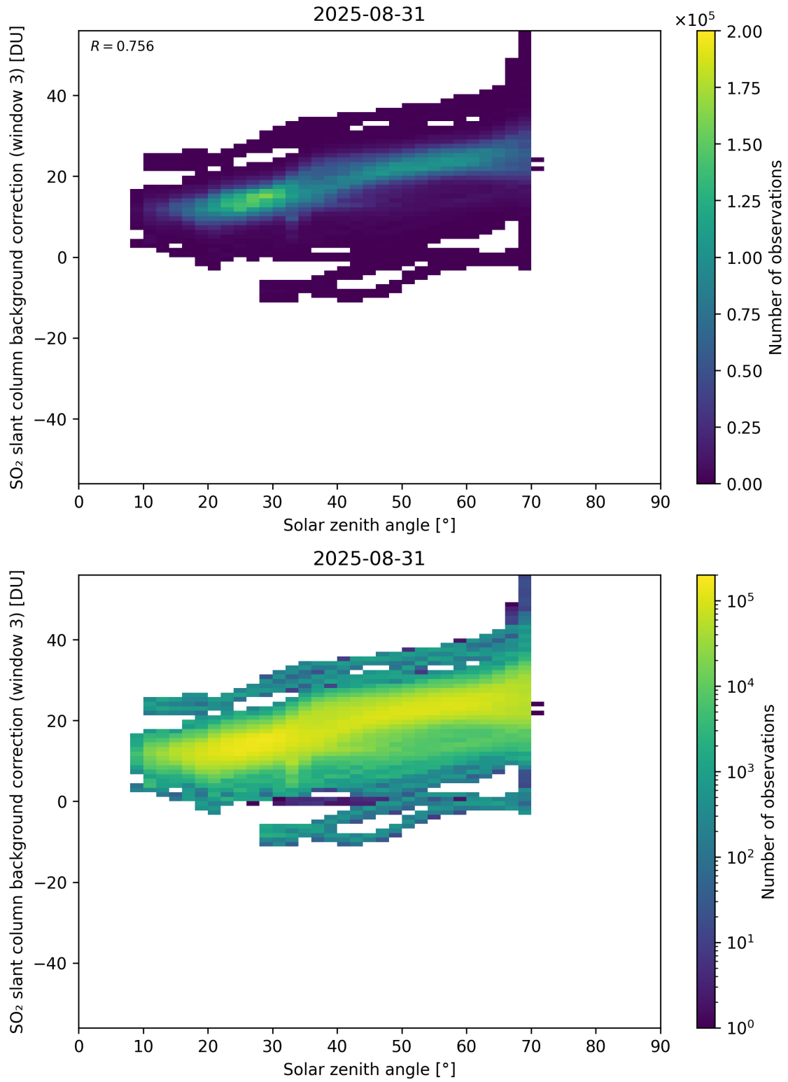
Figure 173: Scatter density plot of “Solar zenith angle” against “SO 2 slant column background correction (window 3)” for 2025-08-30 to 2025-09-01.
