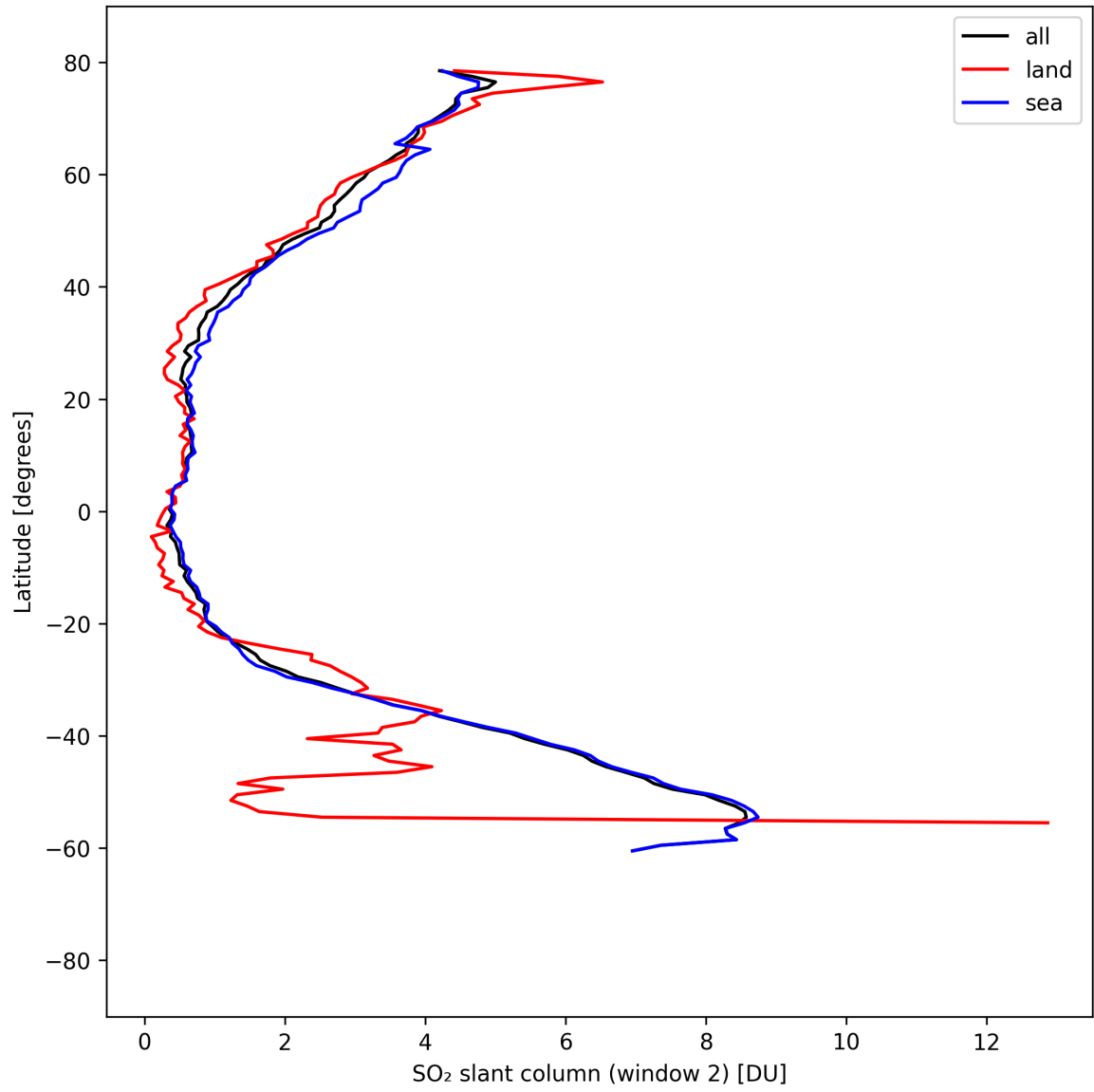
Figure 41: Zonal average of “SO 2 slant column (window 2)” for 2025-08-30 to 2025-09-01.
