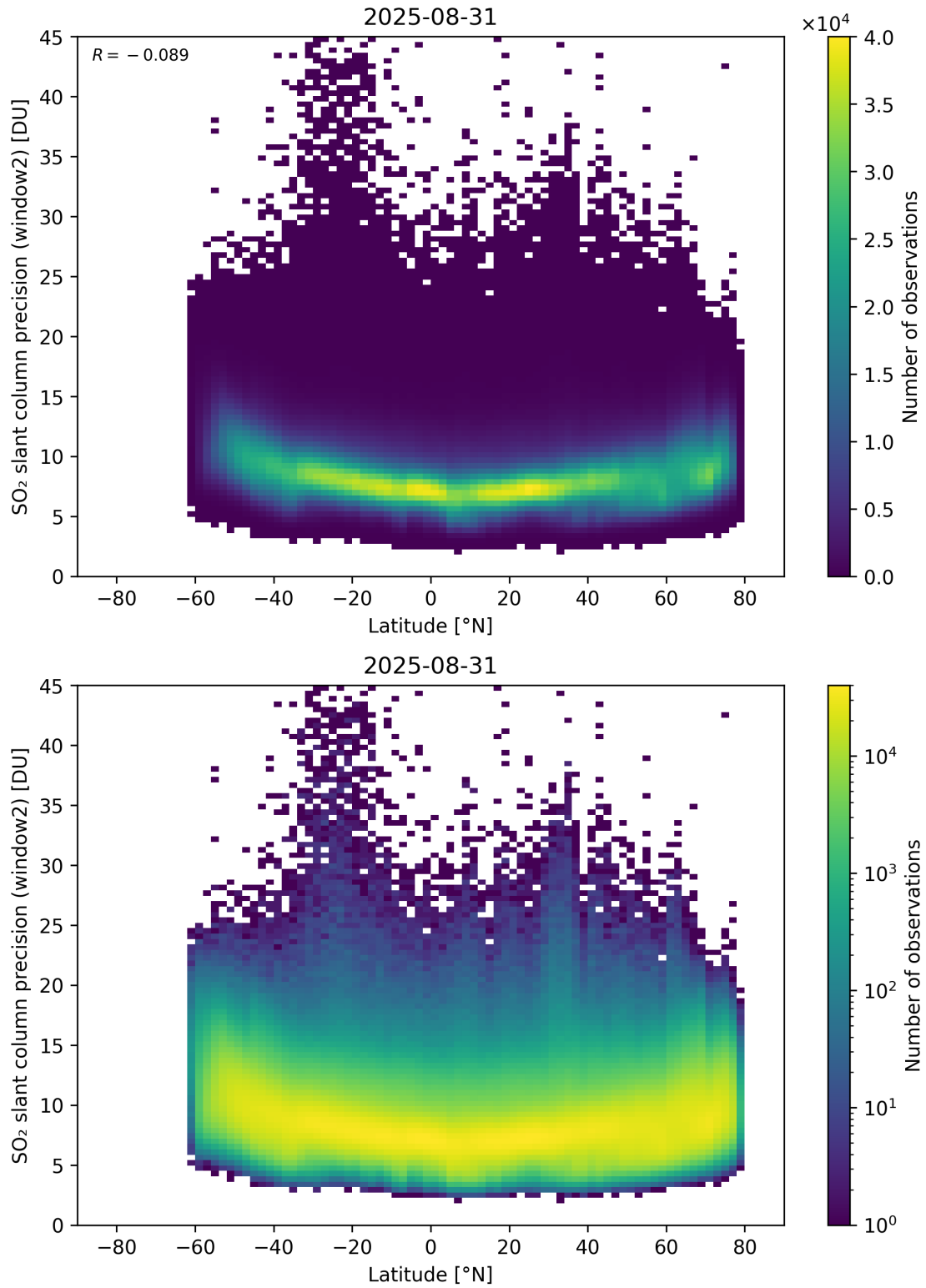
Figure 164: Scatter density plot of “Latitude” against “SO 2 slant column precision (window2)” for 2025-08-30 to 2025-09-01.
