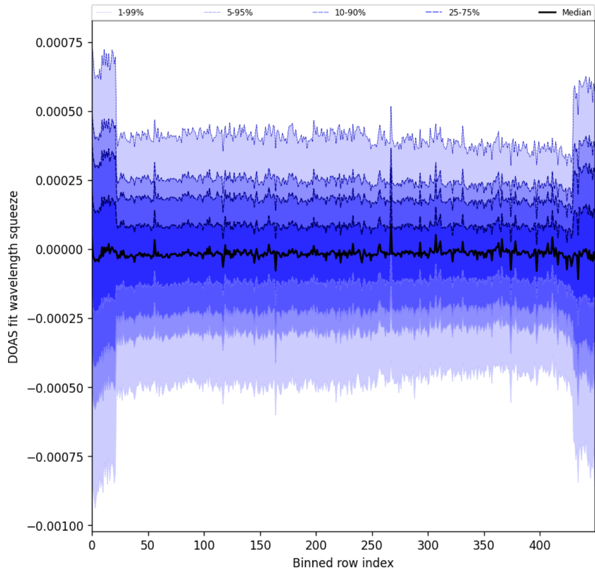
Figure 103: Along track statistics of “DOAS fit wavelength squeeze” for 2025-08-30 to 2025-09-01
