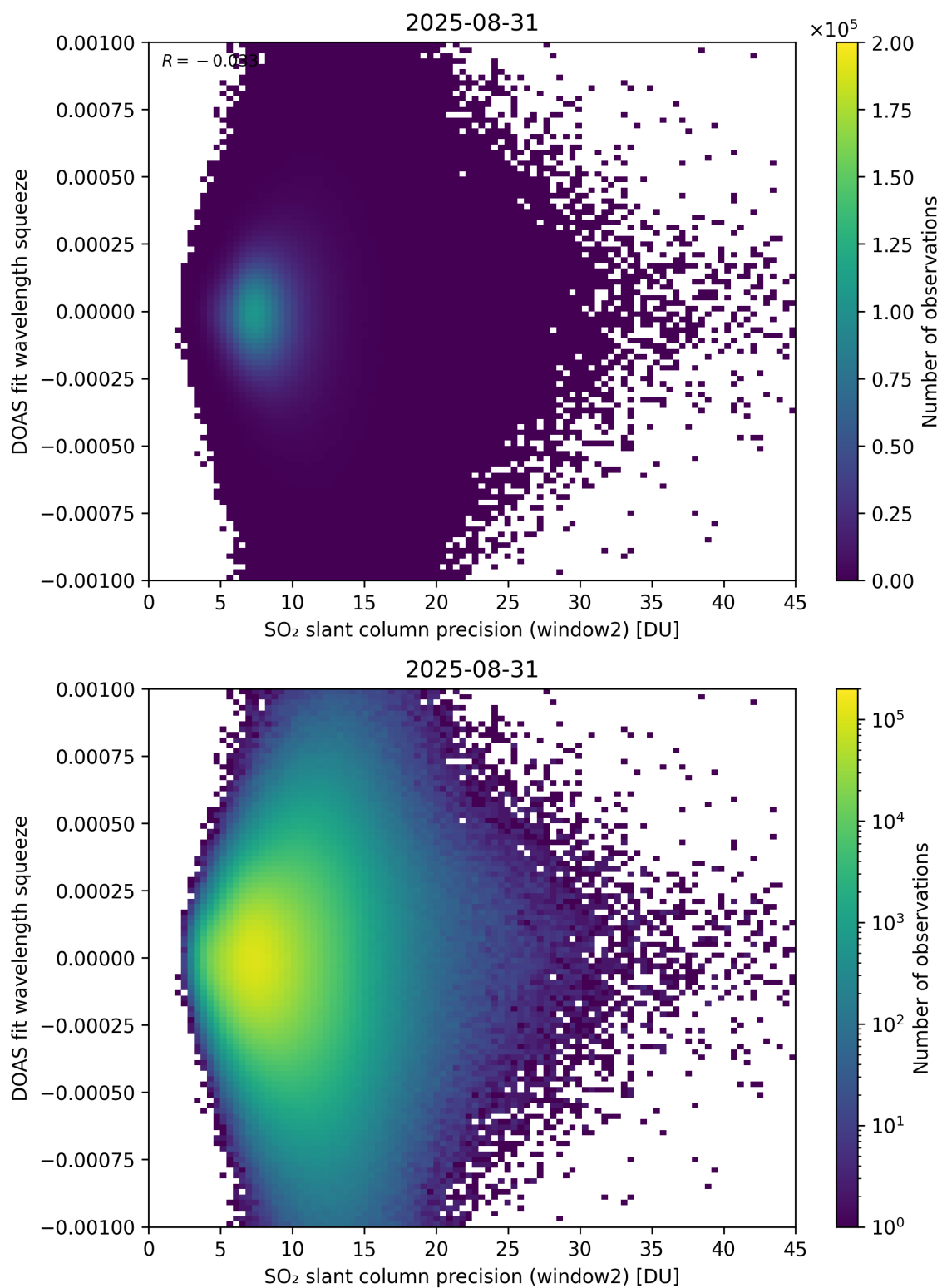
Figure 294: Scatter density plot of “SO 2 slant column precision (window2)” against “DOAS fit wavelength squeeze” for 2025-08-30 to 2025-09-01.
