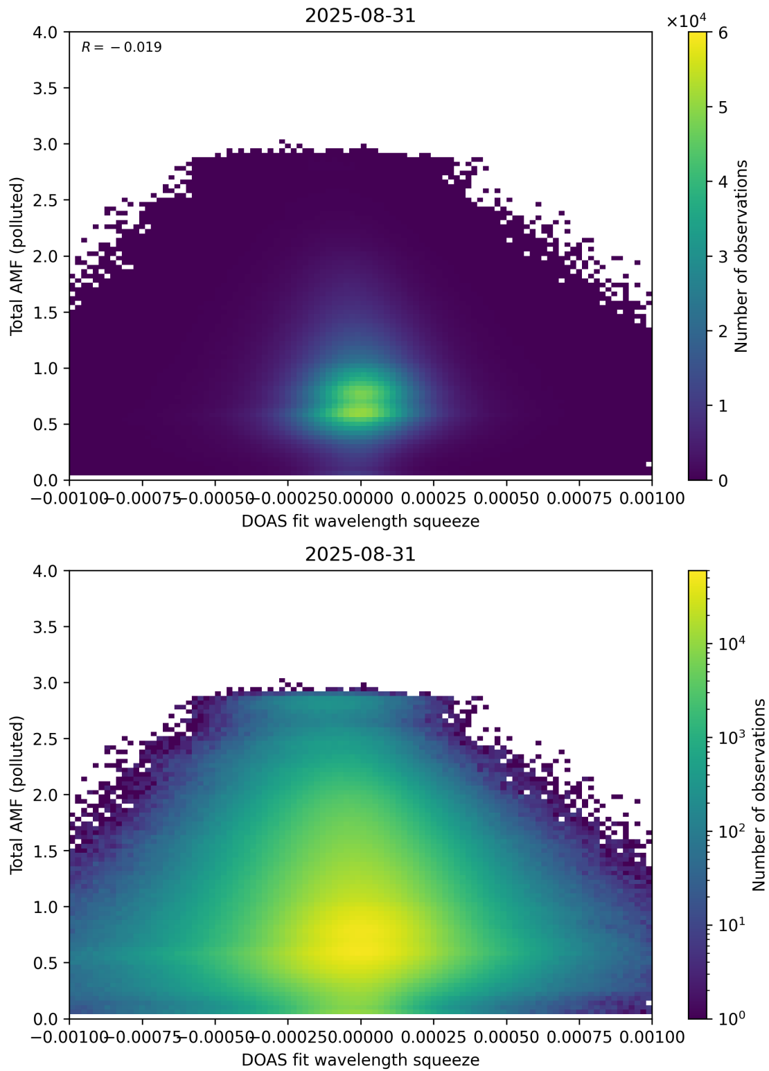
Figure 145: Scatter density plot of “DOAS fit wavelength squeeze” against “Total AMF (polluted)” for 2025-08-30 to 2025-09-01.
