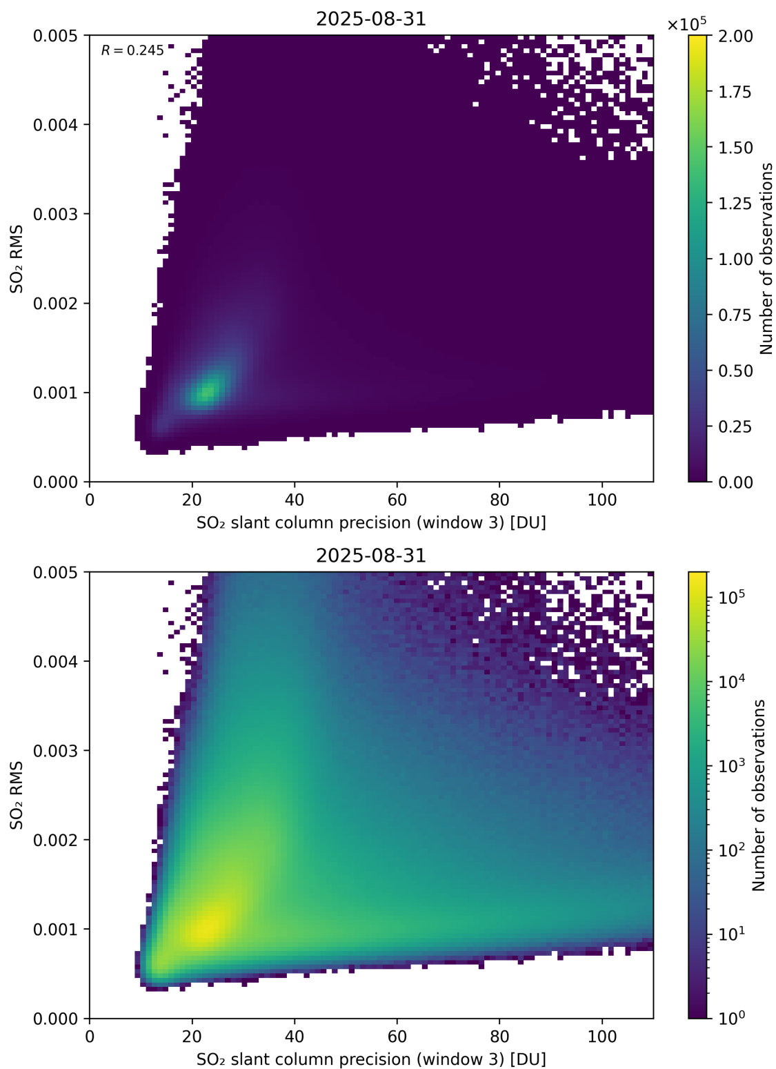
Figure 310: Scatter density plot of “SO 2 slant column precision (window 3)” against “SO 2 RMS” for 2025-08-30 to 2025-09-01.
