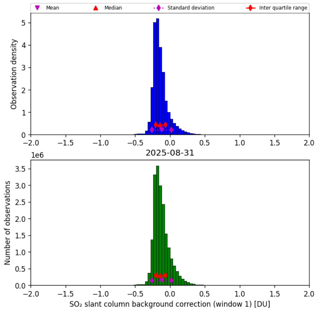
Figure 66: Histogram of “SO 2 slant column background correction (window 1)” for 2025-08-30 to 2025-09-01
