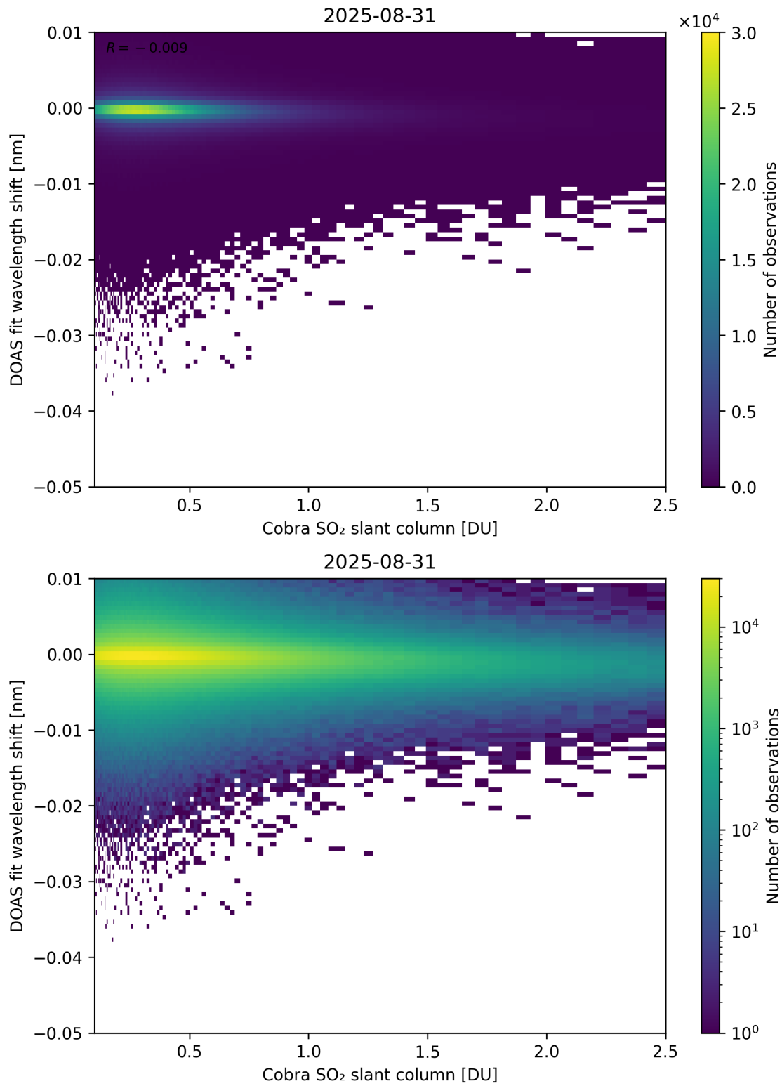
Figure 196: Scatter density plot of “Cobra SO 2 slant column” against “DOAS fit wavelength shift” for 2025-08-30 to 2025-09-01.
