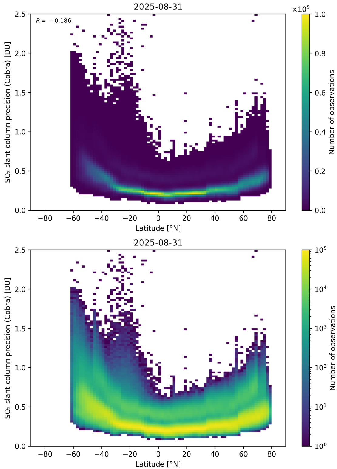
Figure 158: Scatter density plot of “Latitude” against “SO 2 slant column precision (Cobra)” for 2025-08-30 to 2025-09-01.
