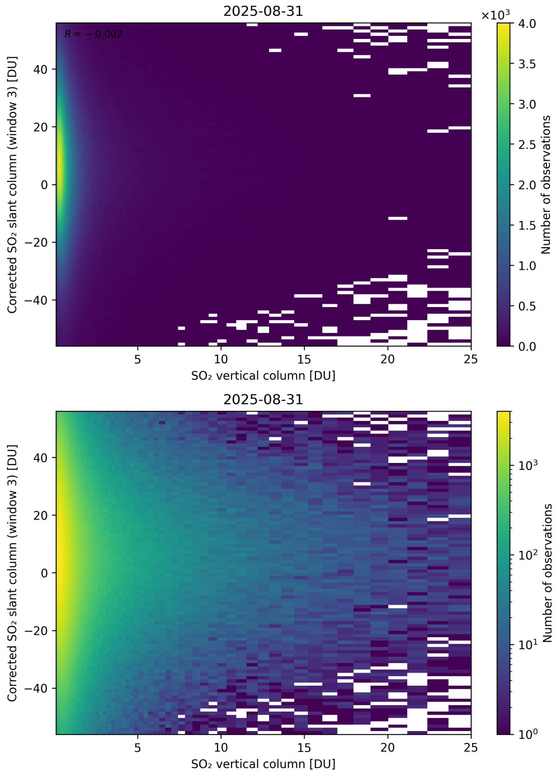
Figure 353: Scatter density plot of “SO 2 vertical column” against “Corrected SO 2 slant column (window 3)” for 2025-08-30 to 2025-09-01.
