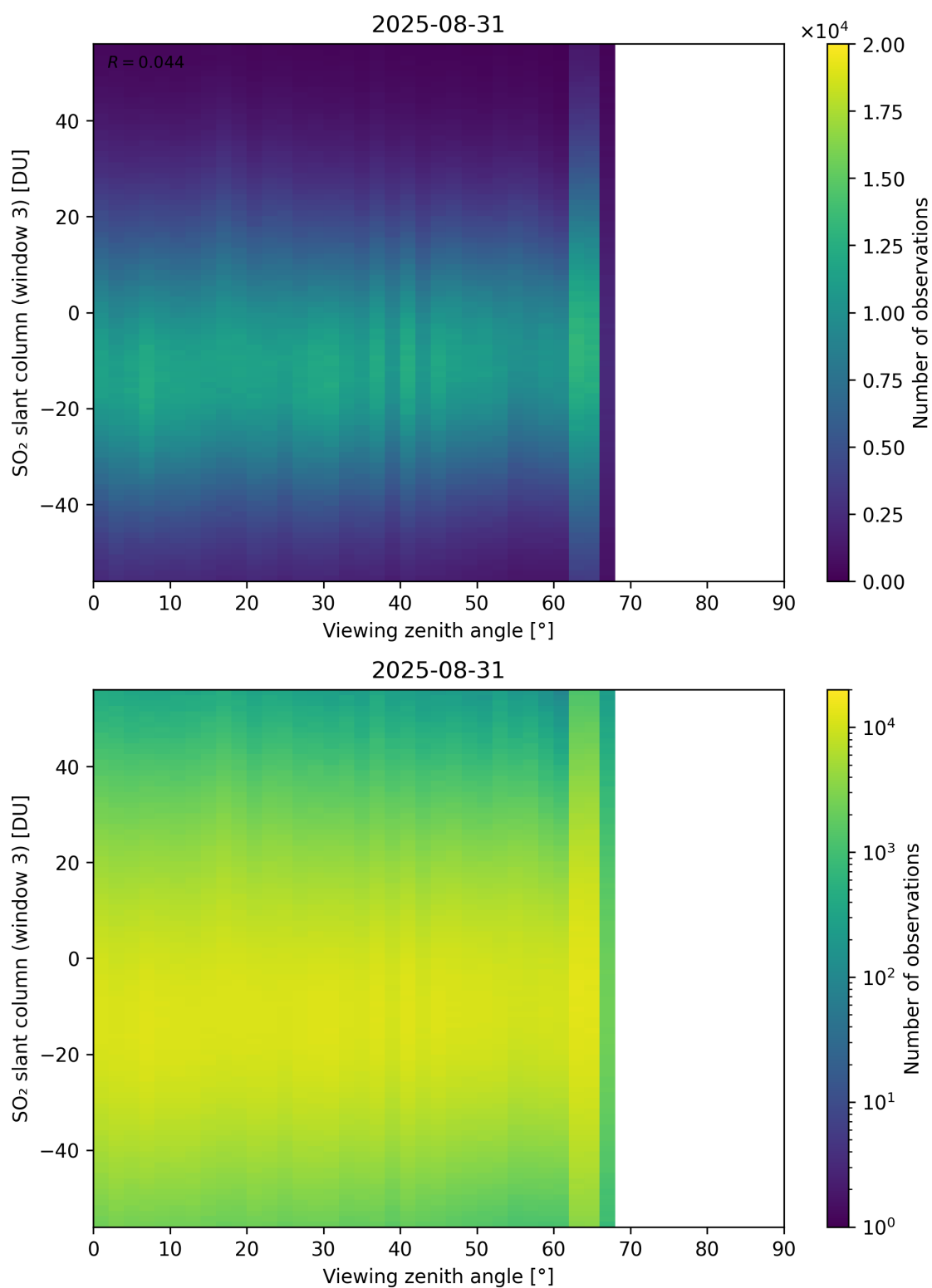
Figure 379: Scatter density plot of “Viewing zenith angle” against “SO 2 slant column (window 3)” for 2025-08-30 to 2025-09-01.
