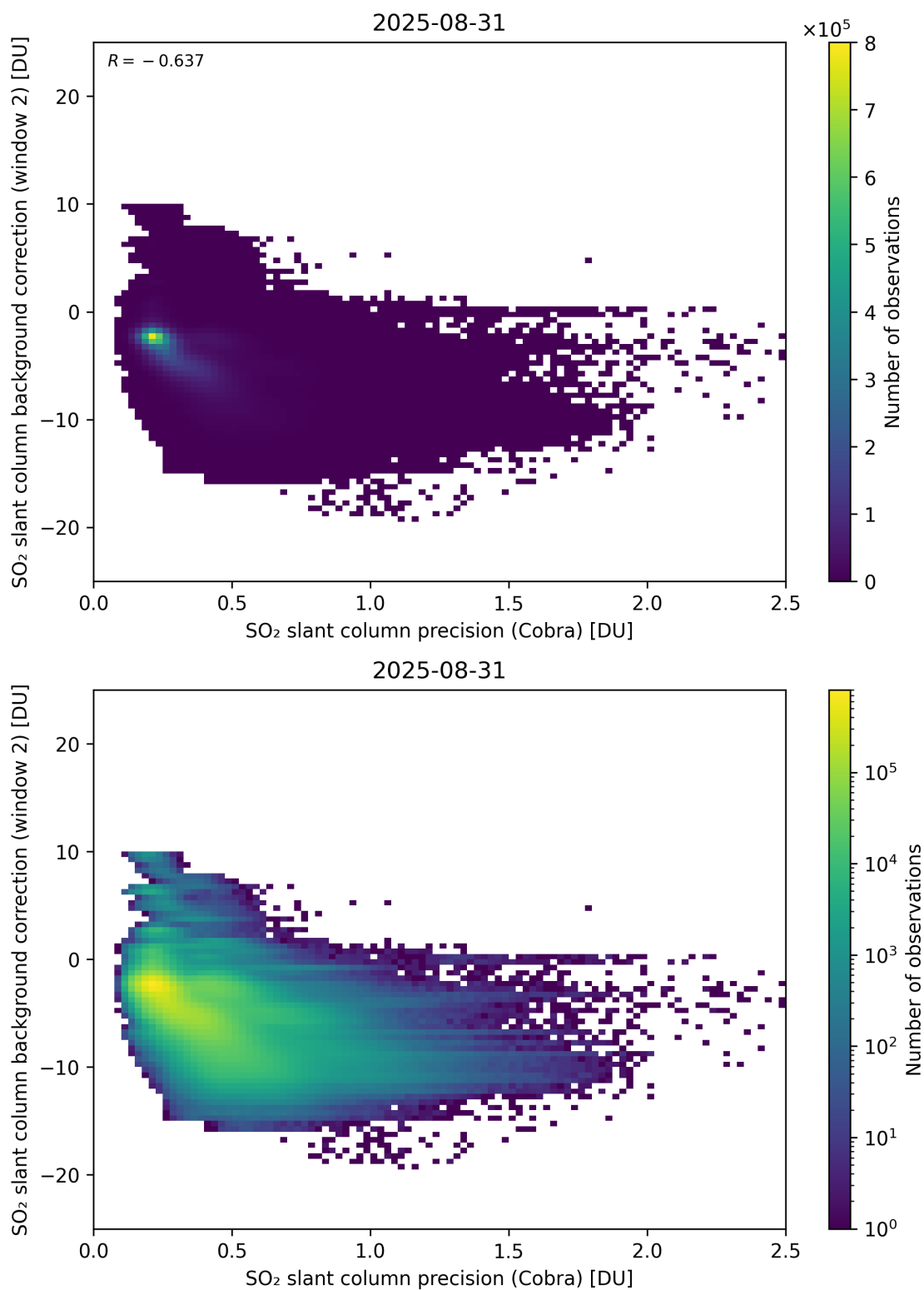
Figure 200: Scatter density plot of “SO 2 slant column precision (Cobra)” against “SO 2 slant column background correction (window 2)” for 2025-08-30 to 2025-09-01.
