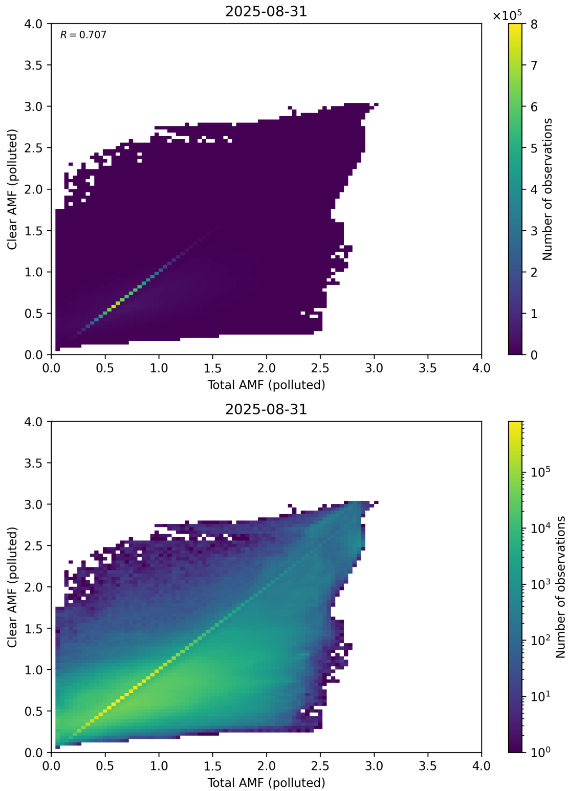
Figure 321: Scatter density plot of “Total AMF (polluted)” against “Clear AMF (polluted)” for 2025-08-30 to 2025-09-01.
