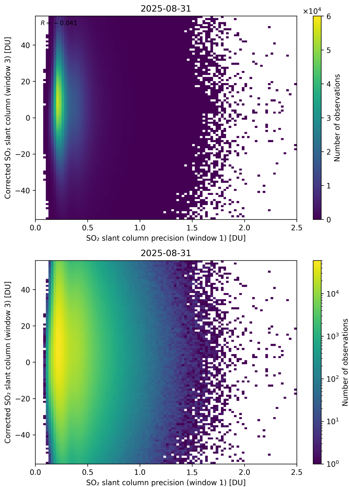
Figure 276: Scatter density plot of “SO 2 slant column precision (window 1)” against “Corrected SO 2 slant column (window 3)” for 2025-08-30 to 2025-09-01.
