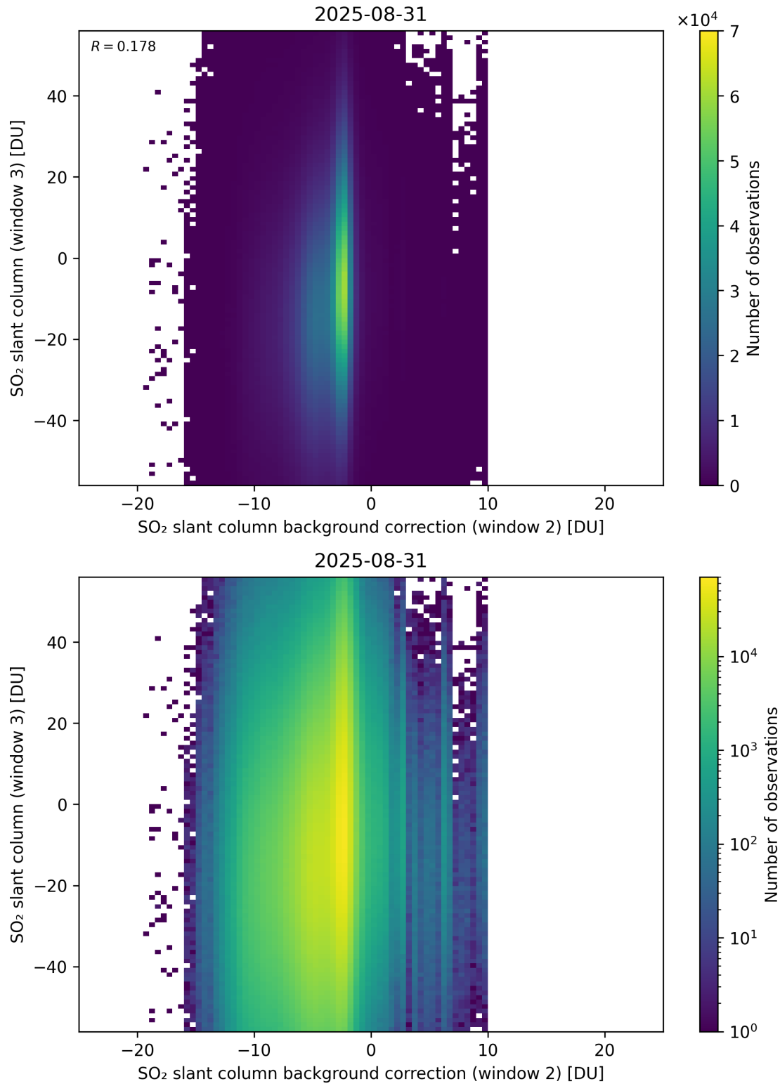
Figure 128: Scatter density plot of “SO 2 slant column background correction (window 2)” against “SO 2 slant column (window 3)” for 2025-08-30 to 2025-09-01.
