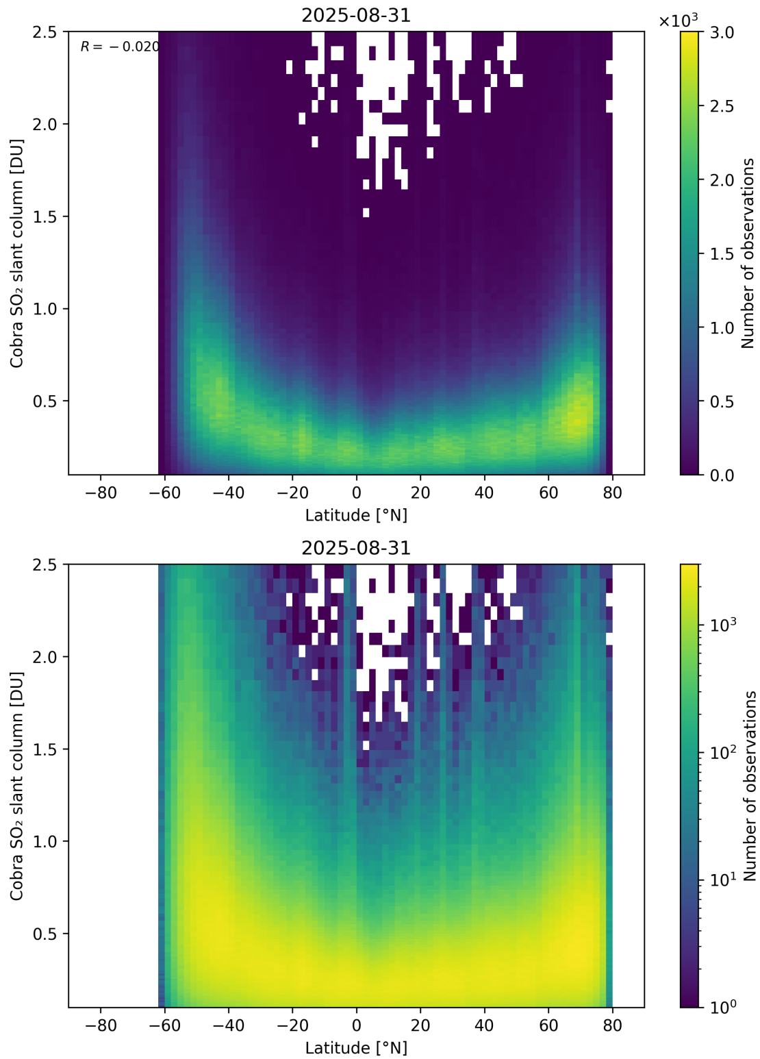
Figure 157: Scatter density plot of “Latitude” against “Cobra SO 2 slant column” for 2025-08-30 to 2025-09-01.
