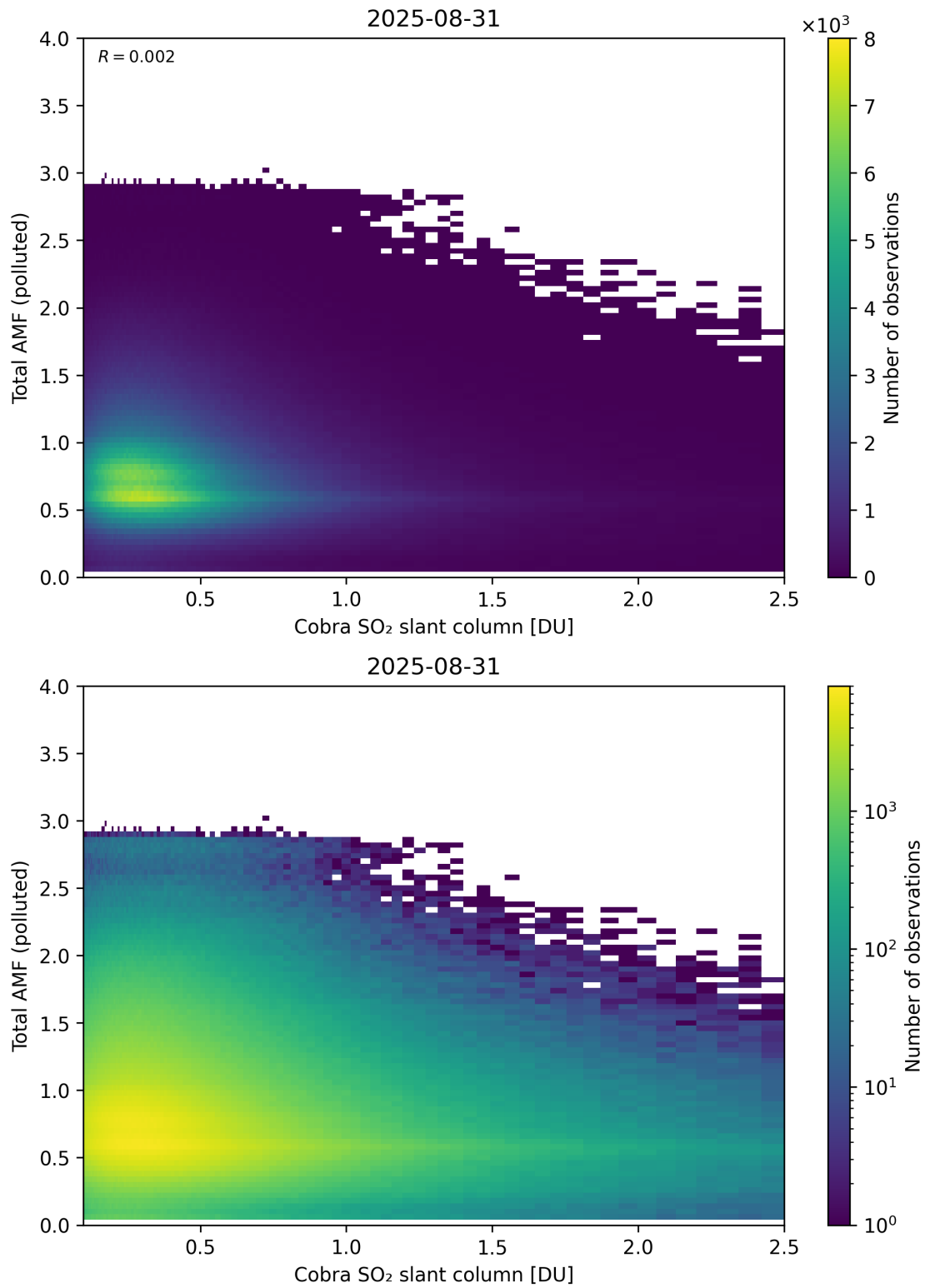
Figure 224: Scatter density plot of “Cobra SO 2 slant column” against “Total AMF (polluted)” for 2025-08-30 to 2025-09-01.
