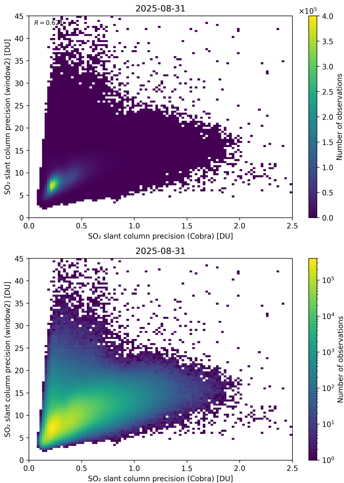
Figure 210: Scatter density plot of “SO 2 slant column precision (Cobra)” against “SO 2 slant column precision (window2)” for 2025-08-30 to 2025-09-01.
