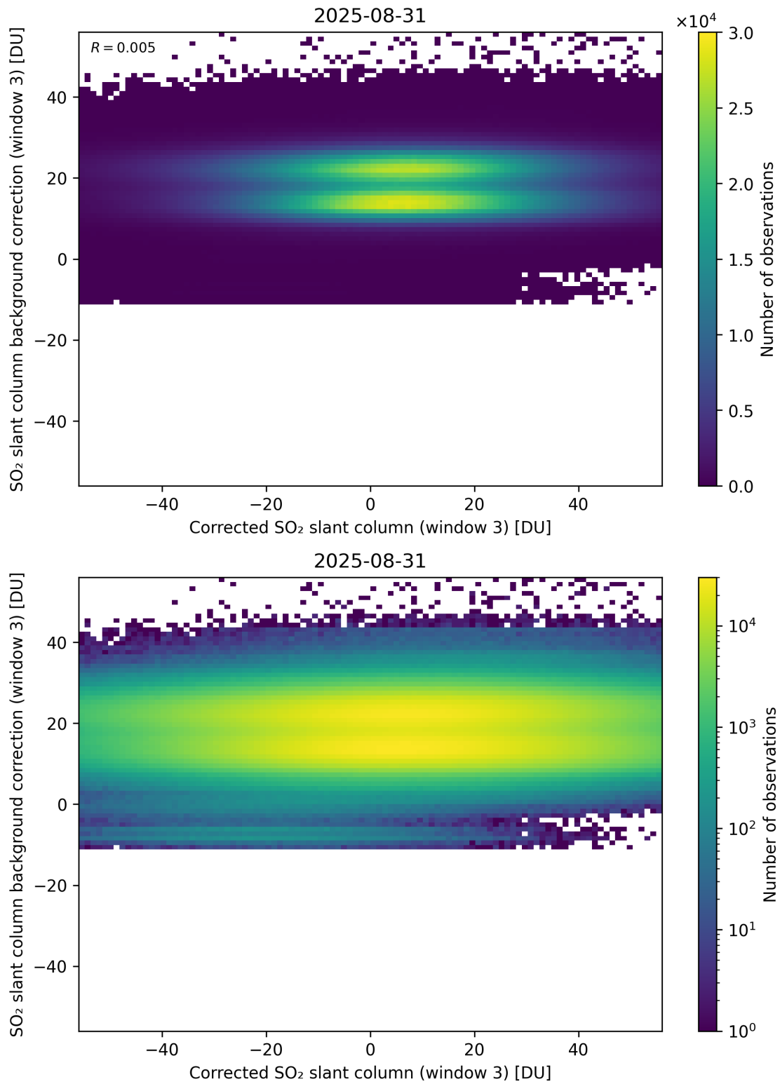
Figure 255: Scatter density plot of “Corrected SO 2 slant column (window 3)” against “SO 2 slant column background correction (window 3)” for 2025-08-30 to 2025-09-01.
