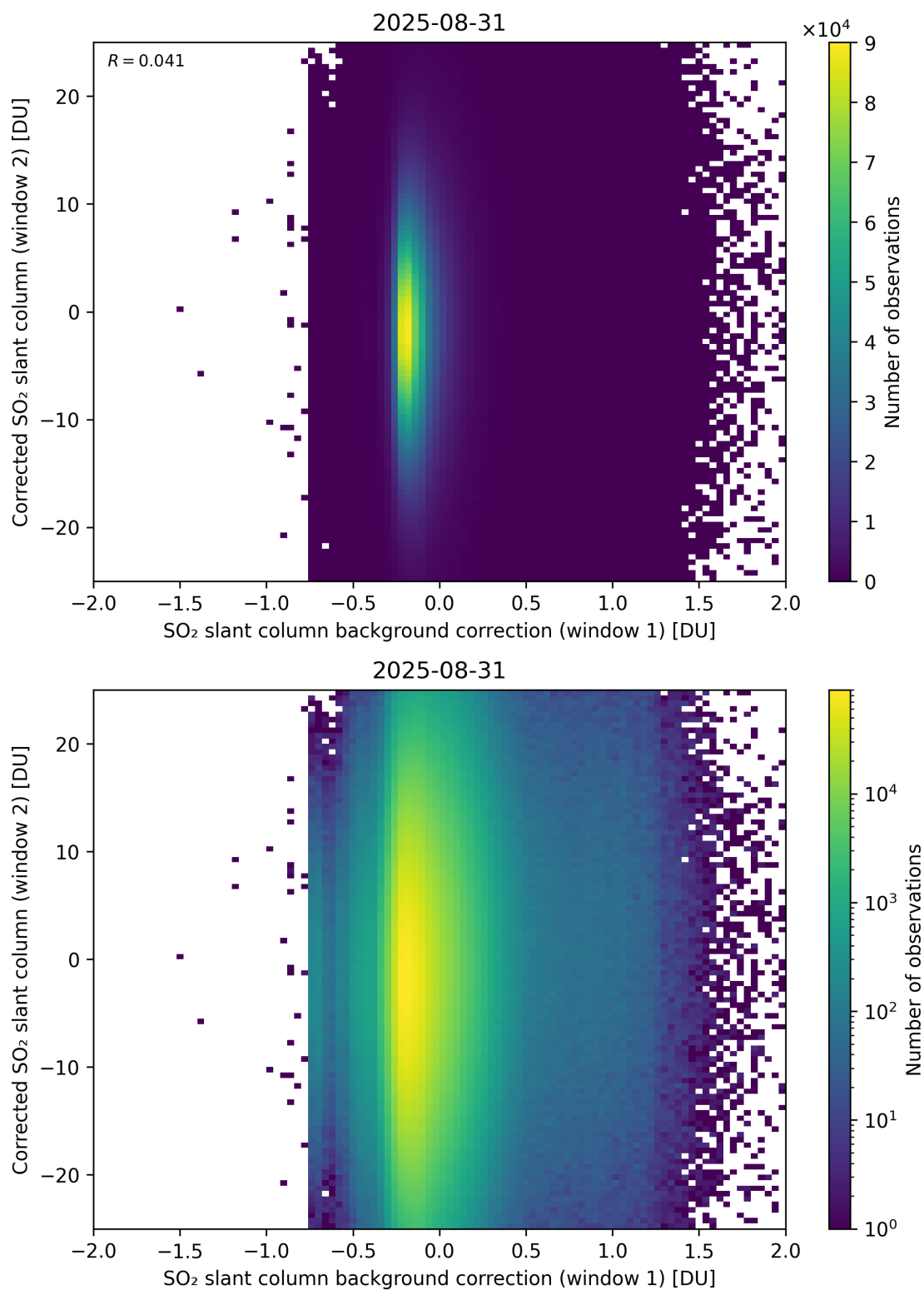
Figure 115: Scatter density plot of “SO 2 slant column background correction (window 1)” against “Corrected SO 2 slant column (window 2)” for 2025-08-30 to 2025-09-01.
