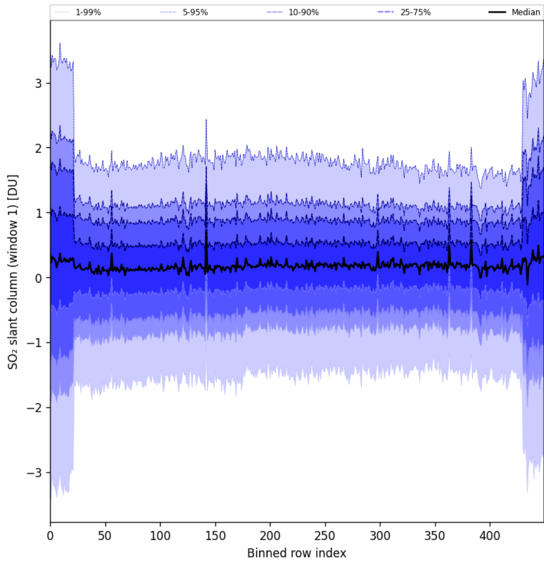
Figure 89: Along track statistics of “SO 2 slant column (window 1)” for 2025-08-30 to 2025-09-01
