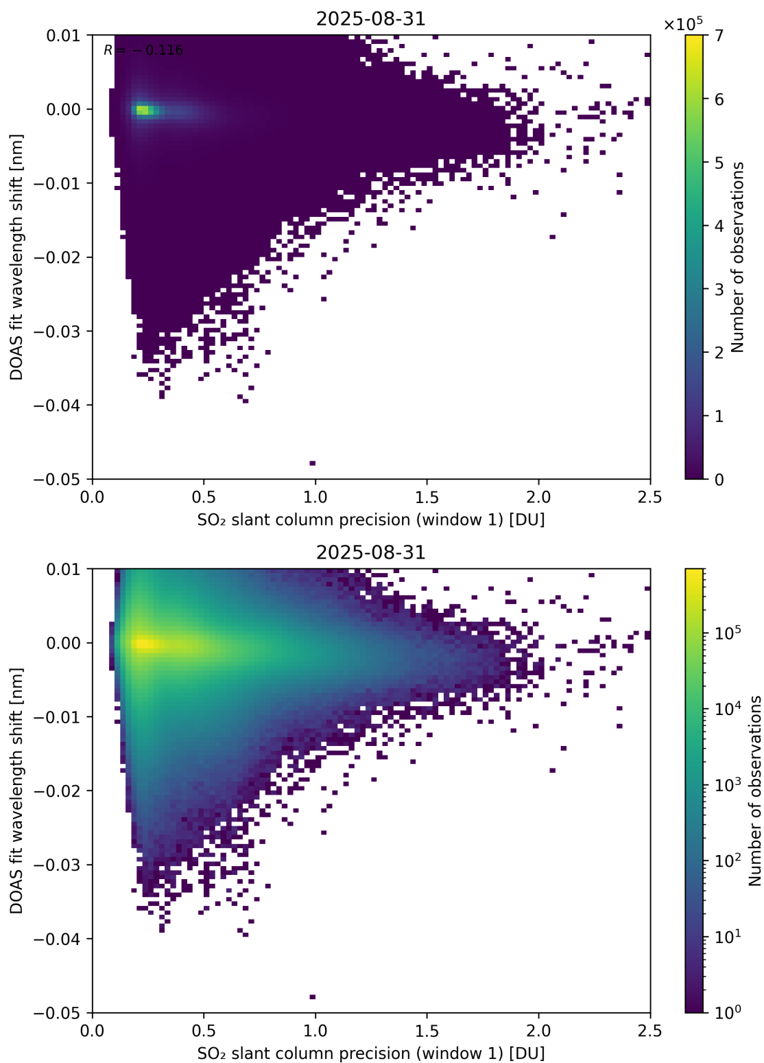
Figure 271: Scatter density plot of “SO 2 slant column precision (window 1)” against “DOAS fit wavelength shift” for 2025-08-30 to 2025-09-01.
