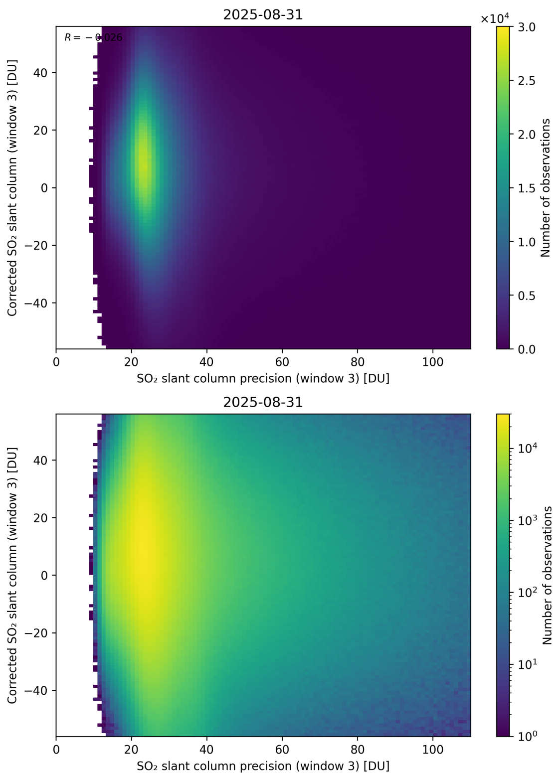
Figure 312: Scatter density plot of “SO 2 slant column precision (window 3)” against “Corrected SO 2 slant column (window 3)” for 2025-08-30 to 2025-09-01.
