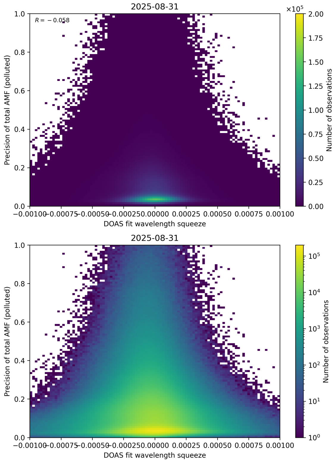
Figure 146: Scatter density plot of “DOAS fit wavelength squeeze” against “Precision of total AMF (polluted)” for 2025-08-30 to 2025-09-01.
