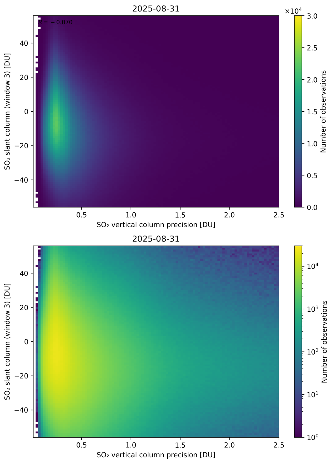
Figure 344: Scatter density plot of “SO 2 vertical column precision” against “SO 2 slant column (window 3)” for 2025-08-30 to 2025-09-01.
