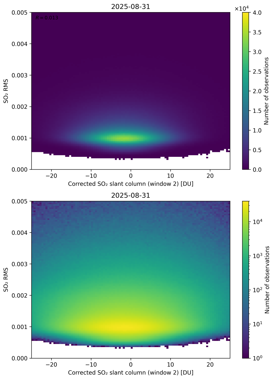
Figure 248: Scatter density plot of “Corrected SO 2 slant column (window 2)” against “SO 2 RMS” for 2025-08-30 to 2025-09-01.
