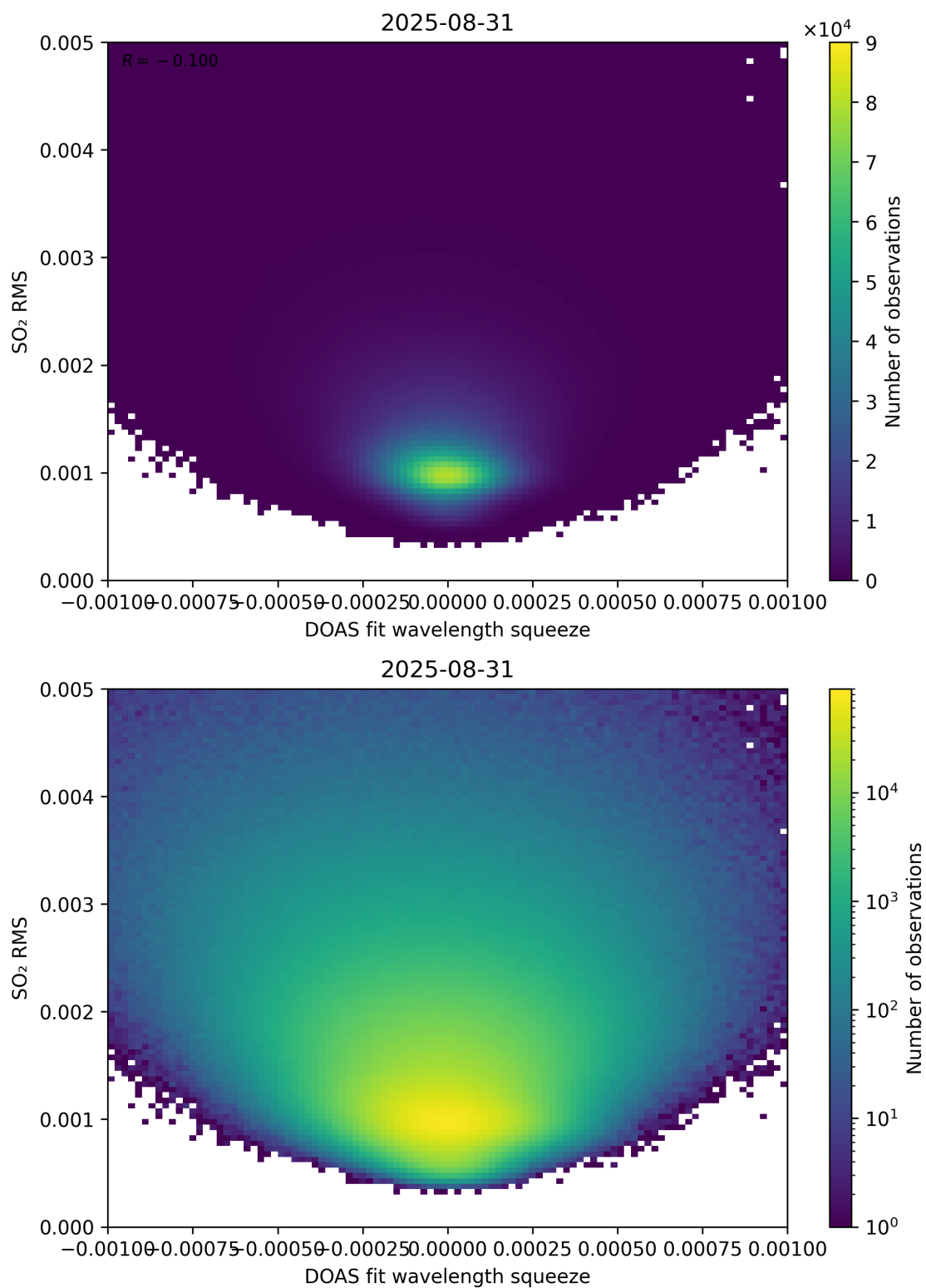
Figure 143: Scatter density plot of “DOAS fit wavelength squeeze” against “SO 2 RMS” for 2025-08-30 to 2025-09-01.
