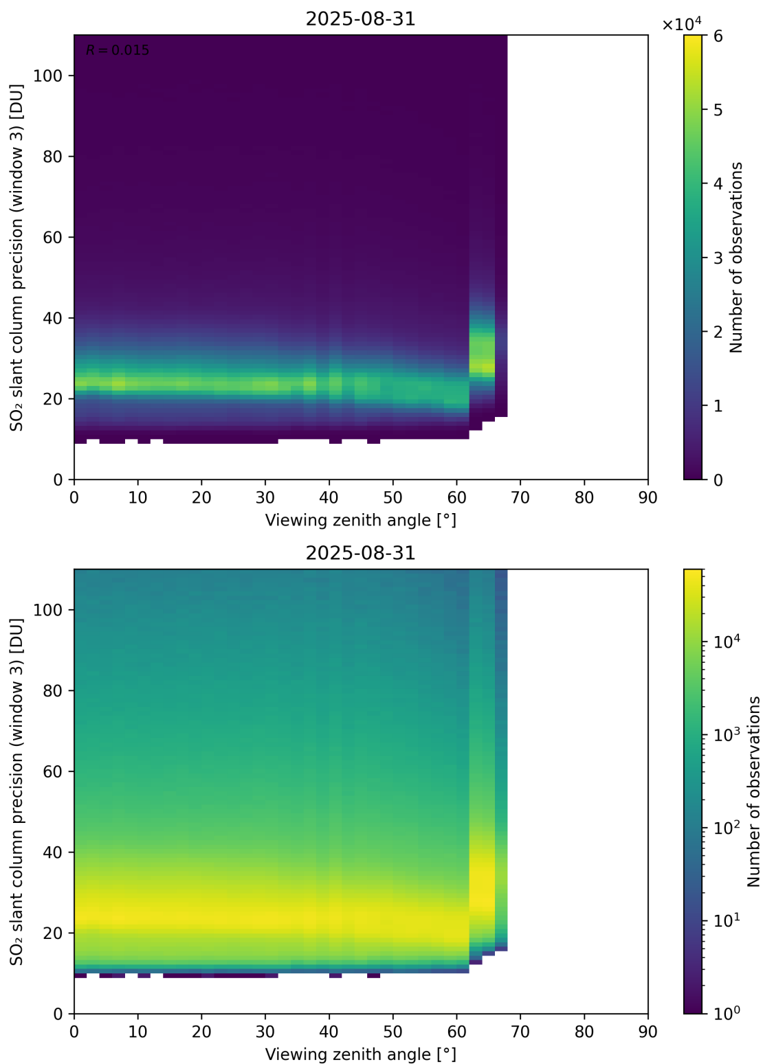
Figure 380: Scatter density plot of “Viewing zenith angle” against “SO 2 slant column precision (window 3)” for 2025-08-30 to 2025-09-01.
