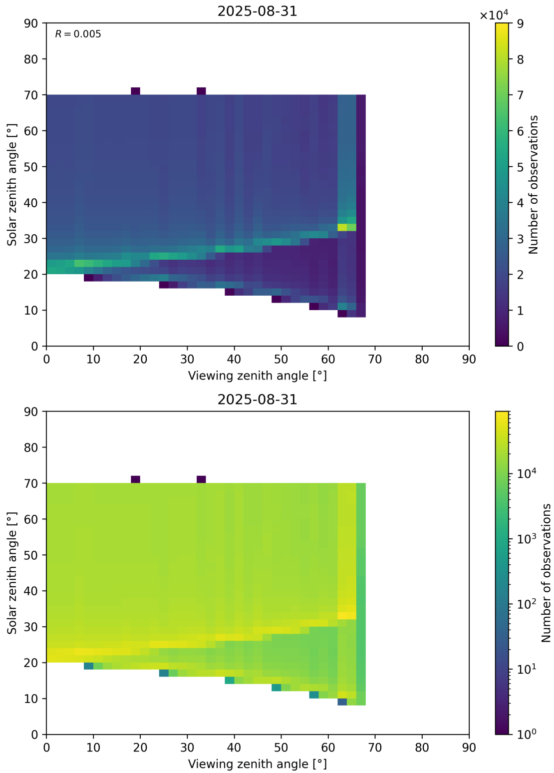
Figure 369: Scatter density plot of “Viewing zenith angle” against “Solar zenith angle” for 2025-08-30 to 2025-09-01.
