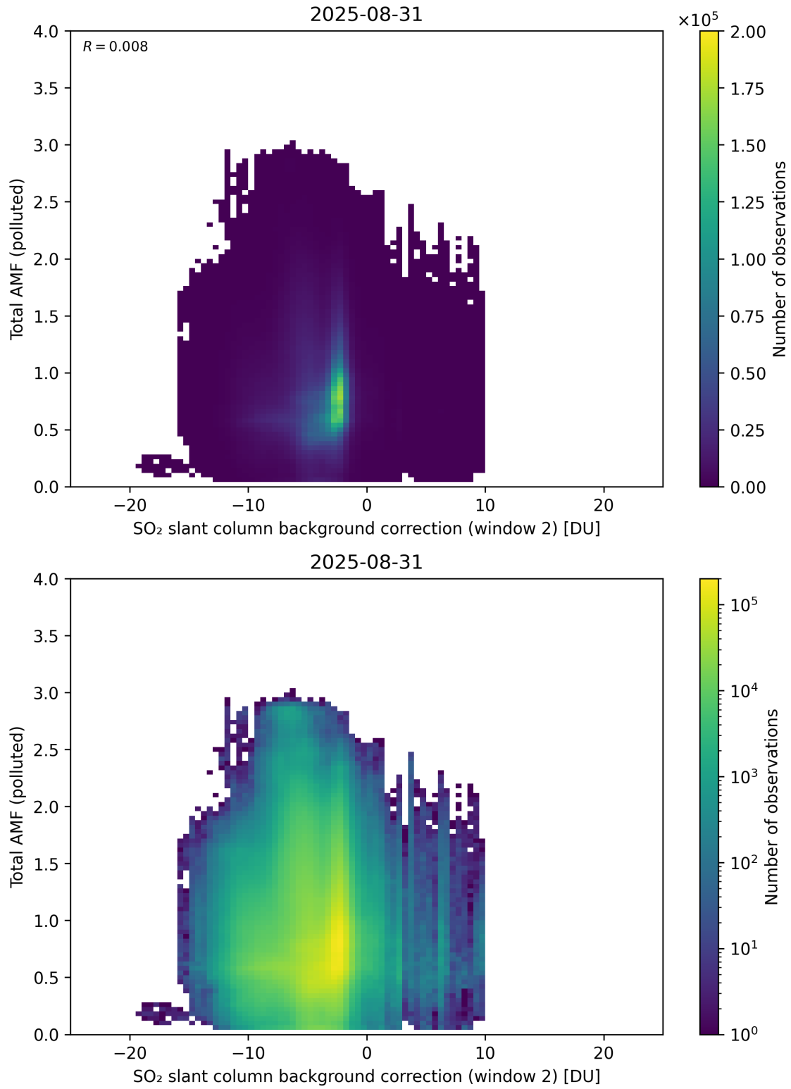
Figure 130: Scatter density plot of “SO 2 slant column background correction (window 2)” against “Total AMF (polluted)” for 2025-08-30 to 2025-09-01.
