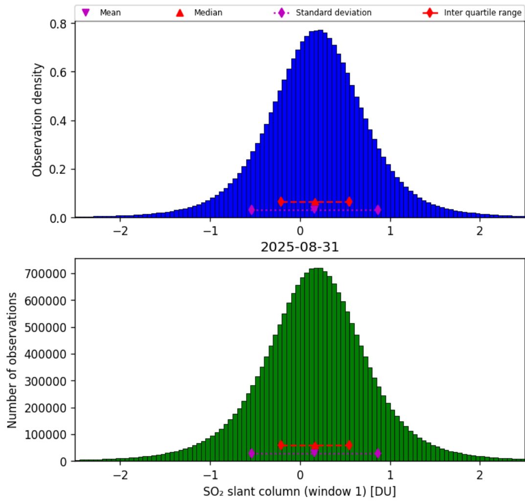
Figure 63: Histogram of “SO 2 slant column (window 1)” for 2025-08-30 to 2025-09-01
