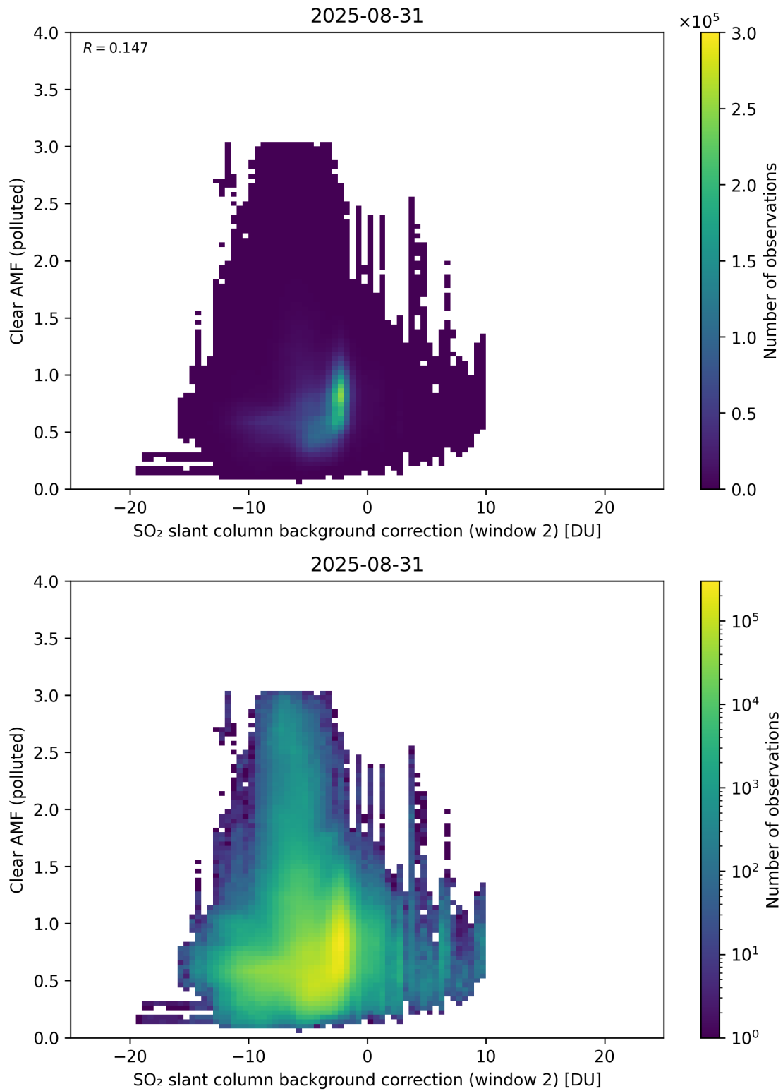
Figure 126: Scatter density plot of “SO 2 slant column background correction (window 2)” against “Clear AMF (polluted)” for 2025-08-30 to 2025-09-01.
