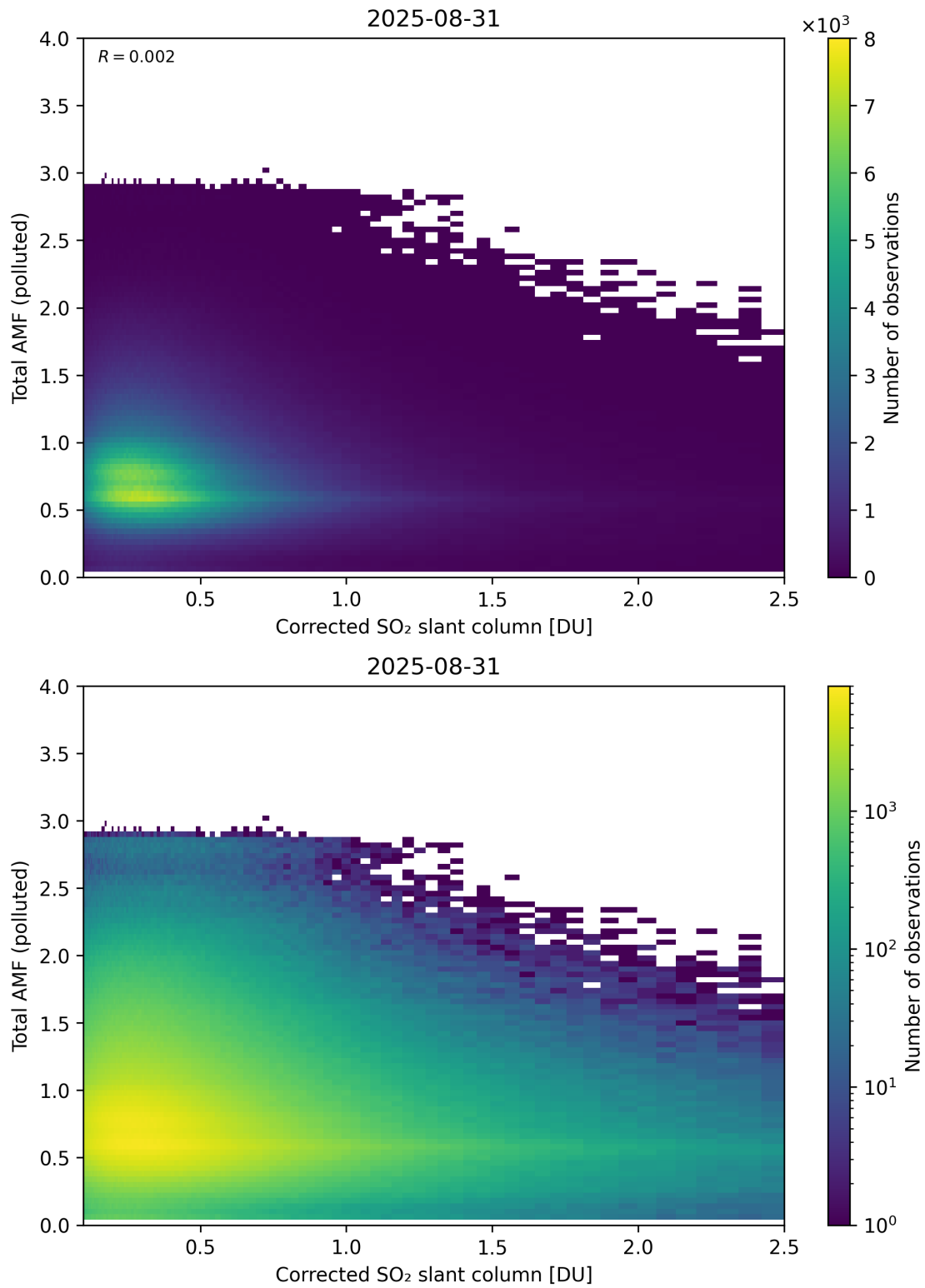
Figure 242: Scatter density plot of “Corrected SO 2 slant column” against “Total AMF (polluted)” for 2025-08-30 to 2025-09-01.
