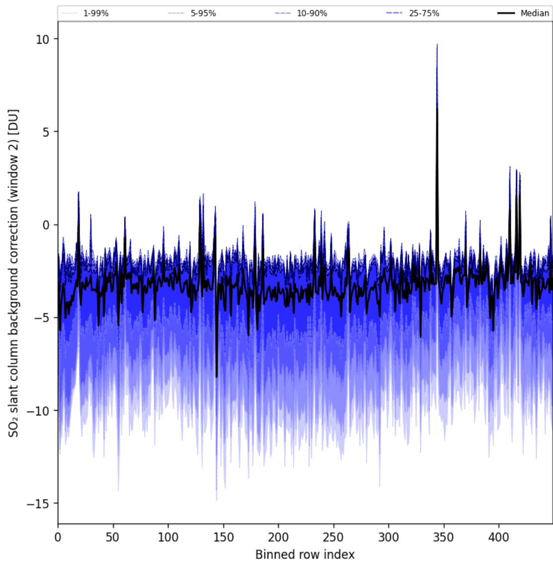
Figure 96: Along track statistics of “SO 2 slant column background correction (window 2)” for 2025-08-30 to 2025-09-01
