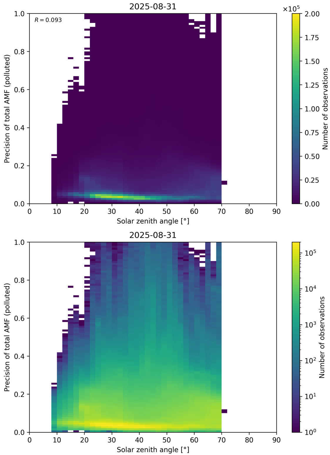
Figure 190: Scatter density plot of “Solar zenith angle” against “Precision of total AMF (polluted)” for 2025-08-30 to 2025-09-01.
