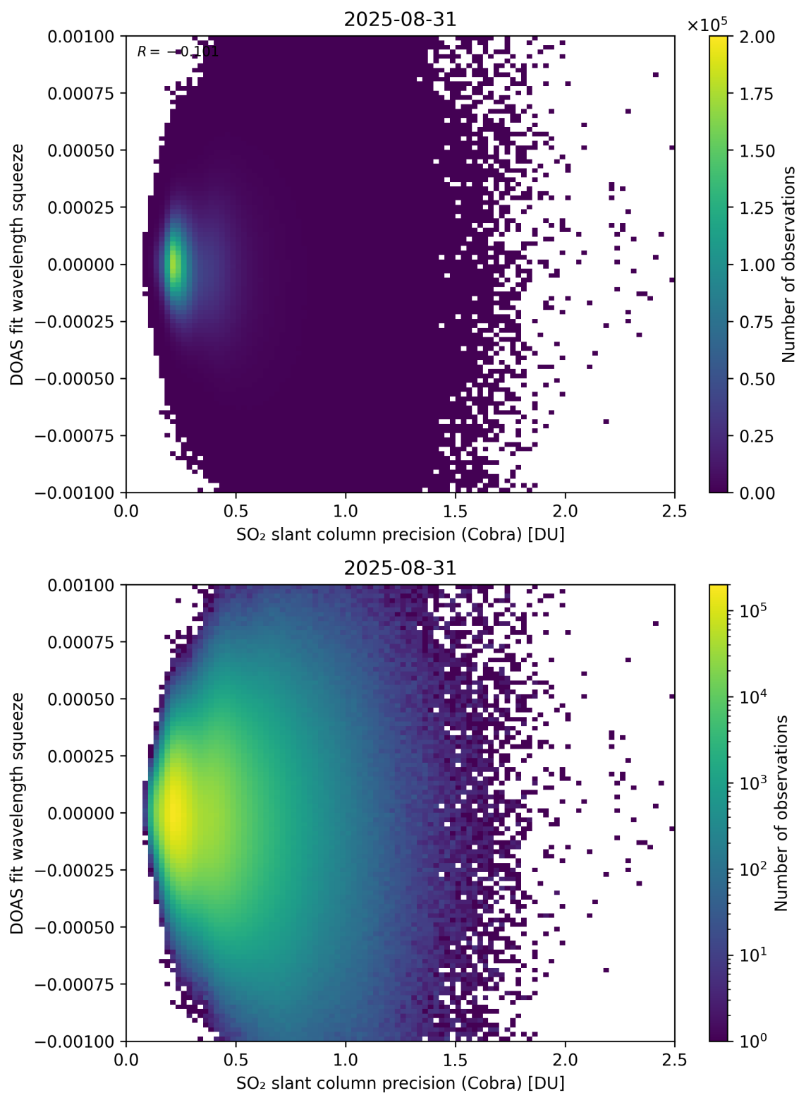
Figure 203: Scatter density plot of “SO 2 slant column precision (Cobra)” against “DOAS fit wavelength squeeze” for 2025-08-30 to 2025-09-01.
