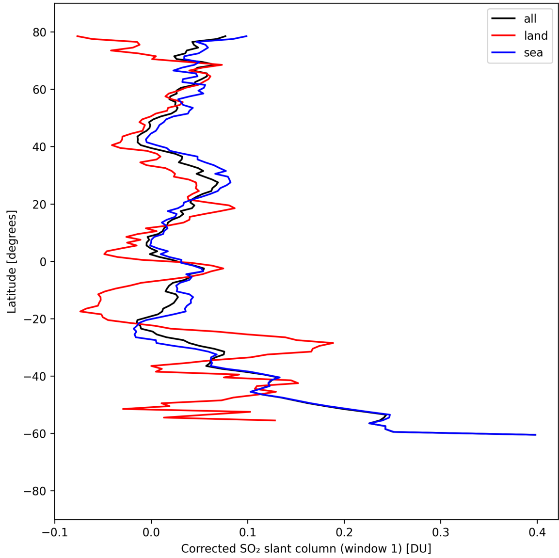
Figure 39: Zonal average of “Corrected SO 2 slant column (window 1)” for 2025-08-30 to 2025-09-01.
