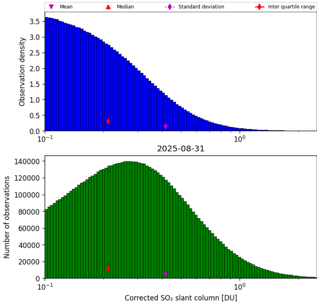
Figure 60: Histogram of "Corrected SO 2 slant column" for 2025-08-30 to 2025-09-01
