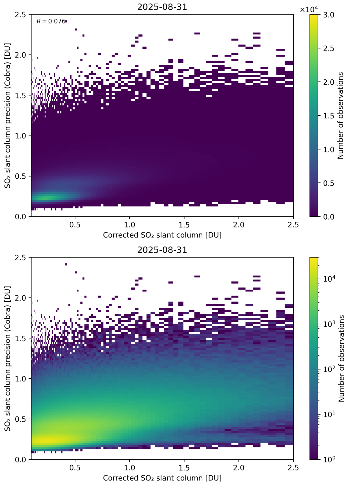
Figure 234: Scatter density plot of “Corrected SO 2 slant column” against “SO 2 slant column precision (Cobra)” for 2025-08-30 to 2025-09-01.
