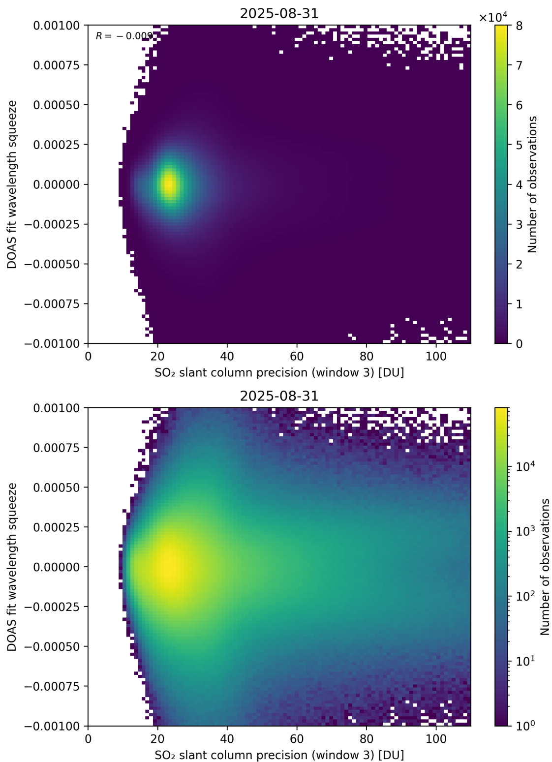
Figure 309: Scatter density plot of “SO 2 slant column precision (window 3)” against “DOAS fit wavelength squeeze” for 2025-08-30 to 2025-09-01.
