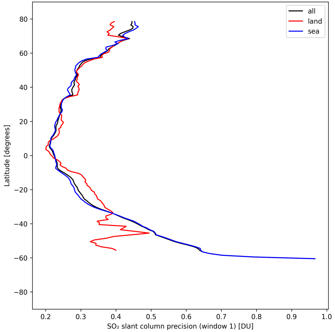
Figure 38: Zonal average of “SO 2 slant column precision (window 1)” for 2025-08-30 to 2025-09-01.
