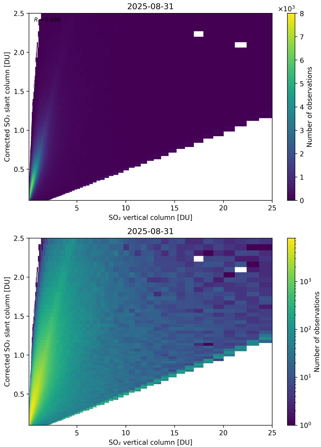
Figure 351: Scatter density plot of “SO 2 vertical column” against “Corrected SO 2 slant column” for 2025-08-30 to 2025-09-01.
