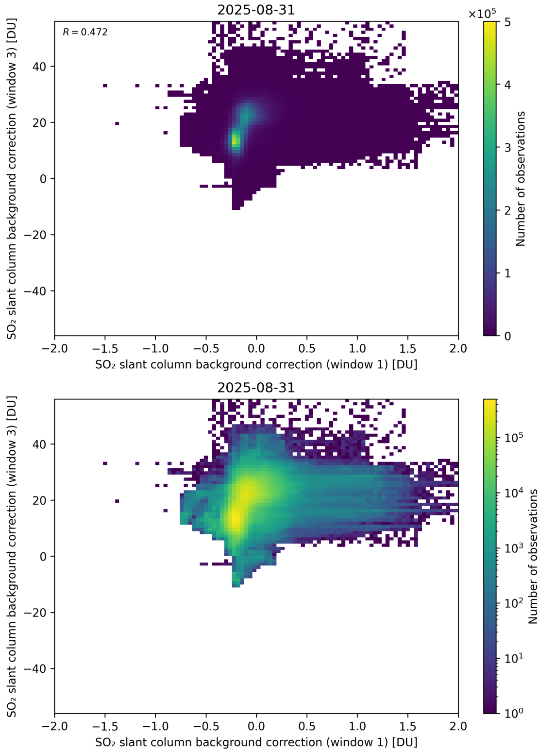
Figure 110: Scatter density plot of “SO 2 slant column background correction (window 1)” against “SO 2 slant column background correction (window 3)” for 2025-08-30 to 2025-09-01.
