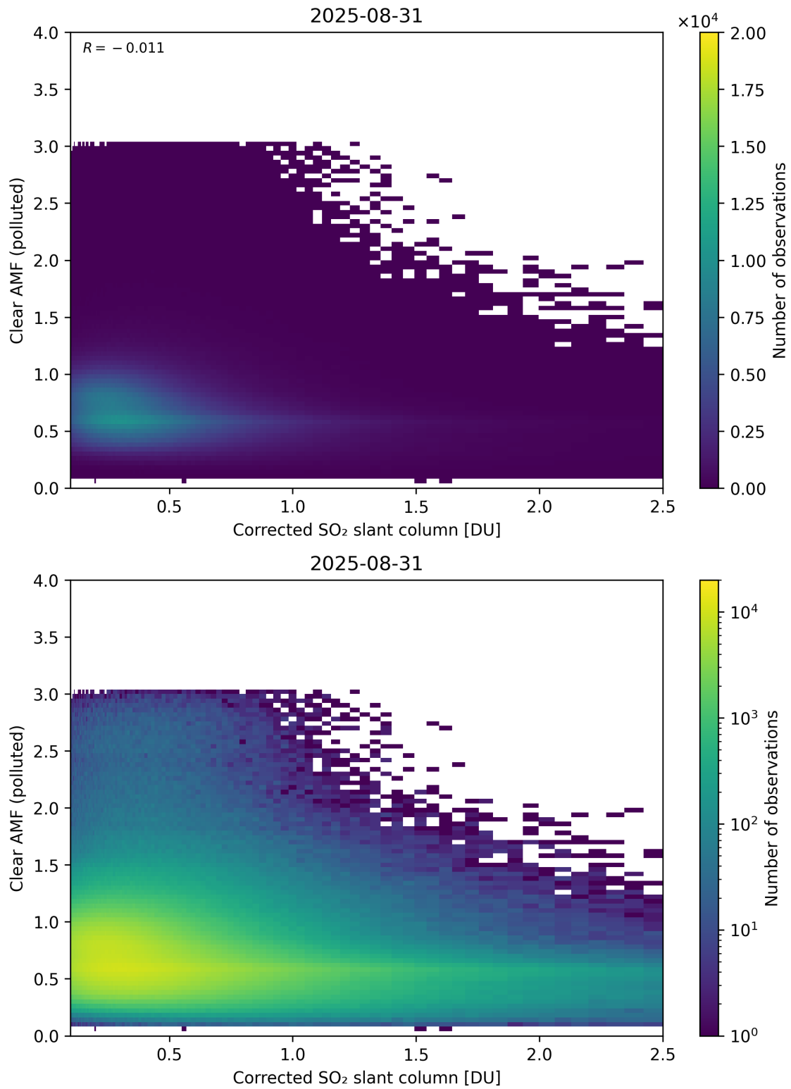
Figure 232: Scatter density plot of “Corrected SO 2 slant column” against “Clear AMF (polluted)” for 2025-08-30 to 2025-09-01.
