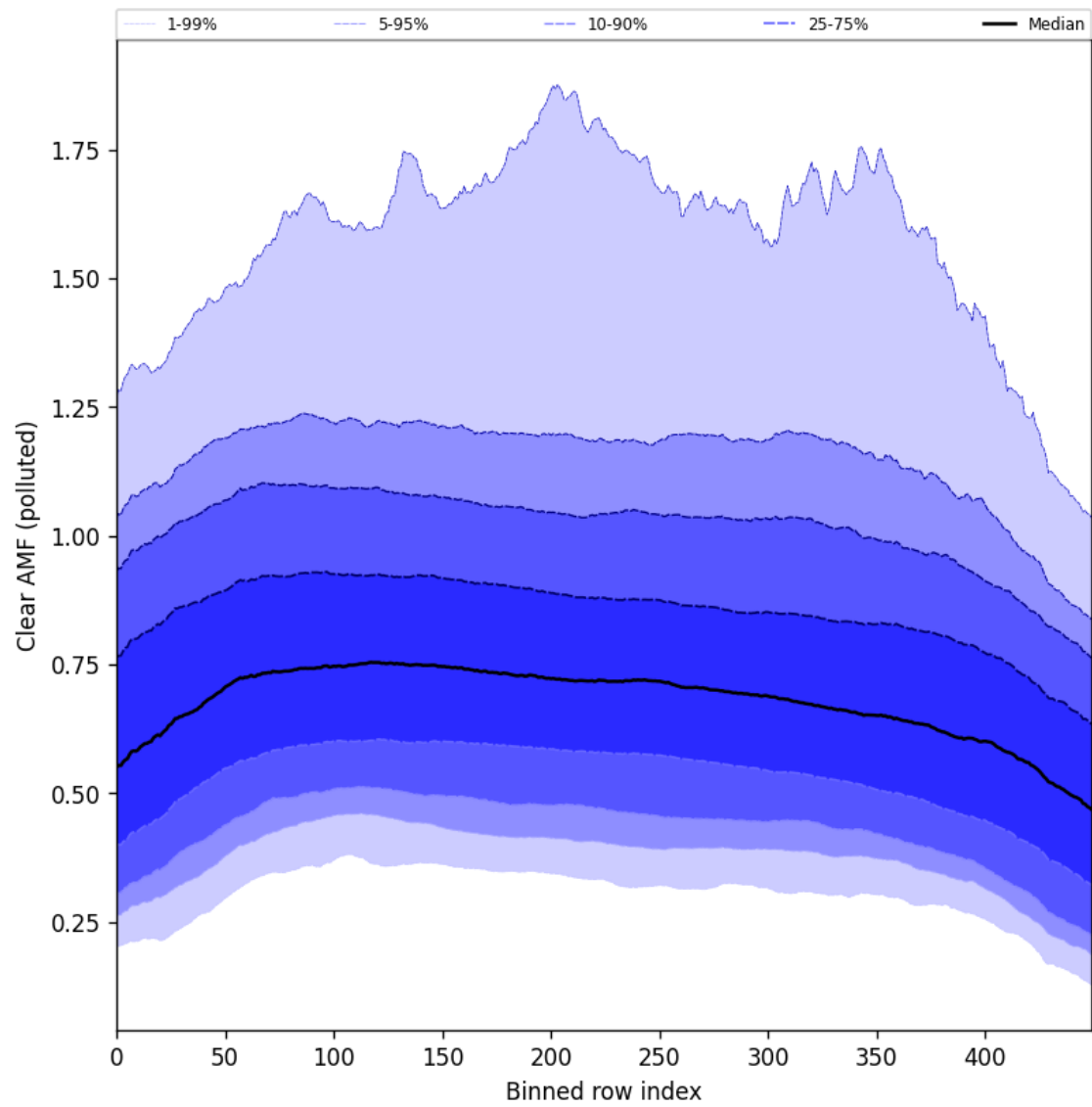
Figure 107: Along track statistics of “Clear AMF (polluted)” for 2025-08-30 to 2025-09-01
