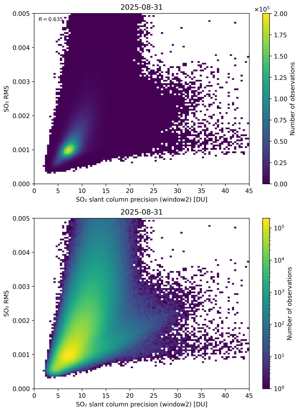
Figure 295: Scatter density plot of “SO 2 slant column precision (window2)” against “SO 2 RMS” for 2025-08-30 to 2025-09-01.
