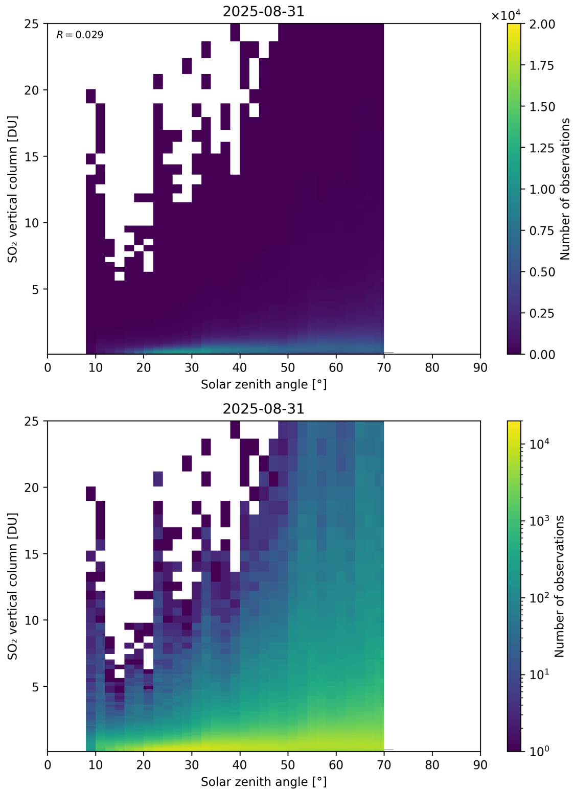
Figure 191: Scatter density plot of “Solar zenith angle” against “SO 2 vertical column” for 2025-08-30 to 2025-09-01.
