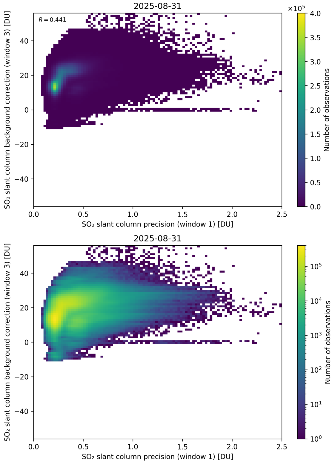
Figure 270: Scatter density plot of “SO 2 slant column precision (window 1)” against “SO 2 slant column background correction (window 3)” for 2025-08-30 to 2025-09-01.
