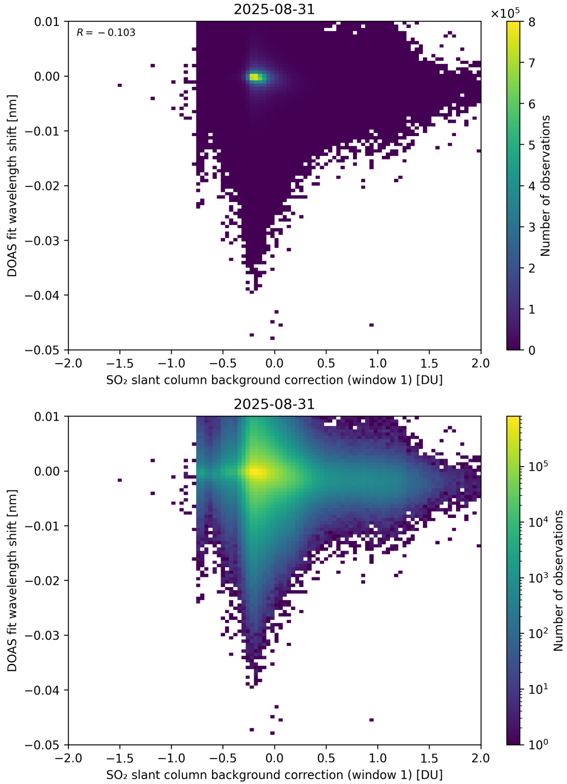
Figure 111: Scatter density plot of “SO 2 slant column background correction (window 1)” against “DOAS fit wavelength shift” for 2025-08-30 to 2025-09-01.
