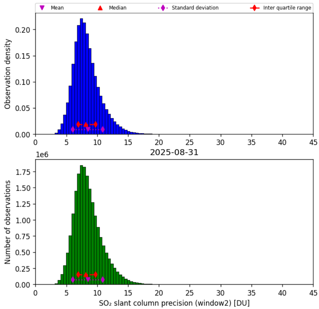
Figure 68: Histogram of “SO 2 slant column precision (window2)” for 2025-08-30 to 2025-09-01
