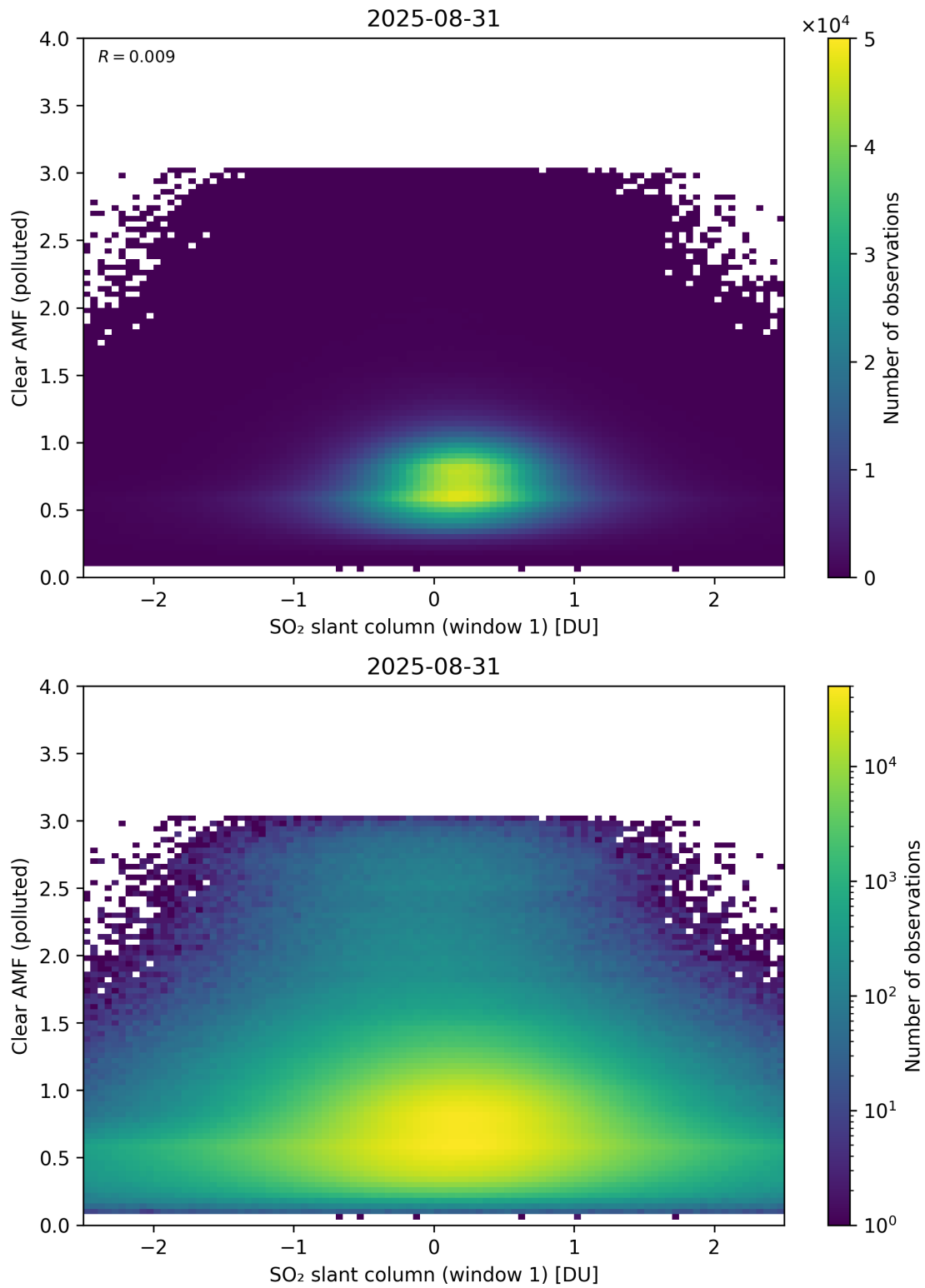
Figure 282: Scatter density plot of “SO 2 slant column (window 1)” against “Clear AMF (polluted)” for 2025-08-30 to 2025-09-01.
