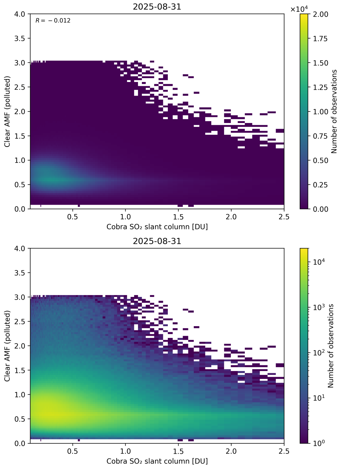
Figure 215: Scatter density plot of “Cobra SO 2 slant column” against “Clear AMF (polluted)” for 2025-08-30 to 2025-09-01.
