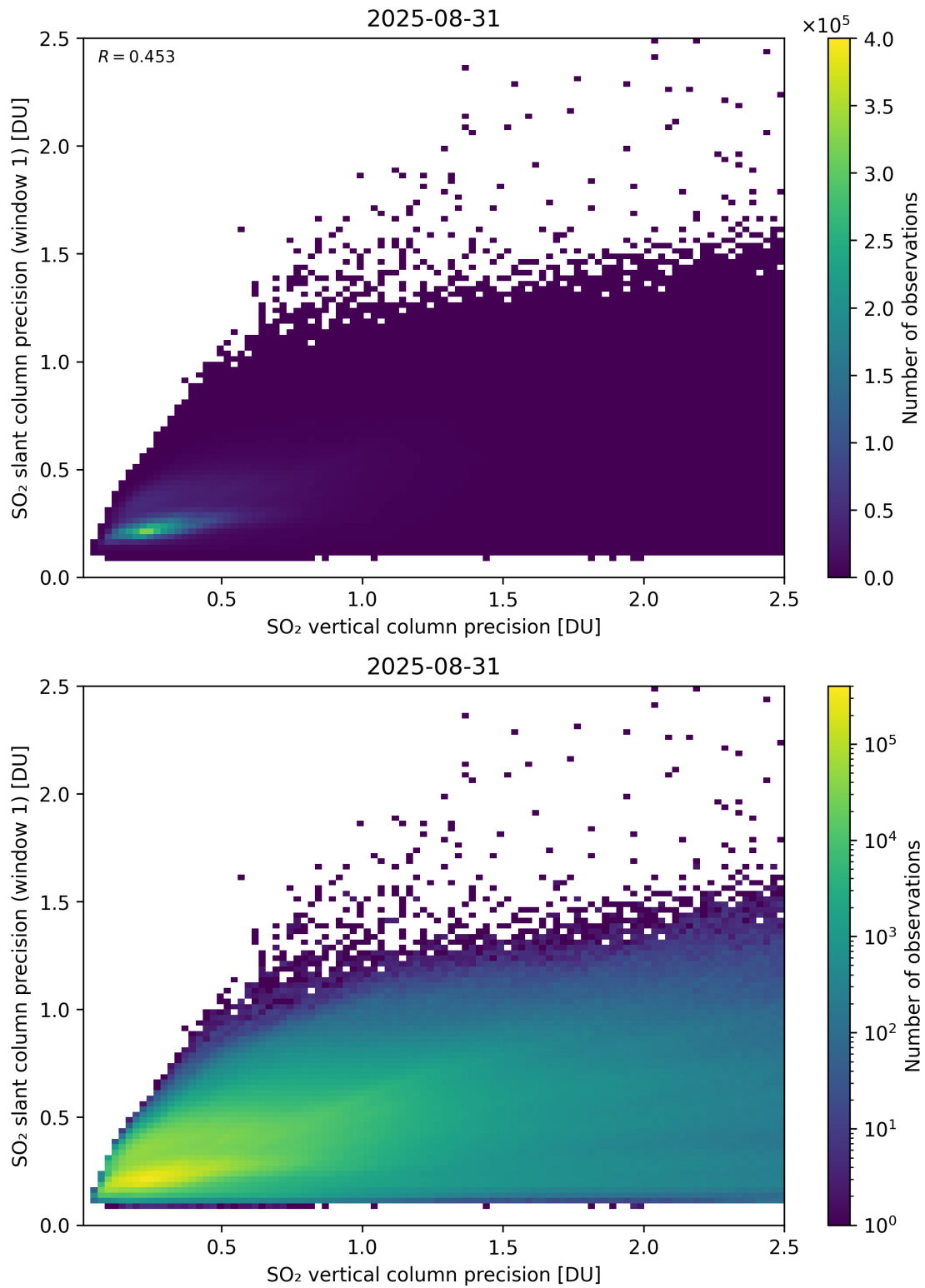
Figure 342: Scatter density plot of “SO 2 vertical column precision” against “SO 2 slant column precision (window 1)” for 2025-08-30 to 2025-09-01.
