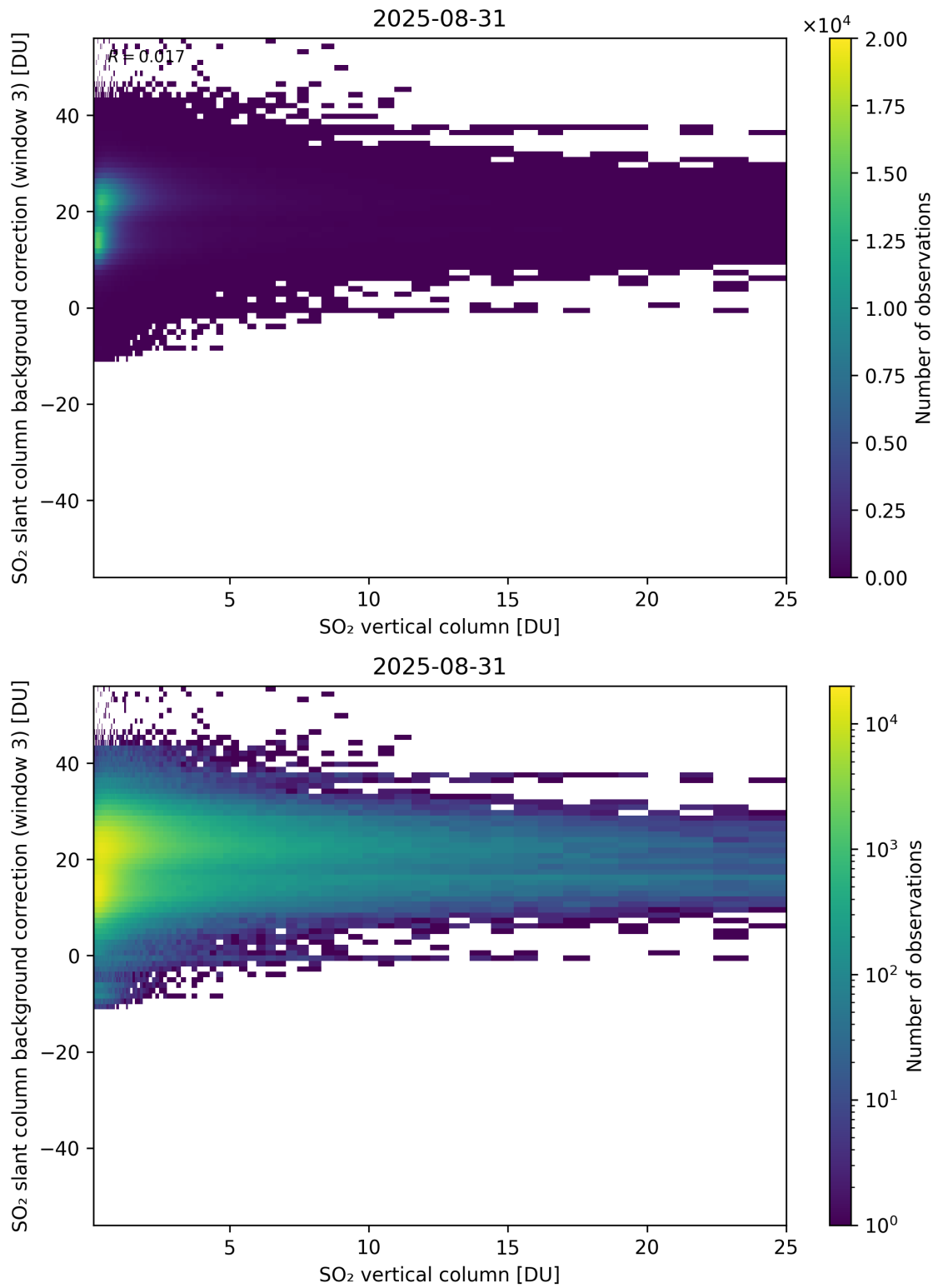
Figure 325: Scatter density plot of “SO 2 vertical column” against “SO 2 slant column background correction (window 3)” for 2025-08-30 to 2025-09-01.
