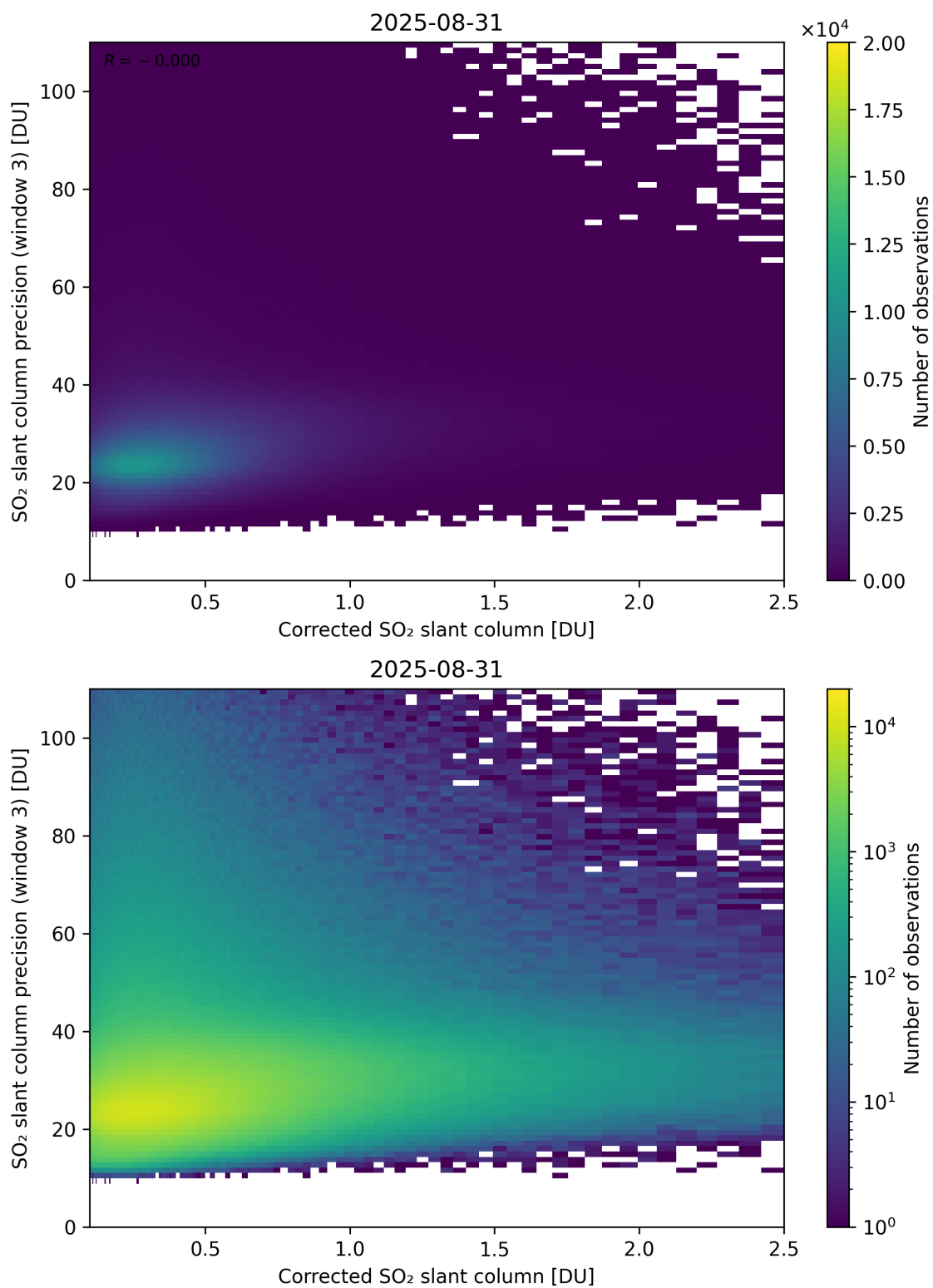
Figure 241: Scatter density plot of “Corrected SO 2 slant column” against “SO 2 slant column precision (window 3)” for 2025-08-30 to 2025-09-01.
