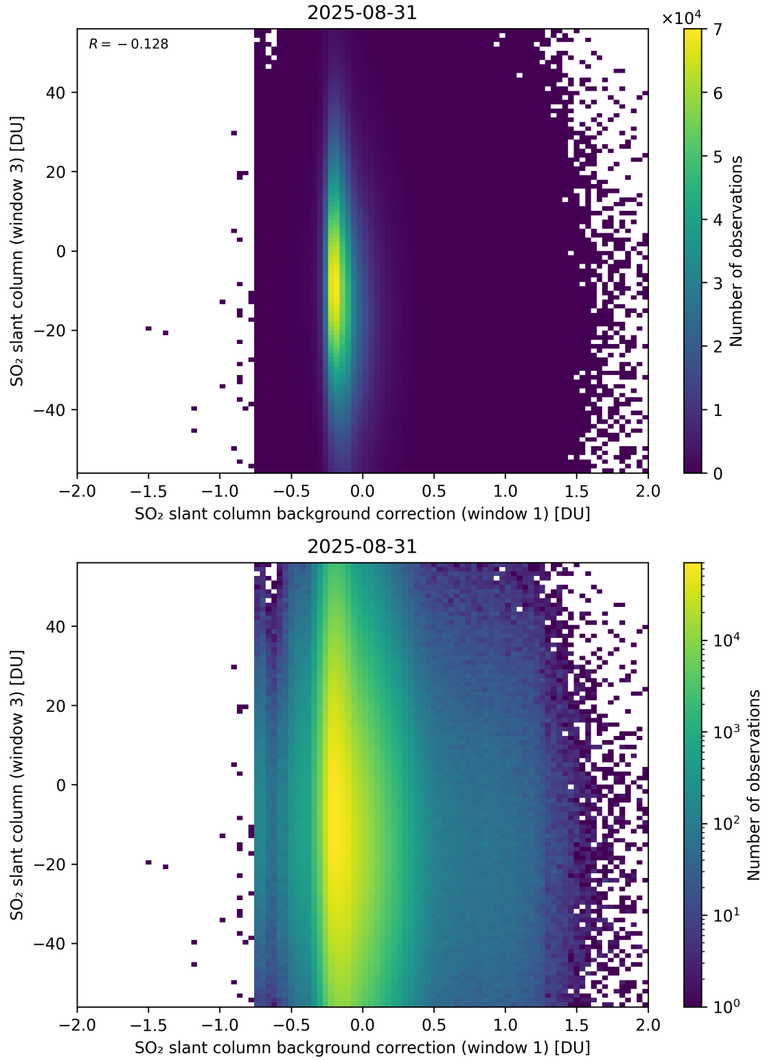
Figure 118: Scatter density plot of “SO 2 slant column background correction (window 1)” against “SO 2 slant column (window 3)” for 2025-08-30 to 2025-09-01.
