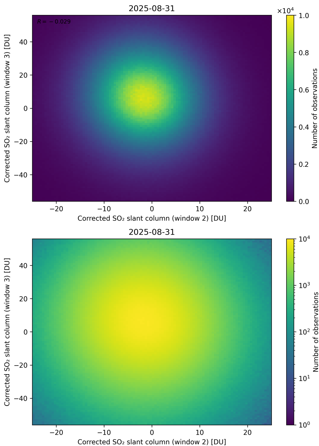
Figure 250: Scatter density plot of “Corrected SO 2 slant column (window 2)” against “Corrected SO 2 slant column (window 3)” for 2025-08-30 to 2025-09-01.
