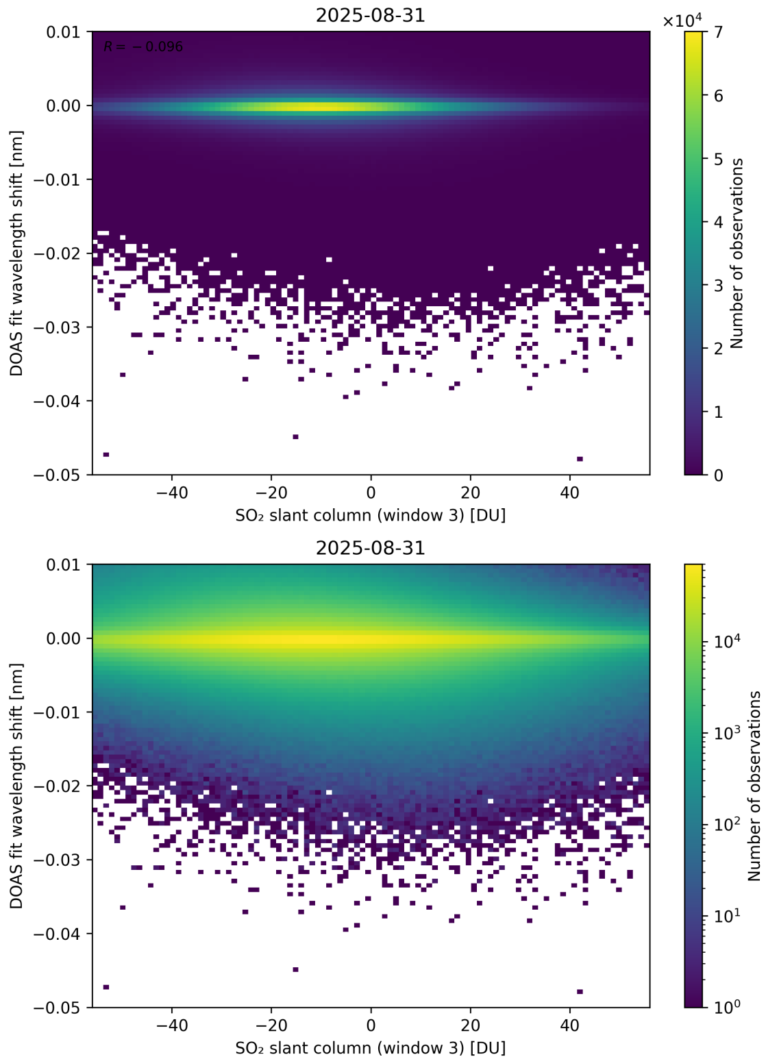
Figure 304: Scatter density plot of “SO 2 slant column (window 3)” against “DOAS fit wavelength shift” for 2025-08-30 to 2025-09-01.
