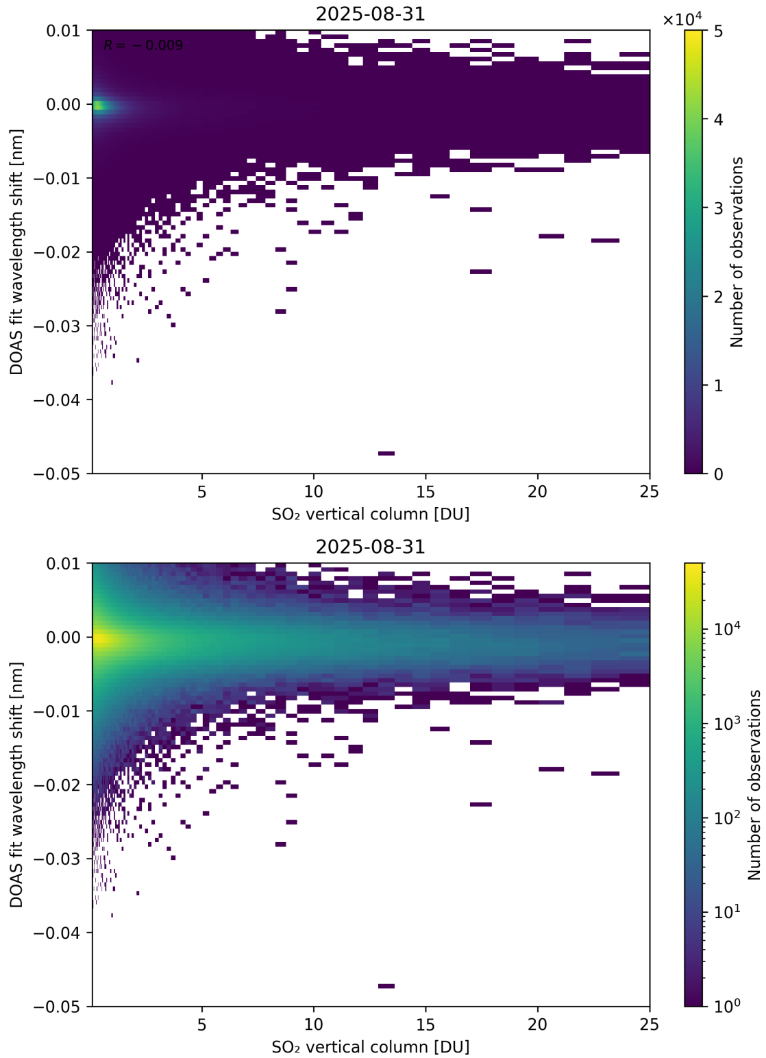
Figure 326: Scatter density plot of “SO 2 vertical column” against “DOAS fit wavelength shift” for 2025-08-30 to 2025-09-01.
