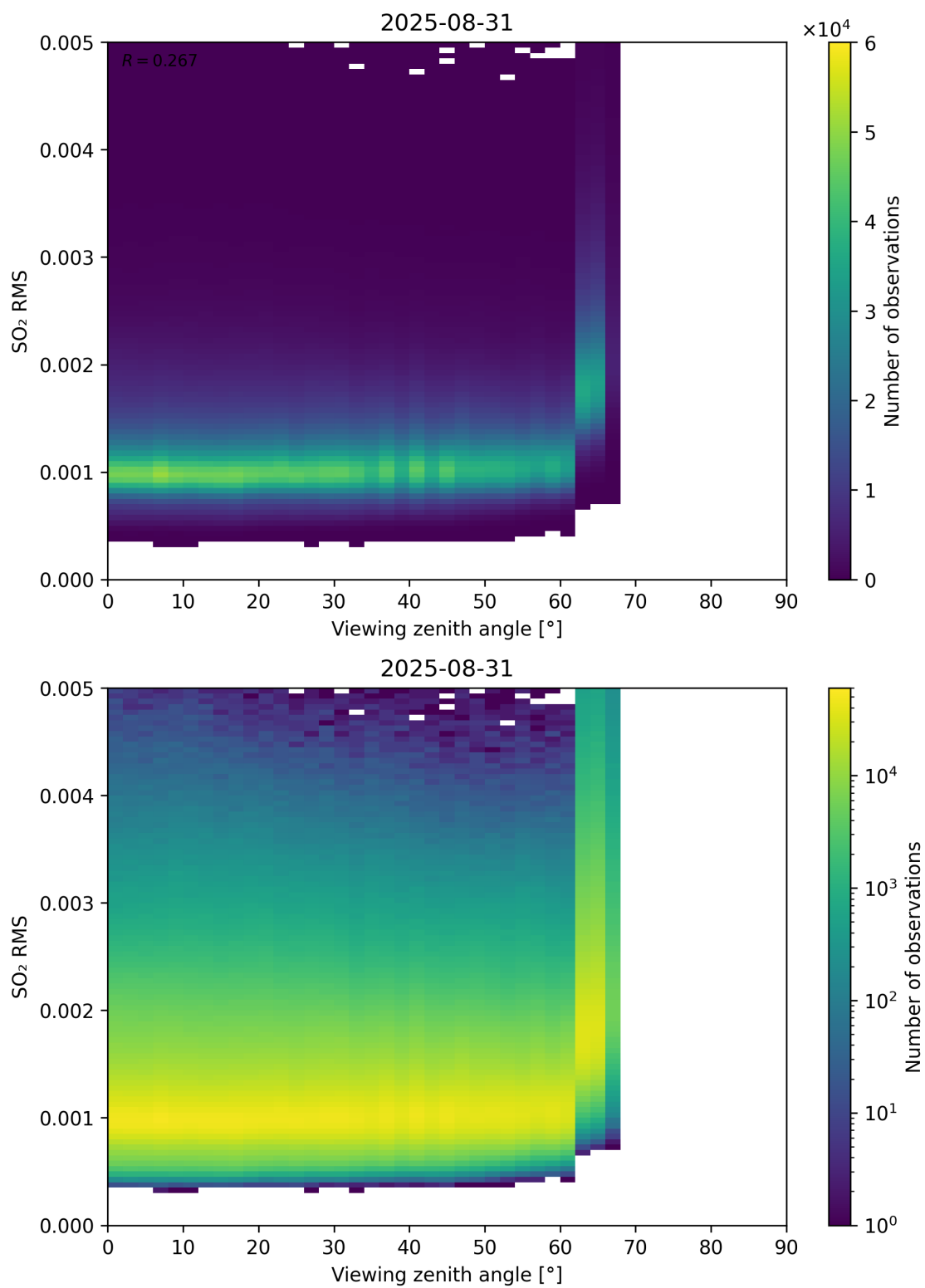
Figure 367: Scatter density plot of “Viewing zenith angle” against “SO 2 RMS” for 2025-08-30 to 2025-09-01.
