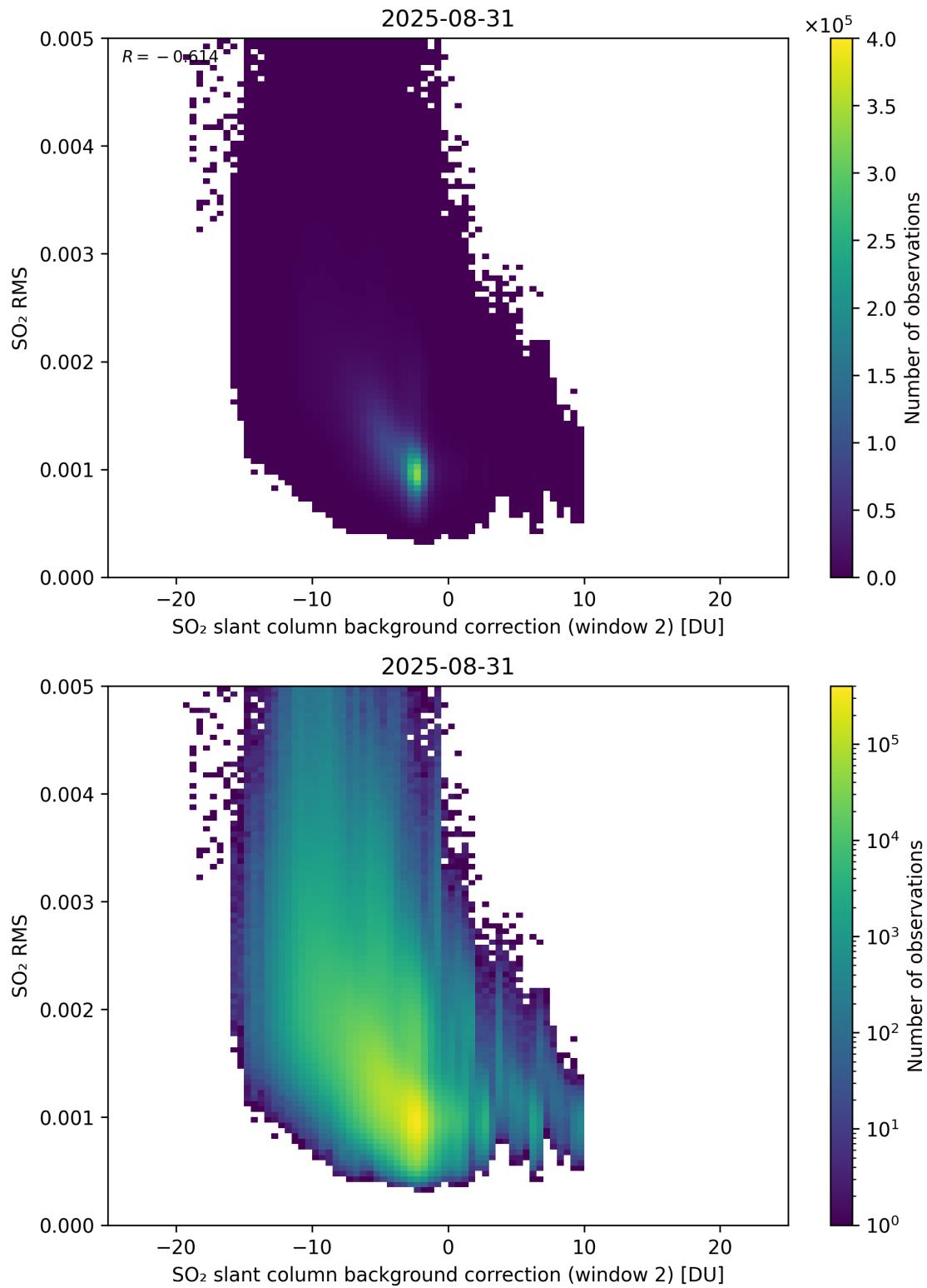
Figure 125: Scatter density plot of “SO 2 slant column background correction (window 2)” against “SO 2 RMS” for 2025-08-30 to 2025-09-01.
