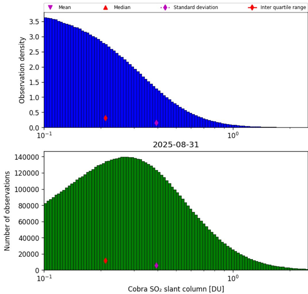
Figure 61: Histogram of “Cobra SO 2 slant column” for 2025-08-30 to 2025-09-01
