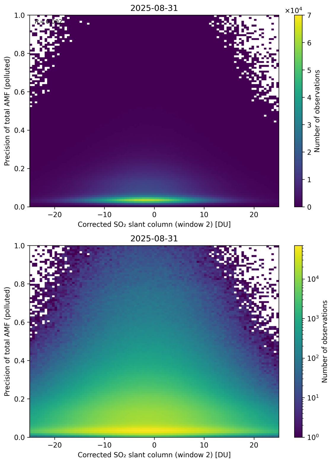
Figure 254: Scatter density plot of “Corrected SO 2 slant column (window 2)” against “Precision of total AMF (polluted)” for 2025-08-30 to 2025-09-01.
