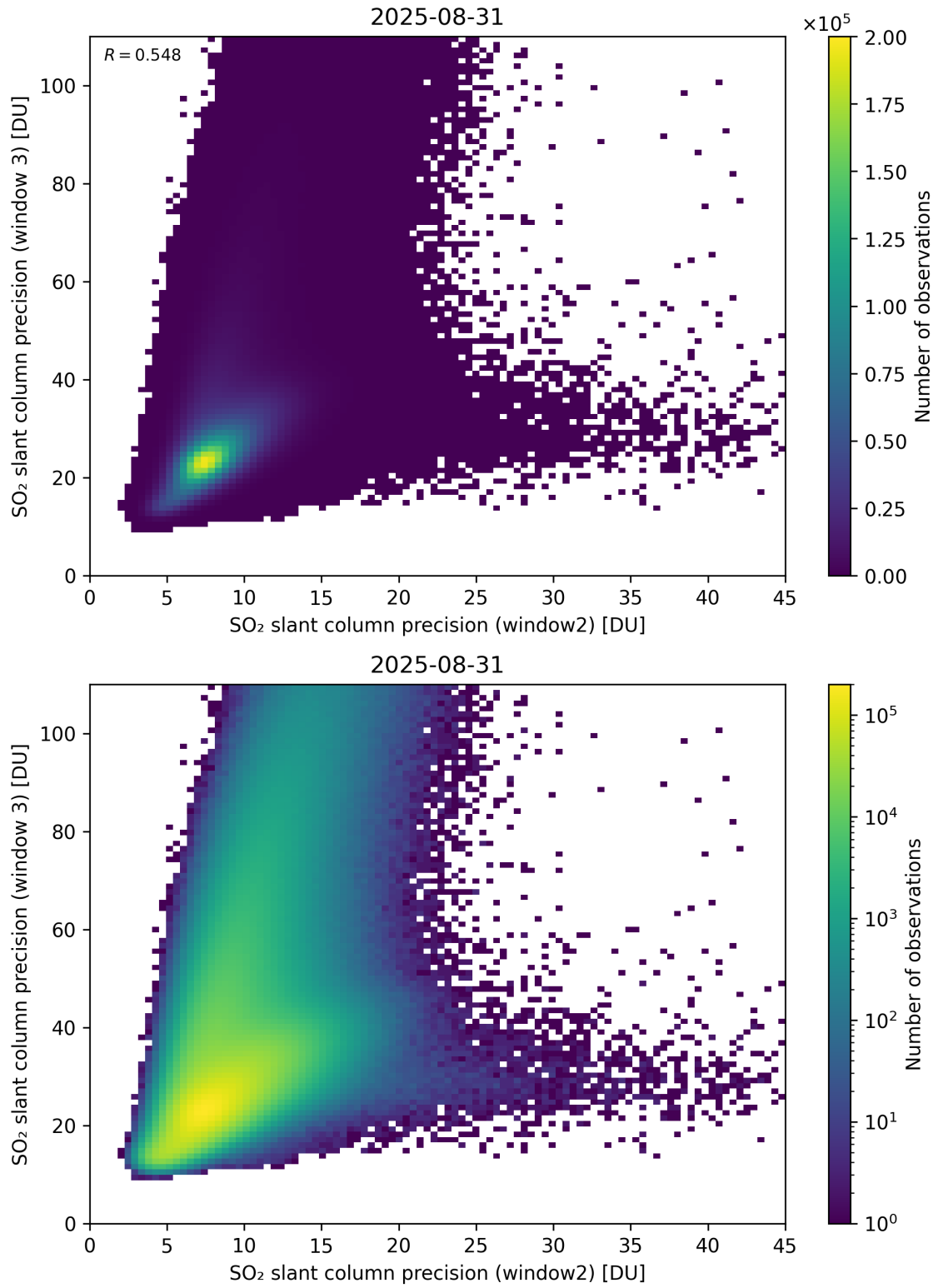
Figure 300: Scatter density plot of “SO 2 slant column precision (window2)” against “SO 2 slant column precision (window 3)” for 2025-08-30 to 2025-09-01.
