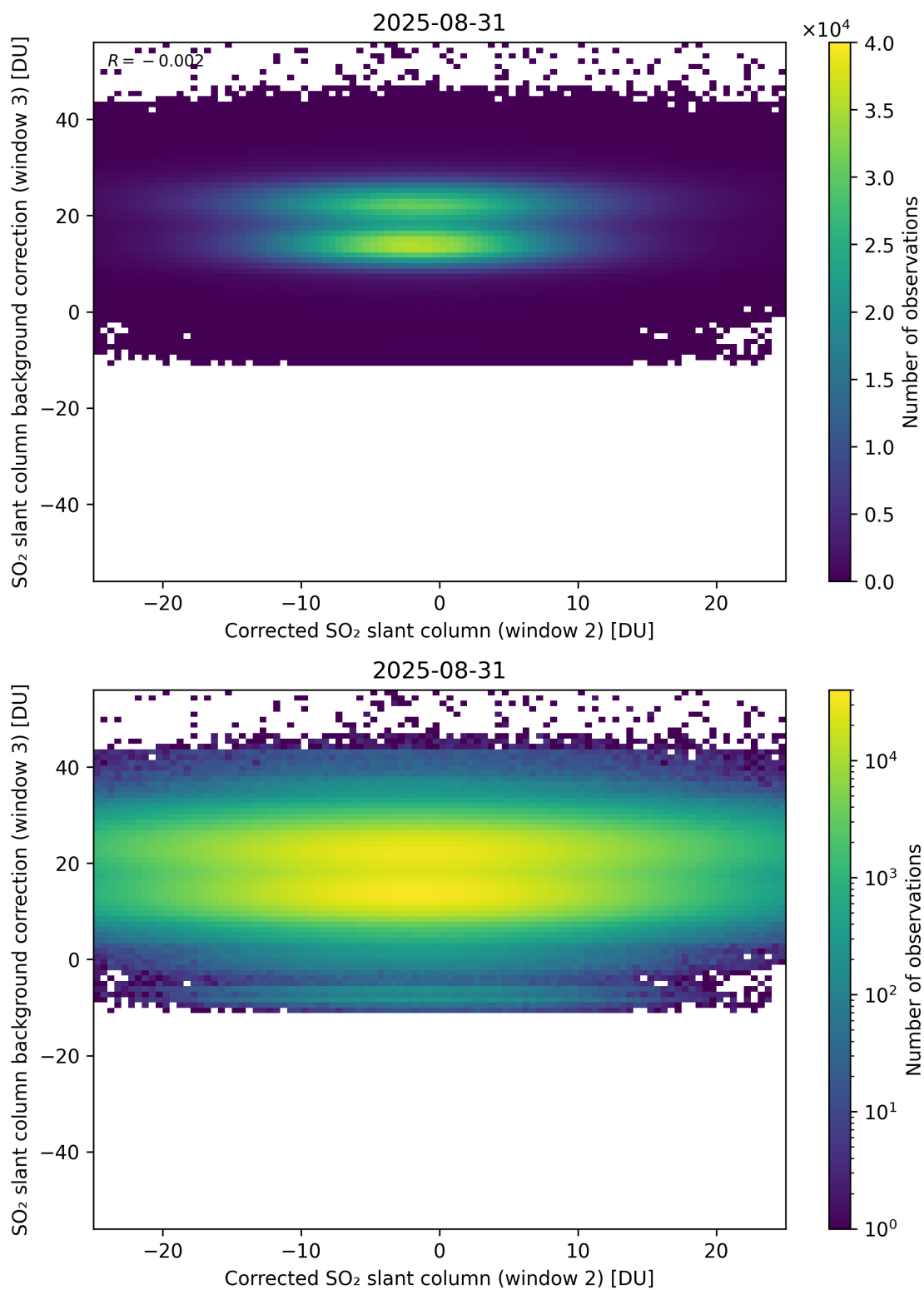
Figure 245: Scatter density plot of “Corrected SO 2 slant column (window 2)” against “SO 2 slant column background correction (window 3)” for 2025-08-30 to 2025-09-01.
