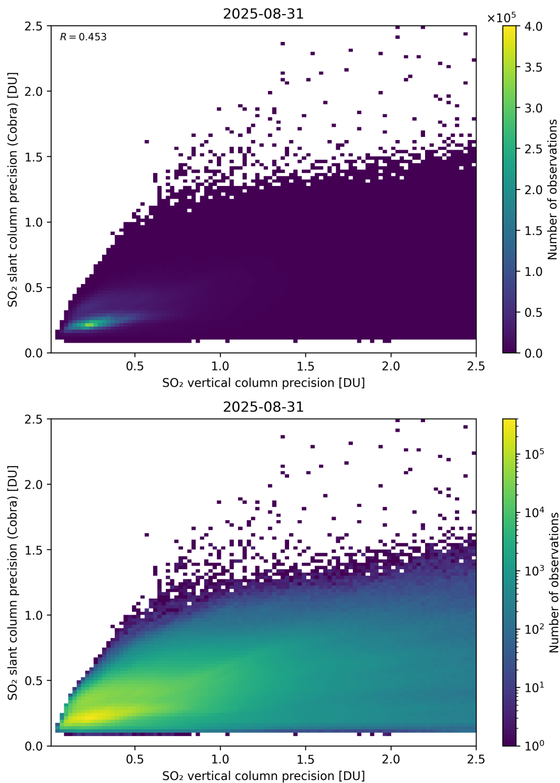
Figure 337: Scatter density plot of “SO 2 vertical column precision” against “SO 2 slant column precision (Cobra)” for 2025-08-30 to 2025-09-01.
