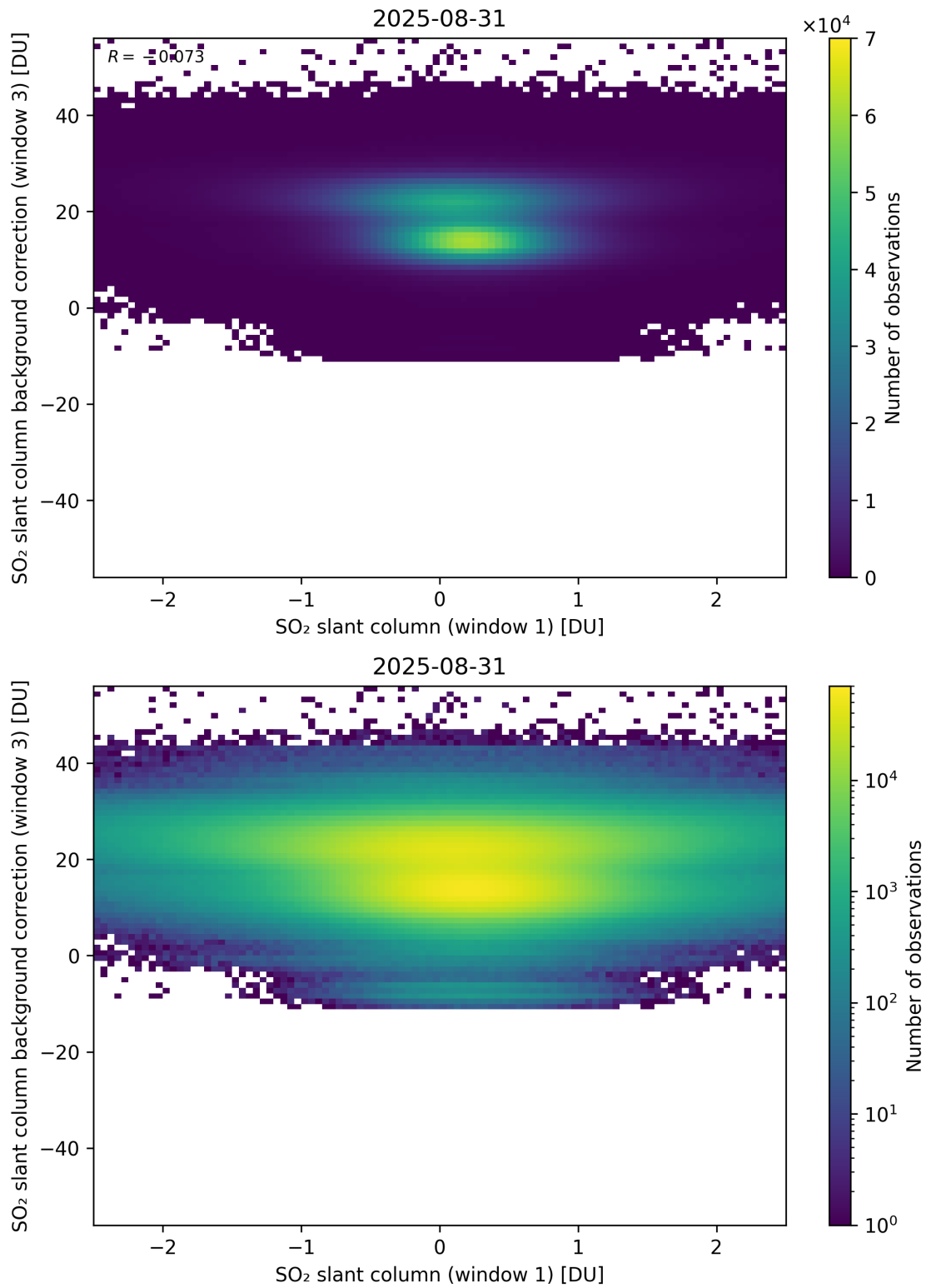
Figure 264: Scatter density plot of “SO 2 slant column (window 1)” against “SO 2 slant column background correction (window 3)” for 2025-08-30 to 2025-09-01.
