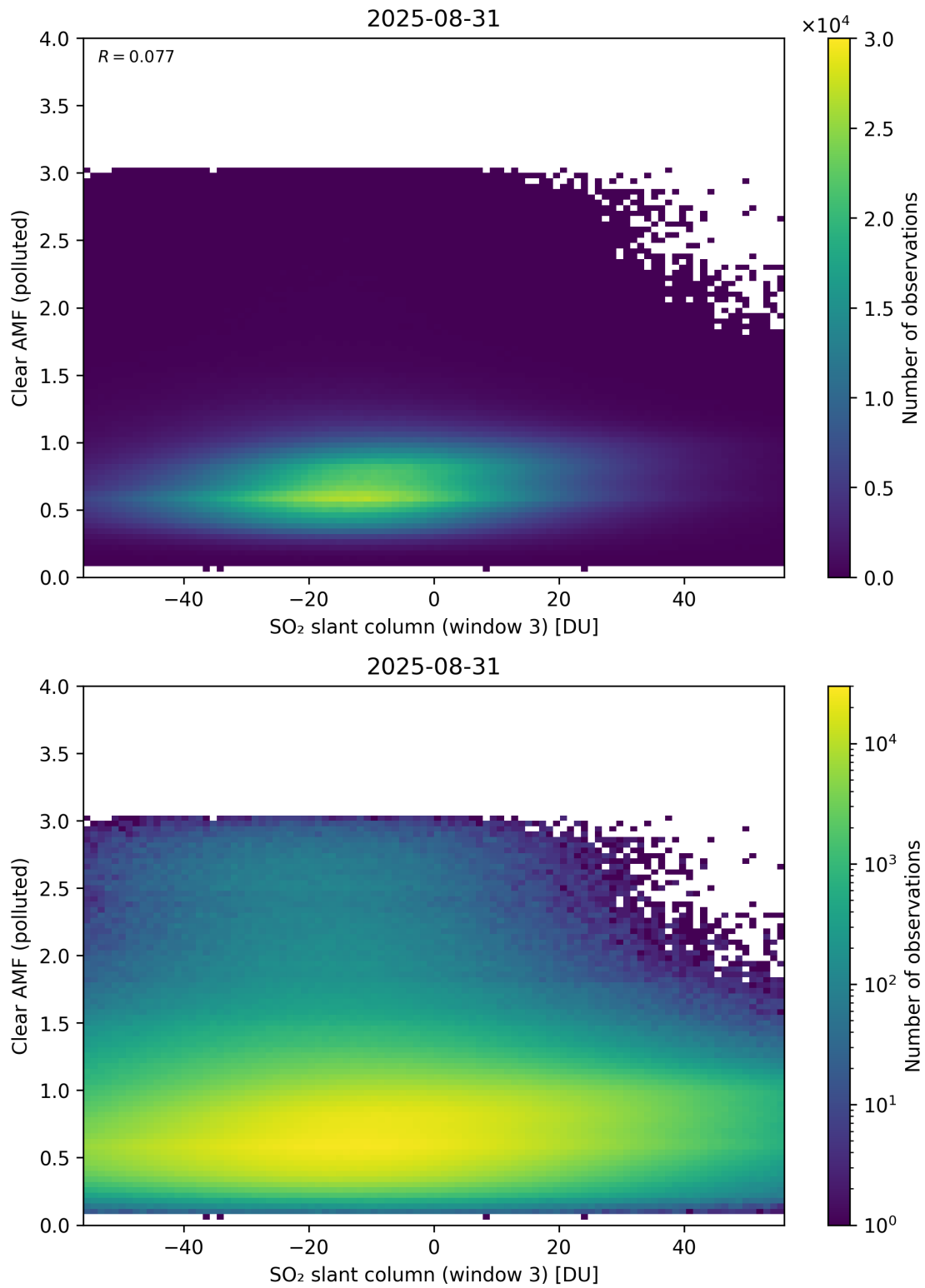
Figure 315: Scatter density plot of “SO 2 slant column (window 3)” against “Clear AMF (polluted)” for 2025-08-30 to 2025-09-01.
