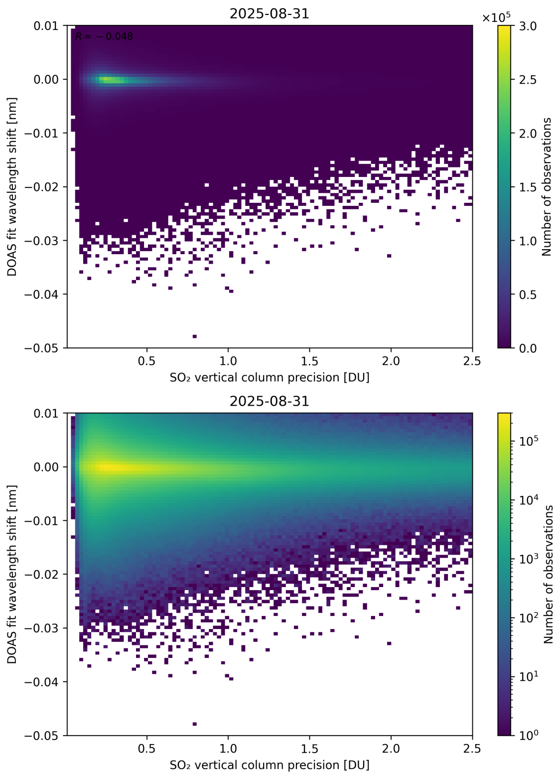
Figure 332: Scatter density plot of “SO 2 vertical column precision” against “DOAS fit wavelength shift” for 2025-08-30 to 2025-09-01.
