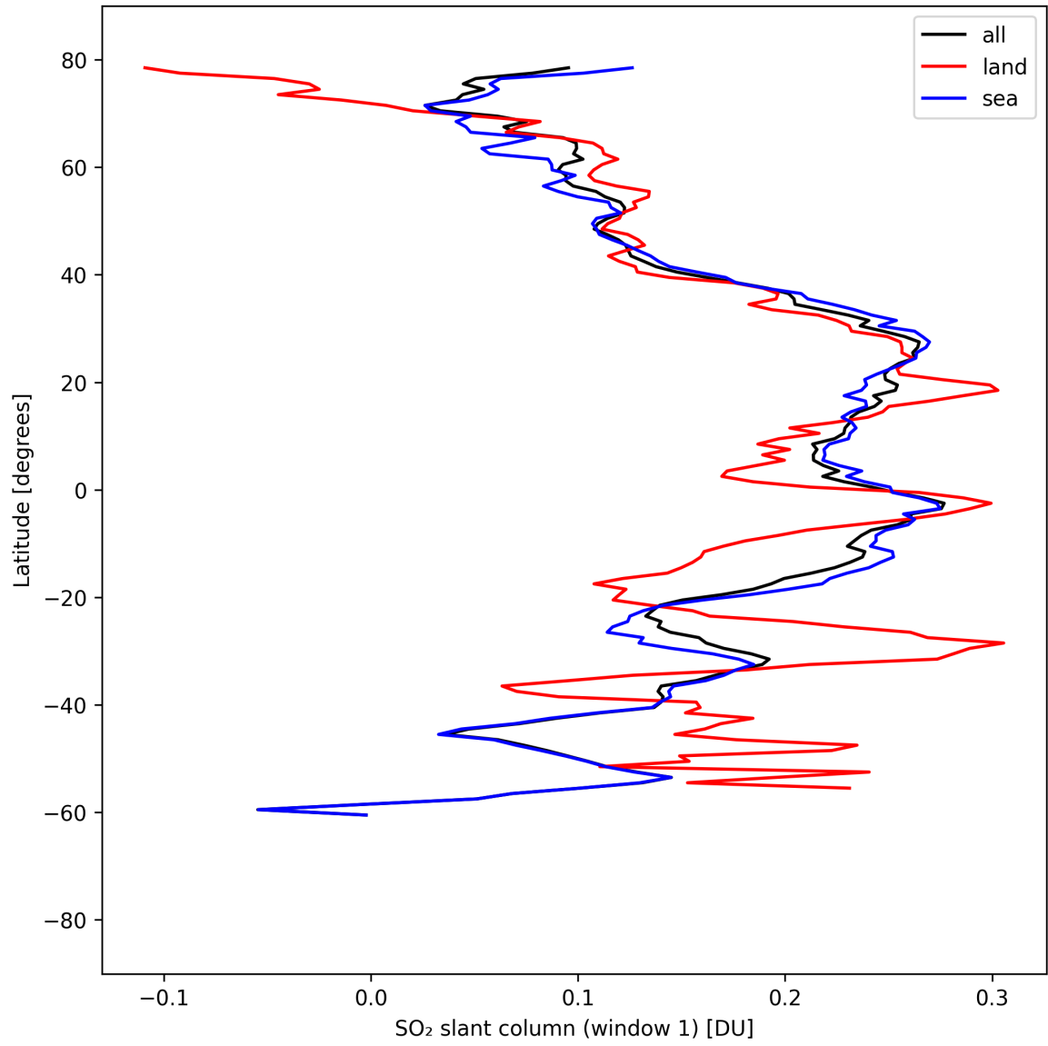
Figure 37: Zonal average of “SO 2 slant column (window 1)” for 2025-08-30 to 2025-09-01.
