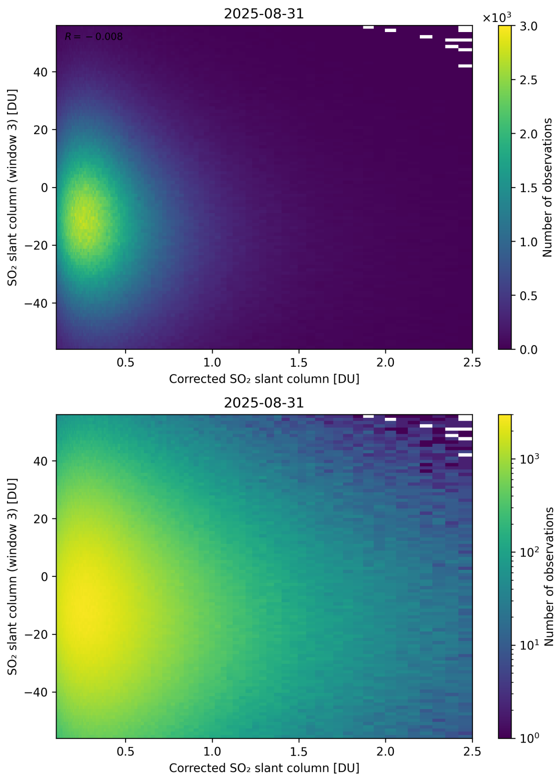
Figure 240: Scatter density plot of “Corrected SO 2 slant column” against “SO 2 slant column (window 3)” for 2025-08-30 to 2025-09-01.
