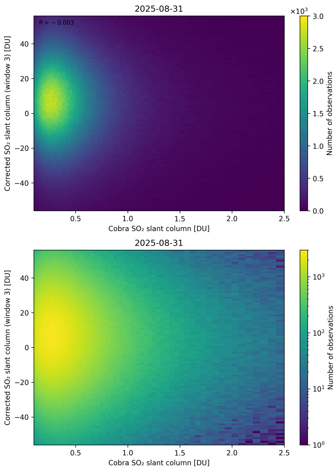
Figure 218: Scatter density plot of “Cobra SO 2 slant column” against “Corrected SO 2 slant column (window 3)” for 2025-08-30 to 2025-09-01.
