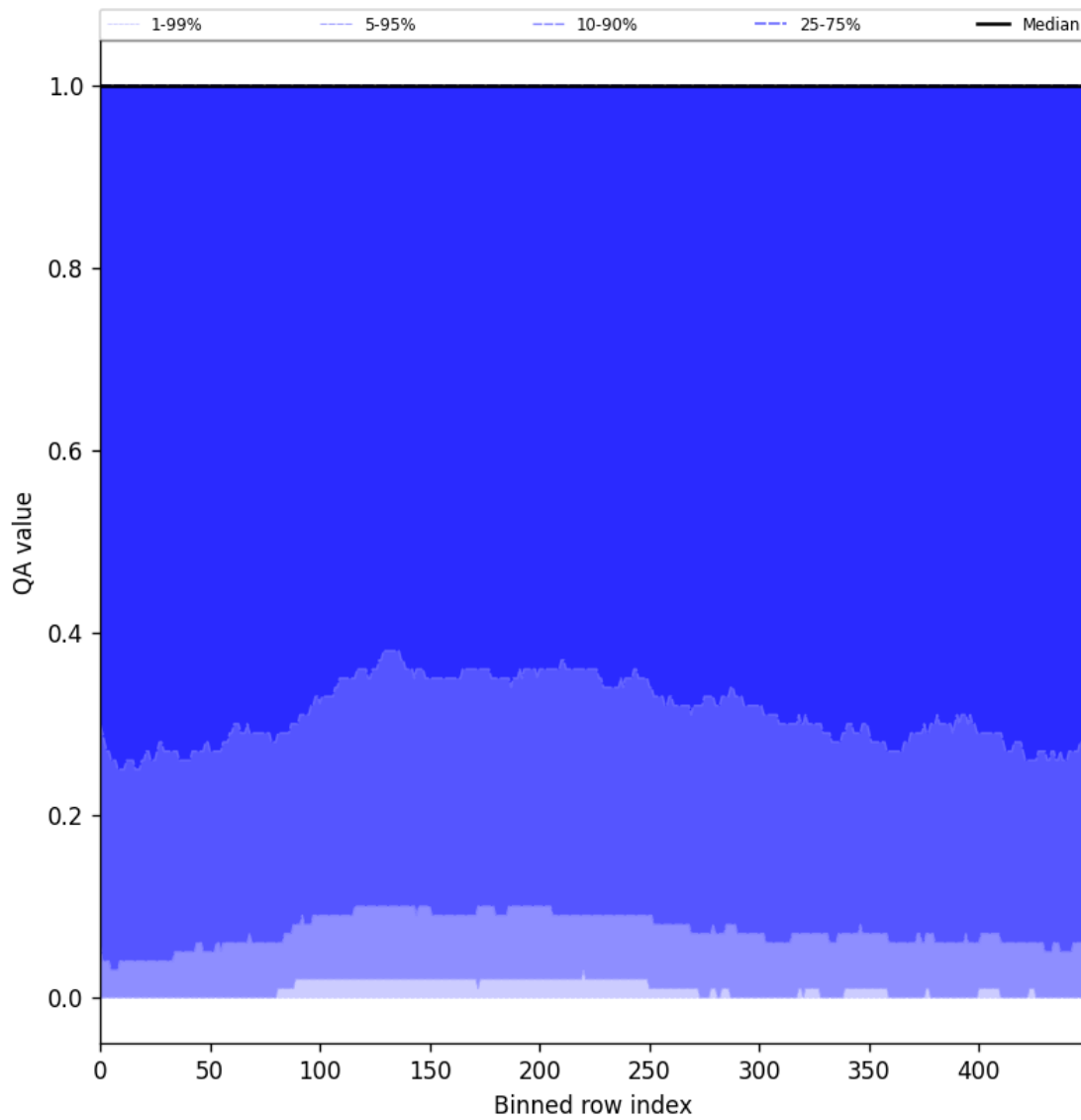
Figure 83: Along track statistics of “QA value” for 2025-08-30 to 2025-09-01
