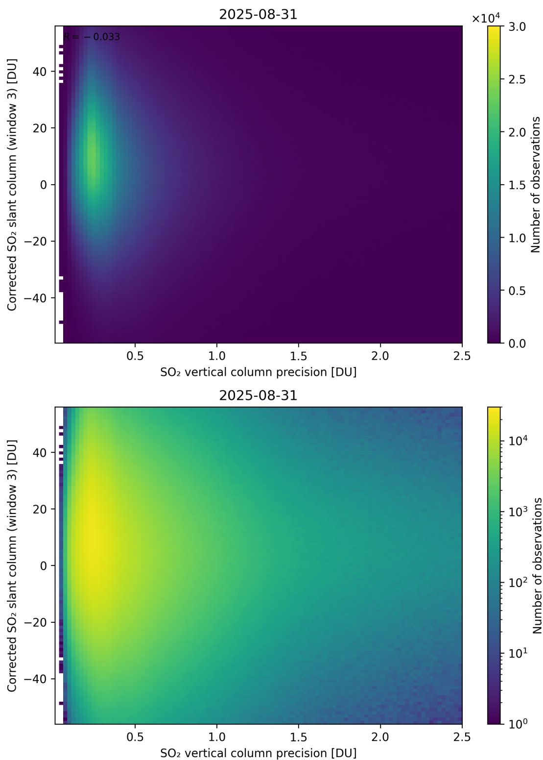
Figure 340: Scatter density plot of “SO 2 vertical column precision” against “Corrected SO 2 slant column (window 3)” for 2025-08-30 to 2025-09-01.
