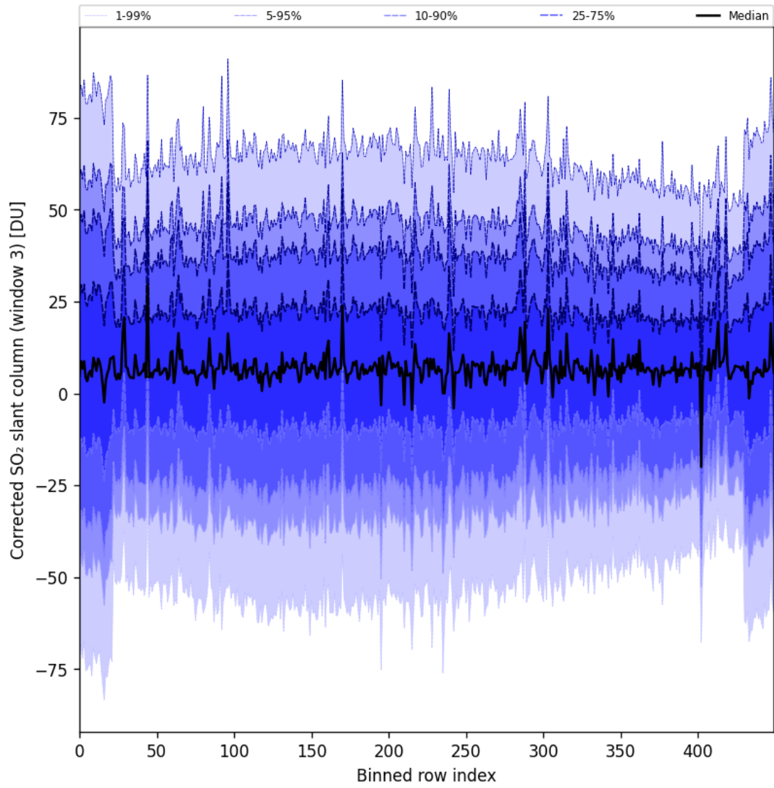
Figure 99: Along track statistics of “Corrected SO 2 slant column (window 3)” for 2025-08-30 to 2025-09-01
