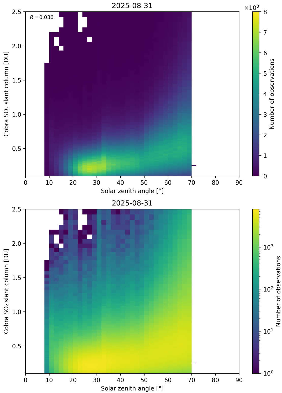
Figure 179: Scatter density plot of “Solar zenith angle” against “Cobra SO 2 slant column” for 2025-08-30 to 2025-09-01.
