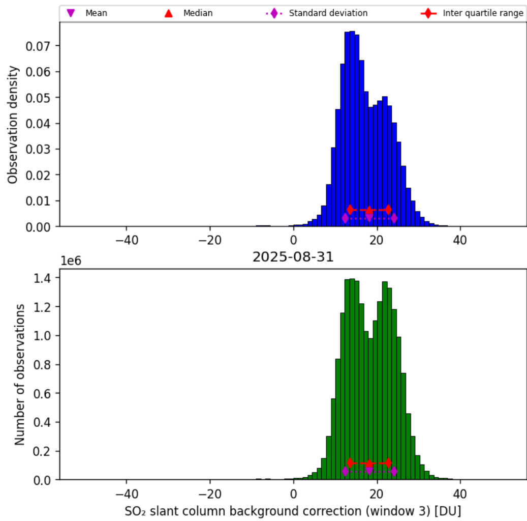
Figure 74: Histogram of “SO 2 slant column background correction (window 3)” for 2025-08-30 to 2025-09-01
