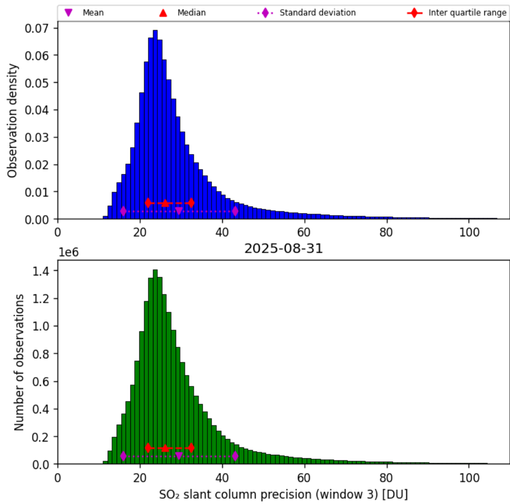
Figure 72: Histogram of “SO 2 slant column precision (window 3)” for 2025-08-30 to 2025-09-01
