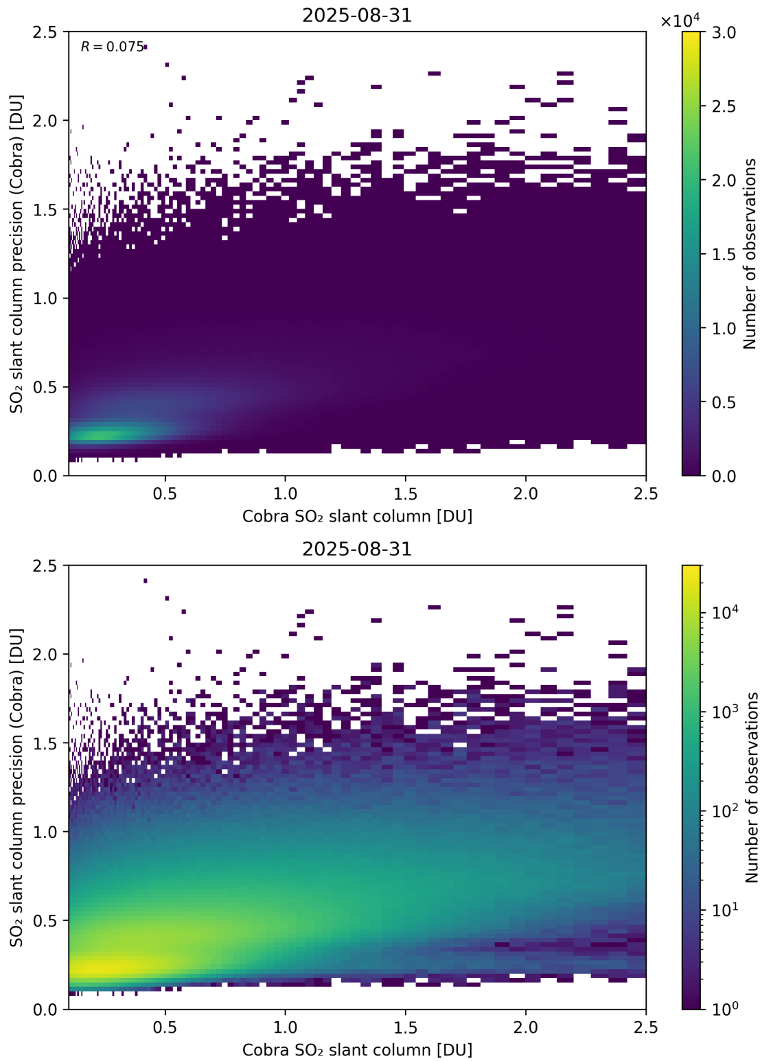
Figure 216: Scatter density plot of “Cobra SO 2 slant column” against “SO 2 slant column precision (Cobra)” for 2025-08-30 to 2025-09-01.
