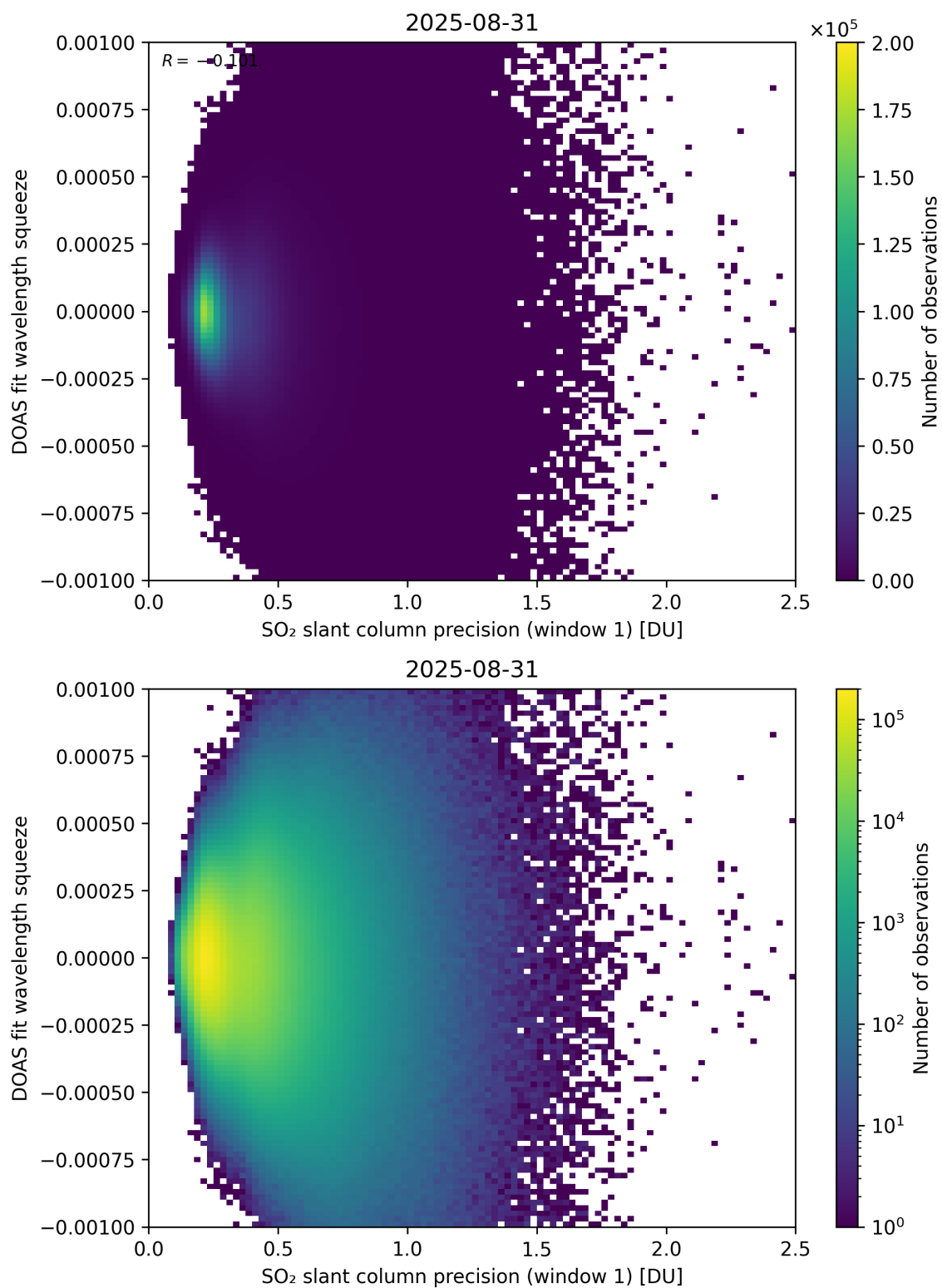
Figure 272: Scatter density plot of “SO 2 slant column precision (window 1)” against “DOAS fit wavelength squeeze” for 2025-08-30 to 2025-09-01.
