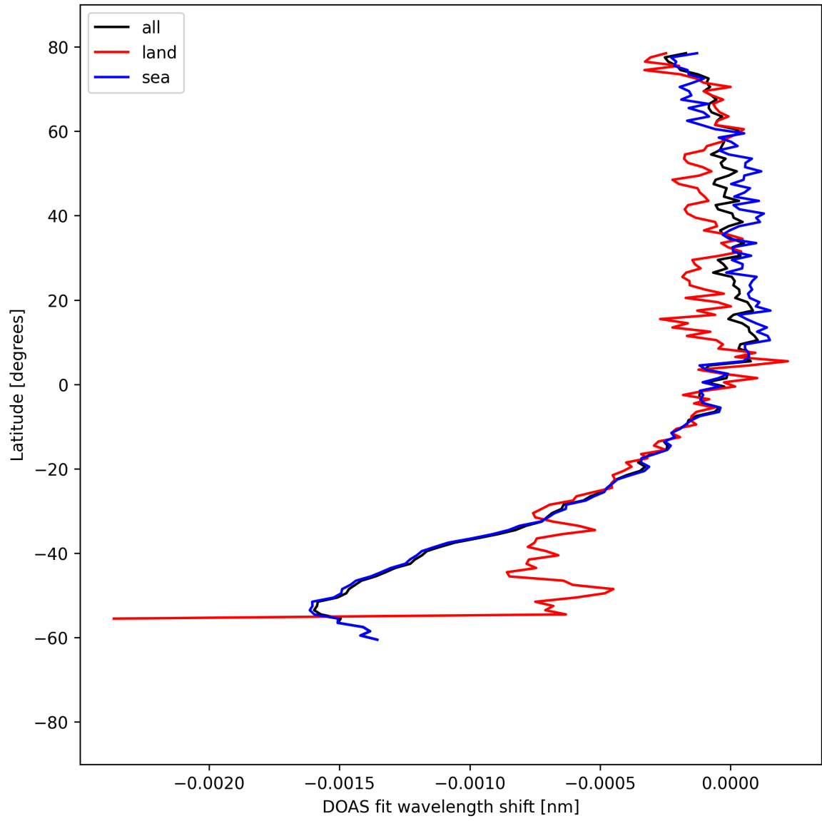
Figure 50: Zonal average of “DOAS fit wavelength shift” for 2025-08-30 to 2025-09-01.
