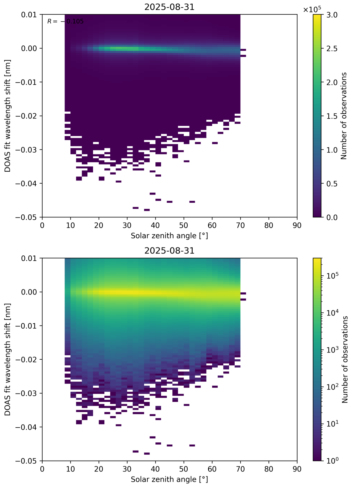
Figure 174: Scatter density plot of “Solar zenith angle” against “DOAS fit wavelength shift” for 2025-08-30 to 2025-09-01.
