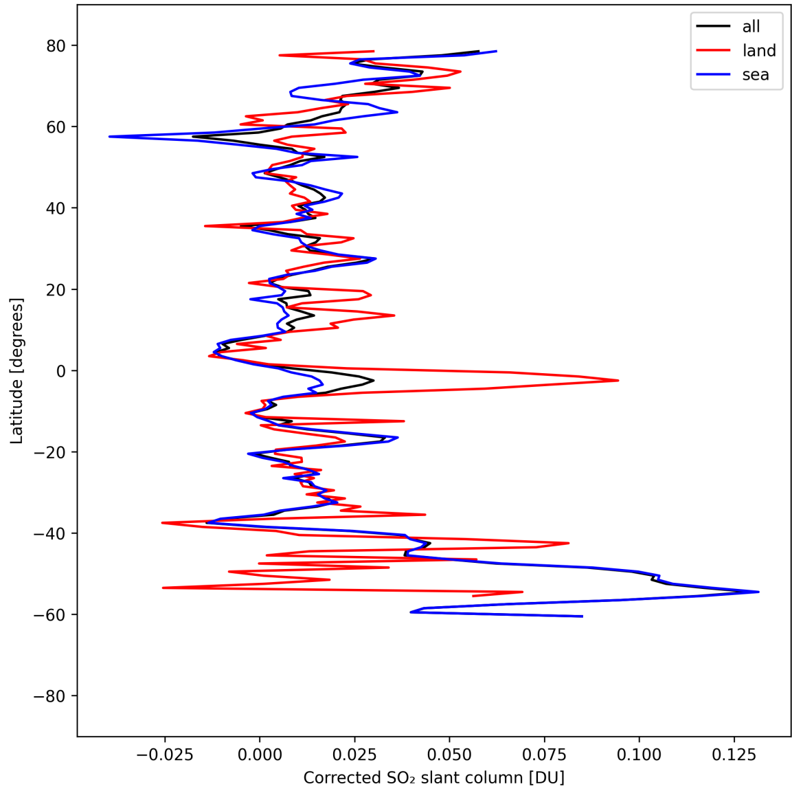
Figure 34: Zonal average of “Corrected SO 2 slant column” for 2025-08-30 to 2025-09-01.
