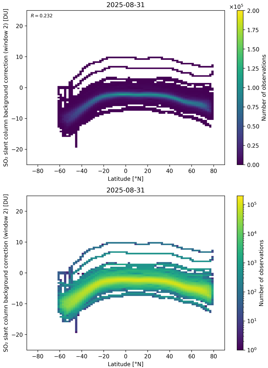
Figure 151: Scatter density plot of “Latitude” against “SO 2 slant column background correction (window 2)” for 2025-08-30 to 2025-09-01.
