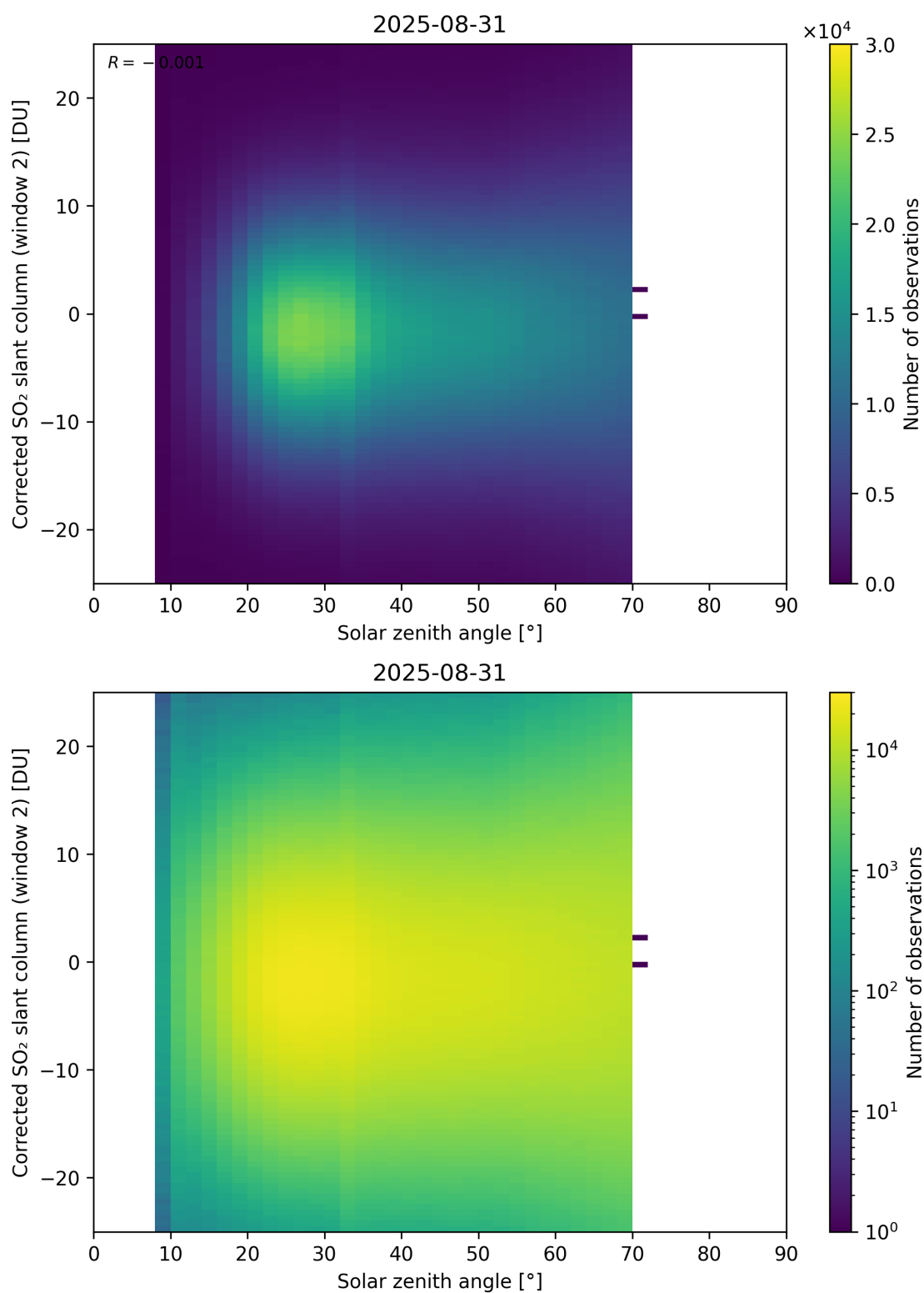
Figure 182: Scatter density plot of “Solar zenith angle” against “Corrected SO 2 slant column (window 2)” for 2025-08-30 to 2025-09-01.
