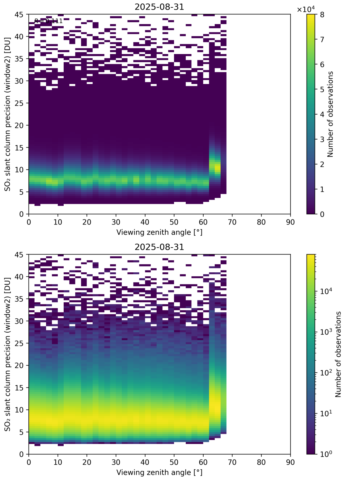
Figure 378: Scatter density plot of “Viewing zenith angle” against “SO 2 slant column precision (window2)” for 2025-08-30 to 2025-09-01.
