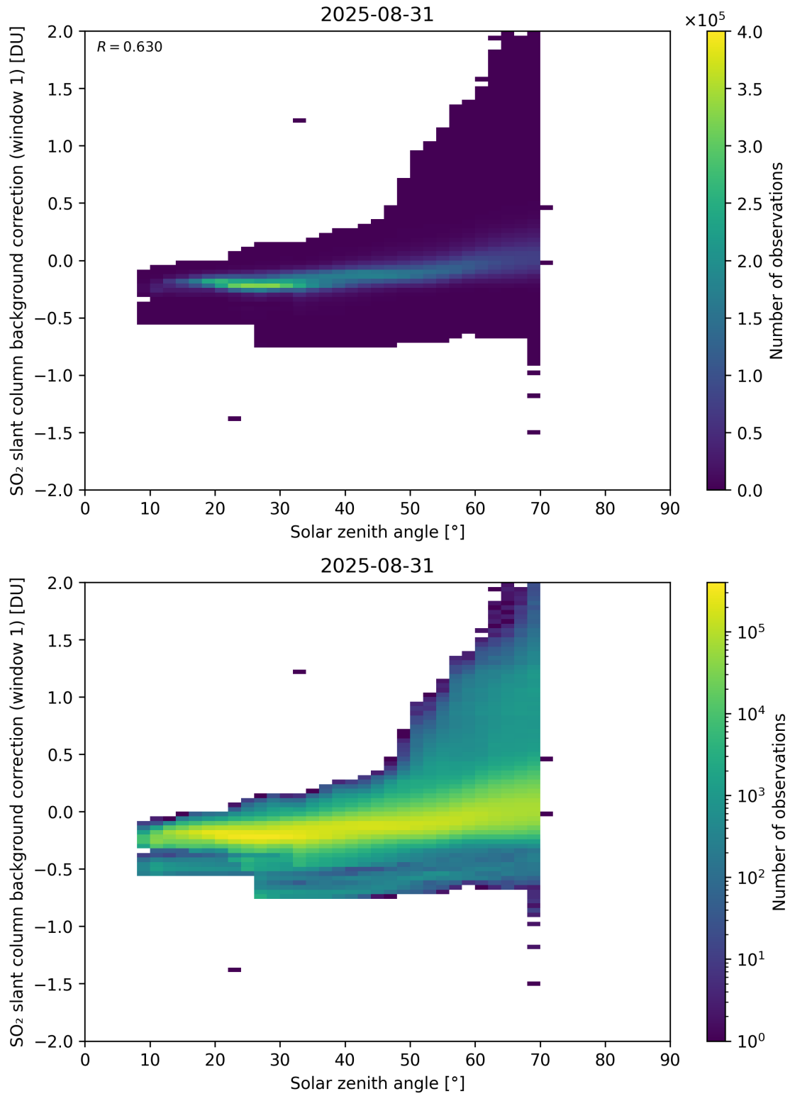
Figure 171: Scatter density plot of “Solar zenith angle” against “SO 2 slant column background correction (window 1)” for 2025-08-30 to 2025-09-01.
