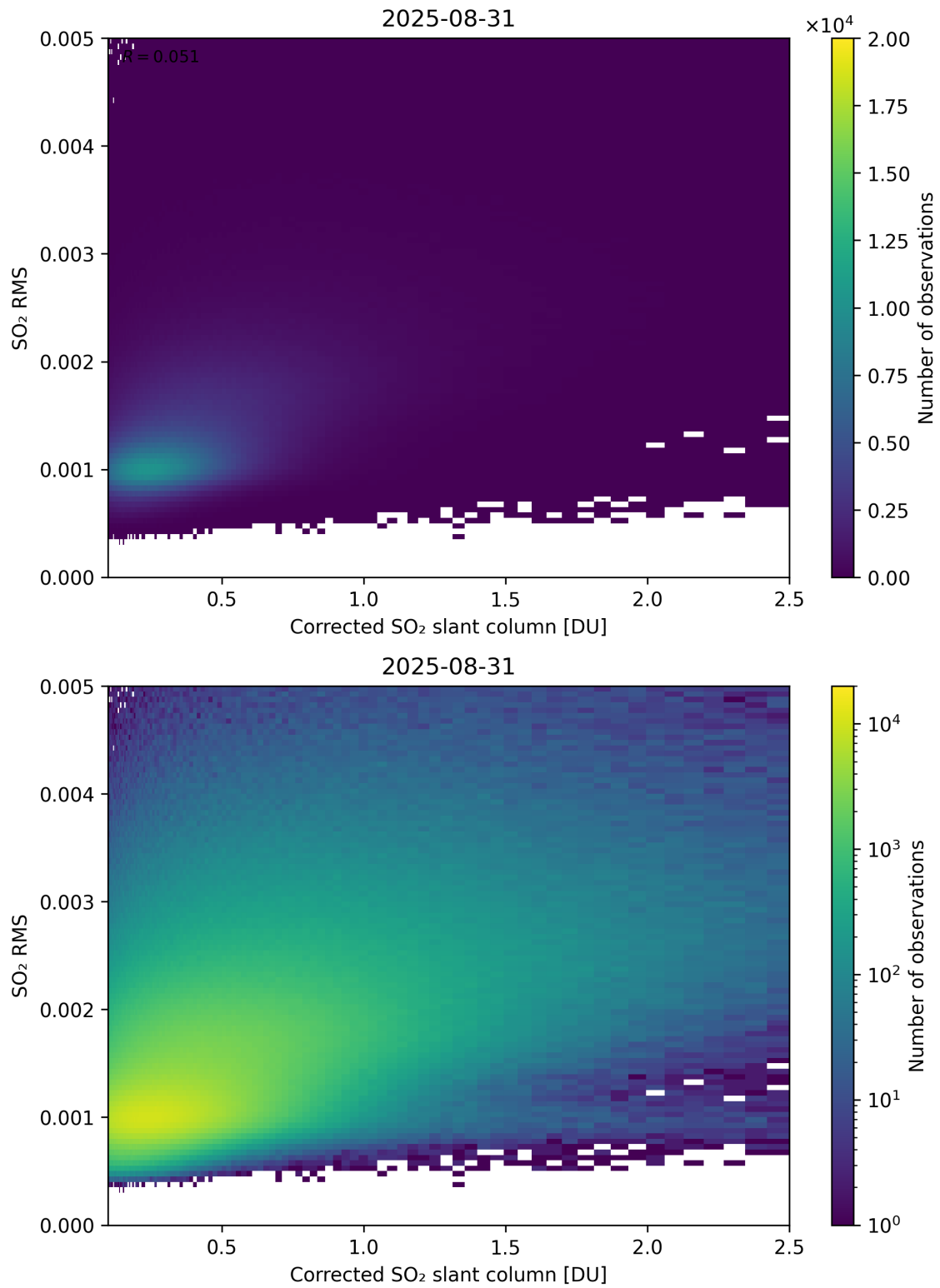
Figure 231: Scatter density plot of “Corrected SO 2 slant column” against “SO 2 RMS” for 2025-08-30 to 2025-09-01.
