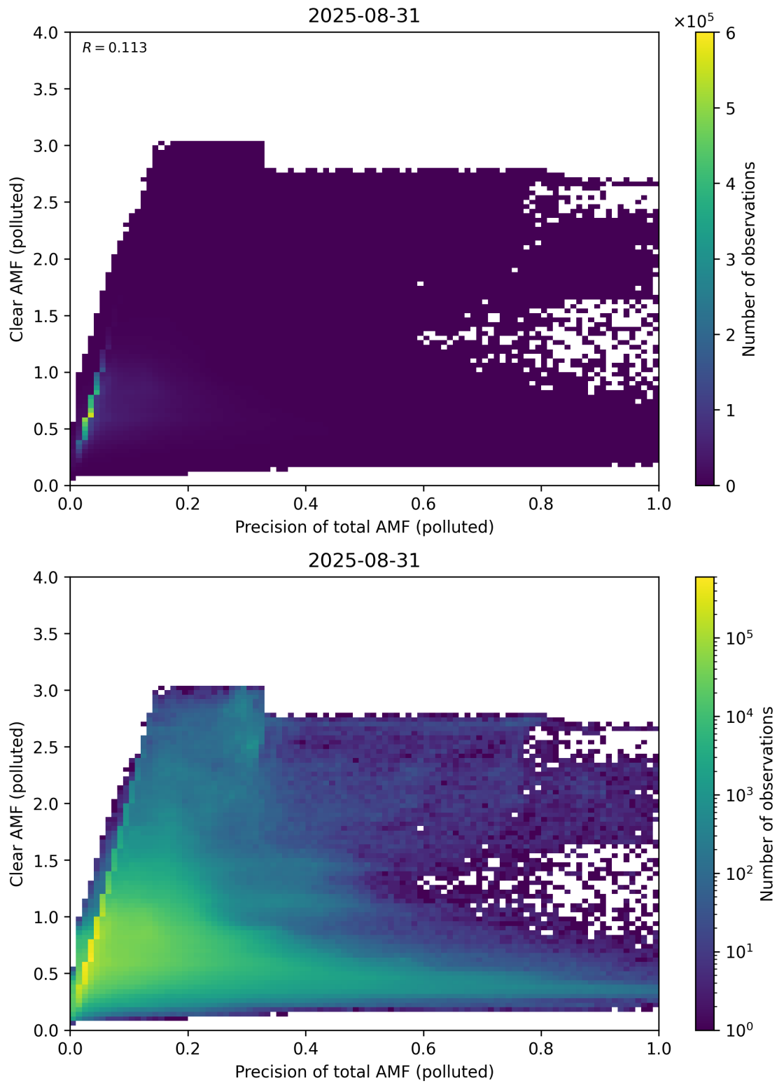
Figure 320: Scatter density plot of “Precision of total AMF (polluted)” against “Clear AMF (polluted)” for 2025-08-30 to 2025-09-01.
