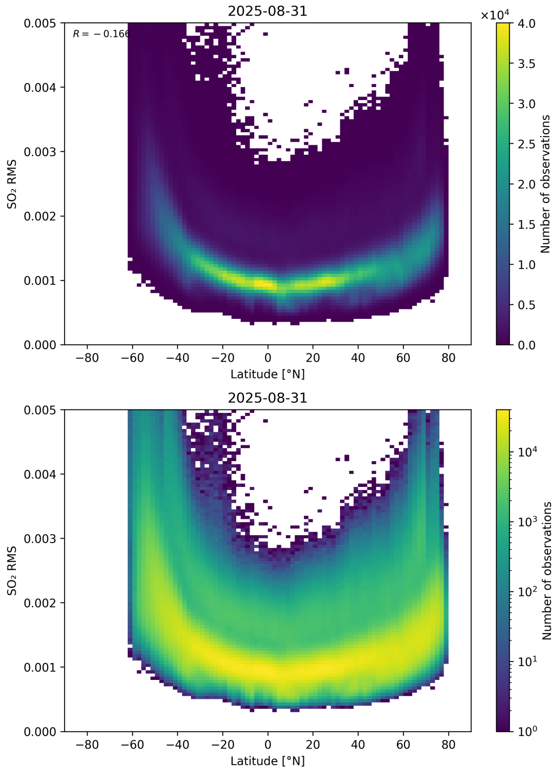
Figure 155: Scatter density plot of “Latitude” against “SO 2 RMS” for 2025-08-30 to 2025-09-01.
