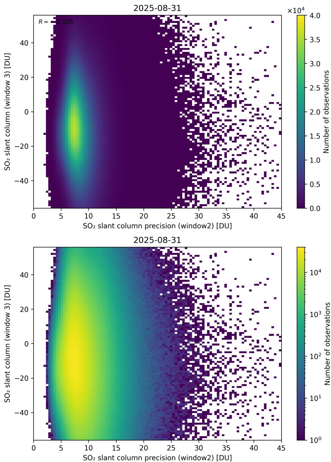
Figure 299: Scatter density plot of “SO 2 slant column precision (window2)” against “SO 2 slant column (window 3)” for 2025-08-30 to 2025-09-01.
