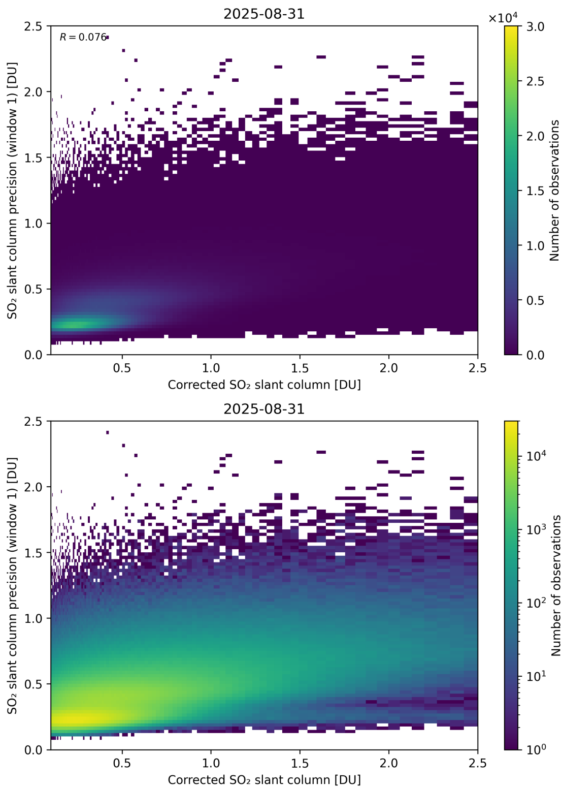
Figure 238: Scatter density plot of “Corrected SO 2 slant column” against “SO 2 slant column precision (window 1)” for 2025-08-30 to 2025-09-01.
