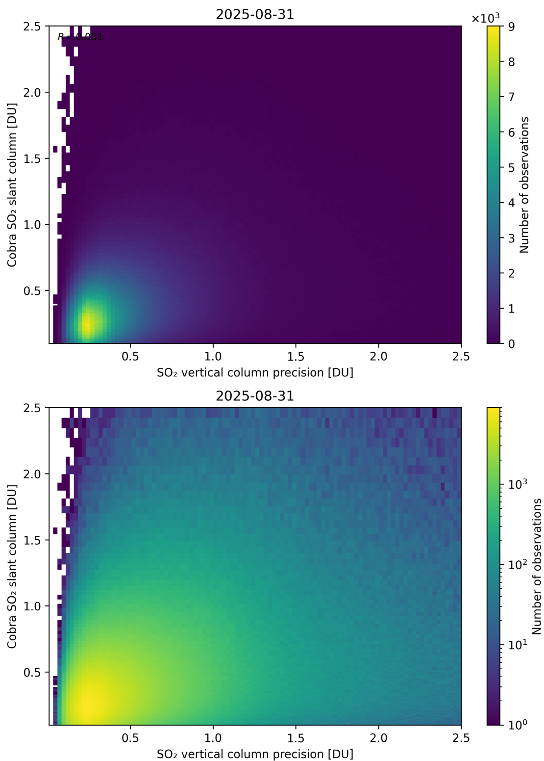
Figure 336: Scatter density plot of “SO 2 vertical column precision” against “Cobra SO 2 slant column” for 2025-08-30 to 2025-09-01.
