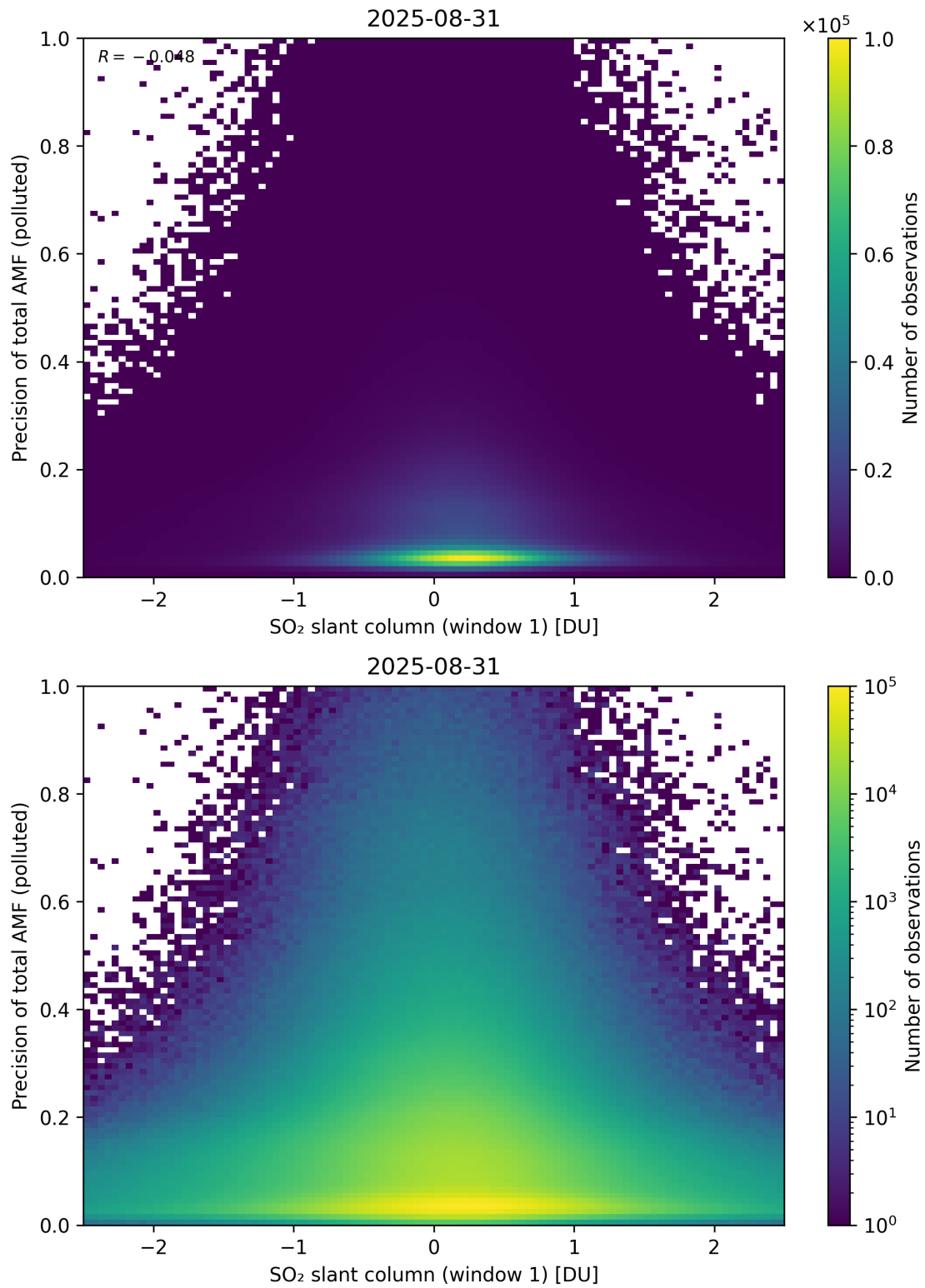
Figure 290: Scatter density plot of “SO 2 slant column (window 1)” against “Precision of total AMF (polluted)” for 2025-08-30 to 2025-09-01.
