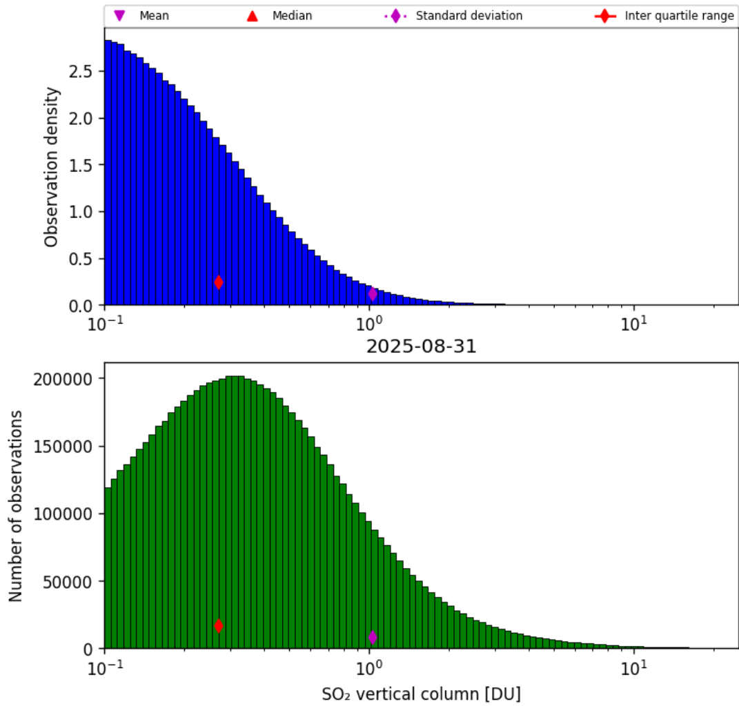
Figure 58: Histogram of “SO 2 vertical column” for 2025-08-30 to 2025-09-01
