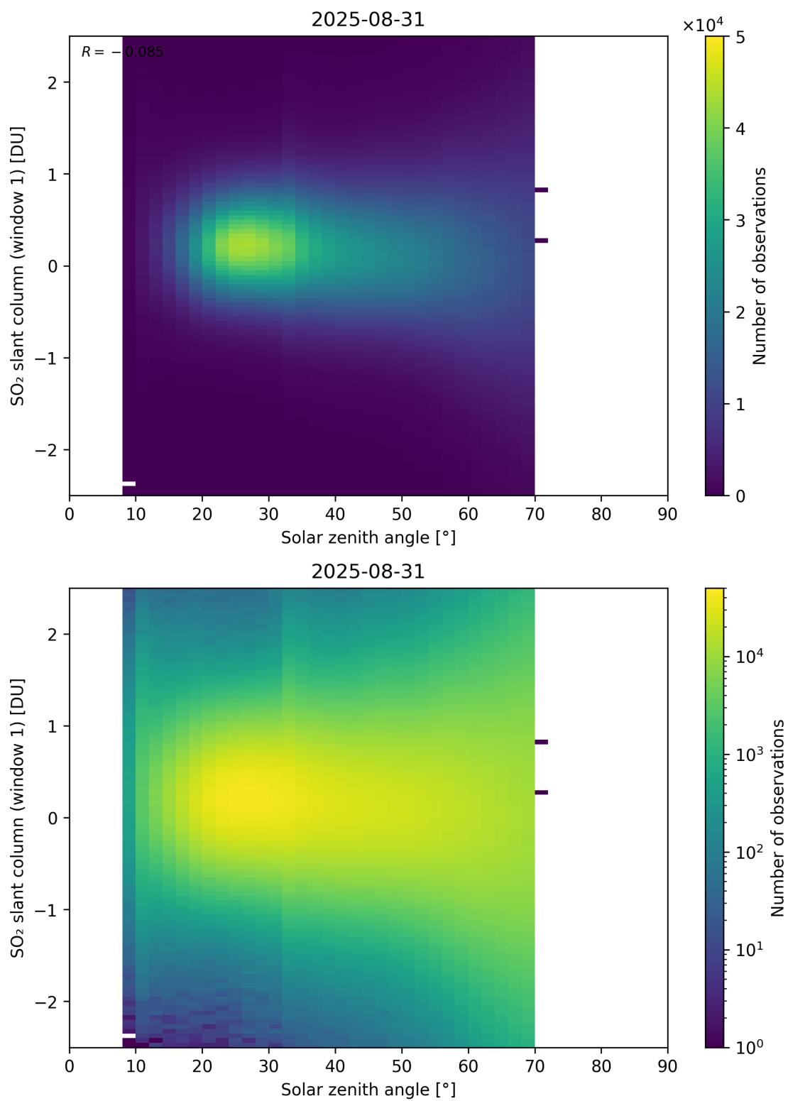
Figure 184: Scatter density plot of “Solar zenith angle” against “SO 2 slant column (window 1)” for 2025-08-30 to 2025-09-01.
