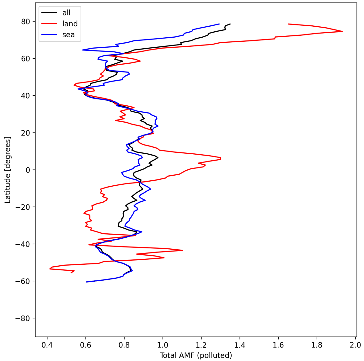
Figure 53: Zonal average of “Total AMF (polluted)” for 2025-08-30 to 2025-09-01.
