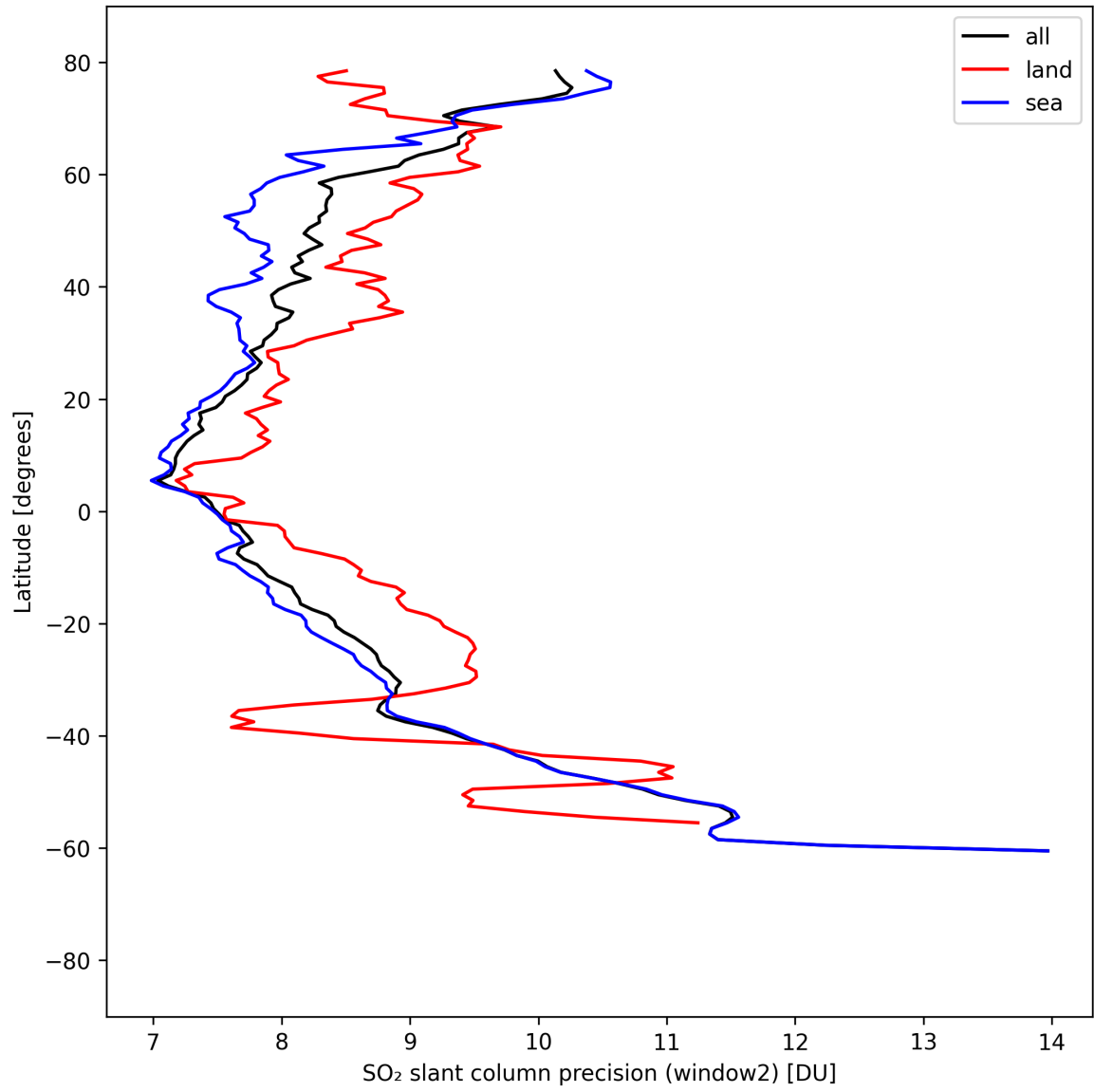
Figure 42: Zonal average of “SO 2 slant column precision (window2)” for 2025-08-30 to 2025-09-01.
