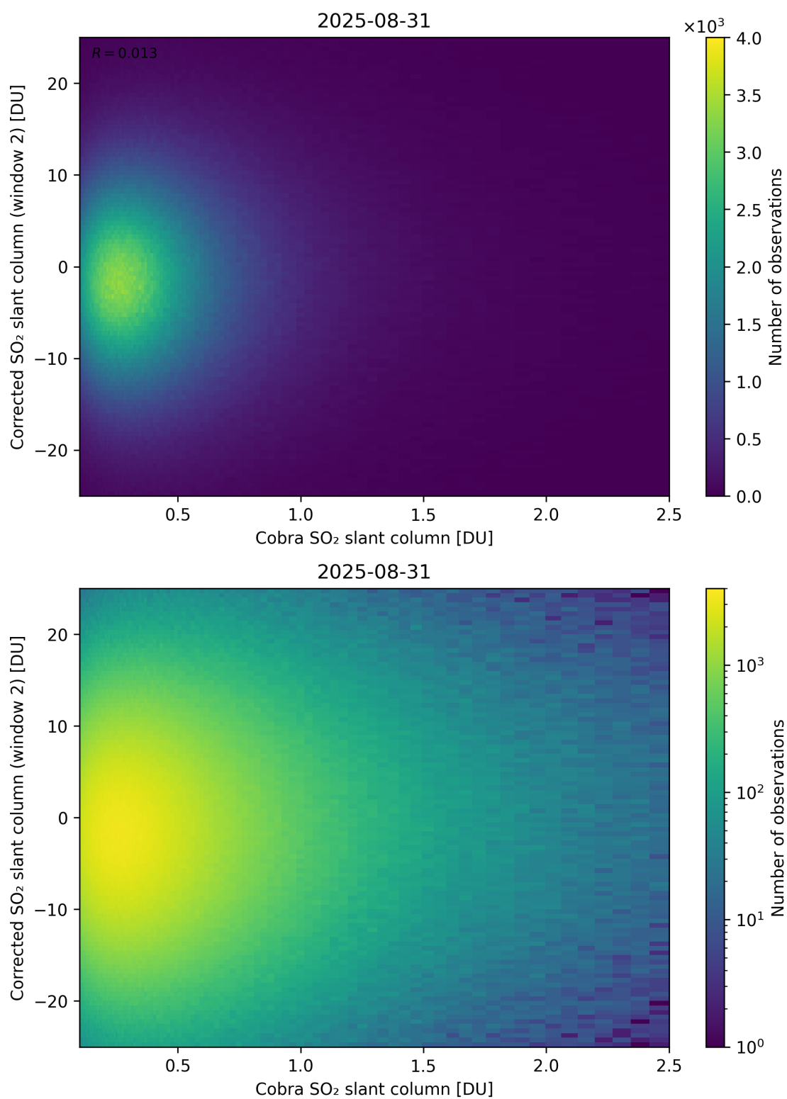
Figure 217: Scatter density plot of “Cobra SO 2 slant column” against “Corrected SO 2 slant column (window 2)” for 2025-08-30 to 2025-09-01.
