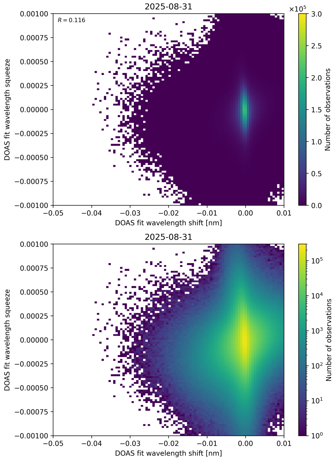
Figure 138: Scatter density plot of “DOAS fit wavelength shift” against “DOAS fit wavelength squeeze” for 2025-08-30 to 2025-09-01.
