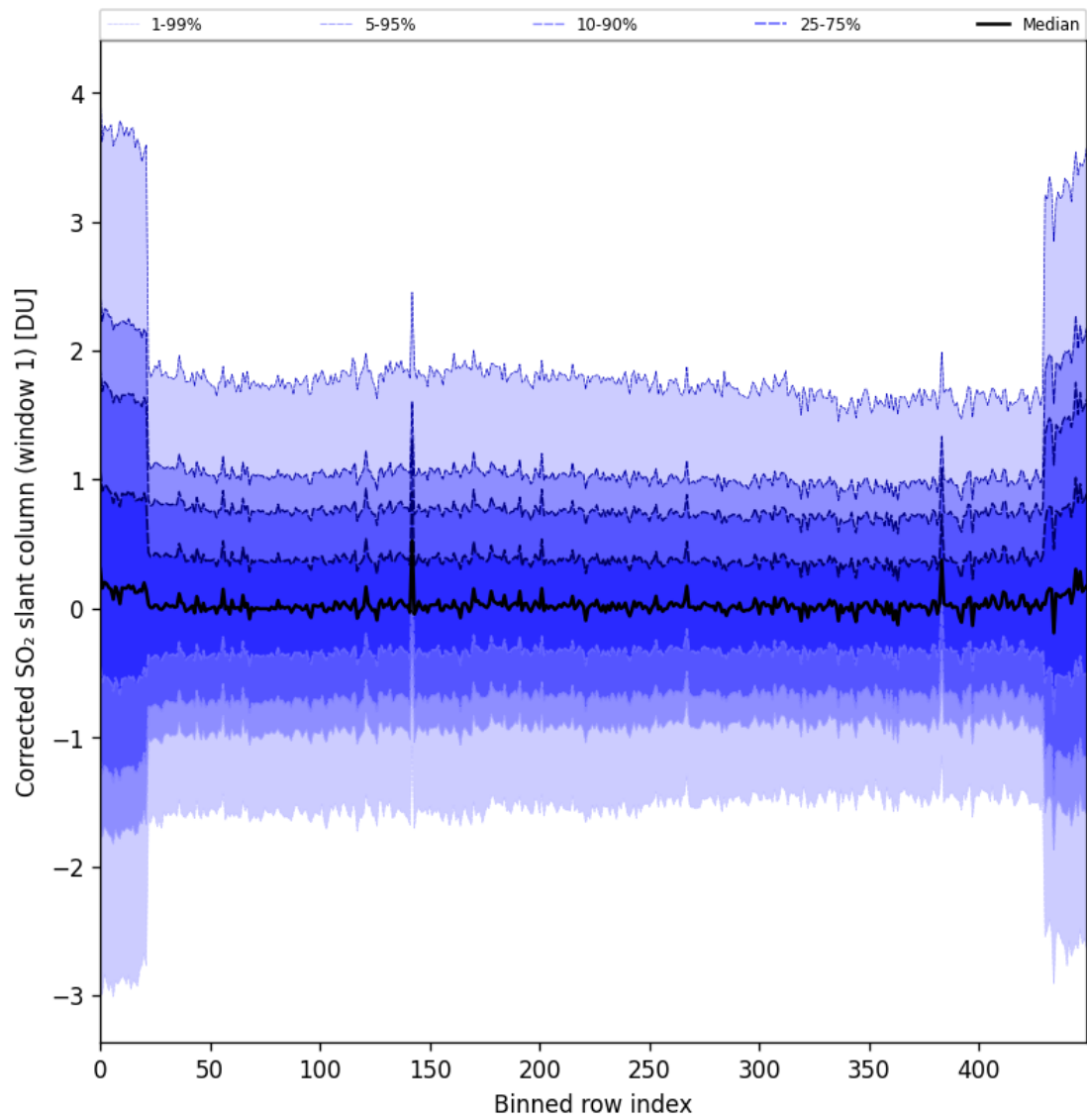
Figure 91: Along track statistics of “Corrected SO 2 slant column (window 1)” for 2025-08-30 to 2025-09-01
