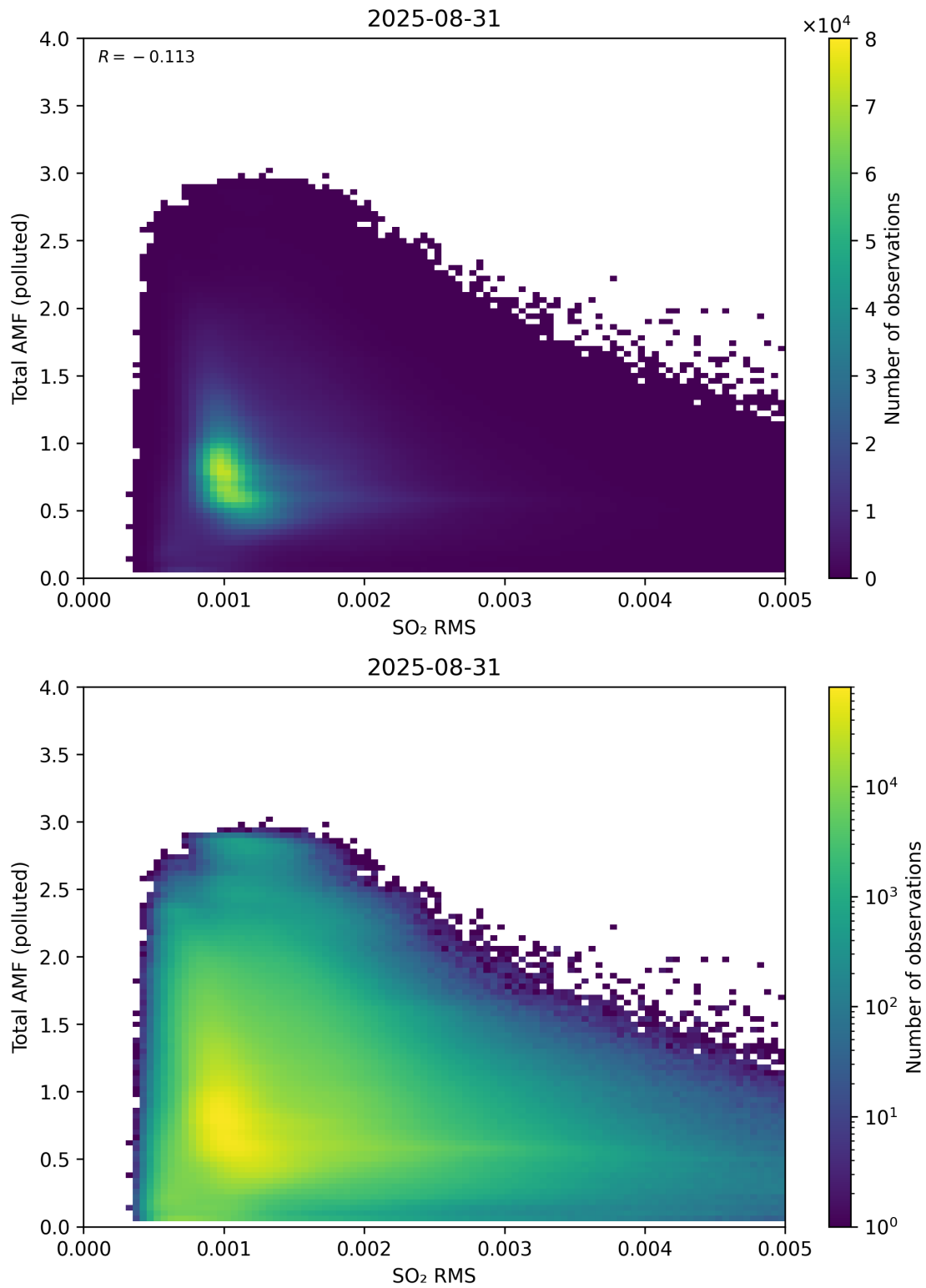
Figure 148: Scatter density plot of “SO 2 RMS” against “Total AMF (polluted)” for 2025-08-30 to 2025-09-01.
