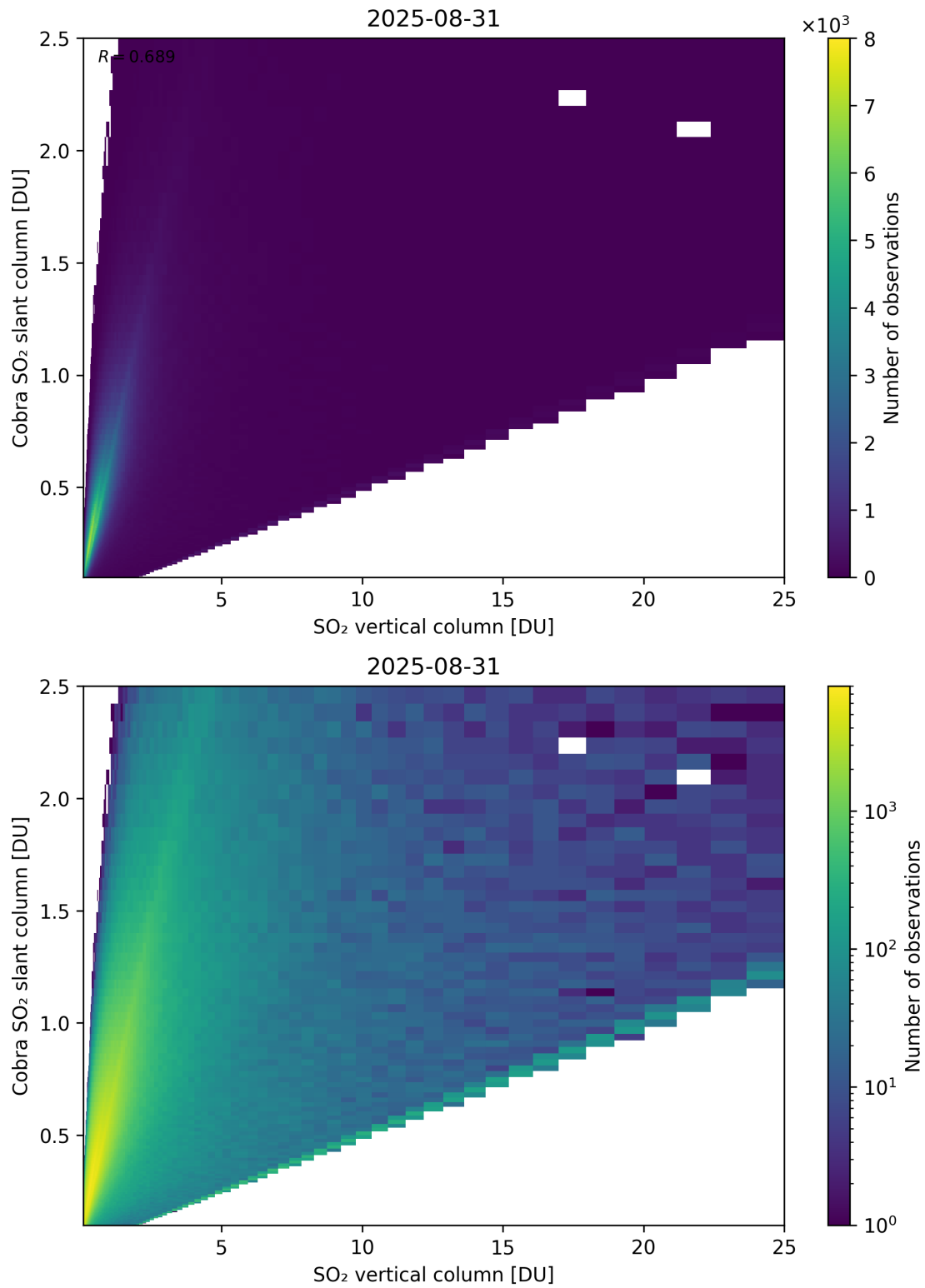
Figure 349: Scatter density plot of “SO 2 vertical column” against “Cobra SO 2 slant column” for 2025-08-30 to 2025-09-01.
