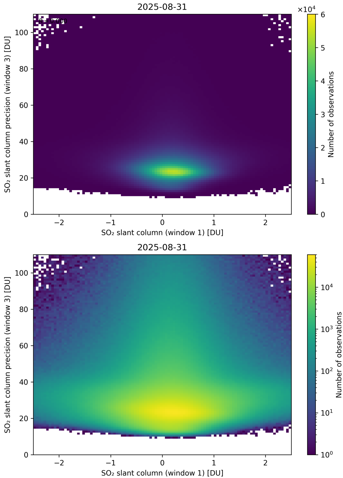
Figure 288: Scatter density plot of “SO 2 slant column (window 1)” against “SO 2 slant column precision (window 3)” for 2025-08-30 to 2025-09-01.
