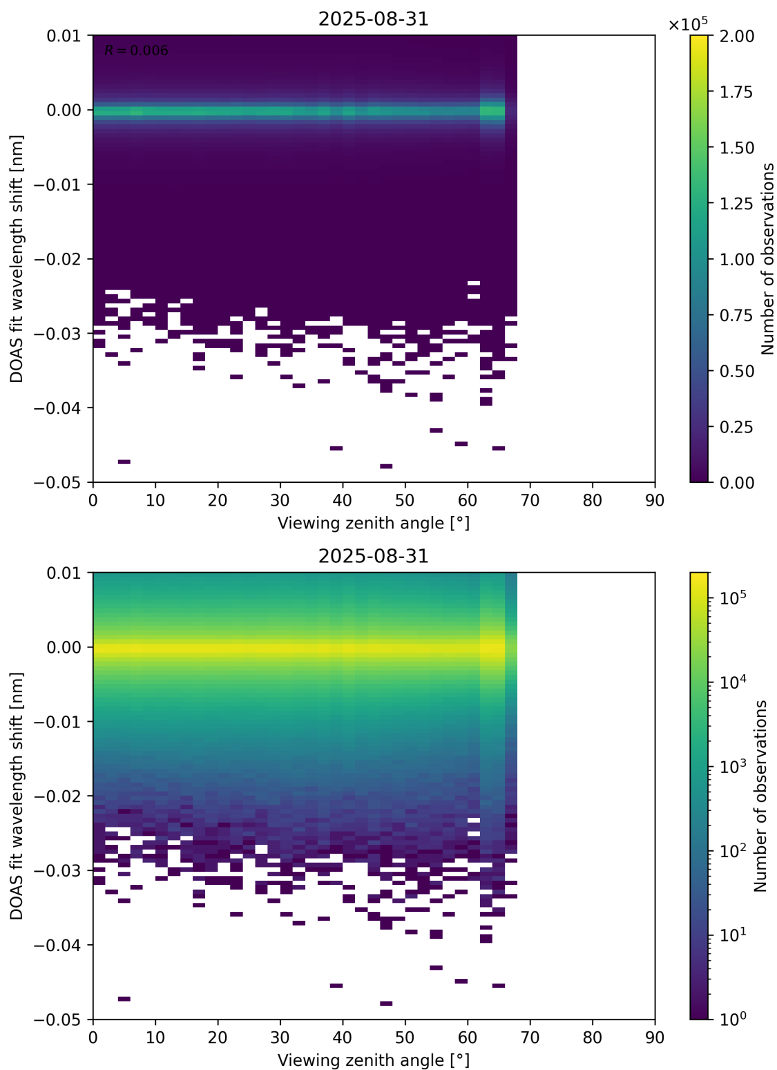
Figure 365: Scatter density plot of “Viewing zenith angle” against “DOAS fit wavelength shift” for 2025-08-30 to 2025-09-01.
