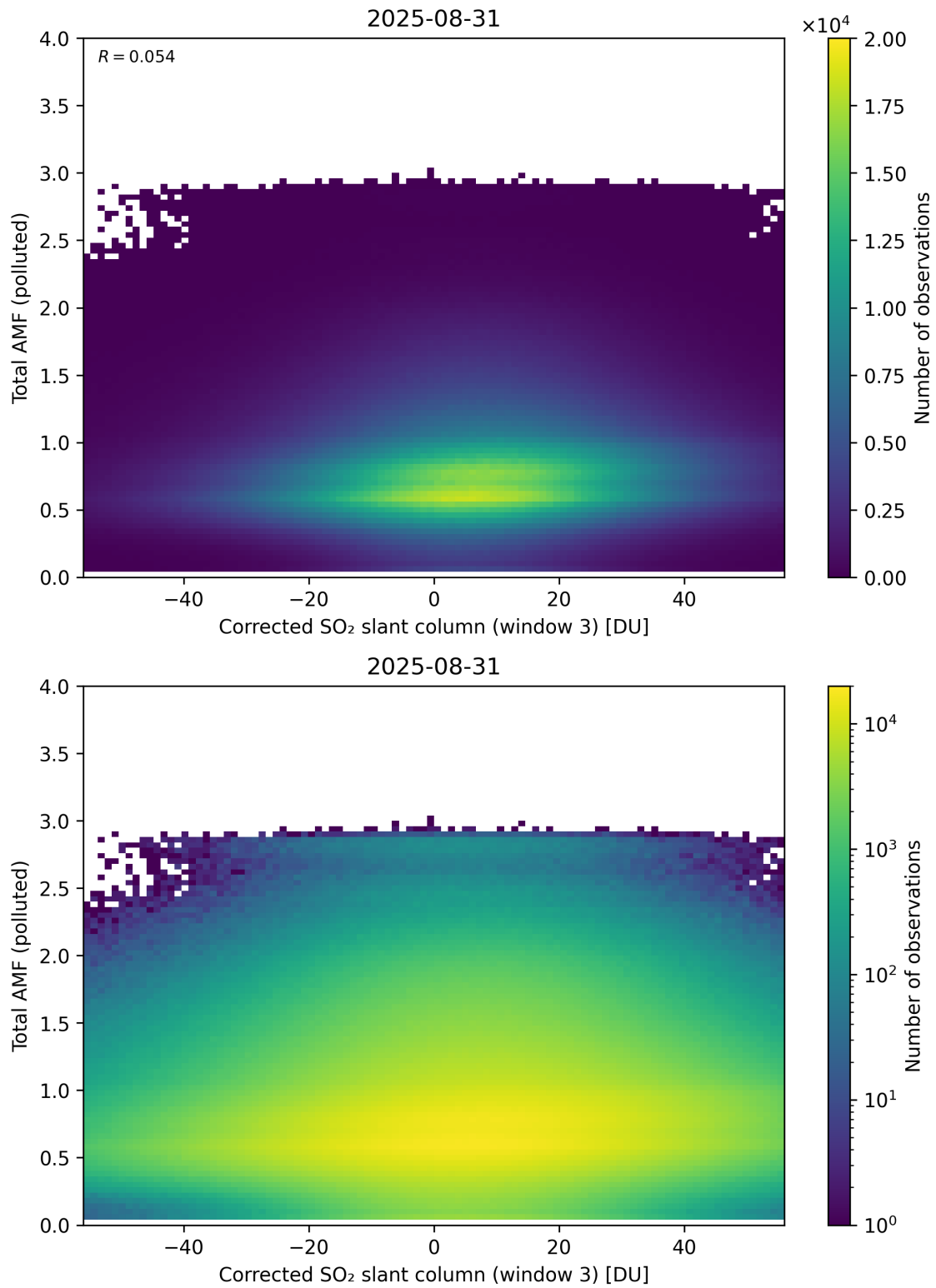
Figure 260: Scatter density plot of “Corrected SO 2 slant column (window 3)” against “Total AMF (polluted)” for 2025-08-30 to 2025-09-01.
