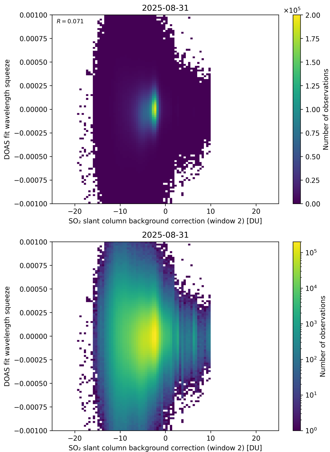
Figure 124: Scatter density plot of “SO 2 slant column background correction (window 2)” against “DOAS fit wavelength squeeze” for 2025-08-30 to 2025-09-01.
