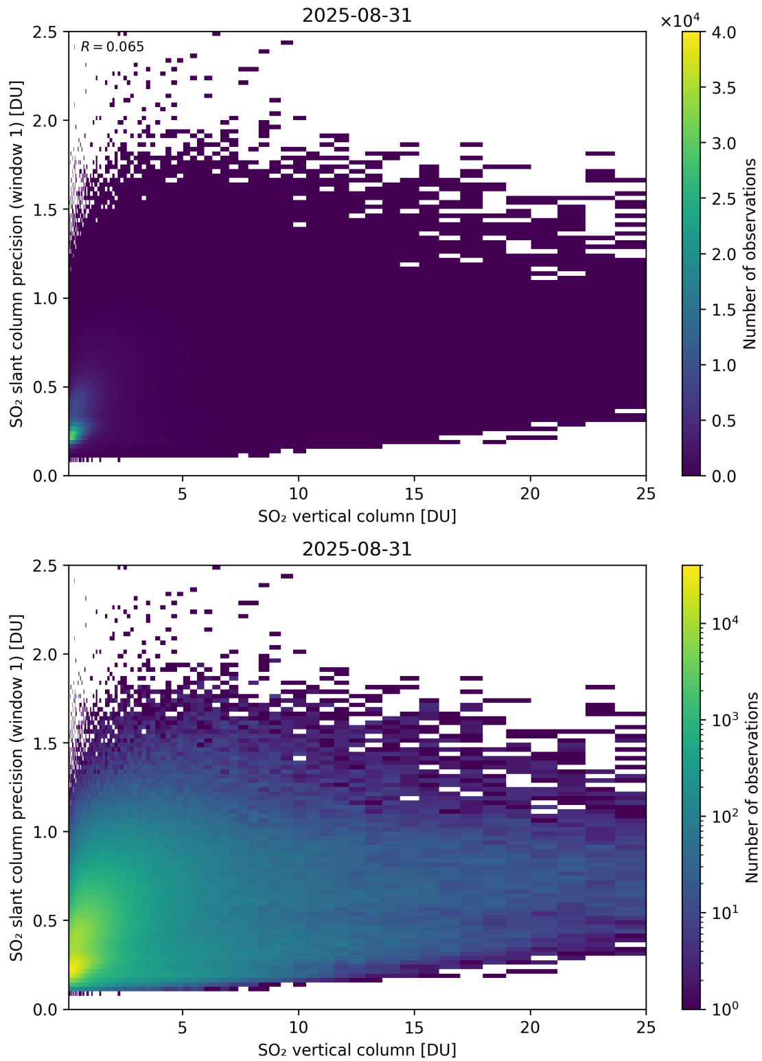
Figure 355: Scatter density plot of “SO 2 vertical column” against “SO 2 slant column precision (window 1)” for 2025-08-30 to 2025-09-01.
