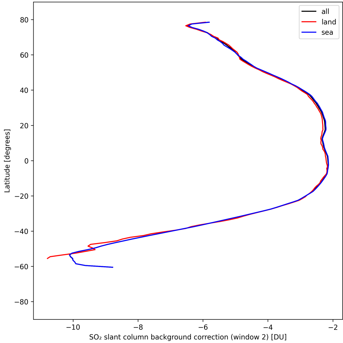
Figure 44: Zonal average of “SO 2 slant column background correction (window 2)” for 2025-08-30 to 2025-09-01.
