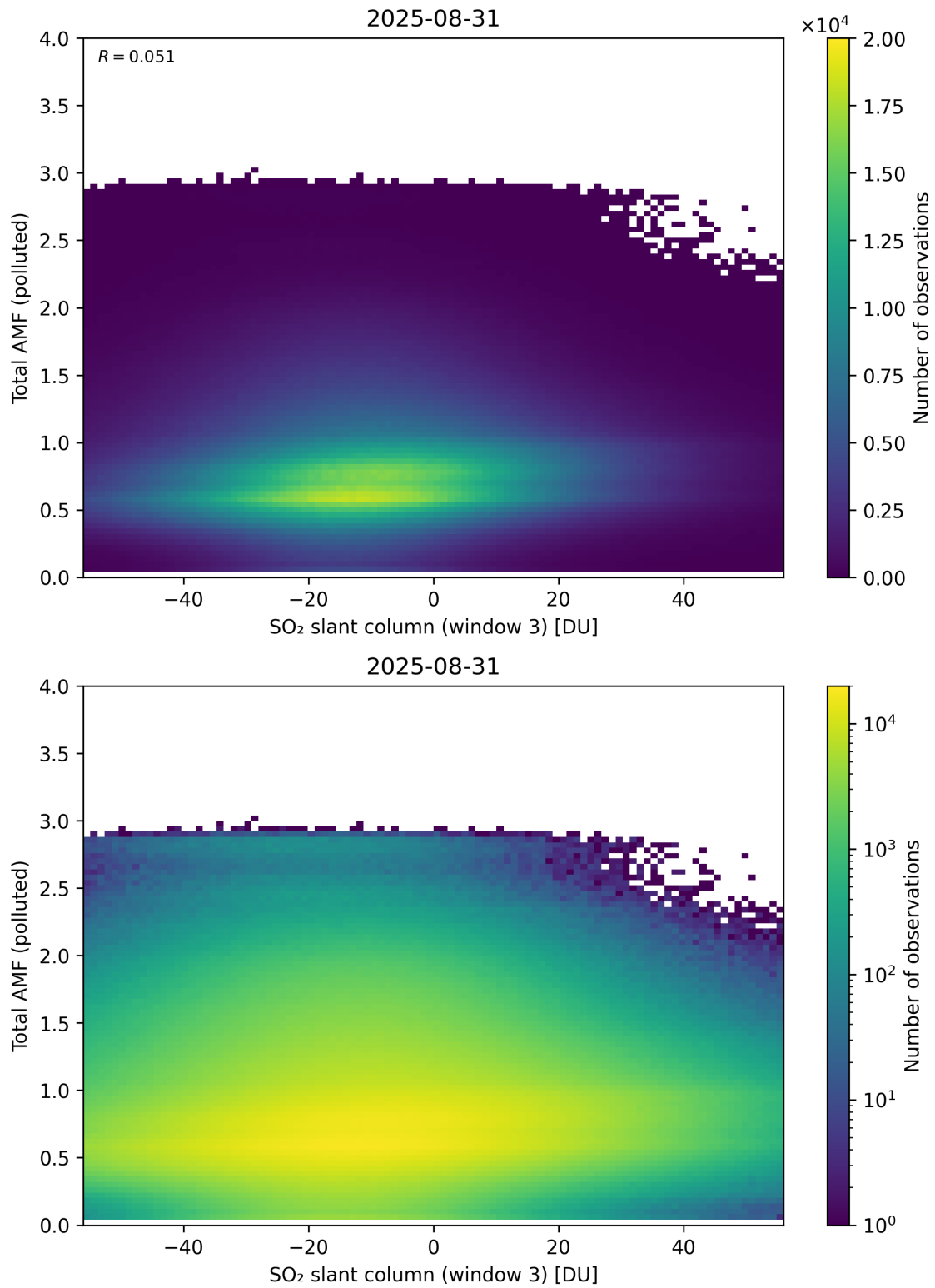
Figure 318: Scatter density plot of “SO 2 slant column (window 3)” against “Total AMF (polluted)” for 2025-08-30 to 2025-09-01.
