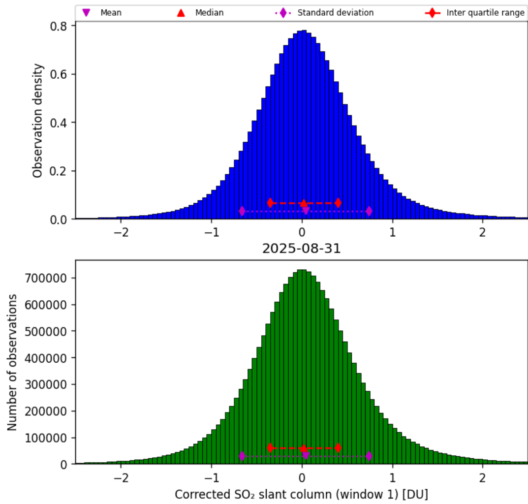
Figure 65: Histogram of “Corrected SO 2 slant column (window 1)” for 2025-08-30 to 2025-09-01
