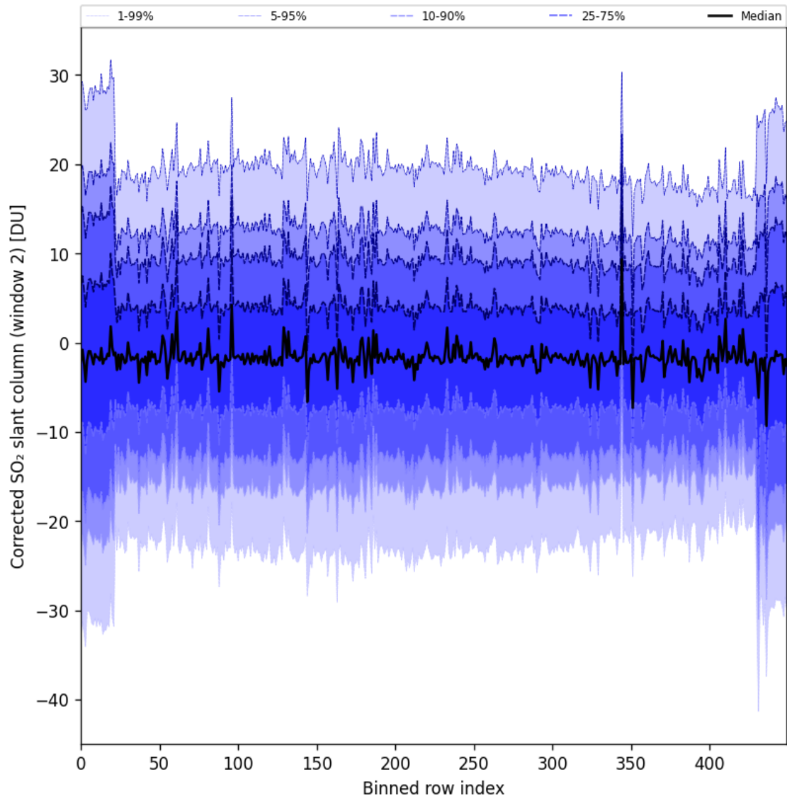
Figure 95: Along track statistics of “Corrected SO 2 slant column (window 2)” for 2025-08-30 to 2025-09-01
