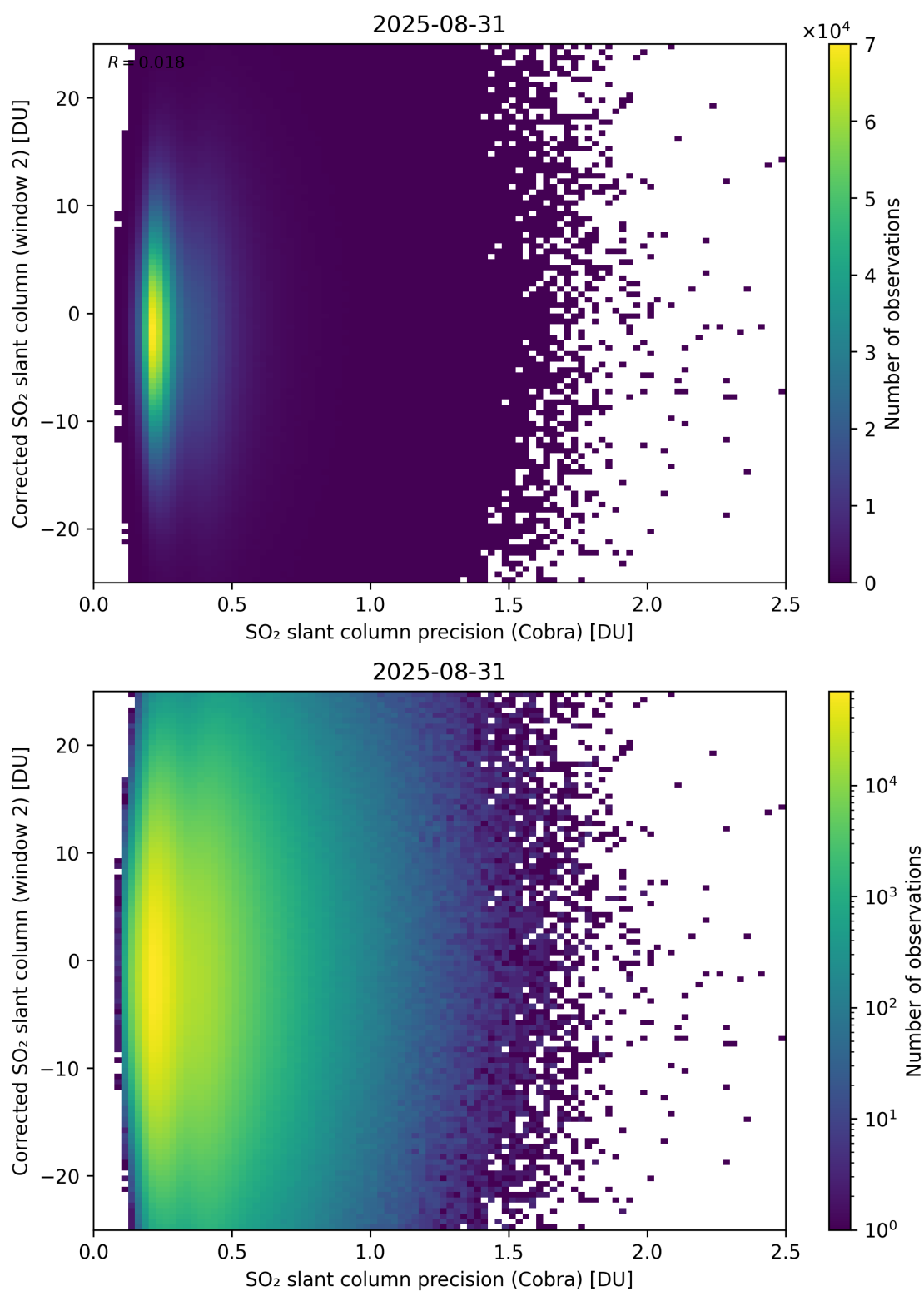
Figure 206: Scatter density plot of “SO 2 slant column precision (Cobra)” against “Corrected SO 2 slant column (window 2)” for 2025-08-30 to 2025-09-01.
