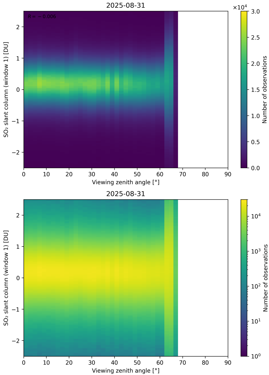
Figure 376: Scatter density plot of “Viewing zenith angle” against “SO 2 slant column (window 1)” for 2025-08-30 to 2025-09-01.
