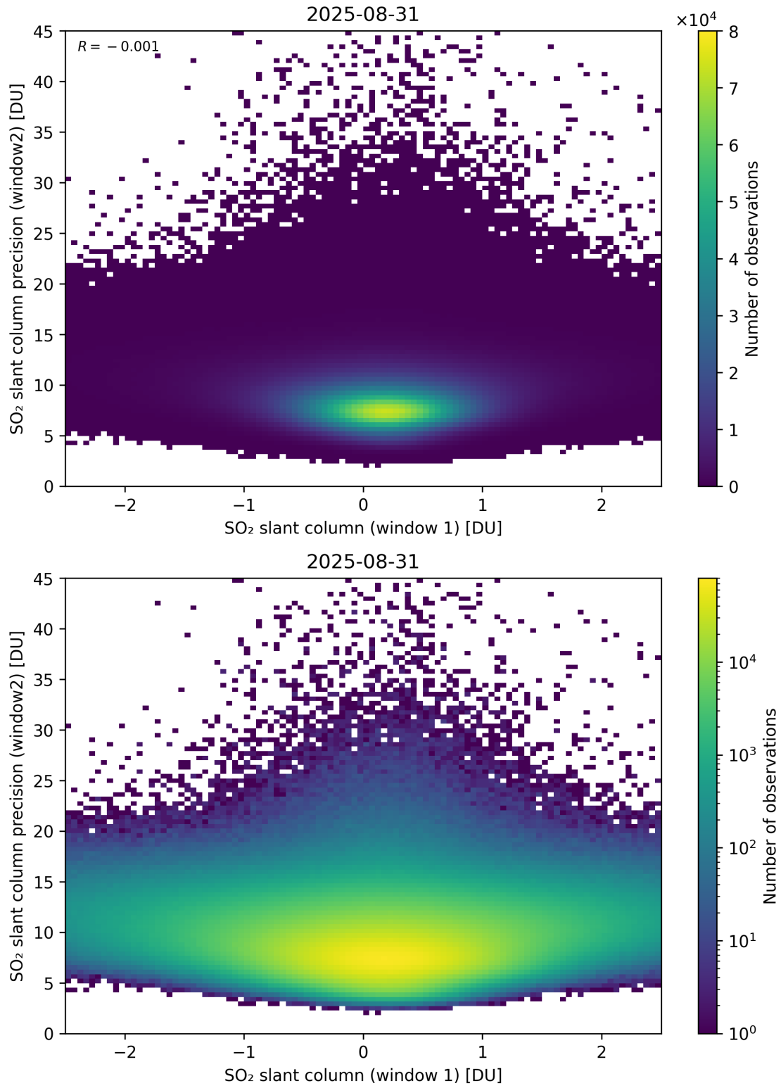
Figure 286: Scatter density plot of “SO 2 slant column (window 1)” against “SO 2 slant column precision (window2)” for 2025-08-30 to 2025-09-01.
