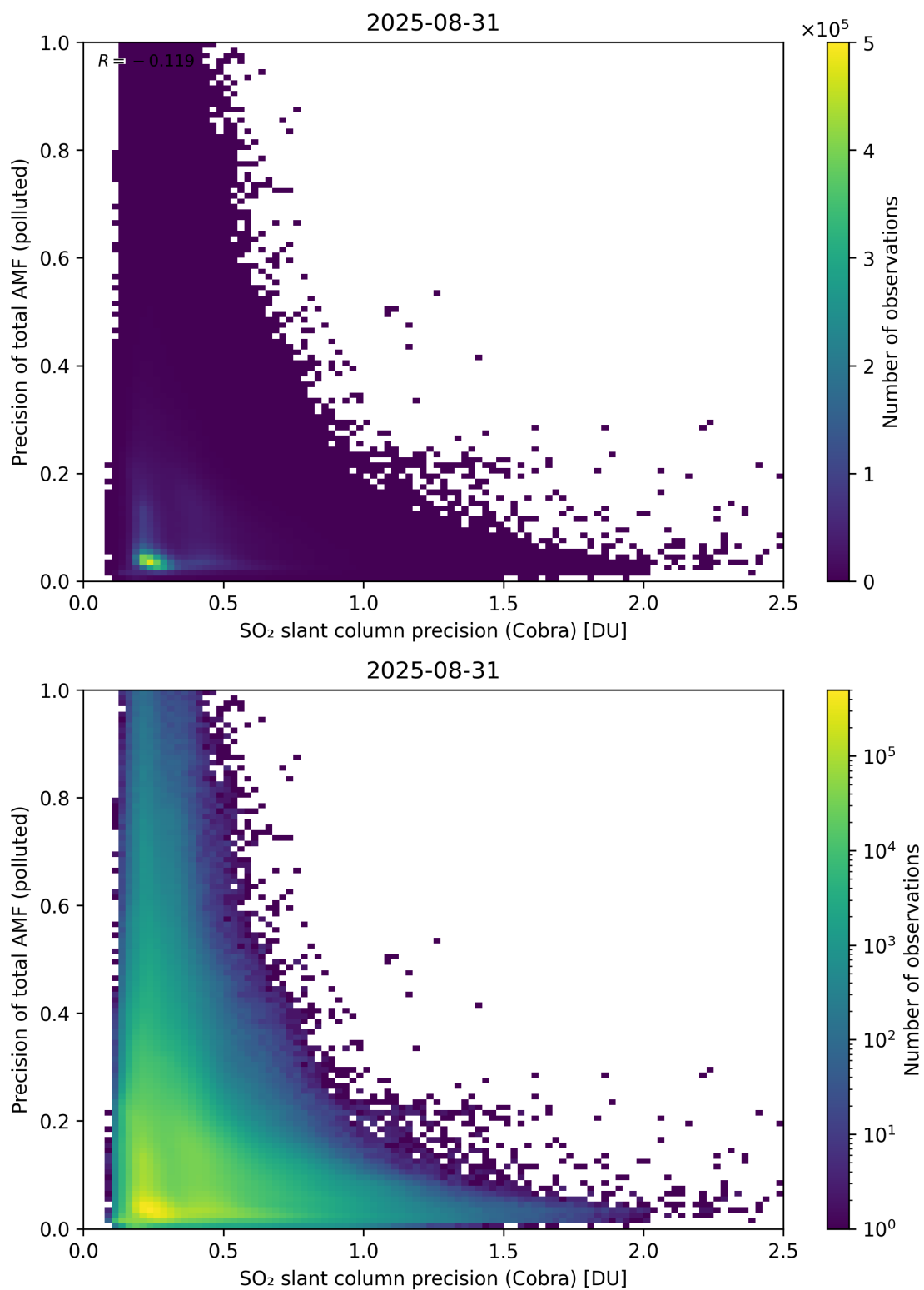
Figure 214: Scatter density plot of “SO 2 slant column precision (Cobra)” against “Precision of total AMF (polluted)” for 2025-08-30 to 2025-09-01.
