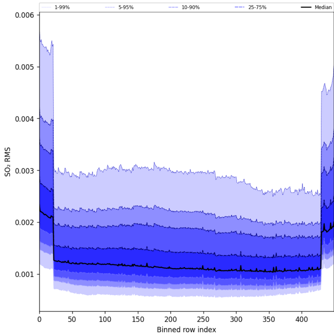
Figure 104: Along track statistics of “SO 2 RMS” for 2025-08-30 to 2025-09-01
