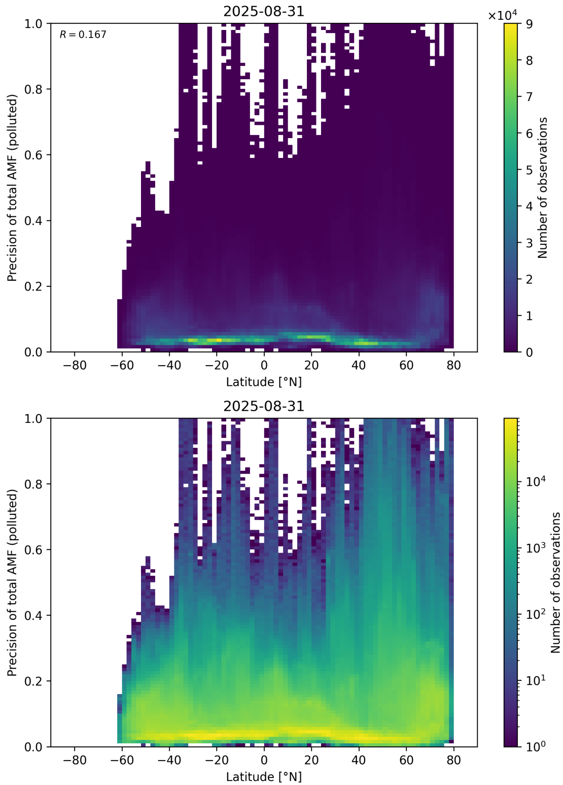
Figure 168: Scatter density plot of “Latitude” against “Precision of total AMF (polluted)” for 2025-08-30 to 2025-09-01.
