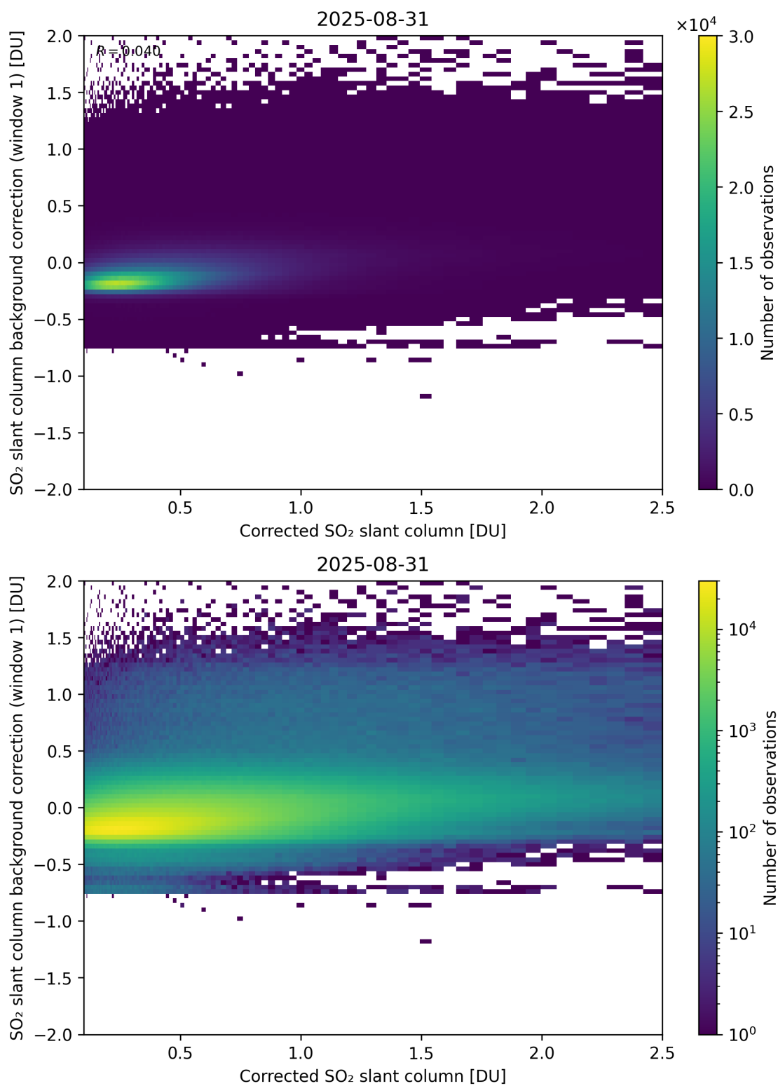
Figure 226: Scatter density plot of “Corrected SO 2 slant column” against “SO 2 slant column background correction (window 1)” for 2025-08-30 to 2025-09-01.
