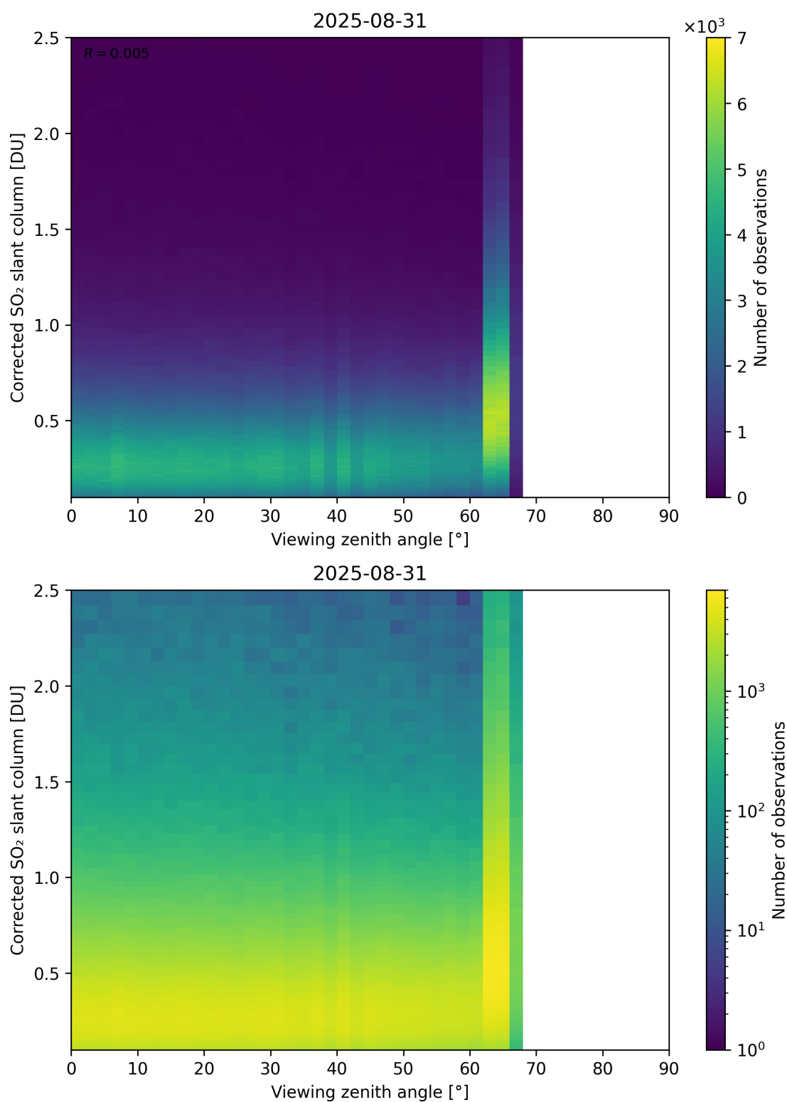
Figure 373: Scatter density plot of “Viewing zenith angle” against “Corrected SO 2 slant column” for 2025-08-30 to 2025-09-01.
