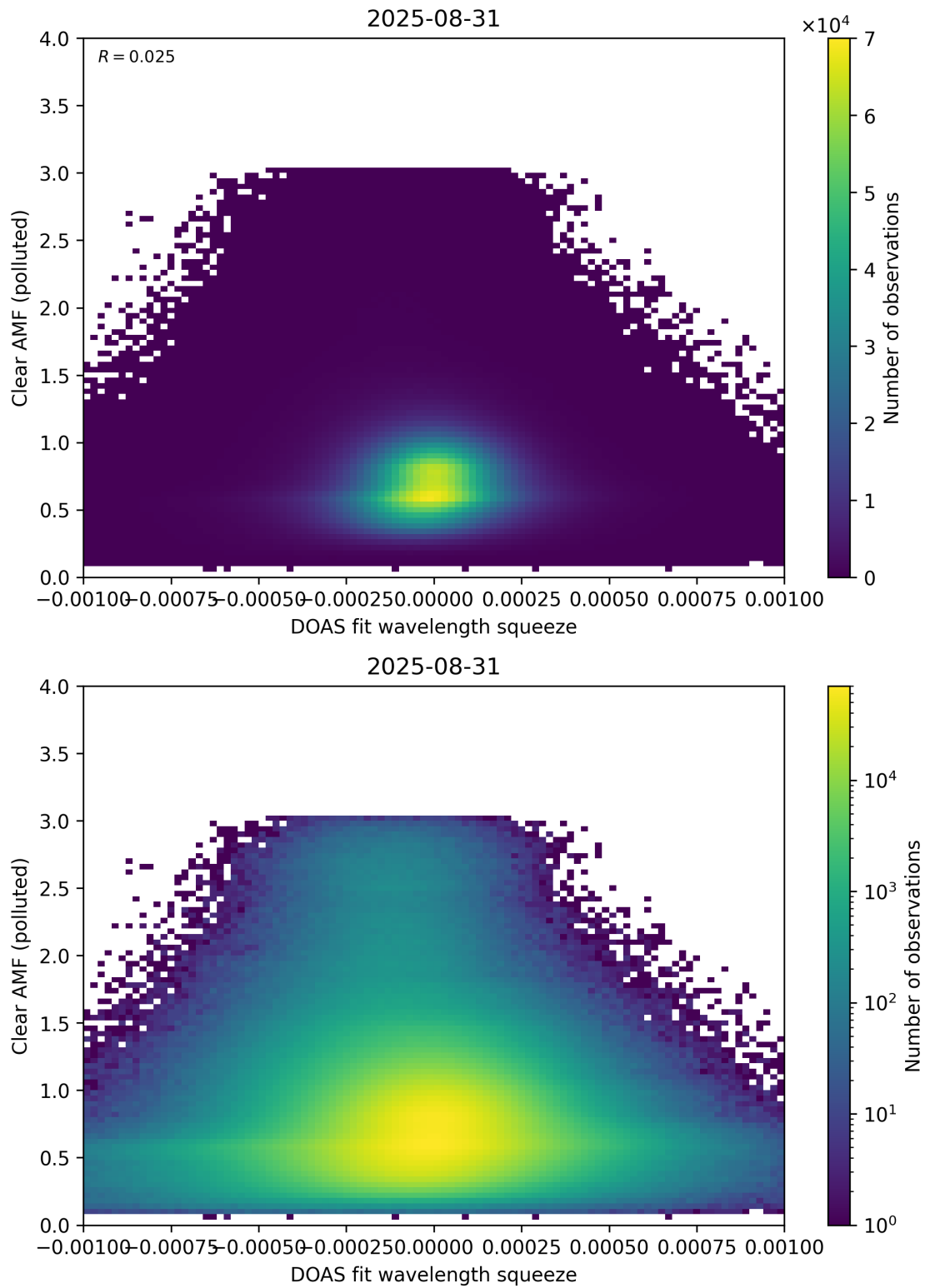
Figure 144: Scatter density plot of “DOAS fit wavelength squeeze” against “Clear AMF (polluted)” for 2025-08-30 to 2025-09-01.
