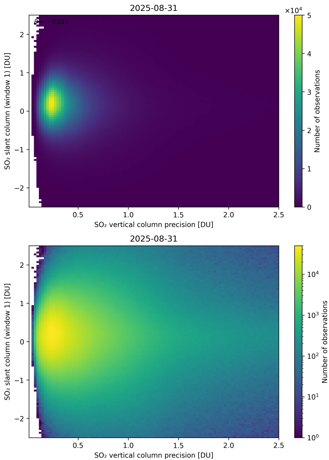
Figure 341: Scatter density plot of “SO 2 vertical column precision” against “SO 2 slant column (window 1)” for 2025-08-30 to 2025-09-01.
