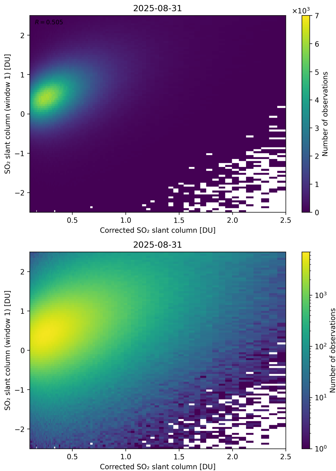
Figure 237: Scatter density plot of “Corrected SO 2 slant column” against “SO 2 slant column (window 1)” for 2025-08-30 to 2025-09-01.
