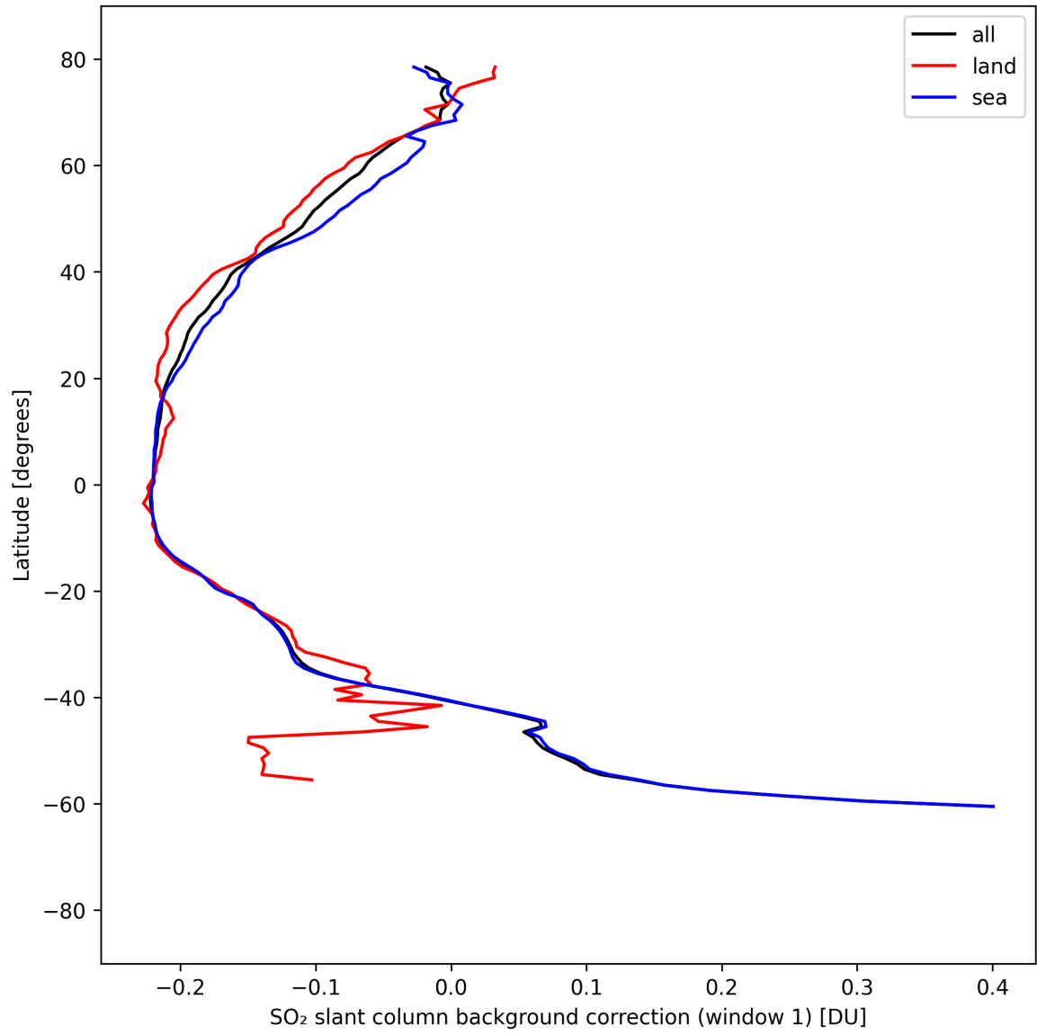
Figure 40: Zonal average of “SO 2 slant column background correction (window 1)” for 2025-08-30 to 2025-09-01.
