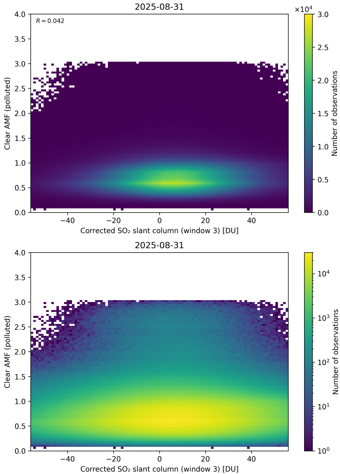
Figure 259: Scatter density plot of “Corrected SO 2 slant column (window 3)” against “Clear AMF (polluted)” for 2025-08-30 to 2025-09-01.
