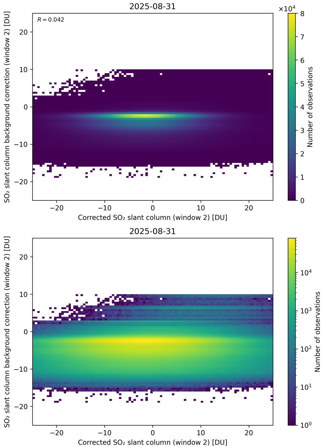
Figure 244: Scatter density plot of “Corrected SO 2 slant column (window 2)” against “SO 2 slant column background correction (window 2)” for 2025-08-30 to 2025-09-01.
