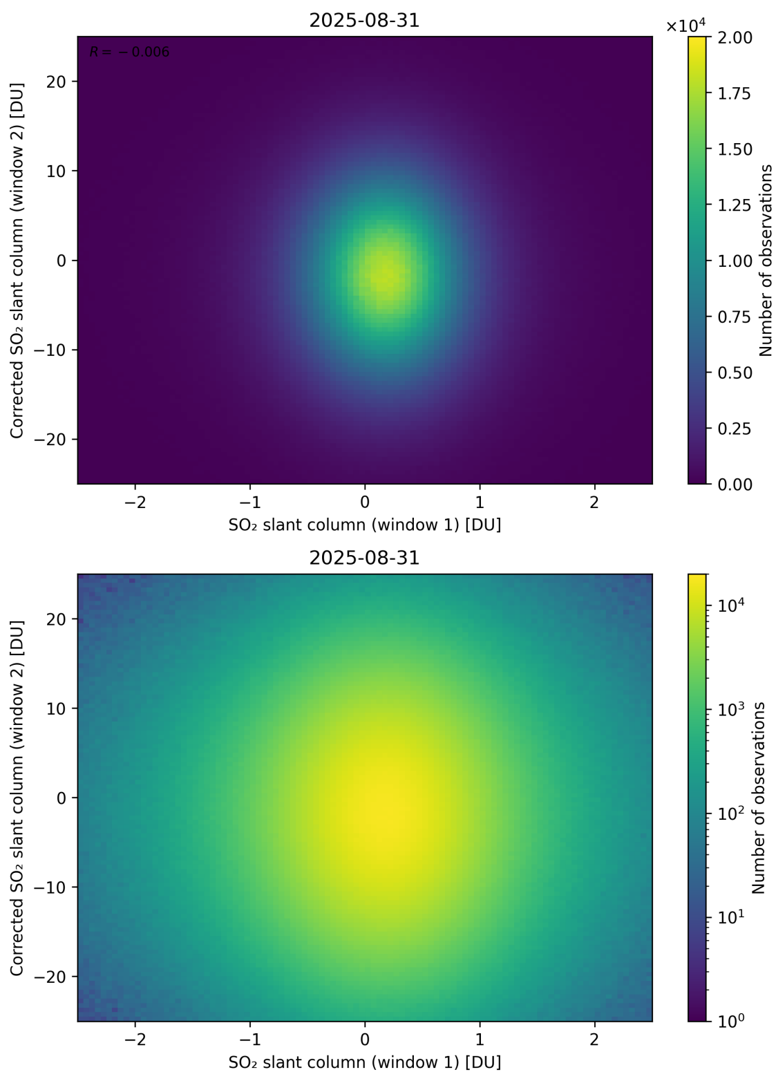
Figure 283: Scatter density plot of “SO 2 slant column (window 1)” against “Corrected SO 2 slant column (window 2)” for 2025-08-30 to 2025-09-01.
