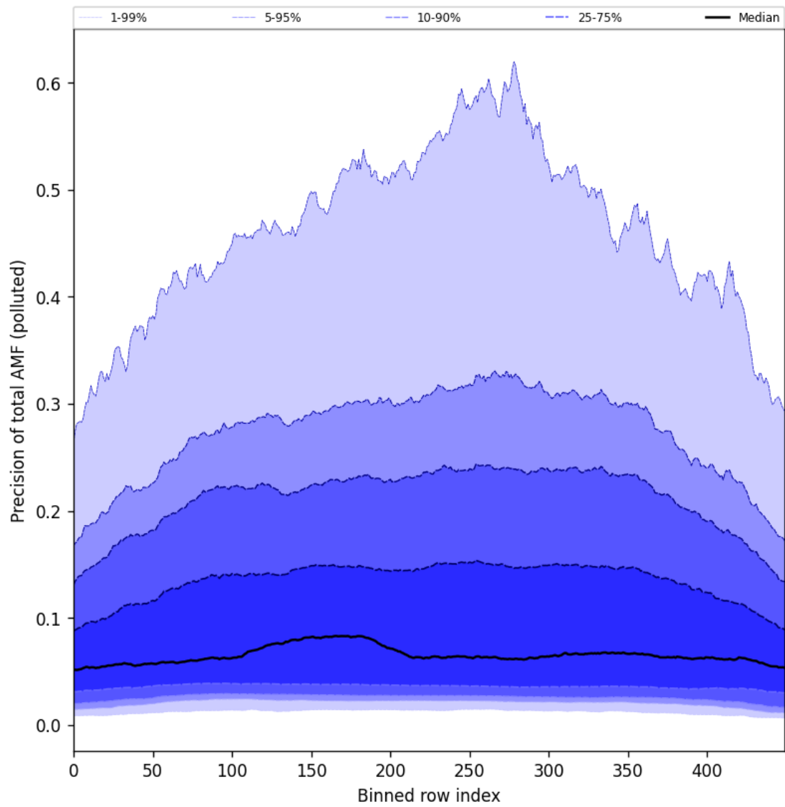
Figure 106: Along track statistics of “Precision of total AMF (polluted)” for 2025-08-30 to 2025-09-01
