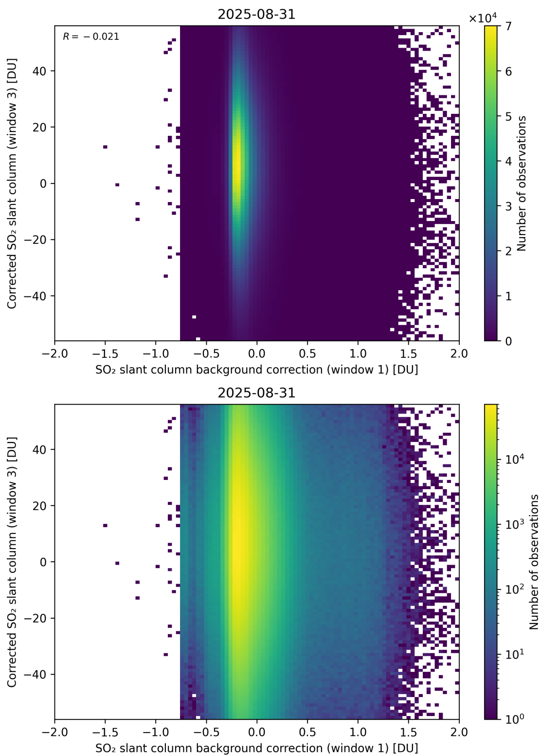
Figure 116: Scatter density plot of “SO 2 slant column background correction (window 1)” against “Corrected SO 2 slant column (window 3)” for 2025-08-30 to 2025-09-01.
