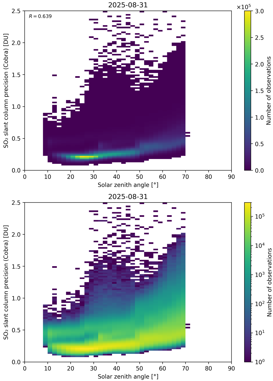
Figure 180: Scatter density plot of “Solar zenith angle” against “SO 2 slant column precision (Cobra)” for 2025-08-30 to 2025-09-01.
