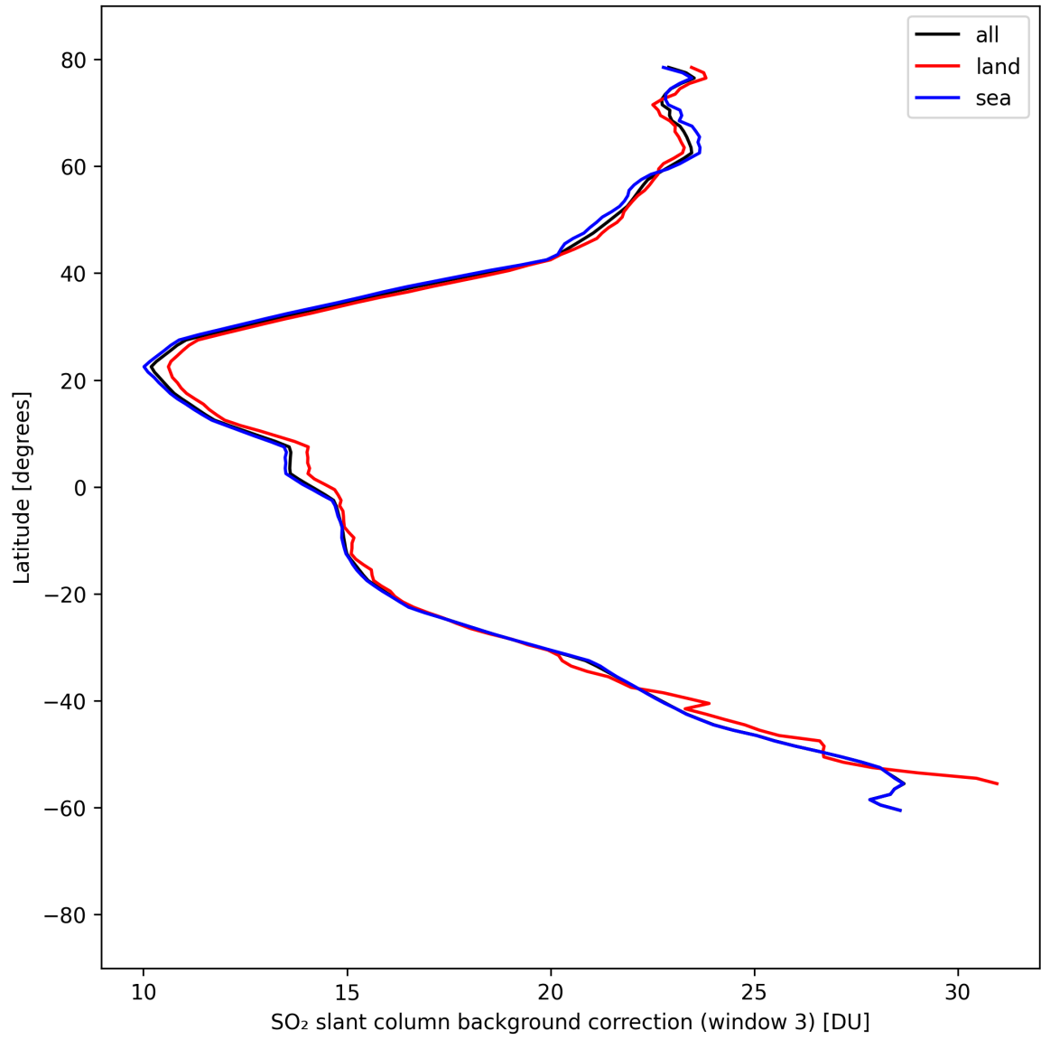
Figure 48: Zonal average of “SO 2 slant column background correction (window 3)” for 2025-08-30 to 2025-09-01.
