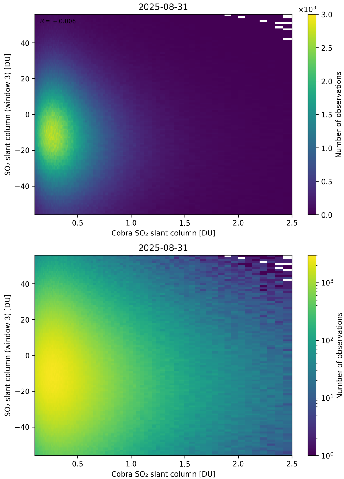
Figure 222: Scatter density plot of “Cobra SO 2 slant column” against “SO 2 slant column (window 3)” for 2025-08-30 to 2025-09-01.
