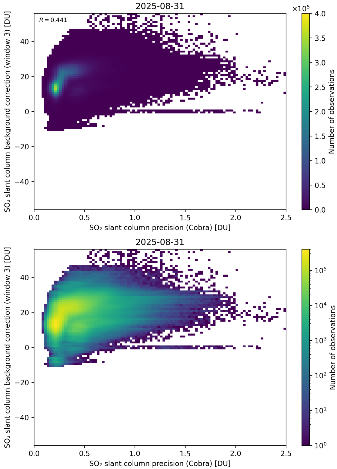
Figure 201: Scatter density plot of “SO 2 slant column precision (Cobra)” against “SO 2 slant column background correction (window 3)” for 2025-08-30 to 2025-09-01.
