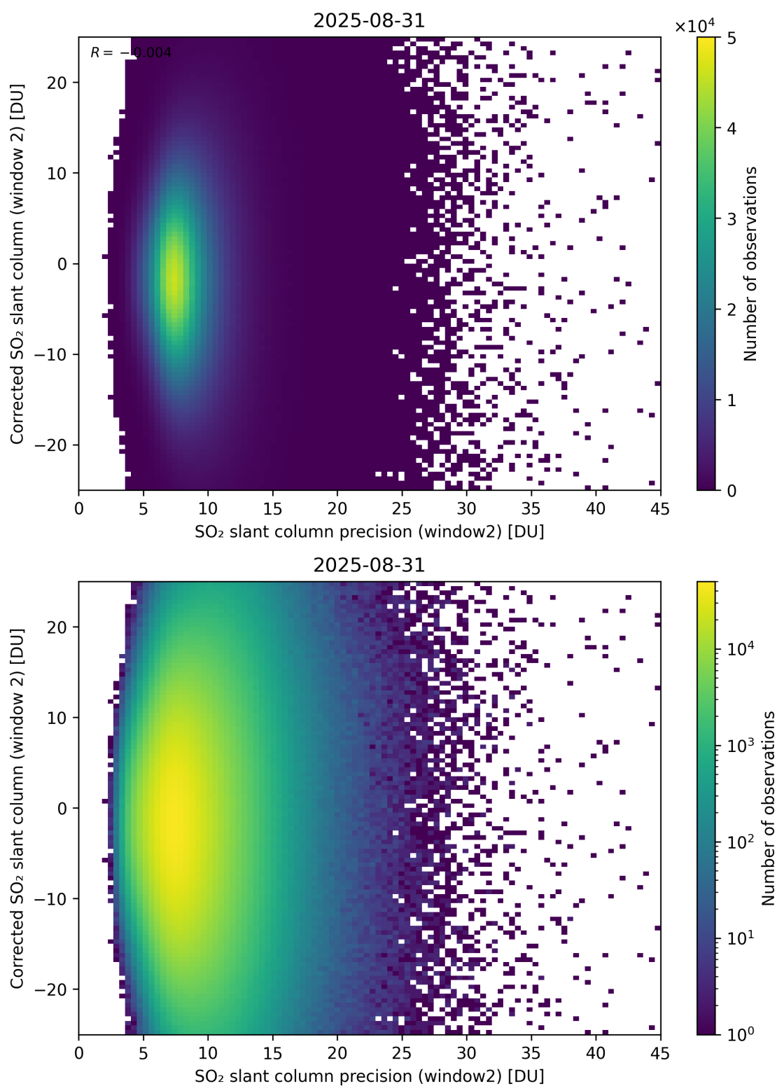
Figure 297: Scatter density plot of “SO 2 slant column precision (window2)” against “Corrected SO 2 slant column (window 2)” for 2025-08-30 to 2025-09-01.
