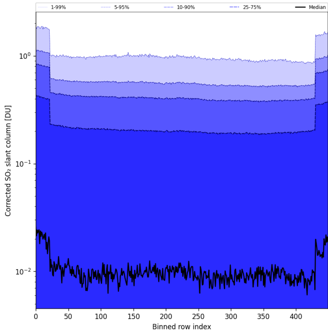
Figure 86: Along track statistics of “Corrected SO 2 slant column” for 2025-08-30 to 2025-09-01
