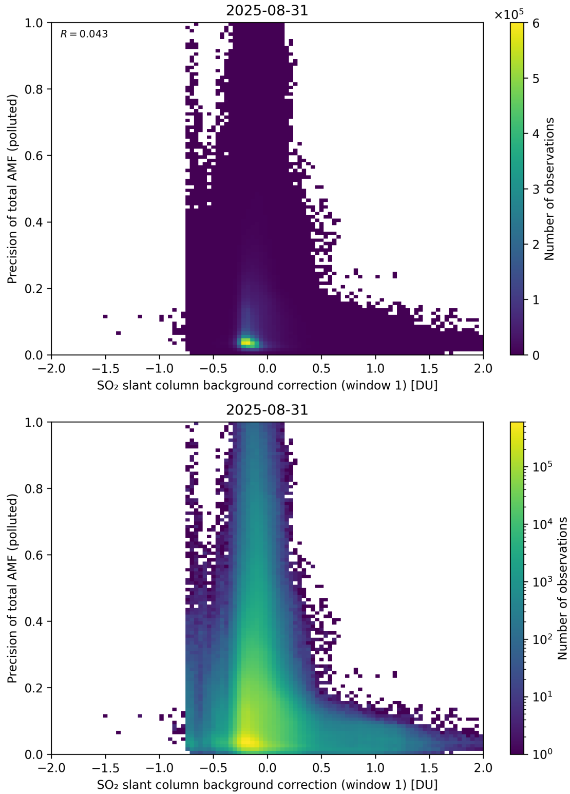
Figure 121: Scatter density plot of “SO 2 slant column background correction (window 1)” against “Precision of total AMF (polluted)” for 2025-08-30 to 2025-09-01.
