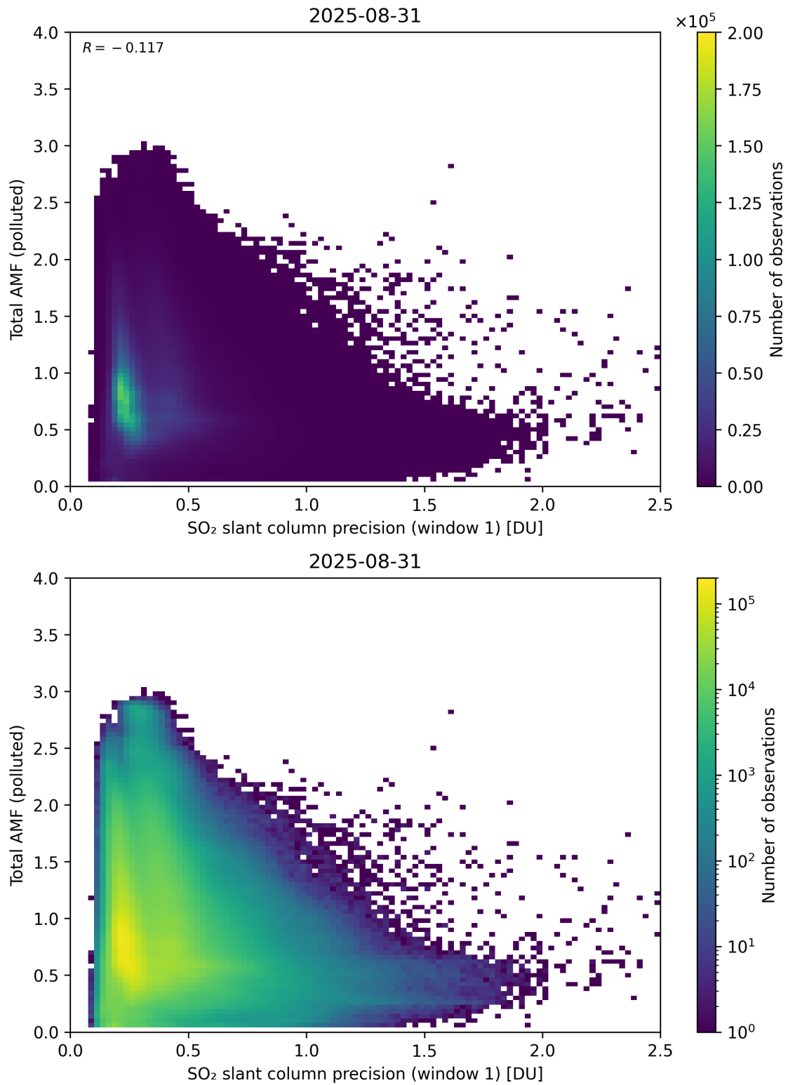
Figure 280: Scatter density plot of “SO 2 slant column precision (window 1)” against “Total AMF (polluted)” for 2025-08-30 to 2025-09-01.
