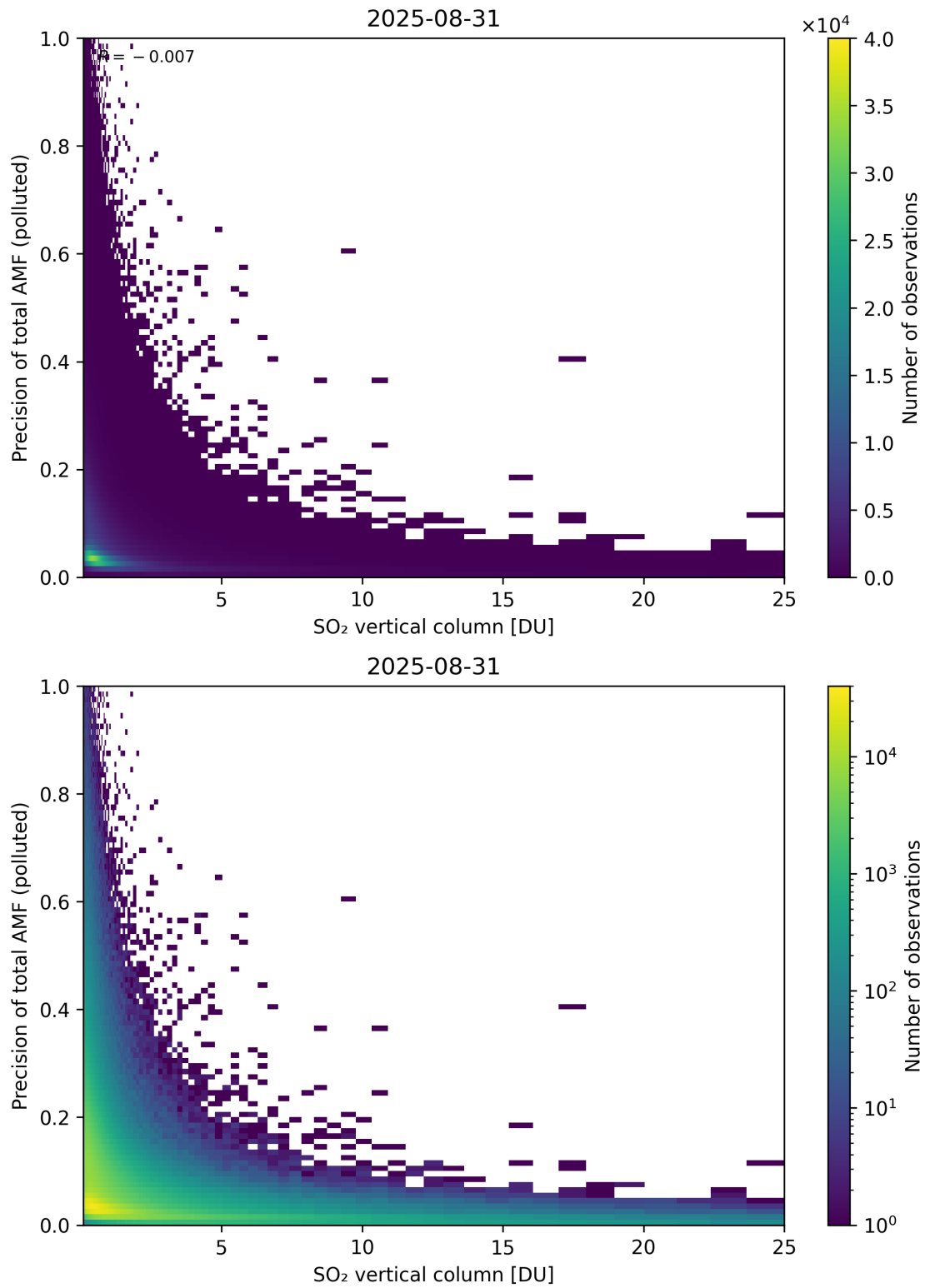
Figure 360: Scatter density plot of “SO 2 vertical column” against “Precision of total AMF (polluted)” for 2025-08-30 to 2025-09-01.
