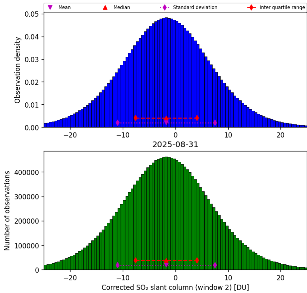
Figure 69: Histogram of “Corrected SO 2 slant column (window 2)” for 2025-08-30 to 2025-09-01
