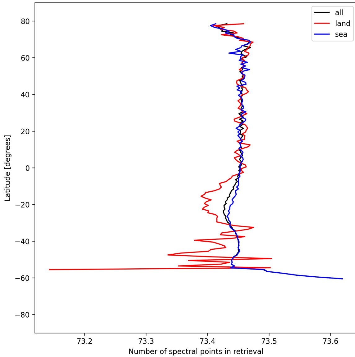
Figure 56: Zonal average of “Number of spectral points in retrieval” for 2025-08-30 to 2025-09-01.
