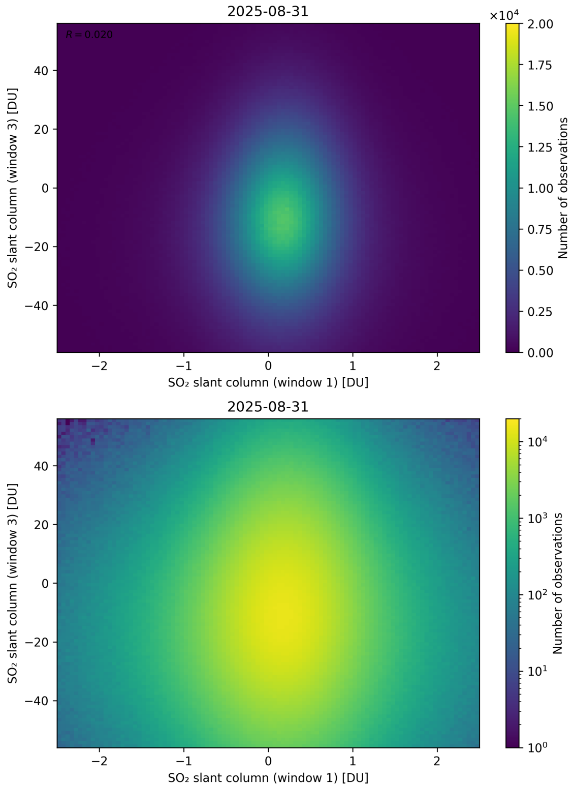
Figure 287: Scatter density plot of “SO 2 slant column (window 1)” against “SO 2 slant column (window 3)” for 2025-08-30 to 2025-09-01.
