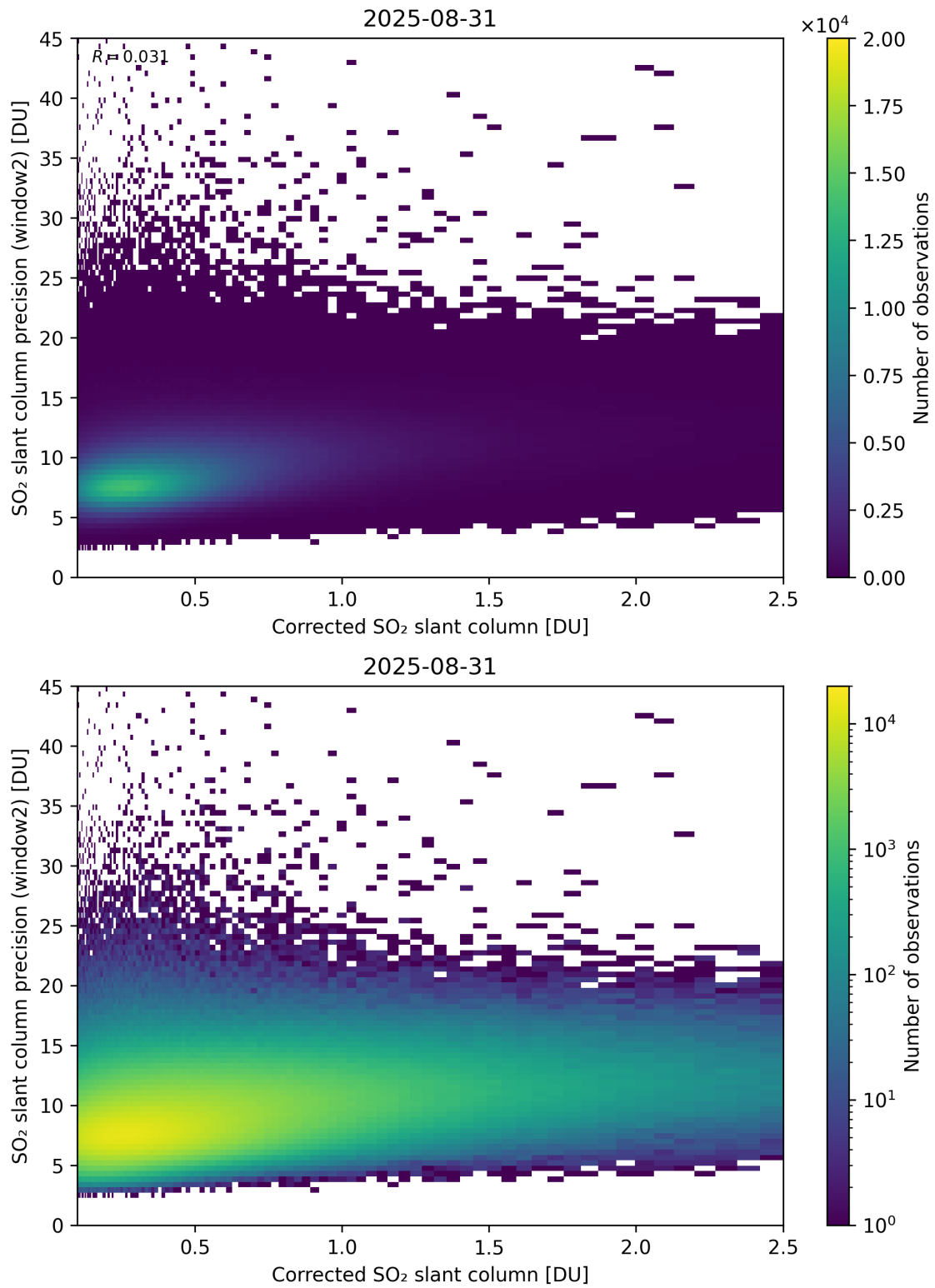
Figure 239: Scatter density plot of “Corrected SO 2 slant column” against “SO 2 slant column precision (window2)” for 2025-08-30 to 2025-09-01.
