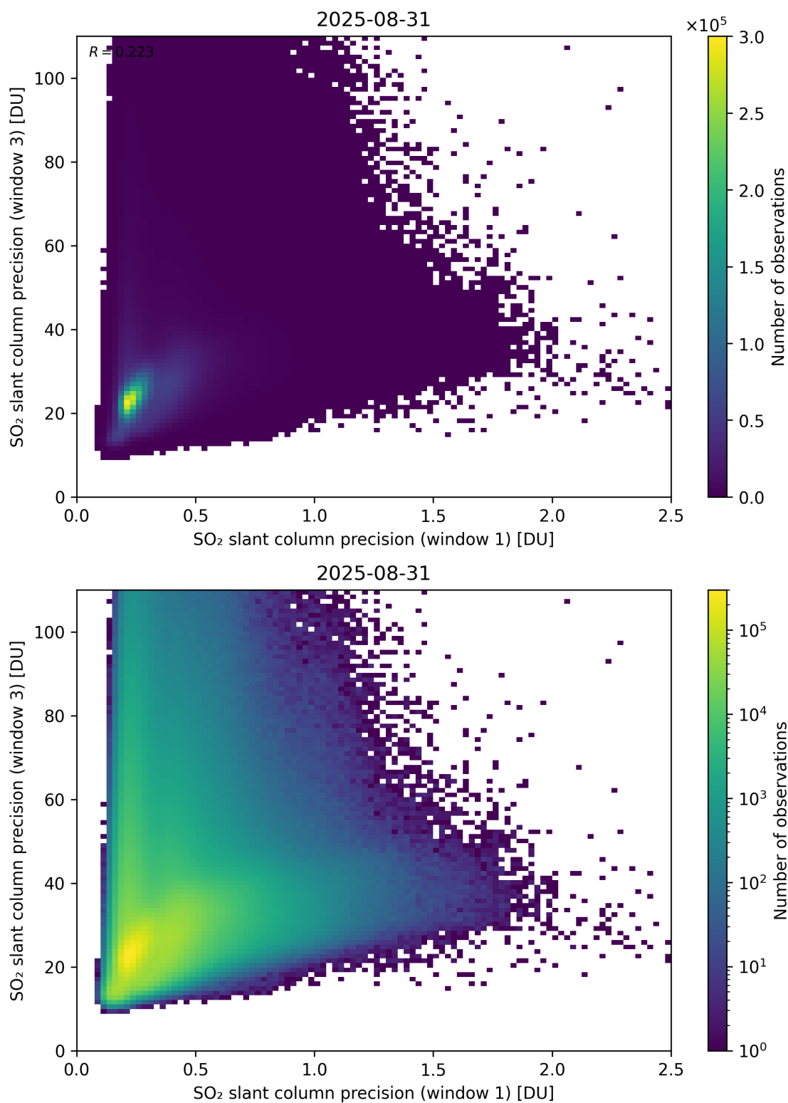
Figure 279: Scatter density plot of “SO 2 slant column precision (window 1)” against “SO 2 slant column precision (window 3)” for 2025-08-30 to 2025-09-01.
