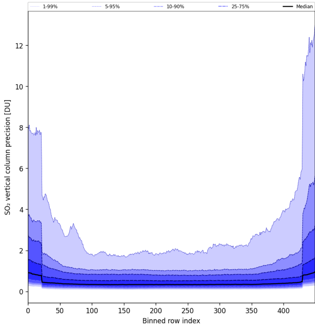
Figure 85: Along track statistics of “SO 2 vertical column precision” for 2025-08-30 to 2025-09-01
