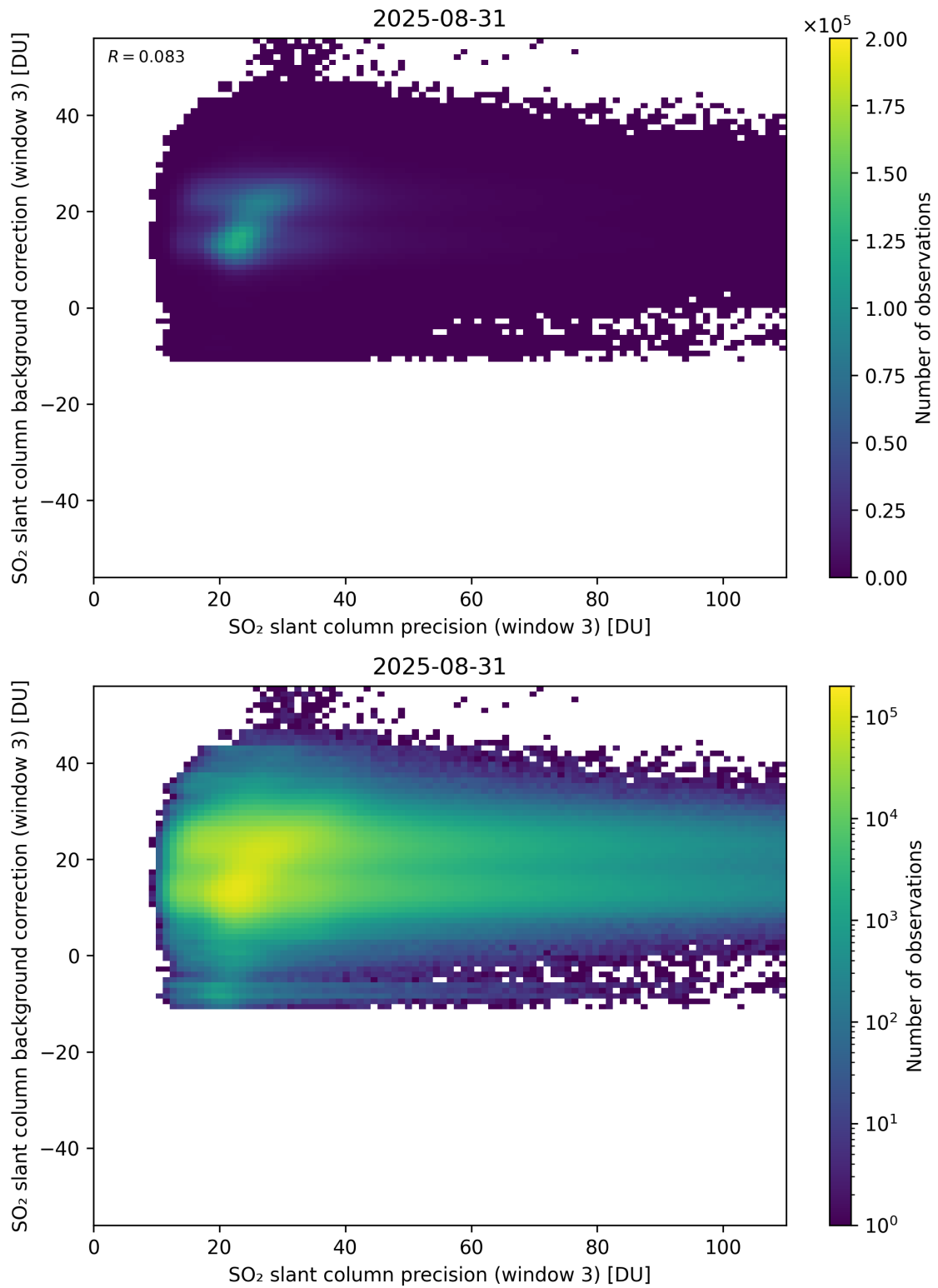
Figure 307: Scatter density plot of “SO 2 slant column precision (window 3)” against “SO 2 slant column background correction (window 3)” for 2025-08-30 to 2025-09-01.
