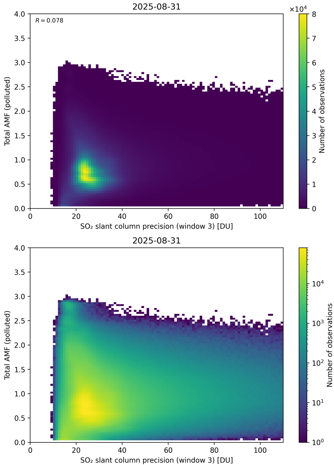
Figure 313: Scatter density plot of “SO 2 slant column precision (window 3)” against “Total AMF (polluted)” for 2025-08-30 to 2025-09-01.
