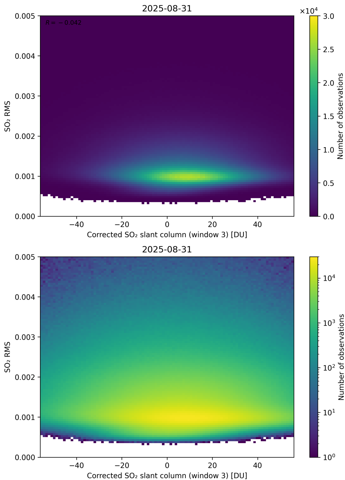
Figure 258: Scatter density plot of “Corrected SO 2 slant column (window 3)” against “SO 2 RMS” for 2025-08-30 to 2025-09-01.
