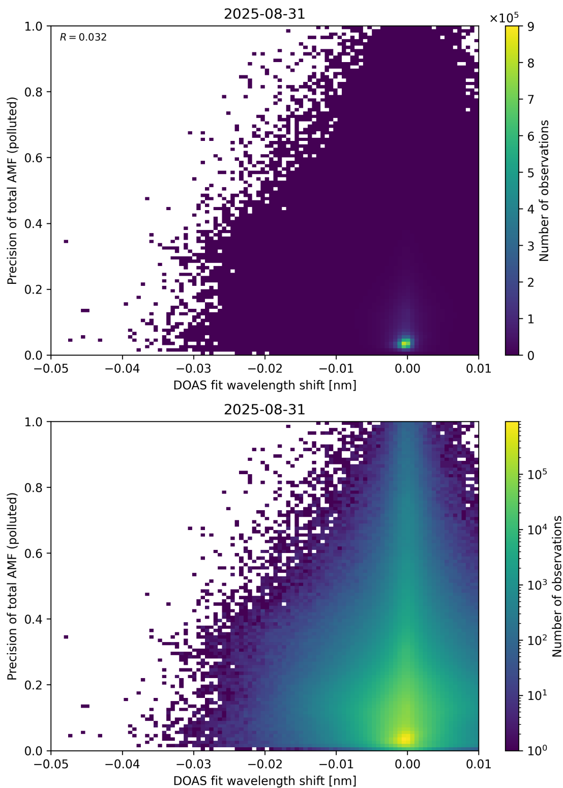
Figure 142: Scatter density plot of “DOAS fit wavelength shift” against “Precision of total AMF (polluted)” for 2025-08-30 to 2025-09-01.
