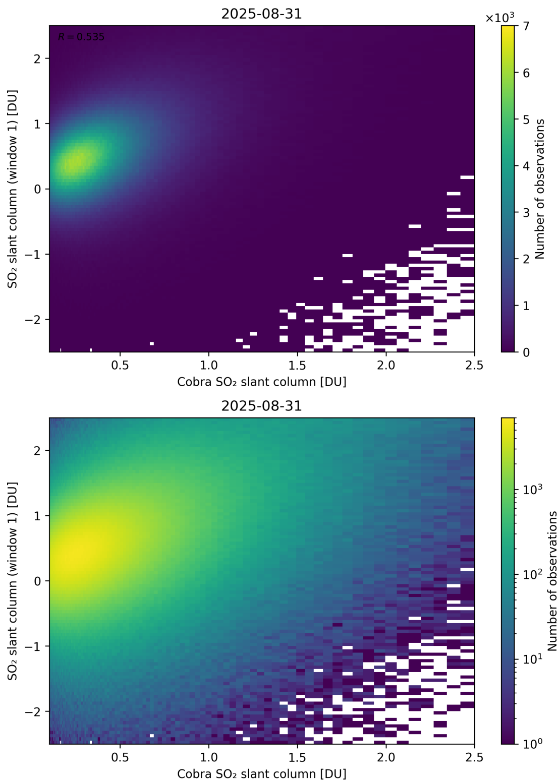
Figure 219: Scatter density plot of “Cobra SO 2 slant column” against “SO 2 slant column (window 1)” for 2025-08-30 to 2025-09-01.
