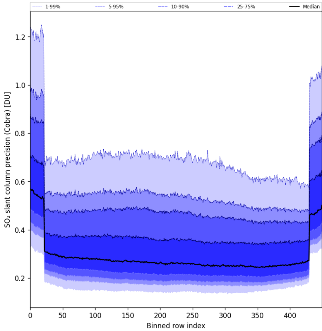
Figure 88: Along track statistics of “SO 2 slant column precision (Cobra)” for 2025-08-30 to 2025-09-01
