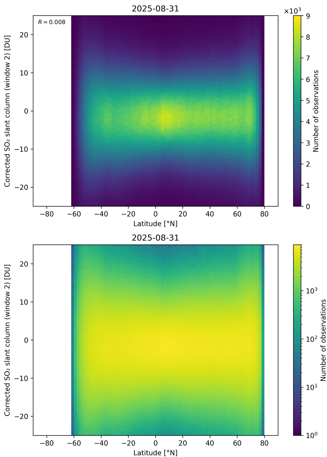
Figure 160: Scatter density plot of “Latitude” against “Corrected SO 2 slant column (window 2)” for 2025-08-30 to 2025-09-01.
