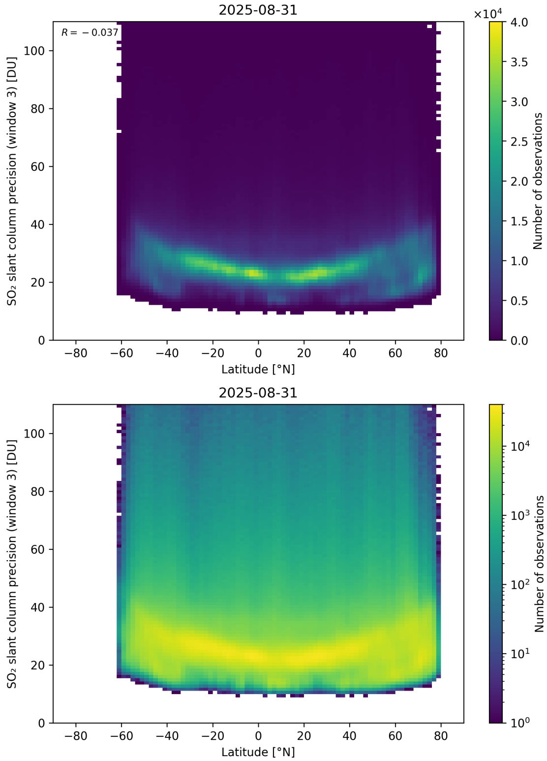
Figure 166: Scatter density plot of “Latitude” against “SO 2 slant column precision (window 3)” for 2025-08-30 to 2025-09-01.
