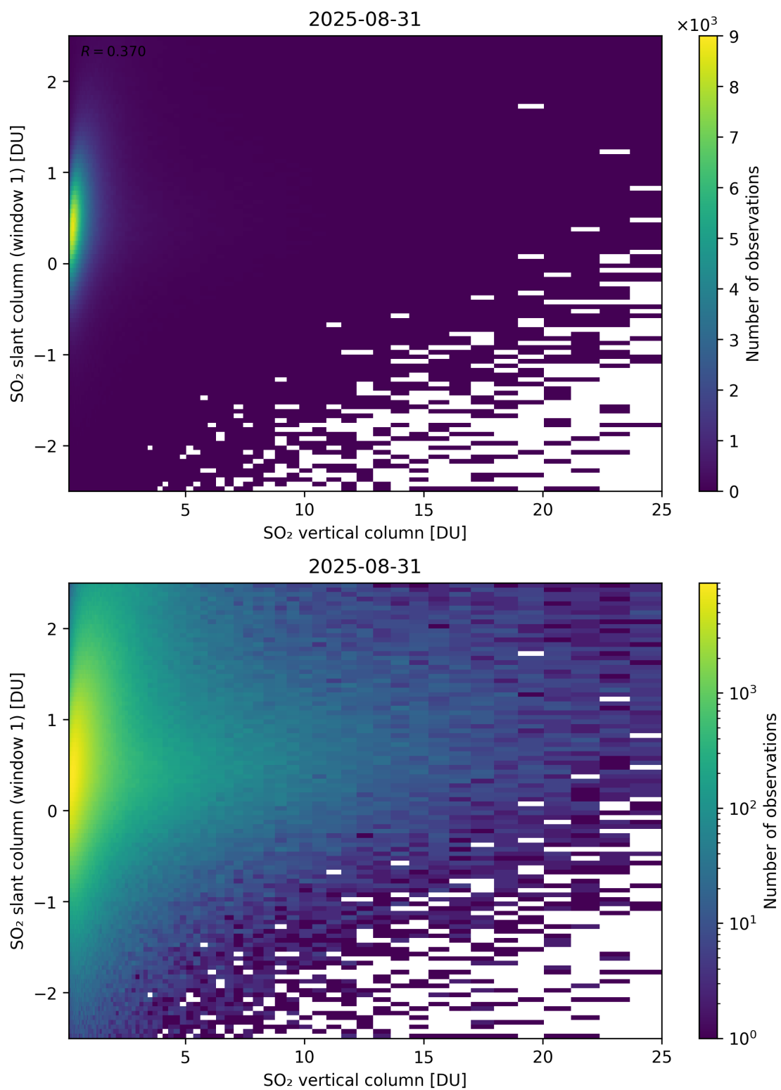
Figure 354: Scatter density plot of “SO 2 vertical column” against “SO 2 slant column (window 1)” for 2025-08-30 to 2025-09-01.
