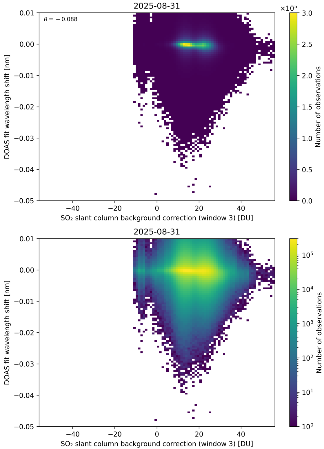
Figure 132: Scatter density plot of “SO 2 slant column background correction (window 3)” against “DOAS fit wavelength shift” for 2025-08-30 to 2025-09-01.
