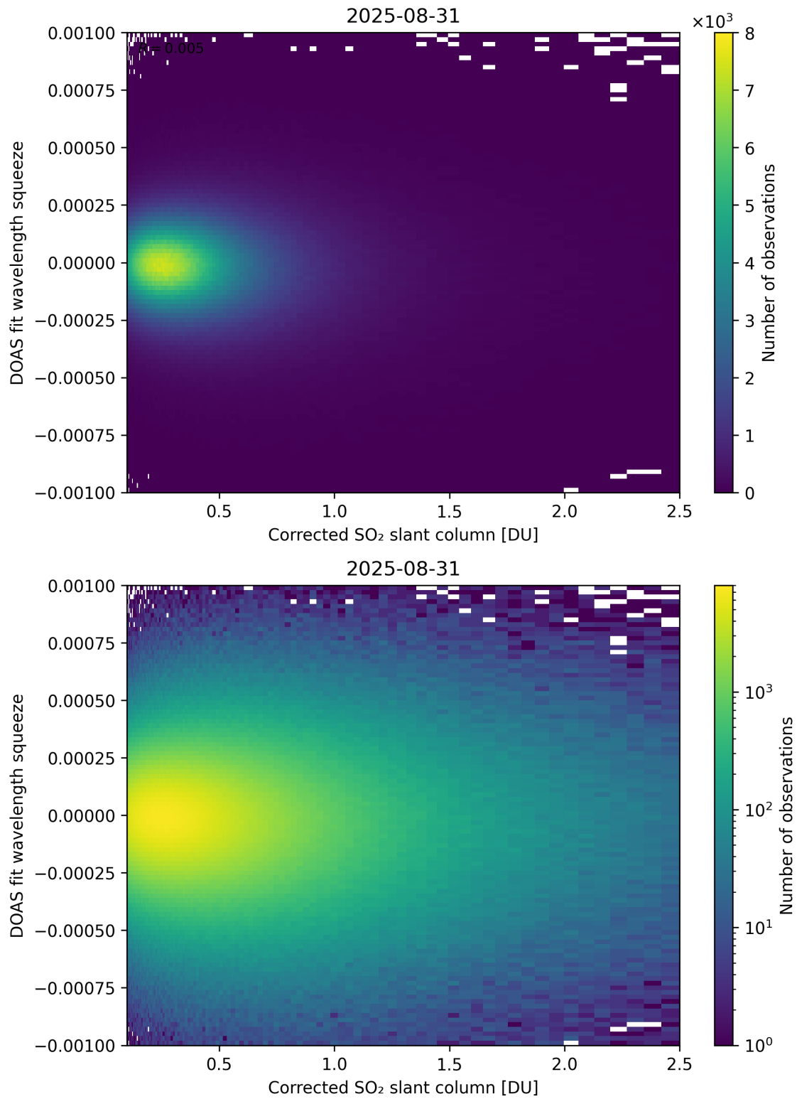
Figure 230: Scatter density plot of "Corrected SO 2 slant column" against "DOAS fit wavelength squeeze" for 2025-08-30 to 2025-09-01.
