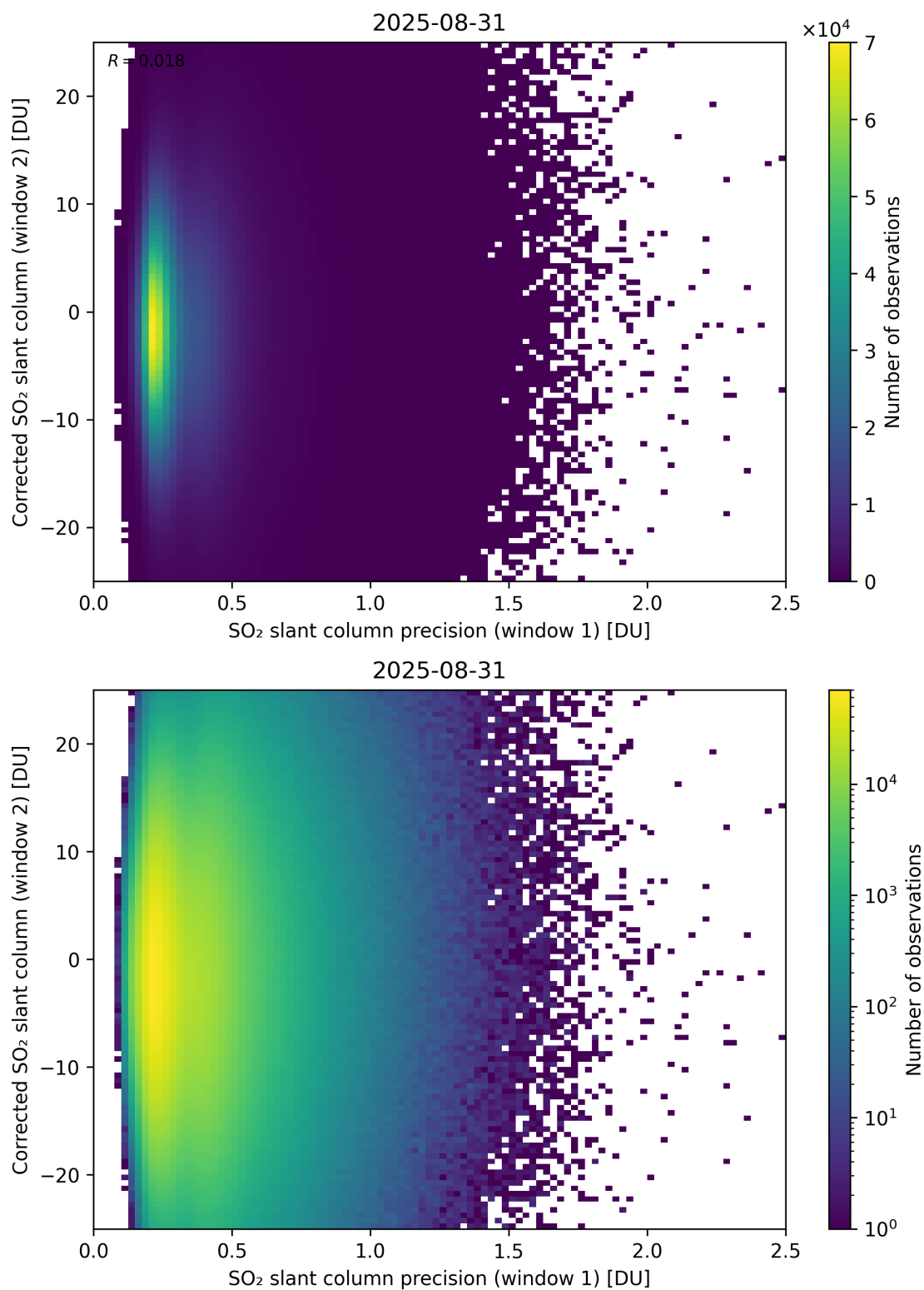
Figure 275: Scatter density plot of “SO 2 slant column precision (window 1)” against “Corrected SO 2 slant column (window 2)” for 2025-08-30 to 2025-09-01.
