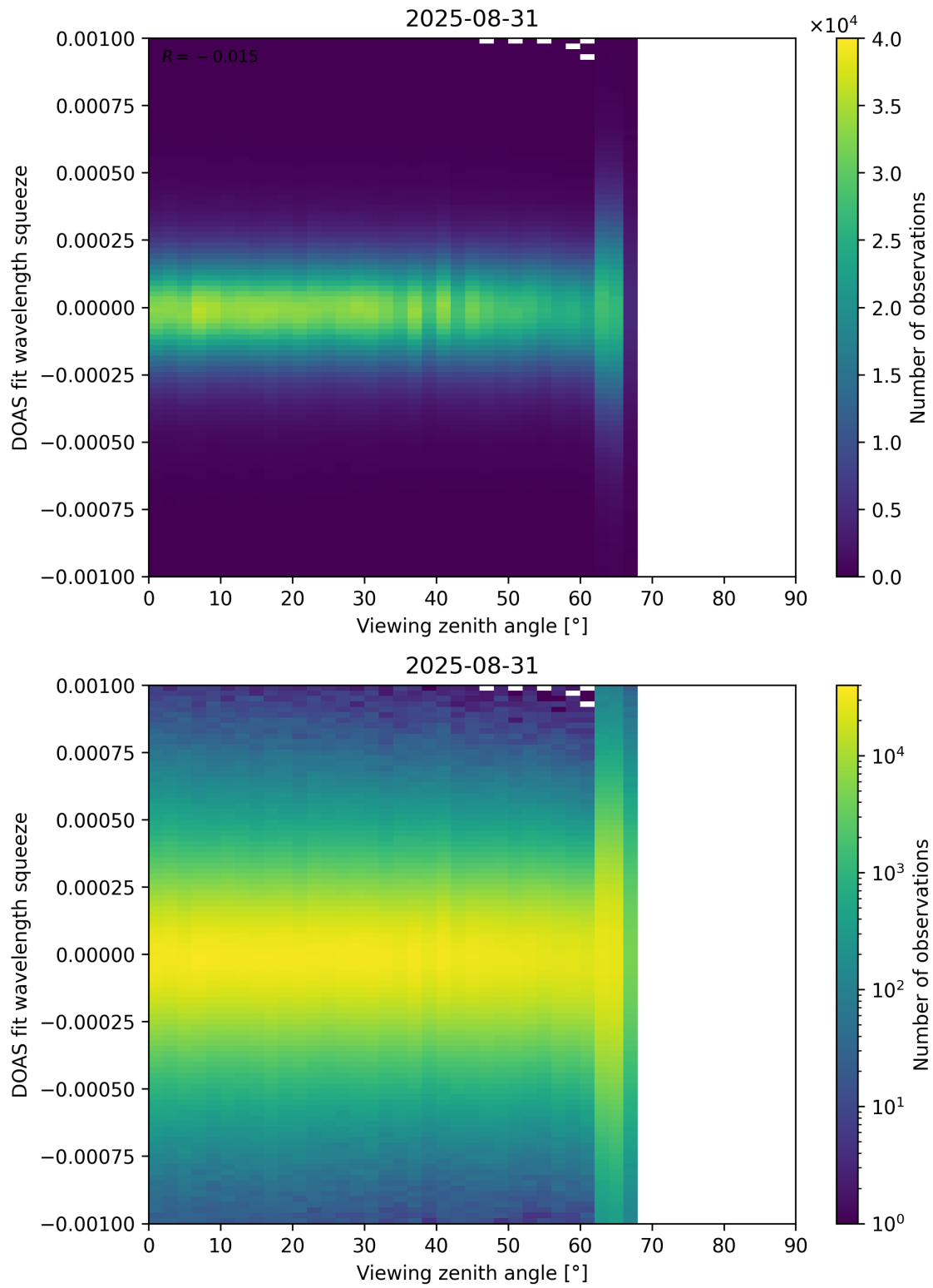
Figure 366: Scatter density plot of “Viewing zenith angle” against “DOAS fit wavelength squeeze” for 2025-08-30 to 2025-09-01.
