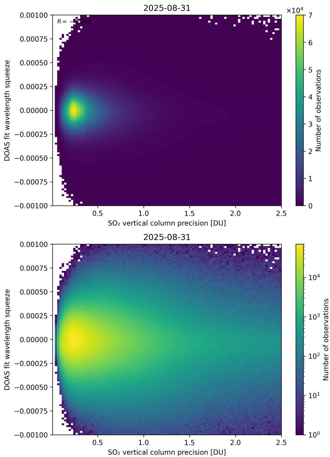
Figure 333: Scatter density plot of “SO 2 vertical column precision” against “DOAS fit wavelength squeeze” for 2025-08-30 to 2025-09-01.
