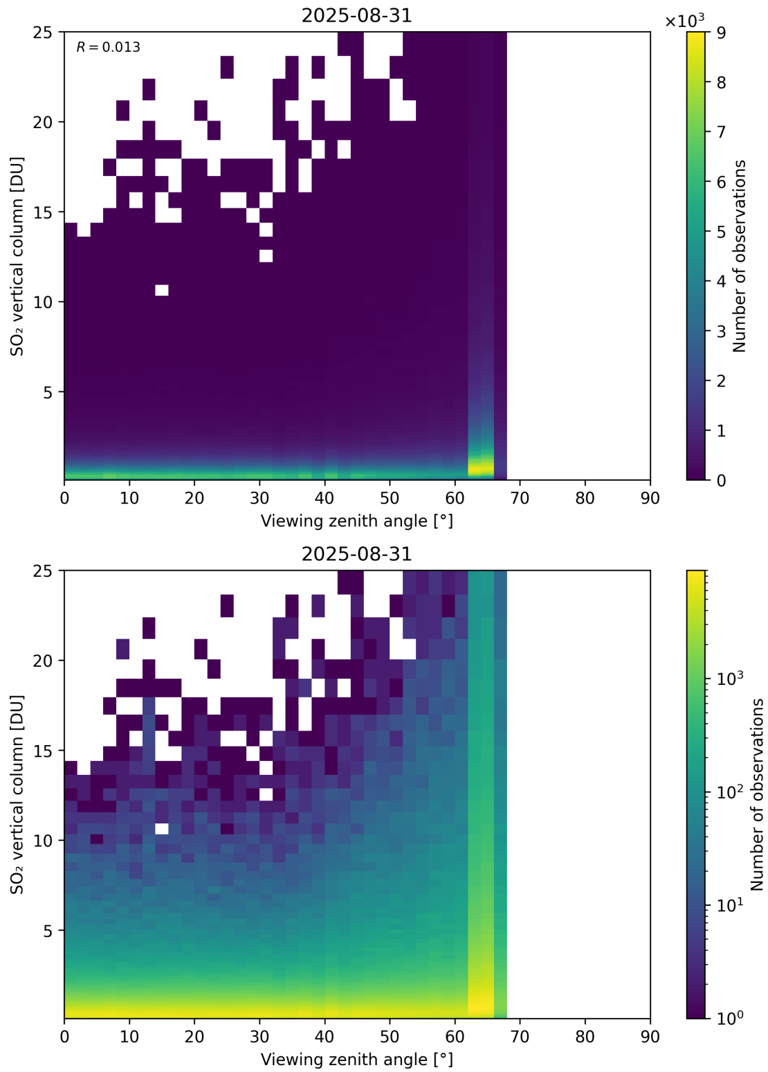
Figure 383: Scatter density plot of “Viewing zenith angle” against “SO 2 vertical column” for 2025-08-30 to 2025-09-01.
