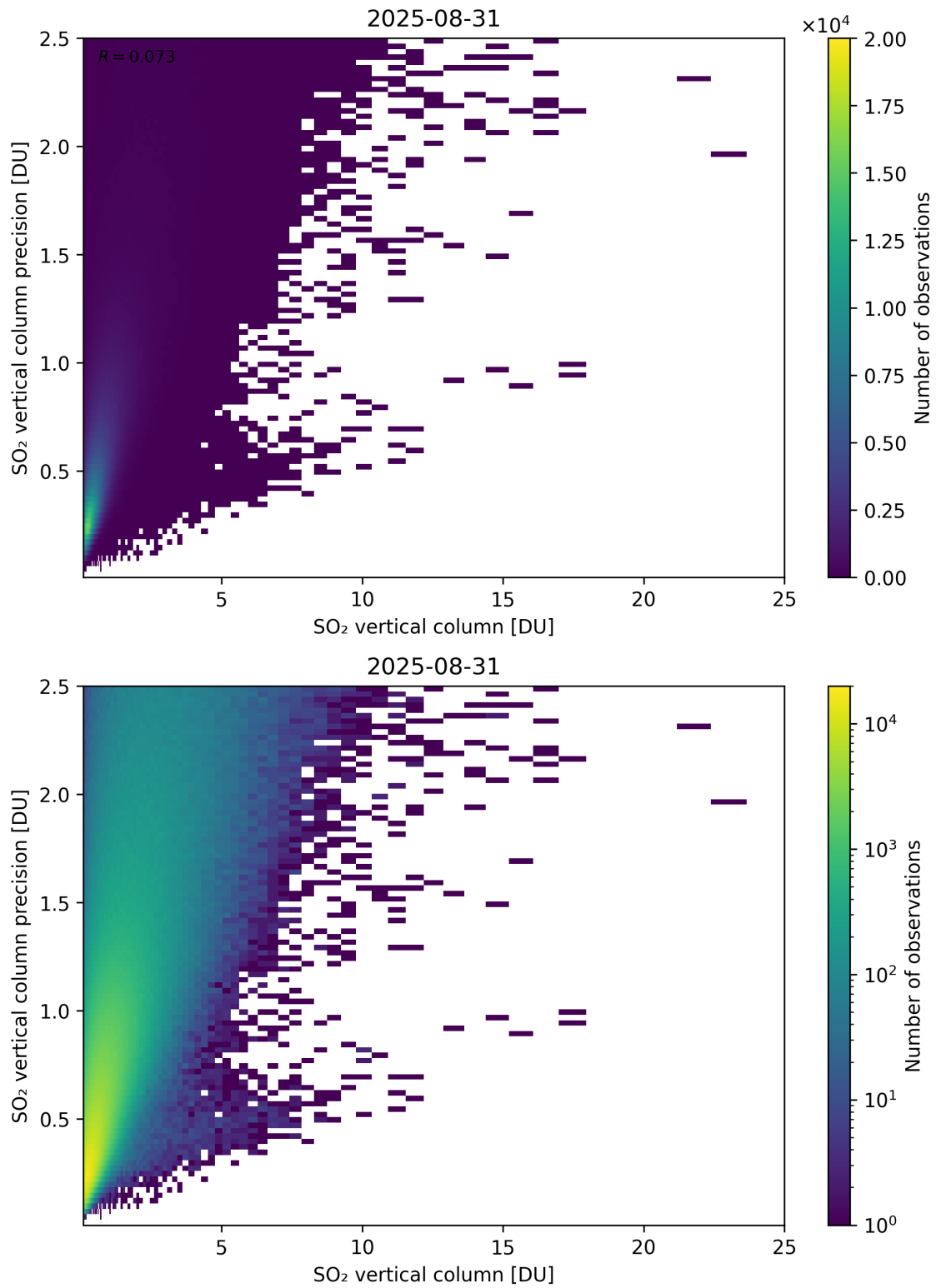
Figure 361: Scatter density plot of “SO 2 vertical column” against “SO 2 vertical column precision” for 2025-08-30 to 2025-09-01.
