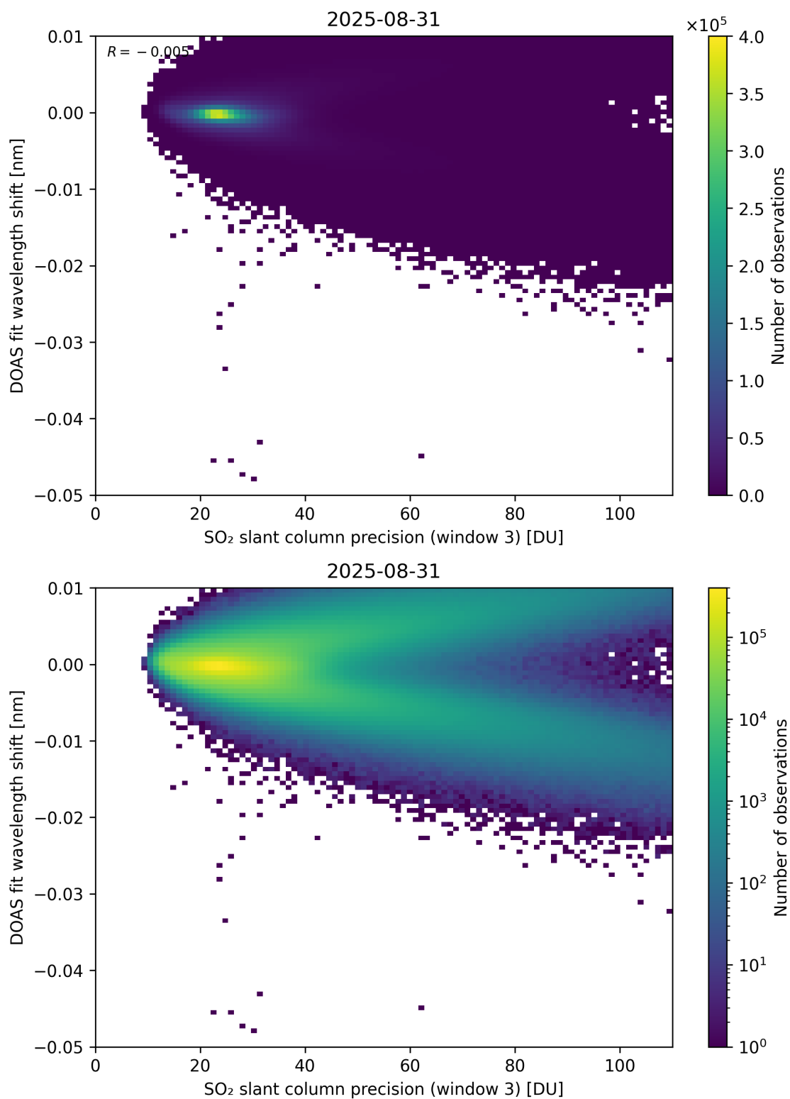
Figure 308: Scatter density plot of “SO 2 slant column precision (window 3)” against “DOAS fit wavelength shift” for 2025-08-30 to 2025-09-01.
