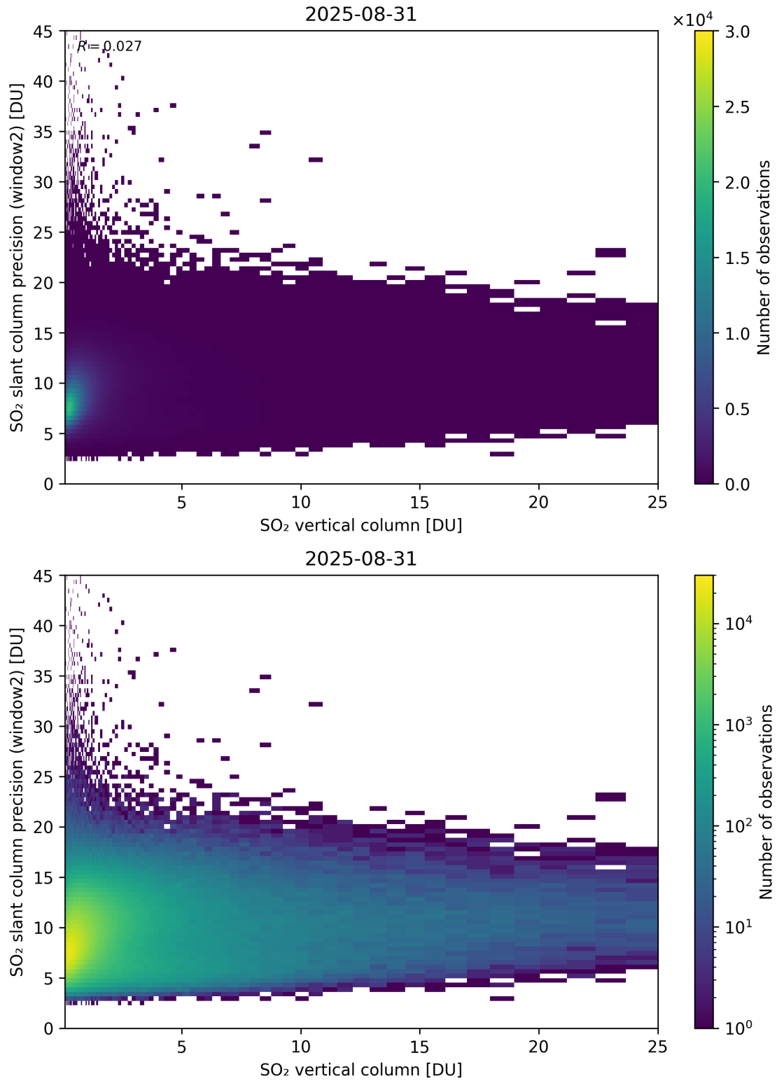
Figure 356: Scatter density plot of “SO 2 vertical column” against “SO 2 slant column precision (window2)” for 2025-08-30 to 2025-09-01.
