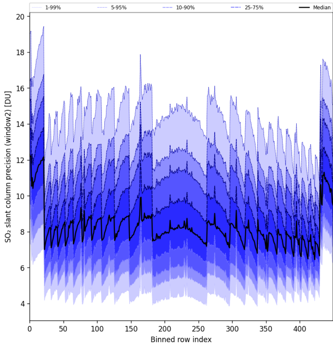
Figure 94: Along track statistics of “SO 2 slant column precision (window2)” for 2025-08-30 to 2025-09-01
