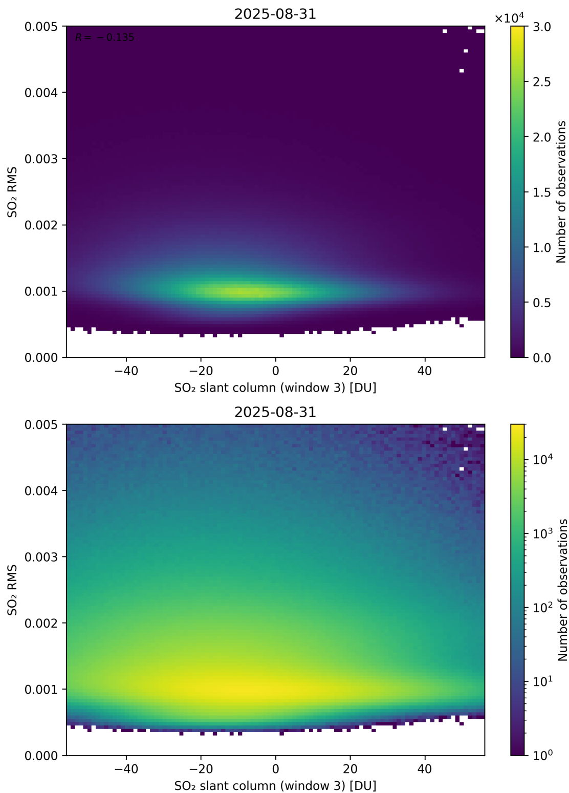
Figure 306: Scatter density plot of “SO 2 slant column (window 3)” against “SO 2 RMS” for 2025-08-30 to 2025-09-01.
