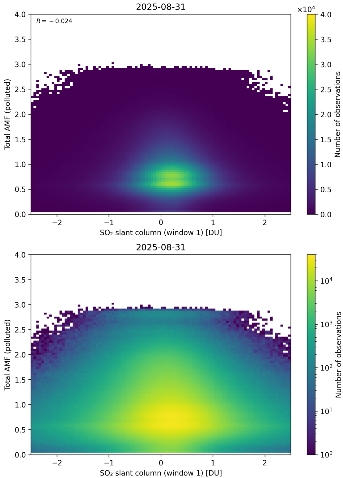
Figure 289: Scatter density plot of “SO 2 slant column (window 1)” against “Total AMF (polluted)” for 2025-08-30 to 2025-09-01.
