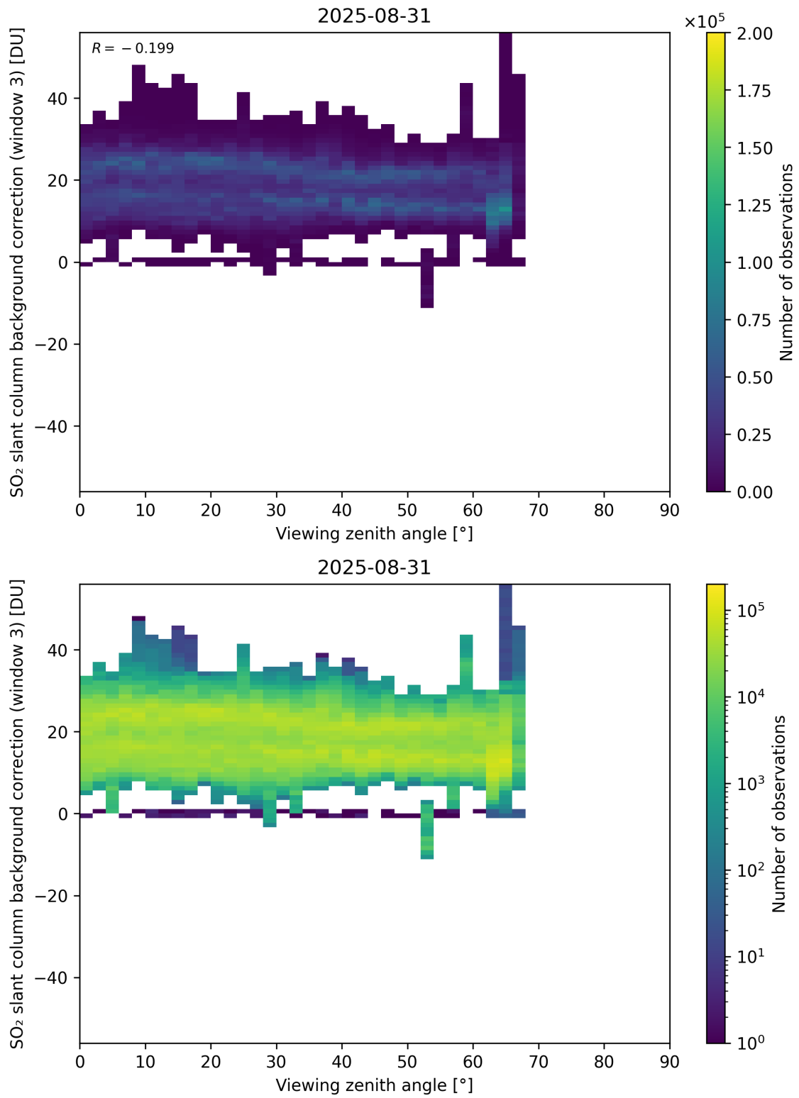
Figure 364: Scatter density plot of “Viewing zenith angle” against “SO 2 slant column background correction (window 3)” for 2025-08-30 to 2025-09-01.
