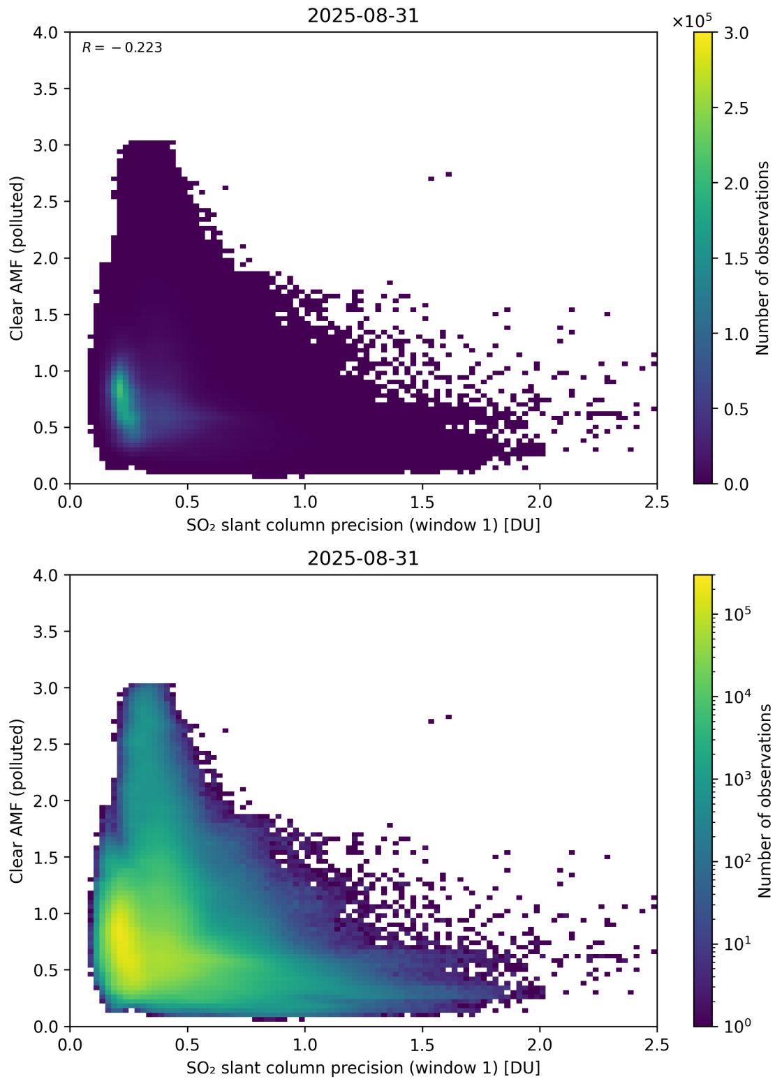
Figure 274: Scatter density plot of “SO 2 slant column precision (window 1)” against “Clear AMF (polluted)” for 2025-08-30 to 2025-09-01.
