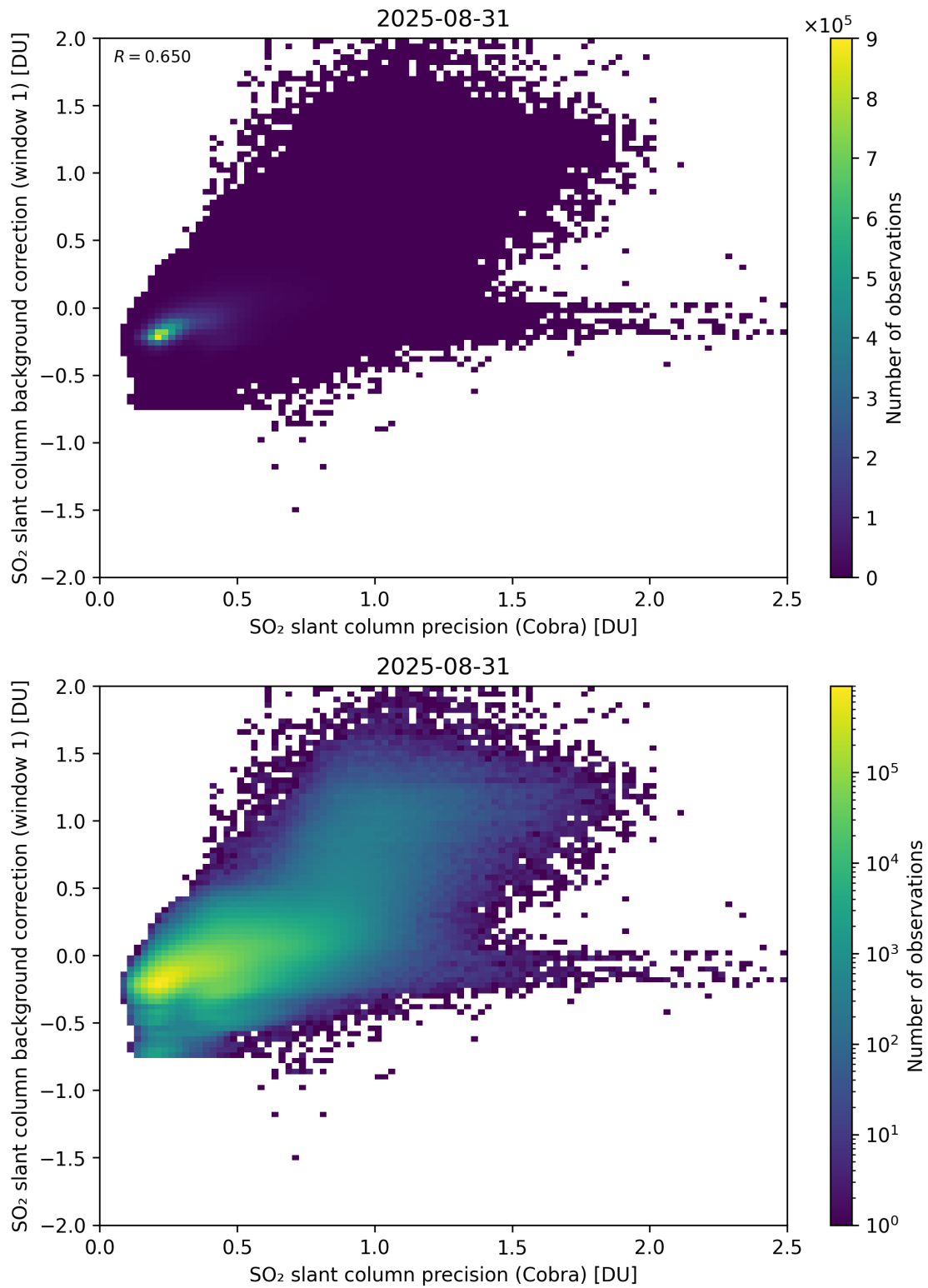
Figure 199: Scatter density plot of “SO 2 slant column precision (Cobra)” against “SO 2 slant column background correction (window 1)” for 2025-08-30 to 2025-09-01.
