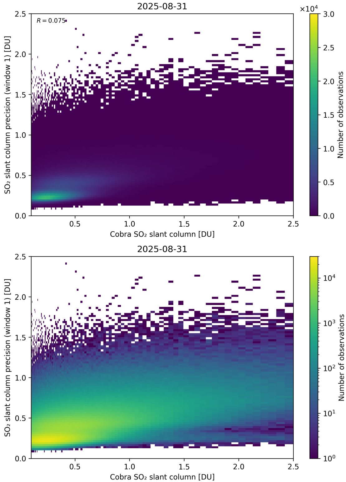
Figure 220: Scatter density plot of “Cobra SO 2 slant column” against “SO 2 slant column precision (window 1)” for 2025-08-30 to 2025-09-01.
