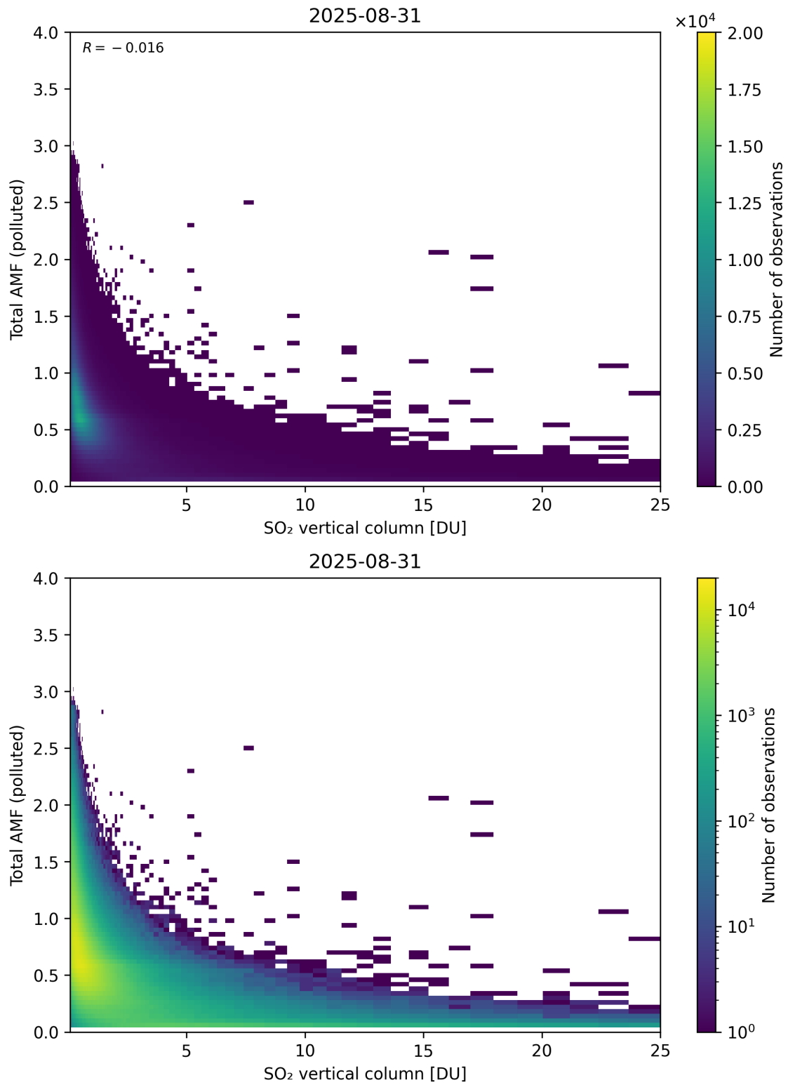
Figure 359: Scatter density plot of “SO 2 vertical column” against “Total AMF (polluted)” for 2025-08-30 to 2025-09-01.
