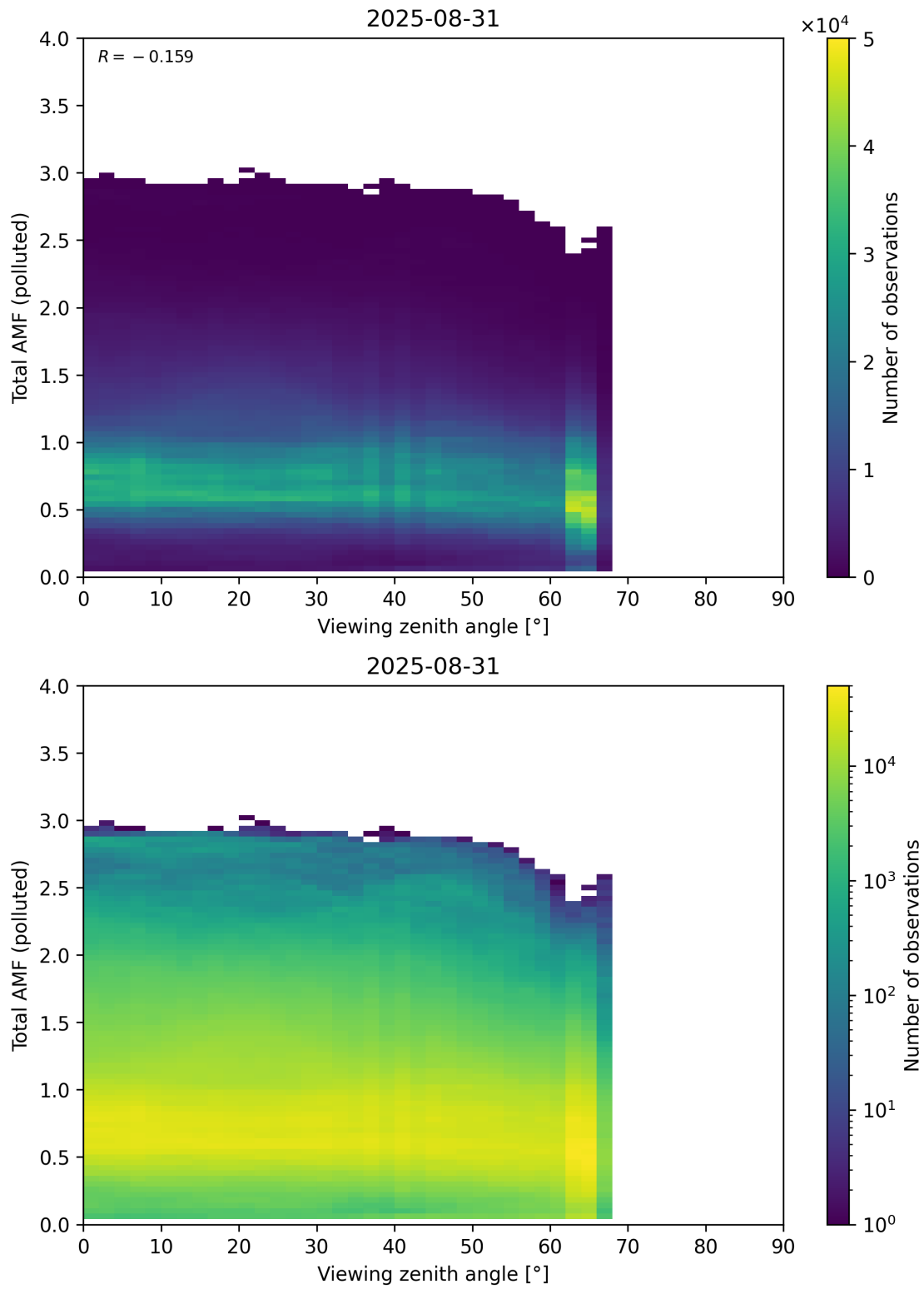
Figure 381: Scatter density plot of “Viewing zenith angle” against “Total AMF (polluted)” for 2025-08-30 to 2025-09-01.
