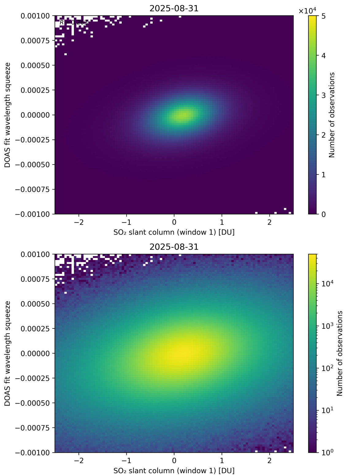
Figure 266: Scatter density plot of “SO 2 slant column (window 1)” against “DOAS fit wavelength squeeze” for 2025-08-30 to 2025-09-01.
