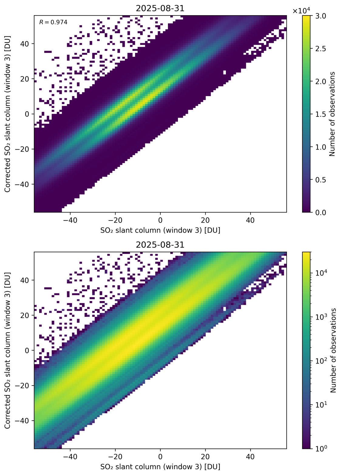
Figure 316: Scatter density plot of “SO 2 slant column (window 3)” against “Corrected SO 2 slant column (window 3)” for 2025-08-30 to 2025-09-01.
