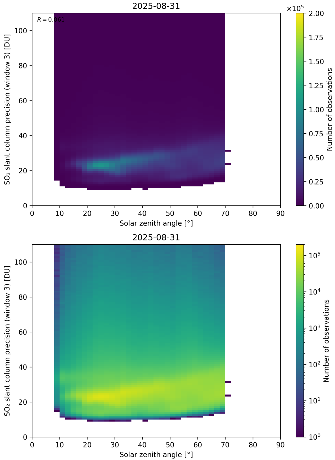
Figure 188: Scatter density plot of “Solar zenith angle” against “SO 2 slant column precision (window 3)” for 2025-08-30 to 2025-09-01.
