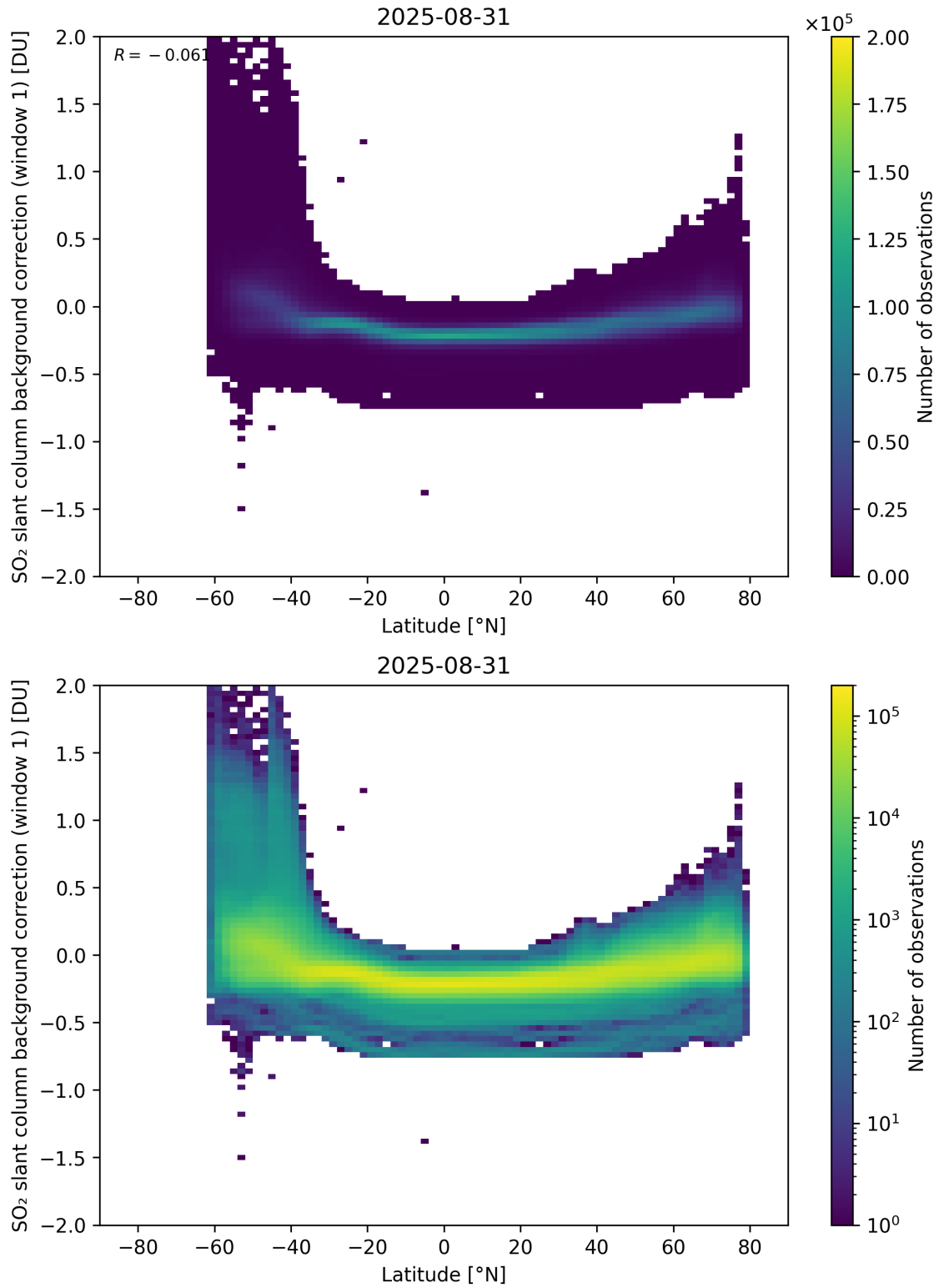
Figure 150: Scatter density plot of “Latitude” against “SO 2 slant column background correction (window 1)” for 2025-08-30 to 2025-09-01.
