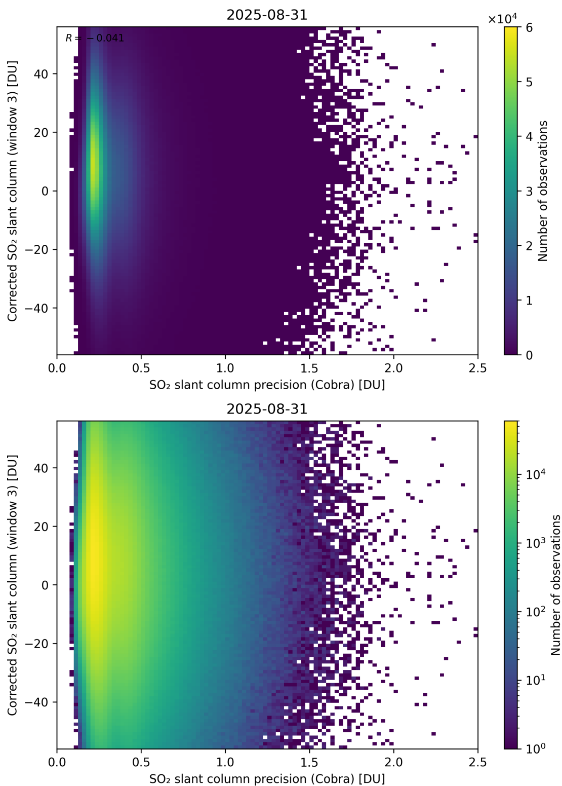
Figure 207: Scatter density plot of “SO 2 slant column precision (Cobra)” against “Corrected SO 2 slant column (window 3)” for 2025-08-30 to 2025-09-01.
