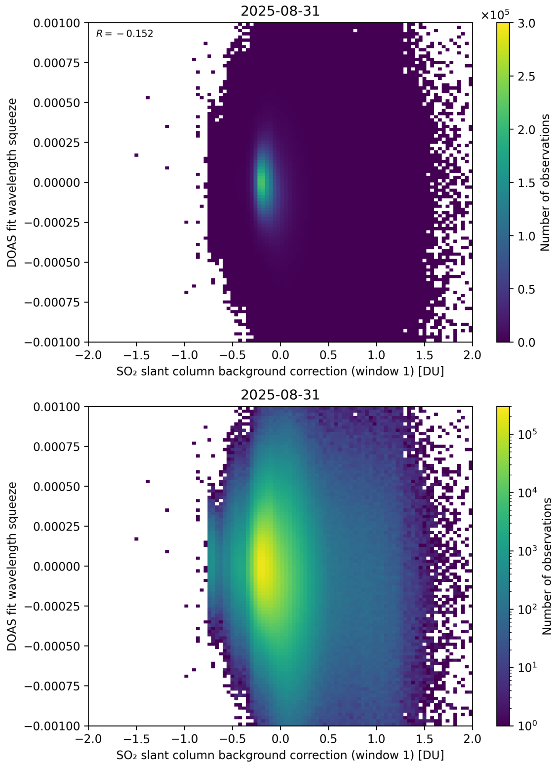
Figure 112: Scatter density plot of “SO 2 slant column background correction (window 1)” against “DOAS fit wavelength squeeze” for 2025-08-30 to 2025-09-01.
