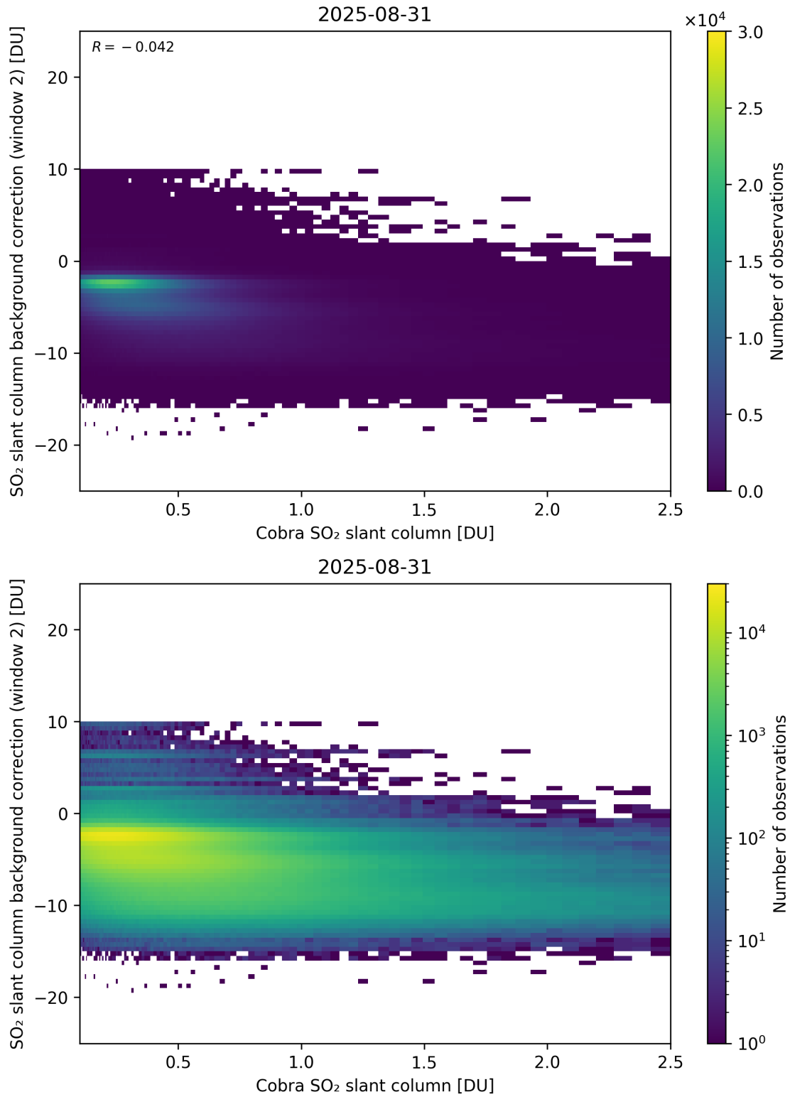
Figure 194: Scatter density plot of “Cobra SO 2 slant column” against “SO 2 slant column background correction (window 2)” for 2025-08-30 to 2025-09-01.
