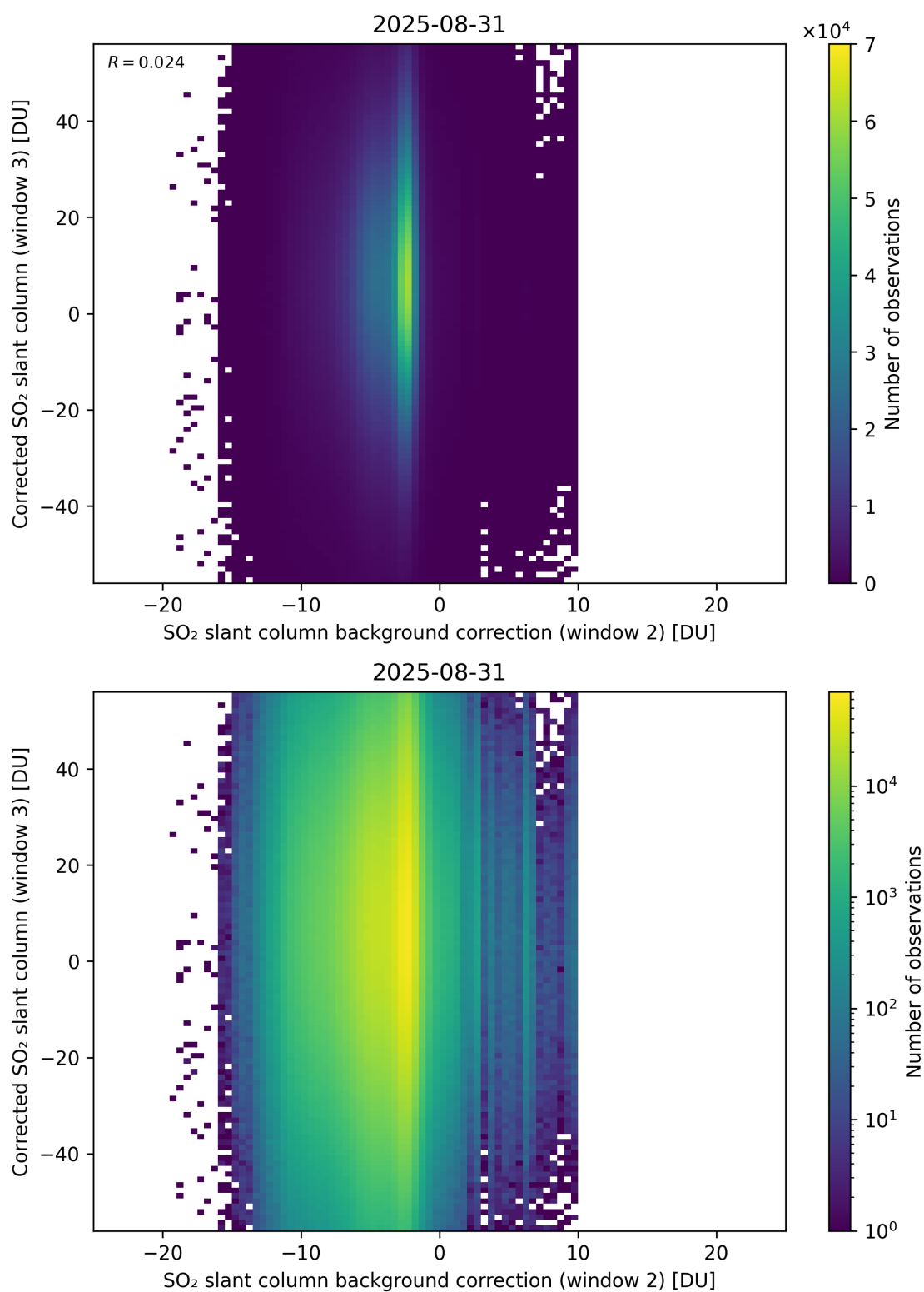
Figure 127: Scatter density plot of “SO 2 slant column background correction (window 2)” against “Corrected SO 2 slant column (window 3)” for 2025-08-30 to 2025-09-01.
