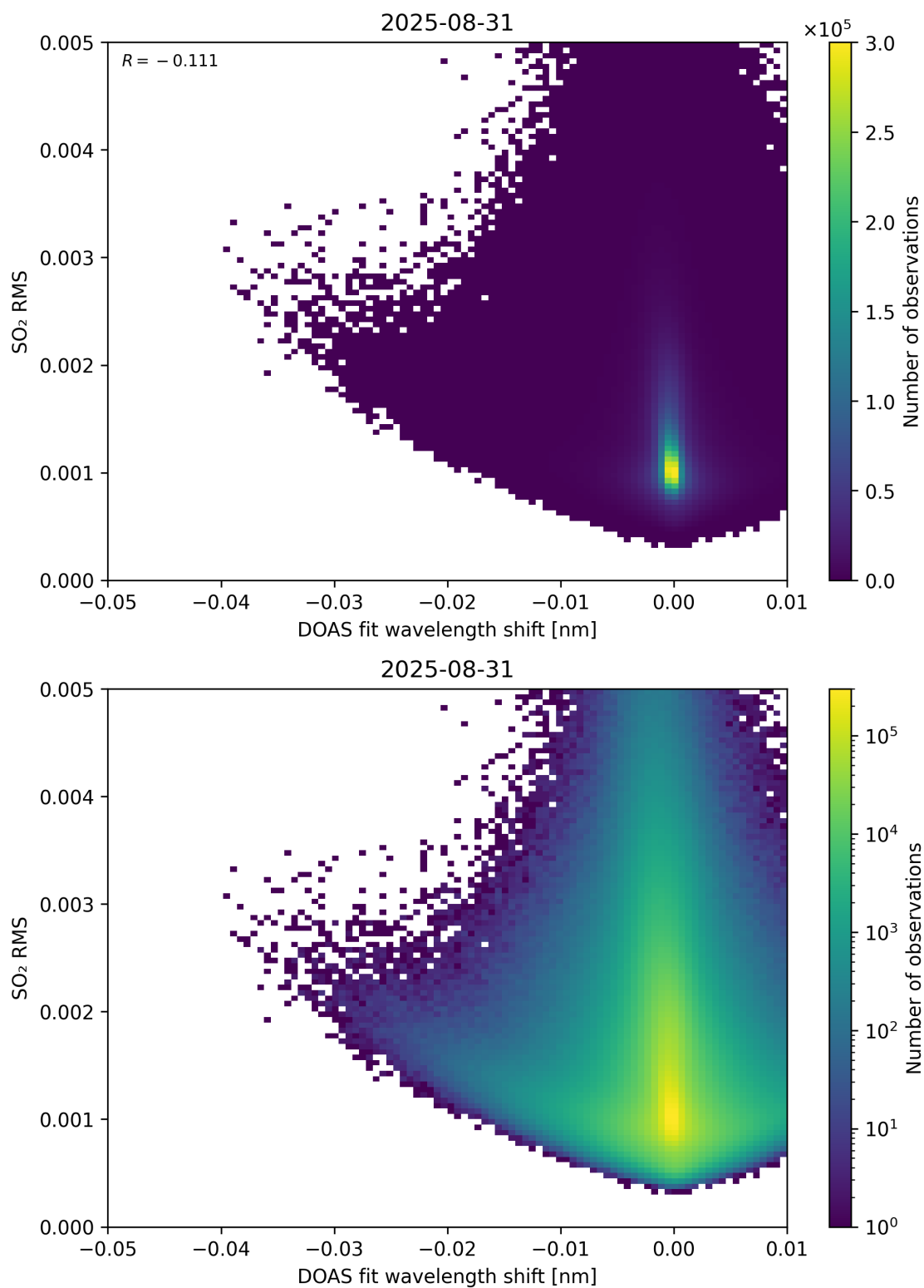
Figure 139: Scatter density plot of “DOAS fit wavelength shift” against “SO 2 RMS” for 2025-08-30 to 2025-09-01.
