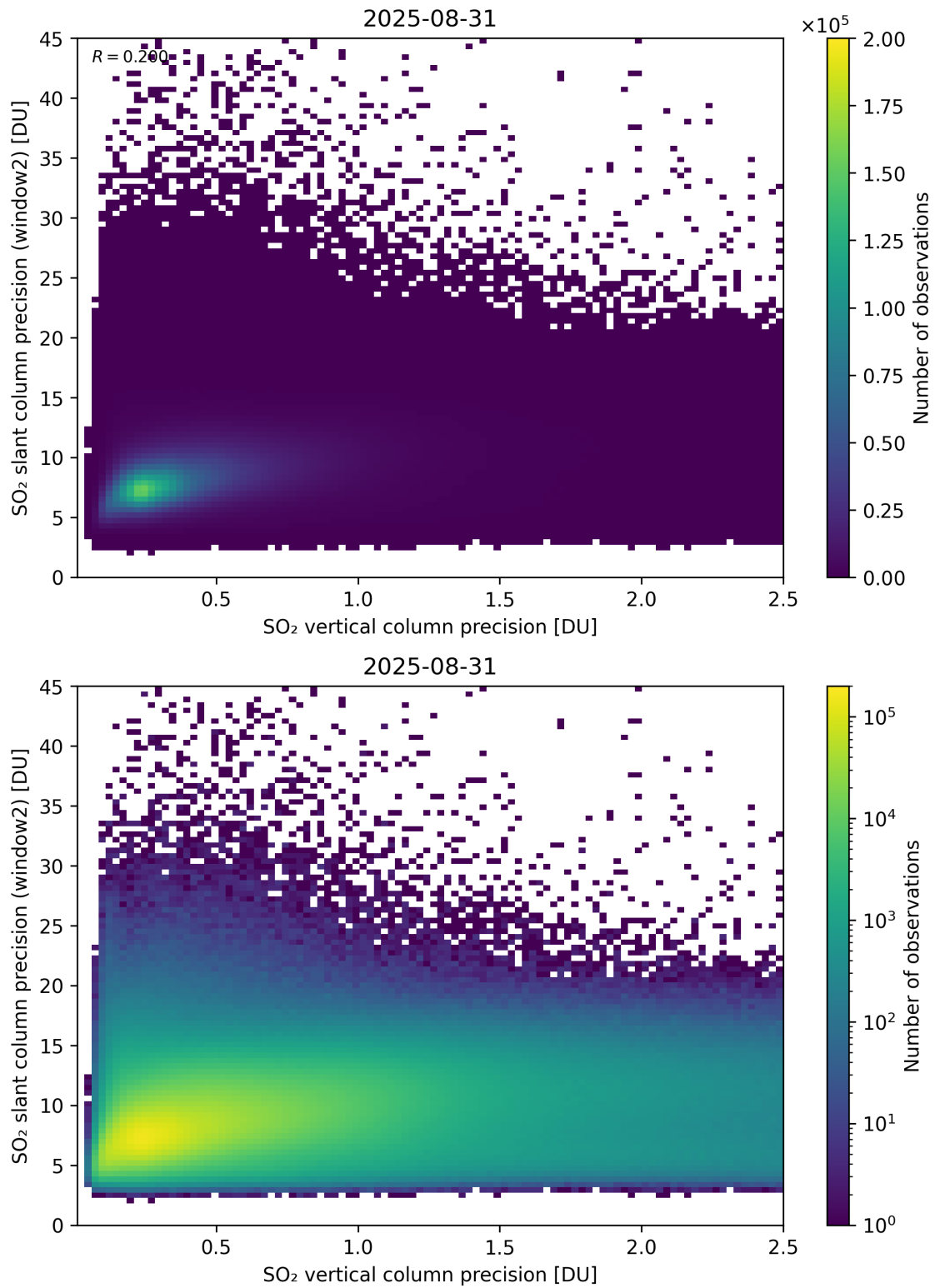
Figure 343: Scatter density plot of “SO 2 vertical column precision” against “SO 2 slant column precision (window2)” for 2025-08-30 to 2025-09-01.
