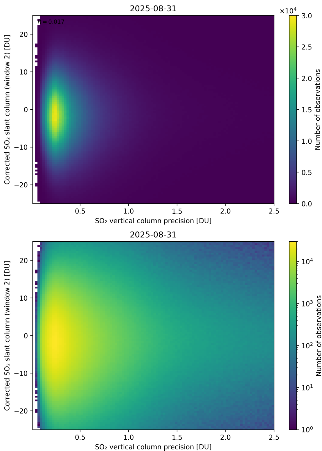
Figure 339: Scatter density plot of “SO 2 vertical column precision” against “Corrected SO 2 slant column (window 2)” for 2025-08-30 to 2025-09-01.
