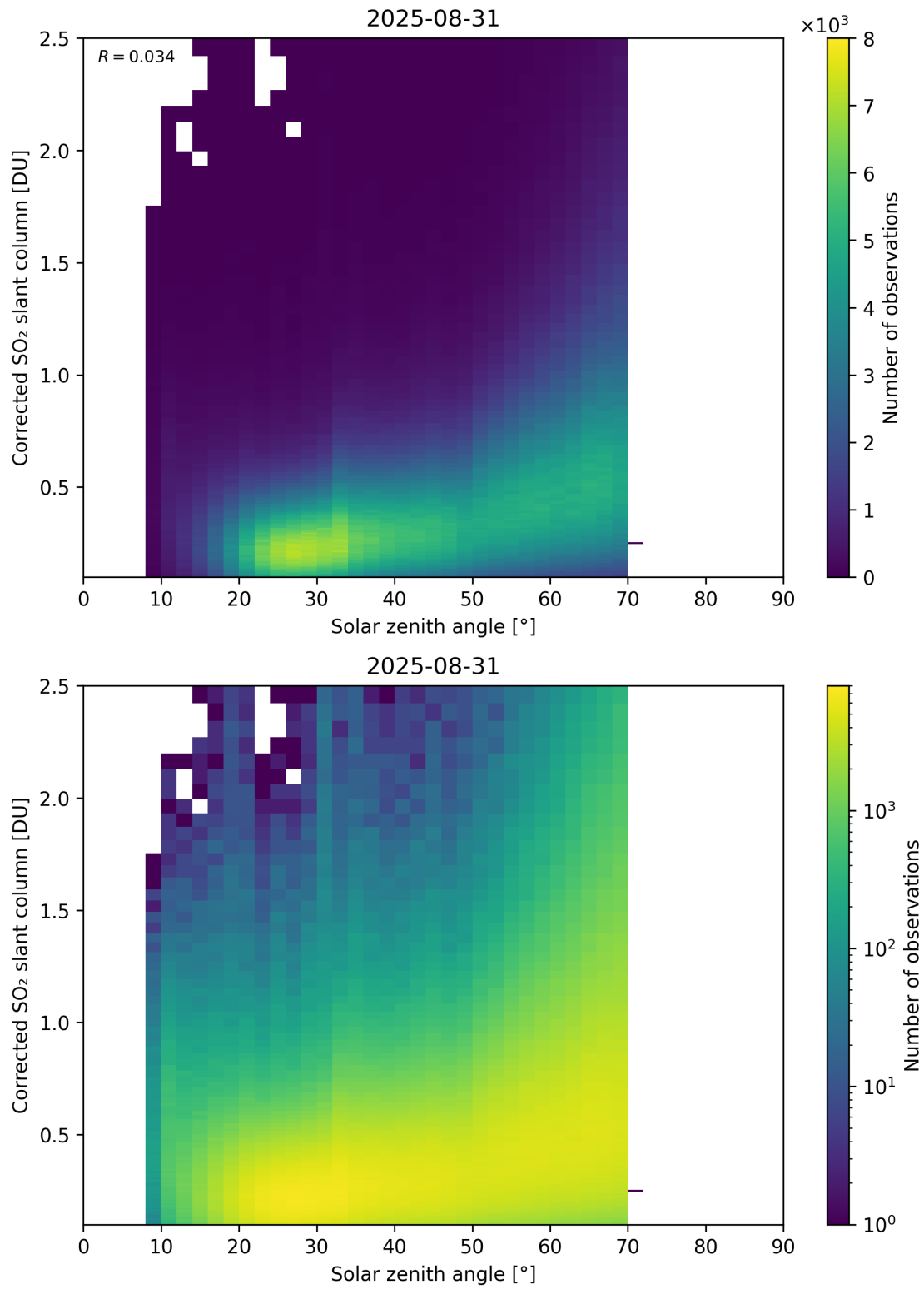
Figure 181: Scatter density plot of “Solar zenith angle” against “Corrected SO 2 slant column” for 2025-08-30 to 2025-09-01.
