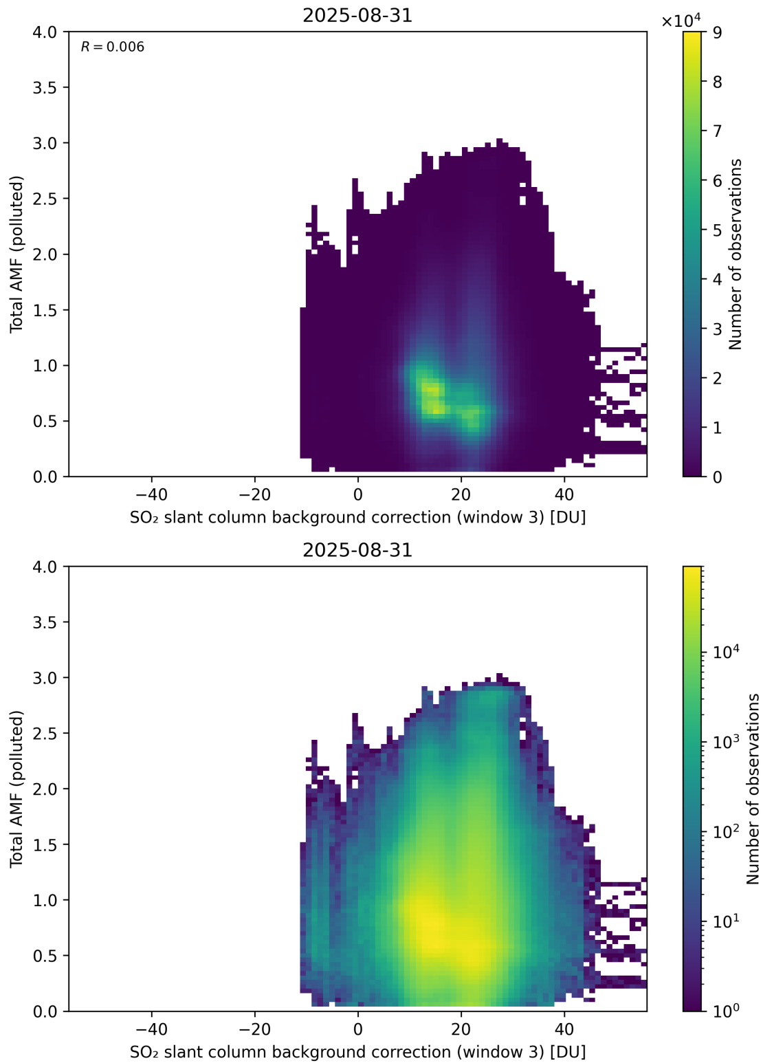
Figure 136: Scatter density plot of “SO 2 slant column background correction (window 3)” against “Total AMF (polluted)” for 2025-08-30 to 2025-09-01.
