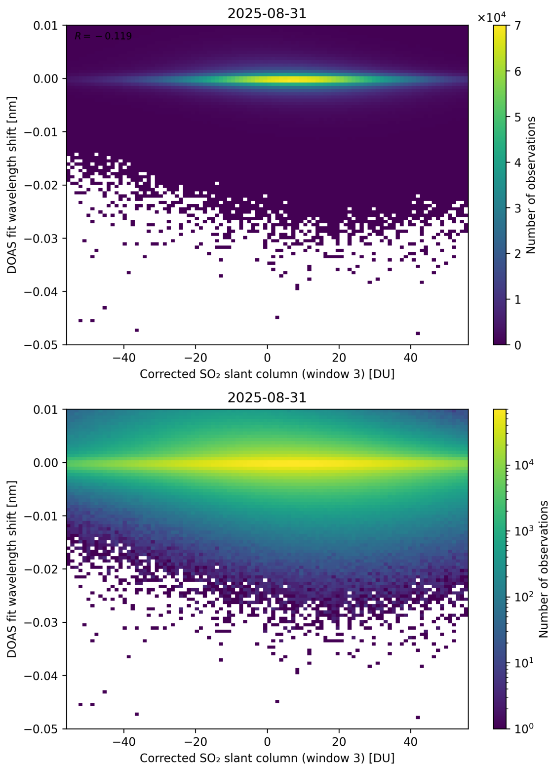
Figure 256: Scatter density plot of “Corrected SO 2 slant column (window 3)” against “DOAS fit wavelength shift” for 2025-08-30 to 2025-09-01.
