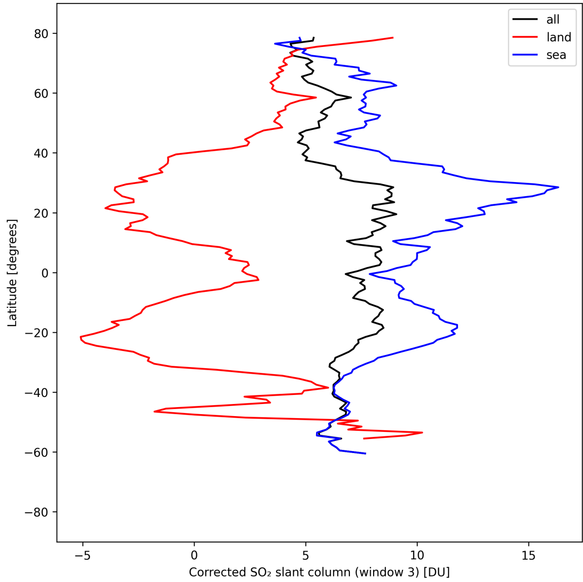
Figure 47: Zonal average of “Corrected SO 2 slant column (window 3)” for 2025-08-30 to 2025-09-01.
