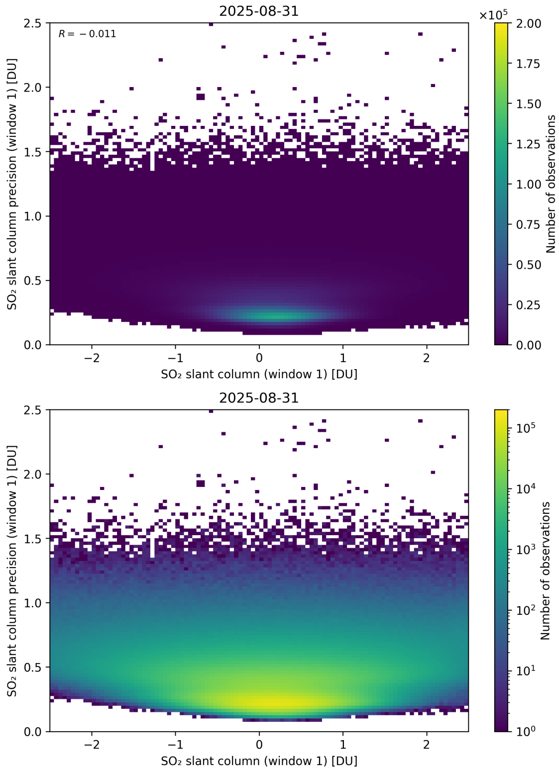
Figure 285: Scatter density plot of “SO 2 slant column (window 1)” against “SO 2 slant column precision (window 1)” for 2025-08-30 to 2025-09-01.
