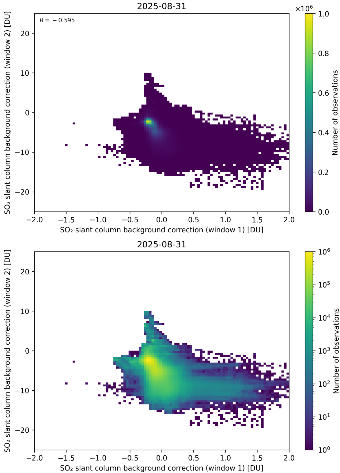
Figure 109: Scatter density plot of “SO 2 slant column background correction (window 1)” against “SO 2 slant column background correction (window 2)” for 2025-08-30 to 2025-09-01.
