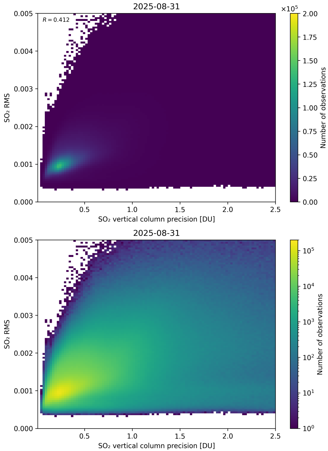
Figure 334: Scatter density plot of “SO 2 vertical column precision” against “SO 2 RMS” for 2025-08-30 to 2025-09-01.
