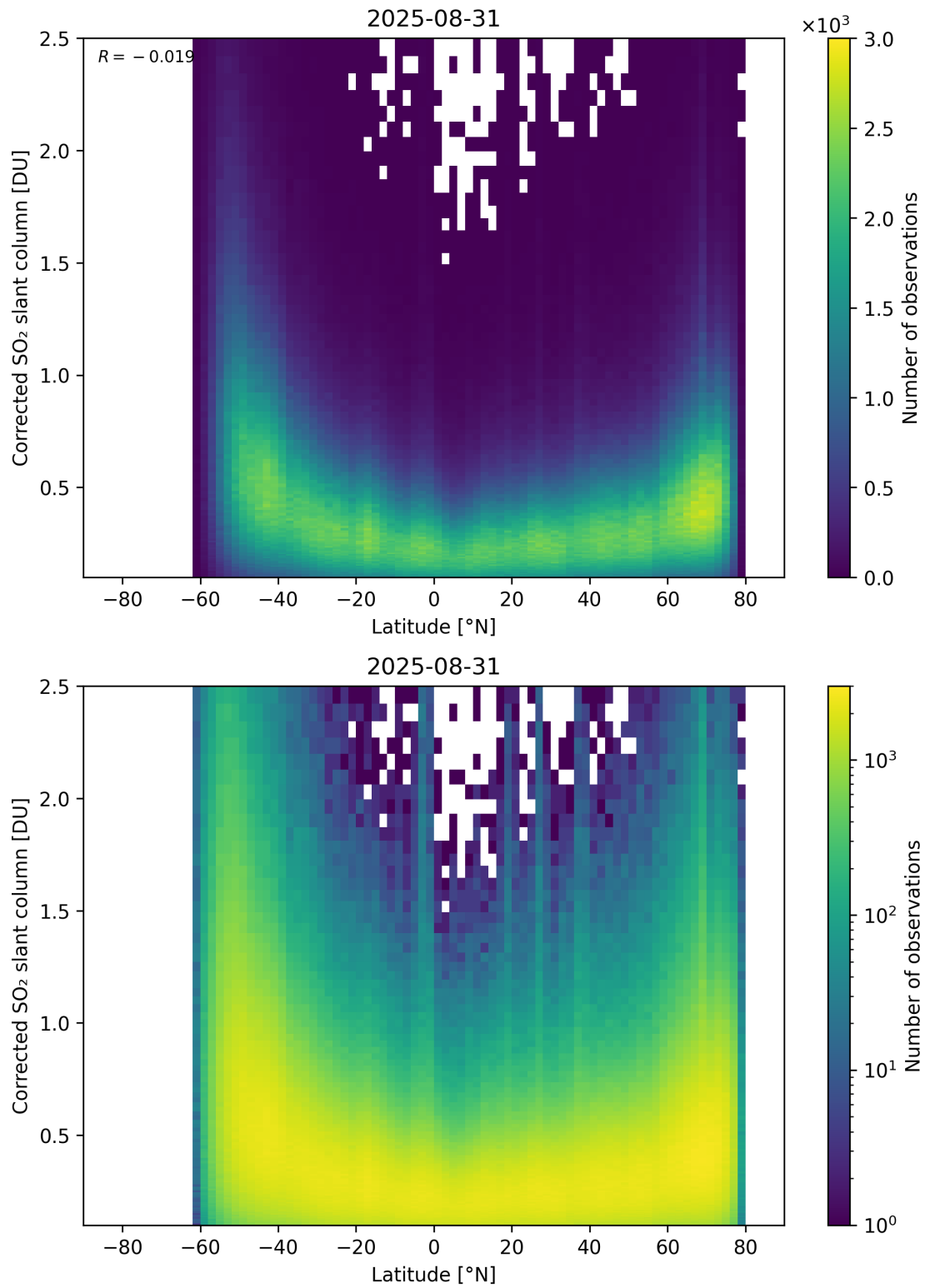
Figure 159: Scatter density plot of “Latitude” against “Corrected SO 2 slant column” for 2025-08-30 to 2025-09-01.
