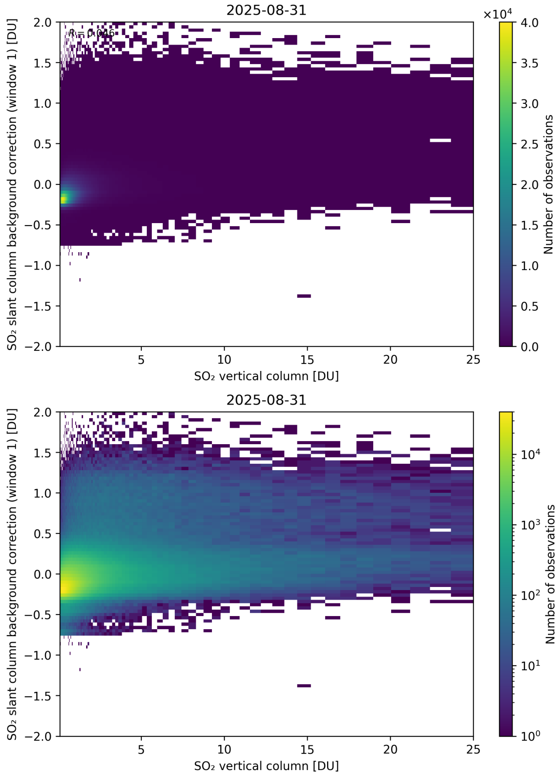
Figure 323: Scatter density plot of “SO 2 vertical column” against “SO 2 slant column background correction (window 1)” for 2025-08-30 to 2025-09-01.
