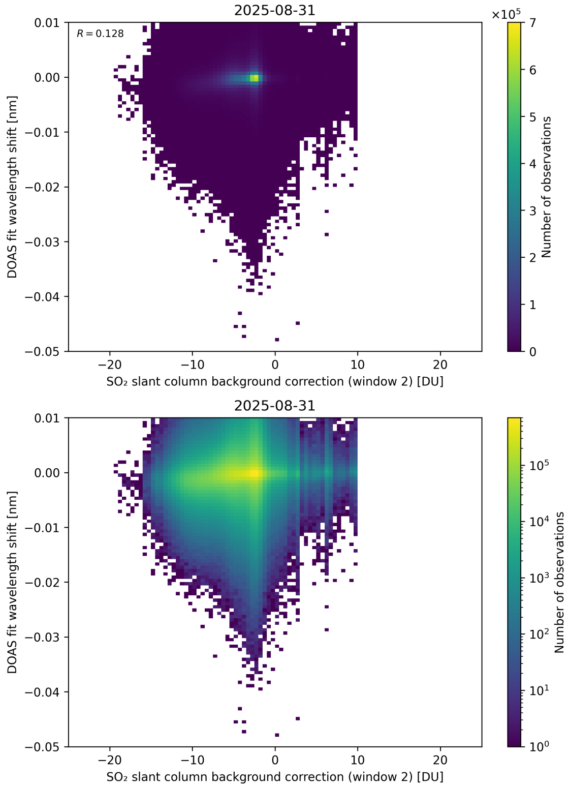
Figure 123: Scatter density plot of “SO 2 slant column background correction (window 2)” against “DOAS fit wavelength shift” for 2025-08-30 to 2025-09-01.
