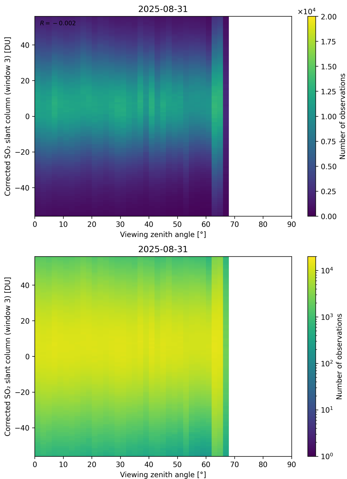
Figure 375: Scatter density plot of “Viewing zenith angle” against “Corrected SO 2 slant column (window 3)” for 2025-08-30 to 2025-09-01.
