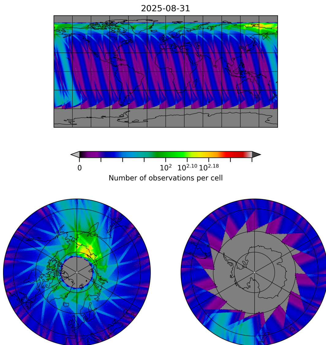
Figure 30: Map of the number of observations for 2025-08-30 to 2025-09-01
