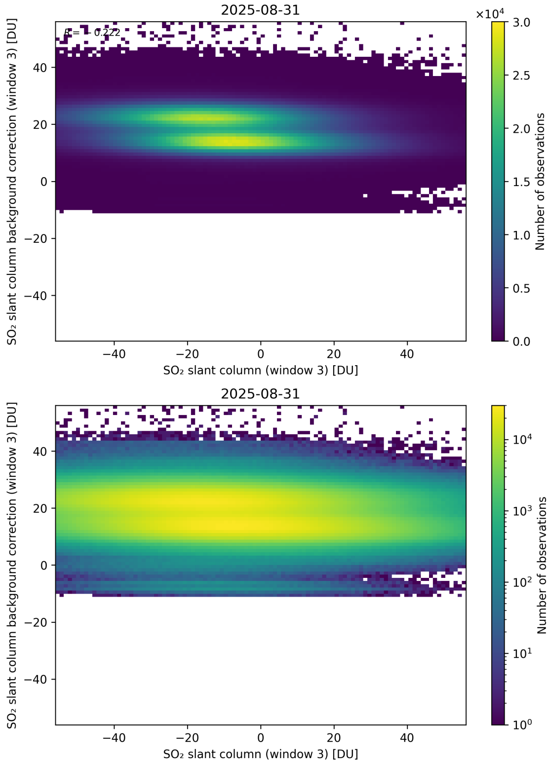
Figure 303: Scatter density plot of “SO 2 slant column (window 3)” against “SO 2 slant column background correction (window 3)” for 2025-08-30 to 2025-09-01.
