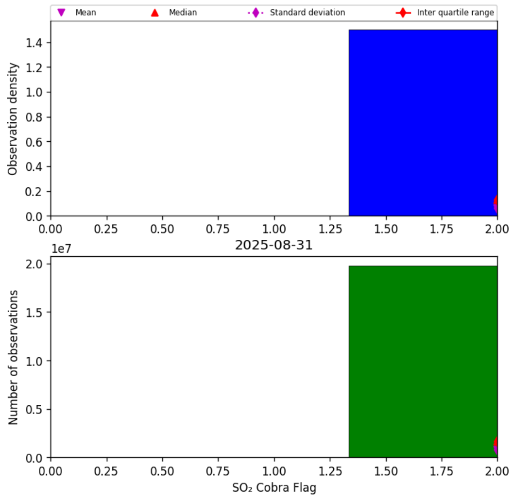
Figure 75: Histogram of "SO 2 Cobra Flag" for 2025-08-30 to 2025-09-01
