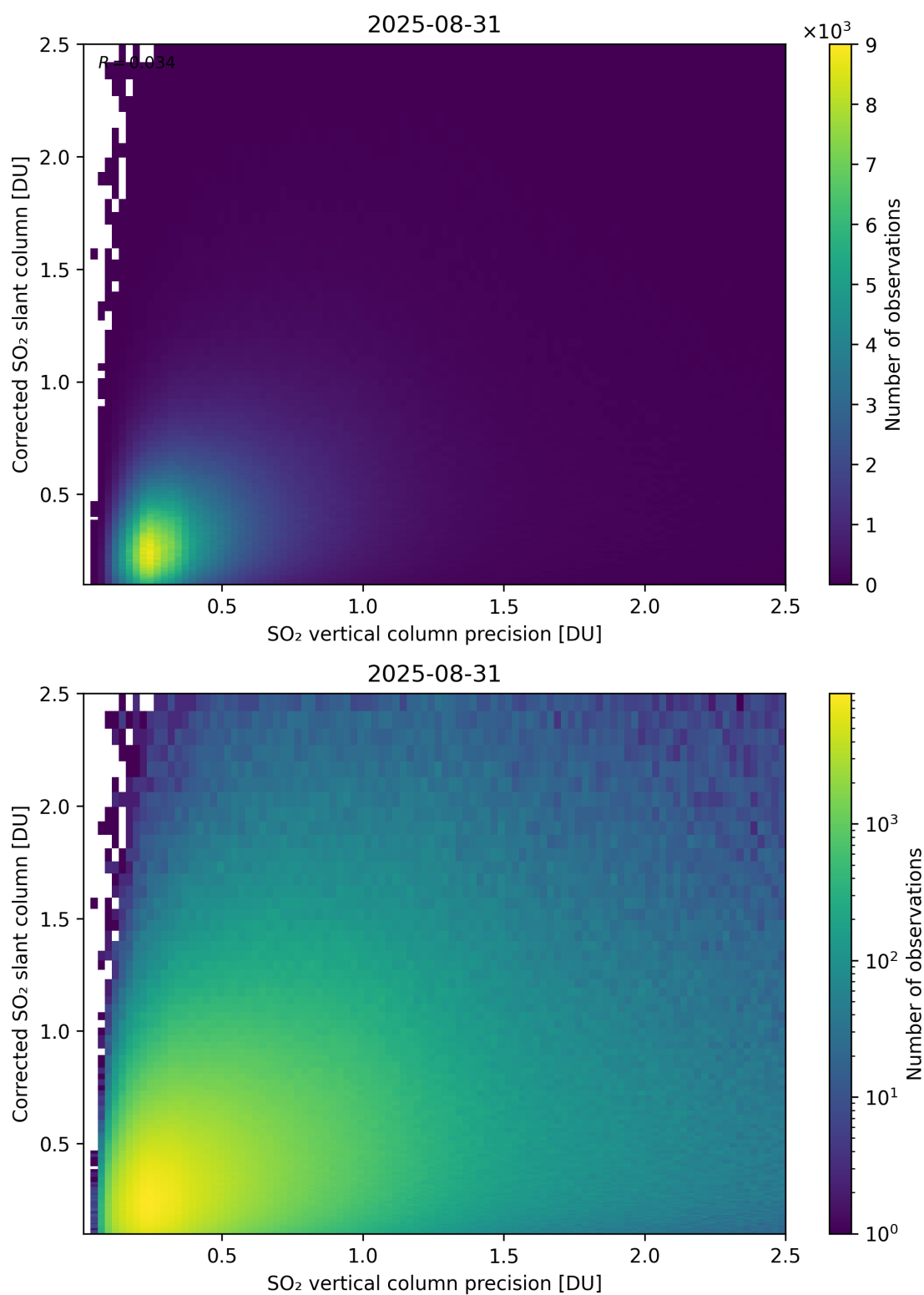
Figure 338: Scatter density plot of “SO 2 vertical column precision” against “Corrected SO 2 slant column” for 2025-08-30 to 2025-09-01.
