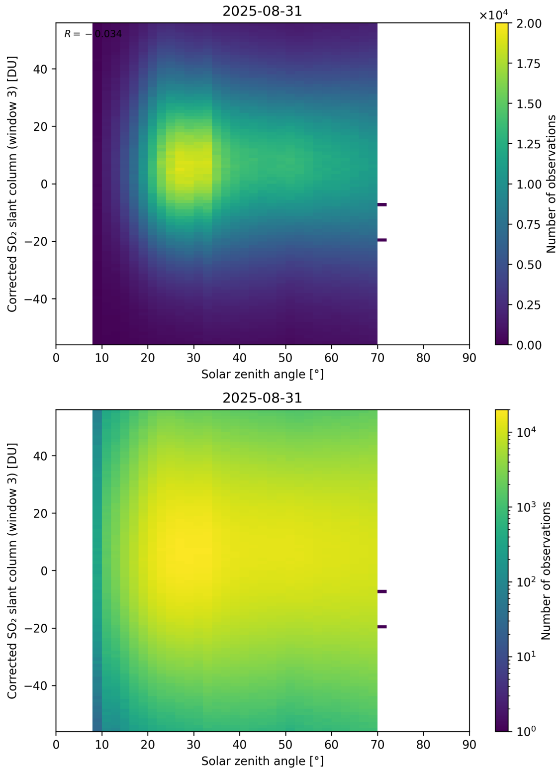
Figure 183: Scatter density plot of “Solar zenith angle” against “Corrected SO 2 slant column (window 3)” for 2025-08-30 to 2025-09-01.
