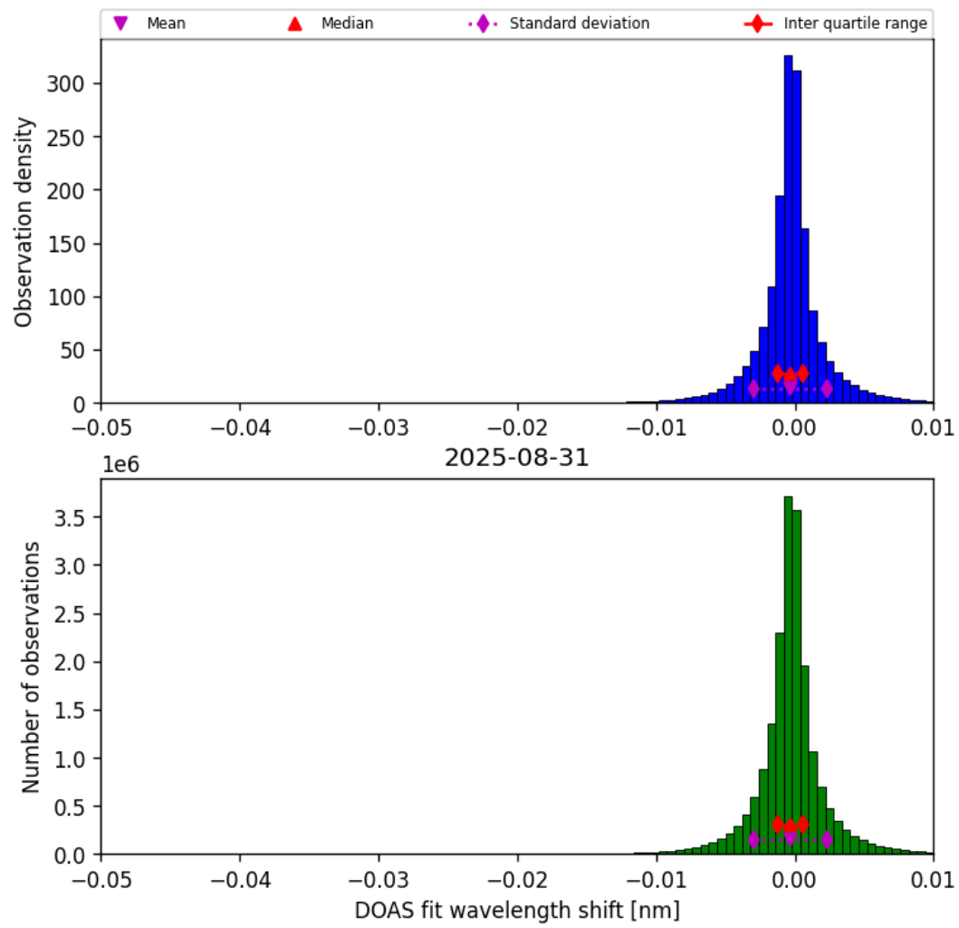
Figure 76: Histogram of “DOAS fit wavelength shift” for 2025-08-30 to 2025-09-01
