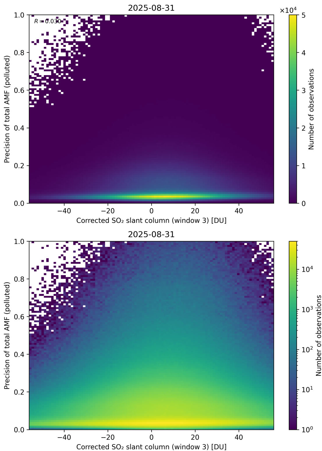
Figure 261: Scatter density plot of “Corrected SO 2 slant column (window 3)” against “Precision of total AMF (polluted)” for 2025-08-30 to 2025-09-01.
