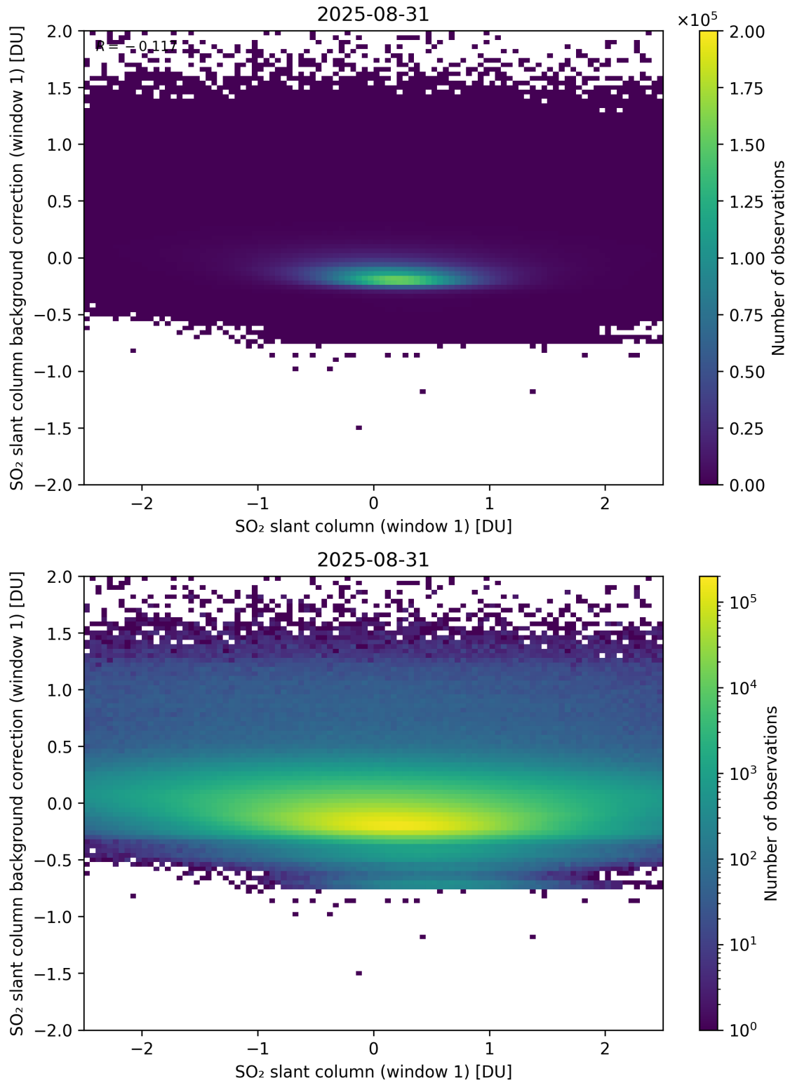
Figure 262: Scatter density plot of “SO 2 slant column (window 1)” against “SO 2 slant column background correction (window 1)” for 2025-08-30 to 2025-09-01.
