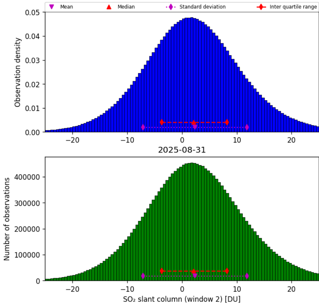
Figure 67: Histogram of “SO 2 slant column (window 2)” for 2025-08-30 to 2025-09-01
