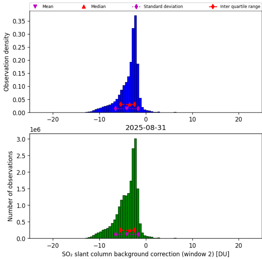
Figure 70: Histogram of “SO 2 slant column background correction (window 2)” for 2025-08-30 to 2025-09-01
