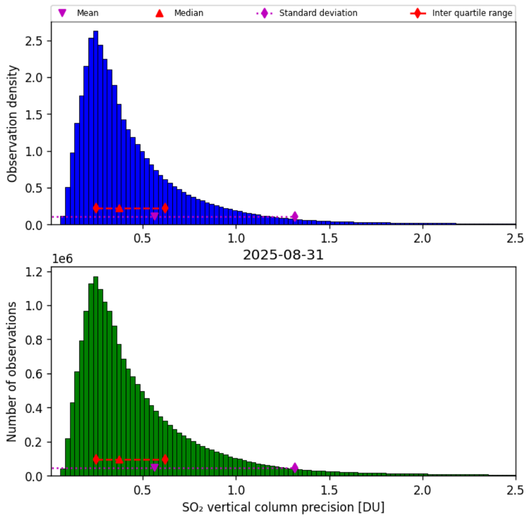
Figure 59: Histogram of “SO 2 vertical column precision” for 2025-08-30 to 2025-09-01
