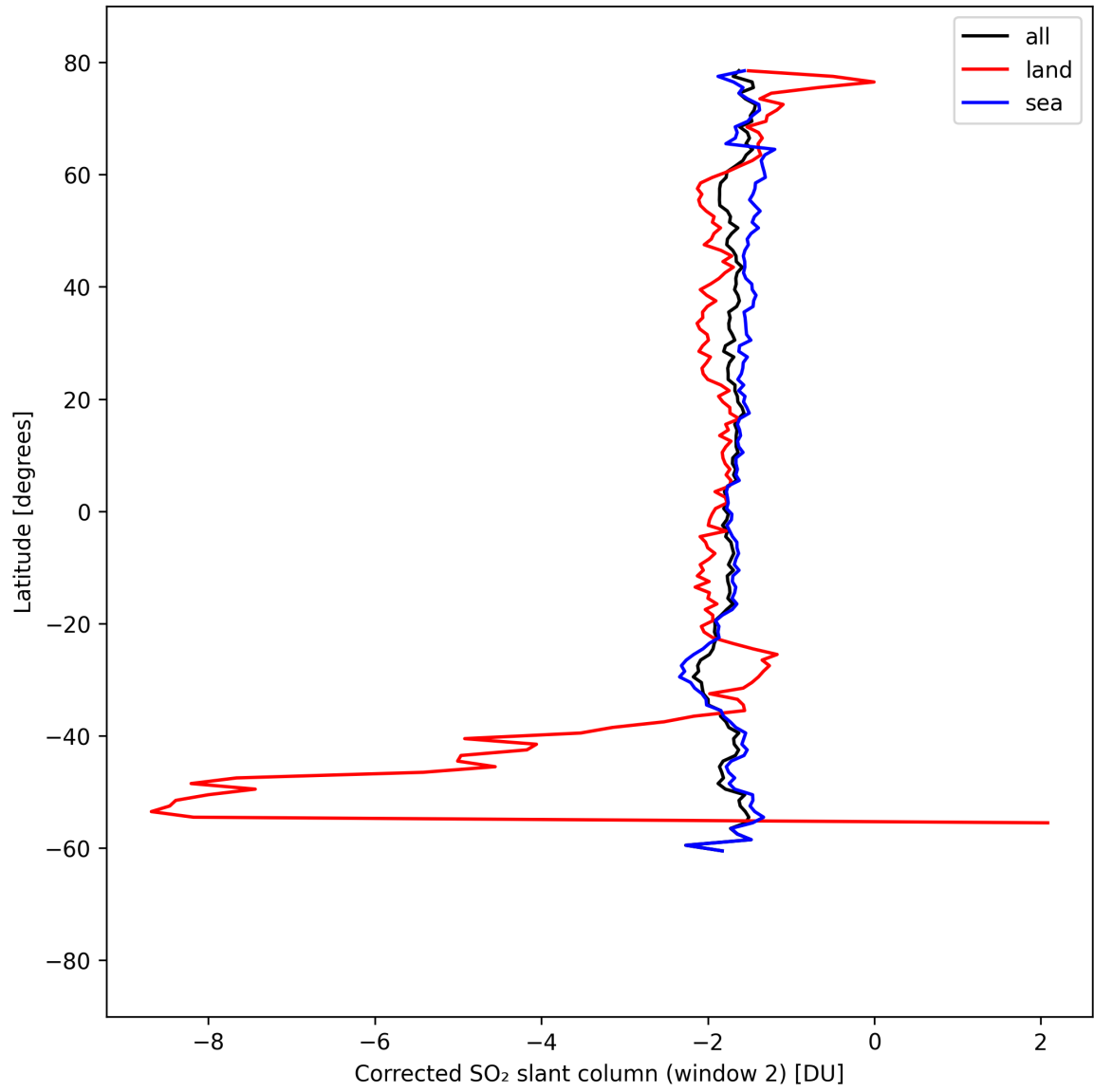
Figure 43: Zonal average of “Corrected SO 2 slant column (window 2)” for 2025-08-30 to 2025-09-01.
