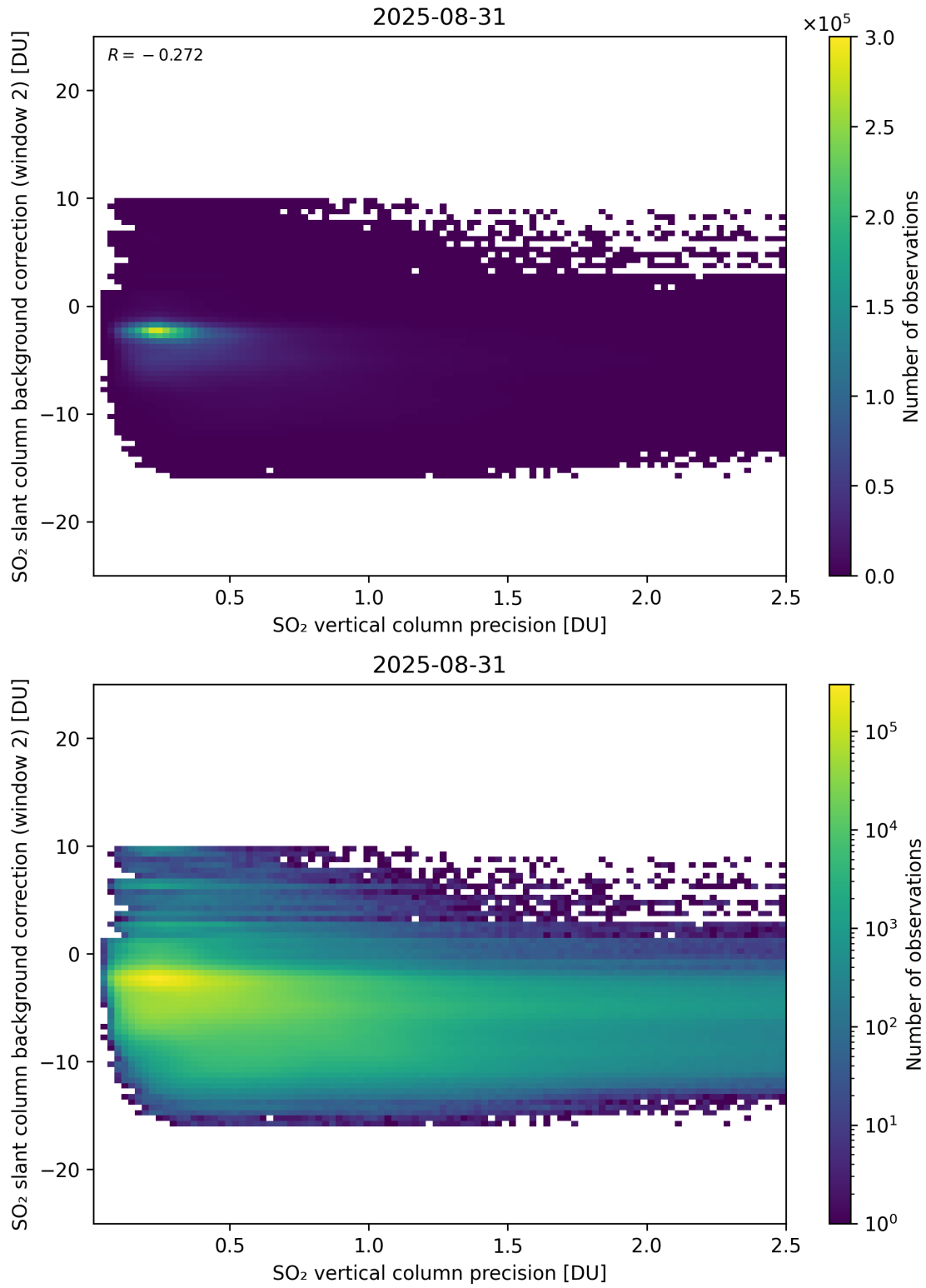
Figure 330: Scatter density plot of “SO 2 vertical column precision” against “SO 2 slant column background correction (window 2)” for 2025-08-30 to 2025-09-01.
