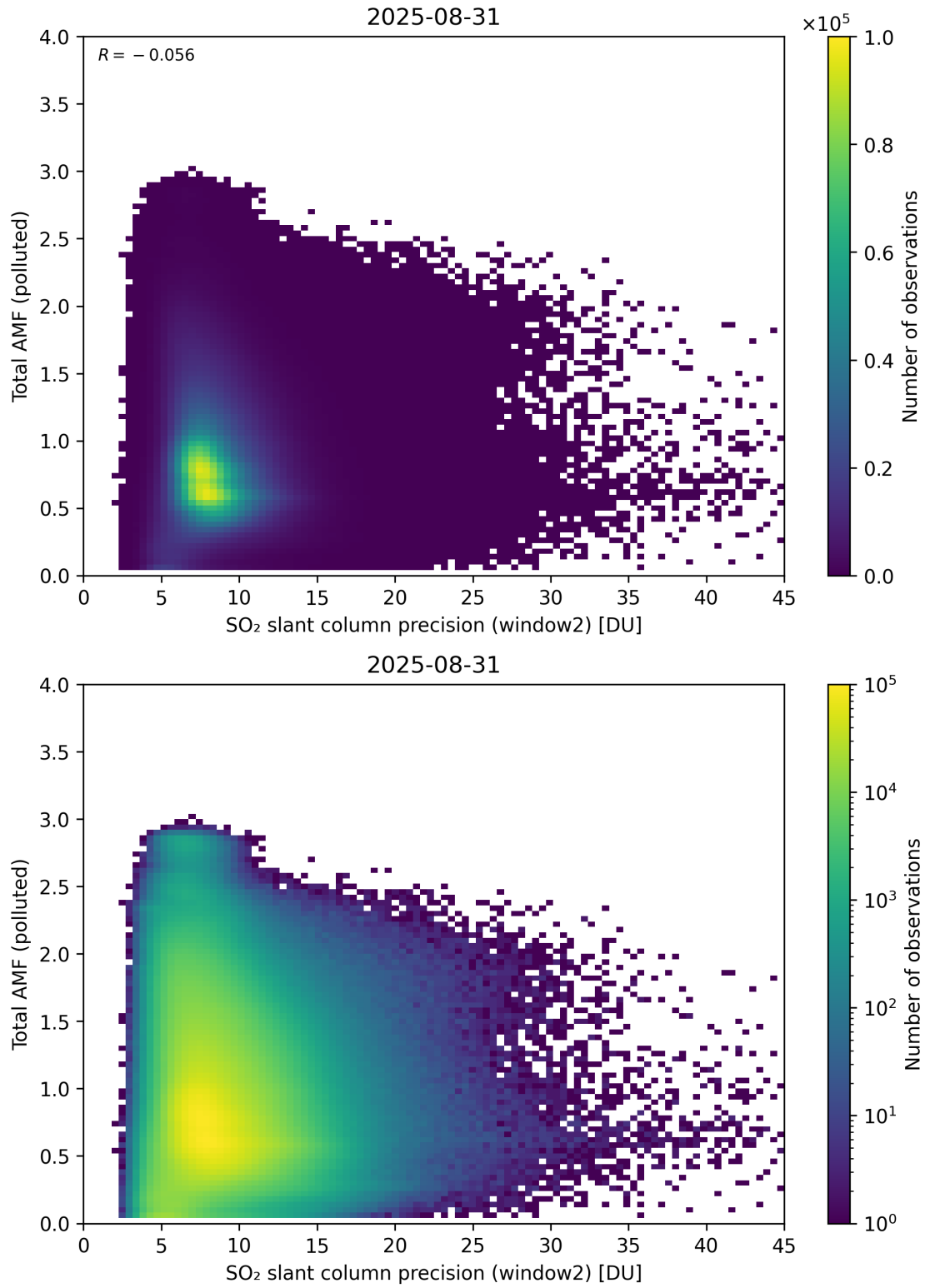
Figure 301: Scatter density plot of “SO 2 slant column precision (window2)” against “Total AMF (polluted)” for 2025-08-30 to 2025-09-01.
