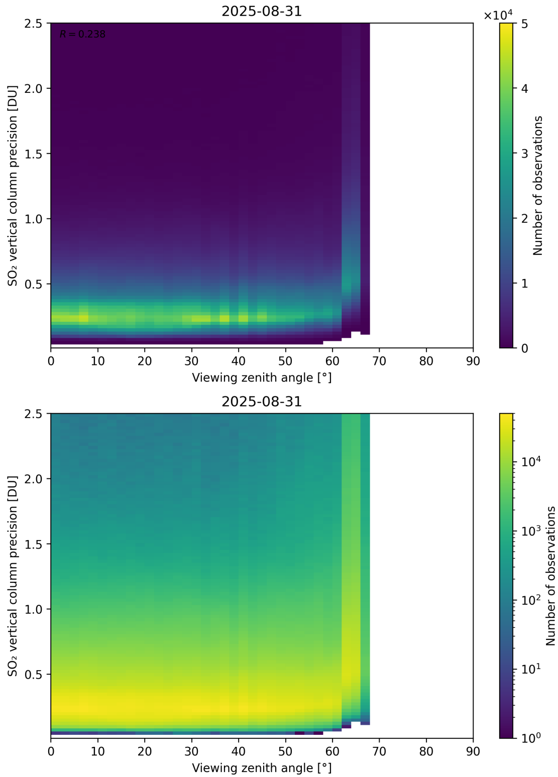
Figure 384: Scatter density plot of “Viewing zenith angle” against “SO 2 vertical column precision” for 2025-08-30 to 2025-09-01.
