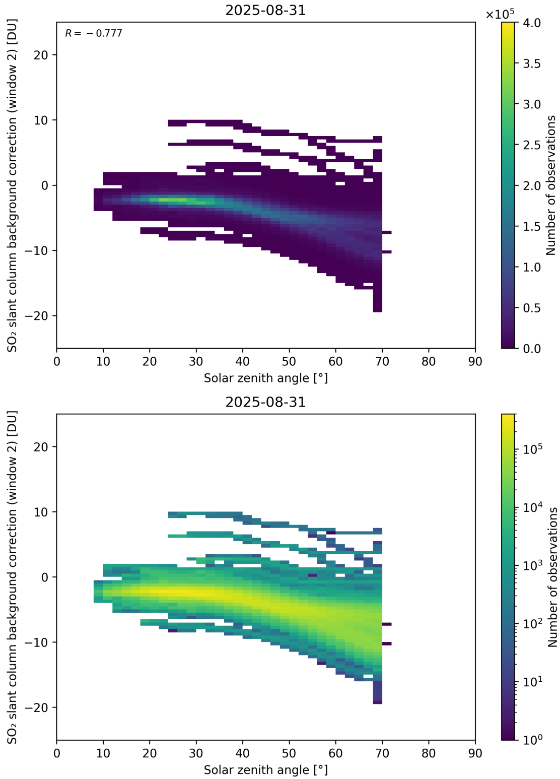
Figure 172: Scatter density plot of “Solar zenith angle” against “SO 2 slant column background correction (window 2)” for 2025-08-30 to 2025-09-01.
