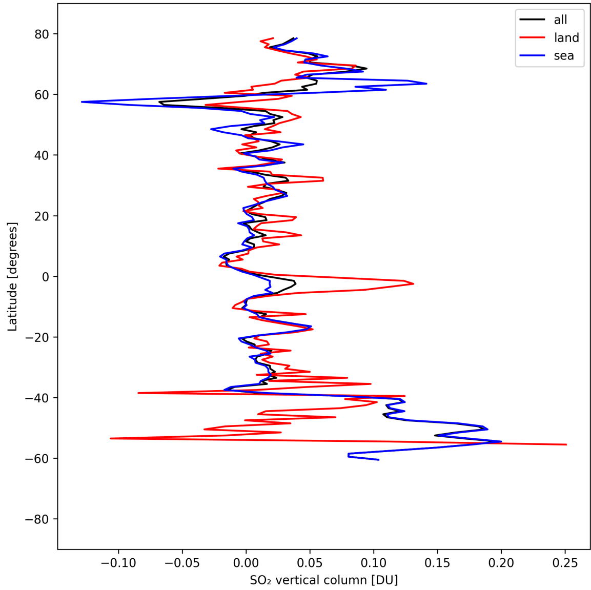
Figure 32: Zonal average of “SO 2 vertical column” for 2025-08-30 to 2025-09-01.
