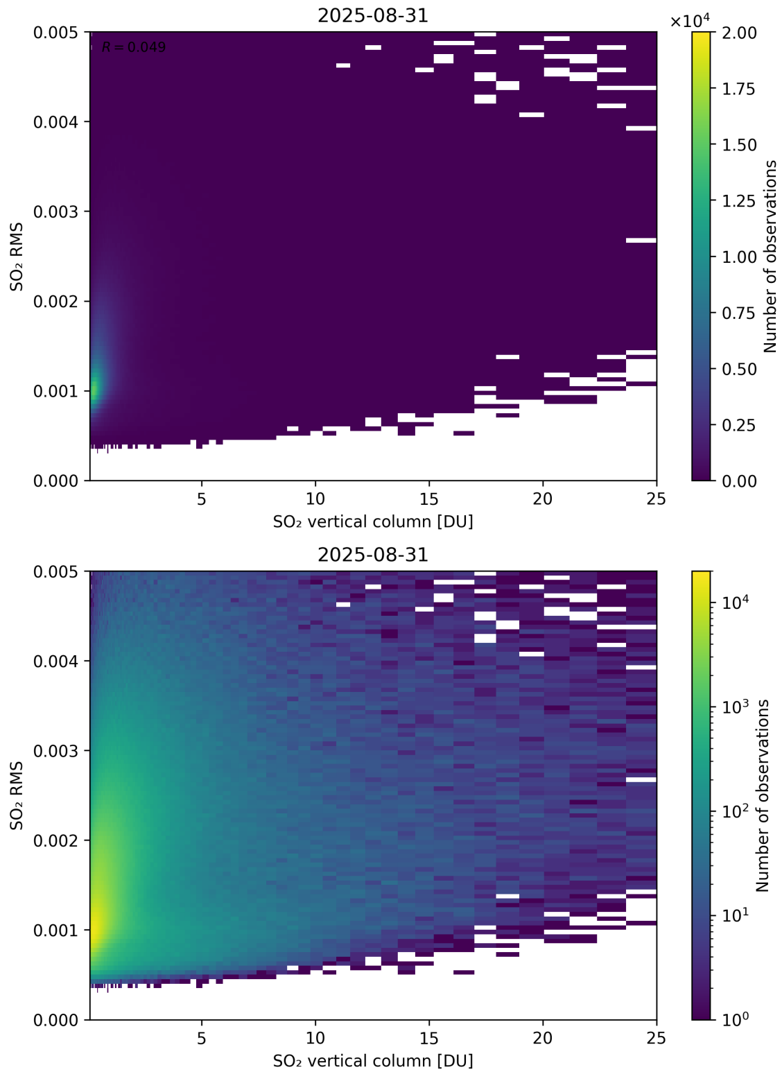
Figure 328: Scatter density plot of “SO 2 vertical column” against “SO 2 RMS” for 2025-08-30 to 2025-09-01.
