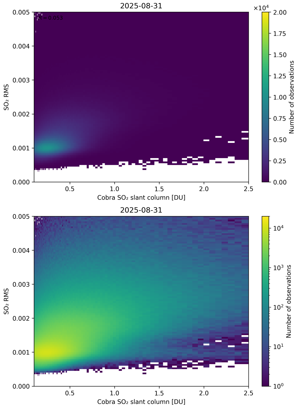
Figure 198: Scatter density plot of “Cobra SO 2 slant column” against “SO 2 RMS” for 2025-08-30 to 2025-09-01.
