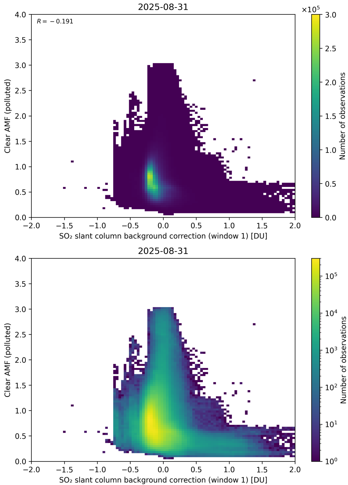
Figure 114: Scatter density plot of “SO 2 slant column background correction (window 1)” against “Clear AMF (polluted)” for 2025-08-30 to 2025-09-01.
