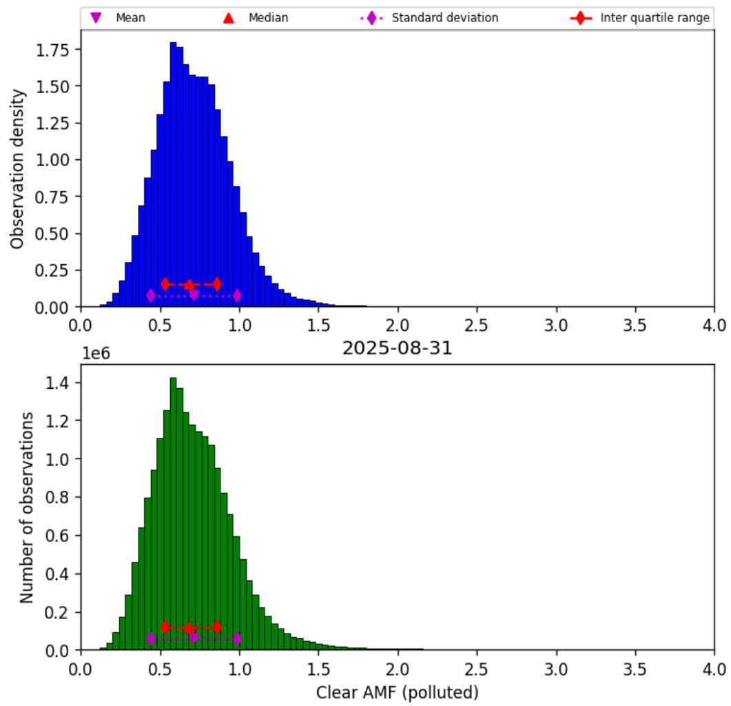
Figure 81: Histogram of “Clear AMF (polluted)” for 2025-08-30 to 2025-09-01
