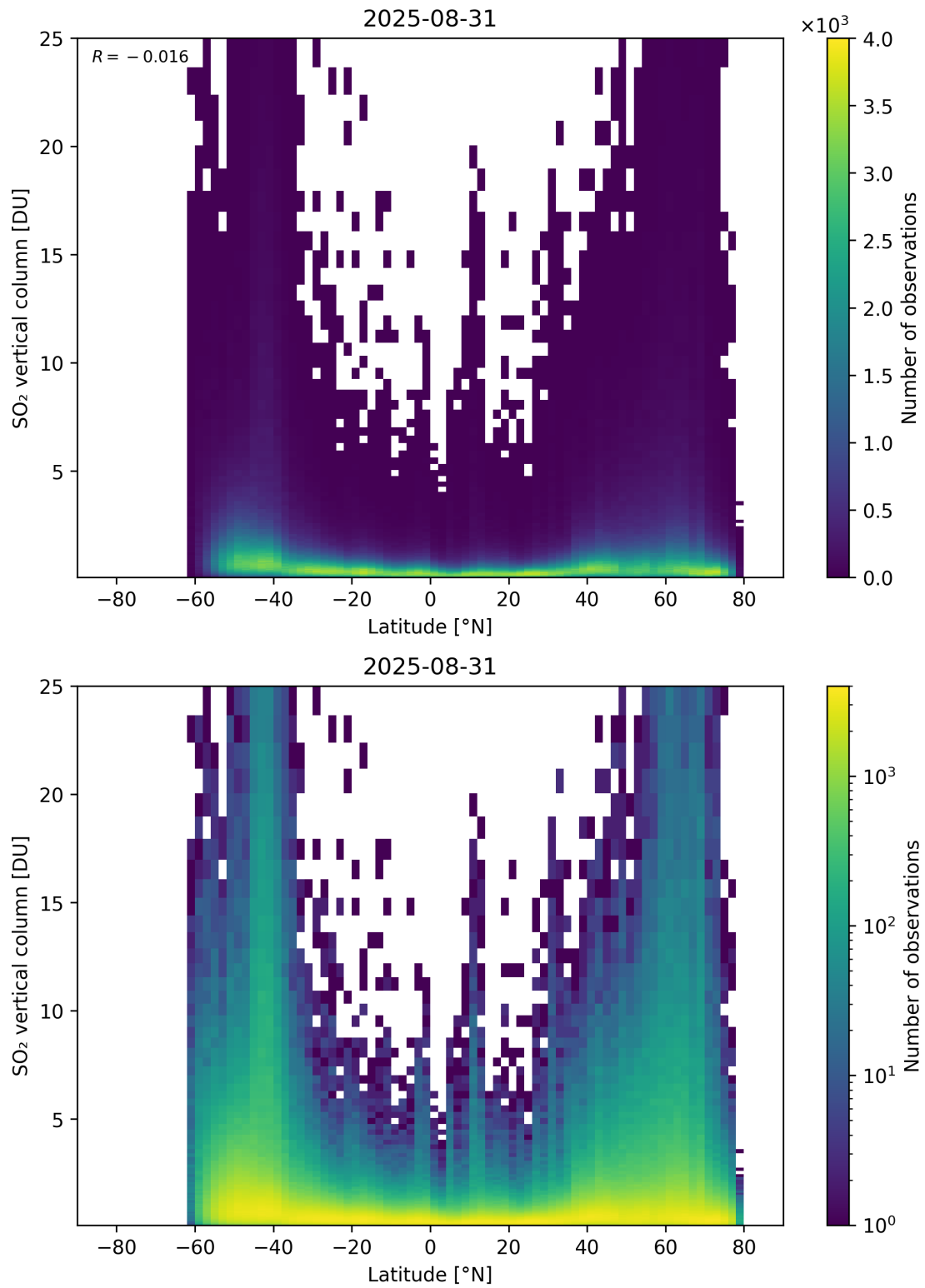
Figure 169: Scatter density plot of “Latitude” against “SO 2 vertical column” for 2025-08-30 to 2025-09-01.
