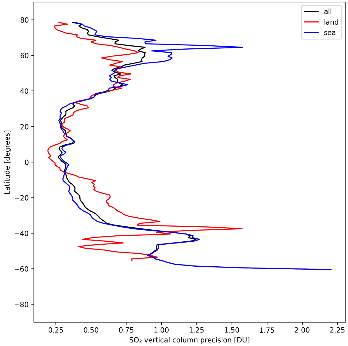
Figure 33: Zonal average of “SO 2 vertical column precision” for 2025-08-30 to 2025-09-01.
