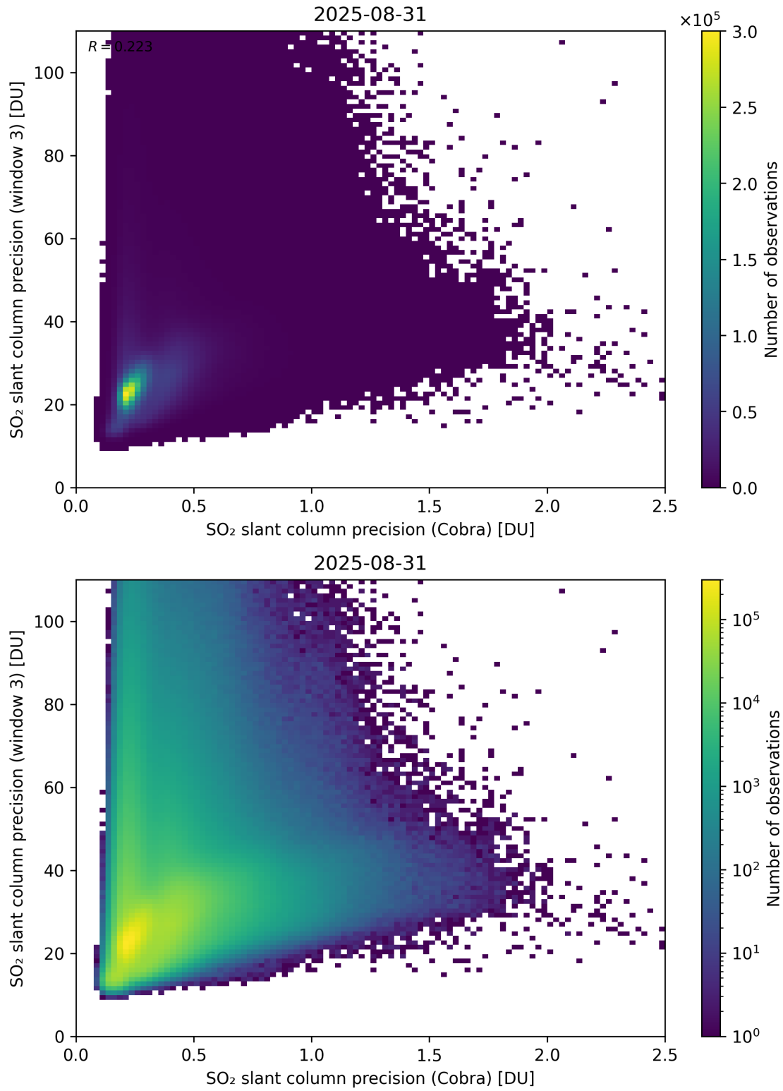
Figure 212: Scatter density plot of “SO 2 slant column precision (Cobra)” against “SO 2 slant column precision (window 3)” for 2025-08-30 to 2025-09-01.
