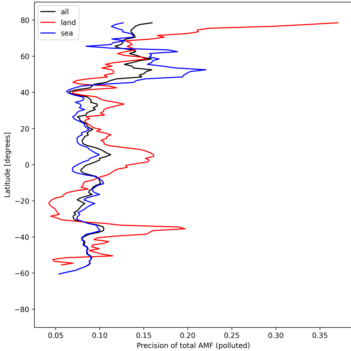
Figure 54: Zonal average of “Precision of total AMF (polluted)” for 2025-08-30 to 2025-09-01.
