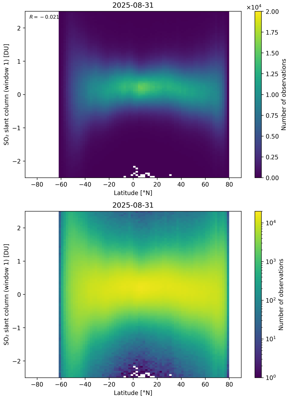
Figure 162: Scatter density plot of “Latitude” against “SO 2 slant column (window 1)” for 2025-08-30 to 2025-09-01.
