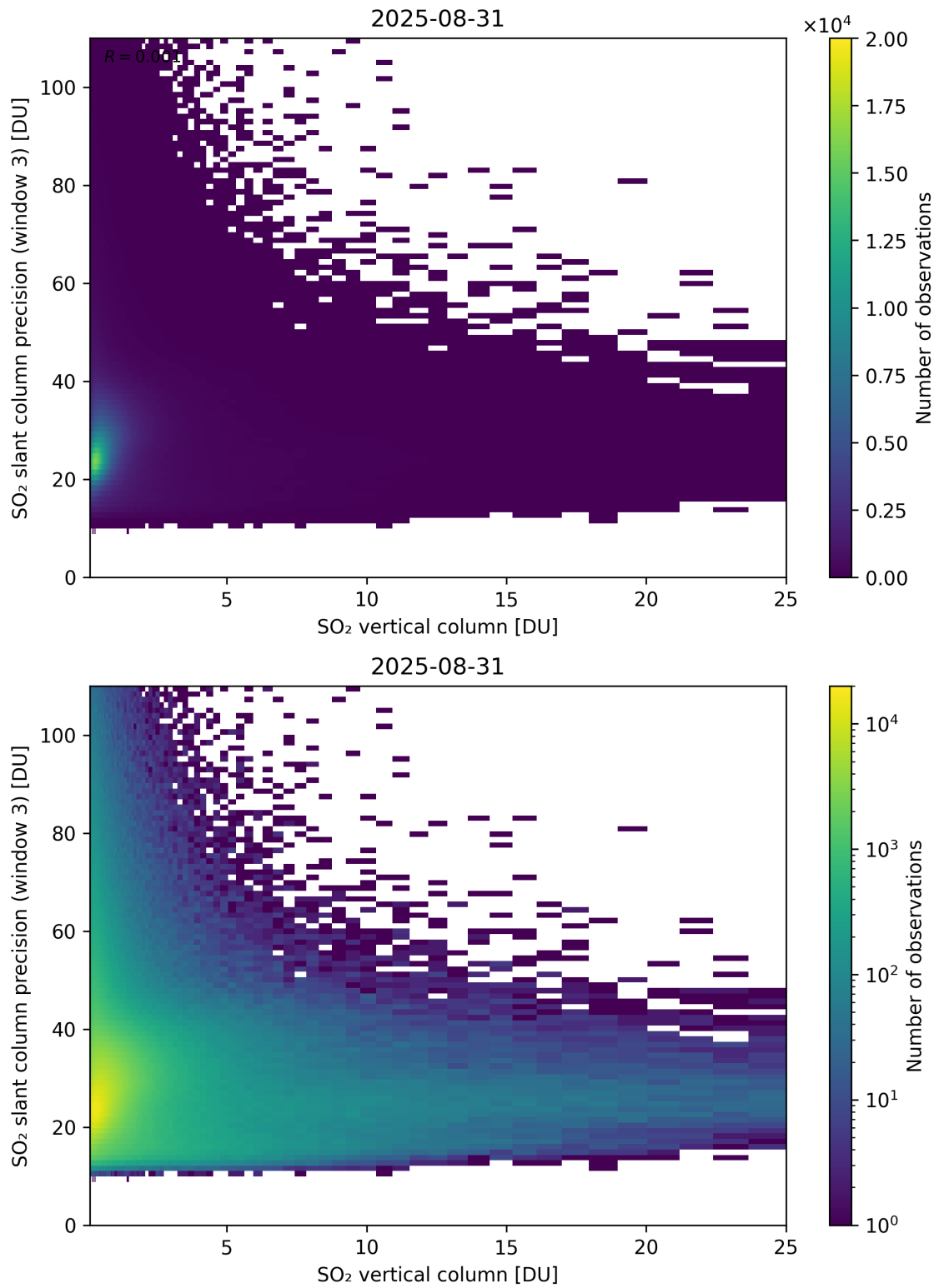
Figure 358: Scatter density plot of “SO 2 vertical column” against “SO 2 slant column precision (window 3)” for 2025-08-30 to 2025-09-01.
