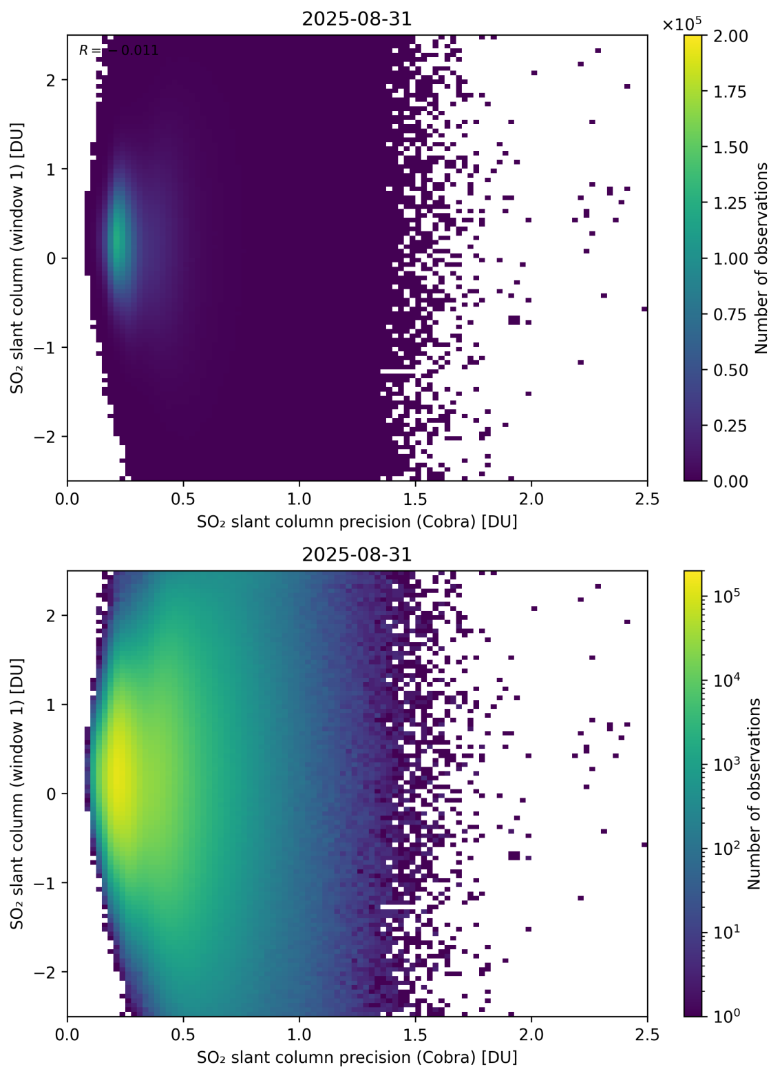
Figure 208: Scatter density plot of “SO 2 slant column precision (Cobra)” against “SO 2 slant column (window 1)” for 2025-08-30 to 2025-09-01.
