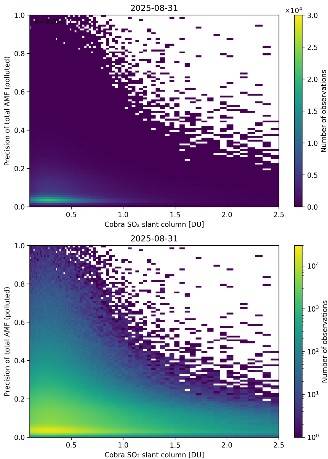
Figure 225: Scatter density plot of “Cobra SO 2 slant column” against “Precision of total AMF (polluted)” for 2025-08-30 to 2025-09-01.
