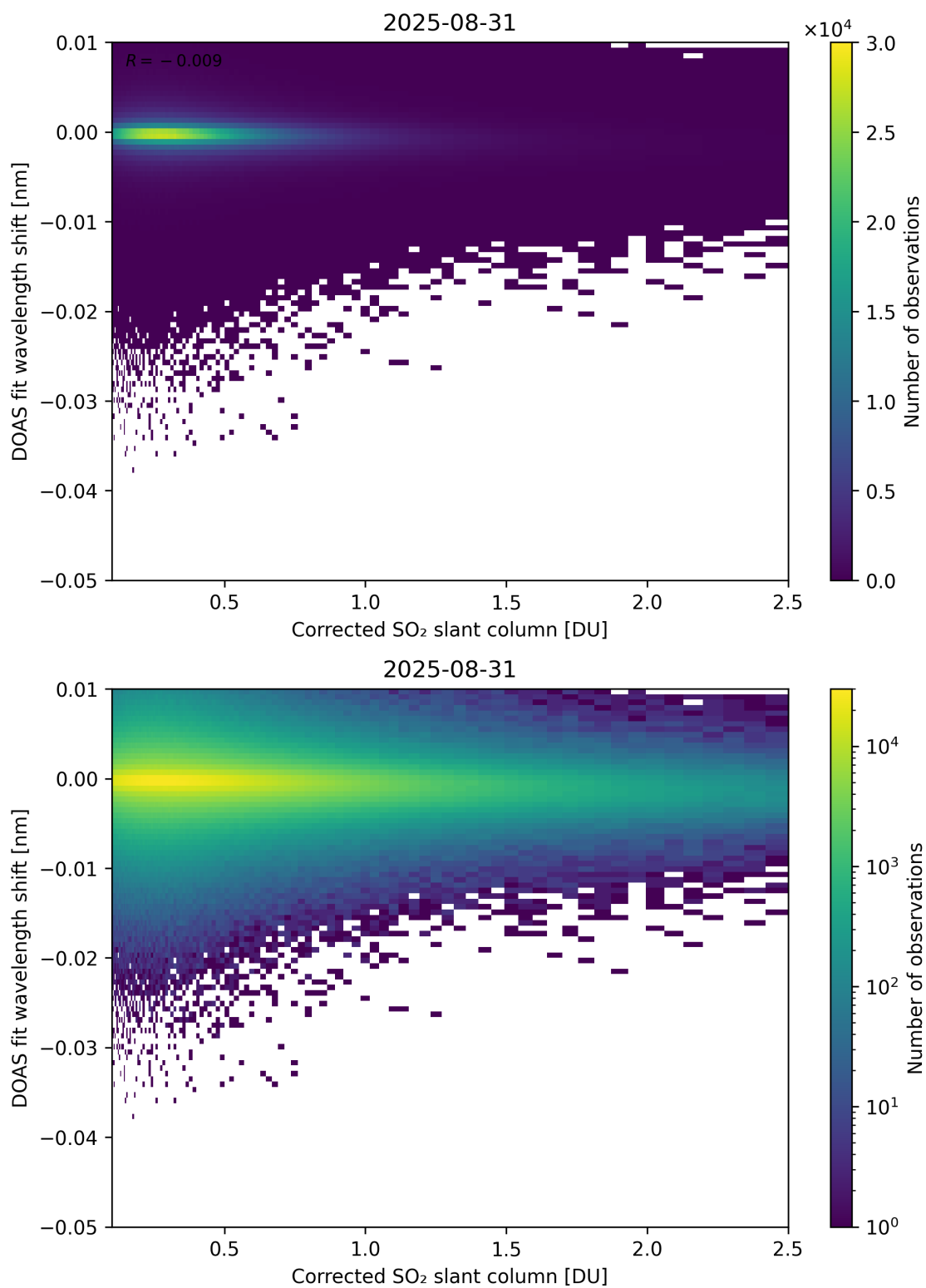
Figure 229: Scatter density plot of “Corrected SO 2 slant column” against “DOAS fit wavelength shift” for 2025-08-30 to 2025-09-01.
