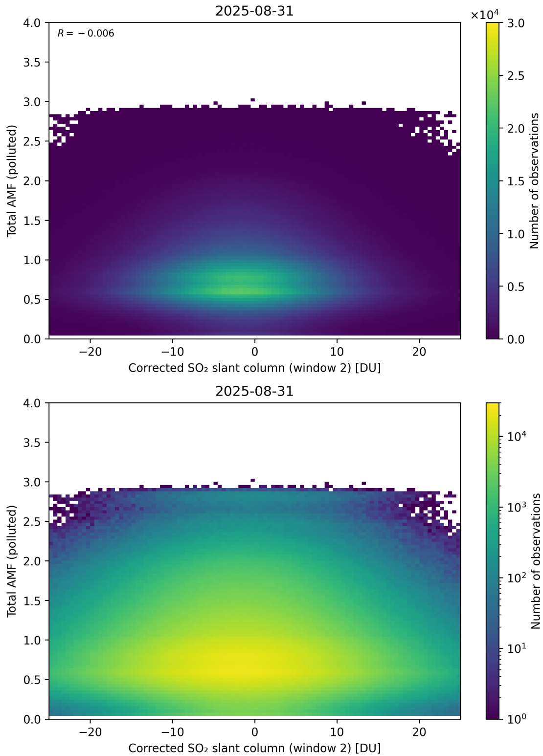
Figure 253: Scatter density plot of “Corrected SO 2 slant column (window 2)” against “Total AMF (polluted)” for 2025-08-30 to 2025-09-01.
