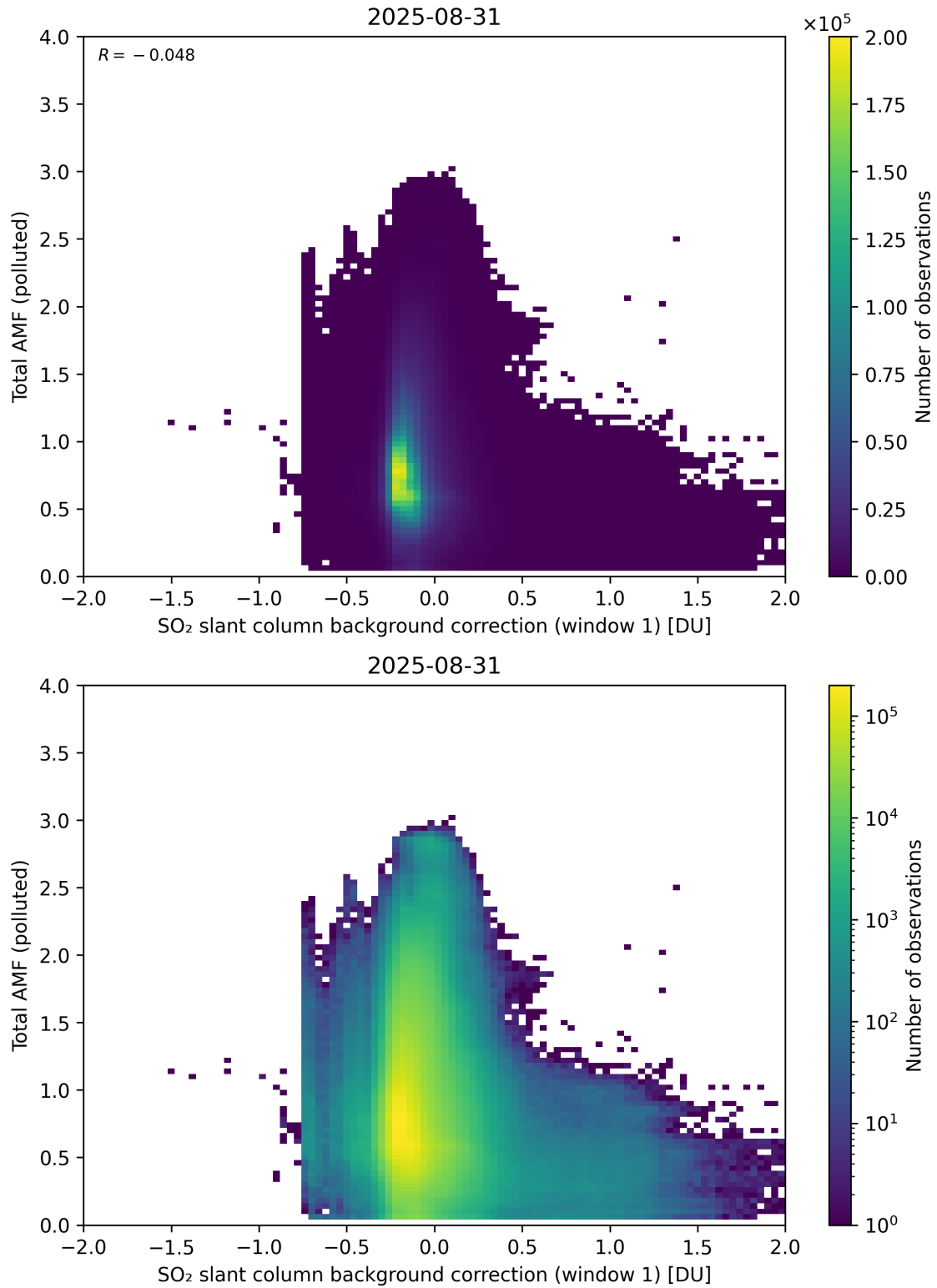
Figure 120: Scatter density plot of “SO 2 slant column background correction (window 1)” against “Total AMF (polluted)” for 2025-08-30 to 2025-09-01.
