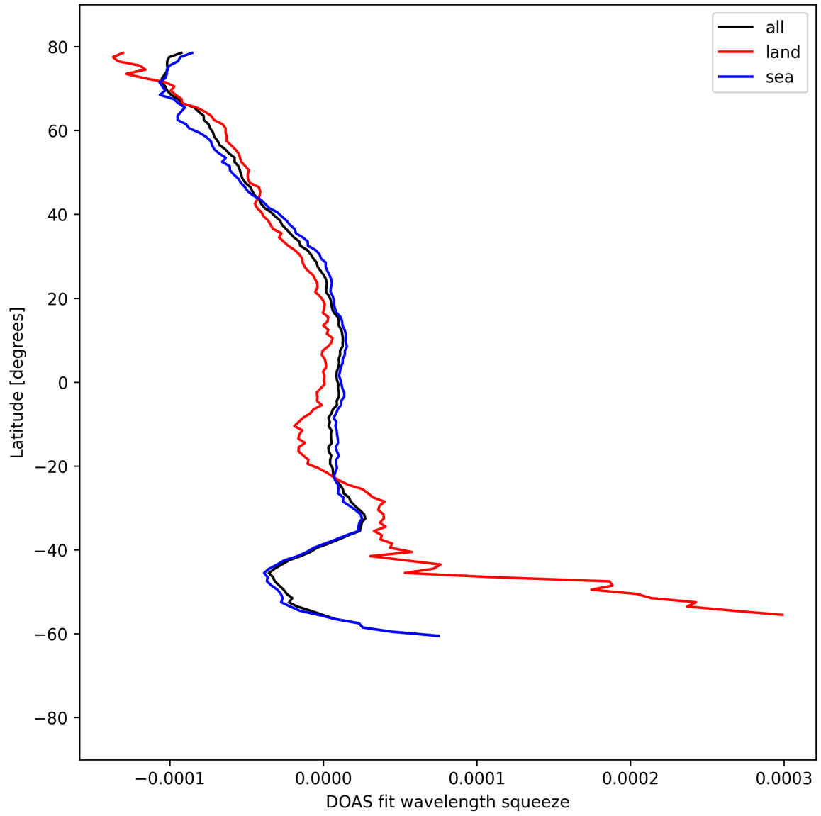
Figure 51: Zonal average of “DOAS fit wavelength squeeze” for 2025-08-30 to 2025-09-01.
