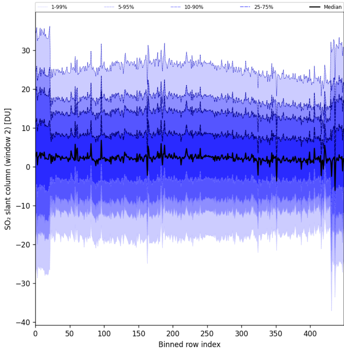
Figure 93: Along track statistics of “SO 2 slant column (window 2)” for 2025-08-30 to 2025-09-01
