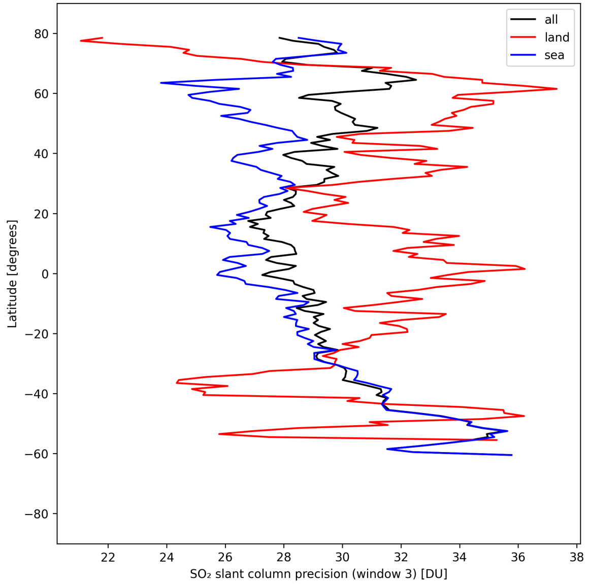
Figure 46: Zonal average of “SO 2 slant column precision (window 3)” for 2025-08-30 to 2025-09-01.
