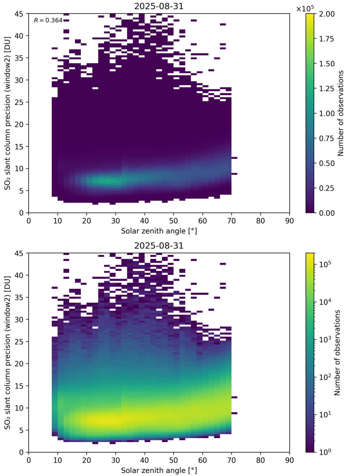
Figure 186: Scatter density plot of “Solar zenith angle” against “SO 2 slant column precision (window2)” for 2025-08-30 to 2025-09-01.
