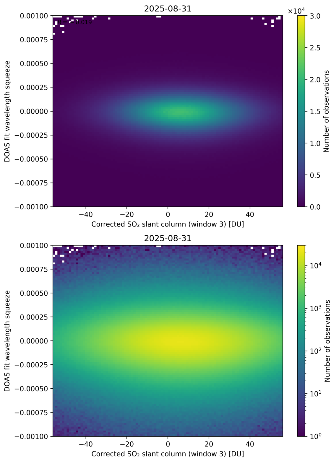
Figure 257: Scatter density plot of “Corrected SO 2 slant column (window 3)” against “DOAS fit wavelength squeeze” for 2025-08-30 to 2025-09-01.
