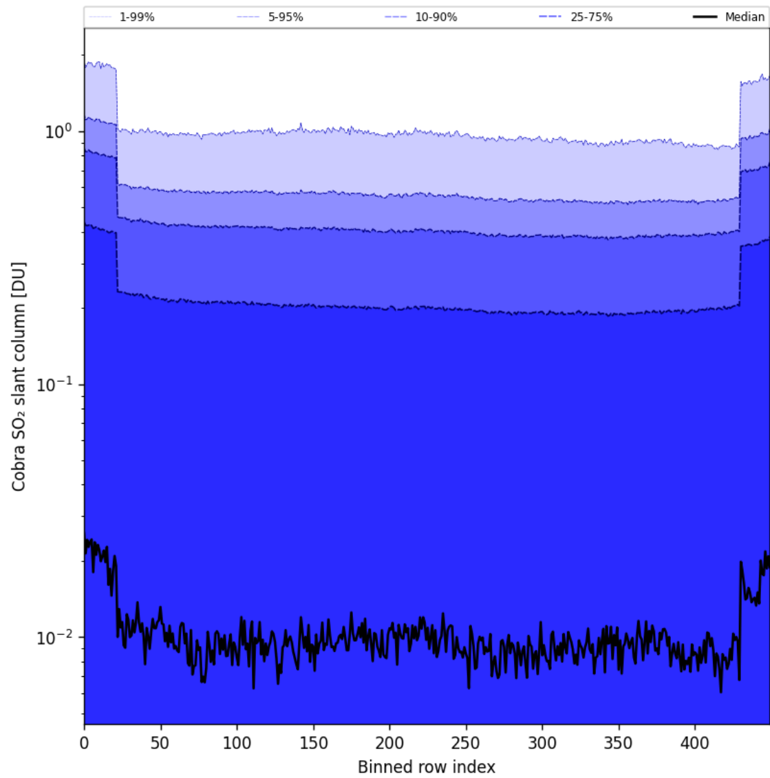
Figure 87: Along track statistics of “Cobra SO 2 slant column” for 2025-08-30 to 2025-09-01
