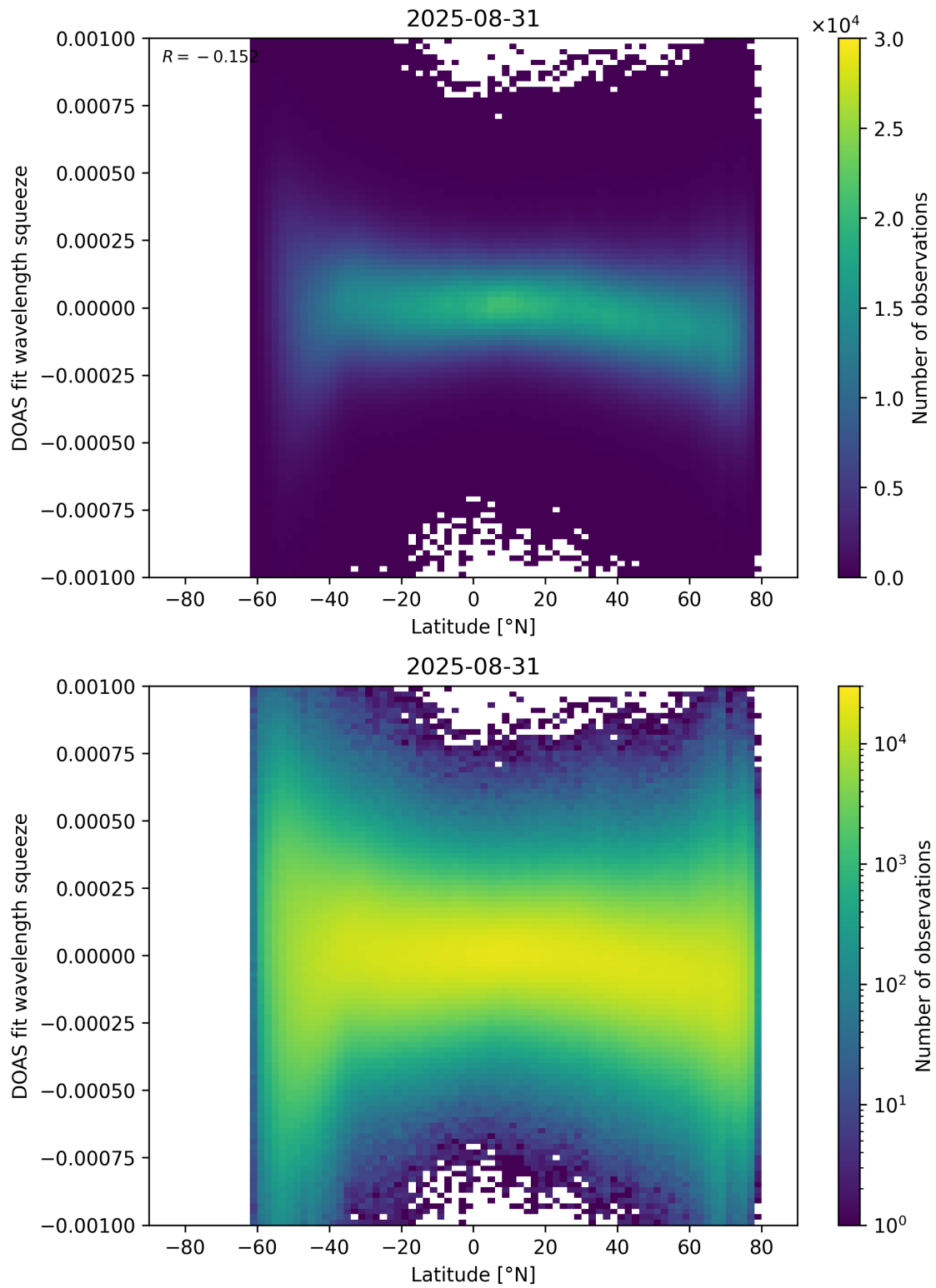
Figure 154: Scatter density plot of “Latitude” against “DOAS fit wavelength squeeze” for 2025-08-30 to 2025-09-01.
