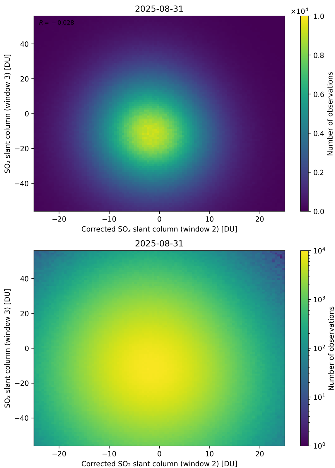
Figure 251: Scatter density plot of “Corrected SO 2 slant column (window 2)” against “SO 2 slant column (window 3)” for 2025-08-30 to 2025-09-01.
