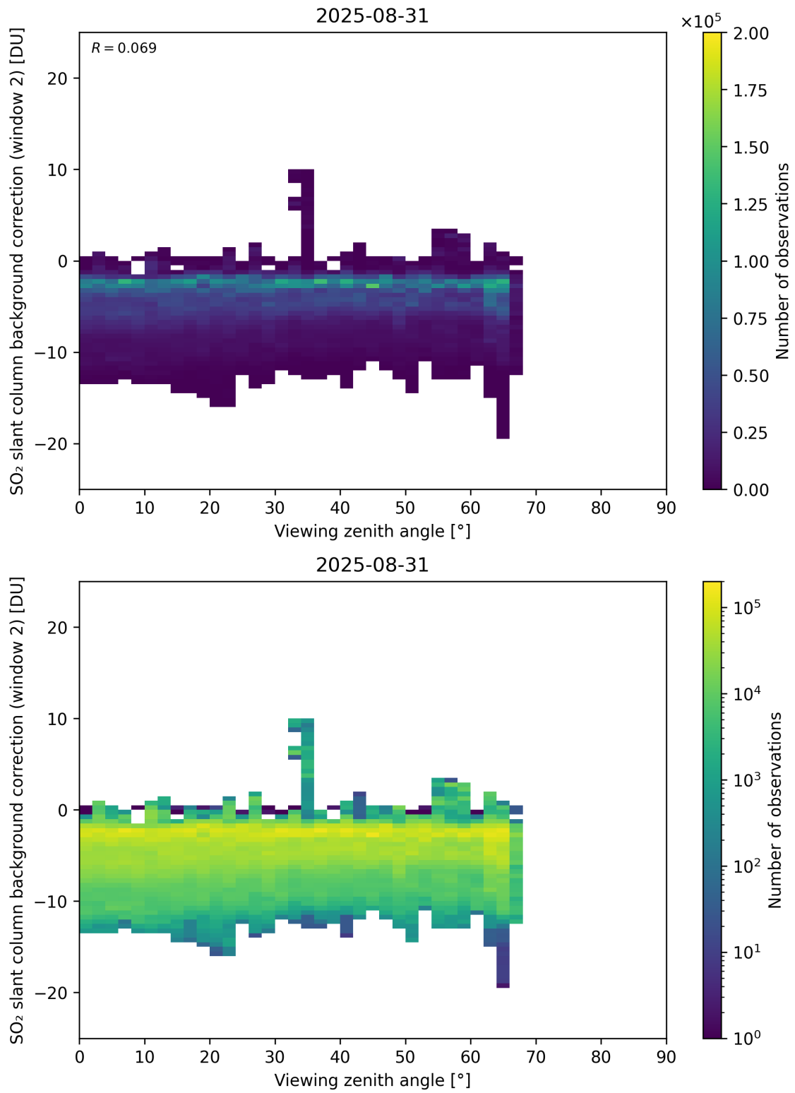
Figure 363: Scatter density plot of “Viewing zenith angle” against “SO 2 slant column background correction (window 2)” for 2025-08-30 to 2025-09-01.
