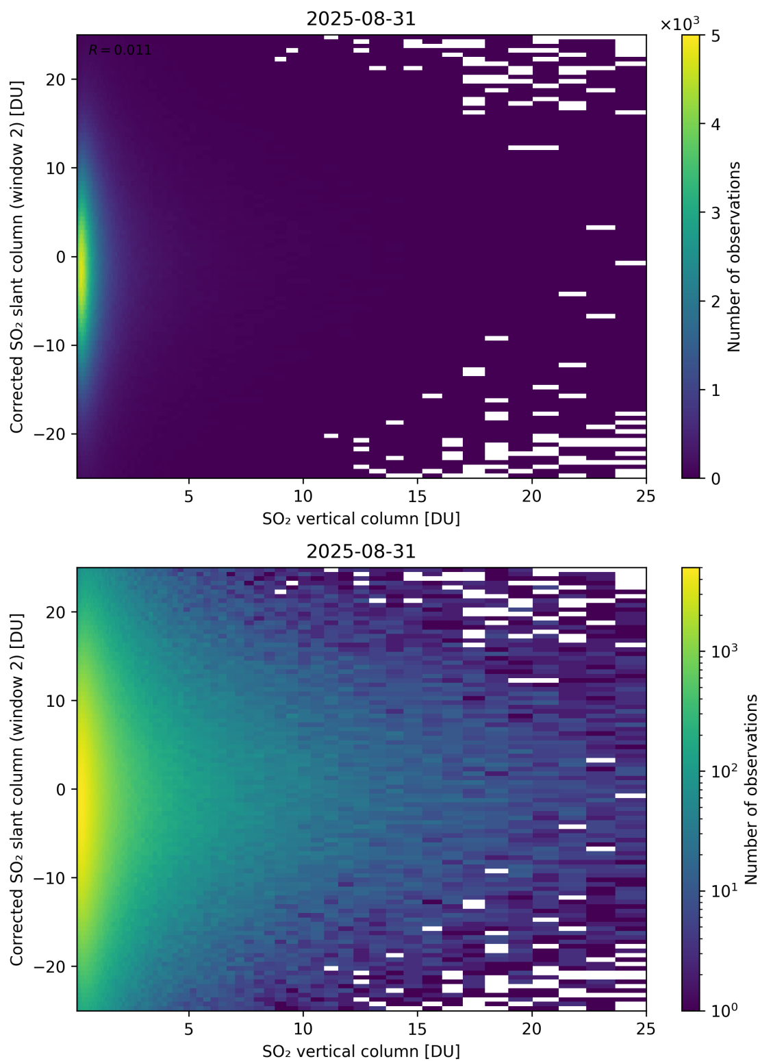
Figure 352: Scatter density plot of “SO 2 vertical column” against “Corrected SO 2 slant column (window 2)” for 2025-08-30 to 2025-09-01.
