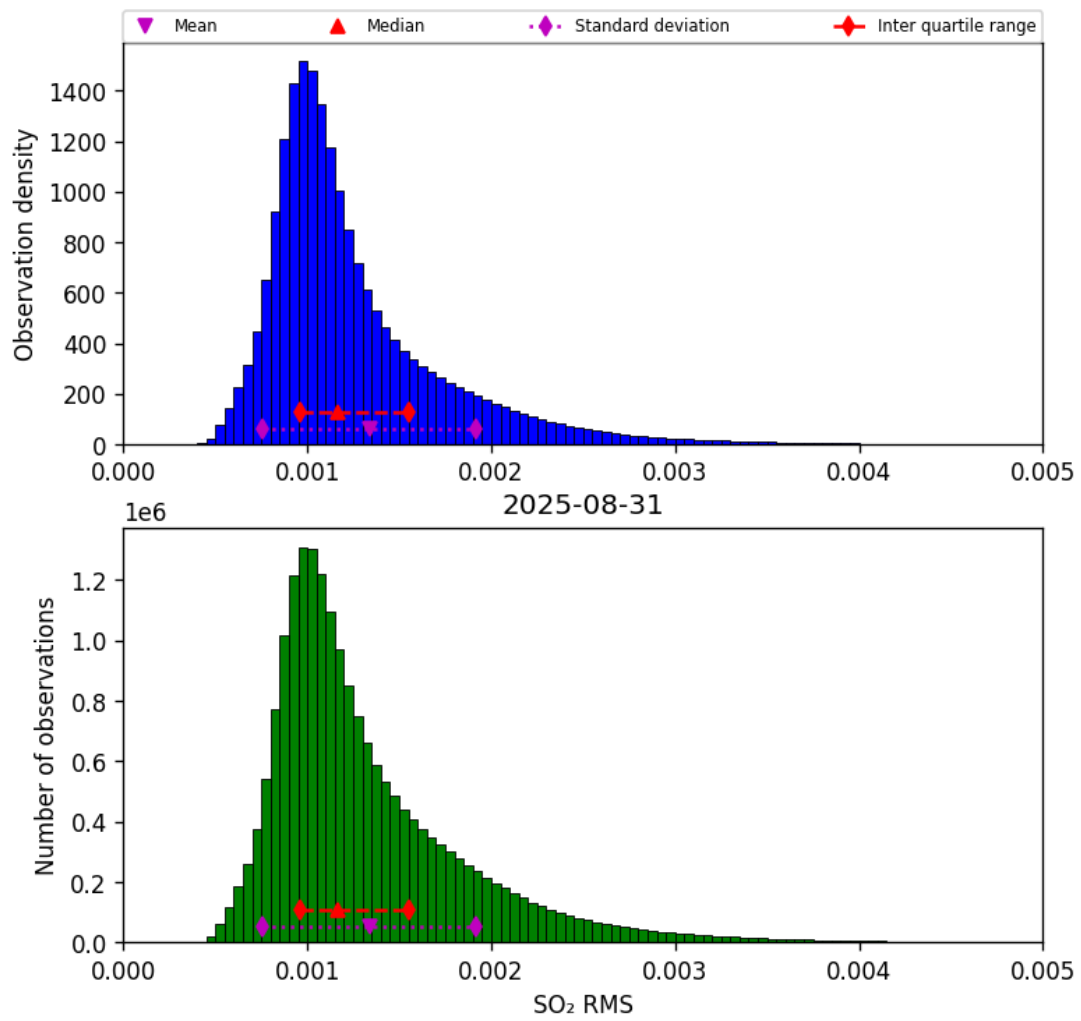
Figure 78: Histogram of “SO 2 RMS” for 2025-08-30 to 2025-09-01
