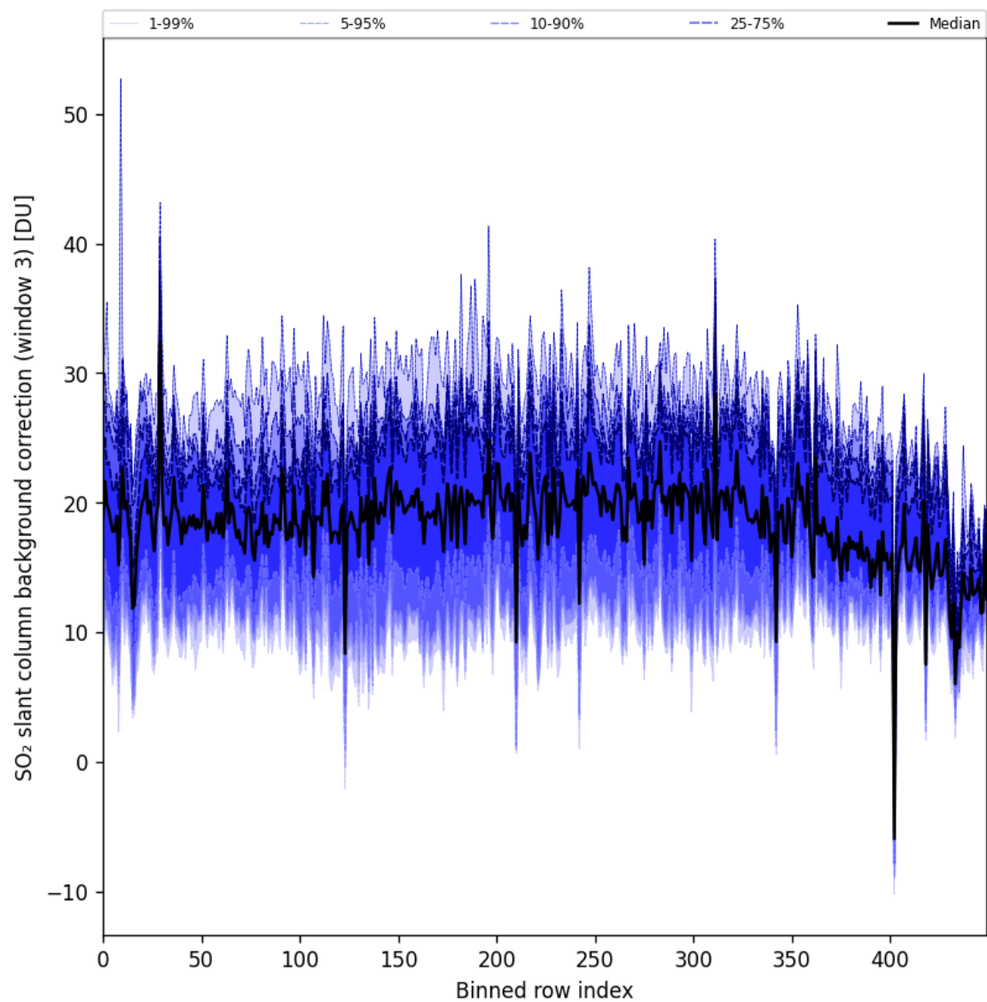
Figure 100: Along track statistics of “SO 2 slant column background correction (window 3)” for 2025-08-30 to 2025-09-01
