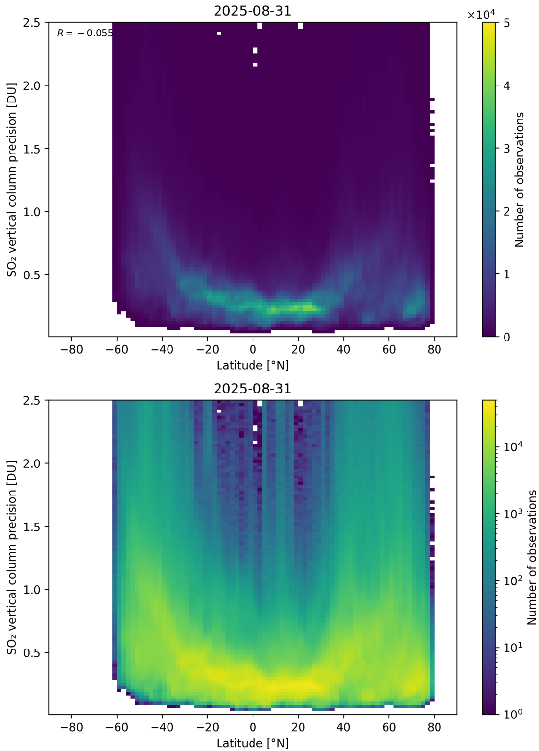
Figure 170: Scatter density plot of “Latitude” against “SO 2 vertical column precision” for 2025-08-30 to 2025-09-01.
