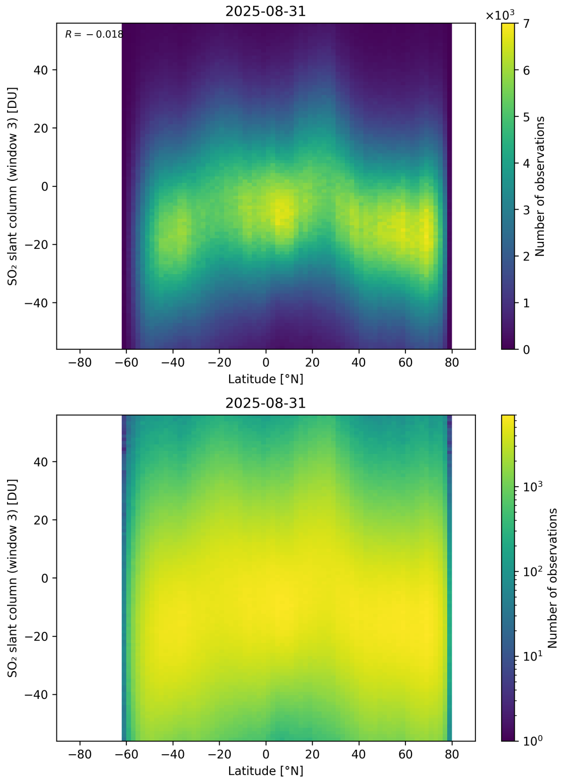
Figure 165: Scatter density plot of “Latitude” against “SO 2 slant column (window 3)” for 2025-08-30 to 2025-09-01.
