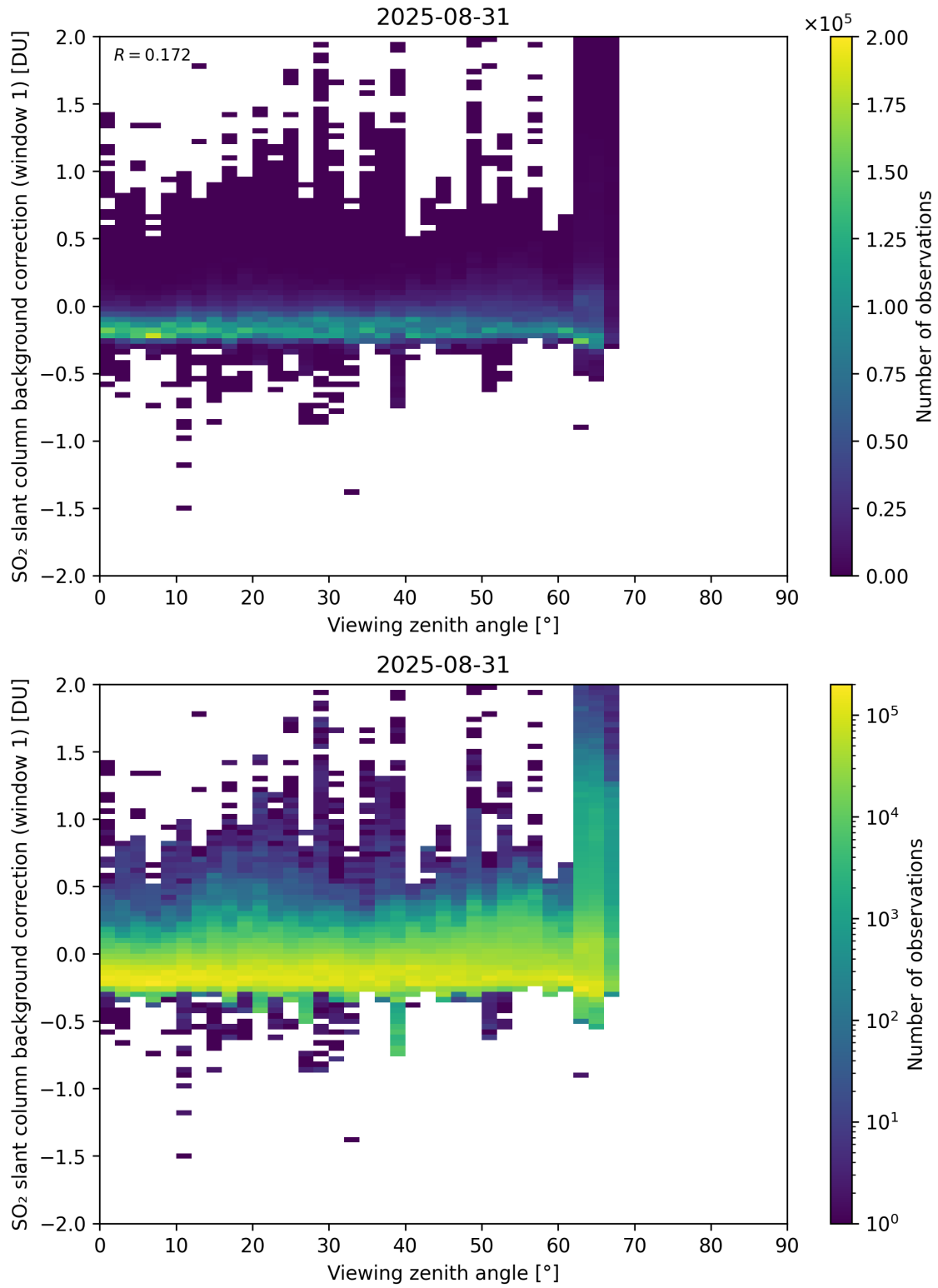
Figure 362: Scatter density plot of “Viewing zenith angle” against “SO 2 slant column background correction (window 1)” for 2025-08-30 to 2025-09-01.
