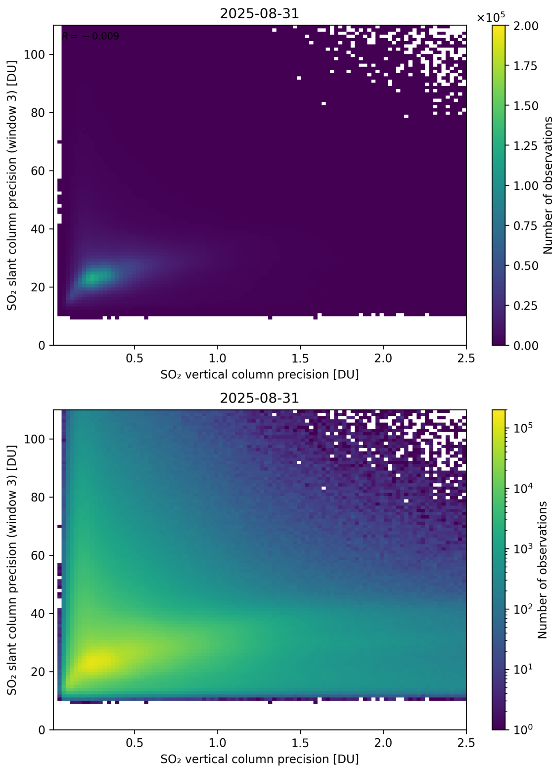
Figure 345: Scatter density plot of “SO 2 vertical column precision” against “SO 2 slant column precision (window 3)” for 2025-08-30 to 2025-09-01.
