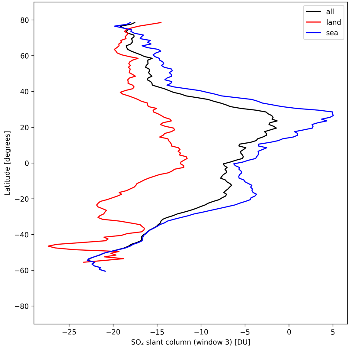
Figure 45: Zonal average of “SO 2 slant column (window 3)” for 2025-08-30 to 2025-09-01.
