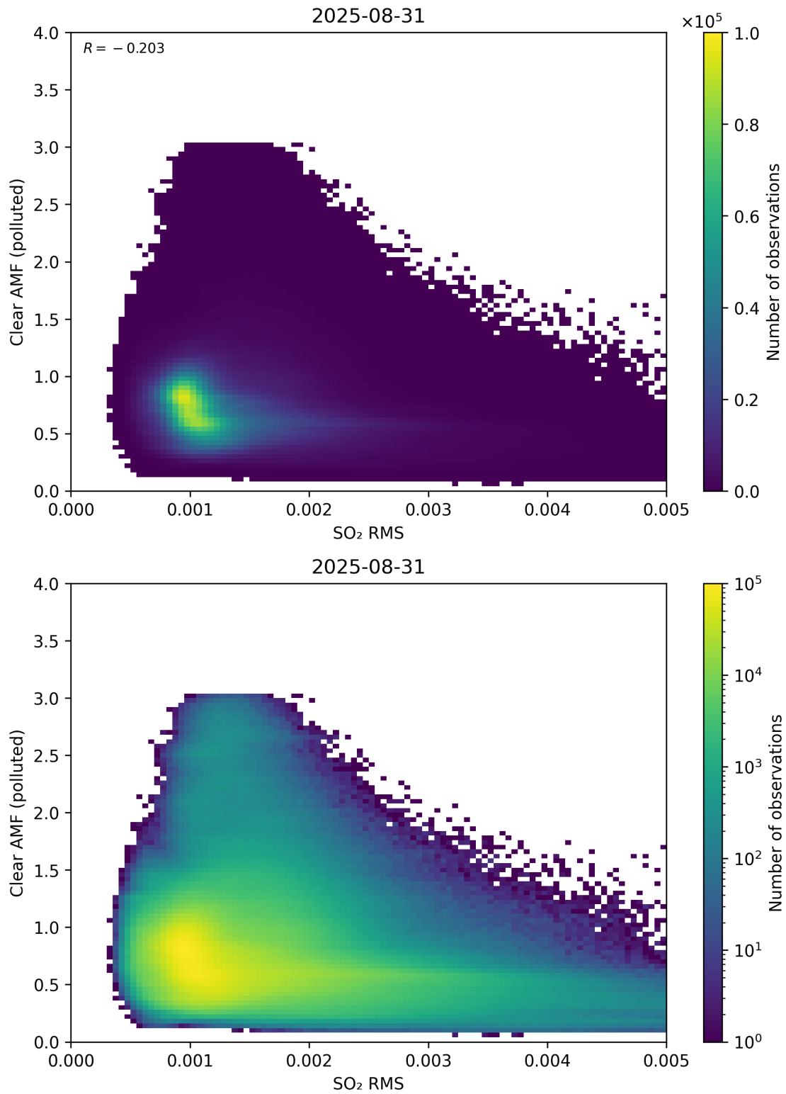
Figure 147: Scatter density plot of “SO 2 RMS” against “Clear AMF (polluted)” for 2025-08-30 to 2025-09-01.
