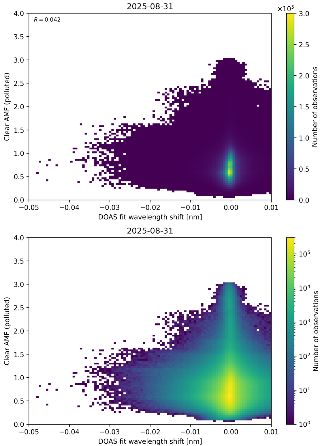
Figure 140: Scatter density plot of “DOAS fit wavelength shift” against “Clear AMF (polluted)” for 2025-08-30 to 2025-09-01.
