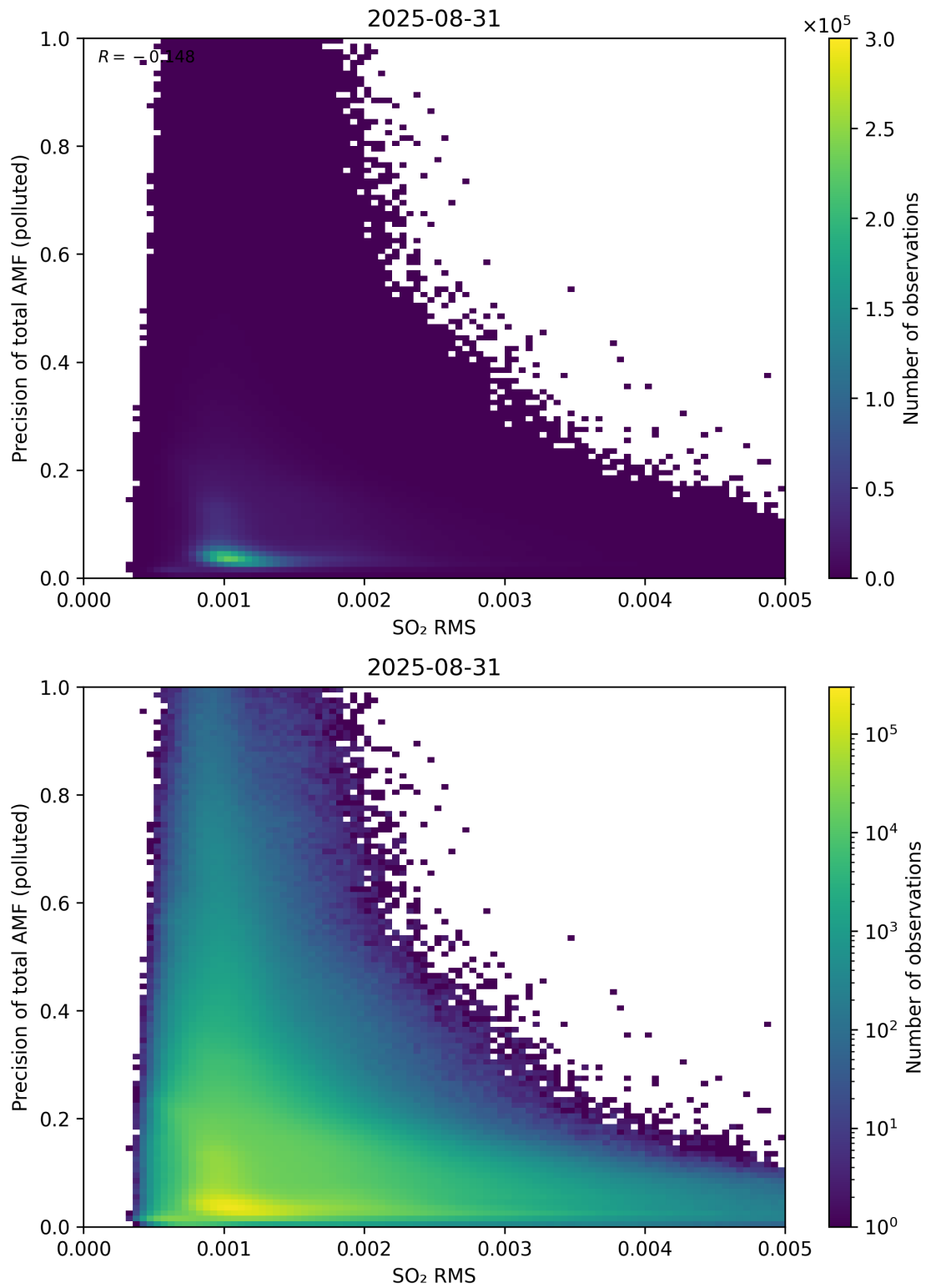
Figure 149: Scatter density plot of “SO 2 RMS” against “Precision of total AMF (polluted)” for 2025-08-30 to 2025-09-01.
