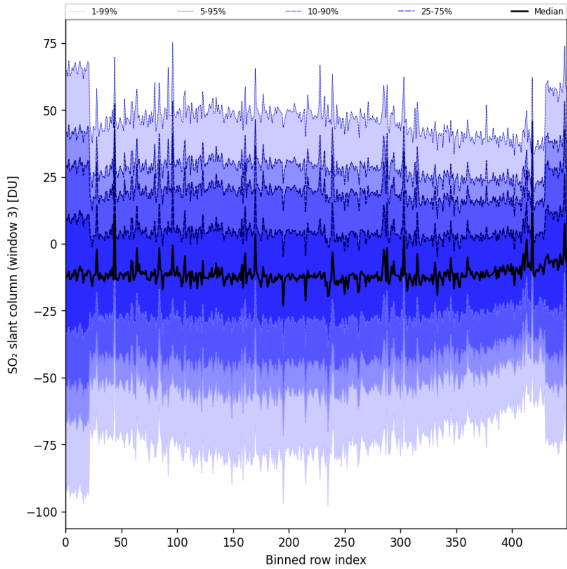
Figure 97: Along track statistics of “SO 2 slant column (window 3)” for 2025-08-30 to 2025-09-01
