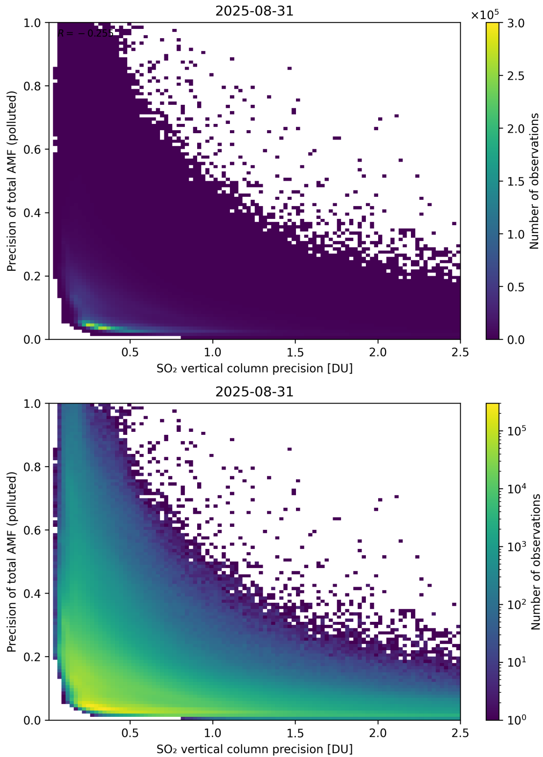
Figure 347: Scatter density plot of “SO 2 vertical column precision” against “Precision of total AMF (polluted)” for 2025-08-30 to 2025-09-01.
