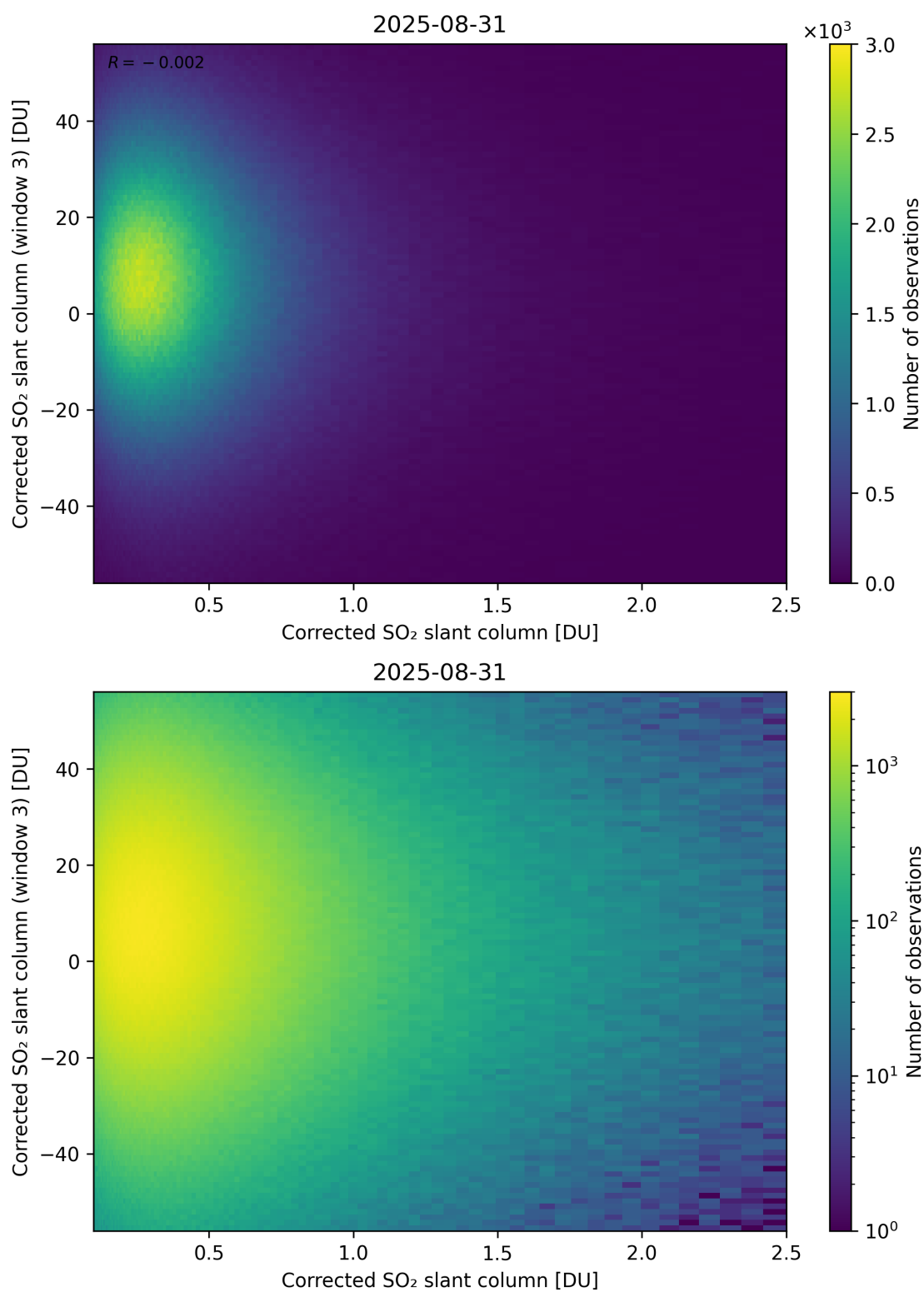
Figure 236: Scatter density plot of “Corrected SO 2 slant column” against “Corrected SO 2 slant column (window 3)” for 2025-08-30 to 2025-09-01.
