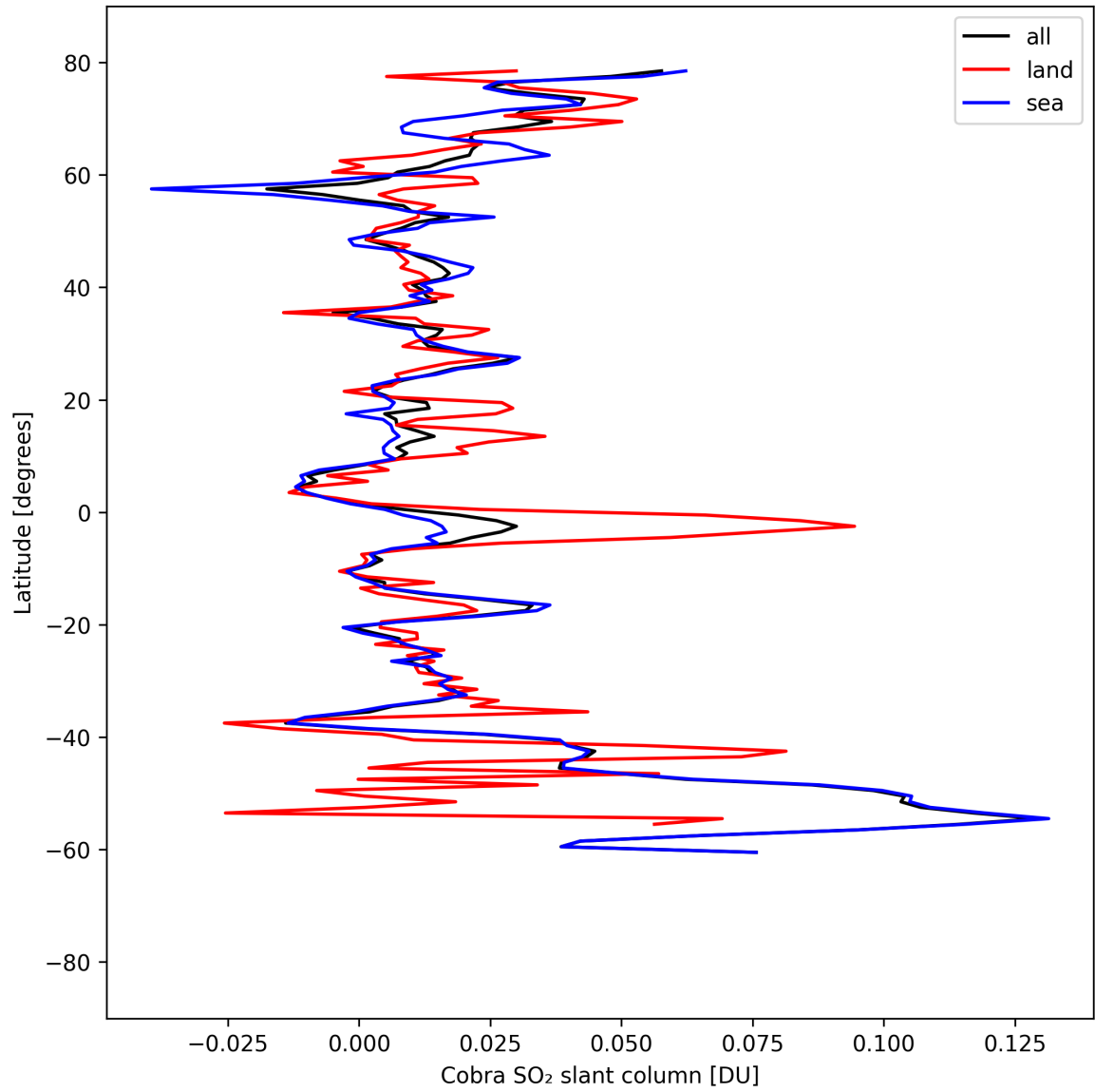
Figure 35: Zonal average of “Cobra SO 2 slant column” for 2025-08-30 to 2025-09-01.
