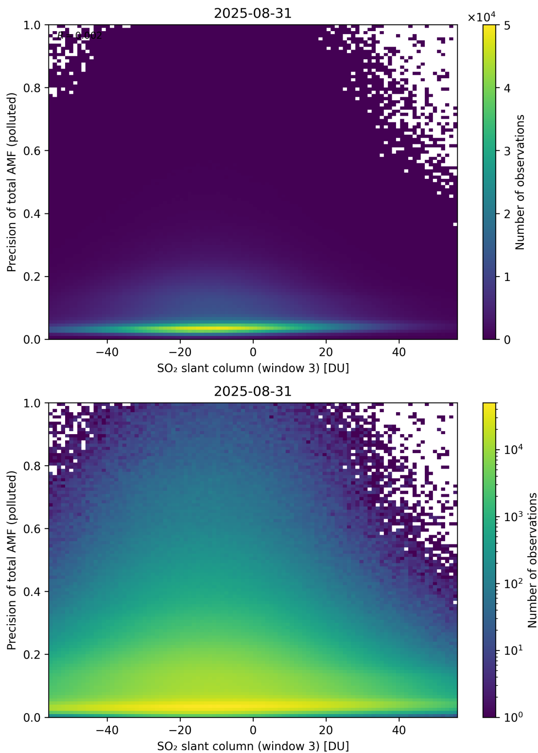
Figure 319: Scatter density plot of “SO 2 slant column (window 3)” against “Precision of total AMF (polluted)” for 2025-08-30 to 2025-09-01.
