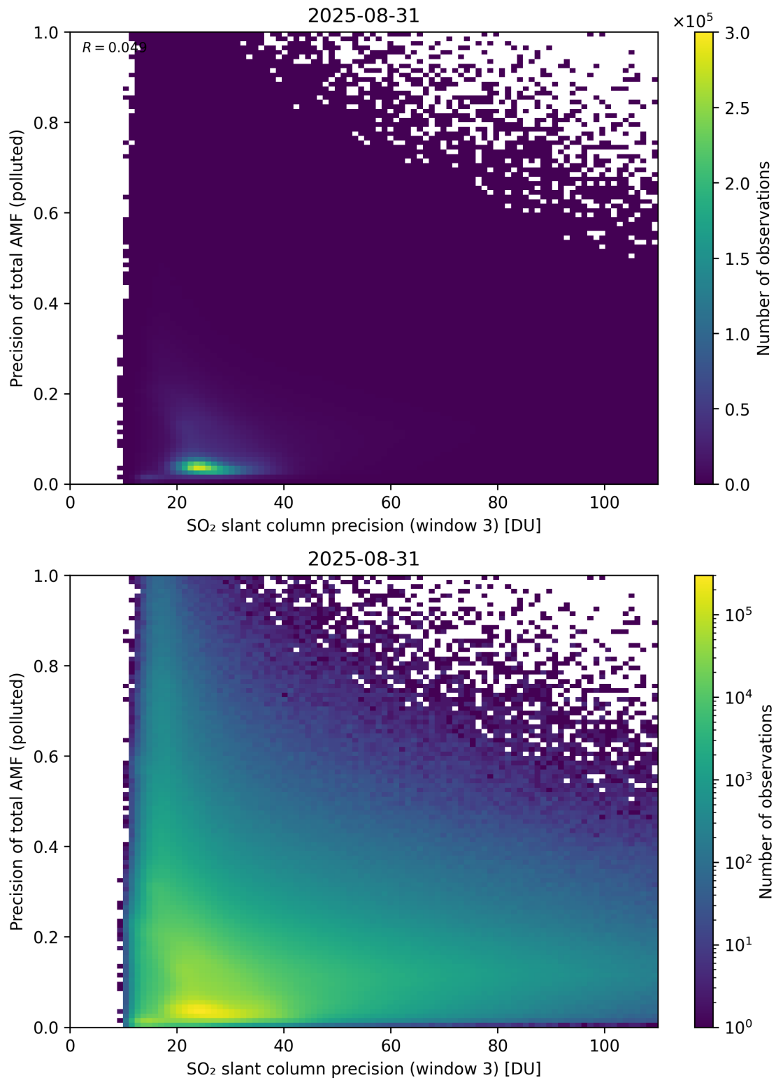
Figure 314: Scatter density plot of “SO 2 slant column precision (window 3)” against “Precision of total AMF (polluted)” for 2025-08-30 to 2025-09-01.
