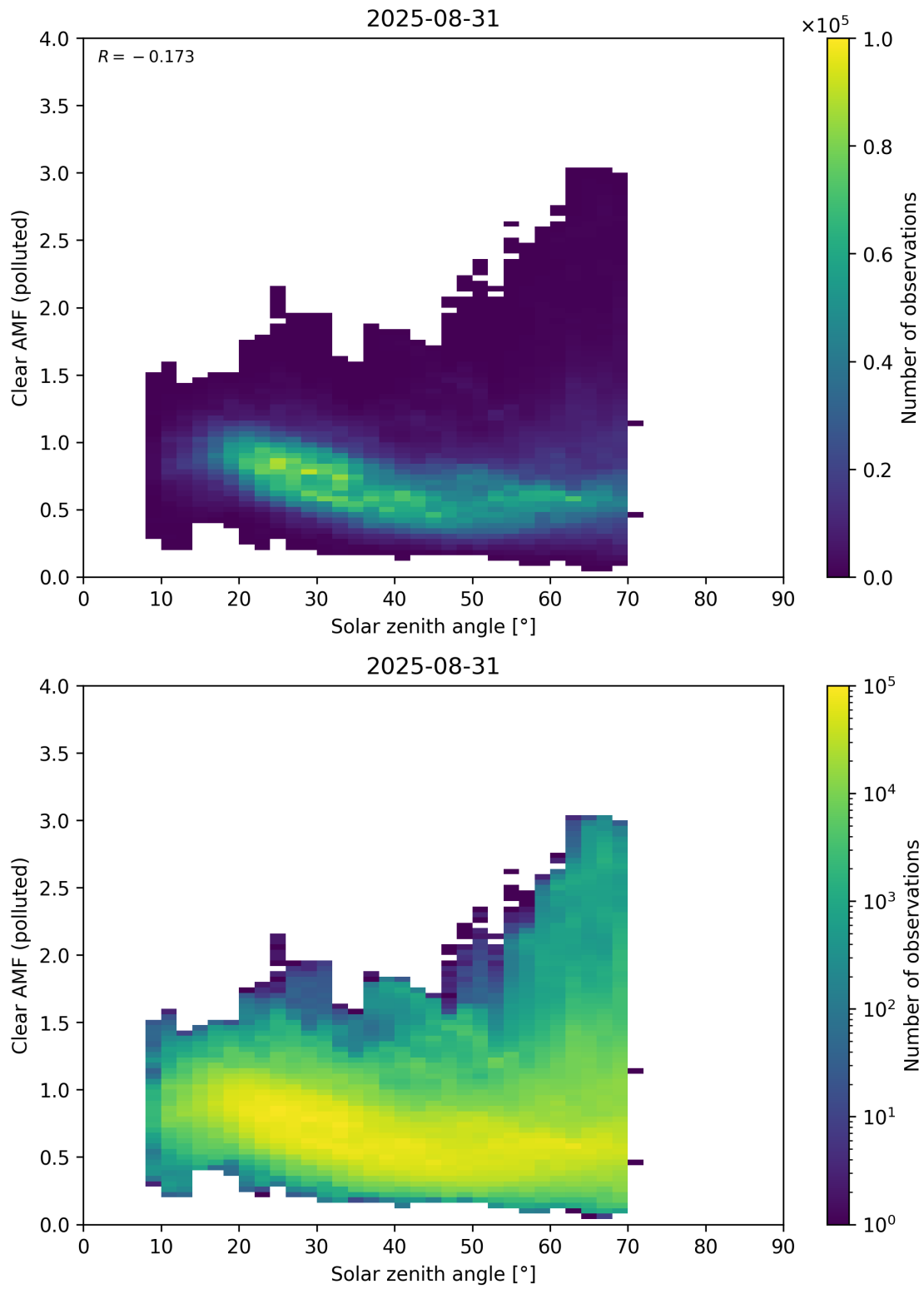
Figure 178: Scatter density plot of “Solar zenith angle” against “Clear AMF (polluted)” for 2025-08-30 to 2025-09-01.
