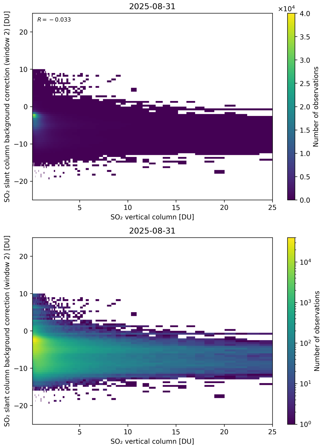
Figure 324: Scatter density plot of “SO 2 vertical column” against “SO 2 slant column background correction (window 2)” for 2025-08-30 to 2025-09-01.
