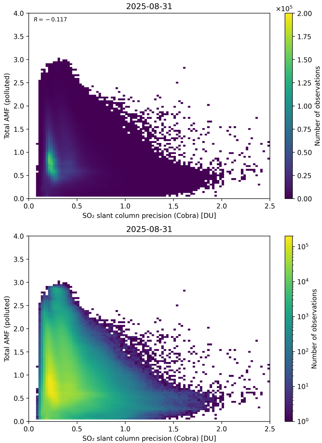
Figure 213: Scatter density plot of “SO 2 slant column precision (Cobra)” against “Total AMF (polluted)” for 2025-08-30 to 2025-09-01.
