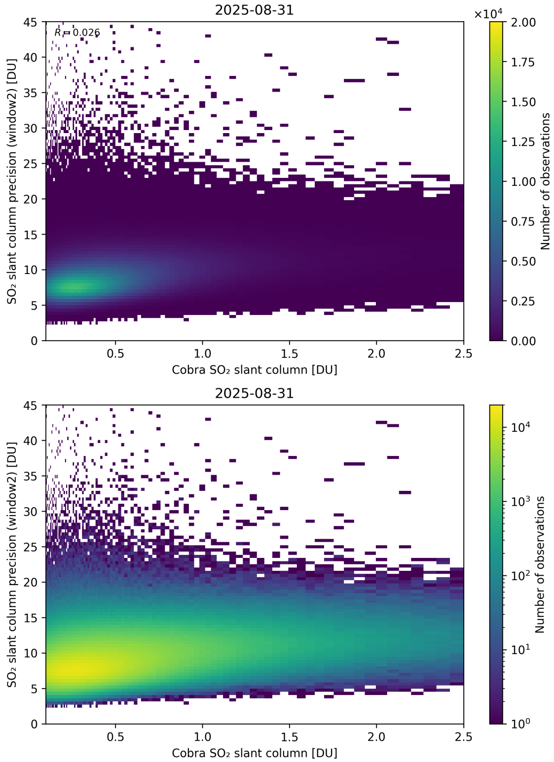
Figure 221: Scatter density plot of “Cobra SO 2 slant column” against “SO 2 slant column precision (window2)” for 2025-08-30 to 2025-09-01.
