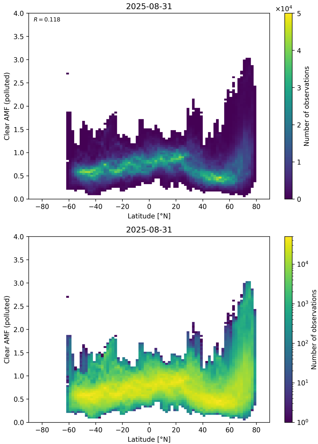
Figure 156: Scatter density plot of “Latitude” against “Clear AMF (polluted)” for 2025-08-30 to 2025-09-01.
