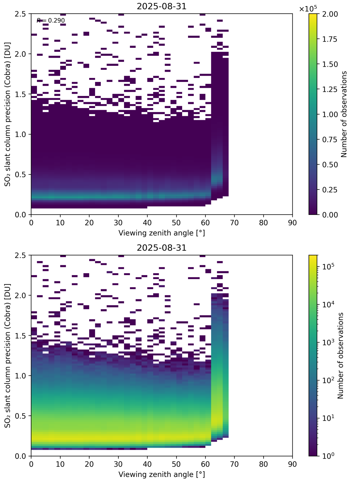
Figure 372: Scatter density plot of “Viewing zenith angle” against “SO 2 slant column precision (Cobra)” for 2025-08-30 to 2025-09-01.
