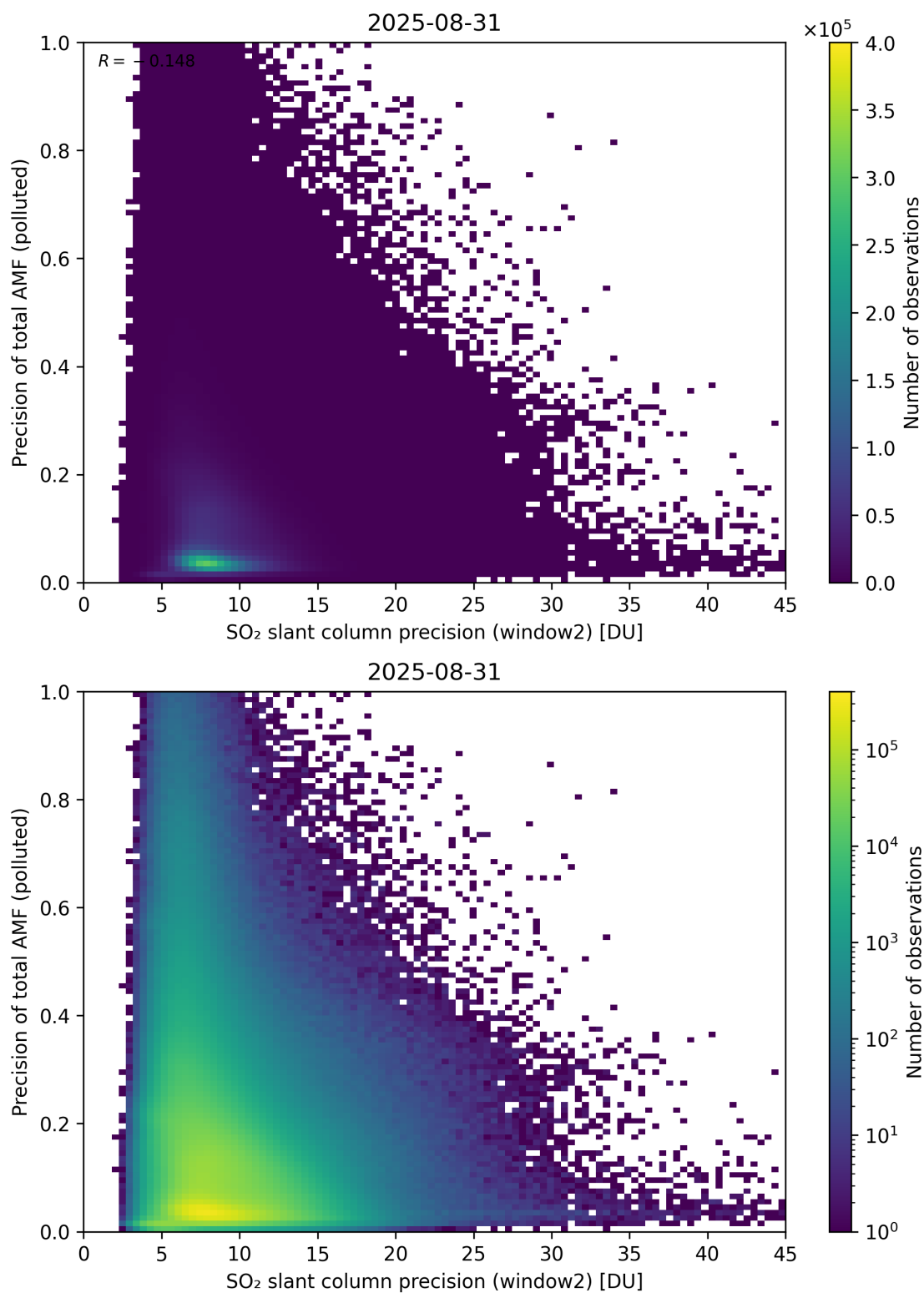
Figure 302: Scatter density plot of “SO 2 slant column precision (window2)” against “Precision of total AMF (polluted)” for 2025-08-30 to 2025-09-01.
