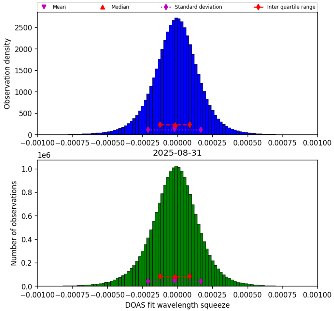
Figure 77: Histogram of “DOAS fit wavelength squeeze” for 2025-08-30 to 2025-09-01
