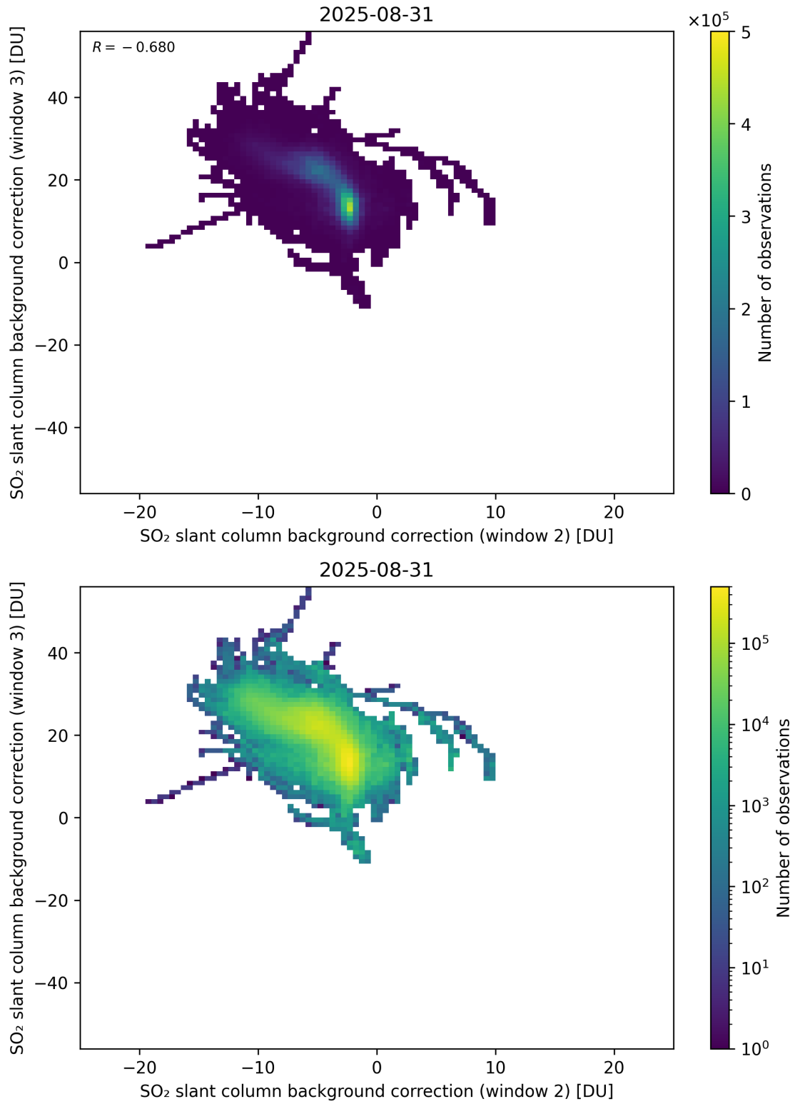
Figure 122: Scatter density plot of “SO 2 slant column background correction (window 2)” against “SO 2 slant column background correction (window 3)” for 2025-08-30 to 2025-09-01.
