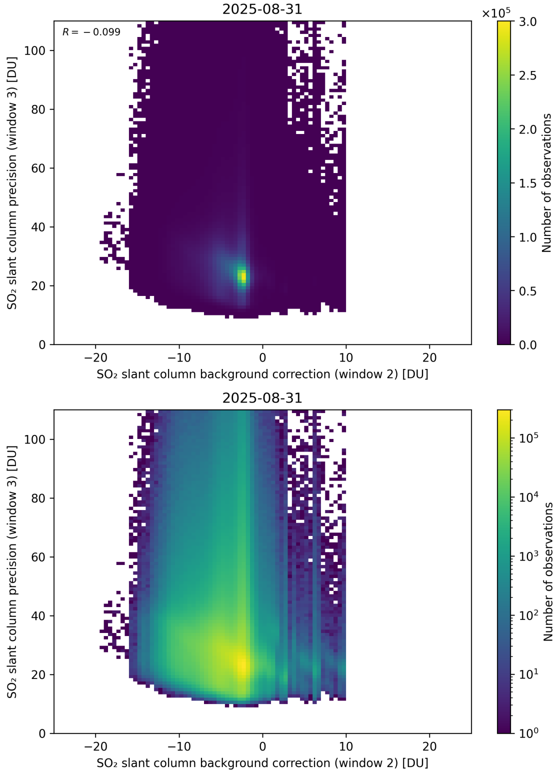
Figure 129: Scatter density plot of “SO 2 slant column background correction (window 2)” against “SO 2 slant column precision (window 3)” for 2025-08-30 to 2025-09-01.
