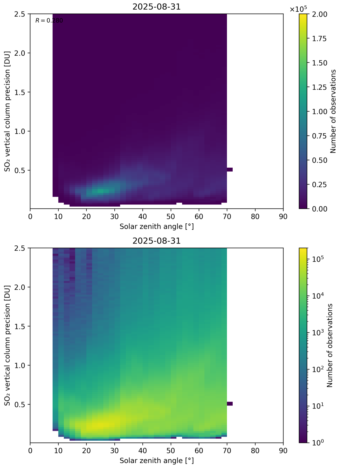
Figure 192: Scatter density plot of “Solar zenith angle” against “SO 2 vertical column precision” for 2025-08-30 to 2025-09-01.
