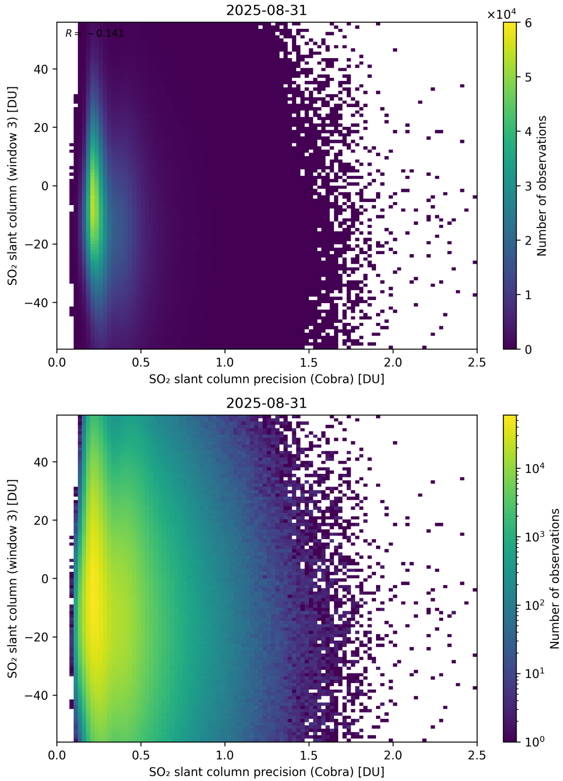
Figure 211: Scatter density plot of “SO 2 slant column precision (Cobra)” against “SO 2 slant column (window 3)” for 2025-08-30 to 2025-09-01.
