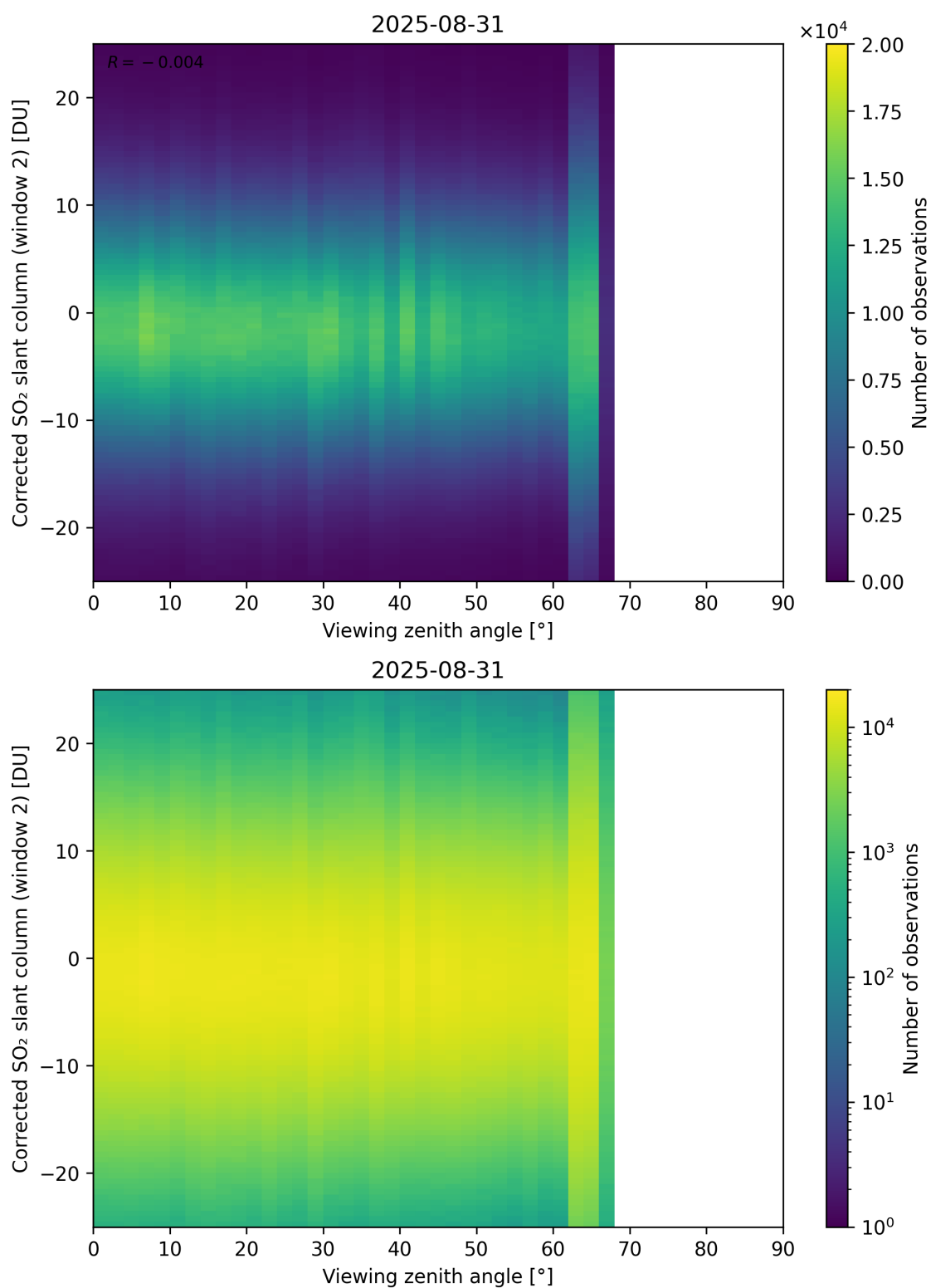
Figure 374: Scatter density plot of “Viewing zenith angle” against “Corrected SO 2 slant column (window 2)” for 2025-08-30 to 2025-09-01.
