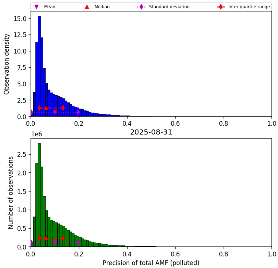
Figure 80: Histogram of “Precision of total AMF (polluted)” for 2025-08-30 to 2025-09-01
