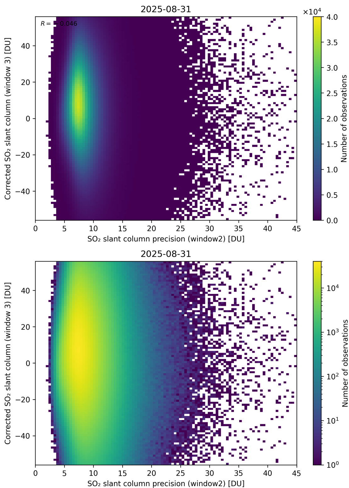
Figure 298: Scatter density plot of “SO 2 slant column precision (window2)” against “Corrected SO 2 slant column (window 3)” for 2025-08-30 to 2025-09-01.
