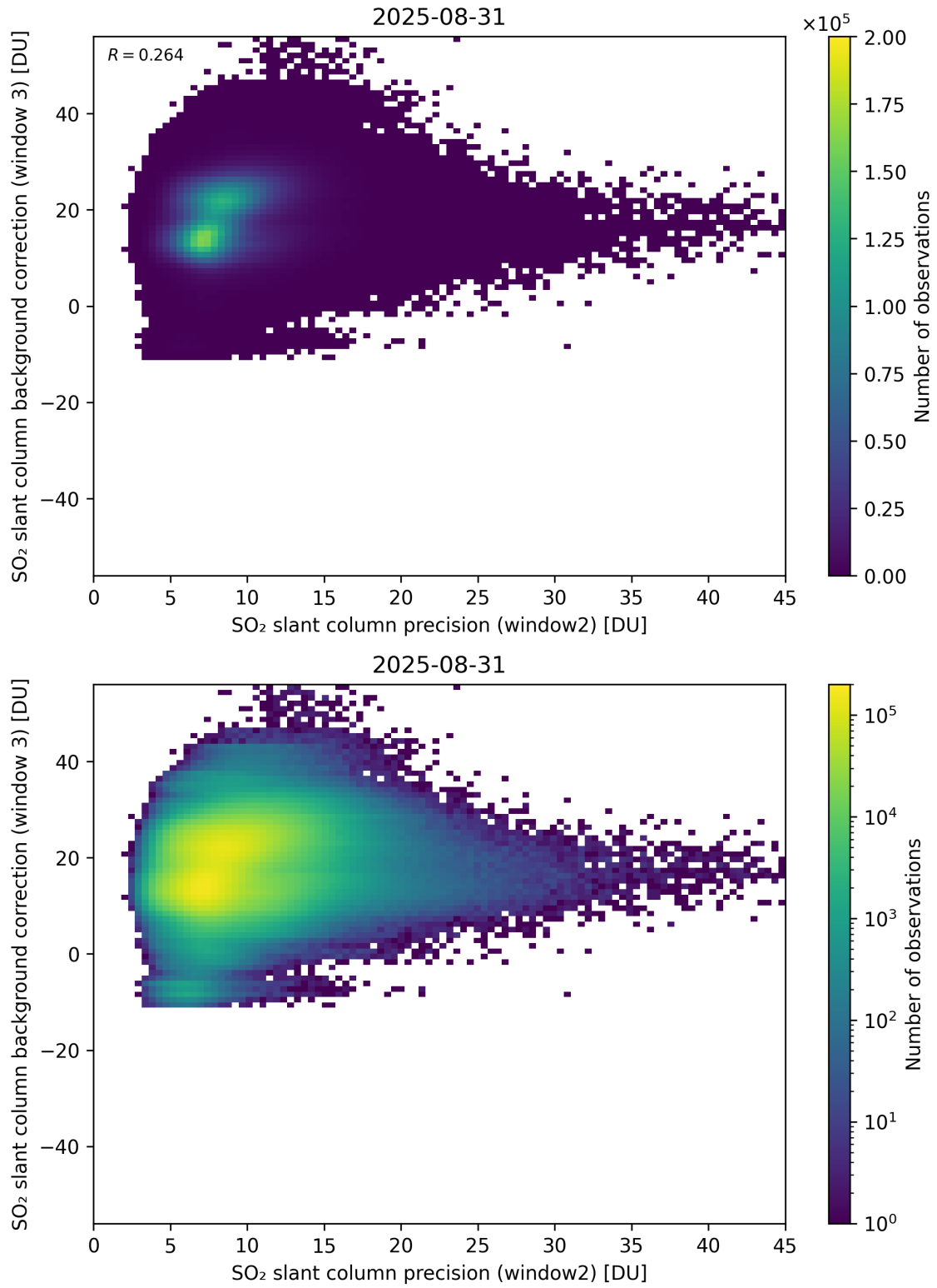
Figure 292: Scatter density plot of “SO 2 slant column precision (window2)” against “SO 2 slant column background correction (window 3)” for 2025-08-30 to 2025-09-01.
