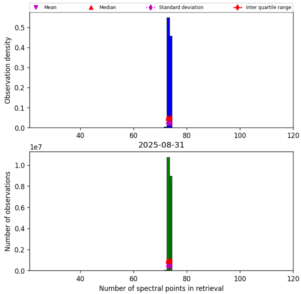
Figure 82: Histogram of “Number of spectral points in retrieval” for 2025-08-30 to 2025-09-01
