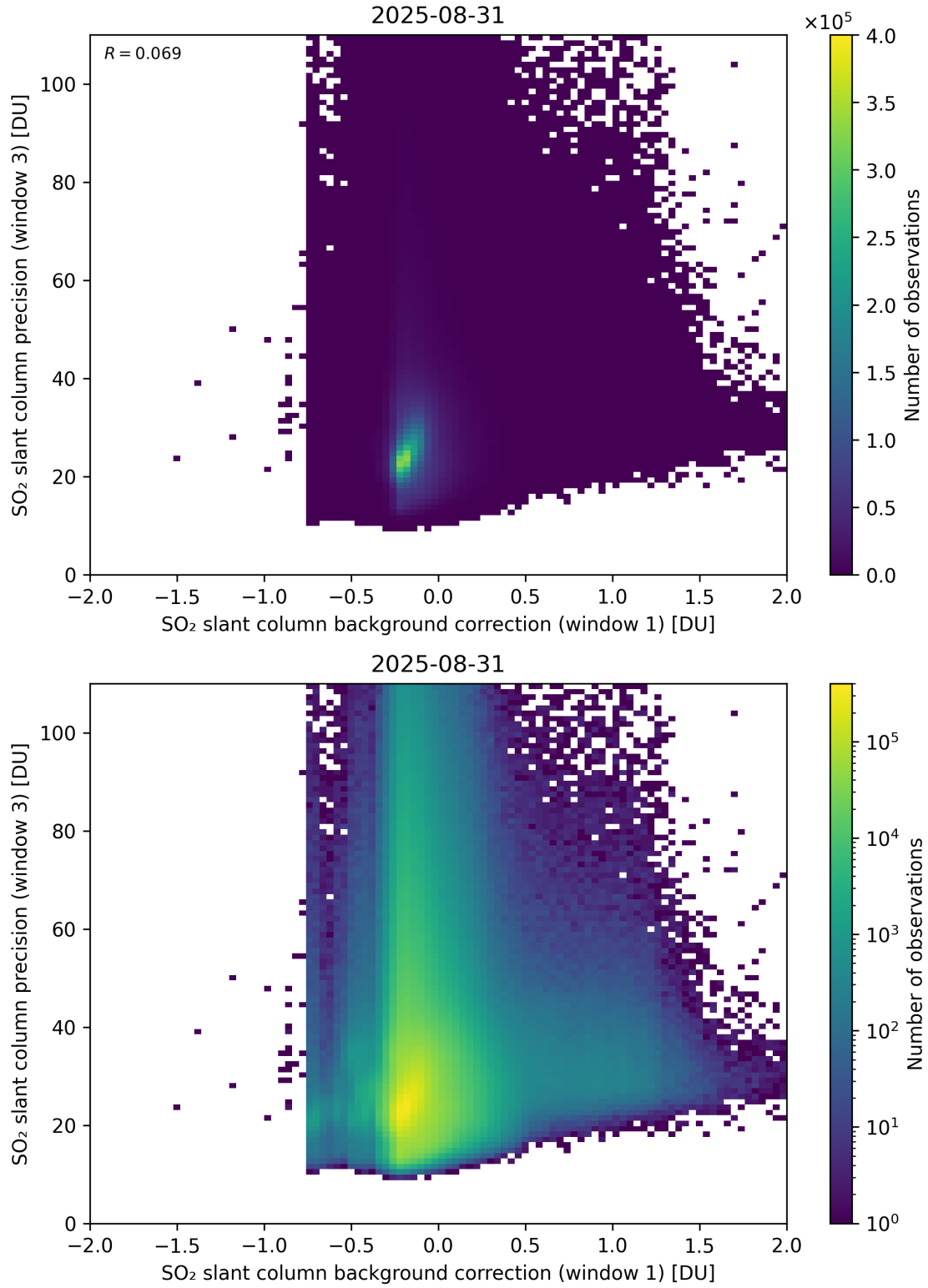
Figure 119: Scatter density plot of “SO 2 slant column background correction (window 1)” against “SO 2 slant column precision (window 3)” for 2025-08-30 to 2025-09-01.
