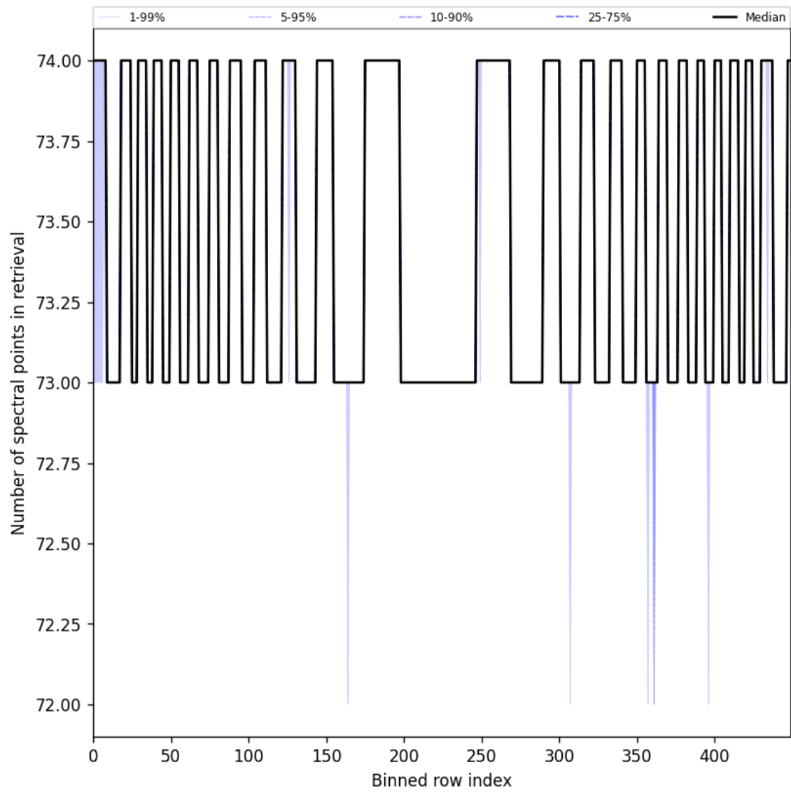
Figure 108: Along track statistics of “Number of spectral points in retrieval” for 2025-08-30 to 2025-09-01
