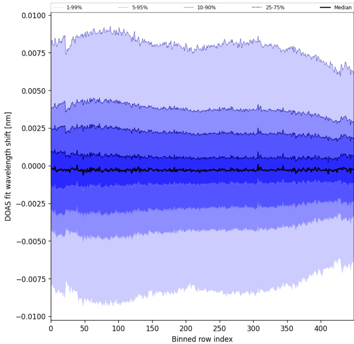
Figure 102: Along track statistics of “DOAS fit wavelength shift” for 2025-08-30 to 2025-09-01
