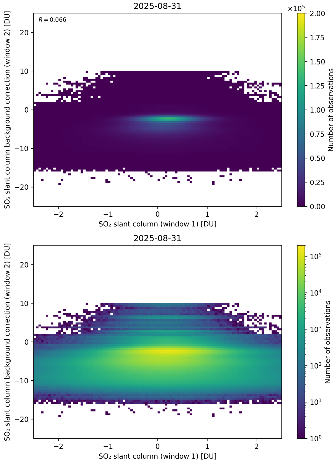
Figure 263: Scatter density plot of “SO 2 slant column (window 1)” against “SO 2 slant column background correction (window 2)” for 2025-08-30 to 2025-09-01.
