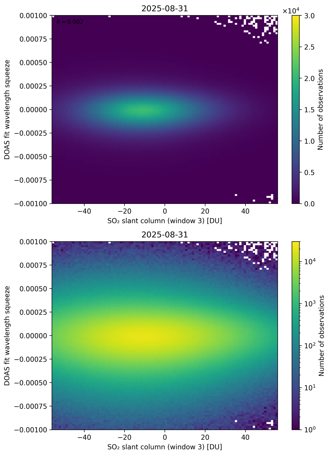
Figure 305: Scatter density plot of “SO 2 slant column (window 3)” against “DOAS fit wavelength squeeze” for 2025-08-30 to 2025-09-01.
