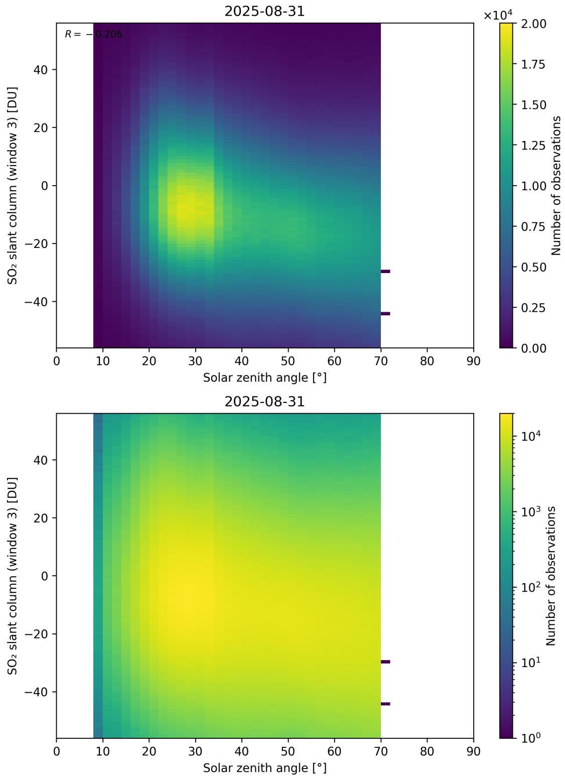
Figure 187: Scatter density plot of “Solar zenith angle” against “SO 2 slant column (window 3)” for 2025-08-30 to 2025-09-01.
