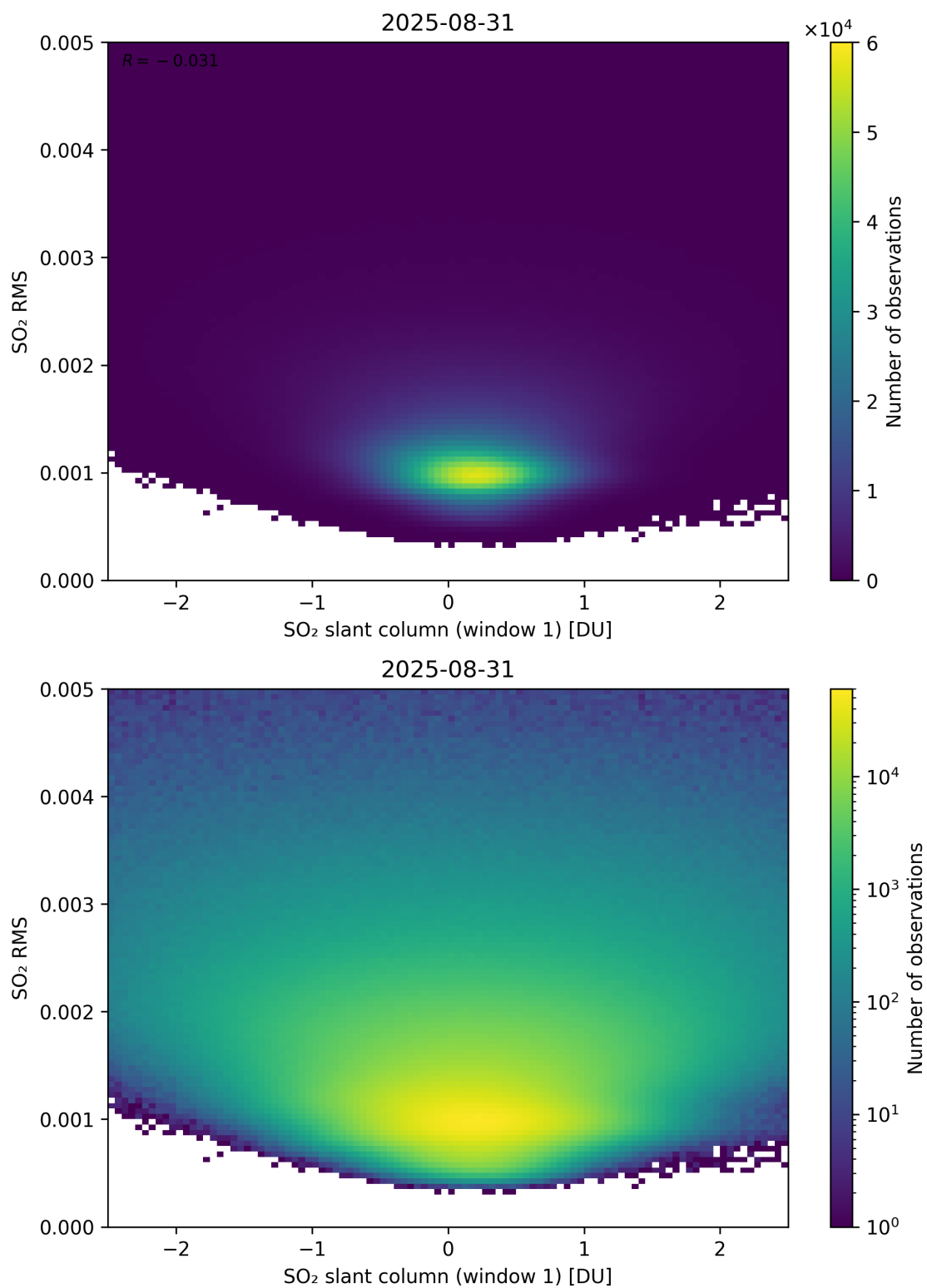
Figure 267: Scatter density plot of “SO 2 slant column (window 1)” against “SO 2 RMS” for 2025-08-30 to 2025-09-01.
