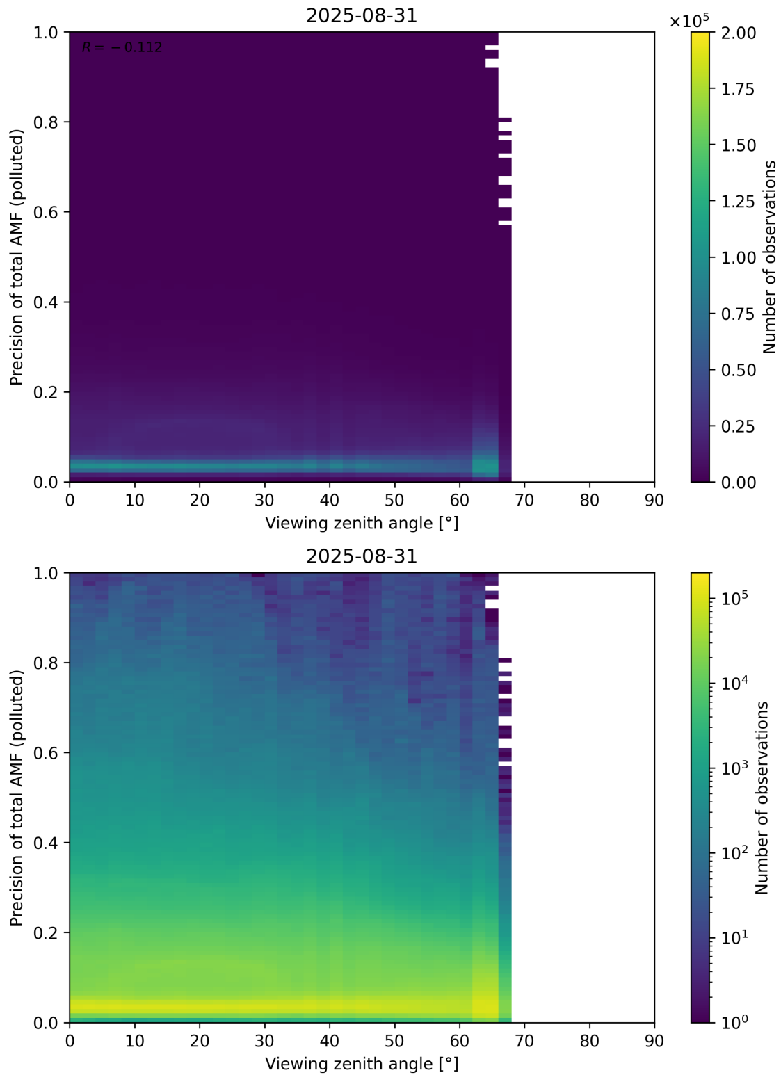
Figure 382: Scatter density plot of “Viewing zenith angle” against “Precision of total AMF (polluted)” for 2025-08-30 to 2025-09-01.
