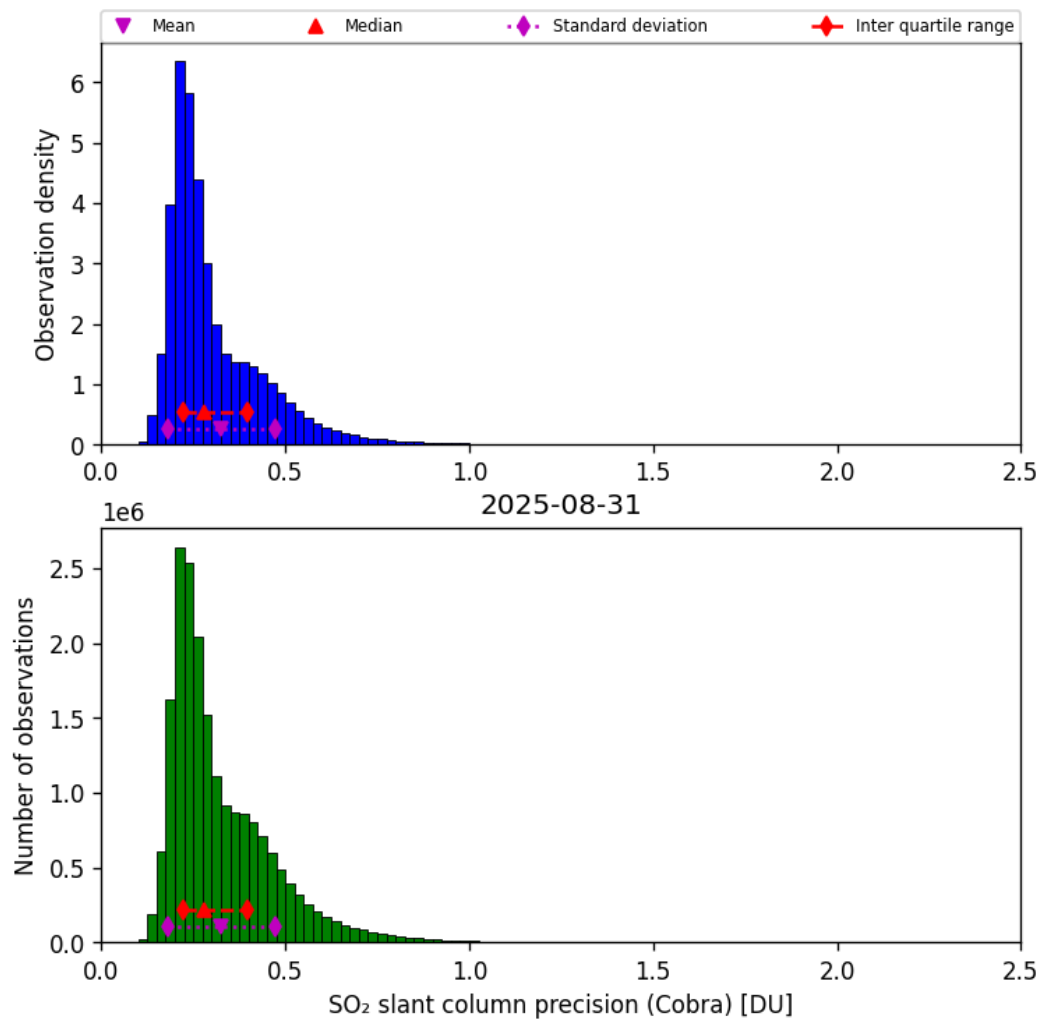
Figure 62: Histogram of “SO 2 slant column precision (Cobra)” for 2025-08-30 to 2025-09-01
