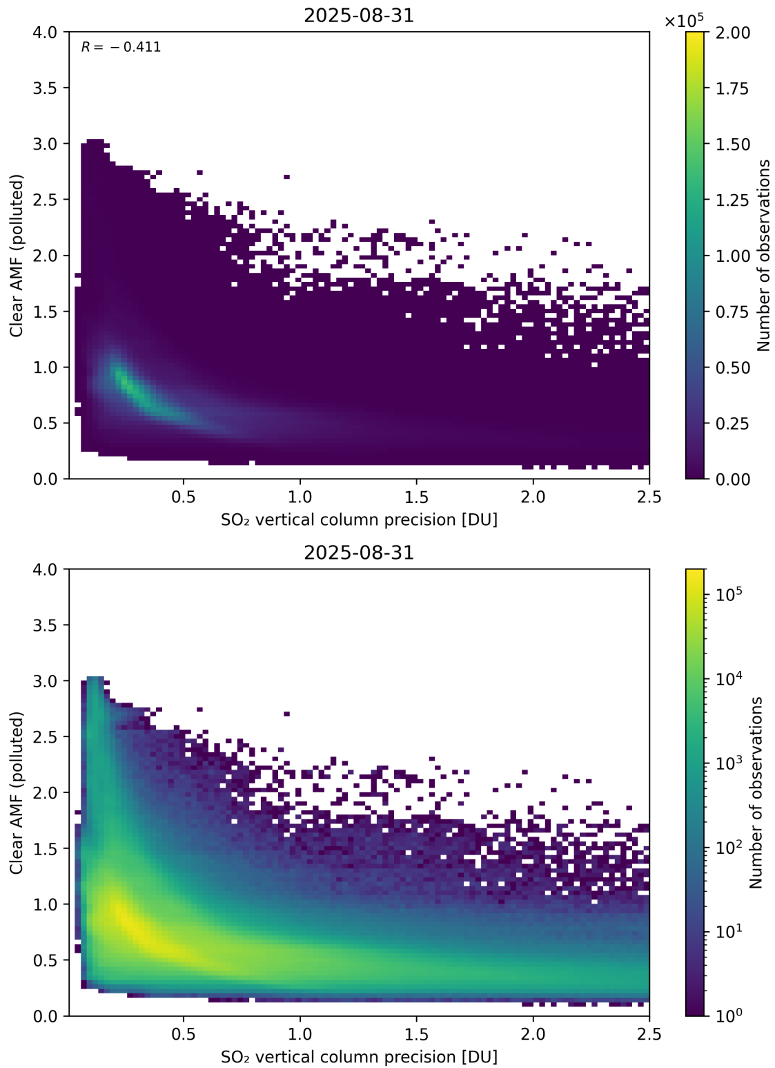
Figure 335: Scatter density plot of “SO 2 vertical column precision” against “Clear AMF (polluted)” for 2025-08-30 to 2025-09-01.
