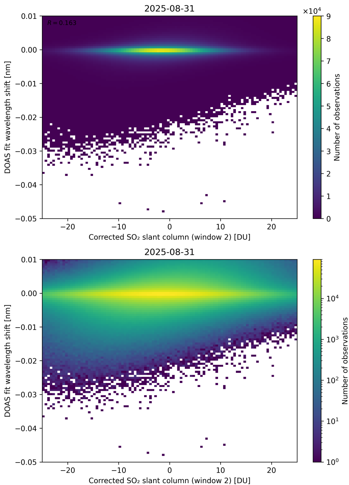
Figure 246: Scatter density plot of “Corrected SO 2 slant column (window 2)” against “DOAS fit wavelength shift” for 2025-08-30 to 2025-09-01.
