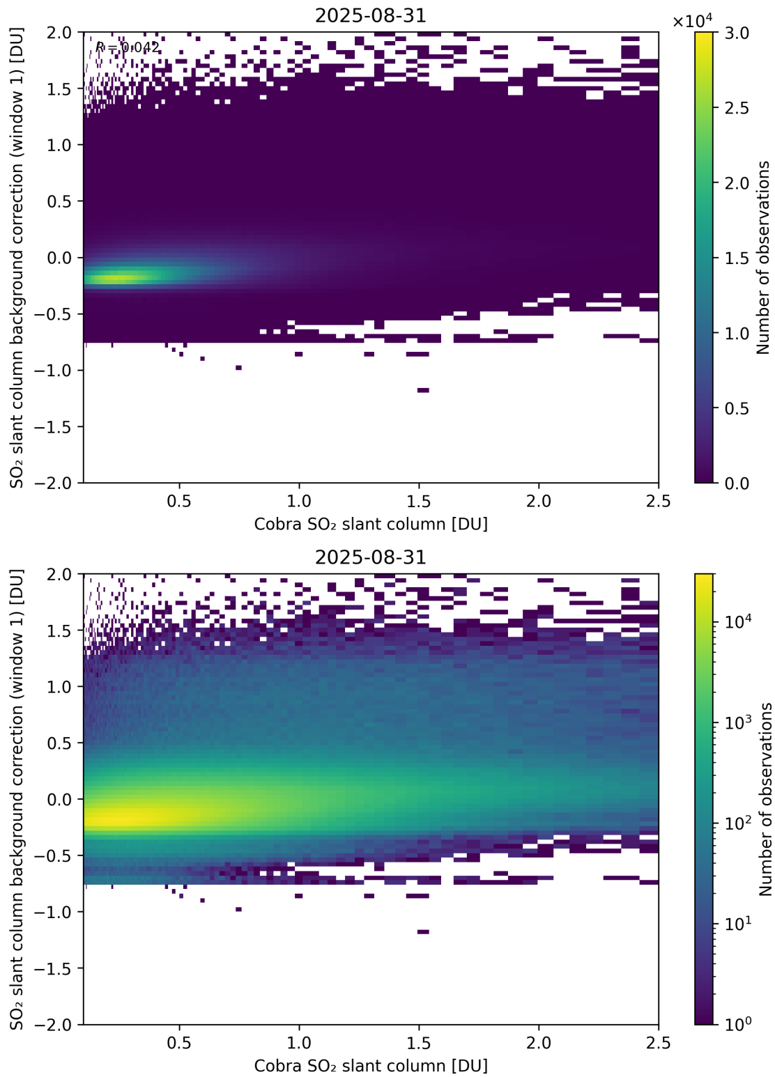
Figure 193: Scatter density plot of “Cobra SO 2 slant column” against “SO 2 slant column background correction (window 1)” for 2025-08-30 to 2025-09-01.
