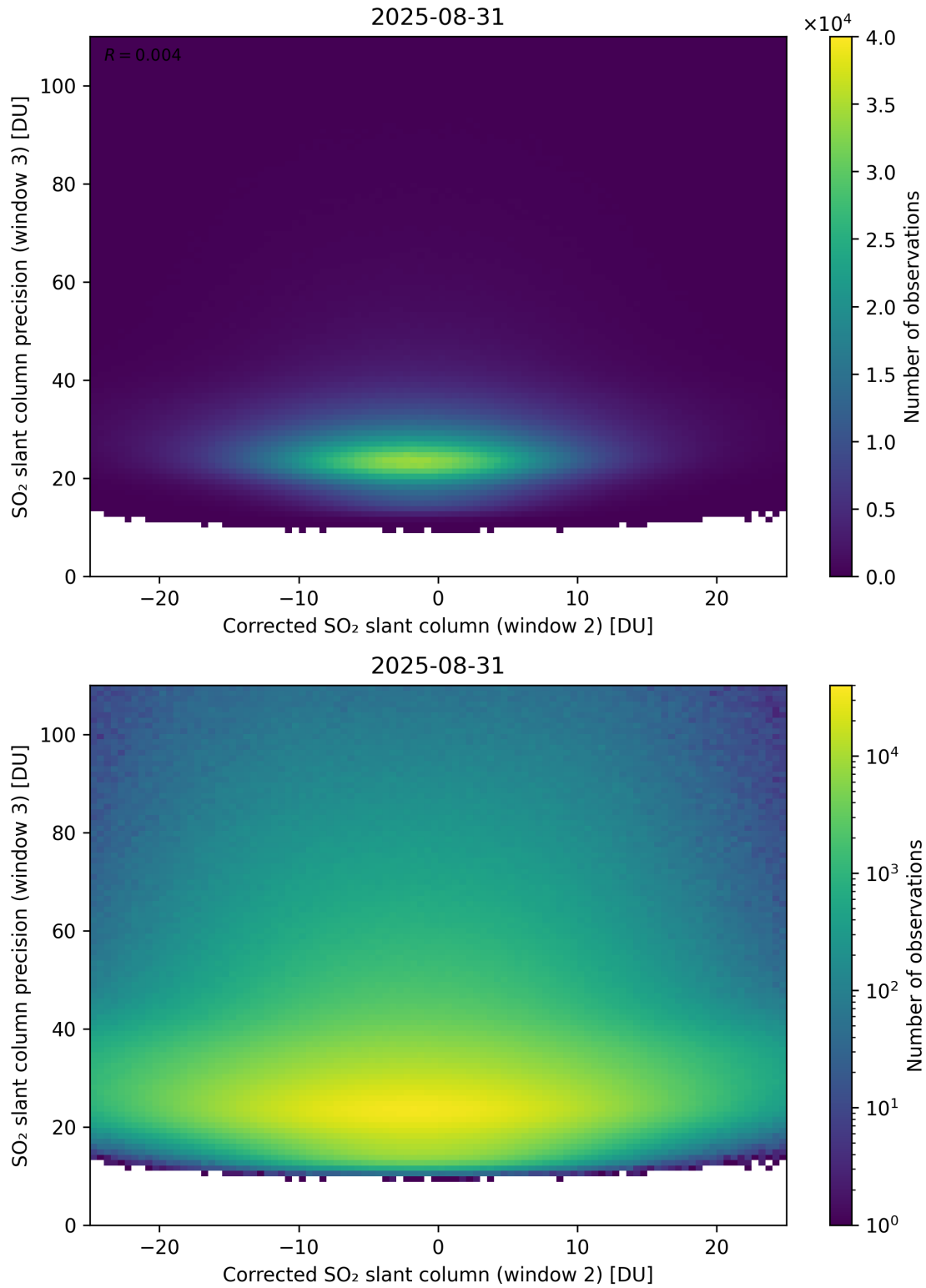
Figure 252: Scatter density plot of “Corrected SO 2 slant column (window 2)” against “SO 2 slant column precision (window 3)” for 2025-08-30 to 2025-09-01.
