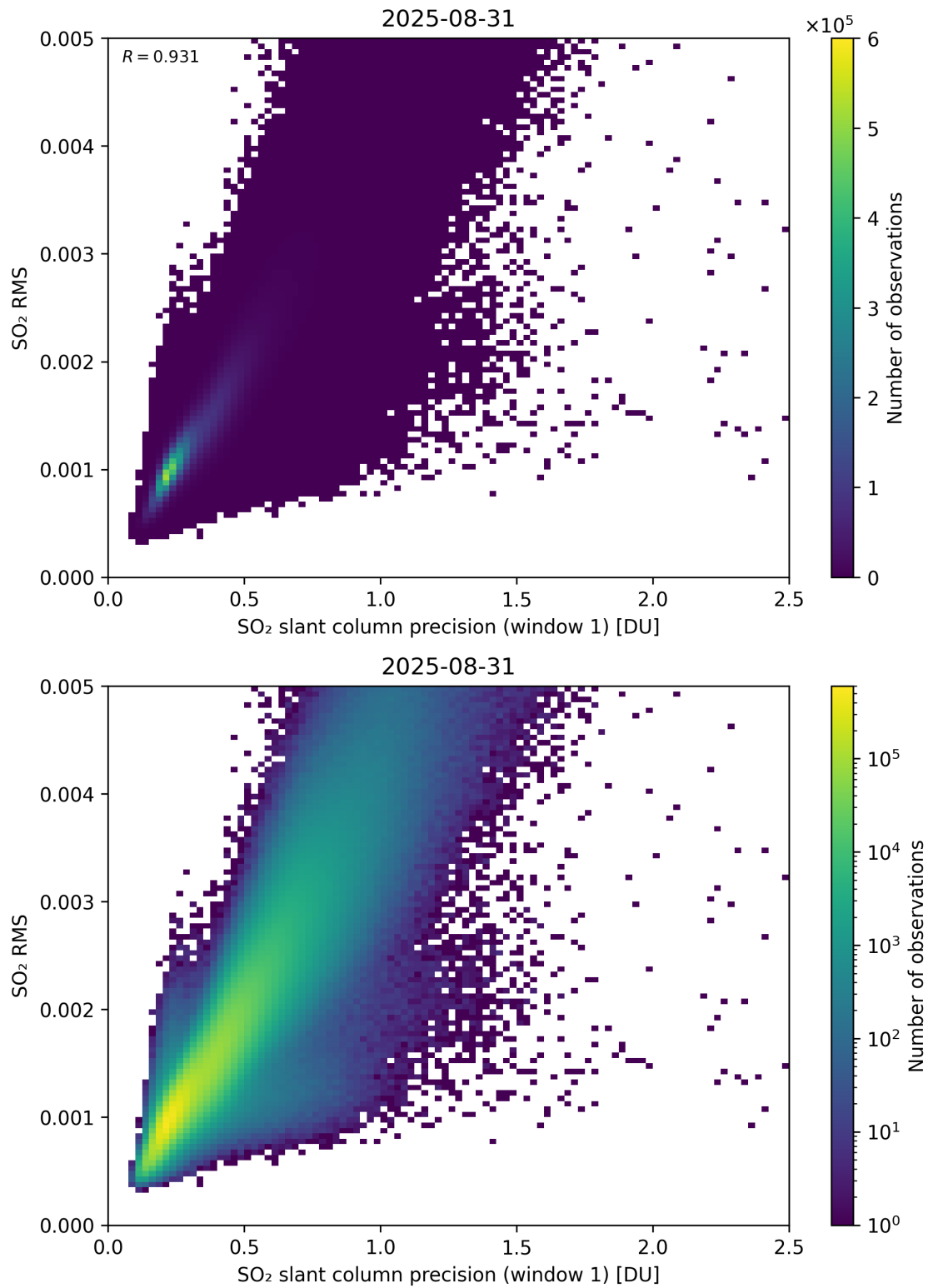
Figure 273: Scatter density plot of “SO 2 slant column precision (window 1)” against “SO 2 RMS” for 2025-08-30 to 2025-09-01.
