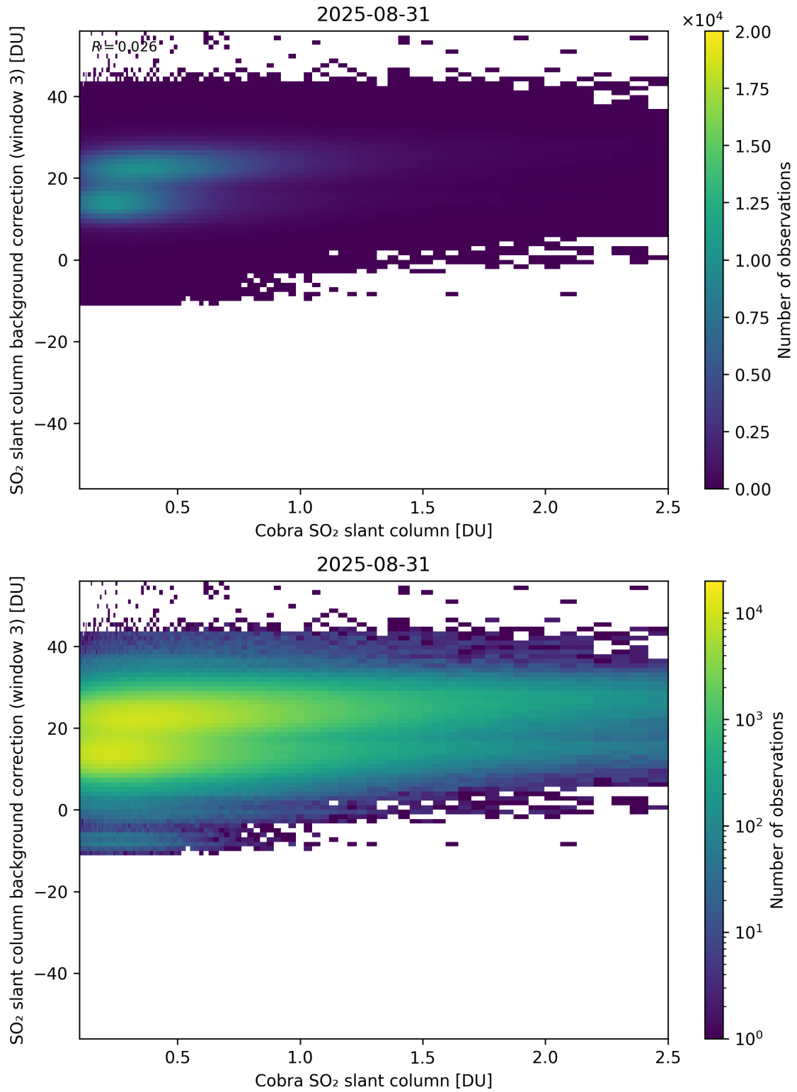
Figure 195: Scatter density plot of “Cobra SO 2 slant column” against “SO 2 slant column background correction (window 3)” for 2025-08-30 to 2025-09-01.
