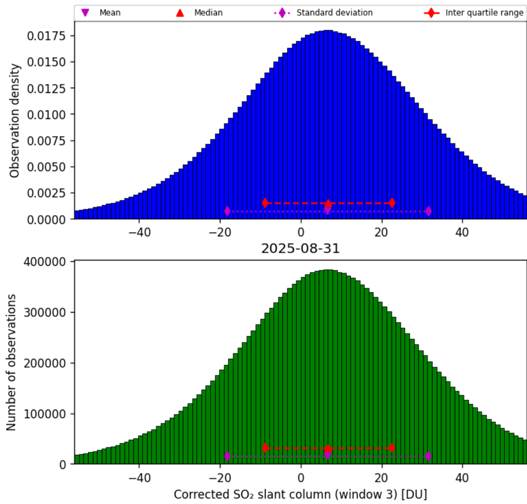
Figure 73: Histogram of “Corrected SO 2 slant column (window 3)” for 2025-08-30 to 2025-09-01
