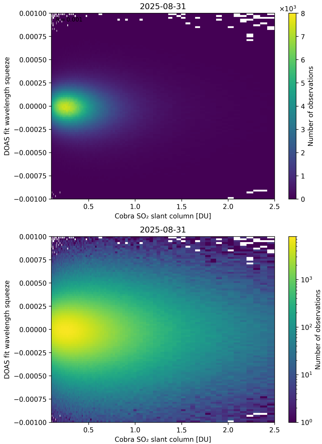
Figure 197: Scatter density plot of “Cobra SO 2 slant column” against “DOAS fit wavelength squeeze” for 2025-08-30 to 2025-09-01.
