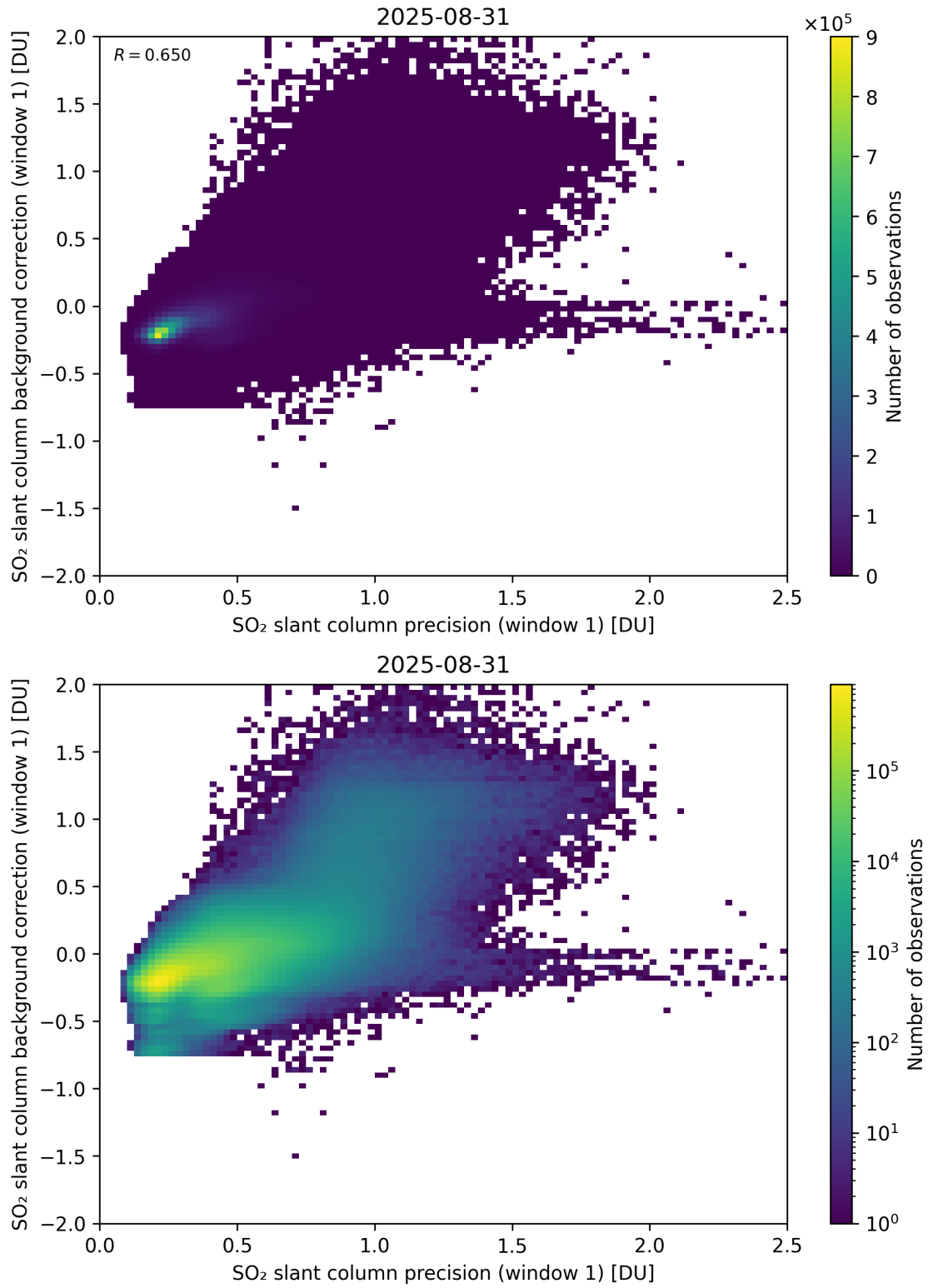
Figure 268: Scatter density plot of “SO 2 slant column precision (window 1)” against “SO 2 slant column background correction (window 1)” for 2025-08-30 to 2025-09-01.
