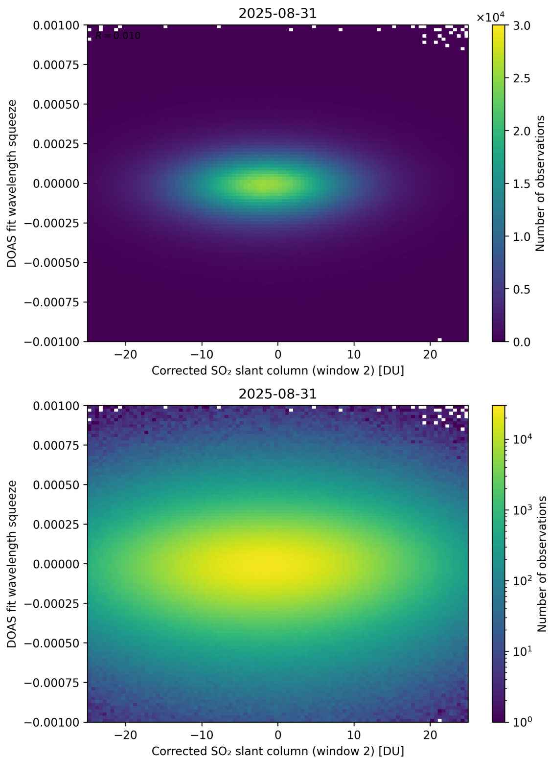
Figure 247: Scatter density plot of “Corrected SO 2 slant column (window 2)” against “DOAS fit wavelength squeeze” for 2025-08-30 to 2025-09-01.
