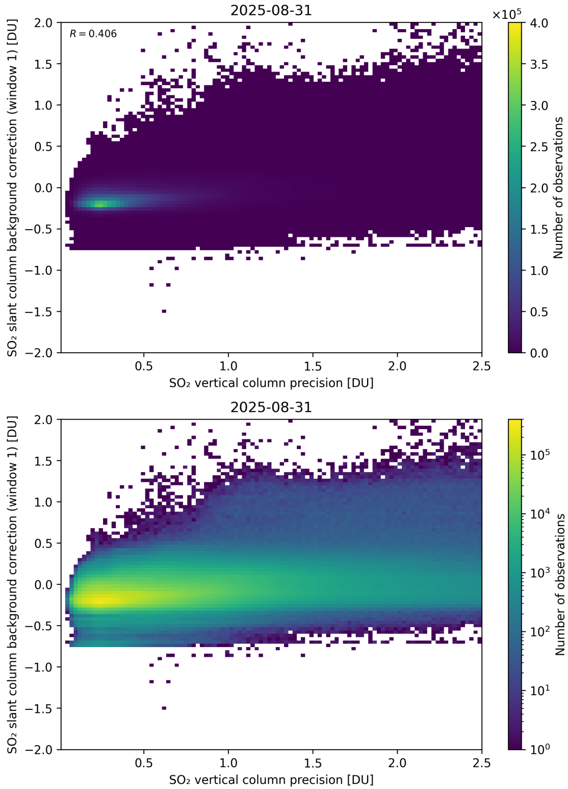
Figure 329: Scatter density plot of “SO 2 vertical column precision” against “SO 2 slant column background correction (window 1)” for 2025-08-30 to 2025-09-01.
