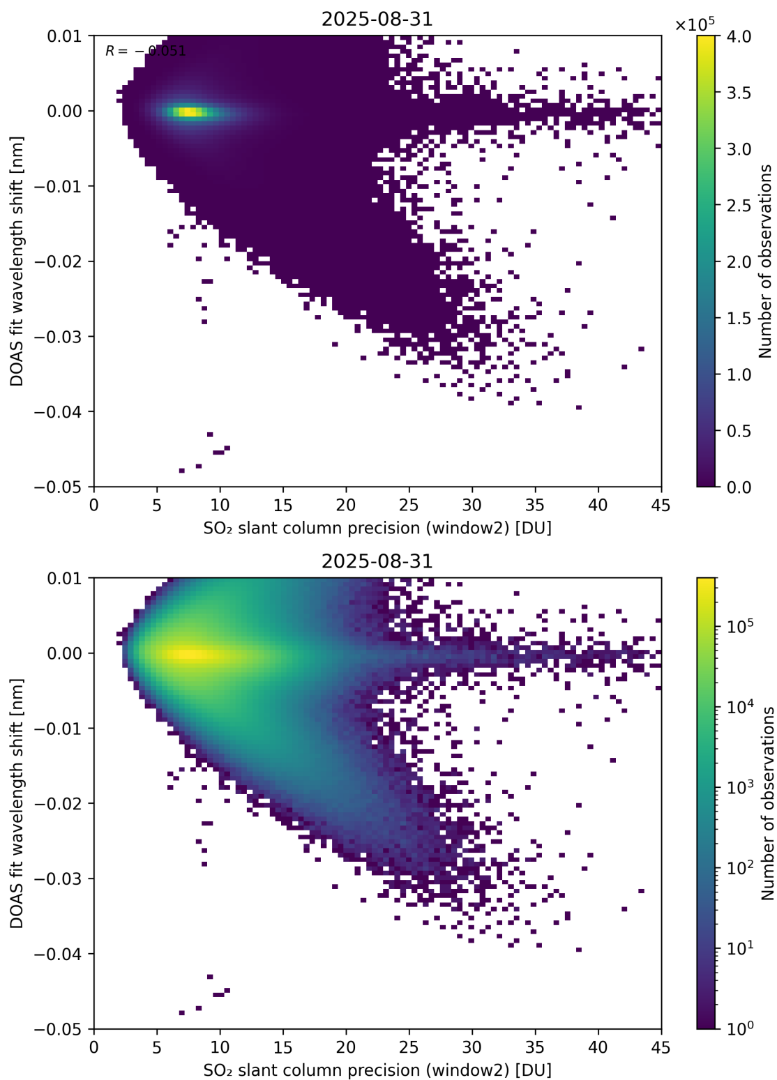
Figure 293: Scatter density plot of “SO 2 slant column precision (window2)” against “DOAS fit wavelength shift” for 2025-08-30 to 2025-09-01.
