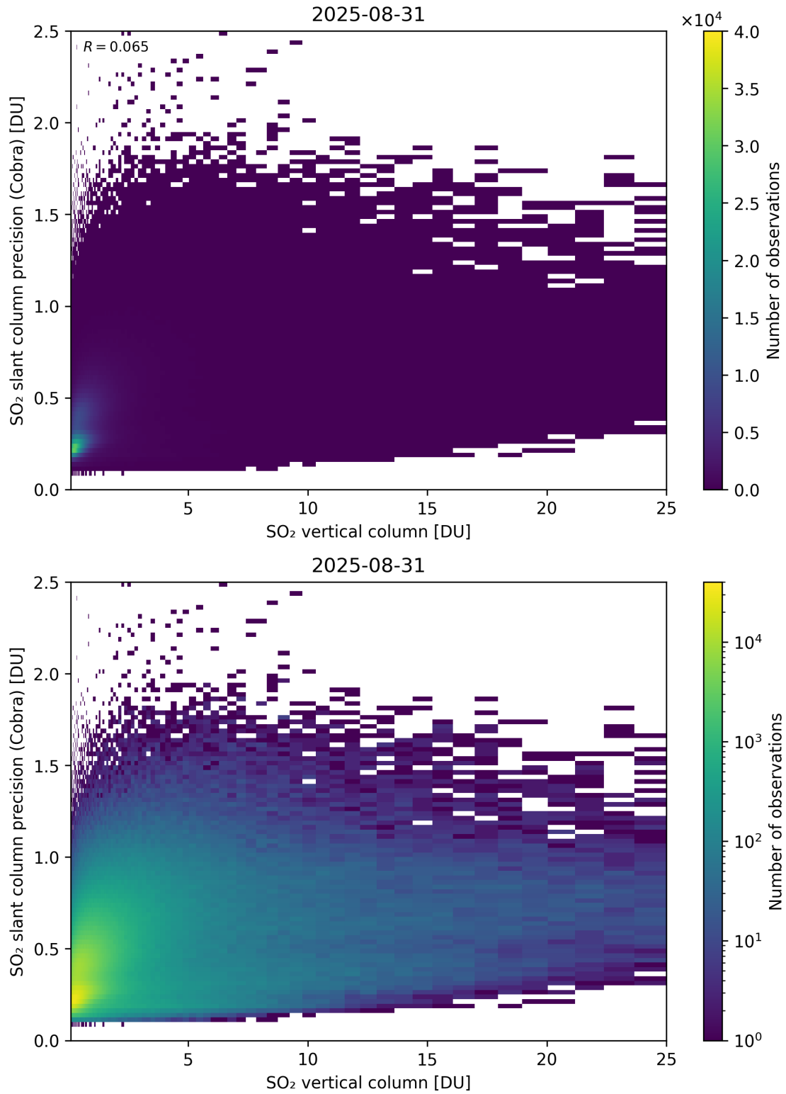
Figure 350: Scatter density plot of “SO 2 vertical column” against “SO 2 slant column precision (Cobra)” for 2025-08-30 to 2025-09-01.
