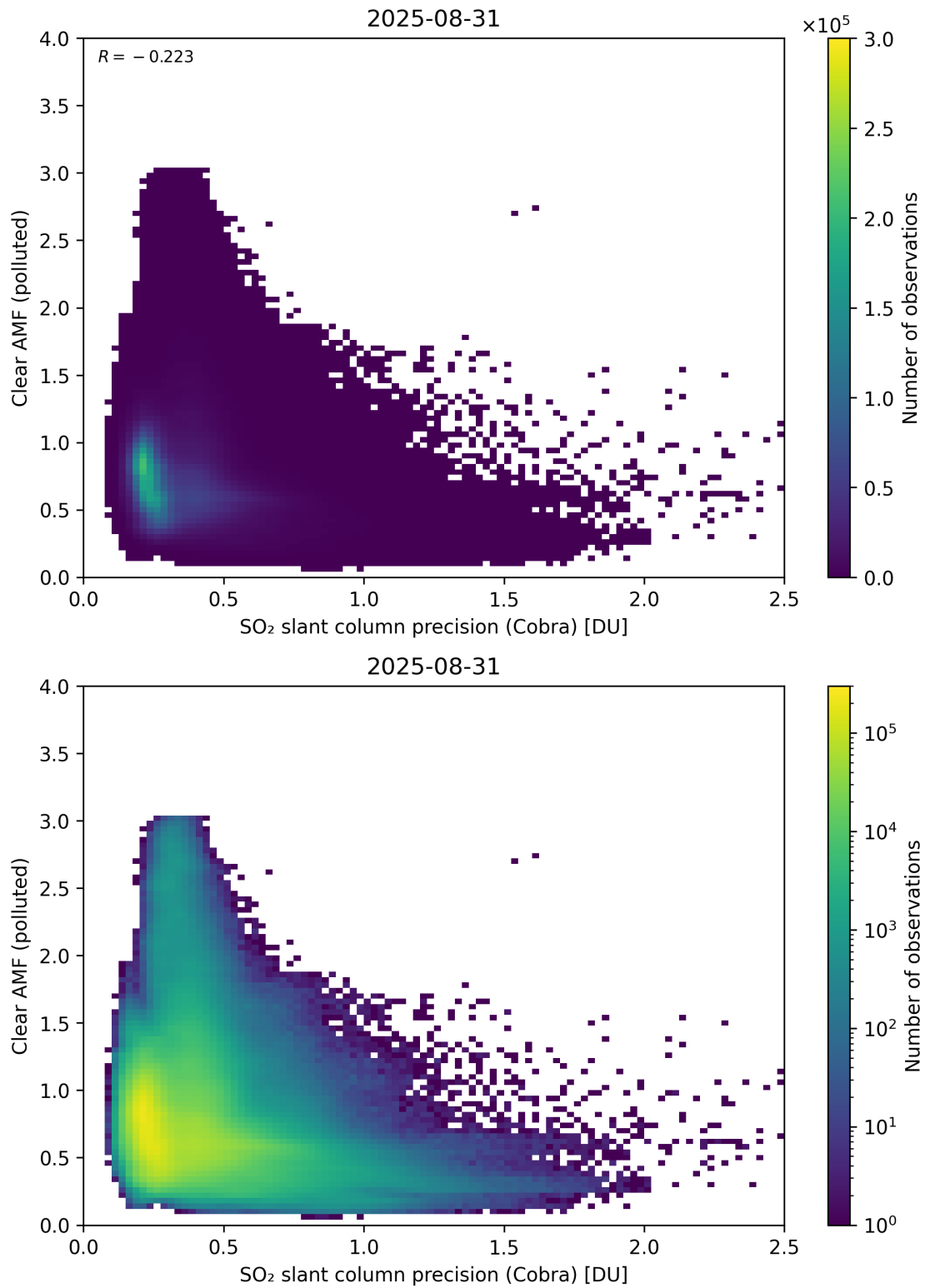
Figure 205: Scatter density plot of “SO 2 slant column precision (Cobra)” against “Clear AMF (polluted)” for 2025-08-30 to 2025-09-01.
