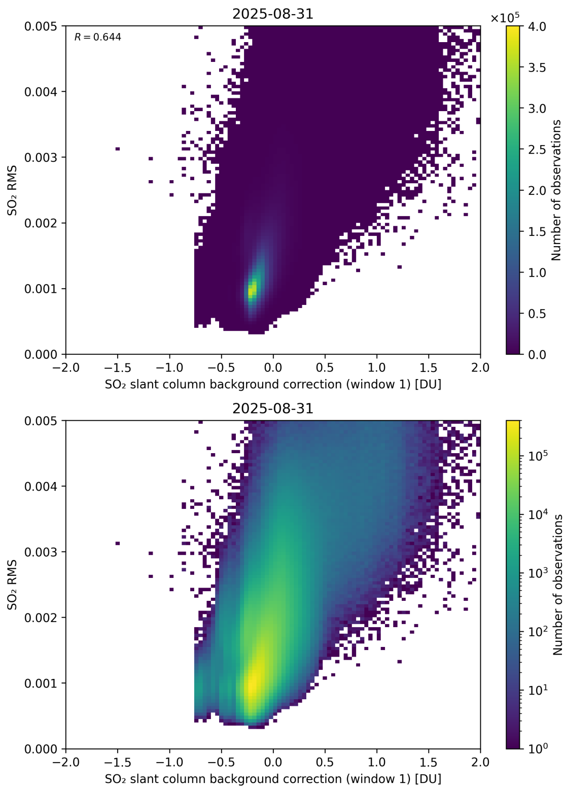
Figure 113: Scatter density plot of “SO 2 slant column background correction (window 1)” against “SO 2 RMS” for 2025-08-30 to 2025-09-01.
