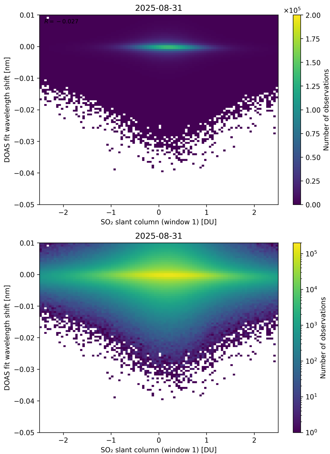
Figure 265: Scatter density plot of “SO 2 slant column (window 1)” against “DOAS fit wavelength shift” for 2025-08-30 to 2025-09-01.
