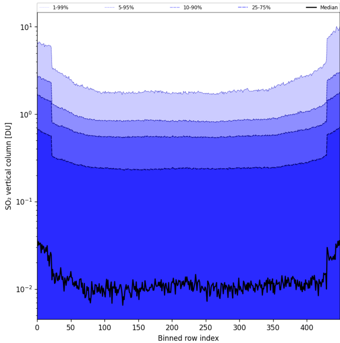
Figure 84: Along track statistics of “SO 2 vertical column” for 2025-08-30 to 2025-09-01
