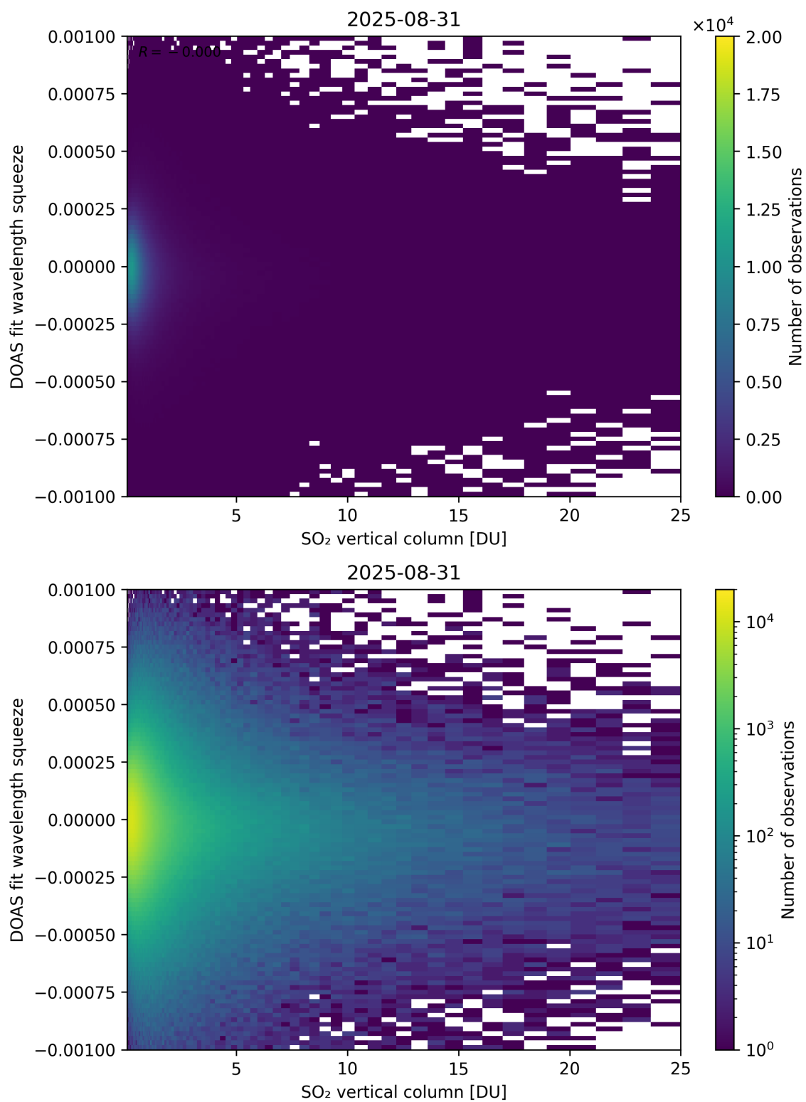
Figure 327: Scatter density plot of “SO 2 vertical column” against “DOAS fit wavelength squeeze” for 2025-08-30 to 2025-09-01.
