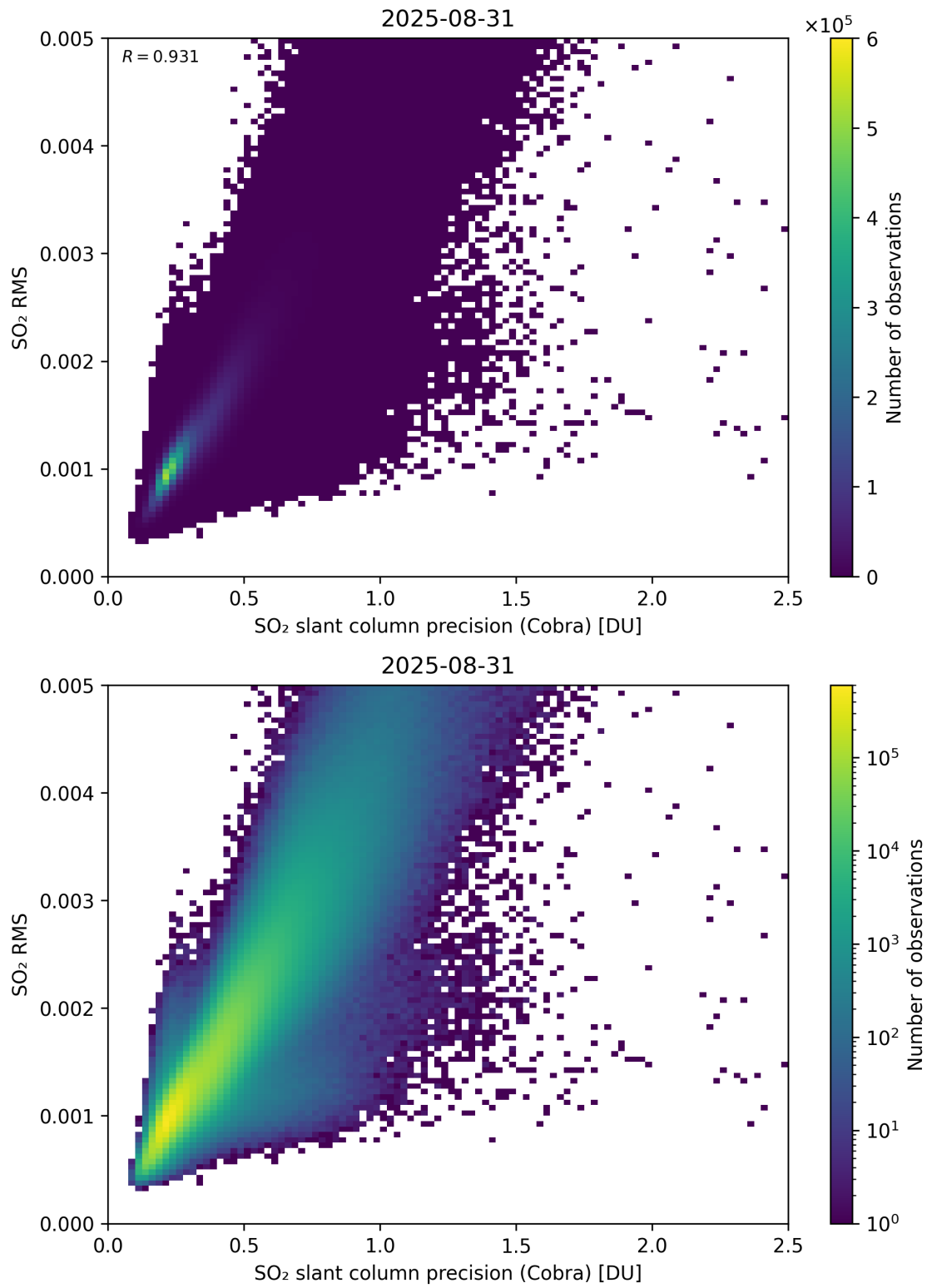
Figure 204: Scatter density plot of “SO 2 slant column precision (Cobra)” against “SO 2 RMS” for 2025-08-30 to 2025-09-01.
