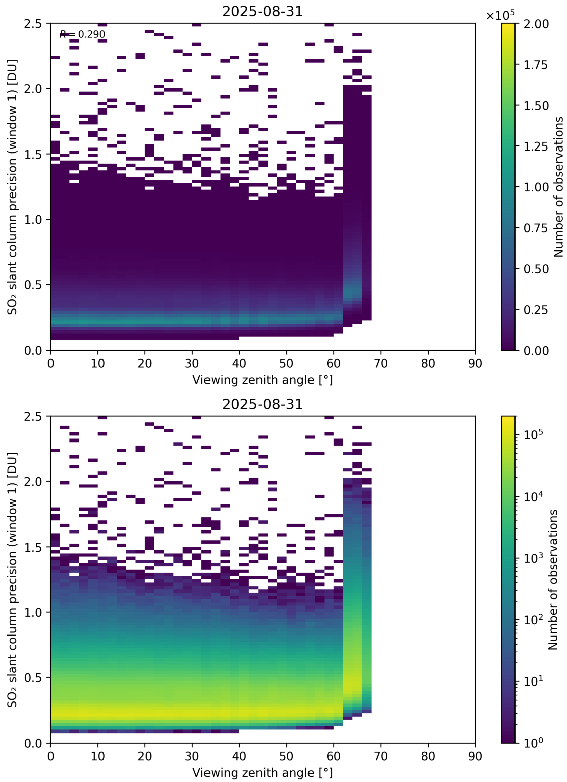
Figure 377: Scatter density plot of “Viewing zenith angle” against “SO 2 slant column precision (window 1)” for 2025-08-30 to 2025-09-01.
