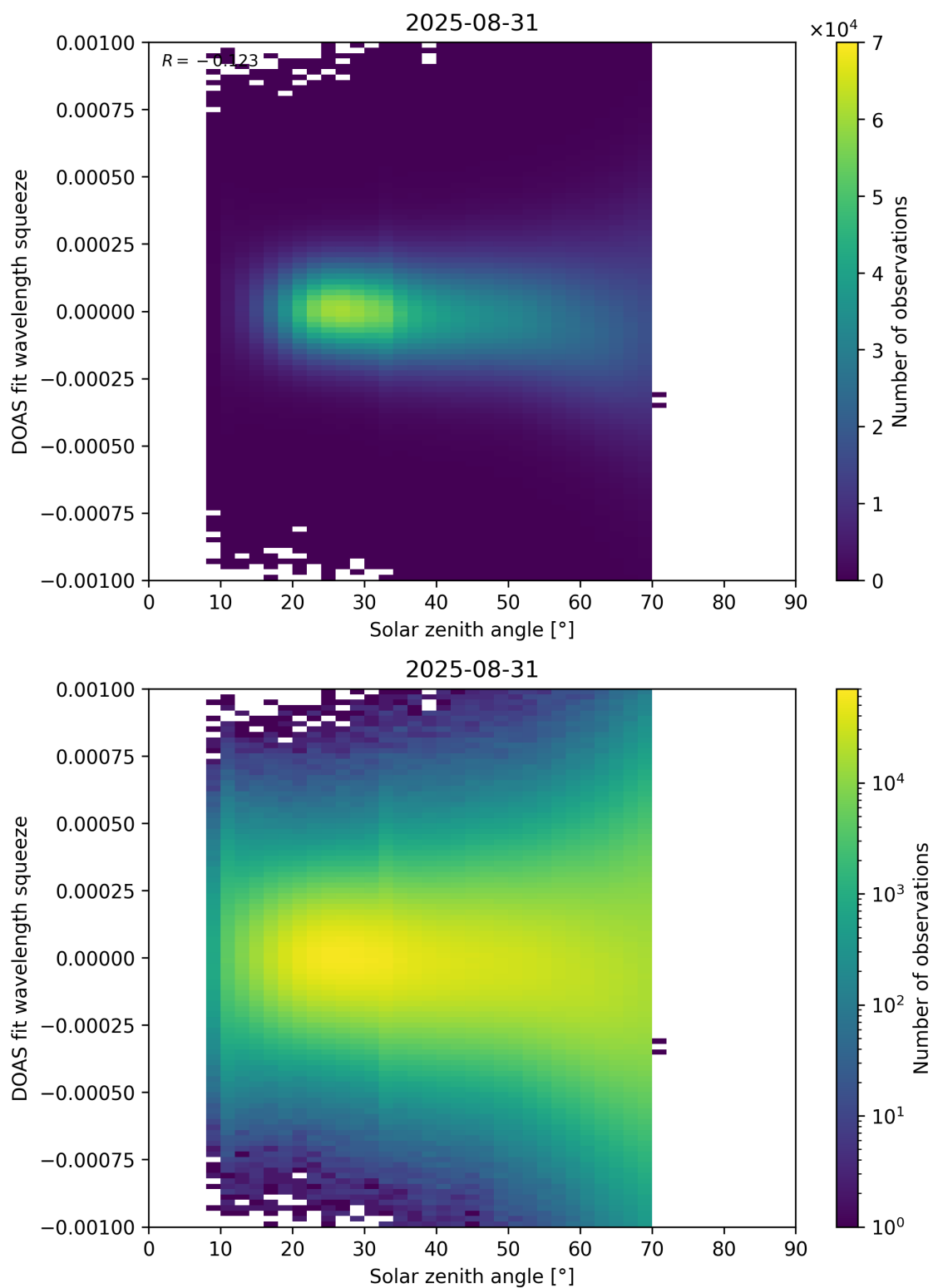
Figure 175: Scatter density plot of “Solar zenith angle” against “DOAS fit wavelength squeeze” for 2025-08-30 to 2025-09-01.
