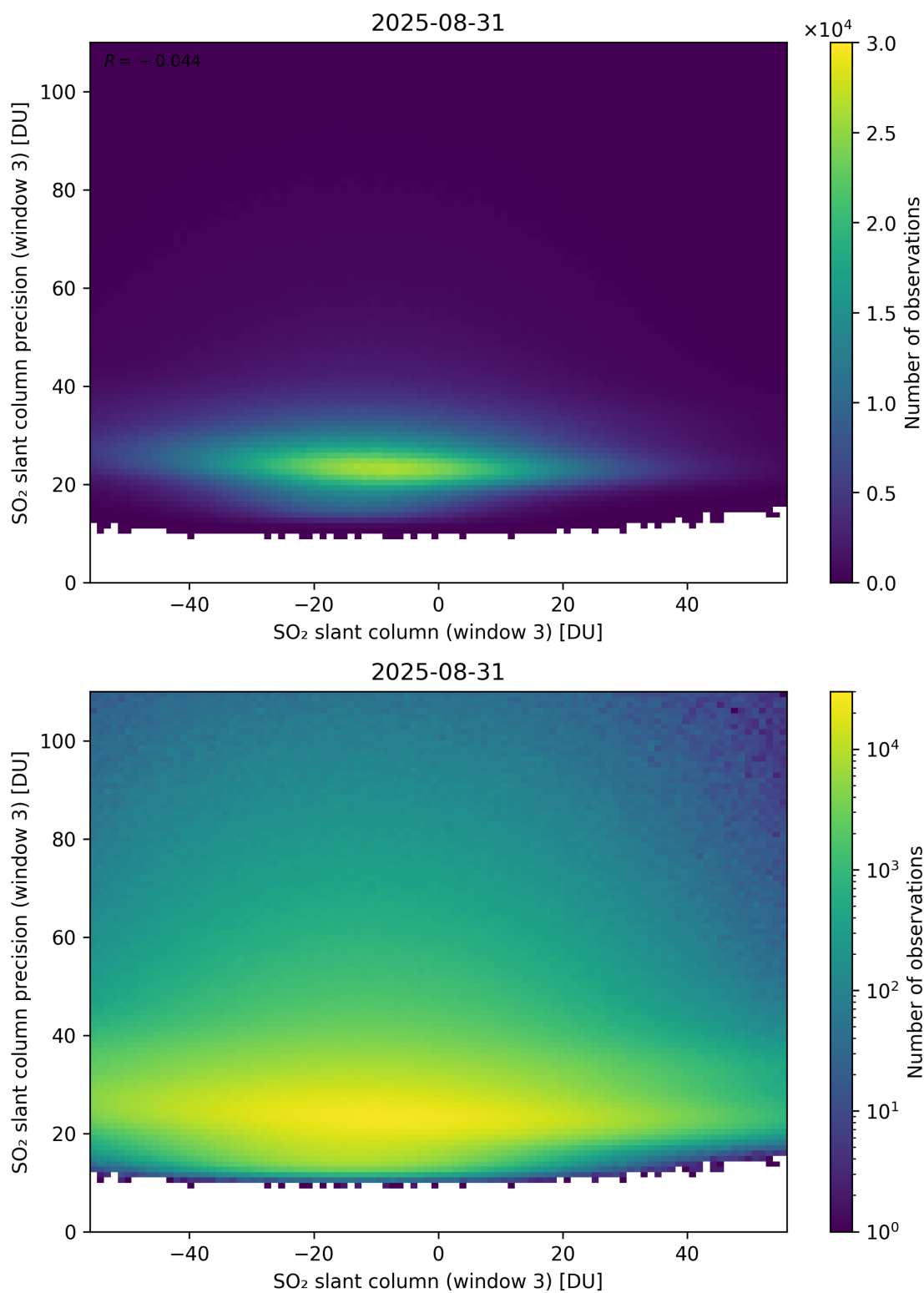
Figure 317: Scatter density plot of “SO 2 slant column (window 3)” against “SO 2 slant column precision (window 3)” for 2025-08-30 to 2025-09-01.
