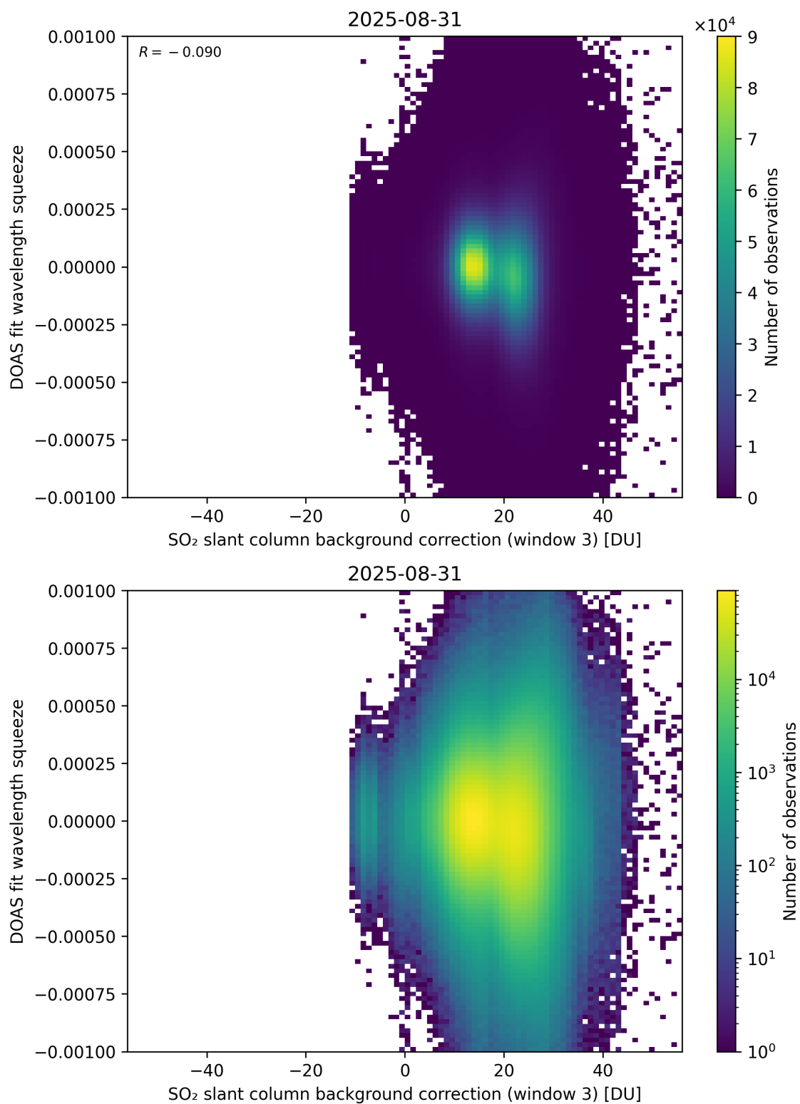
Figure 133: Scatter density plot of “SO 2 slant column background correction (window 3)” against “DOAS fit wavelength squeeze” for 2025-08-30 to 2025-09-01.
