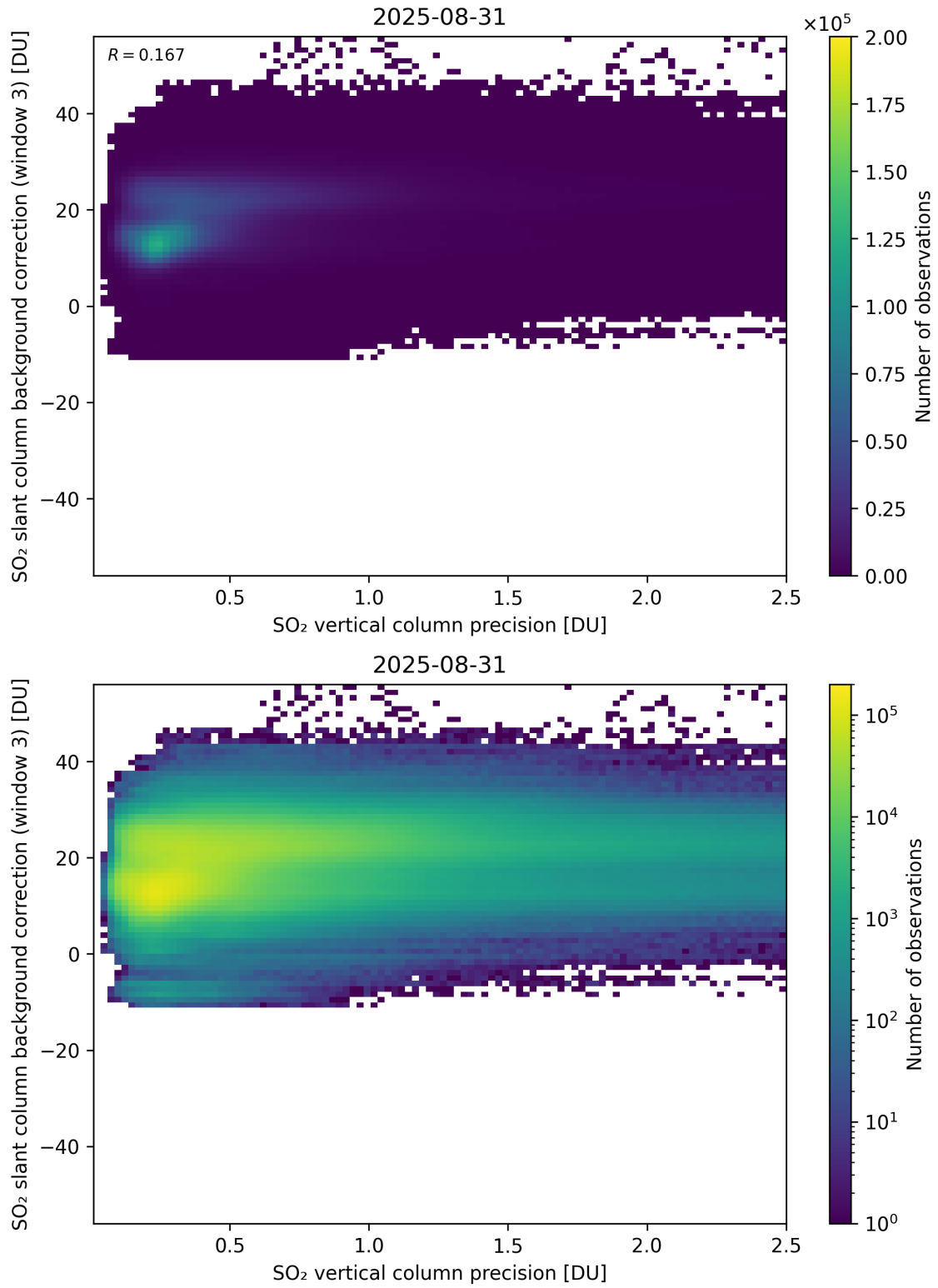
Figure 331: Scatter density plot of “SO 2 vertical column precision” against “SO 2 slant column background correction (window 3)” for 2025-08-30 to 2025-09-01.
