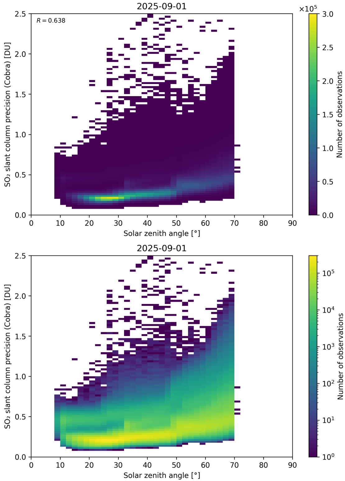
Figure 180: Scatter density plot of “Solar zenith angle” against “SO 2 slant column precision (Cobra)” for 2025-08-31 to 2025-09-02.
