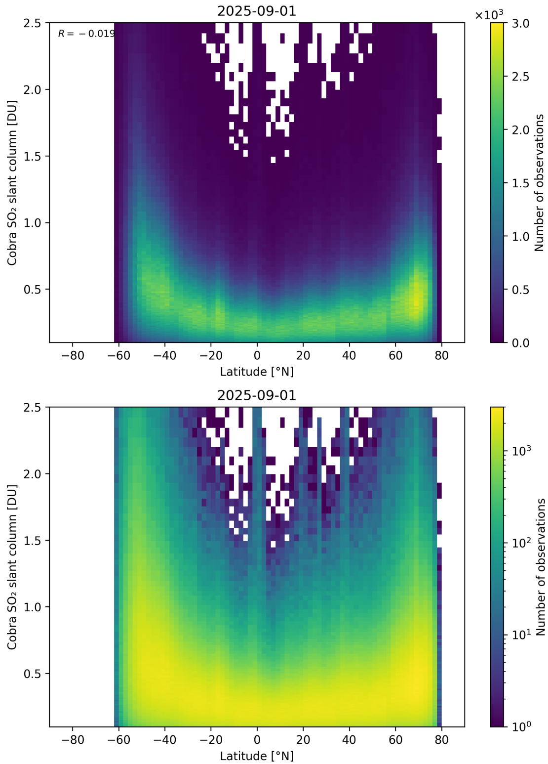
Figure 157: Scatter density plot of “Latitude” against “Cobra SO 2 slant column” for 2025-08-31 to 2025-09-02.
