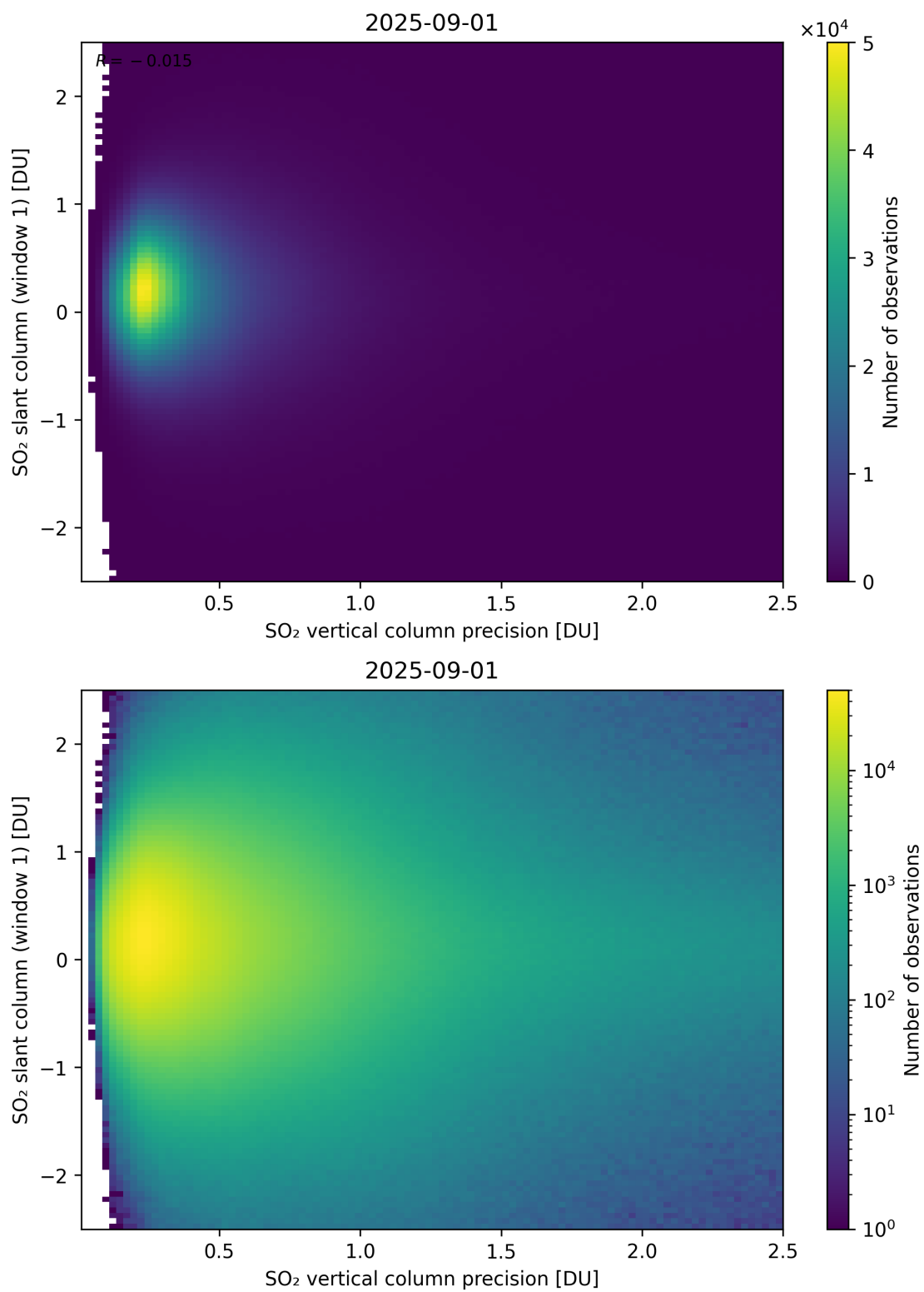
Figure 341: Scatter density plot of “SO 2 vertical column precision” against “SO 2 slant column (window 1)” for 2025-08-31 to 2025-09-02.
