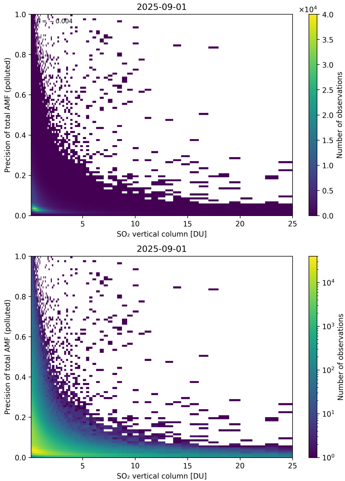
Figure 360: Scatter density plot of “SO 2 vertical column” against “Precision of total AMF (polluted)” for 2025-08-31 to 2025-09-02.
