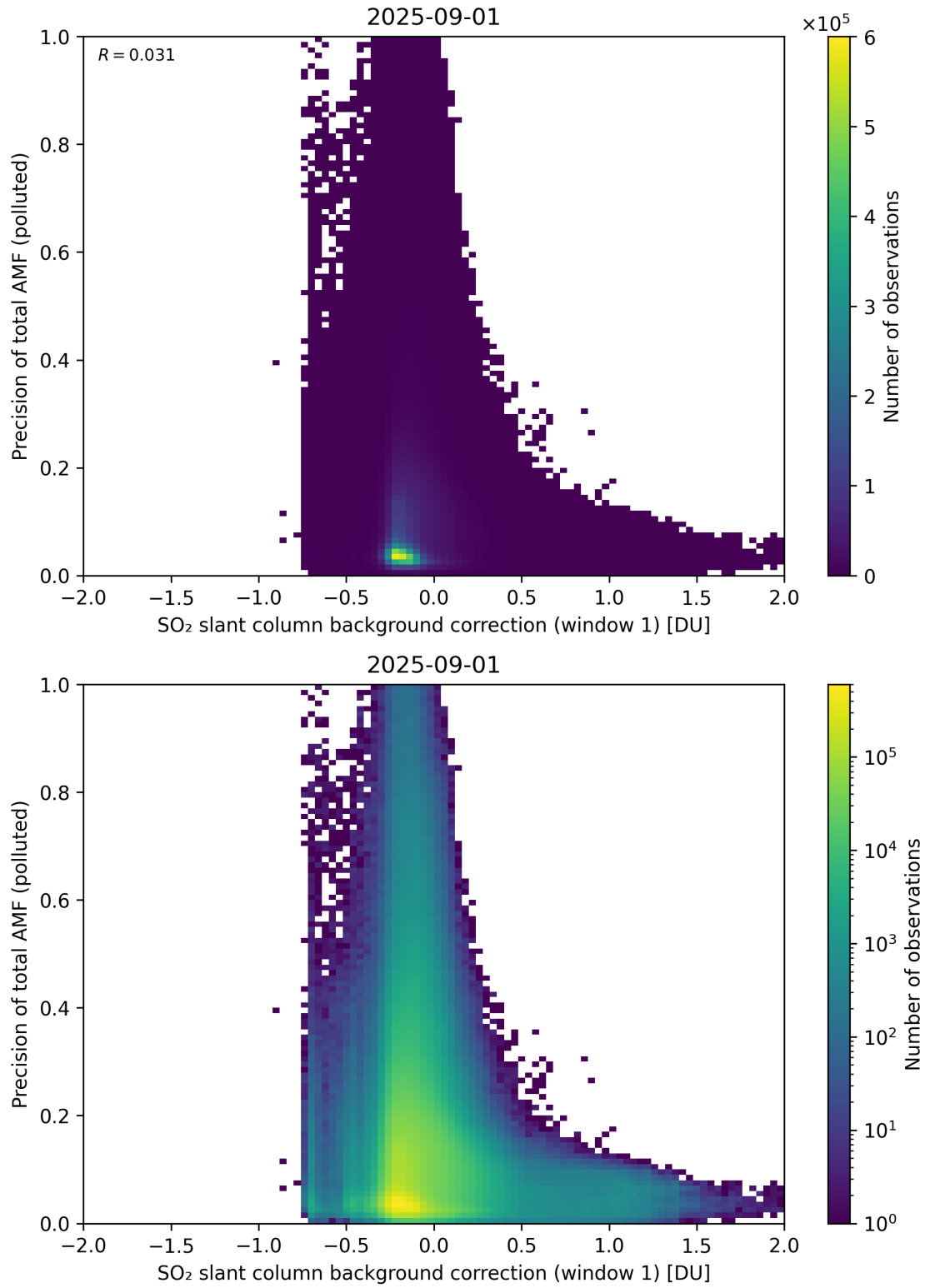
Figure 121: Scatter density plot of “SO 2 slant column background correction (window 1)” against “Precision of total AMF (polluted)” for 2025-08-31 to 2025-09-02.
