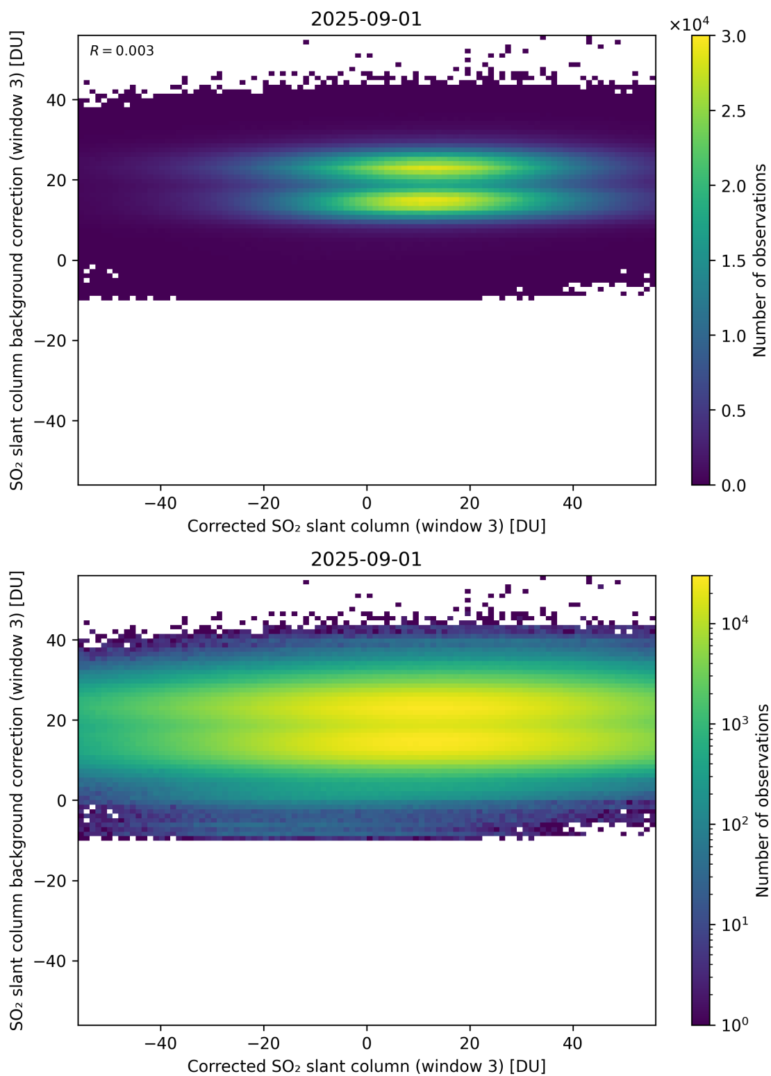
Figure 255: Scatter density plot of “Corrected SO 2 slant column (window 3)” against “SO 2 slant column background correction (window 3)” for 2025-08-31 to 2025-09-02.
