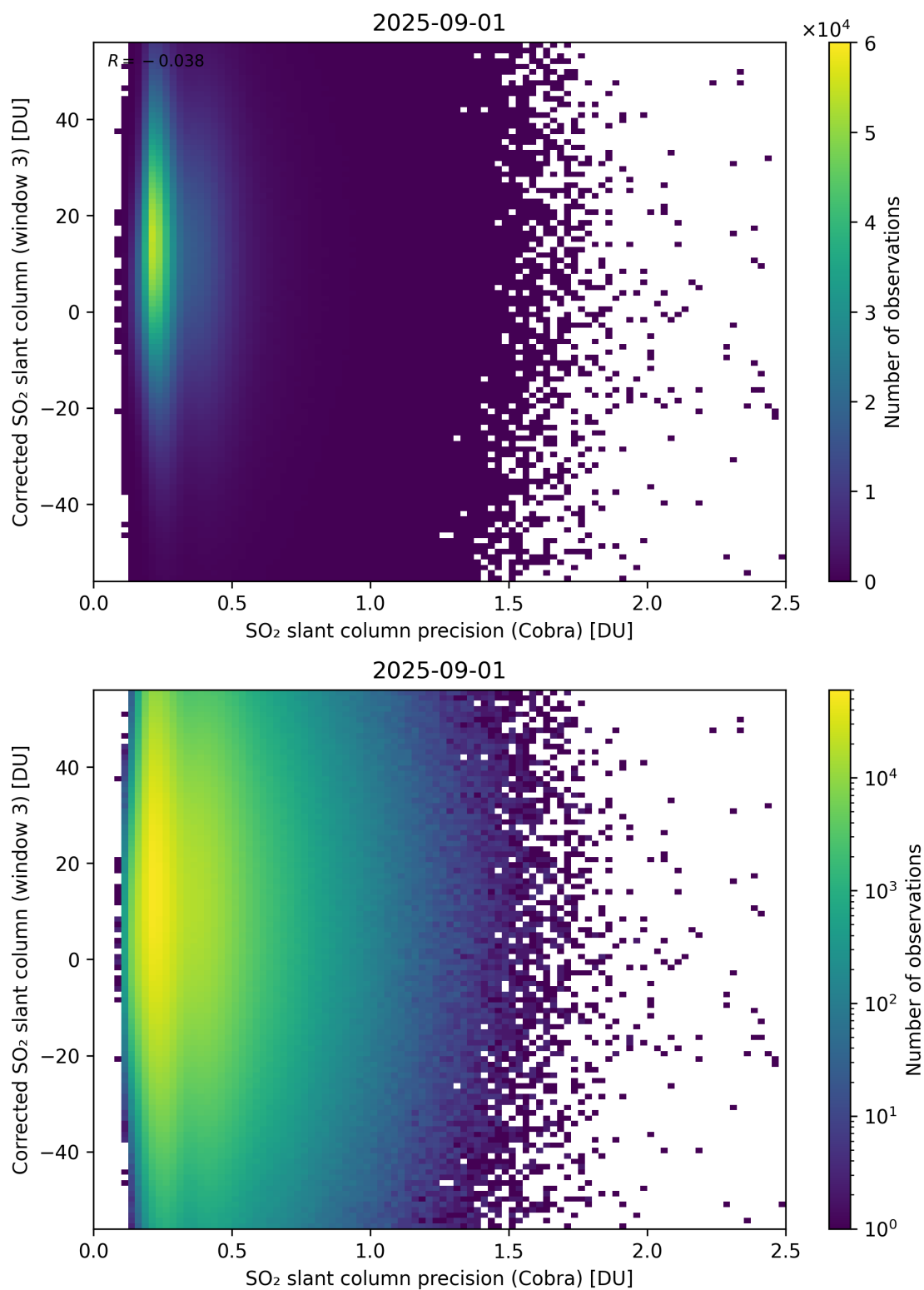
Figure 207: Scatter density plot of “SO 2 slant column precision (Cobra)” against “Corrected SO 2 slant column (window 3)” for 2025-08-31 to 2025-09-02.
