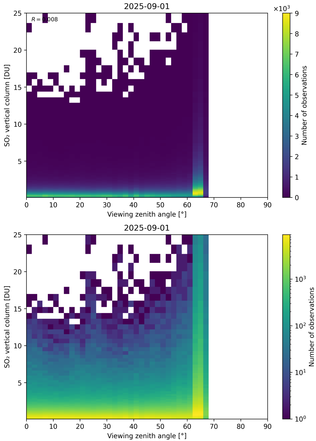
Figure 383: Scatter density plot of “Viewing zenith angle” against “SO 2 vertical column” for 2025-08-31 to 2025-09-02.
