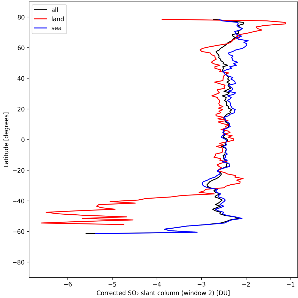
Figure 43: Zonal average of “Corrected SO 2 slant column (window 2)” for 2025-08-31 to 2025-09-02.
