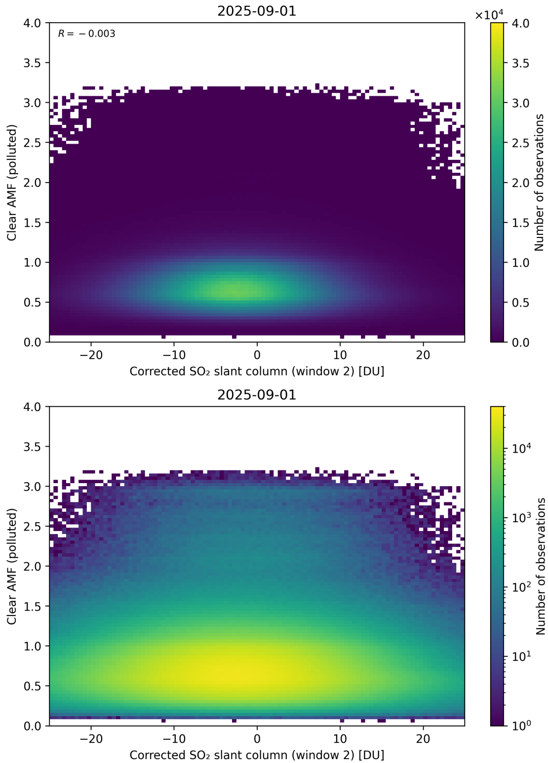
Figure 249: Scatter density plot of “Corrected SO 2 slant column (window 2)” against “Clear AMF (polluted)” for 2025-08-31 to 2025-09-02.
