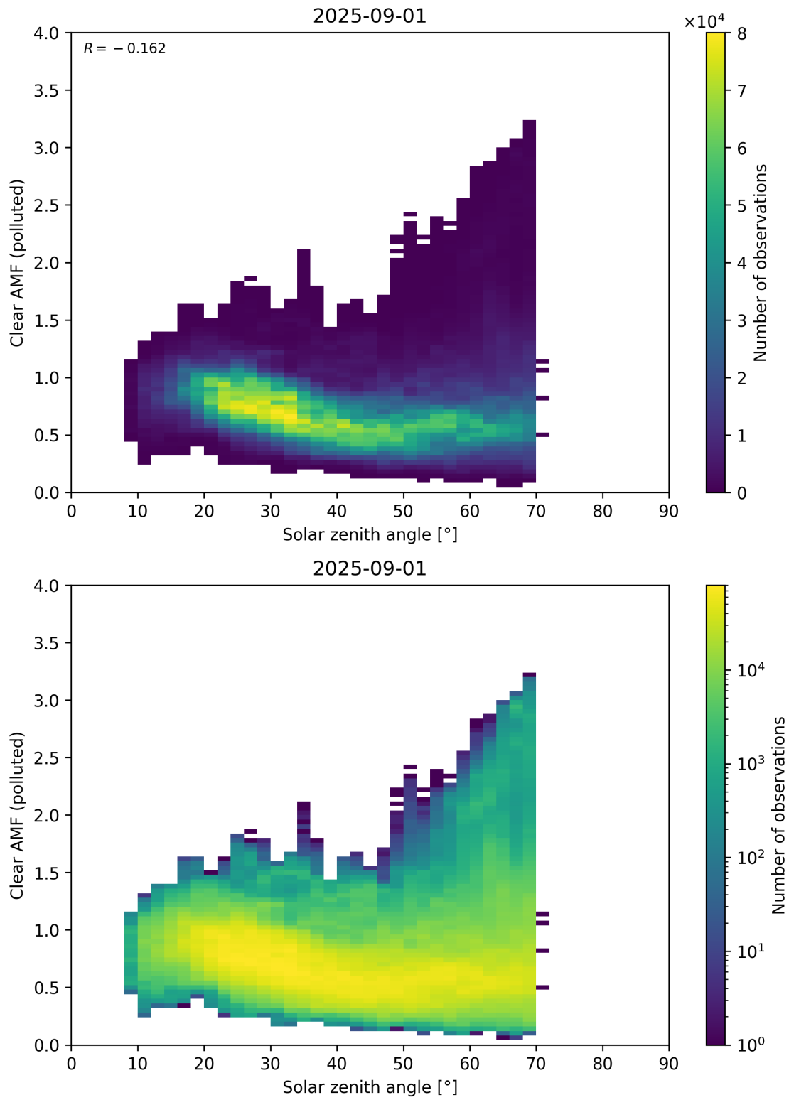
Figure 178: Scatter density plot of “Solar zenith angle” against “Clear AMF (polluted)” for 2025-08-31 to 2025-09-02.
