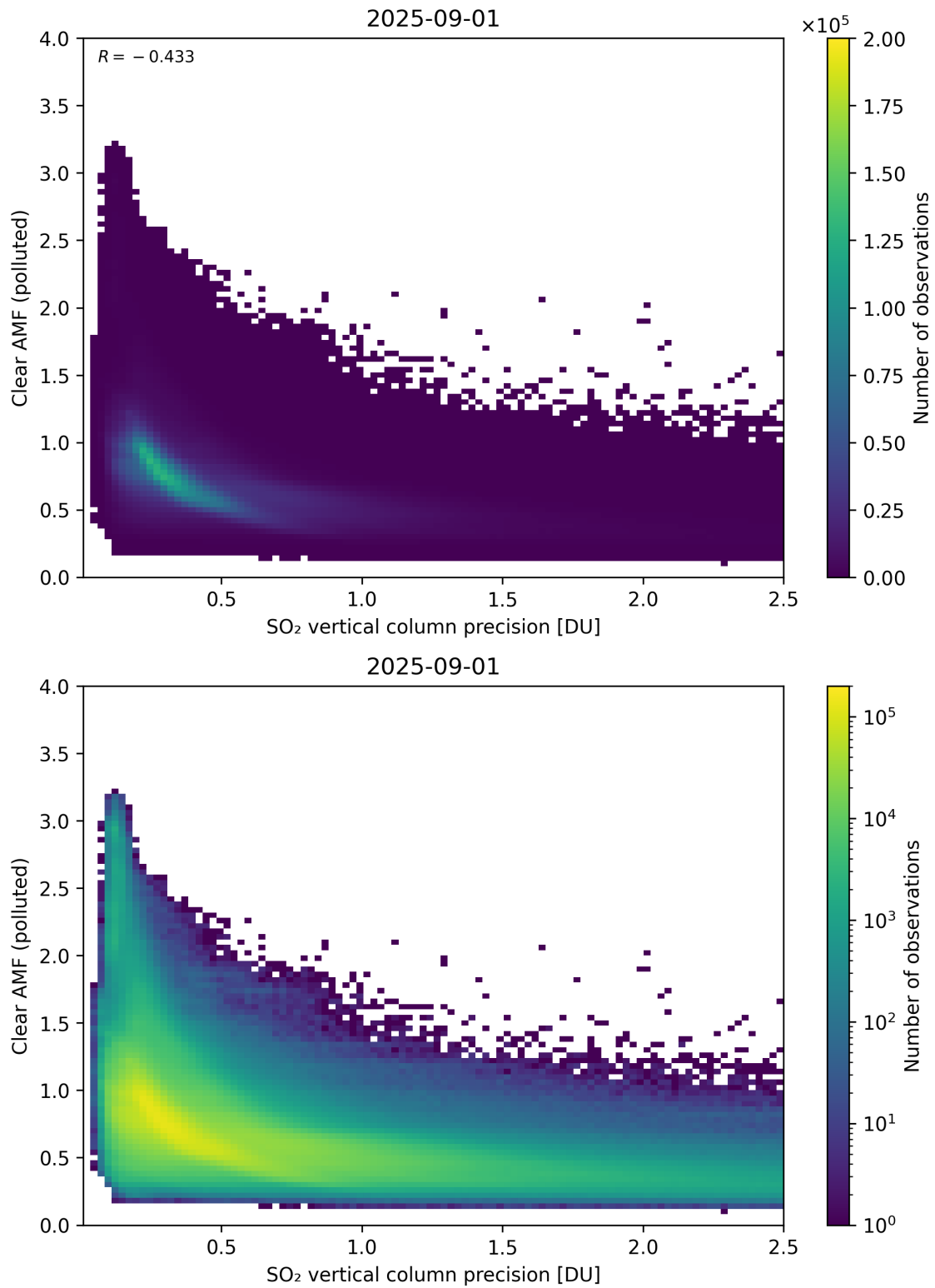
Figure 335: Scatter density plot of “SO 2 vertical column precision” against “Clear AMF (polluted)” for 2025-08-31 to 2025-09-02.
