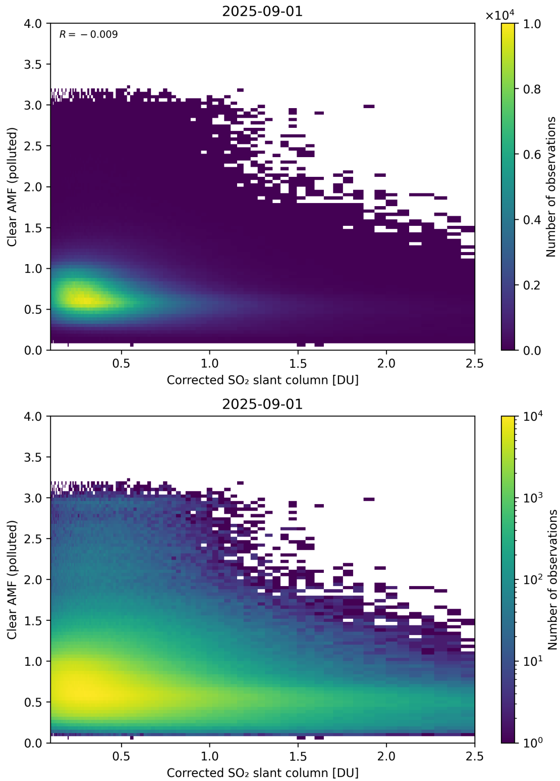
Figure 232: Scatter density plot of “Corrected SO 2 slant column” against “Clear AMF (polluted)” for 2025-08-31 to 2025-09-02.
