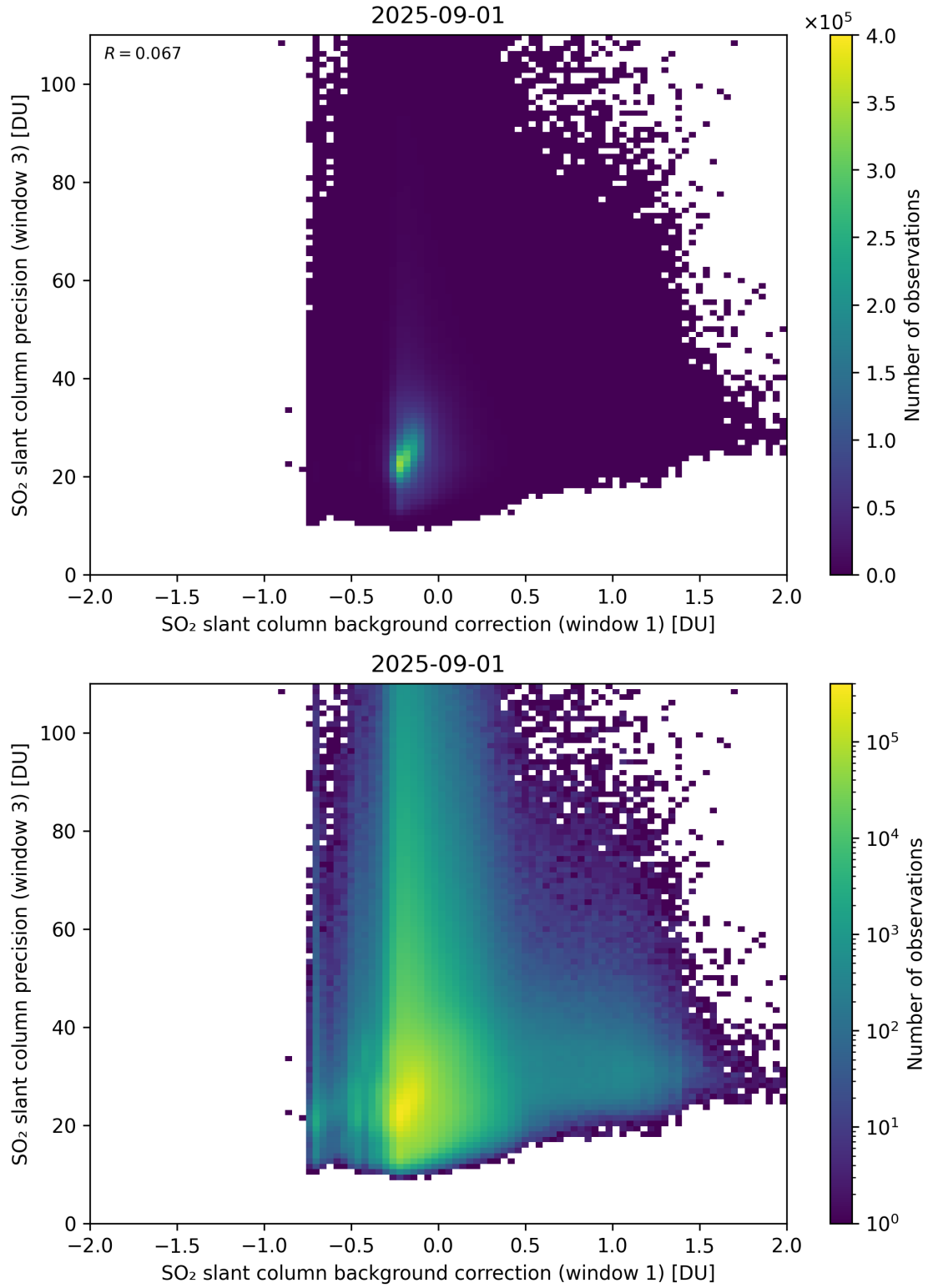
Figure 119: Scatter density plot of “SO 2 slant column background correction (window 1)” against “SO 2 slant column precision (window 3)” for 2025-08-31 to 2025-09-02.
