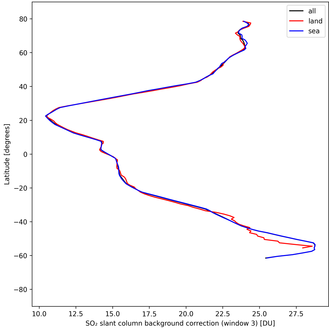
Figure 48: Zonal average of “SO 2 slant column background correction (window 3)” for 2025-08-31 to 2025-09-02.
