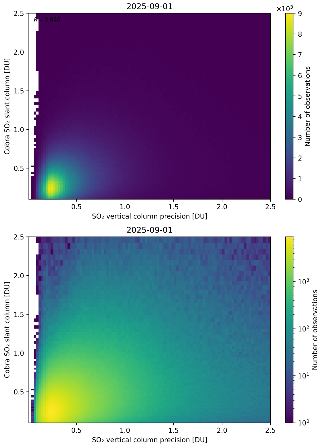
Figure 336: Scatter density plot of “SO 2 vertical column precision” against “Cobra SO 2 slant column” for 2025-08-31 to 2025-09-02.
