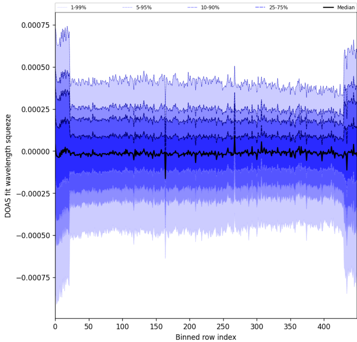
Figure 103: Along track statistics of “DOAS fit wavelength squeeze” for 2025-08-31 to 2025-09-02
