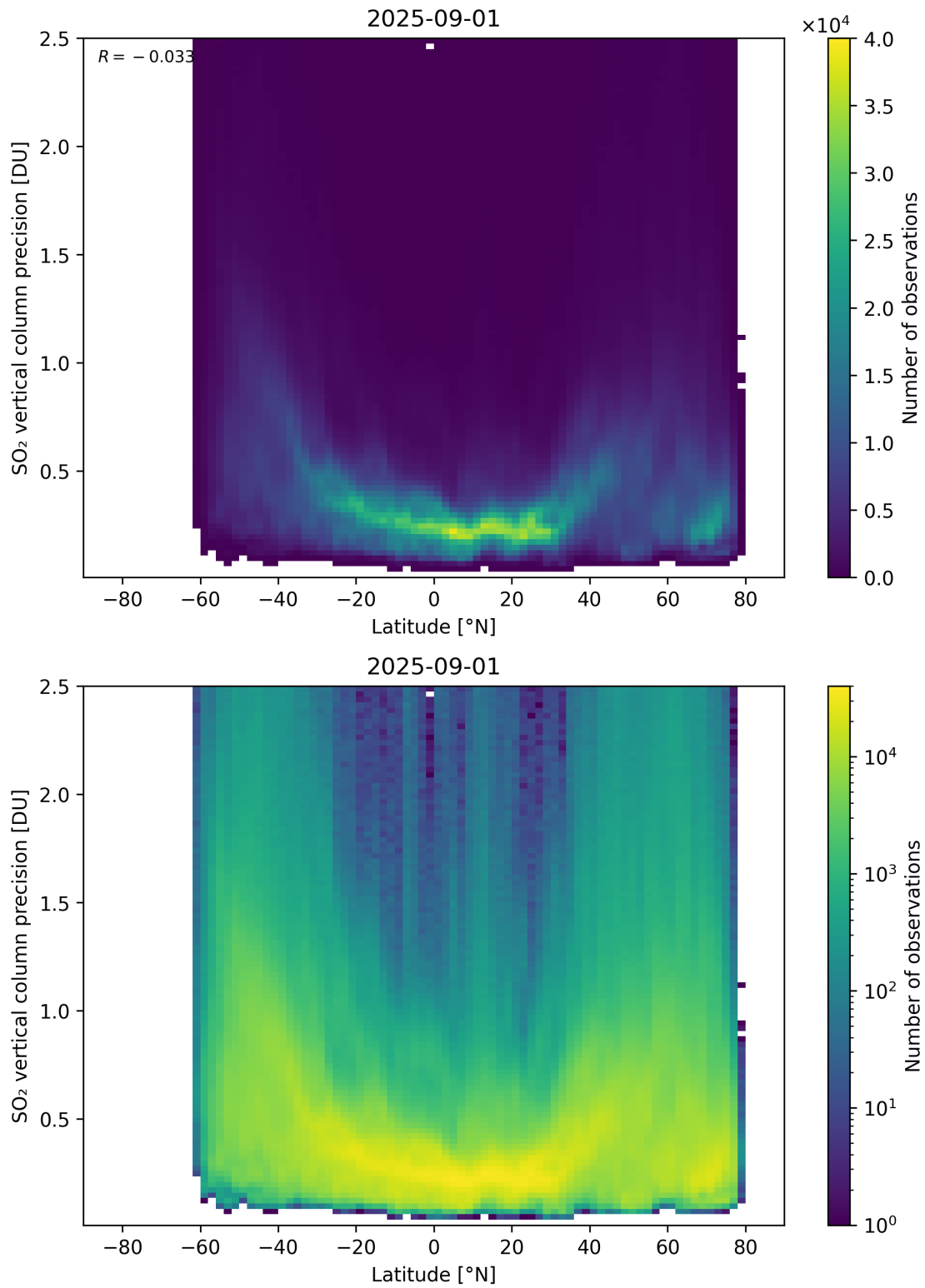
Figure 170: Scatter density plot of “Latitude” against “SO 2 vertical column precision” for 2025-08-31 to 2025-09-02.
