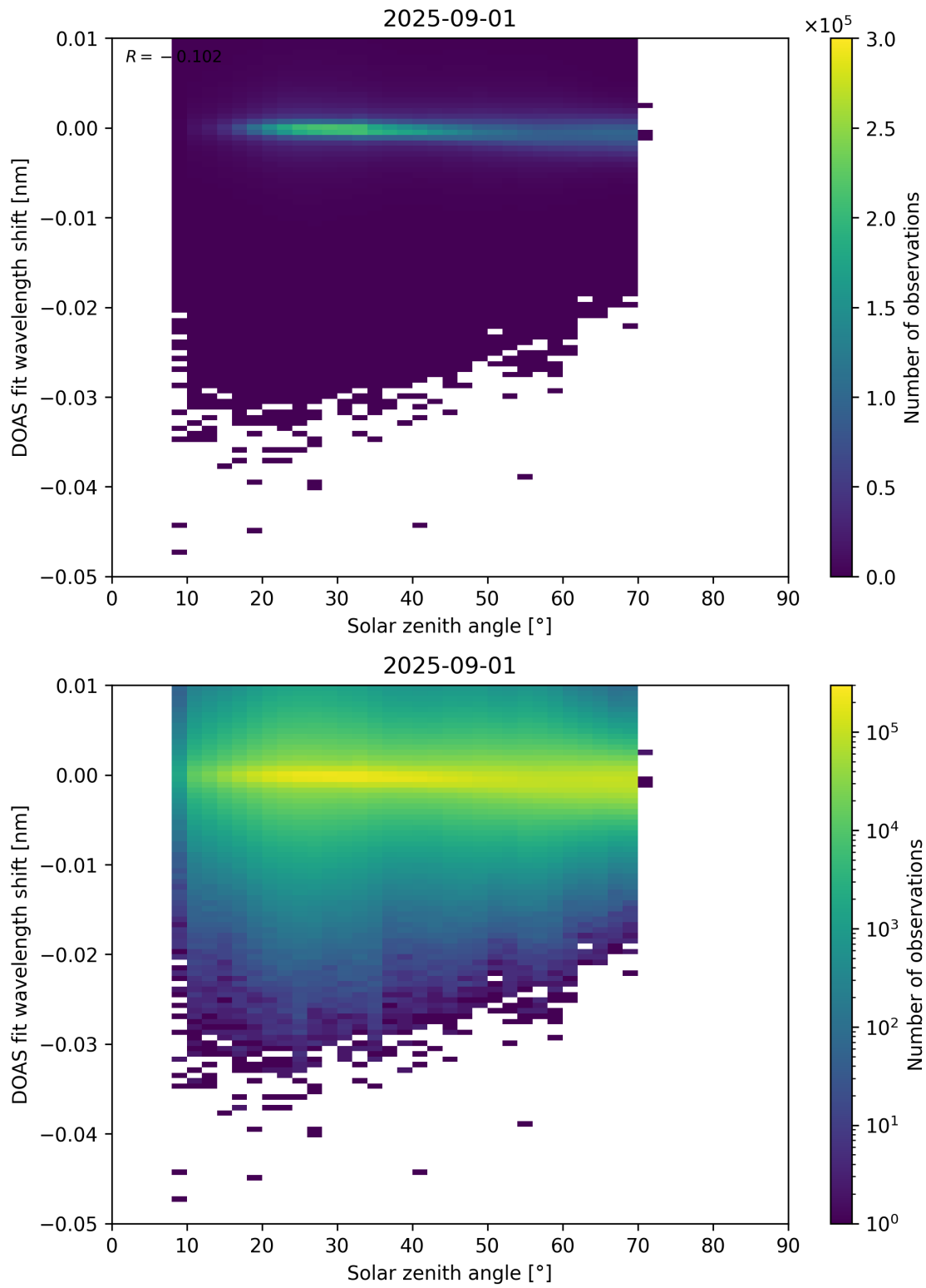
Figure 174: Scatter density plot of “Solar zenith angle” against “DOAS fit wavelength shift” for 2025-08-31 to 2025-09-02.
