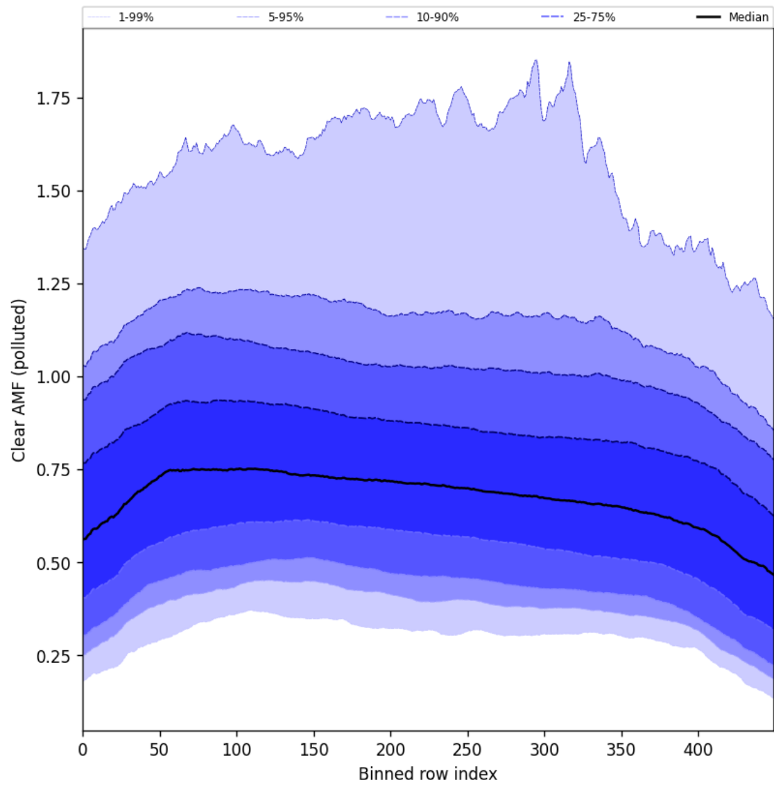
Figure 107: Along track statistics of “Clear AMF (polluted)” for 2025-08-31 to 2025-09-02
