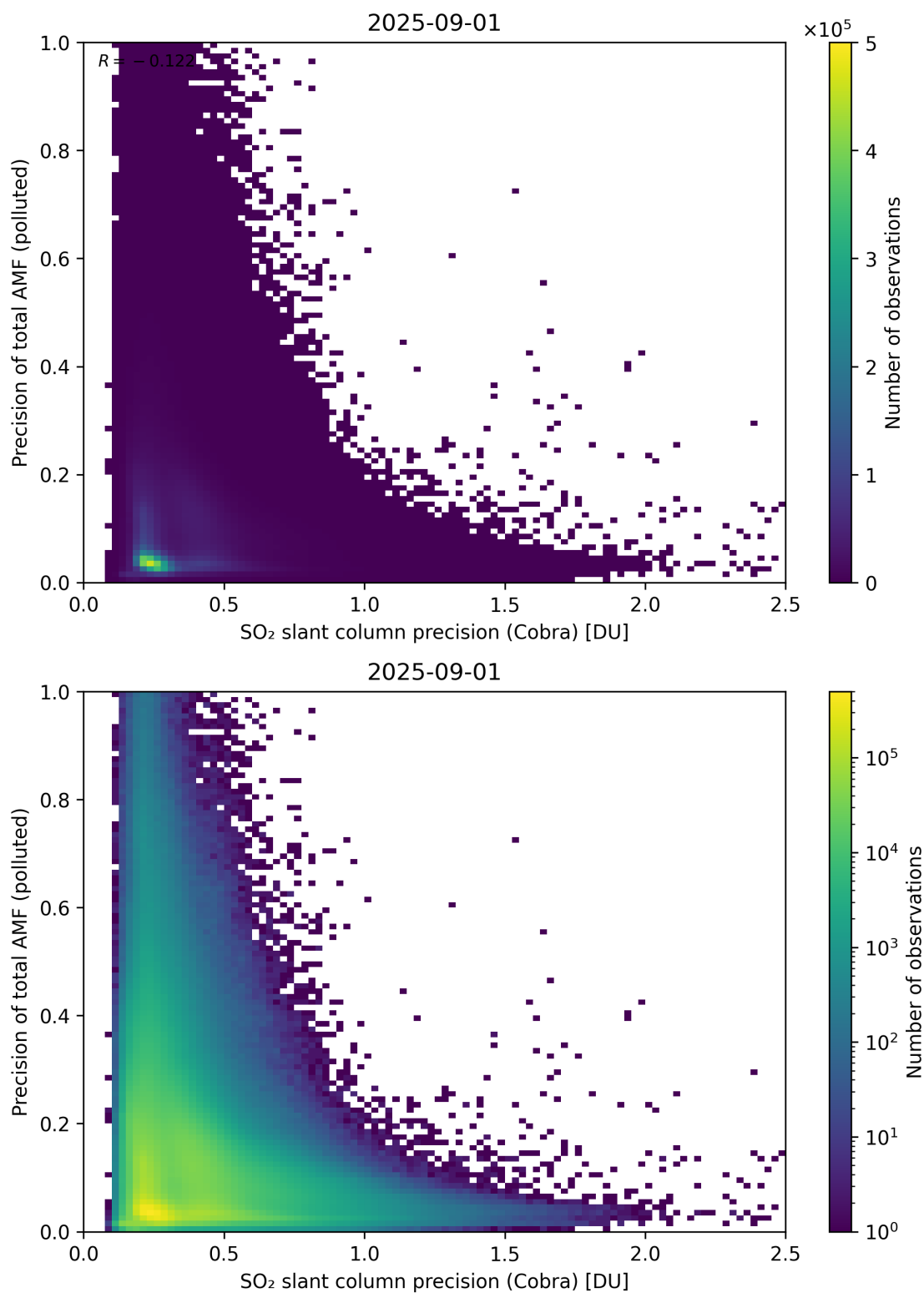
Figure 214: Scatter density plot of “SO 2 slant column precision (Cobra)” against “Precision of total AMF (polluted)” for 2025-08-31 to 2025-09-02.
