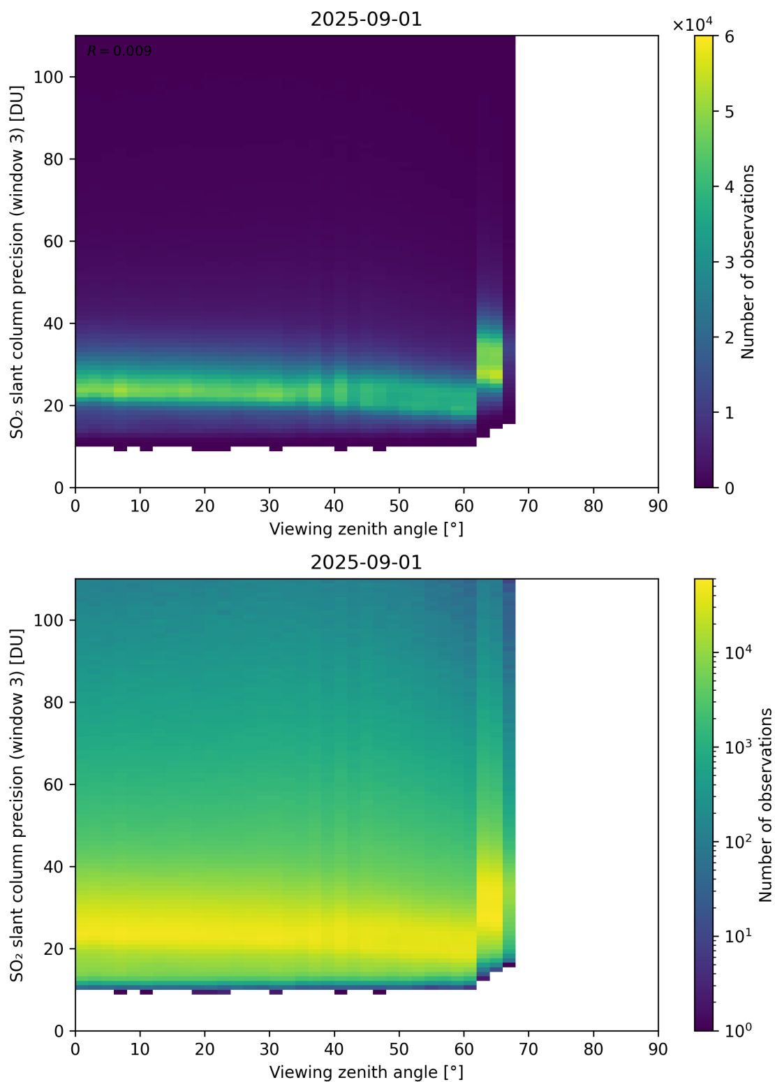
Figure 380: Scatter density plot of “Viewing zenith angle” against “SO 2 slant column precision (window 3)” for 2025-08-31 to 2025-09-02.
