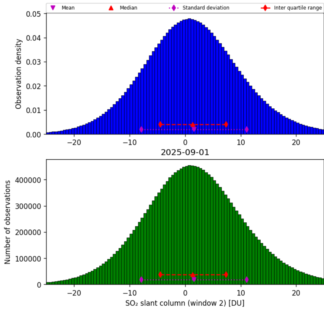
Figure 67: Histogram of “SO 2 slant column (window 2)” for 2025-08-31 to 2025-09-02
