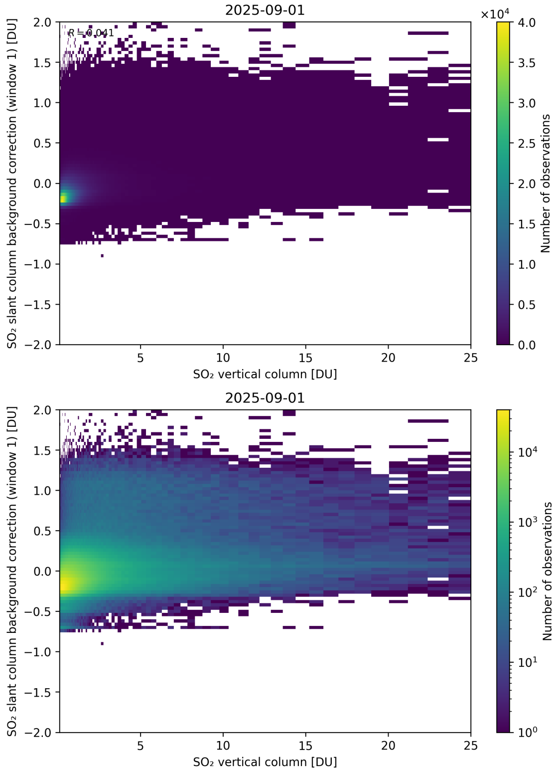
Figure 323: Scatter density plot of “SO 2 vertical column” against “SO 2 slant column background correction (window 1)” for 2025-08-31 to 2025-09-02.
