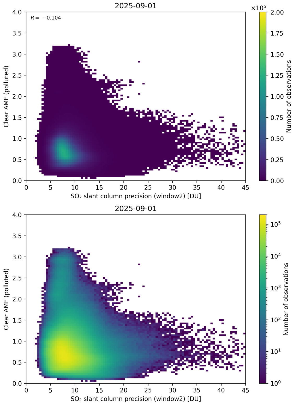
Figure 296: Scatter density plot of “SO 2 slant column precision (window2)” against “Clear AMF (polluted)” for 2025-08-31 to 2025-09-02.
