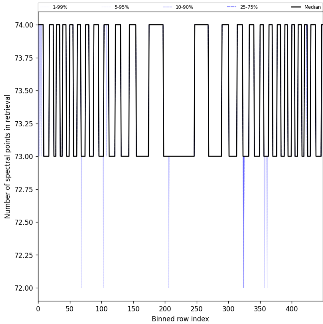
Figure 108: Along track statistics of “Number of spectral points in retrieval” for 2025-08-31 to 2025-09-02
