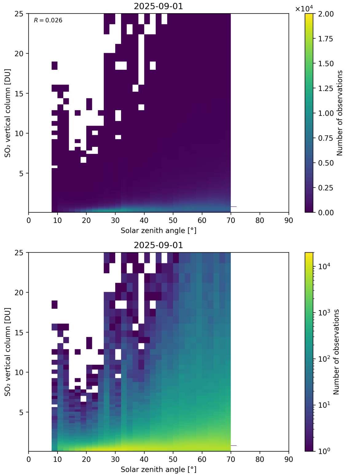
Figure 191: Scatter density plot of “Solar zenith angle” against “SO 2 vertical column” for 2025-08-31 to 2025-09-02.
