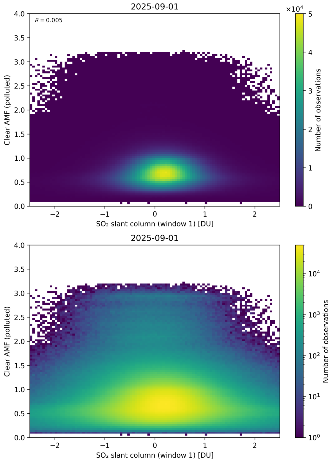
Figure 282: Scatter density plot of “SO 2 slant column (window 1)” against “Clear AMF (polluted)” for 2025-08-31 to 2025-09-02.
