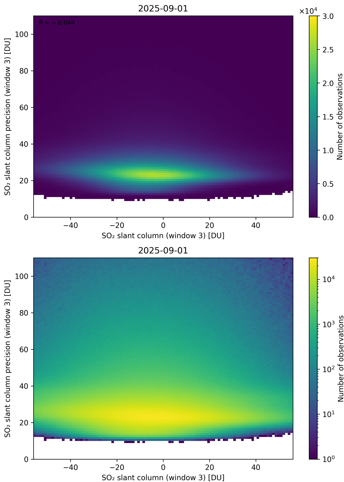
Figure 317: Scatter density plot of “SO 2 slant column (window 3)” against “SO 2 slant column precision (window 3)” for 2025-08-31 to 2025-09-02.
