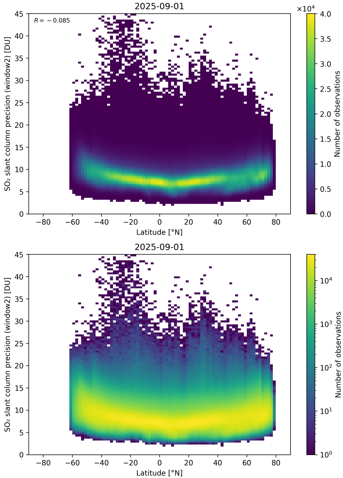
Figure 164: Scatter density plot of “Latitude” against “SO 2 slant column precision (window2)” for 2025-08-31 to 2025-09-02.
