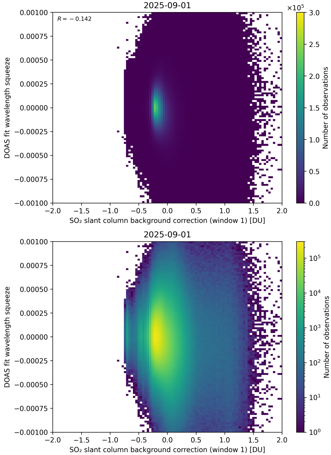
Figure 112: Scatter density plot of “SO 2 slant column background correction (window 1)” against “DOAS fit wavelength squeeze” for 2025-08-31 to 2025-09-02.
