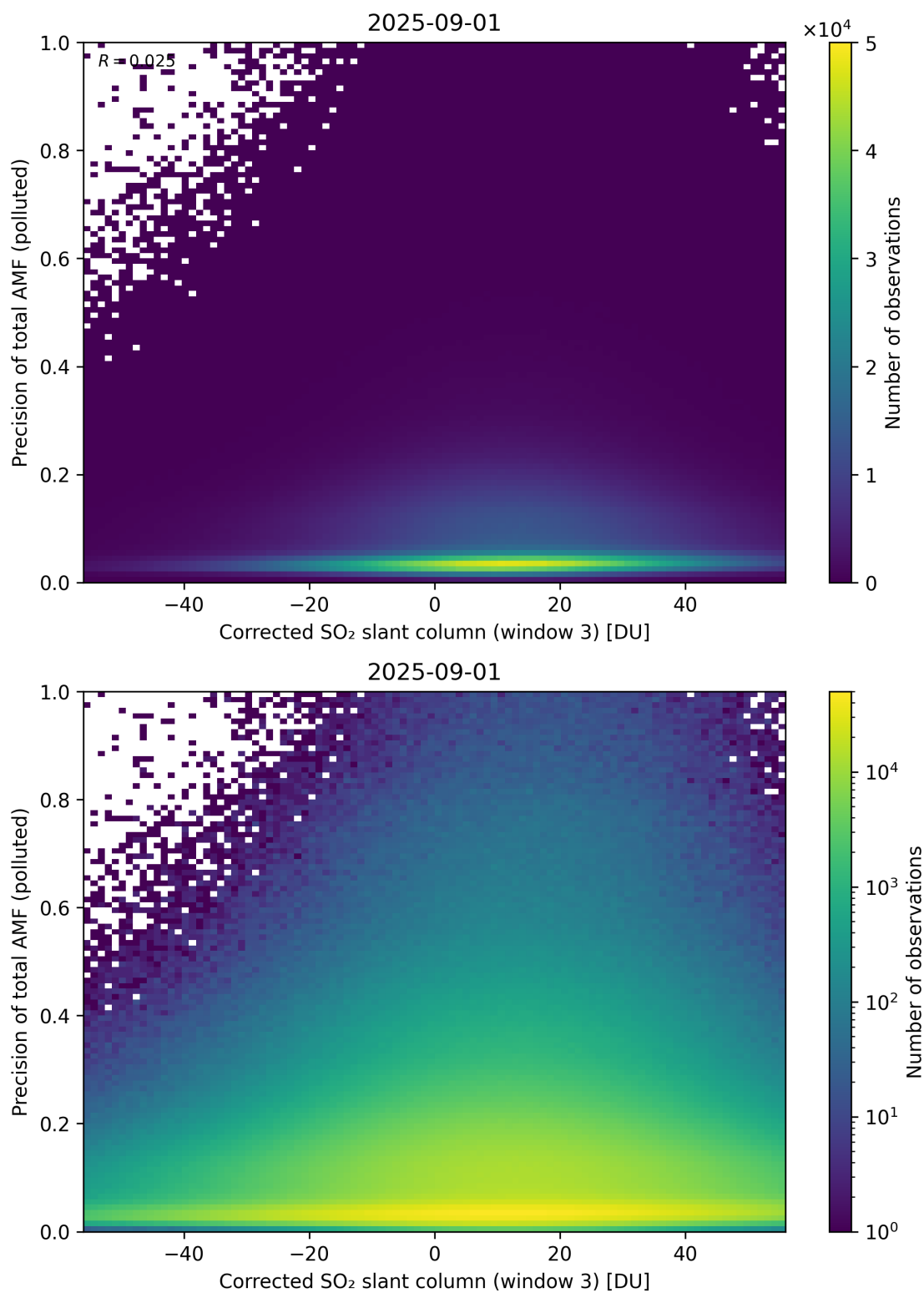
Figure 261: Scatter density plot of “Corrected SO 2 slant column (window 3)” against “Precision of total AMF (polluted)” for 2025-08-31 to 2025-09-02.
