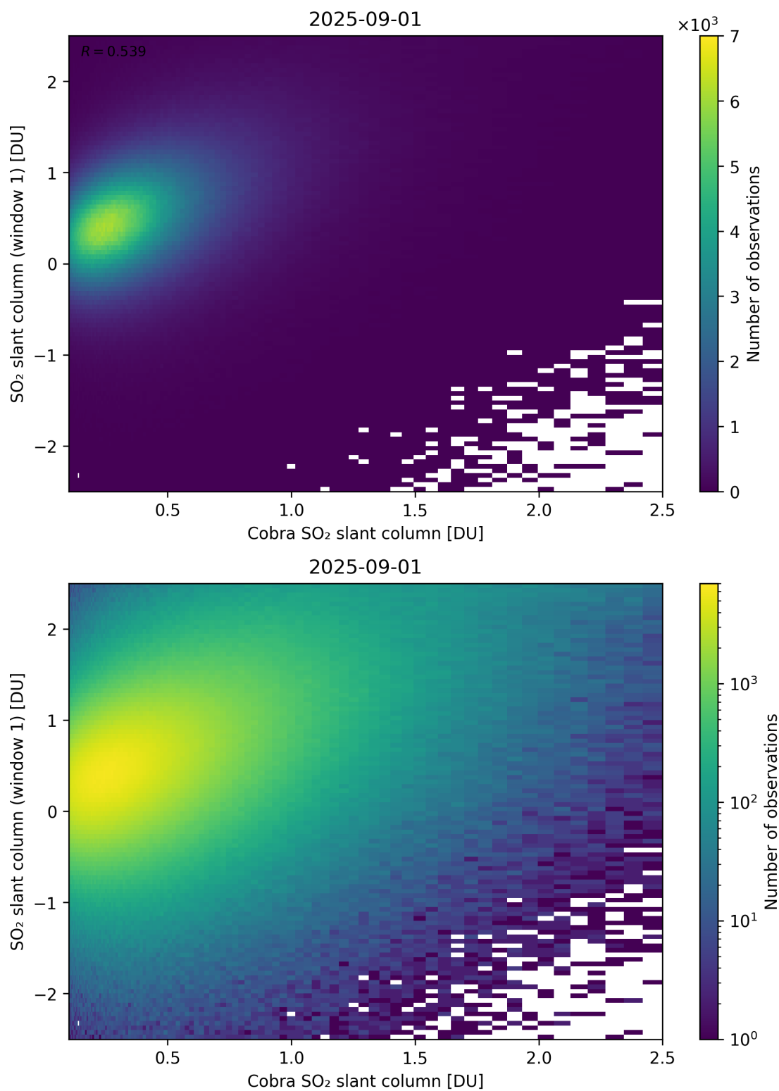
Figure 219: Scatter density plot of “Cobra SO 2 slant column” against “SO 2 slant column (window 1)” for 2025-08-31 to 2025-09-02.
