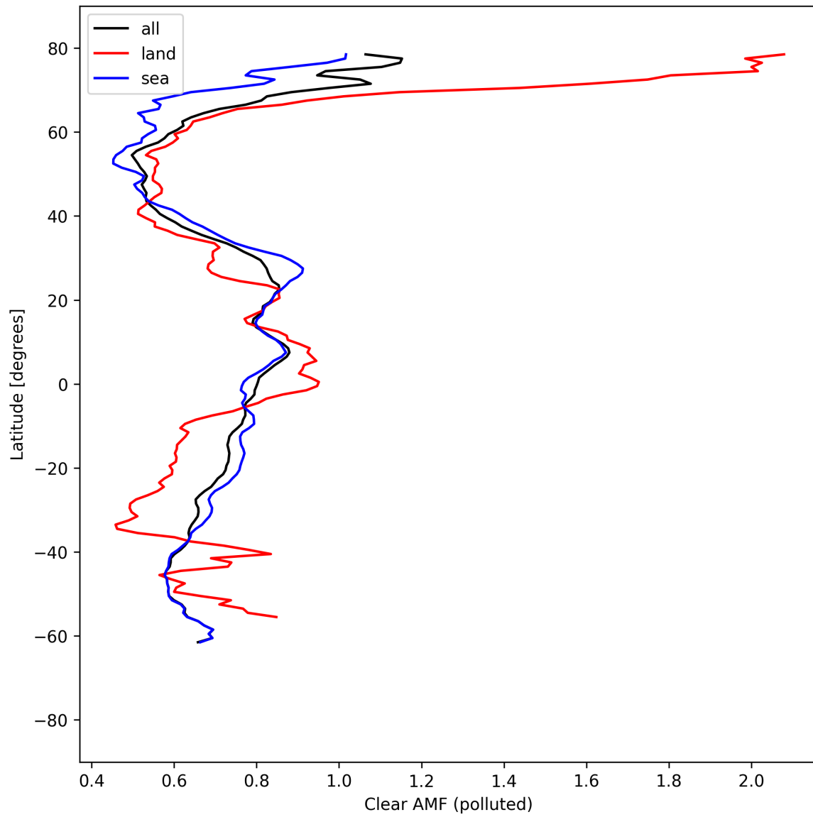
Figure 55: Zonal average of “Clear AMF (polluted)” for 2025-08-31 to 2025-09-02.
