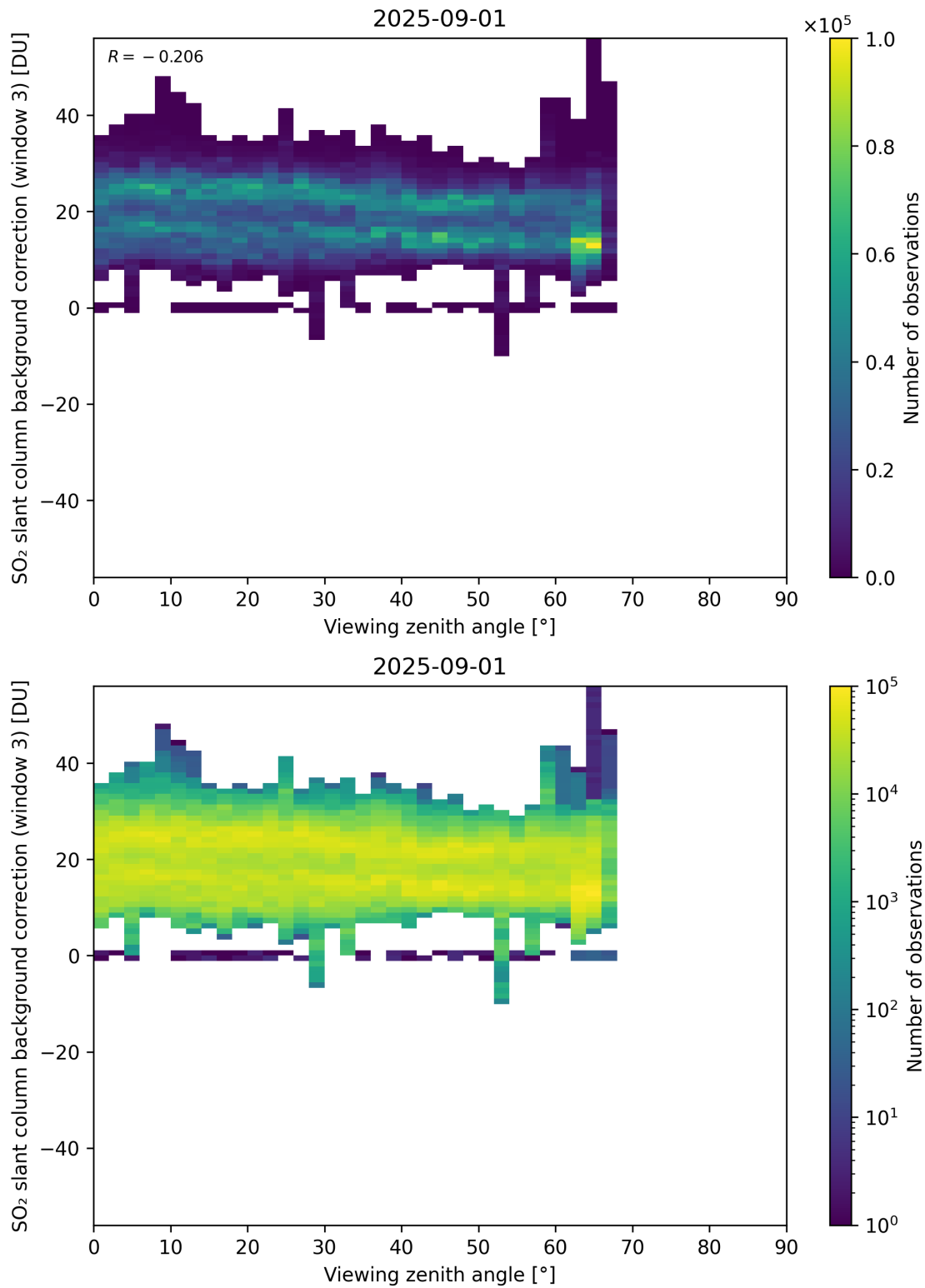
Figure 364: Scatter density plot of “Viewing zenith angle” against “SO 2 slant column background correction (window 3)” for 2025-08-31 to 2025-09-02.
