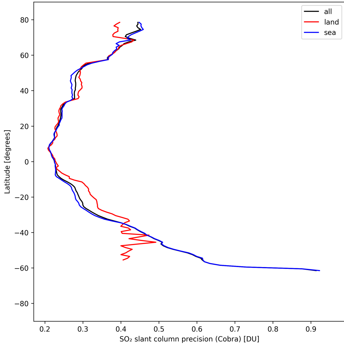
Figure 36: Zonal average of “SO 2 slant column precision (Cobra)” for 2025-08-31 to 2025-09-02.
