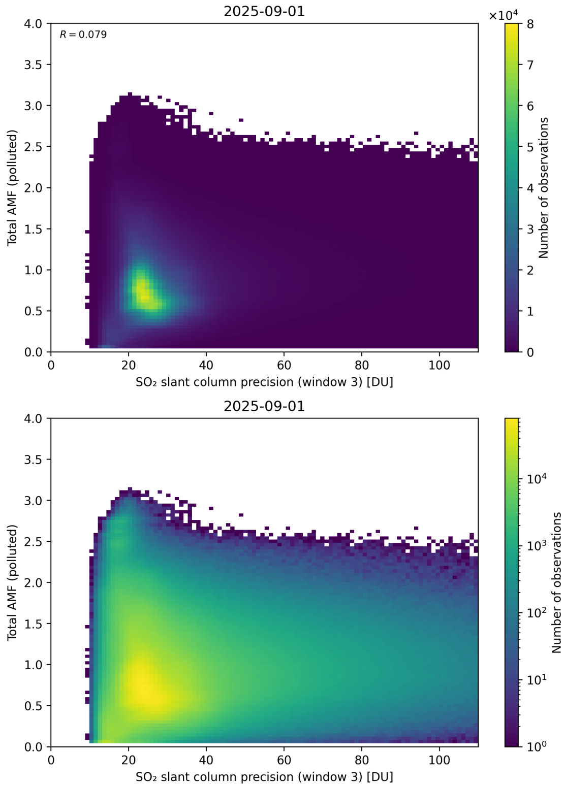
Figure 313: Scatter density plot of “SO 2 slant column precision (window 3)” against “Total AMF (polluted)” for 2025-08-31 to 2025-09-02.
