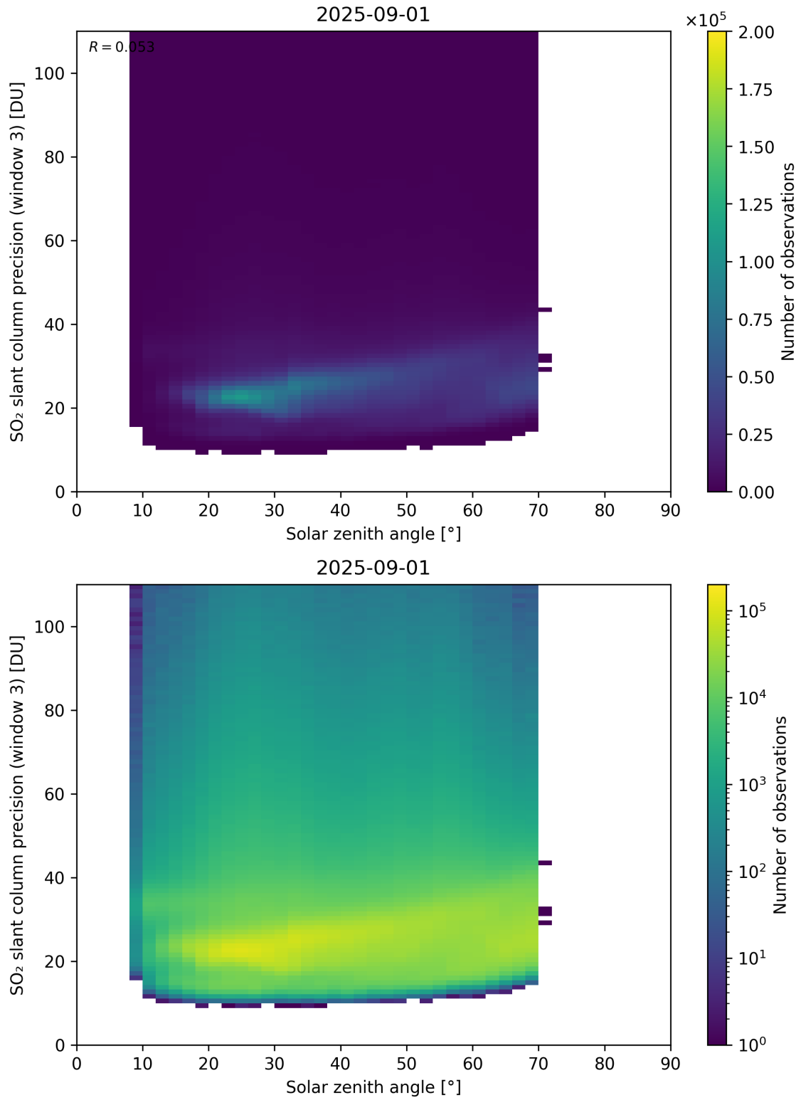
Figure 188: Scatter density plot of “Solar zenith angle” against “SO 2 slant column precision (window 3)” for 2025-08-31 to 2025-09-02.
