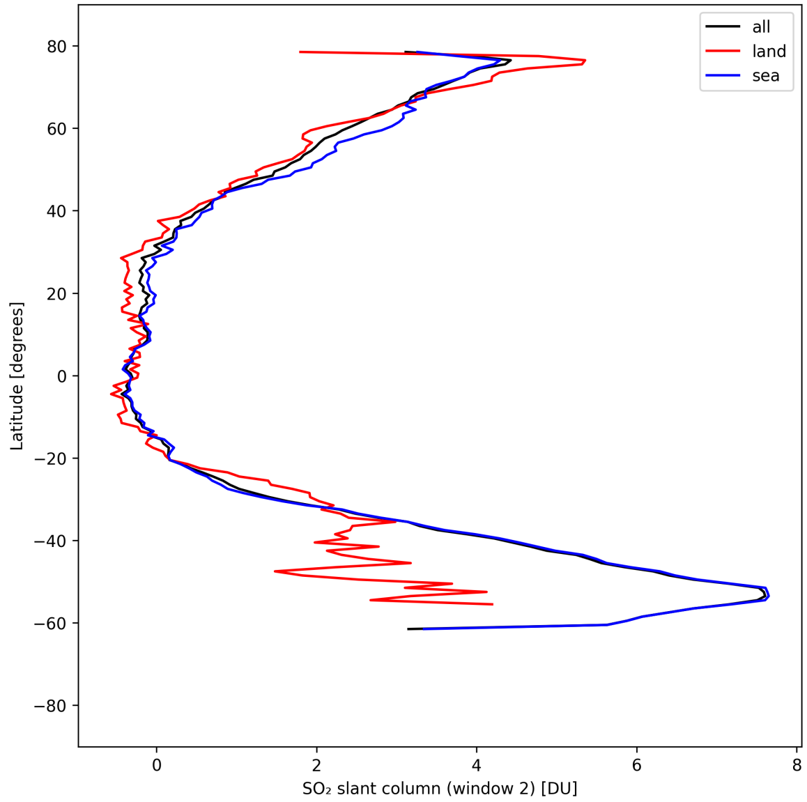
Figure 41: Zonal average of “SO 2 slant column (window 2)” for 2025-08-31 to 2025-09-02.
