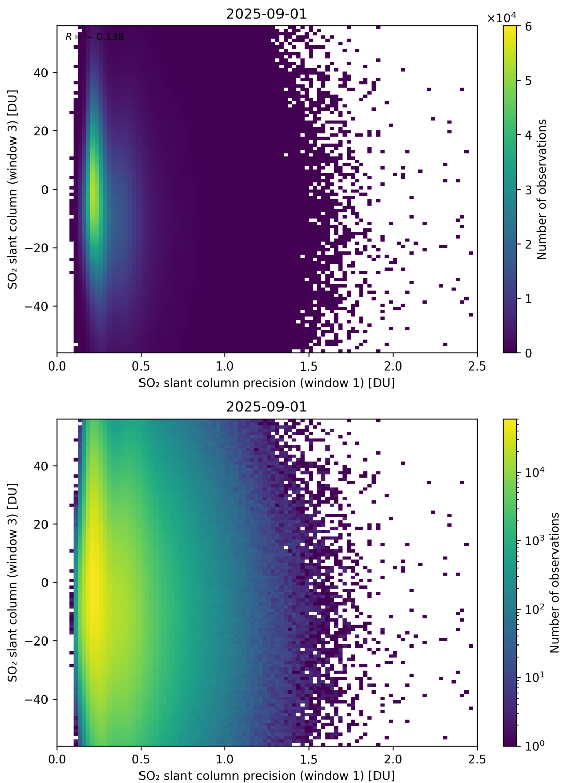
Figure 278: Scatter density plot of “SO 2 slant column precision (window 1)” against “SO 2 slant column (window 3)” for 2025-08-31 to 2025-09-02.
