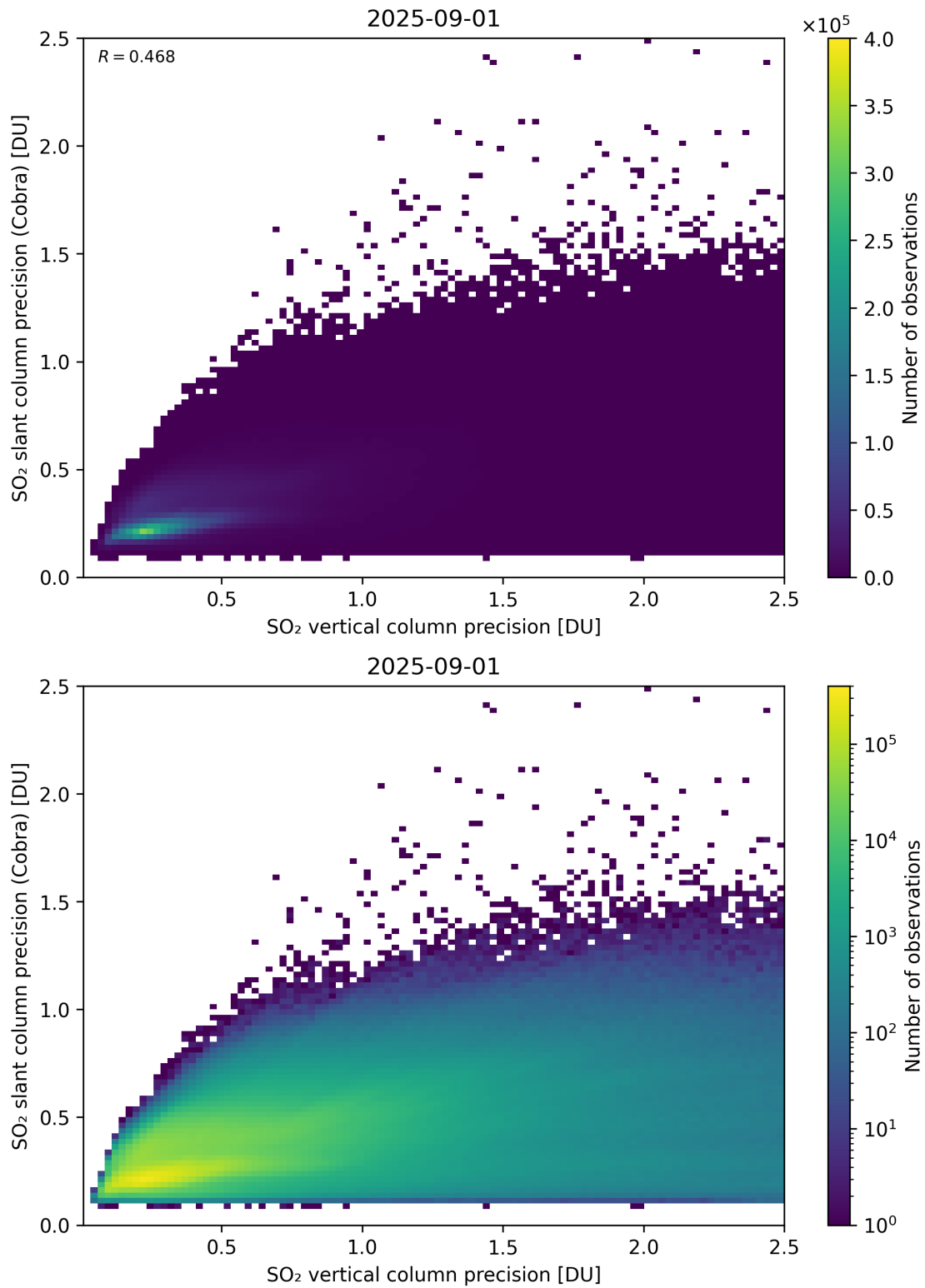
Figure 337: Scatter density plot of “SO 2 vertical column precision” against “SO 2 slant column precision (Cobra)” for 2025-08-31 to 2025-09-02.
