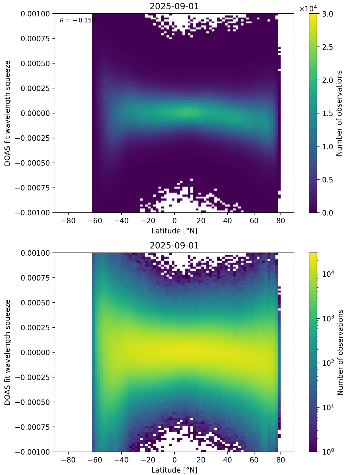
Figure 154: Scatter density plot of “Latitude” against “DOAS fit wavelength squeeze” for 2025-08-31 to 2025-09-02.
