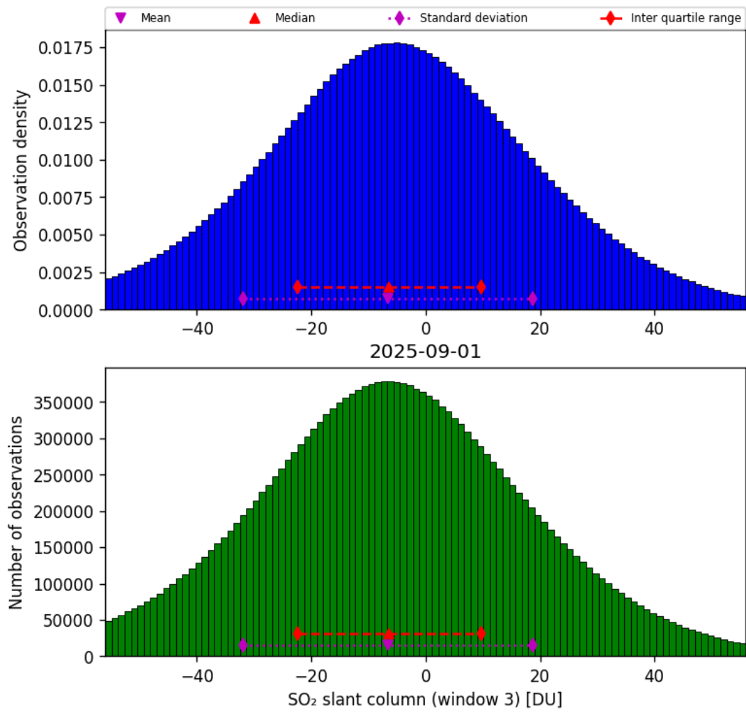
Figure 71: Histogram of “SO 2 slant column (window 3)” for 2025-08-31 to 2025-09-02
