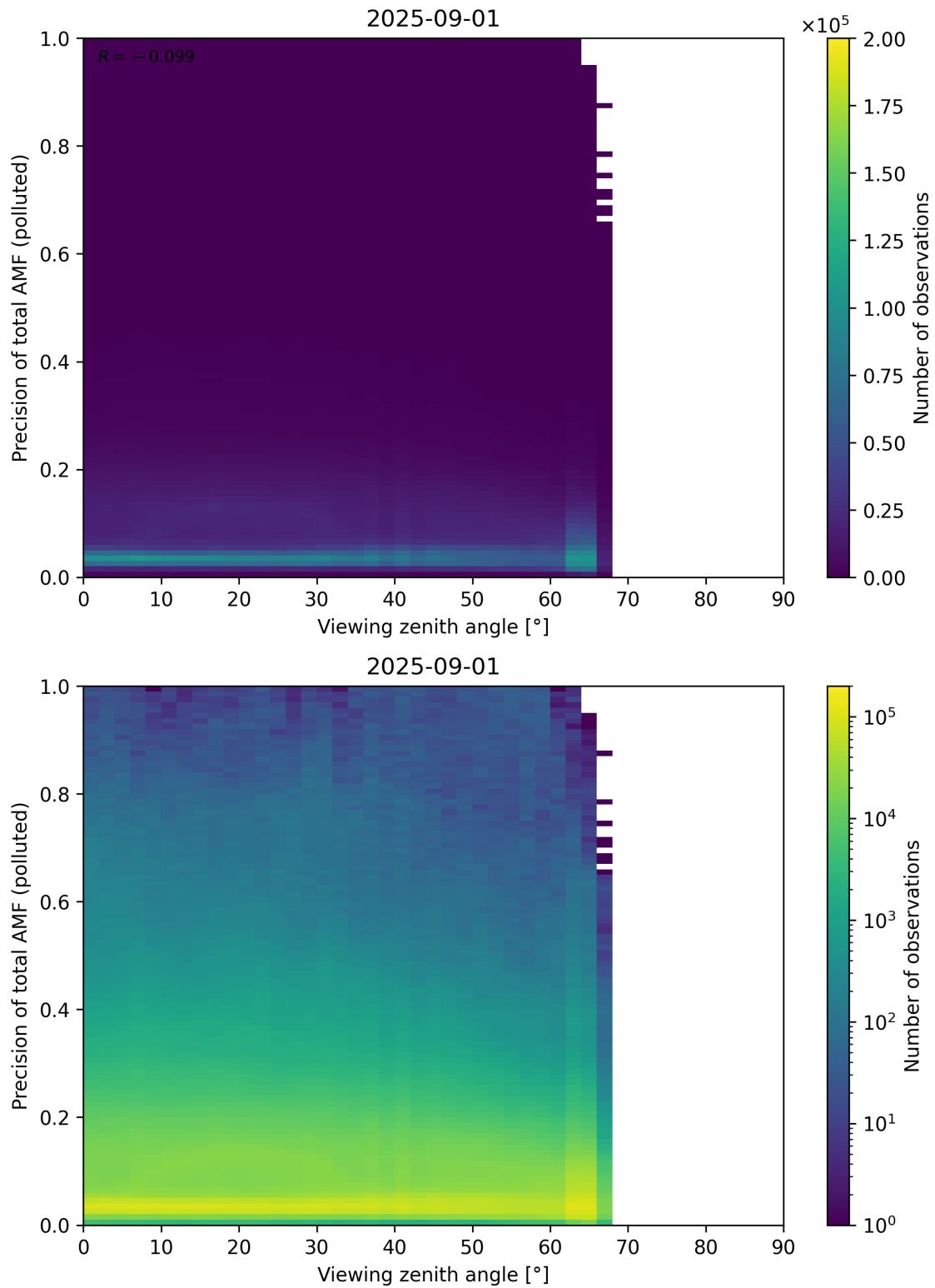
Figure 382: Scatter density plot of “Viewing zenith angle” against “Precision of total AMF (polluted)” for 2025-08-31 to 2025-09-02.
