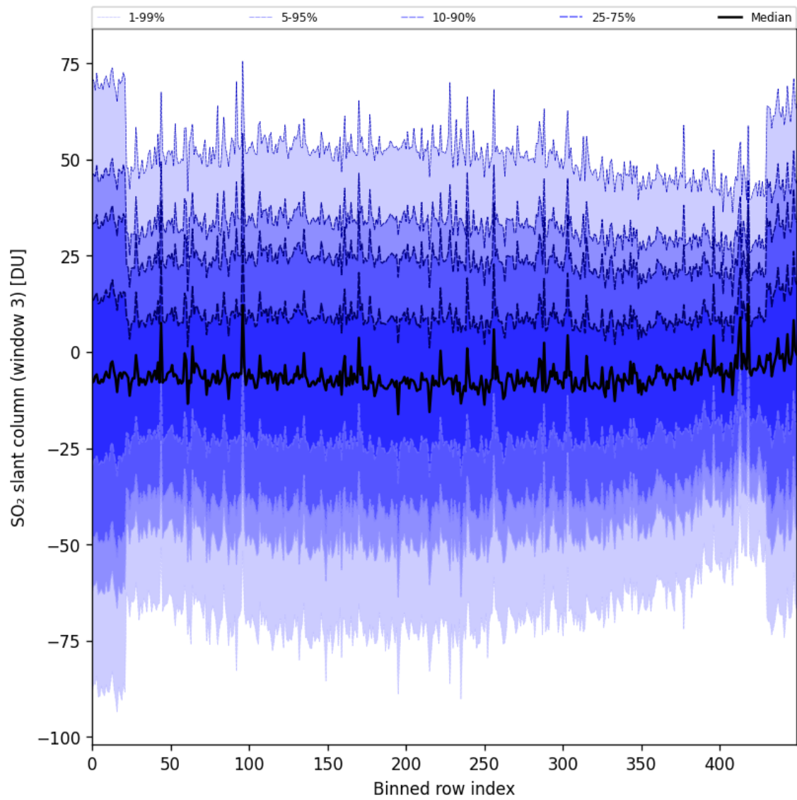
Figure 97: Along track statistics of “SO 2 slant column (window 3)” for 2025-08-31 to 2025-09-02
