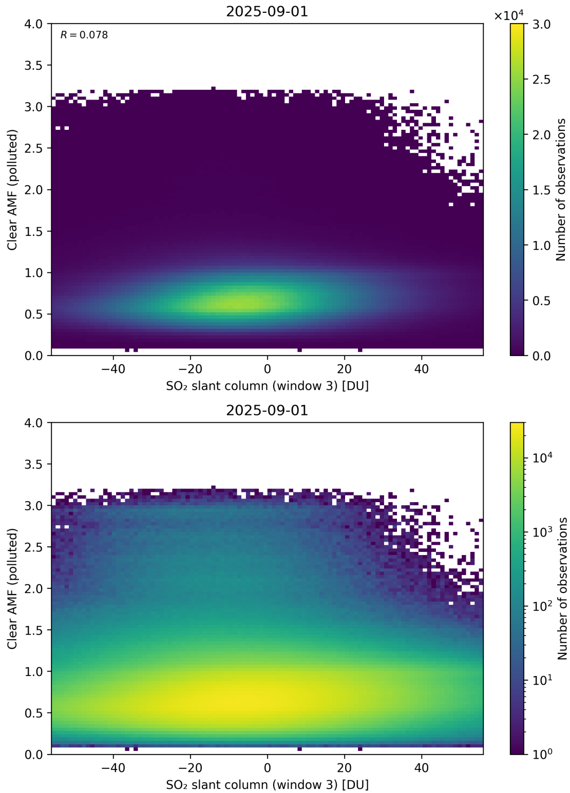
Figure 315: Scatter density plot of “SO 2 slant column (window 3)” against “Clear AMF (polluted)” for 2025-08-31 to 2025-09-02.
