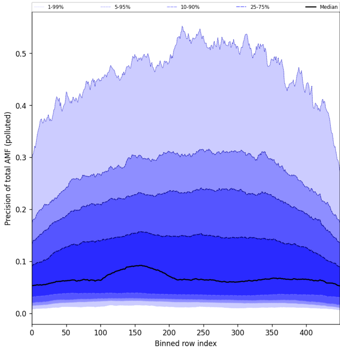
Figure 106: Along track statistics of “Precision of total AMF (polluted)” for 2025-08-31 to 2025-09-02
