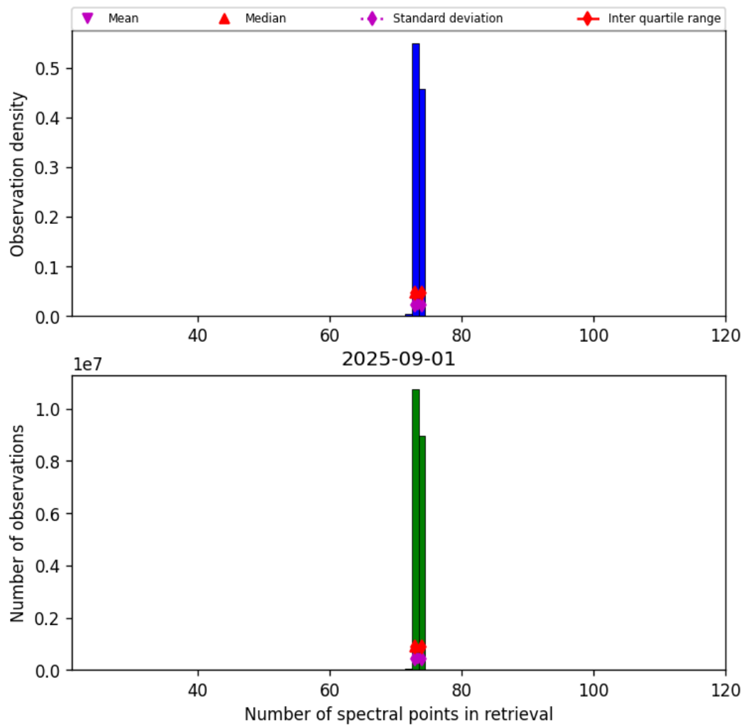
Figure 82: Histogram of “Number of spectral points in retrieval” for 2025-08-31 to 2025-09-02
