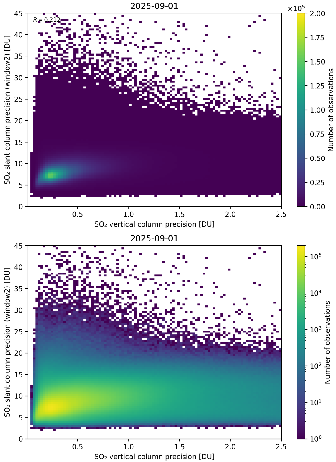
Figure 343: Scatter density plot of “SO 2 vertical column precision” against “SO 2 slant column precision (window2)” for 2025-08-31 to 2025-09-02.
