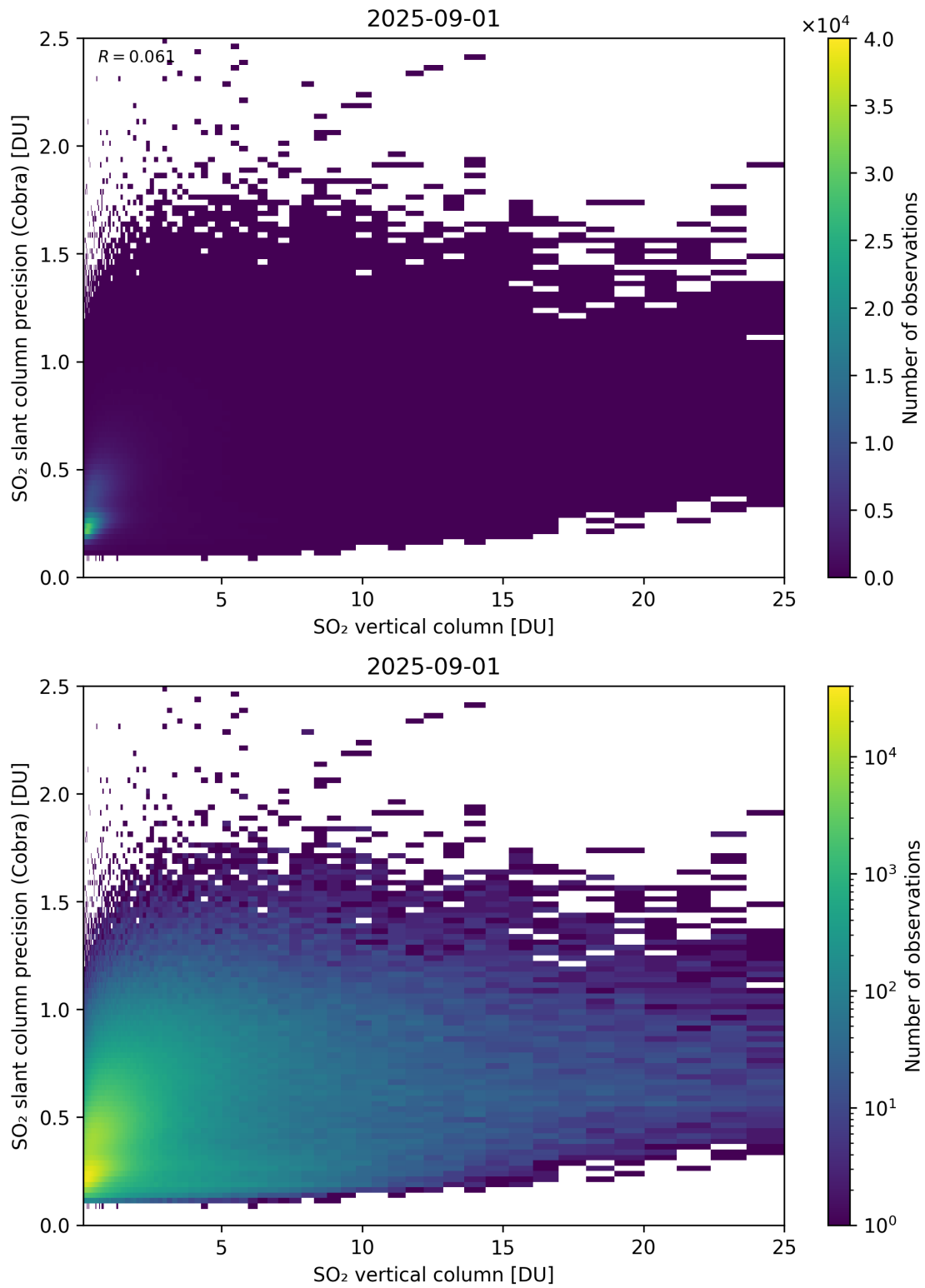
Figure 350: Scatter density plot of “SO 2 vertical column” against “SO 2 slant column precision (Cobra)” for 2025-08-31 to 2025-09-02.
