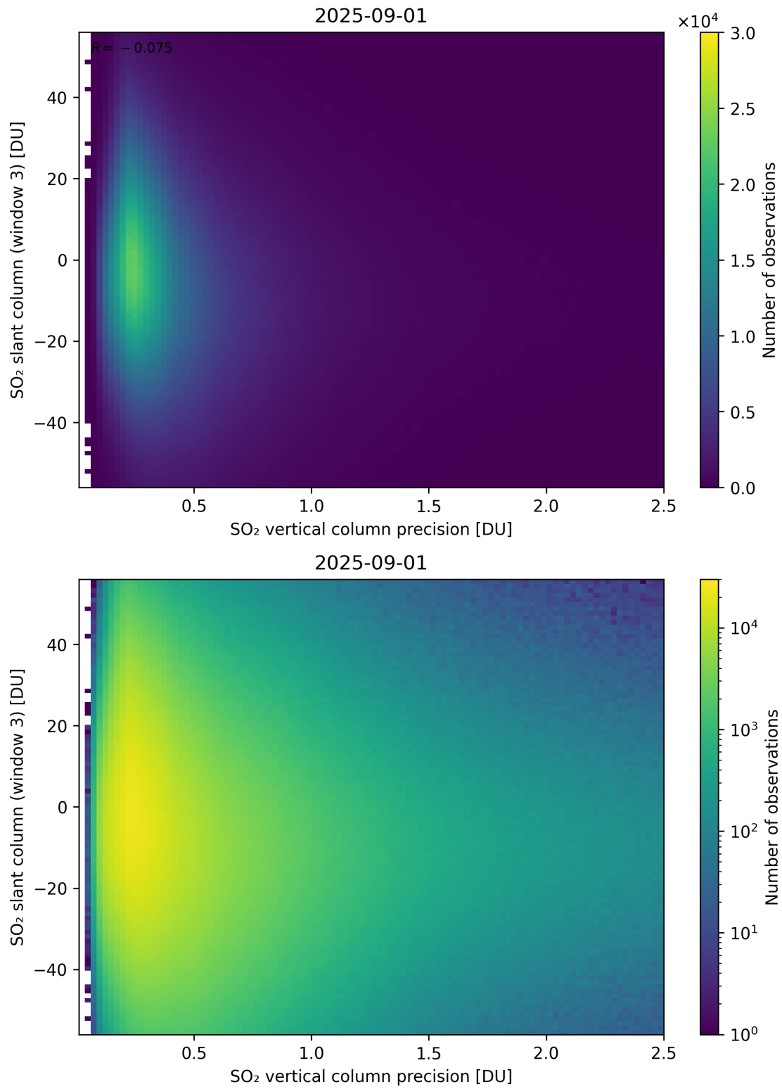
Figure 344: Scatter density plot of “SO 2 vertical column precision” against “SO 2 slant column (window 3)” for 2025-08-31 to 2025-09-02.
