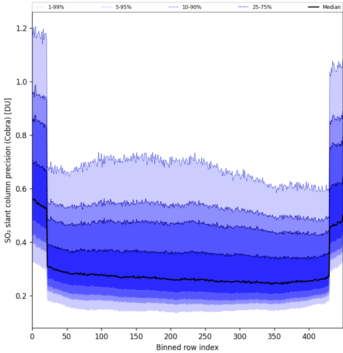
Figure 88: Along track statistics of “SO 2 slant column precision (Cobra)” for 2025-08-31 to 2025-09-02
