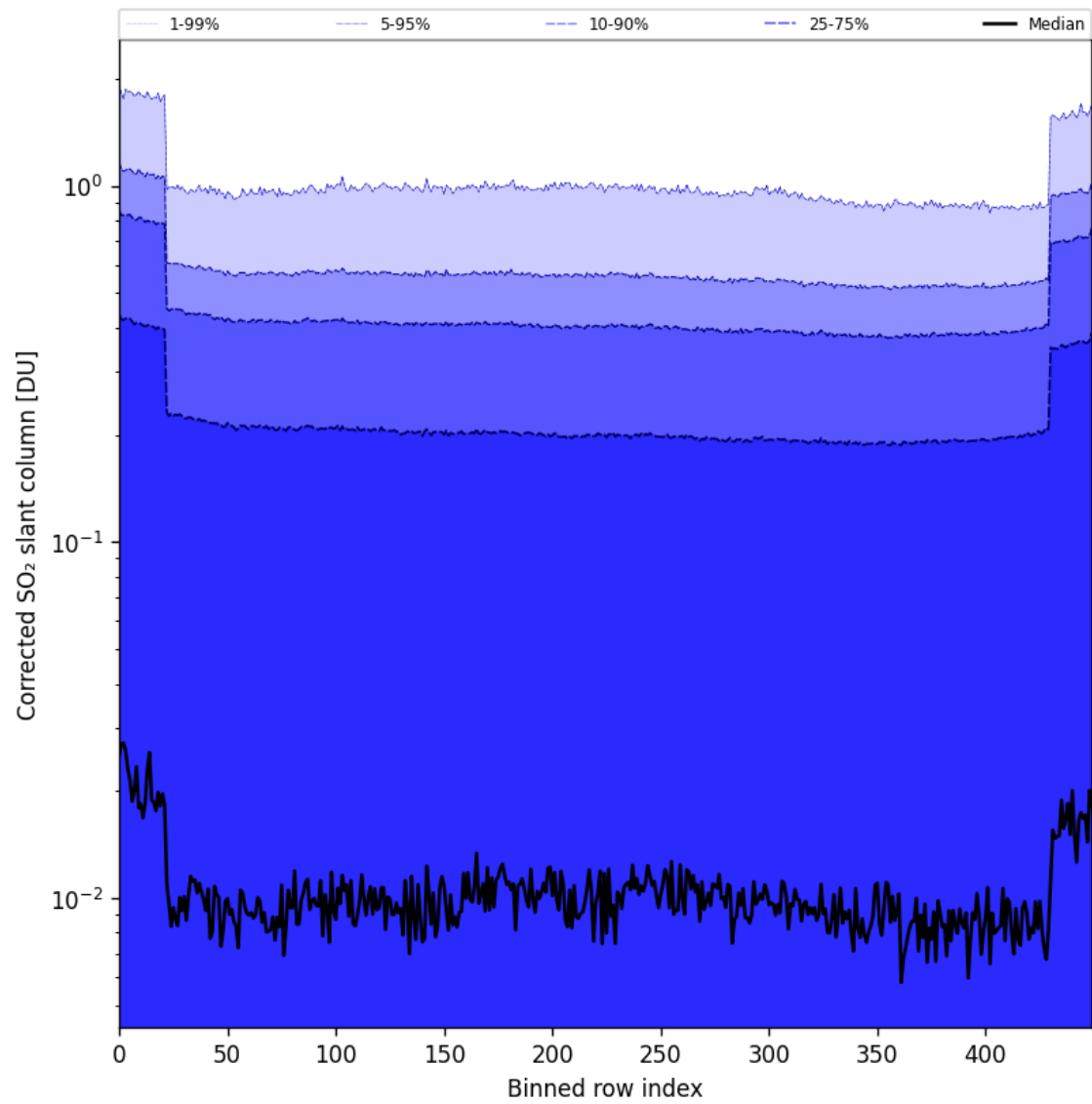
Figure 86: Along track statistics of “Corrected SO 2 slant column” for 2025-08-31 to 2025-09-02
