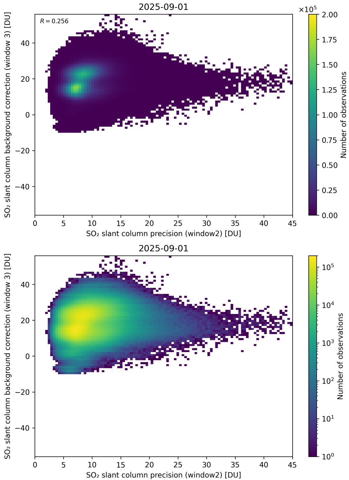
Figure 292: Scatter density plot of “SO 2 slant column precision (window2)” against “SO 2 slant column background correction (window 3)” for 2025-08-31 to 2025-09-02.
