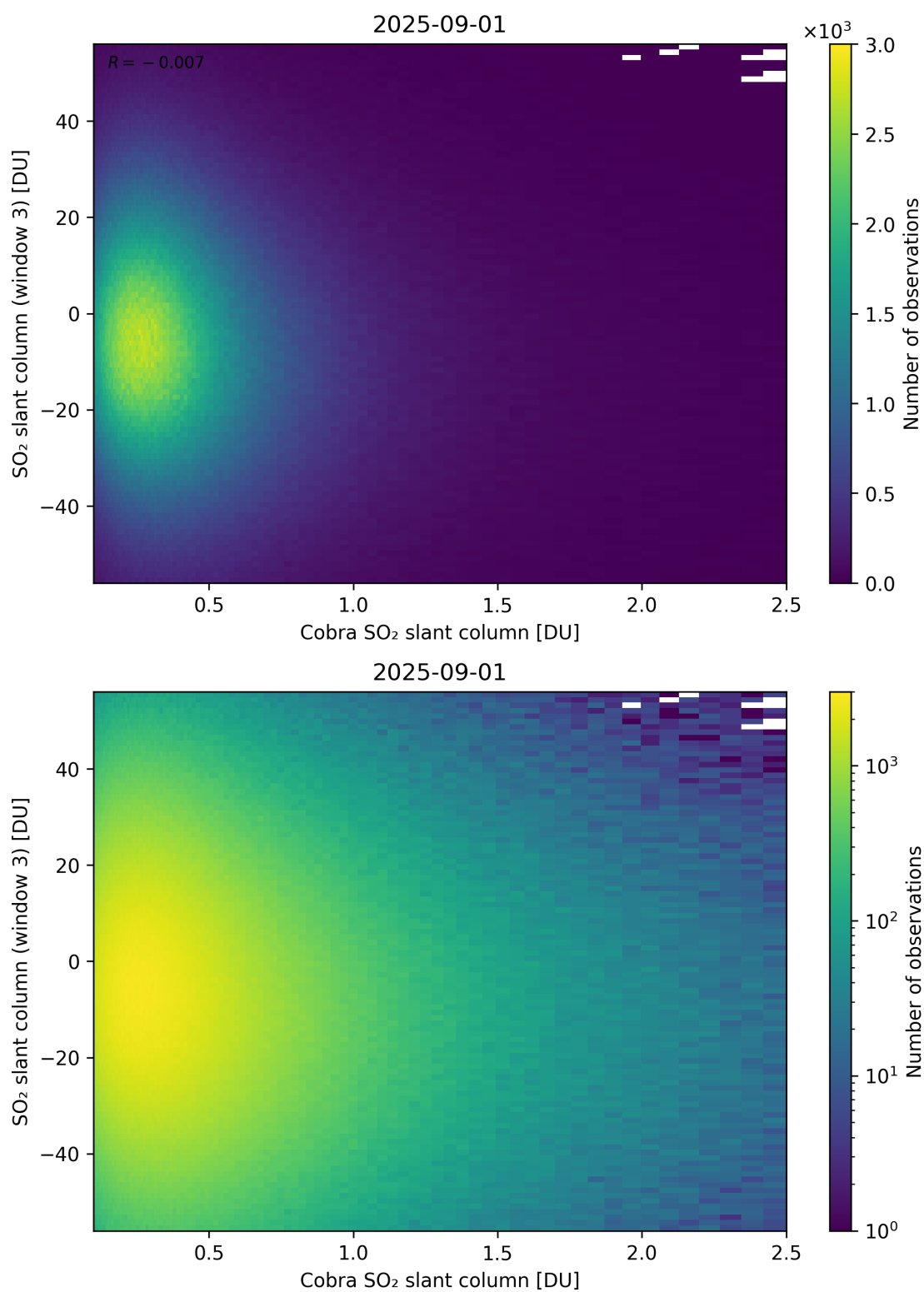
Figure 222: Scatter density plot of “Cobra SO 2 slant column” against “SO 2 slant column (window 3)” for 2025-08-31 to 2025-09-02.
