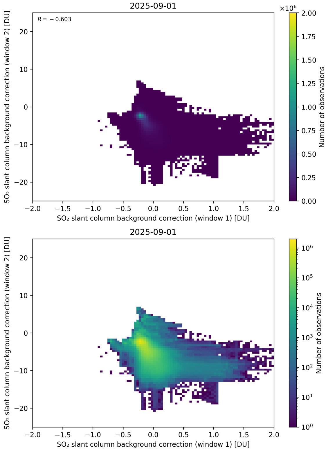
Figure 109: Scatter density plot of “SO 2 slant column background correction (window 1)” against “SO 2 slant column background correction (window 2)” for 2025-08-31 to 2025-09-02.
