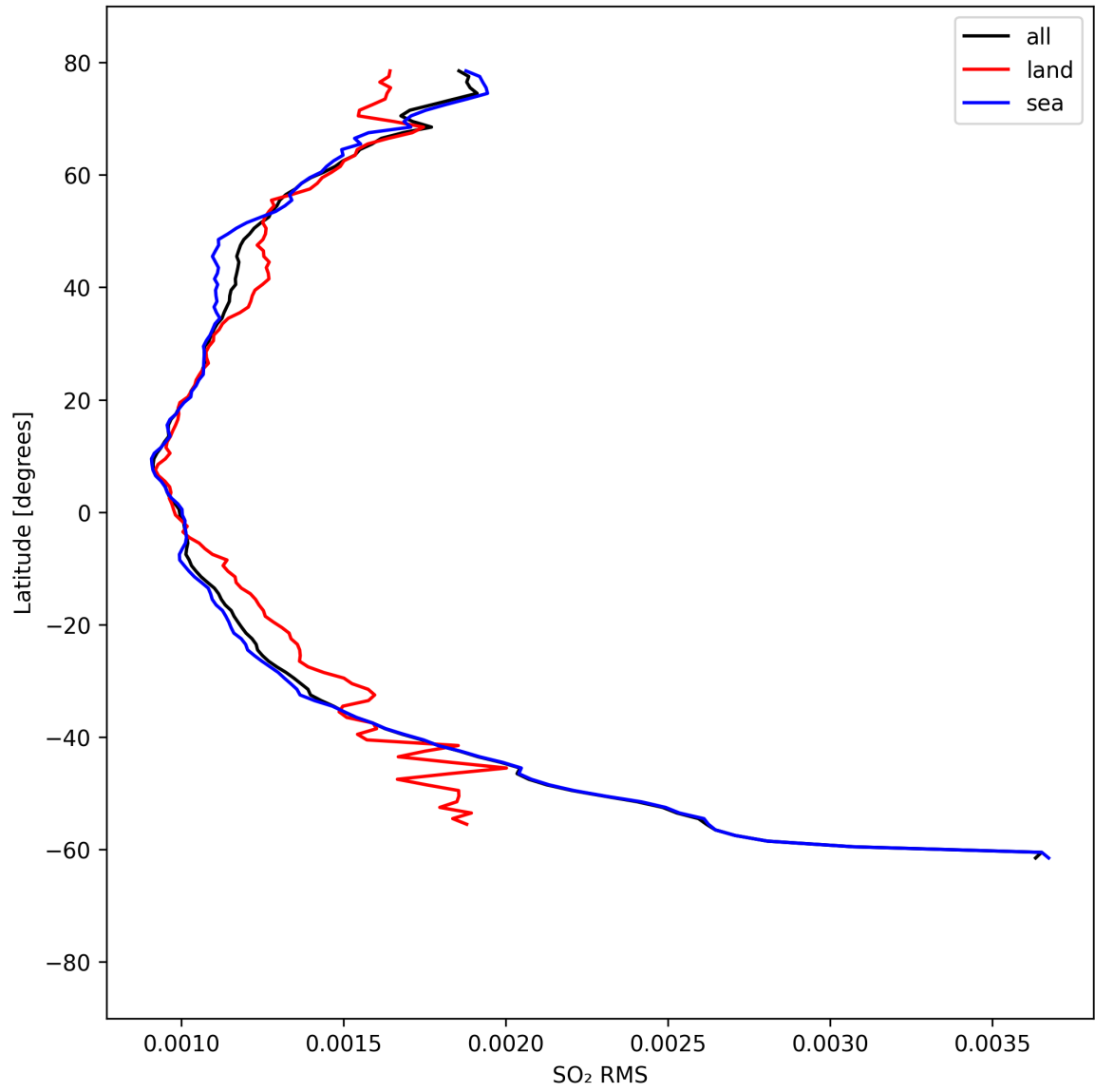
Figure 52: Zonal average of “SO 2 RMS” for 2025-08-31 to 2025-09-02.
