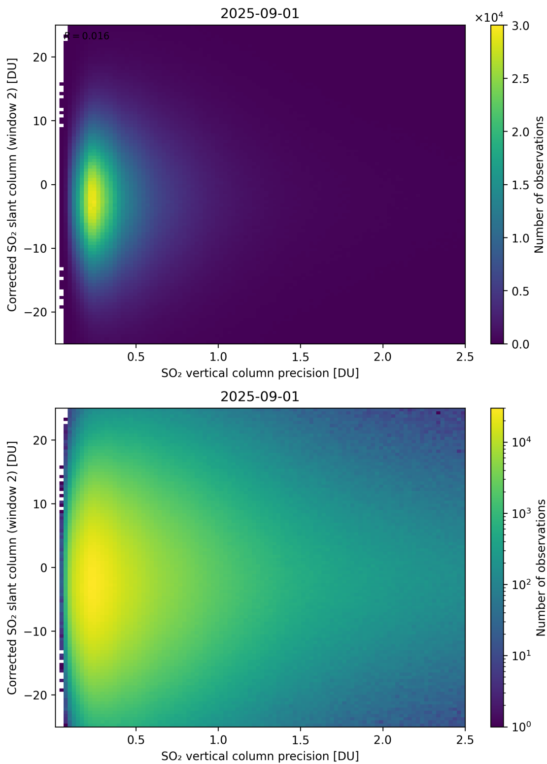
Figure 339: Scatter density plot of “SO 2 vertical column precision” against “Corrected SO 2 slant column (window 2)” for 2025-08-31 to 2025-09-02.
