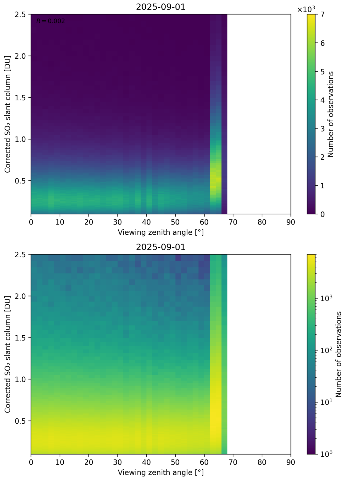
Figure 373: Scatter density plot of “Viewing zenith angle” against “Corrected SO 2 slant column” for 2025-08-31 to 2025-09-02.
