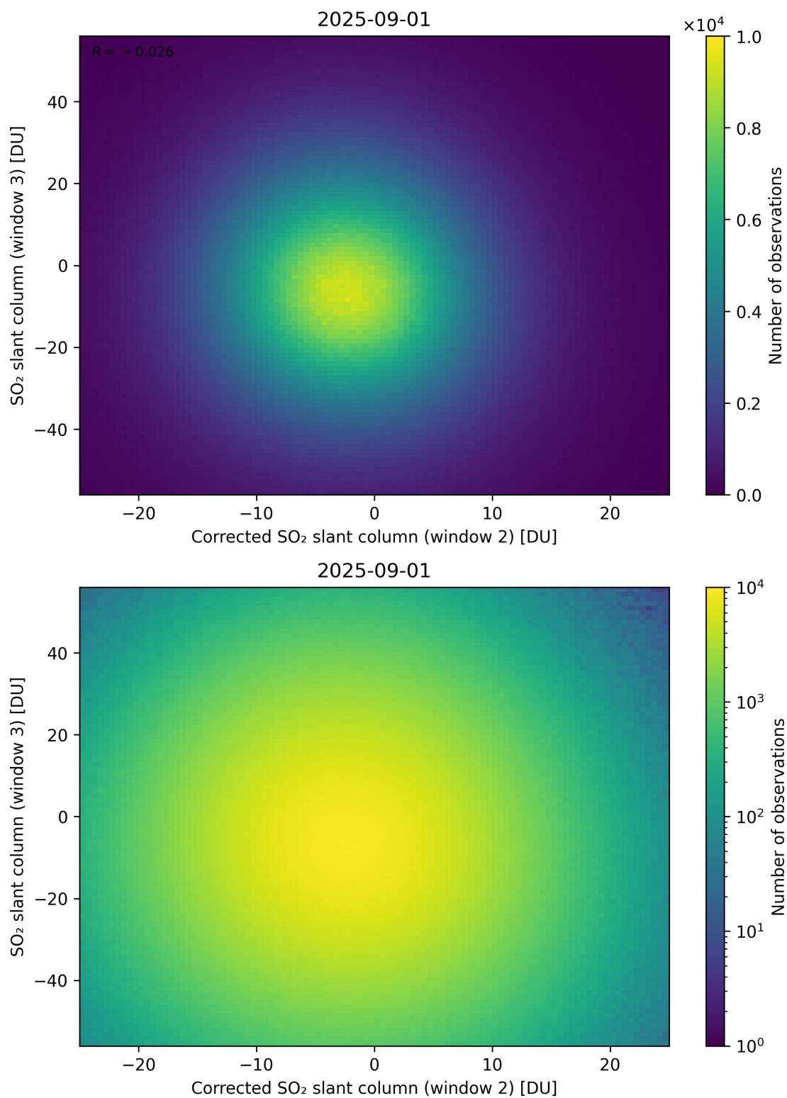
Figure 251: Scatter density plot of “Corrected SO 2 slant column (window 2)” against “SO 2 slant column (window 3)” for 2025-08-31 to 2025-09-02.
