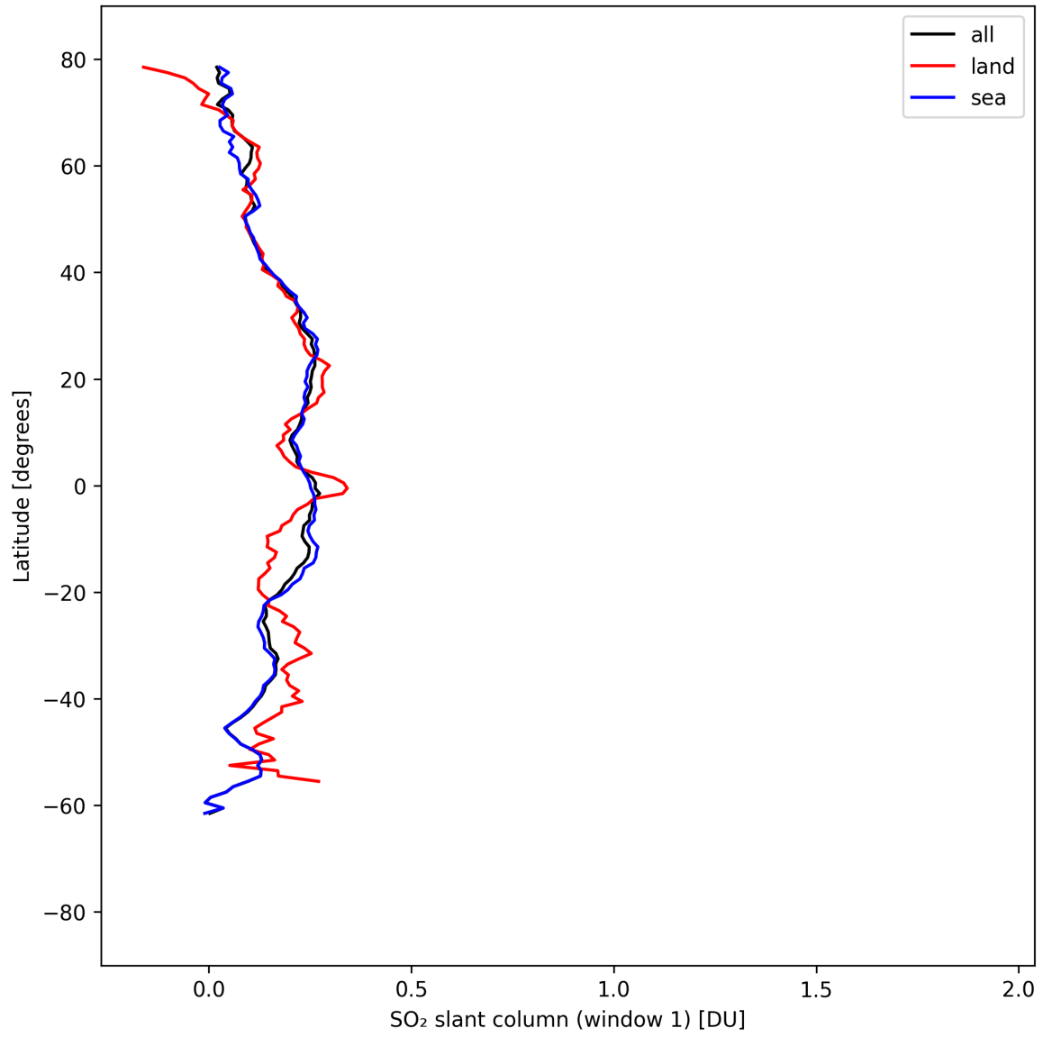
Figure 37: Zonal average of “SO 2 slant column (window 1)” for 2025-08-31 to 2025-09-02.
