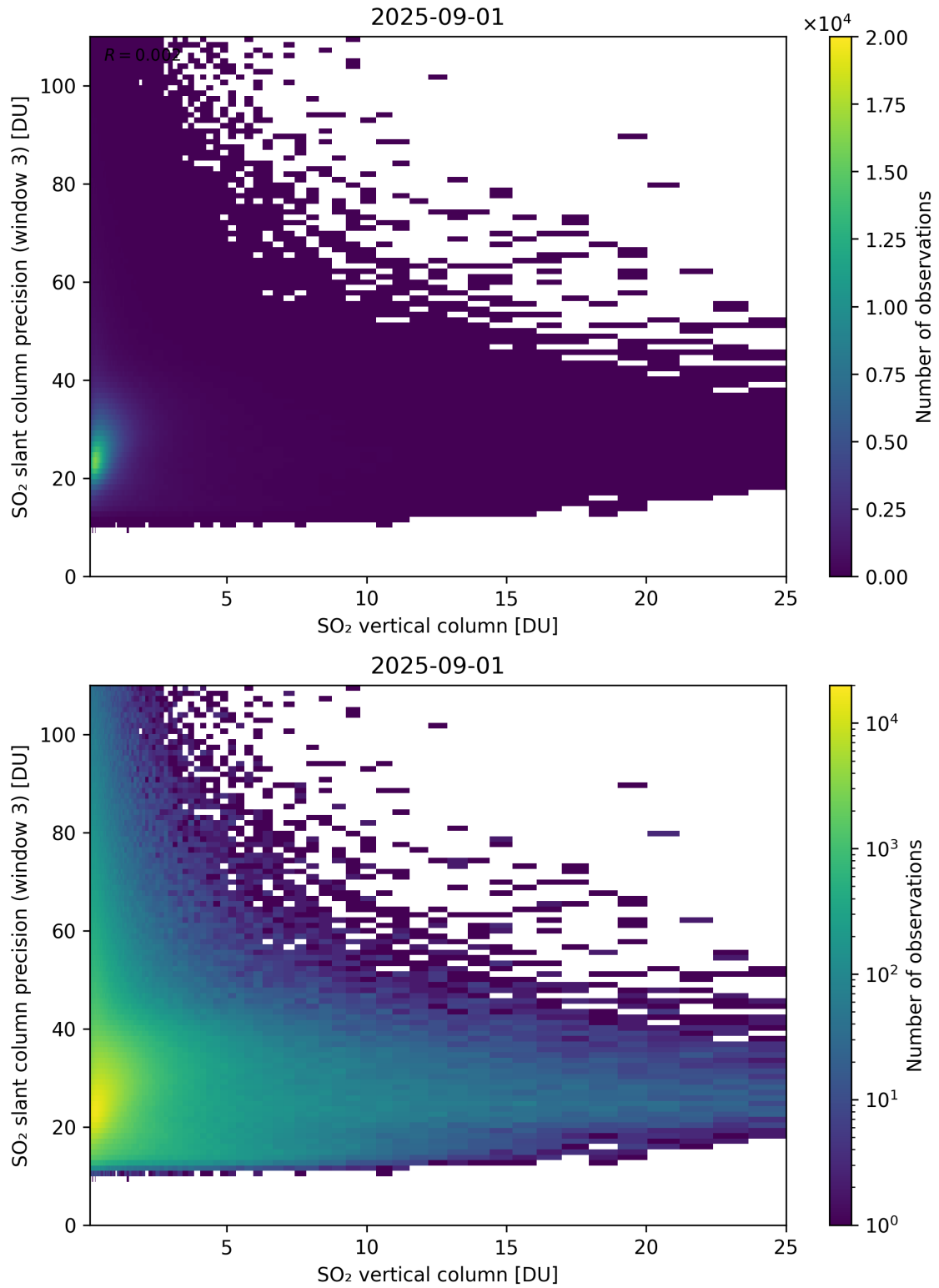
Figure 358: Scatter density plot of “SO 2 vertical column” against “SO 2 slant column precision (window 3)” for 2025-08-31 to 2025-09-02.
