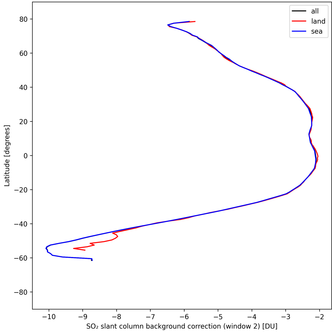
Figure 44: Zonal average of “SO 2 slant column background correction (window 2)” for 2025-08-31 to 2025-09-02.
