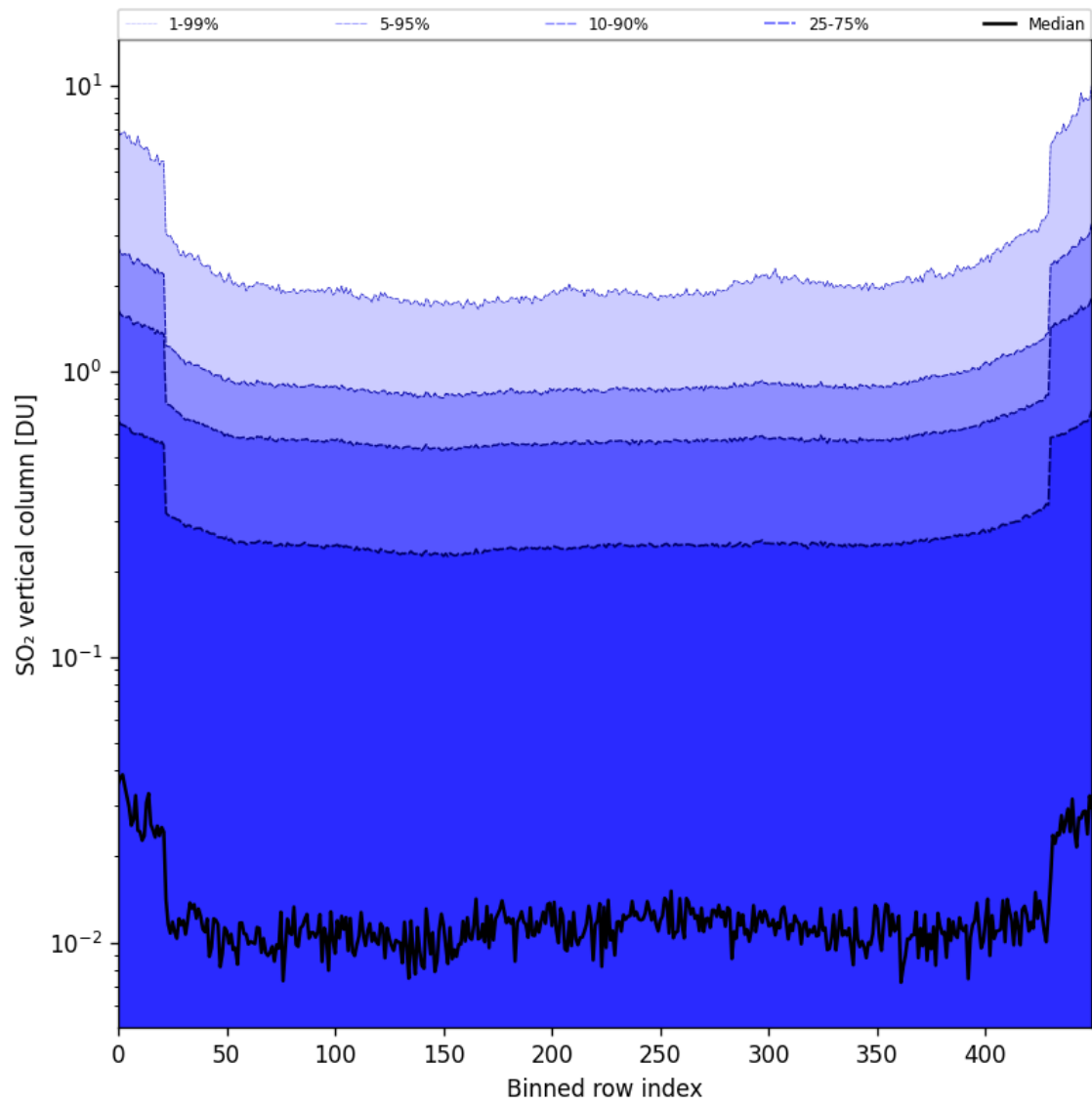
Figure 84: Along track statistics of “SO 2 vertical column” for 2025-08-31 to 2025-09-02
