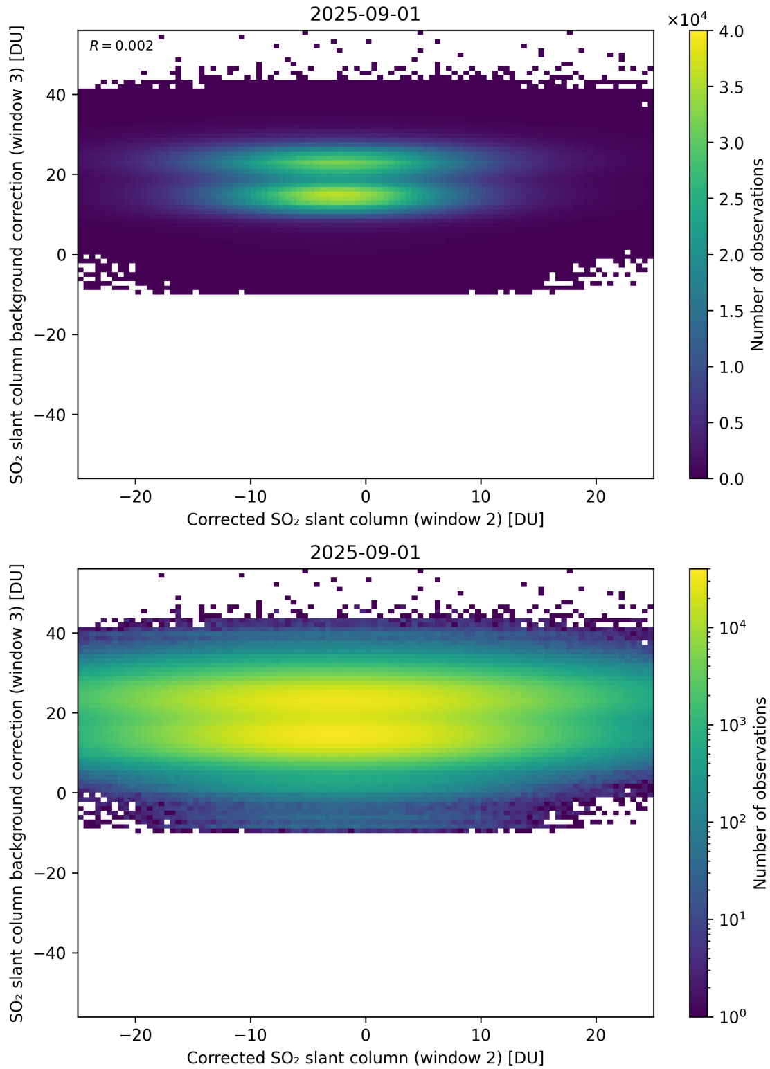
Figure 245: Scatter density plot of “Corrected SO 2 slant column (window 2)” against “SO 2 slant column background correction (window 3)” for 2025-08-31 to 2025-09-02.
