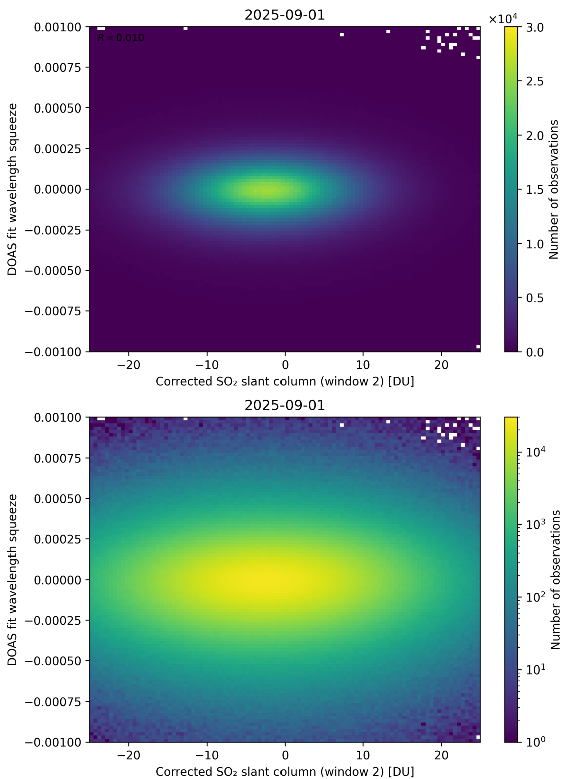
Figure 247: Scatter density plot of “Corrected SO 2 slant column (window 2)” against “DOAS fit wavelength squeeze” for 2025-08-31 to 2025-09-02.
