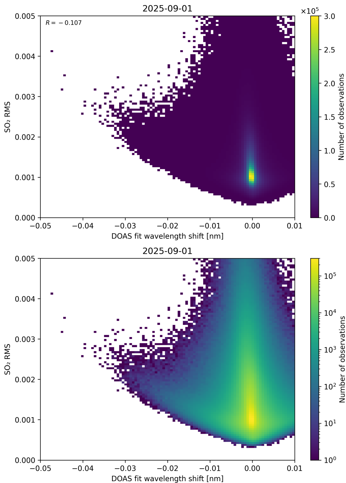
Figure 139: Scatter density plot of “DOAS fit wavelength shift” against “SO 2 RMS” for 2025-08-31 to 2025-09-02.
