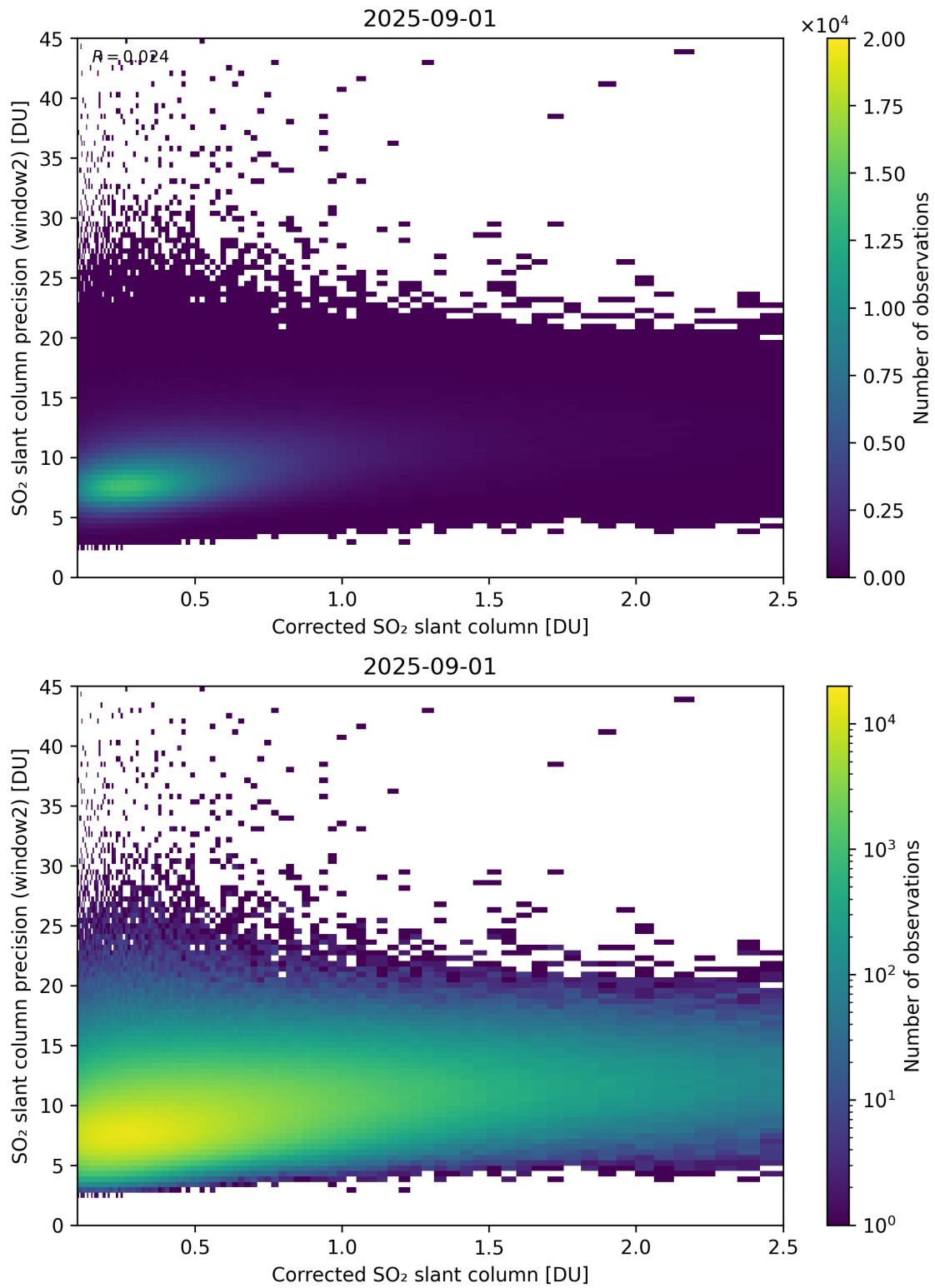
Figure 239: Scatter density plot of “Corrected SO 2 slant column” against “SO 2 slant column precision (window2)” for 2025-08-31 to 2025-09-02.
