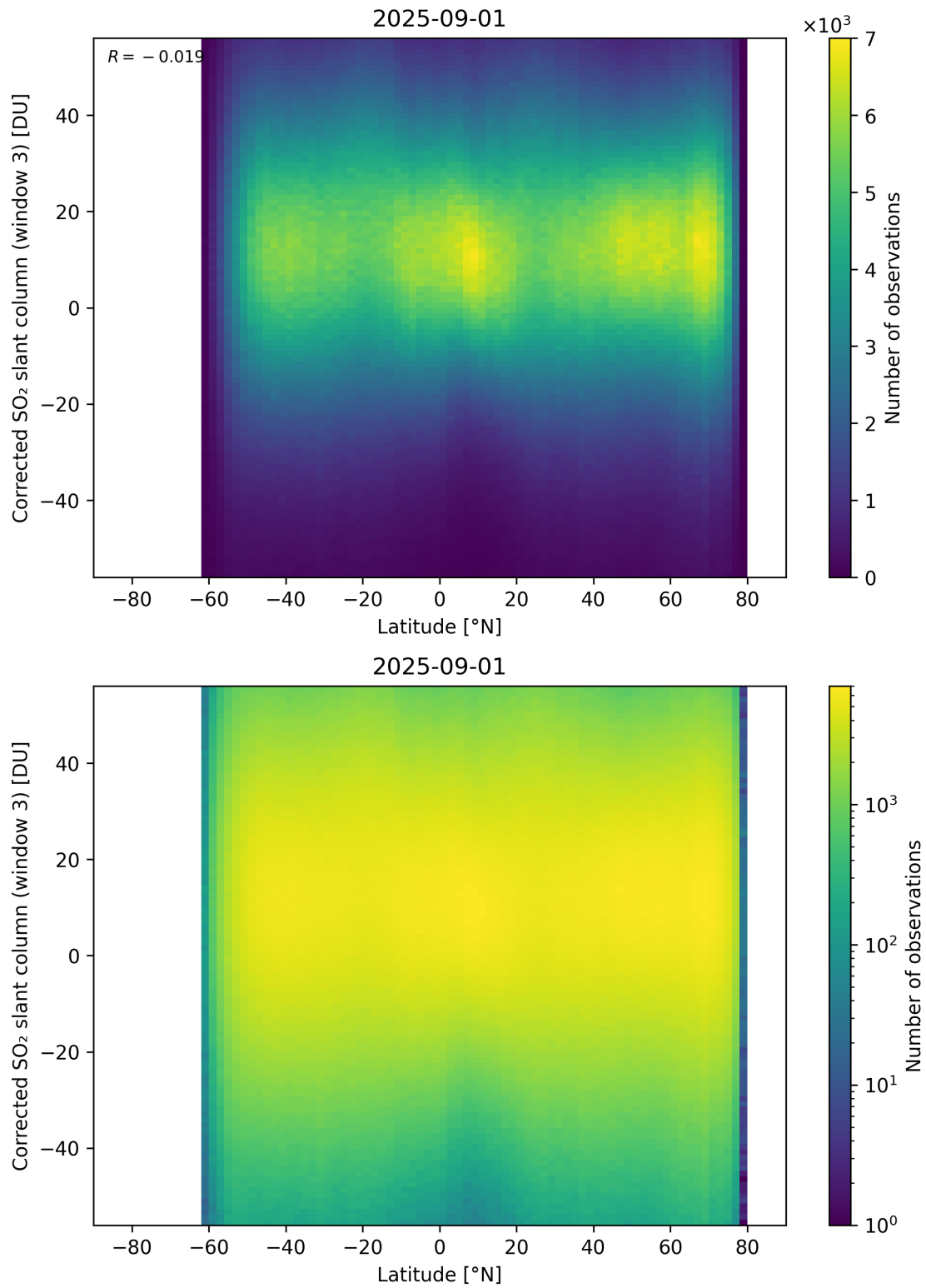
Figure 161: Scatter density plot of “Latitude” against “Corrected SO 2 slant column (window 3)” for 2025-08-31 to 2025-09-02.
