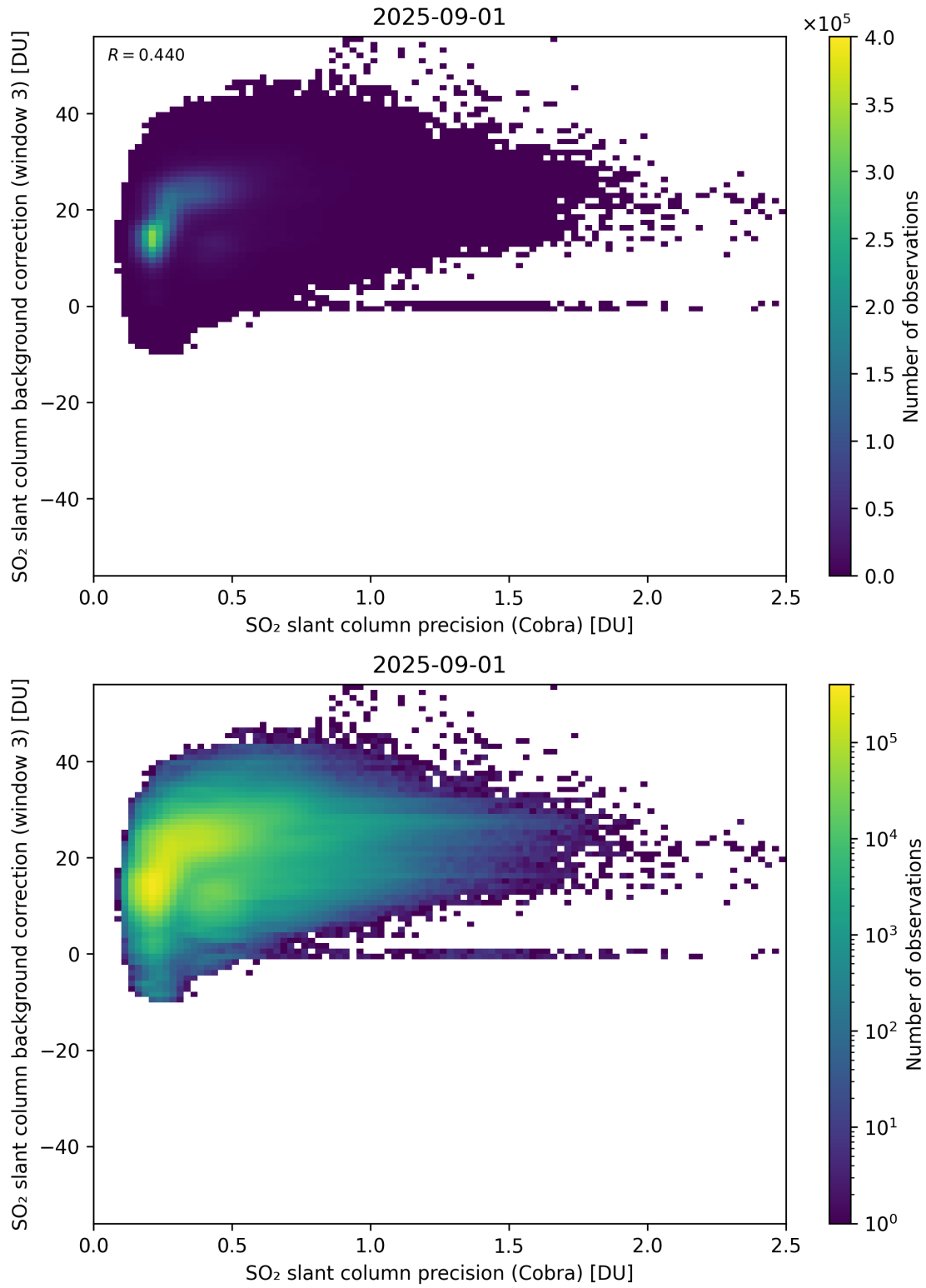
Figure 201: Scatter density plot of “SO 2 slant column precision (Cobra)” against “SO 2 slant column background correction (window 3)” for 2025-08-31 to 2025-09-02.
