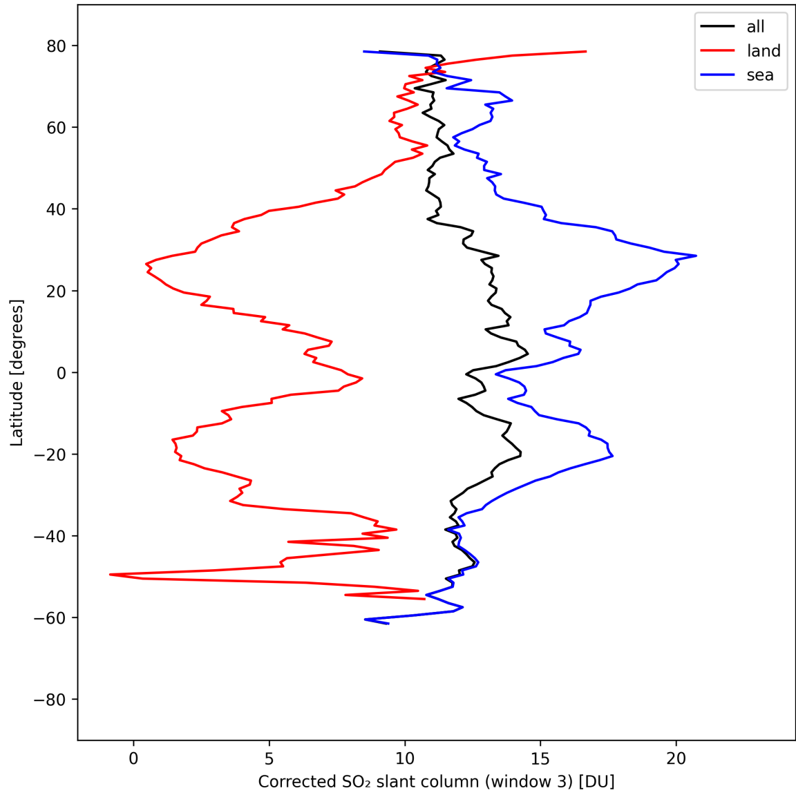
Figure 47: Zonal average of "Corrected SO 2 slant column (window 3)" for 2025-08-31 to 2025-09-02.
