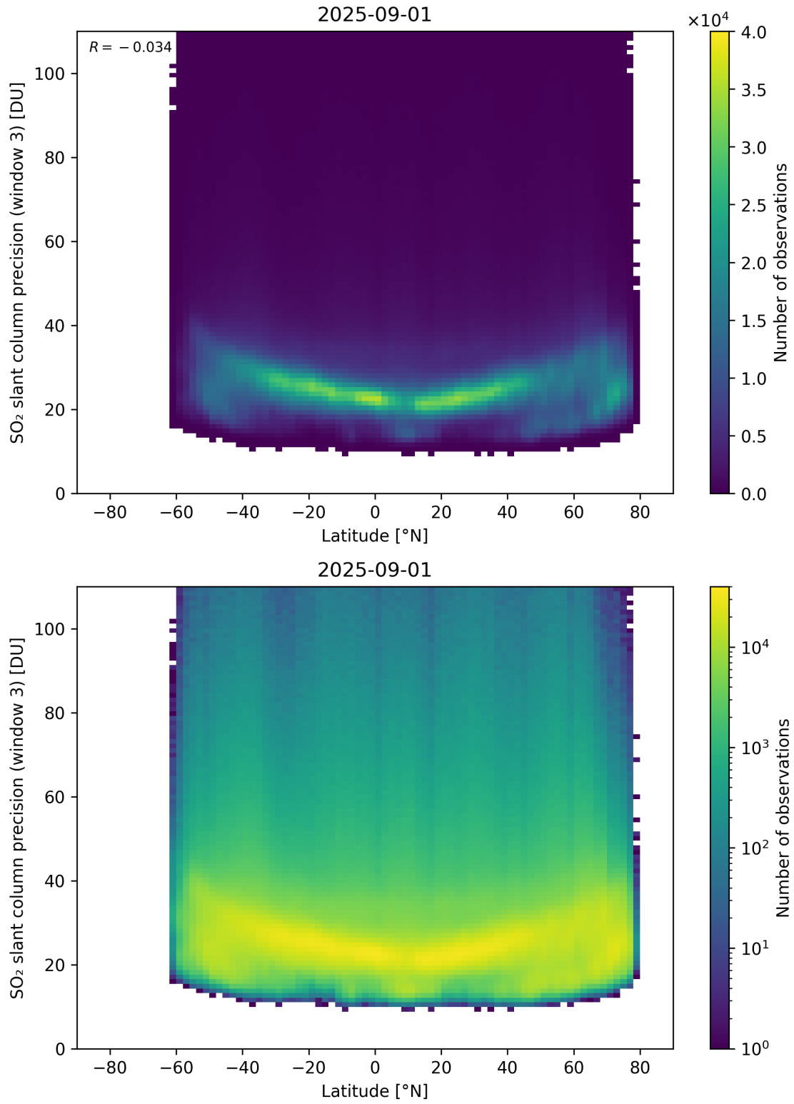
Figure 166: Scatter density plot of “Latitude” against “SO 2 slant column precision (window 3)” for 2025-08-31 to 2025-09-02.
