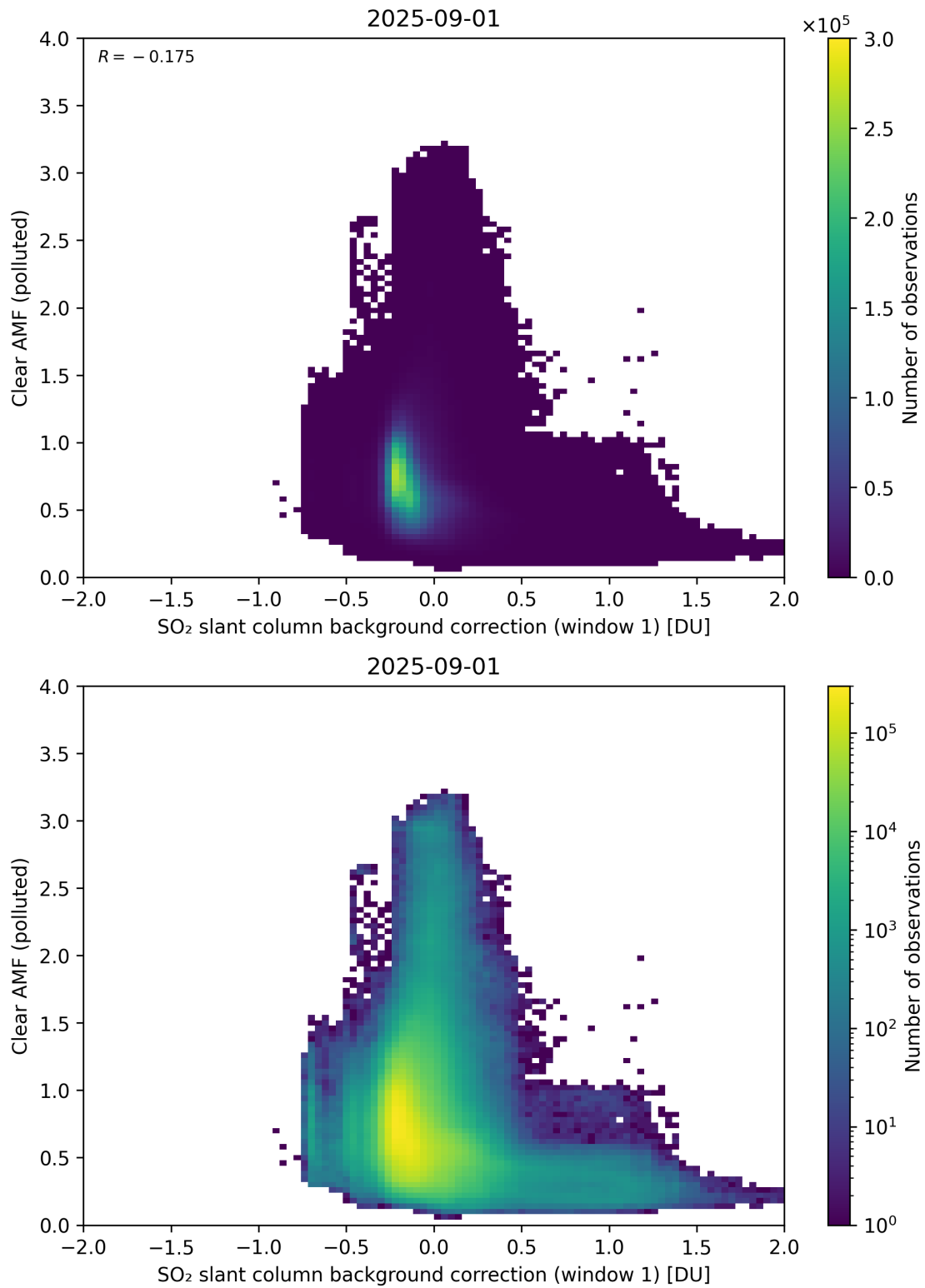
Figure 114: Scatter density plot of “SO 2 slant column background correction (window 1)” against “Clear AMF (polluted)” for 2025-08-31 to 2025-09-02.
