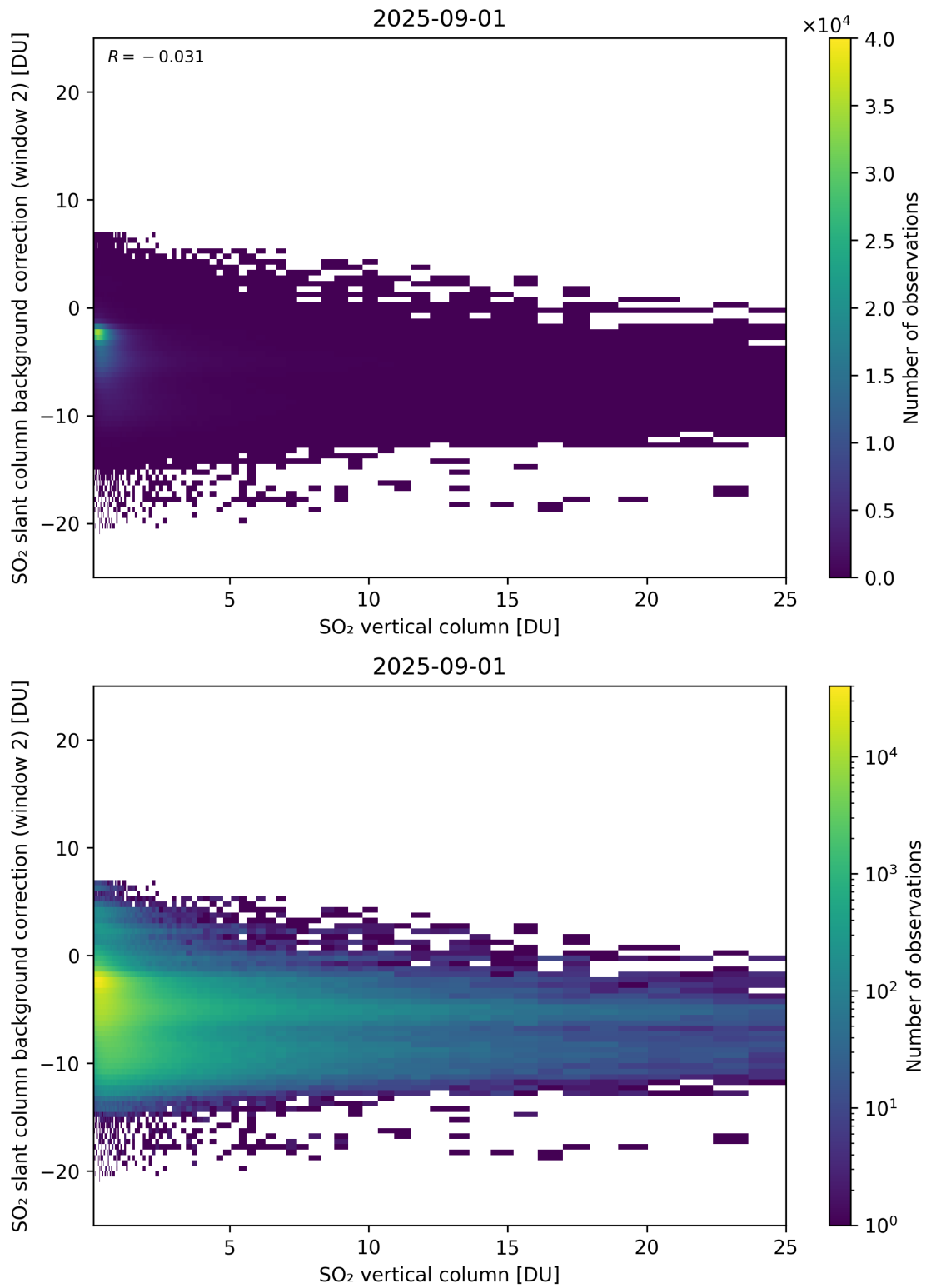
Figure 324: Scatter density plot of “SO 2 vertical column” against “SO 2 slant column background correction (window 2)” for 2025-08-31 to 2025-09-02.
