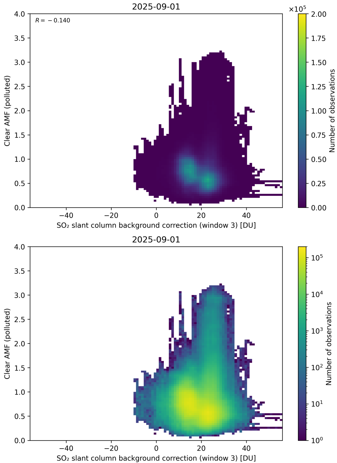
Figure 135: Scatter density plot of “SO 2 slant column background correction (window 3)” against “Clear AMF (polluted)” for 2025-08-31 to 2025-09-02.
