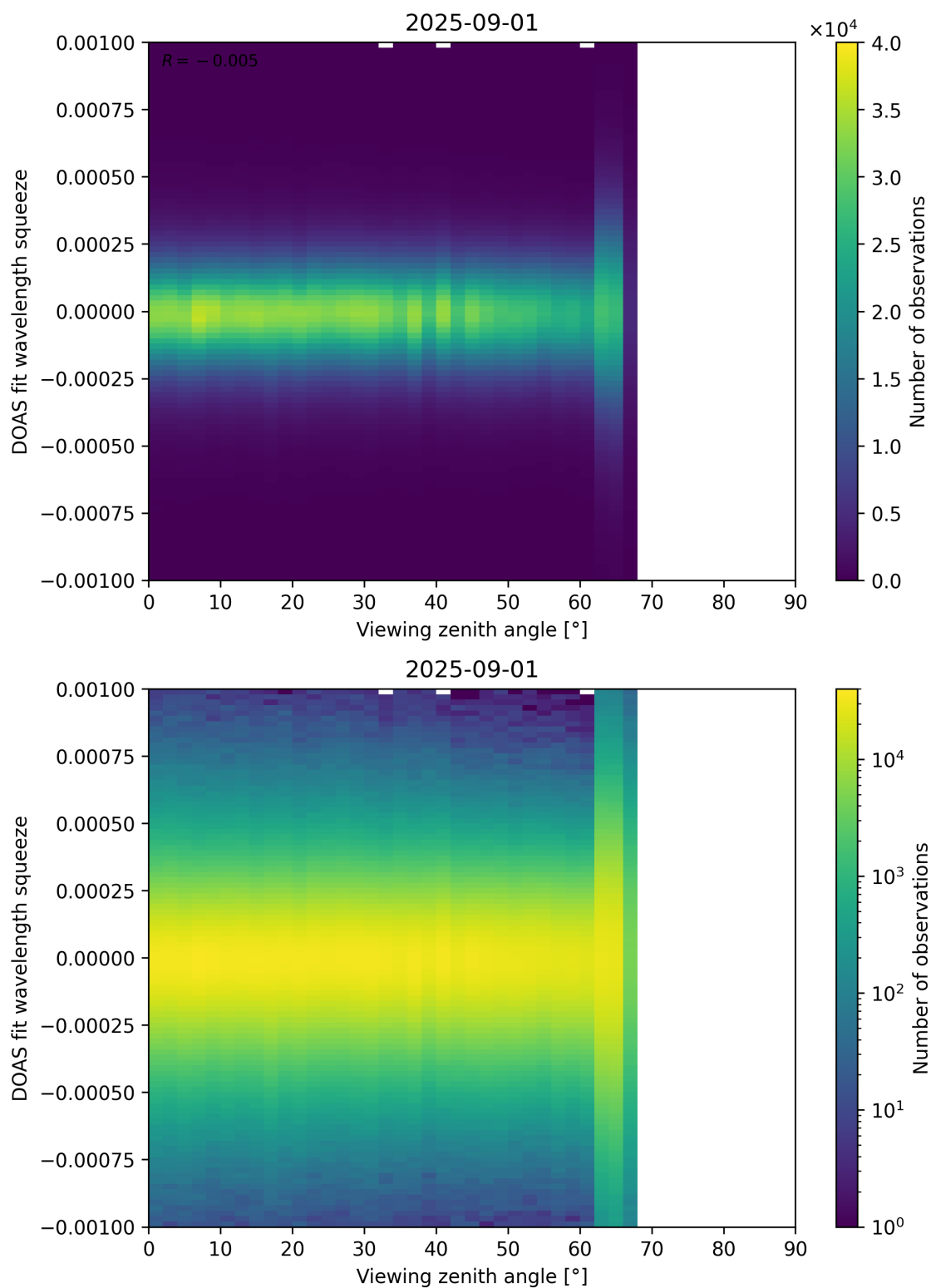
Figure 366: Scatter density plot of “Viewing zenith angle” against “DOAS fit wavelength squeeze” for 2025-08-31 to 2025-09-02.
