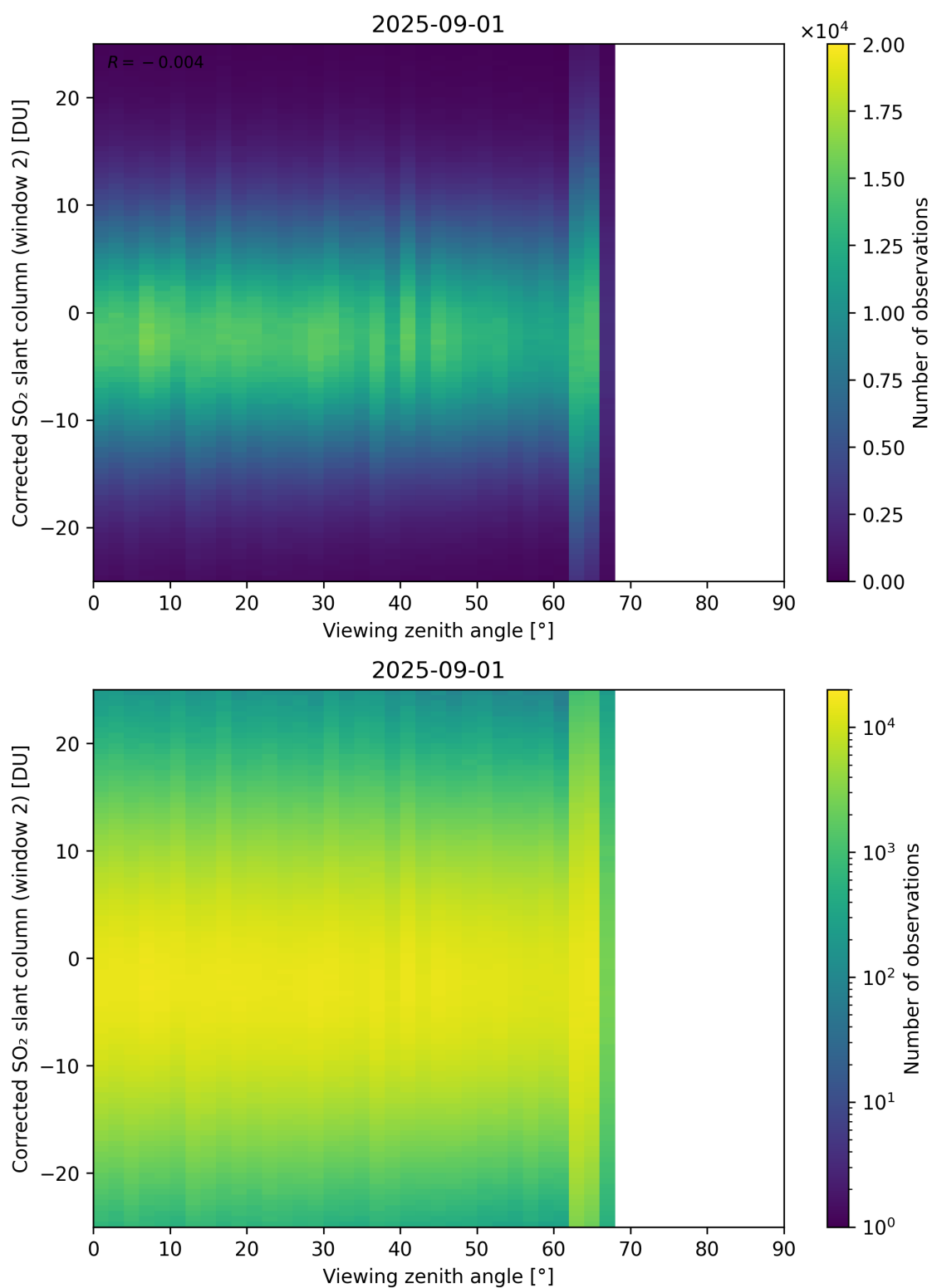
Figure 374: Scatter density plot of “Viewing zenith angle” against “Corrected SO 2 slant column (window 2)” for 2025-08-31 to 2025-09-02.
