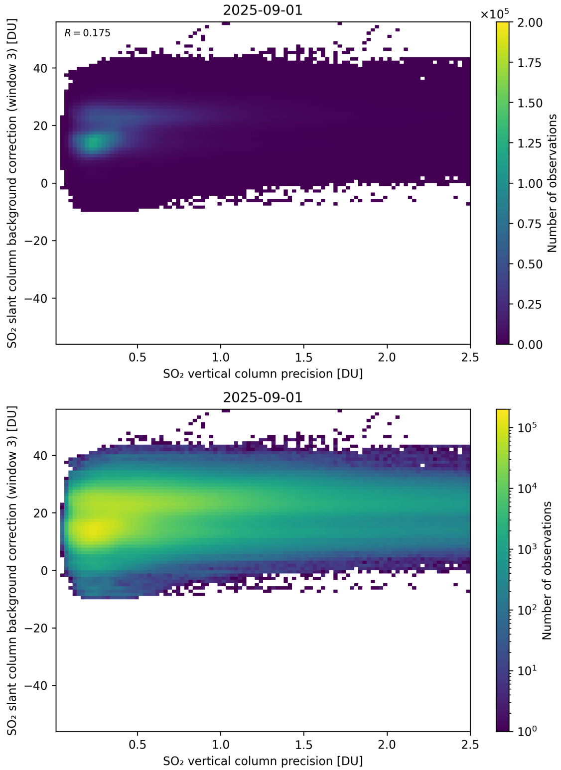
Figure 331: Scatter density plot of “SO 2 vertical column precision” against “SO 2 slant column background correction (window 3)” for 2025-08-31 to 2025-09-02.
