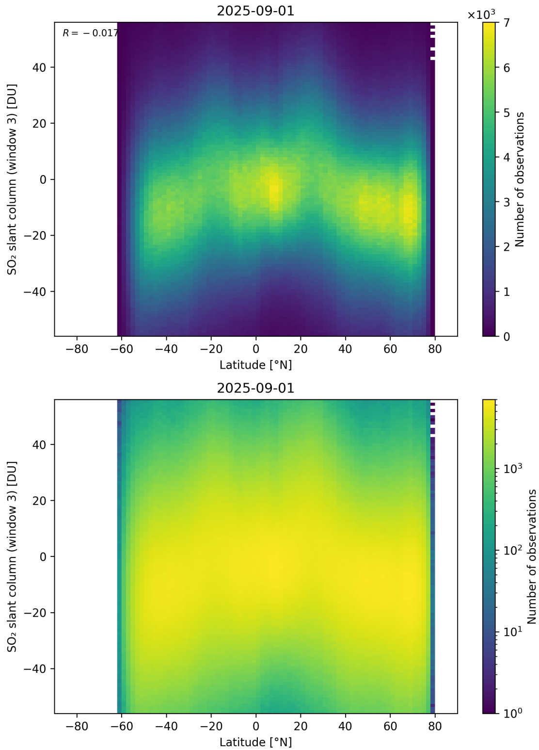
Figure 165: Scatter density plot of “Latitude” against “SO 2 slant column (window 3)” for 2025-08-31 to 2025-09-02.
