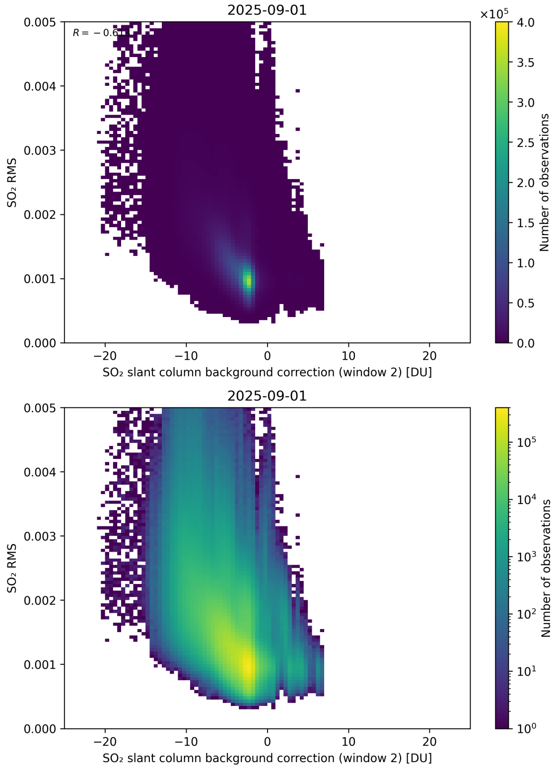
Figure 125: Scatter density plot of “SO 2 slant column background correction (window 2)” against “SO 2 RMS” for 2025-08-31 to 2025-09-02.
