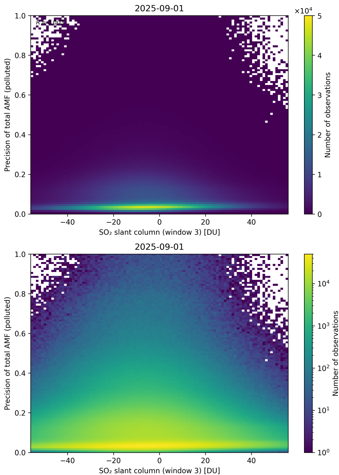
Figure 319: Scatter density plot of “SO 2 slant column (window 3)” against “Precision of total AMF (polluted)” for 2025-08-31 to 2025-09-02.
