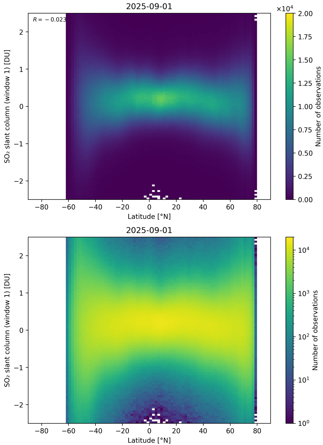
Figure 162: Scatter density plot of “Latitude” against “SO 2 slant column (window 1)” for 2025-08-31 to 2025-09-02.
