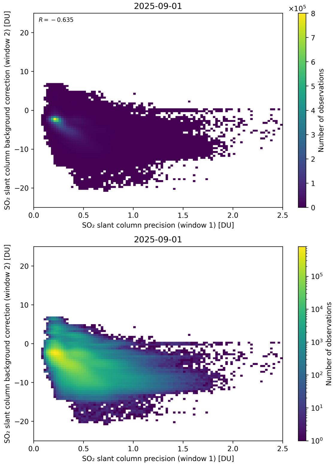
Figure 269: Scatter density plot of “SO 2 slant column precision (window 1)” against “SO 2 slant column background correction (window 2)” for 2025-08-31 to 2025-09-02.
