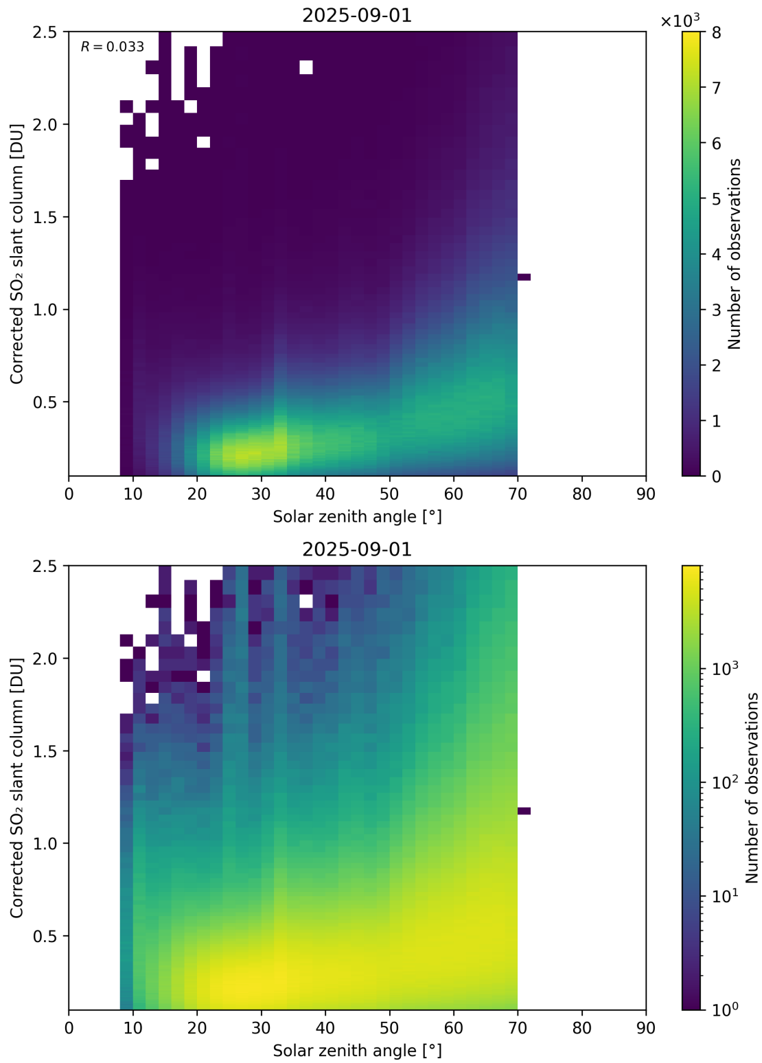
Figure 181: Scatter density plot of “Solar zenith angle” against “Corrected SO 2 slant column” for 2025-08-31 to 2025-09-02.
