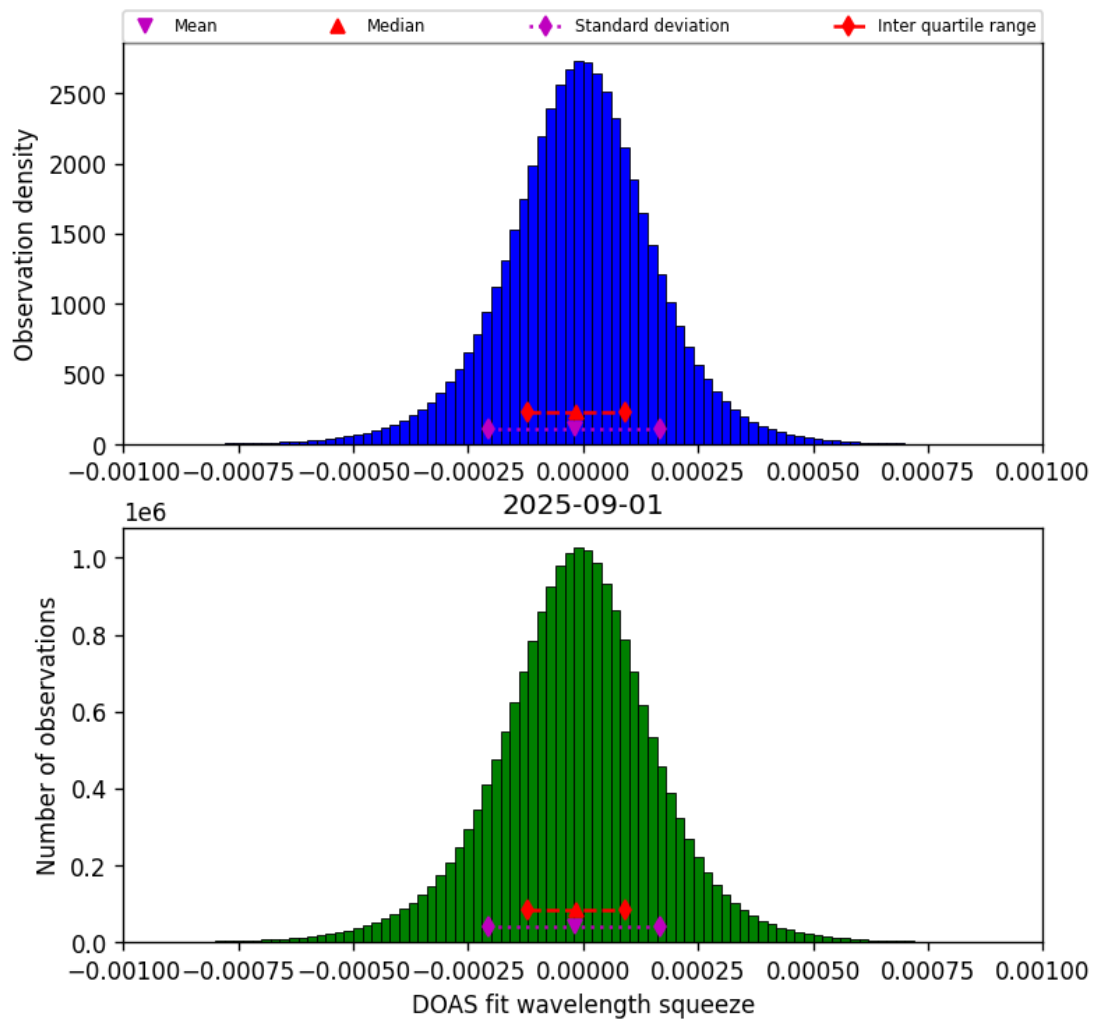
Figure 77: Histogram of “DOAS fit wavelength squeeze” for 2025-08-31 to 2025-09-02
