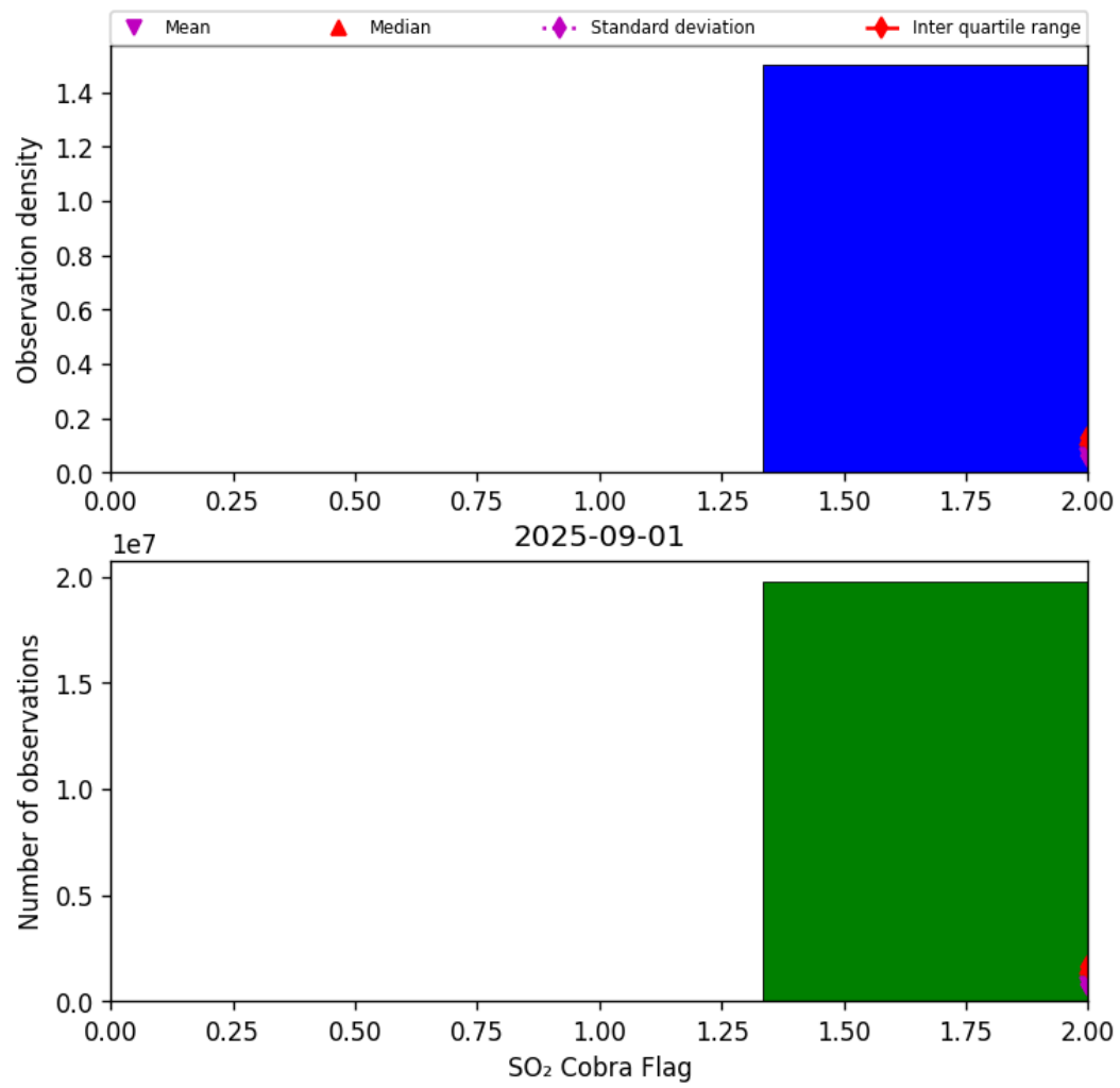
Figure 75: Histogram of “SO 2 Cobra Flag” for 2025-08-31 to 2025-09-02
