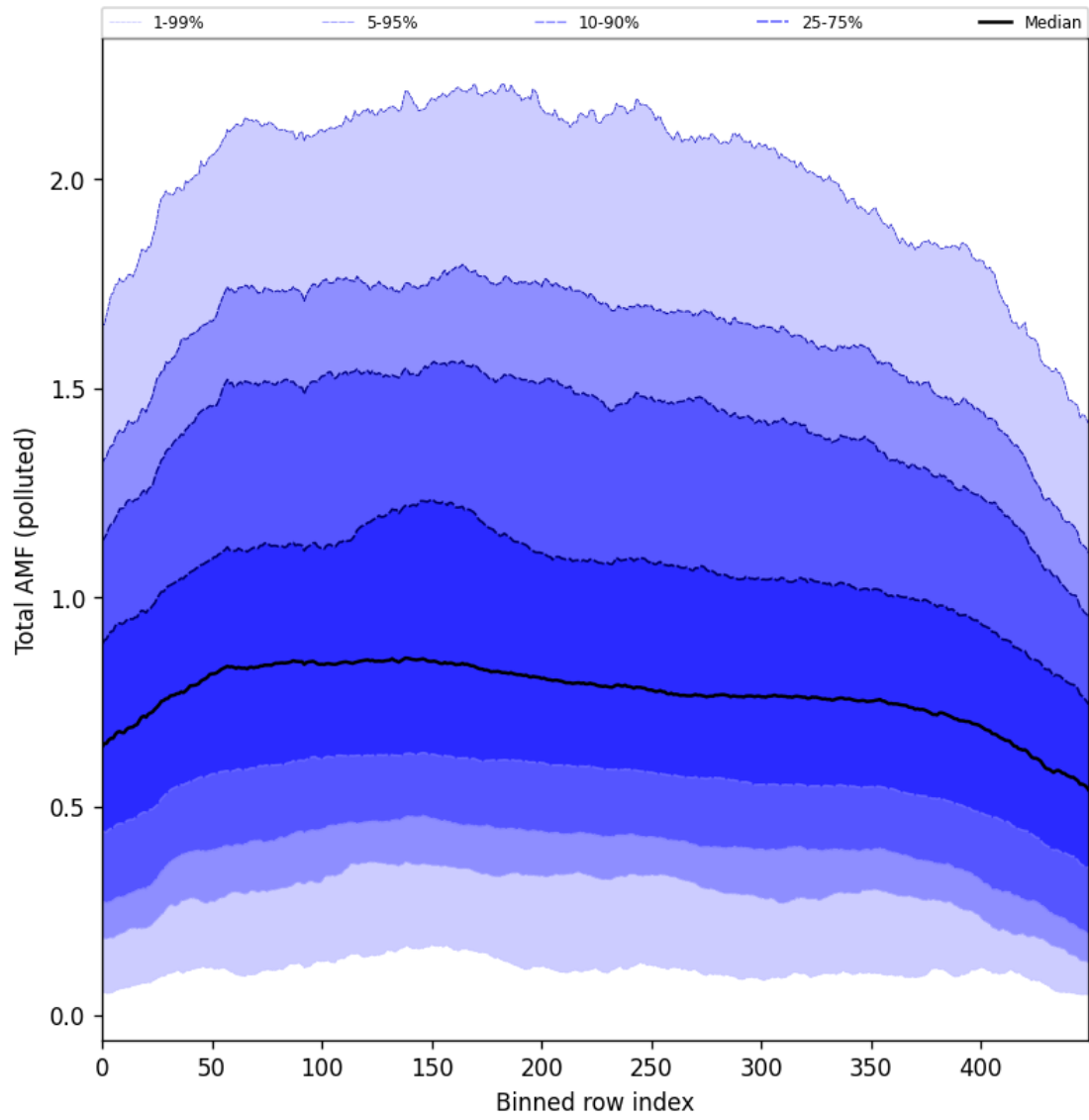
Figure 105: Along track statistics of “Total AMF (polluted)” for 2025-08-31 to 2025-09-02
