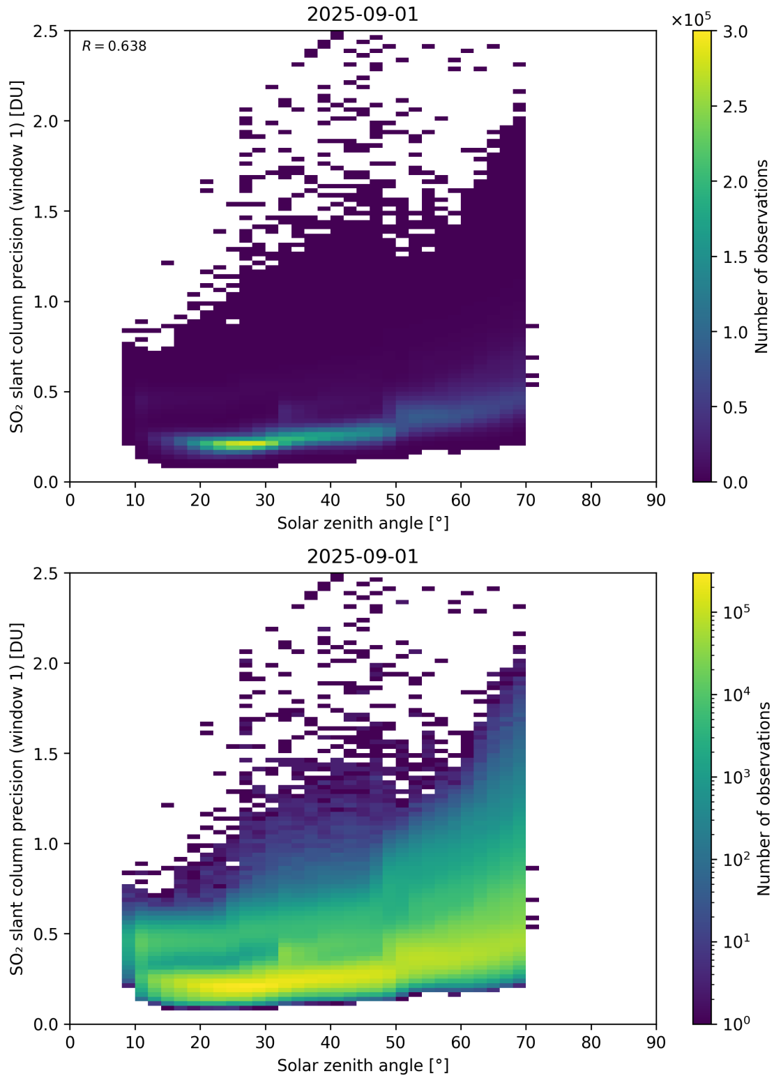
Figure 185: Scatter density plot of “Solar zenith angle” against “SO 2 slant column precision (window 1)” for 2025-08-31 to 2025-09-02.
