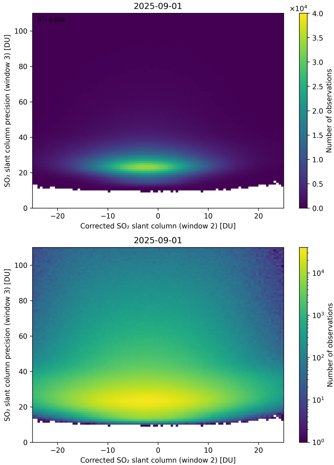
Figure 252: Scatter density plot of “Corrected SO 2 slant column (window 2)” against “SO 2 slant column precision (window 3)” for 2025-08-31 to 2025-09-02.
