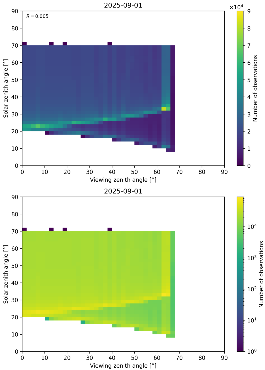
Figure 369: Scatter density plot of “Viewing zenith angle” against “Solar zenith angle” for 2025-08-31 to 2025-09-02.
