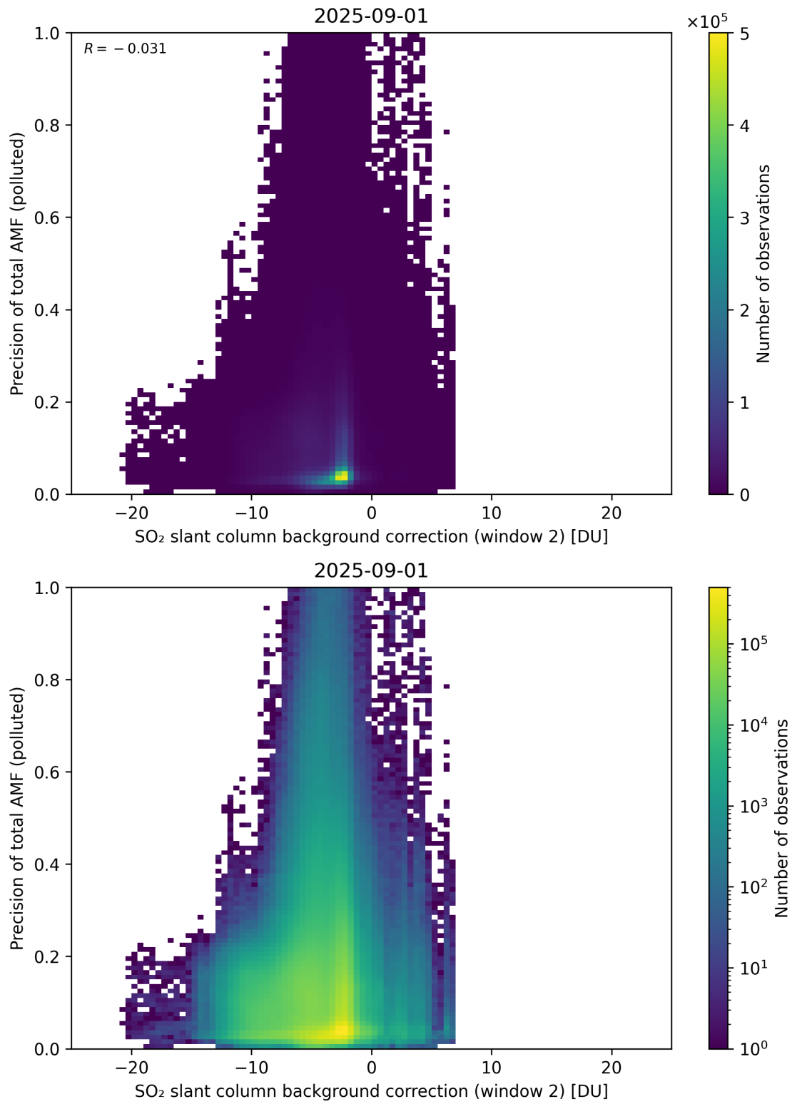
Figure 131: Scatter density plot of “SO 2 slant column background correction (window 2)” against “Precision of total AMF (polluted)” for 2025-08-31 to 2025-09-02.
