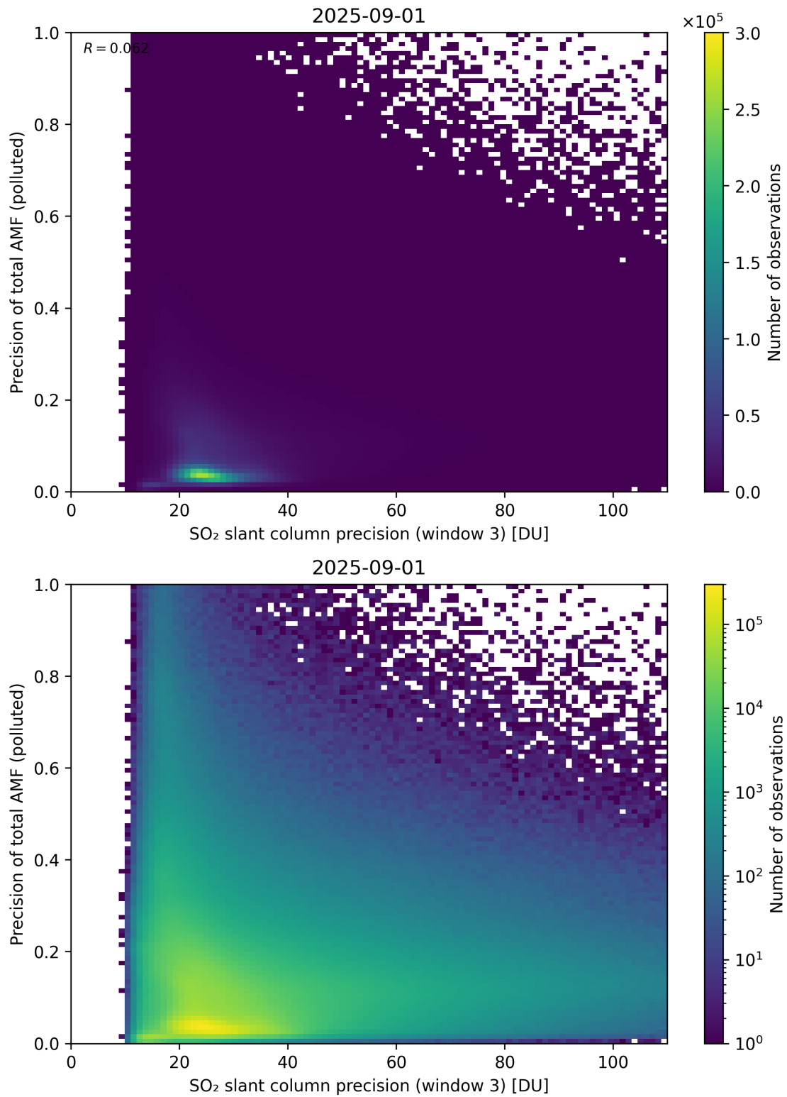
Figure 314: Scatter density plot of “SO 2 slant column precision (window 3)” against “Precision of total AMF (polluted)” for 2025-08-31 to 2025-09-02.
