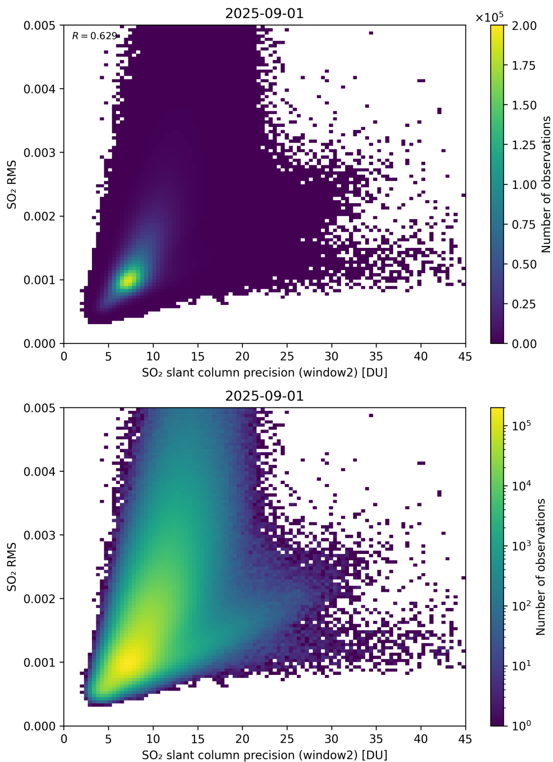
Figure 295: Scatter density plot of “SO 2 slant column precision (window2)” against “SO 2 RMS” for 2025-08-31 to 2025-09-02.
