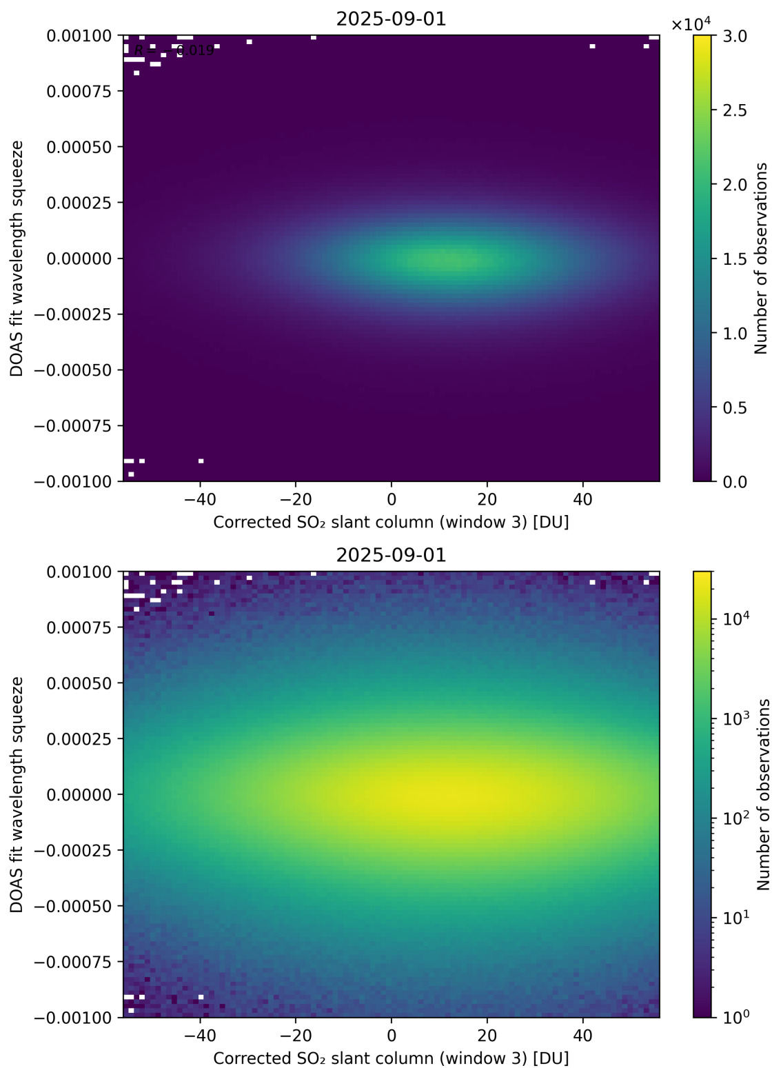
Figure 257: Scatter density plot of “Corrected SO 2 slant column (window 3)” against “DOAS fit wavelength squeeze” for 2025-08-31 to 2025-09-02.
