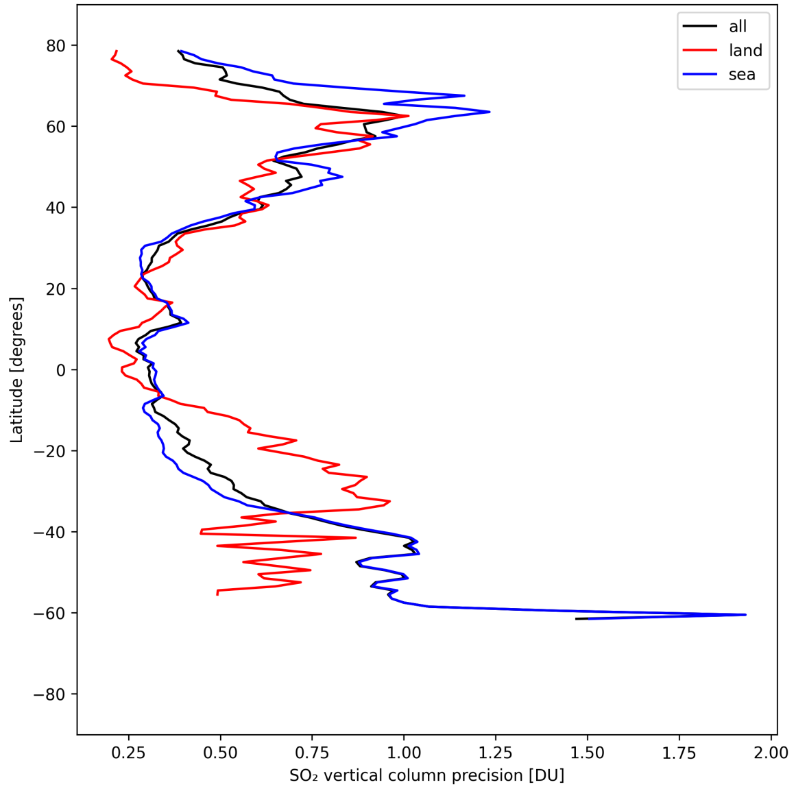
Figure 33: Zonal average of “SO 2 vertical column precision” for 2025-08-31 to 2025-09-02.
