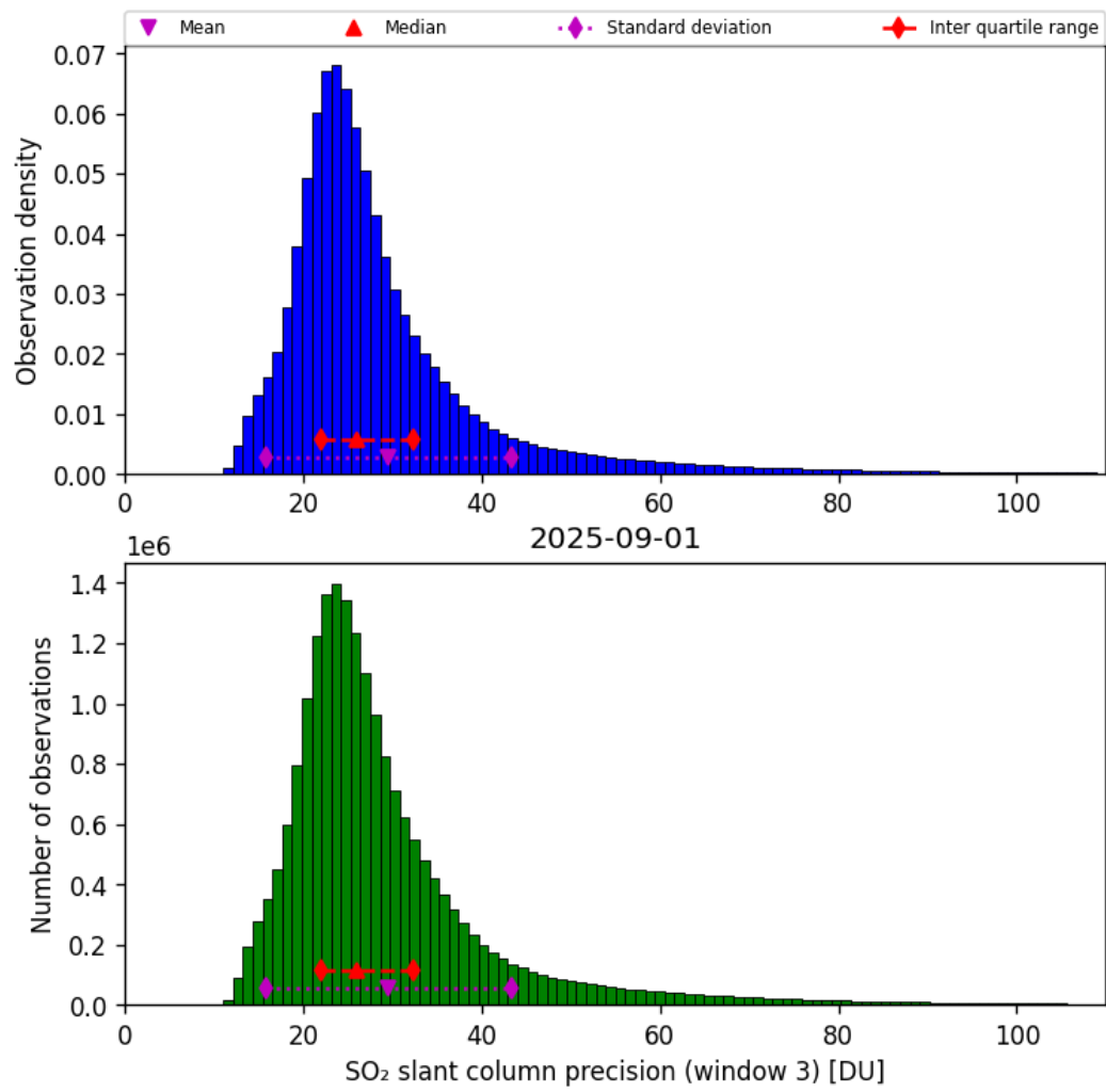
Figure 72: Histogram of “SO 2 slant column precision (window 3)” for 2025-08-31 to 2025-09-02
