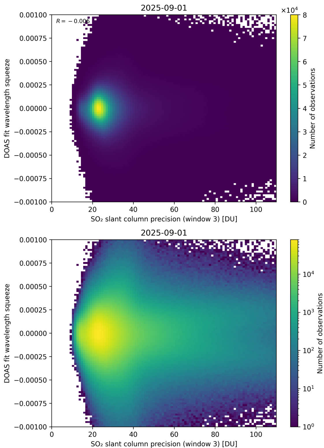
Figure 309: Scatter density plot of “SO 2 slant column precision (window 3)” against “DOAS fit wavelength squeeze” for 2025-08-31 to 2025-09-02.
