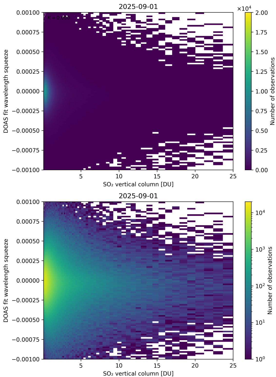
Figure 327: Scatter density plot of “SO 2 vertical column” against “DOAS fit wavelength squeeze” for 2025-08-31 to 2025-09-02.
