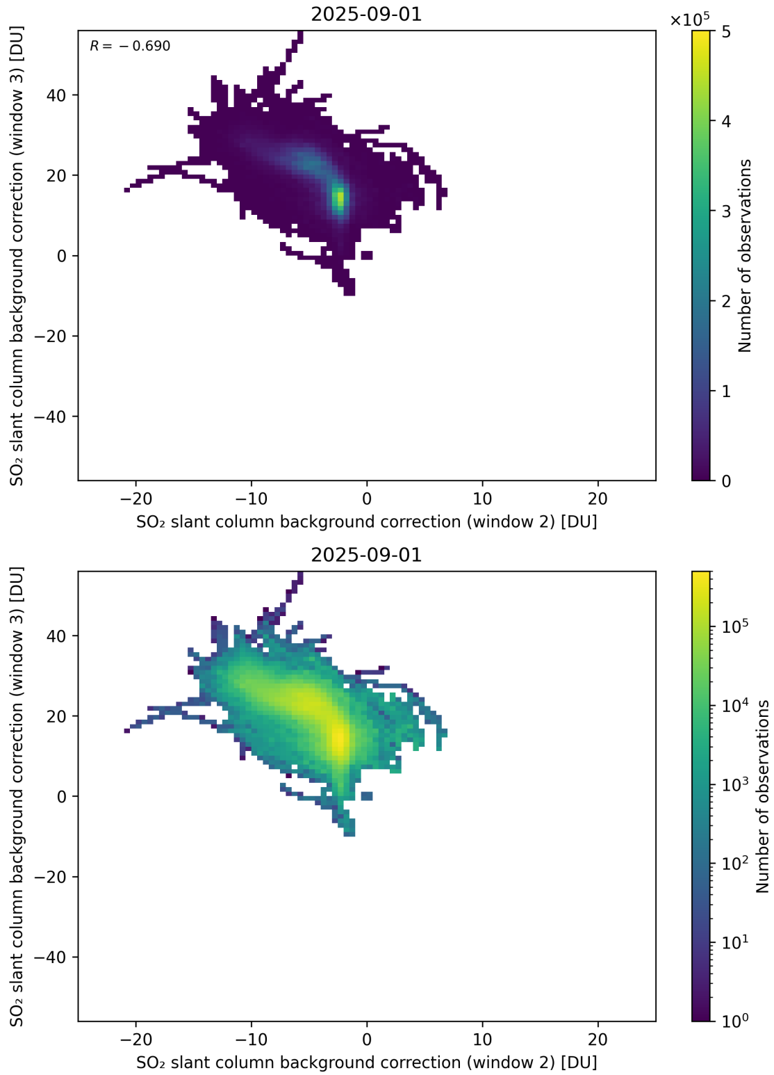
Figure 122: Scatter density plot of “SO 2 slant column background correction (window 2)” against “SO 2 slant column background correction (window 3)” for 2025-08-31 to 2025-09-02.
