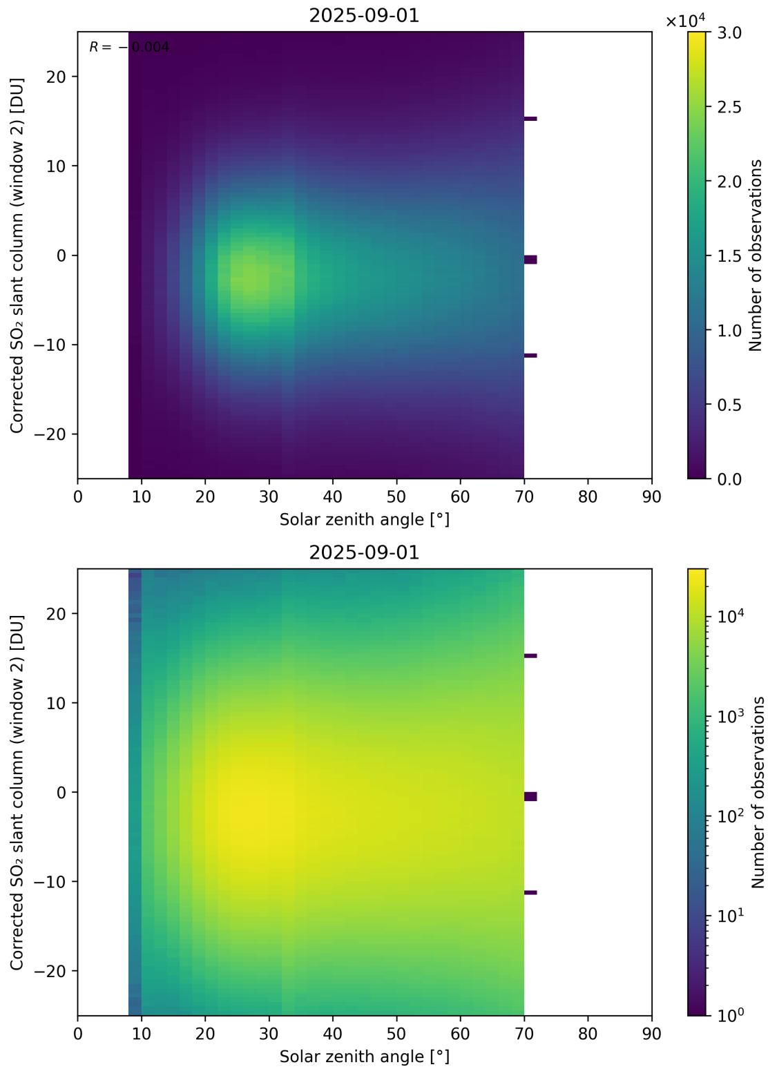
Figure 182: Scatter density plot of “Solar zenith angle” against “Corrected SO 2 slant column (window 2)” for 2025-08-31 to 2025-09-02.
