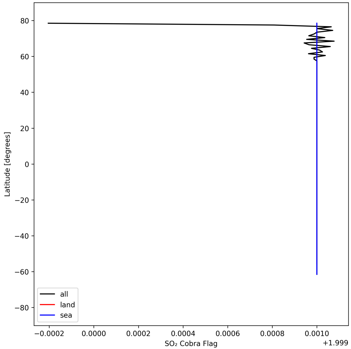
Figure 49: Zonal average of "SO 2 Cobra Flag" for 2025-08-31 to 2025-09-02.
