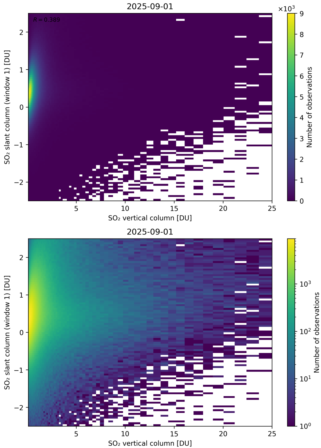
Figure 354: Scatter density plot of “SO 2 vertical column” against “SO 2 slant column (window 1)” for 2025-08-31 to 2025-09-02.
