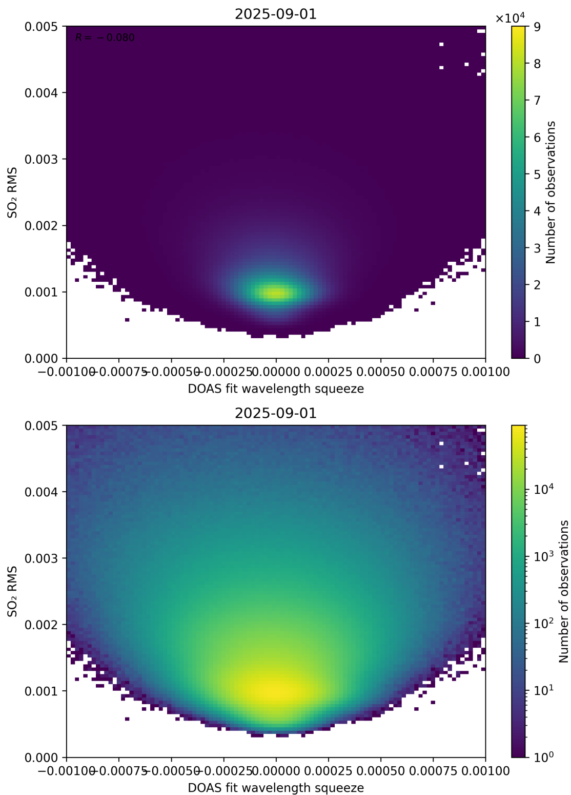
Figure 143: Scatter density plot of “DOAS fit wavelength squeeze” against “SO 2 RMS” for 2025-08-31 to 2025-09-02.
