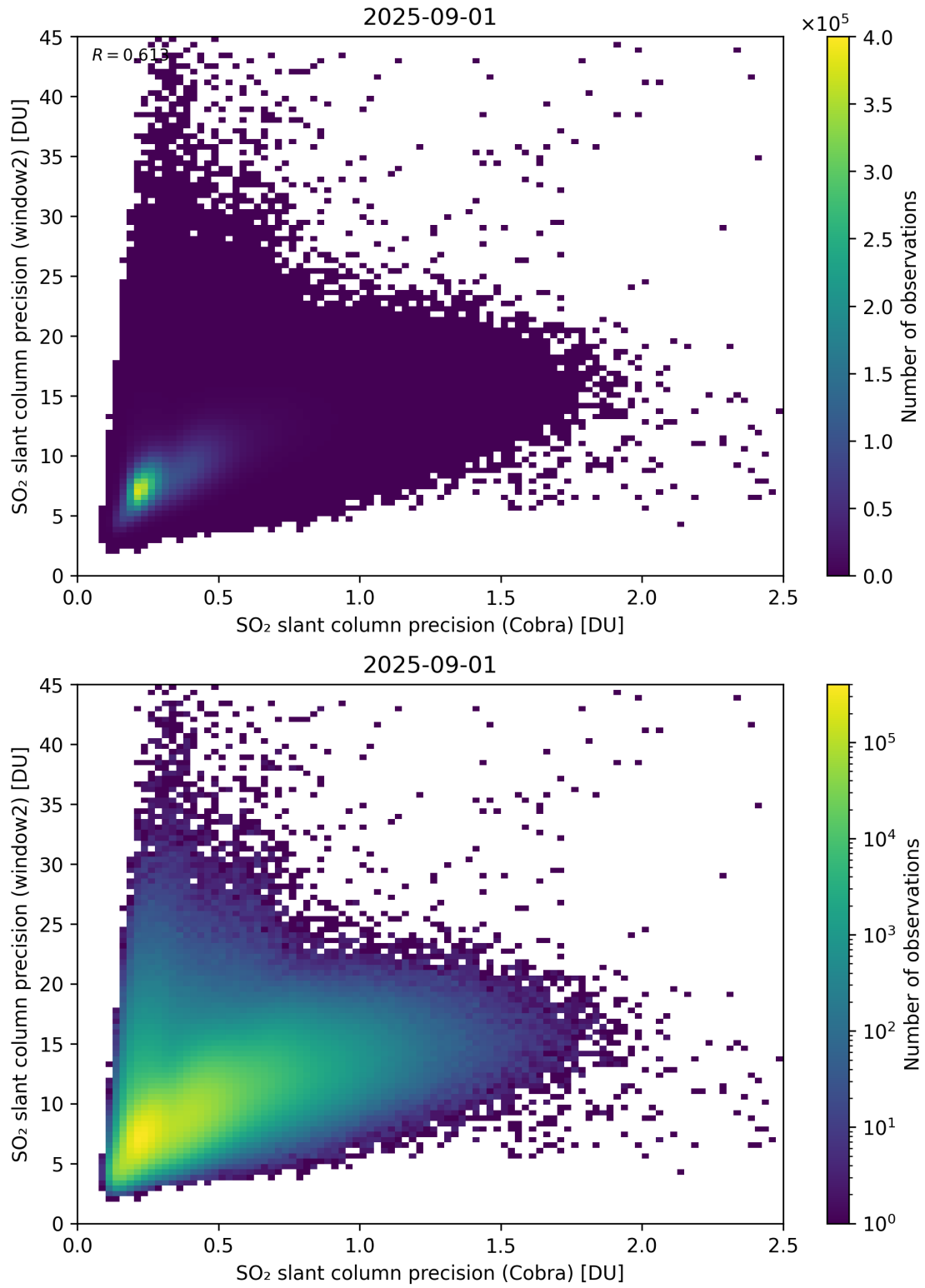
Figure 210: Scatter density plot of “SO 2 slant column precision (Cobra)” against “SO 2 slant column precision (window2)” for 2025-08-31 to 2025-09-02.
