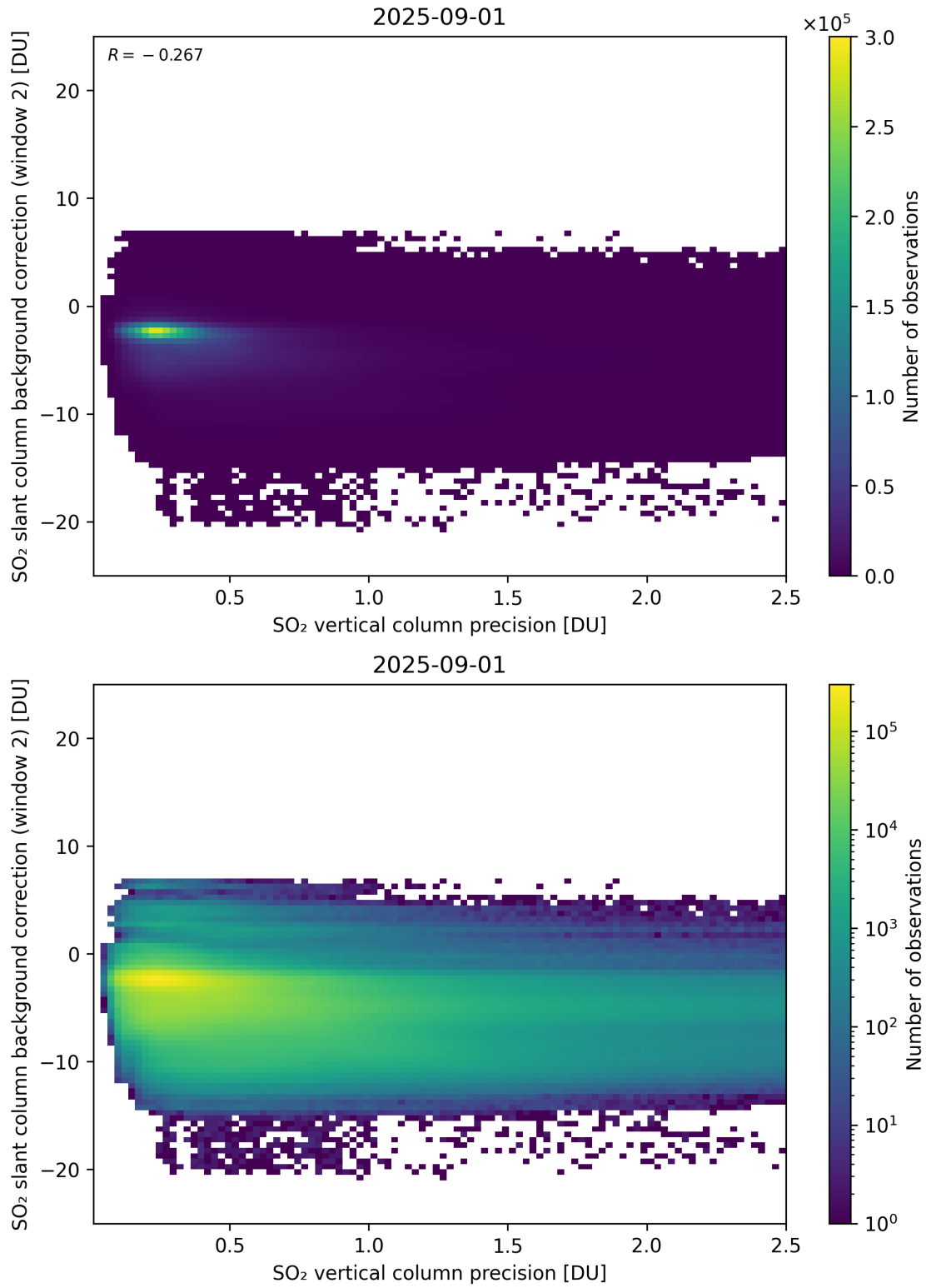
Figure 330: Scatter density plot of “SO 2 vertical column precision” against “SO 2 slant column background correction (window 2)” for 2025-08-31 to 2025-09-02.
