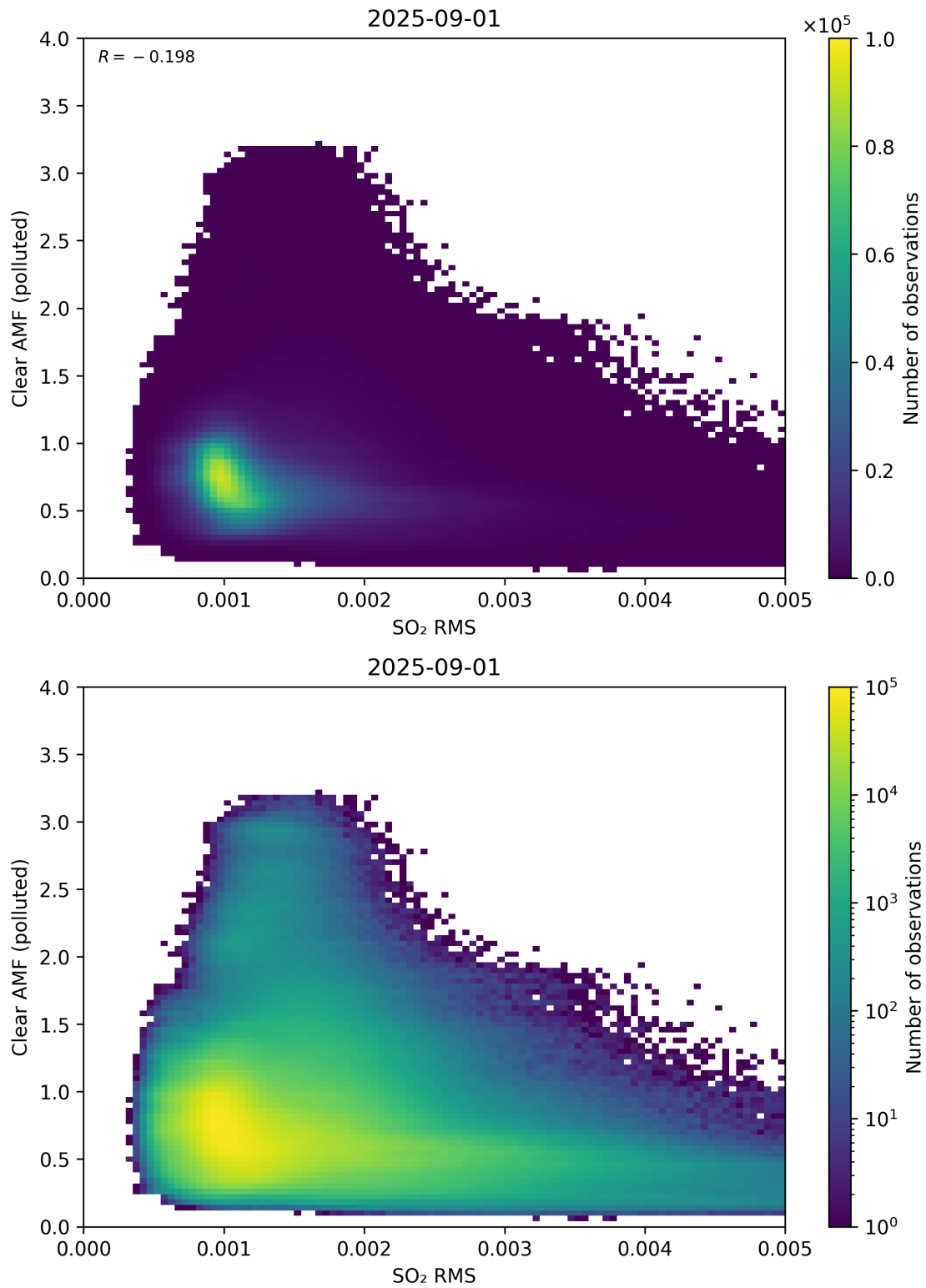
Figure 147: Scatter density plot of “SO 2 RMS” against “Clear AMF (polluted)” for 2025-08-31 to 2025-09-02.
