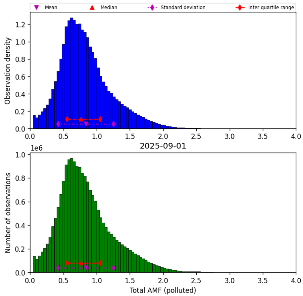
Figure 79: Histogram of “Total AMF (polluted)” for 2025-08-31 to 2025-09-02
