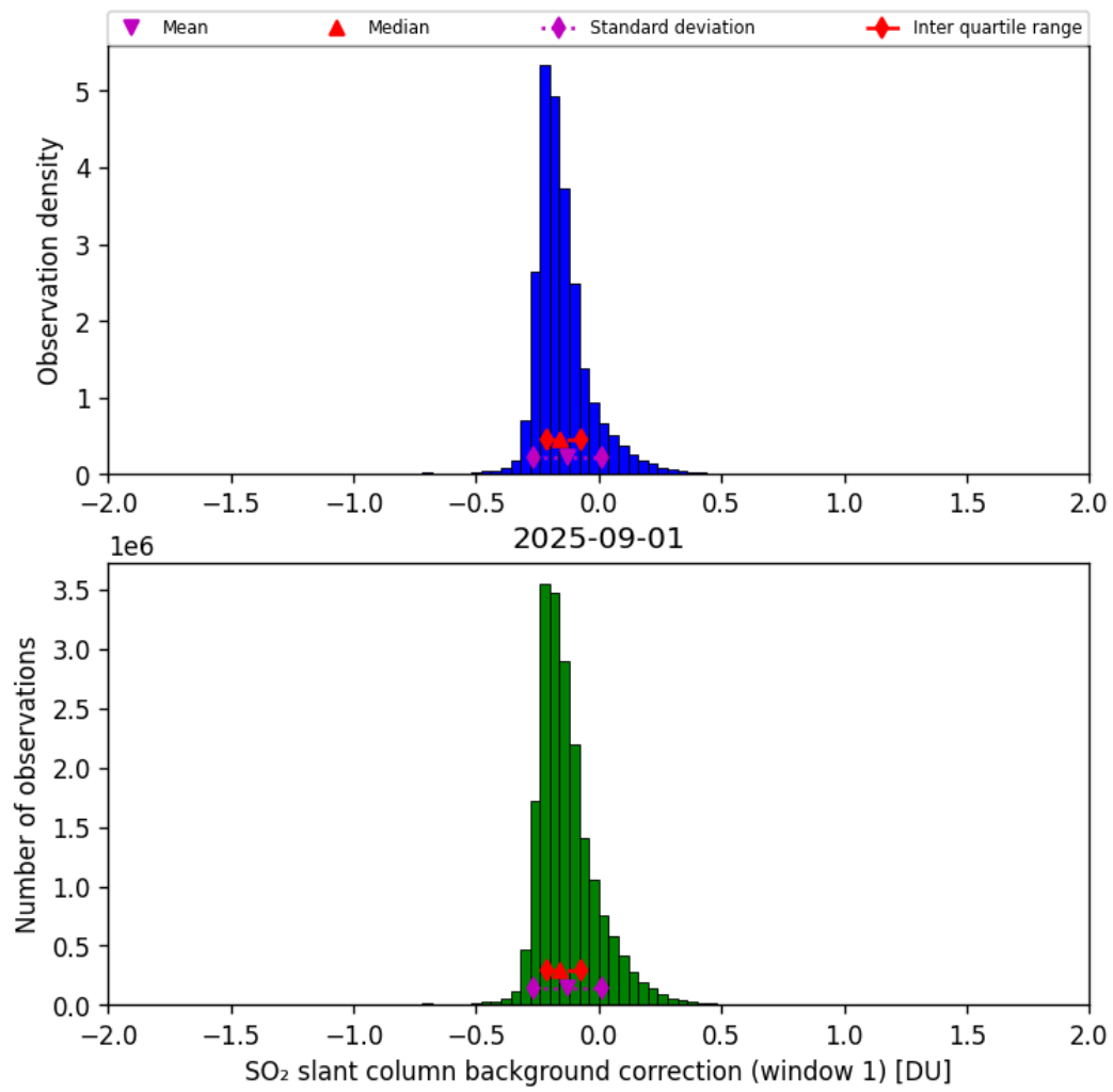
Figure 66: Histogram of “SO 2 slant column background correction (window 1)” for 2025-08-31 to 2025-09-02
