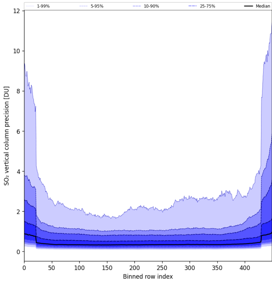
Figure 85: Along track statistics of “SO 2 vertical column precision” for 2025-08-31 to 2025-09-02
