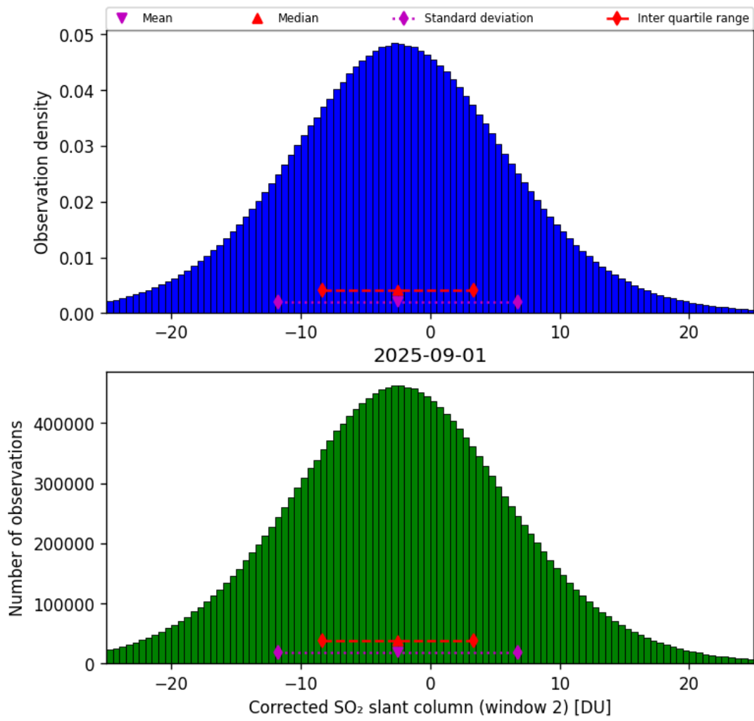
Figure 69: Histogram of “Corrected SO 2 slant column (window 2)” for 2025-08-31 to 2025-09-02
