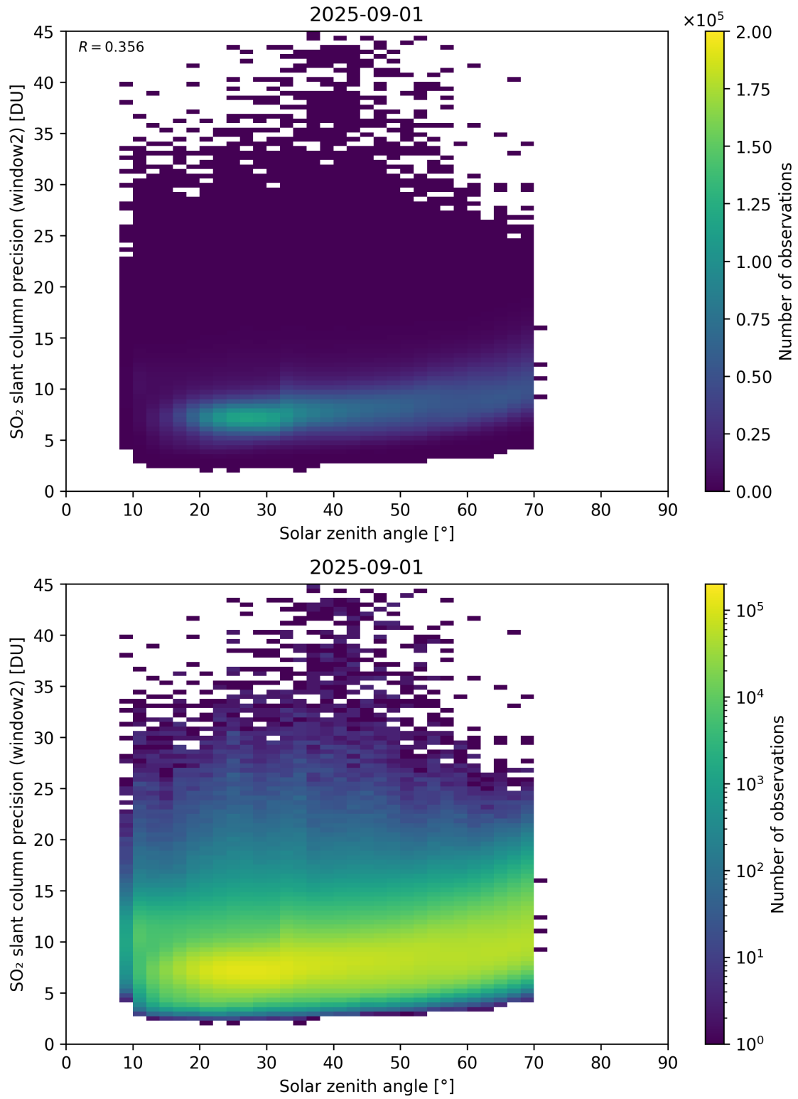
Figure 186: Scatter density plot of “Solar zenith angle” against “SO 2 slant column precision (window2)” for 2025-08-31 to 2025-09-02.
