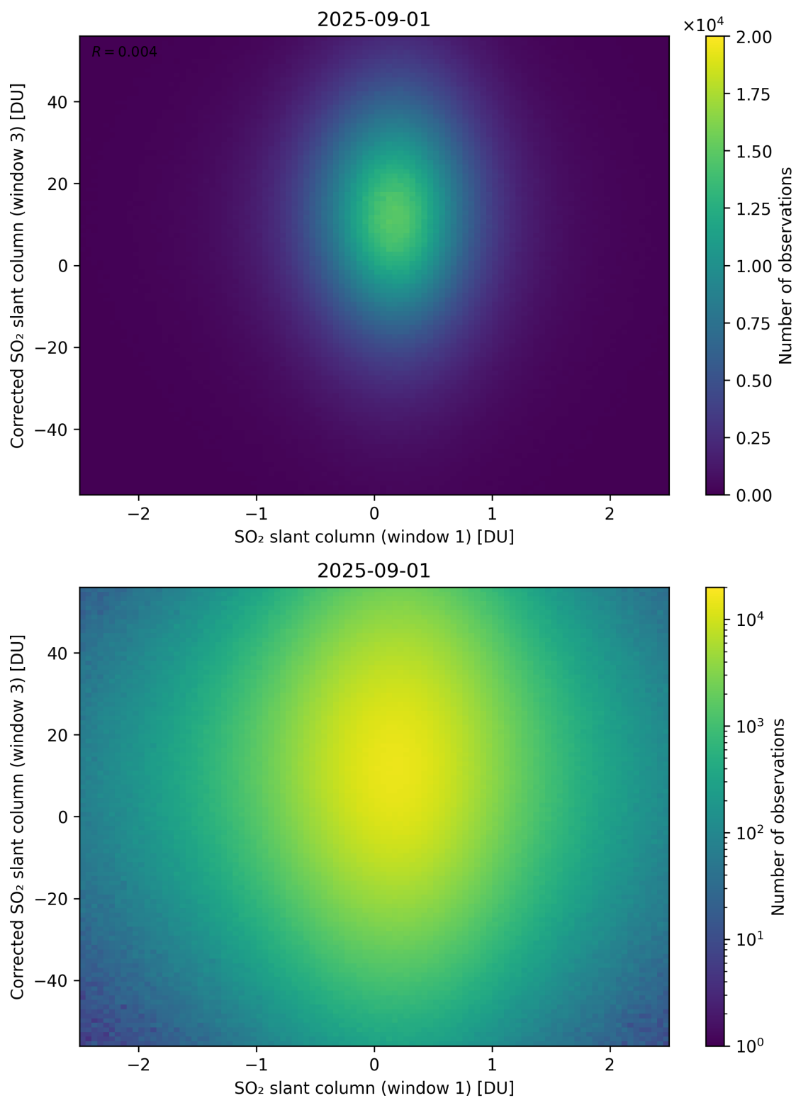
Figure 284: Scatter density plot of “SO 2 slant column (window 1)” against “Corrected SO 2 slant column (window 3)” for 2025-08-31 to 2025-09-02.
