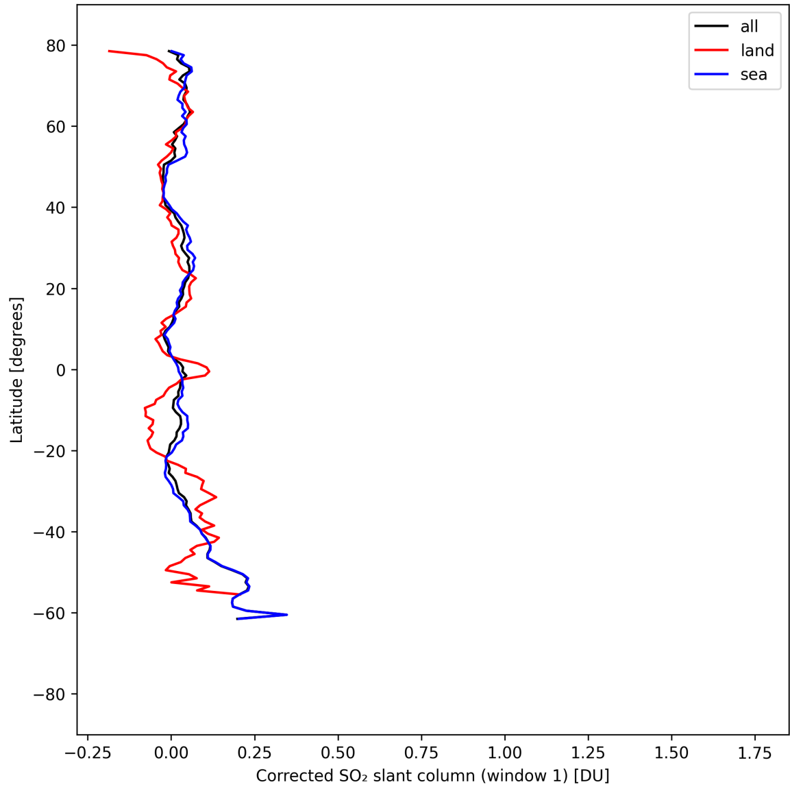
Figure 39: Zonal average of “Corrected SO 2 slant column (window 1)” for 2025-08-31 to 2025-09-02.
