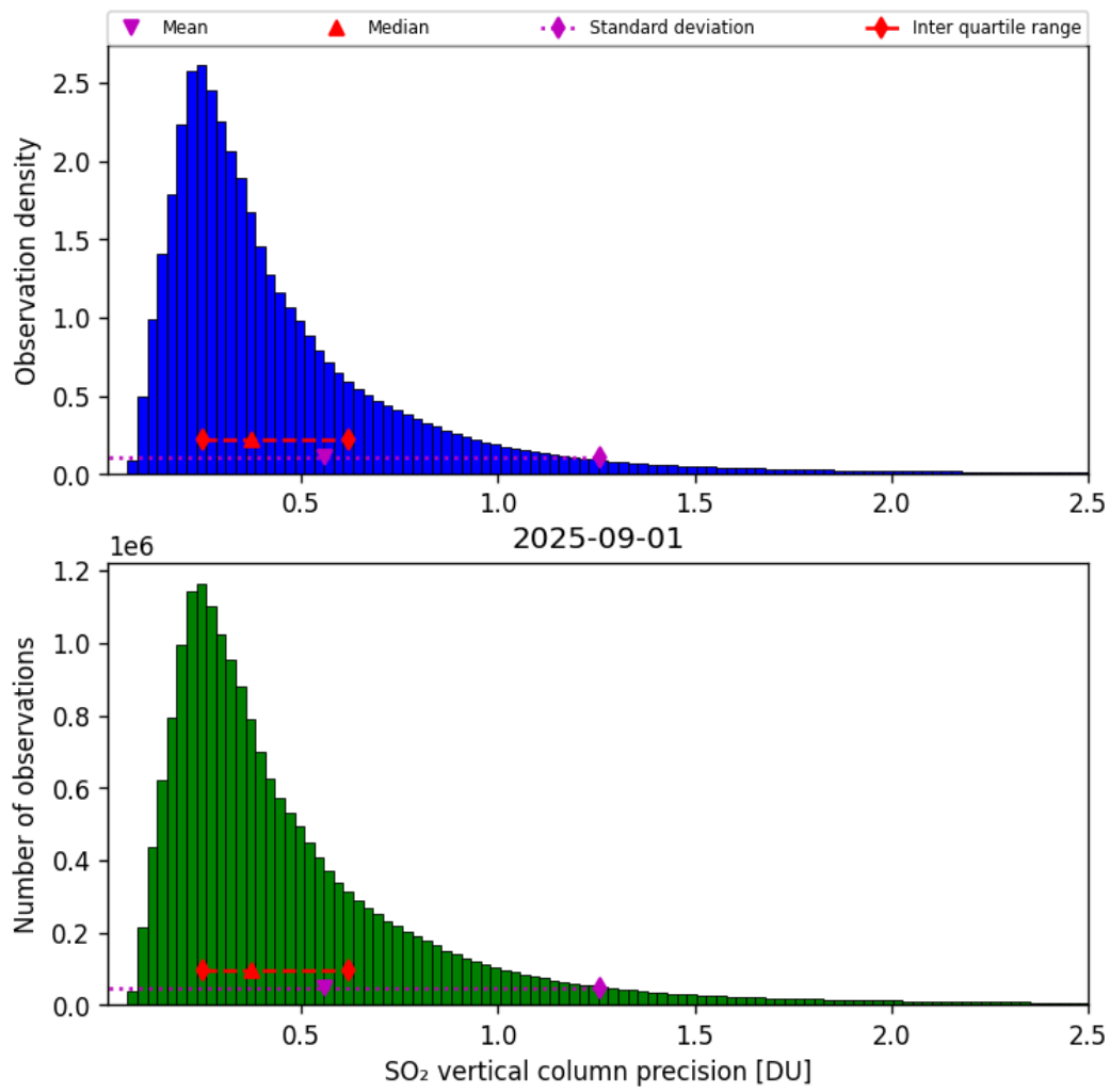
Figure 59: Histogram of “SO 2 vertical column precision” for 2025-08-31 to 2025-09-02
