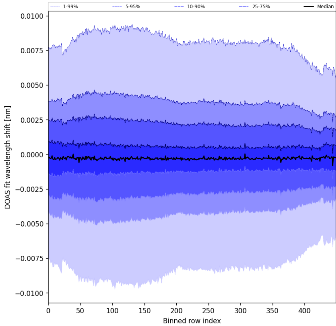
Figure 102: Along track statistics of “DOAS fit wavelength shift” for 2025-08-31 to 2025-09-02
