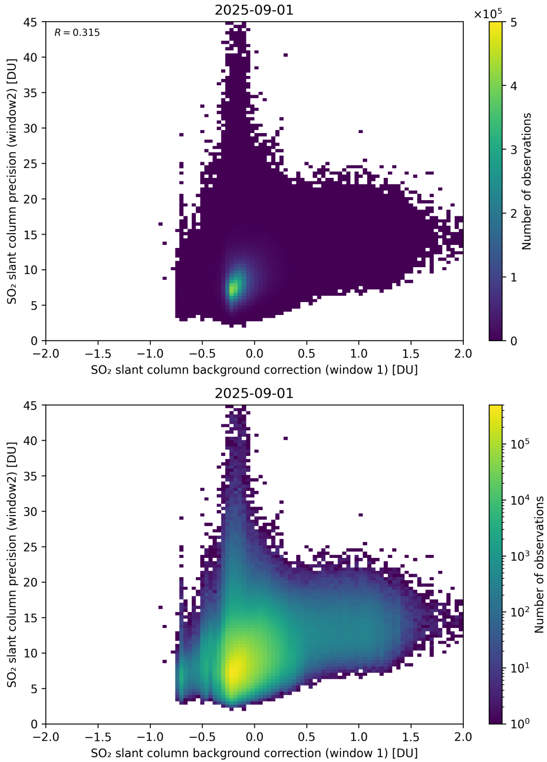
Figure 117: Scatter density plot of “SO 2 slant column background correction (window 1)” against “SO 2 slant column precision (window2)” for 2025-08-31 to 2025-09-02.
