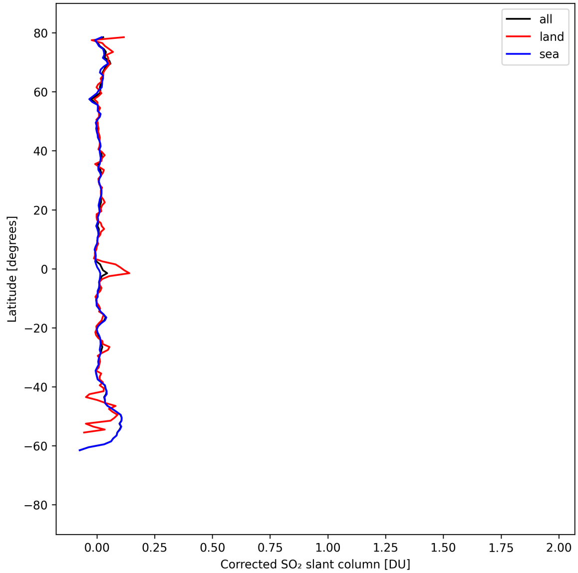
Figure 34: Zonal average of “Corrected SO 2 slant column” for 2025-08-31 to 2025-09-02.
