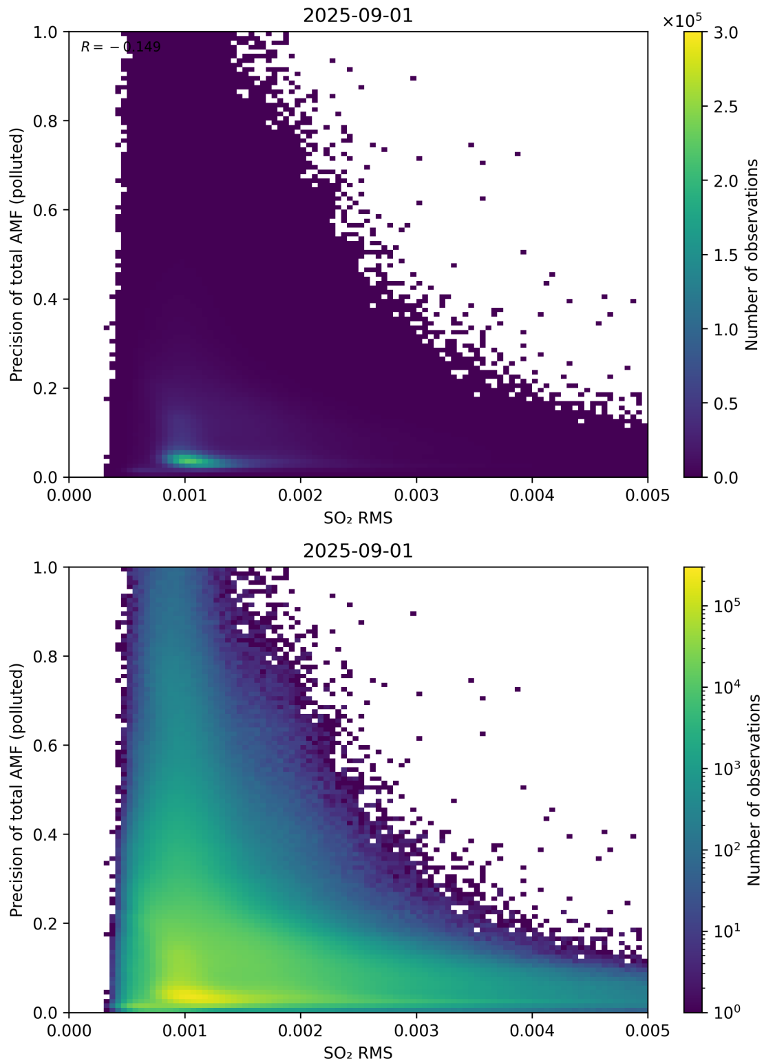
Figure 149: Scatter density plot of “SO 2 RMS” against “Precision of total AMF (polluted)” for 2025-08-31 to 2025-09-02.
