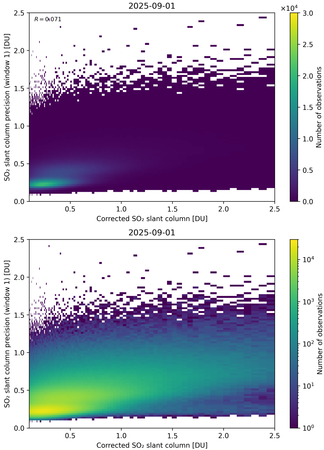
Figure 238: Scatter density plot of “Corrected SO 2 slant column” against “SO 2 slant column precision (window 1)” for 2025-08-31 to 2025-09-02.
