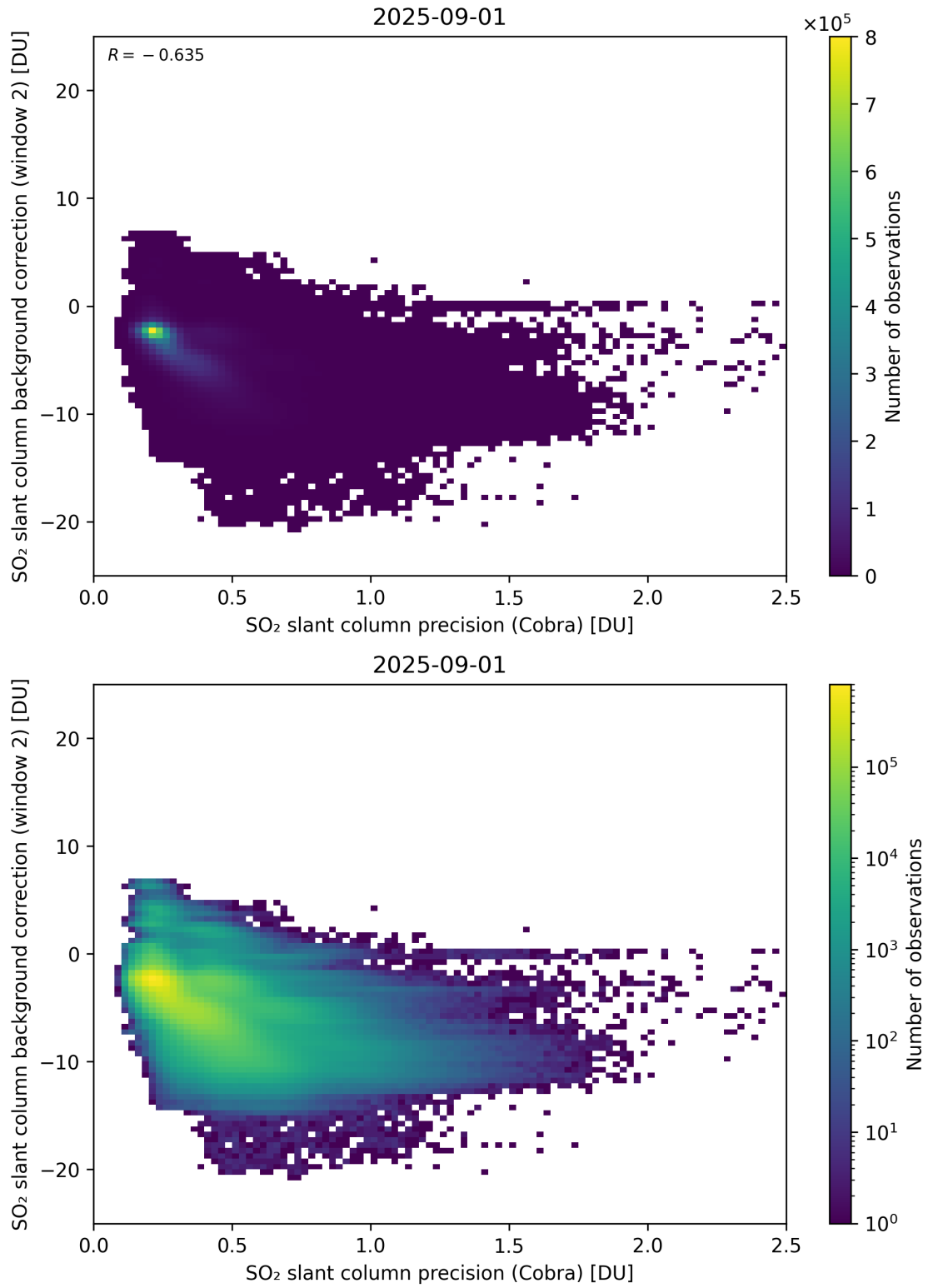
Figure 200: Scatter density plot of “SO 2 slant column precision (Cobra)” against “SO 2 slant column background correction (window 2)” for 2025-08-31 to 2025-09-02.
