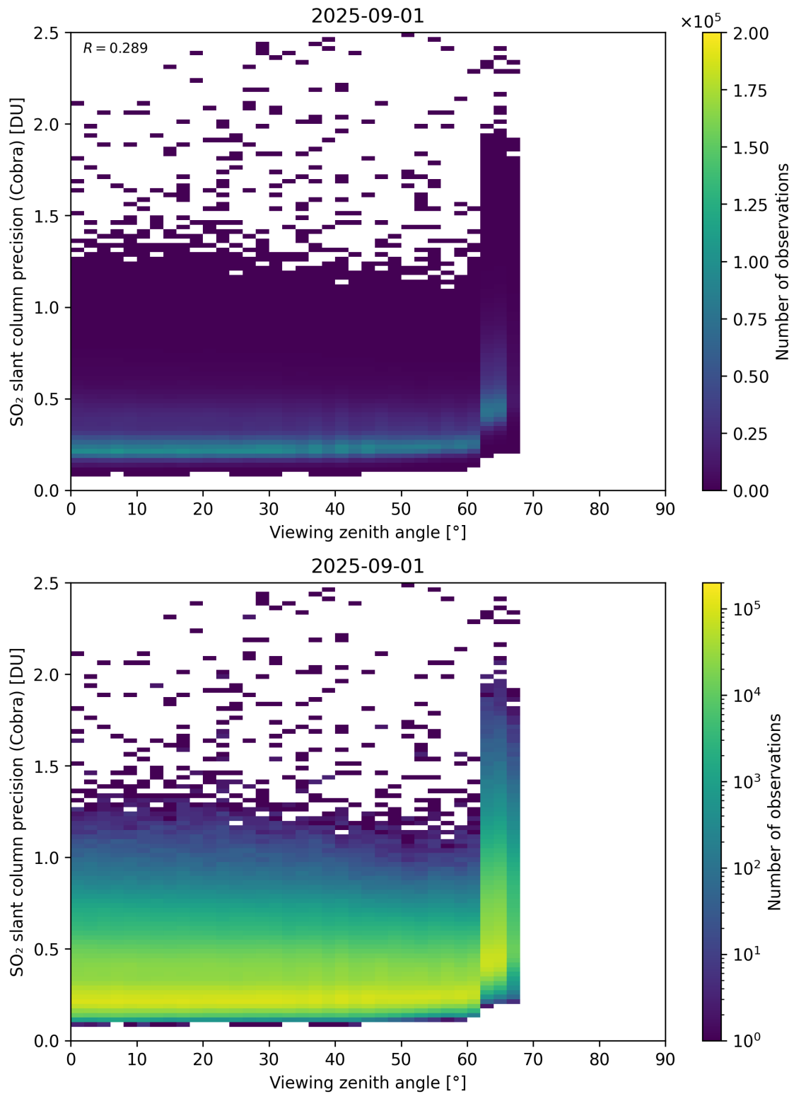
Figure 372: Scatter density plot of “Viewing zenith angle” against “SO 2 slant column precision (Cobra)” for 2025-08-31 to 2025-09-02.
