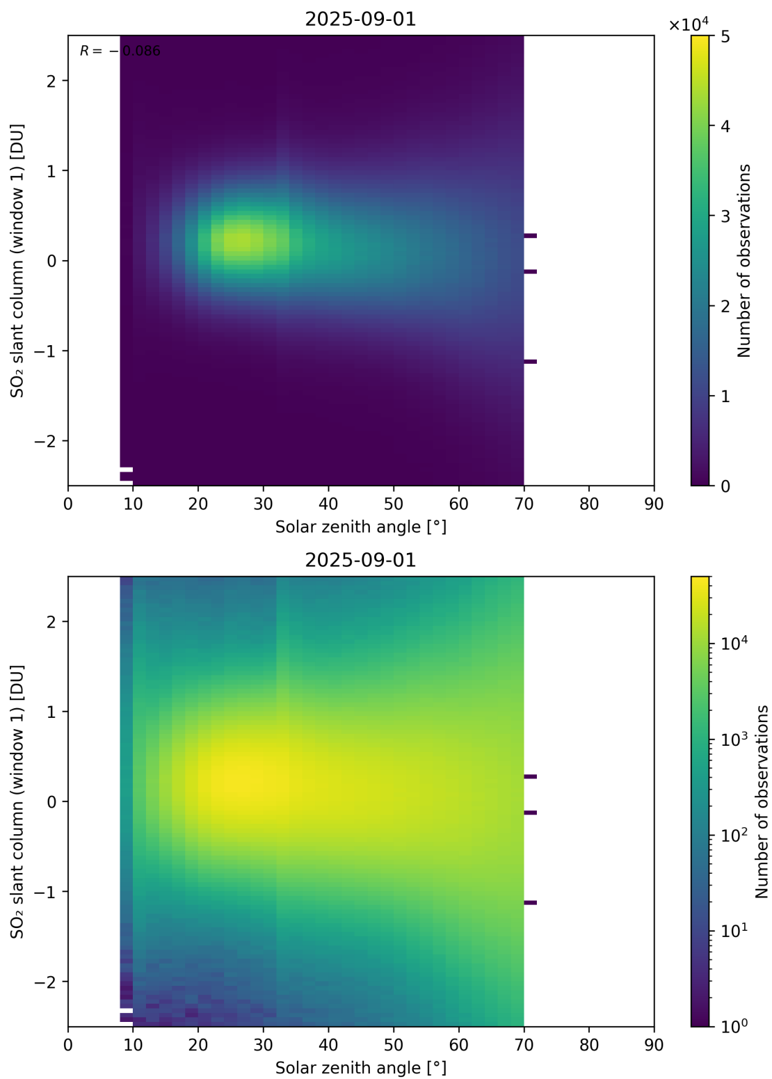
Figure 184: Scatter density plot of “Solar zenith angle” against “SO 2 slant column (window 1)” for 2025-08-31 to 2025-09-02.
