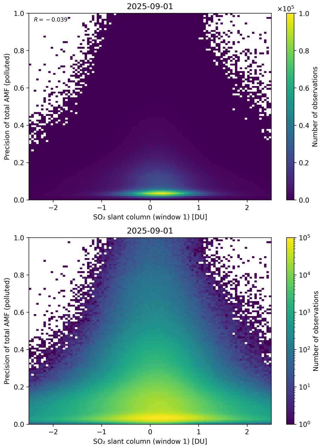
Figure 290: Scatter density plot of “SO 2 slant column (window 1)” against “Precision of total AMF (polluted)” for 2025-08-31 to 2025-09-02.
