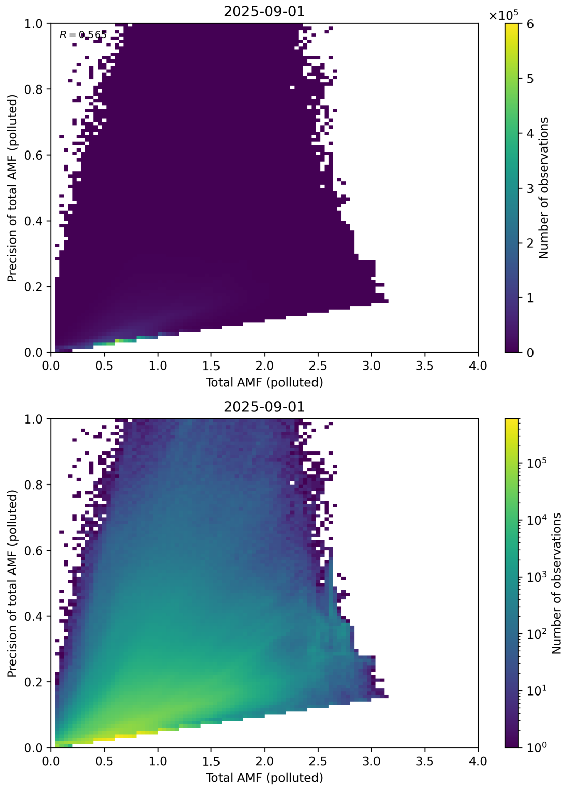
Figure 322: Scatter density plot of “Total AMF (polluted)” against “Precision of total AMF (polluted)” for 2025-08-31 to 2025-09-02.
