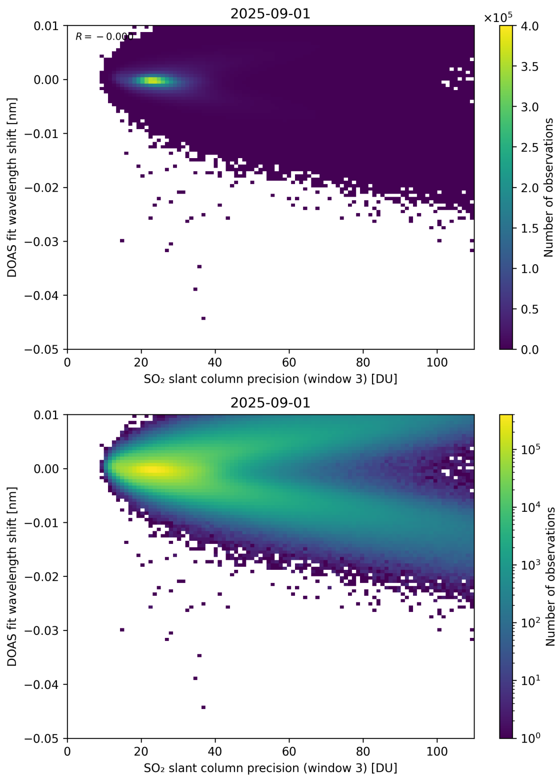
Figure 308: Scatter density plot of “SO 2 slant column precision (window 3)” against “DOAS fit wavelength shift” for 2025-08-31 to 2025-09-02.
