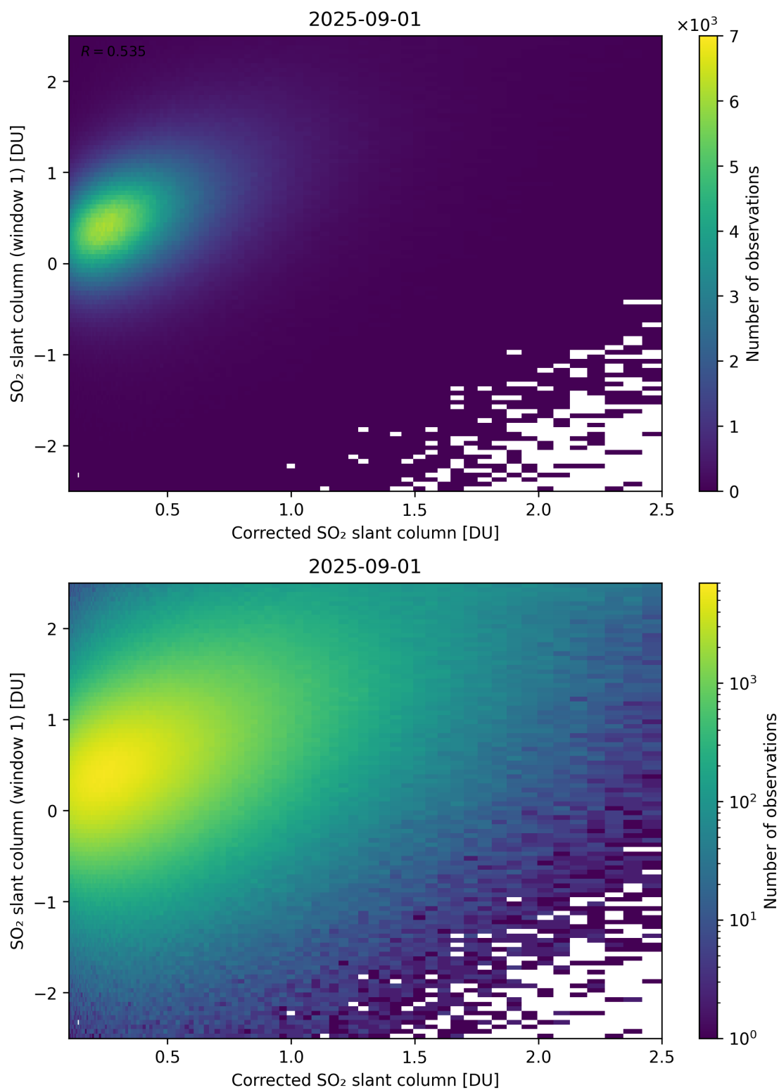
Figure 237: Scatter density plot of “Corrected SO 2 slant column” against “SO 2 slant column (window 1)” for 2025-08-31 to 2025-09-02.
