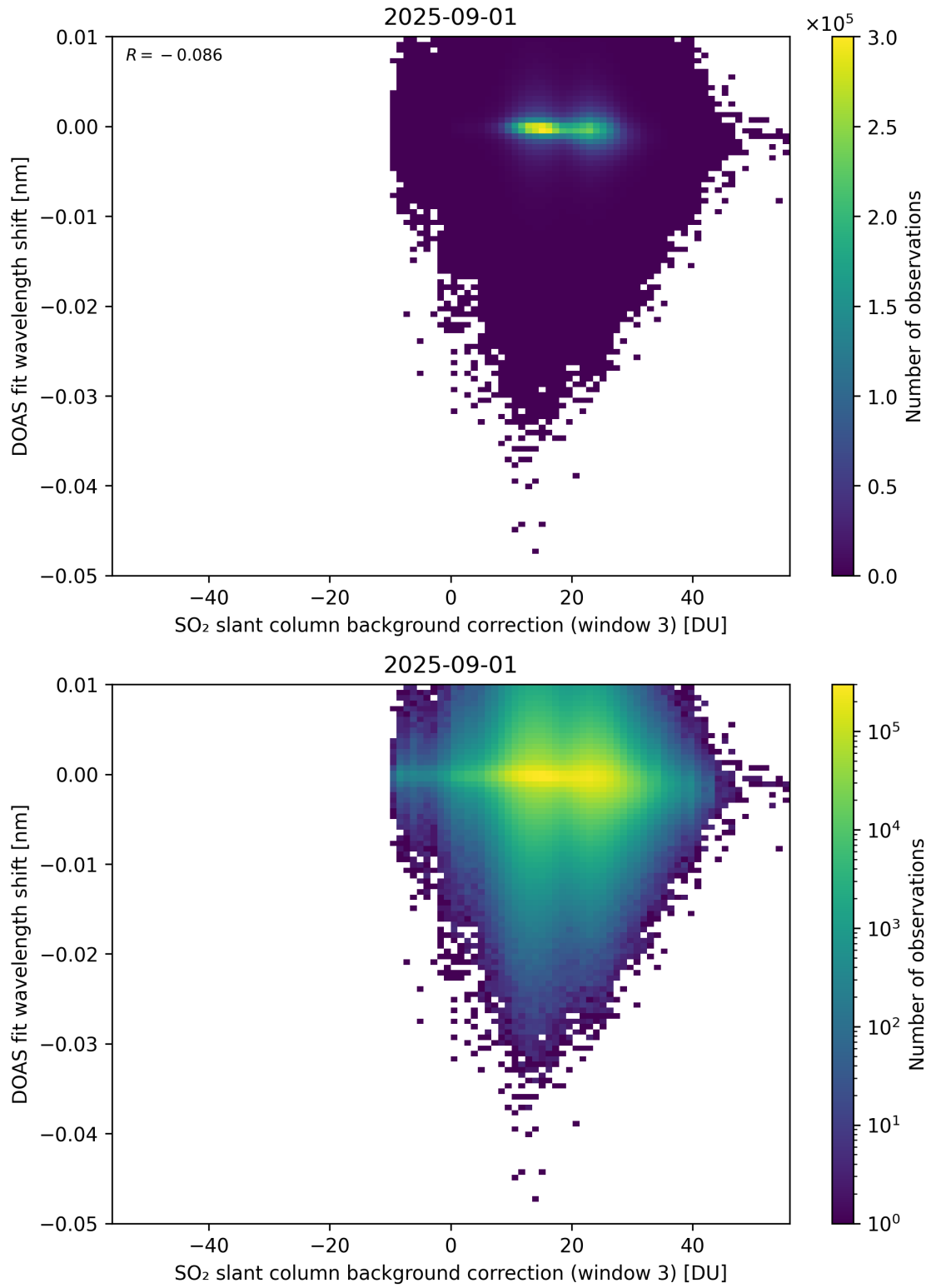
Figure 132: Scatter density plot of “SO 2 slant column background correction (window 3)” against “DOAS fit wavelength shift” for 2025-08-31 to 2025-09-02.
