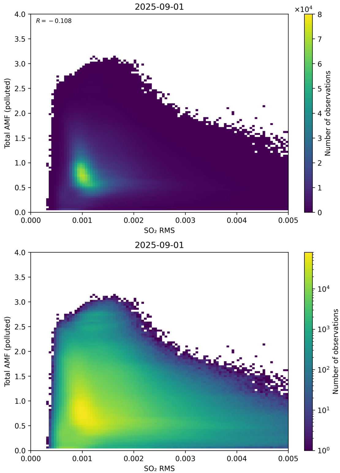
Figure 148: Scatter density plot of “SO 2 RMS” against “Total AMF (polluted)” for 2025-08-31 to 2025-09-02.
