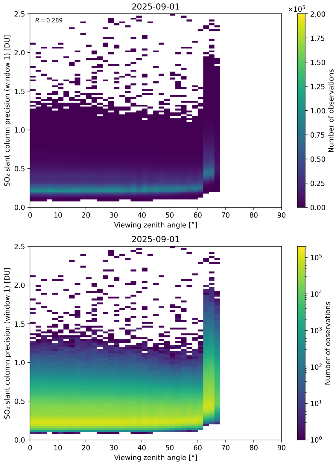
Figure 377: Scatter density plot of “Viewing zenith angle” against “SO 2 slant column precision (window 1)” for 2025-08-31 to 2025-09-02.
