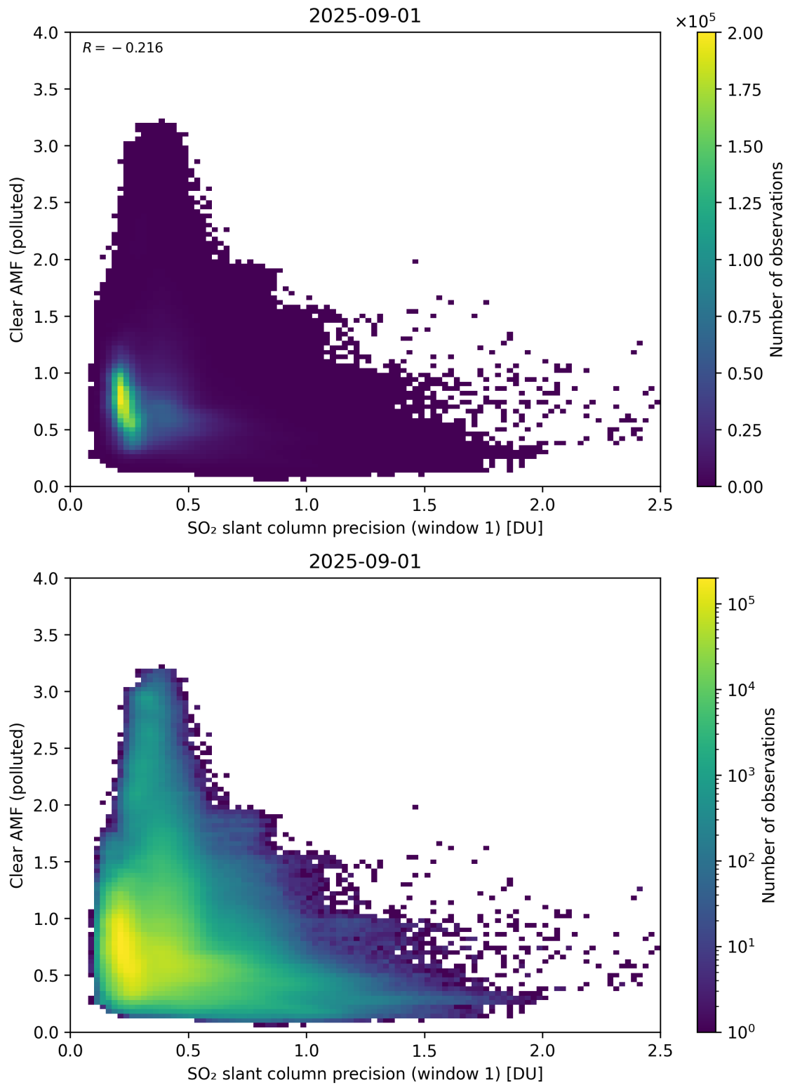
Figure 274: Scatter density plot of “SO 2 slant column precision (window 1)” against “Clear AMF (polluted)” for 2025-08-31 to 2025-09-02.
