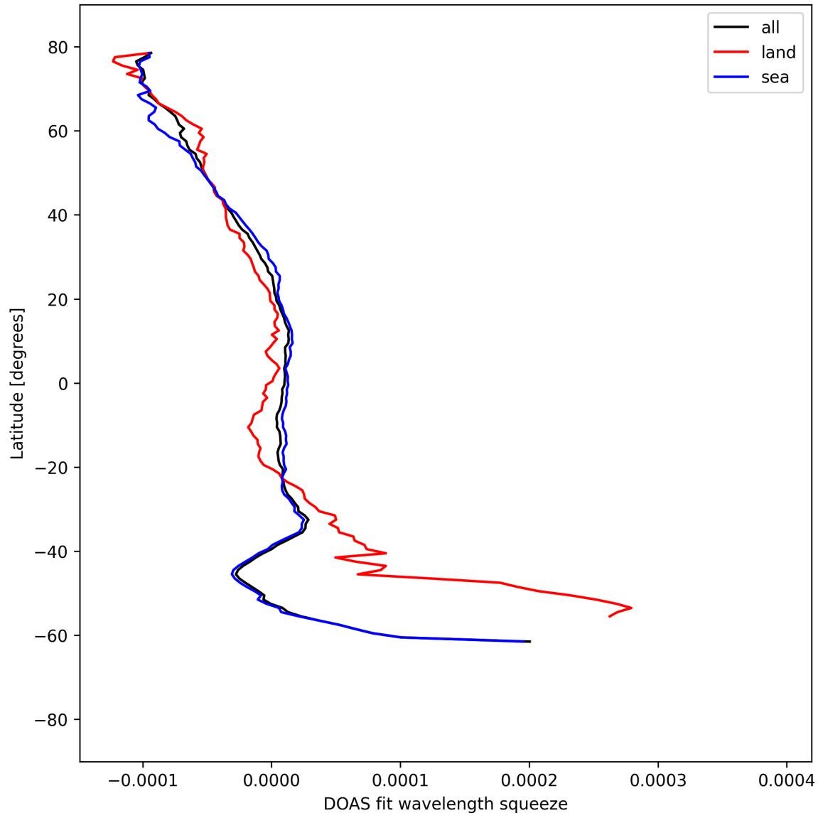
Figure 51: Zonal average of “DOAS fit wavelength squeeze” for 2025-08-31 to 2025-09-02.
