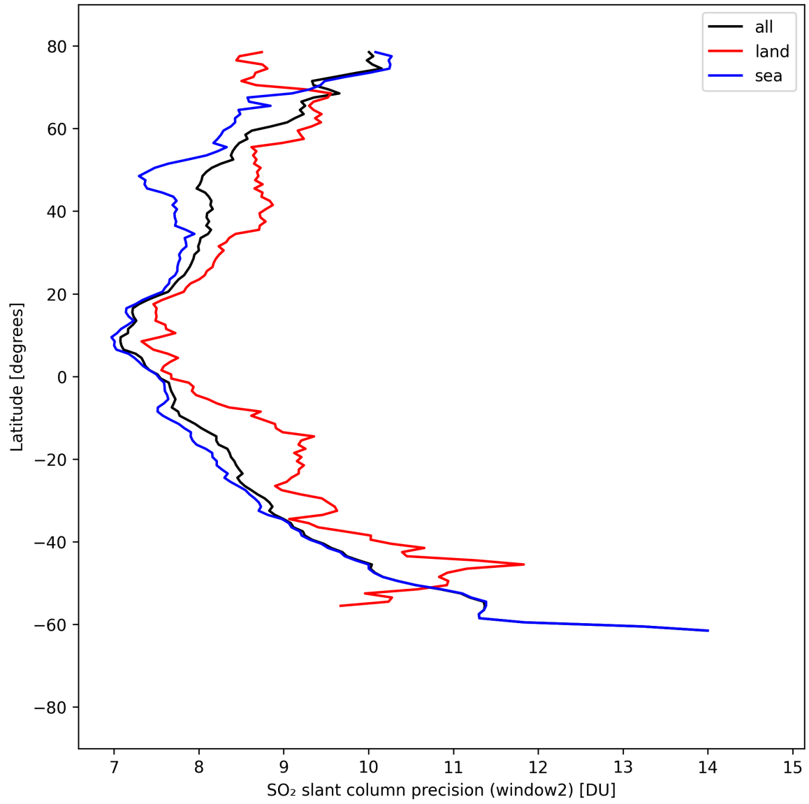
Figure 42: Zonal average of “SO 2 slant column precision (window2)” for 2025-08-31 to 2025-09-02.
