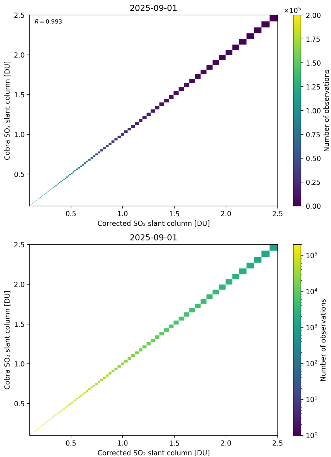
Figure 233: Scatter density plot of “Corrected SO 2 slant column” against “Cobra SO 2 slant column” for 2025-08-31 to 2025-09-02.
