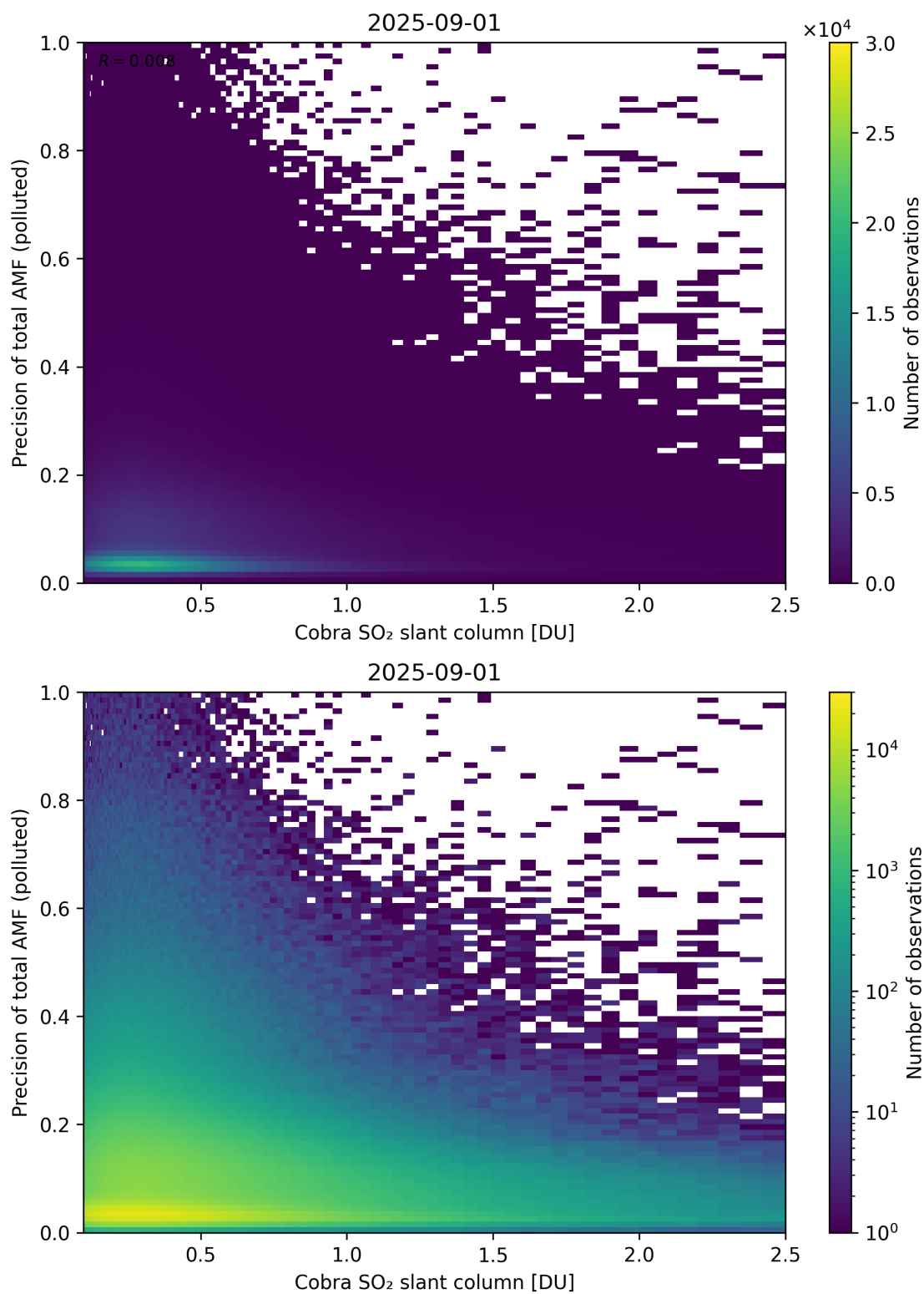
Figure 225: Scatter density plot of “Cobra SO 2 slant column” against “Precision of total AMF (polluted)” for 2025-08-31 to 2025-09-02.
