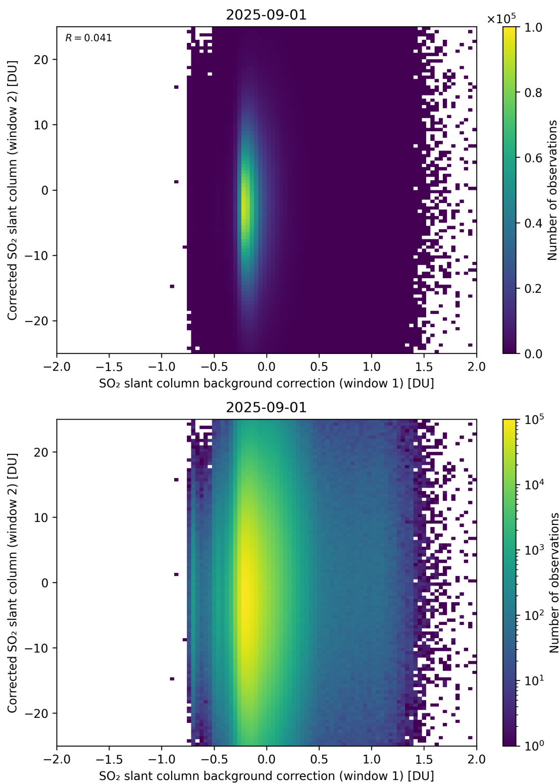
Figure 115: Scatter density plot of “SO 2 slant column background correction (window 1)” against “Corrected SO 2 slant column (window 2)” for 2025-08-31 to 2025-09-02.
