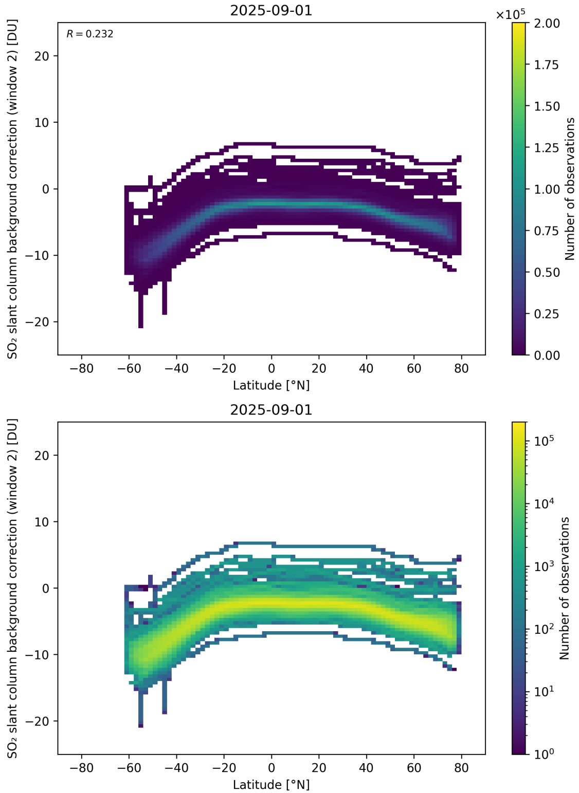
Figure 151: Scatter density plot of “Latitude” against “SO 2 slant column background correction (window 2)” for 2025-08-31 to 2025-09-02.
