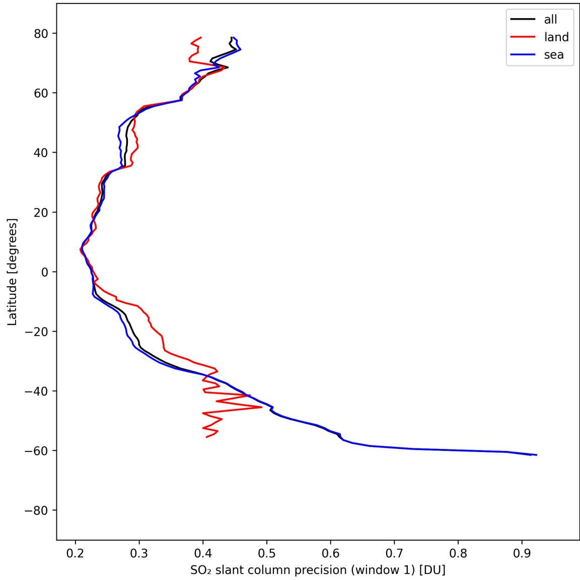
Figure 38: Zonal average of “SO 2 slant column precision (window 1)” for 2025-08-31 to 2025-09-02.
