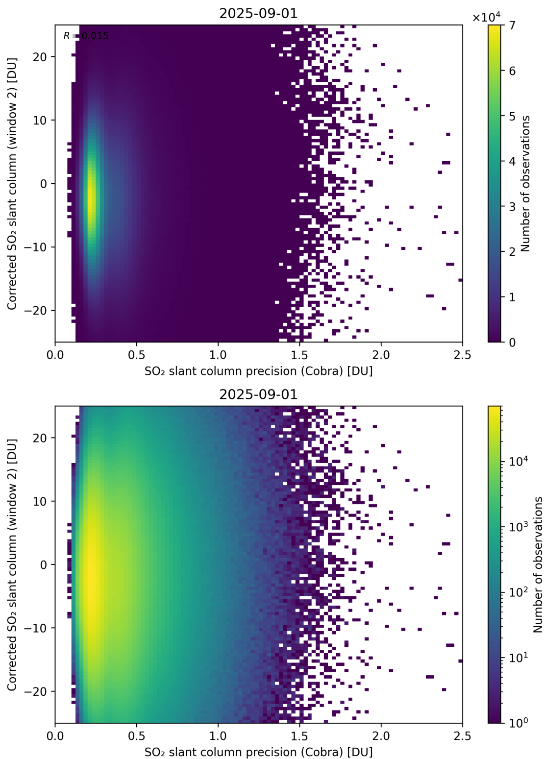
Figure 206: Scatter density plot of “SO 2 slant column precision (Cobra)” against “Corrected SO 2 slant column (window 2)” for 2025-08-31 to 2025-09-02.
