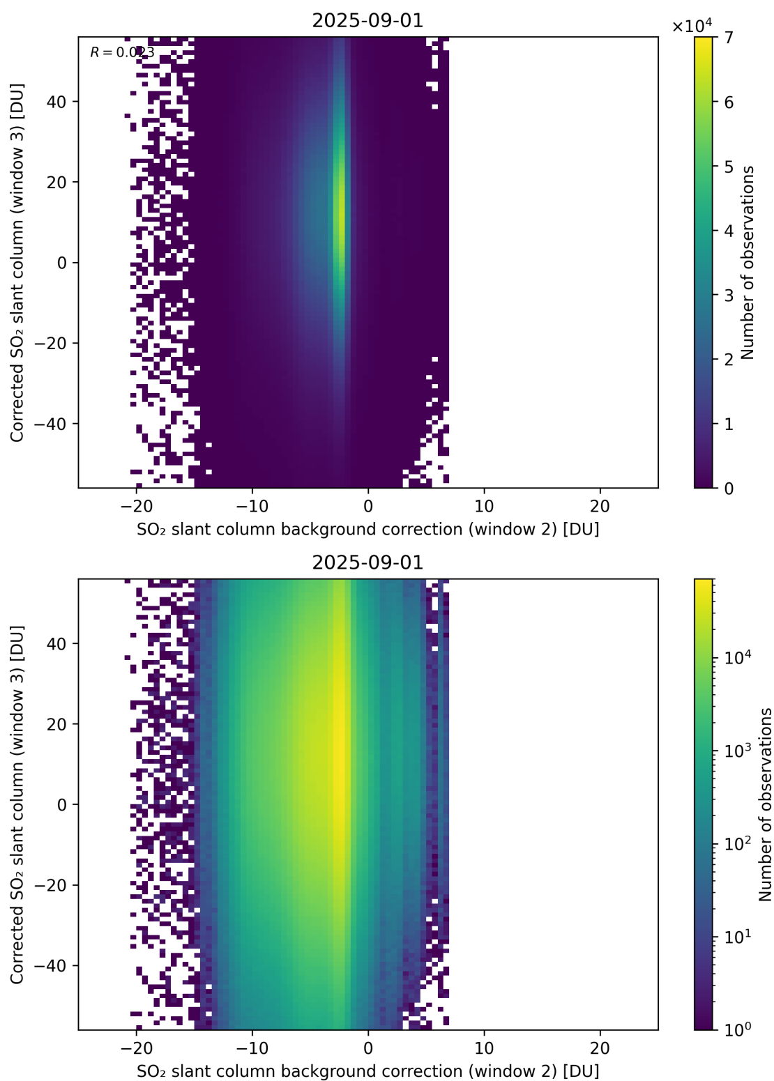
Figure 127: Scatter density plot of “SO 2 slant column background correction (window 2)” against “Corrected SO 2 slant column (window 3)” for 2025-08-31 to 2025-09-02.
