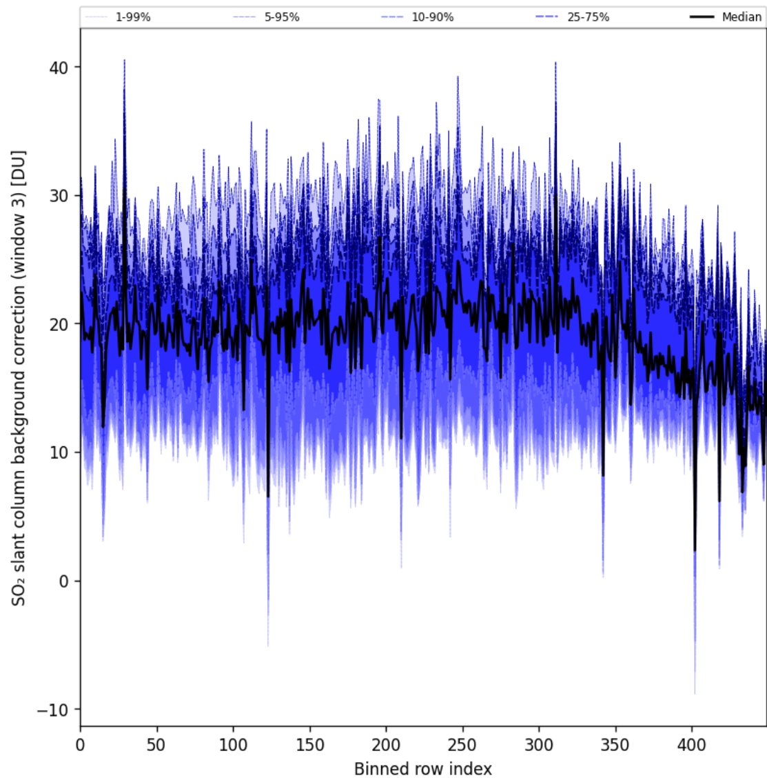
Figure 100: Along track statistics of “SO 2 slant column background correction (window 3)” for 2025-08-31 to 2025-09-02
