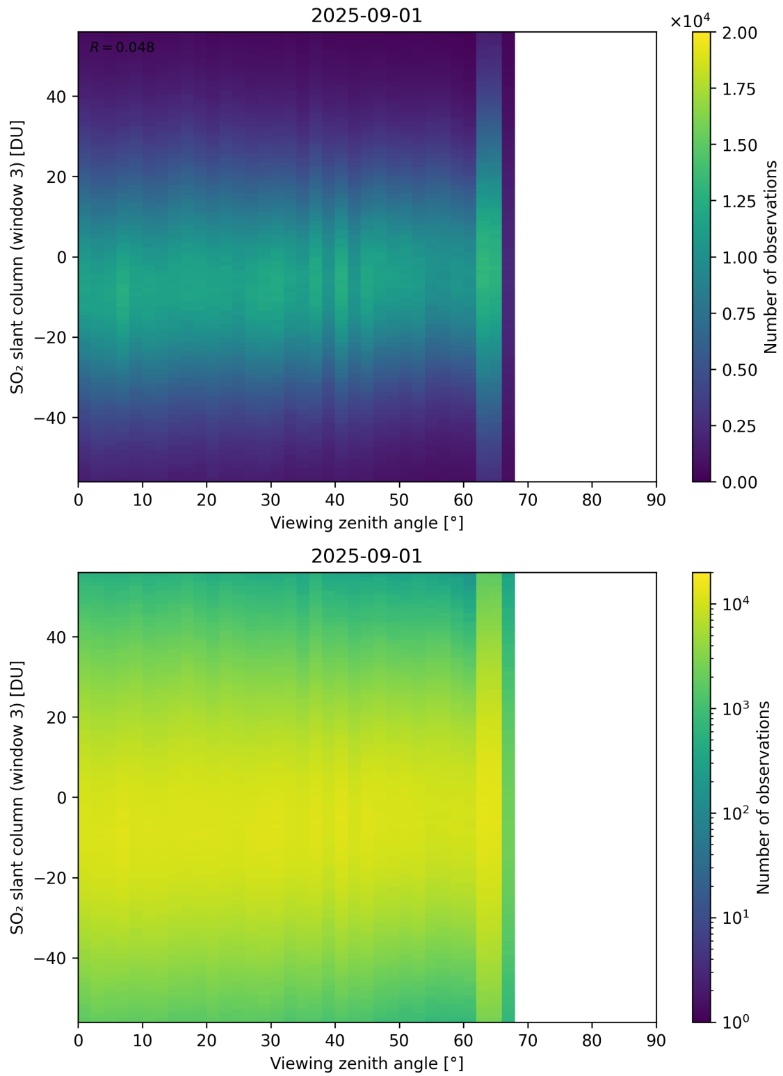
Figure 379: Scatter density plot of “Viewing zenith angle” against “SO 2 slant column (window 3)” for 2025-08-31 to 2025-09-02.
