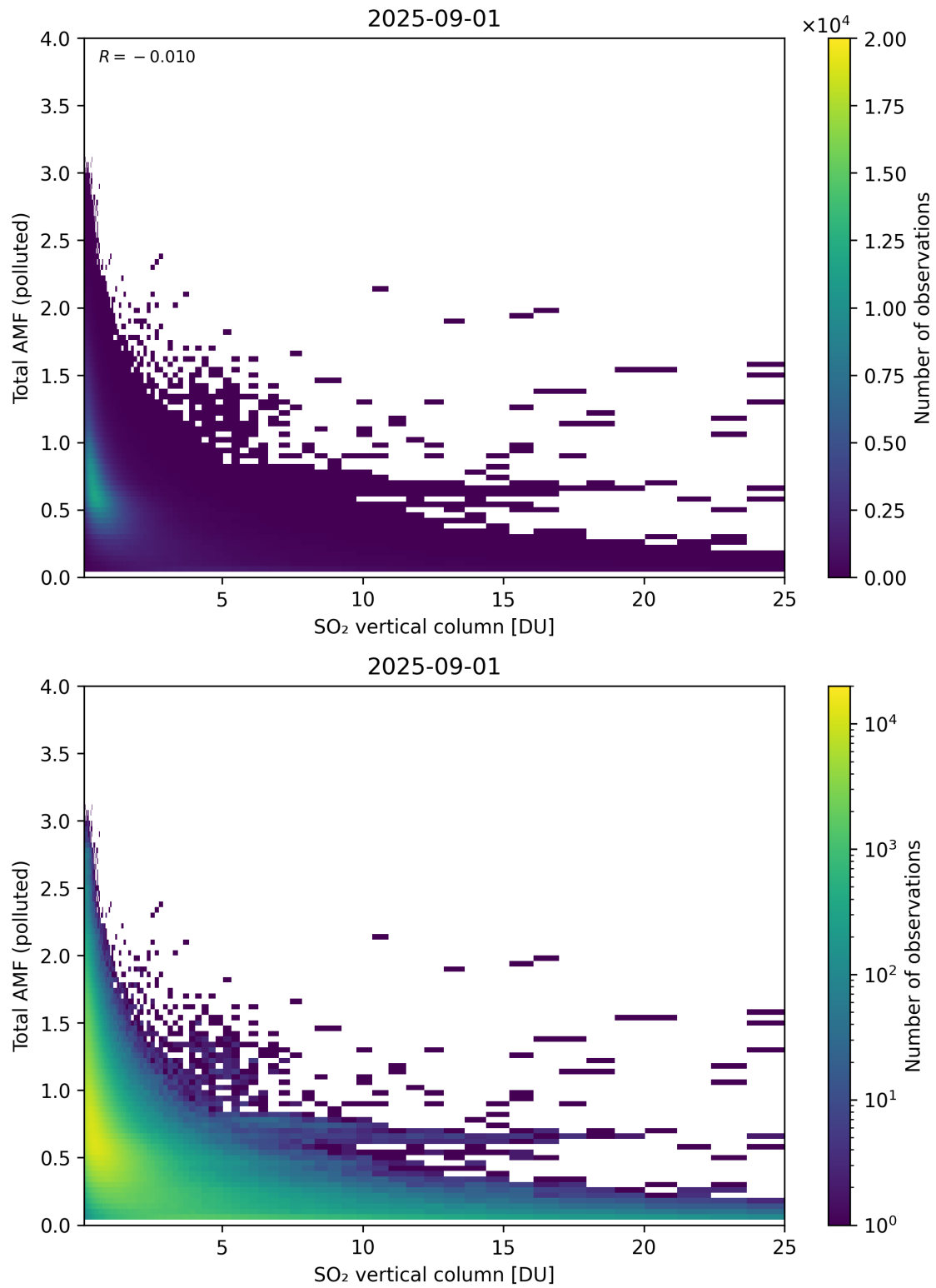
Figure 359: Scatter density plot of “SO 2 vertical column” against “Total AMF (polluted)” for 2025-08-31 to 2025-09-02.
