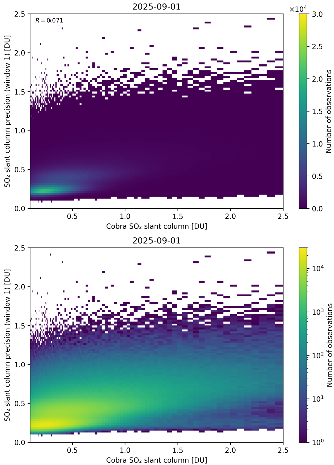
Figure 220: Scatter density plot of “Cobra SO 2 slant column” against “SO 2 slant column precision (window 1)” for 2025-08-31 to 2025-09-02.
