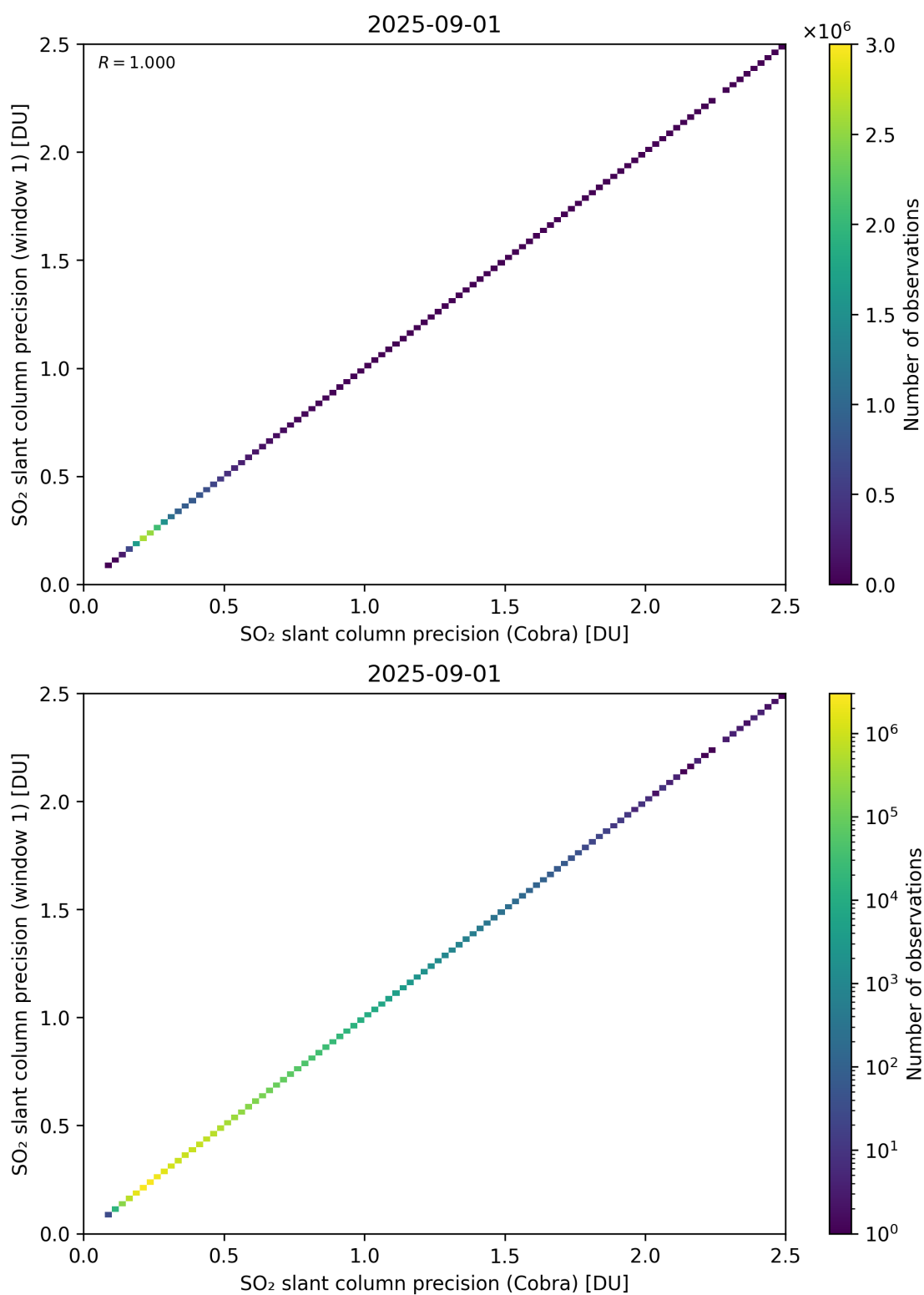
Figure 209: Scatter density plot of “SO 2 slant column precision (Cobra)” against “SO 2 slant column precision (window 1)” for 2025-08-31 to 2025-09-02.
