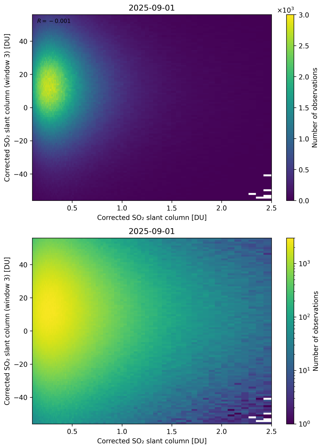
Figure 236: Scatter density plot of “Corrected SO 2 slant column” against “Corrected SO 2 slant column (window 3)” for 2025-08-31 to 2025-09-02.
