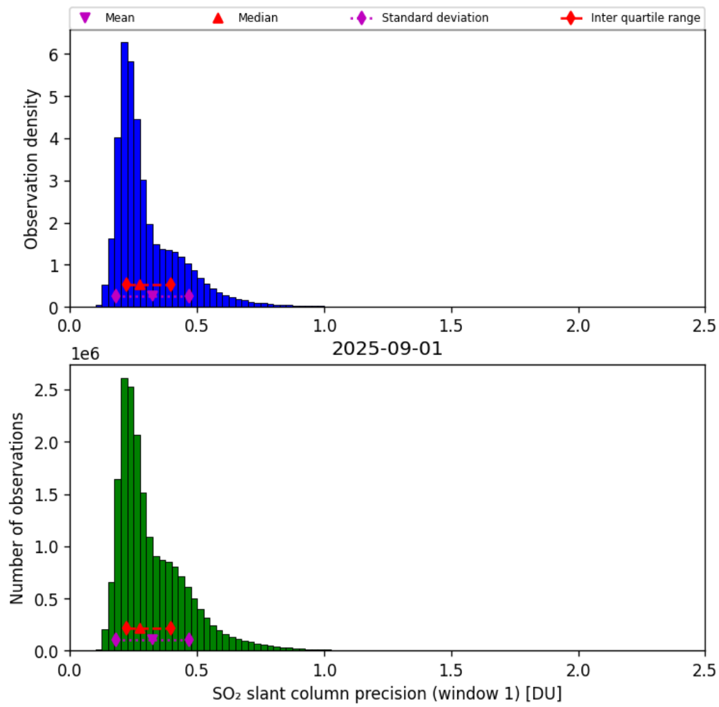
Figure 64: Histogram of “SO 2 slant column precision (window 1)” for 2025-08-31 to 2025-09-02
