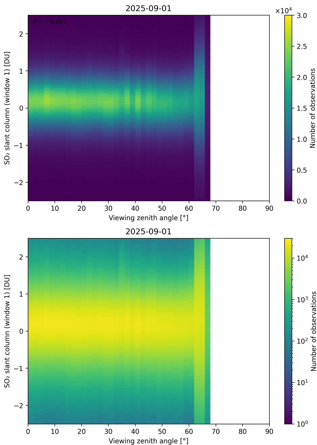
Figure 376: Scatter density plot of “Viewing zenith angle” against “SO 2 slant column (window 1)” for 2025-08-31 to 2025-09-02.
