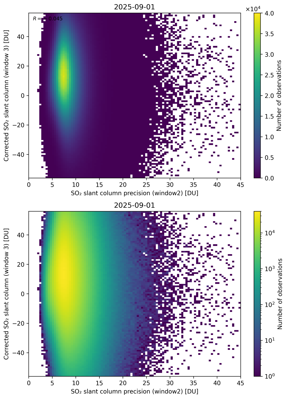
Figure 298: Scatter density plot of “SO 2 slant column precision (window2)” against “Corrected SO 2 slant column (window 3)” for 2025-08-31 to 2025-09-02.
