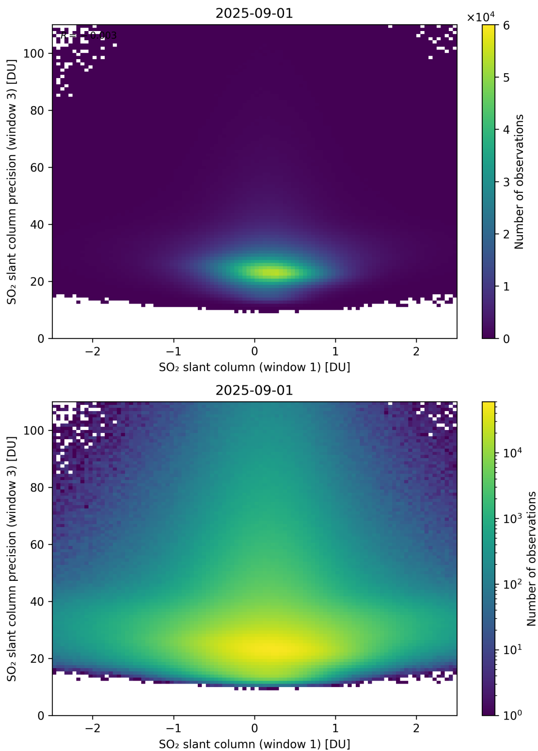
Figure 288: Scatter density plot of “SO 2 slant column (window 1)” against “SO 2 slant column precision (window 3)” for 2025-08-31 to 2025-09-02.
