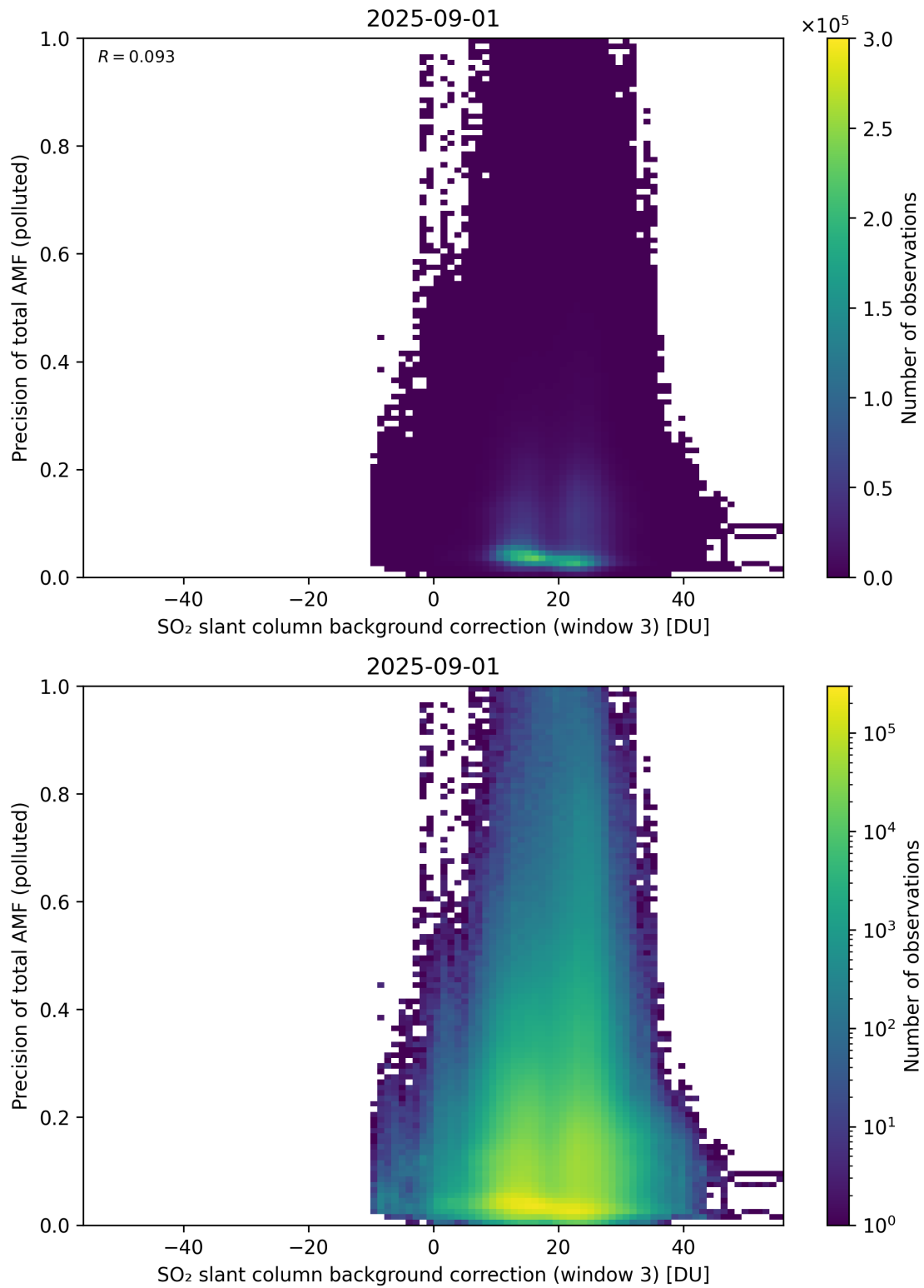
Figure 137: Scatter density plot of “SO 2 slant column background correction (window 3)” against “Precision of total AMF (polluted)” for 2025-08-31 to 2025-09-02.
