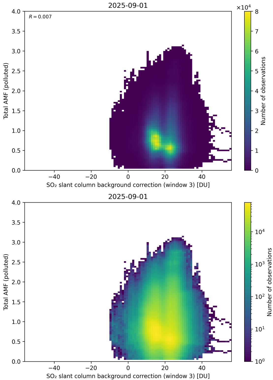
Figure 136: Scatter density plot of “SO 2 slant column background correction (window 3)” against “Total AMF (polluted)” for 2025-08-31 to 2025-09-02.
