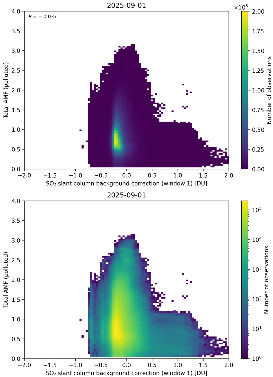
Figure 120: Scatter density plot of “SO 2 slant column background correction (window 1)” against “Total AMF (polluted)” for 2025-08-31 to 2025-09-02.
