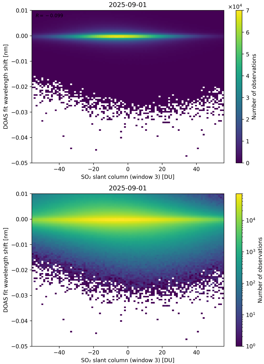
Figure 304: Scatter density plot of “SO 2 slant column (window 3)” against “DOAS fit wavelength shift” for 2025-08-31 to 2025-09-02.
