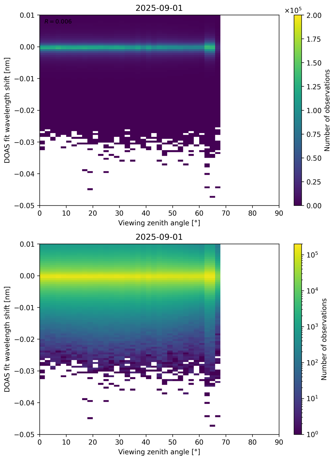
Figure 365: Scatter density plot of “Viewing zenith angle” against “DOAS fit wavelength shift” for 2025-08-31 to 2025-09-02.
