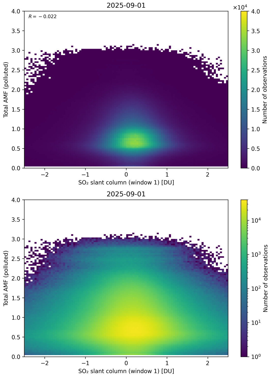
Figure 289: Scatter density plot of “SO 2 slant column (window 1)” against “Total AMF (polluted)” for 2025-08-31 to 2025-09-02.
