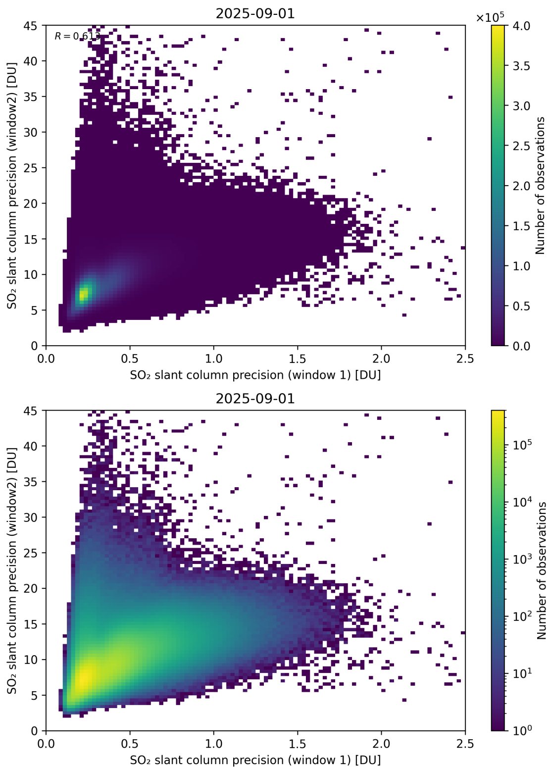
Figure 277: Scatter density plot of “SO 2 slant column precision (window 1)” against “SO 2 slant column precision (window2)” for 2025-08-31 to 2025-09-02.
