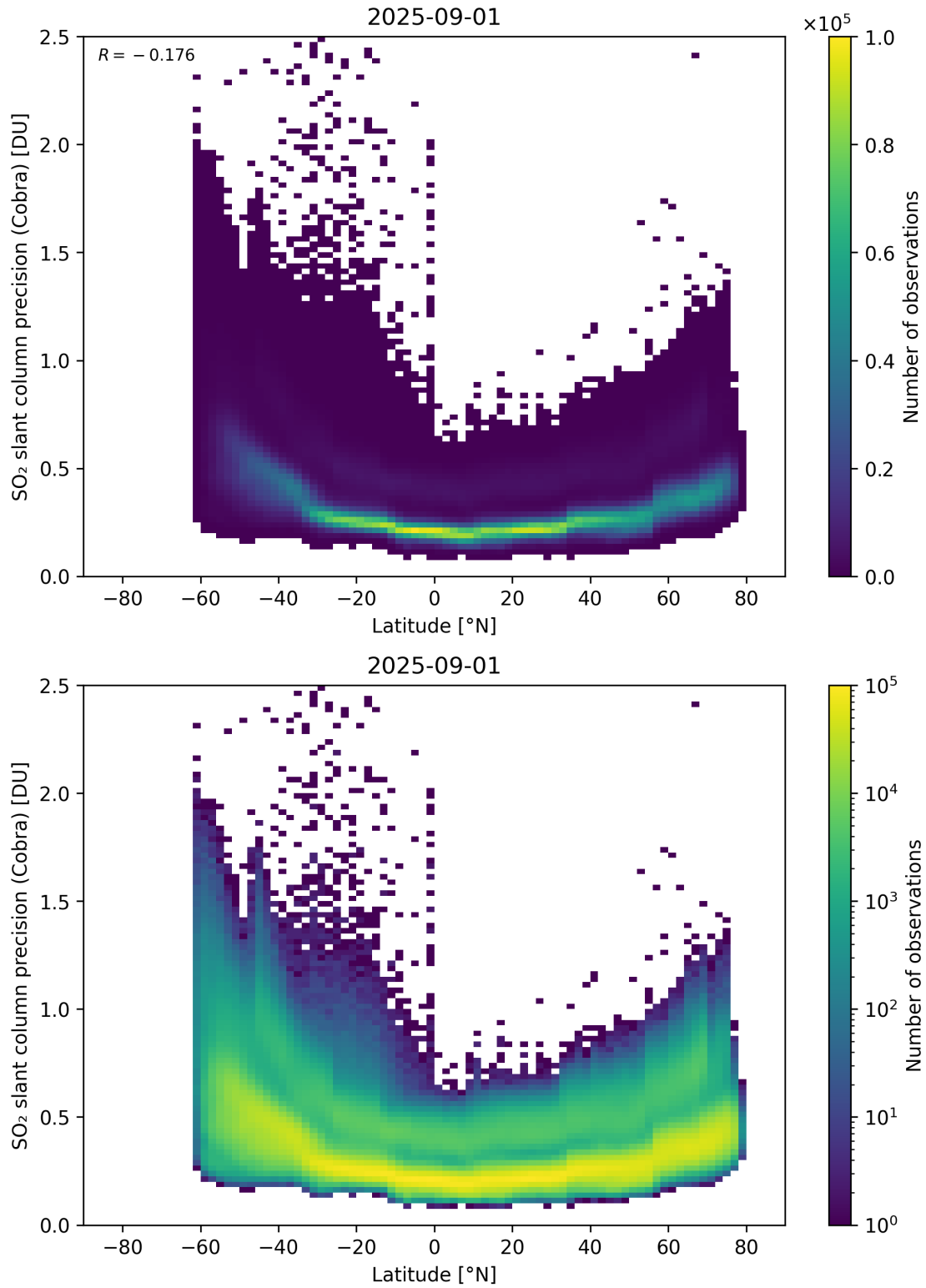
Figure 158: Scatter density plot of “Latitude” against “SO 2 slant column precision (Cobra)” for 2025-08-31 to 2025-09-02.
