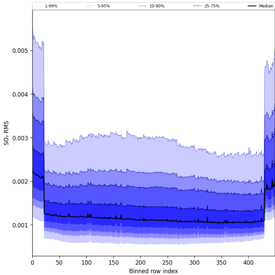
Figure 104: Along track statistics of “SO 2 RMS” for 2025-08-31 to 2025-09-02
