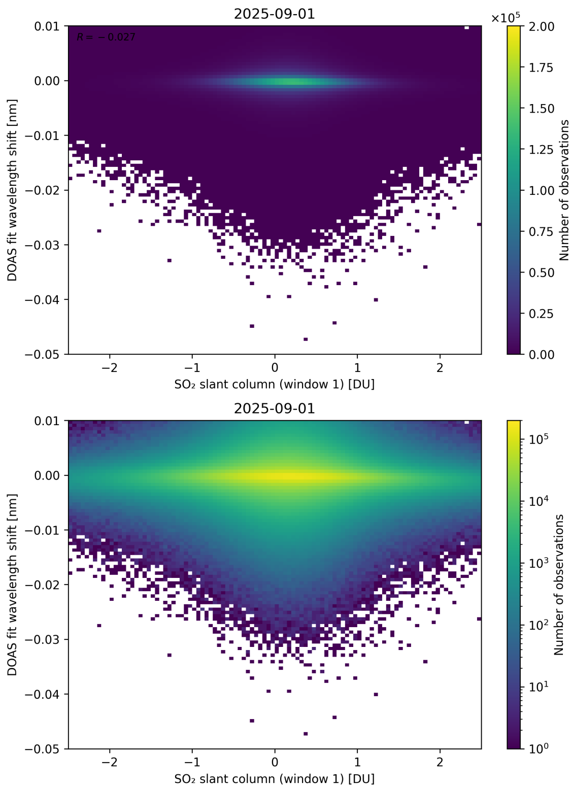
Figure 265: Scatter density plot of “SO 2 slant column (window 1)” against “DOAS fit wavelength shift” for 2025-08-31 to 2025-09-02.
