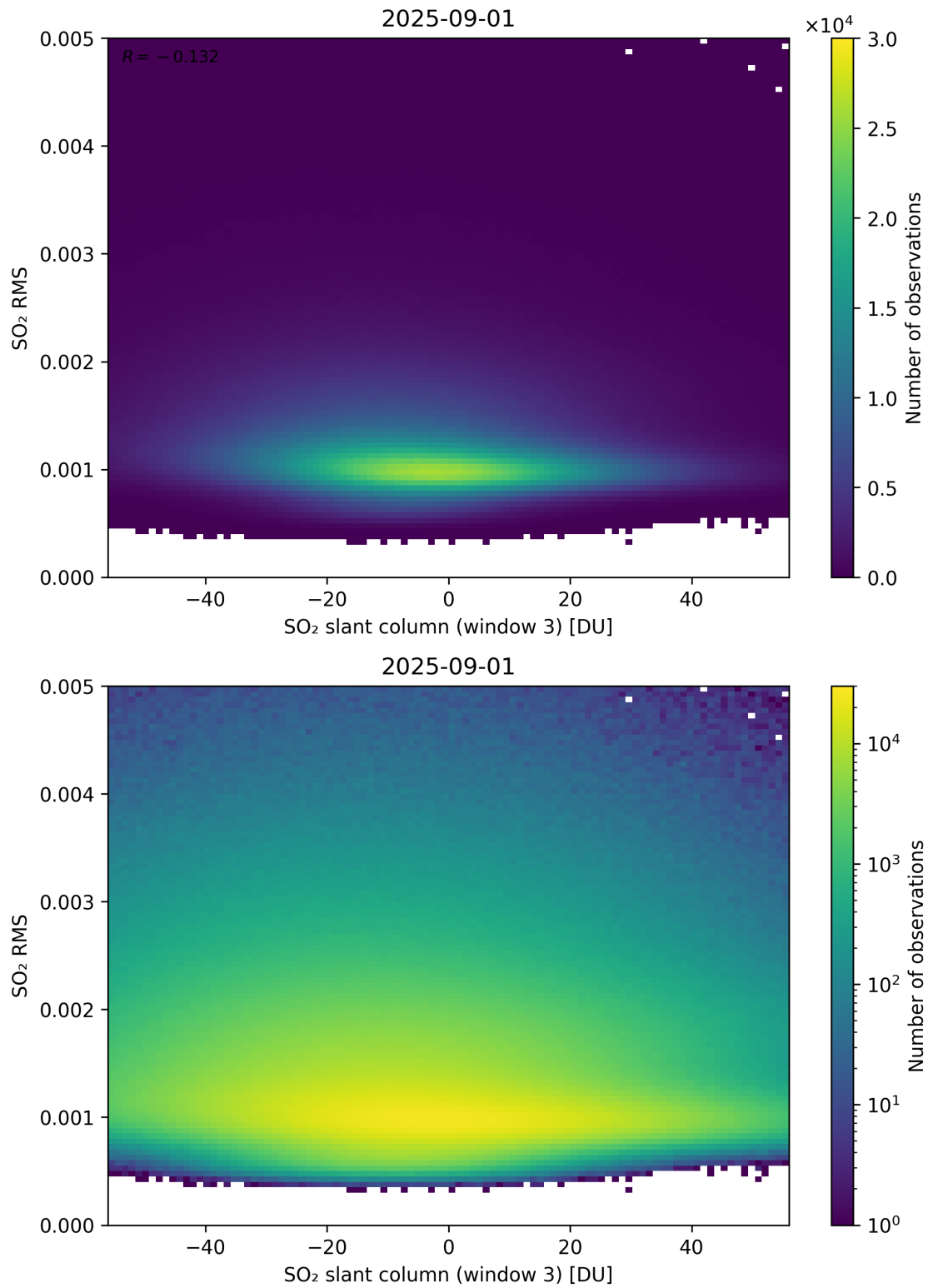
Figure 306: Scatter density plot of “SO 2 slant column (window 3)” against “SO 2 RMS” for 2025-08-31 to 2025-09-02.
