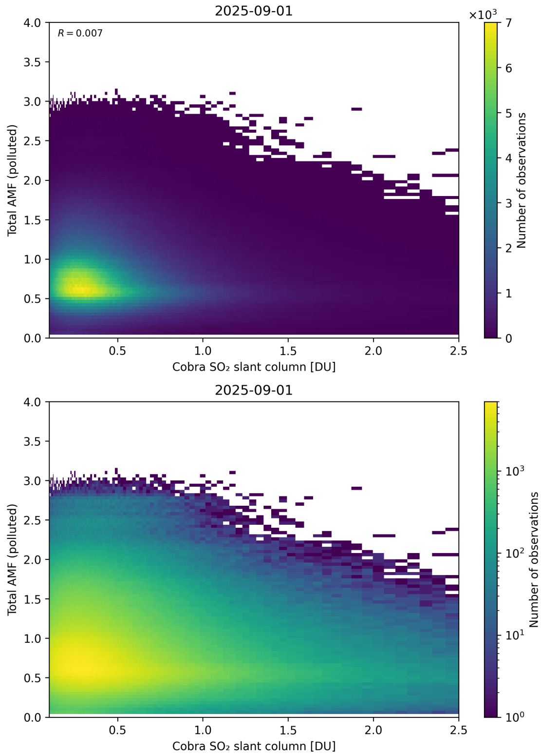
Figure 224: Scatter density plot of “Cobra SO 2 slant column” against “Total AMF (polluted)” for 2025-08-31 to 2025-09-02.
