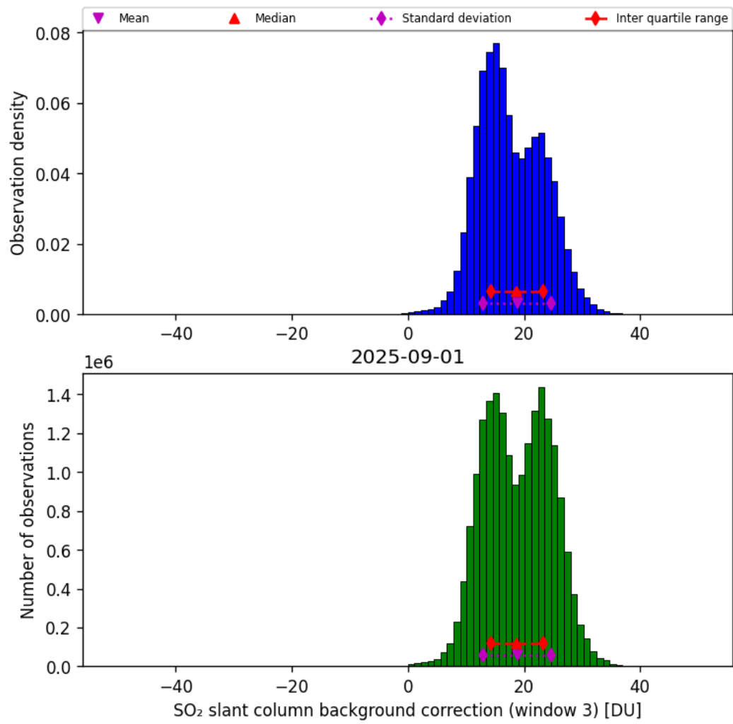
Figure 74: Histogram of “SO 2 slant column background correction (window 3)” for 2025-08-31 to 2025-09-02
