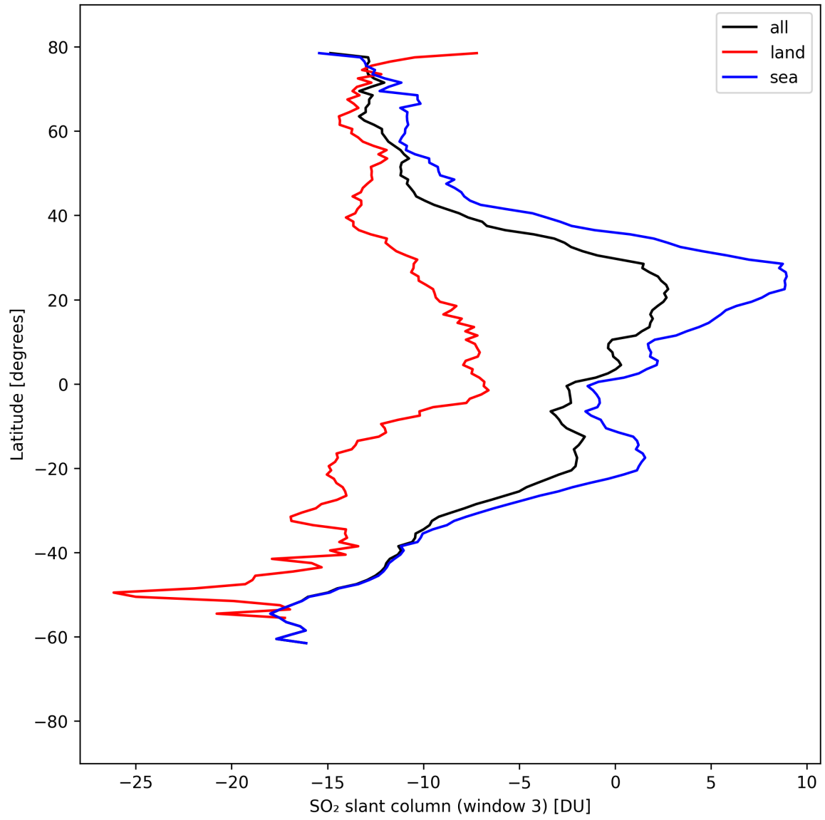
Figure 45: Zonal average of “SO 2 slant column (window 3)” for 2025-08-31 to 2025-09-02.
