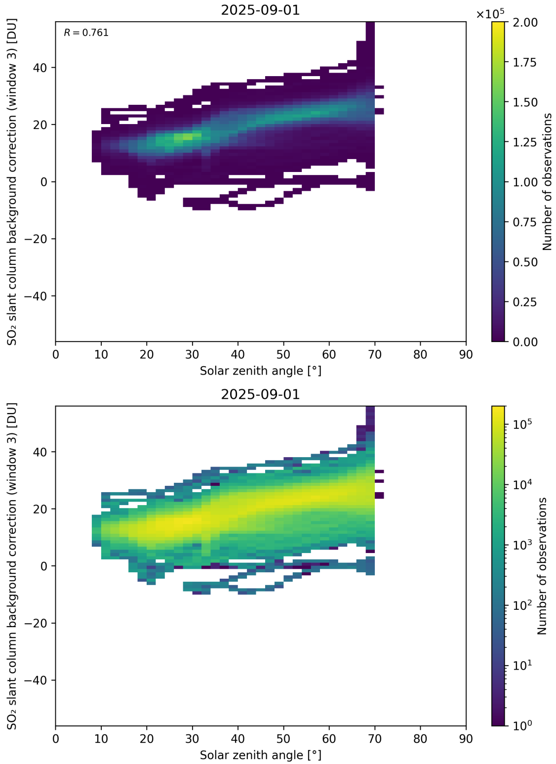
Figure 173: Scatter density plot of “Solar zenith angle” against “SO 2 slant column background correction (window 3)” for 2025-08-31 to 2025-09-02.
