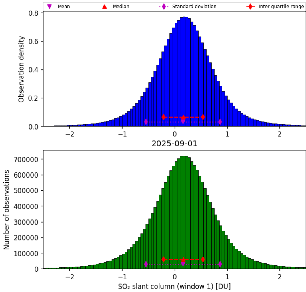
Figure 63: Histogram of “SO 2 slant column (window 1)” for 2025-08-31 to 2025-09-02
