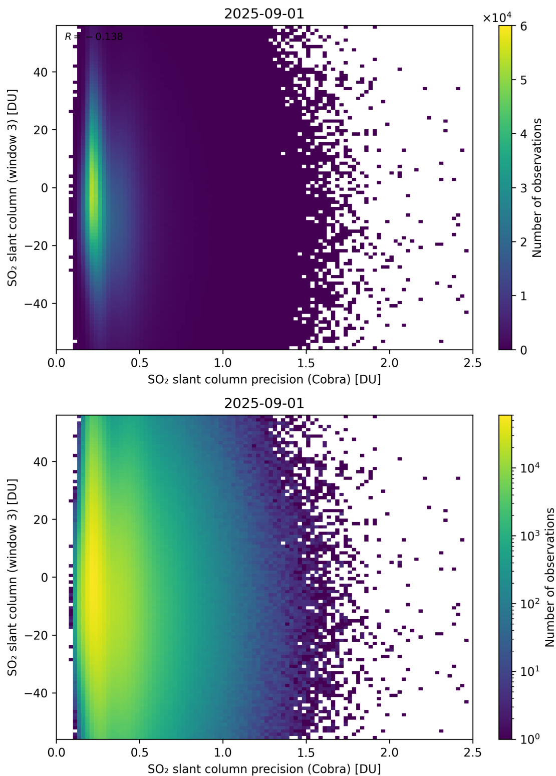
Figure 211: Scatter density plot of “SO 2 slant column precision (Cobra)” against “SO 2 slant column (window 3)” for 2025-08-31 to 2025-09-02.
