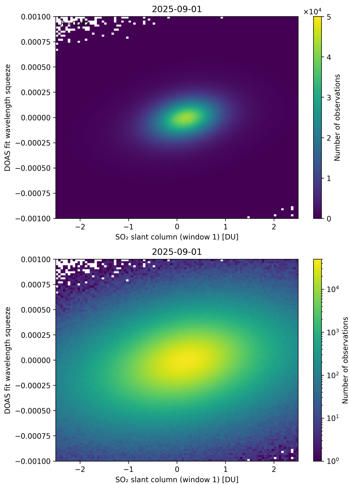
Figure 266: Scatter density plot of “SO 2 slant column (window 1)” against “DOAS fit wavelength squeeze” for 2025-08-31 to 2025-09-02.
