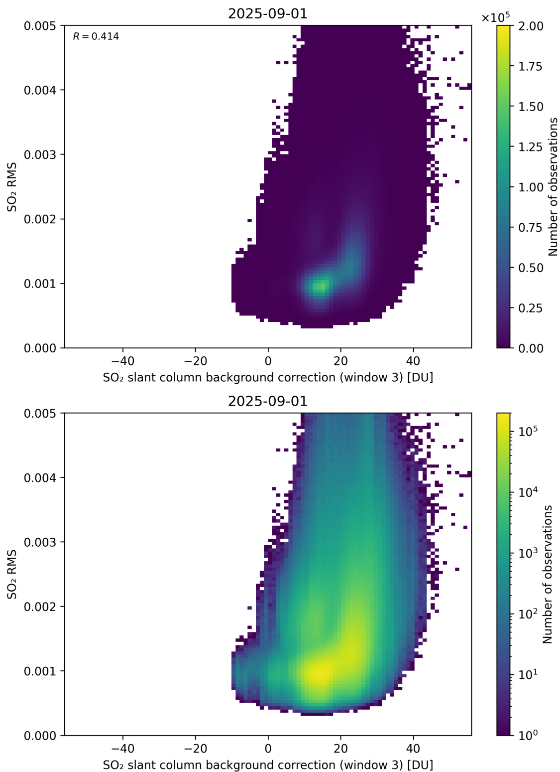
Figure 134: Scatter density plot of “SO 2 slant column background correction (window 3)” against “SO 2 RMS” for 2025-08-31 to 2025-09-02.
