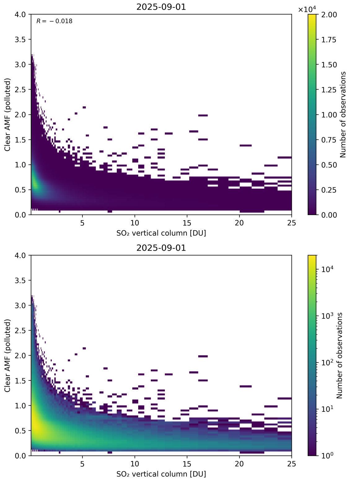
Figure 348: Scatter density plot of “SO 2 vertical column” against “Clear AMF (polluted)” for 2025-08-31 to 2025-09-02.
