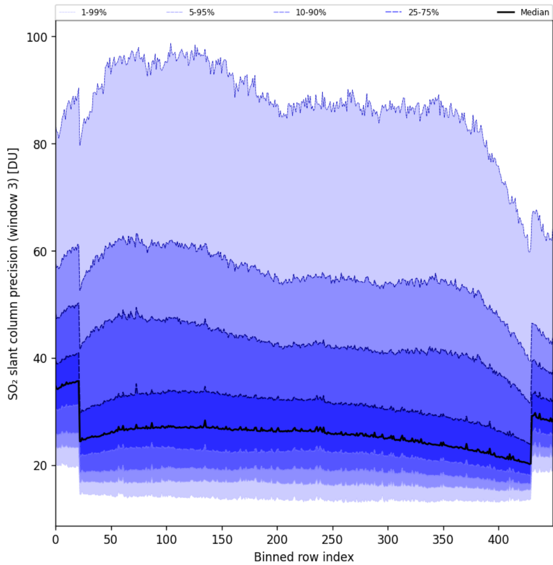
Figure 98: Along track statistics of “SO 2 slant column precision (window 3)” for 2025-08-31 to 2025-09-02
