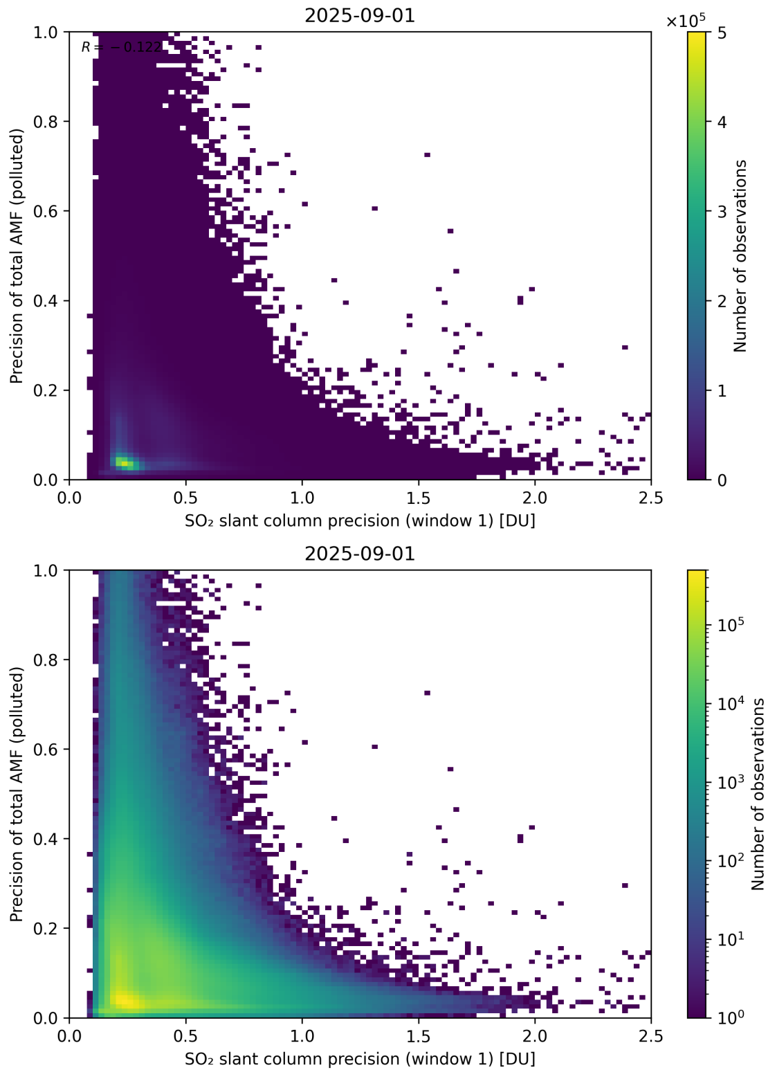
Figure 281: Scatter density plot of “SO 2 slant column precision (window 1)” against “Precision of total AMF (polluted)” for 2025-08-31 to 2025-09-02.
