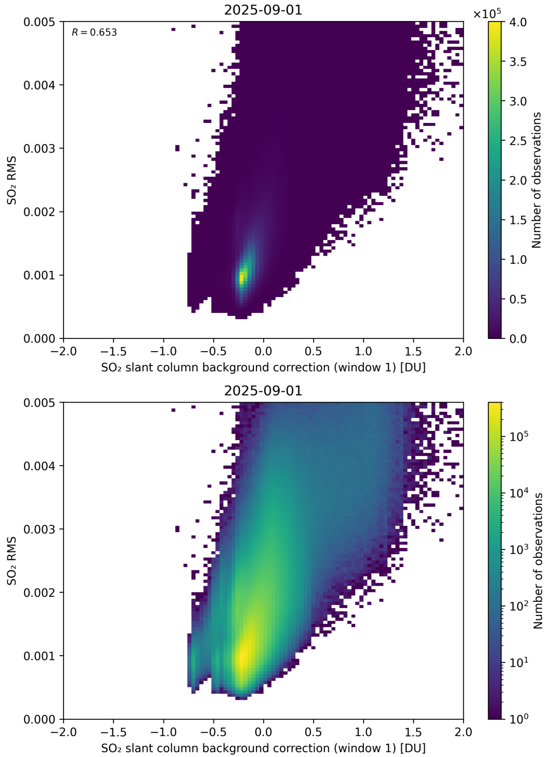
Figure 113: Scatter density plot of “SO 2 slant column background correction (window 1)” against “SO 2 RMS” for 2025-08-31 to 2025-09-02.
