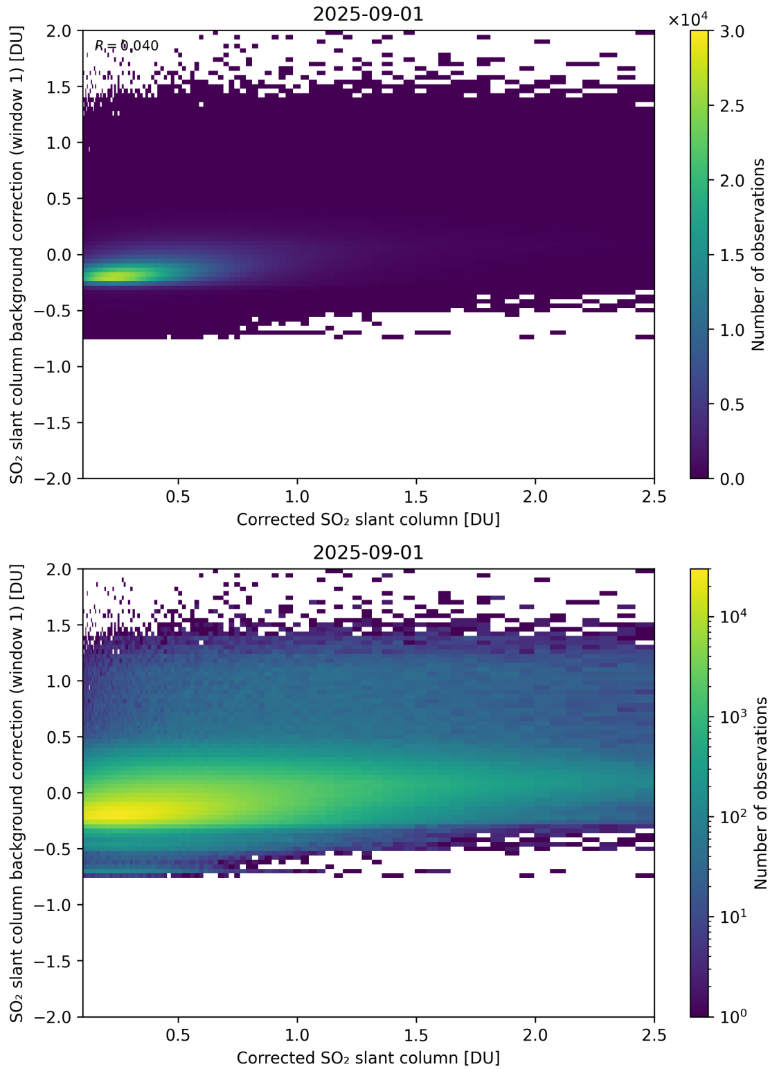
Figure 226: Scatter density plot of “Corrected SO 2 slant column” against “SO 2 slant column background correction (window 1)” for 2025-08-31 to 2025-09-02.
