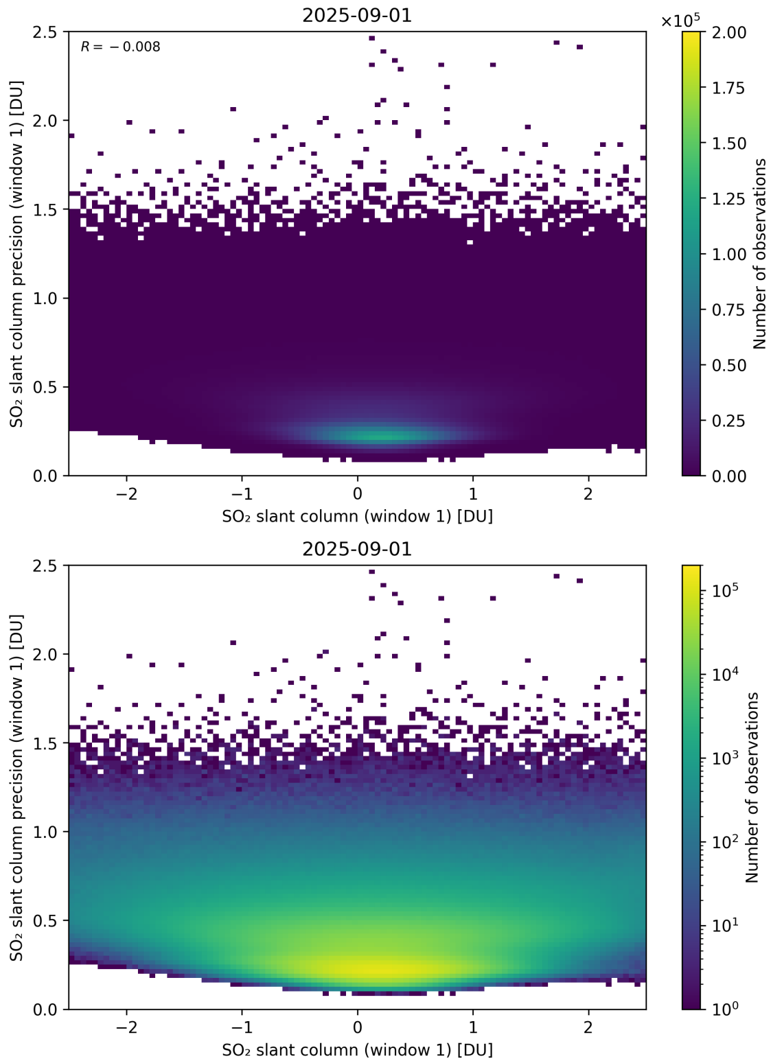
Figure 285: Scatter density plot of “SO 2 slant column (window 1)” against “SO 2 slant column precision (window 1)” for 2025-08-31 to 2025-09-02.
