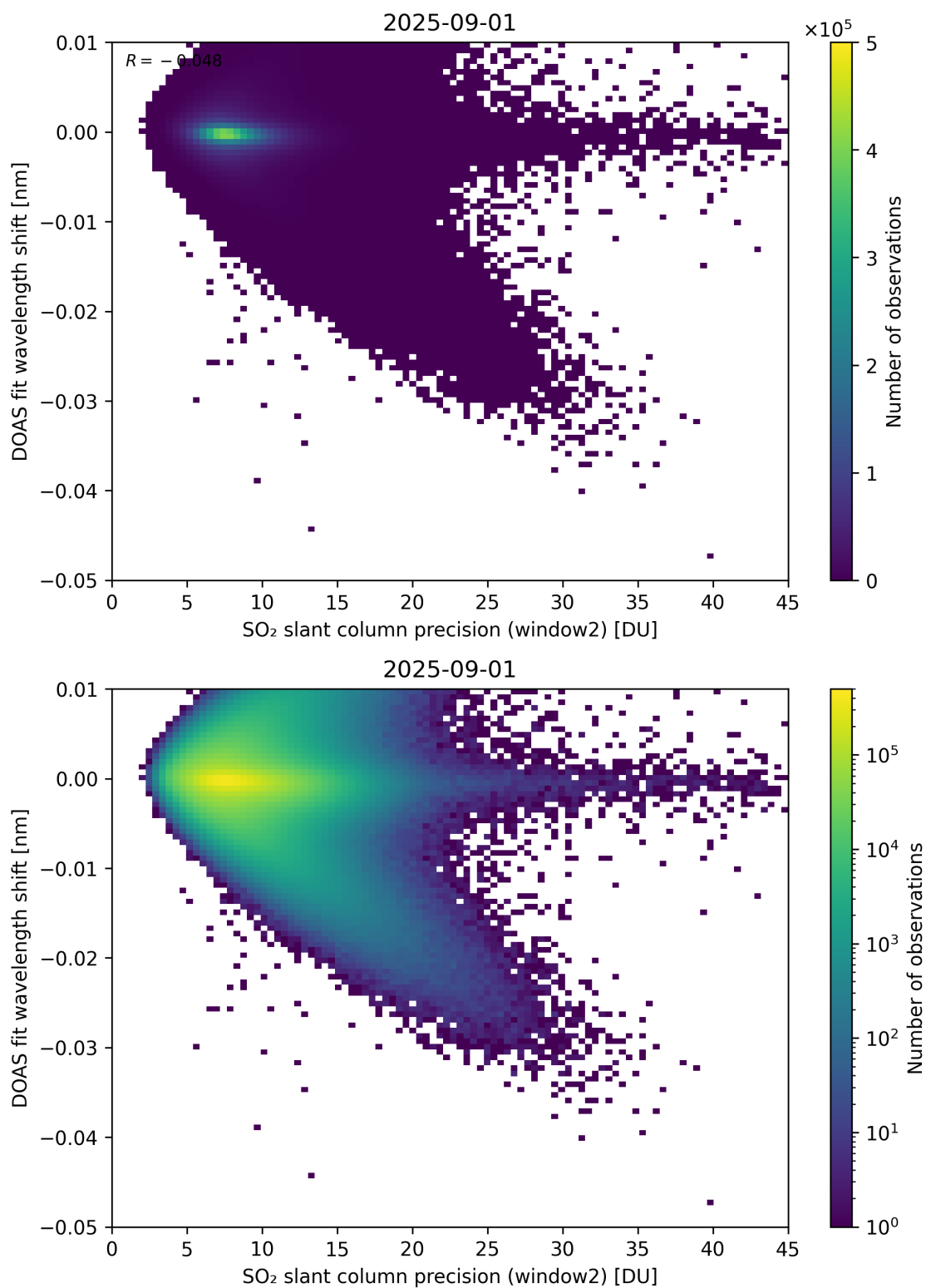
Figure 293: Scatter density plot of “SO 2 slant column precision (window2)” against “DOAS fit wavelength shift” for 2025-08-31 to 2025-09-02.
