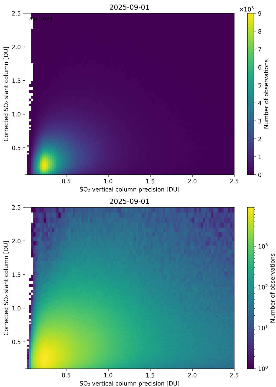
Figure 338: Scatter density plot of “SO 2 vertical column precision” against “Corrected SO 2 slant column” for 2025-08-31 to 2025-09-02.
