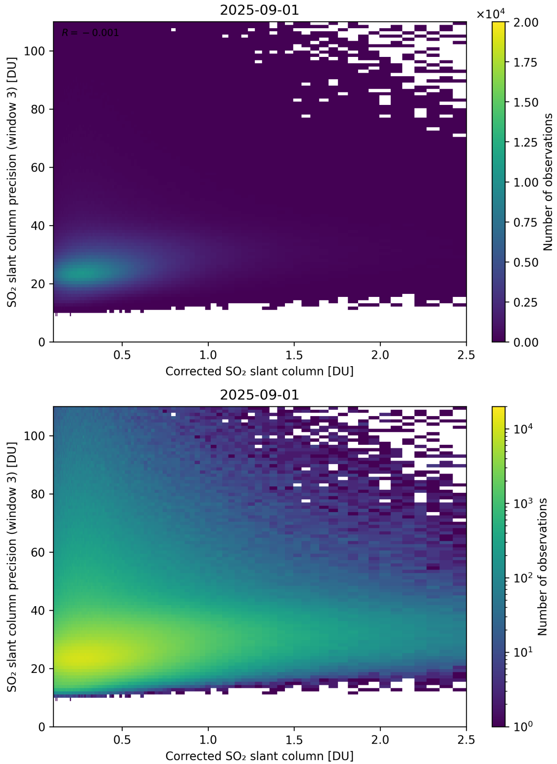
Figure 241: Scatter density plot of “Corrected SO 2 slant column” against “SO 2 slant column precision (window 3)” for 2025-08-31 to 2025-09-02.
