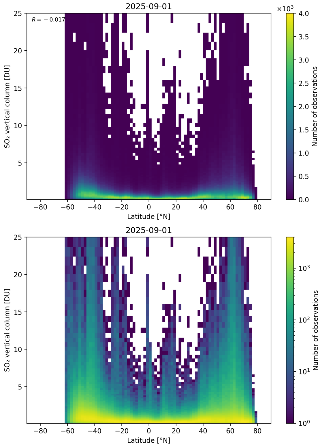
Figure 169: Scatter density plot of “Latitude” against “SO 2 vertical column” for 2025-08-31 to 2025-09-02.
