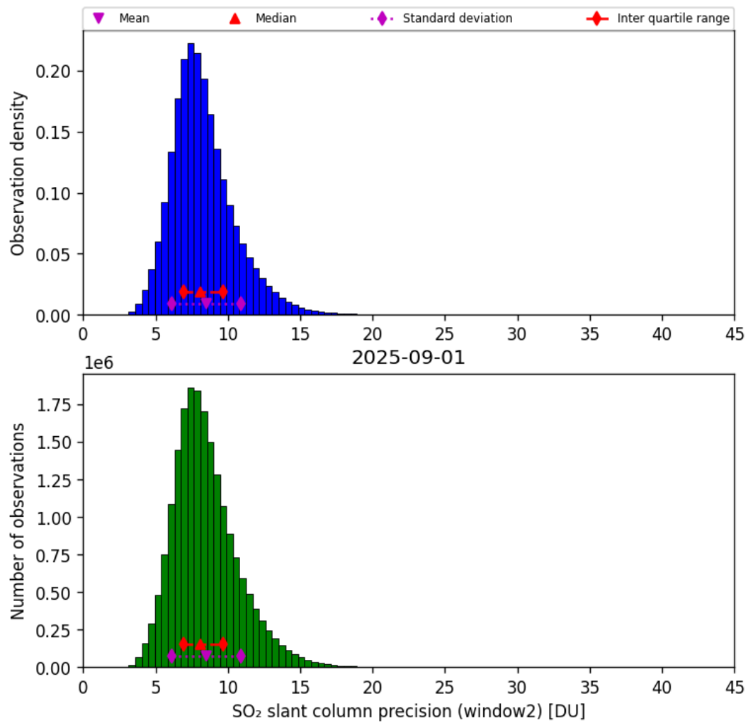
Figure 68: Histogram of “SO 2 slant column precision (window2)” for 2025-08-31 to 2025-09-02
