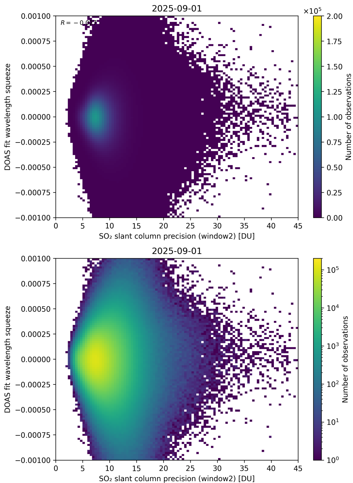
Figure 294: Scatter density plot of “SO 2 slant column precision (window2)” against “DOAS fit wavelength squeeze” for 2025-08-31 to 2025-09-02.
