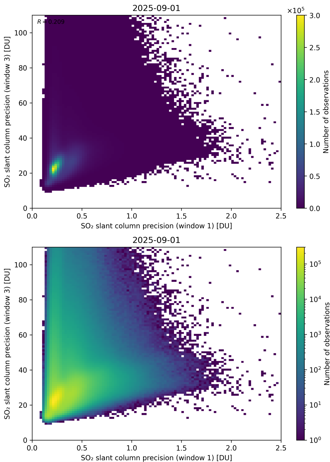
Figure 279: Scatter density plot of “SO 2 slant column precision (window 1)” against “SO 2 slant column precision (window 3)” for 2025-08-31 to 2025-09-02.
