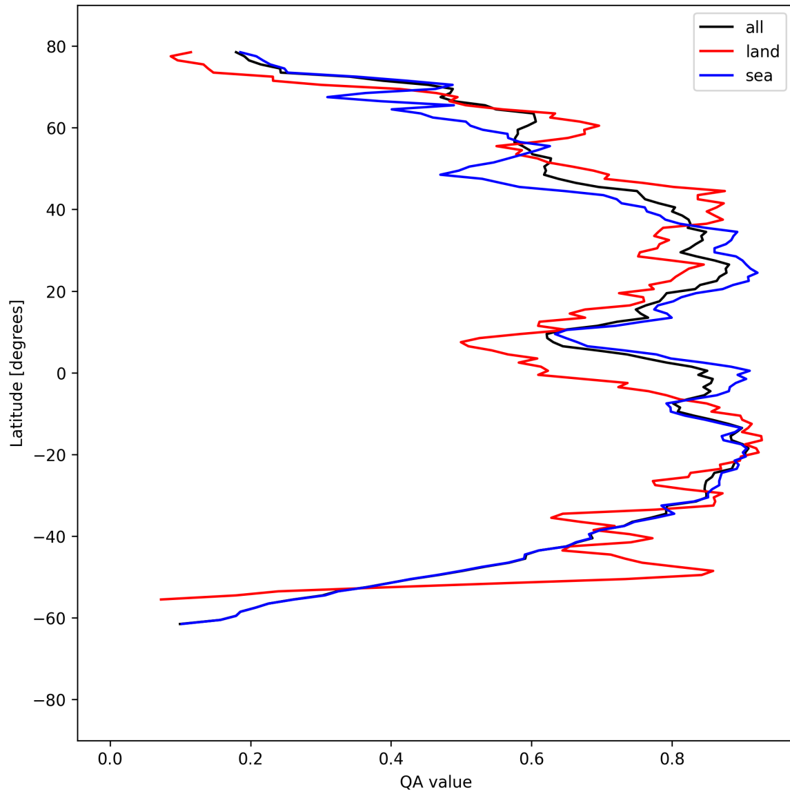
Figure 31: Zonal average of “QA value” for 2025-08-31 to 2025-09-02.
