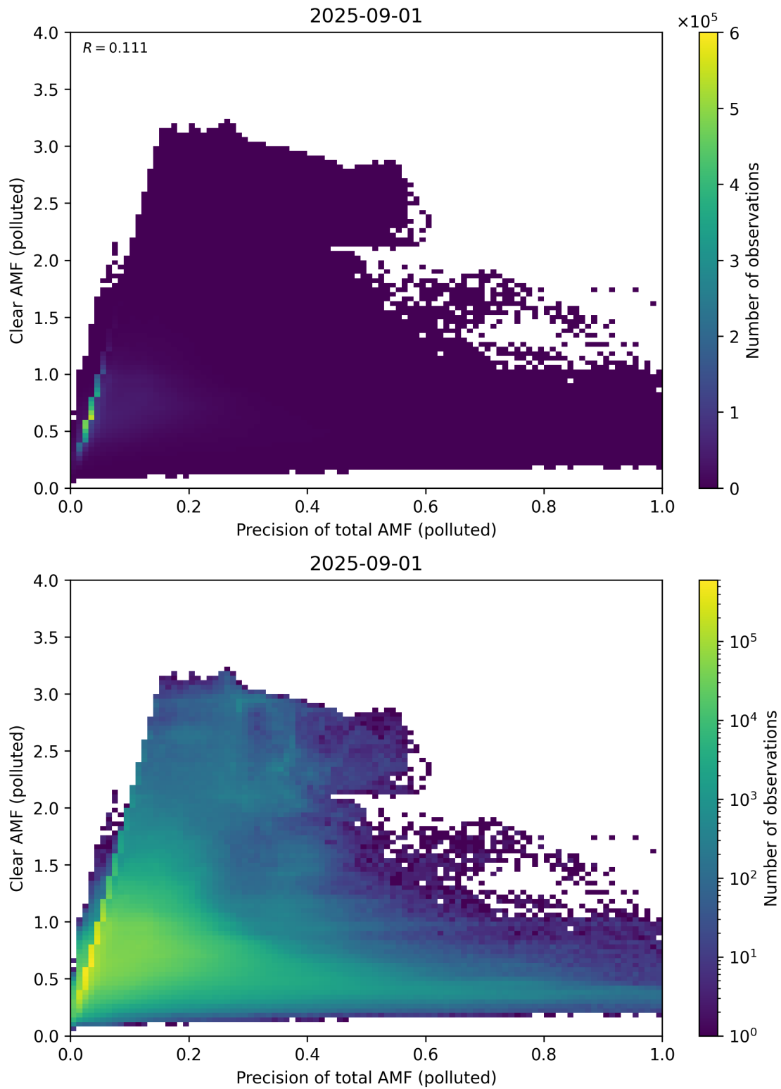
Figure 320: Scatter density plot of “Precision of total AMF (polluted)” against “Clear AMF (polluted)” for 2025-08-31 to 2025-09-02.
