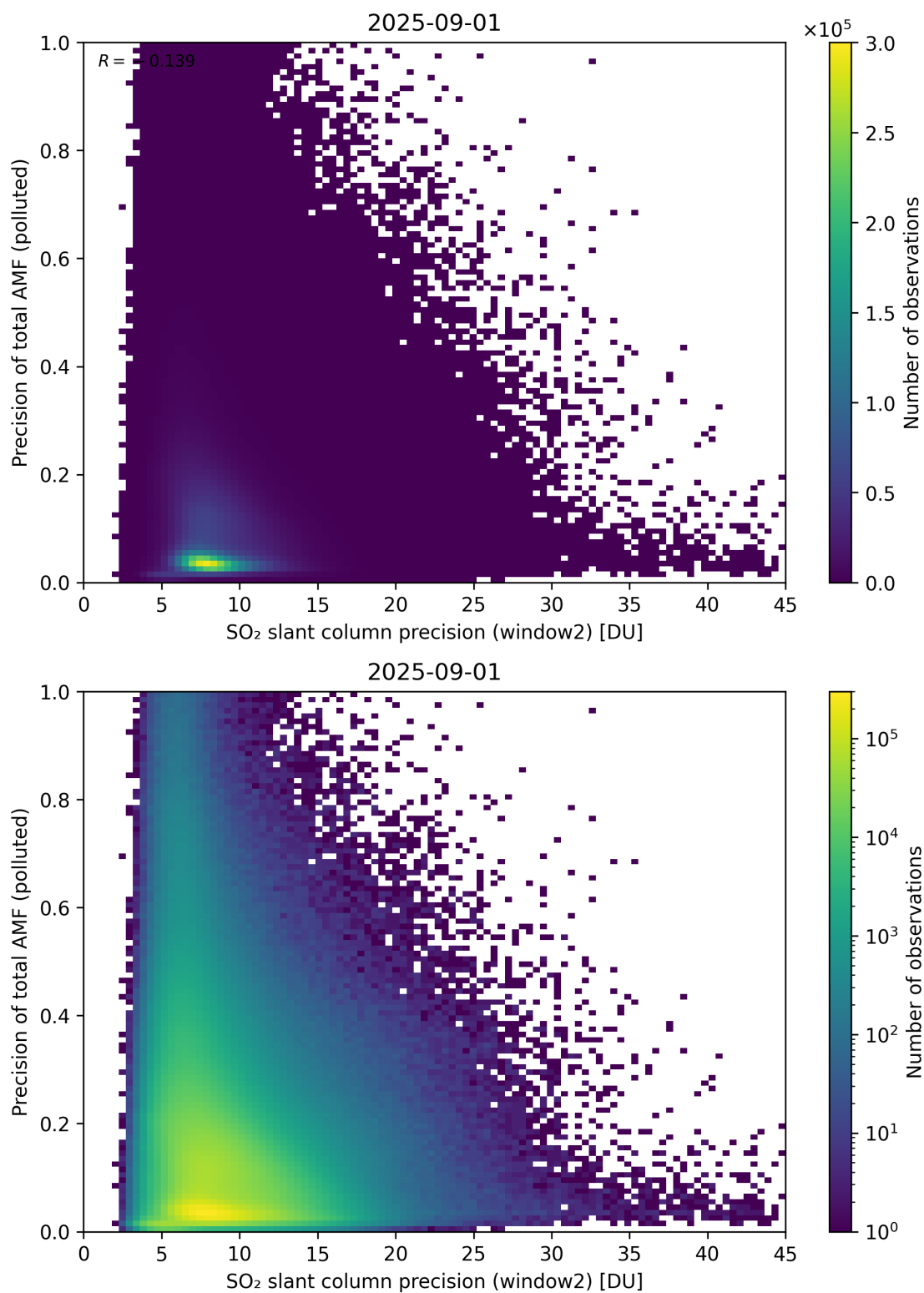
Figure 302: Scatter density plot of “SO 2 slant column precision (window2)” against “Precision of total AMF (polluted)” for 2025-08-31 to 2025-09-02.
