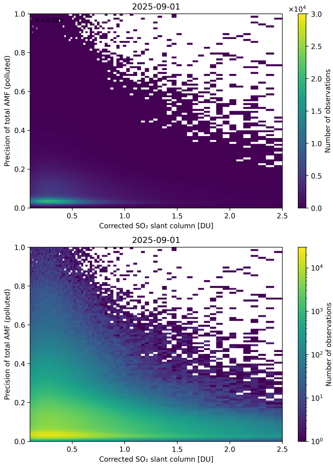
Figure 243: Scatter density plot of “Corrected SO 2 slant column” against “Precision of total AMF (polluted)” for 2025-08-31 to 2025-09-02.
