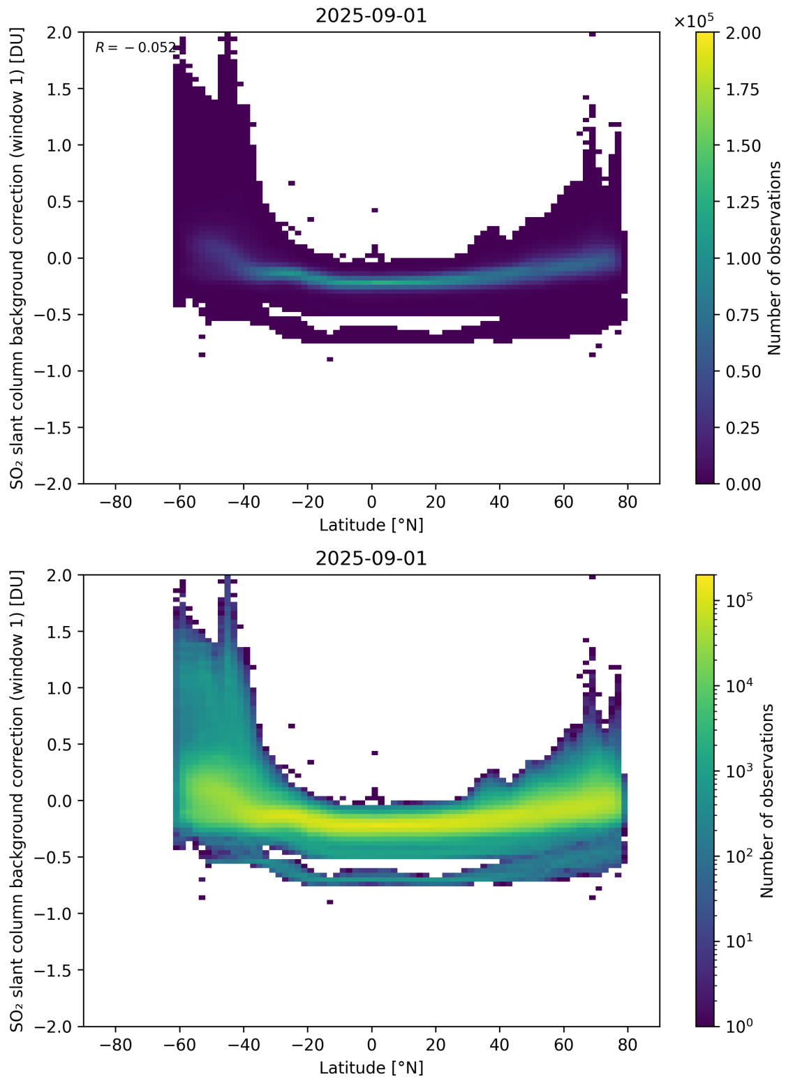
Figure 150: Scatter density plot of “Latitude” against “SO 2 slant column background correction (window 1)” for 2025-08-31 to 2025-09-02.
