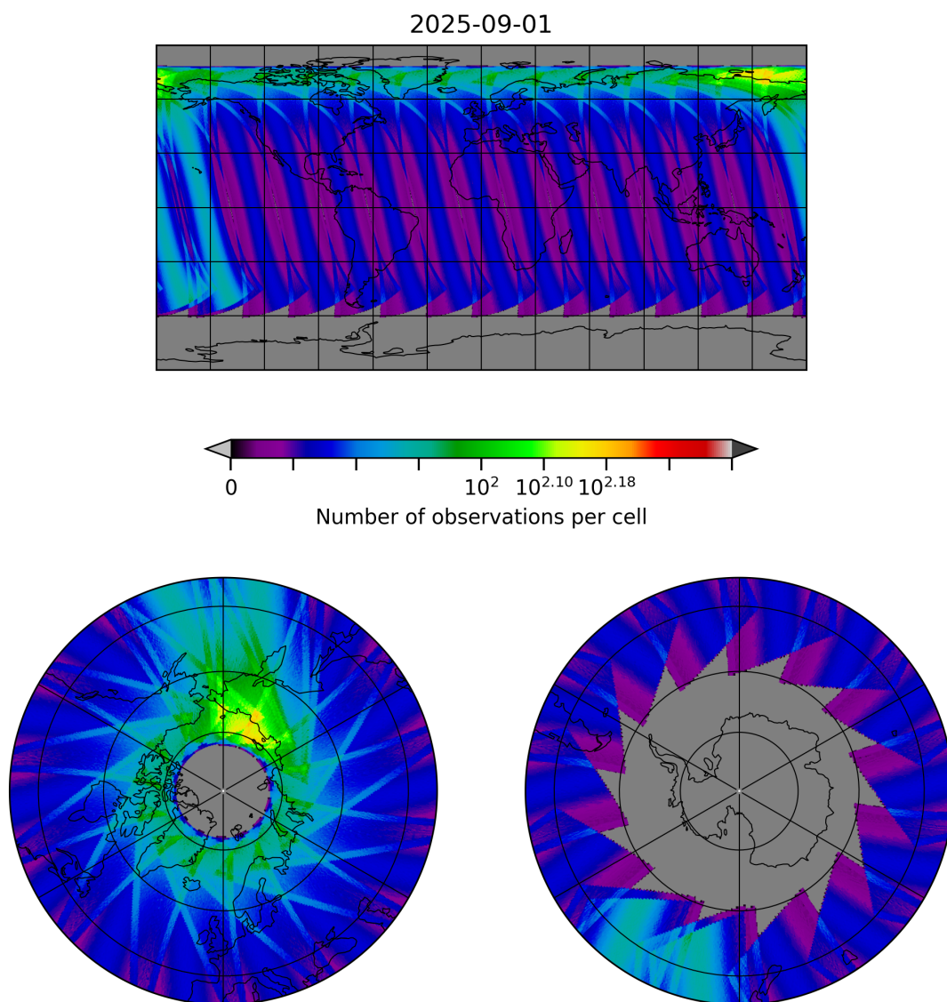
Figure 30: Map of the number of observations for 2025-08-31 to 2025-09-02
