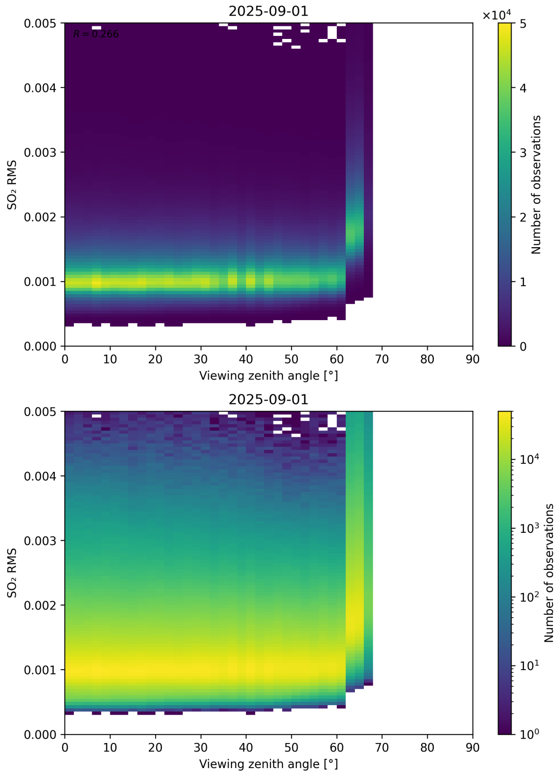
Figure 367: Scatter density plot of “Viewing zenith angle” against “SO 2 RMS” for 2025-08-31 to 2025-09-02.
