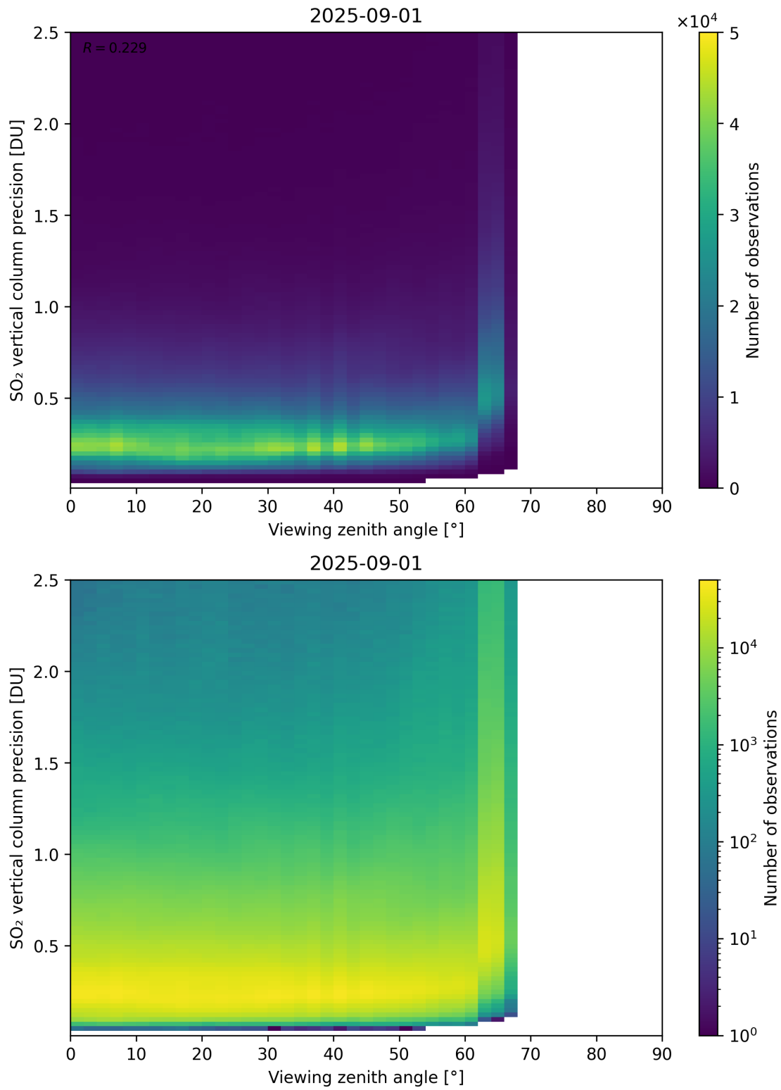
Figure 384: Scatter density plot of “Viewing zenith angle” against “SO 2 vertical column precision” for 2025-08-31 to 2025-09-02.
