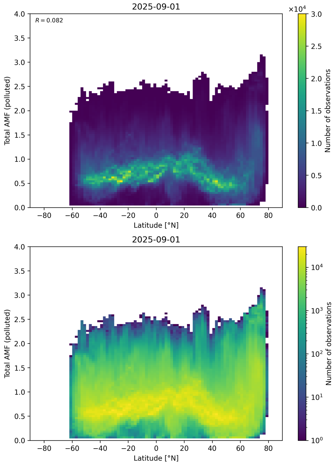
Figure 167: Scatter density plot of “Latitude” against “Total AMF (polluted)” for 2025-08-31 to 2025-09-02.
