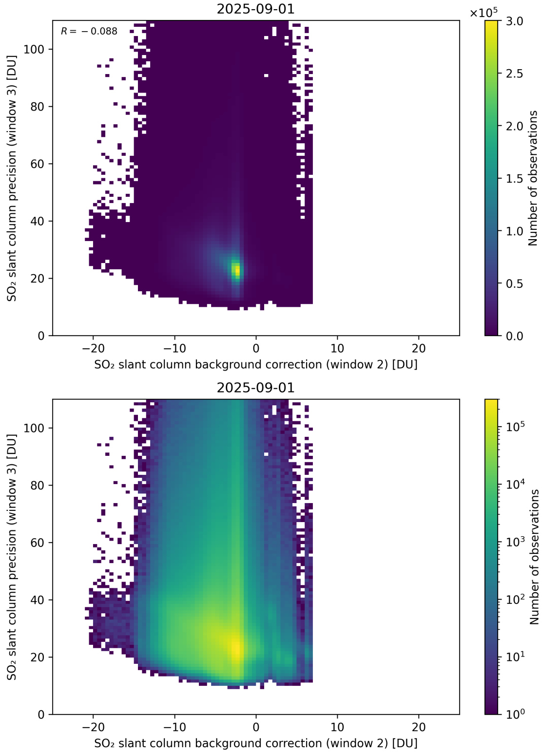
Figure 129: Scatter density plot of “SO 2 slant column background correction (window 2)” against “SO 2 slant column precision (window 3)” for 2025-08-31 to 2025-09-02.
