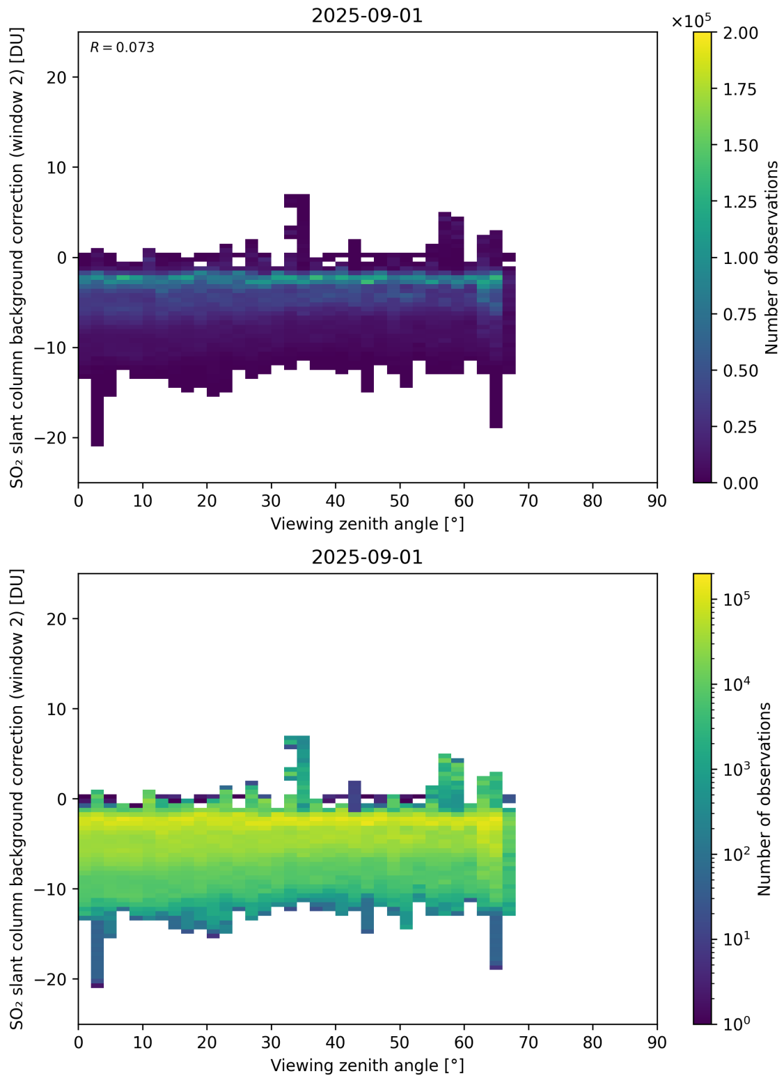
Figure 363: Scatter density plot of “Viewing zenith angle” against “SO 2 slant column background correction (window 2)” for 2025-08-31 to 2025-09-02.
