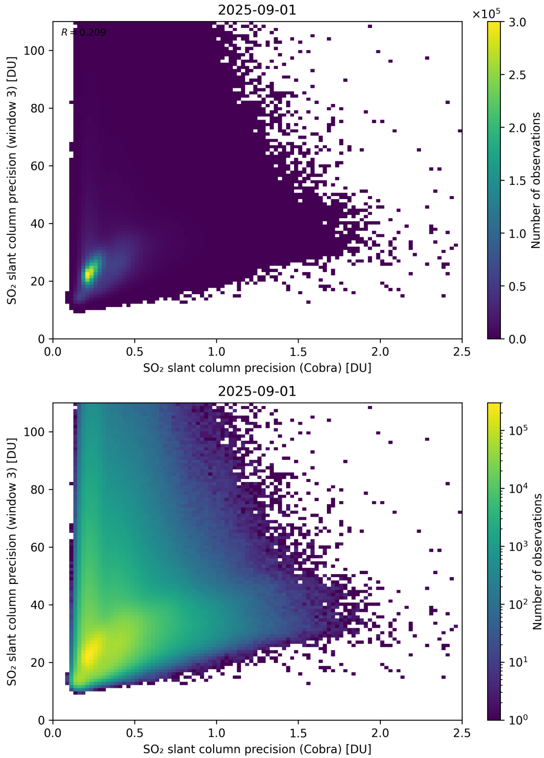
Figure 212: Scatter density plot of “SO 2 slant column precision (Cobra)” against “SO 2 slant column precision (window 3)” for 2025-08-31 to 2025-09-02.
