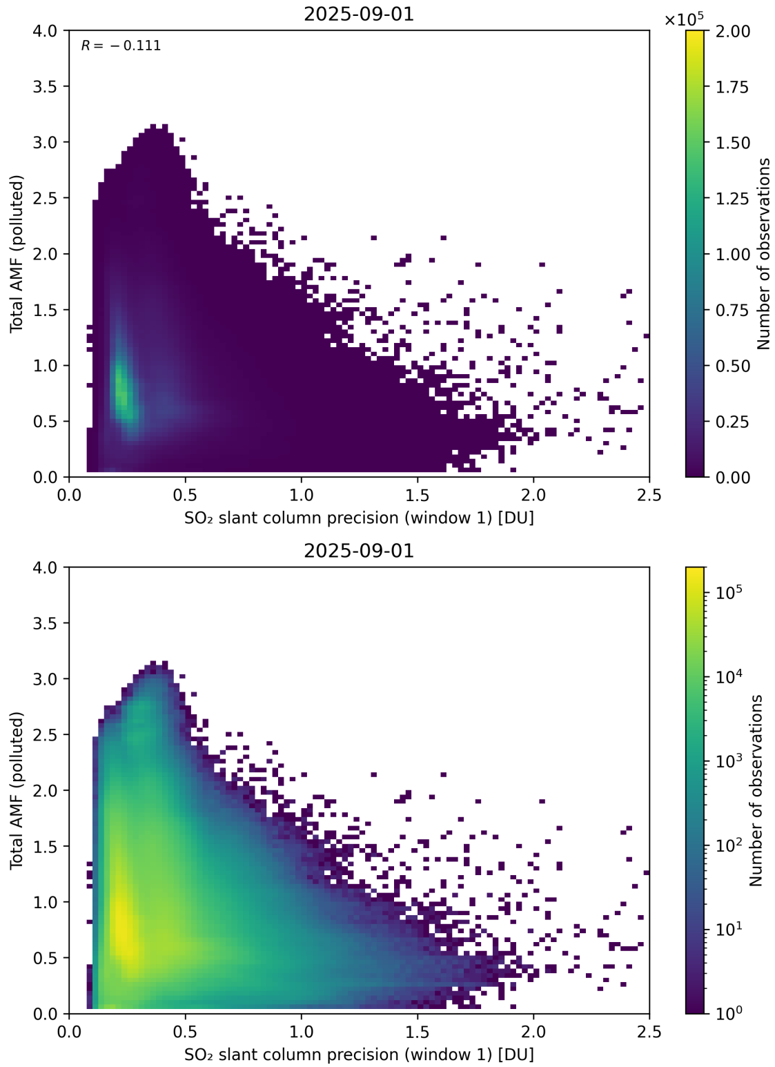
Figure 280: Scatter density plot of “SO 2 slant column precision (window 1)” against “Total AMF (polluted)” for 2025-08-31 to 2025-09-02.
