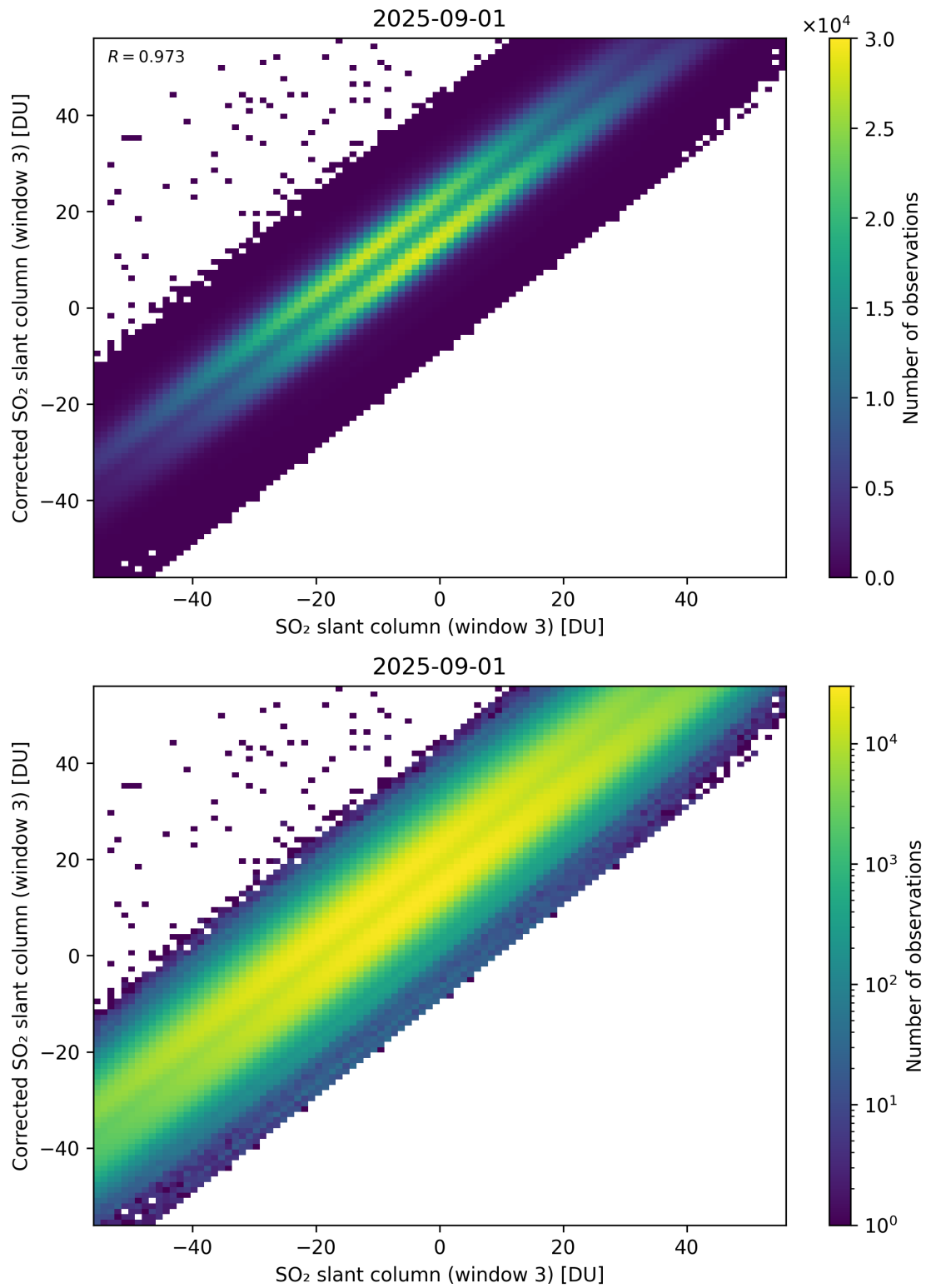
Figure 316: Scatter density plot of “SO 2 slant column (window 3)” against “Corrected SO 2 slant column (window 3)” for 2025-08-31 to 2025-09-02.
