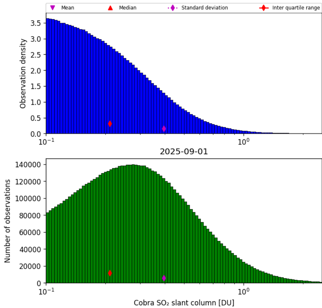
Figure 61: Histogram of “Cobra SO 2 slant column” for 2025-08-31 to 2025-09-02
