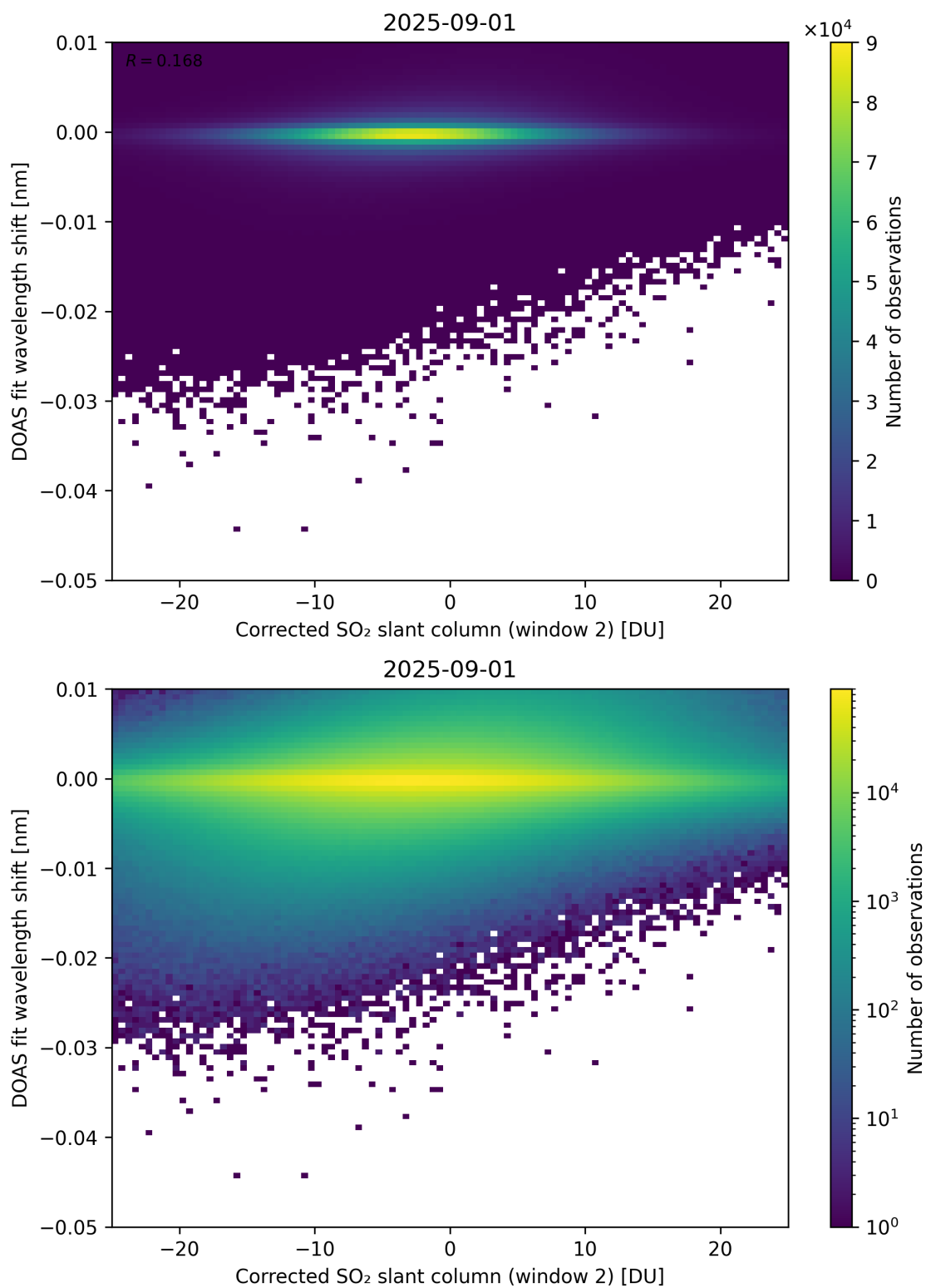
Figure 246: Scatter density plot of “Corrected SO 2 slant column (window 2)” against “DOAS fit wavelength shift” for 2025-08-31 to 2025-09-02.
