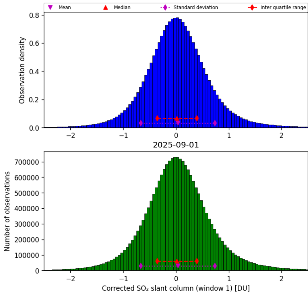
Figure 65: Histogram of “Corrected SO 2 slant column (window 1)” for 2025-08-31 to 2025-09-02
