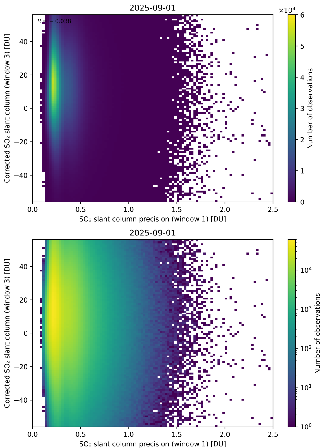
Figure 276: Scatter density plot of “SO 2 slant column precision (window 1)” against “Corrected SO 2 slant column (window 3)” for 2025-08-31 to 2025-09-02.
