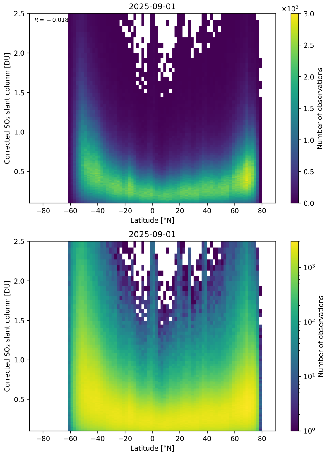
Figure 159: Scatter density plot of “Latitude” against “Corrected SO 2 slant column” for 2025-08-31 to 2025-09-02.
