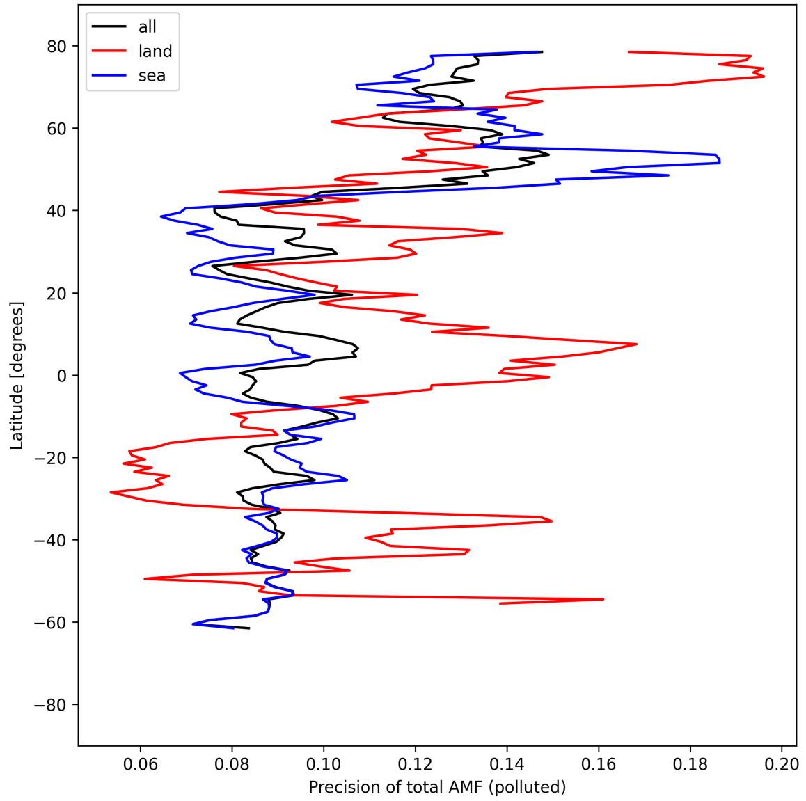
Figure 54: Zonal average of “Precision of total AMF (polluted)” for 2025-08-31 to 2025-09-02.
