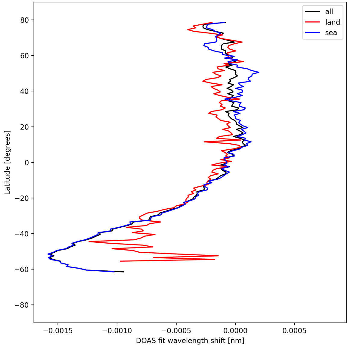
Figure 50: Zonal average of “DOAS fit wavelength shift” for 2025-08-31 to 2025-09-02.
