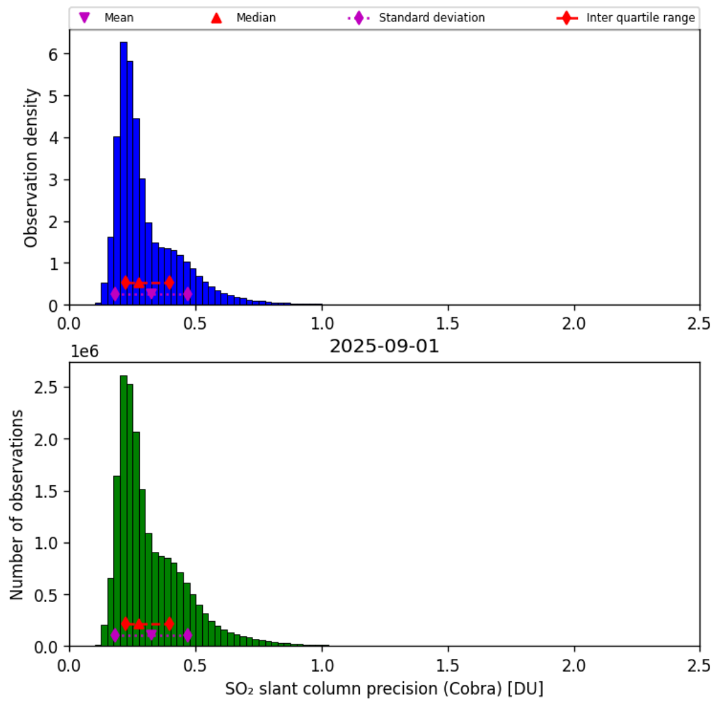
Figure 62: Histogram of “SO 2 slant column precision (Cobra)” for 2025-08-31 to 2025-09-02
