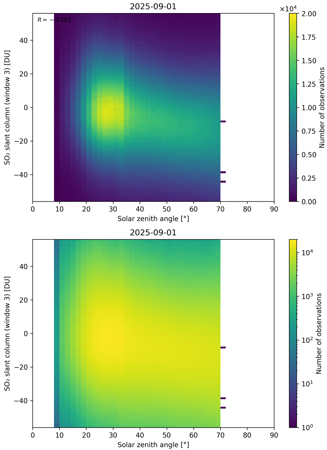
Figure 187: Scatter density plot of “Solar zenith angle” against “SO 2 slant column (window 3)” for 2025-08-31 to 2025-09-02.
