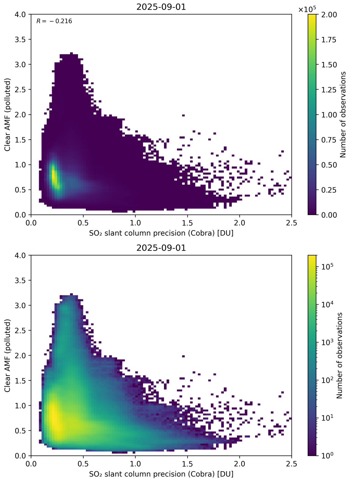
Figure 205: Scatter density plot of “SO 2 slant column precision (Cobra)” against “Clear AMF (polluted)” for 2025-08-31 to 2025-09-02.
