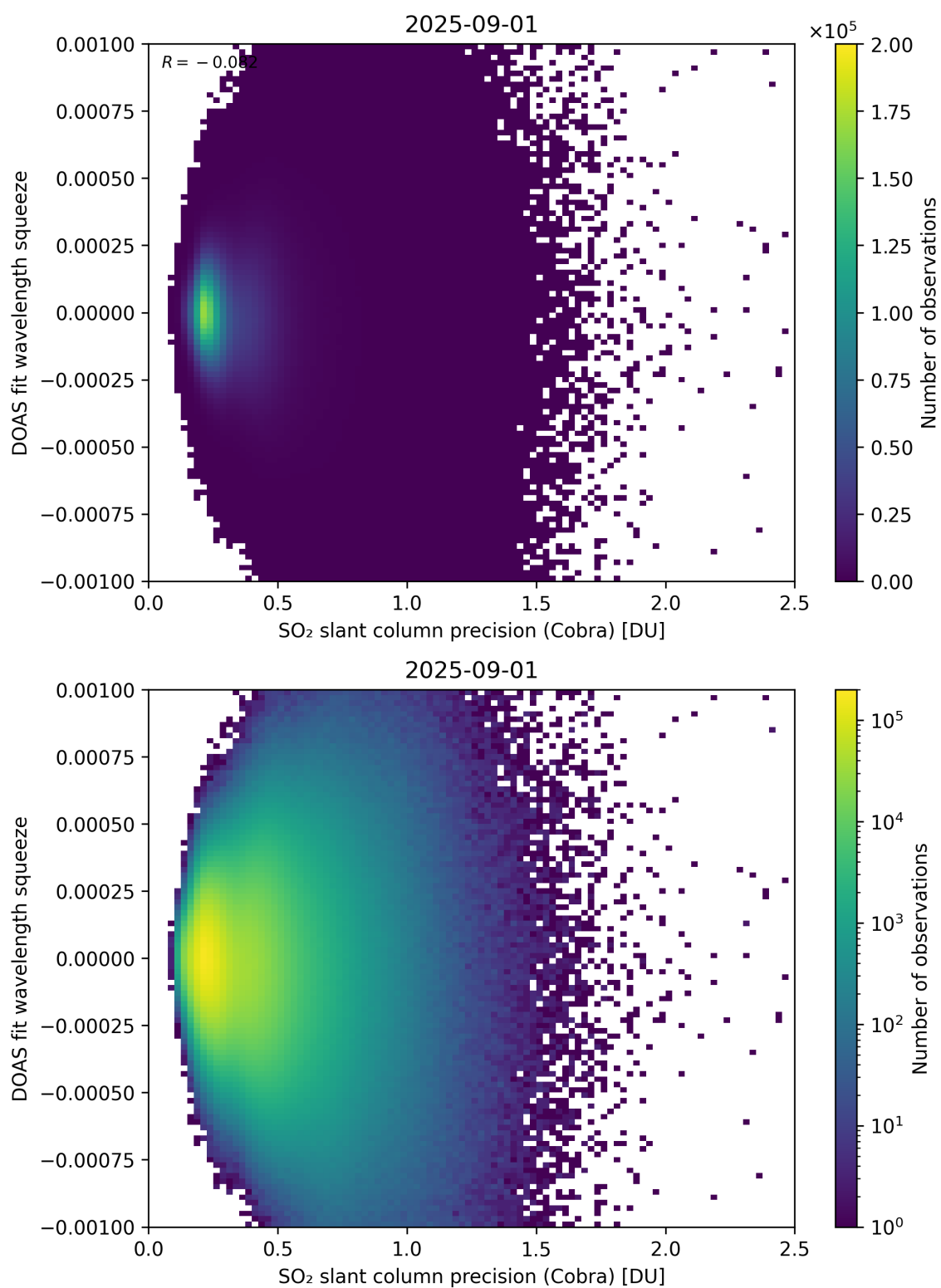
Figure 203: Scatter density plot of “SO 2 slant column precision (Cobra)” against “DOAS fit wavelength squeeze” for 2025-08-31 to 2025-09-02.
