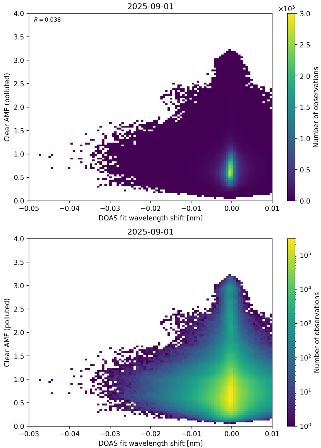
Figure 140: Scatter density plot of “DOAS fit wavelength shift” against “Clear AMF (polluted)” for 2025-08-31 to 2025-09-02.
