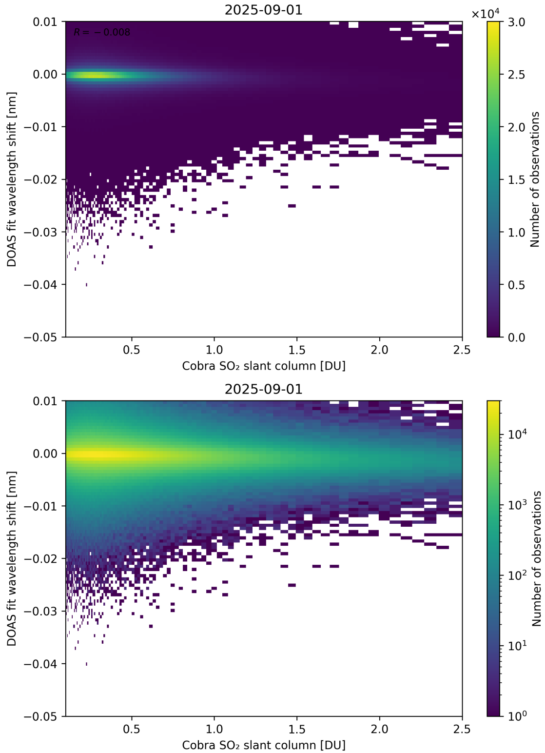
Figure 196: Scatter density plot of “Cobra SO 2 slant column” against “DOAS fit wavelength shift” for 2025-08-31 to 2025-09-02.
