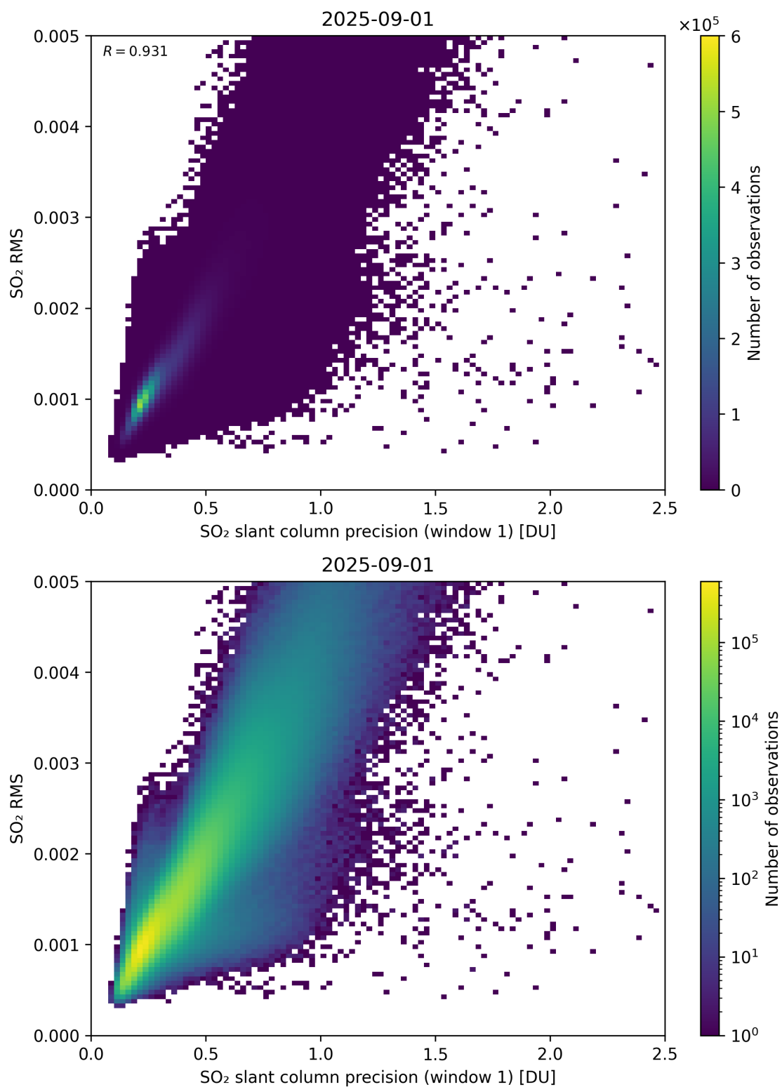
Figure 273: Scatter density plot of “SO 2 slant column precision (window 1)” against “SO 2 RMS” for 2025-08-31 to 2025-09-02.
