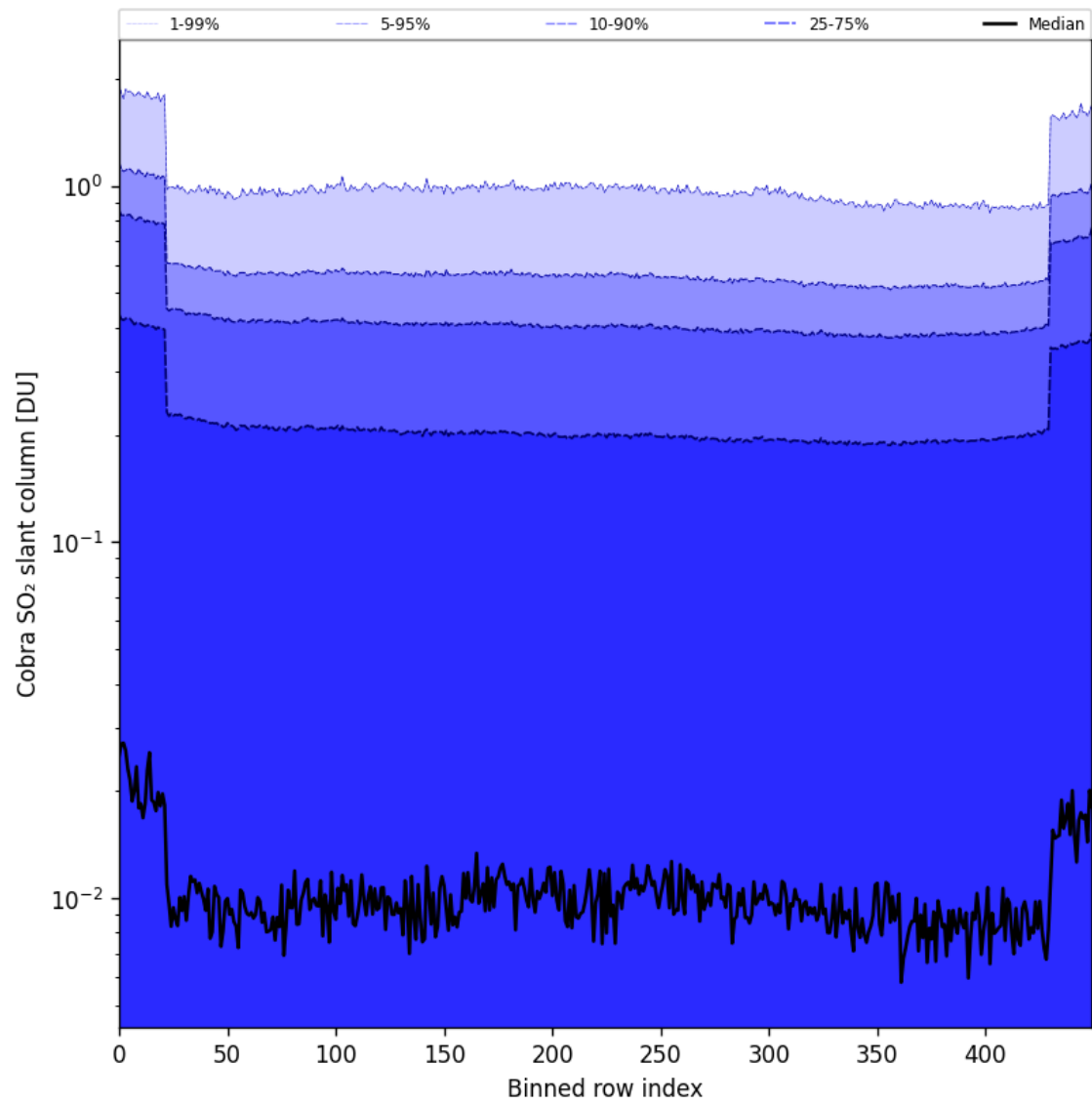
Figure 87: Along track statistics of “Cobra SO 2 slant column” for 2025-08-31 to 2025-09-02
