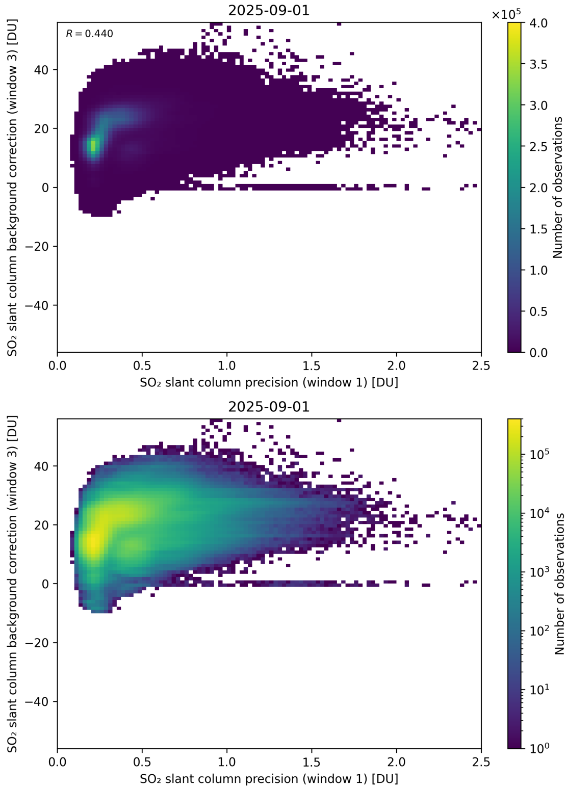
Figure 270: Scatter density plot of “SO 2 slant column precision (window 1)” against “SO 2 slant column background correction (window 3)” for 2025-08-31 to 2025-09-02.
