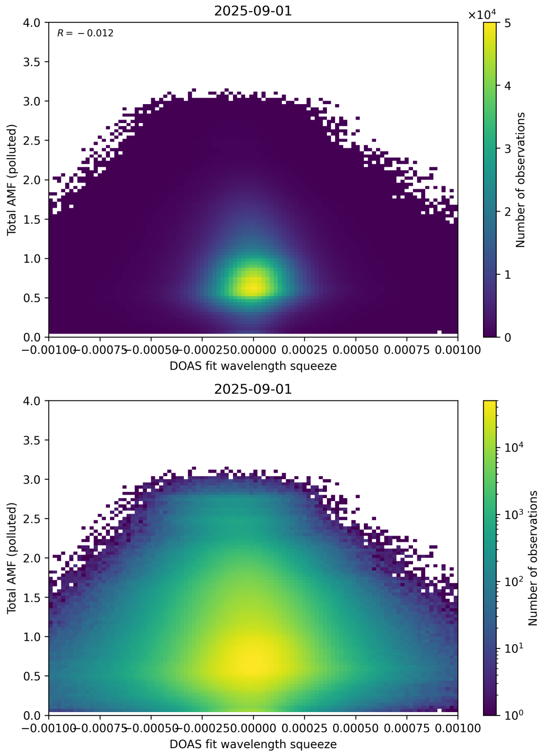
Figure 145: Scatter density plot of “DOAS fit wavelength squeeze” against “Total AMF (polluted)” for 2025-08-31 to 2025-09-02.
