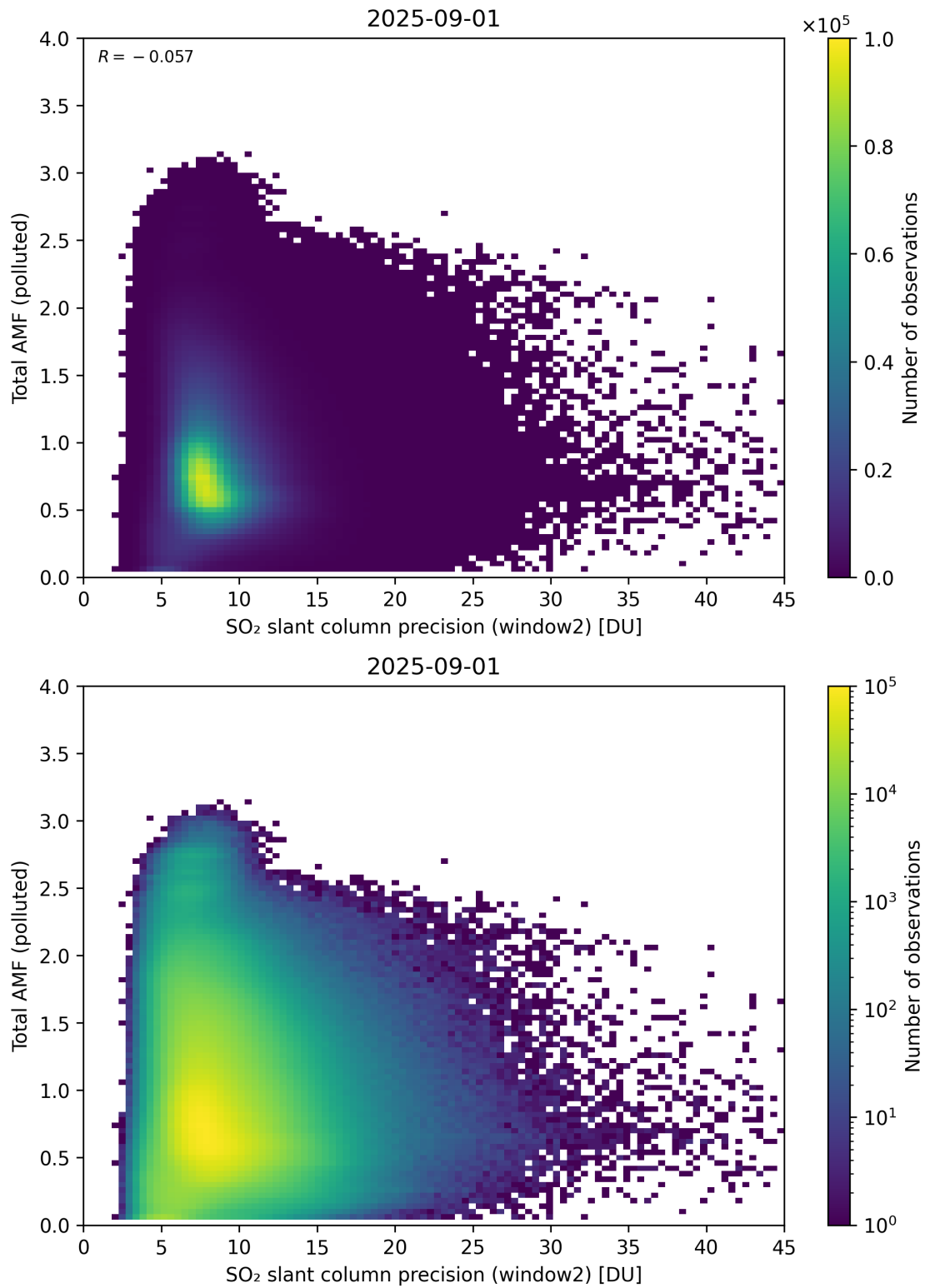
Figure 301: Scatter density plot of “SO 2 slant column precision (window2)” against “Total AMF (polluted)” for 2025-08-31 to 2025-09-02.
