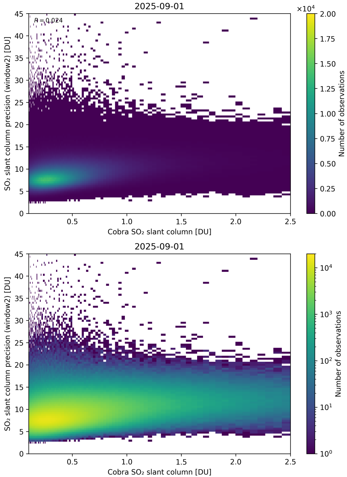
Figure 221: Scatter density plot of “Cobra SO 2 slant column” against “SO 2 slant column precision (window2)” for 2025-08-31 to 2025-09-02.
