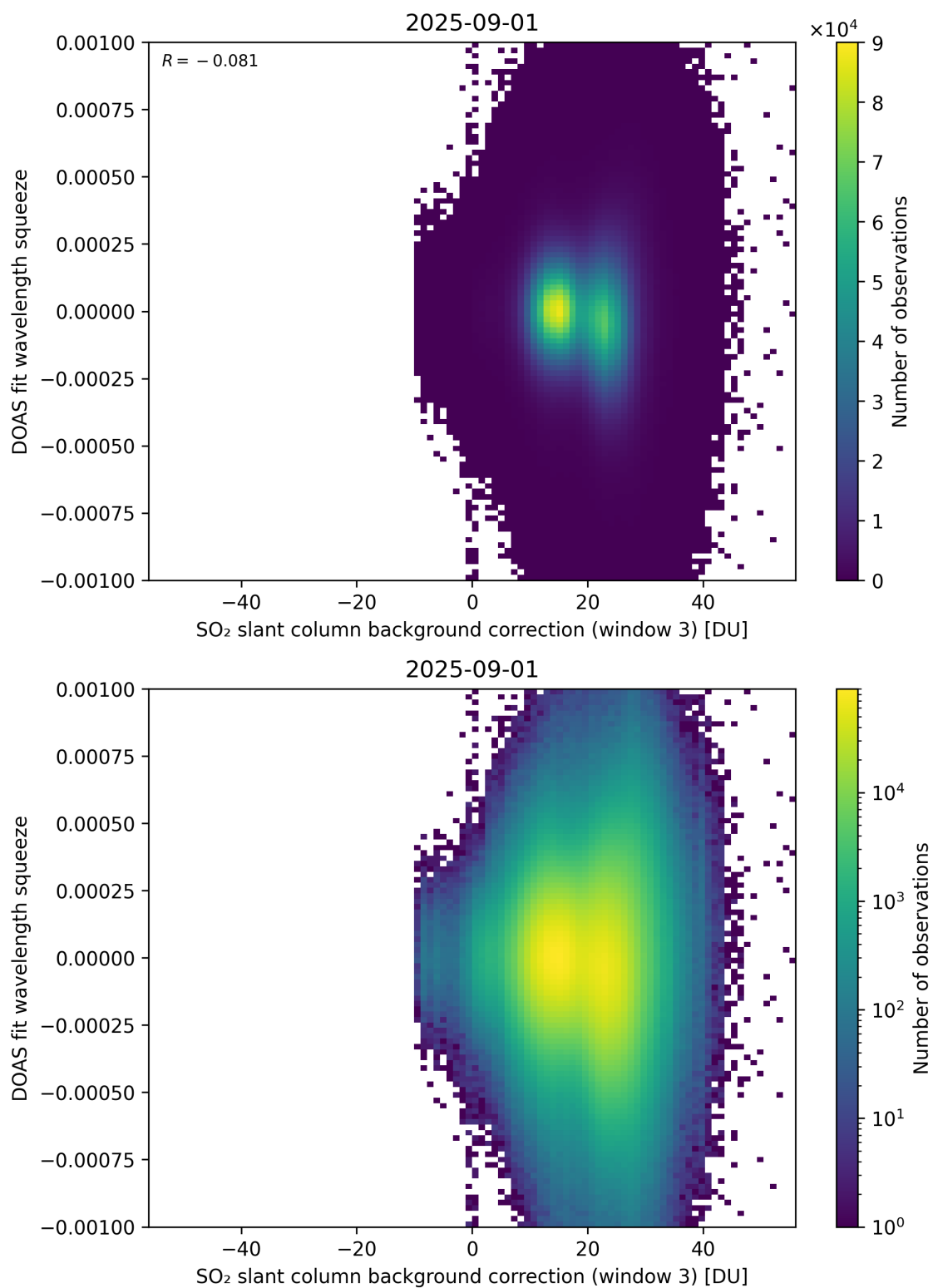
Figure 133: Scatter density plot of “SO 2 slant column background correction (window 3)” against “DOAS fit wavelength squeeze” for 2025-08-31 to 2025-09-02.
