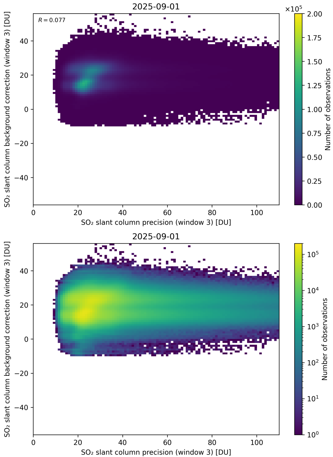
Figure 307: Scatter density plot of “SO 2 slant column precision (window 3)” against “SO 2 slant column background correction (window 3)” for 2025-08-31 to 2025-09-02.
