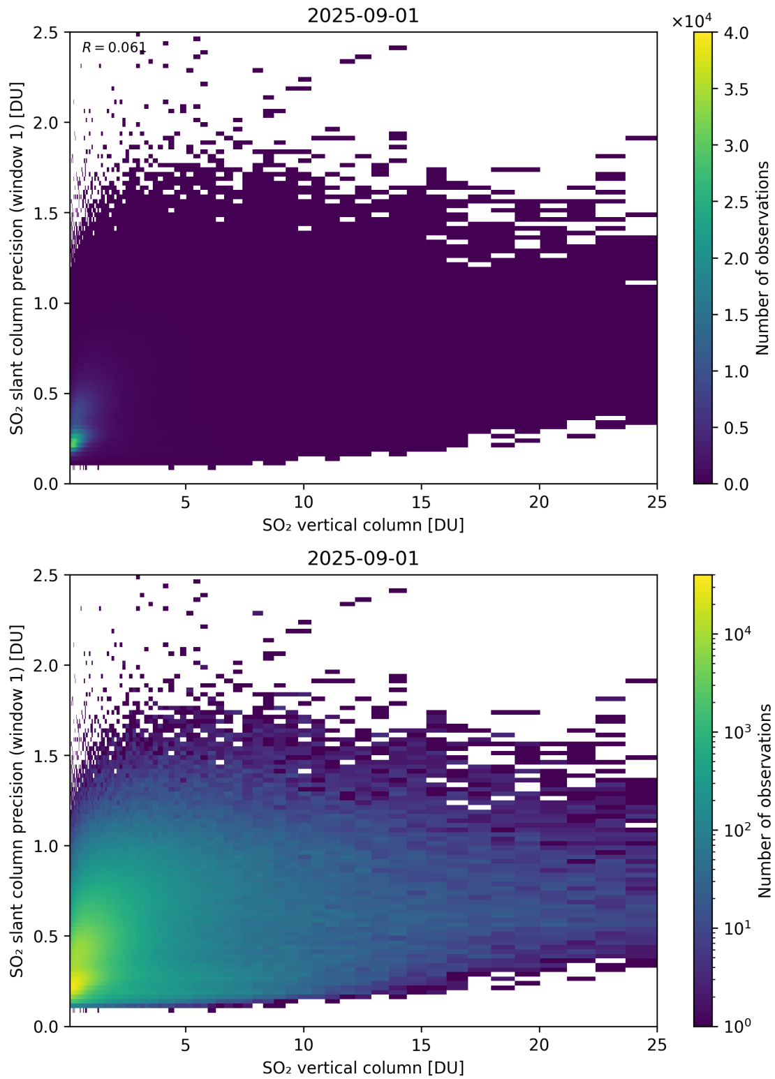
Figure 355: Scatter density plot of “SO 2 vertical column” against “SO 2 slant column precision (window 1)” for 2025-08-31 to 2025-09-02.
