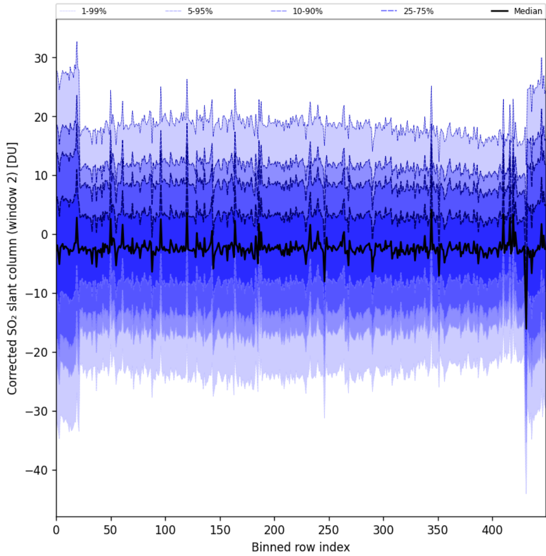
Figure 95: Along track statistics of “Corrected SO 2 slant column (window 2)” for 2025-08-31 to 2025-09-02
