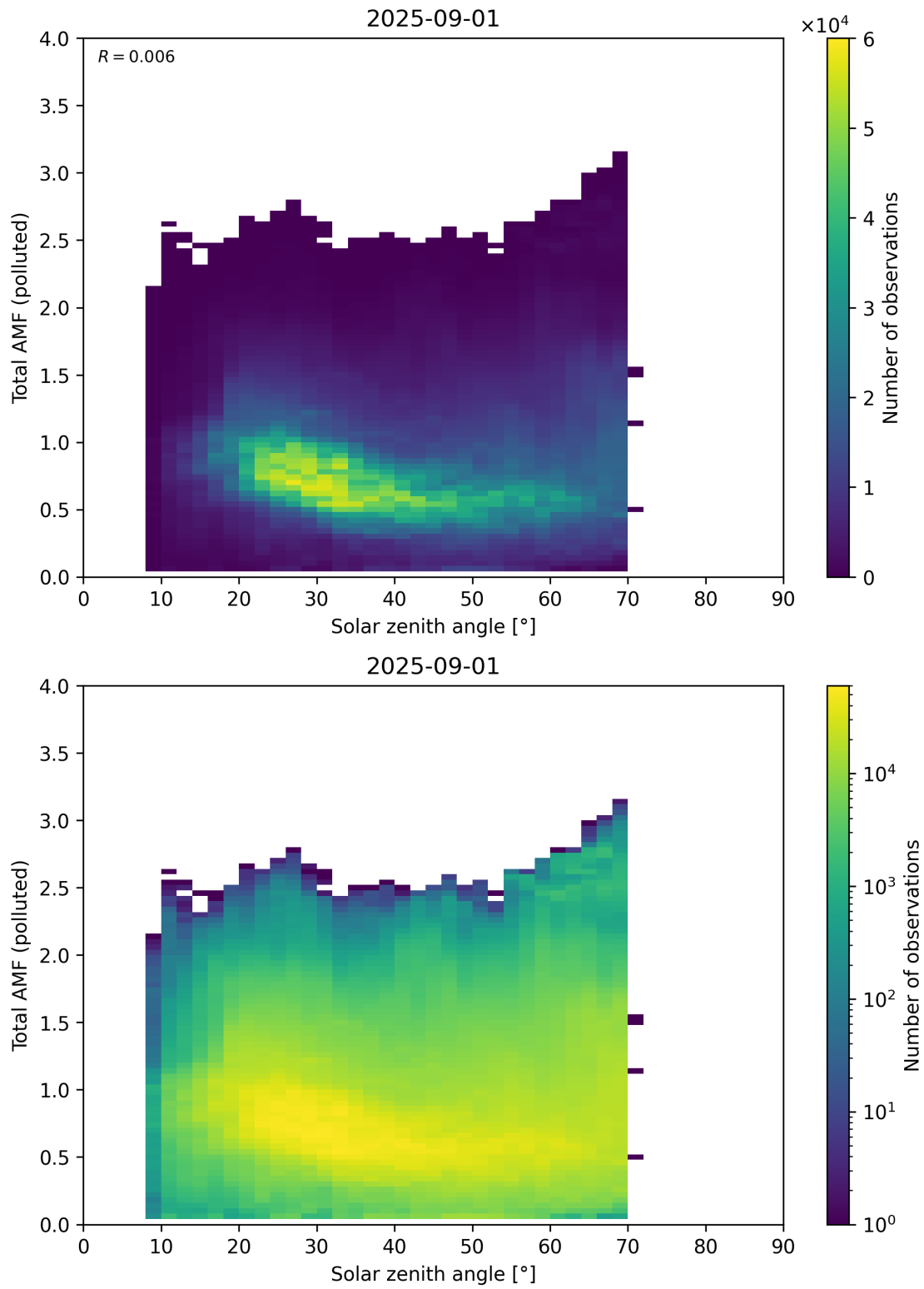
Figure 189: Scatter density plot of “Solar zenith angle” against “Total AMF (polluted)” for 2025-08-31 to 2025-09-02.
