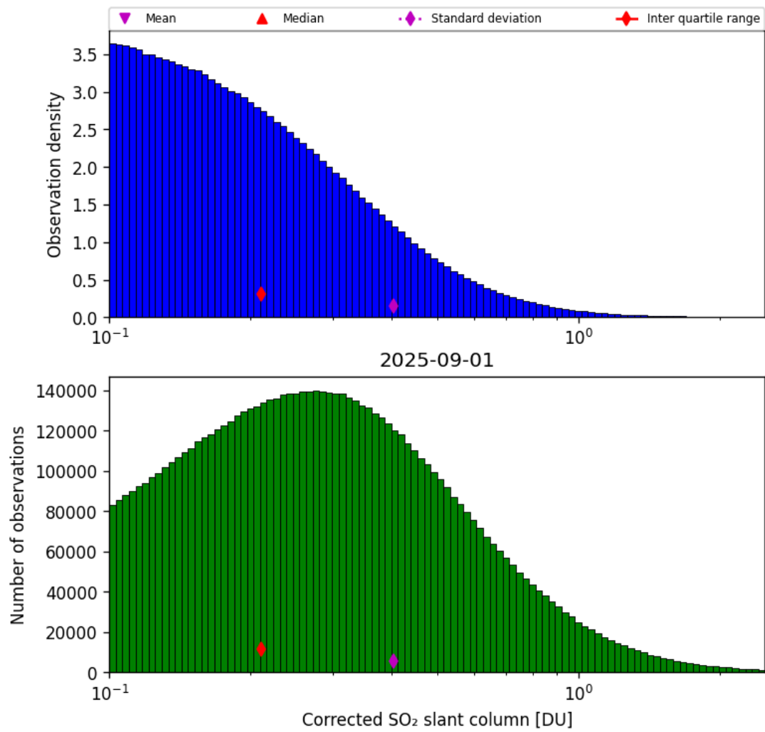
Figure 60: Histogram of “Corrected SO 2 slant column” for 2025-08-31 to 2025-09-02
