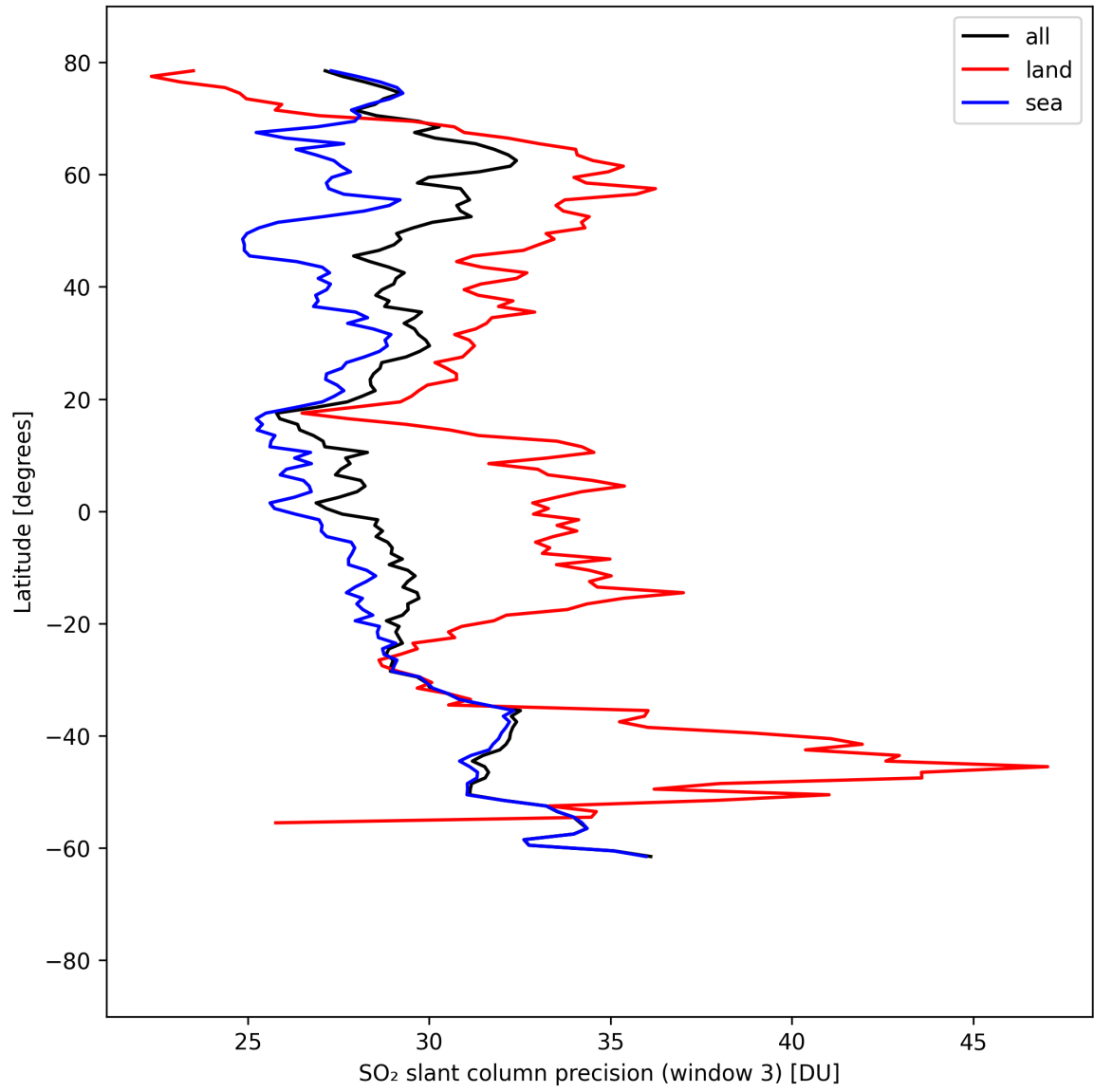
Figure 46: Zonal average of “SO 2 slant column precision (window 3)” for 2025-08-31 to 2025-09-02.
