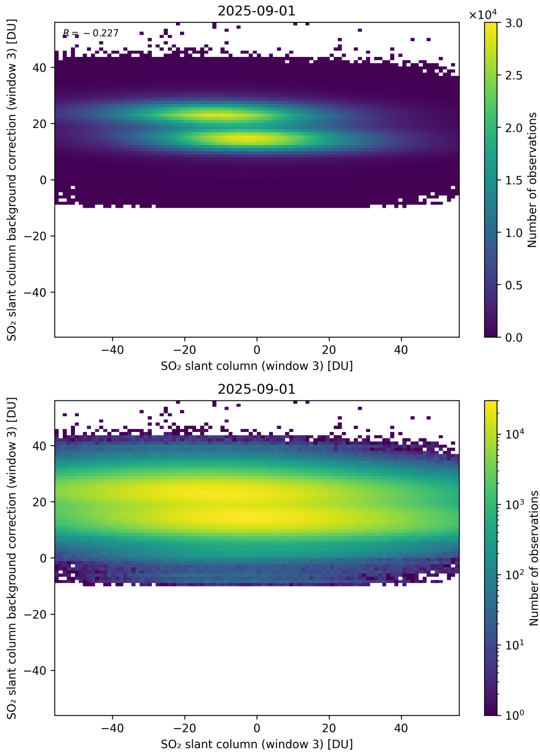
Figure 303: Scatter density plot of “SO 2 slant column (window 3)” against “SO 2 slant column background correction (window 3)” for 2025-08-31 to 2025-09-02.
