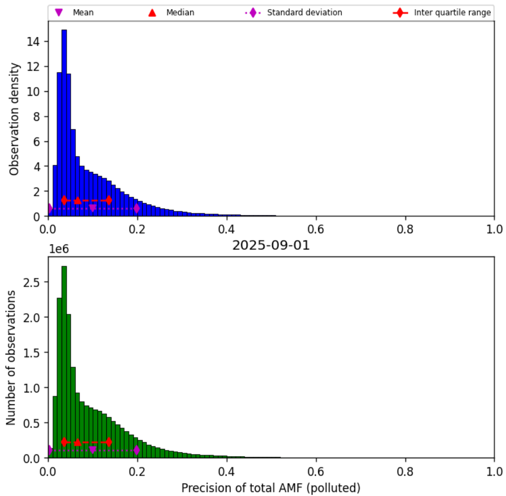
Figure 80: Histogram of “Precision of total AMF (polluted)” for 2025-08-31 to 2025-09-02
