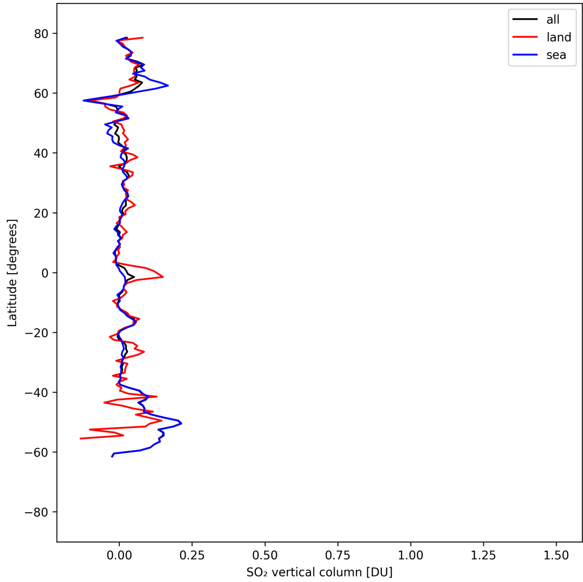
Figure 32: Zonal average of “SO 2 vertical column” for 2025-08-31 to 2025-09-02.
