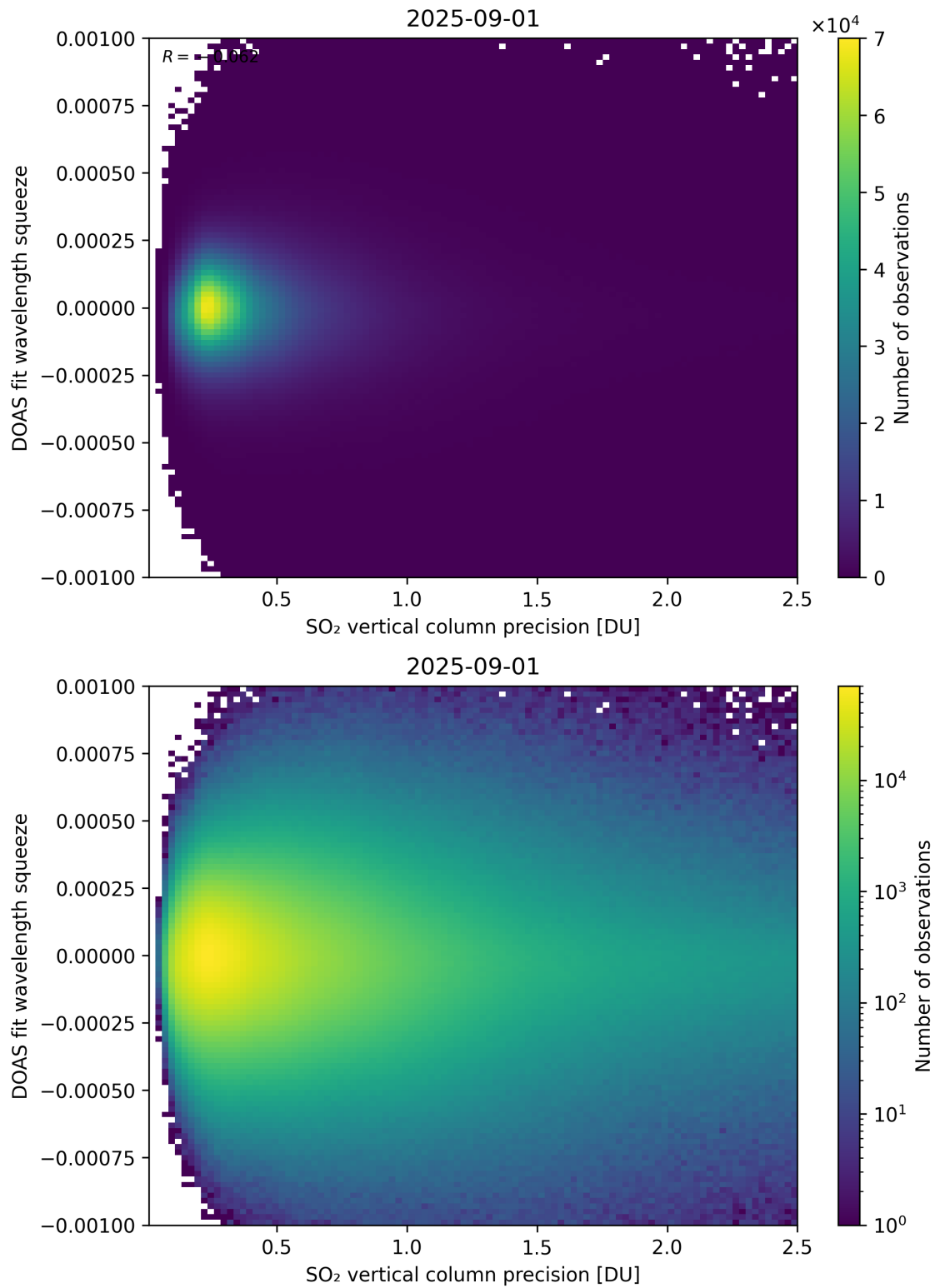
Figure 333: Scatter density plot of “SO 2 vertical column precision” against “DOAS fit wavelength squeeze” for 2025-08-31 to 2025-09-02.
