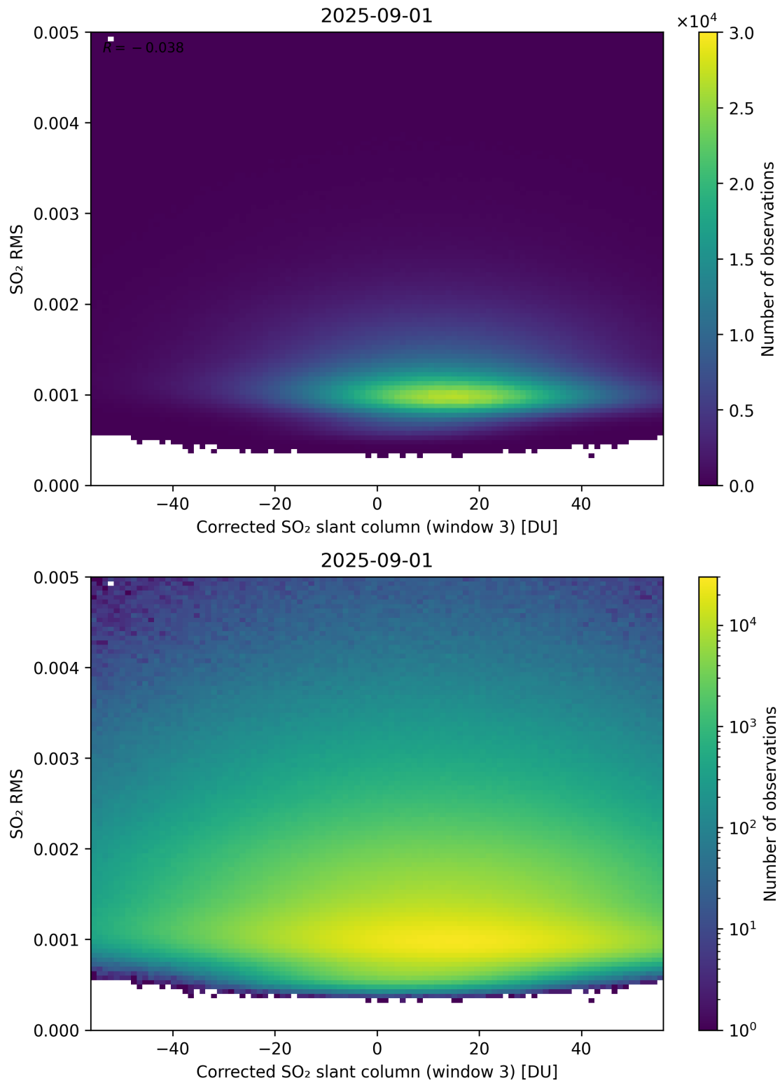
Figure 258: Scatter density plot of “Corrected SO 2 slant column (window 3)” against “SO 2 RMS” for 2025-08-31 to 2025-09-02.
