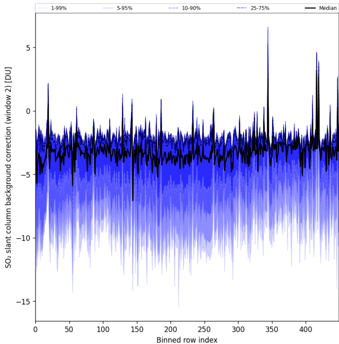
Figure 96: Along track statistics of “SO 2 slant column background correction (window 2)” for 2025-08-31 to 2025-09-02
