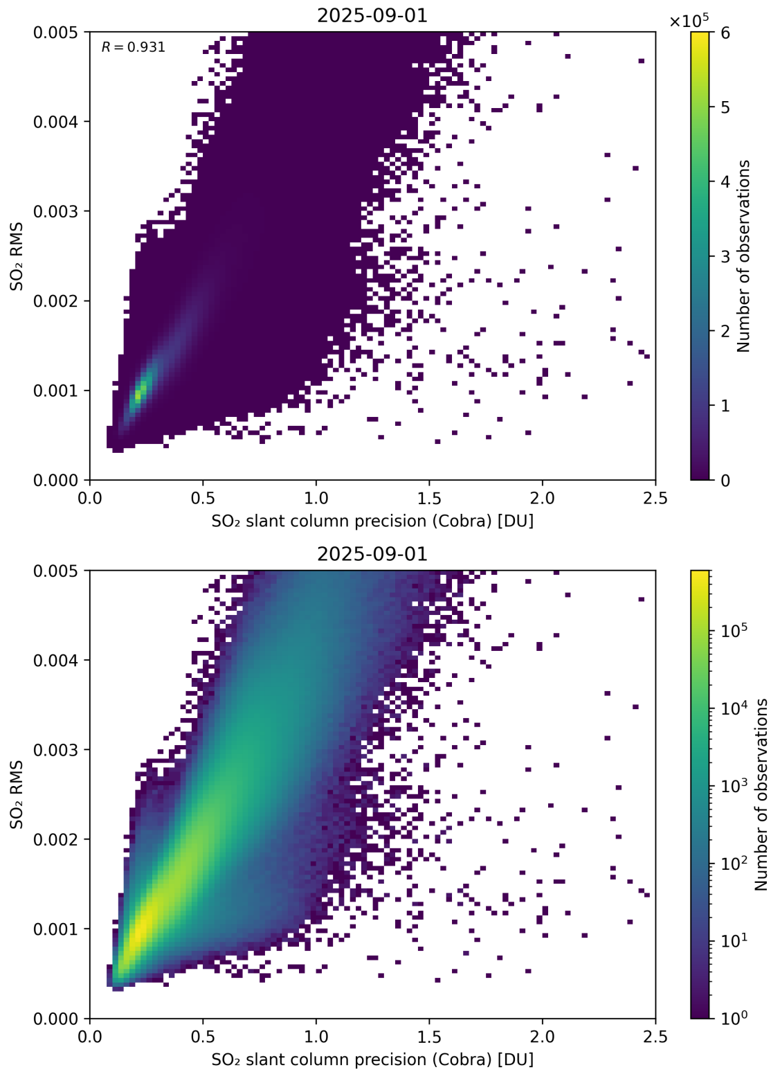
Figure 204: Scatter density plot of “SO 2 slant column precision (Cobra)” against “SO 2 RMS” for 2025-08-31 to 2025-09-02.
