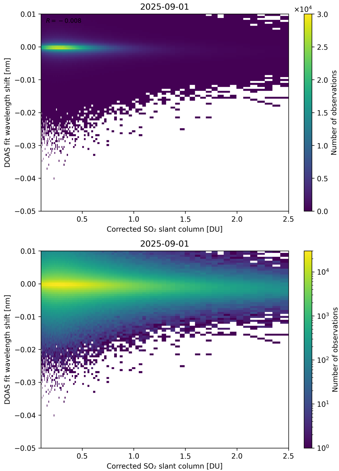
Figure 229: Scatter density plot of “Corrected SO 2 slant column” against “DOAS fit wavelength shift” for 2025-08-31 to 2025-09-02.
