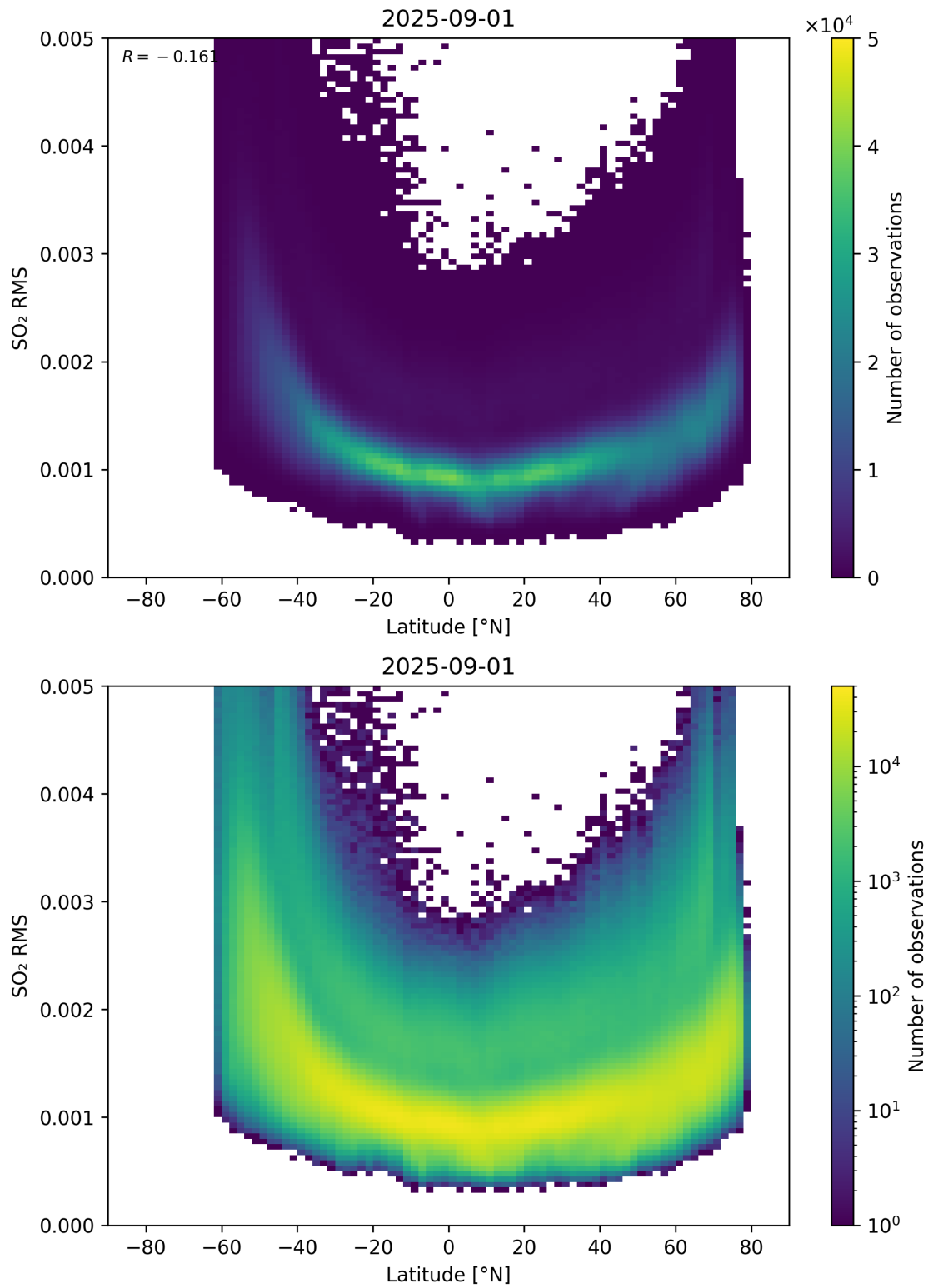
Figure 155: Scatter density plot of “Latitude” against “SO 2 RMS” for 2025-08-31 to 2025-09-02.
