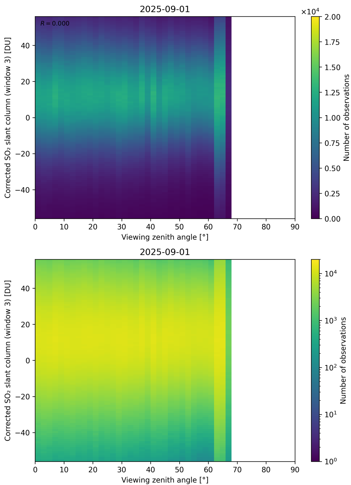
Figure 375: Scatter density plot of “Viewing zenith angle” against “Corrected SO 2 slant column (window 3)” for 2025-08-31 to 2025-09-02.
