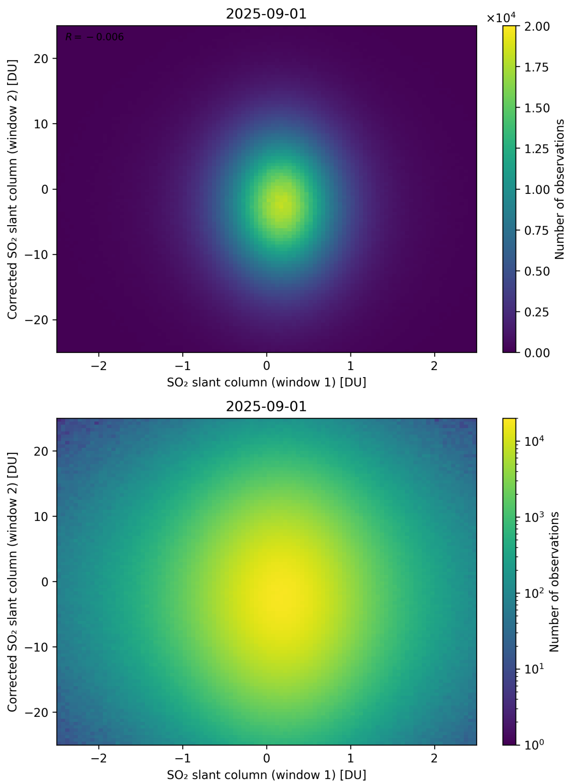
Figure 283: Scatter density plot of “SO 2 slant column (window 1)” against “Corrected SO 2 slant column (window 2)” for 2025-08-31 to 2025-09-02.
