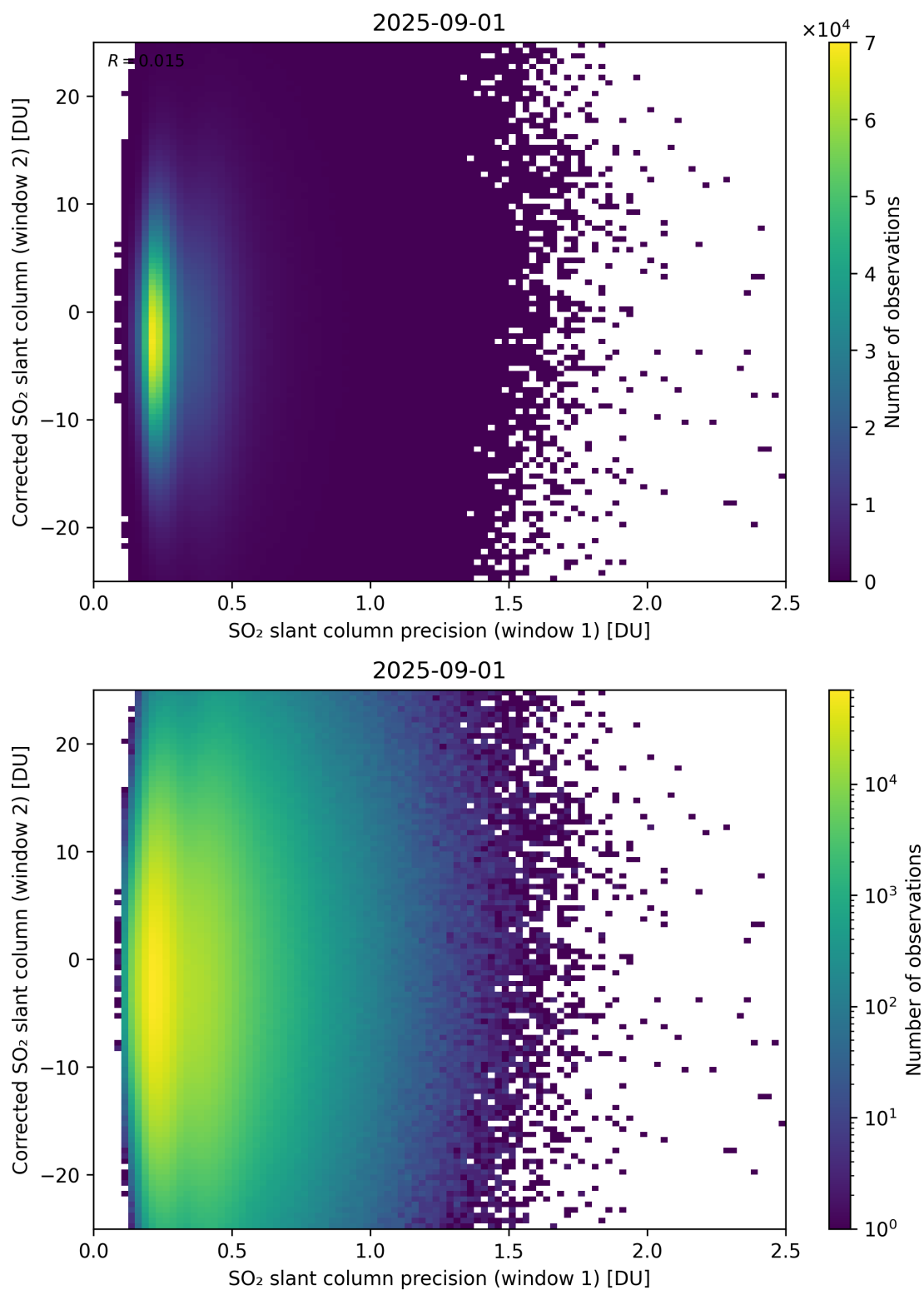
Figure 275: Scatter density plot of “SO 2 slant column precision (window 1)” against “Corrected SO 2 slant column (window 2)” for 2025-08-31 to 2025-09-02.
