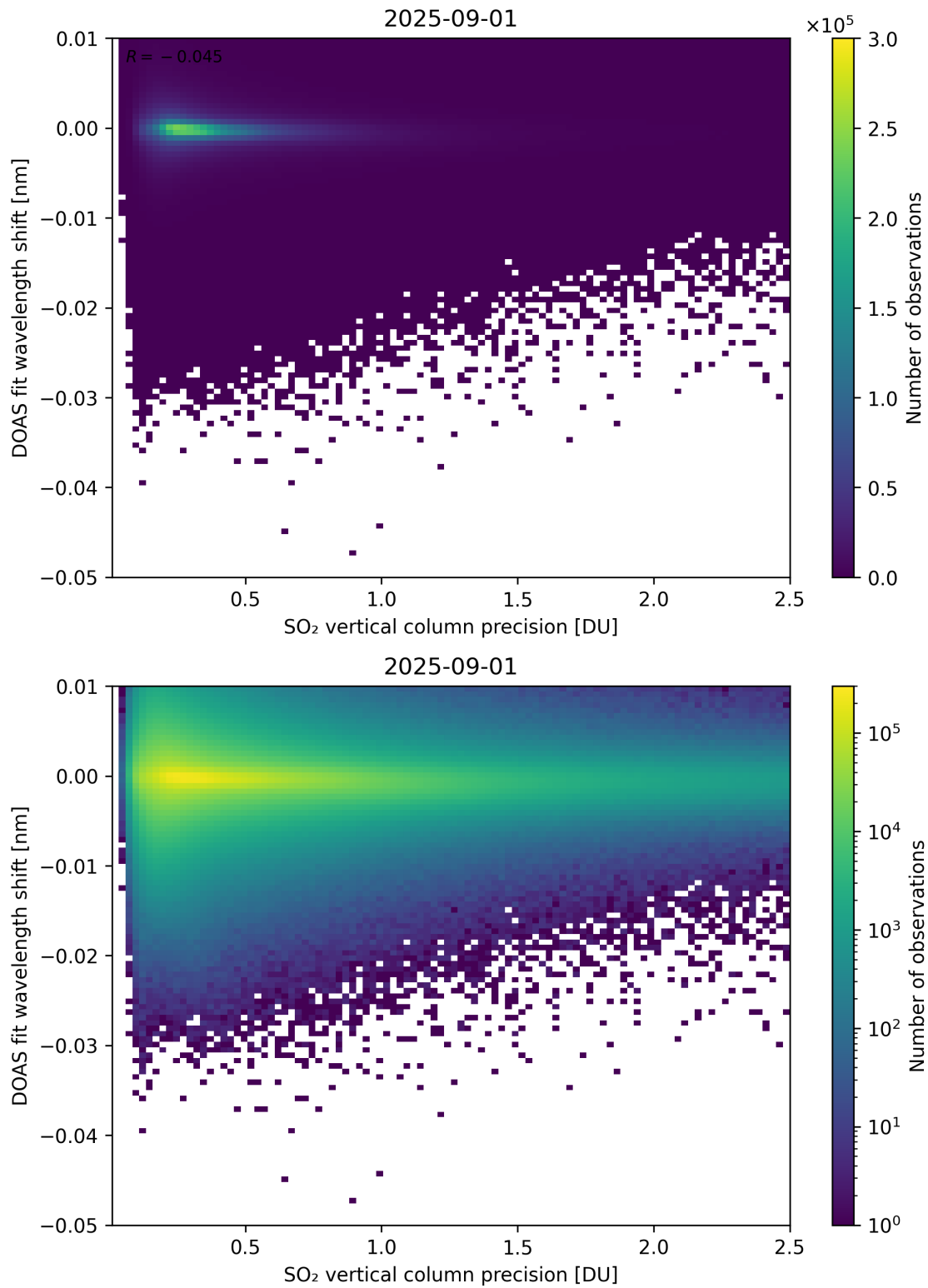
Figure 332: Scatter density plot of “SO 2 vertical column precision” against “DOAS fit wavelength shift” for 2025-08-31 to 2025-09-02.
