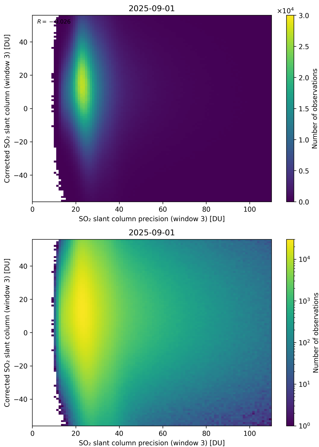
Figure 312: Scatter density plot of “SO 2 slant column precision (window 3)” against “Corrected SO 2 slant column (window 3)” for 2025-08-31 to 2025-09-02.
