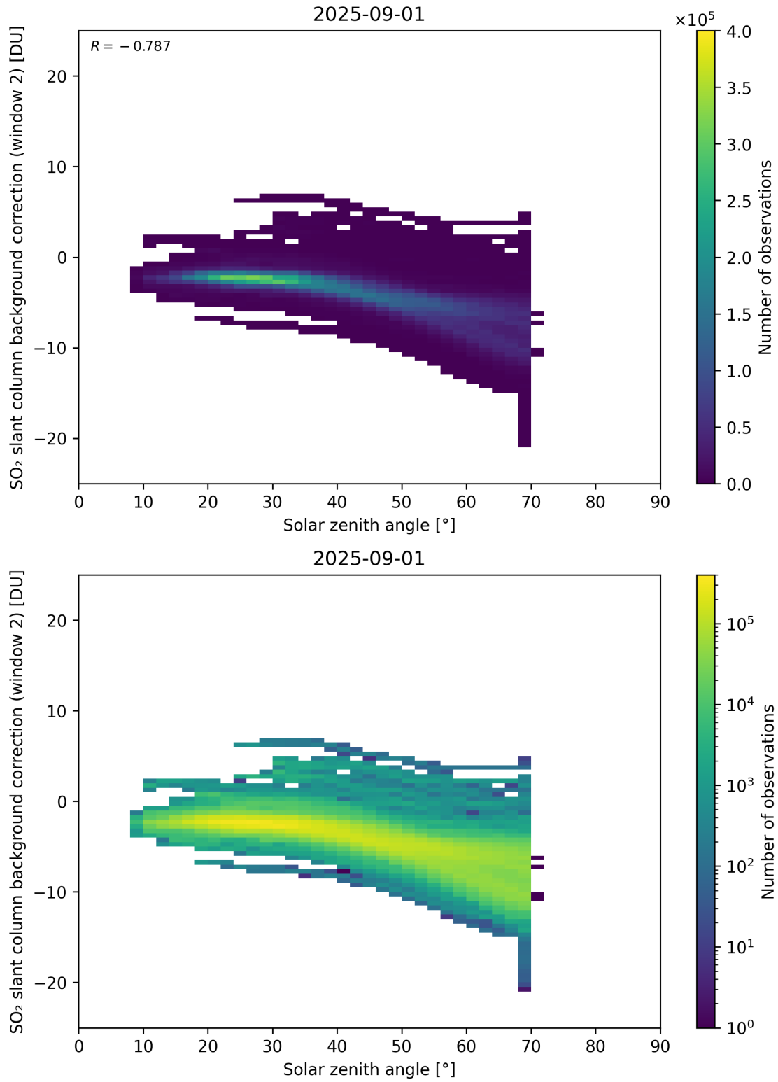
Figure 172: Scatter density plot of “Solar zenith angle” against “SO 2 slant column background correction (window 2)” for 2025-08-31 to 2025-09-02.
