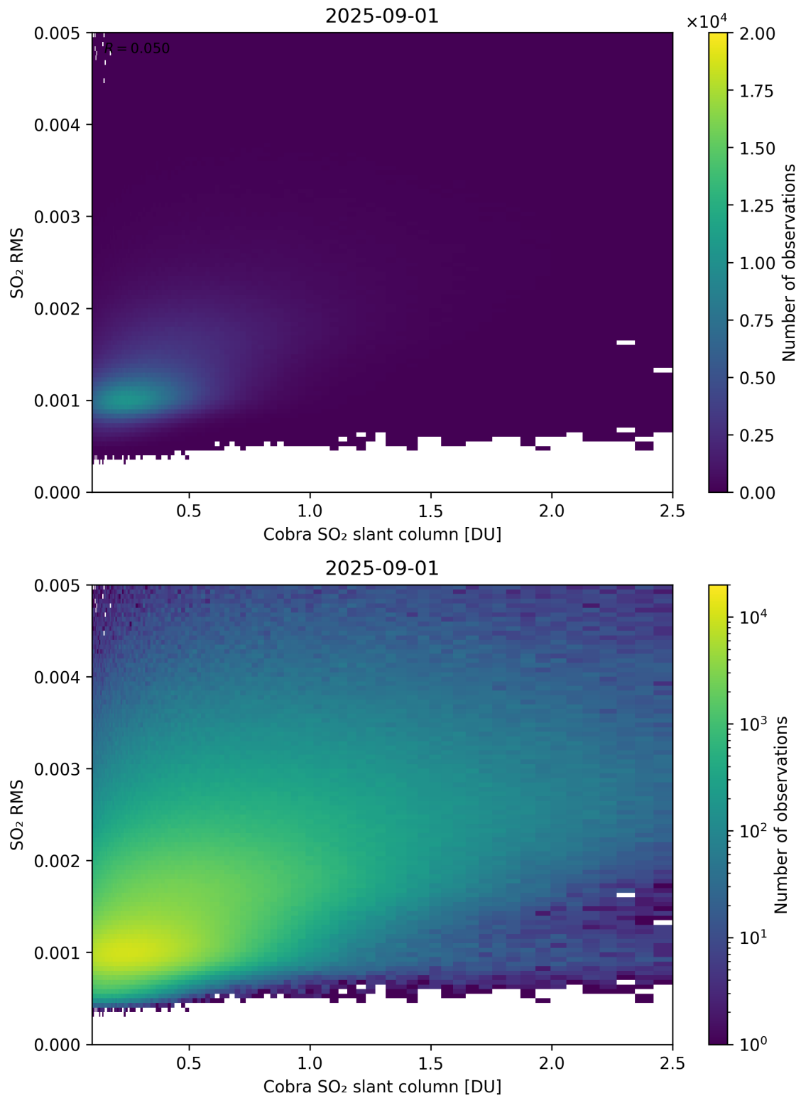
Figure 198: Scatter density plot of “Cobra SO 2 slant column” against “SO 2 RMS” for 2025-08-31 to 2025-09-02.
