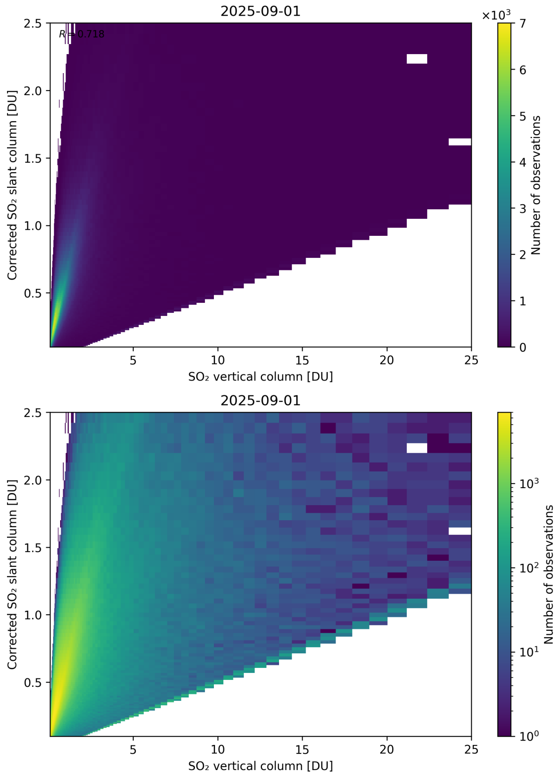
Figure 351: Scatter density plot of “SO 2 vertical column” against “Corrected SO 2 slant column” for 2025-08-31 to 2025-09-02.
