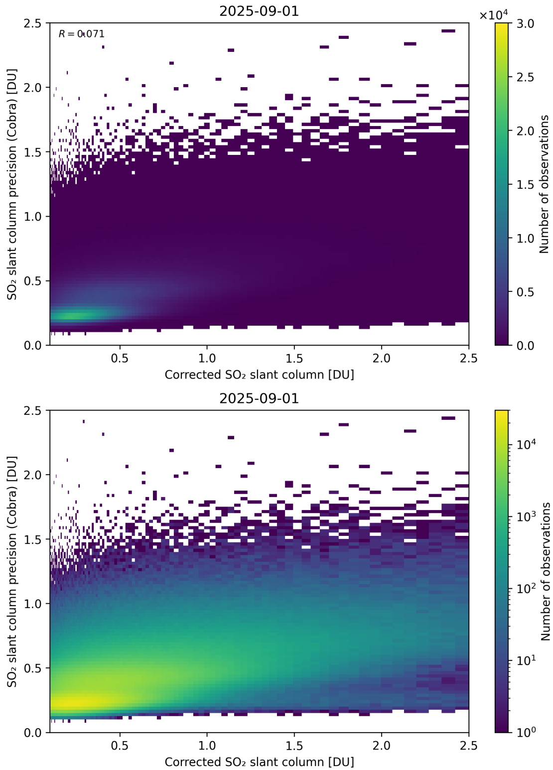
Figure 234: Scatter density plot of “Corrected SO 2 slant column” against “SO 2 slant column precision (Cobra)” for 2025-08-31 to 2025-09-02.
