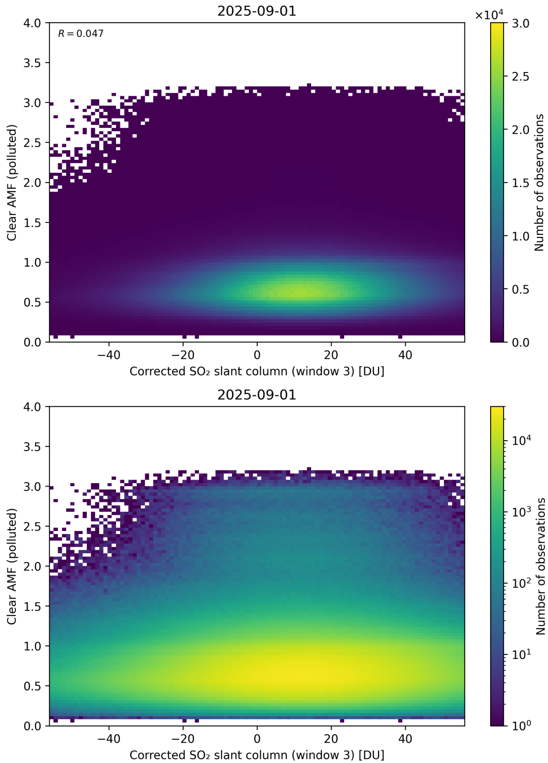
Figure 259: Scatter density plot of “Corrected SO 2 slant column (window 3)” against “Clear AMF (polluted)” for 2025-08-31 to 2025-09-02.
