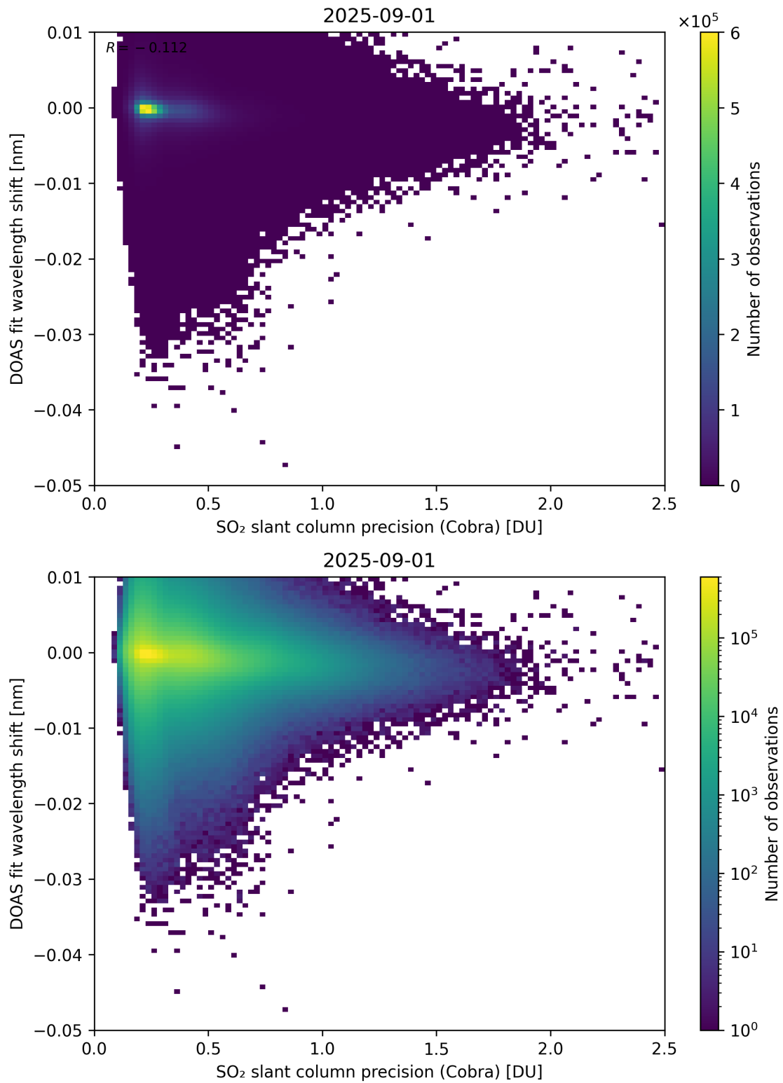
Figure 202: Scatter density plot of “SO 2 slant column precision (Cobra)” against “DOAS fit wavelength shift” for 2025-08-31 to 2025-09-02.
