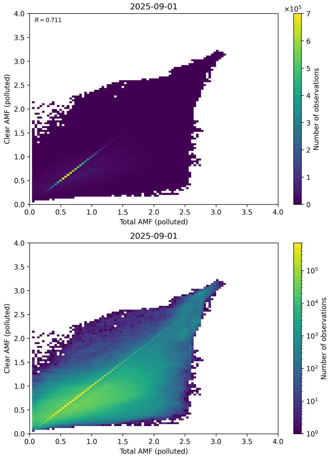
Figure 321: Scatter density plot of “Total AMF (polluted)” against “Clear AMF (polluted)” for 2025-08-31 to 2025-09-02.
