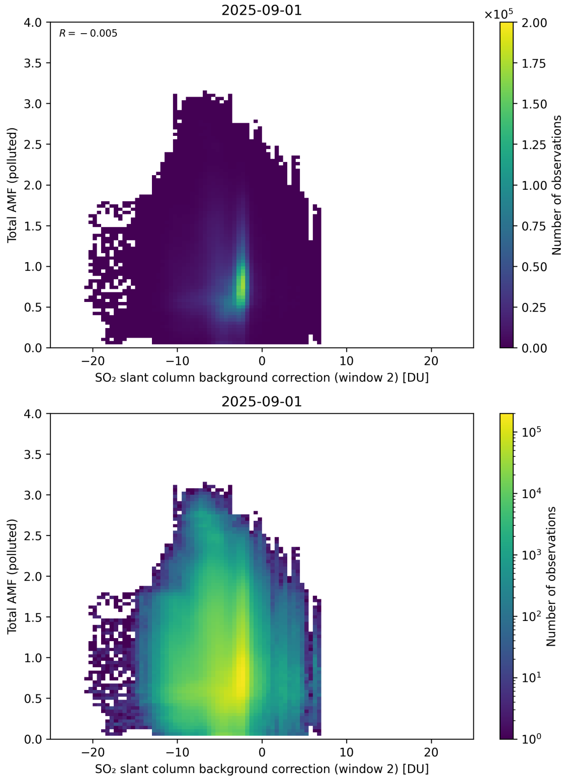
Figure 130: Scatter density plot of “SO 2 slant column background correction (window 2)” against “Total AMF (polluted)” for 2025-08-31 to 2025-09-02.
