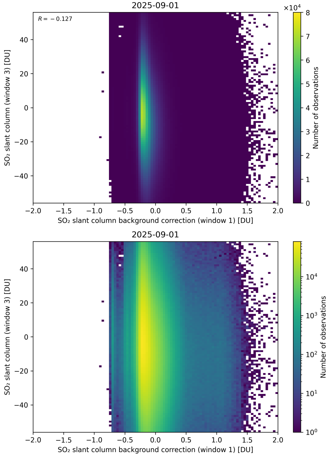
Figure 118: Scatter density plot of “SO 2 slant column background correction (window 1)” against “SO 2 slant column (window 3)” for 2025-08-31 to 2025-09-02.
