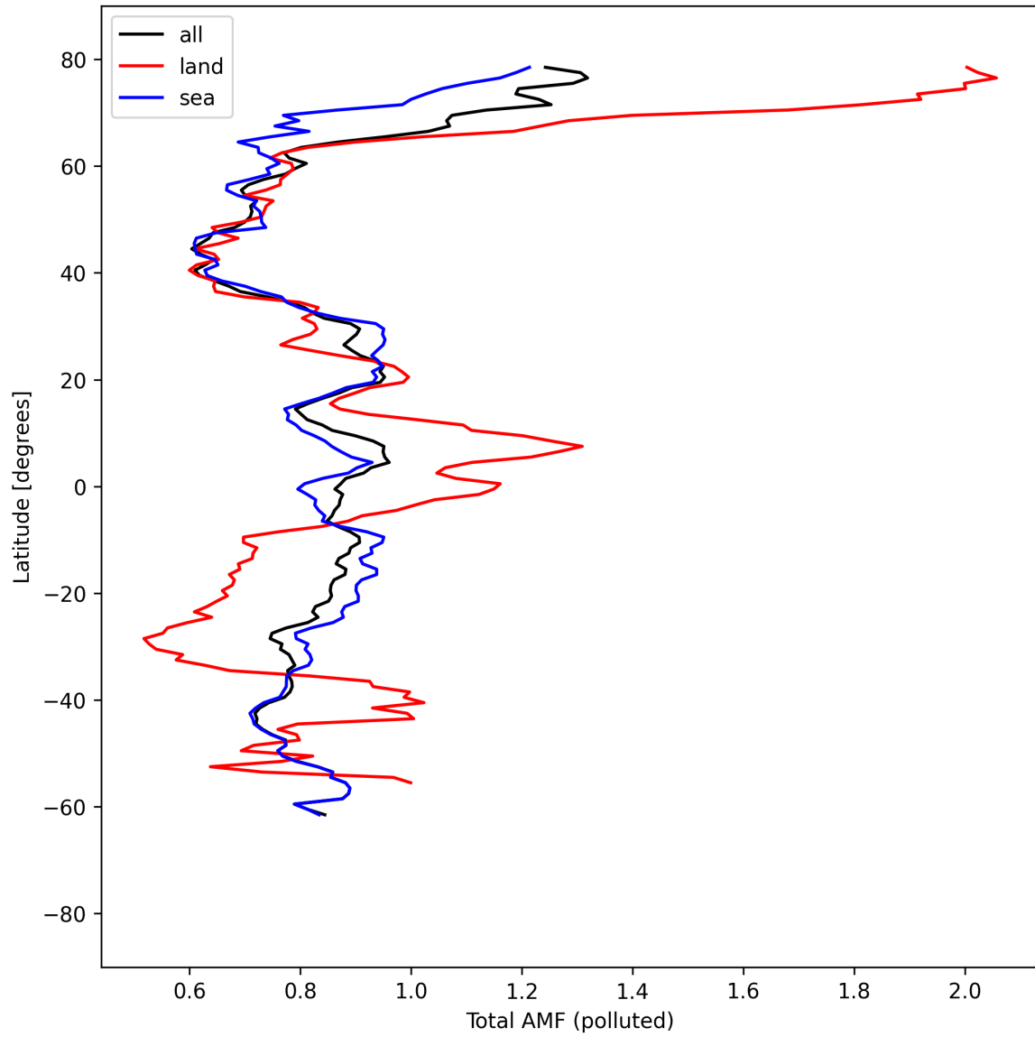
Figure 53: Zonal average of “Total AMF (polluted)” for 2025-08-31 to 2025-09-02.
