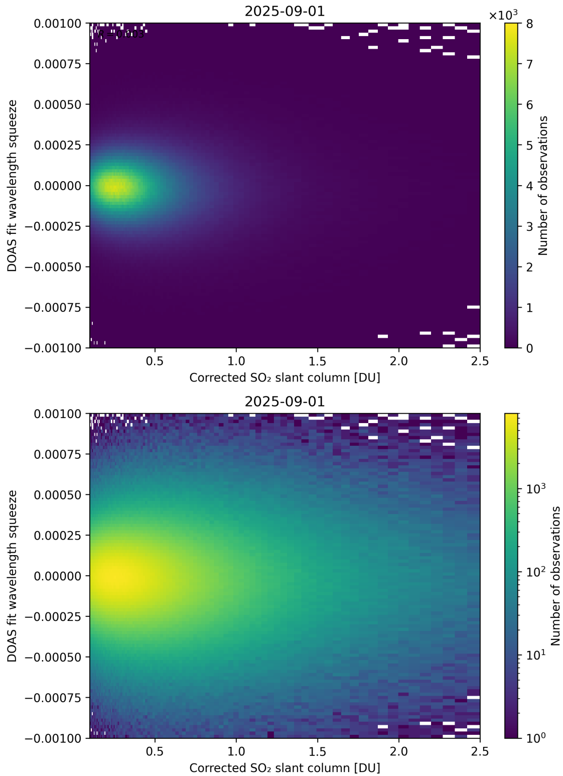
Figure 230: Scatter density plot of “Corrected SO 2 slant column” against “DOAS fit wavelength squeeze” for 2025-08-31 to 2025-09-02.
