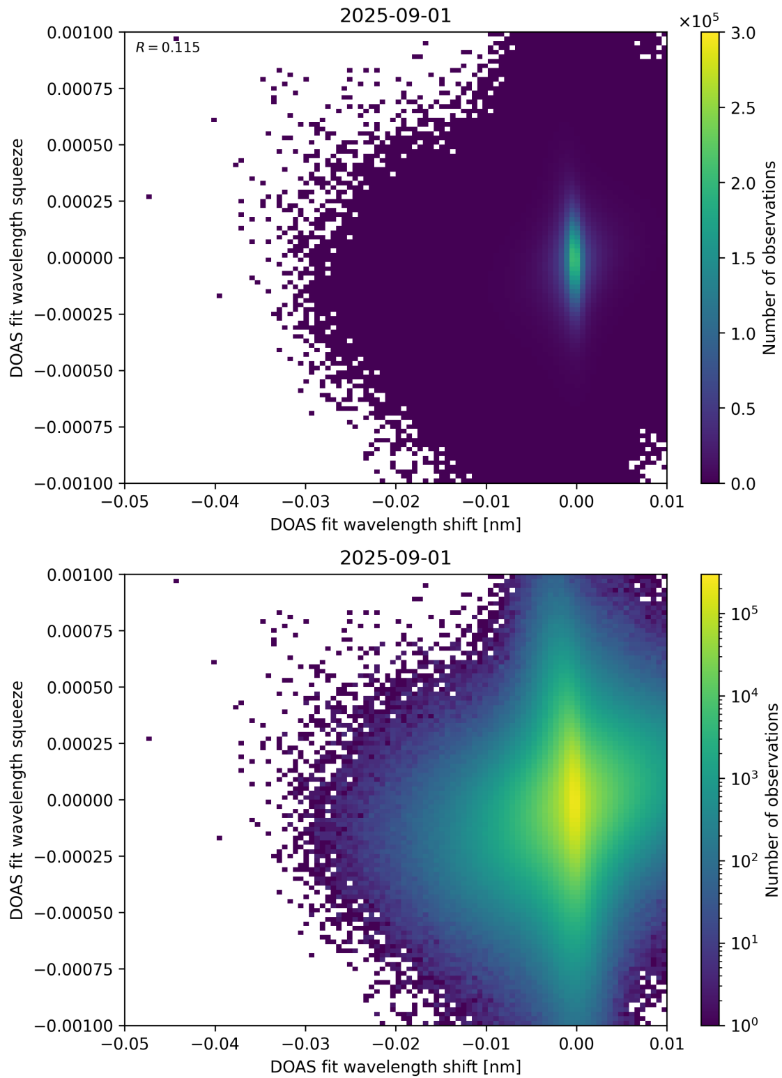
Figure 138: Scatter density plot of “DOAS fit wavelength shift” against “DOAS fit wavelength squeeze” for 2025-08-31 to 2025-09-02.
