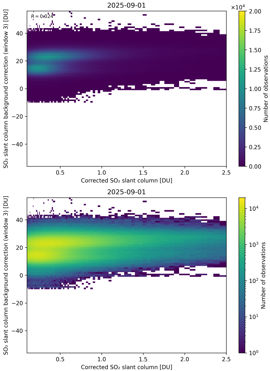
Figure 228: Scatter density plot of “Corrected SO 2 slant column” against “SO 2 slant column background correction (window 3)” for 2025-08-31 to 2025-09-02.
