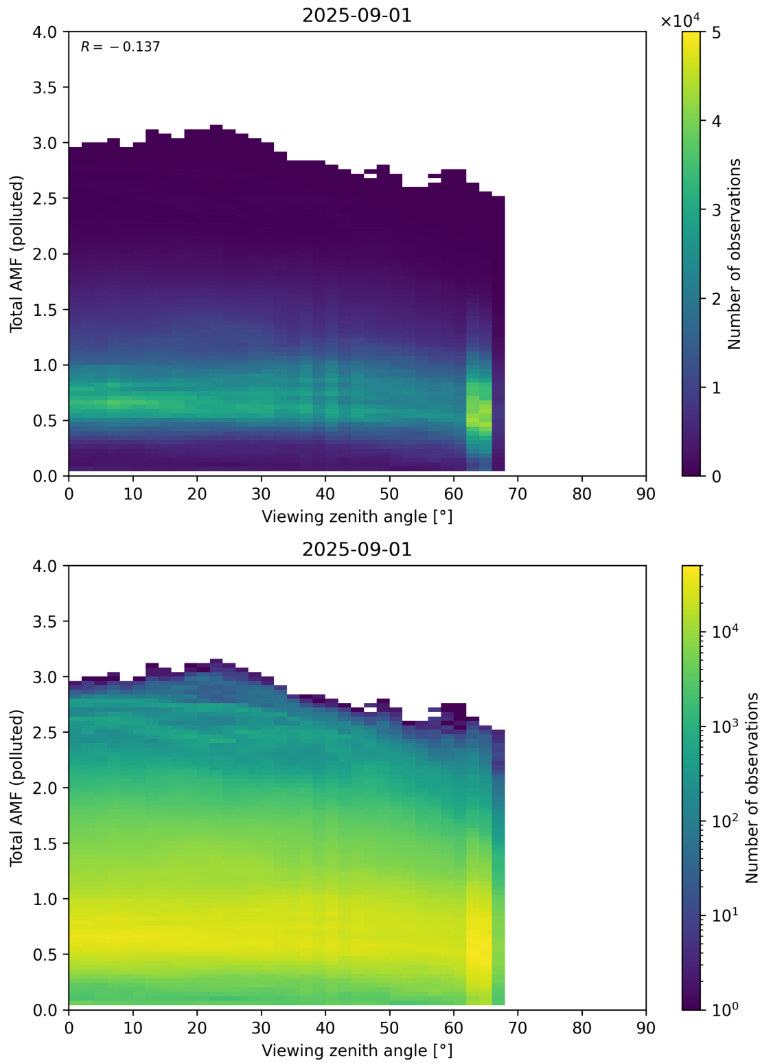
Figure 381: Scatter density plot of “Viewing zenith angle” against “Total AMF (polluted)” for 2025-08-31 to 2025-09-02.
