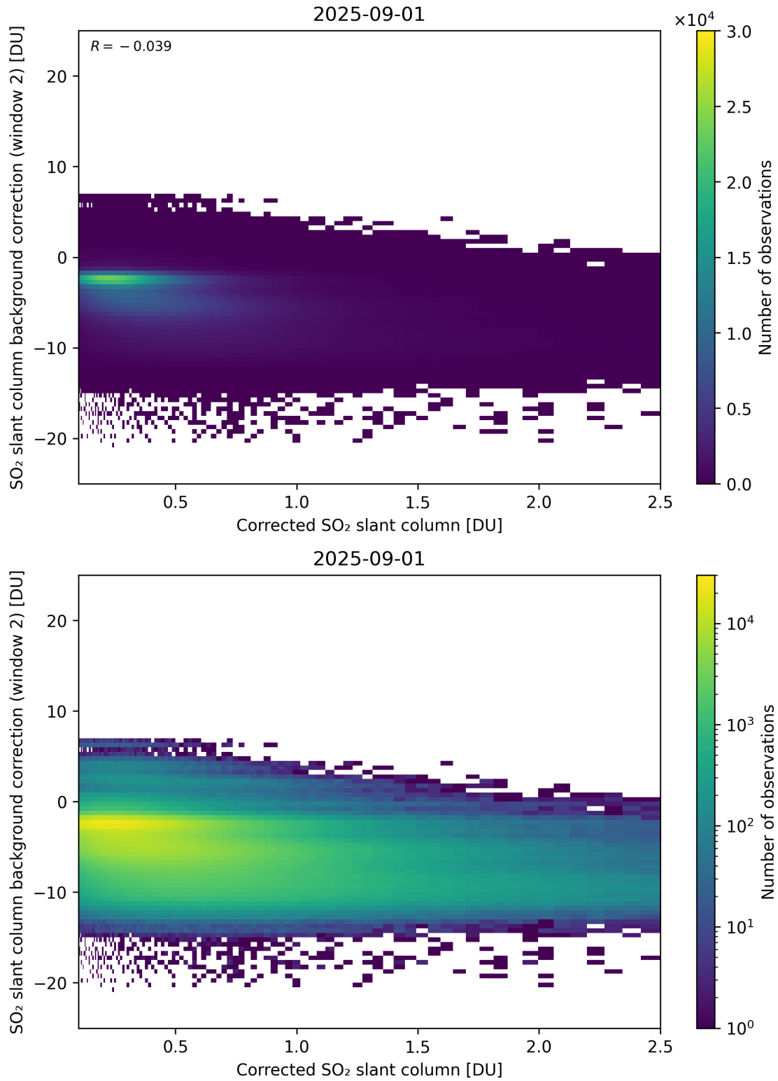
Figure 227: Scatter density plot of “Corrected SO 2 slant column” against “SO 2 slant column background correction (window 2)” for 2025-08-31 to 2025-09-02.
