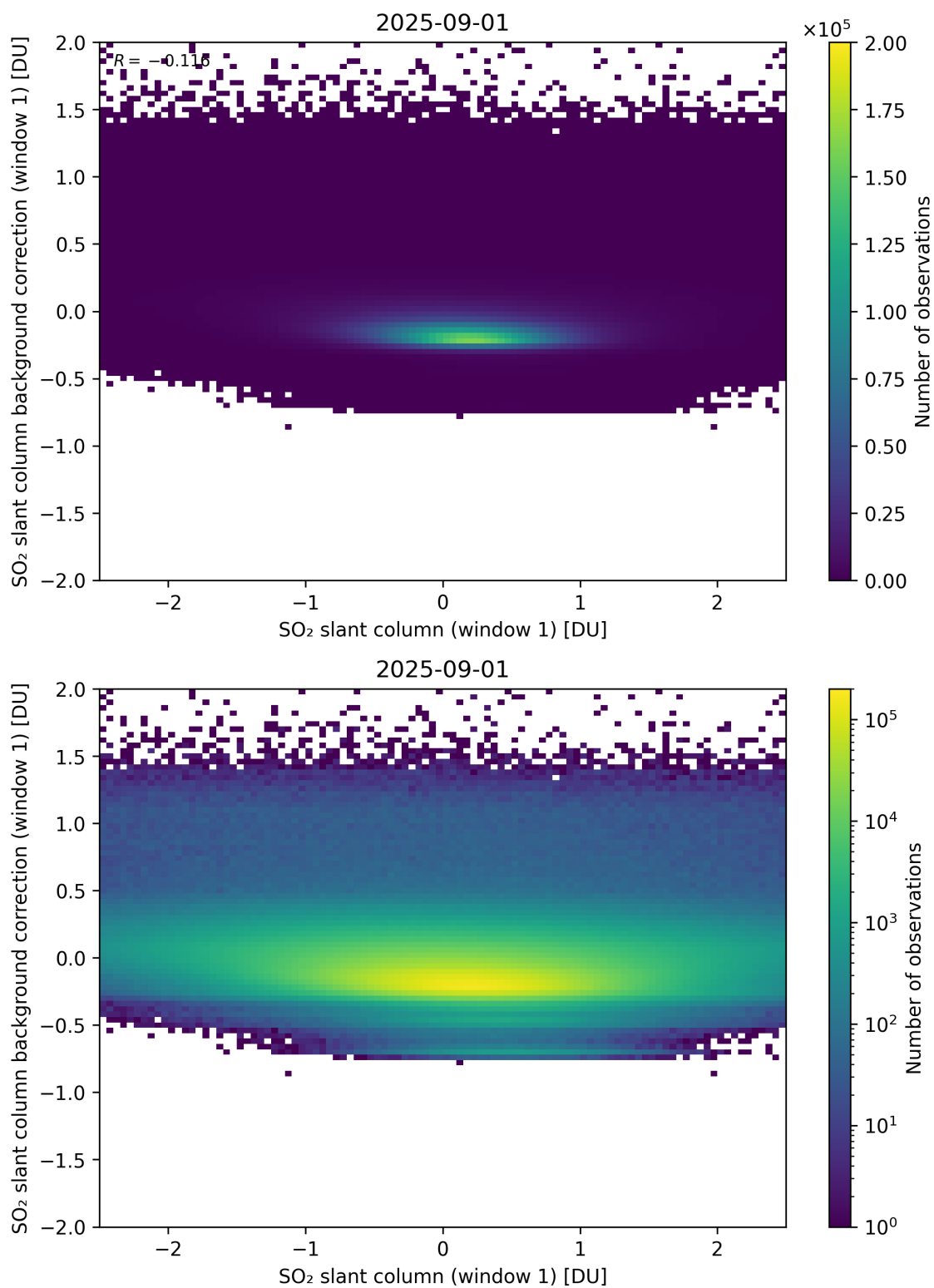
Figure 262: Scatter density plot of “SO 2 slant column (window 1)” against “SO 2 slant column background correction (window 1)” for 2025-08-31 to 2025-09-02.
