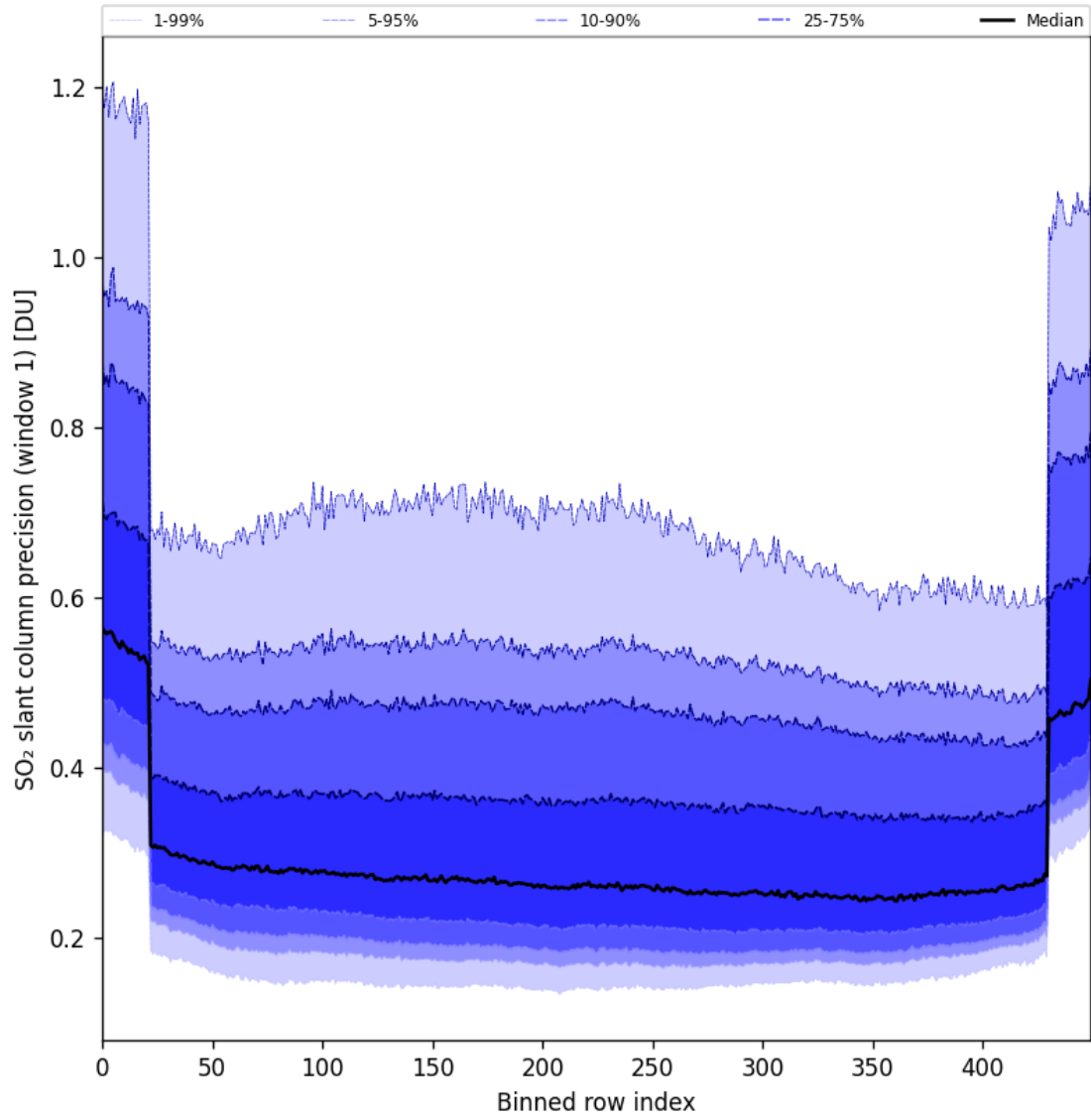
Figure 90: Along track statistics of “SO 2 slant column precision (window 1)” for 2025-08-31 to 2025-09-02
