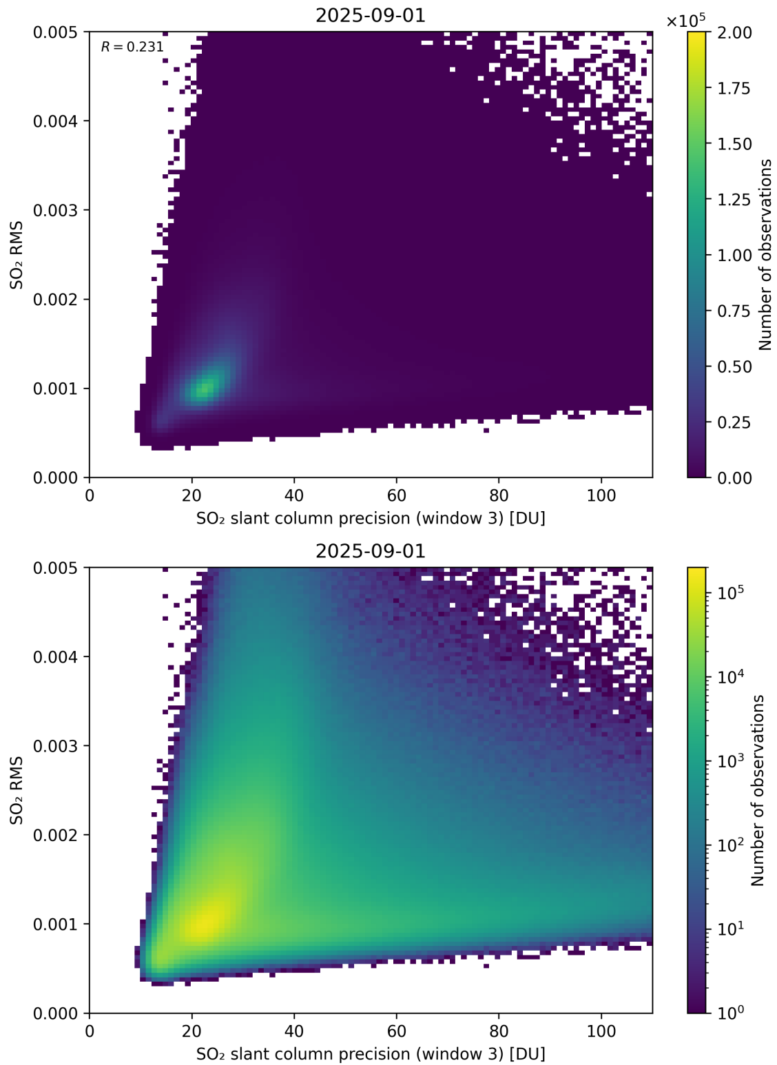
Figure 310: Scatter density plot of “SO 2 slant column precision (window 3)” against “SO 2 RMS” for 2025-08-31 to 2025-09-02.
