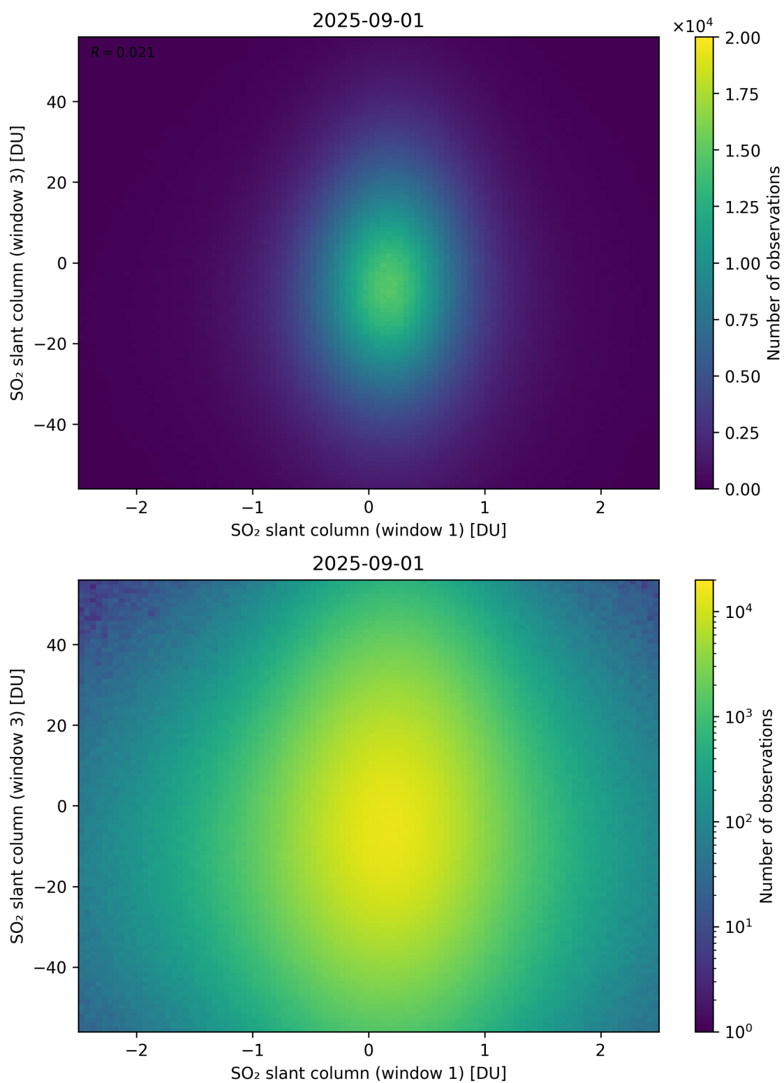
Figure 287: Scatter density plot of “SO 2 slant column (window 1)” against “SO 2 slant column (window 3)” for 2025-08-31 to 2025-09-02.
