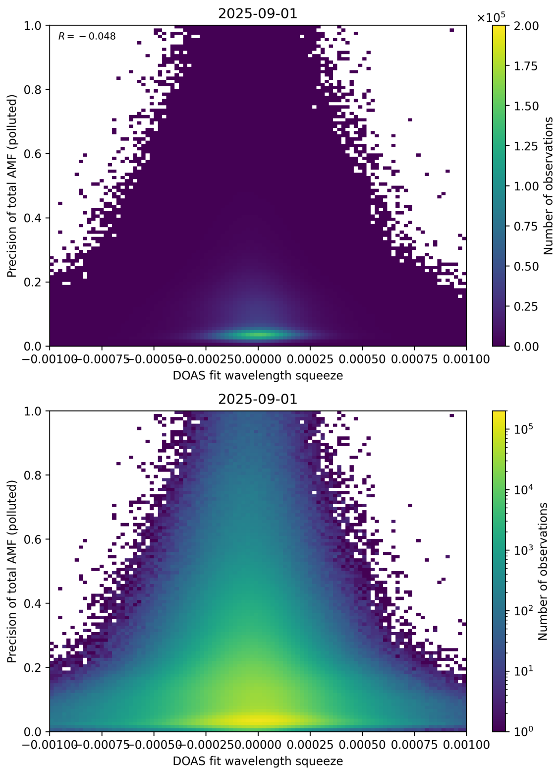
Figure 146: Scatter density plot of “DOAS fit wavelength squeeze” against “Precision of total AMF (polluted)” for 2025-08-31 to 2025-09-02.
