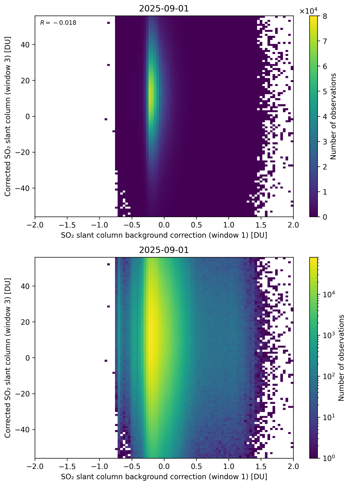
Figure 116: Scatter density plot of “SO 2 slant column background correction (window 1)” against “Corrected SO 2 slant column (window 3)” for 2025-08-31 to 2025-09-02.
