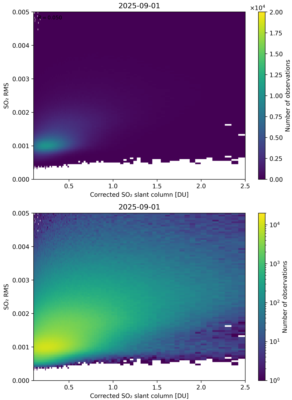
Figure 231: Scatter density plot of “Corrected SO 2 slant column” against “SO 2 RMS” for 2025-08-31 to 2025-09-02.
