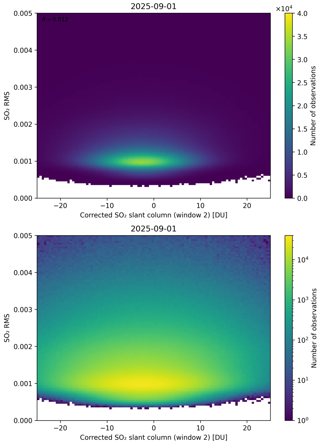
Figure 248: Scatter density plot of “Corrected SO 2 slant column (window 2)” against “SO 2 RMS” for 2025-08-31 to 2025-09-02.
