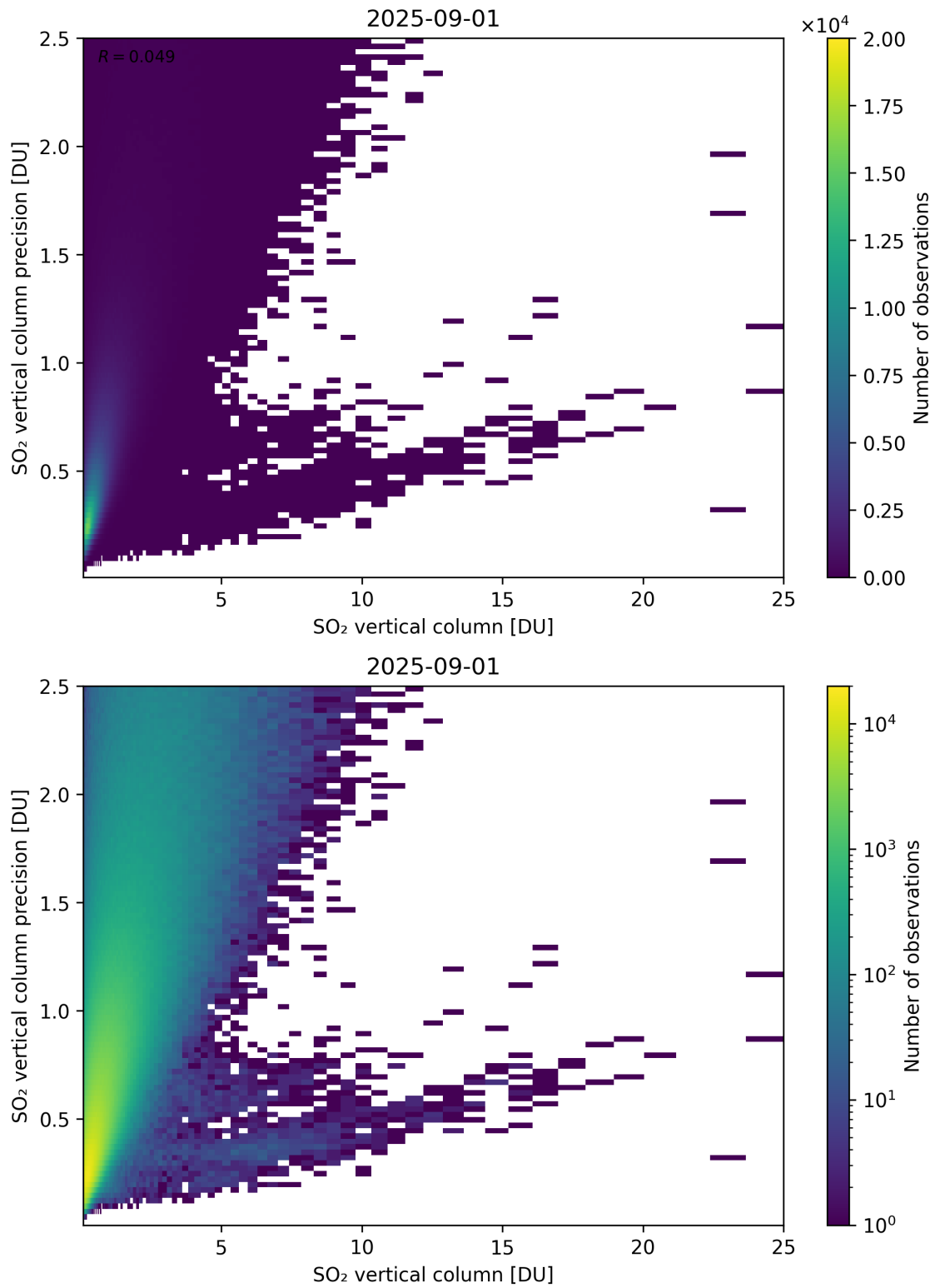
Figure 361: Scatter density plot of “SO 2 vertical column” against “SO 2 vertical column precision” for 2025-08-31 to 2025-09-02.
