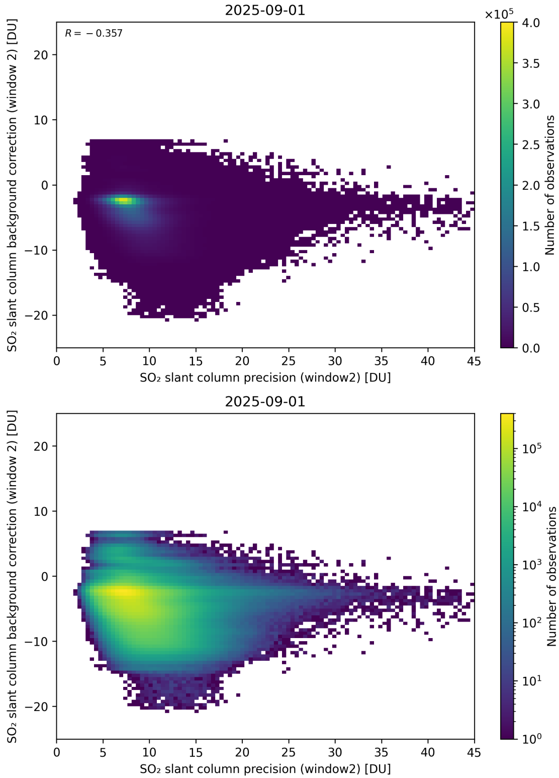
Figure 291: Scatter density plot of “SO 2 slant column precision (window2)” against “SO 2 slant column background correction (window 2)” for 2025-08-31 to 2025-09-02.
