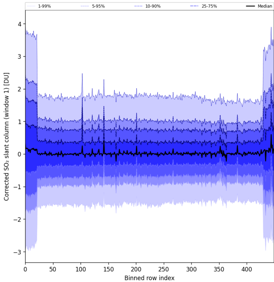
Figure 91: Along track statistics of “Corrected SO 2 slant column (window 1)” for 2025-08-31 to 2025-09-02
