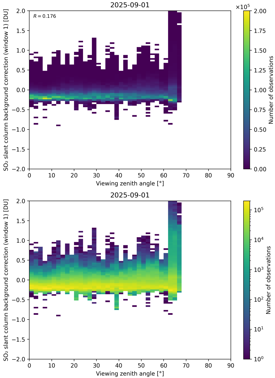
Figure 362: Scatter density plot of “Viewing zenith angle” against “SO 2 slant column background correction (window 1)” for 2025-08-31 to 2025-09-02.
