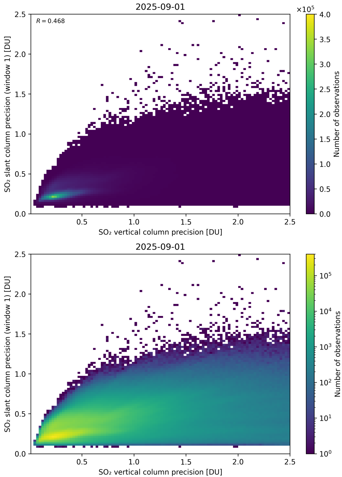
Figure 342: Scatter density plot of “SO 2 vertical column precision” against “SO 2 slant column precision (window 1)” for 2025-08-31 to 2025-09-02.
