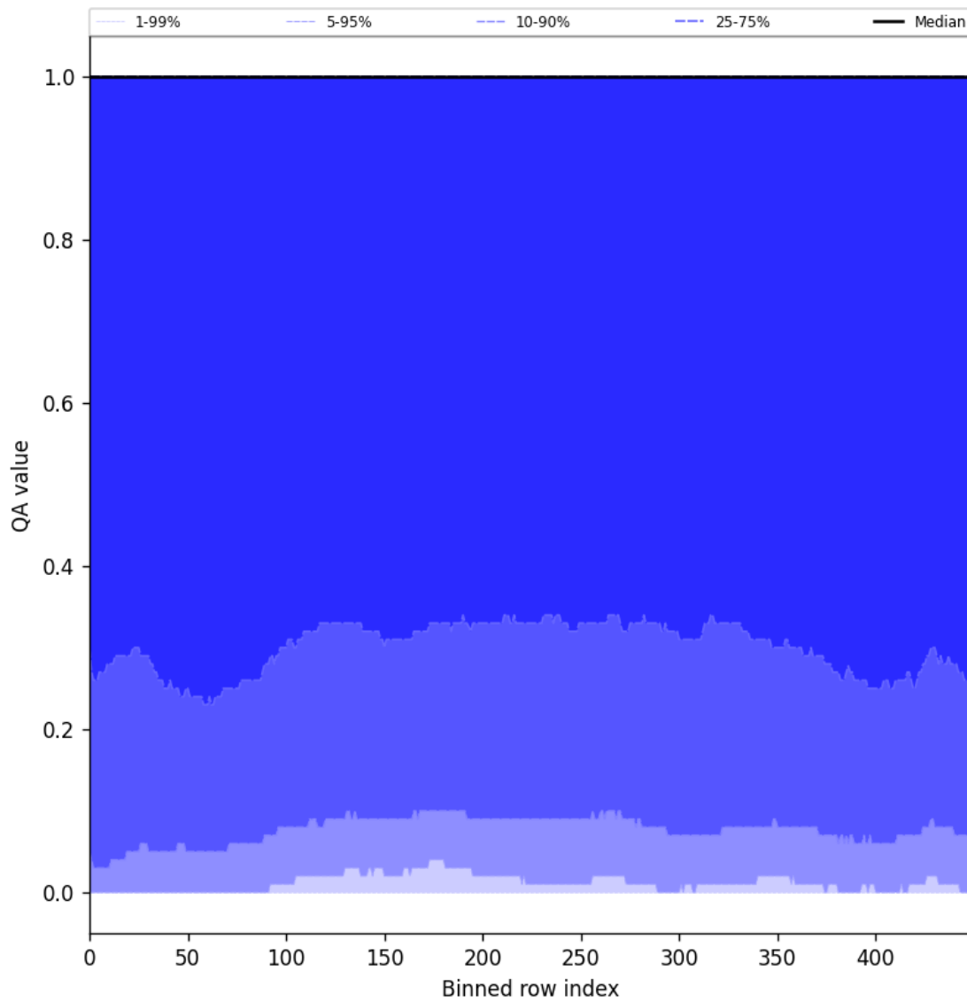
Figure 83: Along track statistics of “QA value” for 2025-08-31 to 2025-09-02
