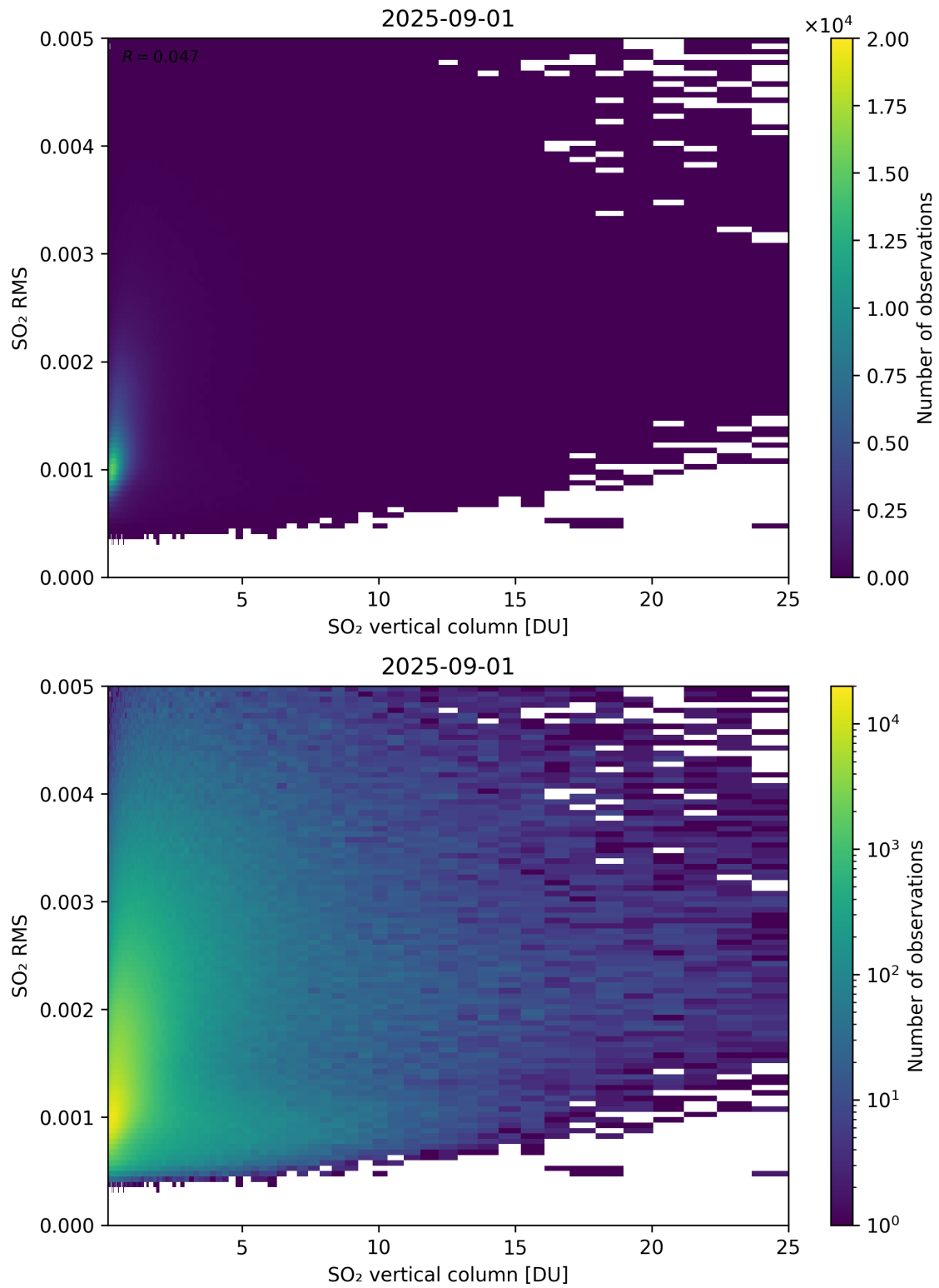
Figure 328: Scatter density plot of “SO 2 vertical column” against “SO 2 RMS” for 2025-08-31 to 2025-09-02.
