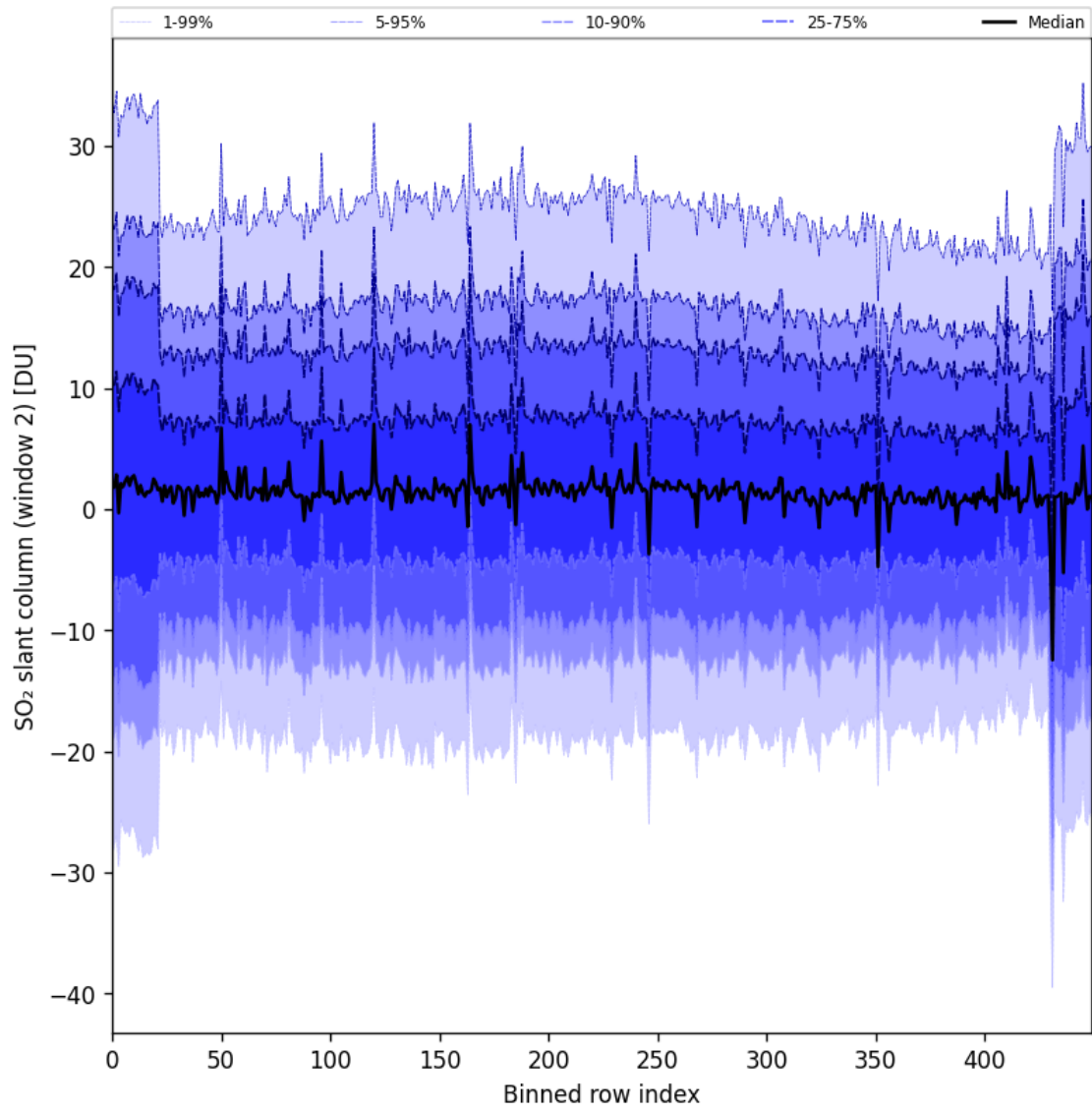
Figure 93: Along track statistics of “SO 2 slant column (window 2)” for 2025-08-31 to 2025-09-02
