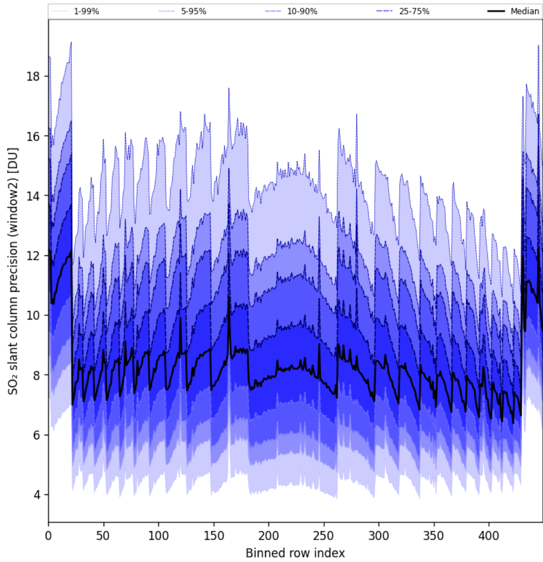
Figure 94: Along track statistics of “SO 2 slant column precision (window2)” for 2025-08-31 to 2025-09-02
