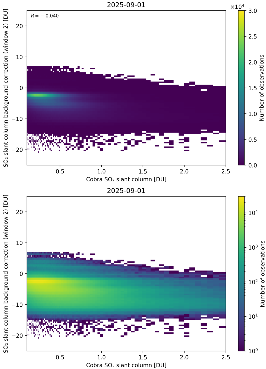
Figure 194: Scatter density plot of “Cobra SO 2 slant column” against “SO 2 slant column background correction (window 2)” for 2025-08-31 to 2025-09-02.
