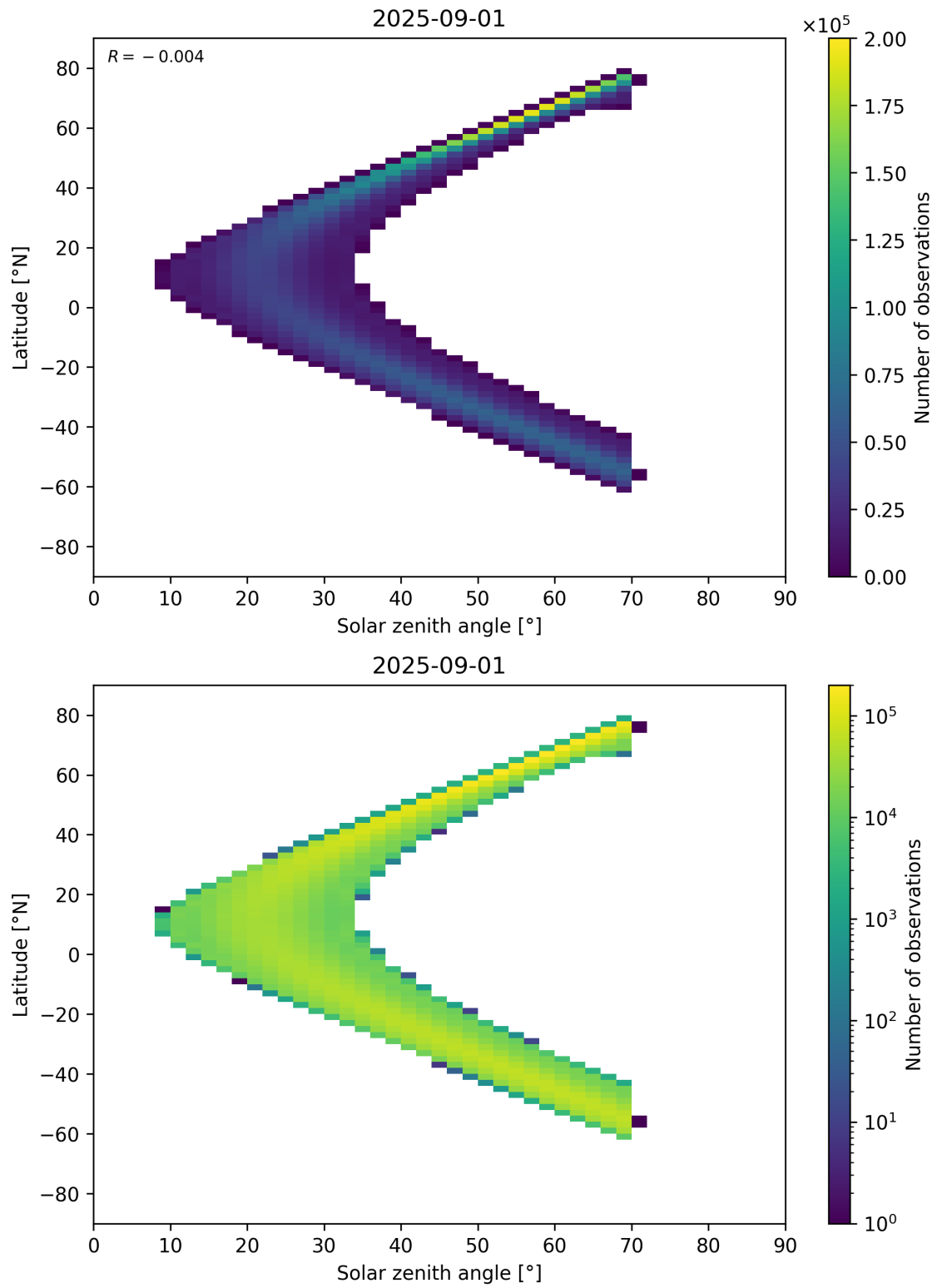
Figure 177: Scatter density plot of “Solar zenith angle” against “Latitude” for 2025-08-31 to 2025-09-02.
