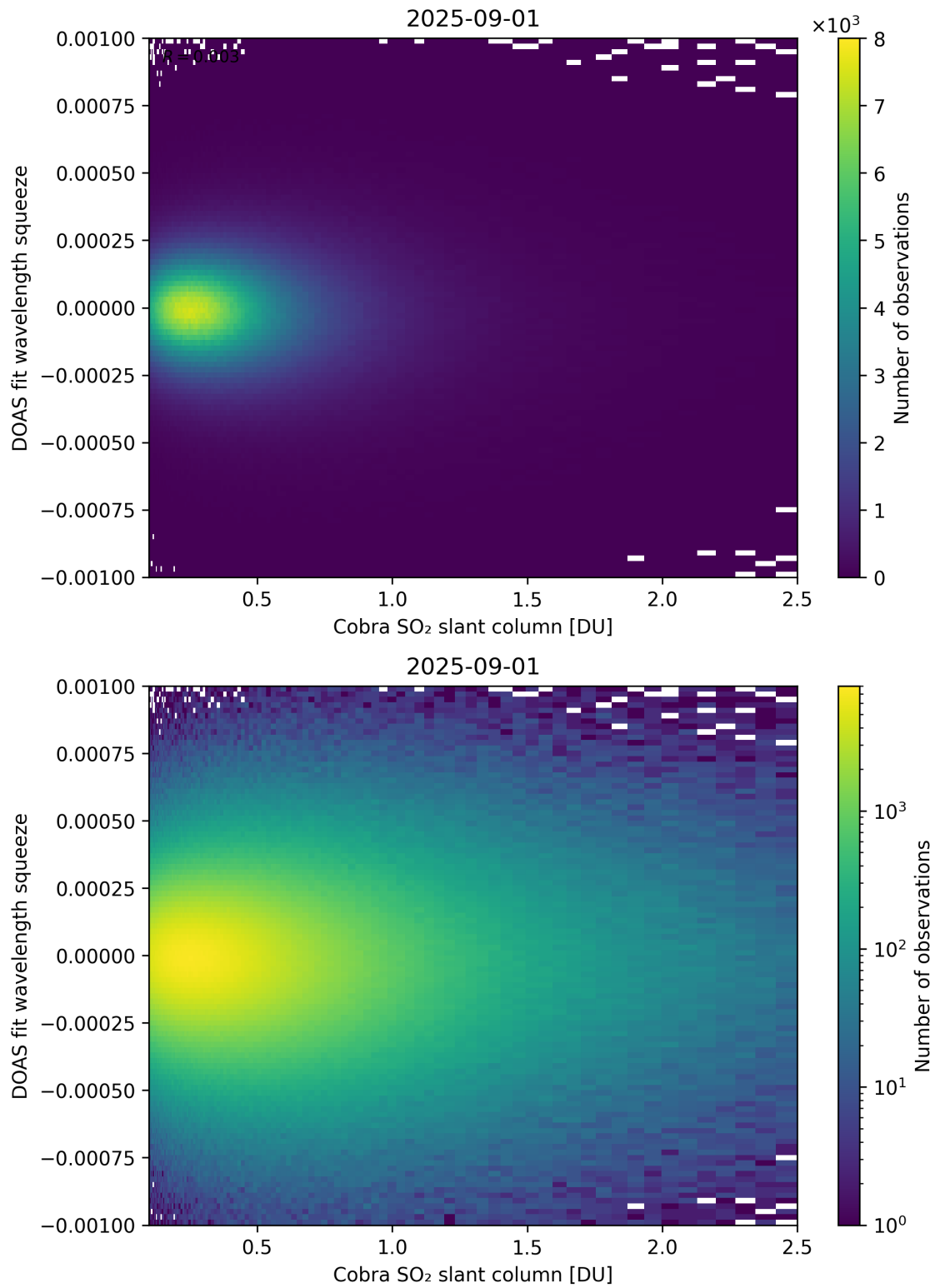
Figure 197: Scatter density plot of “Cobra SO 2 slant column” against “DOAS fit wavelength squeeze” for 2025-08-31 to 2025-09-02.
