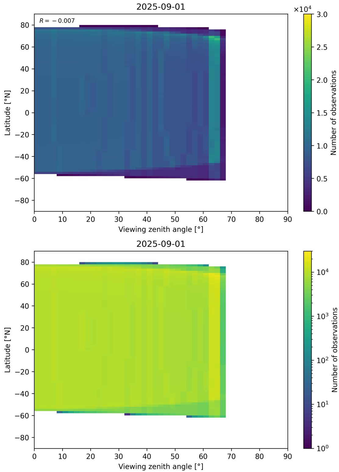
Figure 368: Scatter density plot of “Viewing zenith angle” against “Latitude” for 2025-08-31 to 2025-09-02.
