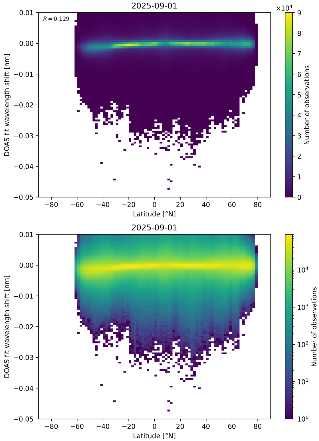
Figure 153: Scatter density plot of “Latitude” against “DOAS fit wavelength shift” for 2025-08-31 to 2025-09-02.
