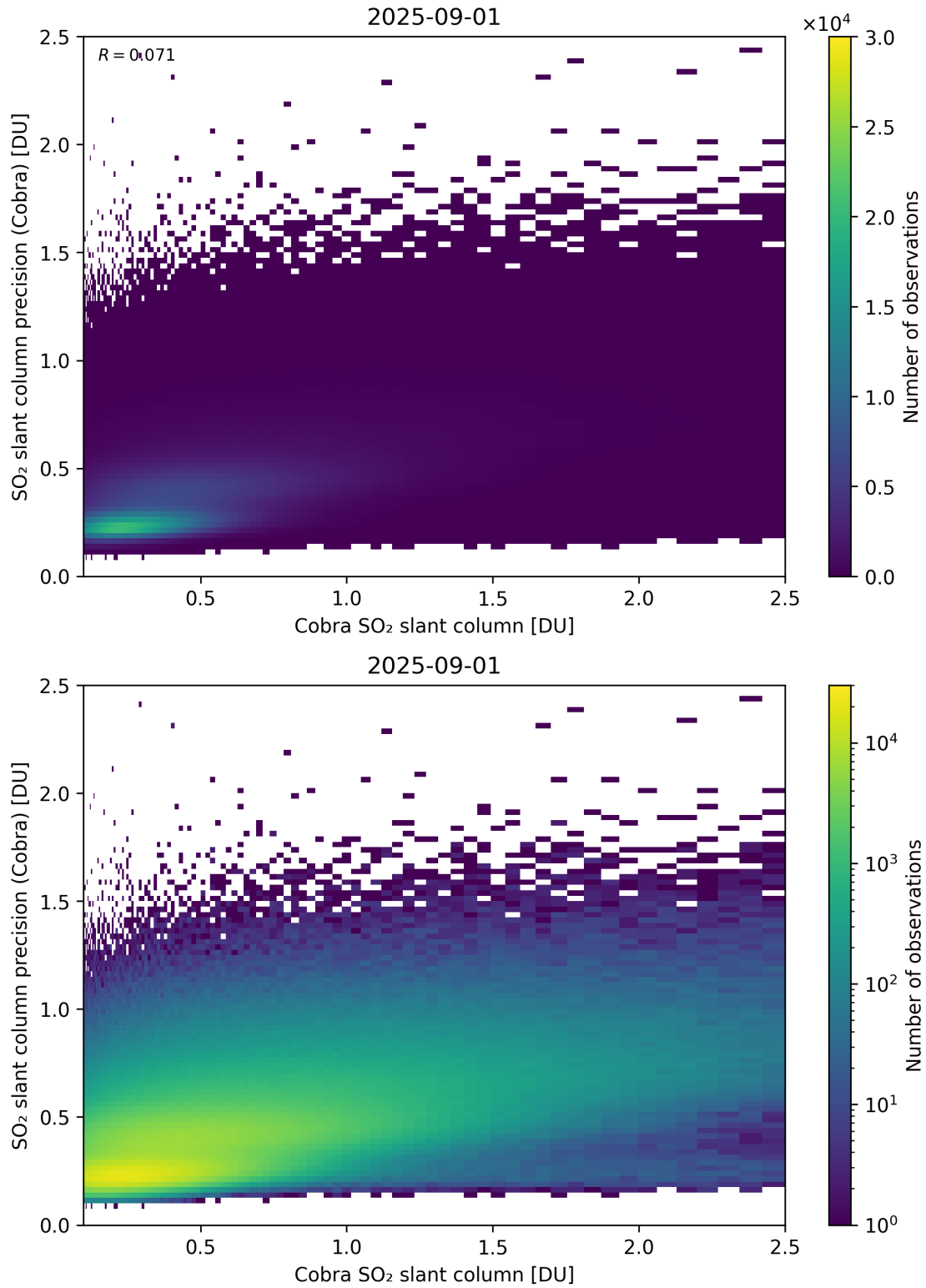
Figure 216: Scatter density plot of “Cobra SO 2 slant column” against “SO 2 slant column precision (Cobra)” for 2025-08-31 to 2025-09-02.
