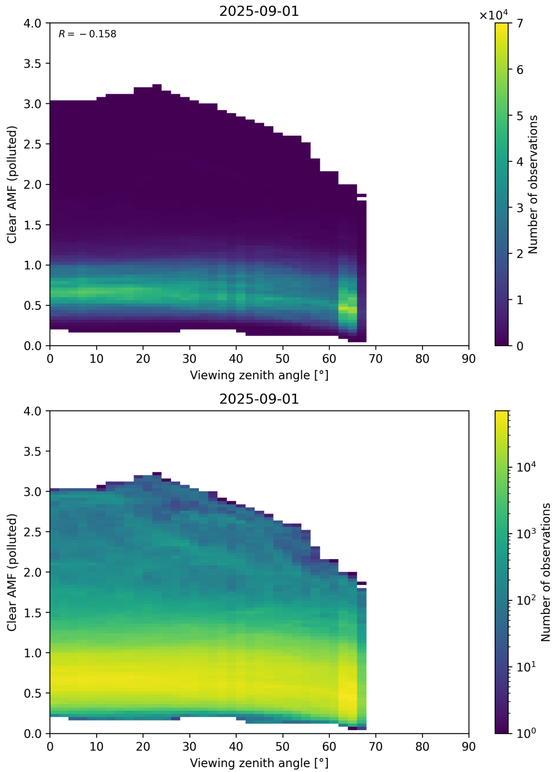
Figure 370: Scatter density plot of “Viewing zenith angle” against “Clear AMF (polluted)” for 2025-08-31 to 2025-09-02.
