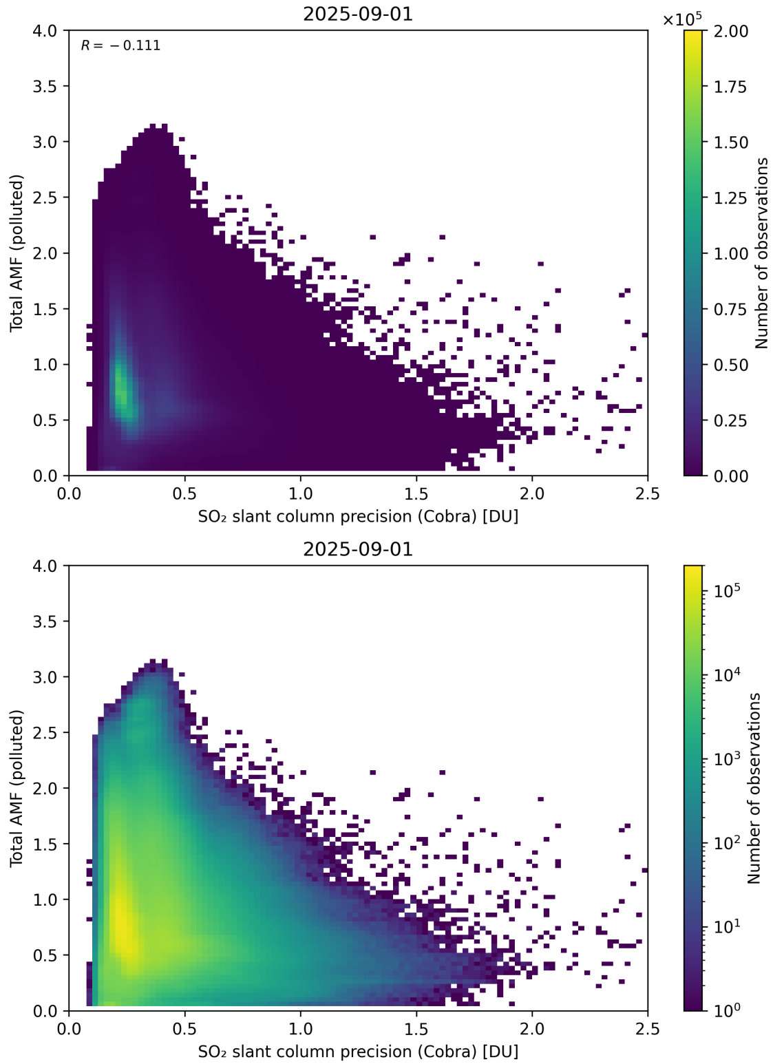
Figure 213: Scatter density plot of “SO 2 slant column precision (Cobra)” against “Total AMF (polluted)” for 2025-08-31 to 2025-09-02.
