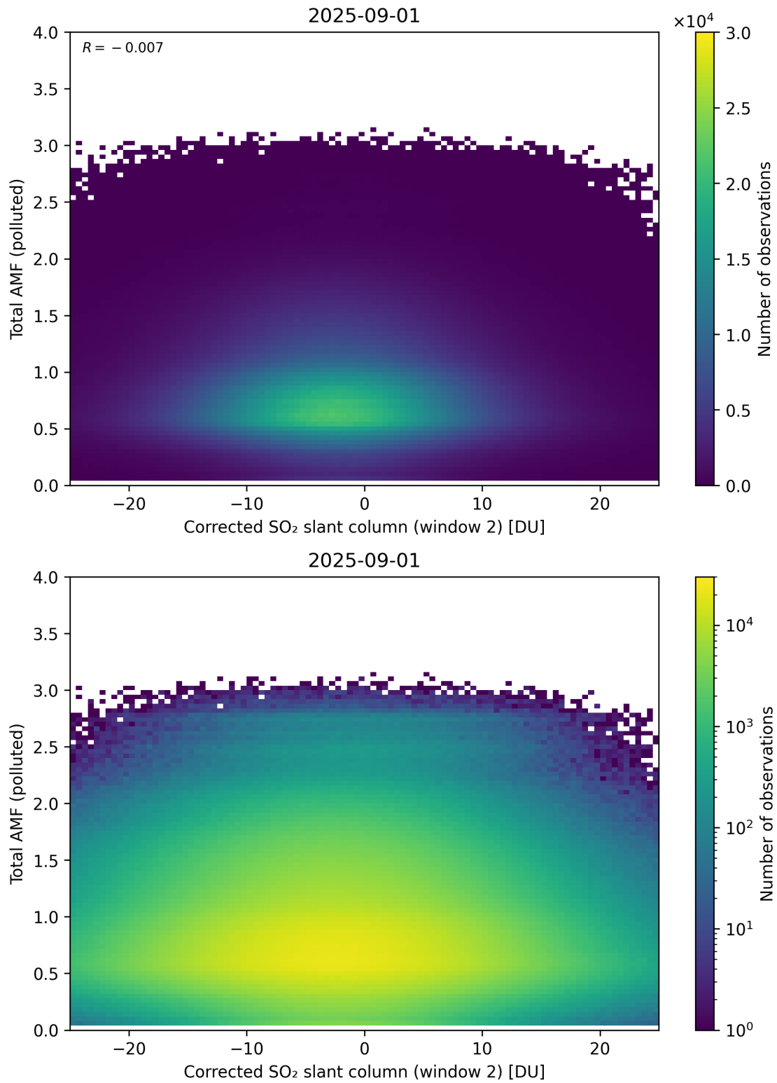
Figure 253: Scatter density plot of “Corrected SO 2 slant column (window 2)” against “Total AMF (polluted)” for 2025-08-31 to 2025-09-02.
