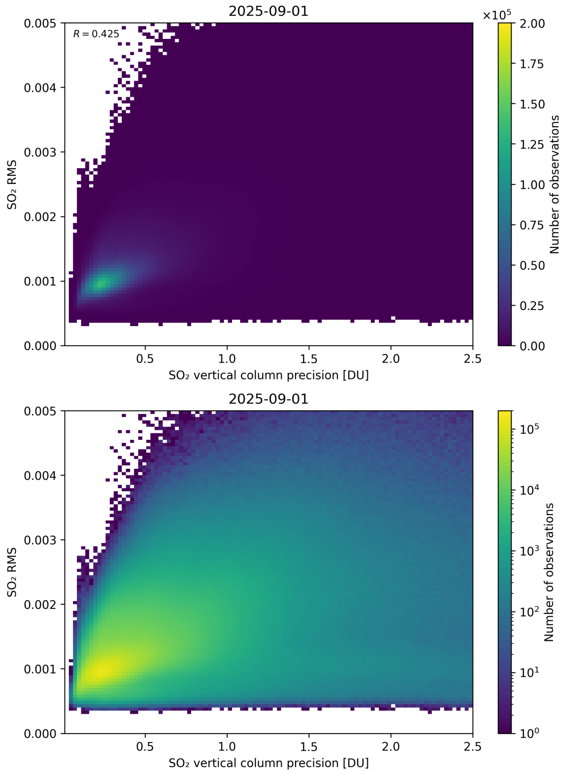
Figure 334: Scatter density plot of “SO 2 vertical column precision” against “SO 2 RMS” for 2025-08-31 to 2025-09-02.
