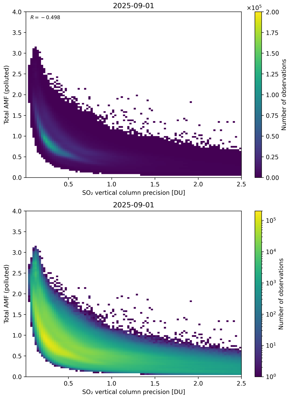
Figure 346: Scatter density plot of “SO 2 vertical column precision” against “Total AMF (polluted)” for 2025-08-31 to 2025-09-02.
