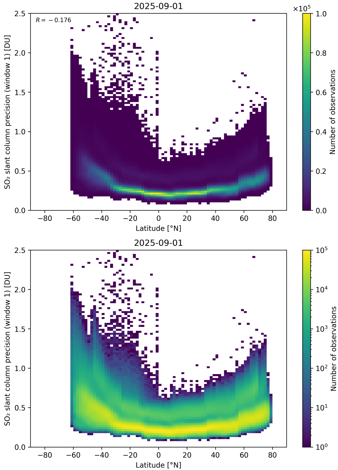
Figure 163: Scatter density plot of “Latitude” against “SO 2 slant column precision (window 1)” for 2025-08-31 to 2025-09-02.
