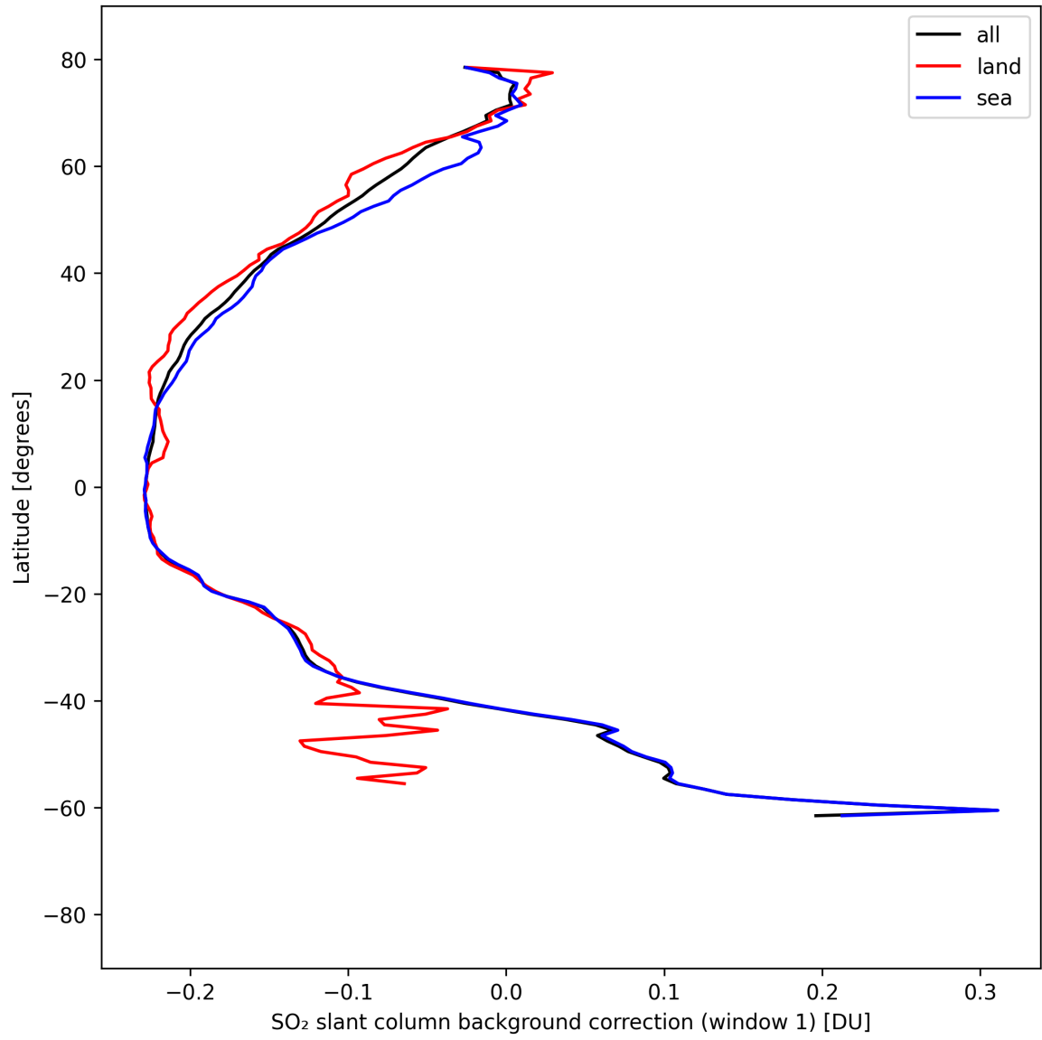
Figure 40: Zonal average of “SO 2 slant column background correction (window 1)” for 2025-08-31 to 2025-09-02.
