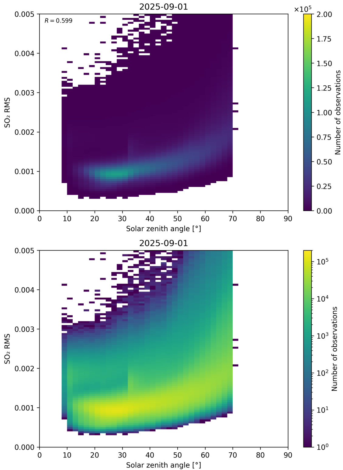
Figure 176: Scatter density plot of “Solar zenith angle” against “SO 2 RMS” for 2025-08-31 to 2025-09-02.
