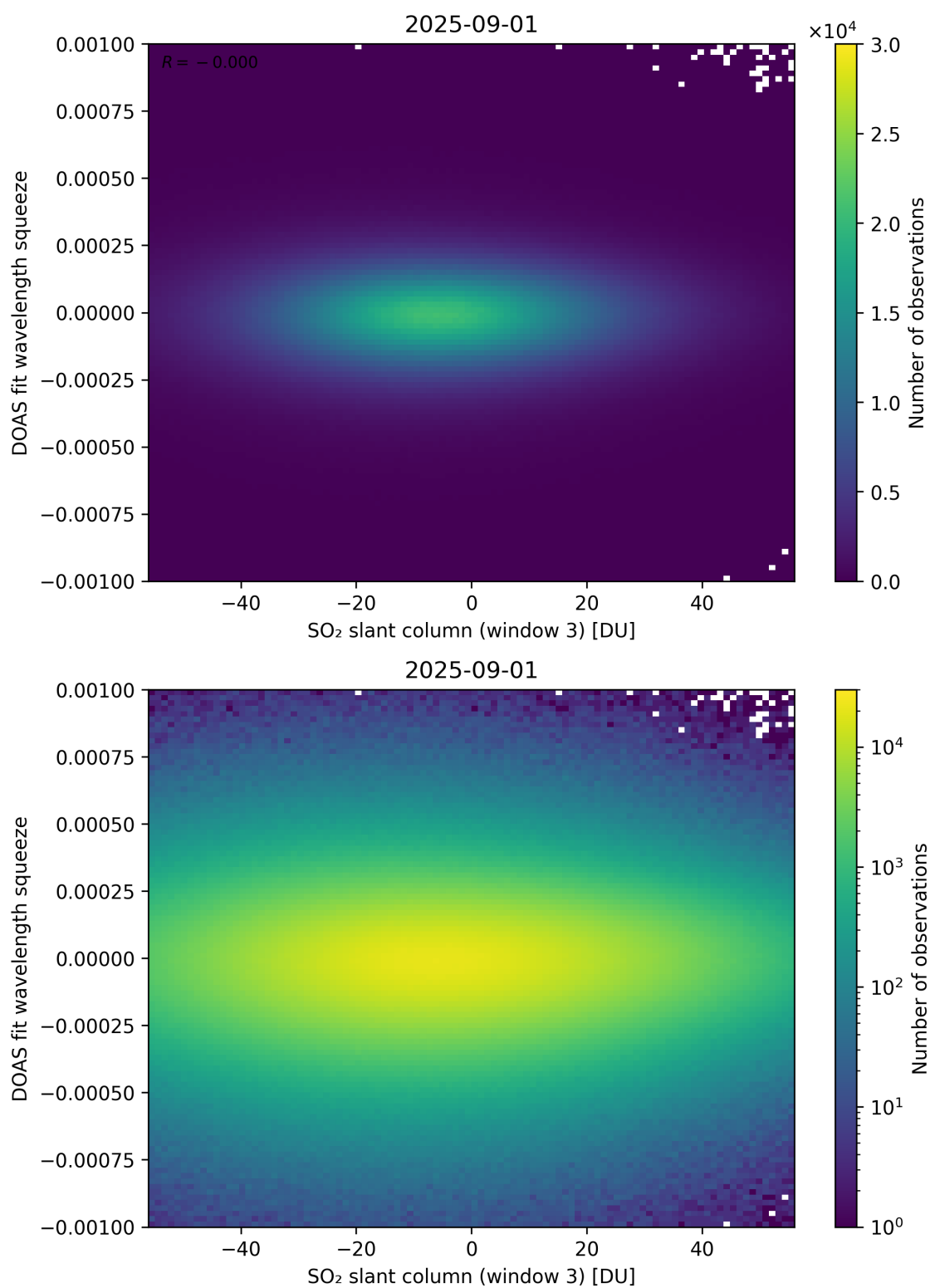
Figure 305: Scatter density plot of “SO 2 slant column (window 3)” against “DOAS fit wavelength squeeze” for 2025-08-31 to 2025-09-02.
