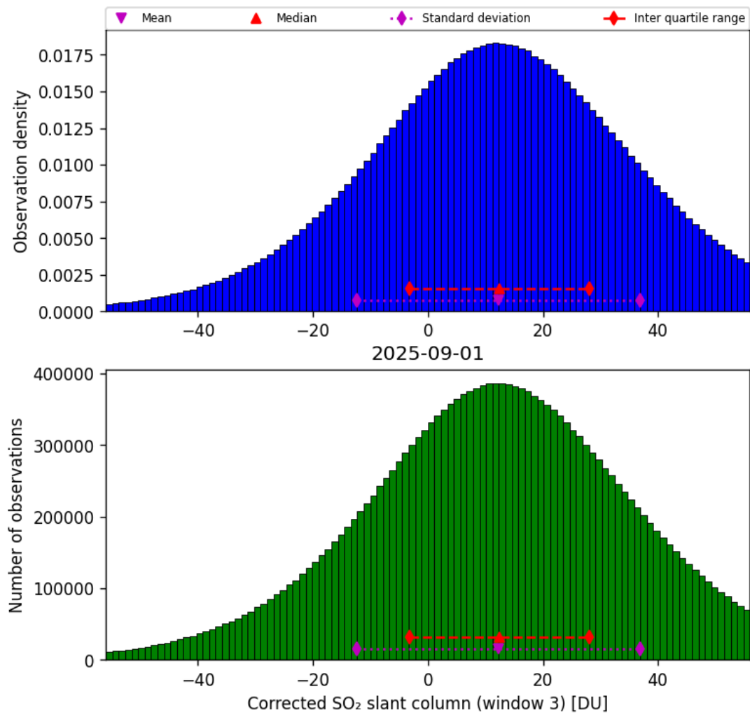
Figure 73: Histogram of “Corrected SO 2 slant column (window 3)” for 2025-08-31 to 2025-09-02
