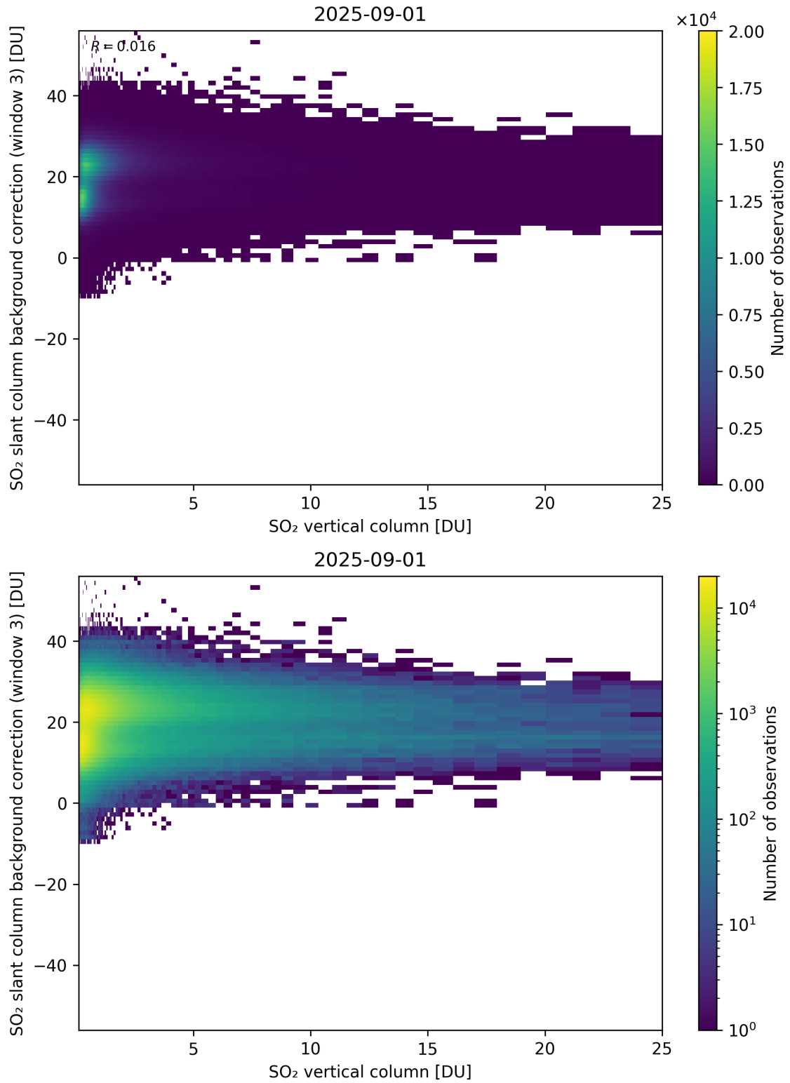
Figure 325: Scatter density plot of “SO 2 vertical column” against “SO 2 slant column background correction (window 3)” for 2025-08-31 to 2025-09-02.
