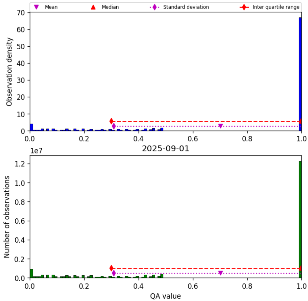
Figure 57: Histogram of “QA value” for 2025-08-31 to 2025-09-02
