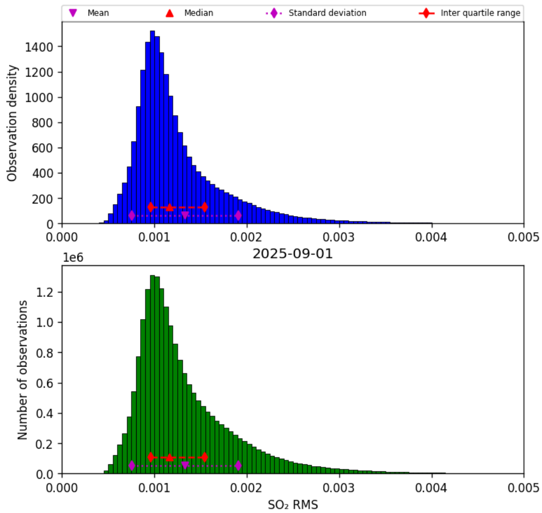
Figure 78: Histogram of “SO 2 RMS” for 2025-08-31 to 2025-09-02
