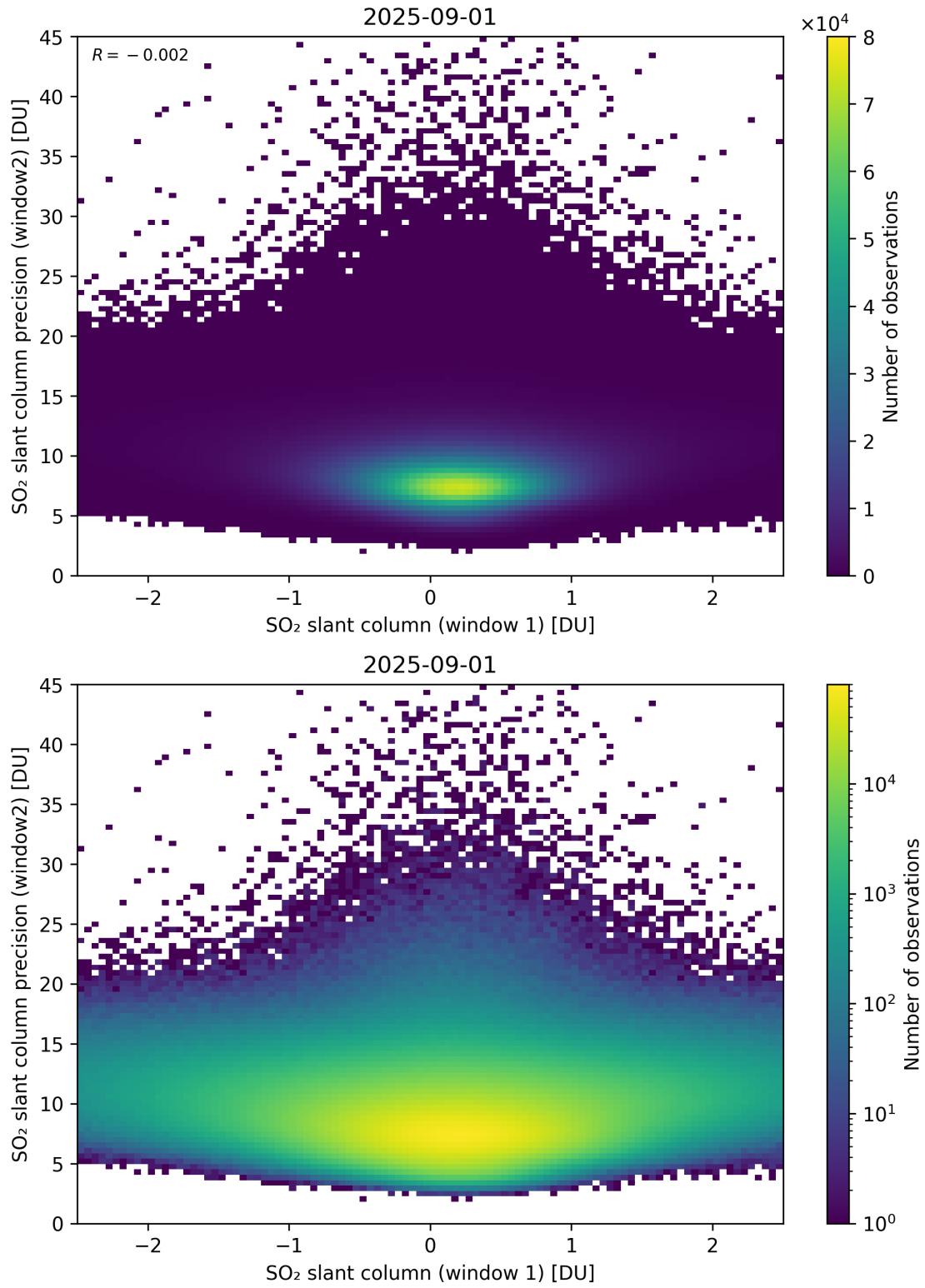
Figure 286: Scatter density plot of “SO 2 slant column (window 1)” against “SO 2 slant column precision (window2)” for 2025-08-31 to 2025-09-02.
