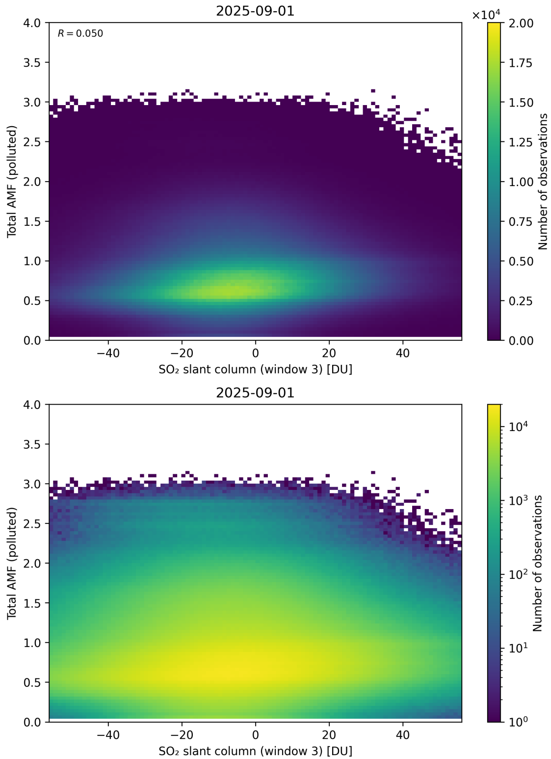
Figure 318: Scatter density plot of “SO 2 slant column (window 3)” against “Total AMF (polluted)” for 2025-08-31 to 2025-09-02.
