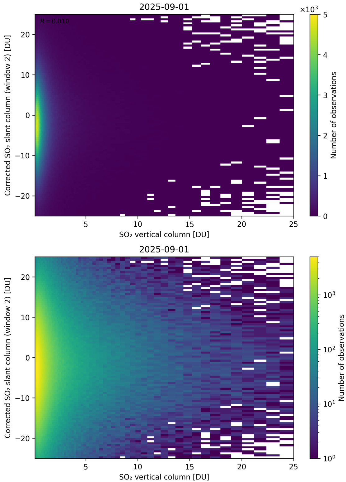
Figure 352: Scatter density plot of “SO 2 vertical column” against “Corrected SO 2 slant column (window 2)” for 2025-08-31 to 2025-09-02.
