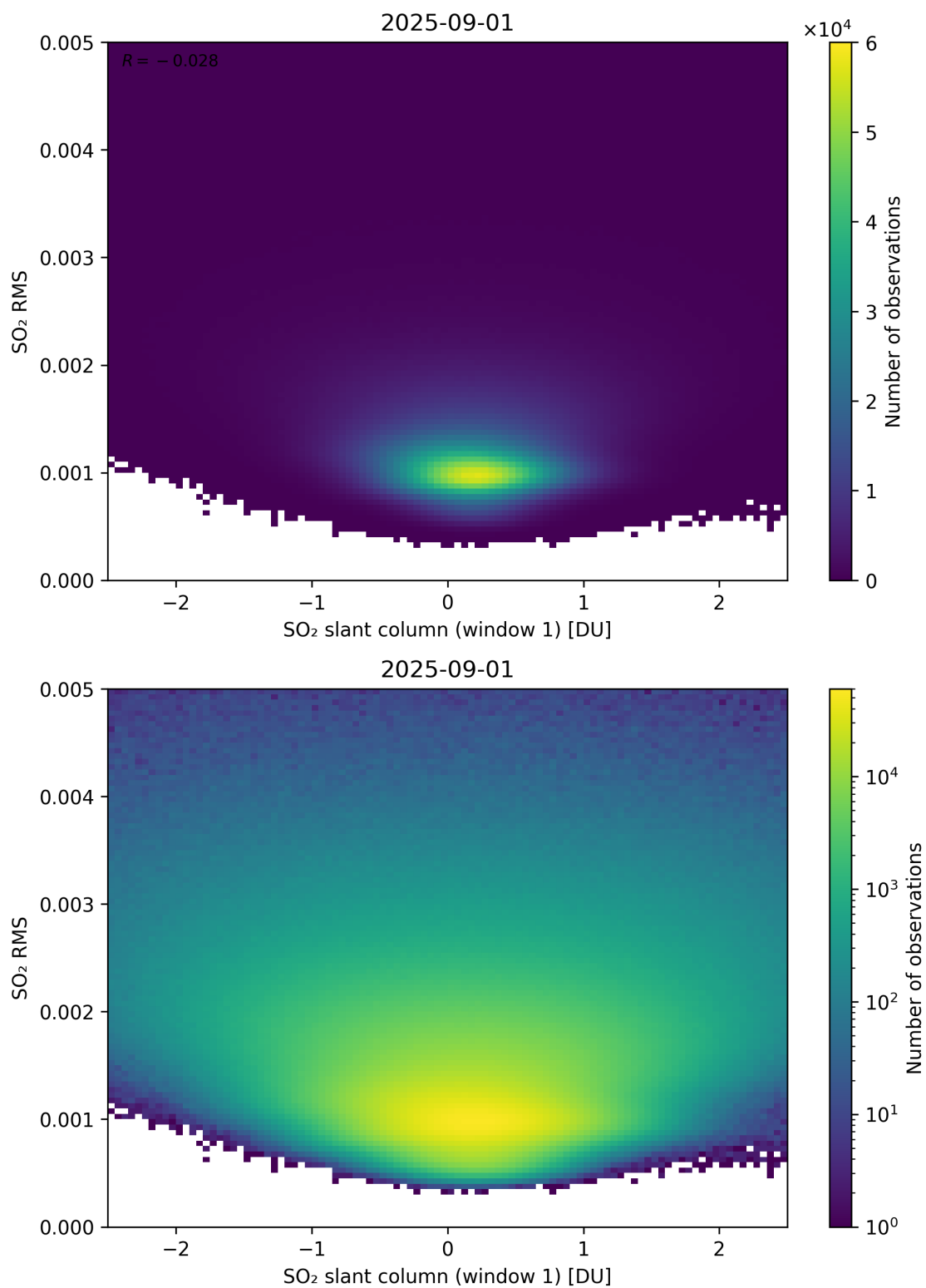
Figure 267: Scatter density plot of “SO 2 slant column (window 1)” against “SO 2 RMS” for 2025-08-31 to 2025-09-02.
