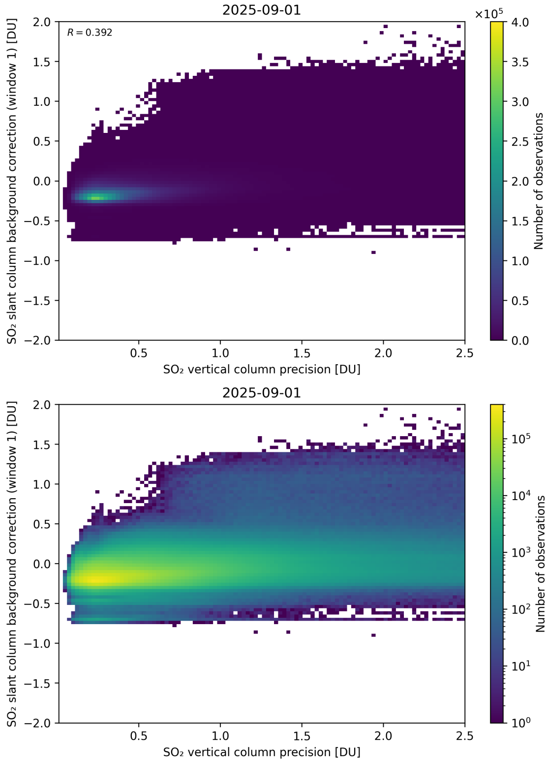
Figure 329: Scatter density plot of “SO 2 vertical column precision” against “SO 2 slant column background correction (window 1)” for 2025-08-31 to 2025-09-02.
