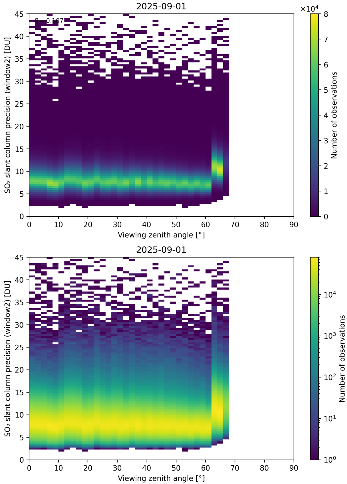
Figure 378: Scatter density plot of “Viewing zenith angle” against “SO 2 slant column precision (window2)” for 2025-08-31 to 2025-09-02.
