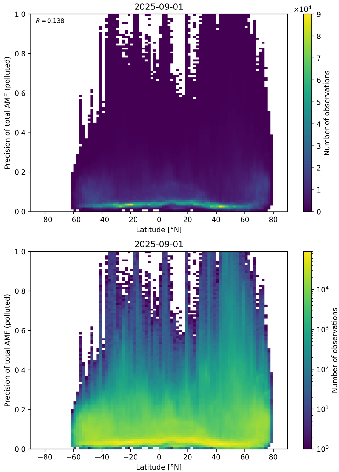
Figure 168: Scatter density plot of “Latitude” against “Precision of total AMF (polluted)” for 2025-08-31 to 2025-09-02.
