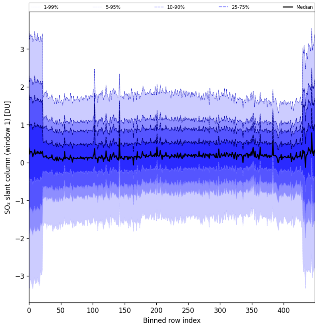
Figure 89: Along track statistics of “SO 2 slant column (window 1)” for 2025-08-31 to 2025-09-02
