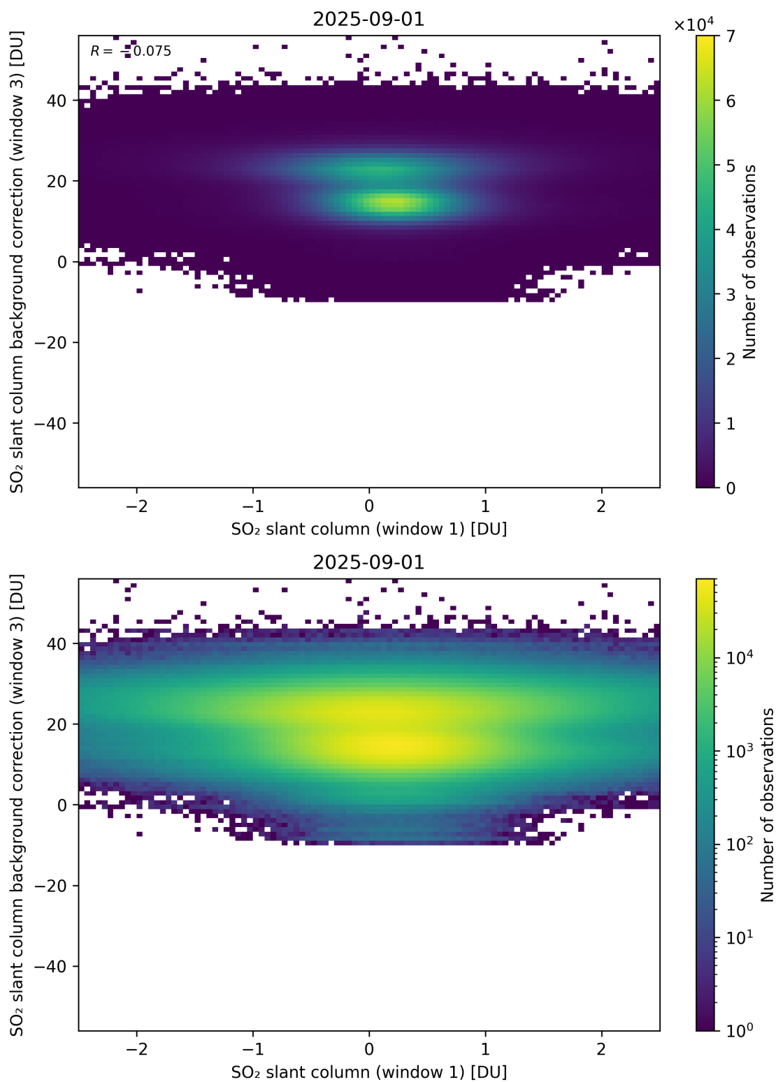
Figure 264: Scatter density plot of “SO 2 slant column (window 1)” against “SO 2 slant column background correction (window 3)” for 2025-08-31 to 2025-09-02.
