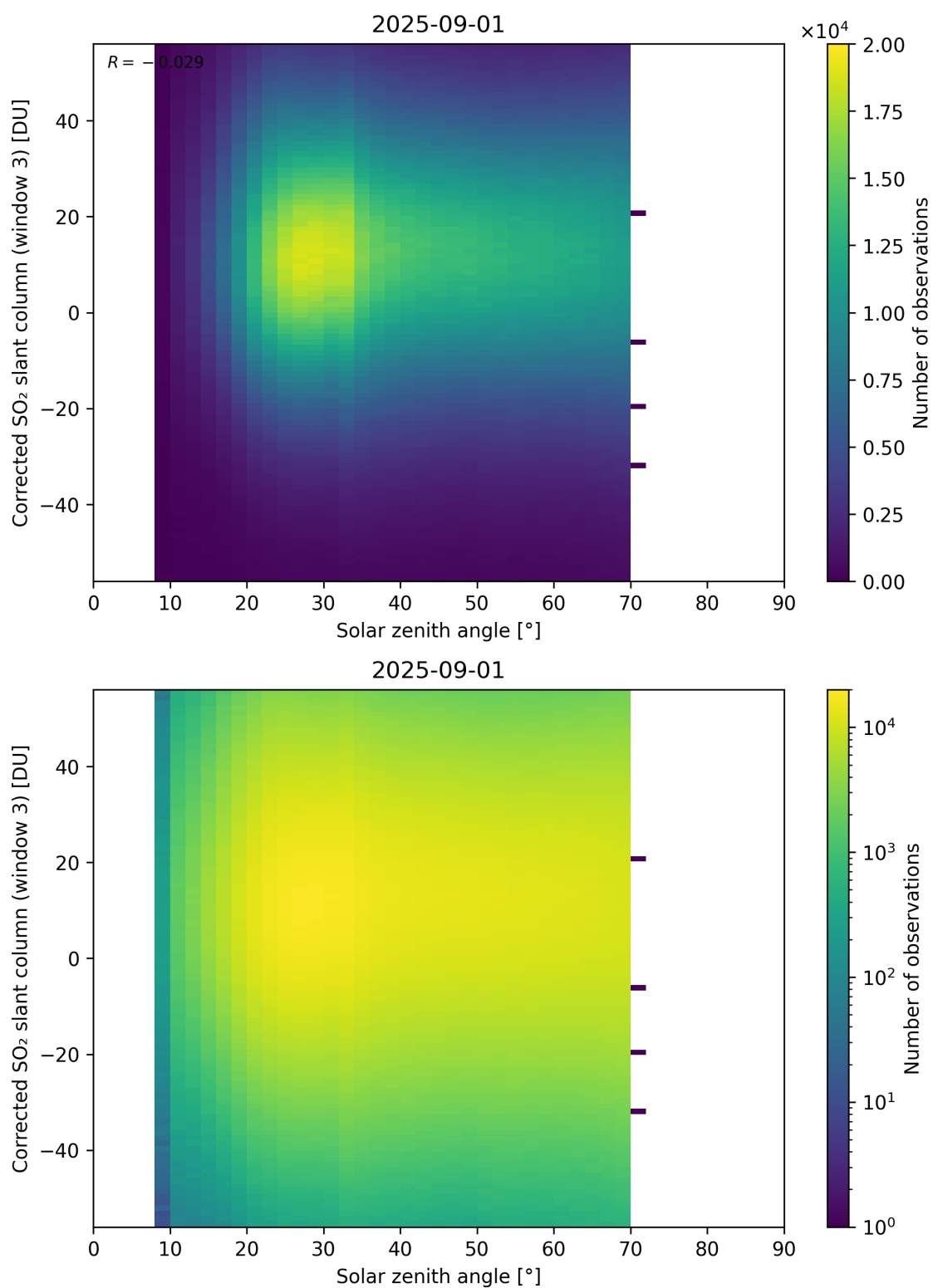
Figure 183: Scatter density plot of “Solar zenith angle” against “Corrected SO 2 slant column (window 3)” for 2025-08-31 to 2025-09-02.
