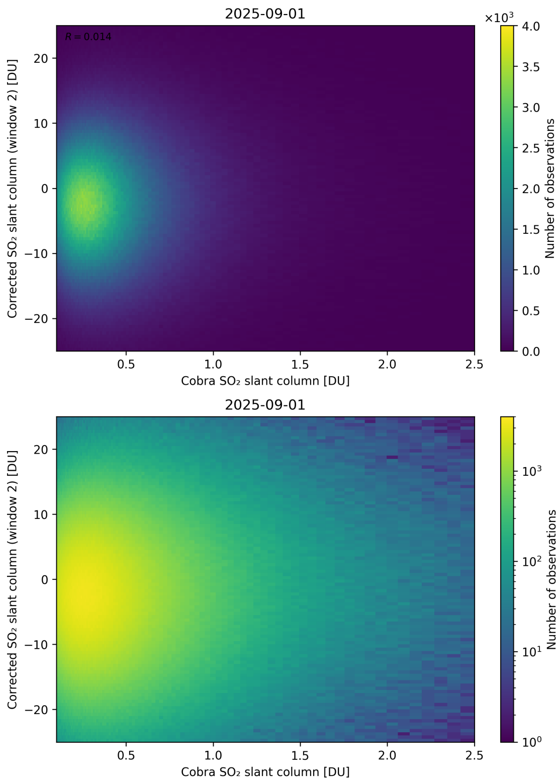
Figure 217: Scatter density plot of “Cobra SO 2 slant column” against “Corrected SO 2 slant column (window 2)” for 2025-08-31 to 2025-09-02.
