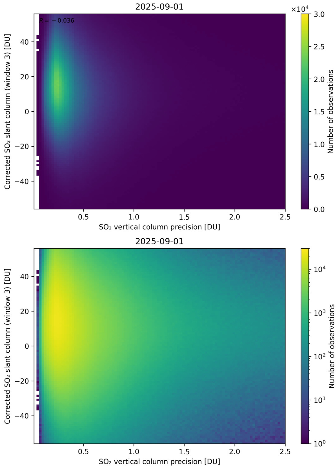
Figure 340: Scatter density plot of “SO 2 vertical column precision” against “Corrected SO 2 slant column (window 3)” for 2025-08-31 to 2025-09-02.
