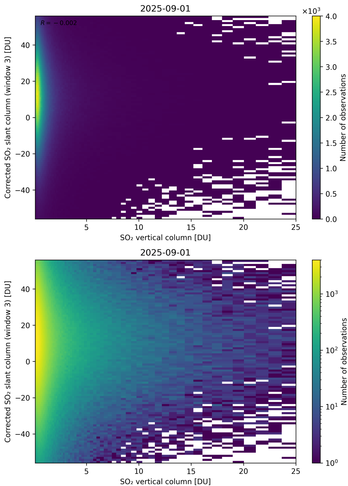
Figure 353: Scatter density plot of “SO 2 vertical column” against “Corrected SO 2 slant column (window 3)” for 2025-08-31 to 2025-09-02.
