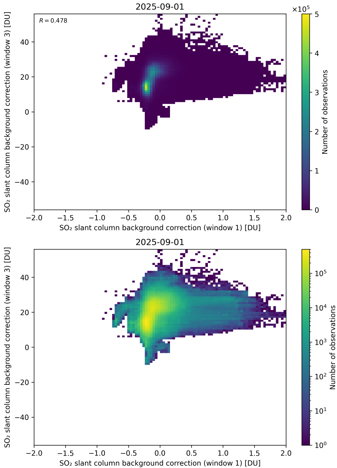
Figure 110: Scatter density plot of “SO 2 slant column background correction (window 1)” against “SO 2 slant column background correction (window 3)” for 2025-08-31 to 2025-09-02.
