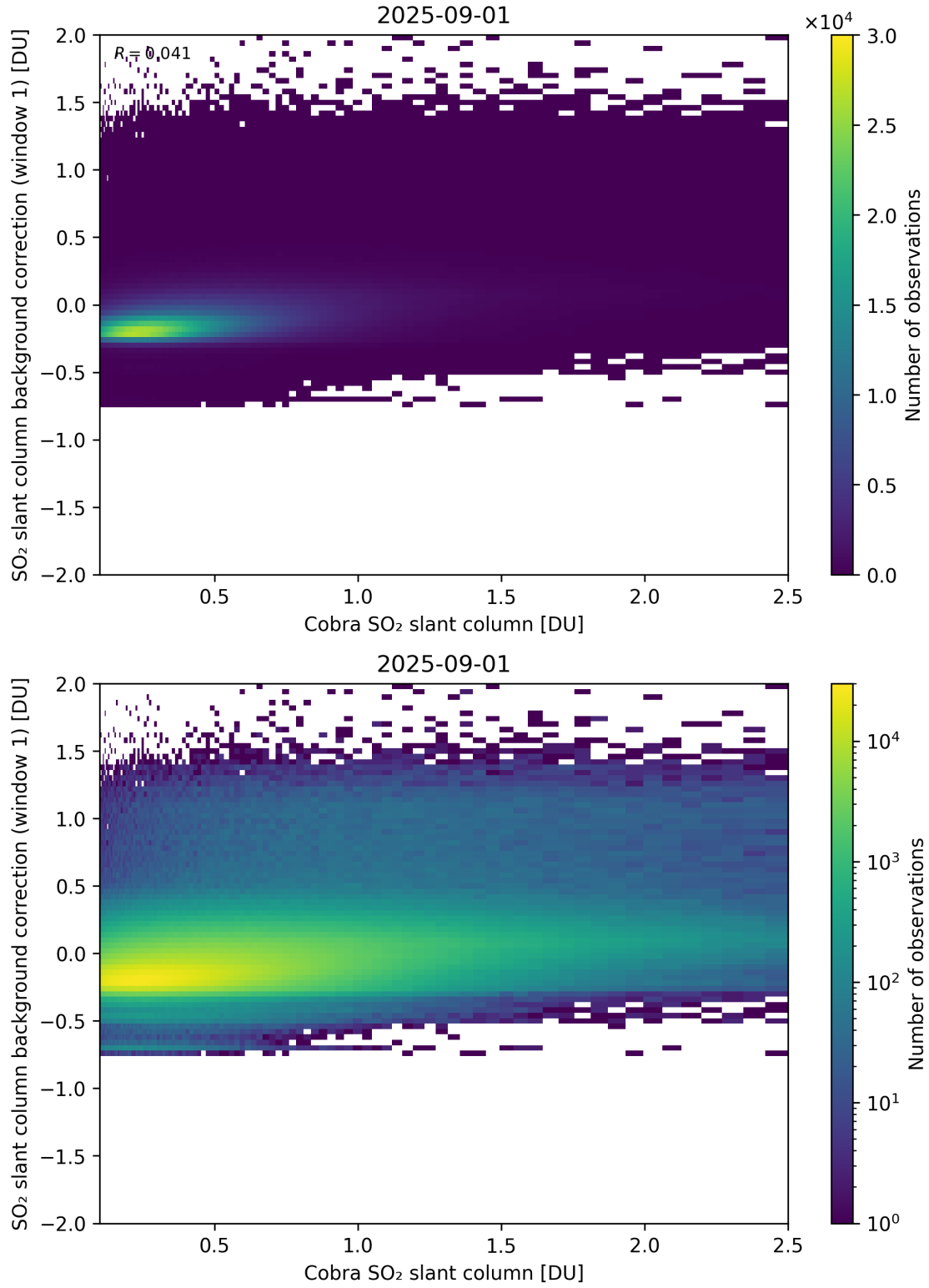
Figure 193: Scatter density plot of “Cobra SO 2 slant column” against “SO 2 slant column background correction (window 1)” for 2025-08-31 to 2025-09-02.
