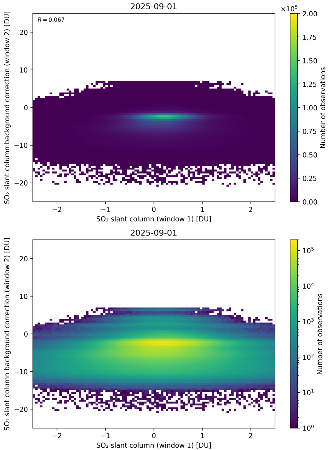
Figure 263: Scatter density plot of “SO 2 slant column (window 1)” against “SO 2 slant column background correction (window 2)” for 2025-08-31 to 2025-09-02.
