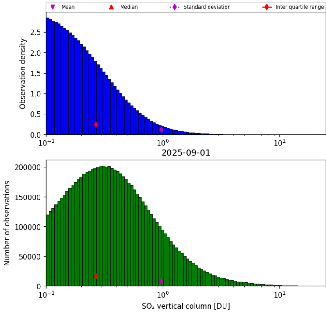
Figure 58: Histogram of “SO 2 vertical column” for 2025-08-31 to 2025-09-02
