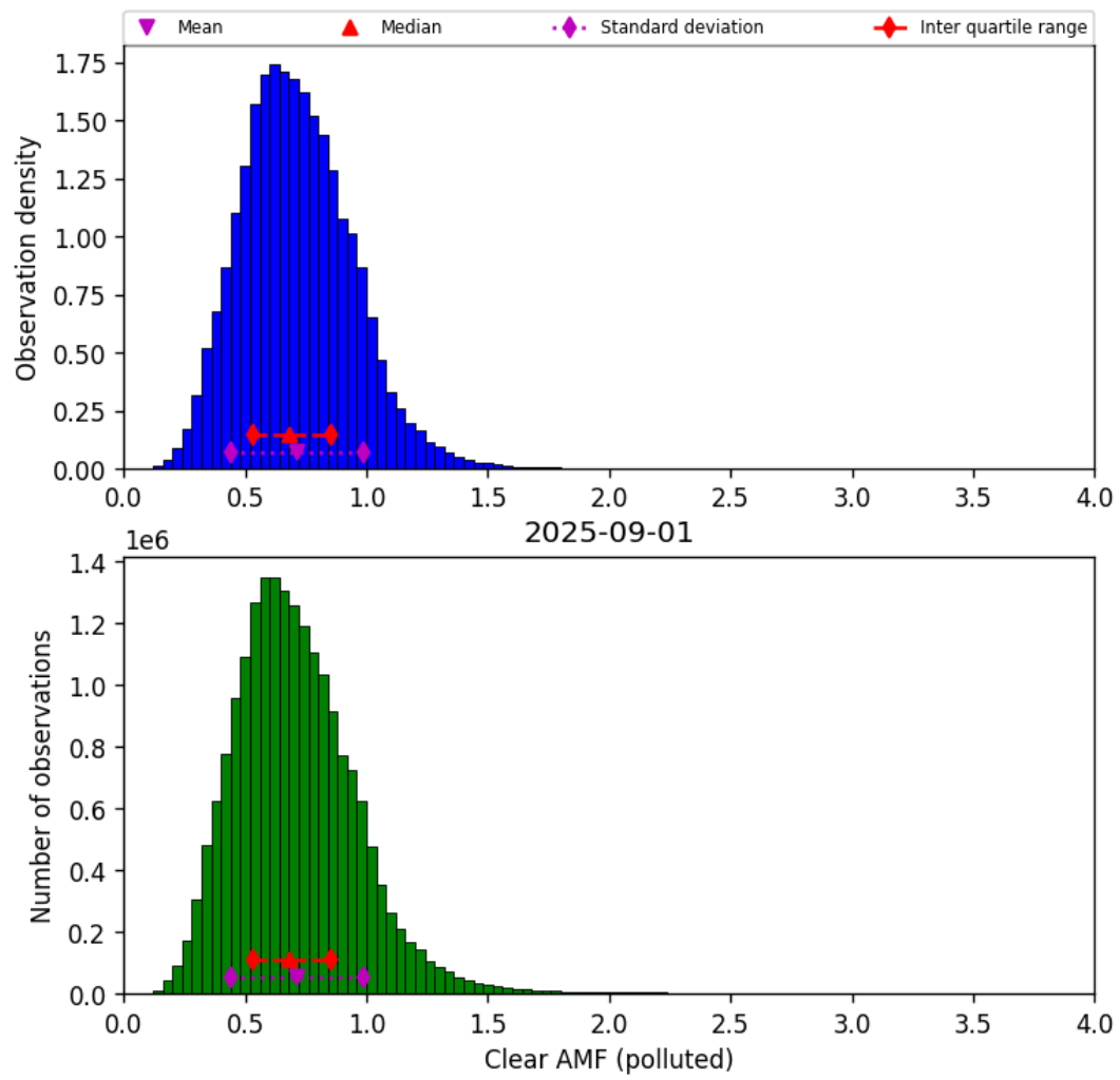
Figure 81: Histogram of “Clear AMF (polluted)” for 2025-08-31 to 2025-09-02
