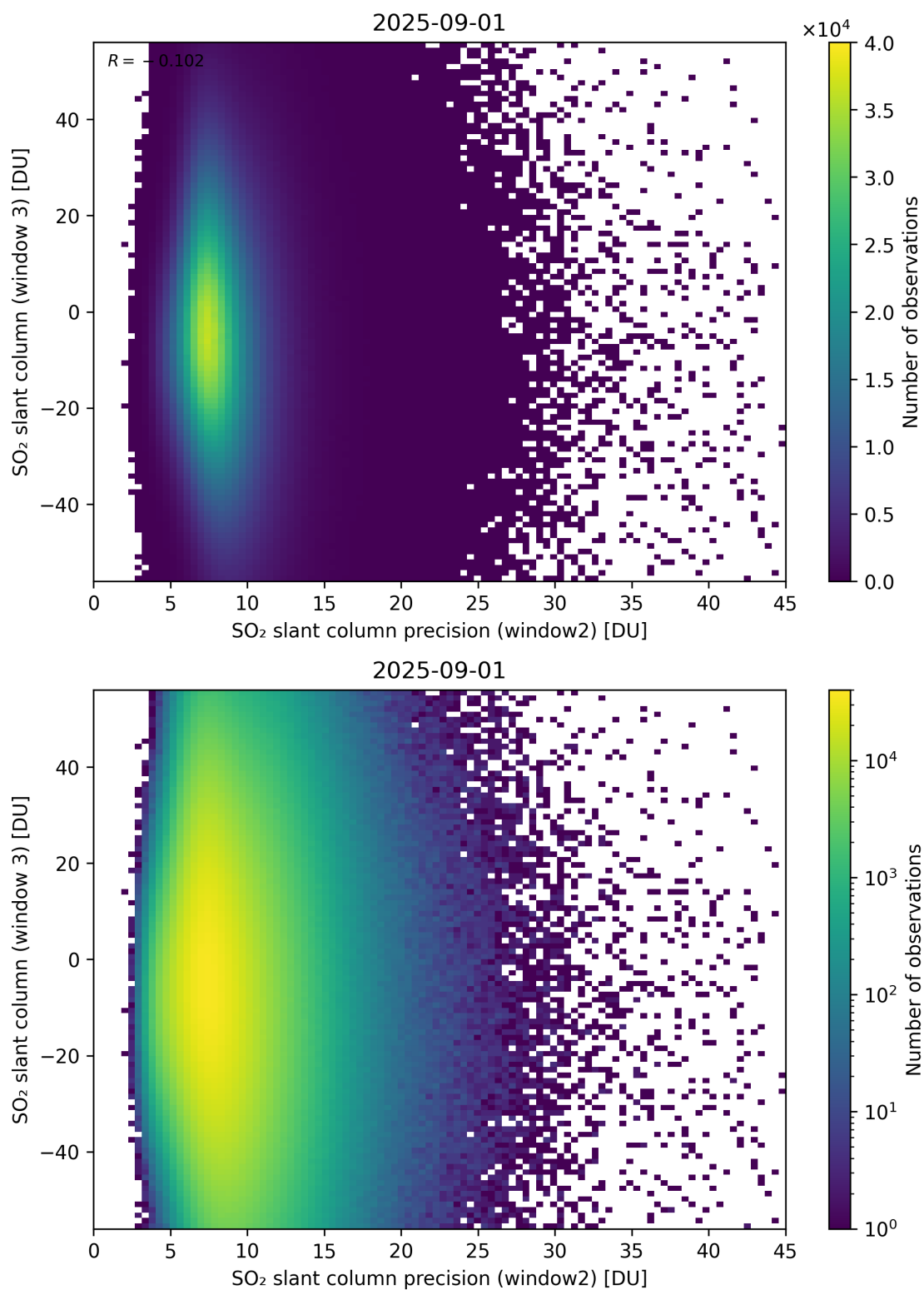
Figure 299: Scatter density plot of “SO 2 slant column precision (window2)” against “SO 2 slant column (window 3)” for 2025-08-31 to 2025-09-02.
