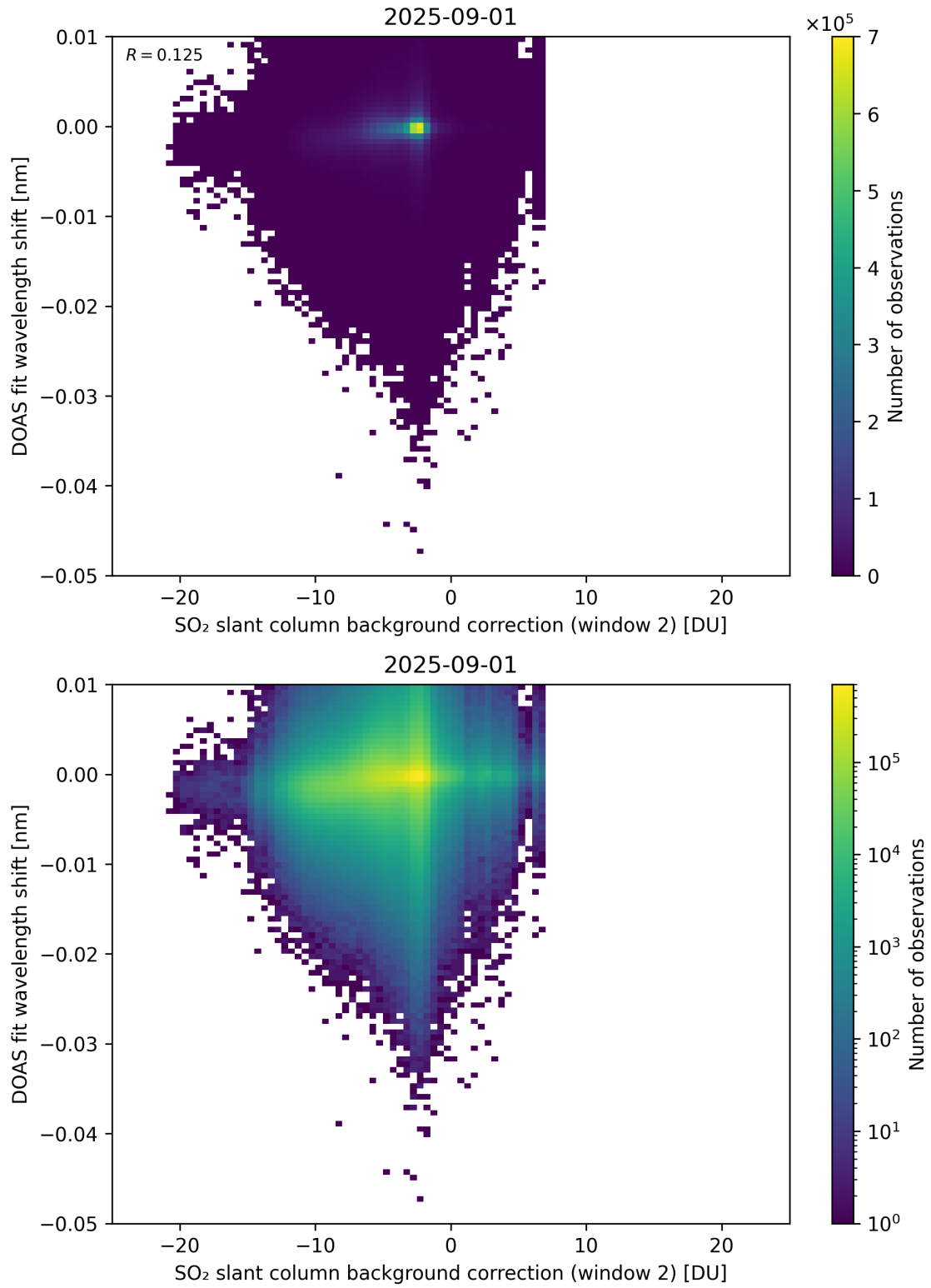
Figure 123: Scatter density plot of “SO 2 slant column background correction (window 2)” against “DOAS fit wavelength shift” for 2025-08-31 to 2025-09-02.
