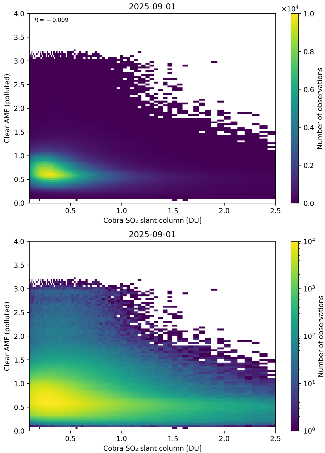
Figure 215: Scatter density plot of “Cobra SO 2 slant column” against “Clear AMF (polluted)” for 2025-08-31 to 2025-09-02.
