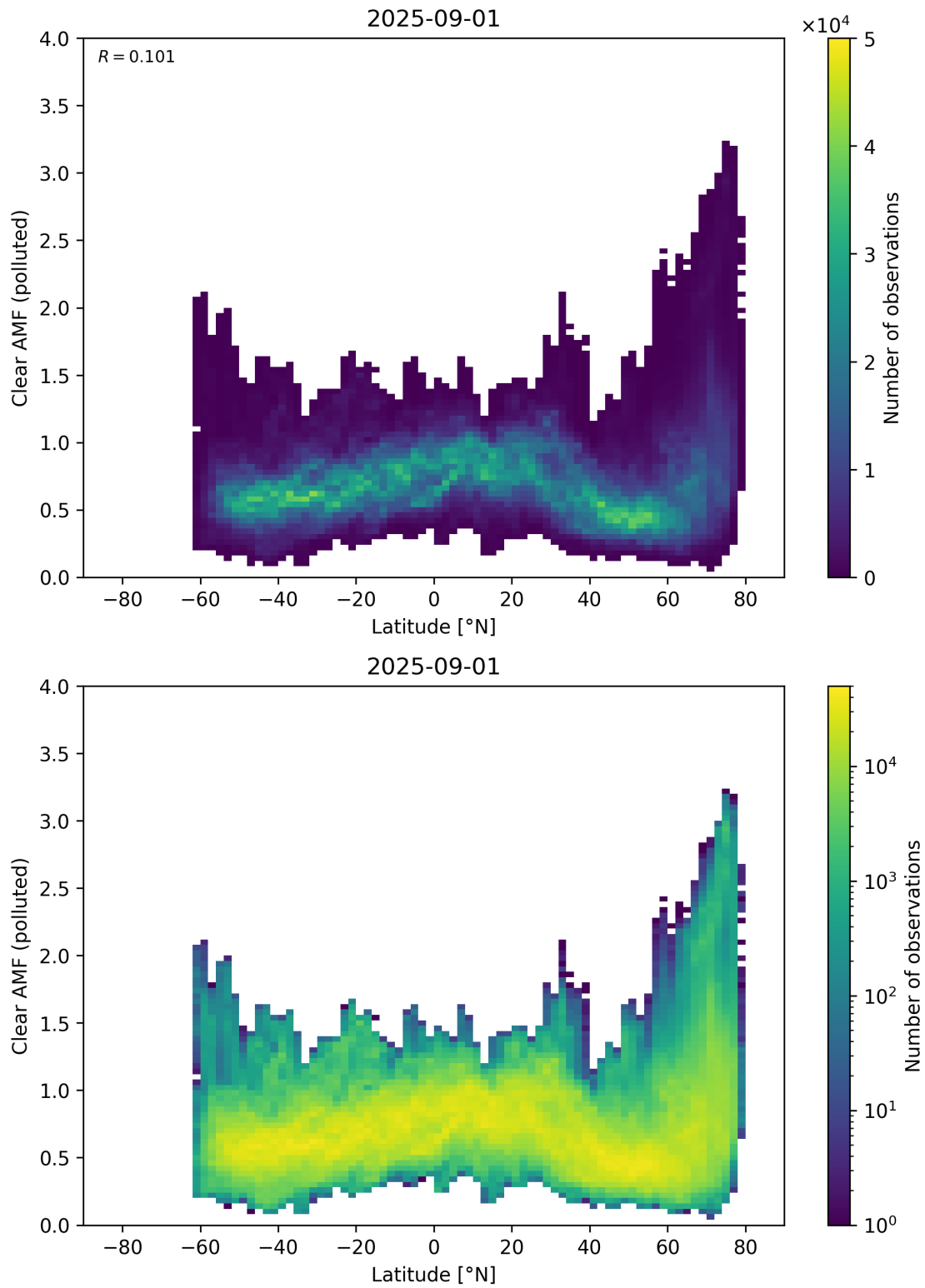
Figure 156: Scatter density plot of “Latitude” against “Clear AMF (polluted)” for 2025-08-31 to 2025-09-02.
