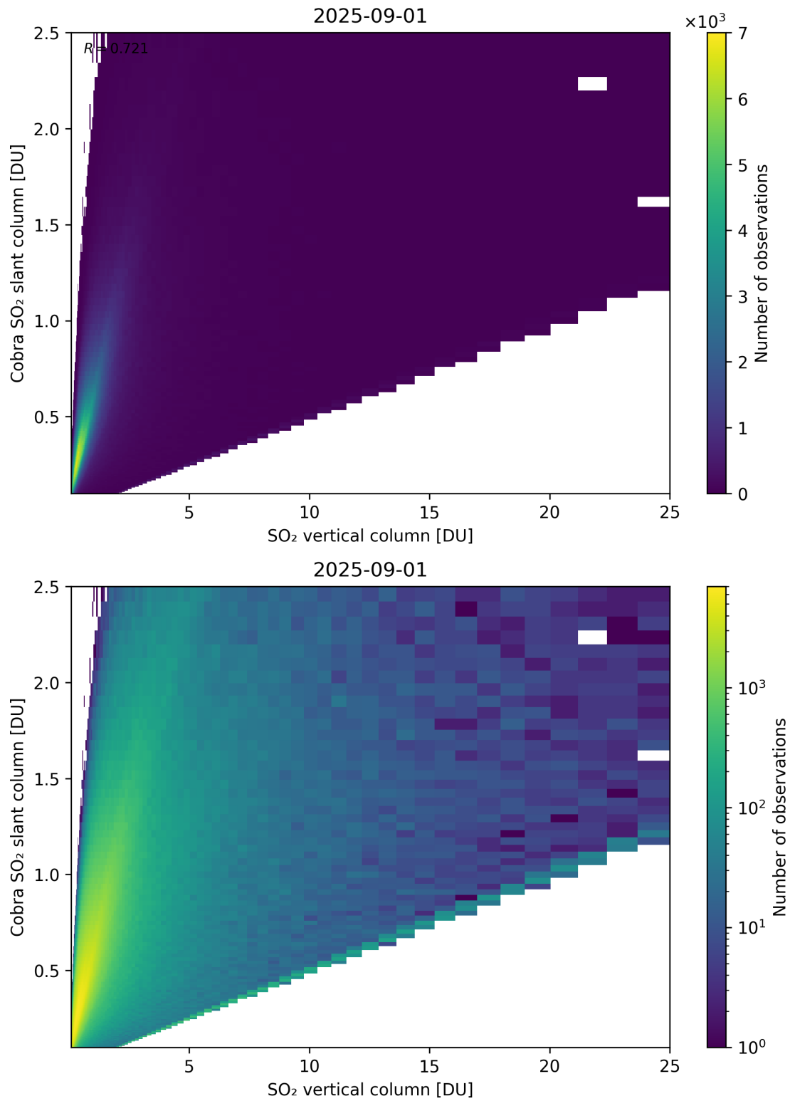
Figure 349: Scatter density plot of “SO 2 vertical column” against “Cobra SO 2 slant column” for 2025-08-31 to 2025-09-02.
