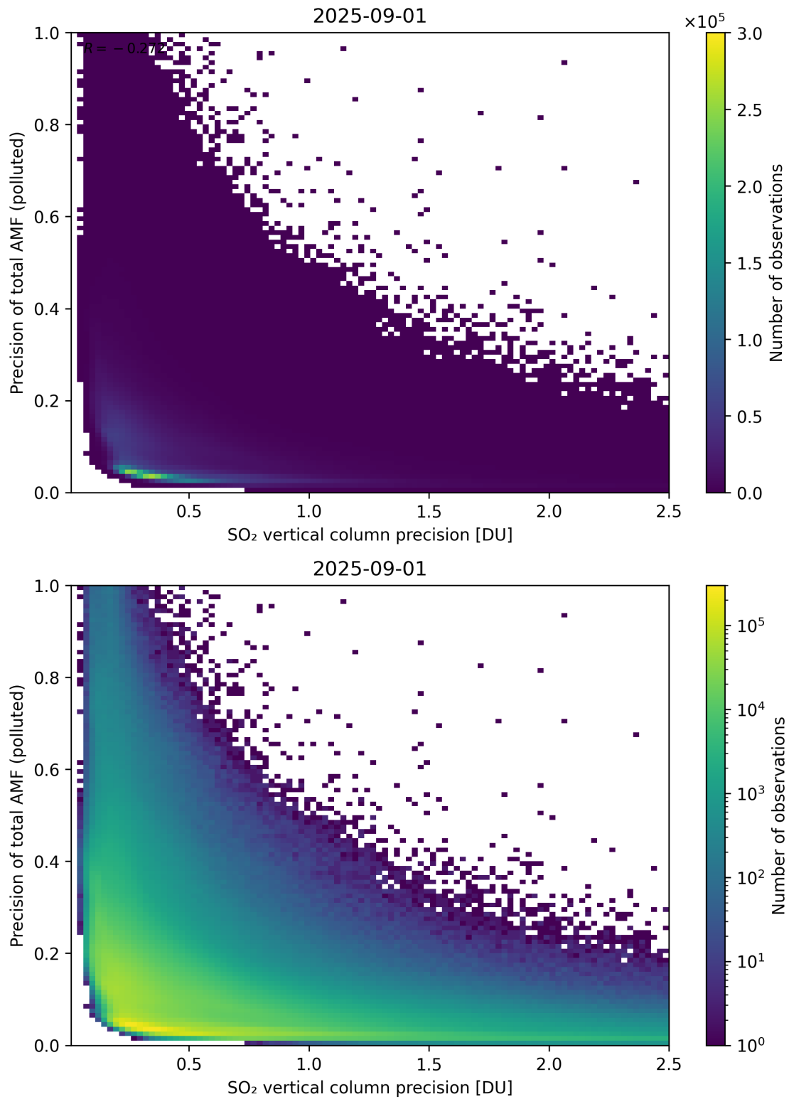
Figure 347: Scatter density plot of “SO 2 vertical column precision” against “Precision of total AMF (polluted)” for 2025-08-31 to 2025-09-02.
