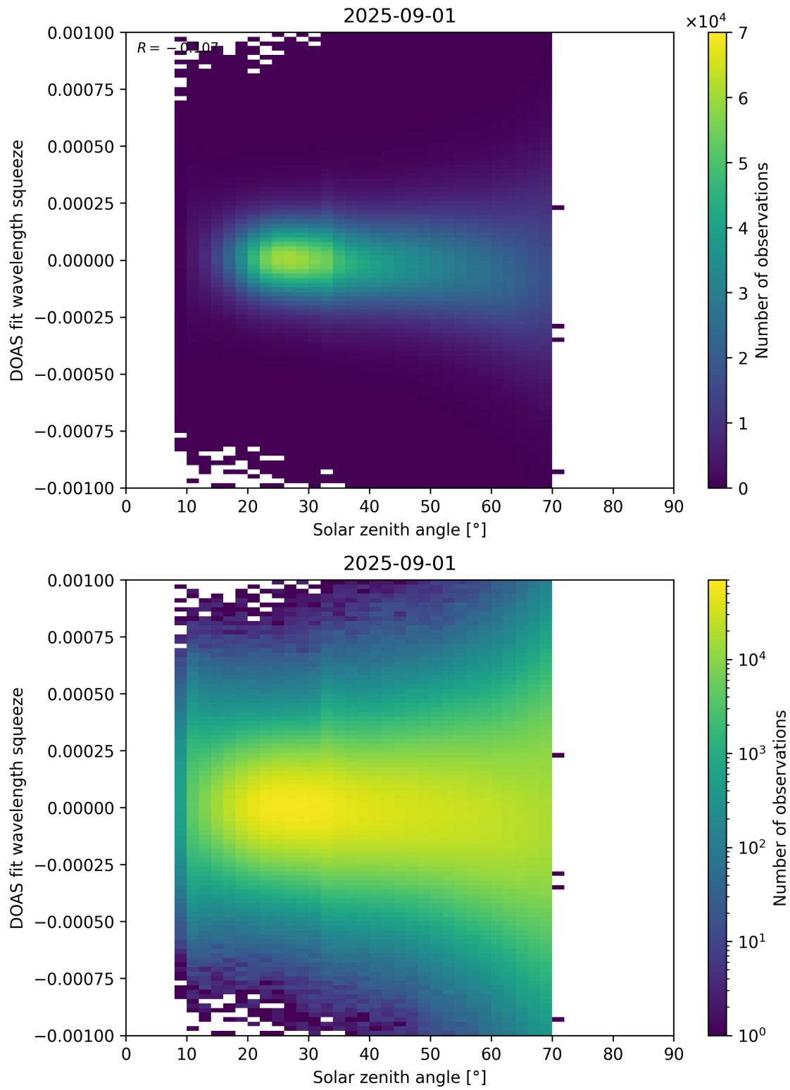
Figure 175: Scatter density plot of “Solar zenith angle” against “DOAS fit wavelength squeeze” for 2025-08-31 to 2025-09-02.
