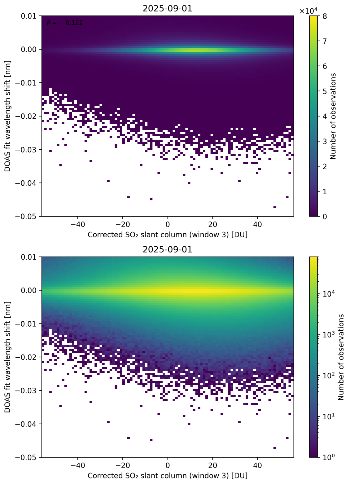
Figure 256: Scatter density plot of “Corrected SO 2 slant column (window 3)” against “DOAS fit wavelength shift” for 2025-08-31 to 2025-09-02.
