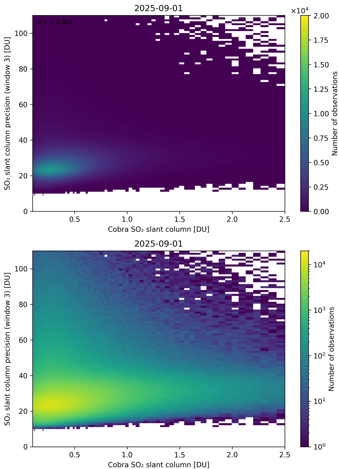
Figure 223: Scatter density plot of “Cobra SO 2 slant column” against “SO 2 slant column precision (window 3)” for 2025-08-31 to 2025-09-02.
