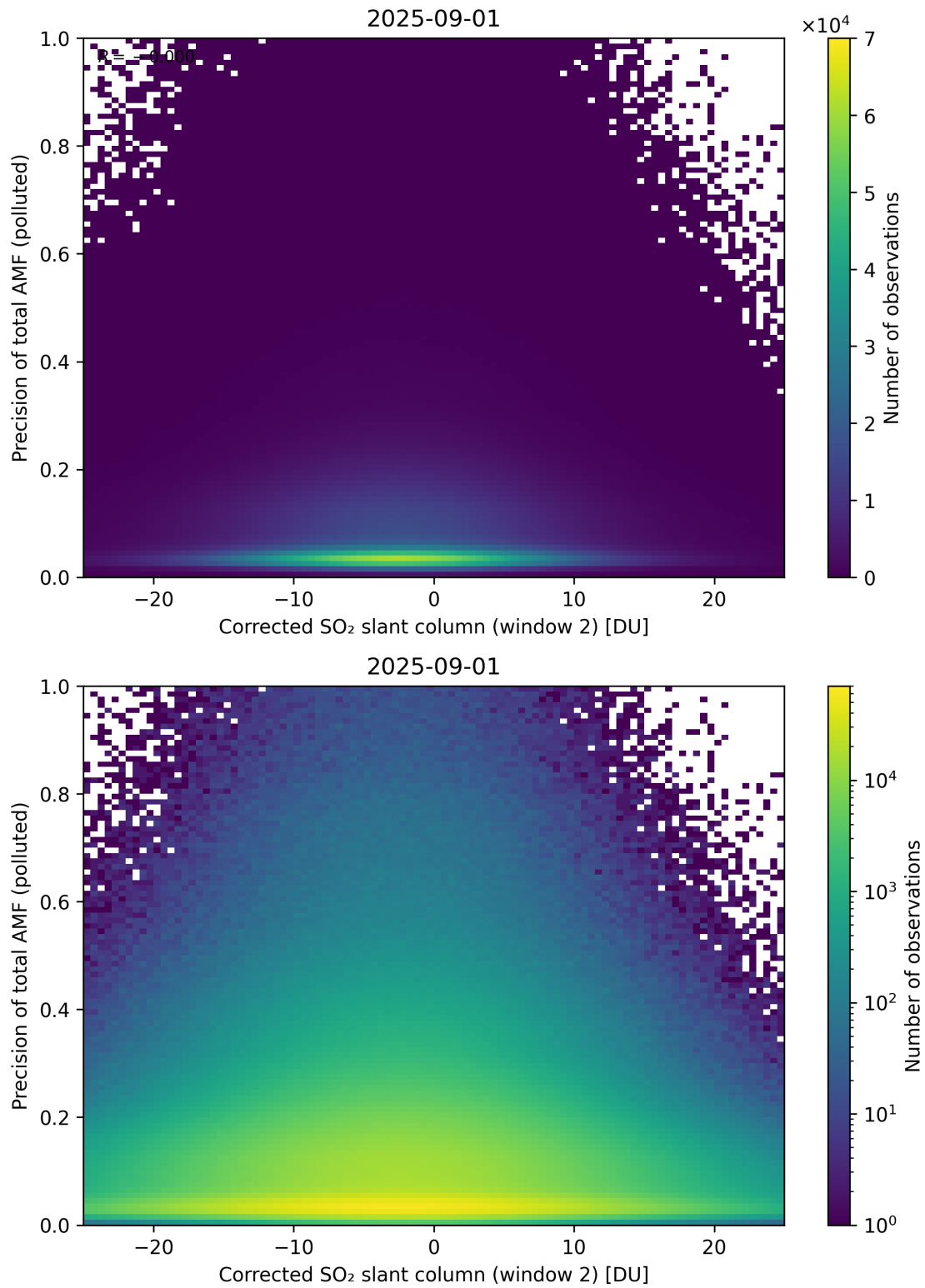
Figure 254: Scatter density plot of “Corrected SO 2 slant column (window 2)” against “Precision of total AMF (polluted)” for 2025-08-31 to 2025-09-02.
