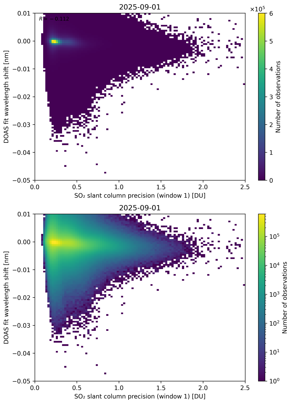
Figure 271: Scatter density plot of “SO 2 slant column precision (window 1)” against “DOAS fit wavelength shift” for 2025-08-31 to 2025-09-02.
