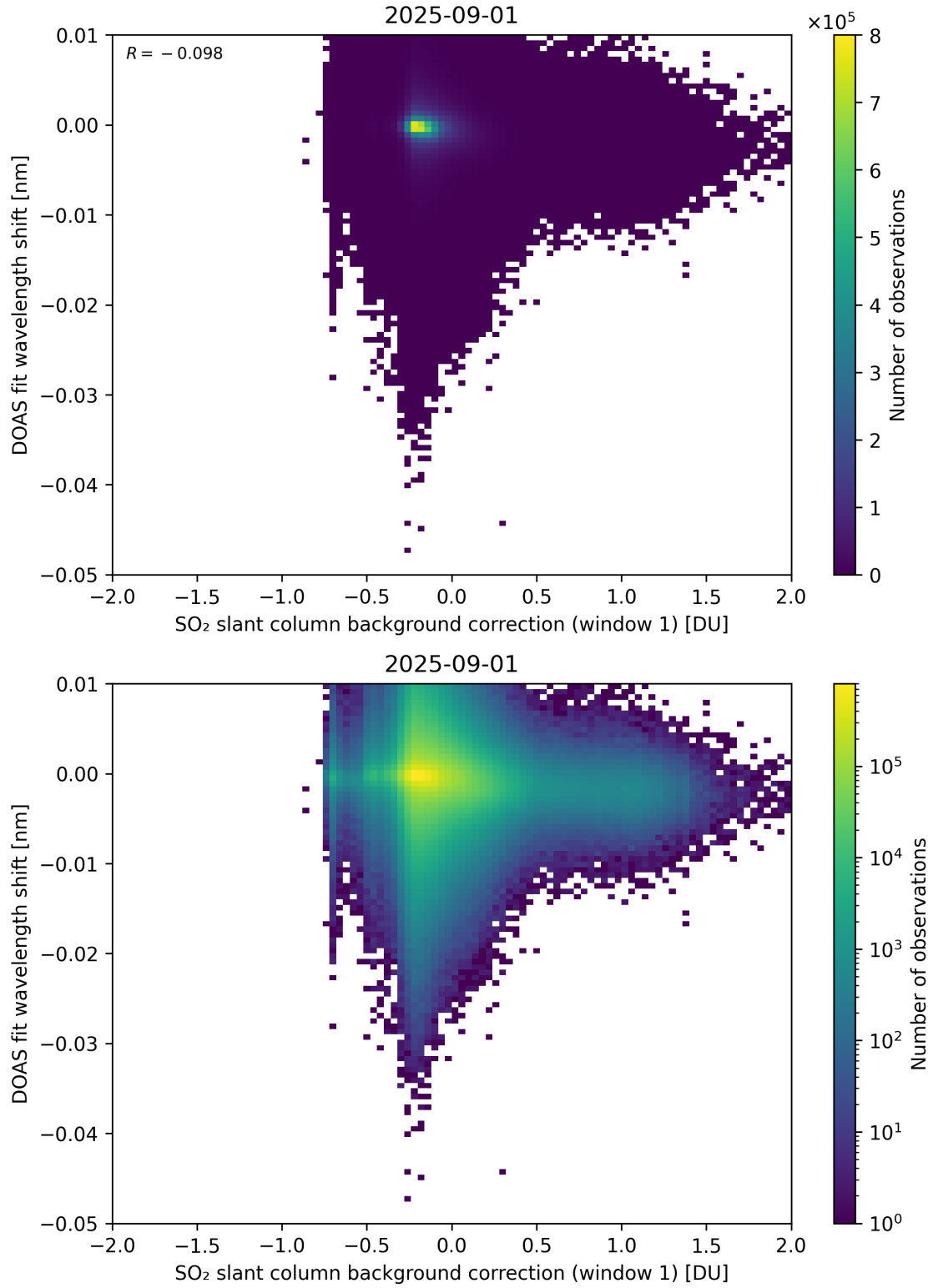
Figure 111: Scatter density plot of “SO 2 slant column background correction (window 1)” against “DOAS fit wavelength shift” for 2025-08-31 to 2025-09-02.
