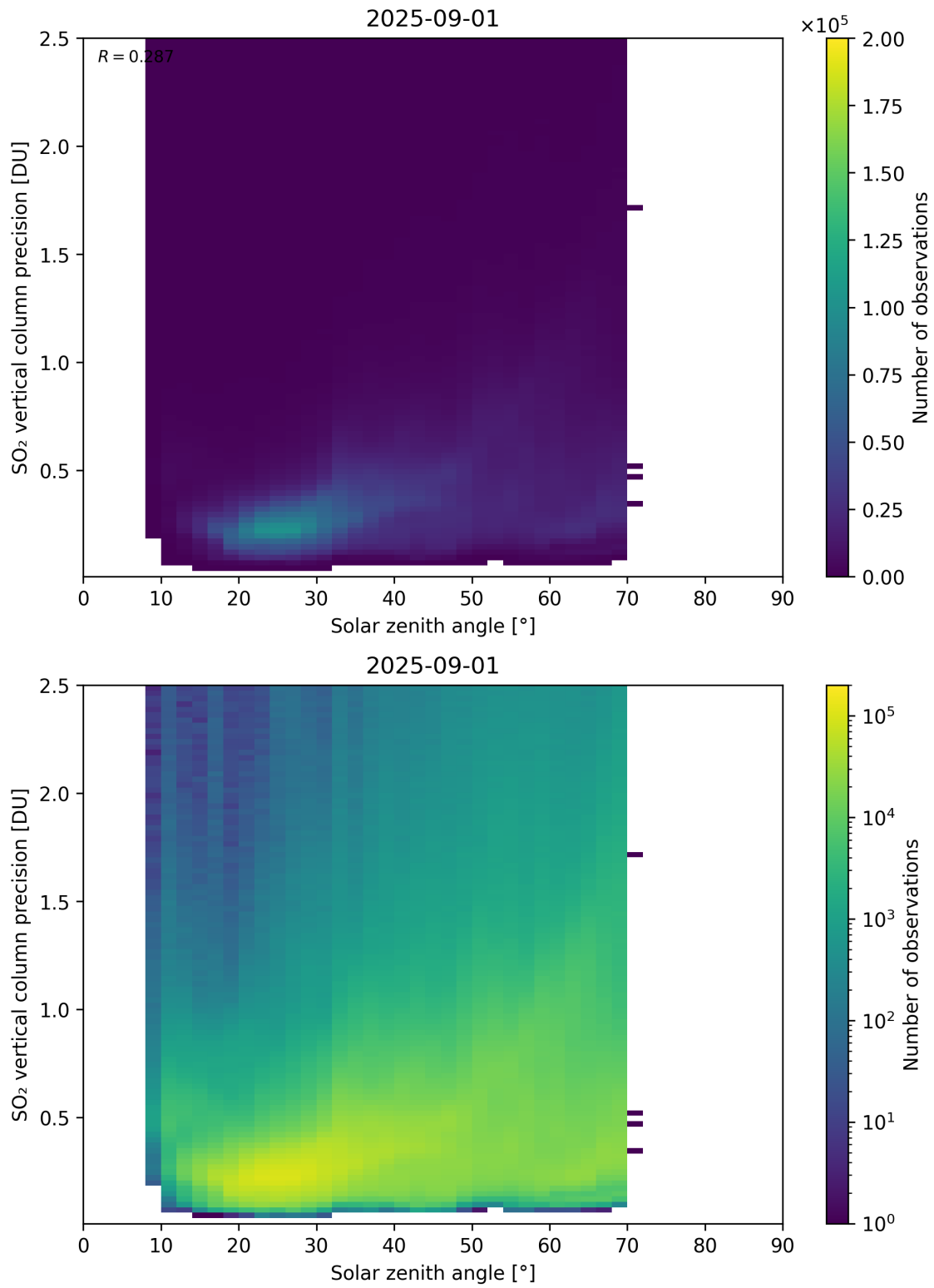
Figure 192: Scatter density plot of “Solar zenith angle” against “SO 2 vertical column precision” for 2025-08-31 to 2025-09-02.
