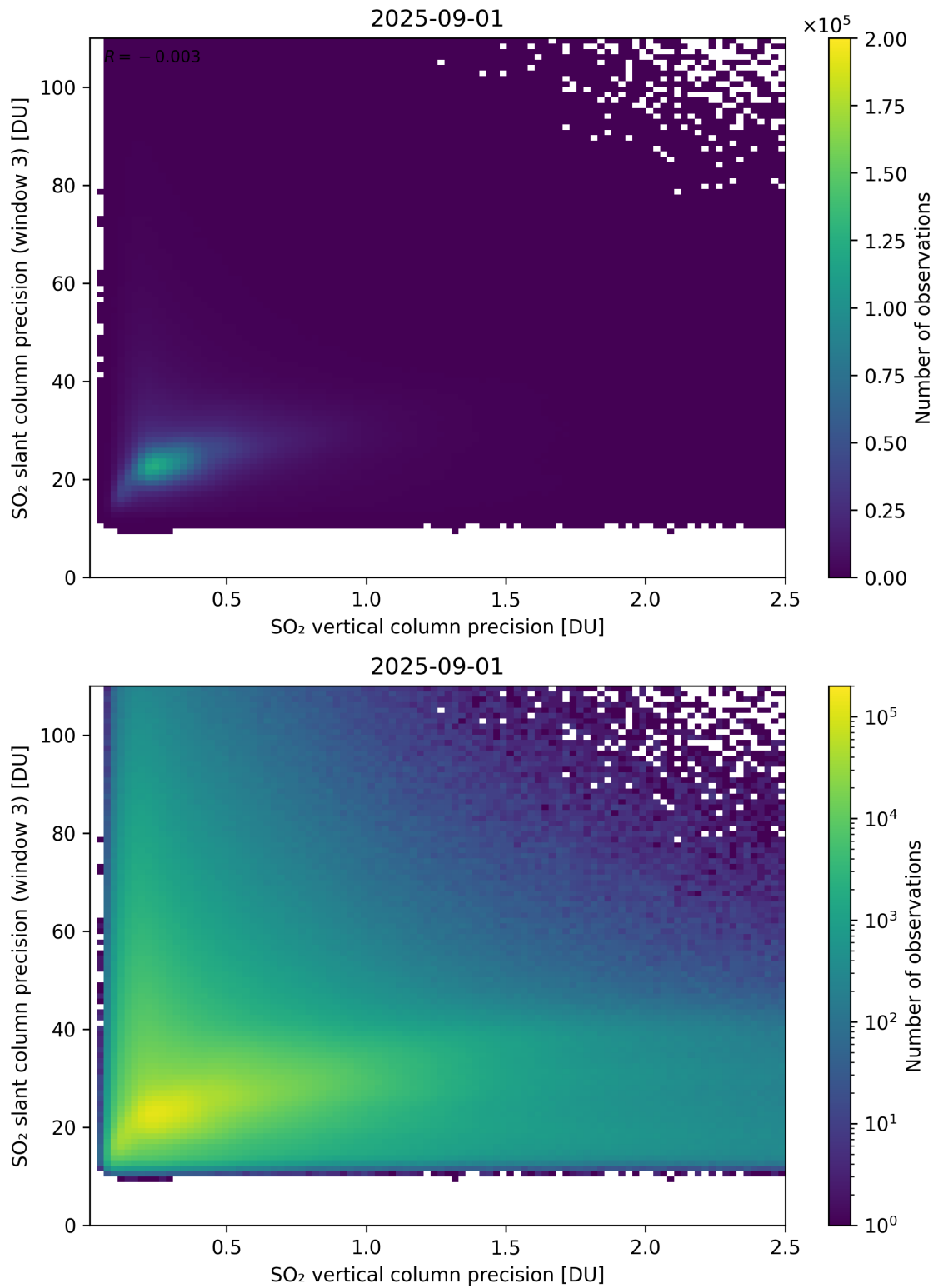
Figure 345: Scatter density plot of “SO 2 vertical column precision” against “SO 2 slant column precision (window 3)” for 2025-08-31 to 2025-09-02.
