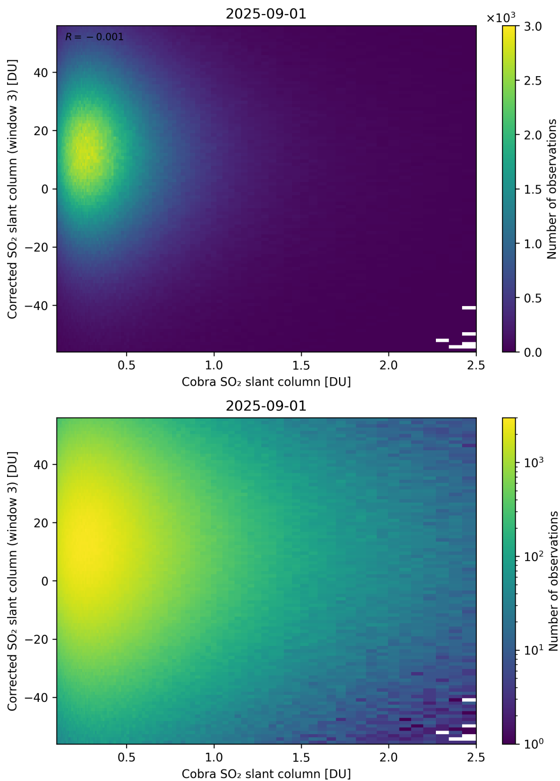
Figure 218: Scatter density plot of “Cobra SO 2 slant column” against “Corrected SO 2 slant column (window 3)” for 2025-08-31 to 2025-09-02.
