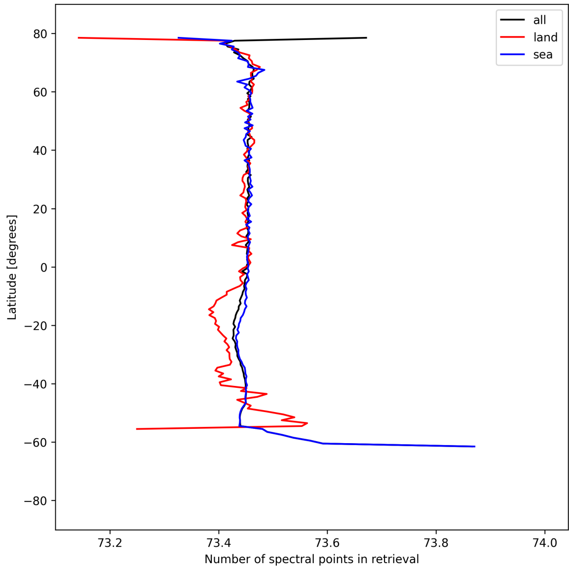
Figure 56: Zonal average of “Number of spectral points in retrieval” for 2025-08-31 to 2025-09-02.
