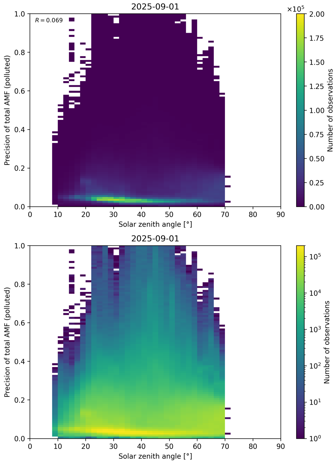
Figure 190: Scatter density plot of “Solar zenith angle” against “Precision of total AMF (polluted)” for 2025-08-31 to 2025-09-02.
