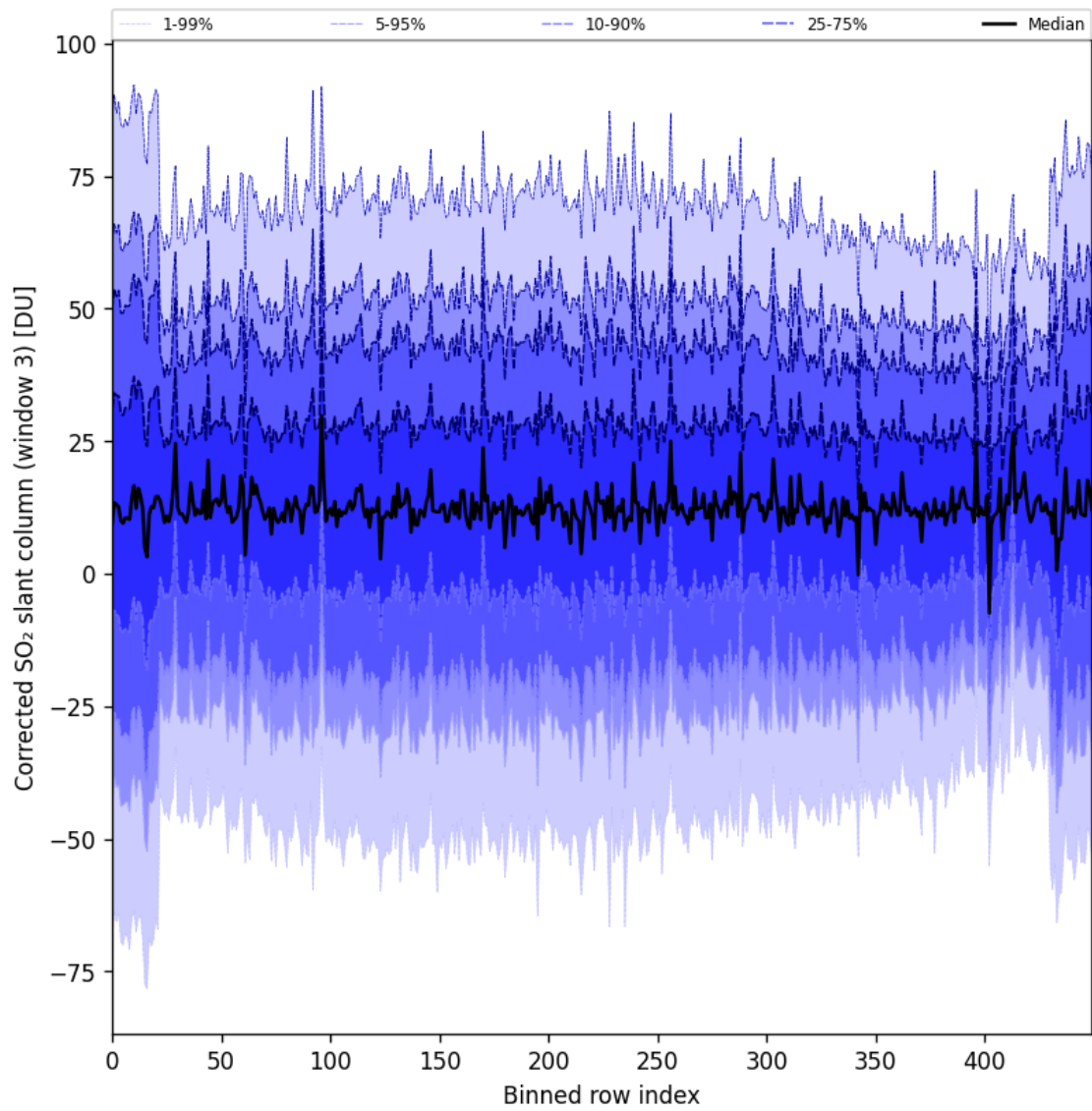
Figure 99: Along track statistics of “Corrected SO 2 slant column (window 3)” for 2025-08-31 to 2025-09-02
