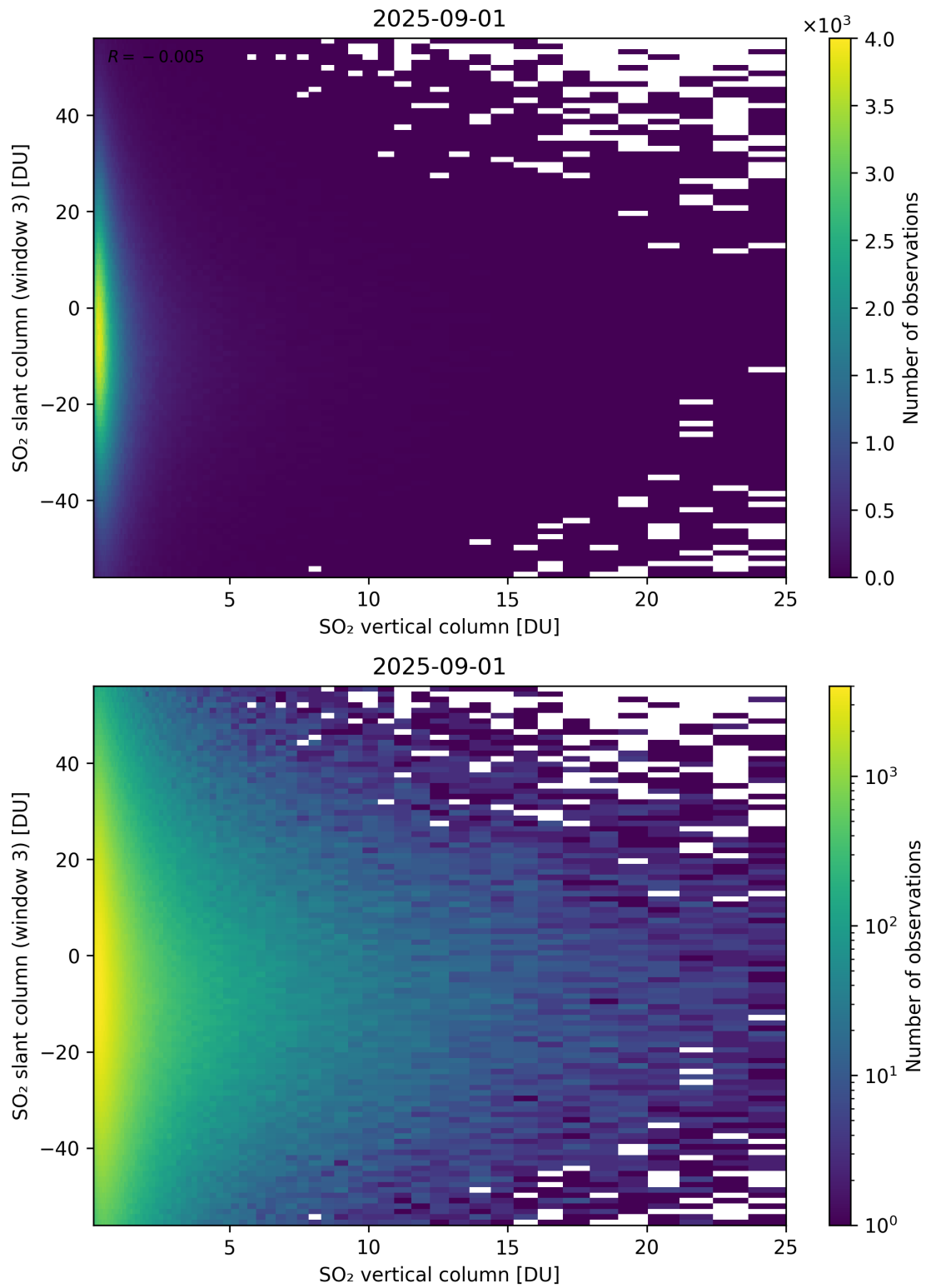
Figure 357: Scatter density plot of “SO 2 vertical column” against “SO 2 slant column (window 3)” for 2025-08-31 to 2025-09-02.
