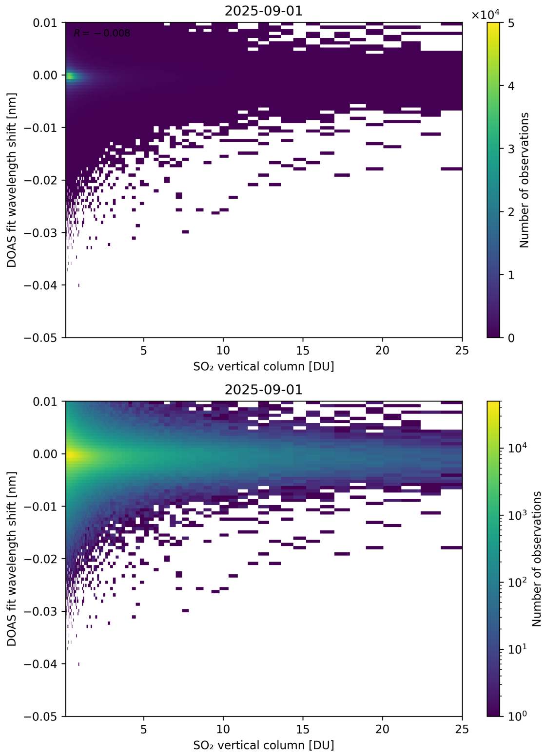
Figure 326: Scatter density plot of “SO 2 vertical column” against “DOAS fit wavelength shift” for 2025-08-31 to 2025-09-02.
