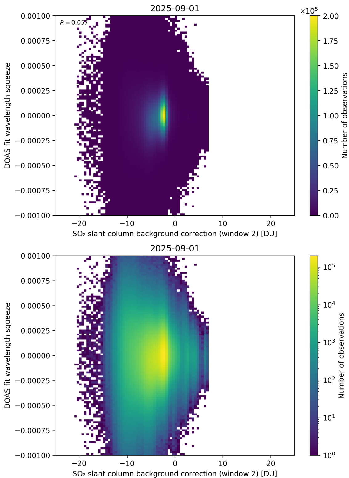
Figure 124: Scatter density plot of “SO 2 slant column background correction (window 2)” against “DOAS fit wavelength squeeze” for 2025-08-31 to 2025-09-02.
