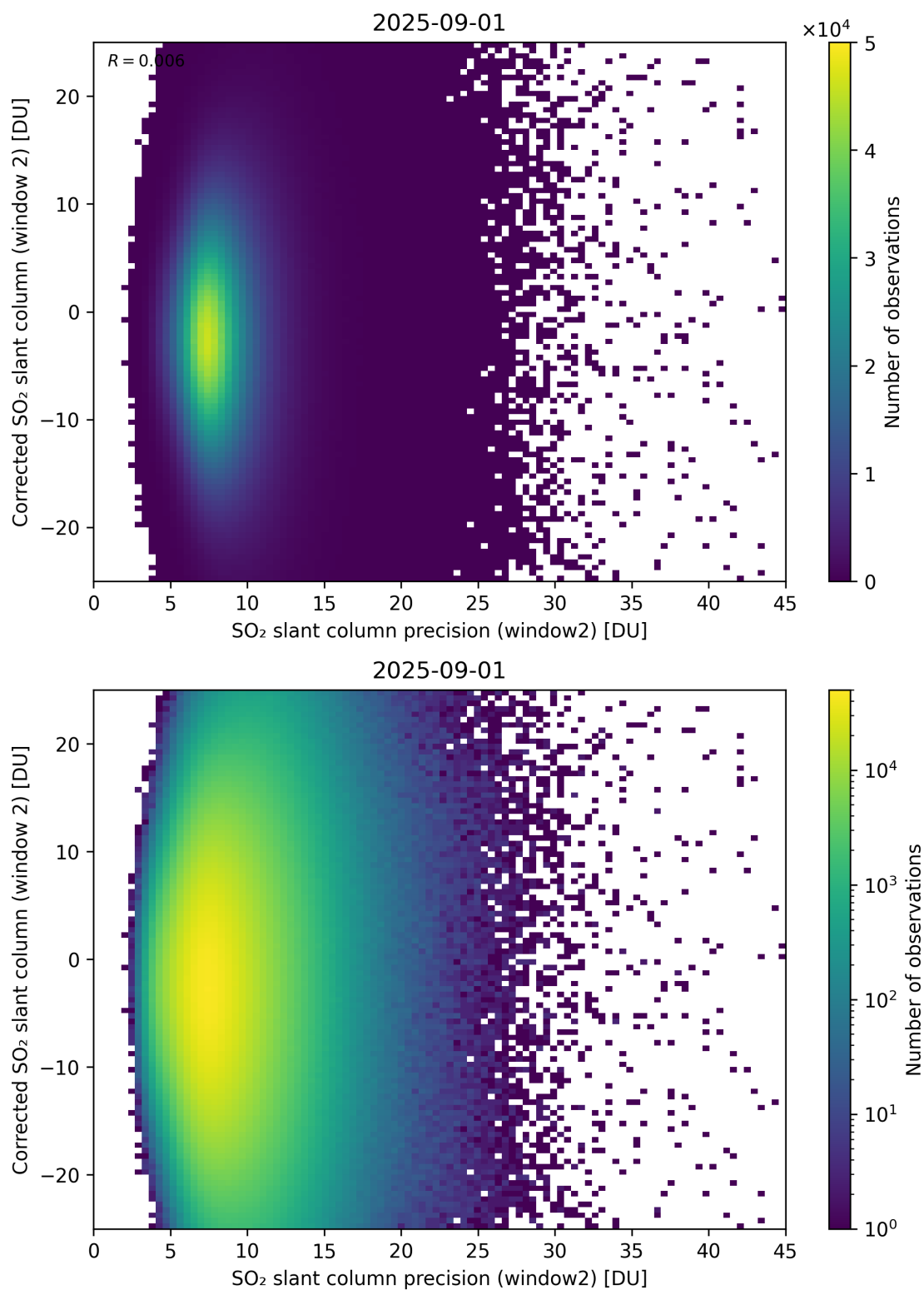
Figure 297: Scatter density plot of “SO 2 slant column precision (window2)” against “Corrected SO 2 slant column (window 2)” for 2025-08-31 to 2025-09-02.
