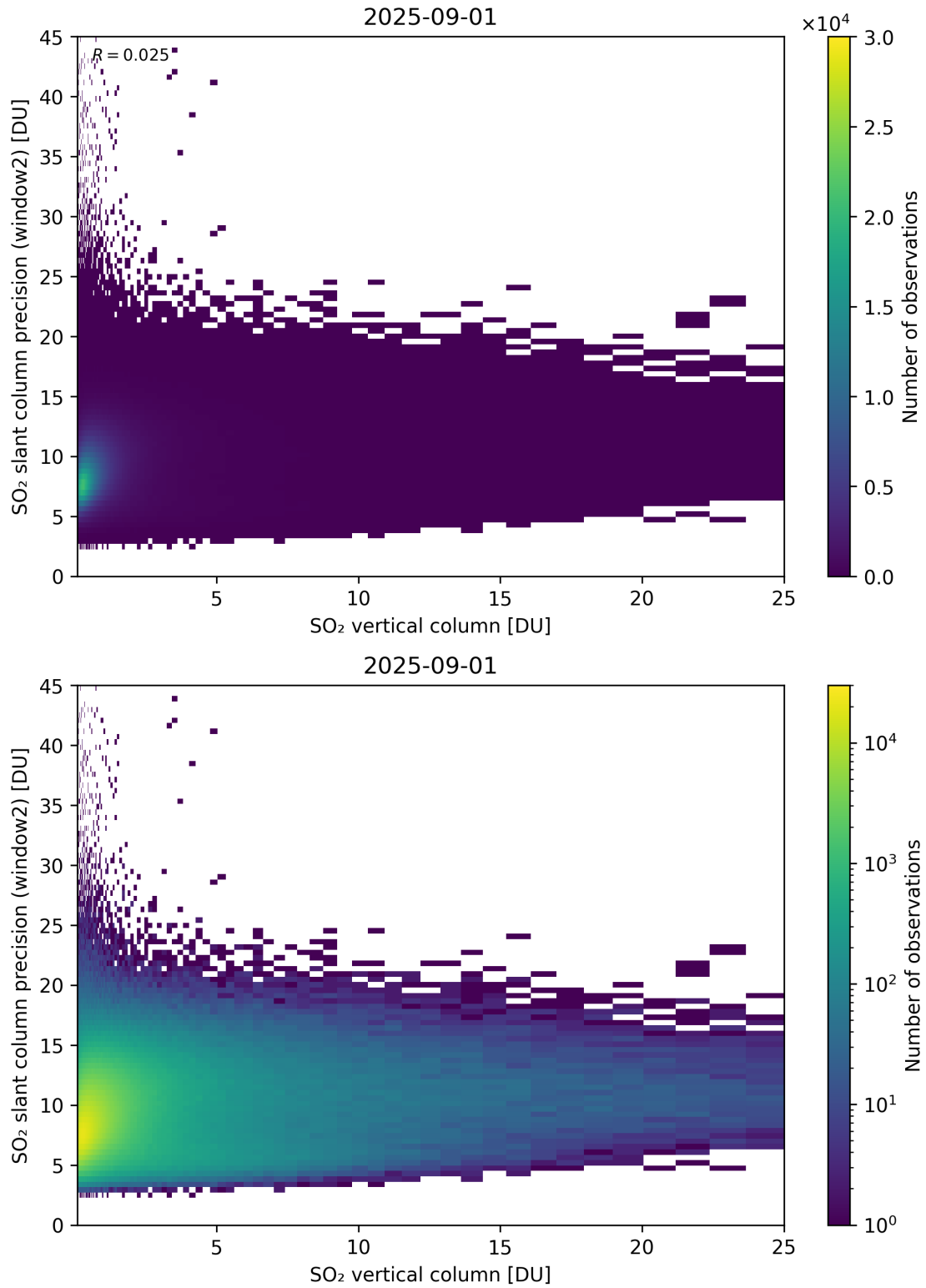
Figure 356: Scatter density plot of “SO 2 vertical column” against “SO 2 slant column precision (window2)” for 2025-08-31 to 2025-09-02.
