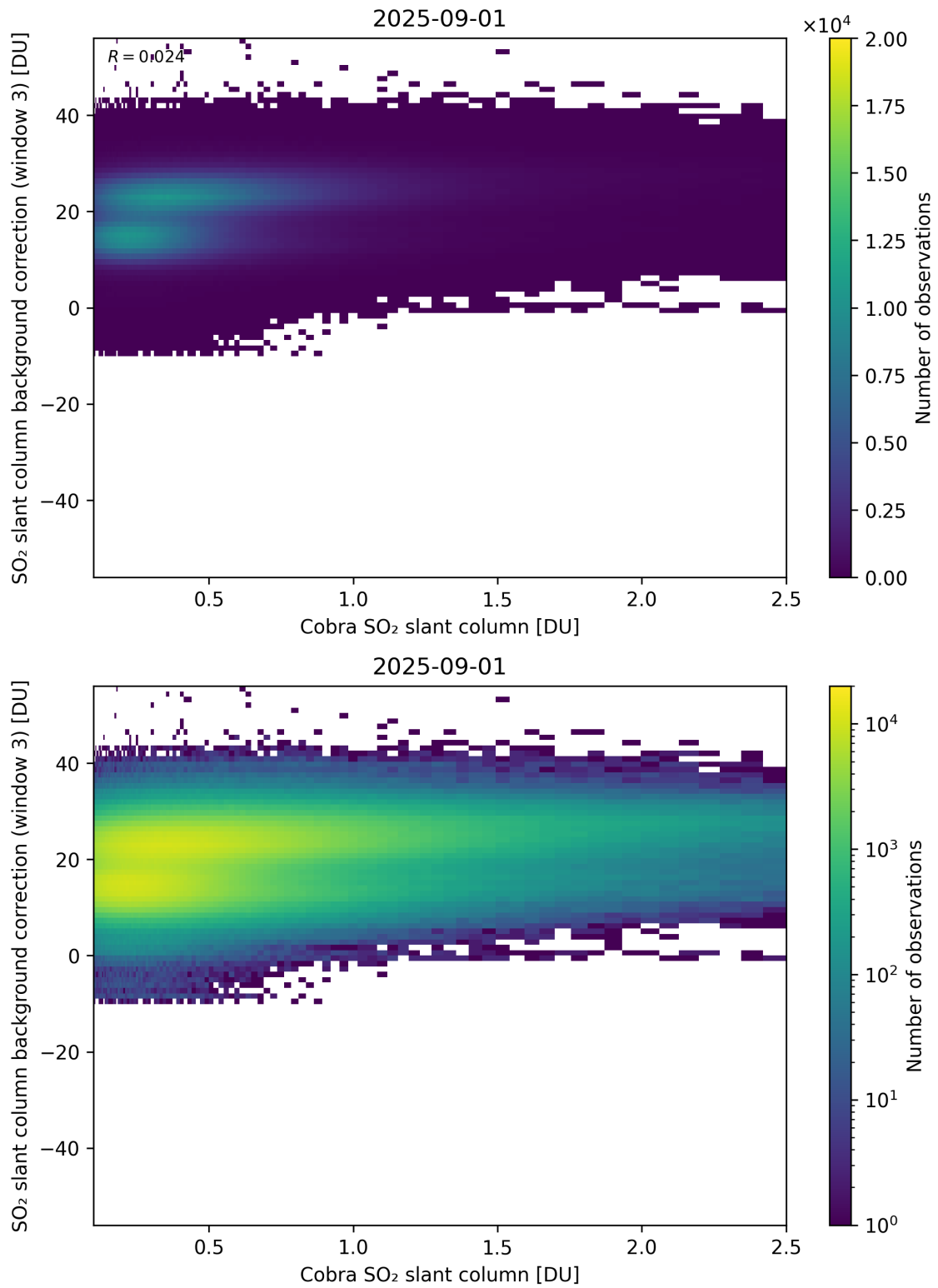
Figure 195: Scatter density plot of “Cobra SO 2 slant column” against “SO 2 slant column background correction (window 3)” for 2025-08-31 to 2025-09-02.
