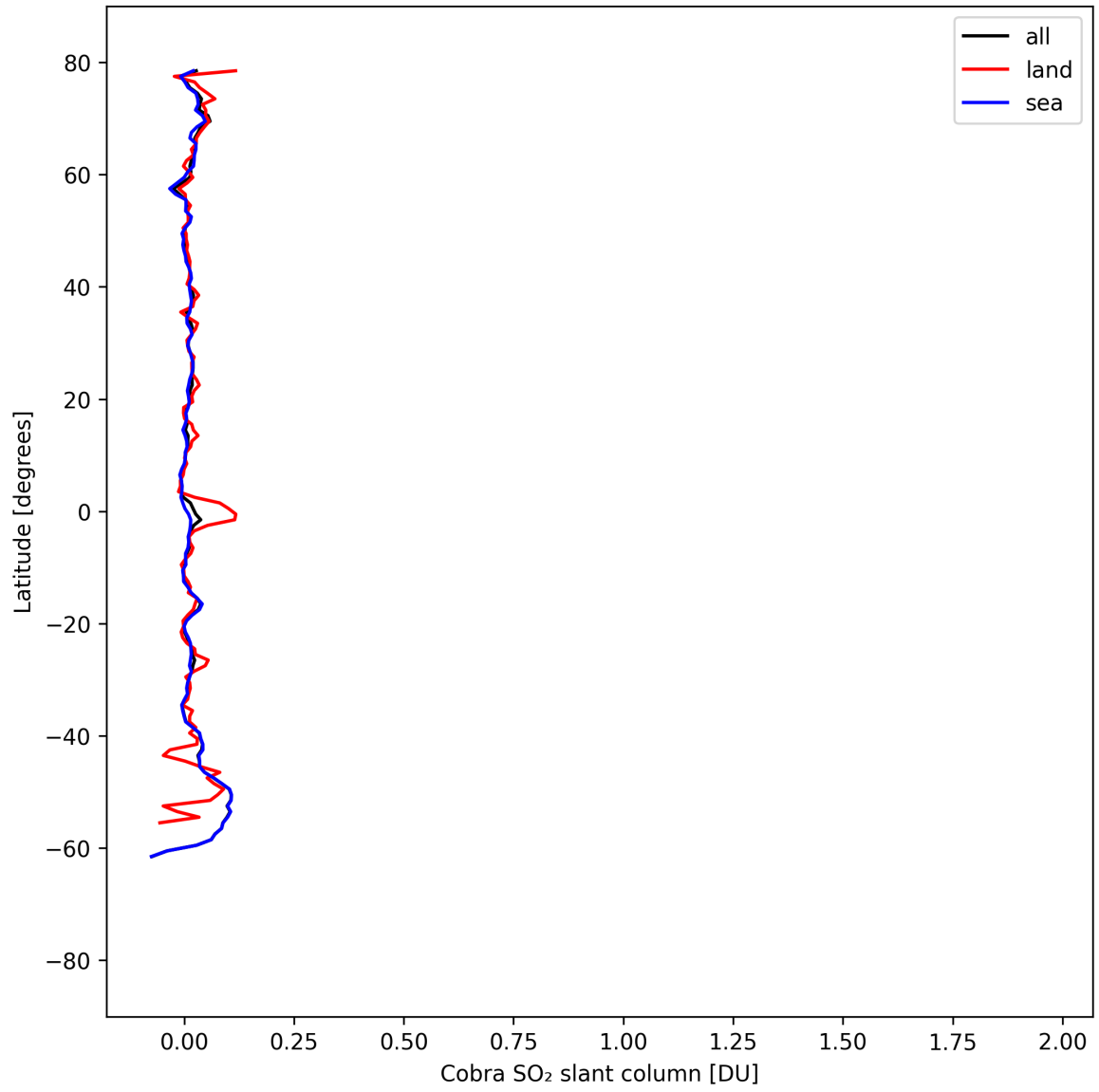
Figure 35: Zonal average of “Cobra SO 2 slant column” for 2025-08-31 to 2025-09-02.
