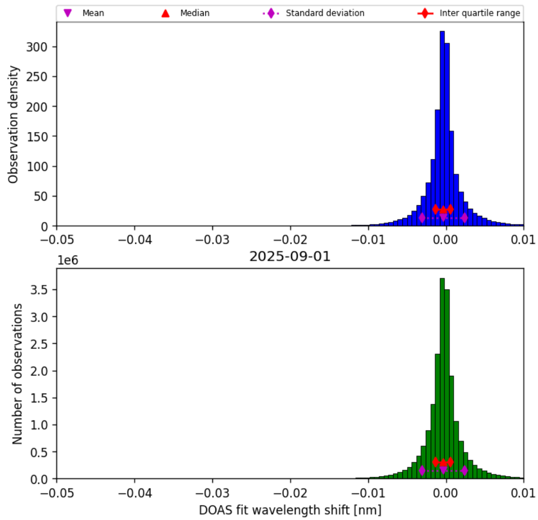
Figure 76: Histogram of “DOAS fit wavelength shift” for 2025-08-31 to 2025-09-02
