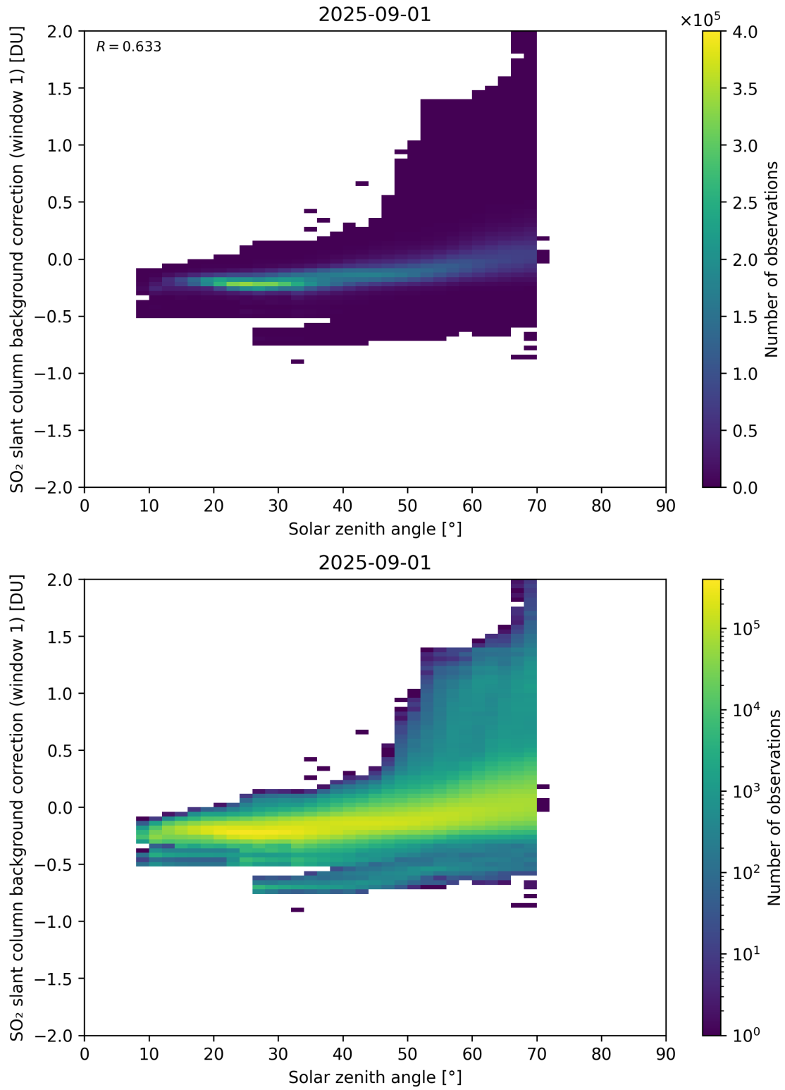
Figure 171: Scatter density plot of “Solar zenith angle” against “SO 2 slant column background correction (window 1)” for 2025-08-31 to 2025-09-02.
