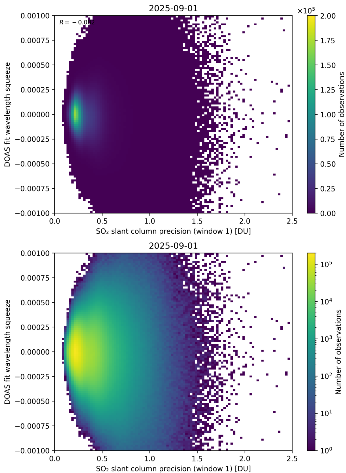
Figure 272: Scatter density plot of “SO 2 slant column precision (window 1)” against “DOAS fit wavelength squeeze” for 2025-08-31 to 2025-09-02.
