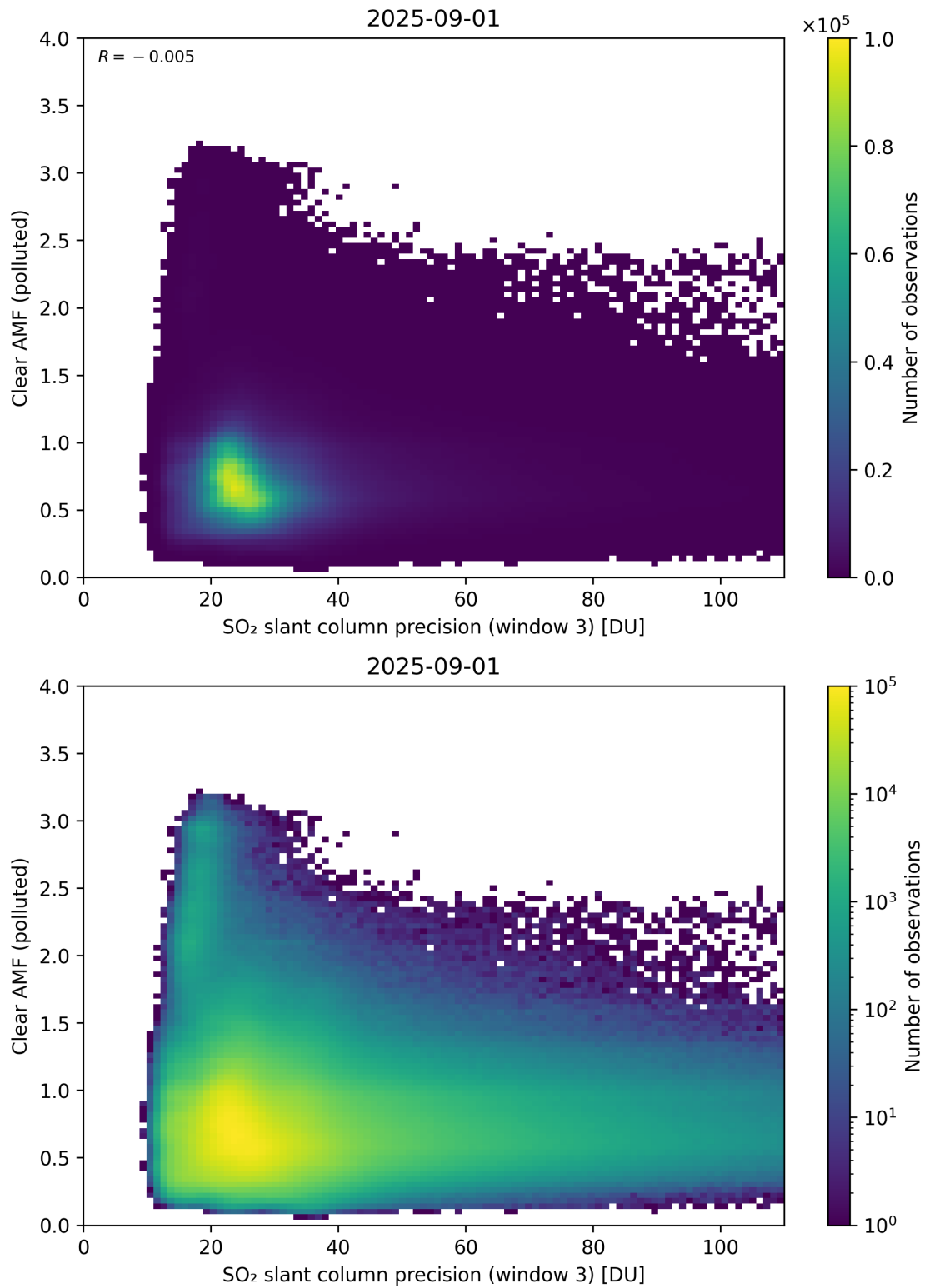
Figure 311: Scatter density plot of “SO 2 slant column precision (window 3)” against “Clear AMF (polluted)” for 2025-08-31 to 2025-09-02.
