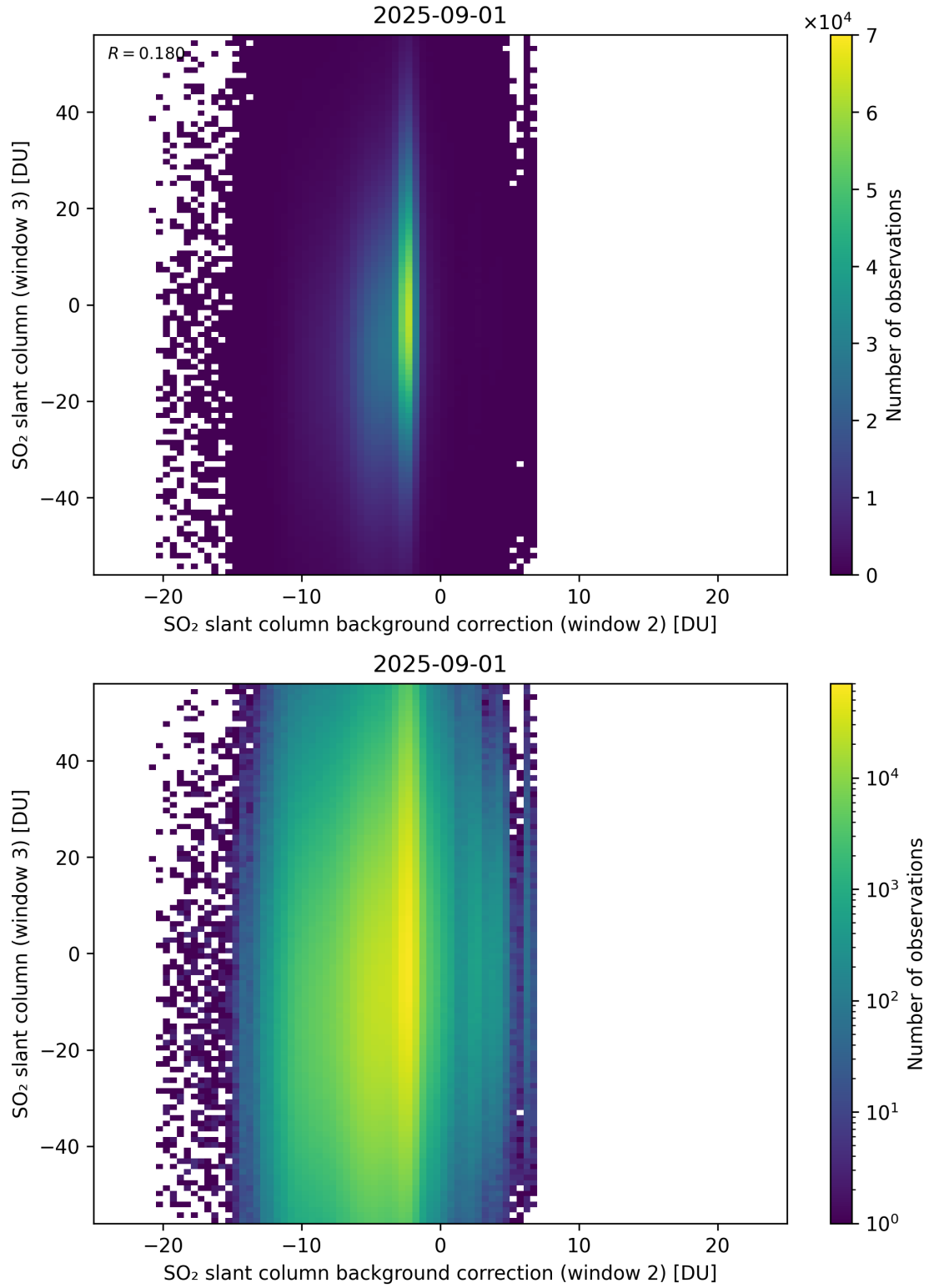
Figure 128: Scatter density plot of “SO 2 slant column background correction (window 2)” against “SO 2 slant column (window 3)” for 2025-08-31 to 2025-09-02.
