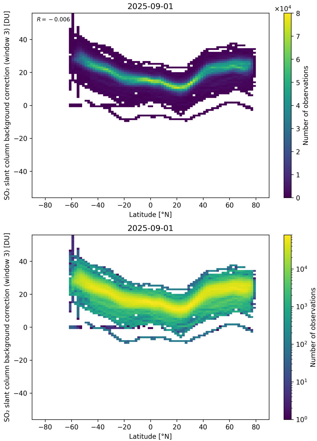
Figure 152: Scatter density plot of “Latitude” against “SO 2 slant column background correction (window 3)” for 2025-08-31 to 2025-09-02.
