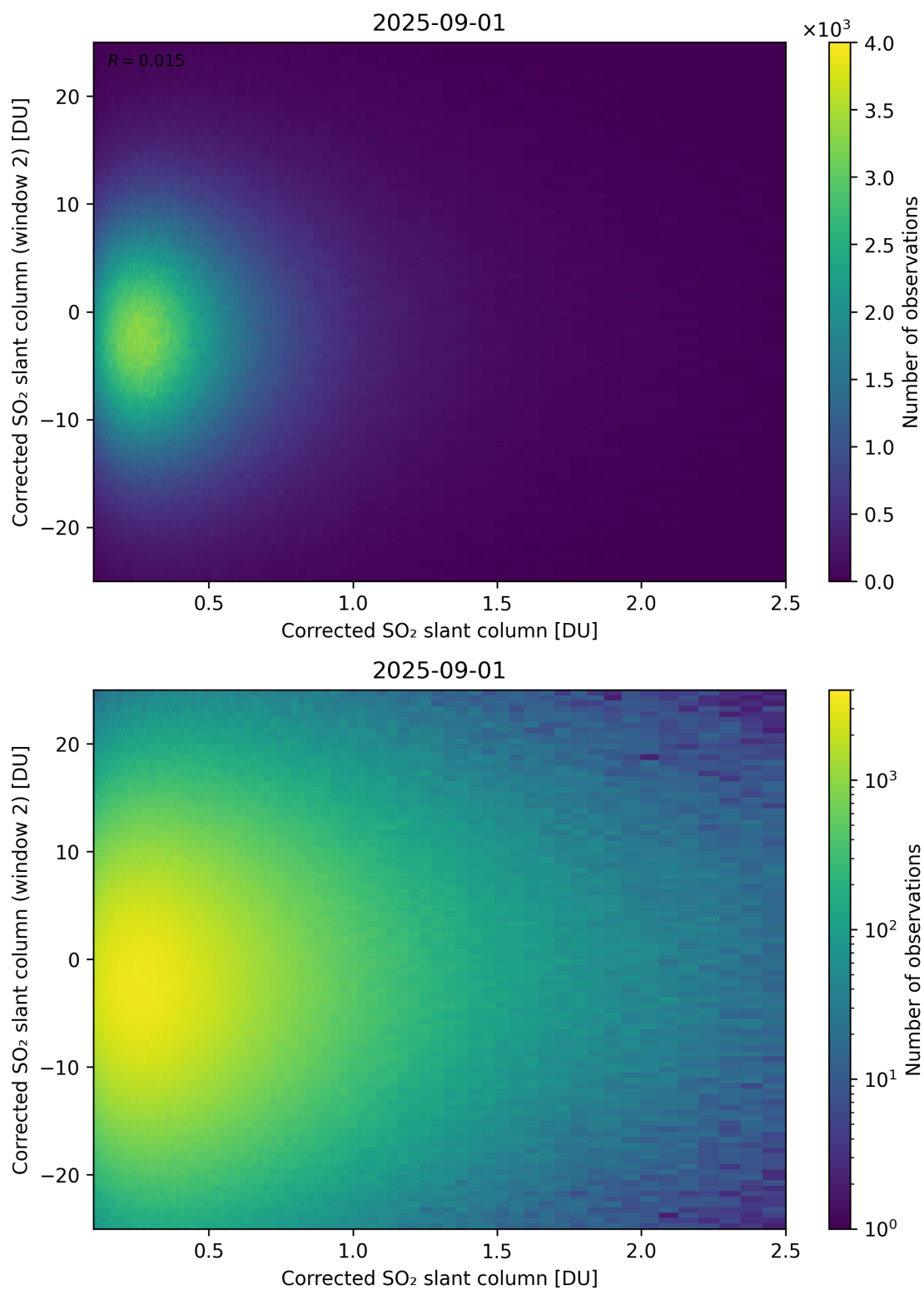
Figure 235: Scatter density plot of “Corrected SO 2 slant column” against “Corrected SO 2 slant column (window 2)” for 2025-08-31 to 2025-09-02.
