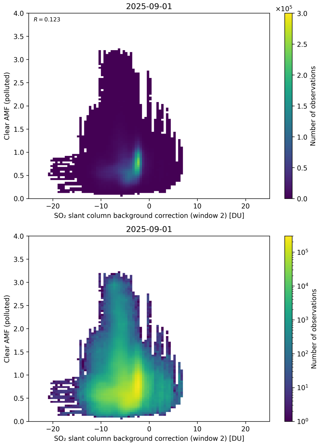
Figure 126: Scatter density plot of “SO 2 slant column background correction (window 2)” against “Clear AMF (polluted)” for 2025-08-31 to 2025-09-02.
