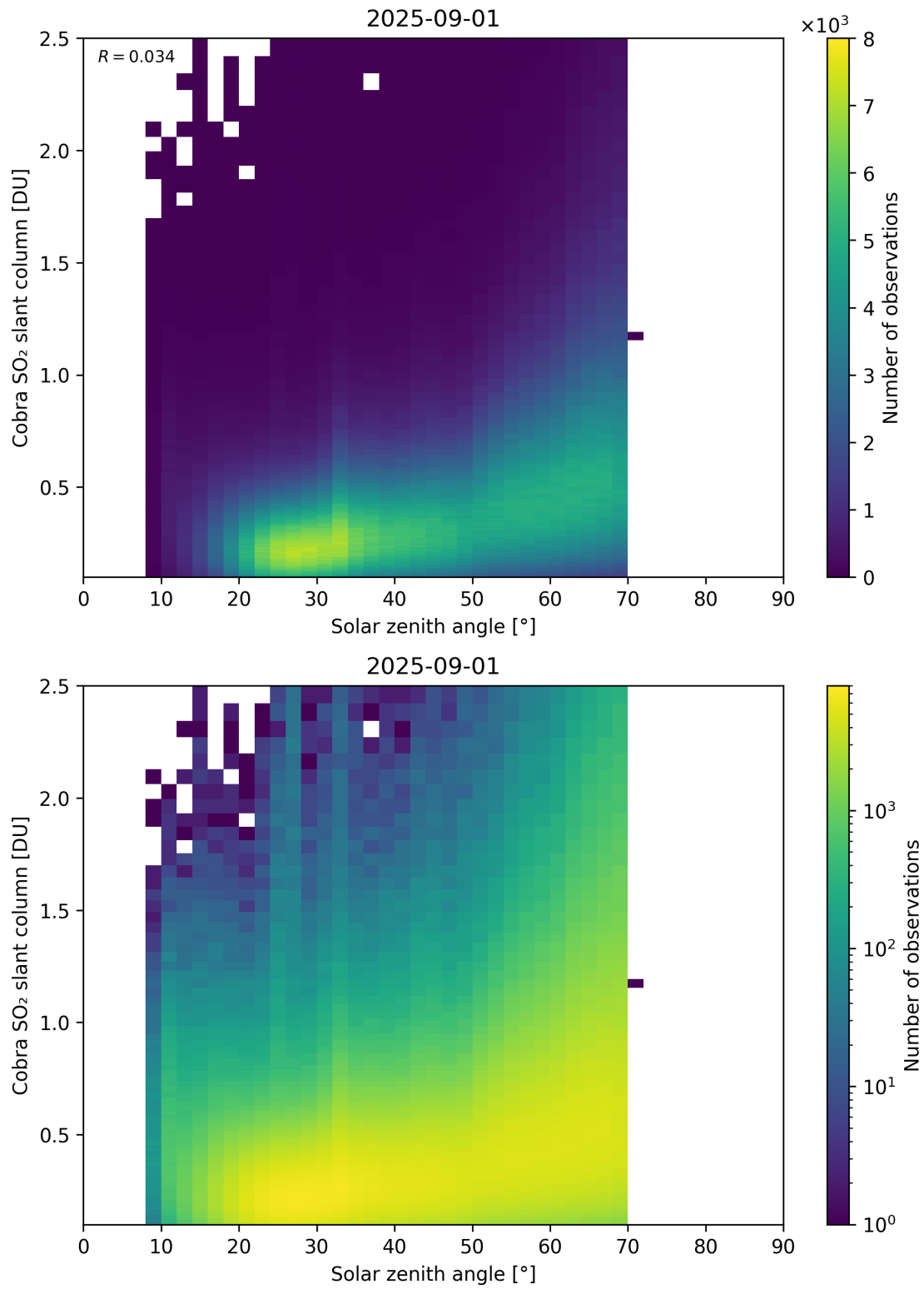
Figure 179: Scatter density plot of “Solar zenith angle” against “Cobra SO 2 slant column” for 2025-08-31 to 2025-09-02.
