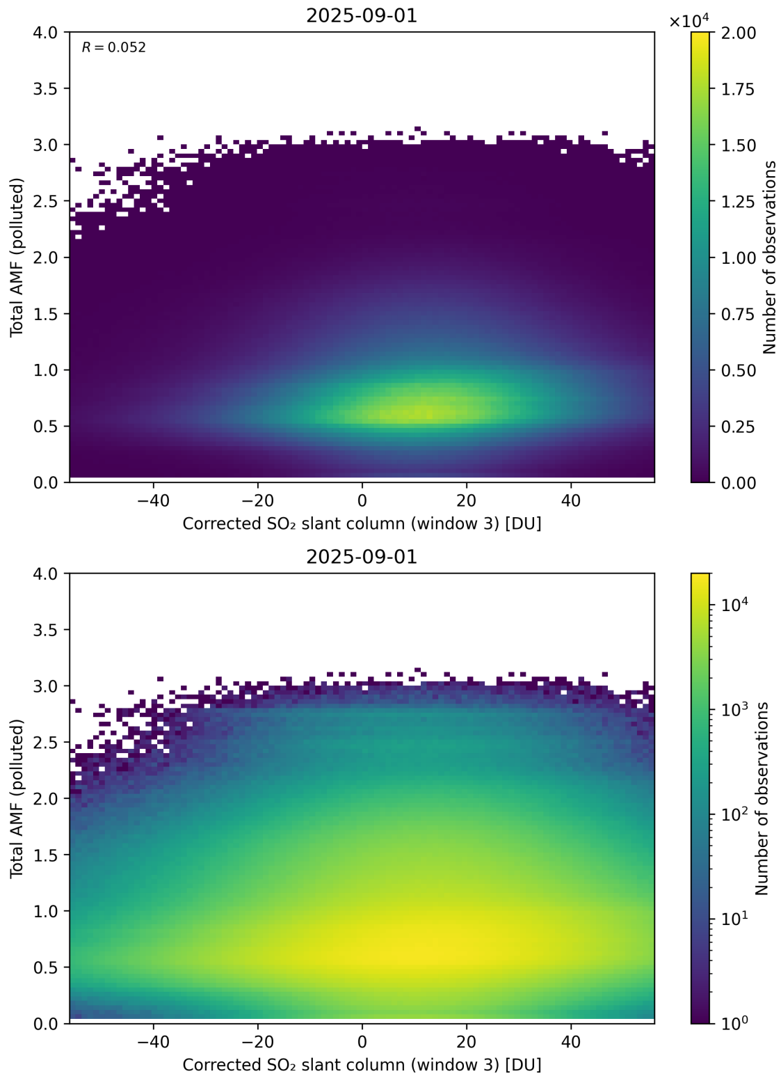
Figure 260: Scatter density plot of “Corrected SO 2 slant column (window 3)” against “Total AMF (polluted)” for 2025-08-31 to 2025-09-02.
