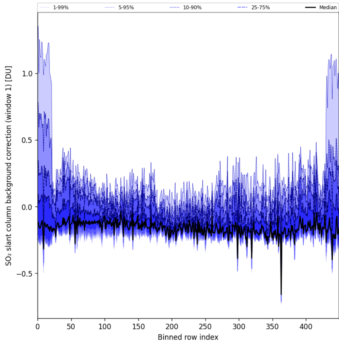
Figure 92: Along track statistics of “SO 2 slant column background correction (window 1)” for 2025-08-31 to 2025-09-02
