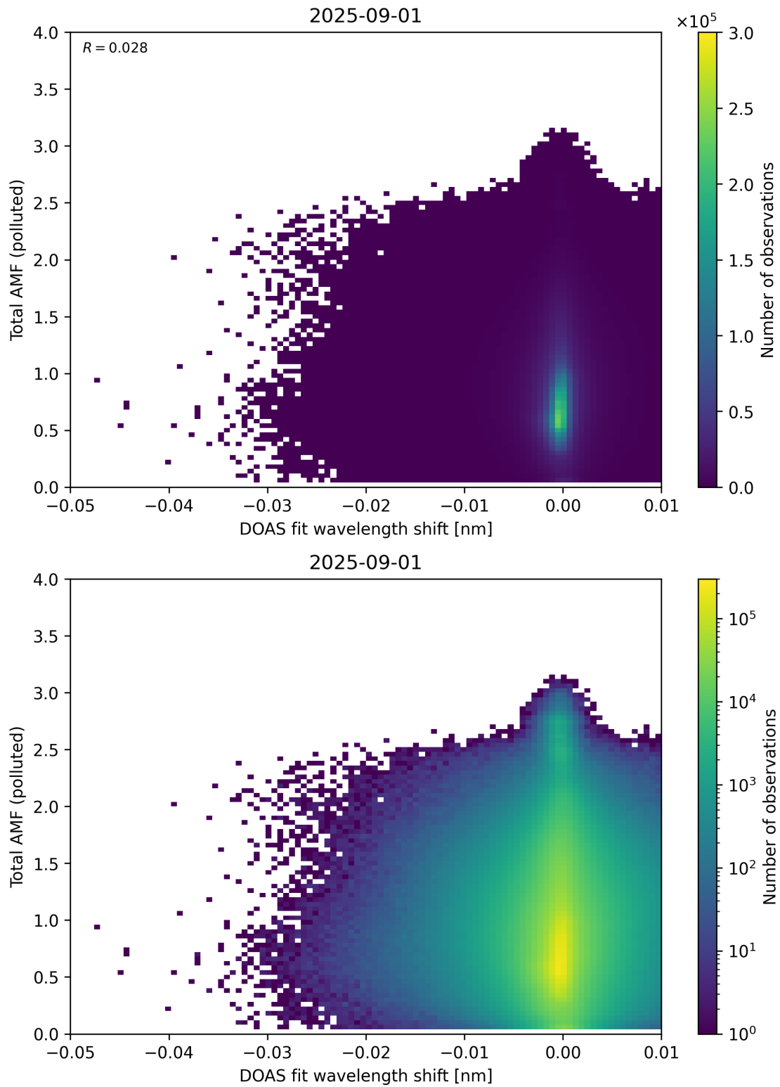
Figure 141: Scatter density plot of “DOAS fit wavelength shift” against “Total AMF (polluted)” for 2025-08-31 to 2025-09-02.
