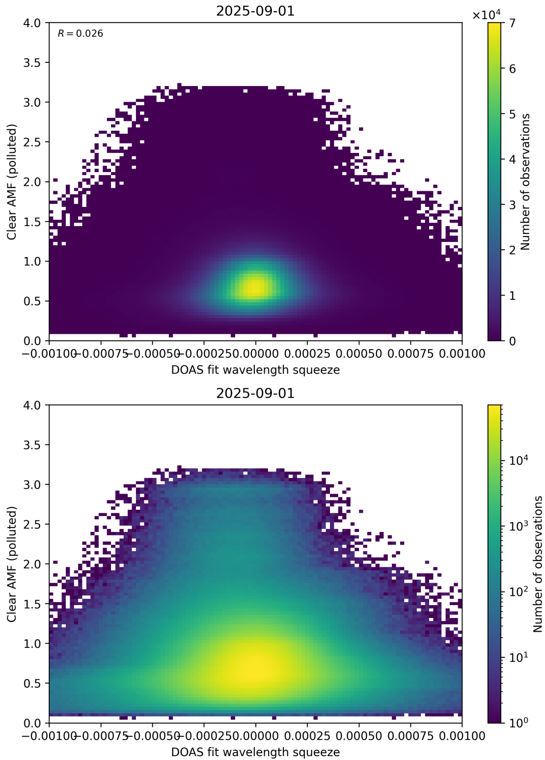
Figure 144: Scatter density plot of “DOAS fit wavelength squeeze” against “Clear AMF (polluted)” for 2025-08-31 to 2025-09-02.
