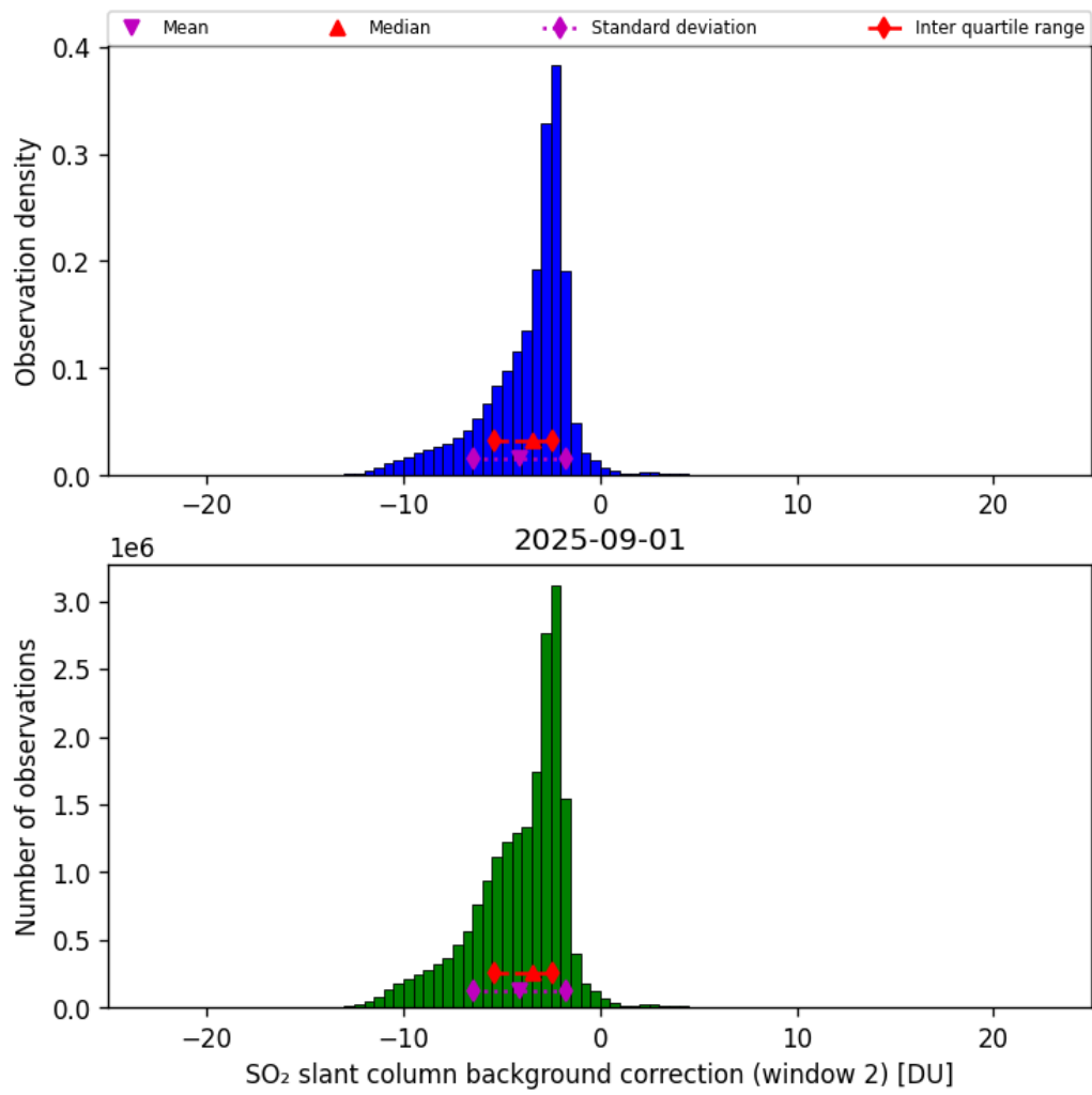
Figure 70: Histogram of “SO 2 slant column background correction (window 2)” for 2025-08-31 to 2025-09-02
