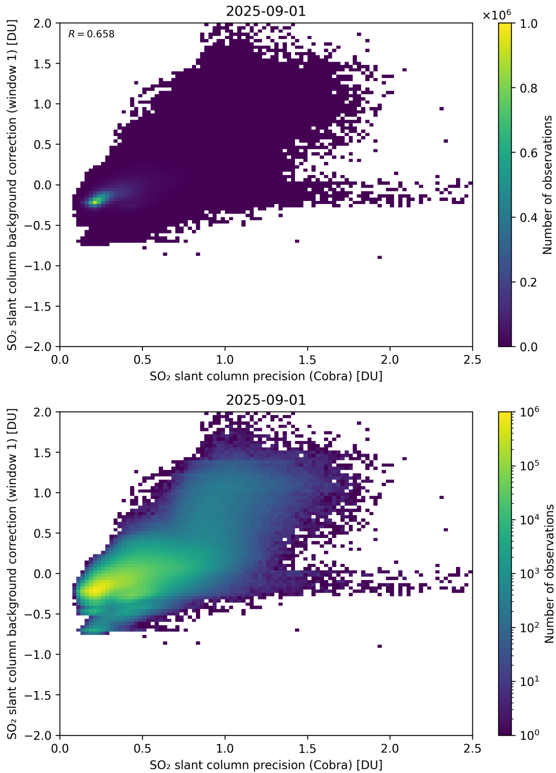
Figure 199: Scatter density plot of “SO 2 slant column precision (Cobra)” against “SO 2 slant column background correction (window 1)” for 2025-08-31 to 2025-09-02.
