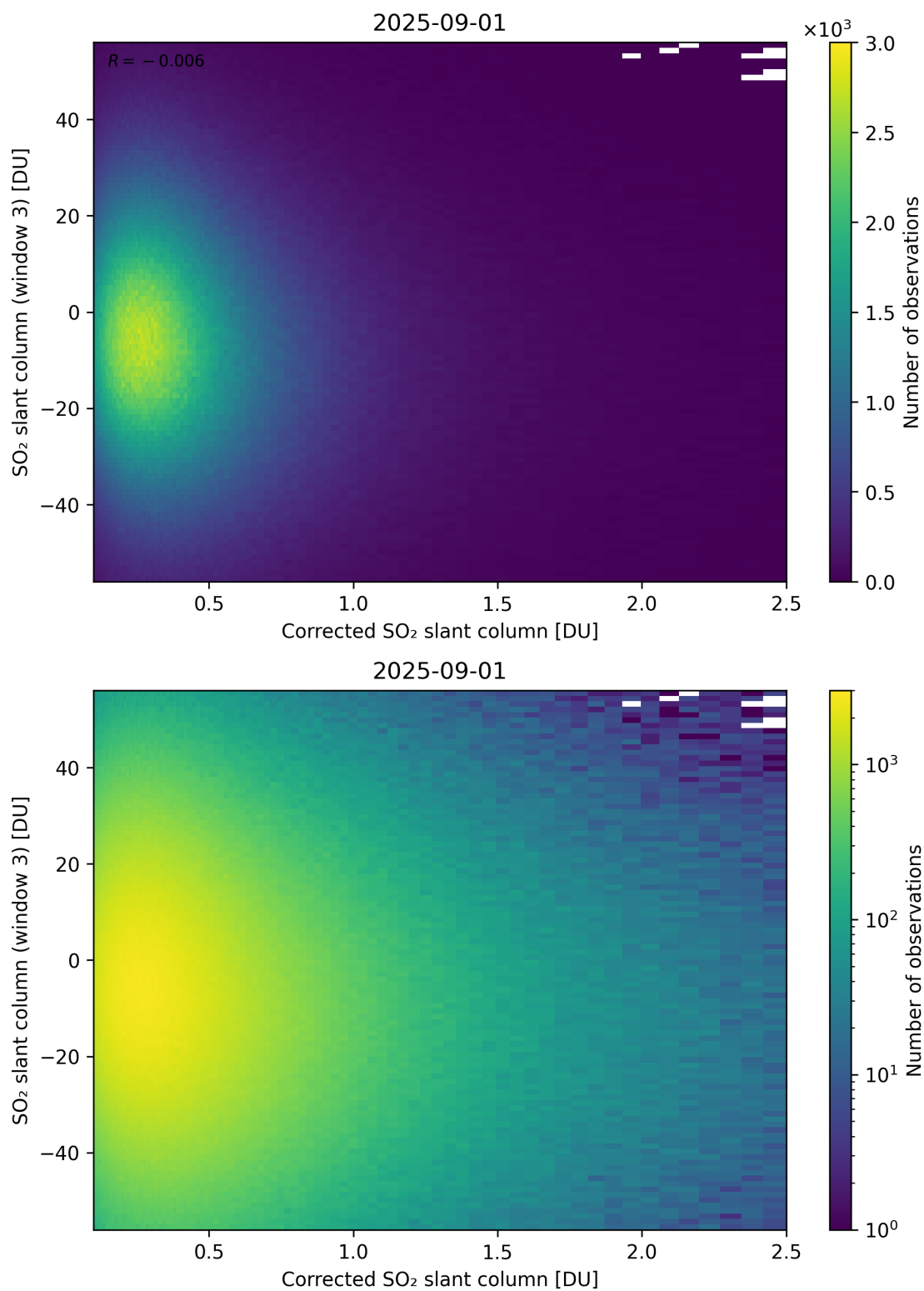
Figure 240: Scatter density plot of “Corrected SO 2 slant column” against “SO 2 slant column (window 3)” for 2025-08-31 to 2025-09-02.
