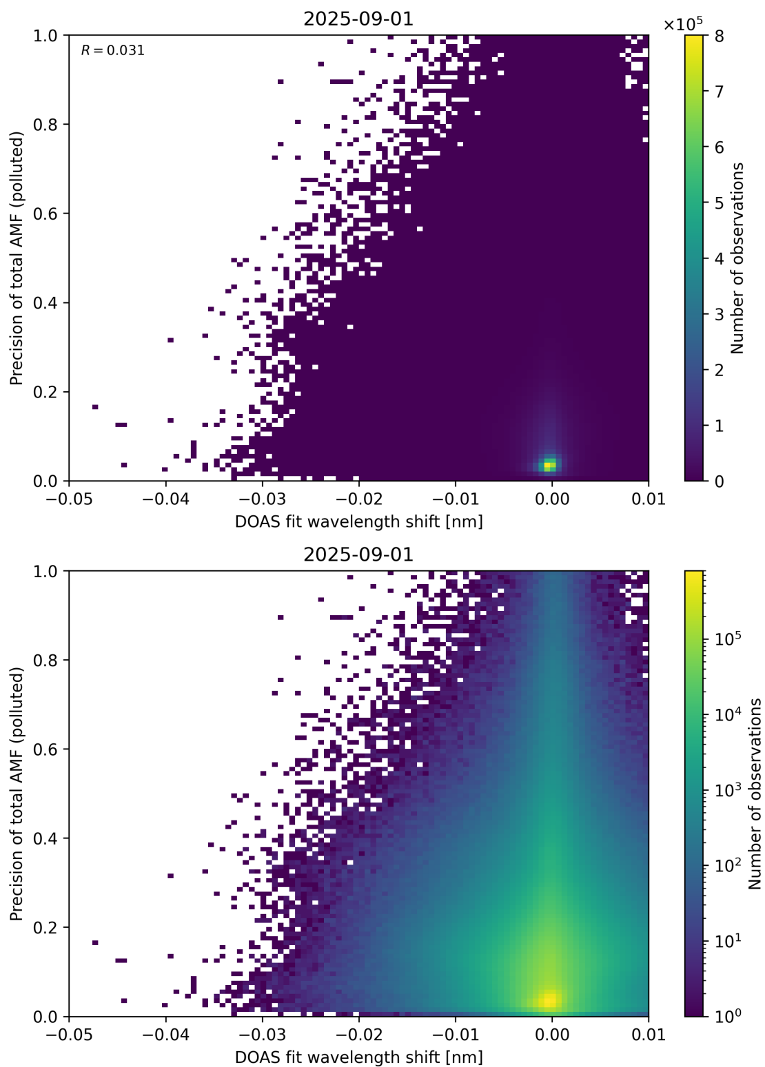
Figure 142: Scatter density plot of “DOAS fit wavelength shift” against “Precision of total AMF (polluted)” for 2025-08-31 to 2025-09-02.
