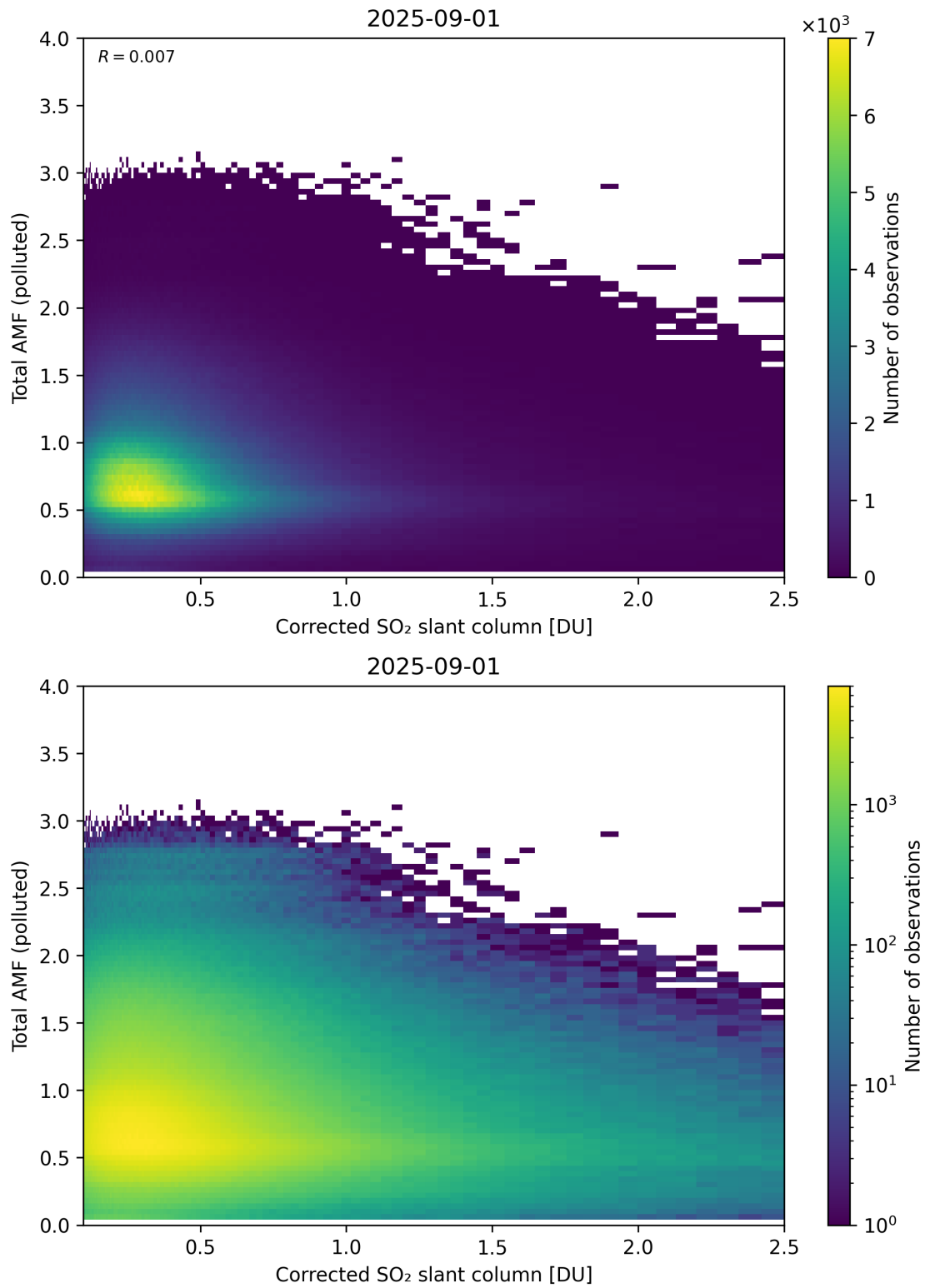
Figure 242: Scatter density plot of “Corrected SO 2 slant column” against “Total AMF (polluted)” for 2025-08-31 to 2025-09-02.
