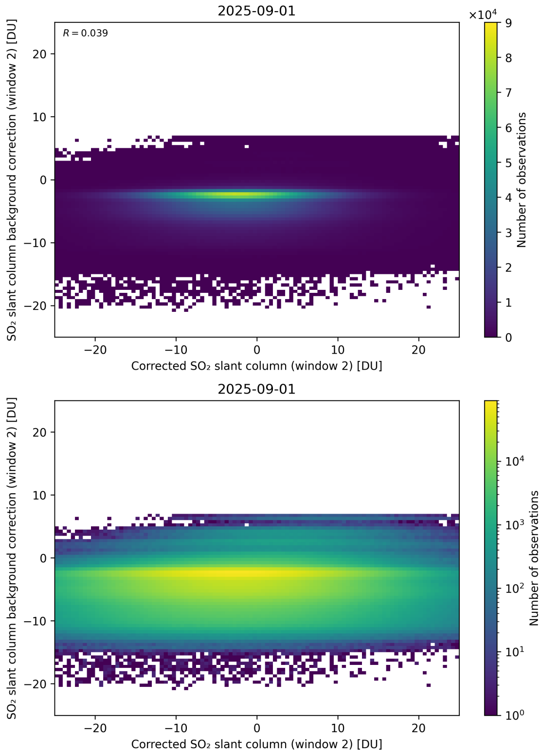
Figure 244: Scatter density plot of “Corrected SO 2 slant column (window 2)” against “SO 2 slant column background correction (window 2)” for 2025-08-31 to 2025-09-02.
