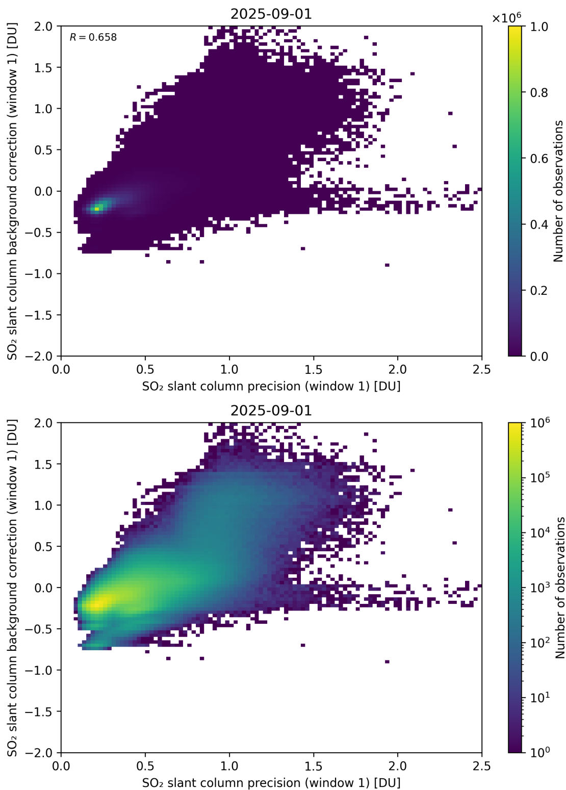
Figure 268: Scatter density plot of “SO 2 slant column precision (window 1)” against “SO 2 slant column background correction (window 1)” for 2025-08-31 to 2025-09-02.
