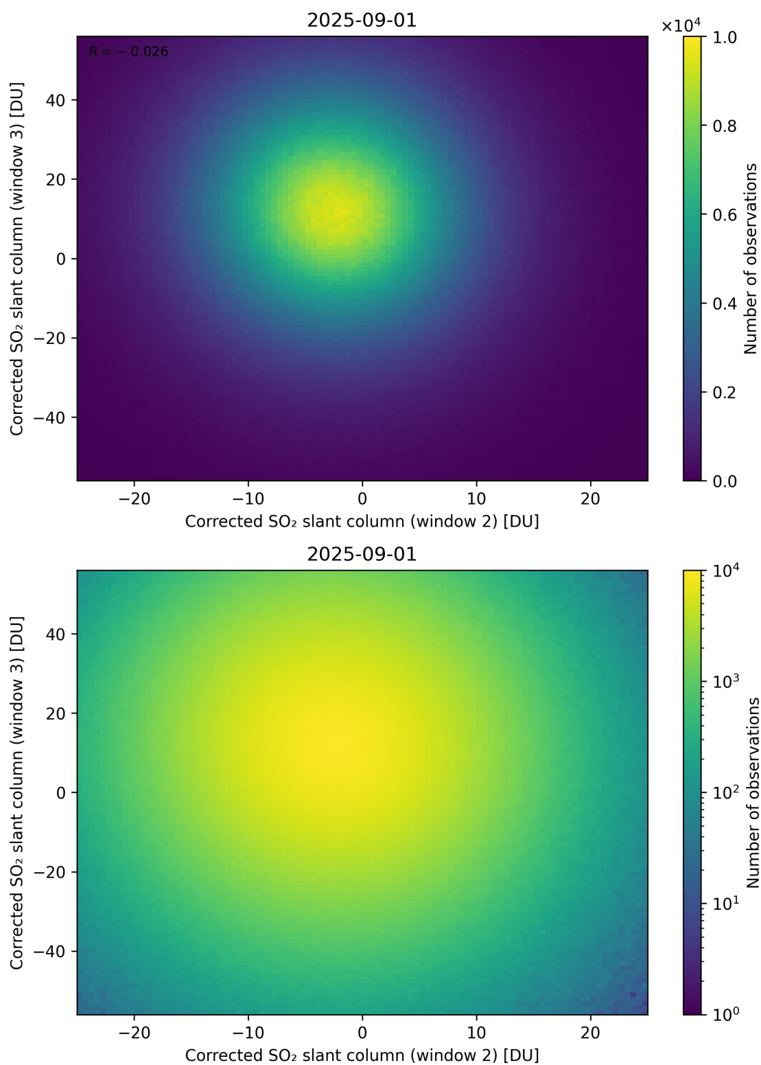
Figure 250: Scatter density plot of “Corrected SO 2 slant column (window 2)” against “Corrected SO 2 slant column (window 3)” for 2025-08-31 to 2025-09-02.
