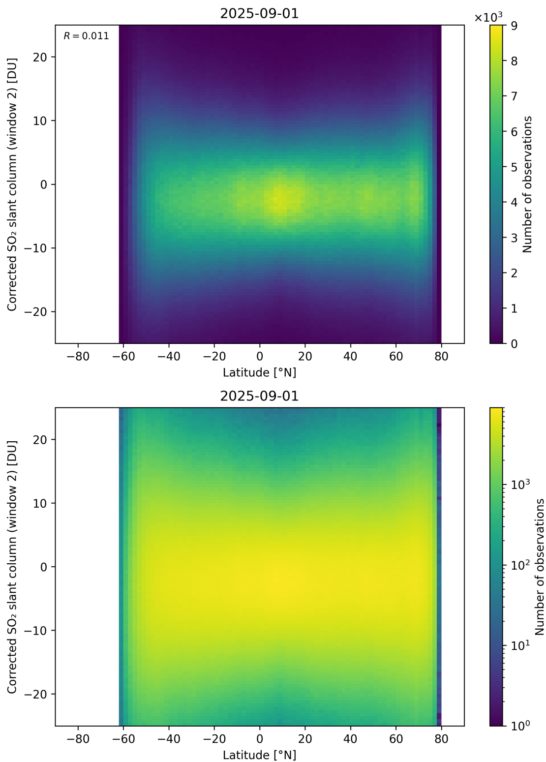
Figure 160: Scatter density plot of “Latitude” against “Corrected SO 2 slant column (window 2)” for 2025-08-31 to 2025-09-02.
