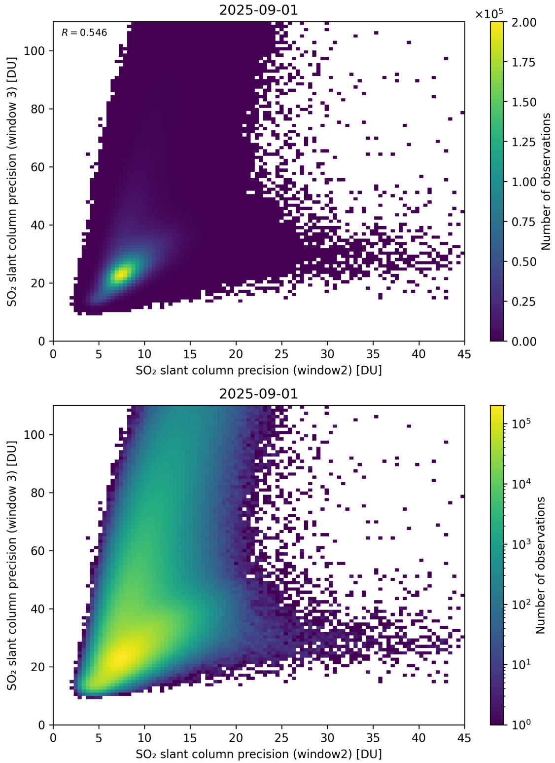
Figure 300: Scatter density plot of “SO 2 slant column precision (window2)” against “SO 2 slant column precision (window 3)” for 2025-08-31 to 2025-09-02.
