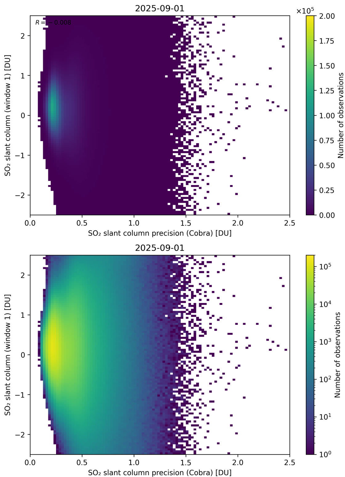
Figure 208: Scatter density plot of “SO 2 slant column precision (Cobra)” against “SO 2 slant column (window 1)” for 2025-08-31 to 2025-09-02.
