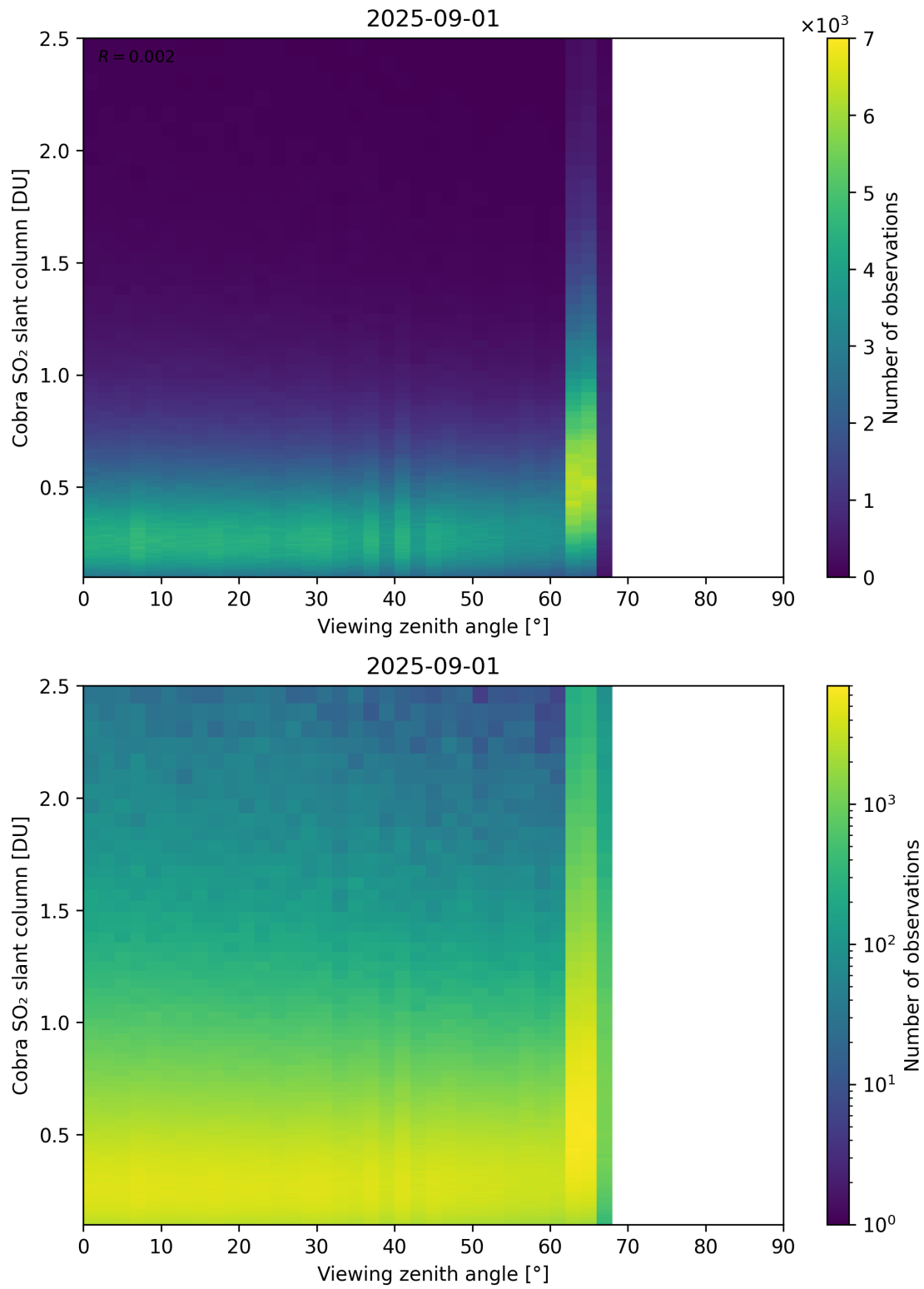
Figure 371: Scatter density plot of “Viewing zenith angle” against “Cobra SO 2 slant column” for 2025-08-31 to 2025-09-02.
