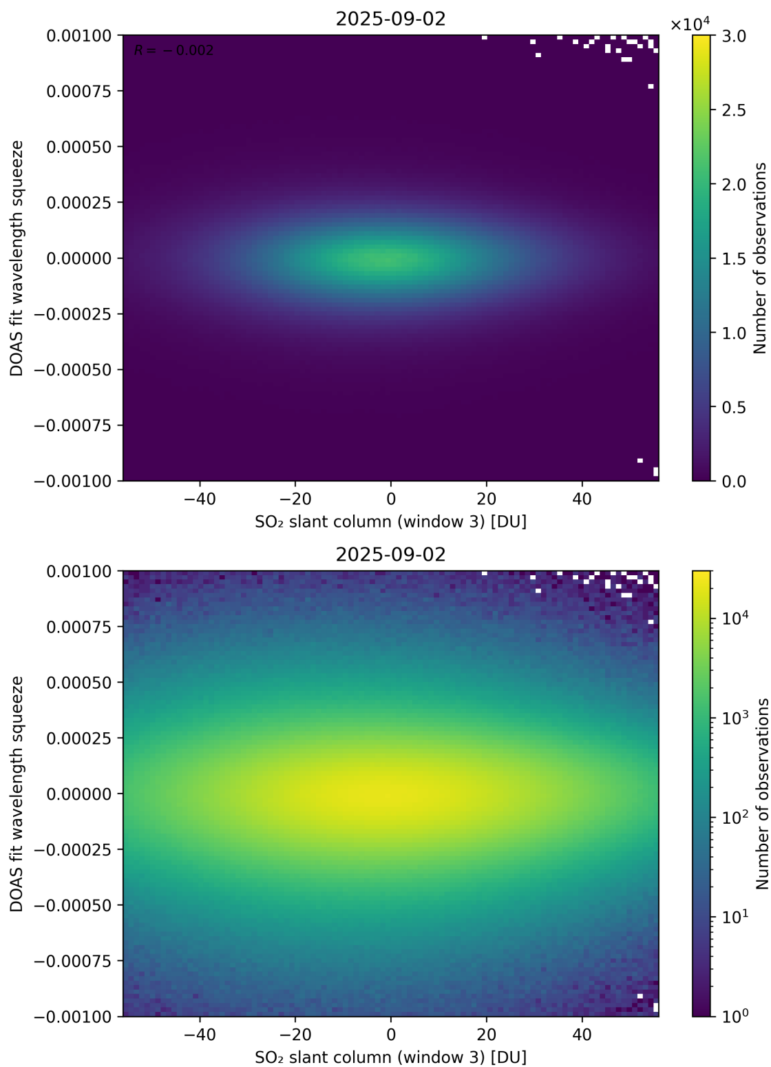
Figure 305: Scatter density plot of “SO 2 slant column (window 3)” against “DOAS fit wavelength squeeze” for 2025-09-01 to 2025-09-03.
