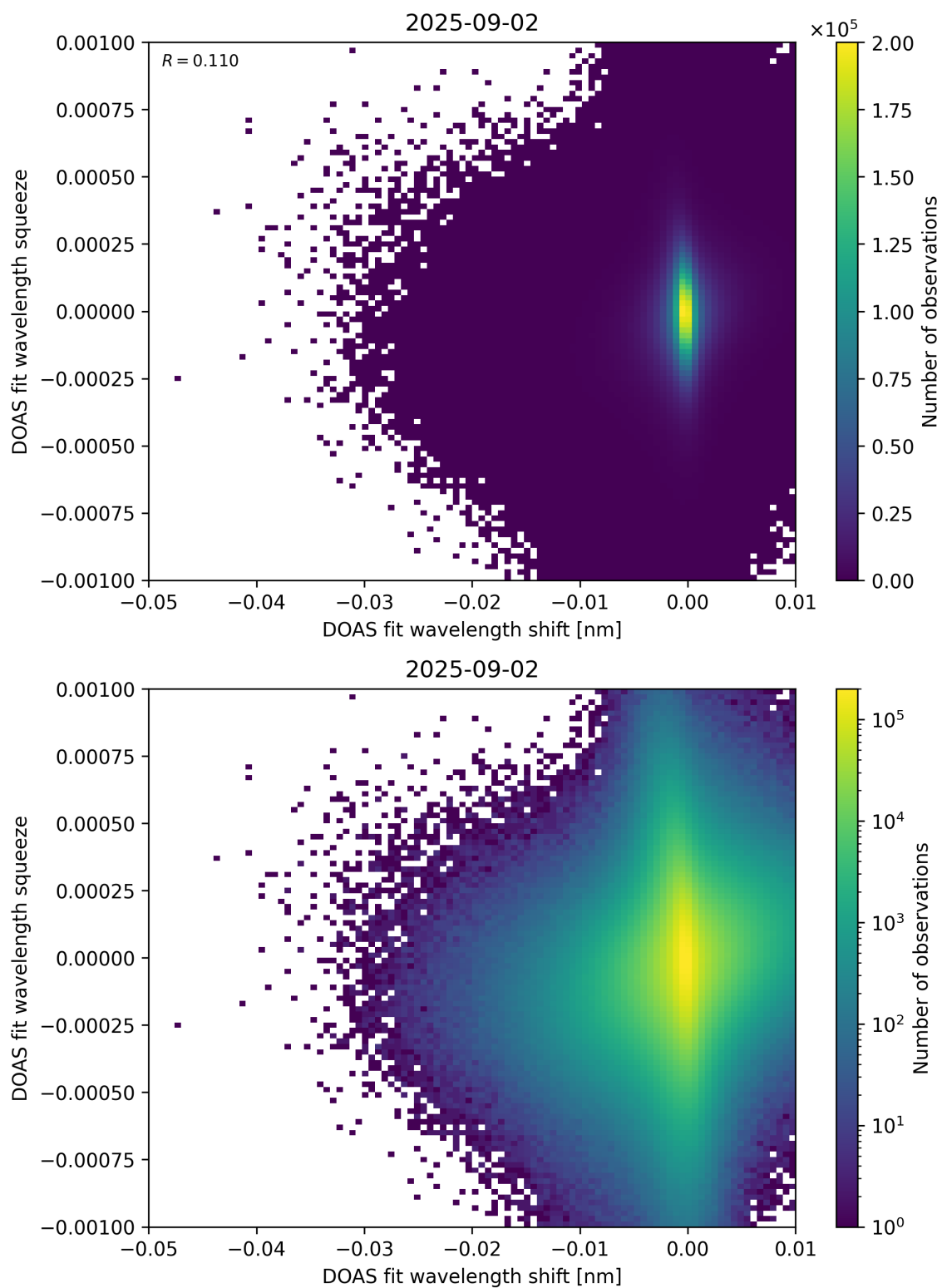
Figure 138: Scatter density plot of “DOAS fit wavelength shift” against “DOAS fit wavelength squeeze” for 2025-09-01 to 2025-09-03.
