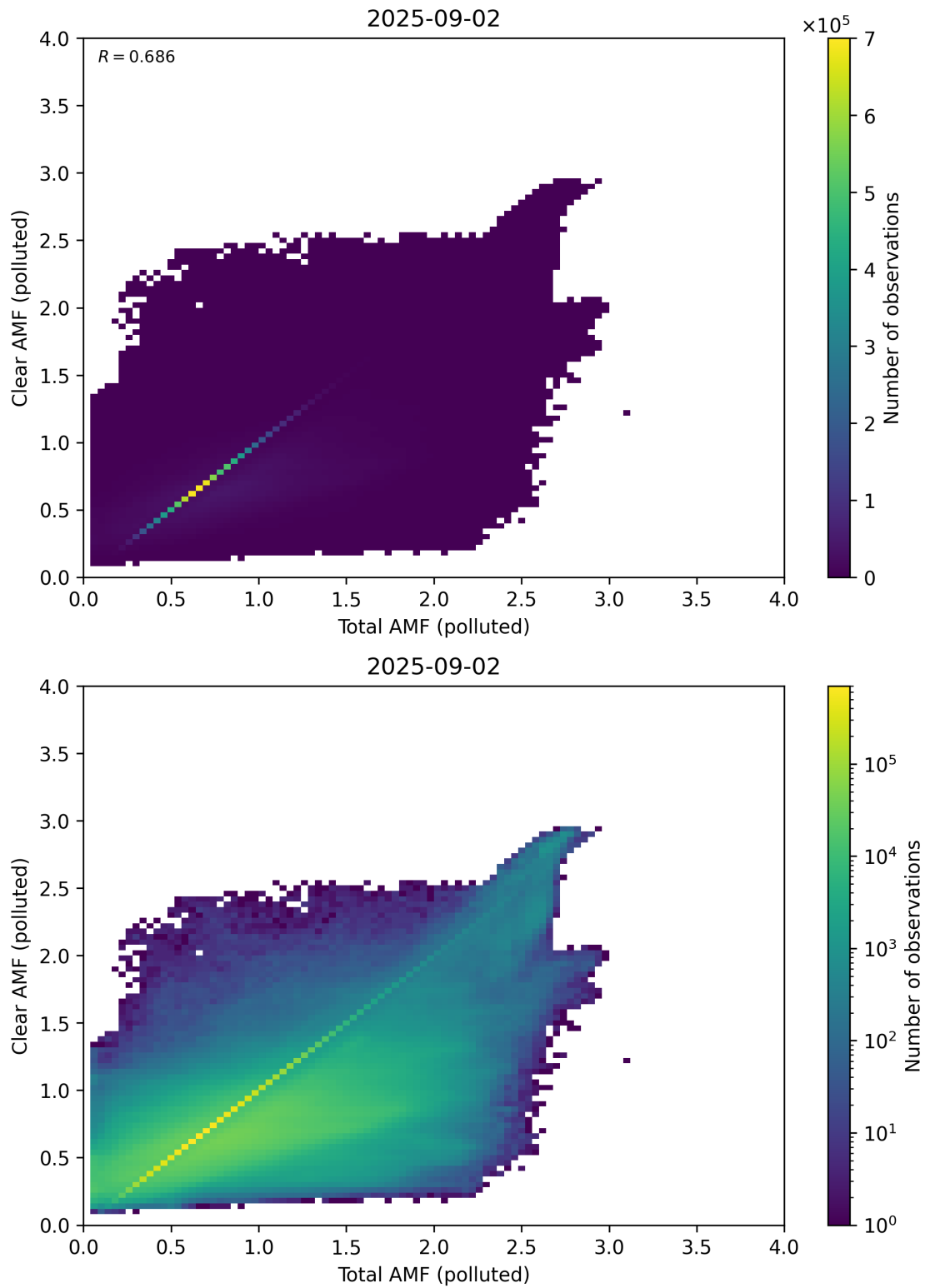
Figure 321: Scatter density plot of “Total AMF (polluted)” against “Clear AMF (polluted)” for 2025-09-01 to 2025-09-03.
