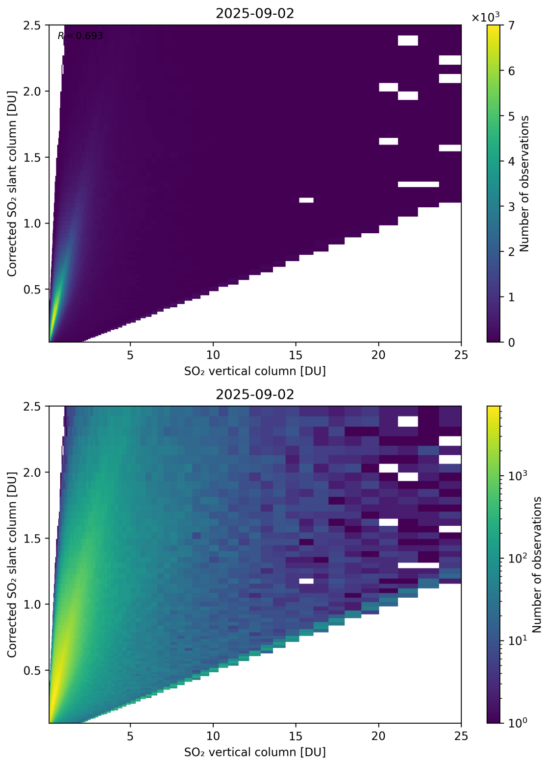
Figure 351: Scatter density plot of “SO 2 vertical column” against “Corrected SO 2 slant column” for 2025-09-01 to 2025-09-03.
