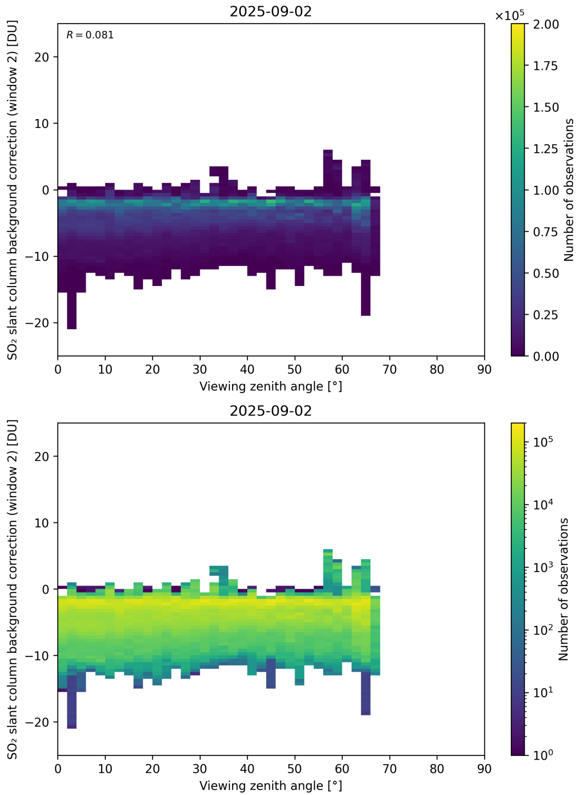
Figure 363: Scatter density plot of “Viewing zenith angle” against “SO 2 slant column background correction (window 2)” for 2025-09-01 to 2025-09-03.
