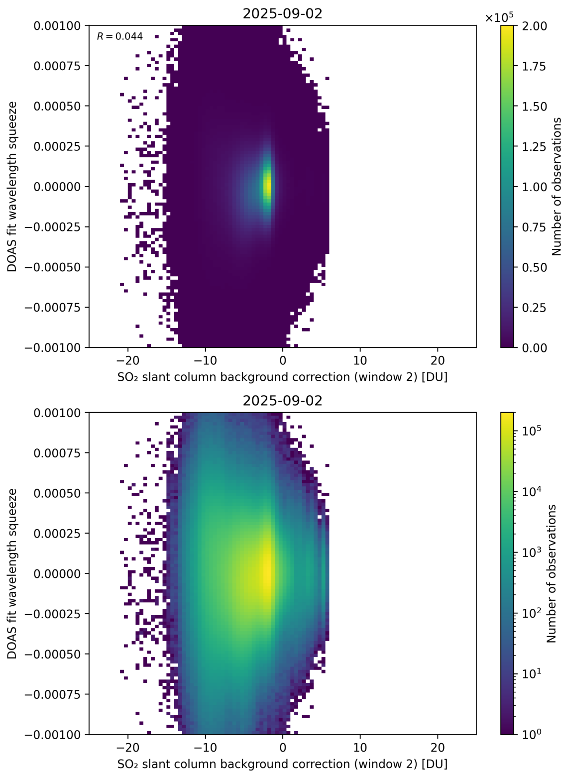
Figure 124: Scatter density plot of “SO 2 slant column background correction (window 2)” against “DOAS fit wavelength squeeze” for 2025-09-01 to 2025-09-03.
