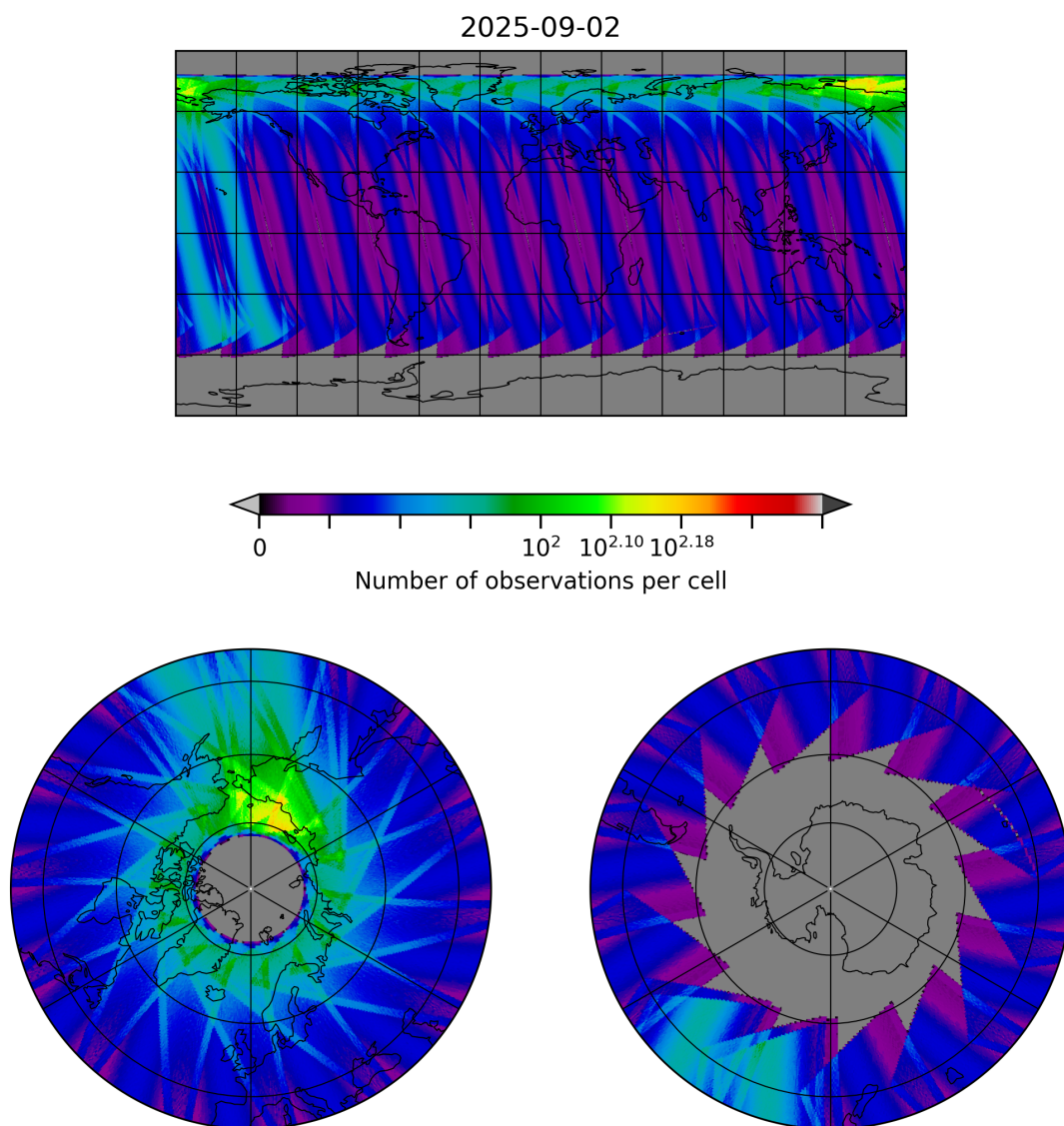
Figure 30: Map of the number of observations for 2025-09-01 to 2025-09-03
