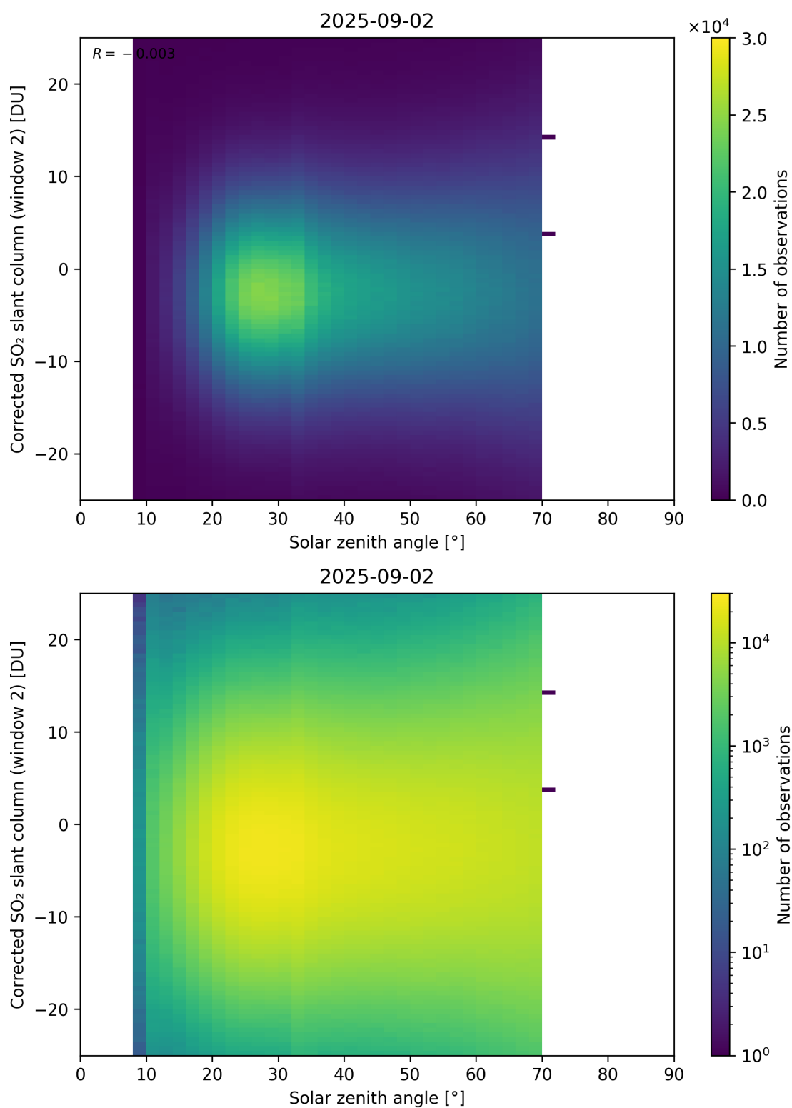
Figure 182: Scatter density plot of “Solar zenith angle” against “Corrected SO 2 slant column (window 2)” for 2025-09-01 to 2025-09-03.
