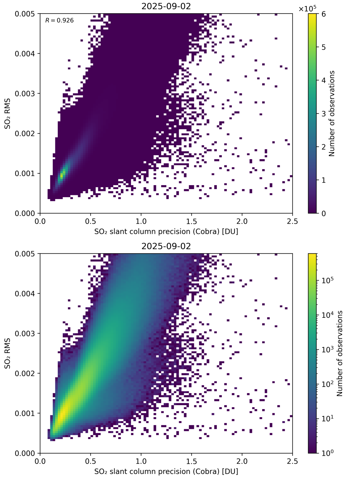
Figure 204: Scatter density plot of “SO 2 slant column precision (Cobra)” against “SO 2 RMS” for 2025-09-01 to 2025-09-03.
