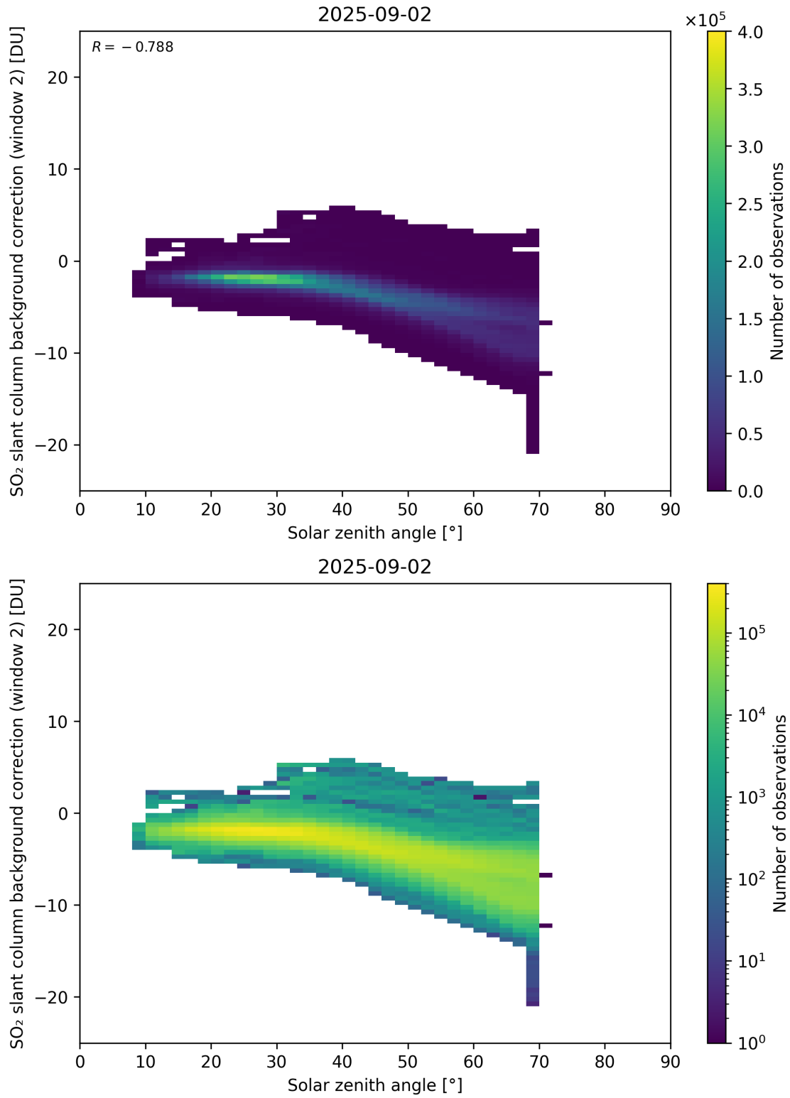
Figure 172: Scatter density plot of “Solar zenith angle” against “SO 2 slant column background correction (window 2)” for 2025-09-01 to 2025-09-03.
