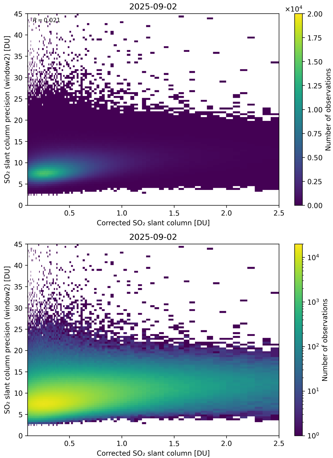
Figure 239: Scatter density plot of “Corrected SO 2 slant column” against “SO 2 slant column precision (window2)” for 2025-09-01 to 2025-09-03.
