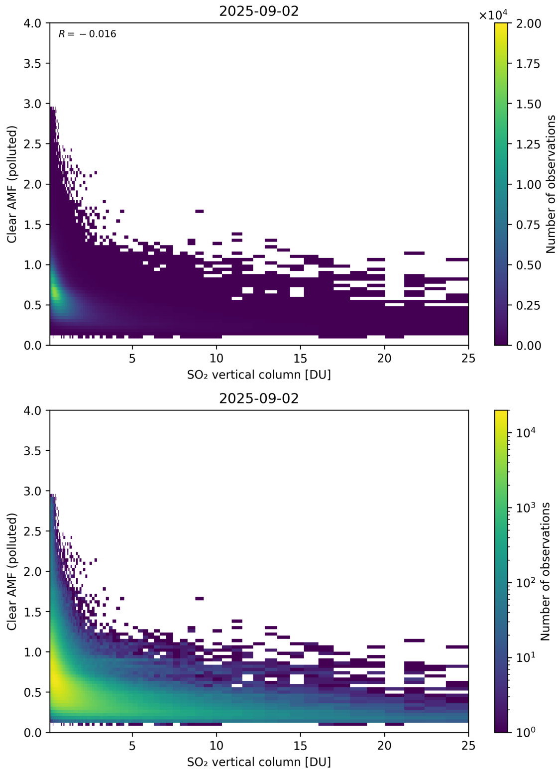
Figure 348: Scatter density plot of “SO 2 vertical column” against “Clear AMF (polluted)” for 2025-09-01 to 2025-09-03.
