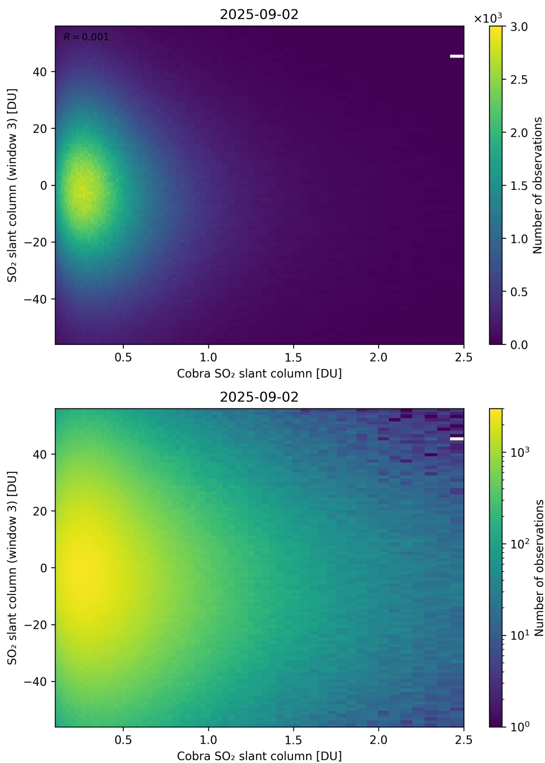
Figure 222: Scatter density plot of “Cobra SO 2 slant column” against “SO 2 slant column (window 3)” for 2025-09-01 to 2025-09-03.
