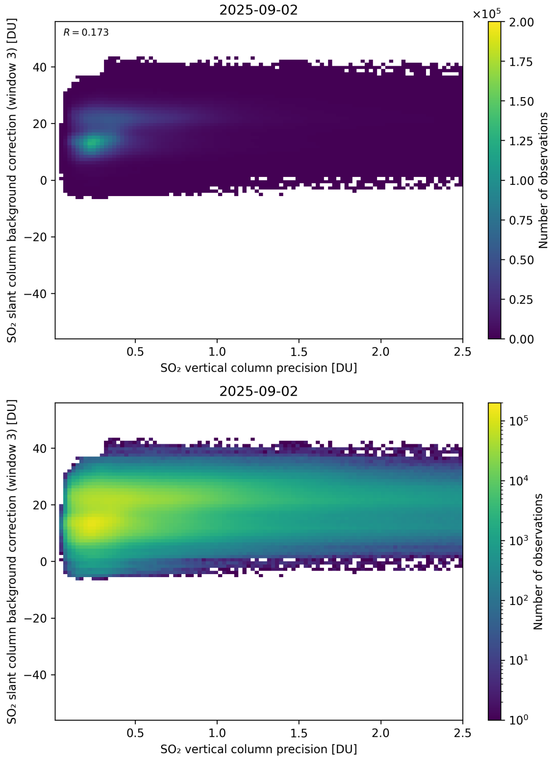
Figure 331: Scatter density plot of “SO 2 vertical column precision” against “SO 2 slant column background correction (window 3)” for 2025-09-01 to 2025-09-03.
