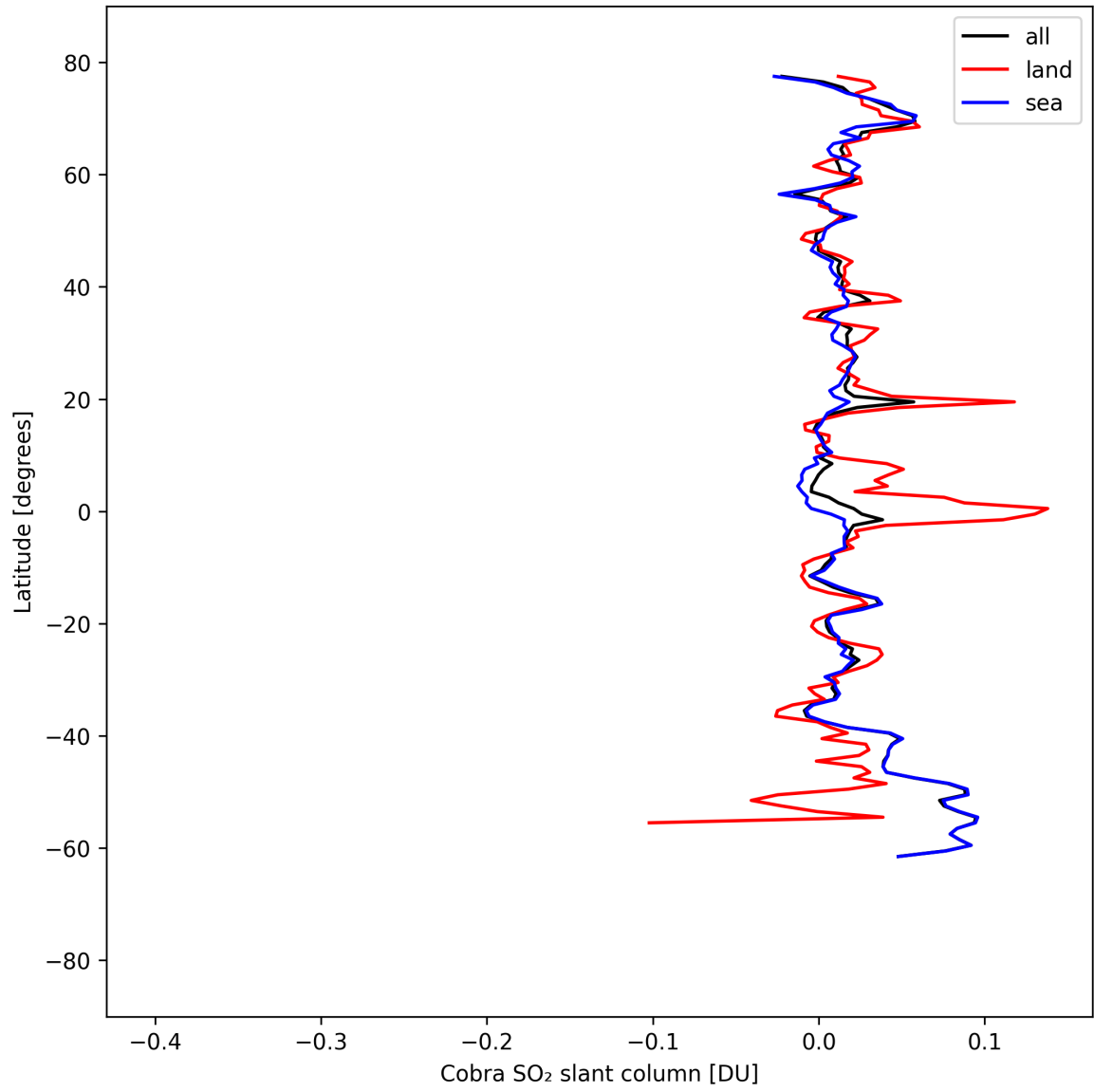
Figure 35: Zonal average of “Cobra SO 2 slant column” for 2025-09-01 to 2025-09-03.
