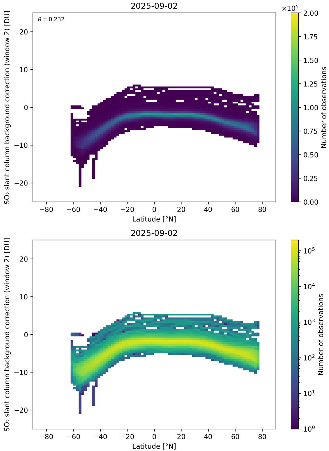
Figure 151: Scatter density plot of “Latitude” against “SO 2 slant column background correction (window 2)” for 2025-09-01 to 2025-09-03.
