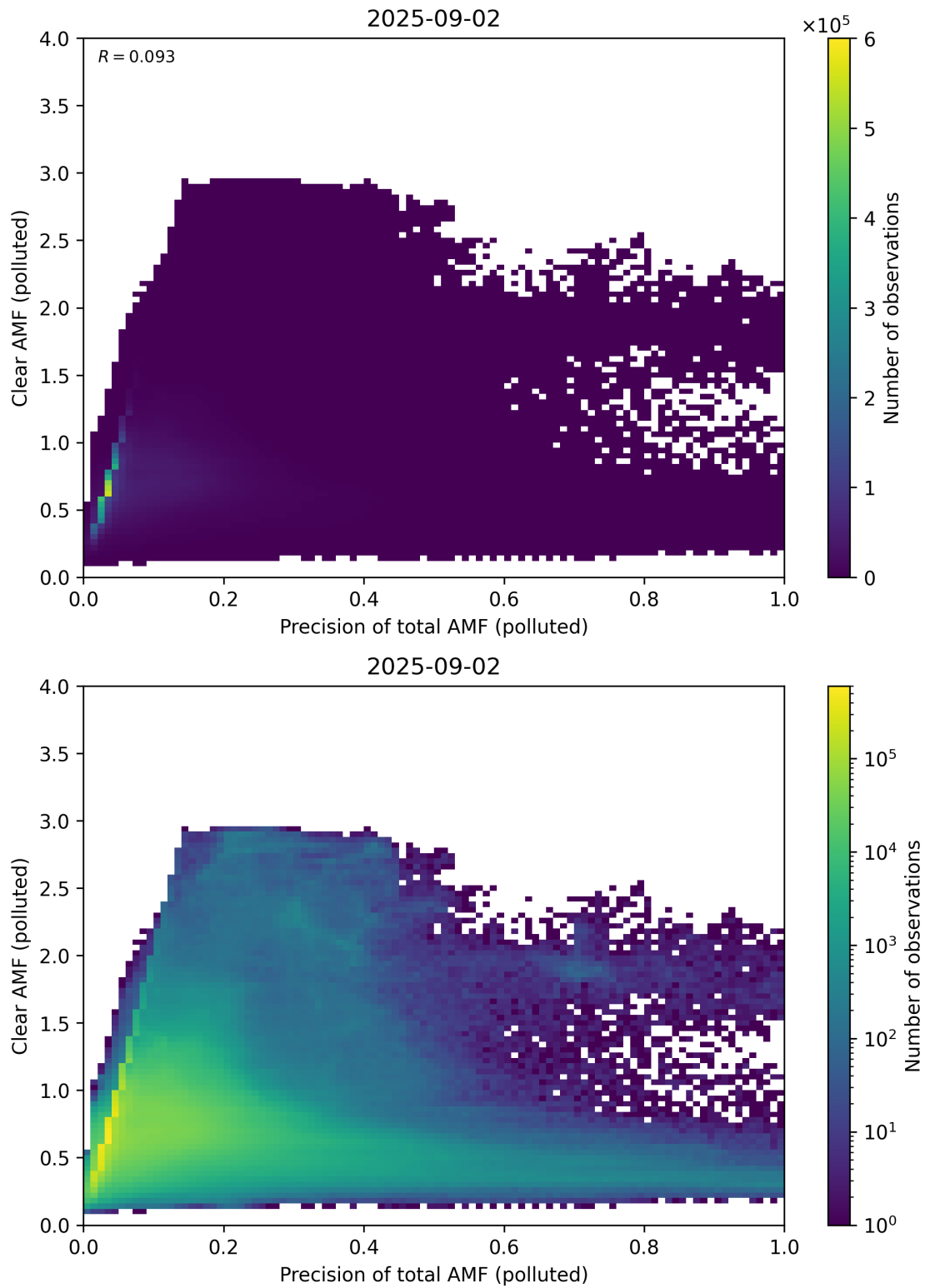
Figure 320: Scatter density plot of “Precision of total AMF (polluted)” against “Clear AMF (polluted)” for 2025-09-01 to 2025-09-03.
