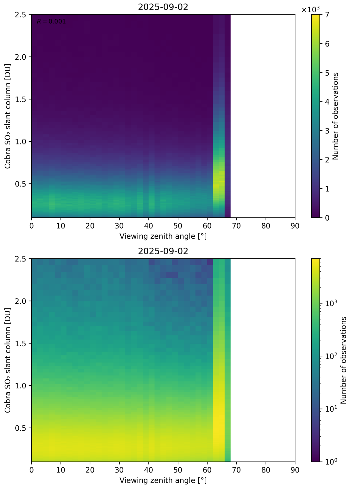
Figure 371: Scatter density plot of “Viewing zenith angle” against “Cobra SO 2 slant column” for 2025-09-01 to 2025-09-03.
