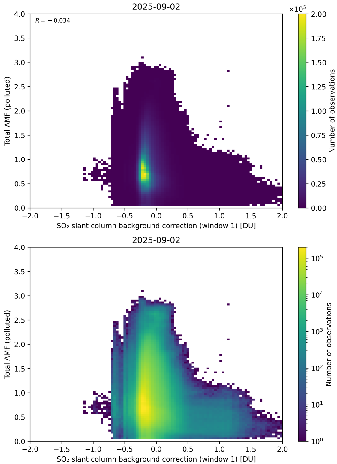
Figure 120: Scatter density plot of “SO 2 slant column background correction (window 1)” against “Total AMF (polluted)” for 2025-09-01 to 2025-09-03.
