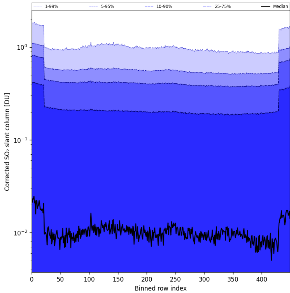
Figure 86: Along track statistics of “Corrected SO 2 slant column” for 2025-09-01 to 2025-09-03
