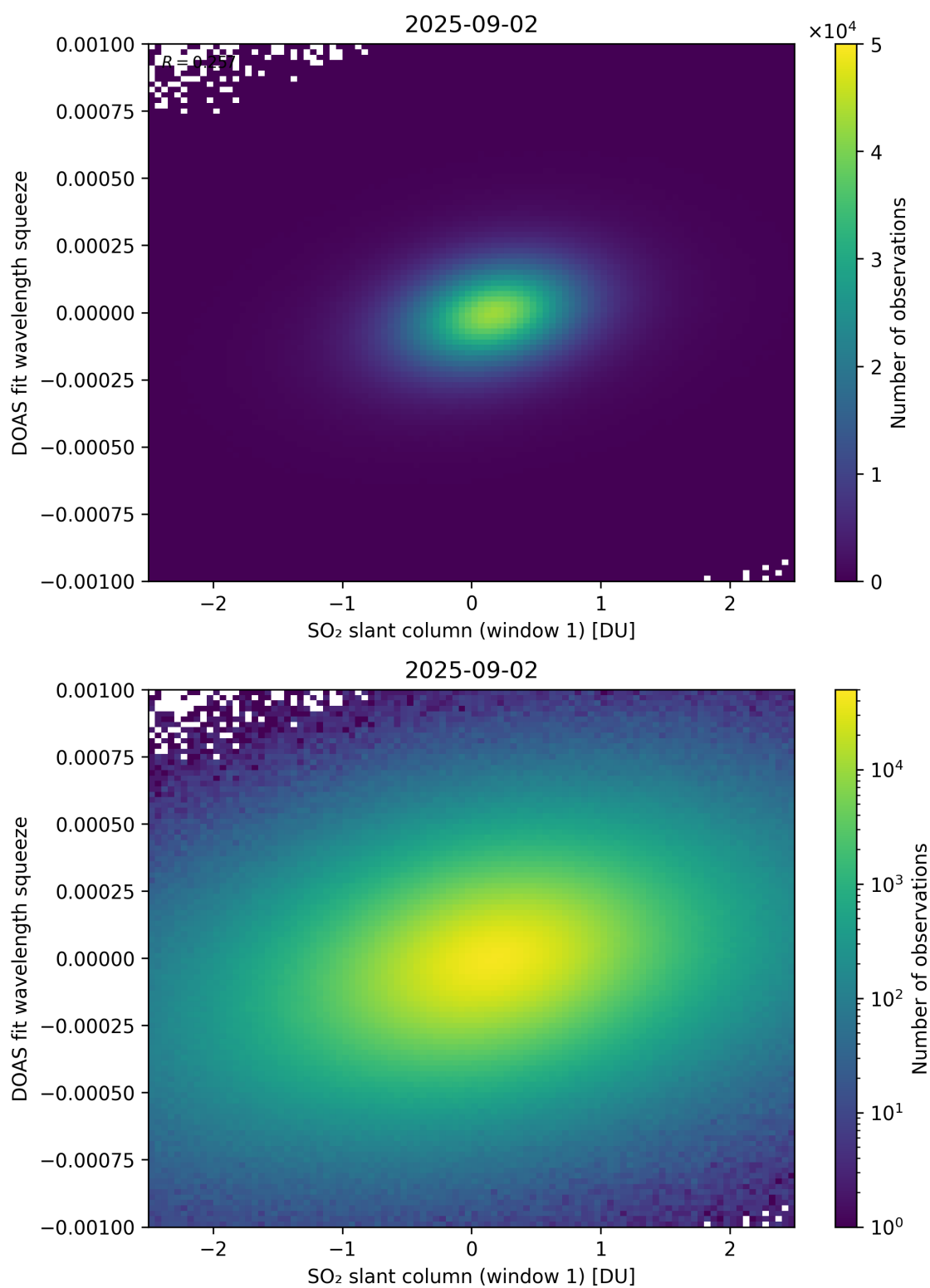
Figure 266: Scatter density plot of “SO 2 slant column (window 1)” against “DOAS fit wavelength squeeze” for 2025-09-01 to 2025-09-03.
