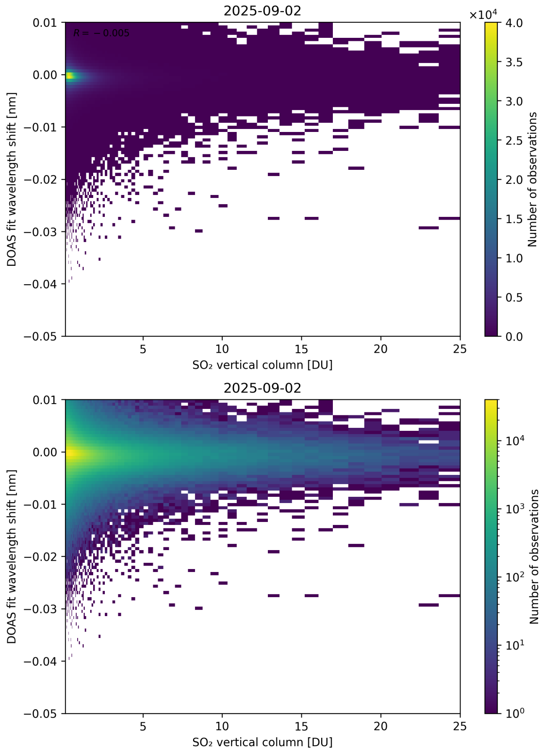
Figure 326: Scatter density plot of “SO 2 vertical column” against “DOAS fit wavelength shift” for 2025-09-01 to 2025-09-03.
