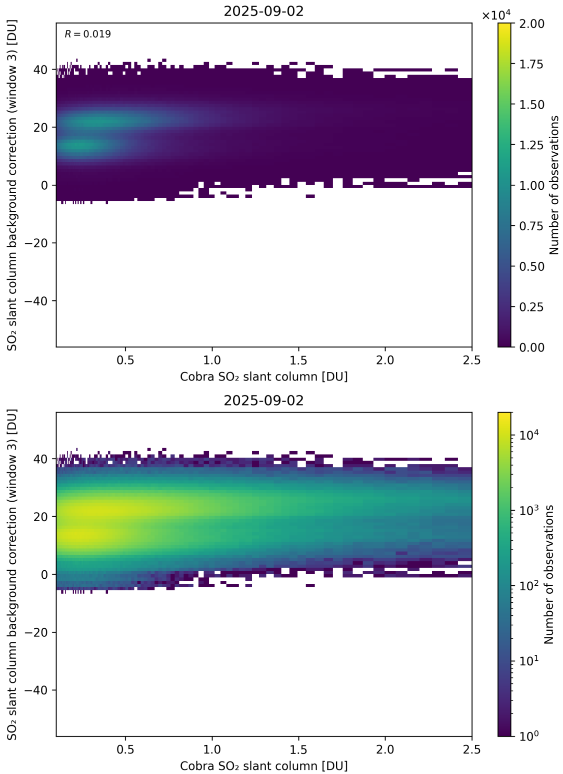
Figure 195: Scatter density plot of “Cobra SO 2 slant column” against “SO 2 slant column background correction (window 3)” for 2025-09-01 to 2025-09-03.
