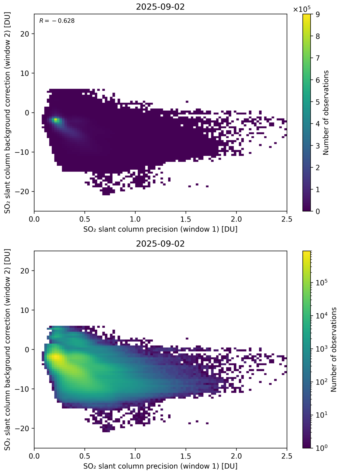
Figure 269: Scatter density plot of “SO 2 slant column precision (window 1)” against “SO 2 slant column background correction (window 2)” for 2025-09-01 to 2025-09-03.
