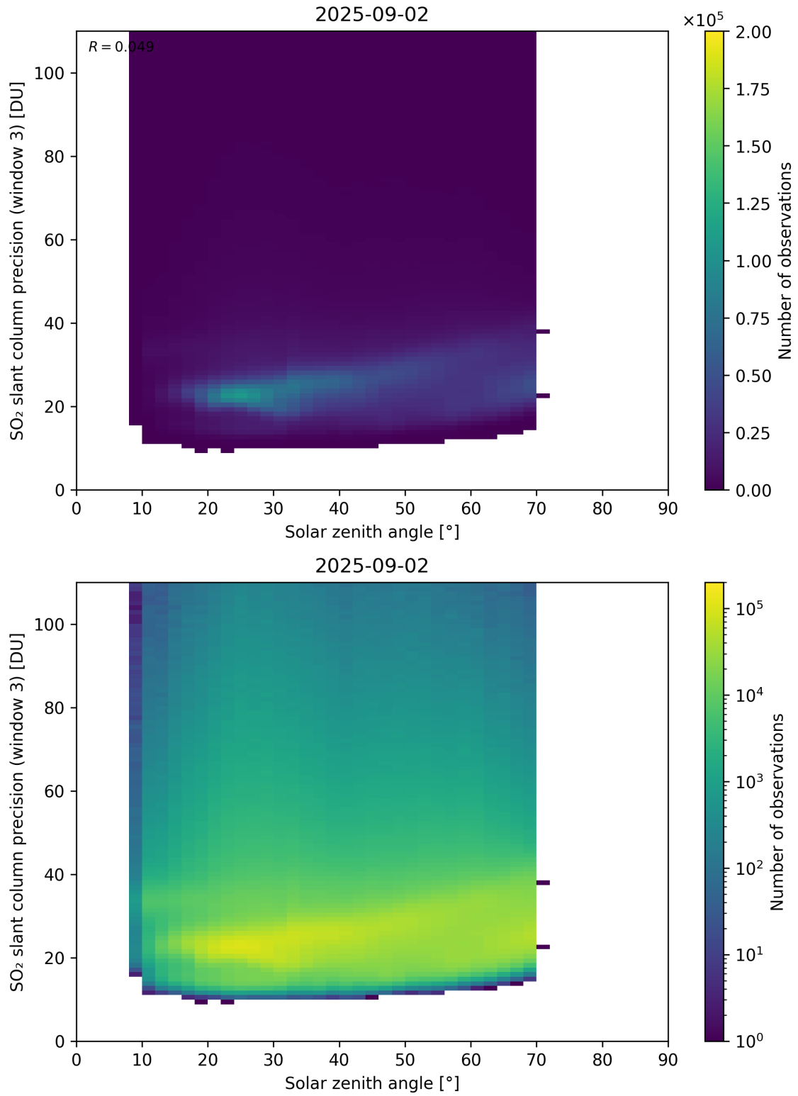
Figure 188: Scatter density plot of “Solar zenith angle” against “SO 2 slant column precision (window 3)” for 2025-09-01 to 2025-09-03.
