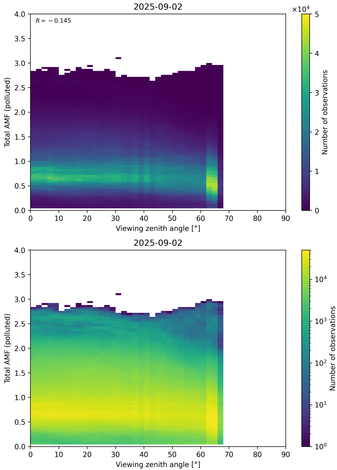
Figure 381: Scatter density plot of “Viewing zenith angle” against “Total AMF (polluted)” for 2025-09-01 to 2025-09-03.
