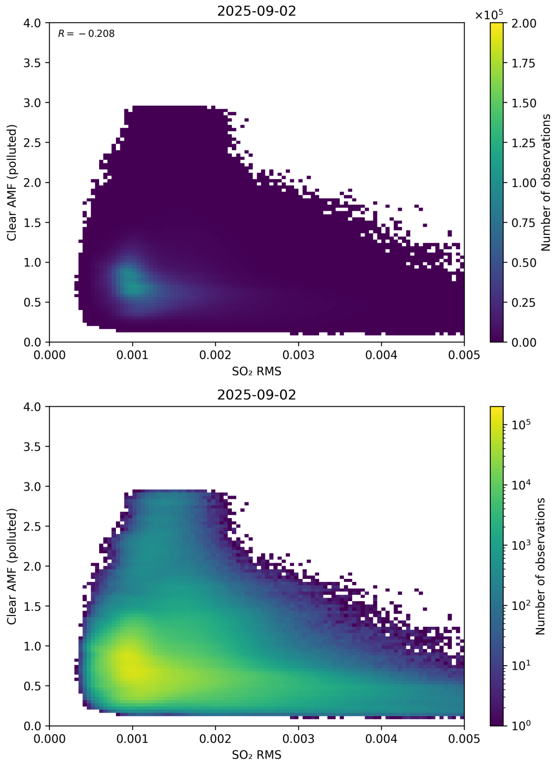
Figure 147: Scatter density plot of “SO 2 RMS” against “Clear AMF (polluted)” for 2025-09-01 to 2025-09-03.
