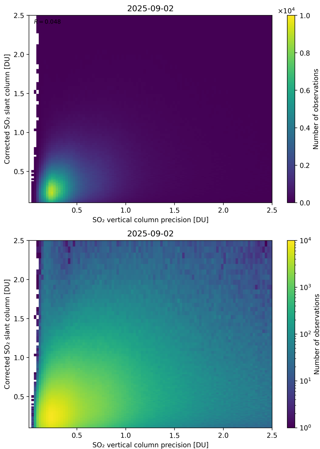
Figure 338: Scatter density plot of “SO 2 vertical column precision” against “Corrected SO 2 slant column” for 2025-09-01 to 2025-09-03.
