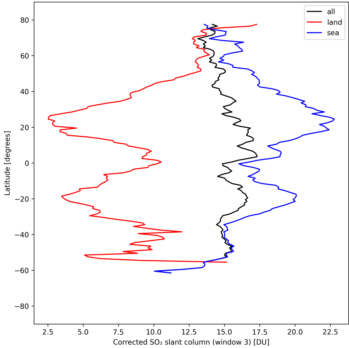
Figure 47: Zonal average of “Corrected SO 2 slant column (window 3)” for 2025-09-01 to 2025-09-03.
