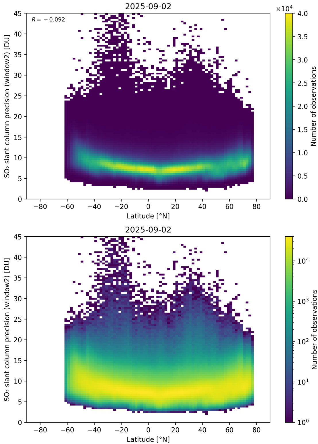
Figure 164: Scatter density plot of “Latitude” against “SO 2 slant column precision (window2)” for 2025-09-01 to 2025-09-03.
