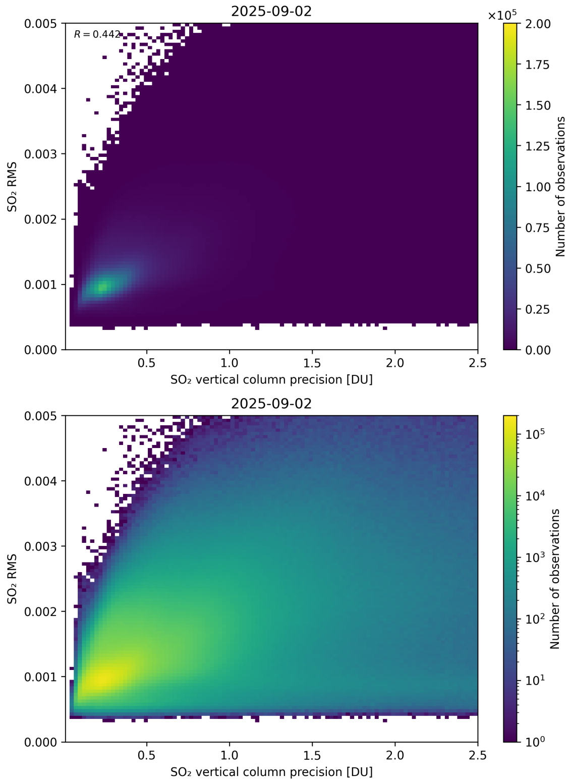
Figure 334: Scatter density plot of “SO 2 vertical column precision” against “SO 2 RMS” for 2025-09-01 to 2025-09-03.
