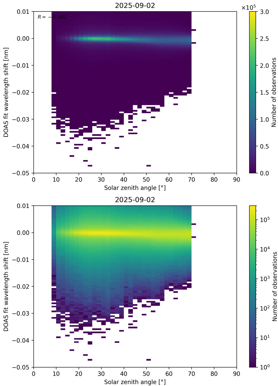
Figure 174: Scatter density plot of “Solar zenith angle” against “DOAS fit wavelength shift” for 2025-09-01 to 2025-09-03.
