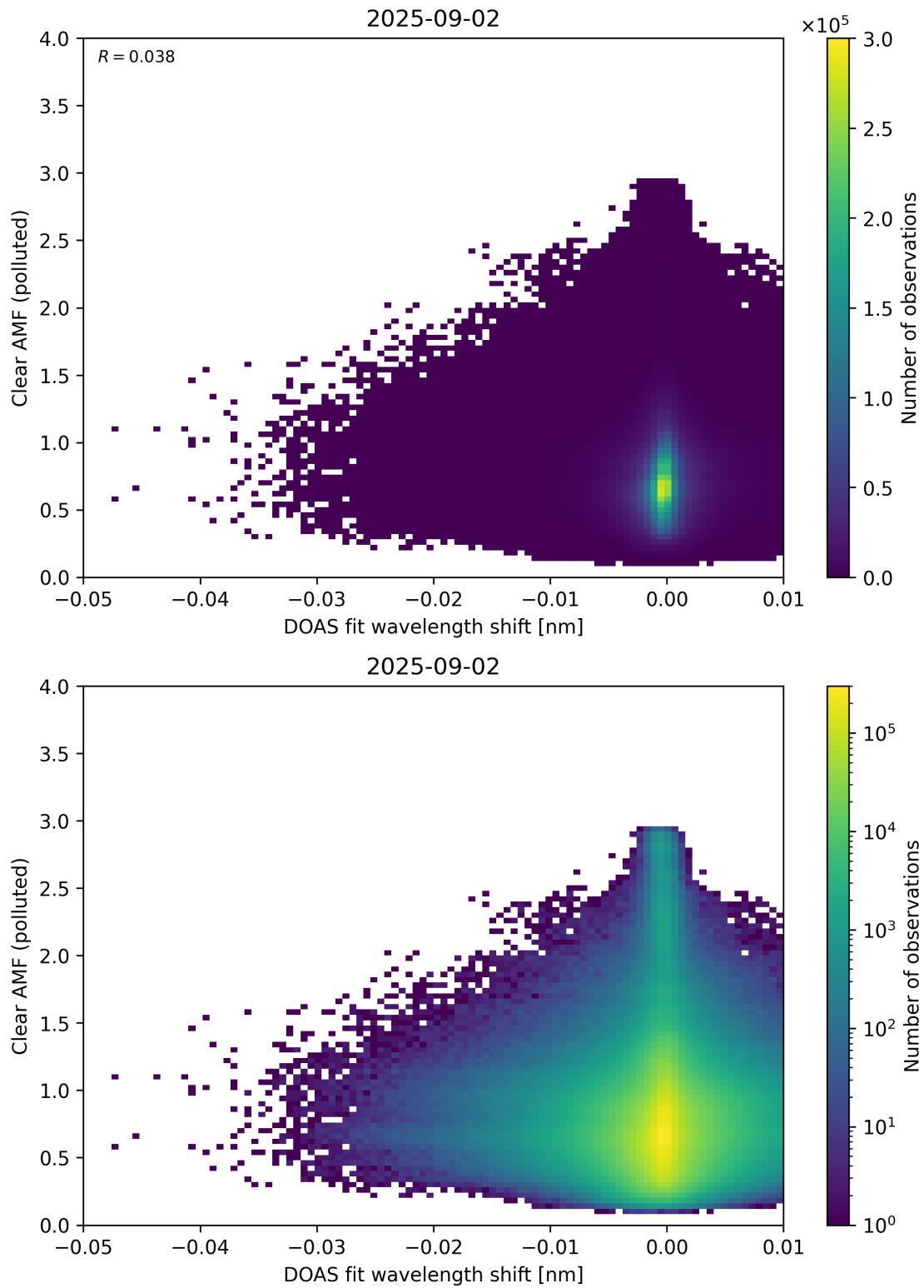
Figure 140: Scatter density plot of “DOAS fit wavelength shift” against “Clear AMF (polluted)” for 2025-09-01 to 2025-09-03.
