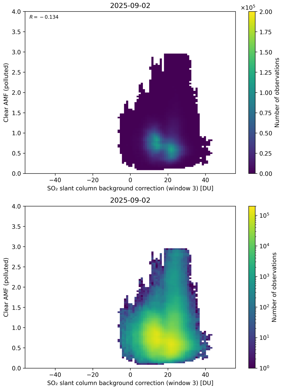
Figure 135: Scatter density plot of “SO 2 slant column background correction (window 3)” against “Clear AMF (polluted)” for 2025-09-01 to 2025-09-03.
