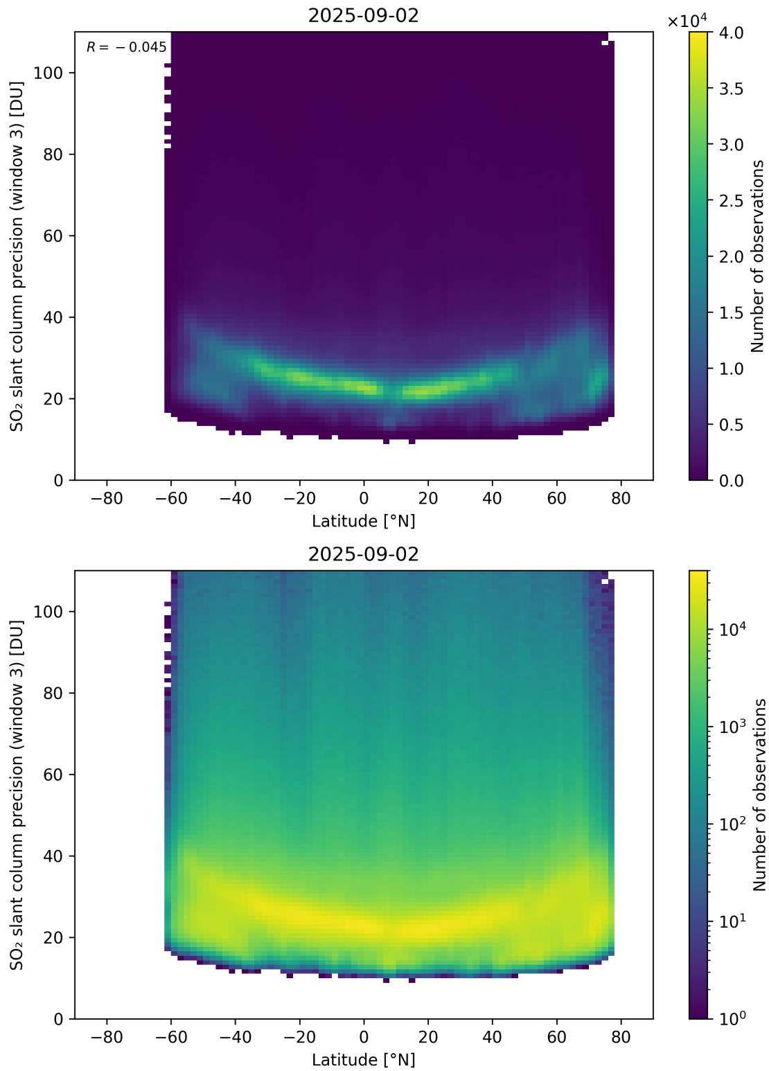
Figure 166: Scatter density plot of “Latitude” against “SO 2 slant column precision (window 3)” for 2025-09-01 to 2025-09-03.
