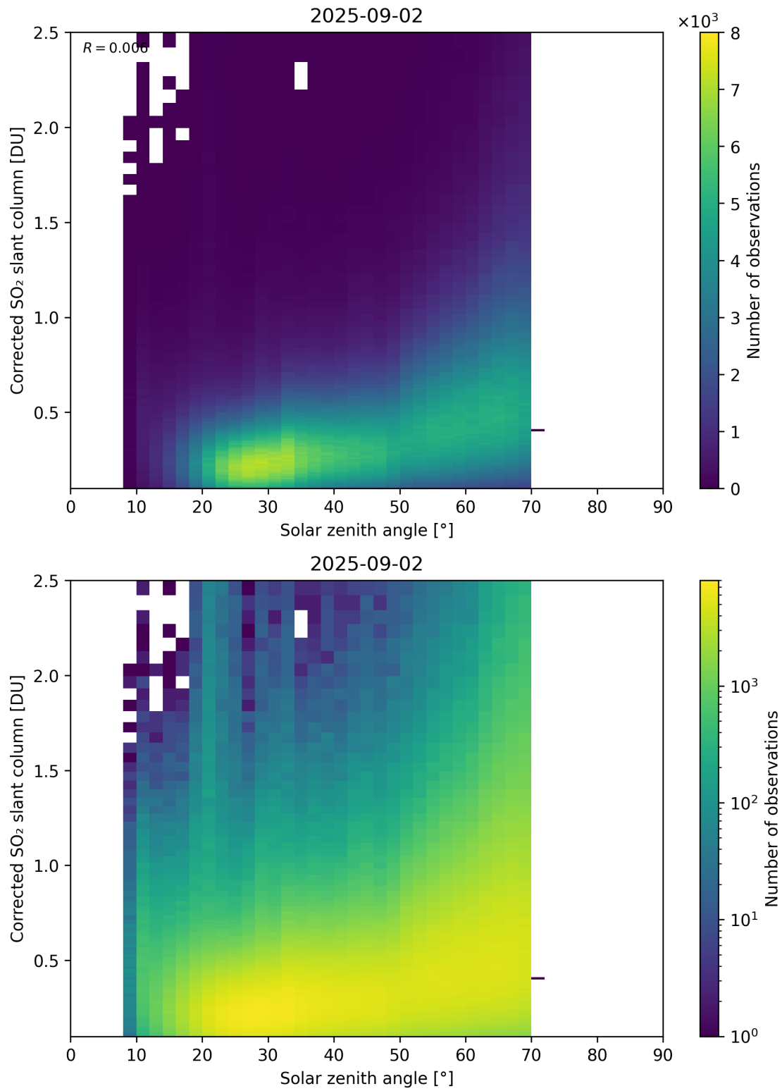
Figure 181: Scatter density plot of “Solar zenith angle” against “Corrected SO 2 slant column” for 2025-09-01 to 2025-09-03.
