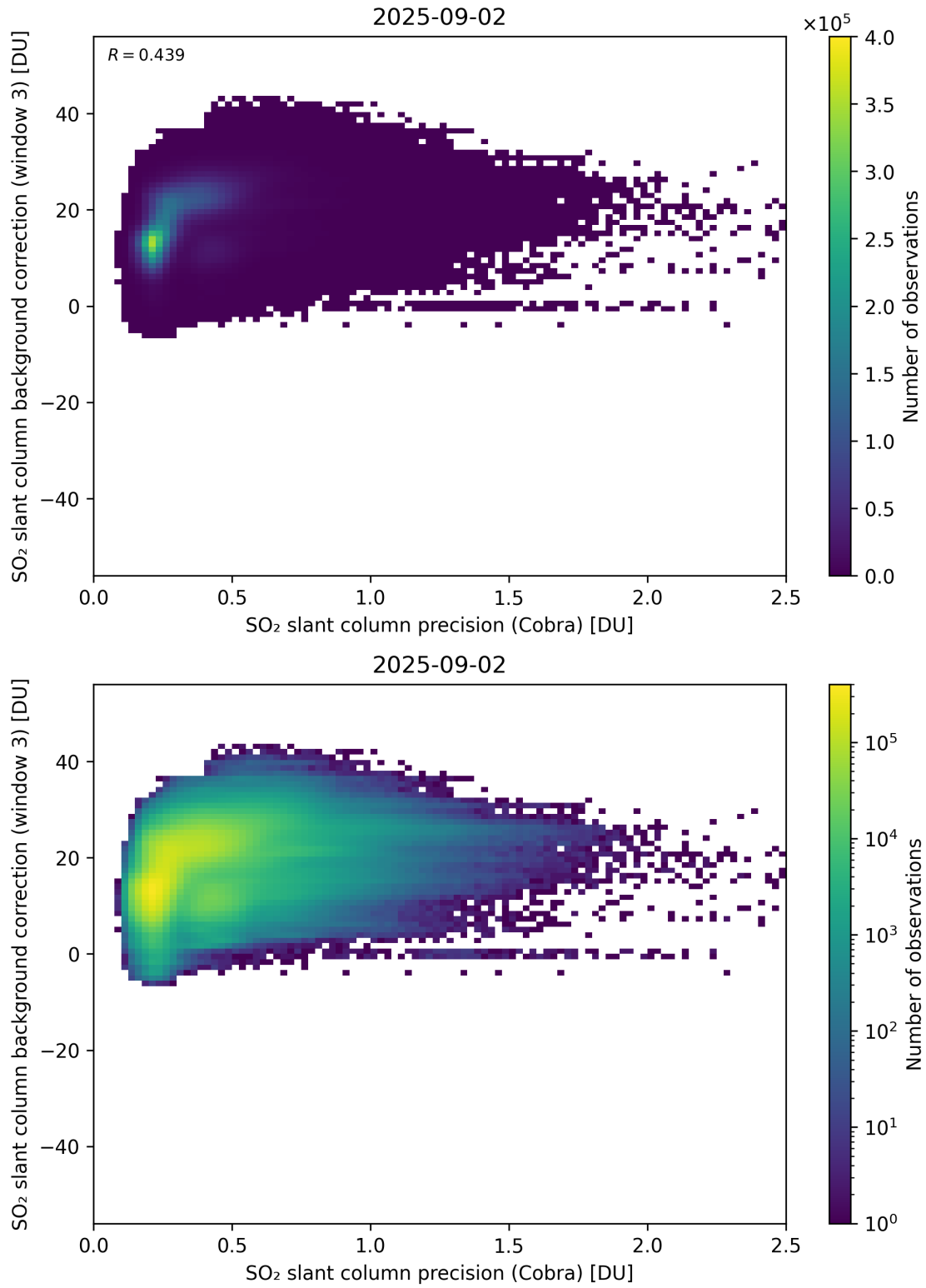
Figure 201: Scatter density plot of “SO 2 slant column precision (Cobra)” against “SO 2 slant column background correction (window 3)” for 2025-09-01 to 2025-09-03.
