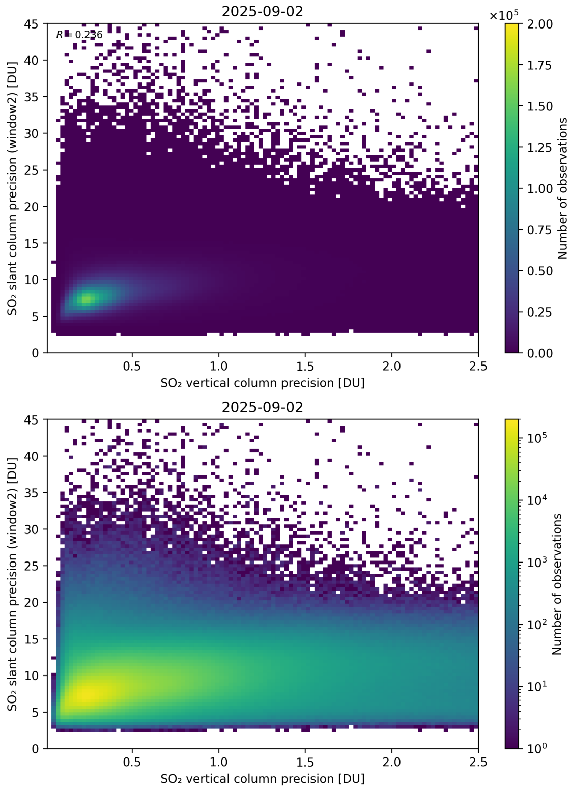
Figure 343: Scatter density plot of “SO 2 vertical column precision” against “SO 2 slant column precision (window2)” for 2025-09-01 to 2025-09-03.
