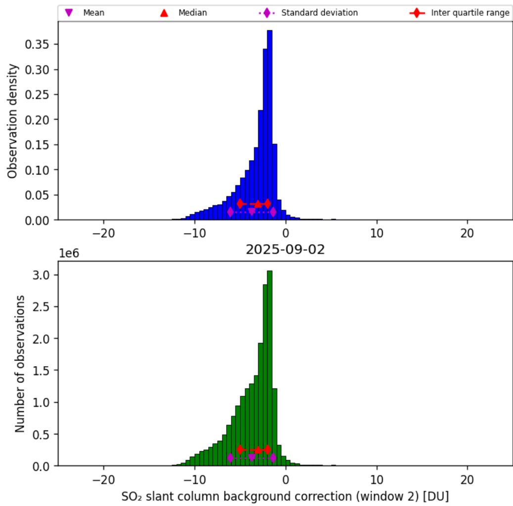
Figure 70: Histogram of “SO 2 slant column background correction (window 2)” for 2025-09-01 to 2025-09-03
