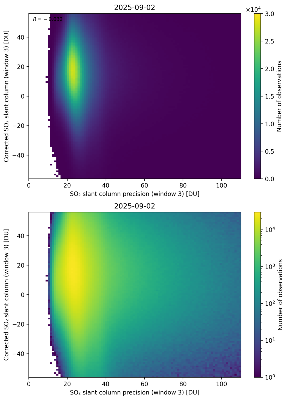
Figure 312: Scatter density plot of “SO 2 slant column precision (window 3)” against “Corrected SO 2 slant column (window 3)” for 2025-09-01 to 2025-09-03.
