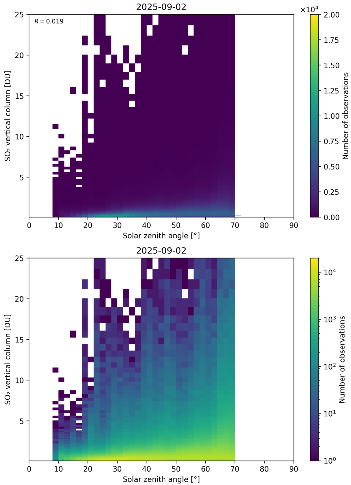
Figure 191: Scatter density plot of “Solar zenith angle” against “SO 2 vertical column” for 2025-09-01 to 2025-09-03.
