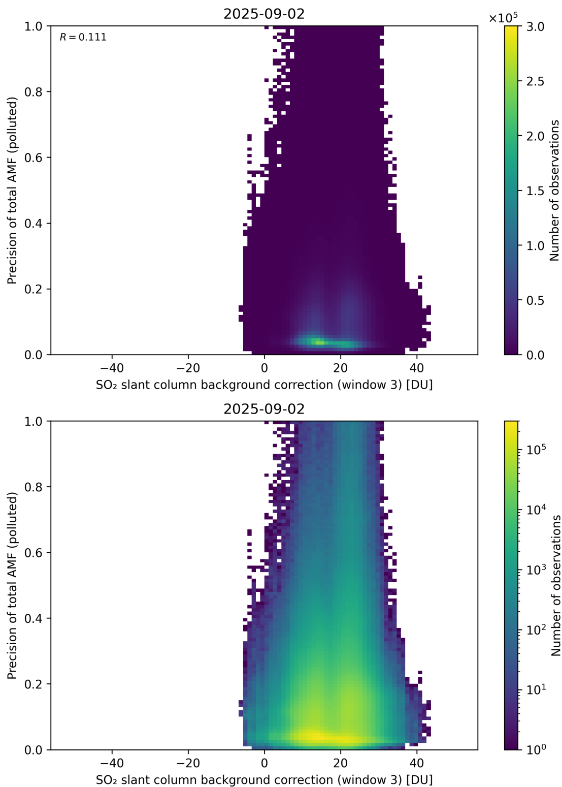
Figure 137: Scatter density plot of “SO 2 slant column background correction (window 3)” against “Precision of total AMF (polluted)” for 2025-09-01 to 2025-09-03.
