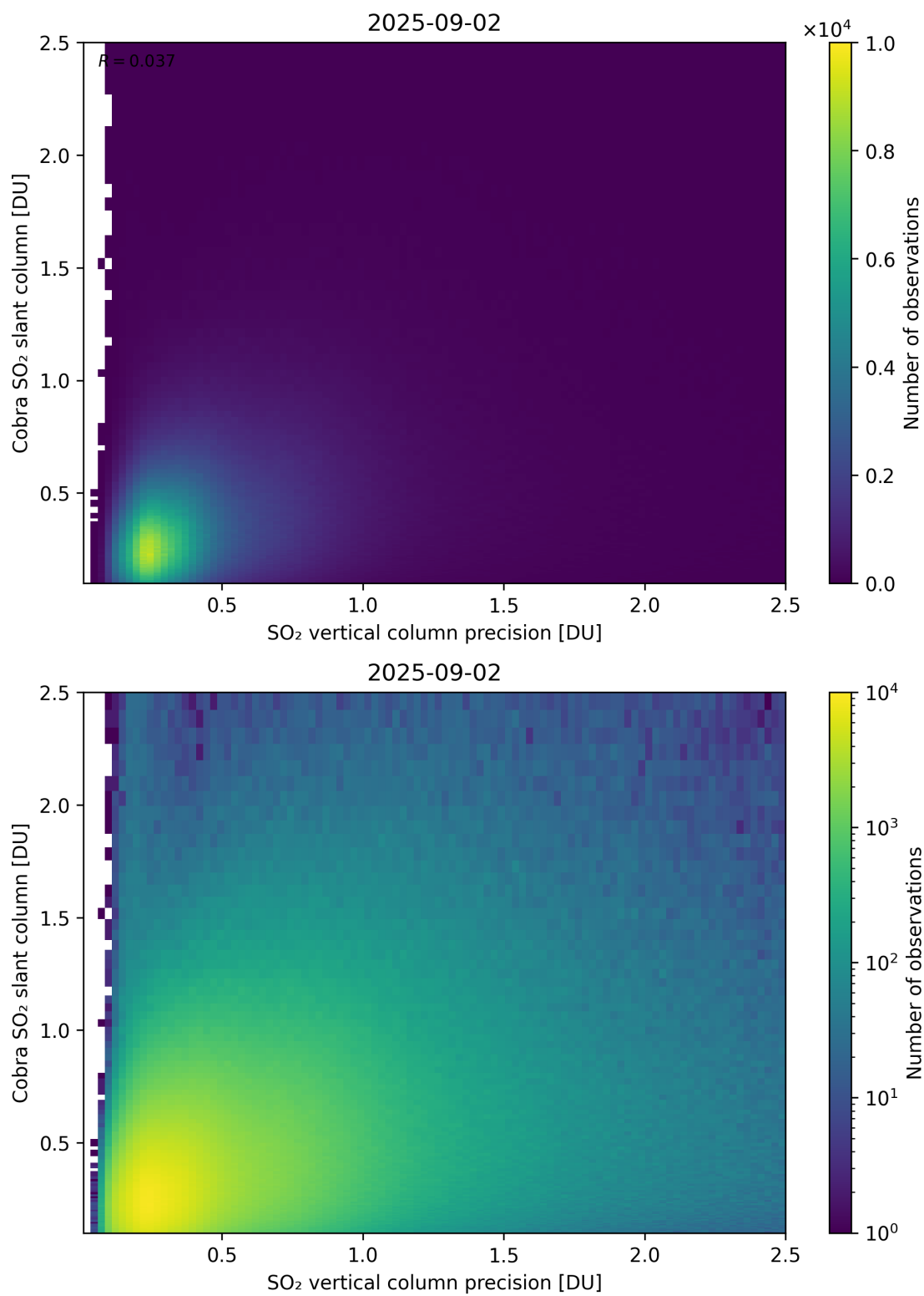
Figure 336: Scatter density plot of “SO 2 vertical column precision” against “Cobra SO 2 slant column” for 2025-09-01 to 2025-09-03.
