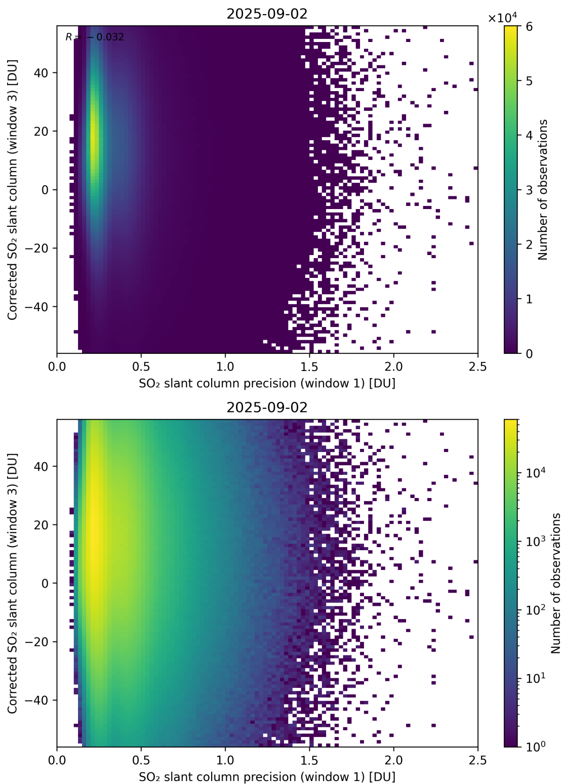
Figure 276: Scatter density plot of “SO 2 slant column precision (window 1)” against “Corrected SO 2 slant column (window 3)” for 2025-09-01 to 2025-09-03.
