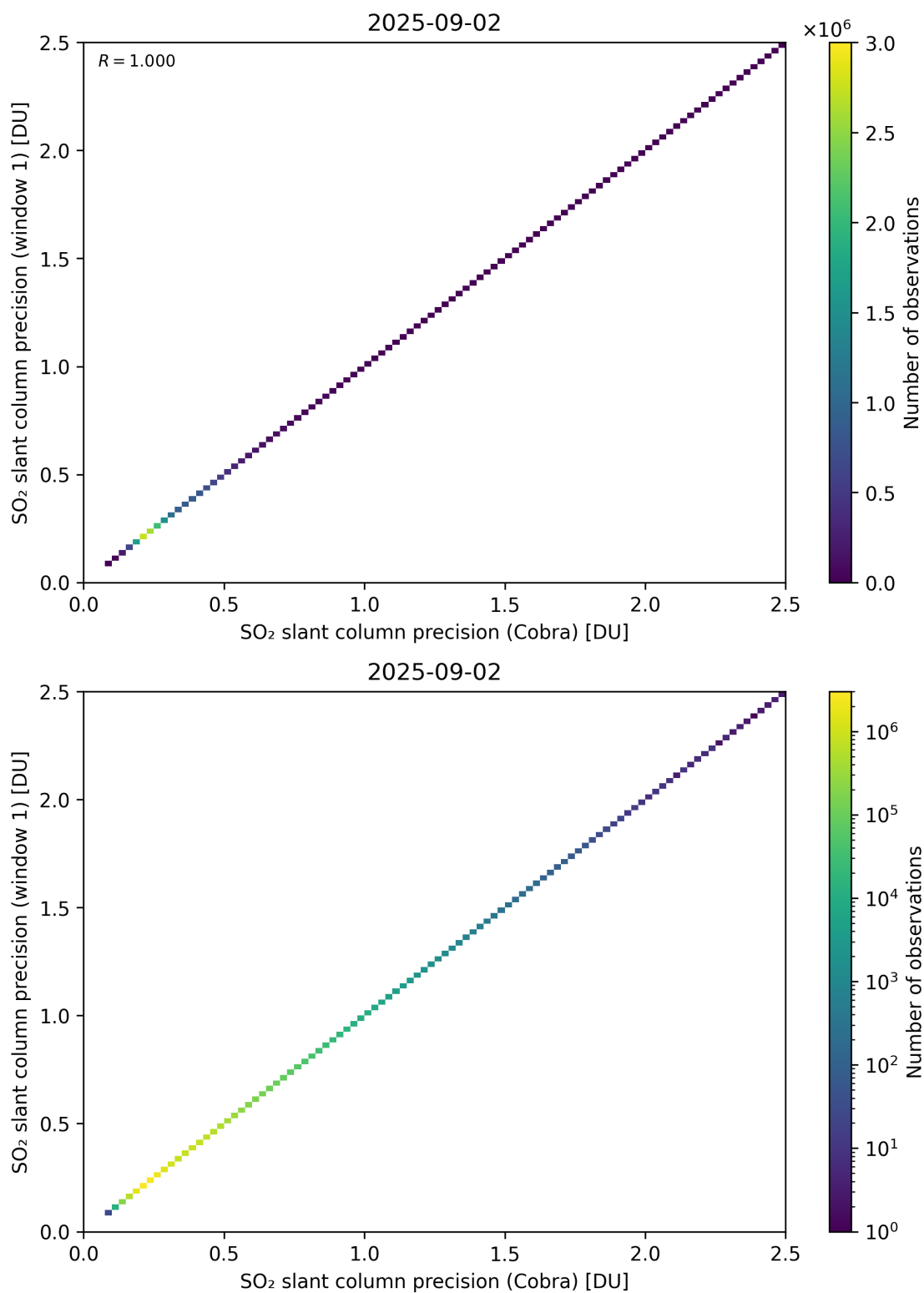
Figure 209: Scatter density plot of “SO 2 slant column precision (Cobra)” against “SO 2 slant column precision (window 1)” for 2025-09-01 to 2025-09-03.
