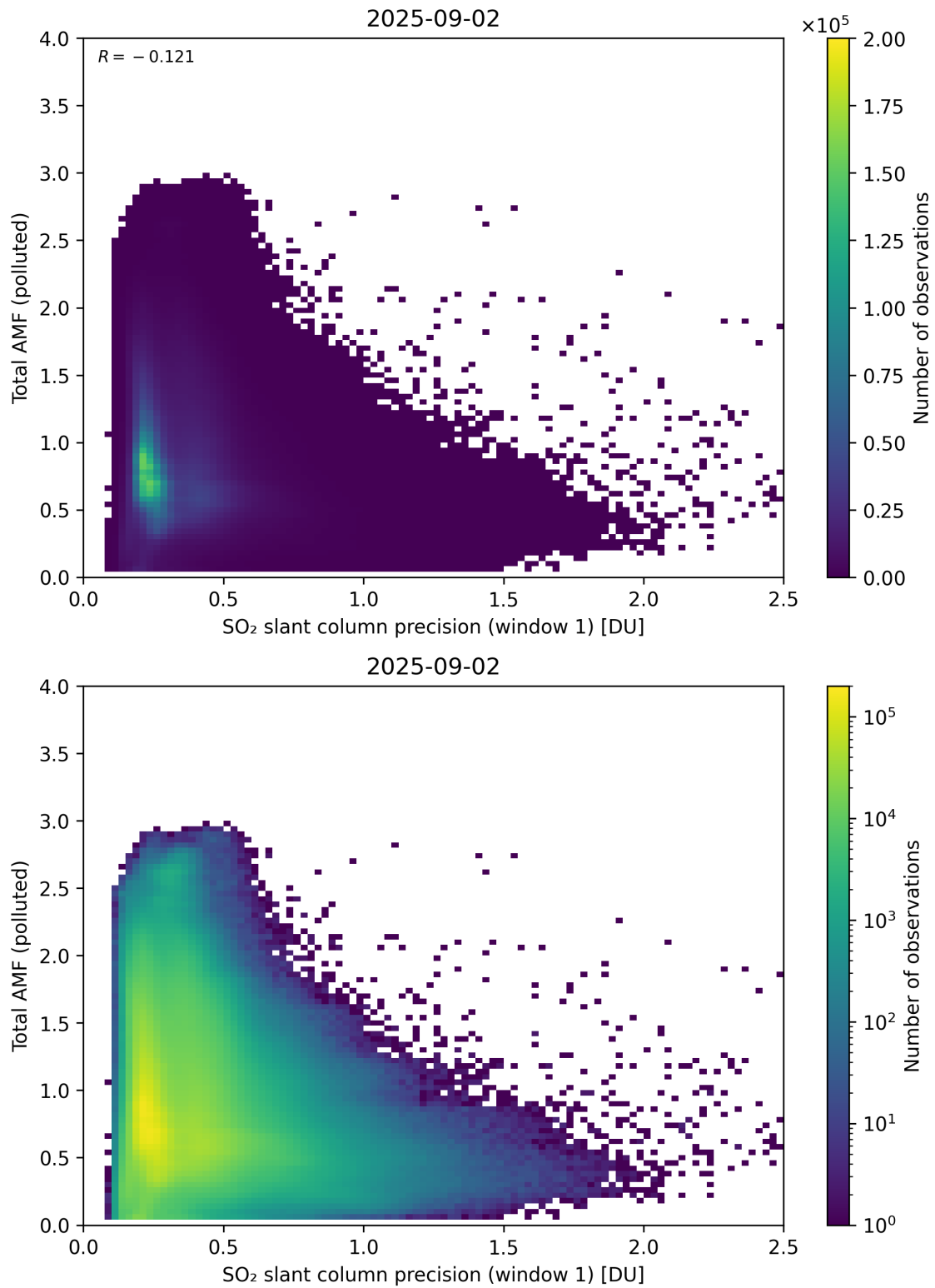
Figure 280: Scatter density plot of “SO 2 slant column precision (window 1)” against “Total AMF (polluted)” for 2025-09-01 to 2025-09-03.
