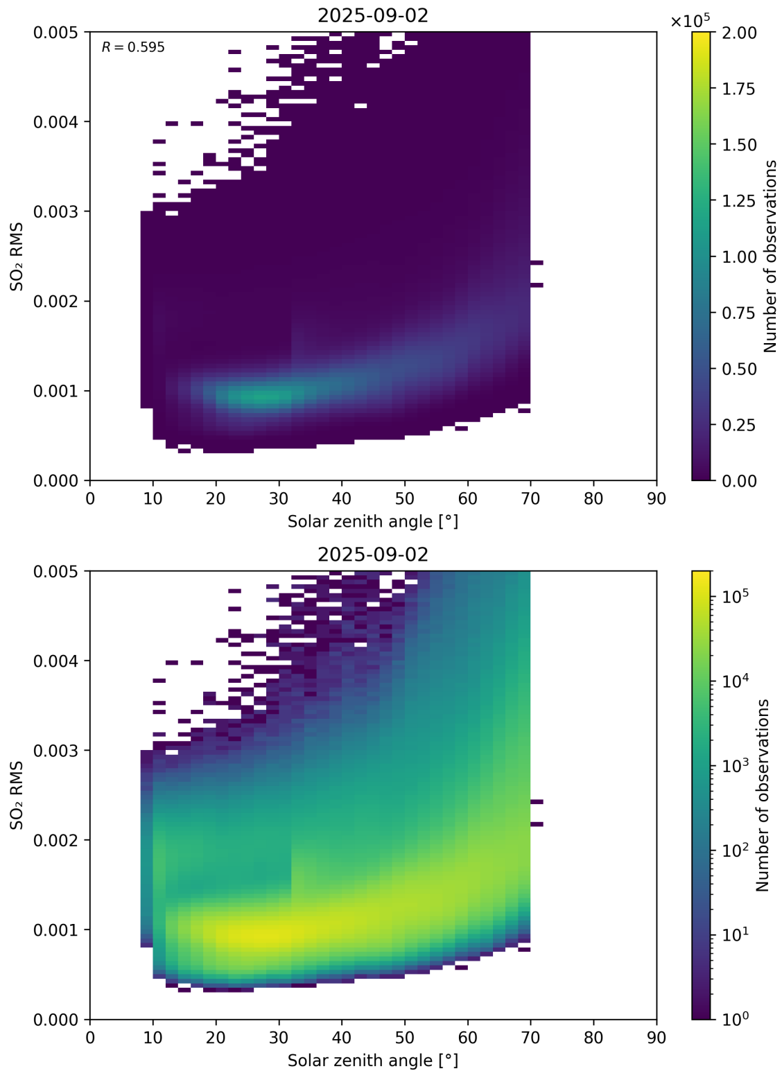
Figure 176: Scatter density plot of “Solar zenith angle” against “SO 2 RMS” for 2025-09-01 to 2025-09-03.
