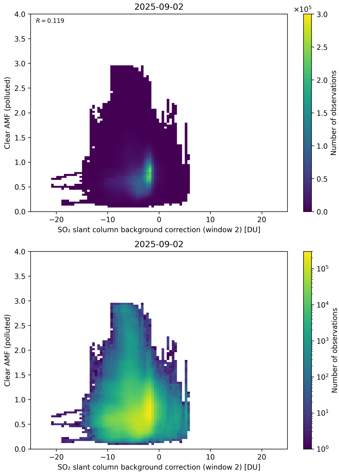
Figure 126: Scatter density plot of “SO 2 slant column background correction (window 2)” against “Clear AMF (polluted)” for 2025-09-01 to 2025-09-03.
