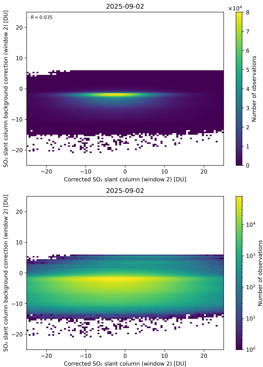
Figure 244: Scatter density plot of “Corrected SO 2 slant column (window 2)” against “SO 2 slant column background correction (window 2)” for 2025-09-01 to 2025-09-03.
