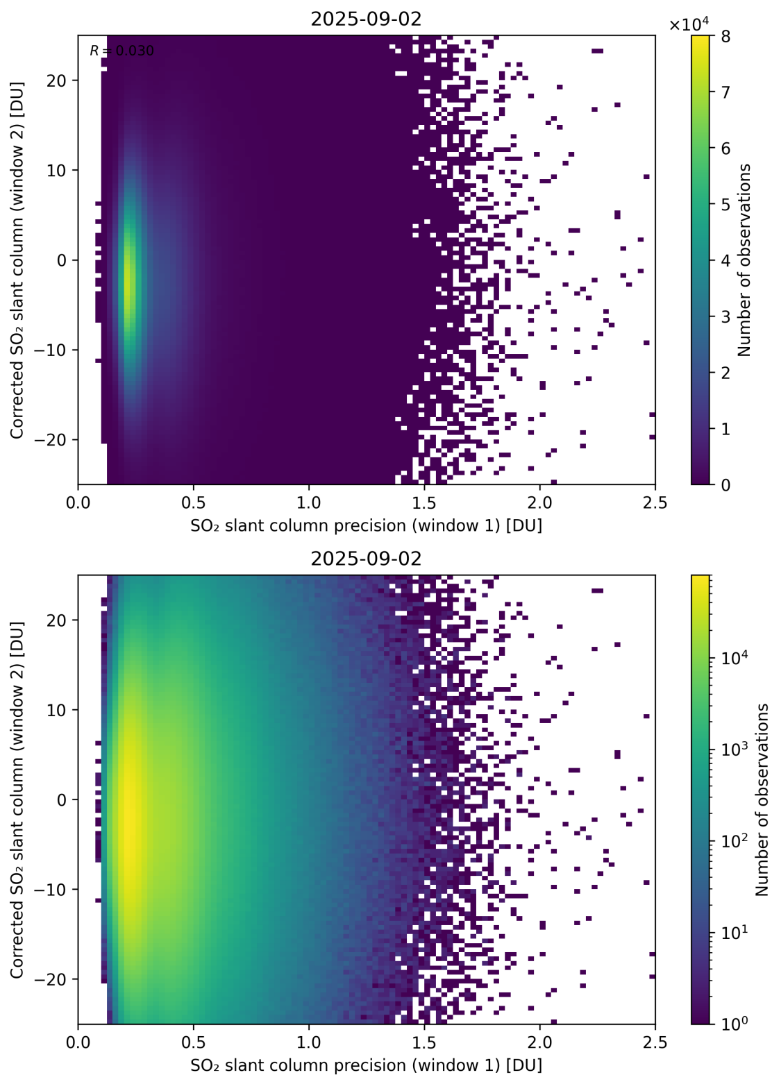
Figure 275: Scatter density plot of “SO 2 slant column precision (window 1)” against “Corrected SO 2 slant column (window 2)” for 2025-09-01 to 2025-09-03.
