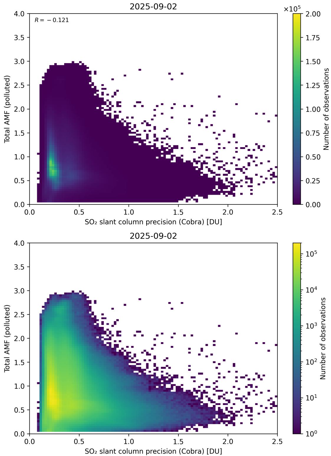
Figure 213: Scatter density plot of “SO 2 slant column precision (Cobra)” against “Total AMF (polluted)” for 2025-09-01 to 2025-09-03.
