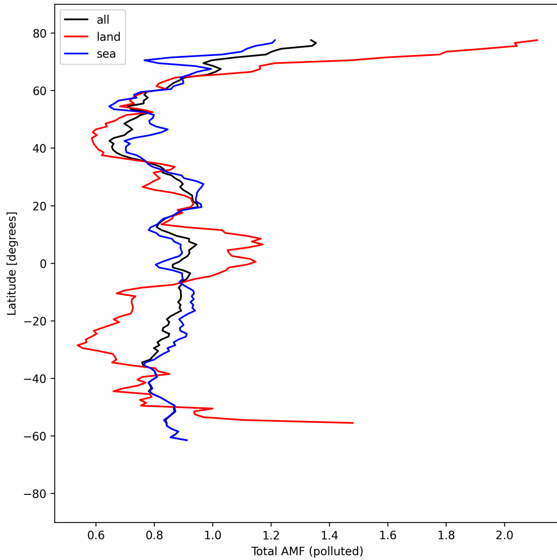
Figure 53: Zonal average of “Total AMF (polluted)” for 2025-09-01 to 2025-09-03.
