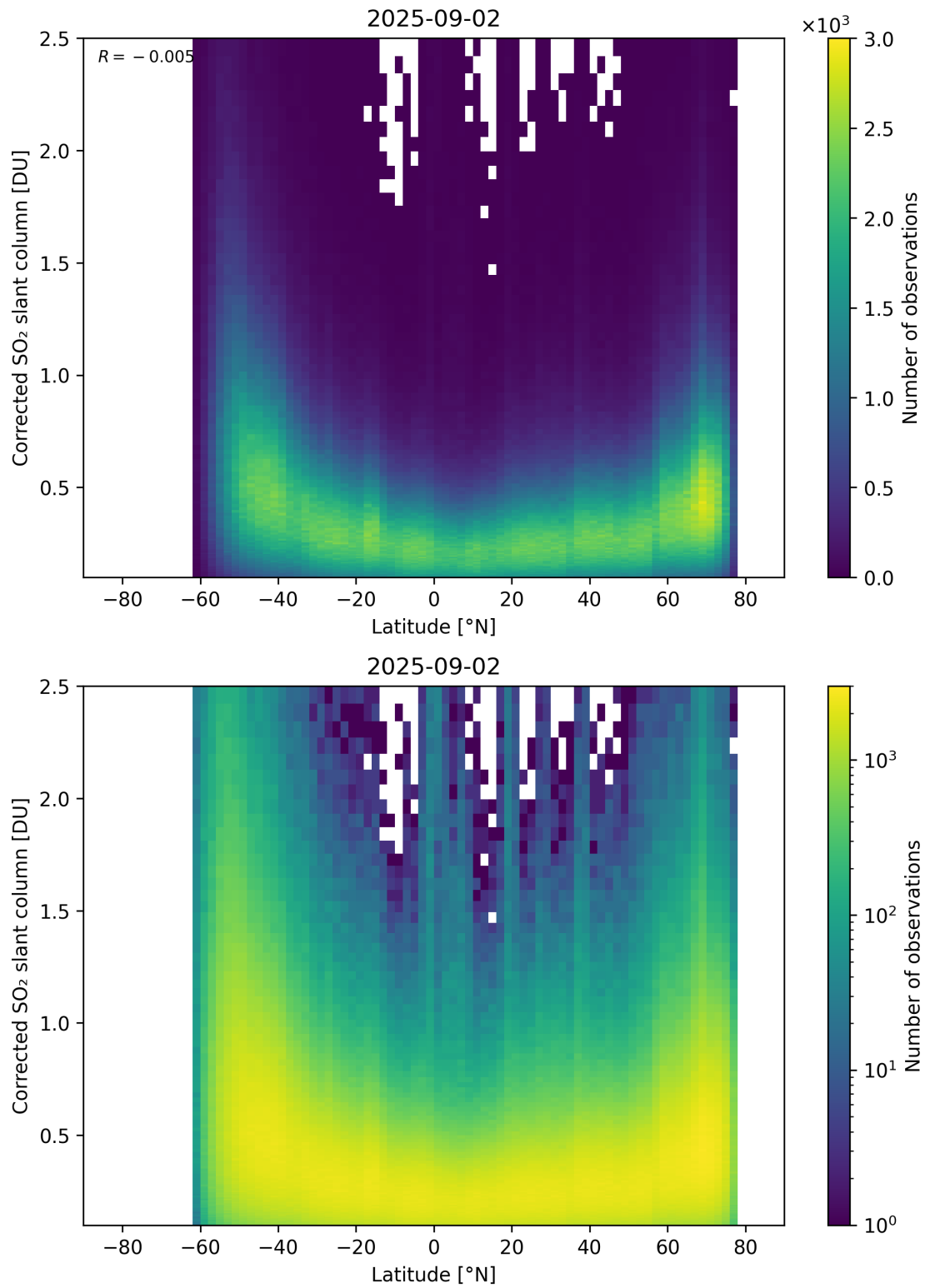
Figure 159: Scatter density plot of “Latitude” against “Corrected SO 2 slant column” for 2025-09-01 to 2025-09-03.
