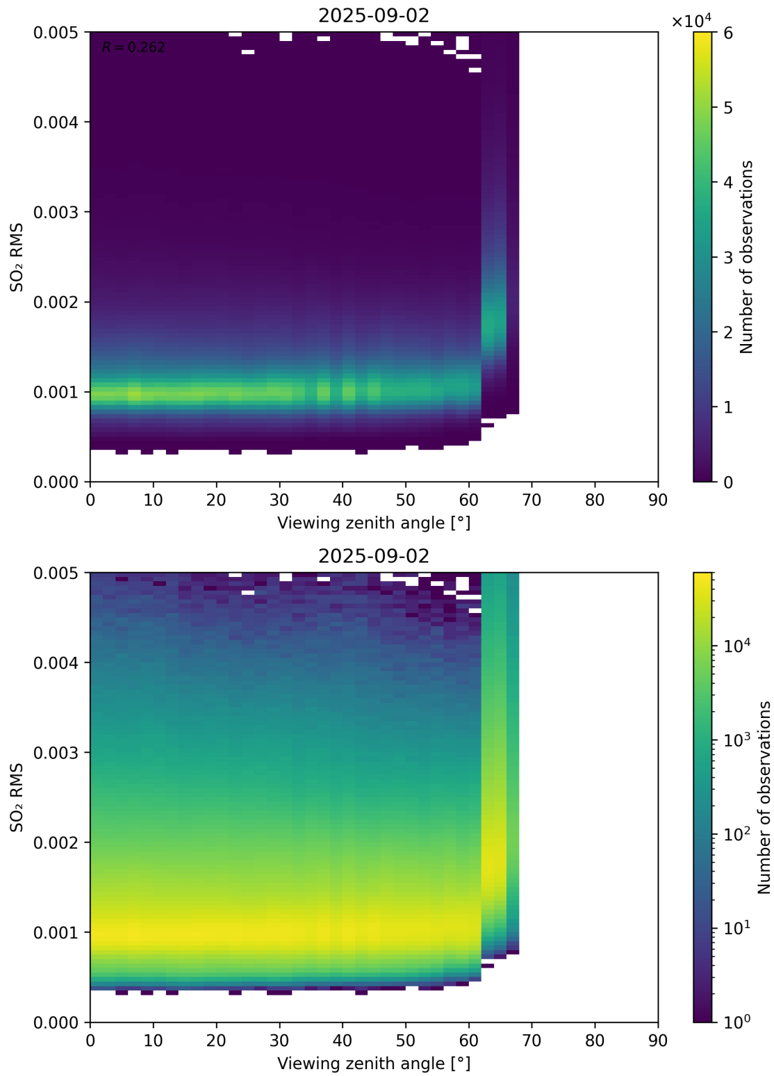
Figure 367: Scatter density plot of “Viewing zenith angle” against “SO 2 RMS” for 2025-09-01 to 2025-09-03.
