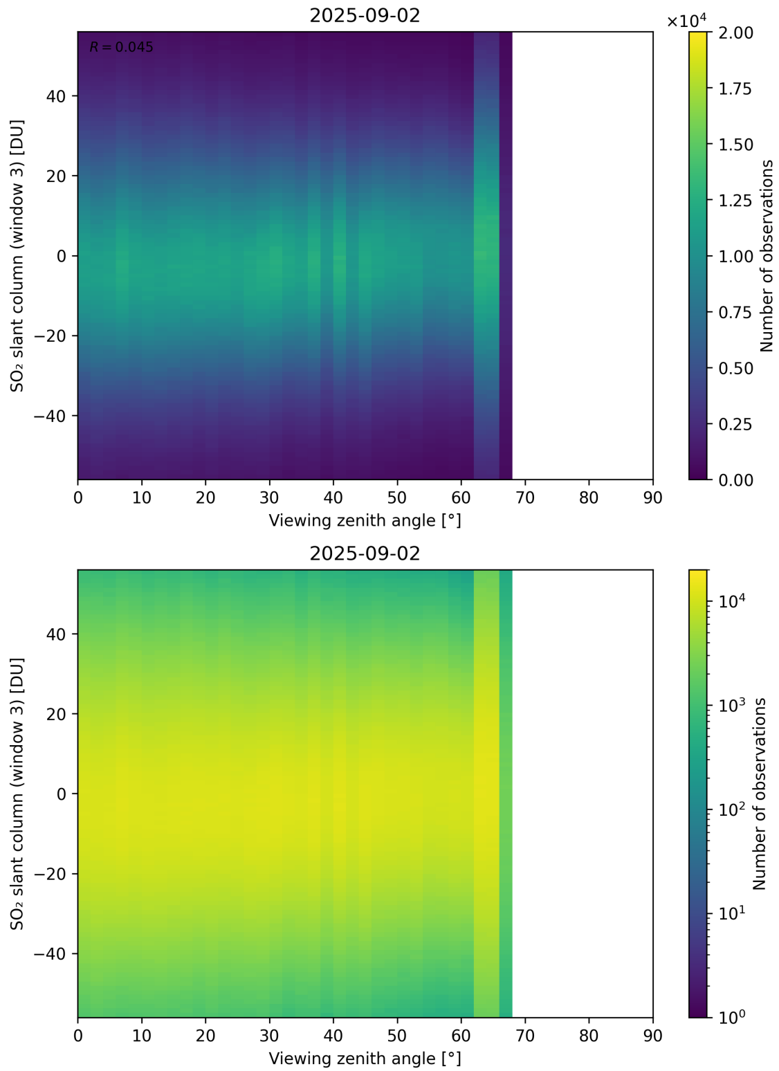
Figure 379: Scatter density plot of “Viewing zenith angle” against “SO 2 slant column (window 3)” for 2025-09-01 to 2025-09-03.
