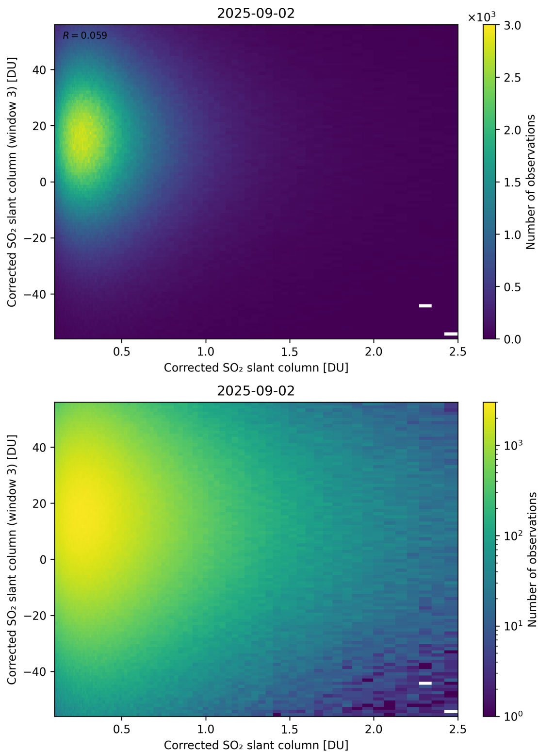
Figure 236: Scatter density plot of “Corrected SO 2 slant column” against “Corrected SO 2 slant column (window 3)” for 2025-09-01 to 2025-09-03.
