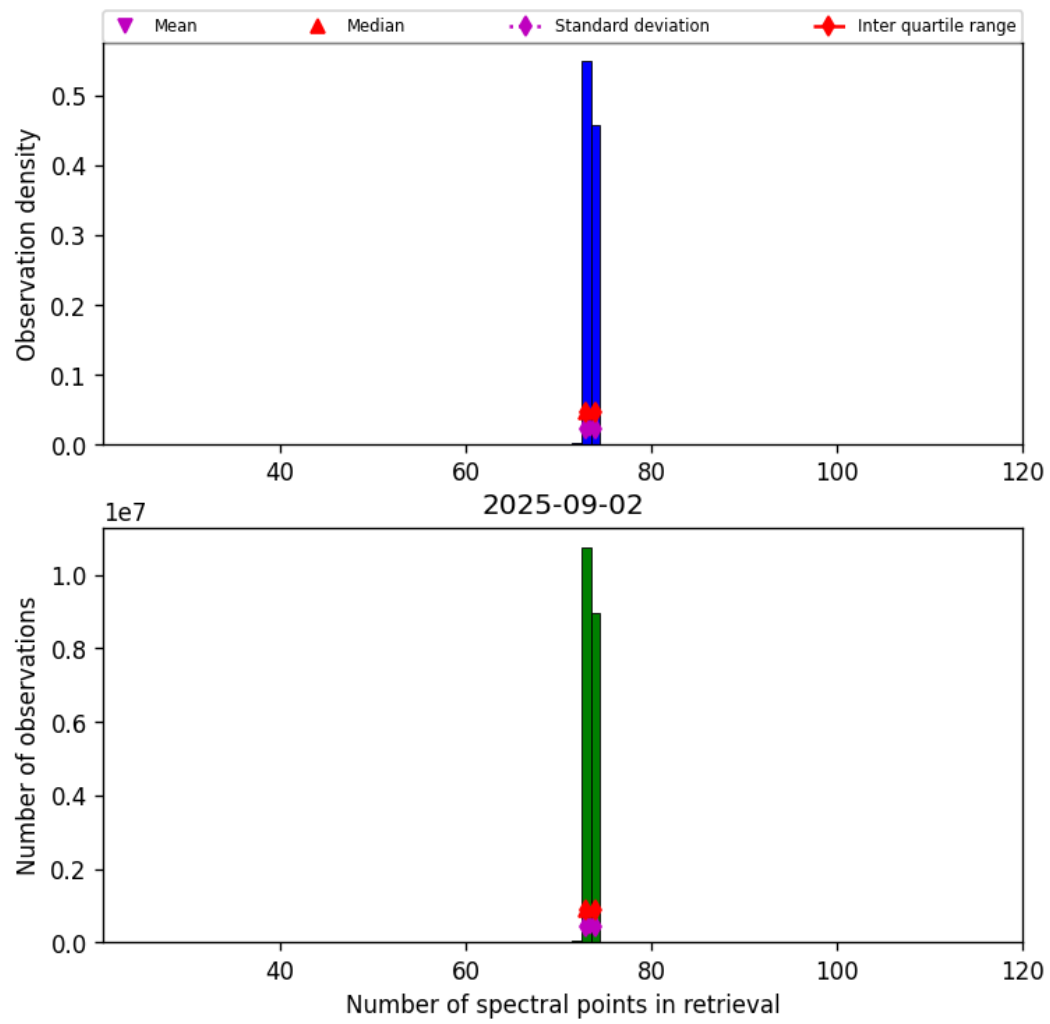
Figure 82: Histogram of “Number of spectral points in retrieval” for 2025-09-01 to 2025-09-03
