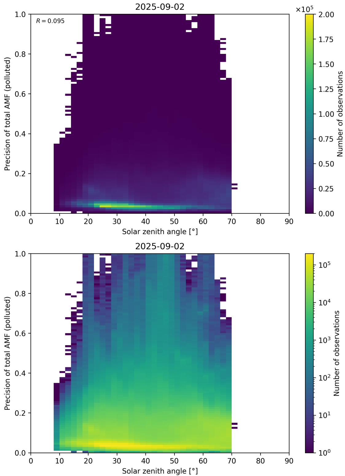
Figure 190: Scatter density plot of “Solar zenith angle” against “Precision of total AMF (polluted)” for 2025-09-01 to 2025-09-03.
