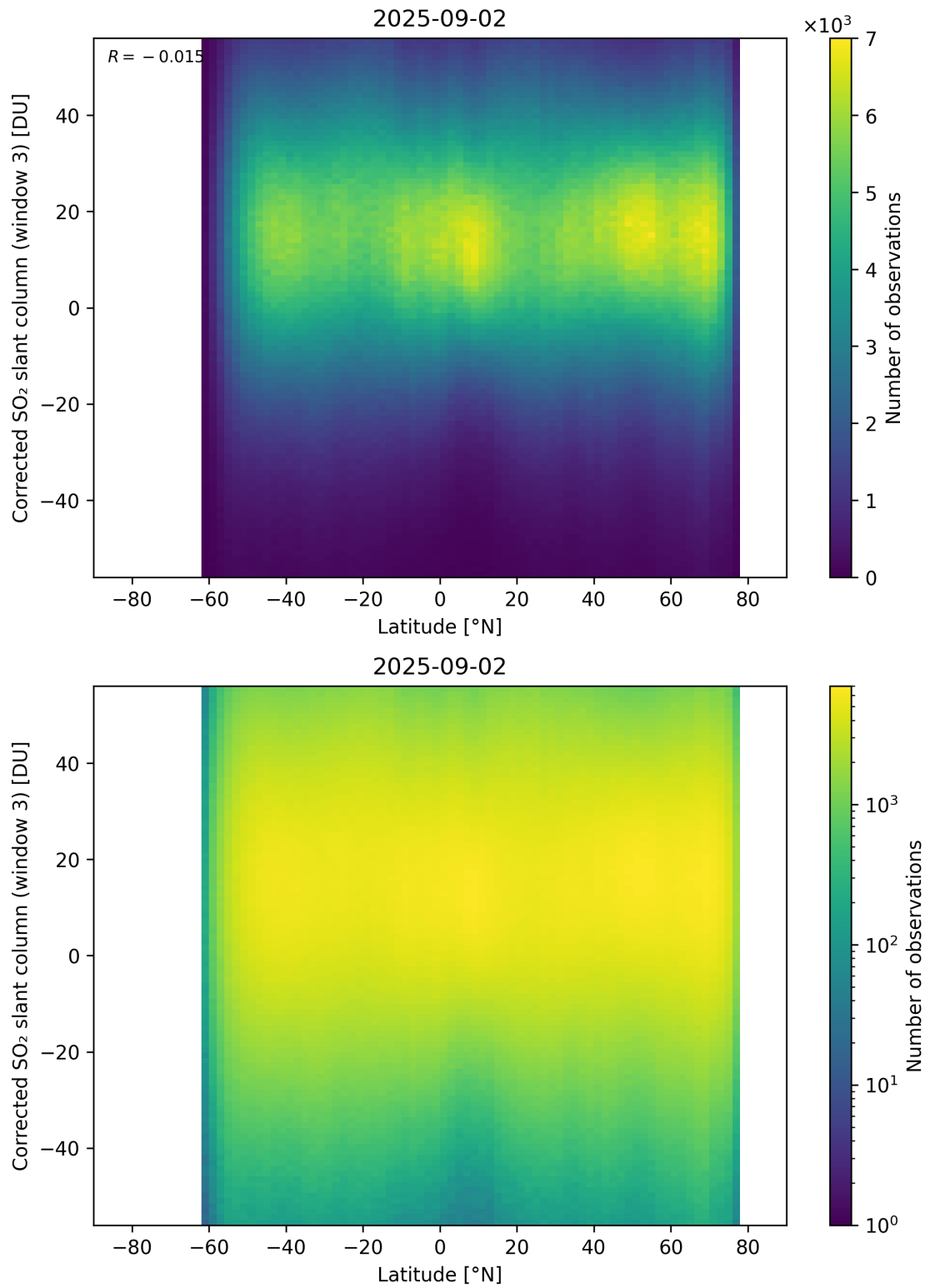
Figure 161: Scatter density plot of “Latitude” against “Corrected SO 2 slant column (window 3)” for 2025-09-01 to 2025-09-03.
