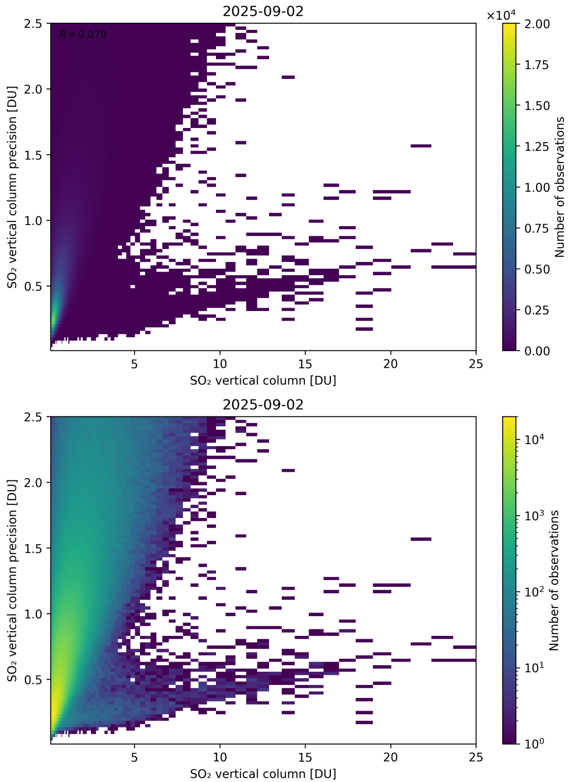
Figure 361: Scatter density plot of “SO 2 vertical column” against “SO 2 vertical column precision” for 2025-09-01 to 2025-09-03.
