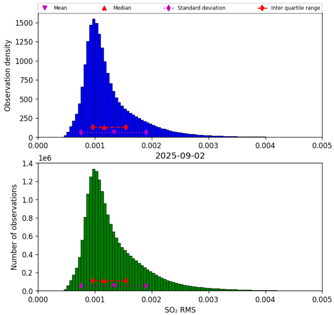
Figure 78: Histogram of “SO 2 RMS” for 2025-09-01 to 2025-09-03
