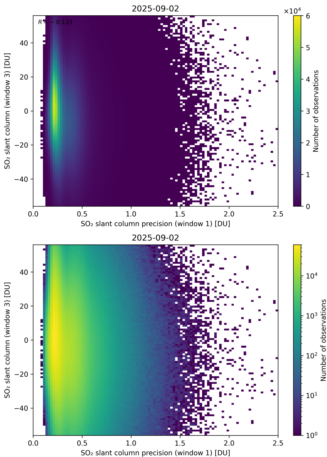
Figure 278: Scatter density plot of “SO 2 slant column precision (window 1)” against “SO 2 slant column (window 3)” for 2025-09-01 to 2025-09-03.
