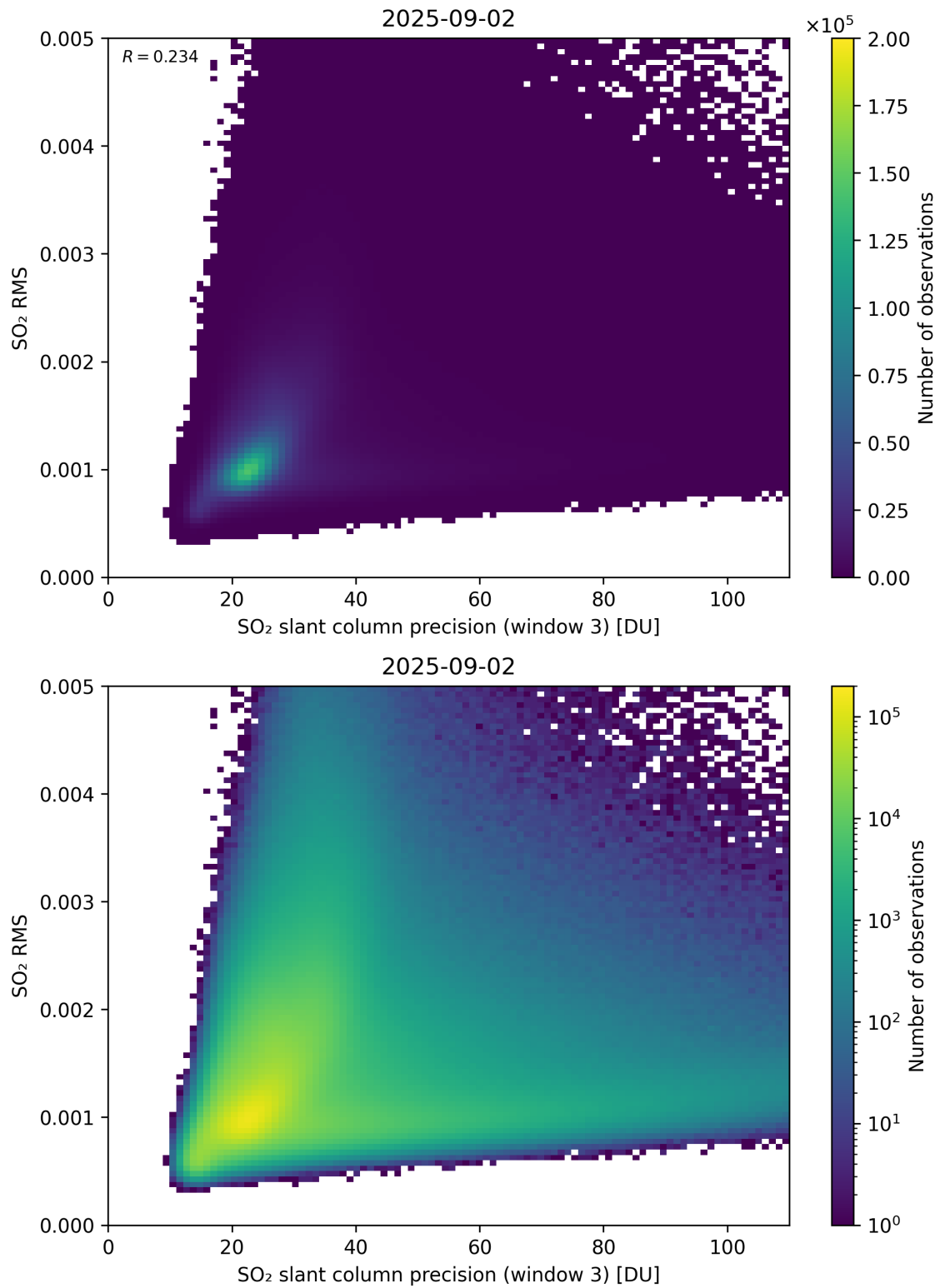
Figure 310: Scatter density plot of “SO 2 slant column precision (window 3)” against “SO 2 RMS” for 2025-09-01 to 2025-09-03.
