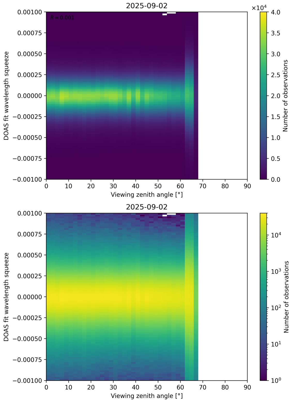
Figure 366: Scatter density plot of “Viewing zenith angle” against “DOAS fit wavelength squeeze” for 2025-09-01 to 2025-09-03.
