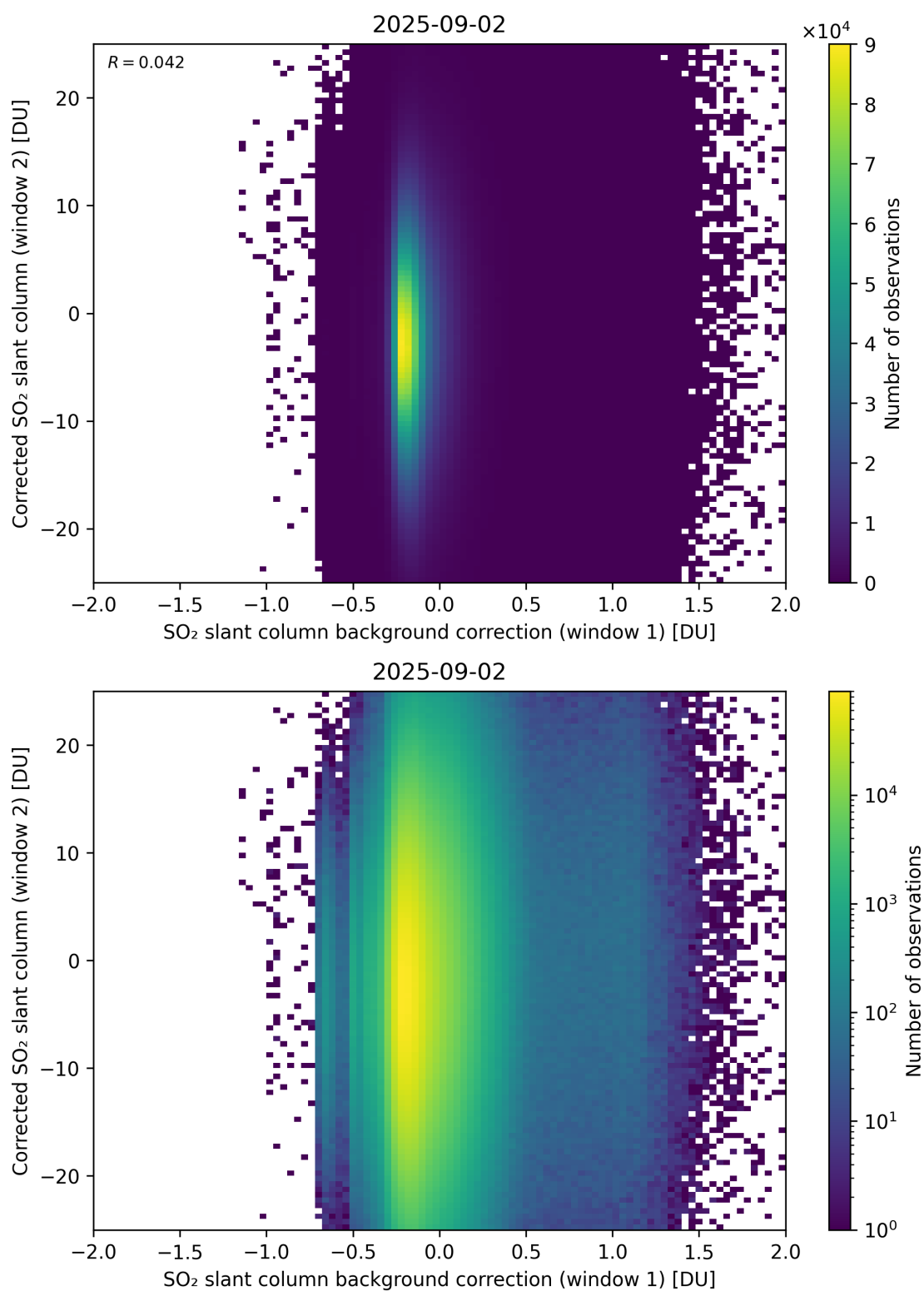
Figure 115: Scatter density plot of “SO 2 slant column background correction (window 1)” against “Corrected SO 2 slant column (window 2)” for 2025-09-01 to 2025-09-03.
