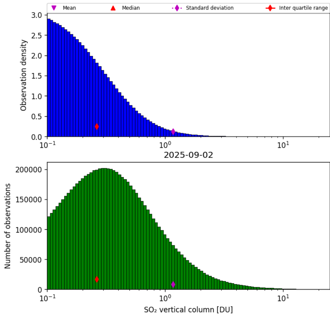
Figure 58: Histogram of “SO 2 vertical column” for 2025-09-01 to 2025-09-03
