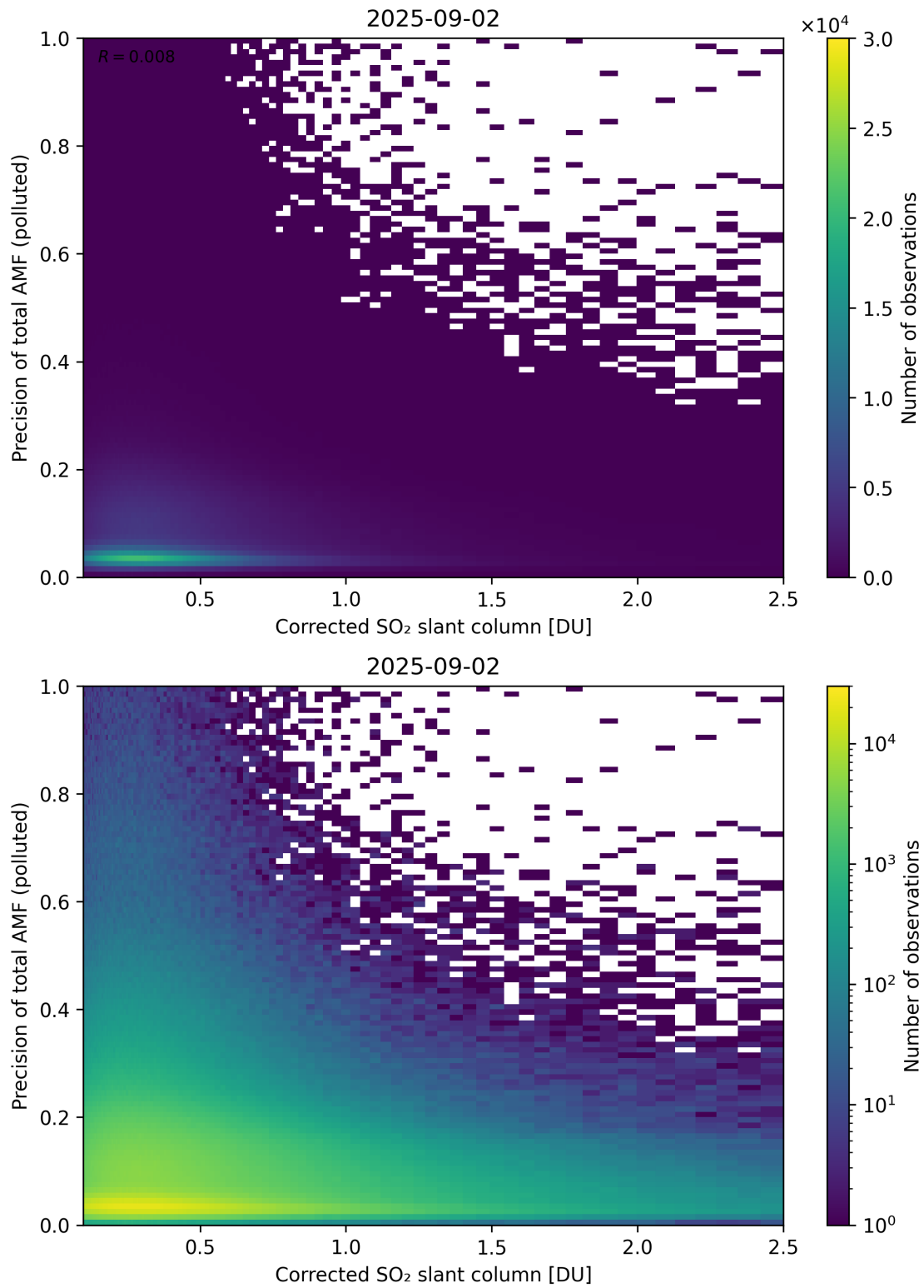
Figure 243: Scatter density plot of “Corrected SO 2 slant column” against “Precision of total AMF (polluted)” for 2025-09-01 to 2025-09-03.
