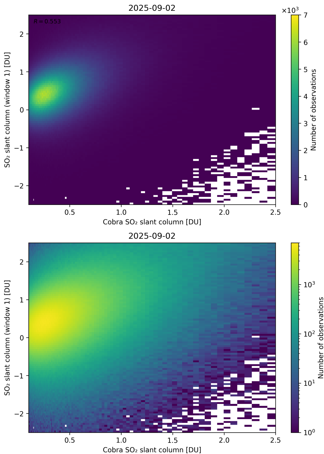
Figure 219: Scatter density plot of “Cobra SO 2 slant column” against “SO 2 slant column (window 1)” for 2025-09-01 to 2025-09-03.
