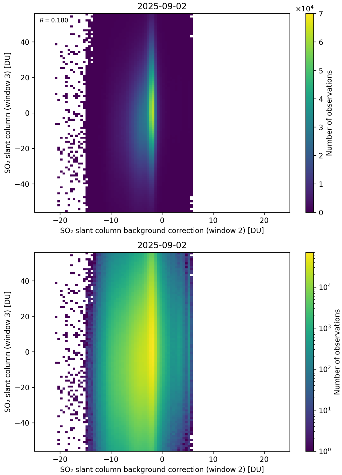
Figure 128: Scatter density plot of “SO 2 slant column background correction (window 2)” against “SO 2 slant column (window 3)” for 2025-09-01 to 2025-09-03.
