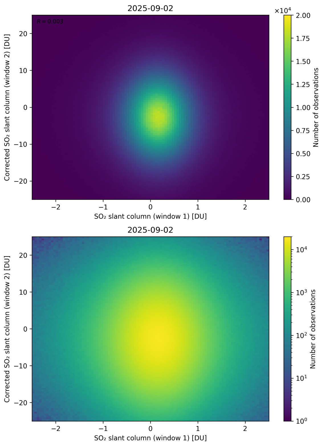
Figure 283: Scatter density plot of “SO 2 slant column (window 1)” against “Corrected SO 2 slant column (window 2)” for 2025-09-01 to 2025-09-03.
