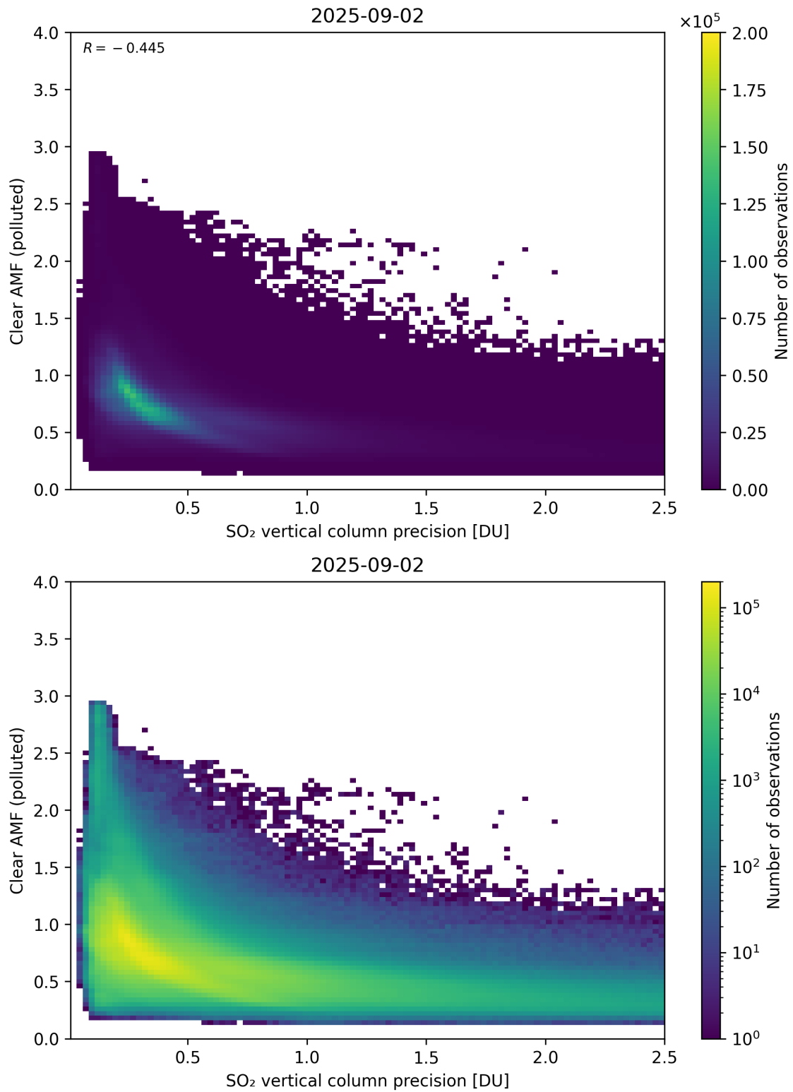
Figure 335: Scatter density plot of “SO 2 vertical column precision” against “Clear AMF (polluted)” for 2025-09-01 to 2025-09-03.
