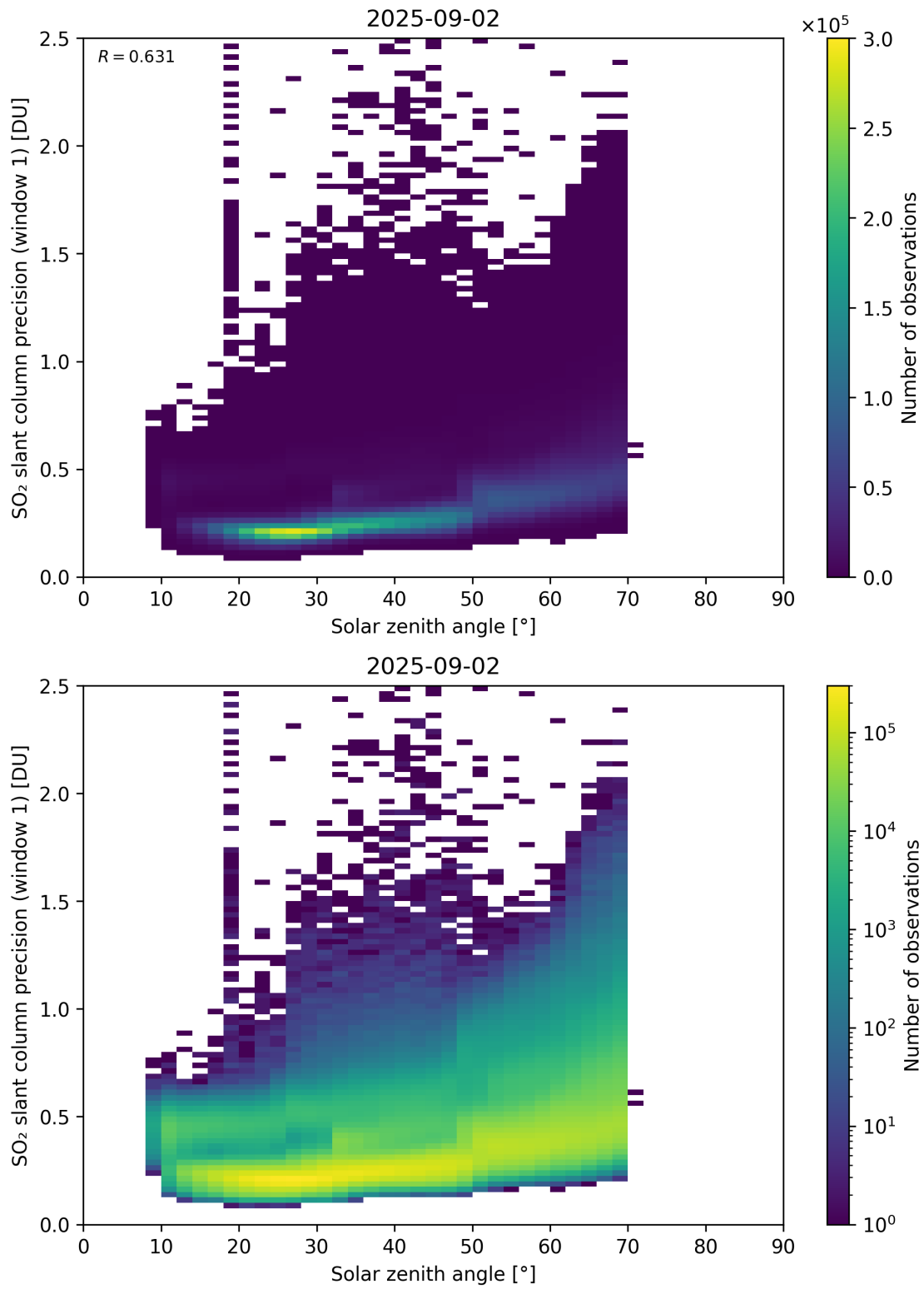
Figure 185: Scatter density plot of “Solar zenith angle” against “SO 2 slant column precision (window 1)” for 2025-09-01 to 2025-09-03.
