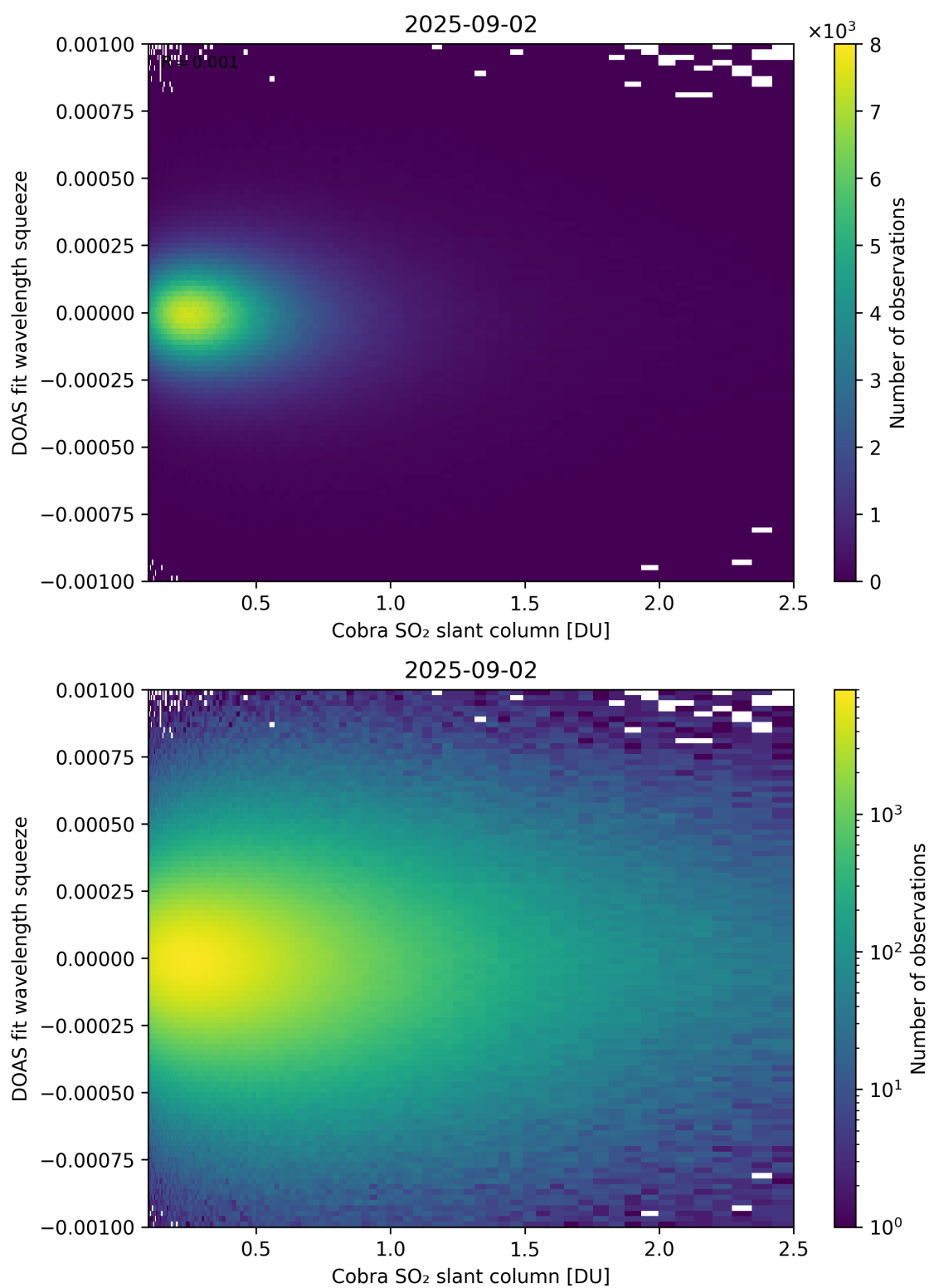
Figure 197: Scatter density plot of “Cobra SO 2 slant column” against “DOAS fit wavelength squeeze” for 2025-09-01 to 2025-09-03.
