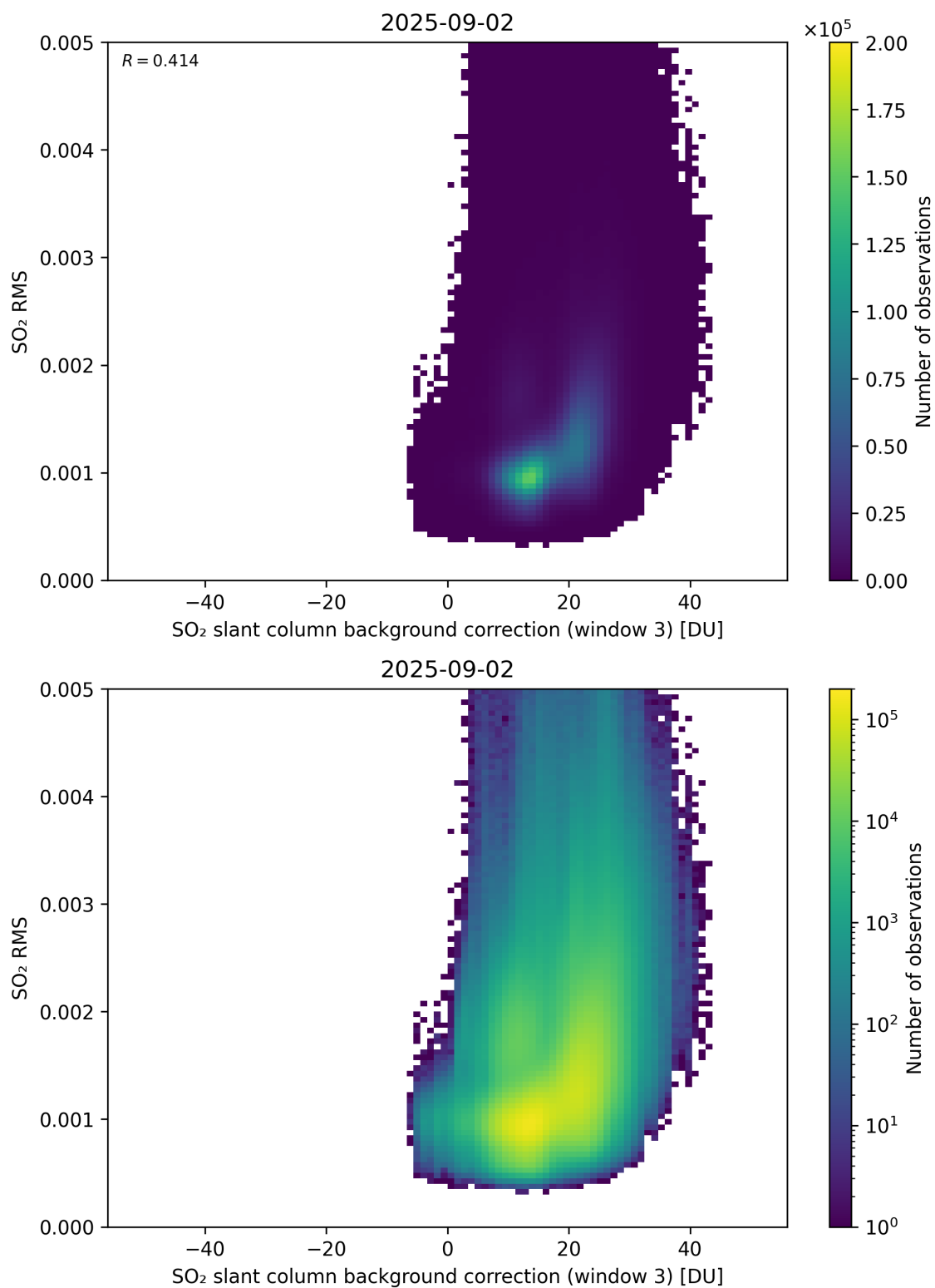
Figure 134: Scatter density plot of “SO 2 slant column background correction (window 3)” against “SO 2 RMS” for 2025-09-01 to 2025-09-03.
