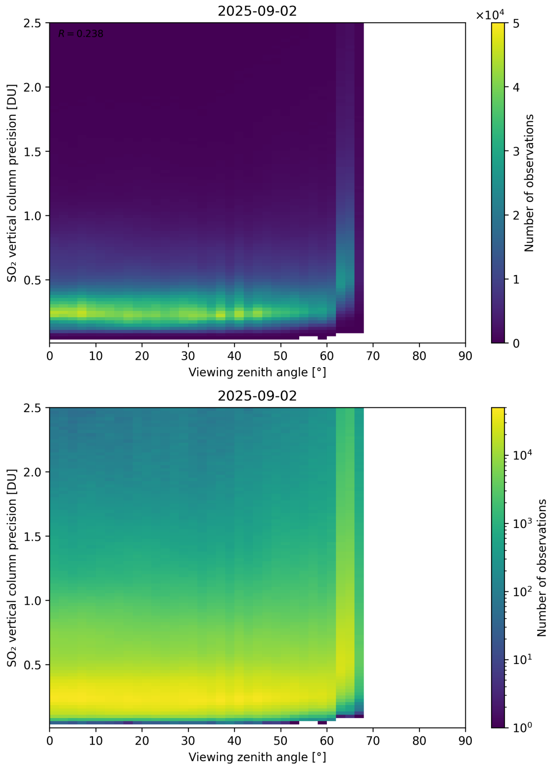
Figure 384: Scatter density plot of “Viewing zenith angle” against “SO 2 vertical column precision” for 2025-09-01 to 2025-09-03.
