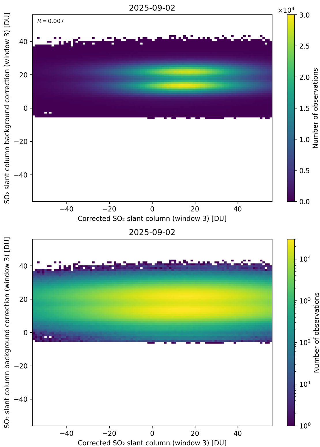
Figure 255: Scatter density plot of “Corrected SO 2 slant column (window 3)” against “SO 2 slant column background correction (window 3)” for 2025-09-01 to 2025-09-03.
