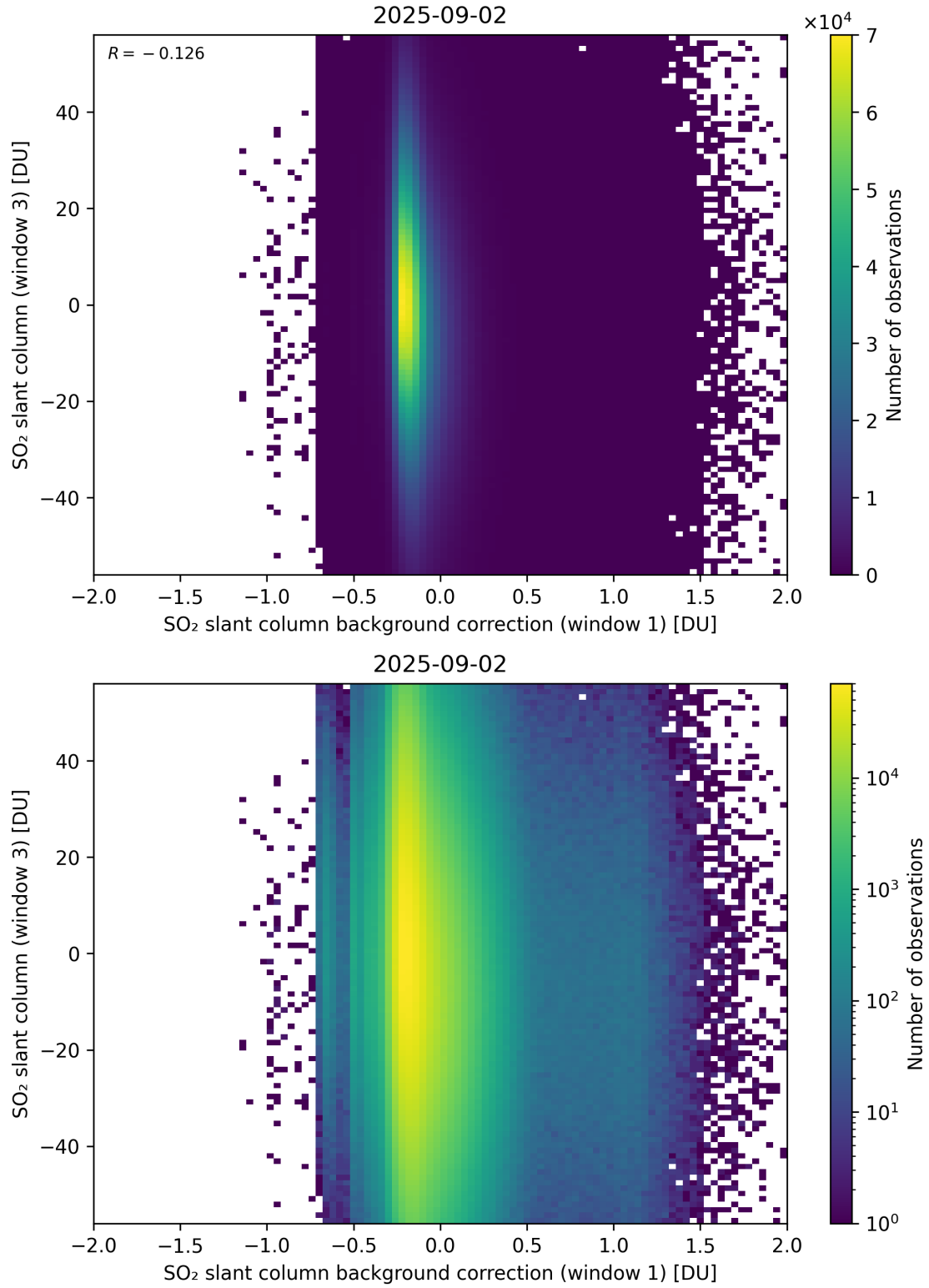
Figure 118: Scatter density plot of “SO 2 slant column background correction (window 1)” against “SO 2 slant column (window 3)” for 2025-09-01 to 2025-09-03.
