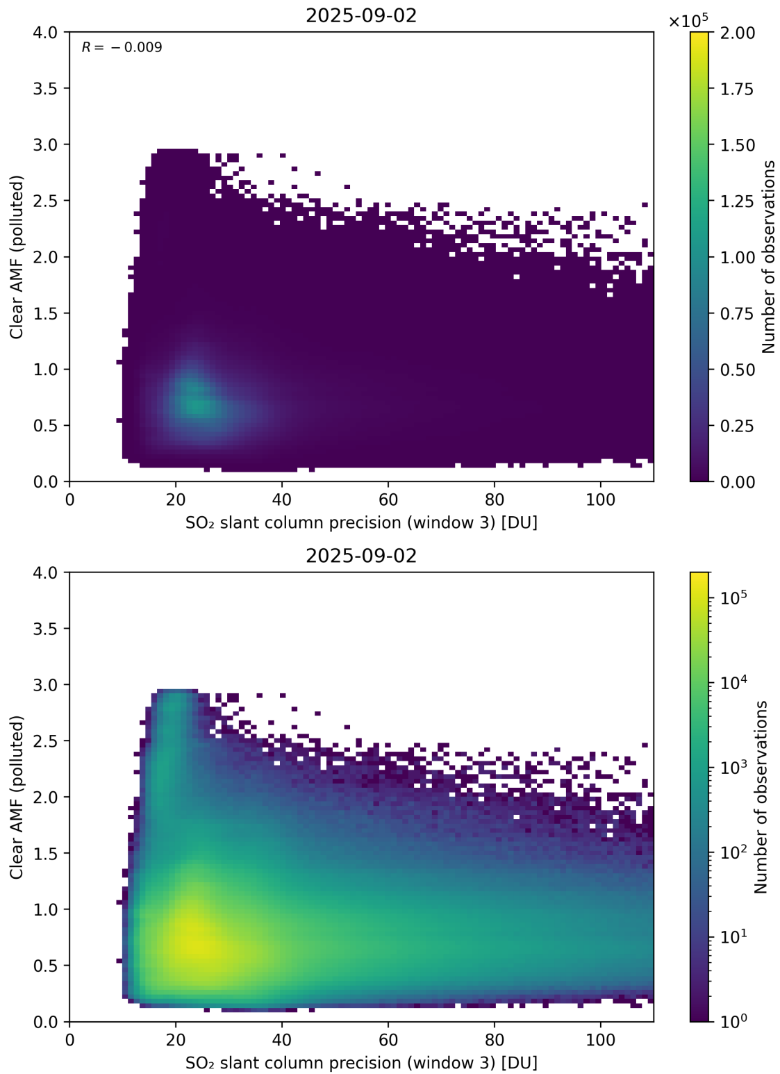
Figure 311: Scatter density plot of “SO 2 slant column precision (window 3)” against “Clear AMF (polluted)” for 2025-09-01 to 2025-09-03.
