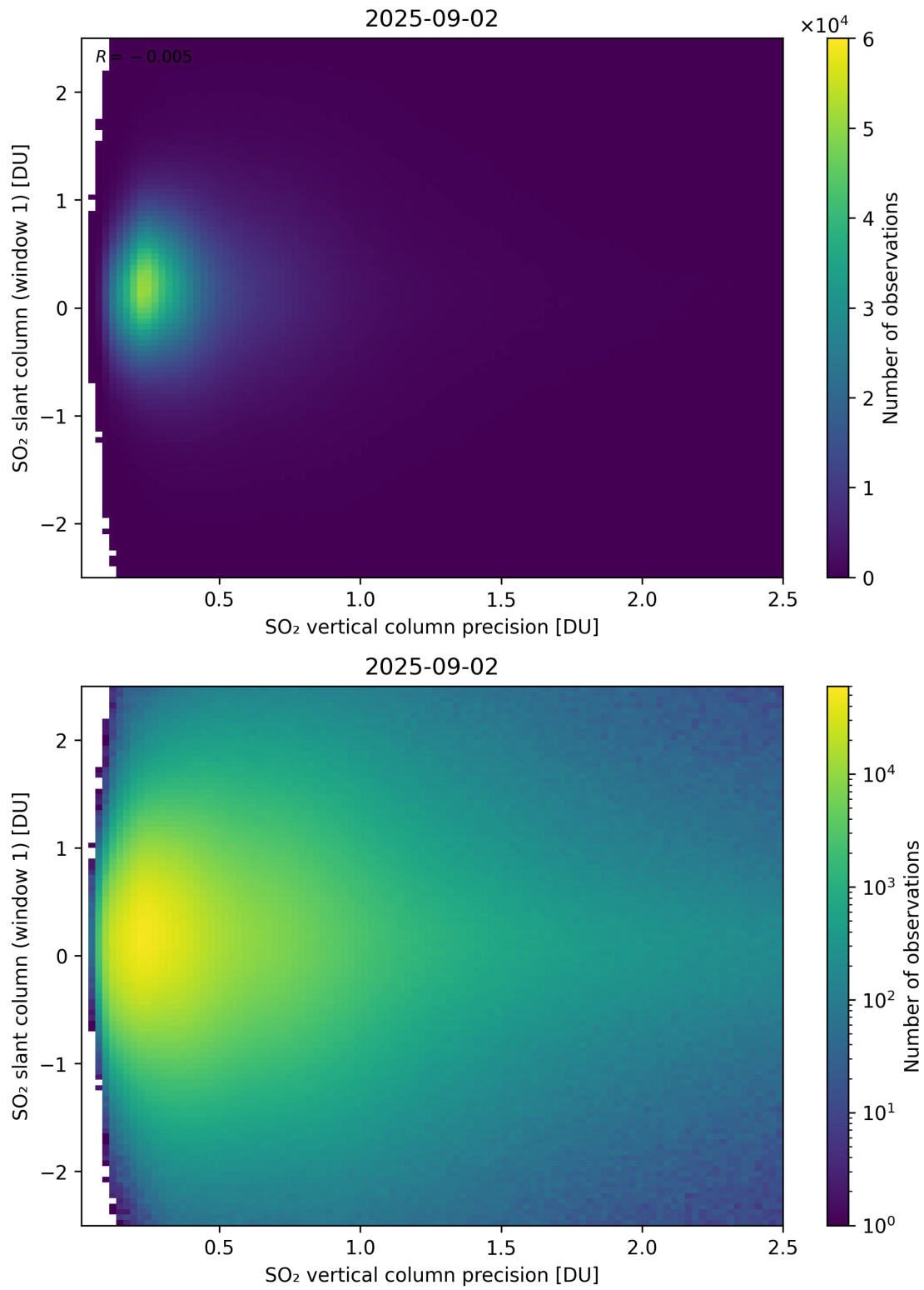
Figure 341: Scatter density plot of “SO 2 vertical column precision” against “SO 2 slant column (window 1)” for 2025-09-01 to 2025-09-03.
