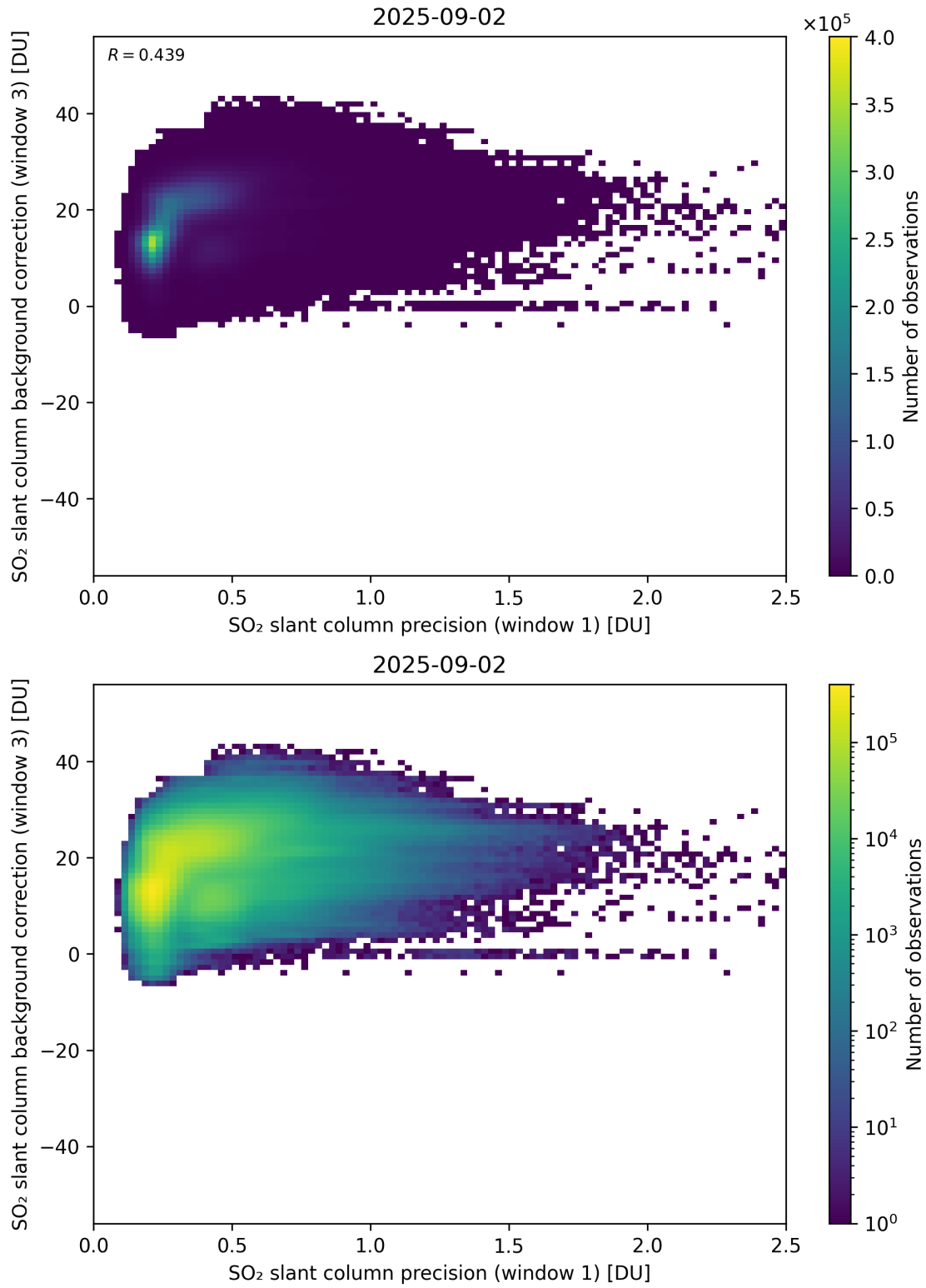
Figure 270: Scatter density plot of “SO 2 slant column precision (window 1)” against “SO 2 slant column background correction (window 3)” for 2025-09-01 to 2025-09-03.
