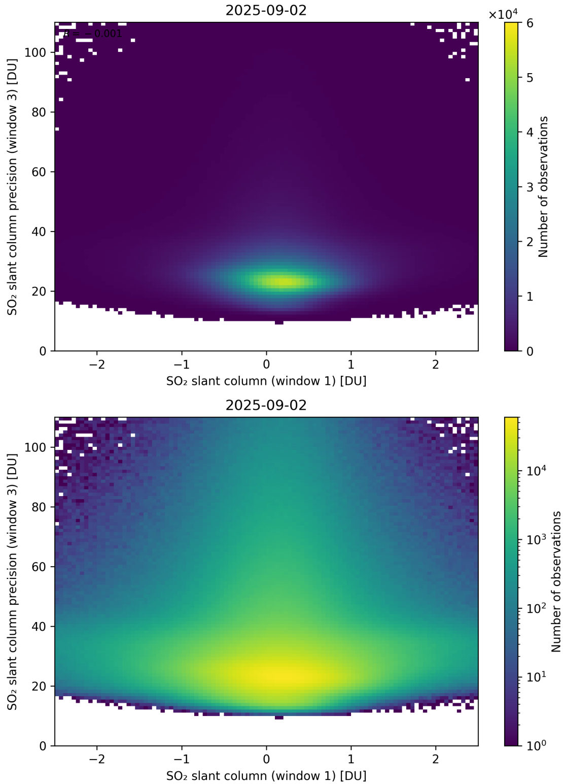
Figure 288: Scatter density plot of “SO 2 slant column (window 1)” against “SO 2 slant column precision (window 3)” for 2025-09-01 to 2025-09-03.
