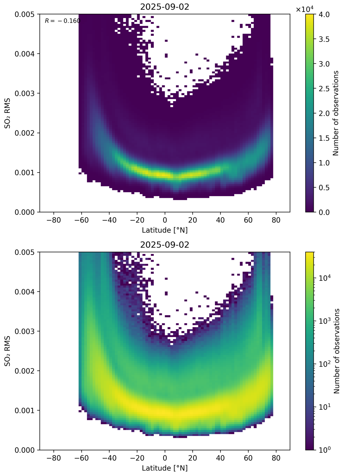
Figure 155: Scatter density plot of “Latitude” against “SO 2 RMS” for 2025-09-01 to 2025-09-03.
