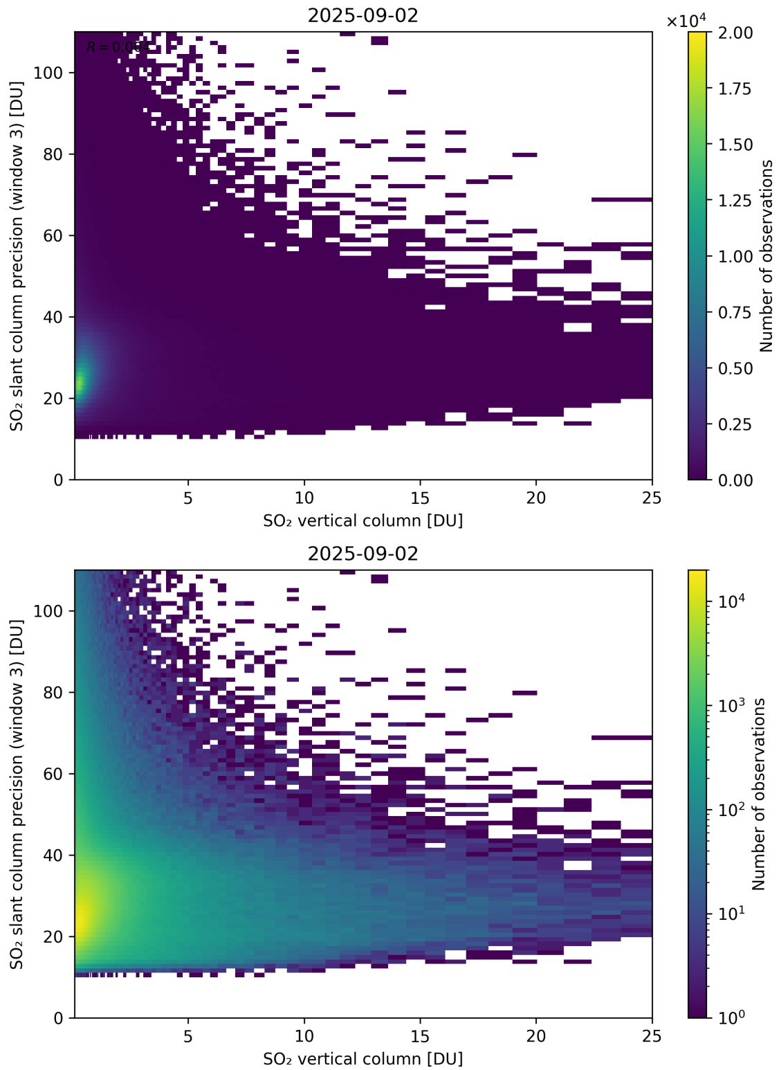
Figure 358: Scatter density plot of “SO 2 vertical column” against “SO 2 slant column precision (window 3)” for 2025-09-01 to 2025-09-03.
