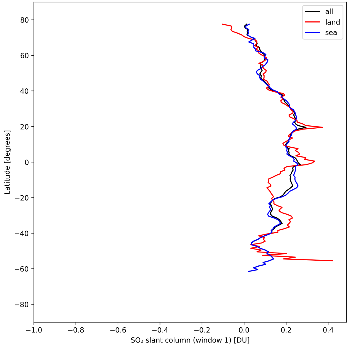
Figure 37: Zonal average of “SO 2 slant column (window 1)” for 2025-09-01 to 2025-09-03.
