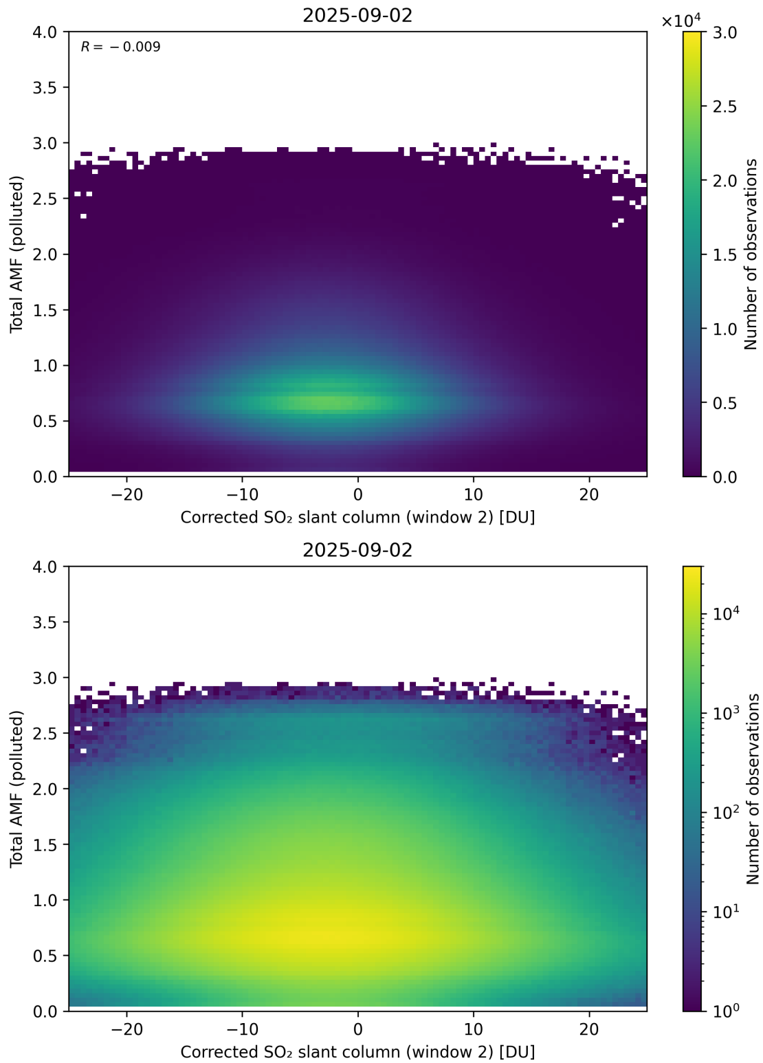
Figure 253: Scatter density plot of “Corrected SO 2 slant column (window 2)” against “Total AMF (polluted)” for 2025-09-01 to 2025-09-03.
