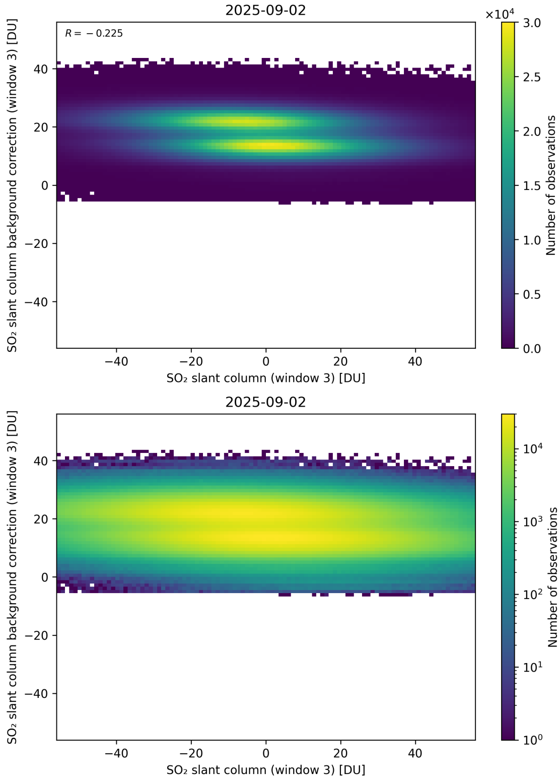
Figure 303: Scatter density plot of “SO 2 slant column (window 3)” against “SO 2 slant column background correction (window 3)” for 2025-09-01 to 2025-09-03.
