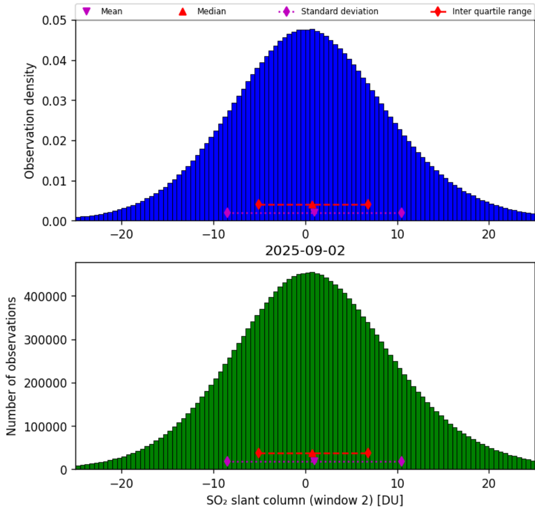
Figure 67: Histogram of “SO 2 slant column (window 2)” for 2025-09-01 to 2025-09-03
