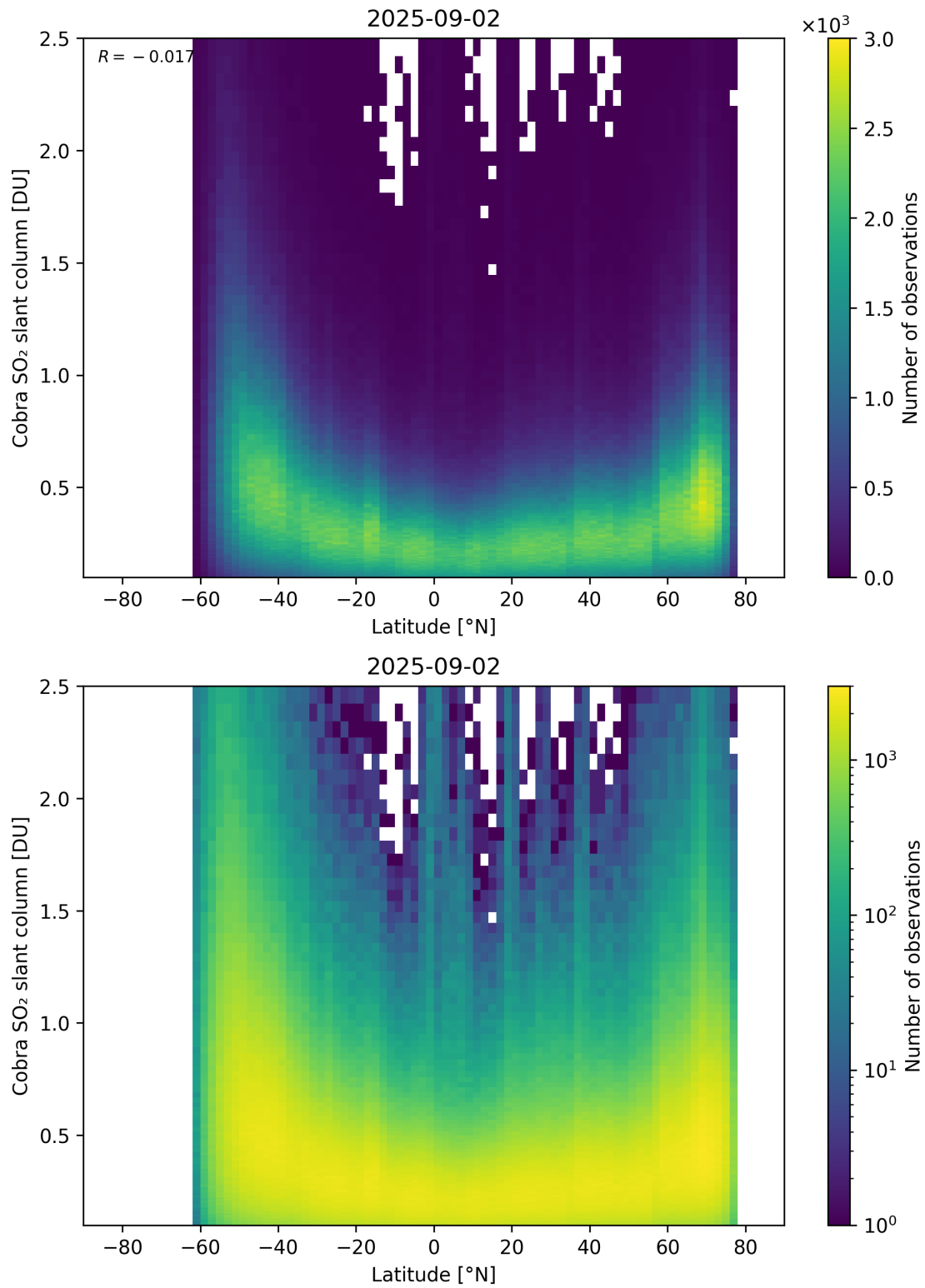
Figure 157: Scatter density plot of “Latitude” against “Cobra SO 2 slant column” for 2025-09-01 to 2025-09-03.
