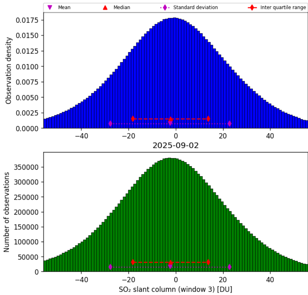
Figure 71: Histogram of “SO 2 slant column (window 3)” for 2025-09-01 to 2025-09-03
