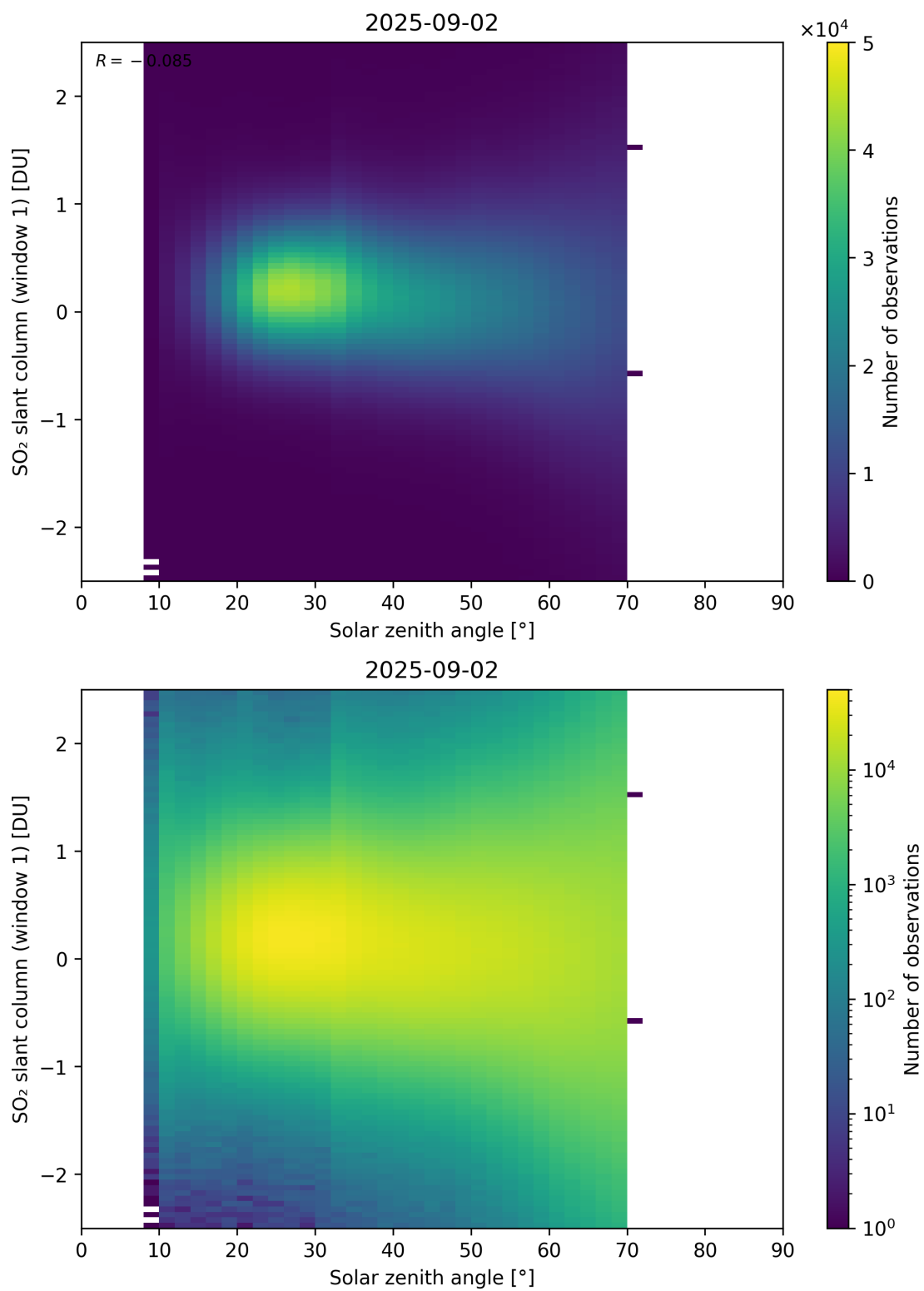
Figure 184: Scatter density plot of “Solar zenith angle” against “SO 2 slant column (window 1)” for 2025-09-01 to 2025-09-03.
