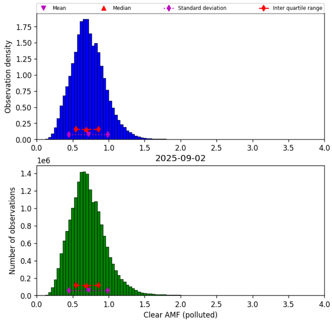
Figure 81: Histogram of “Clear AMF (polluted)” for 2025-09-01 to 2025-09-03
