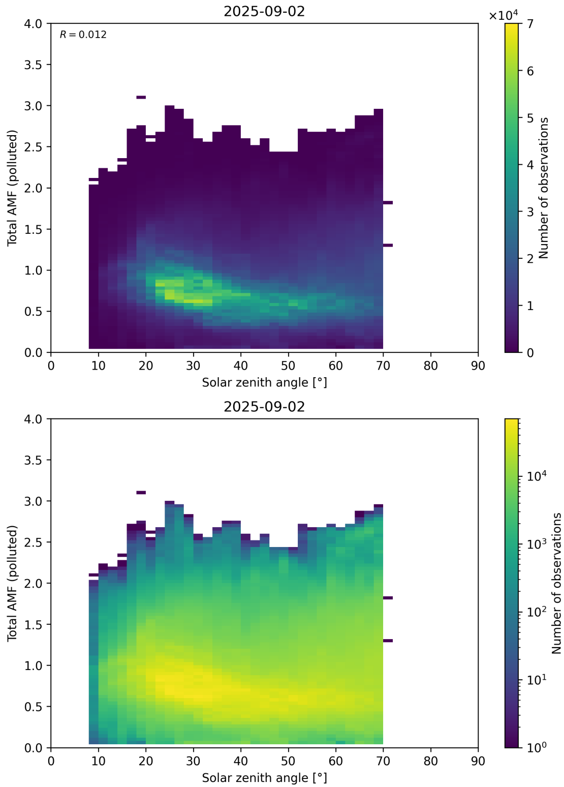
Figure 189: Scatter density plot of “Solar zenith angle” against “Total AMF (polluted)” for 2025-09-01 to 2025-09-03.
