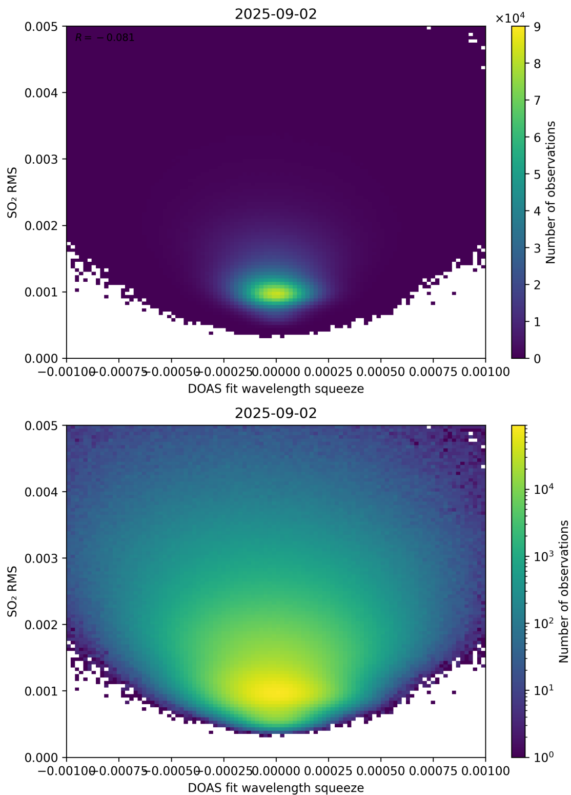
Figure 143: Scatter density plot of “DOAS fit wavelength squeeze” against “SO 2 RMS” for 2025-09-01 to 2025-09-03.
