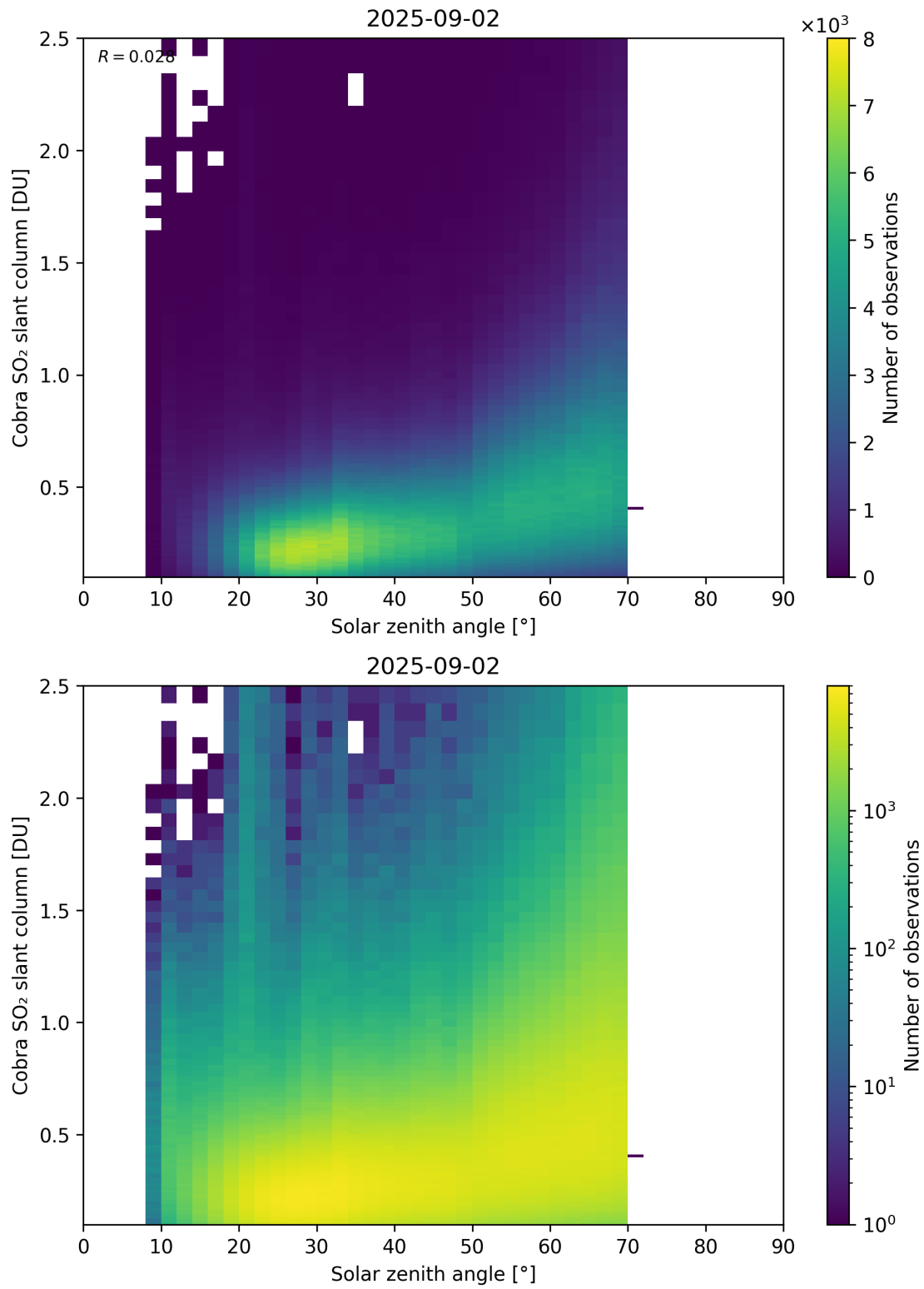
Figure 179: Scatter density plot of “Solar zenith angle” against “Cobra SO 2 slant column” for 2025-09-01 to 2025-09-03.
