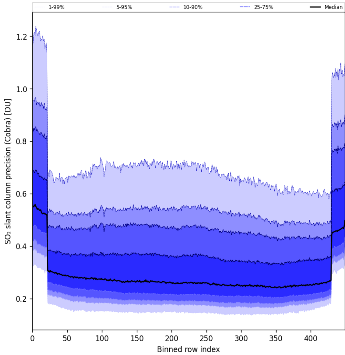
Figure 88: Along track statistics of “SO 2 slant column precision (Cobra)” for 2025-09-01 to 2025-09-03
