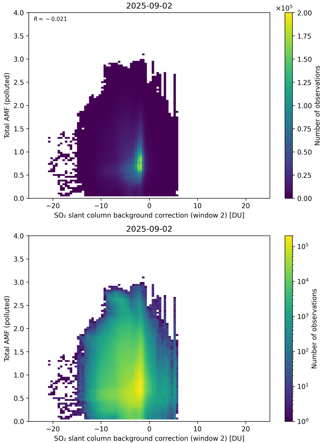
Figure 130: Scatter density plot of “SO 2 slant column background correction (window 2)” against “Total AMF (polluted)” for 2025-09-01 to 2025-09-03.
