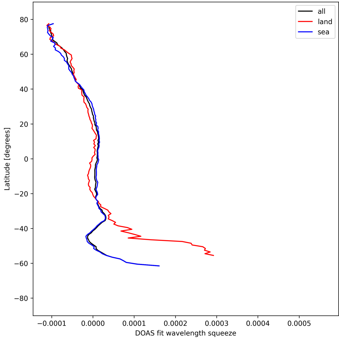
Figure 51: Zonal average of “DOAS fit wavelength squeeze” for 2025-09-01 to 2025-09-03.
