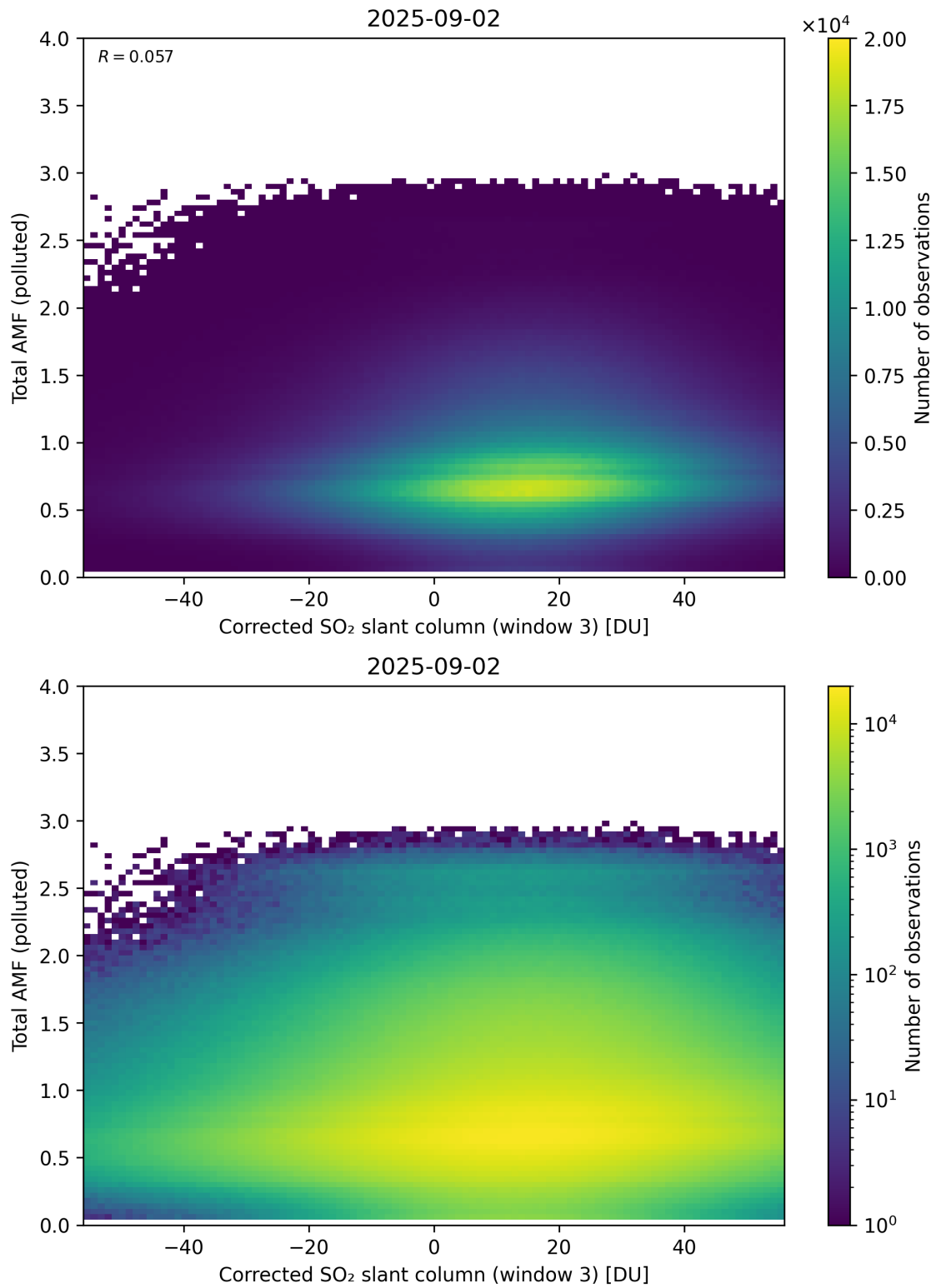
Figure 260: Scatter density plot of “Corrected SO 2 slant column (window 3)” against “Total AMF (polluted)” for 2025-09-01 to 2025-09-03.
