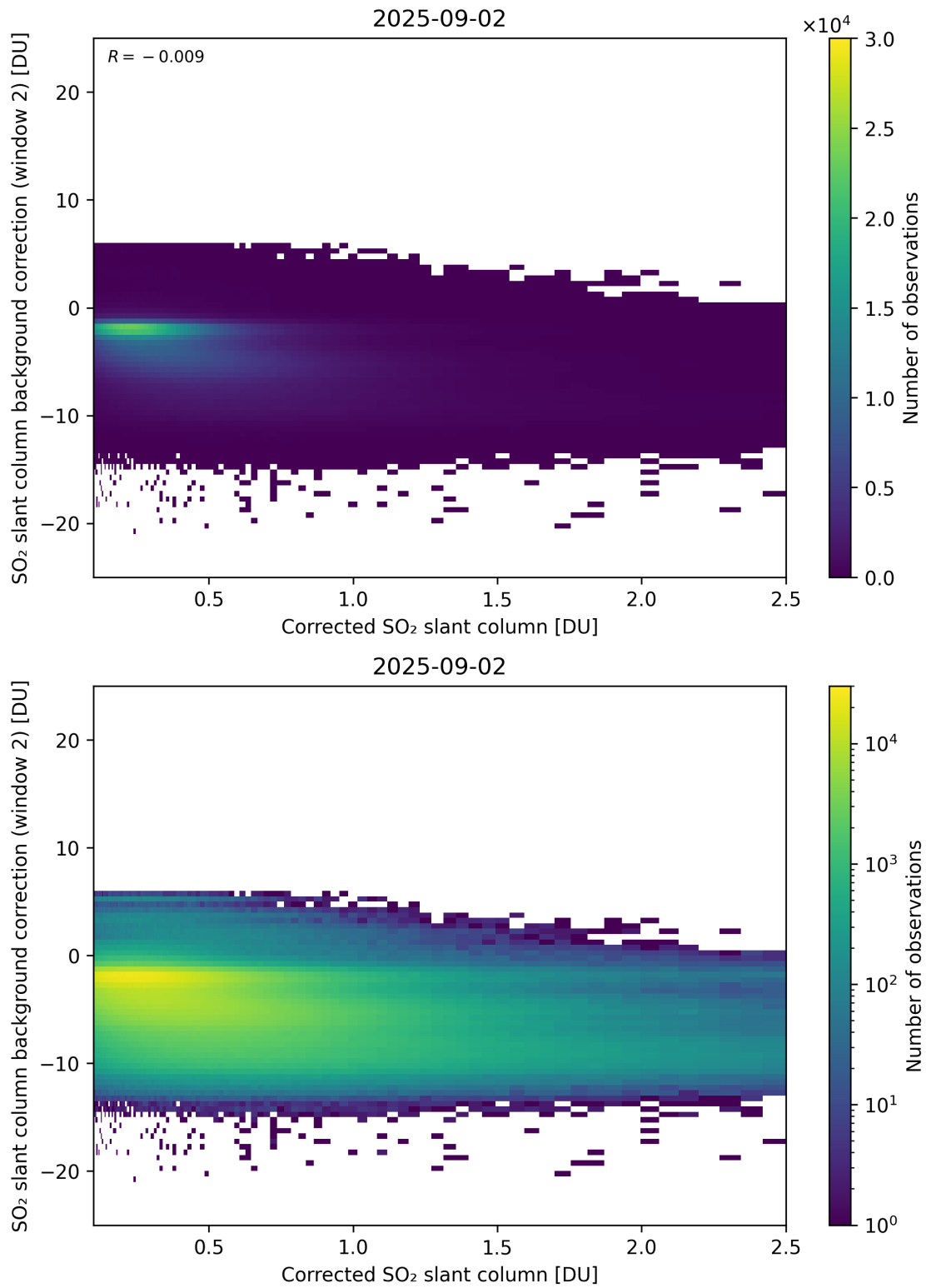
Figure 227: Scatter density plot of “Corrected SO 2 slant column” against “SO 2 slant column background correction (window 2)” for 2025-09-01 to 2025-09-03.
