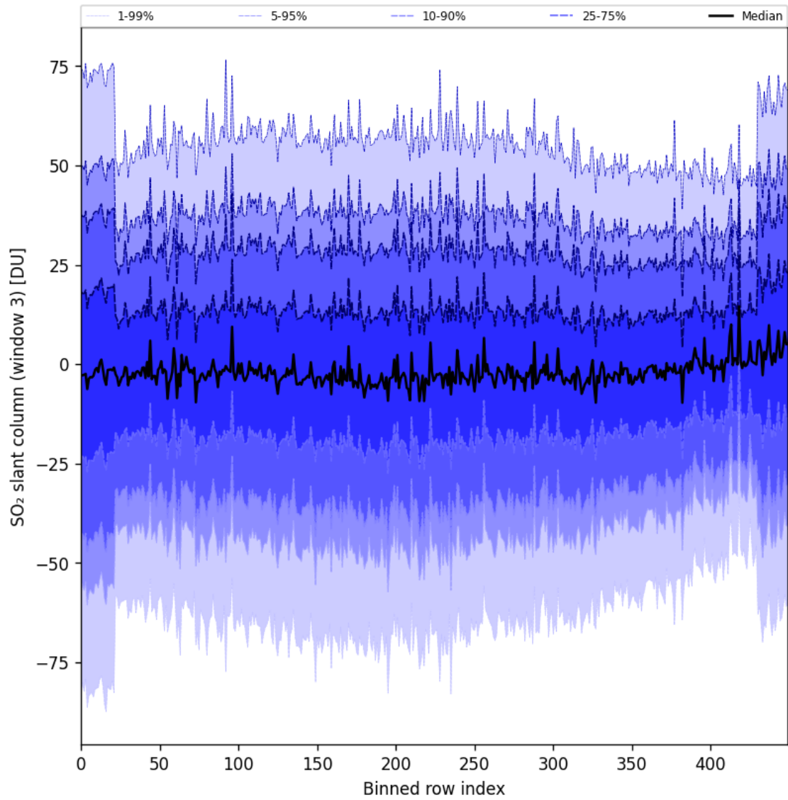
Figure 97: Along track statistics of “SO 2 slant column (window 3)” for 2025-09-01 to 2025-09-03
