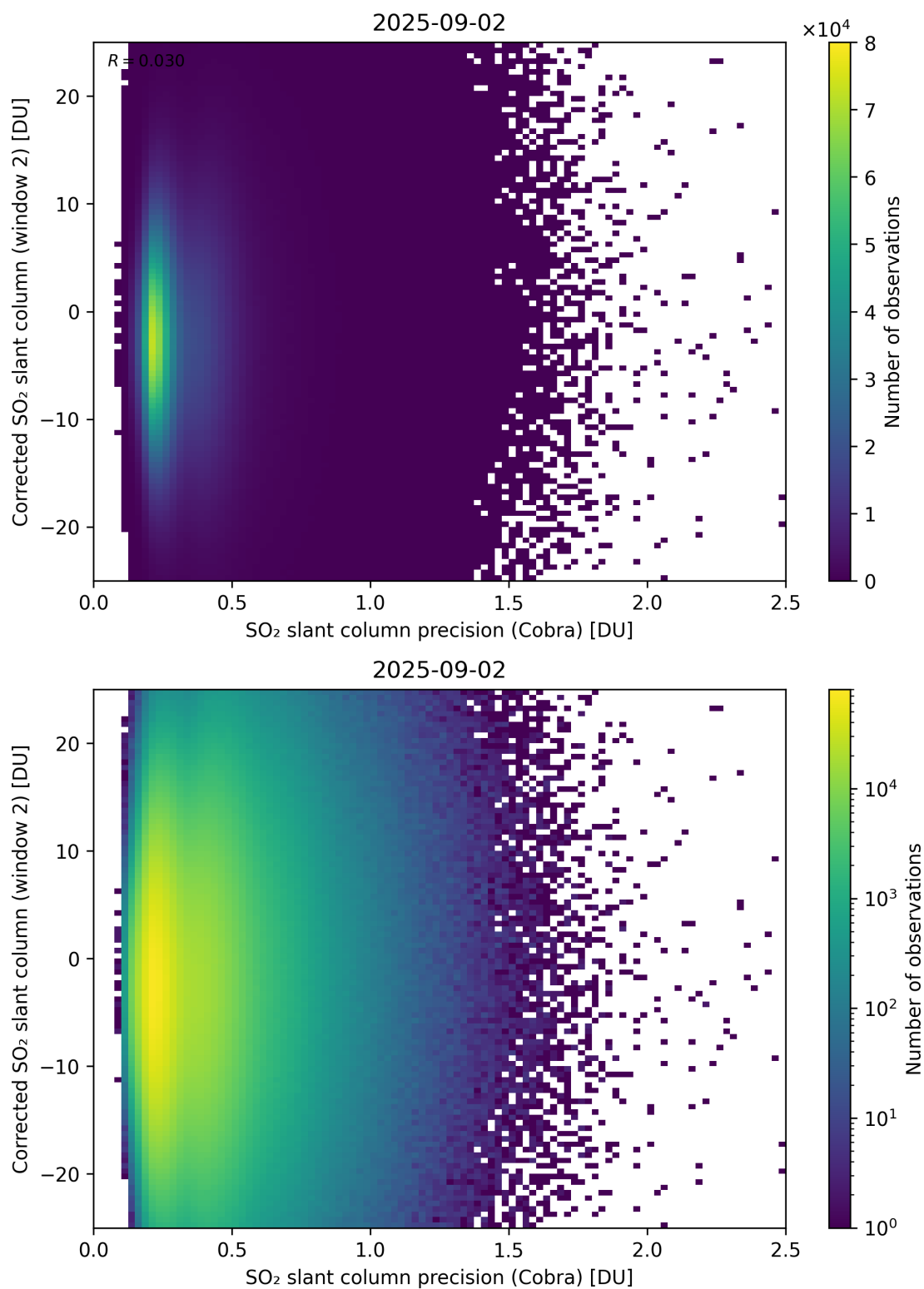
Figure 206: Scatter density plot of “SO 2 slant column precision (Cobra)” against “Corrected SO 2 slant column (window 2)” for 2025-09-01 to 2025-09-03.
