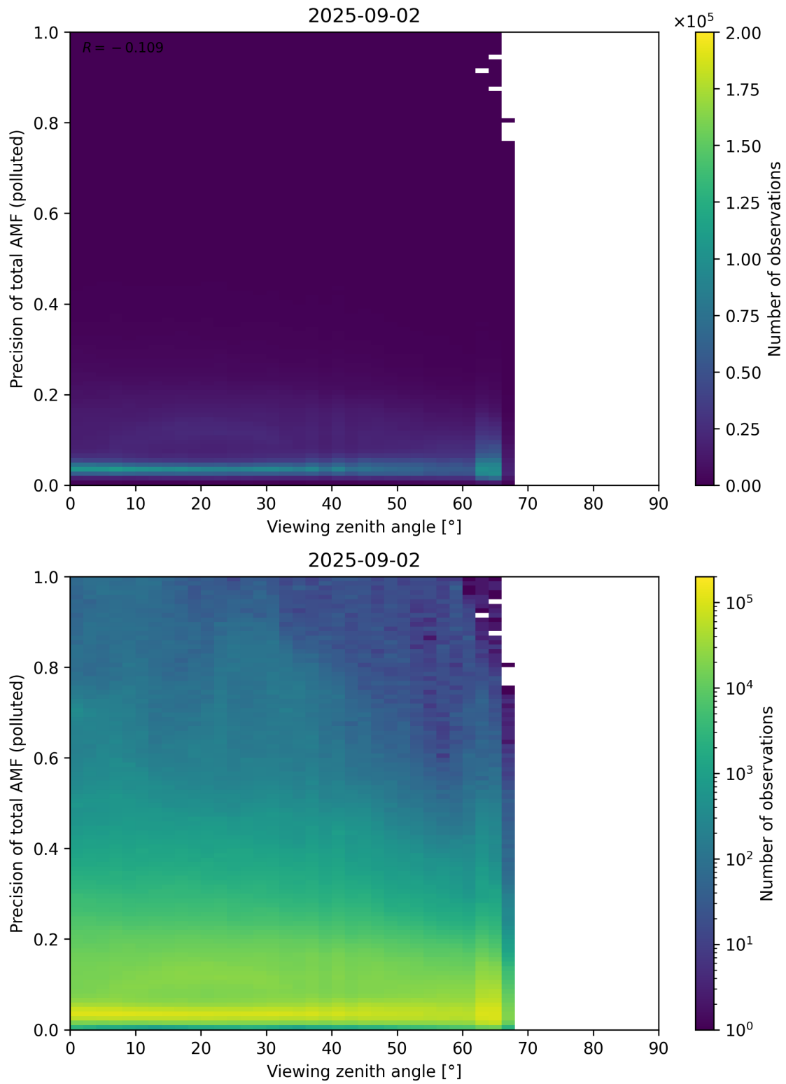
Figure 382: Scatter density plot of “Viewing zenith angle” against “Precision of total AMF (polluted)” for 2025-09-01 to 2025-09-03.
