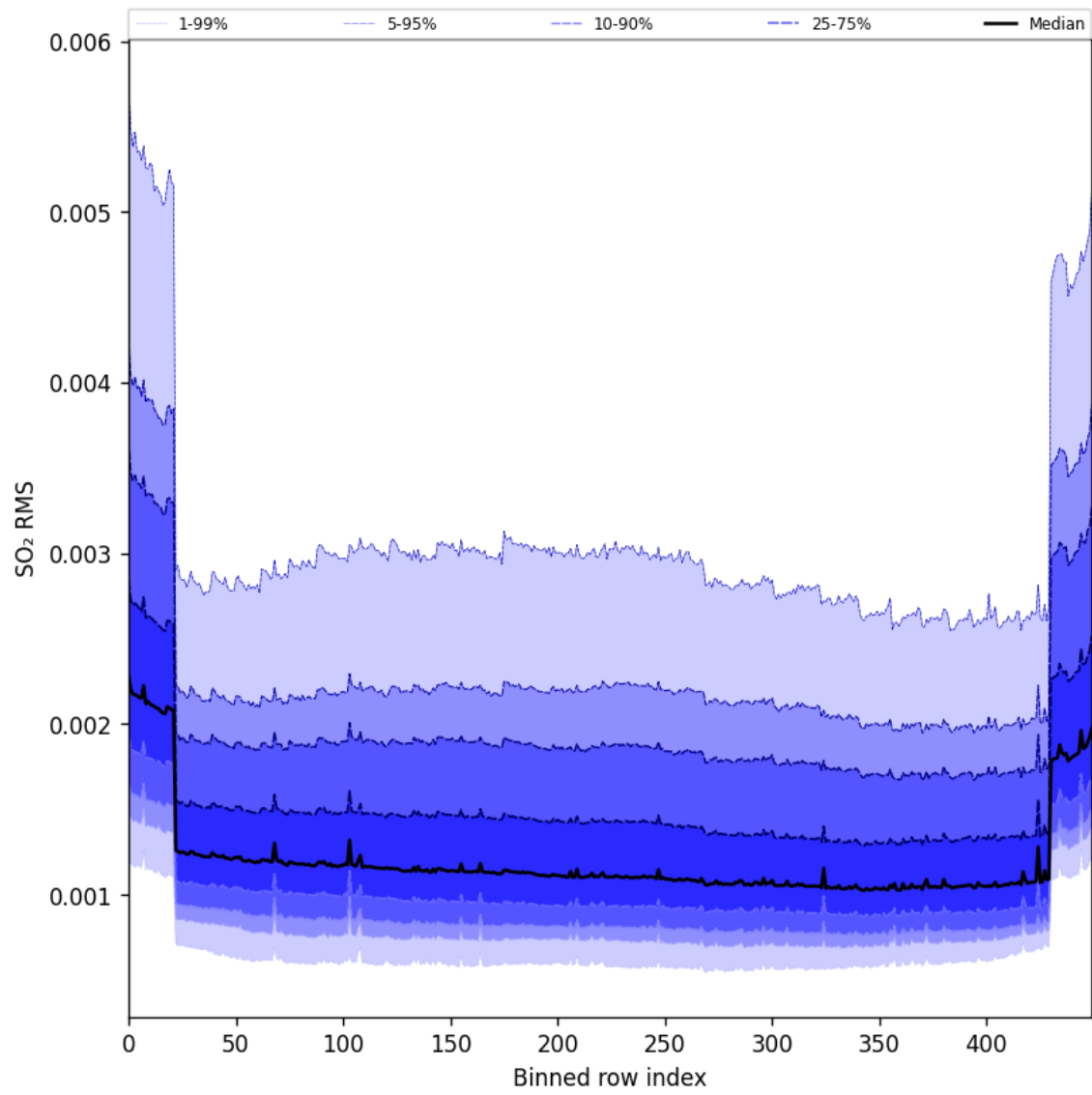
Figure 104: Along track statistics of “SO 2 RMS” for 2025-09-01 to 2025-09-03
