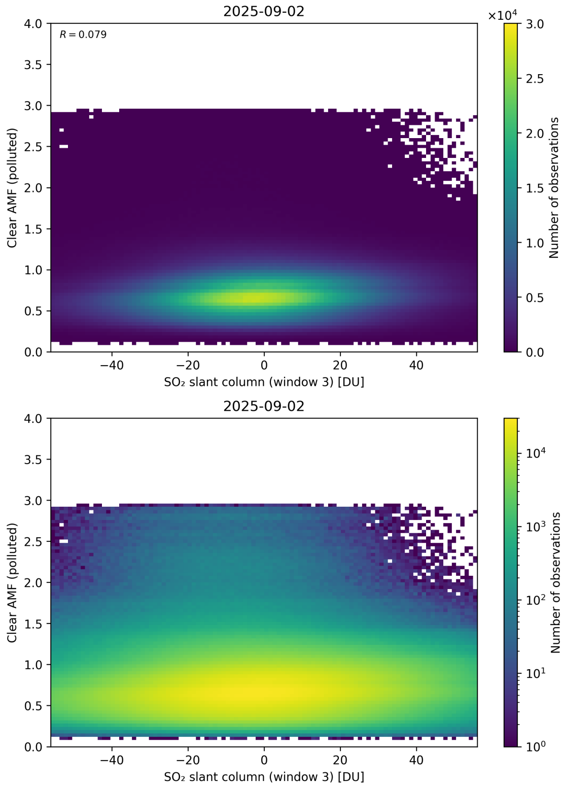
Figure 315: Scatter density plot of “SO 2 slant column (window 3)” against “Clear AMF (polluted)” for 2025-09-01 to 2025-09-03.
