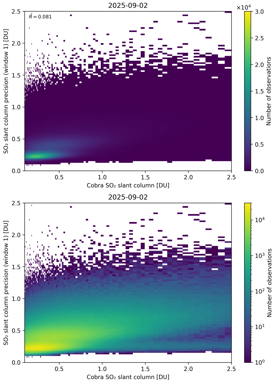
Figure 220: Scatter density plot of “Cobra SO 2 slant column” against “SO 2 slant column precision (window 1)” for 2025-09-01 to 2025-09-03.
