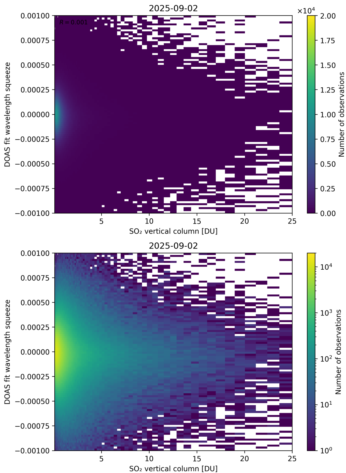
Figure 327: Scatter density plot of “SO 2 vertical column” against “DOAS fit wavelength squeeze” for 2025-09-01 to 2025-09-03.
