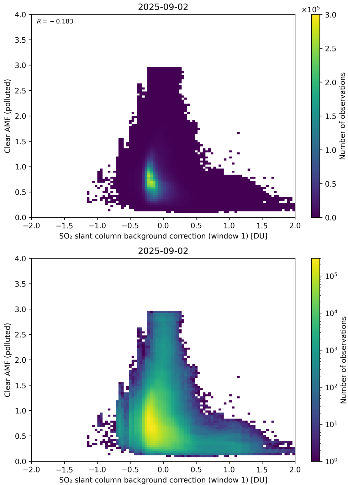
Figure 114: Scatter density plot of “SO 2 slant column background correction (window 1)” against “Clear AMF (polluted)” for 2025-09-01 to 2025-09-03.
