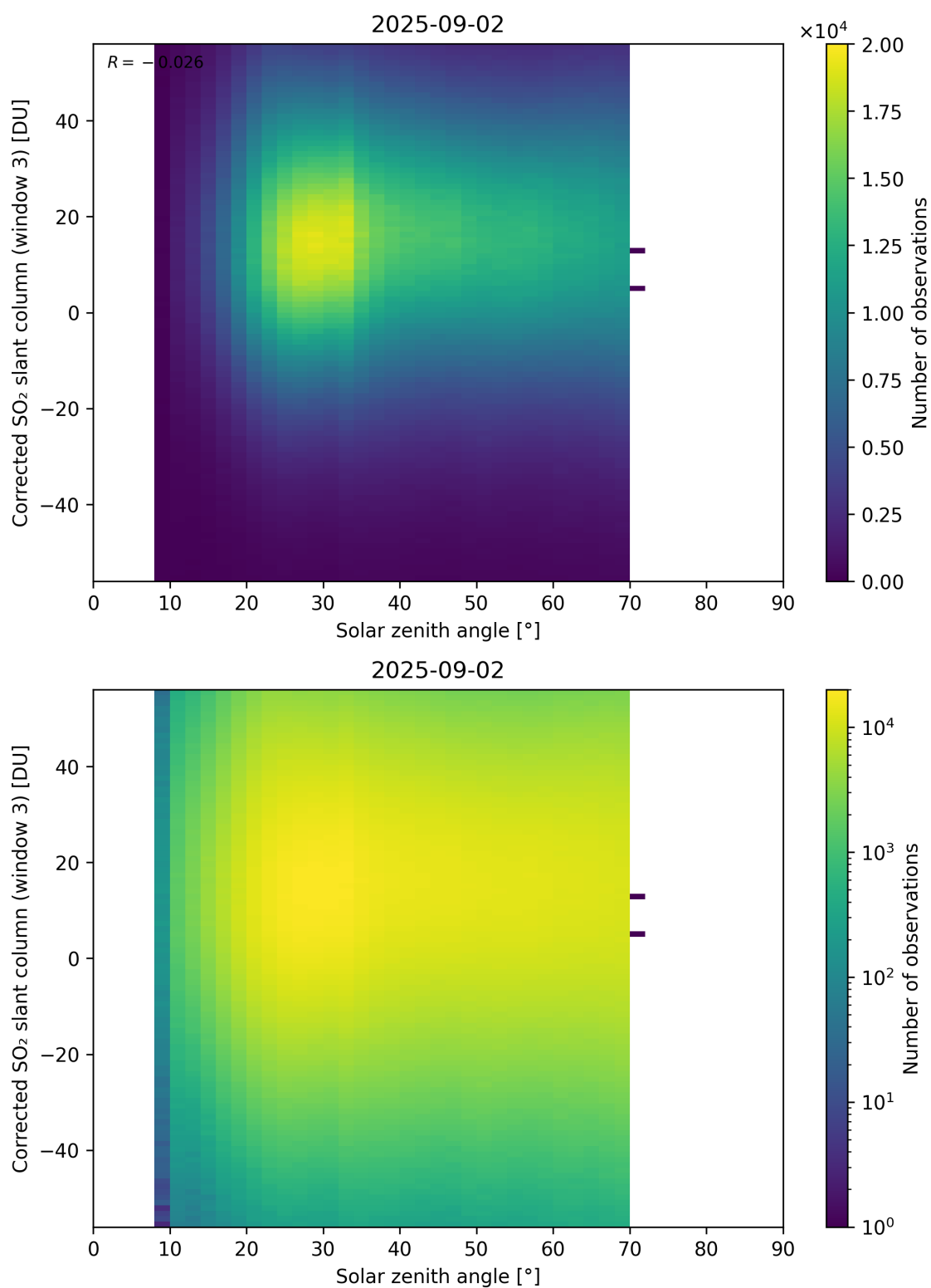
Figure 183: Scatter density plot of “Solar zenith angle” against “Corrected SO 2 slant column (window 3)” for 2025-09-01 to 2025-09-03.
