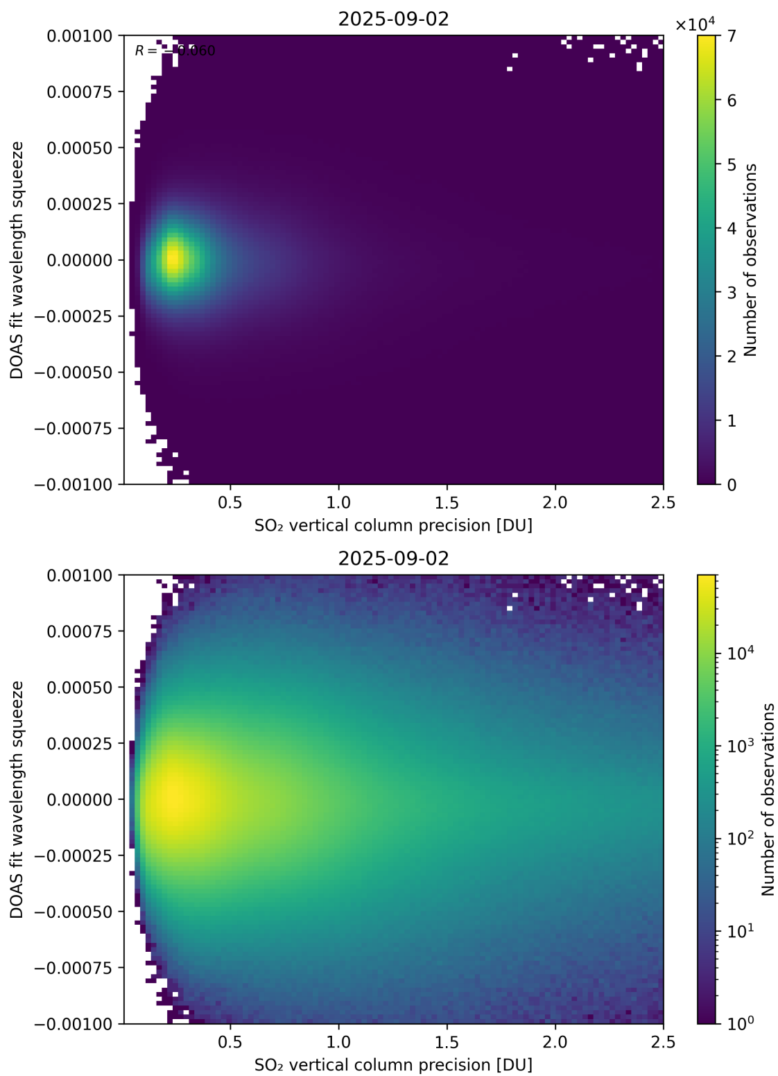
Figure 333: Scatter density plot of “SO 2 vertical column precision” against “DOAS fit wavelength squeeze” for 2025-09-01 to 2025-09-03.
