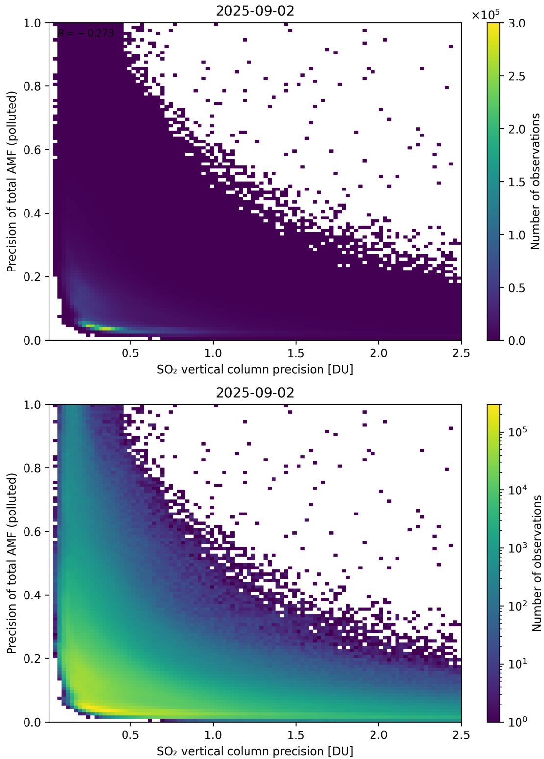
Figure 347: Scatter density plot of “SO 2 vertical column precision” against “Precision of total AMF (polluted)” for 2025-09-01 to 2025-09-03.
