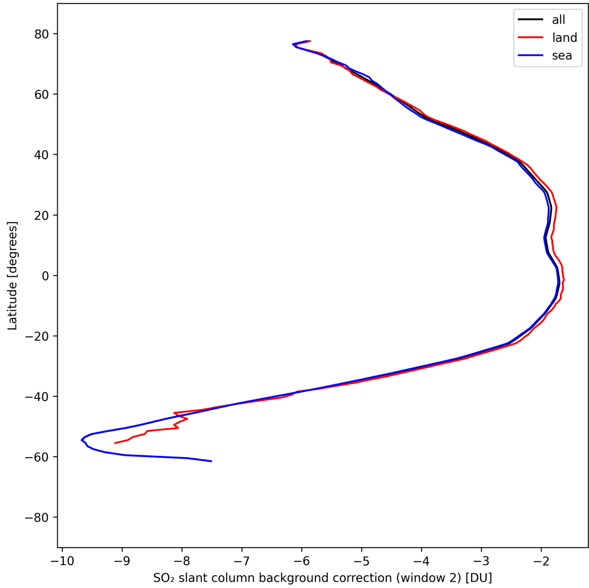
Figure 44: Zonal average of “SO 2 slant column background correction (window 2)” for 2025-09-01 to 2025-09-03.
