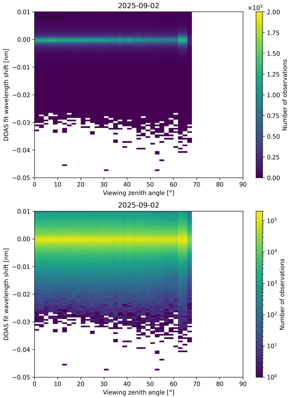
Figure 365: Scatter density plot of “Viewing zenith angle” against “DOAS fit wavelength shift” for 2025-09-01 to 2025-09-03.
