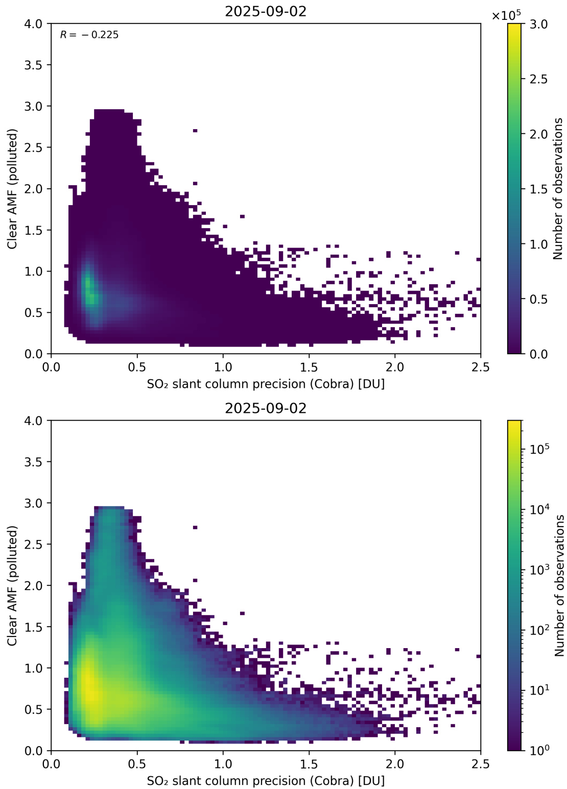
Figure 205: Scatter density plot of “SO 2 slant column precision (Cobra)” against “Clear AMF (polluted)” for 2025-09-01 to 2025-09-03.
