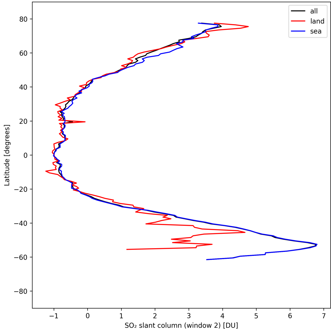
Figure 41: Zonal average of “SO 2 slant column (window 2)” for 2025-09-01 to 2025-09-03.
