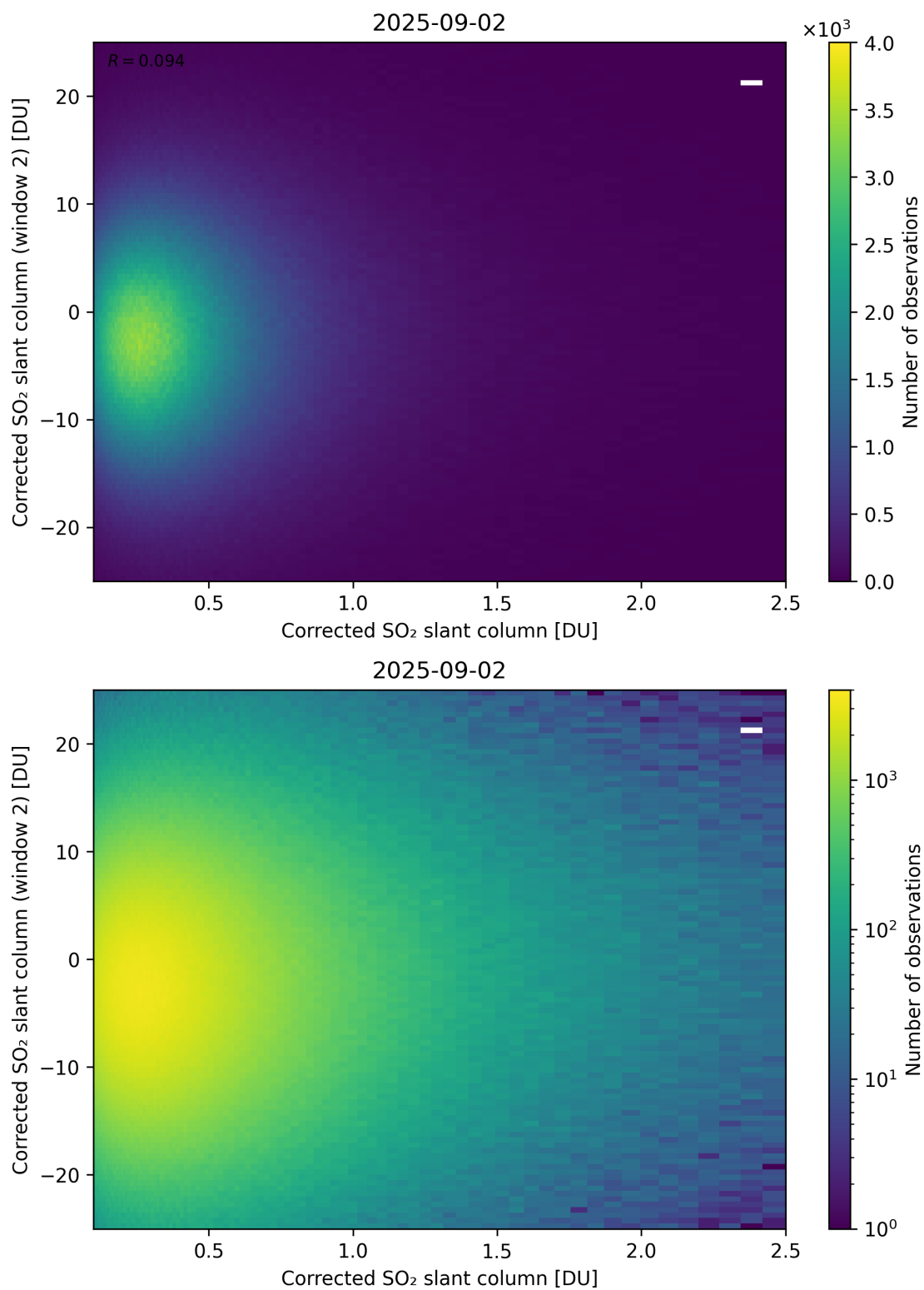
Figure 235: Scatter density plot of “Corrected SO 2 slant column” against “Corrected SO 2 slant column (window 2)” for 2025-09-01 to 2025-09-03.
