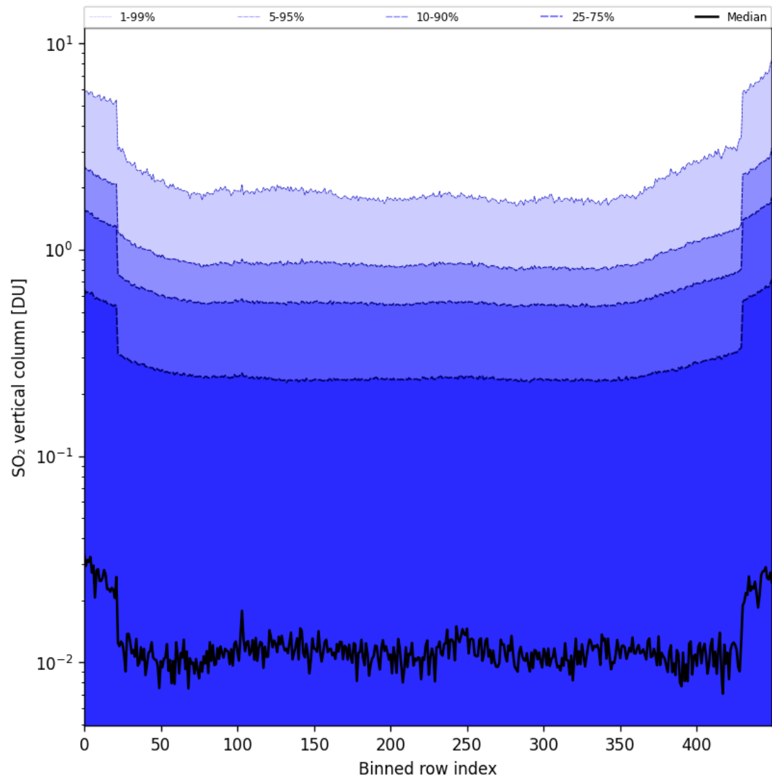
Figure 84: Along track statistics of “SO 2 vertical column” for 2025-09-01 to 2025-09-03
