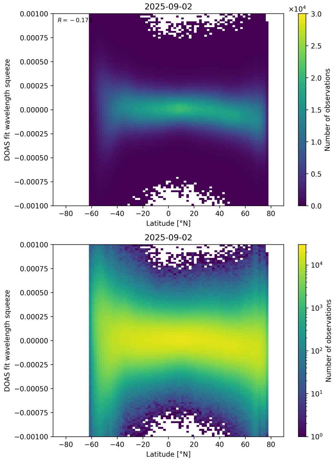
Figure 154: Scatter density plot of “Latitude” against “DOAS fit wavelength squeeze” for 2025-09-01 to 2025-09-03.
