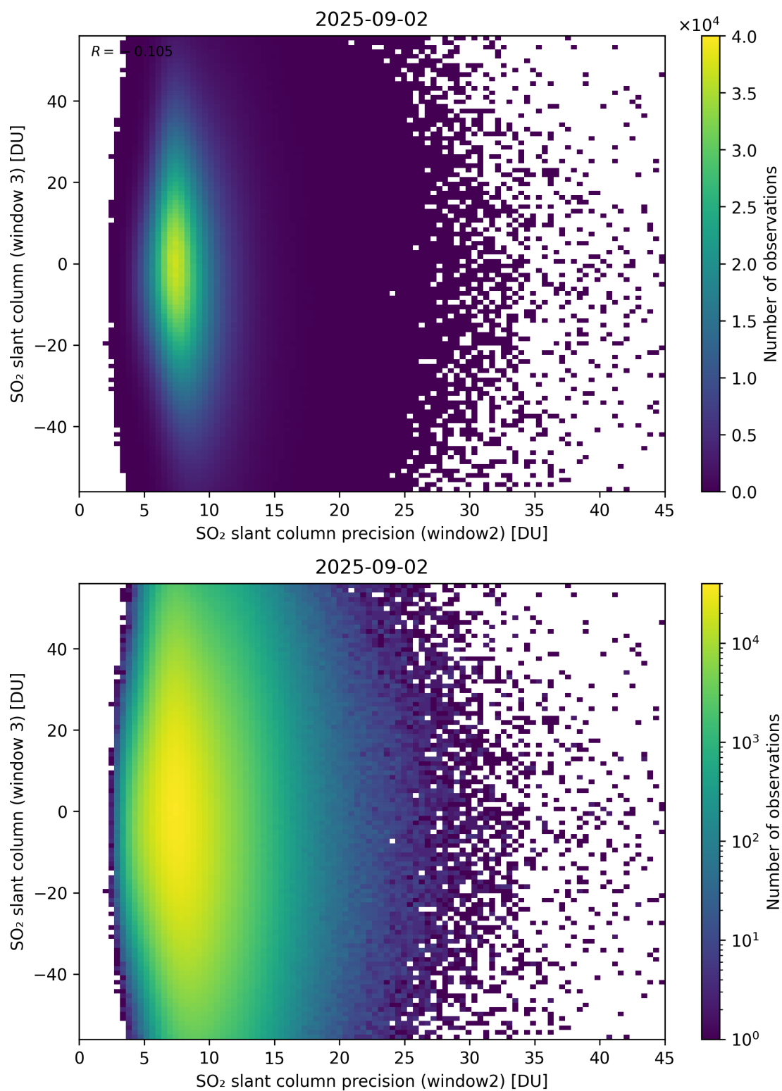
Figure 299: Scatter density plot of “SO 2 slant column precision (window2)” against “SO 2 slant column (window 3)” for 2025-09-01 to 2025-09-03.
