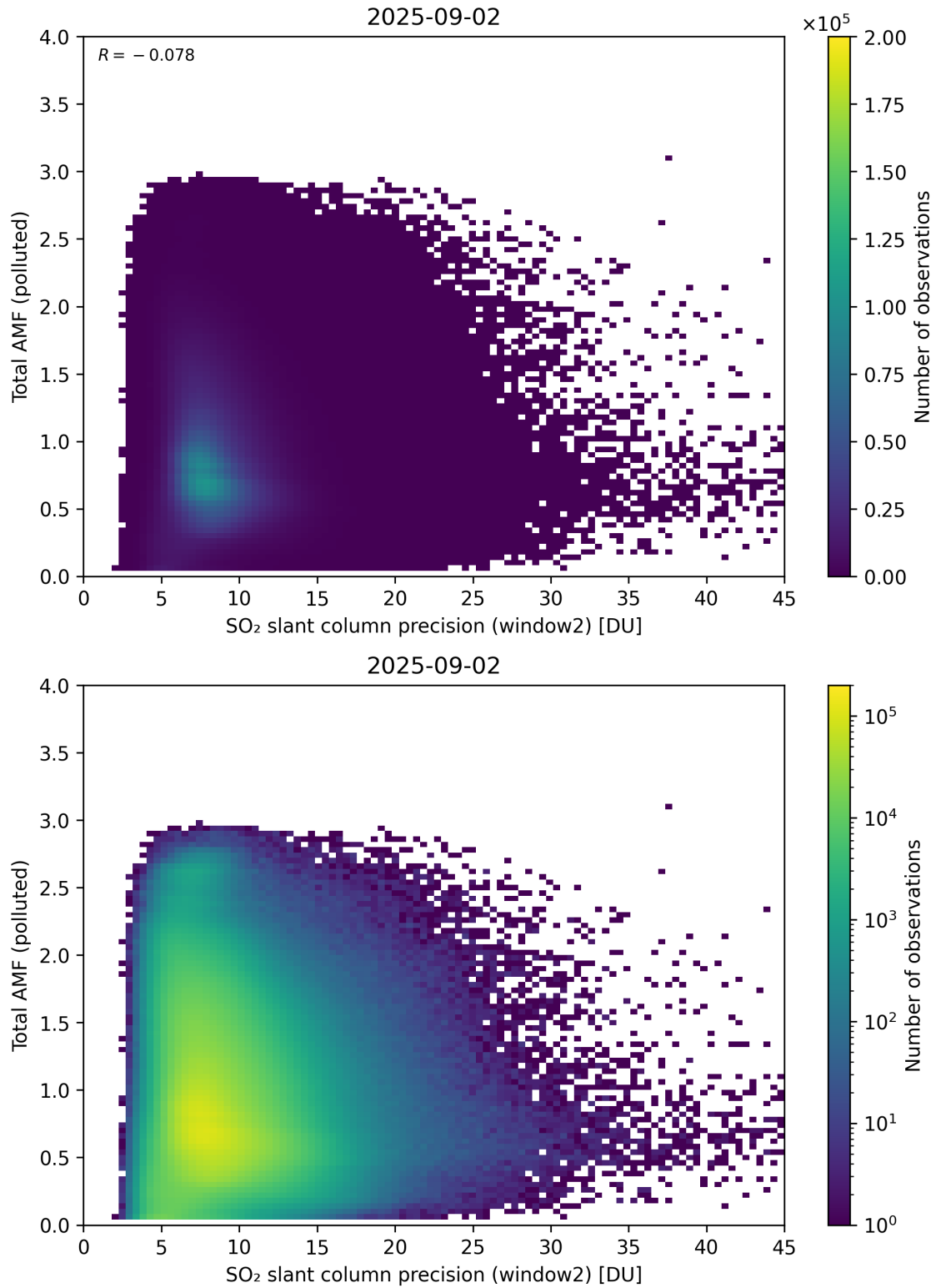
Figure 301: Scatter density plot of “SO 2 slant column precision (window2)” against “Total AMF (polluted)” for 2025-09-01 to 2025-09-03.
