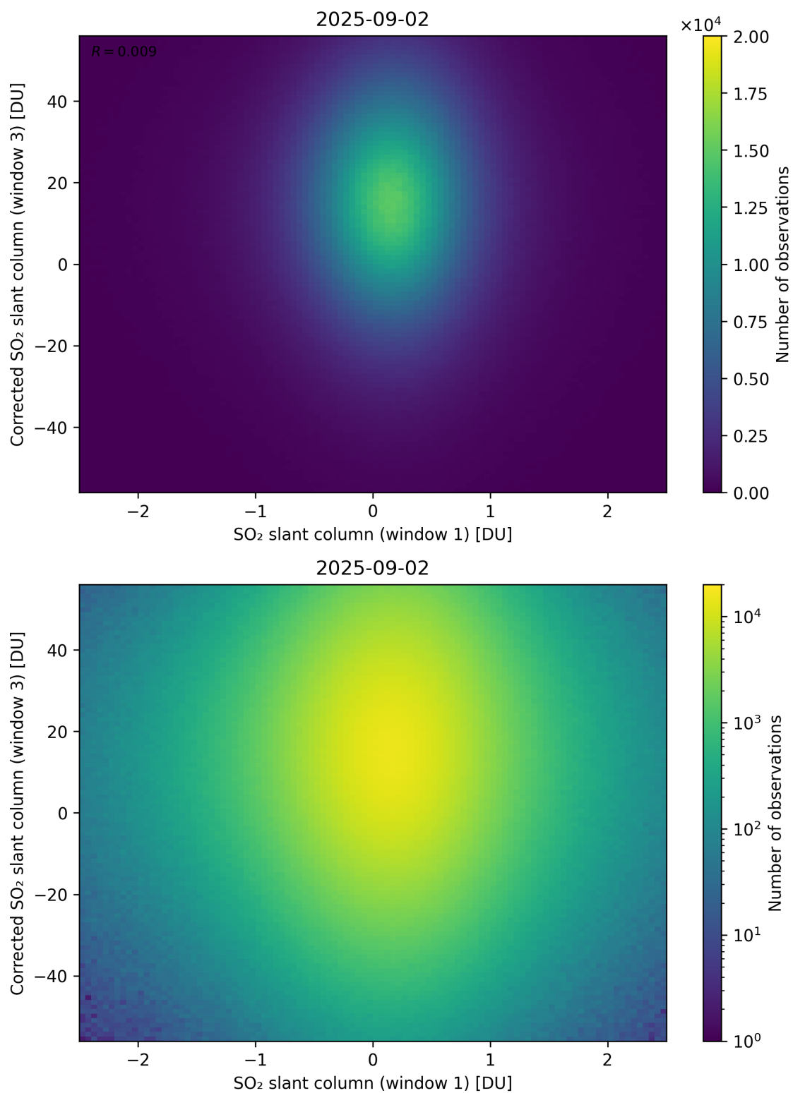
Figure 284: Scatter density plot of “SO 2 slant column (window 1)” against “Corrected SO 2 slant column (window 3)” for 2025-09-01 to 2025-09-03.
