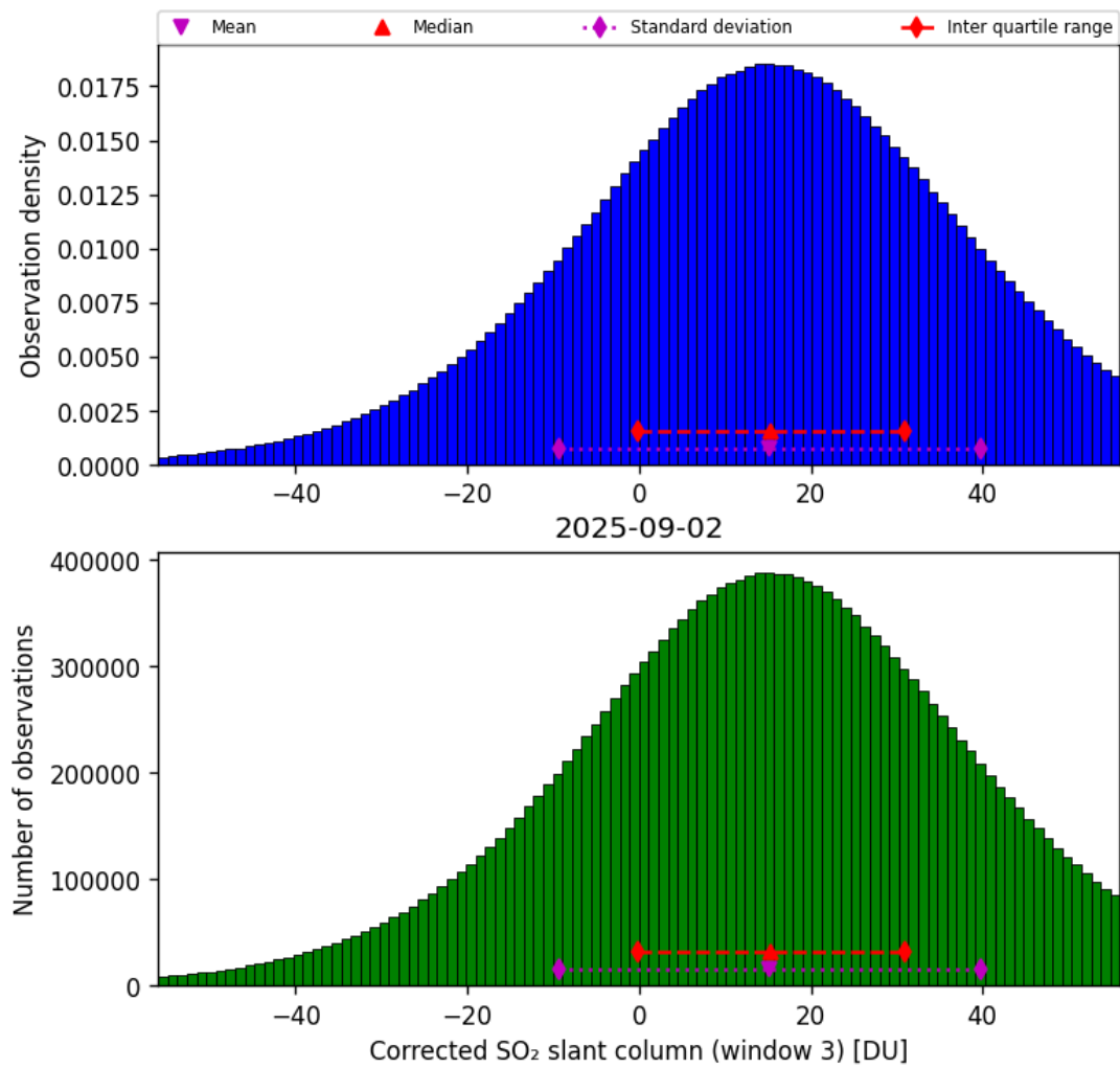
Figure 73: Histogram of “Corrected SO 2 slant column (window 3)” for 2025-09-01 to 2025-09-03
