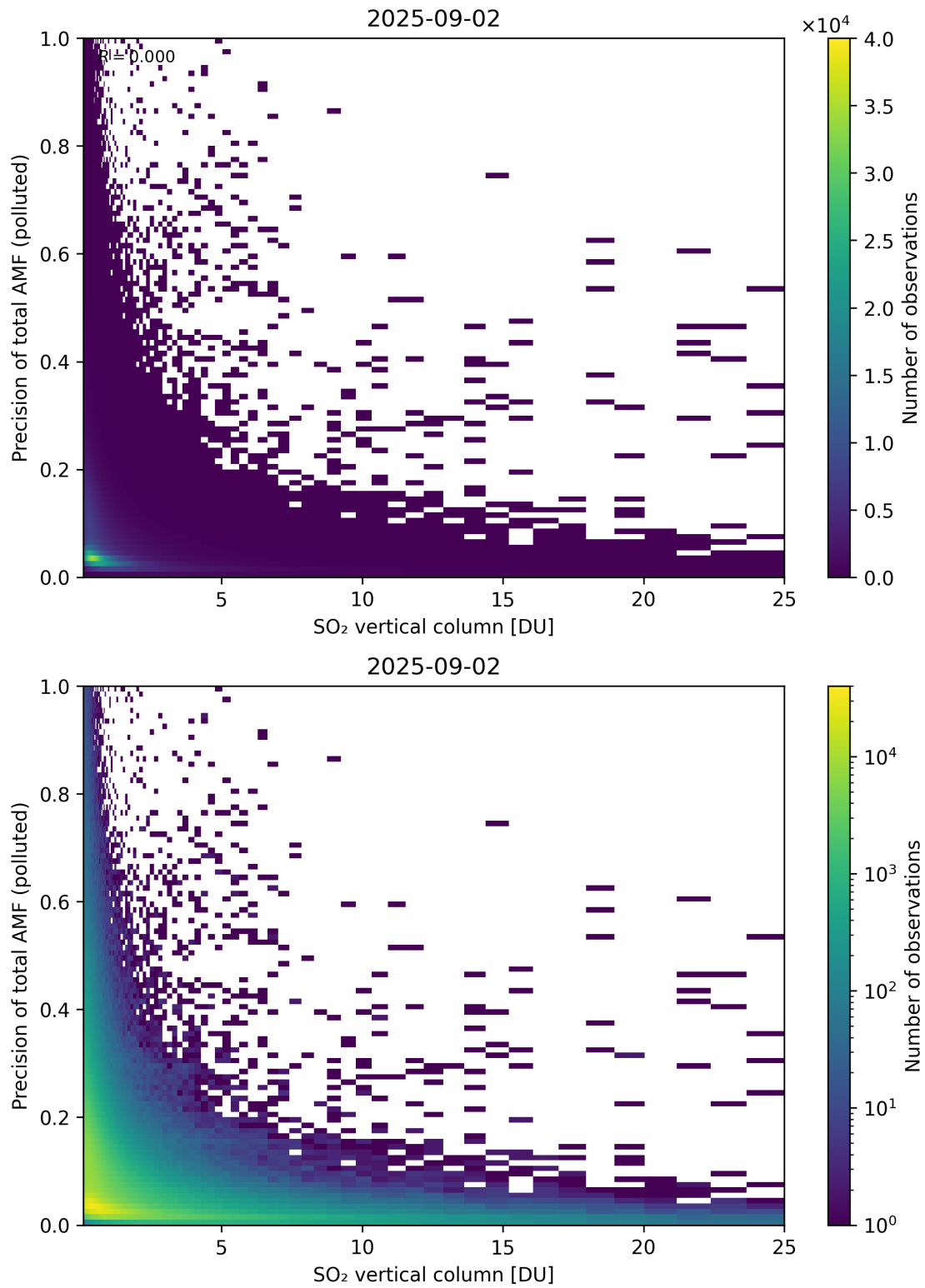
Figure 360: Scatter density plot of “SO 2 vertical column” against “Precision of total AMF (polluted)” for 2025-09-01 to 2025-09-03.
