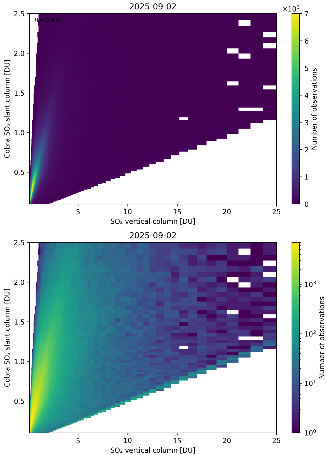
Figure 349: Scatter density plot of “SO 2 vertical column” against “Cobra SO 2 slant column” for 2025-09-01 to 2025-09-03.
