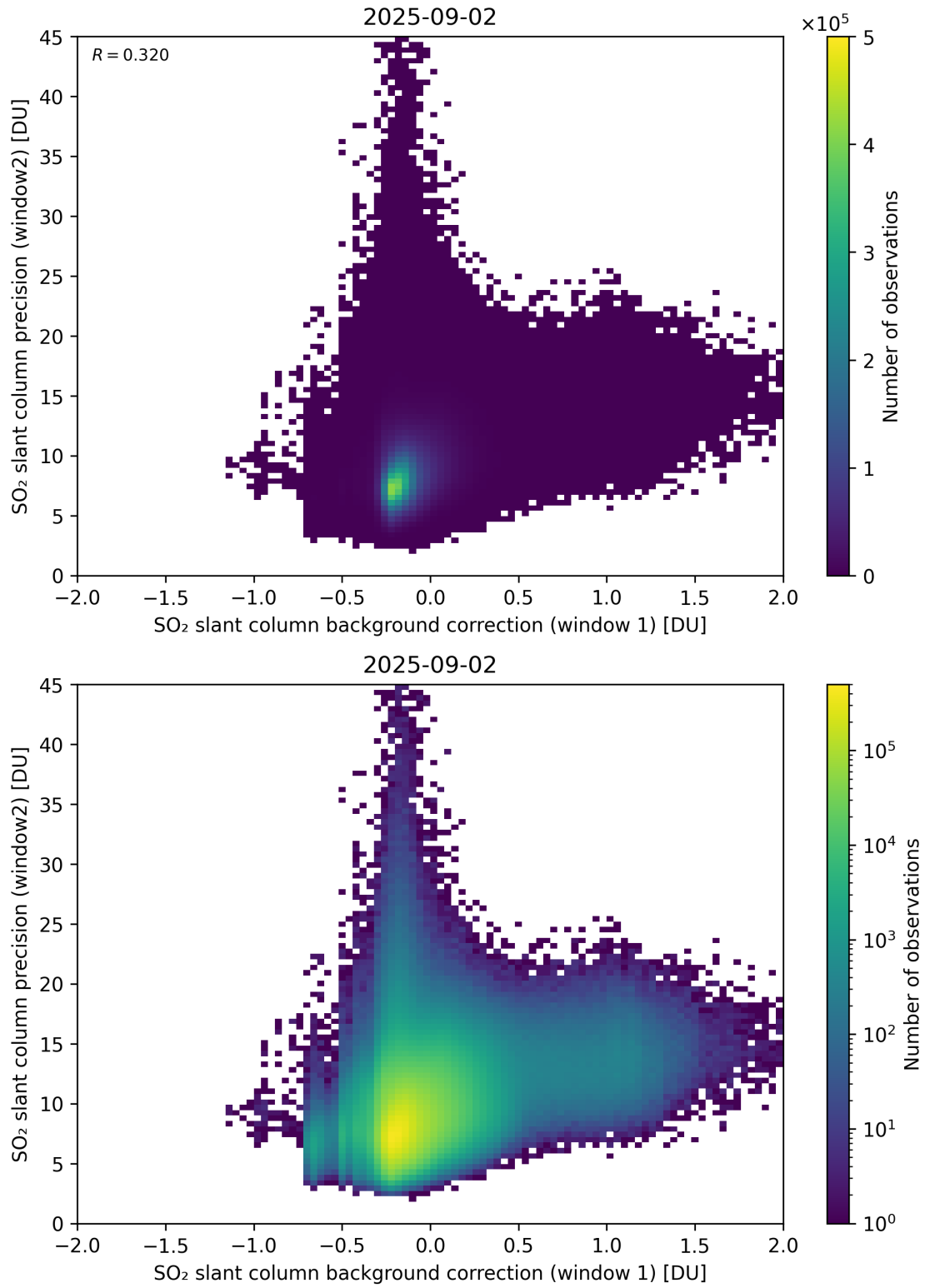
Figure 117: Scatter density plot of “SO 2 slant column background correction (window 1)” against “SO 2 slant column precision (window2)” for 2025-09-01 to 2025-09-03.
