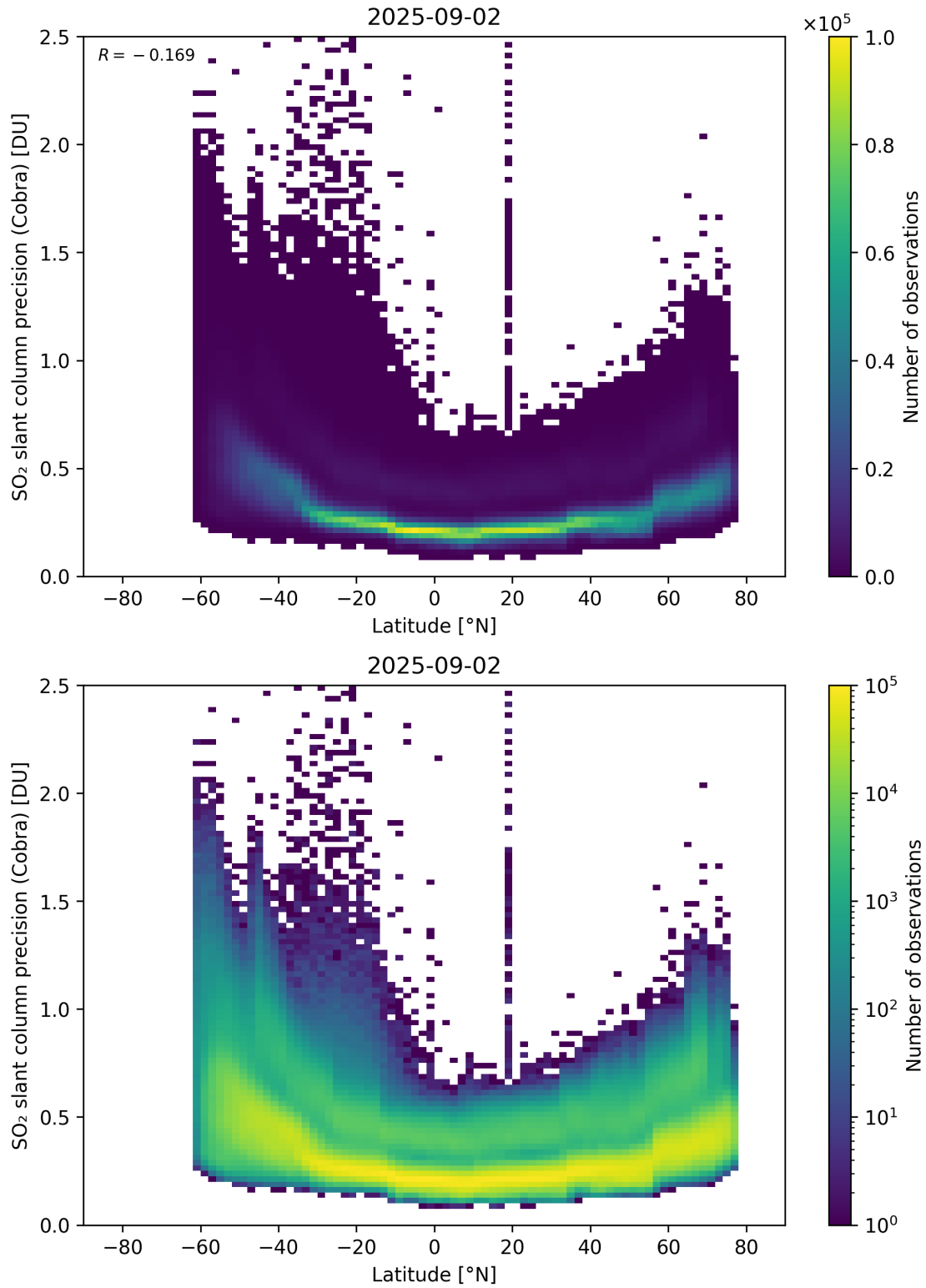
Figure 158: Scatter density plot of “Latitude” against “SO 2 slant column precision (Cobra)” for 2025-09-01 to 2025-09-03.
