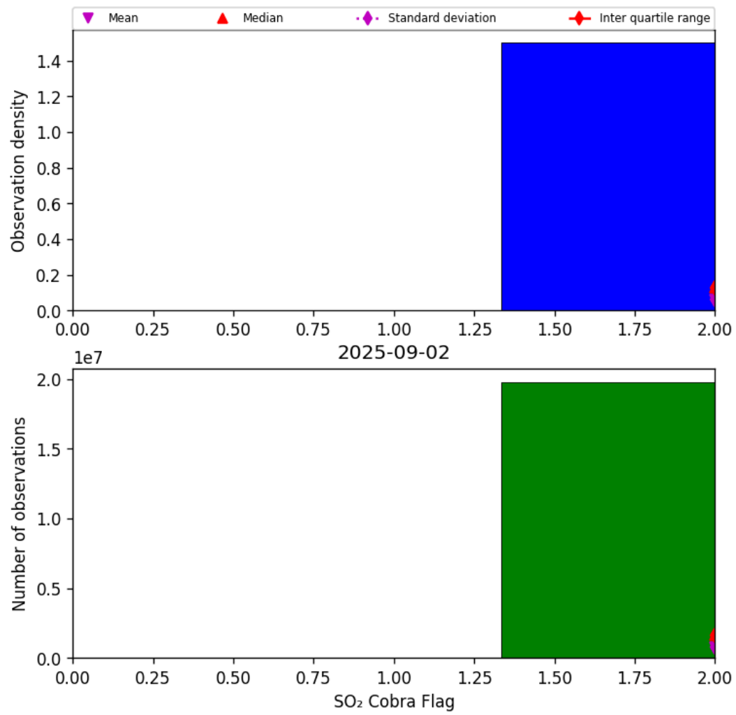
Figure 75: Histogram of “SO 2 Cobra Flag” for 2025-09-01 to 2025-09-03
