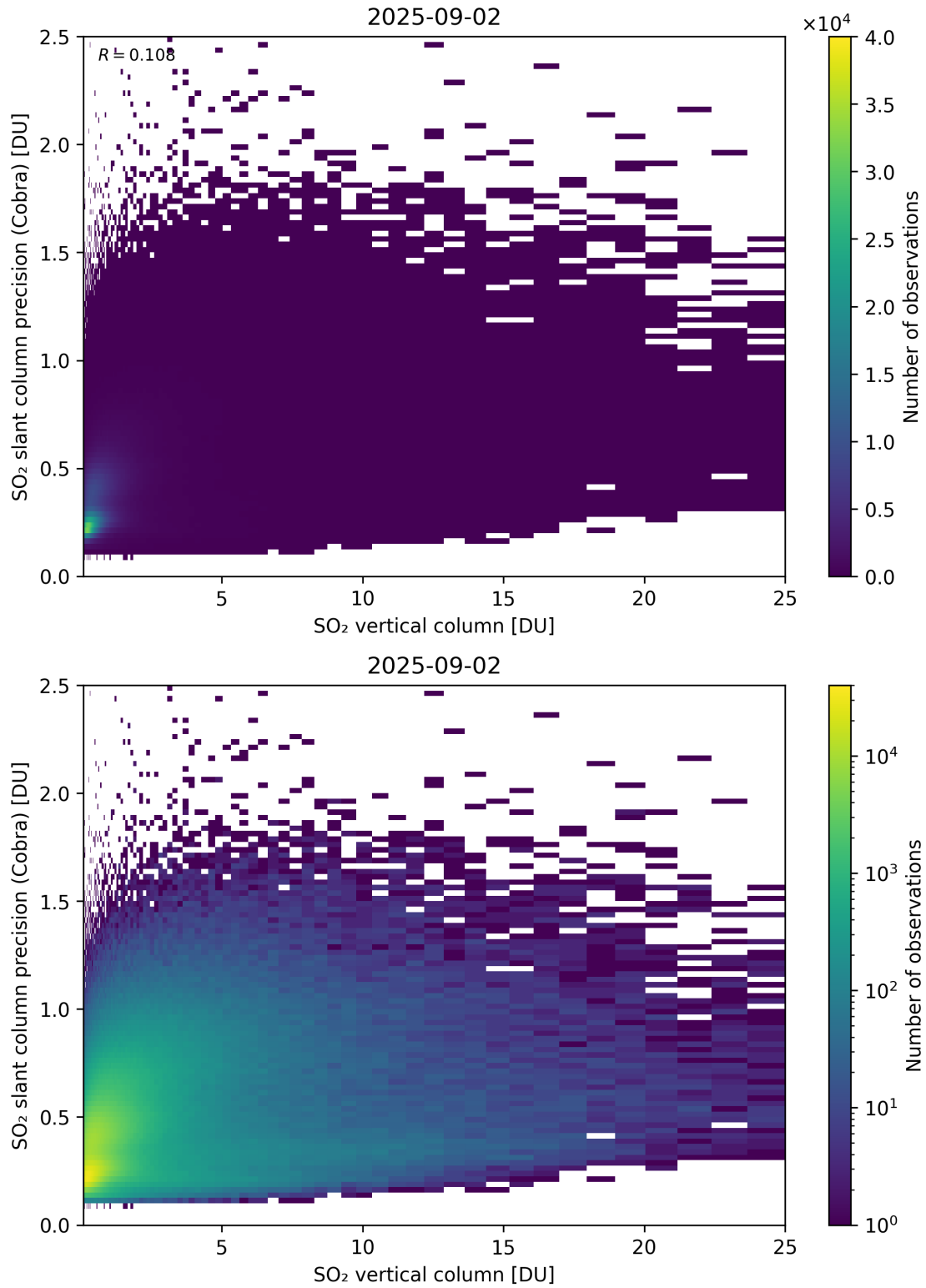
Figure 350: Scatter density plot of “SO 2 vertical column” against “SO 2 slant column precision (Cobra)” for 2025-09-01 to 2025-09-03.
