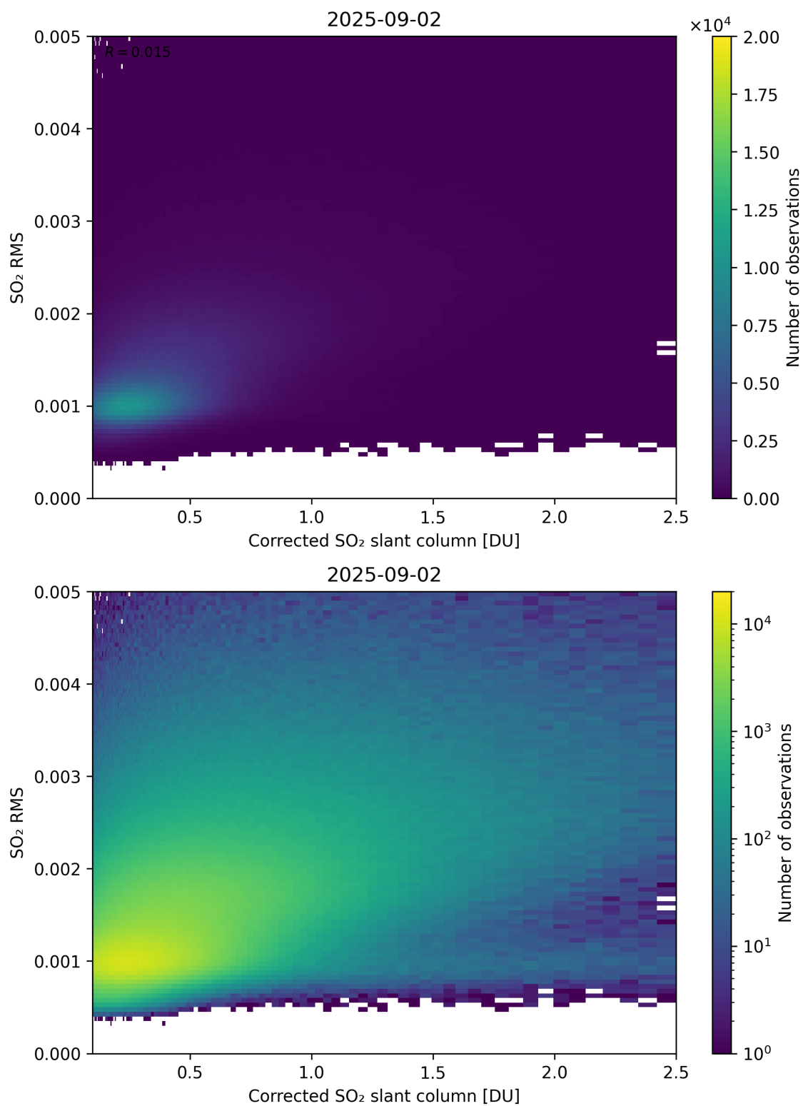
Figure 231: Scatter density plot of “Corrected SO 2 slant column” against “SO 2 RMS” for 2025-09-01 to 2025-09-03.
