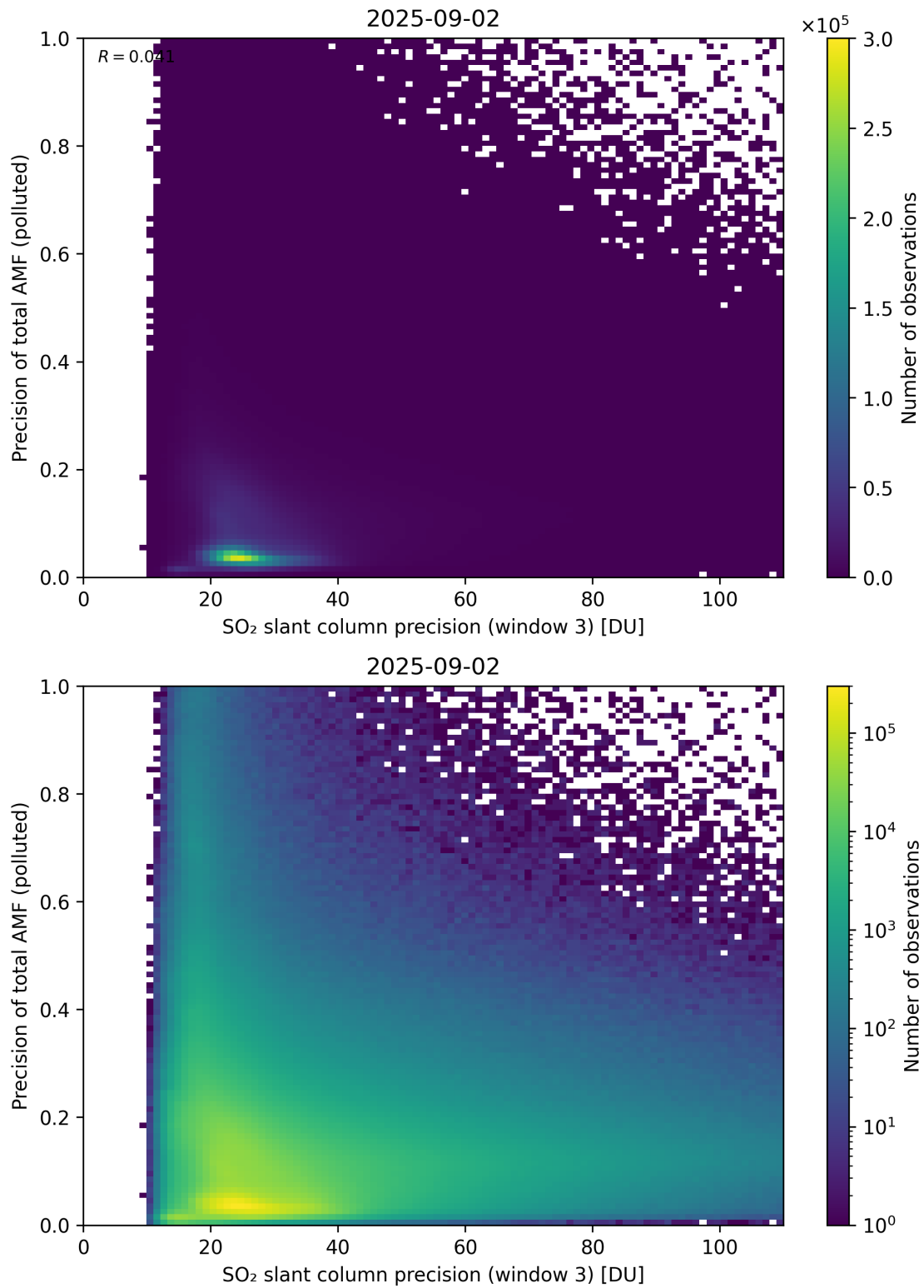
Figure 314: Scatter density plot of “SO 2 slant column precision (window 3)” against “Precision of total AMF (polluted)” for 2025-09-01 to 2025-09-03.
