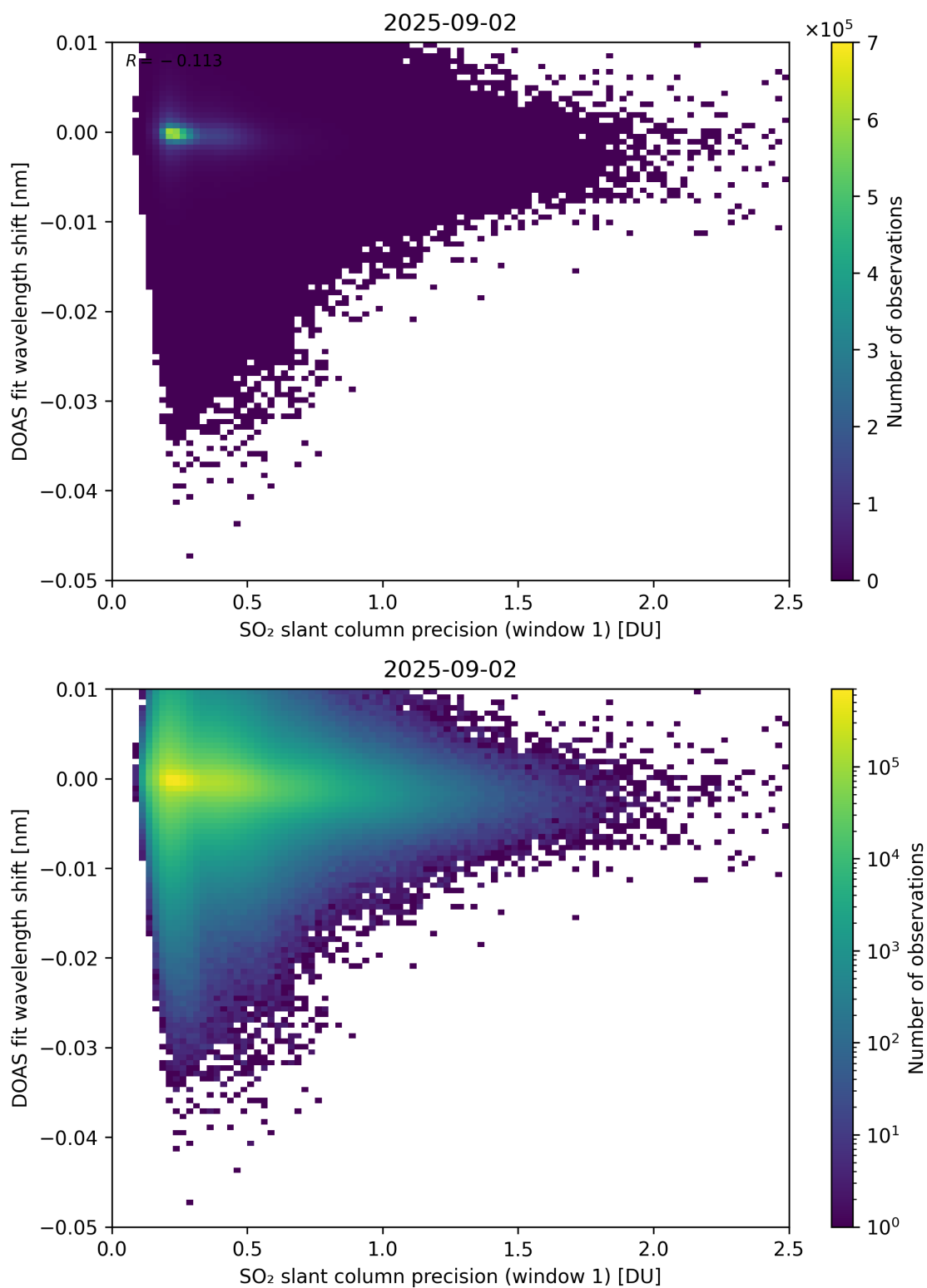
Figure 271: Scatter density plot of “SO 2 slant column precision (window 1)” against “DOAS fit wavelength shift” for 2025-09-01 to 2025-09-03.
