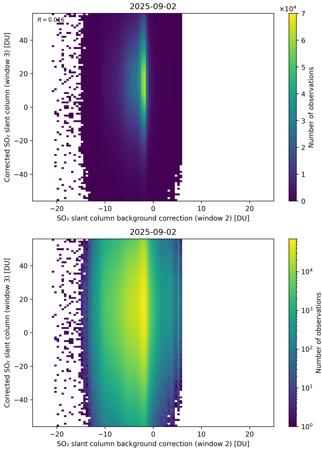
Figure 127: Scatter density plot of “SO 2 slant column background correction (window 2)” against “Corrected SO 2 slant column (window 3)” for 2025-09-01 to 2025-09-03.
