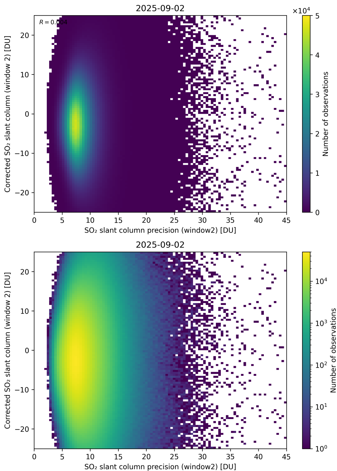
Figure 297: Scatter density plot of “SO 2 slant column precision (window2)” against “Corrected SO 2 slant column (window 2)” for 2025-09-01 to 2025-09-03.
