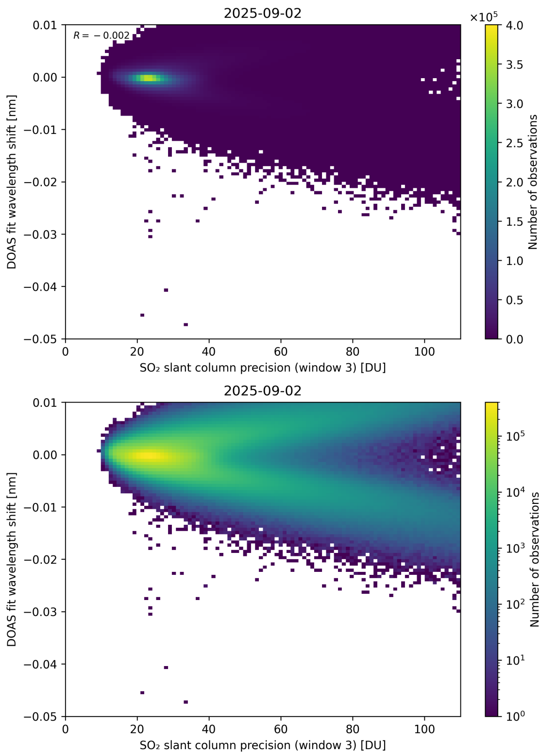
Figure 308: Scatter density plot of “SO 2 slant column precision (window 3)” against “DOAS fit wavelength shift” for 2025-09-01 to 2025-09-03.
