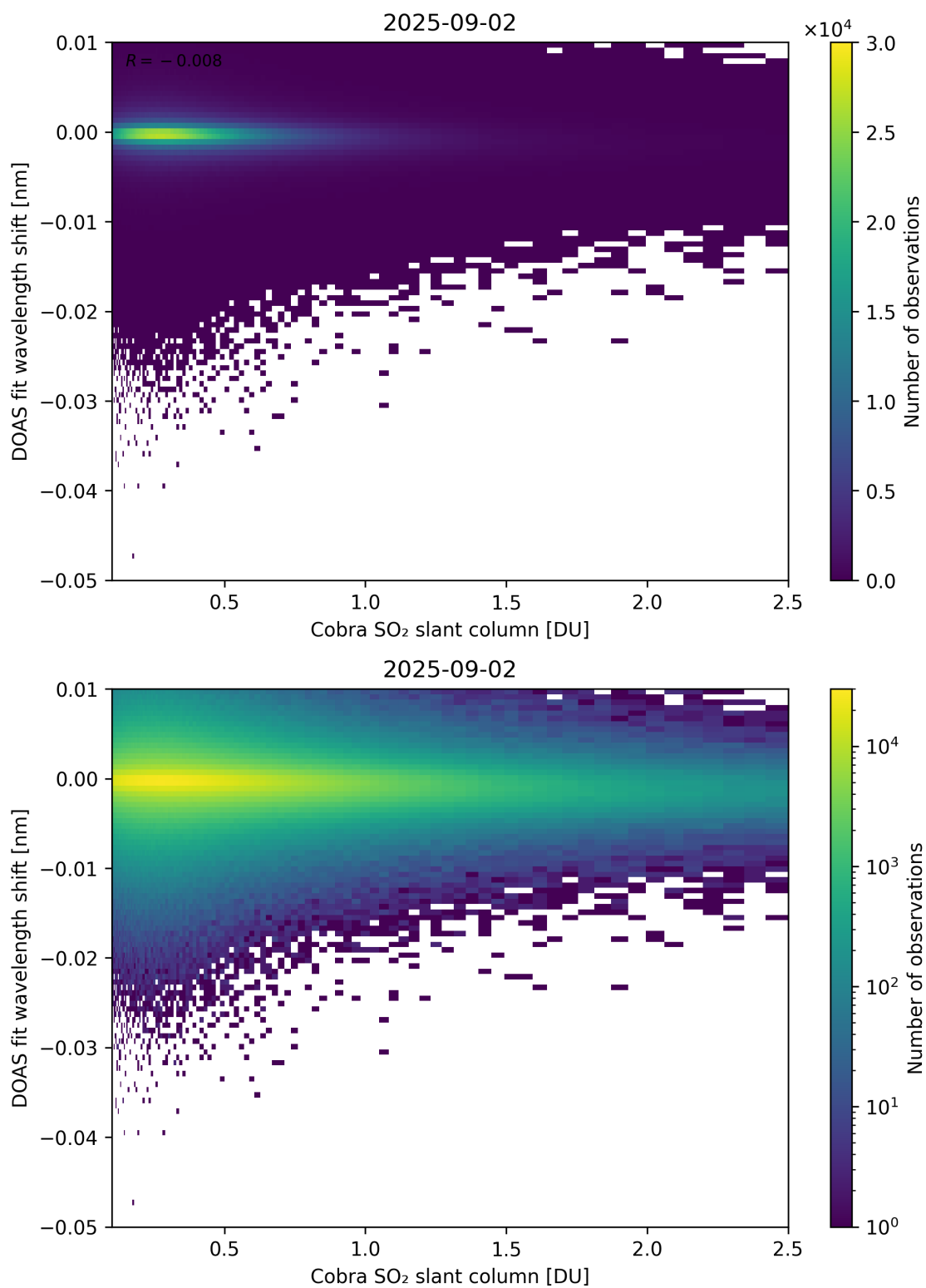
Figure 196: Scatter density plot of “Cobra SO 2 slant column” against “DOAS fit wavelength shift” for 2025-09-01 to 2025-09-03.
