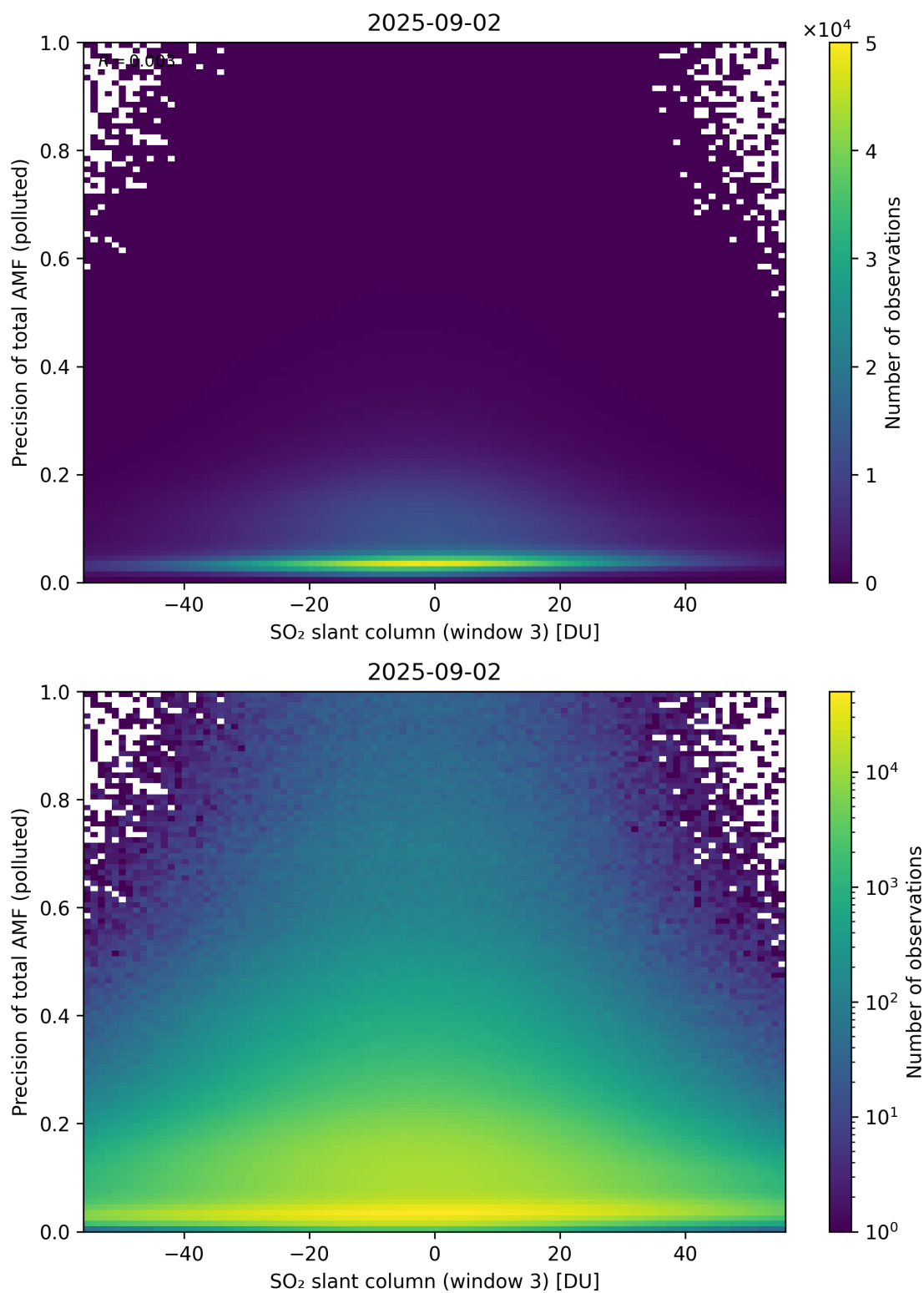
Figure 319: Scatter density plot of “SO 2 slant column (window 3)” against “Precision of total AMF (polluted)” for 2025-09-01 to 2025-09-03.
