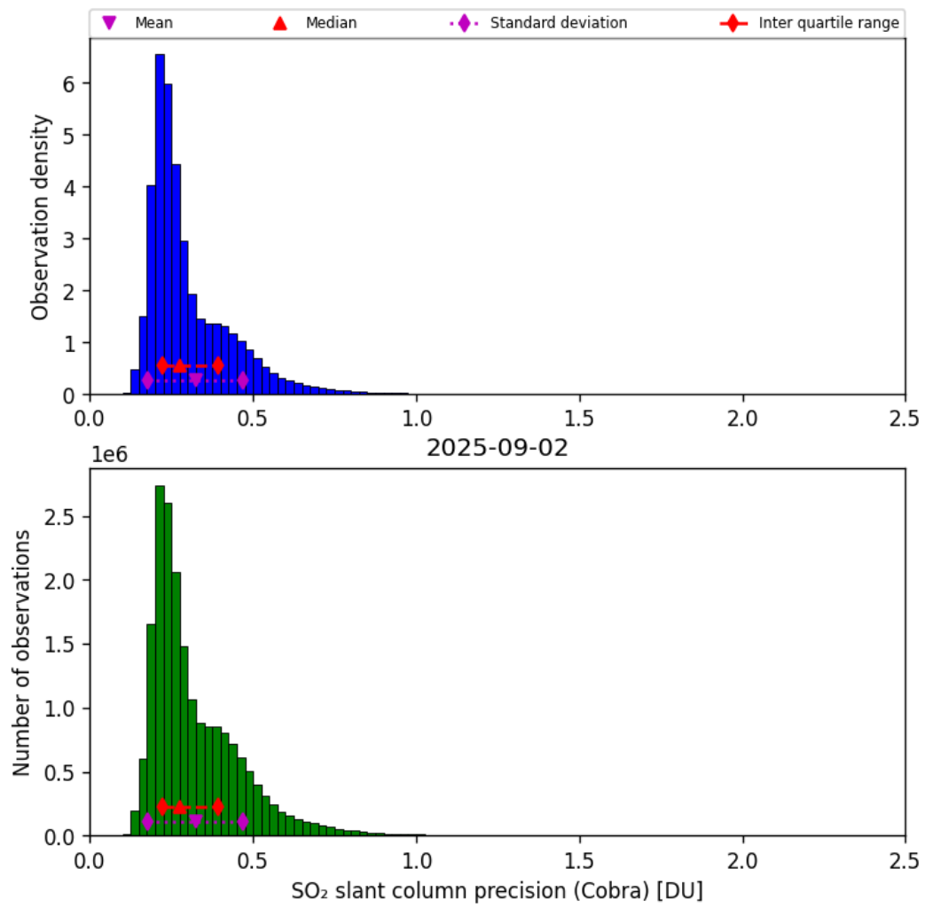
Figure 62: Histogram of “SO 2 slant column precision (Cobra)” for 2025-09-01 to 2025-09-03
