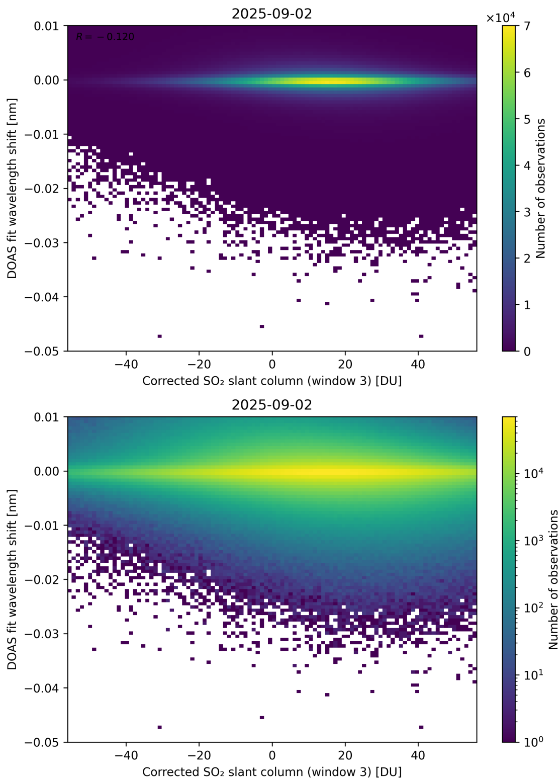
Figure 256: Scatter density plot of “Corrected SO 2 slant column (window 3)” against “DOAS fit wavelength shift” for 2025-09-01 to 2025-09-03.
