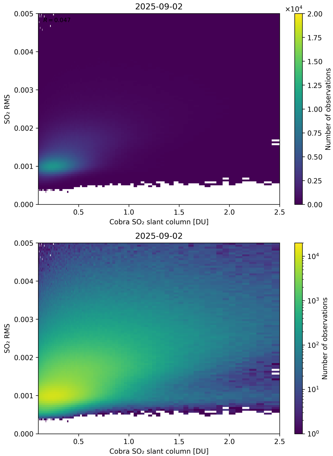
Figure 198: Scatter density plot of “Cobra SO 2 slant column” against “SO 2 RMS” for 2025-09-01 to 2025-09-03.
