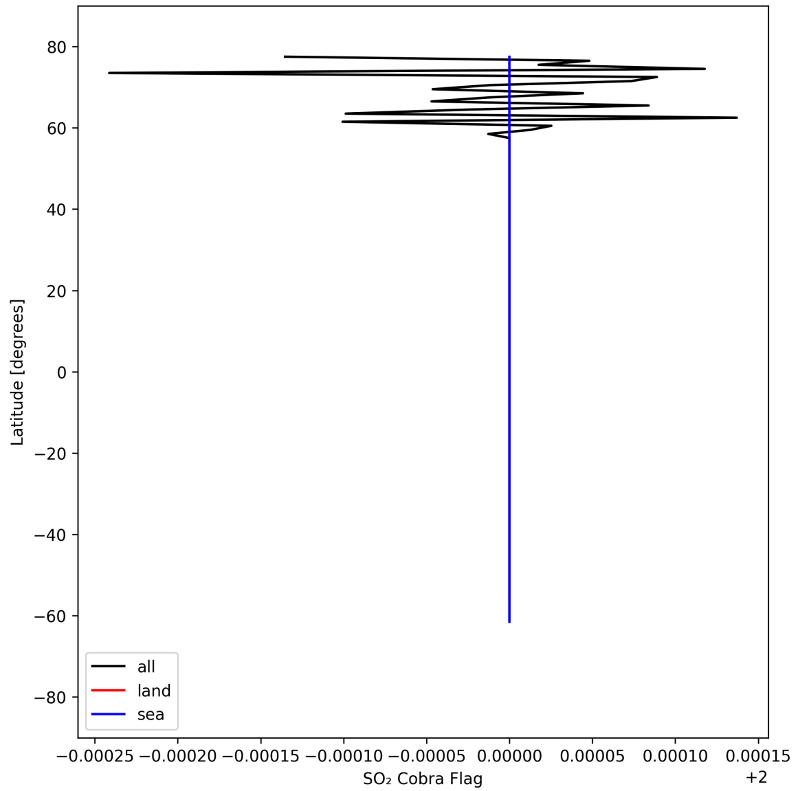
Figure 49: Zonal average of "SO 2 Cobra Flag" for 2025-09-01 to 2025-09-03.
