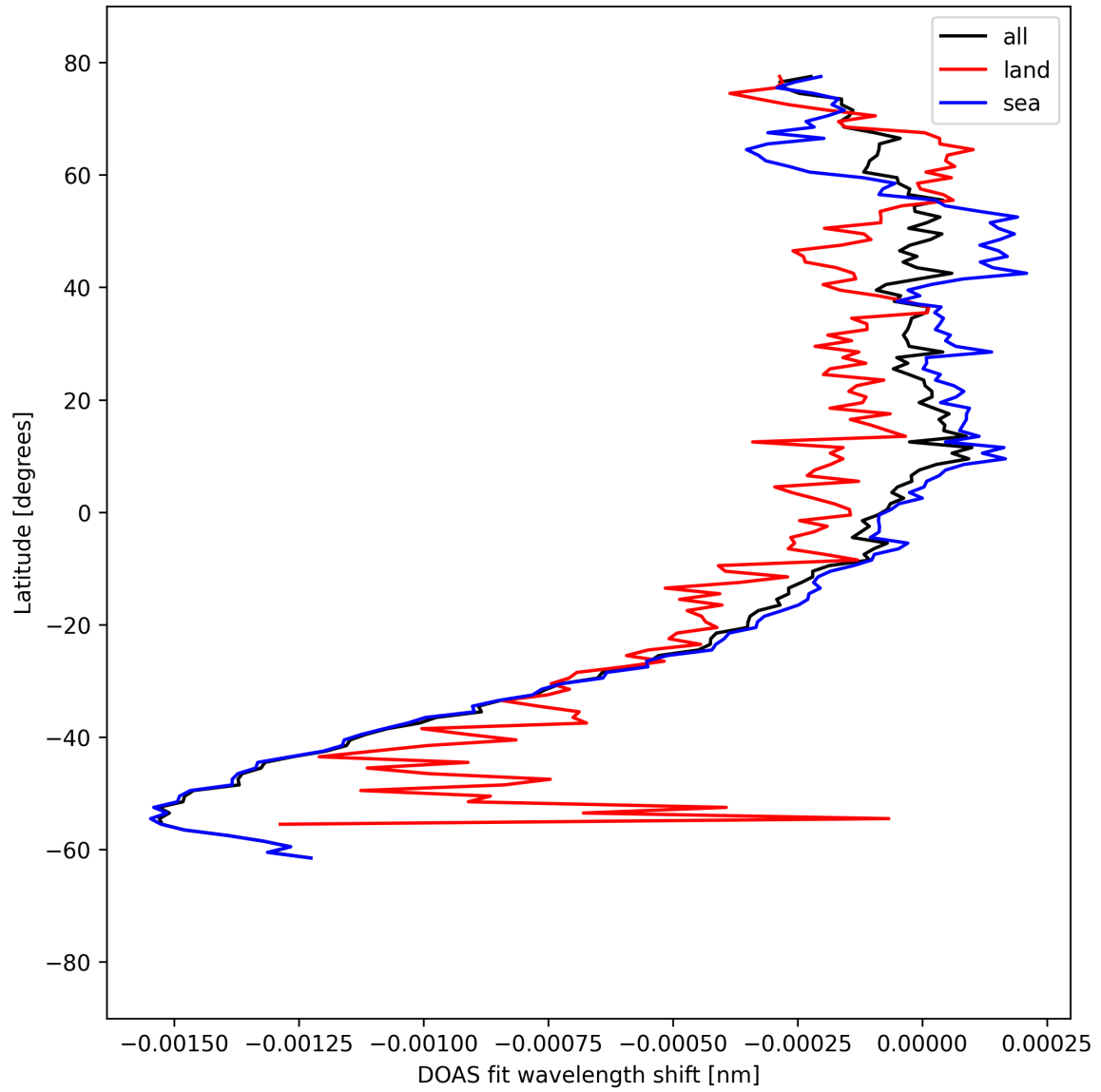
Figure 50: Zonal average of “DOAS fit wavelength shift” for 2025-09-01 to 2025-09-03.
