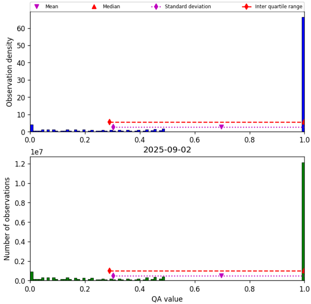
Figure 57: Histogram of “QA value” for 2025-09-01 to 2025-09-03
