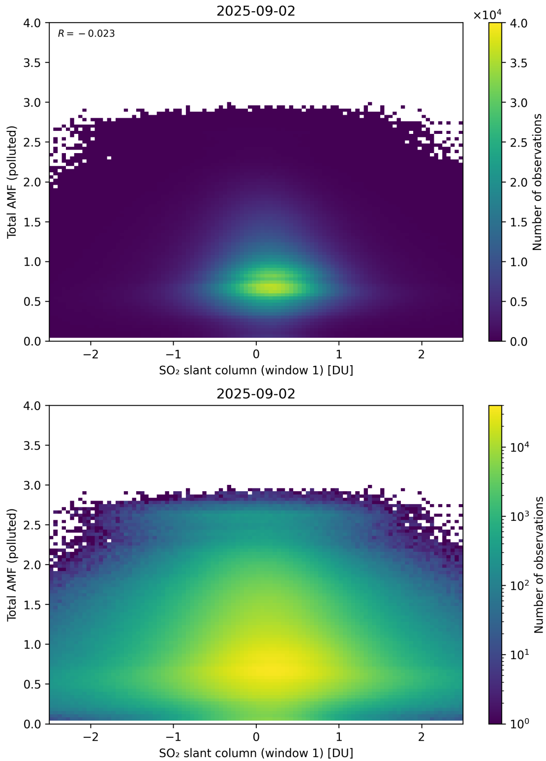
Figure 289: Scatter density plot of “SO 2 slant column (window 1)” against “Total AMF (polluted)” for 2025-09-01 to 2025-09-03.
