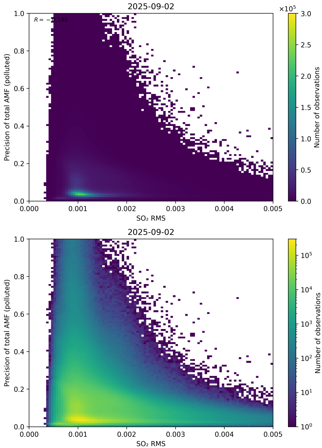
Figure 149: Scatter density plot of “SO 2 RMS” against “Precision of total AMF (polluted)” for 2025-09-01 to 2025-09-03.
