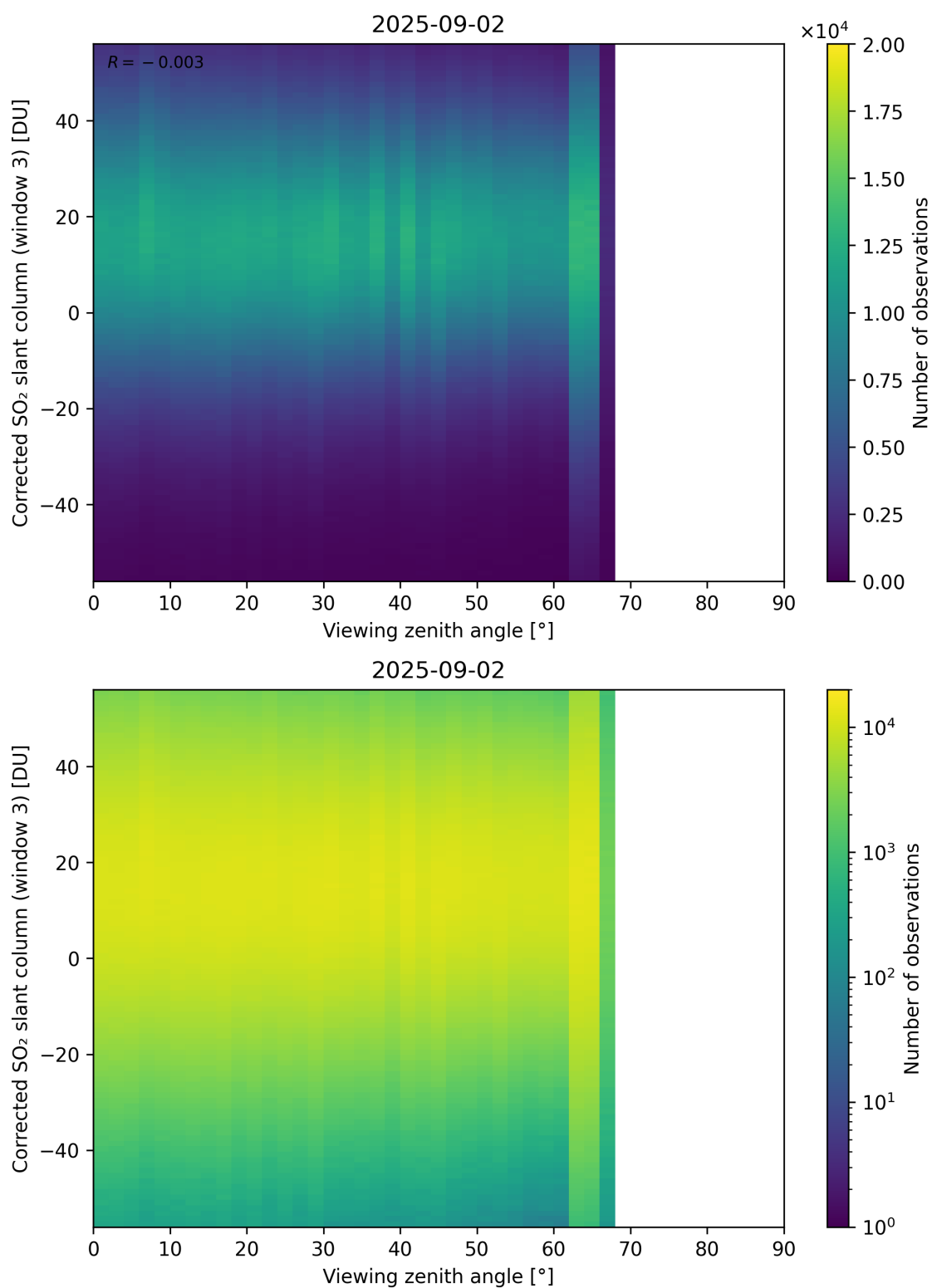
Figure 375: Scatter density plot of “Viewing zenith angle” against “Corrected SO 2 slant column (window 3)” for 2025-09-01 to 2025-09-03.
