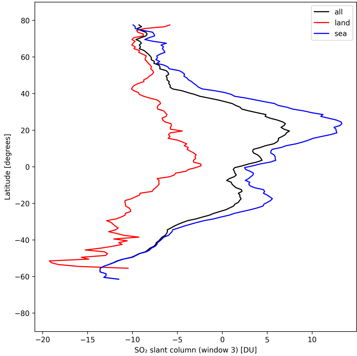
Figure 45: Zonal average of “SO 2 slant column (window 3)” for 2025-09-01 to 2025-09-03.
