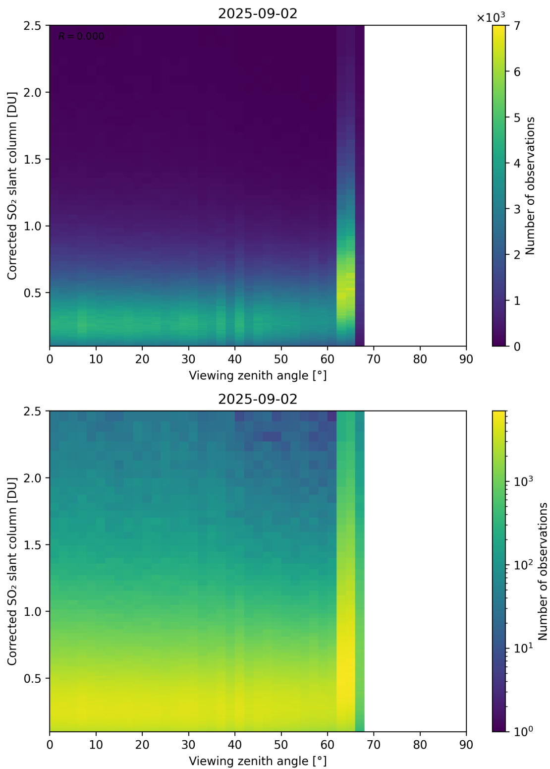
Figure 373: Scatter density plot of “Viewing zenith angle” against “Corrected SO 2 slant column” for 2025-09-01 to 2025-09-03.
