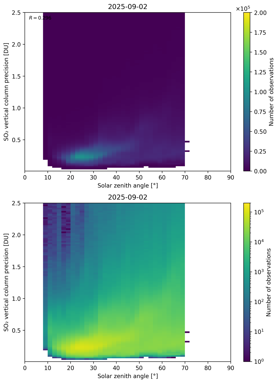
Figure 192: Scatter density plot of “Solar zenith angle” against “SO 2 vertical column precision” for 2025-09-01 to 2025-09-03.
