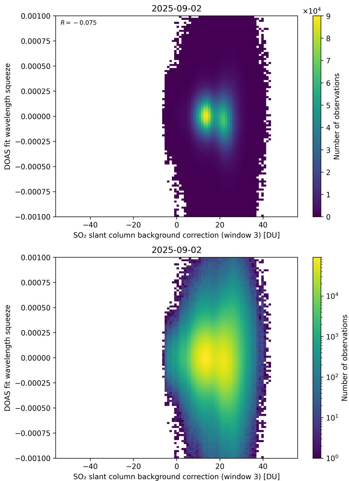
Figure 133: Scatter density plot of “SO 2 slant column background correction (window 3)” against “DOAS fit wavelength squeeze” for 2025-09-01 to 2025-09-03.
