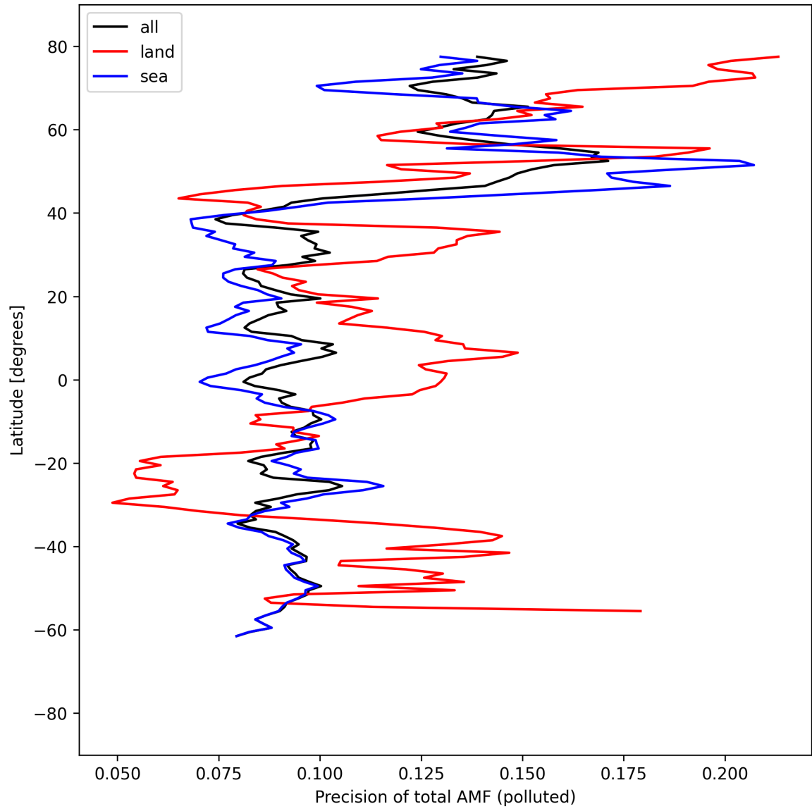
Figure 54: Zonal average of “Precision of total AMF (polluted)” for 2025-09-01 to 2025-09-03.
