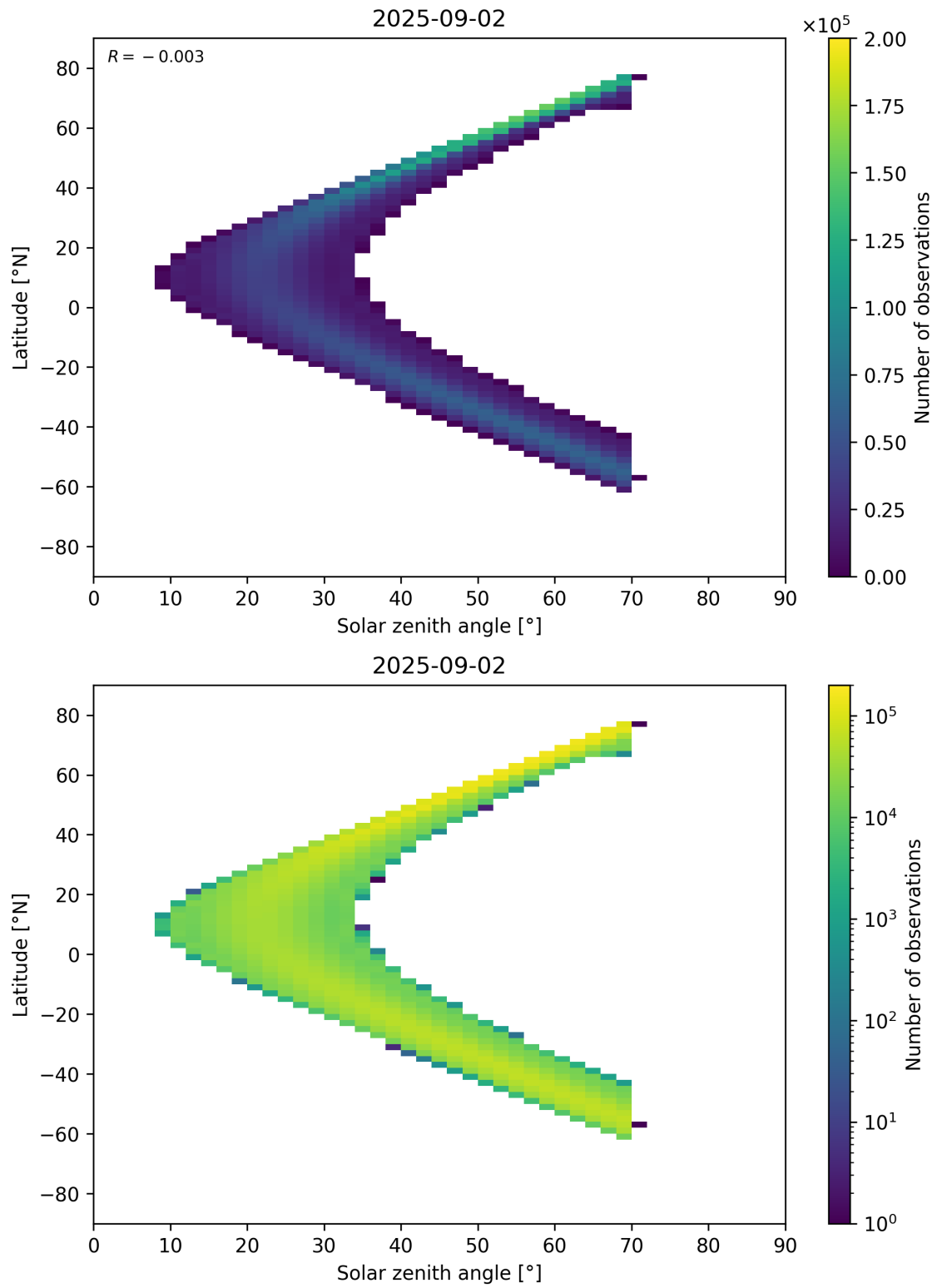
Figure 177: Scatter density plot of “Solar zenith angle” against “Latitude” for 2025-09-01 to 2025-09-03.
