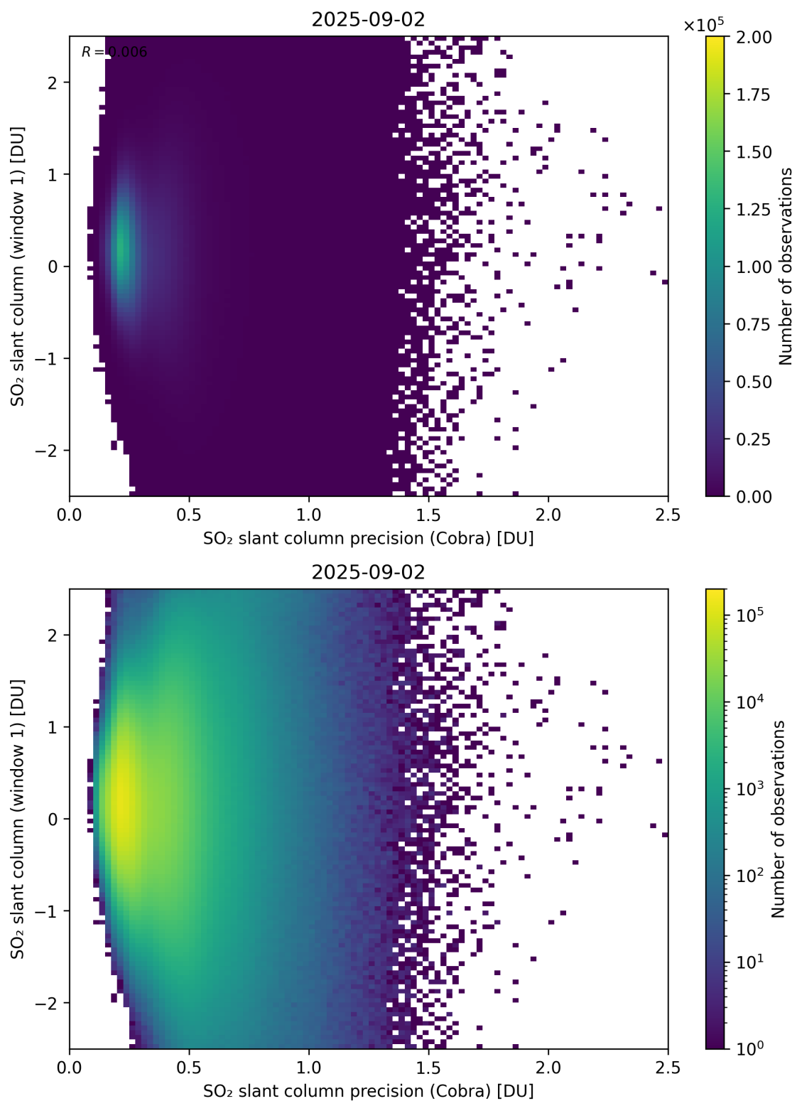
Figure 208: Scatter density plot of “SO 2 slant column precision (Cobra)” against “SO 2 slant column (window 1)” for 2025-09-01 to 2025-09-03.
