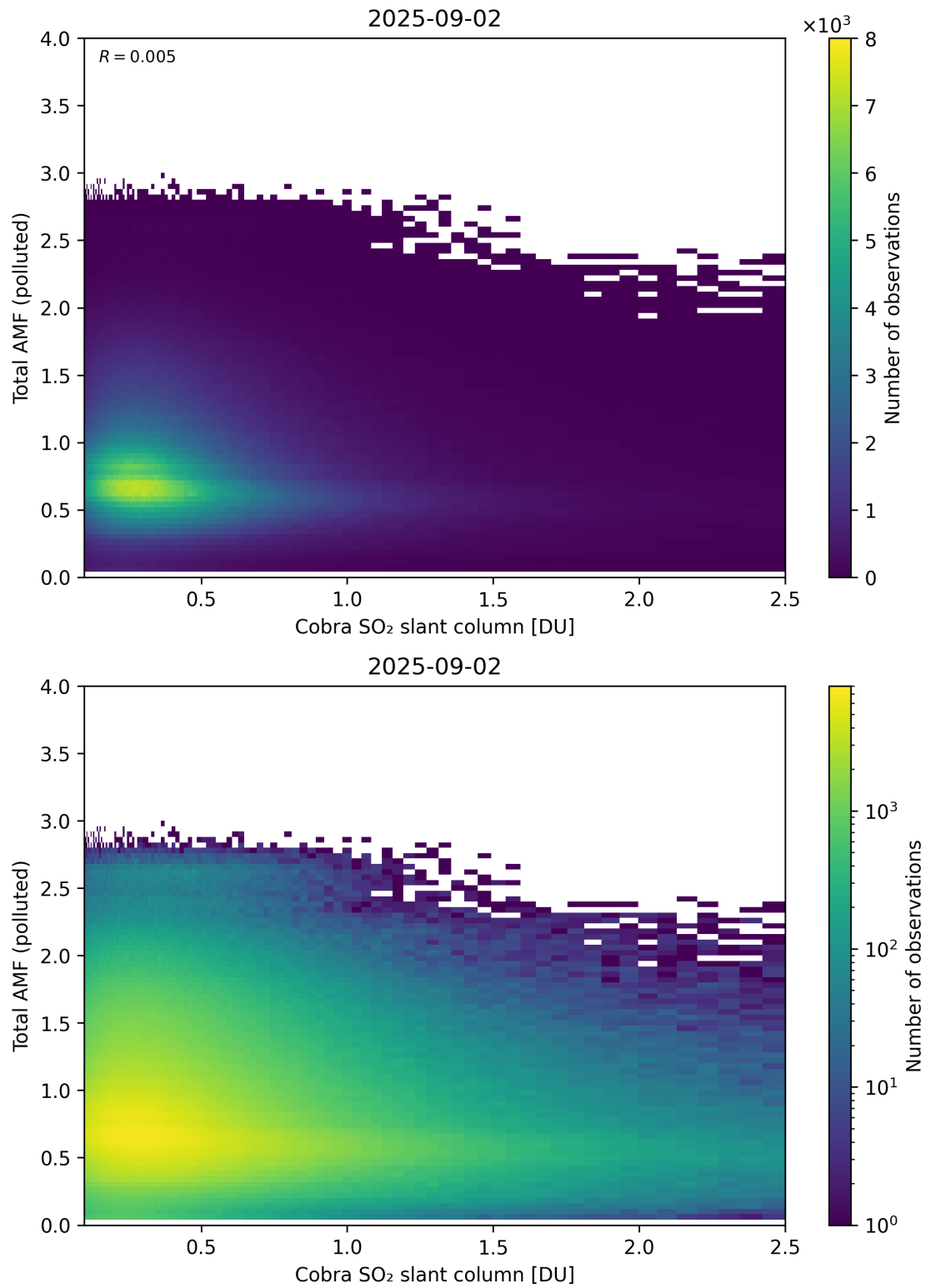
Figure 224: Scatter density plot of “Cobra SO 2 slant column” against “Total AMF (polluted)” for 2025-09-01 to 2025-09-03.
