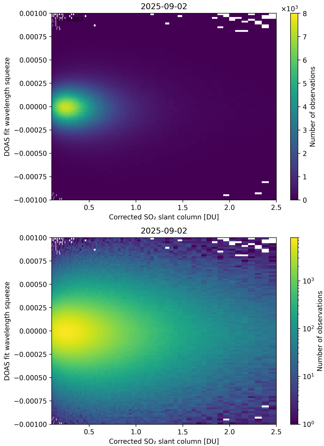
Figure 230: Scatter density plot of “Corrected SO 2 slant column” against “DOAS fit wavelength squeeze” for 2025-09-01 to 2025-09-03.
