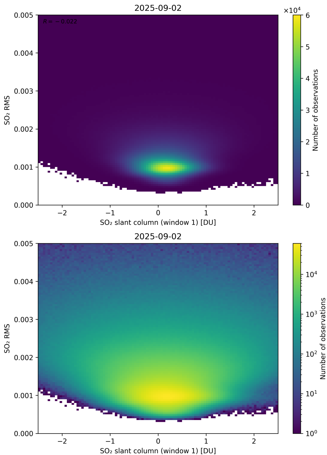
Figure 267: Scatter density plot of “SO 2 slant column (window 1)” against “SO 2 RMS” for 2025-09-01 to 2025-09-03.
