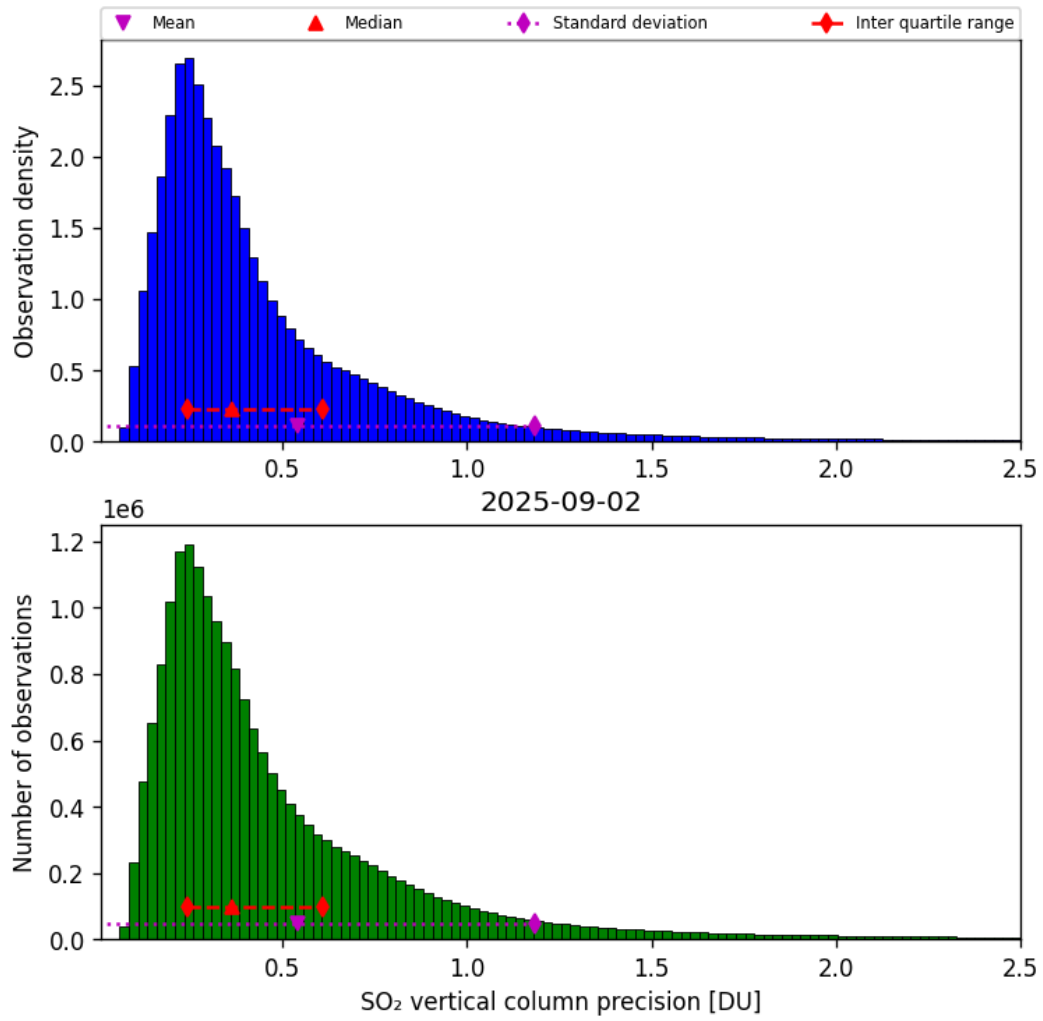
Figure 59: Histogram of “SO 2 vertical column precision” for 2025-09-01 to 2025-09-03
