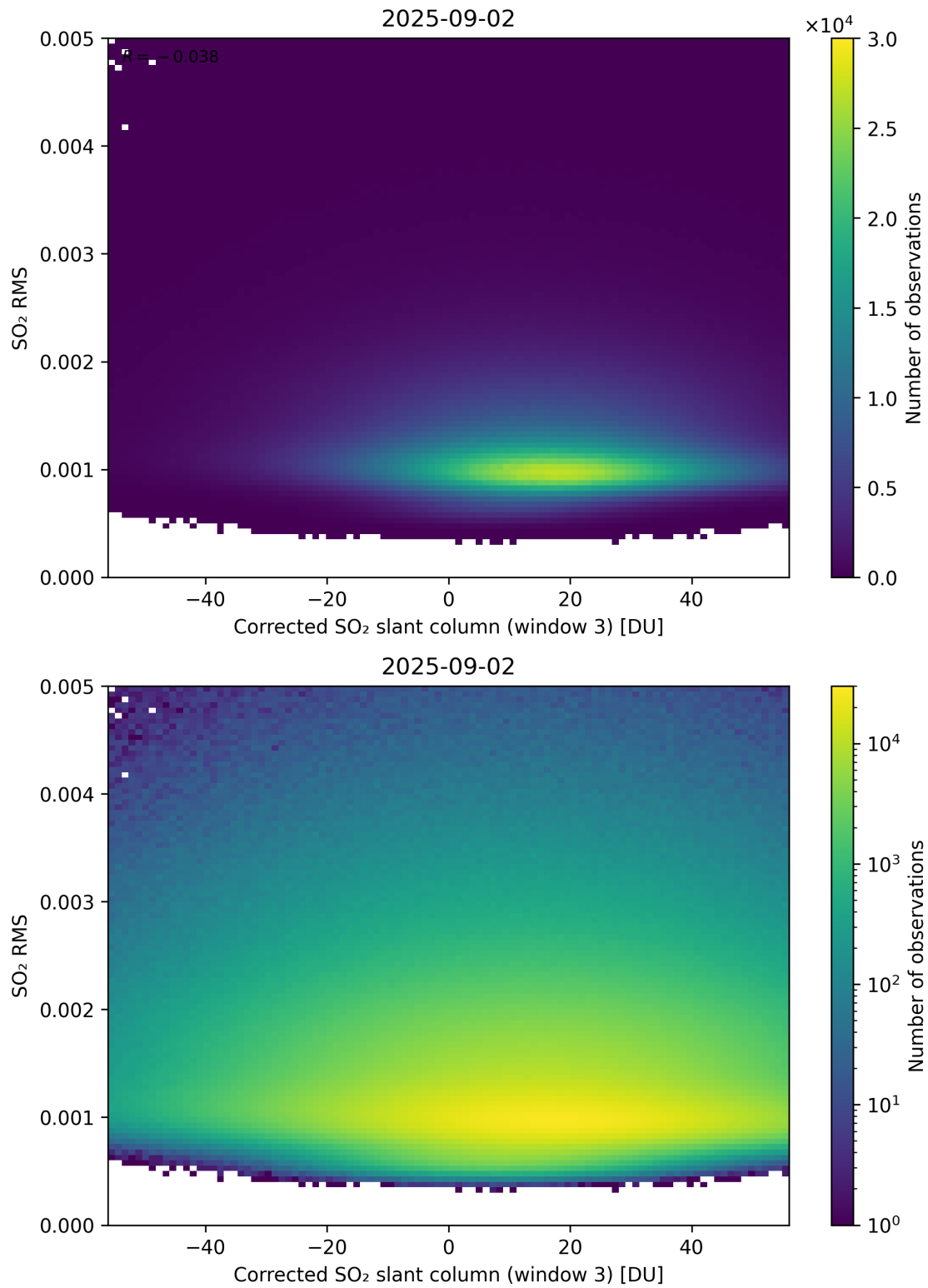
Figure 258: Scatter density plot of “Corrected SO 2 slant column (window 3)” against “SO 2 RMS” for 2025-09-01 to 2025-09-03.
