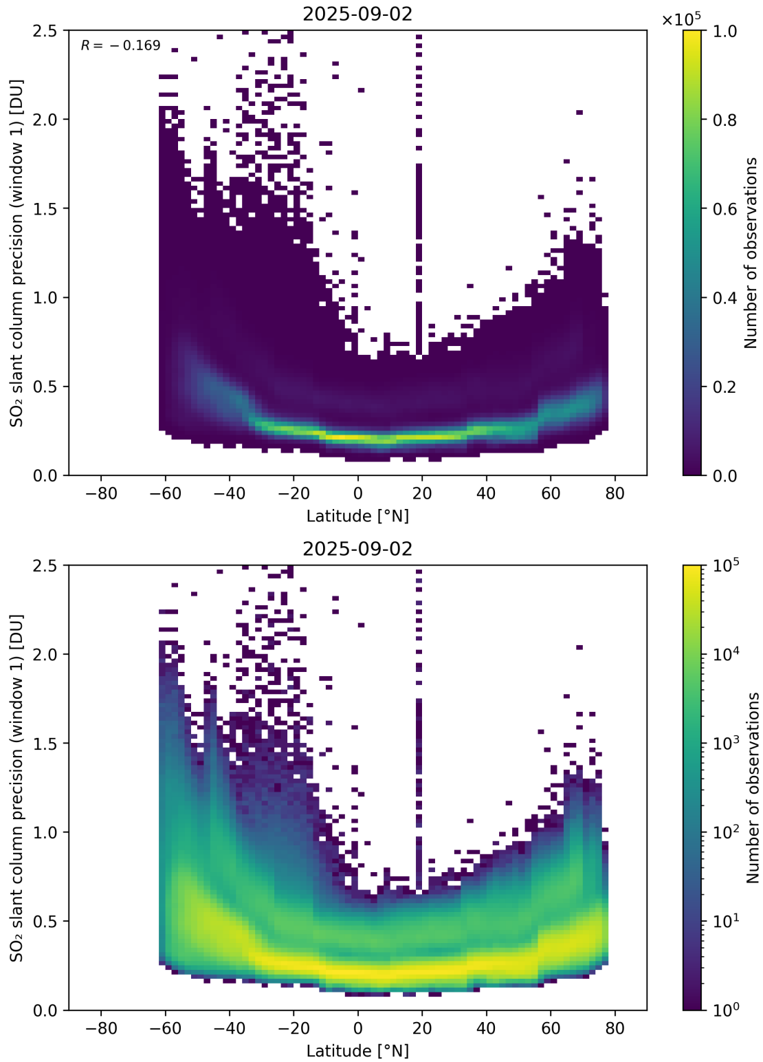
Figure 163: Scatter density plot of “Latitude” against “SO 2 slant column precision (window 1)” for 2025-09-01 to 2025-09-03.
