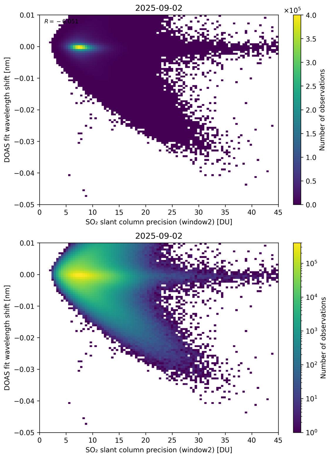
Figure 293: Scatter density plot of “SO 2 slant column precision (window2)” against “DOAS fit wavelength shift” for 2025-09-01 to 2025-09-03.
