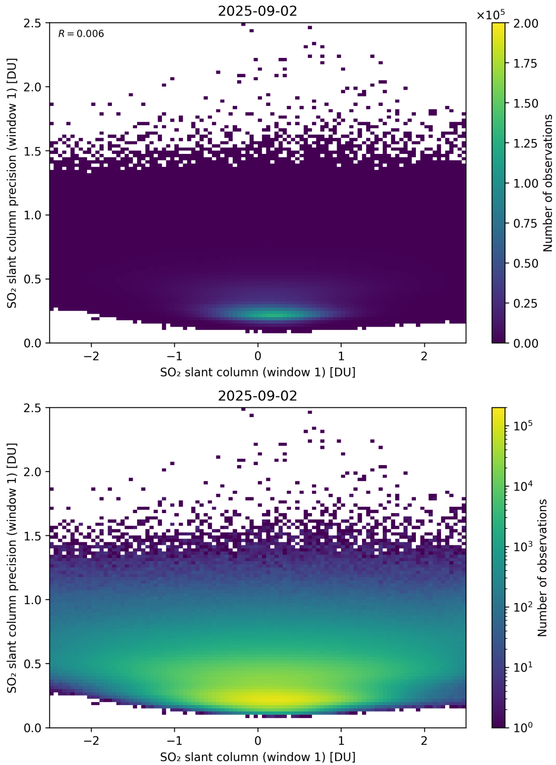
Figure 285: Scatter density plot of “SO 2 slant column (window 1)” against “SO 2 slant column precision (window 1)” for 2025-09-01 to 2025-09-03.
