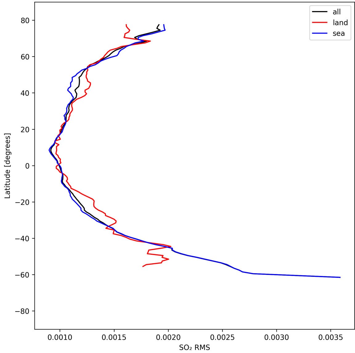
Figure 52: Zonal average of “SO 2 RMS” for 2025-09-01 to 2025-09-03.
