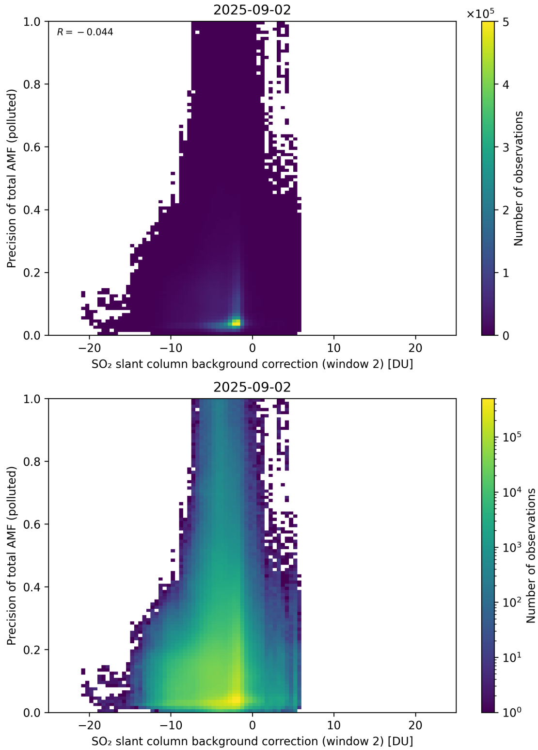
Figure 131: Scatter density plot of “SO 2 slant column background correction (window 2)” against “Precision of total AMF (polluted)” for 2025-09-01 to 2025-09-03.
