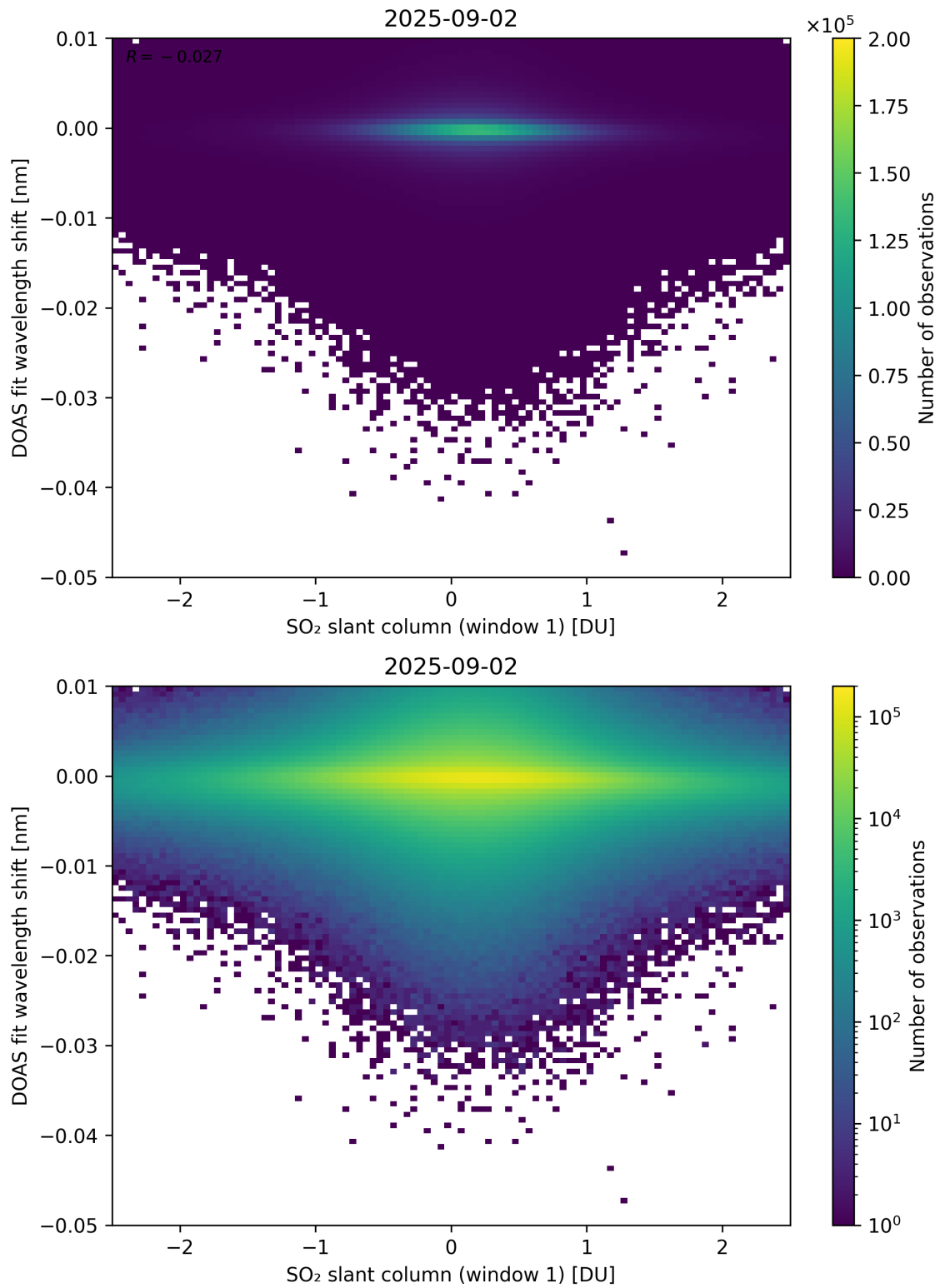
Figure 265: Scatter density plot of “SO 2 slant column (window 1)” against “DOAS fit wavelength shift” for 2025-09-01 to 2025-09-03.
