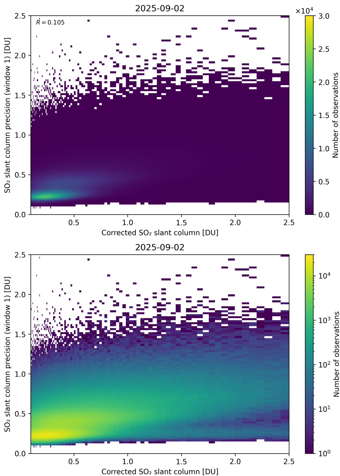
Figure 238: Scatter density plot of “Corrected SO 2 slant column” against “SO 2 slant column precision (window 1)” for 2025-09-01 to 2025-09-03.
