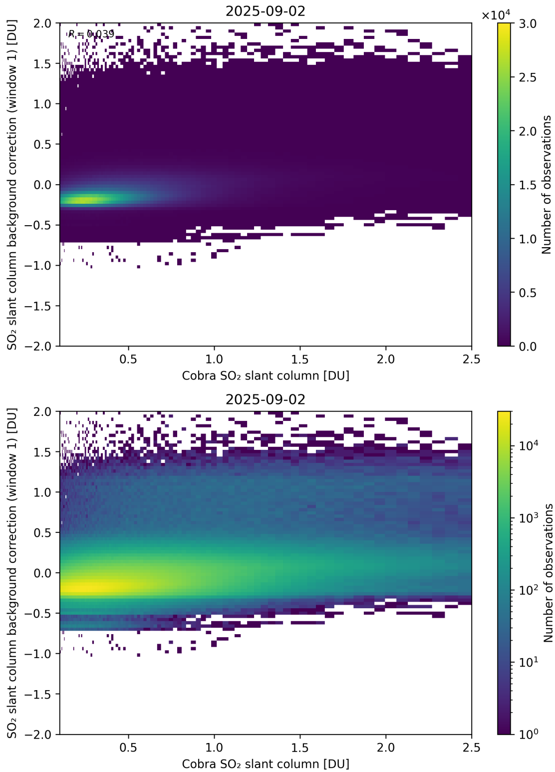
Figure 193: Scatter density plot of “Cobra SO 2 slant column” against “SO 2 slant column background correction (window 1)” for 2025-09-01 to 2025-09-03.
