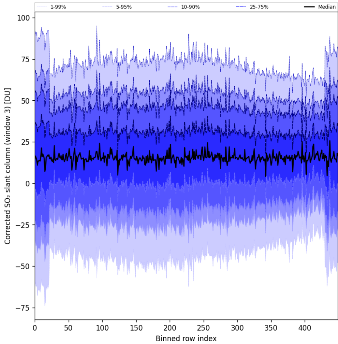
Figure 99: Along track statistics of “Corrected SO 2 slant column (window 3)” for 2025-09-01 to 2025-09-03
