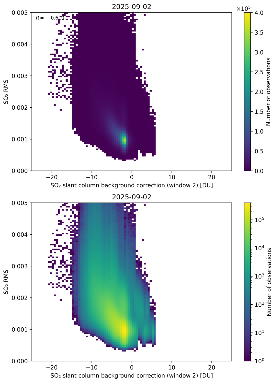
Figure 125: Scatter density plot of “SO 2 slant column background correction (window 2)” against “SO 2 RMS” for 2025-09-01 to 2025-09-03.
