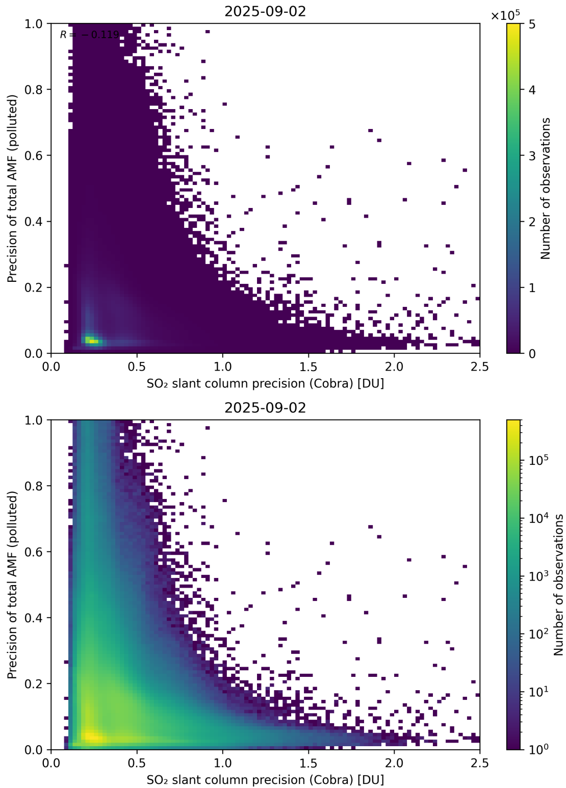
Figure 214: Scatter density plot of “SO 2 slant column precision (Cobra)” against “Precision of total AMF (polluted)” for 2025-09-01 to 2025-09-03.
