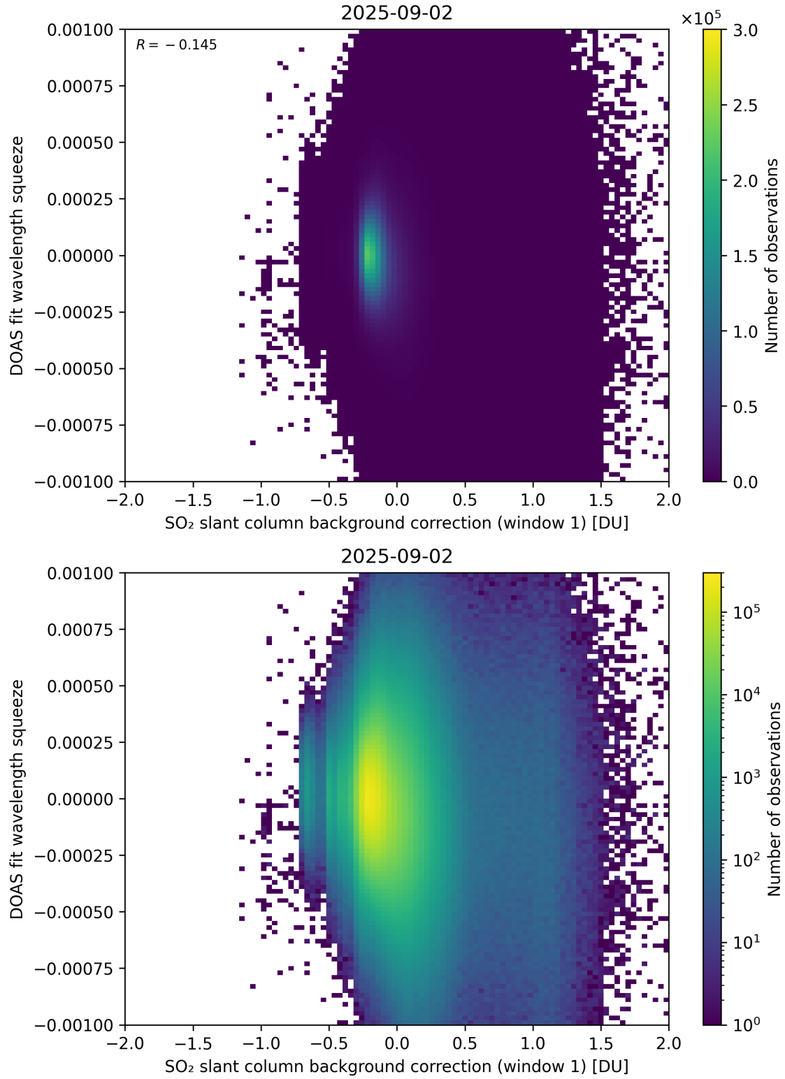
Figure 112: Scatter density plot of “SO 2 slant column background correction (window 1)” against “DOAS fit wavelength squeeze” for 2025-09-01 to 2025-09-03.
