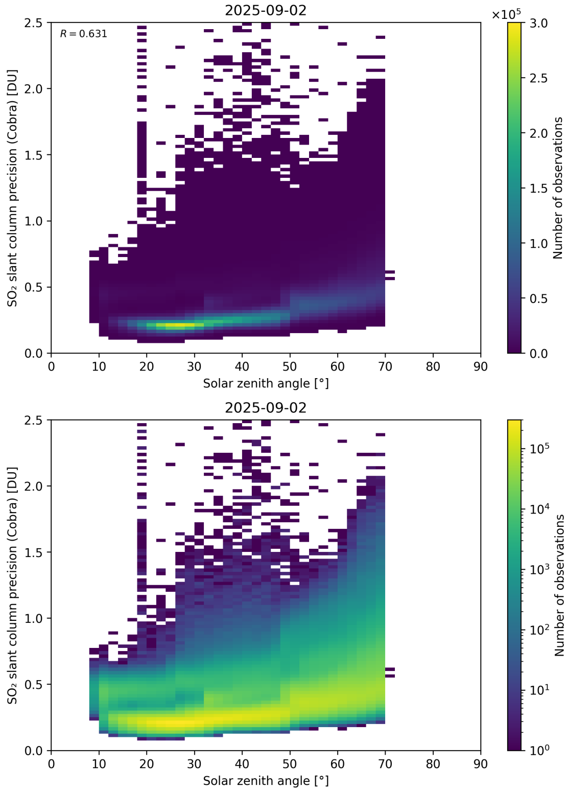
Figure 180: Scatter density plot of “Solar zenith angle” against “SO 2 slant column precision (Cobra)” for 2025-09-01 to 2025-09-03.
