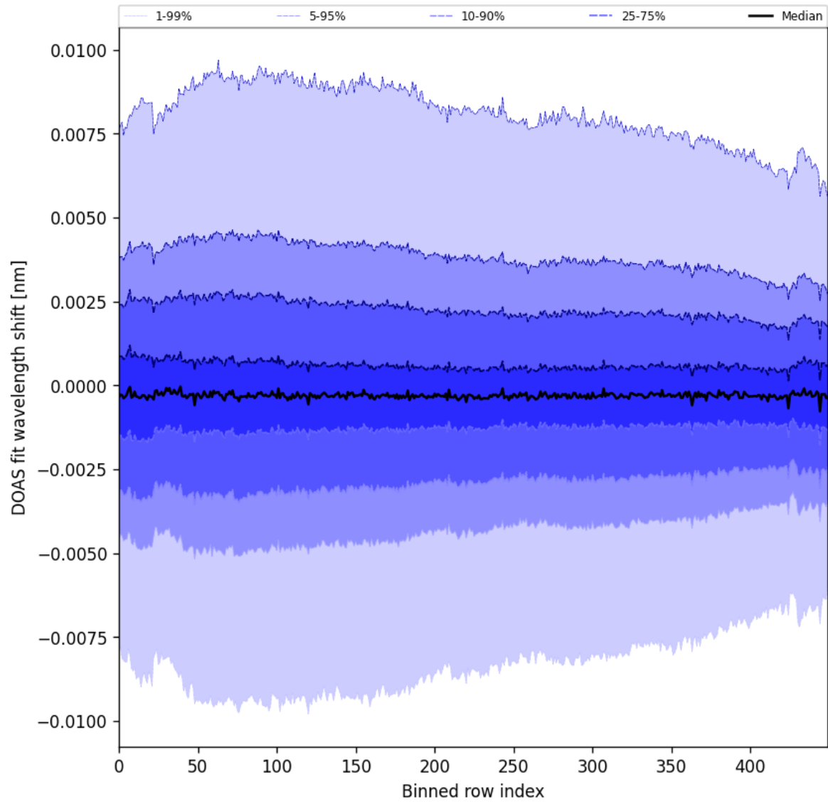
Figure 102: Along track statistics of “DOAS fit wavelength shift” for 2025-09-01 to 2025-09-03
