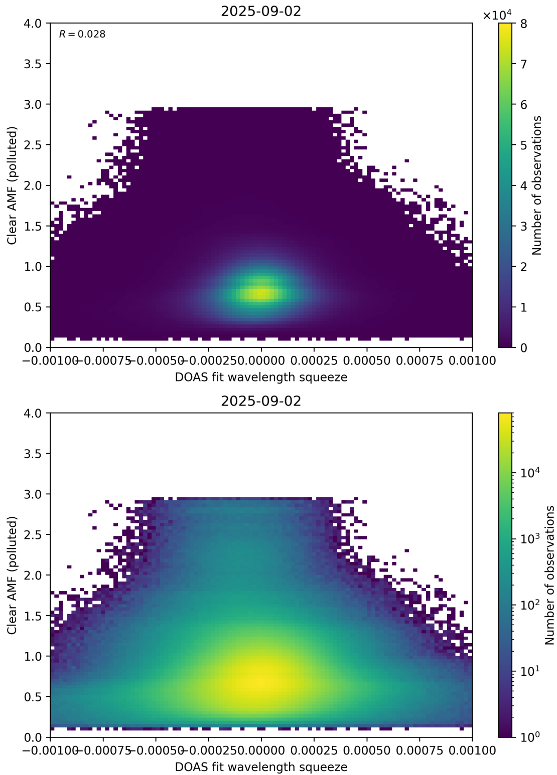
Figure 144: Scatter density plot of “DOAS fit wavelength squeeze” against “Clear AMF (polluted)” for 2025-09-01 to 2025-09-03.
