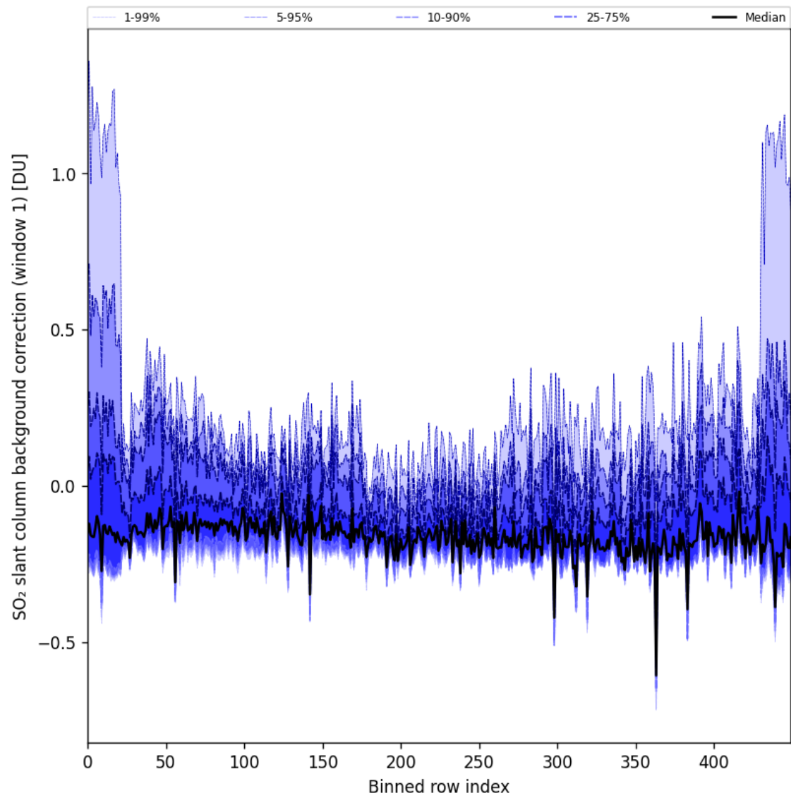
Figure 92: Along track statistics of “SO 2 slant column background correction (window 1)” for 2025-09-01 to 2025-09-03
