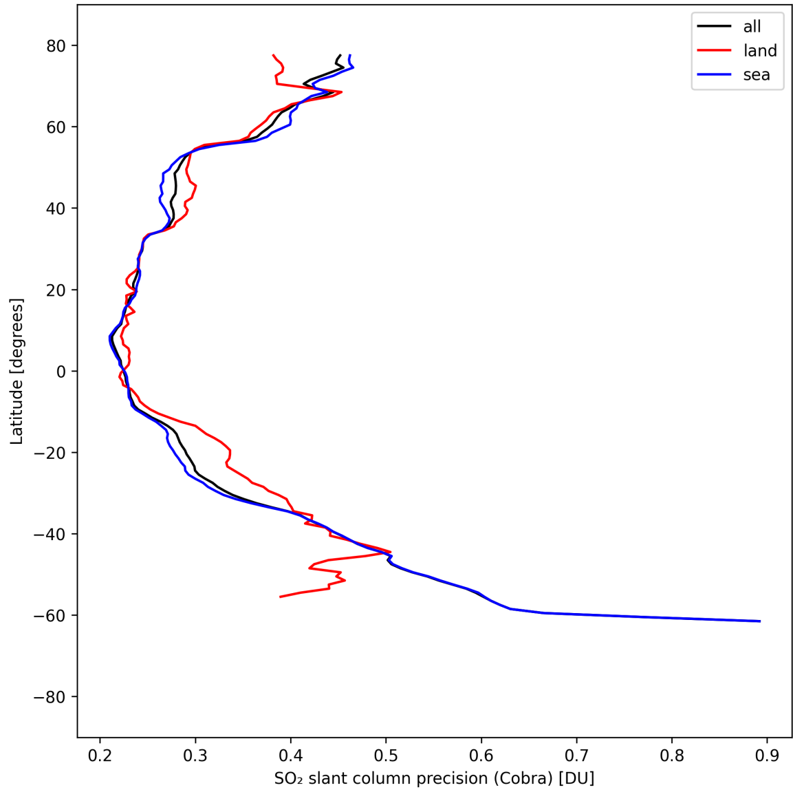
Figure 36: Zonal average of “SO 2 slant column precision (Cobra)” for 2025-09-01 to 2025-09-03.
