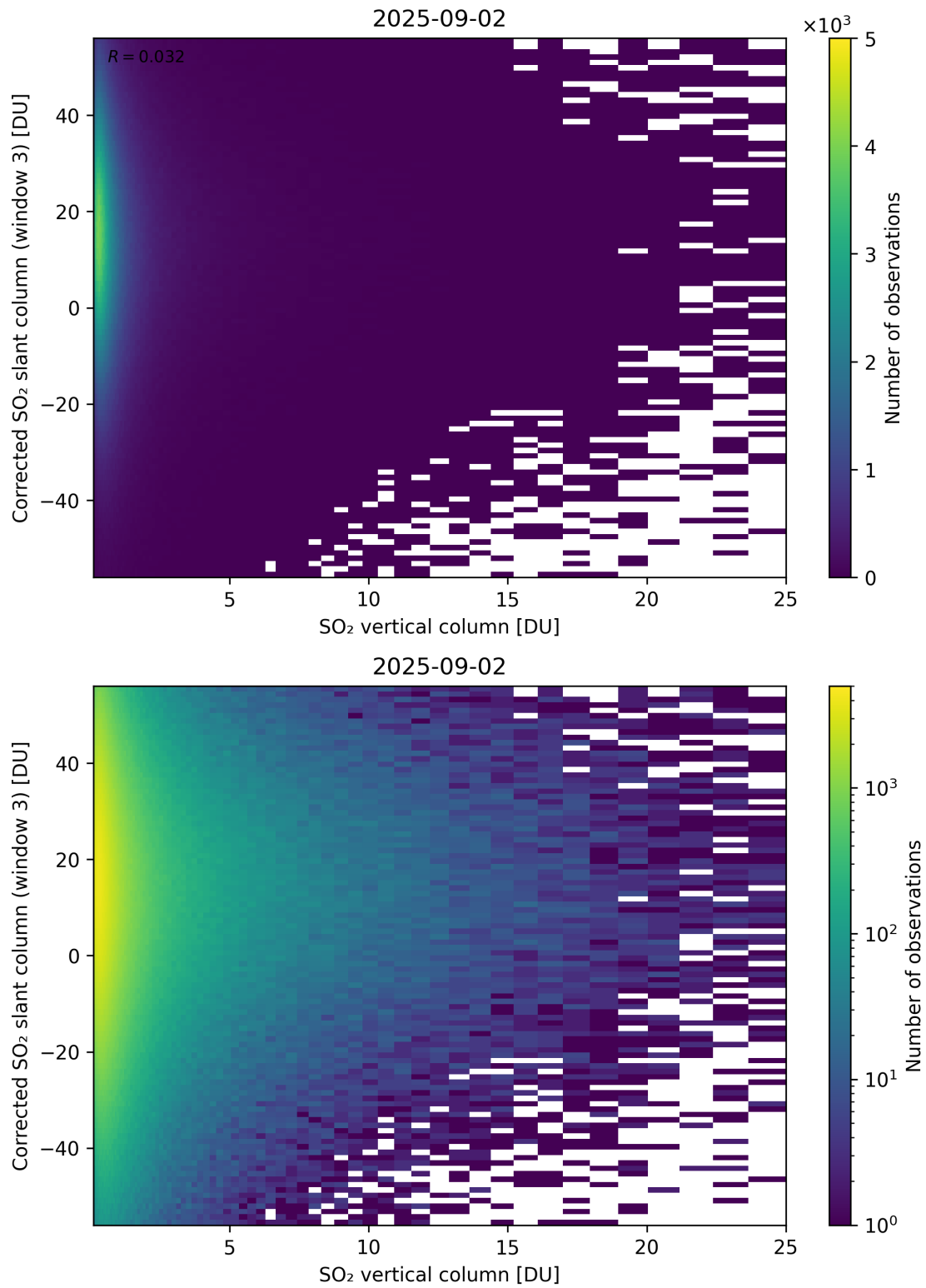
Figure 353: Scatter density plot of “SO 2 vertical column” against “Corrected SO 2 slant column (window 3)” for 2025-09-01 to 2025-09-03.
