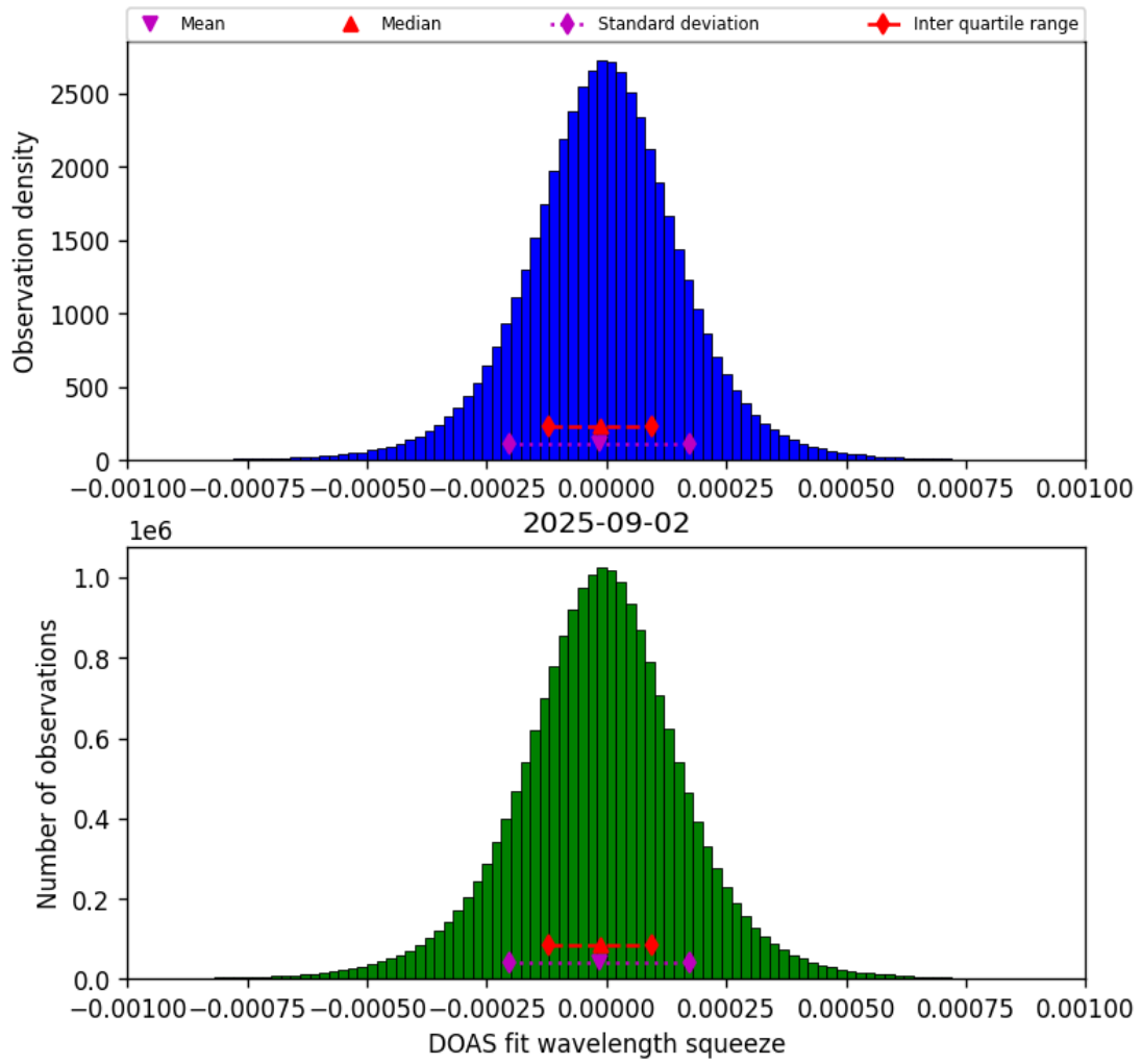
Figure 77: Histogram of “DOAS fit wavelength squeeze” for 2025-09-01 to 2025-09-03
