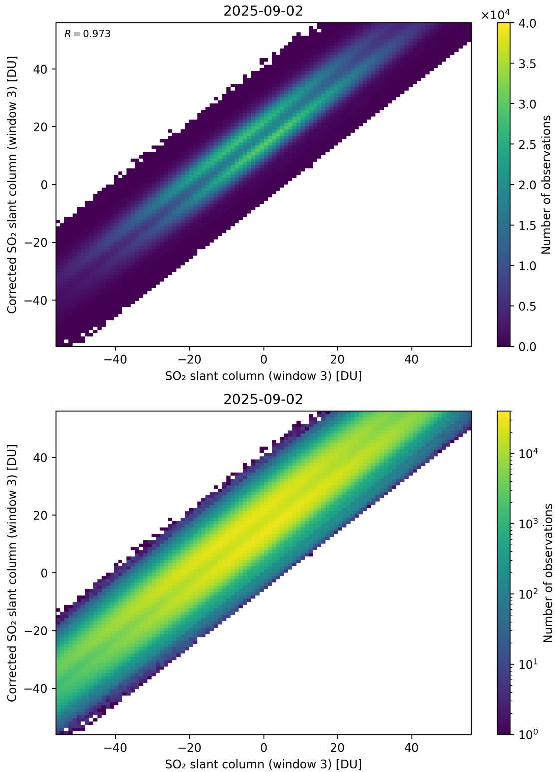
Figure 316: Scatter density plot of “SO 2 slant column (window 3)” against “Corrected SO 2 slant column (window 3)” for 2025-09-01 to 2025-09-03.
