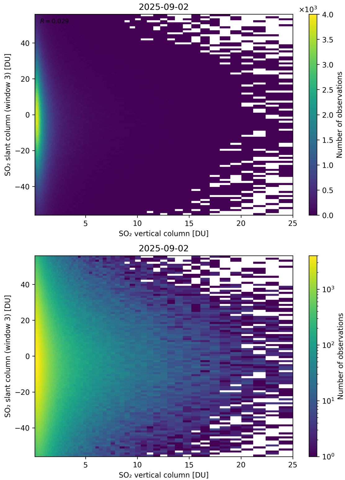
Figure 357: Scatter density plot of “SO 2 vertical column” against “SO 2 slant column (window 3)” for 2025-09-01 to 2025-09-03.
