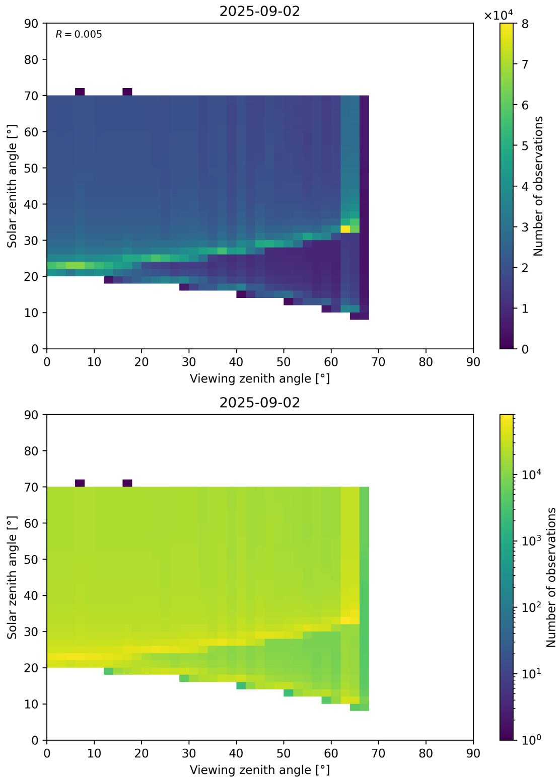
Figure 369: Scatter density plot of “Viewing zenith angle” against “Solar zenith angle” for 2025-09-01 to 2025-09-03.
