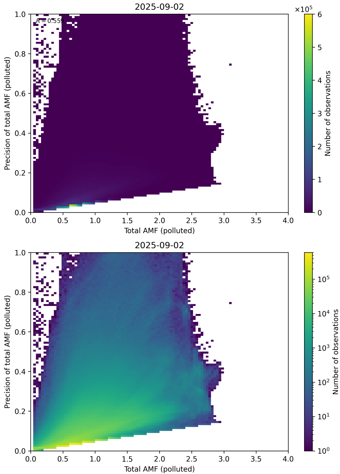
Figure 322: Scatter density plot of “Total AMF (polluted)” against “Precision of total AMF (polluted)” for 2025-09-01 to 2025-09-03.
