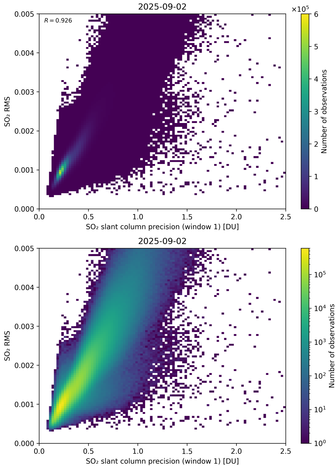
Figure 273: Scatter density plot of “SO 2 slant column precision (window 1)” against “SO 2 RMS” for 2025-09-01 to 2025-09-03.
