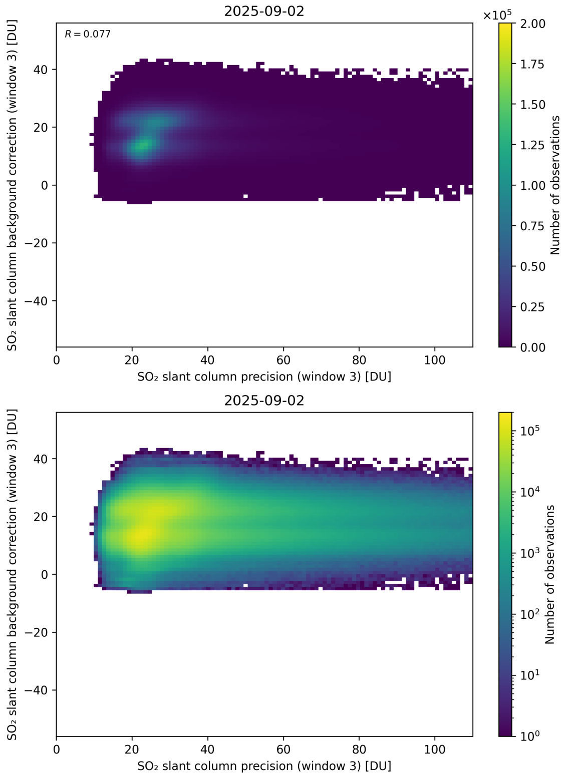
Figure 307: Scatter density plot of “SO 2 slant column precision (window 3)” against “SO 2 slant column background correction (window 3)” for 2025-09-01 to 2025-09-03.
