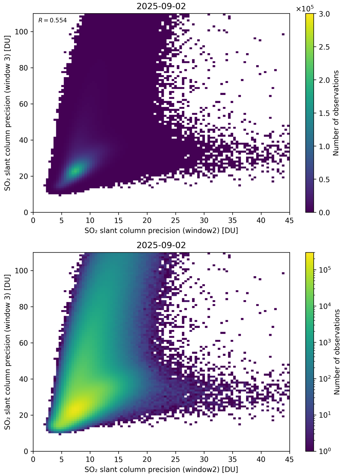
Figure 300: Scatter density plot of “SO 2 slant column precision (window2)” against “SO 2 slant column precision (window 3)” for 2025-09-01 to 2025-09-03.
