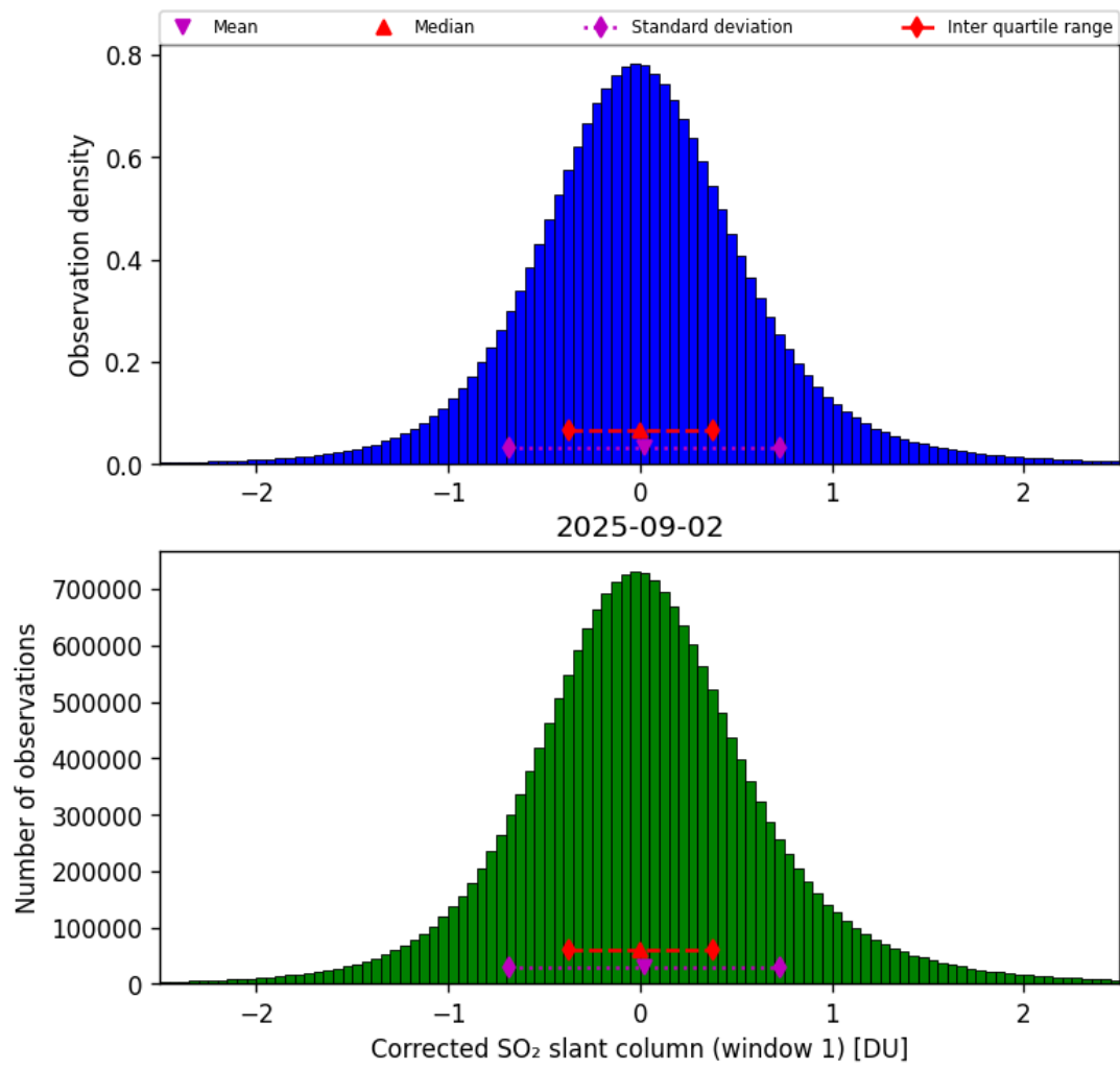
Figure 65: Histogram of “Corrected SO 2 slant column (window 1)” for 2025-09-01 to 2025-09-03
