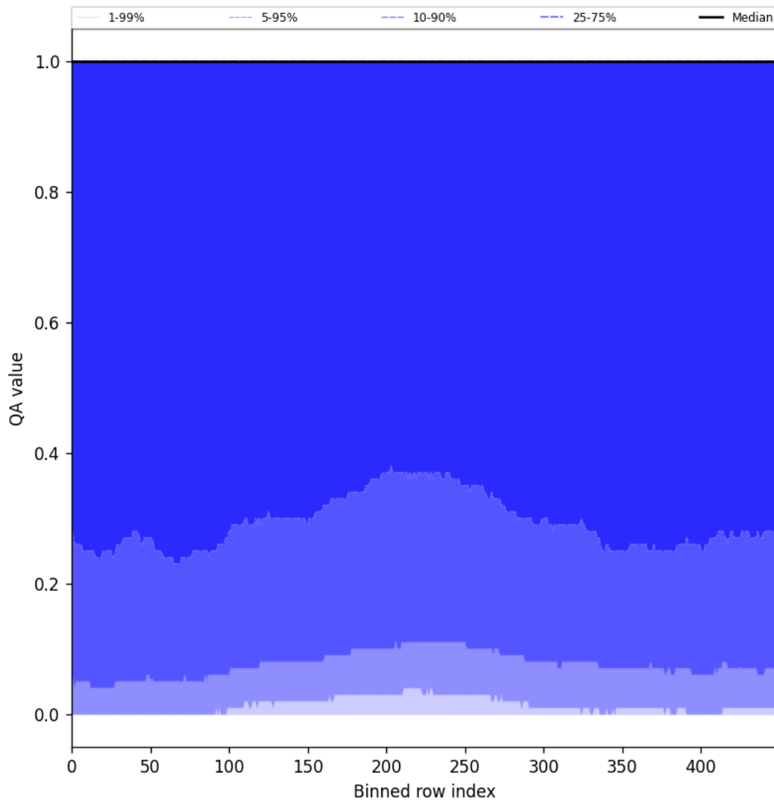
Figure 83: Along track statistics of “QA value” for 2025-09-01 to 2025-09-03
