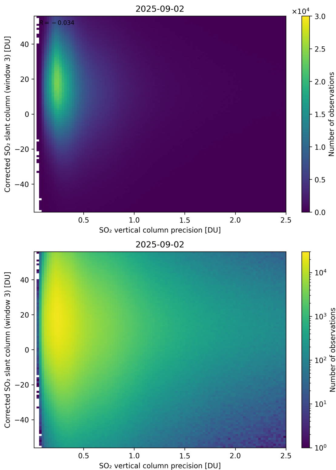
Figure 340: Scatter density plot of “SO 2 vertical column precision” against “Corrected SO 2 slant column (window 3)” for 2025-09-01 to 2025-09-03.
