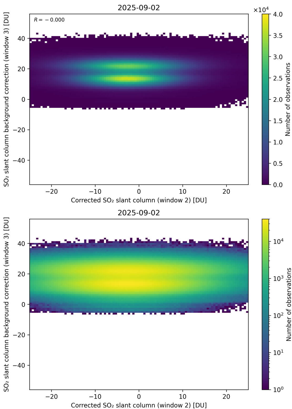
Figure 245: Scatter density plot of “Corrected SO 2 slant column (window 2)” against “SO 2 slant column background correction (window 3)” for 2025-09-01 to 2025-09-03.
