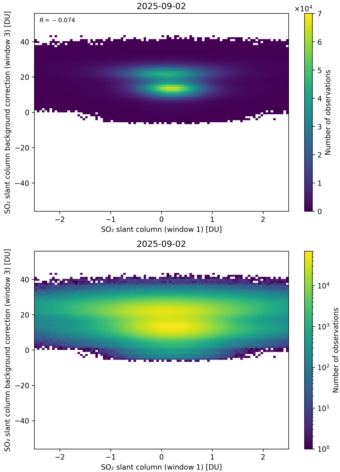
Figure 264: Scatter density plot of “SO 2 slant column (window 1)” against “SO 2 slant column background correction (window 3)” for 2025-09-01 to 2025-09-03.
