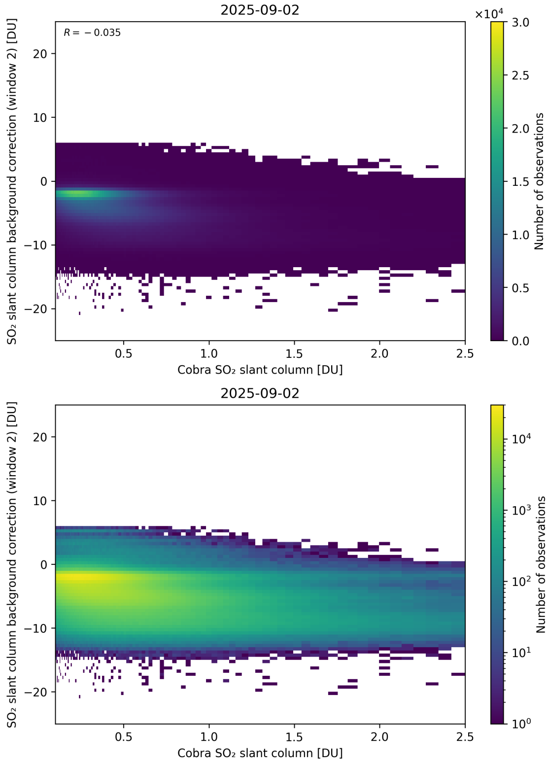
Figure 194: Scatter density plot of “Cobra SO 2 slant column” against “SO 2 slant column background correction (window 2)” for 2025-09-01 to 2025-09-03.
