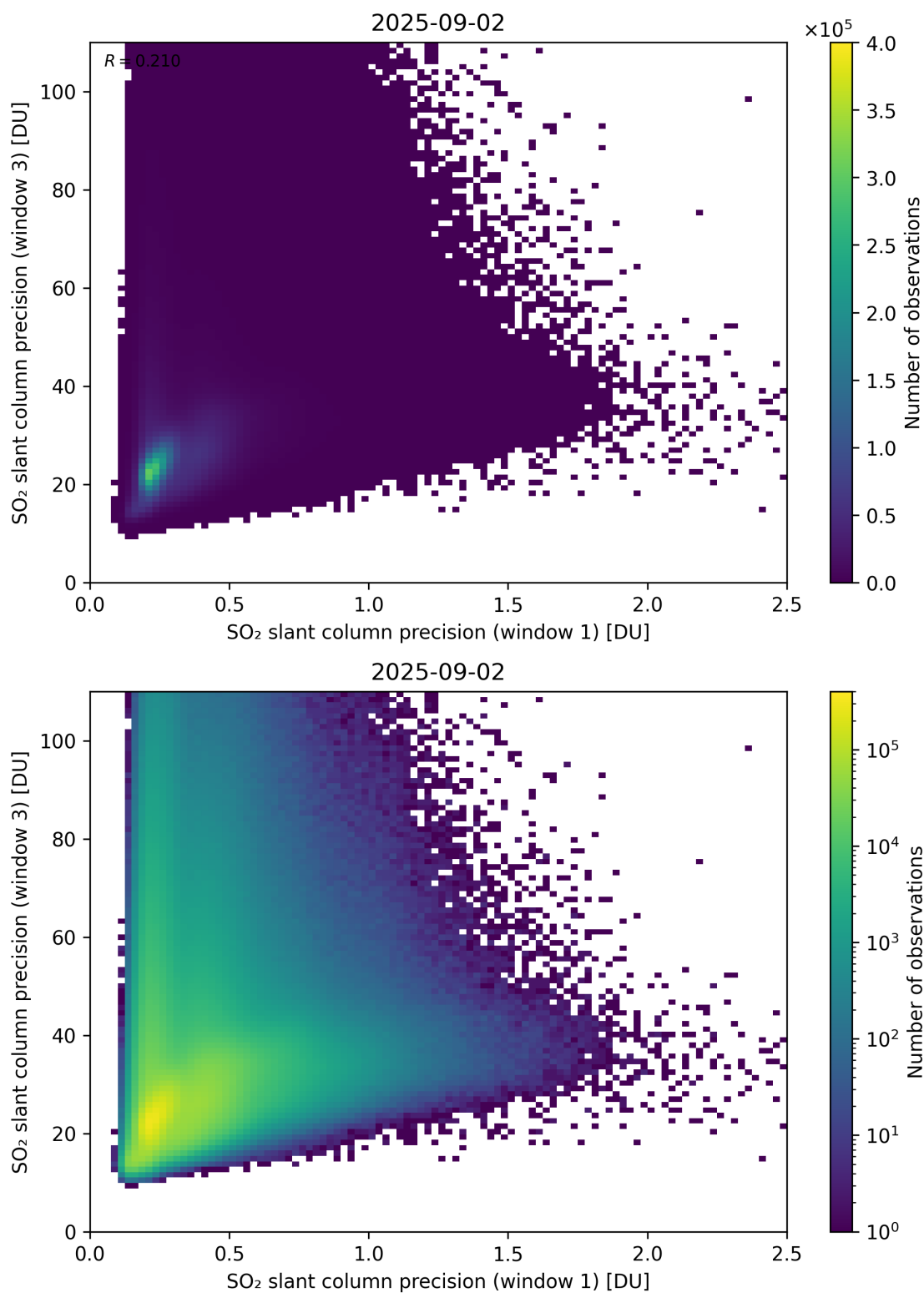
Figure 279: Scatter density plot of “SO 2 slant column precision (window 1)” against “SO 2 slant column precision (window 3)” for 2025-09-01 to 2025-09-03.
