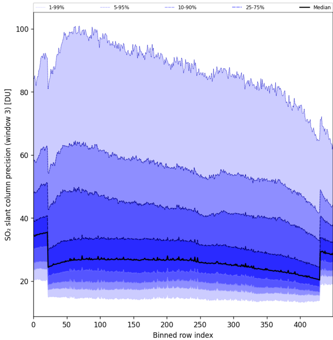
Figure 98: Along track statistics of “SO 2 slant column precision (window 3)” for 2025-09-01 to 2025-09-03
