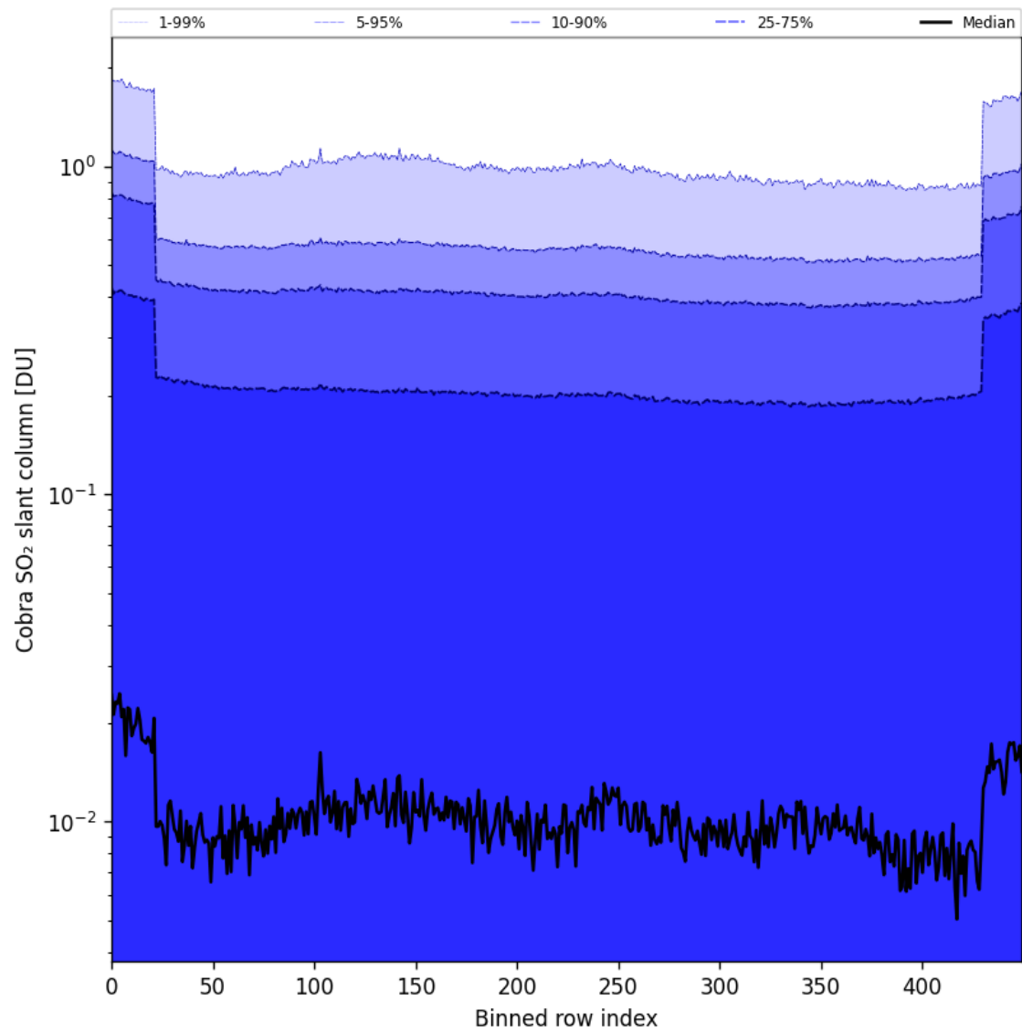
Figure 87: Along track statistics of “Cobra SO 2 slant column” for 2025-09-01 to 2025-09-03
