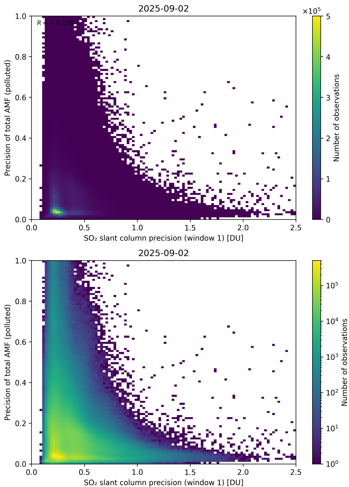
Figure 281: Scatter density plot of “SO 2 slant column precision (window 1)” against “Precision of total AMF (polluted)” for 2025-09-01 to 2025-09-03.
