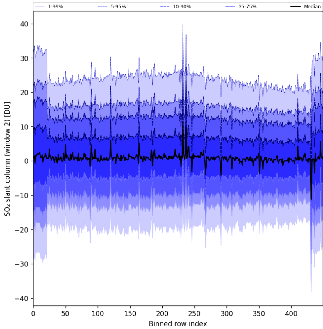
Figure 93: Along track statistics of “SO 2 slant column (window 2)” for 2025-09-01 to 2025-09-03
