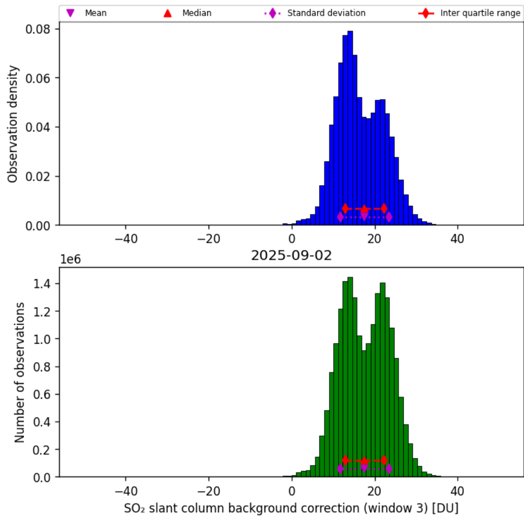
Figure 74: Histogram of “SO 2 slant column background correction (window 3)” for 2025-09-01 to 2025-09-03
