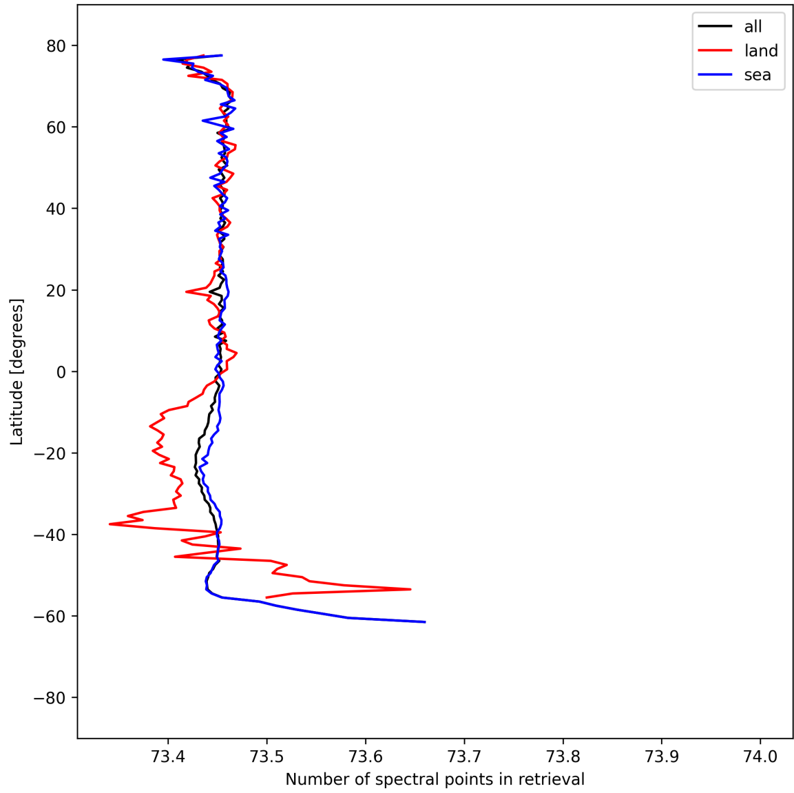
Figure 56: Zonal average of “Number of spectral points in retrieval” for 2025-09-01 to 2025-09-03.
