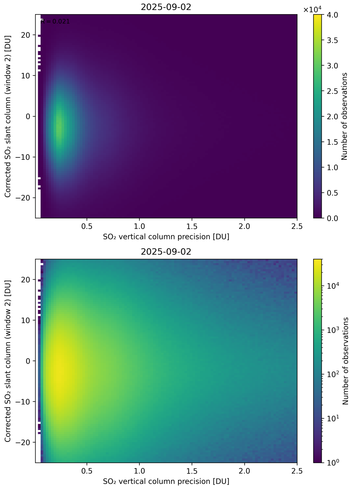
Figure 339: Scatter density plot of “SO 2 vertical column precision” against “Corrected SO 2 slant column (window 2)” for 2025-09-01 to 2025-09-03.
