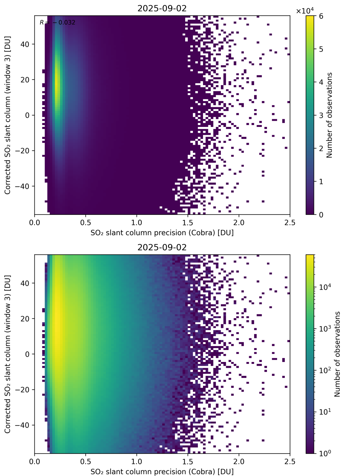
Figure 207: Scatter density plot of “SO 2 slant column precision (Cobra)” against “Corrected SO 2 slant column (window 3)” for 2025-09-01 to 2025-09-03.
