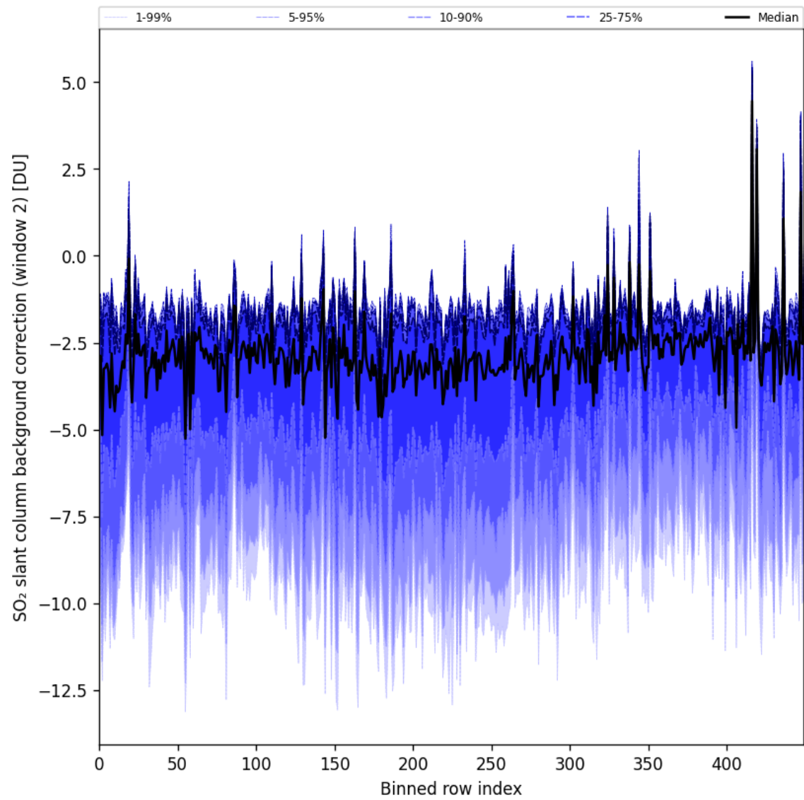
Figure 96: Along track statistics of “SO 2 slant column background correction (window 2)” for 2025-09-01 to 2025-09-03
