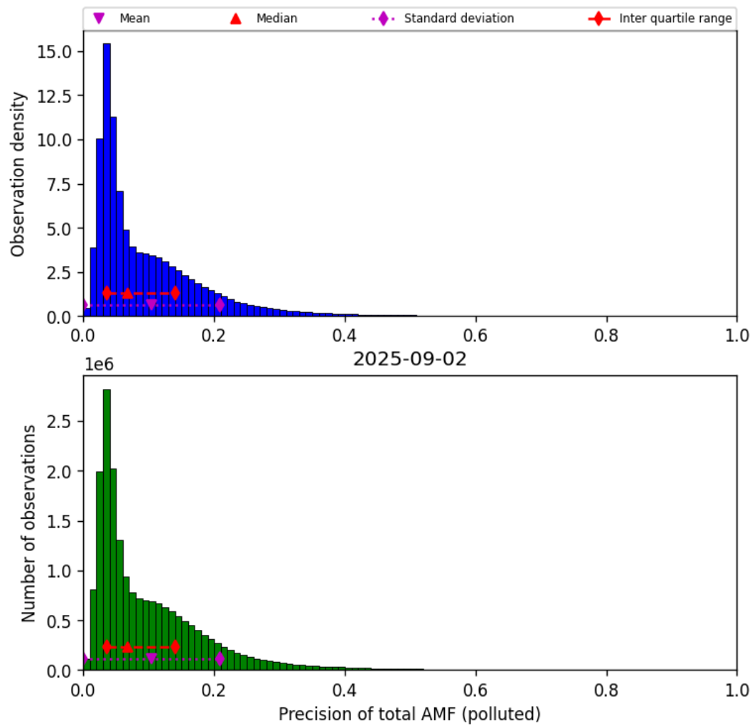
Figure 80: Histogram of “Precision of total AMF (polluted)” for 2025-09-01 to 2025-09-03
