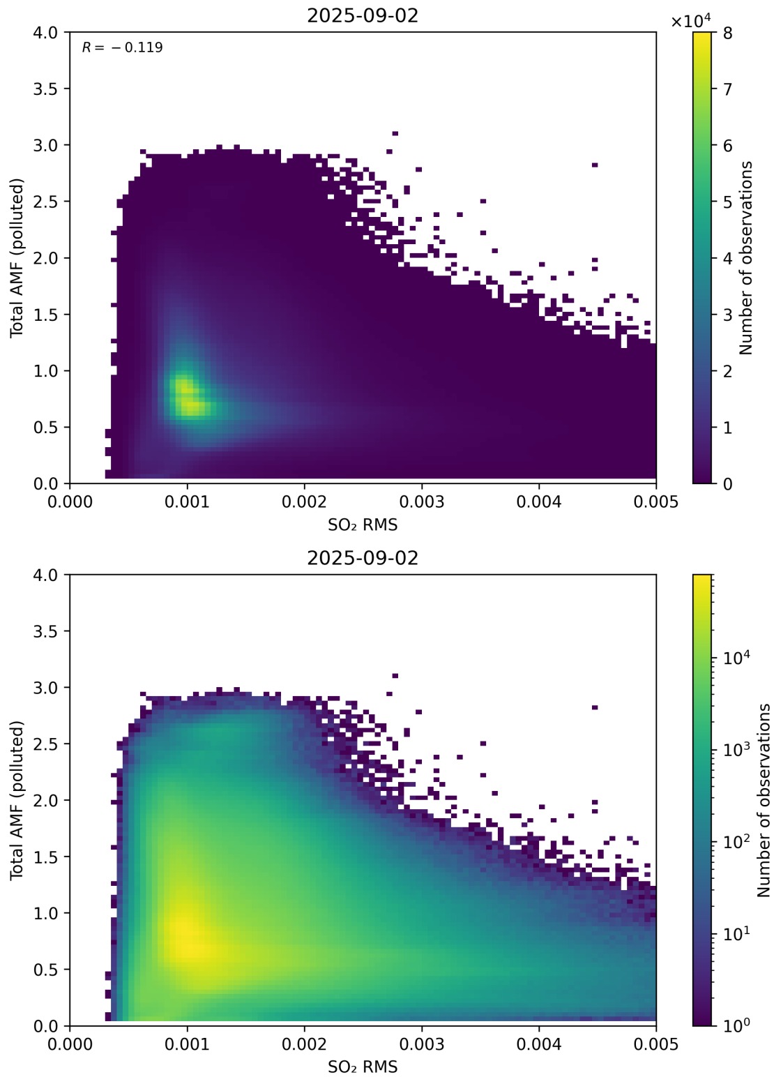
Figure 148: Scatter density plot of “SO 2 RMS” against “Total AMF (polluted)” for 2025-09-01 to 2025-09-03.
