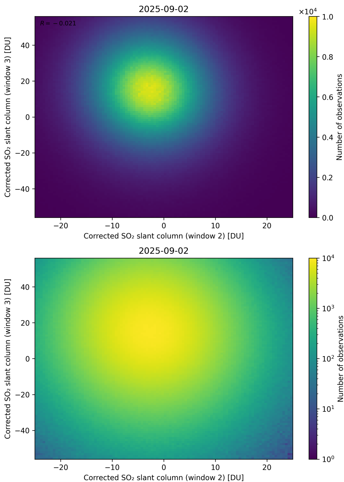
Figure 250: Scatter density plot of “Corrected SO 2 slant column (window 2)” against “Corrected SO 2 slant column (window 3)” for 2025-09-01 to 2025-09-03.
