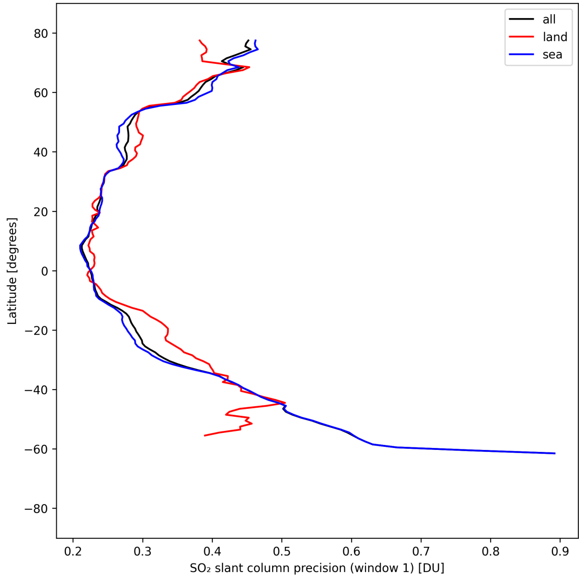
Figure 38: Zonal average of “SO 2 slant column precision (window 1)” for 2025-09-01 to 2025-09-03.
