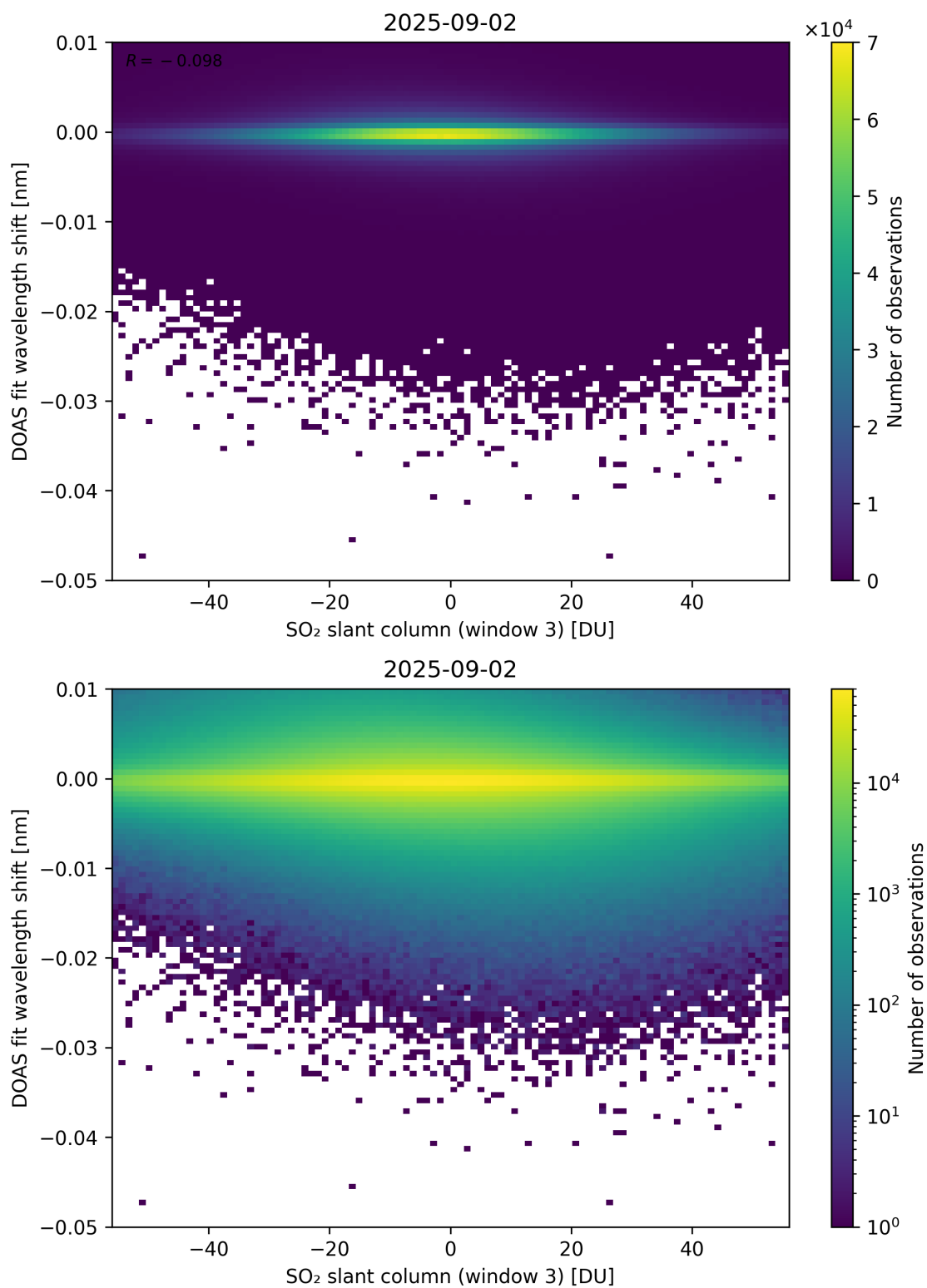
Figure 304: Scatter density plot of “SO 2 slant column (window 3)” against “DOAS fit wavelength shift” for 2025-09-01 to 2025-09-03.
