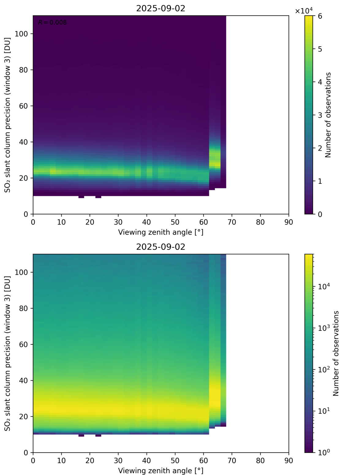
Figure 380: Scatter density plot of “Viewing zenith angle” against “SO 2 slant column precision (window 3)” for 2025-09-01 to 2025-09-03.
