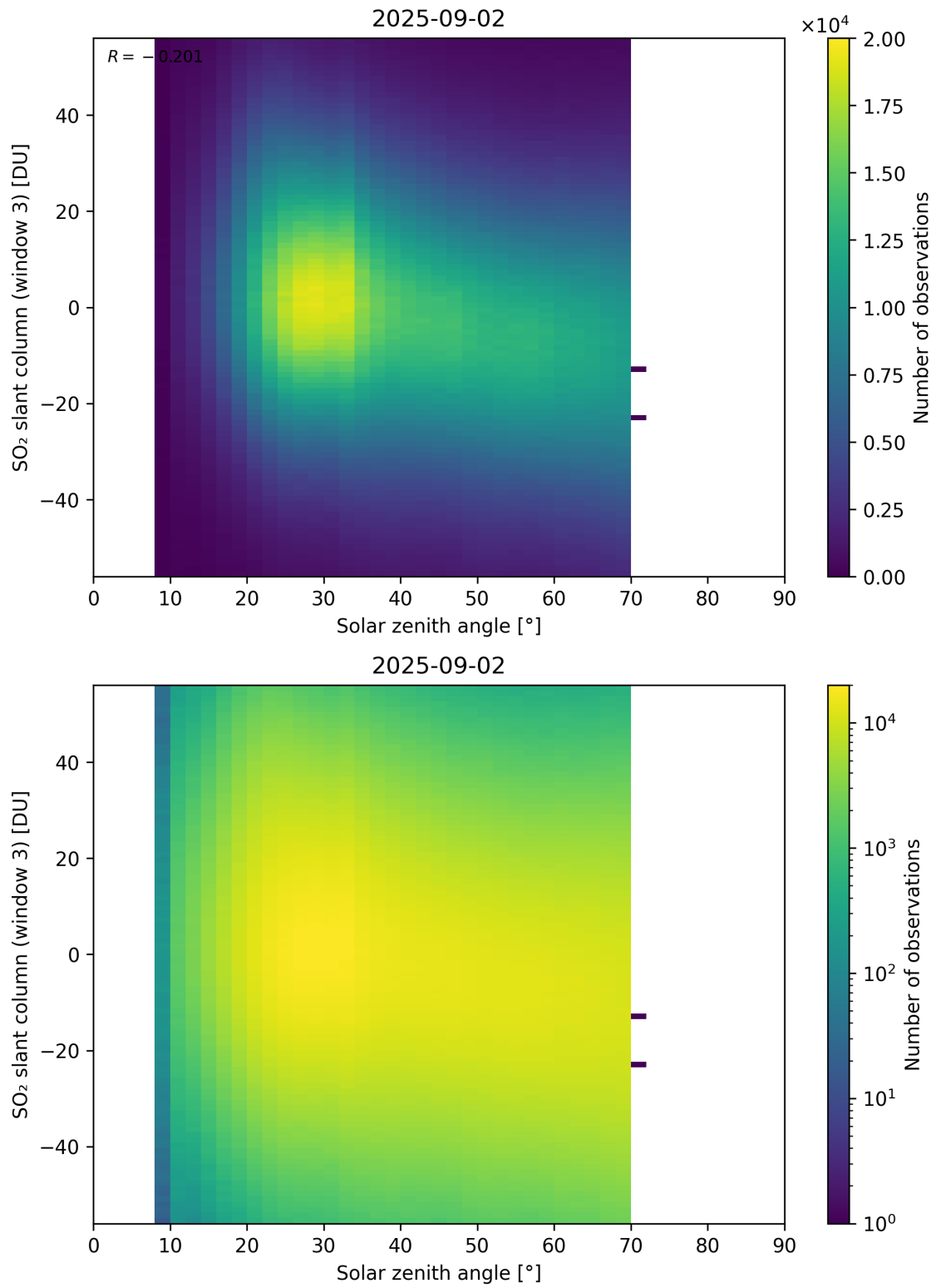
Figure 187: Scatter density plot of “Solar zenith angle” against “SO 2 slant column (window 3)” for 2025-09-01 to 2025-09-03.
