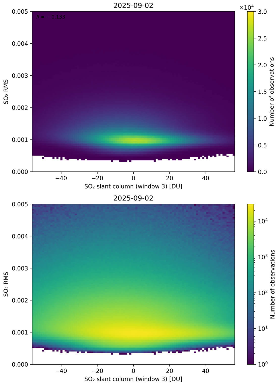
Figure 306: Scatter density plot of “SO 2 slant column (window 3)” against “SO 2 RMS” for 2025-09-01 to 2025-09-03.
