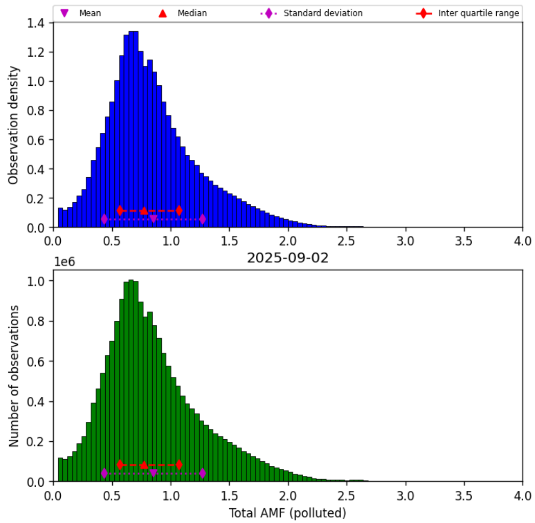
Figure 79: Histogram of “Total AMF (polluted)” for 2025-09-01 to 2025-09-03
