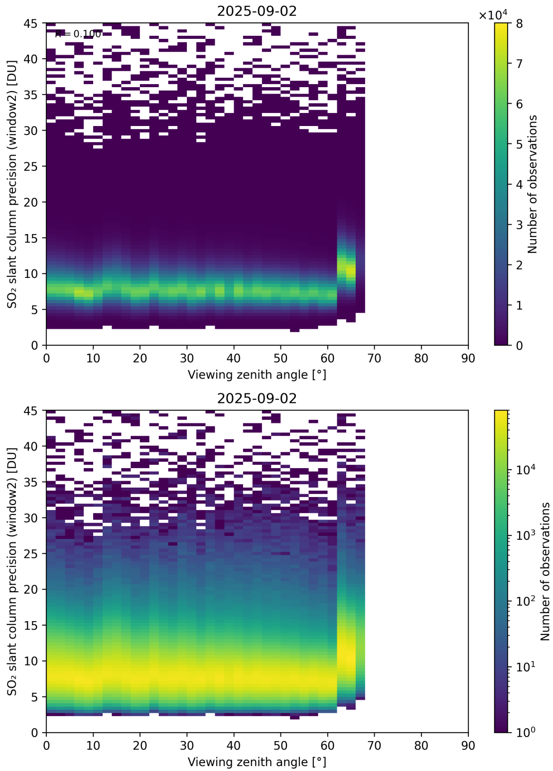
Figure 378: Scatter density plot of “Viewing zenith angle” against “SO 2 slant column precision (window2)” for 2025-09-01 to 2025-09-03.
