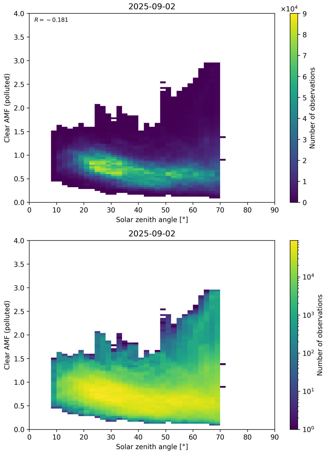
Figure 178: Scatter density plot of “Solar zenith angle” against “Clear AMF (polluted)” for 2025-09-01 to 2025-09-03.
