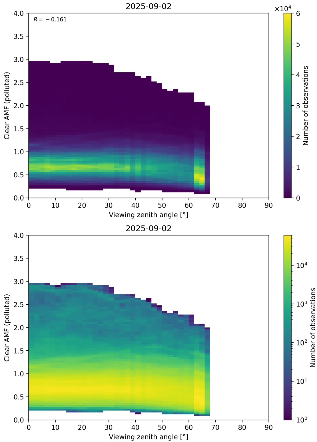
Figure 370: Scatter density plot of “Viewing zenith angle” against “Clear AMF (polluted)” for 2025-09-01 to 2025-09-03.
