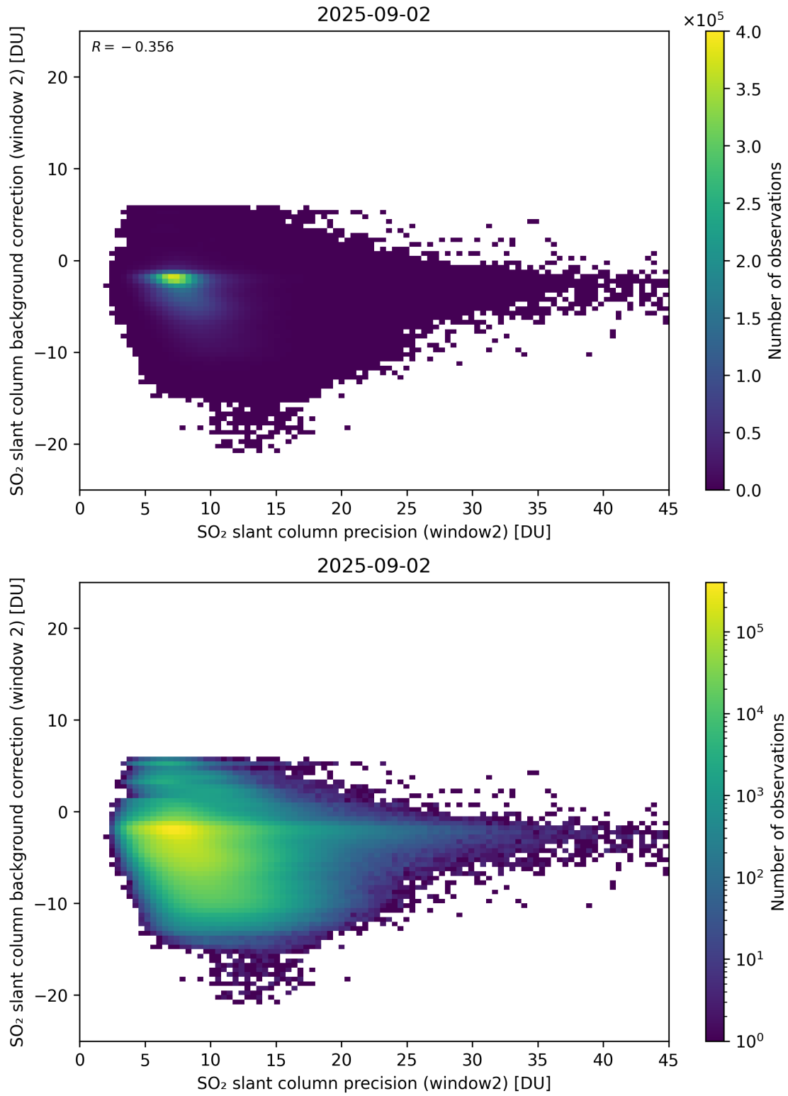
Figure 291: Scatter density plot of “SO 2 slant column precision (window2)” against “SO 2 slant column background correction (window 2)” for 2025-09-01 to 2025-09-03.
