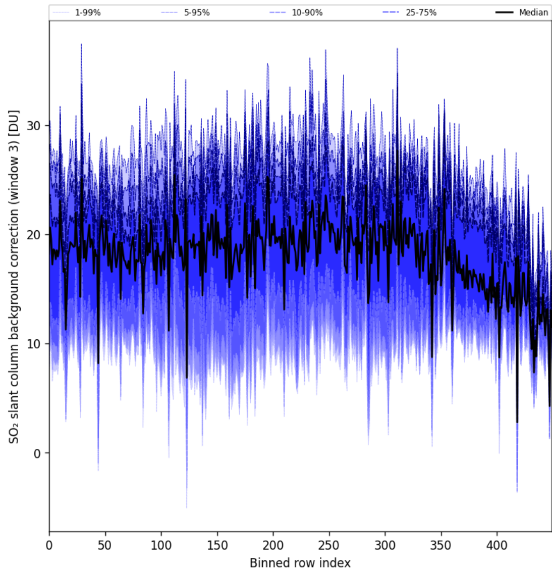
Figure 100: Along track statistics of “SO 2 slant column background correction (window 3)” for 2025-09-01 to 2025-09-03
