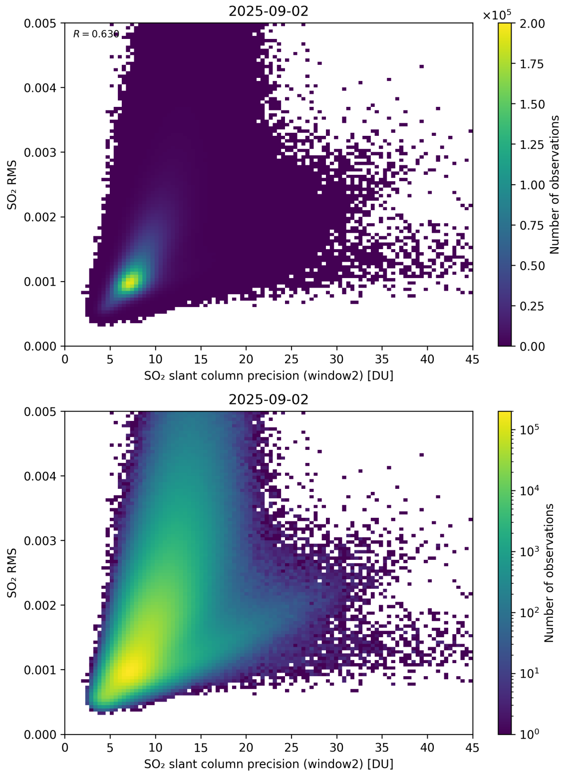
Figure 295: Scatter density plot of “SO 2 slant column precision (window2)” against “SO 2 RMS” for 2025-09-01 to 2025-09-03.
