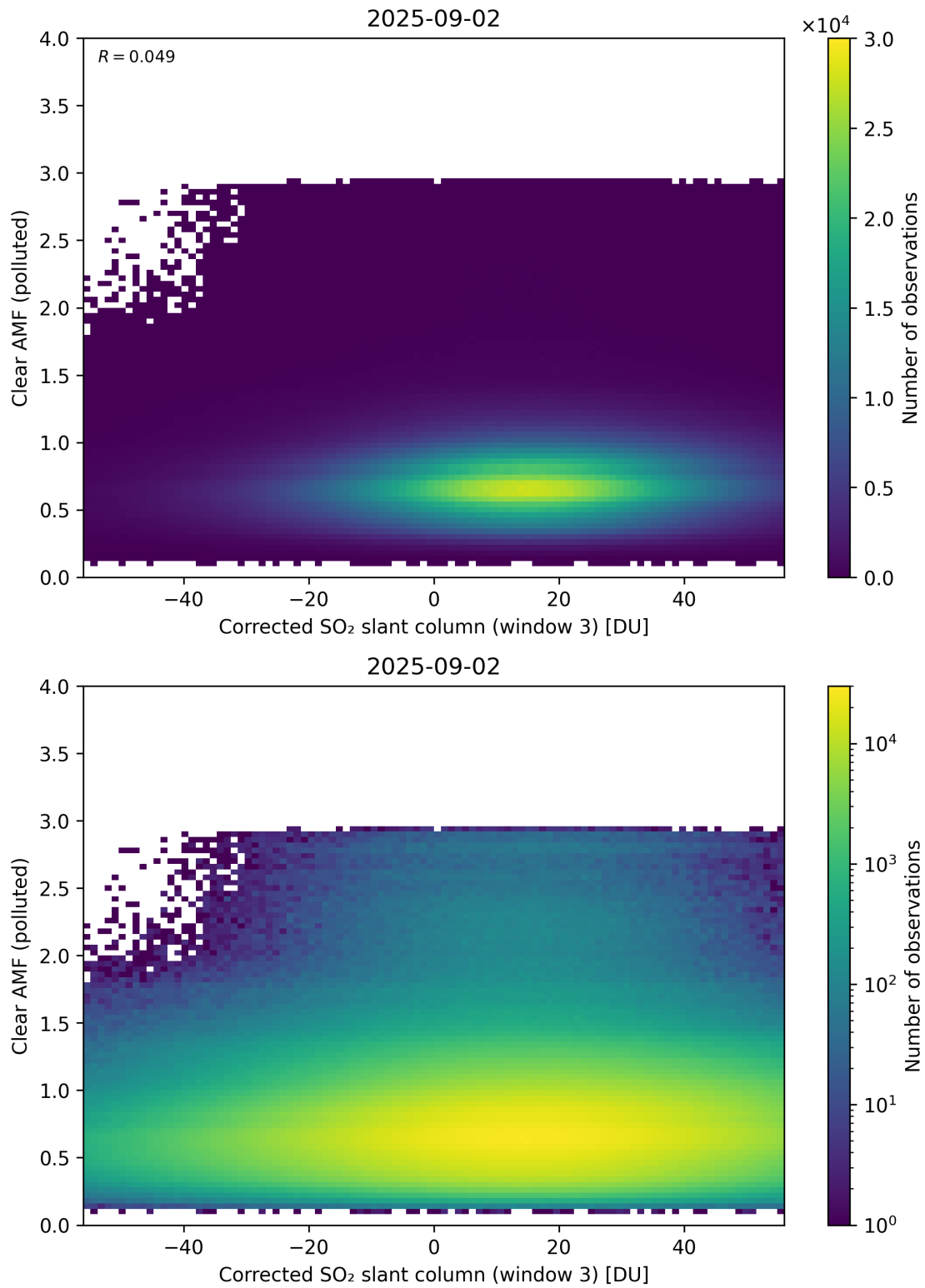
Figure 259: Scatter density plot of “Corrected SO 2 slant column (window 3)” against “Clear AMF (polluted)” for 2025-09-01 to 2025-09-03.
