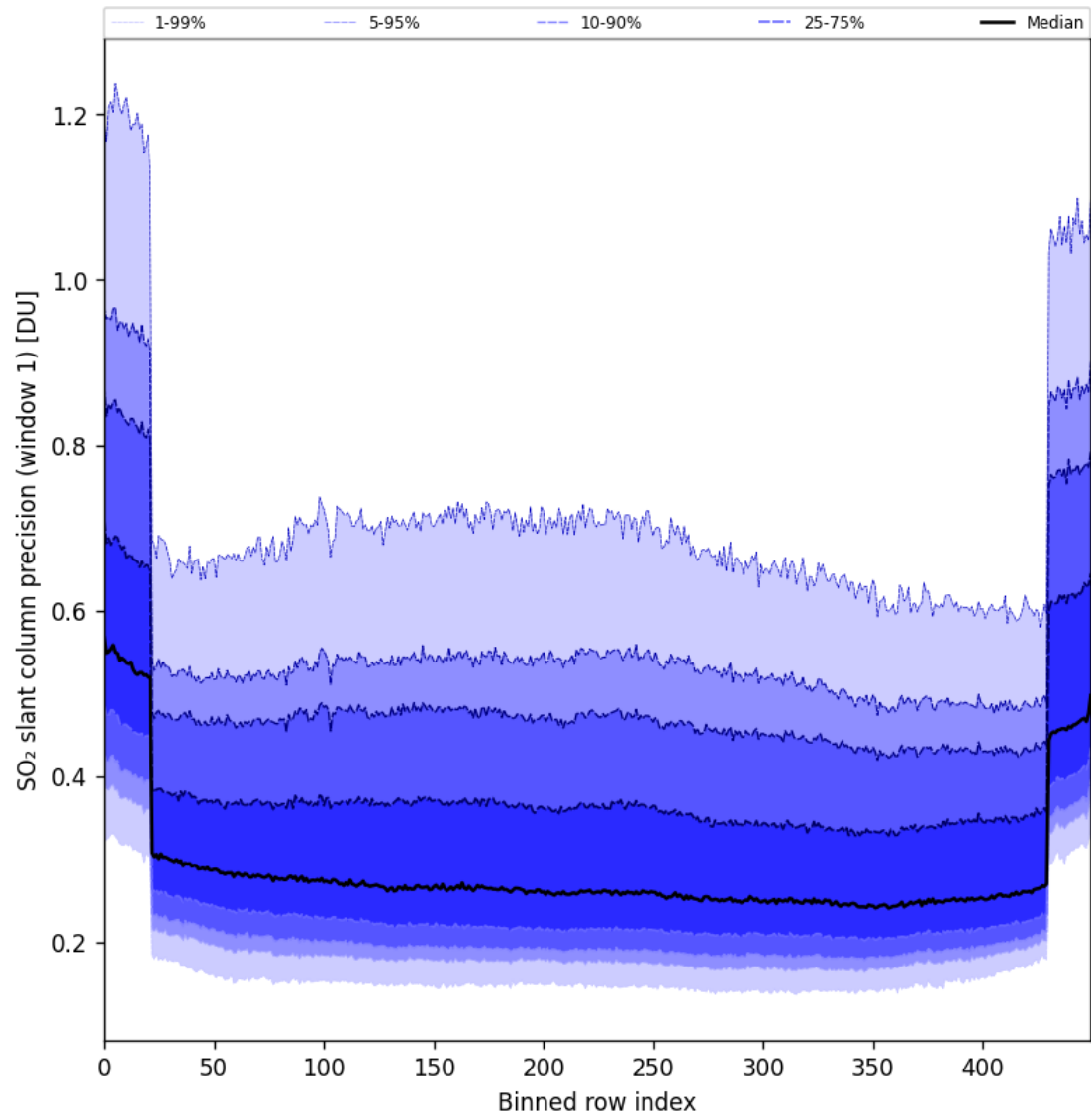
Figure 90: Along track statistics of “SO 2 slant column precision (window 1)” for 2025-09-01 to 2025-09-03
