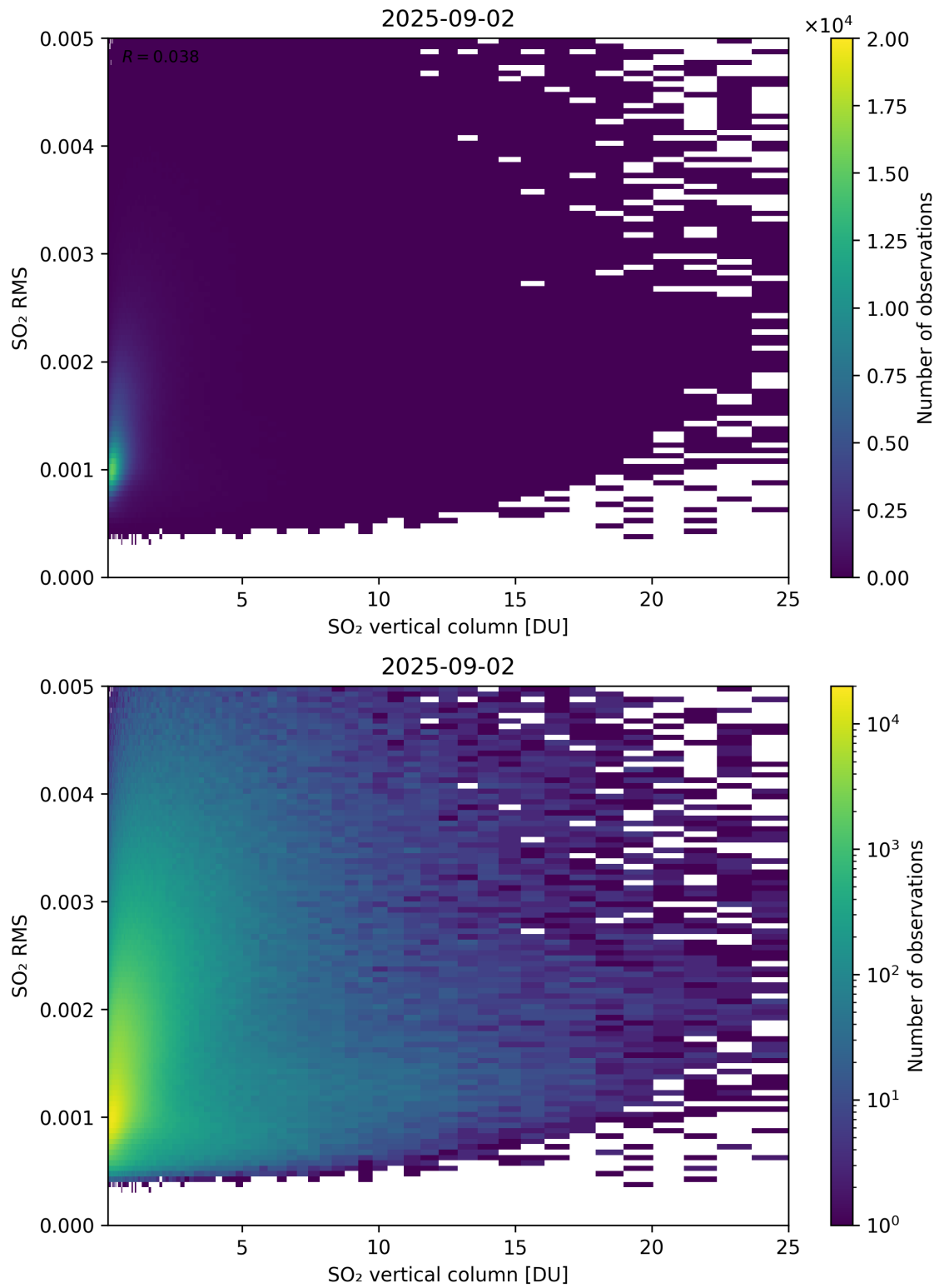
Figure 328: Scatter density plot of “SO 2 vertical column” against “SO 2 RMS” for 2025-09-01 to 2025-09-03.
