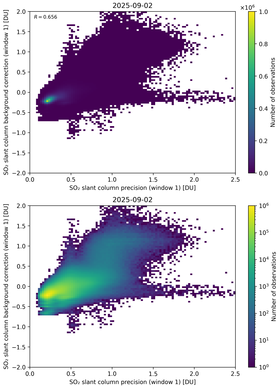
Figure 268: Scatter density plot of “SO 2 slant column precision (window 1)” against “SO 2 slant column background correction (window 1)” for 2025-09-01 to 2025-09-03.
