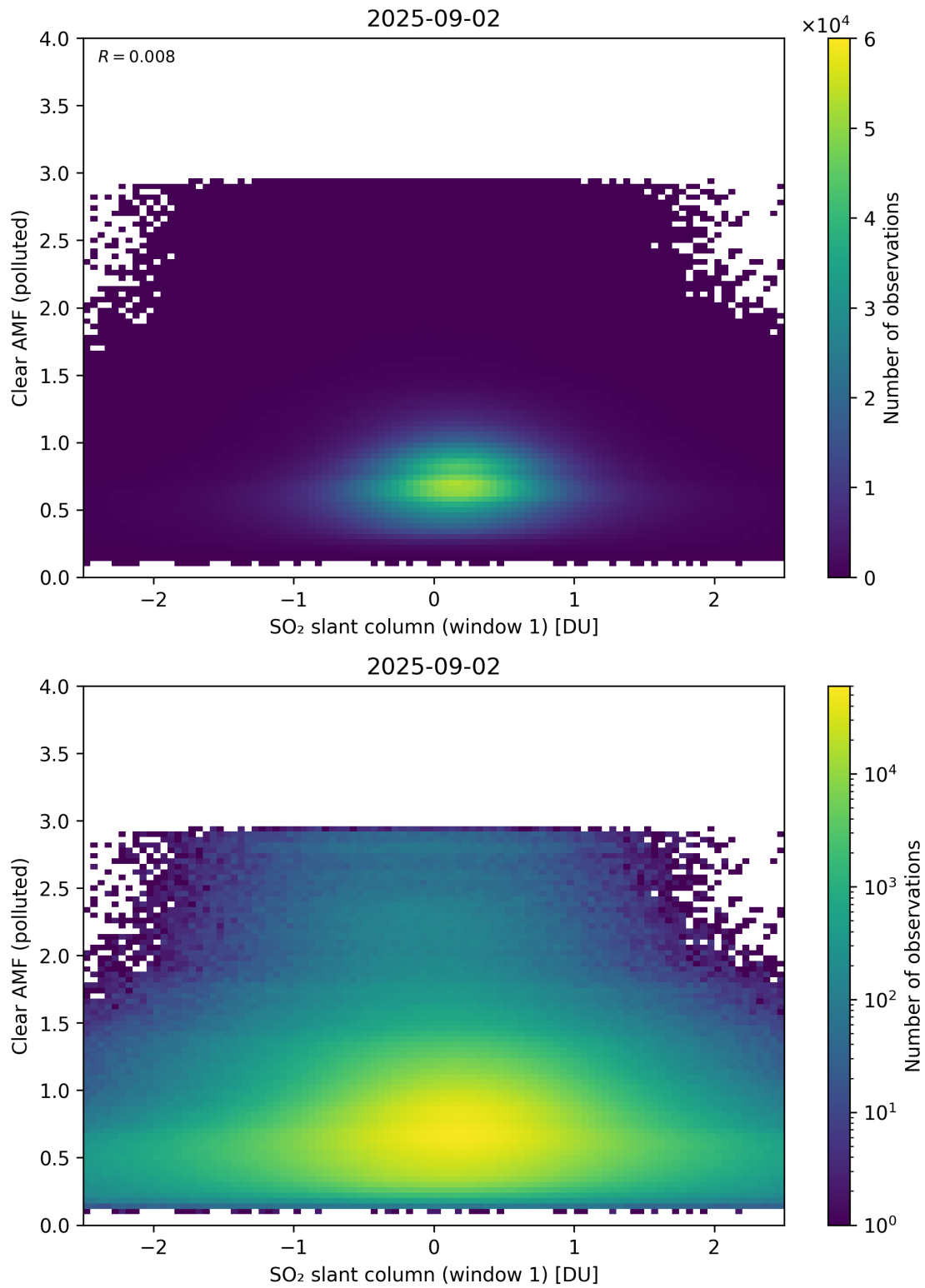
Figure 282: Scatter density plot of “SO 2 slant column (window 1)” against “Clear AMF (polluted)” for 2025-09-01 to 2025-09-03.
