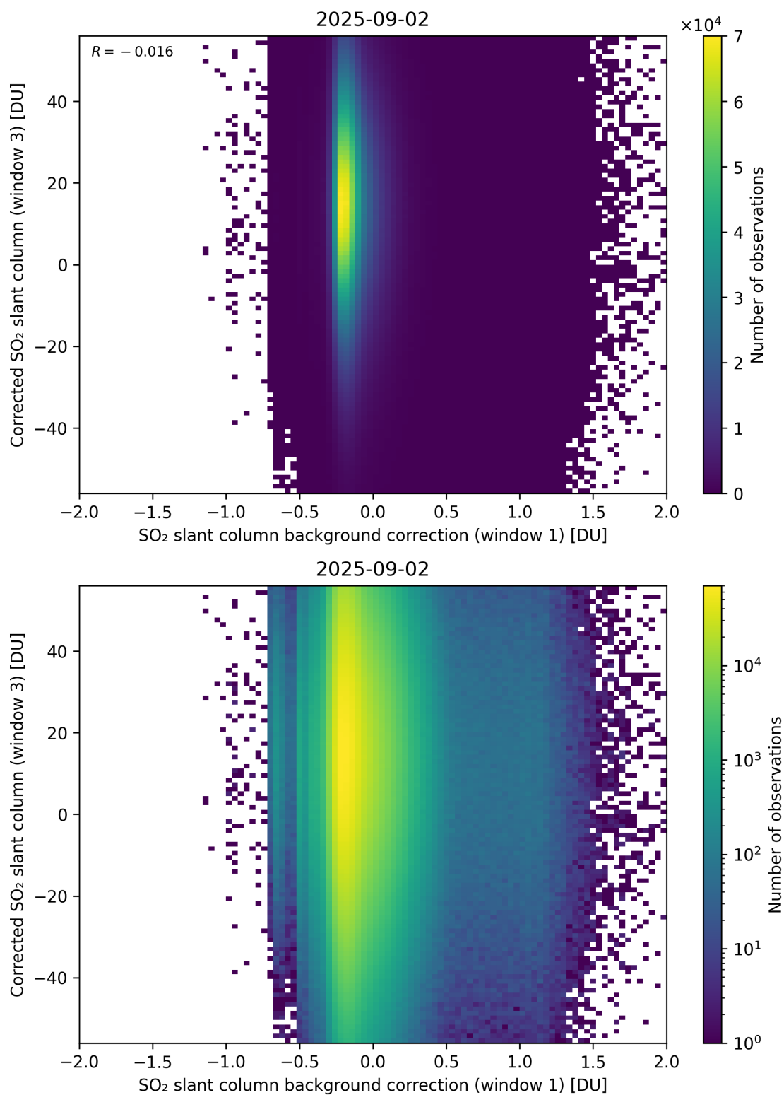
Figure 116: Scatter density plot of “SO 2 slant column background correction (window 1)” against “Corrected SO 2 slant column (window 3)” for 2025-09-01 to 2025-09-03.
