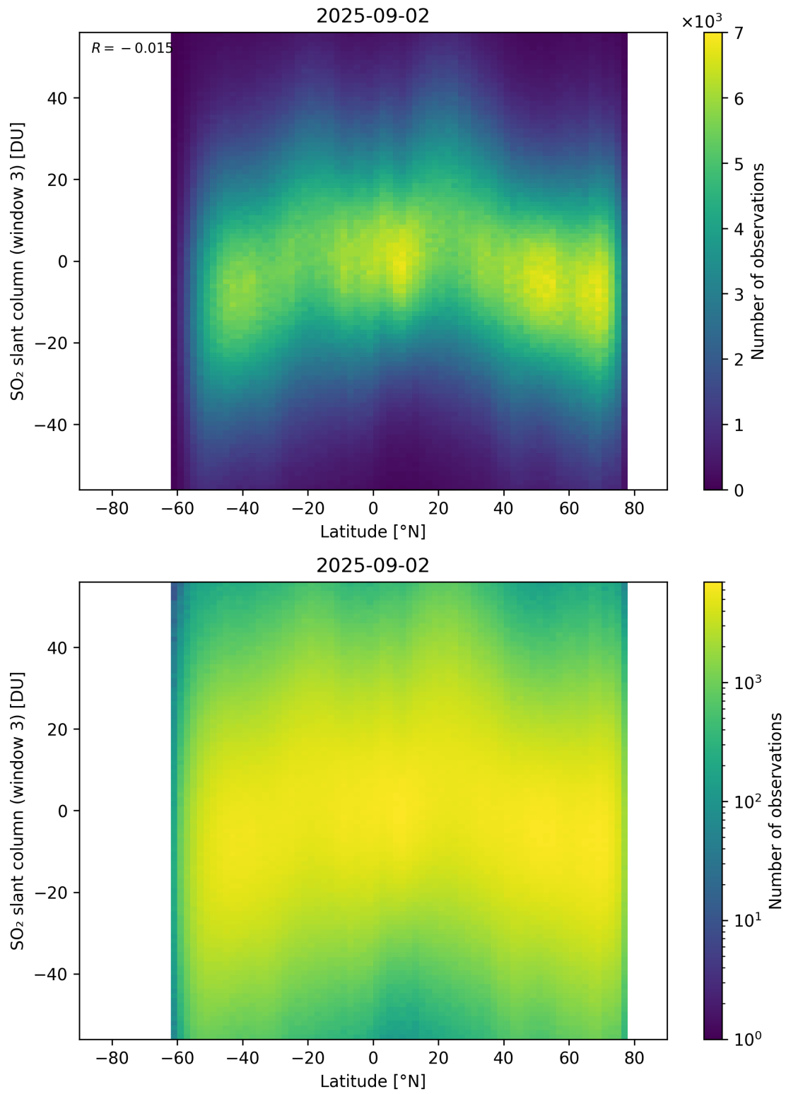
Figure 165: Scatter density plot of “Latitude” against “SO 2 slant column (window 3)” for 2025-09-01 to 2025-09-03.
