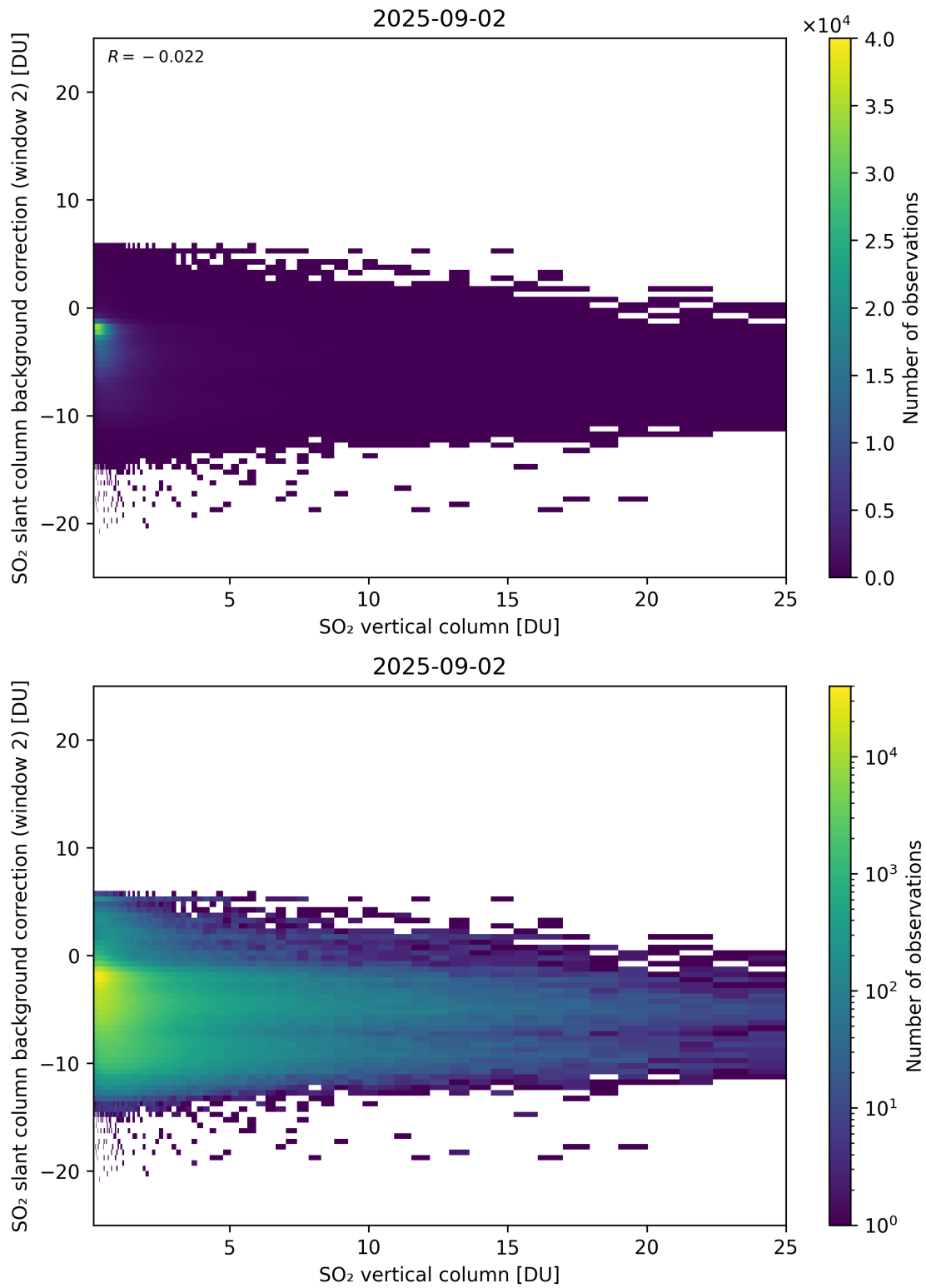
Figure 324: Scatter density plot of “SO 2 vertical column” against “SO 2 slant column background correction (window 2)” for 2025-09-01 to 2025-09-03.
