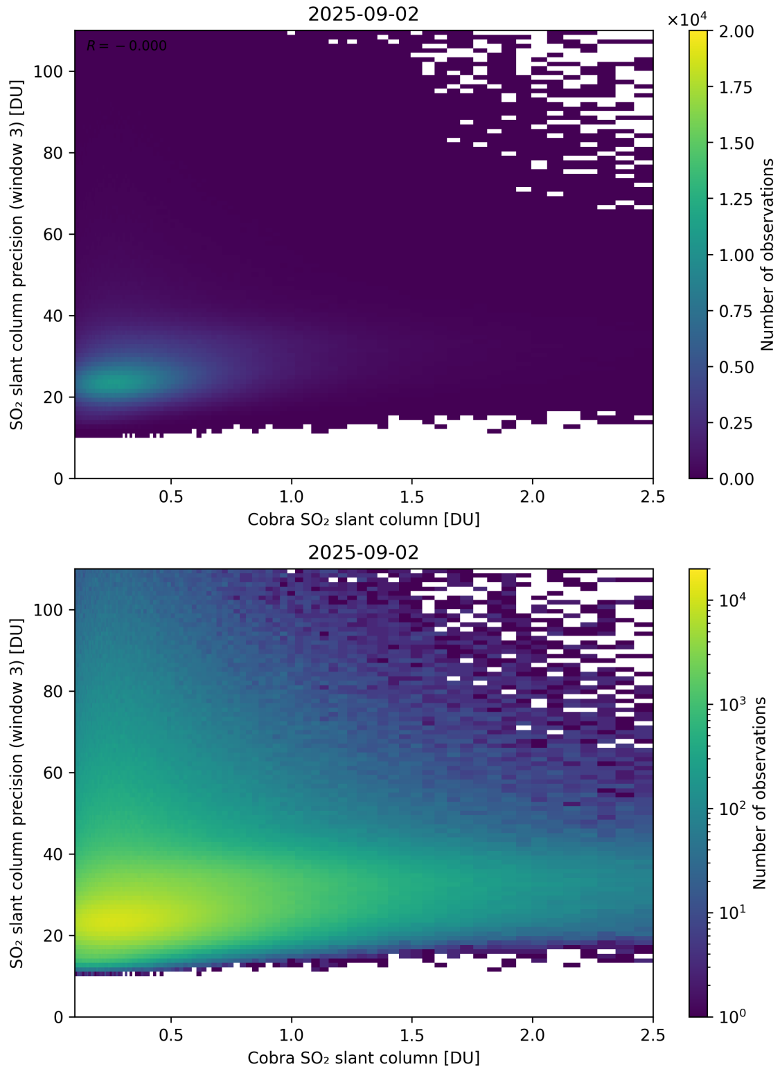
Figure 223: Scatter density plot of “Cobra SO 2 slant column” against “SO 2 slant column precision (window 3)” for 2025-09-01 to 2025-09-03.
