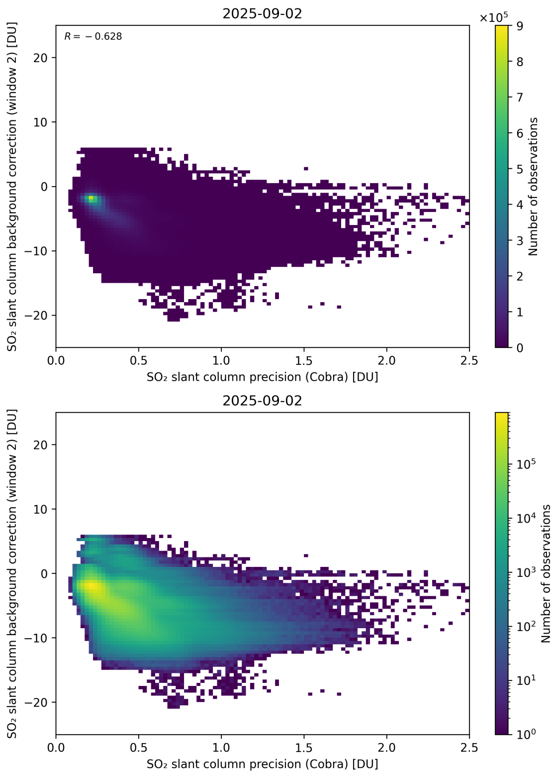
Figure 200: Scatter density plot of “SO 2 slant column precision (Cobra)” against “SO 2 slant column background correction (window 2)” for 2025-09-01 to 2025-09-03.
