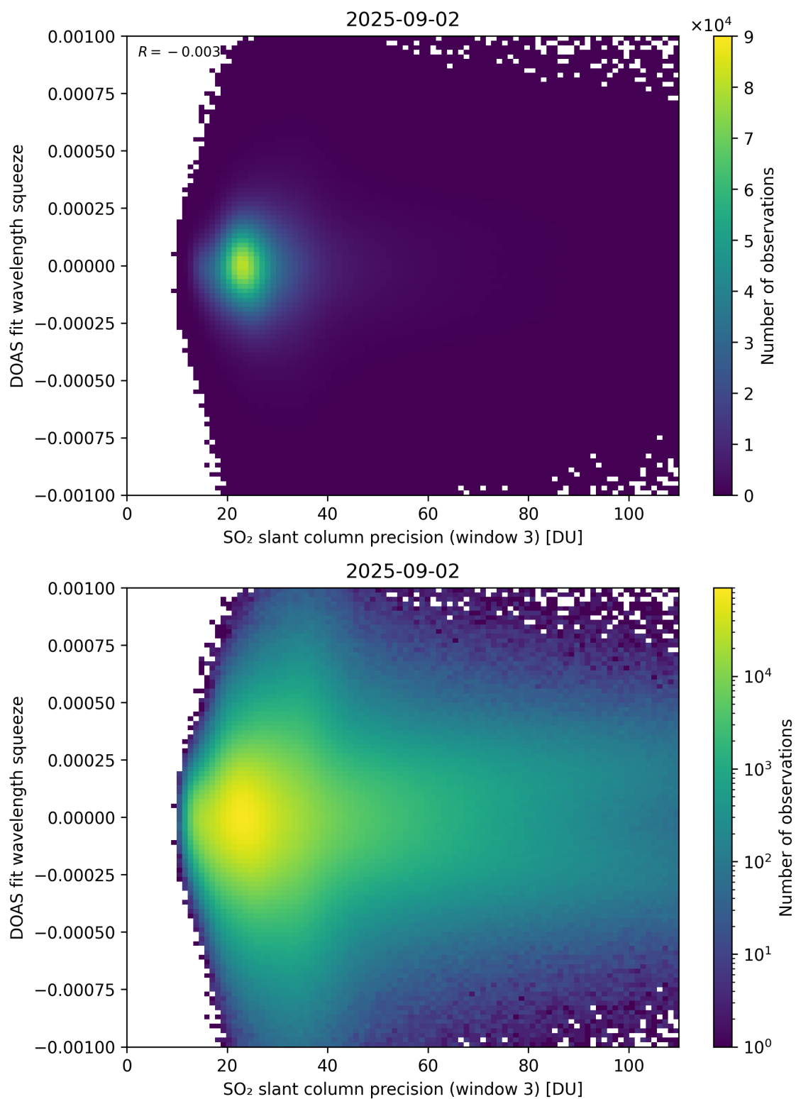
Figure 309: Scatter density plot of “SO 2 slant column precision (window 3)” against “DOAS fit wavelength squeeze” for 2025-09-01 to 2025-09-03.
