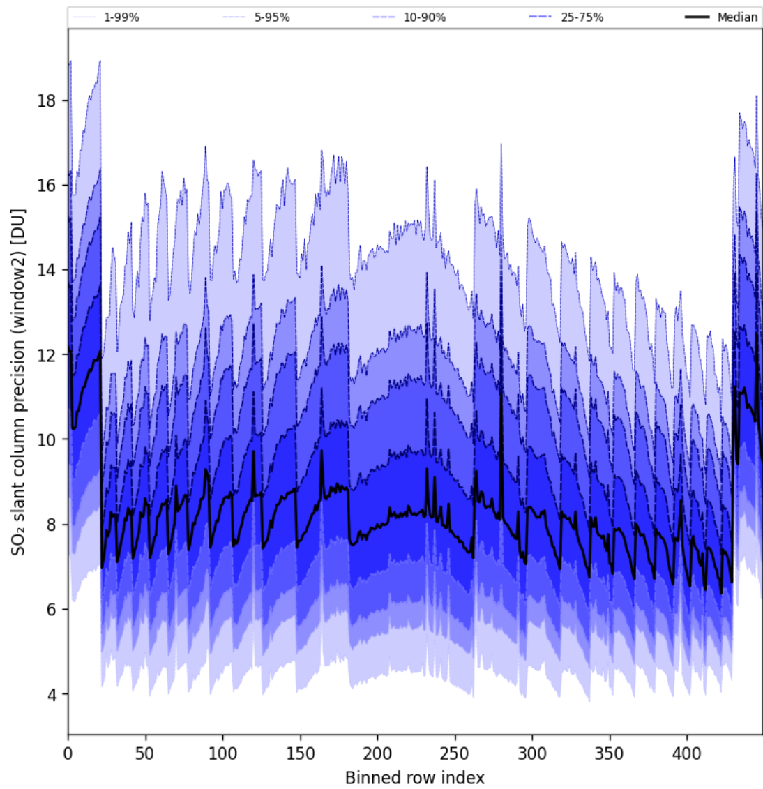
Figure 94: Along track statistics of “SO 2 slant column precision (window2)” for 2025-09-01 to 2025-09-03
