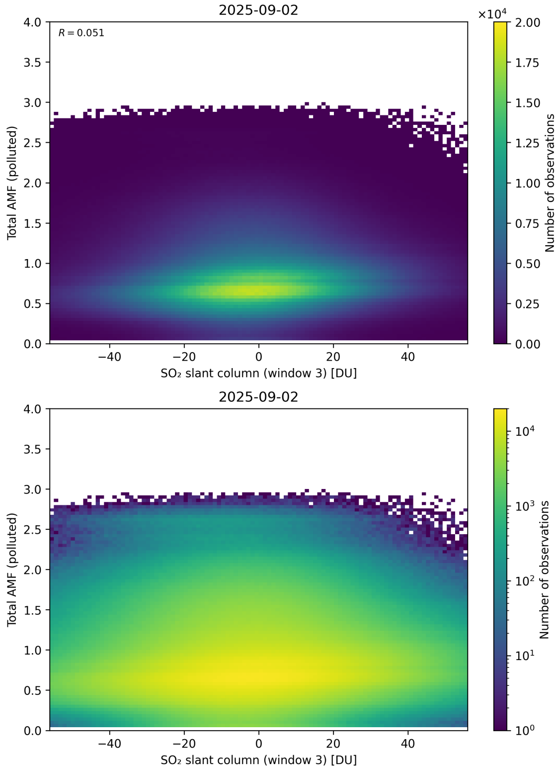
Figure 318: Scatter density plot of “SO 2 slant column (window 3)” against “Total AMF (polluted)” for 2025-09-01 to 2025-09-03.
