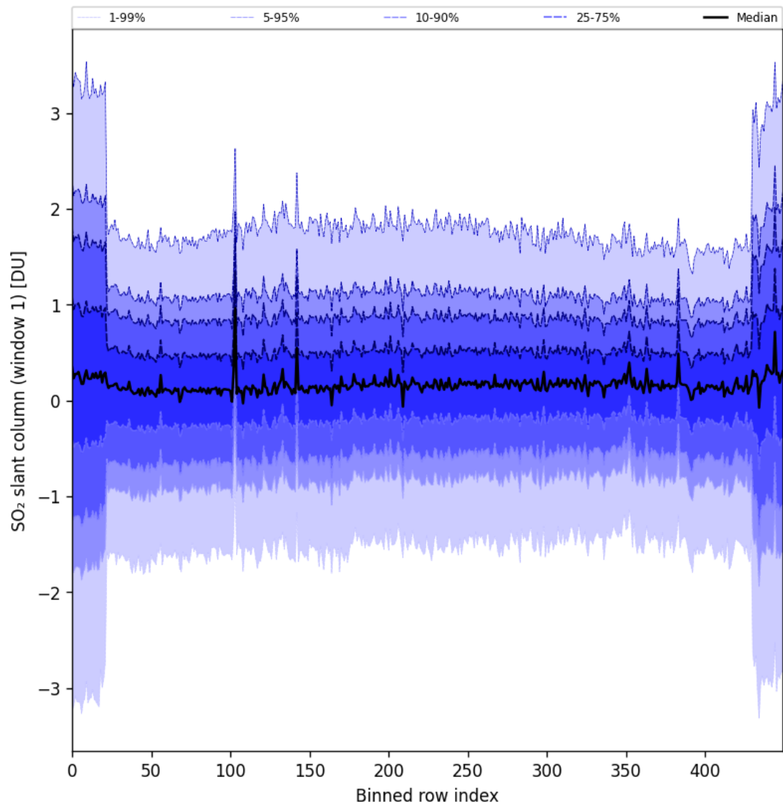
Figure 89: Along track statistics of “SO 2 slant column (window 1)” for 2025-09-01 to 2025-09-03
