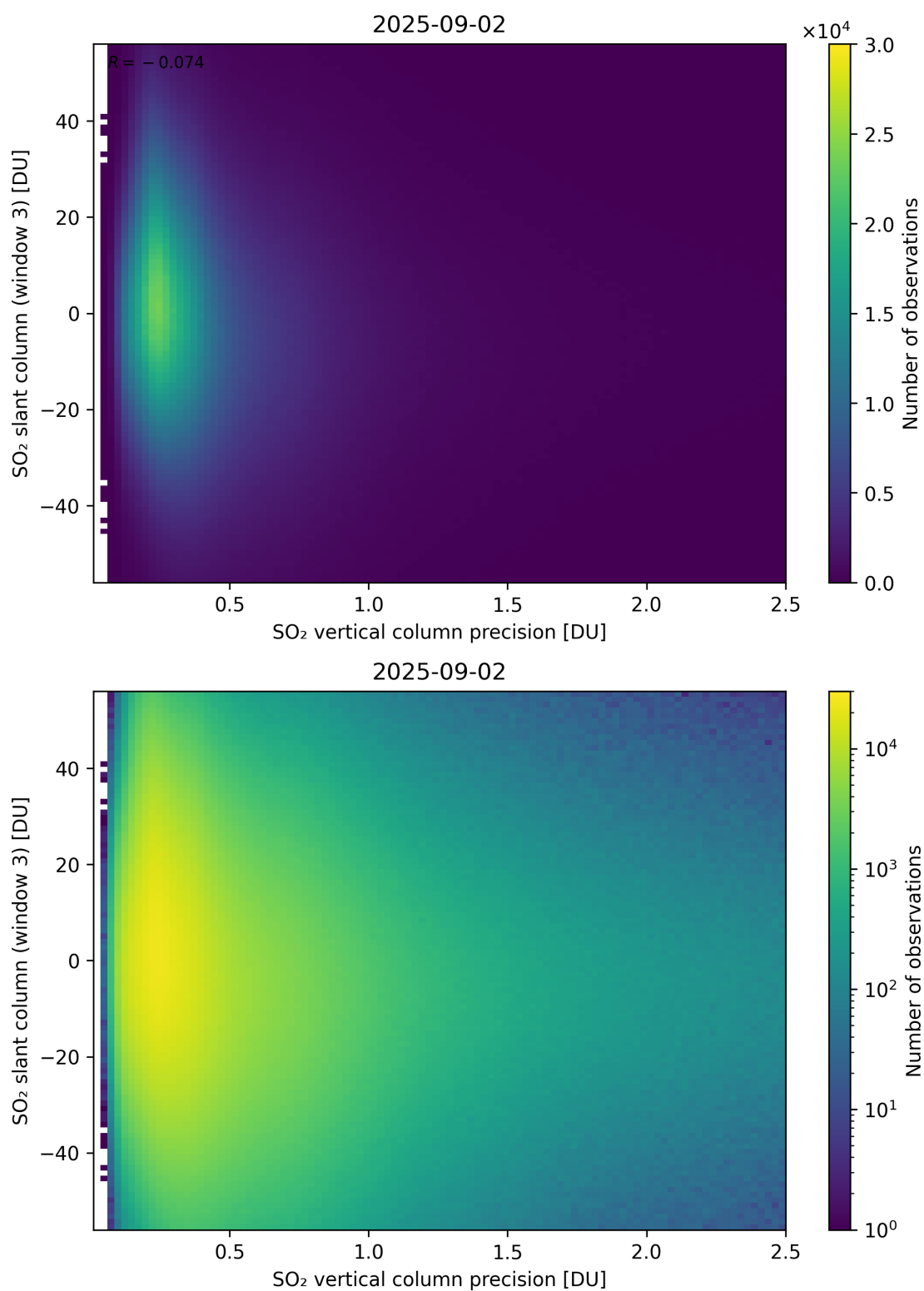
Figure 344: Scatter density plot of “SO 2 vertical column precision” against “SO 2 slant column (window 3)” for 2025-09-01 to 2025-09-03.
