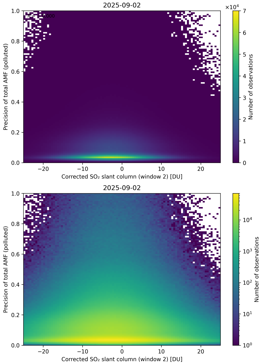
Figure 254: Scatter density plot of “Corrected SO 2 slant column (window 2)” against “Precision of total AMF (polluted)” for 2025-09-01 to 2025-09-03.
