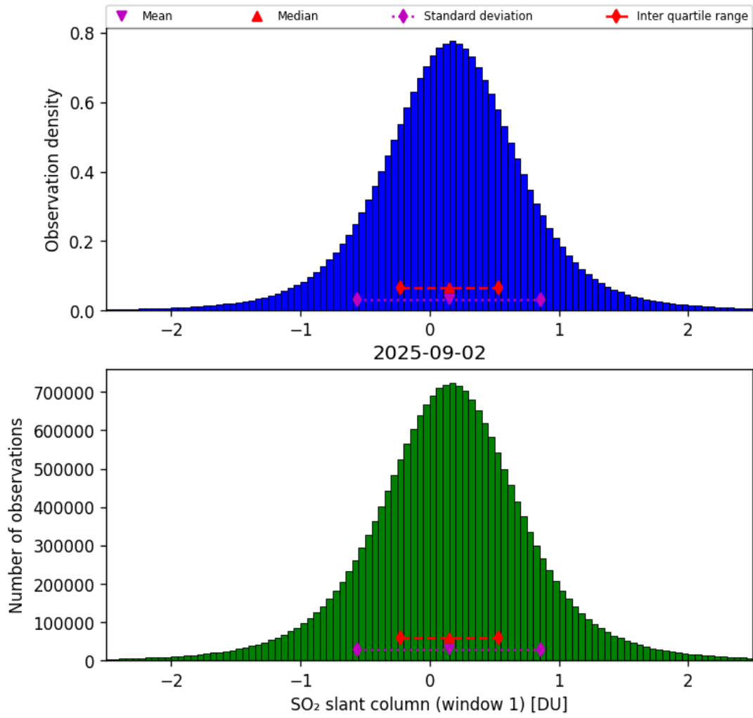
Figure 63: Histogram of “SO 2 slant column (window 1)” for 2025-09-01 to 2025-09-03
