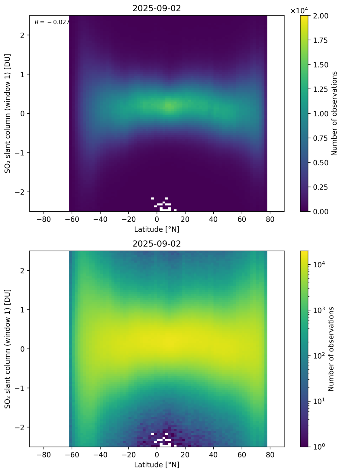
Figure 162: Scatter density plot of “Latitude” against “SO 2 slant column (window 1)” for 2025-09-01 to 2025-09-03.
