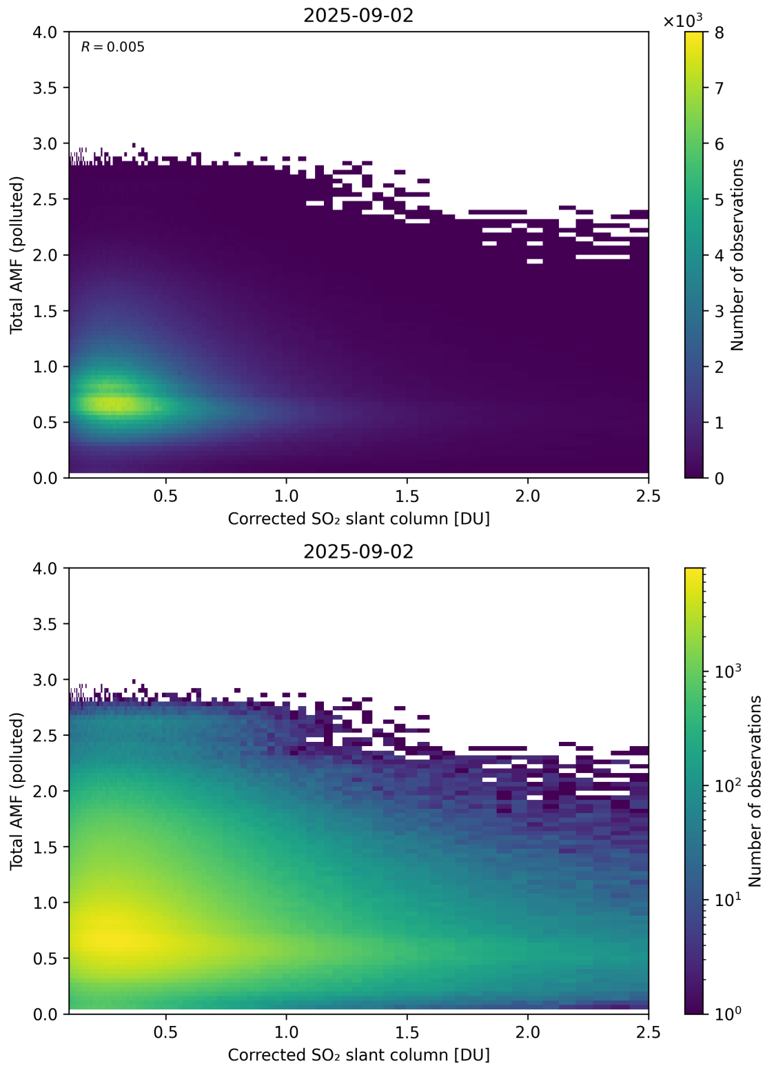
Figure 242: Scatter density plot of “Corrected SO 2 slant column” against “Total AMF (polluted)” for 2025-09-01 to 2025-09-03.
