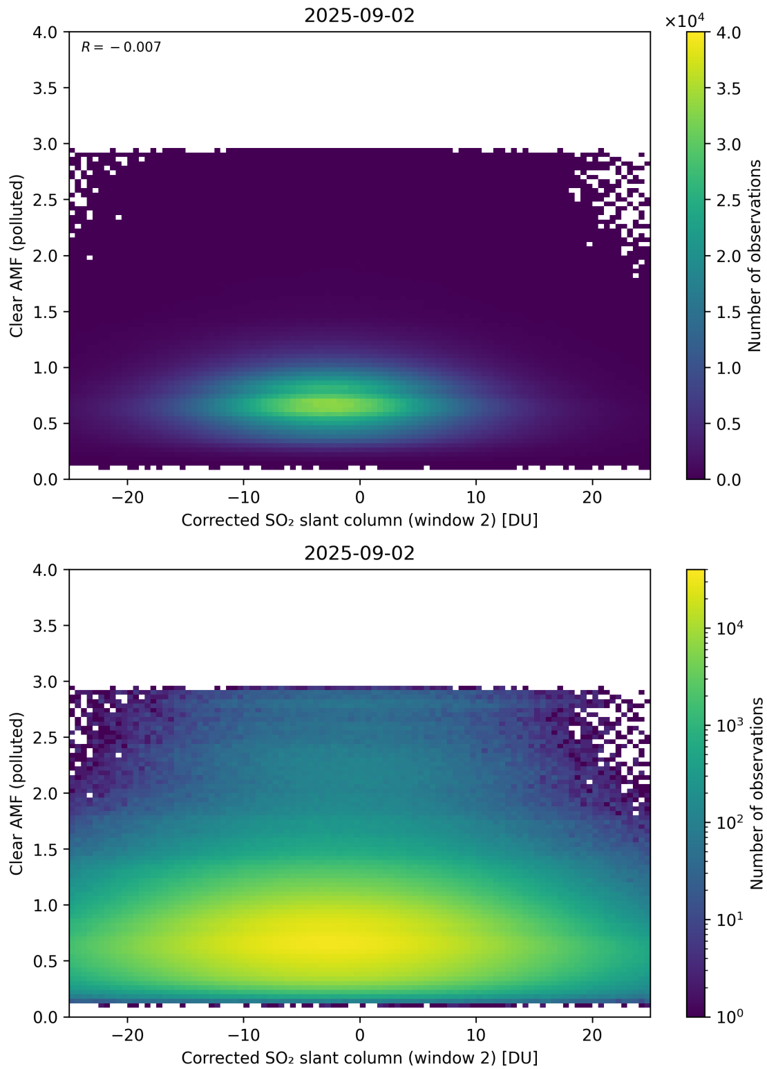
Figure 249: Scatter density plot of “Corrected SO 2 slant column (window 2)” against “Clear AMF (polluted)” for 2025-09-01 to 2025-09-03.
