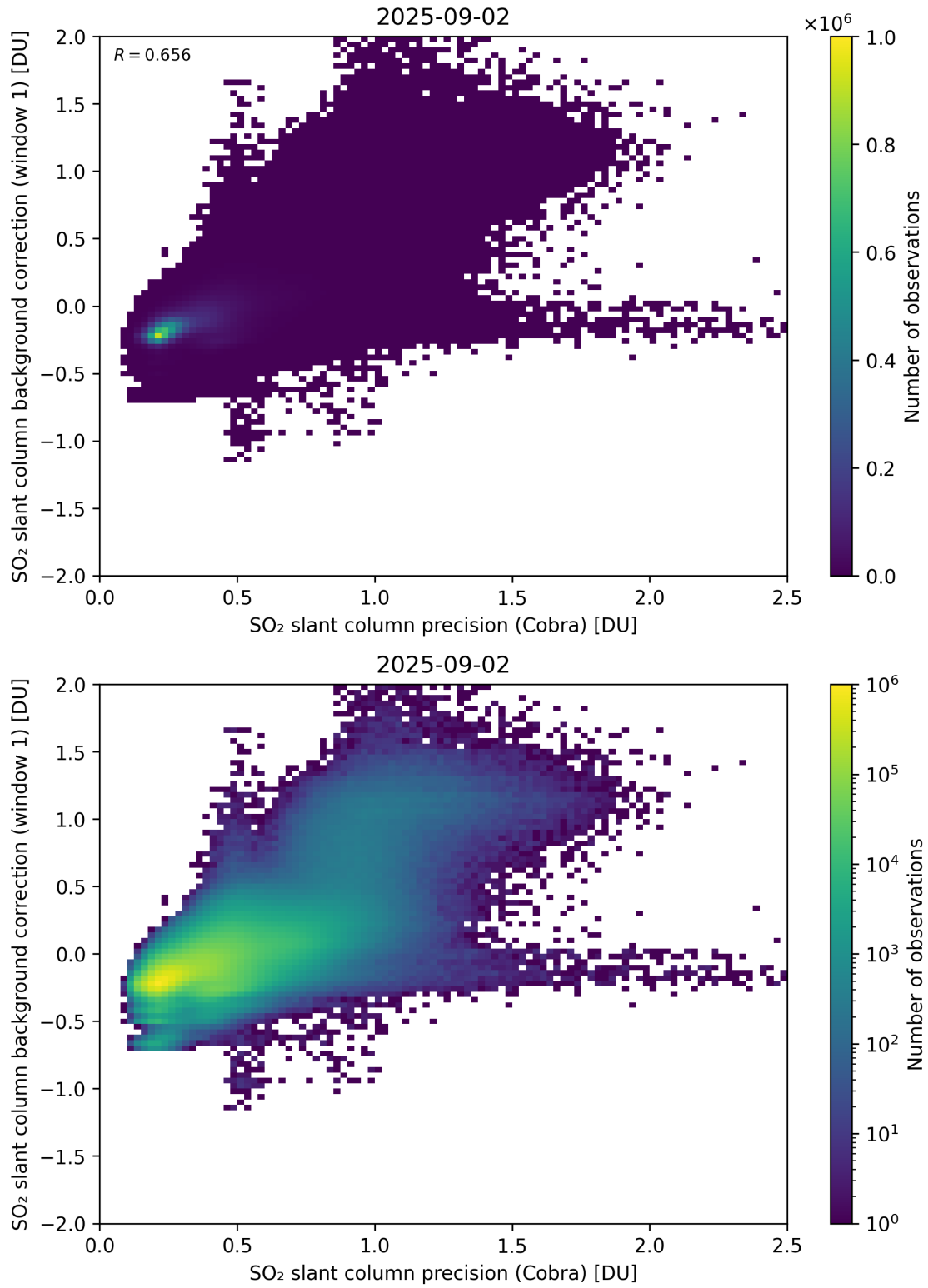
Figure 199: Scatter density plot of “SO 2 slant column precision (Cobra)” against “SO 2 slant column background correction (window 1)” for 2025-09-01 to 2025-09-03.
