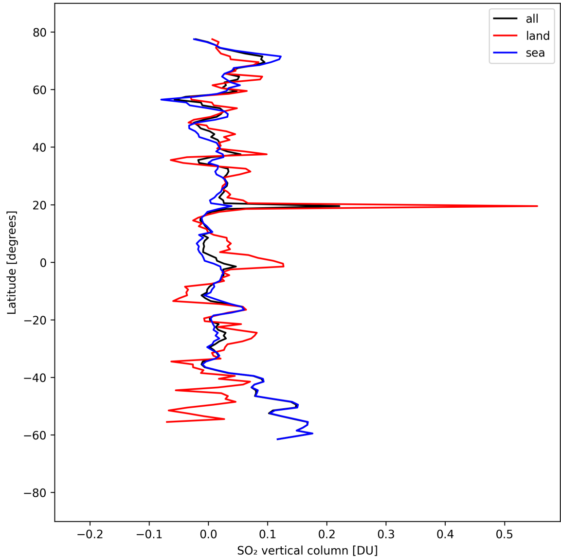
Figure 32: Zonal average of “SO 2 vertical column” for 2025-09-01 to 2025-09-03.
