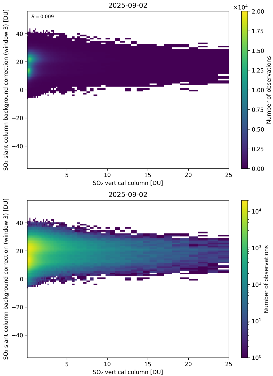
Figure 325: Scatter density plot of “SO 2 vertical column” against “SO 2 slant column background correction (window 3)” for 2025-09-01 to 2025-09-03.
