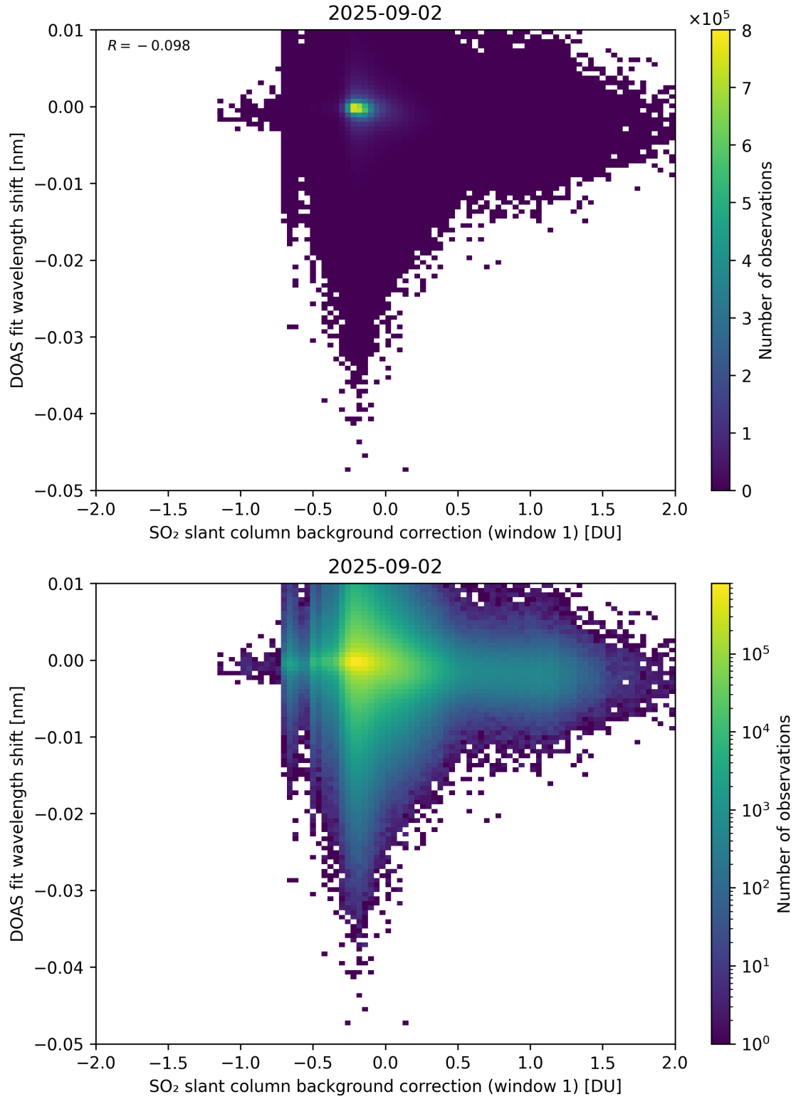
Figure 111: Scatter density plot of “SO 2 slant column background correction (window 1)” against “DOAS fit wavelength shift” for 2025-09-01 to 2025-09-03.
