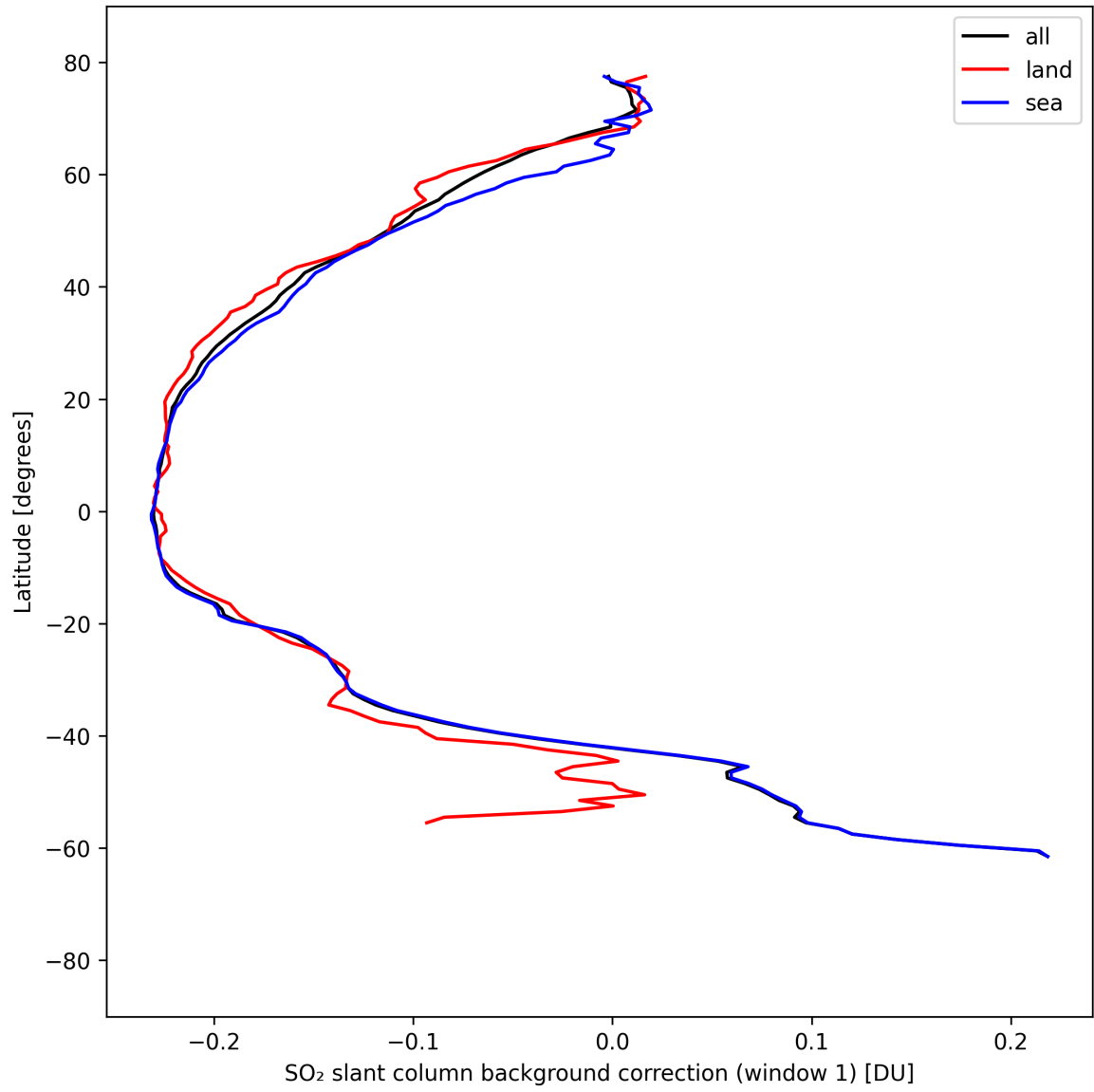
Figure 40: Zonal average of “SO 2 slant column background correction (window 1)” for 2025-09-01 to 2025-09-03.
