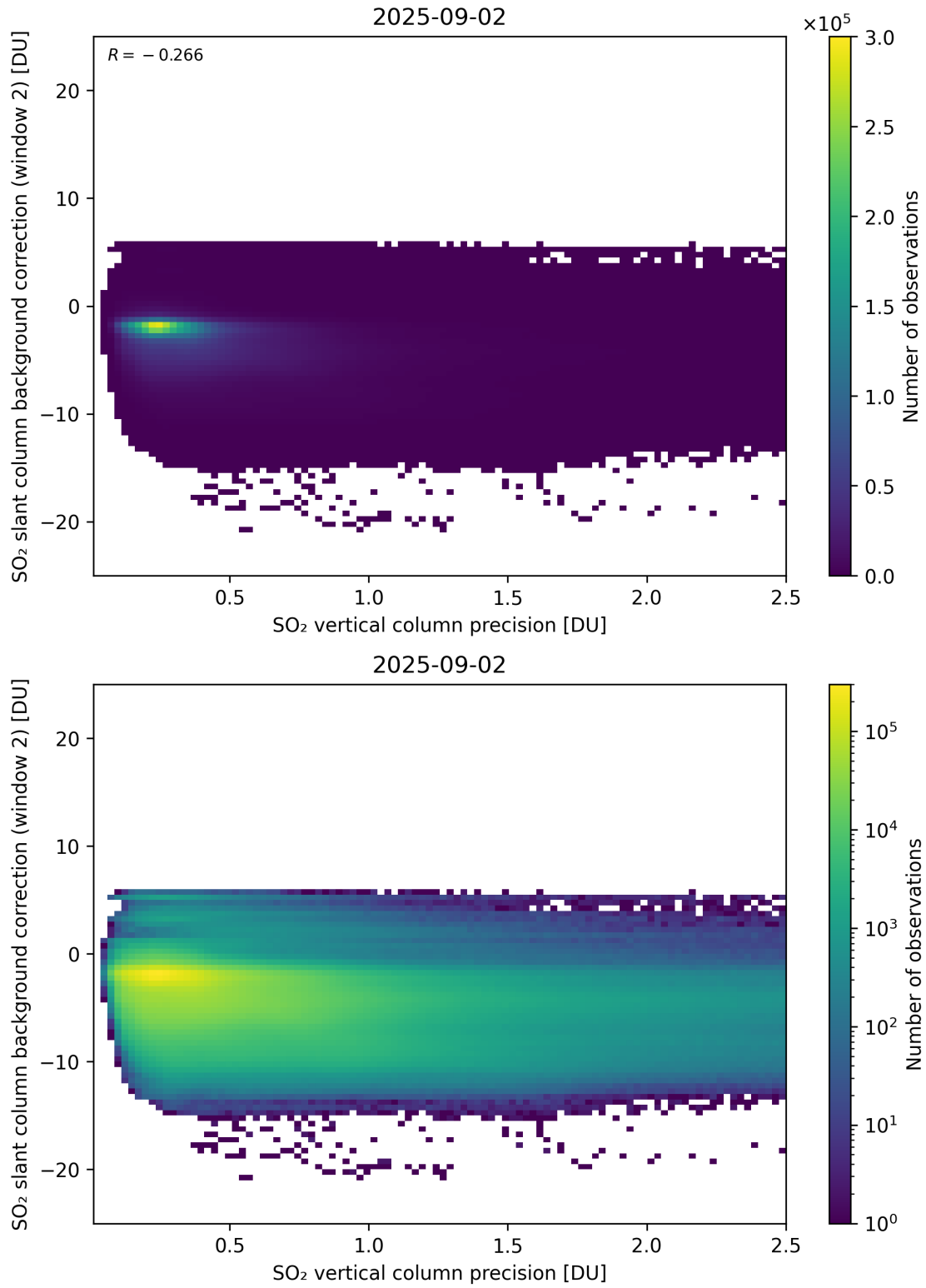
Figure 330: Scatter density plot of “SO 2 vertical column precision” against “SO 2 slant column background correction (window 2)” for 2025-09-01 to 2025-09-03.
