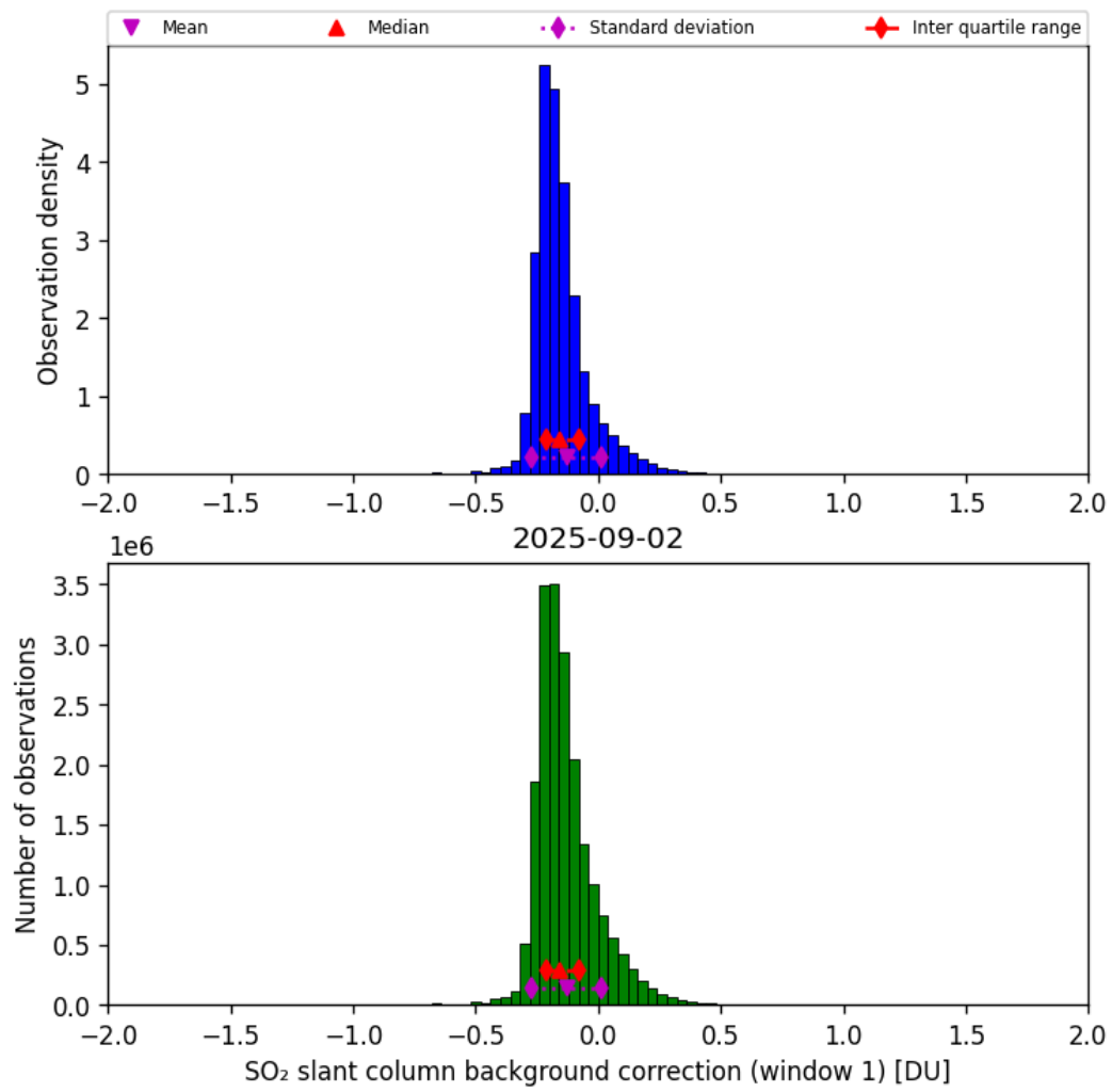
Figure 66: Histogram of “SO 2 slant column background correction (window 1)” for 2025-09-01 to 2025-09-03
