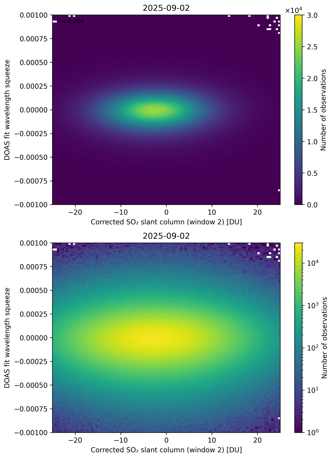
Figure 247: Scatter density plot of “Corrected SO 2 slant column (window 2)” against “DOAS fit wavelength squeeze” for 2025-09-01 to 2025-09-03.
