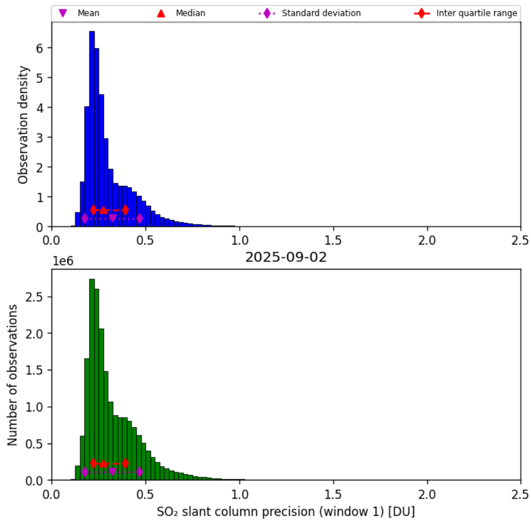
Figure 64: Histogram of “SO 2 slant column precision (window 1)” for 2025-09-01 to 2025-09-03
