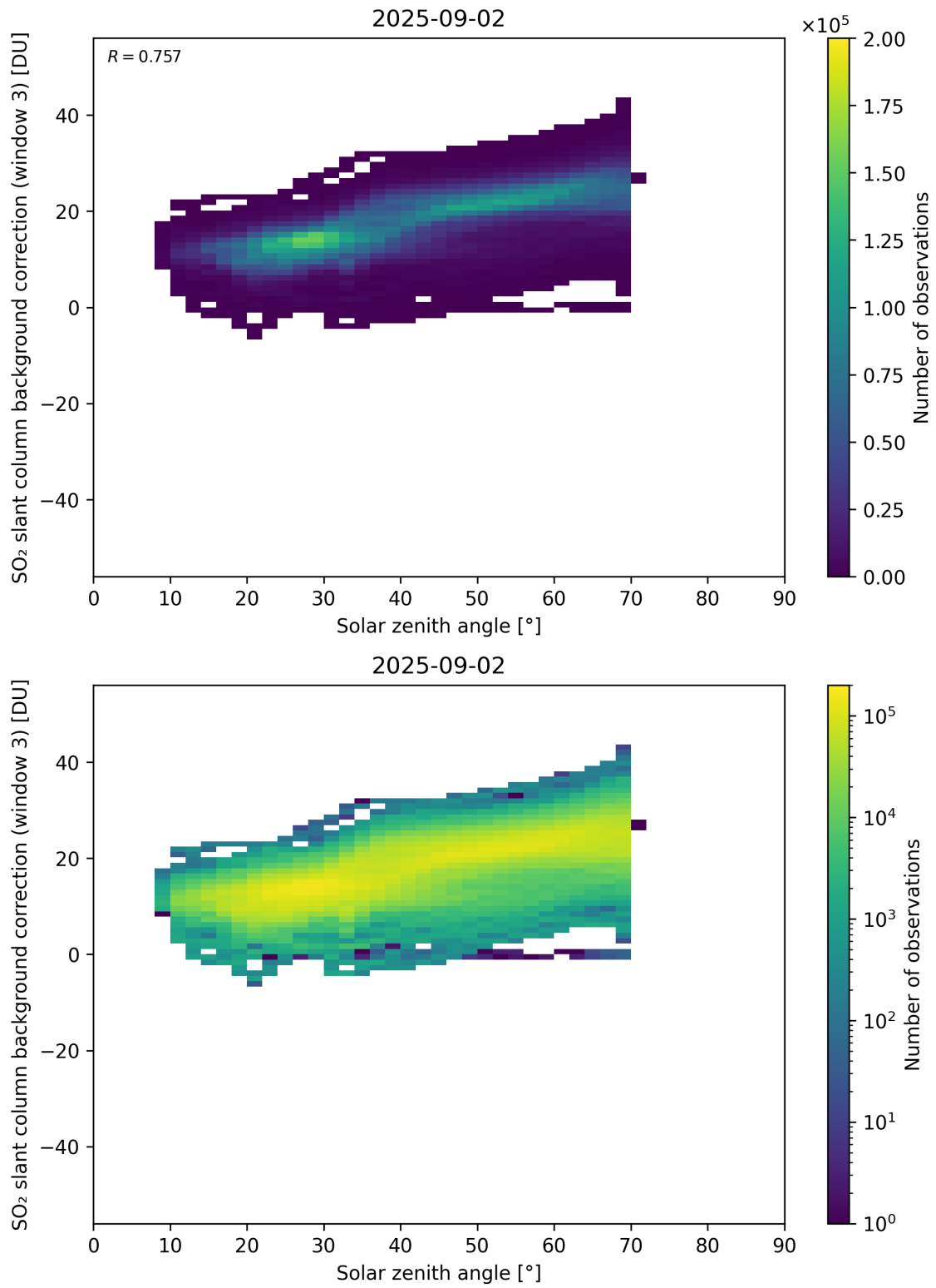
Figure 173: Scatter density plot of “Solar zenith angle” against “SO 2 slant column background correction (window 3)” for 2025-09-01 to 2025-09-03.
