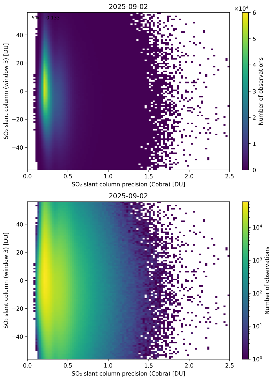
Figure 211: Scatter density plot of “SO 2 slant column precision (Cobra)” against “SO 2 slant column (window 3)” for 2025-09-01 to 2025-09-03.
