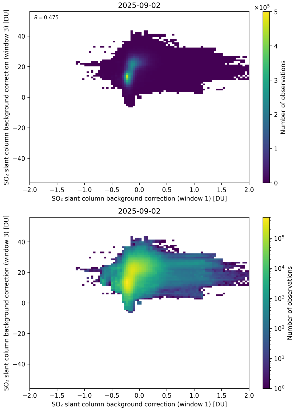
Figure 110: Scatter density plot of “SO 2 slant column background correction (window 1)” against “SO 2 slant column background correction (window 3)” for 2025-09-01 to 2025-09-03.
