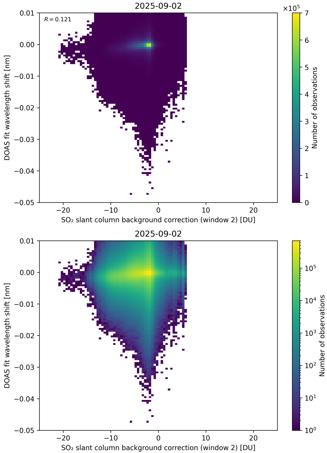
Figure 123: Scatter density plot of “SO 2 slant column background correction (window 2)” against “DOAS fit wavelength shift” for 2025-09-01 to 2025-09-03.
