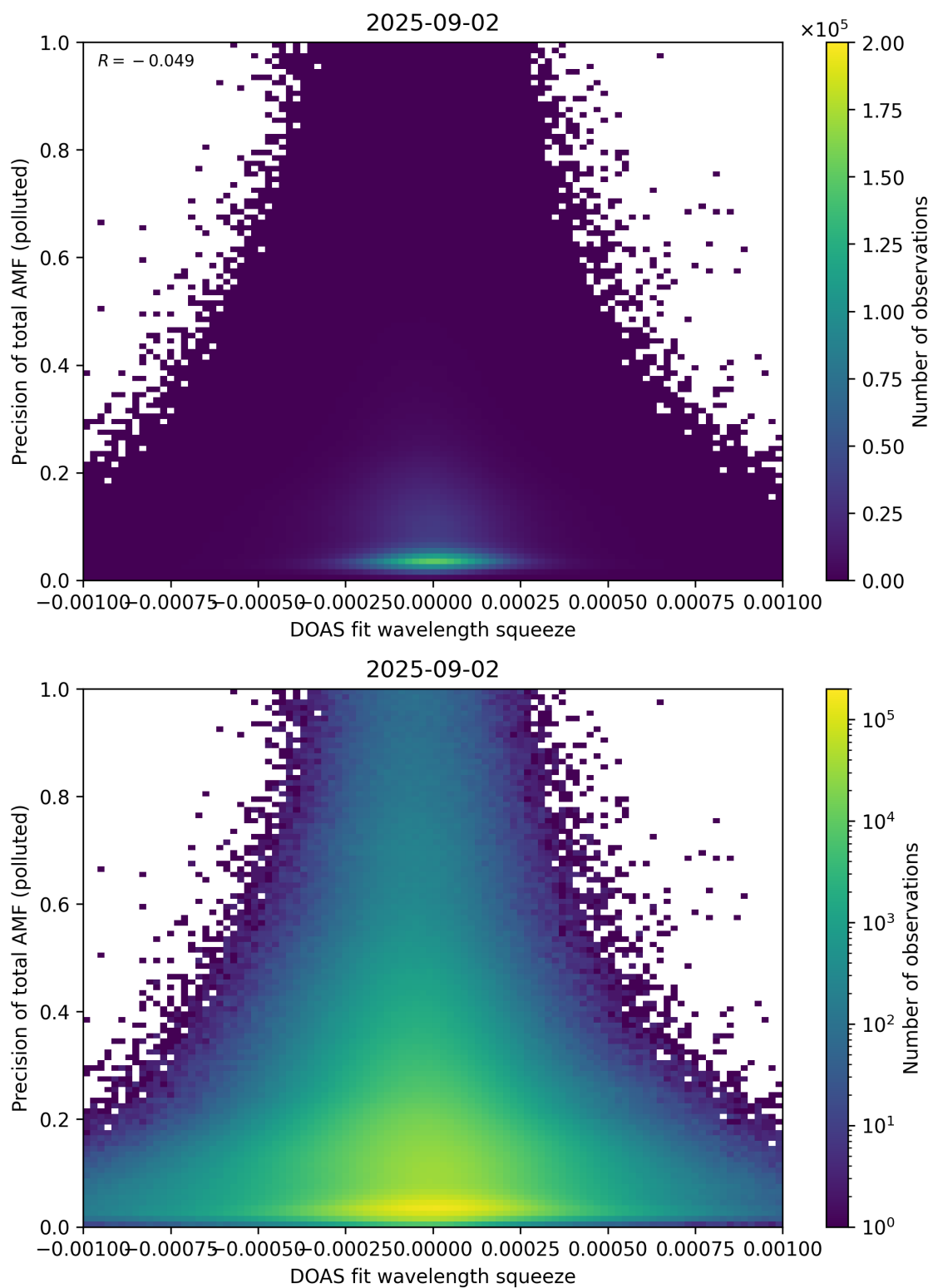
Figure 146: Scatter density plot of “DOAS fit wavelength squeeze” against “Precision of total AMF (polluted)” for 2025-09-01 to 2025-09-03.
