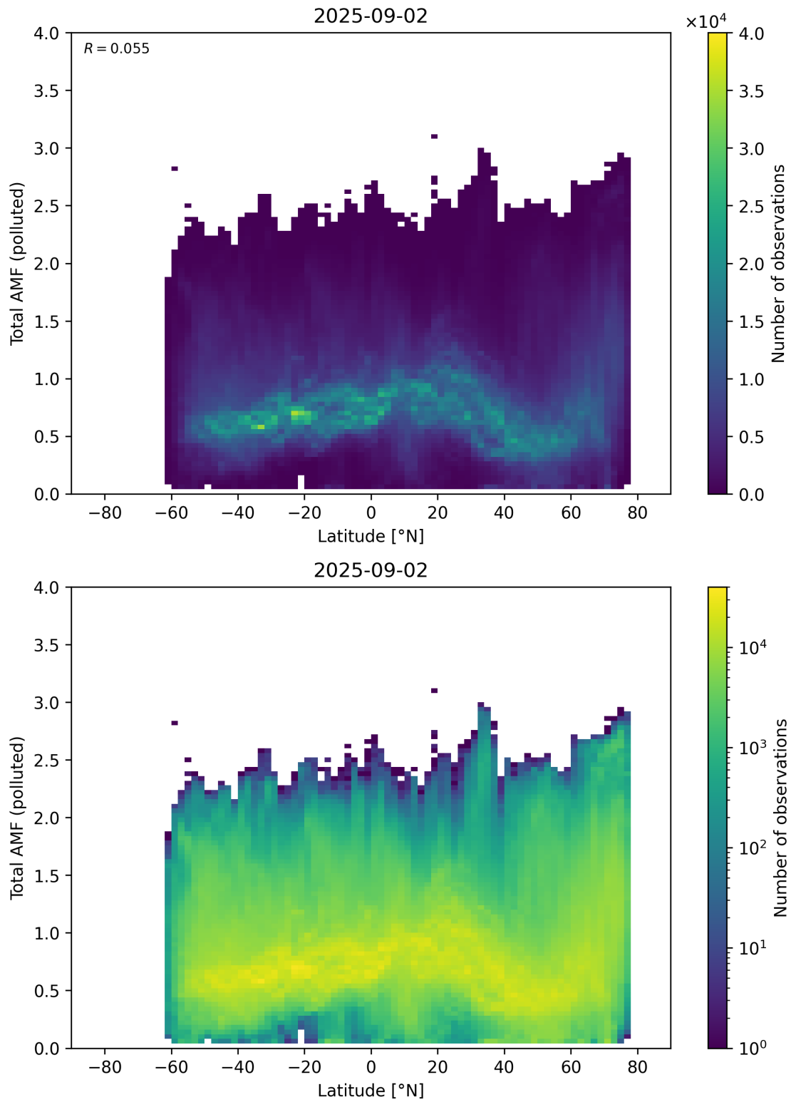
Figure 167: Scatter density plot of “Latitude” against “Total AMF (polluted)” for 2025-09-01 to 2025-09-03.
