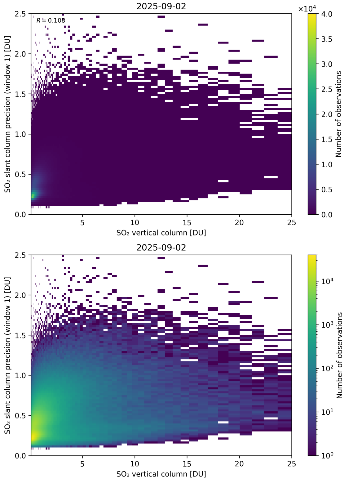
Figure 355: Scatter density plot of “SO 2 vertical column” against “SO 2 slant column precision (window 1)” for 2025-09-01 to 2025-09-03.
