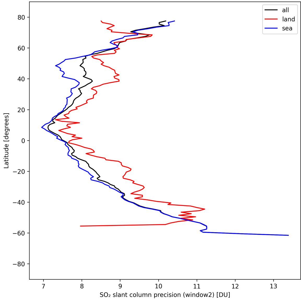
Figure 42: Zonal average of "SO 2 slant column precision (window2)" for 2025-09-01 to 2025-09-03.
