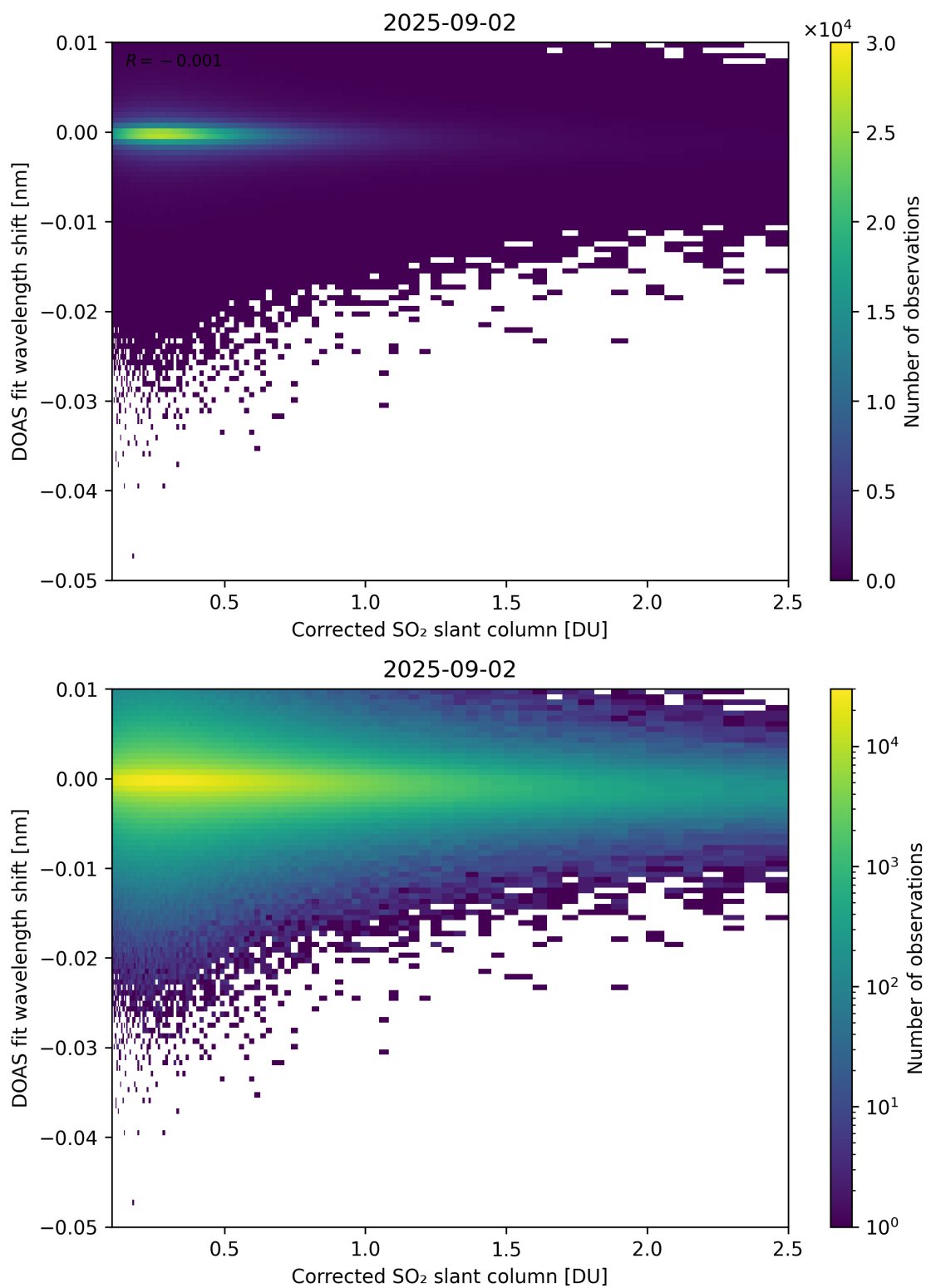
Figure 229: Scatter density plot of “Corrected SO 2 slant column” against “DOAS fit wavelength shift” for 2025-09-01 to 2025-09-03.
