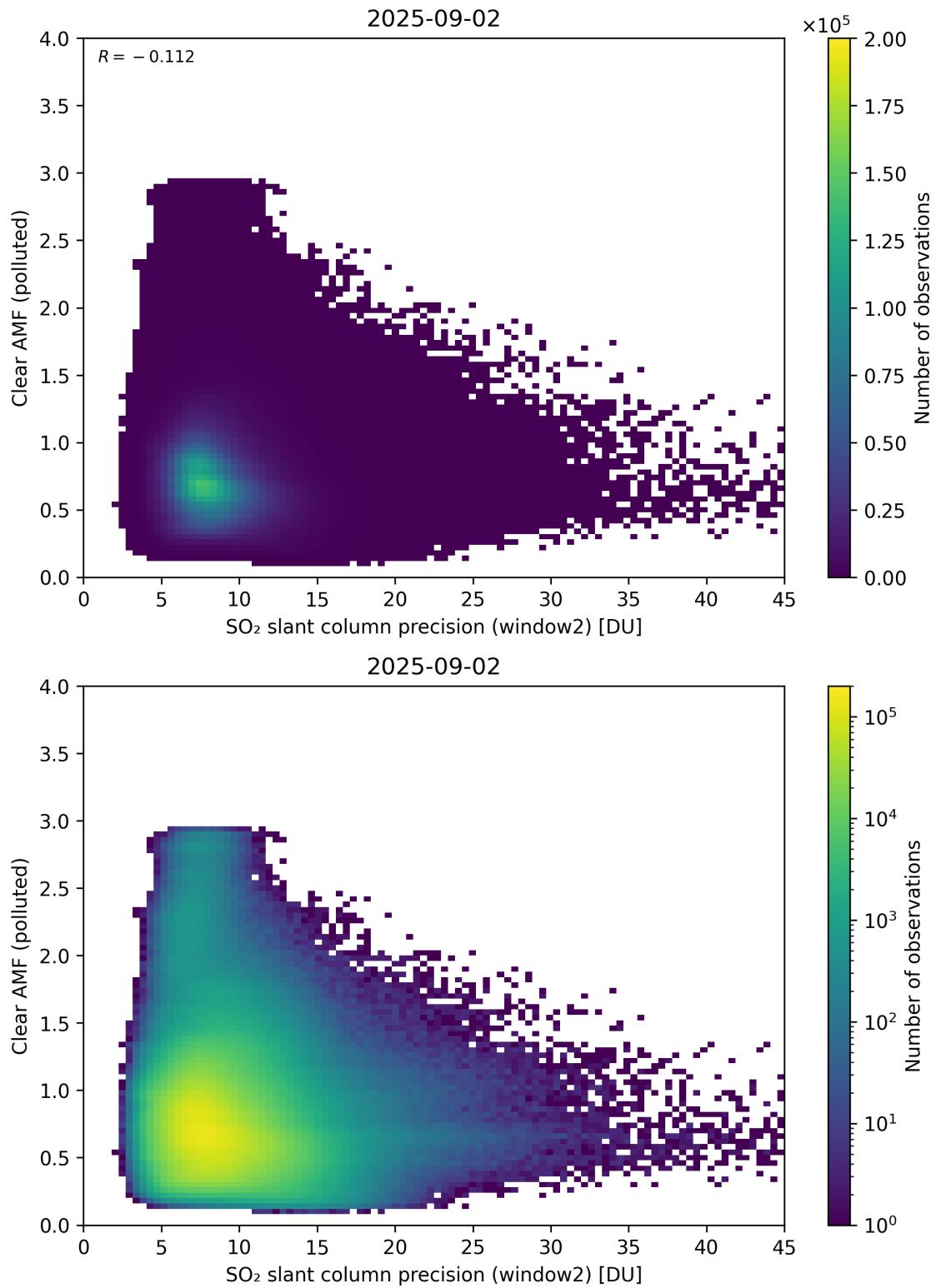
Figure 296: Scatter density plot of “SO 2 slant column precision (window2)” against “Clear AMF (polluted)” for 2025-09-01 to 2025-09-03.
