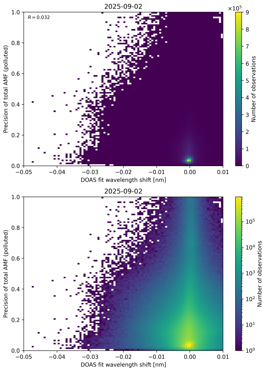
Figure 142: Scatter density plot of “DOAS fit wavelength shift” against “Precision of total AMF (polluted)” for 2025-09-01 to 2025-09-03.
