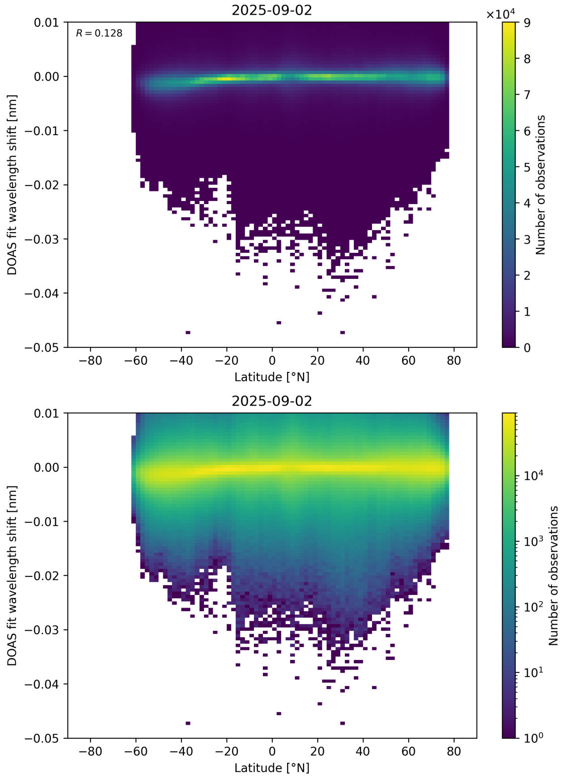
Figure 153: Scatter density plot of “Latitude” against “DOAS fit wavelength shift” for 2025-09-01 to 2025-09-03.
