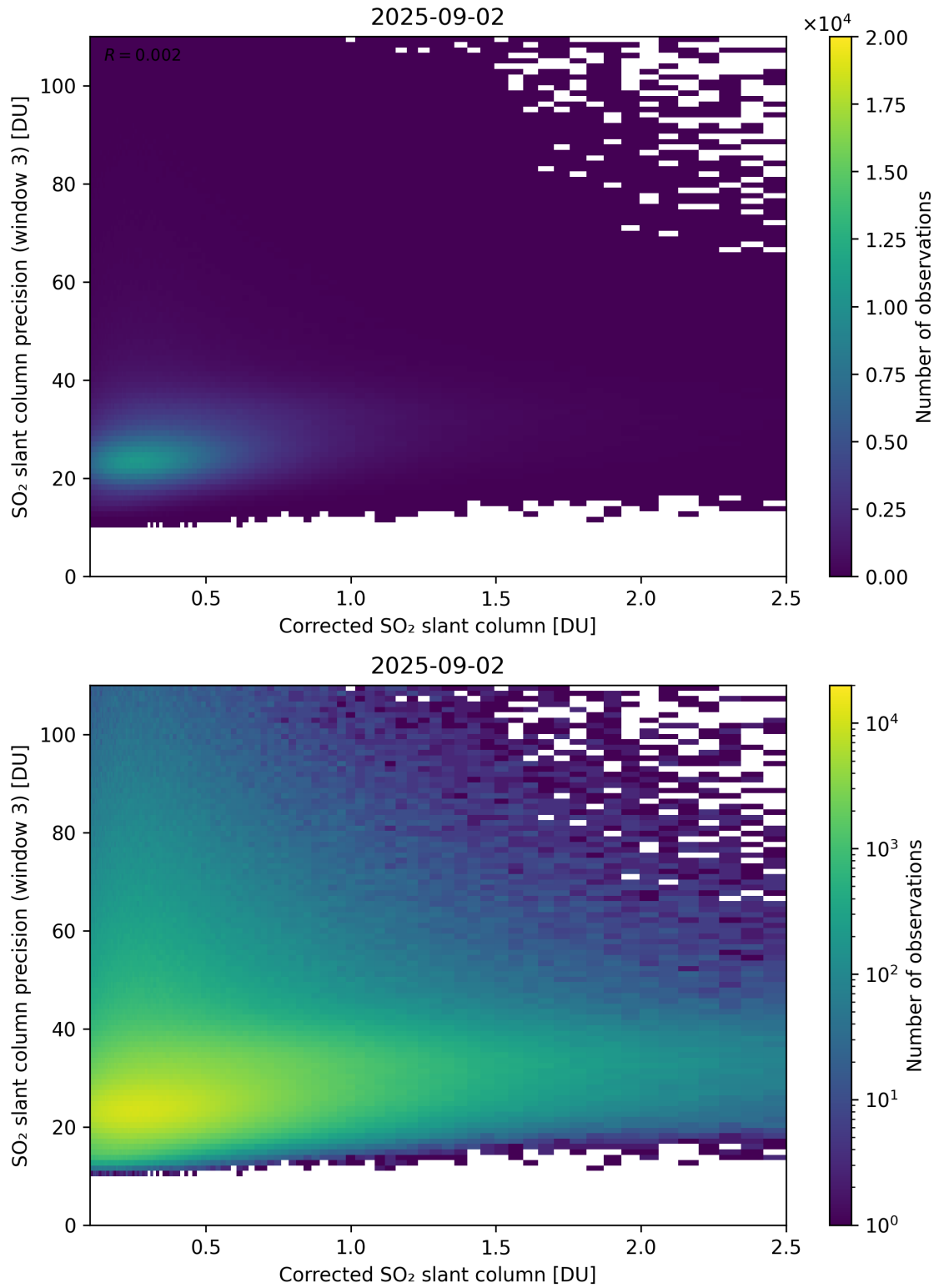
Figure 241: Scatter density plot of “Corrected SO 2 slant column” against “SO 2 slant column precision (window 3)” for 2025-09-01 to 2025-09-03.
