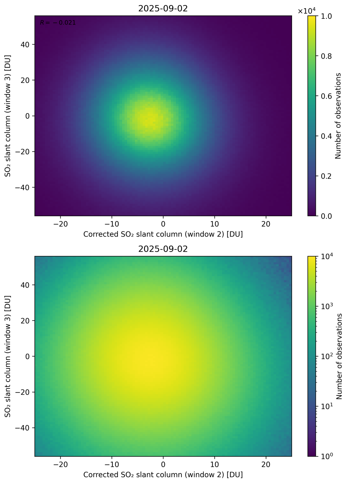
Figure 251: Scatter density plot of “Corrected SO 2 slant column (window 2)” against “SO 2 slant column (window 3)” for 2025-09-01 to 2025-09-03.
