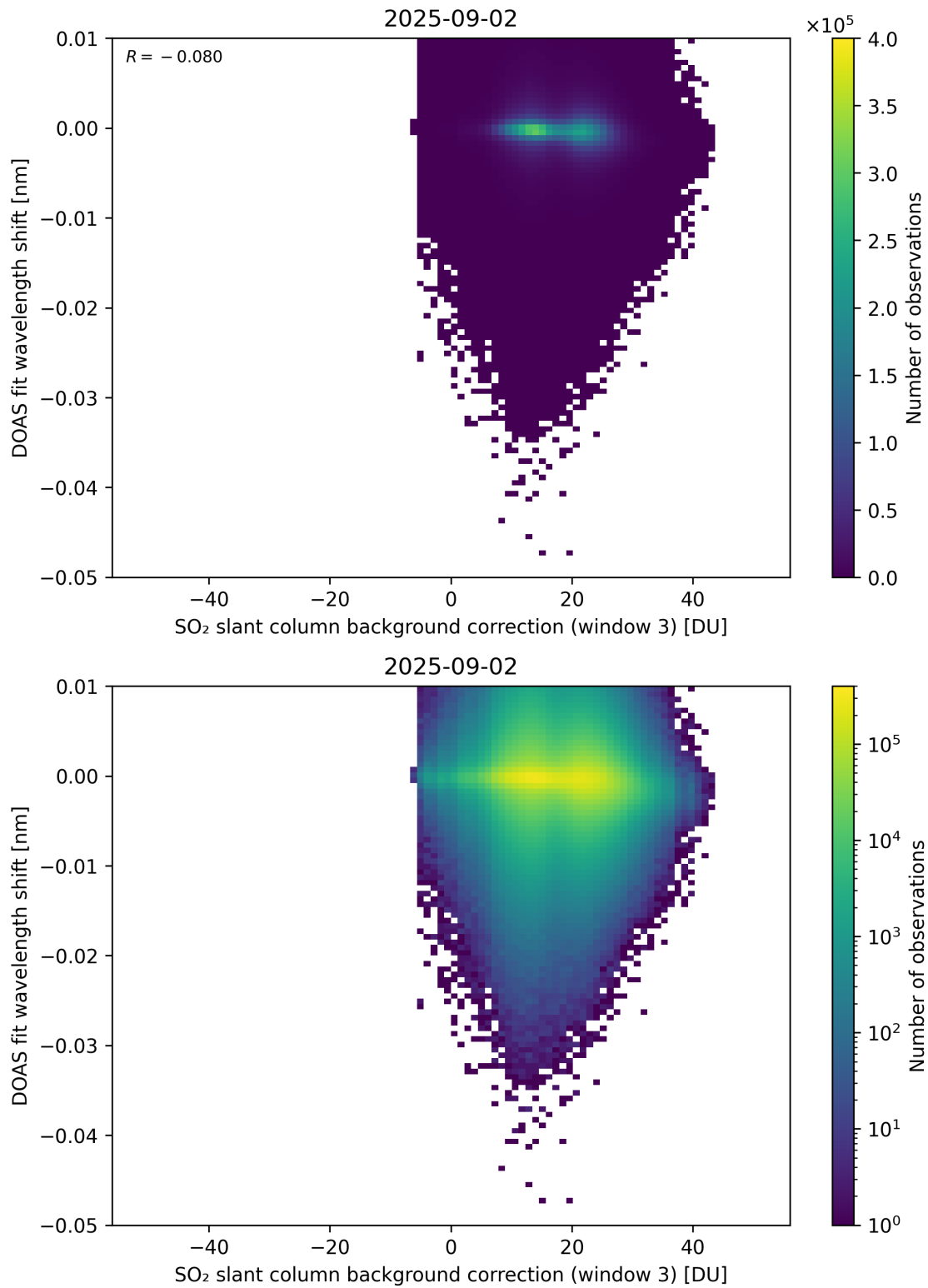
Figure 132: Scatter density plot of “SO 2 slant column background correction (window 3)” against “DOAS fit wavelength shift” for 2025-09-01 to 2025-09-03.
