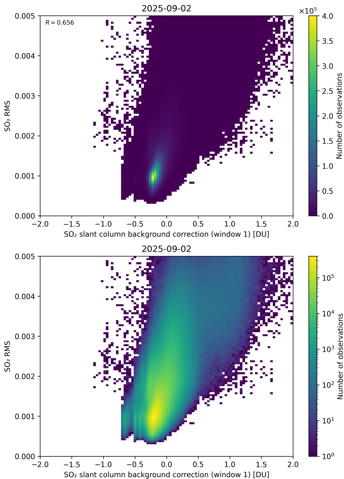
Figure 113: Scatter density plot of “SO 2 slant column background correction (window 1)” against “SO 2 RMS” for 2025-09-01 to 2025-09-03.
