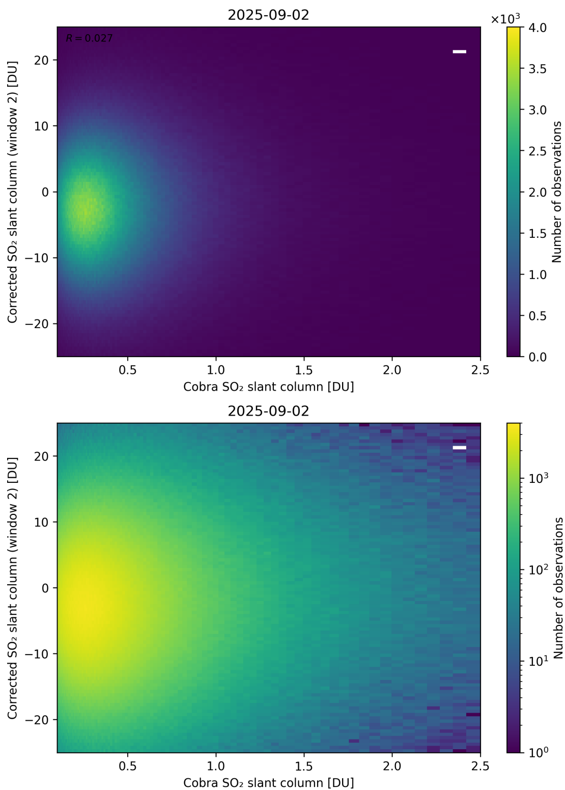
Figure 217: Scatter density plot of “Cobra SO 2 slant column” against “Corrected SO 2 slant column (window 2)” for 2025-09-01 to 2025-09-03.
