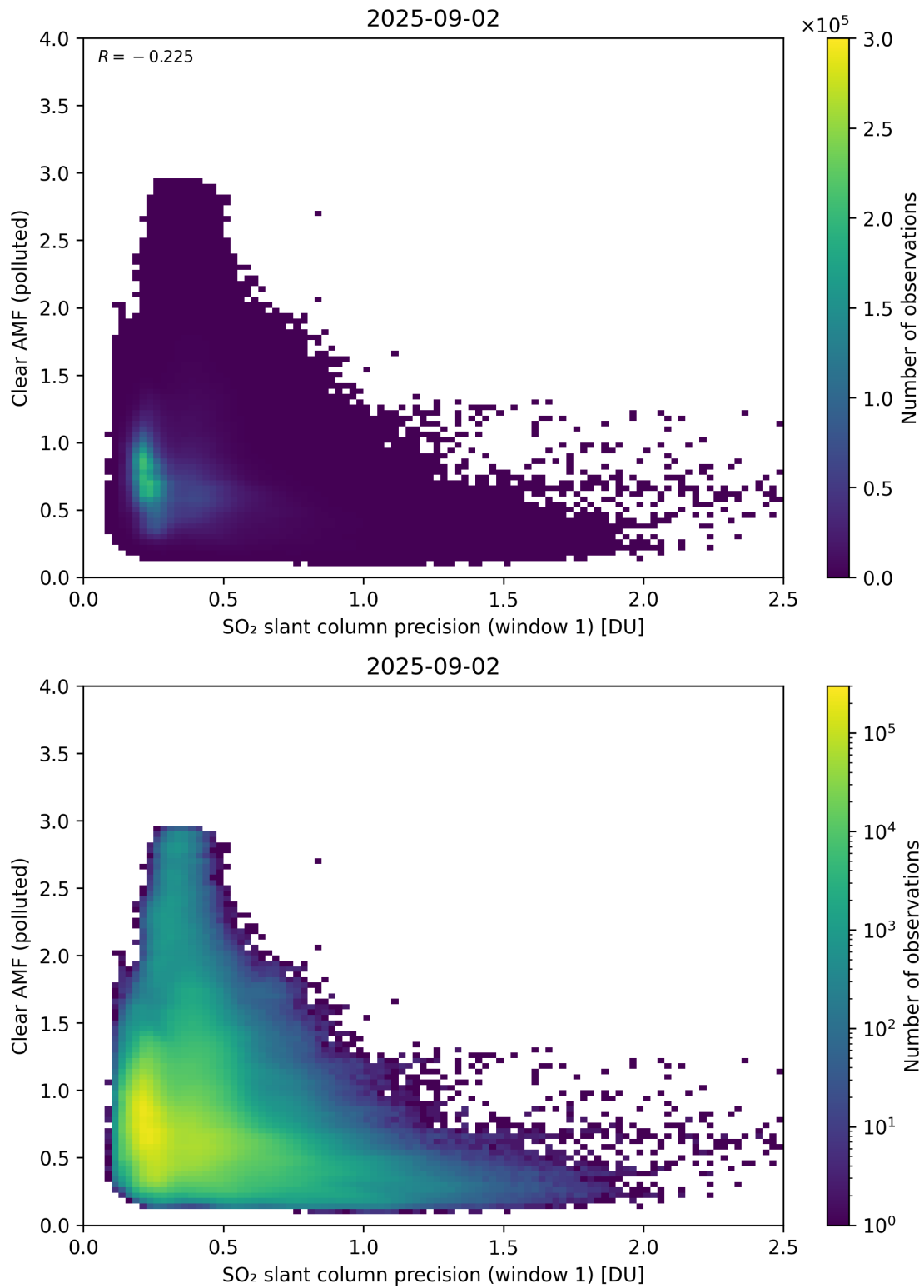
Figure 274: Scatter density plot of “SO 2 slant column precision (window 1)” against “Clear AMF (polluted)” for 2025-09-01 to 2025-09-03.
