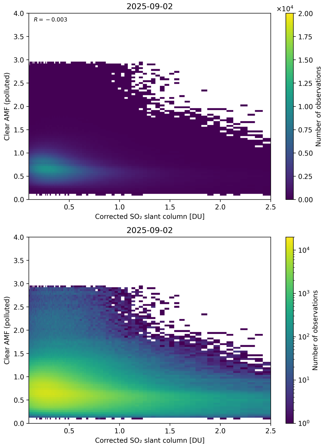
Figure 232: Scatter density plot of “Corrected SO 2 slant column” against “Clear AMF (polluted)” for 2025-09-01 to 2025-09-03.
