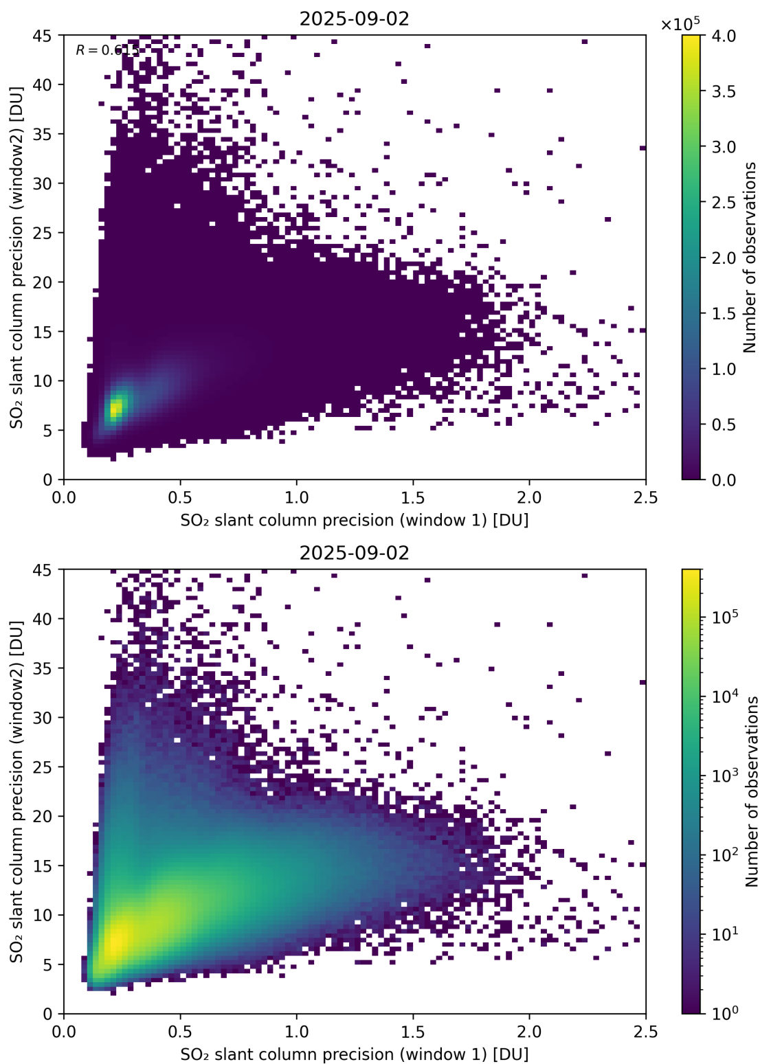
Figure 277: Scatter density plot of “SO 2 slant column precision (window 1)” against “SO 2 slant column precision (window2)” for 2025-09-01 to 2025-09-03.
