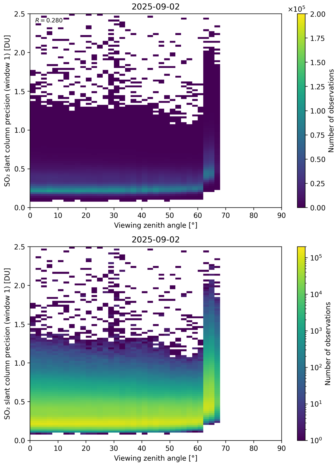
Figure 377: Scatter density plot of “Viewing zenith angle” against “SO 2 slant column precision (window 1)” for 2025-09-01 to 2025-09-03.
