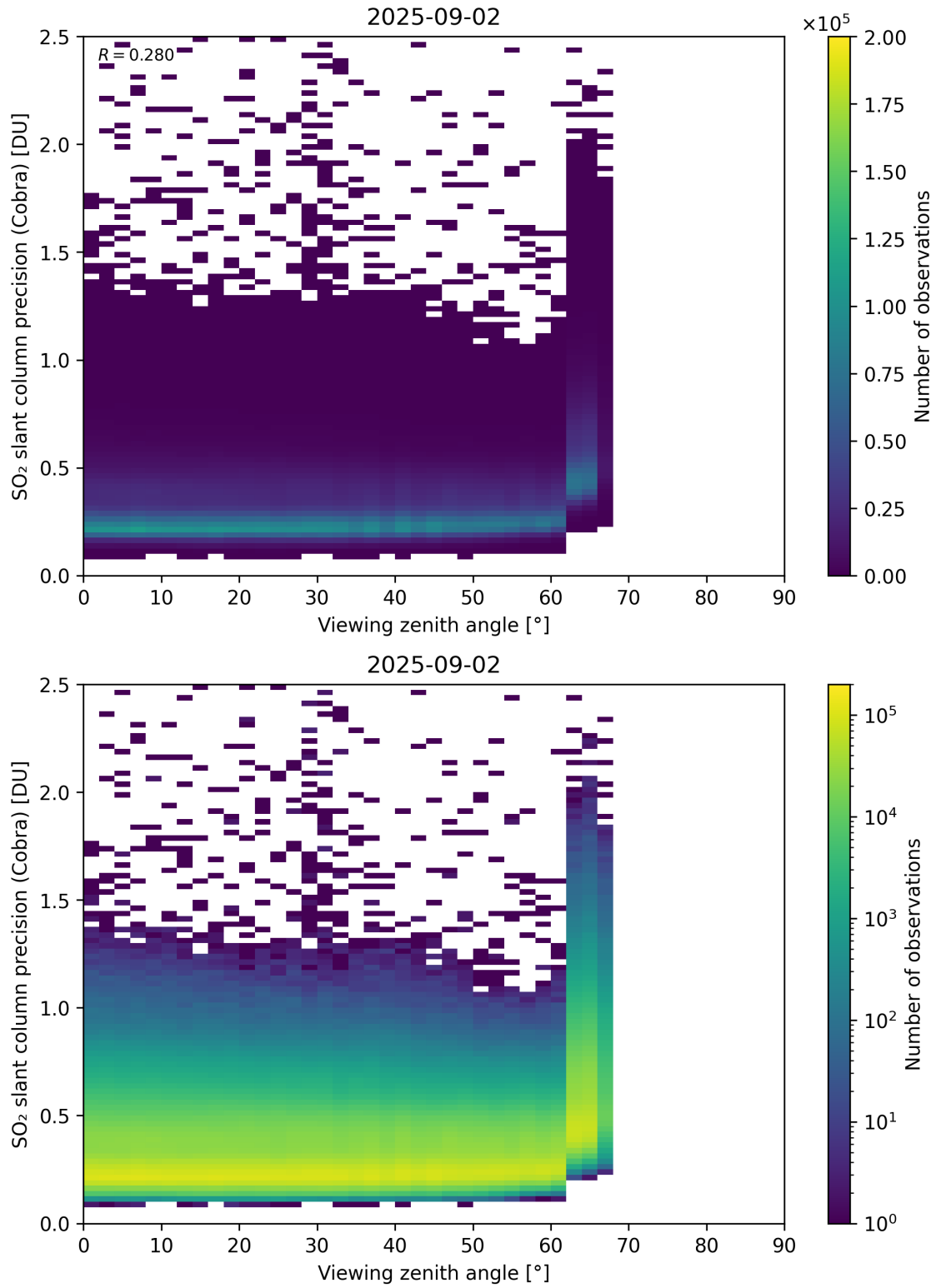
Figure 372: Scatter density plot of “Viewing zenith angle” against “SO 2 slant column precision (Cobra)” for 2025-09-01 to 2025-09-03.
