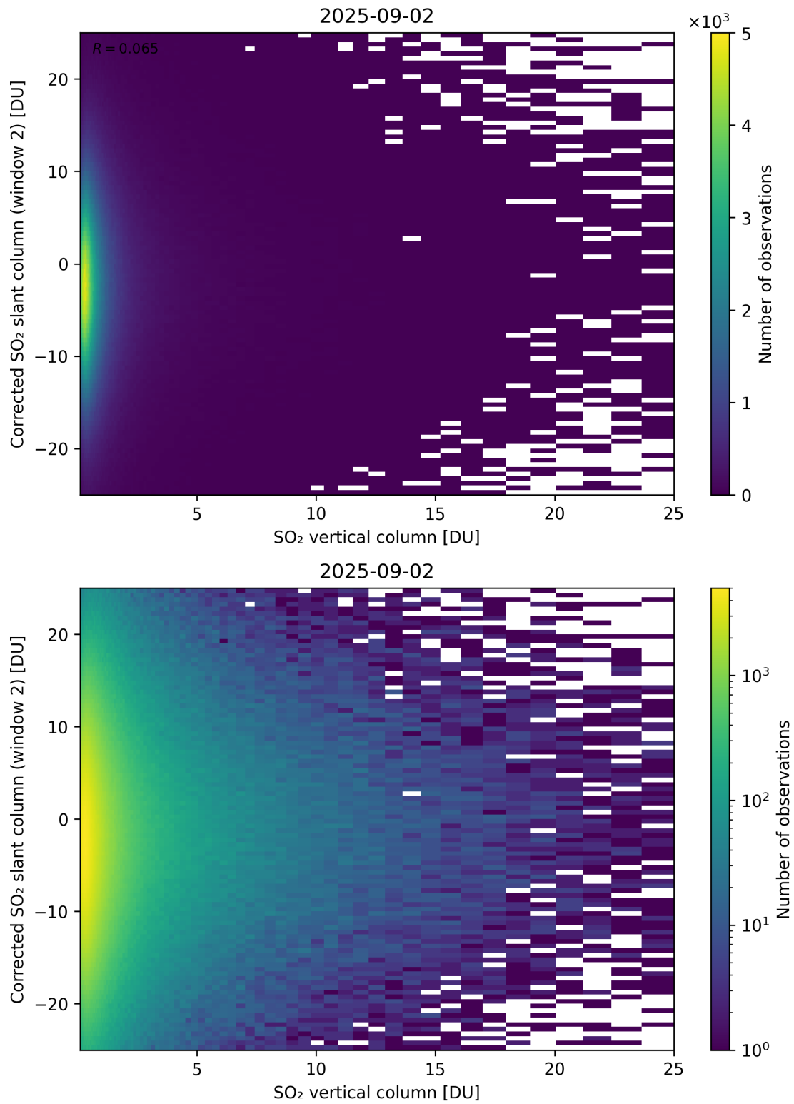
Figure 352: Scatter density plot of “SO 2 vertical column” against “Corrected SO 2 slant column (window 2)” for 2025-09-01 to 2025-09-03.
