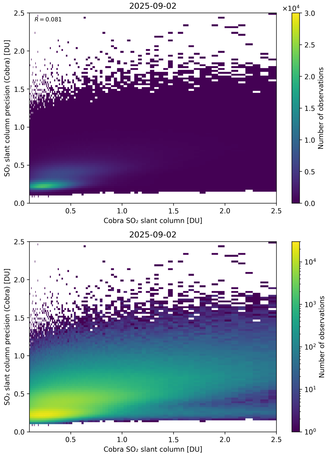
Figure 216: Scatter density plot of “Cobra SO 2 slant column” against “SO 2 slant column precision (Cobra)” for 2025-09-01 to 2025-09-03.
