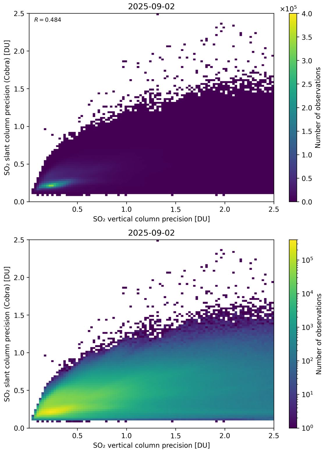
Figure 337: Scatter density plot of “SO 2 vertical column precision” against “SO 2 slant column precision (Cobra)” for 2025-09-01 to 2025-09-03.
