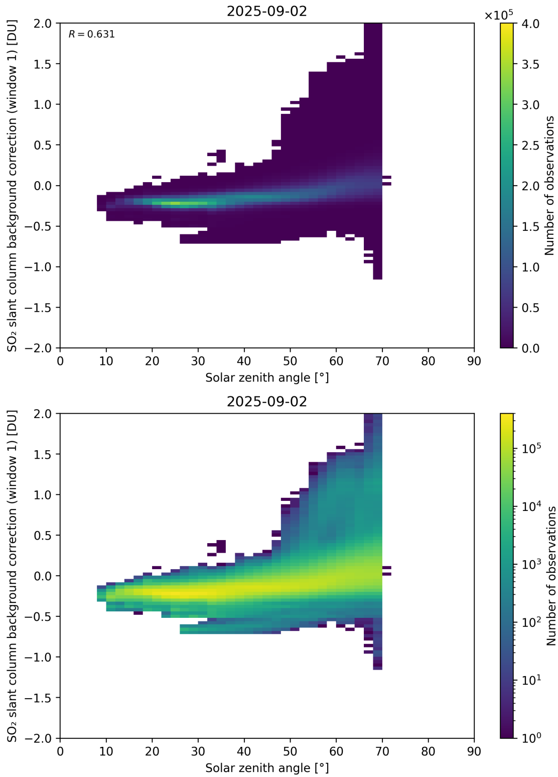
Figure 171: Scatter density plot of “Solar zenith angle” against “SO 2 slant column background correction (window 1)” for 2025-09-01 to 2025-09-03.
