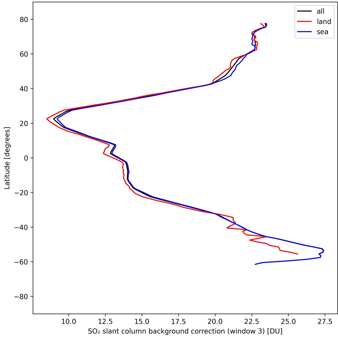
Figure 48: Zonal average of “SO 2 slant column background correction (window 3)” for 2025-09-01 to 2025-09-03.
