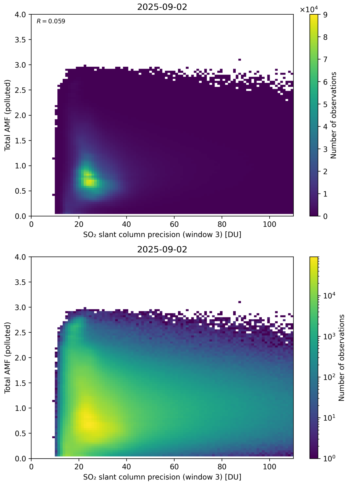
Figure 313: Scatter density plot of “SO 2 slant column precision (window 3)” against “Total AMF (polluted)” for 2025-09-01 to 2025-09-03.
