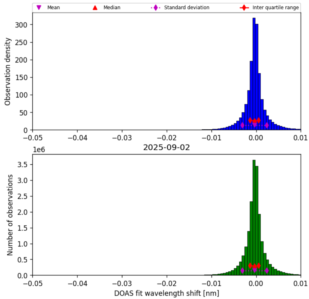
Figure 76: Histogram of “DOAS fit wavelength shift” for 2025-09-01 to 2025-09-03
