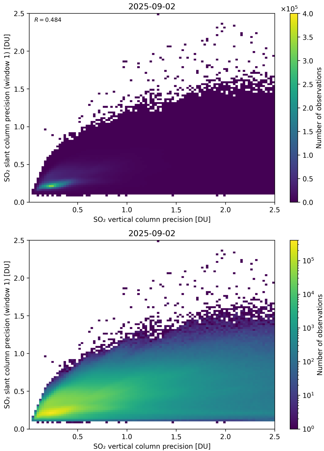
Figure 342: Scatter density plot of “SO 2 vertical column precision” against “SO 2 slant column precision (window 1)” for 2025-09-01 to 2025-09-03.
