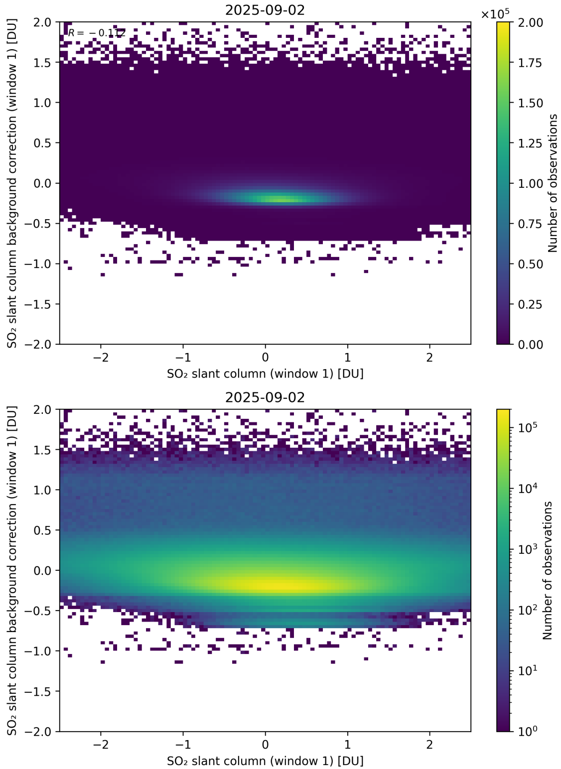
Figure 262: Scatter density plot of “SO 2 slant column (window 1)” against “SO 2 slant column background correction (window 1)” for 2025-09-01 to 2025-09-03.
