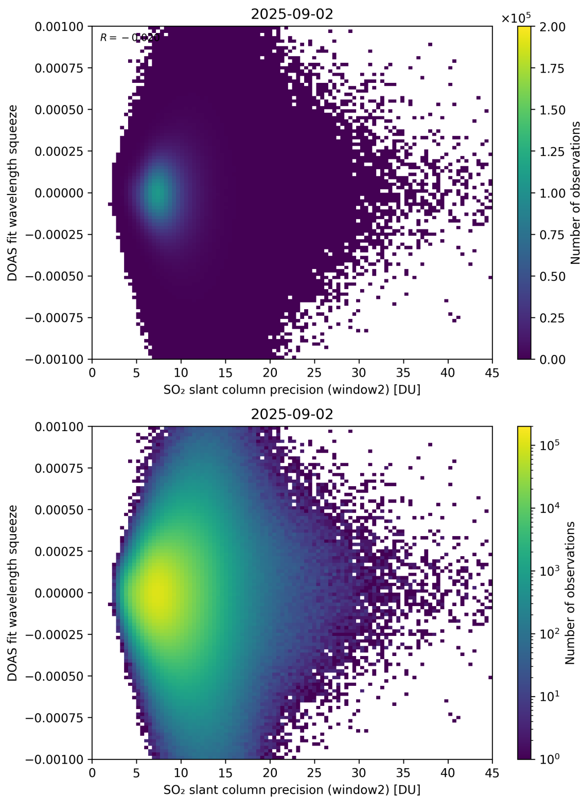
Figure 294: Scatter density plot of “SO 2 slant column precision (window2)” against “DOAS fit wavelength squeeze” for 2025-09-01 to 2025-09-03.
