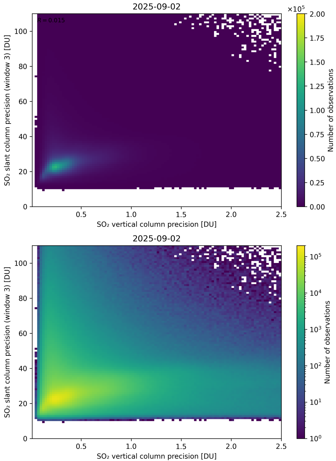
Figure 345: Scatter density plot of “SO 2 vertical column precision” against “SO 2 slant column precision (window 3)” for 2025-09-01 to 2025-09-03.
