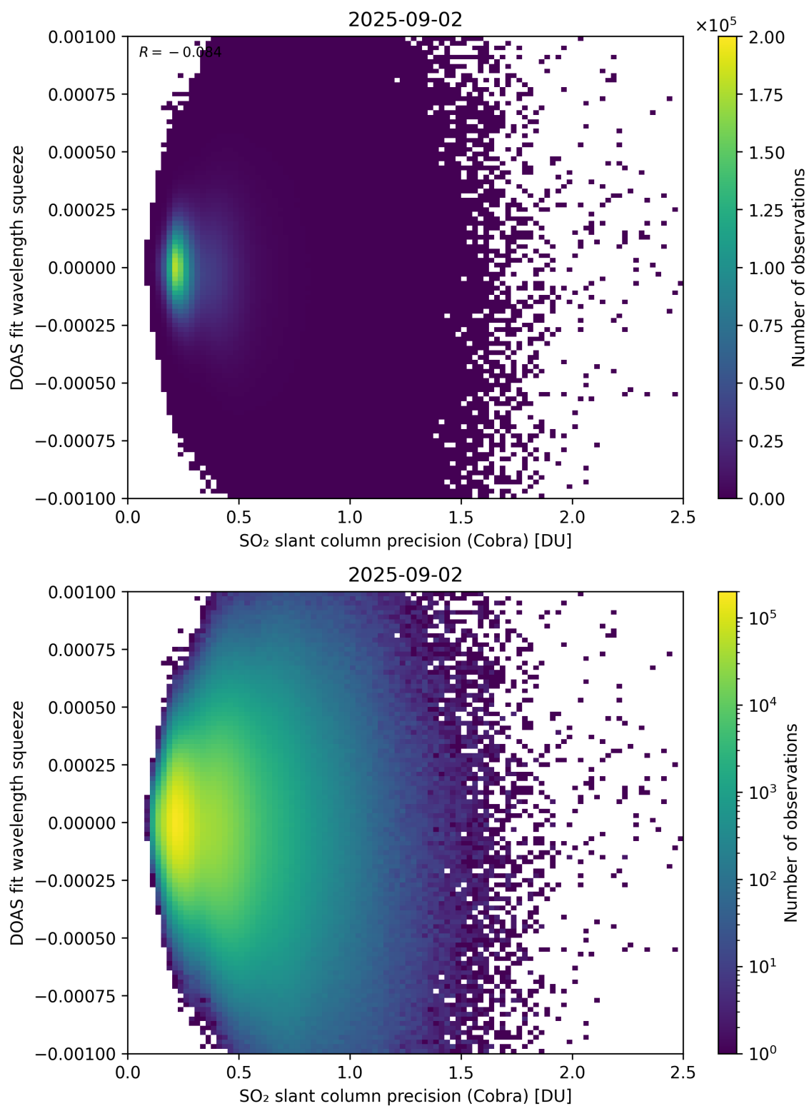
Figure 203: Scatter density plot of “SO 2 slant column precision (Cobra)” against “DOAS fit wavelength squeeze” for 2025-09-01 to 2025-09-03.
