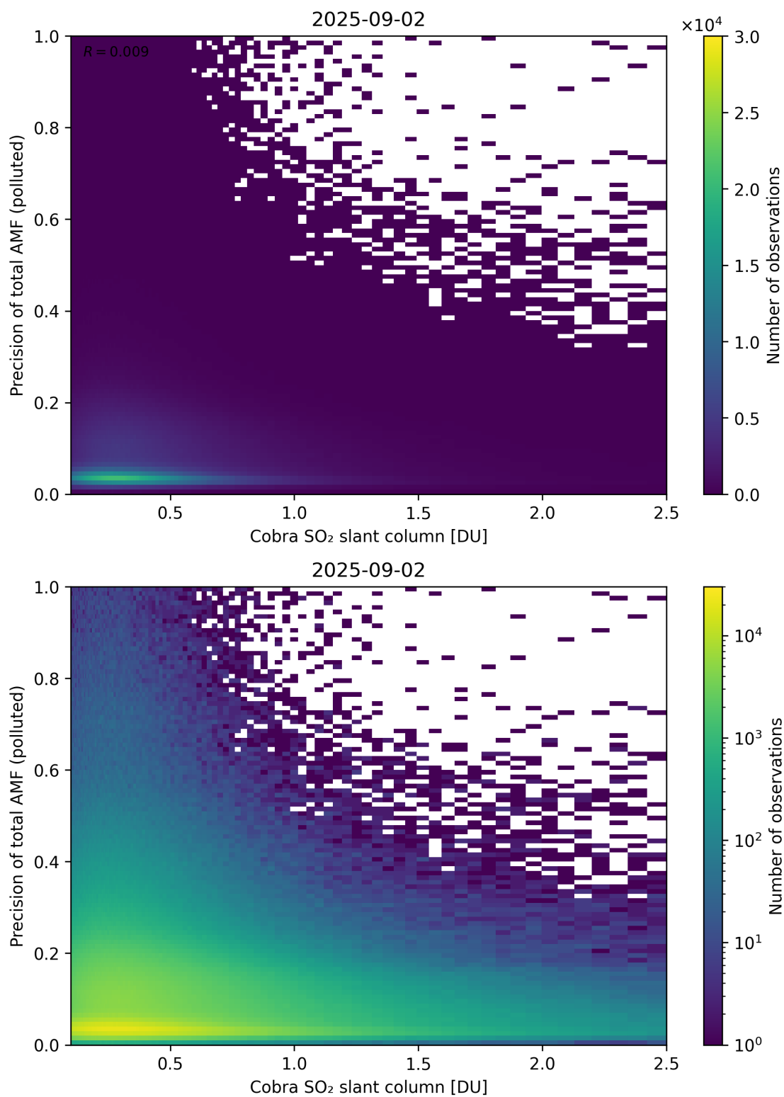
Figure 225: Scatter density plot of “Cobra SO 2 slant column” against “Precision of total AMF (polluted)” for 2025-09-01 to 2025-09-03.
