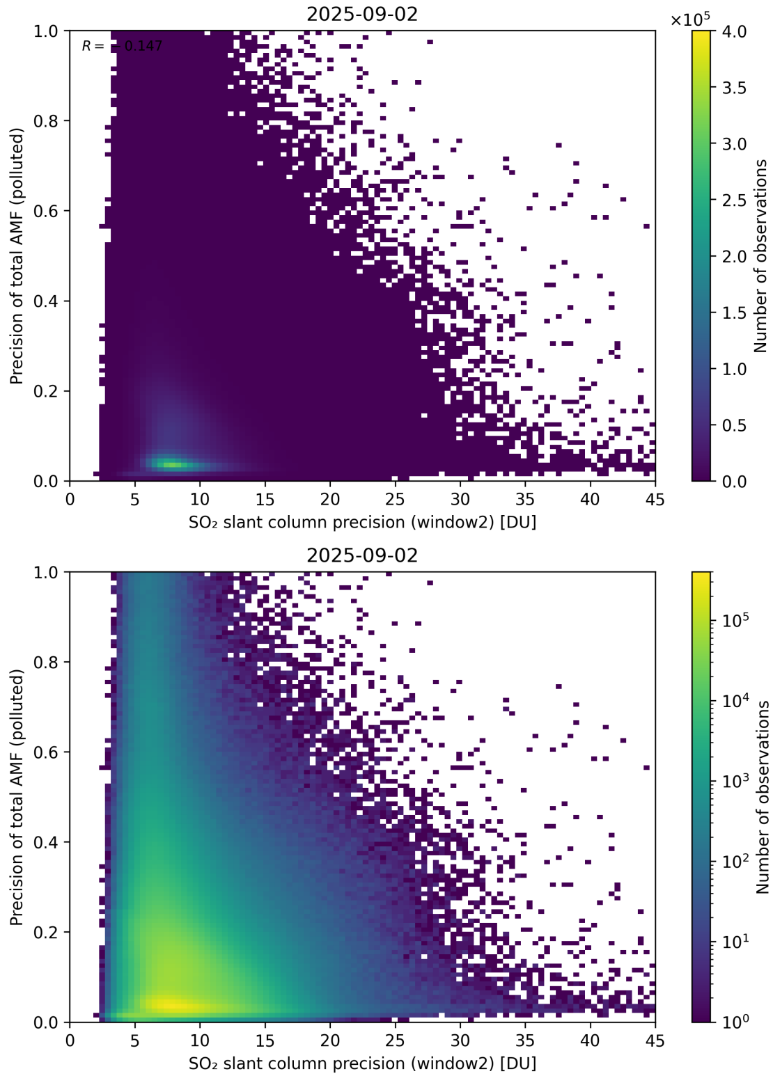
Figure 302: Scatter density plot of “SO 2 slant column precision (window2)” against “Precision of total AMF (polluted)” for 2025-09-01 to 2025-09-03.
