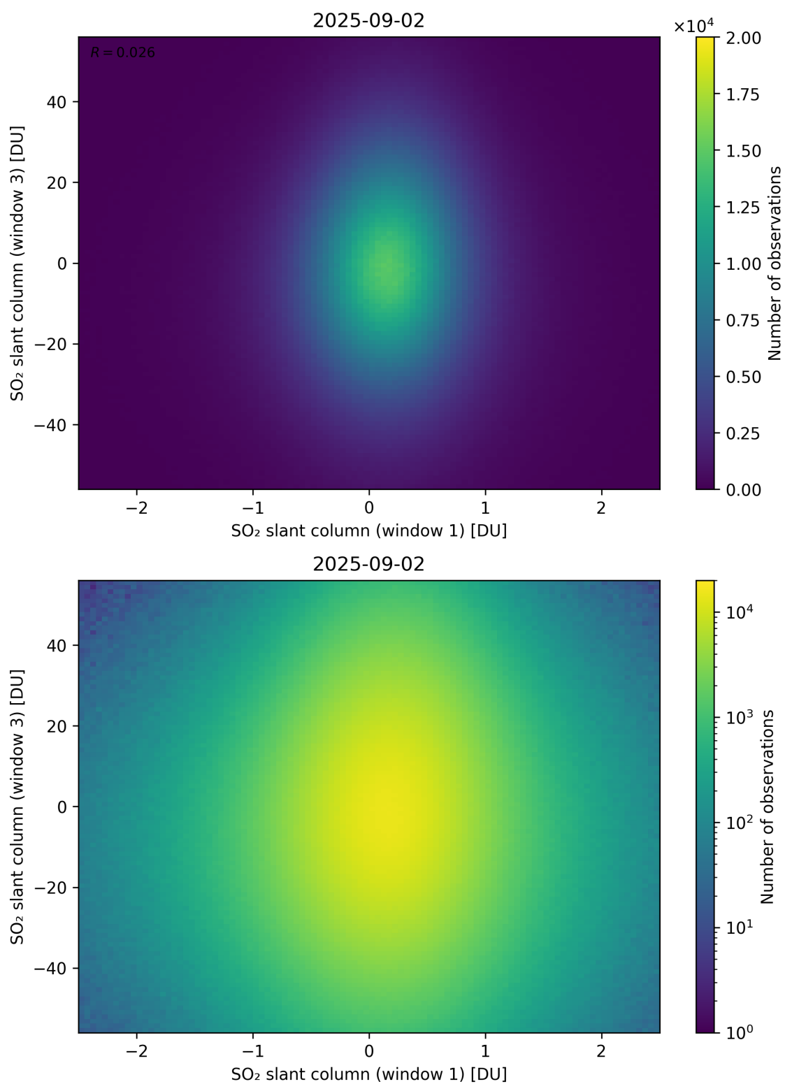
Figure 287: Scatter density plot of “SO 2 slant column (window 1)” against “SO 2 slant column (window 3)” for 2025-09-01 to 2025-09-03.
