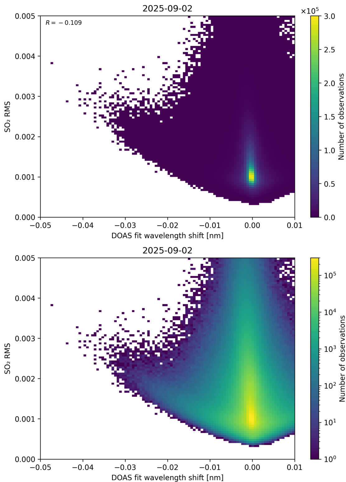
Figure 139: Scatter density plot of “DOAS fit wavelength shift” against “SO 2 RMS” for 2025-09-01 to 2025-09-03.
