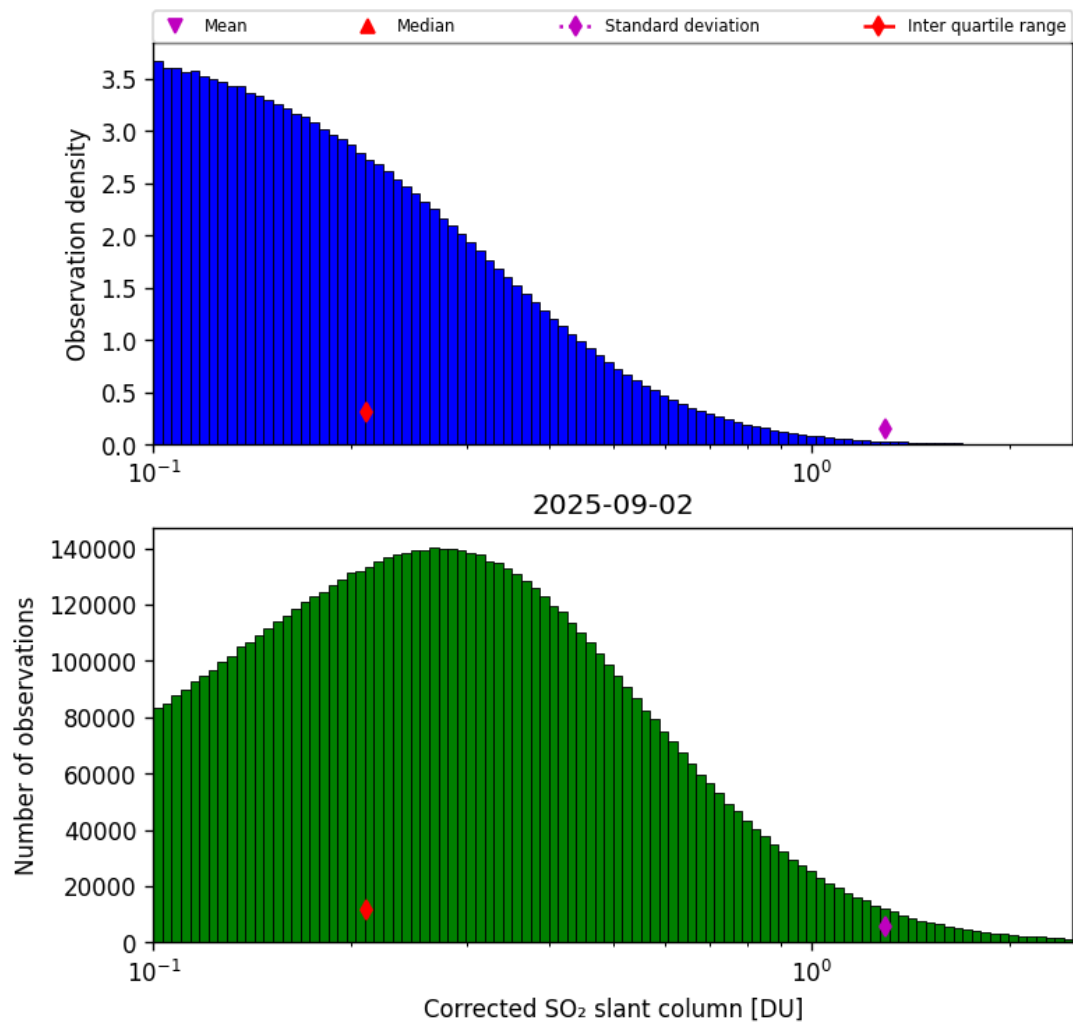
Figure 60: Histogram of “Corrected SO 2 slant column” for 2025-09-01 to 2025-09-03
