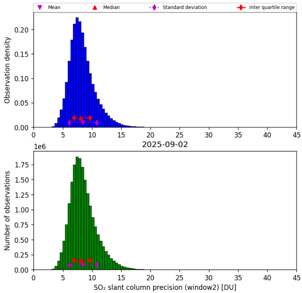
Figure 68: Histogram of “SO 2 slant column precision (window2)” for 2025-09-01 to 2025-09-03
