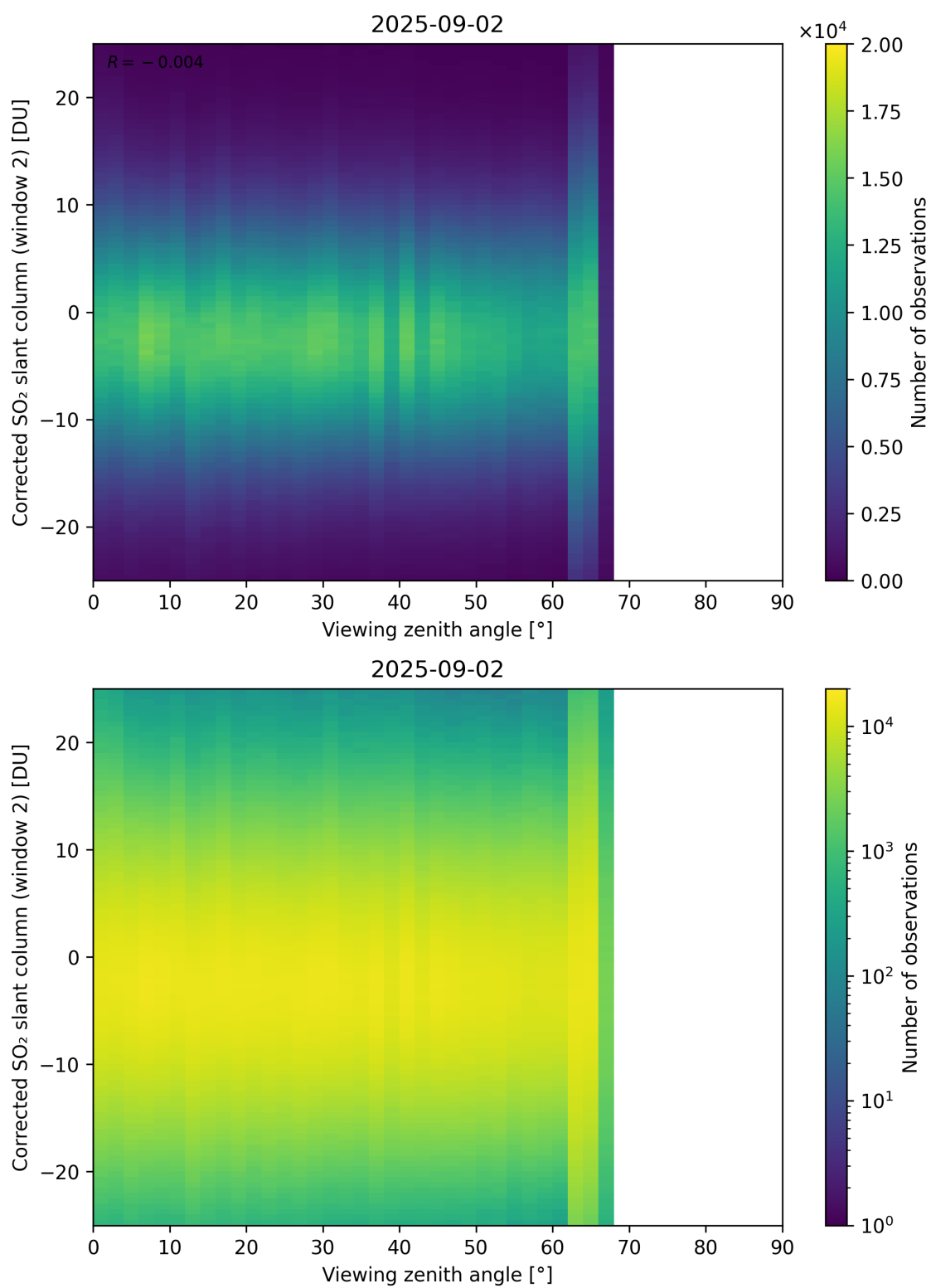
Figure 374: Scatter density plot of “Viewing zenith angle” against “Corrected SO 2 slant column (window 2)” for 2025-09-01 to 2025-09-03.
