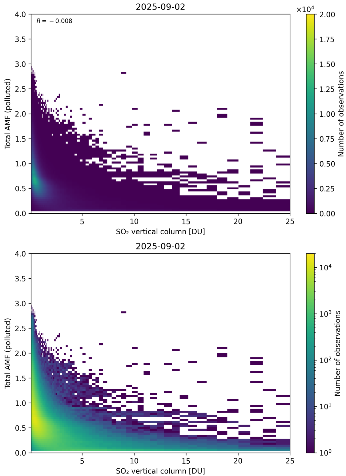
Figure 359: Scatter density plot of “SO 2 vertical column” against “Total AMF (polluted)” for 2025-09-01 to 2025-09-03.
