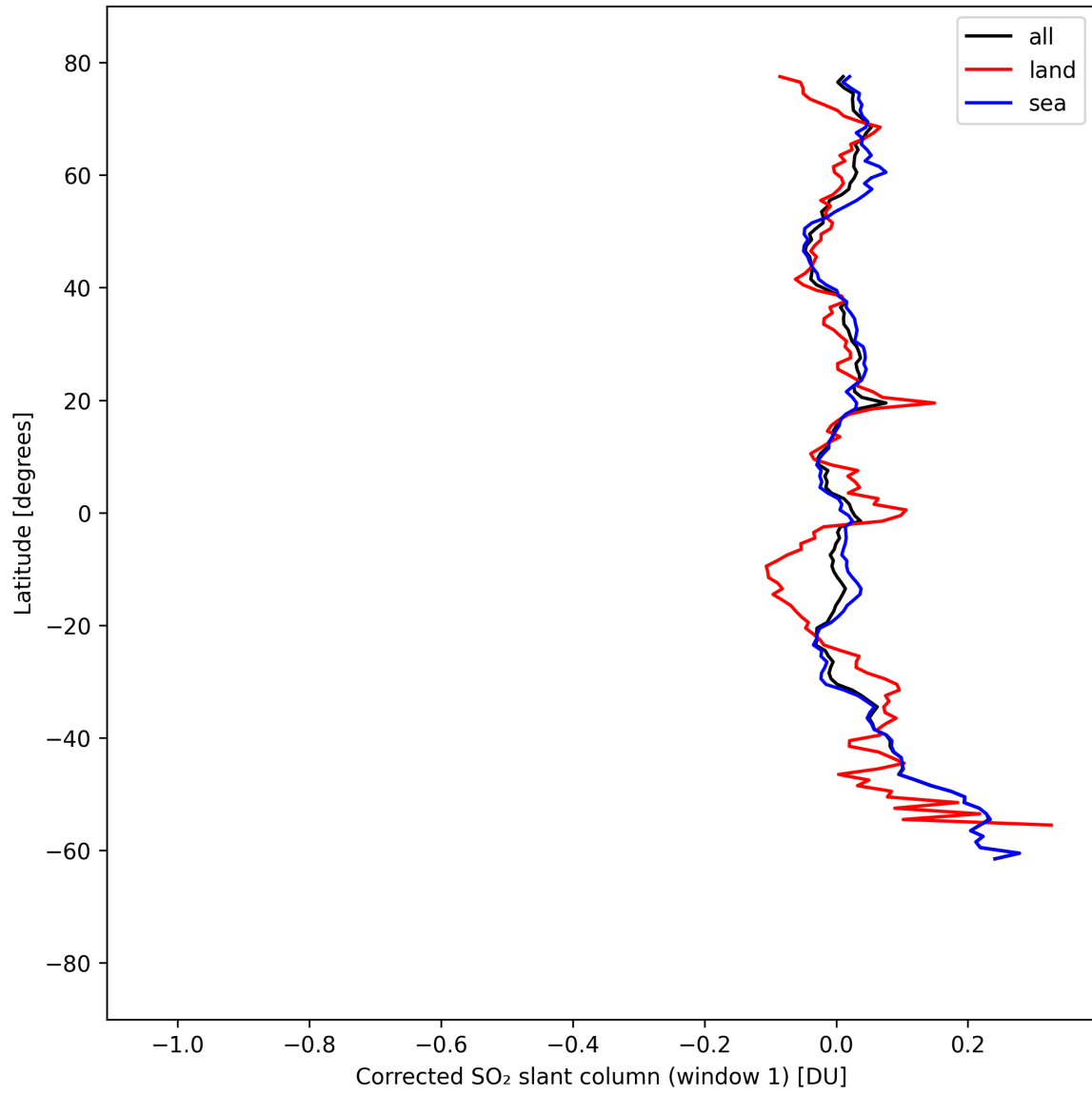
Figure 39: Zonal average of “Corrected SO 2 slant column (window 1)” for 2025-09-01 to 2025-09-03.
