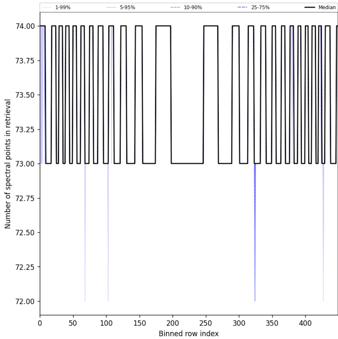
Figure 108: Along track statistics of “Number of spectral points in retrieval” for 2025-09-01 to 2025-09-03
