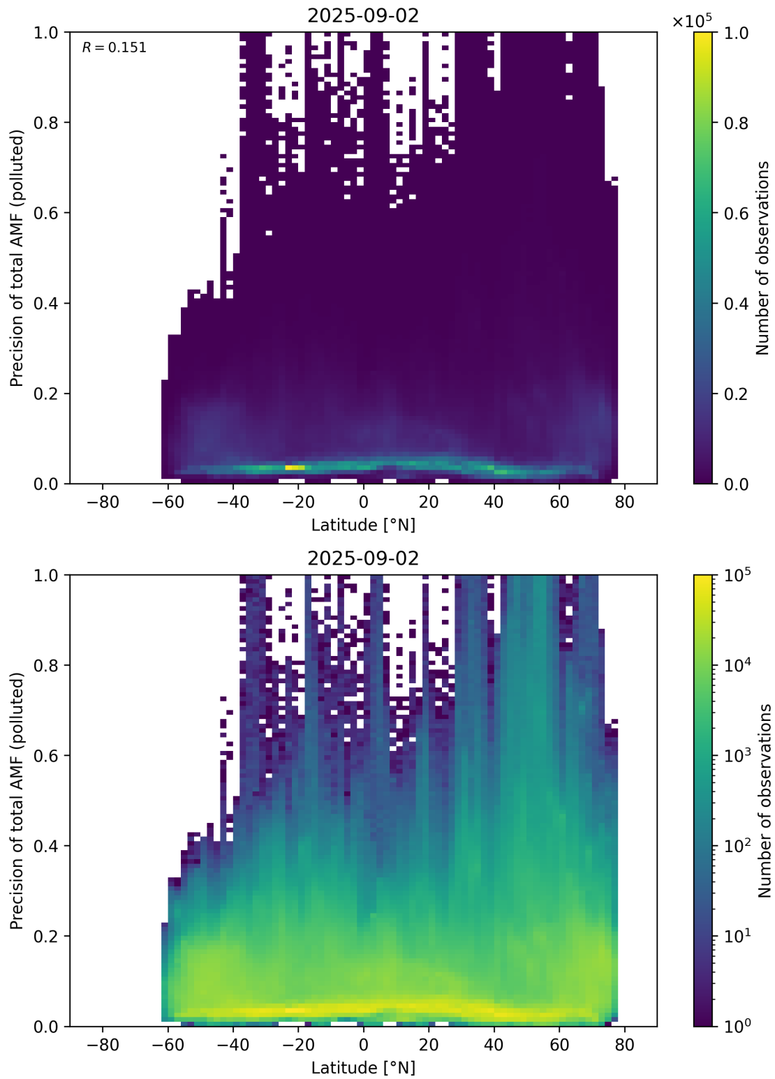
Figure 168: Scatter density plot of “Latitude” against “Precision of total AMF (polluted)” for 2025-09-01 to 2025-09-03.
