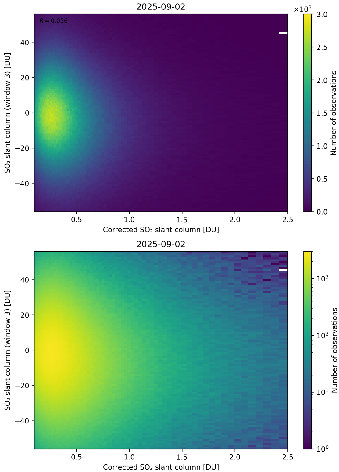
Figure 240: Scatter density plot of “Corrected SO 2 slant column” against “SO 2 slant column (window 3)” for 2025-09-01 to 2025-09-03.
