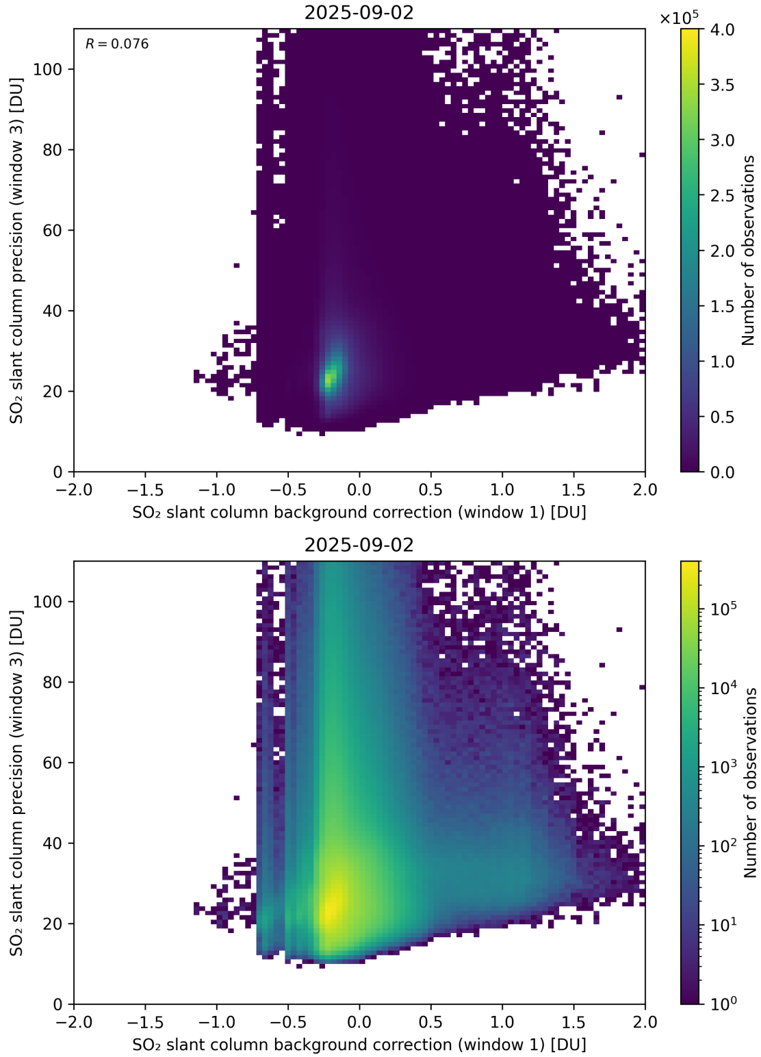
Figure 119: Scatter density plot of “SO 2 slant column background correction (window 1)” against “SO 2 slant column precision (window 3)” for 2025-09-01 to 2025-09-03.
