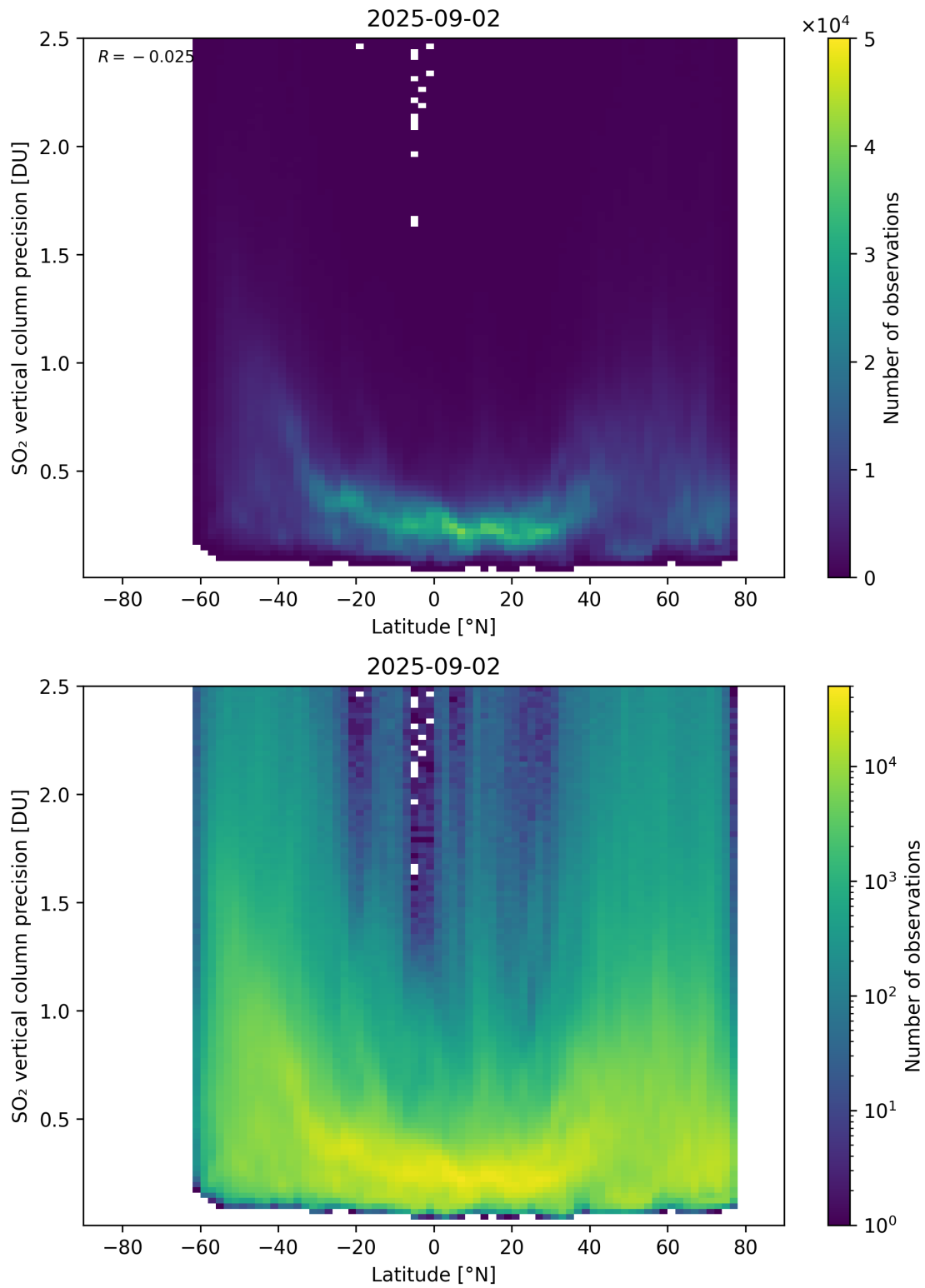
Figure 170: Scatter density plot of “Latitude” against “SO 2 vertical column precision” for 2025-09-01 to 2025-09-03.
