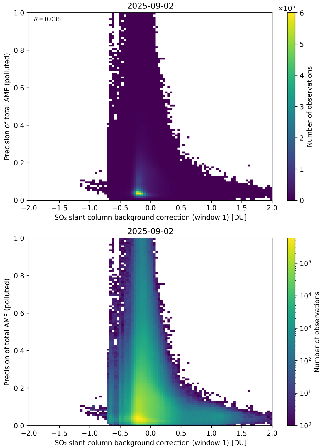
Figure 121: Scatter density plot of “SO 2 slant column background correction (window 1)” against “Precision of total AMF (polluted)” for 2025-09-01 to 2025-09-03.
