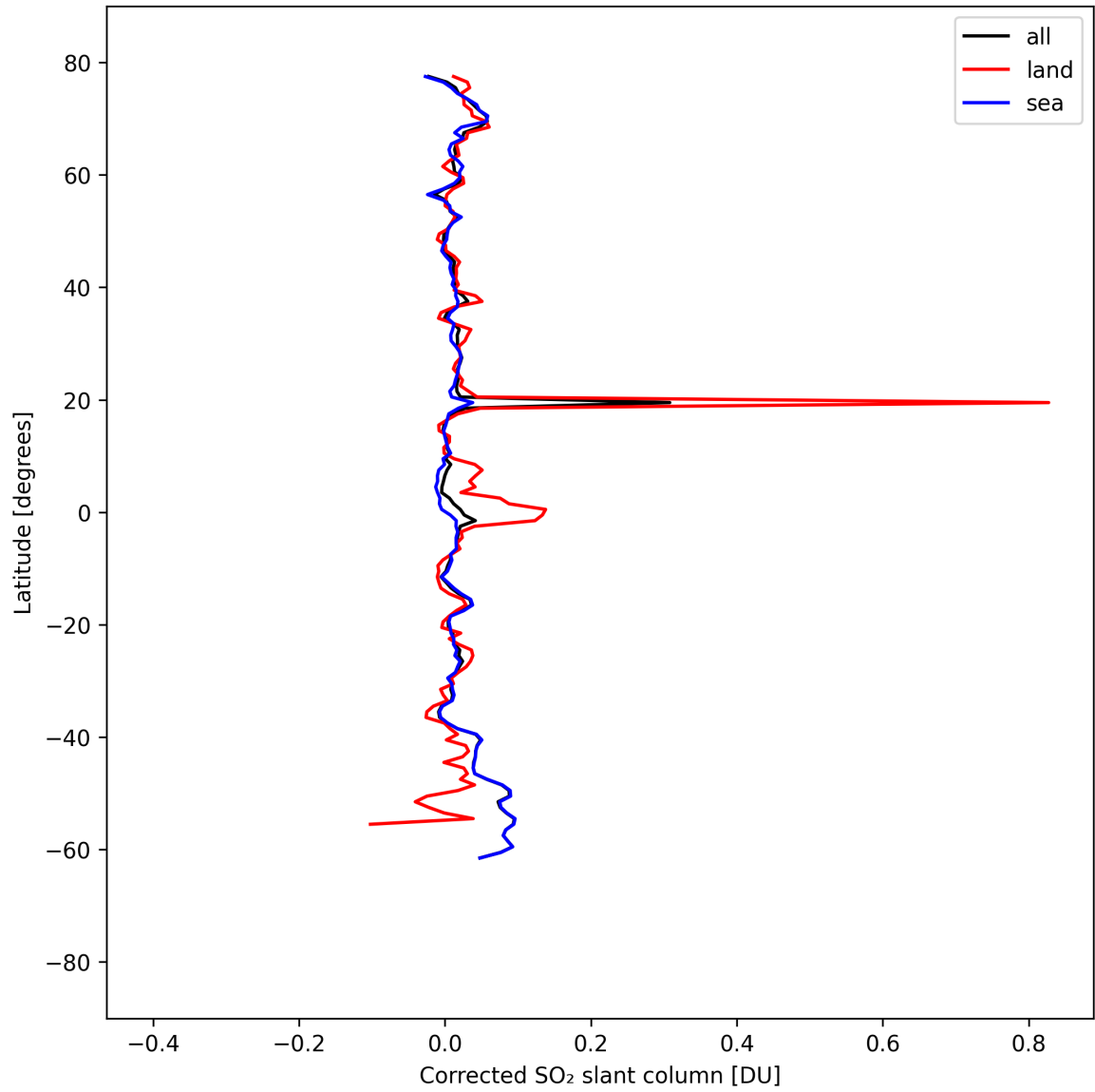
Figure 34: Zonal average of "Corrected SO 2 slant column" for 2025-09-01 to 2025-09-03.
