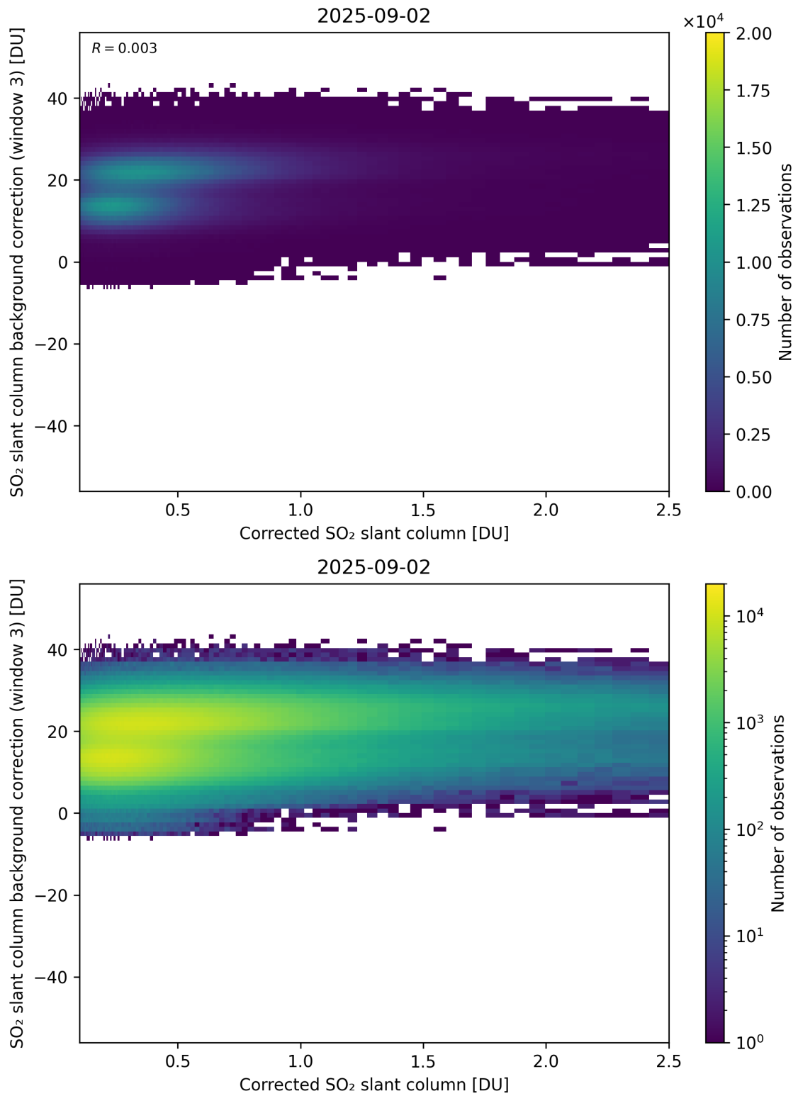
Figure 228: Scatter density plot of “Corrected SO 2 slant column” against “SO 2 slant column background correction (window 3)” for 2025-09-01 to 2025-09-03.
