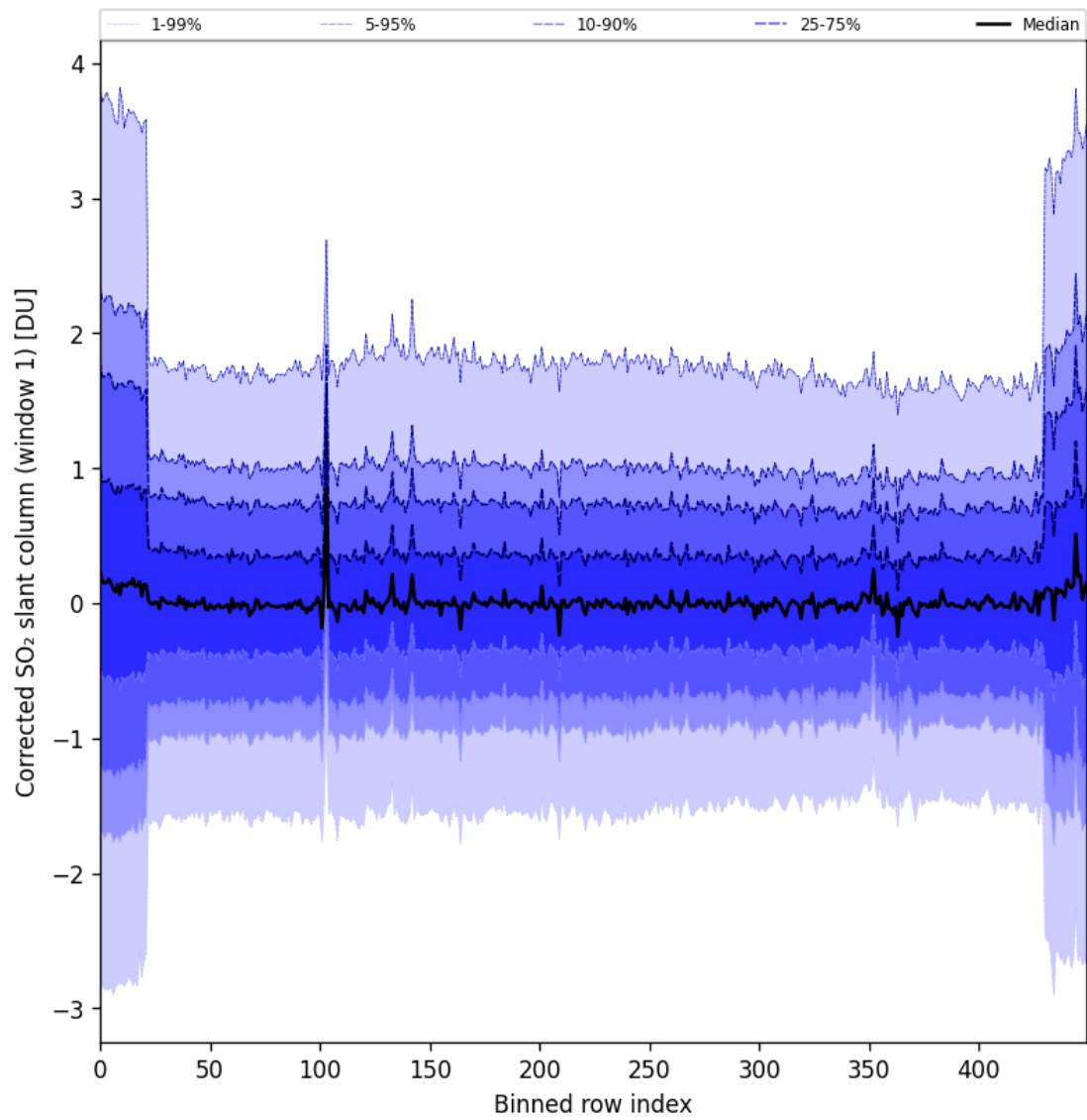
Figure 91: Along track statistics of “Corrected SO 2 slant column (window 1)” for 2025-09-01 to 2025-09-03
