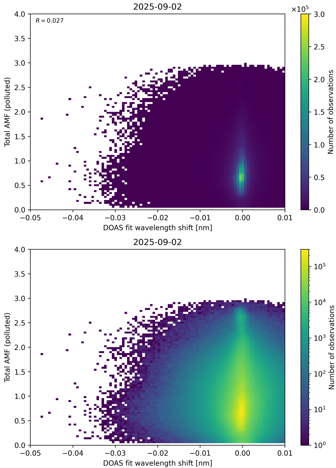
Figure 141: Scatter density plot of “DOAS fit wavelength shift” against “Total AMF (polluted)” for 2025-09-01 to 2025-09-03.
