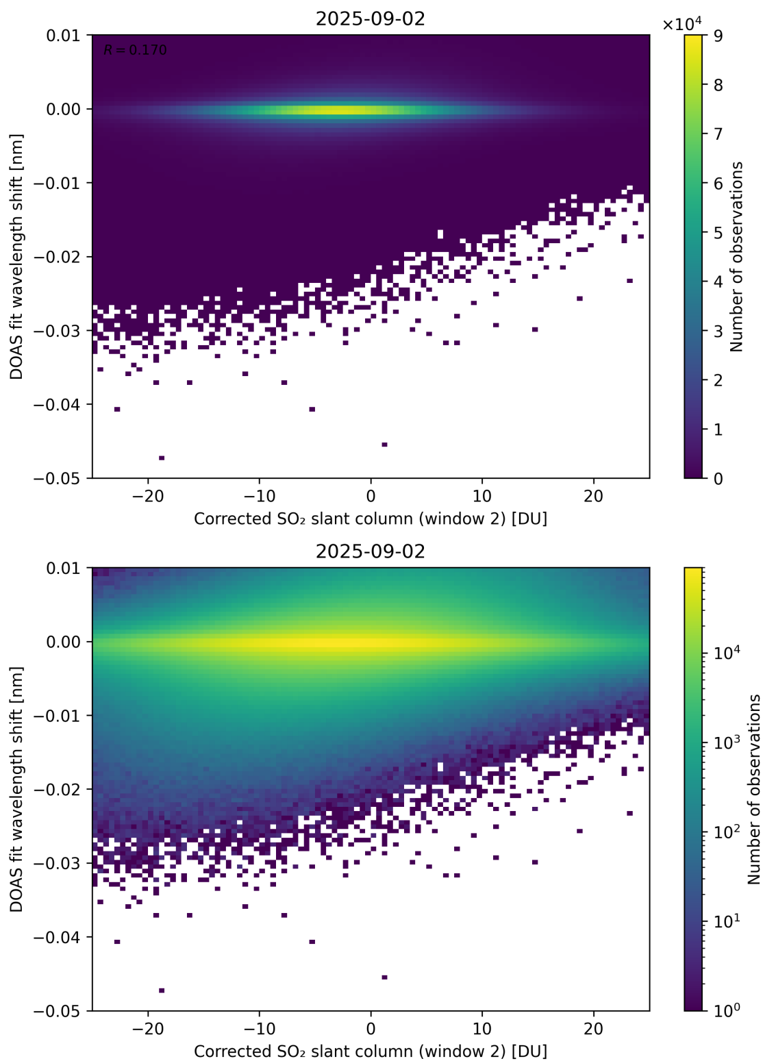
Figure 246: Scatter density plot of “Corrected SO 2 slant column (window 2)” against “DOAS fit wavelength shift” for 2025-09-01 to 2025-09-03.
