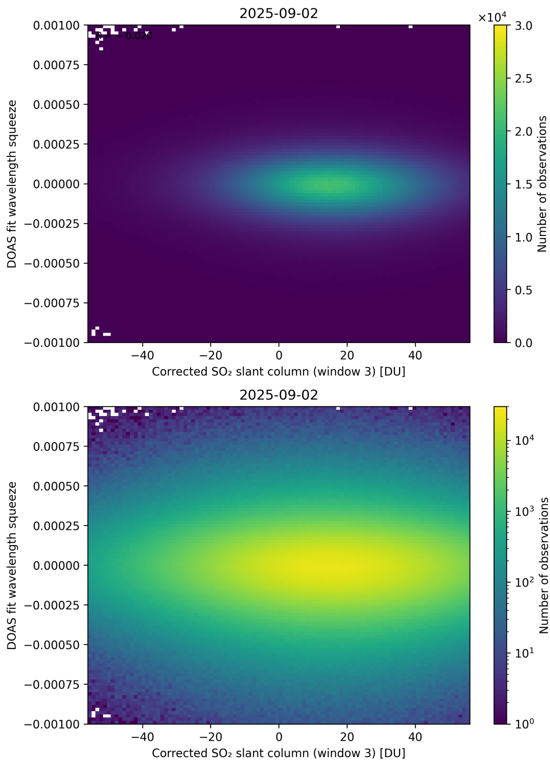
Figure 257: Scatter density plot of “Corrected SO 2 slant column (window 3)” against “DOAS fit wavelength squeeze” for 2025-09-01 to 2025-09-03.
