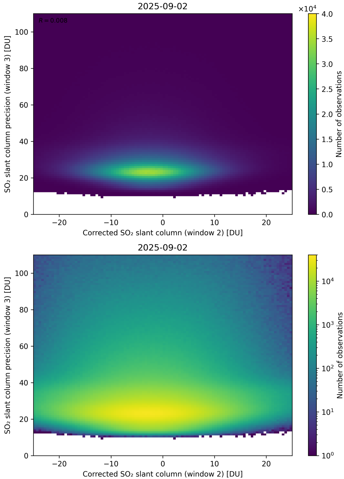
Figure 252: Scatter density plot of “Corrected SO 2 slant column (window 2)” against “SO 2 slant column precision (window 3)” for 2025-09-01 to 2025-09-03.
