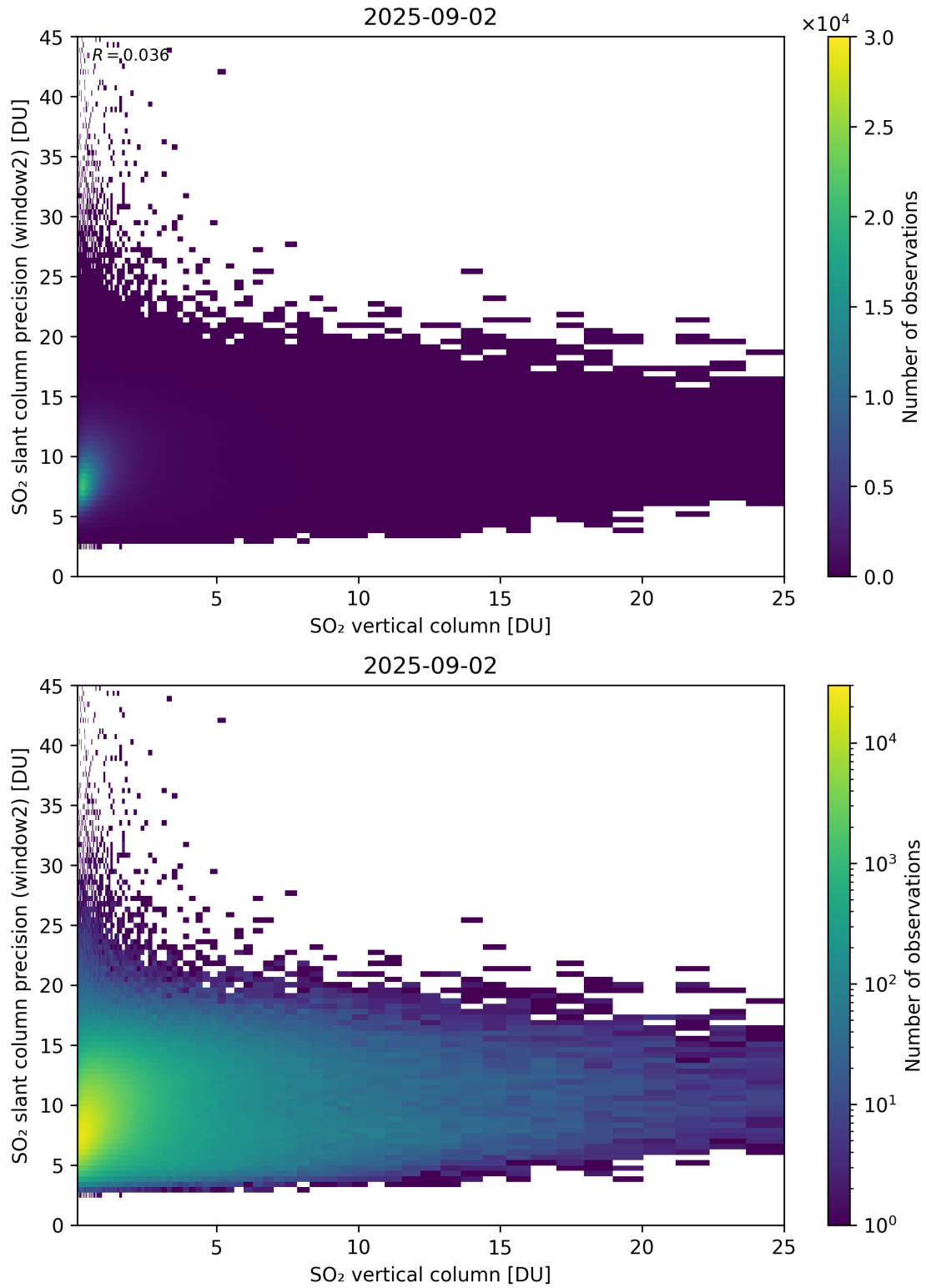
Figure 356: Scatter density plot of “SO 2 vertical column” against “SO 2 slant column precision (window2)” for 2025-09-01 to 2025-09-03.
