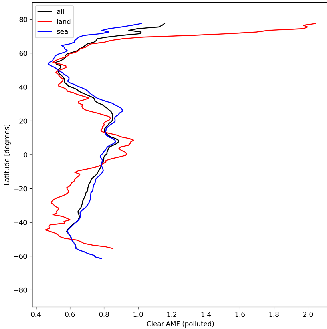
Figure 55: Zonal average of “Clear AMF (polluted)” for 2025-09-01 to 2025-09-03.
