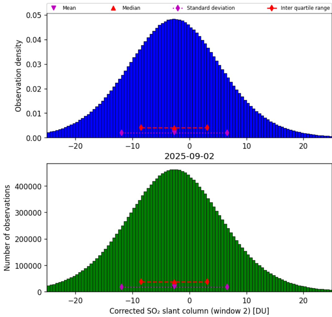
Figure 69: Histogram of “Corrected SO 2 slant column (window 2)” for 2025-09-01 to 2025-09-03
