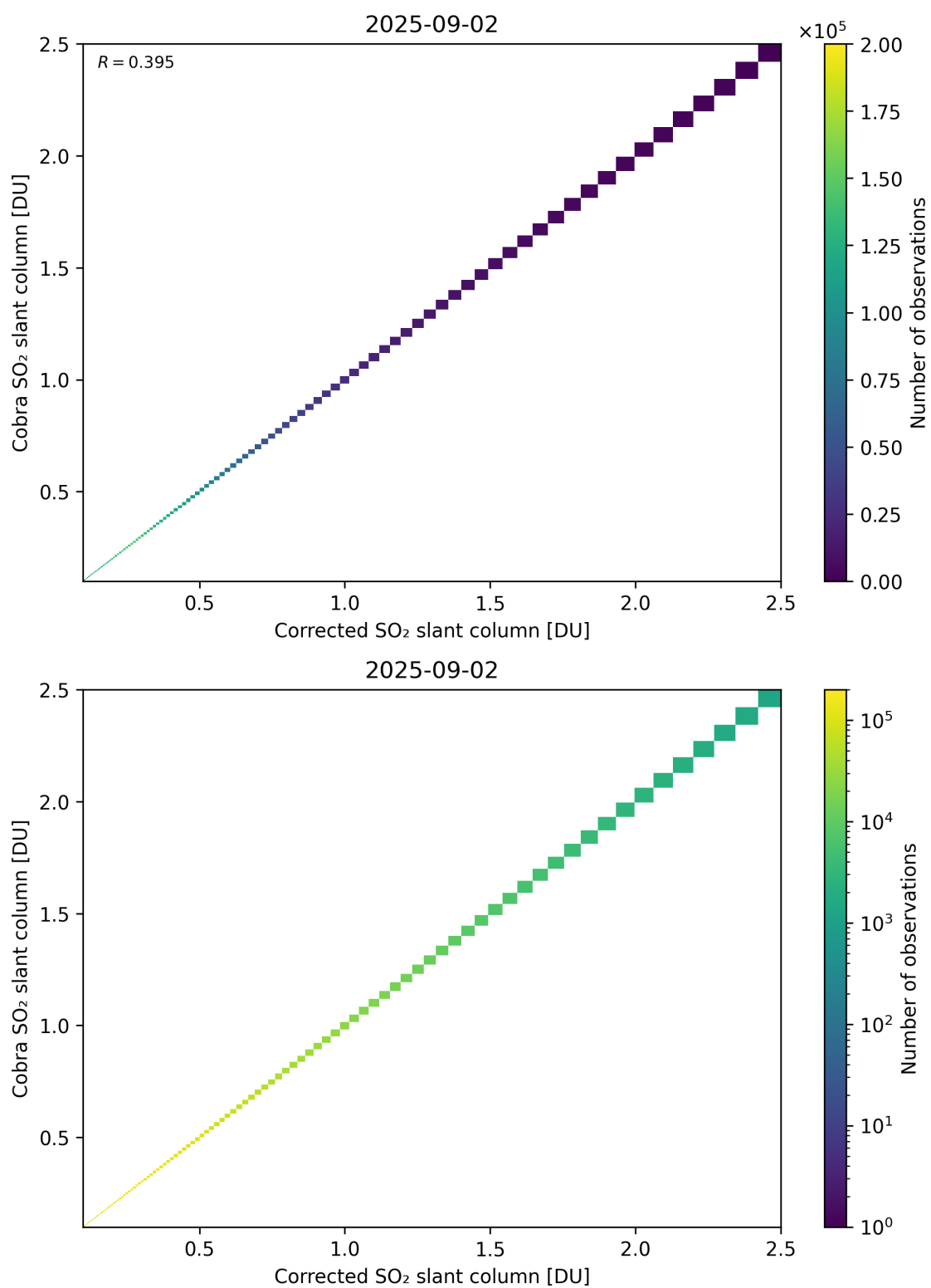
Figure 233: Scatter density plot of “Corrected SO 2 slant column” against “Cobra SO 2 slant column” for 2025-09-01 to 2025-09-03.
