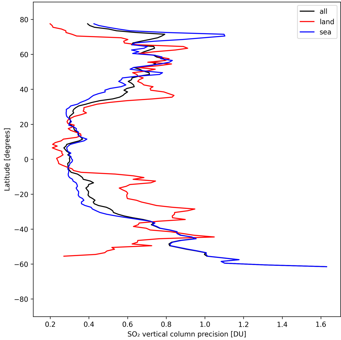
Figure 33: Zonal average of “SO 2 vertical column precision” for 2025-09-01 to 2025-09-03.
