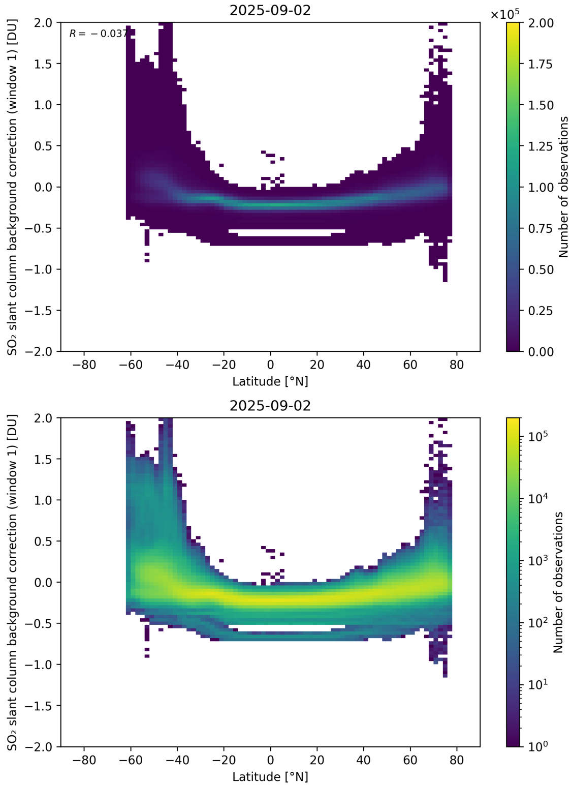
Figure 150: Scatter density plot of “Latitude” against “SO 2 slant column background correction (window 1)” for 2025-09-01 to 2025-09-03.
