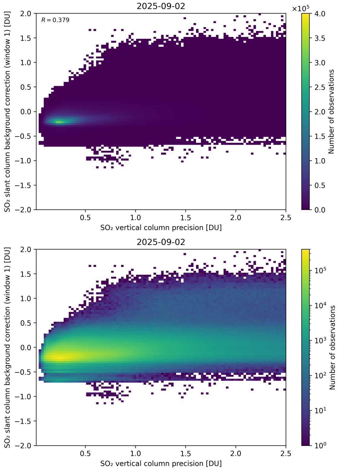
Figure 329: Scatter density plot of “SO 2 vertical column precision” against “SO 2 slant column background correction (window 1)” for 2025-09-01 to 2025-09-03.
