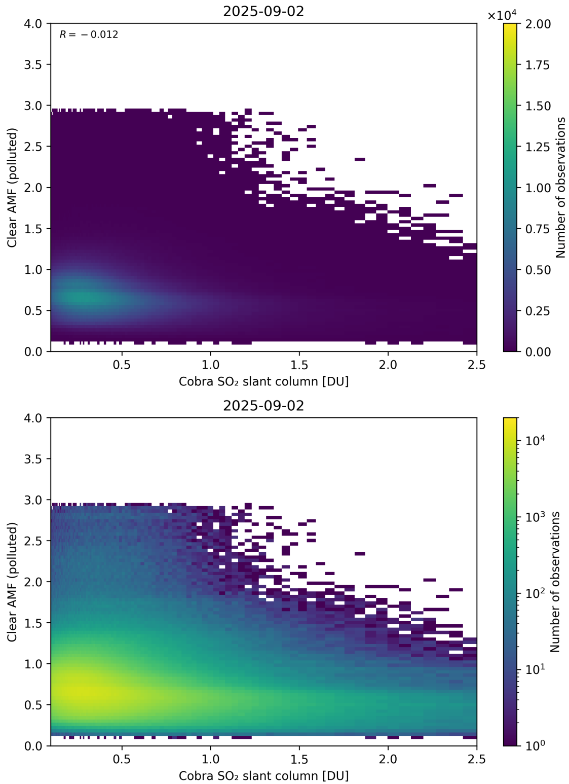
Figure 215: Scatter density plot of “Cobra SO 2 slant column” against “Clear AMF (polluted)” for 2025-09-01 to 2025-09-03.
