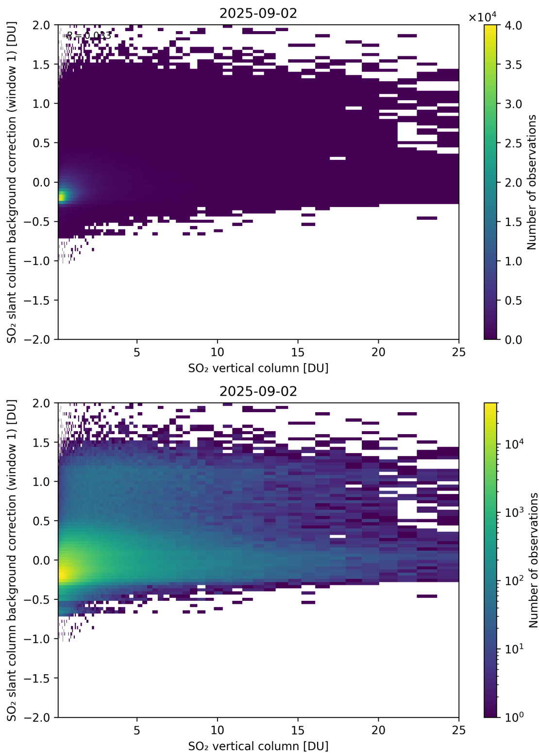
Figure 323: Scatter density plot of “SO 2 vertical column” against “SO 2 slant column background correction (window 1)” for 2025-09-01 to 2025-09-03.
