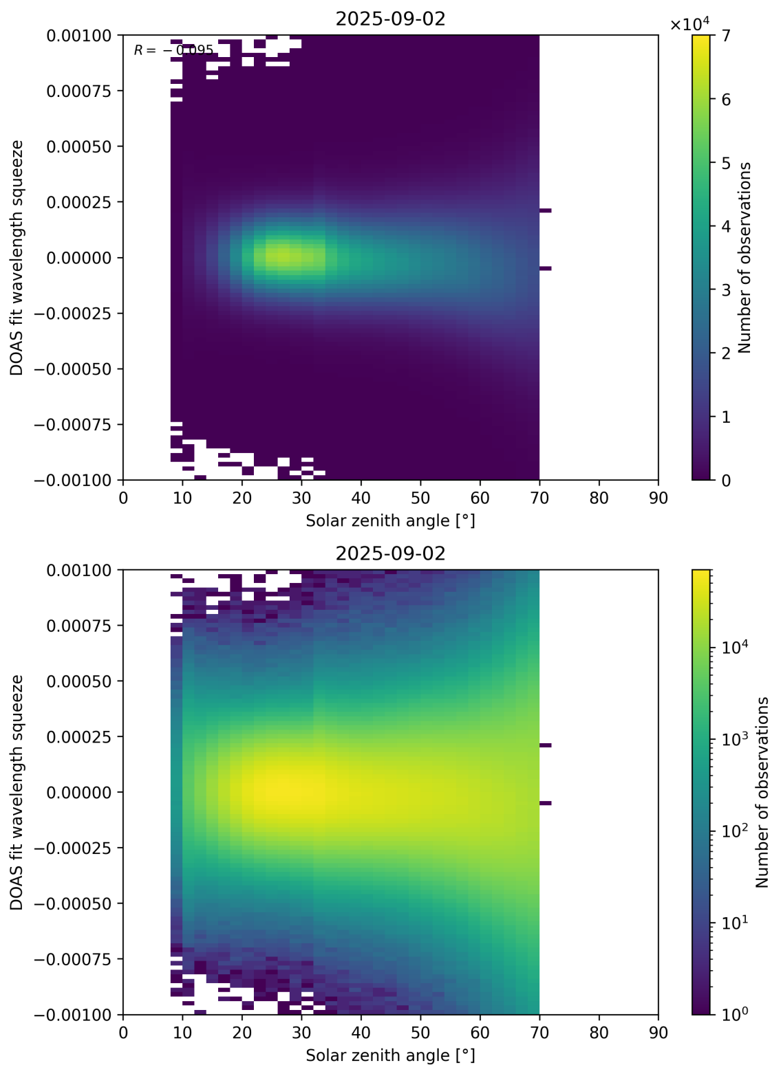
Figure 175: Scatter density plot of “Solar zenith angle” against “DOAS fit wavelength squeeze” for 2025-09-01 to 2025-09-03.
