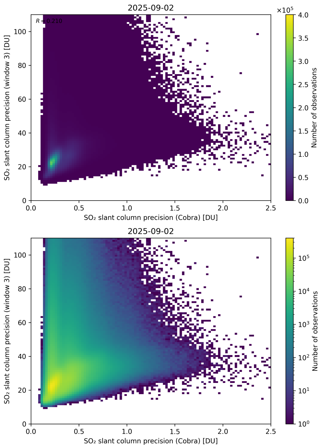
Figure 212: Scatter density plot of “SO 2 slant column precision (Cobra)” against “SO 2 slant column precision (window 3)” for 2025-09-01 to 2025-09-03.
