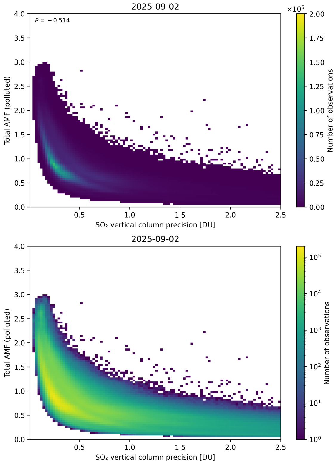
Figure 346: Scatter density plot of “SO 2 vertical column precision” against “Total AMF (polluted)” for 2025-09-01 to 2025-09-03.
