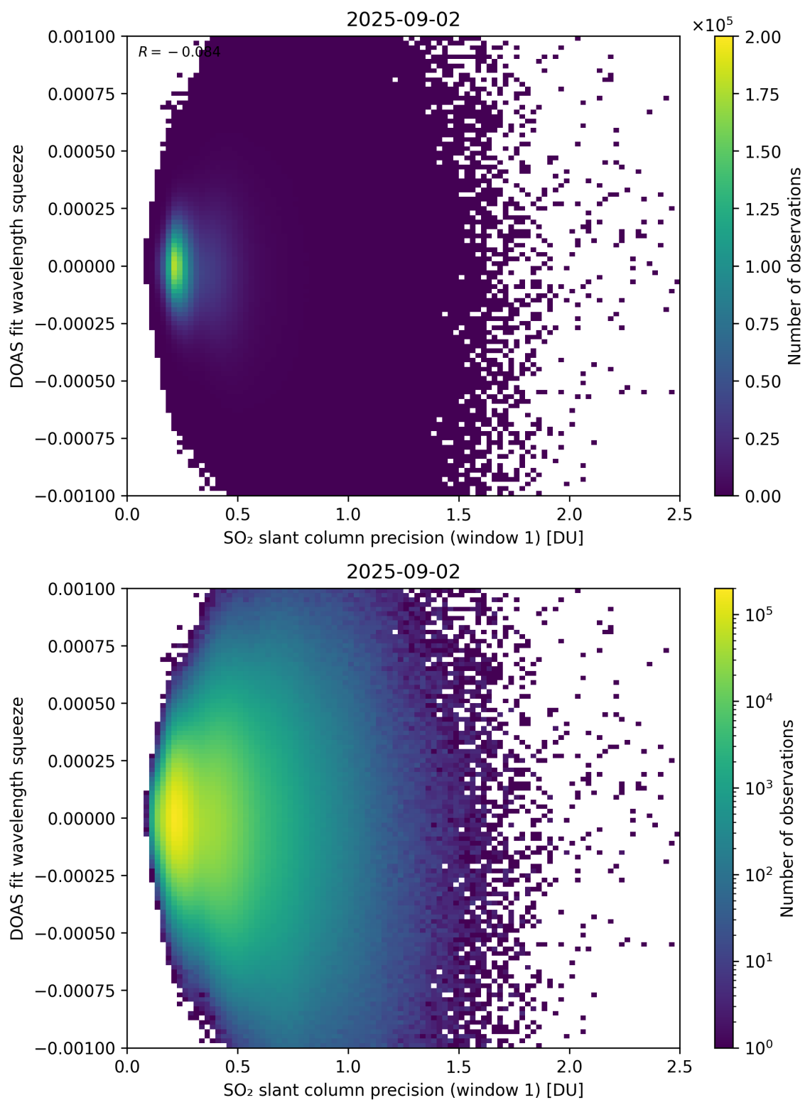
Figure 272: Scatter density plot of “SO 2 slant column precision (window 1)” against “DOAS fit wavelength squeeze” for 2025-09-01 to 2025-09-03.
