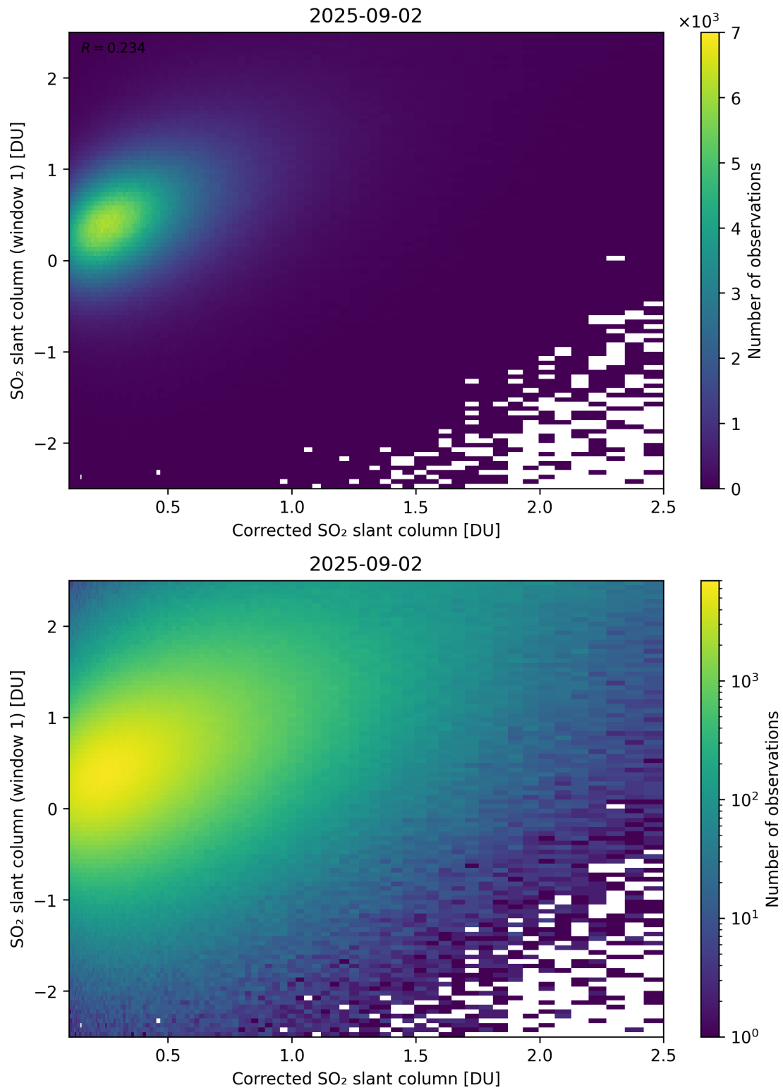
Figure 237: Scatter density plot of “Corrected SO 2 slant column” against “SO 2 slant column (window 1)” for 2025-09-01 to 2025-09-03.
