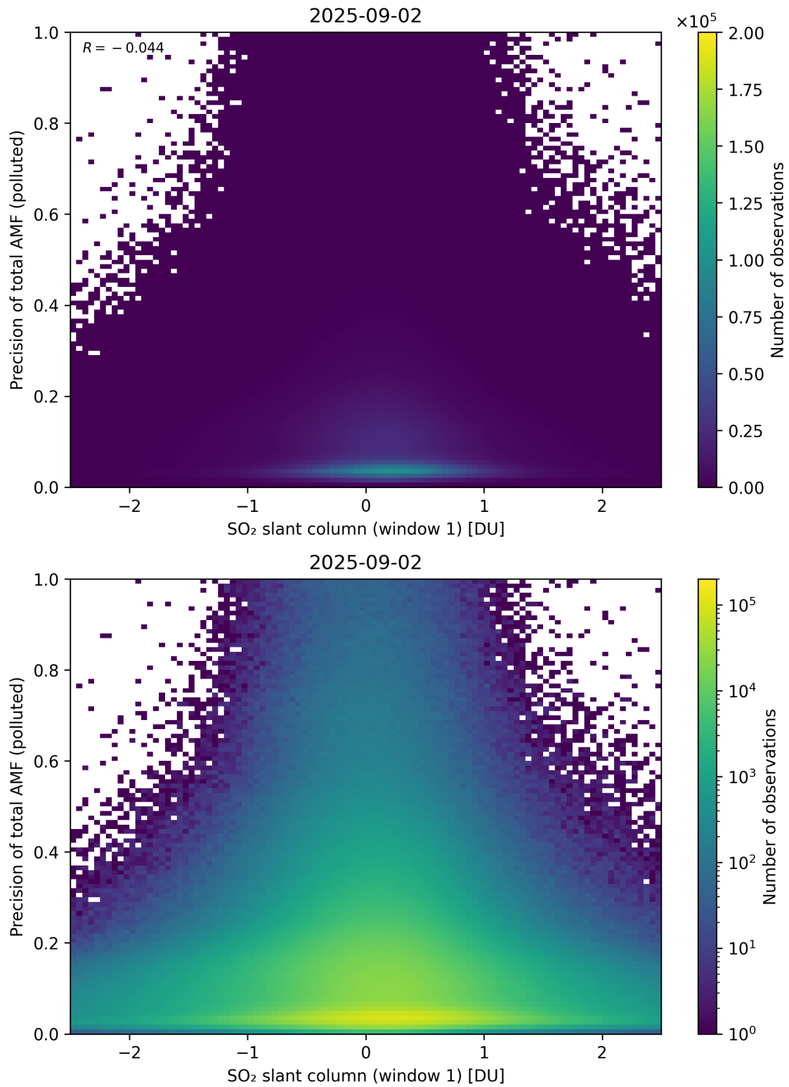
Figure 290: Scatter density plot of “SO 2 slant column (window 1)” against “Precision of total AMF (polluted)” for 2025-09-01 to 2025-09-03.
