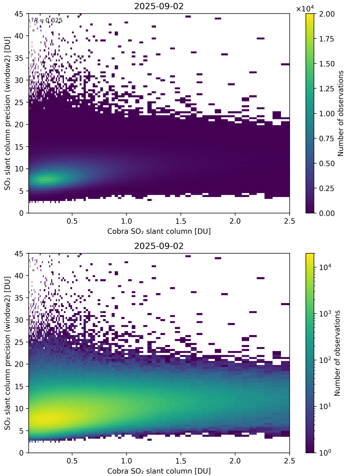
Figure 221: Scatter density plot of “Cobra SO 2 slant column” against “SO 2 slant column precision (window2)” for 2025-09-01 to 2025-09-03.
