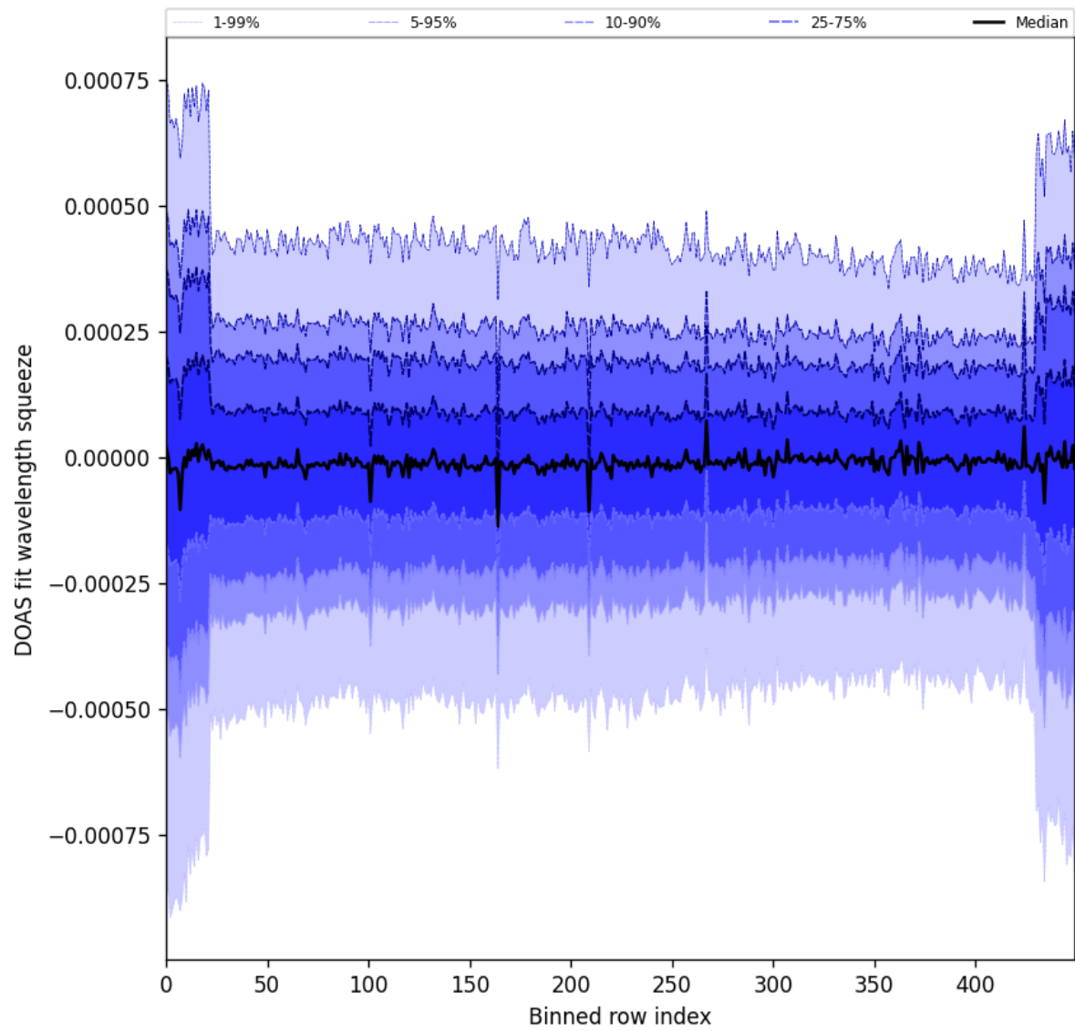
Figure 103: Along track statistics of “DOAS fit wavelength squeeze” for 2025-09-01 to 2025-09-03
