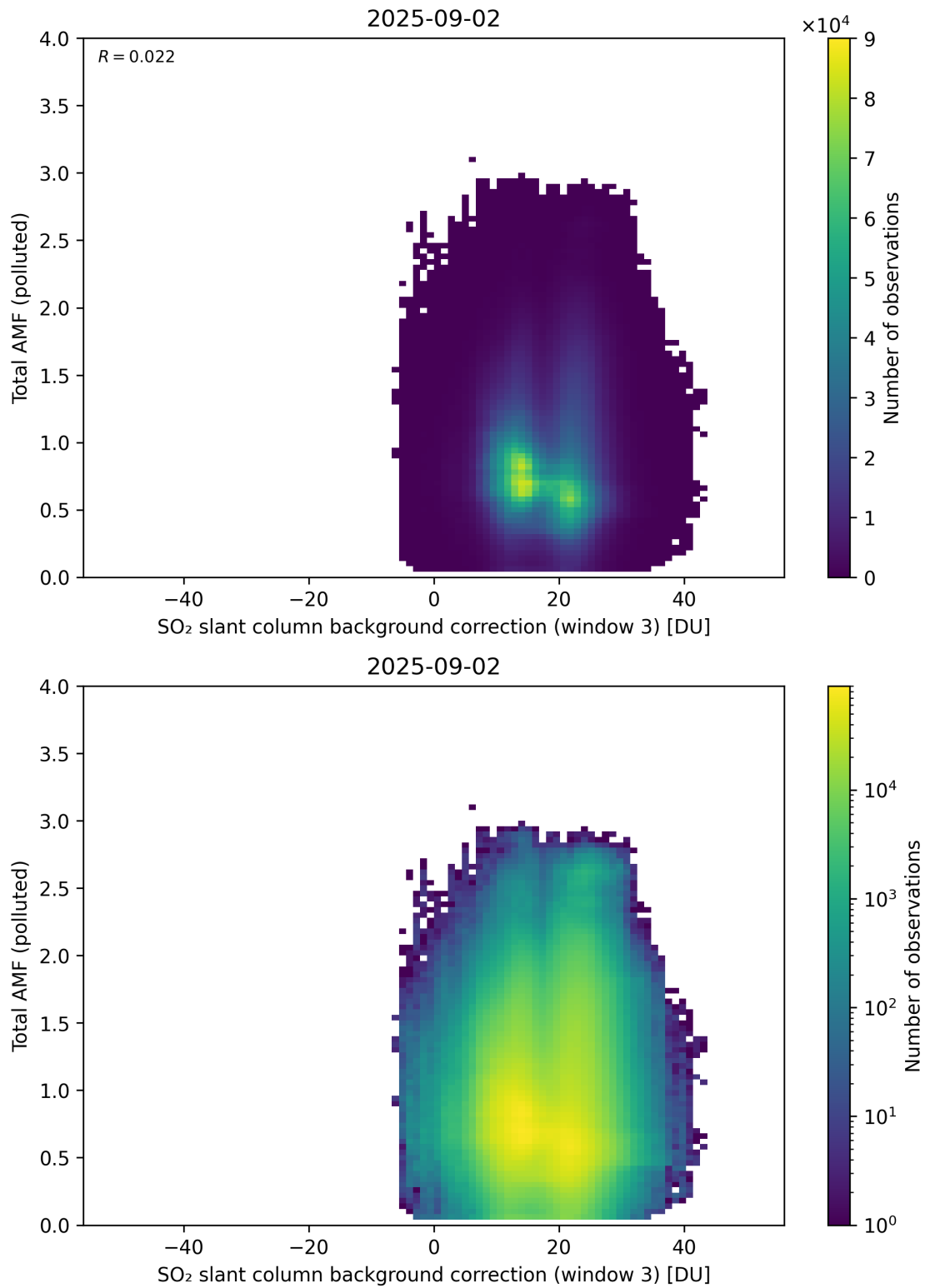
Figure 136: Scatter density plot of “SO 2 slant column background correction (window 3)” against “Total AMF (polluted)” for 2025-09-01 to 2025-09-03.
