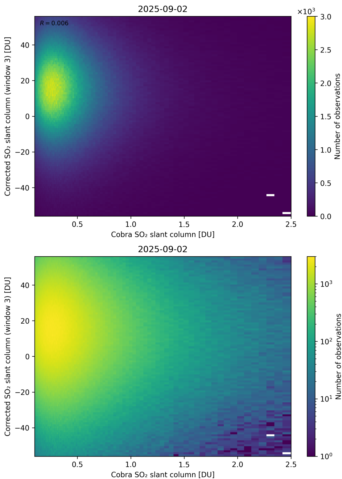
Figure 218: Scatter density plot of “Cobra SO 2 slant column” against “Corrected SO 2 slant column (window 3)” for 2025-09-01 to 2025-09-03.
