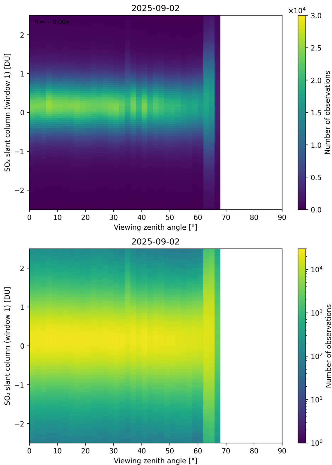
Figure 376: Scatter density plot of “Viewing zenith angle” against “SO 2 slant column (window 1)” for 2025-09-01 to 2025-09-03.
