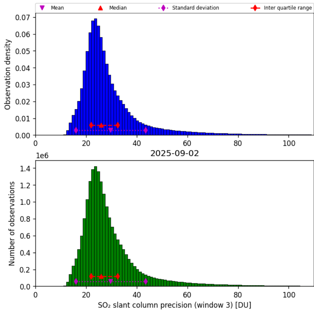
Figure 72: Histogram of “SO 2 slant column precision (window 3)” for 2025-09-01 to 2025-09-03
