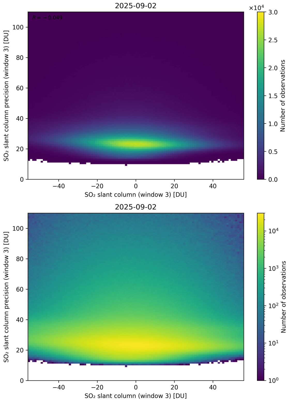
Figure 317: Scatter density plot of “SO 2 slant column (window 3)” against “SO 2 slant column precision (window 3)” for 2025-09-01 to 2025-09-03.
