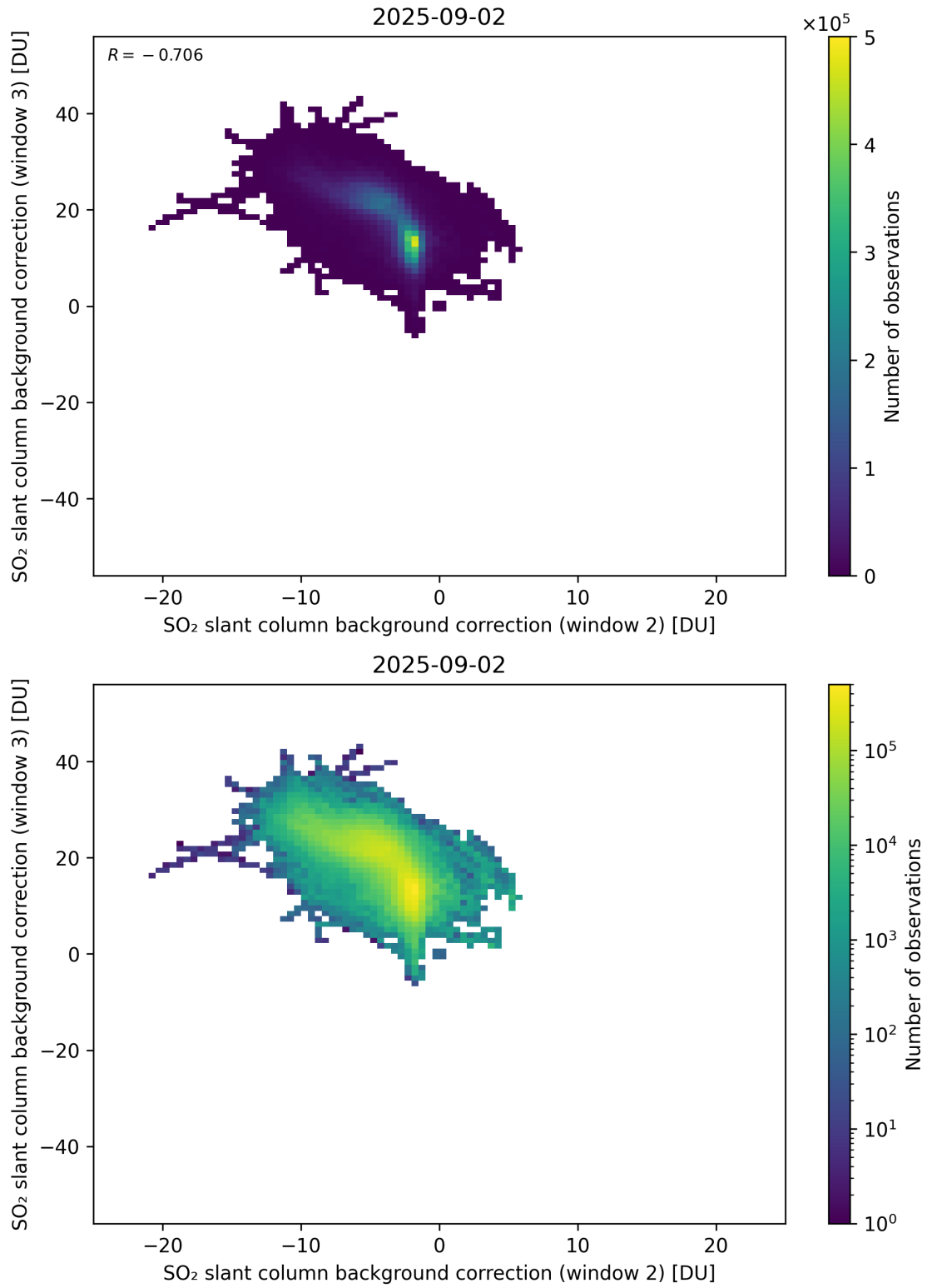
Figure 122: Scatter density plot of “SO 2 slant column background correction (window 2)” against “SO 2 slant column background correction (window 3)” for 2025-09-01 to 2025-09-03.
