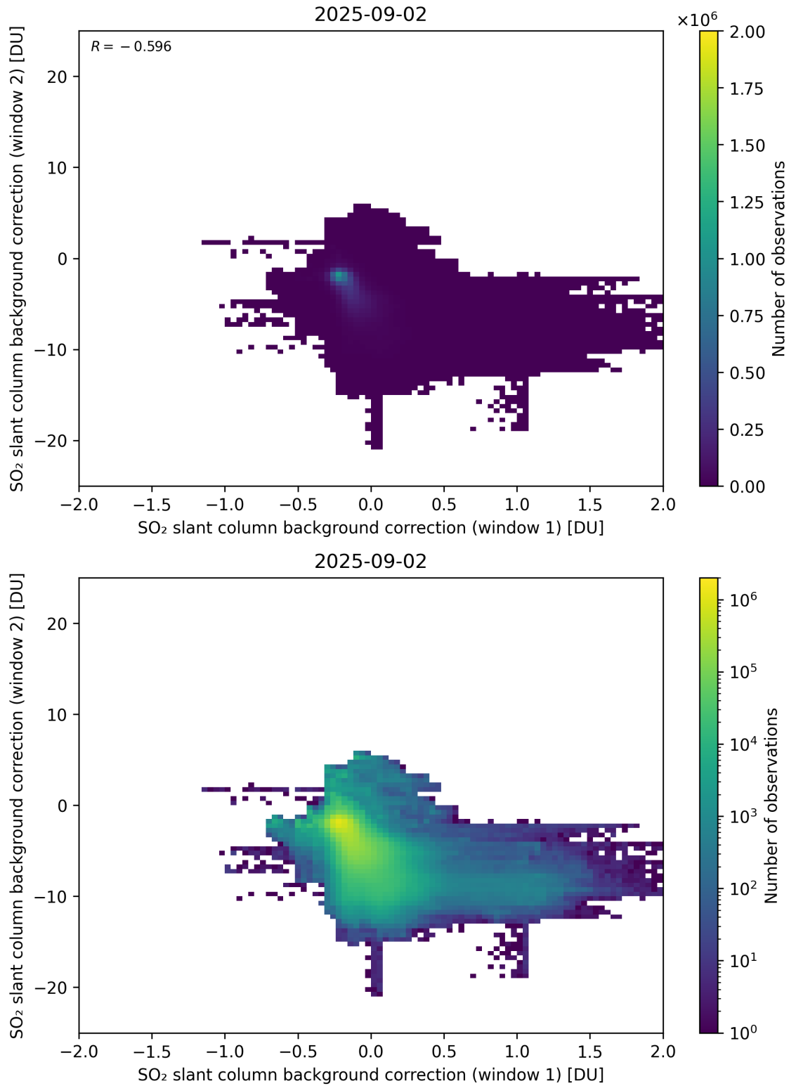
Figure 109: Scatter density plot of “SO 2 slant column background correction (window 1)” against “SO 2 slant column background correction (window 2)” for 2025-09-01 to 2025-09-03.
