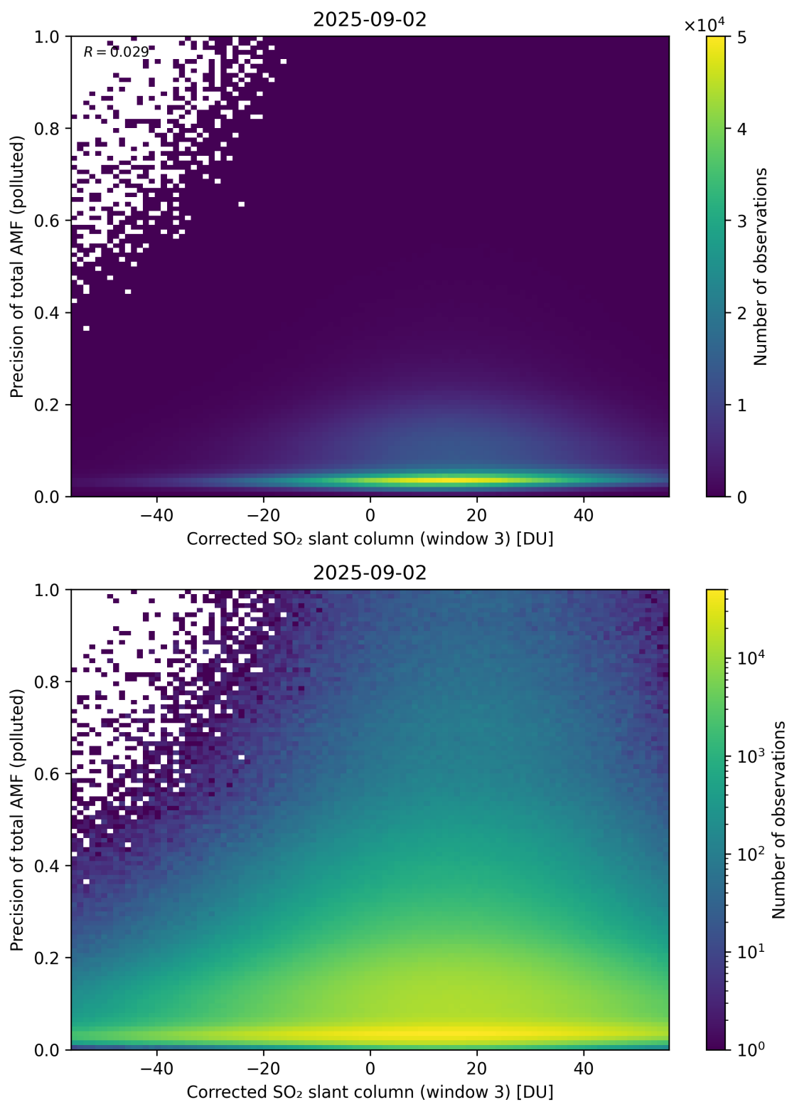
Figure 261: Scatter density plot of “Corrected SO 2 slant column (window 3)” against “Precision of total AMF (polluted)” for 2025-09-01 to 2025-09-03.
