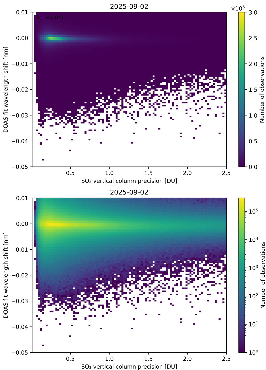
Figure 332: Scatter density plot of “SO 2 vertical column precision” against “DOAS fit wavelength shift” for 2025-09-01 to 2025-09-03.
