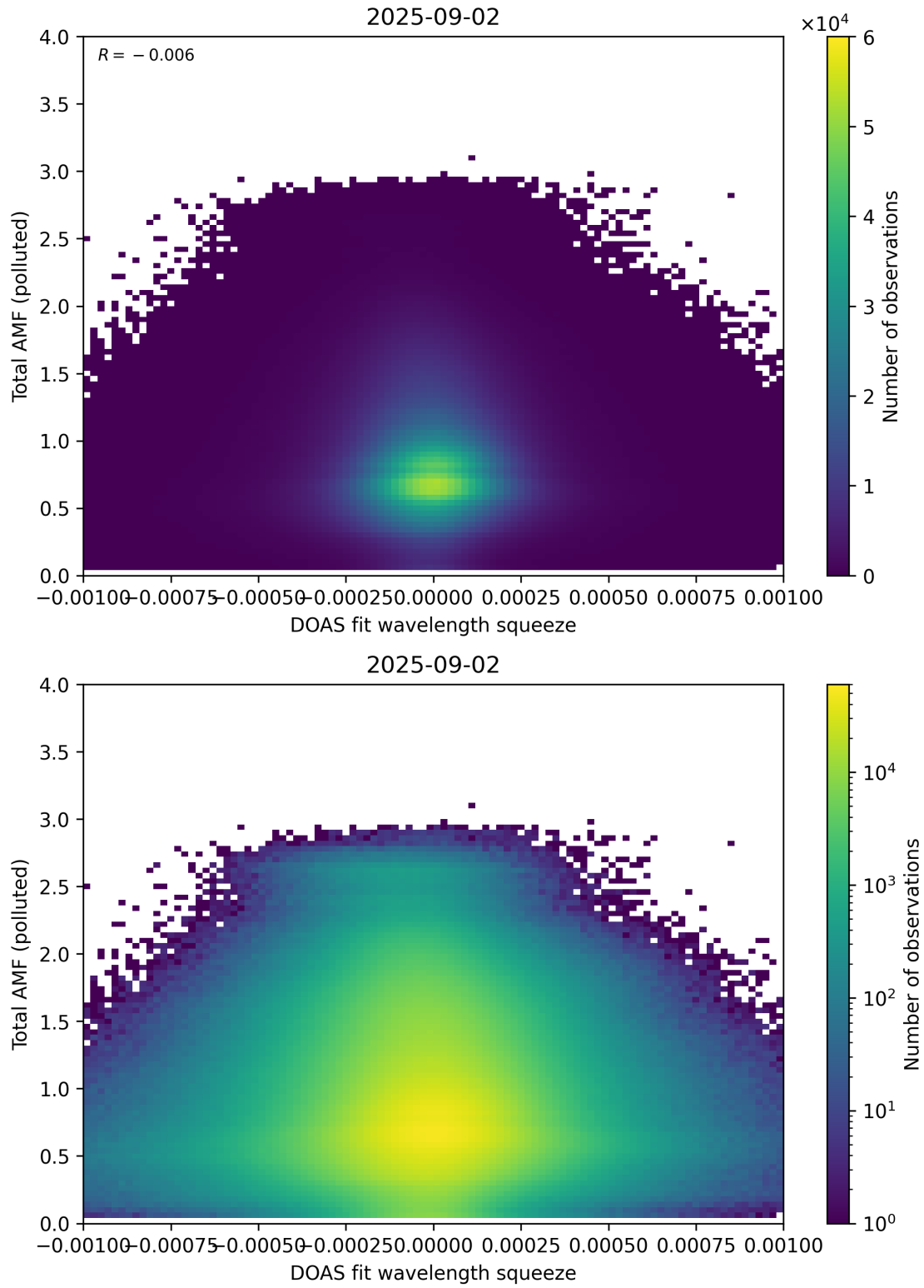
Figure 145: Scatter density plot of “DOAS fit wavelength squeeze” against “Total AMF (polluted)” for 2025-09-01 to 2025-09-03.
