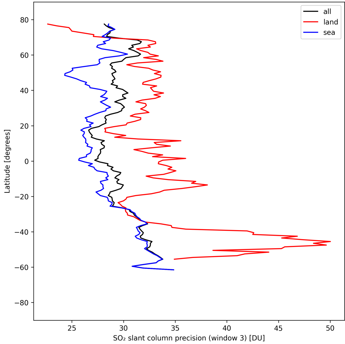
Figure 46: Zonal average of “SO 2 slant column precision (window 3)” for 2025-09-01 to 2025-09-03.
