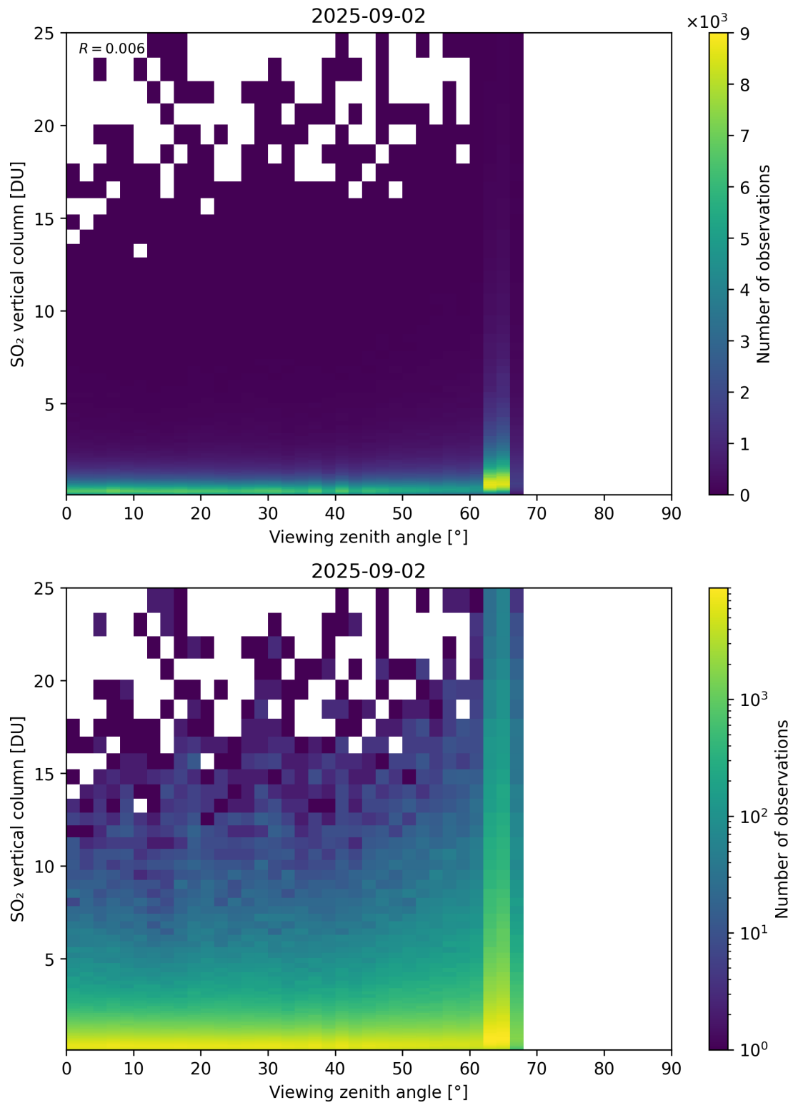
Figure 383: Scatter density plot of “Viewing zenith angle” against “SO 2 vertical column” for 2025-09-01 to 2025-09-03.
