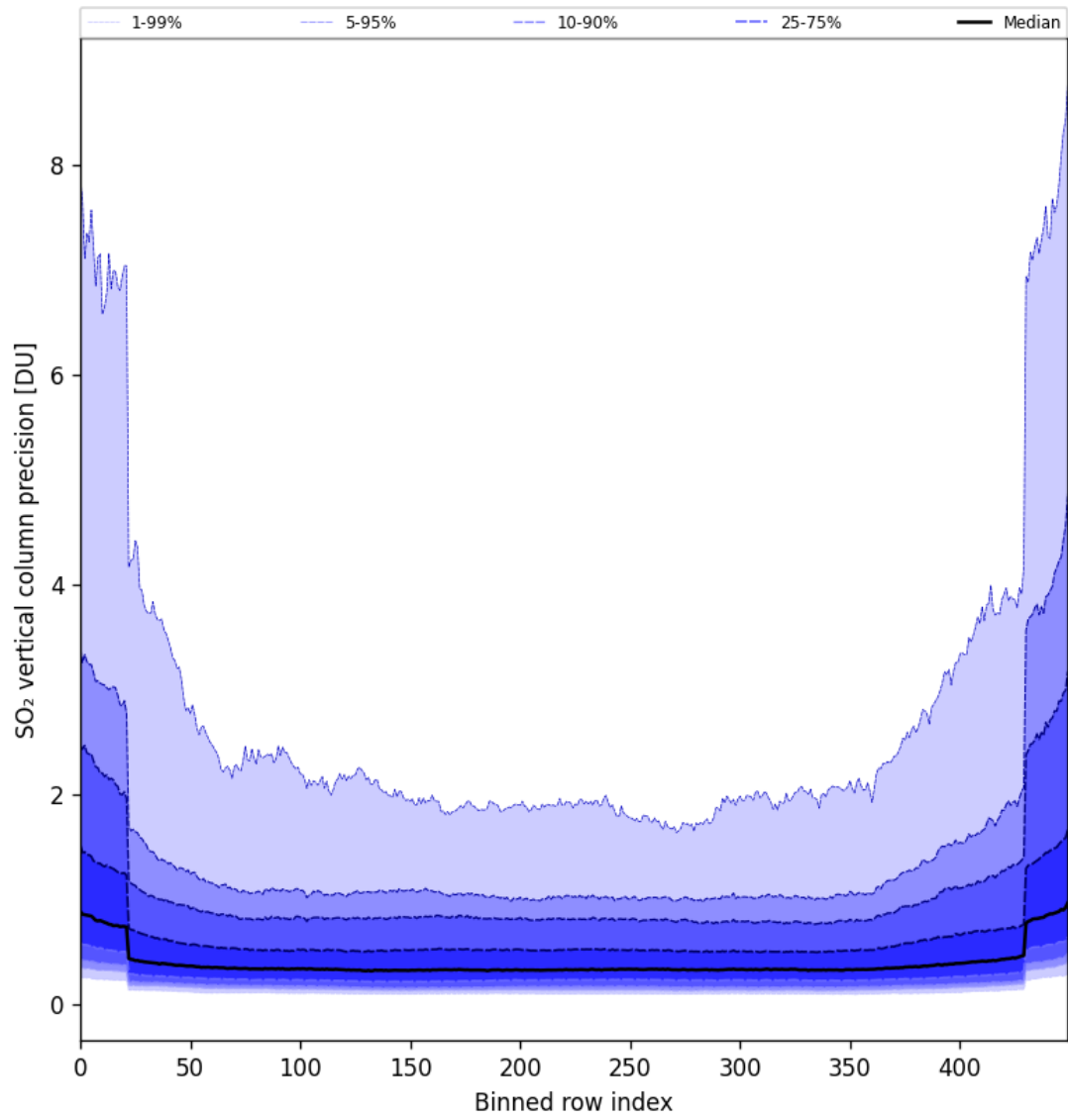
Figure 85: Along track statistics of “SO 2 vertical column precision” for 2025-09-01 to 2025-09-03
