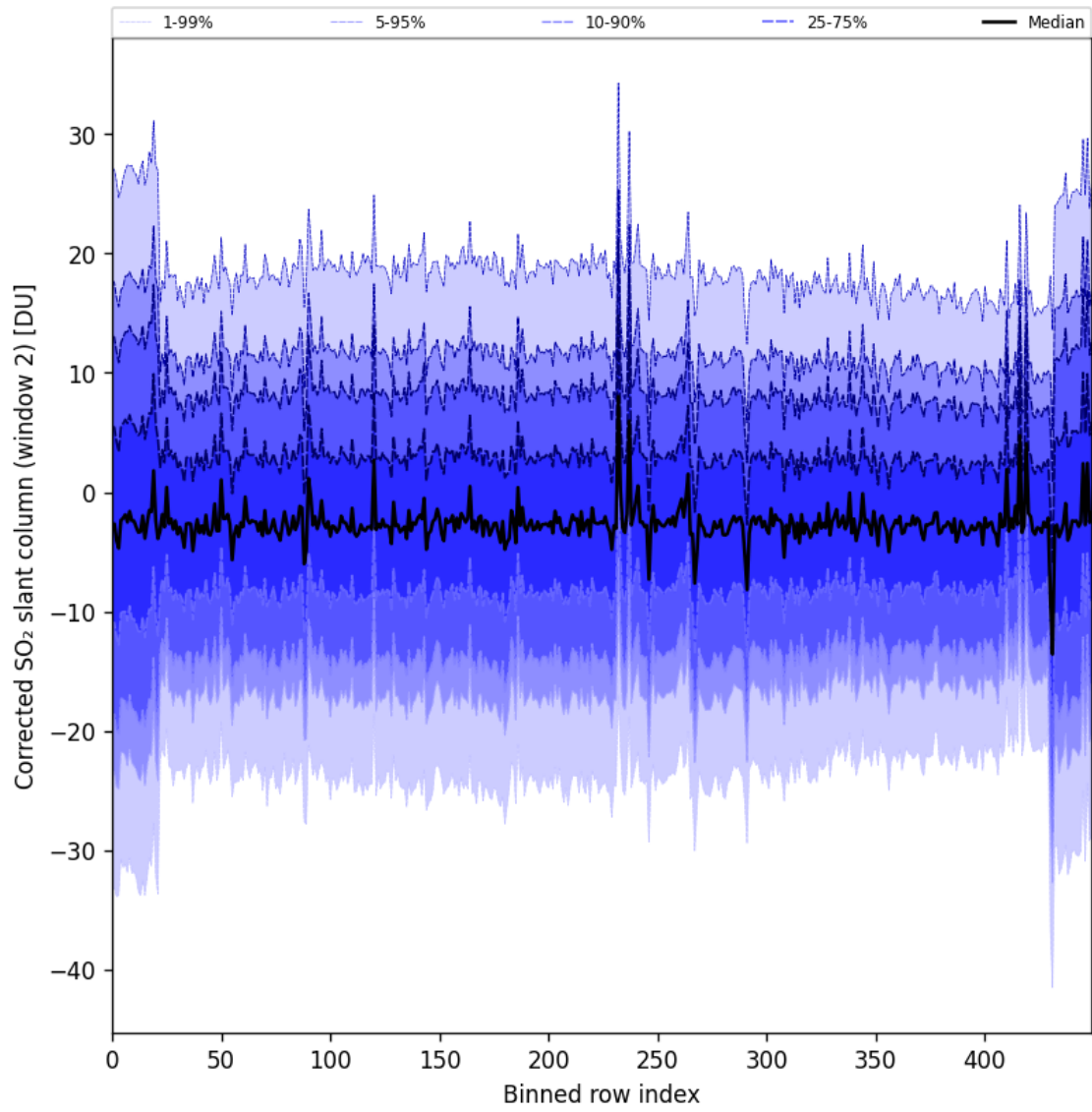
Figure 95: Along track statistics of “Corrected SO 2 slant column (window 2)” for 2025-09-01 to 2025-09-03
