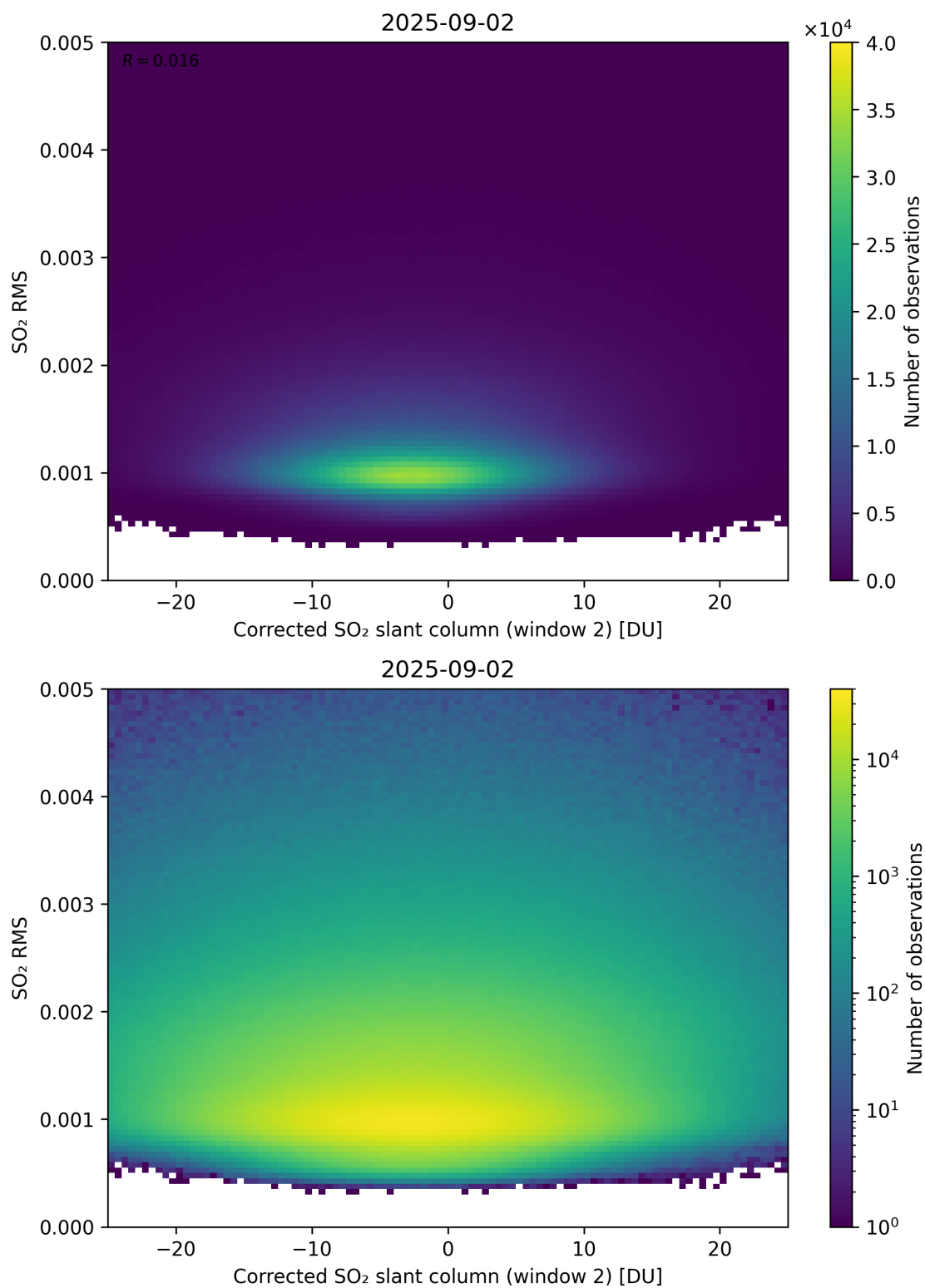
Figure 248: Scatter density plot of “Corrected SO 2 slant column (window 2)” against “SO 2 RMS” for 2025-09-01 to 2025-09-03.
