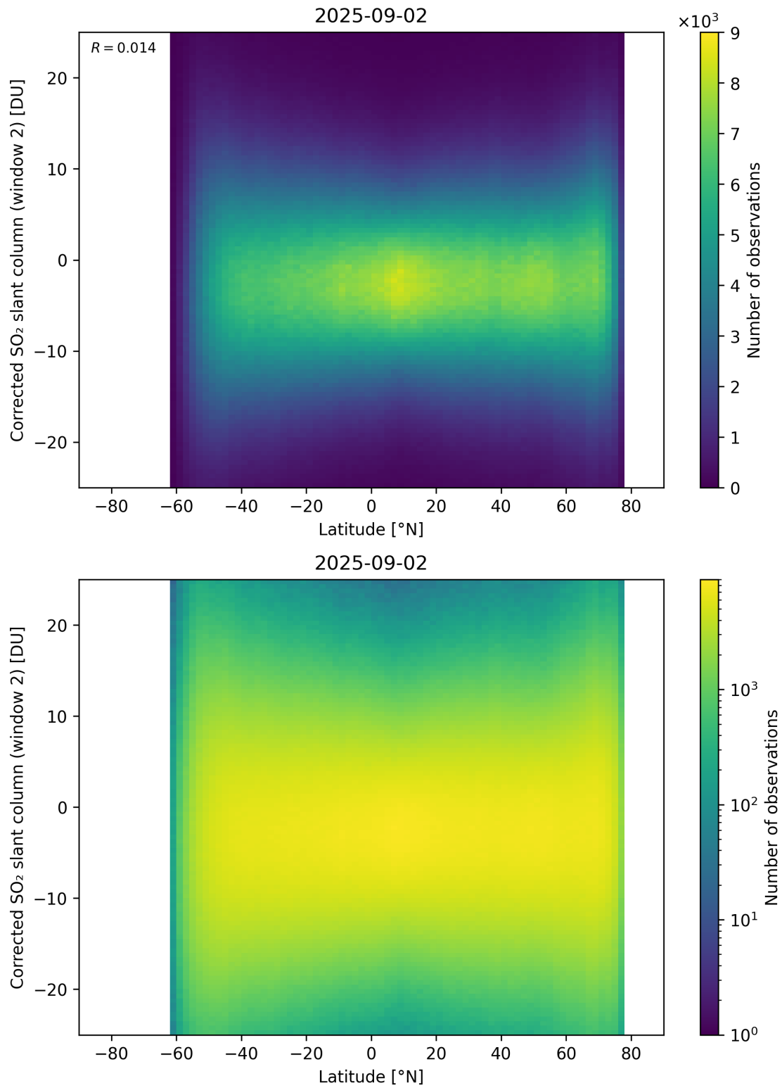
Figure 160: Scatter density plot of “Latitude” against “Corrected SO 2 slant column (window 2)” for 2025-09-01 to 2025-09-03.
