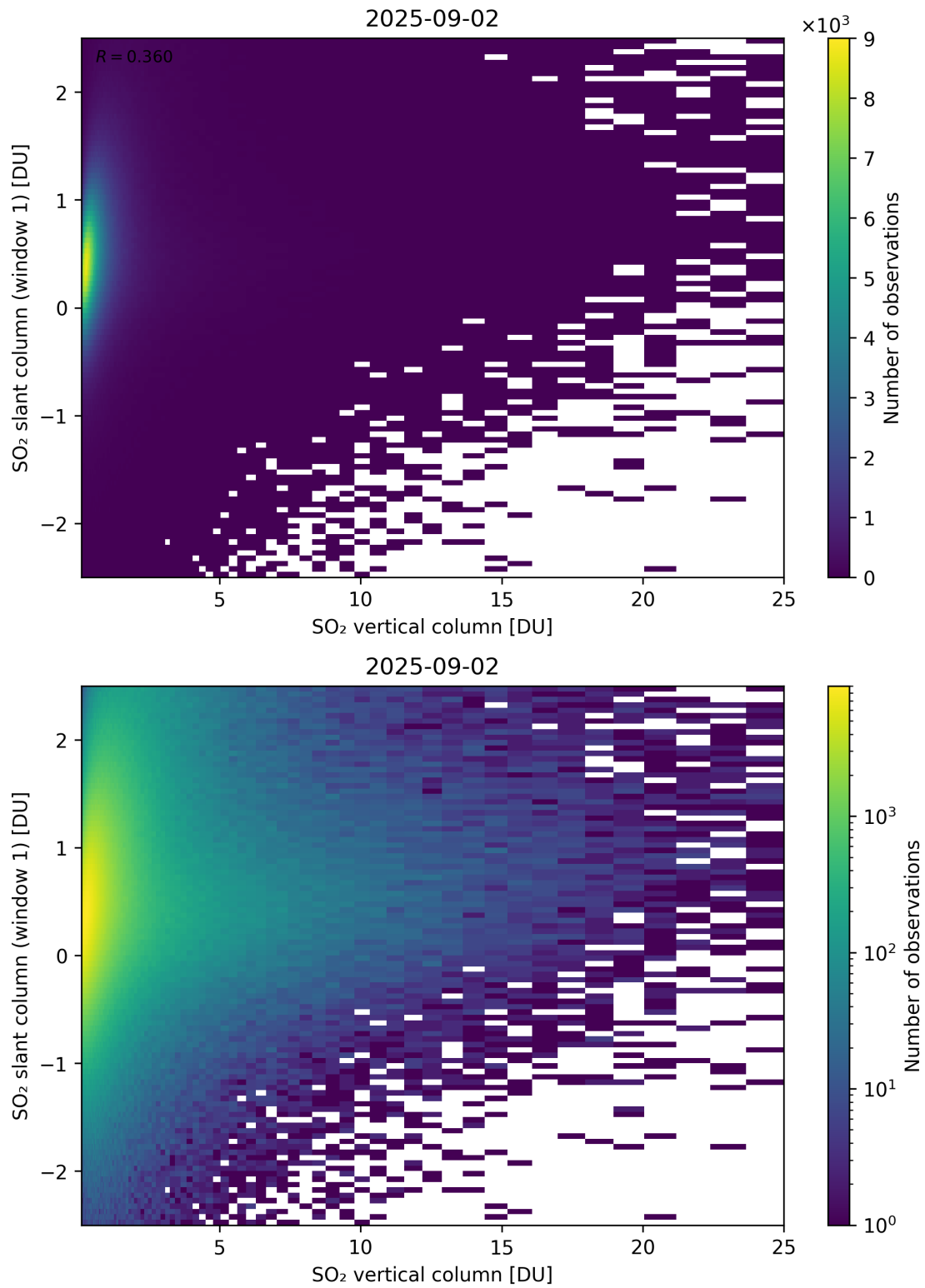
Figure 354: Scatter density plot of “SO 2 vertical column” against “SO 2 slant column (window 1)” for 2025-09-01 to 2025-09-03.
