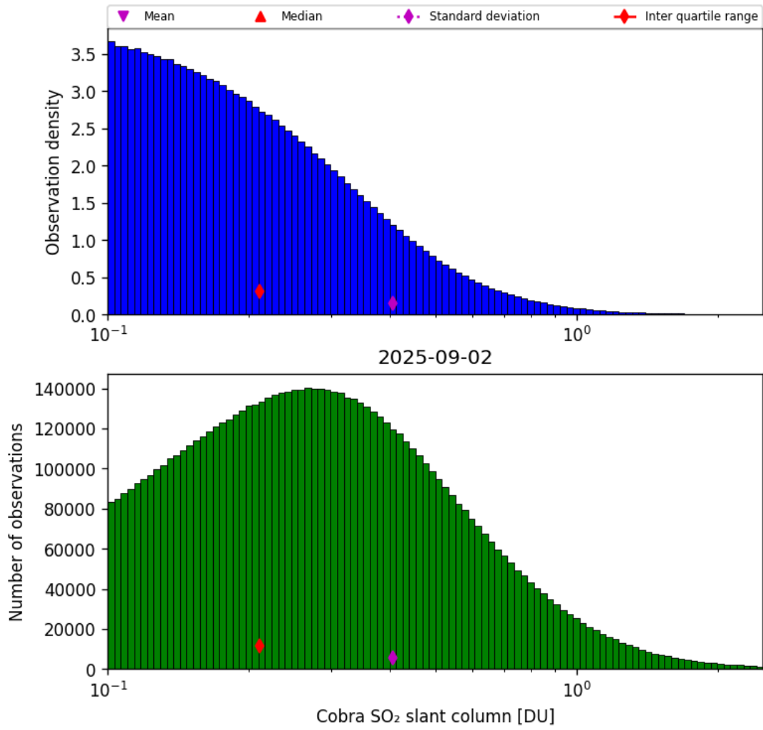
Figure 61: Histogram of “Cobra SO 2 slant column” for 2025-09-01 to 2025-09-03
