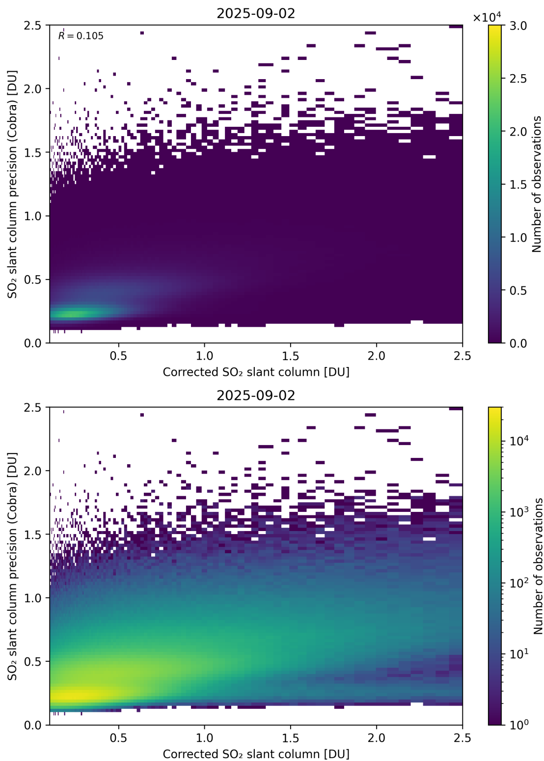
Figure 234: Scatter density plot of “Corrected SO 2 slant column” against “SO 2 slant column precision (Cobra)” for 2025-09-01 to 2025-09-03.
