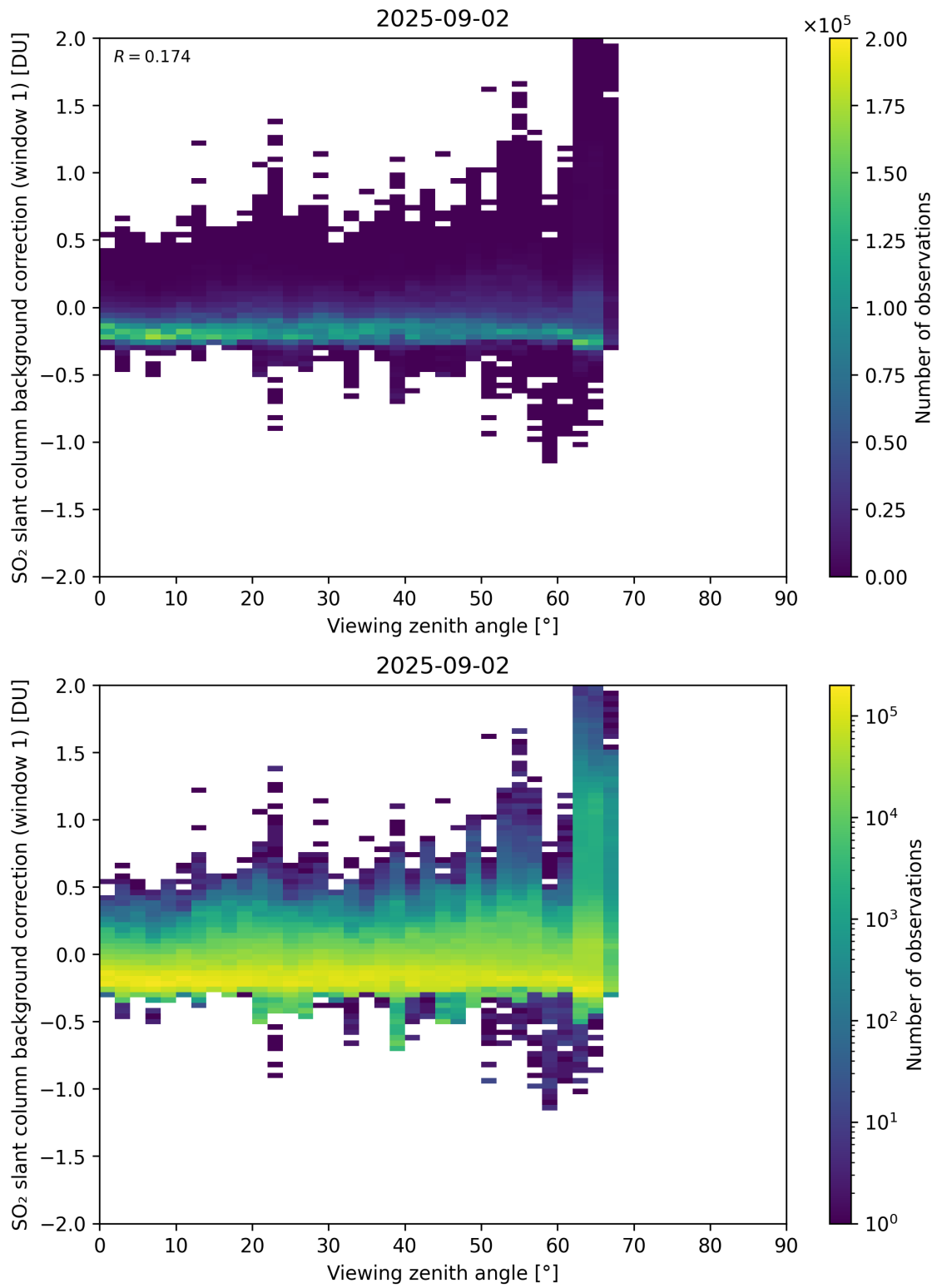
Figure 362: Scatter density plot of “Viewing zenith angle” against “SO 2 slant column background correction (window 1)” for 2025-09-01 to 2025-09-03.
