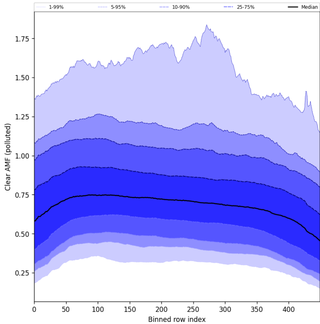
Figure 107: Along track statistics of “Clear AMF (polluted)” for 2025-09-01 to 2025-09-03
