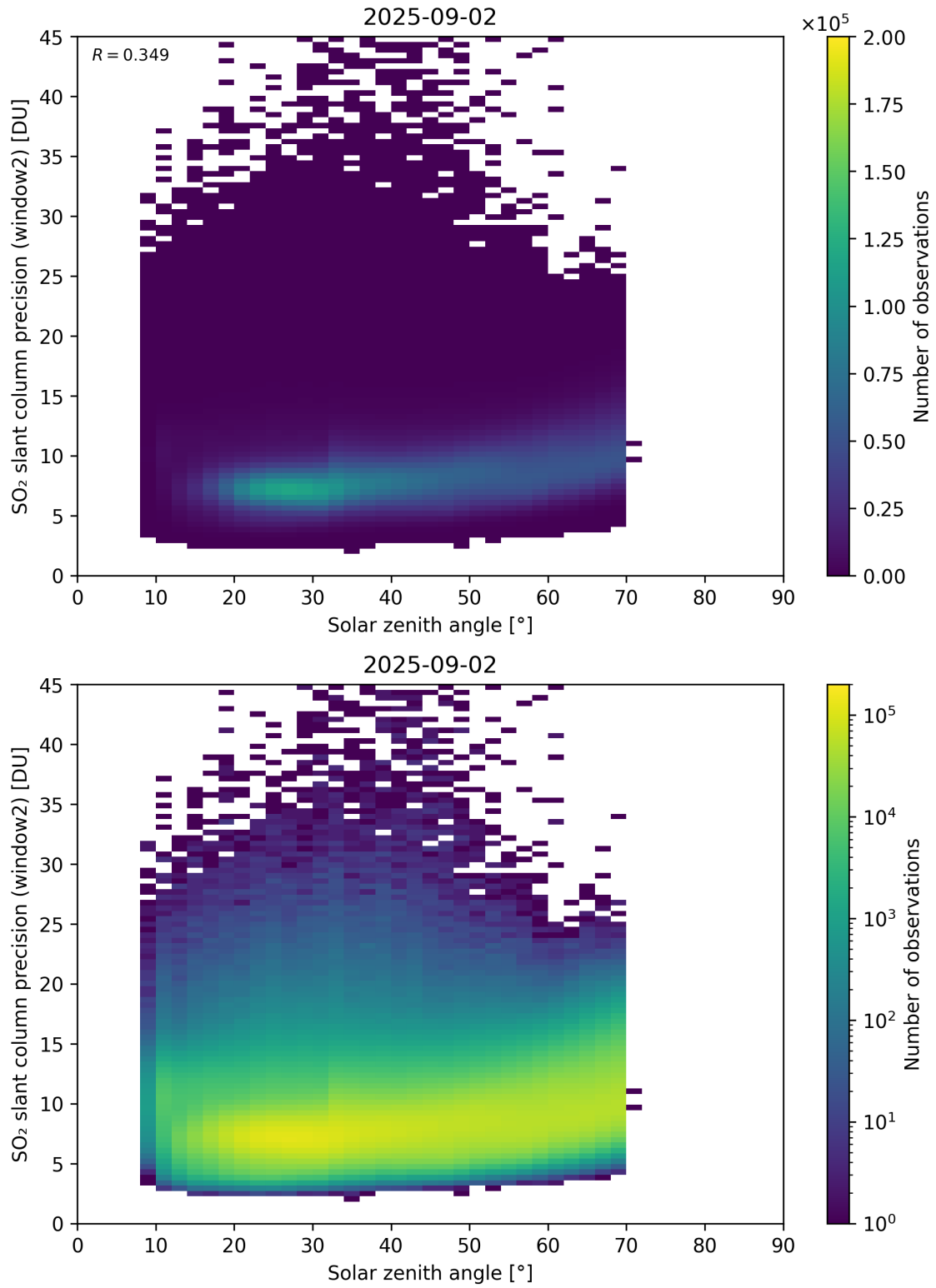
Figure 186: Scatter density plot of “Solar zenith angle” against “SO 2 slant column precision (window2)” for 2025-09-01 to 2025-09-03.
