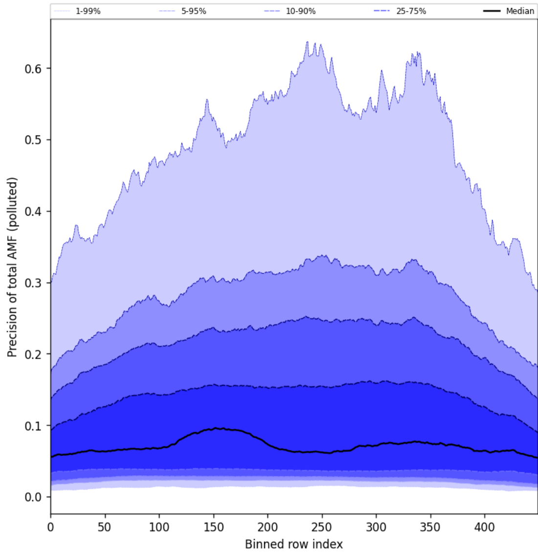
Figure 106: Along track statistics of “Precision of total AMF (polluted)” for 2025-09-01 to 2025-09-03
