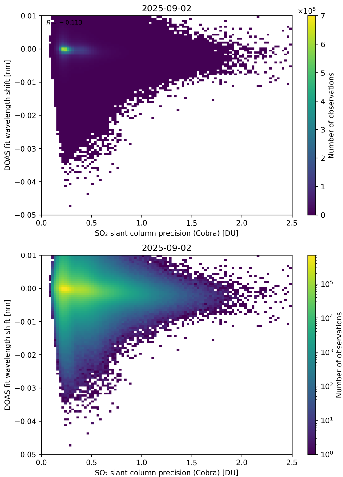
Figure 202: Scatter density plot of “SO 2 slant column precision (Cobra)” against “DOAS fit wavelength shift” for 2025-09-01 to 2025-09-03.
