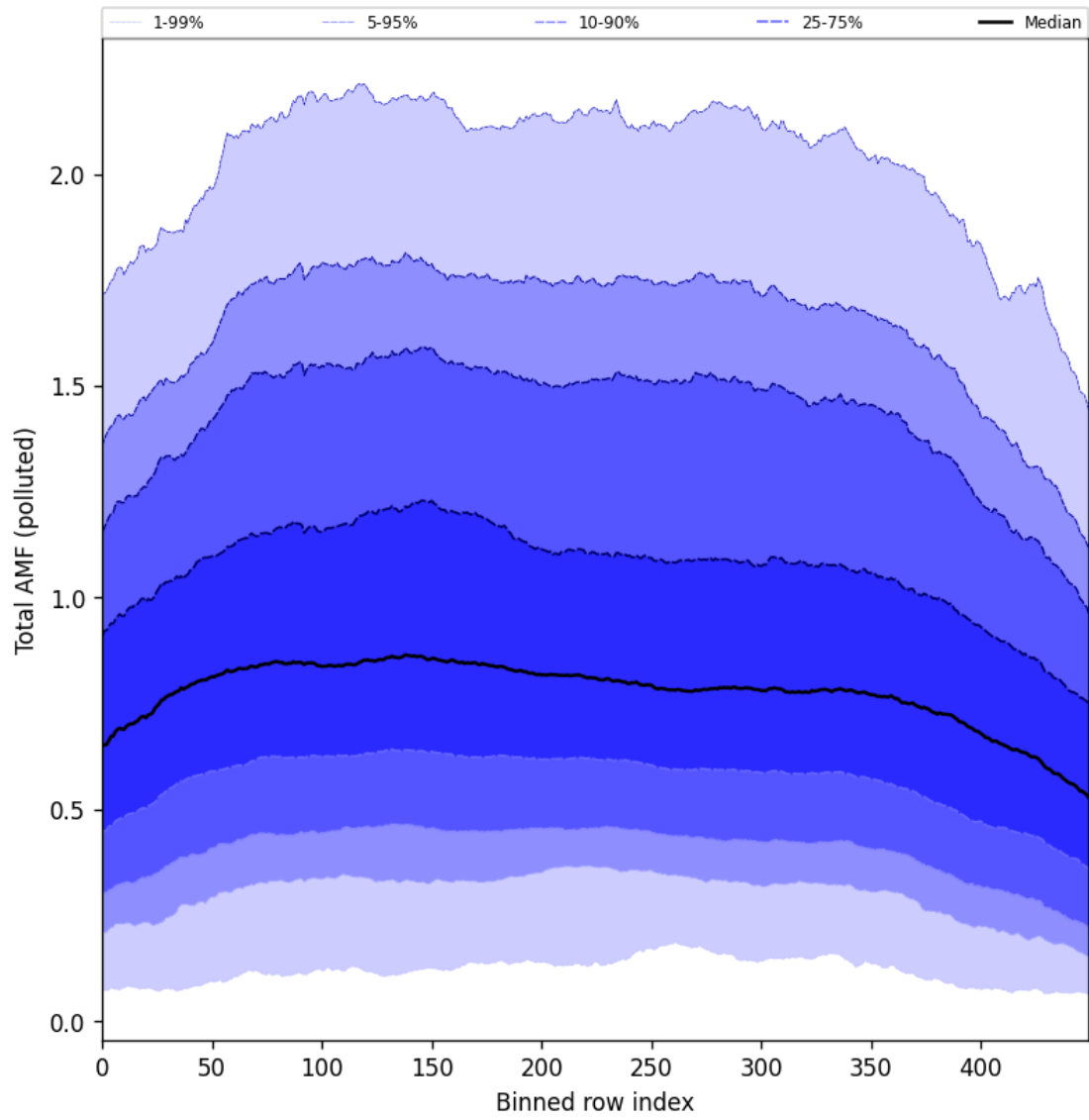
Figure 105: Along track statistics of “Total AMF (polluted)” for 2025-09-01 to 2025-09-03
