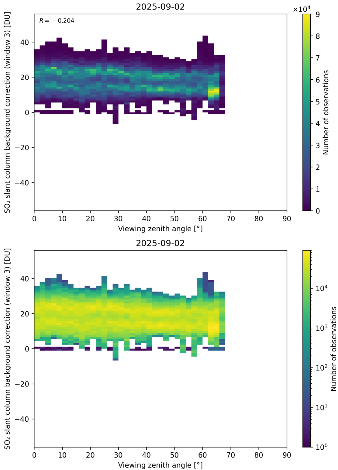
Figure 364: Scatter density plot of “Viewing zenith angle” against “SO 2 slant column background correction (window 3)” for 2025-09-01 to 2025-09-03.
