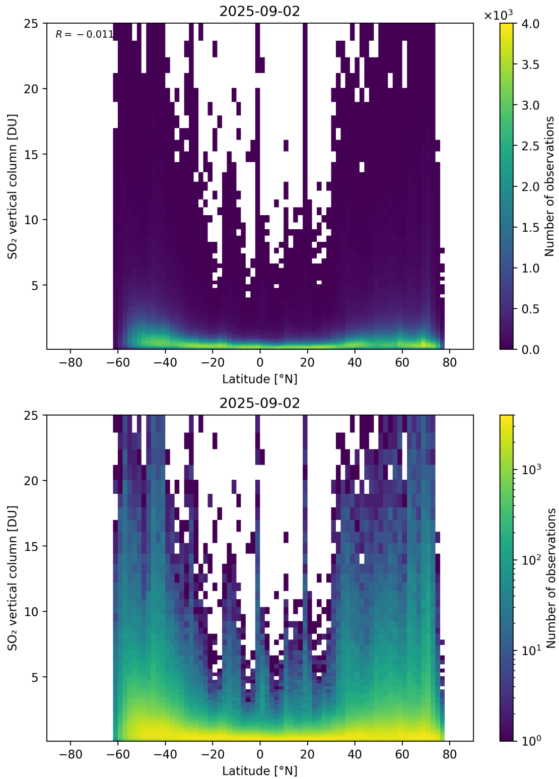
Figure 169: Scatter density plot of “Latitude” against “SO 2 vertical column” for 2025-09-01 to 2025-09-03.
