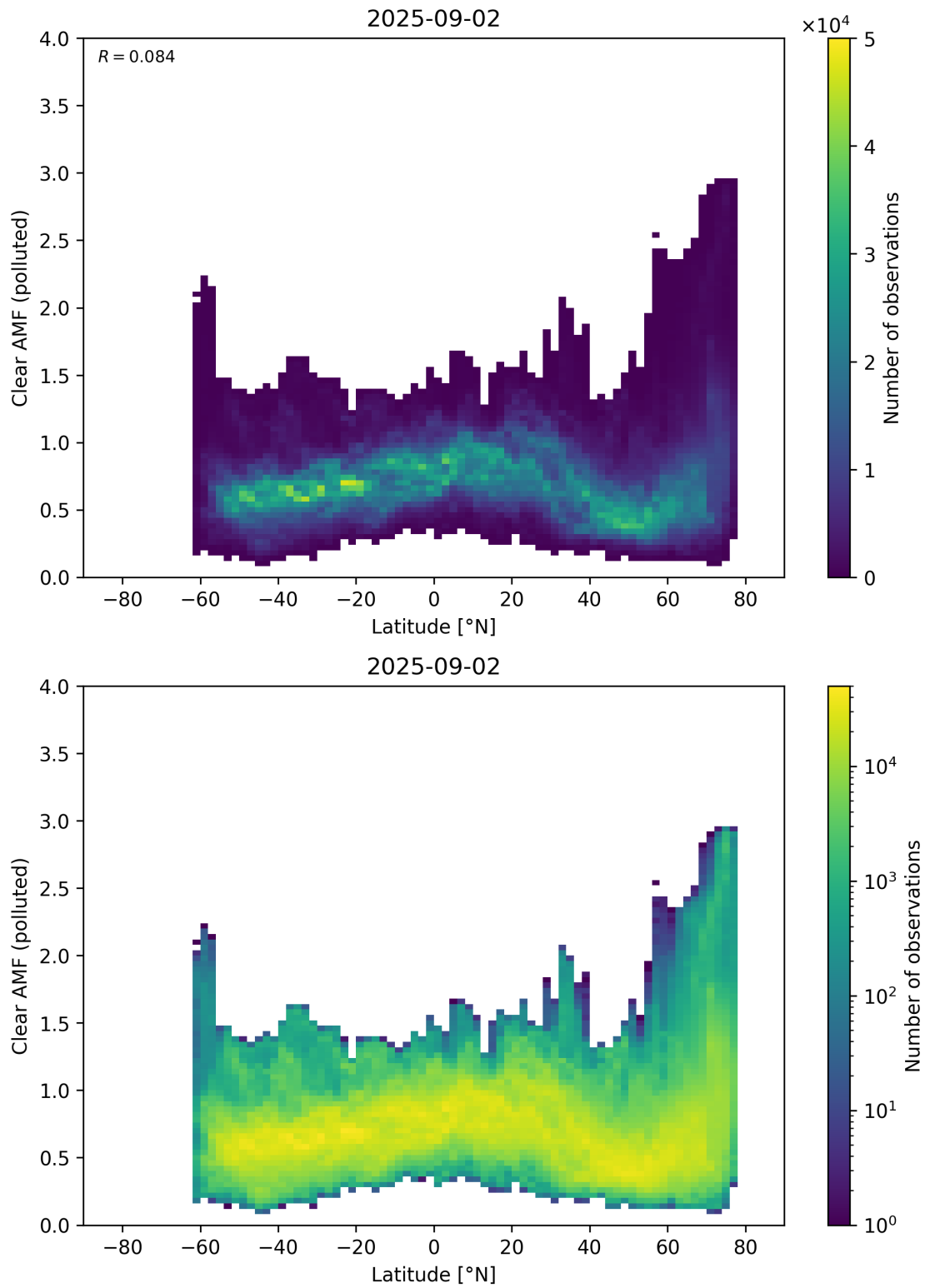
Figure 156: Scatter density plot of “Latitude” against “Clear AMF (polluted)” for 2025-09-01 to 2025-09-03.
