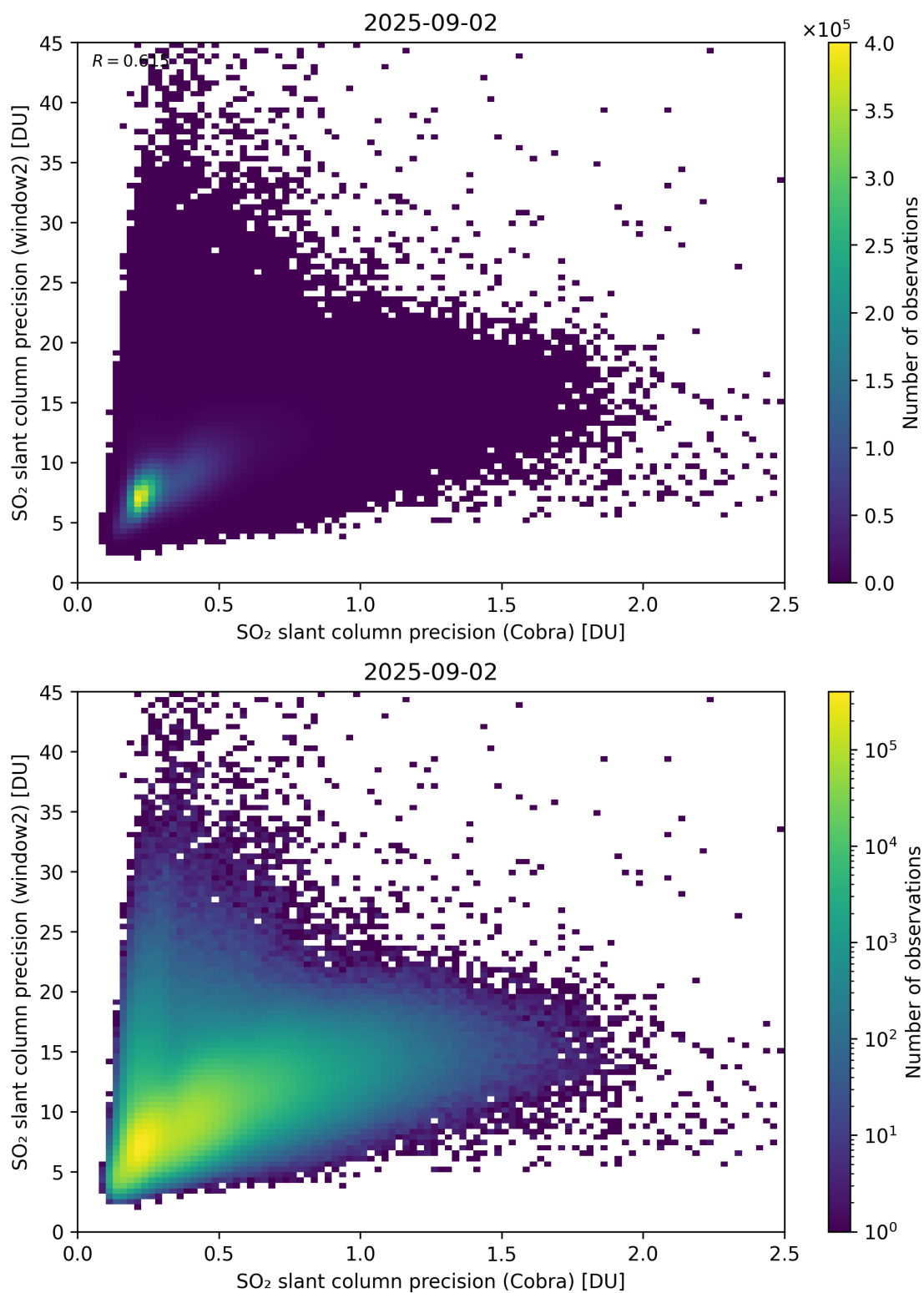
Figure 210: Scatter density plot of “SO 2 slant column precision (Cobra)” against “SO 2 slant column precision (window2)” for 2025-09-01 to 2025-09-03.
