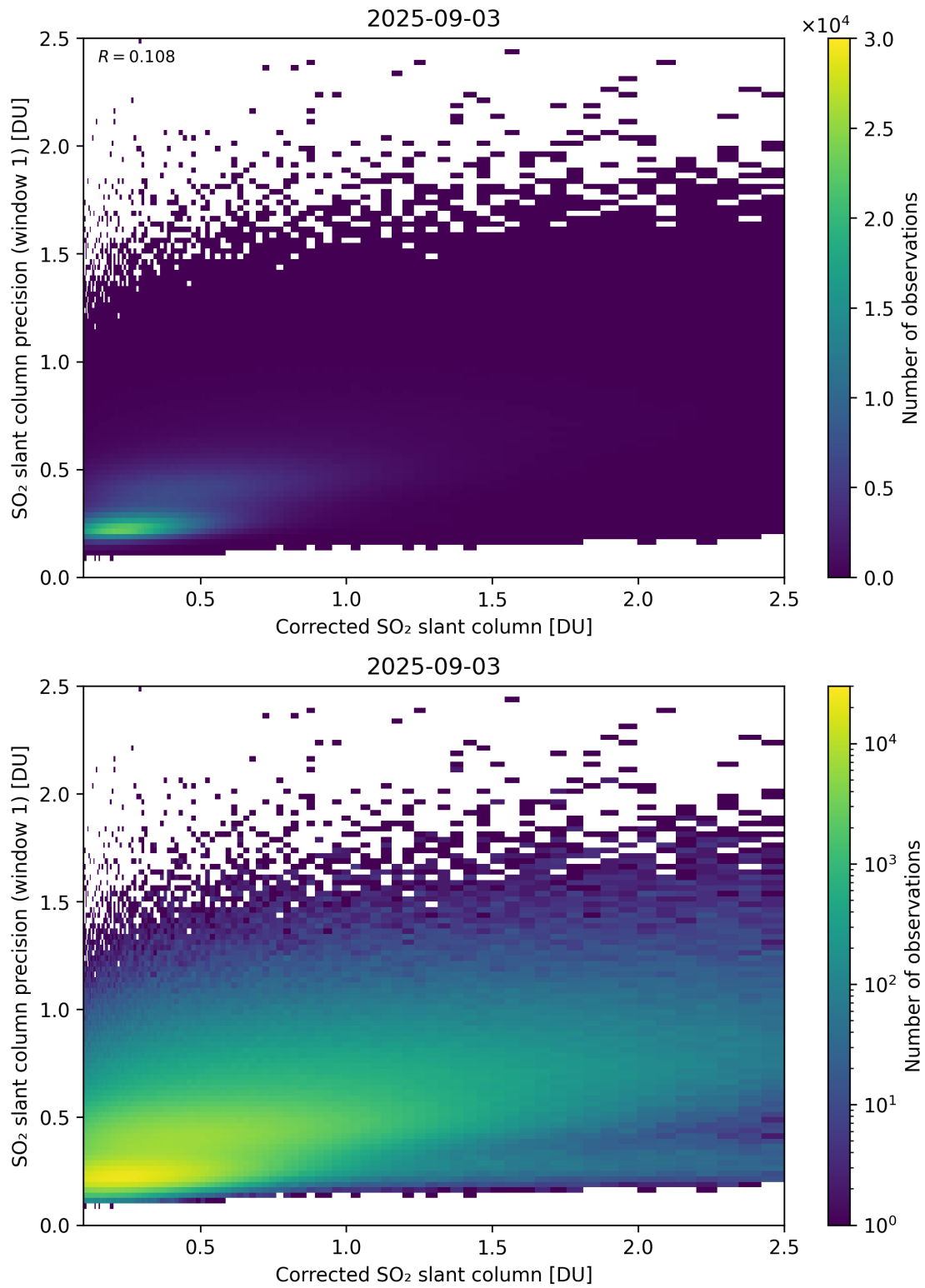
Figure 238: Scatter density plot of “Corrected SO 2 slant column” against “SO 2 slant column precision (window 1)” for 2025-09-02 to 2025-09-04.
