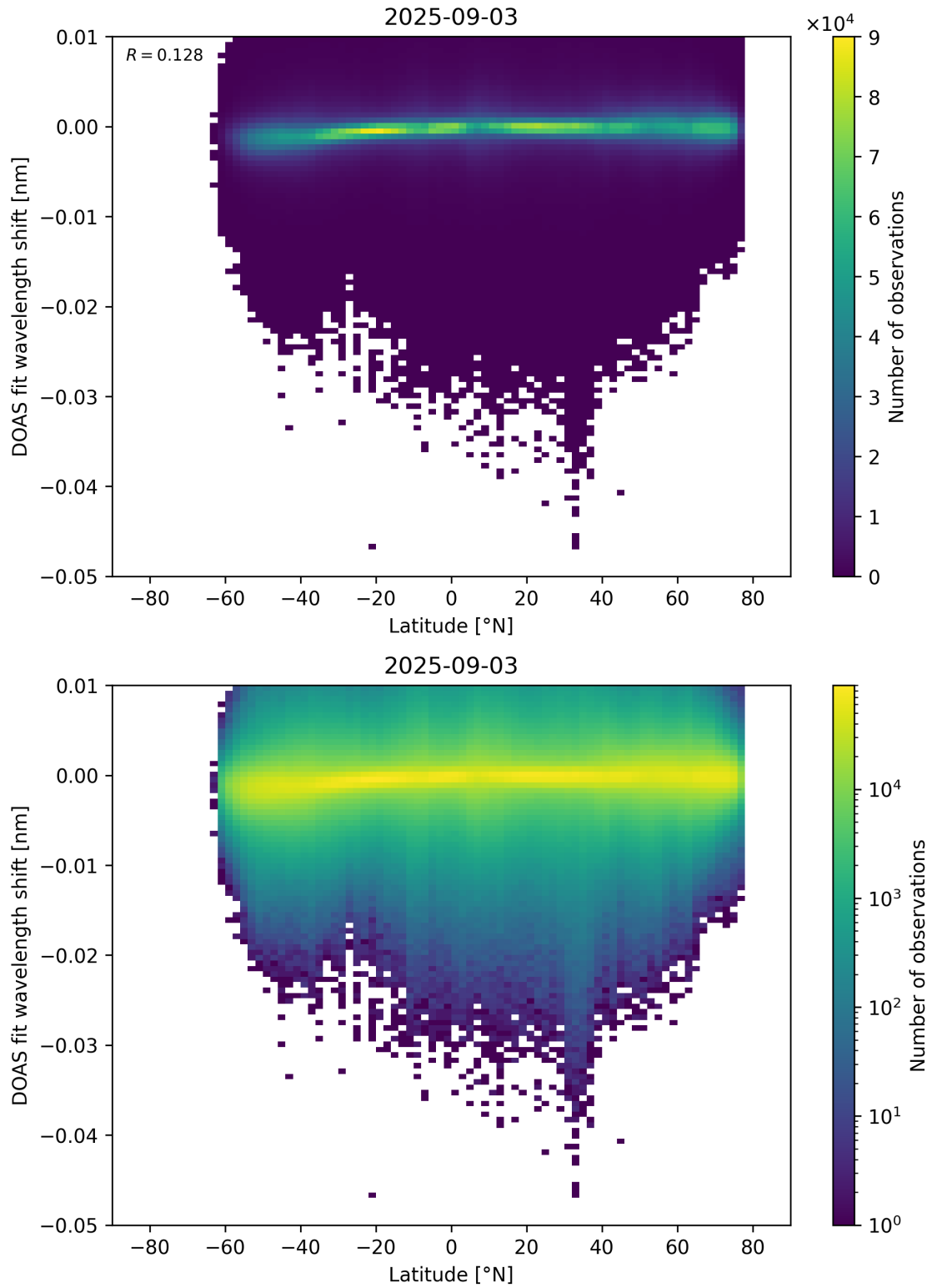
Figure 153: Scatter density plot of “Latitude” against “DOAS fit wavelength shift” for 2025-09-02 to 2025-09-04.
