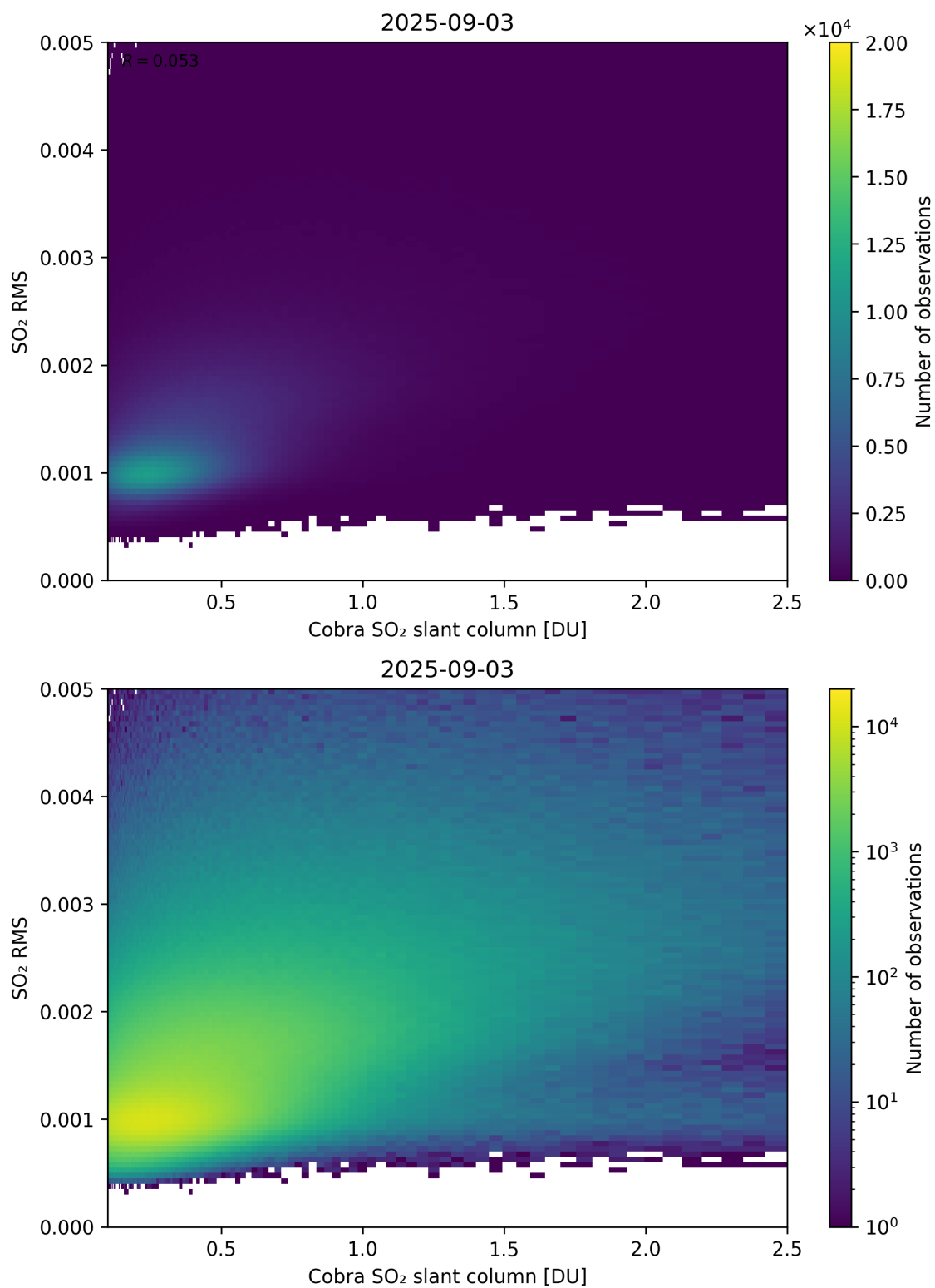
Figure 198: Scatter density plot of “Cobra SO 2 slant column” against “SO 2 RMS” for 2025-09-02 to 2025-09-04.
