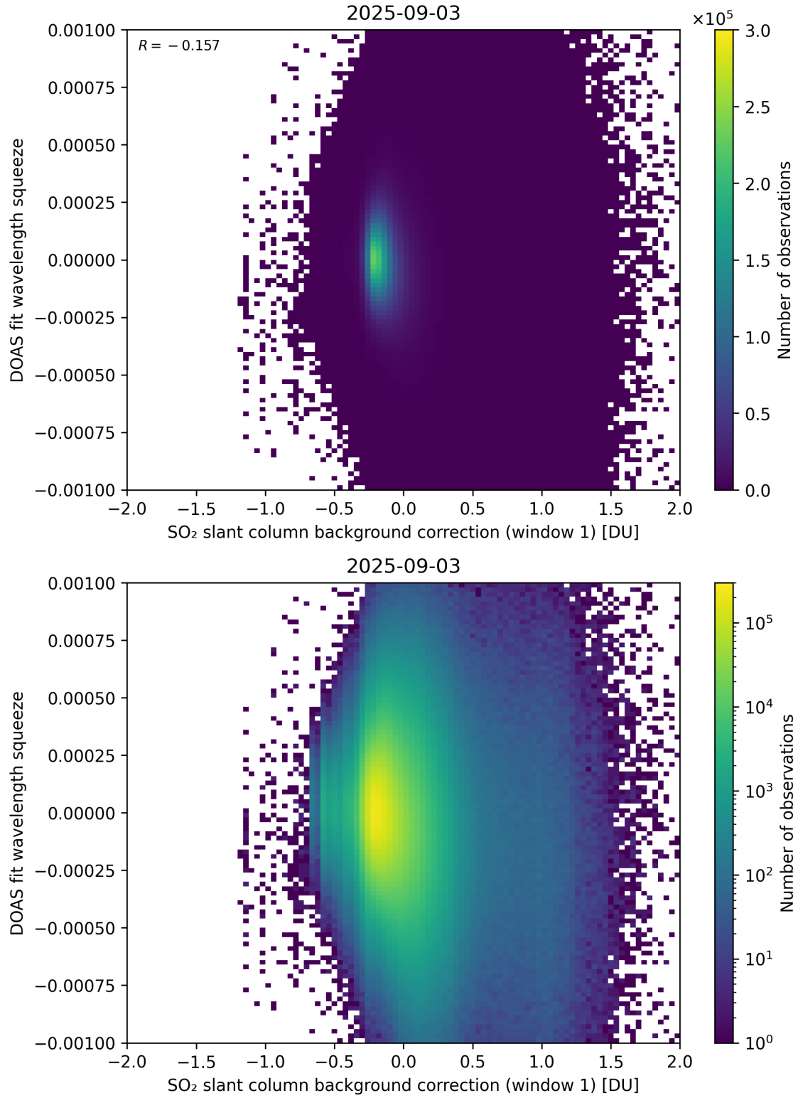
Figure 112: Scatter density plot of “SO 2 slant column background correction (window 1)” against “DOAS fit wavelength squeeze” for 2025-09-02 to 2025-09-04.
