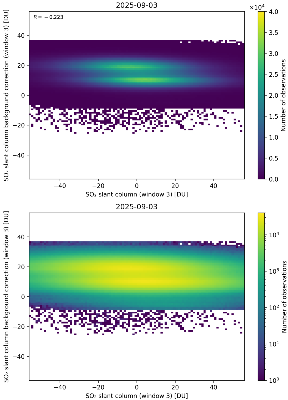
Figure 303: Scatter density plot of “SO 2 slant column (window 3)” against “SO 2 slant column background correction (window 3)” for 2025-09-02 to 2025-09-04.
