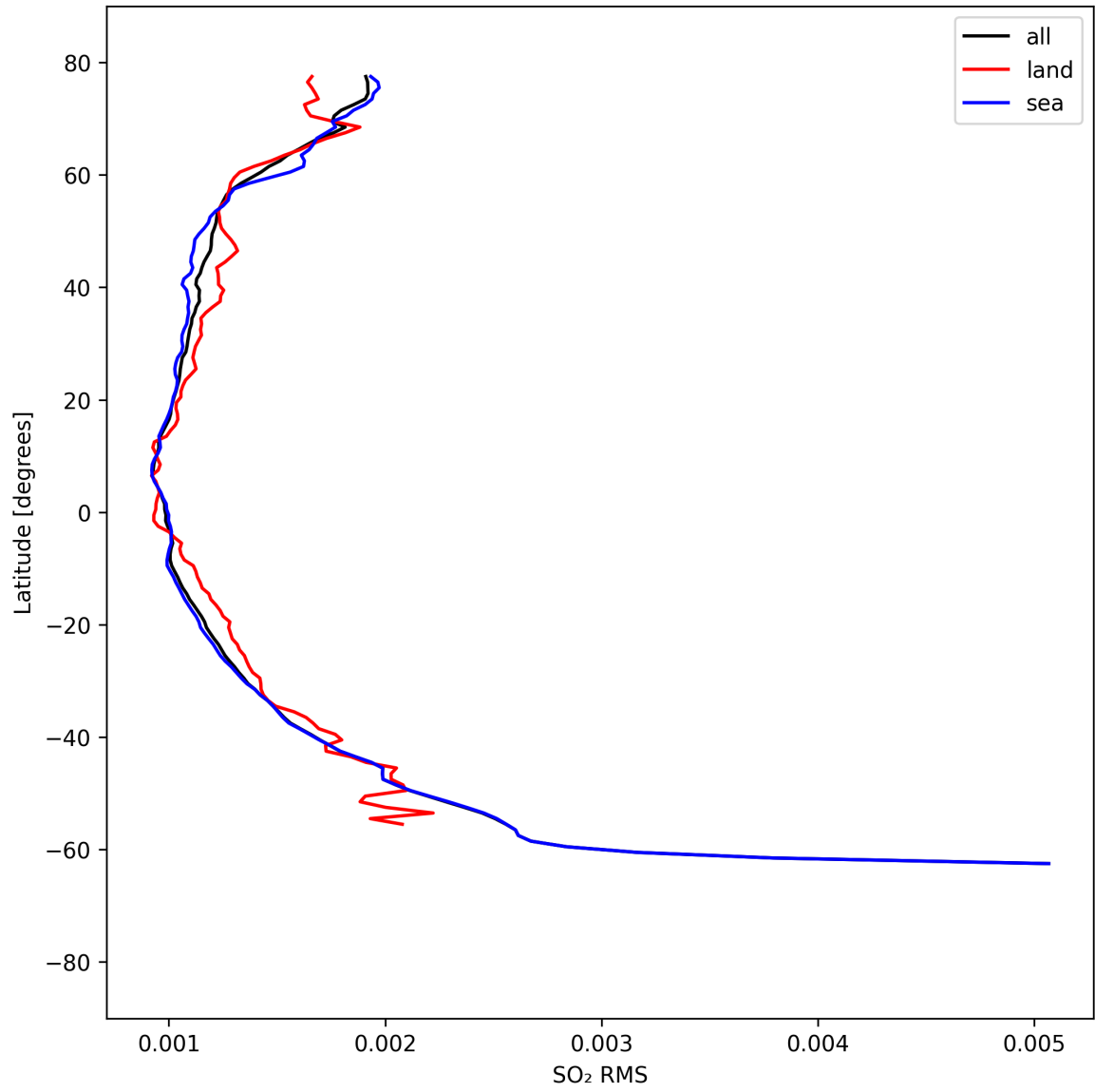
Figure 52: Zonal average of “SO 2 RMS” for 2025-09-02 to 2025-09-04.
