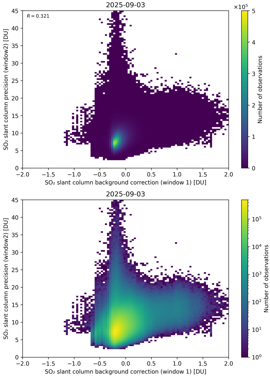
Figure 117: Scatter density plot of “SO 2 slant column background correction (window 1)” against “SO 2 slant column precision (window2)” for 2025-09-02 to 2025-09-04.
