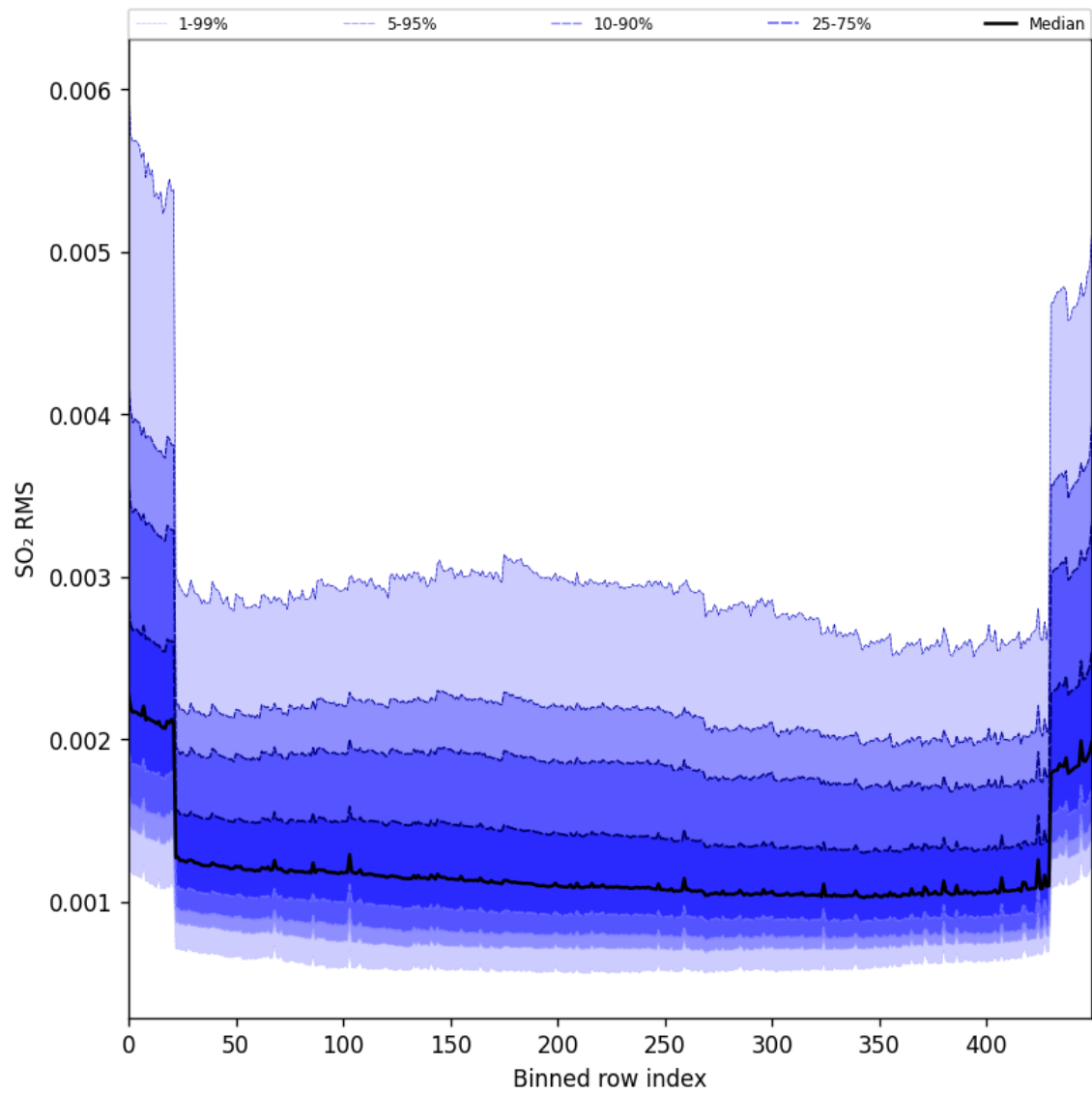
Figure 104: Along track statistics of “SO 2 RMS” for 2025-09-02 to 2025-09-04
