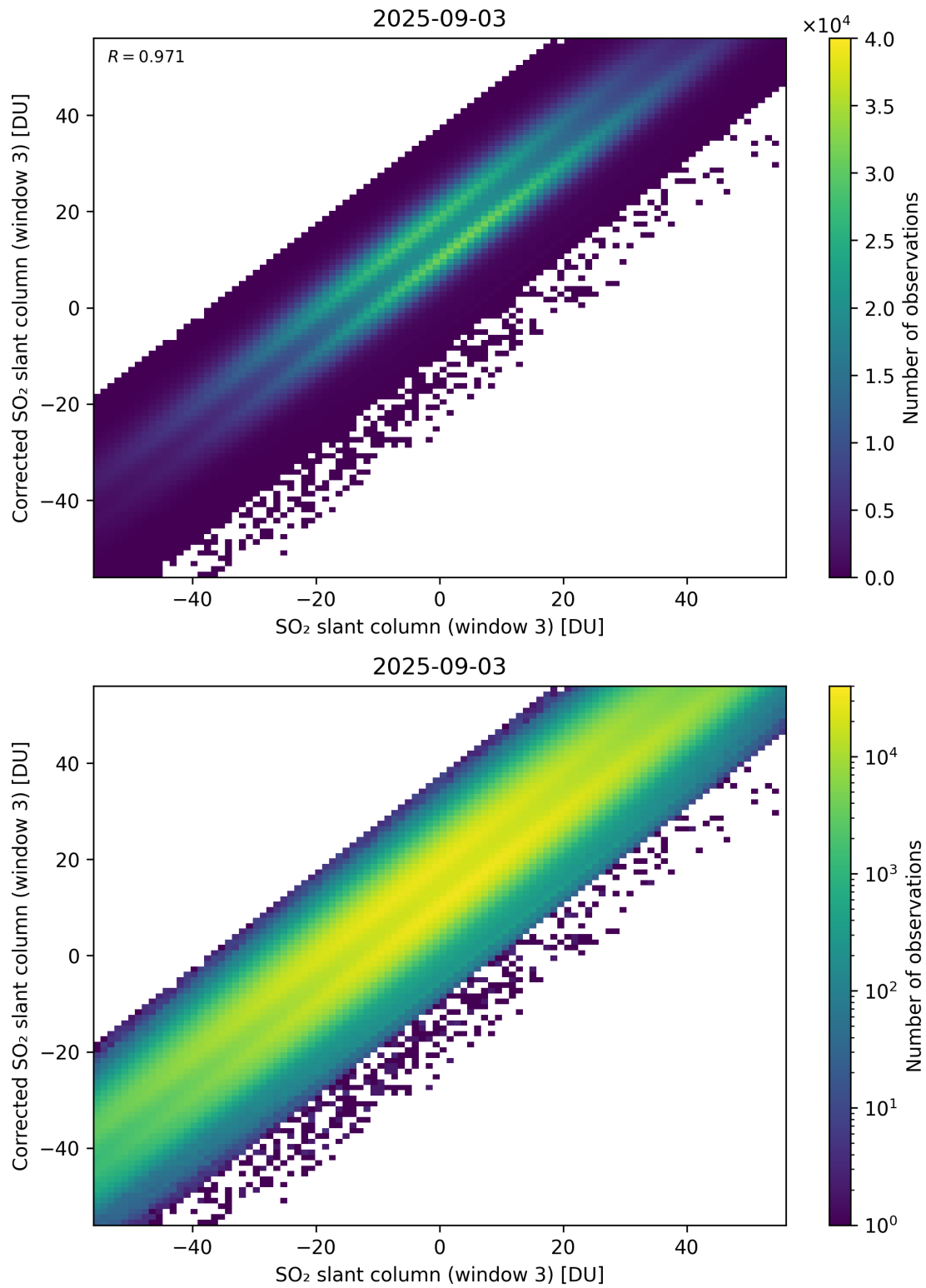
Figure 316: Scatter density plot of “SO 2 slant column (window 3)” against “Corrected SO 2 slant column (window 3)” for 2025-09-02 to 2025-09-04.
