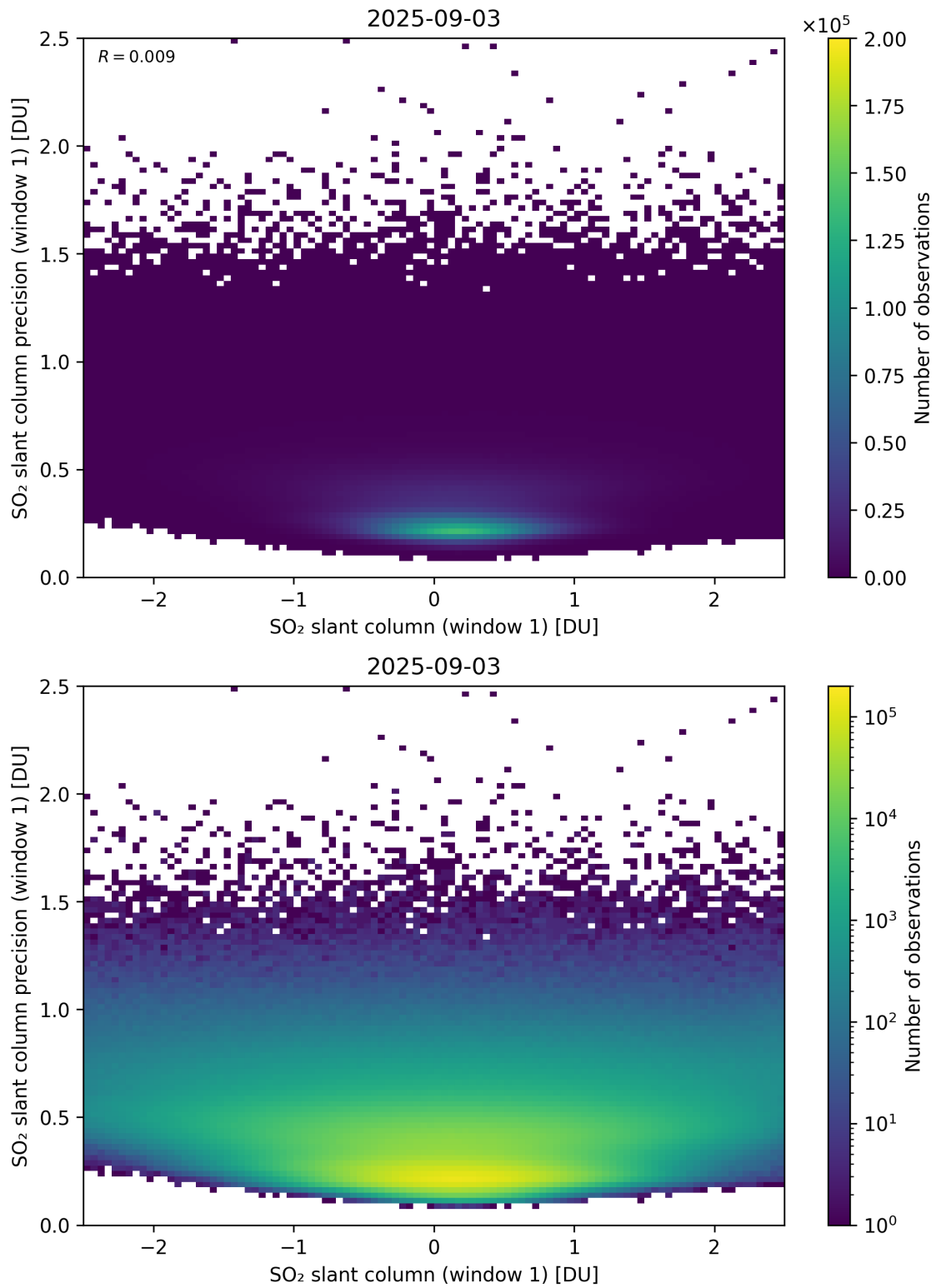
Figure 285: Scatter density plot of “SO 2 slant column (window 1)” against “SO 2 slant column precision (window 1)” for 2025-09-02 to 2025-09-04.
