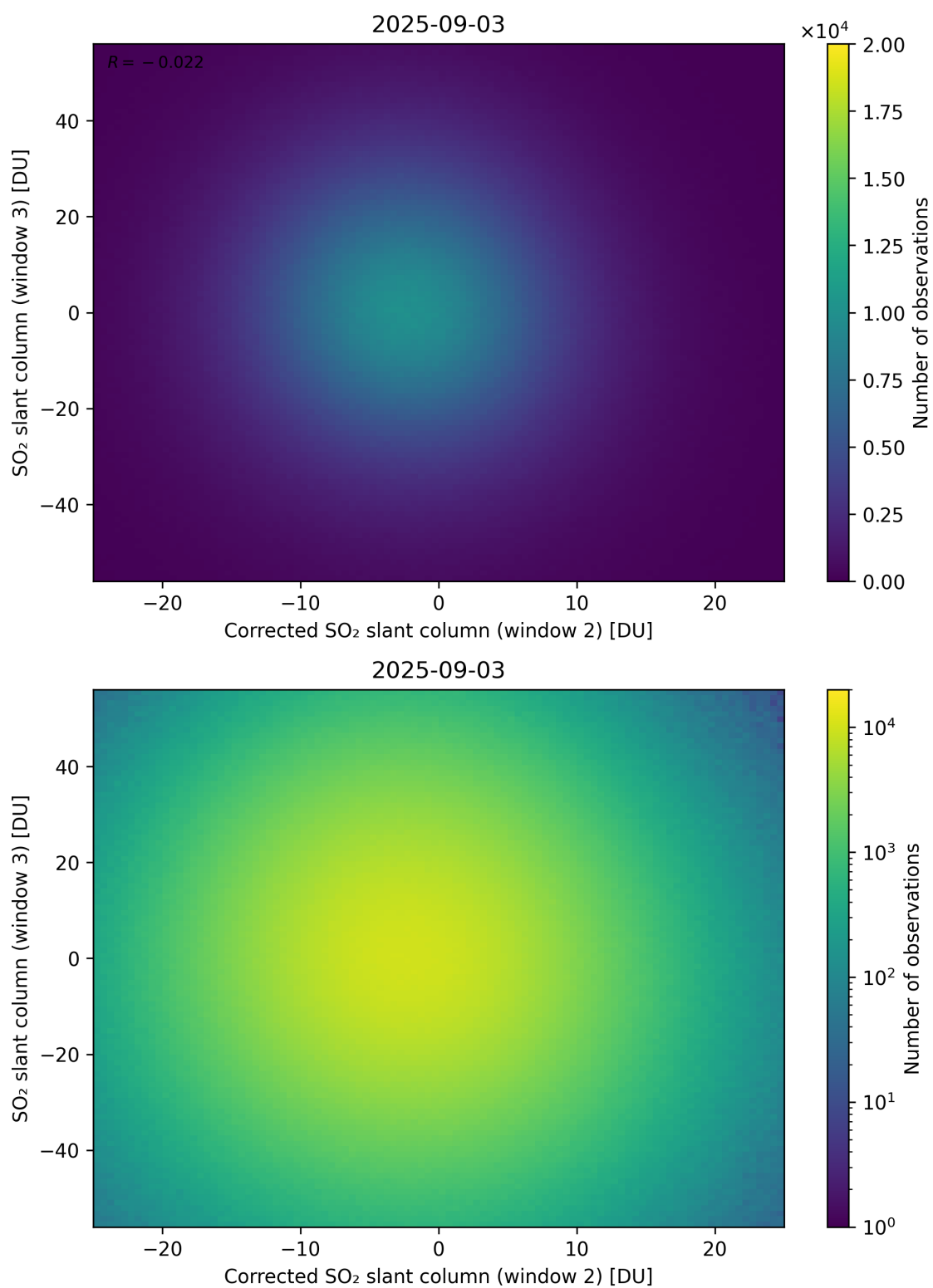
Figure 251: Scatter density plot of “Corrected SO 2 slant column (window 2)” against “SO 2 slant column (window 3)” for 2025-09-02 to 2025-09-04.
