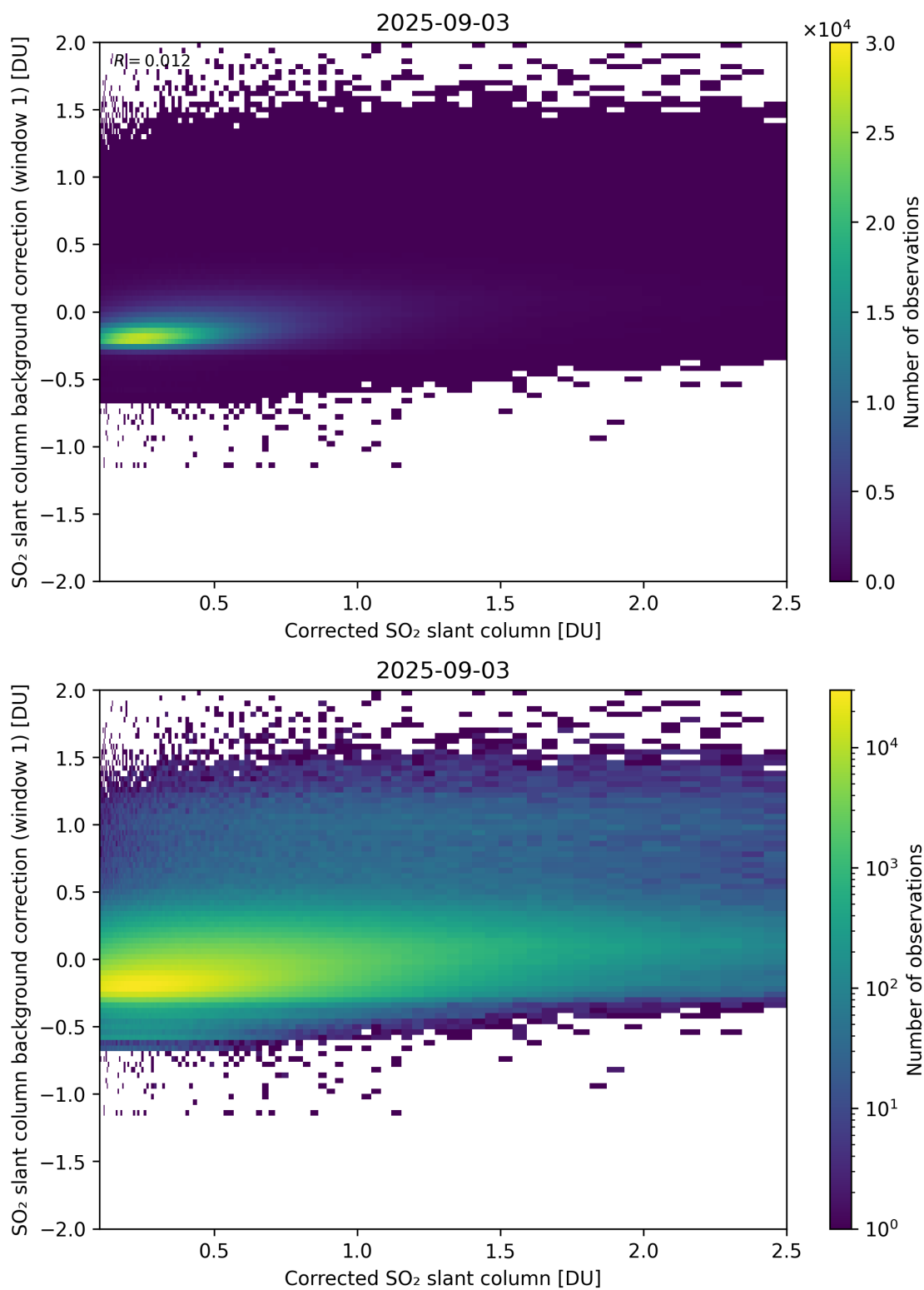
Figure 226: Scatter density plot of “Corrected SO 2 slant column” against “SO 2 slant column background correction (window 1)” for 2025-09-02 to 2025-09-04.
