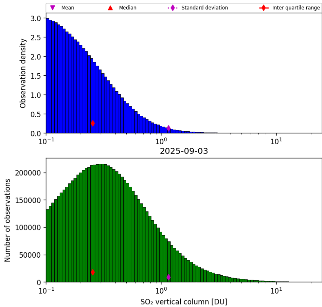
Figure 58: Histogram of “SO 2 vertical column” for 2025-09-02 to 2025-09-04
