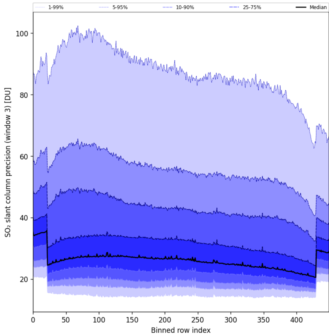
Figure 98: Along track statistics of “SO 2 slant column precision (window 3)” for 2025-09-02 to 2025-09-04
