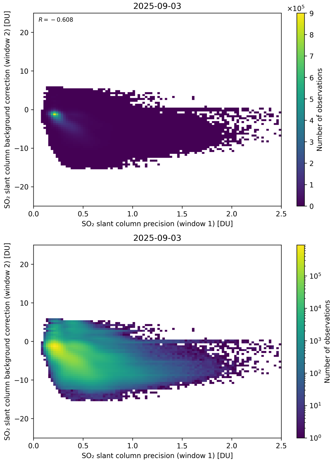
Figure 269: Scatter density plot of “SO 2 slant column precision (window 1)” against “SO 2 slant column background correction (window 2)” for 2025-09-02 to 2025-09-04.
