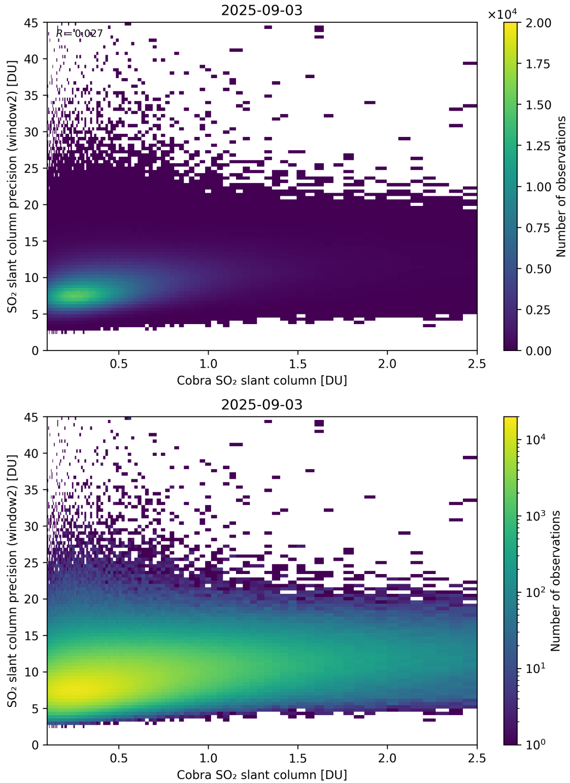
Figure 221: Scatter density plot of “Cobra SO 2 slant column” against “SO 2 slant column precision (window2)” for 2025-09-02 to 2025-09-04.
