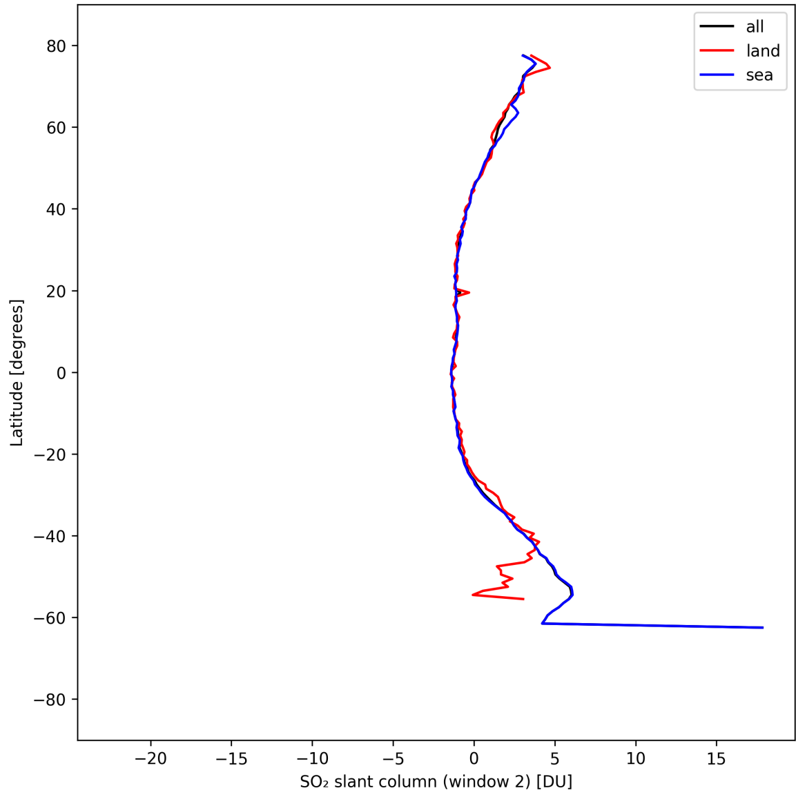
Figure 41: Zonal average of “SO 2 slant column (window 2)” for 2025-09-02 to 2025-09-04.
