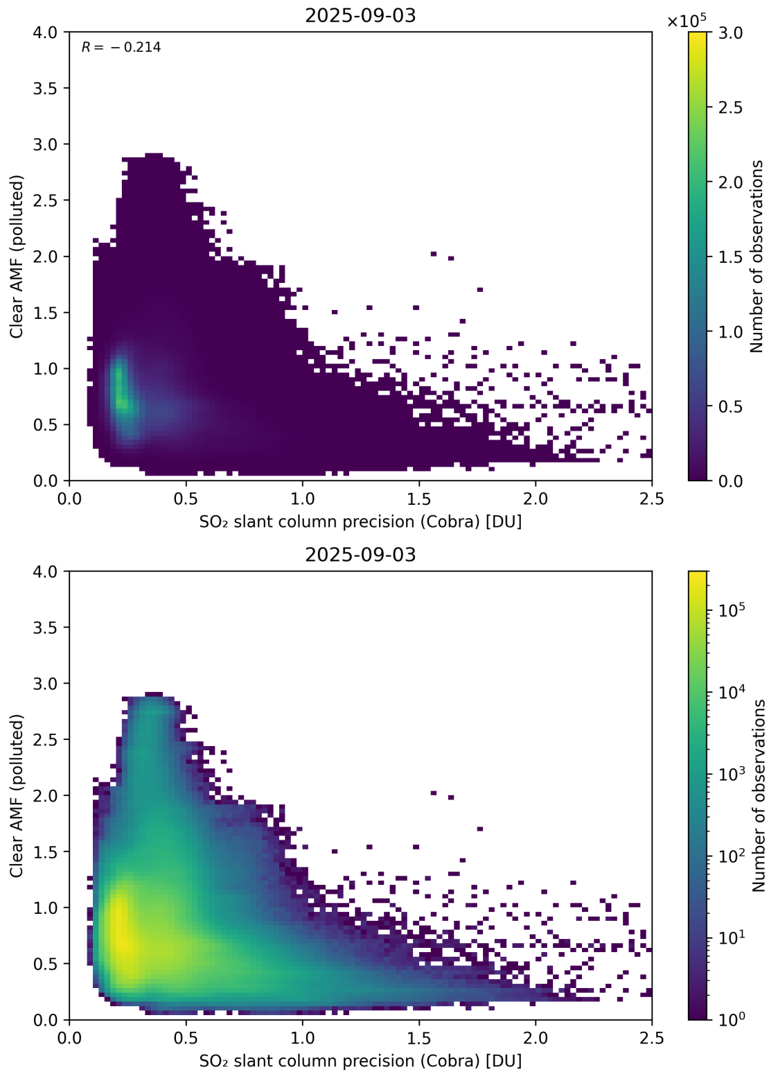
Figure 205: Scatter density plot of “SO 2 slant column precision (Cobra)” against “Clear AMF (polluted)” for 2025-09-02 to 2025-09-04.
