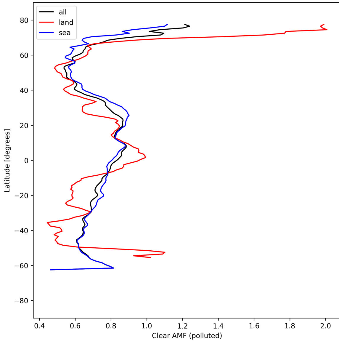
Figure 55: Zonal average of “Clear AMF (polluted)” for 2025-09-02 to 2025-09-04.
