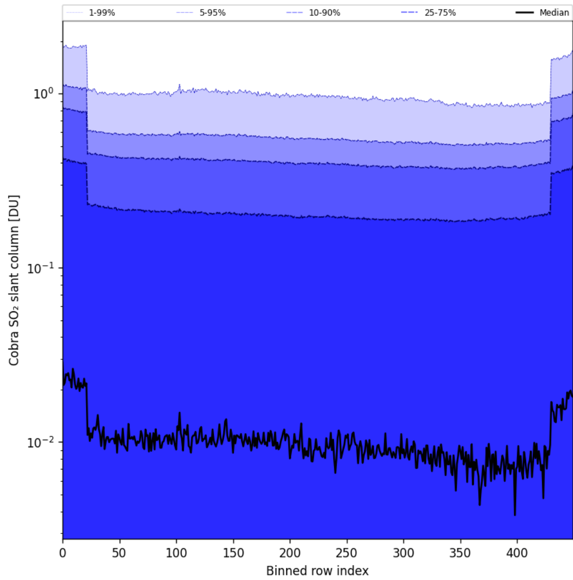
Figure 87: Along track statistics of “Cobra SO 2 slant column” for 2025-09-02 to 2025-09-04
