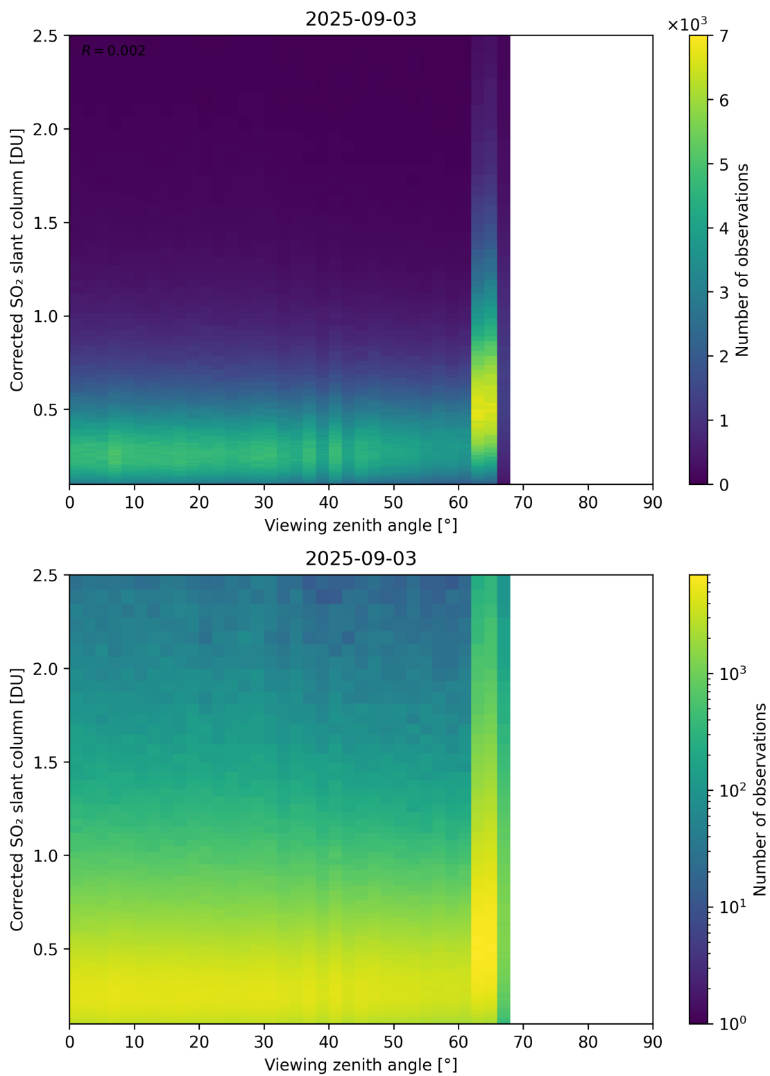
Figure 373: Scatter density plot of “Viewing zenith angle” against “Corrected SO 2 slant column” for 2025-09-02 to 2025-09-04.
