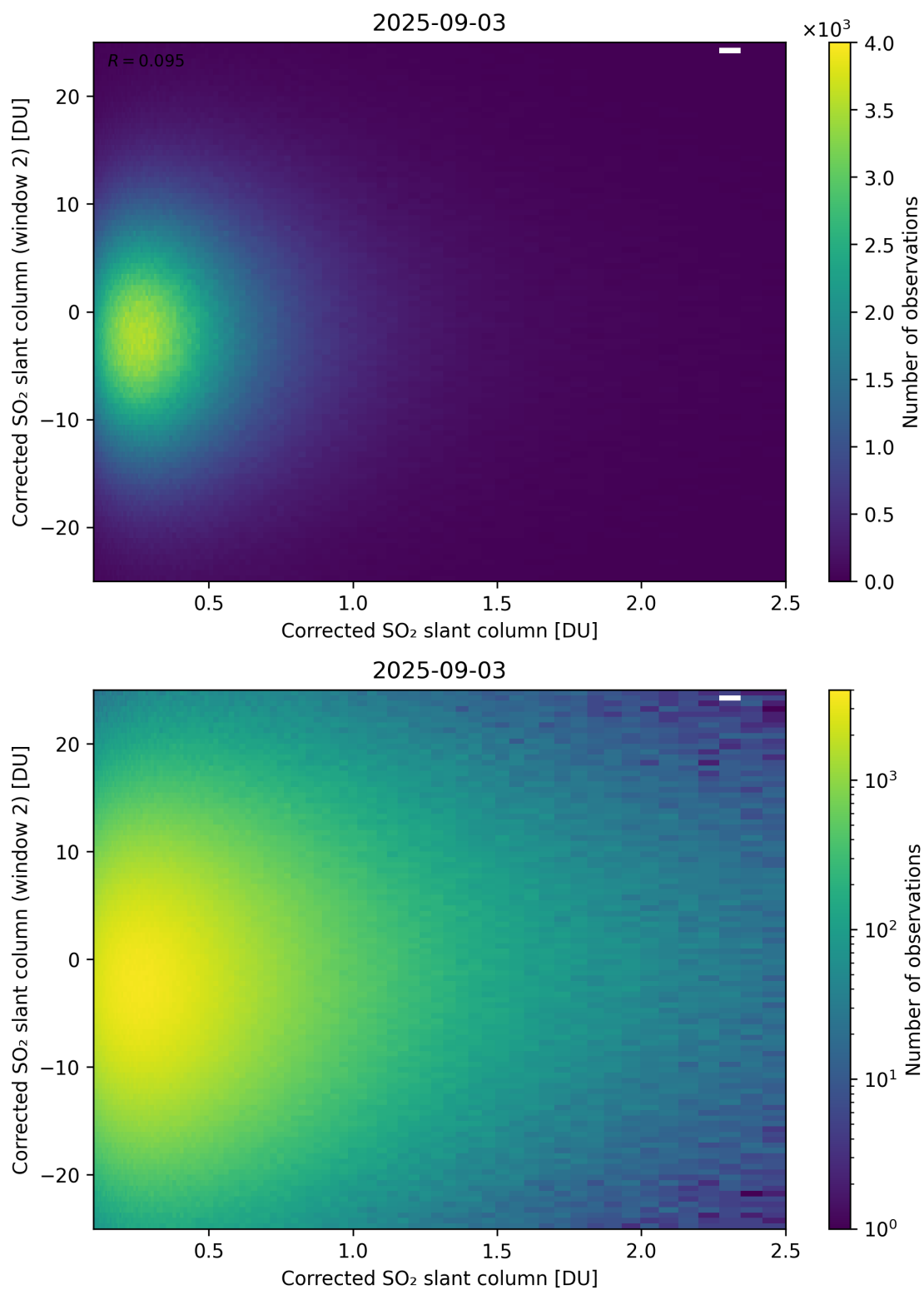
Figure 235: Scatter density plot of “Corrected SO 2 slant column” against “Corrected SO 2 slant column (window 2)” for 2025-09-02 to 2025-09-04.
