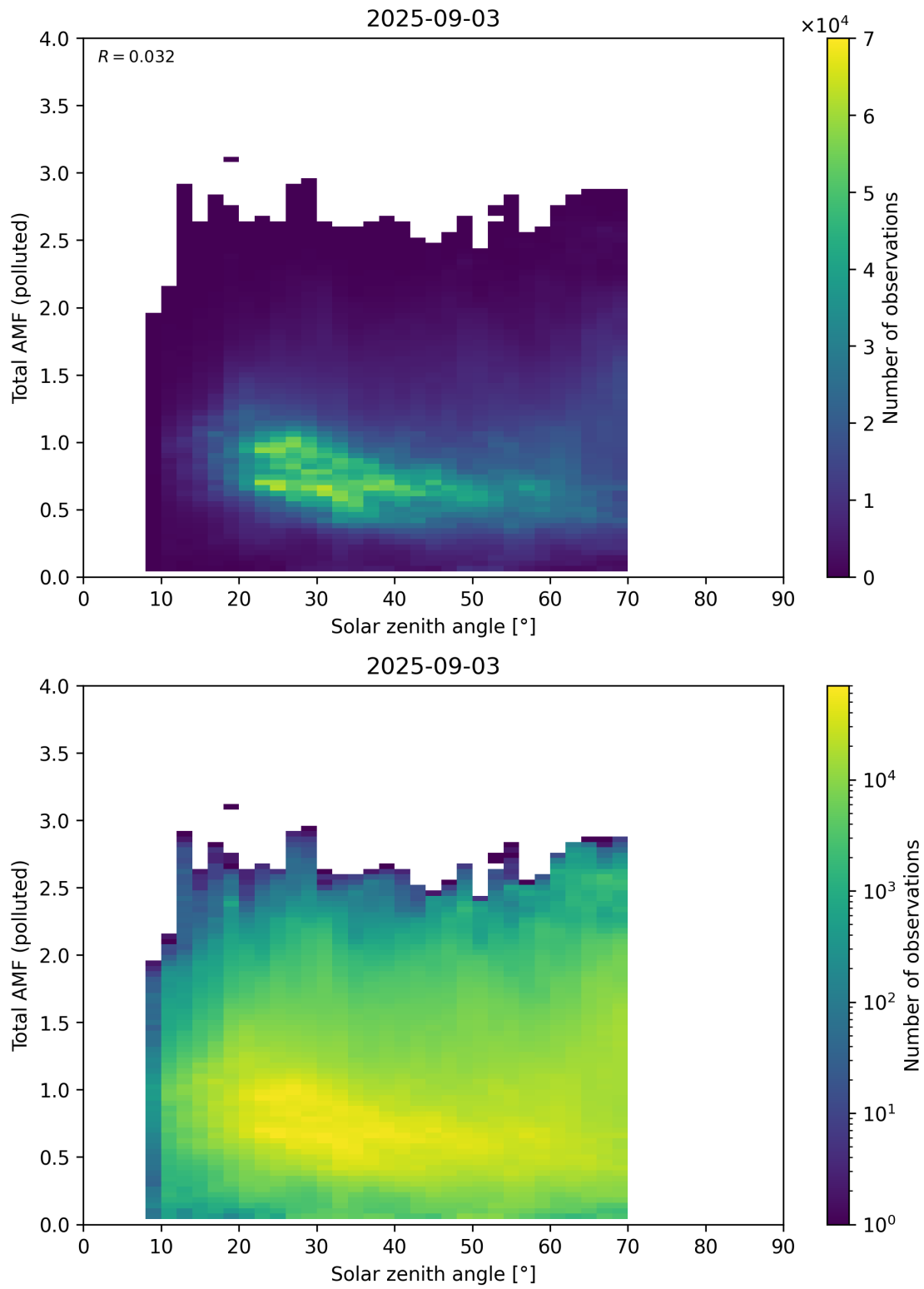
Figure 189: Scatter density plot of “Solar zenith angle” against “Total AMF (polluted)” for 2025-09-02 to 2025-09-04.
