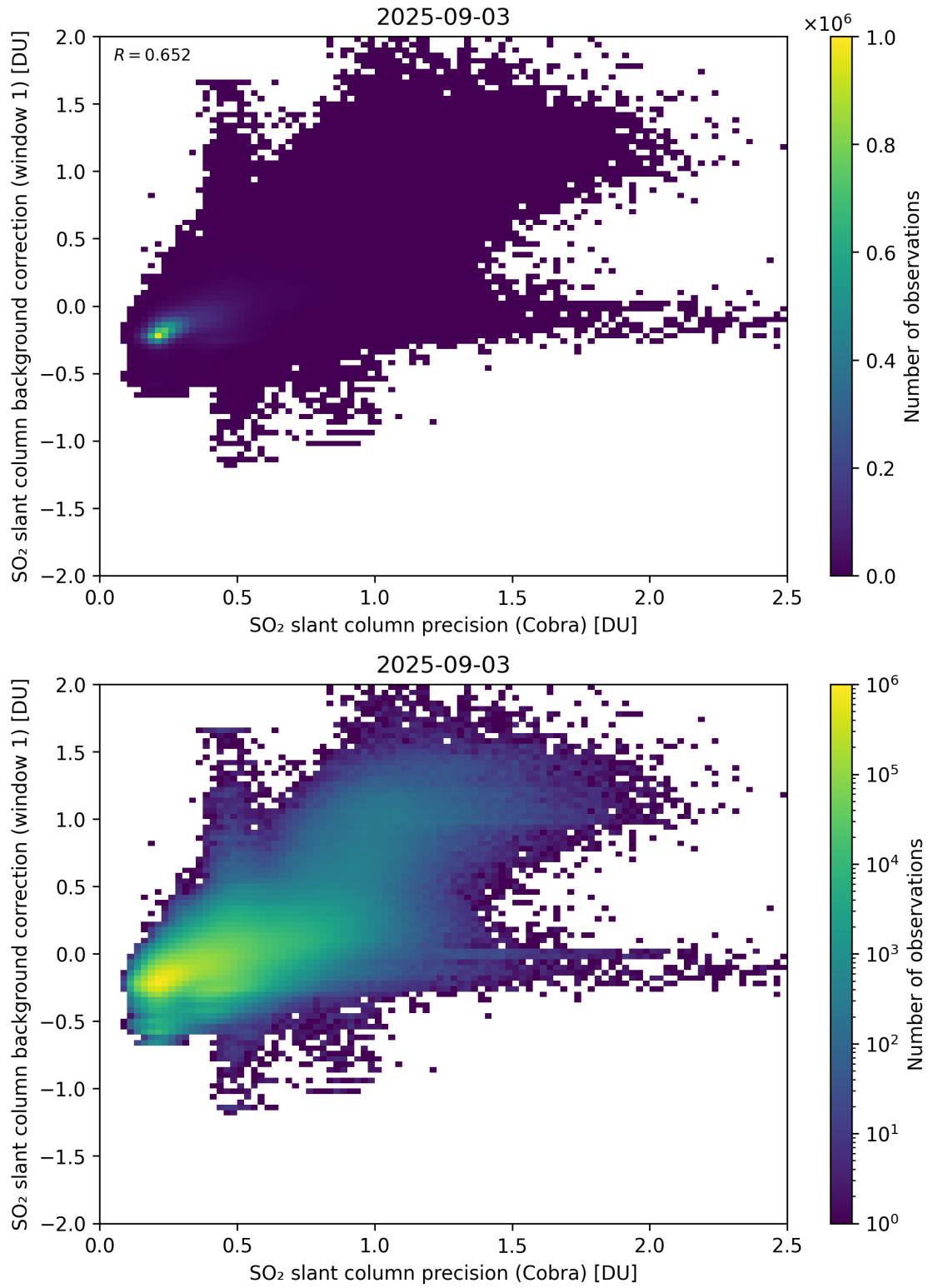
Figure 199: Scatter density plot of “SO 2 slant column precision (Cobra)” against “SO 2 slant column background correction (window 1)” for 2025-09-02 to 2025-09-04.
