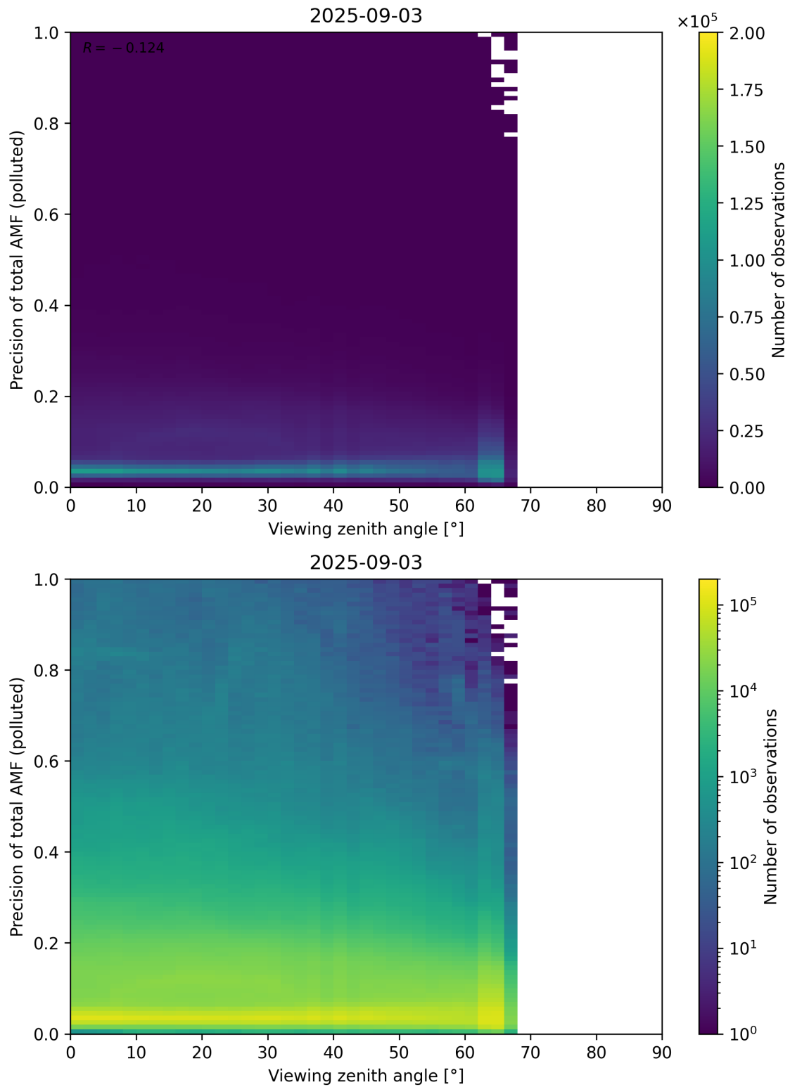
Figure 382: Scatter density plot of “Viewing zenith angle” against “Precision of total AMF (polluted)” for 2025-09-02 to 2025-09-04.
