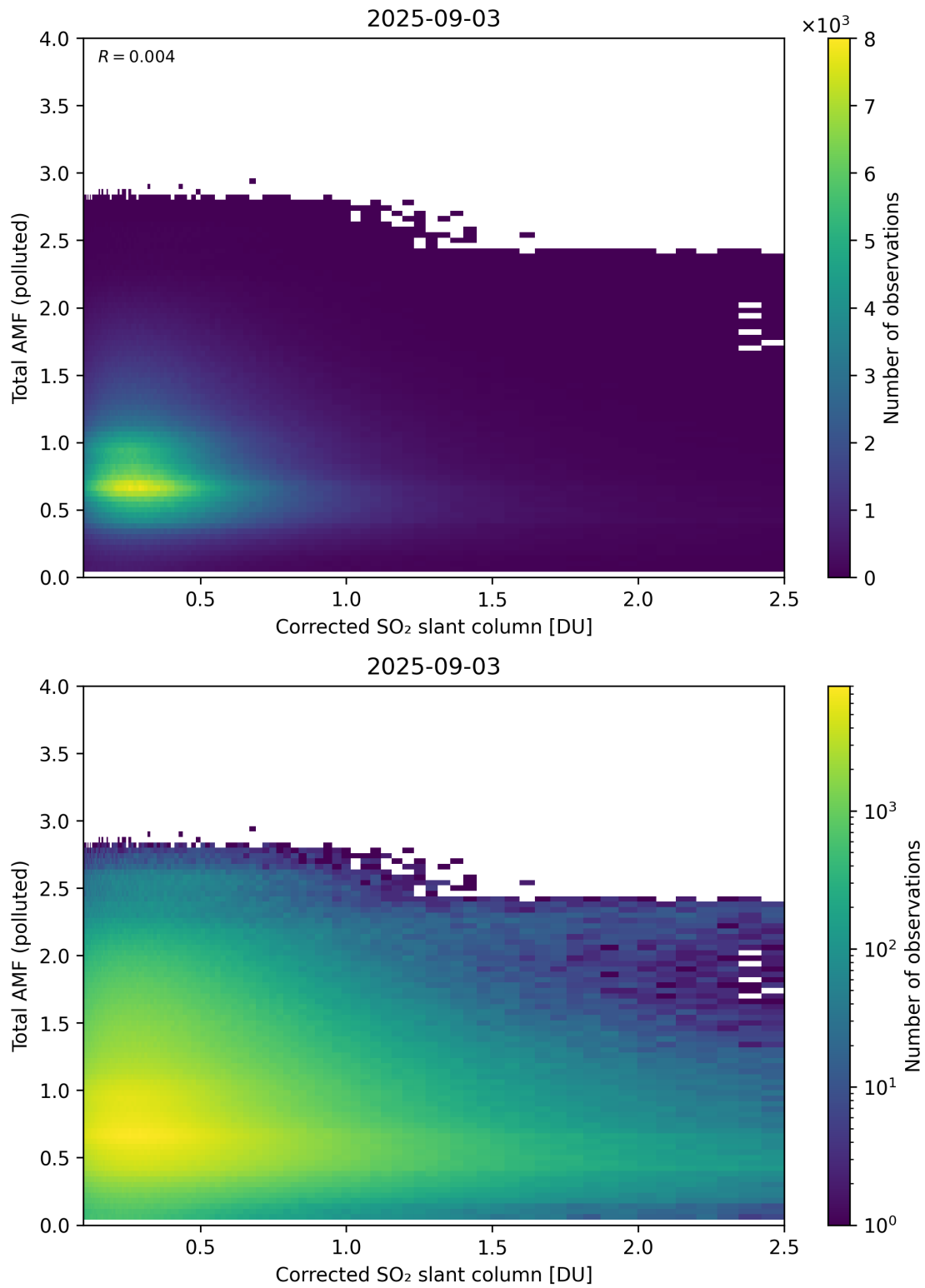
Figure 242: Scatter density plot of “Corrected SO 2 slant column” against “Total AMF (polluted)” for 2025-09-02 to 2025-09-04.
