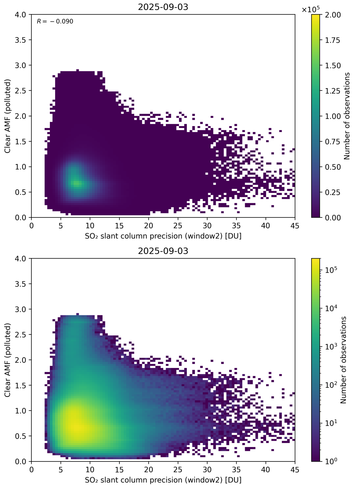
Figure 296: Scatter density plot of “SO 2 slant column precision (window2)” against “Clear AMF (polluted)” for 2025-09-02 to 2025-09-04.
