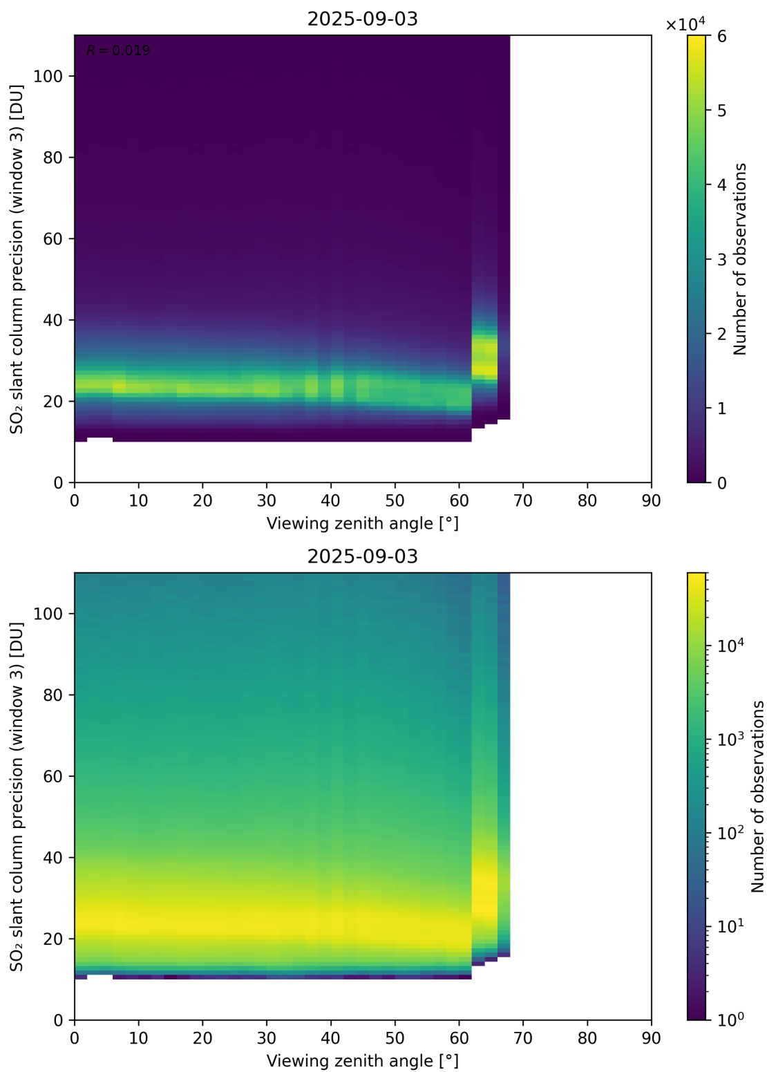
Figure 380: Scatter density plot of “Viewing zenith angle” against “SO 2 slant column precision (window 3)” for 2025-09-02 to 2025-09-04.
