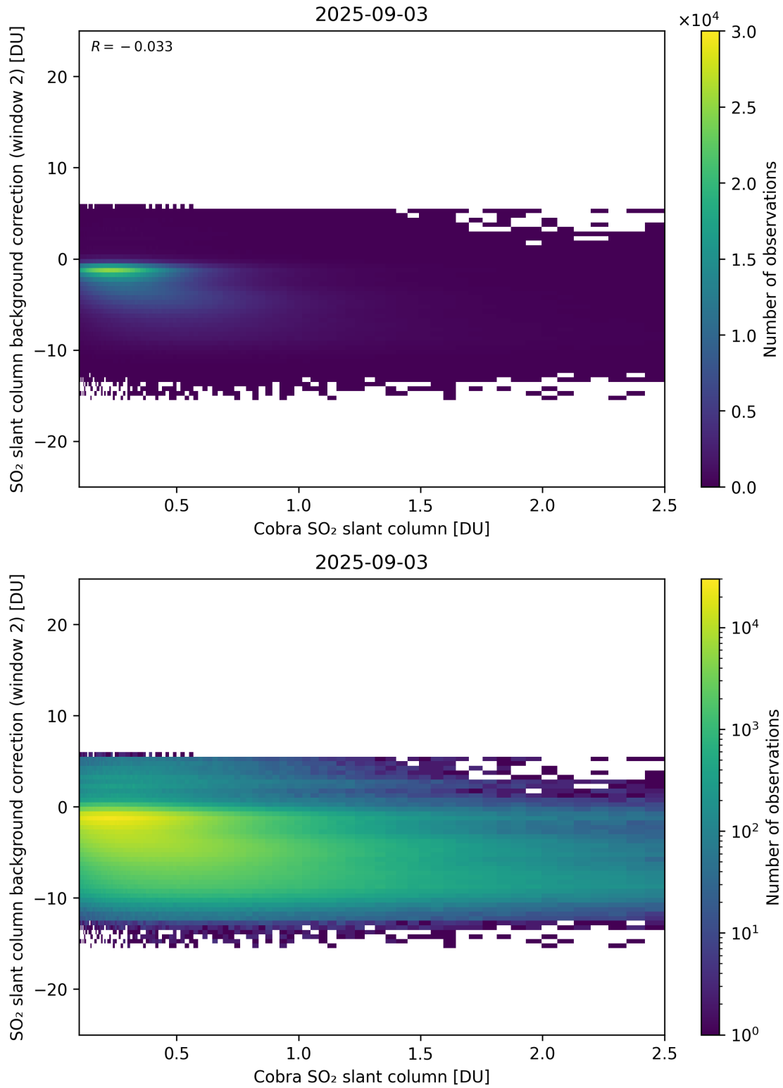
Figure 194: Scatter density plot of “Cobra SO 2 slant column” against “SO 2 slant column background correction (window 2)” for 2025-09-02 to 2025-09-04.
