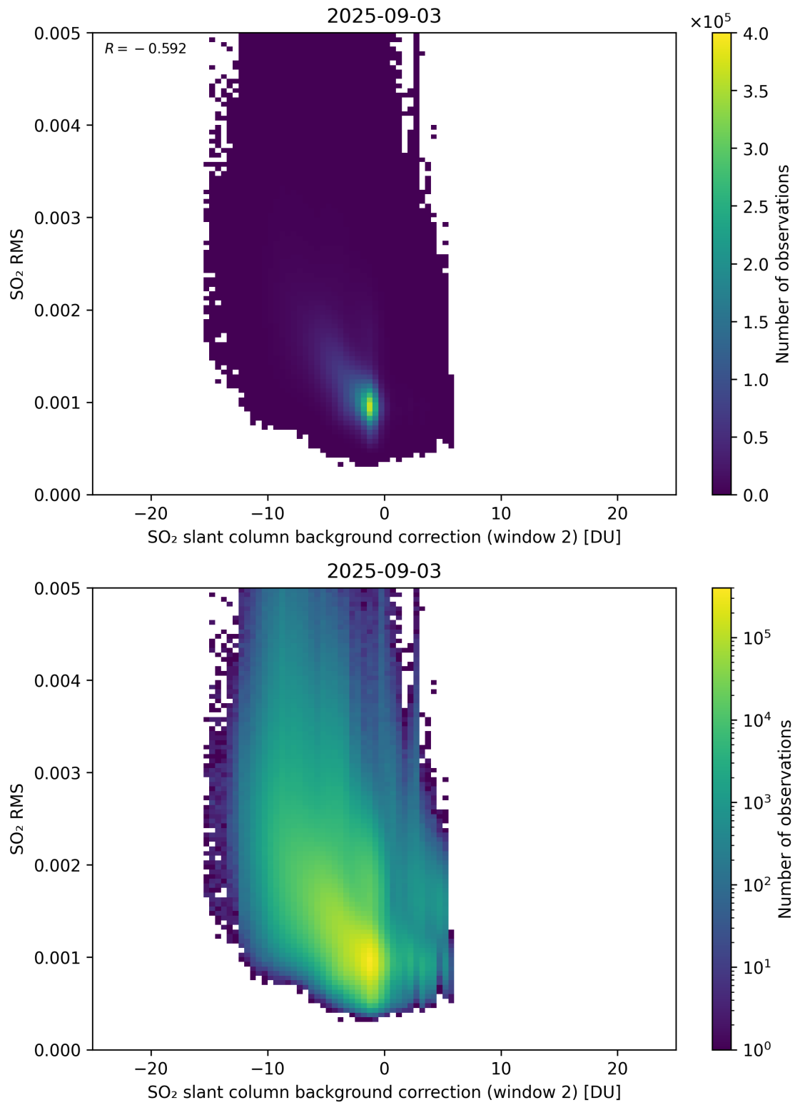
Figure 125: Scatter density plot of “SO 2 slant column background correction (window 2)” against “SO 2 RMS” for 2025-09-02 to 2025-09-04.
