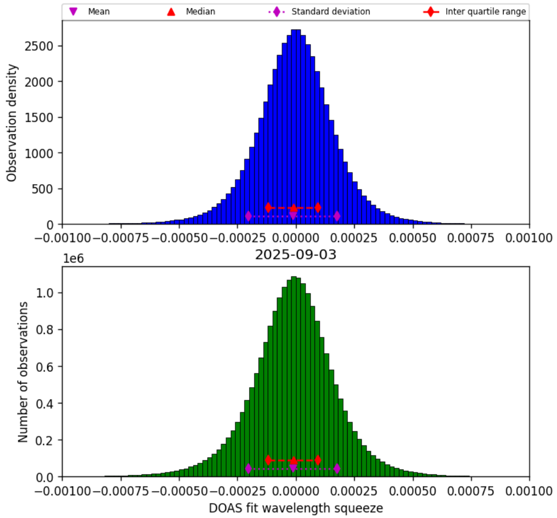
Figure 77: Histogram of “DOAS fit wavelength squeeze” for 2025-09-02 to 2025-09-04
