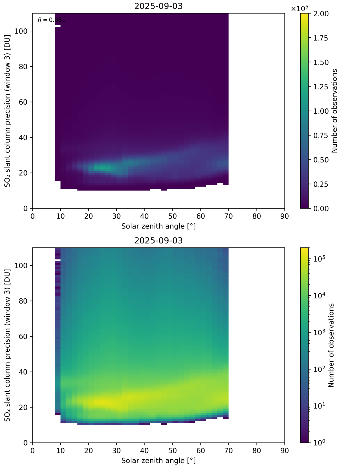
Figure 188: Scatter density plot of “Solar zenith angle” against “SO 2 slant column precision (window 3)” for 2025-09-02 to 2025-09-04.
