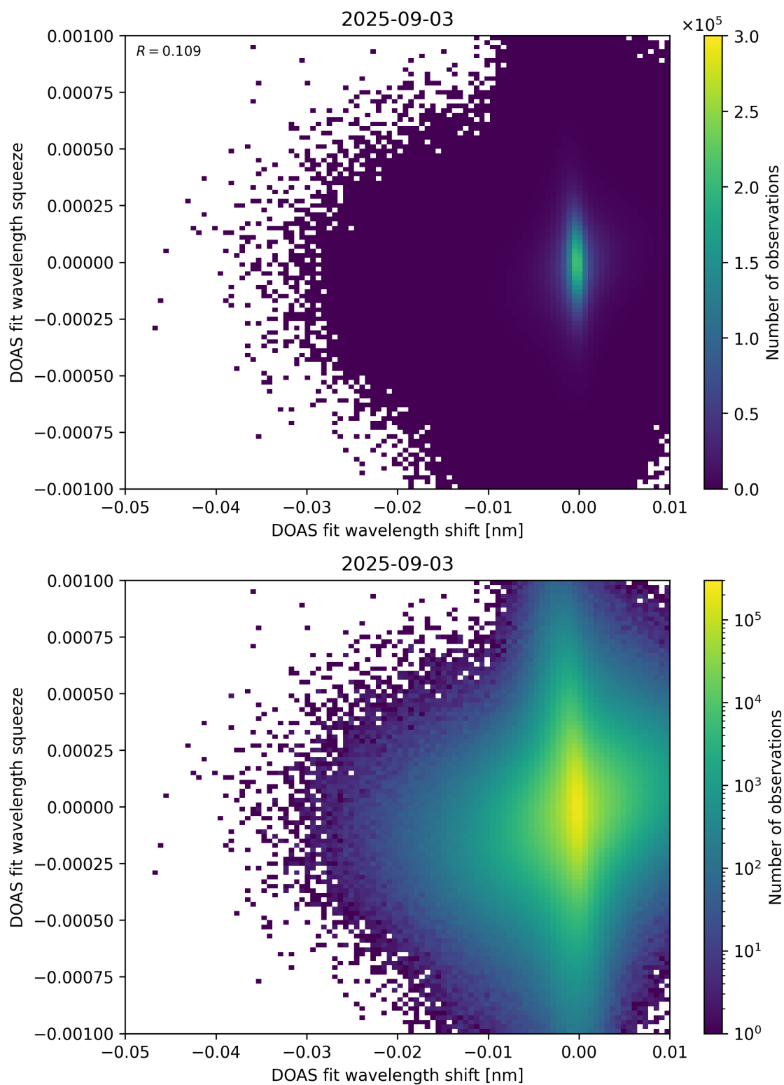
Figure 138: Scatter density plot of “DOAS fit wavelength shift” against “DOAS fit wavelength squeeze” for 2025-09-02 to 2025-09-04.
