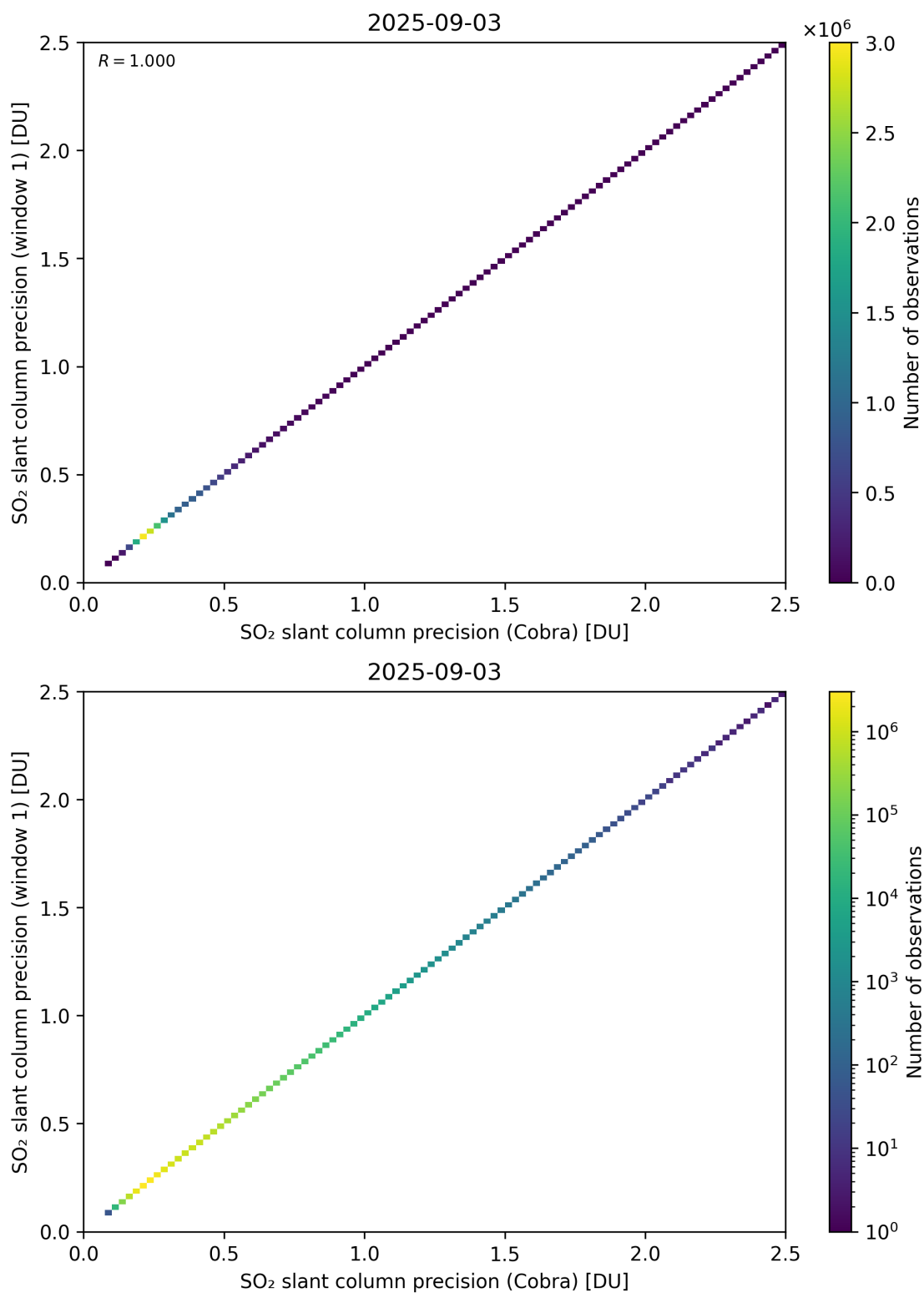
Figure 209: Scatter density plot of “SO 2 slant column precision (Cobra)” against “SO 2 slant column precision (window 1)” for 2025-09-02 to 2025-09-04.
