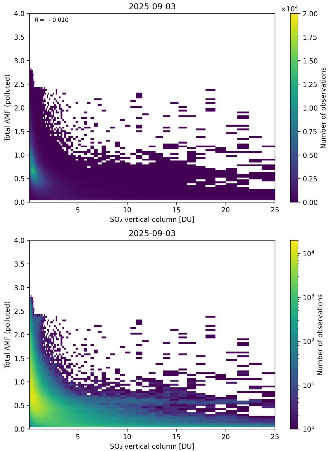
Figure 359: Scatter density plot of “SO 2 vertical column” against “Total AMF (polluted)” for 2025-09-02 to 2025-09-04.
