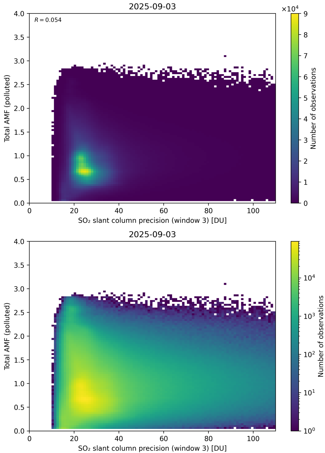
Figure 313: Scatter density plot of “SO 2 slant column precision (window 3)” against “Total AMF (polluted)” for 2025-09-02 to 2025-09-04.
