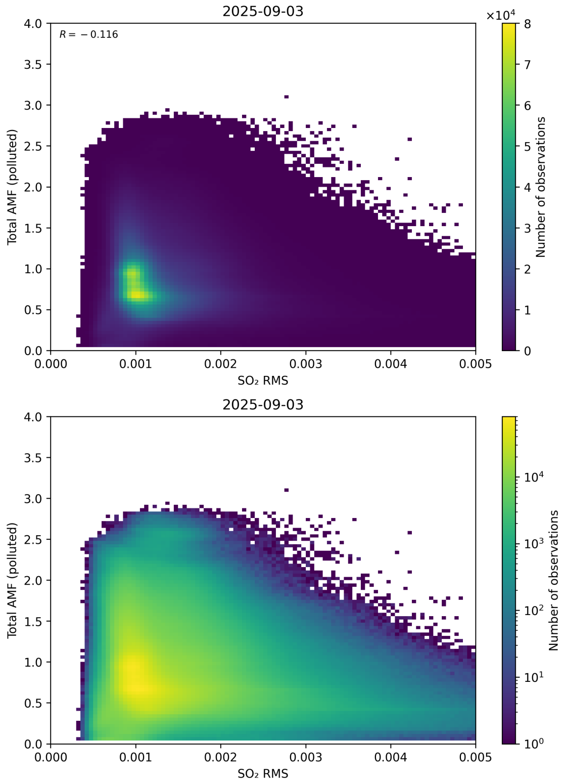
Figure 148: Scatter density plot of “SO 2 RMS” against “Total AMF (polluted)” for 2025-09-02 to 2025-09-04.
