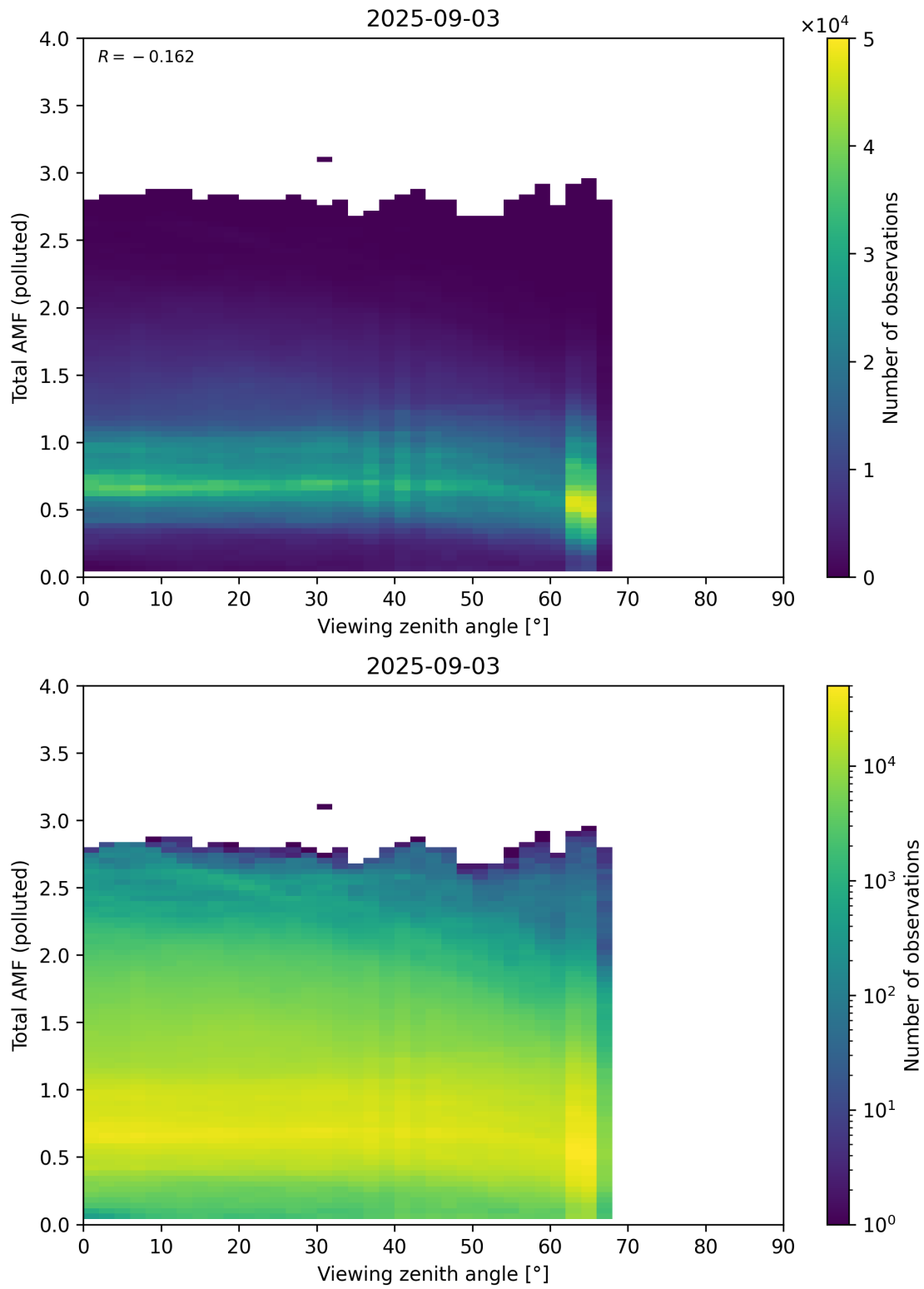
Figure 381: Scatter density plot of “Viewing zenith angle” against “Total AMF (polluted)” for 2025-09-02 to 2025-09-04.
