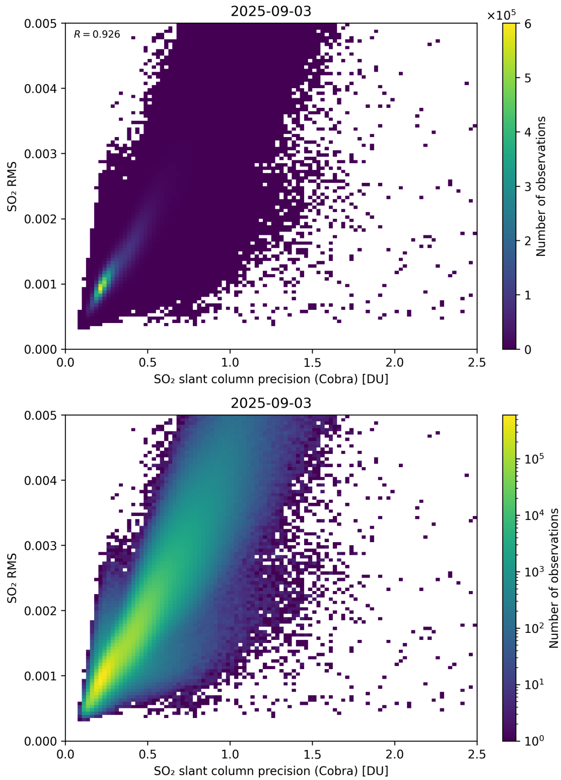
Figure 204: Scatter density plot of “SO 2 slant column precision (Cobra)” against “SO 2 RMS” for 2025-09-02 to 2025-09-04.
