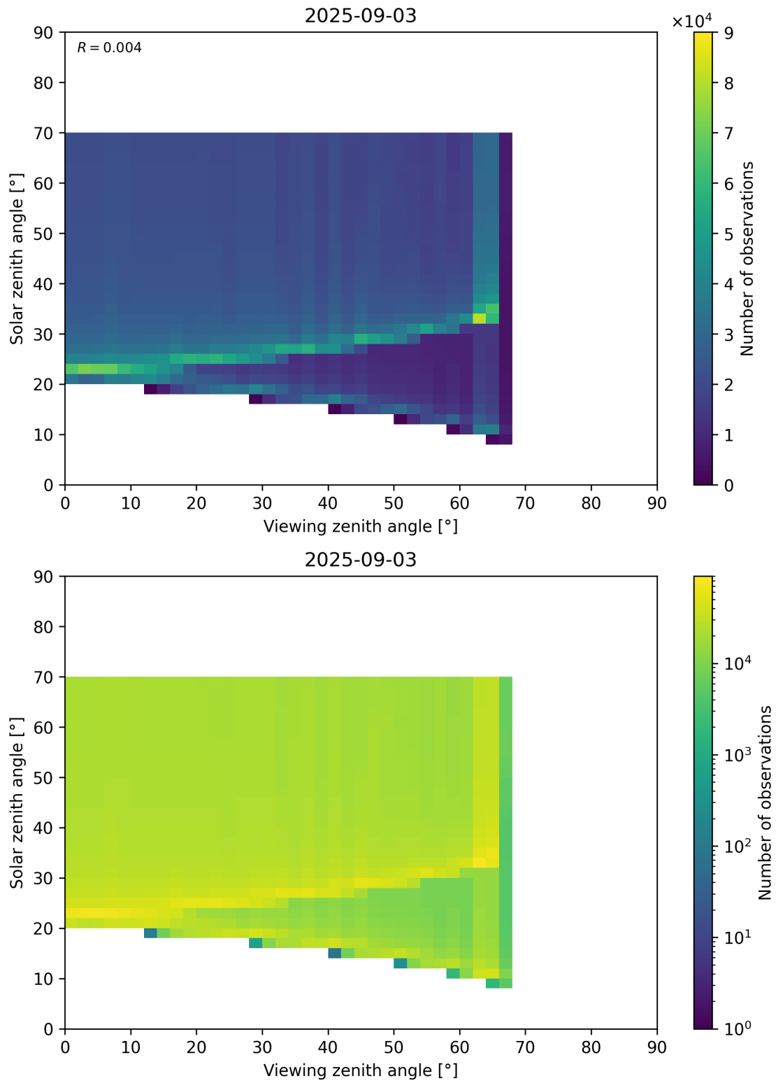
Figure 369: Scatter density plot of “Viewing zenith angle” against “Solar zenith angle” for 2025-09-02 to 2025-09-04.
