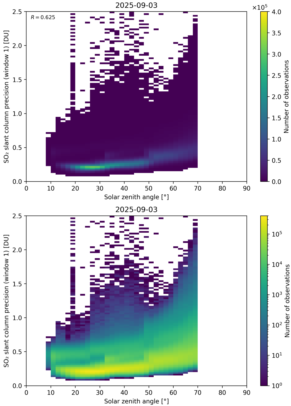
Figure 185: Scatter density plot of “Solar zenith angle” against “SO 2 slant column precision (window 1)” for 2025-09-02 to 2025-09-04.
