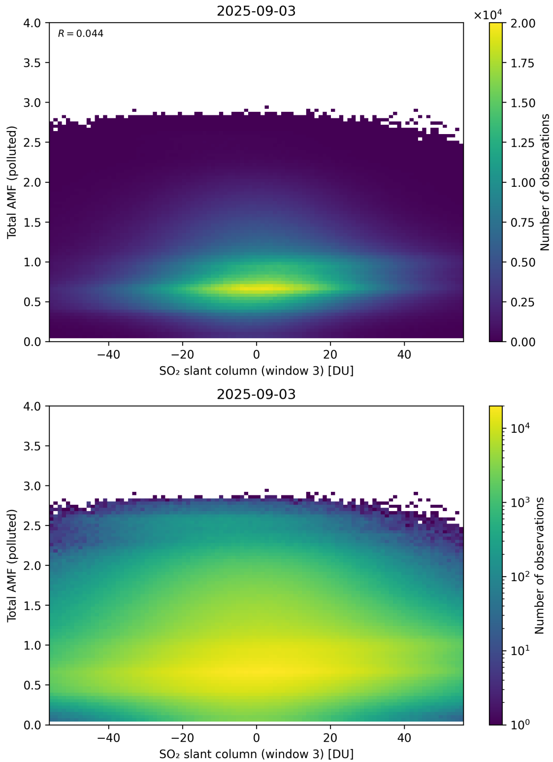
Figure 318: Scatter density plot of “SO 2 slant column (window 3)” against “Total AMF (polluted)” for 2025-09-02 to 2025-09-04.
