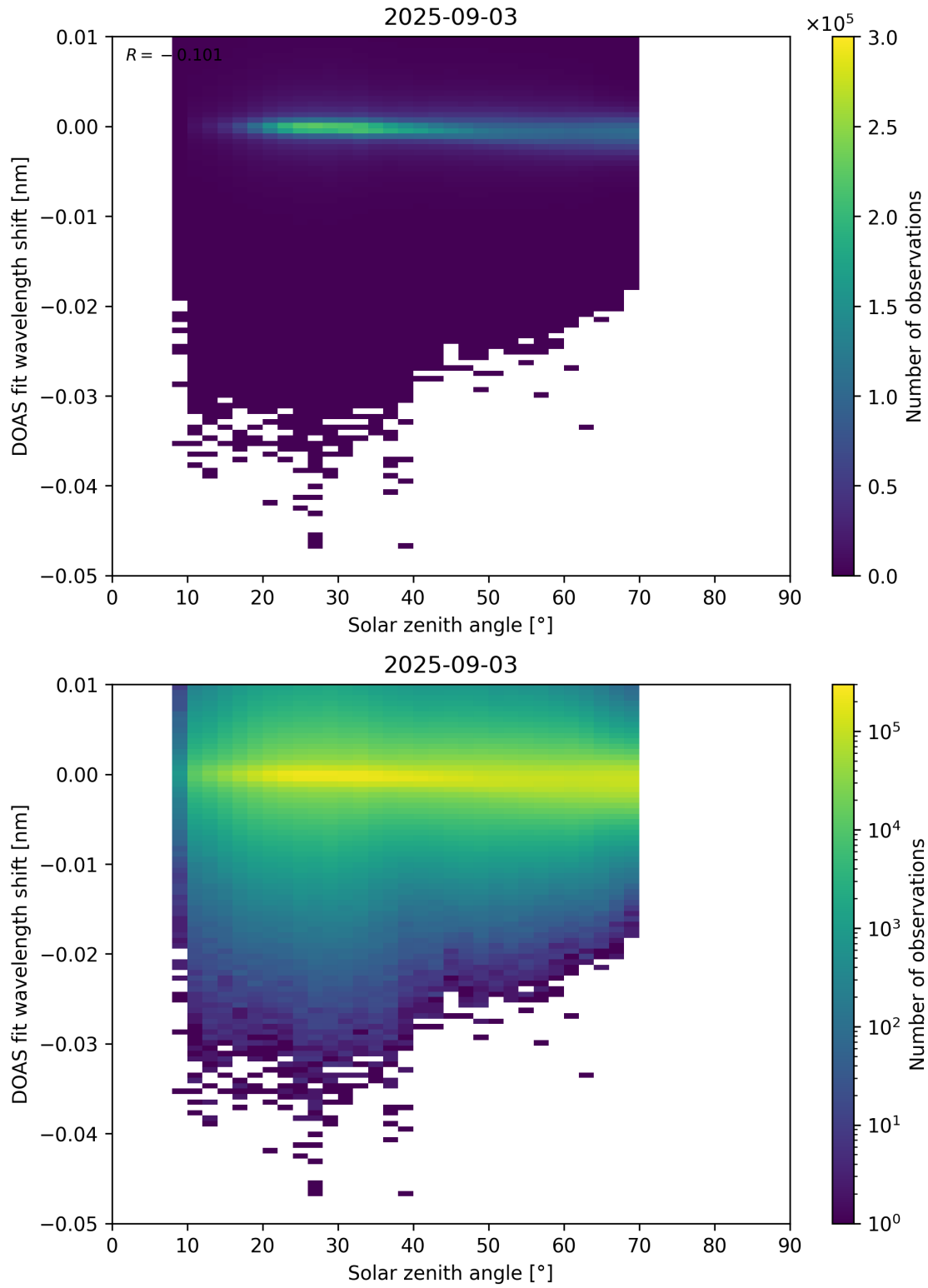
Figure 174: Scatter density plot of “Solar zenith angle” against “DOAS fit wavelength shift” for 2025-09-02 to 2025-09-04.
