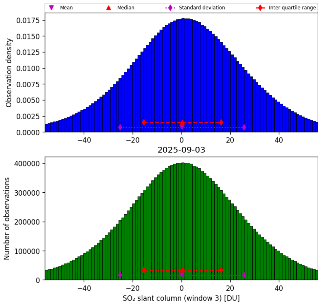
Figure 71: Histogram of “SO 2 slant column (window 3)” for 2025-09-02 to 2025-09-04
