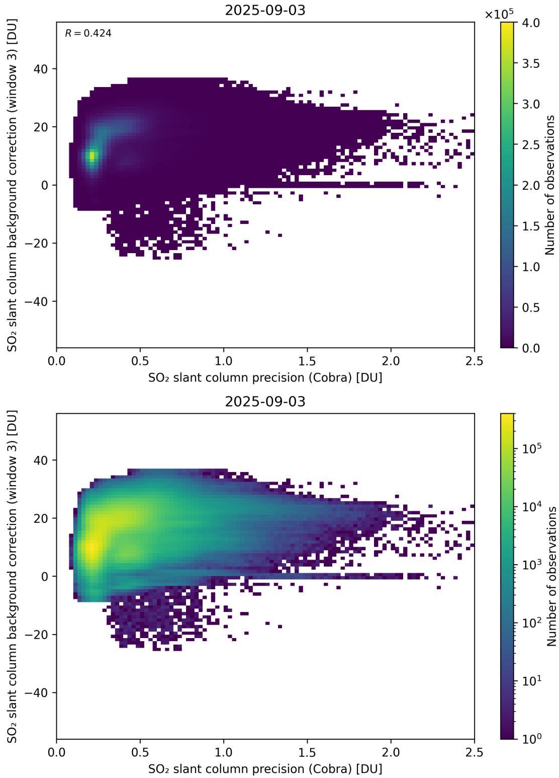
Figure 201: Scatter density plot of “SO 2 slant column precision (Cobra)” against “SO 2 slant column background correction (window 3)” for 2025-09-02 to 2025-09-04.
