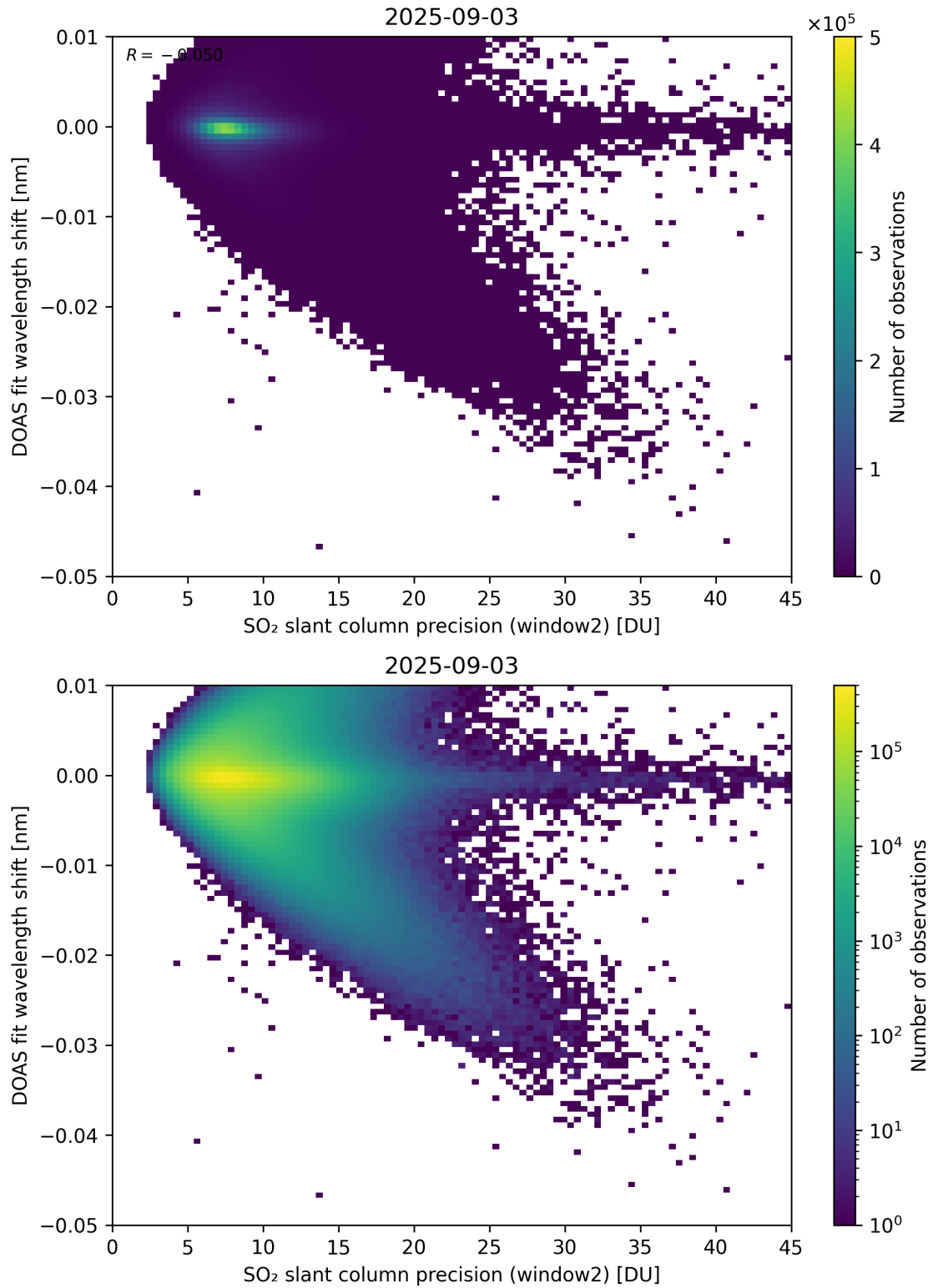
Figure 293: Scatter density plot of “SO 2 slant column precision (window2)” against “DOAS fit wavelength shift” for 2025-09-02 to 2025-09-04.
