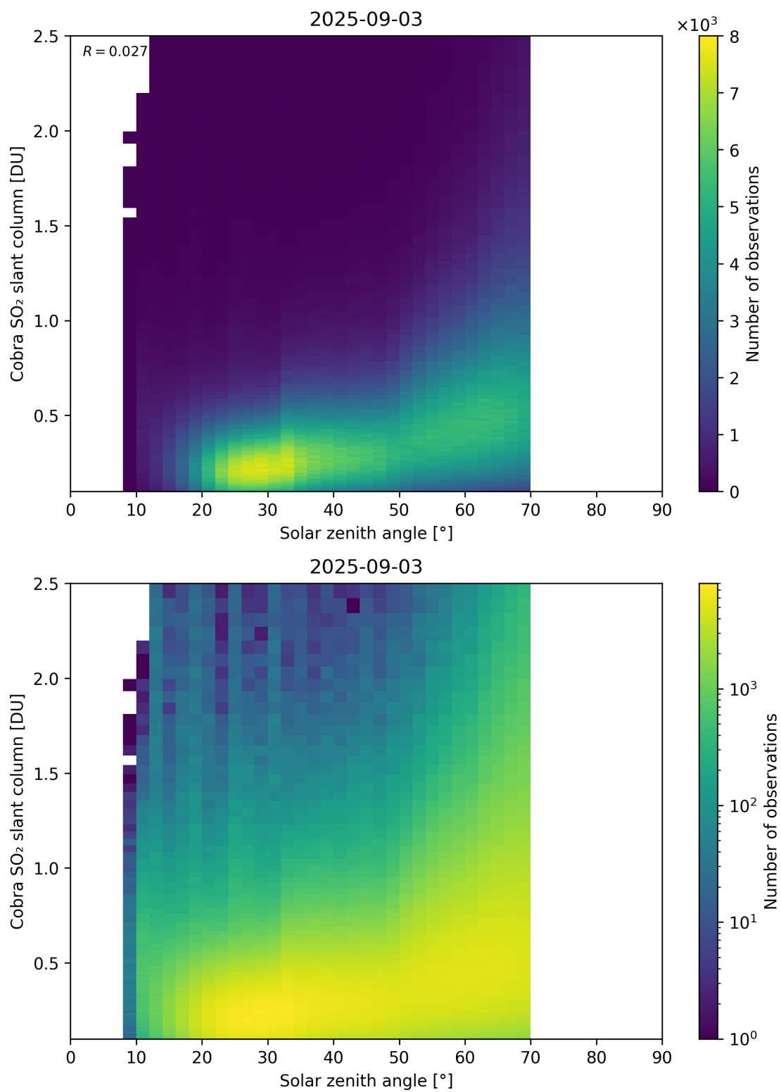
Figure 179: Scatter density plot of “Solar zenith angle” against “Cobra SO 2 slant column” for 2025-09-02 to 2025-09-04.
