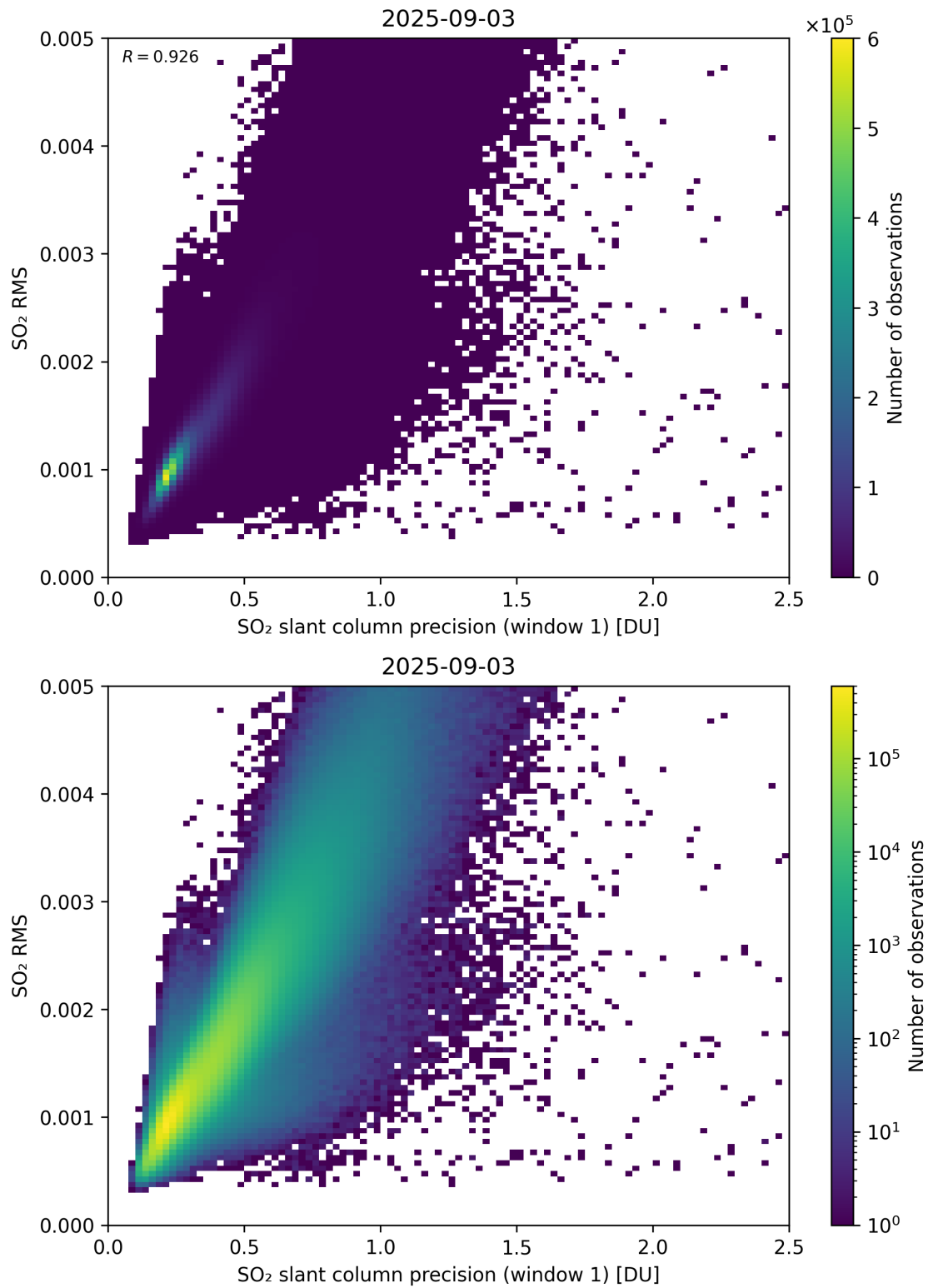
Figure 273: Scatter density plot of “SO 2 slant column precision (window 1)” against “SO 2 RMS” for 2025-09-02 to 2025-09-04.
