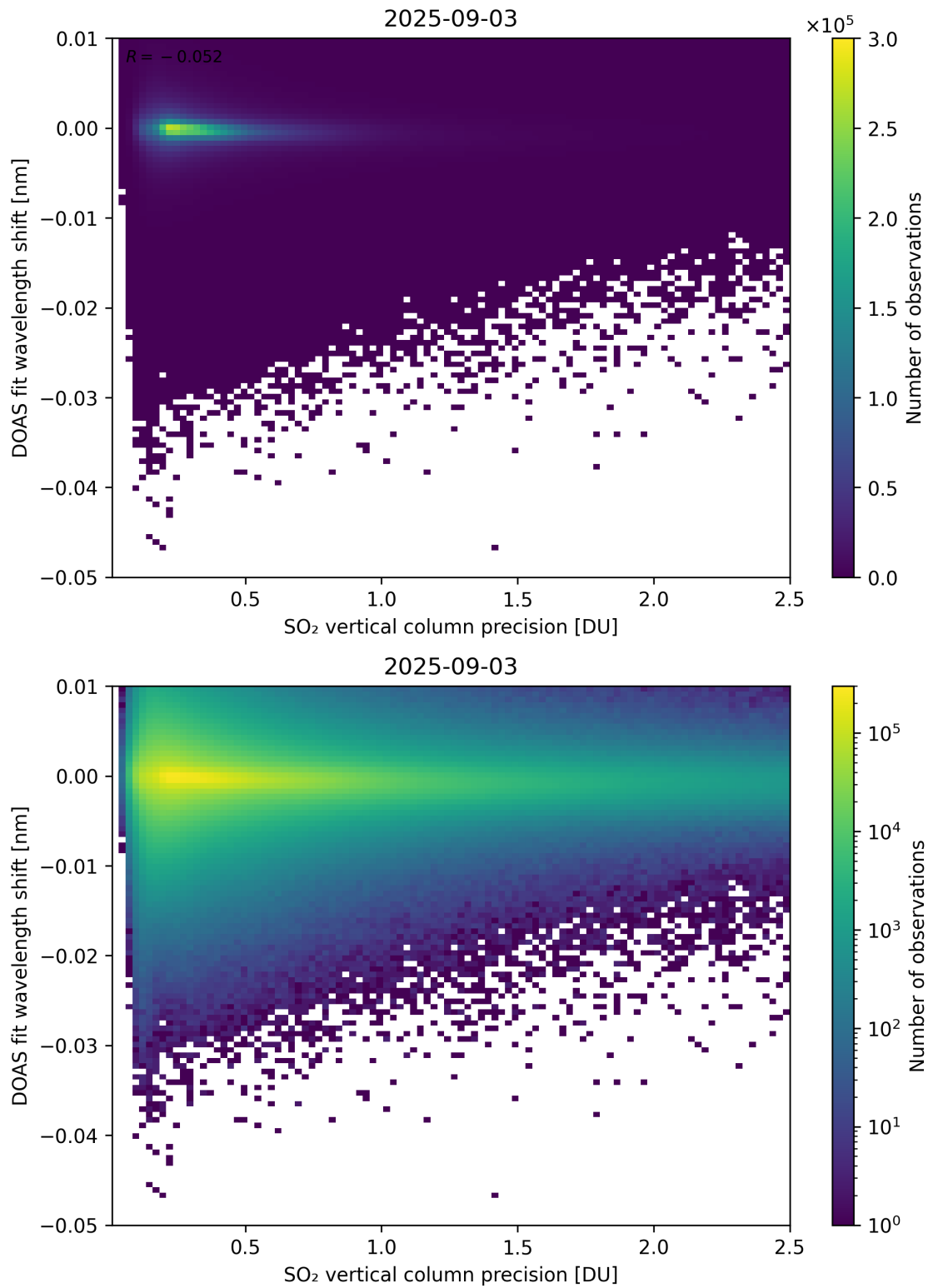
Figure 332: Scatter density plot of “SO 2 vertical column precision” against “DOAS fit wavelength shift” for 2025-09-02 to 2025-09-04.
