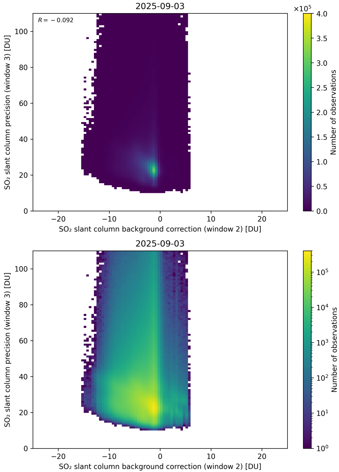
Figure 129: Scatter density plot of “SO 2 slant column background correction (window 2)” against “SO 2 slant column precision (window 3)” for 2025-09-02 to 2025-09-04.
