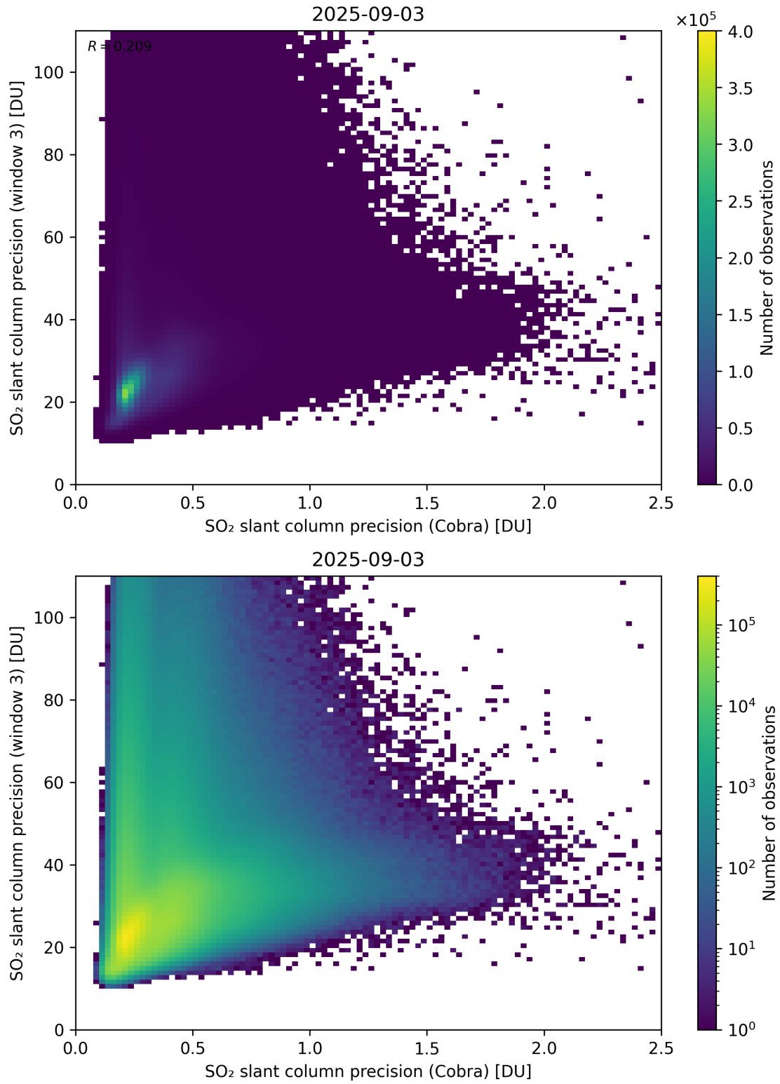
Figure 212: Scatter density plot of “SO 2 slant column precision (Cobra)” against “SO 2 slant column precision (window 3)” for 2025-09-02 to 2025-09-04.
