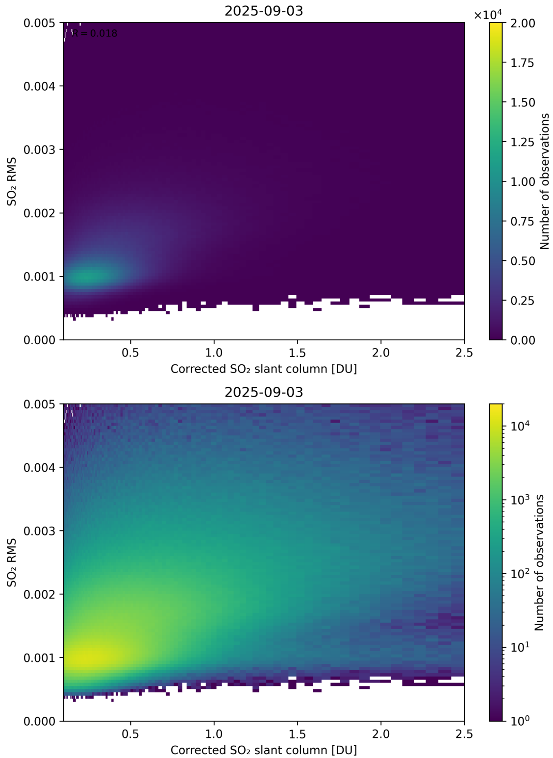
Figure 231: Scatter density plot of “Corrected SO 2 slant column” against “SO 2 RMS” for 2025-09-02 to 2025-09-04.
