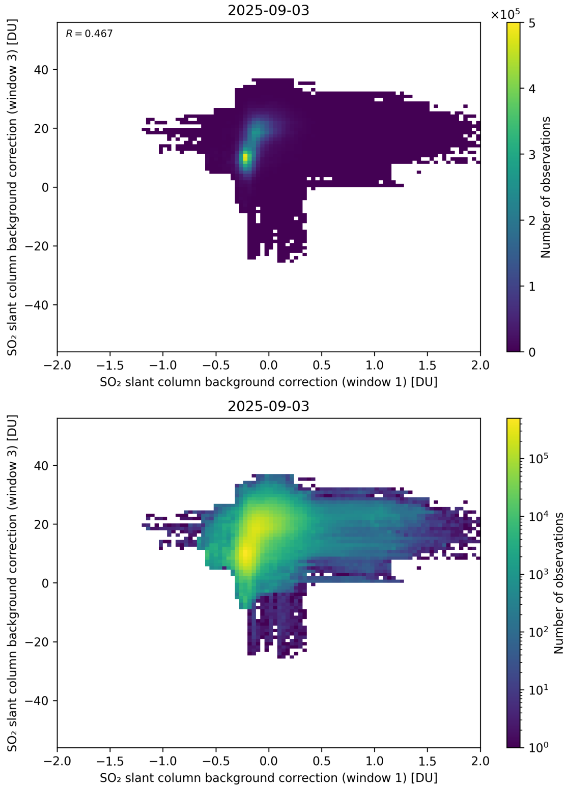
Figure 110: Scatter density plot of “SO 2 slant column background correction (window 1)” against “SO 2 slant column background correction (window 3)” for 2025-09-02 to 2025-09-04.
