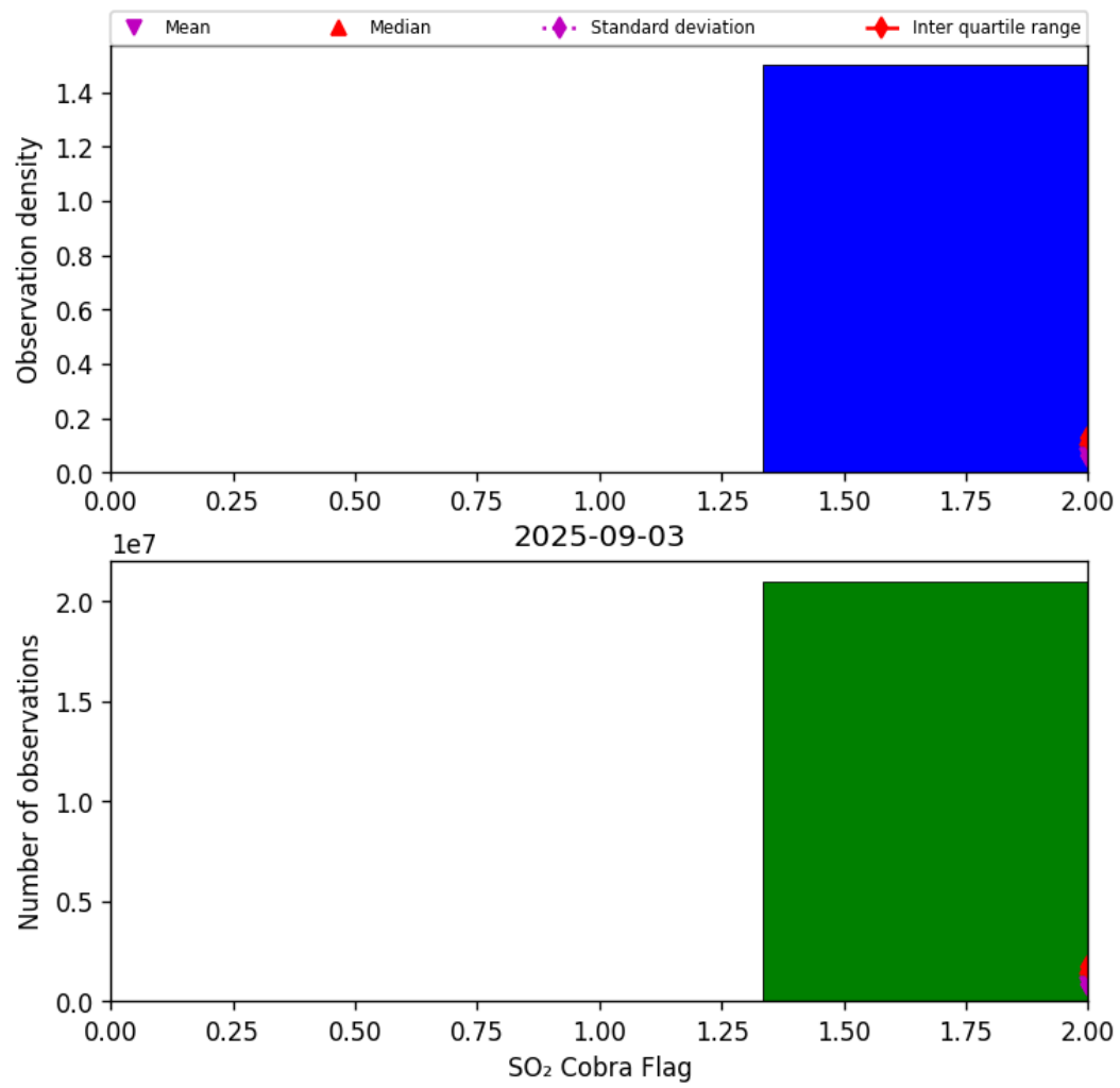
Figure 75: Histogram of “SO 2 Cobra Flag” for 2025-09-02 to 2025-09-04
