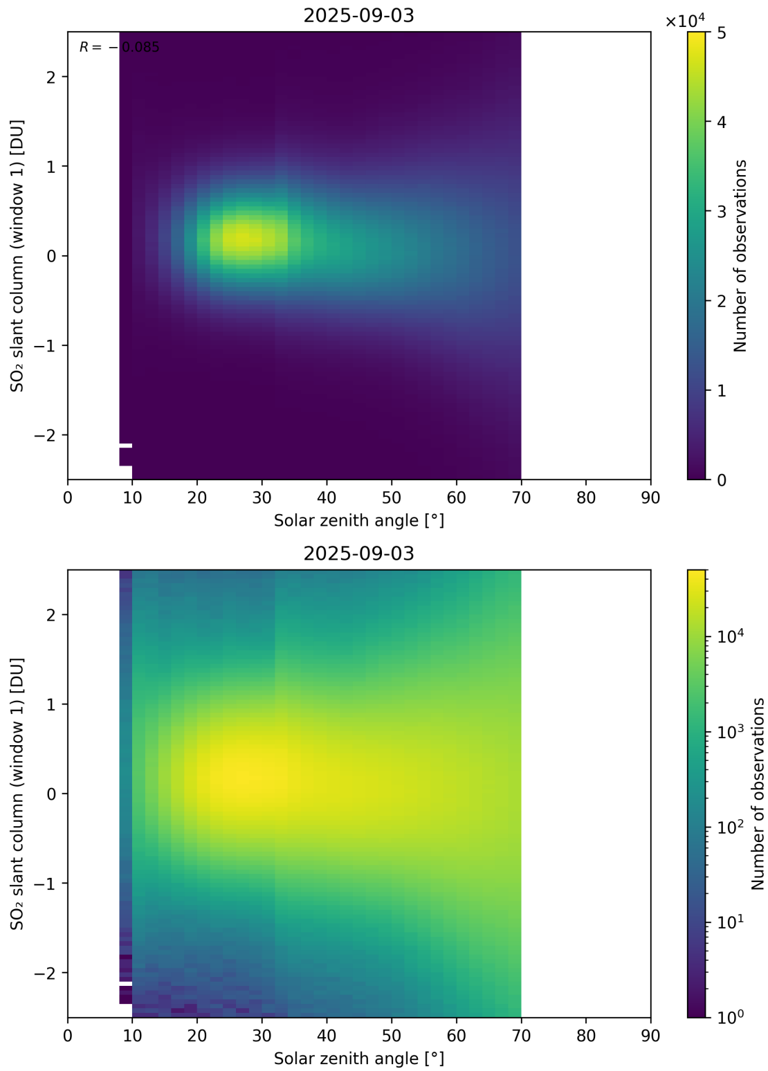
Figure 184: Scatter density plot of “Solar zenith angle” against “SO 2 slant column (window 1)” for 2025-09-02 to 2025-09-04.
