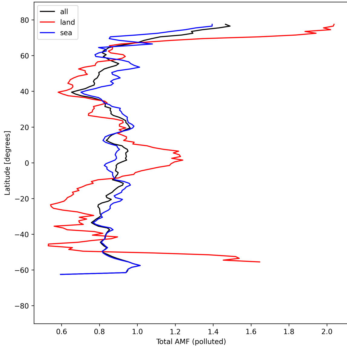
Figure 53: Zonal average of “Total AMF (polluted)” for 2025-09-02 to 2025-09-04.
