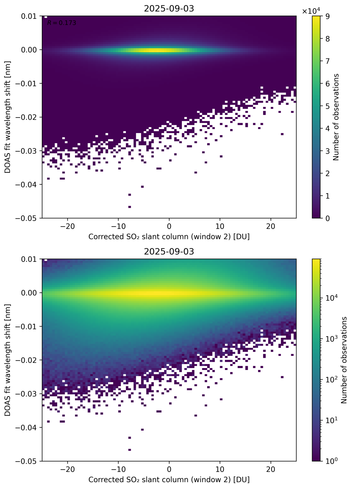
Figure 246: Scatter density plot of “Corrected SO 2 slant column (window 2)” against “DOAS fit wavelength shift” for 2025-09-02 to 2025-09-04.
