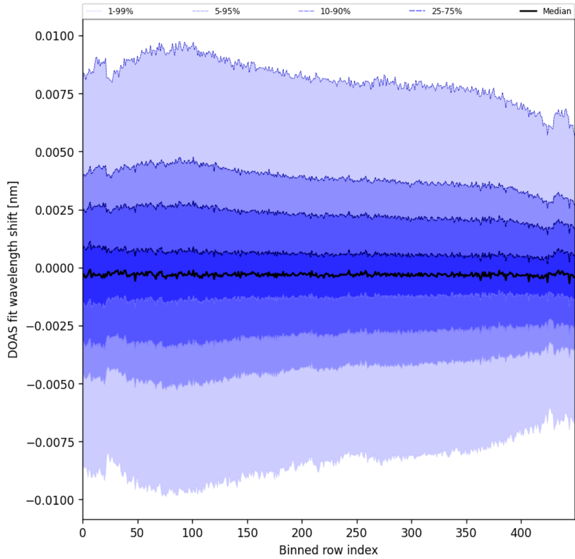
Figure 102: Along track statistics of “DOAS fit wavelength shift” for 2025-09-02 to 2025-09-04
