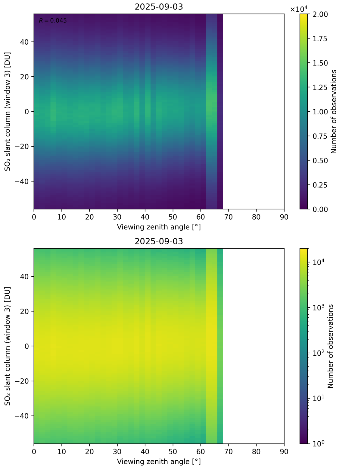
Figure 379: Scatter density plot of “Viewing zenith angle” against “SO 2 slant column (window 3)” for 2025-09-02 to 2025-09-04.
