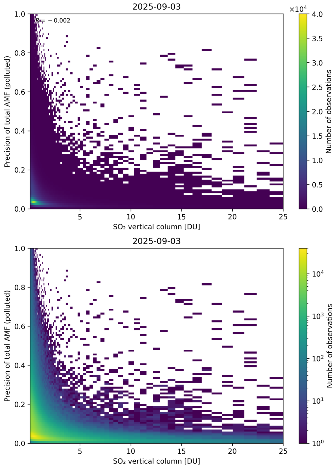
Figure 360: Scatter density plot of “SO 2 vertical column” against “Precision of total AMF (polluted)” for 2025-09-02 to 2025-09-04.
