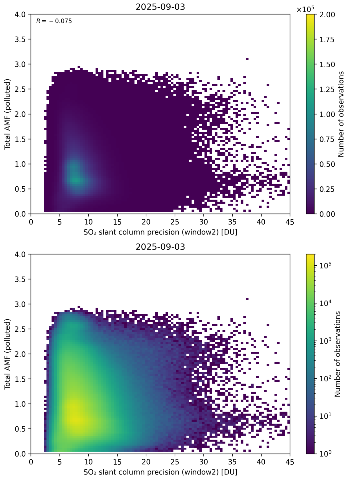
Figure 301: Scatter density plot of “SO 2 slant column precision (window2)” against “Total AMF (polluted)” for 2025-09-02 to 2025-09-04.
