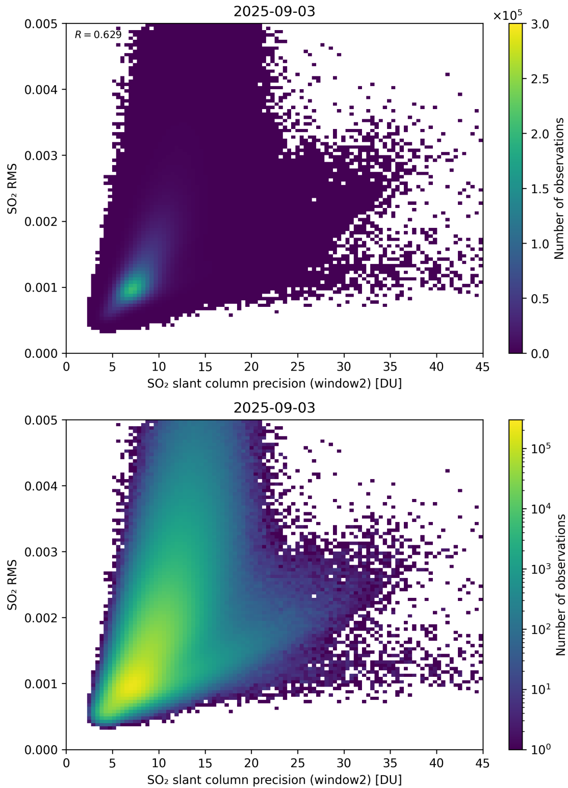
Figure 295: Scatter density plot of “SO 2 slant column precision (window2)” against “SO 2 RMS” for 2025-09-02 to 2025-09-04.
