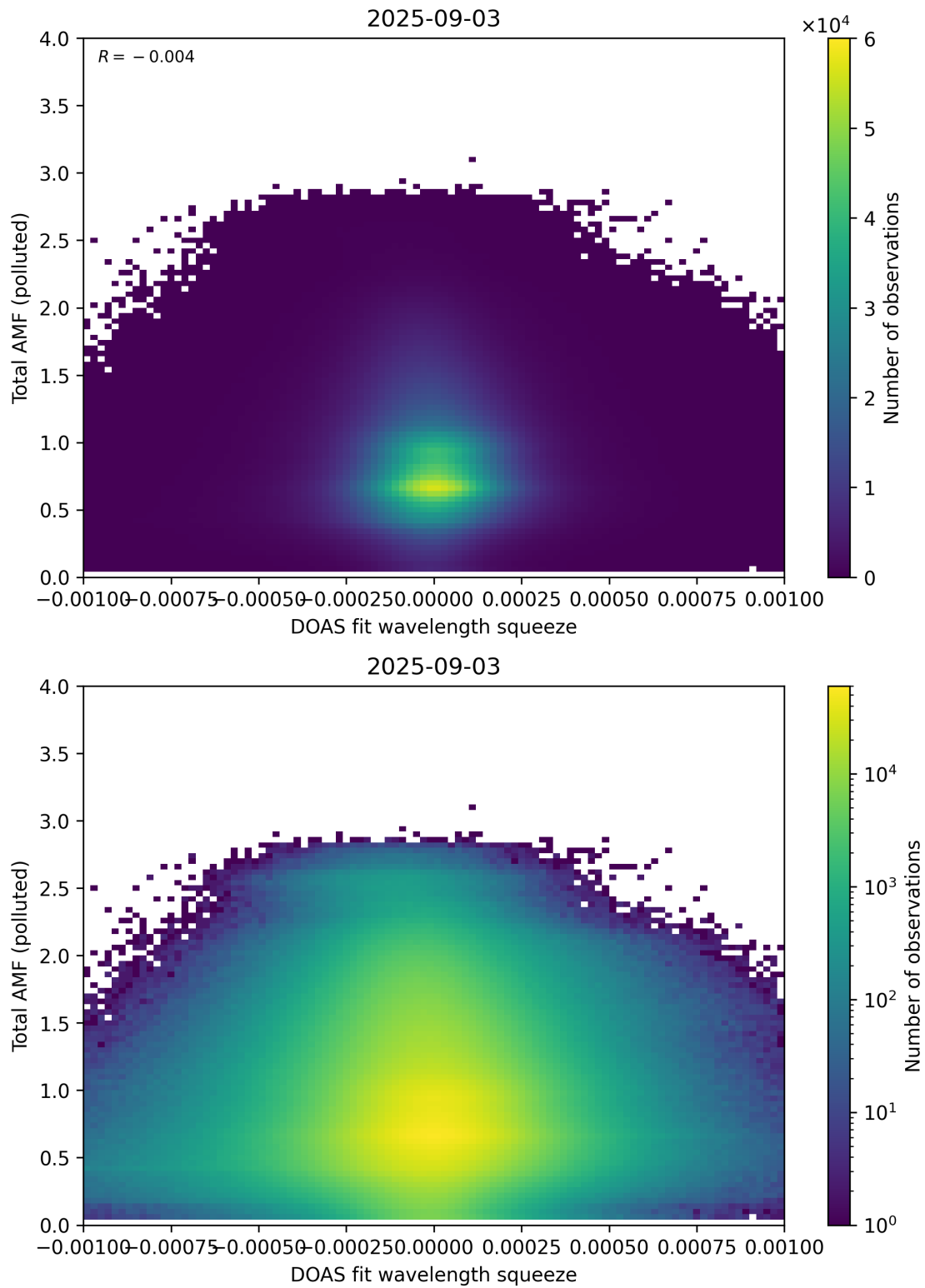
Figure 145: Scatter density plot of “DOAS fit wavelength squeeze” against “Total AMF (polluted)” for 2025-09-02 to 2025-09-04.
