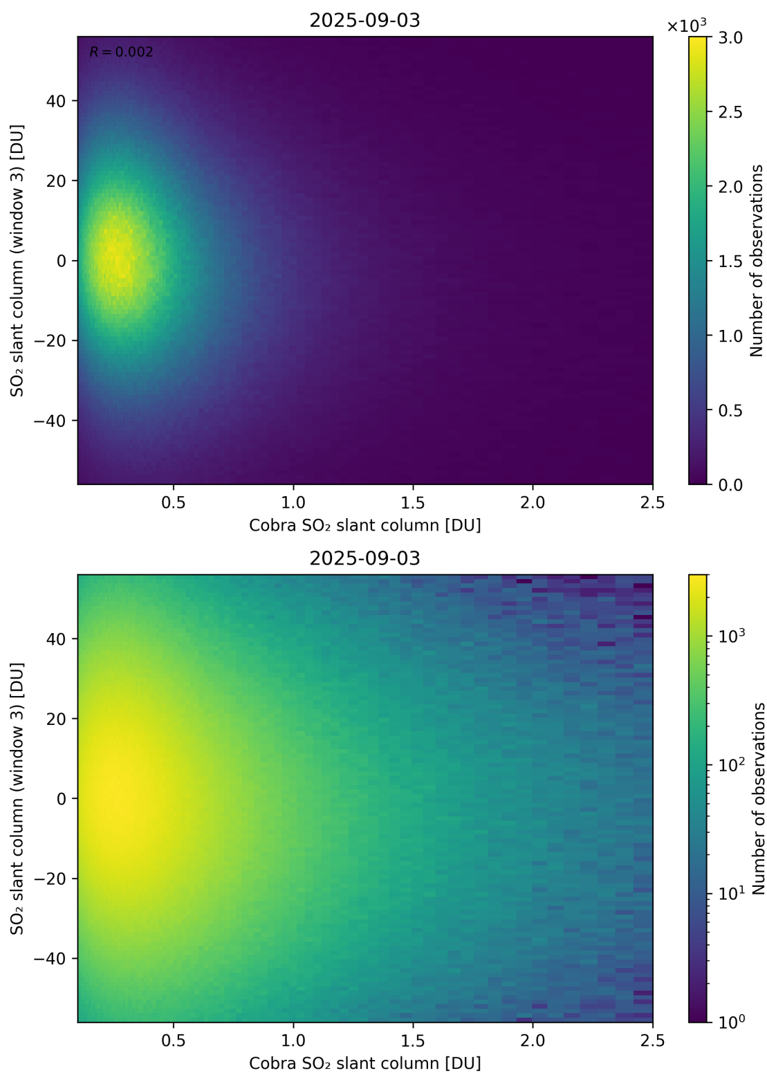
Figure 222: Scatter density plot of “Cobra SO 2 slant column” against “SO 2 slant column (window 3)” for 2025-09-02 to 2025-09-04.
