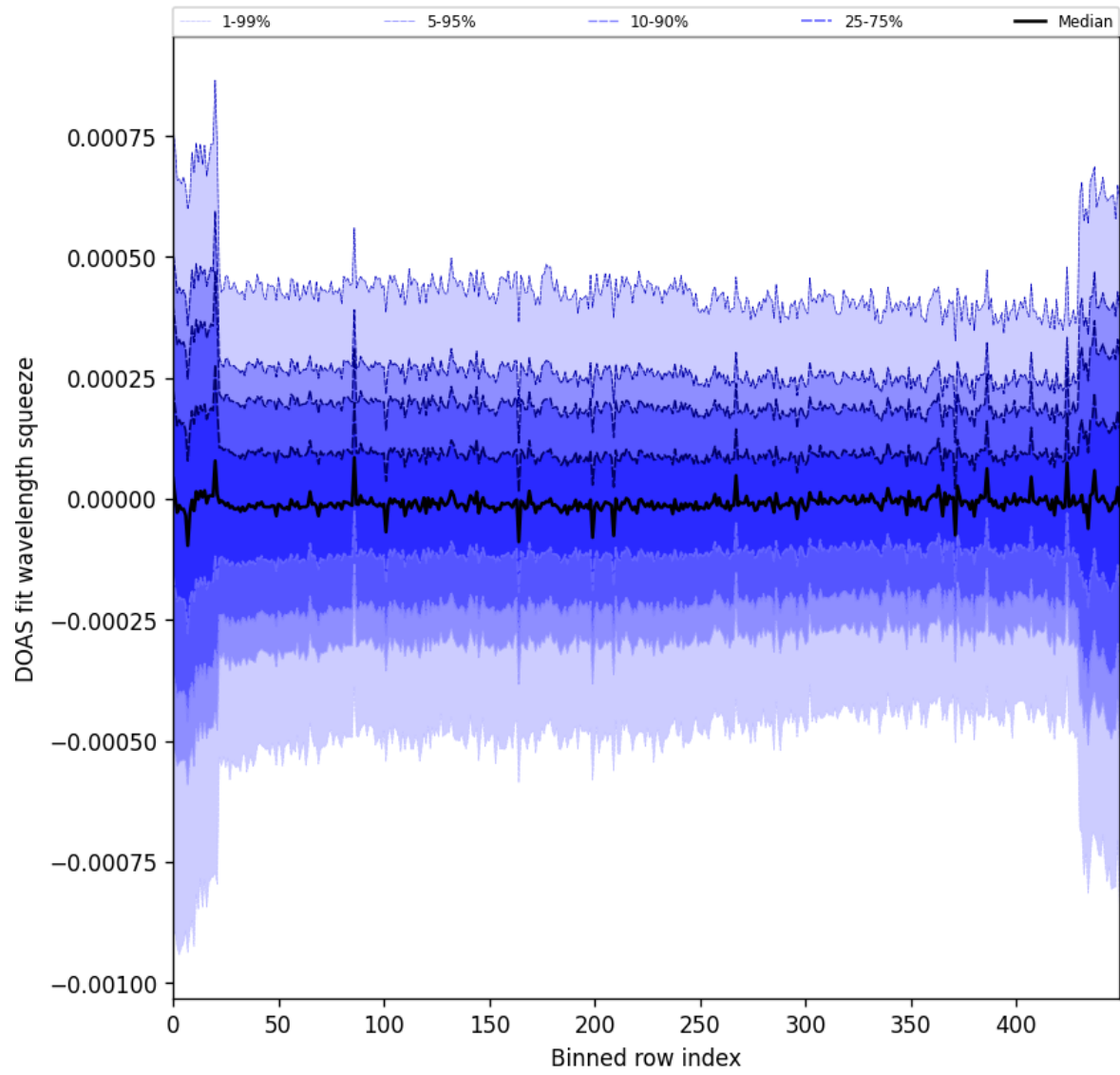
Figure 103: Along track statistics of “DOAS fit wavelength squeeze” for 2025-09-02 to 2025-09-04
