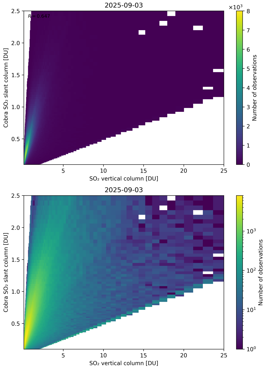
Figure 349: Scatter density plot of “SO 2 vertical column” against “Cobra SO 2 slant column” for 2025-09-02 to 2025-09-04.
