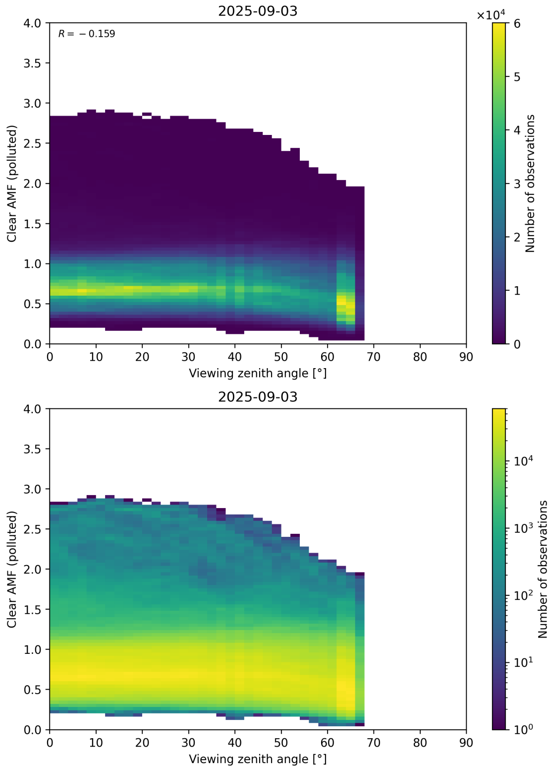
Figure 370: Scatter density plot of “Viewing zenith angle” against “Clear AMF (polluted)” for 2025-09-02 to 2025-09-04.
