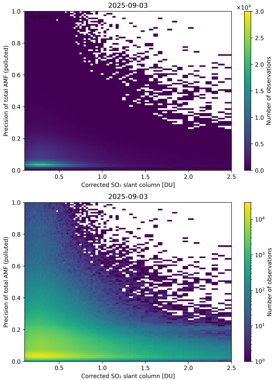
Figure 243: Scatter density plot of “Corrected SO 2 slant column” against “Precision of total AMF (polluted)” for 2025-09-02 to 2025-09-04.
