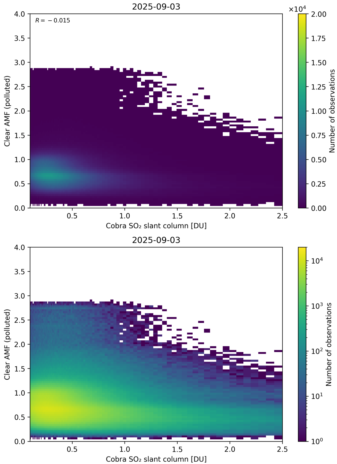
Figure 215: Scatter density plot of “Cobra SO 2 slant column” against “Clear AMF (polluted)” for 2025-09-02 to 2025-09-04.
