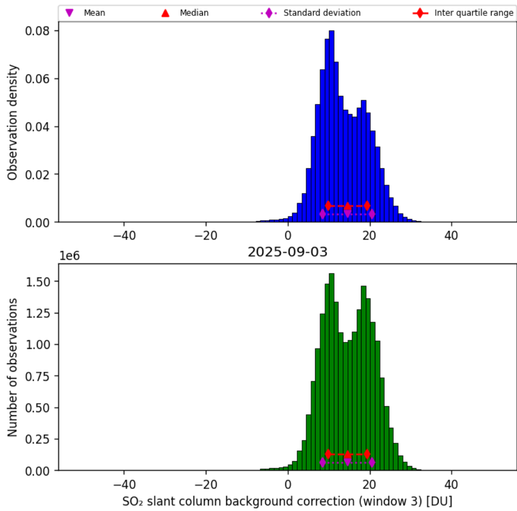
Figure 74: Histogram of “SO 2 slant column background correction (window 3)” for 2025-09-02 to 2025-09-04
