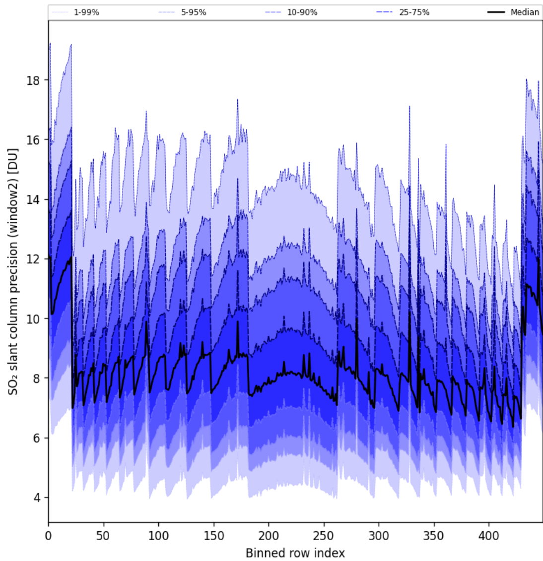
Figure 94: Along track statistics of “SO 2 slant column precision (window2)” for 2025-09-02 to 2025-09-04
