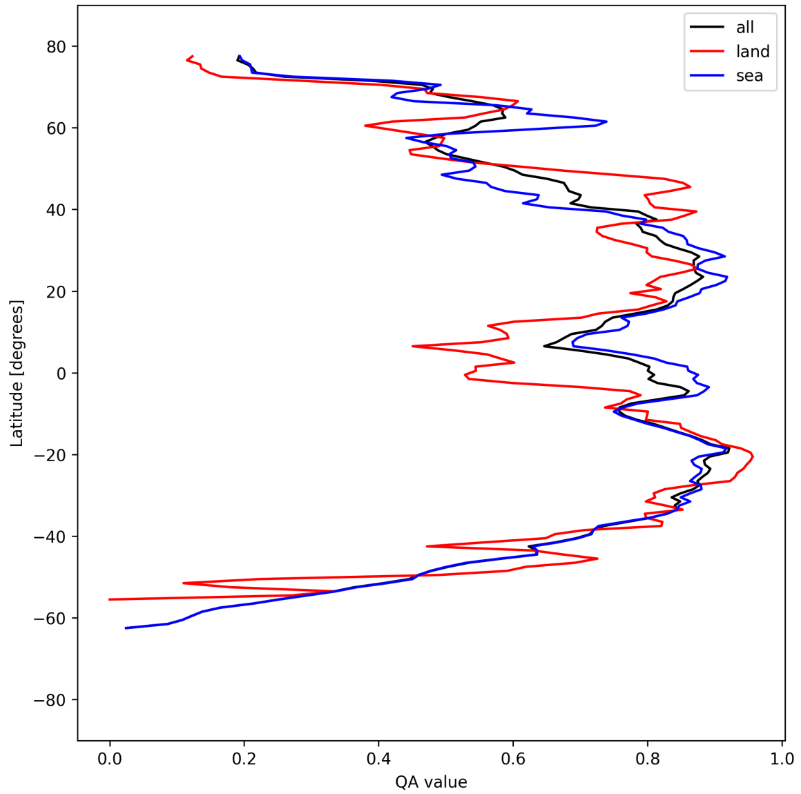
Figure 31: Zonal average of “QA value” for 2025-09-02 to 2025-09-04.
