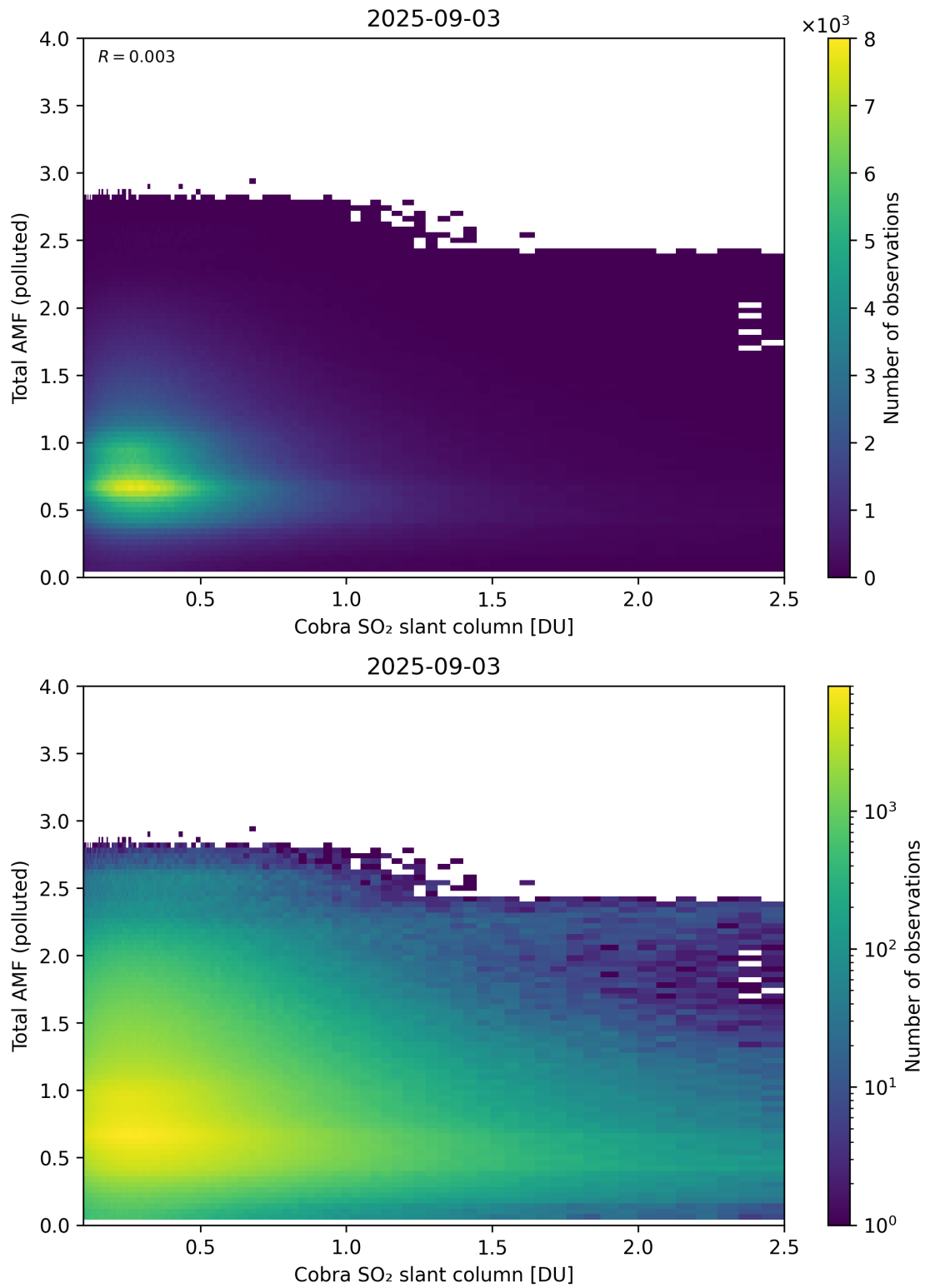
Figure 224: Scatter density plot of “Cobra SO 2 slant column” against “Total AMF (polluted)” for 2025-09-02 to 2025-09-04.
