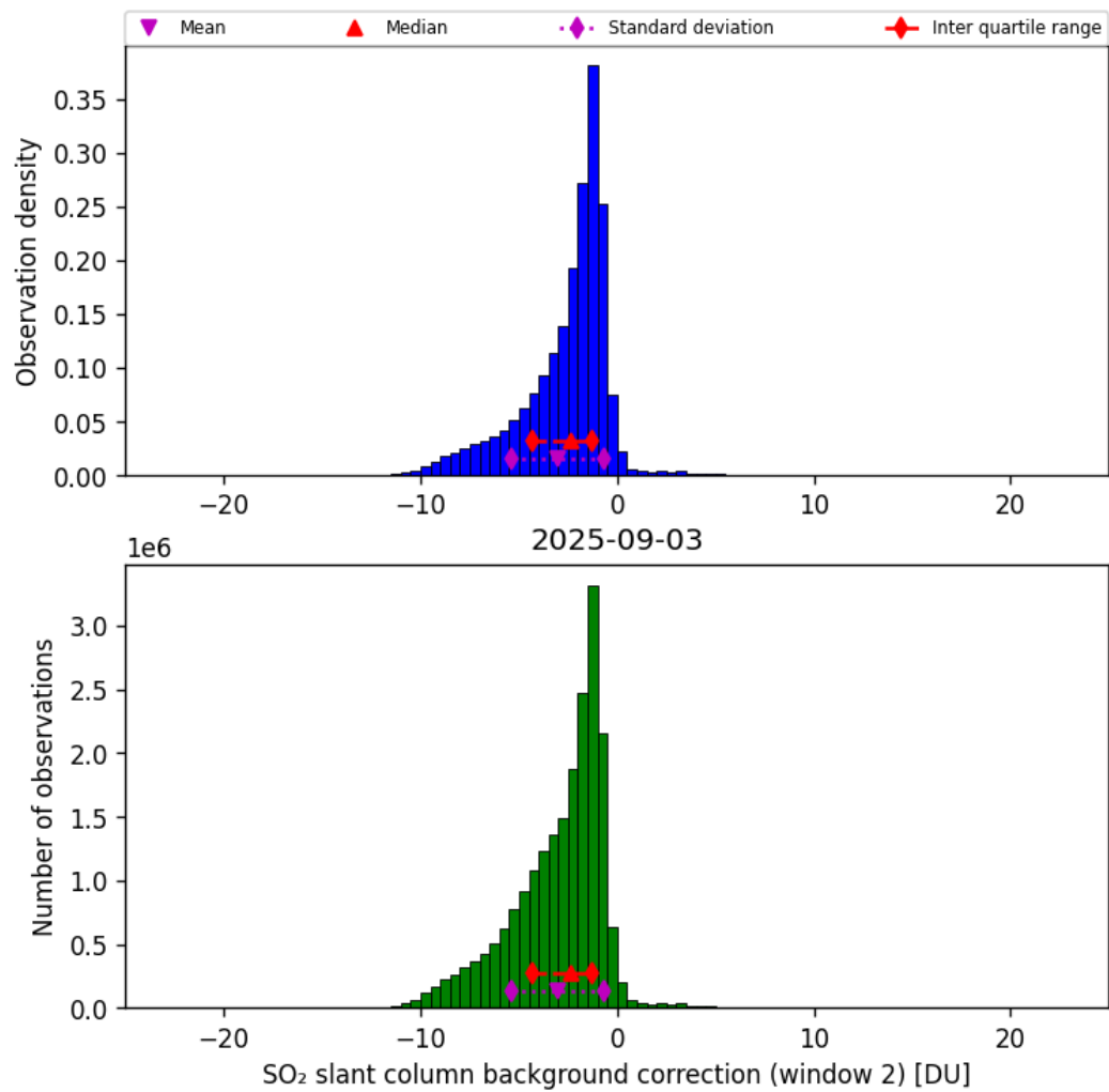
Figure 70: Histogram of “SO 2 slant column background correction (window 2)” for 2025-09-02 to 2025-09-04
