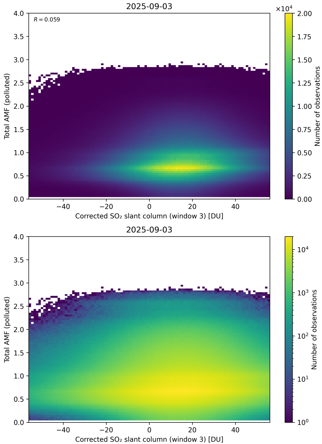
Figure 260: Scatter density plot of “Corrected SO 2 slant column (window 3)” against “Total AMF (polluted)” for 2025-09-02 to 2025-09-04.
