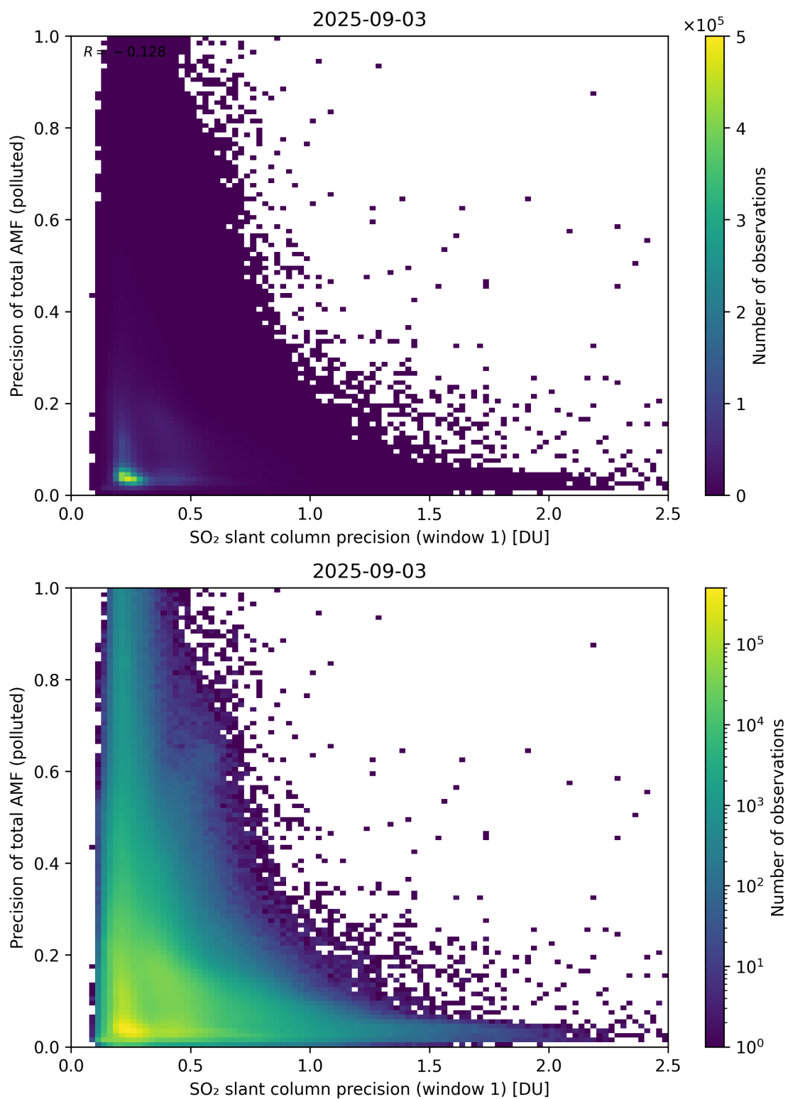
Figure 281: Scatter density plot of “SO 2 slant column precision (window 1)” against “Precision of total AMF (polluted)” for 2025-09-02 to 2025-09-04.
