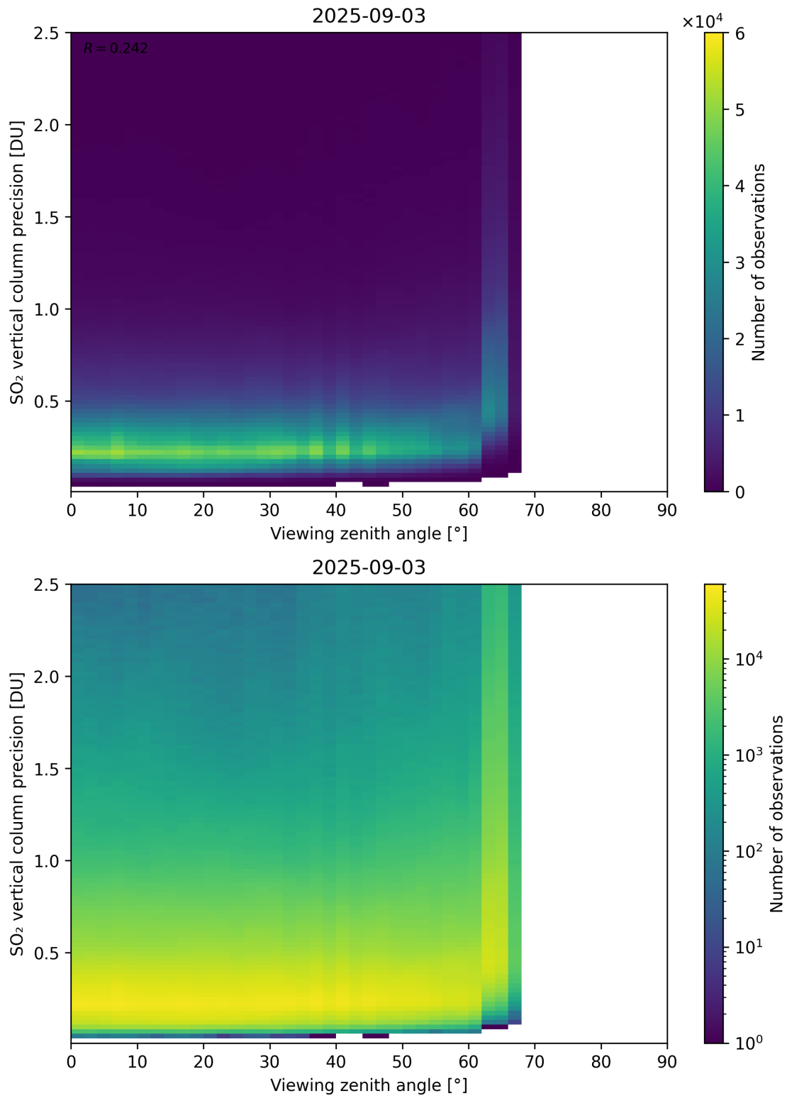
Figure 384: Scatter density plot of “Viewing zenith angle” against “SO 2 vertical column precision” for 2025-09-02 to 2025-09-04.
