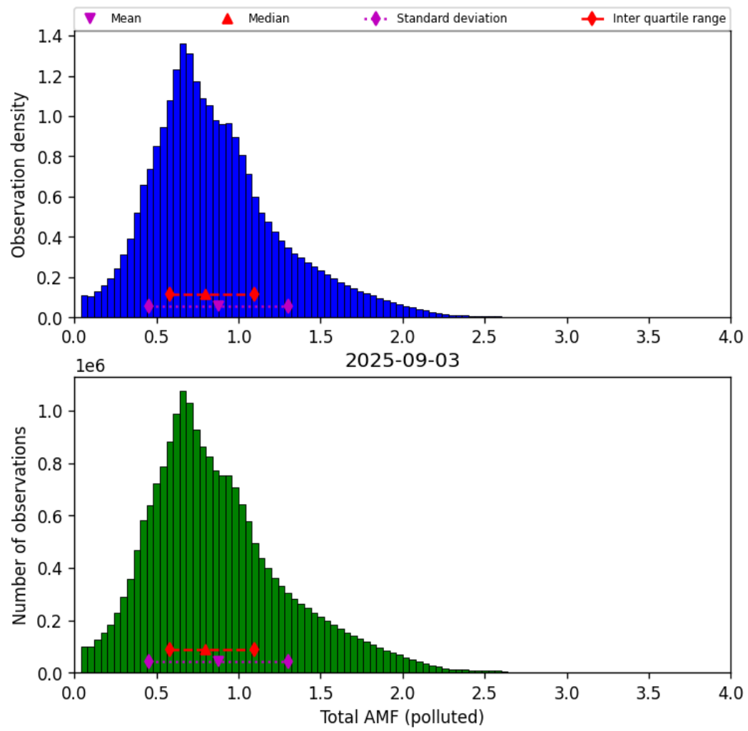
Figure 79: Histogram of “Total AMF (polluted)” for 2025-09-02 to 2025-09-04
