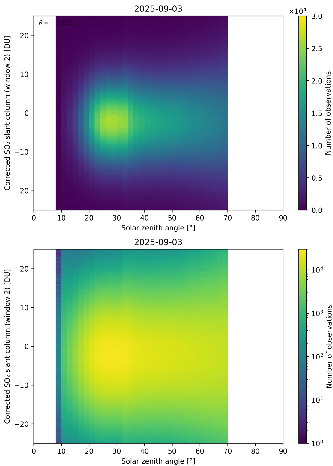
Figure 182: Scatter density plot of “Solar zenith angle” against “Corrected SO 2 slant column (window 2)” for 2025-09-02 to 2025-09-04.
