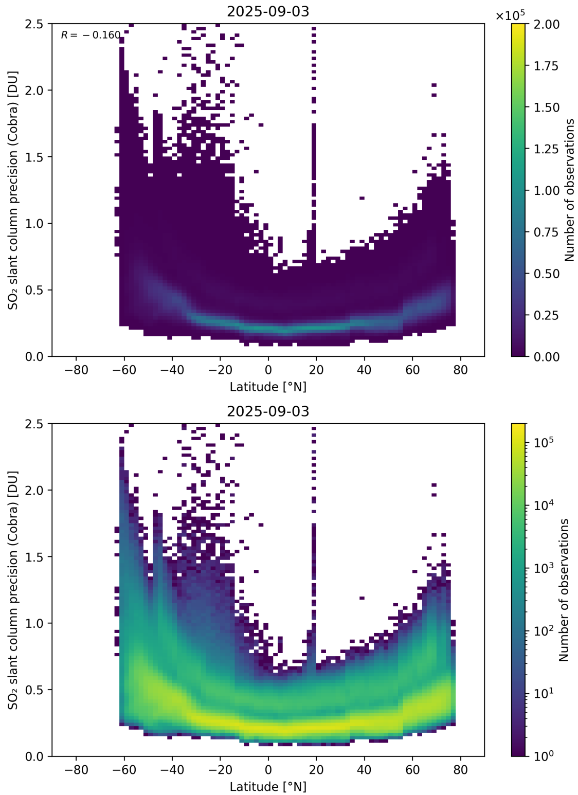
Figure 158: Scatter density plot of “Latitude” against “SO 2 slant column precision (Cobra)” for 2025-09-02 to 2025-09-04.
