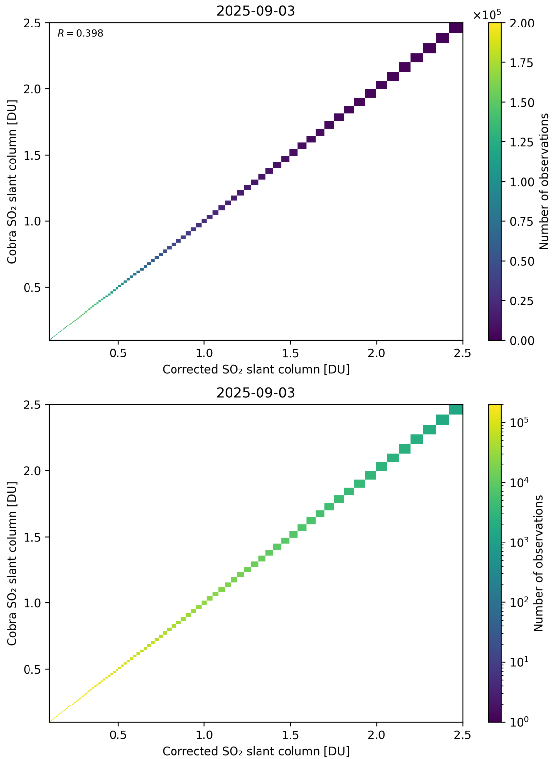
Figure 233: Scatter density plot of “Corrected SO 2 slant column” against “Cobra SO 2 slant column” for 2025-09-02 to 2025-09-04.
