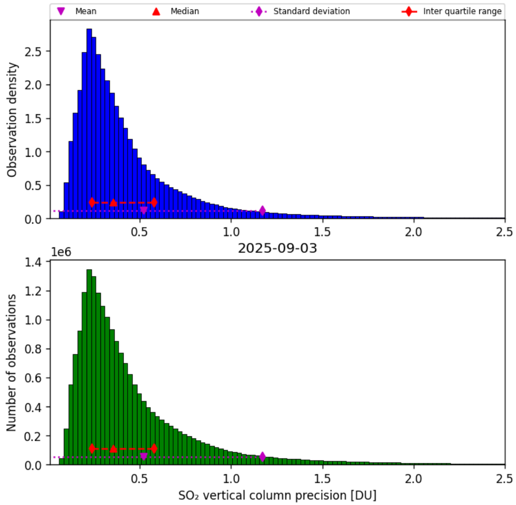
Figure 59: Histogram of “SO 2 vertical column precision” for 2025-09-02 to 2025-09-04
