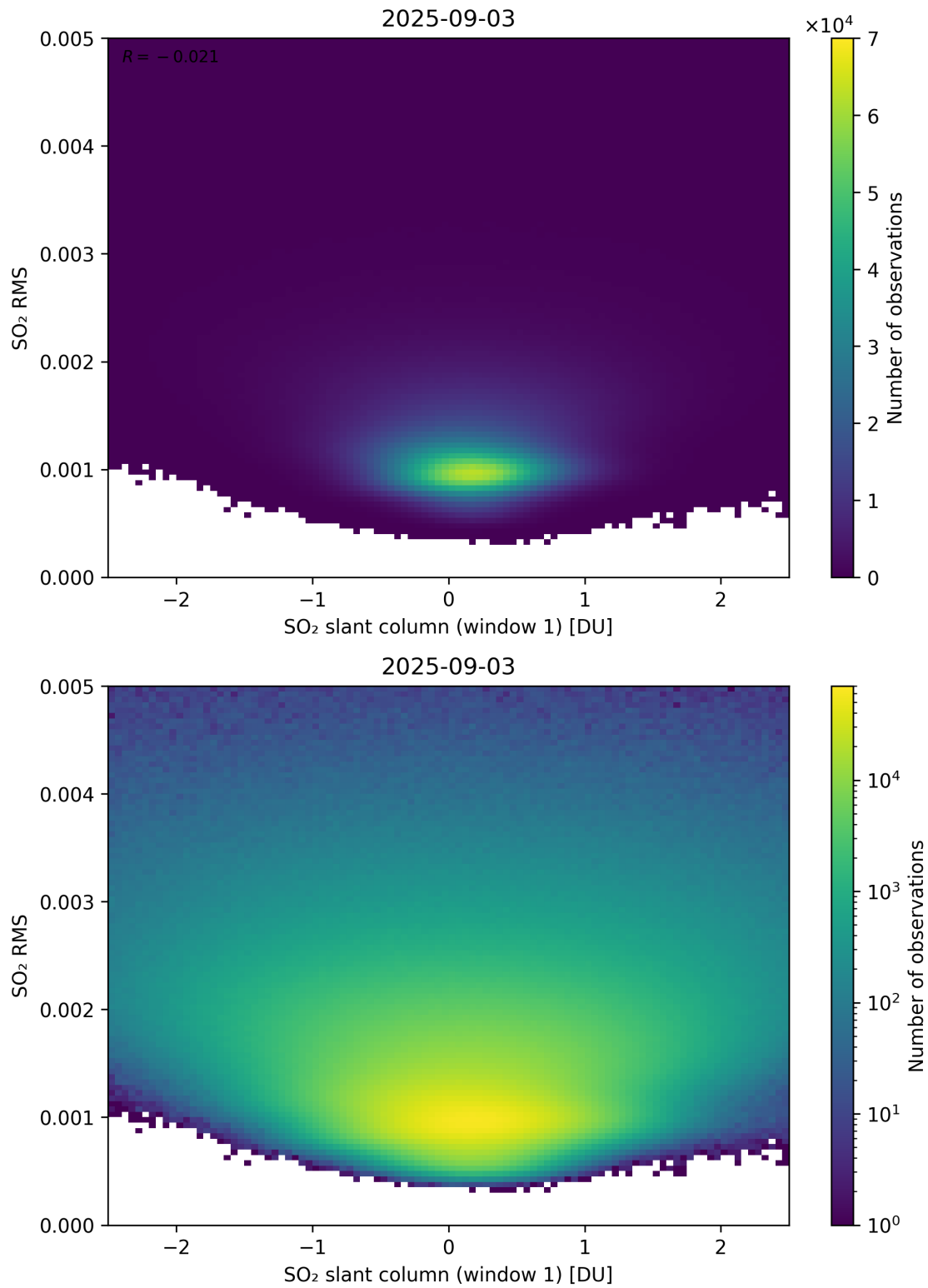
Figure 267: Scatter density plot of “SO 2 slant column (window 1)” against “SO 2 RMS” for 2025-09-02 to 2025-09-04.
