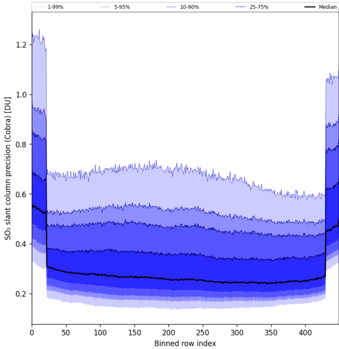
Figure 88: Along track statistics of “SO 2 slant column precision (Cobra)” for 2025-09-02 to 2025-09-04
