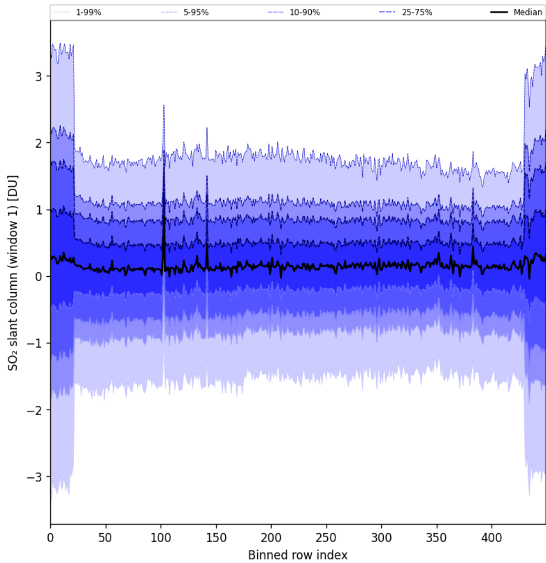
Figure 89: Along track statistics of “SO 2 slant column (window 1)” for 2025-09-02 to 2025-09-04
