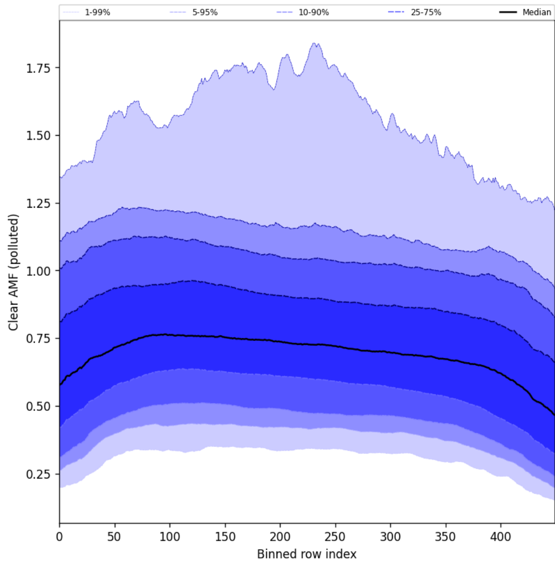
Figure 107: Along track statistics of “Clear AMF (polluted)” for 2025-09-02 to 2025-09-04
