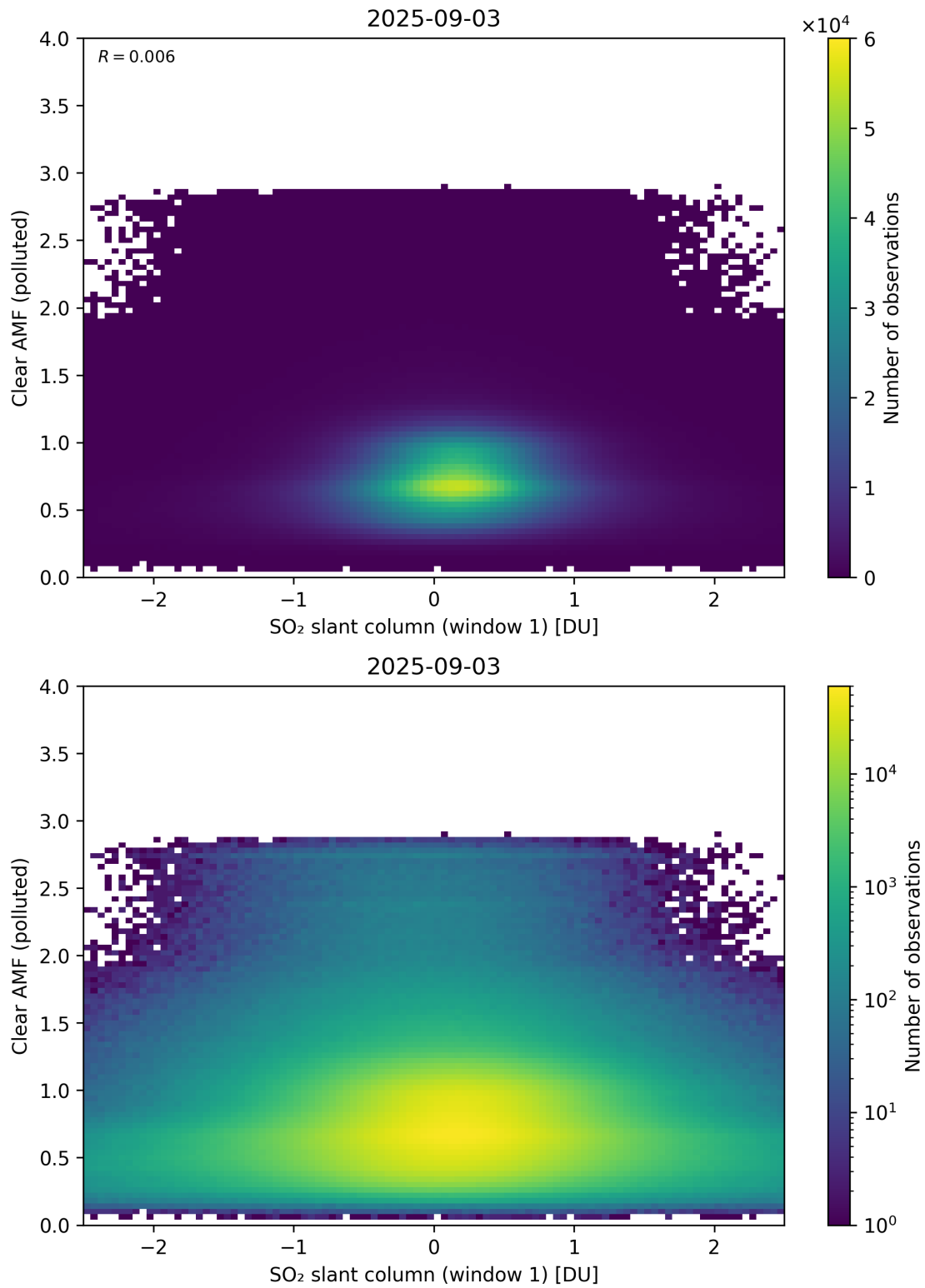
Figure 282: Scatter density plot of “SO 2 slant column (window 1)” against “Clear AMF (polluted)” for 2025-09-02 to 2025-09-04.
