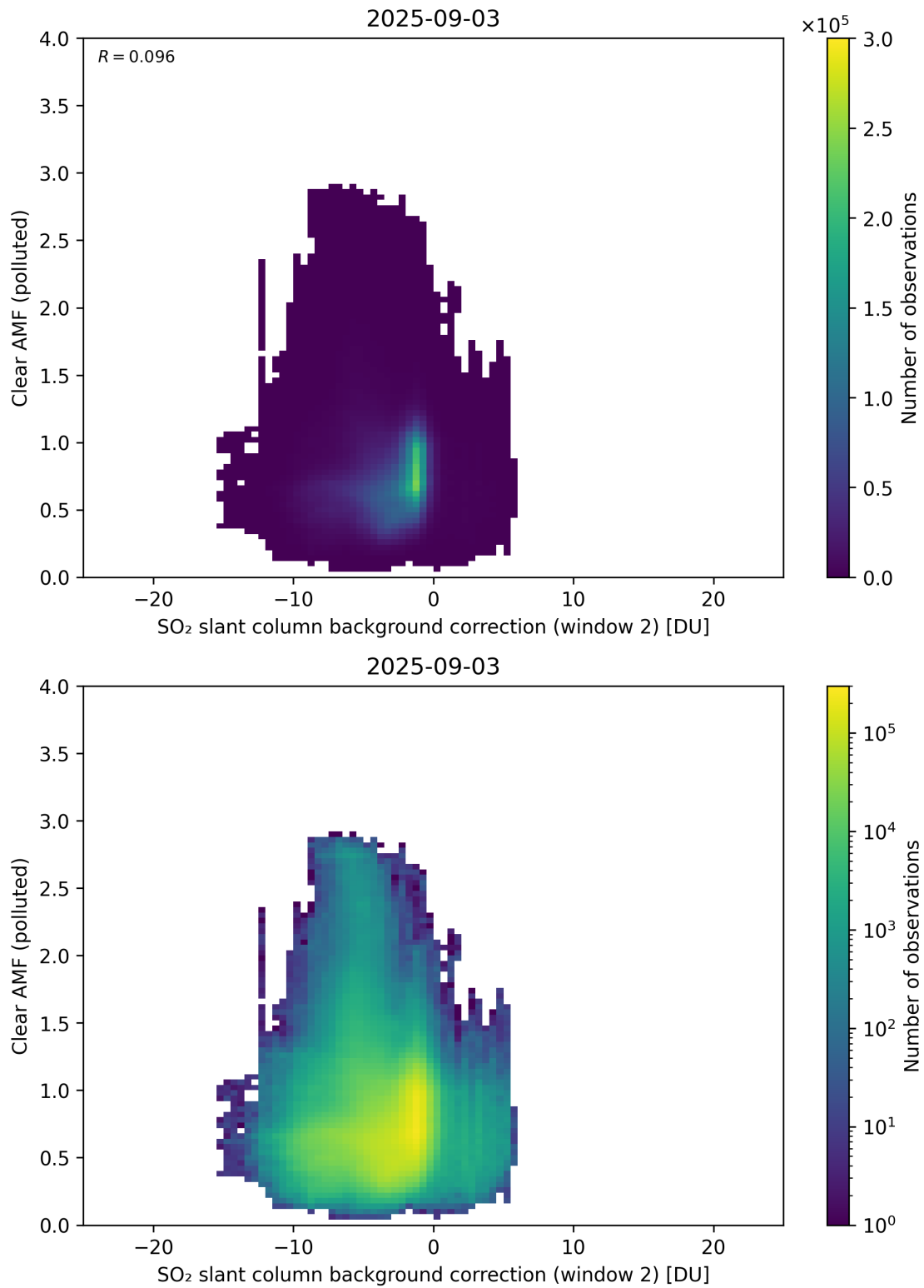
Figure 126: Scatter density plot of “SO 2 slant column background correction (window 2)” against “Clear AMF (polluted)” for 2025-09-02 to 2025-09-04.
