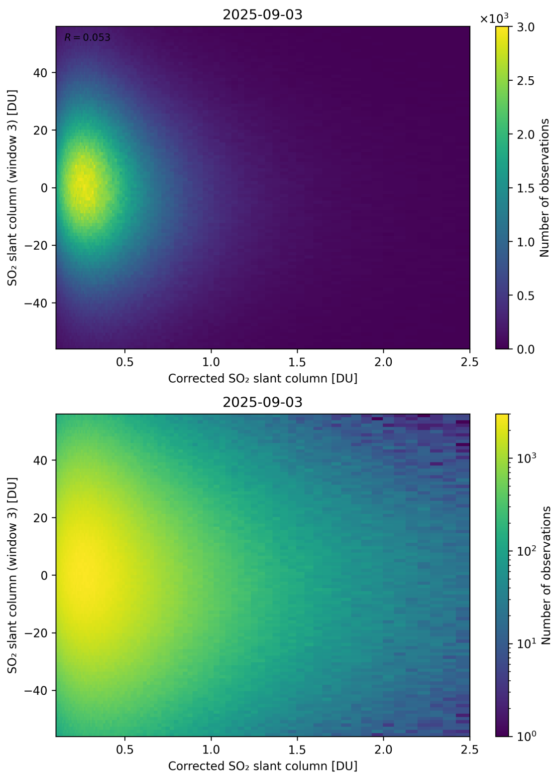
Figure 240: Scatter density plot of “Corrected SO 2 slant column” against “SO 2 slant column (window 3)” for 2025-09-02 to 2025-09-04.
