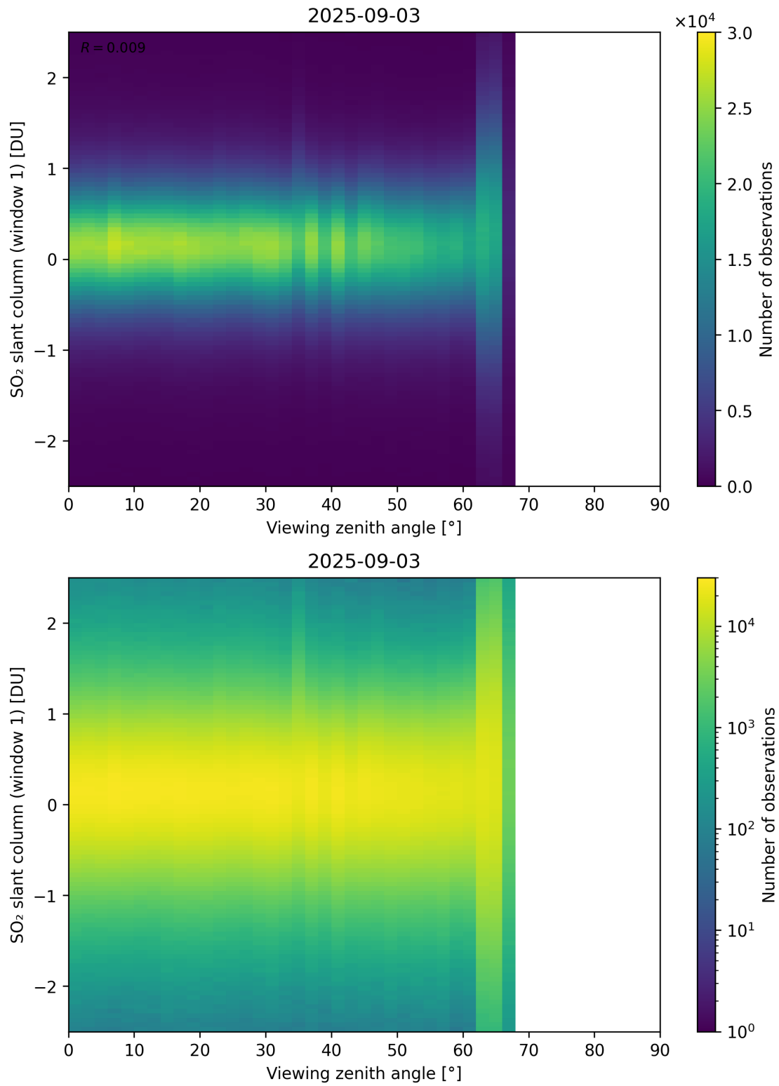
Figure 376: Scatter density plot of “Viewing zenith angle” against “SO 2 slant column (window 1)” for 2025-09-02 to 2025-09-04.
