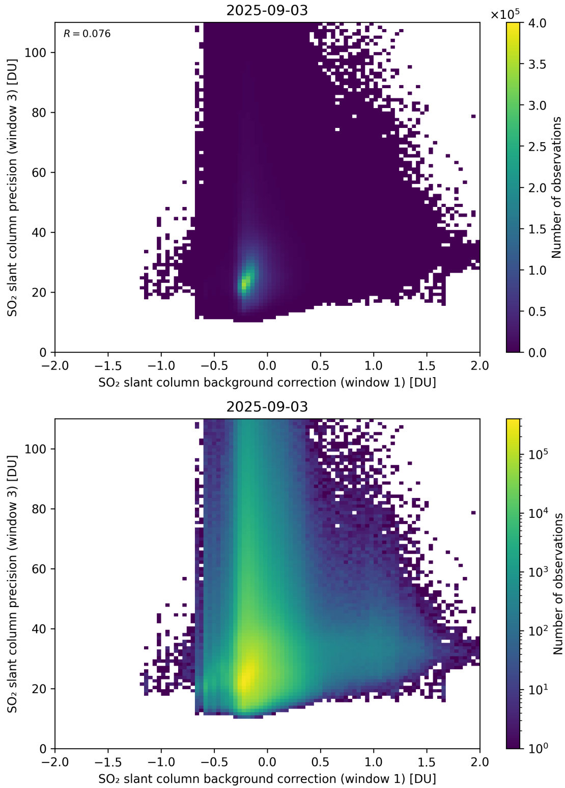
Figure 119: Scatter density plot of “SO 2 slant column background correction (window 1)” against “SO 2 slant column precision (window 3)” for 2025-09-02 to 2025-09-04.
