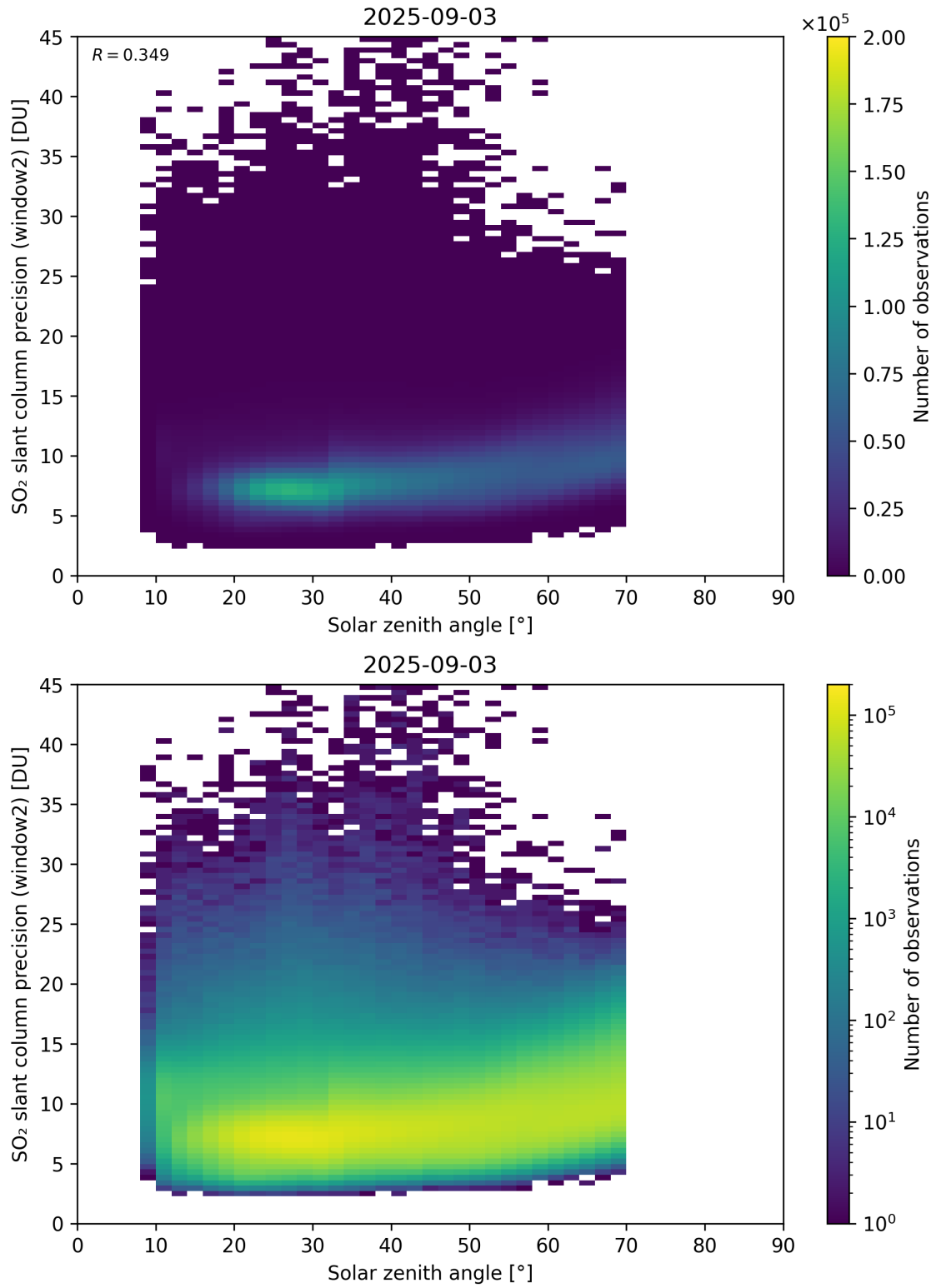
Figure 186: Scatter density plot of “Solar zenith angle” against “SO 2 slant column precision (window2)” for 2025-09-02 to 2025-09-04.
