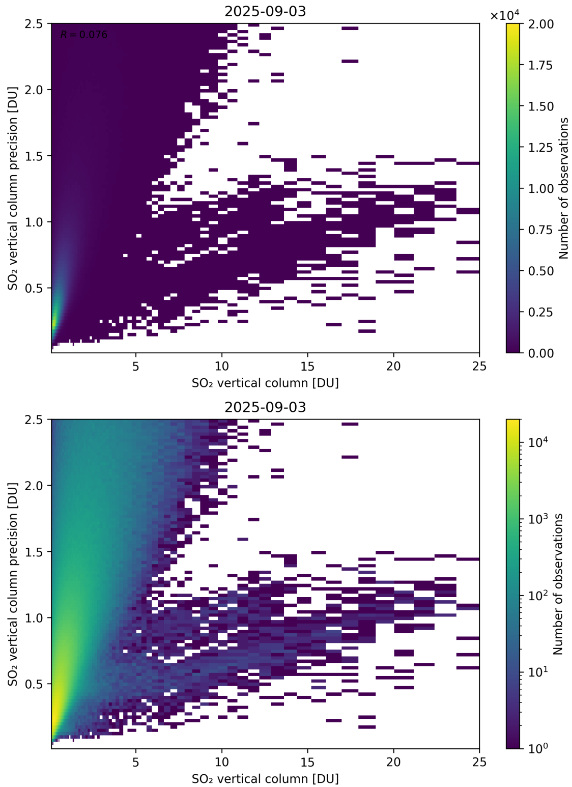
Figure 361: Scatter density plot of “SO 2 vertical column” against “SO 2 vertical column precision” for 2025-09-02 to 2025-09-04.
