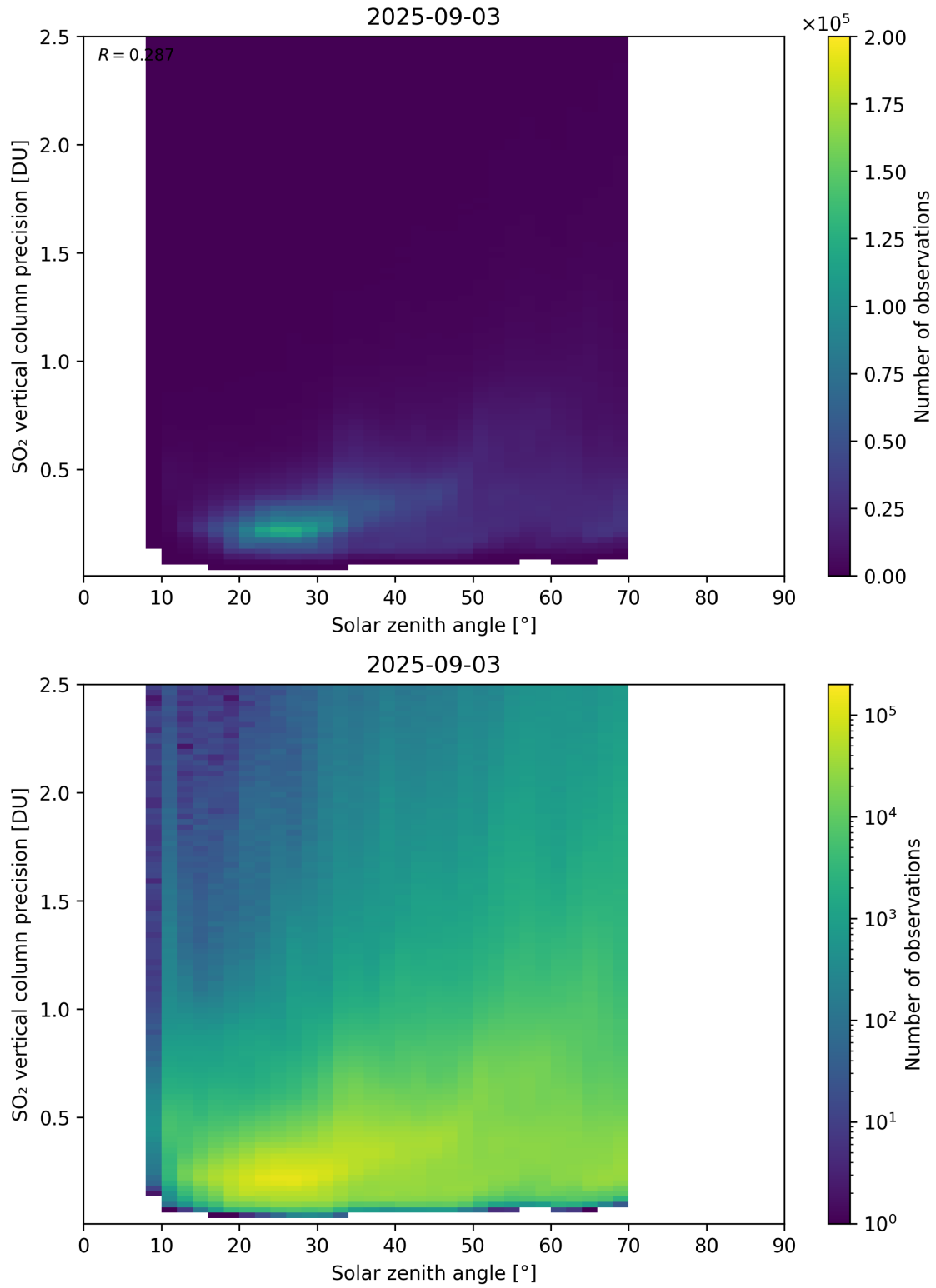
Figure 192: Scatter density plot of “Solar zenith angle” against “SO 2 vertical column precision” for 2025-09-02 to 2025-09-04.
