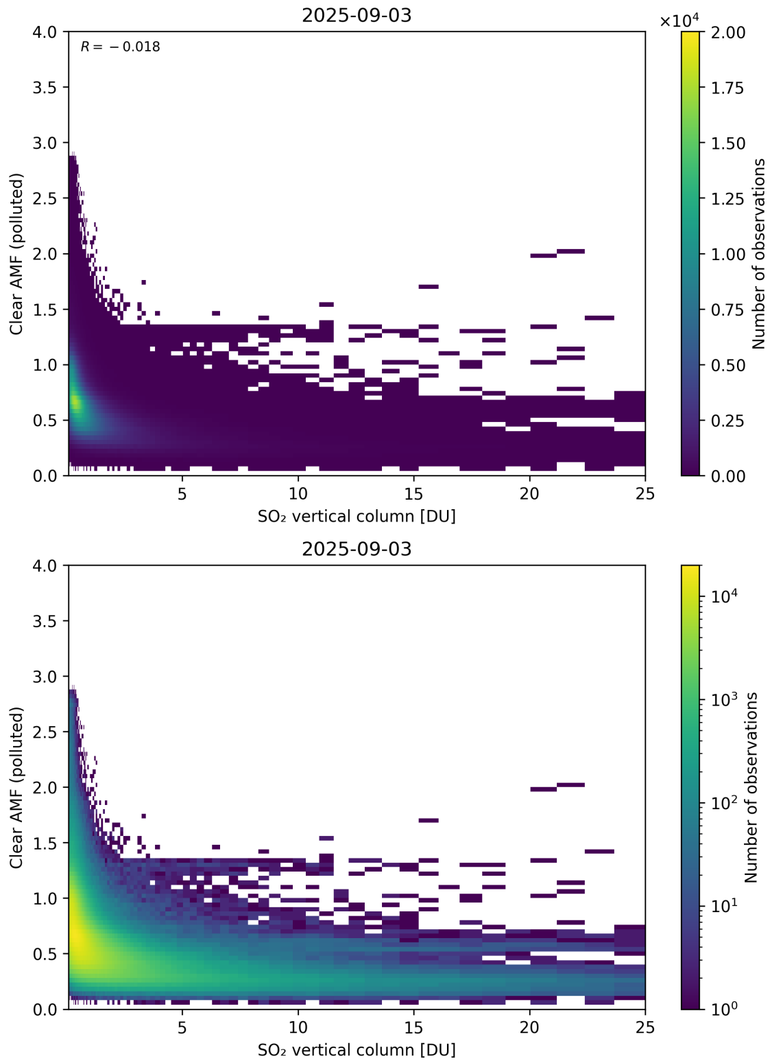
Figure 348: Scatter density plot of “SO 2 vertical column” against “Clear AMF (polluted)” for 2025-09-02 to 2025-09-04.
