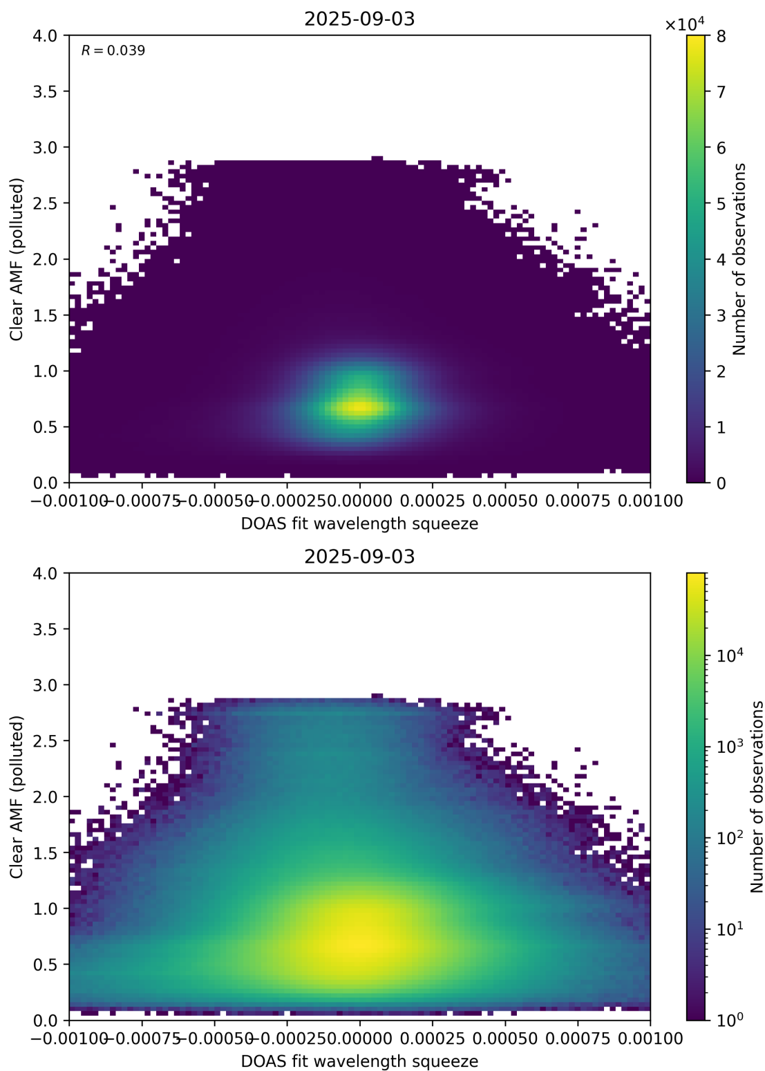
Figure 144: Scatter density plot of “DOAS fit wavelength squeeze” against “Clear AMF (polluted)” for 2025-09-02 to 2025-09-04.
