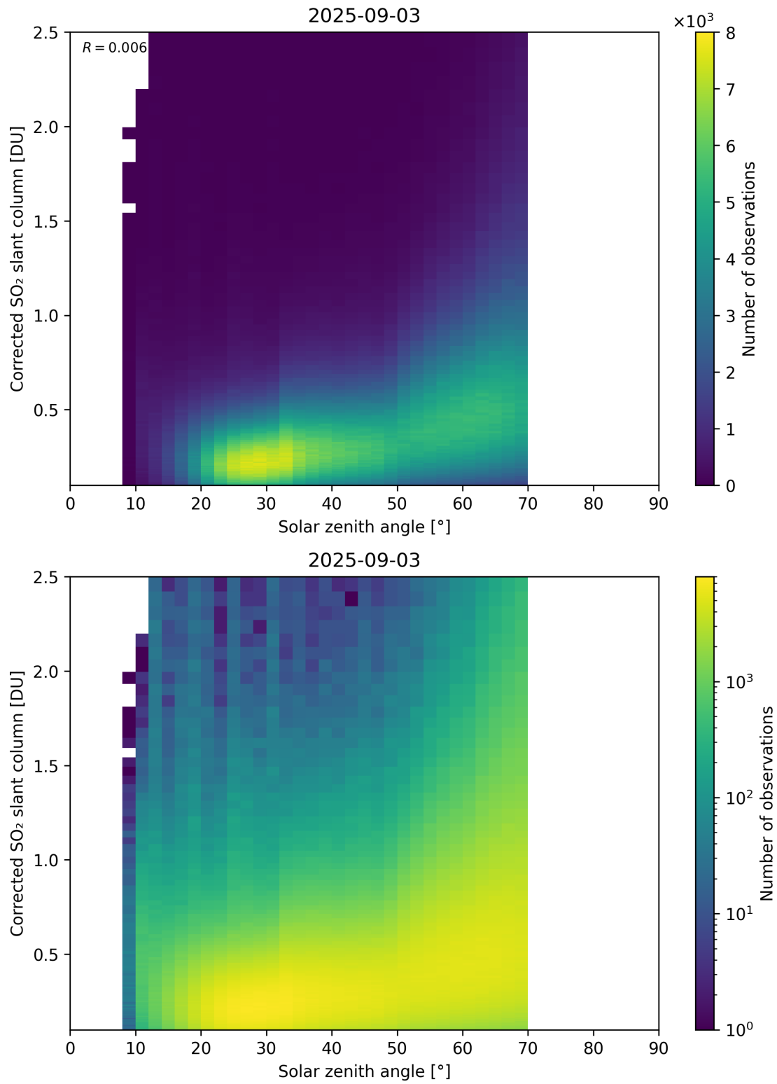
Figure 181: Scatter density plot of “Solar zenith angle” against “Corrected SO 2 slant column” for 2025-09-02 to 2025-09-04.
