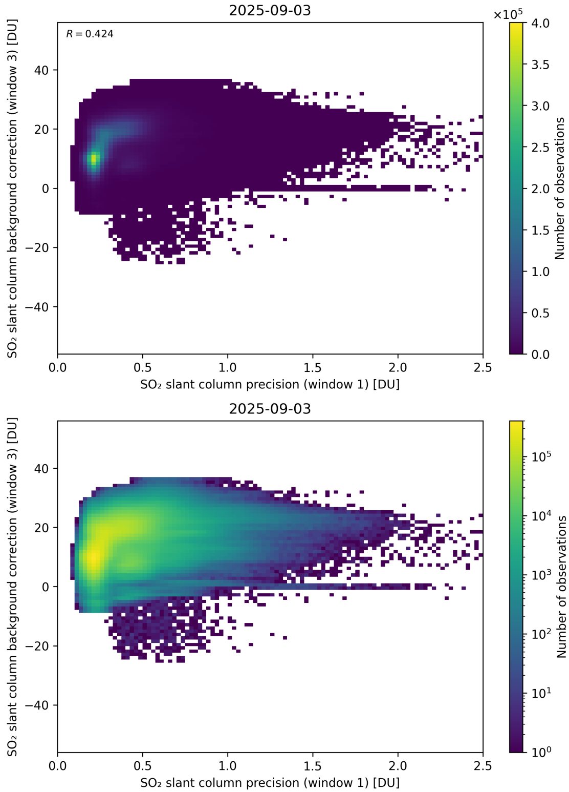
Figure 270: Scatter density plot of “SO 2 slant column precision (window 1)” against “SO 2 slant column background correction (window 3)” for 2025-09-02 to 2025-09-04.
