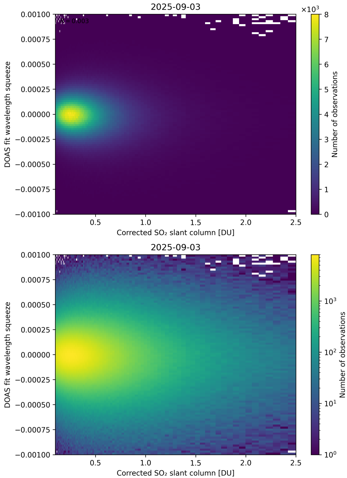
Figure 230: Scatter density plot of "Corrected SO 2 slant column" against "DOAS fit wavelength squeeze" for 2025-09-02 to 2025-09-04.
