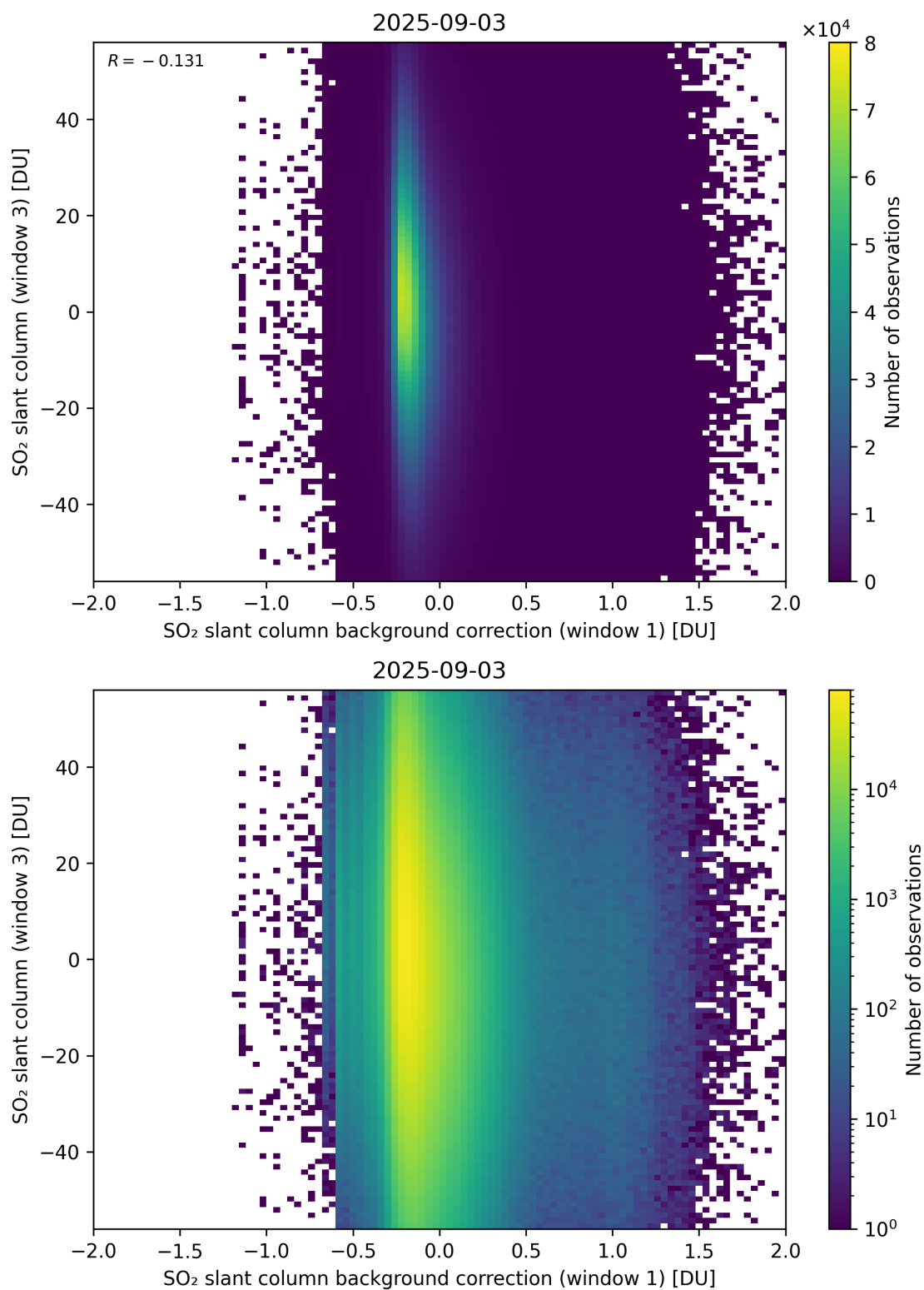
Figure 118: Scatter density plot of “SO 2 slant column background correction (window 1)” against “SO 2 slant column (window 3)” for 2025-09-02 to 2025-09-04.
