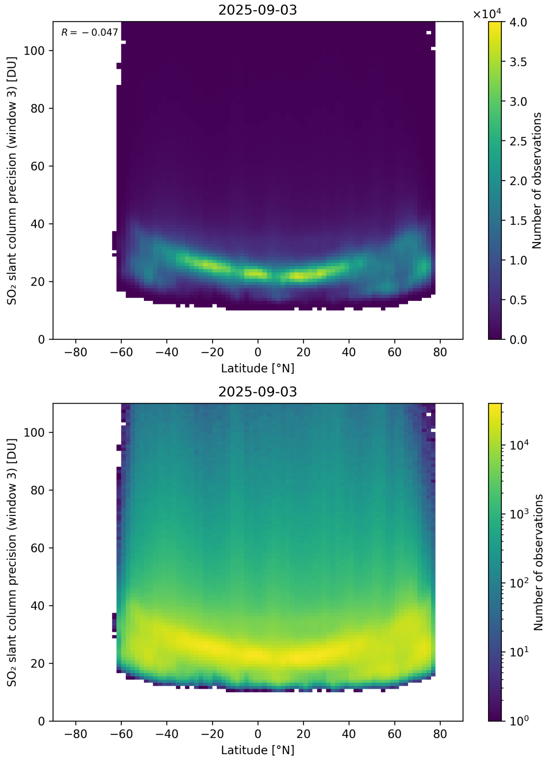
Figure 166: Scatter density plot of “Latitude” against “SO 2 slant column precision (window 3)” for 2025-09-02 to 2025-09-04.
