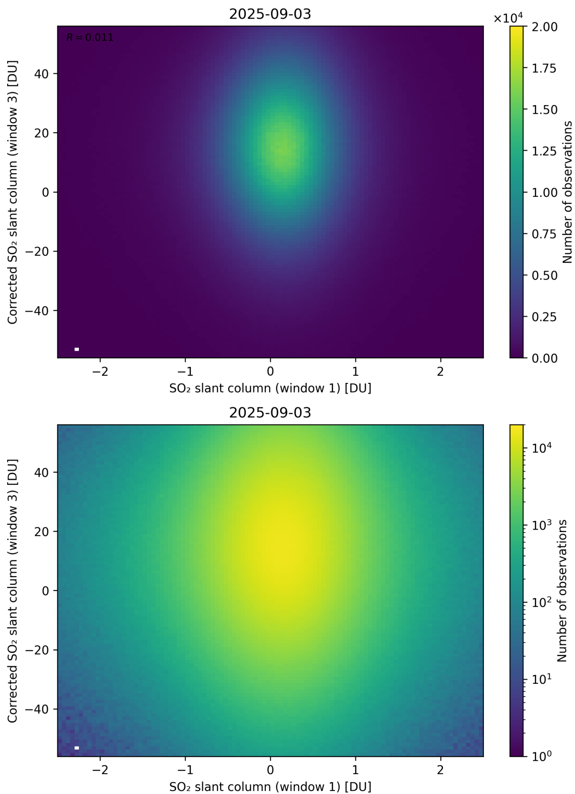
Figure 284: Scatter density plot of “SO 2 slant column (window 1)” against “Corrected SO 2 slant column (window 3)” for 2025-09-02 to 2025-09-04.
