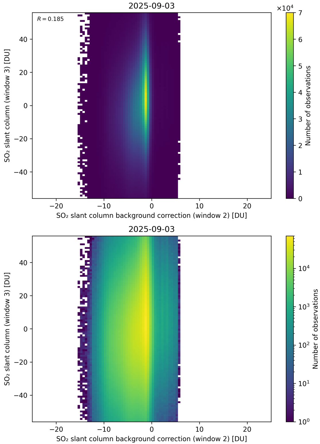
Figure 128: Scatter density plot of “SO 2 slant column background correction (window 2)” against “SO 2 slant column (window 3)” for 2025-09-02 to 2025-09-04.
