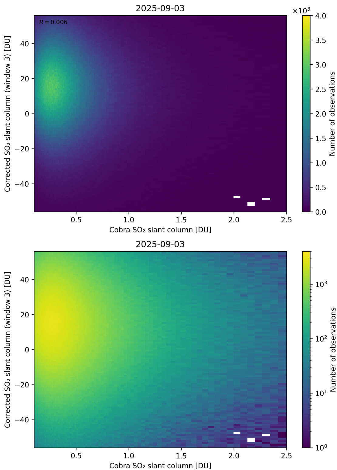
Figure 218: Scatter density plot of “Cobra SO 2 slant column” against “Corrected SO 2 slant column (window 3)” for 2025-09-02 to 2025-09-04.
