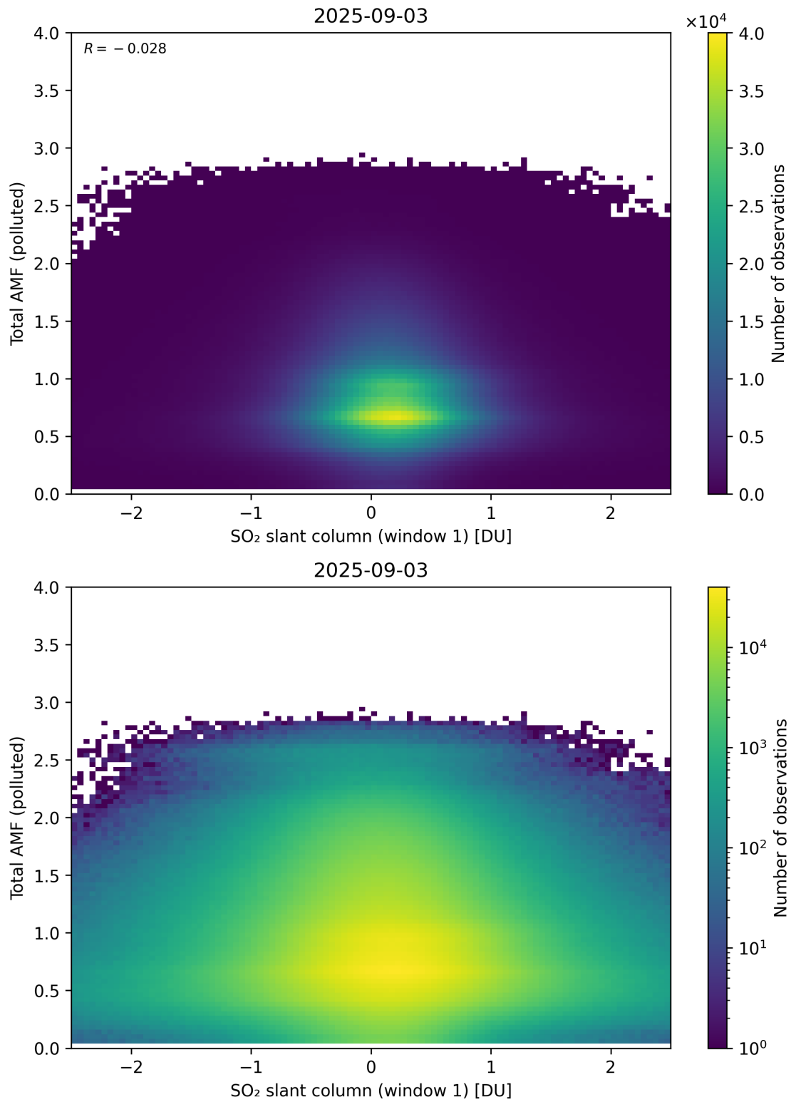
Figure 289: Scatter density plot of “SO 2 slant column (window 1)” against “Total AMF (polluted)” for 2025-09-02 to 2025-09-04.
