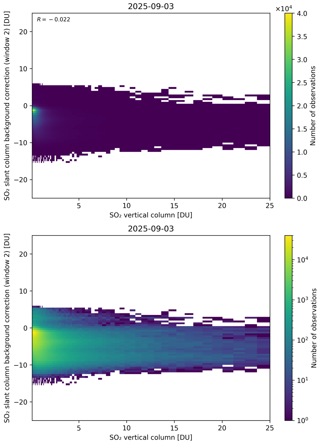
Figure 324: Scatter density plot of “SO 2 vertical column” against “SO 2 slant column background correction (window 2)” for 2025-09-02 to 2025-09-04.
