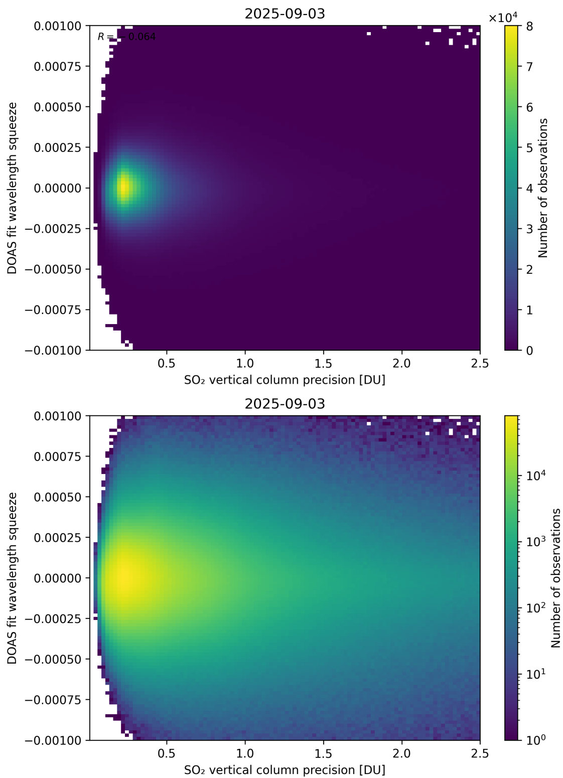
Figure 333: Scatter density plot of “SO 2 vertical column precision” against “DOAS fit wavelength squeeze” for 2025-09-02 to 2025-09-04.
