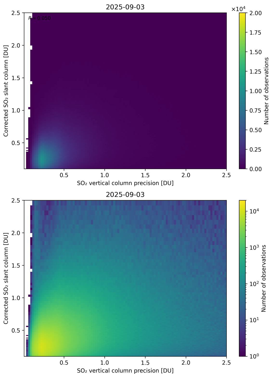
Figure 338: Scatter density plot of “SO 2 vertical column precision” against “Corrected SO 2 slant column” for 2025-09-02 to 2025-09-04.
