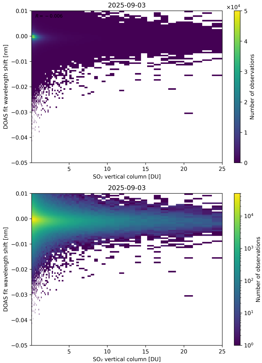
Figure 326: Scatter density plot of “SO 2 vertical column” against “DOAS fit wavelength shift” for 2025-09-02 to 2025-09-04.
