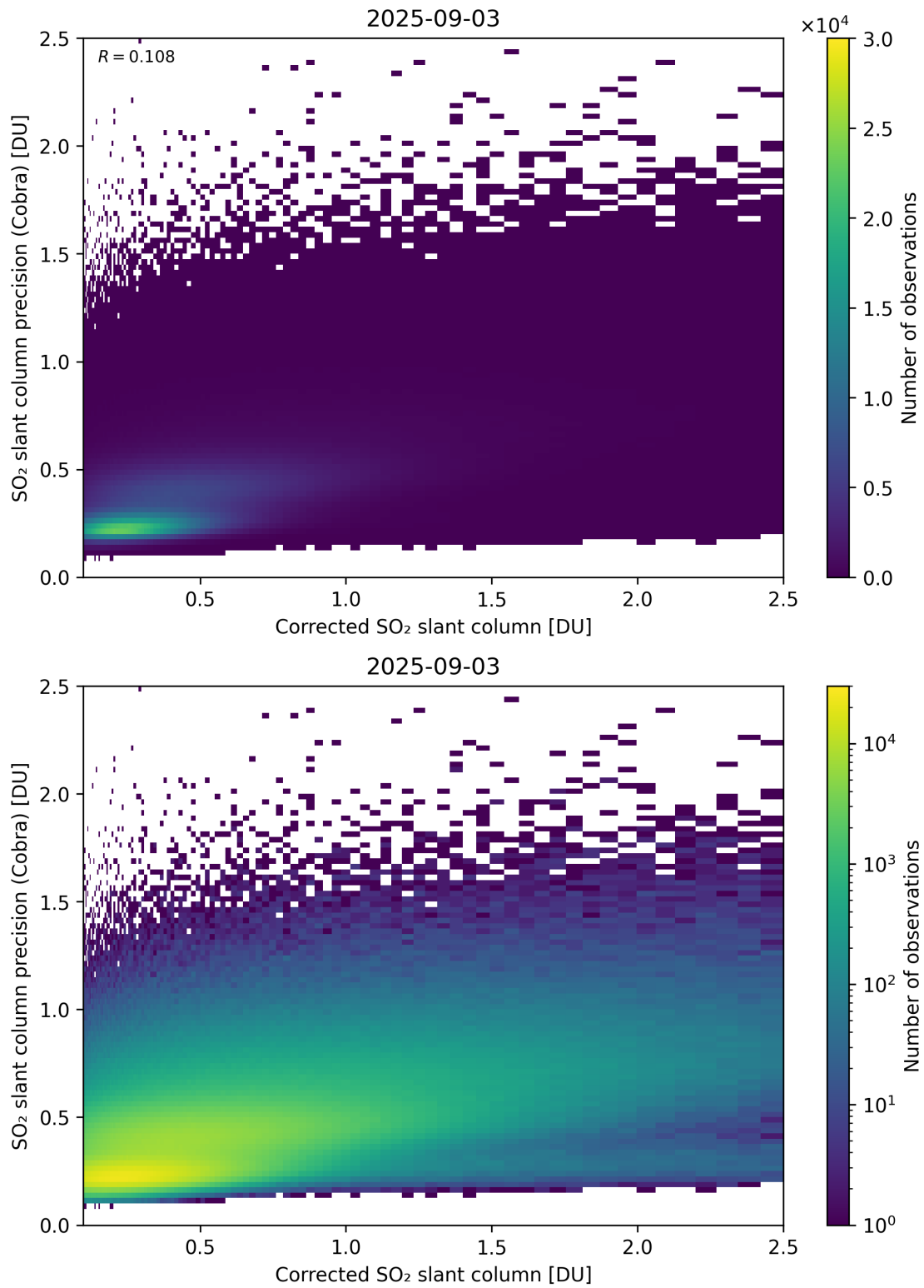
Figure 234: Scatter density plot of “Corrected SO 2 slant column” against “SO 2 slant column precision (Cobra)” for 2025-09-02 to 2025-09-04.
