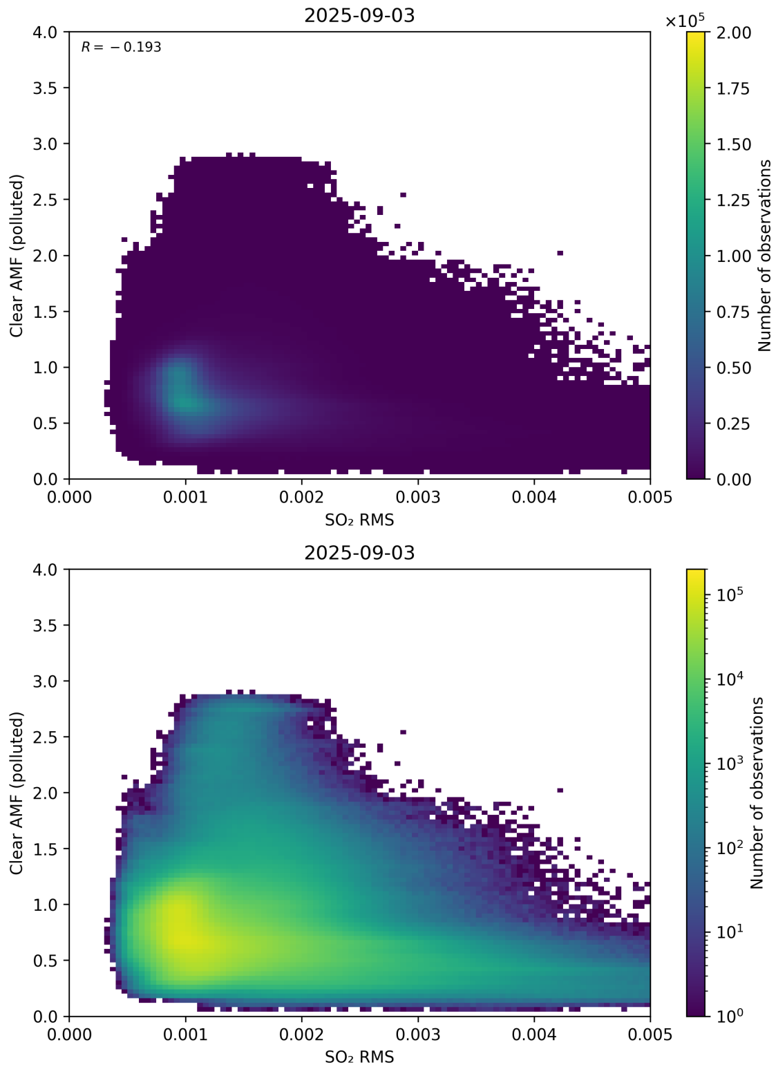
Figure 147: Scatter density plot of “SO 2 RMS” against “Clear AMF (polluted)” for 2025-09-02 to 2025-09-04.
