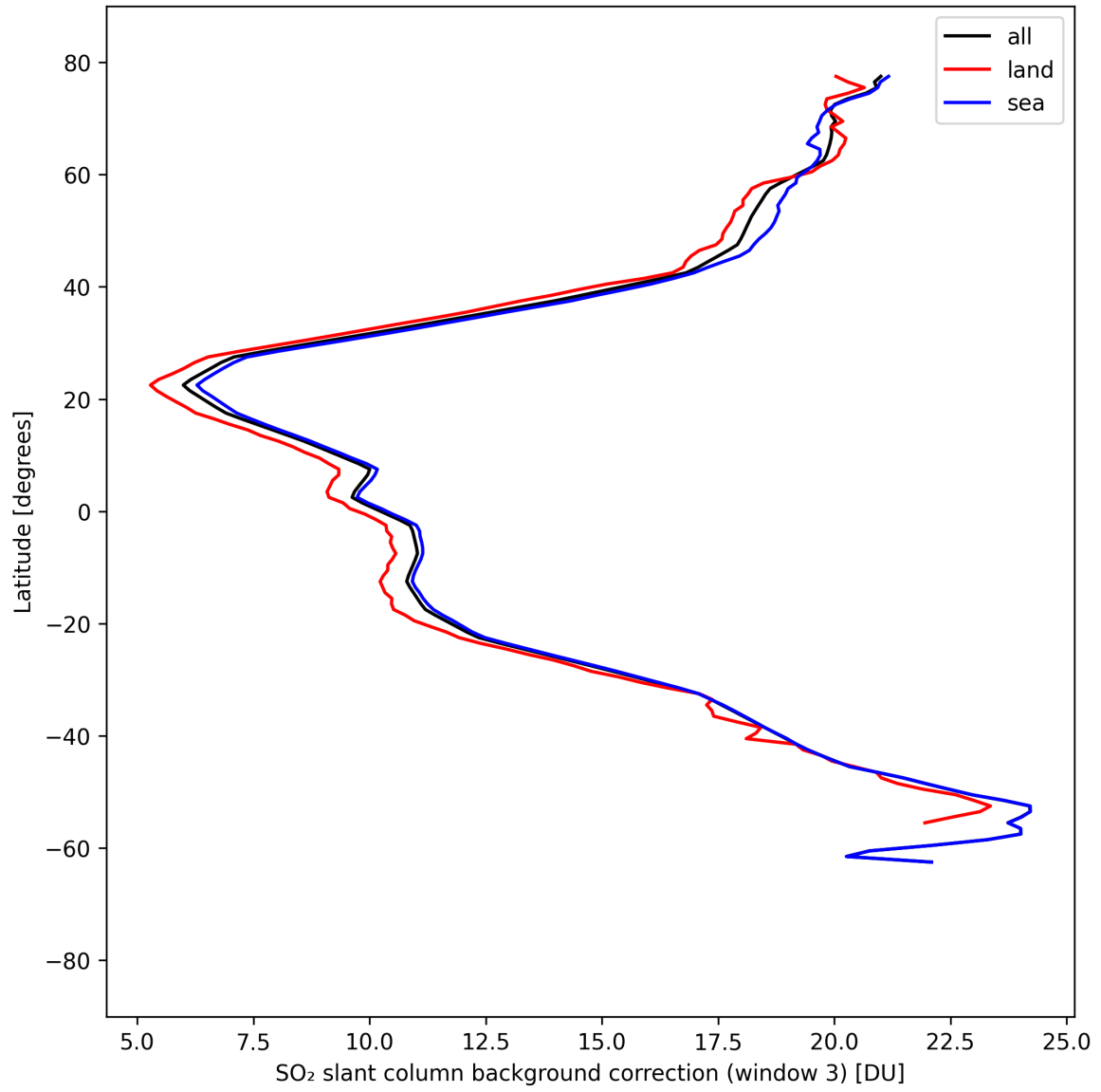
Figure 48: Zonal average of “SO 2 slant column background correction (window 3)” for 2025-09-02 to 2025-09-04.
