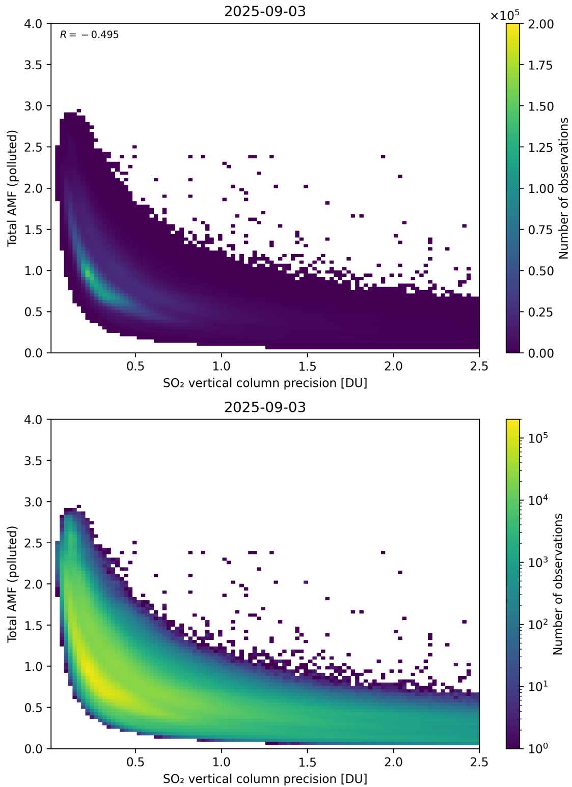
Figure 346: Scatter density plot of “SO 2 vertical column precision” against “Total AMF (polluted)” for 2025-09-02 to 2025-09-04.
