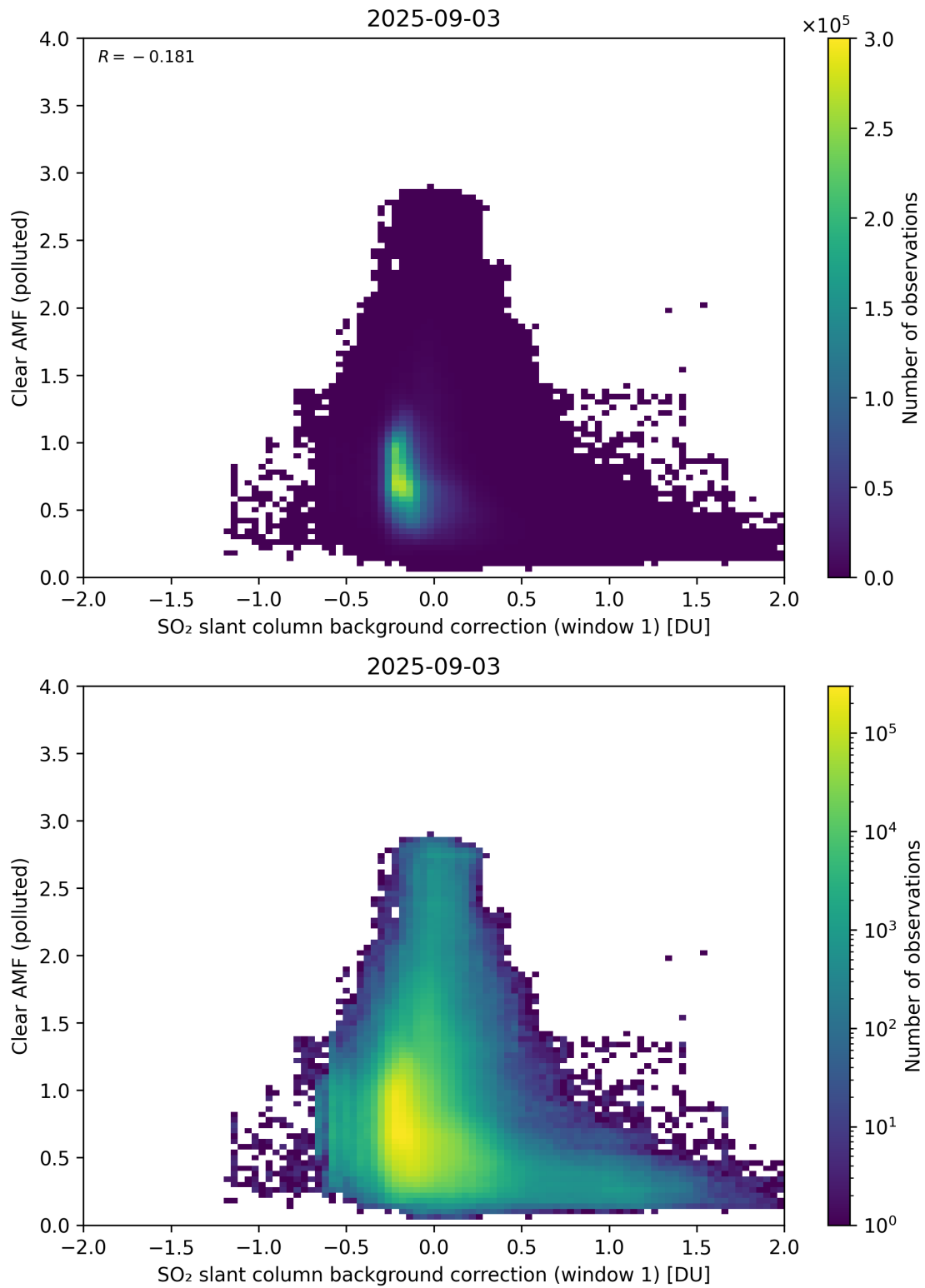
Figure 114: Scatter density plot of “SO 2 slant column background correction (window 1)” against “Clear AMF (polluted)” for 2025-09-02 to 2025-09-04.
