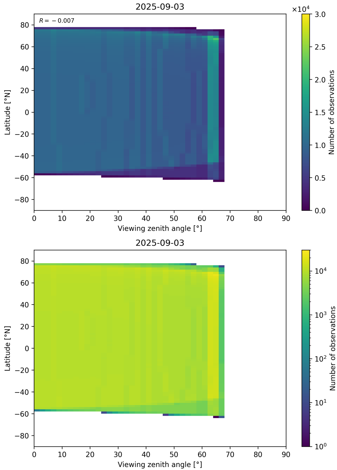
Figure 368: Scatter density plot of “Viewing zenith angle” against “Latitude” for 2025-09-02 to 2025-09-04.
