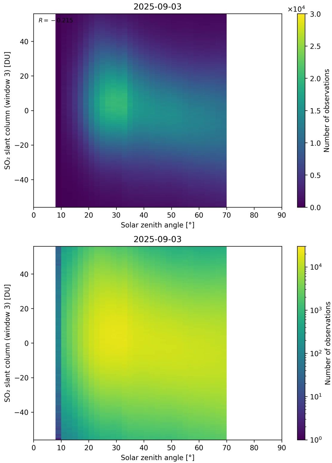
Figure 187: Scatter density plot of “Solar zenith angle” against “SO 2 slant column (window 3)” for 2025-09-02 to 2025-09-04.
