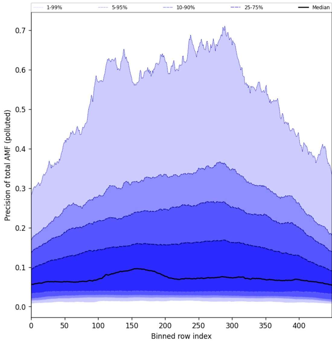
Figure 106: Along track statistics of “Precision of total AMF (polluted)” for 2025-09-02 to 2025-09-04
