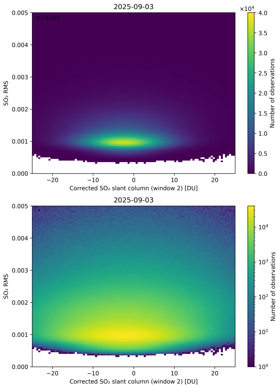
Figure 248: Scatter density plot of “Corrected SO 2 slant column (window 2)” against “SO 2 RMS” for 2025-09-02 to 2025-09-04.
