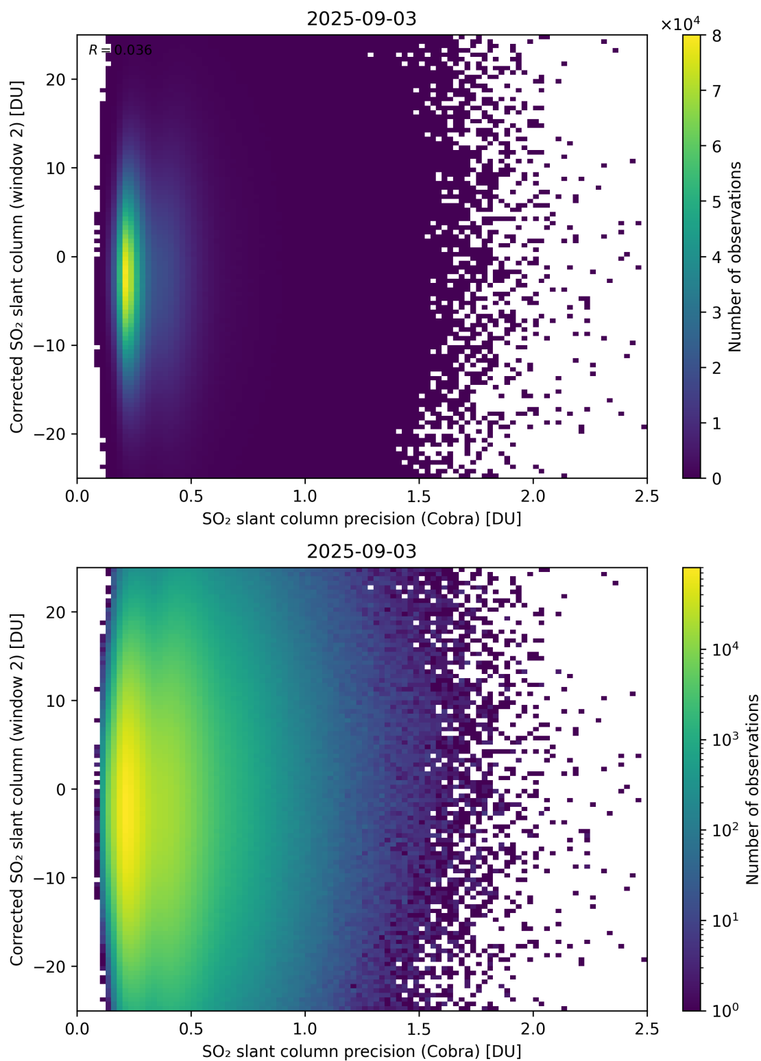
Figure 206: Scatter density plot of “SO 2 slant column precision (Cobra)” against “Corrected SO 2 slant column (window 2)” for 2025-09-02 to 2025-09-04.
