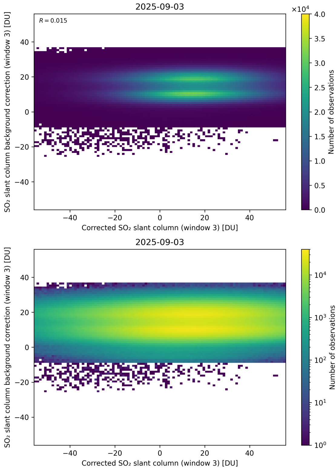
Figure 255: Scatter density plot of “Corrected SO 2 slant column (window 3)” against “SO 2 slant column background correction (window 3)” for 2025-09-02 to 2025-09-04.
