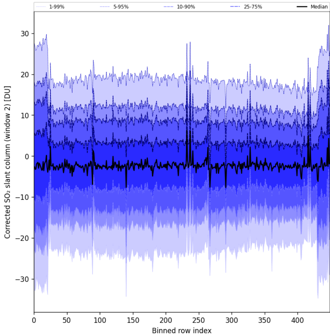
Figure 95: Along track statistics of “Corrected SO 2 slant column (window 2)” for 2025-09-02 to 2025-09-04
