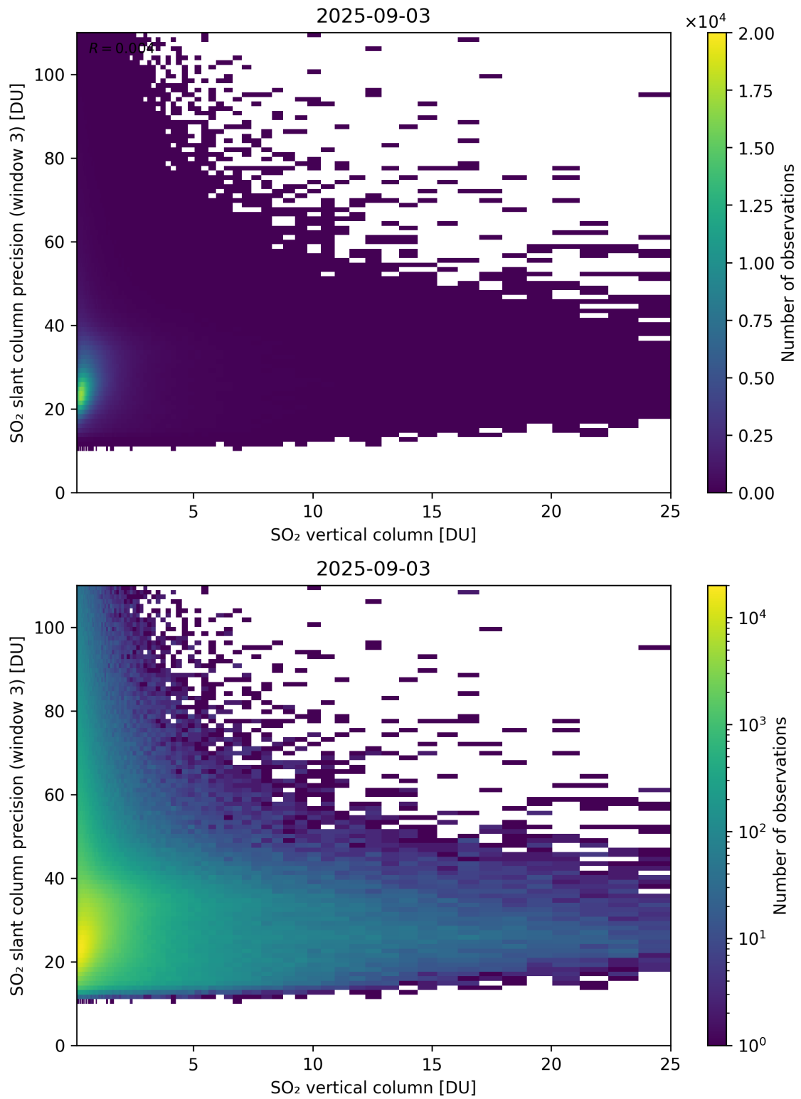
Figure 358: Scatter density plot of “SO 2 vertical column” against “SO 2 slant column precision (window 3)” for 2025-09-02 to 2025-09-04.
