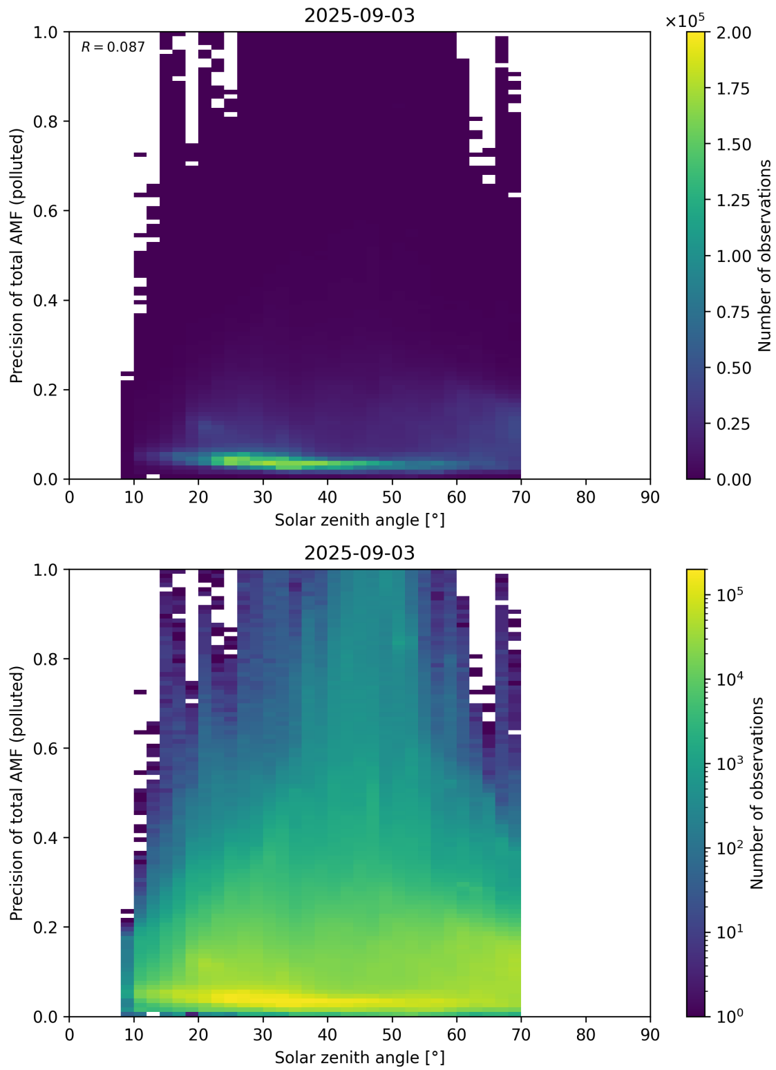
Figure 190: Scatter density plot of “Solar zenith angle” against “Precision of total AMF (polluted)” for 2025-09-02 to 2025-09-04.
