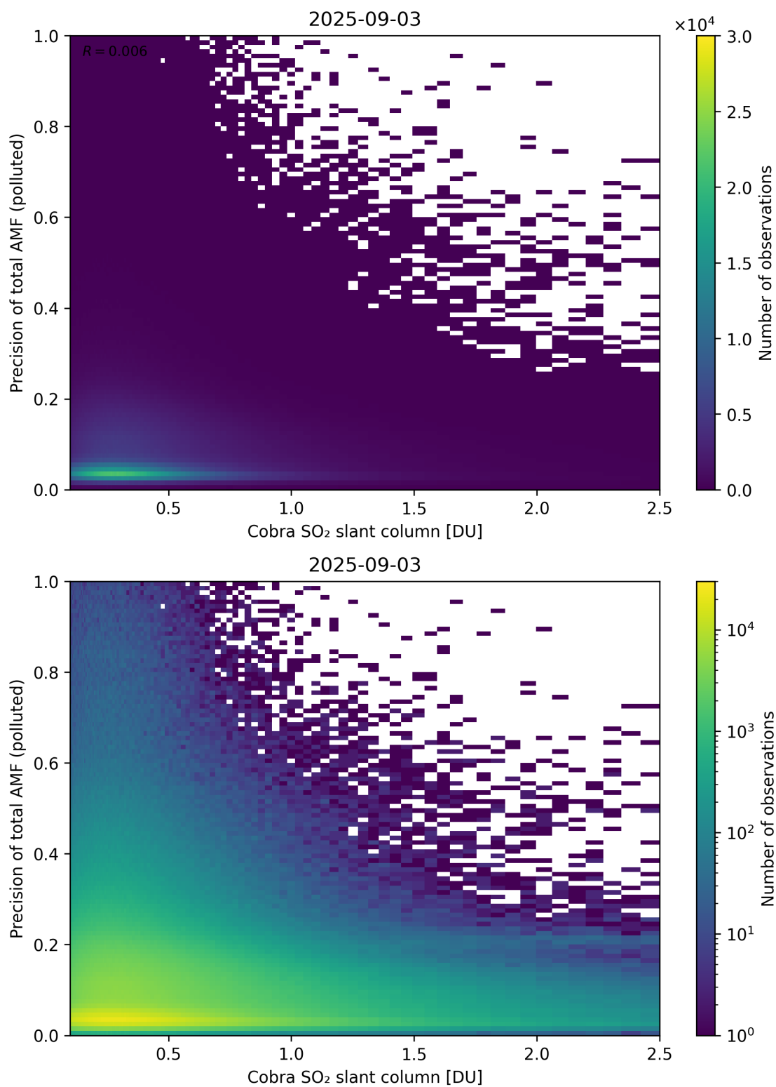
Figure 225: Scatter density plot of “Cobra SO 2 slant column” against “Precision of total AMF (polluted)” for 2025-09-02 to 2025-09-04.
