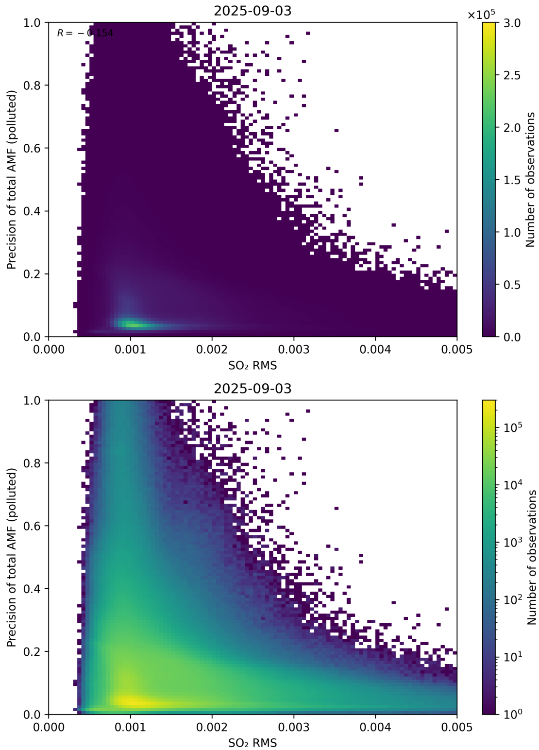
Figure 149: Scatter density plot of “SO 2 RMS” against “Precision of total AMF (polluted)” for 2025-09-02 to 2025-09-04.
