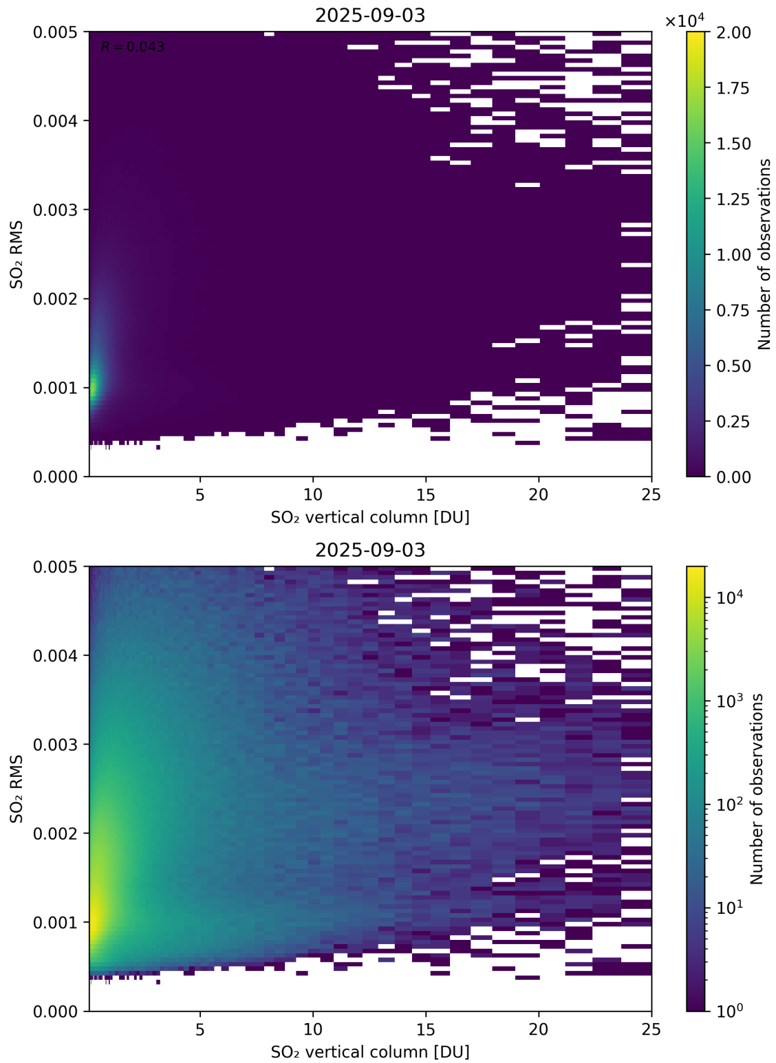
Figure 328: Scatter density plot of “SO 2 vertical column” against “SO 2 RMS” for 2025-09-02 to 2025-09-04.
