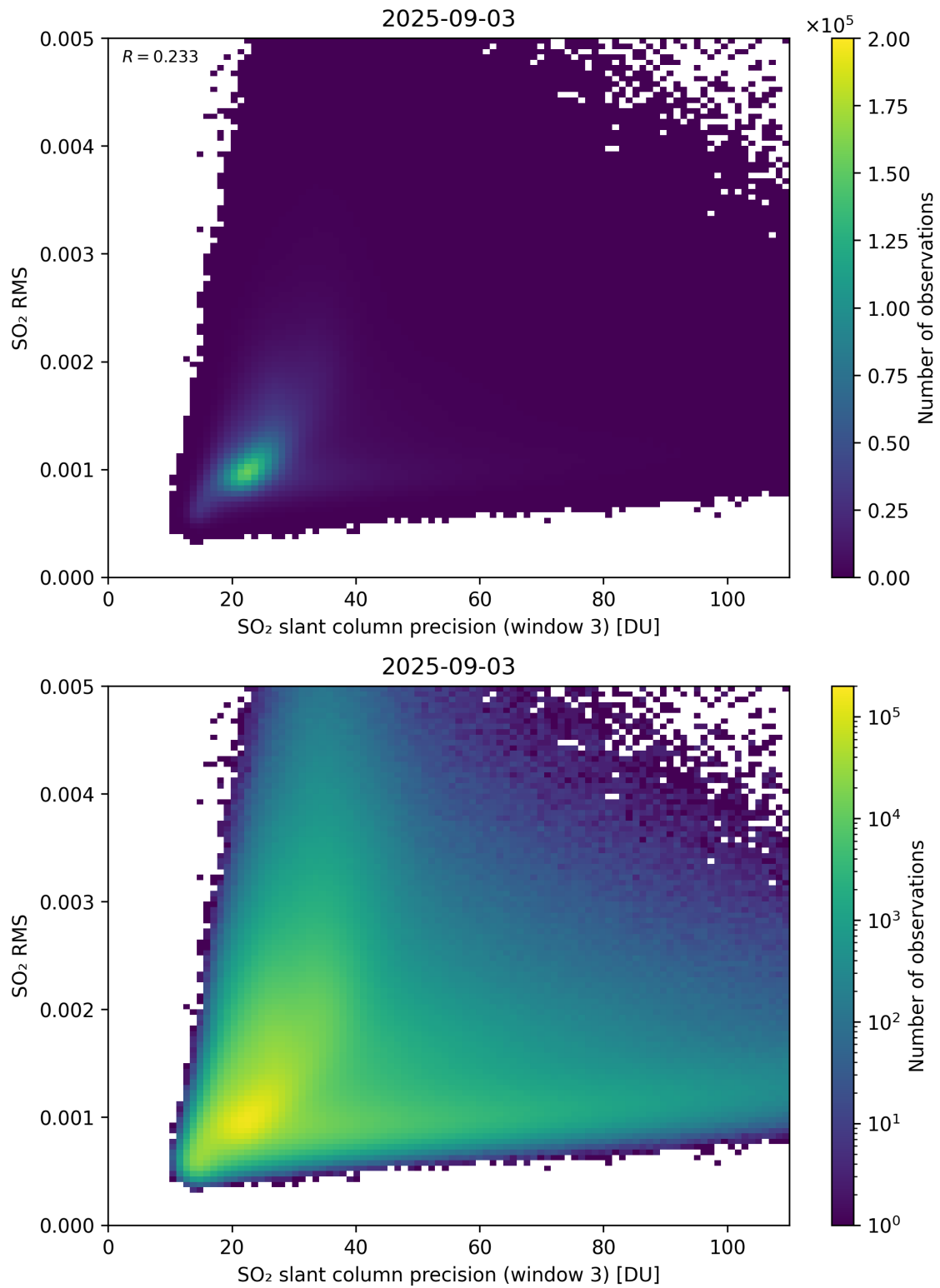
Figure 310: Scatter density plot of “SO 2 slant column precision (window 3)” against “SO 2 RMS” for 2025-09-02 to 2025-09-04.
