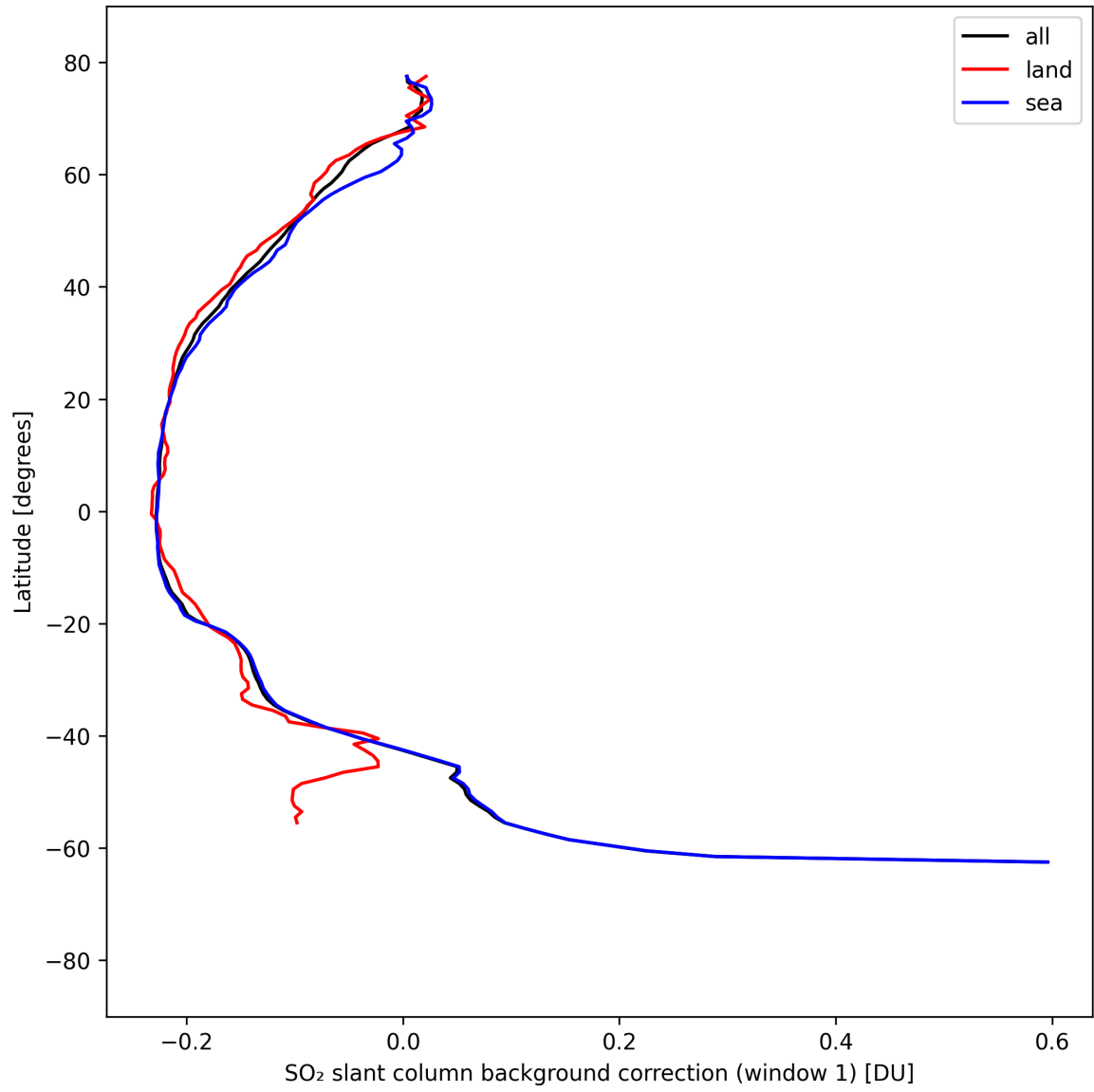
Figure 40: Zonal average of “SO 2 slant column background correction (window 1)” for 2025-09-02 to 2025-09-04.
