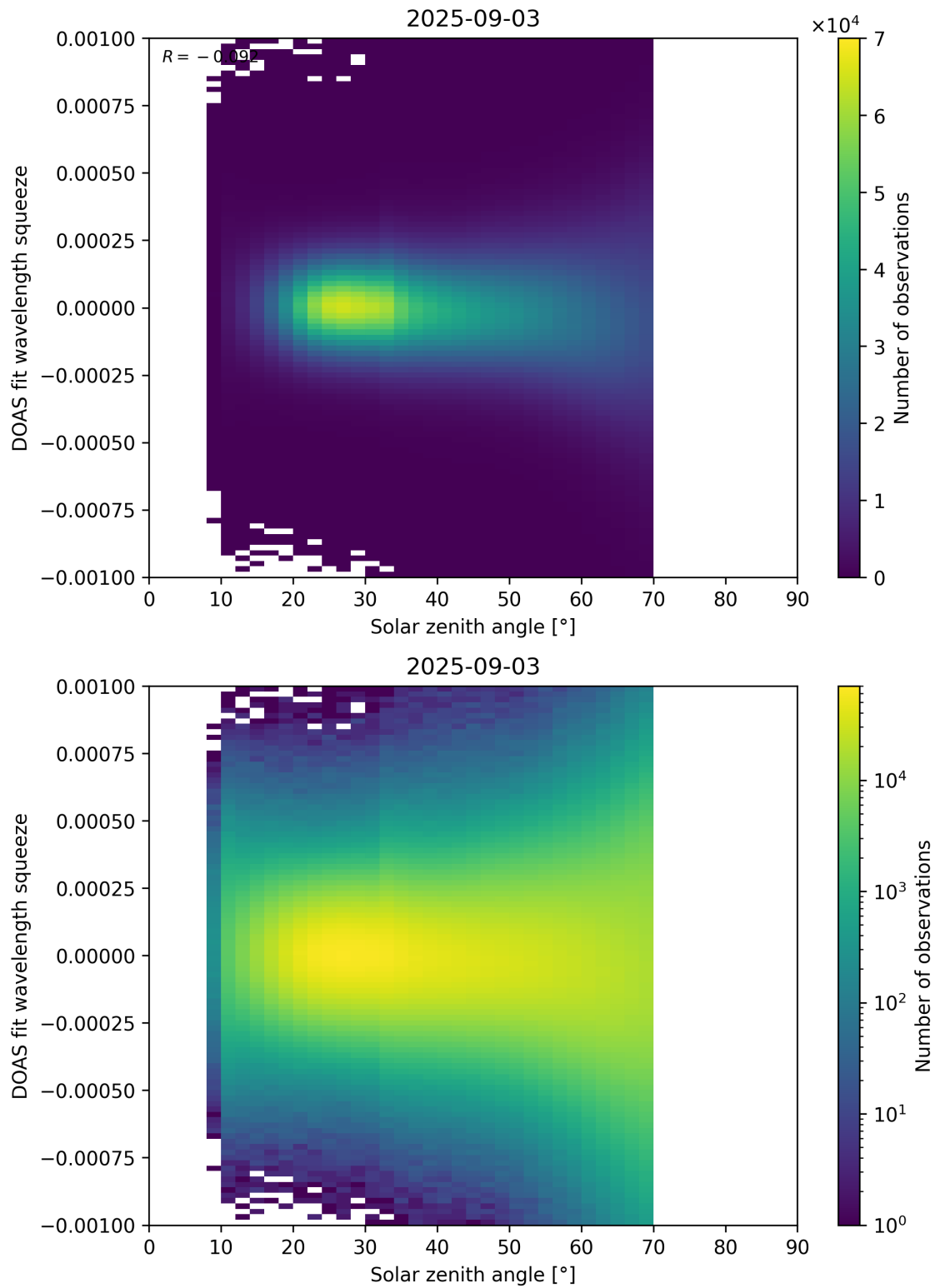
Figure 175: Scatter density plot of “Solar zenith angle” against “DOAS fit wavelength squeeze” for 2025-09-02 to 2025-09-04.
