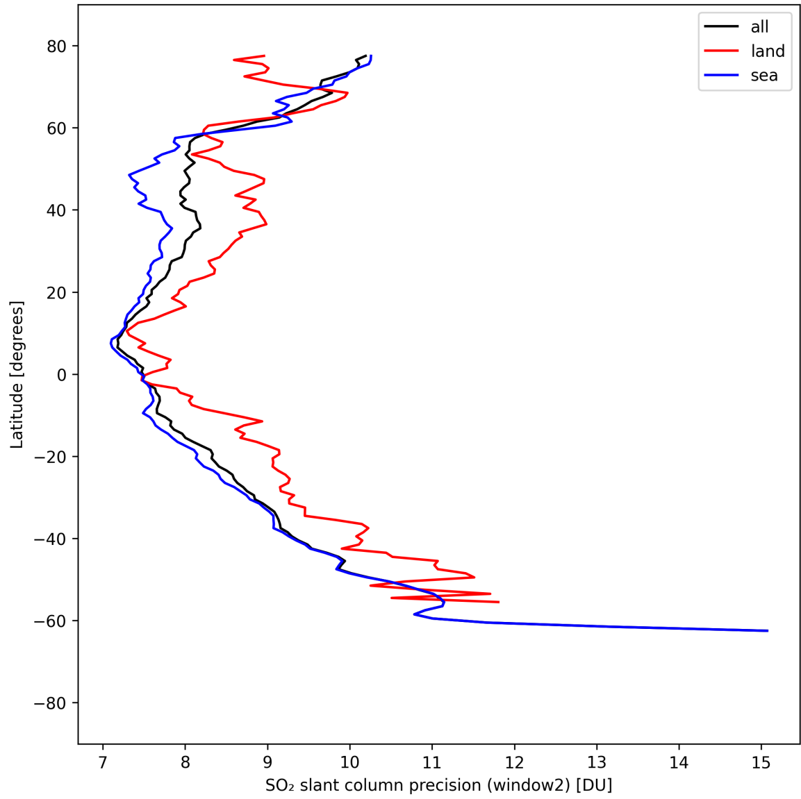
Figure 42: Zonal average of “SO 2 slant column precision (window2)” for 2025-09-02 to 2025-09-04.
