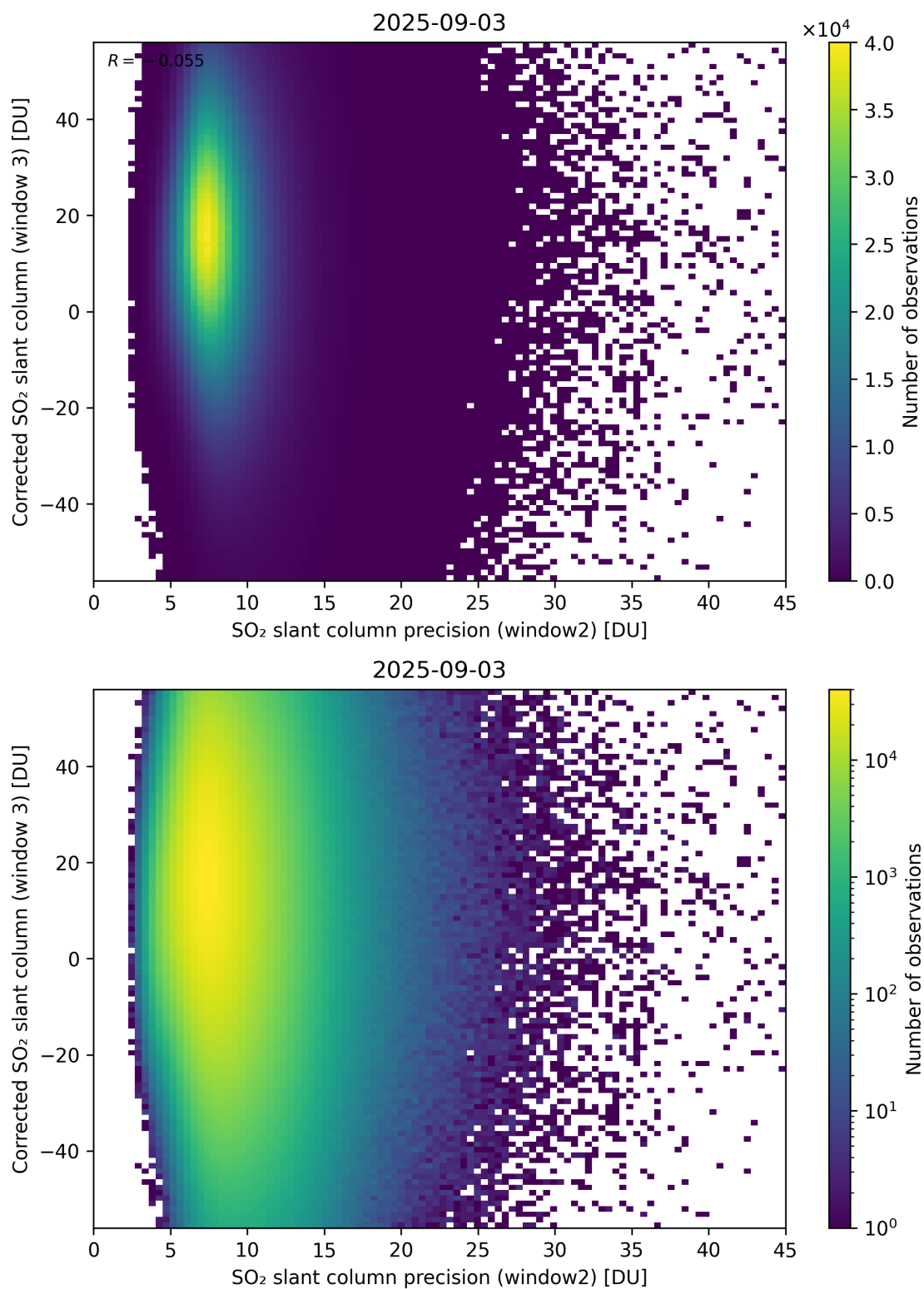
Figure 298: Scatter density plot of “SO 2 slant column precision (window2)” against “Corrected SO 2 slant column (window 3)” for 2025-09-02 to 2025-09-04.
