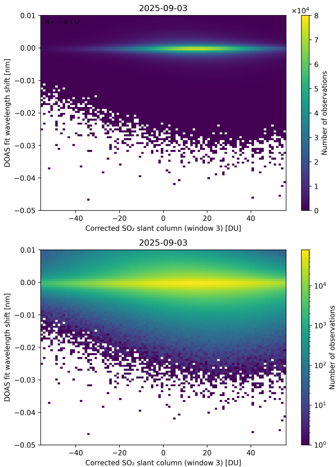
Figure 256: Scatter density plot of “Corrected SO 2 slant column (window 3)” against “DOAS fit wavelength shift” for 2025-09-02 to 2025-09-04.
