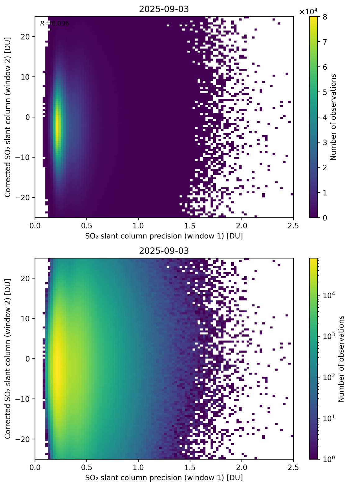
Figure 275: Scatter density plot of “SO 2 slant column precision (window 1)” against “Corrected SO 2 slant column (window 2)” for 2025-09-02 to 2025-09-04.
