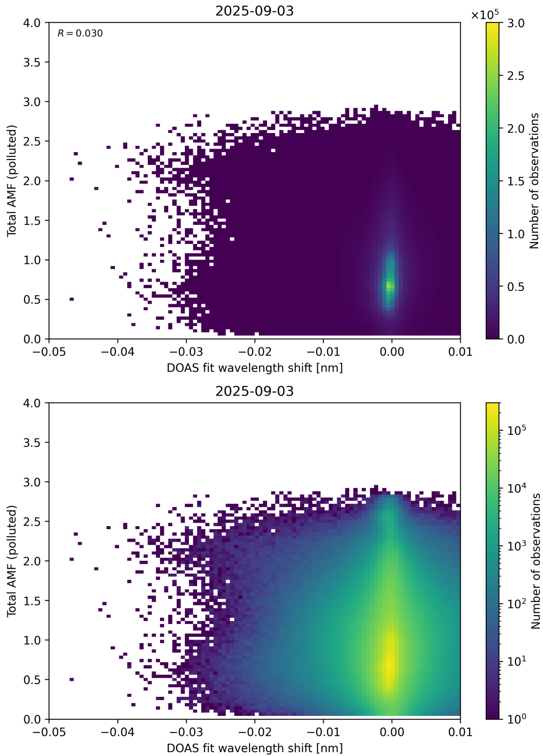
Figure 141: Scatter density plot of “DOAS fit wavelength shift” against “Total AMF (polluted)” for 2025-09-02 to 2025-09-04.
