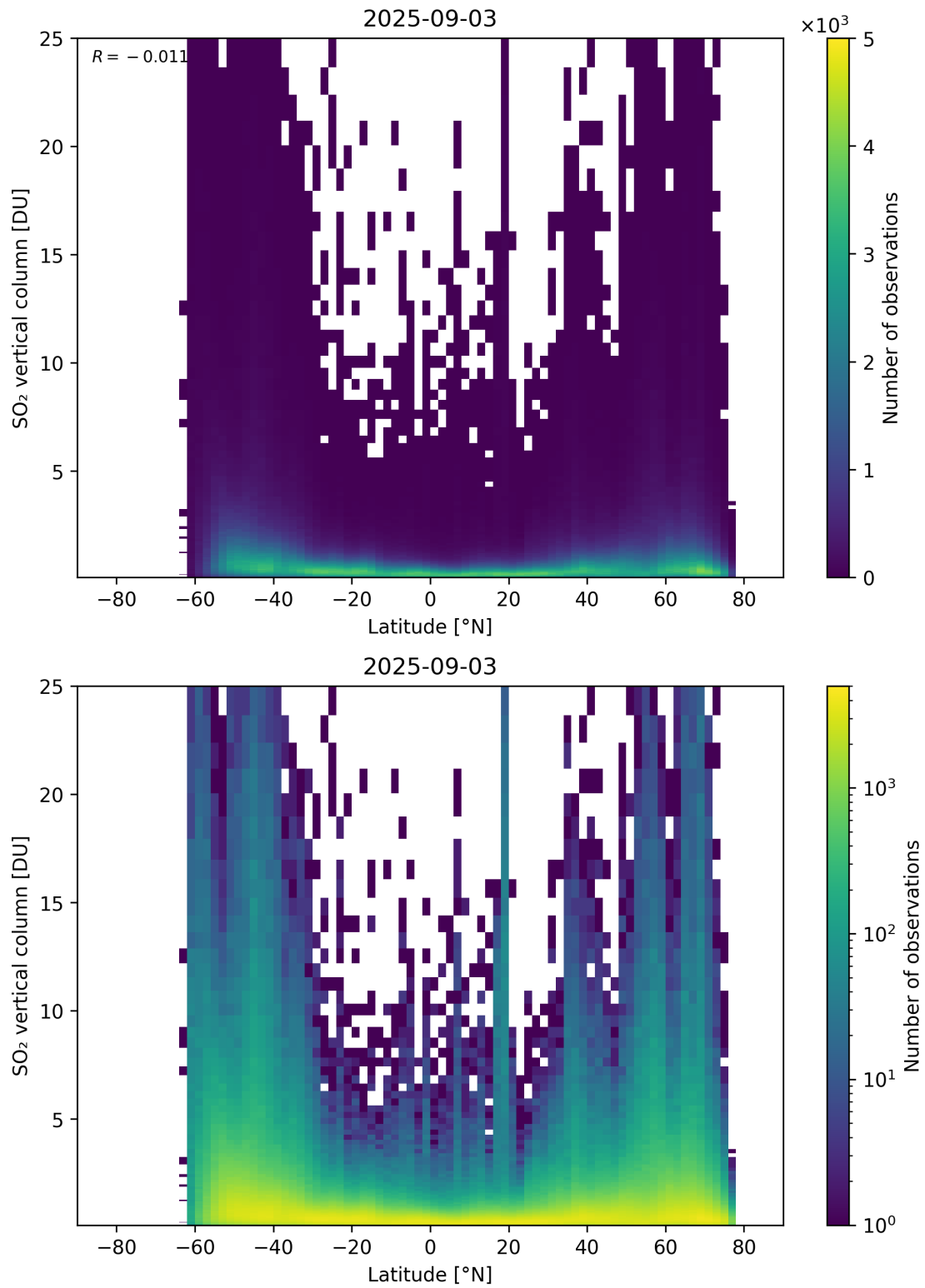
Figure 169: Scatter density plot of “Latitude” against “SO 2 vertical column” for 2025-09-02 to 2025-09-04.
