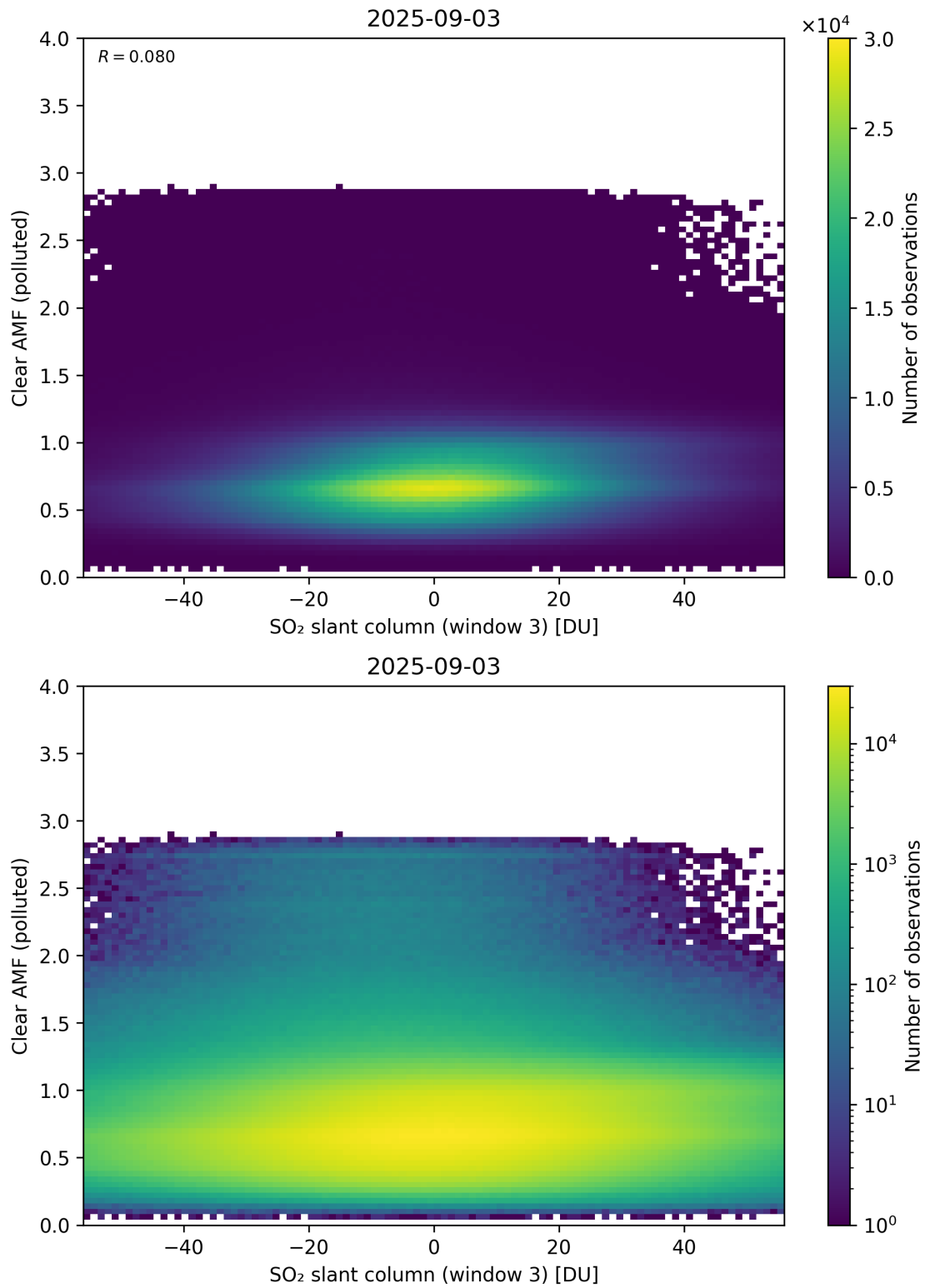
Figure 315: Scatter density plot of “SO 2 slant column (window 3)” against “Clear AMF (polluted)” for 2025-09-02 to 2025-09-04.
