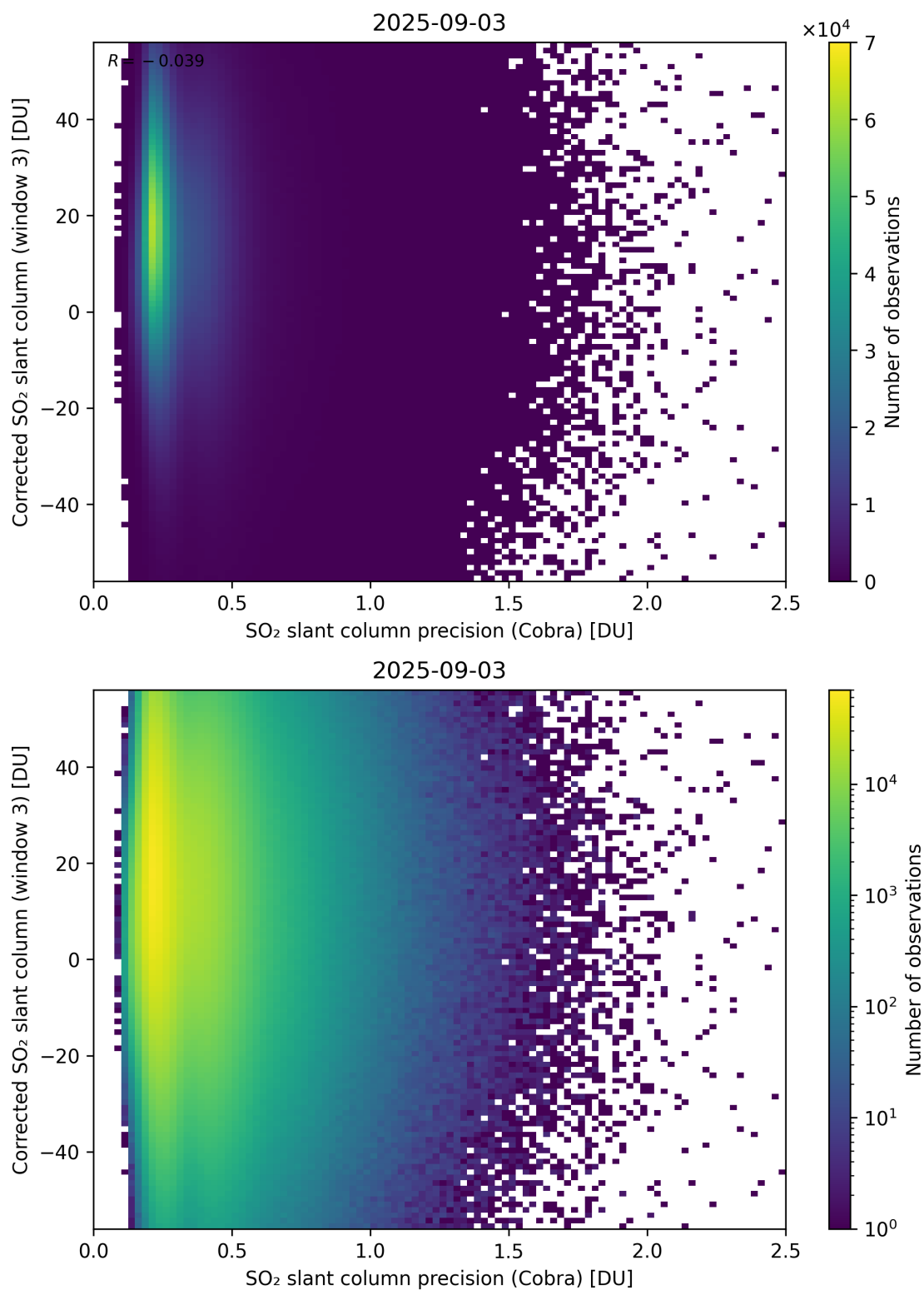
Figure 207: Scatter density plot of “SO 2 slant column precision (Cobra)” against “Corrected SO 2 slant column (window 3)” for 2025-09-02 to 2025-09-04.
