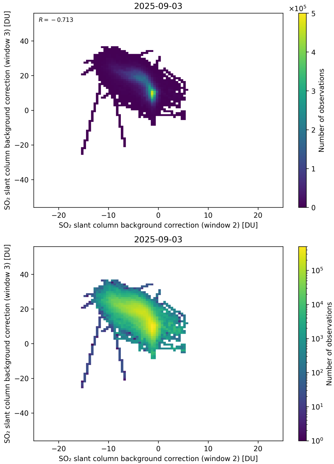
Figure 122: Scatter density plot of “SO 2 slant column background correction (window 2)” against “SO 2 slant column background correction (window 3)” for 2025-09-02 to 2025-09-04.
