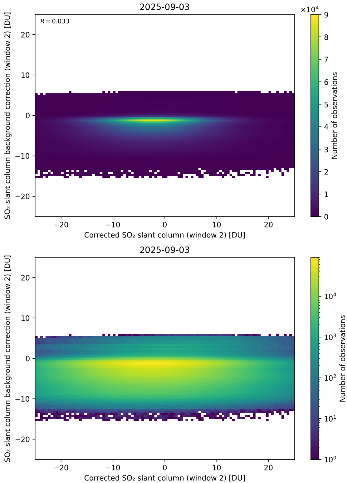
Figure 244: Scatter density plot of “Corrected SO 2 slant column (window 2)” against “SO 2 slant column background correction (window 2)” for 2025-09-02 to 2025-09-04.
