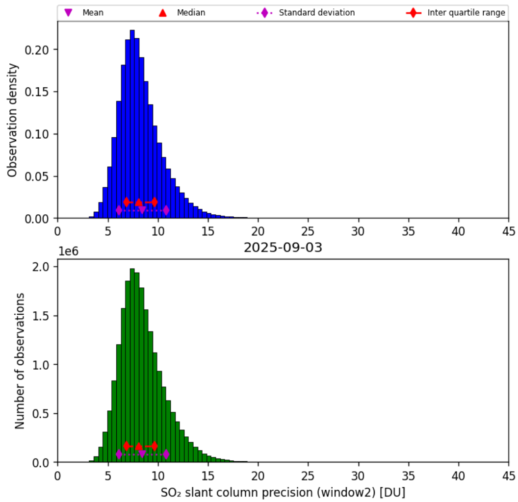
Figure 68: Histogram of “SO 2 slant column precision (window2)” for 2025-09-02 to 2025-09-04
