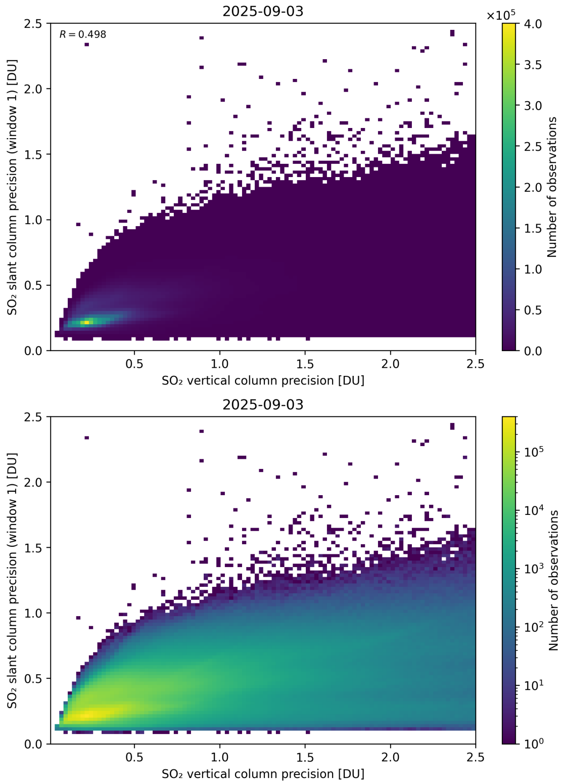
Figure 342: Scatter density plot of “SO 2 vertical column precision” against “SO 2 slant column precision (window 1)” for 2025-09-02 to 2025-09-04.
