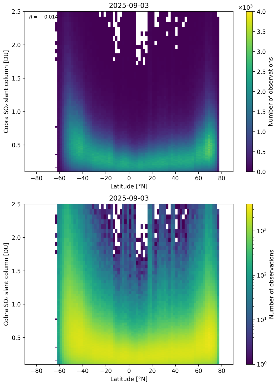
Figure 157: Scatter density plot of “Latitude” against “Cobra SO 2 slant column” for 2025-09-02 to 2025-09-04.
