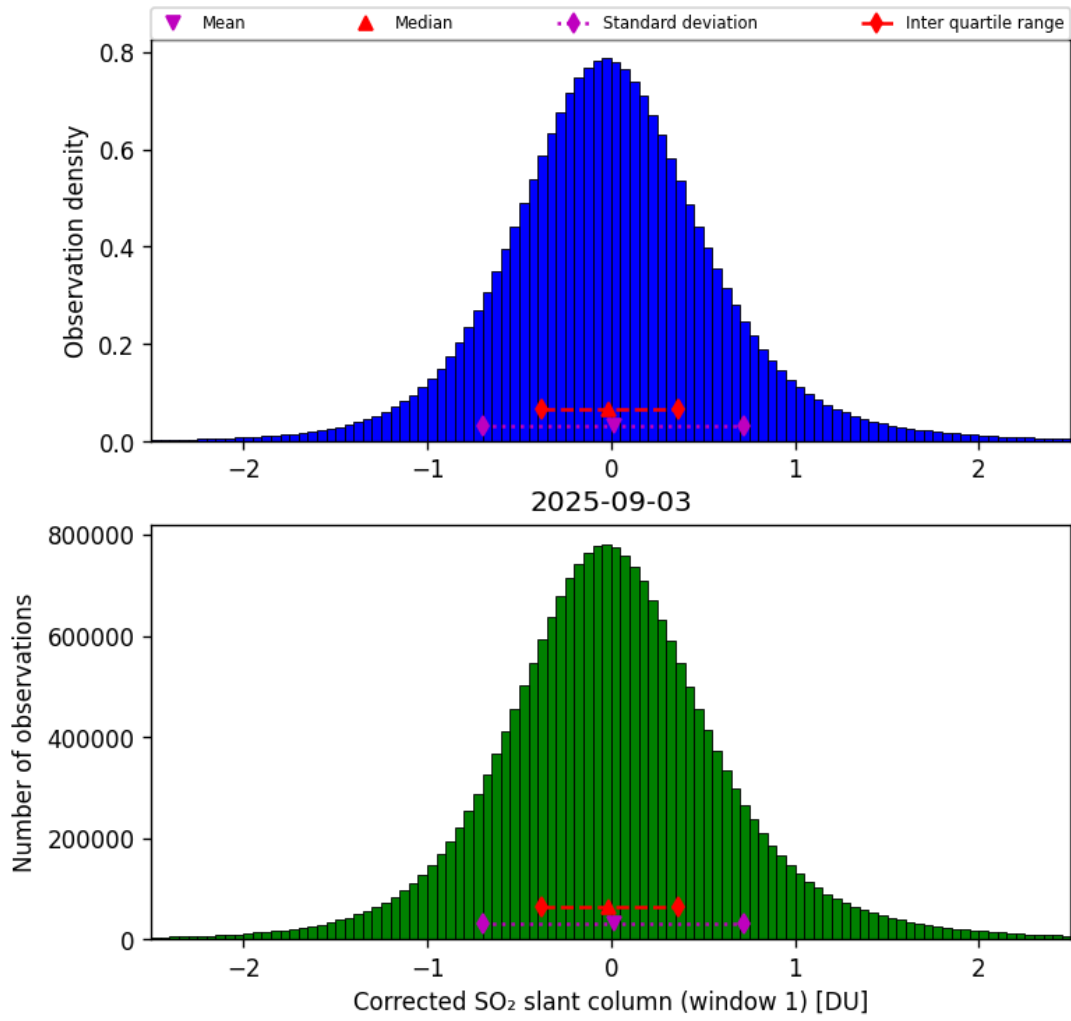
Figure 65: Histogram of “Corrected SO 2 slant column (window 1)” for 2025-09-02 to 2025-09-04
