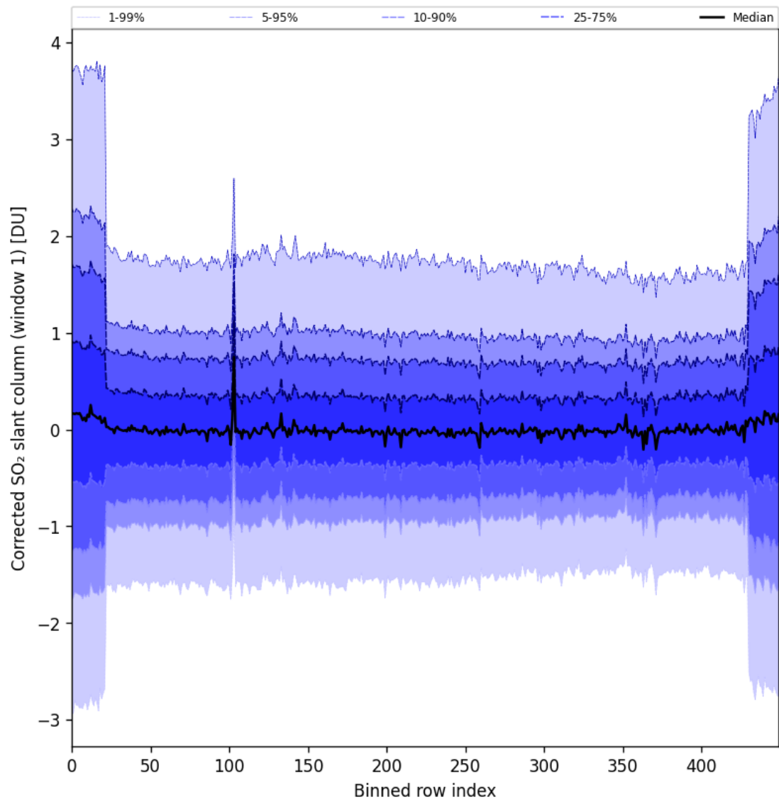
Figure 91: Along track statistics of “Corrected SO 2 slant column (window 1)” for 2025-09-02 to 2025-09-04
