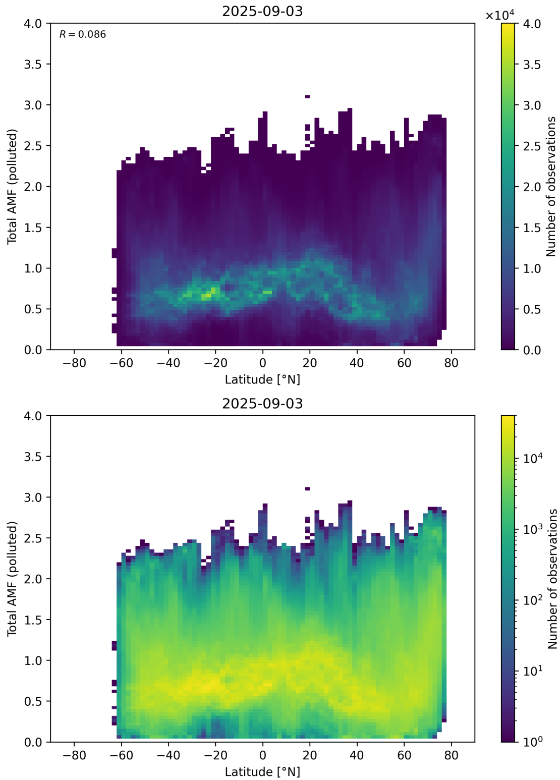
Figure 167: Scatter density plot of “Latitude” against “Total AMF (polluted)” for 2025-09-02 to 2025-09-04.
