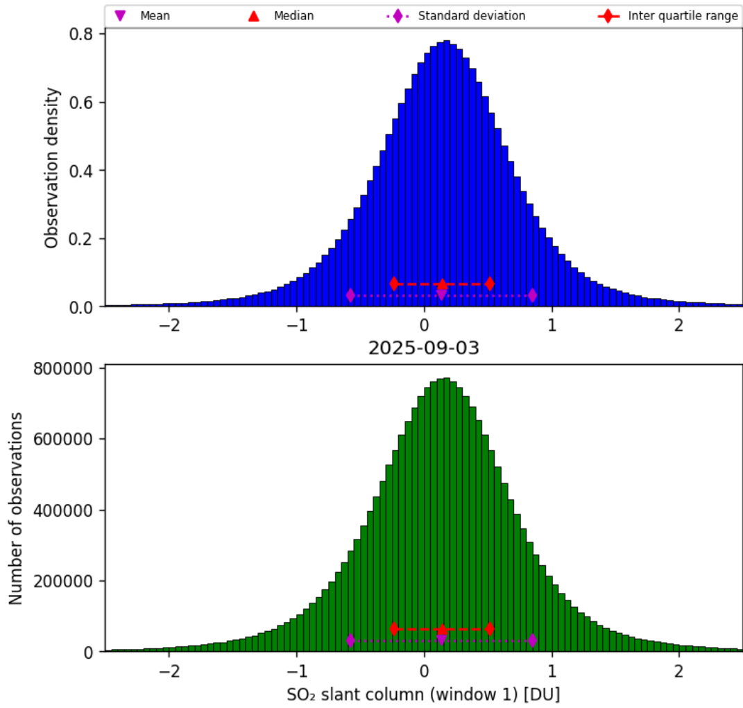
Figure 63: Histogram of “SO 2 slant column (window 1)” for 2025-09-02 to 2025-09-04
