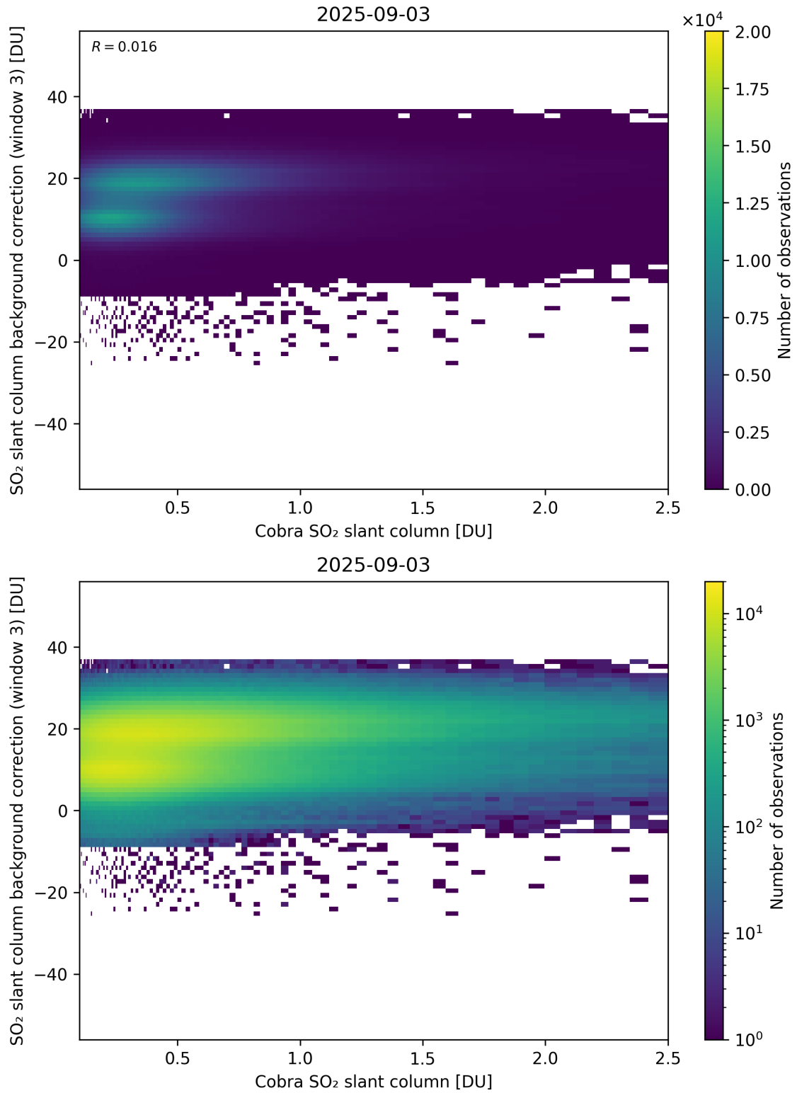
Figure 195: Scatter density plot of “Cobra SO 2 slant column” against “SO 2 slant column background correction (window 3)” for 2025-09-02 to 2025-09-04.
