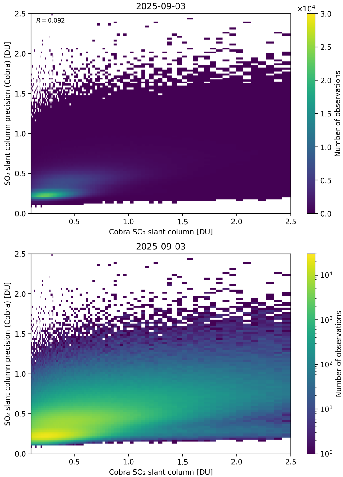
Figure 216: Scatter density plot of “Cobra SO 2 slant column” against “SO 2 slant column precision (Cobra)” for 2025-09-02 to 2025-09-04.
