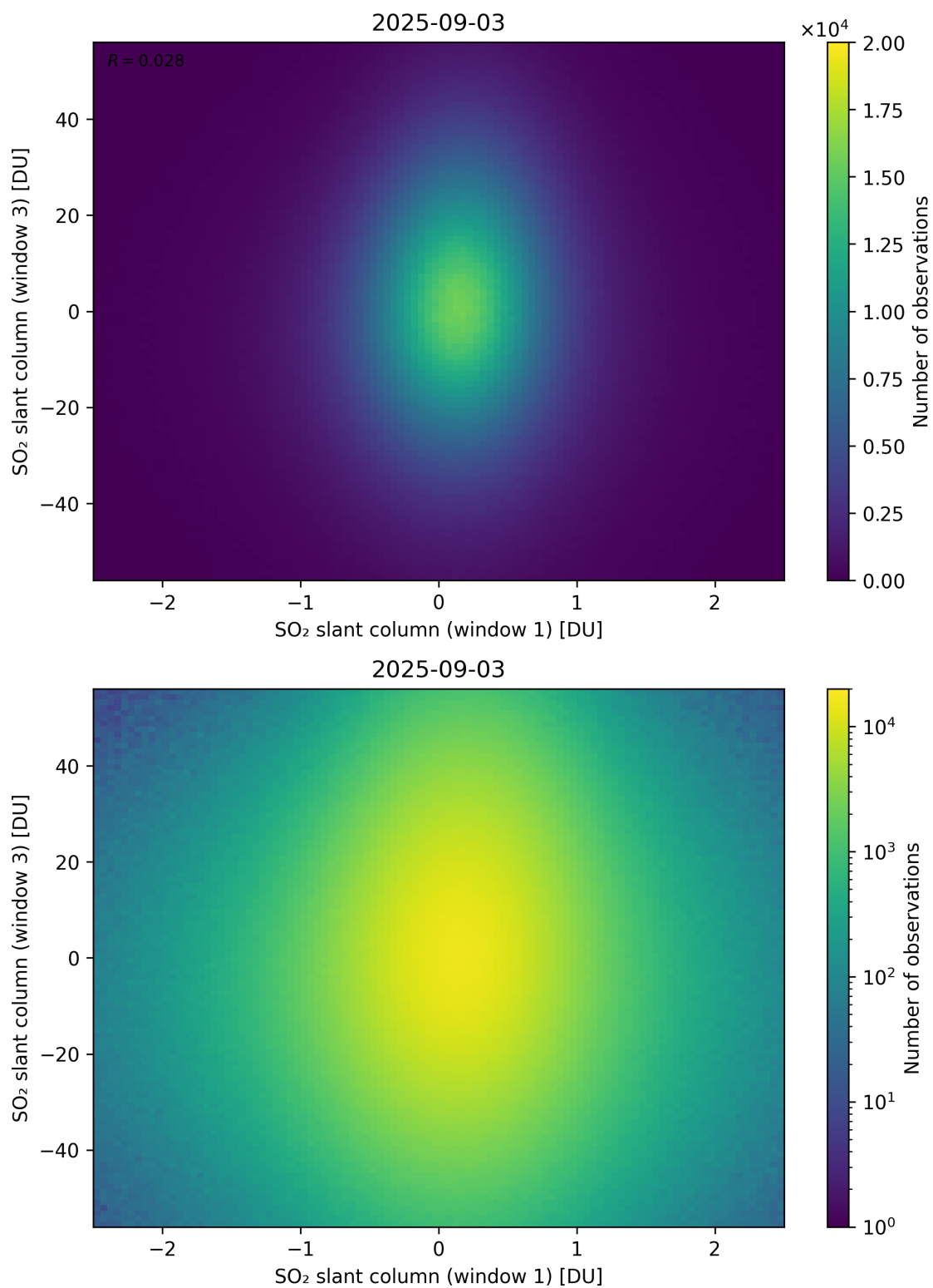
Figure 287: Scatter density plot of “SO 2 slant column (window 1)” against “SO 2 slant column (window 3)” for 2025-09-02 to 2025-09-04.
