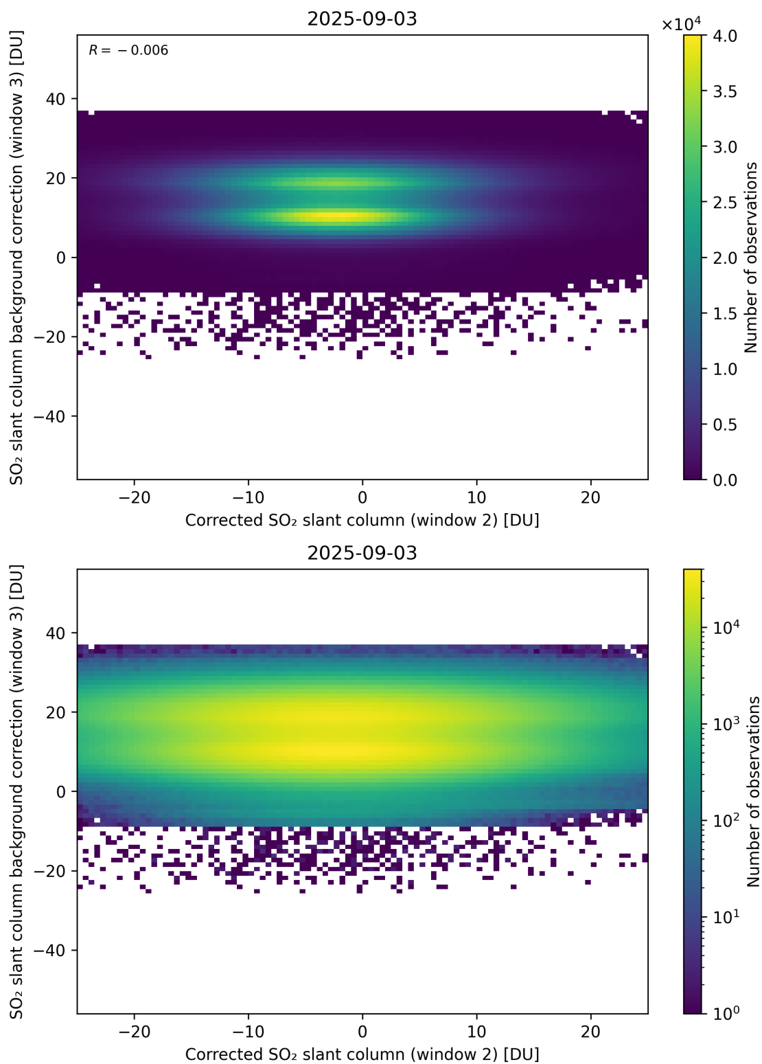
Figure 245: Scatter density plot of “Corrected SO 2 slant column (window 2)” against “SO 2 slant column background correction (window 3)” for 2025-09-02 to 2025-09-04.
