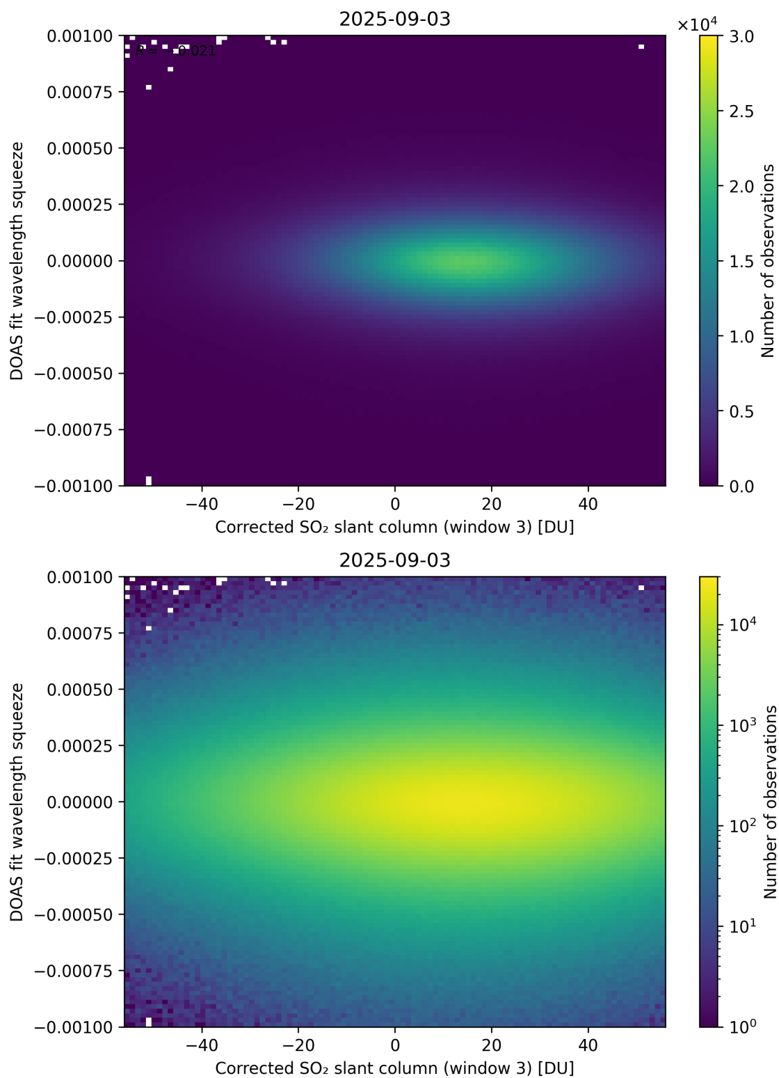
Figure 257: Scatter density plot of “Corrected SO 2 slant column (window 3)” against “DOAS fit wavelength squeeze” for 2025-09-02 to 2025-09-04.
