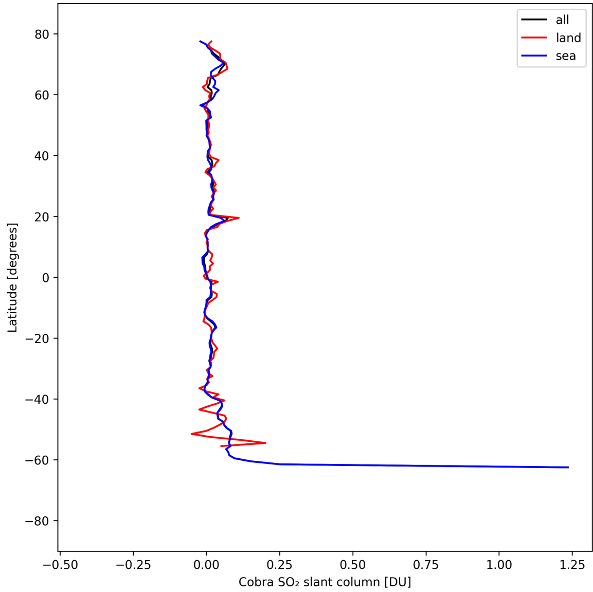
Figure 35: Zonal average of “Cobra SO 2 slant column” for 2025-09-02 to 2025-09-04.
