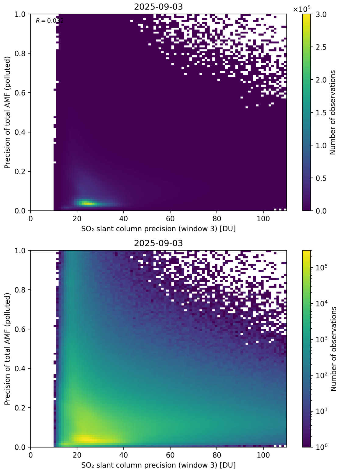
Figure 314: Scatter density plot of “SO 2 slant column precision (window 3)” against “Precision of total AMF (polluted)” for 2025-09-02 to 2025-09-04.
