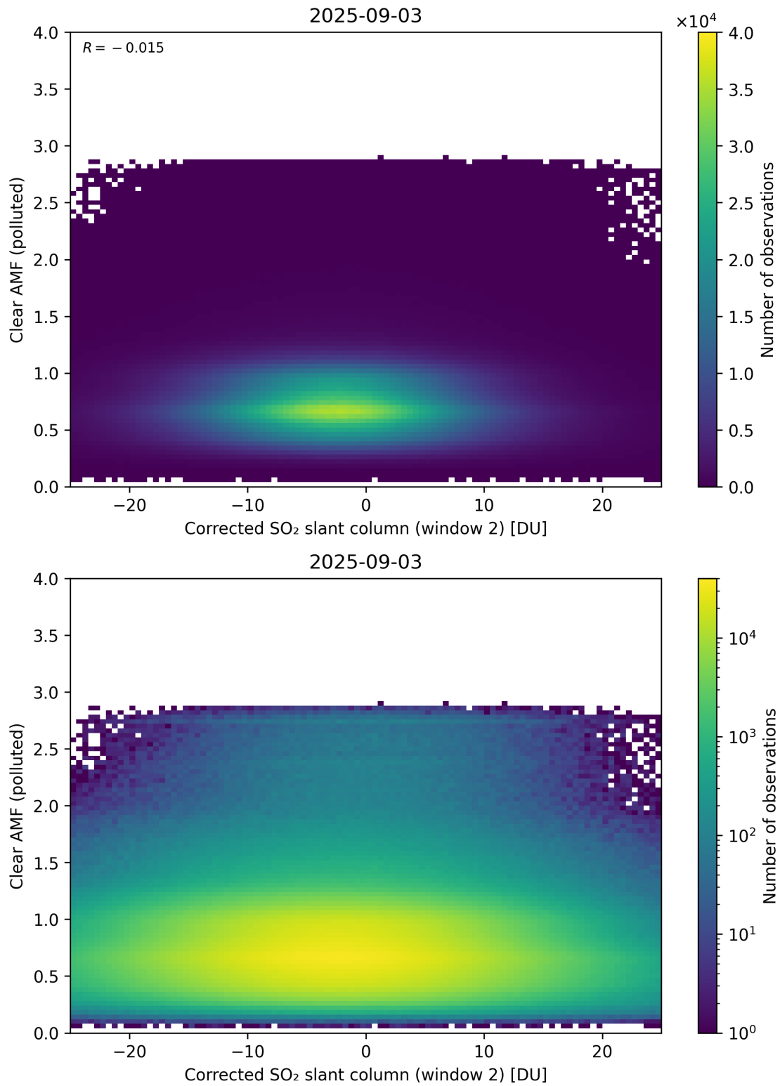
Figure 249: Scatter density plot of “Corrected SO 2 slant column (window 2)” against “Clear AMF (polluted)” for 2025-09-02 to 2025-09-04.
