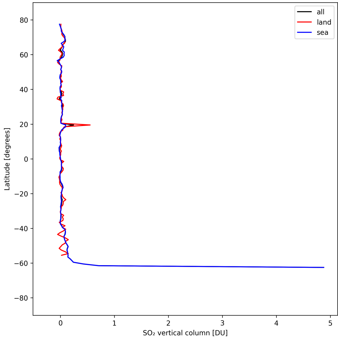
Figure 32: Zonal average of “SO 2 vertical column” for 2025-09-02 to 2025-09-04.
