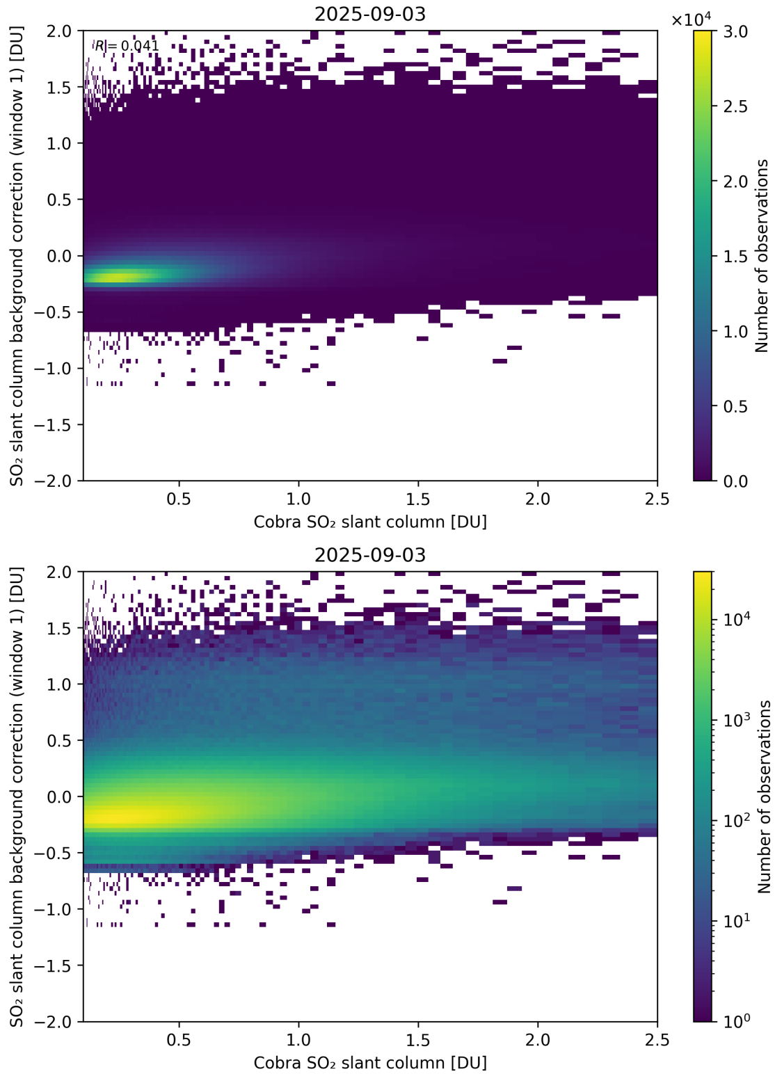
Figure 193: Scatter density plot of “Cobra SO 2 slant column” against “SO 2 slant column background correction (window 1)” for 2025-09-02 to 2025-09-04.
