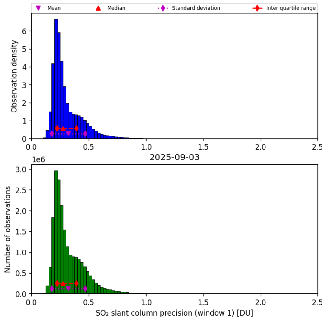
Figure 64: Histogram of “SO 2 slant column precision (window 1)” for 2025-09-02 to 2025-09-04
