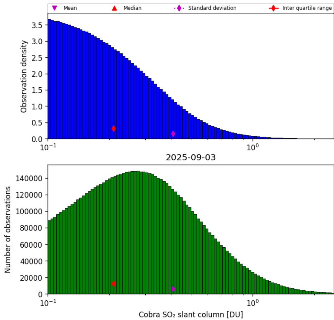
Figure 61: Histogram of “Cobra SO 2 slant column” for 2025-09-02 to 2025-09-04
