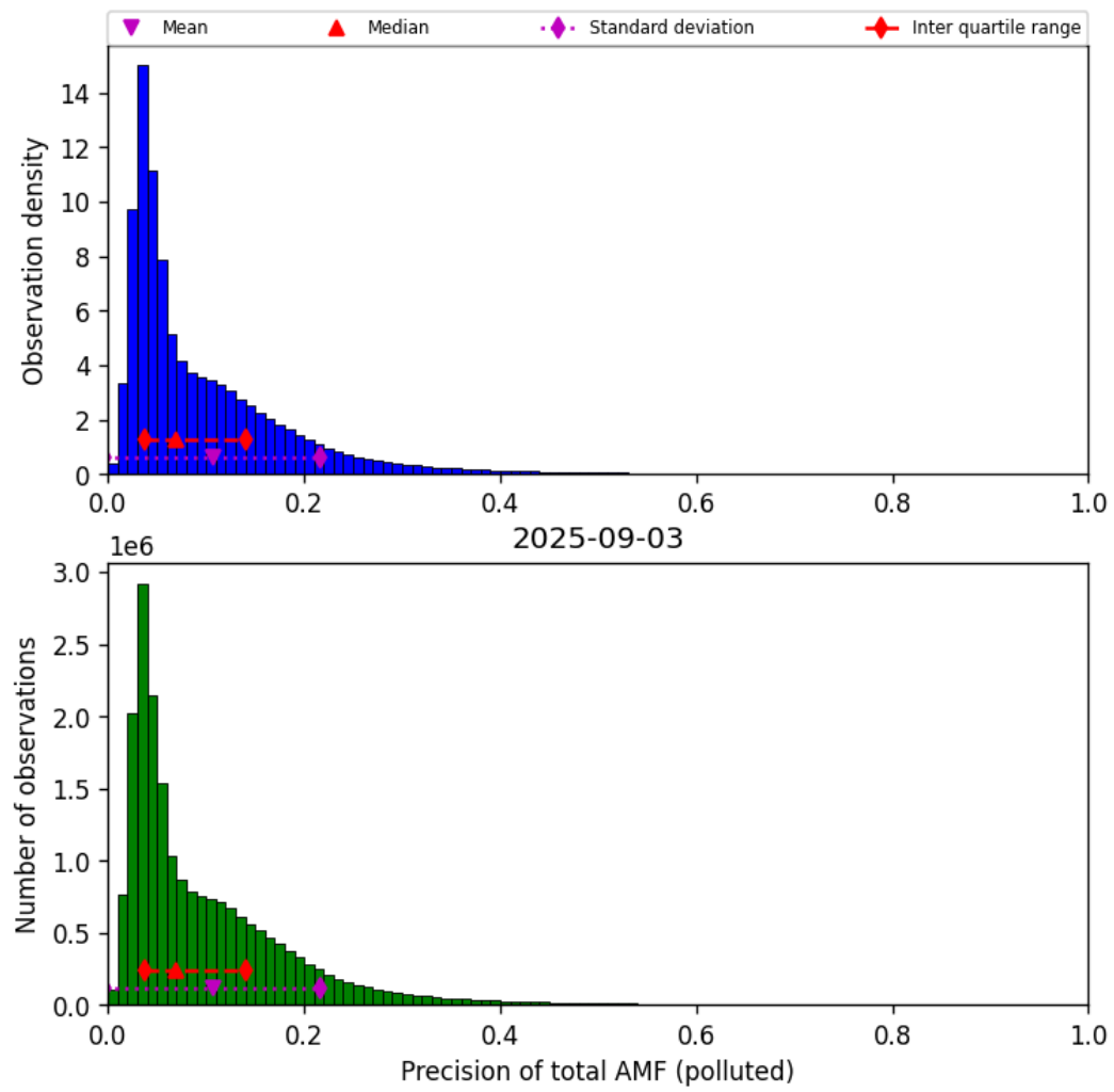
Figure 80: Histogram of “Precision of total AMF (polluted)” for 2025-09-02 to 2025-09-04
