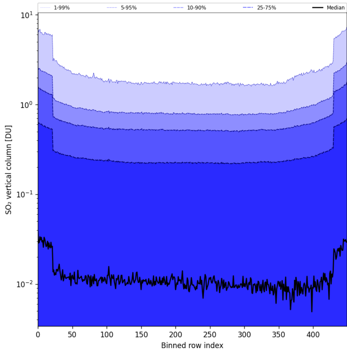
Figure 84: Along track statistics of “SO 2 vertical column” for 2025-09-02 to 2025-09-04
