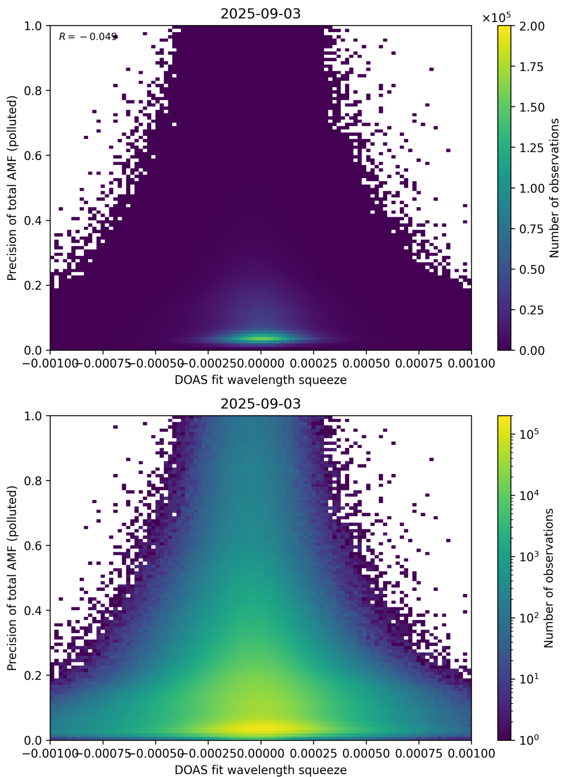
Figure 146: Scatter density plot of “DOAS fit wavelength squeeze” against “Precision of total AMF (polluted)” for 2025-09-02 to 2025-09-04.
