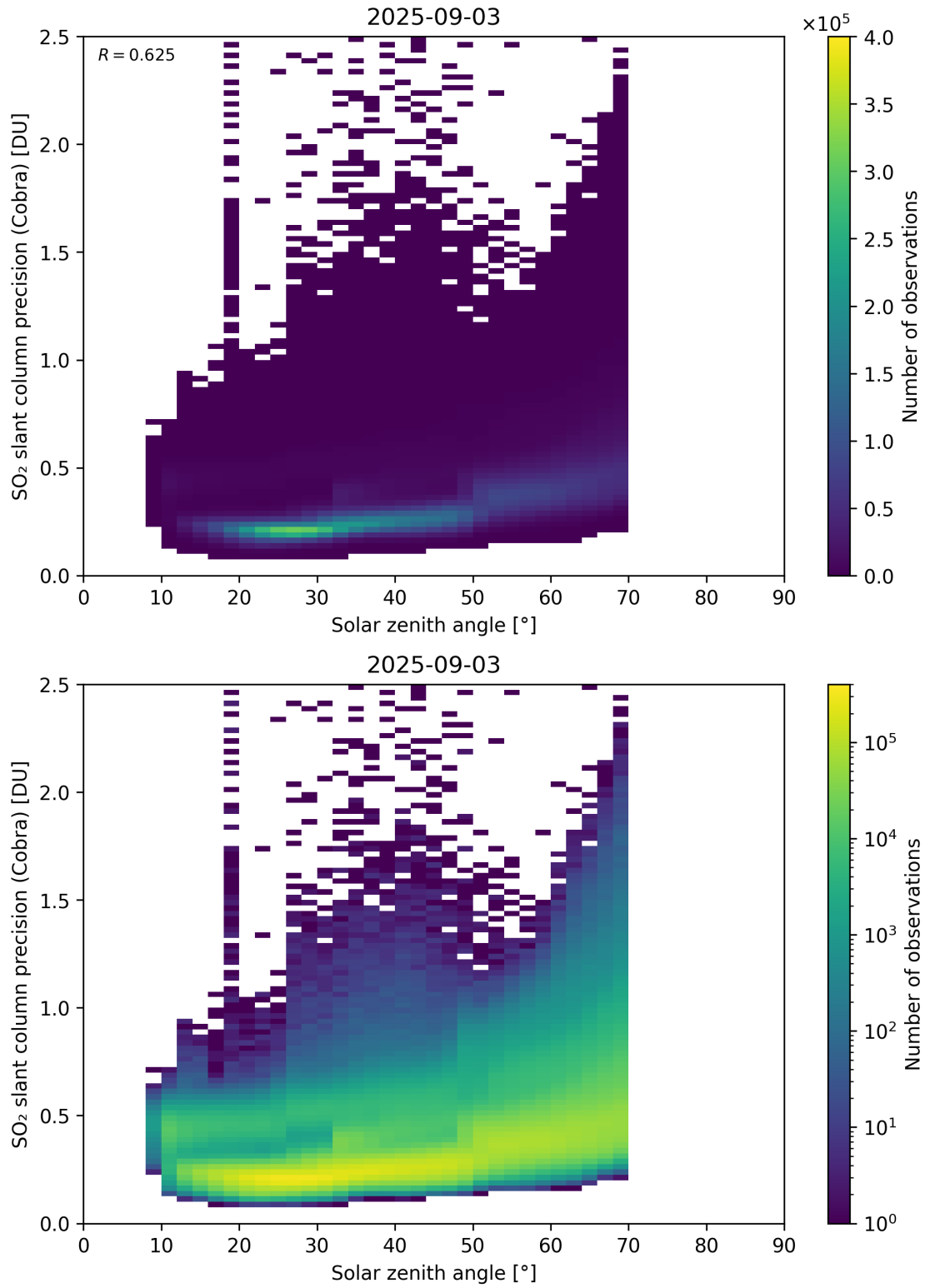
Figure 180: Scatter density plot of “Solar zenith angle” against “SO 2 slant column precision (Cobra)” for 2025-09-02 to 2025-09-04.
