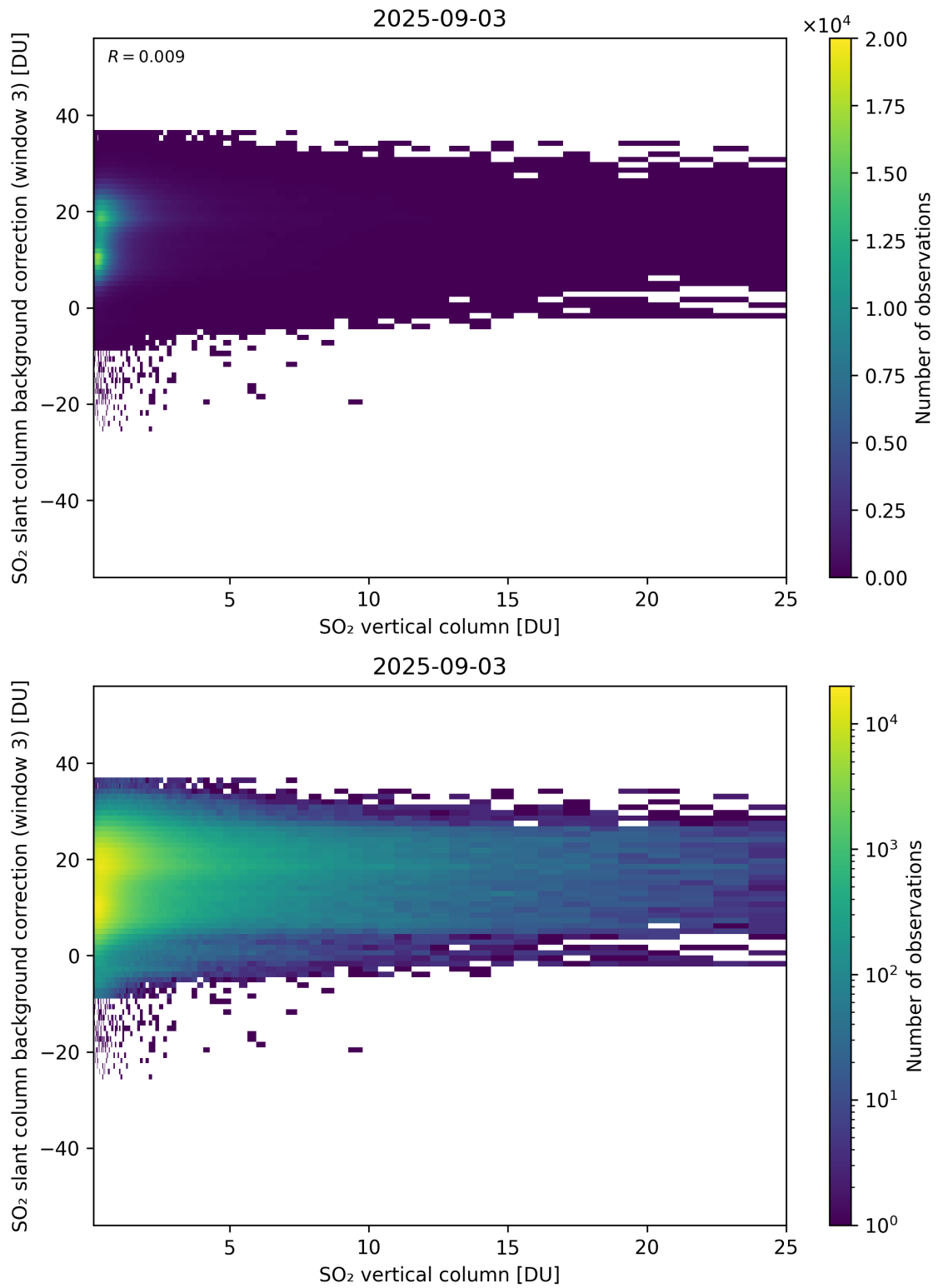
Figure 325: Scatter density plot of “SO 2 vertical column” against “SO 2 slant column background correction (window 3)” for 2025-09-02 to 2025-09-04.
