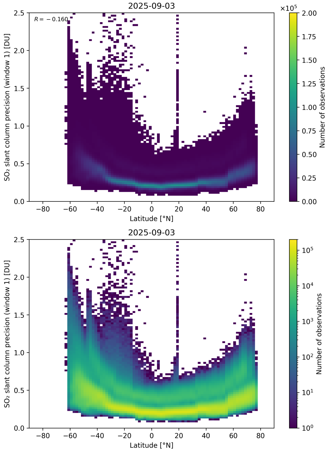
Figure 163: Scatter density plot of “Latitude” against “SO 2 slant column precision (window 1)” for 2025-09-02 to 2025-09-04.
