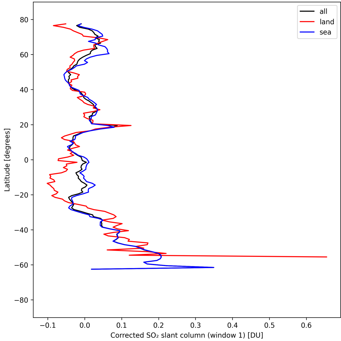
Figure 39: Zonal average of “Corrected SO 2 slant column (window 1)” for 2025-09-02 to 2025-09-04.
