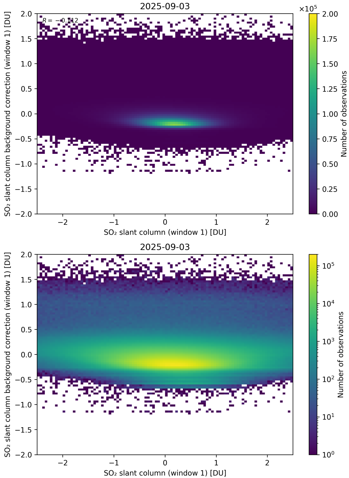
Figure 262: Scatter density plot of “SO 2 slant column (window 1)” against “SO 2 slant column background correction (window 1)” for 2025-09-02 to 2025-09-04.
