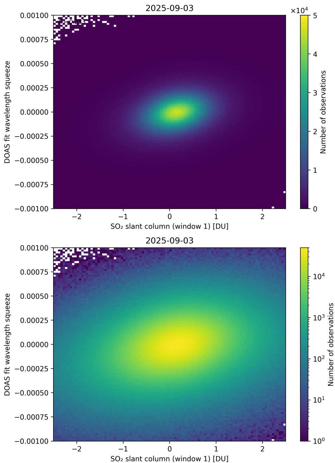
Figure 266: Scatter density plot of “SO 2 slant column (window 1)” against “DOAS fit wavelength squeeze” for 2025-09-02 to 2025-09-04.
