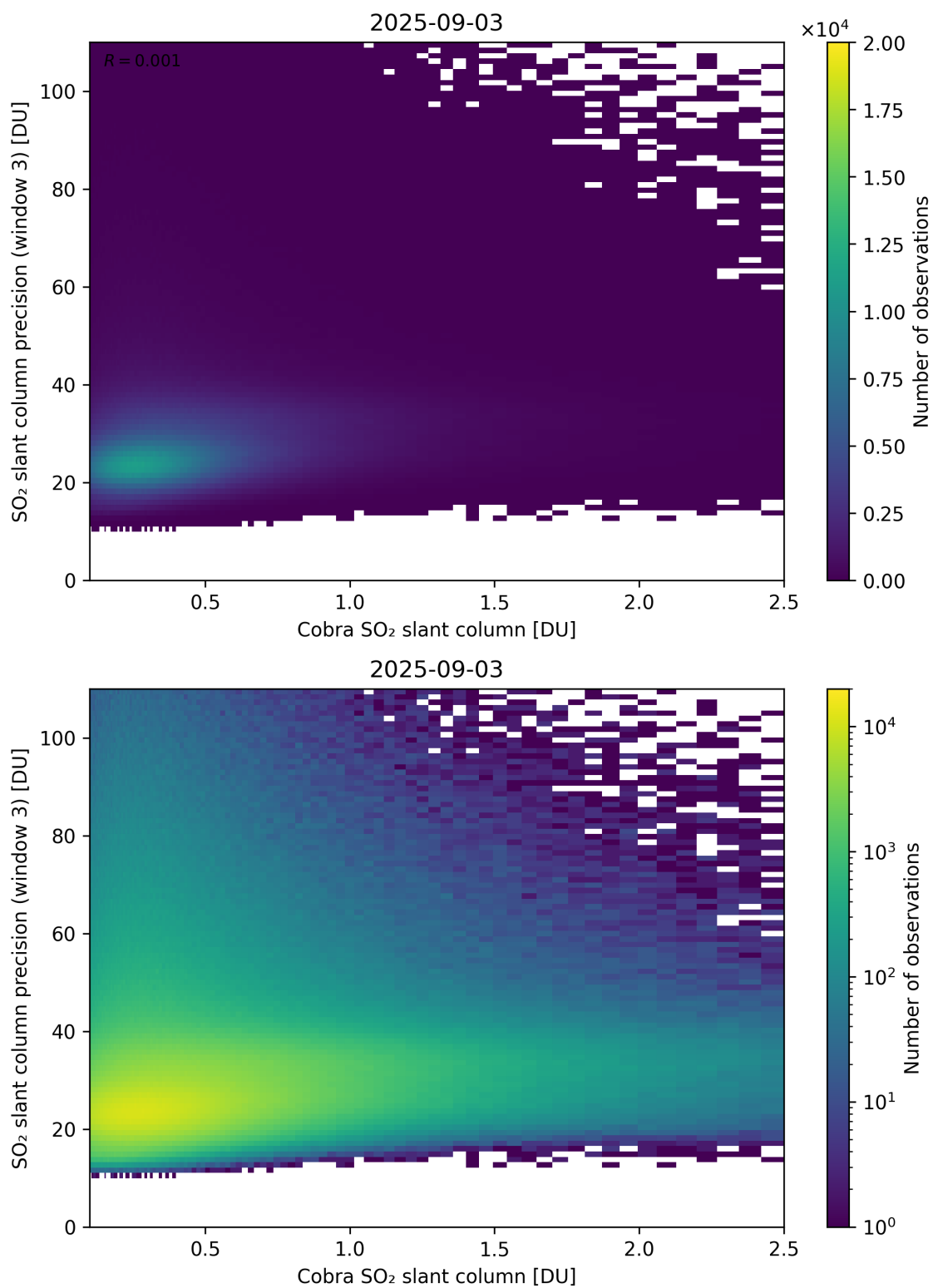
Figure 223: Scatter density plot of “Cobra SO 2 slant column” against “SO 2 slant column precision (window 3)” for 2025-09-02 to 2025-09-04.
