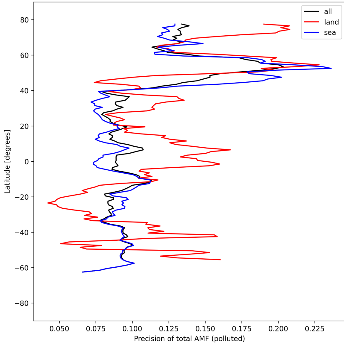
Figure 54: Zonal average of “Precision of total AMF (polluted)” for 2025-09-02 to 2025-09-04.
