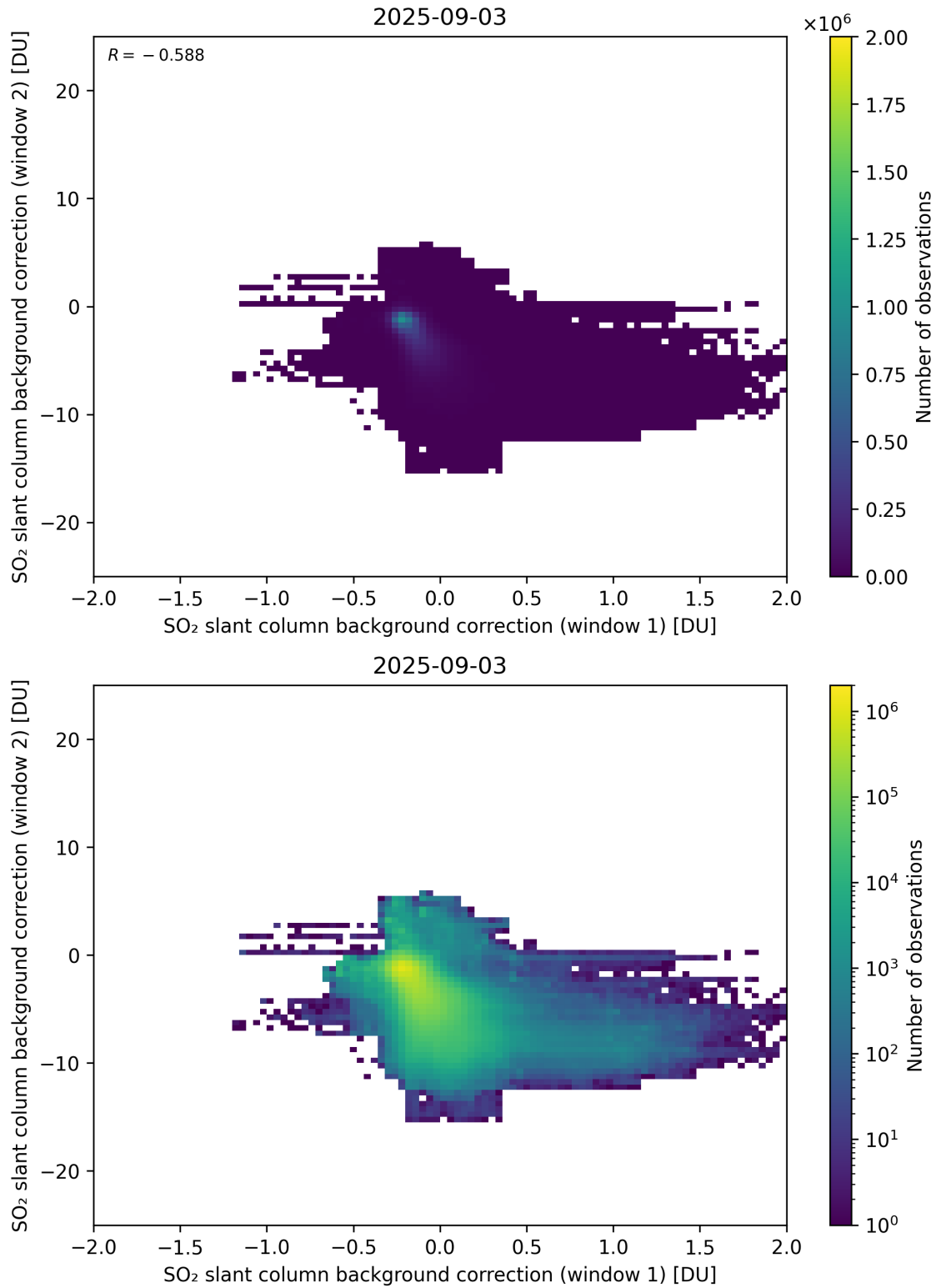
Figure 109: Scatter density plot of “SO 2 slant column background correction (window 1)” against “SO 2 slant column background correction (window 2)” for 2025-09-02 to 2025-09-04.
