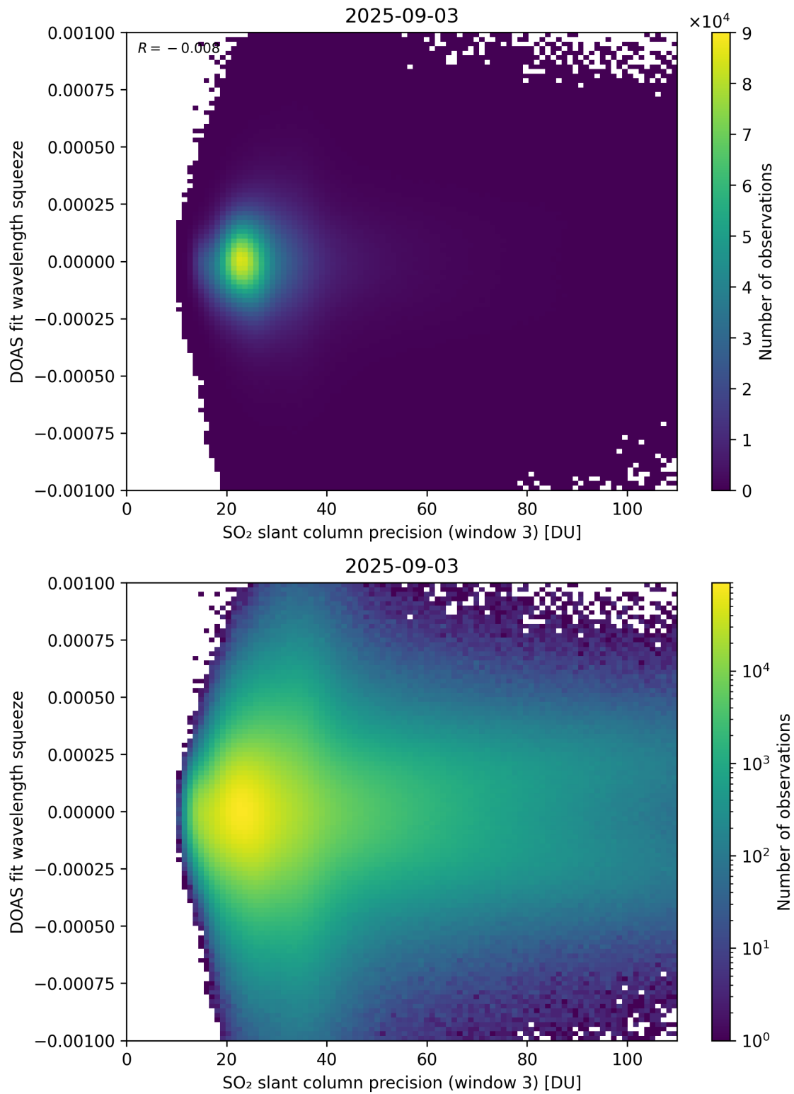
Figure 309: Scatter density plot of “SO 2 slant column precision (window 3)” against “DOAS fit wavelength squeeze” for 2025-09-02 to 2025-09-04.
