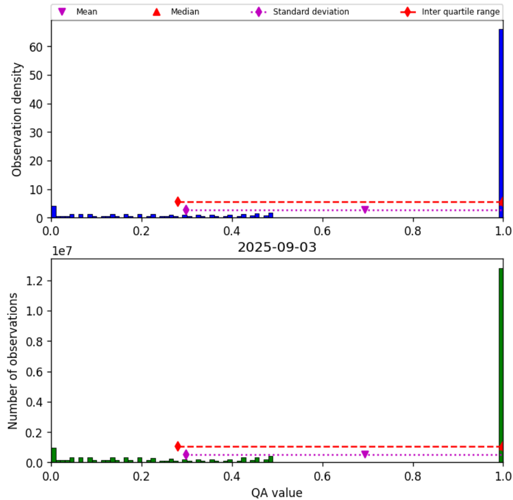
Figure 57: Histogram of “QA value” for 2025-09-02 to 2025-09-04
