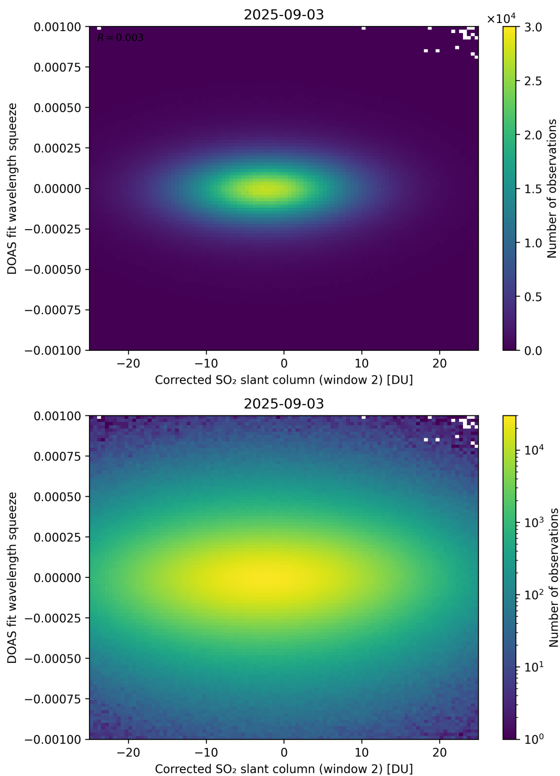
Figure 247: Scatter density plot of “Corrected SO 2 slant column (window 2)” against “DOAS fit wavelength squeeze” for 2025-09-02 to 2025-09-04.
