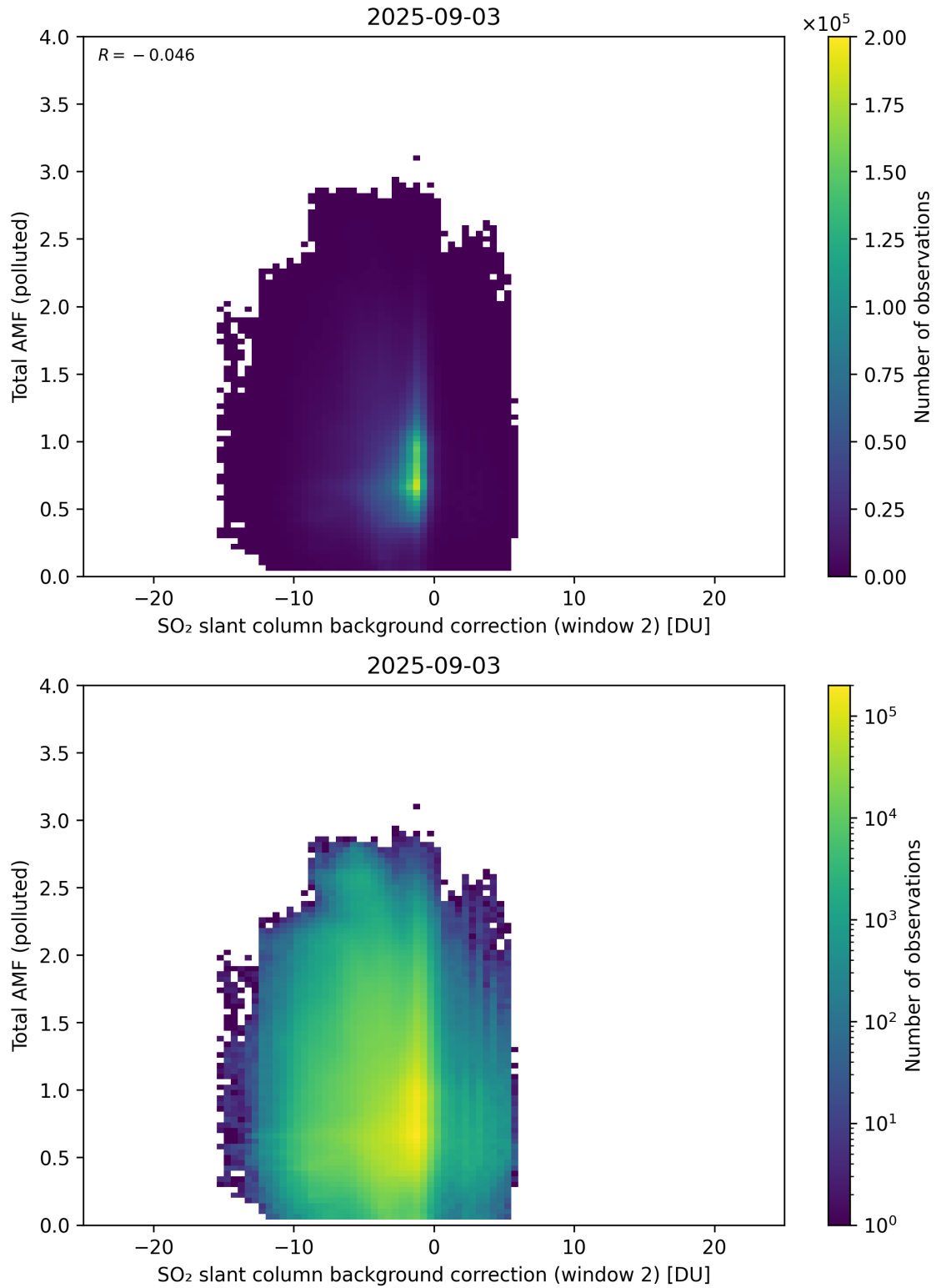
Figure 130: Scatter density plot of “SO 2 slant column background correction (window 2)” against “Total AMF (polluted)” for 2025-09-02 to 2025-09-04.
