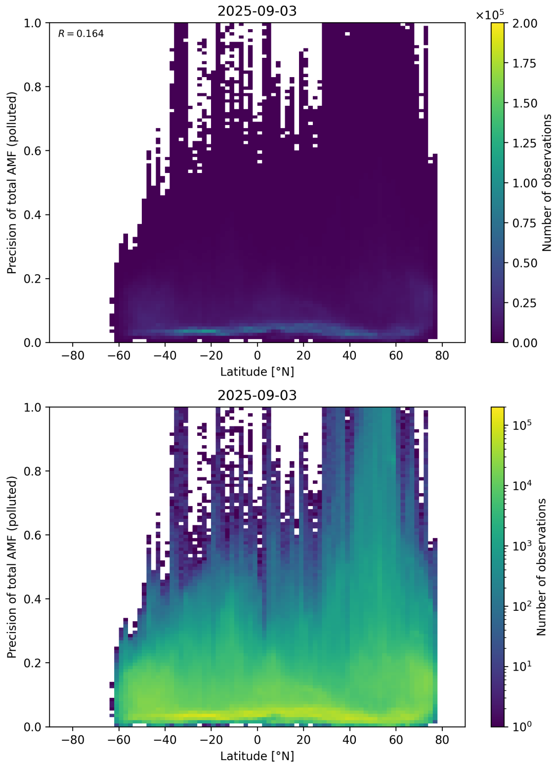
Figure 168: Scatter density plot of “Latitude” against “Precision of total AMF (polluted)” for 2025-09-02 to 2025-09-04.
