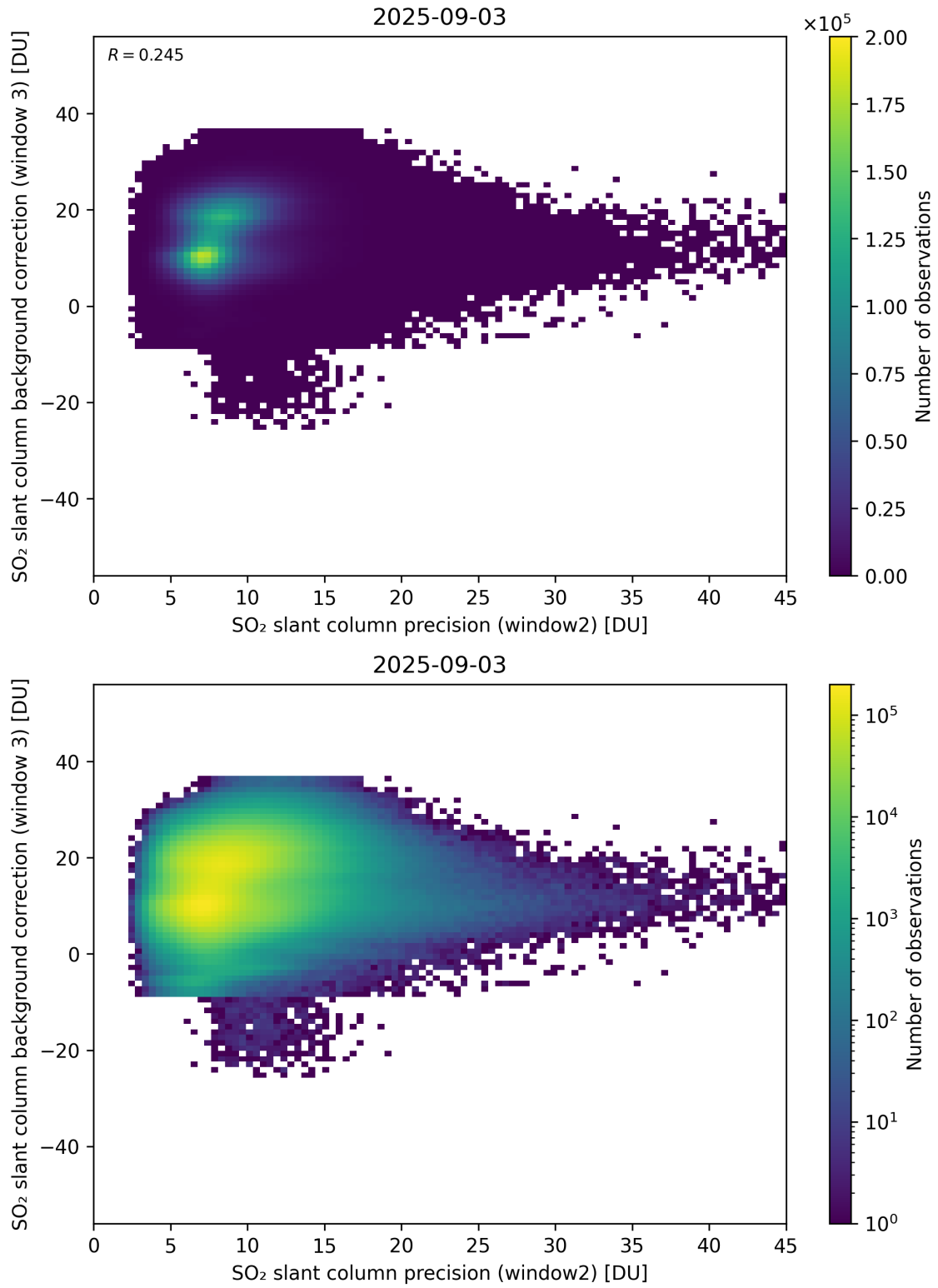
Figure 292: Scatter density plot of “SO 2 slant column precision (window2)” against “SO 2 slant column background correction (window 3)” for 2025-09-02 to 2025-09-04.
