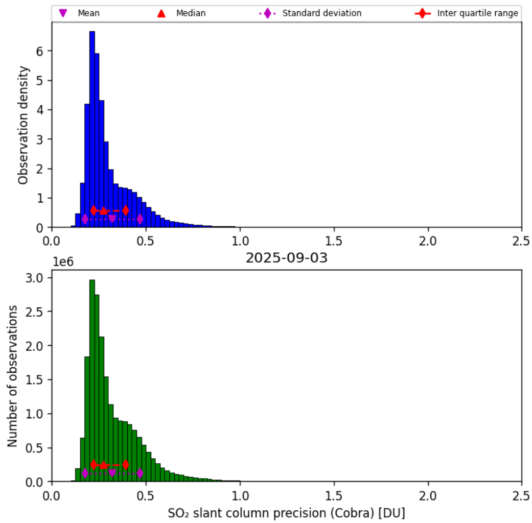
Figure 62: Histogram of “SO 2 slant column precision (Cobra)” for 2025-09-02 to 2025-09-04
