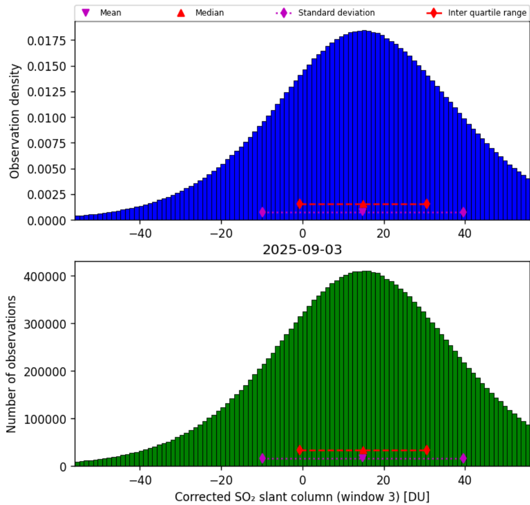
Figure 73: Histogram of “Corrected SO 2 slant column (window 3)” for 2025-09-02 to 2025-09-04
