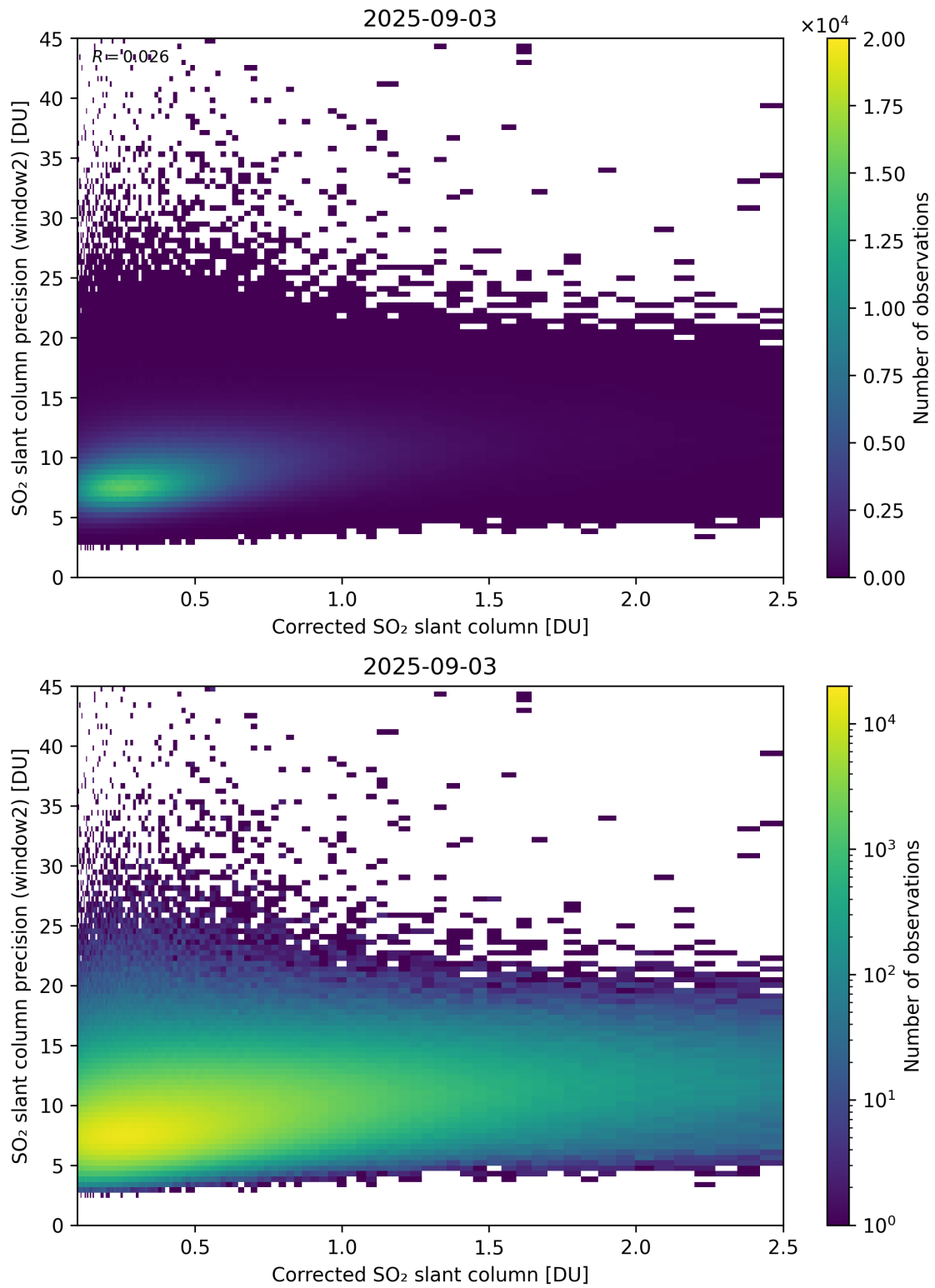
Figure 239: Scatter density plot of “Corrected SO 2 slant column” against “SO 2 slant column precision (window2)” for 2025-09-02 to 2025-09-04.
