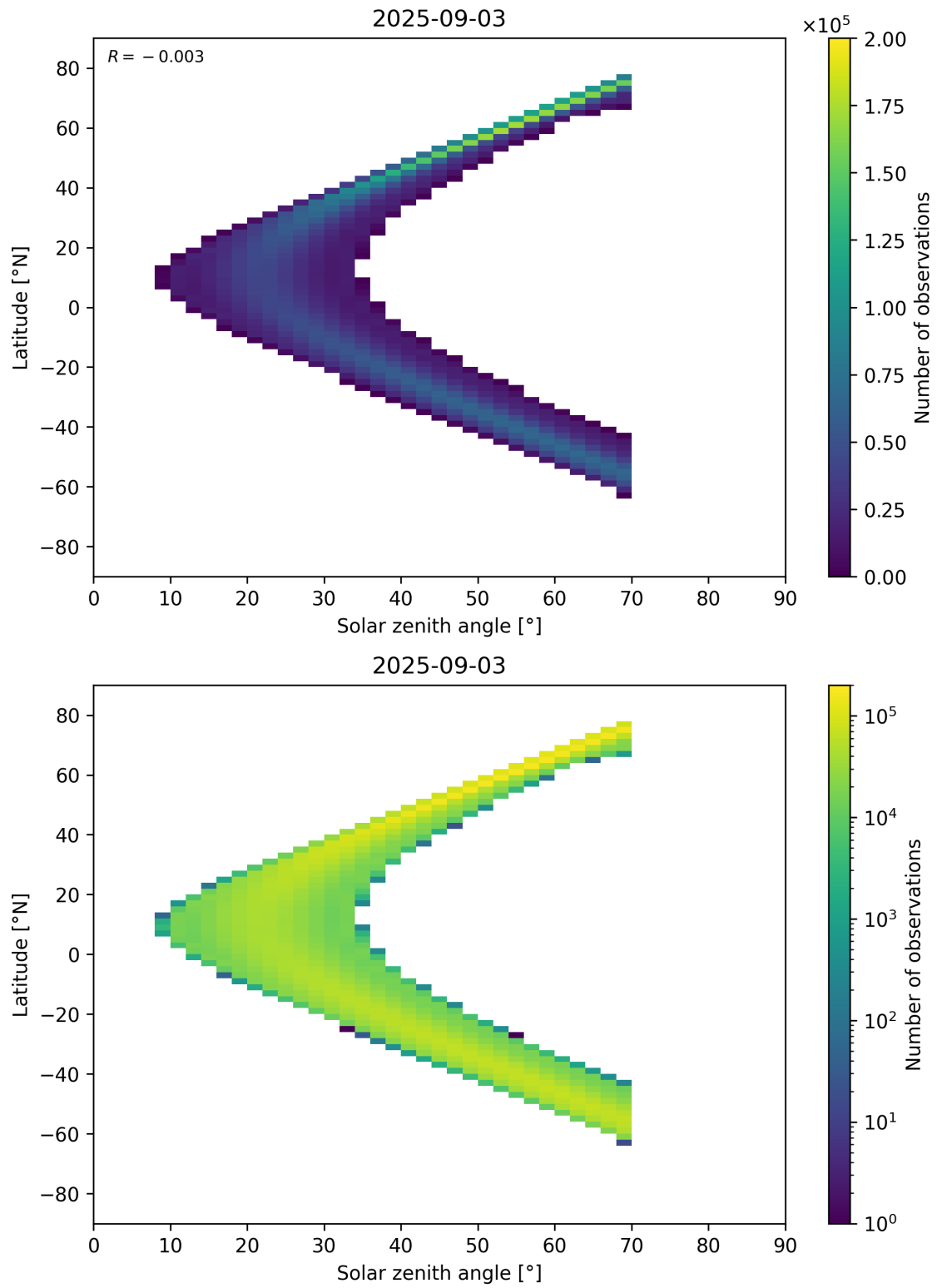
Figure 177: Scatter density plot of “Solar zenith angle” against “Latitude” for 2025-09-02 to 2025-09-04.
