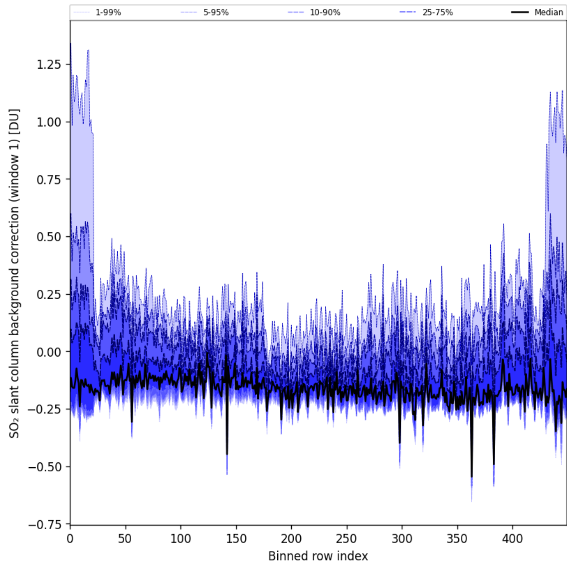
Figure 92: Along track statistics of “SO 2 slant column background correction (window 1)” for 2025-09-02 to 2025-09-04
