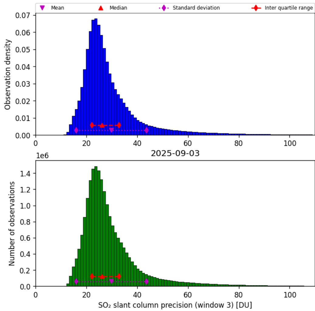
Figure 72: Histogram of “SO 2 slant column precision (window 3)” for 2025-09-02 to 2025-09-04
