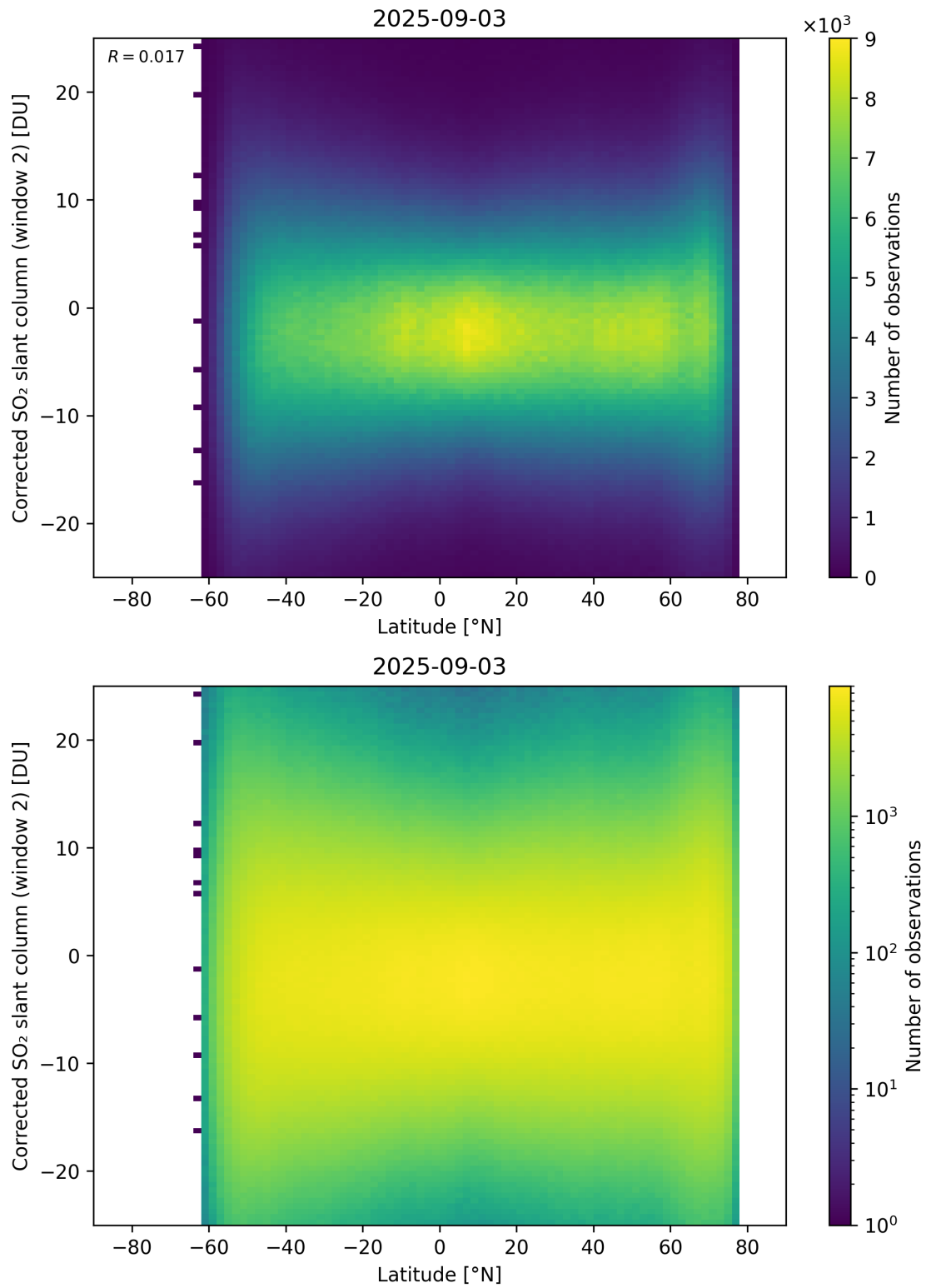
Figure 160: Scatter density plot of “Latitude” against “Corrected SO 2 slant column (window 2)” for 2025-09-02 to 2025-09-04.
