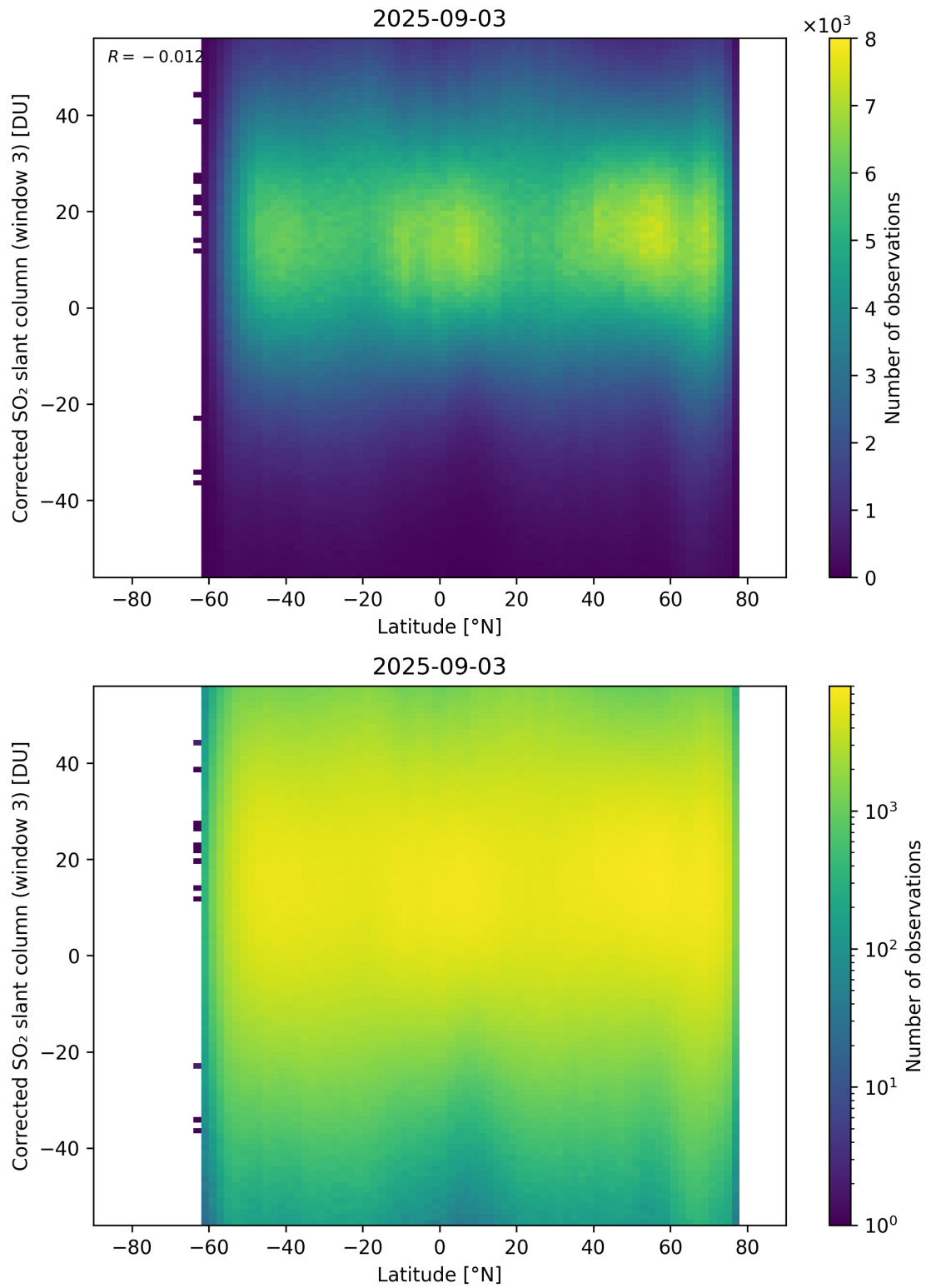
Figure 161: Scatter density plot of “Latitude” against “Corrected SO 2 slant column (window 3)” for 2025-09-02 to 2025-09-04.
