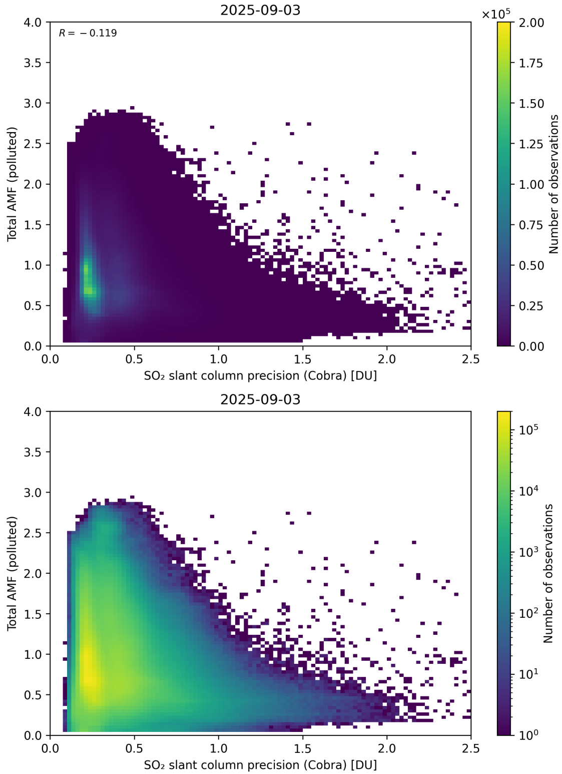
Figure 213: Scatter density plot of “SO 2 slant column precision (Cobra)” against “Total AMF (polluted)” for 2025-09-02 to 2025-09-04.
