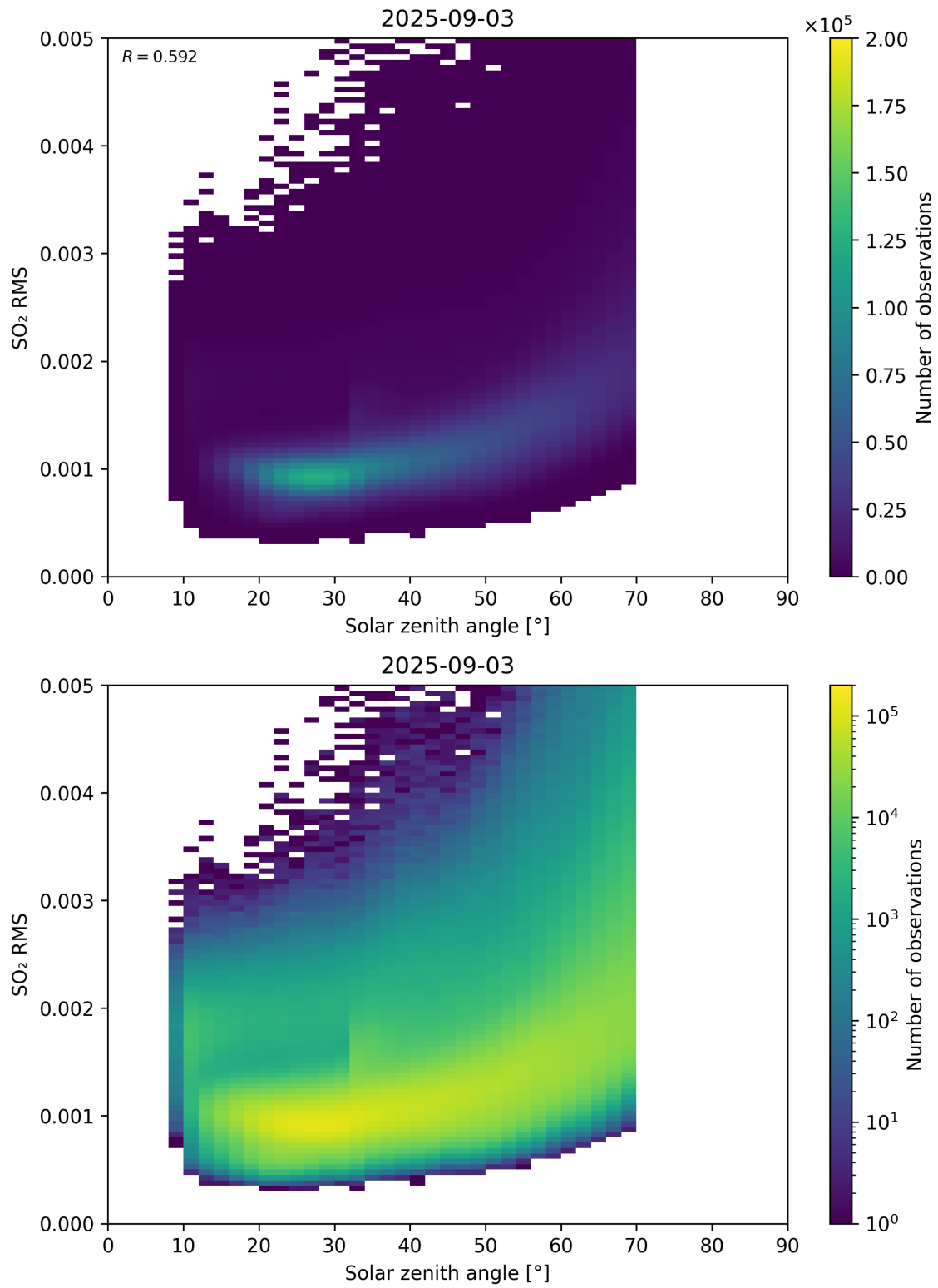
Figure 176: Scatter density plot of “Solar zenith angle” against “SO 2 RMS” for 2025-09-02 to 2025-09-04.
