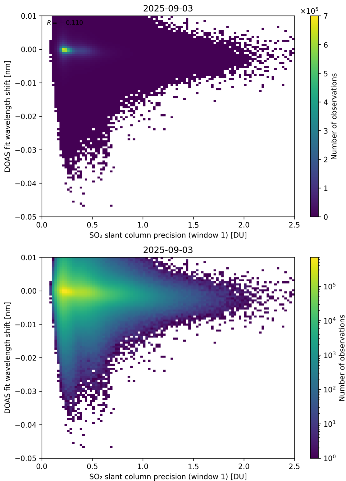
Figure 271: Scatter density plot of “SO 2 slant column precision (window 1)” against “DOAS fit wavelength shift” for 2025-09-02 to 2025-09-04.
