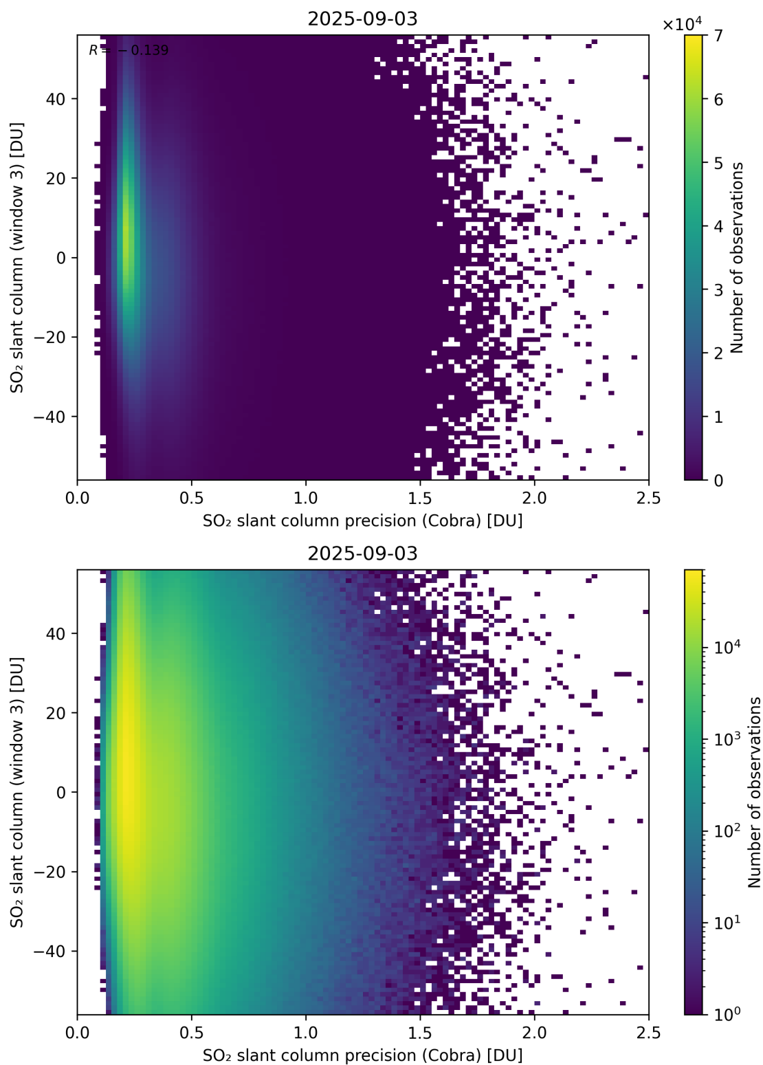
Figure 211: Scatter density plot of “SO 2 slant column precision (Cobra)” against “SO 2 slant column (window 3)” for 2025-09-02 to 2025-09-04.
