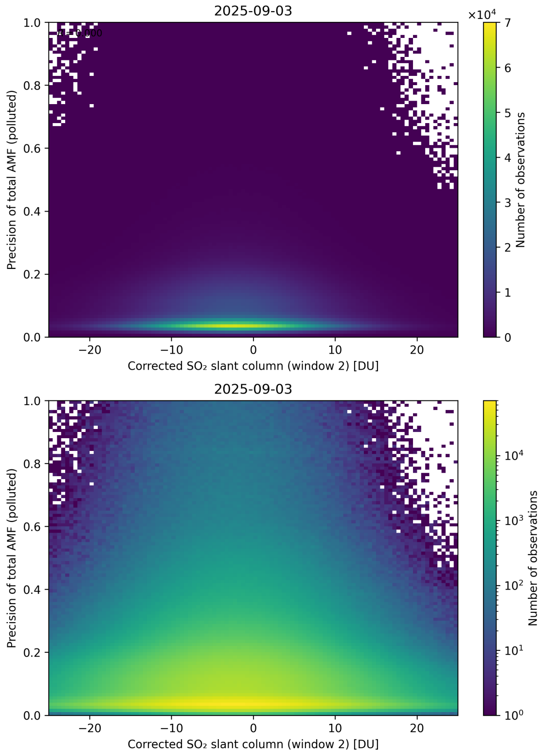
Figure 254: Scatter density plot of “Corrected SO 2 slant column (window 2)” against “Precision of total AMF (polluted)” for 2025-09-02 to 2025-09-04.
