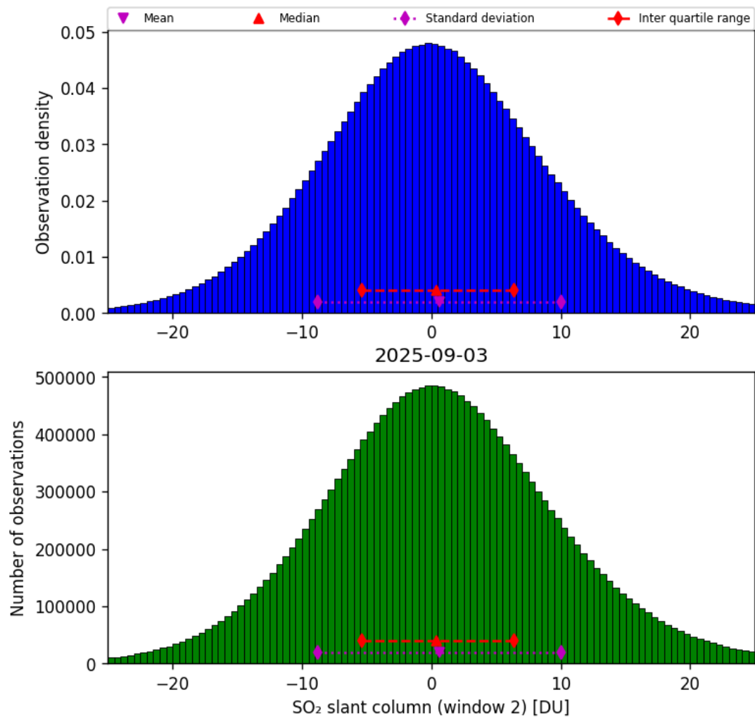
Figure 67: Histogram of “SO 2 slant column (window 2)” for 2025-09-02 to 2025-09-04
