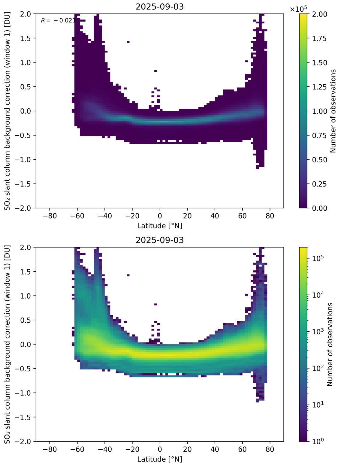
Figure 150: Scatter density plot of “Latitude” against “SO 2 slant column background correction (window 1)” for 2025-09-02 to 2025-09-04.
