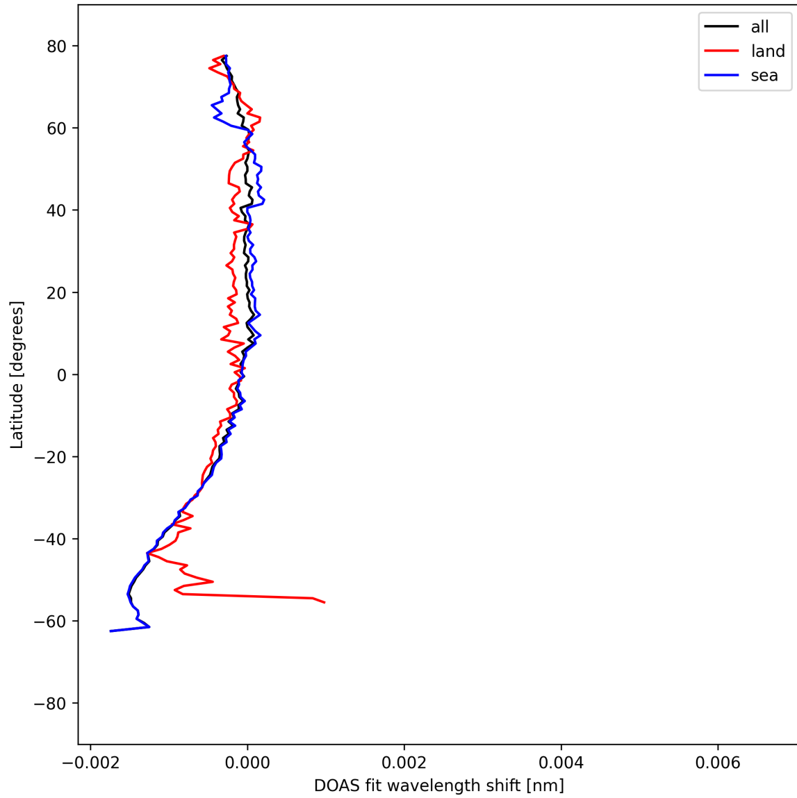
Figure 50: Zonal average of “DOAS fit wavelength shift” for 2025-09-02 to 2025-09-04.
