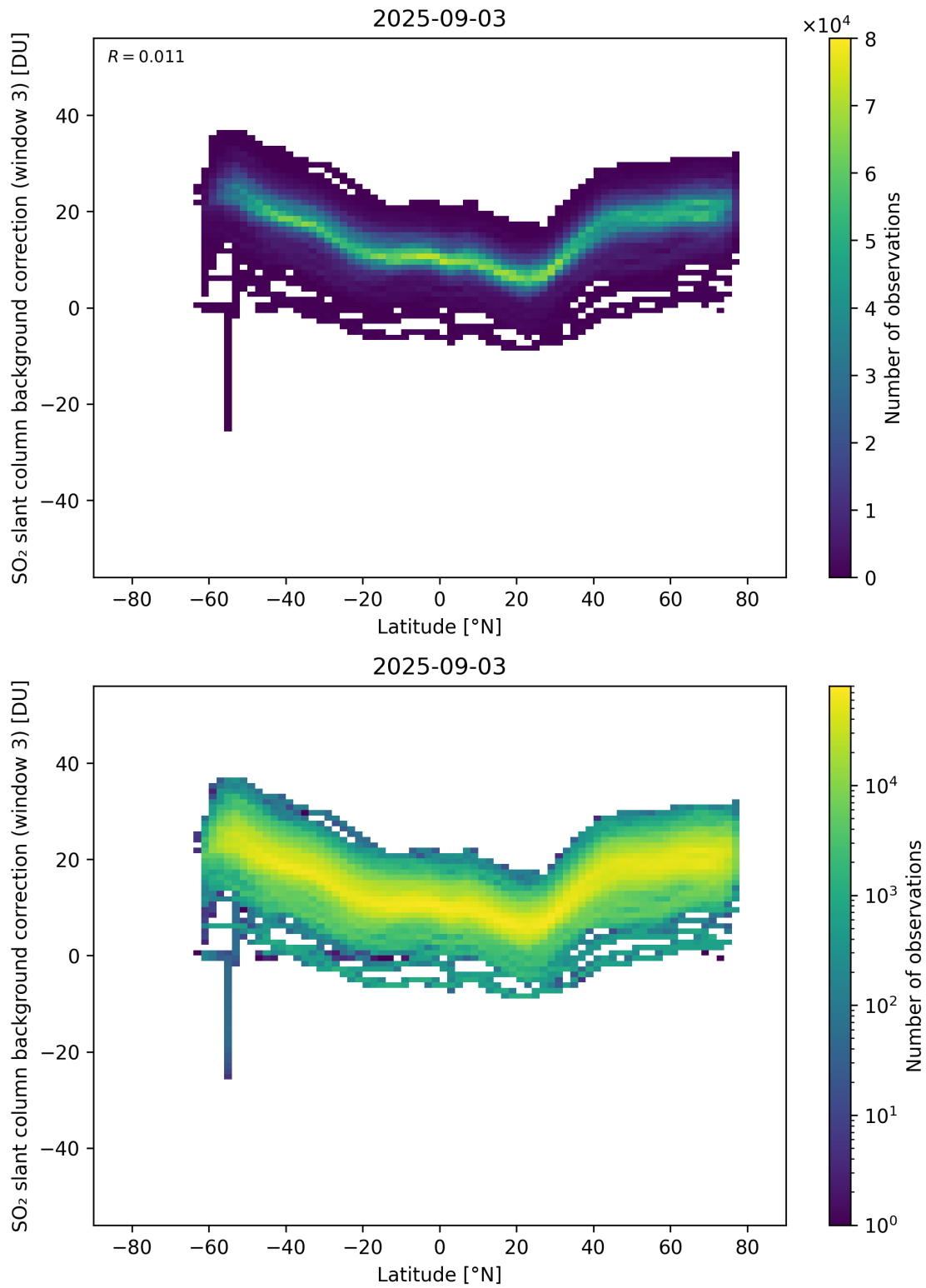
Figure 152: Scatter density plot of “Latitude” against “SO 2 slant column background correction (window 3)” for 2025-09-02 to 2025-09-04.
