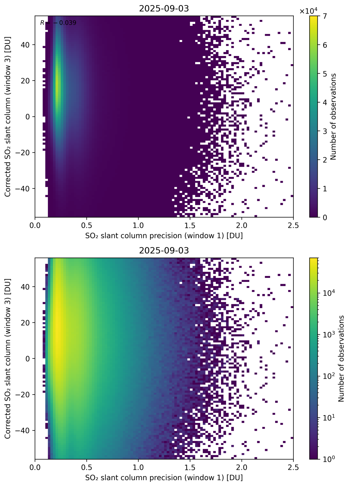
Figure 276: Scatter density plot of “SO 2 slant column precision (window 1)” against “Corrected SO 2 slant column (window 3)” for 2025-09-02 to 2025-09-04.
