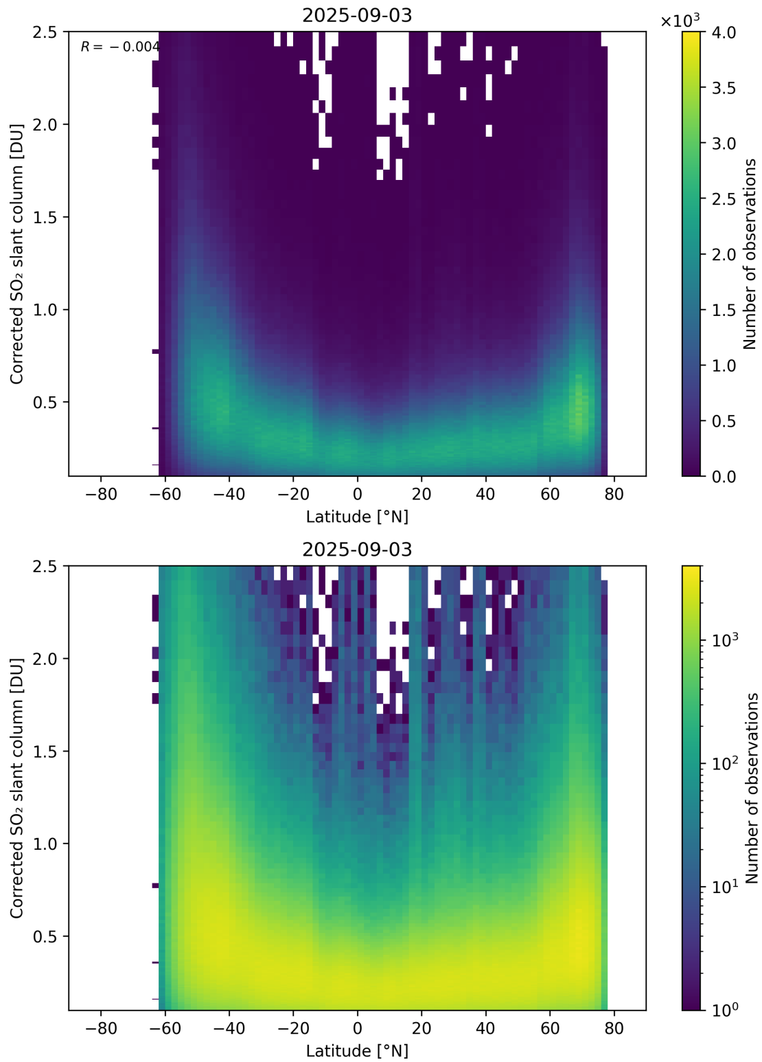
Figure 159: Scatter density plot of “Latitude” against “Corrected SO 2 slant column” for 2025-09-02 to 2025-09-04.
