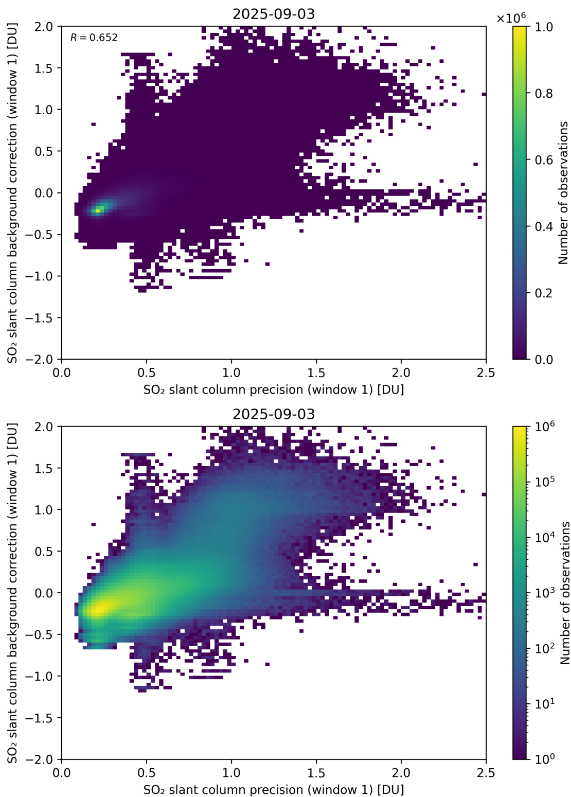
Figure 268: Scatter density plot of “SO 2 slant column precision (window 1)” against “SO 2 slant column background correction (window 1)” for 2025-09-02 to 2025-09-04.
