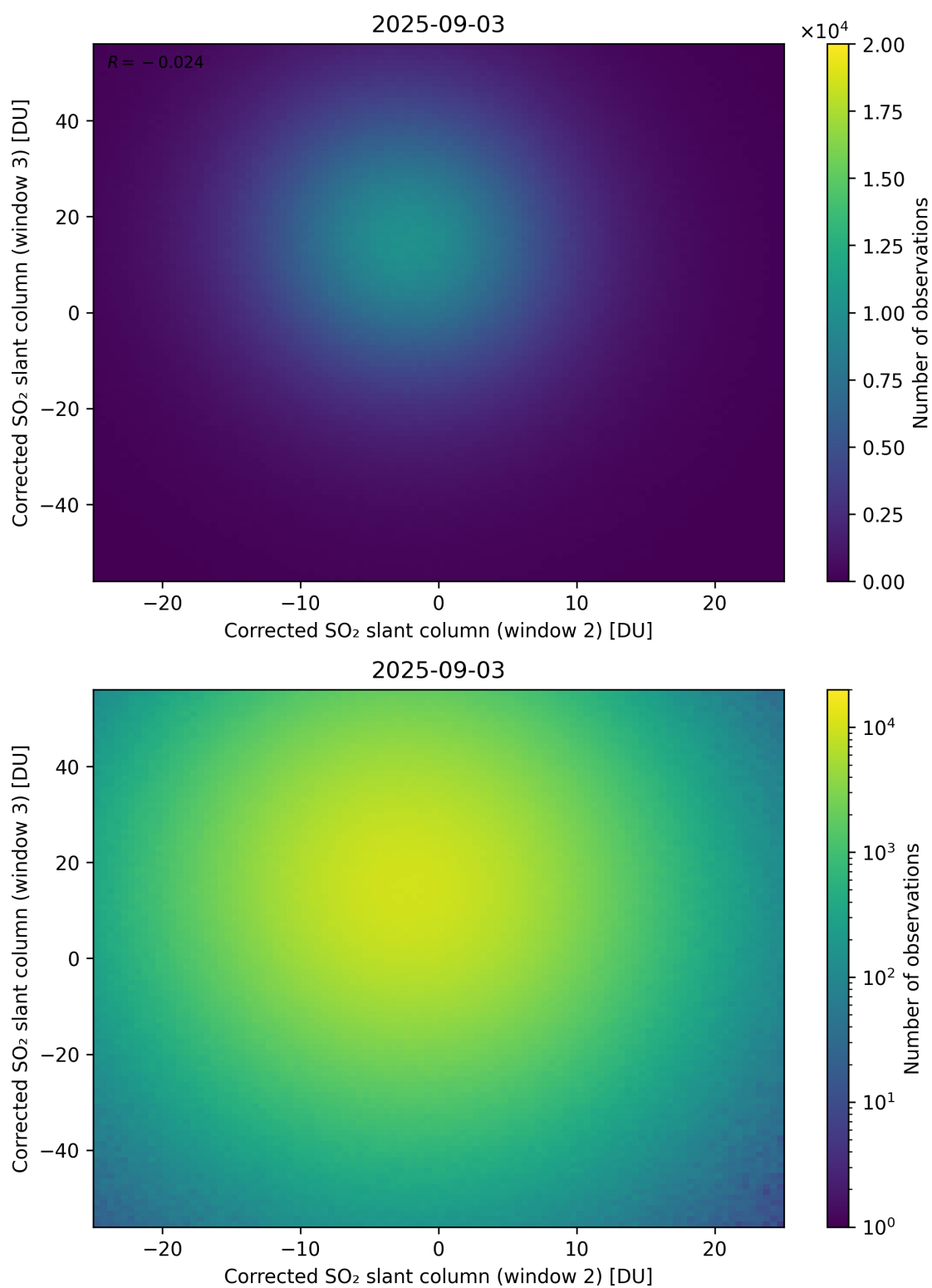
Figure 250: Scatter density plot of “Corrected SO 2 slant column (window 2)” against “Corrected SO 2 slant column (window 3)” for 2025-09-02 to 2025-09-04.
