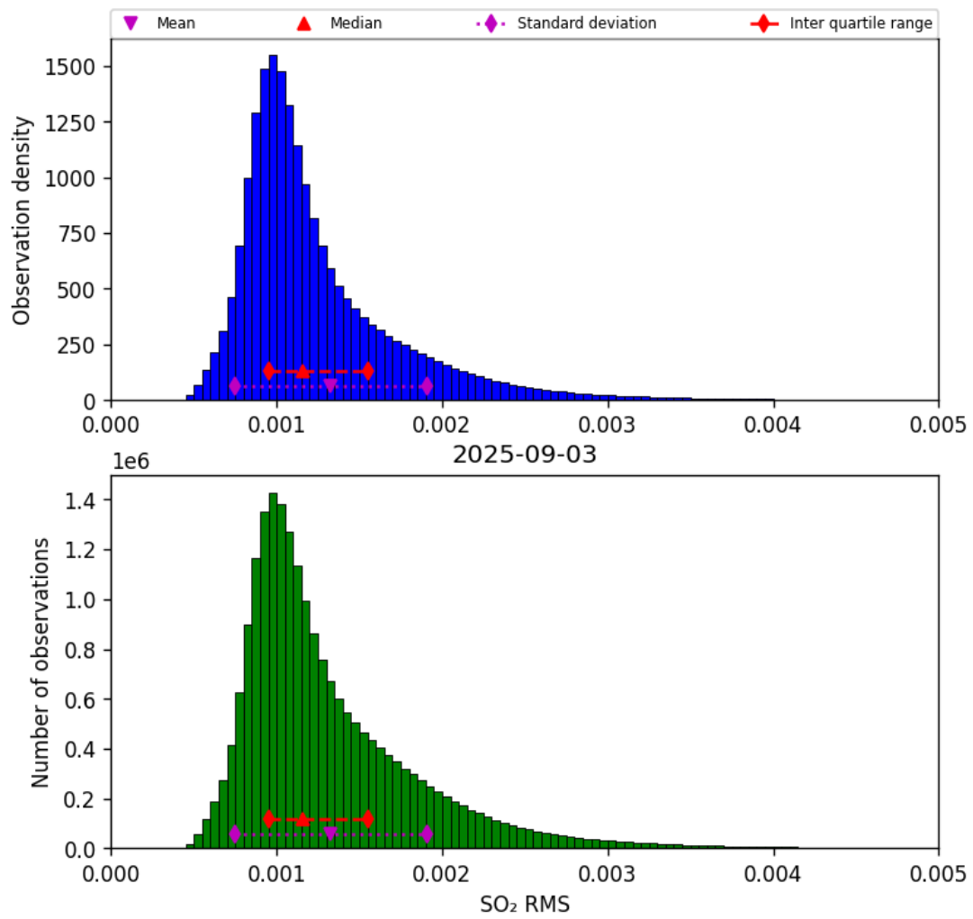
Figure 78: Histogram of “SO 2 RMS” for 2025-09-02 to 2025-09-04
