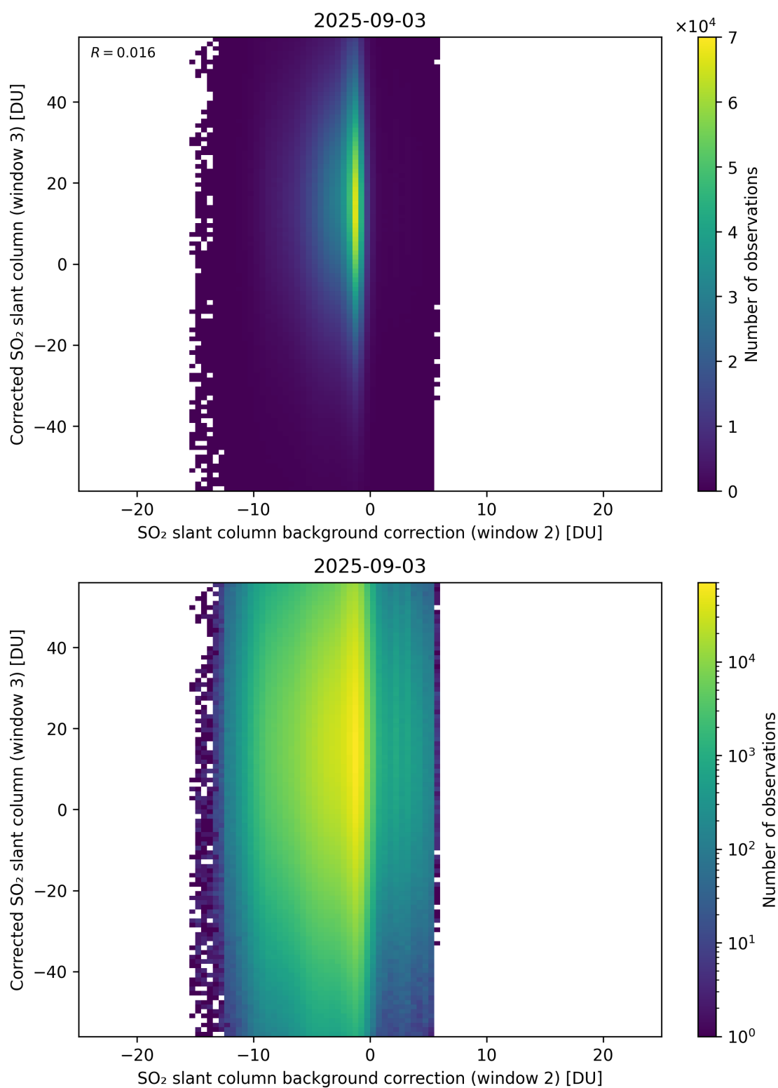
Figure 127: Scatter density plot of “SO 2 slant column background correction (window 2)” against “Corrected SO 2 slant column (window 3)” for 2025-09-02 to 2025-09-04.
