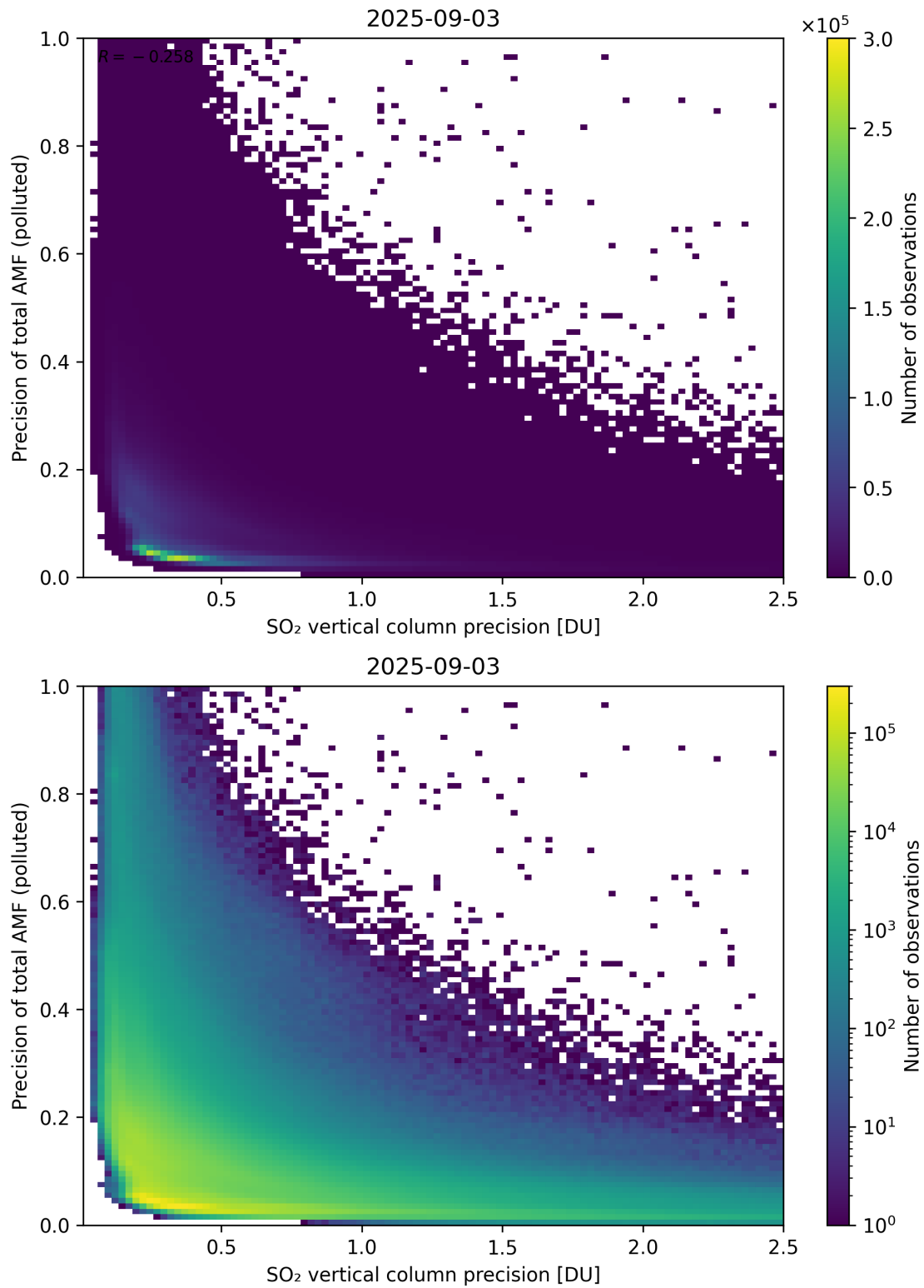
Figure 347: Scatter density plot of “SO 2 vertical column precision” against “Precision of total AMF (polluted)” for 2025-09-02 to 2025-09-04.
