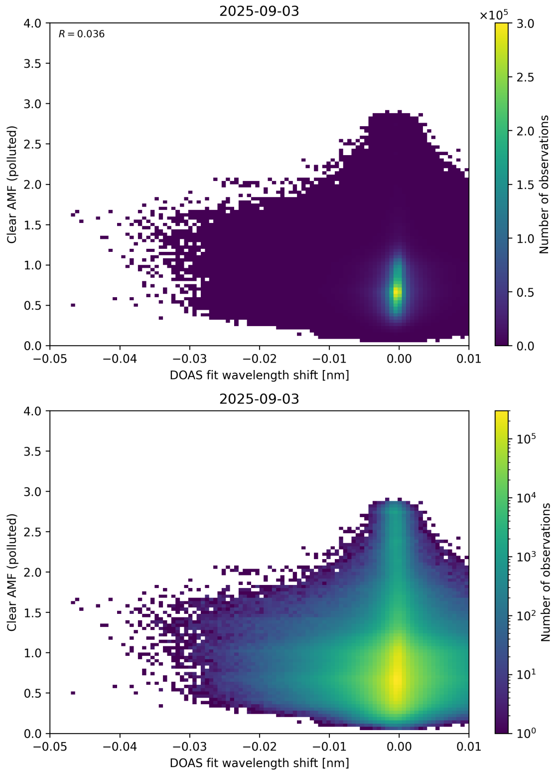
Figure 140: Scatter density plot of “DOAS fit wavelength shift” against “Clear AMF (polluted)” for 2025-09-02 to 2025-09-04.
