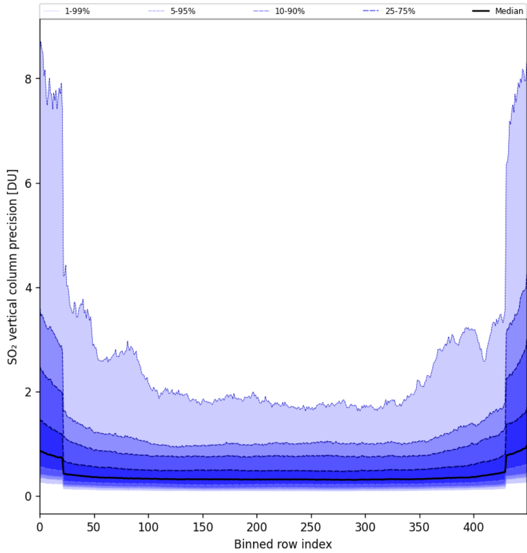
Figure 85: Along track statistics of “SO 2 vertical column precision” for 2025-09-02 to 2025-09-04
