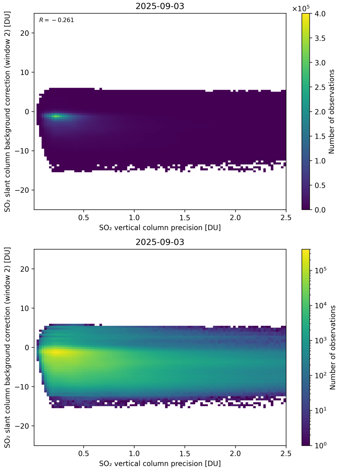
Figure 330: Scatter density plot of “SO 2 vertical column precision” against “SO 2 slant column background correction (window 2)” for 2025-09-02 to 2025-09-04.
