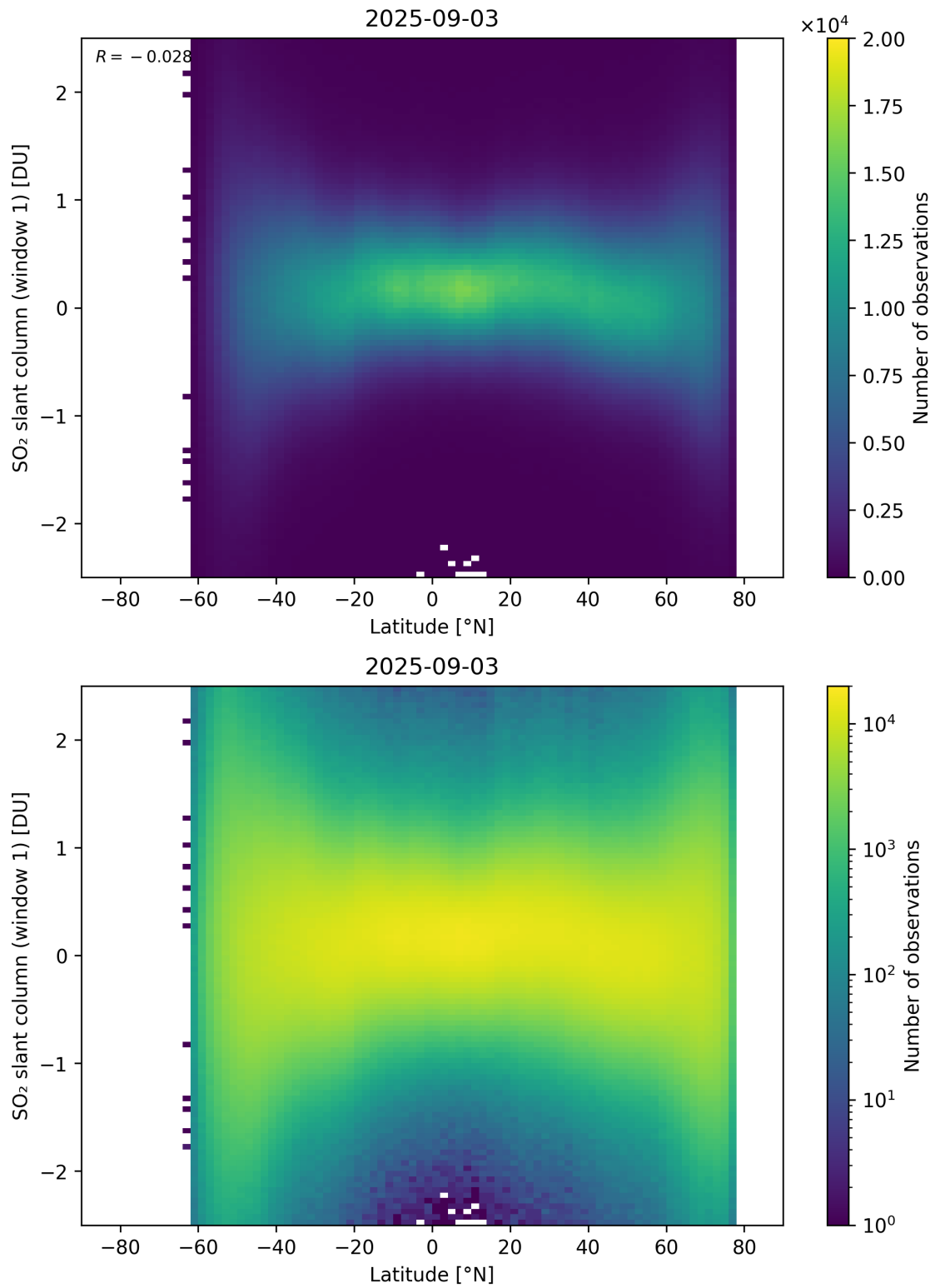
Figure 162: Scatter density plot of “Latitude” against “SO 2 slant column (window 1)” for 2025-09-02 to 2025-09-04.
