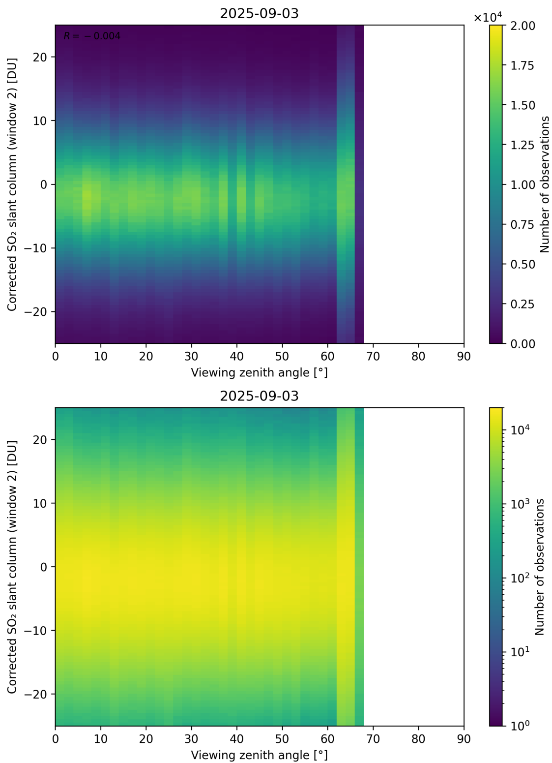
Figure 374: Scatter density plot of “Viewing zenith angle” against “Corrected SO 2 slant column (window 2)” for 2025-09-02 to 2025-09-04.
