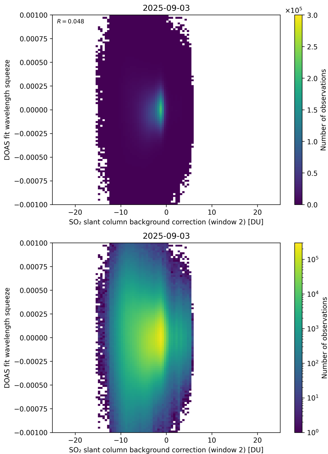
Figure 124: Scatter density plot of “SO 2 slant column background correction (window 2)” against “DOAS fit wavelength squeeze” for 2025-09-02 to 2025-09-04.
