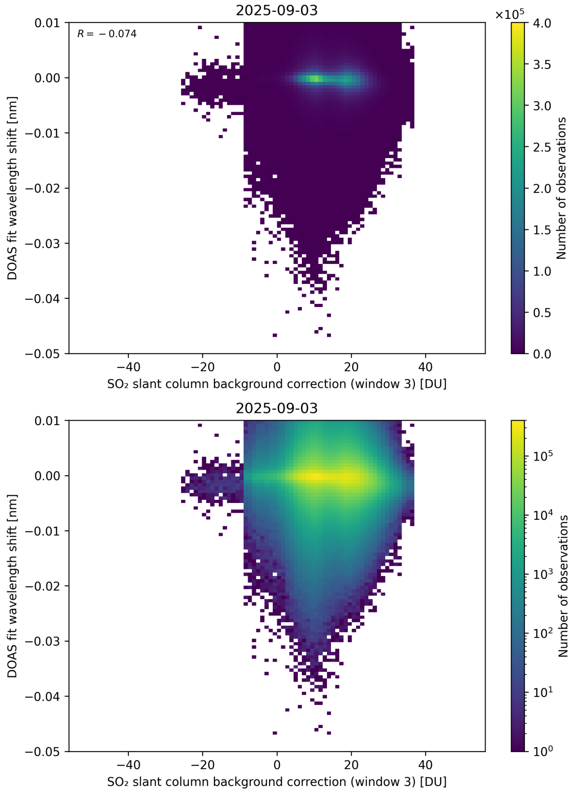
Figure 132: Scatter density plot of “SO 2 slant column background correction (window 3)” against “DOAS fit wavelength shift” for 2025-09-02 to 2025-09-04.
