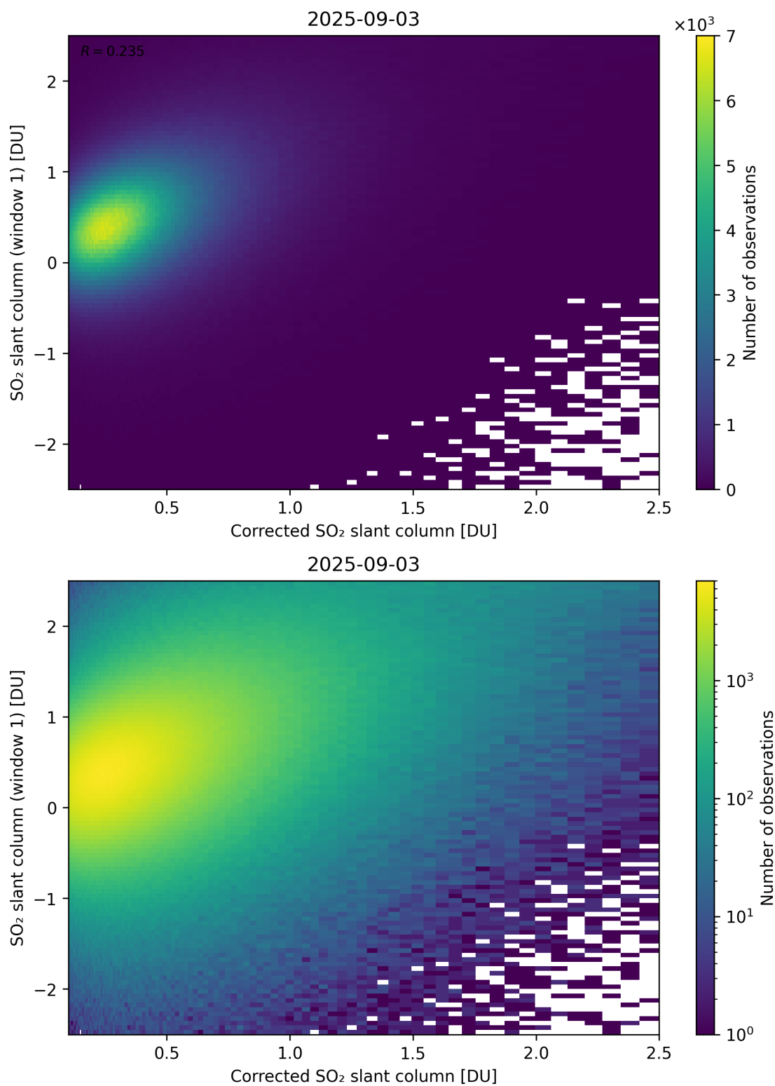
Figure 237: Scatter density plot of “Corrected SO 2 slant column” against “SO 2 slant column (window 1)” for 2025-09-02 to 2025-09-04.
