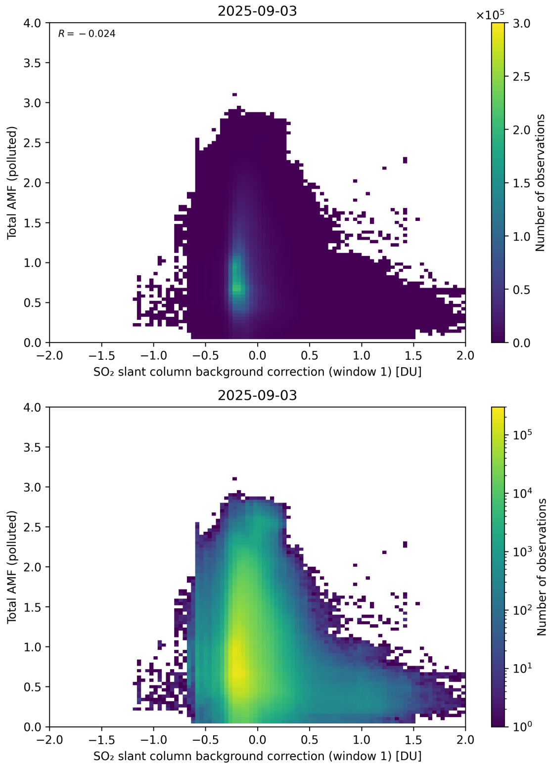
Figure 120: Scatter density plot of “SO 2 slant column background correction (window 1)” against “Total AMF (polluted)” for 2025-09-02 to 2025-09-04.
