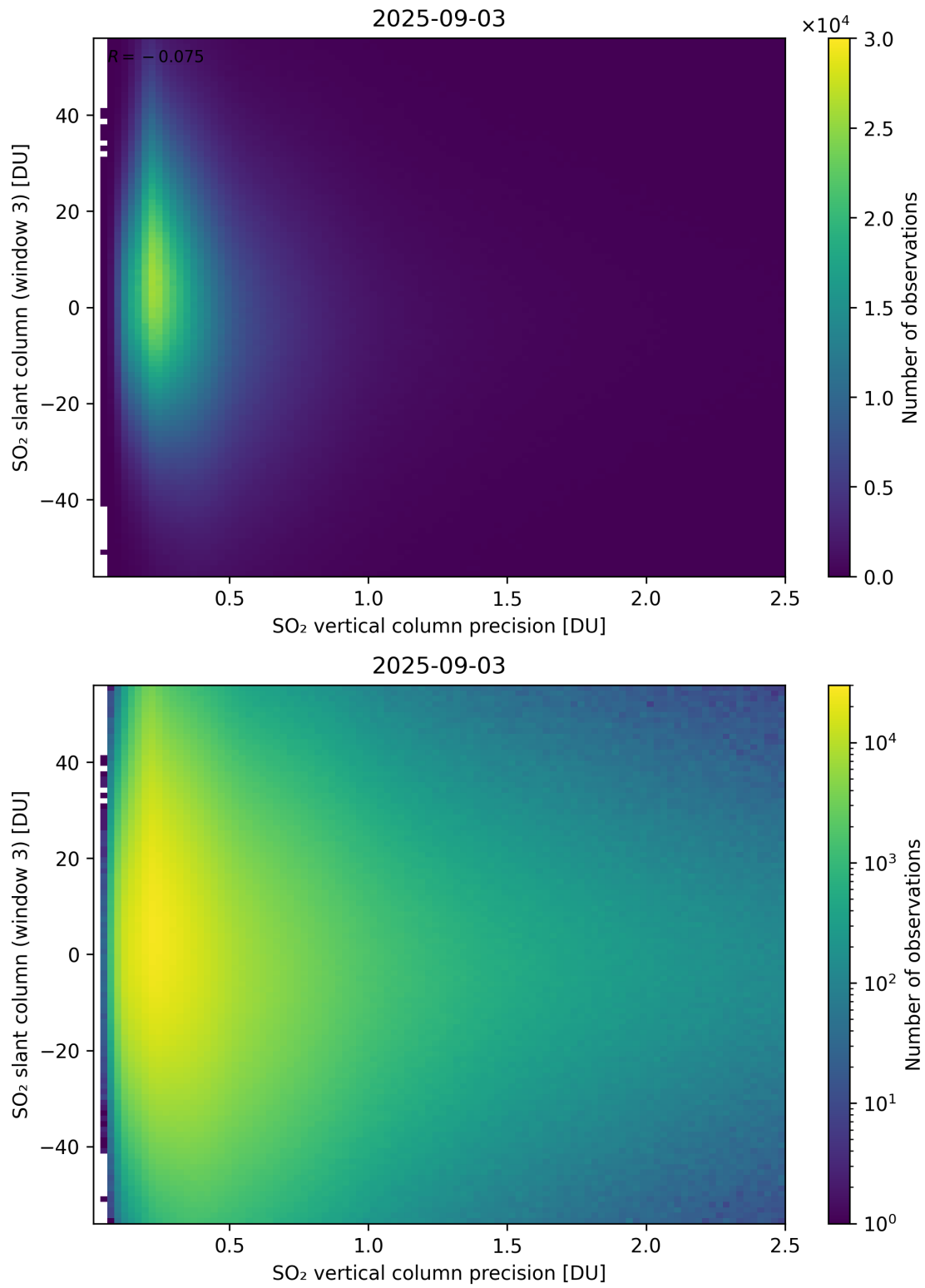
Figure 344: Scatter density plot of “SO 2 vertical column precision” against “SO 2 slant column (window 3)” for 2025-09-02 to 2025-09-04.
