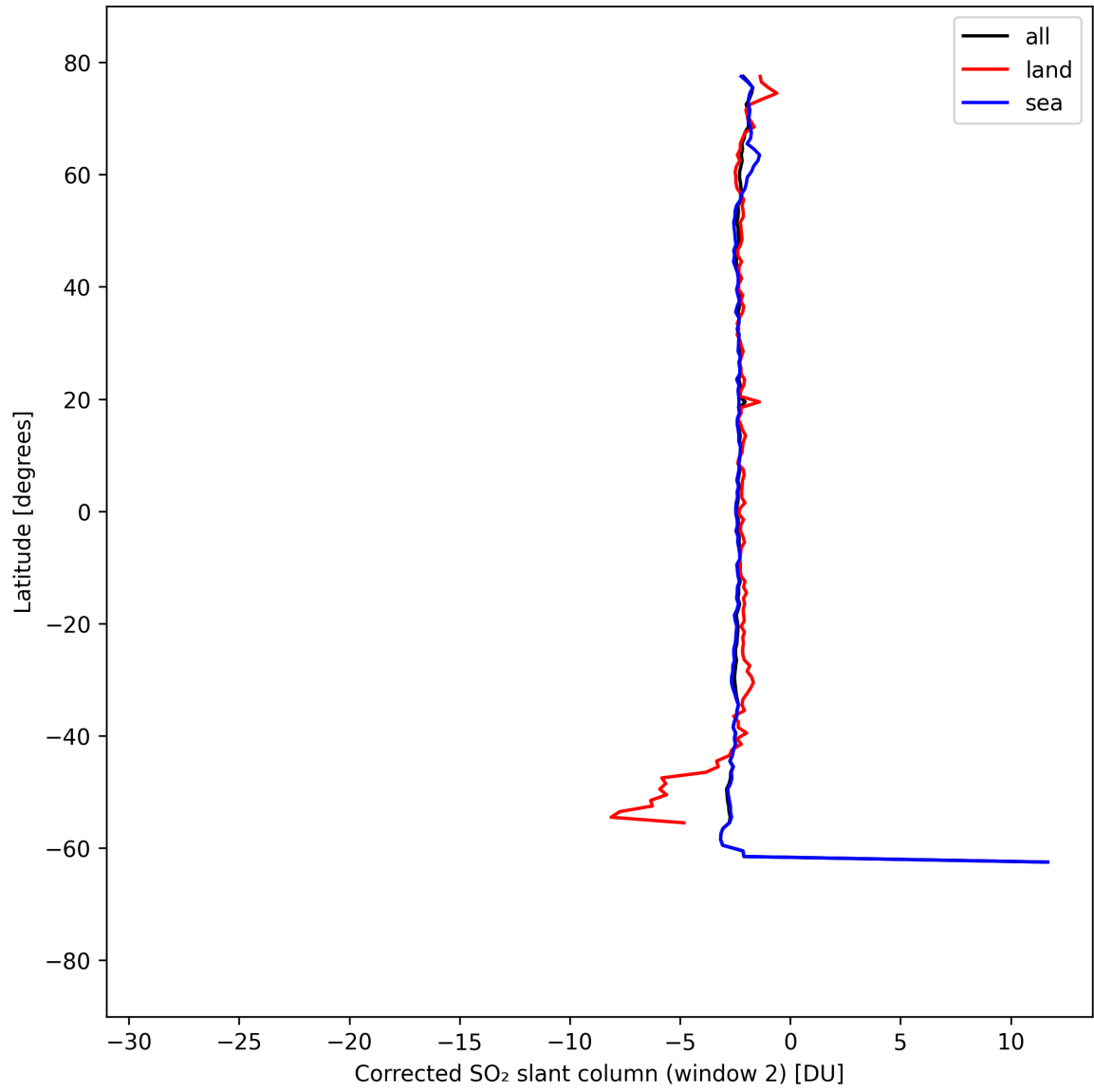
Figure 43: Zonal average of “Corrected SO 2 slant column (window 2)” for 2025-09-02 to 2025-09-04.
