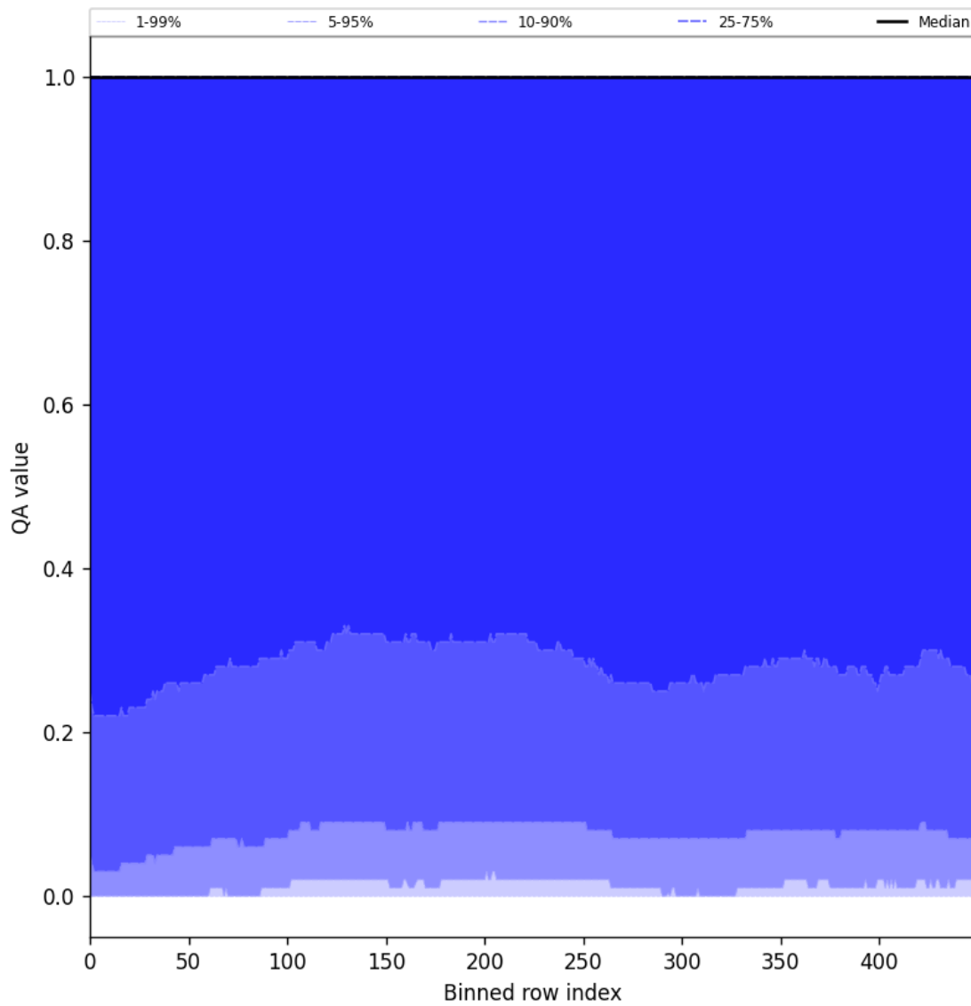
Figure 83: Along track statistics of “QA value” for 2025-09-02 to 2025-09-04
