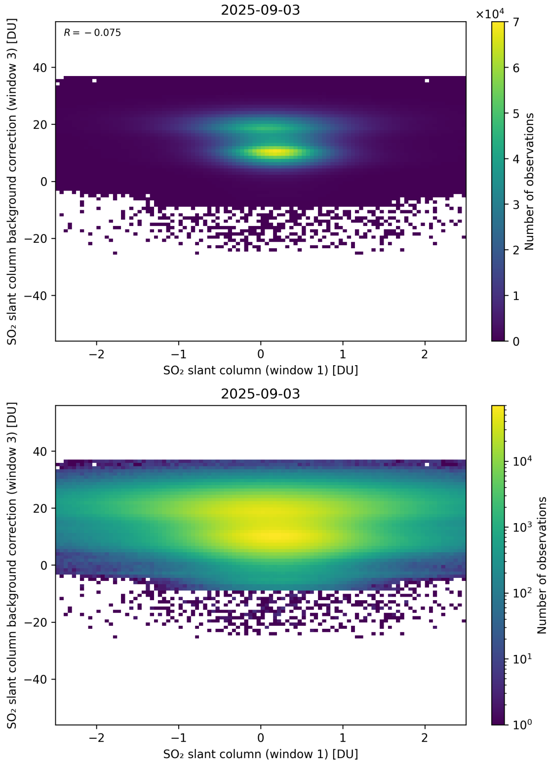
Figure 264: Scatter density plot of “SO 2 slant column (window 1)” against “SO 2 slant column background correction (window 3)” for 2025-09-02 to 2025-09-04.
