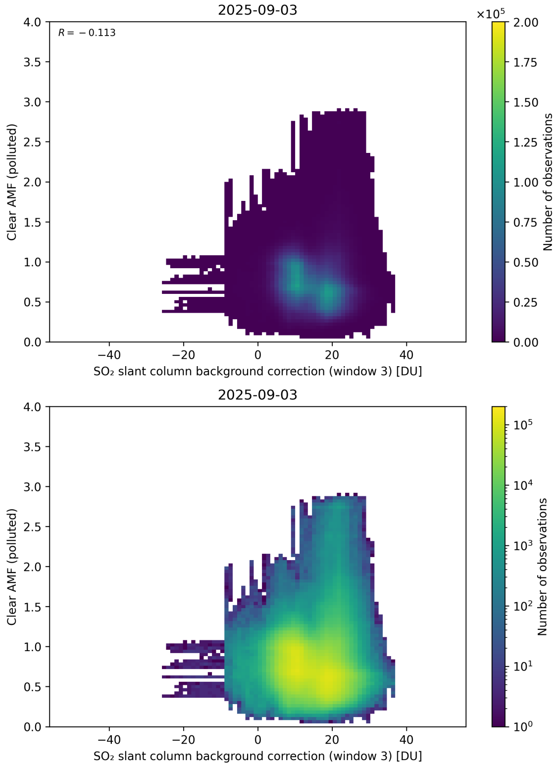
Figure 135: Scatter density plot of “SO 2 slant column background correction (window 3)” against “Clear AMF (polluted)” for 2025-09-02 to 2025-09-04.
