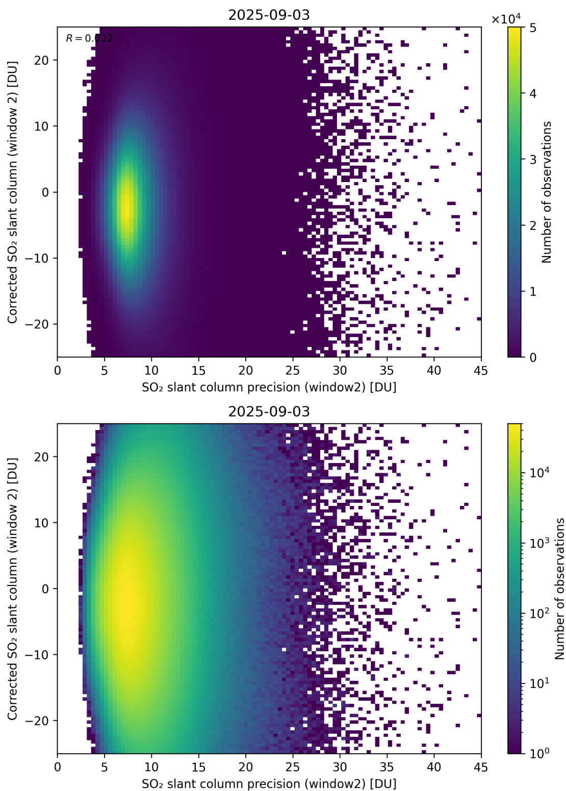
Figure 297: Scatter density plot of “SO 2 slant column precision (window2)” against “Corrected SO 2 slant column (window 2)” for 2025-09-02 to 2025-09-04.
