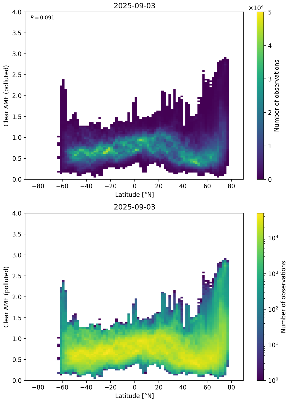
Figure 156: Scatter density plot of “Latitude” against “Clear AMF (polluted)” for 2025-09-02 to 2025-09-04.
