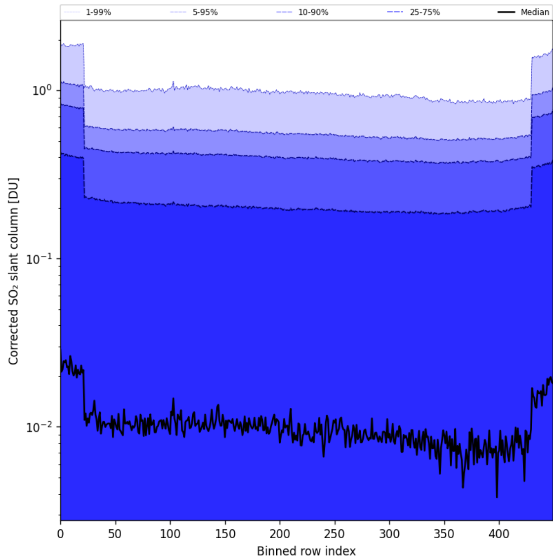
Figure 86: Along track statistics of “Corrected SO 2 slant column” for 2025-09-02 to 2025-09-04
