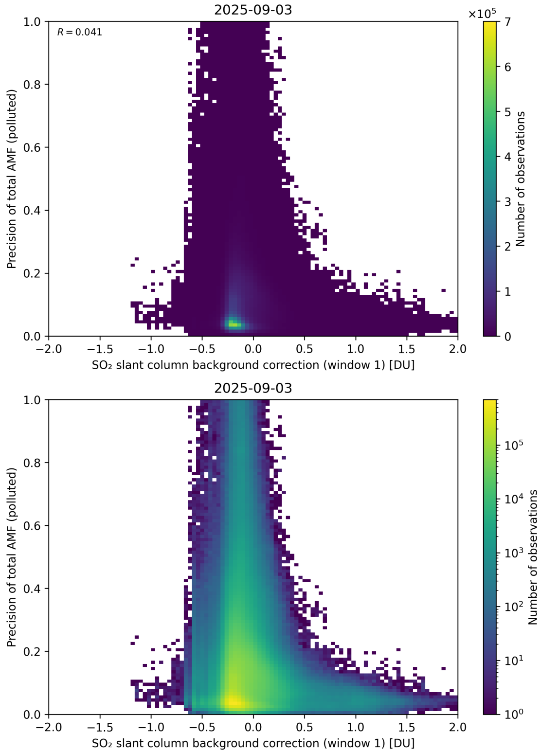
Figure 121: Scatter density plot of “SO 2 slant column background correction (window 1)” against “Precision of total AMF (polluted)” for 2025-09-02 to 2025-09-04.
