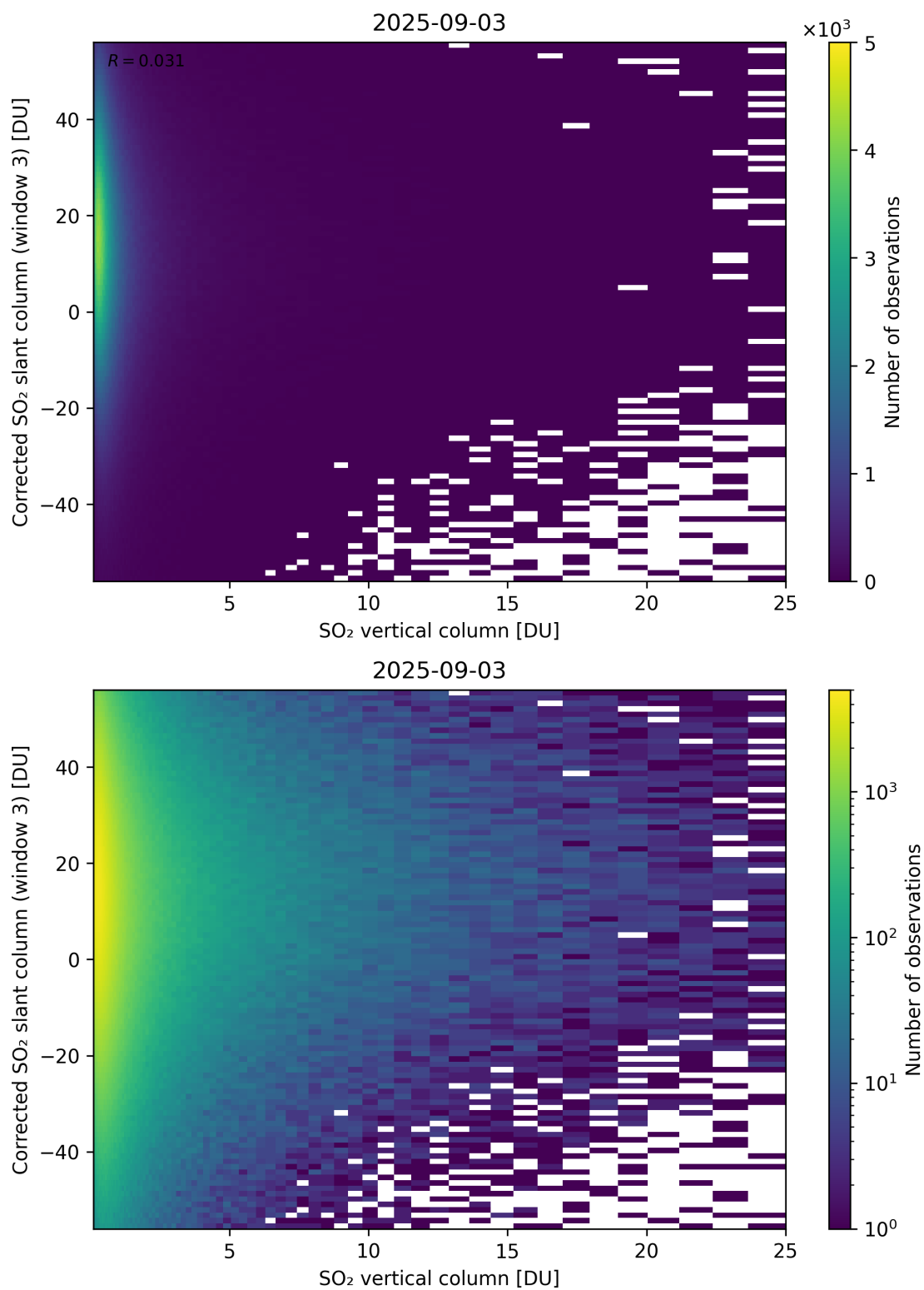
Figure 353: Scatter density plot of “SO 2 vertical column” against “Corrected SO 2 slant column (window 3)” for 2025-09-02 to 2025-09-04.
