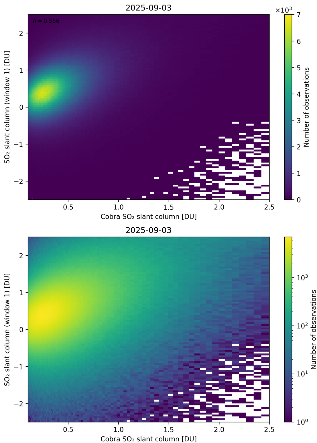
Figure 219: Scatter density plot of “Cobra SO 2 slant column” against “SO 2 slant column (window 1)” for 2025-09-02 to 2025-09-04.
