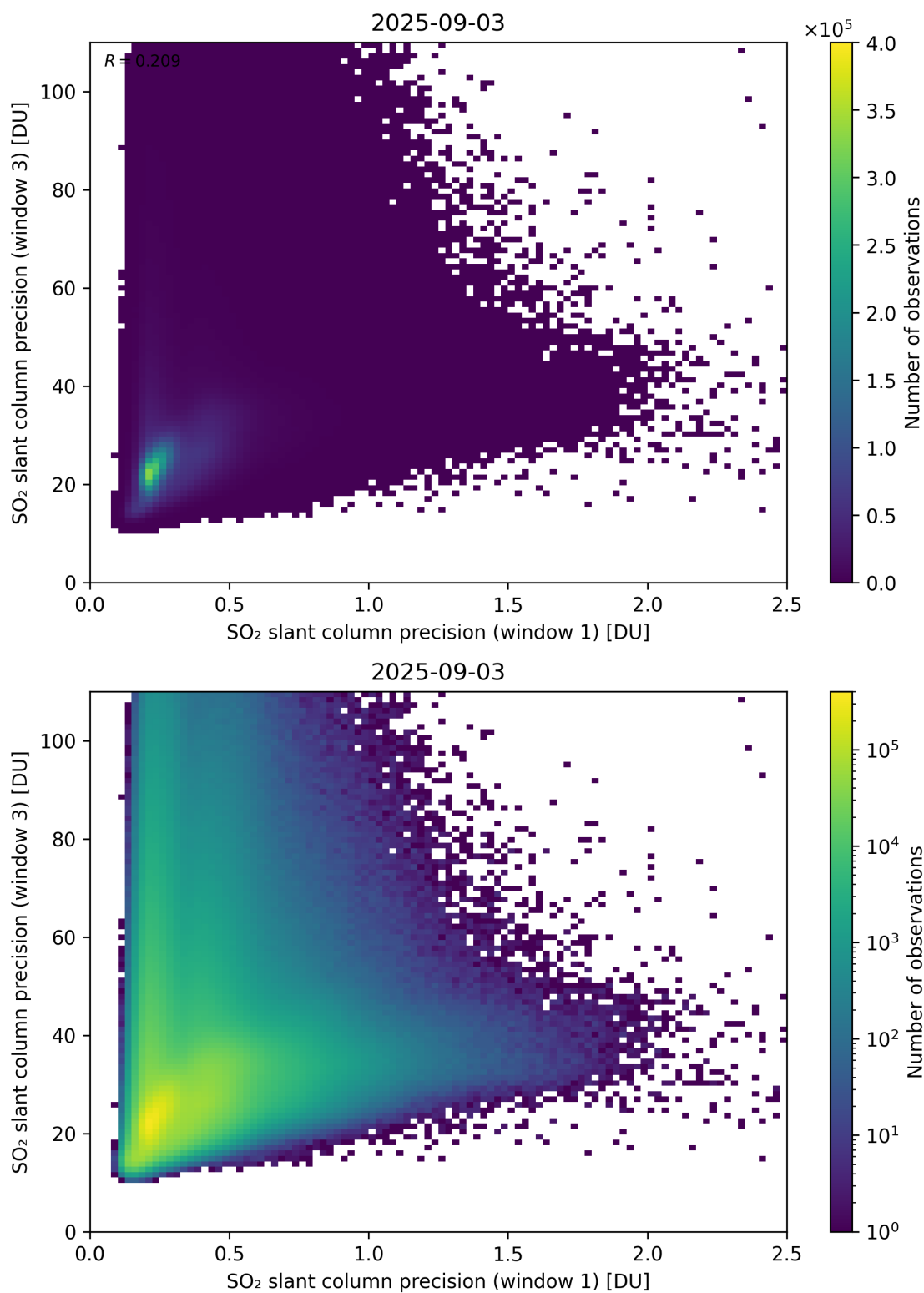
Figure 279: Scatter density plot of “SO 2 slant column precision (window 1)” against “SO 2 slant column precision (window 3)” for 2025-09-02 to 2025-09-04.
