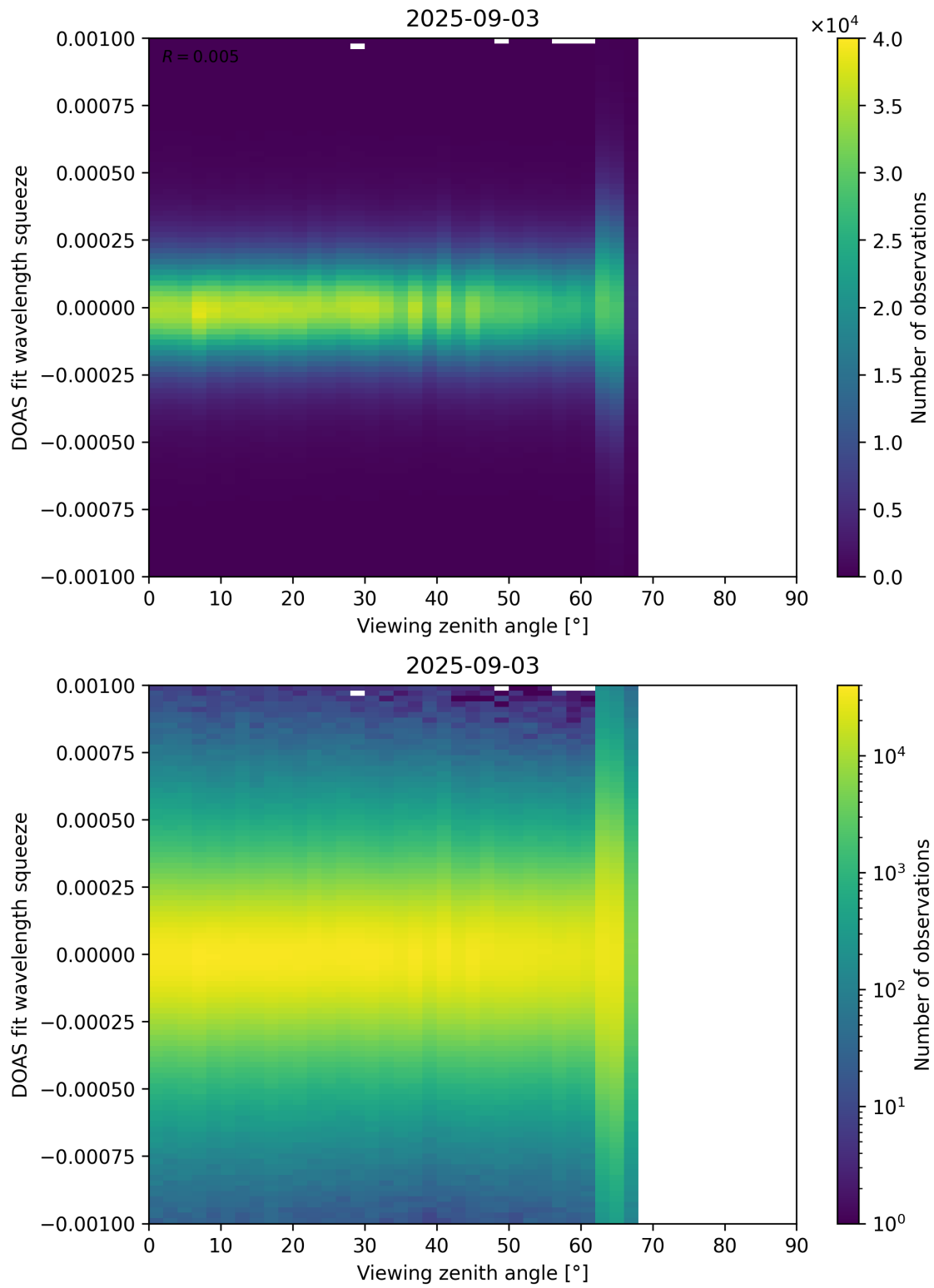
Figure 366: Scatter density plot of “Viewing zenith angle” against “DOAS fit wavelength squeeze” for 2025-09-02 to 2025-09-04.
