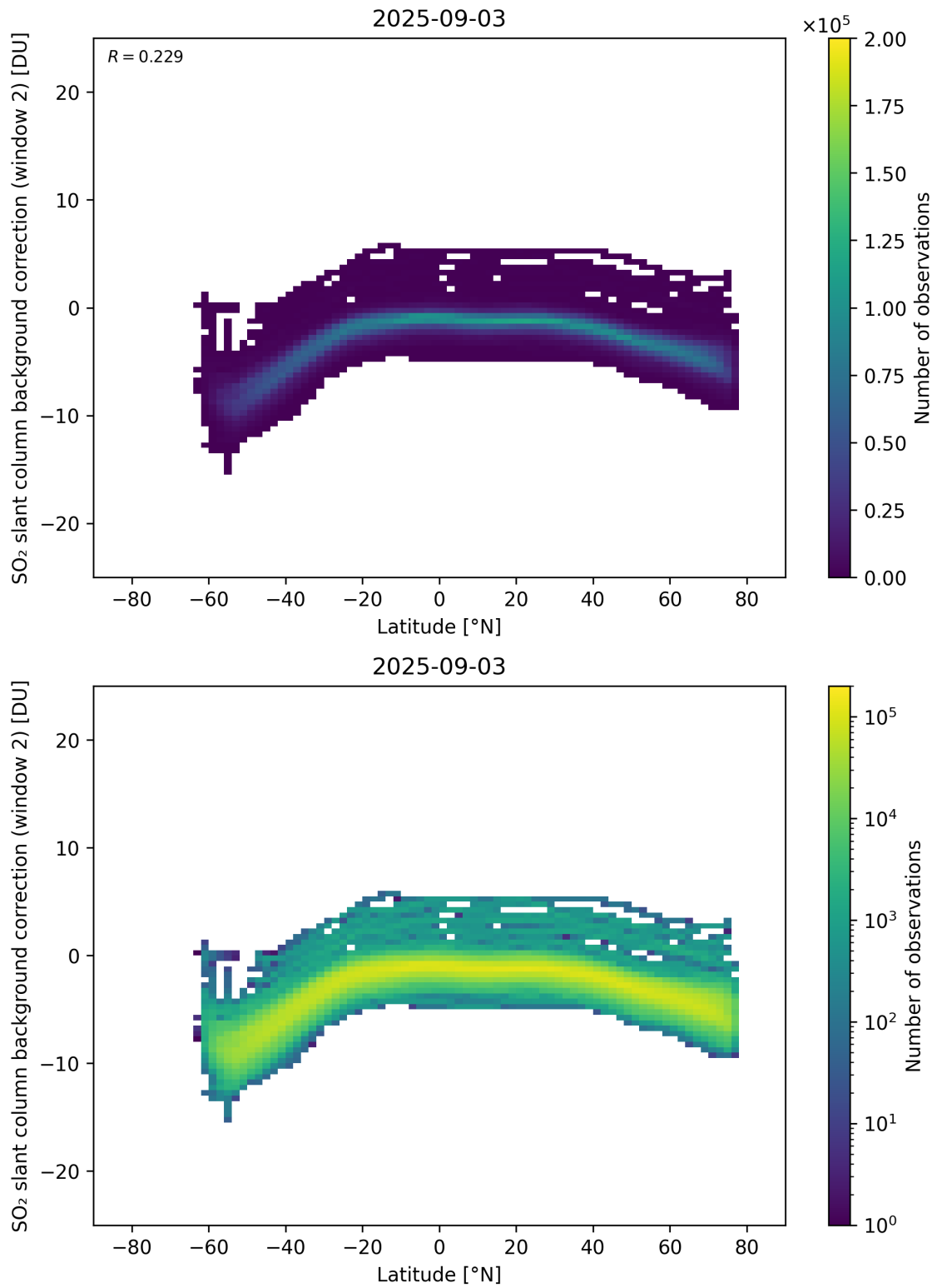
Figure 151: Scatter density plot of “Latitude” against “SO 2 slant column background correction (window 2)” for 2025-09-02 to 2025-09-04.
