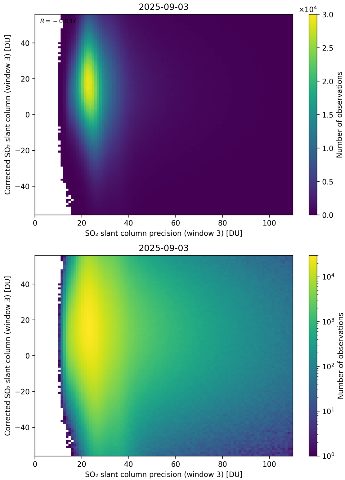
Figure 312: Scatter density plot of “SO 2 slant column precision (window 3)” against “Corrected SO 2 slant column (window 3)” for 2025-09-02 to 2025-09-04.
