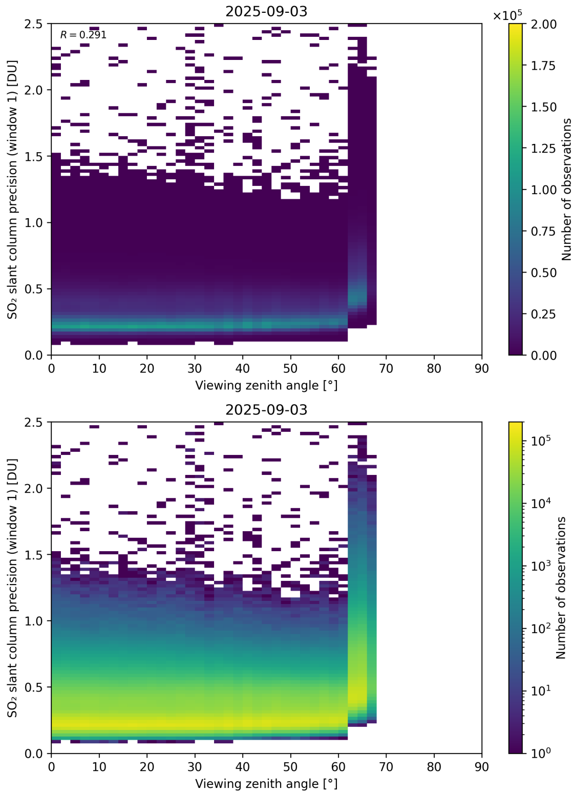
Figure 377: Scatter density plot of “Viewing zenith angle” against “SO 2 slant column precision (window 1)” for 2025-09-02 to 2025-09-04.
