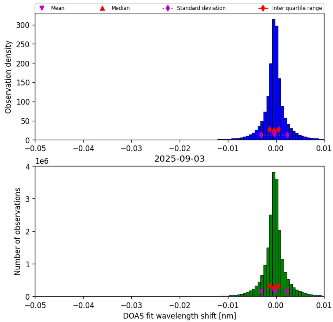
Figure 76: Histogram of “DOAS fit wavelength shift” for 2025-09-02 to 2025-09-04
