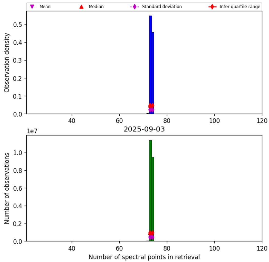
Figure 82: Histogram of “Number of spectral points in retrieval” for 2025-09-02 to 2025-09-04
