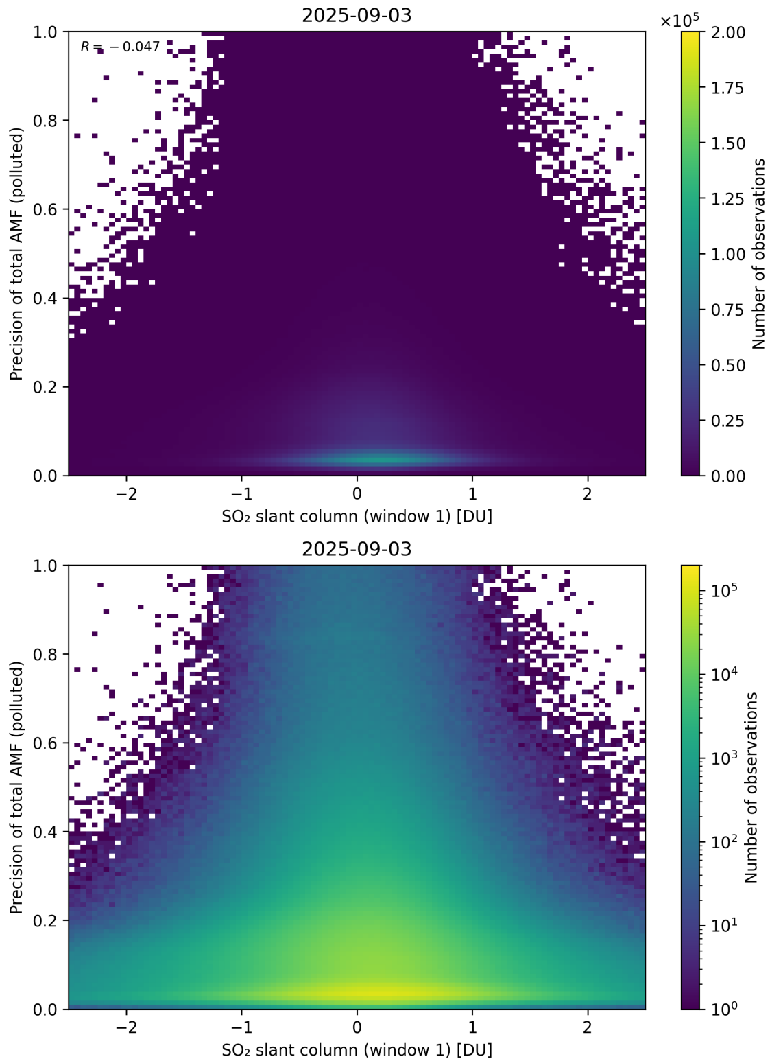
Figure 290: Scatter density plot of “SO 2 slant column (window 1)” against “Precision of total AMF (polluted)” for 2025-09-02 to 2025-09-04.
