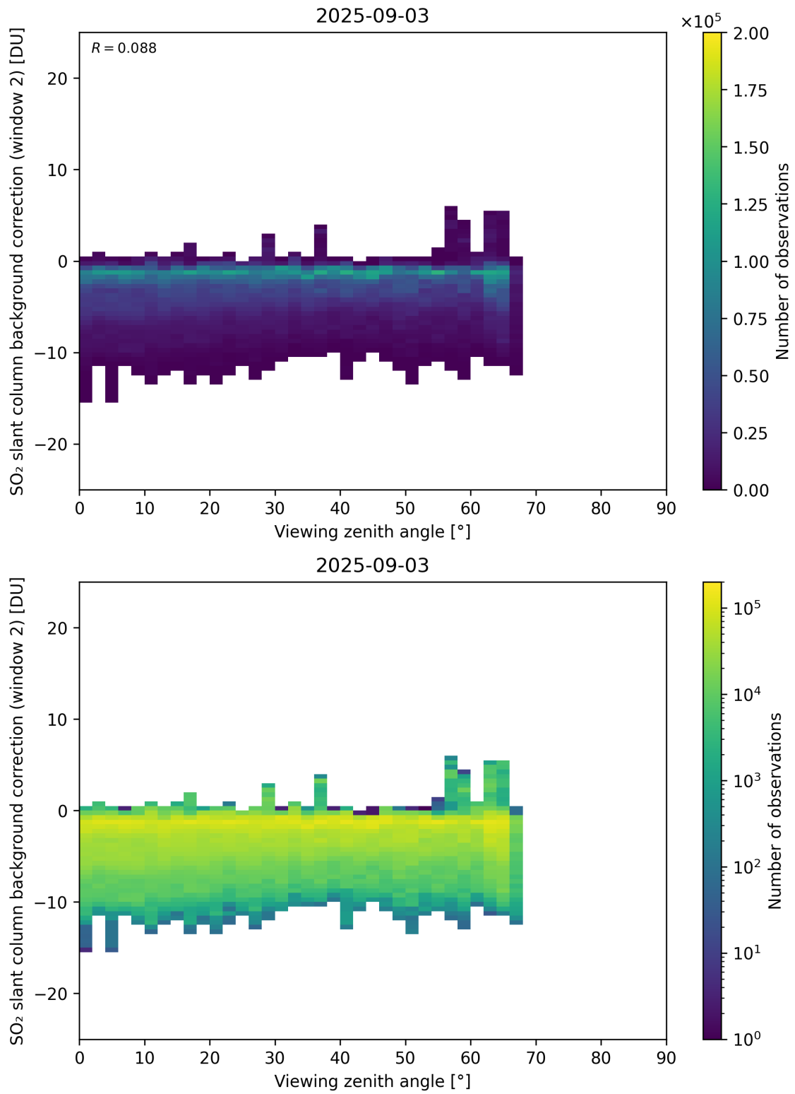
Figure 363: Scatter density plot of “Viewing zenith angle” against “SO 2 slant column background correction (window 2)” for 2025-09-02 to 2025-09-04.
