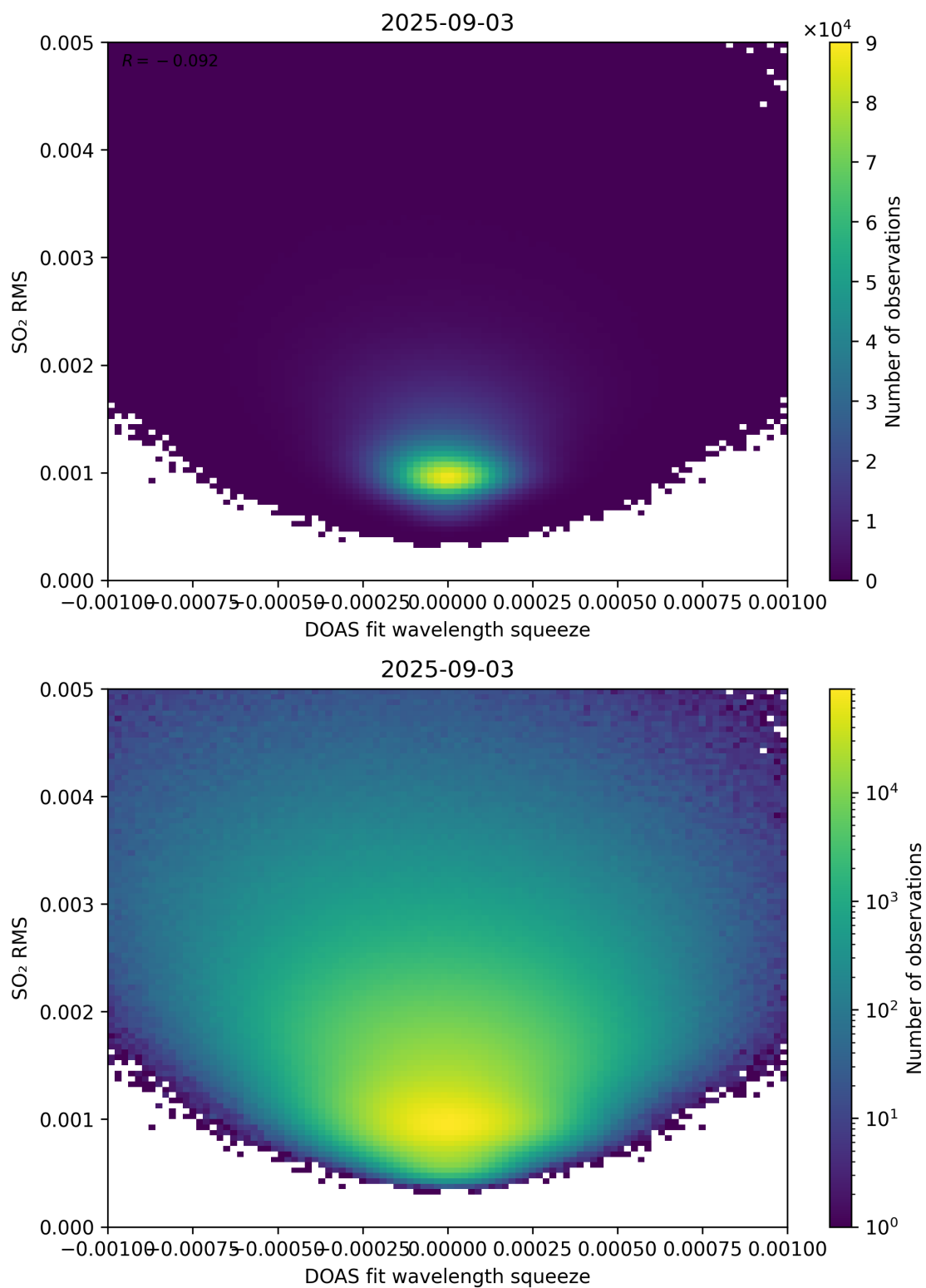
Figure 143: Scatter density plot of “DOAS fit wavelength squeeze” against “SO 2 RMS” for 2025-09-02 to 2025-09-04.
