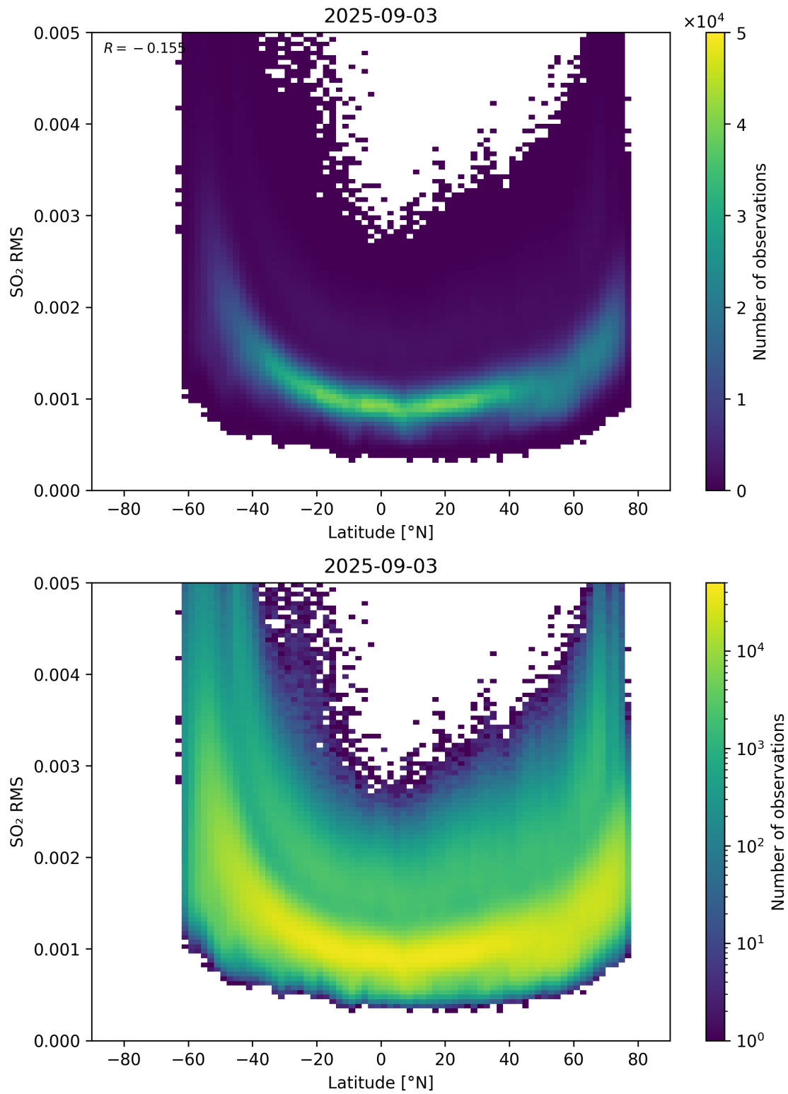
Figure 155: Scatter density plot of “Latitude” against “SO 2 RMS” for 2025-09-02 to 2025-09-04.
