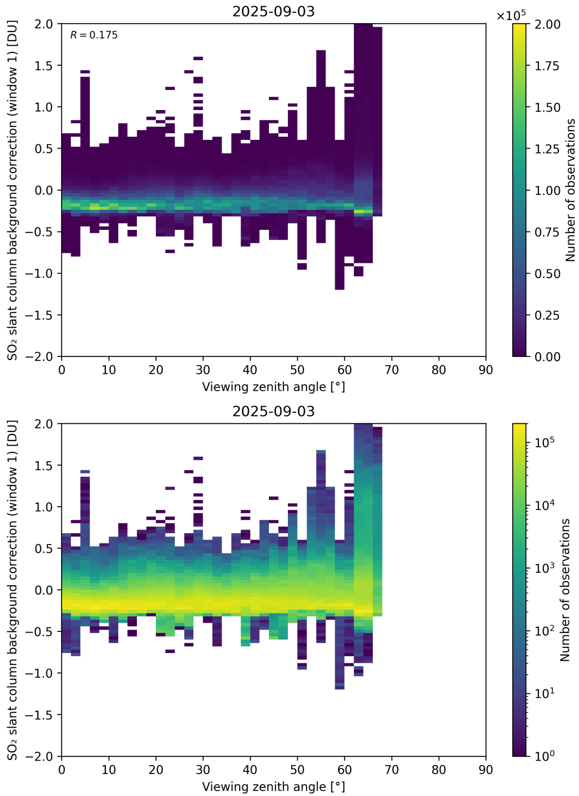
Figure 362: Scatter density plot of “Viewing zenith angle” against “SO 2 slant column background correction (window 1)” for 2025-09-02 to 2025-09-04.
