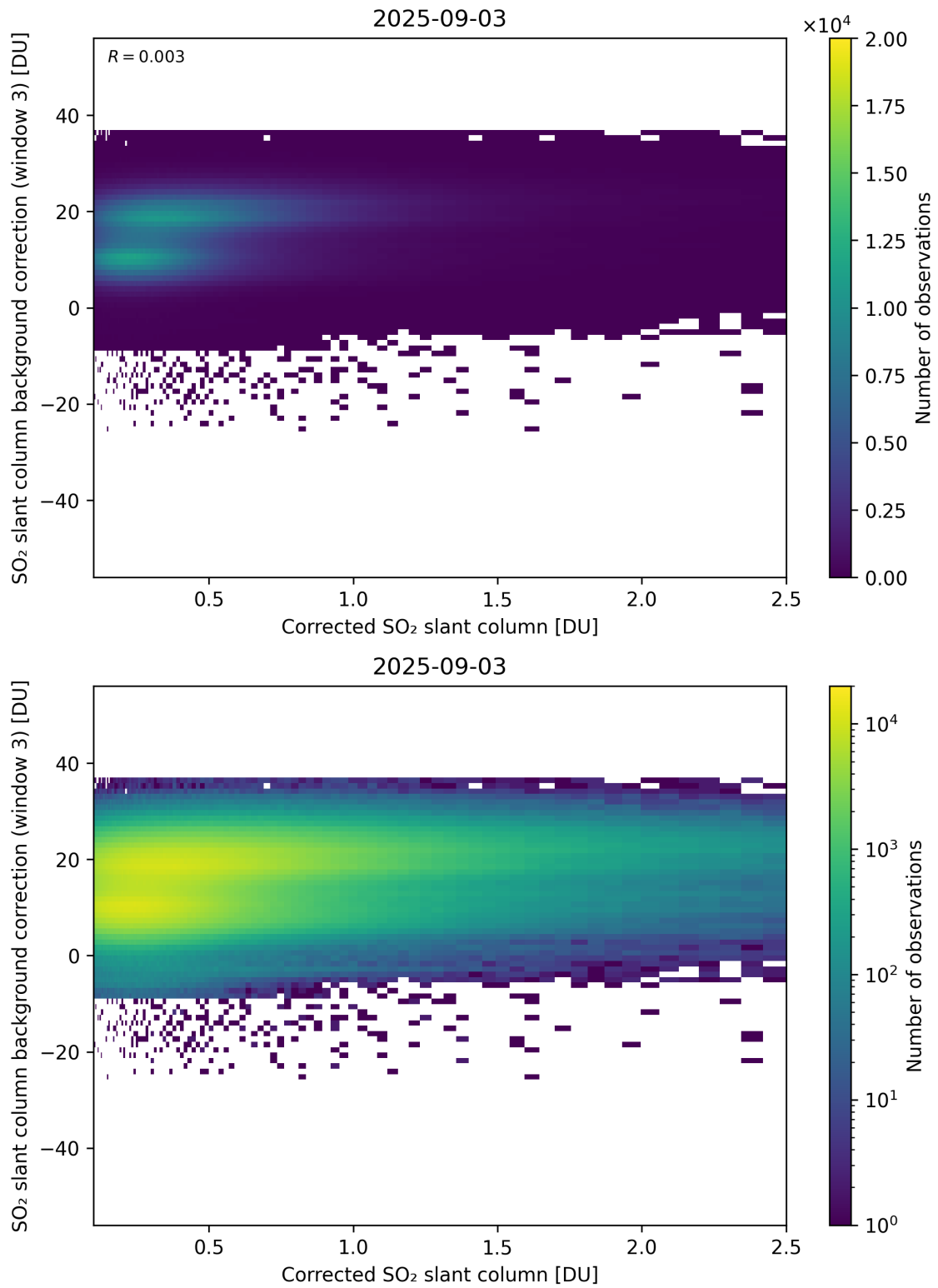
Figure 228: Scatter density plot of “Corrected SO 2 slant column” against “SO 2 slant column background correction (window 3)” for 2025-09-02 to 2025-09-04.
