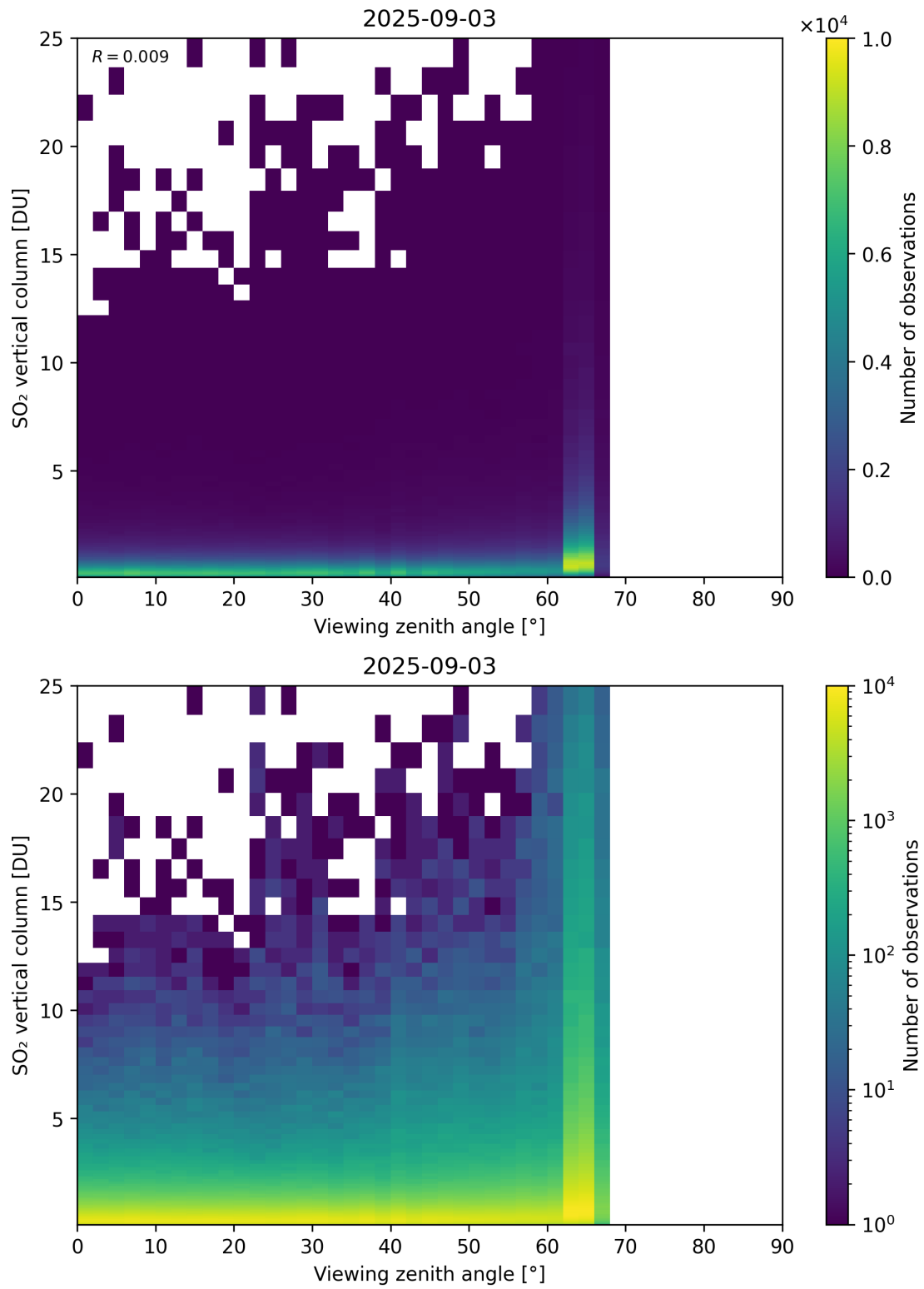
Figure 383: Scatter density plot of “Viewing zenith angle” against “SO 2 vertical column” for 2025-09-02 to 2025-09-04.
