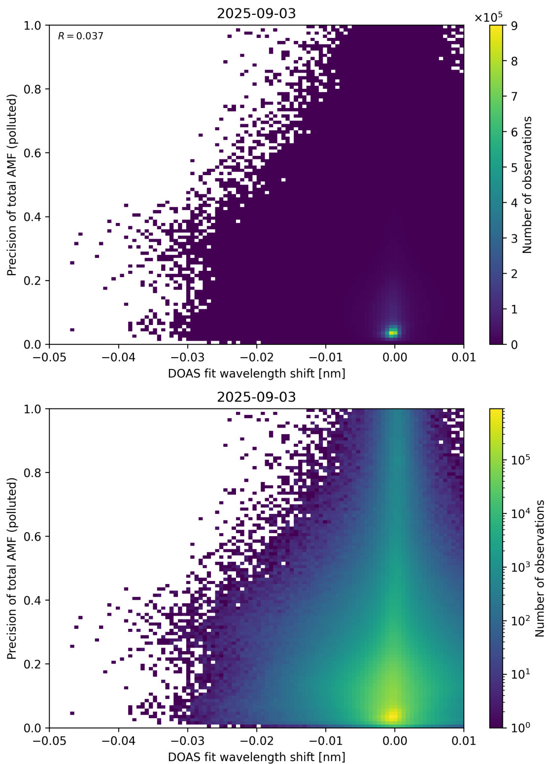
Figure 142: Scatter density plot of “DOAS fit wavelength shift” against “Precision of total AMF (polluted)” for 2025-09-02 to 2025-09-04.
