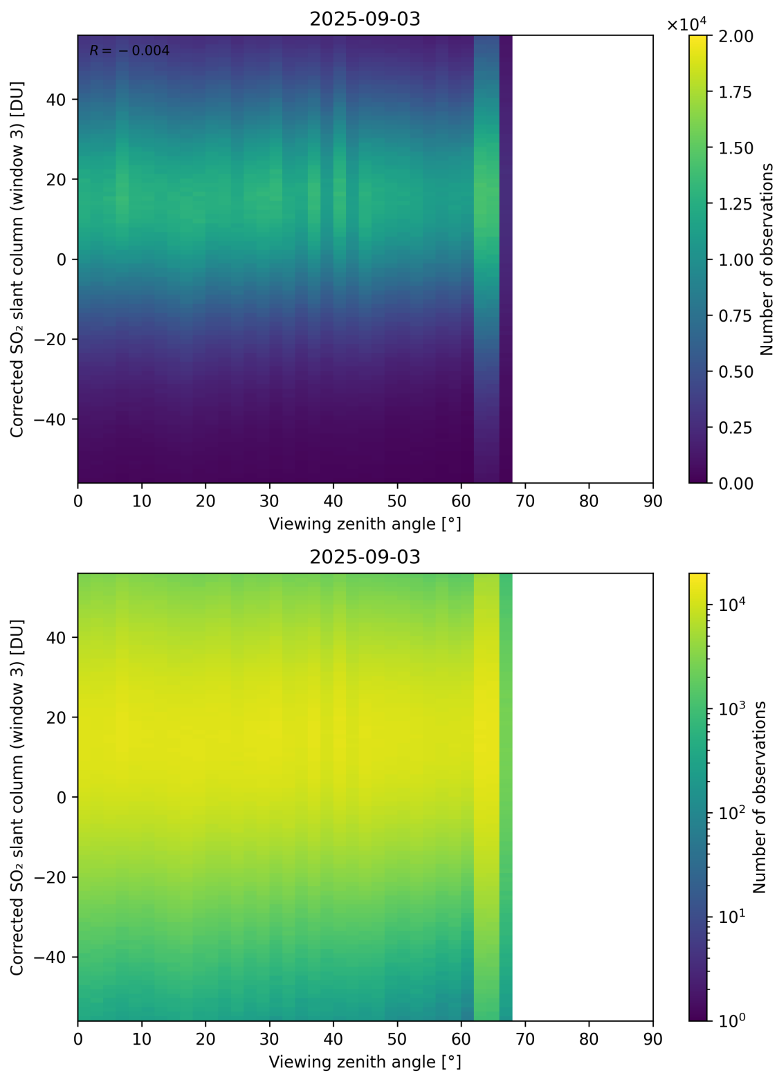
Figure 375: Scatter density plot of “Viewing zenith angle” against “Corrected SO 2 slant column (window 3)” for 2025-09-02 to 2025-09-04.
