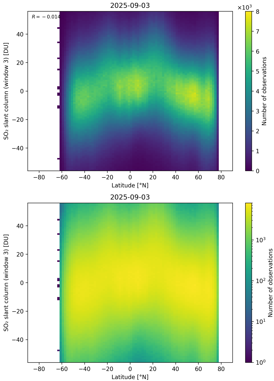
Figure 165: Scatter density plot of “Latitude” against “SO 2 slant column (window 3)” for 2025-09-02 to 2025-09-04.
