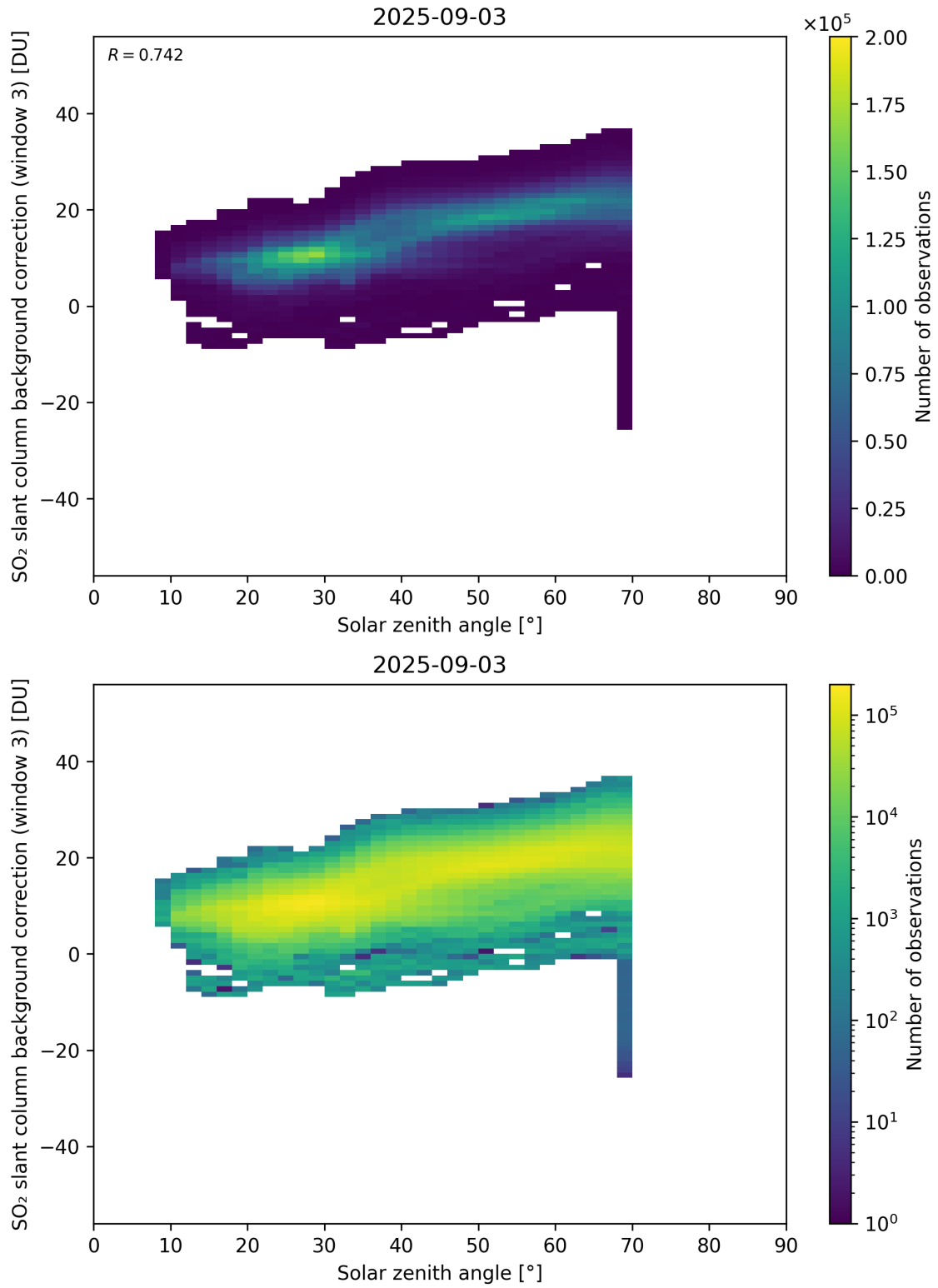
Figure 173: Scatter density plot of “Solar zenith angle” against “SO 2 slant column background correction (window 3)” for 2025-09-02 to 2025-09-04.
