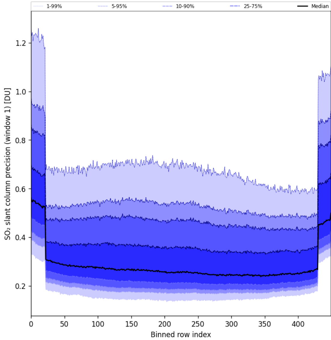
Figure 90: Along track statistics of “SO 2 slant column precision (window 1)” for 2025-09-02 to 2025-09-04
