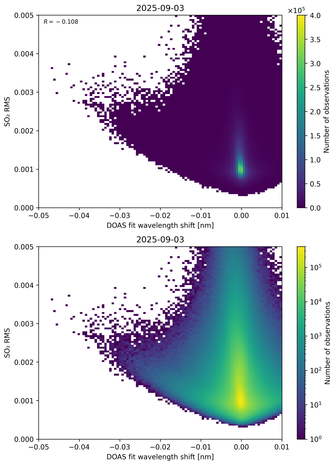
Figure 139: Scatter density plot of “DOAS fit wavelength shift” against “SO 2 RMS” for 2025-09-02 to 2025-09-04.
