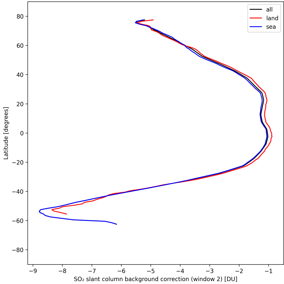
Figure 44: Zonal average of “SO 2 slant column background correction (window 2)” for 2025-09-02 to 2025-09-04.
