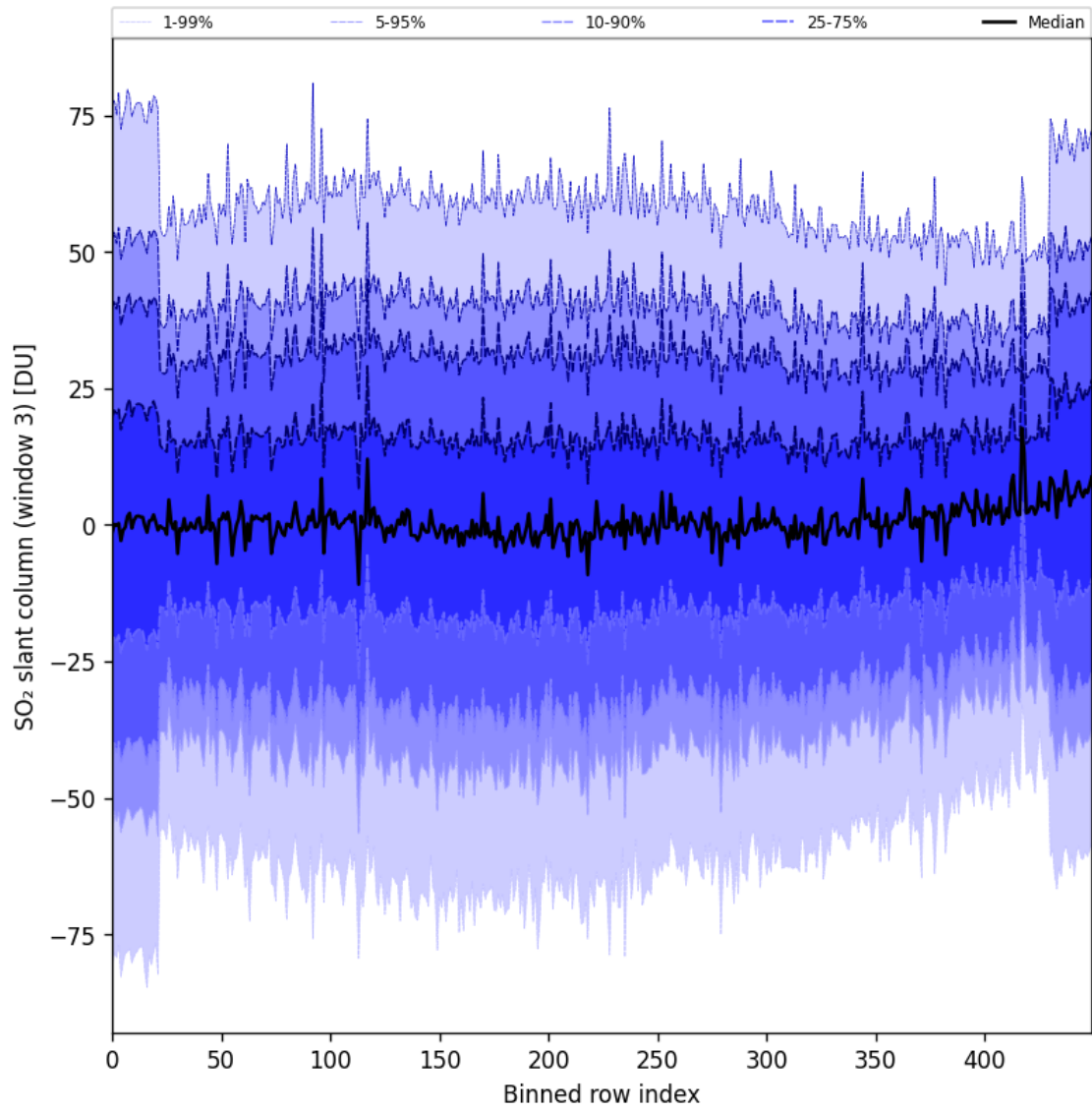
Figure 97: Along track statistics of “SO 2 slant column (window 3)” for 2025-09-02 to 2025-09-04
