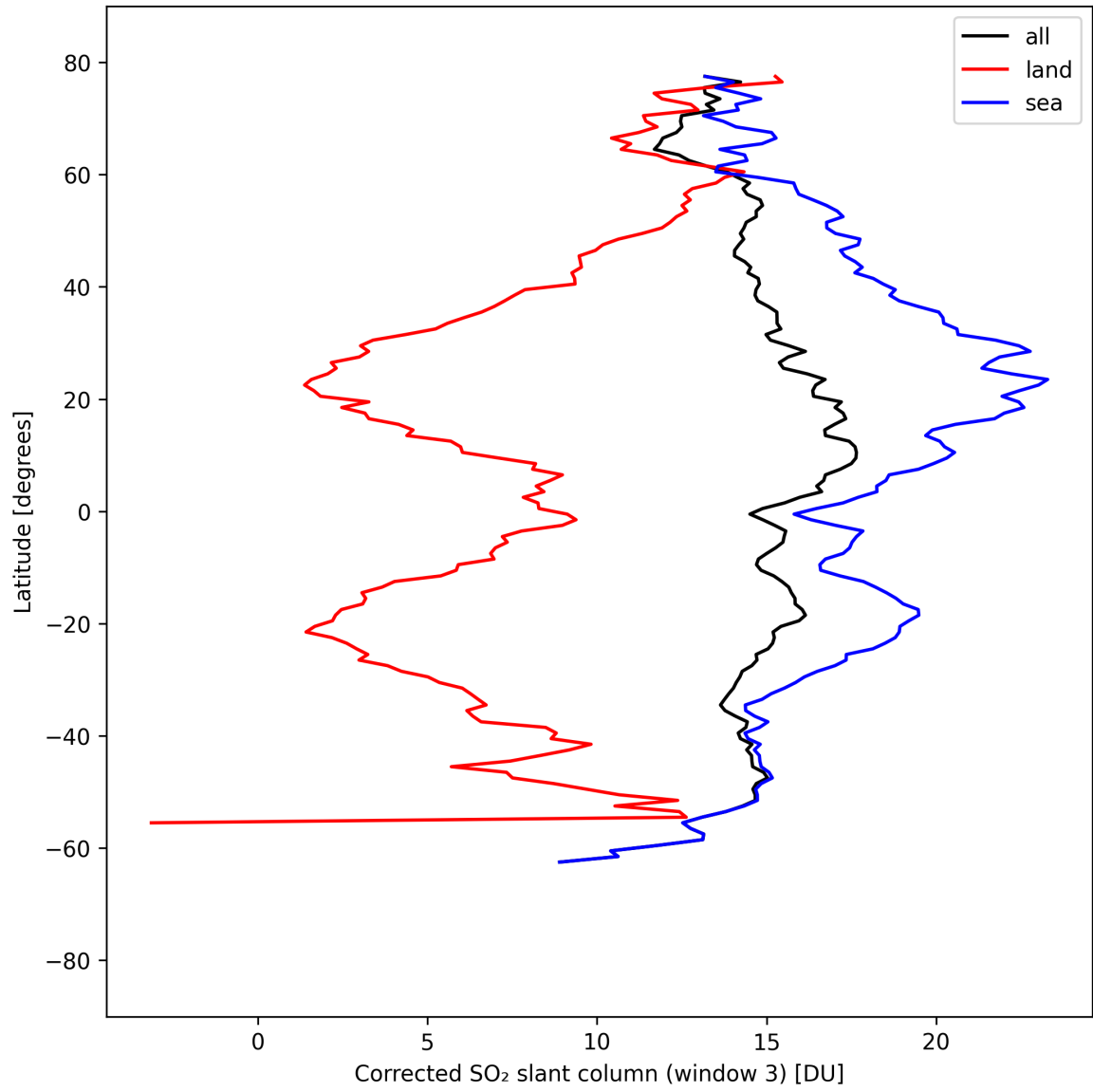
Figure 47: Zonal average of “Corrected SO 2 slant column (window 3)” for 2025-09-02 to 2025-09-04.
