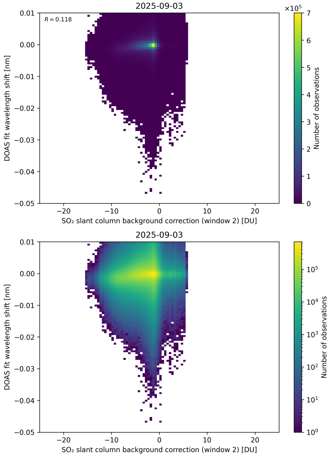
Figure 123: Scatter density plot of “SO 2 slant column background correction (window 2)” against “DOAS fit wavelength shift” for 2025-09-02 to 2025-09-04.
