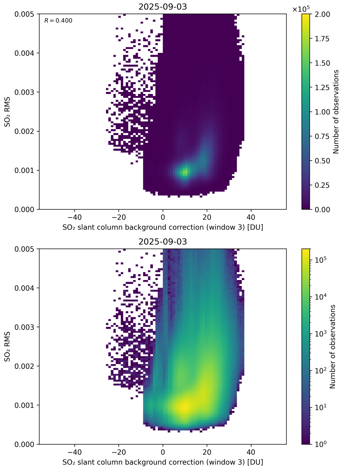
Figure 134: Scatter density plot of “SO 2 slant column background correction (window 3)” against “SO 2 RMS” for 2025-09-02 to 2025-09-04.
