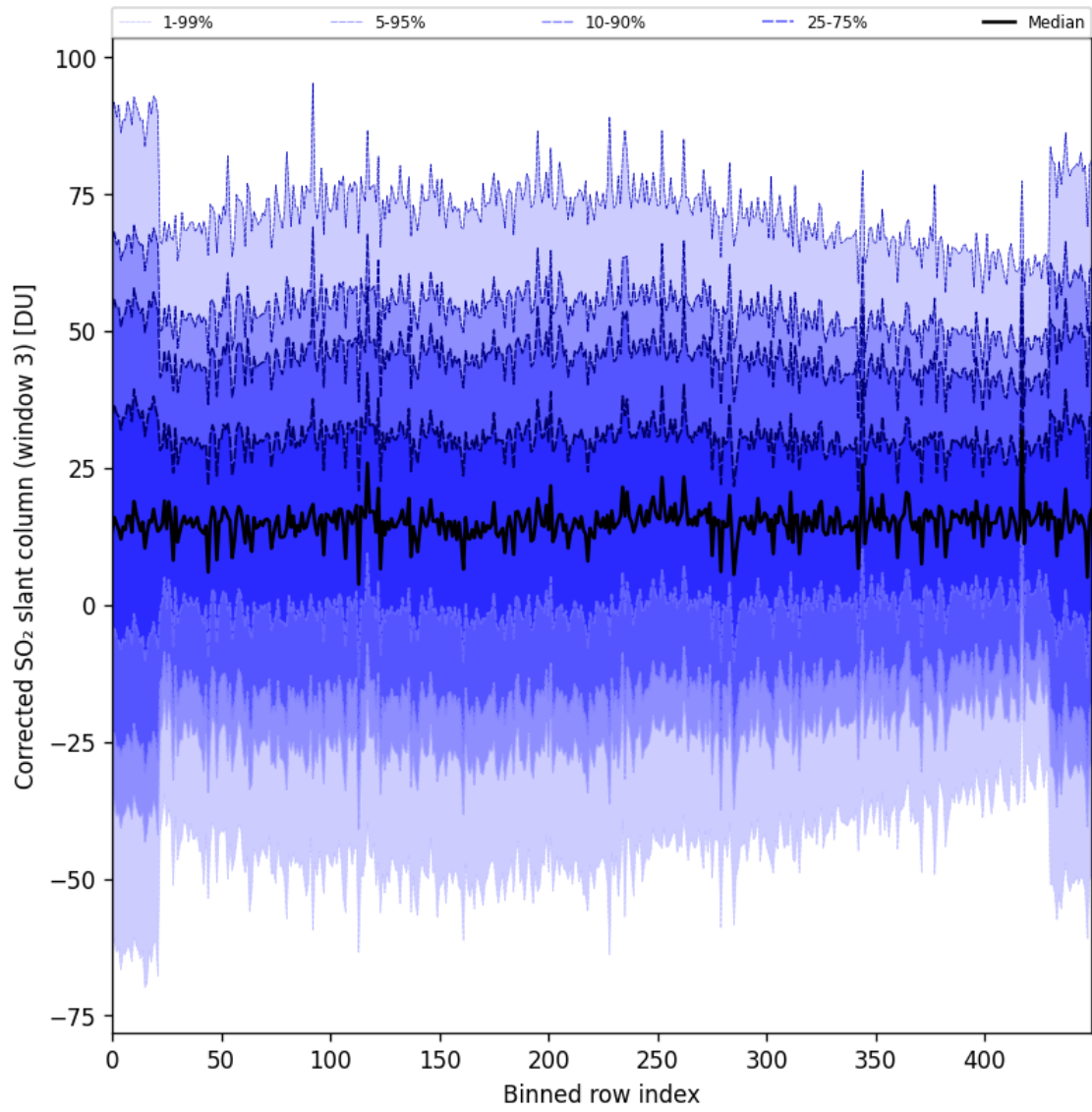
Figure 99: Along track statistics of “Corrected SO 2 slant column (window 3)” for 2025-09-02 to 2025-09-04
