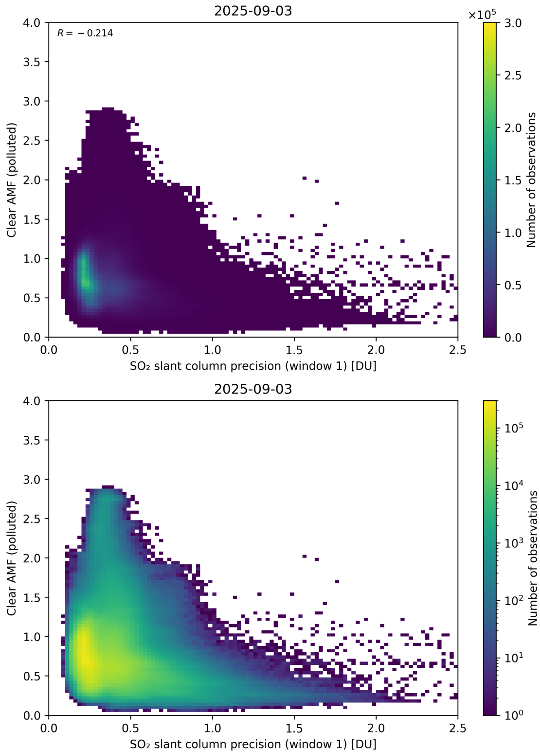
Figure 274: Scatter density plot of “SO 2 slant column precision (window 1)” against “Clear AMF (polluted)” for 2025-09-02 to 2025-09-04.
