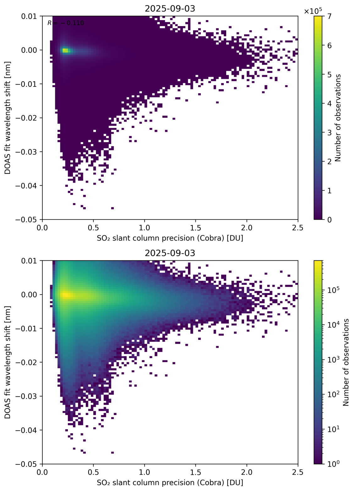
Figure 202: Scatter density plot of “SO 2 slant column precision (Cobra)” against “DOAS fit wavelength shift” for 2025-09-02 to 2025-09-04.
