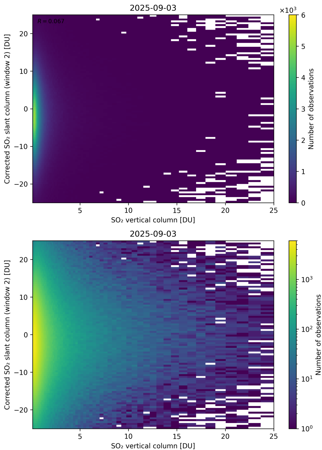
Figure 352: Scatter density plot of “SO 2 vertical column” against “Corrected SO 2 slant column (window 2)” for 2025-09-02 to 2025-09-04.
