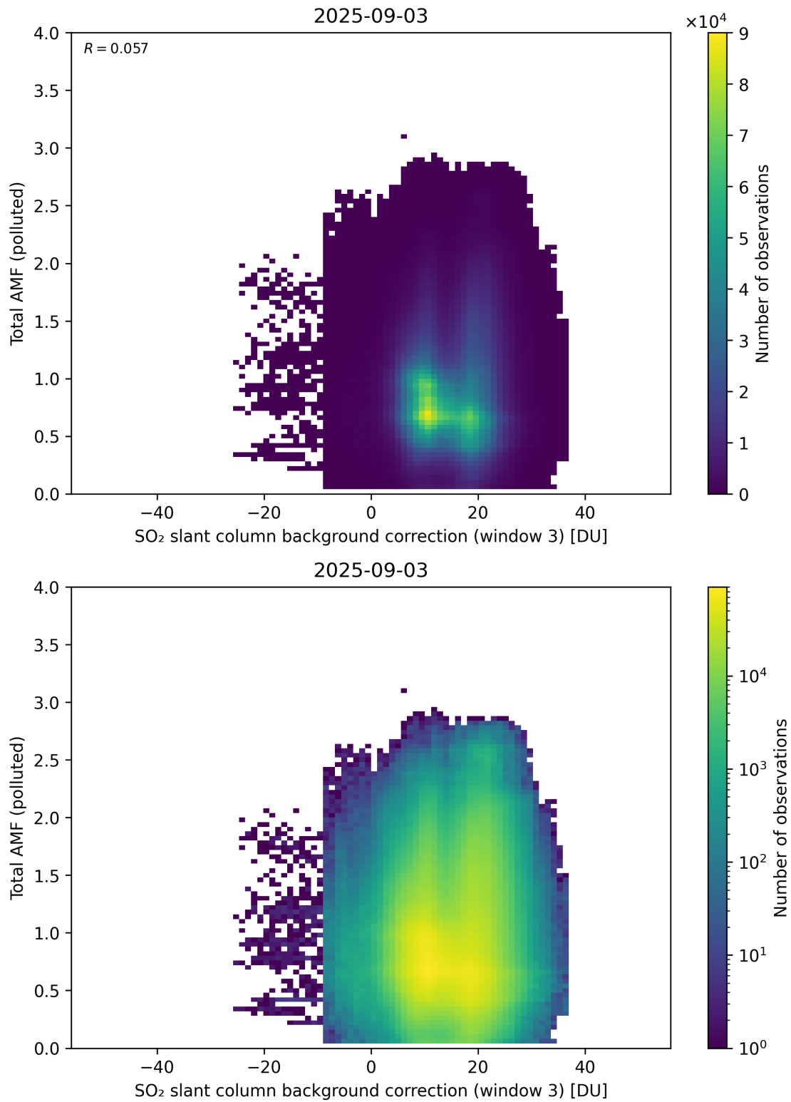
Figure 136: Scatter density plot of “SO 2 slant column background correction (window 3)” against “Total AMF (polluted)” for 2025-09-02 to 2025-09-04.
