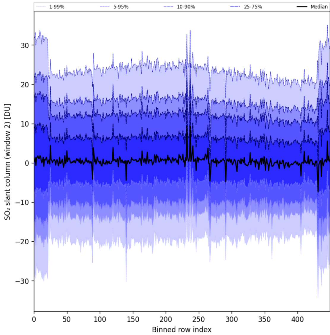
Figure 93: Along track statistics of “SO 2 slant column (window 2)” for 2025-09-02 to 2025-09-04
