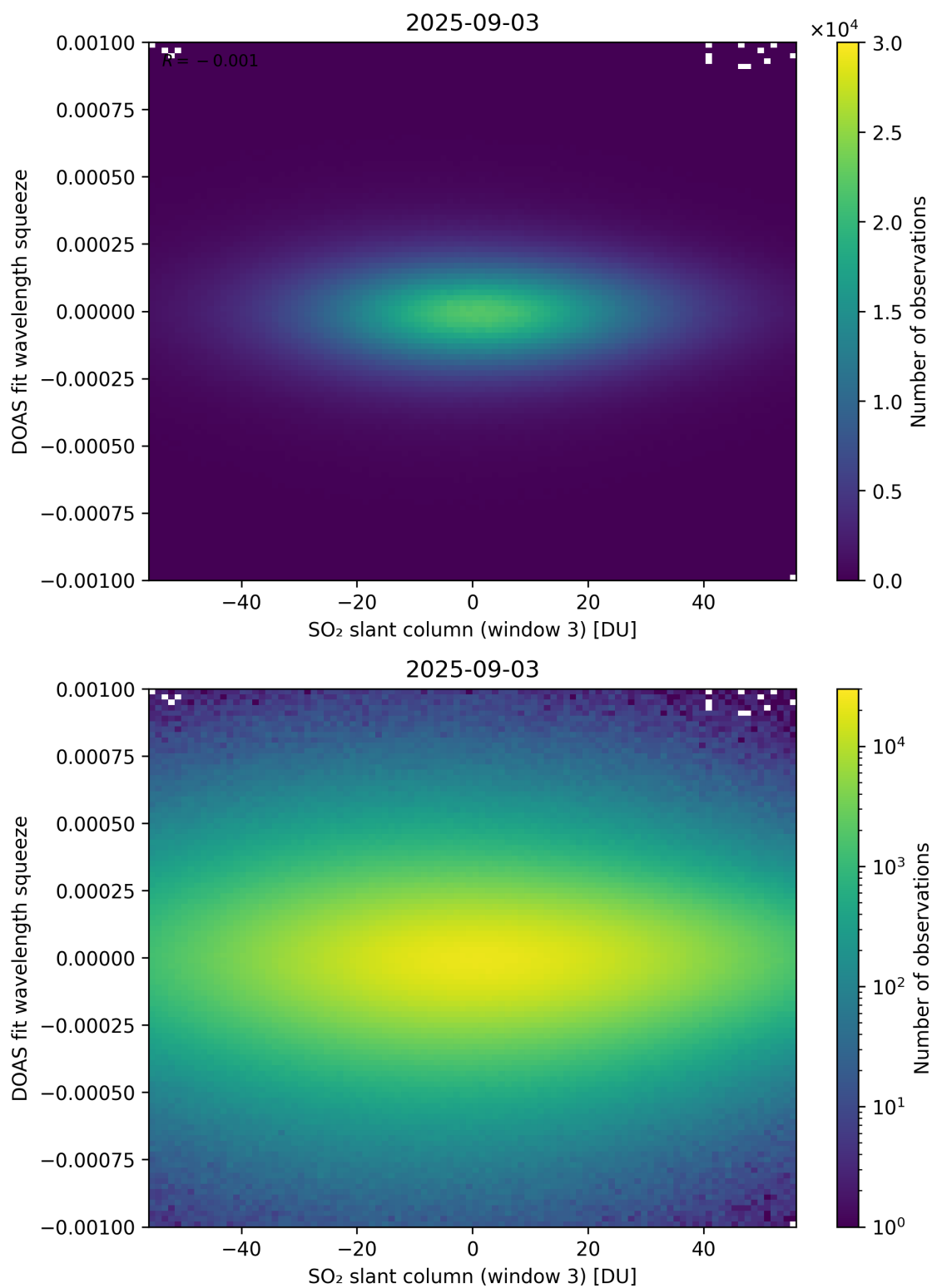
Figure 305: Scatter density plot of “SO 2 slant column (window 3)” against “DOAS fit wavelength squeeze” for 2025-09-02 to 2025-09-04.
