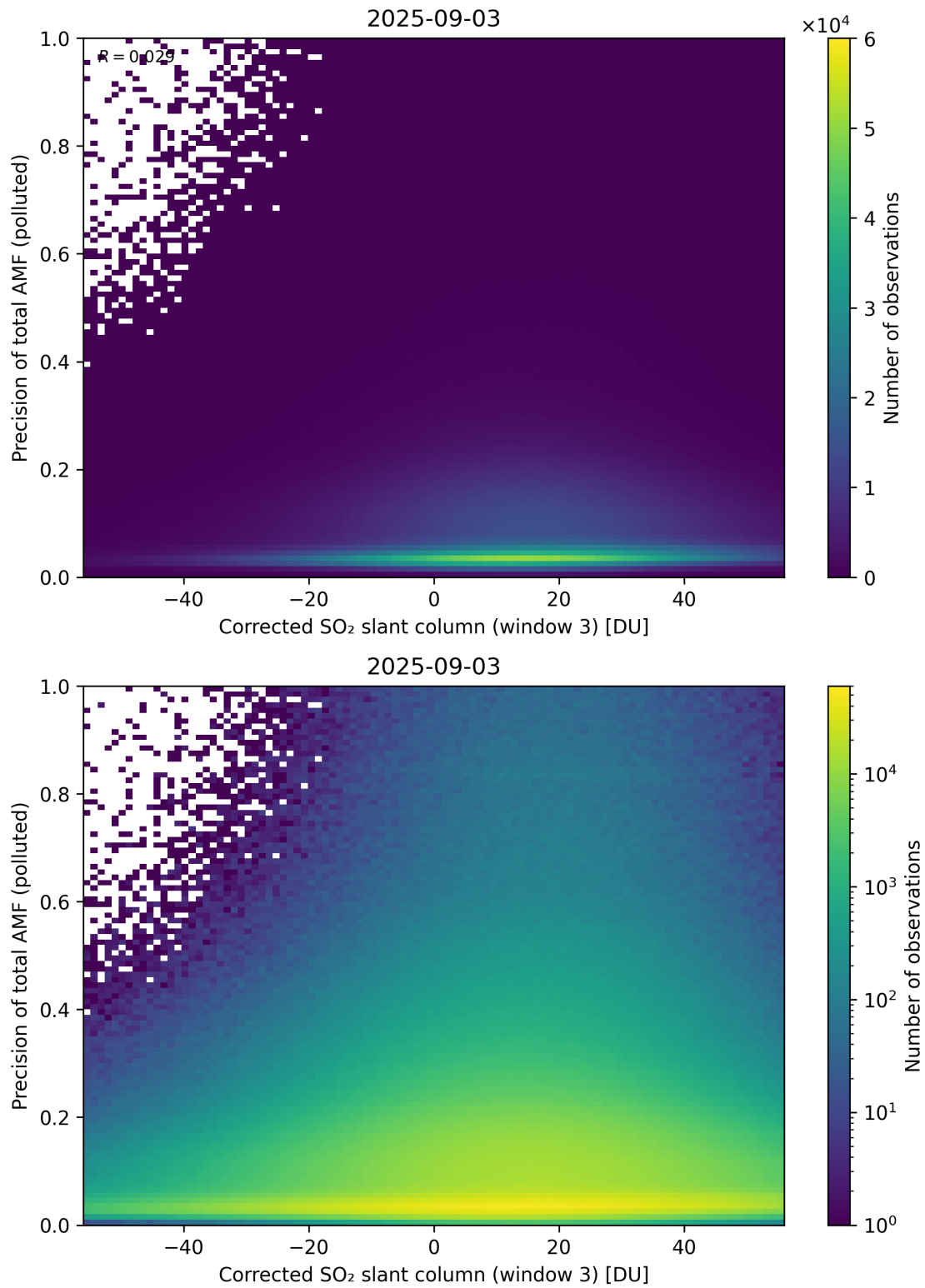
Figure 261: Scatter density plot of “Corrected SO 2 slant column (window 3)” against “Precision of total AMF (polluted)” for 2025-09-02 to 2025-09-04.
