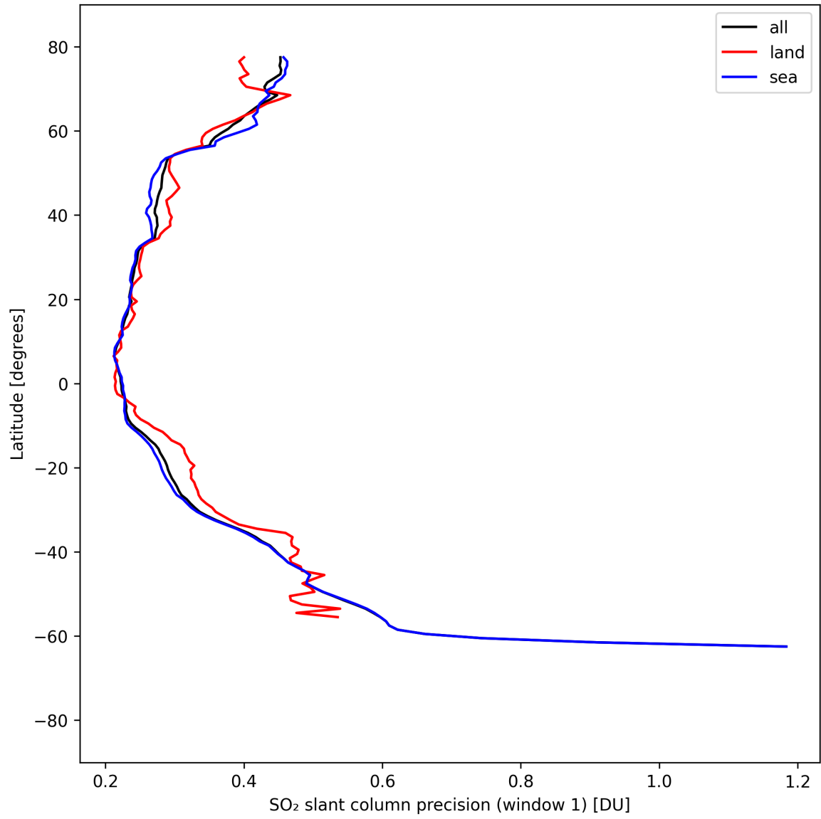
Figure 38: Zonal average of “SO 2 slant column precision (window 1)” for 2025-09-02 to 2025-09-04.
