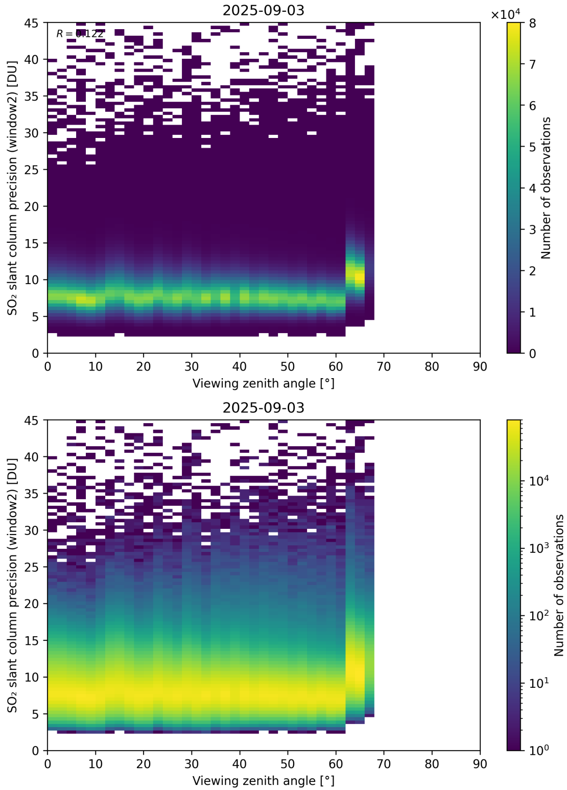
Figure 378: Scatter density plot of “Viewing zenith angle” against “SO 2 slant column precision (window2)” for 2025-09-02 to 2025-09-04.
