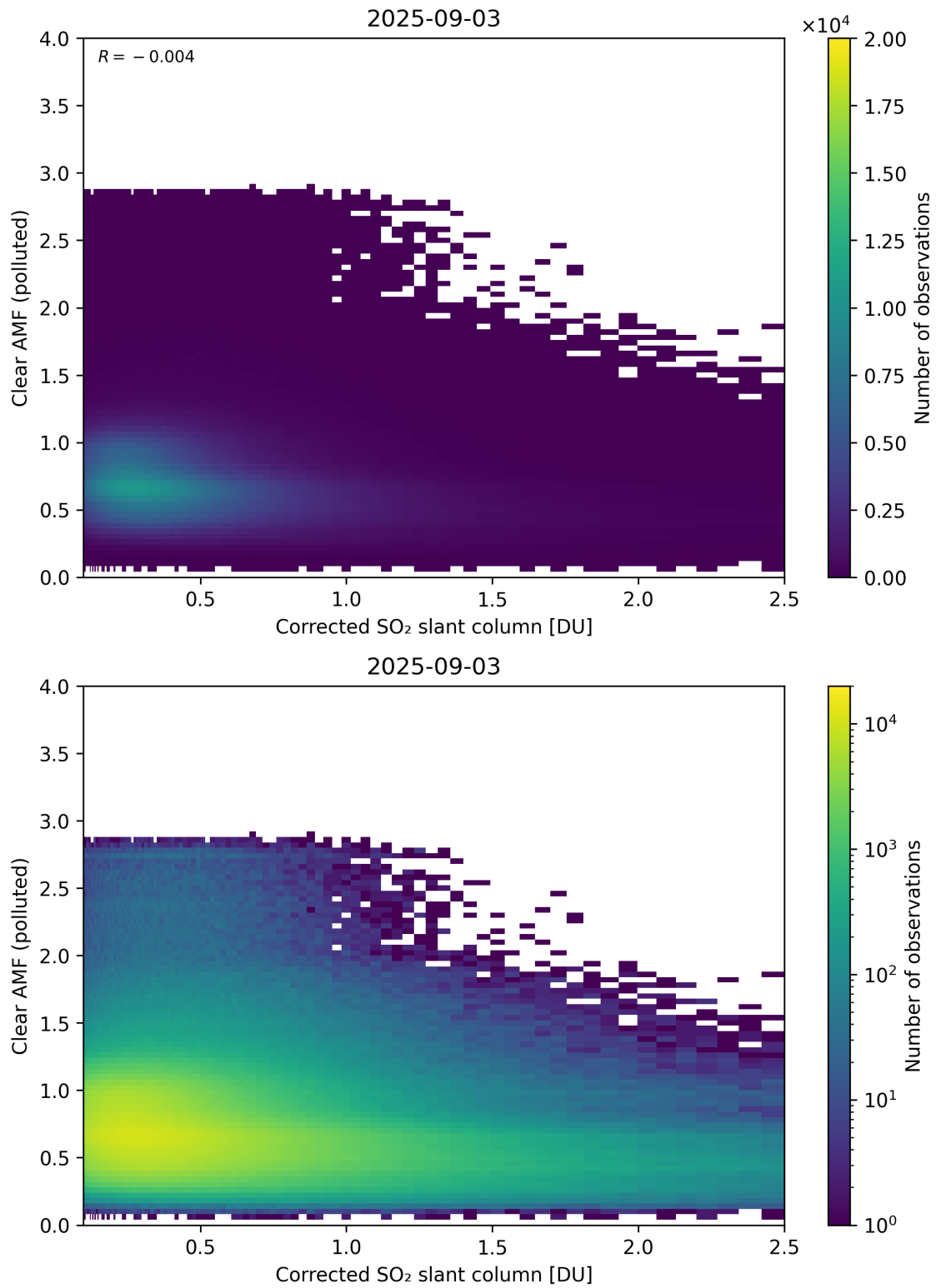
Figure 232: Scatter density plot of “Corrected SO 2 slant column” against “Clear AMF (polluted)” for 2025-09-02 to 2025-09-04.
