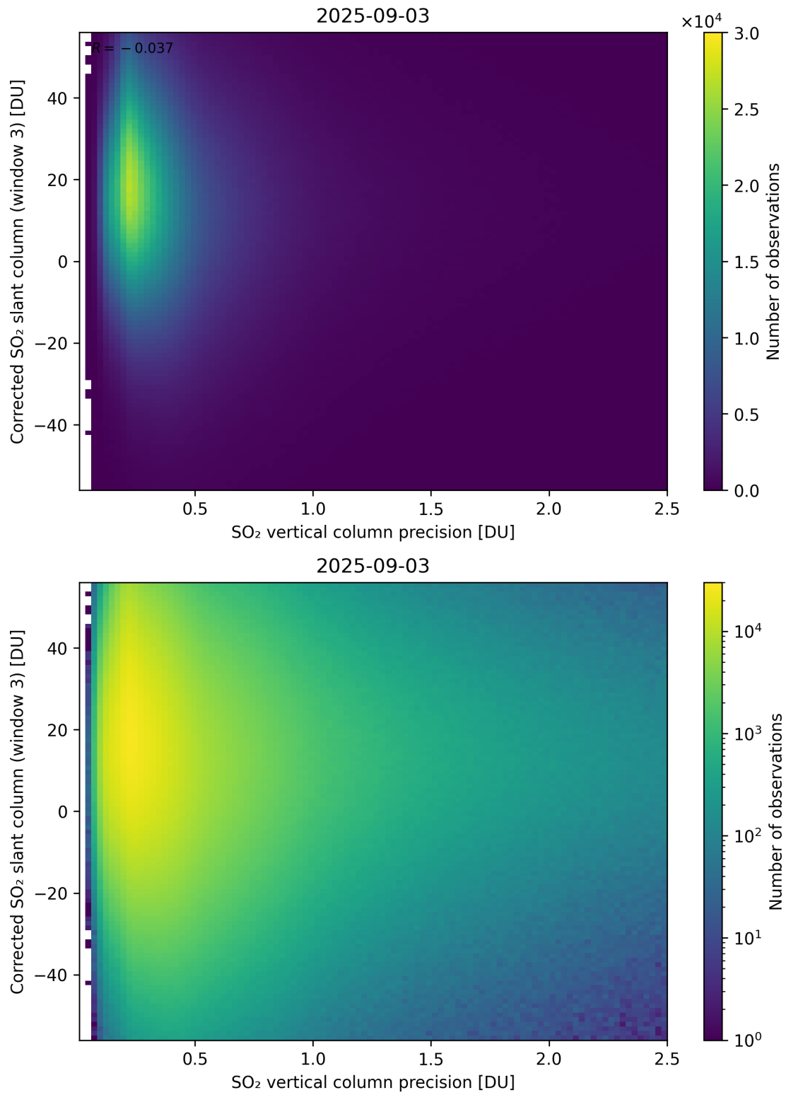
Figure 340: Scatter density plot of “SO 2 vertical column precision” against “Corrected SO 2 slant column (window 3)” for 2025-09-02 to 2025-09-04.
