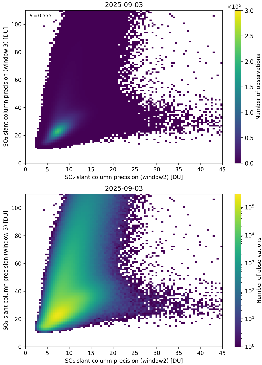
Figure 300: Scatter density plot of “SO 2 slant column precision (window2)” against “SO 2 slant column precision (window 3)” for 2025-09-02 to 2025-09-04.
