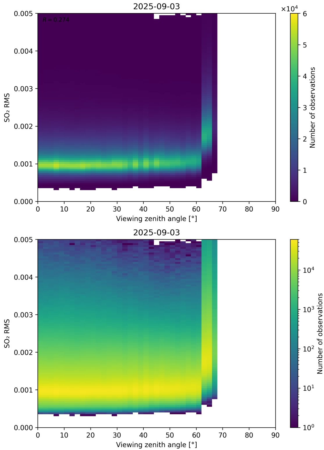
Figure 367: Scatter density plot of “Viewing zenith angle” against “SO 2 RMS” for 2025-09-02 to 2025-09-04.
