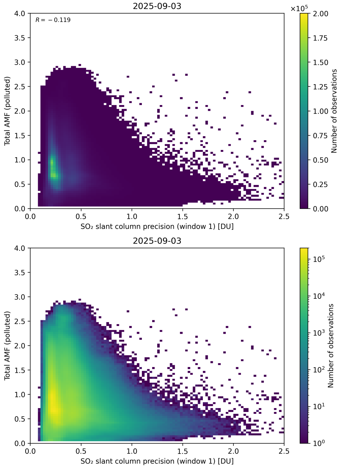
Figure 280: Scatter density plot of “SO 2 slant column precision (window 1)” against “Total AMF (polluted)” for 2025-09-02 to 2025-09-04.
