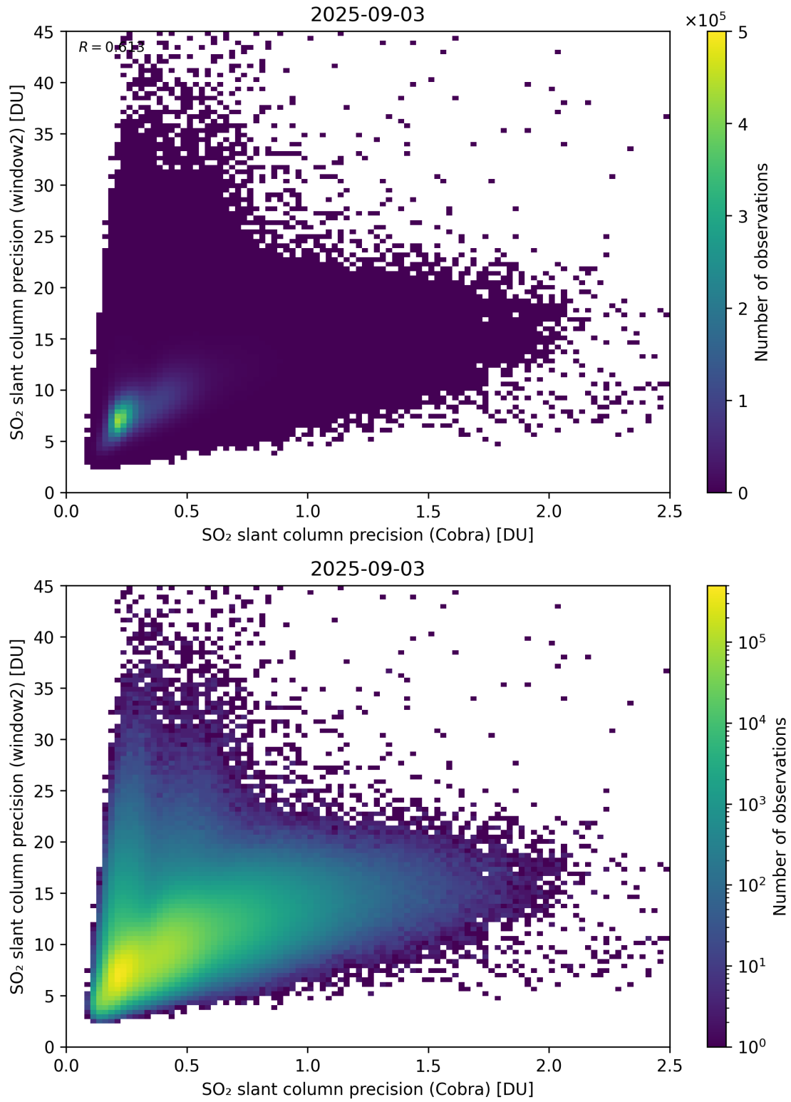
Figure 210: Scatter density plot of “SO 2 slant column precision (Cobra)” against “SO 2 slant column precision (window2)” for 2025-09-02 to 2025-09-04.
