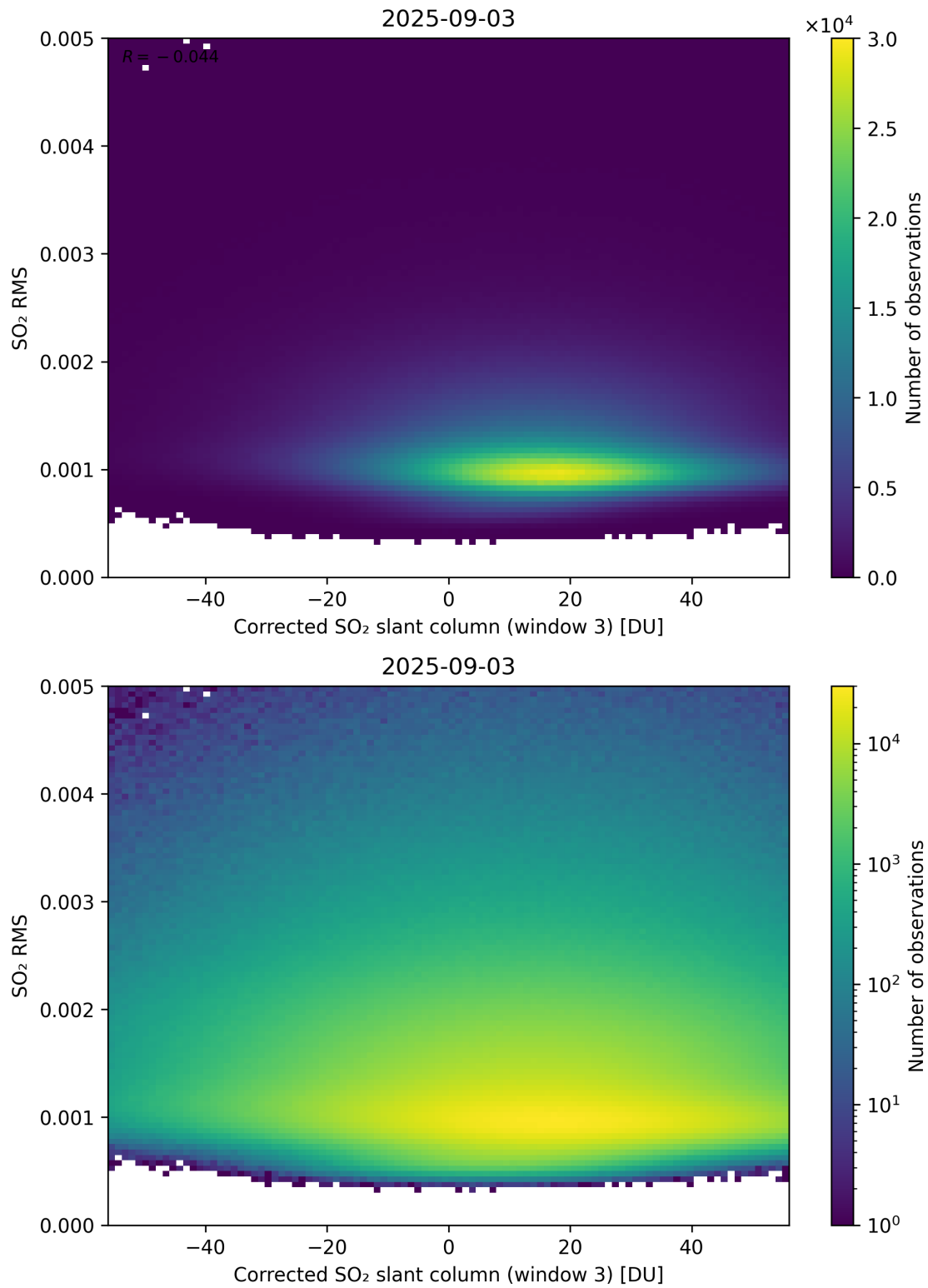
Figure 258: Scatter density plot of “Corrected SO 2 slant column (window 3)” against “SO 2 RMS” for 2025-09-02 to 2025-09-04.
