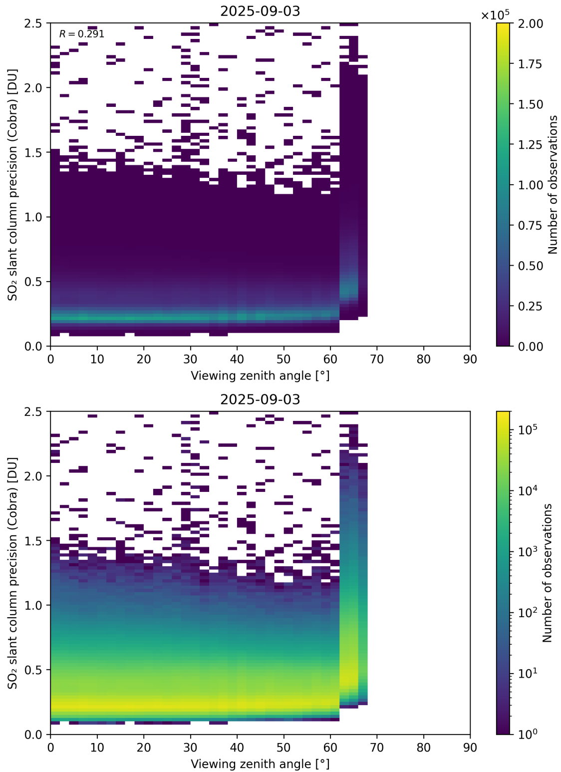
Figure 372: Scatter density plot of “Viewing zenith angle” against “SO 2 slant column precision (Cobra)” for 2025-09-02 to 2025-09-04.
