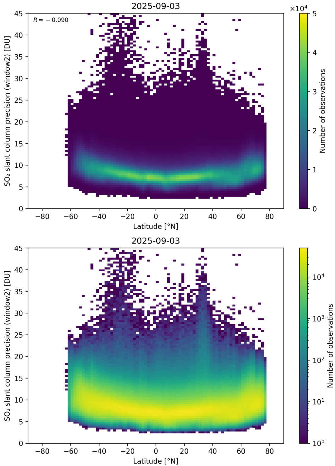
Figure 164: Scatter density plot of “Latitude” against “SO 2 slant column precision (window2)” for 2025-09-02 to 2025-09-04.
