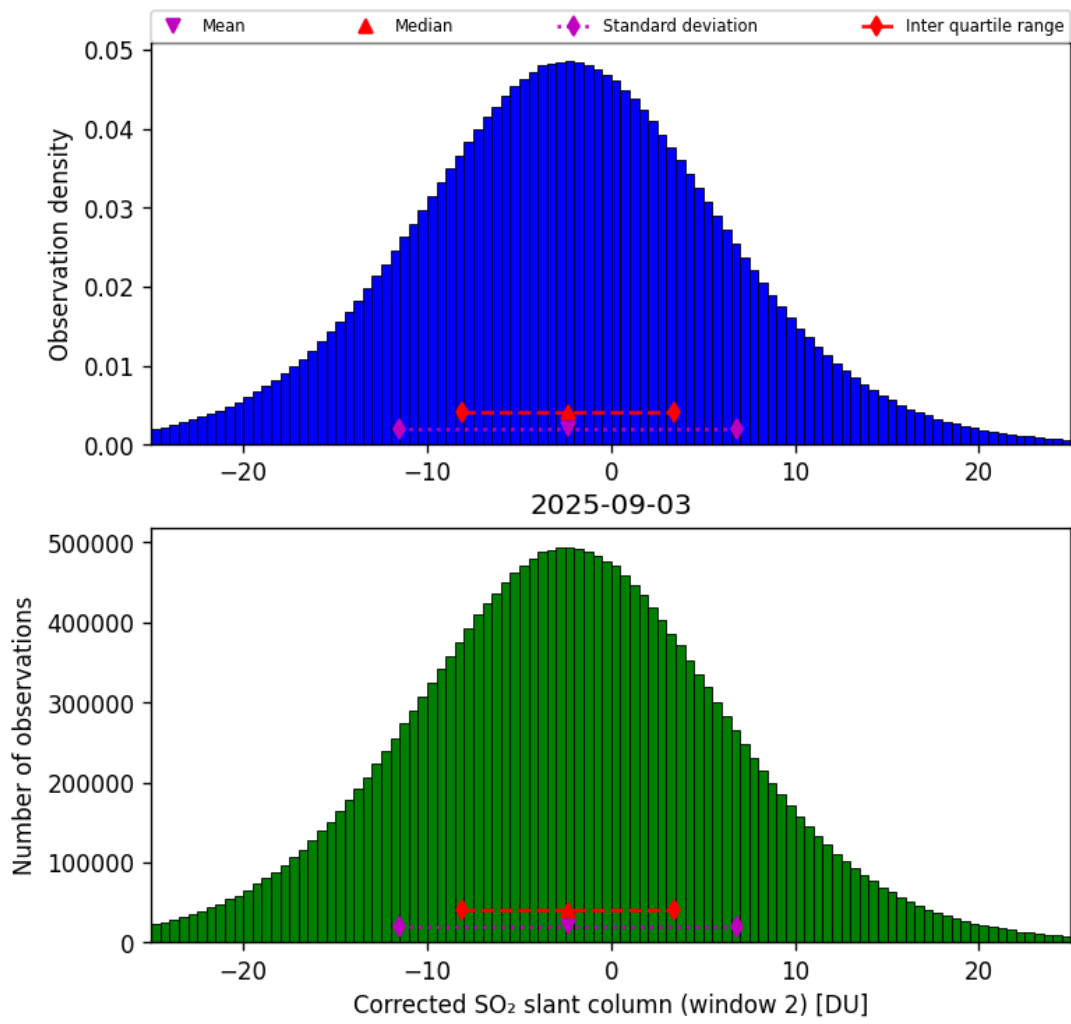
Figure 69: Histogram of “Corrected SO 2 slant column (window 2)” for 2025-09-02 to 2025-09-04
