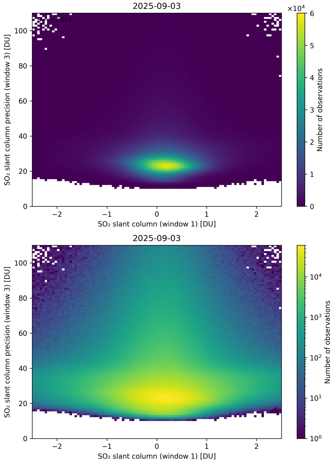
Figure 288: Scatter density plot of “SO 2 slant column (window 1)” against “SO 2 slant column precision (window 3)” for 2025-09-02 to 2025-09-04.
