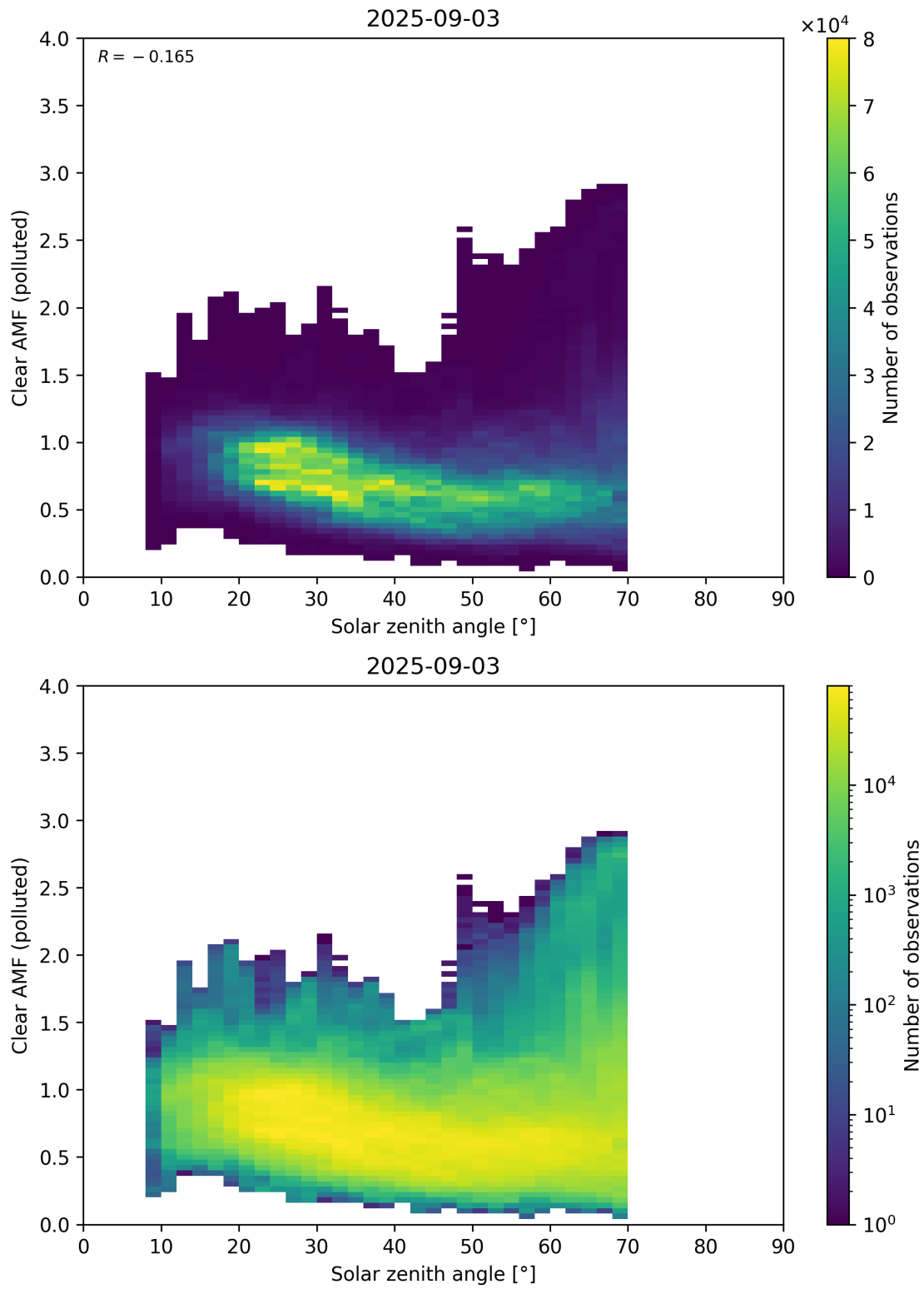
Figure 178: Scatter density plot of “Solar zenith angle” against “Clear AMF (polluted)” for 2025-09-02 to 2025-09-04.
