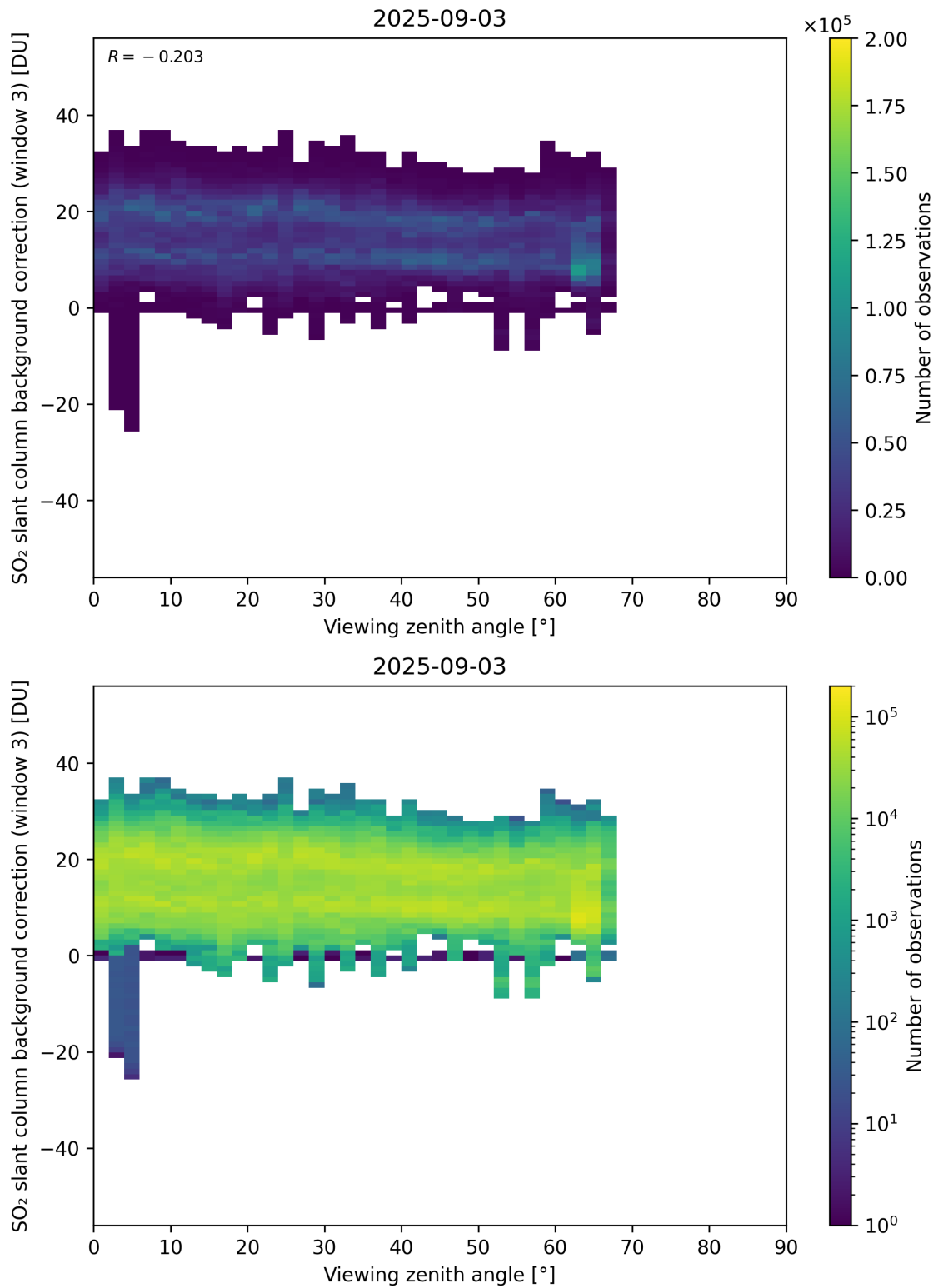
Figure 364: Scatter density plot of “Viewing zenith angle” against “SO 2 slant column background correction (window 3)” for 2025-09-02 to 2025-09-04.
