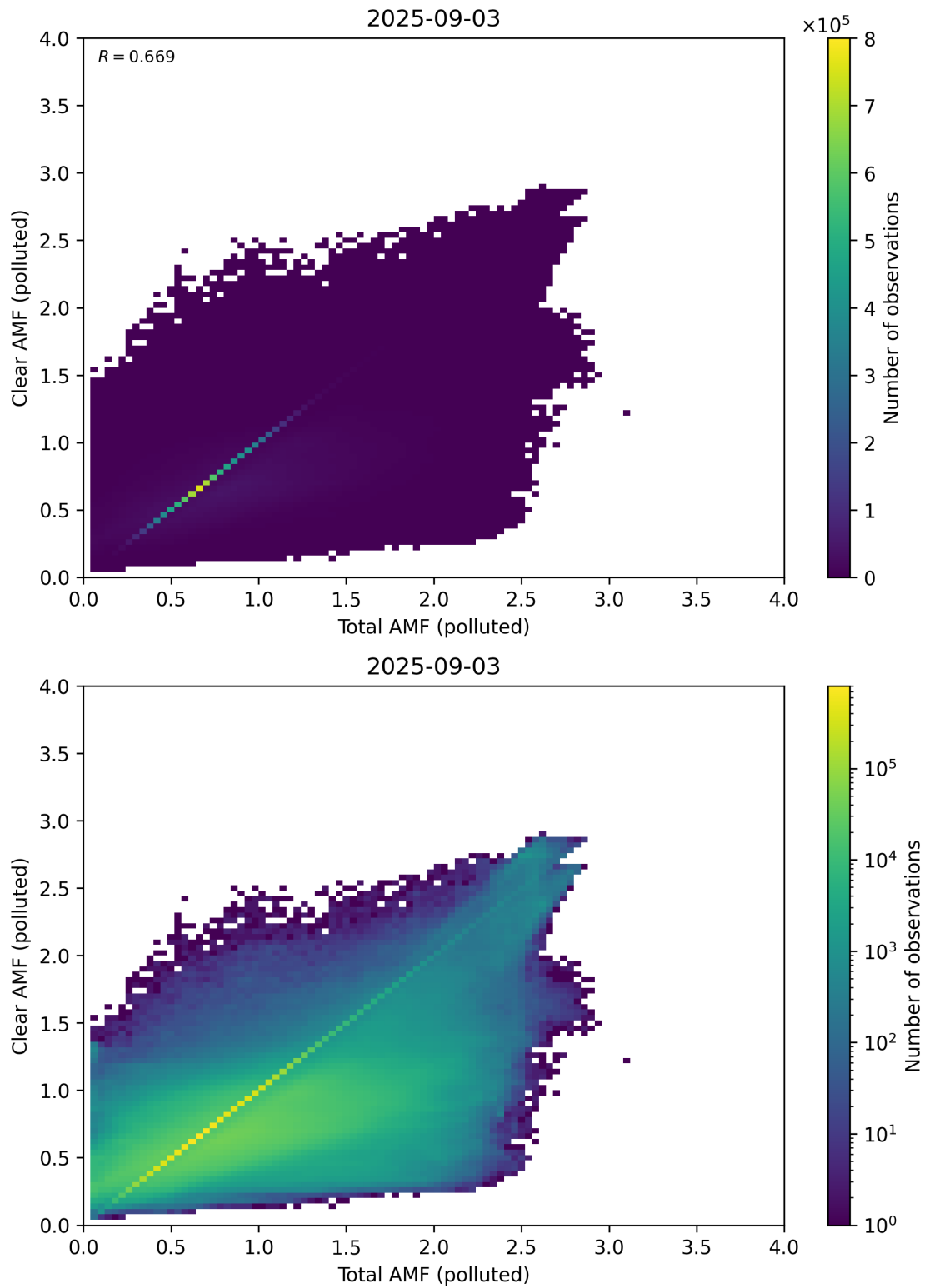
Figure 321: Scatter density plot of “Total AMF (polluted)” against “Clear AMF (polluted)” for 2025-09-02 to 2025-09-04.
