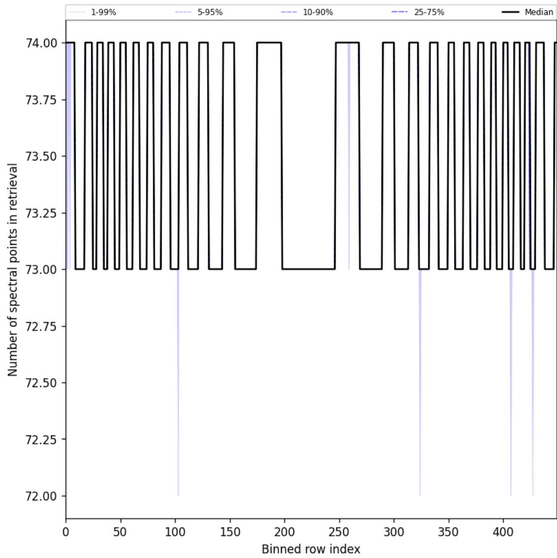
Figure 108: Along track statistics of “Number of spectral points in retrieval” for 2025-09-02 to 2025-09-04
