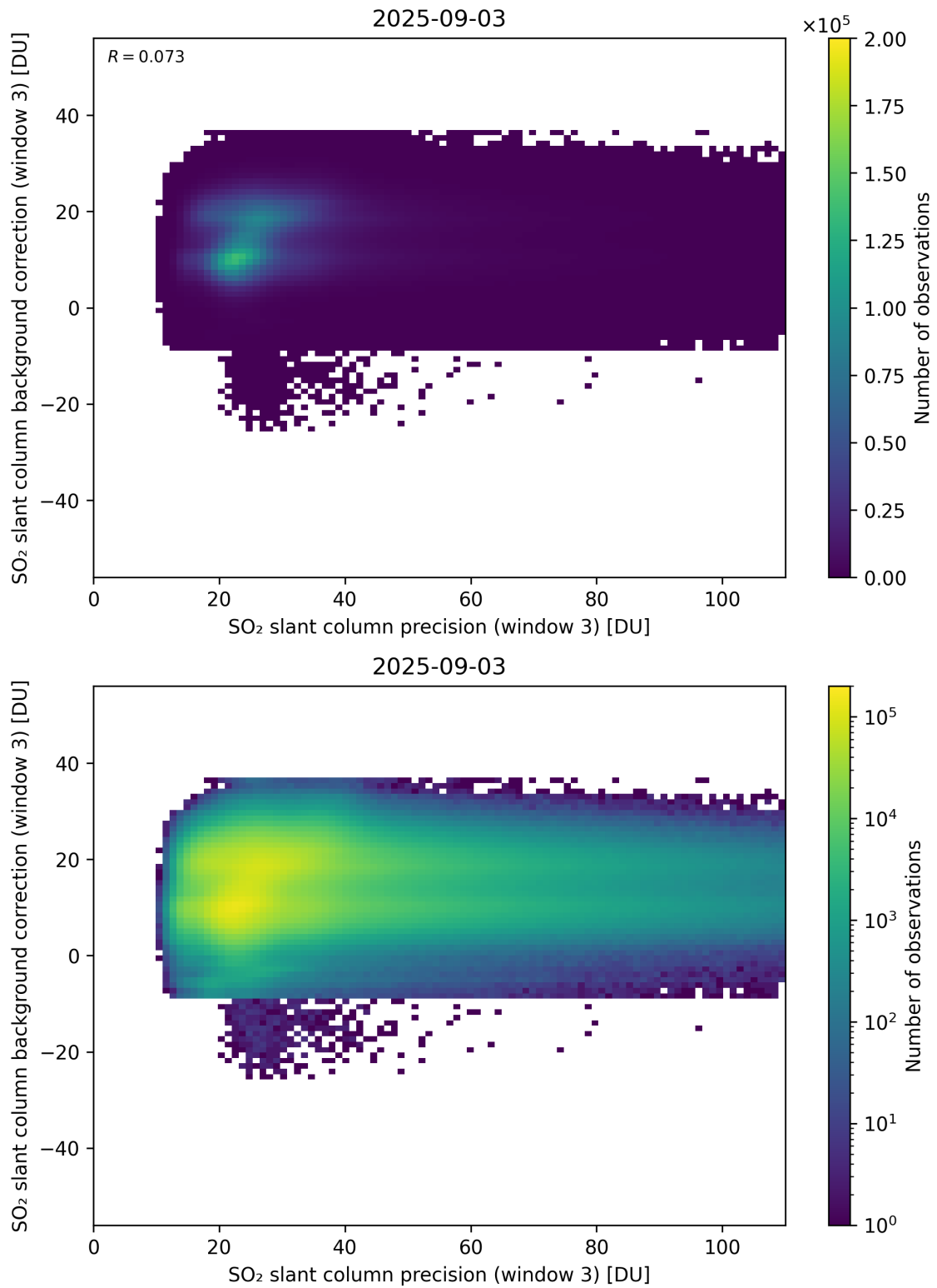
Figure 307: Scatter density plot of “SO 2 slant column precision (window 3)” against “SO 2 slant column background correction (window 3)” for 2025-09-02 to 2025-09-04.
