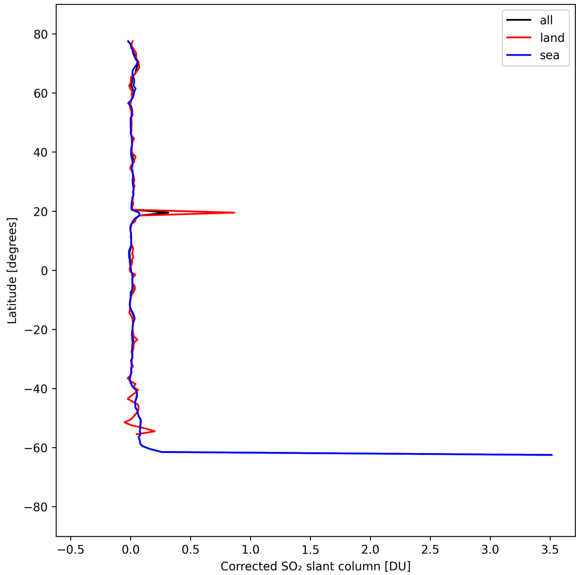
Figure 34: Zonal average of “Corrected SO 2 slant column” for 2025-09-02 to 2025-09-04.
