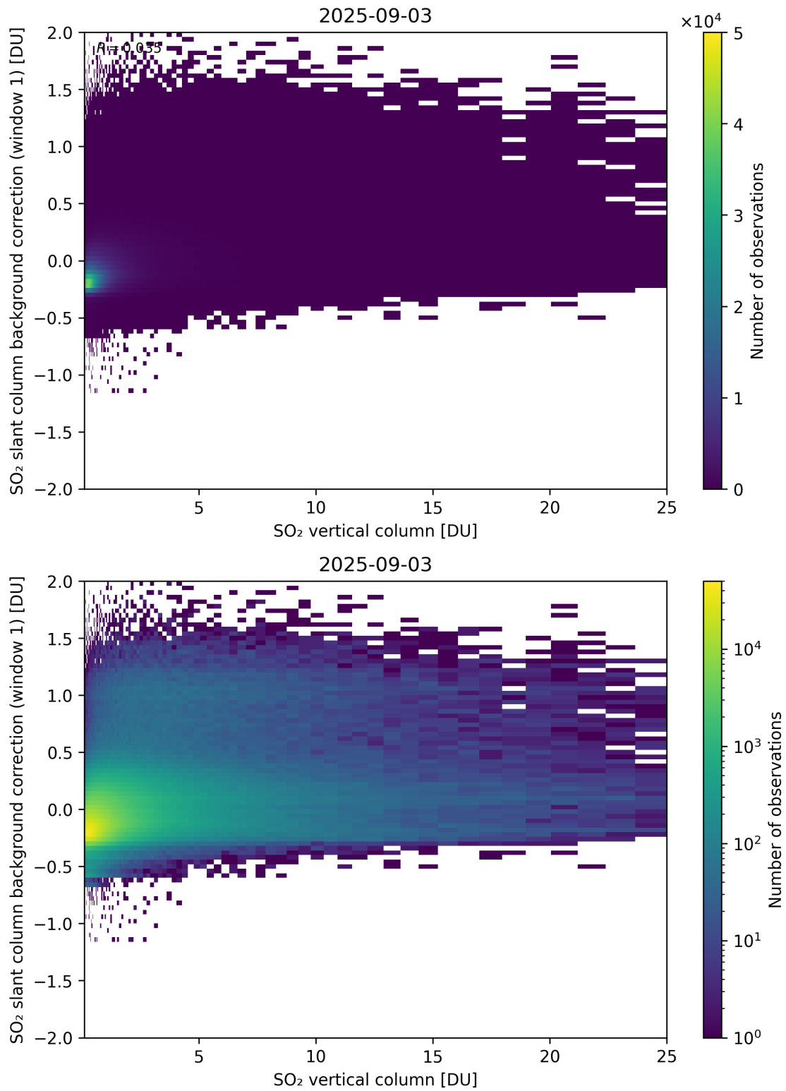
Figure 323: Scatter density plot of “SO 2 vertical column” against “SO 2 slant column background correction (window 1)” for 2025-09-02 to 2025-09-04.
