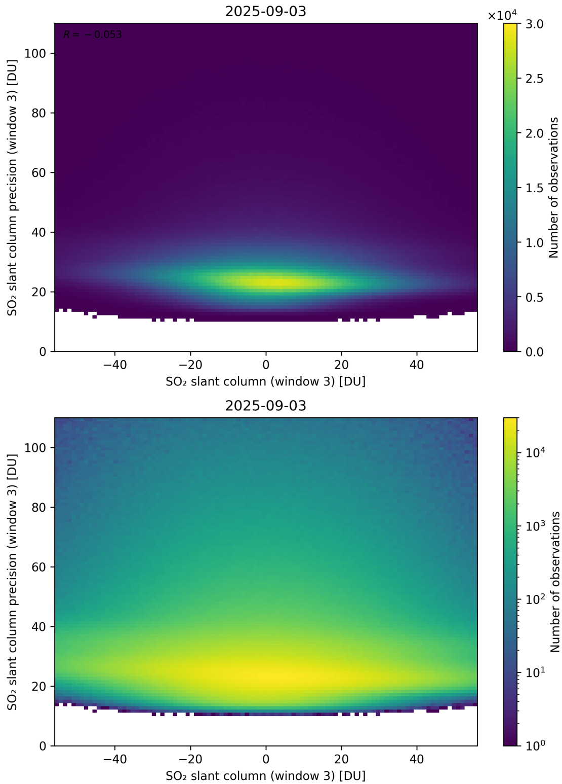
Figure 317: Scatter density plot of “SO 2 slant column (window 3)” against “SO 2 slant column precision (window 3)” for 2025-09-02 to 2025-09-04.
