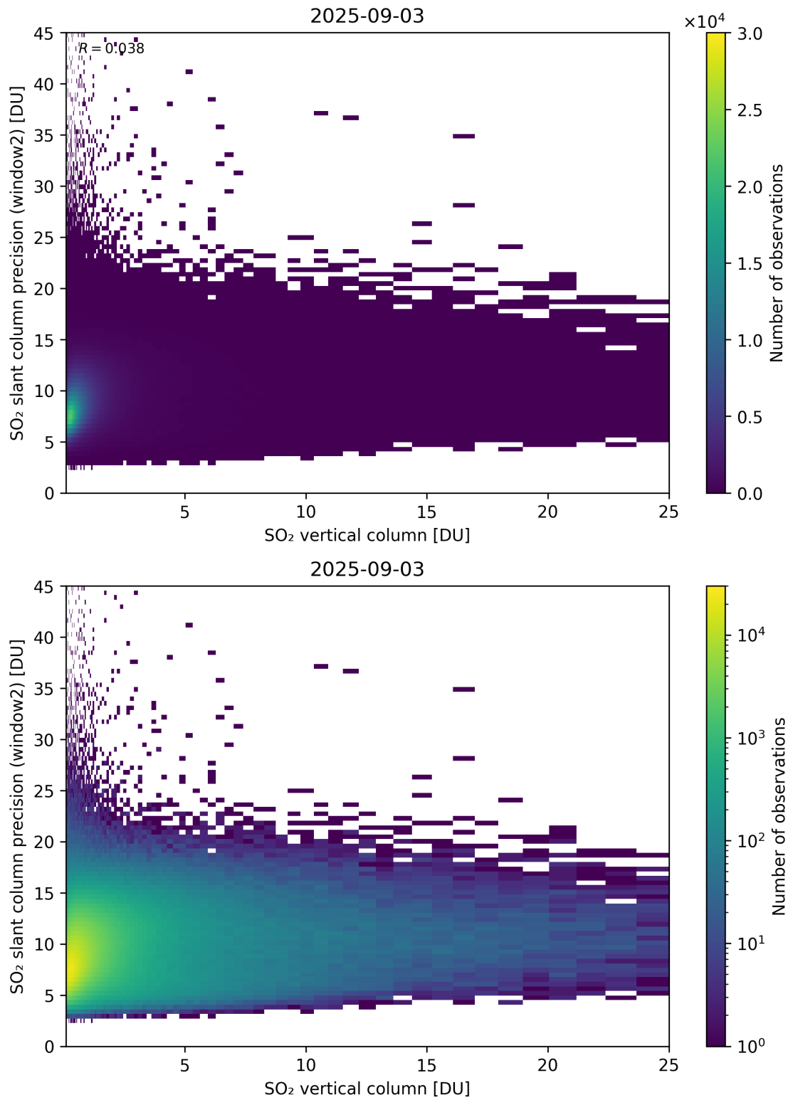
Figure 356: Scatter density plot of “SO 2 vertical column” against “SO 2 slant column precision (window2)” for 2025-09-02 to 2025-09-04.
