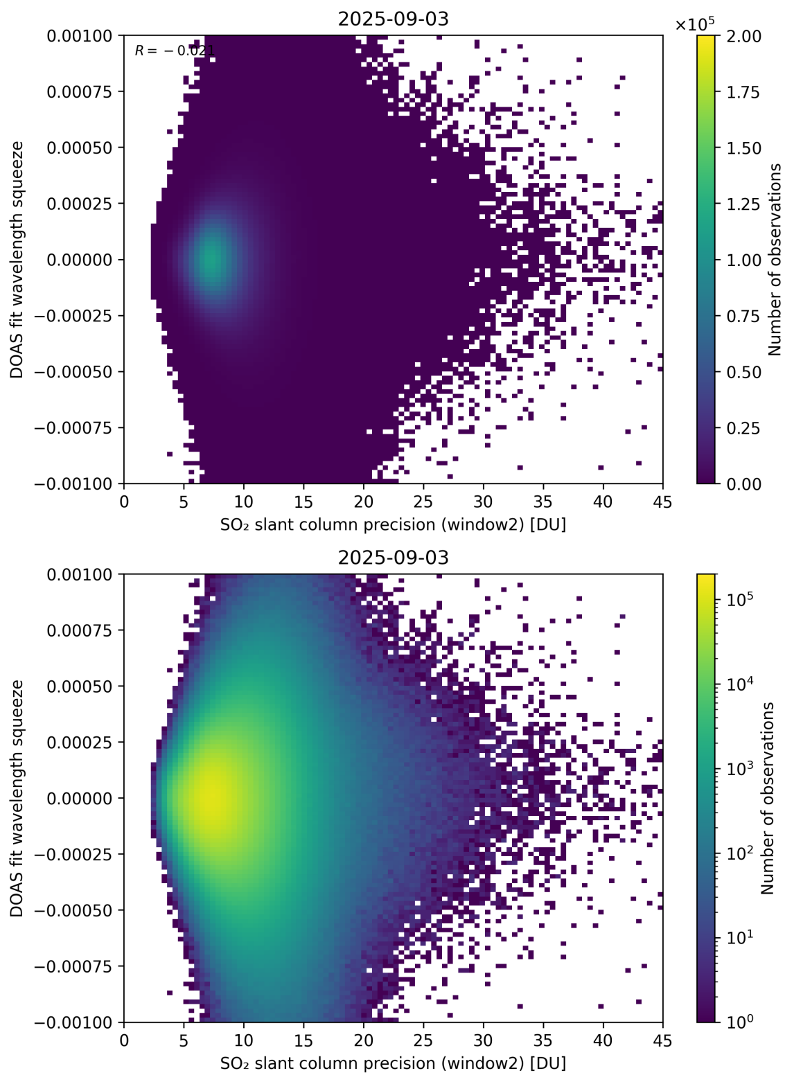
Figure 294: Scatter density plot of “SO 2 slant column precision (window2)” against “DOAS fit wavelength squeeze” for 2025-09-02 to 2025-09-04.
