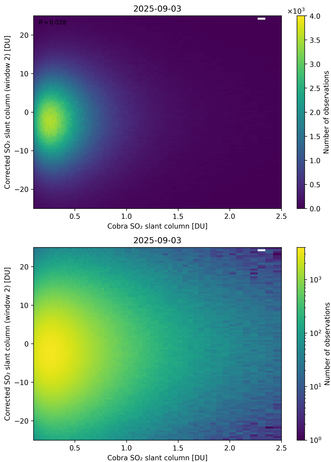
Figure 217: Scatter density plot of “Cobra SO 2 slant column” against “Corrected SO 2 slant column (window 2)” for 2025-09-02 to 2025-09-04.
