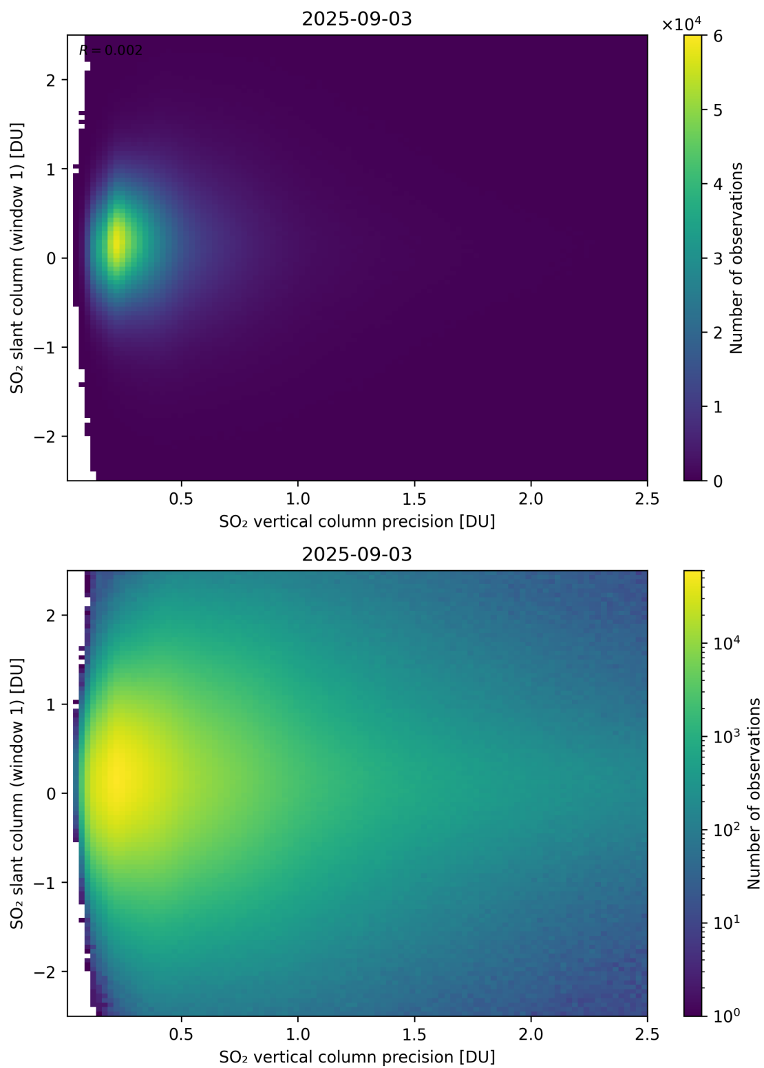
Figure 341: Scatter density plot of “SO 2 vertical column precision” against “SO 2 slant column (window 1)” for 2025-09-02 to 2025-09-04.
