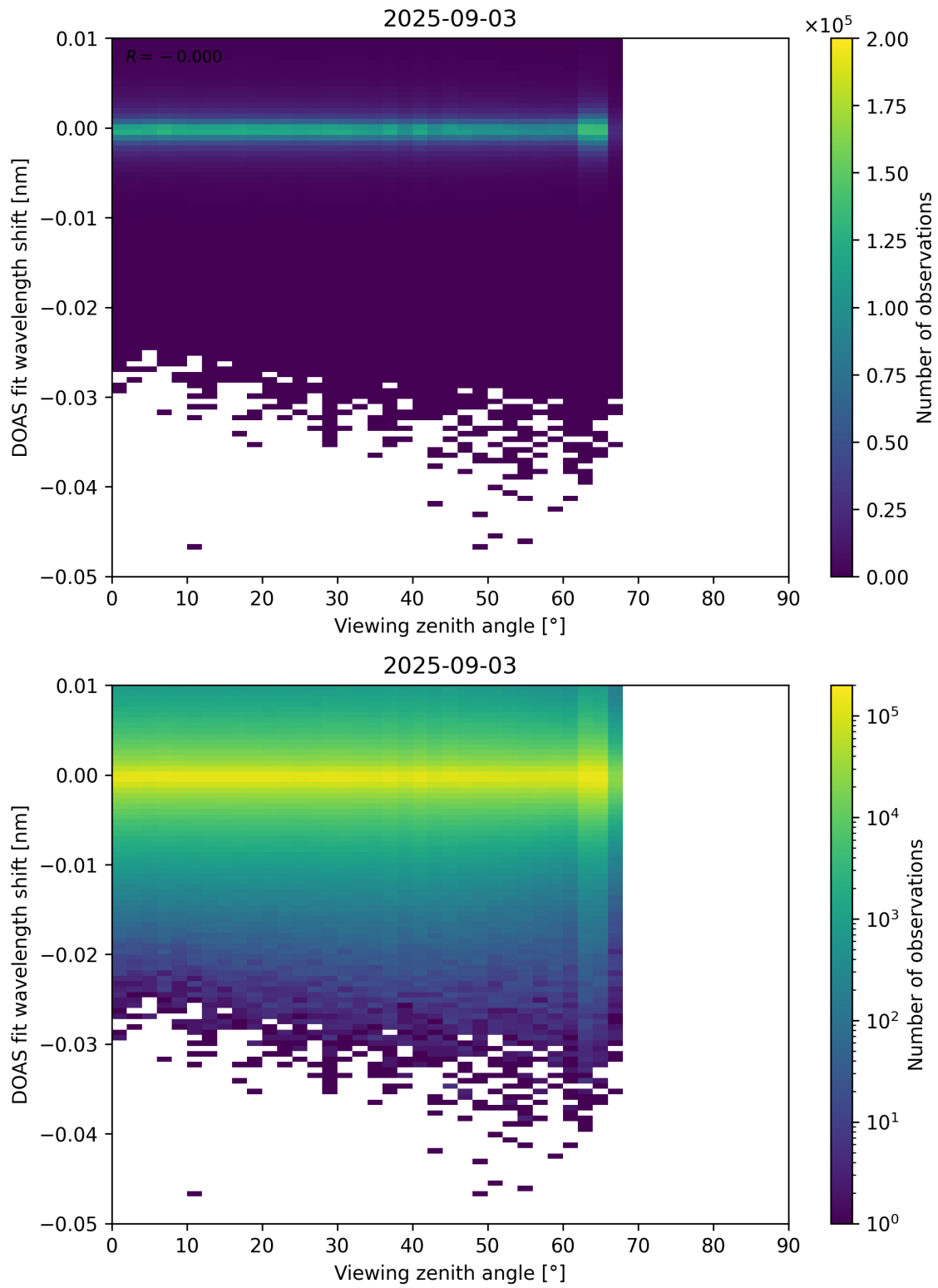
Figure 365: Scatter density plot of “Viewing zenith angle” against “DOAS fit wavelength shift” for 2025-09-02 to 2025-09-04.
