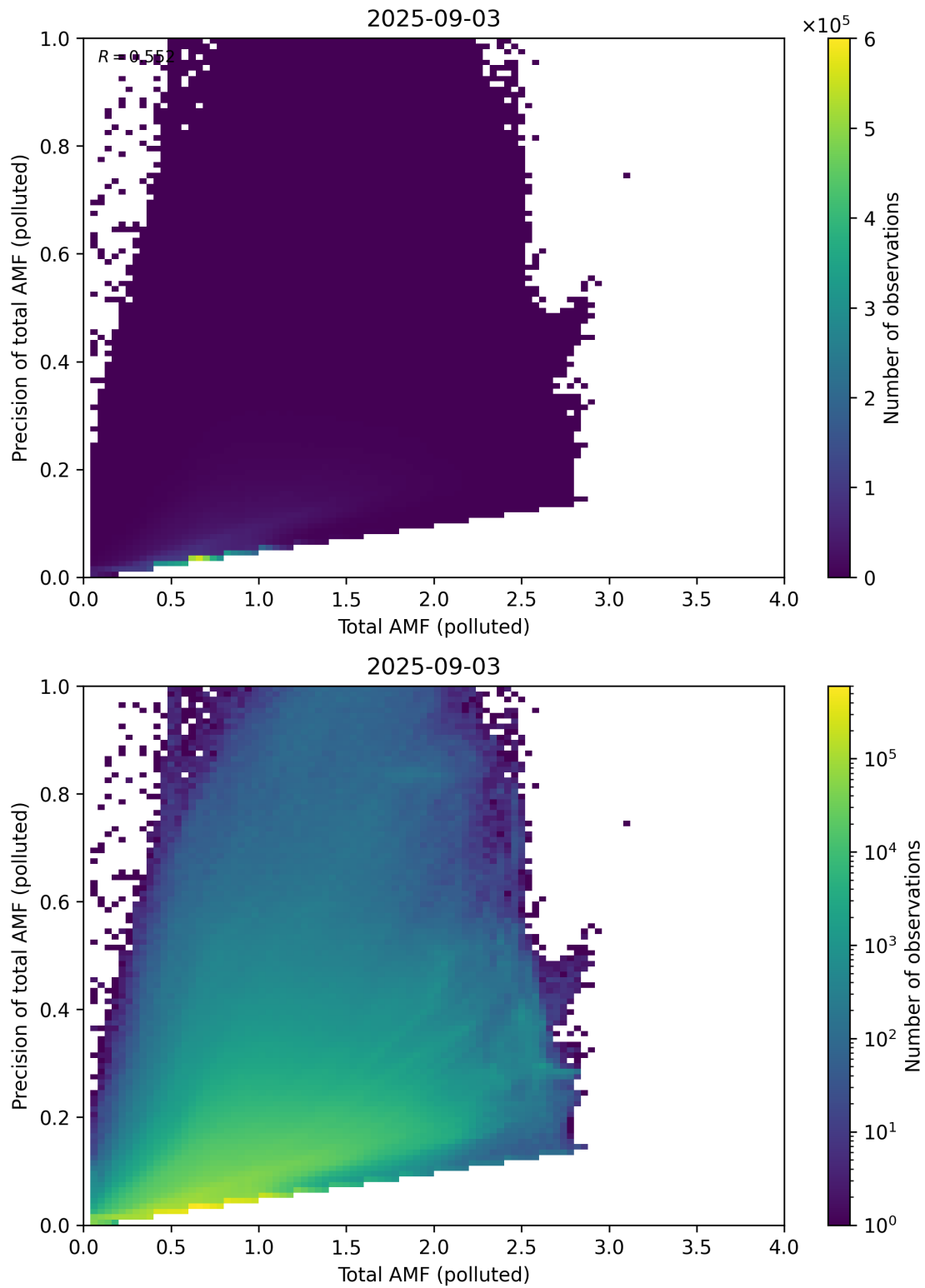
Figure 322: Scatter density plot of “Total AMF (polluted)” against “Precision of total AMF (polluted)” for 2025-09-02 to 2025-09-04.
