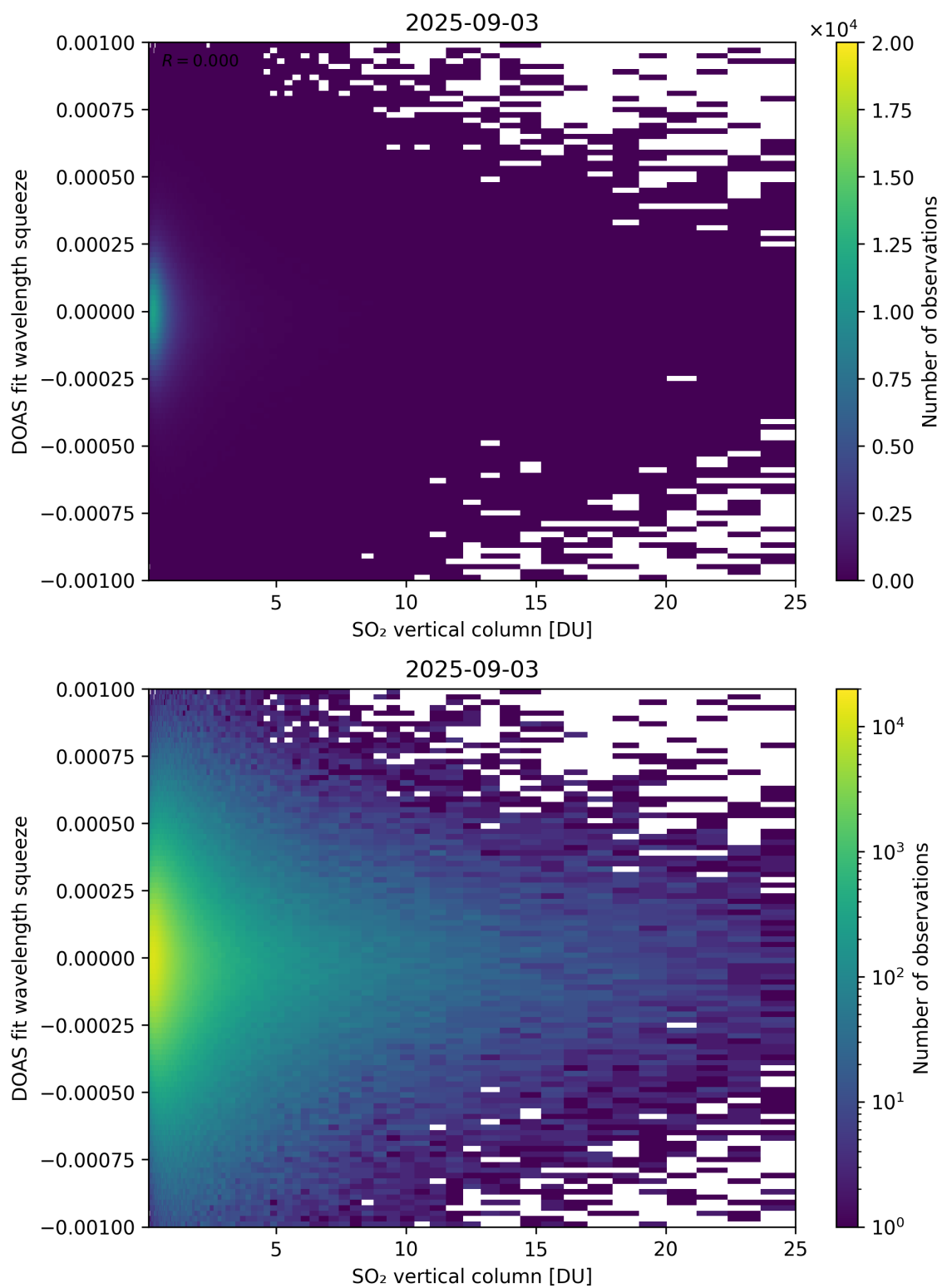
Figure 327: Scatter density plot of “SO 2 vertical column” against “DOAS fit wavelength squeeze” for 2025-09-02 to 2025-09-04.
