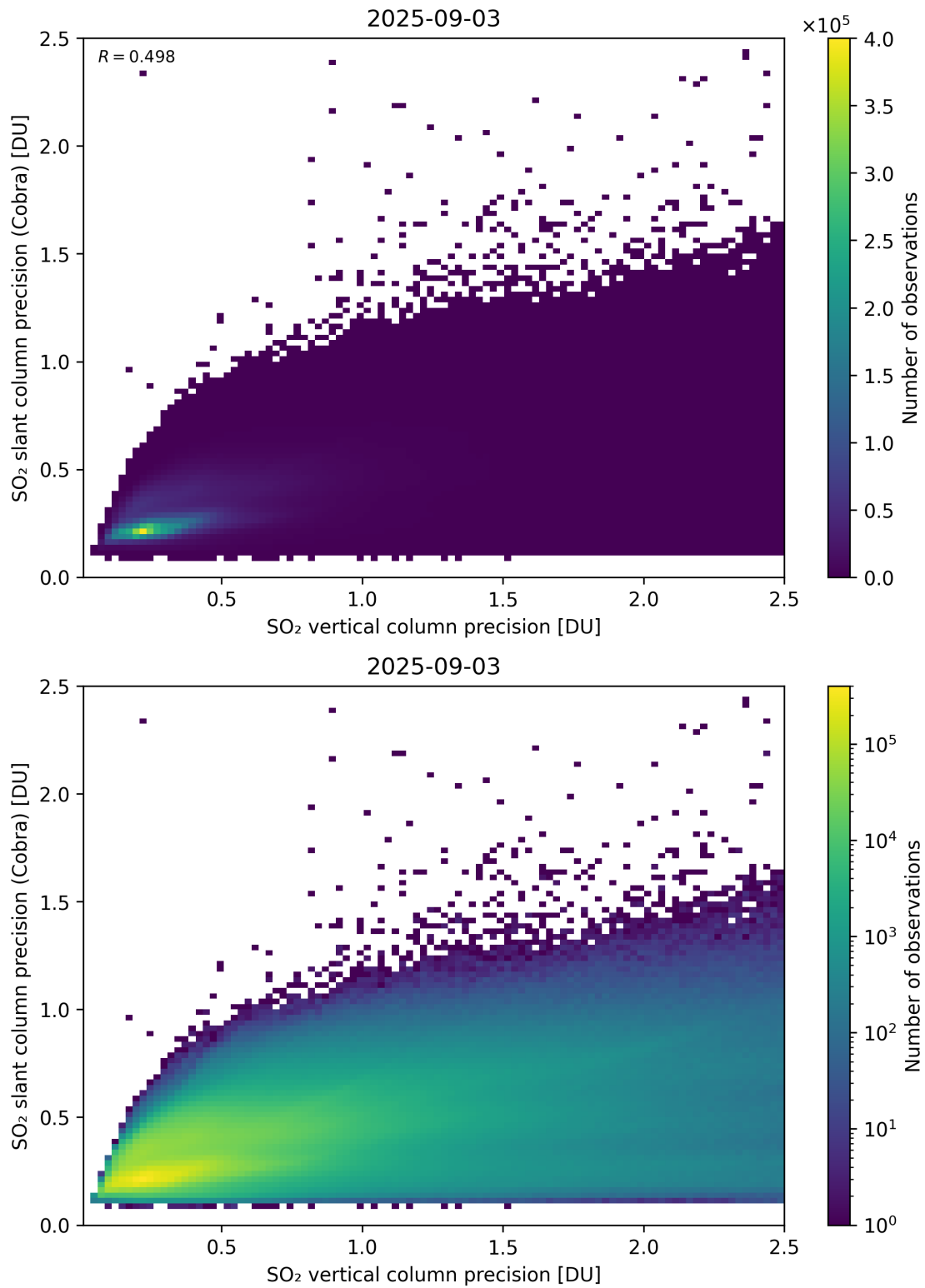
Figure 337: Scatter density plot of “SO 2 vertical column precision” against “SO 2 slant column precision (Cobra)” for 2025-09-02 to 2025-09-04.
