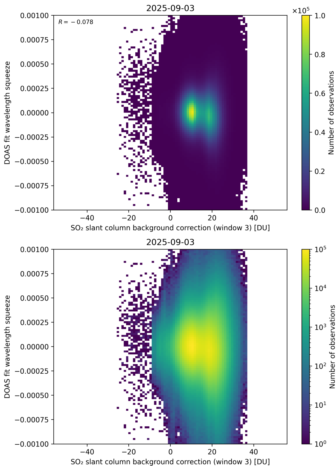
Figure 133: Scatter density plot of “SO 2 slant column background correction (window 3)” against “DOAS fit wavelength squeeze” for 2025-09-02 to 2025-09-04.
