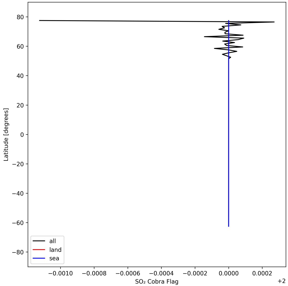
Figure 49: Zonal average of “SO 2 Cobra Flag” for 2025-09-02 to 2025-09-04.
