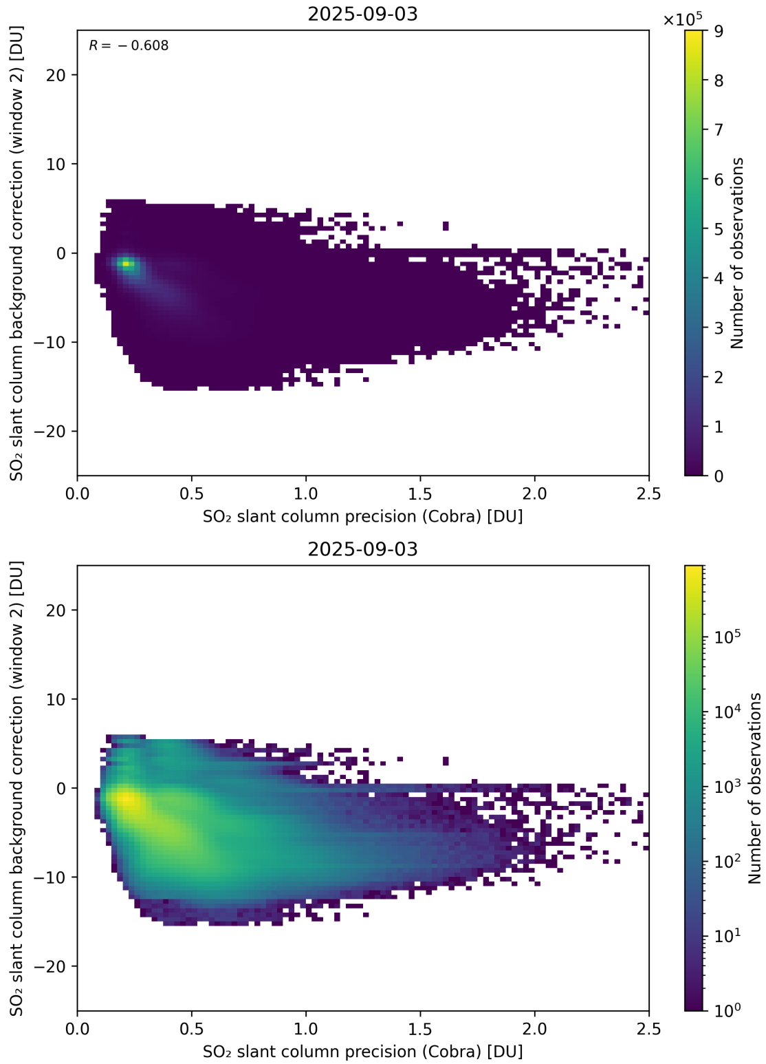
Figure 200: Scatter density plot of “SO 2 slant column precision (Cobra)” against “SO 2 slant column background correction (window 2)” for 2025-09-02 to 2025-09-04.
