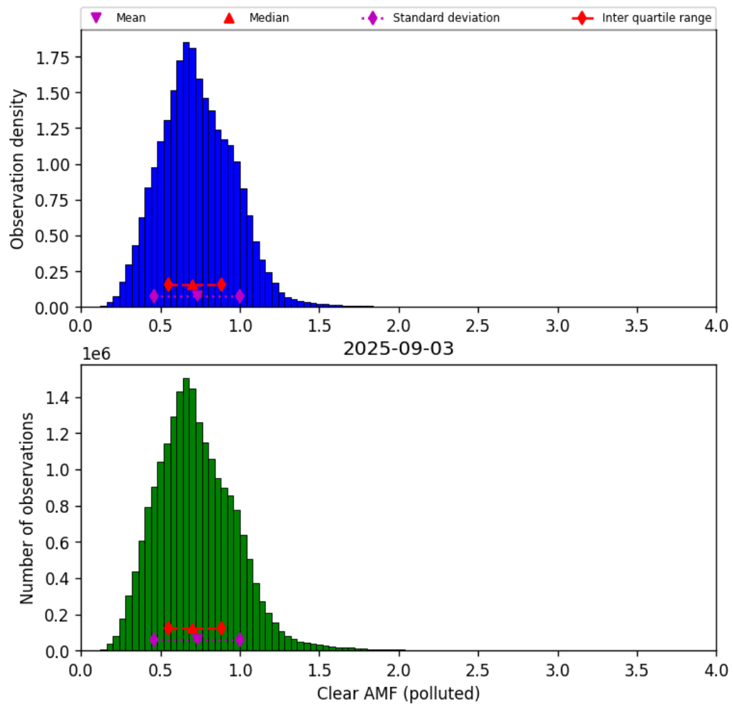
Figure 81: Histogram of “Clear AMF (polluted)” for 2025-09-02 to 2025-09-04
