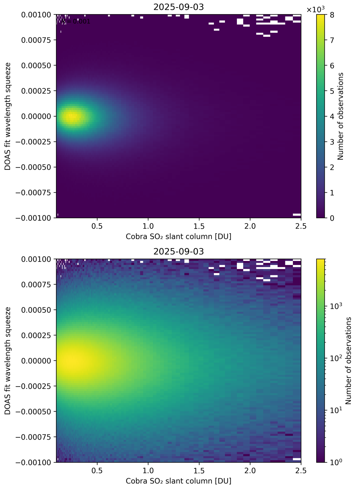
Figure 197: Scatter density plot of “Cobra SO 2 slant column” against “DOAS fit wavelength squeeze” for 2025-09-02 to 2025-09-04.
