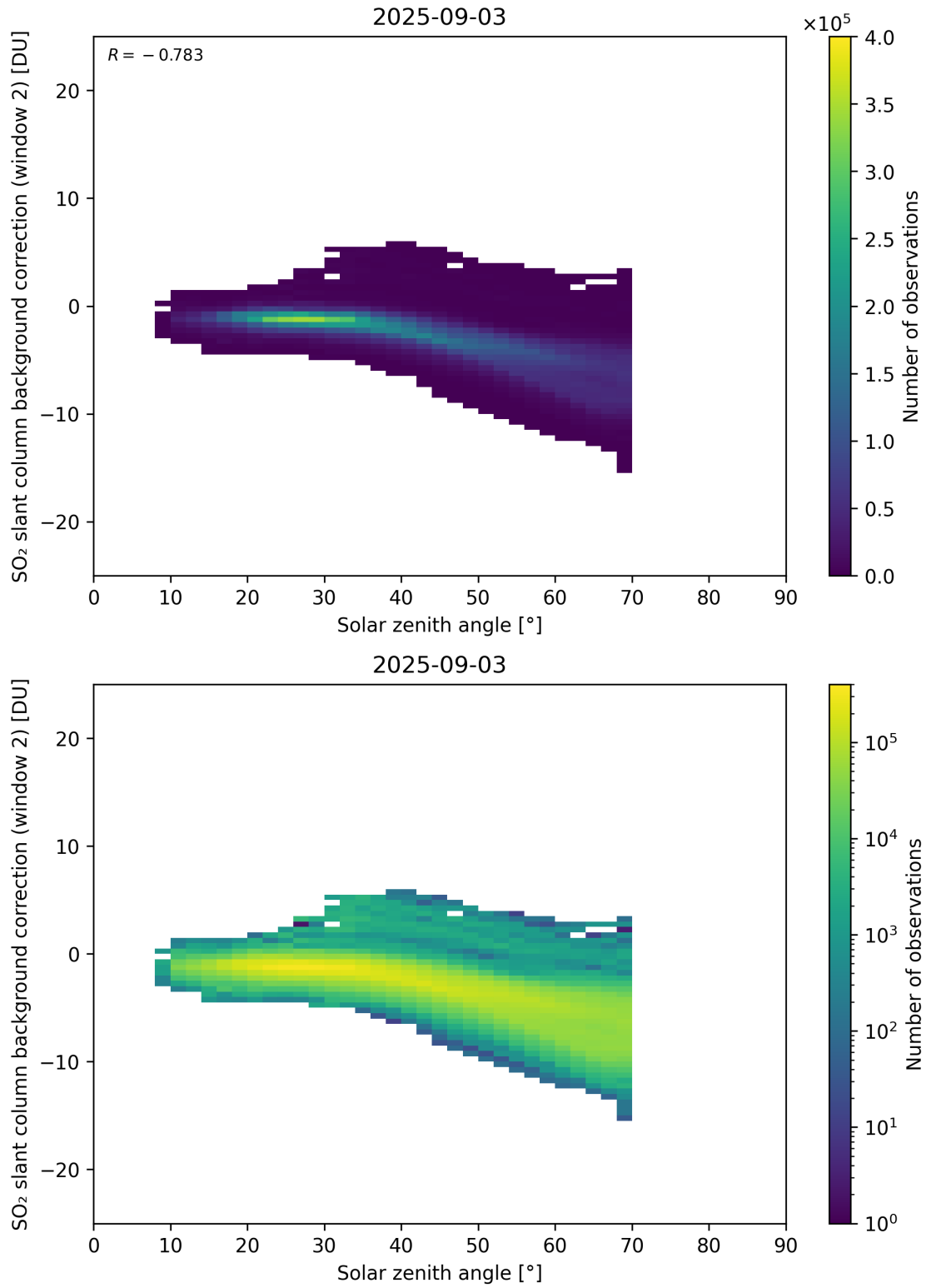
Figure 172: Scatter density plot of “Solar zenith angle” against “SO 2 slant column background correction (window 2)” for 2025-09-02 to 2025-09-04.
