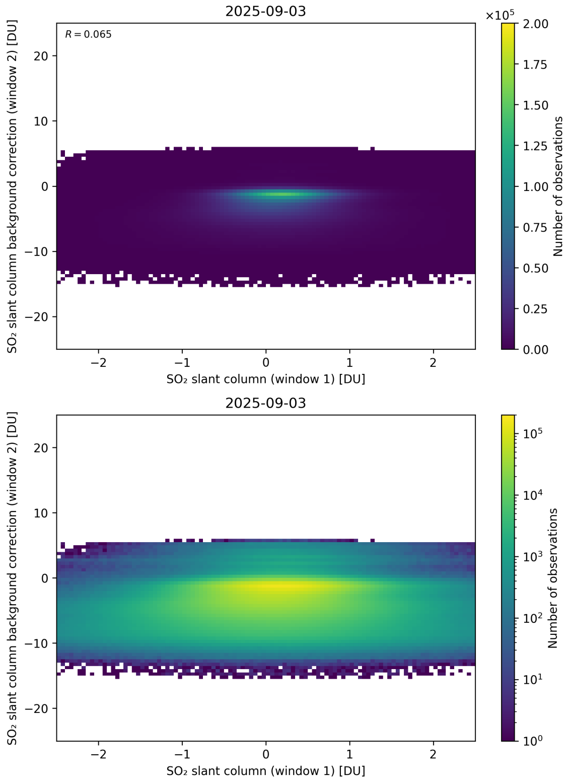
Figure 263: Scatter density plot of “SO 2 slant column (window 1)” against “SO 2 slant column background correction (window 2)” for 2025-09-02 to 2025-09-04.
