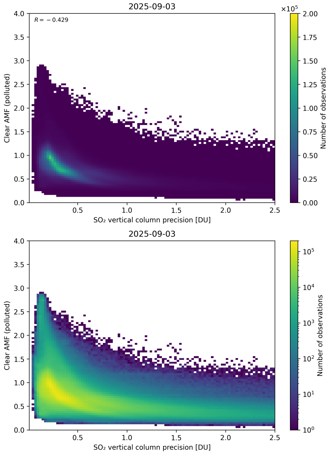
Figure 335: Scatter density plot of “SO 2 vertical column precision” against “Clear AMF (polluted)” for 2025-09-02 to 2025-09-04.
