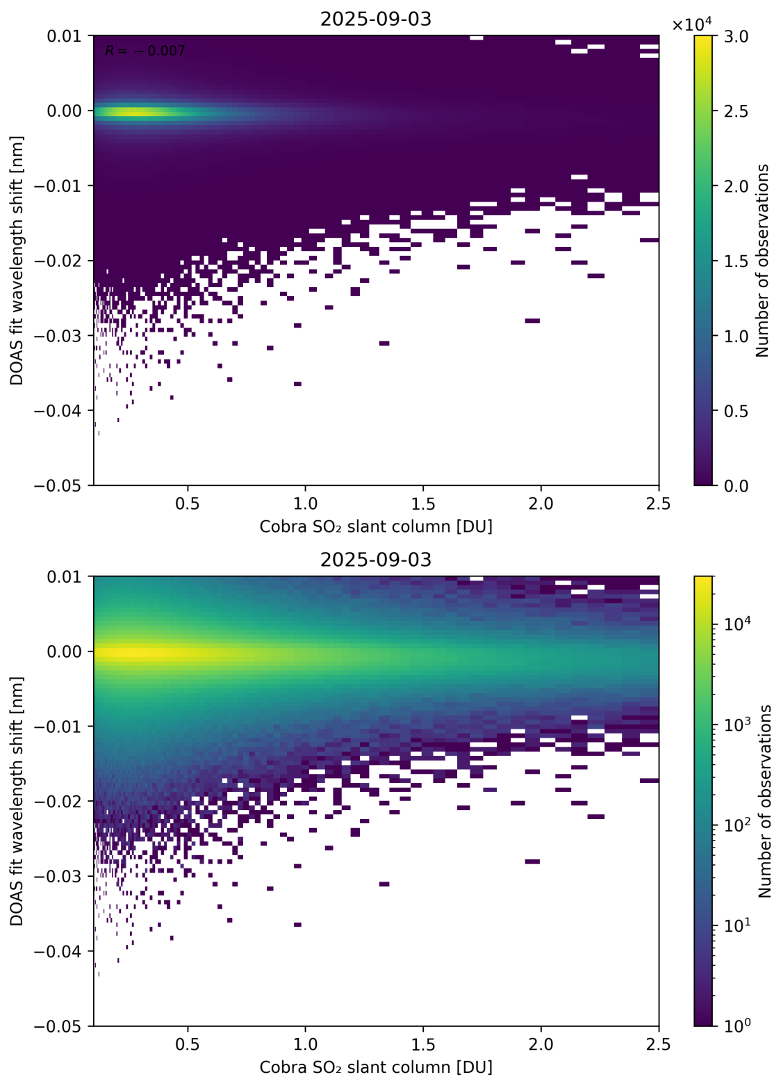
Figure 196: Scatter density plot of “Cobra SO 2 slant column” against “DOAS fit wavelength shift” for 2025-09-02 to 2025-09-04.
