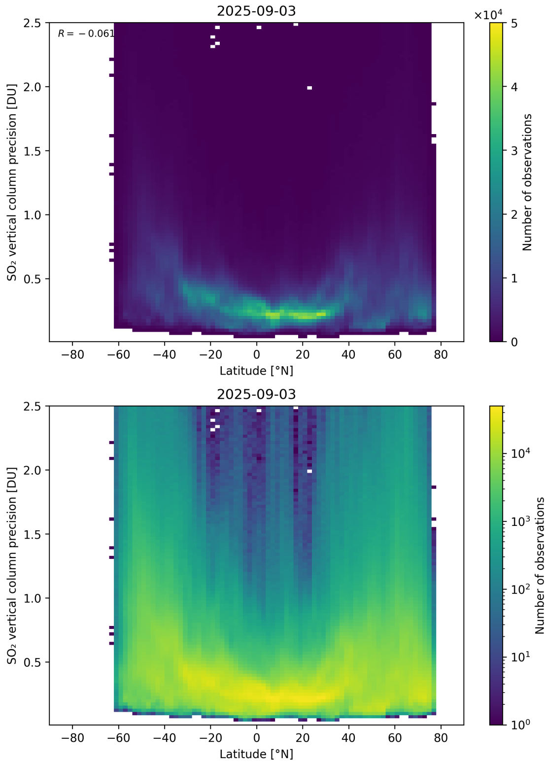
Figure 170: Scatter density plot of “Latitude” against “SO 2 vertical column precision” for 2025-09-02 to 2025-09-04.
