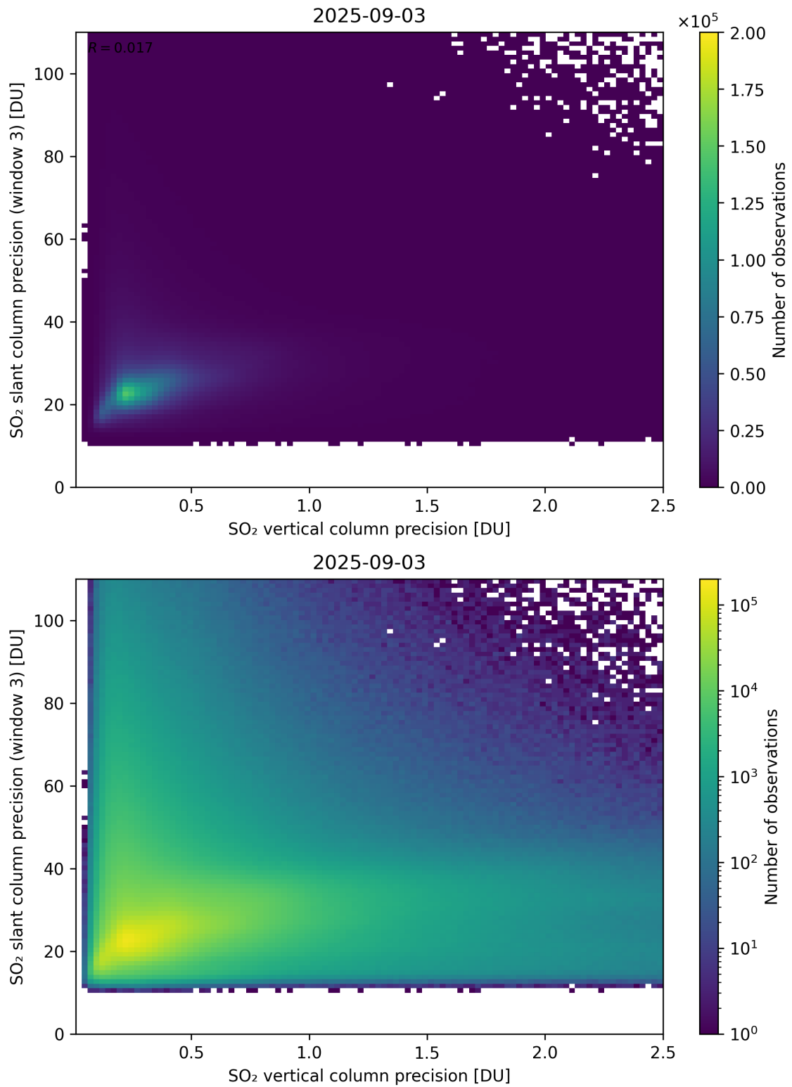
Figure 345: Scatter density plot of “SO 2 vertical column precision” against “SO 2 slant column precision (window 3)” for 2025-09-02 to 2025-09-04.
