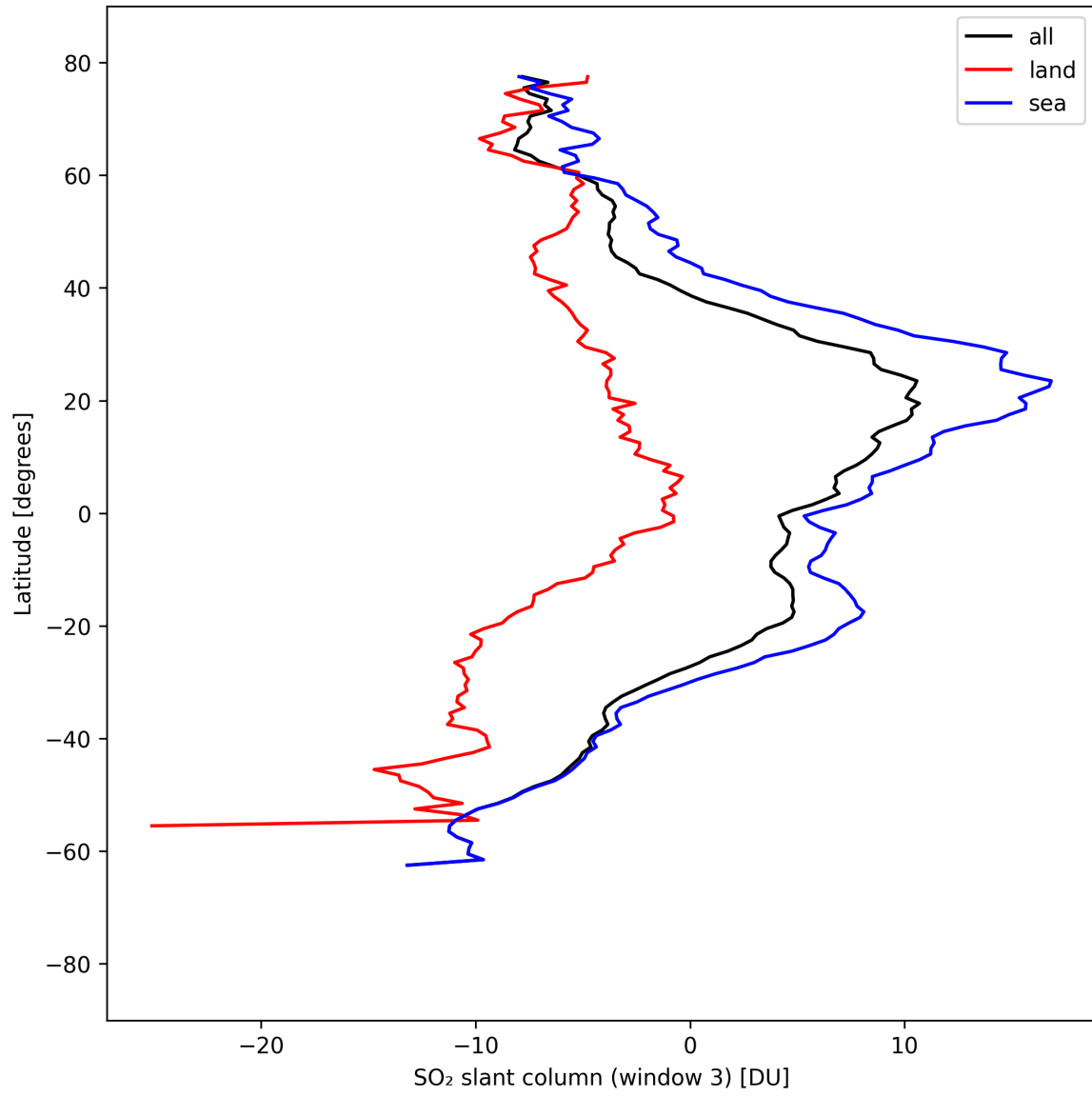
Figure 45: Zonal average of “SO 2 slant column (window 3)” for 2025-09-02 to 2025-09-04.
