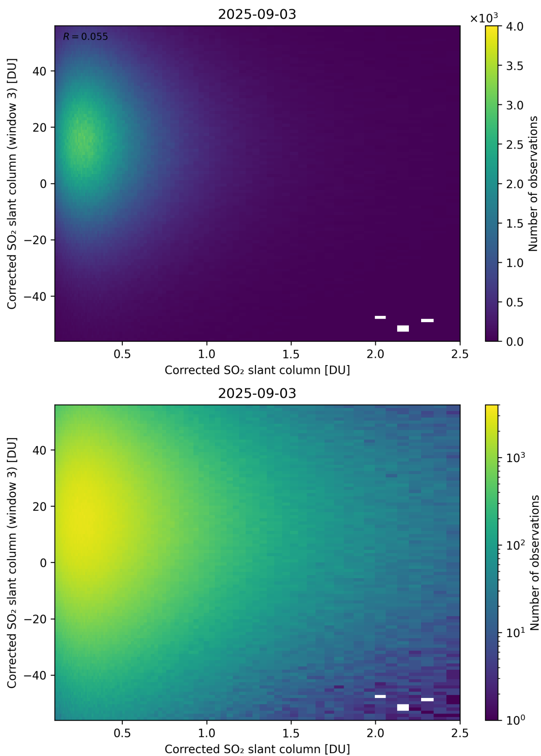
Figure 236: Scatter density plot of “Corrected SO 2 slant column” against “Corrected SO 2 slant column (window 3)” for 2025-09-02 to 2025-09-04.
