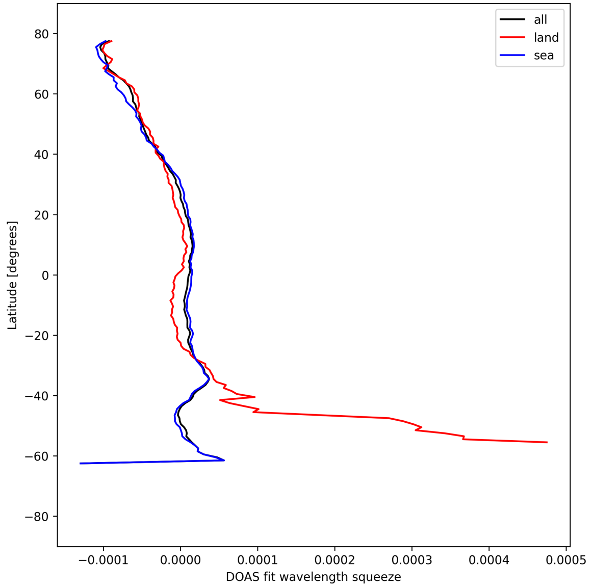
Figure 51: Zonal average of “DOAS fit wavelength squeeze” for 2025-09-02 to 2025-09-04.
