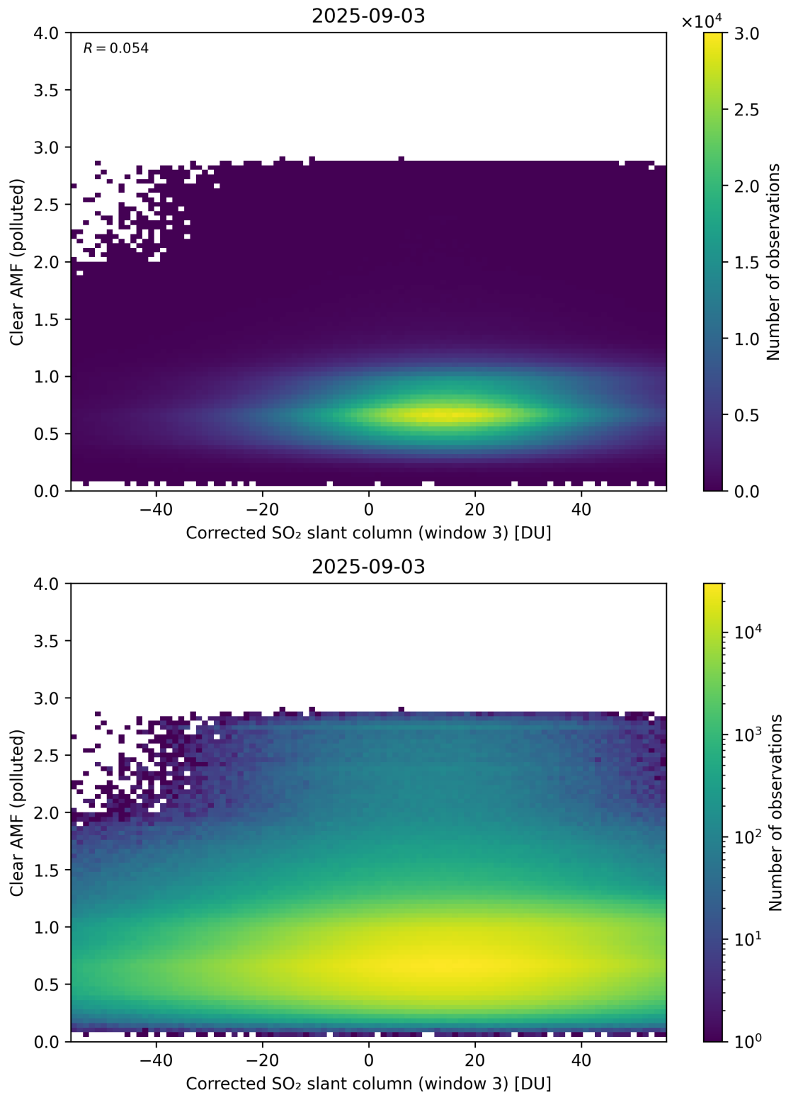
Figure 259: Scatter density plot of “Corrected SO 2 slant column (window 3)” against “Clear AMF (polluted)” for 2025-09-02 to 2025-09-04.
