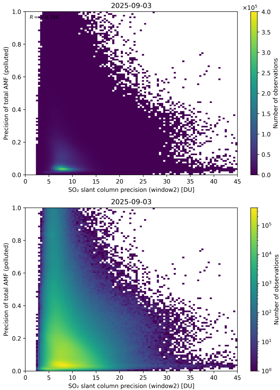
Figure 302: Scatter density plot of “SO 2 slant column precision (window2)” against “Precision of total AMF (polluted)” for 2025-09-02 to 2025-09-04.
