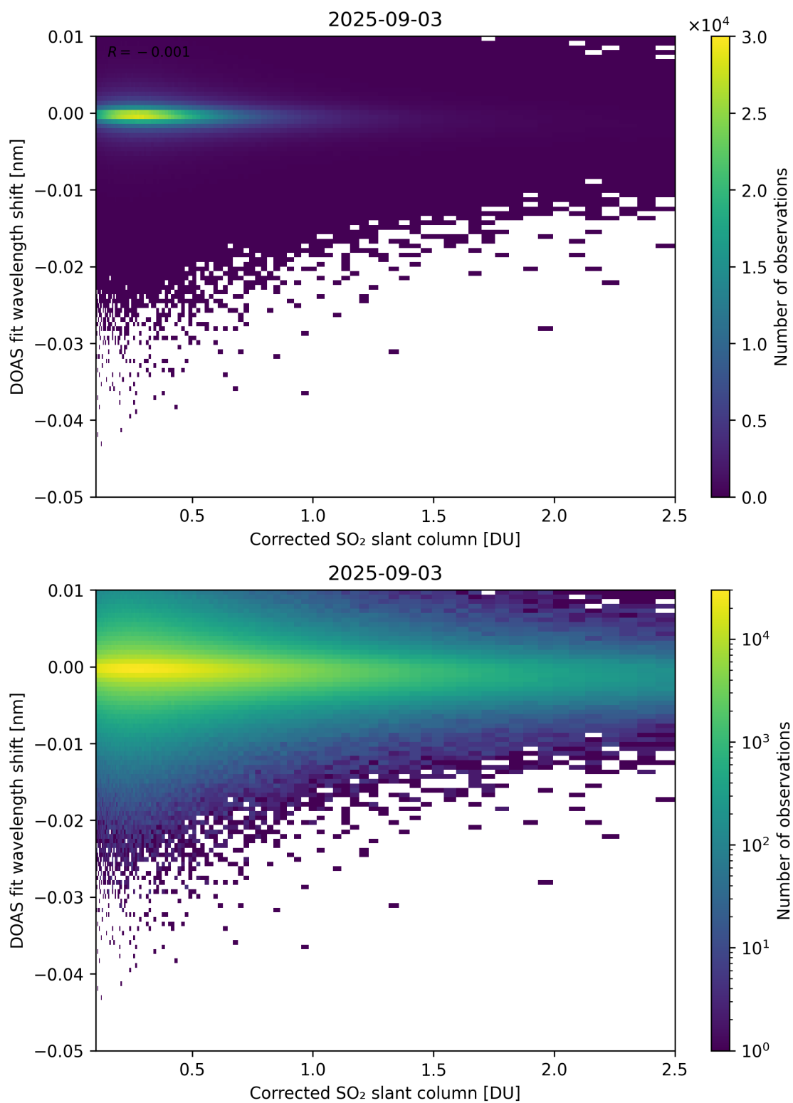
Figure 229: Scatter density plot of “Corrected SO 2 slant column” against “DOAS fit wavelength shift” for 2025-09-02 to 2025-09-04.
