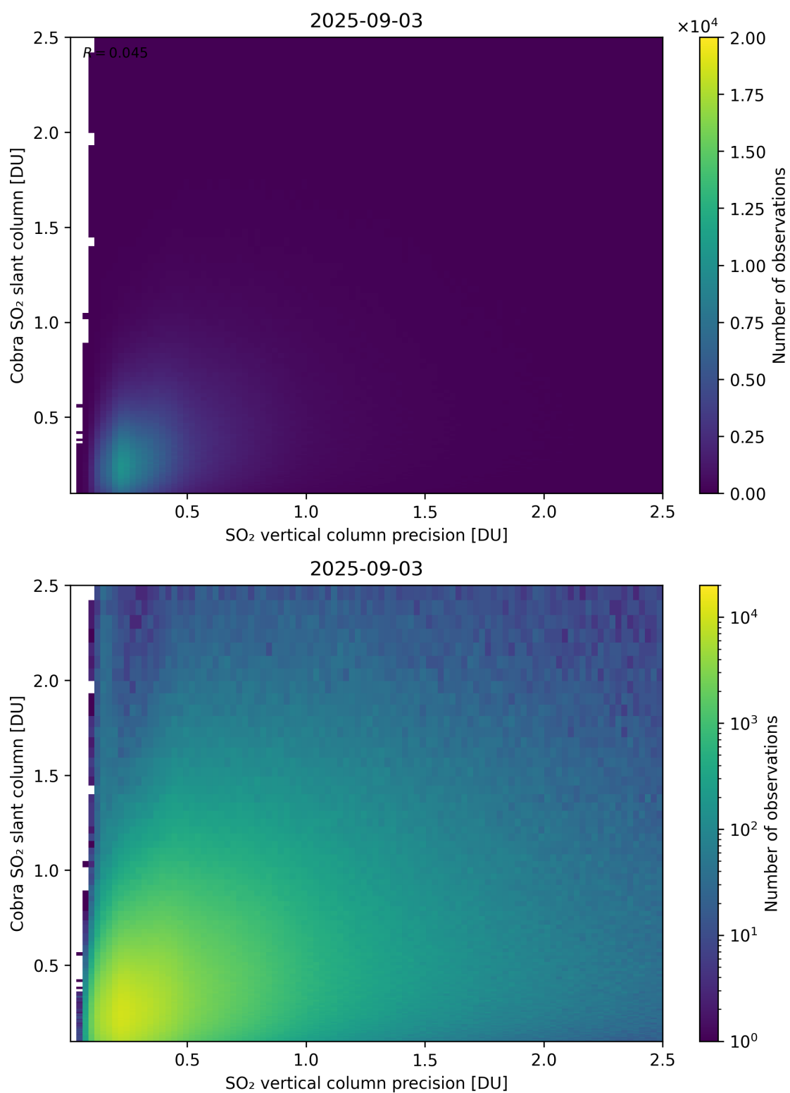
Figure 336: Scatter density plot of “SO 2 vertical column precision” against “Cobra SO 2 slant column” for 2025-09-02 to 2025-09-04.
