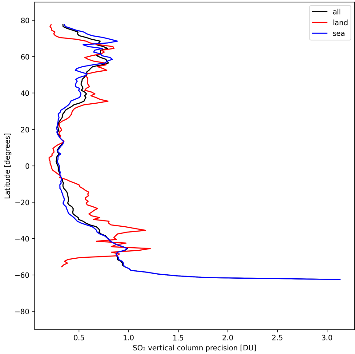
Figure 33: Zonal average of “SO 2 vertical column precision” for 2025-09-02 to 2025-09-04.
