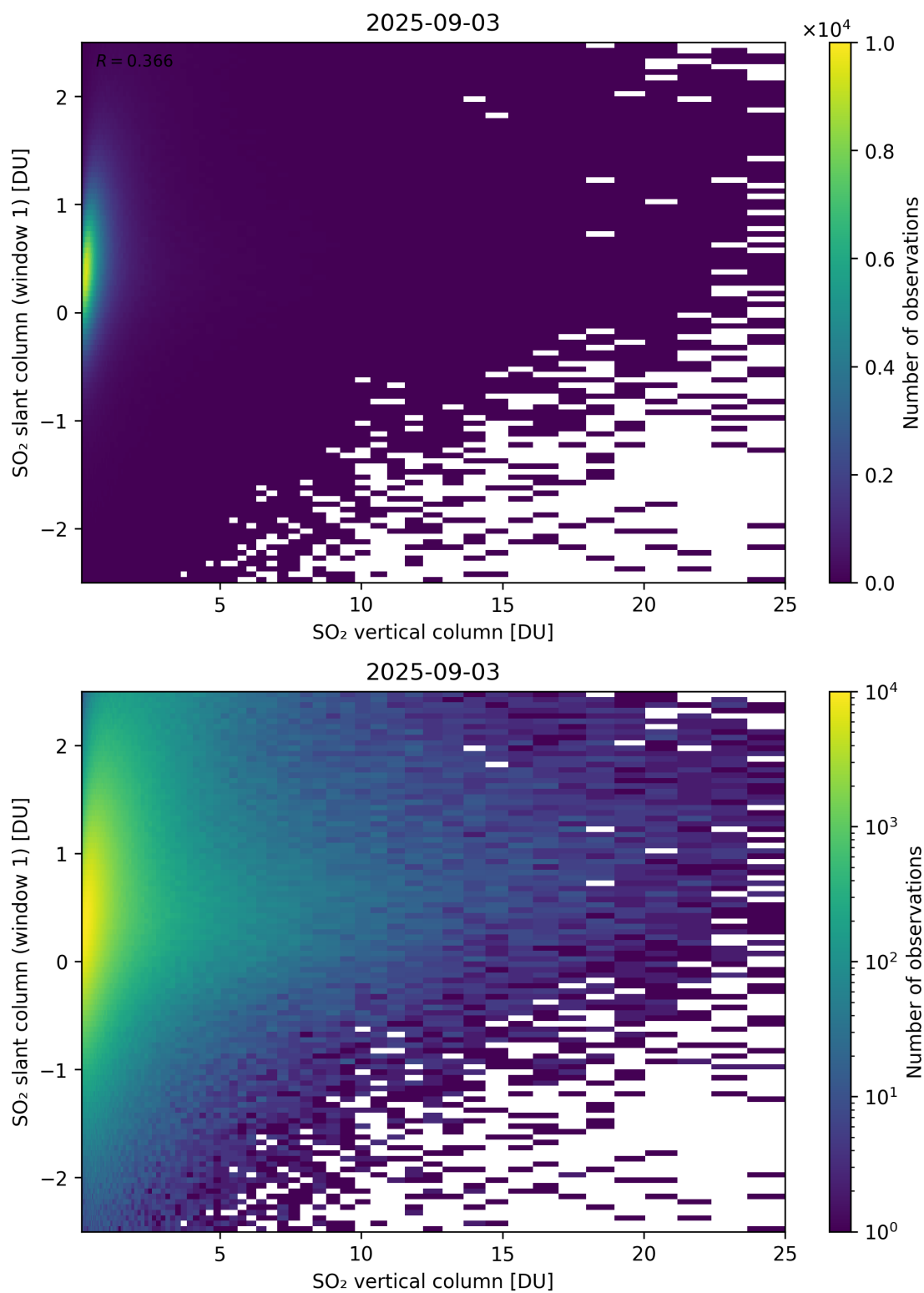
Figure 354: Scatter density plot of “SO 2 vertical column” against “SO 2 slant column (window 1)” for 2025-09-02 to 2025-09-04.
