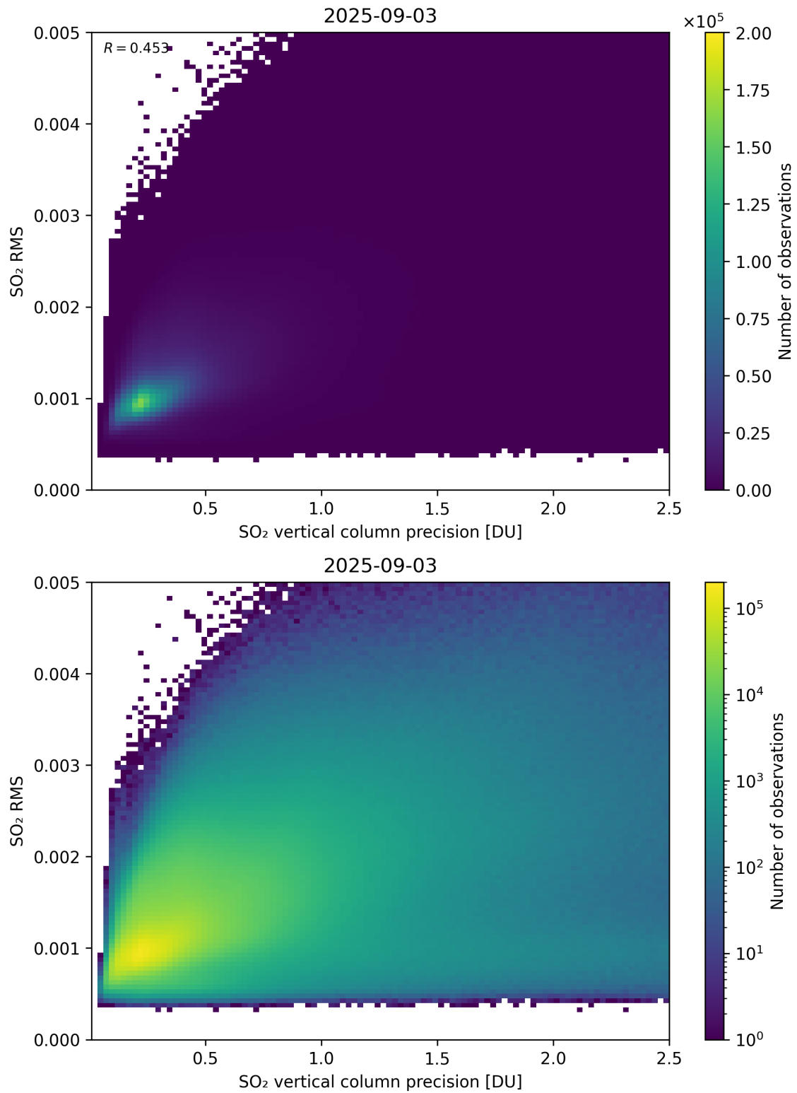
Figure 334: Scatter density plot of “SO 2 vertical column precision” against “SO 2 RMS” for 2025-09-02 to 2025-09-04.
