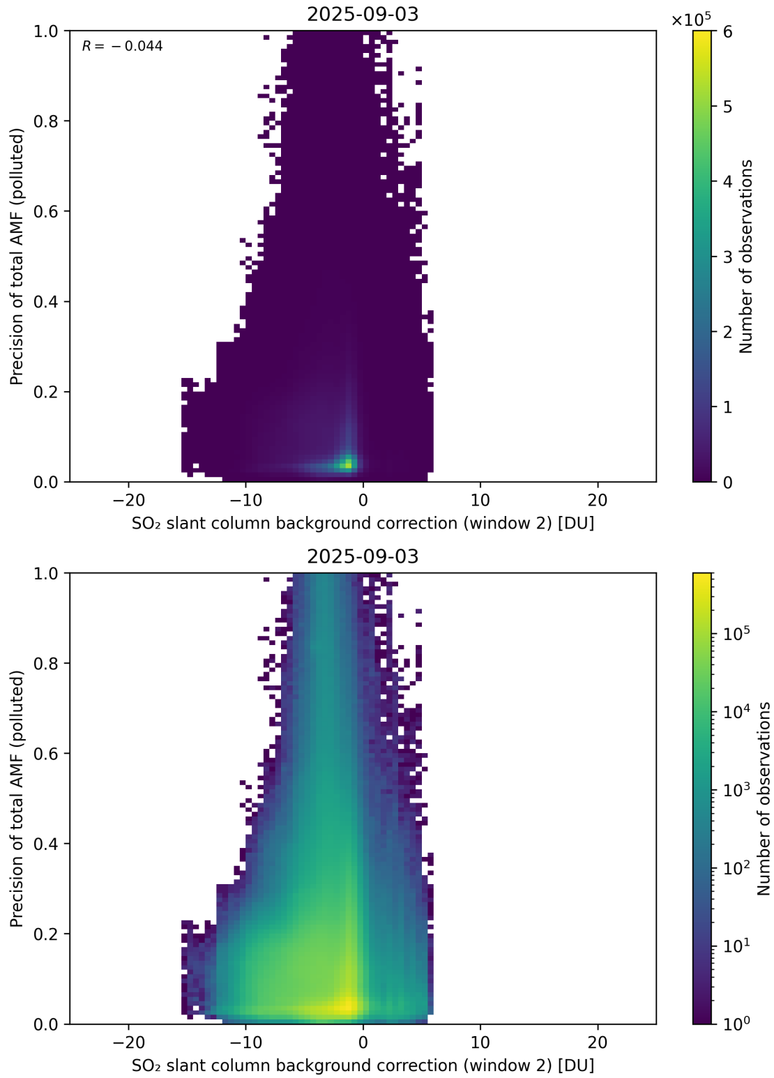
Figure 131: Scatter density plot of “SO 2 slant column background correction (window 2)” against “Precision of total AMF (polluted)” for 2025-09-02 to 2025-09-04.
