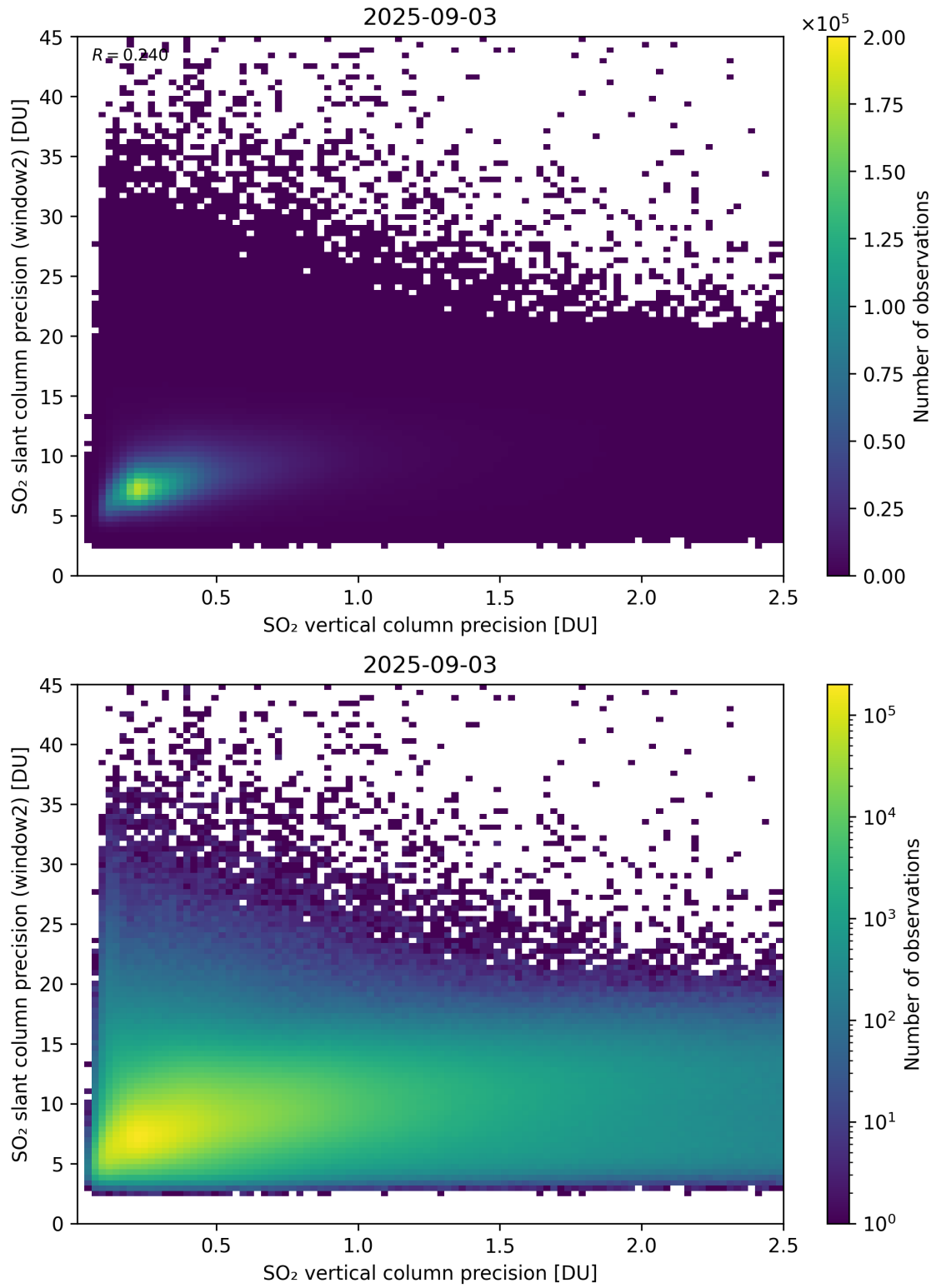
Figure 343: Scatter density plot of “SO 2 vertical column precision” against “SO 2 slant column precision (window2)” for 2025-09-02 to 2025-09-04.
