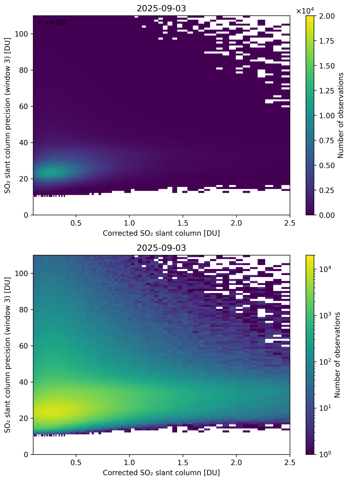
Figure 241: Scatter density plot of “Corrected SO 2 slant column” against “SO 2 slant column precision (window 3)” for 2025-09-02 to 2025-09-04.
