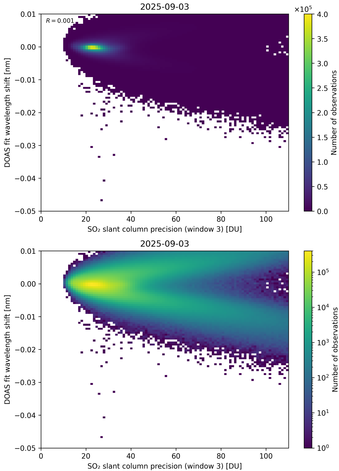
Figure 308: Scatter density plot of “SO 2 slant column precision (window 3)” against “DOAS fit wavelength shift” for 2025-09-02 to 2025-09-04.
