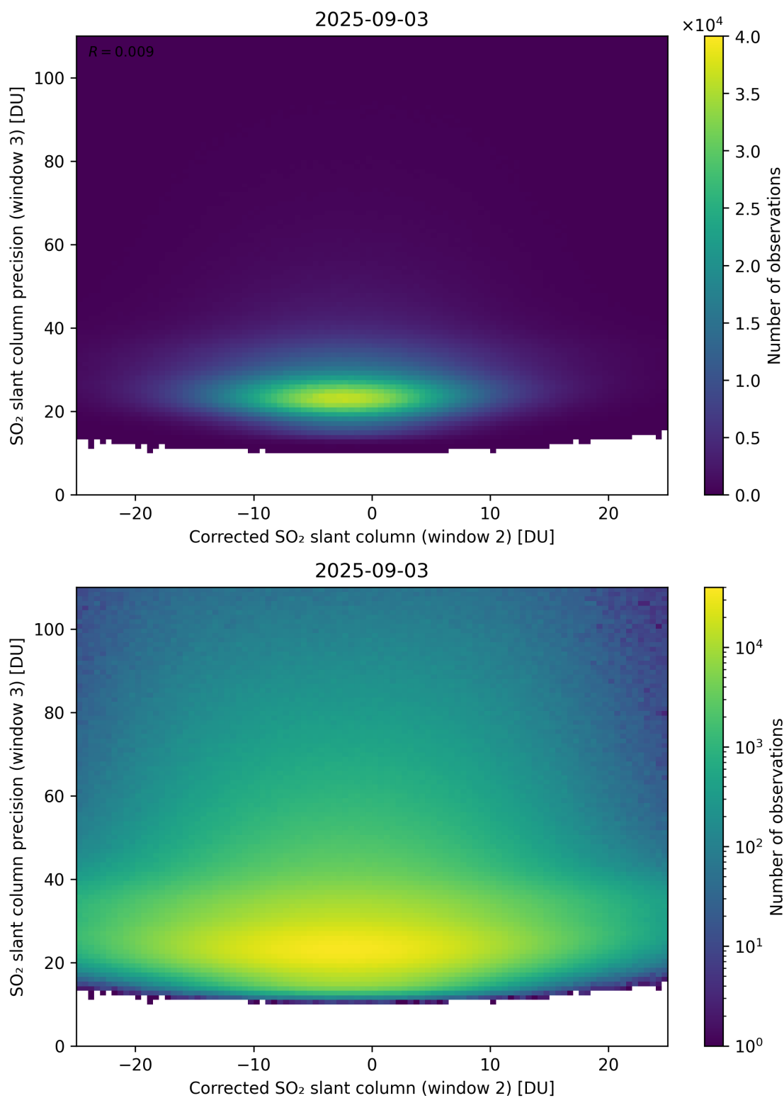
Figure 252: Scatter density plot of “Corrected SO 2 slant column (window 2)” against “SO 2 slant column precision (window 3)” for 2025-09-02 to 2025-09-04.
