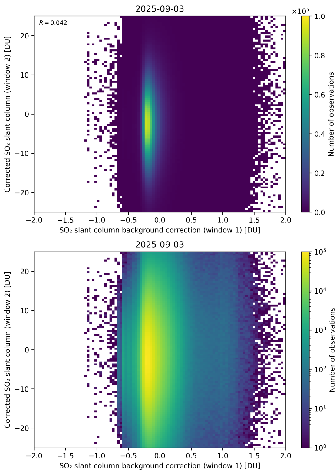
Figure 115: Scatter density plot of “SO 2 slant column background correction (window 1)” against “Corrected SO 2 slant column (window 2)” for 2025-09-02 to 2025-09-04.
