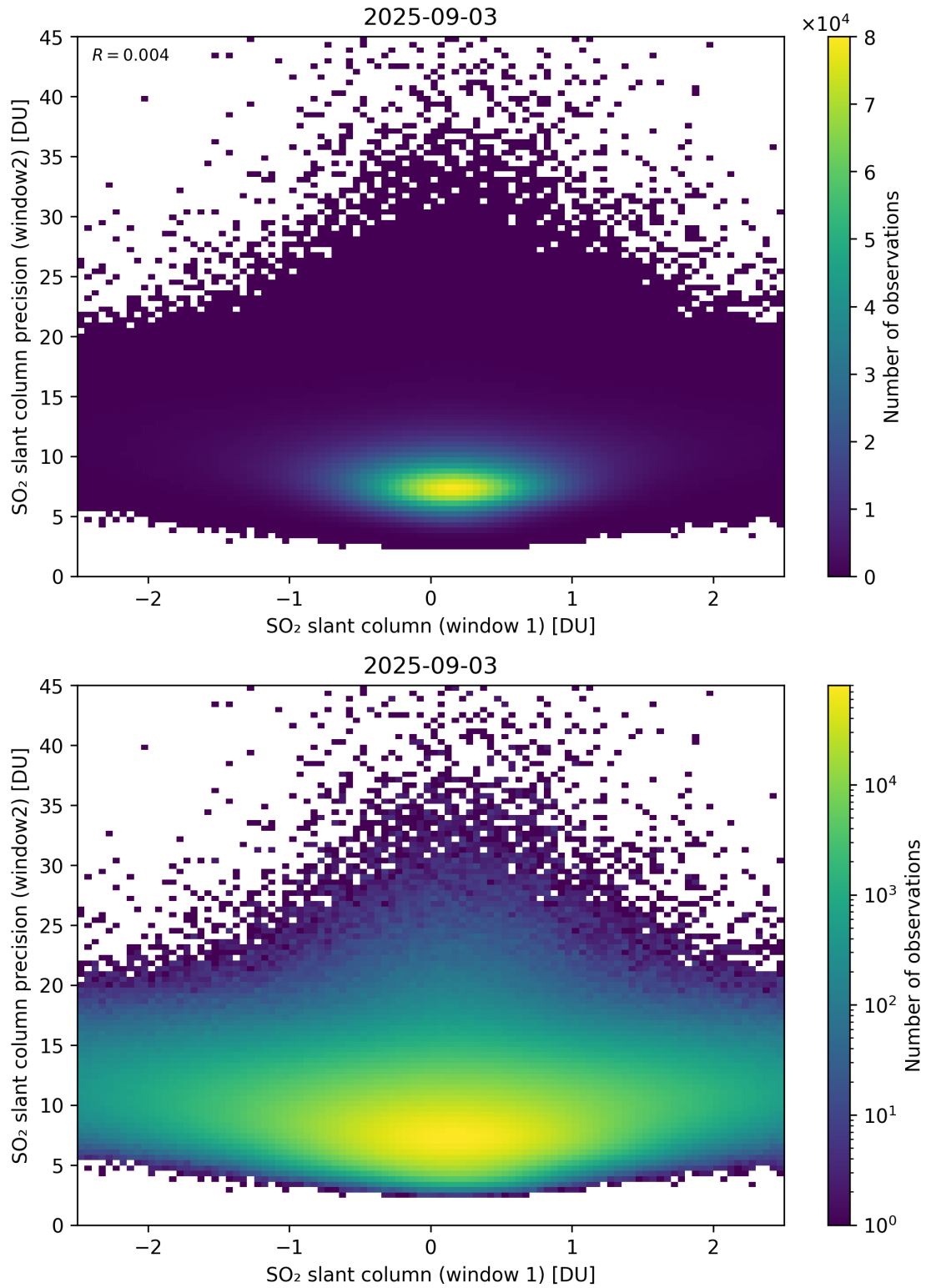
Figure 286: Scatter density plot of “SO 2 slant column (window 1)” against “SO 2 slant column precision (window2)” for 2025-09-02 to 2025-09-04.
