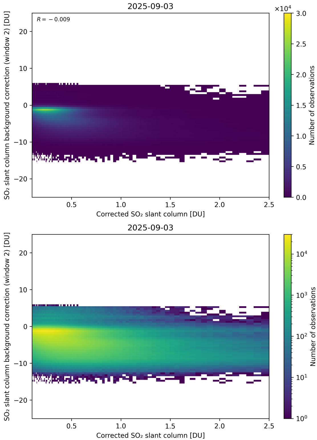
Figure 227: Scatter density plot of “Corrected SO 2 slant column” against “SO 2 slant column background correction (window 2)” for 2025-09-02 to 2025-09-04.
