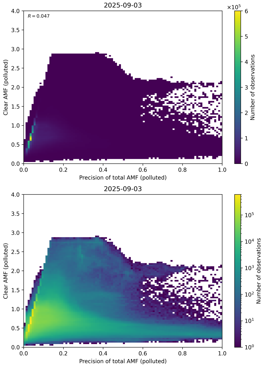
Figure 320: Scatter density plot of “Precision of total AMF (polluted)” against “Clear AMF (polluted)” for 2025-09-02 to 2025-09-04.
