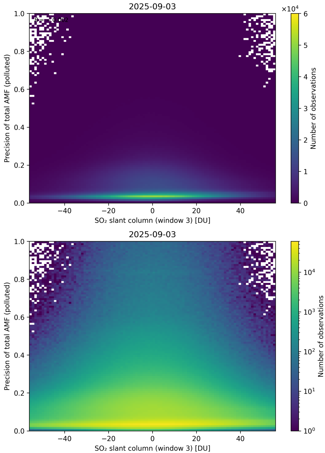
Figure 319: Scatter density plot of “SO 2 slant column (window 3)” against “Precision of total AMF (polluted)” for 2025-09-02 to 2025-09-04.
