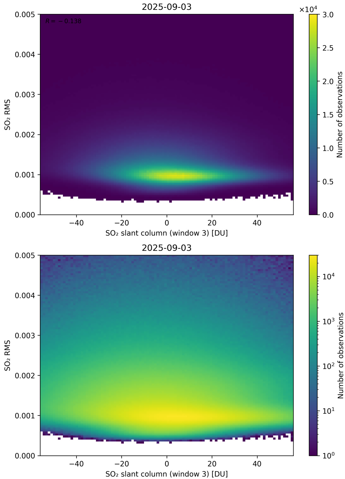
Figure 306: Scatter density plot of “SO 2 slant column (window 3)” against “SO 2 RMS” for 2025-09-02 to 2025-09-04.
