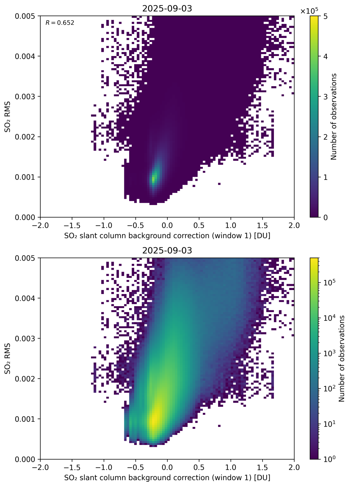
Figure 113: Scatter density plot of “SO 2 slant column background correction (window 1)” against “SO 2 RMS” for 2025-09-02 to 2025-09-04.
