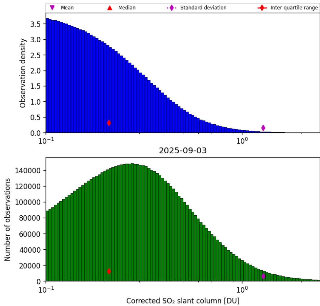
Figure 60: Histogram of “Corrected SO 2 slant column” for 2025-09-02 to 2025-09-04
