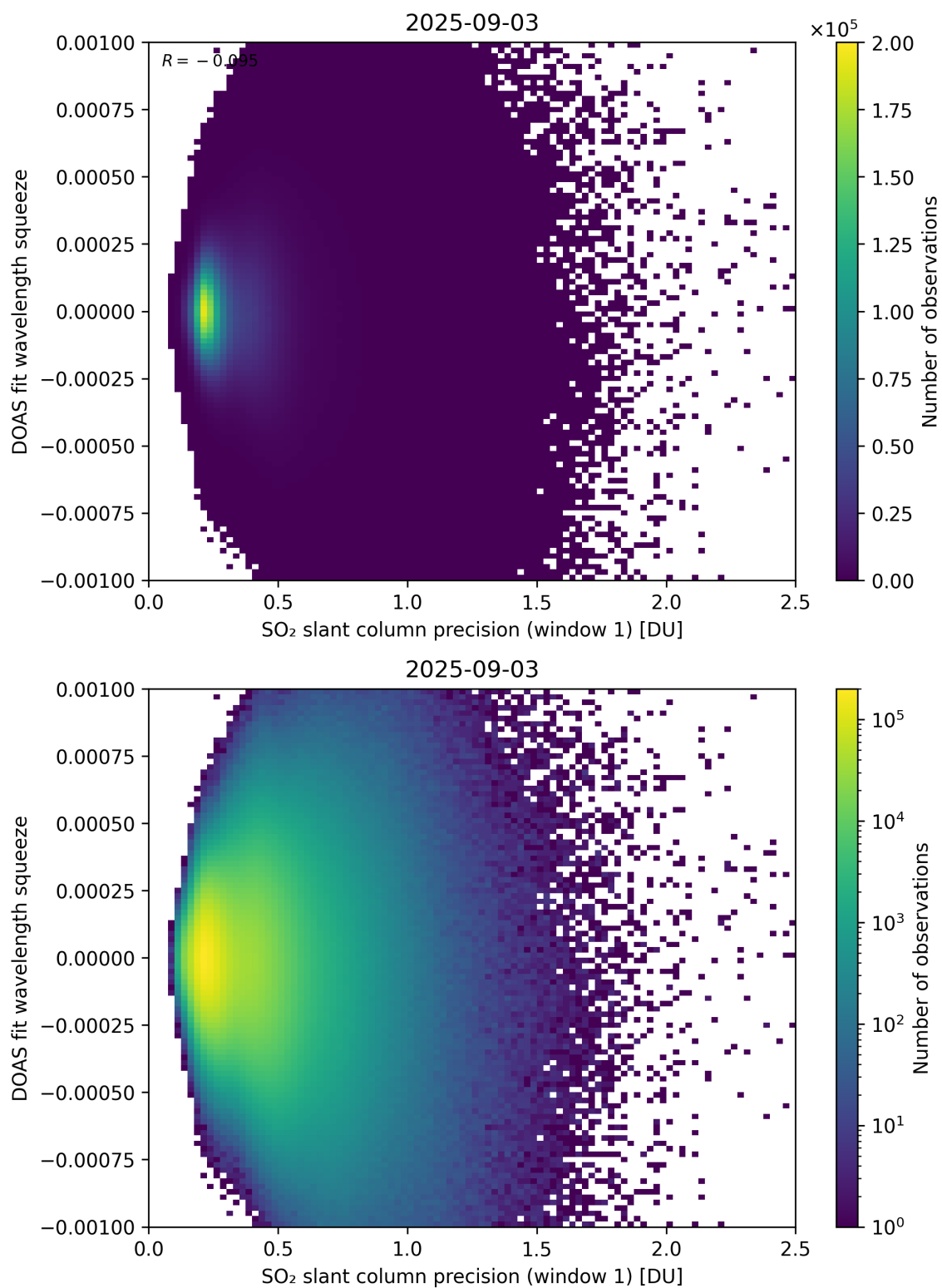
Figure 272: Scatter density plot of “SO 2 slant column precision (window 1)” against “DOAS fit wavelength squeeze” for 2025-09-02 to 2025-09-04.
