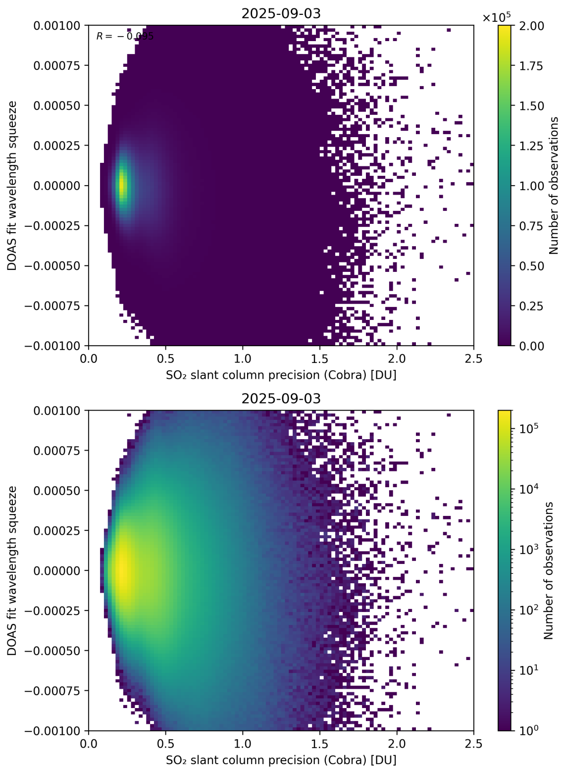
Figure 203: Scatter density plot of “SO 2 slant column precision (Cobra)” against “DOAS fit wavelength squeeze” for 2025-09-02 to 2025-09-04.
