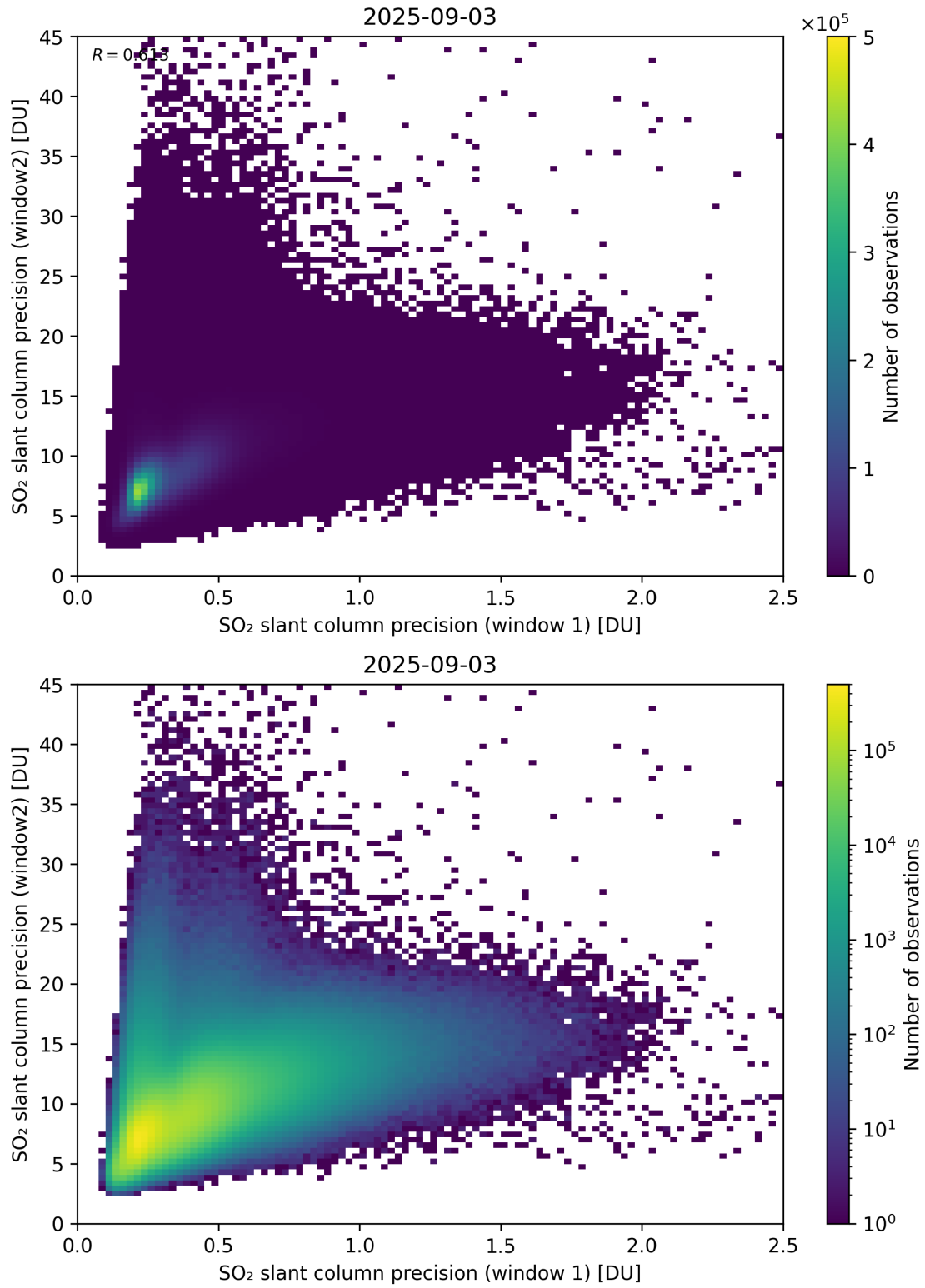
Figure 277: Scatter density plot of “SO 2 slant column precision (window 1)” against “SO 2 slant column precision (window2)” for 2025-09-02 to 2025-09-04.
