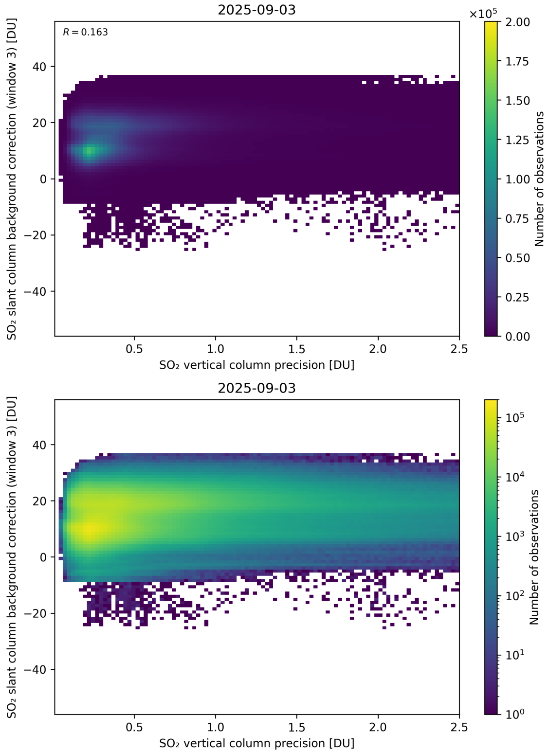
Figure 331: Scatter density plot of “SO 2 vertical column precision” against “SO 2 slant column background correction (window 3)” for 2025-09-02 to 2025-09-04.
