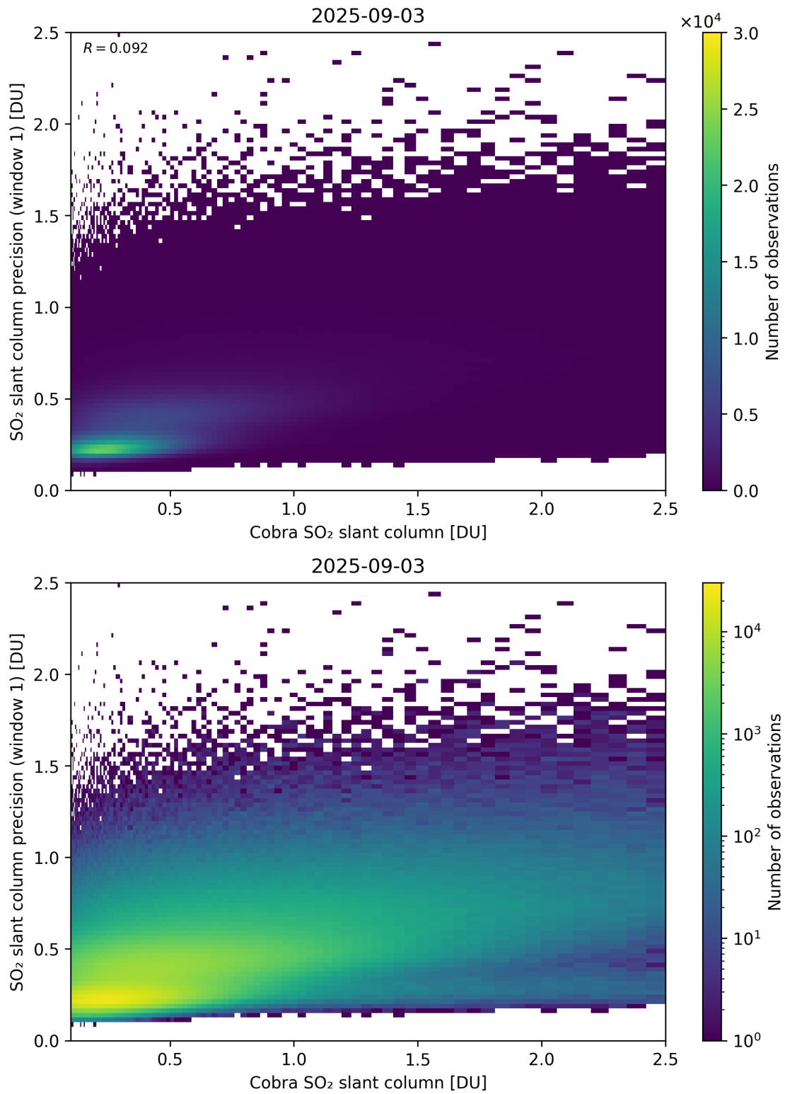
Figure 220: Scatter density plot of “Cobra SO 2 slant column” against “SO 2 slant column precision (window 1)” for 2025-09-02 to 2025-09-04.
