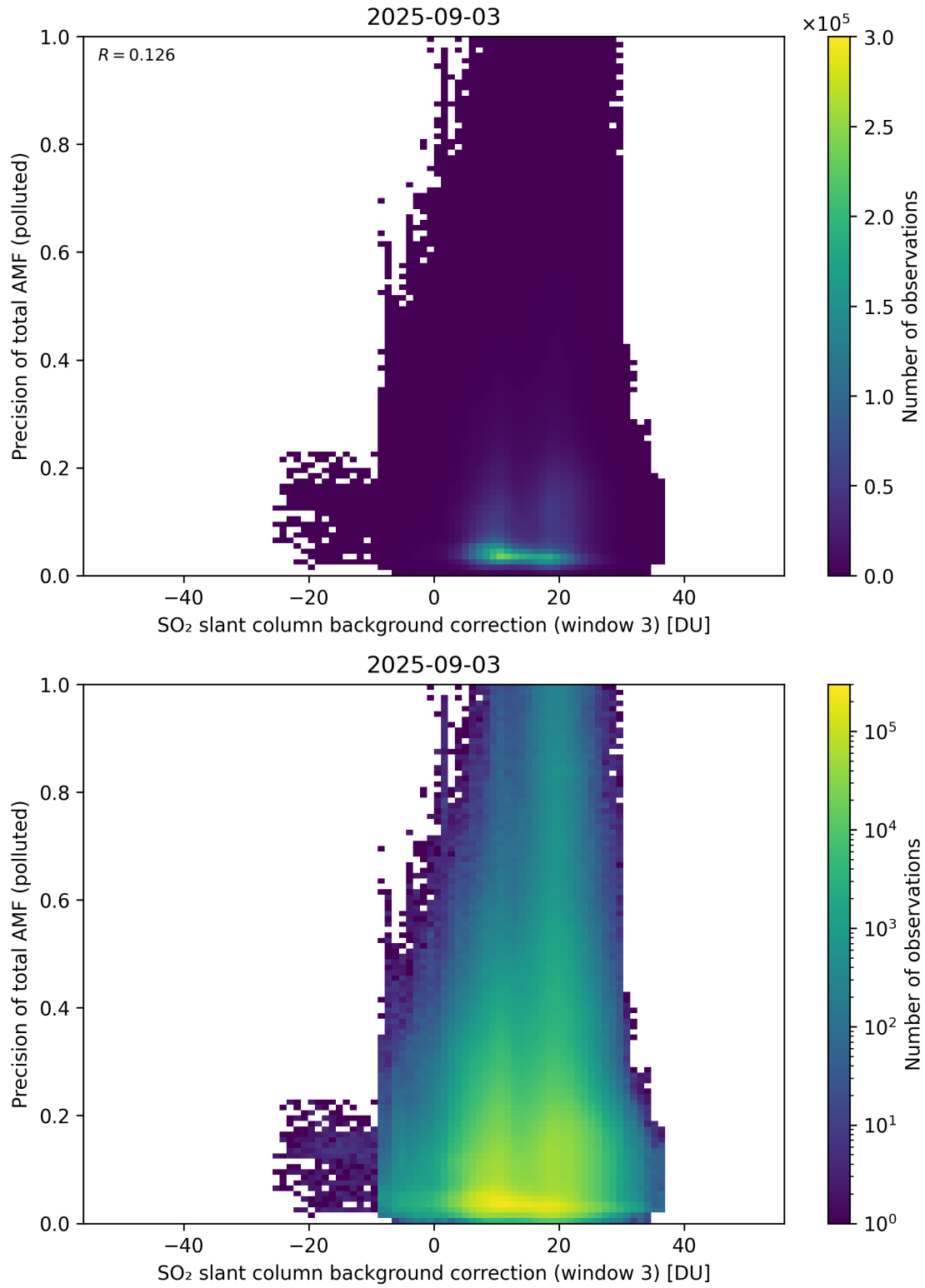
Figure 137: Scatter density plot of “SO 2 slant column background correction (window 3)” against “Precision of total AMF (polluted)” for 2025-09-02 to 2025-09-04.
