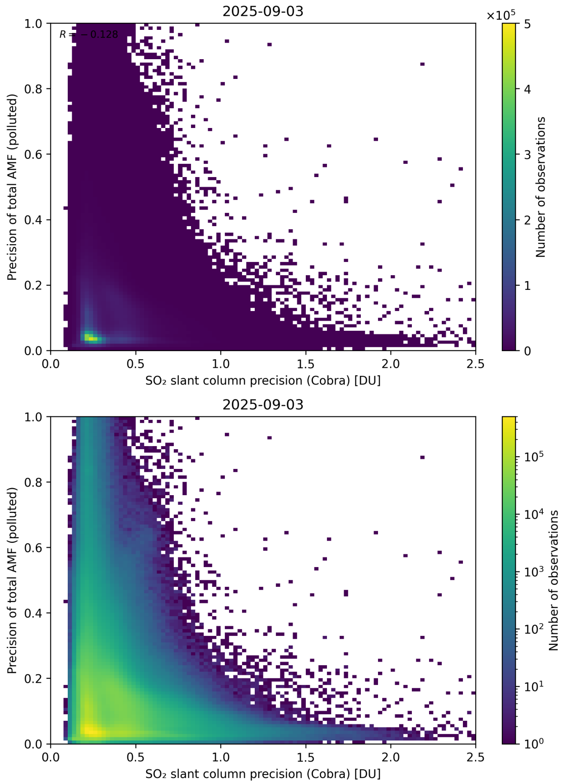
Figure 214: Scatter density plot of “SO 2 slant column precision (Cobra)” against “Precision of total AMF (polluted)” for 2025-09-02 to 2025-09-04.
