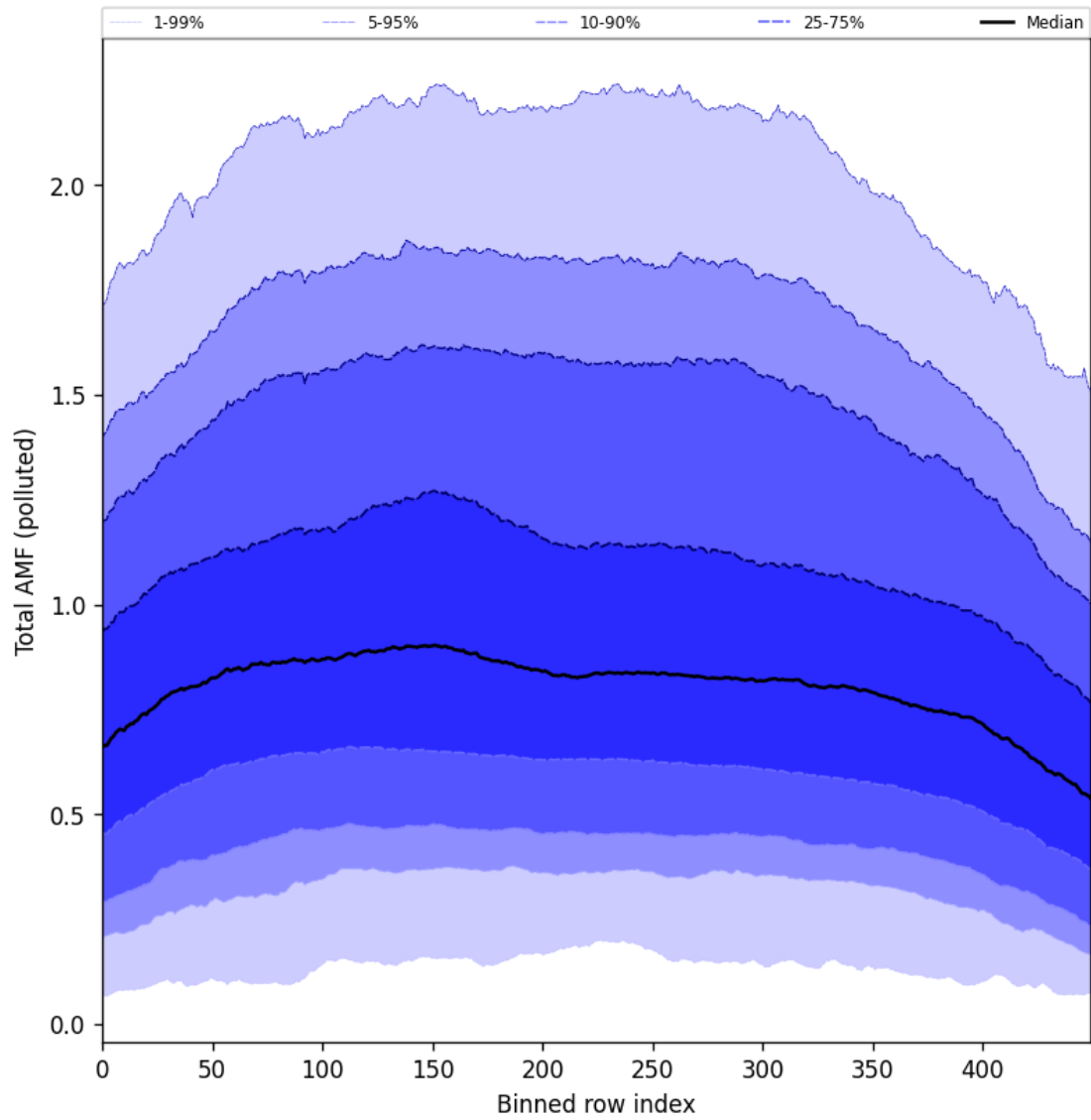
Figure 105: Along track statistics of “Total AMF (polluted)” for 2025-09-02 to 2025-09-04
