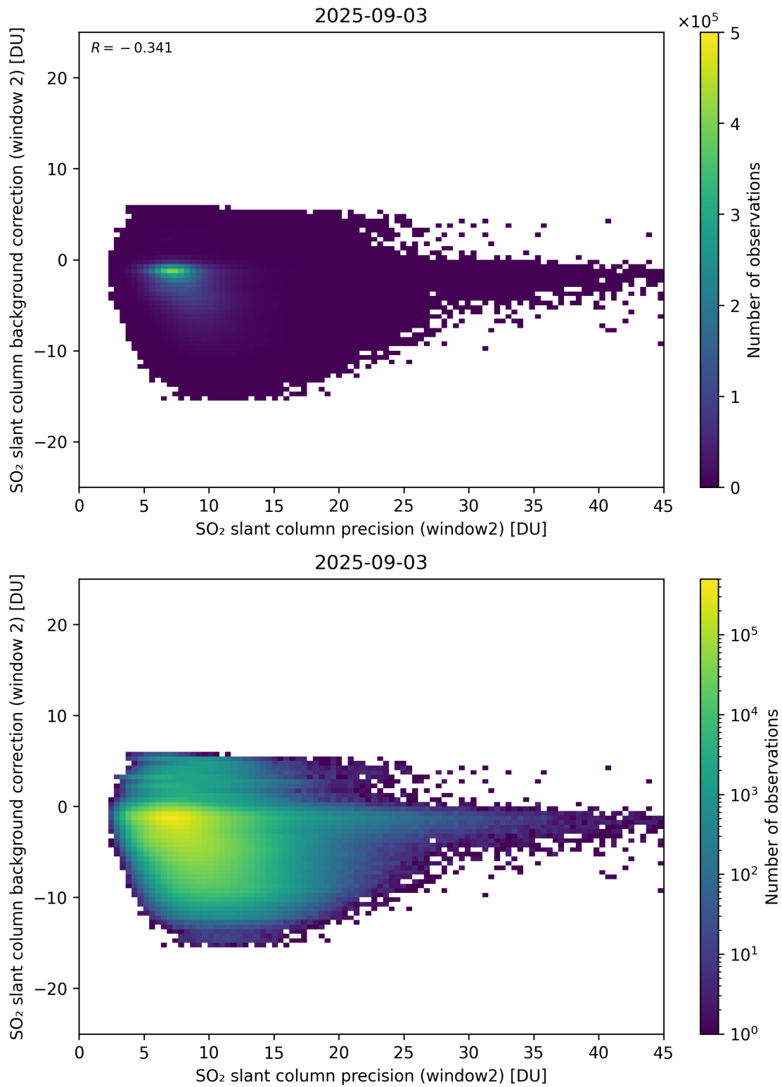
Figure 291: Scatter density plot of “SO 2 slant column precision (window2)” against “SO 2 slant column background correction (window 2)” for 2025-09-02 to 2025-09-04.
