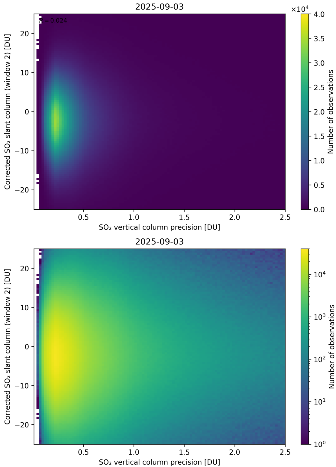
Figure 339: Scatter density plot of “SO 2 vertical column precision” against “Corrected SO 2 slant column (window 2)” for 2025-09-02 to 2025-09-04.
