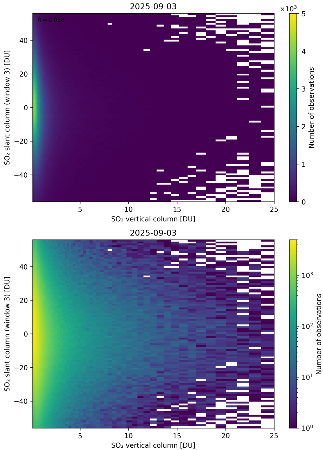
Figure 357: Scatter density plot of “SO 2 vertical column” against “SO 2 slant column (window 3)” for 2025-09-02 to 2025-09-04.
