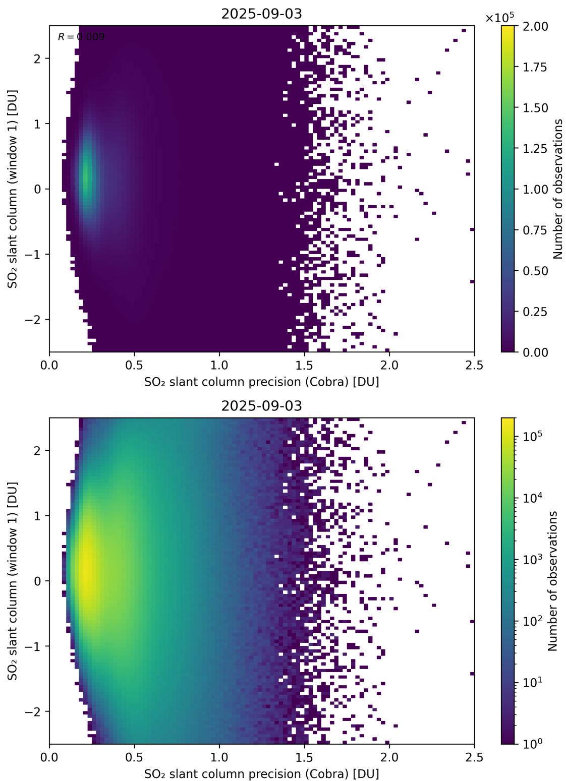
Figure 208: Scatter density plot of “SO 2 slant column precision (Cobra)” against “SO 2 slant column (window 1)” for 2025-09-02 to 2025-09-04.
