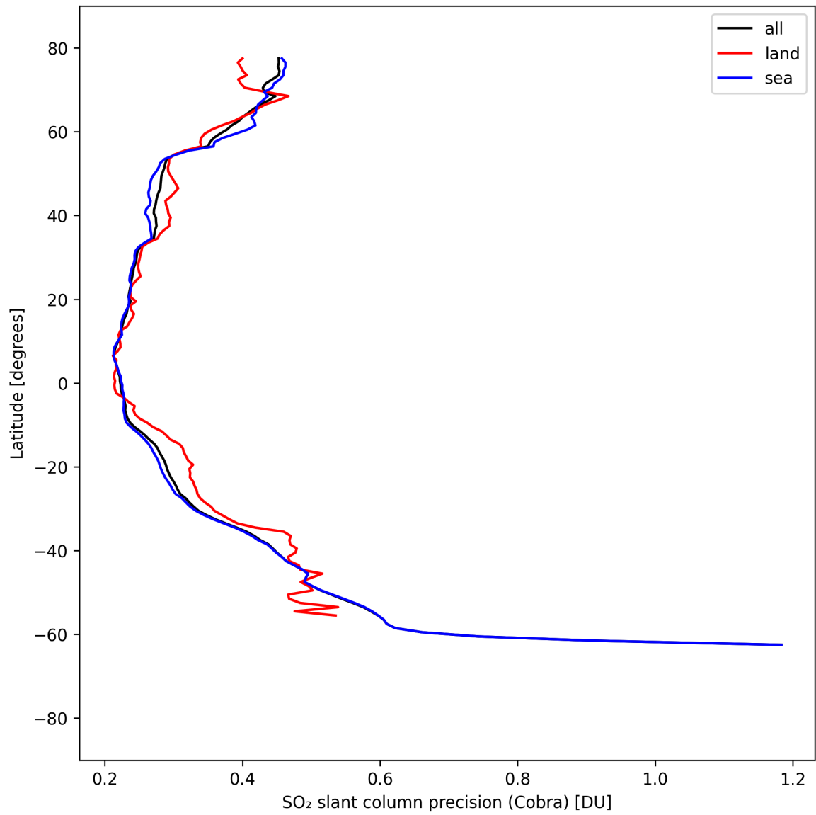
Figure 36: Zonal average of “SO 2 slant column precision (Cobra)” for 2025-09-02 to 2025-09-04.
