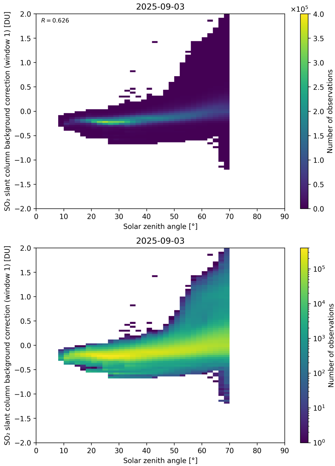
Figure 171: Scatter density plot of “Solar zenith angle” against “SO 2 slant column background correction (window 1)” for 2025-09-02 to 2025-09-04.
