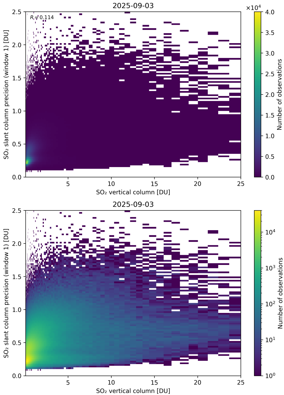
Figure 355: Scatter density plot of “SO 2 vertical column” against “SO 2 slant column precision (window 1)” for 2025-09-02 to 2025-09-04.
