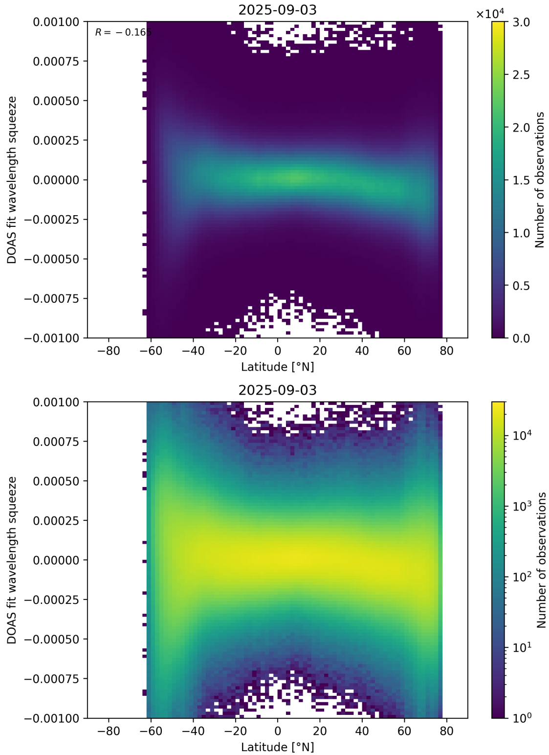
Figure 154: Scatter density plot of “Latitude” against “DOAS fit wavelength squeeze” for 2025-09-02 to 2025-09-04.
