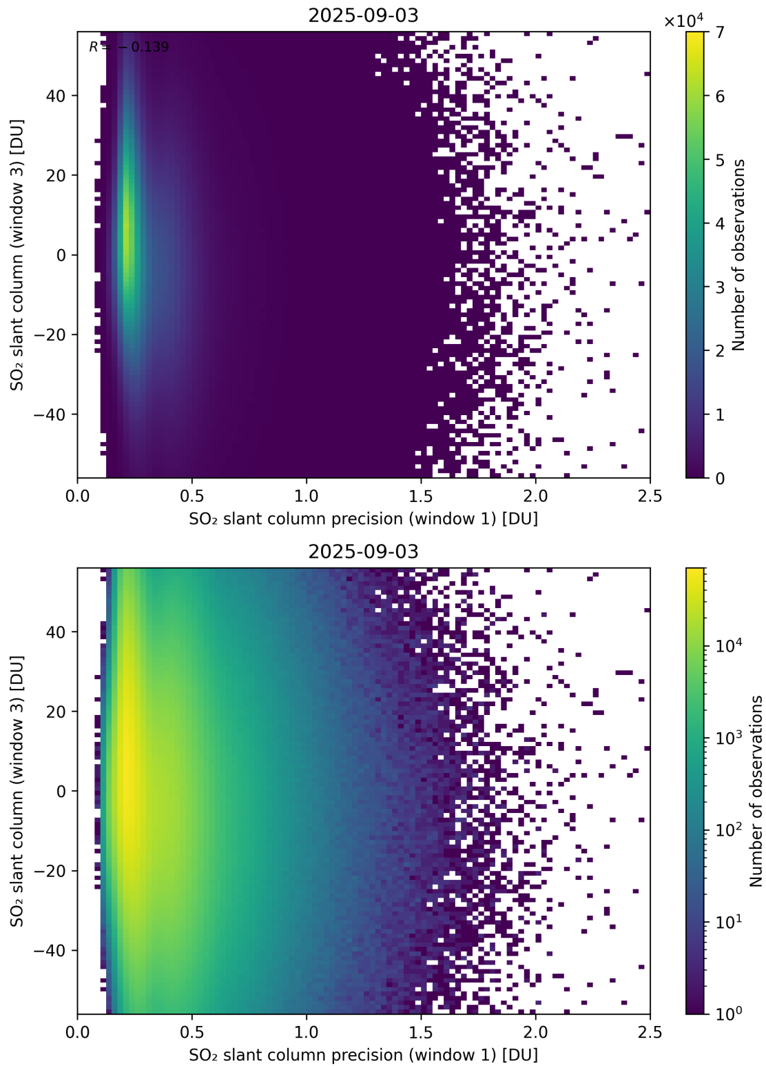
Figure 278: Scatter density plot of “SO 2 slant column precision (window 1)” against “SO 2 slant column (window 3)” for 2025-09-02 to 2025-09-04.
