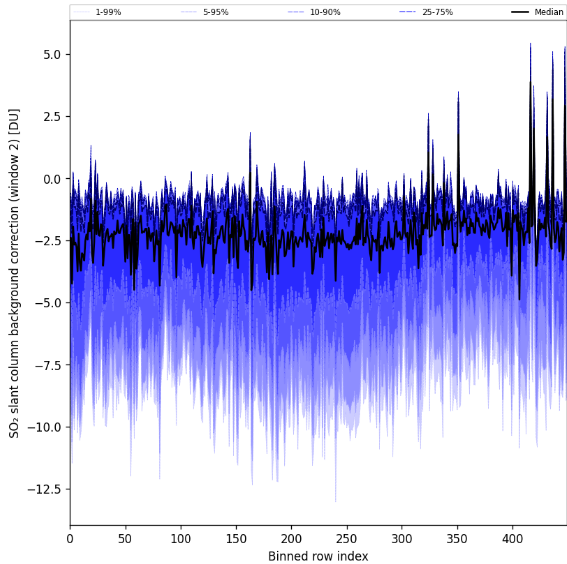
Figure 96: Along track statistics of “SO 2 slant column background correction (window 2)” for 2025-09-02 to 2025-09-04
