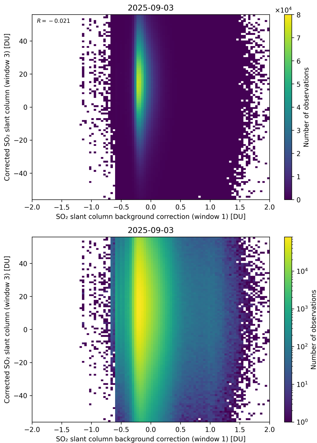
Figure 116: Scatter density plot of “SO 2 slant column background correction (window 1)” against “Corrected SO 2 slant column (window 3)” for 2025-09-02 to 2025-09-04.
