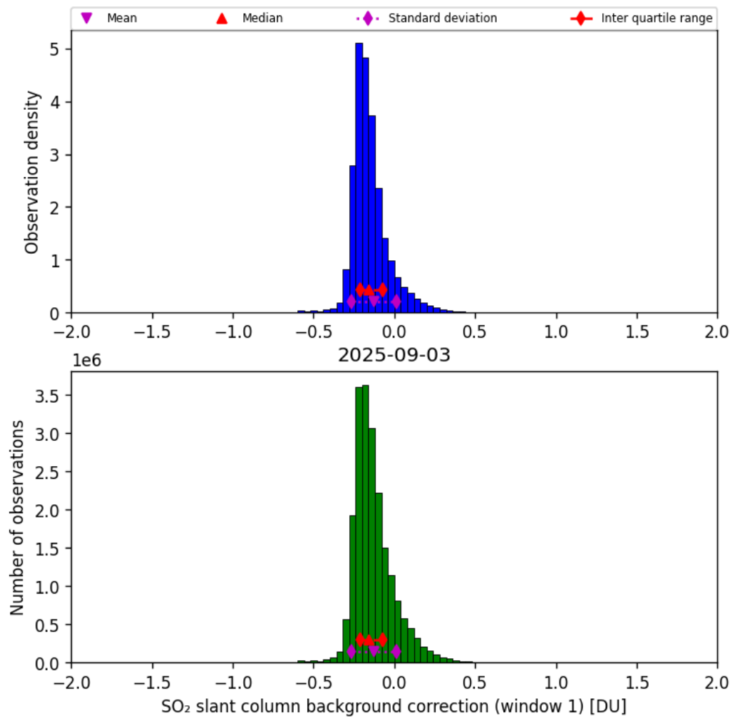
Figure 66: Histogram of “SO 2 slant column background correction (window 1)” for 2025-09-02 to 2025-09-04
