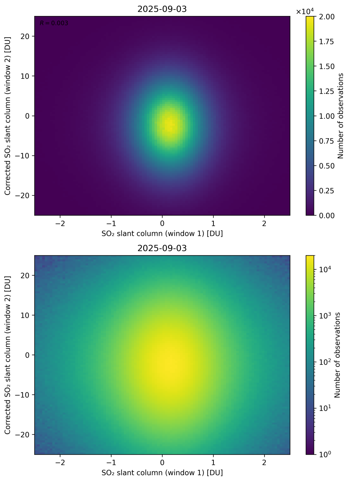
Figure 283: Scatter density plot of “SO 2 slant column (window 1)” against “Corrected SO 2 slant column (window 2)” for 2025-09-02 to 2025-09-04.
