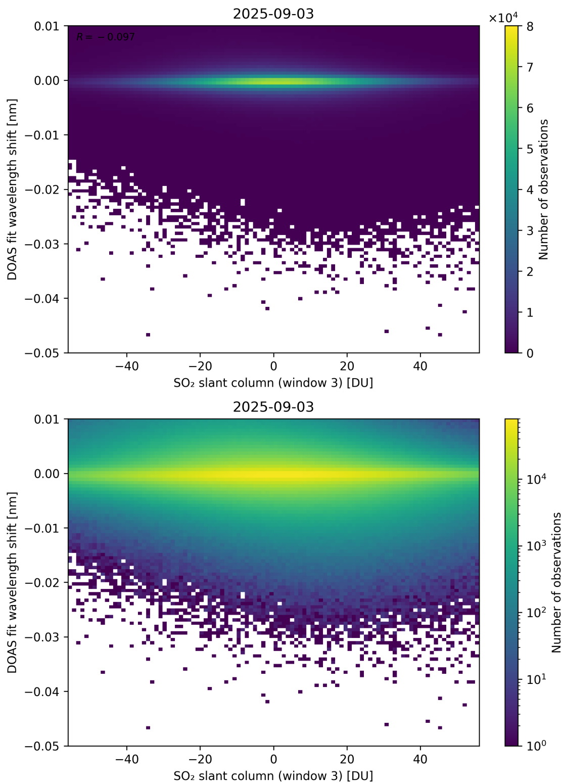
Figure 304: Scatter density plot of “SO 2 slant column (window 3)” against “DOAS fit wavelength shift” for 2025-09-02 to 2025-09-04.
