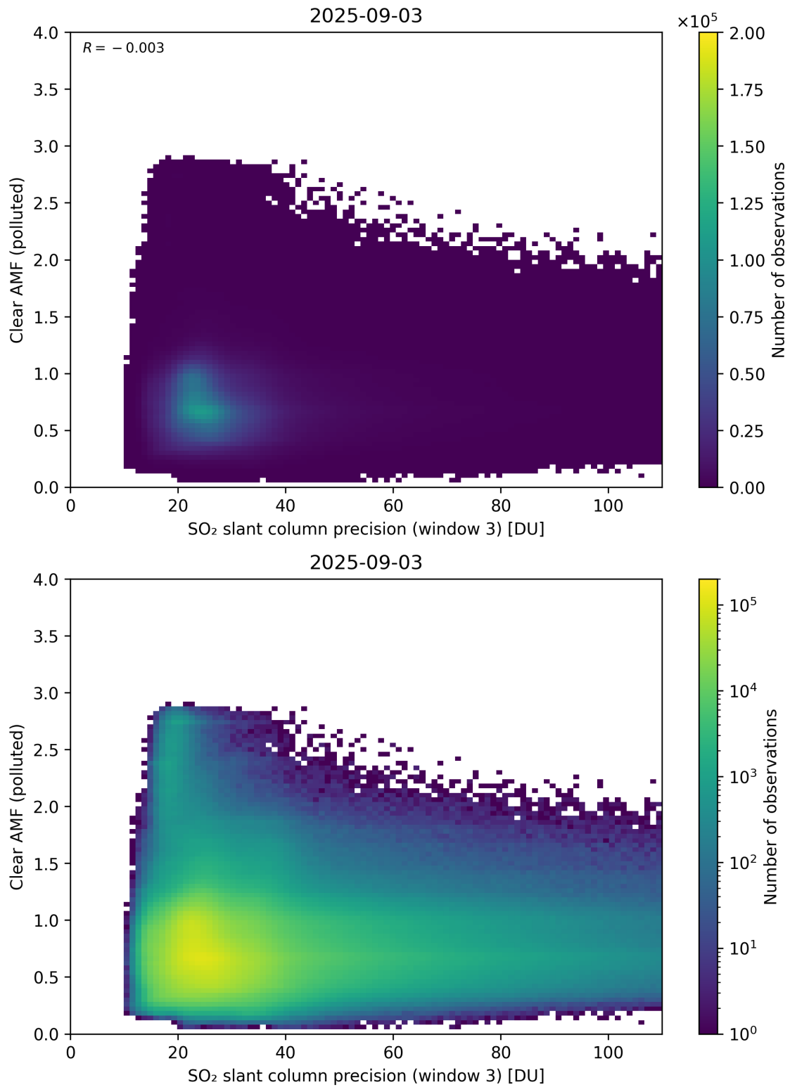
Figure 311: Scatter density plot of “SO 2 slant column precision (window 3)” against “Clear AMF (polluted)” for 2025-09-02 to 2025-09-04.
