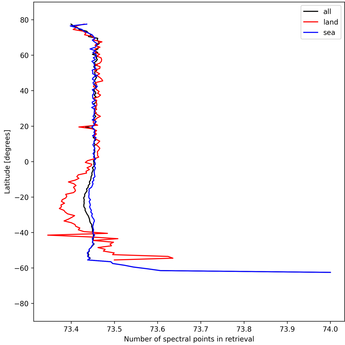
Figure 56: Zonal average of “Number of spectral points in retrieval” for 2025-09-02 to 2025-09-04.
