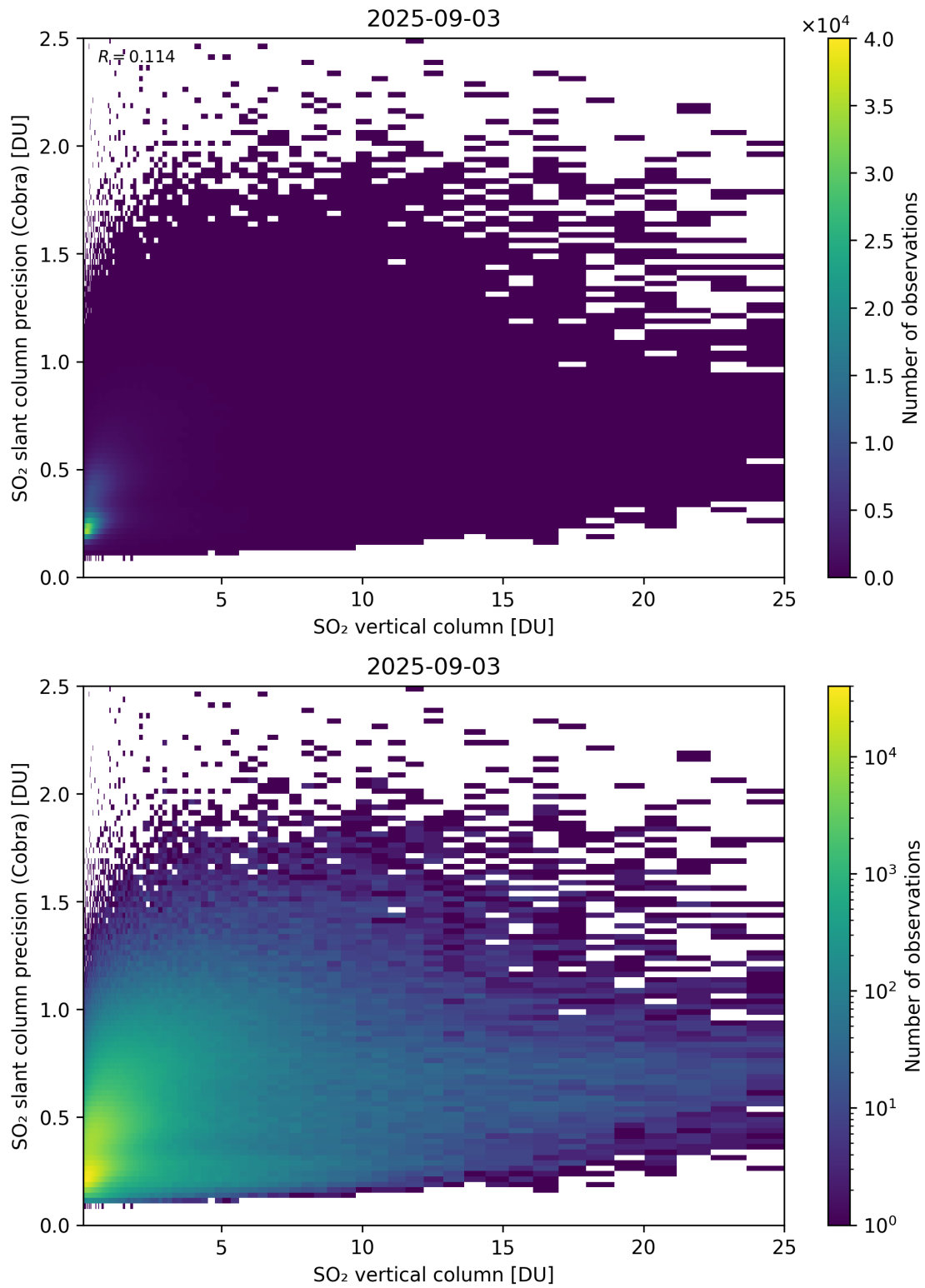
Figure 350: Scatter density plot of “SO 2 vertical column” against “SO 2 slant column precision (Cobra)” for 2025-09-02 to 2025-09-04.
