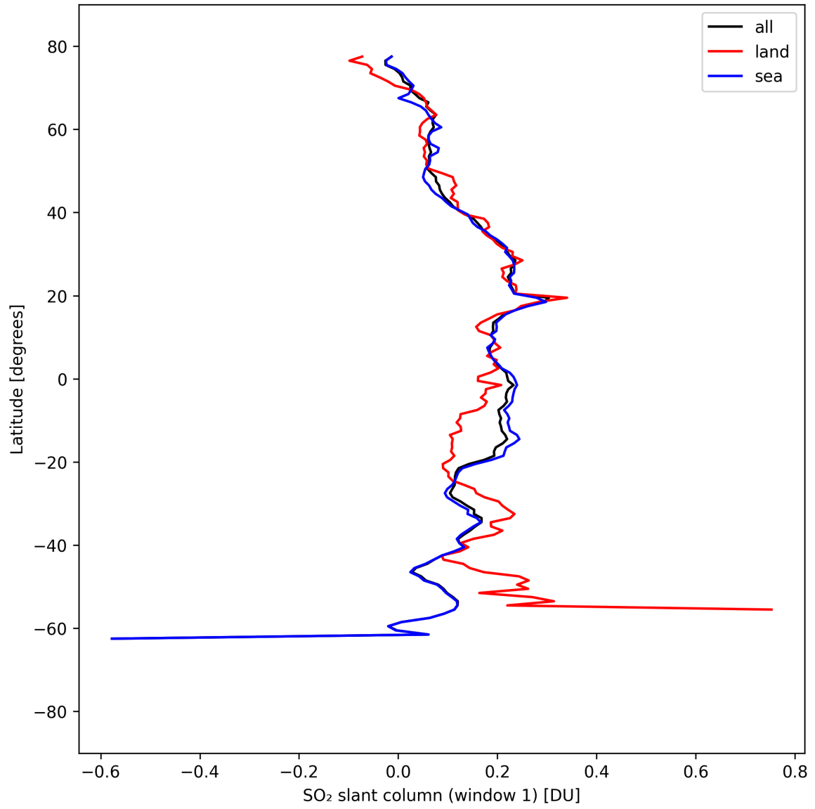
Figure 37: Zonal average of “SO 2 slant column (window 1)” for 2025-09-02 to 2025-09-04.
