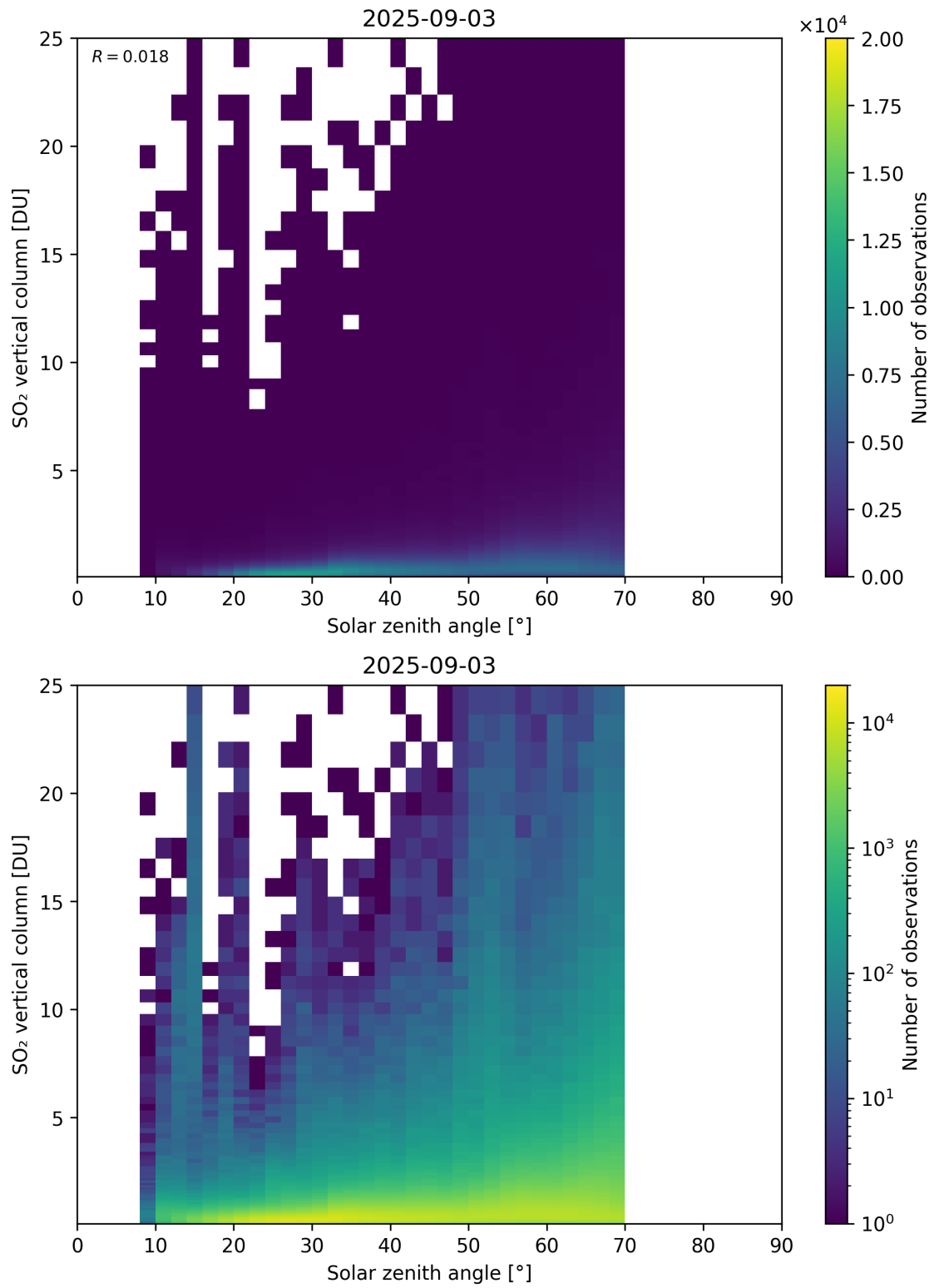
Figure 191: Scatter density plot of “Solar zenith angle” against “SO 2 vertical column” for 2025-09-02 to 2025-09-04.
