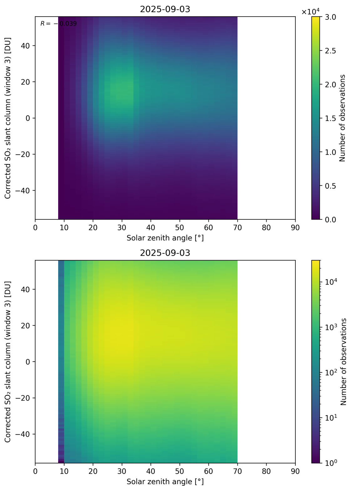
Figure 183: Scatter density plot of “Solar zenith angle” against “Corrected SO 2 slant column (window 3)” for 2025-09-02 to 2025-09-04.
