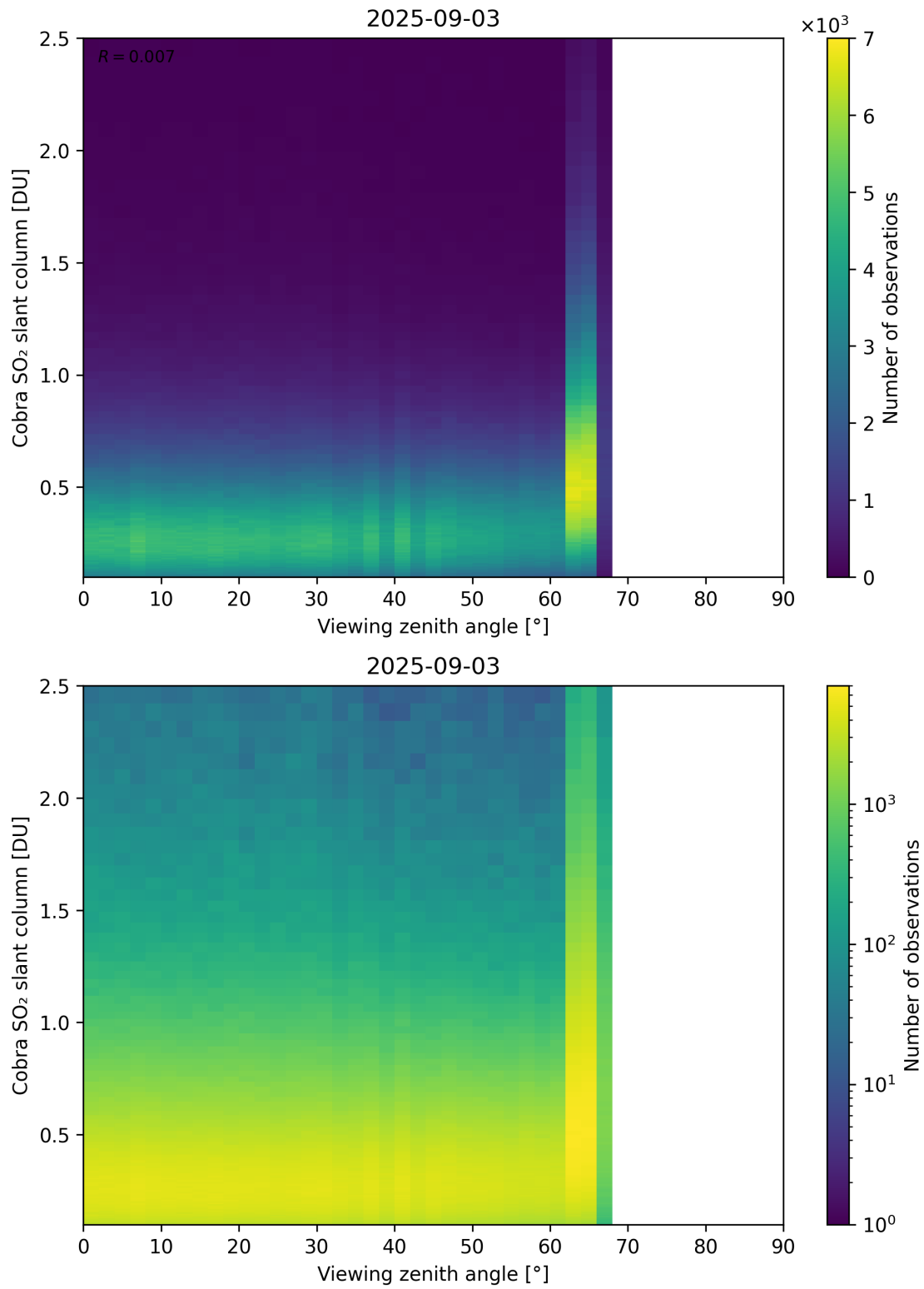
Figure 371: Scatter density plot of “Viewing zenith angle” against “Cobra SO 2 slant column” for 2025-09-02 to 2025-09-04.
