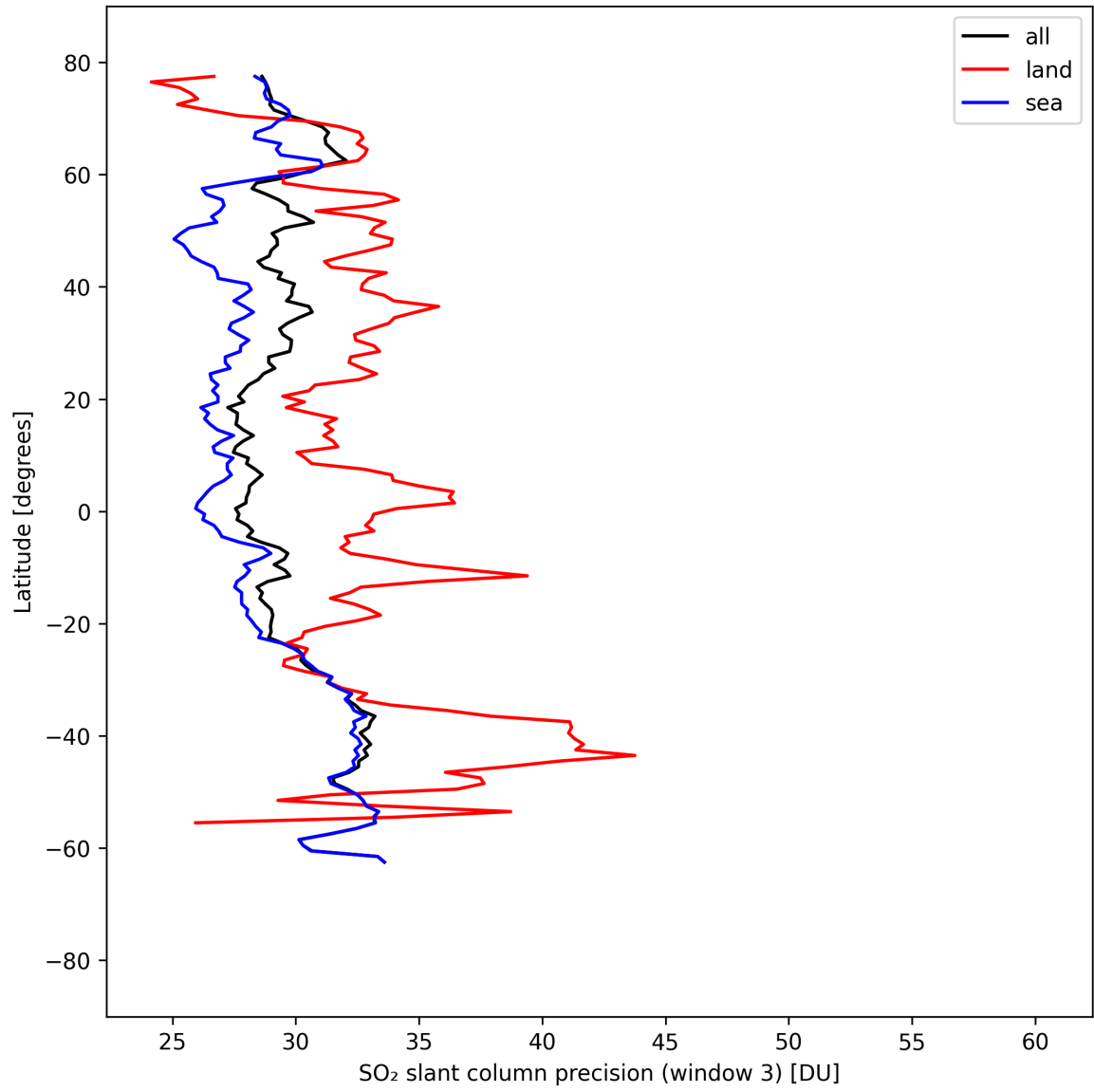
Figure 46: Zonal average of “SO 2 slant column precision (window 3)” for 2025-09-02 to 2025-09-04.
