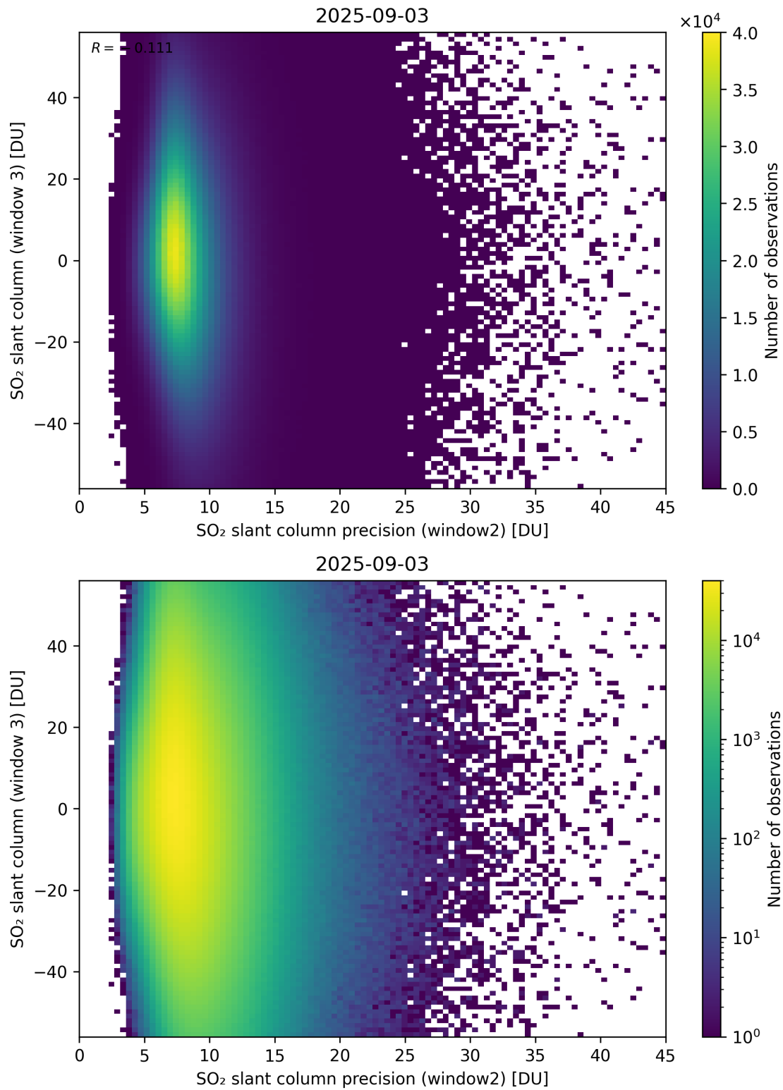
Figure 299: Scatter density plot of “SO 2 slant column precision (window2)” against “SO 2 slant column (window 3)” for 2025-09-02 to 2025-09-04.
