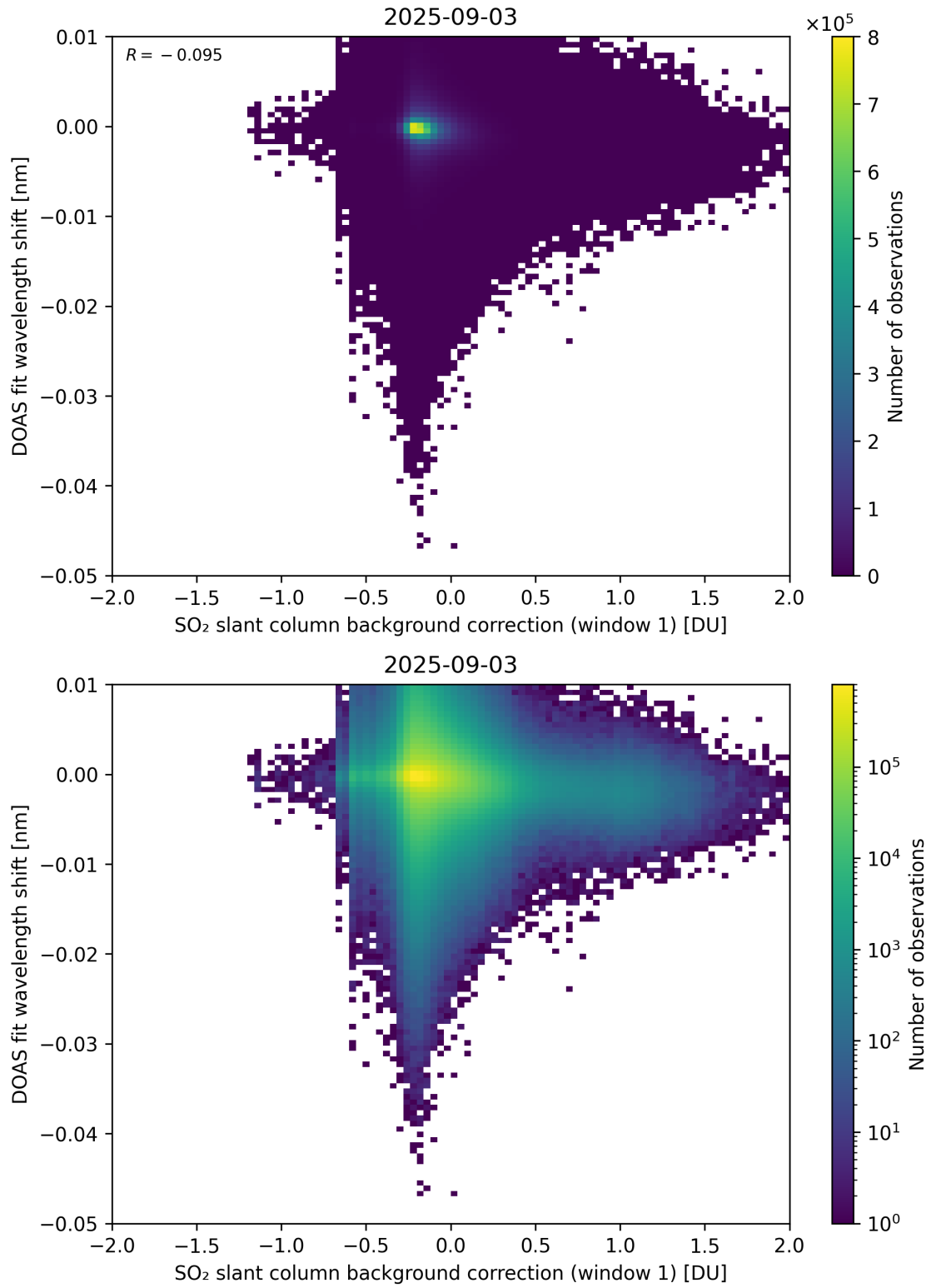
Figure 111: Scatter density plot of “SO 2 slant column background correction (window 1)” against “DOAS fit wavelength shift” for 2025-09-02 to 2025-09-04.
