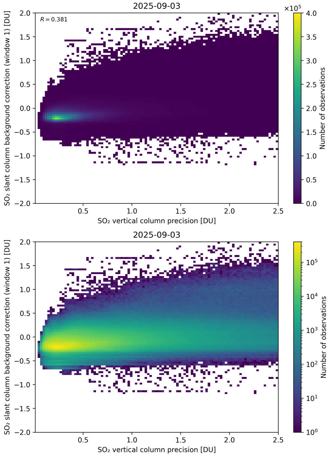
Figure 329: Scatter density plot of “SO 2 vertical column precision” against “SO 2 slant column background correction (window 1)” for 2025-09-02 to 2025-09-04.
