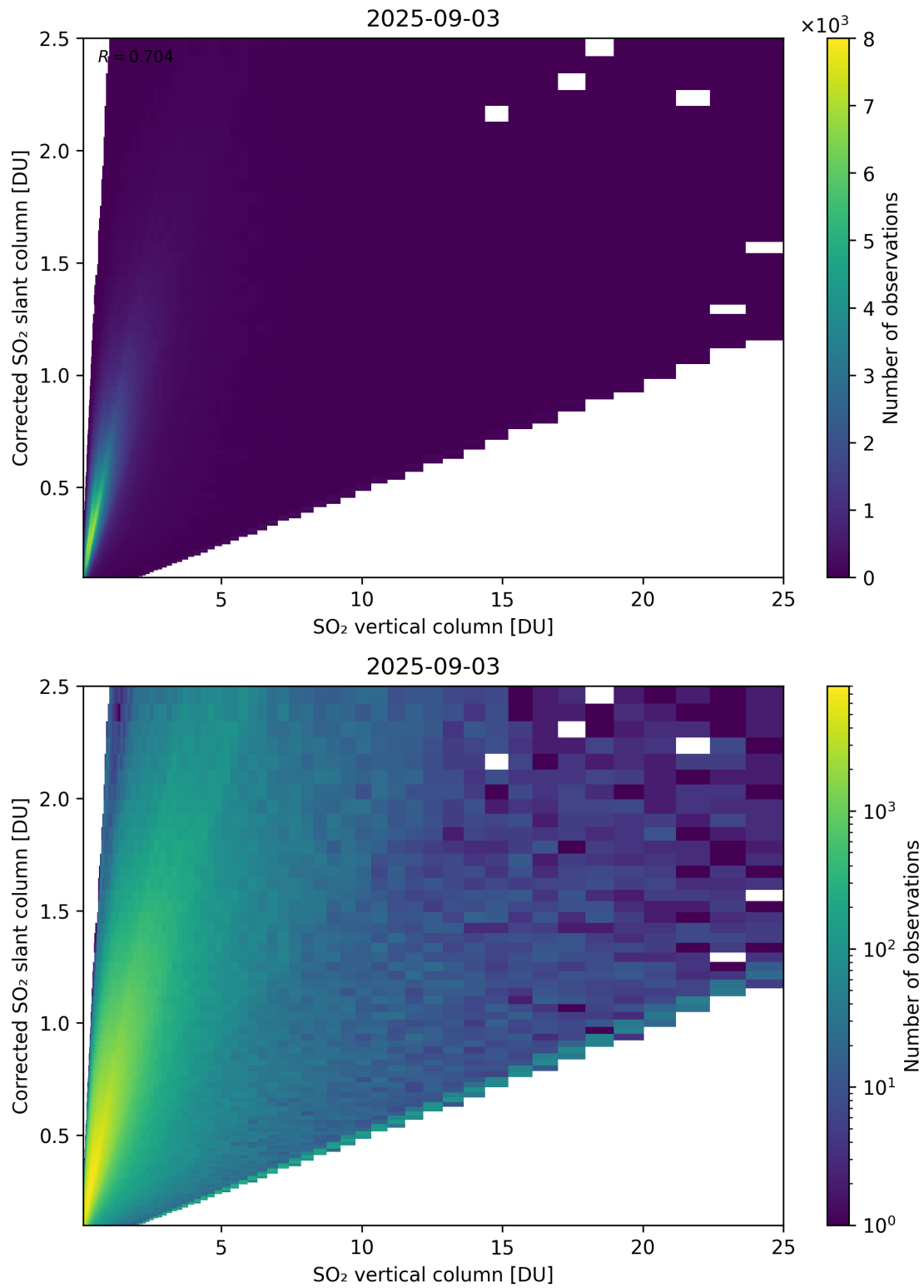
Figure 351: Scatter density plot of “SO 2 vertical column” against “Corrected SO 2 slant column” for 2025-09-02 to 2025-09-04.
