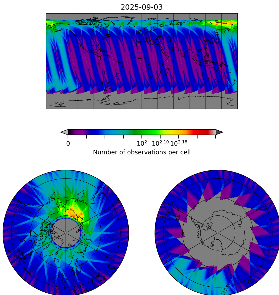
Figure 30: Map of the number of observations for 2025-09-02 to 2025-09-04
