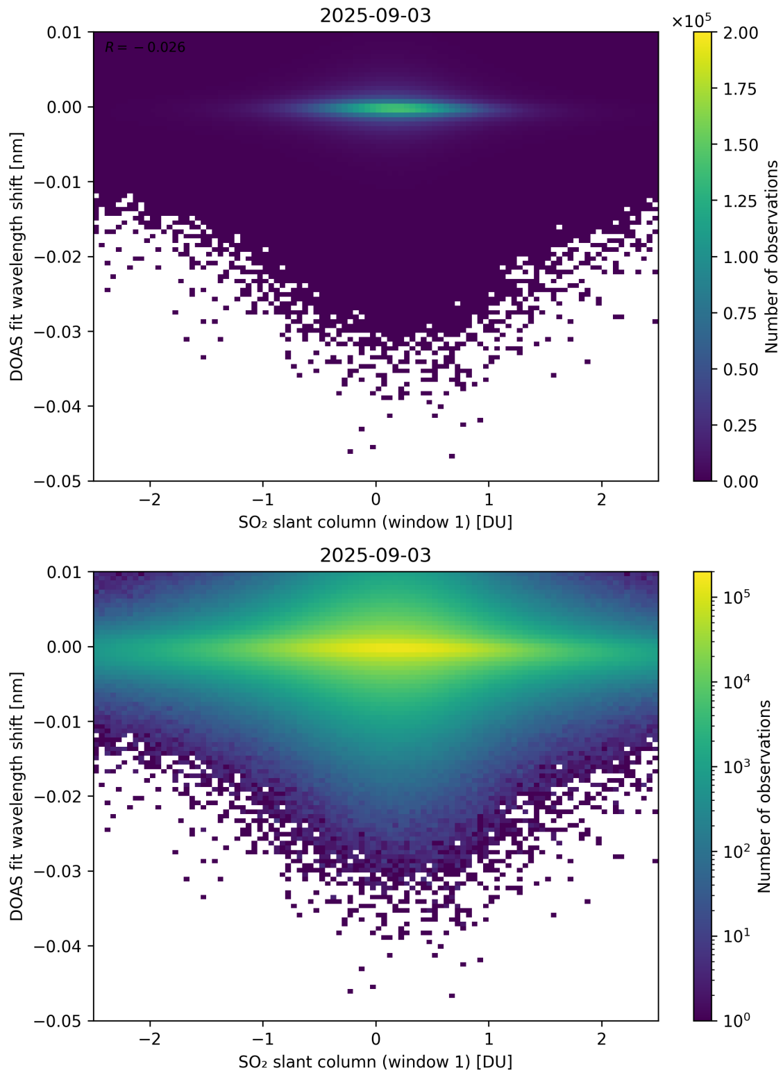
Figure 265: Scatter density plot of “SO 2 slant column (window 1)” against “DOAS fit wavelength shift” for 2025-09-02 to 2025-09-04.
