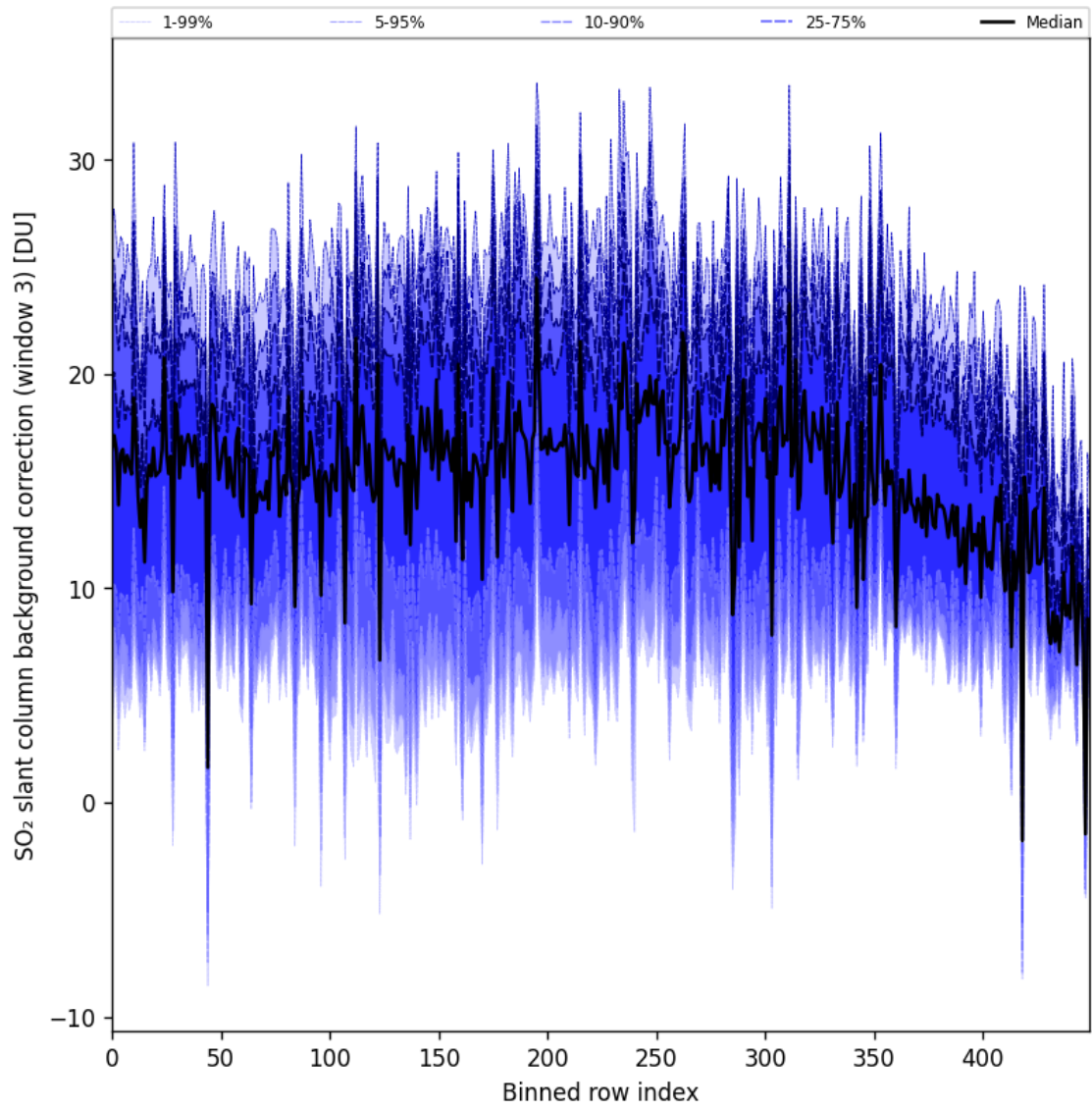
Figure 100: Along track statistics of “SO 2 slant column background correction (window 3)” for 2025-09-02 to 2025-09-04
