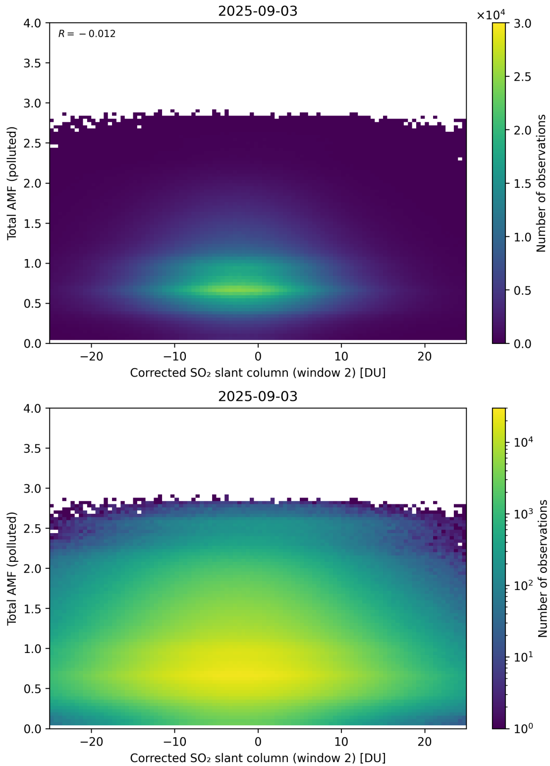
Figure 253: Scatter density plot of “Corrected SO 2 slant column (window 2)” against “Total AMF (polluted)” for 2025-09-02 to 2025-09-04.
