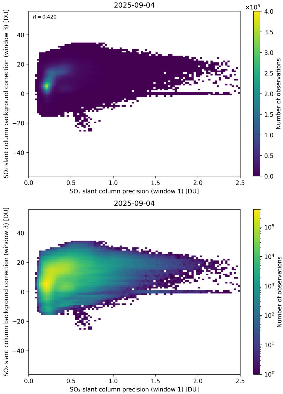
Figure 270: Scatter density plot of “SO 2 slant column precision (window 1)” against “SO 2 slant column background correction (window 3)” for 2025-09-04 to 2025-09-05.
