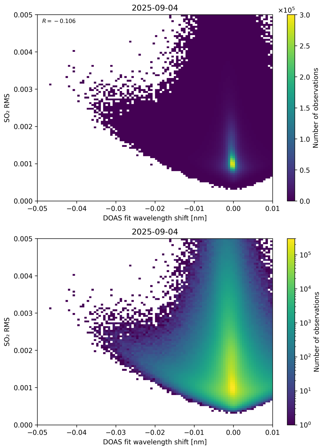
Figure 139: Scatter density plot of “DOAS fit wavelength shift” against “SO 2 RMS” for 2025-09-04 to 2025-09-05.
