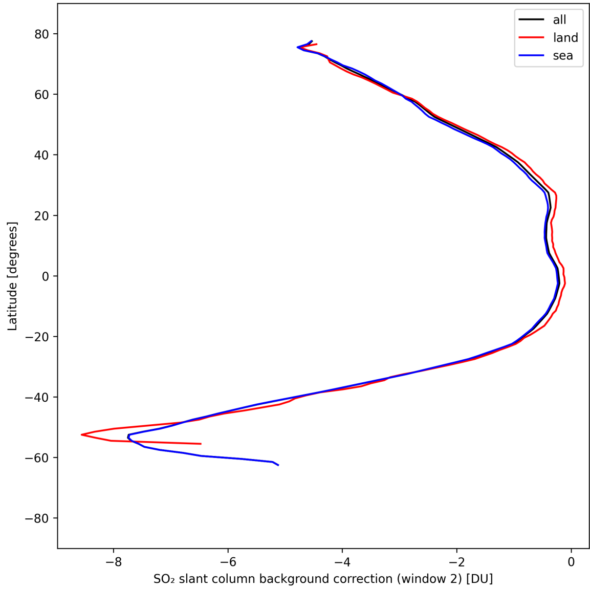
Figure 44: Zonal average of “SO 2 slant column background correction (window 2)” for 2025-09-04 to 2025-09-05.
