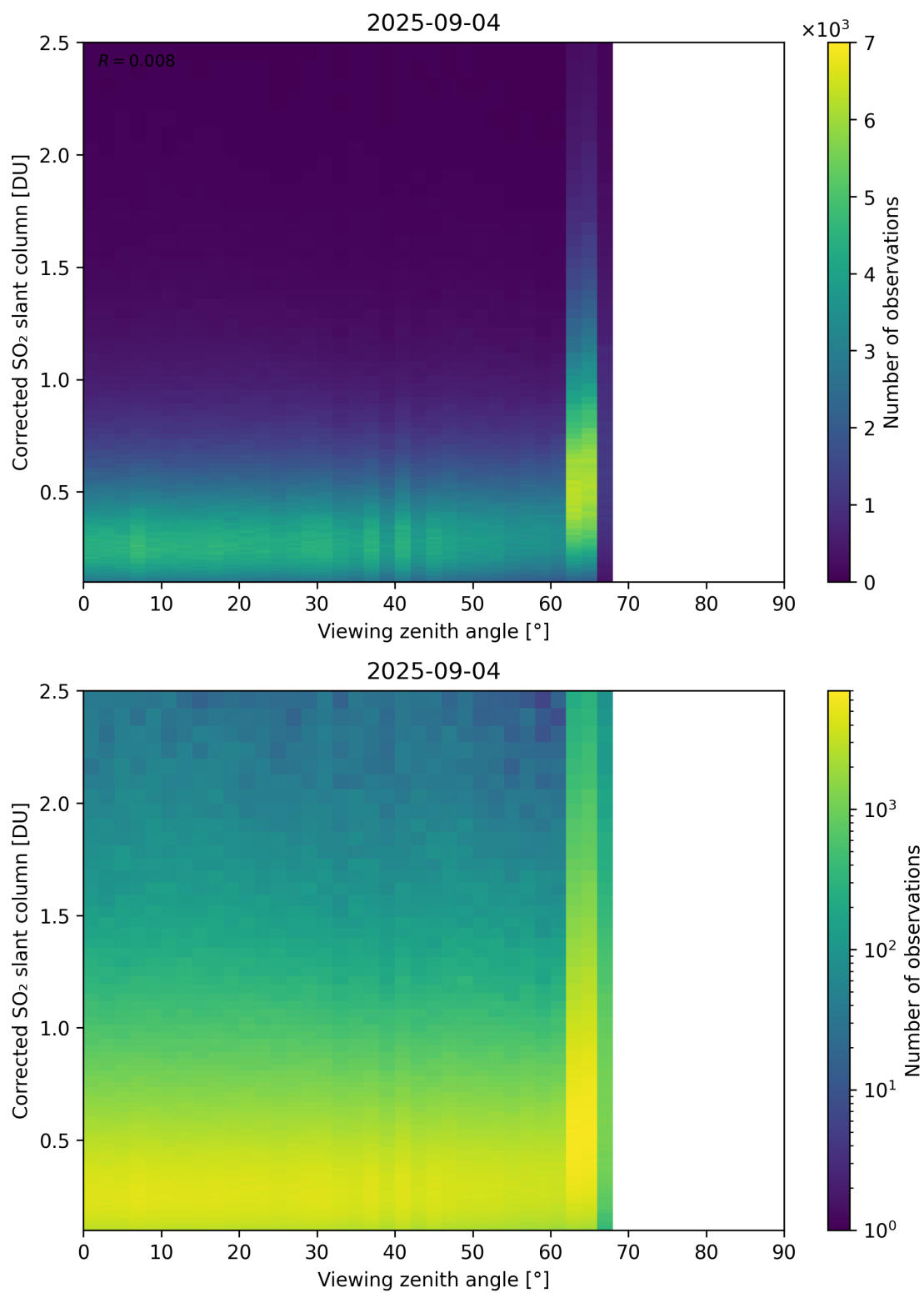
Figure 373: Scatter density plot of “Viewing zenith angle” against “Corrected SO 2 slant column” for 2025-09-04 to 2025-09-05.
