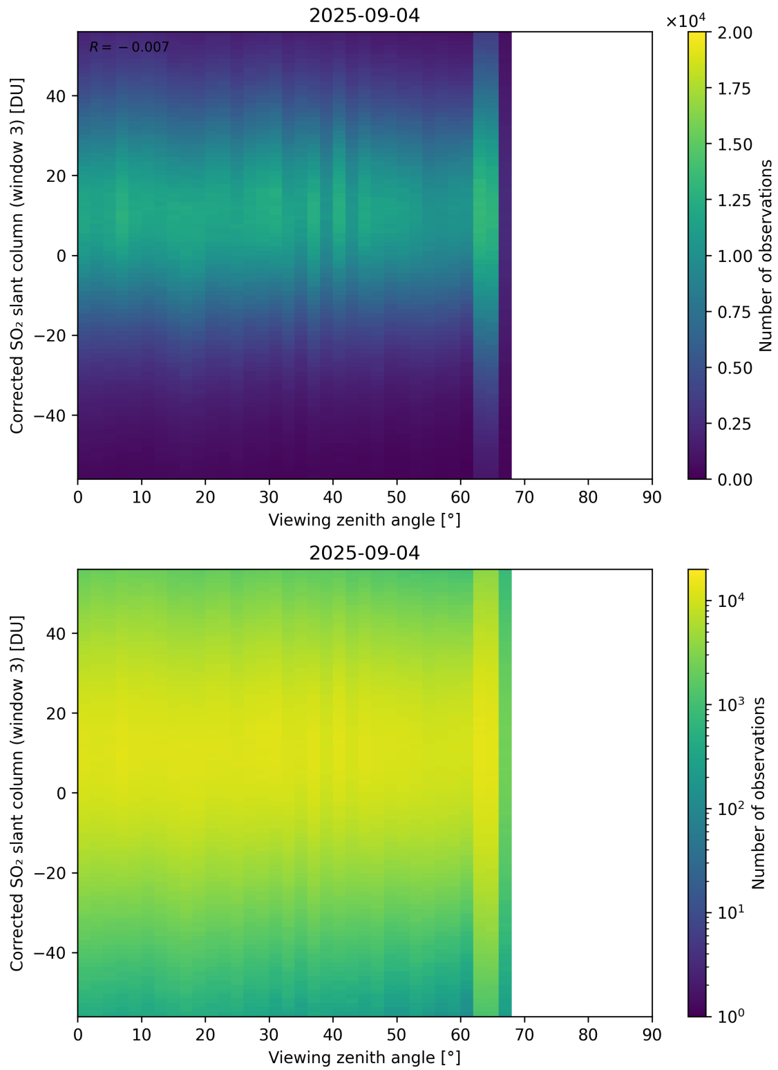
Figure 375: Scatter density plot of “Viewing zenith angle” against “Corrected SO 2 slant column (window 3)” for 2025-09-04 to 2025-09-05.
