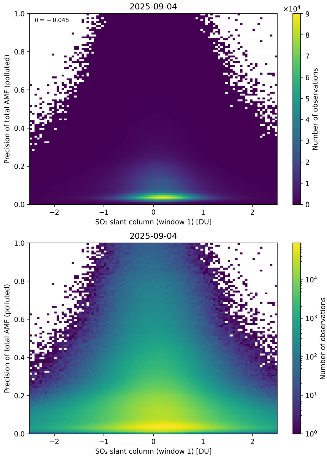
Figure 290: Scatter density plot of “SO 2 slant column (window 1)” against “Precision of total AMF (polluted)” for 2025-09-04 to 2025-09-05.
