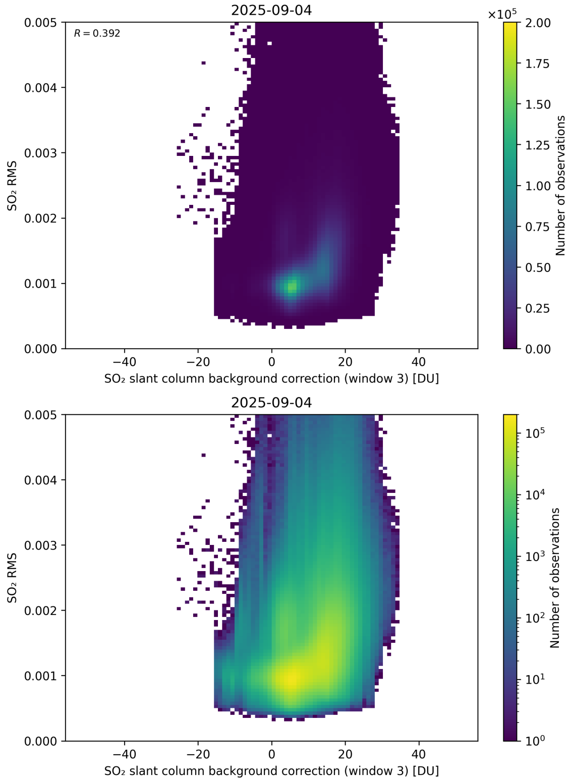
Figure 134: Scatter density plot of “SO 2 slant column background correction (window 3)” against “SO 2 RMS” for 2025-09-04 to 2025-09-05.
