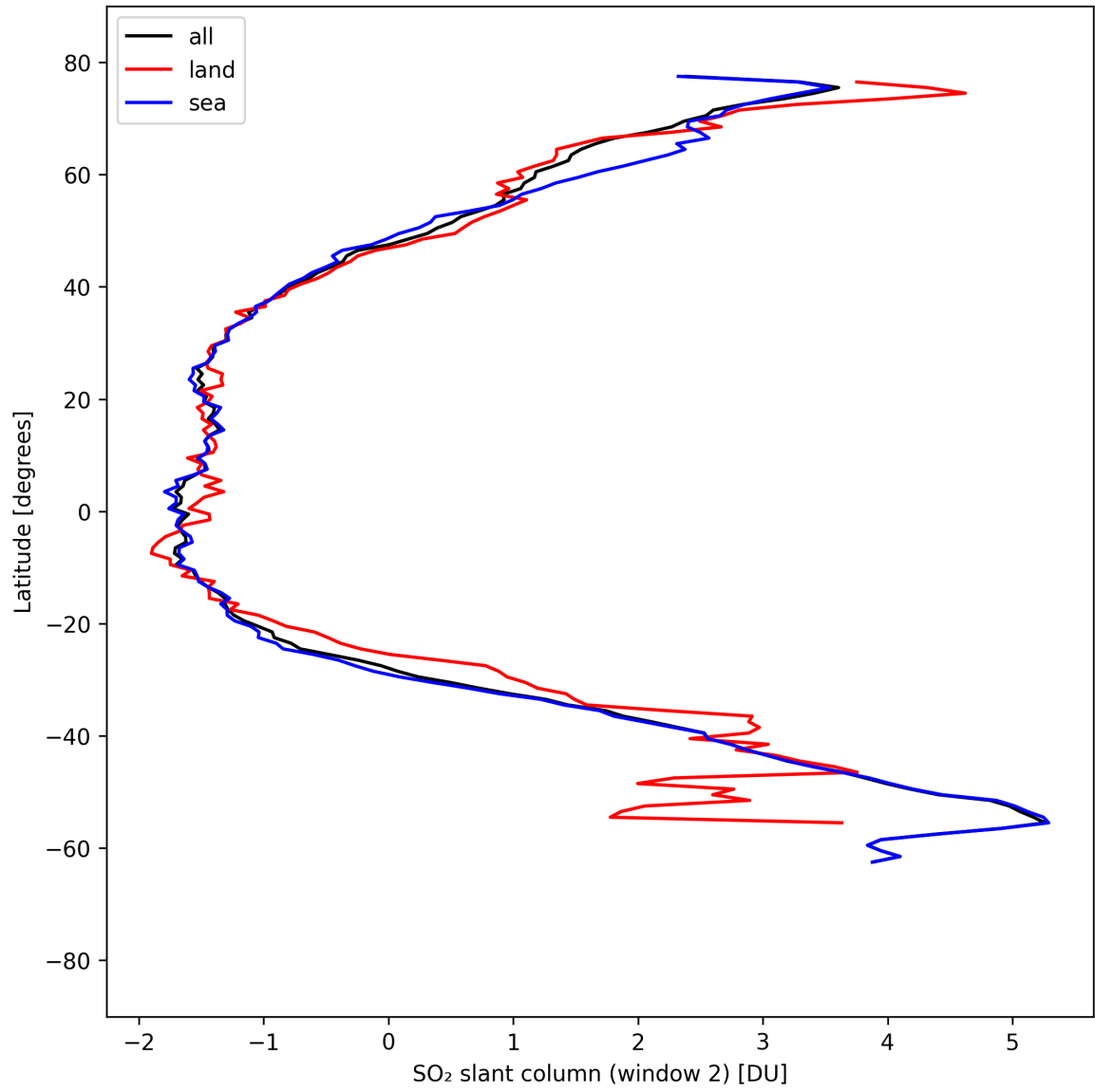
Figure 41: Zonal average of “SO 2 slant column (window 2)” for 2025-09-04 to 2025-09-05.
