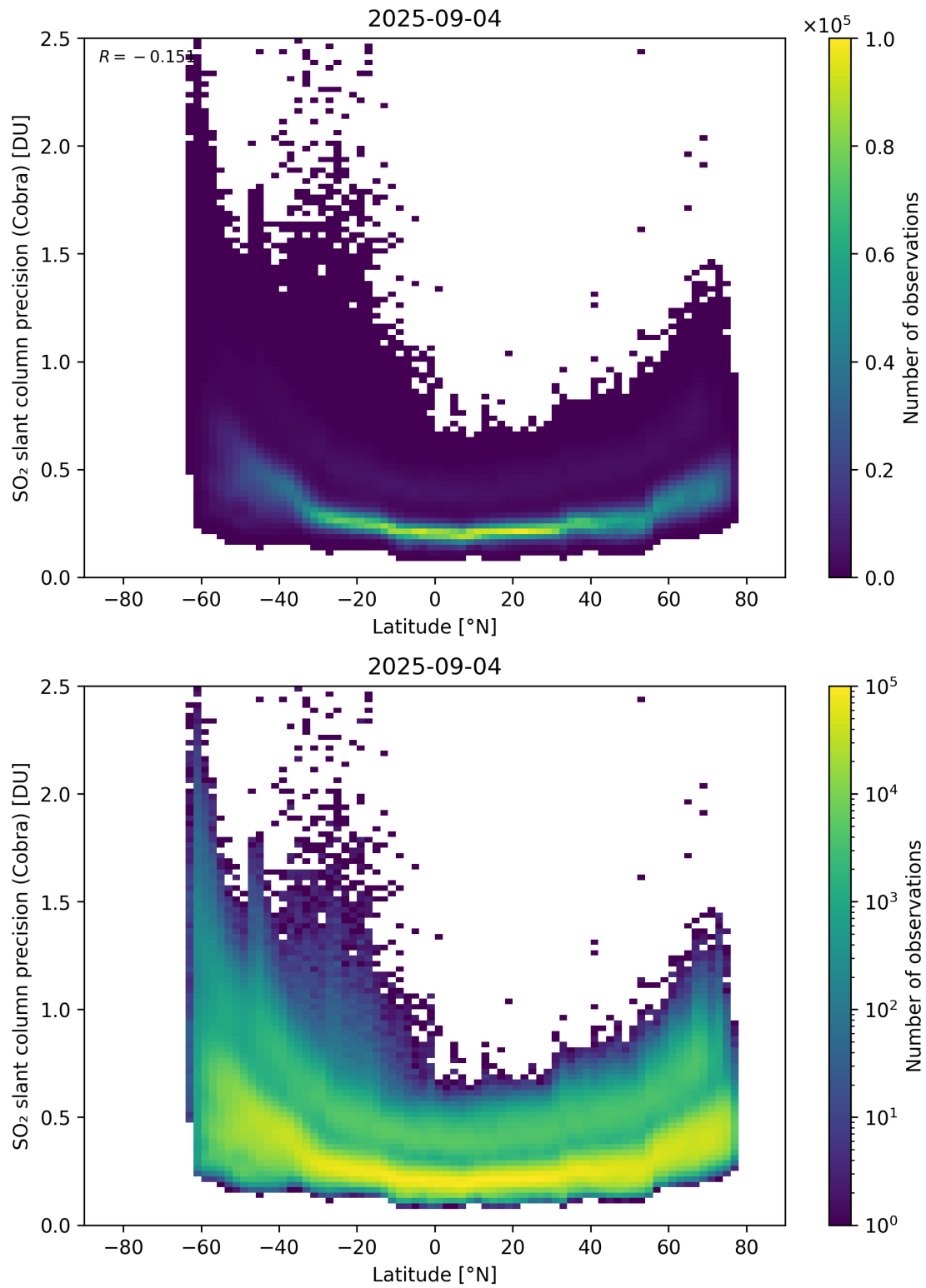
Figure 158: Scatter density plot of “Latitude” against “SO 2 slant column precision (Cobra)” for 2025-09-04 to 2025-09-05.
