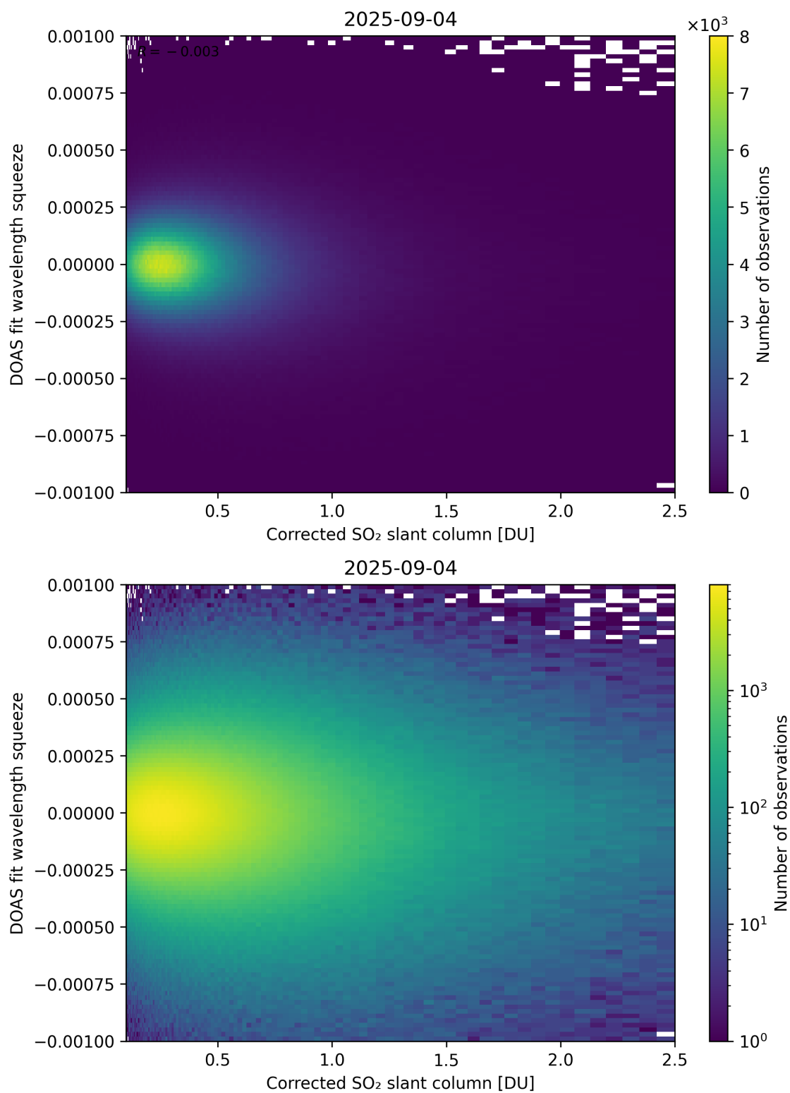
Figure 230: Scatter density plot of “Corrected SO 2 slant column” against “DOAS fit wavelength squeeze” for 2025-09-04 to 2025-09-05.
