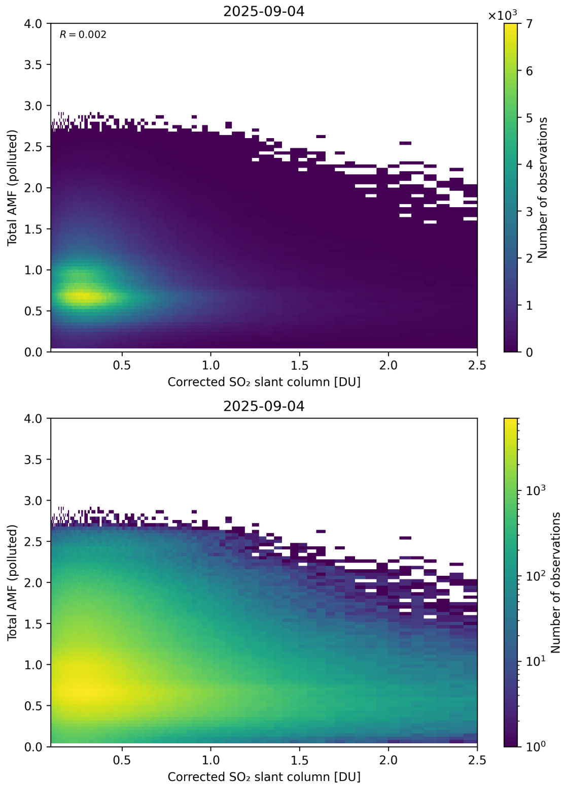
Figure 242: Scatter density plot of “Corrected SO 2 slant column” against “Total AMF (polluted)” for 2025-09-04 to 2025-09-05.
