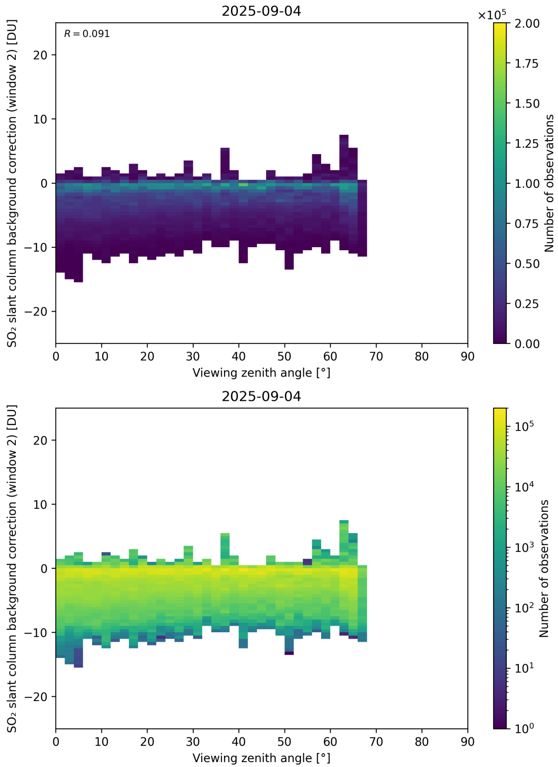
Figure 363: Scatter density plot of “Viewing zenith angle” against “SO 2 slant column background correction (window 2)” for 2025-09-04 to 2025-09-05.
