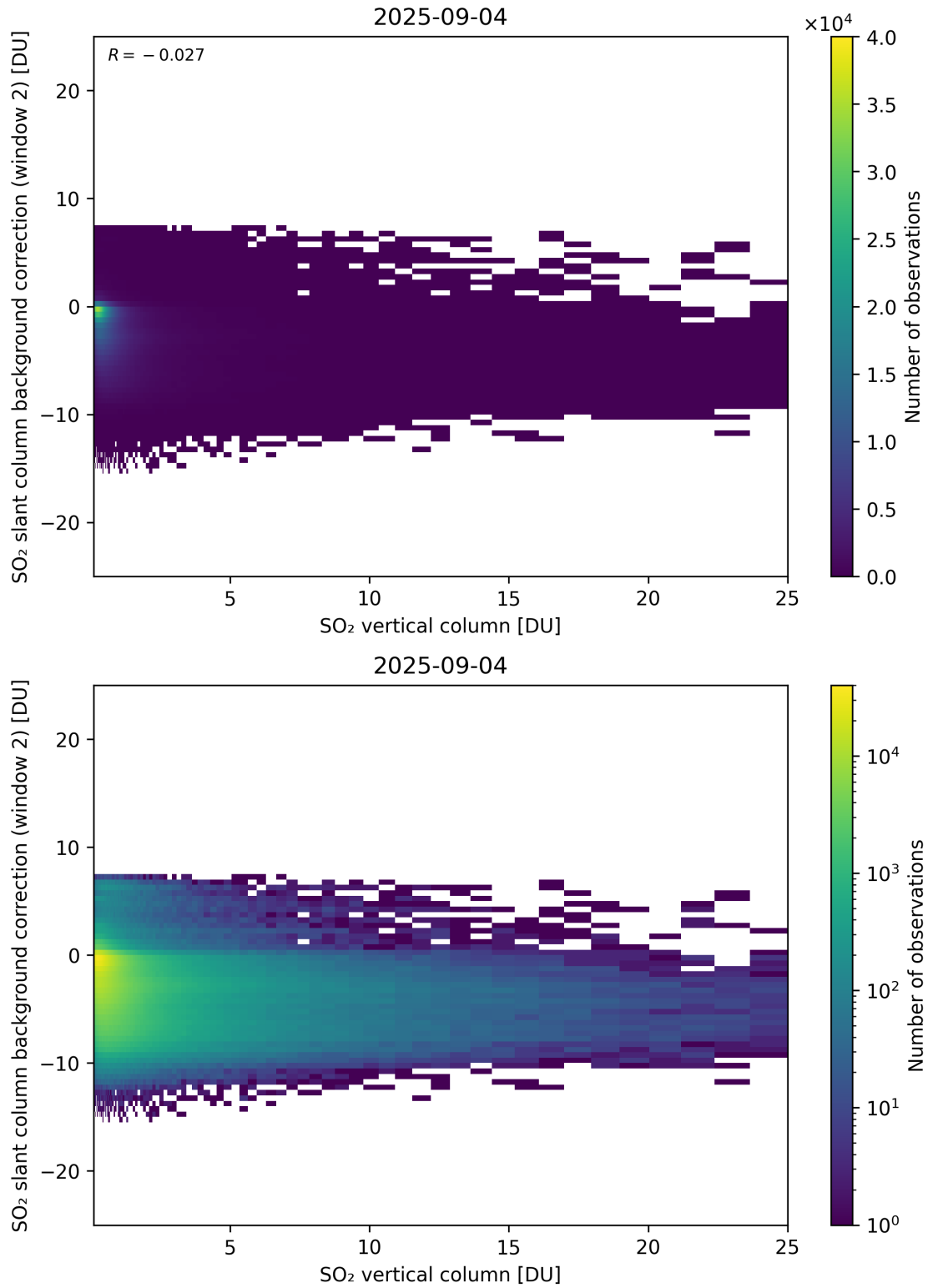
Figure 324: Scatter density plot of “SO 2 vertical column” against “SO 2 slant column background correction (window 2)” for 2025-09-04 to 2025-09-05.
