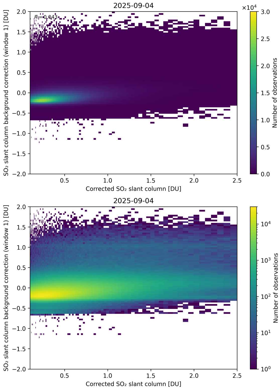
Figure 226: Scatter density plot of “Corrected SO 2 slant column” against “SO 2 slant column background correction (window 1)” for 2025-09-04 to 2025-09-05.
