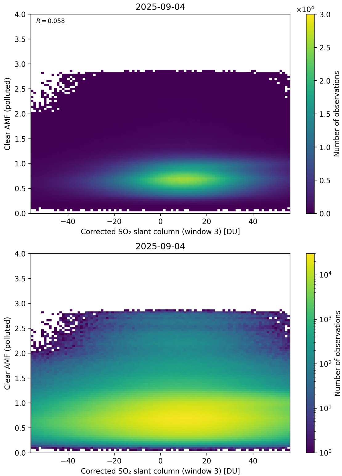
Figure 259: Scatter density plot of “Corrected SO 2 slant column (window 3)” against “Clear AMF (polluted)” for 2025-09-04 to 2025-09-05.
