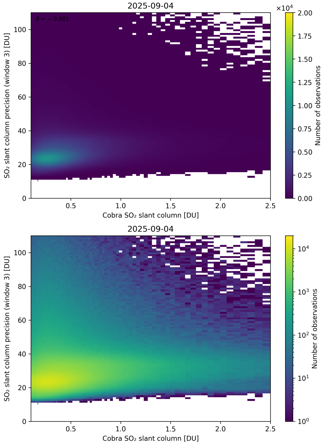
Figure 223: Scatter density plot of “Cobra SO 2 slant column” against “SO 2 slant column precision (window 3)” for 2025-09-04 to 2025-09-05.
