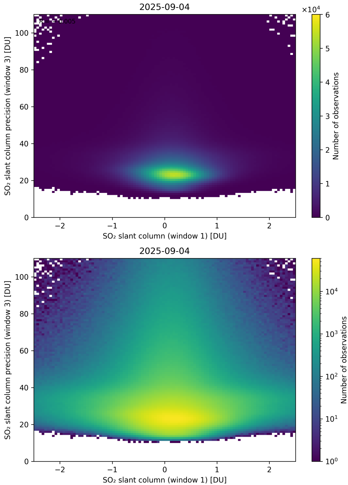
Figure 288: Scatter density plot of “SO 2 slant column (window 1)” against “SO 2 slant column precision (window 3)” for 2025-09-04 to 2025-09-05.
