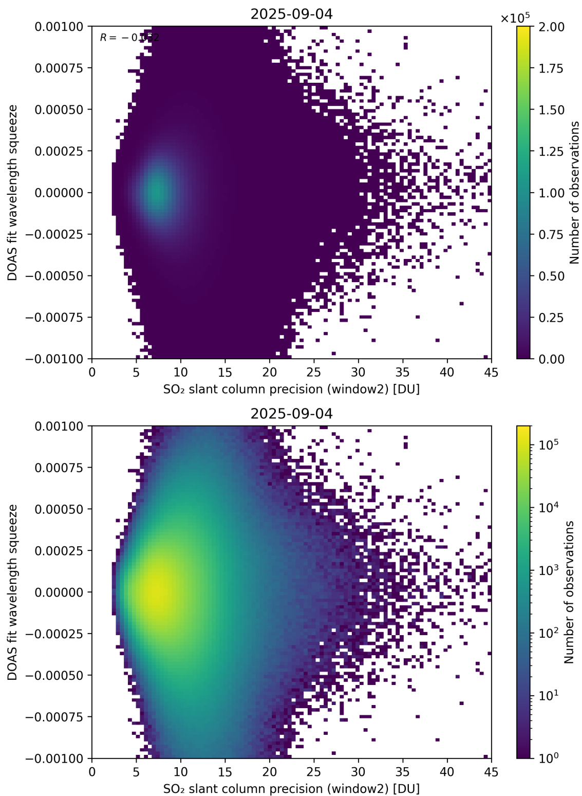
Figure 294: Scatter density plot of “SO 2 slant column precision (window2)” against “DOAS fit wavelength squeeze” for 2025-09-04 to 2025-09-05.
