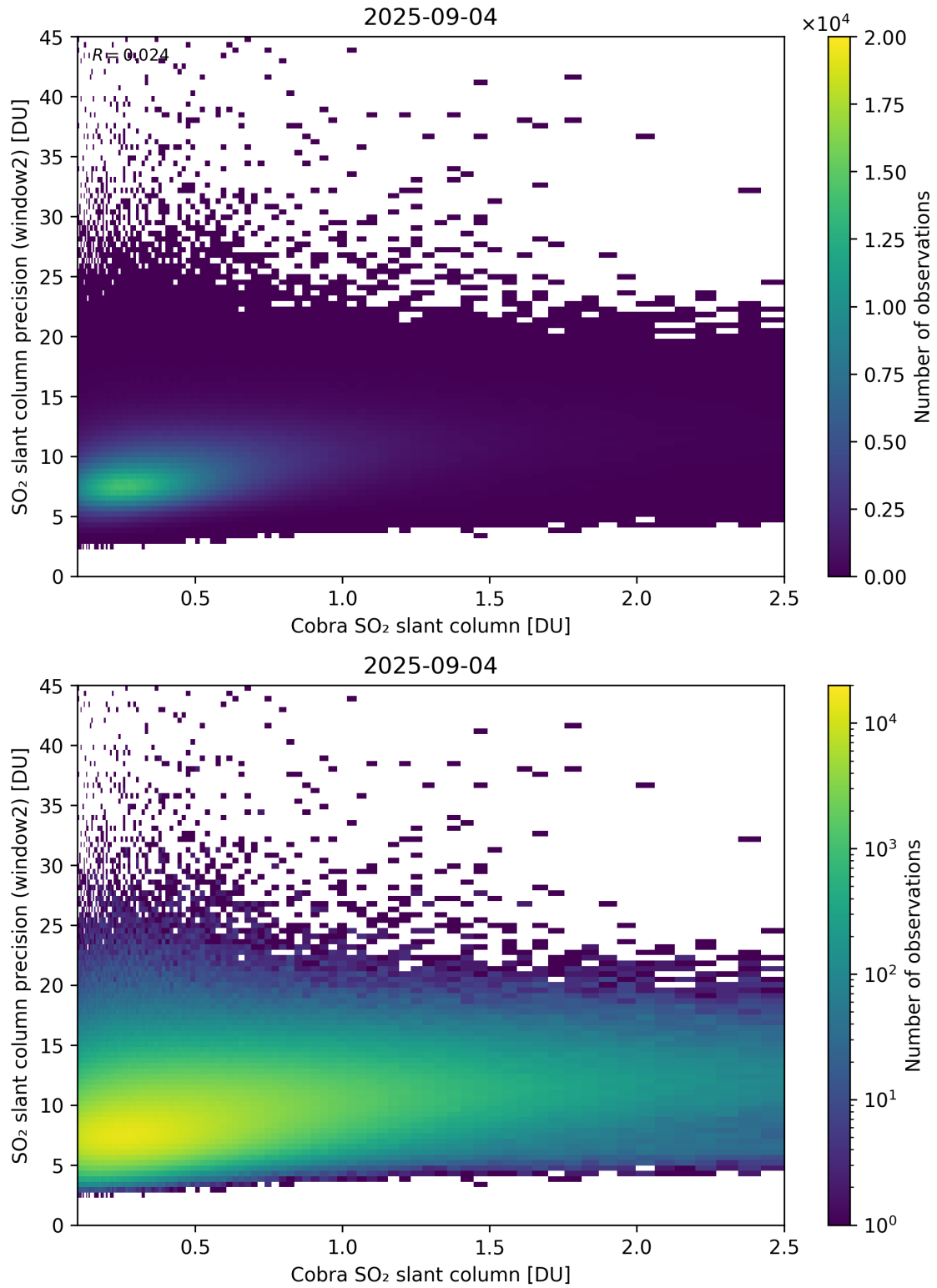
Figure 221: Scatter density plot of “Cobra SO 2 slant column” against “SO 2 slant column precision (window2)” for 2025-09-04 to 2025-09-05.
