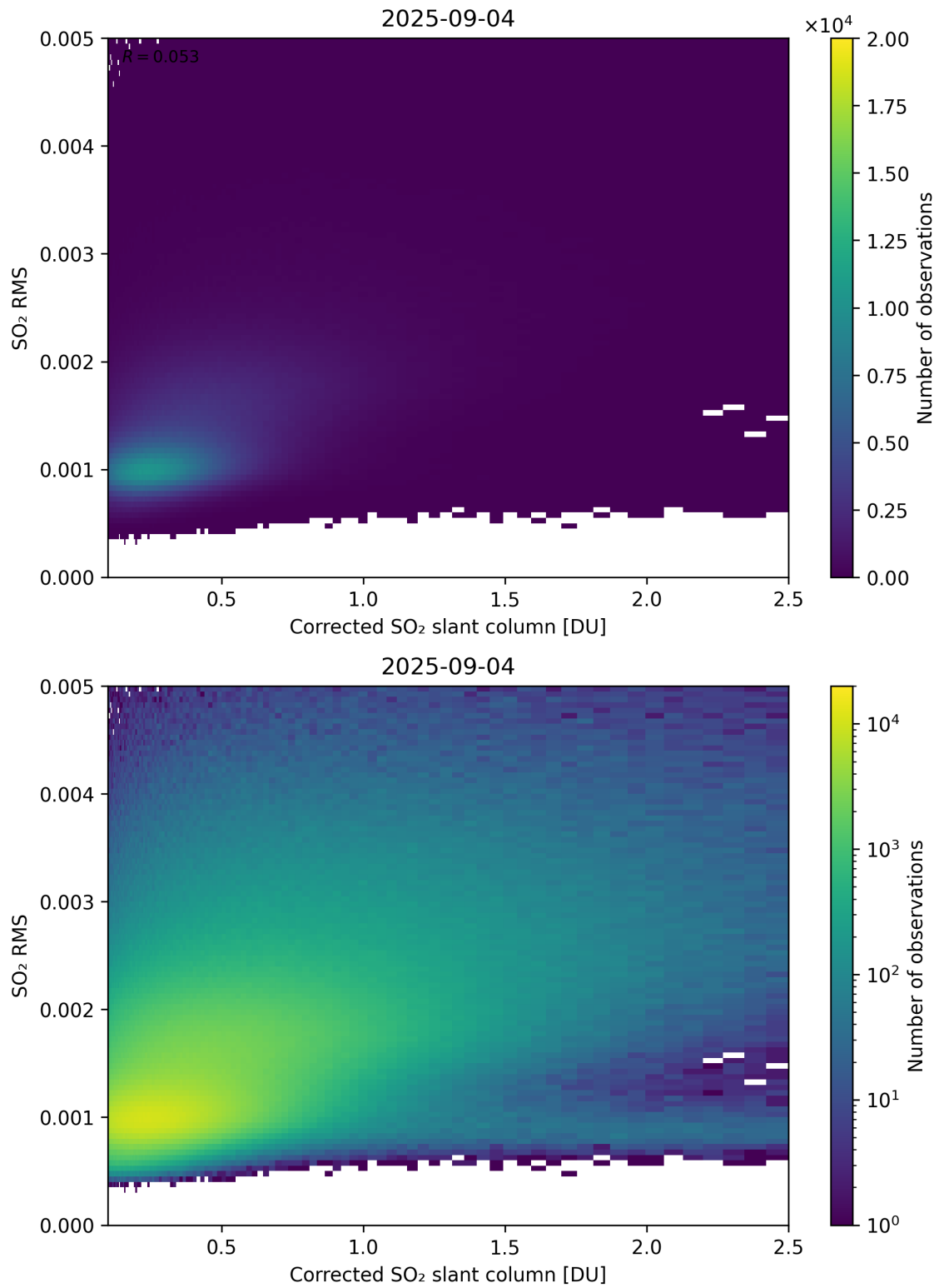
Figure 231: Scatter density plot of “Corrected SO 2 slant column” against “SO 2 RMS” for 2025-09-04 to 2025-09-05.
