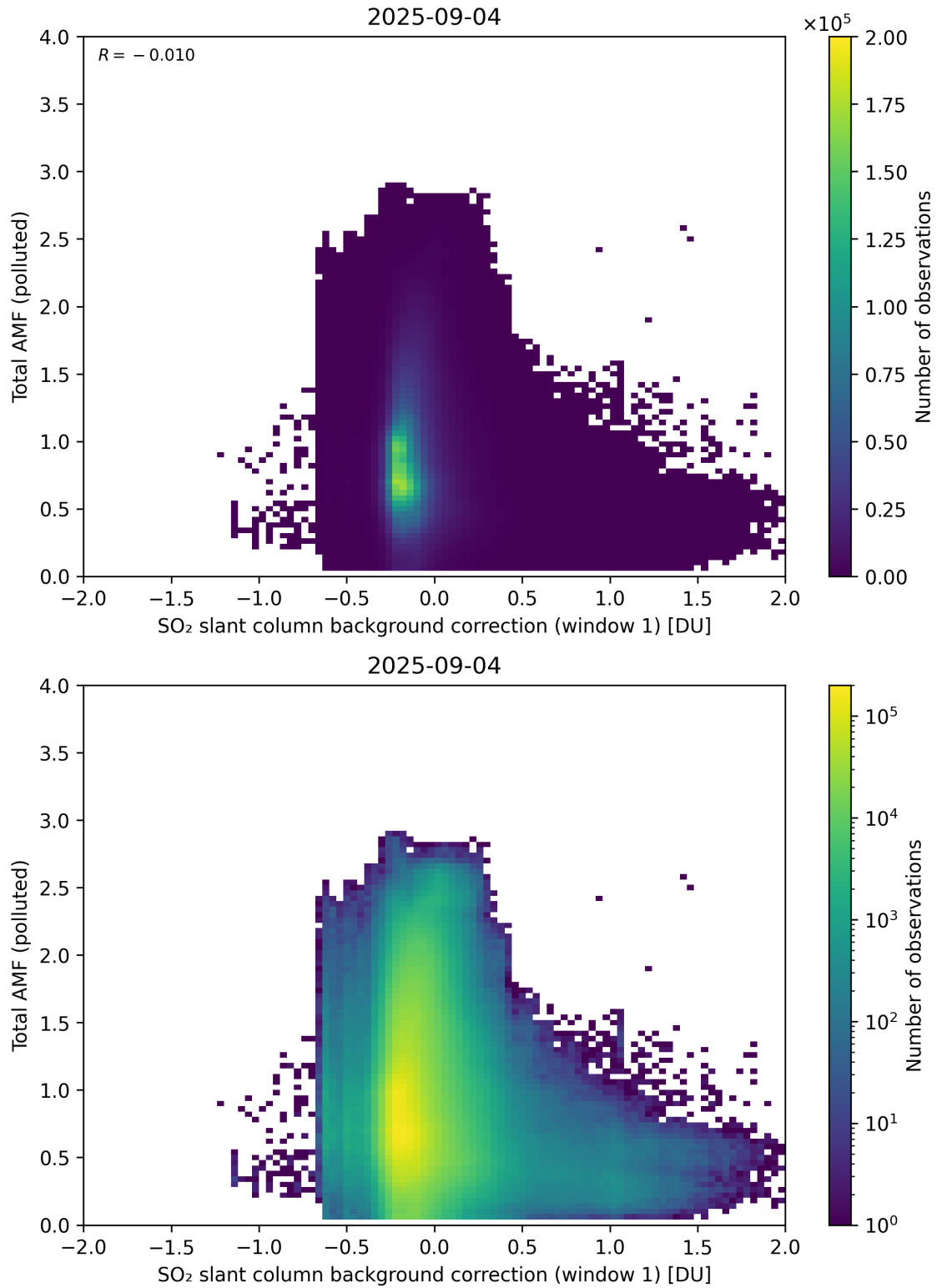
Figure 120: Scatter density plot of “SO 2 slant column background correction (window 1)” against “Total AMF (polluted)” for 2025-09-04 to 2025-09-05.
