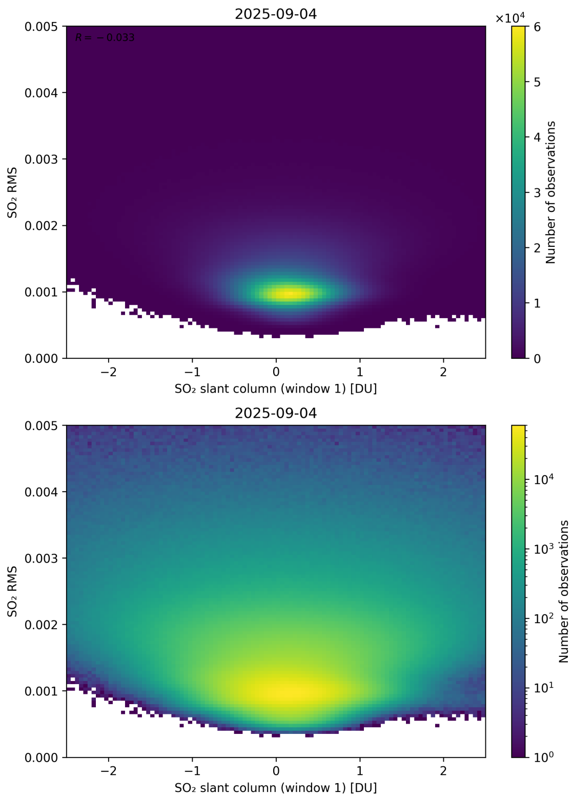
Figure 267: Scatter density plot of “SO 2 slant column (window 1)” against “SO 2 RMS” for 2025-09-04 to 2025-09-05.
