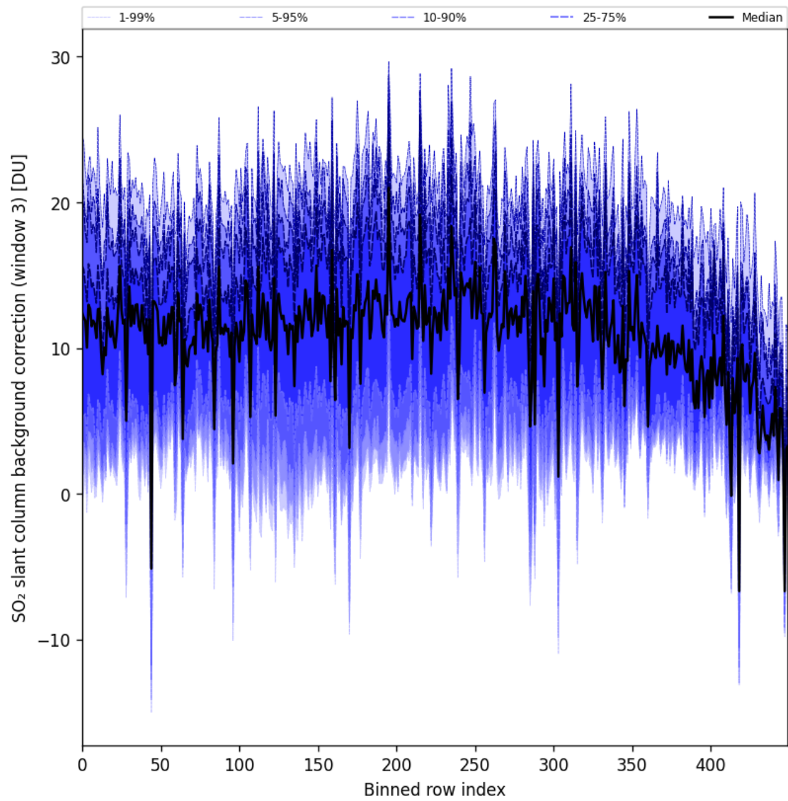
Figure 100: Along track statistics of “SO 2 slant column background correction (window 3)” for 2025-09-04 to 2025-09-05
