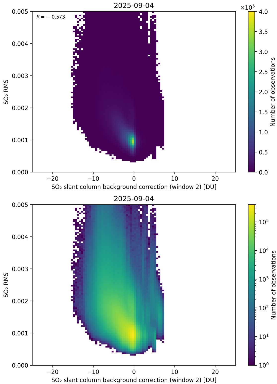
Figure 125: Scatter density plot of “SO 2 slant column background correction (window 2)” against “SO 2 RMS” for 2025-09-04 to 2025-09-05.
