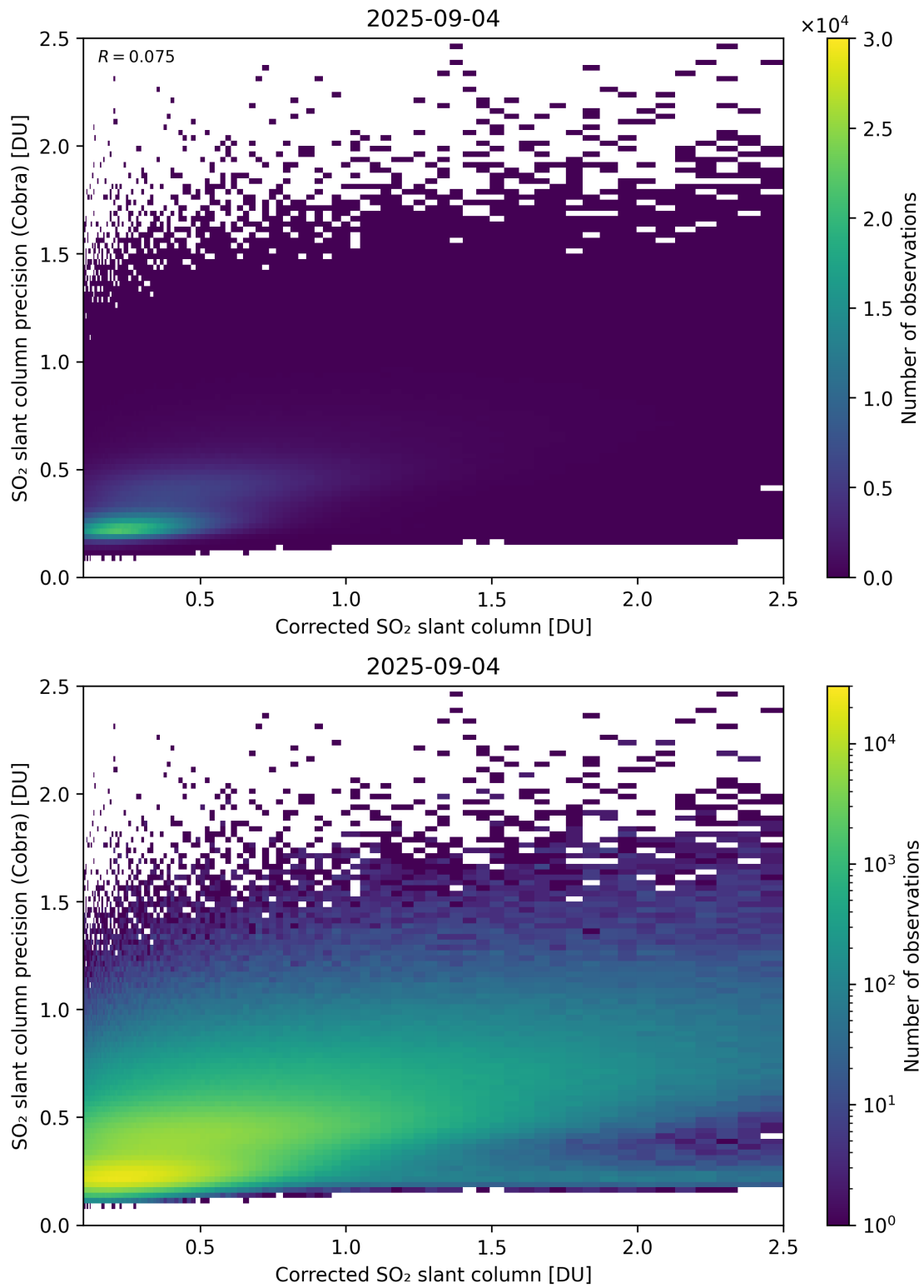
Figure 234: Scatter density plot of “Corrected SO 2 slant column” against “SO 2 slant column precision (Cobra)” for 2025-09-04 to 2025-09-05.
