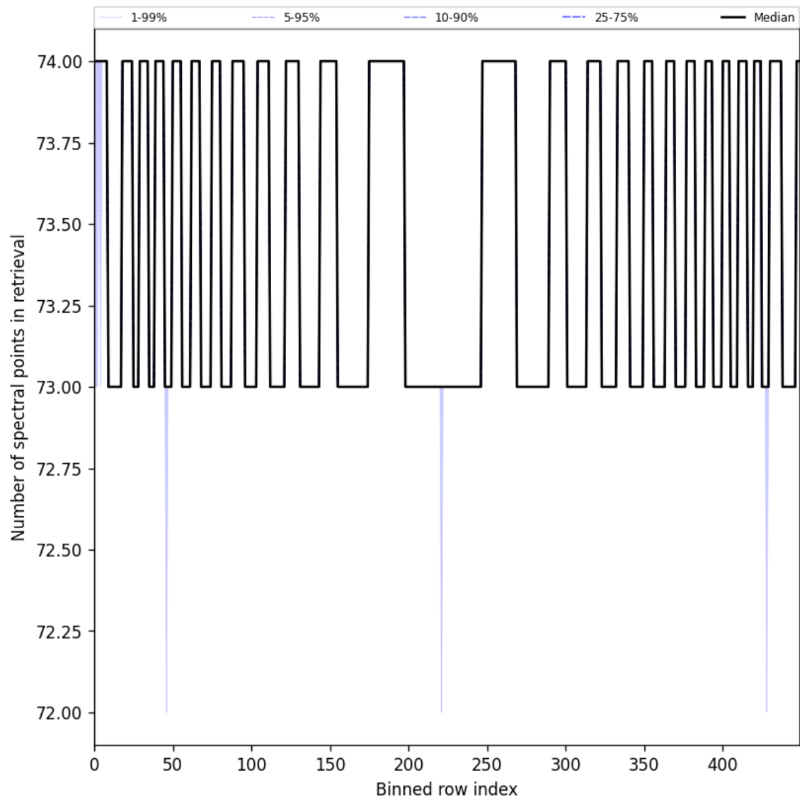
Figure 108: Along track statistics of “Number of spectral points in retrieval” for 2025-09-04 to 2025-09-05
