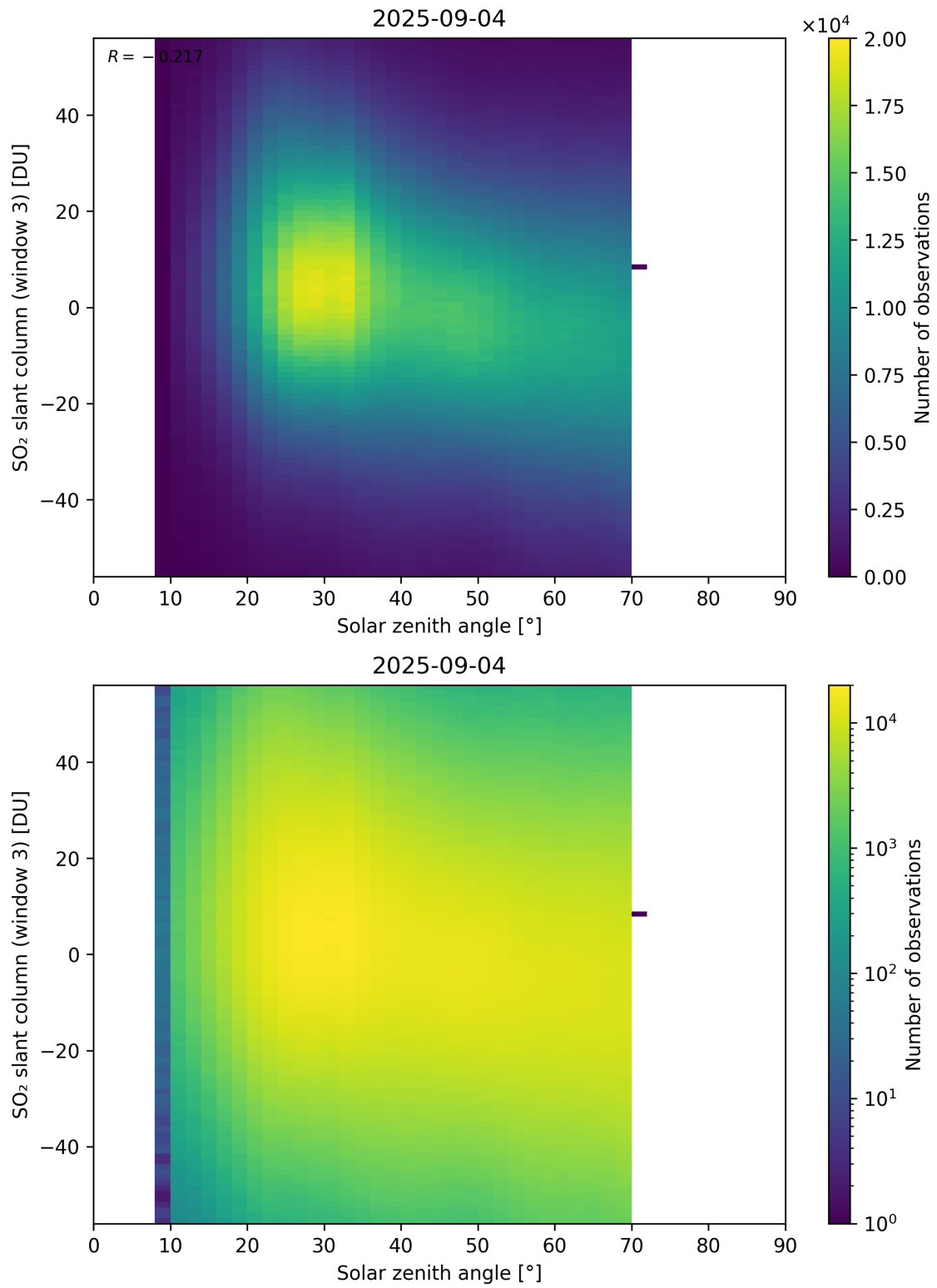
Figure 187: Scatter density plot of “Solar zenith angle” against “SO 2 slant column (window 3)” for 2025-09-04 to 2025-09-05.
