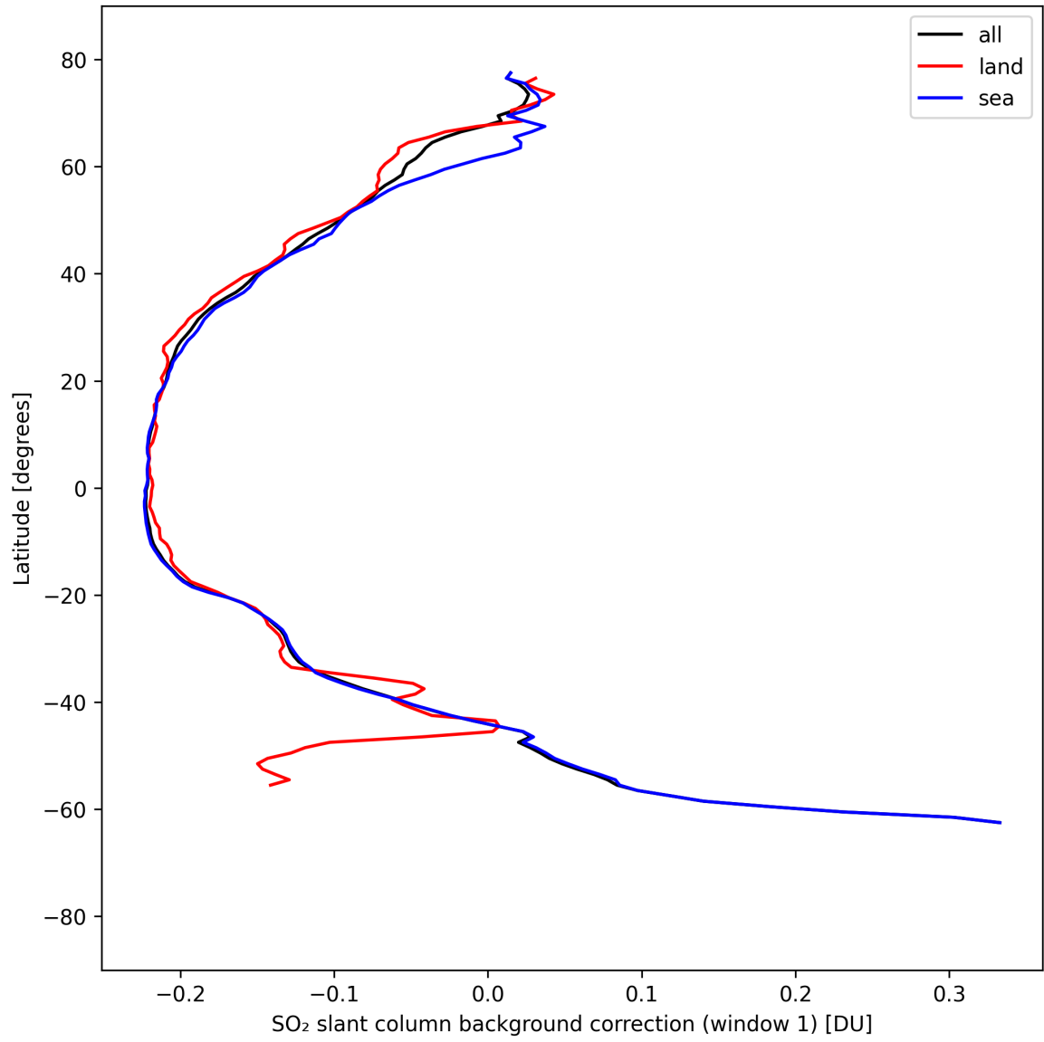
Figure 40: Zonal average of “SO 2 slant column background correction (window 1)” for 2025-09-04 to 2025-09-05.
