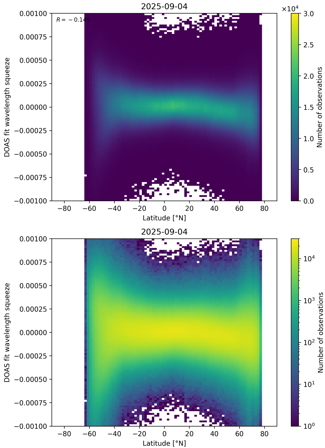
Figure 154: Scatter density plot of “Latitude” against “DOAS fit wavelength squeeze” for 2025-09-04 to 2025-09-05.
