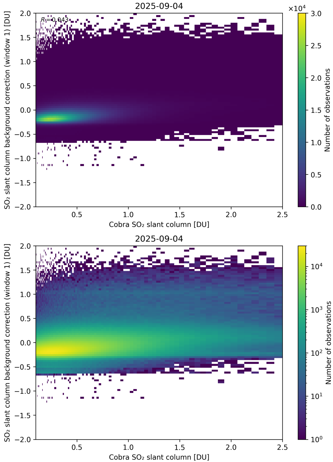
Figure 193: Scatter density plot of “Cobra SO 2 slant column” against “SO 2 slant column background correction (window 1)” for 2025-09-04 to 2025-09-05.
