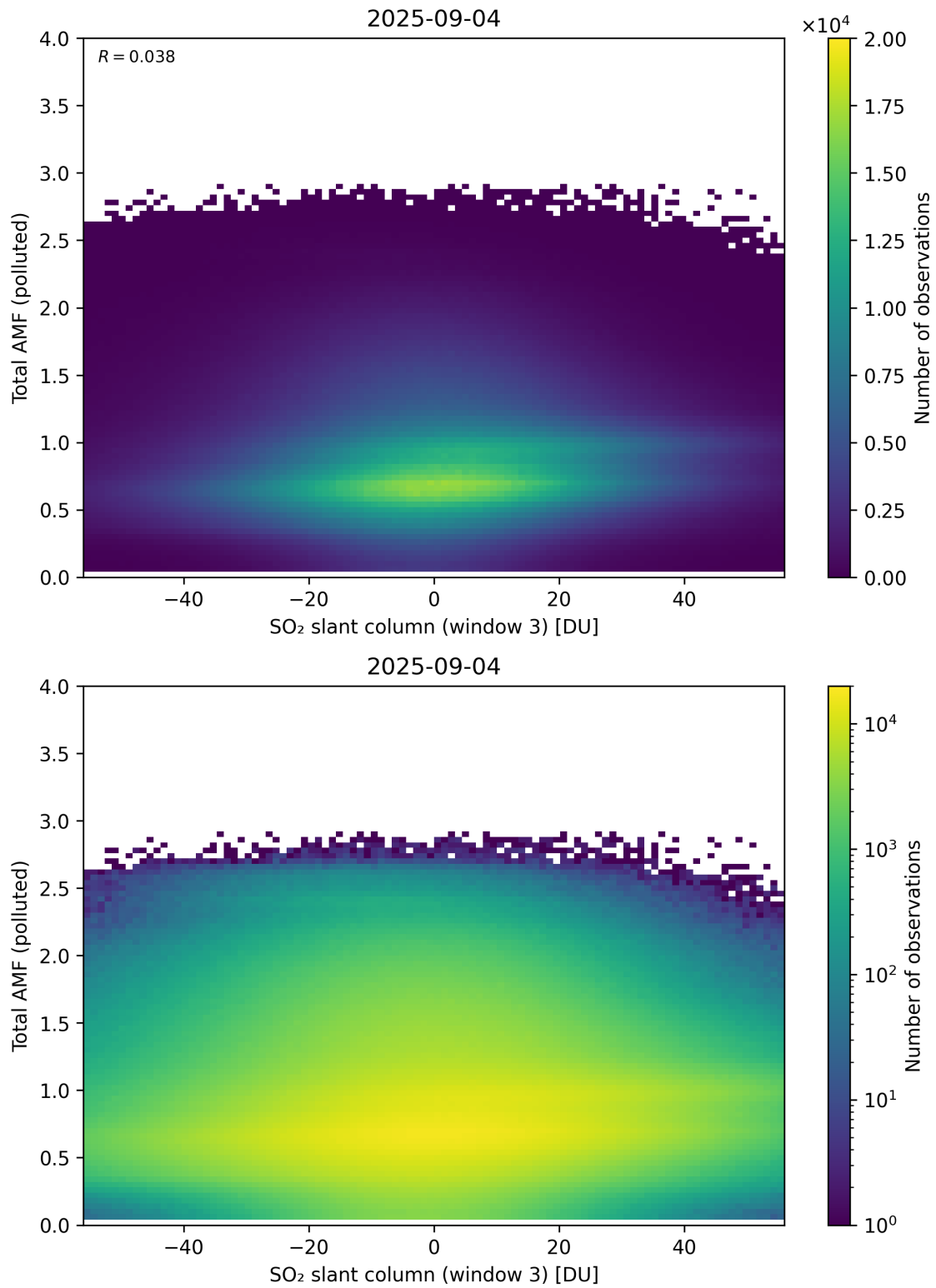
Figure 318: Scatter density plot of “SO 2 slant column (window 3)” against “Total AMF (polluted)” for 2025-09-04 to 2025-09-05.
