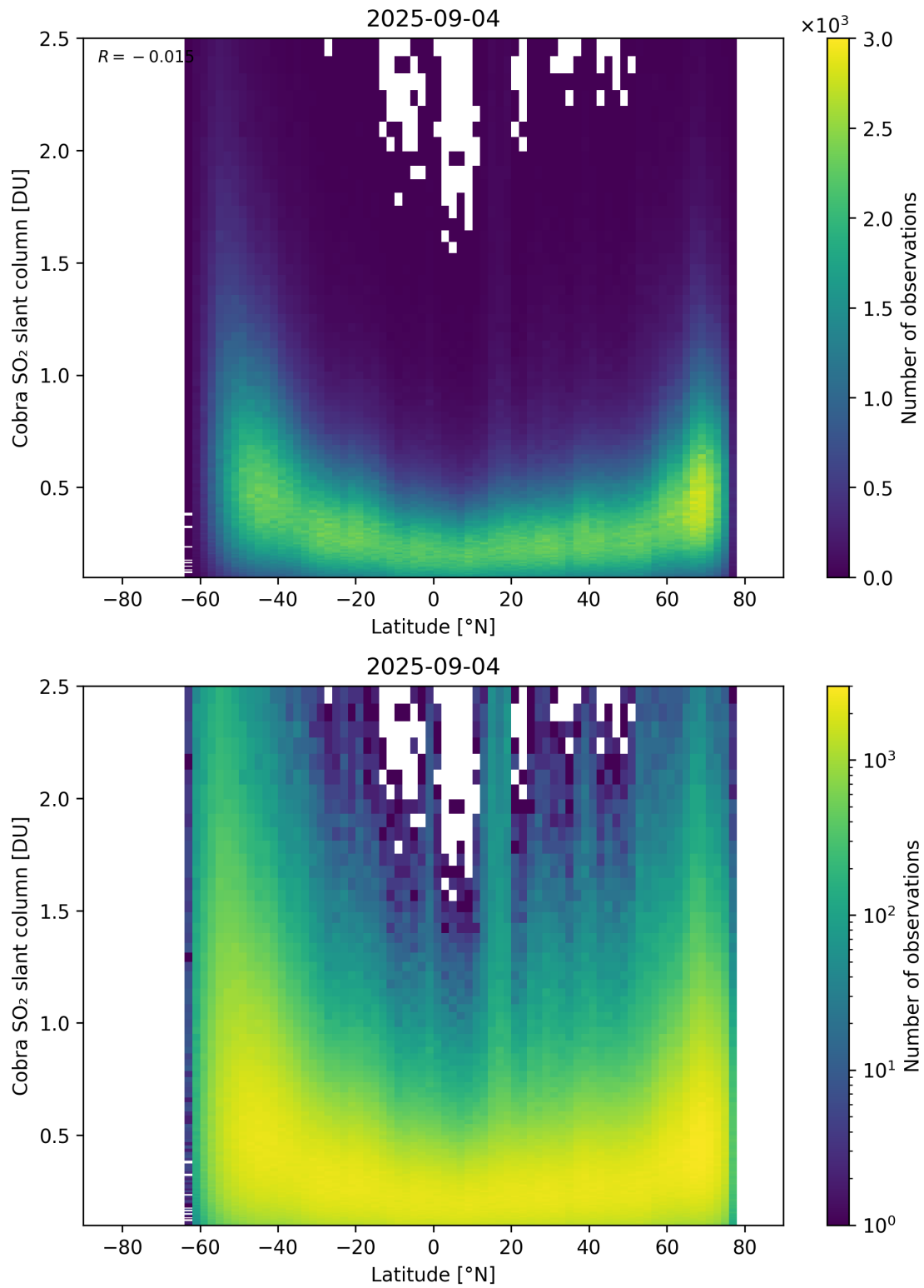
Figure 157: Scatter density plot of “Latitude” against “Cobra SO 2 slant column” for 2025-09-04 to 2025-09-05.
