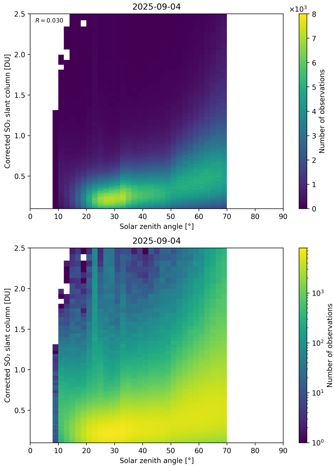
Figure 181: Scatter density plot of “Solar zenith angle” against “Corrected SO 2 slant column” for 2025-09-04 to 2025-09-05.
