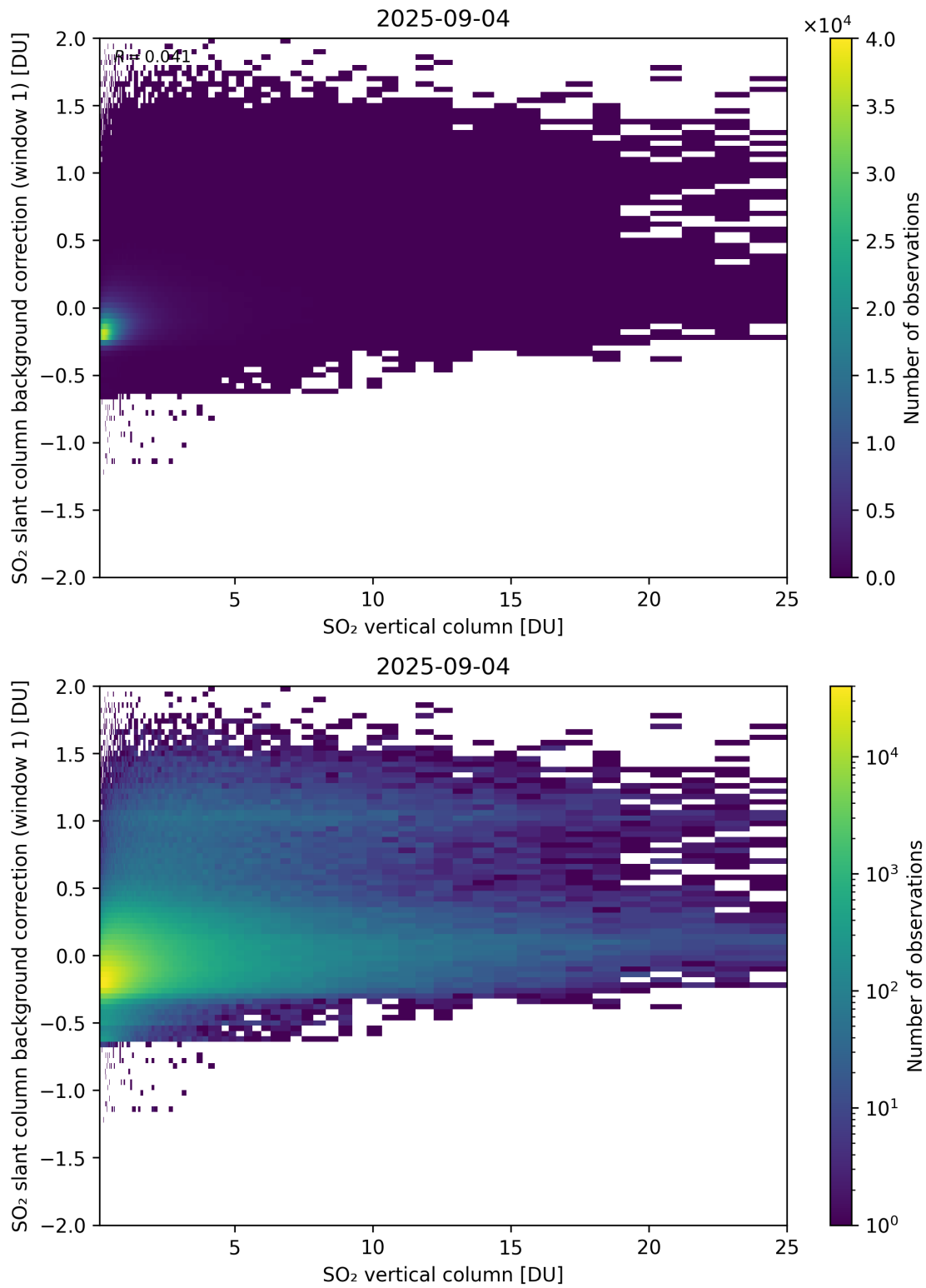
Figure 323: Scatter density plot of “SO 2 vertical column” against “SO 2 slant column background correction (window 1)” for 2025-09-04 to 2025-09-05.
