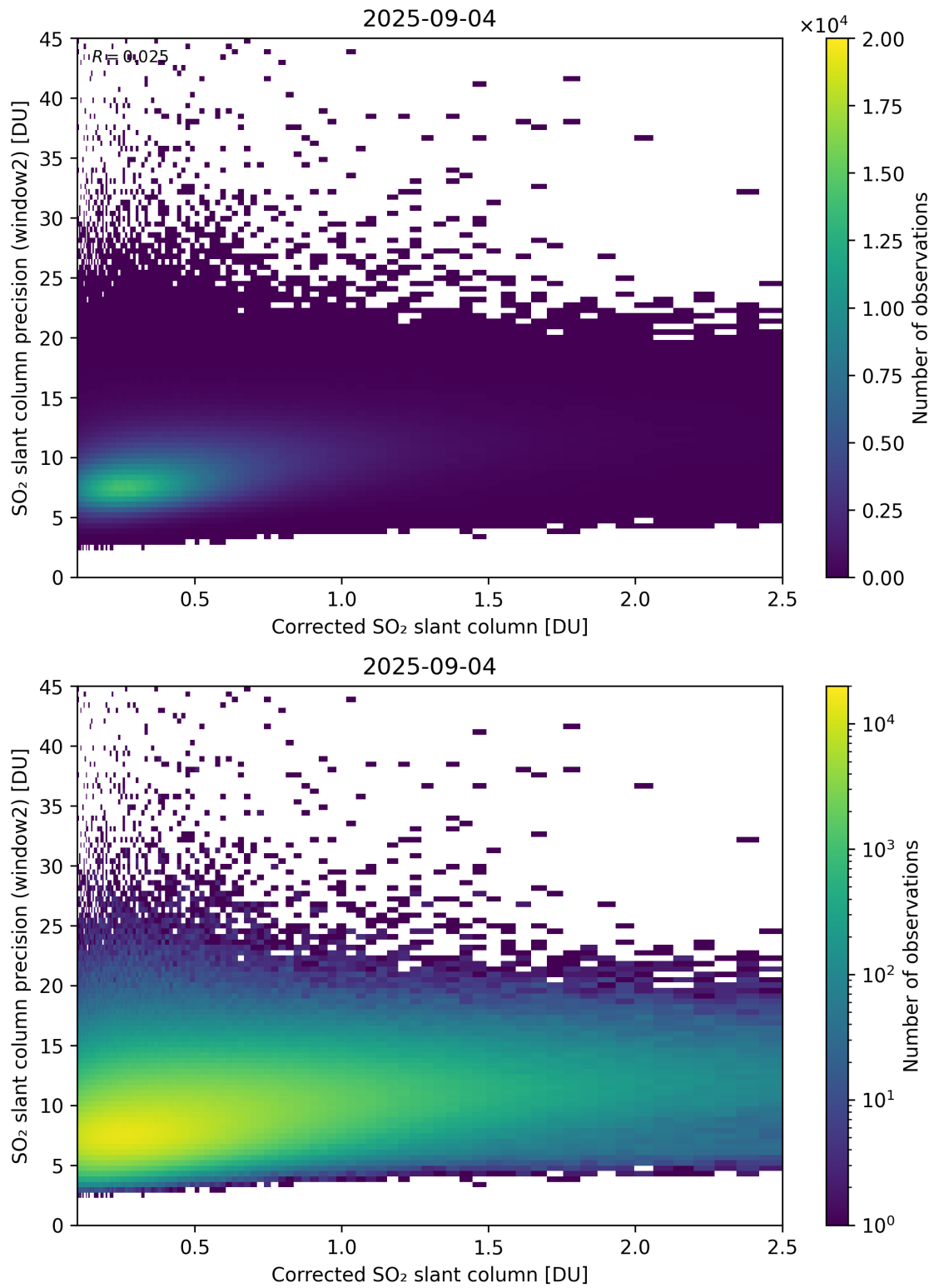
Figure 239: Scatter density plot of “Corrected SO 2 slant column” against “SO 2 slant column precision (window2)” for 2025-09-04 to 2025-09-05.
