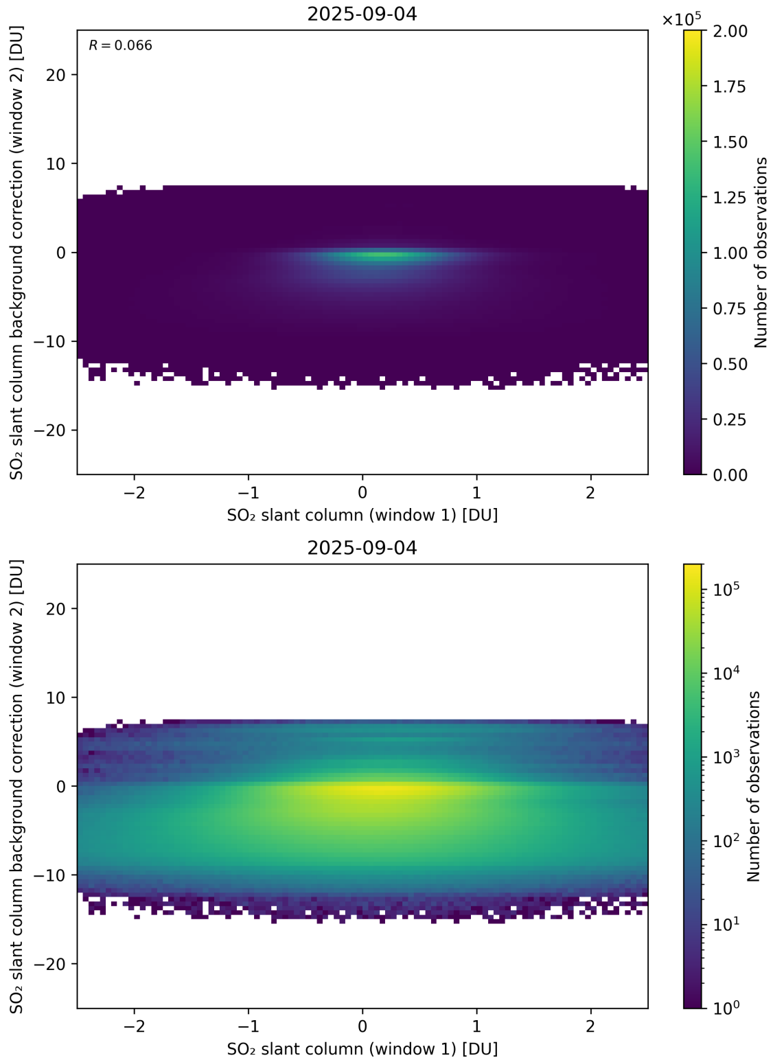
Figure 263: Scatter density plot of “SO 2 slant column (window 1)” against “SO 2 slant column background correction (window 2)” for 2025-09-04 to 2025-09-05.
