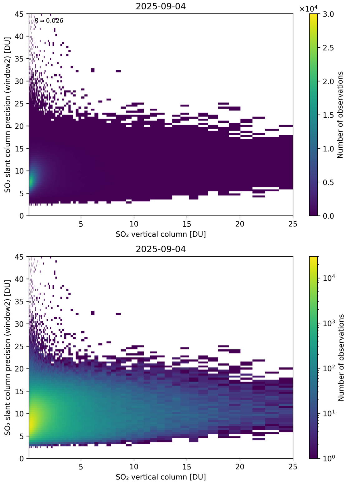
Figure 356: Scatter density plot of “SO 2 vertical column” against “SO 2 slant column precision (window2)” for 2025-09-04 to 2025-09-05.
