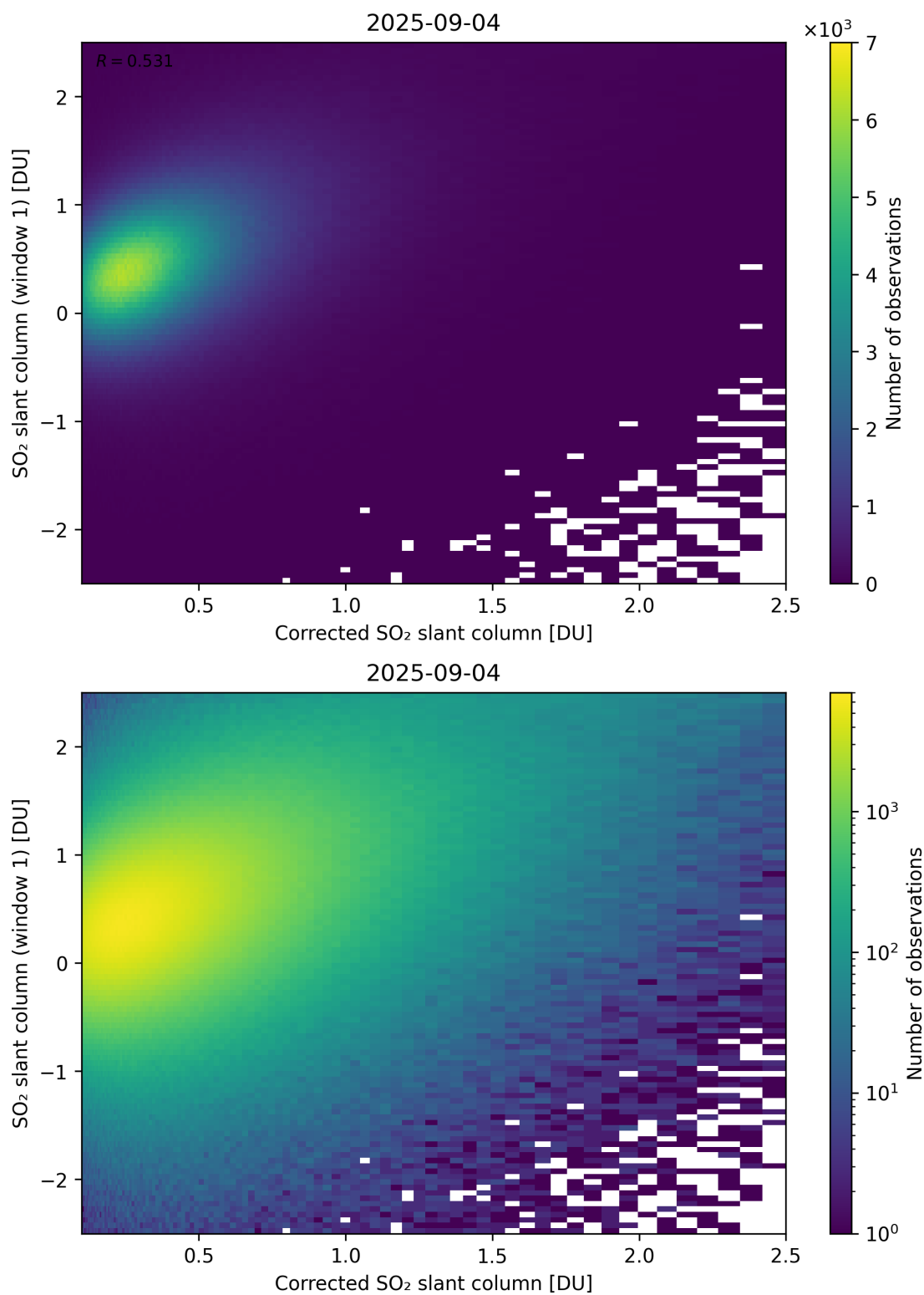
Figure 237: Scatter density plot of “Corrected SO 2 slant column” against “SO 2 slant column (window 1)” for 2025-09-04 to 2025-09-05.
