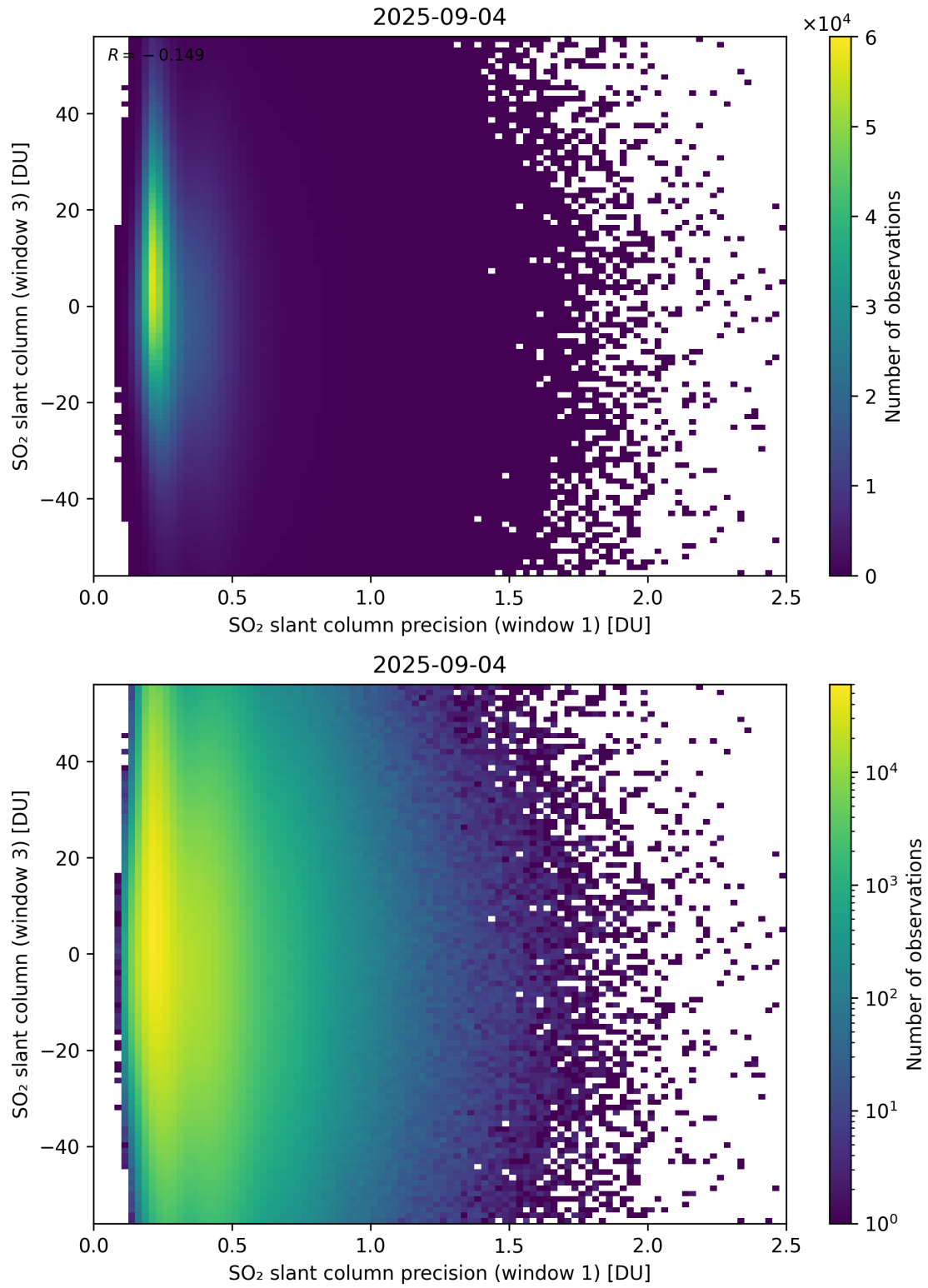
Figure 278: Scatter density plot of “SO 2 slant column precision (window 1)” against “SO 2 slant column (window 3)” for 2025-09-04 to 2025-09-05.
