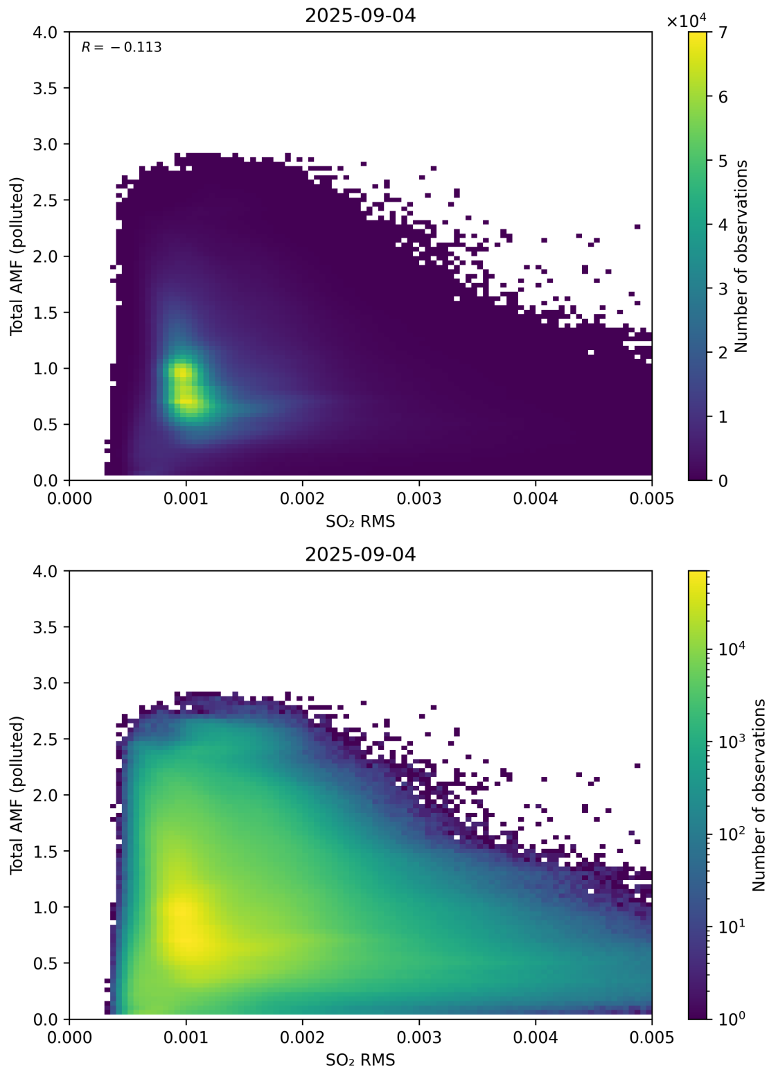
Figure 148: Scatter density plot of “SO 2 RMS” against “Total AMF (polluted)” for 2025-09-04 to 2025-09-05.
