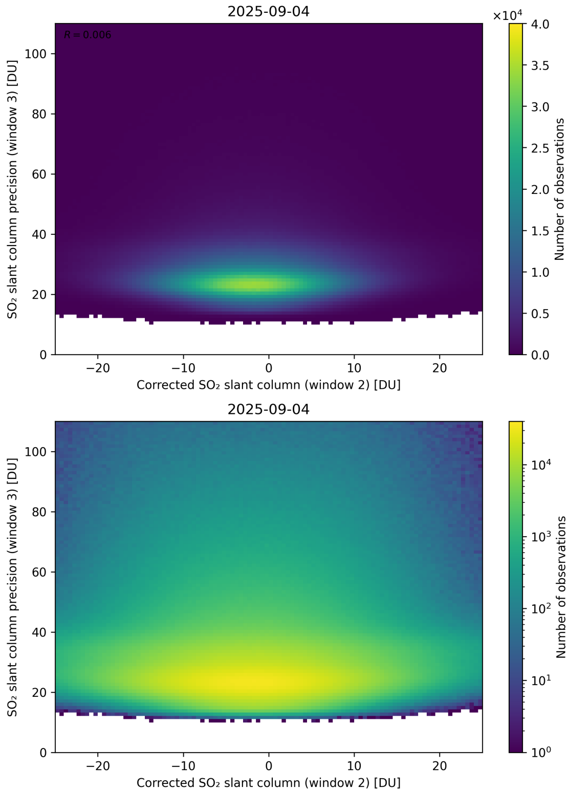
Figure 252: Scatter density plot of “Corrected SO 2 slant column (window 2)” against “SO 2 slant column precision (window 3)” for 2025-09-04 to 2025-09-05.
