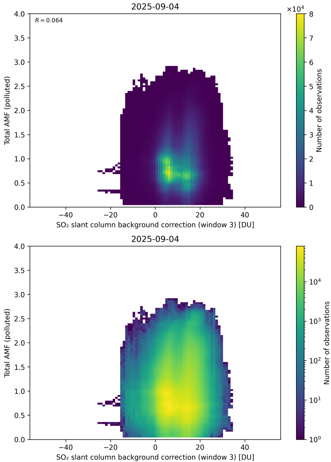
Figure 136: Scatter density plot of “SO 2 slant column background correction (window 3)” against “Total AMF (polluted)” for 2025-09-04 to 2025-09-05.
