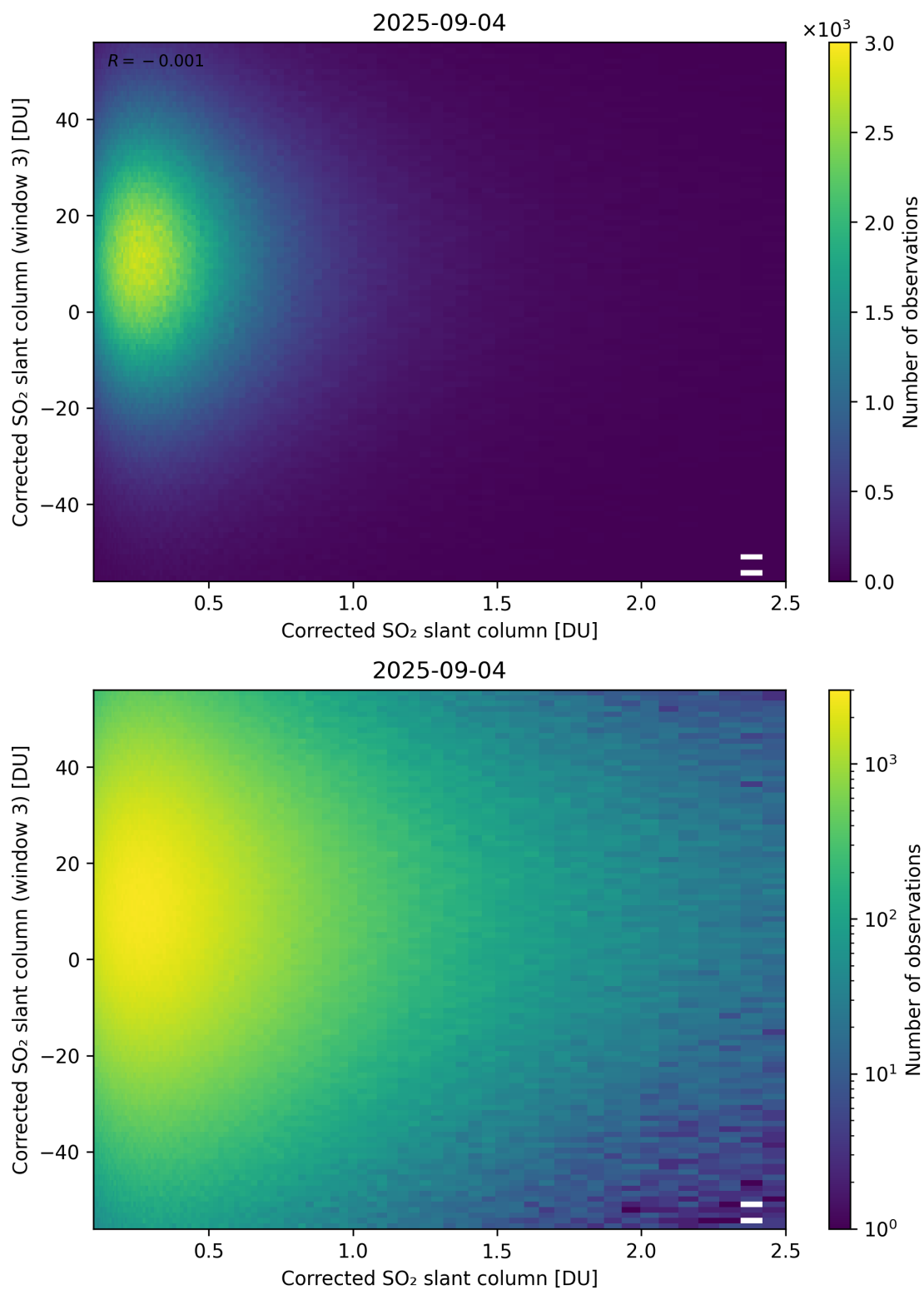
Figure 236: Scatter density plot of “Corrected SO 2 slant column” against “Corrected SO 2 slant column (window 3)” for 2025-09-04 to 2025-09-05.
