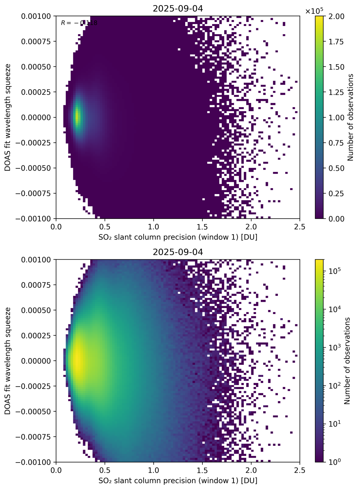
Figure 272: Scatter density plot of “SO 2 slant column precision (window 1)” against “DOAS fit wavelength squeeze” for 2025-09-04 to 2025-09-05.
