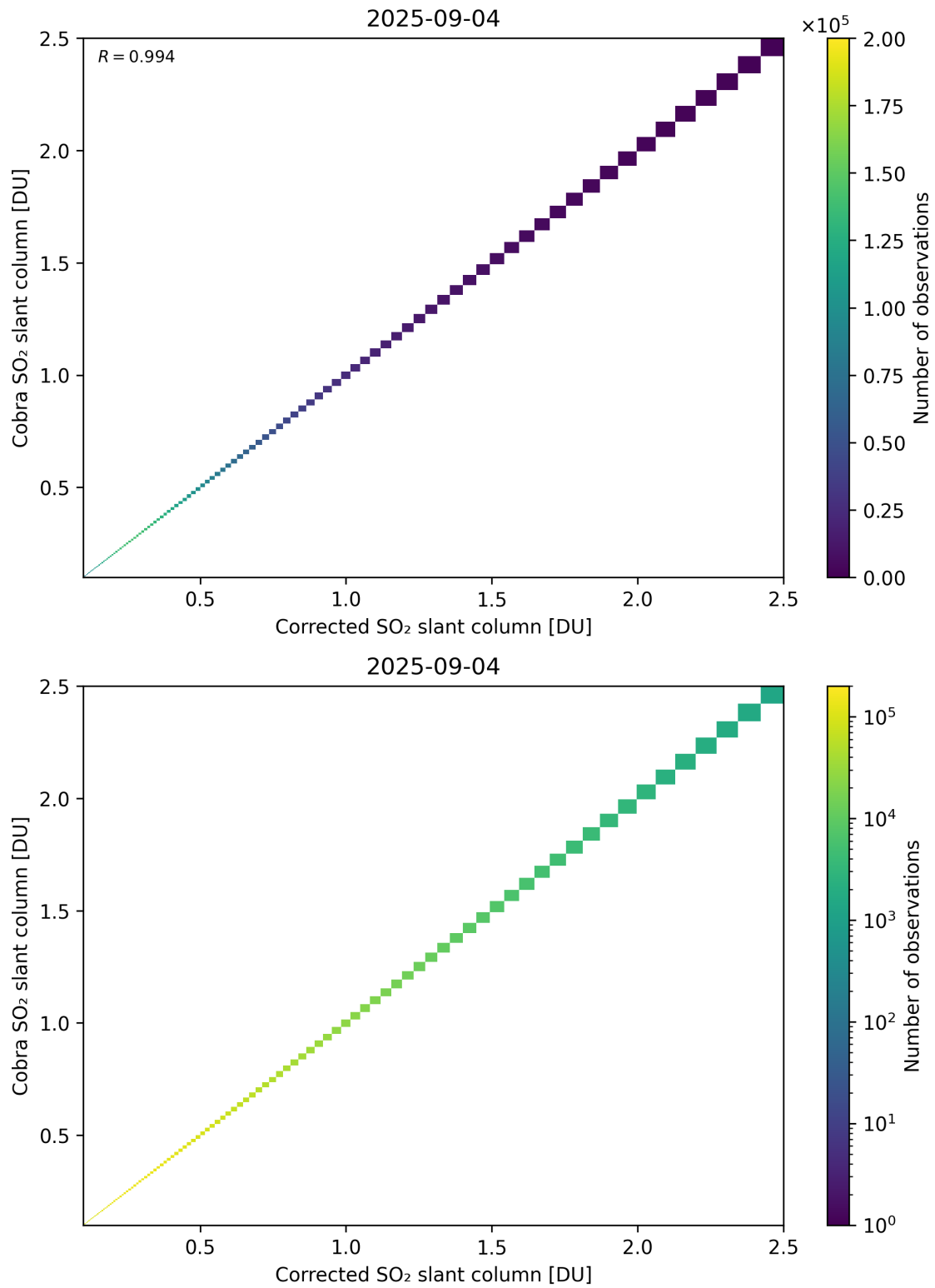
Figure 233: Scatter density plot of “Corrected SO 2 slant column” against “Cobra SO 2 slant column” for 2025-09-04 to 2025-09-05.
