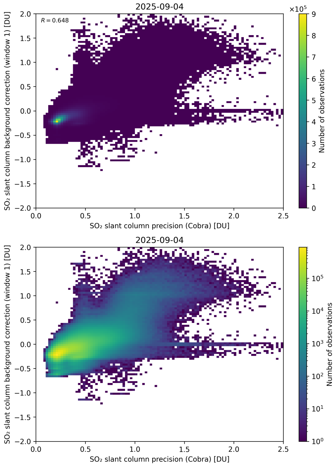
Figure 199: Scatter density plot of “SO 2 slant column precision (Cobra)” against “SO 2 slant column background correction (window 1)” for 2025-09-04 to 2025-09-05.
