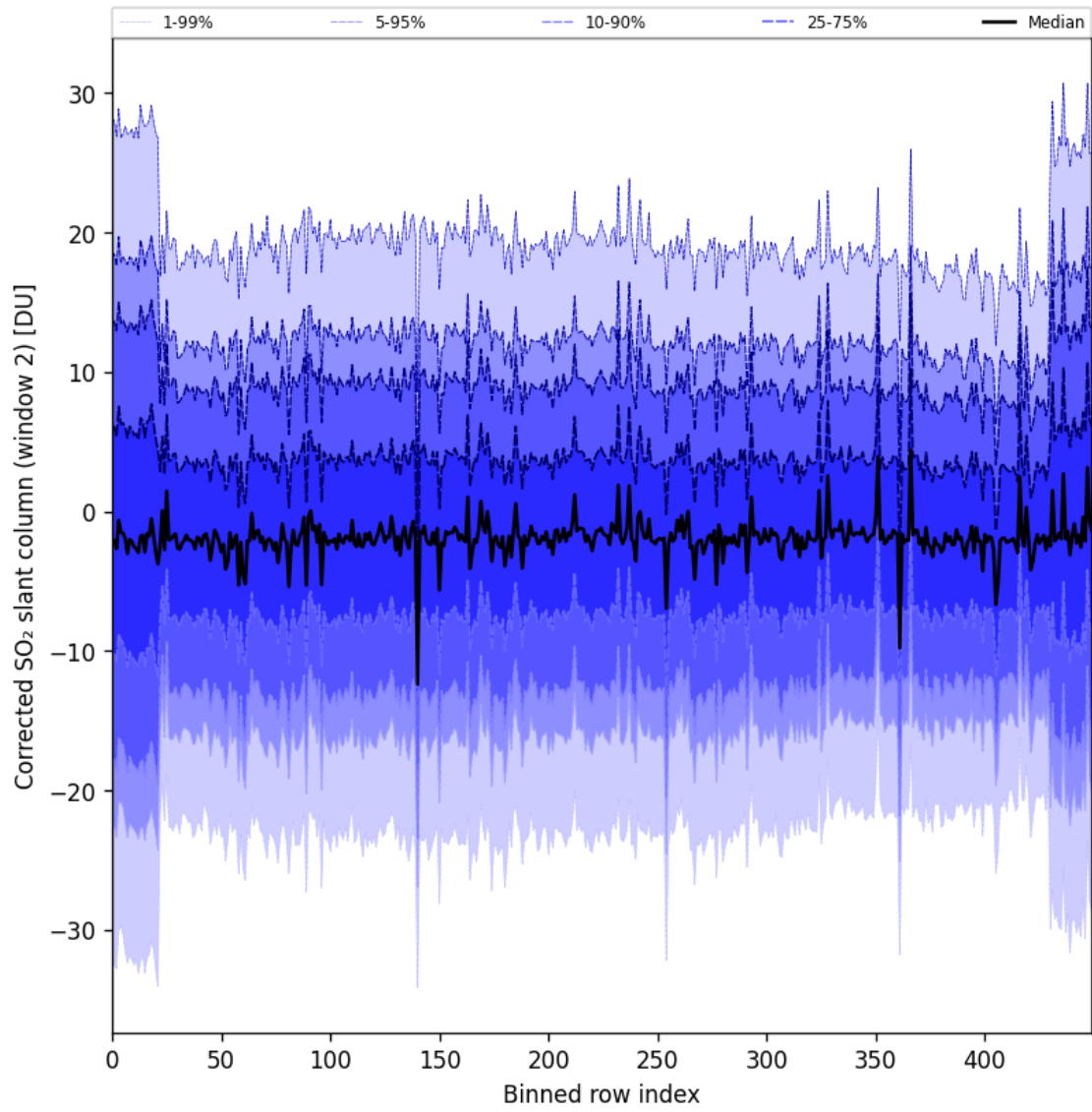
Figure 95: Along track statistics of “Corrected SO 2 slant column (window 2)” for 2025-09-04 to 2025-09-05
