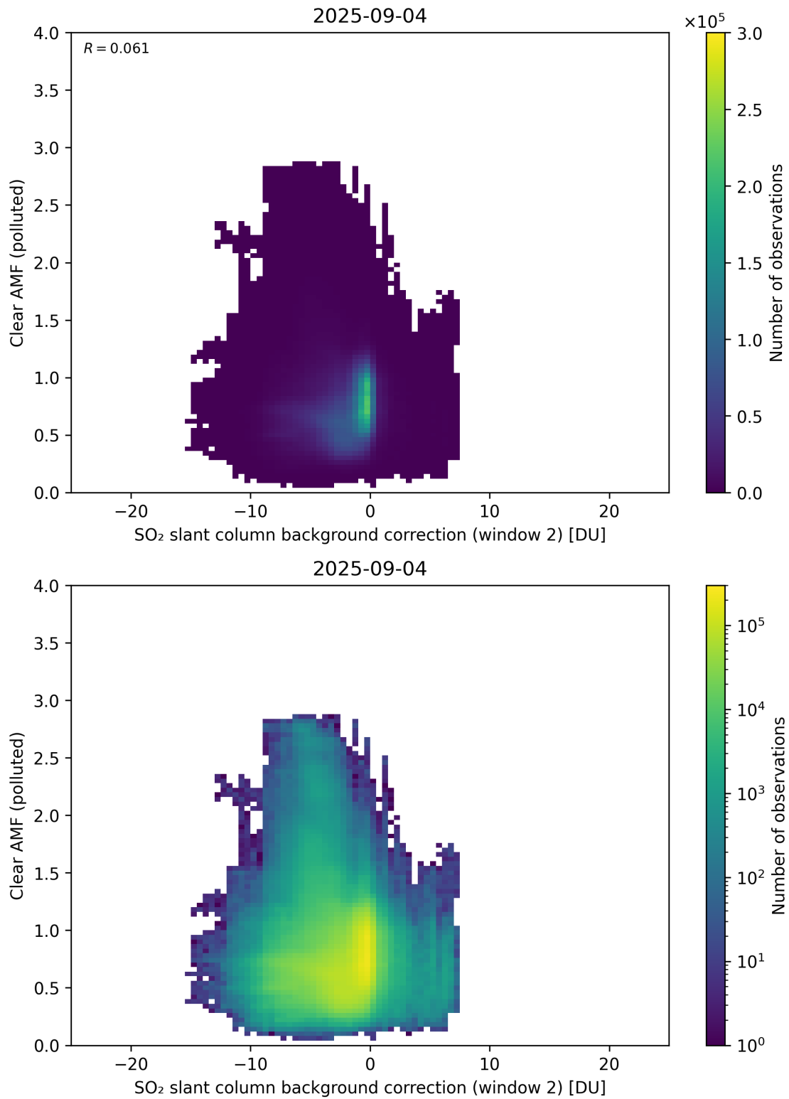
Figure 126: Scatter density plot of “SO 2 slant column background correction (window 2)” against “Clear AMF (polluted)” for 2025-09-04 to 2025-09-05.
