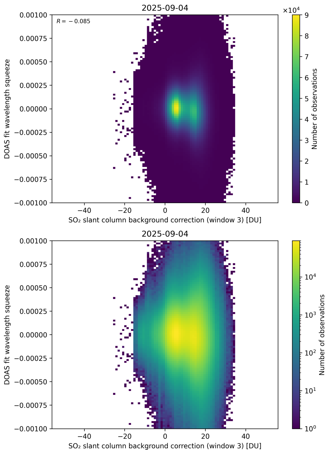
Figure 133: Scatter density plot of “SO 2 slant column background correction (window 3)” against “DOAS fit wavelength squeeze” for 2025-09-04 to 2025-09-05.
