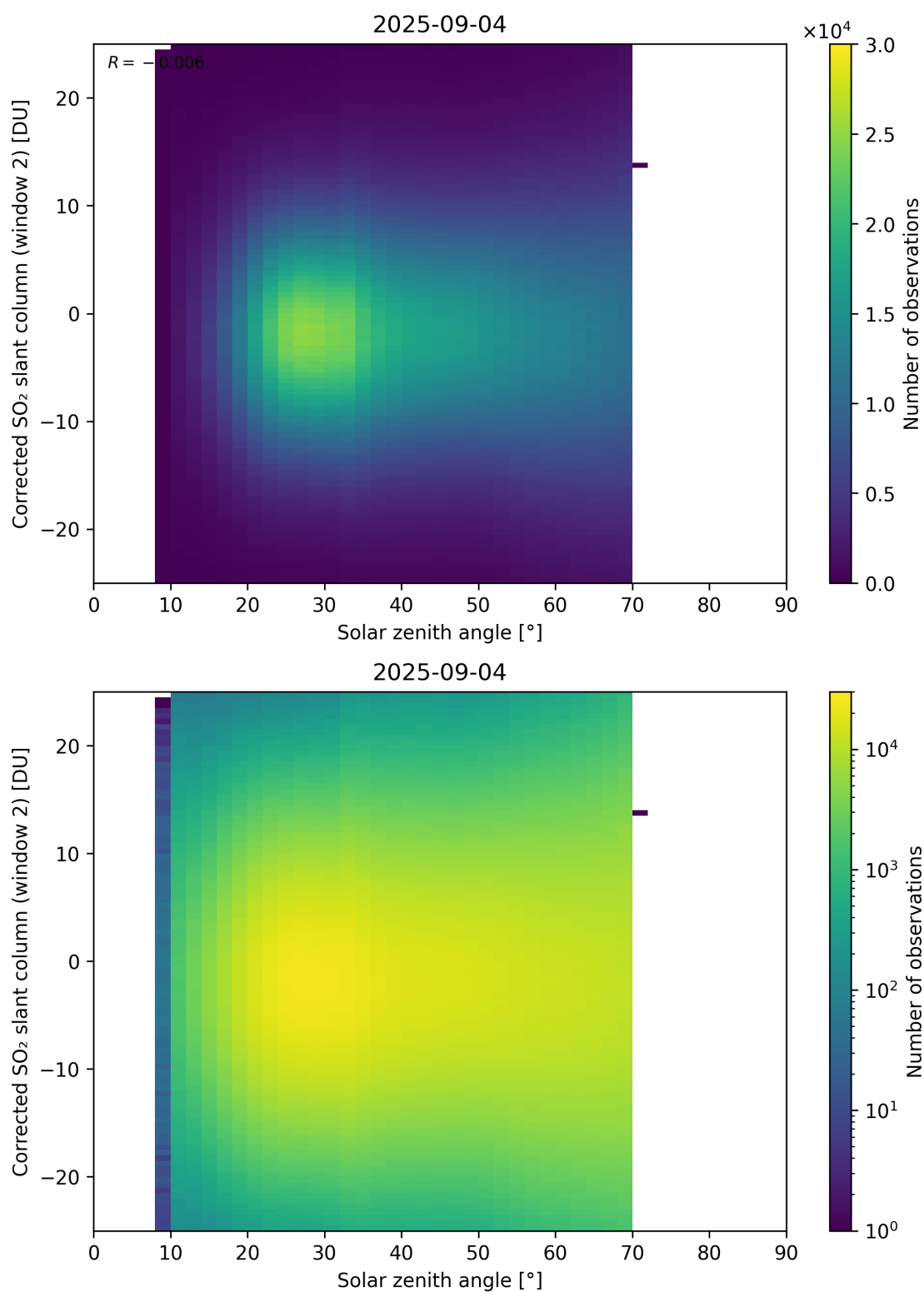
Figure 182: Scatter density plot of “Solar zenith angle” against “Corrected SO 2 slant column (window 2)” for 2025-09-04 to 2025-09-05.
