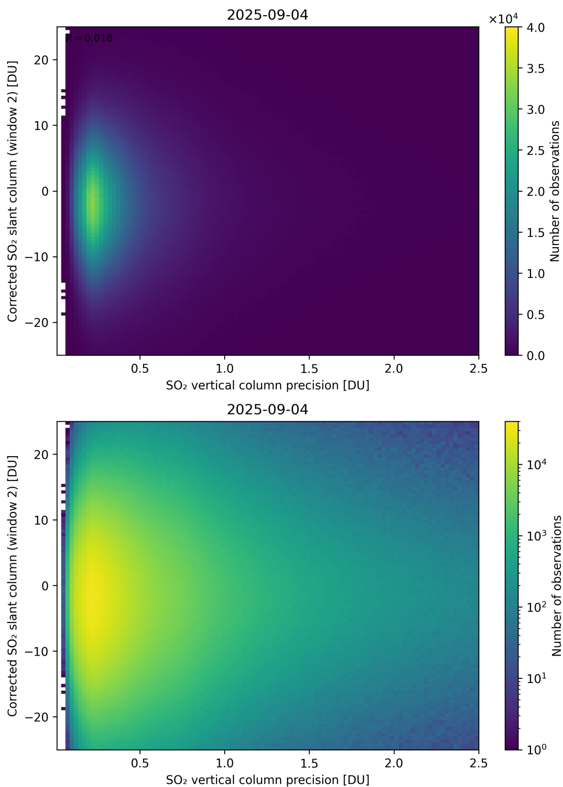
Figure 339: Scatter density plot of “SO 2 vertical column precision” against “Corrected SO 2 slant column (window 2)” for 2025-09-04 to 2025-09-05.
