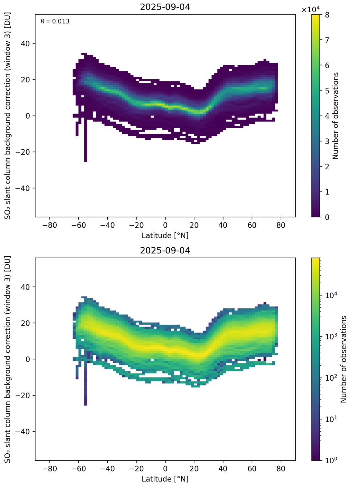
Figure 152: Scatter density plot of “Latitude” against “SO 2 slant column background correction (window 3)” for 2025-09-04 to 2025-09-05.
