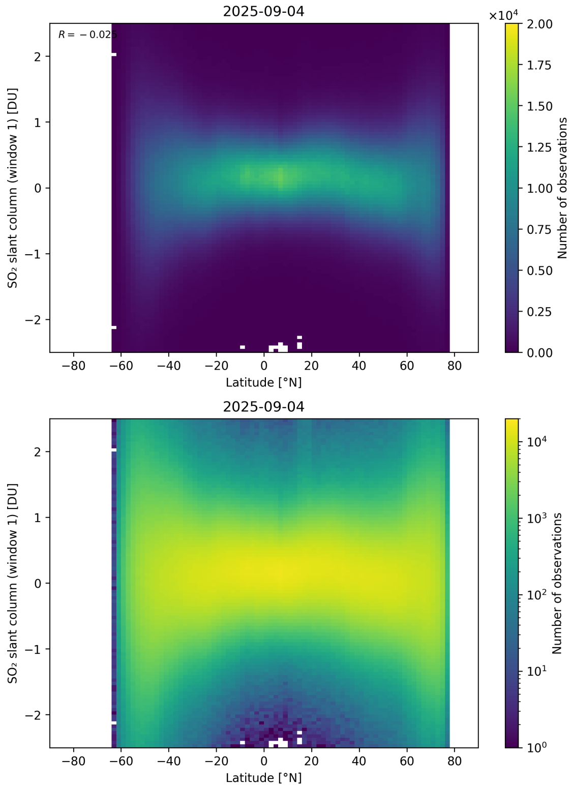
Figure 162: Scatter density plot of “Latitude” against “SO 2 slant column (window 1)” for 2025-09-04 to 2025-09-05.
