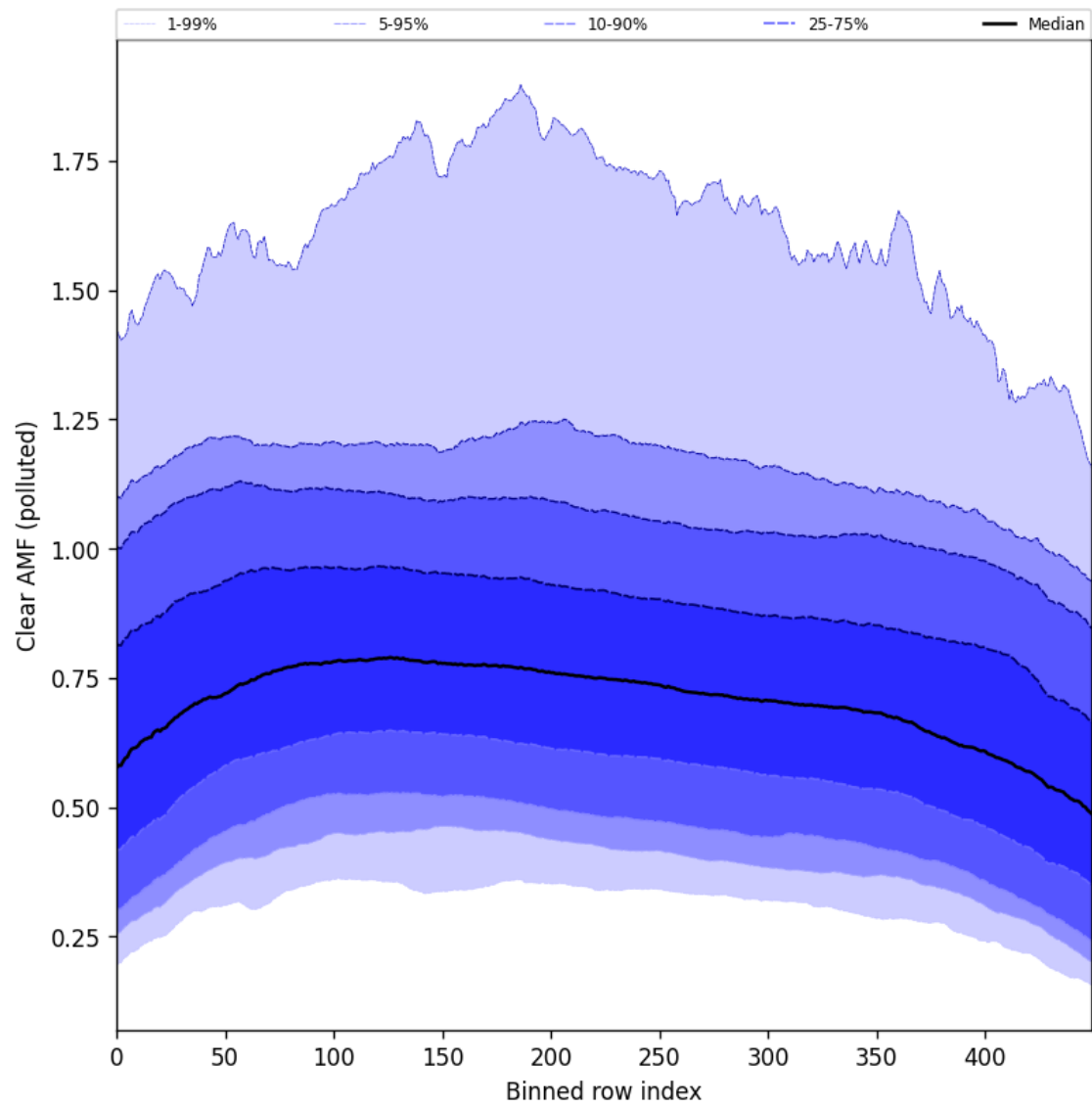
Figure 107: Along track statistics of “Clear AMF (polluted)” for 2025-09-04 to 2025-09-05
