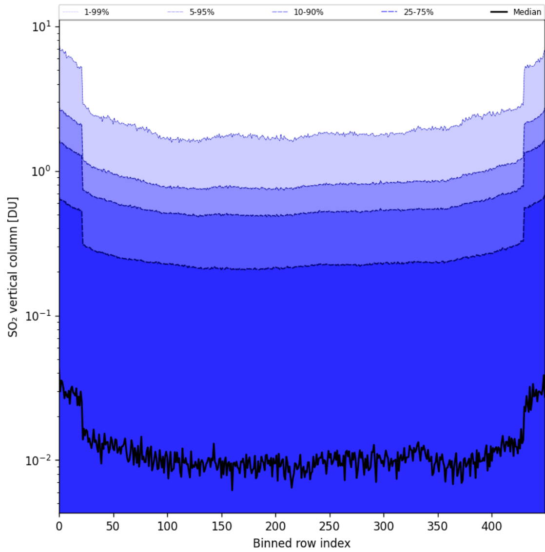
Figure 84: Along track statistics of “SO 2 vertical column” for 2025-09-04 to 2025-09-05
