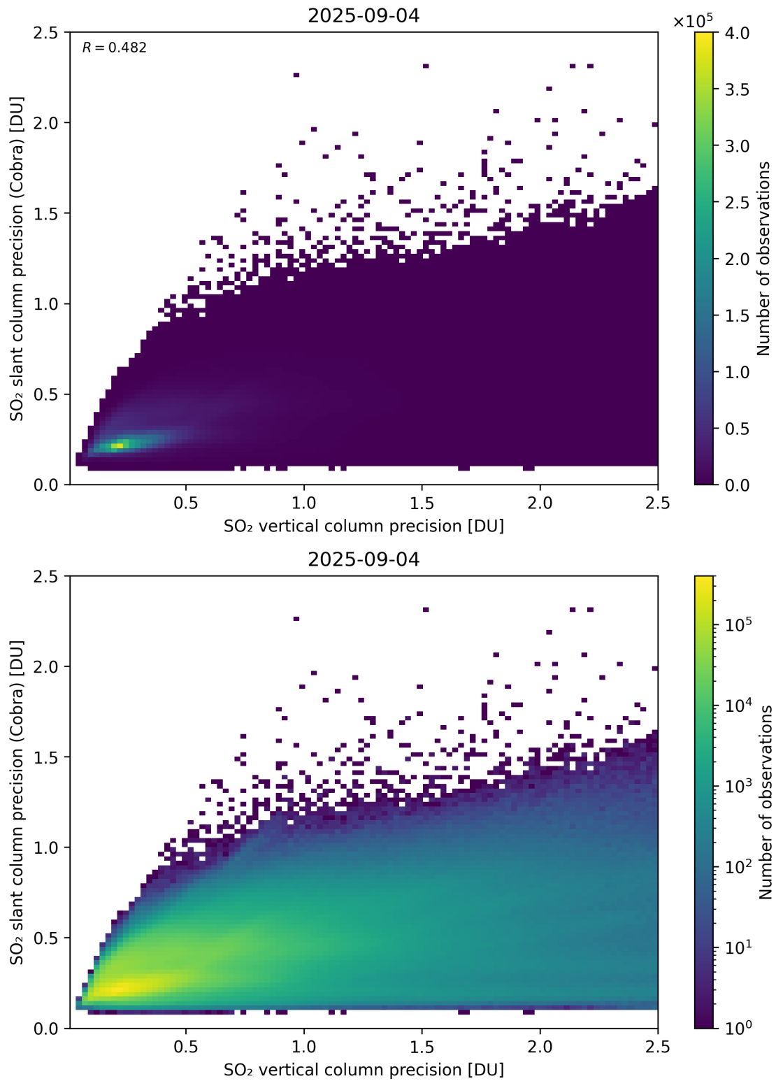
Figure 337: Scatter density plot of “SO 2 vertical column precision” against “SO 2 slant column precision (Cobra)” for 2025-09-04 to 2025-09-05.
