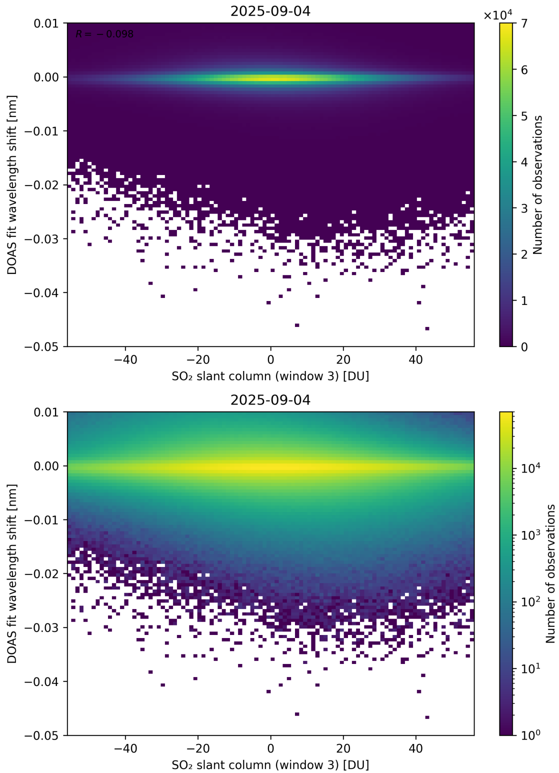
Figure 304: Scatter density plot of “SO 2 slant column (window 3)” against “DOAS fit wavelength shift” for 2025-09-04 to 2025-09-05.
