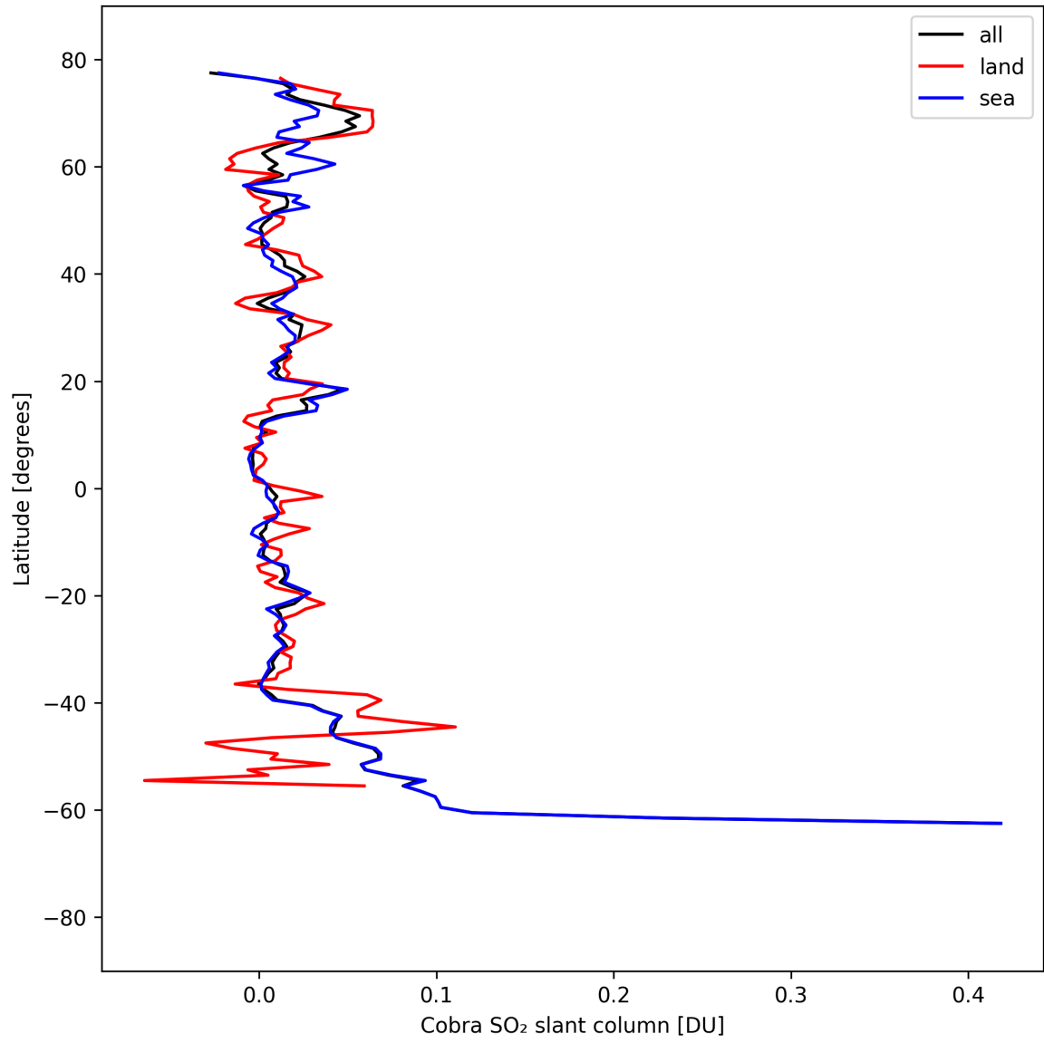
Figure 35: Zonal average of “Cobra SO 2 slant column” for 2025-09-04 to 2025-09-05.
