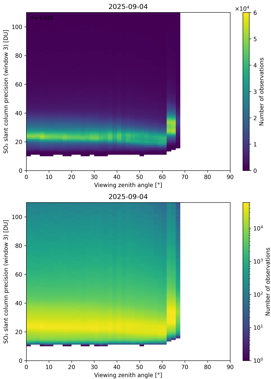
Figure 380: Scatter density plot of “Viewing zenith angle” against “SO 2 slant column precision (window 3)” for 2025-09-04 to 2025-09-05.
