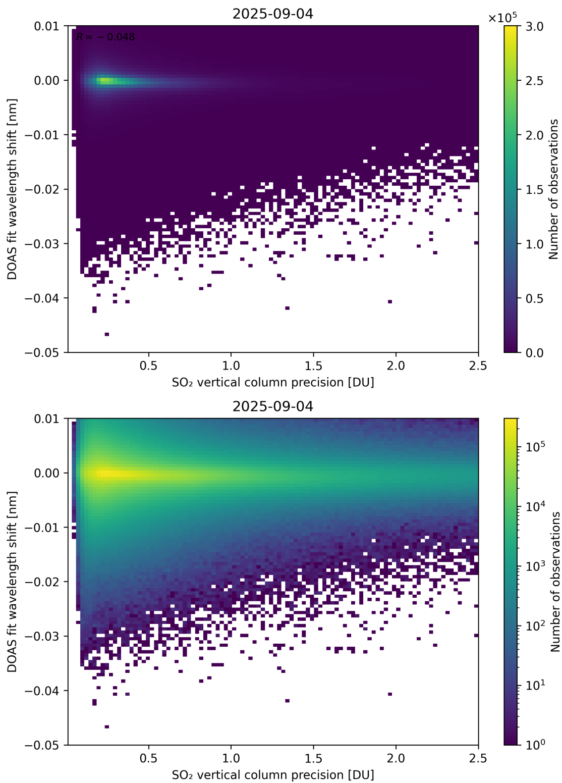
Figure 332: Scatter density plot of “SO 2 vertical column precision” against “DOAS fit wavelength shift” for 2025-09-04 to 2025-09-05.
