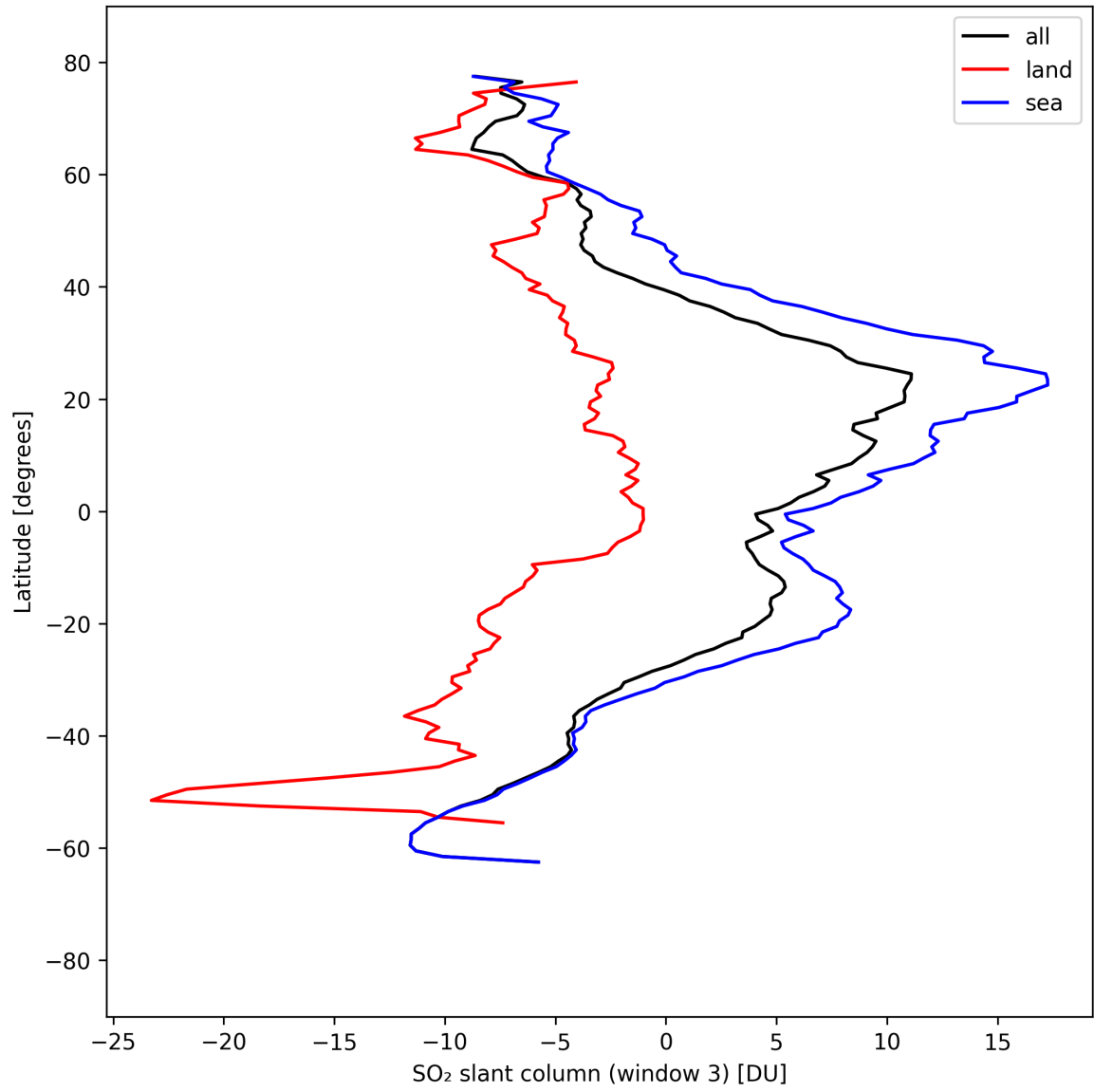
Figure 45: Zonal average of “SO 2 slant column (window 3)” for 2025-09-04 to 2025-09-05.
