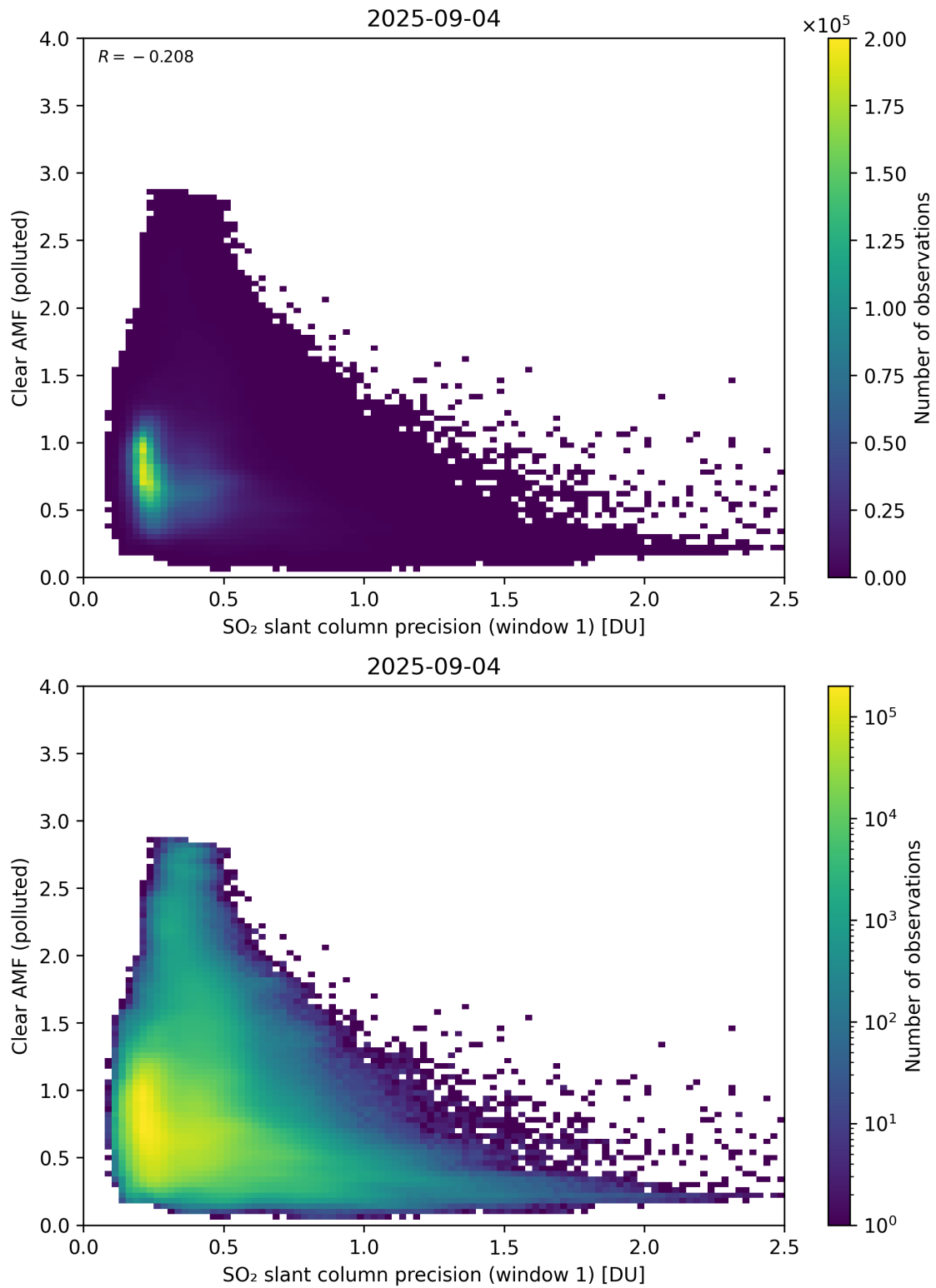
Figure 274: Scatter density plot of “SO 2 slant column precision (window 1)” against “Clear AMF (polluted)” for 2025-09-04 to 2025-09-05.
