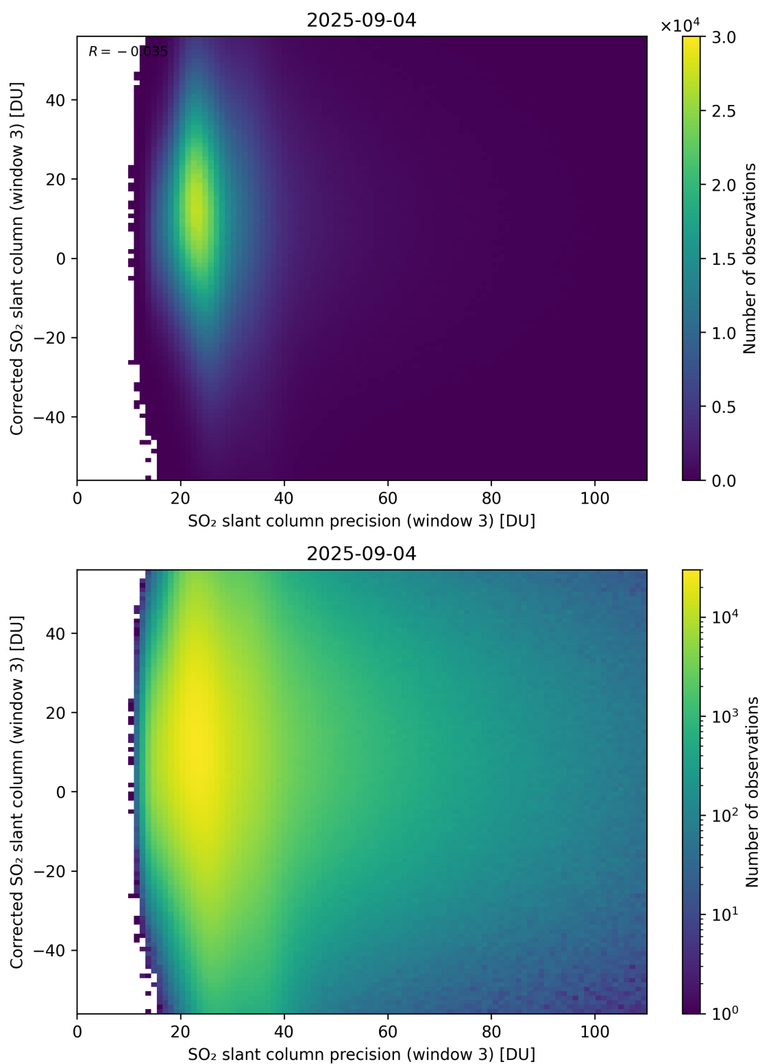
Figure 312: Scatter density plot of “SO 2 slant column precision (window 3)” against “Corrected SO 2 slant column (window 3)” for 2025-09-04 to 2025-09-05.
