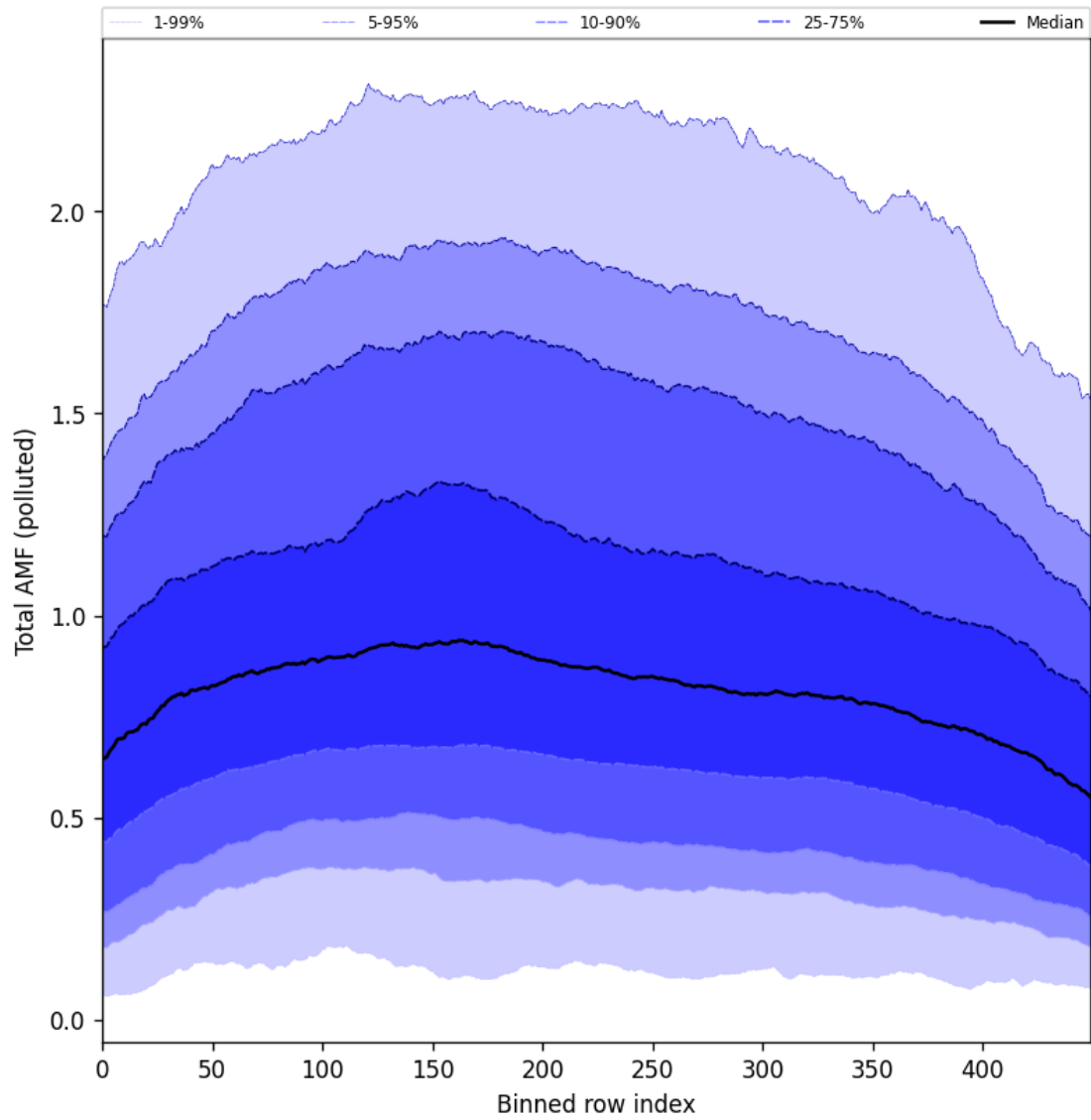
Figure 105: Along track statistics of “Total AMF (polluted)” for 2025-09-04 to 2025-09-05
