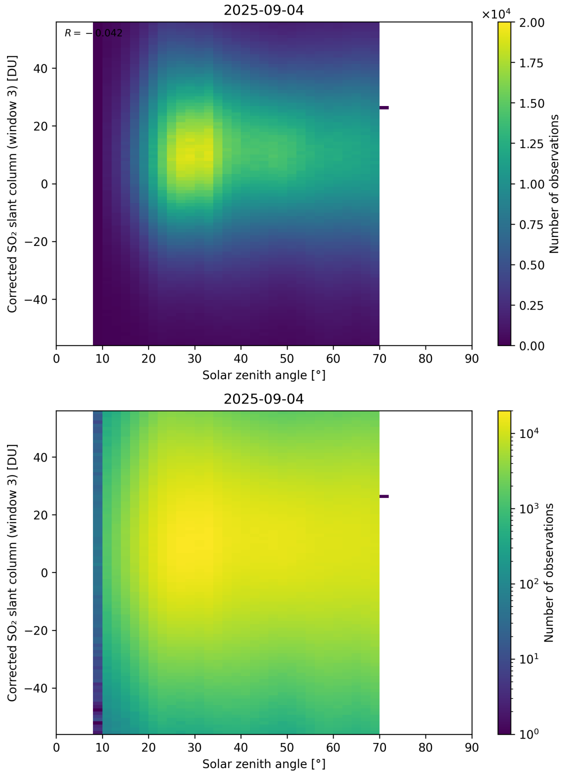
Figure 183: Scatter density plot of “Solar zenith angle” against “Corrected SO 2 slant column (window 3)” for 2025-09-04 to 2025-09-05.
