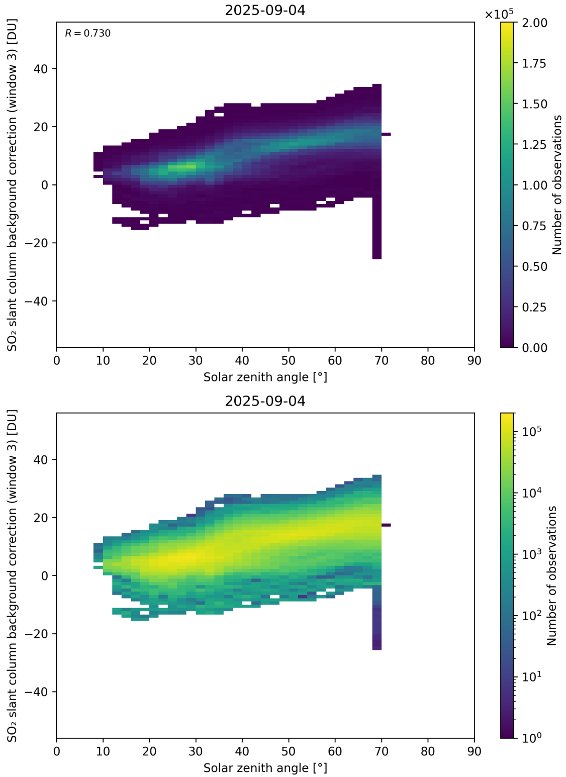
Figure 173: Scatter density plot of “Solar zenith angle” against “SO 2 slant column background correction (window 3)” for 2025-09-04 to 2025-09-05.
