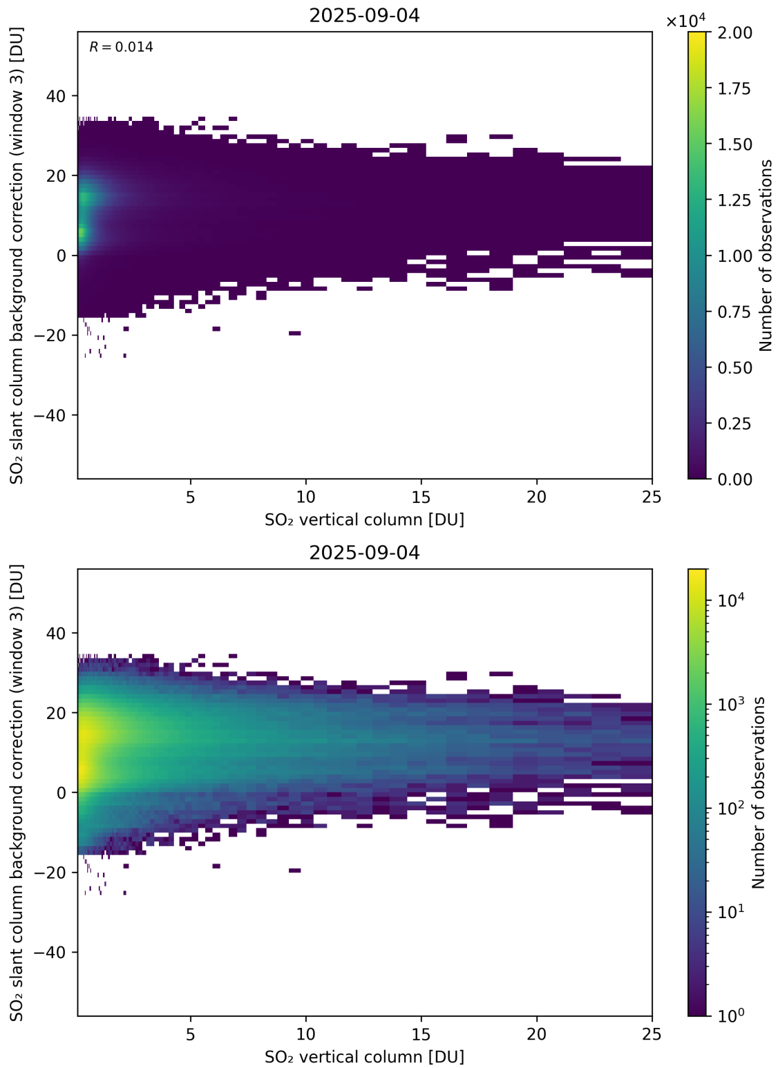
Figure 325: Scatter density plot of “SO 2 vertical column” against “SO 2 slant column background correction (window 3)” for 2025-09-04 to 2025-09-05.
