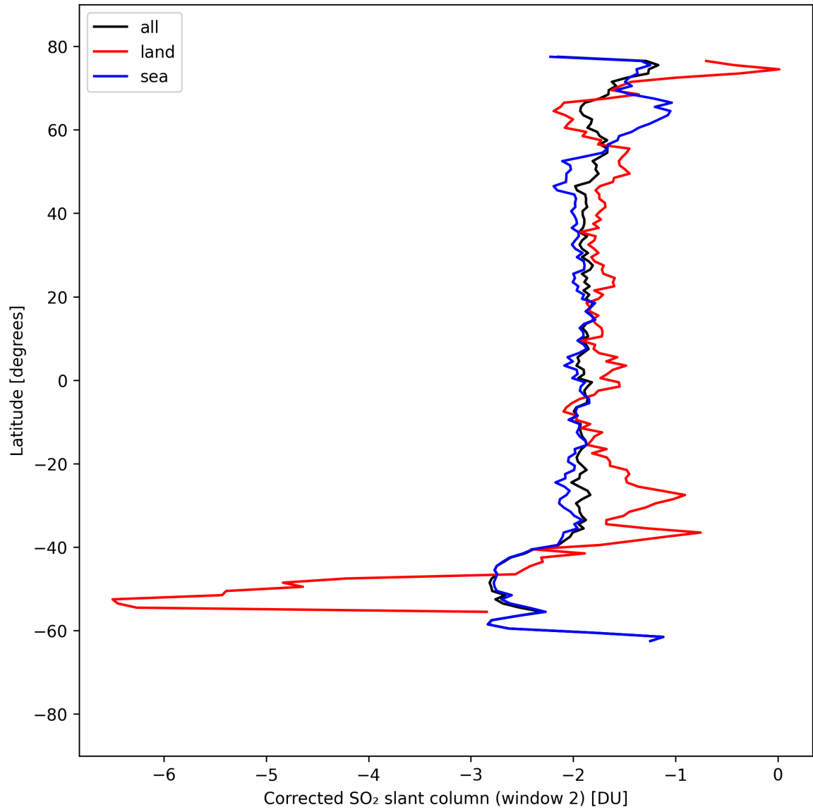
Figure 43: Zonal average of “Corrected SO 2 slant column (window 2)” for 2025-09-04 to 2025-09-05.
