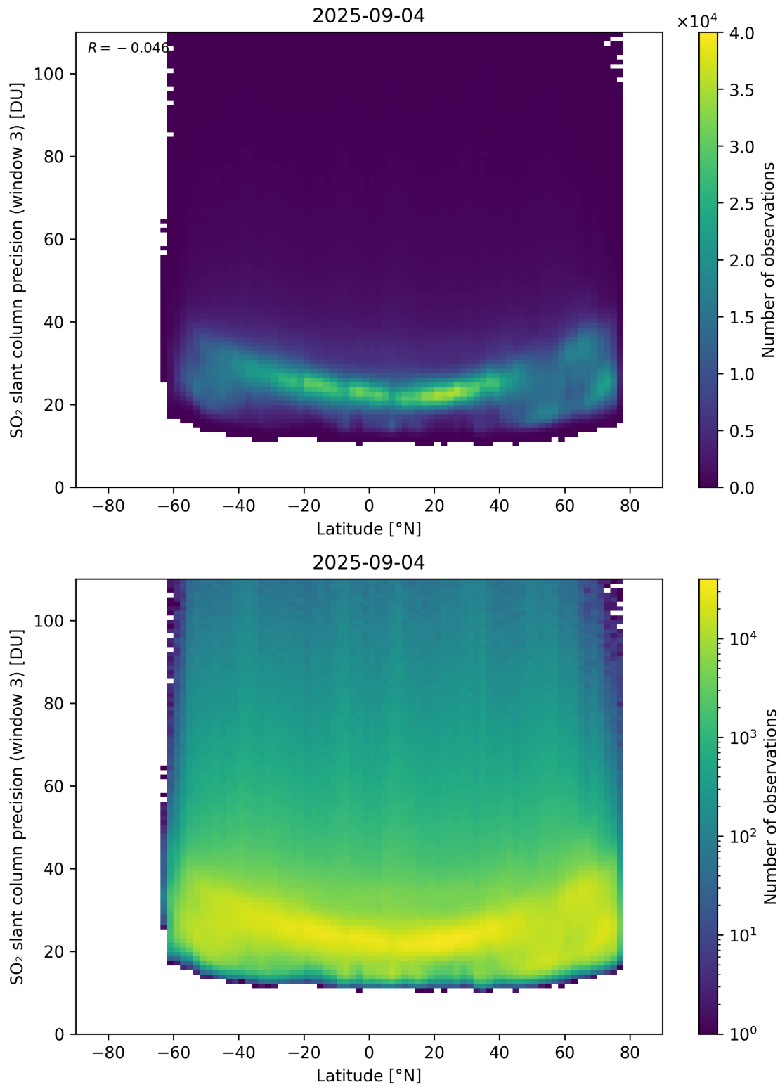
Figure 166: Scatter density plot of “Latitude” against “SO 2 slant column precision (window 3)” for 2025-09-04 to 2025-09-05.
