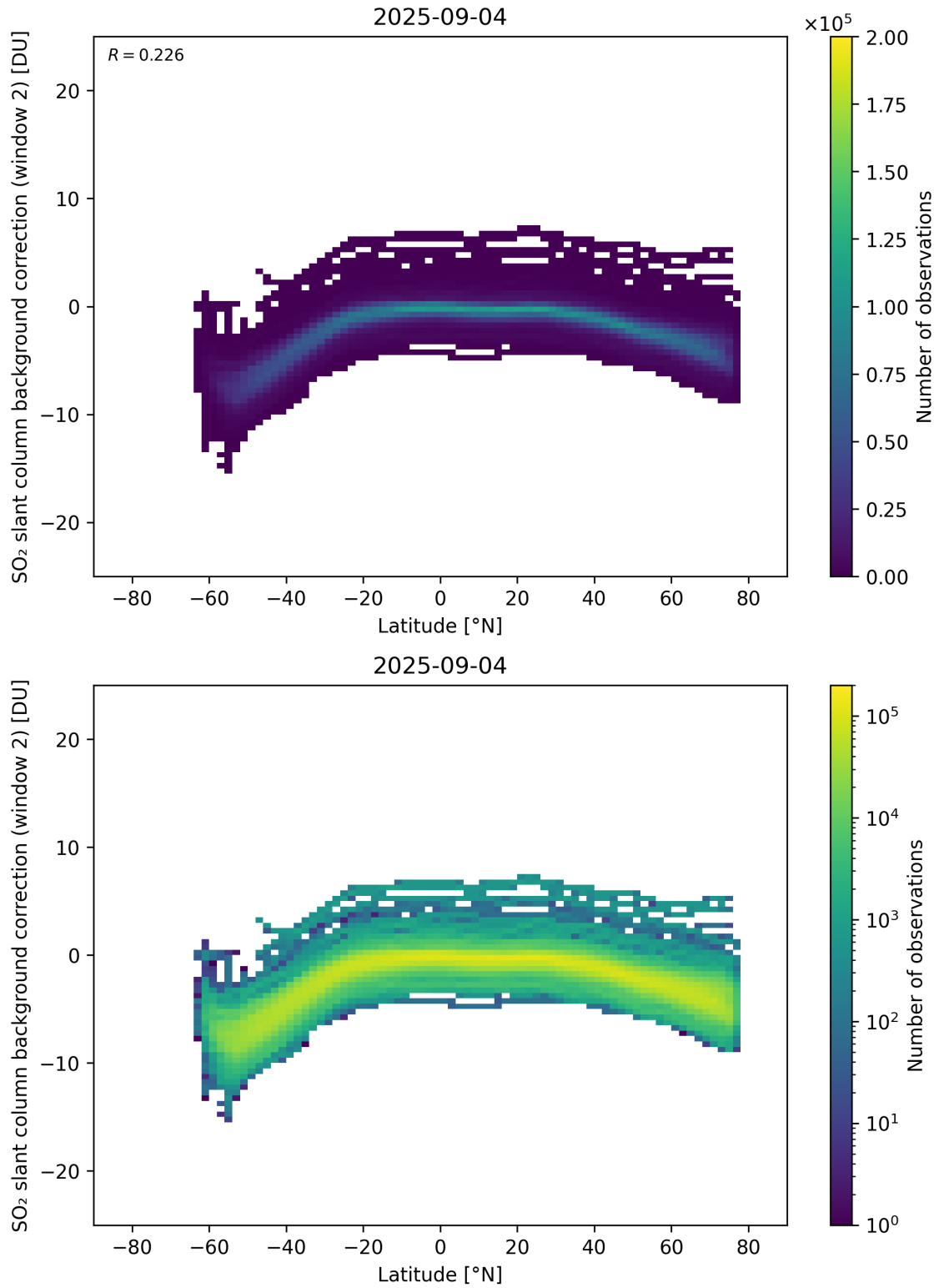
Figure 151: Scatter density plot of “Latitude” against “SO 2 slant column background correction (window 2)” for 2025-09-04 to 2025-09-05.
