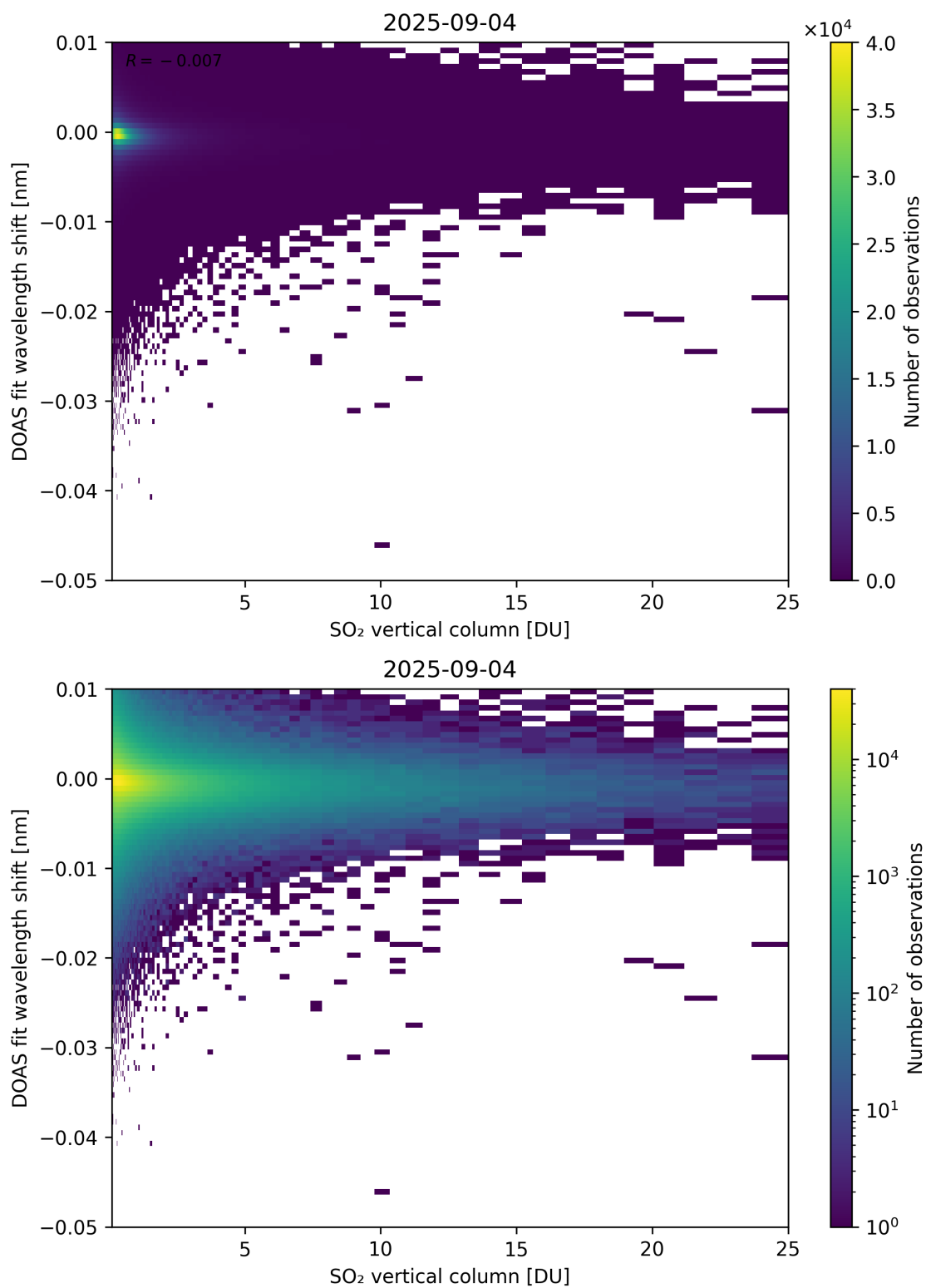
Figure 326: Scatter density plot of “SO 2 vertical column” against “DOAS fit wavelength shift” for 2025-09-04 to 2025-09-05.
