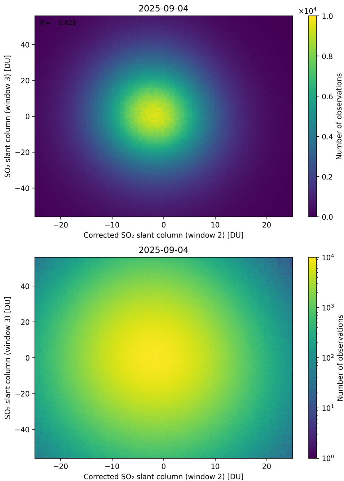
Figure 251: Scatter density plot of “Corrected SO 2 slant column (window 2)” against “SO 2 slant column (window 3)” for 2025-09-04 to 2025-09-05.
