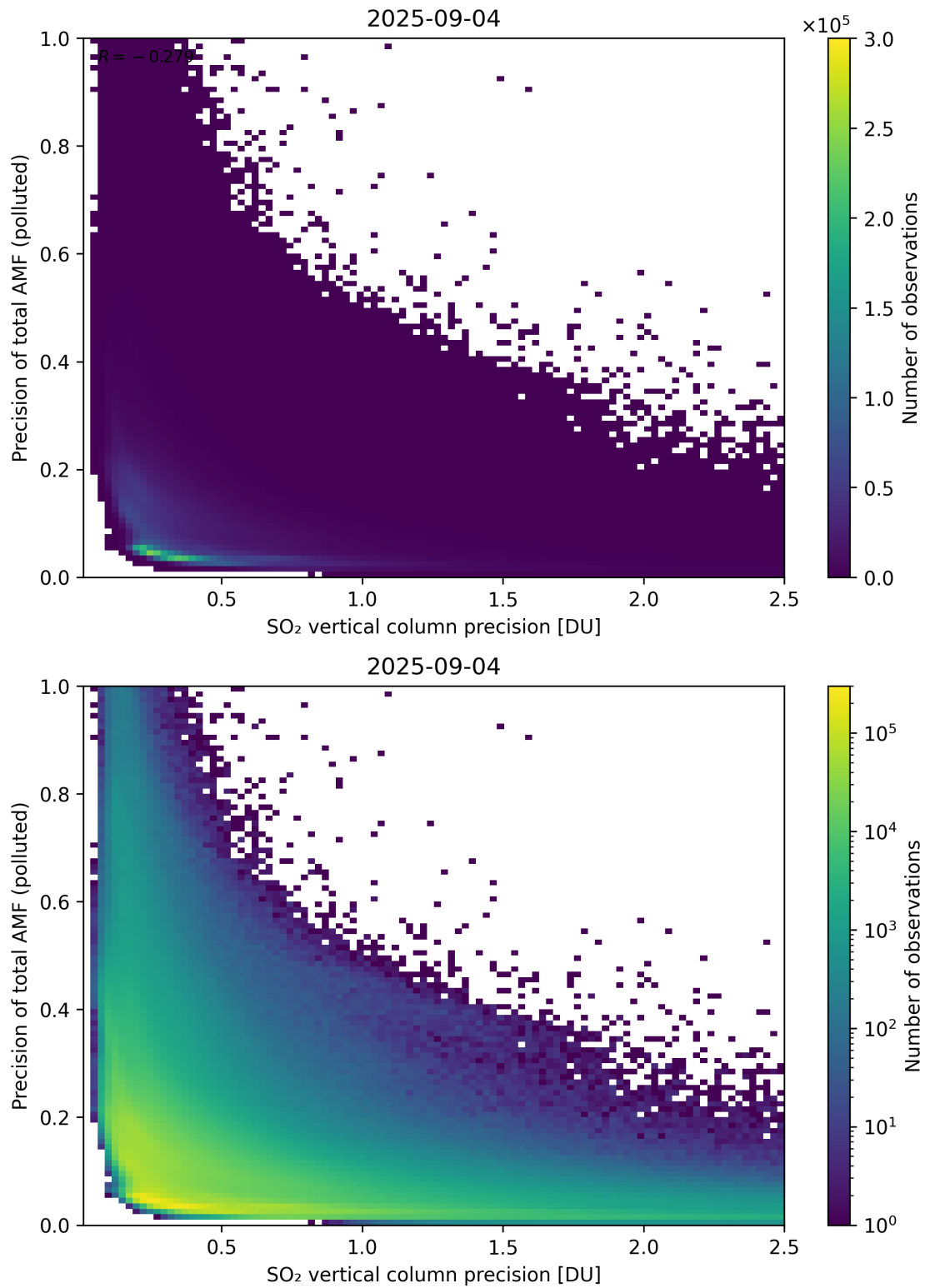
Figure 347: Scatter density plot of “SO 2 vertical column precision” against “Precision of total AMF (polluted)” for 2025-09-04 to 2025-09-05.
