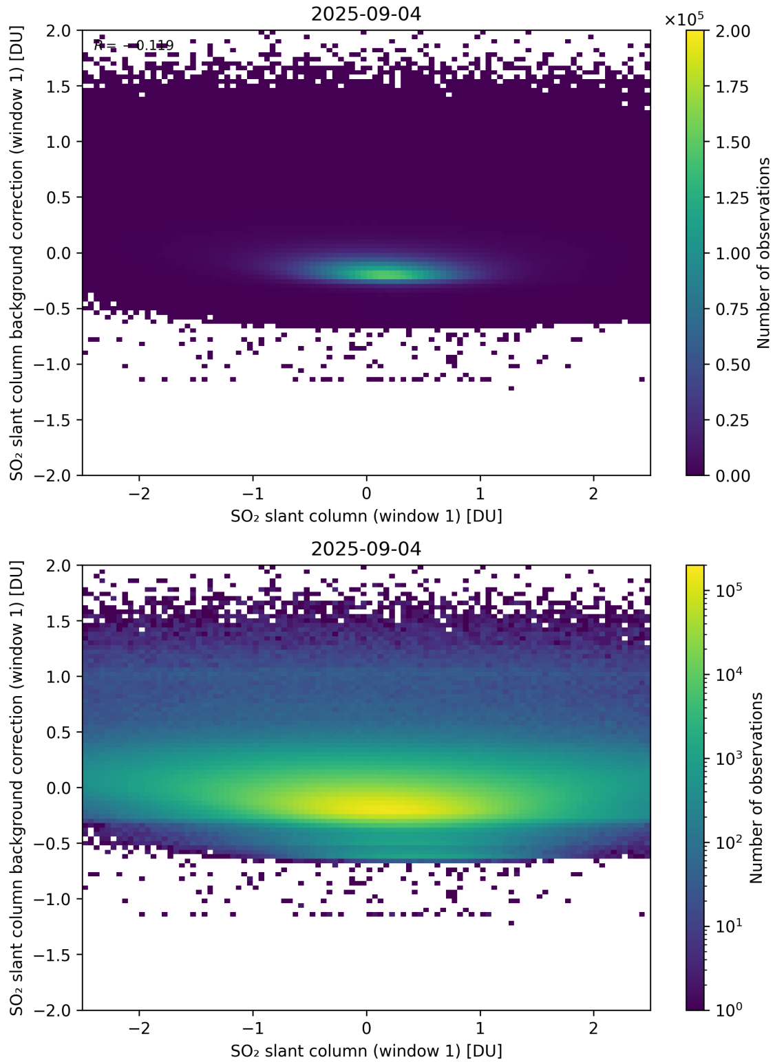
Figure 262: Scatter density plot of “SO 2 slant column (window 1)” against “SO 2 slant column background correction (window 1)” for 2025-09-04 to 2025-09-05.
