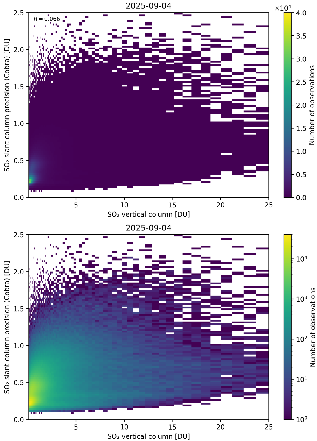
Figure 350: Scatter density plot of “SO 2 vertical column” against “SO 2 slant column precision (Cobra)” for 2025-09-04 to 2025-09-05.
