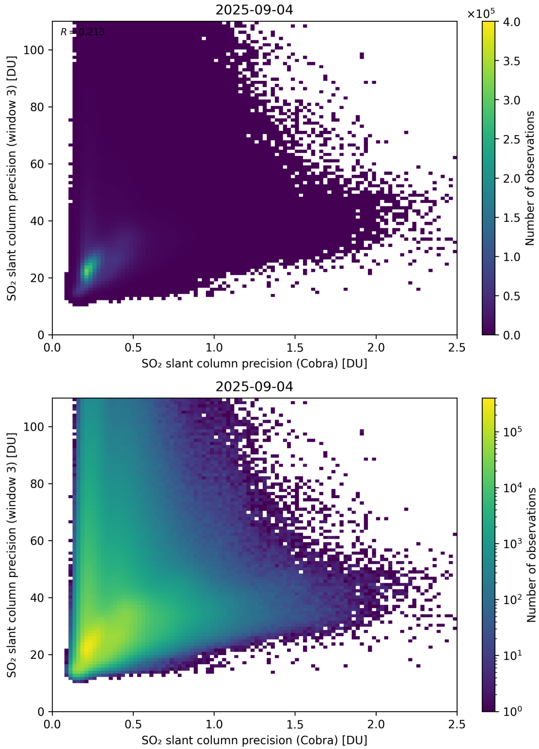
Figure 212: Scatter density plot of “SO 2 slant column precision (Cobra)” against “SO 2 slant column precision (window 3)” for 2025-09-04 to 2025-09-05.
