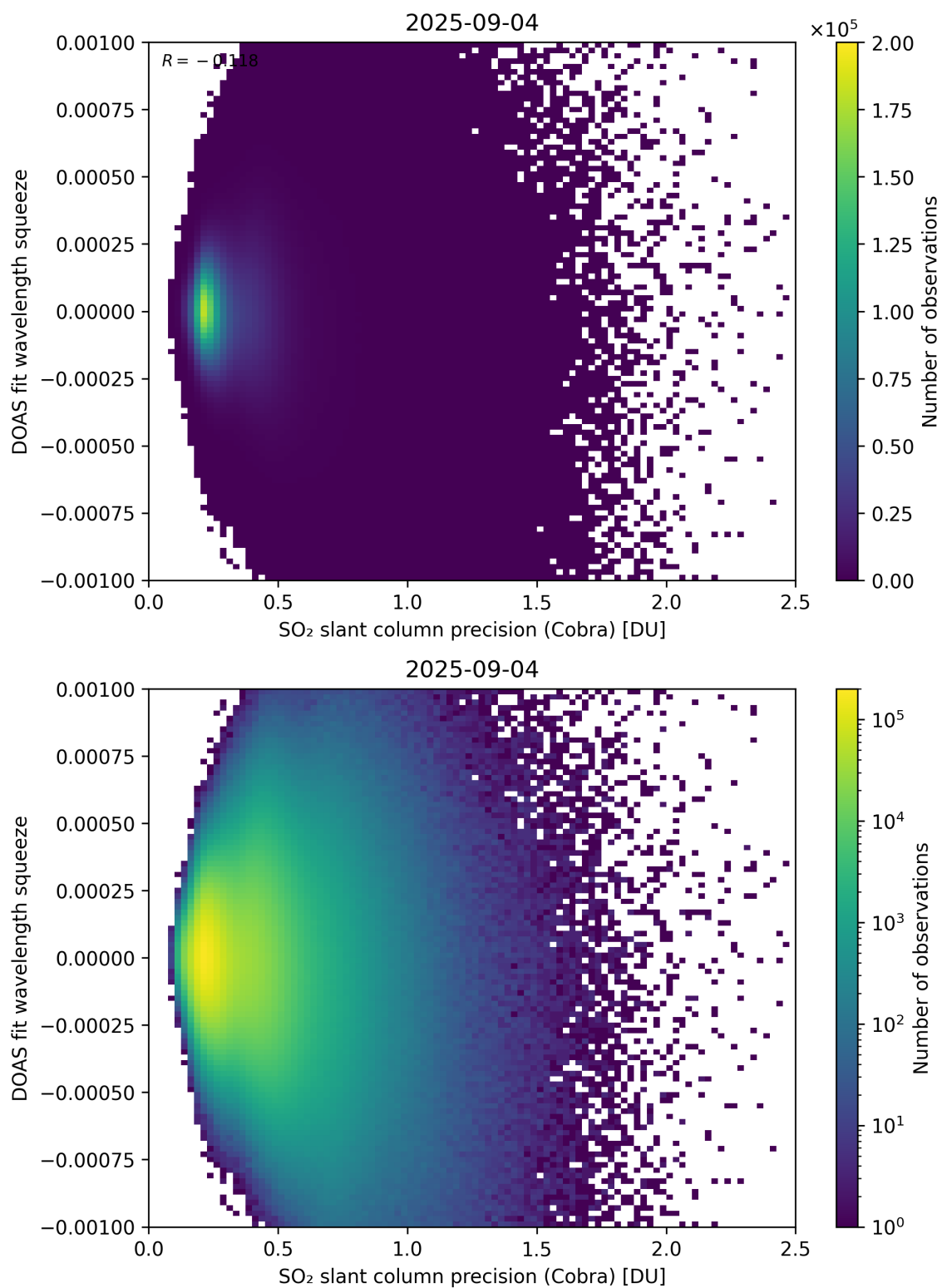
Figure 203: Scatter density plot of “SO 2 slant column precision (Cobra)” against “DOAS fit wavelength squeeze” for 2025-09-04 to 2025-09-05.
