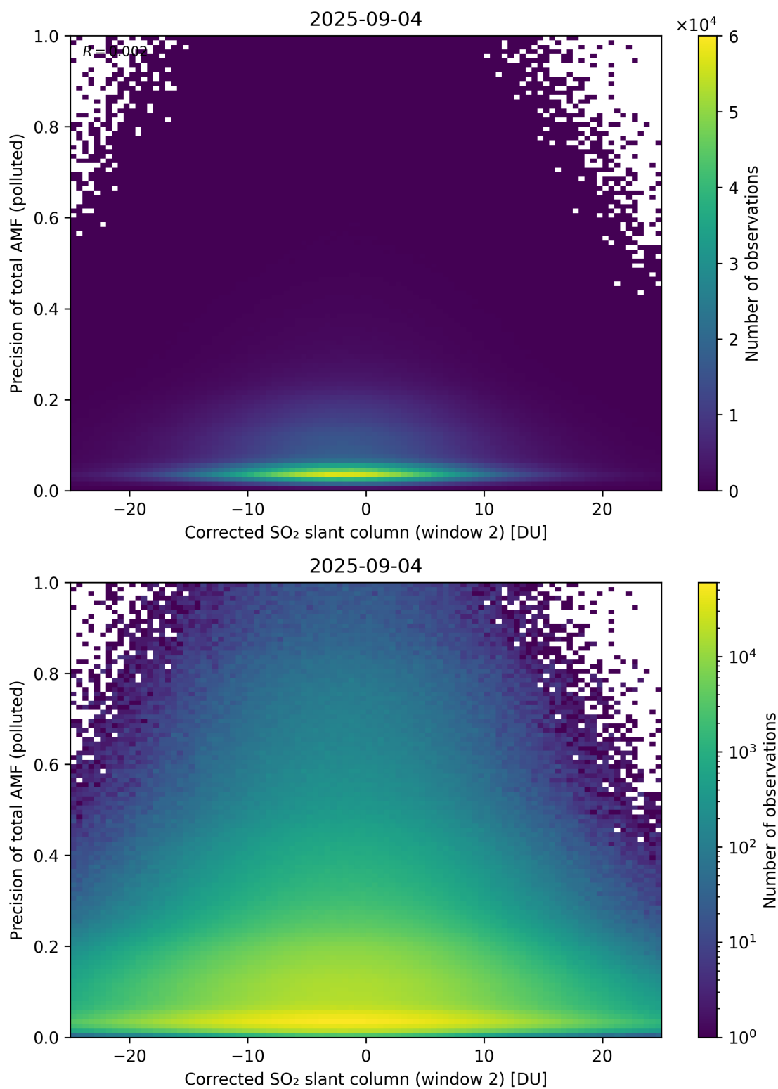
Figure 254: Scatter density plot of “Corrected SO 2 slant column (window 2)” against “Precision of total AMF (polluted)” for 2025-09-04 to 2025-09-05.
