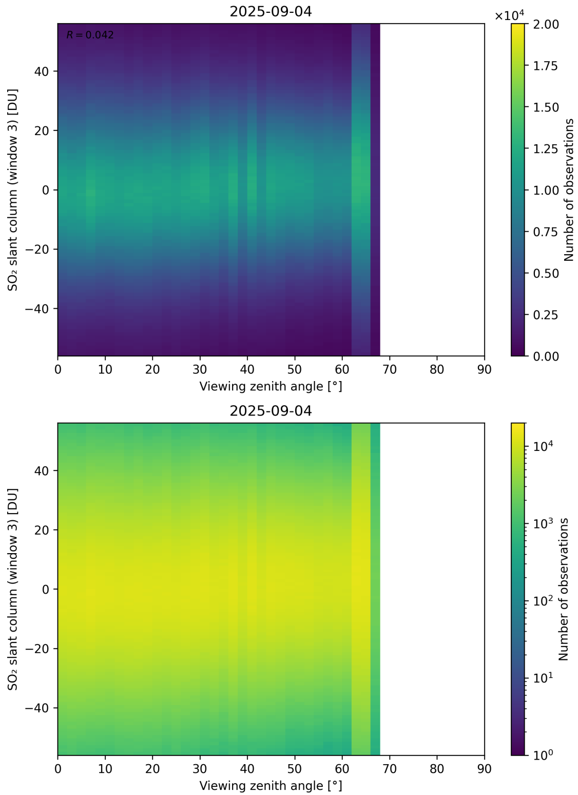
Figure 379: Scatter density plot of “Viewing zenith angle” against “SO 2 slant column (window 3)” for 2025-09-04 to 2025-09-05.
