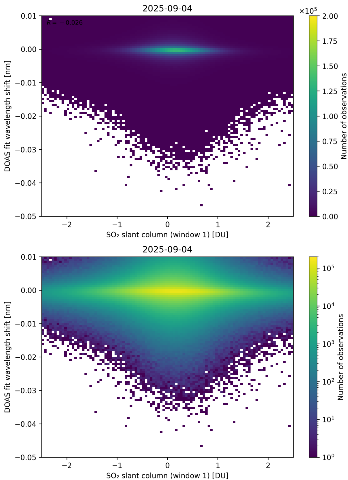
Figure 265: Scatter density plot of “SO 2 slant column (window 1)” against “DOAS fit wavelength shift” for 2025-09-04 to 2025-09-05.
