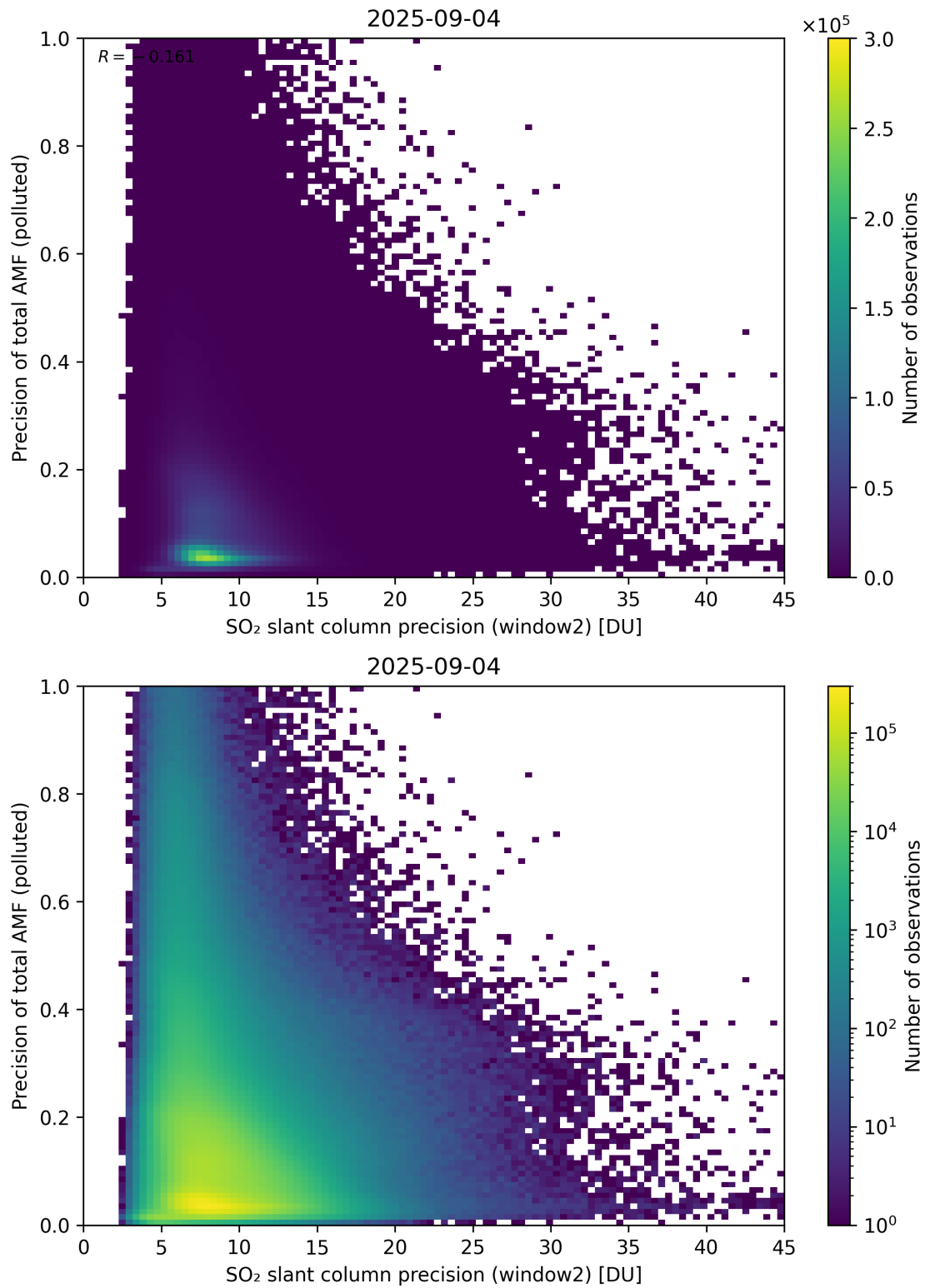
Figure 302: Scatter density plot of “SO 2 slant column precision (window2)” against “Precision of total AMF (polluted)” for 2025-09-04 to 2025-09-05.
