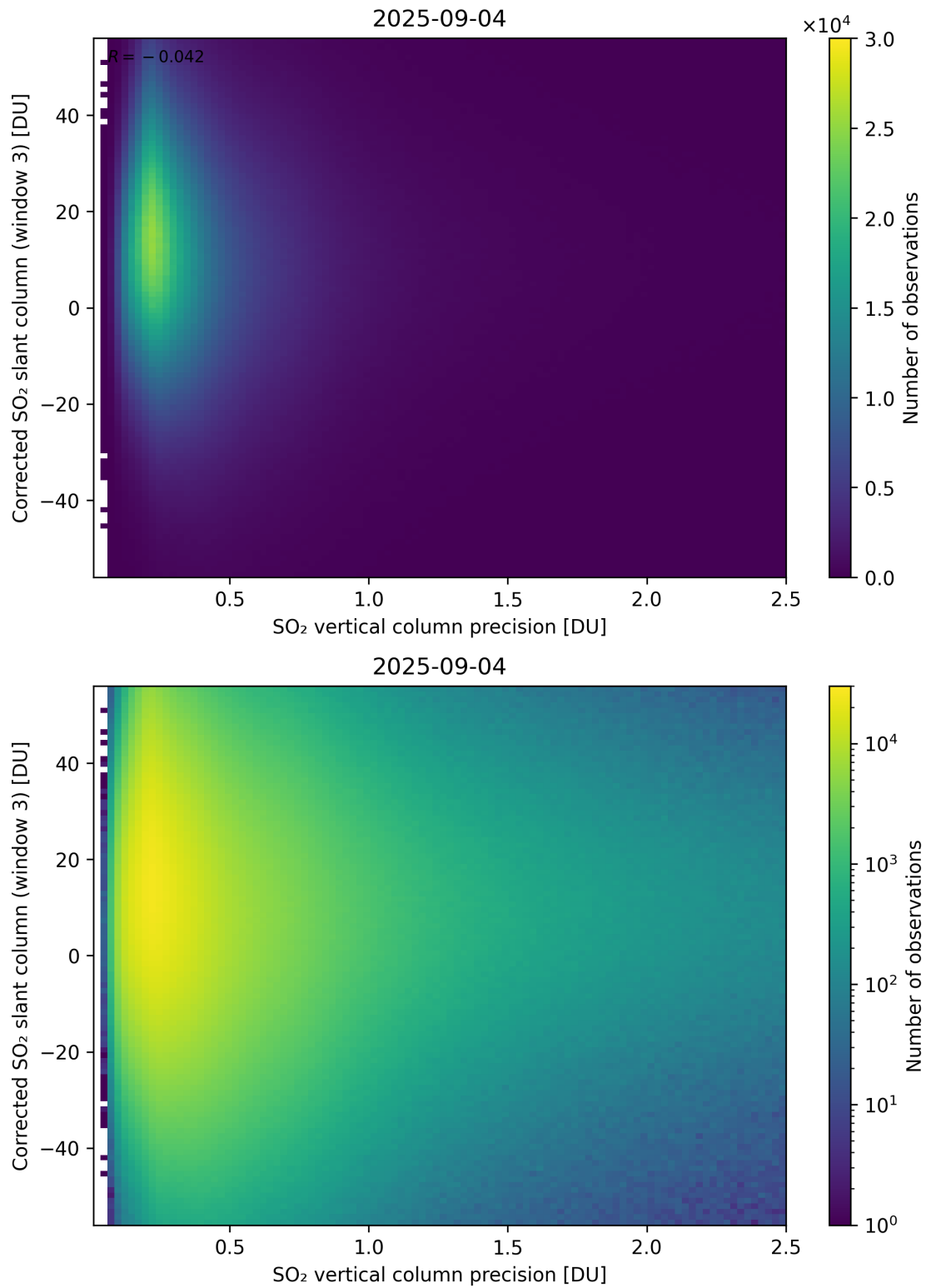
Figure 340: Scatter density plot of “SO 2 vertical column precision” against “Corrected SO 2 slant column (window 3)” for 2025-09-04 to 2025-09-05.
