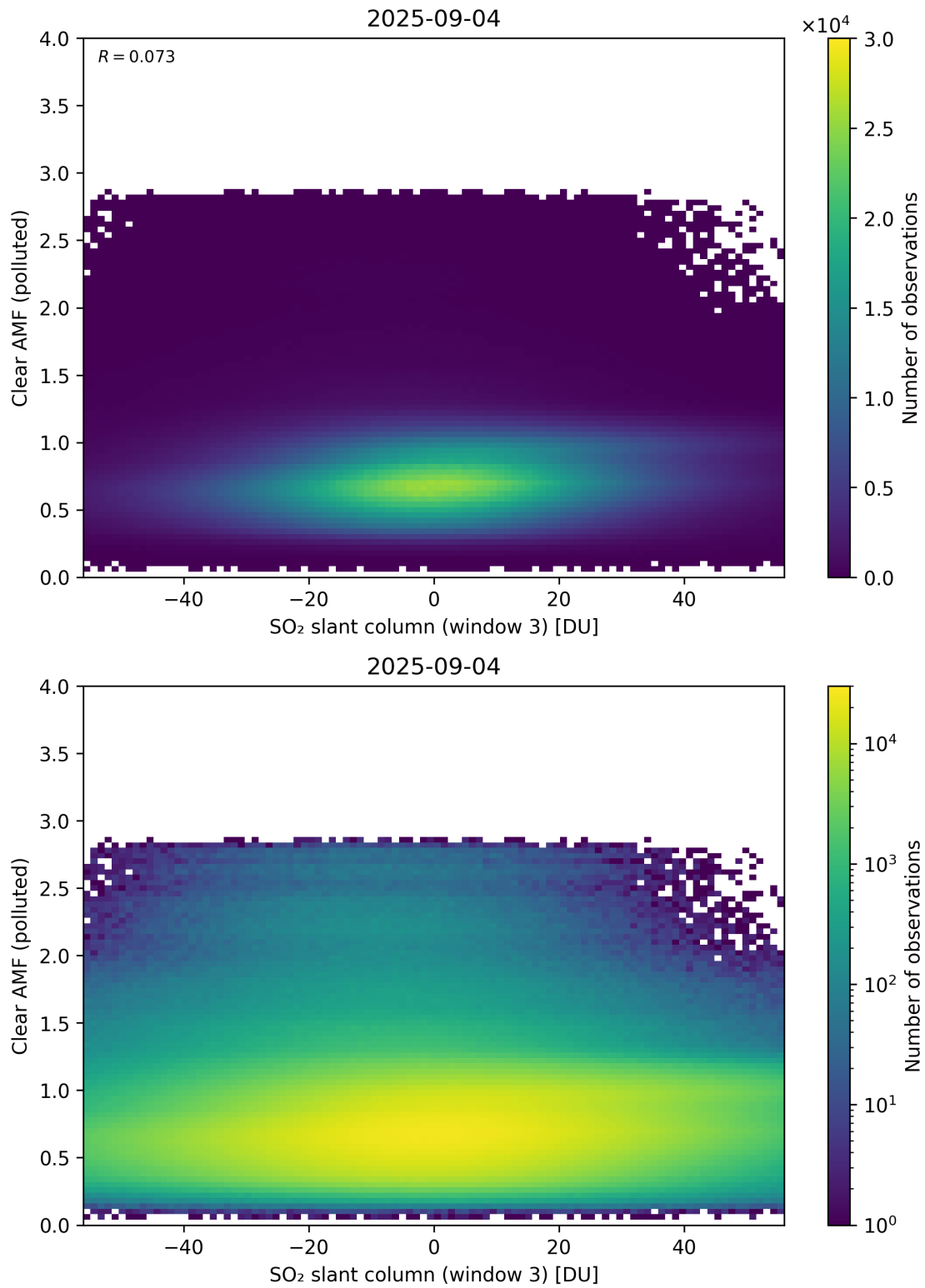
Figure 315: Scatter density plot of “SO 2 slant column (window 3)” against “Clear AMF (polluted)” for 2025-09-04 to 2025-09-05.
