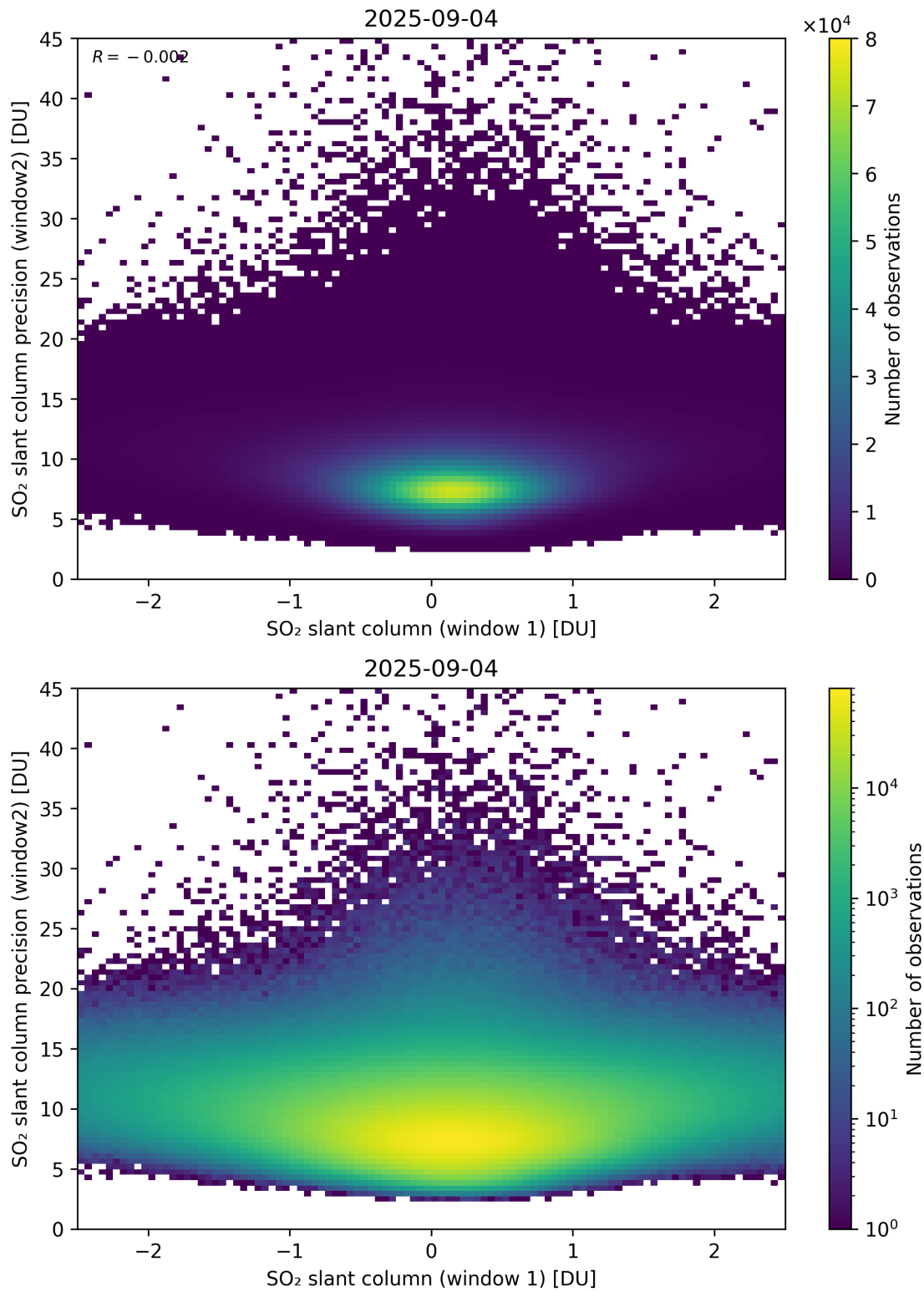
Figure 286: Scatter density plot of “SO 2 slant column (window 1)” against “SO 2 slant column precision (window2)” for 2025-09-04 to 2025-09-05.
