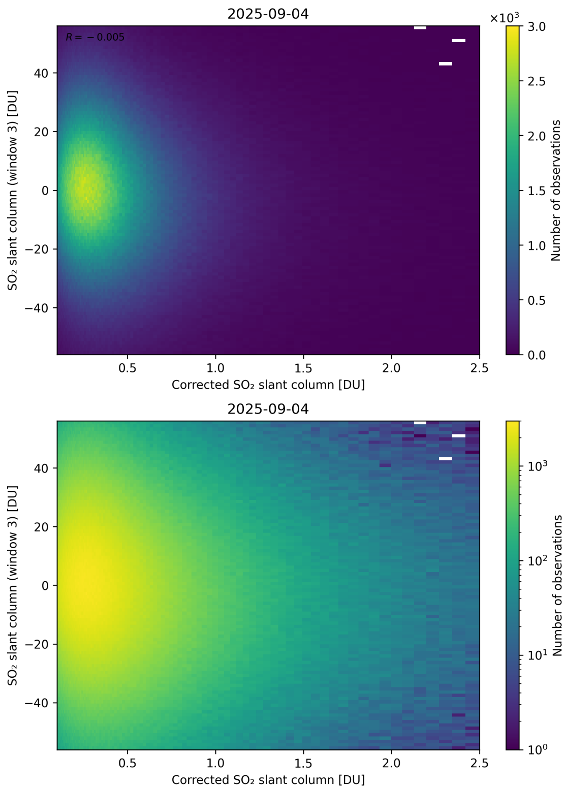
Figure 240: Scatter density plot of “Corrected SO 2 slant column” against “SO 2 slant column (window 3)” for 2025-09-04 to 2025-09-05.
