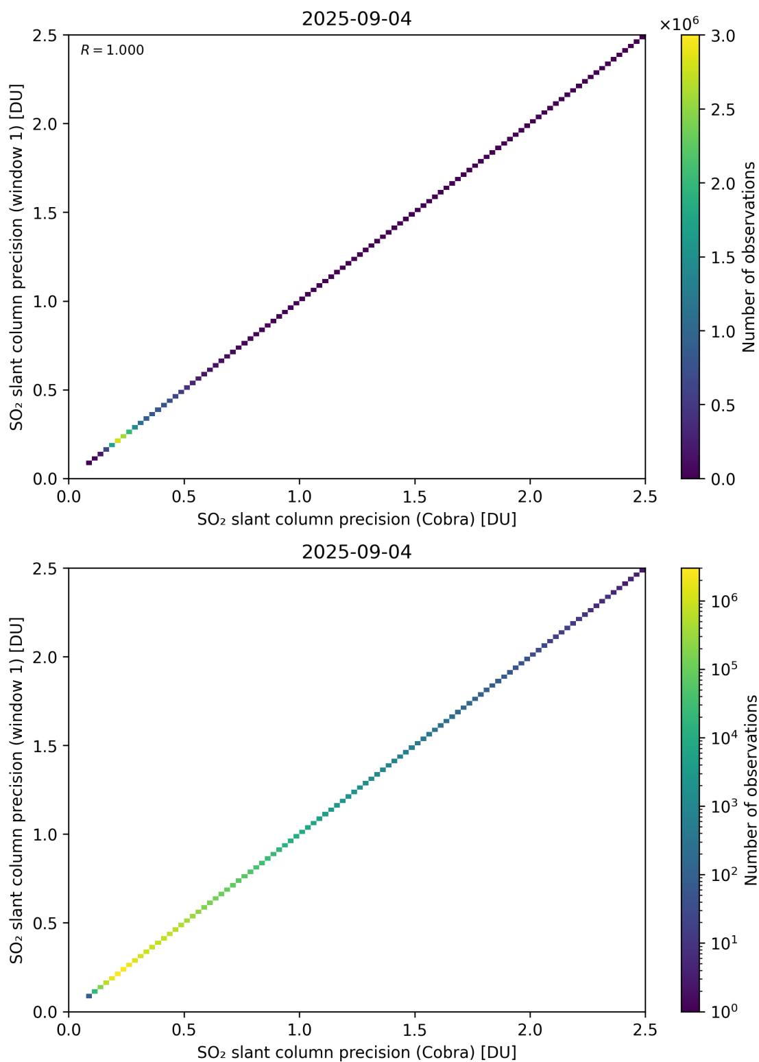
Figure 209: Scatter density plot of “SO 2 slant column precision (Cobra)” against “SO 2 slant column precision (window 1)” for 2025-09-04 to 2025-09-05.
