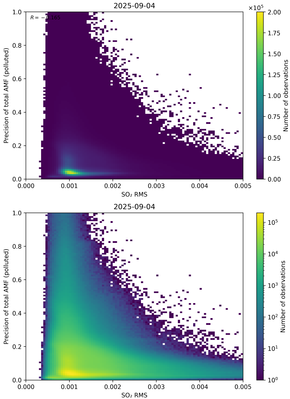
Figure 149: Scatter density plot of “SO 2 RMS” against “Precision of total AMF (polluted)” for 2025-09-04 to 2025-09-05.
