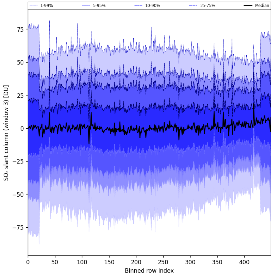
Figure 97: Along track statistics of “SO 2 slant column (window 3)” for 2025-09-04 to 2025-09-05
