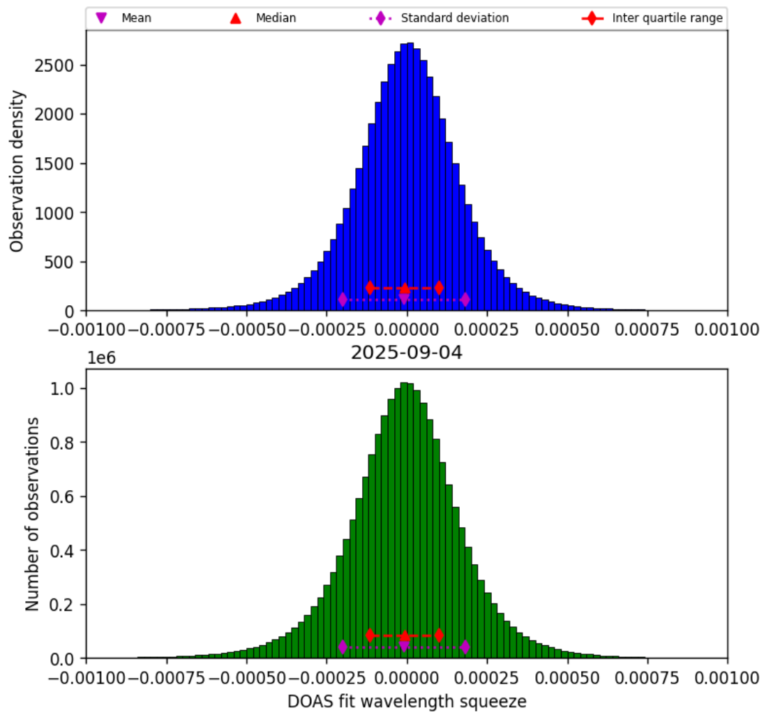
Figure 77: Histogram of “DOAS fit wavelength squeeze” for 2025-09-04 to 2025-09-05
