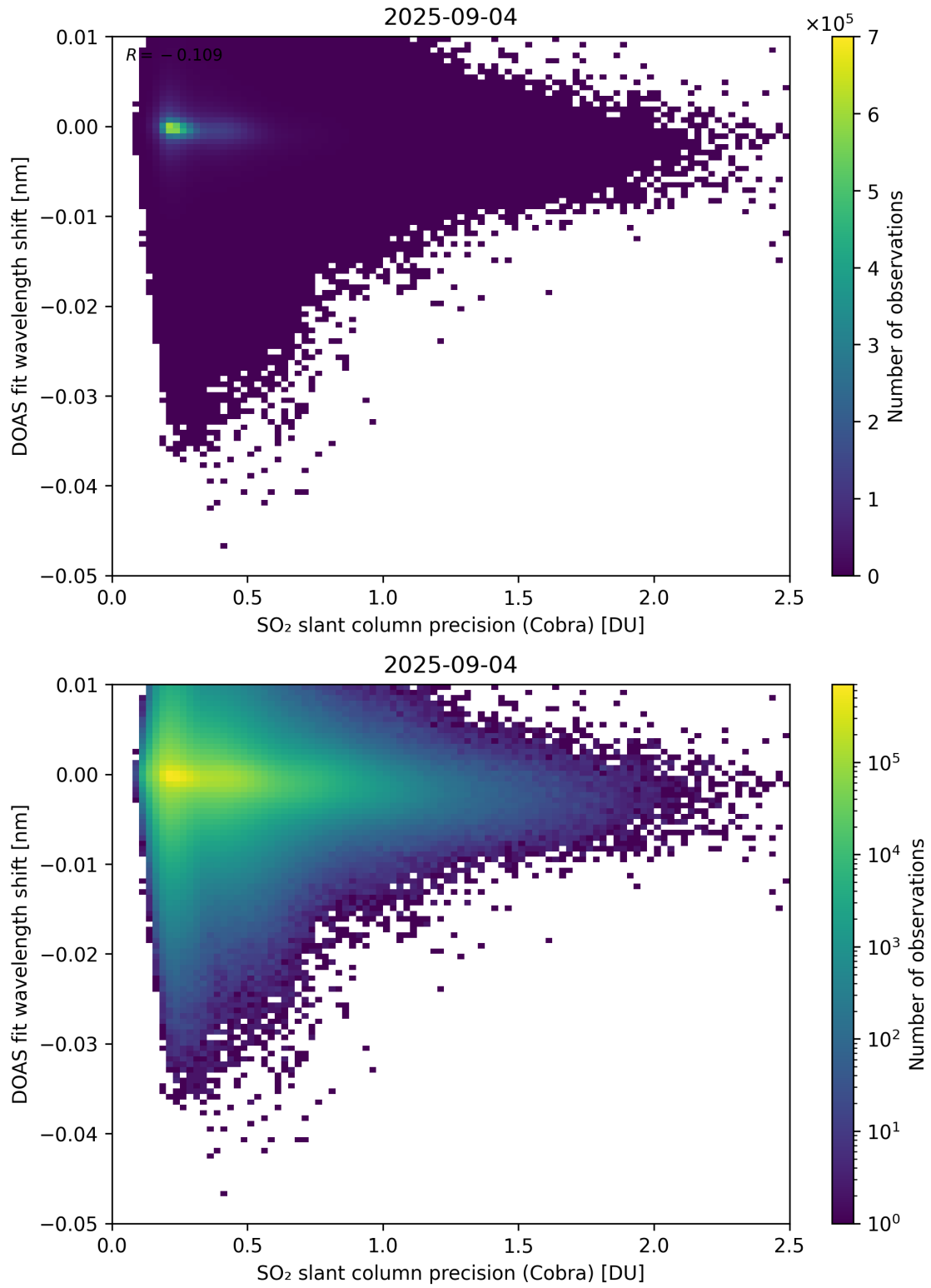
Figure 202: Scatter density plot of “SO 2 slant column precision (Cobra)” against “DOAS fit wavelength shift” for 2025-09-04 to 2025-09-05.
