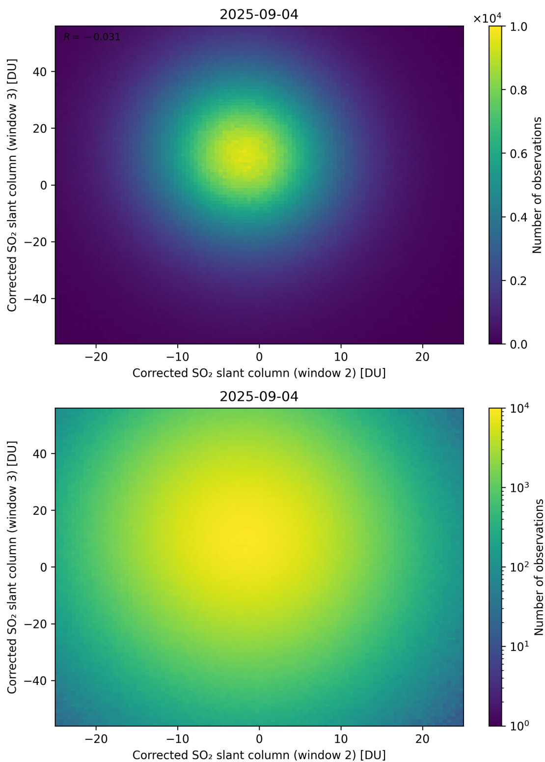
Figure 250: Scatter density plot of “Corrected SO 2 slant column (window 2)” against “Corrected SO 2 slant column (window 3)” for 2025-09-04 to 2025-09-05.
