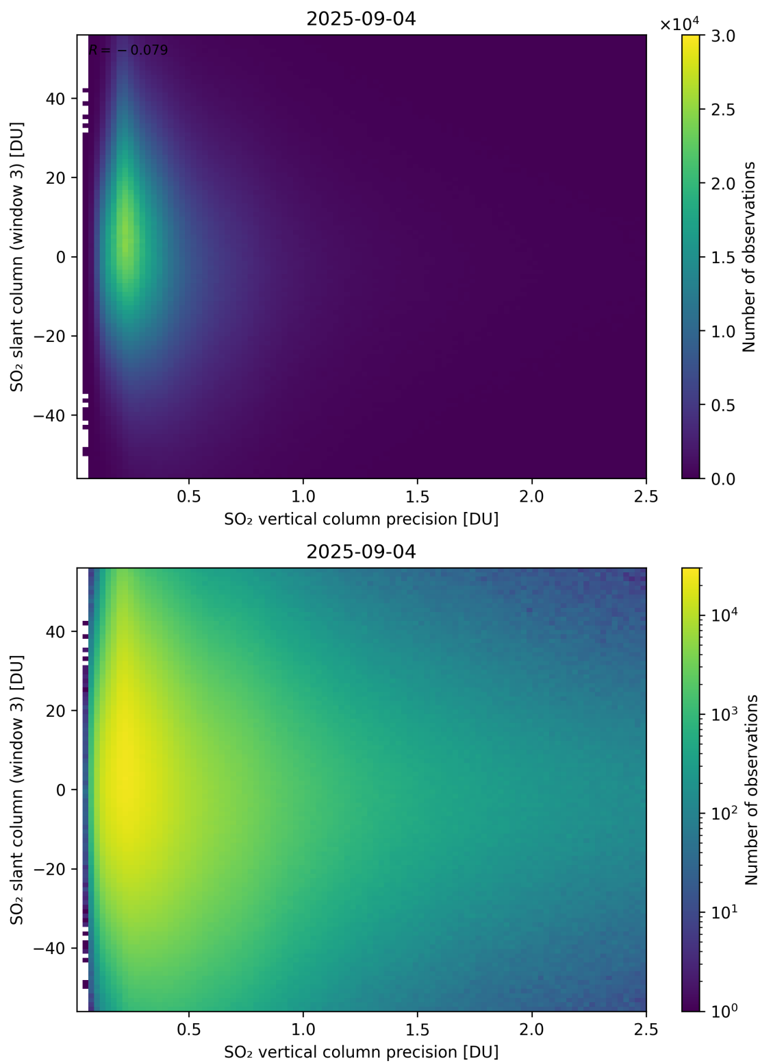
Figure 344: Scatter density plot of “SO 2 vertical column precision” against “SO 2 slant column (window 3)” for 2025-09-04 to 2025-09-05.
