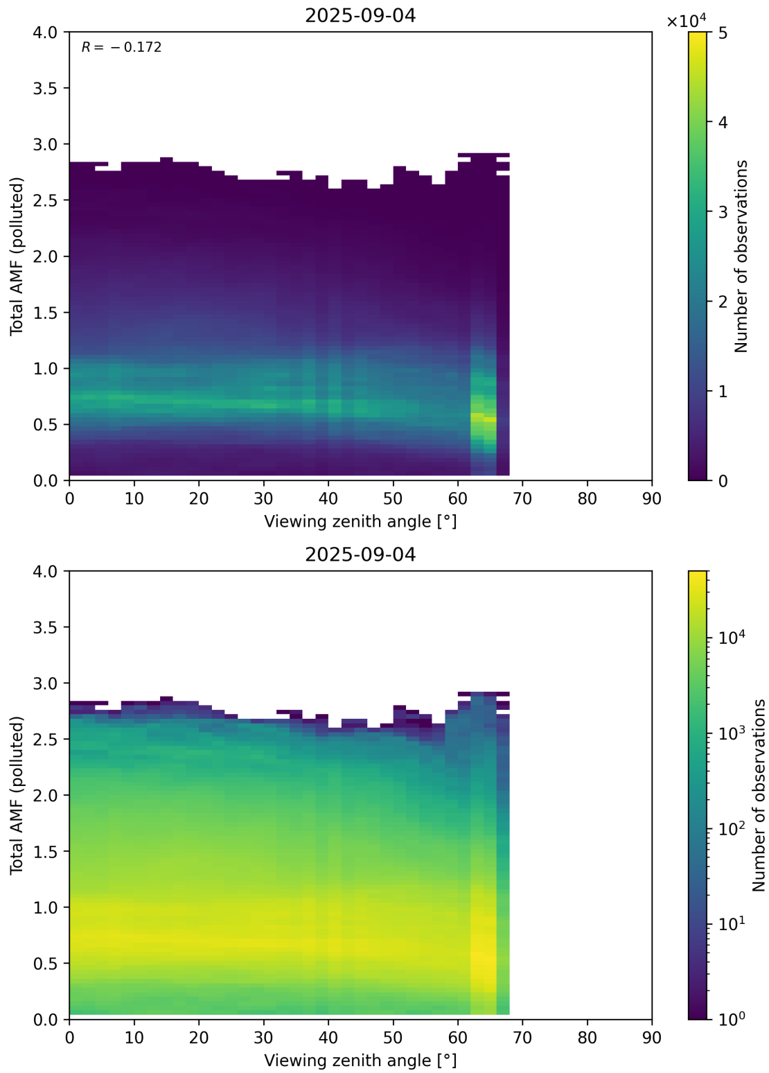
Figure 381: Scatter density plot of “Viewing zenith angle” against “Total AMF (polluted)” for 2025-09-04 to 2025-09-05.
