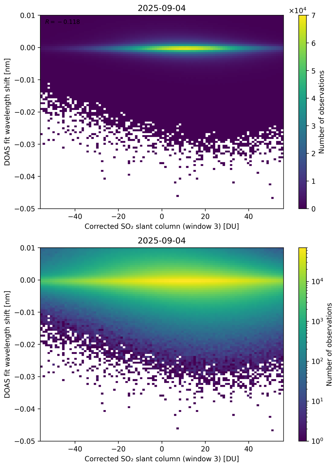
Figure 256: Scatter density plot of “Corrected SO 2 slant column (window 3)” against “DOAS fit wavelength shift” for 2025-09-04 to 2025-09-05.
