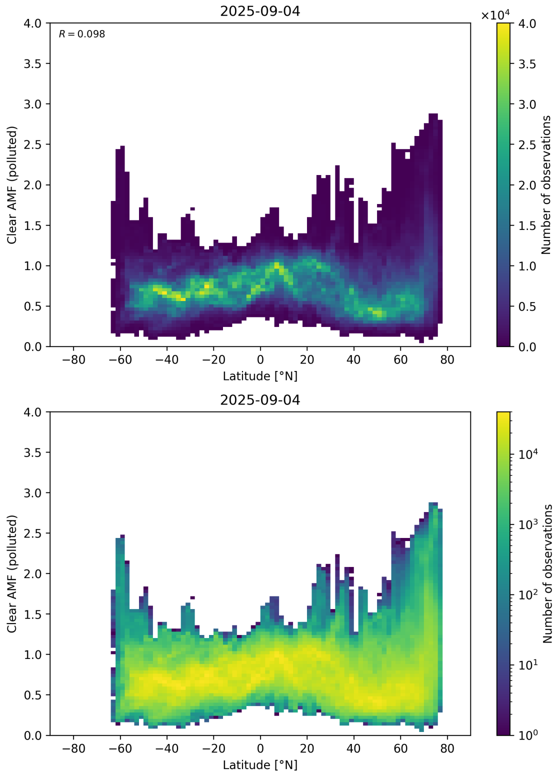
Figure 156: Scatter density plot of “Latitude” against “Clear AMF (polluted)” for 2025-09-04 to 2025-09-05.
