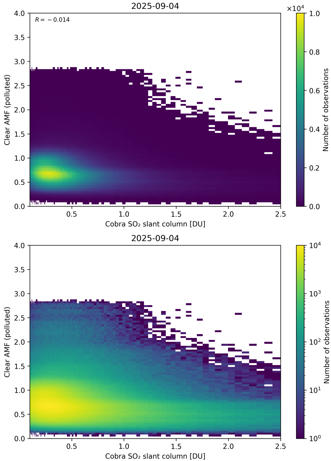
Figure 215: Scatter density plot of “Cobra SO 2 slant column” against “Clear AMF (polluted)” for 2025-09-04 to 2025-09-05.
