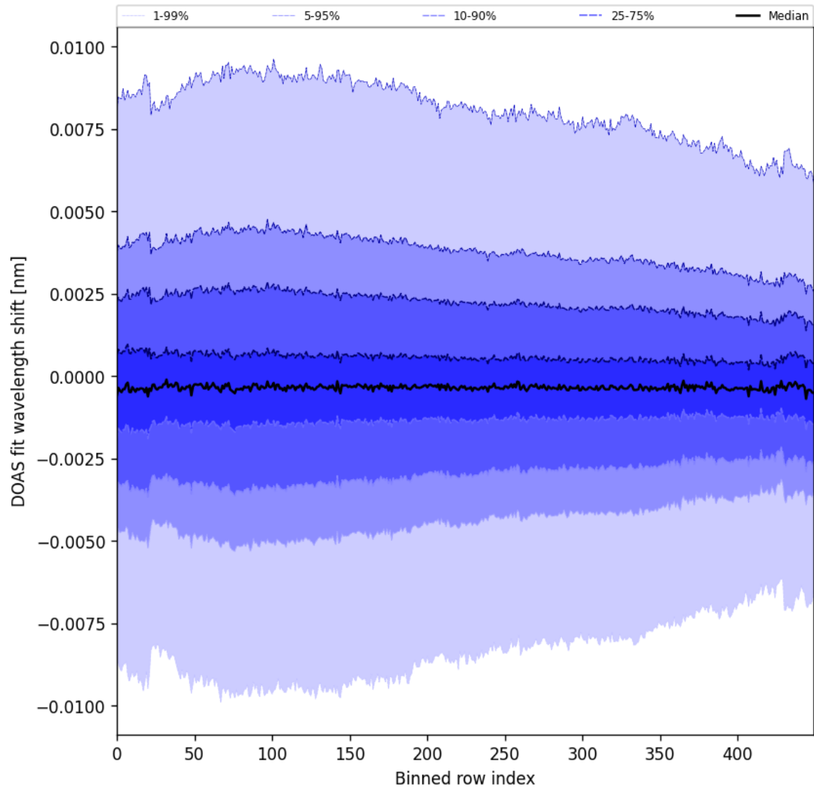
Figure 102: Along track statistics of “DOAS fit wavelength shift” for 2025-09-04 to 2025-09-05
