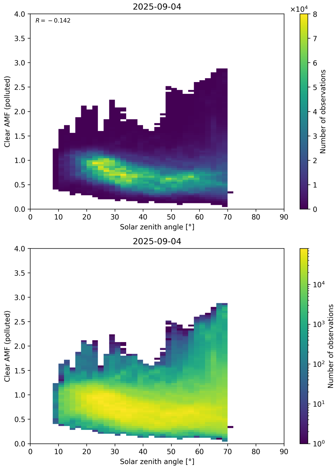
Figure 178: Scatter density plot of “Solar zenith angle” against “Clear AMF (polluted)” for 2025-09-04 to 2025-09-05.
