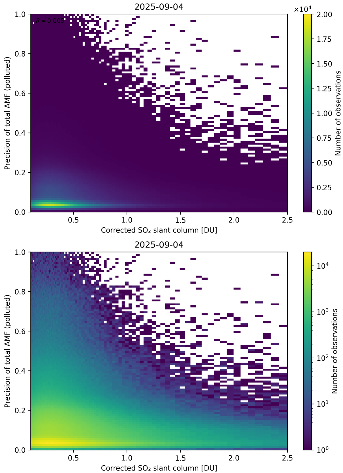
Figure 243: Scatter density plot of “Corrected SO 2 slant column” against “Precision of total AMF (polluted)” for 2025-09-04 to 2025-09-05.
