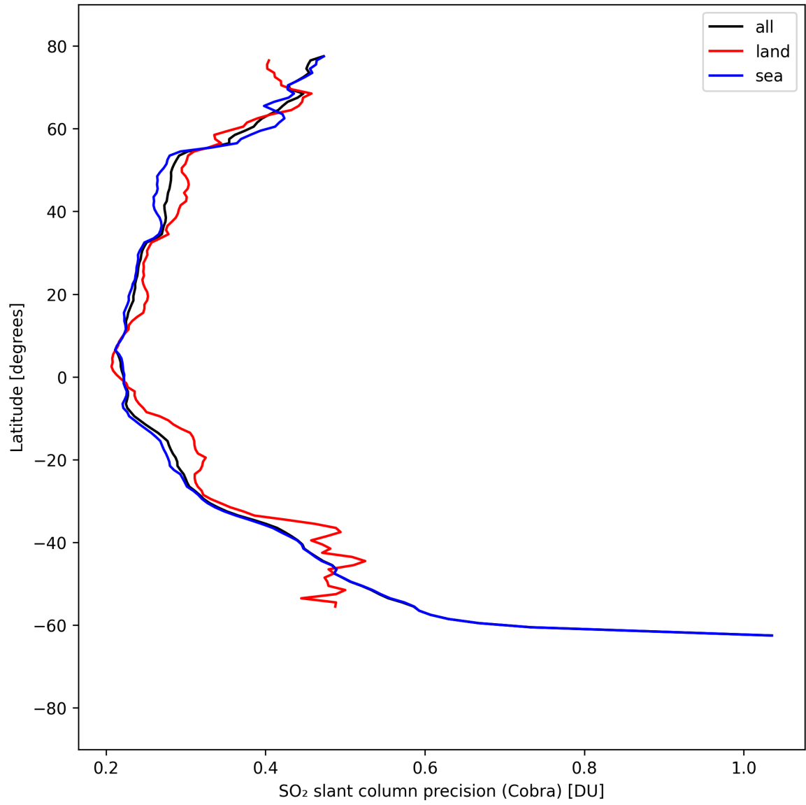
Figure 36: Zonal average of “SO 2 slant column precision (Cobra)” for 2025-09-04 to 2025-09-05.
