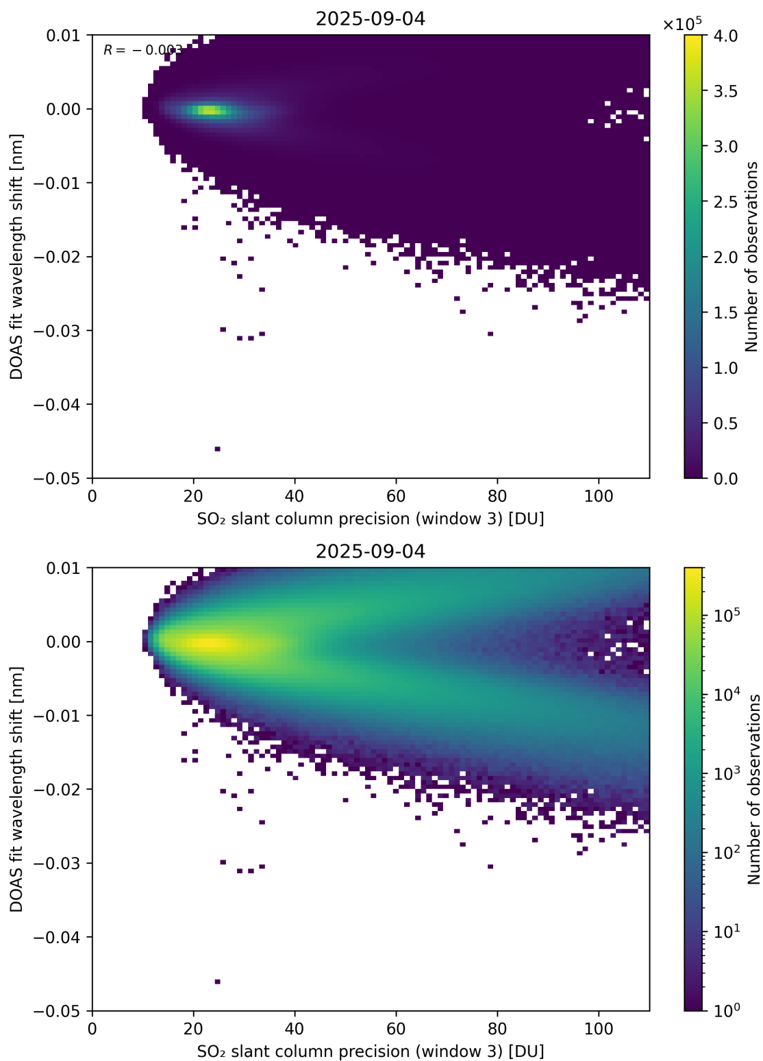
Figure 308: Scatter density plot of “SO 2 slant column precision (window 3)” against “DOAS fit wavelength shift” for 2025-09-04 to 2025-09-05.
