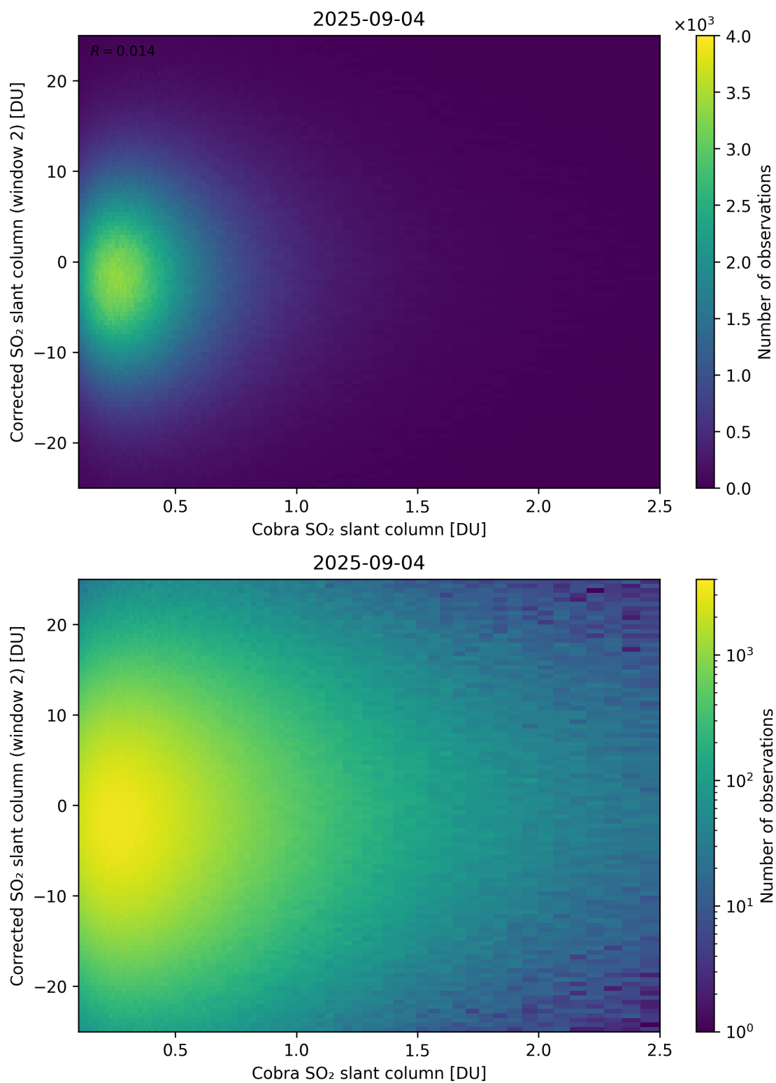
Figure 217: Scatter density plot of “Cobra SO 2 slant column” against “Corrected SO 2 slant column (window 2)” for 2025-09-04 to 2025-09-05.
