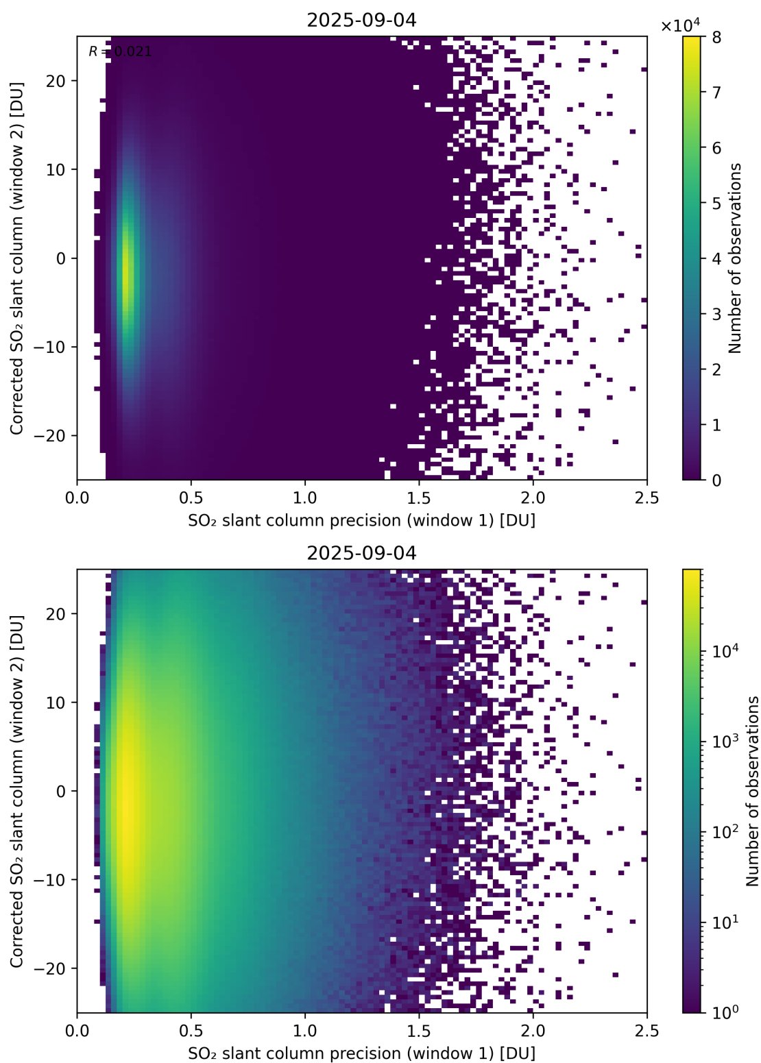
Figure 275: Scatter density plot of “SO 2 slant column precision (window 1)” against “Corrected SO 2 slant column (window 2)” for 2025-09-04 to 2025-09-05.
