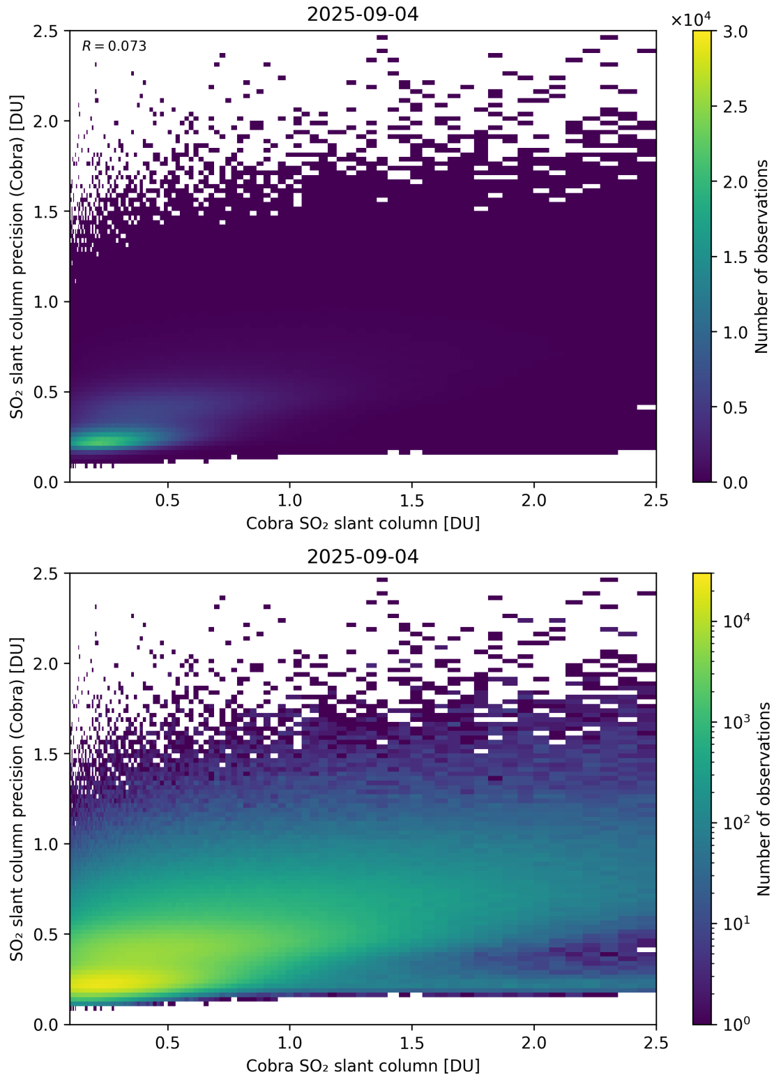
Figure 216: Scatter density plot of “Cobra SO 2 slant column” against “SO 2 slant column precision (Cobra)” for 2025-09-04 to 2025-09-05.
