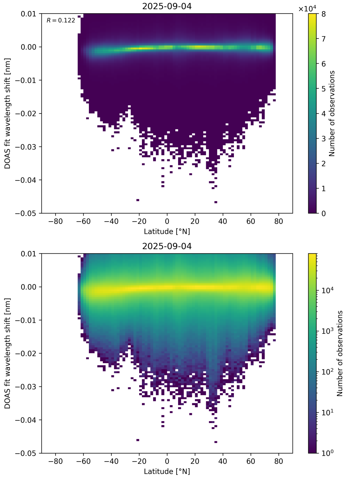
Figure 153: Scatter density plot of “Latitude” against “DOAS fit wavelength shift” for 2025-09-04 to 2025-09-05.
