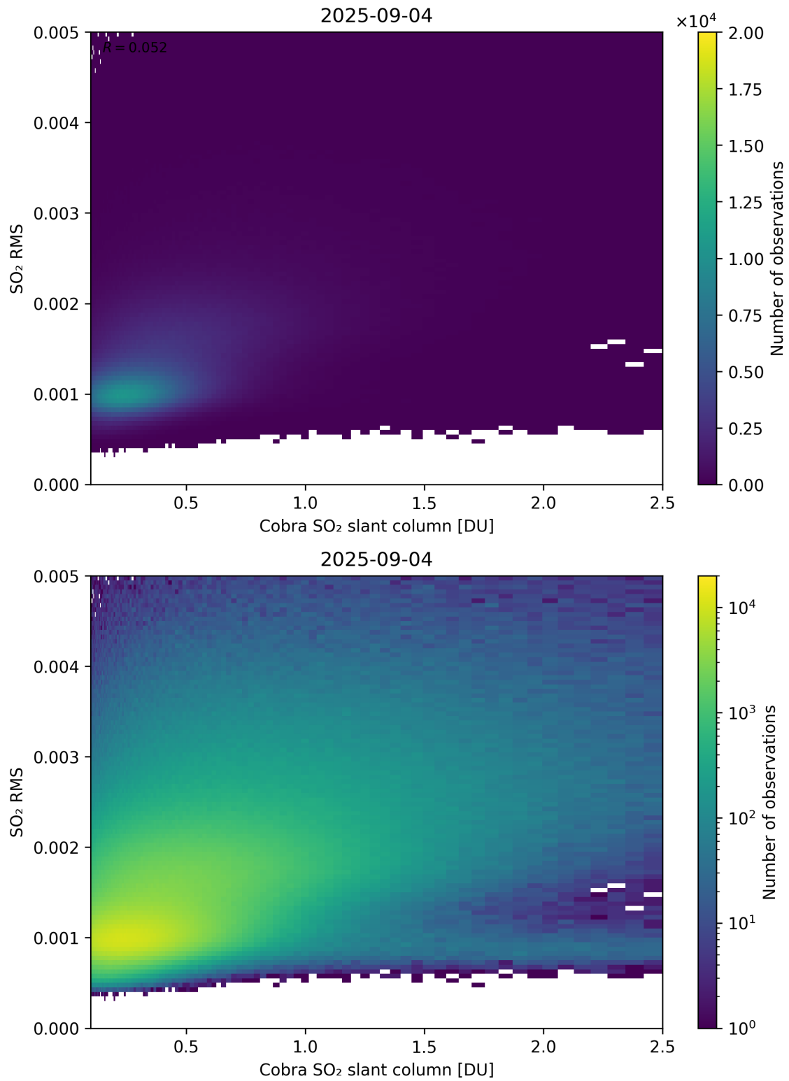
Figure 198: Scatter density plot of “Cobra SO 2 slant column” against “SO 2 RMS” for 2025-09-04 to 2025-09-05.
