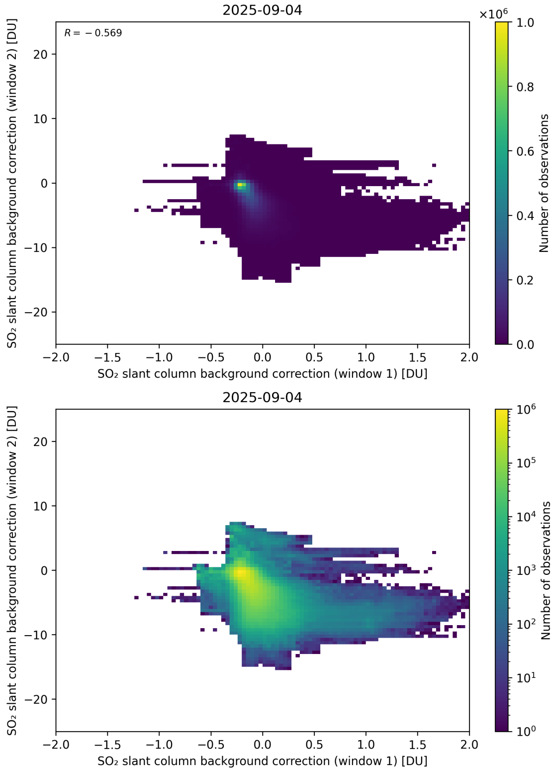
Figure 109: Scatter density plot of “SO 2 slant column background correction (window 1)” against “SO 2 slant column background correction (window 2)” for 2025-09-04 to 2025-09-05.
