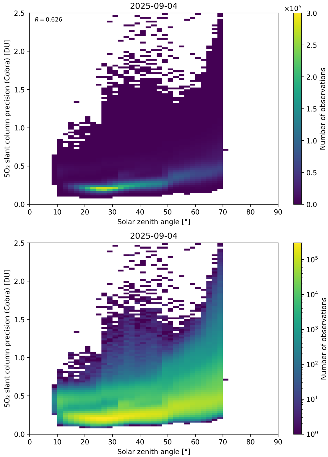
Figure 180: Scatter density plot of “Solar zenith angle” against “SO 2 slant column precision (Cobra)” for 2025-09-04 to 2025-09-05.
