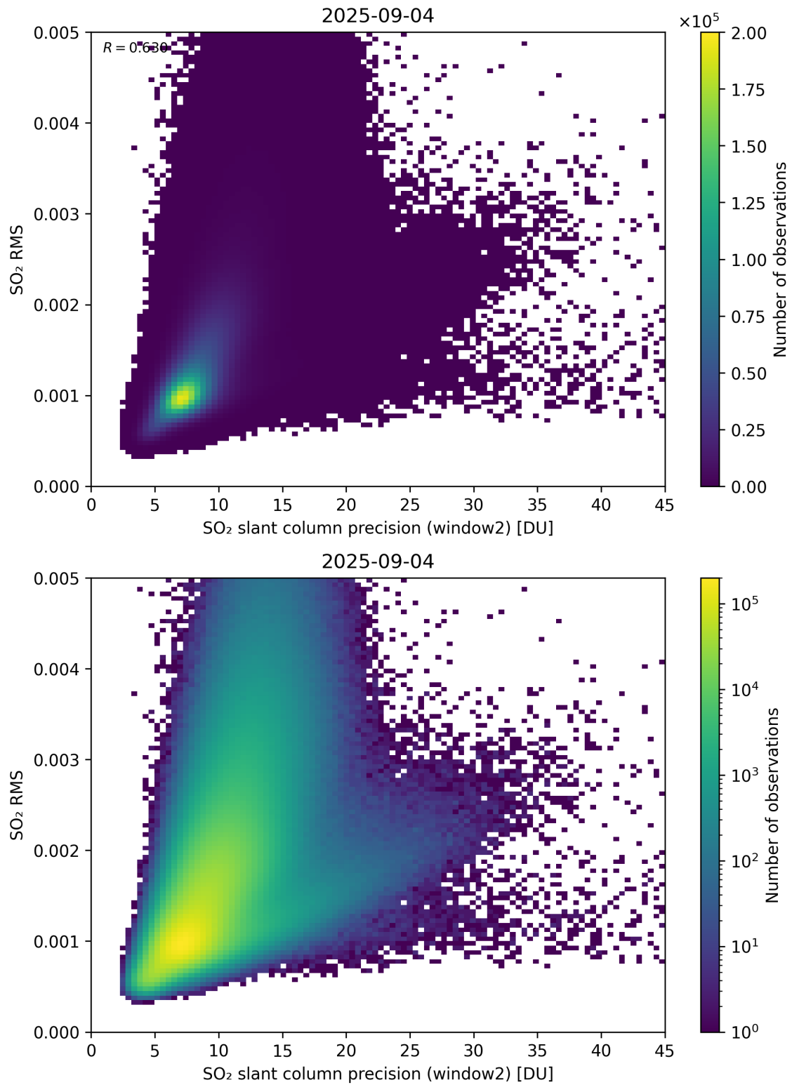
Figure 295: Scatter density plot of “SO 2 slant column precision (window2)” against “SO 2 RMS” for 2025-09-04 to 2025-09-05.
