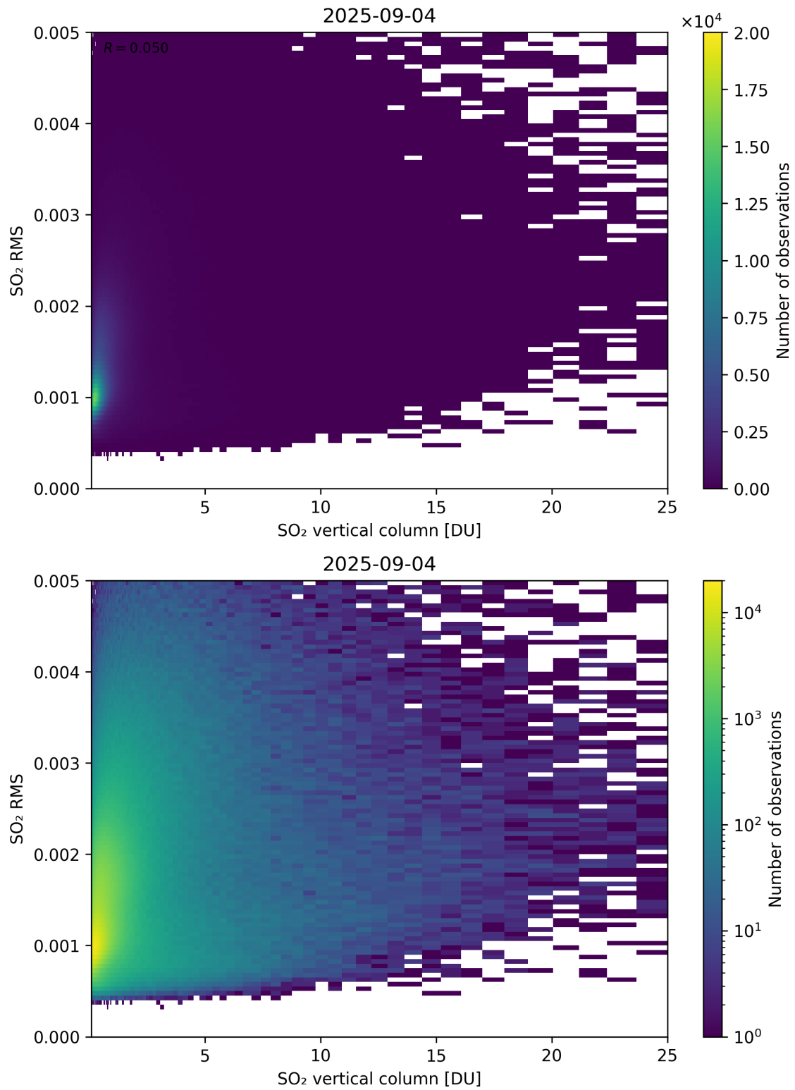
Figure 328: Scatter density plot of “SO 2 vertical column” against “SO 2 RMS” for 2025-09-04 to 2025-09-05.
