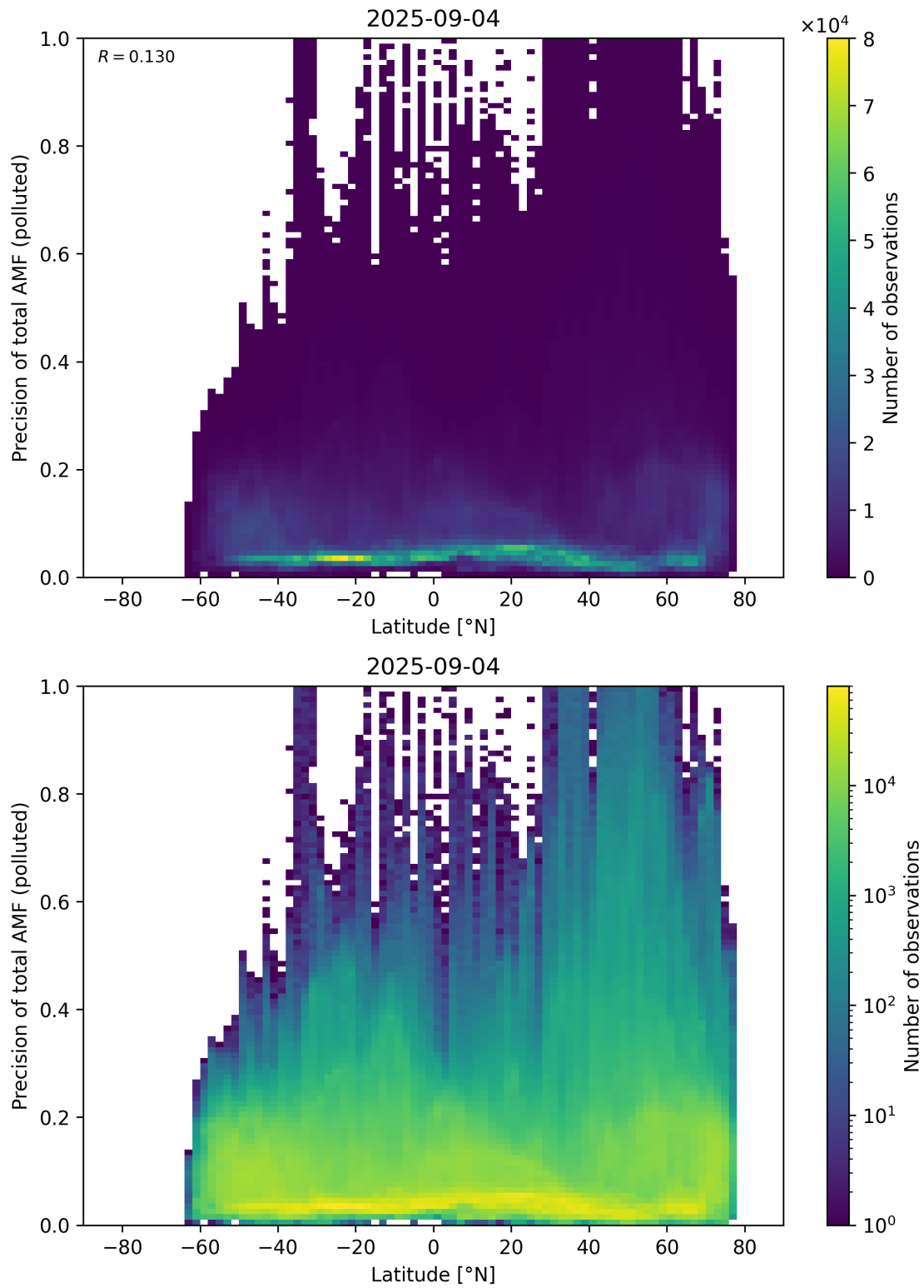
Figure 168: Scatter density plot of “Latitude” against “Precision of total AMF (polluted)” for 2025-09-04 to 2025-09-05.
