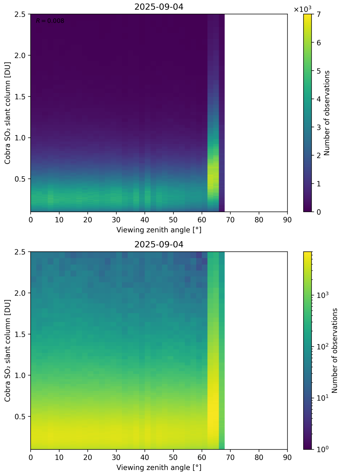
Figure 371: Scatter density plot of “Viewing zenith angle” against “Cobra SO 2 slant column” for 2025-09-04 to 2025-09-05.
