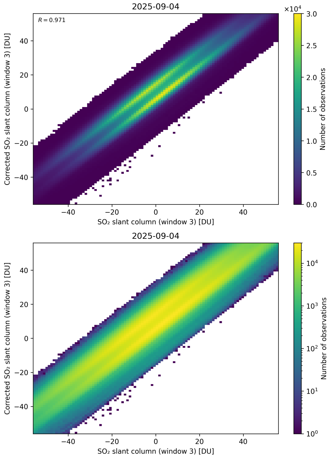
Figure 316: Scatter density plot of “SO 2 slant column (window 3)” against “Corrected SO 2 slant column (window 3)” for 2025-09-04 to 2025-09-05.
