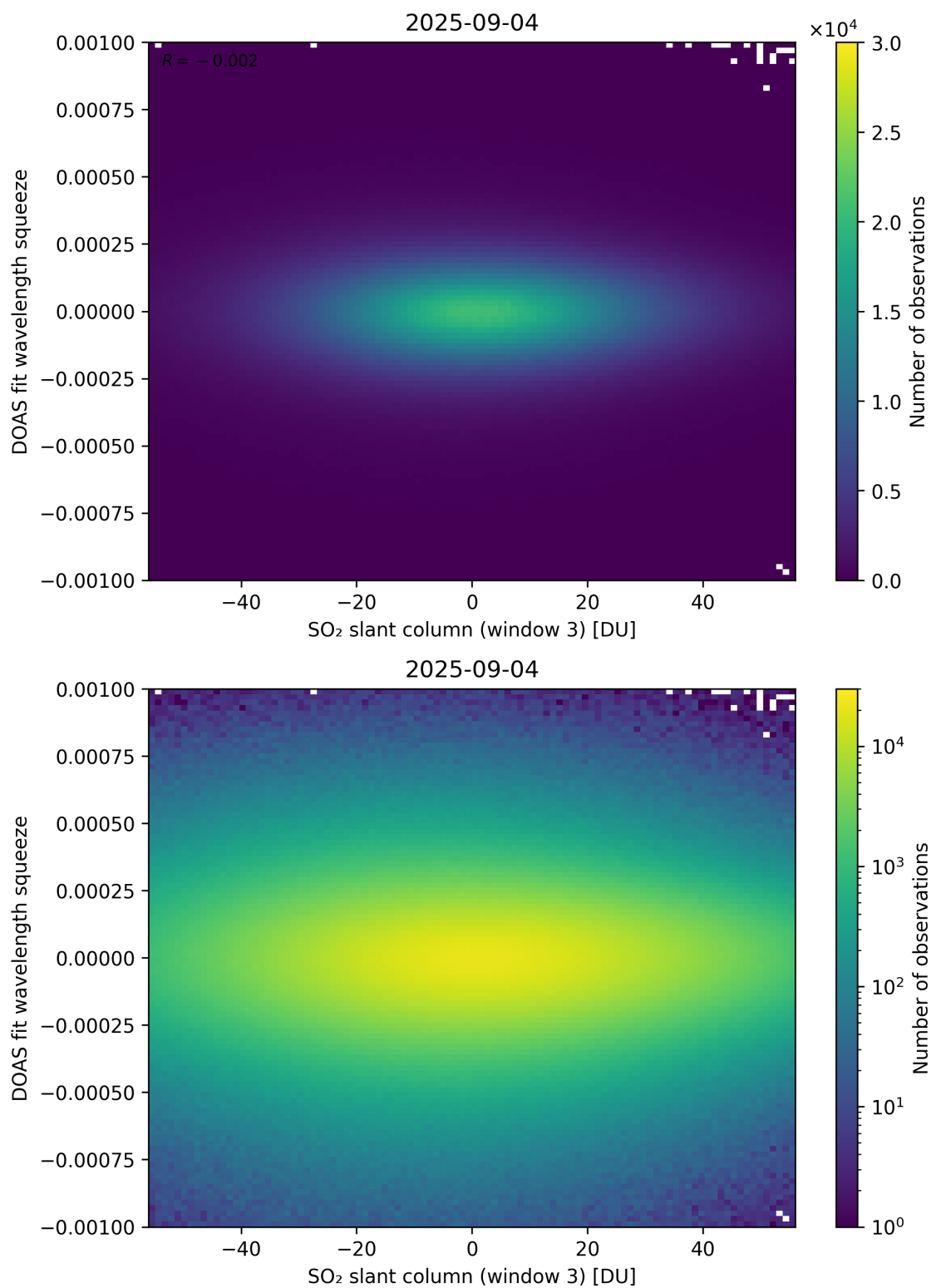
Figure 305: Scatter density plot of “SO 2 slant column (window 3)” against “DOAS fit wavelength squeeze” for 2025-09-04 to 2025-09-05.
