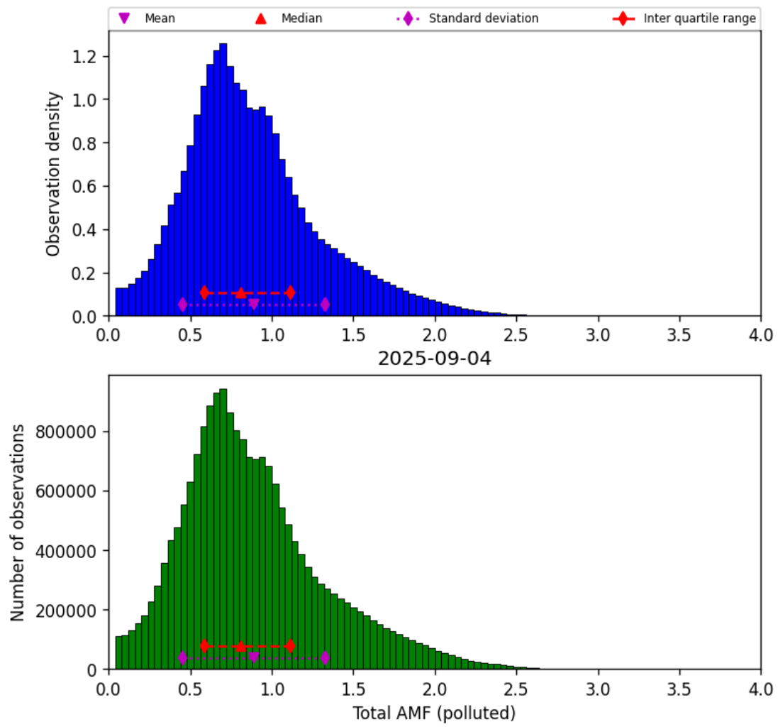
Figure 79: Histogram of “Total AMF (polluted)” for 2025-09-04 to 2025-09-05
