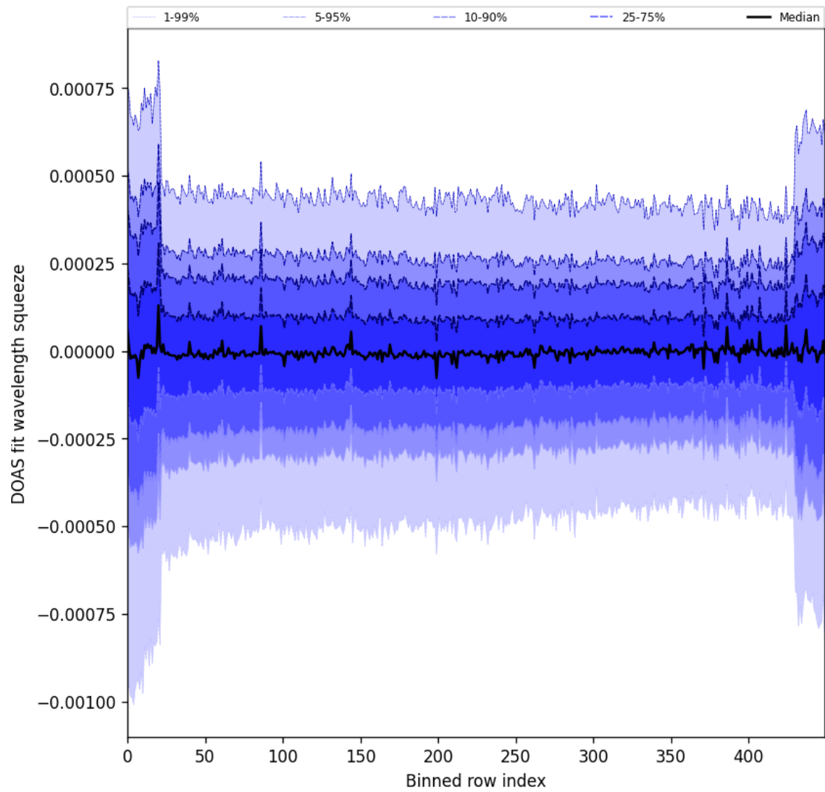
Figure 103: Along track statistics of “DOAS fit wavelength squeeze” for 2025-09-04 to 2025-09-05
