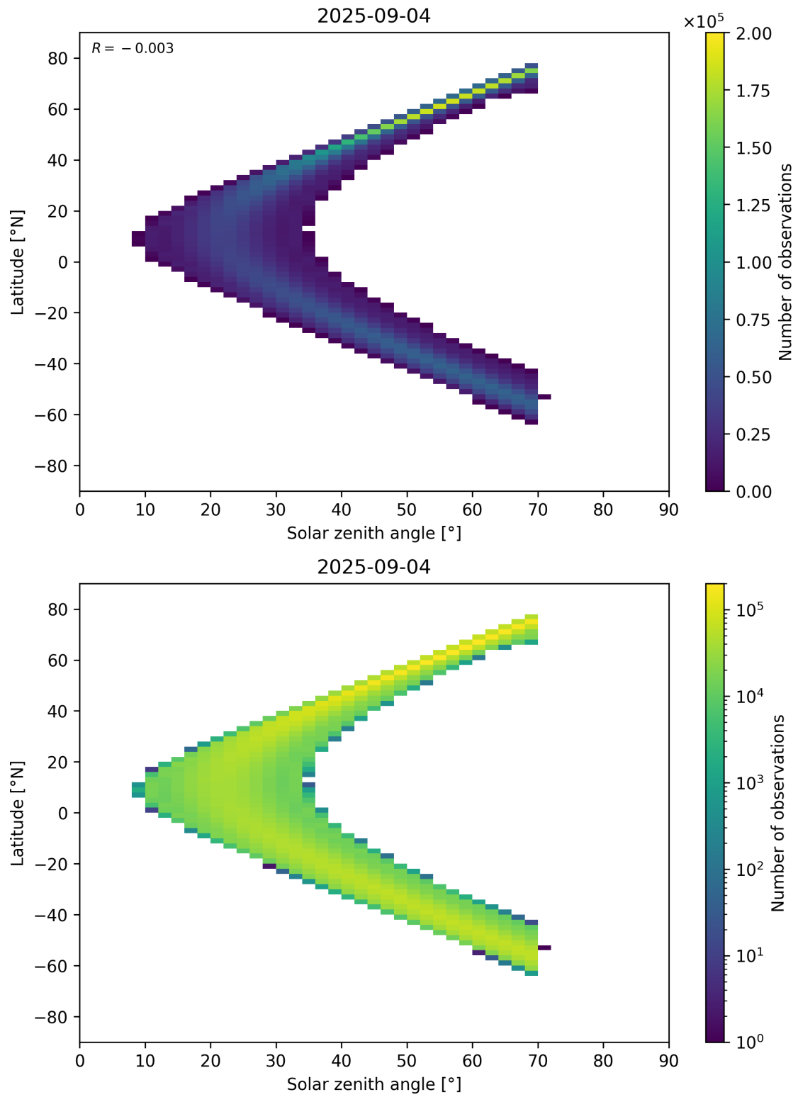
Figure 177: Scatter density plot of “Solar zenith angle” against “Latitude” for 2025-09-04 to 2025-09-05.
