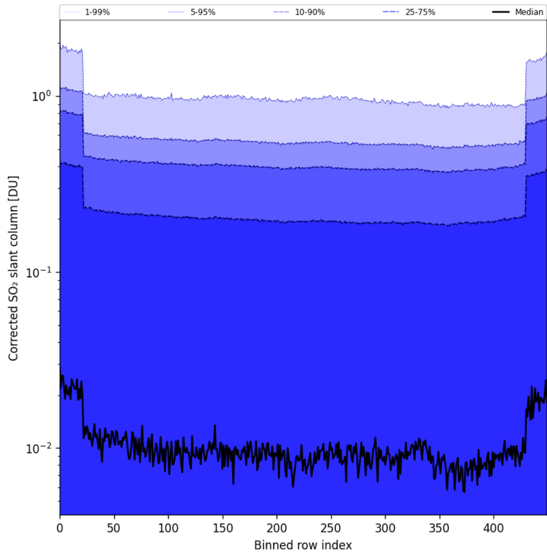
Figure 86: Along track statistics of “Corrected SO 2 slant column” for 2025-09-04 to 2025-09-05
