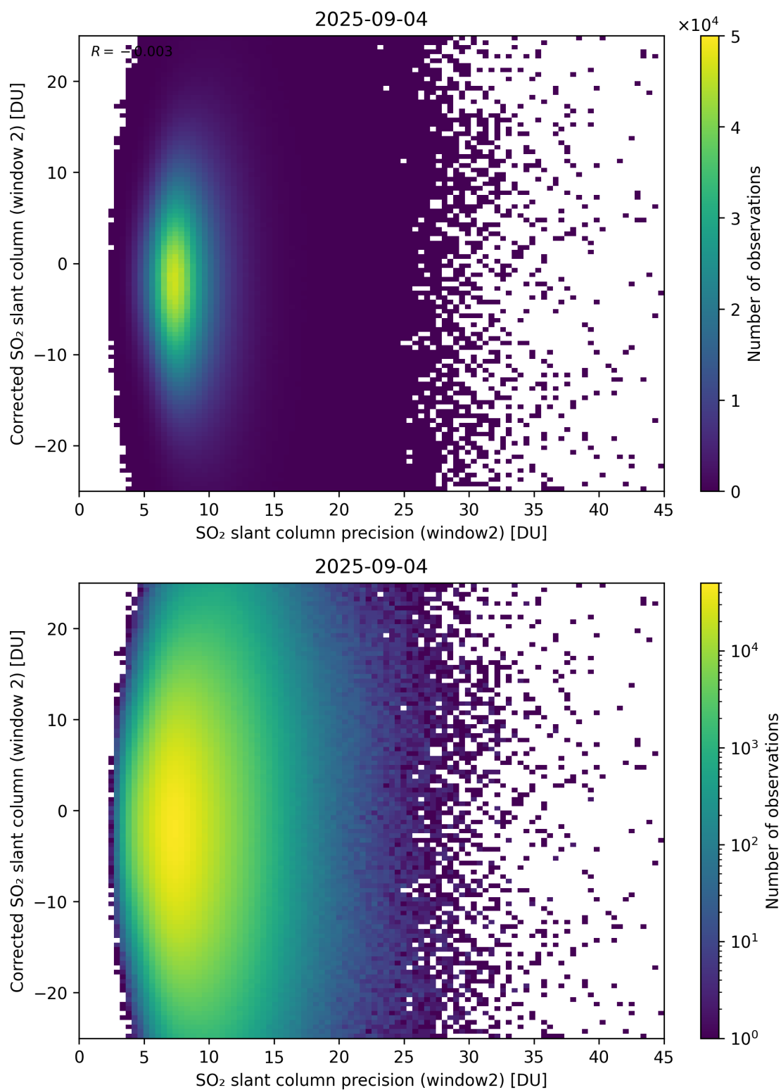
Figure 297: Scatter density plot of “SO 2 slant column precision (window2)” against “Corrected SO 2 slant column (window 2)” for 2025-09-04 to 2025-09-05.
