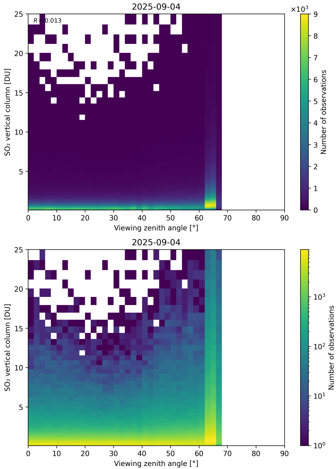
Figure 383: Scatter density plot of “Viewing zenith angle” against “SO 2 vertical column” for 2025-09-04 to 2025-09-05.
