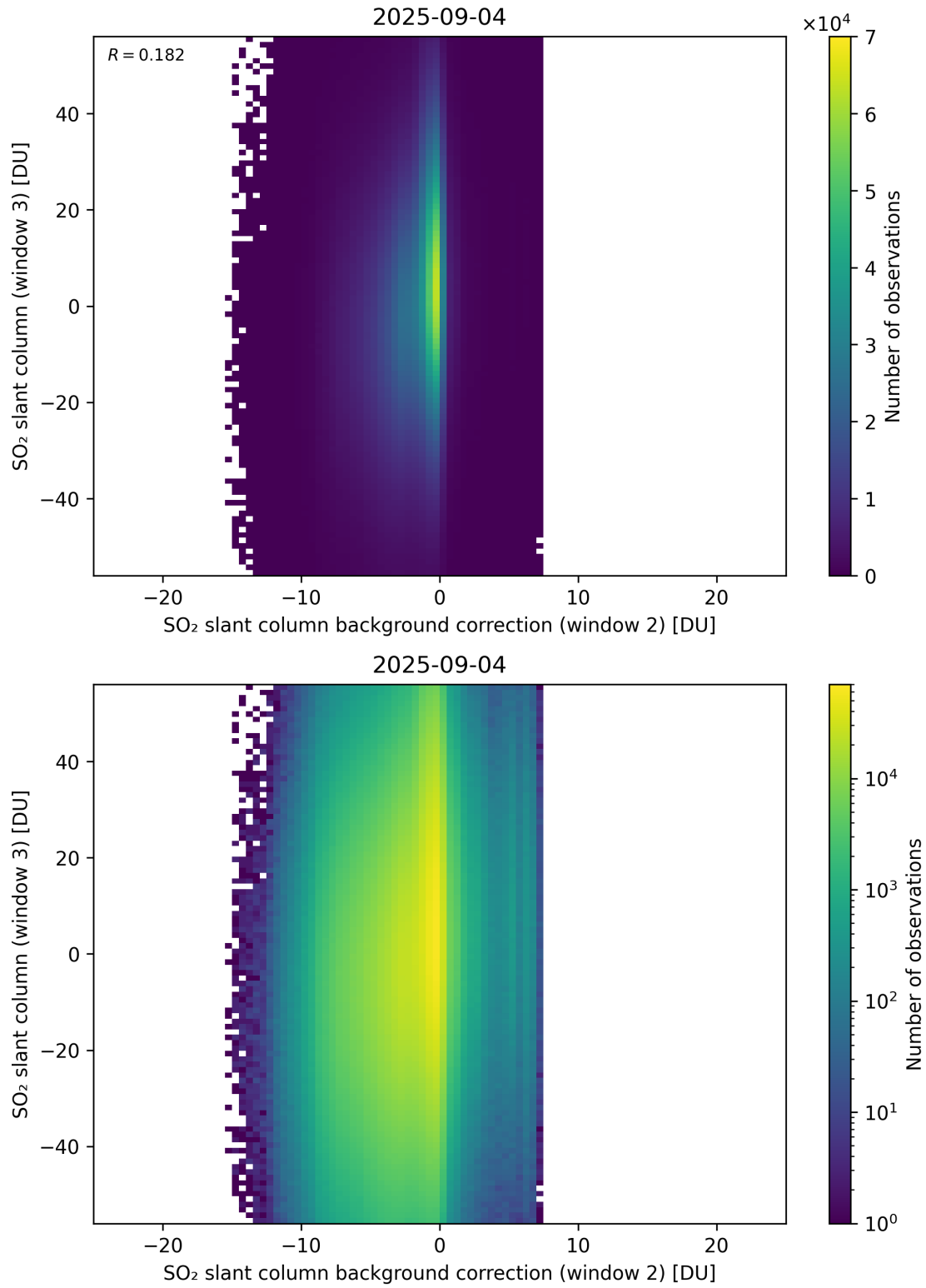
Figure 128: Scatter density plot of “SO 2 slant column background correction (window 2)” against “SO 2 slant column (window 3)” for 2025-09-04 to 2025-09-05.
