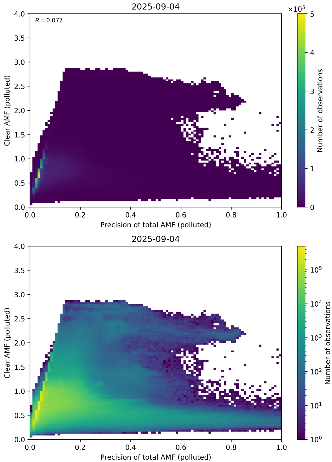
Figure 320: Scatter density plot of “Precision of total AMF (polluted)” against “Clear AMF (polluted)” for 2025-09-04 to 2025-09-05.
