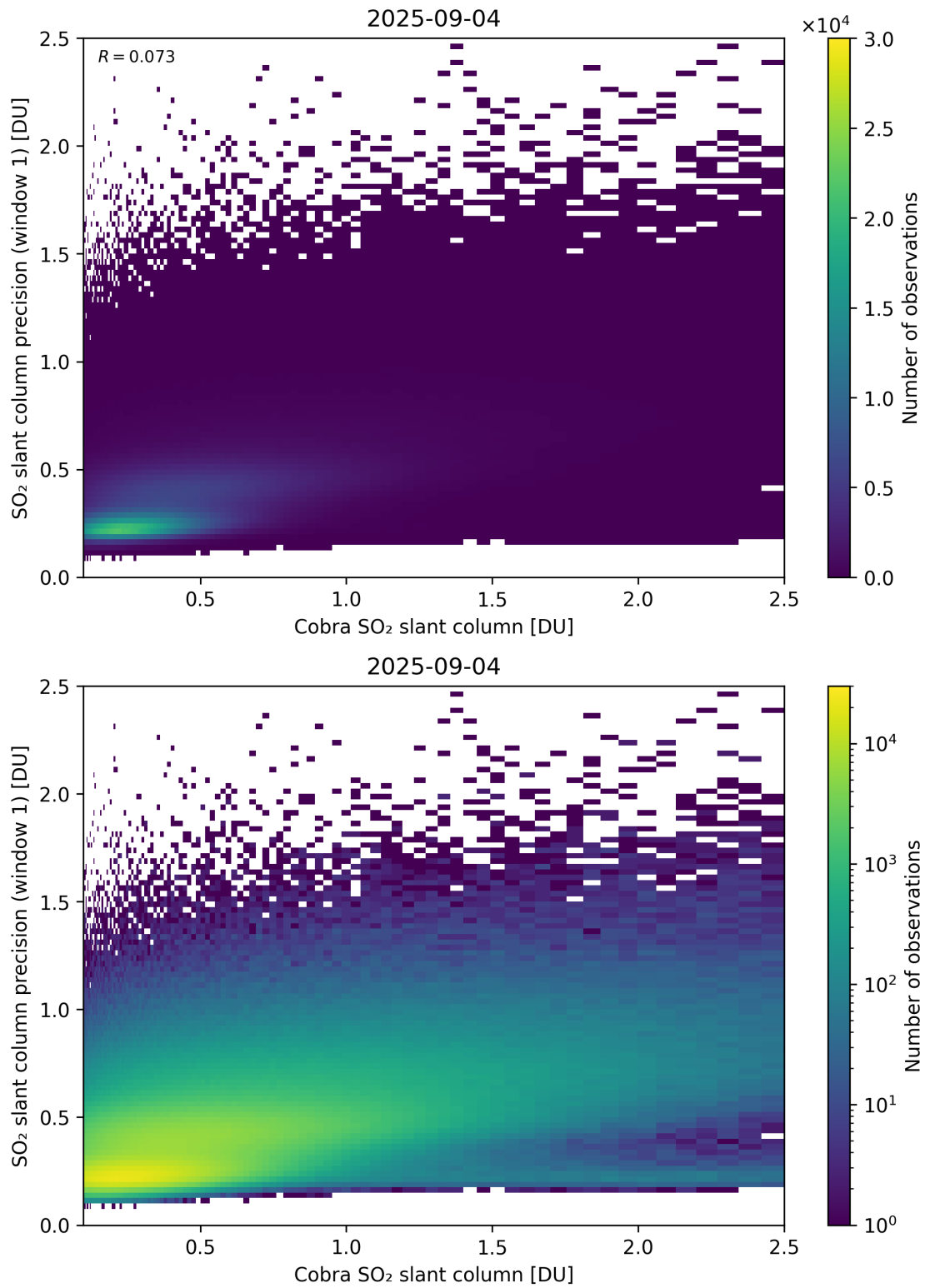
Figure 220: Scatter density plot of “Cobra SO 2 slant column” against “SO 2 slant column precision (window 1)” for 2025-09-04 to 2025-09-05.
