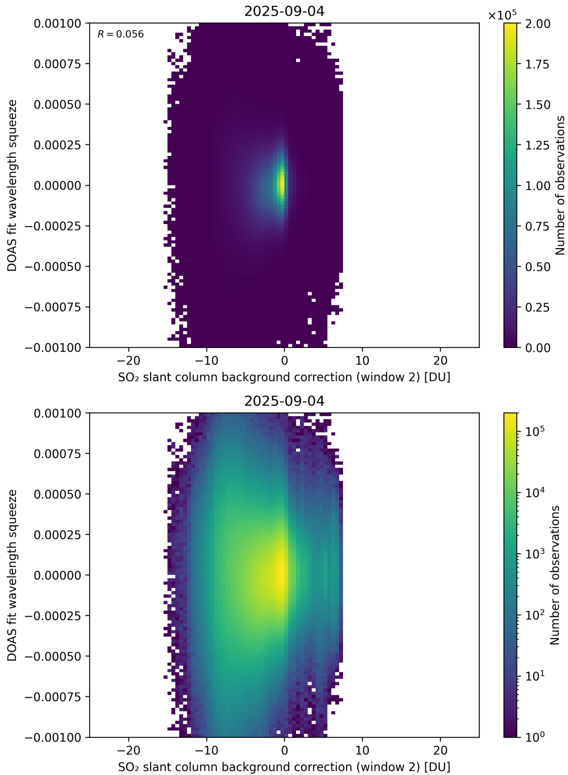
Figure 124: Scatter density plot of “SO 2 slant column background correction (window 2)” against “DOAS fit wavelength squeeze” for 2025-09-04 to 2025-09-05.
