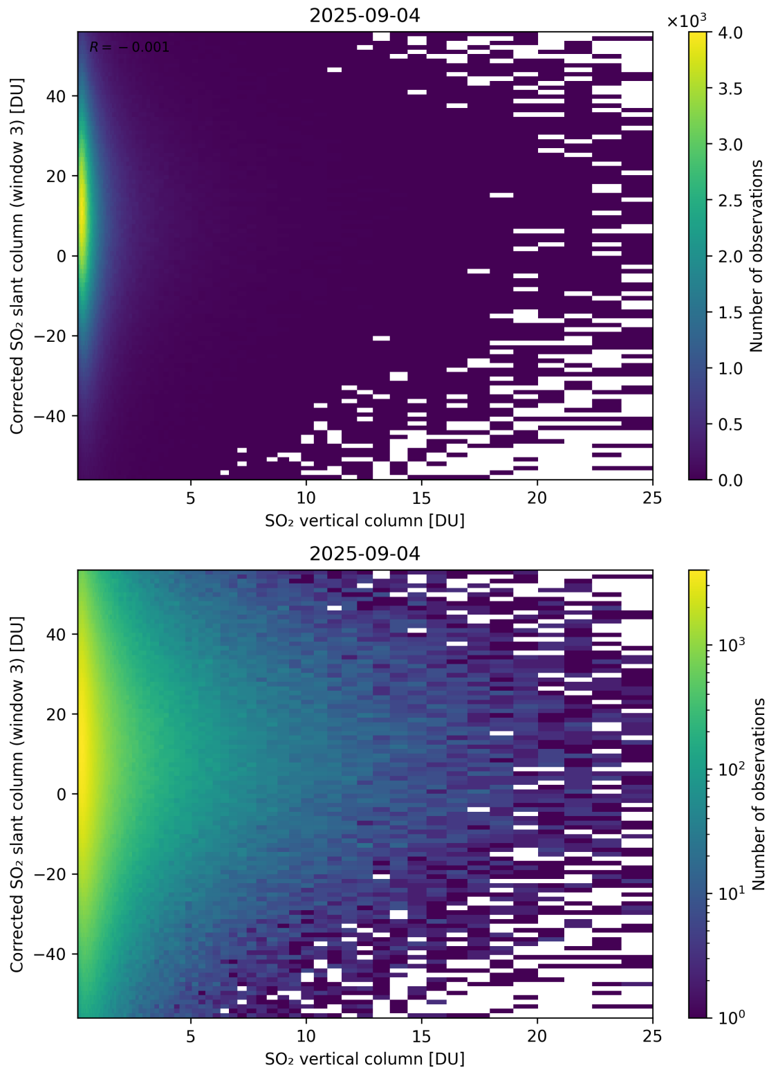
Figure 353: Scatter density plot of “SO 2 vertical column” against “Corrected SO 2 slant column (window 3)” for 2025-09-04 to 2025-09-05.
