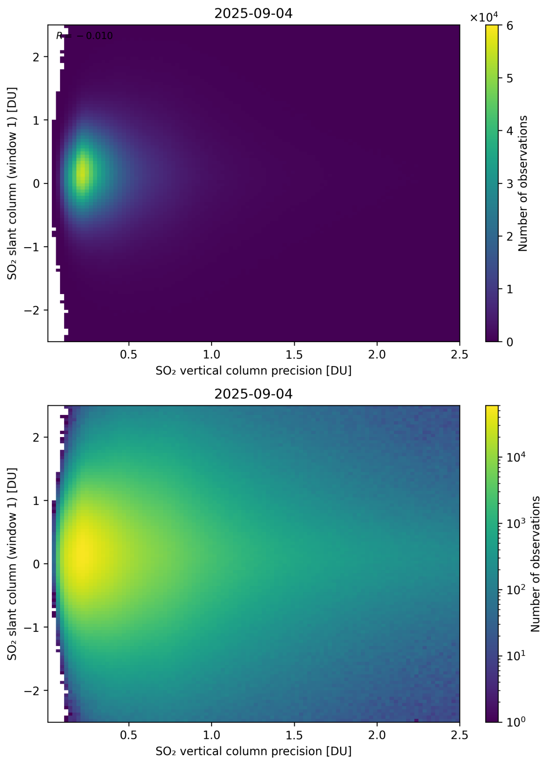
Figure 341: Scatter density plot of “SO 2 vertical column precision” against “SO 2 slant column (window 1)” for 2025-09-04 to 2025-09-05.
