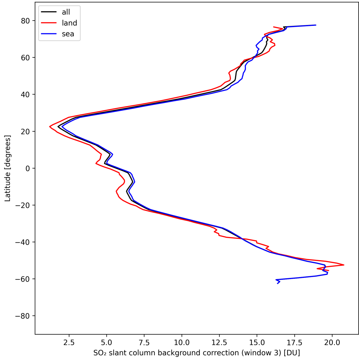
Figure 48: Zonal average of “SO 2 slant column background correction (window 3)” for 2025-09-04 to 2025-09-05.
