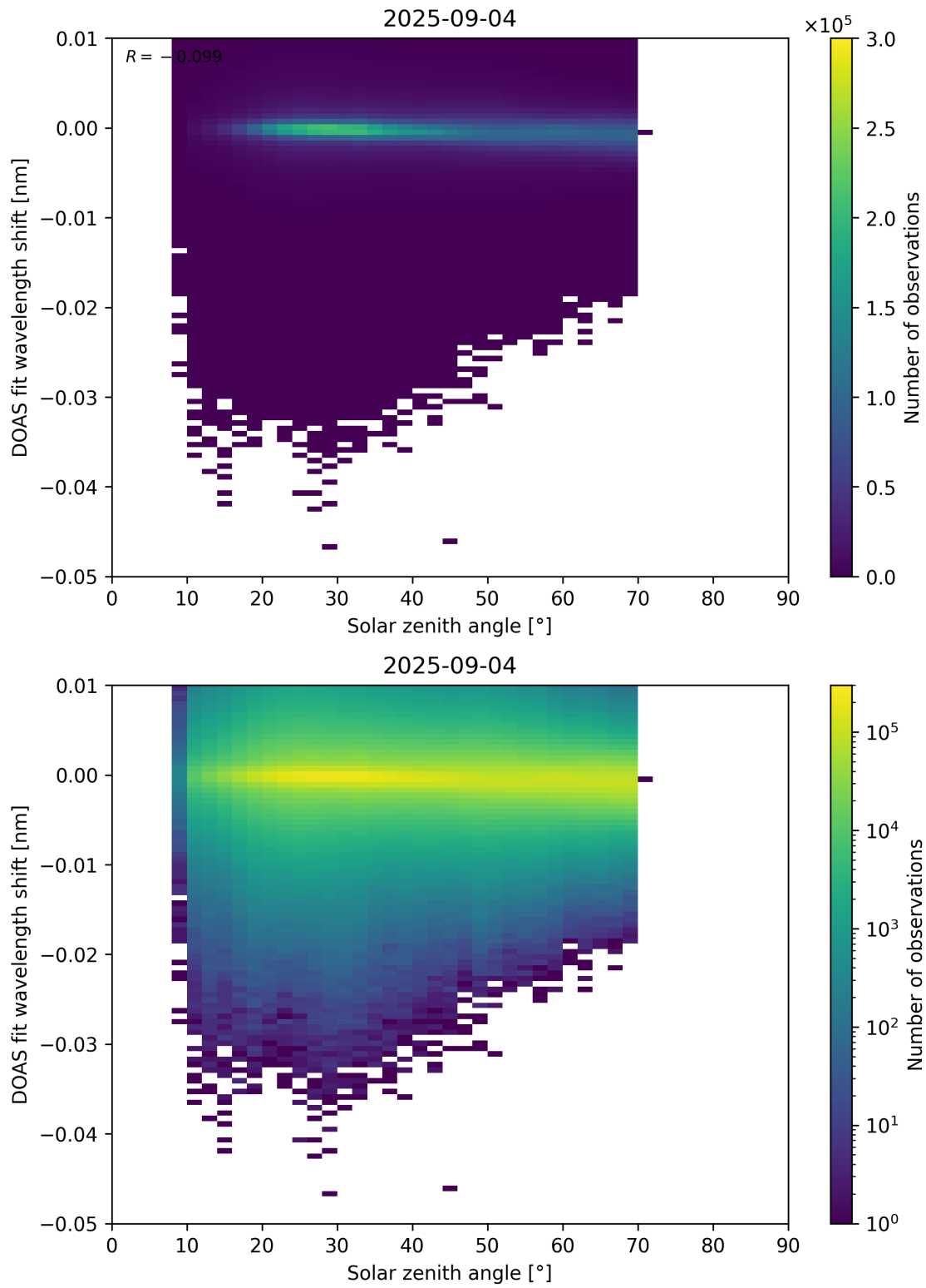
Figure 174: Scatter density plot of “Solar zenith angle” against “DOAS fit wavelength shift” for 2025-09-04 to 2025-09-05.
