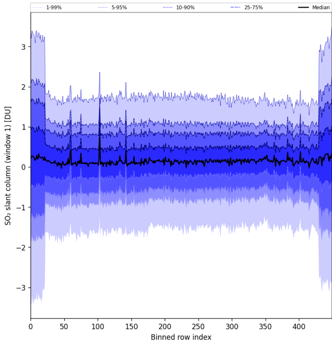
Figure 89: Along track statistics of “SO 2 slant column (window 1)” for 2025-09-04 to 2025-09-05
