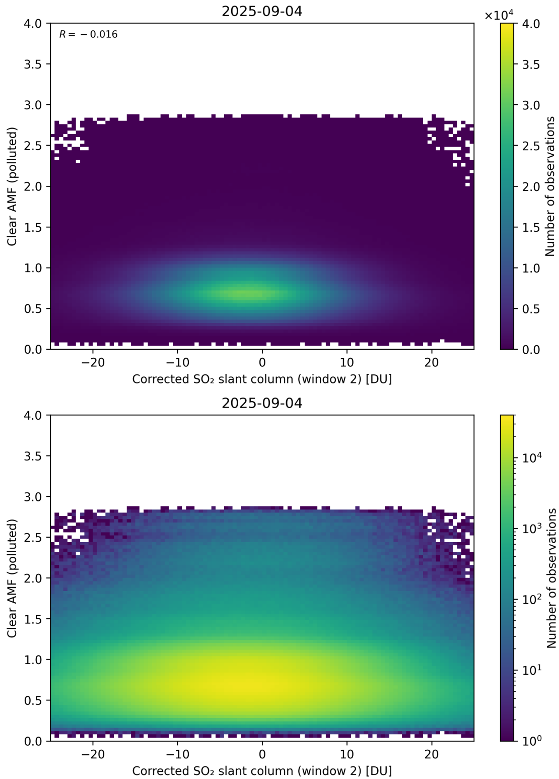
Figure 249: Scatter density plot of “Corrected SO 2 slant column (window 2)” against “Clear AMF (polluted)” for 2025-09-04 to 2025-09-05.
