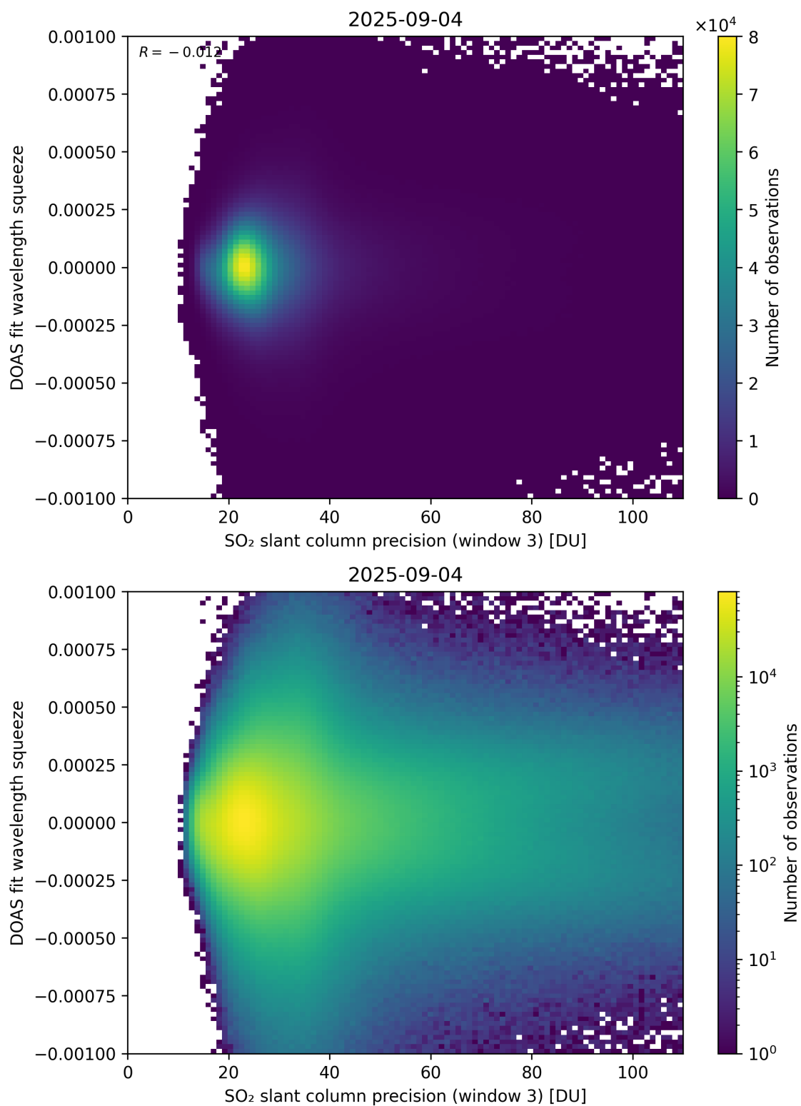
Figure 309: Scatter density plot of “SO 2 slant column precision (window 3)” against “DOAS fit wavelength squeeze” for 2025-09-04 to 2025-09-05.
