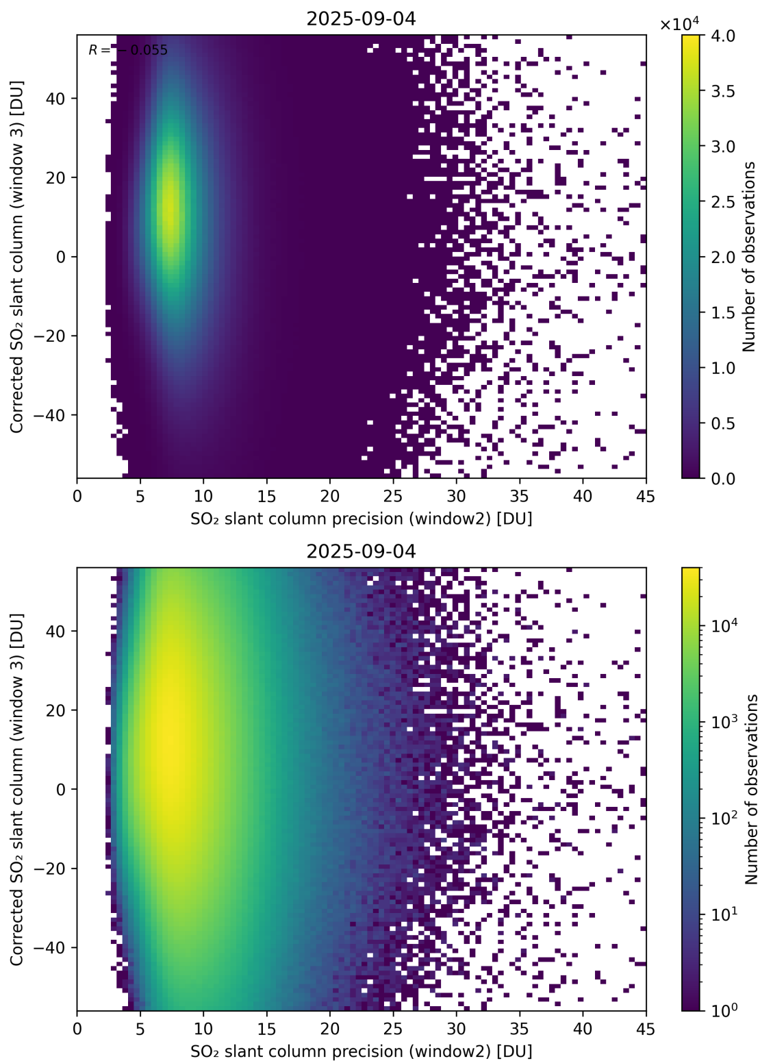
Figure 298: Scatter density plot of “SO 2 slant column precision (window2)” against “Corrected SO 2 slant column (window 3)” for 2025-09-04 to 2025-09-05.
