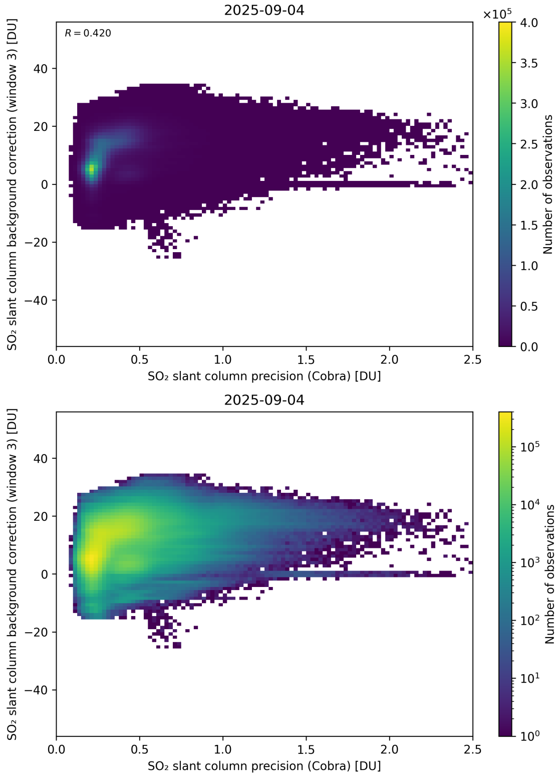
Figure 201: Scatter density plot of “SO 2 slant column precision (Cobra)” against “SO 2 slant column background correction (window 3)” for 2025-09-04 to 2025-09-05.
