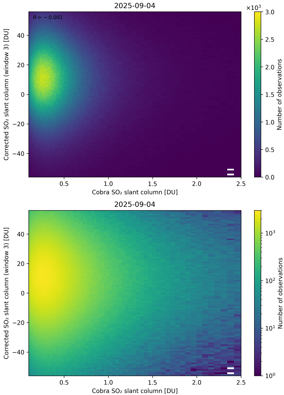
Figure 218: Scatter density plot of “Cobra SO 2 slant column” against “Corrected SO 2 slant column (window 3)” for 2025-09-04 to 2025-09-05.
