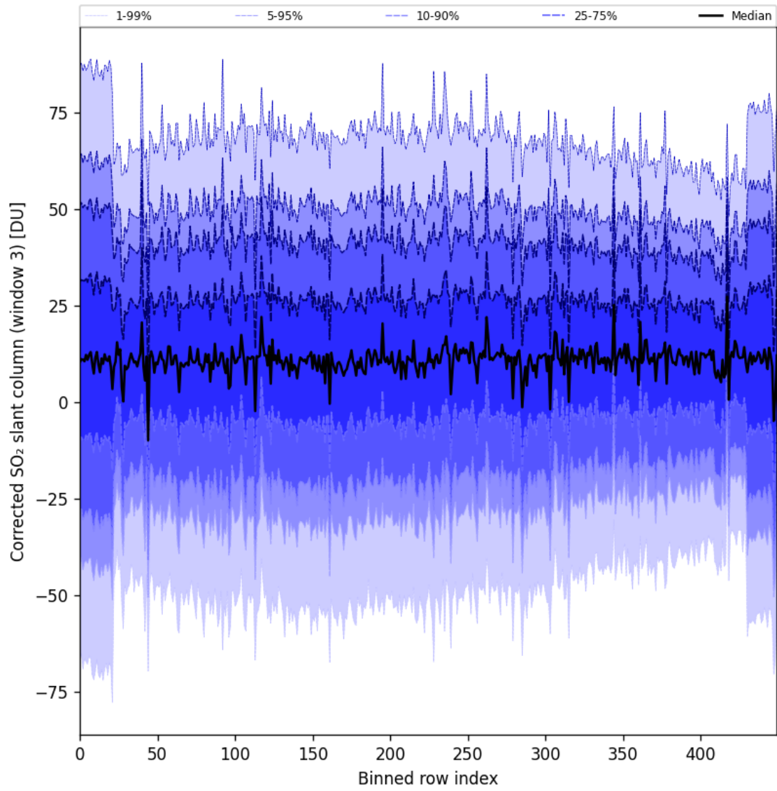
Figure 99: Along track statistics of “Corrected SO 2 slant column (window 3)” for 2025-09-04 to 2025-09-05
