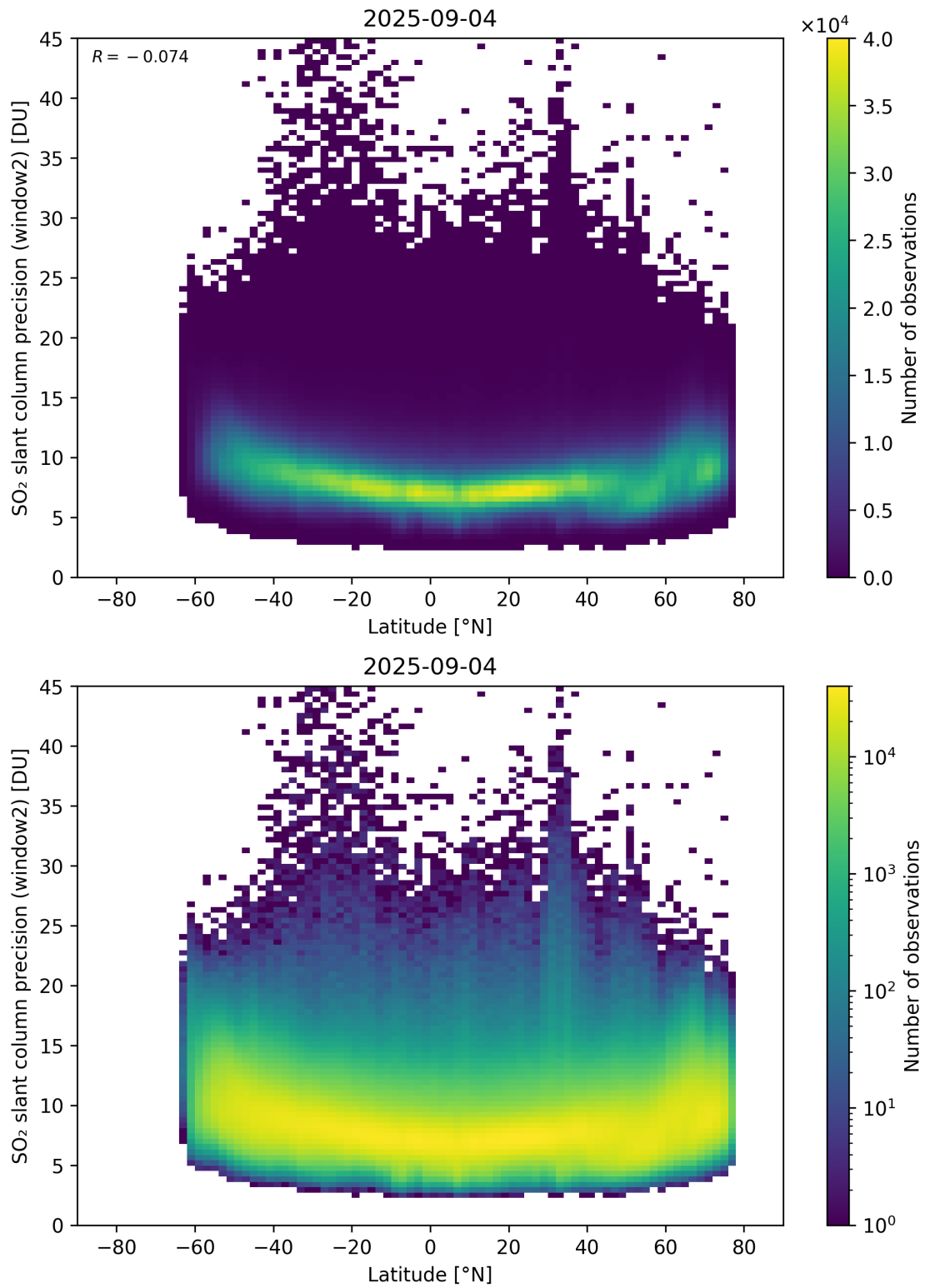
Figure 164: Scatter density plot of “Latitude” against “SO 2 slant column precision (window2)” for 2025-09-04 to 2025-09-05.
