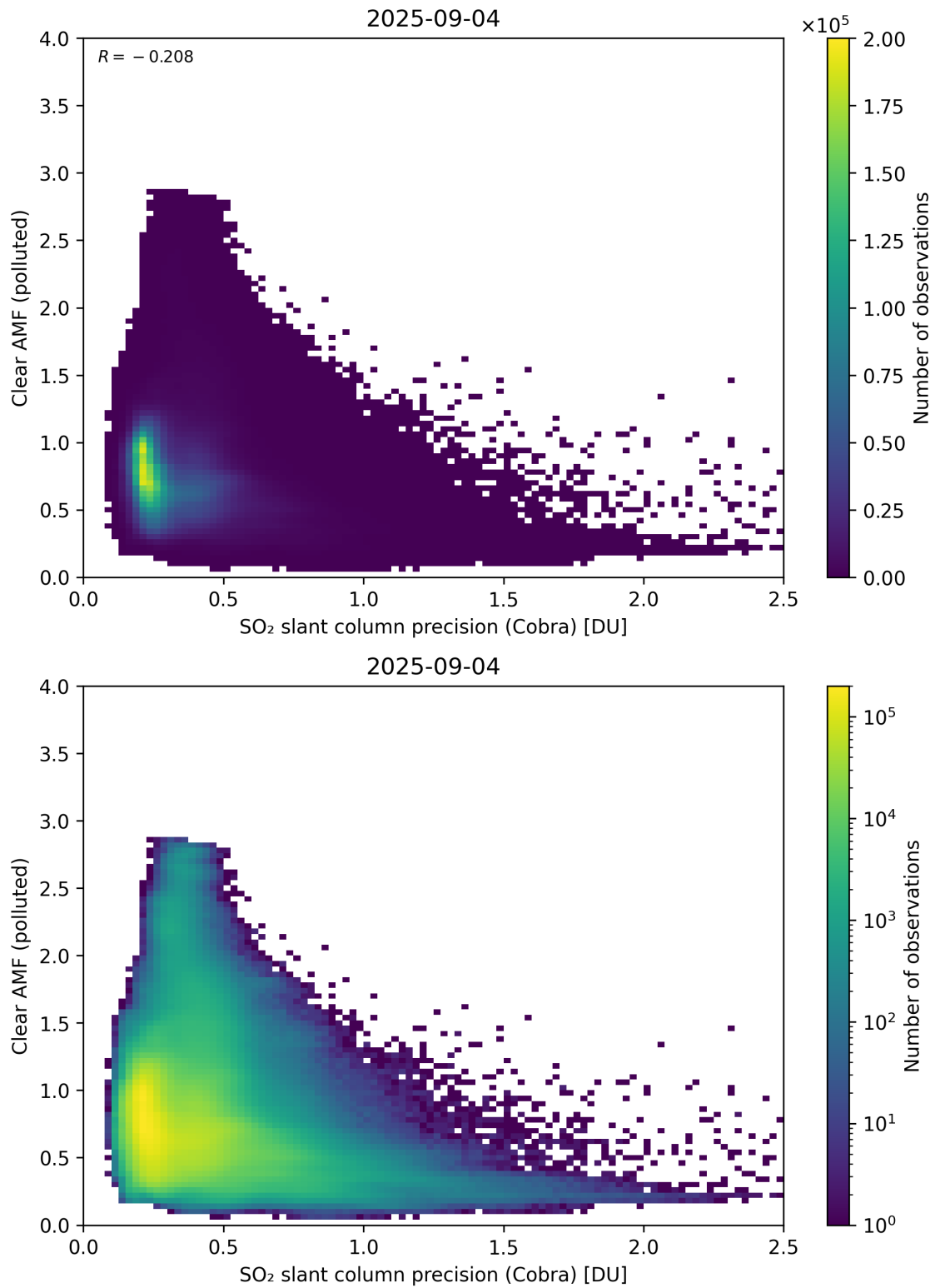
Figure 205: Scatter density plot of “SO 2 slant column precision (Cobra)” against “Clear AMF (polluted)” for 2025-09-04 to 2025-09-05.
