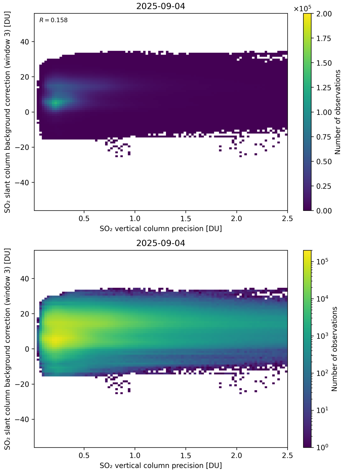
Figure 331: Scatter density plot of “SO 2 vertical column precision” against “SO 2 slant column background correction (window 3)” for 2025-09-04 to 2025-09-05.
