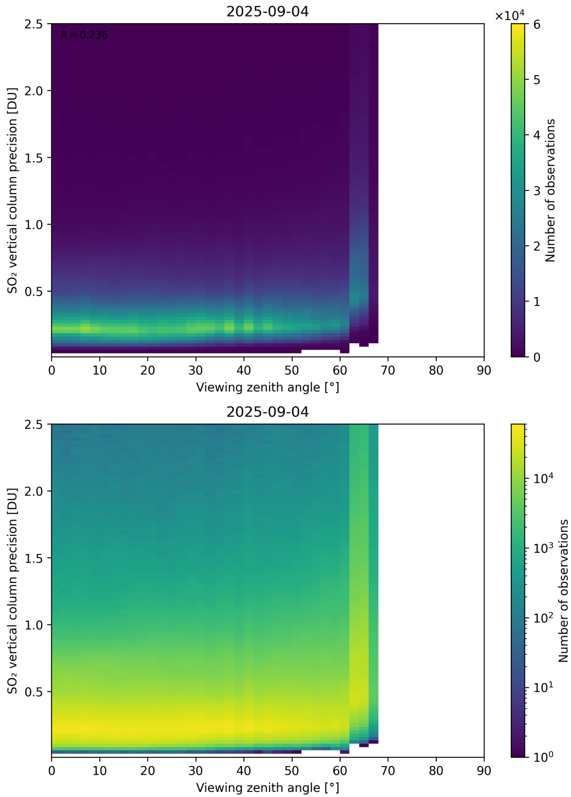
Figure 384: Scatter density plot of “Viewing zenith angle” against “SO 2 vertical column precision” for 2025-09-04 to 2025-09-05.
