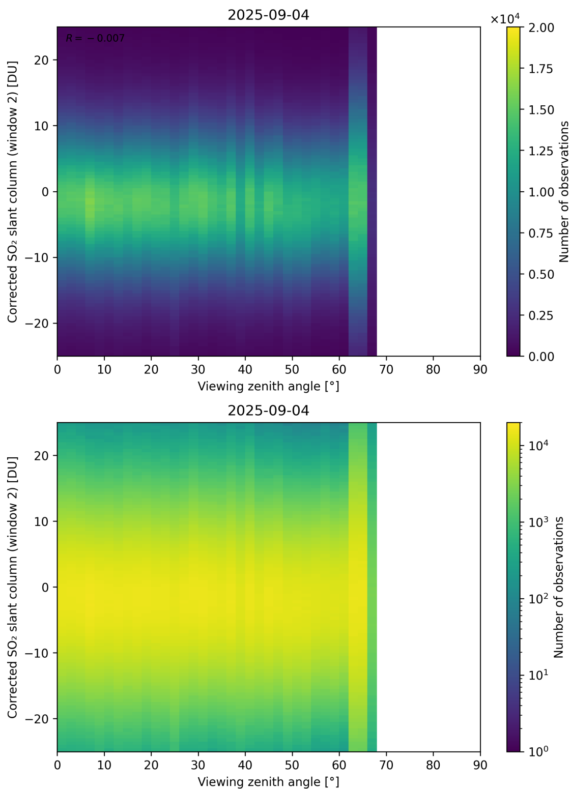
Figure 374: Scatter density plot of “Viewing zenith angle” against “Corrected SO 2 slant column (window 2)” for 2025-09-04 to 2025-09-05.
