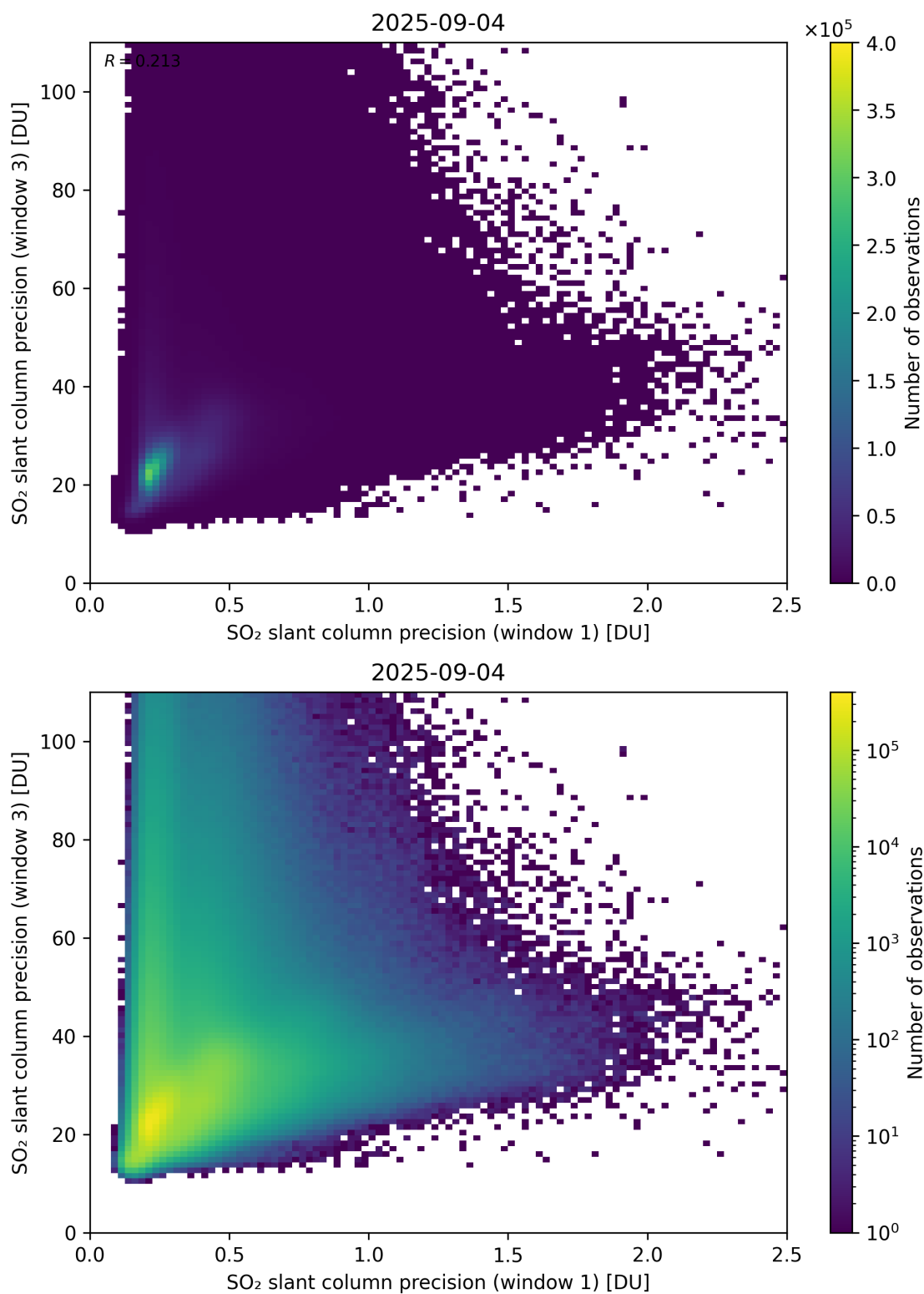
Figure 279: Scatter density plot of “SO 2 slant column precision (window 1)” against “SO 2 slant column precision (window 3)” for 2025-09-04 to 2025-09-05.
