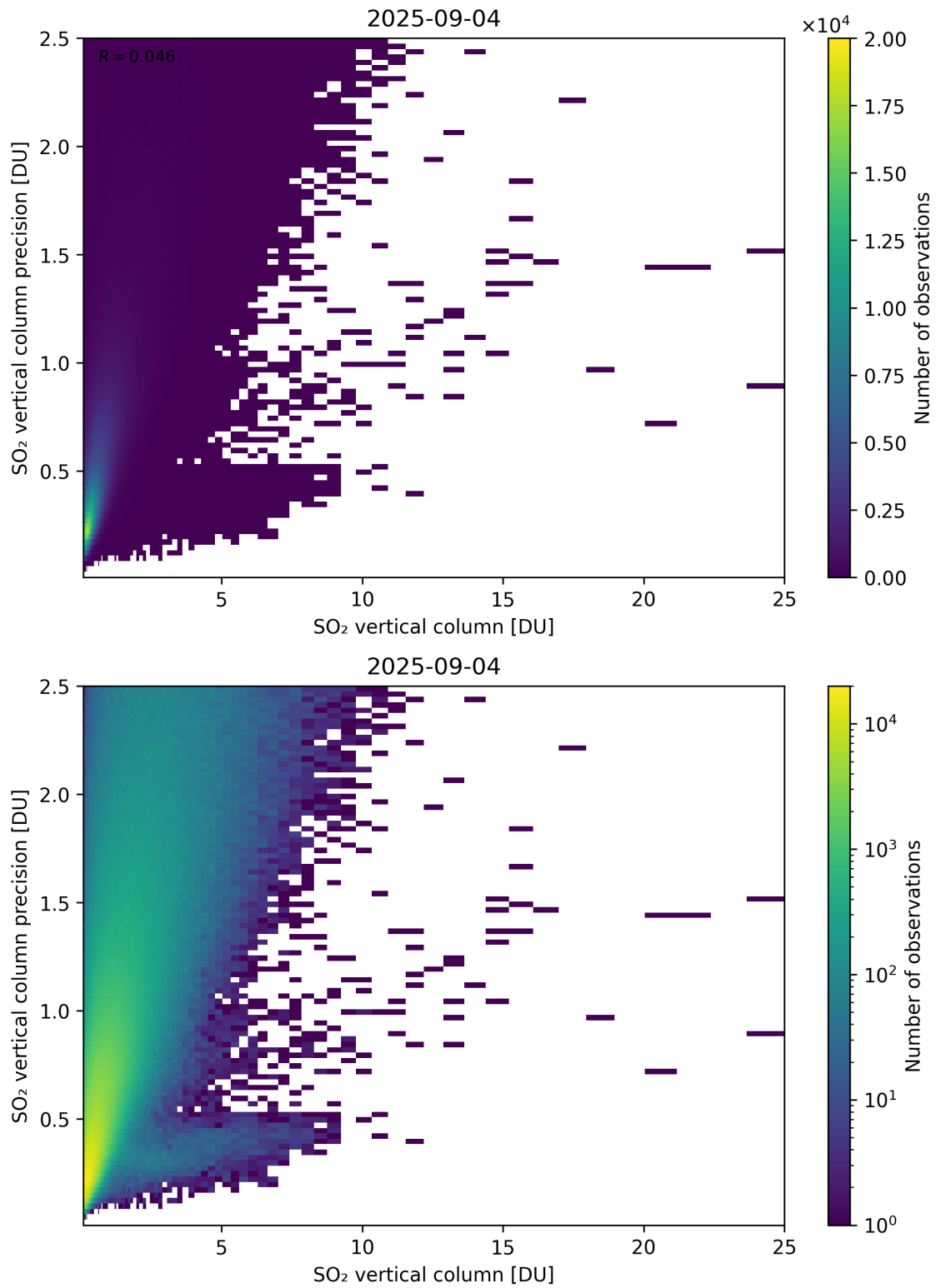
Figure 361: Scatter density plot of “SO 2 vertical column” against “SO 2 vertical column precision” for 2025-09-04 to 2025-09-05.
