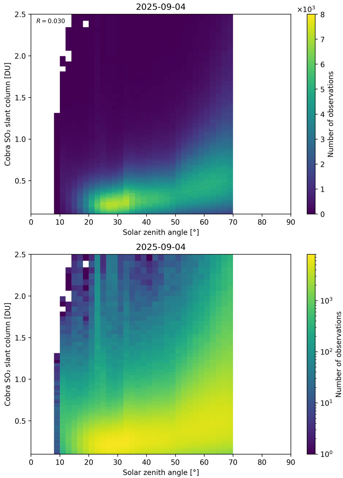
Figure 179: Scatter density plot of “Solar zenith angle” against “Cobra SO 2 slant column” for 2025-09-04 to 2025-09-05.
