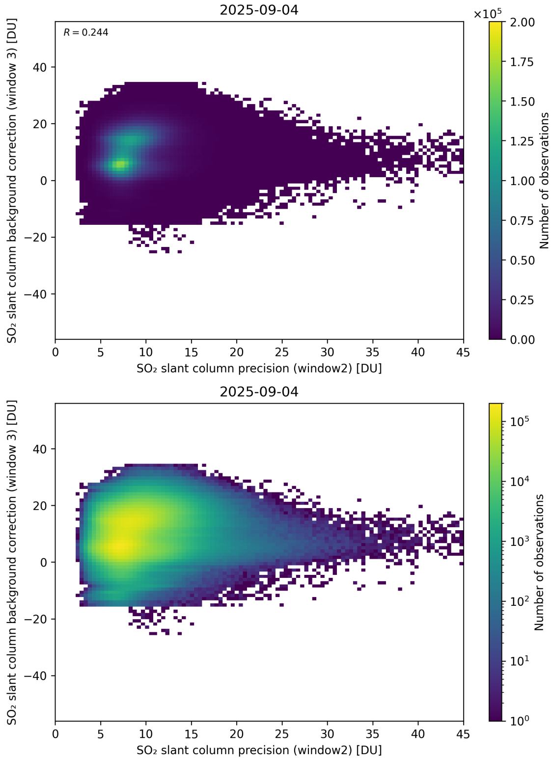
Figure 292: Scatter density plot of “SO 2 slant column precision (window2)” against “SO 2 slant column background correction (window 3)” for 2025-09-04 to 2025-09-05.
