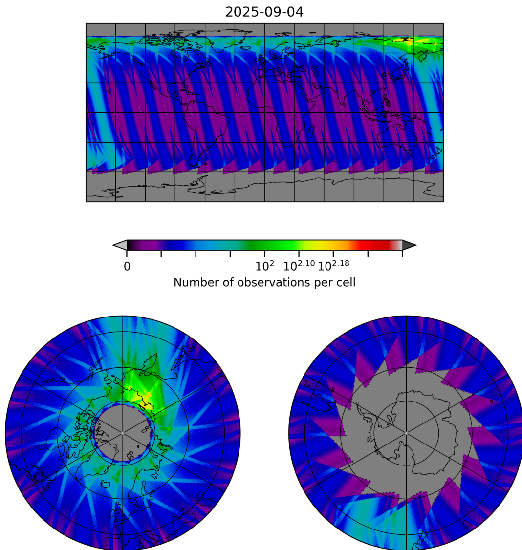
Figure 30: Map of the number of observations for 2025-09-04 to 2025-09-05
