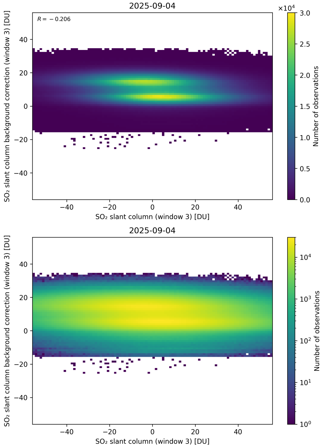
Figure 303: Scatter density plot of “SO 2 slant column (window 3)” against “SO 2 slant column background correction (window 3)” for 2025-09-04 to 2025-09-05.
