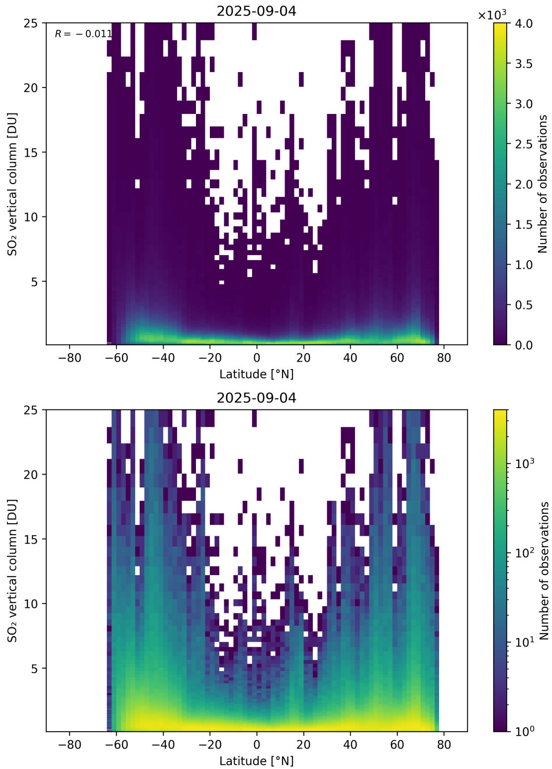
Figure 169: Scatter density plot of “Latitude” against “SO 2 vertical column” for 2025-09-04 to 2025-09-05.
