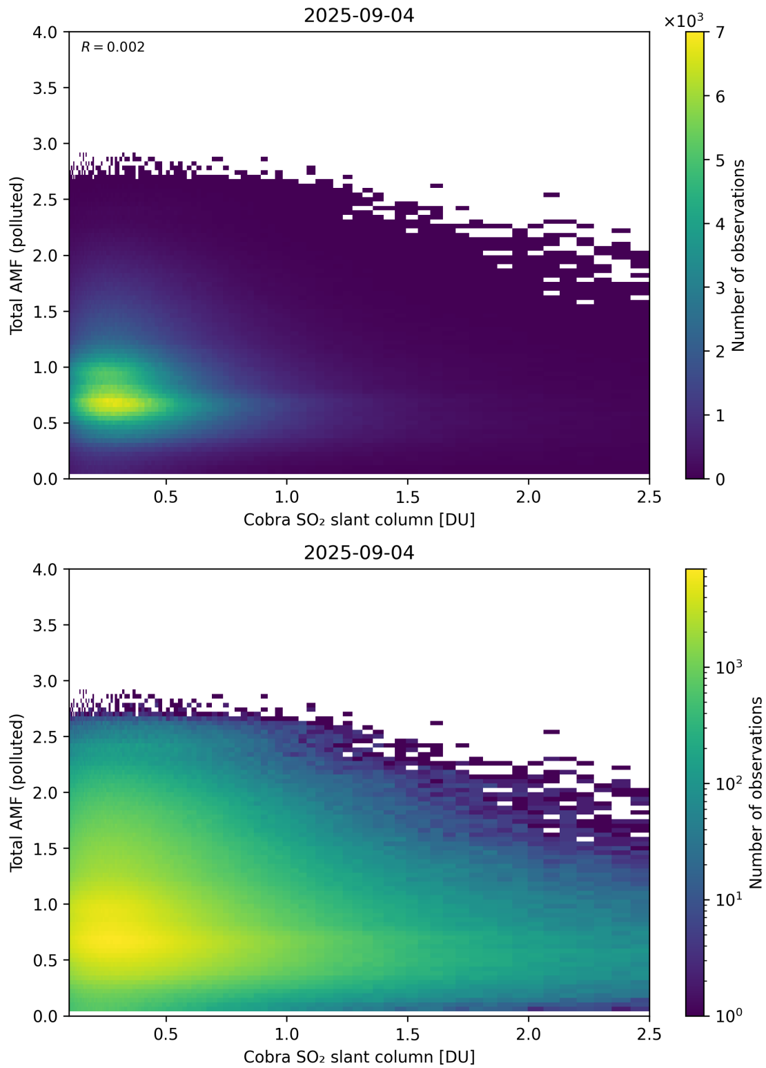
Figure 224: Scatter density plot of “Cobra SO 2 slant column” against “Total AMF (polluted)” for 2025-09-04 to 2025-09-05.
