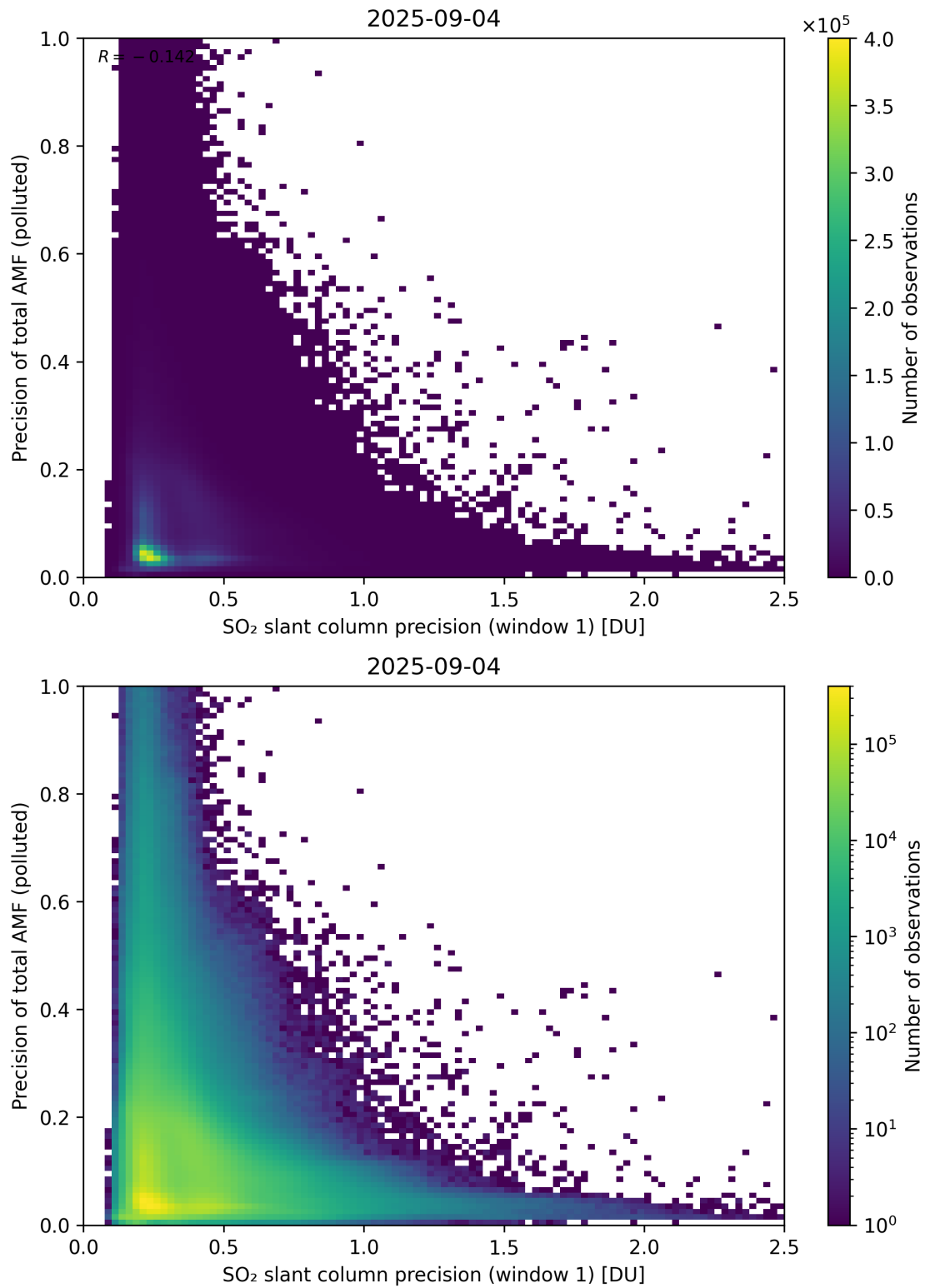
Figure 281: Scatter density plot of “SO 2 slant column precision (window 1)” against “Precision of total AMF (polluted)” for 2025-09-04 to 2025-09-05.
