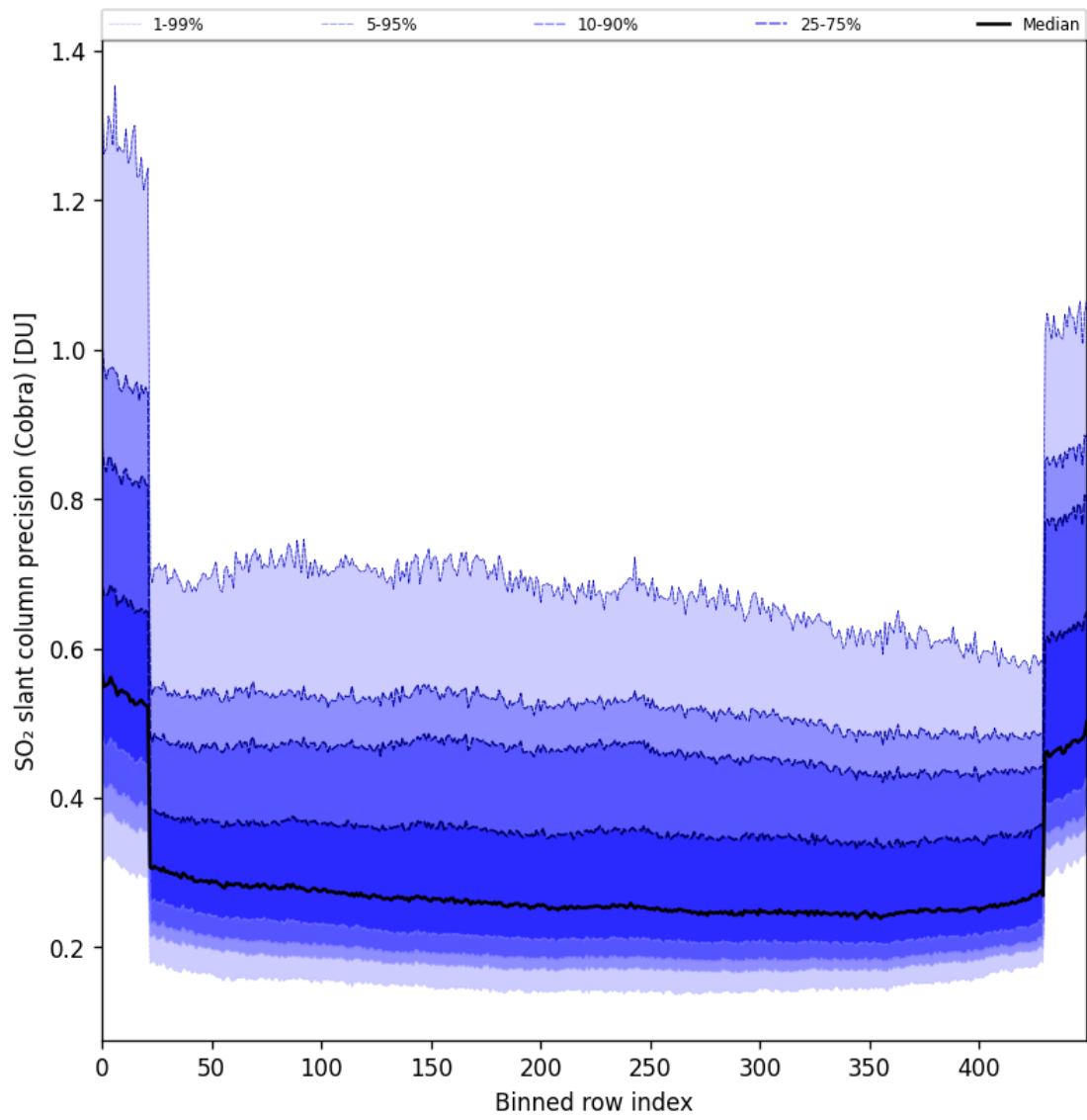
Figure 88: Along track statistics of “SO 2 slant column precision (Cobra)” for 2025-09-04 to 2025-09-05
