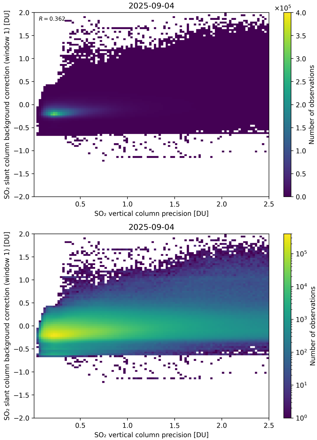
Figure 329: Scatter density plot of “SO 2 vertical column precision” against “SO 2 slant column background correction (window 1)” for 2025-09-04 to 2025-09-05.
