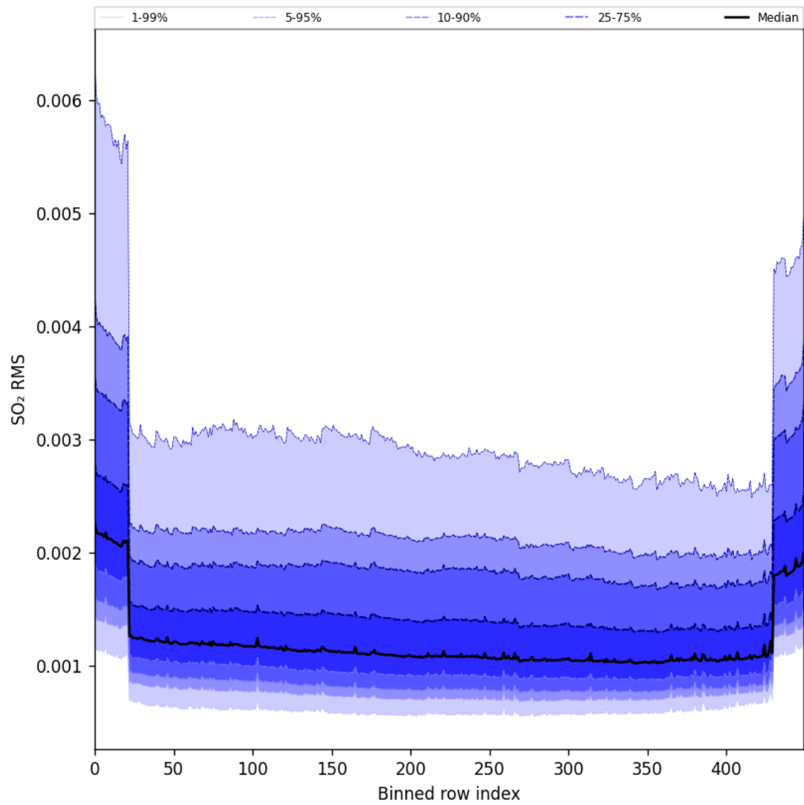
Figure 104: Along track statistics of “SO 2 RMS” for 2025-09-04 to 2025-09-05
