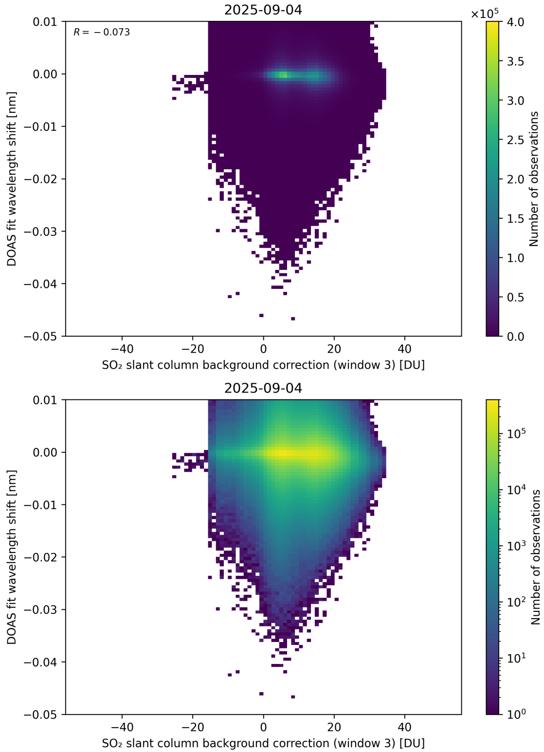
Figure 132: Scatter density plot of “SO 2 slant column background correction (window 3)” against “DOAS fit wavelength shift” for 2025-09-04 to 2025-09-05.
