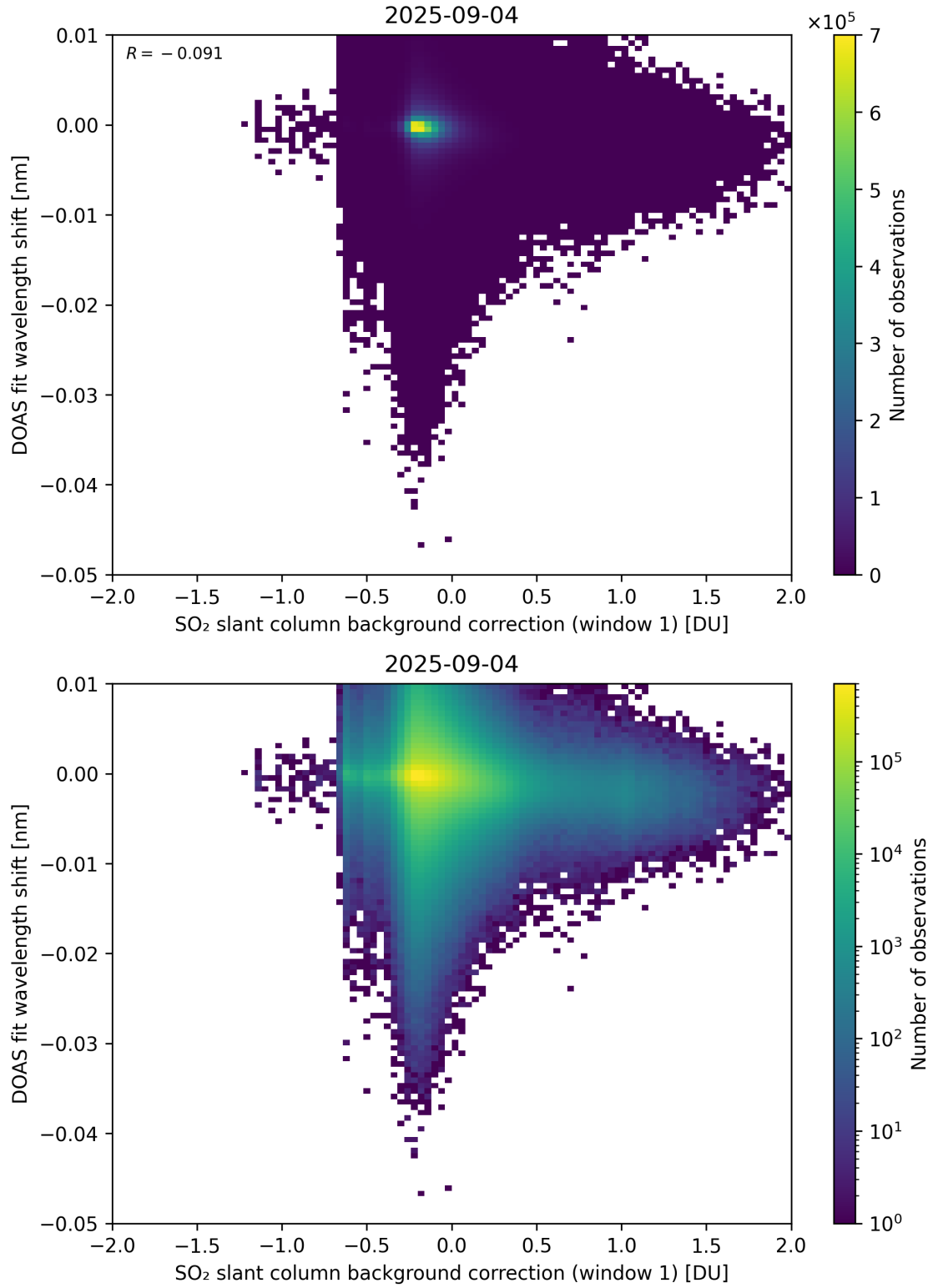
Figure 111: Scatter density plot of “SO 2 slant column background correction (window 1)” against “DOAS fit wavelength shift” for 2025-09-04 to 2025-09-05.
