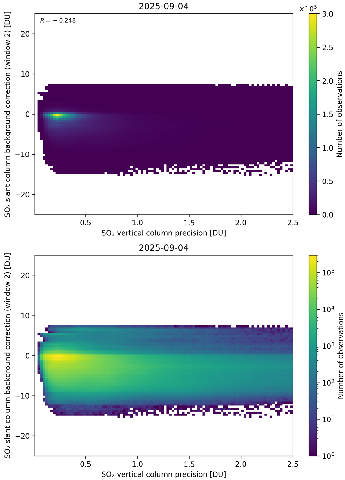
Figure 330: Scatter density plot of “SO 2 vertical column precision” against “SO 2 slant column background correction (window 2)” for 2025-09-04 to 2025-09-05.
