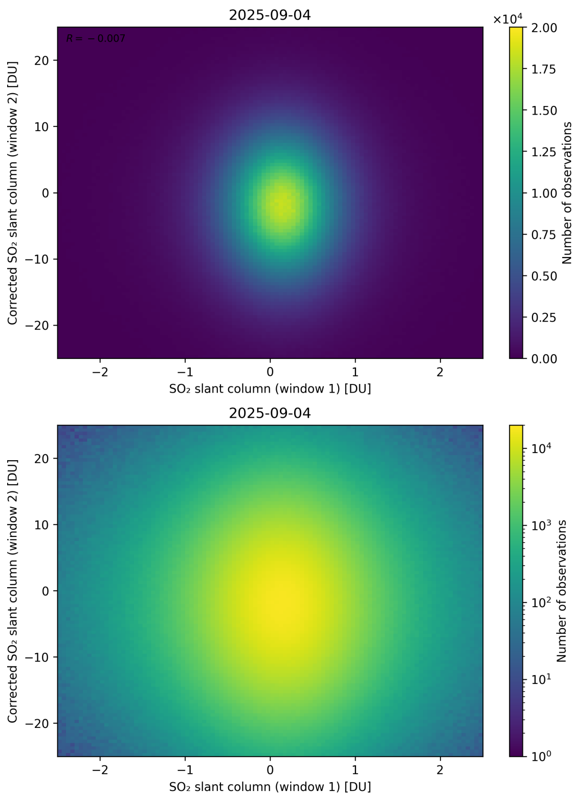
Figure 283: Scatter density plot of “SO 2 slant column (window 1)” against “Corrected SO 2 slant column (window 2)” for 2025-09-04 to 2025-09-05.
