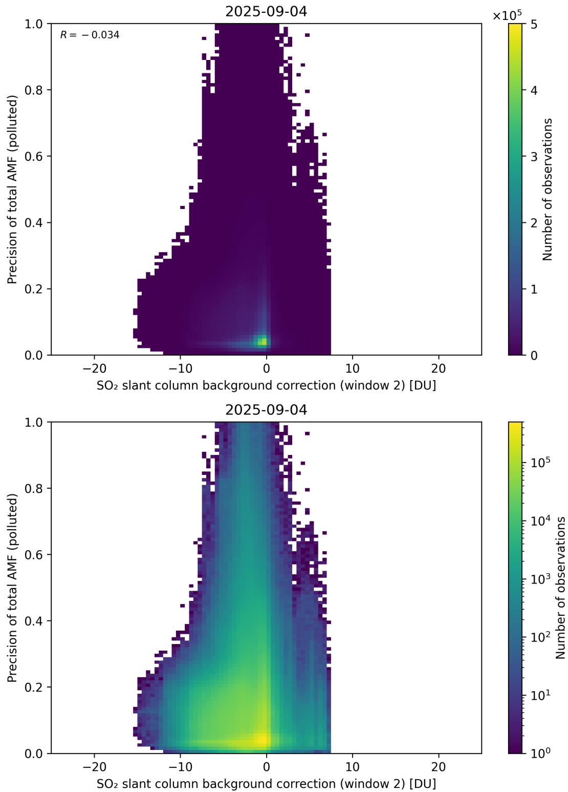
Figure 131: Scatter density plot of “SO 2 slant column background correction (window 2)” against “Precision of total AMF (polluted)” for 2025-09-04 to 2025-09-05.
