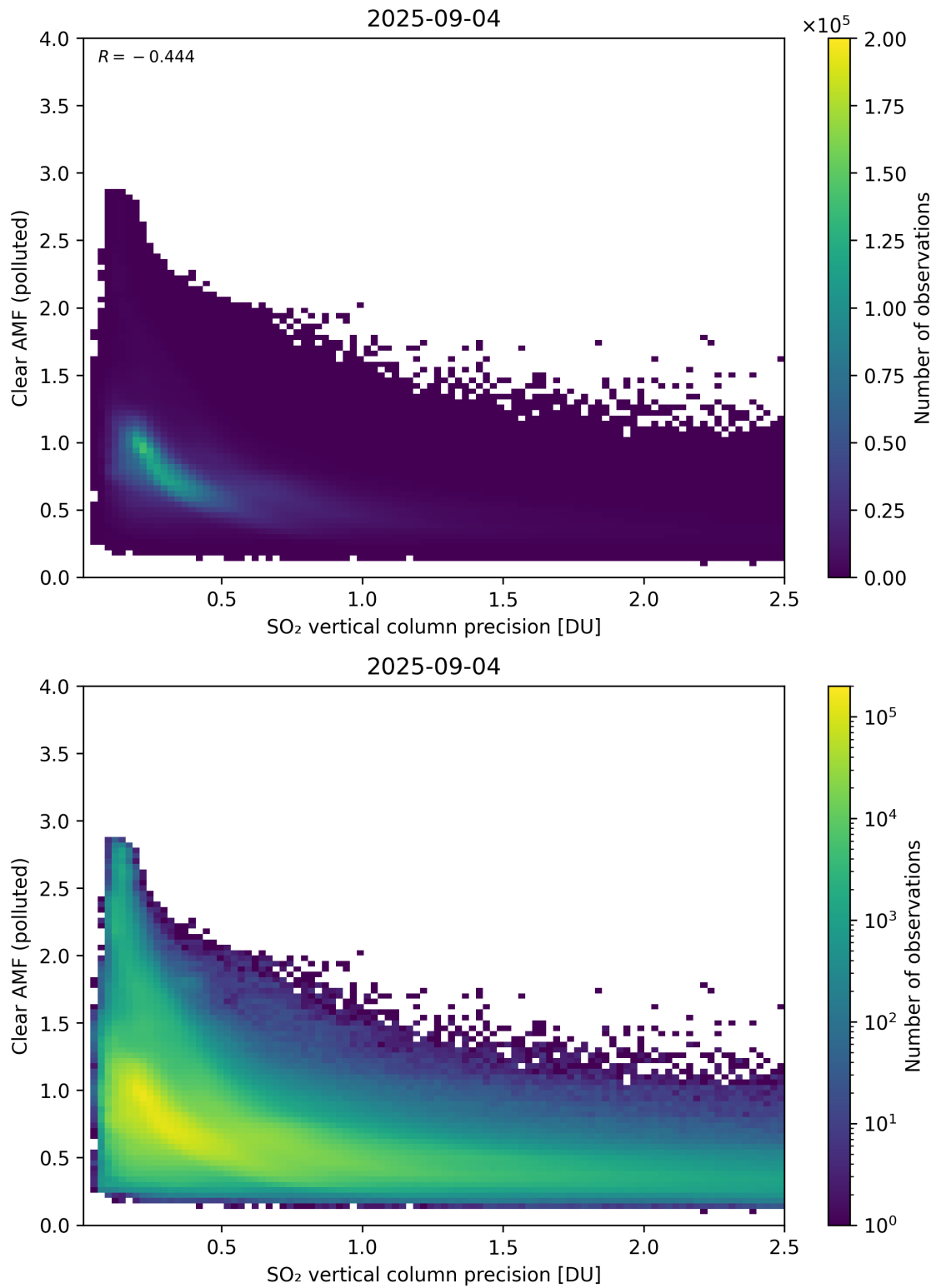
Figure 335: Scatter density plot of “SO 2 vertical column precision” against “Clear AMF (polluted)” for 2025-09-04 to 2025-09-05.
