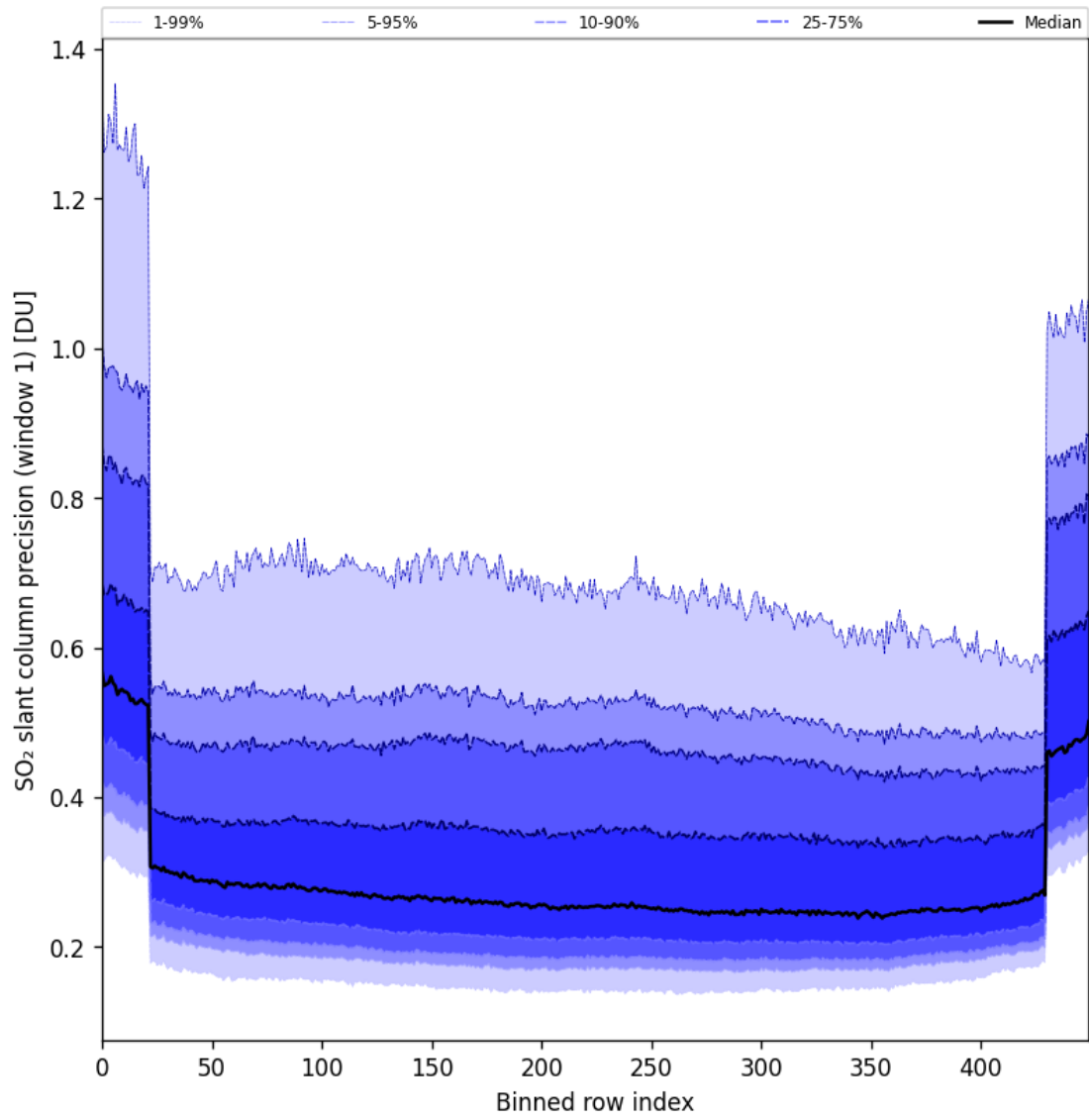
Figure 90: Along track statistics of “SO 2 slant column precision (window 1)” for 2025-09-04 to 2025-09-05
