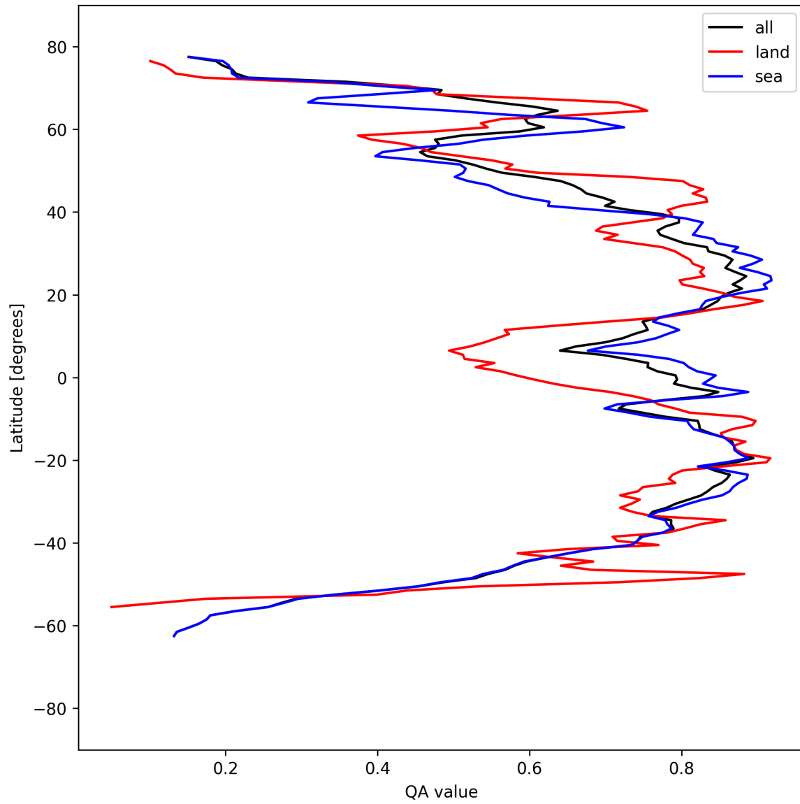
Figure 31: Zonal average of “QA value” for 2025-09-04 to 2025-09-05.
