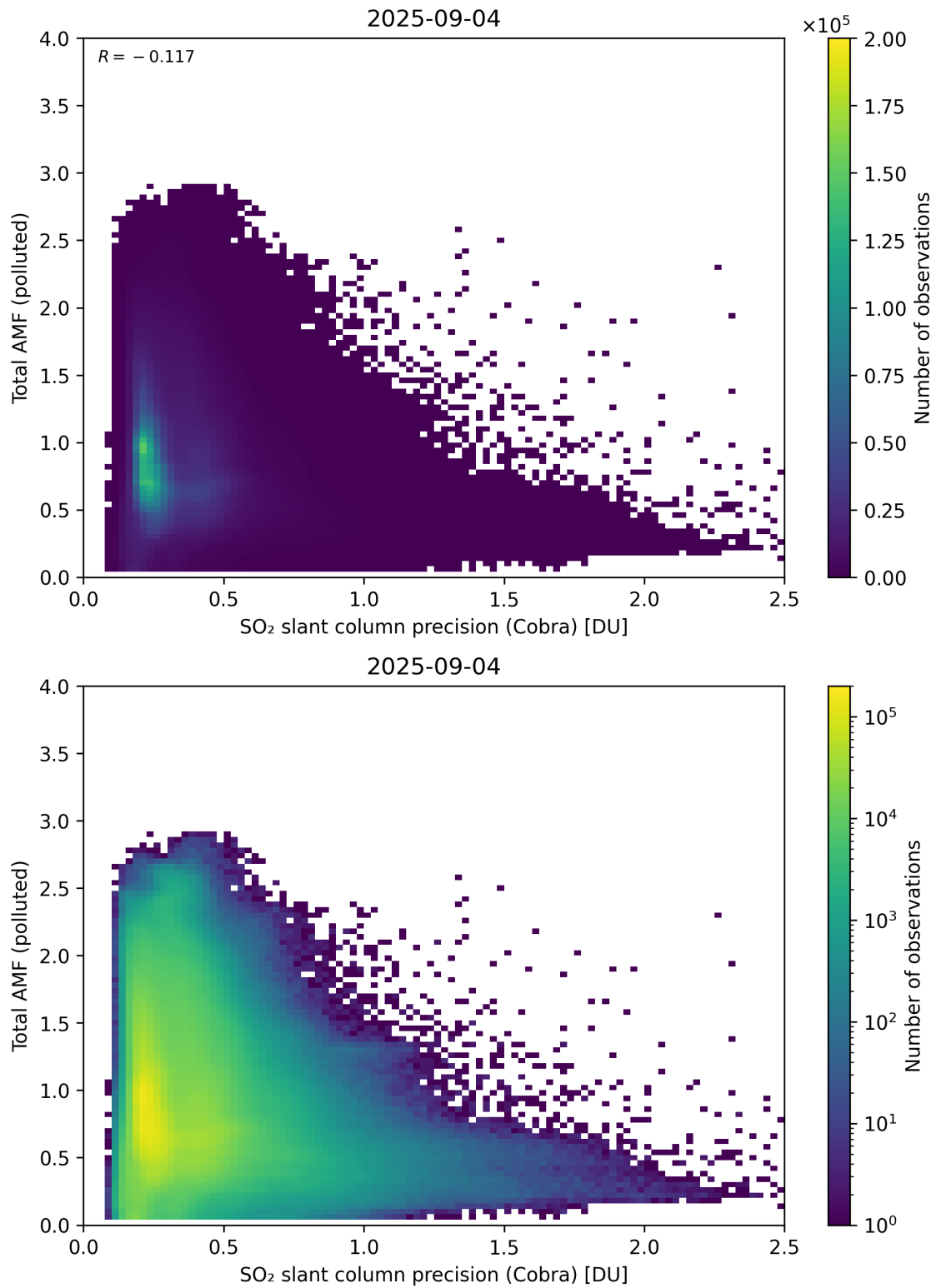
Figure 213: Scatter density plot of “SO 2 slant column precision (Cobra)” against “Total AMF (polluted)” for 2025-09-04 to 2025-09-05.
