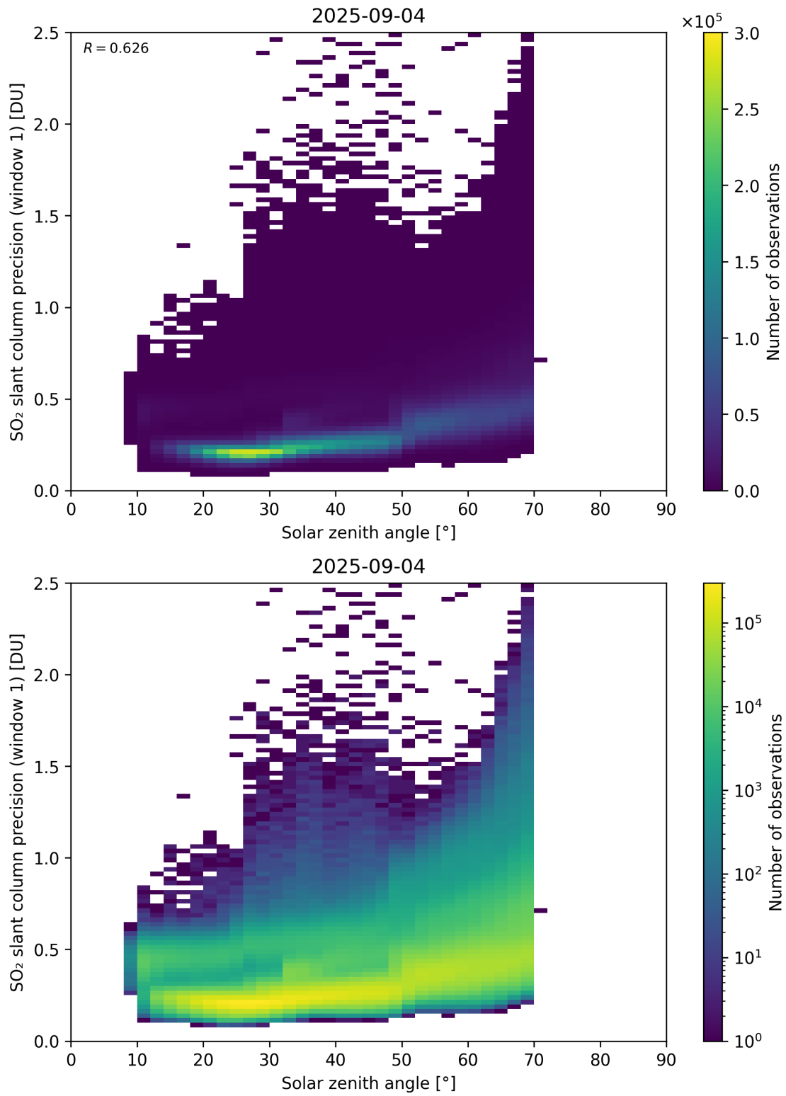
Figure 185: Scatter density plot of “Solar zenith angle” against “SO 2 slant column precision (window 1)” for 2025-09-04 to 2025-09-05.
