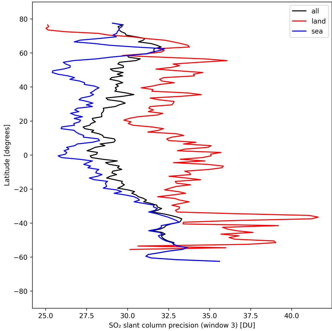
Figure 46: Zonal average of “SO 2 slant column precision (window 3)” for 2025-09-04 to 2025-09-05.
