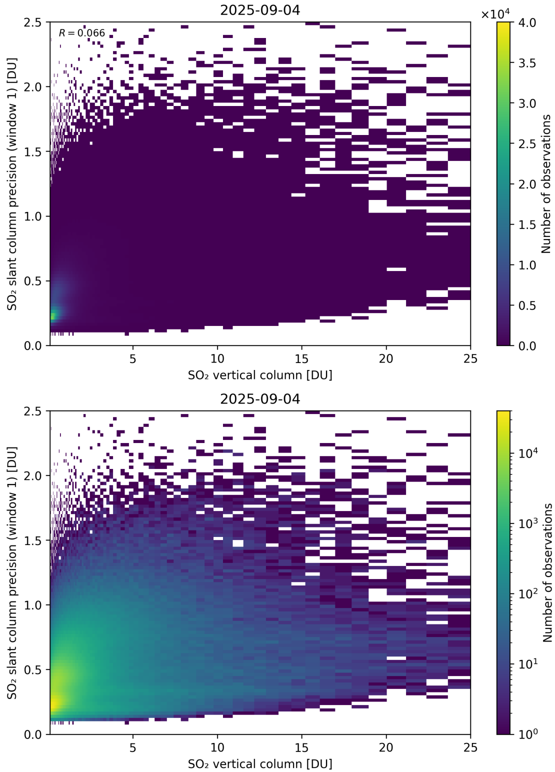
Figure 355: Scatter density plot of “SO 2 vertical column” against “SO 2 slant column precision (window 1)” for 2025-09-04 to 2025-09-05.
