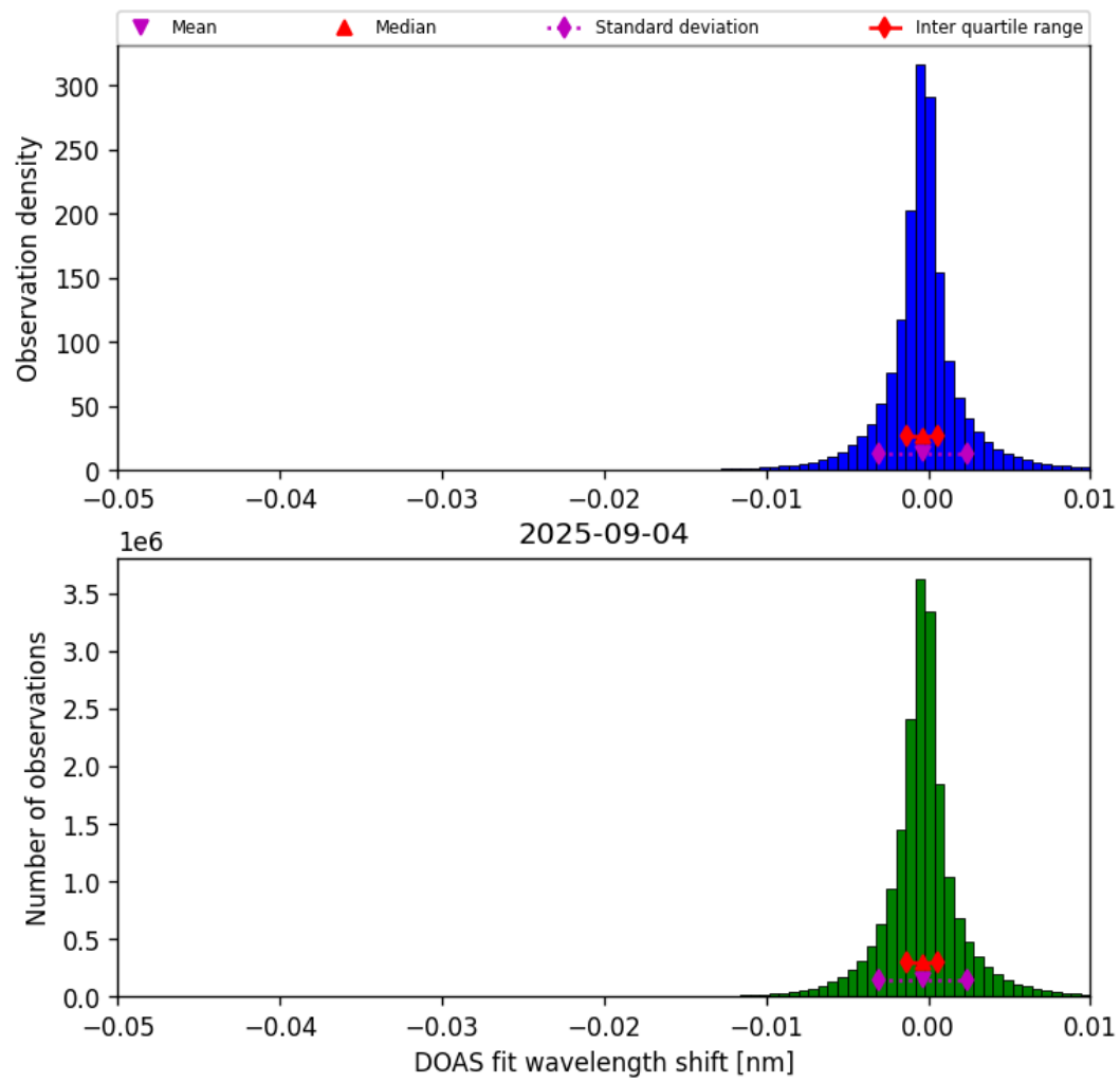
Figure 76: Histogram of “DOAS fit wavelength shift” for 2025-09-04 to 2025-09-05
