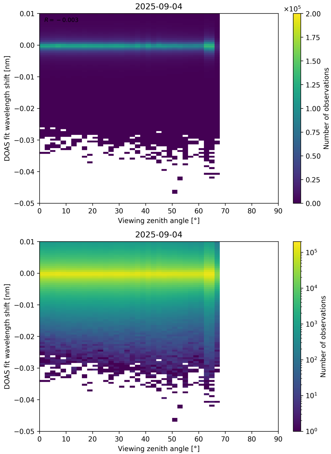
Figure 365: Scatter density plot of “Viewing zenith angle” against “DOAS fit wavelength shift” for 2025-09-04 to 2025-09-05.
