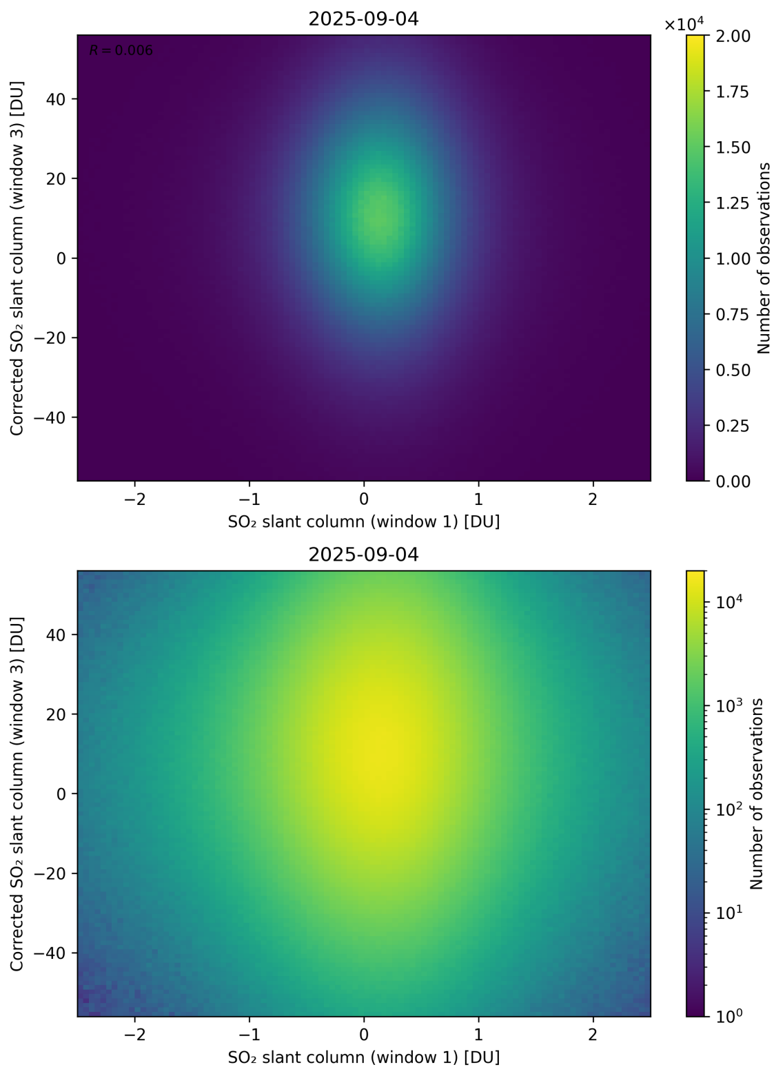
Figure 284: Scatter density plot of “SO 2 slant column (window 1)” against “Corrected SO 2 slant column (window 3)” for 2025-09-04 to 2025-09-05.
