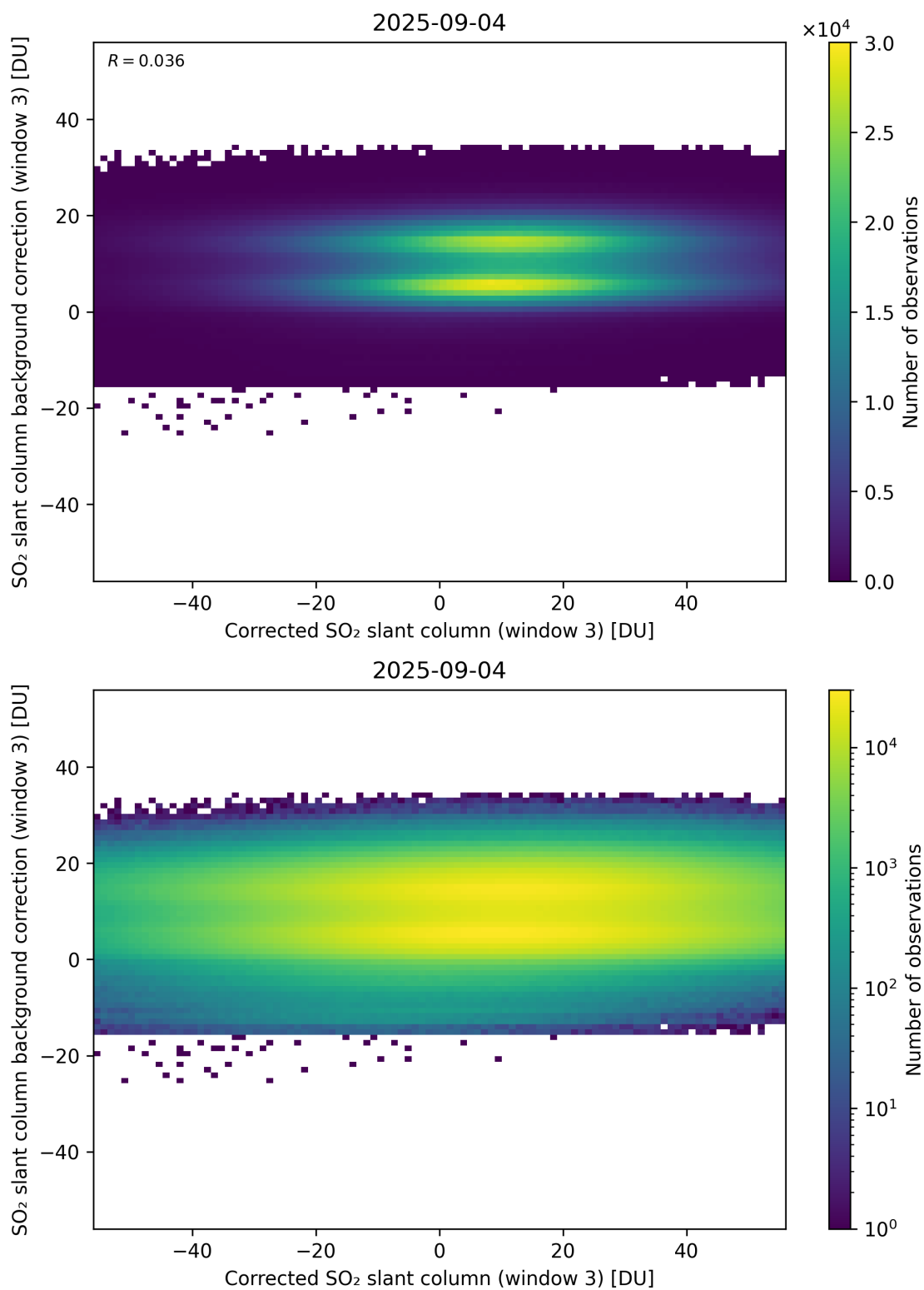
Figure 255: Scatter density plot of “Corrected SO 2 slant column (window 3)” against “SO 2 slant column background correction (window 3)” for 2025-09-04 to 2025-09-05.
