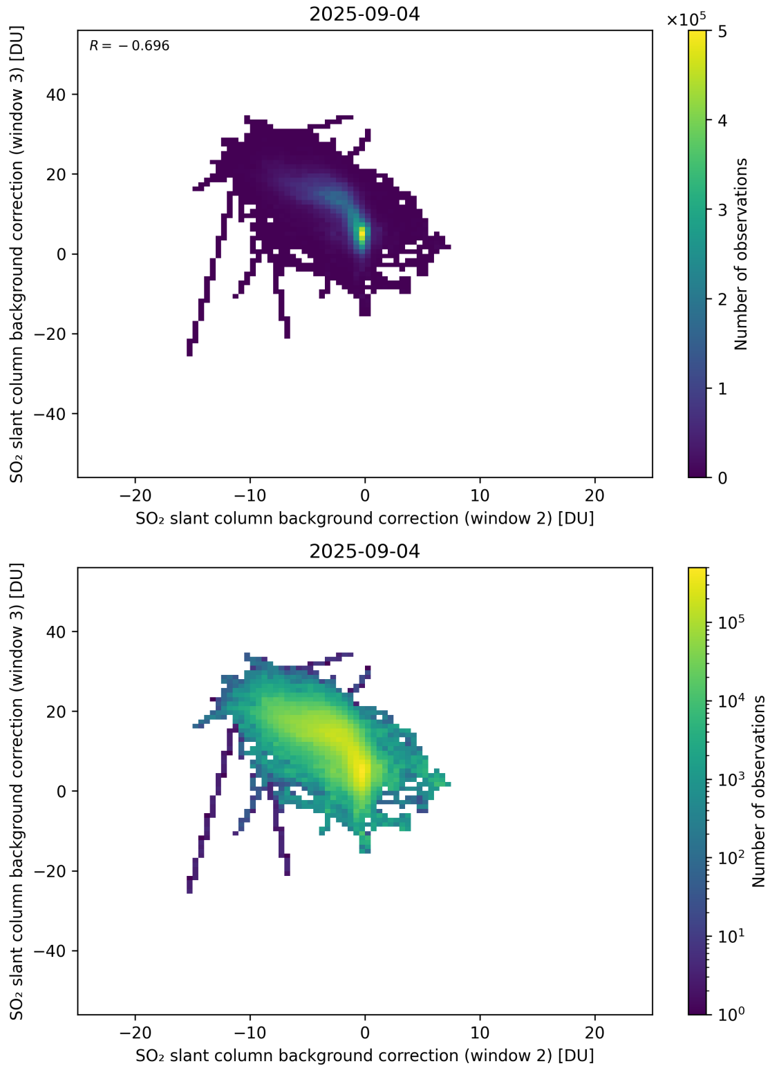
Figure 122: Scatter density plot of “SO 2 slant column background correction (window 2)” against “SO 2 slant column background correction (window 3)” for 2025-09-04 to 2025-09-05.
