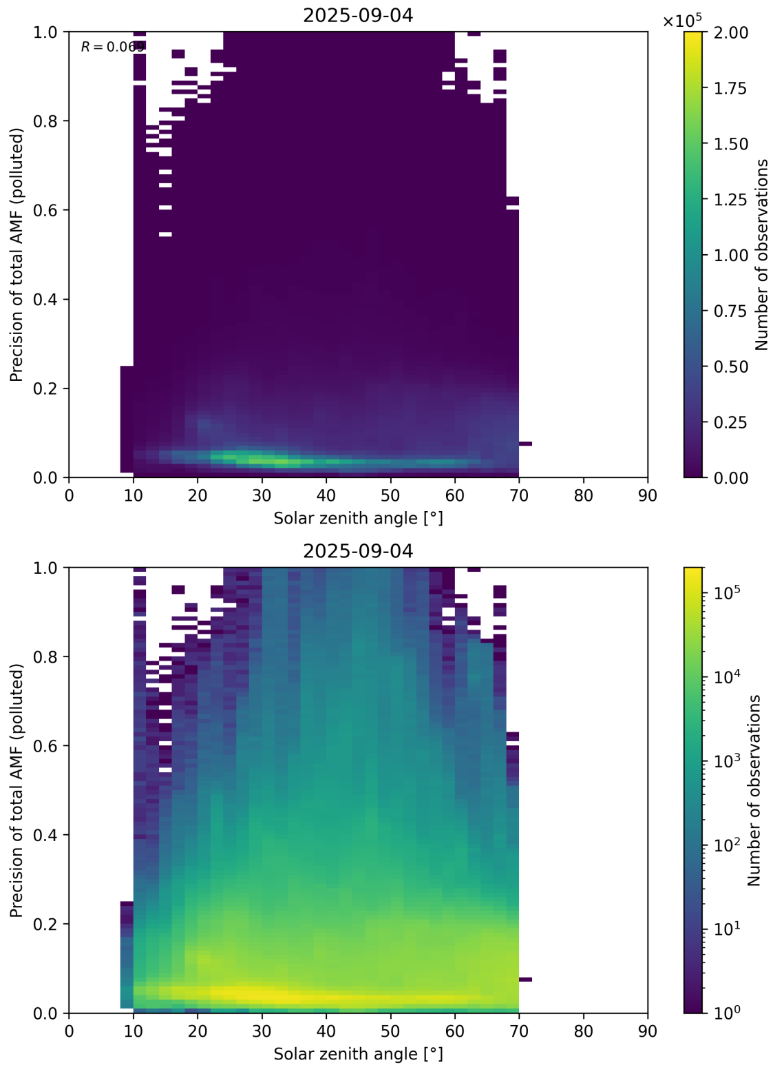
Figure 190: Scatter density plot of “Solar zenith angle” against “Precision of total AMF (polluted)” for 2025-09-04 to 2025-09-05.
