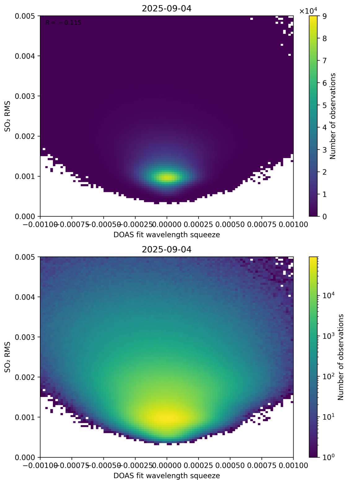
Figure 143: Scatter density plot of “DOAS fit wavelength squeeze” against “SO 2 RMS” for 2025-09-04 to 2025-09-05.
