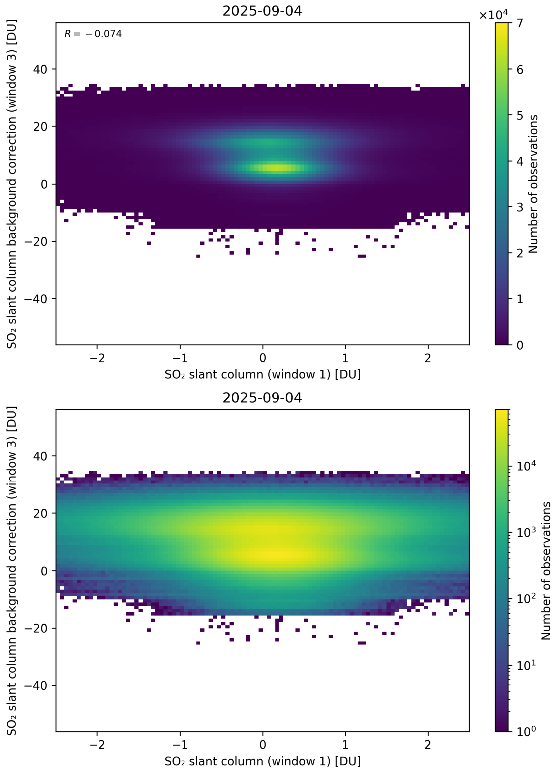
Figure 264: Scatter density plot of “SO 2 slant column (window 1)” against “SO 2 slant column background correction (window 3)” for 2025-09-04 to 2025-09-05.
