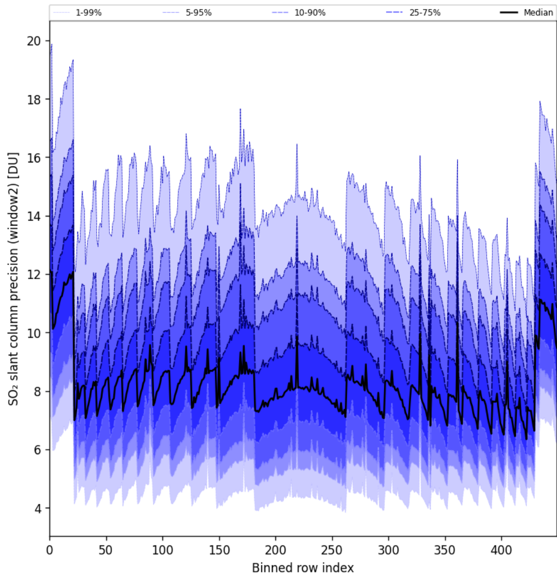
Figure 94: Along track statistics of “SO 2 slant column precision (window2)” for 2025-09-04 to 2025-09-05
