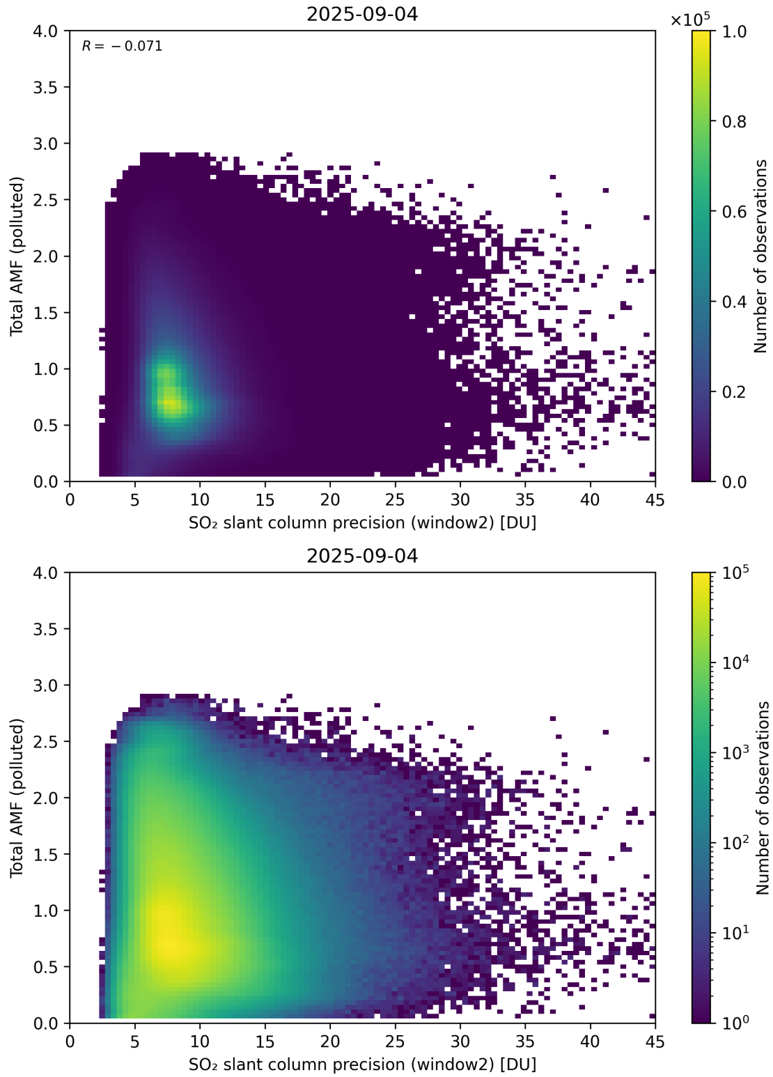
Figure 301: Scatter density plot of “SO 2 slant column precision (window2)” against “Total AMF (polluted)” for 2025-09-04 to 2025-09-05.
