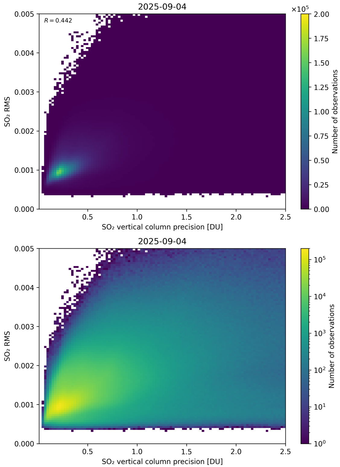
Figure 334: Scatter density plot of “SO 2 vertical column precision” against “SO 2 RMS” for 2025-09-04 to 2025-09-05.
