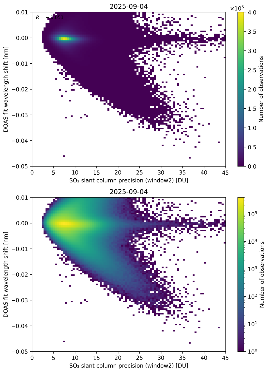
Figure 293: Scatter density plot of “SO 2 slant column precision (window2)” against “DOAS fit wavelength shift” for 2025-09-04 to 2025-09-05.
