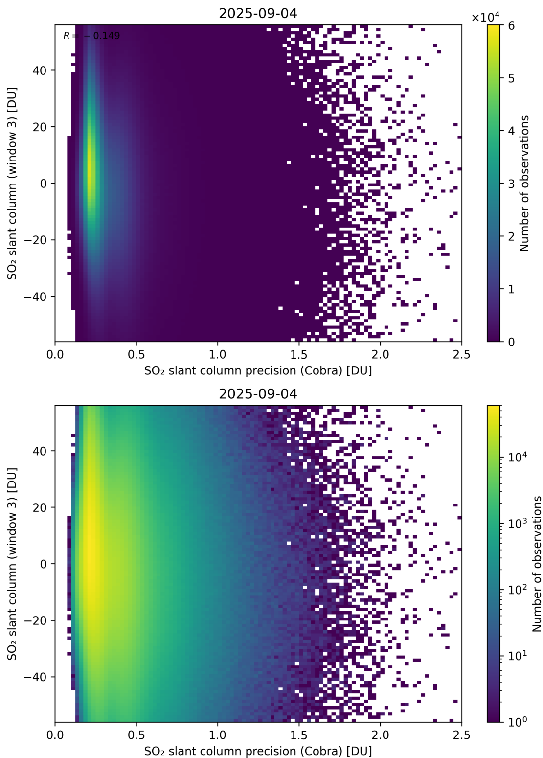
Figure 211: Scatter density plot of “SO 2 slant column precision (Cobra)” against “SO 2 slant column (window 3)” for 2025-09-04 to 2025-09-05.
