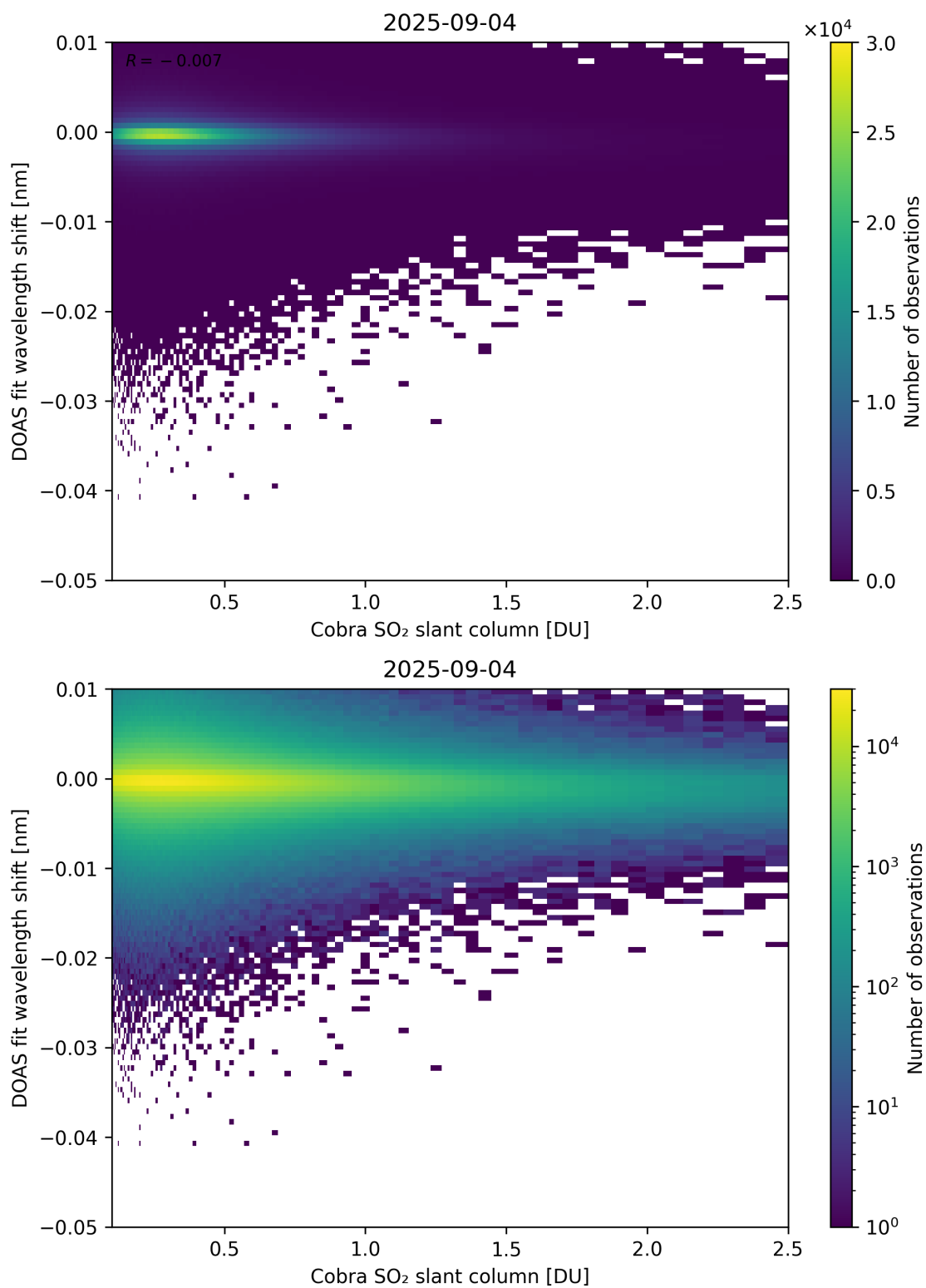
Figure 196: Scatter density plot of “Cobra SO 2 slant column” against “DOAS fit wavelength shift” for 2025-09-04 to 2025-09-05.
