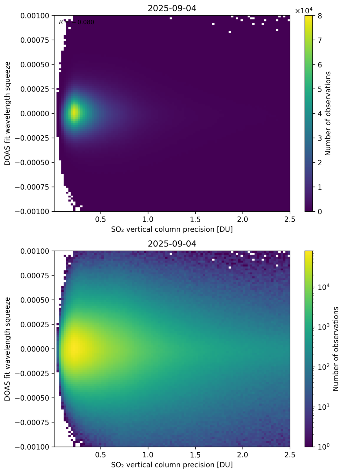
Figure 333: Scatter density plot of “SO 2 vertical column precision” against “DOAS fit wavelength squeeze” for 2025-09-04 to 2025-09-05.
