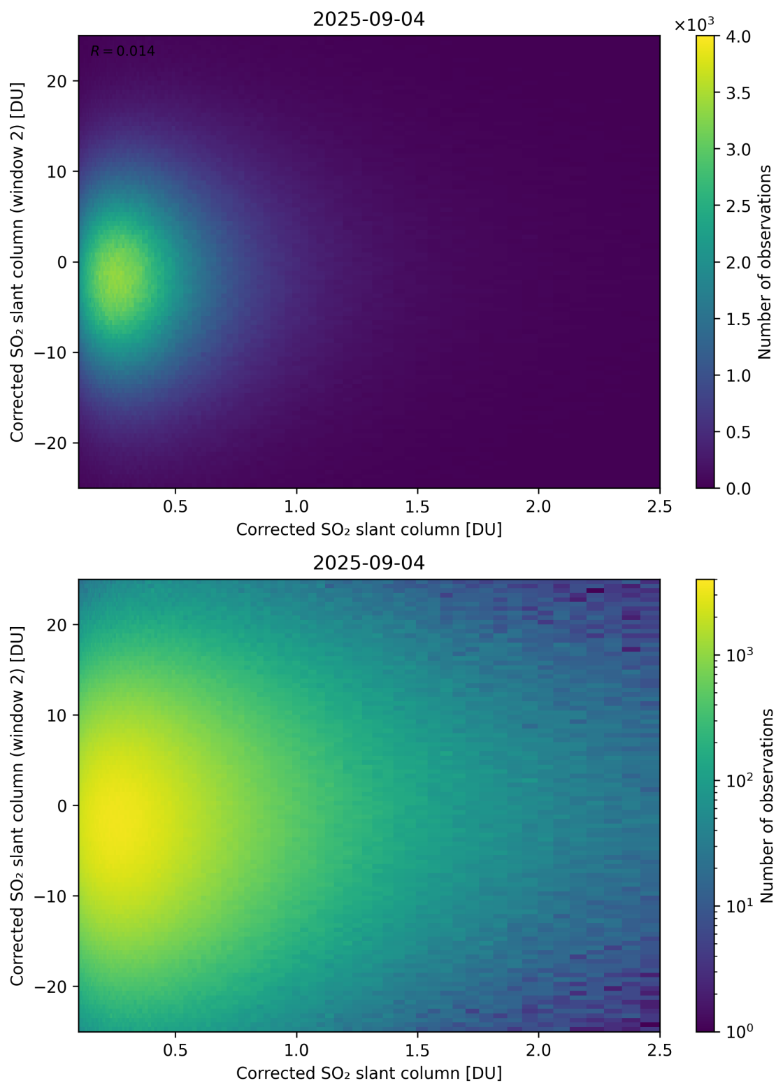
Figure 235: Scatter density plot of “Corrected SO 2 slant column” against “Corrected SO 2 slant column (window 2)” for 2025-09-04 to 2025-09-05.
