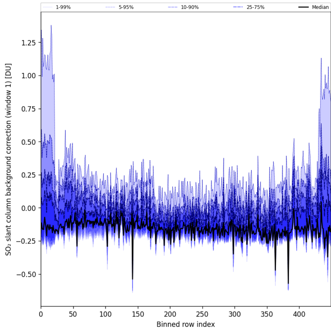
Figure 92: Along track statistics of “SO 2 slant column background correction (window 1)” for 2025-09-04 to 2025-09-05
