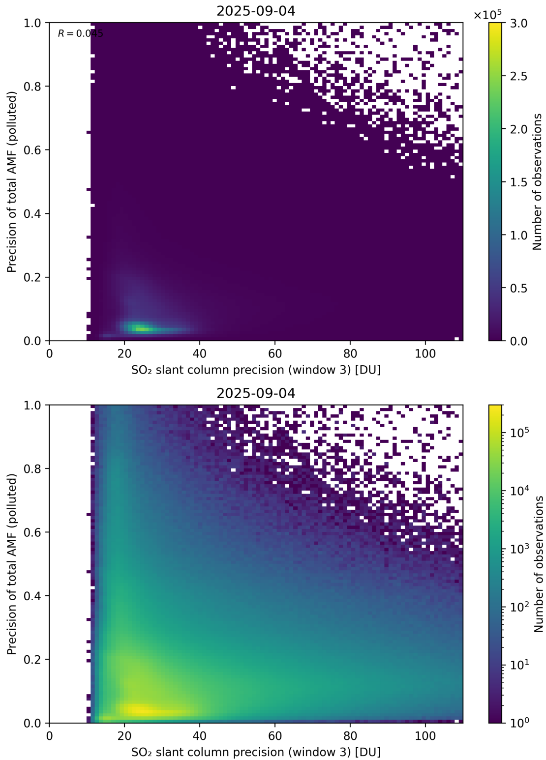
Figure 314: Scatter density plot of “SO 2 slant column precision (window 3)” against “Precision of total AMF (polluted)” for 2025-09-04 to 2025-09-05.
