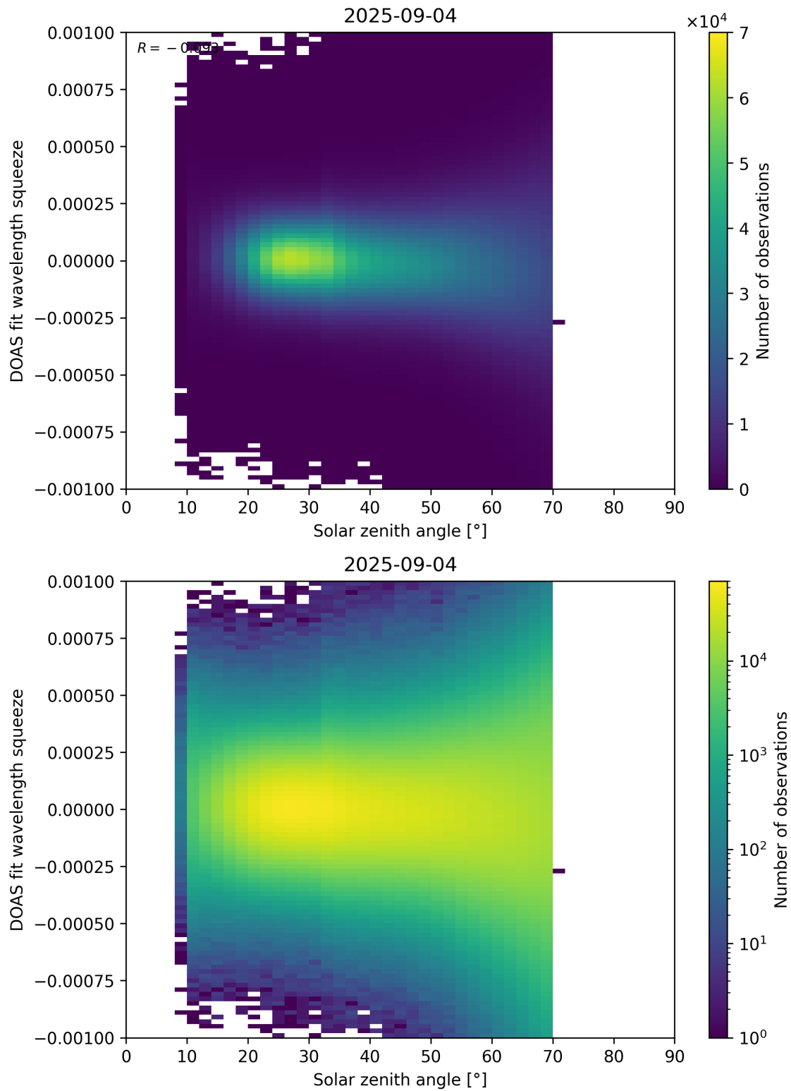
Figure 175: Scatter density plot of “Solar zenith angle” against “DOAS fit wavelength squeeze” for 2025-09-04 to 2025-09-05.
