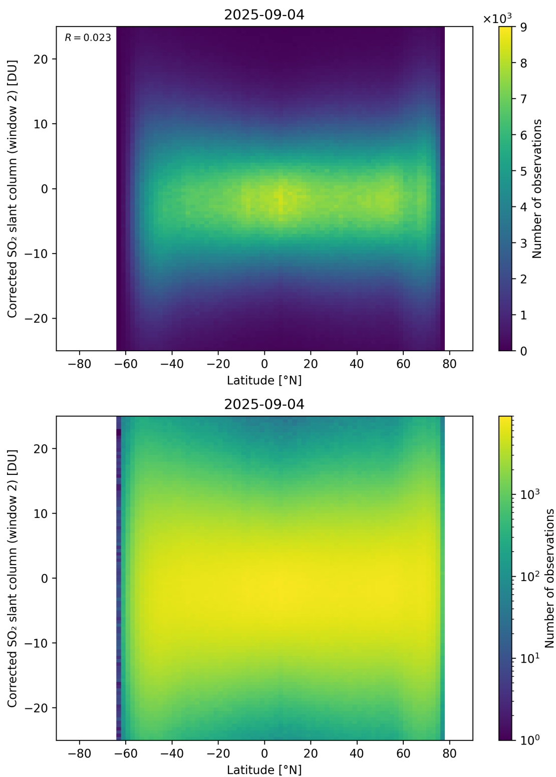
Figure 160: Scatter density plot of “Latitude” against “Corrected SO 2 slant column (window 2)” for 2025-09-04 to 2025-09-05.
