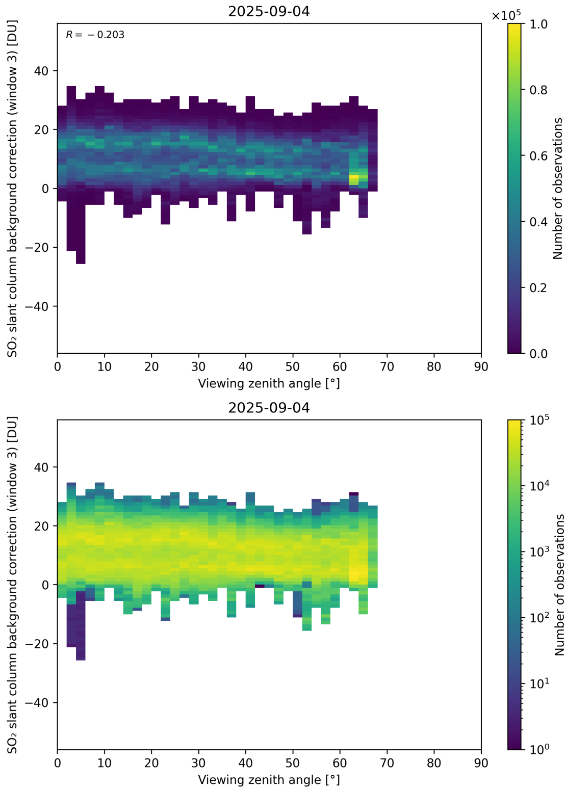
Figure 364: Scatter density plot of “Viewing zenith angle” against “SO 2 slant column background correction (window 3)” for 2025-09-04 to 2025-09-05.
