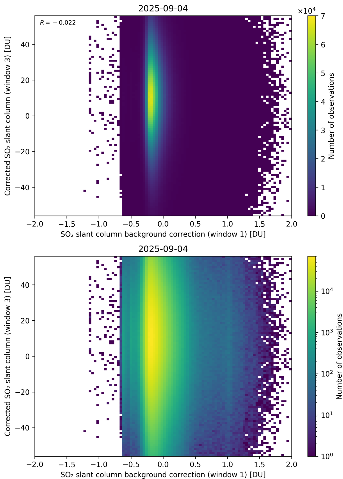
Figure 116: Scatter density plot of “SO 2 slant column background correction (window 1)” against “Corrected SO 2 slant column (window 3)” for 2025-09-04 to 2025-09-05.
