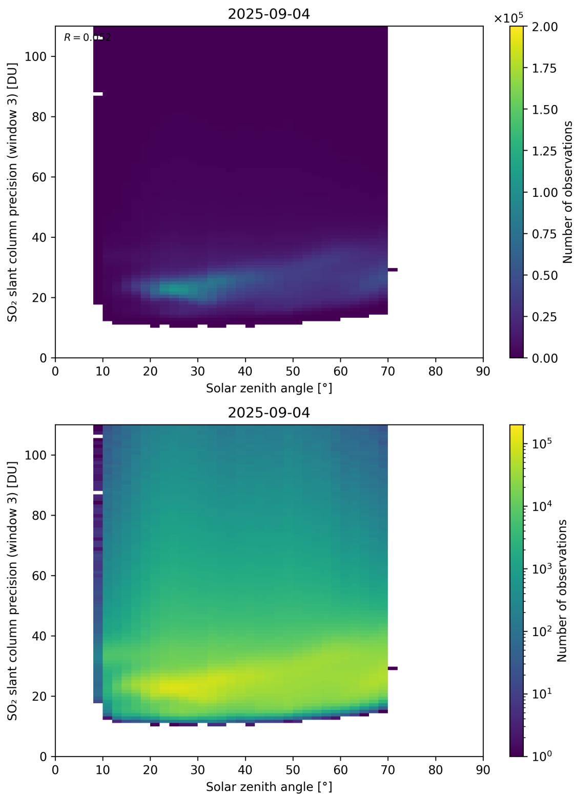
Figure 188: Scatter density plot of “Solar zenith angle” against “SO 2 slant column precision (window 3)” for 2025-09-04 to 2025-09-05.
