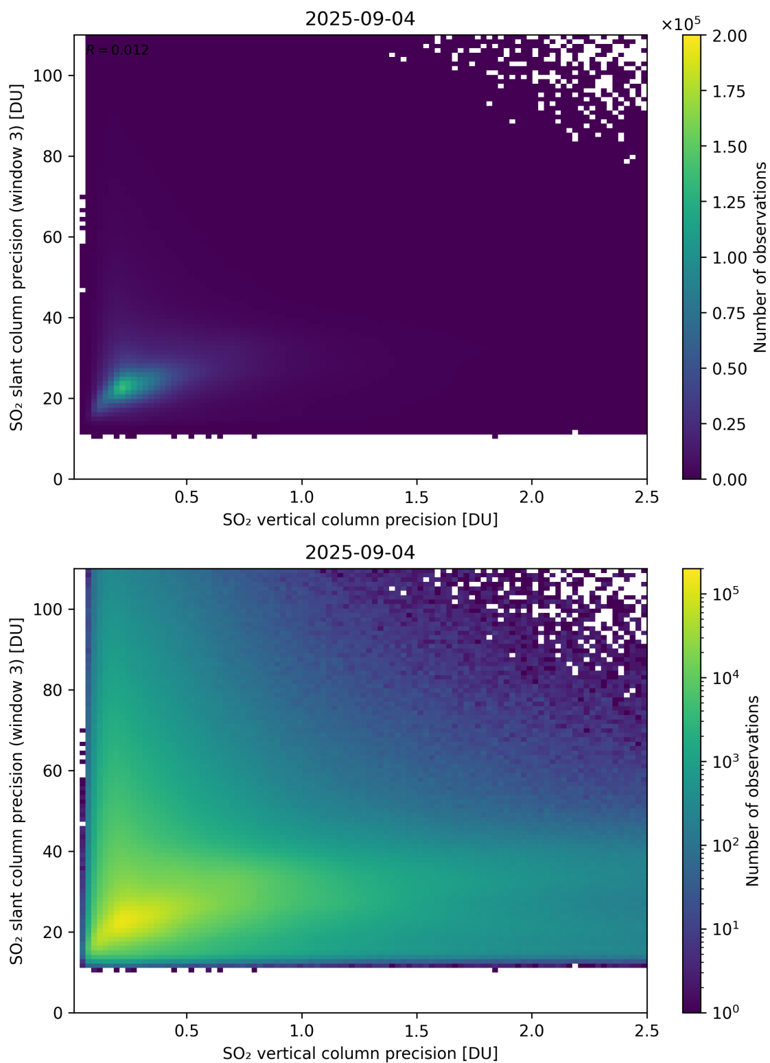
Figure 345: Scatter density plot of “SO 2 vertical column precision” against “SO 2 slant column precision (window 3)” for 2025-09-04 to 2025-09-05.
