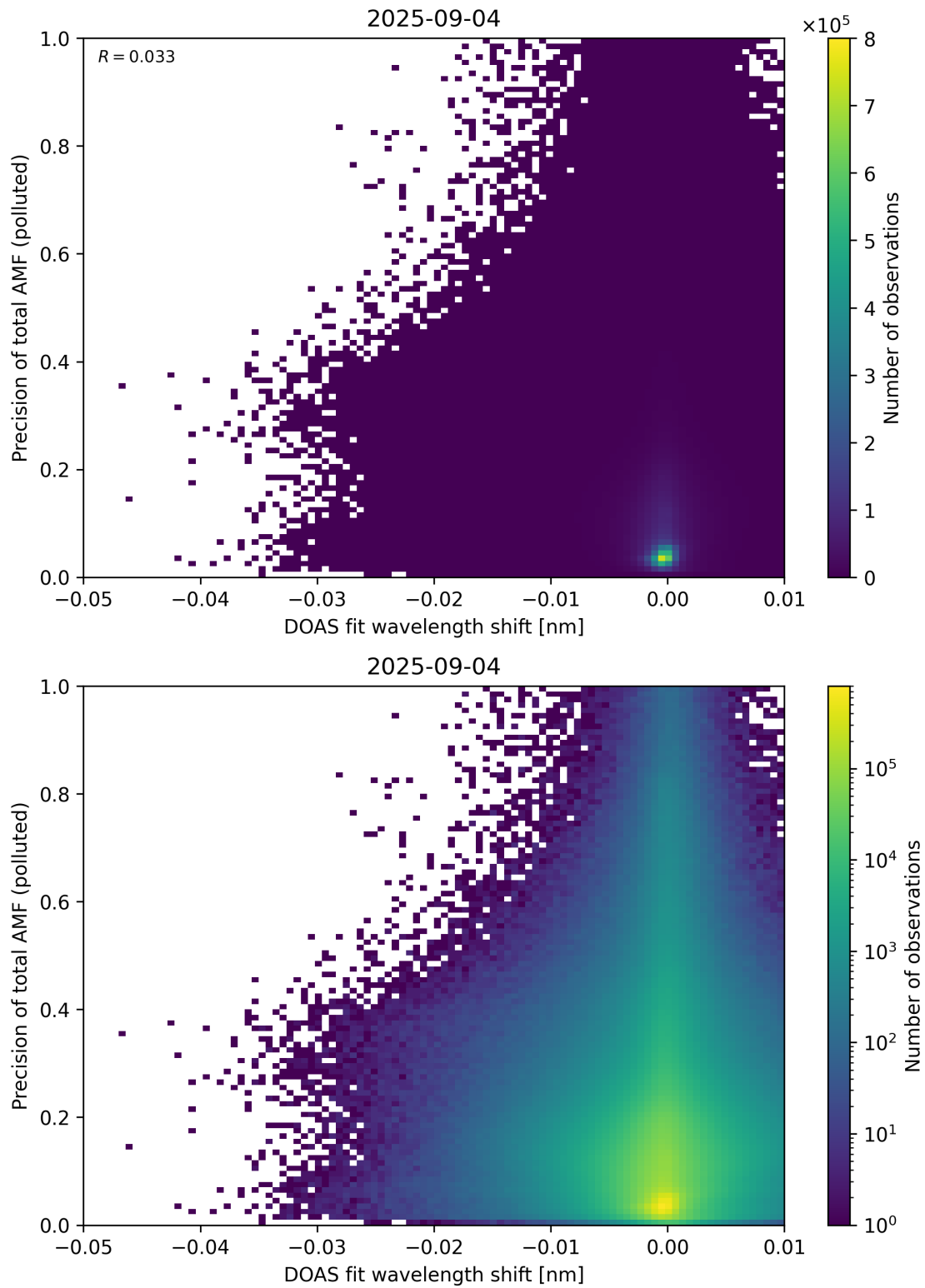
Figure 142: Scatter density plot of “DOAS fit wavelength shift” against “Precision of total AMF (polluted)” for 2025-09-04 to 2025-09-05.
