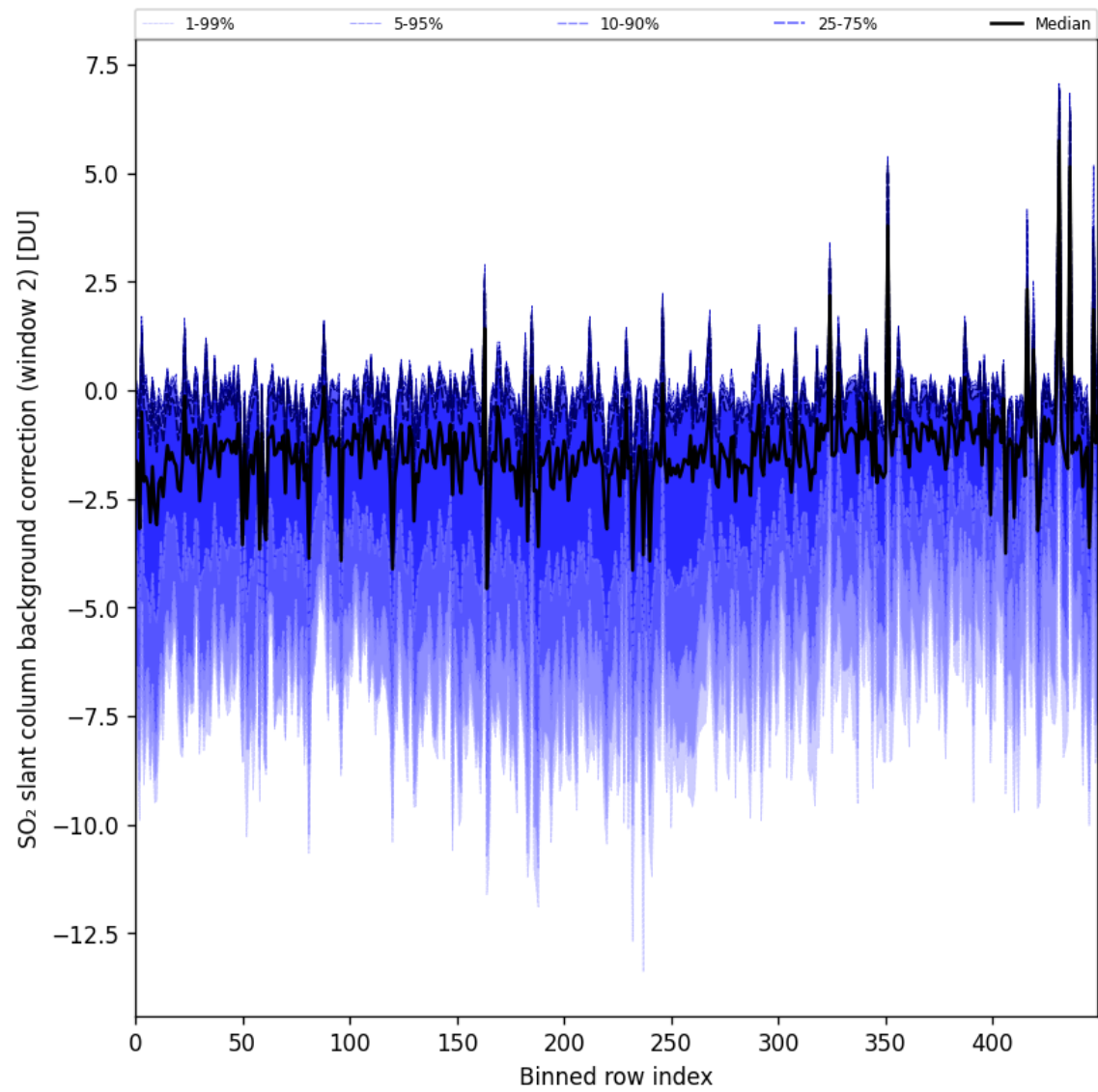
Figure 96: Along track statistics of “SO 2 slant column background correction (window 2)” for 2025-09-04 to 2025-09-05
