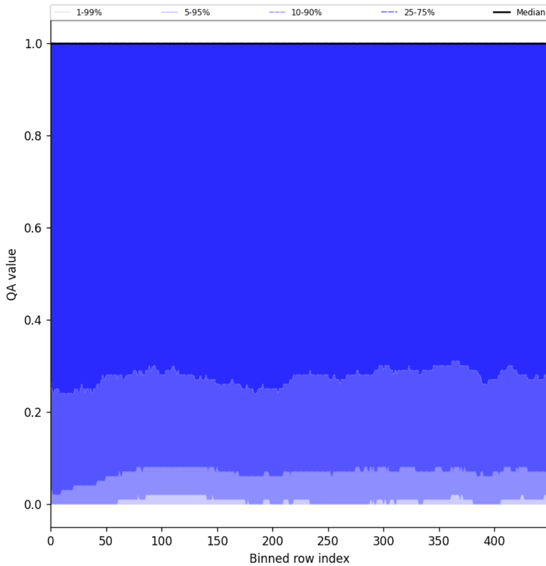
Figure 83: Along track statistics of “QA value” for 2025-09-04 to 2025-09-05
