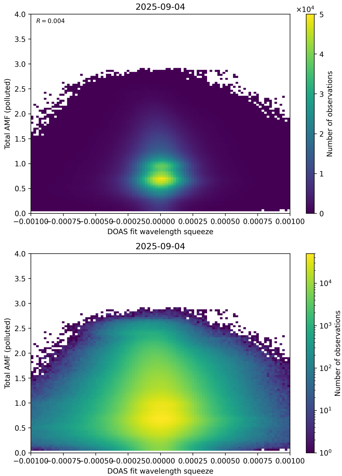
Figure 145: Scatter density plot of “DOAS fit wavelength squeeze” against “Total AMF (polluted)” for 2025-09-04 to 2025-09-05.
