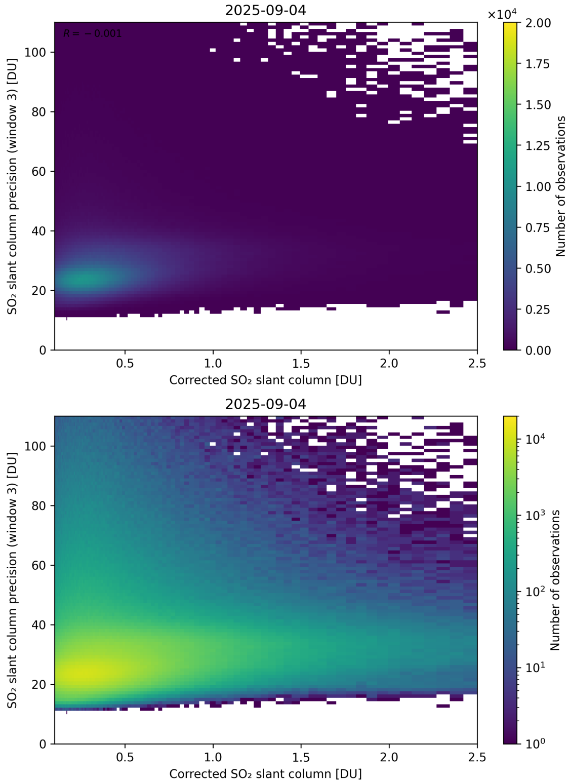
Figure 241: Scatter density plot of “Corrected SO 2 slant column” against “SO 2 slant column precision (window 3)” for 2025-09-04 to 2025-09-05.
