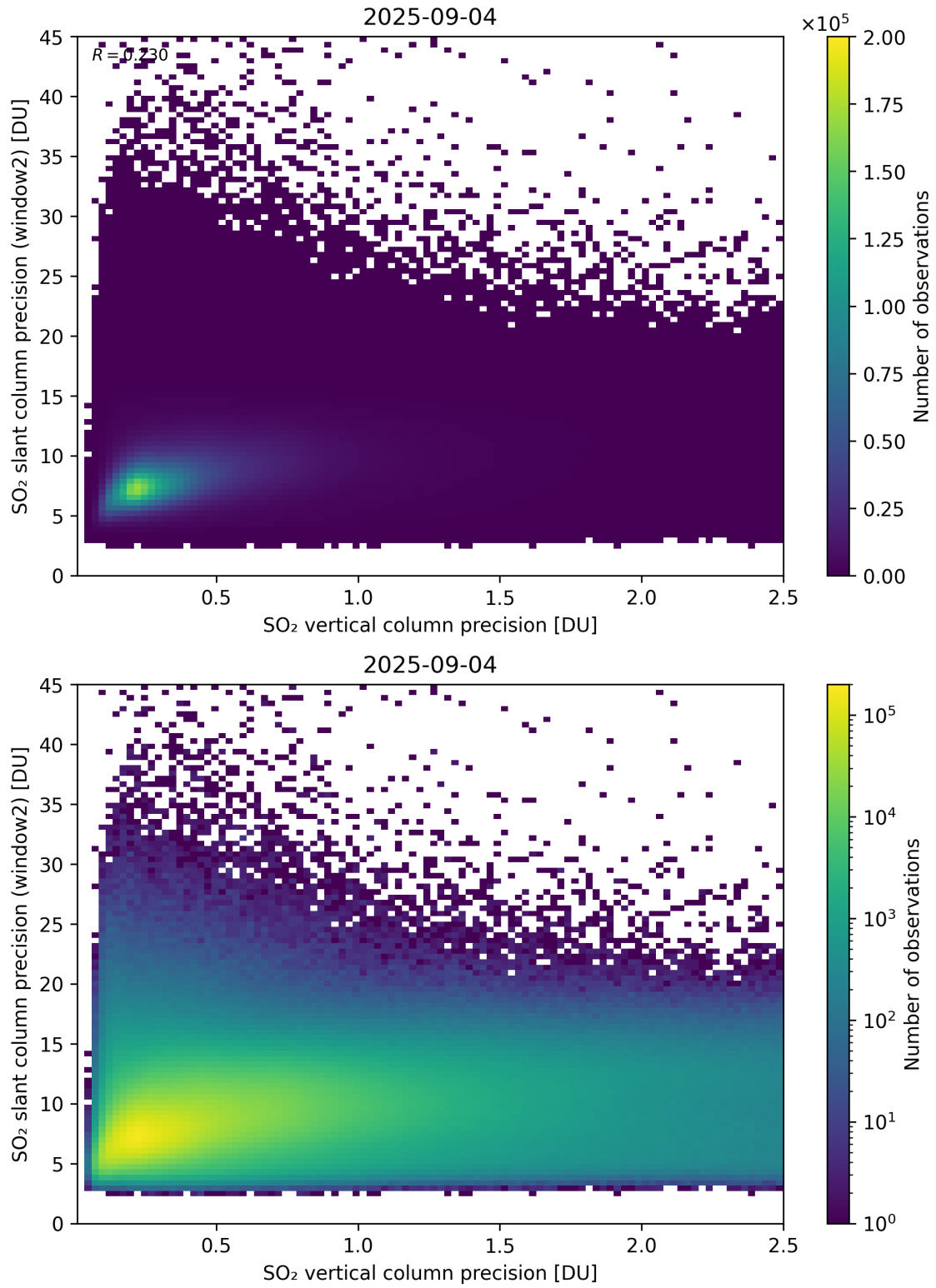
Figure 343: Scatter density plot of “SO 2 vertical column precision” against “SO 2 slant column precision (window2)” for 2025-09-04 to 2025-09-05.
