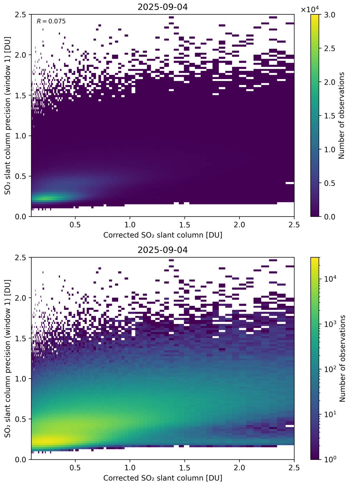
Figure 238: Scatter density plot of “Corrected SO 2 slant column” against “SO 2 slant column precision (window 1)” for 2025-09-04 to 2025-09-05.
