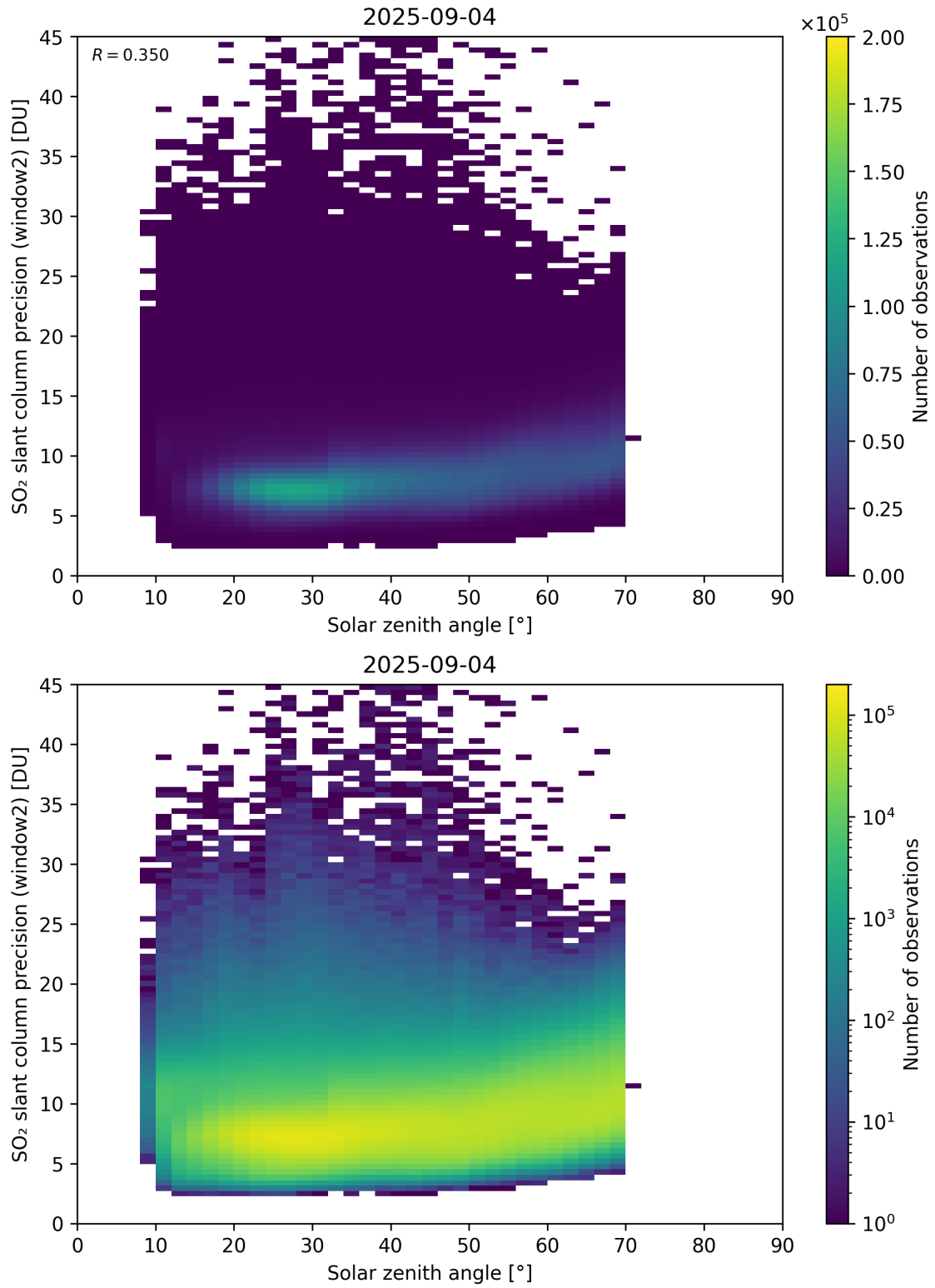
Figure 186: Scatter density plot of “Solar zenith angle” against “SO 2 slant column precision (window2)” for 2025-09-04 to 2025-09-05.
