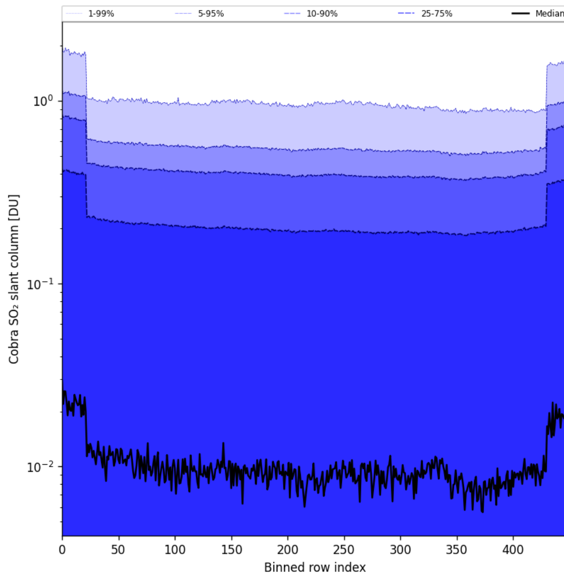
Figure 87: Along track statistics of "Cobra SO 2 slant column" for 2025-09-04 to 2025-09-05
