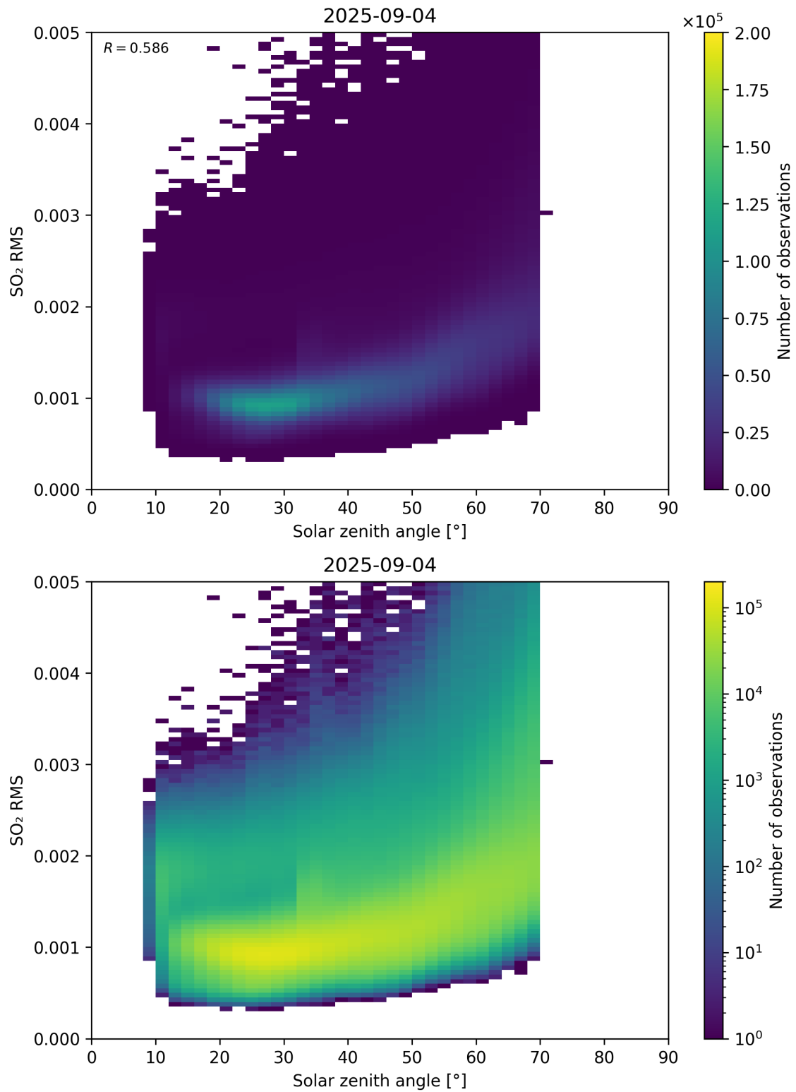
Figure 176: Scatter density plot of “Solar zenith angle” against “SO 2 RMS” for 2025-09-04 to 2025-09-05.
