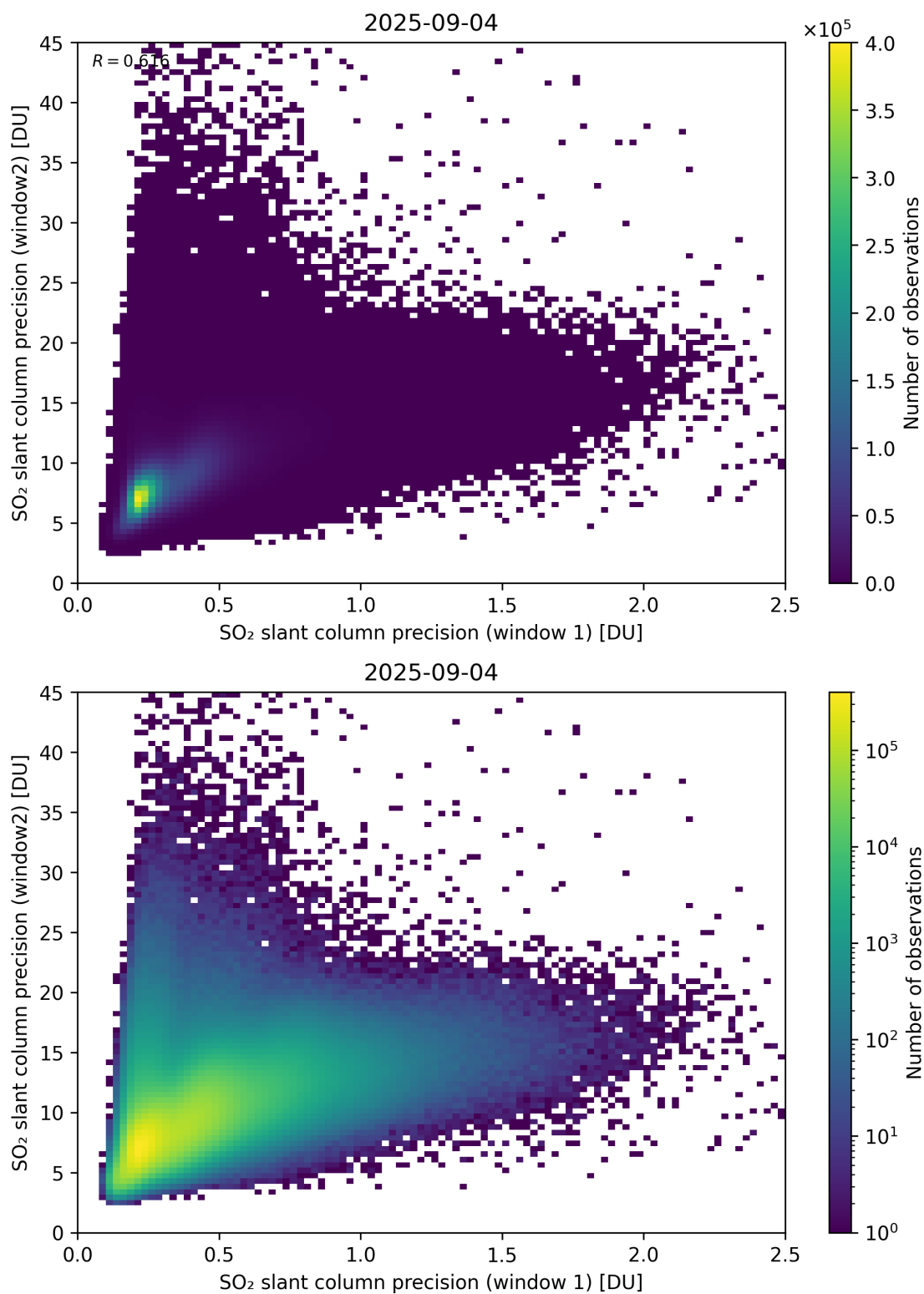
Figure 277: Scatter density plot of “SO 2 slant column precision (window 1)” against “SO 2 slant column precision (window2)” for 2025-09-04 to 2025-09-05.
