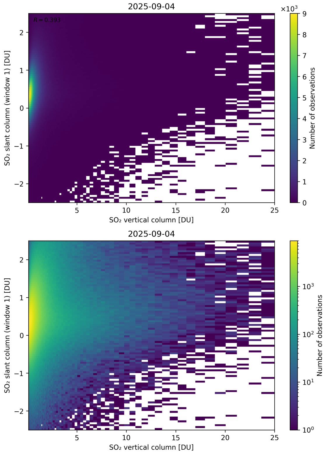
Figure 354: Scatter density plot of “SO 2 vertical column” against “SO 2 slant column (window 1)” for 2025-09-04 to 2025-09-05.
