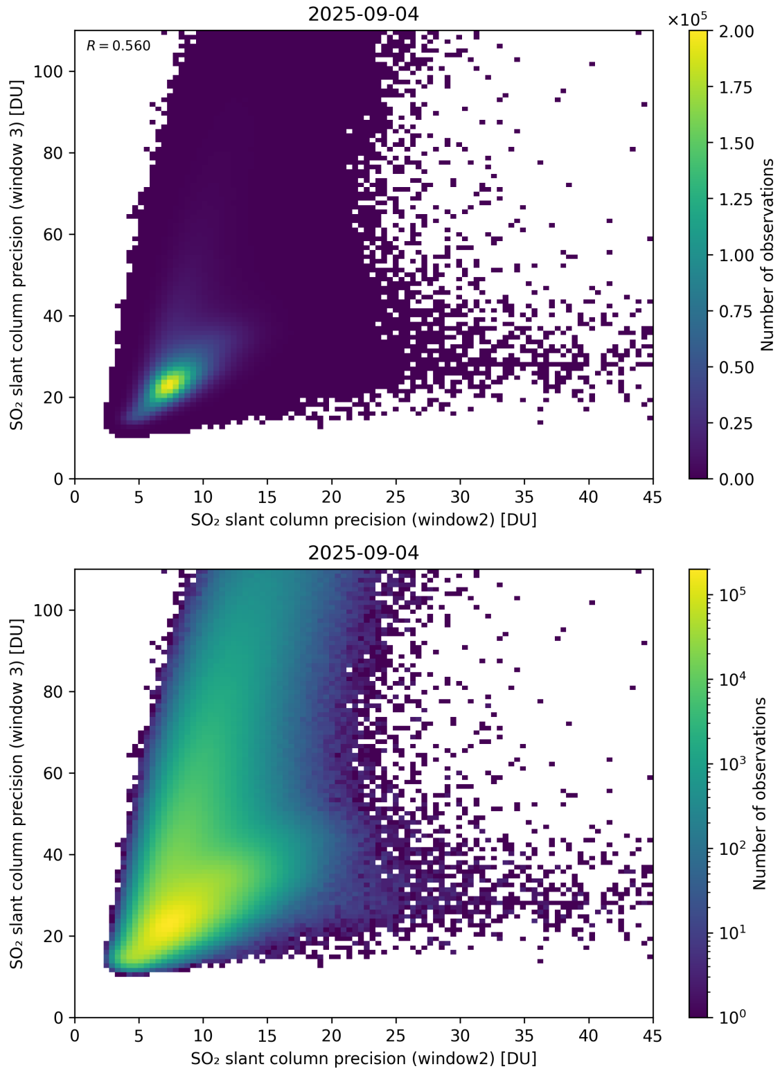
Figure 300: Scatter density plot of “SO 2 slant column precision (window2)” against “SO 2 slant column precision (window 3)” for 2025-09-04 to 2025-09-05.
