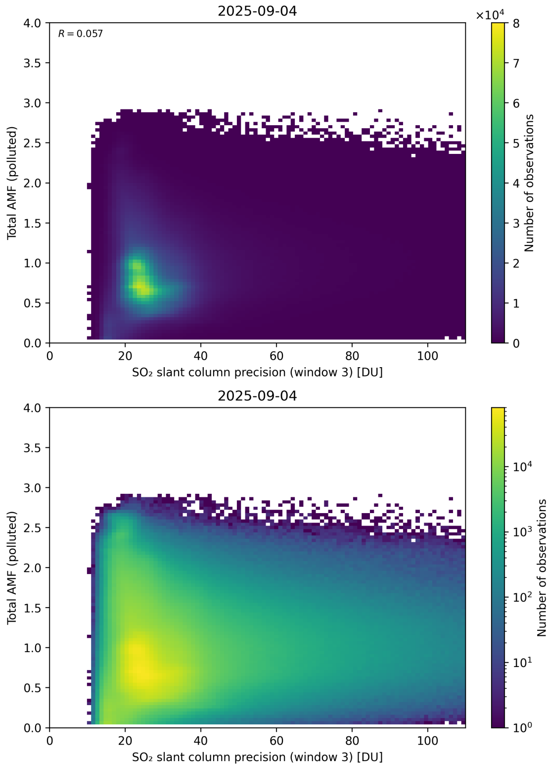
Figure 313: Scatter density plot of “SO 2 slant column precision (window 3)” against “Total AMF (polluted)” for 2025-09-04 to 2025-09-05.
