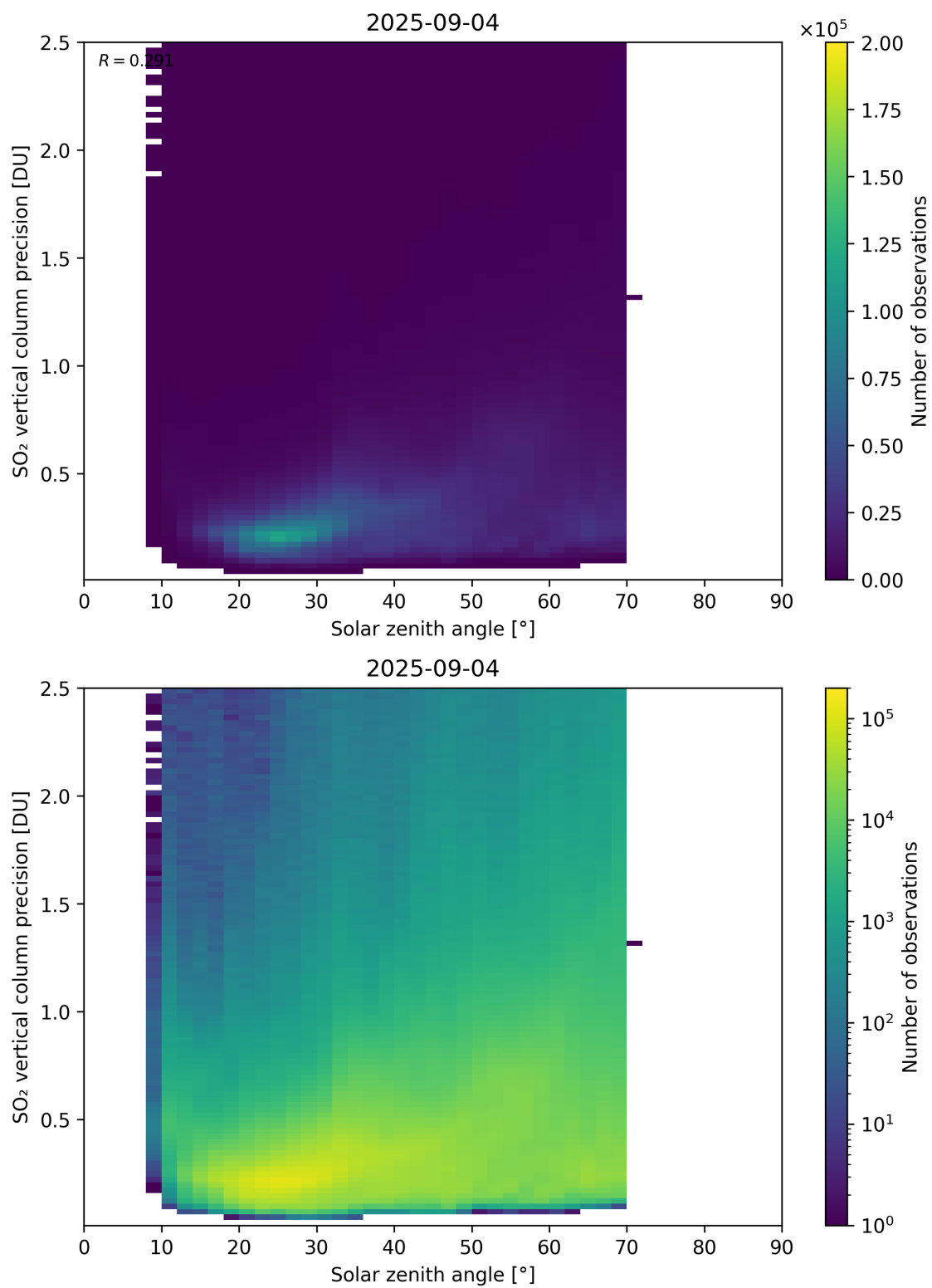
Figure 192: Scatter density plot of “Solar zenith angle” against “SO 2 vertical column precision” for 2025-09-04 to 2025-09-05.
