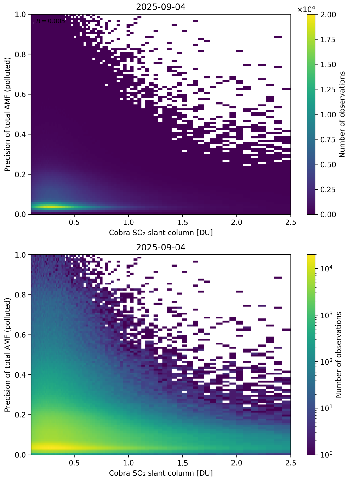
Figure 225: Scatter density plot of “Cobra SO 2 slant column” against “Precision of total AMF (polluted)” for 2025-09-04 to 2025-09-05.
