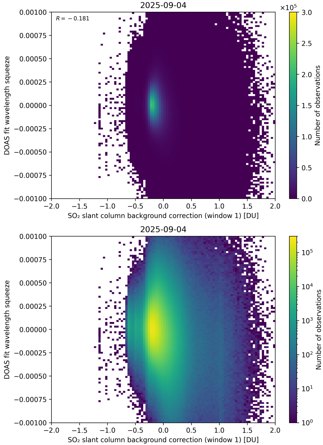
Figure 112: Scatter density plot of “SO 2 slant column background correction (window 1)” against “DOAS fit wavelength squeeze” for 2025-09-04 to 2025-09-05.
