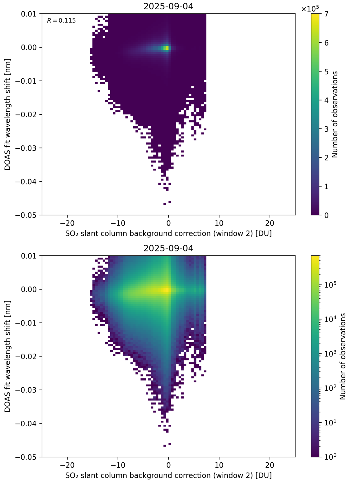
Figure 123: Scatter density plot of “SO 2 slant column background correction (window 2)” against “DOAS fit wavelength shift” for 2025-09-04 to 2025-09-05.
