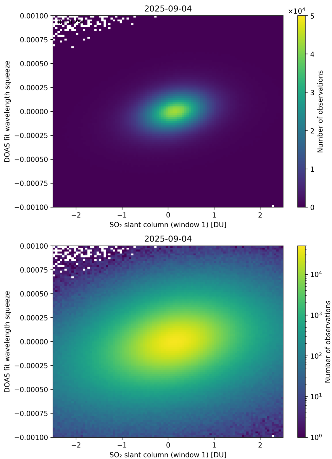
Figure 266: Scatter density plot of “SO 2 slant column (window 1)” against “DOAS fit wavelength squeeze” for 2025-09-04 to 2025-09-05.
