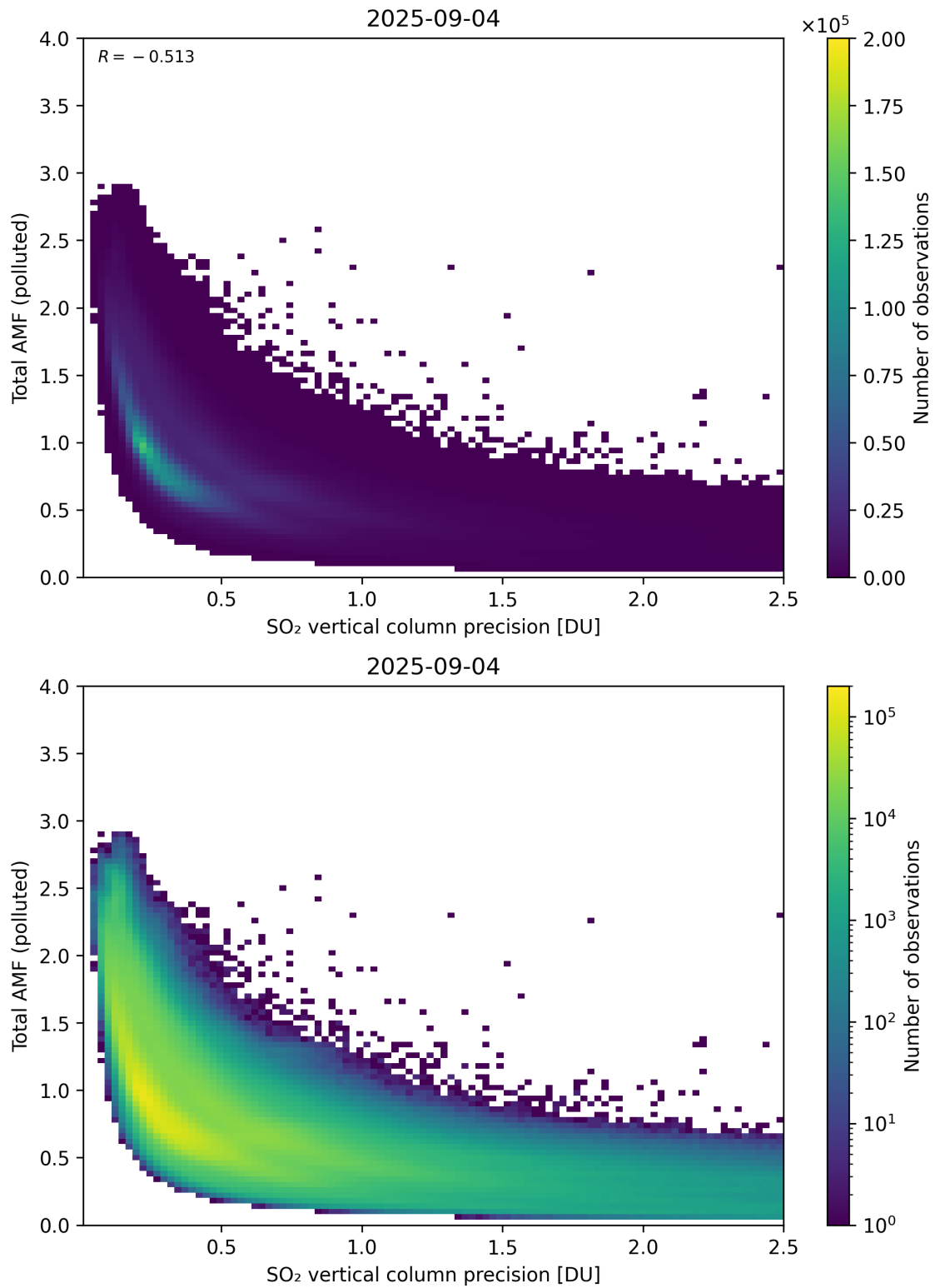
Figure 346: Scatter density plot of “SO 2 vertical column precision” against “Total AMF (polluted)” for 2025-09-04 to 2025-09-05.
