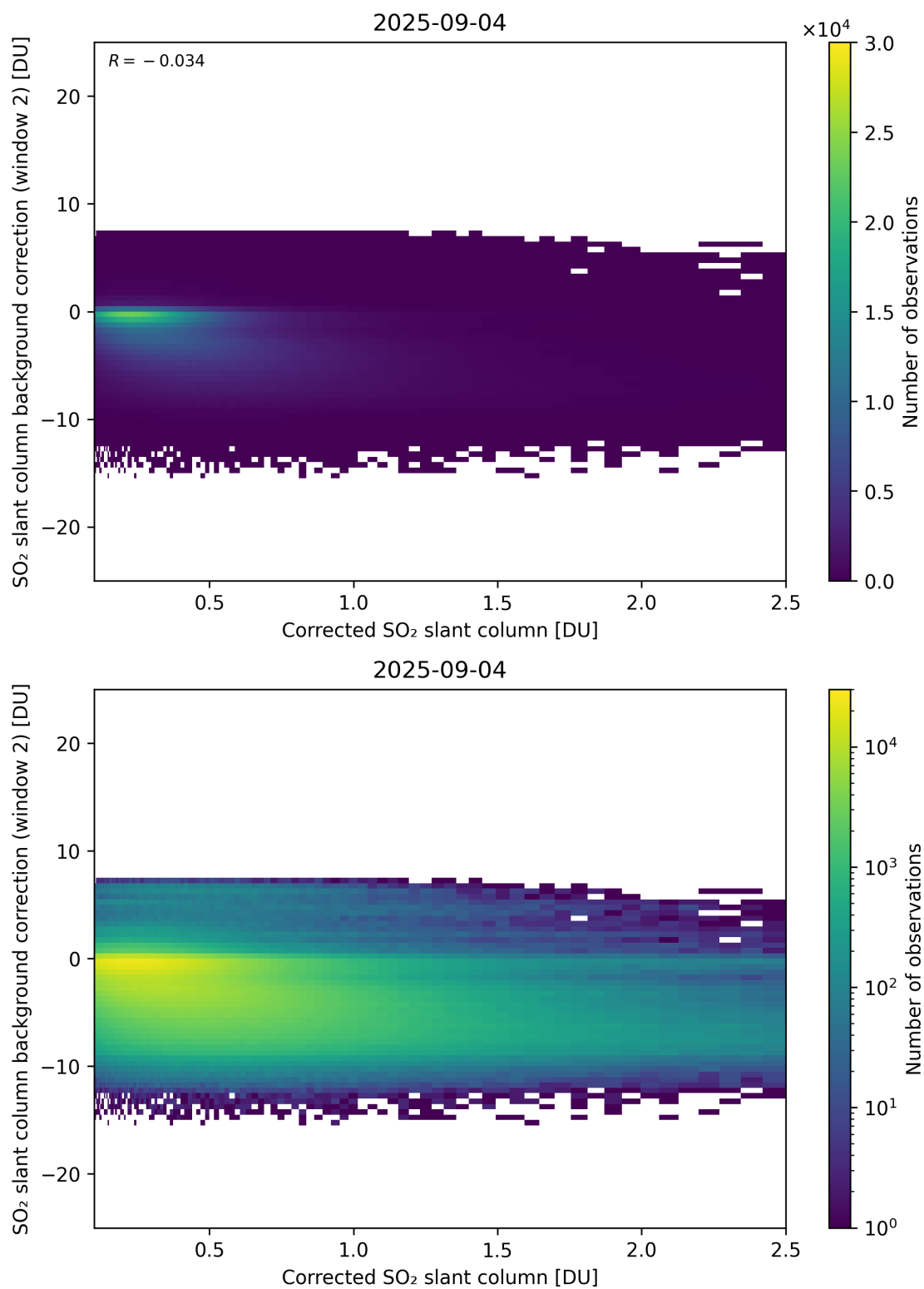
Figure 227: Scatter density plot of “Corrected SO 2 slant column” against “SO 2 slant column background correction (window 2)” for 2025-09-04 to 2025-09-05.
