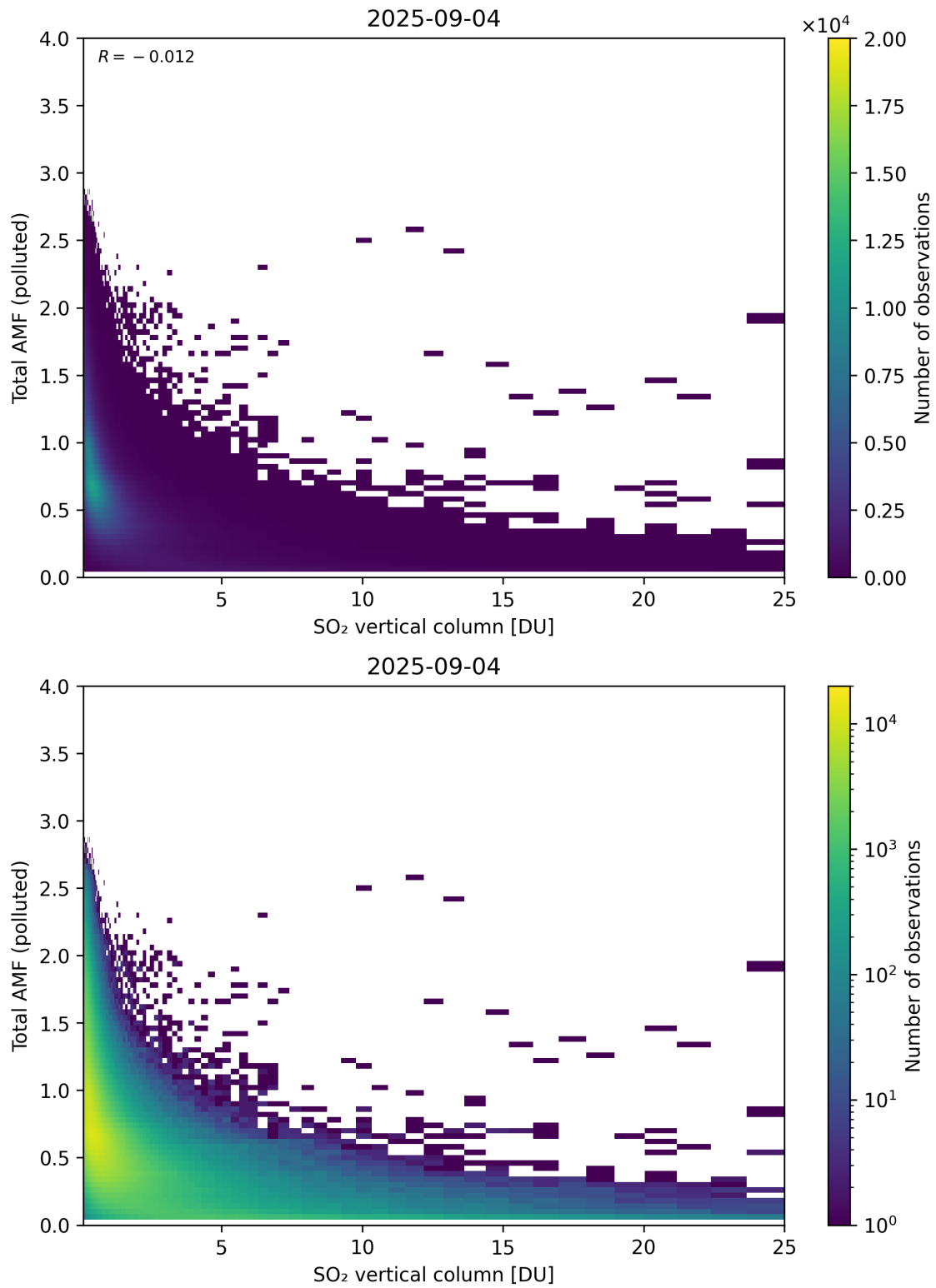
Figure 359: Scatter density plot of “SO 2 vertical column” against “Total AMF (polluted)” for 2025-09-04 to 2025-09-05.
