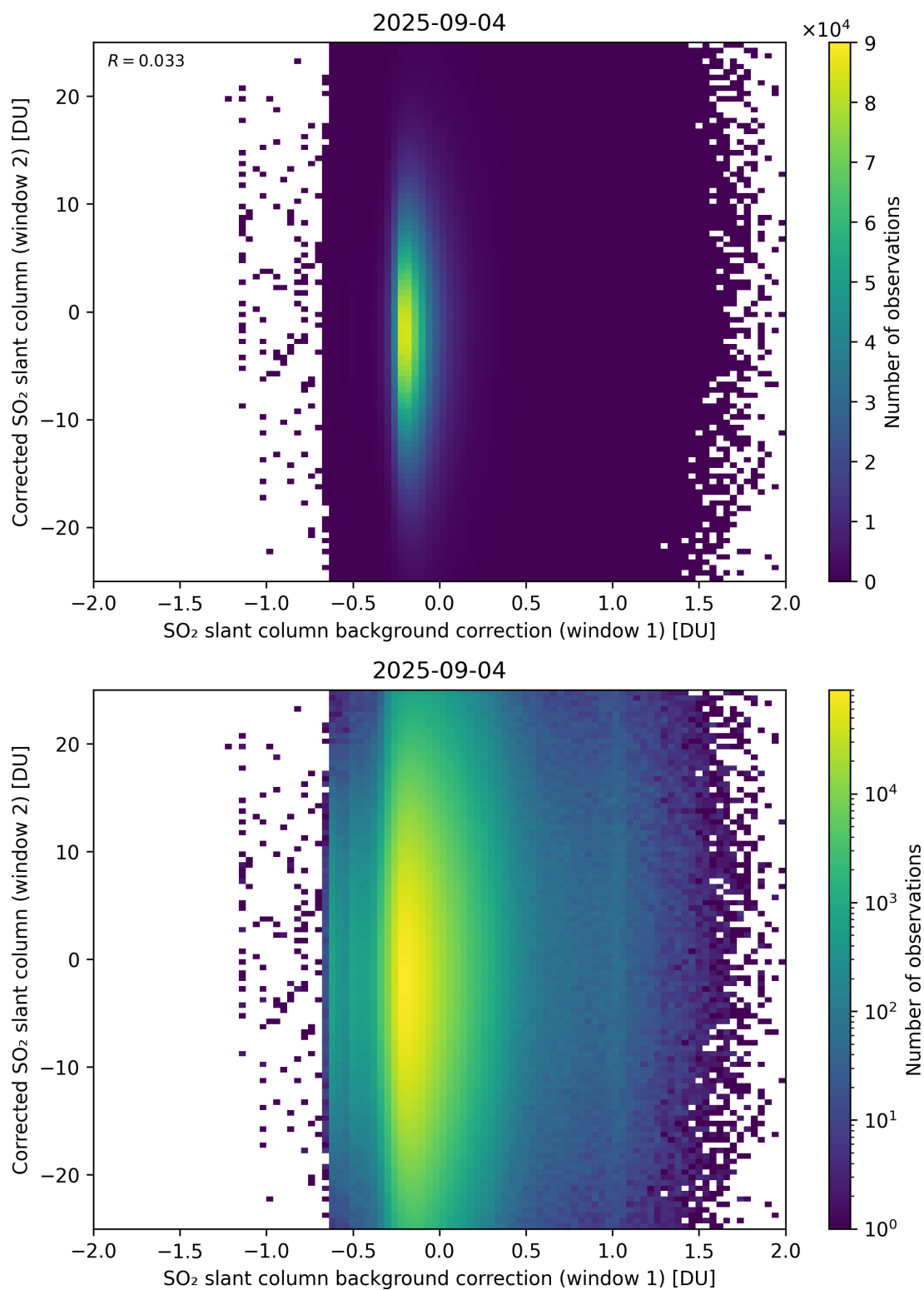
Figure 115: Scatter density plot of “SO 2 slant column background correction (window 1)” against “Corrected SO 2 slant column (window 2)” for 2025-09-04 to 2025-09-05.
