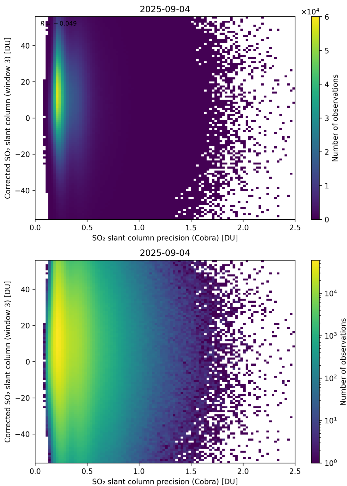
Figure 207: Scatter density plot of “SO 2 slant column precision (Cobra)” against “Corrected SO 2 slant column (window 3)” for 2025-09-04 to 2025-09-05.
