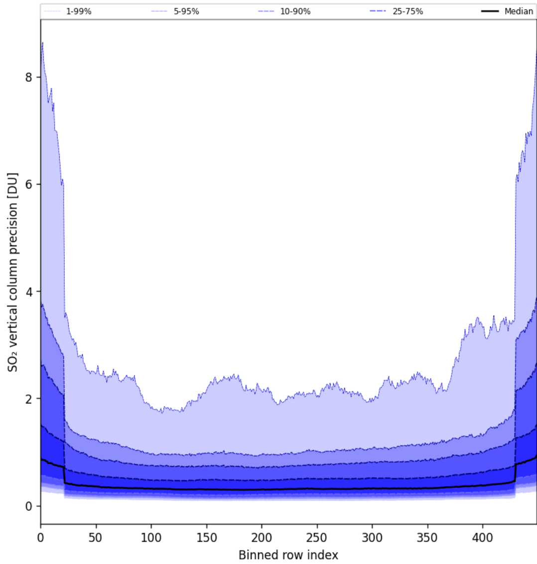
Figure 85: Along track statistics of “SO 2 vertical column precision” for 2025-09-04 to 2025-09-05
