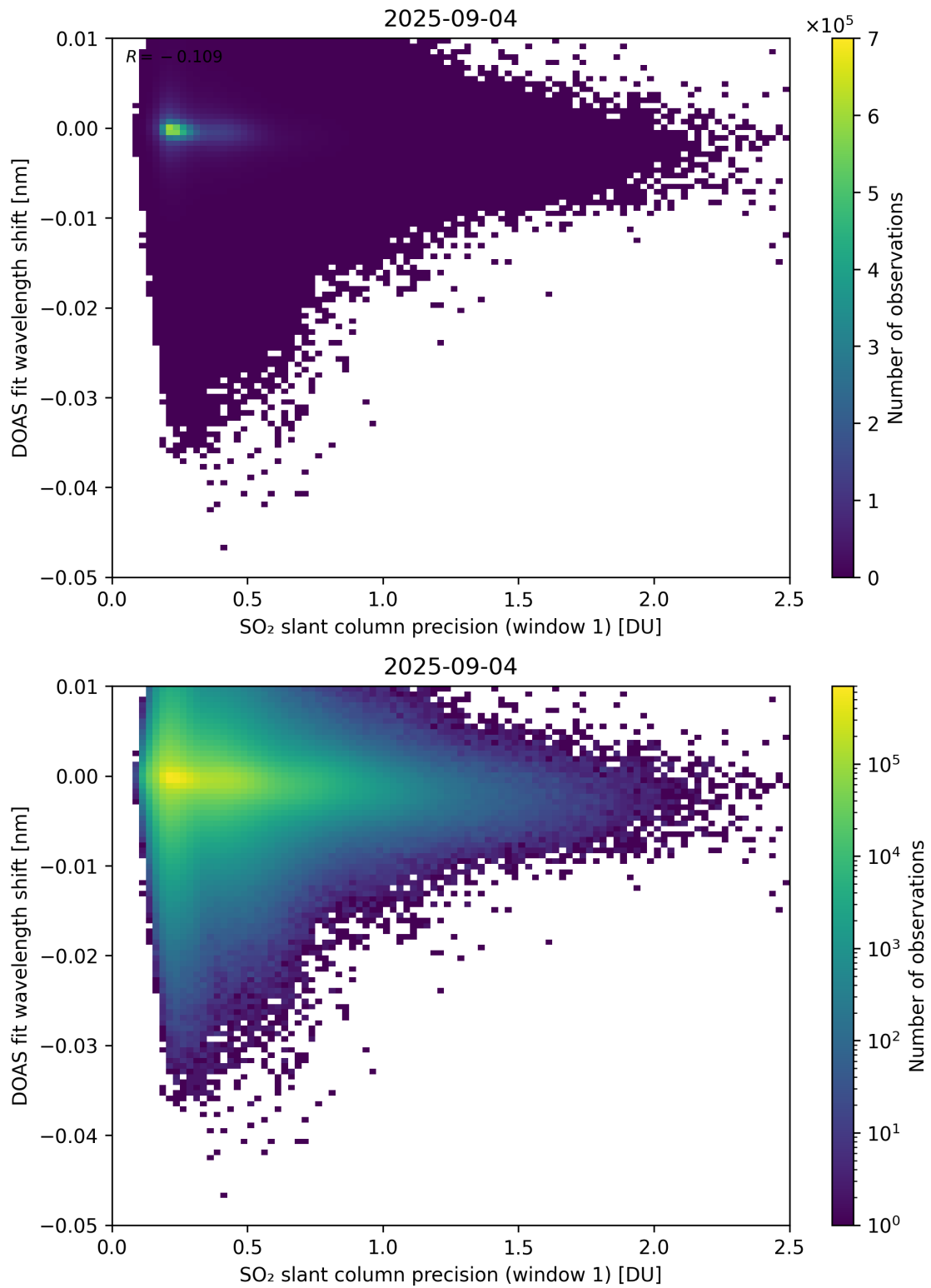
Figure 271: Scatter density plot of “SO 2 slant column precision (window 1)” against “DOAS fit wavelength shift” for 2025-09-04 to 2025-09-05.
