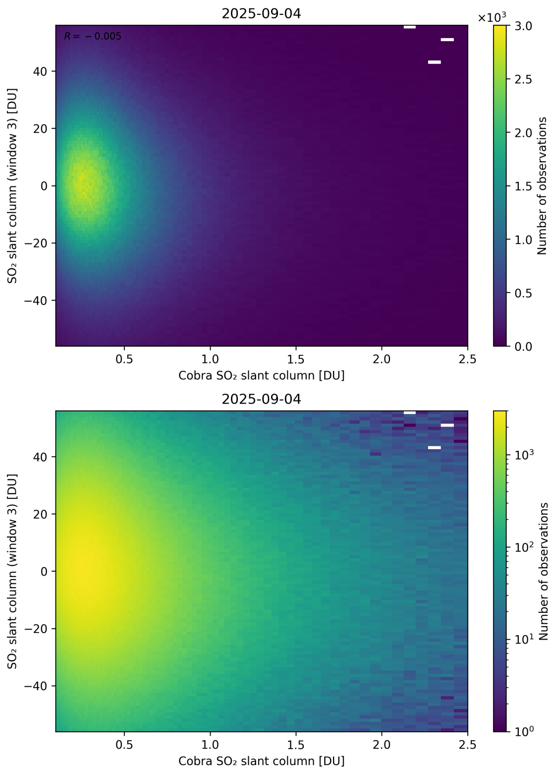
Figure 222: Scatter density plot of “Cobra SO 2 slant column” against “SO 2 slant column (window 3)” for 2025-09-04 to 2025-09-05.
