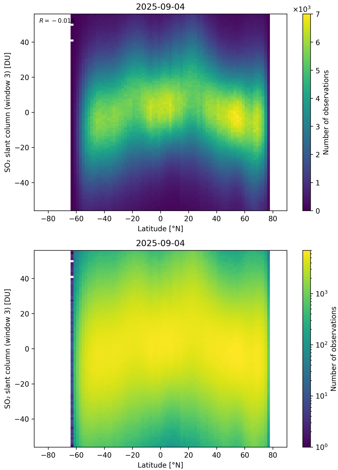
Figure 165: Scatter density plot of “Latitude” against “SO 2 slant column (window 3)” for 2025-09-04 to 2025-09-05.
