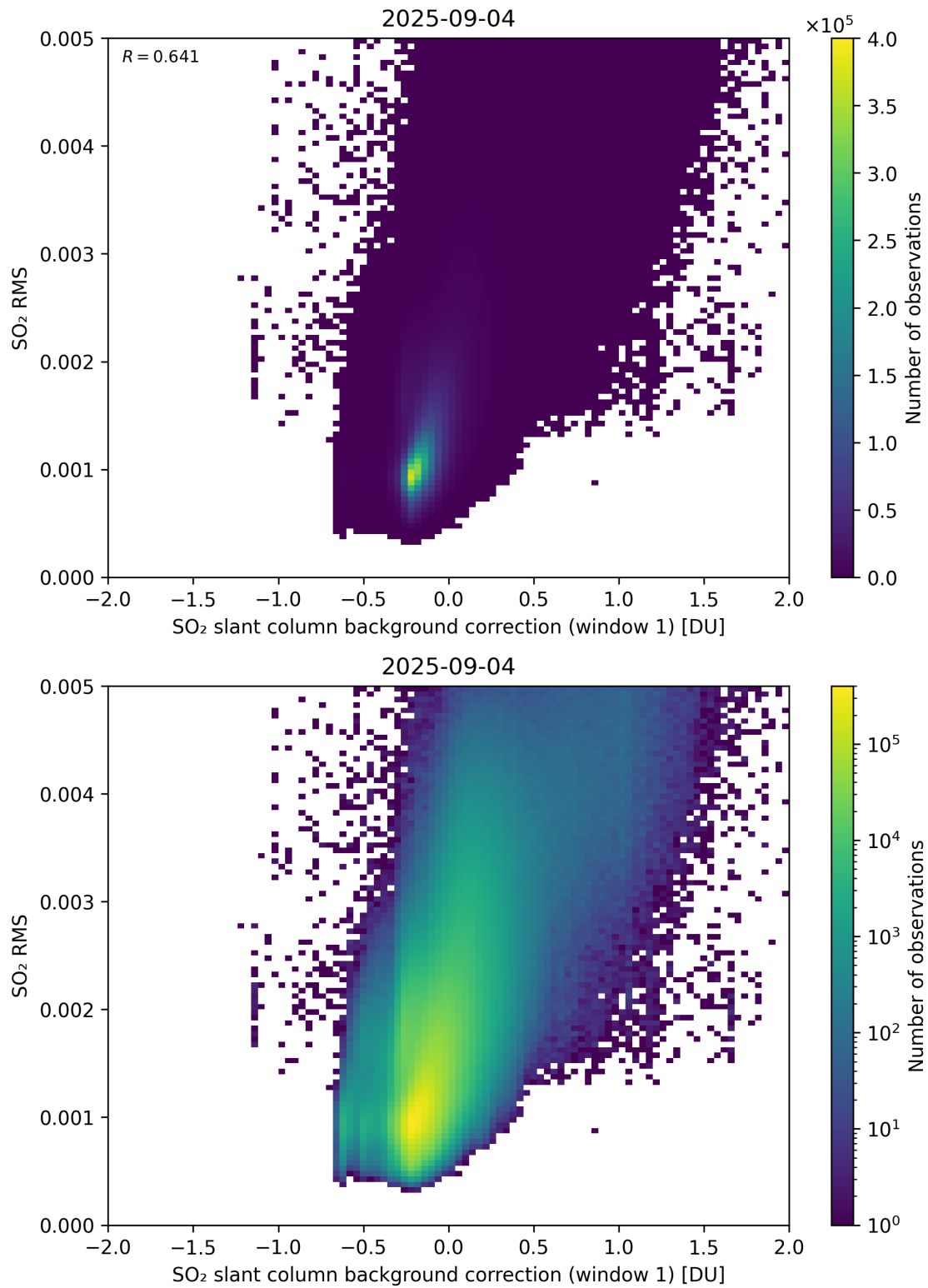
Figure 113: Scatter density plot of “SO 2 slant column background correction (window 1)” against “SO 2 RMS” for 2025-09-04 to 2025-09-05.
