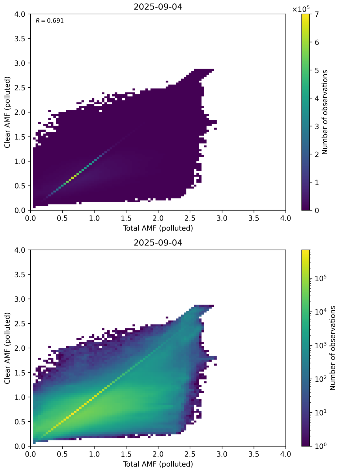
Figure 321: Scatter density plot of “Total AMF (polluted)” against “Clear AMF (polluted)” for 2025-09-04 to 2025-09-05.
