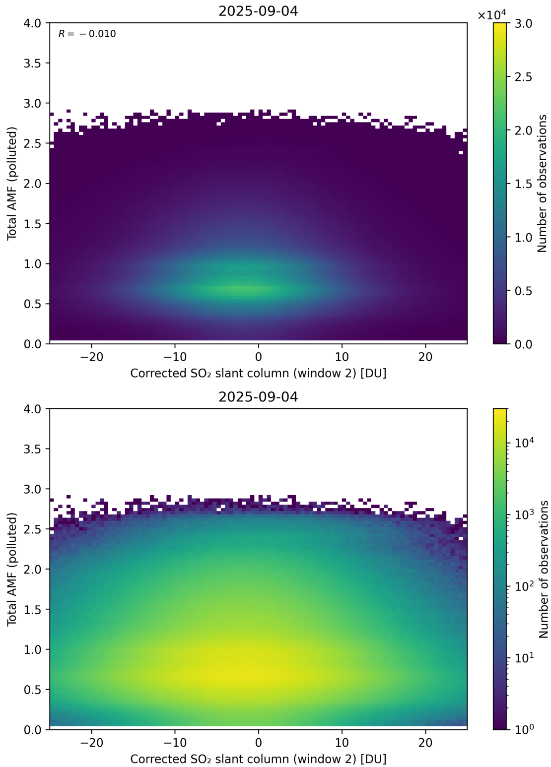
Figure 253: Scatter density plot of “Corrected SO 2 slant column (window 2)” against “Total AMF (polluted)” for 2025-09-04 to 2025-09-05.
