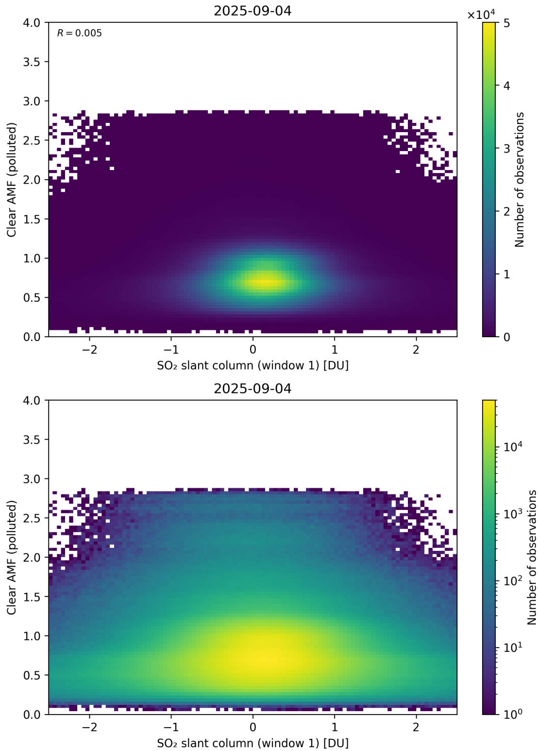
Figure 282: Scatter density plot of “SO 2 slant column (window 1)” against “Clear AMF (polluted)” for 2025-09-04 to 2025-09-05.
