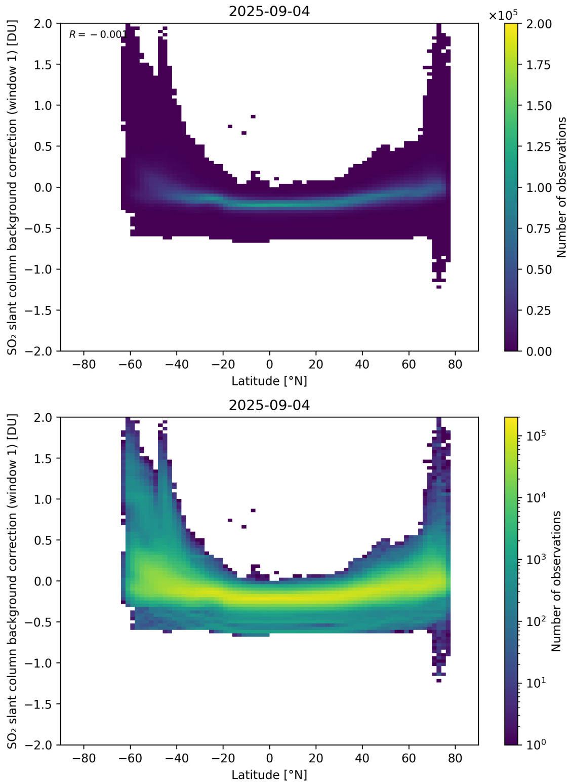
Figure 150: Scatter density plot of “Latitude” against “SO 2 slant column background correction (window 1)” for 2025-09-04 to 2025-09-05.
