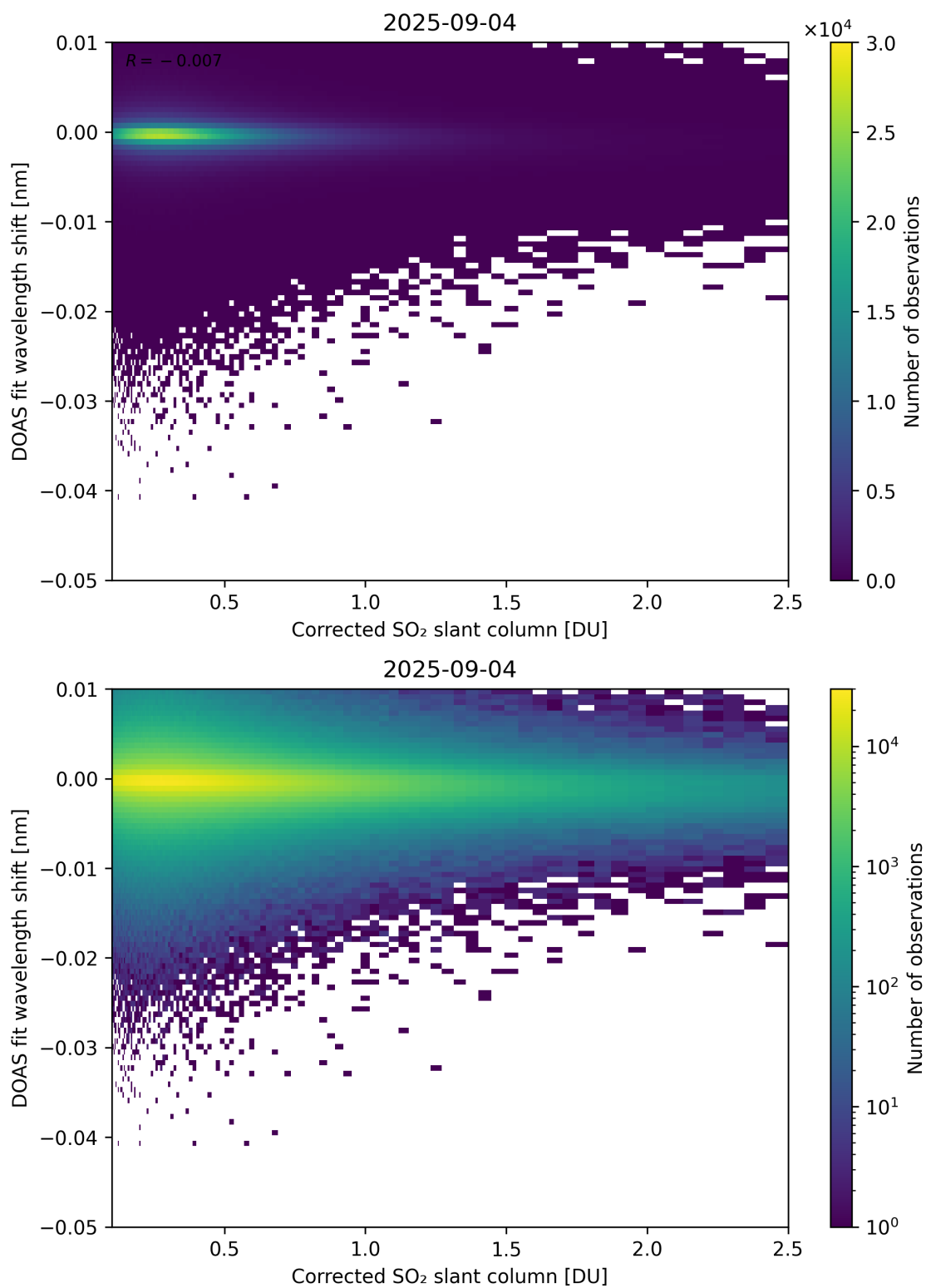
Figure 229: Scatter density plot of “Corrected SO 2 slant column” against “DOAS fit wavelength shift” for 2025-09-04 to 2025-09-05.
