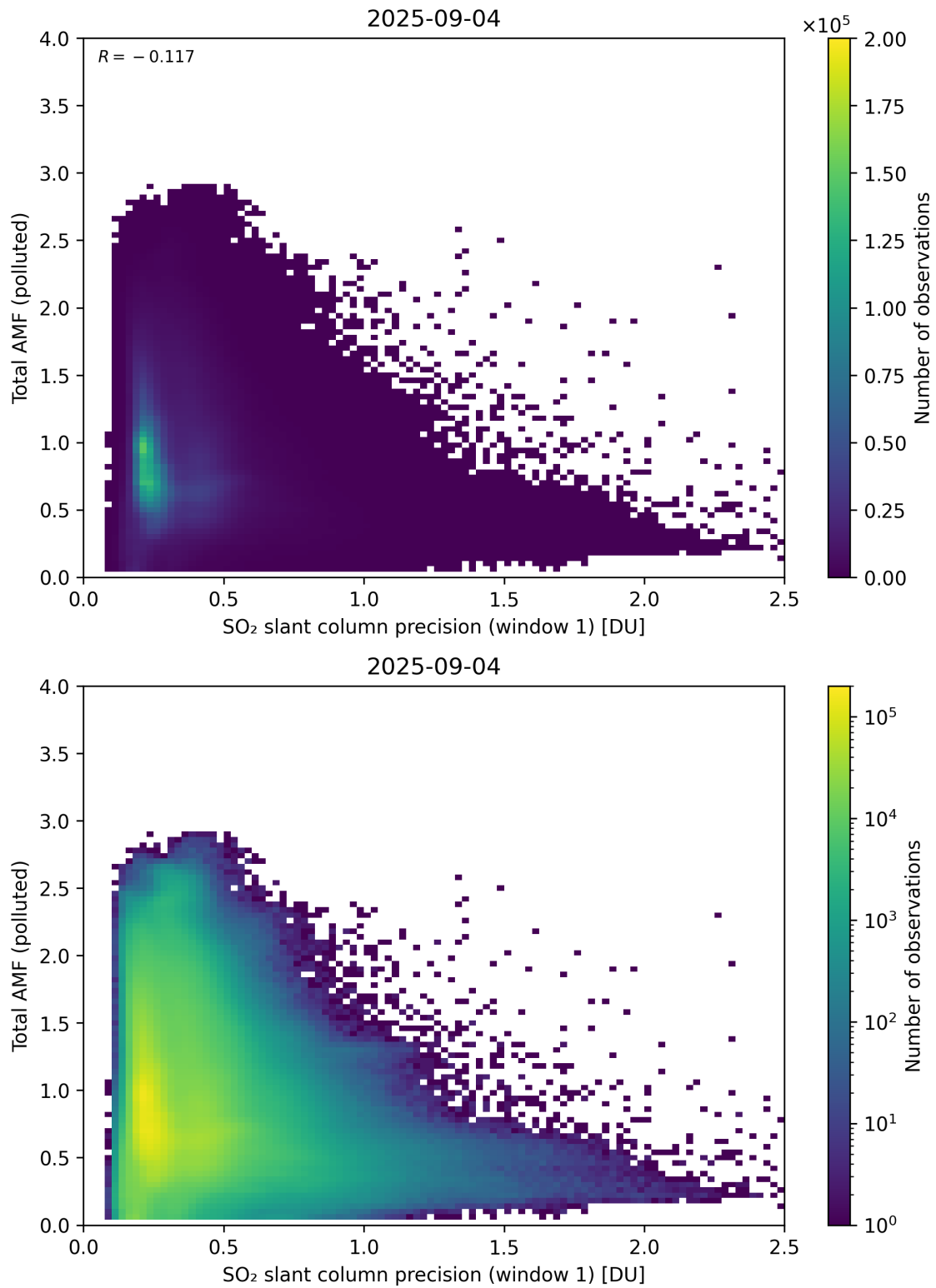
Figure 280: Scatter density plot of “SO 2 slant column precision (window 1)” against “Total AMF (polluted)” for 2025-09-04 to 2025-09-05.
