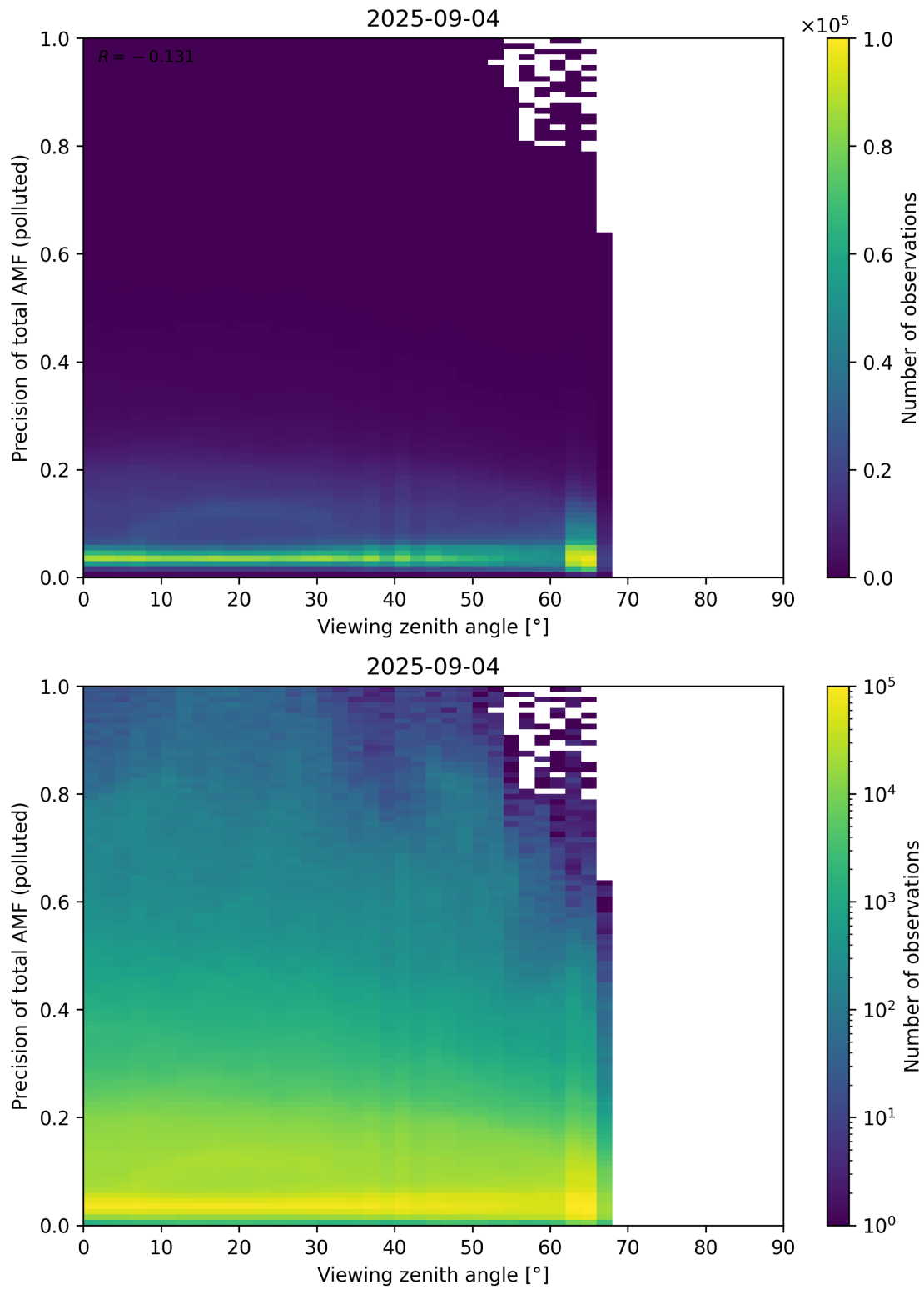
Figure 382: Scatter density plot of “Viewing zenith angle” against “Precision of total AMF (polluted)” for 2025-09-04 to 2025-09-05.
