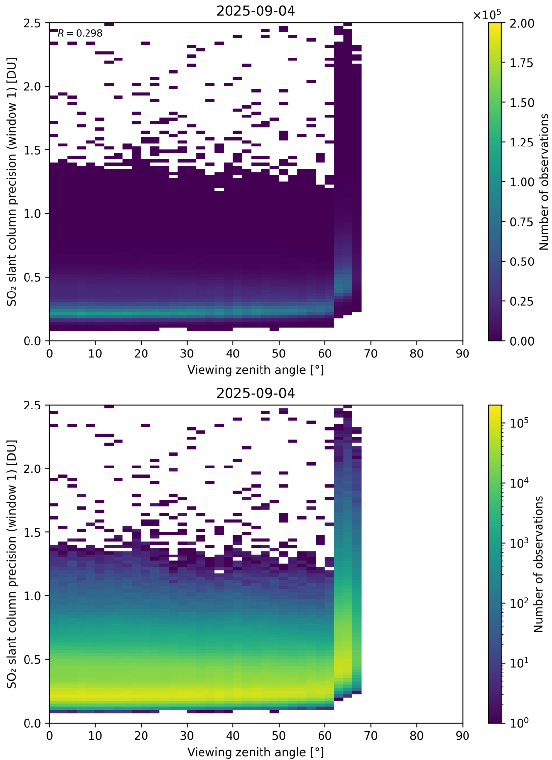
Figure 377: Scatter density plot of “Viewing zenith angle” against “SO 2 slant column precision (window 1)” for 2025-09-04 to 2025-09-05.
