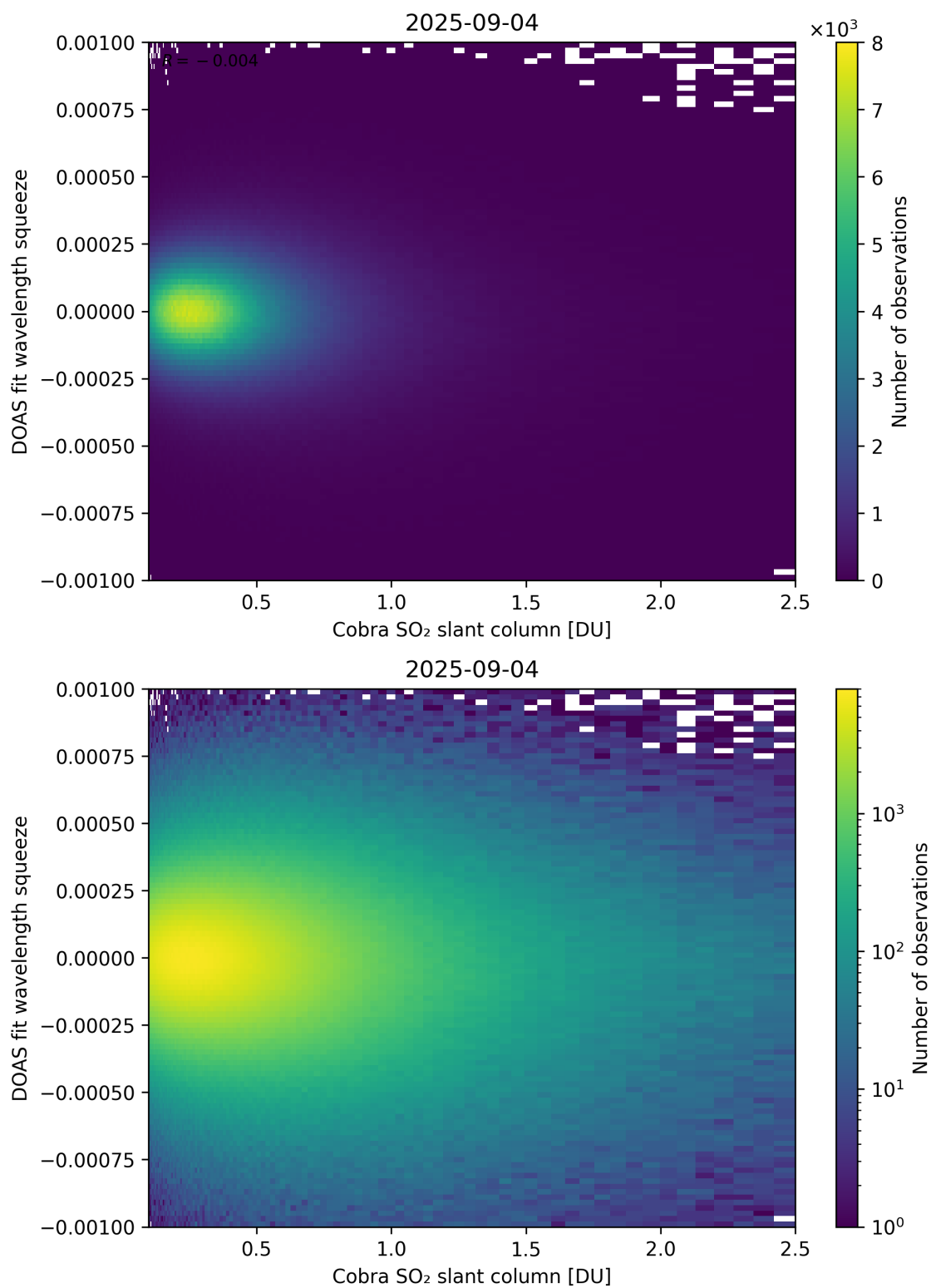
Figure 197: Scatter density plot of “Cobra SO 2 slant column” against “DOAS fit wavelength squeeze” for 2025-09-04 to 2025-09-05.
