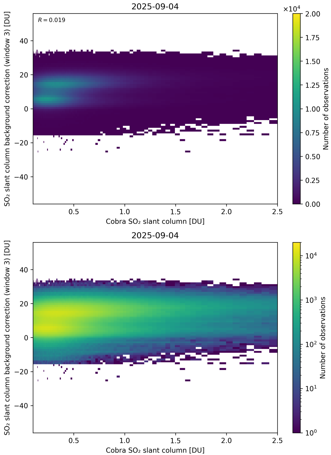
Figure 195: Scatter density plot of “Cobra SO 2 slant column” against “SO 2 slant column background correction (window 3)” for 2025-09-04 to 2025-09-05.
