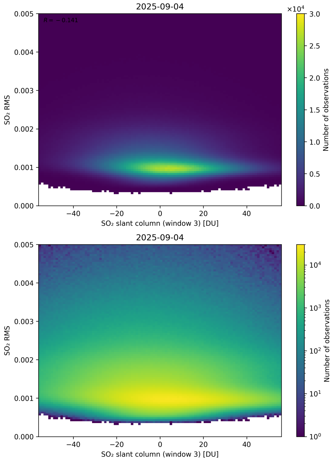
Figure 306: Scatter density plot of “SO 2 slant column (window 3)” against “SO 2 RMS” for 2025-09-04 to 2025-09-05.
