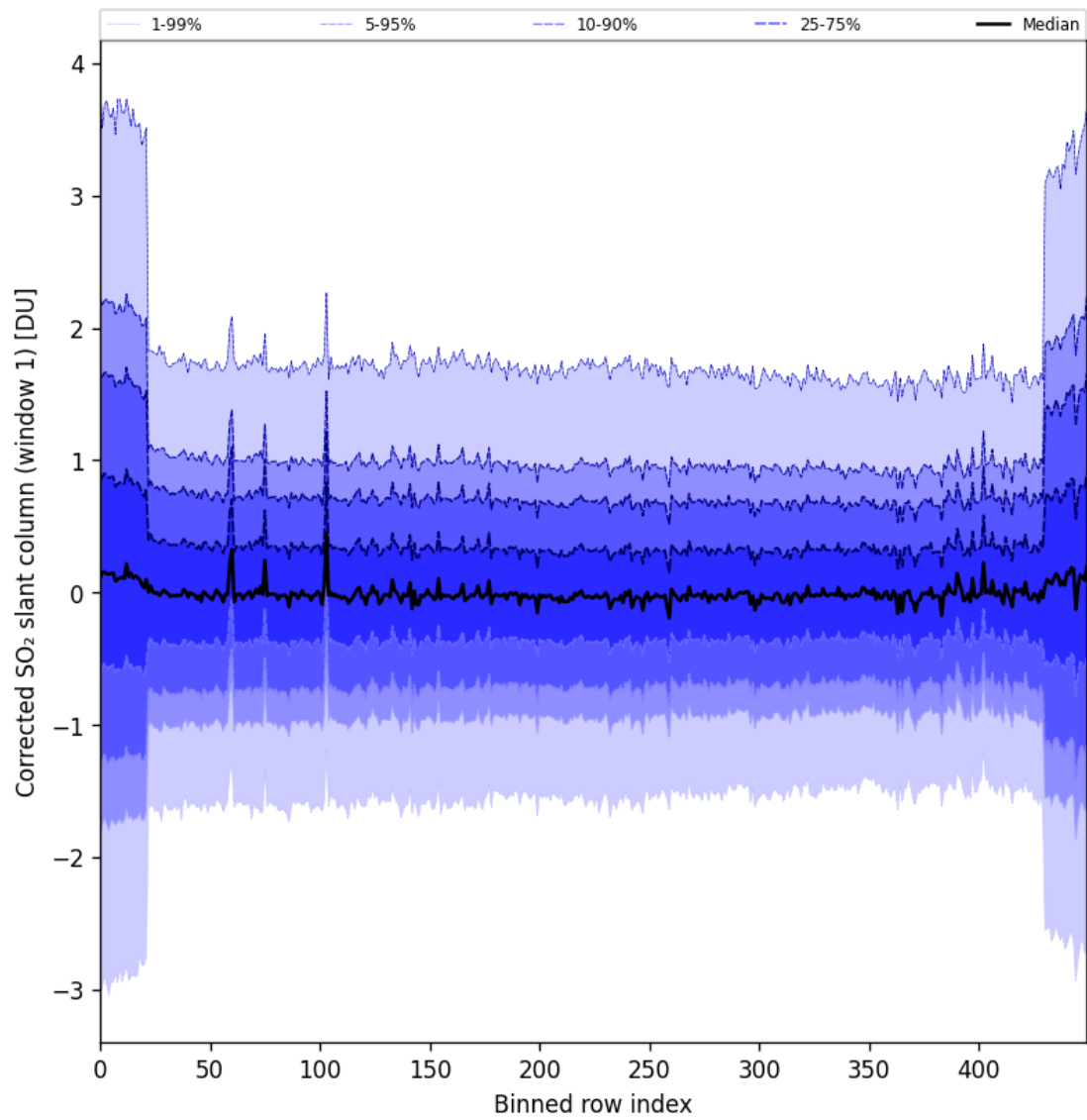
Figure 91: Along track statistics of “Corrected SO 2 slant column (window 1)” for 2025-09-04 to 2025-09-05
