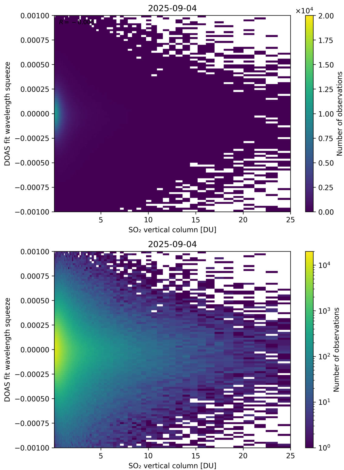
Figure 327: Scatter density plot of “SO 2 vertical column” against “DOAS fit wavelength squeeze” for 2025-09-04 to 2025-09-05.
