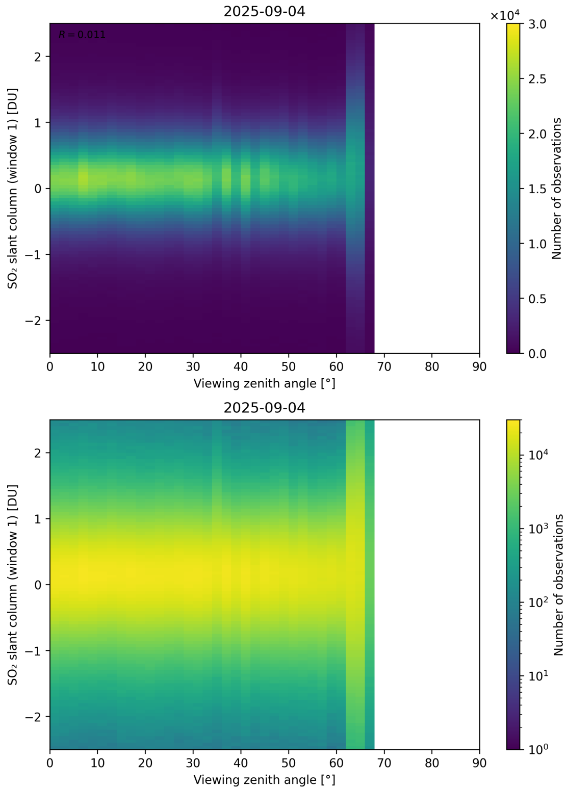
Figure 376: Scatter density plot of “Viewing zenith angle” against “SO 2 slant column (window 1)” for 2025-09-04 to 2025-09-05.
