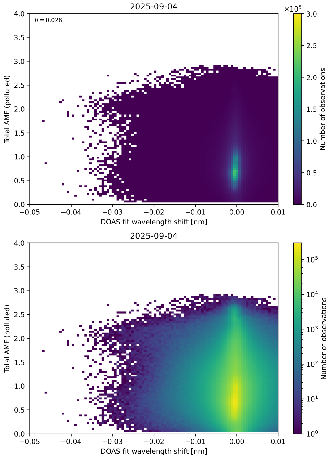
Figure 141: Scatter density plot of “DOAS fit wavelength shift” against “Total AMF (polluted)” for 2025-09-04 to 2025-09-05.
