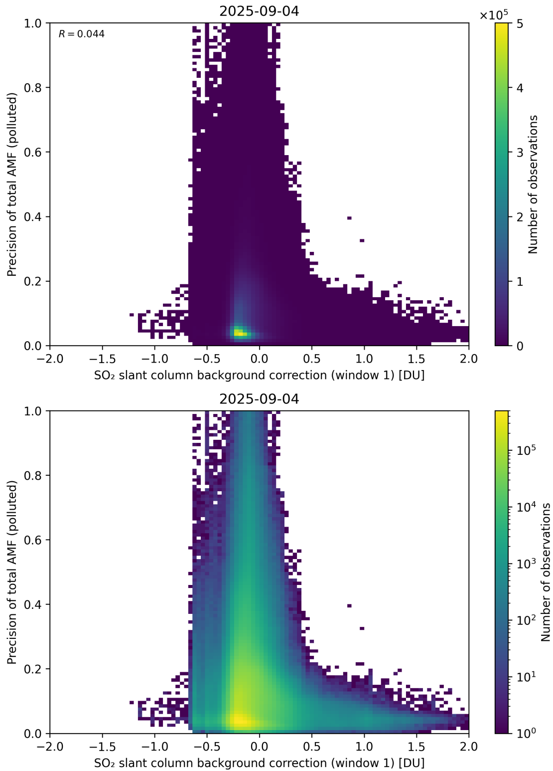
Figure 121: Scatter density plot of “SO 2 slant column background correction (window 1)” against “Precision of total AMF (polluted)” for 2025-09-04 to 2025-09-05.
