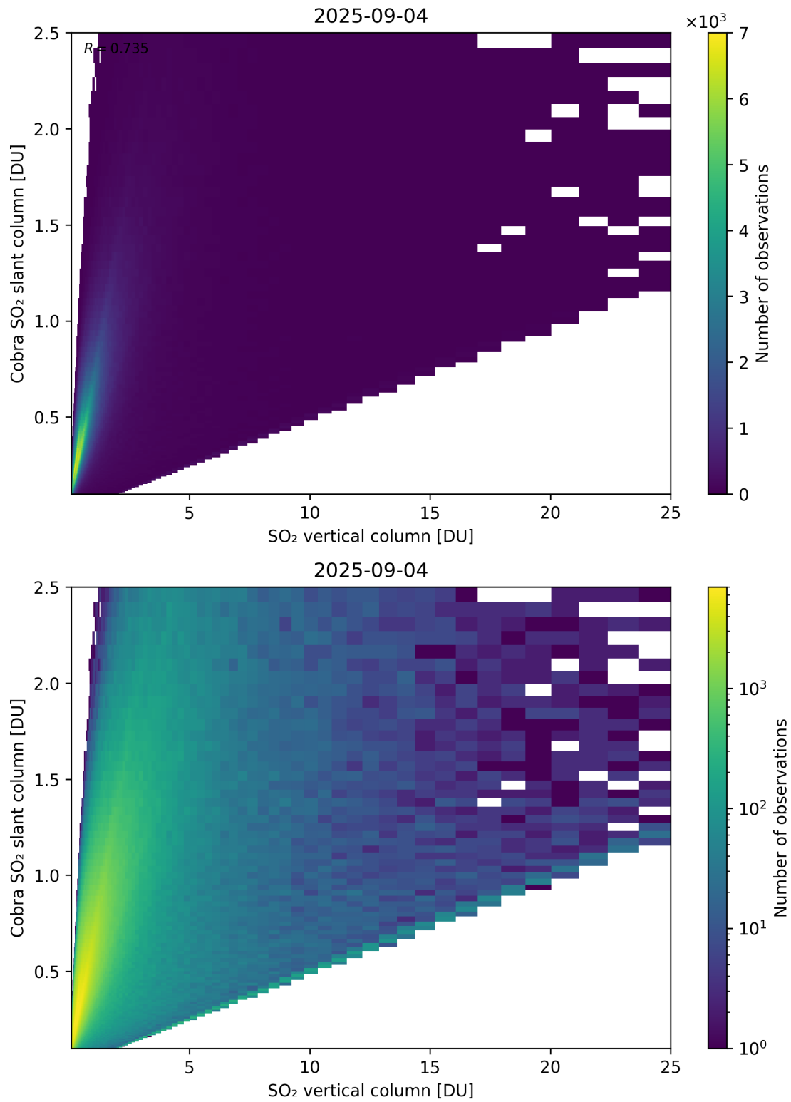
Figure 349: Scatter density plot of “SO 2 vertical column” against “Cobra SO 2 slant column” for 2025-09-04 to 2025-09-05.
