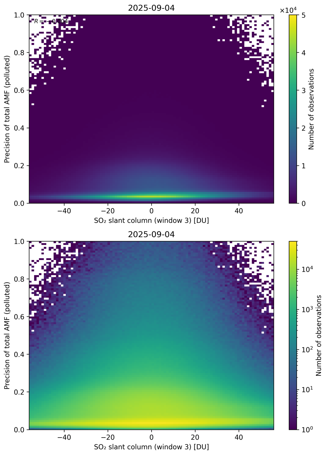
Figure 319: Scatter density plot of “SO 2 slant column (window 3)” against “Precision of total AMF (polluted)” for 2025-09-04 to 2025-09-05.
