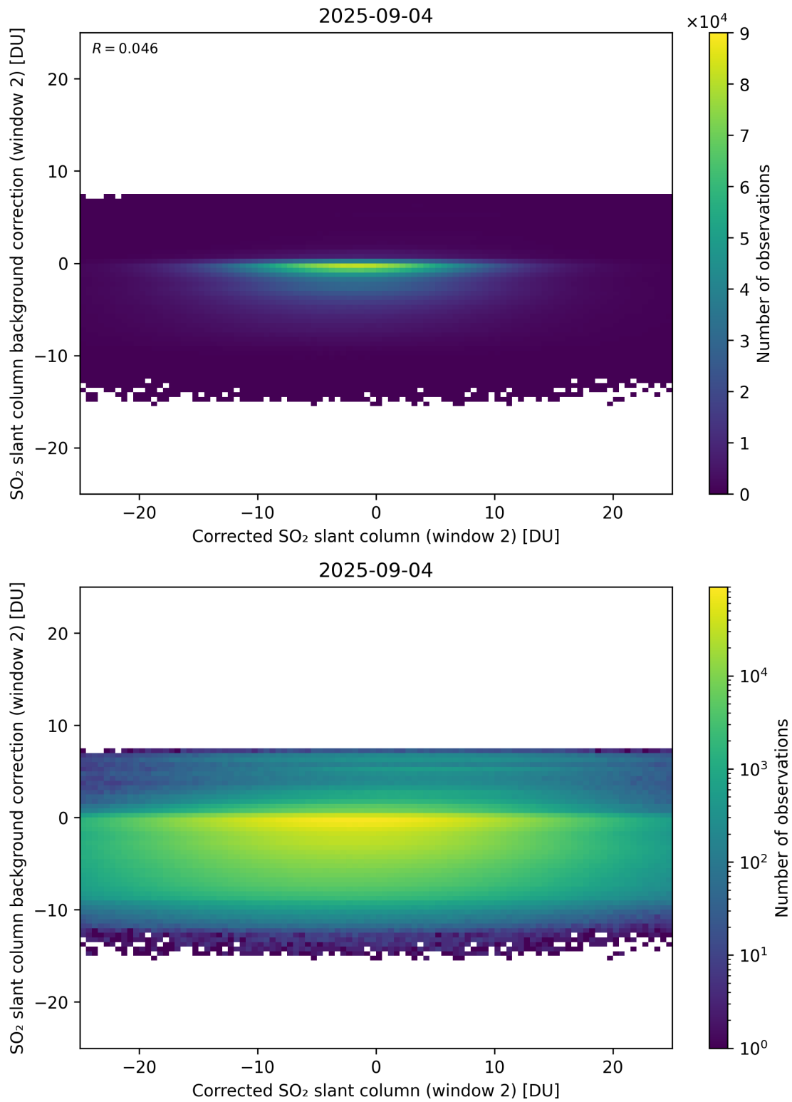
Figure 244: Scatter density plot of “Corrected SO 2 slant column (window 2)” against “SO 2 slant column background correction (window 2)” for 2025-09-04 to 2025-09-05.
