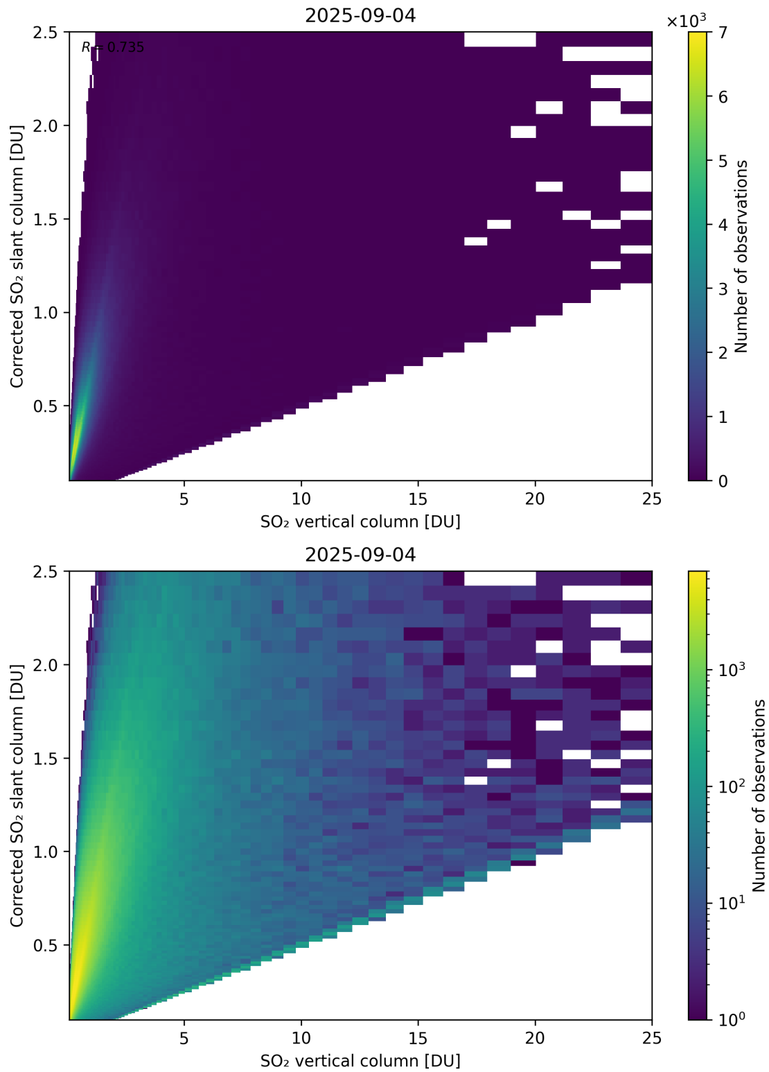
Figure 351: Scatter density plot of “SO 2 vertical column” against “Corrected SO 2 slant column” for 2025-09-04 to 2025-09-05.
