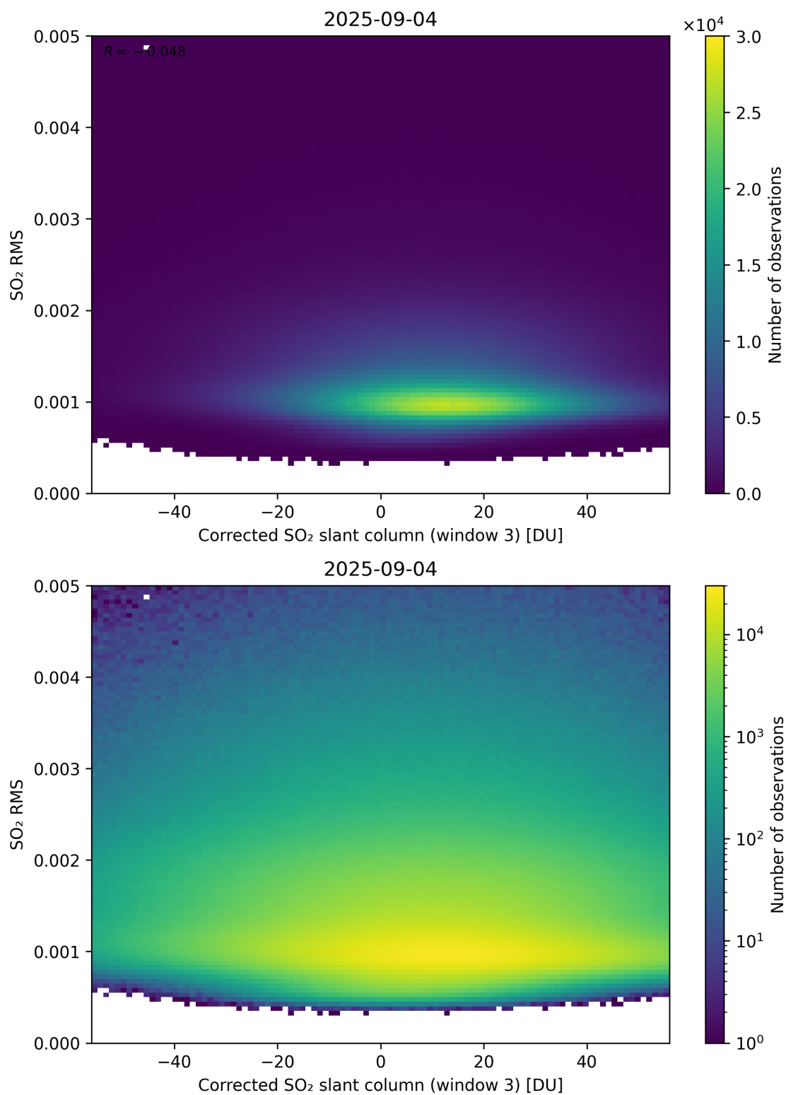
Figure 258: Scatter density plot of “Corrected SO 2 slant column (window 3)” against “SO 2 RMS” for 2025-09-04 to 2025-09-05.
