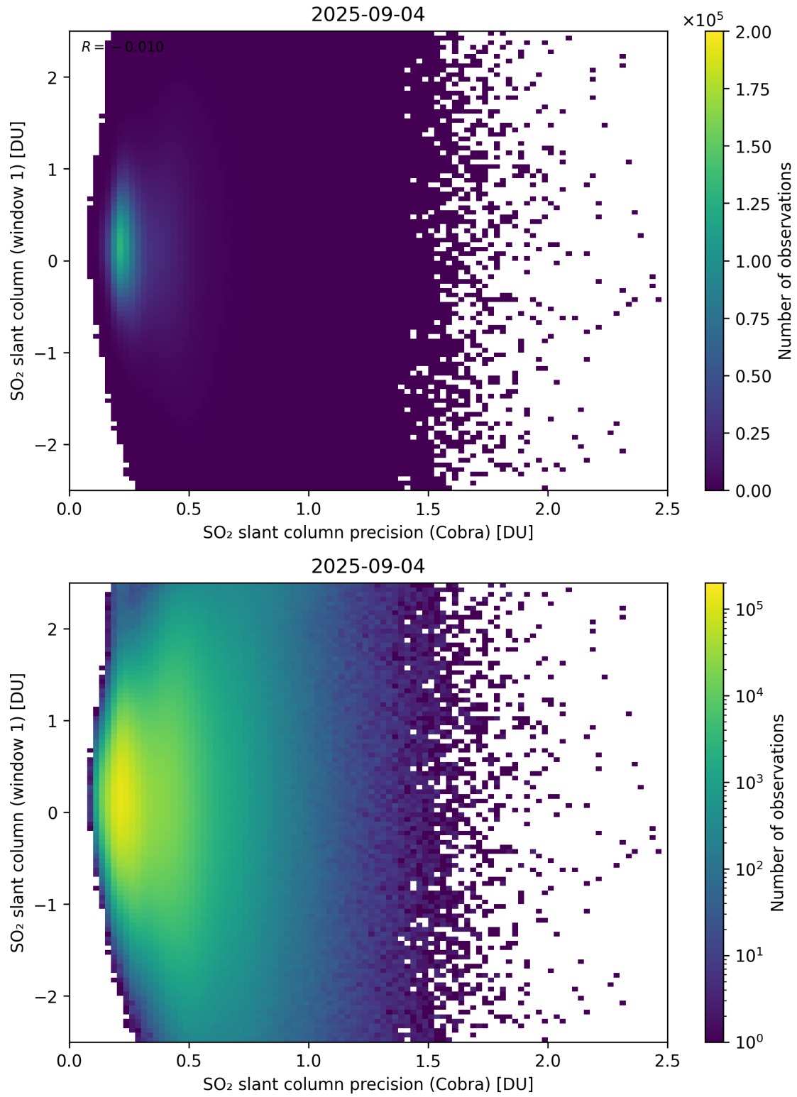
Figure 208: Scatter density plot of “SO 2 slant column precision (Cobra)” against “SO 2 slant column (window 1)” for 2025-09-04 to 2025-09-05.
