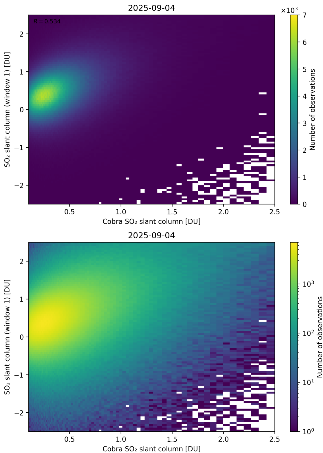
Figure 219: Scatter density plot of “Cobra SO 2 slant column” against “SO 2 slant column (window 1)” for 2025-09-04 to 2025-09-05.
