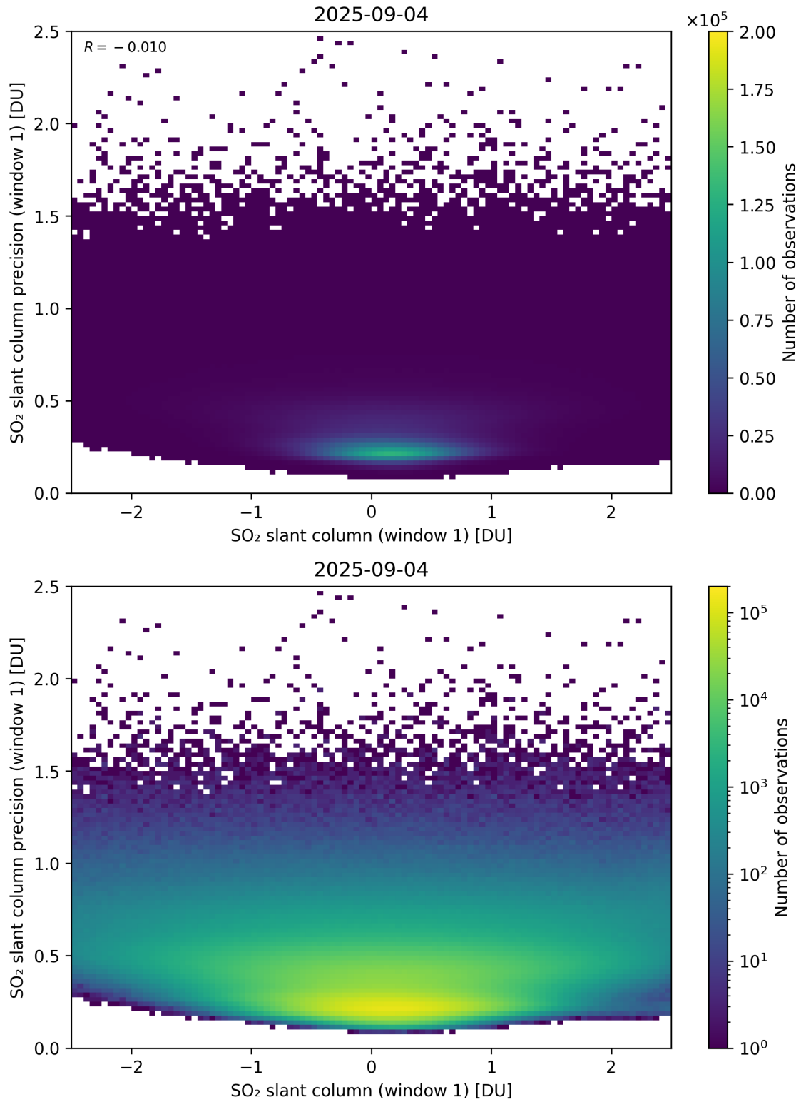
Figure 285: Scatter density plot of “SO 2 slant column (window 1)” against “SO 2 slant column precision (window 1)” for 2025-09-04 to 2025-09-05.
