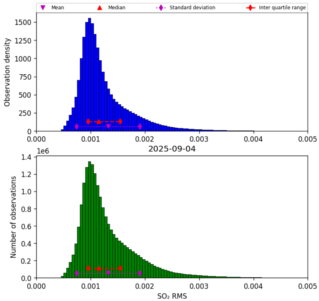
Figure 78: Histogram of “SO 2 RMS” for 2025-09-04 to 2025-09-05
