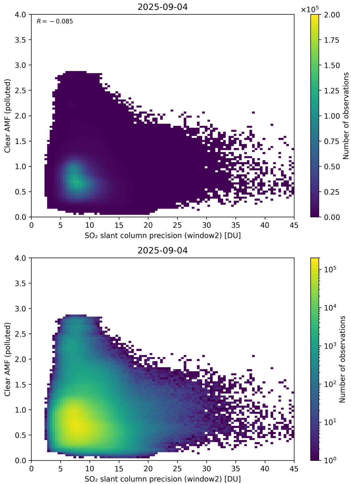
Figure 296: Scatter density plot of “SO 2 slant column precision (window2)” against “Clear AMF (polluted)” for 2025-09-04 to 2025-09-05.
