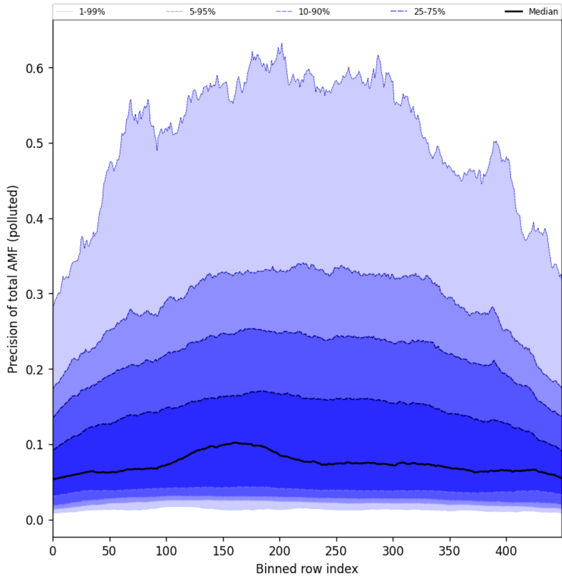
Figure 106: Along track statistics of “Precision of total AMF (polluted)” for 2025-09-04 to 2025-09-05
