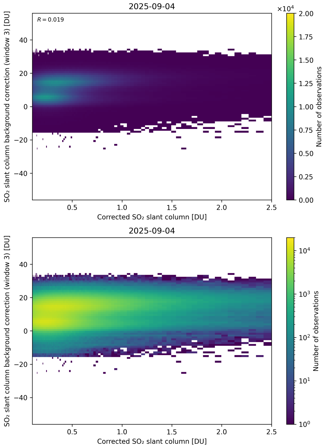
Figure 228: Scatter density plot of “Corrected SO 2 slant column” against “SO 2 slant column background correction (window 3)” for 2025-09-04 to 2025-09-05.
