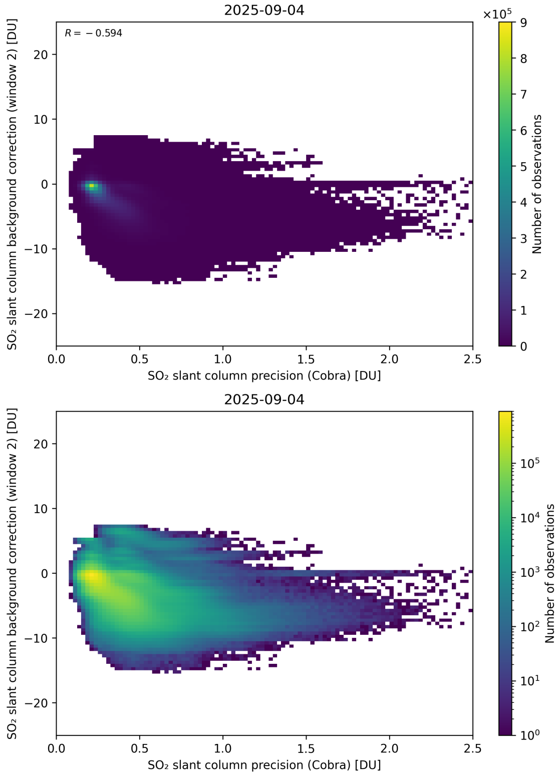
Figure 200: Scatter density plot of “SO 2 slant column precision (Cobra)” against “SO 2 slant column background correction (window 2)” for 2025-09-04 to 2025-09-05.
