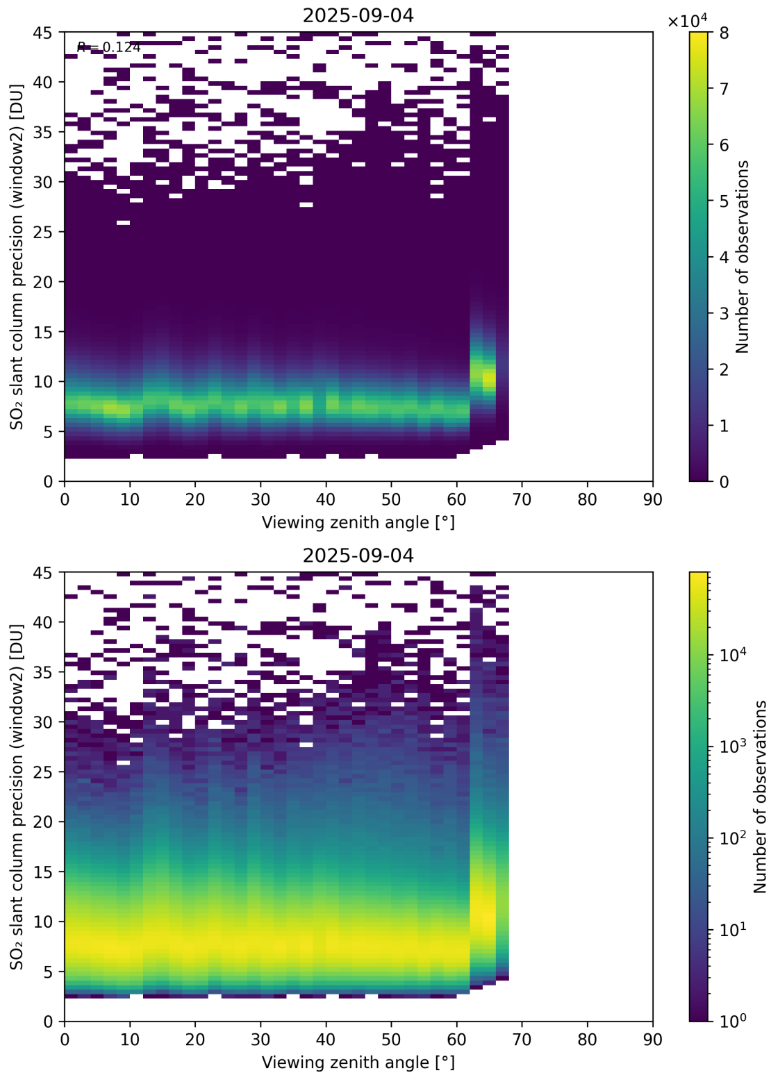
Figure 378: Scatter density plot of “Viewing zenith angle” against “SO 2 slant column precision (window2)” for 2025-09-04 to 2025-09-05.
