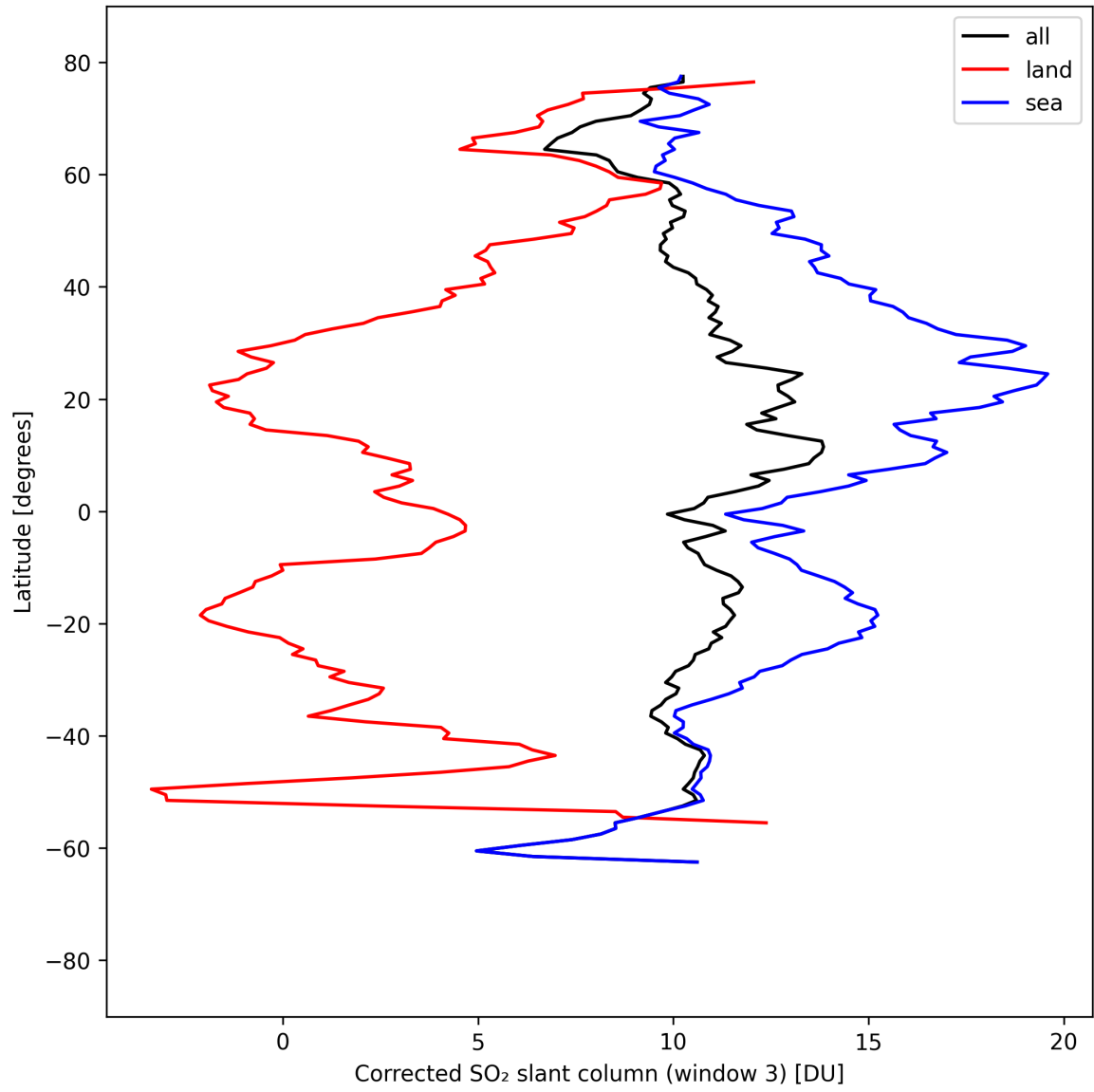
Figure 47: Zonal average of “Corrected SO 2 slant column (window 3)” for 2025-09-04 to 2025-09-05.
