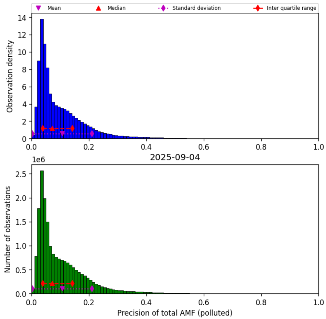
Figure 80: Histogram of “Precision of total AMF (polluted)” for 2025-09-04 to 2025-09-05
