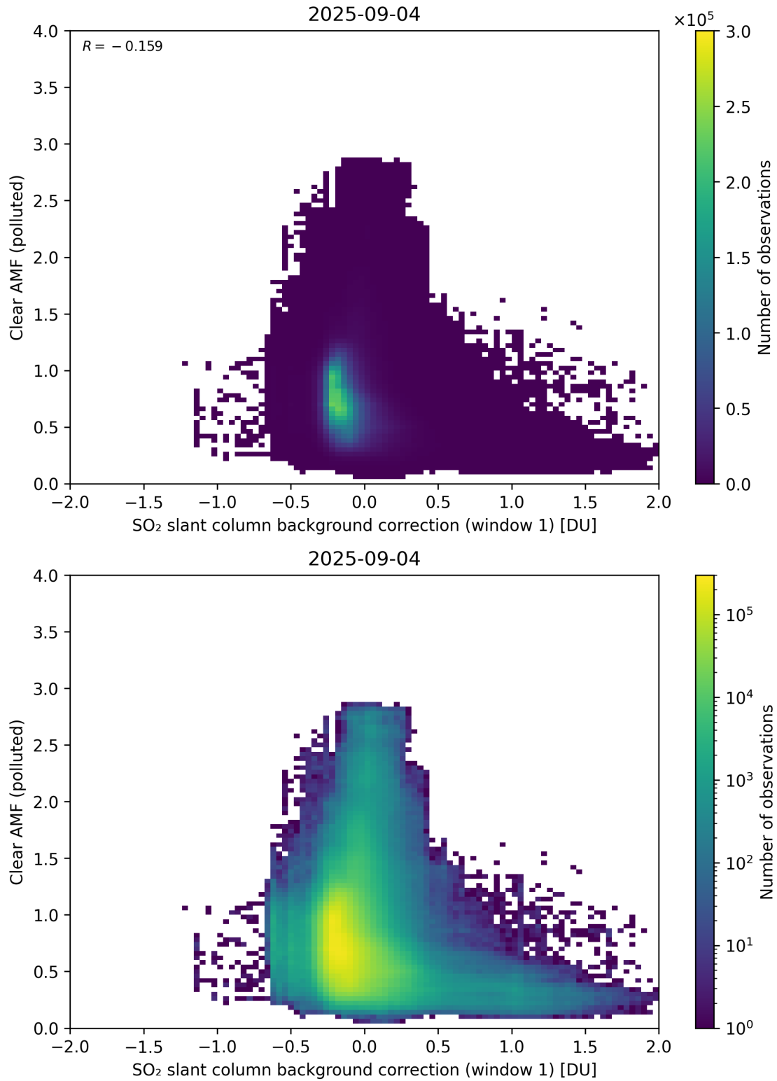
Figure 114: Scatter density plot of “SO 2 slant column background correction (window 1)” against “Clear AMF (polluted)” for 2025-09-04 to 2025-09-05.
