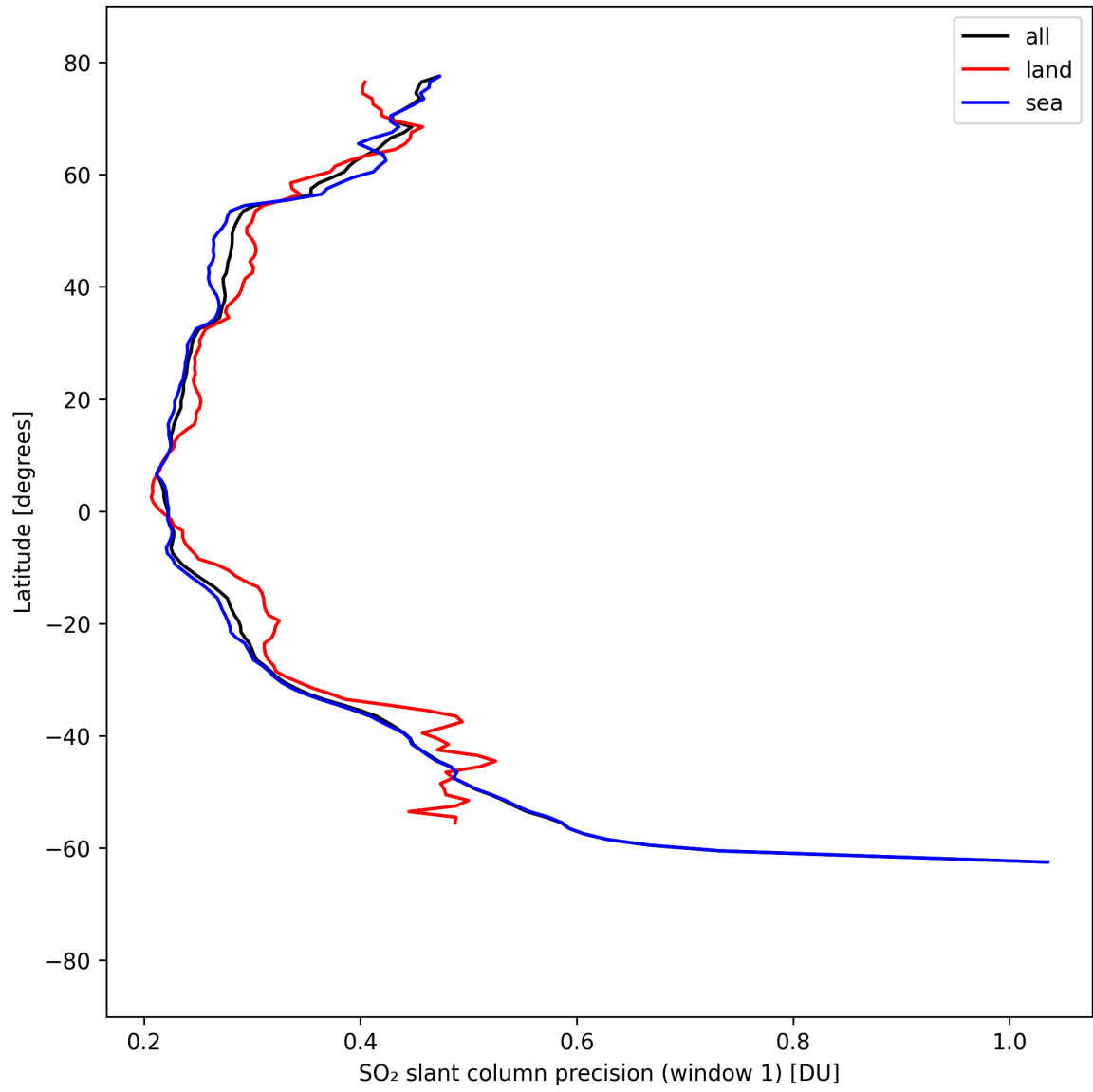
Figure 38: Zonal average of “SO 2 slant column precision (window 1)” for 2025-09-04 to 2025-09-05.
