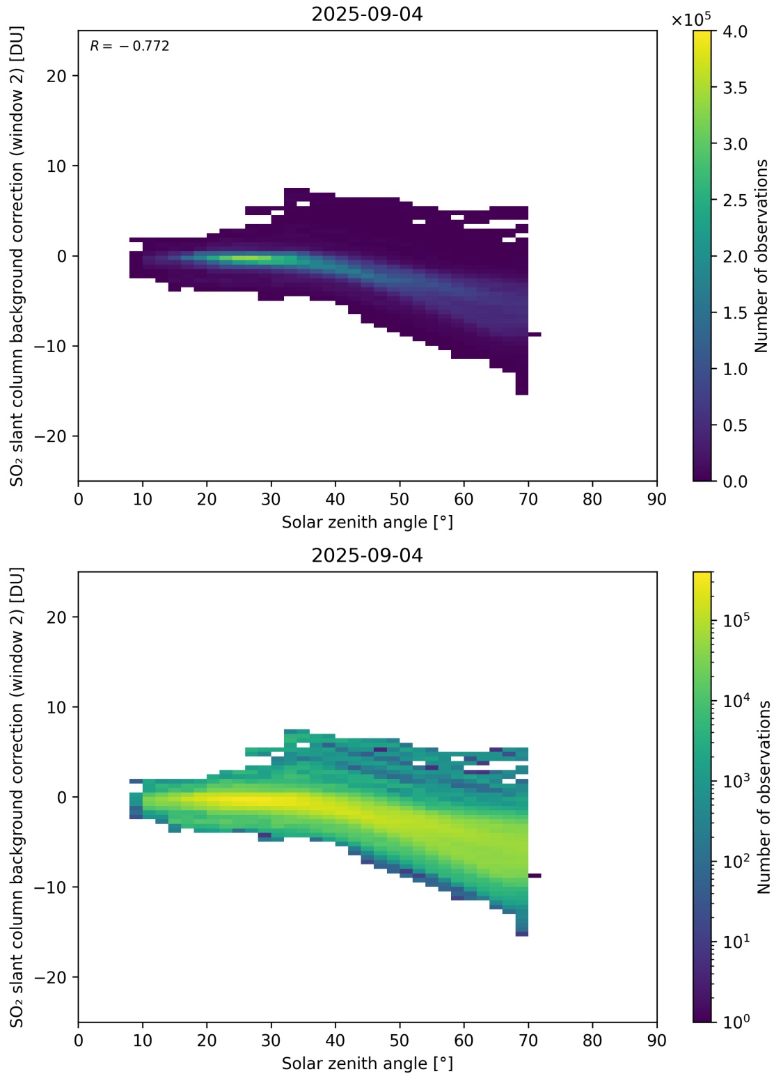
Figure 172: Scatter density plot of “Solar zenith angle” against “SO 2 slant column background correction (window 2)” for 2025-09-04 to 2025-09-05.
