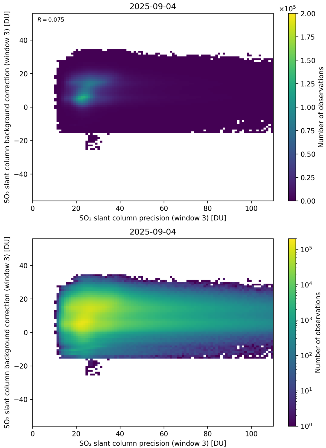
Figure 307: Scatter density plot of “SO 2 slant column precision (window 3)” against “SO 2 slant column background correction (window 3)” for 2025-09-04 to 2025-09-05.
