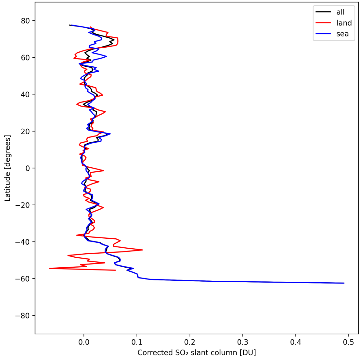
Figure 34: Zonal average of “Corrected SO 2 slant column” for 2025-09-04 to 2025-09-05.
