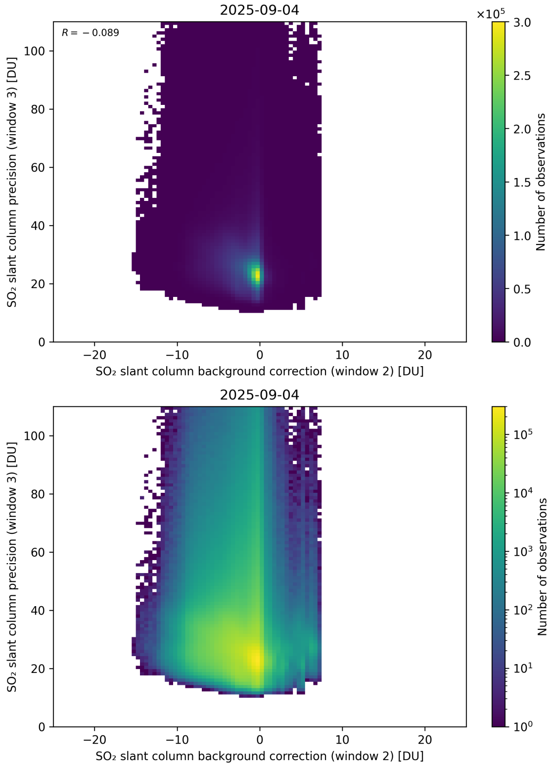
Figure 129: Scatter density plot of “SO 2 slant column background correction (window 2)” against “SO 2 slant column precision (window 3)” for 2025-09-04 to 2025-09-05.
