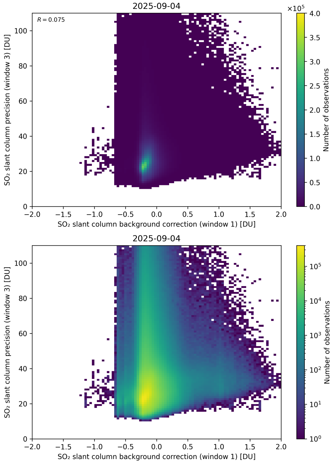
Figure 119: Scatter density plot of “SO 2 slant column background correction (window 1)” against “SO 2 slant column precision (window 3)” for 2025-09-04 to 2025-09-05.
