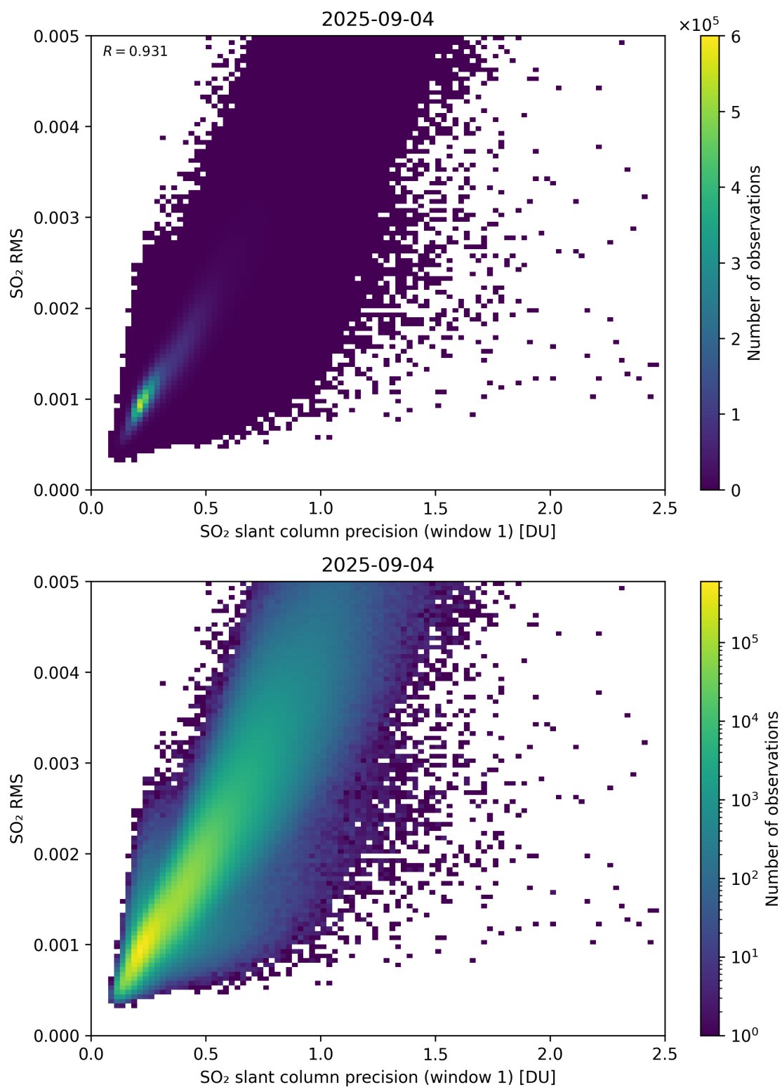
Figure 273: Scatter density plot of “SO 2 slant column precision (window 1)” against “SO 2 RMS” for 2025-09-04 to 2025-09-05.
