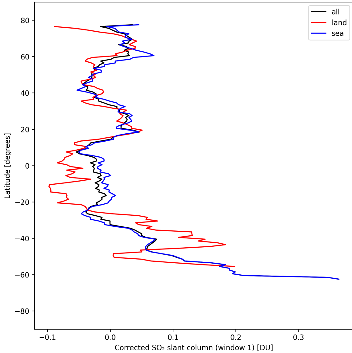
Figure 39: Zonal average of “Corrected SO 2 slant column (window 1)” for 2025-09-04 to 2025-09-05.
