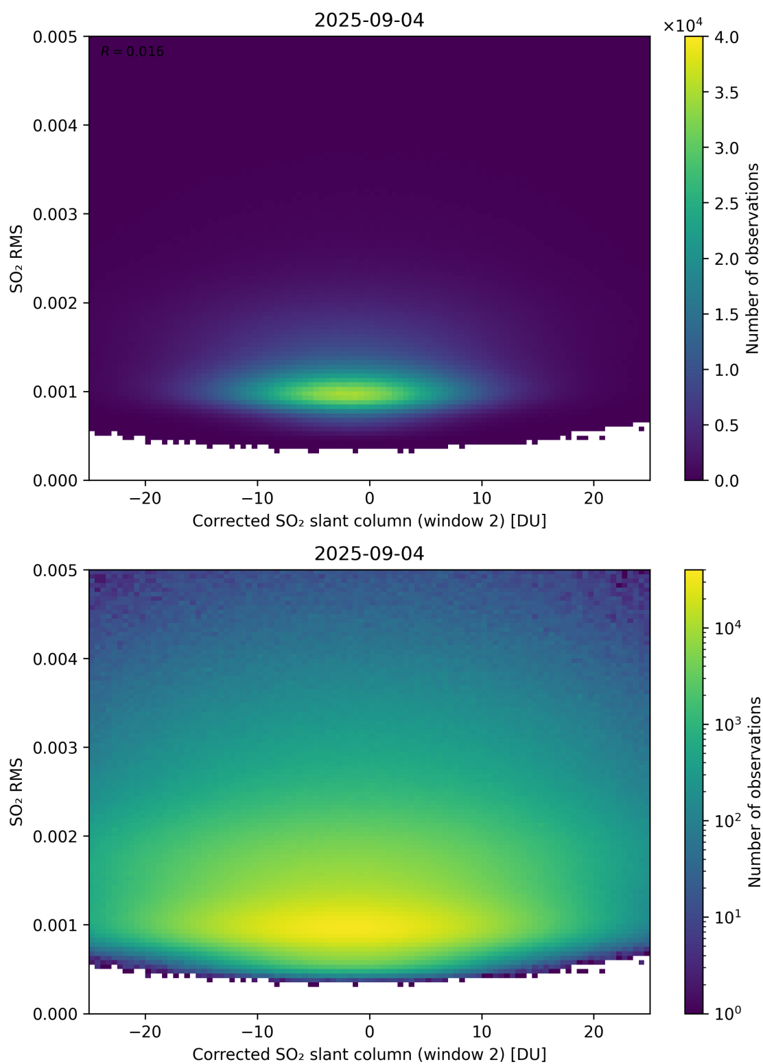
Figure 248: Scatter density plot of “Corrected SO 2 slant column (window 2)” against “SO 2 RMS” for 2025-09-04 to 2025-09-05.
