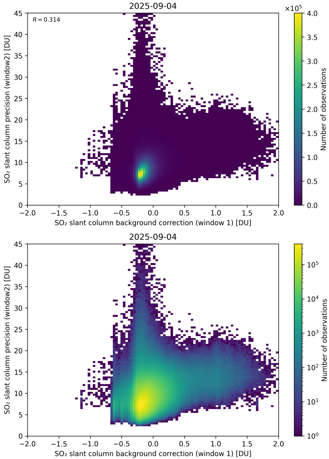
Figure 117: Scatter density plot of “SO 2 slant column background correction (window 1)” against “SO 2 slant column precision (window2)” for 2025-09-04 to 2025-09-05.
