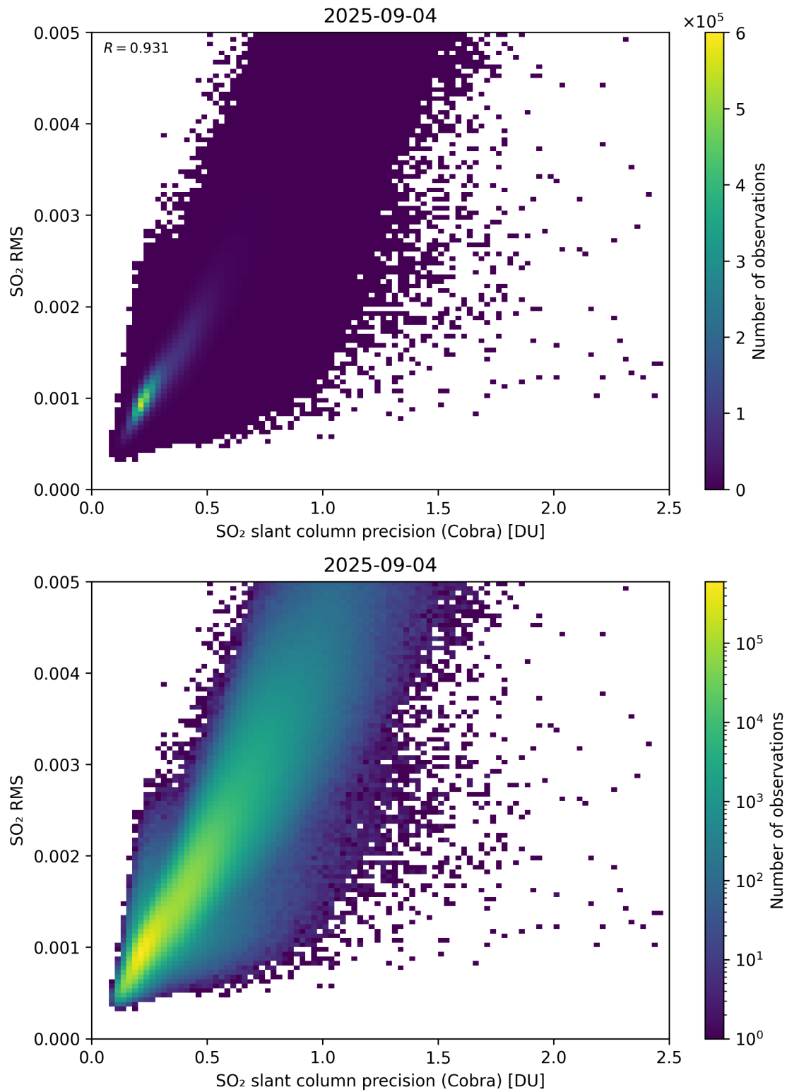
Figure 204: Scatter density plot of “SO 2 slant column precision (Cobra)” against “SO 2 RMS” for 2025-09-04 to 2025-09-05.
