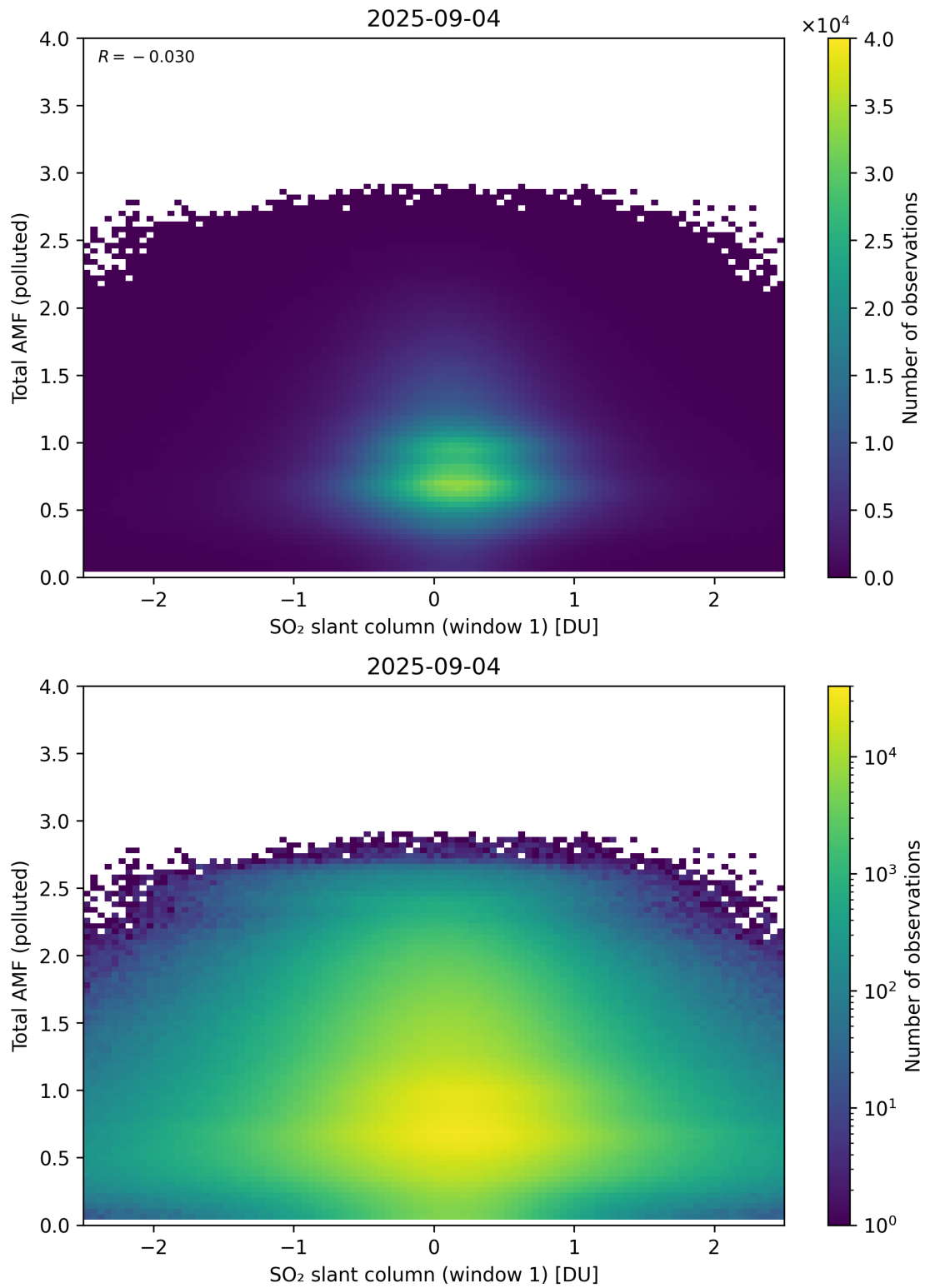
Figure 289: Scatter density plot of “SO 2 slant column (window 1)” against “Total AMF (polluted)” for 2025-09-04 to 2025-09-05.
