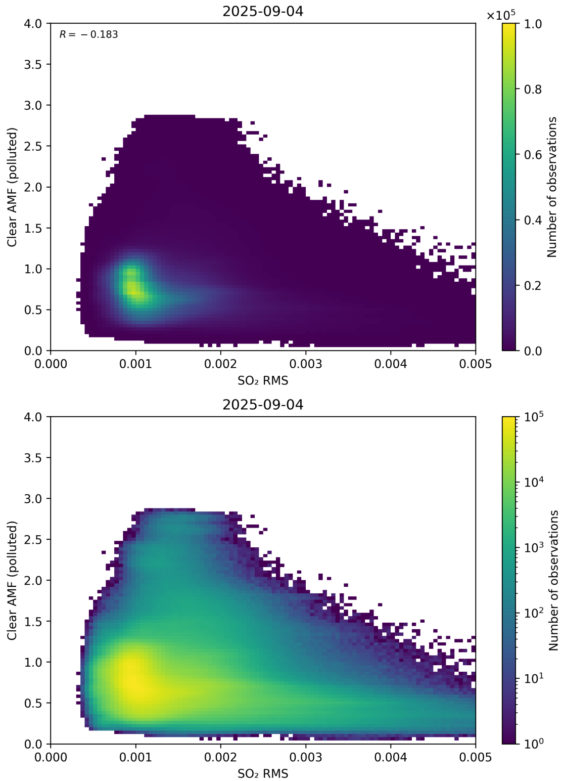
Figure 147: Scatter density plot of “SO 2 RMS” against “Clear AMF (polluted)” for 2025-09-04 to 2025-09-05.
