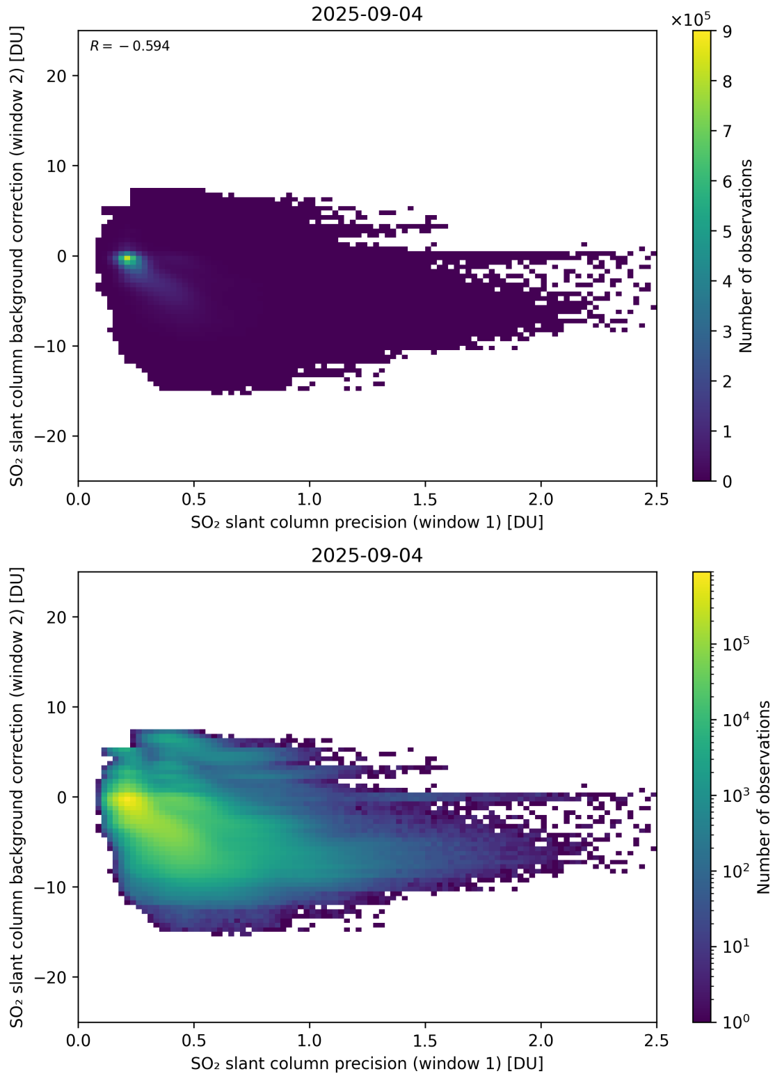
Figure 269: Scatter density plot of “SO 2 slant column precision (window 1)” against “SO 2 slant column background correction (window 2)” for 2025-09-04 to 2025-09-05.
