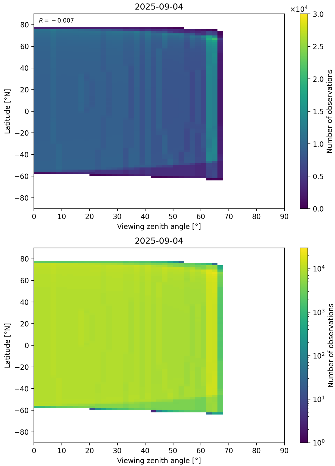
Figure 368: Scatter density plot of “Viewing zenith angle” against “Latitude” for 2025-09-04 to 2025-09-05.
