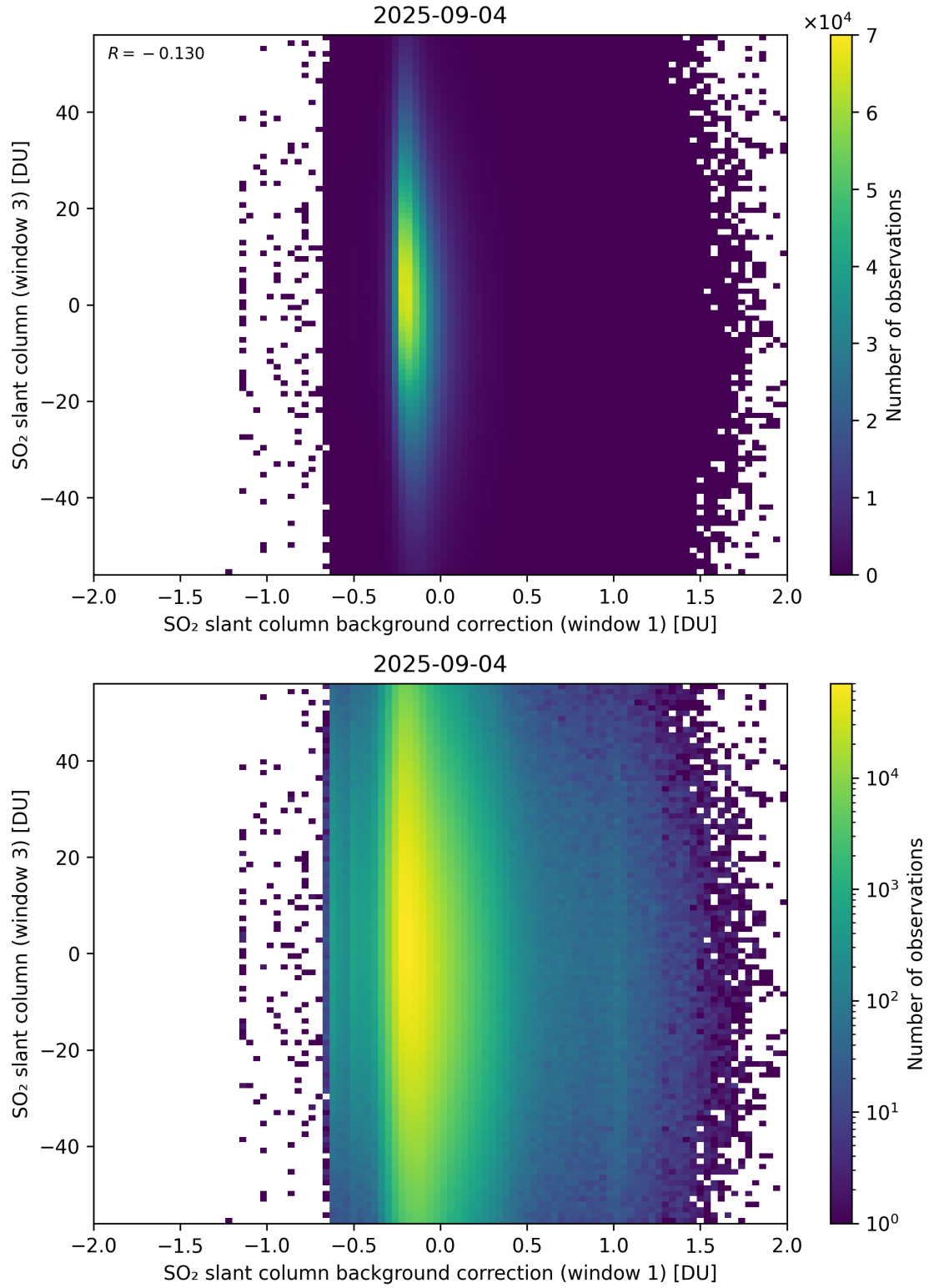
Figure 118: Scatter density plot of “SO 2 slant column background correction (window 1)” against “SO 2 slant column (window 3)” for 2025-09-04 to 2025-09-05.
