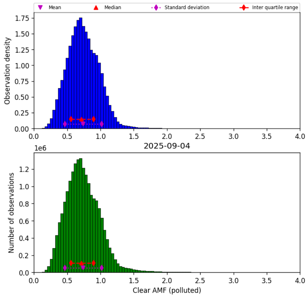
Figure 81: Histogram of “Clear AMF (polluted)” for 2025-09-04 to 2025-09-05
