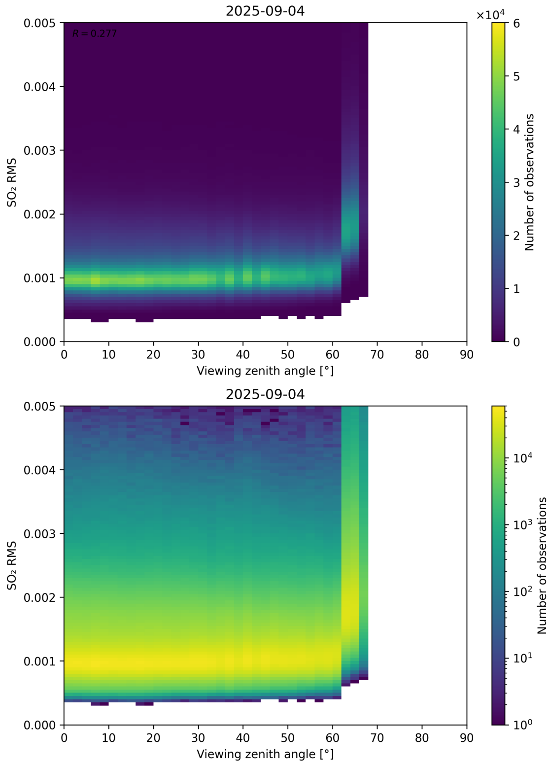
Figure 367: Scatter density plot of “Viewing zenith angle” against “SO 2 RMS” for 2025-09-04 to 2025-09-05.
