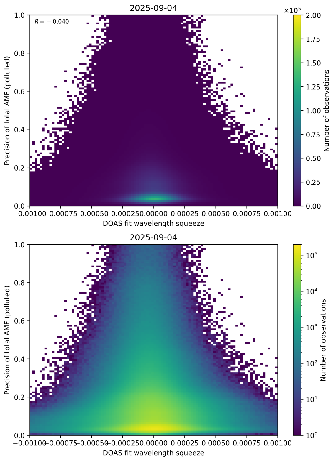
Figure 146: Scatter density plot of “DOAS fit wavelength squeeze” against “Precision of total AMF (polluted)” for 2025-09-04 to 2025-09-05.
