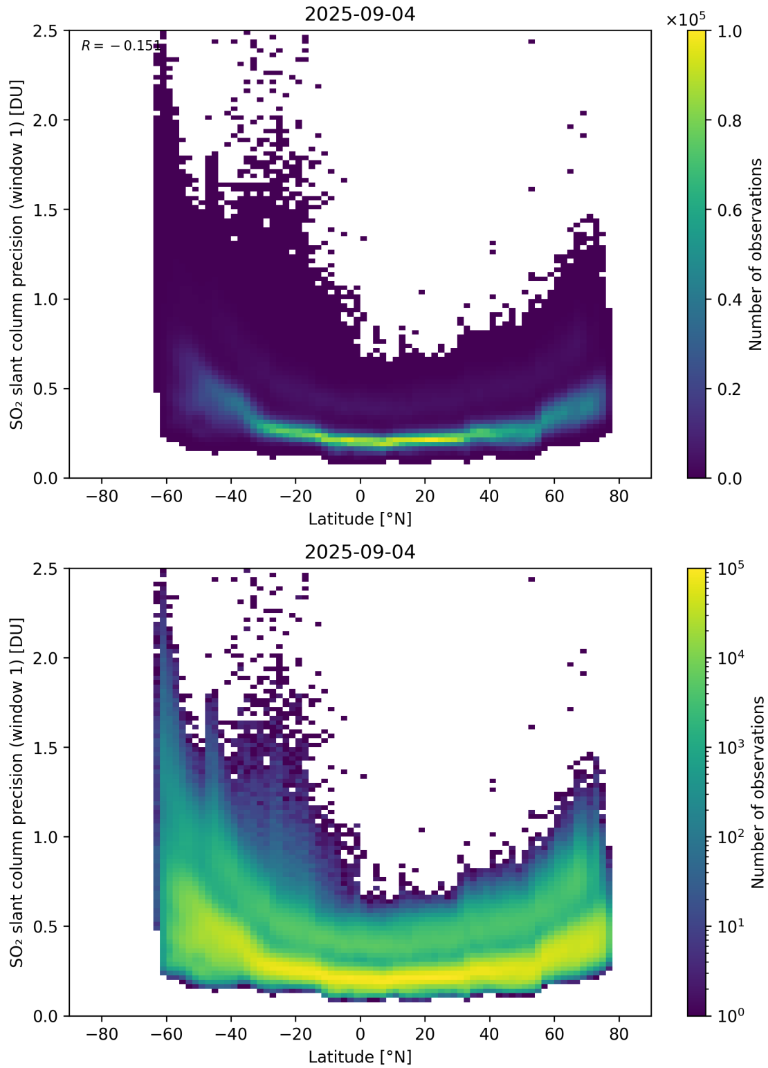
Figure 163: Scatter density plot of “Latitude” against “SO 2 slant column precision (window 1)” for 2025-09-04 to 2025-09-05.
