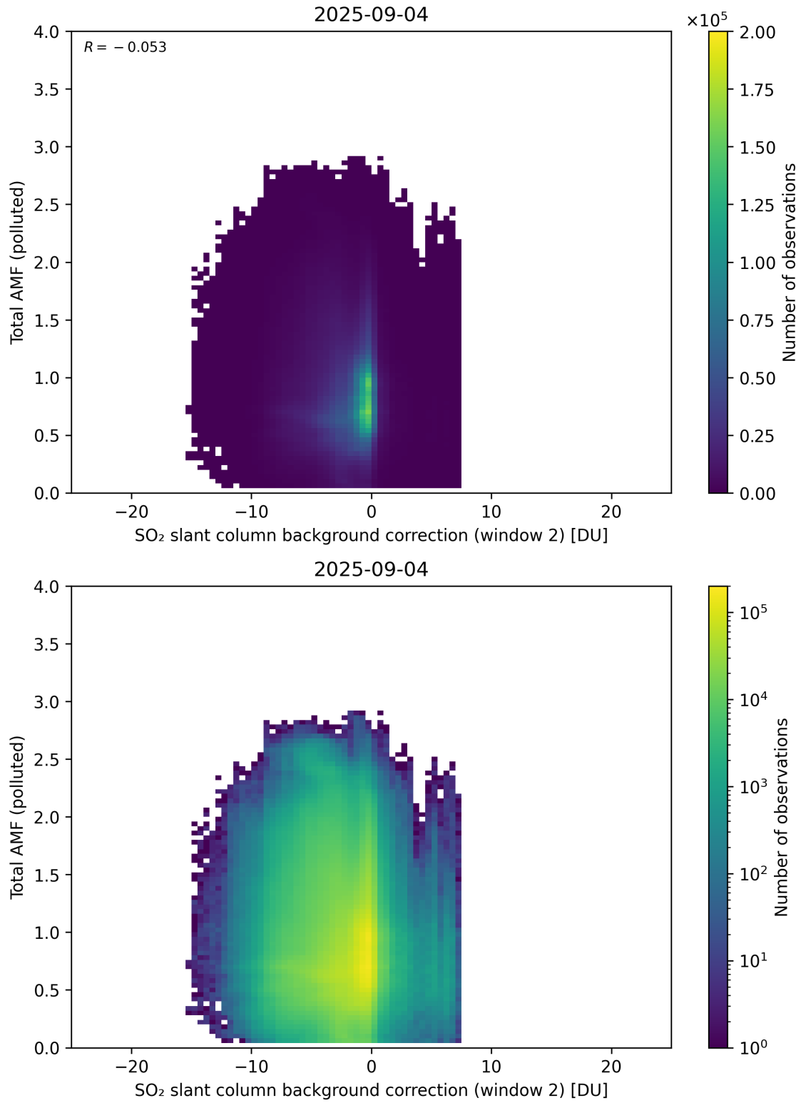
Figure 130: Scatter density plot of “SO 2 slant column background correction (window 2)” against “Total AMF (polluted)” for 2025-09-04 to 2025-09-05.
