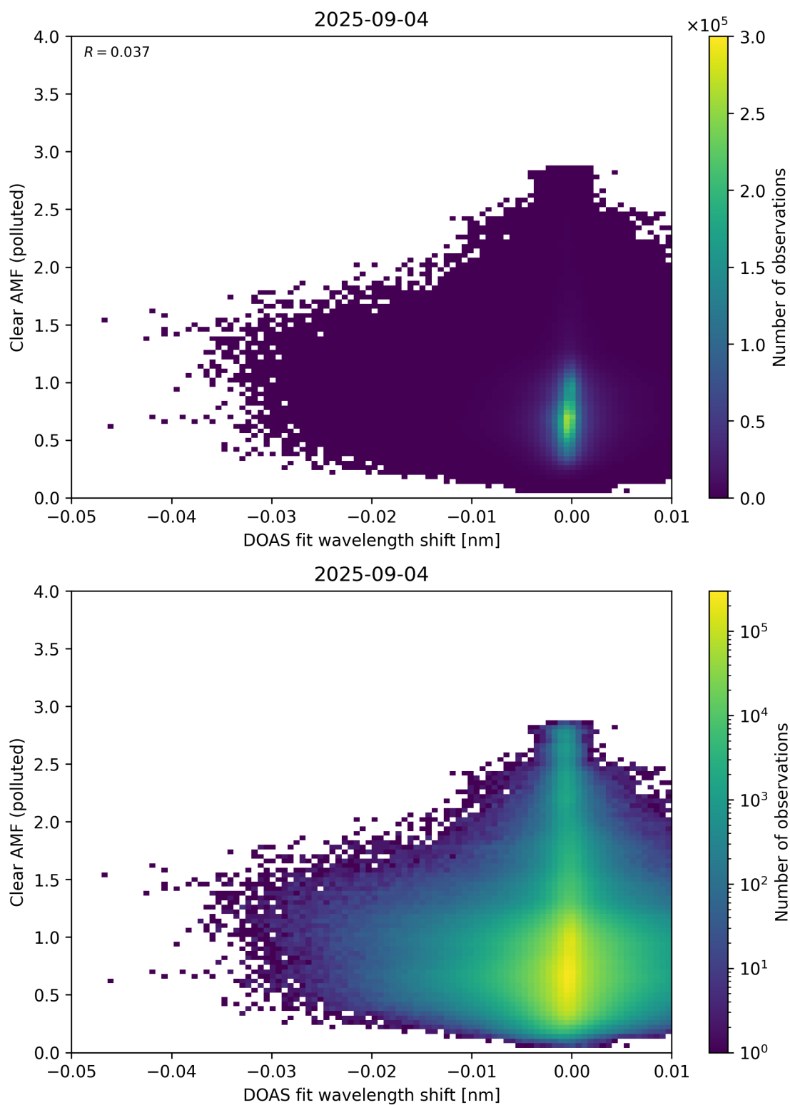
Figure 140: Scatter density plot of “DOAS fit wavelength shift” against “Clear AMF (polluted)” for 2025-09-04 to 2025-09-05.
