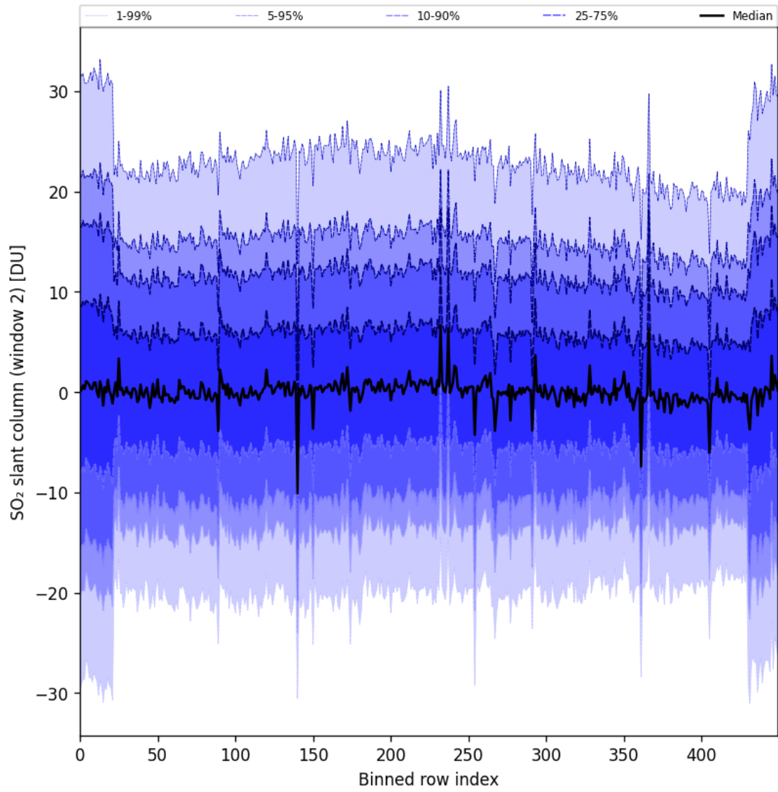
Figure 93: Along track statistics of “SO 2 slant column (window 2)” for 2025-09-04 to 2025-09-05
