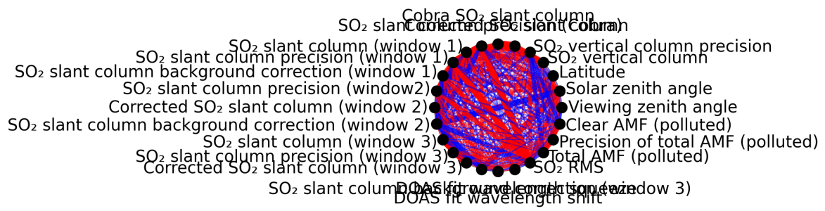
Figure 1: Map of correlation graph for 2025-09-04 to 2025-09-05.
