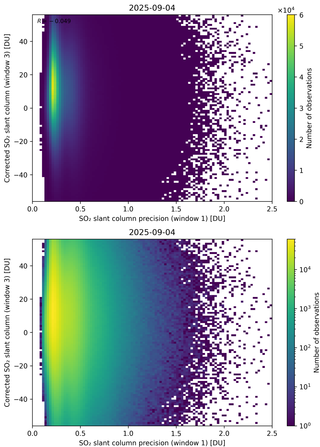
Figure 276: Scatter density plot of “SO 2 slant column precision (window 1)” against “Corrected SO 2 slant column (window 3)” for 2025-09-04 to 2025-09-05.
