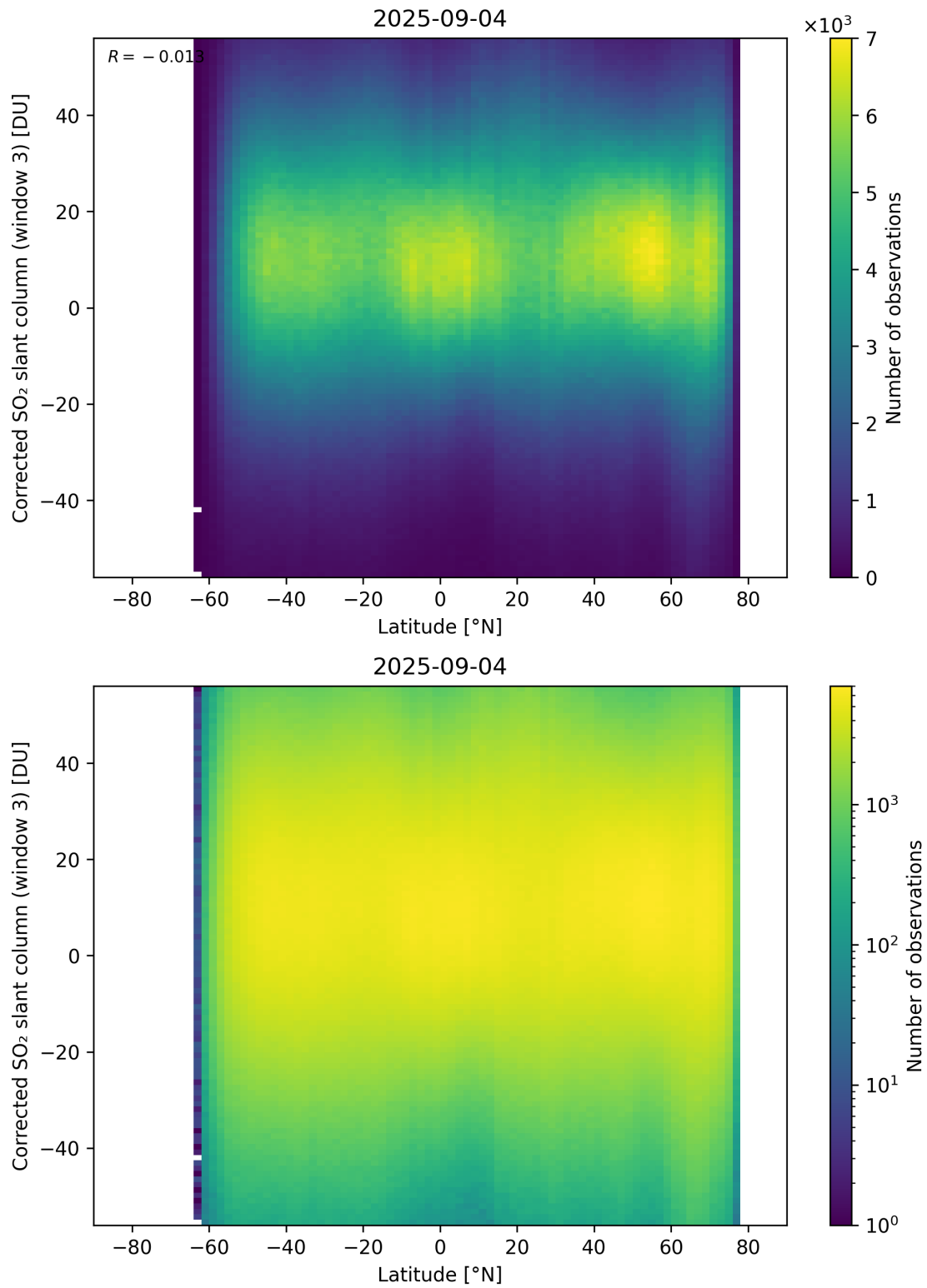
Figure 161: Scatter density plot of “Latitude” against “Corrected SO 2 slant column (window 3)” for 2025-09-04 to 2025-09-05.
