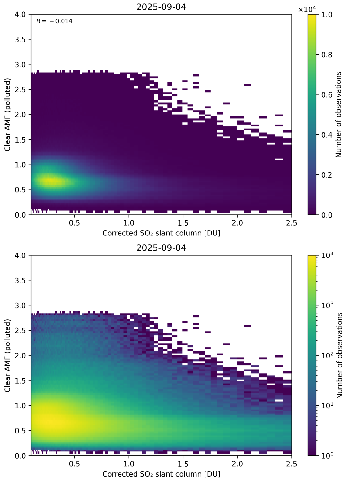
Figure 232: Scatter density plot of “Corrected SO 2 slant column” against “Clear AMF (polluted)” for 2025-09-04 to 2025-09-05.
