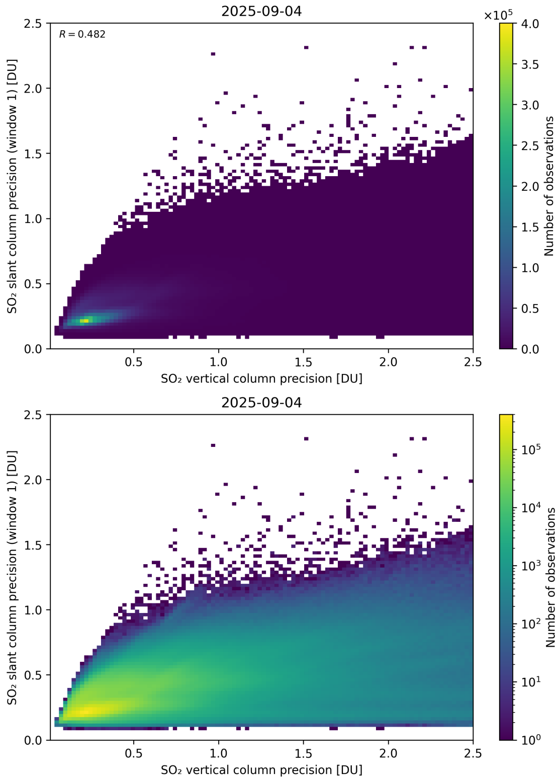
Figure 342: Scatter density plot of “SO 2 vertical column precision” against “SO 2 slant column precision (window 1)” for 2025-09-04 to 2025-09-05.
