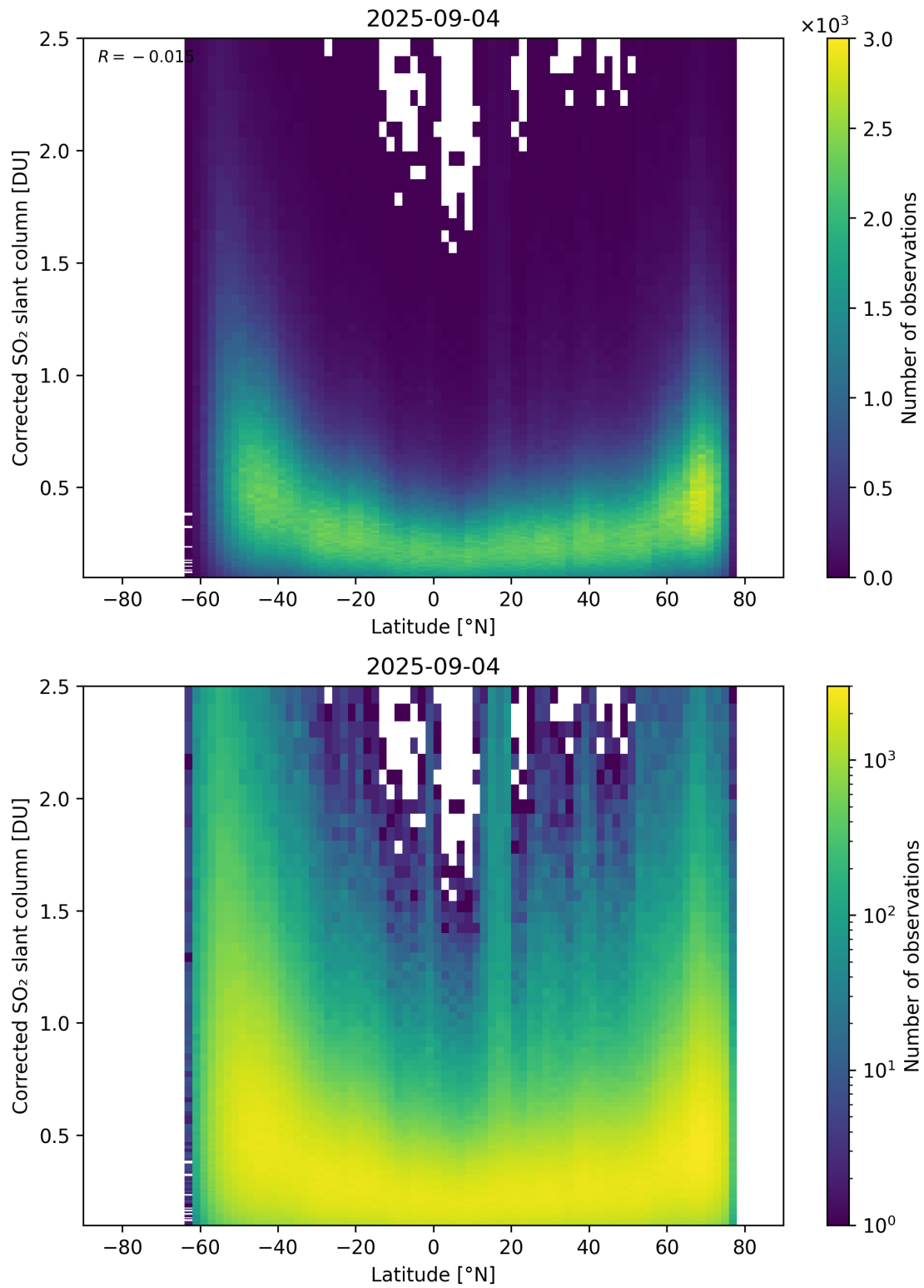
Figure 159: Scatter density plot of “Latitude” against “Corrected SO 2 slant column” for 2025-09-04 to 2025-09-05.
