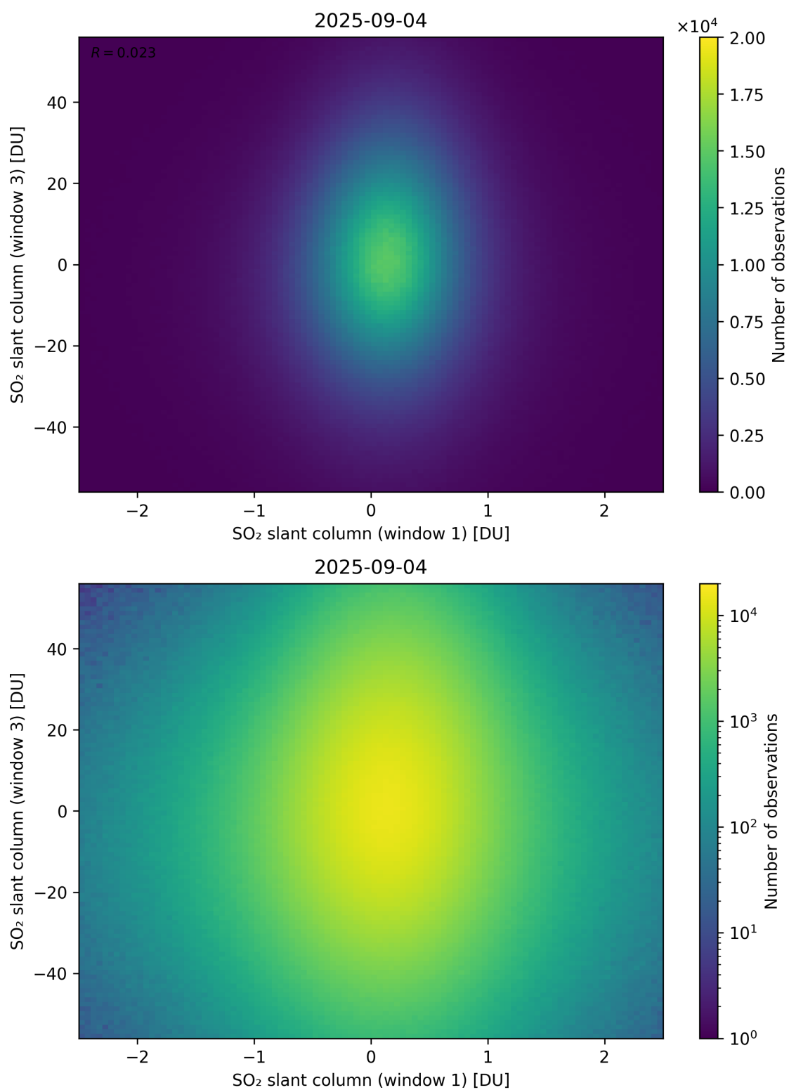
Figure 287: Scatter density plot of “SO 2 slant column (window 1)” against “SO 2 slant column (window 3)” for 2025-09-04 to 2025-09-05.
