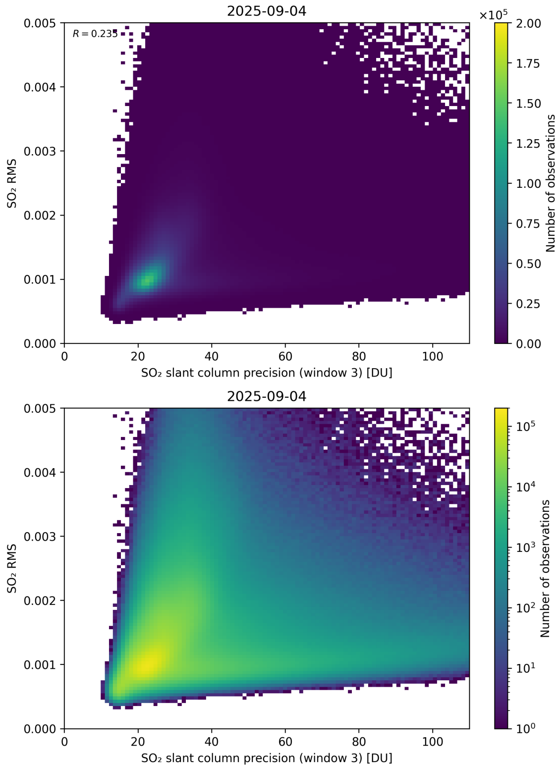
Figure 310: Scatter density plot of “SO 2 slant column precision (window 3)” against “SO 2 RMS” for 2025-09-04 to 2025-09-05.
