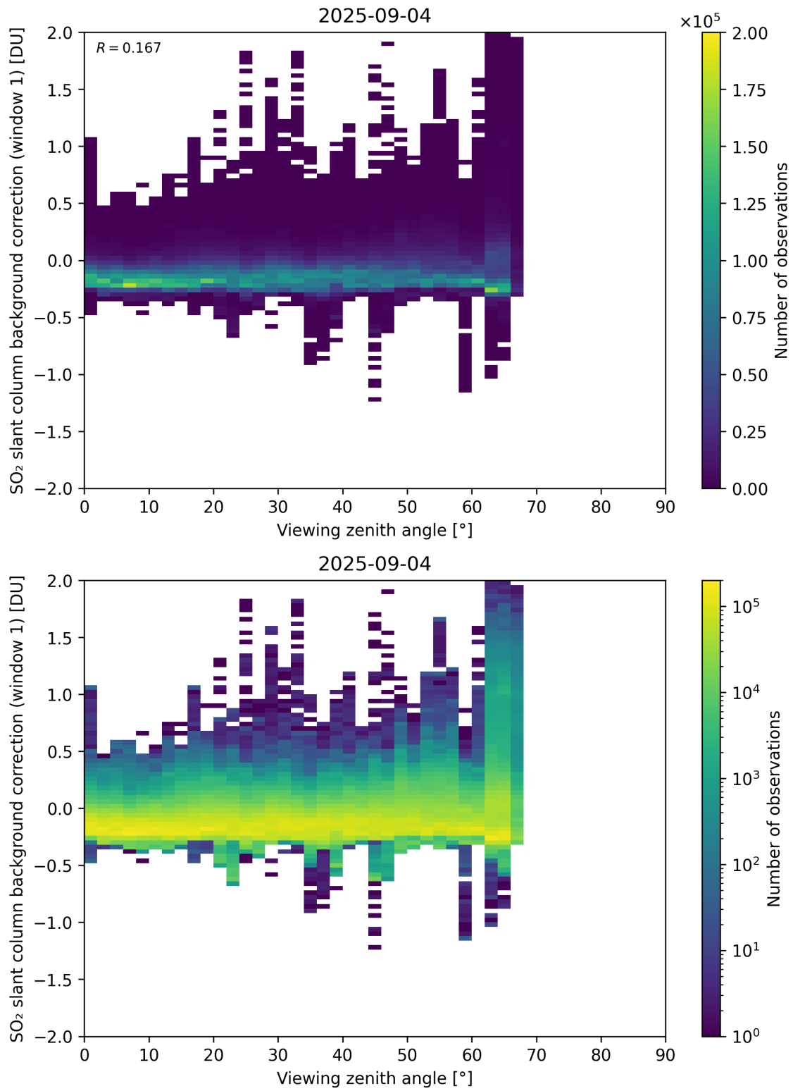
Figure 362: Scatter density plot of “Viewing zenith angle” against “SO 2 slant column background correction (window 1)” for 2025-09-04 to 2025-09-05.
