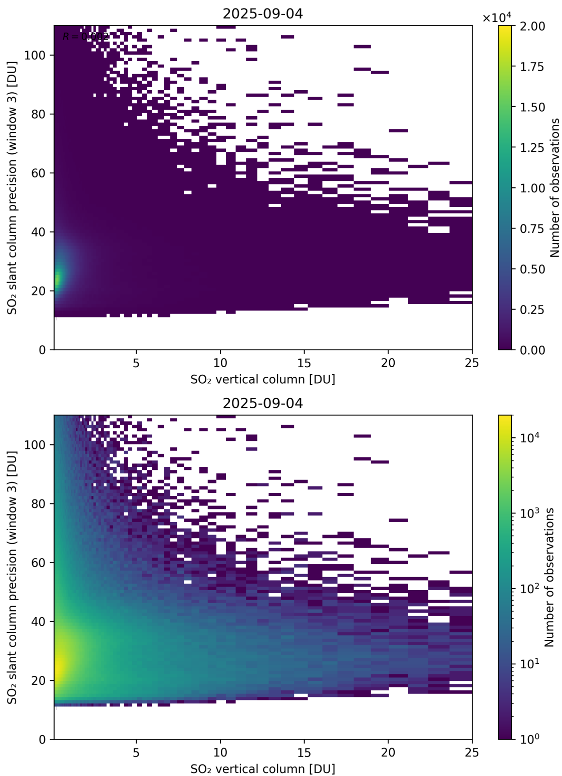
Figure 358: Scatter density plot of “SO 2 vertical column” against “SO 2 slant column precision (window 3)” for 2025-09-04 to 2025-09-05.
