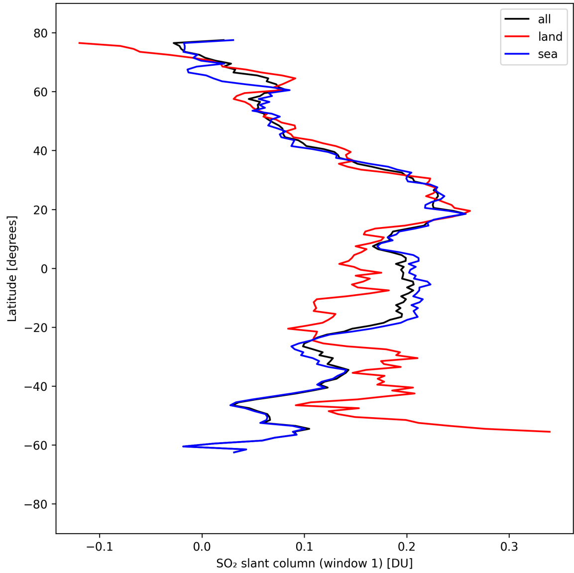
Figure 37: Zonal average of “SO 2 slant column (window 1)” for 2025-09-04 to 2025-09-05.
