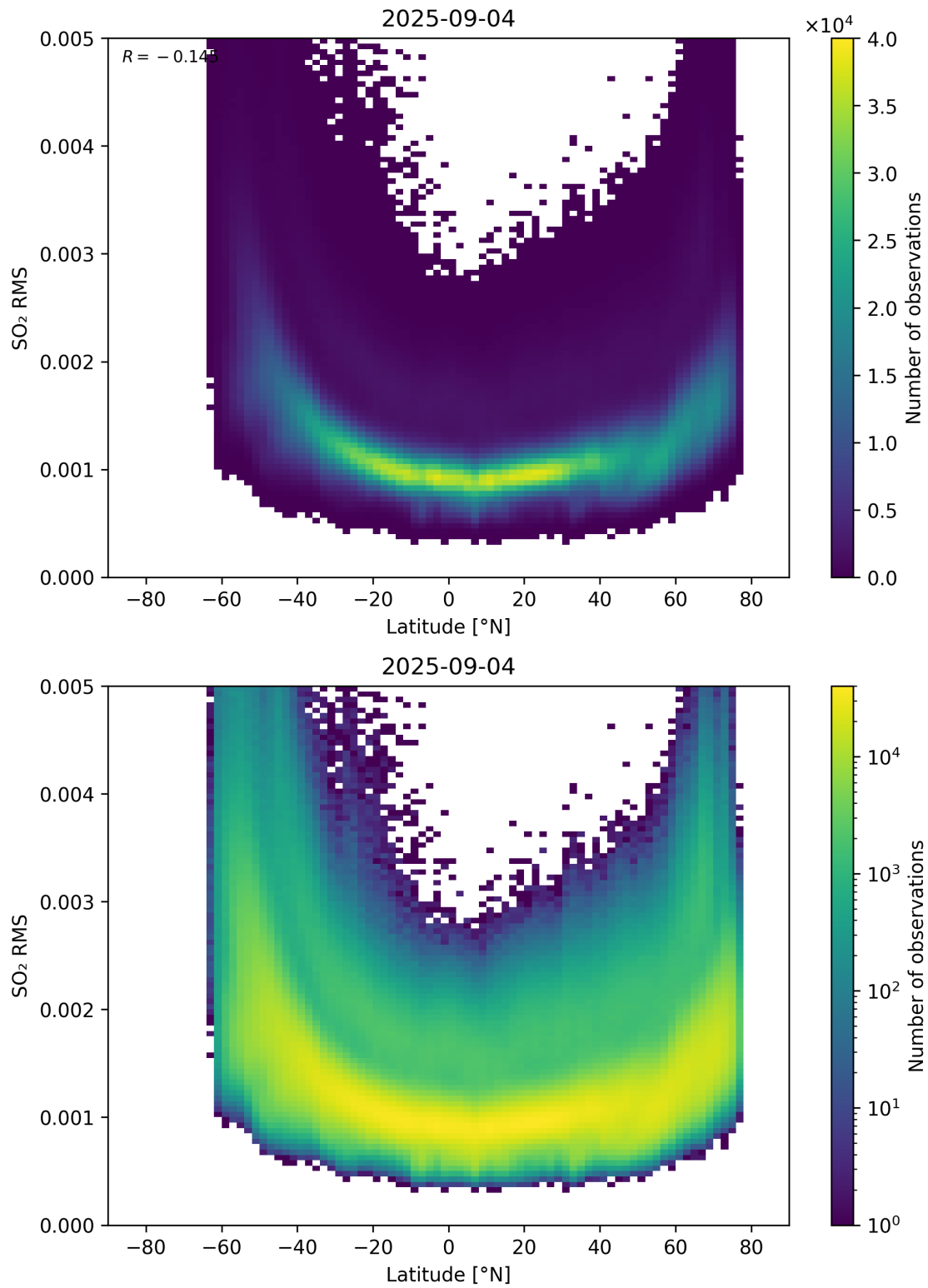
Figure 155: Scatter density plot of “Latitude” against “SO 2 RMS” for 2025-09-04 to 2025-09-05.
