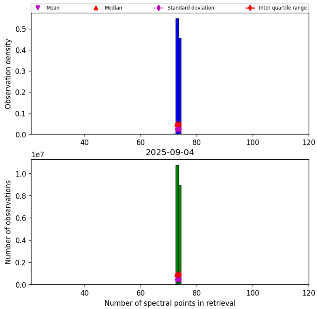
Figure 82: Histogram of “Number of spectral points in retrieval” for 2025-09-04 to 2025-09-05
