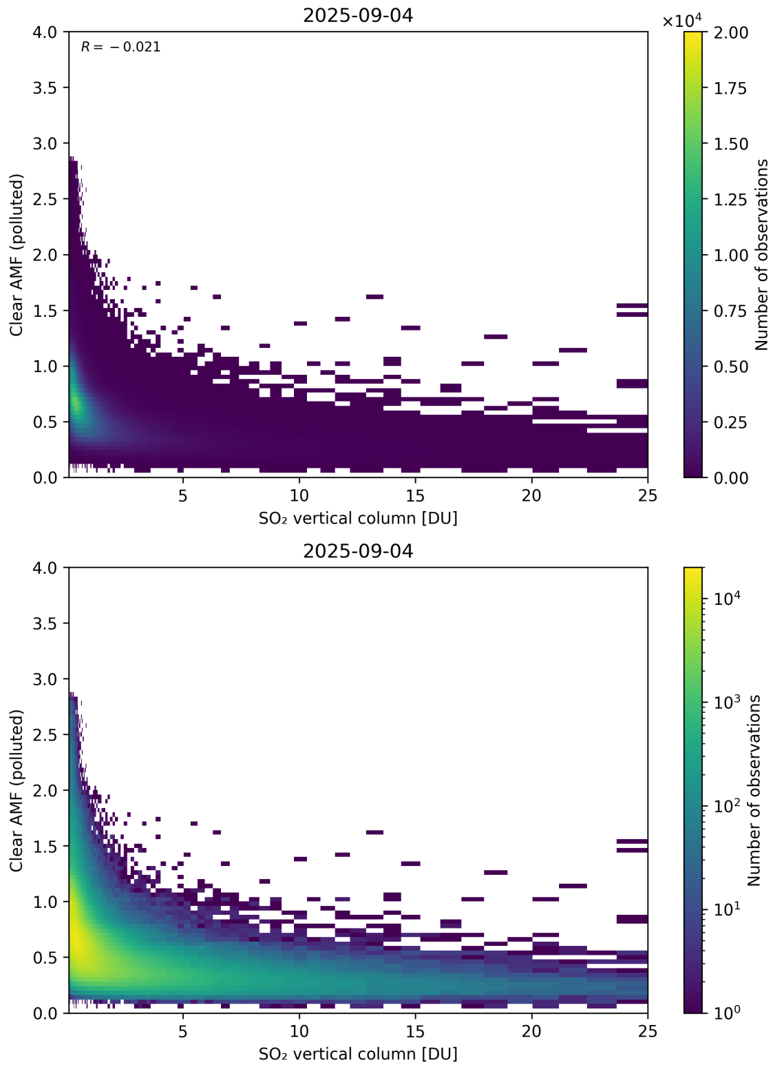
Figure 348: Scatter density plot of “SO 2 vertical column” against “Clear AMF (polluted)” for 2025-09-04 to 2025-09-05.
