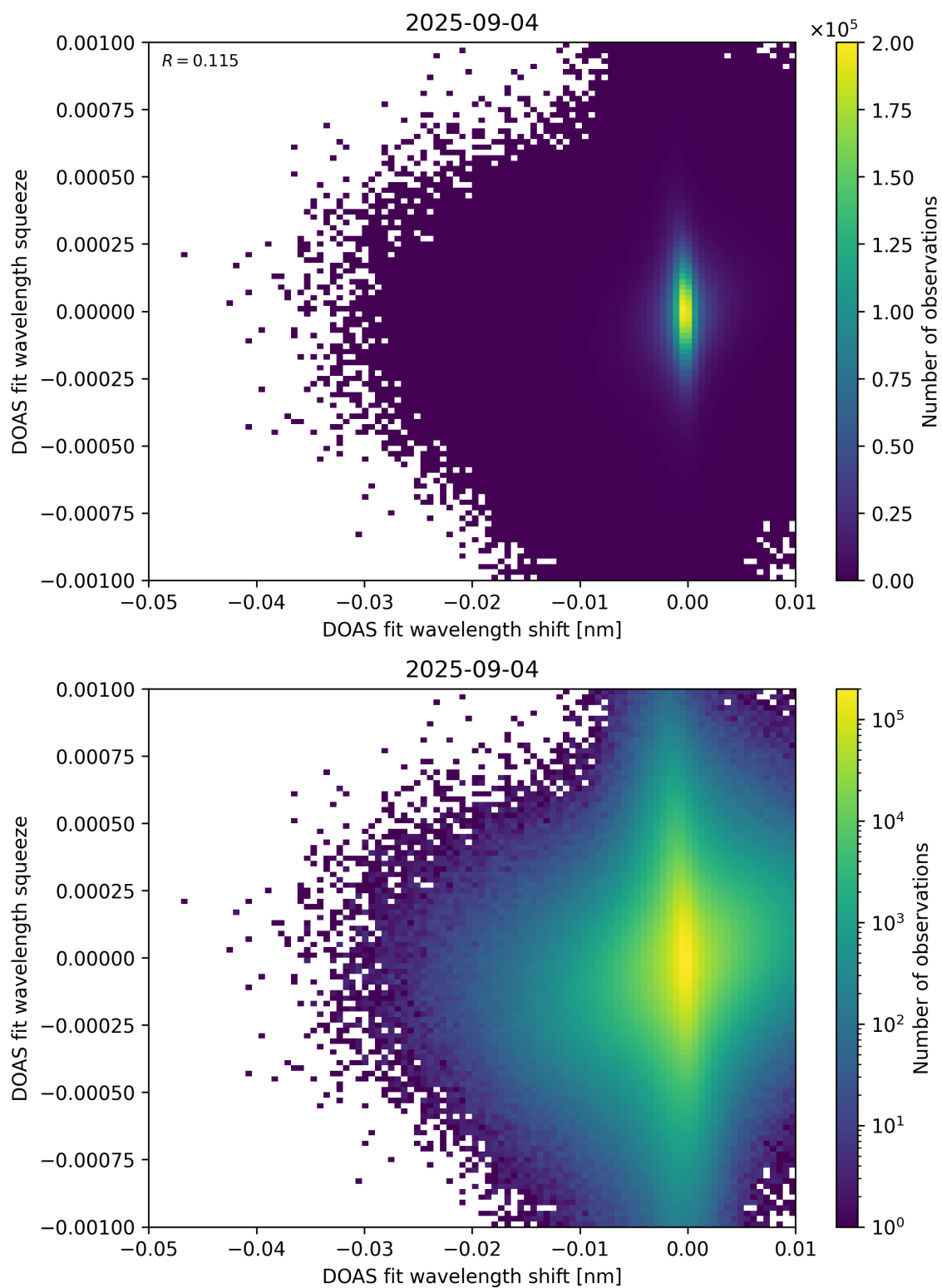
Figure 138: Scatter density plot of “DOAS fit wavelength shift” against “DOAS fit wavelength squeeze” for 2025-09-04 to 2025-09-05.
