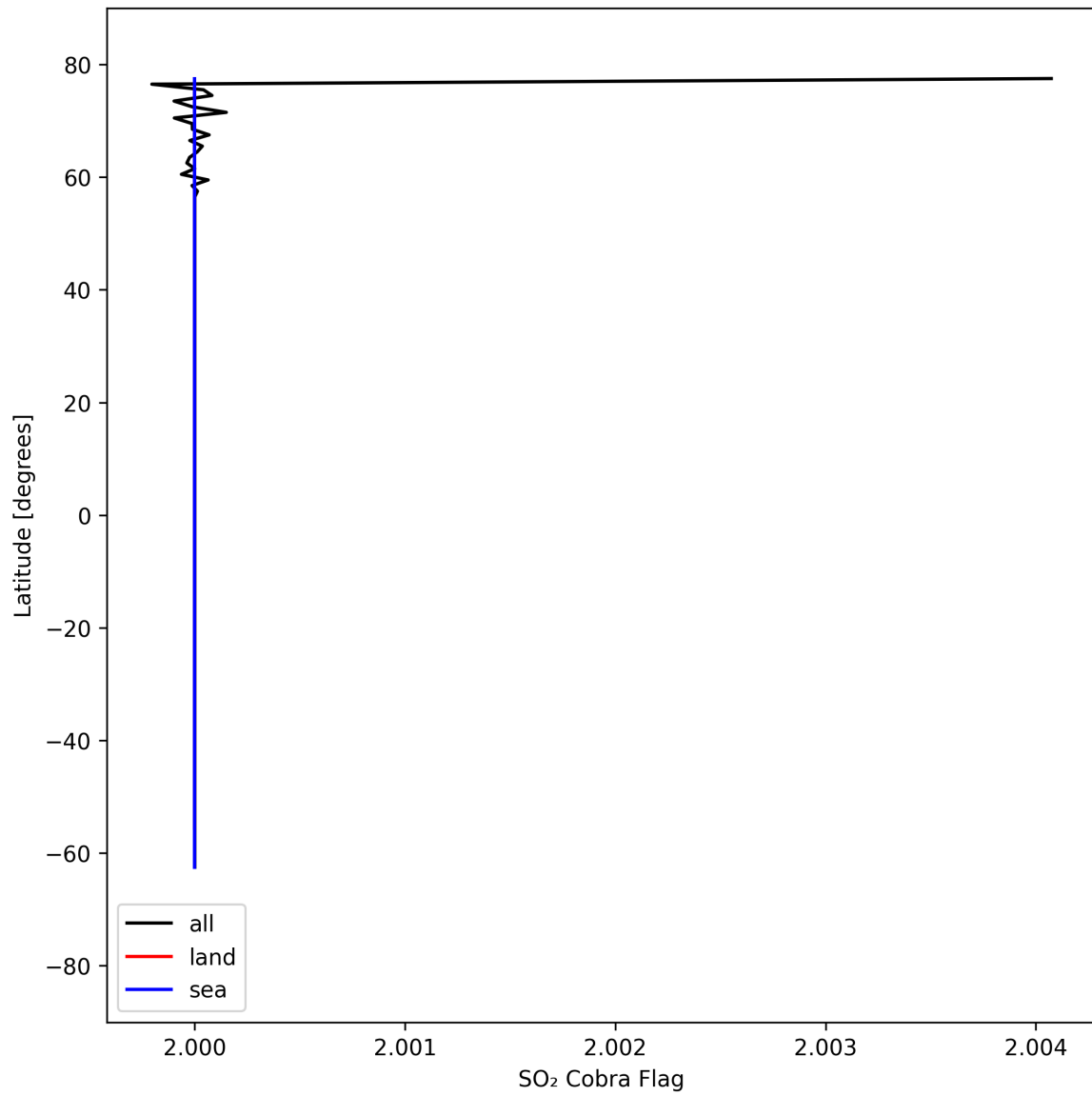
Figure 49: Zonal average of “SO 2 Cobra Flag” for 2025-09-04 to 2025-09-05.
