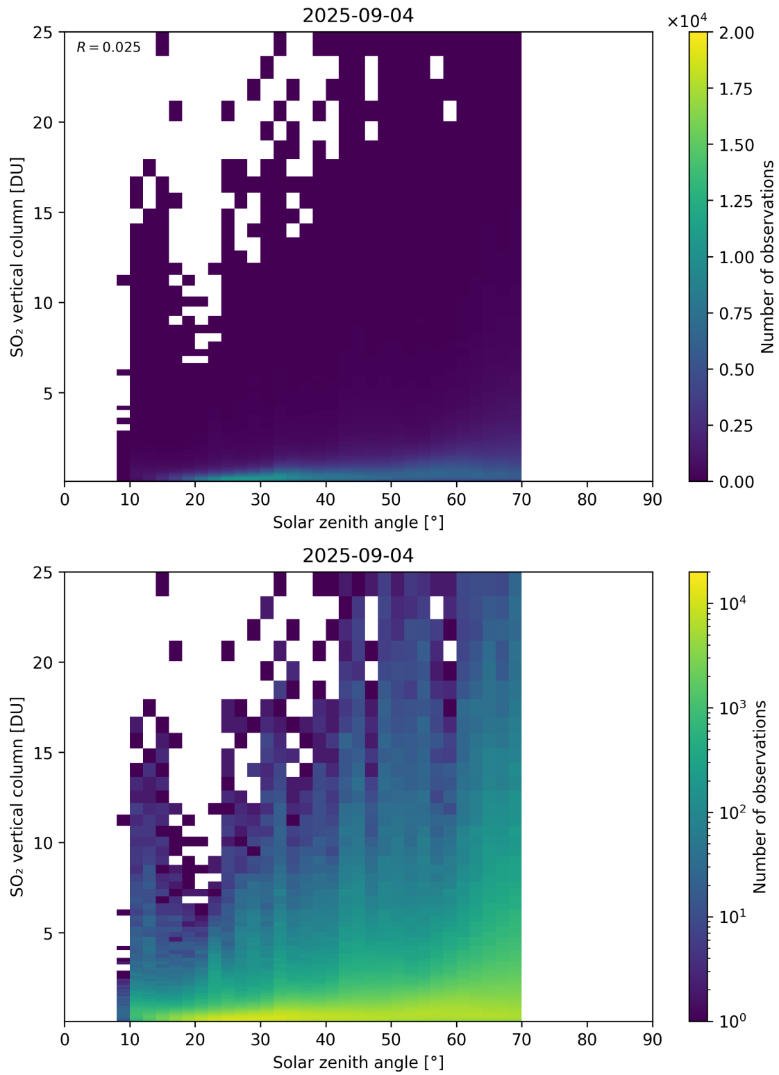
Figure 191: Scatter density plot of “Solar zenith angle” against “SO 2 vertical column” for 2025-09-04 to 2025-09-05.
