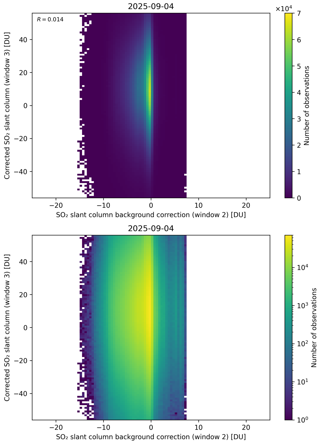
Figure 127: Scatter density plot of “SO 2 slant column background correction (window 2)” against “Corrected SO 2 slant column (window 3)” for 2025-09-04 to 2025-09-05.
