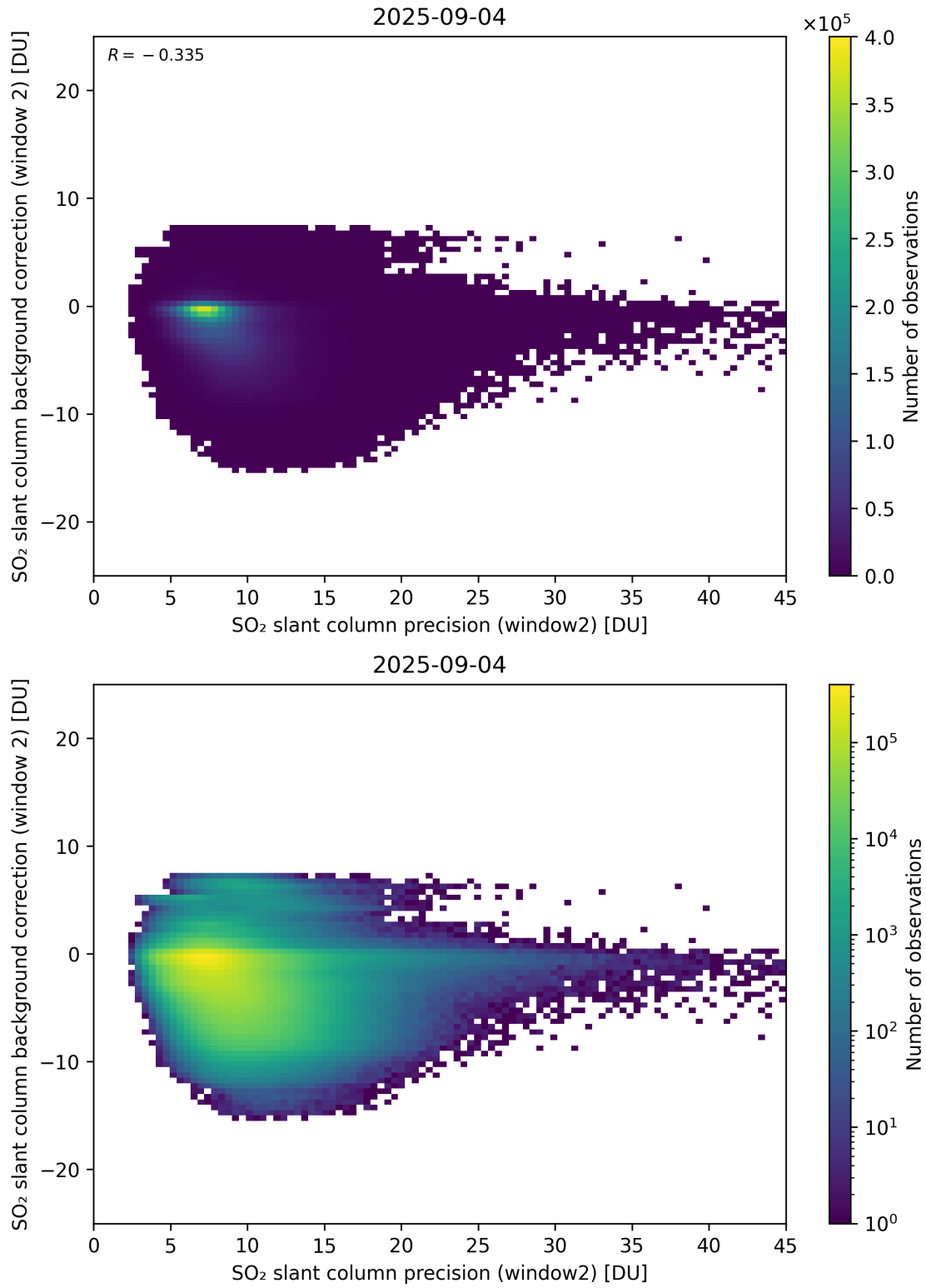
Figure 291: Scatter density plot of “SO 2 slant column precision (window2)” against “SO 2 slant column background correction (window 2)” for 2025-09-04 to 2025-09-05.
