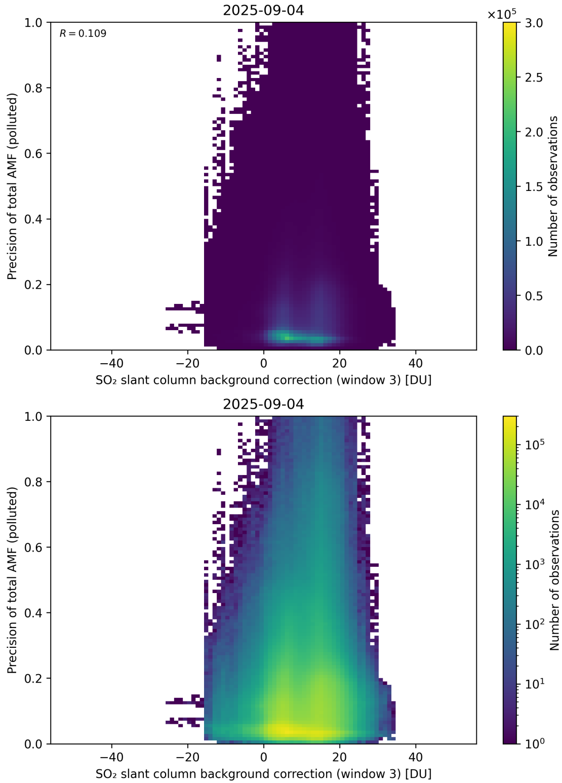
Figure 137: Scatter density plot of “SO 2 slant column background correction (window 3)” against “Precision of total AMF (polluted)” for 2025-09-04 to 2025-09-05.
