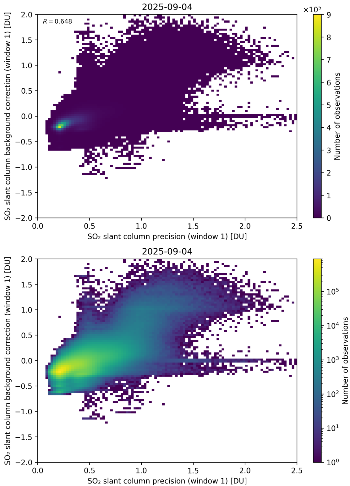
Figure 268: Scatter density plot of “SO 2 slant column precision (window 1)” against “SO 2 slant column background correction (window 1)” for 2025-09-04 to 2025-09-05.
