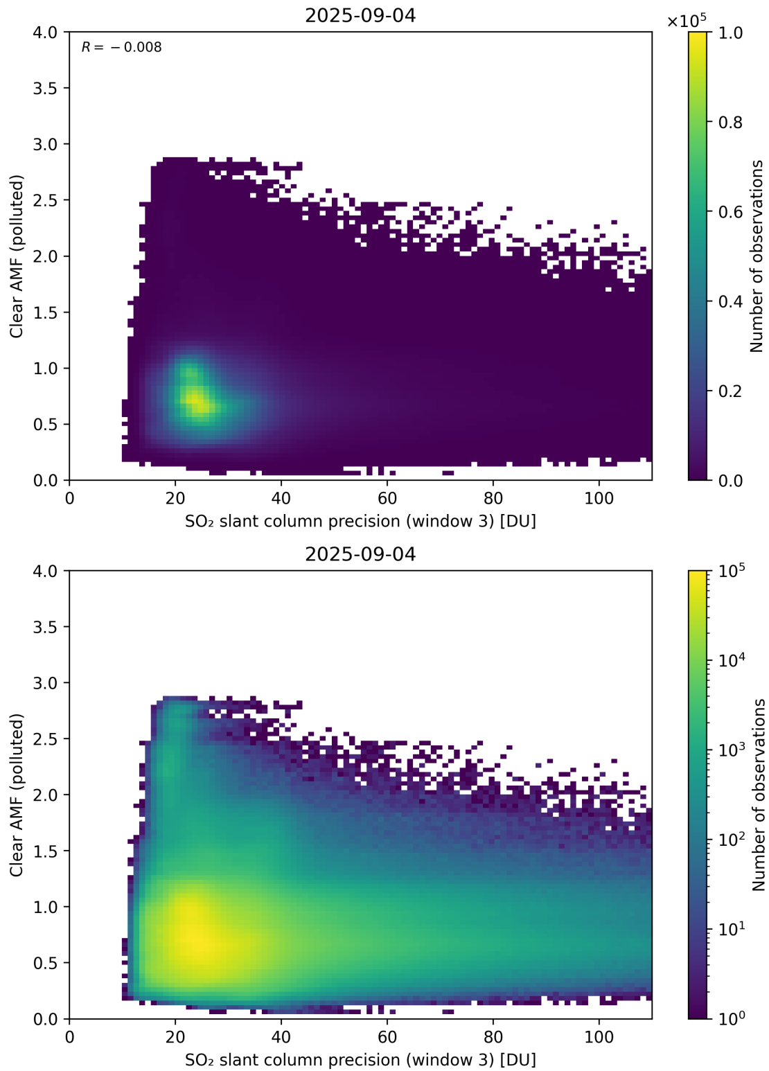
Figure 311: Scatter density plot of “SO 2 slant column precision (window 3)” against “Clear AMF (polluted)” for 2025-09-04 to 2025-09-05.
