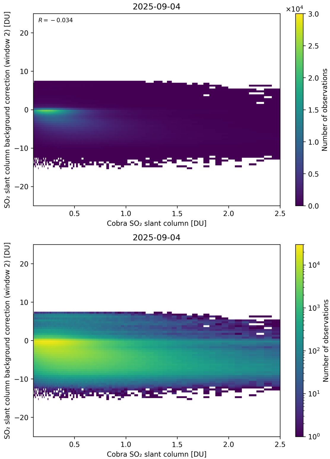
Figure 194: Scatter density plot of “Cobra SO 2 slant column” against “SO 2 slant column background correction (window 2)” for 2025-09-04 to 2025-09-05.
