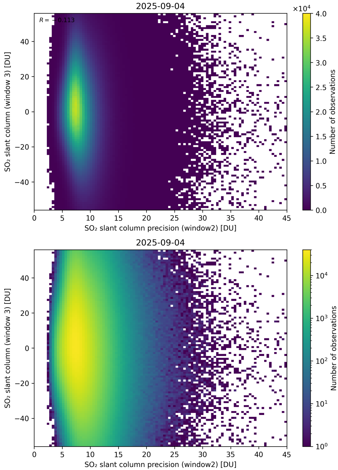
Figure 299: Scatter density plot of “SO 2 slant column precision (window2)” against “SO 2 slant column (window 3)” for 2025-09-04 to 2025-09-05.
