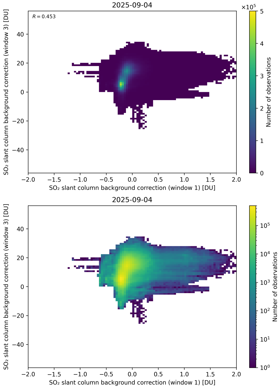
Figure 110: Scatter density plot of “SO 2 slant column background correction (window 1)” against “SO 2 slant column background correction (window 3)” for 2025-09-04 to 2025-09-05.
