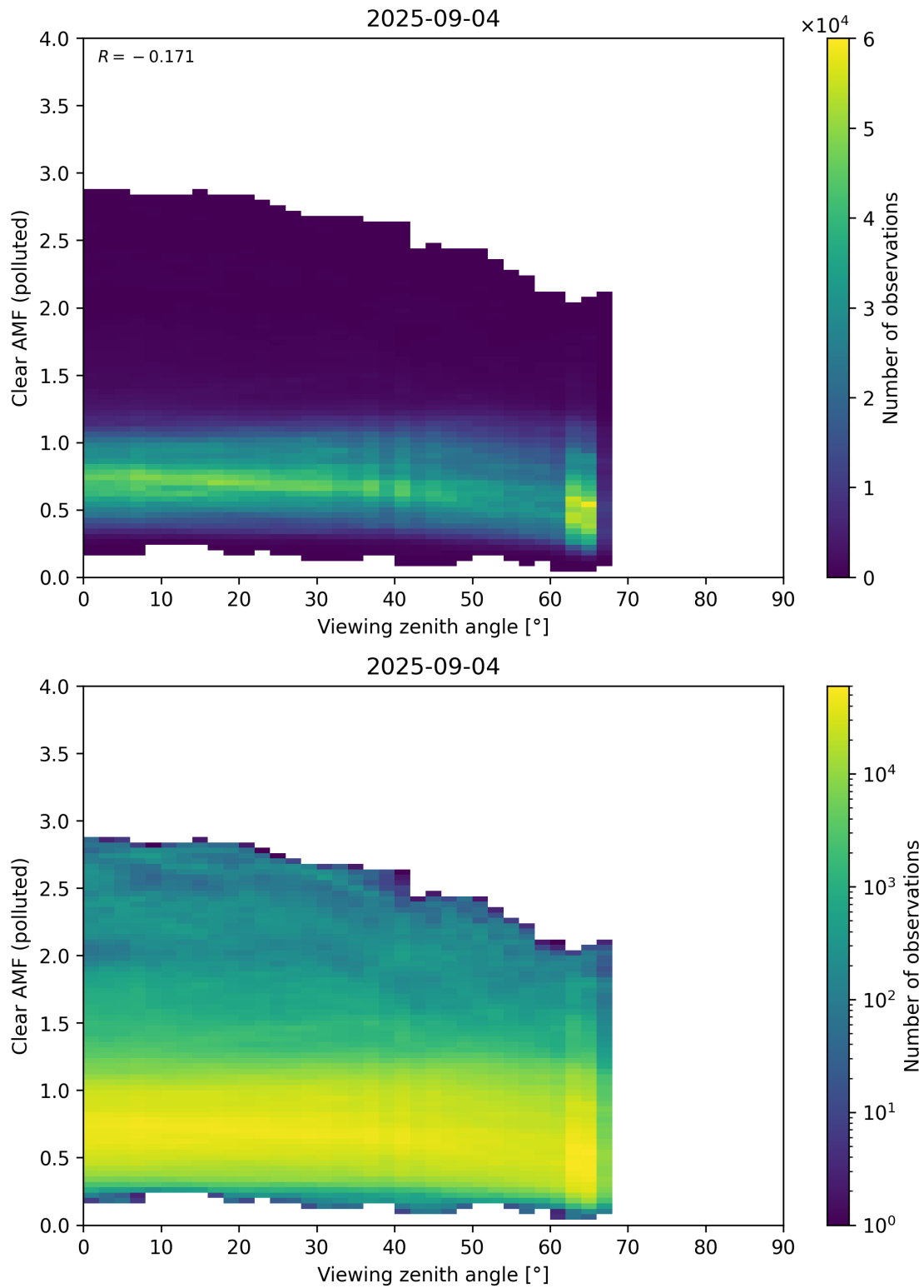
Figure 370: Scatter density plot of “Viewing zenith angle” against “Clear AMF (polluted)” for 2025-09-04 to 2025-09-05.
