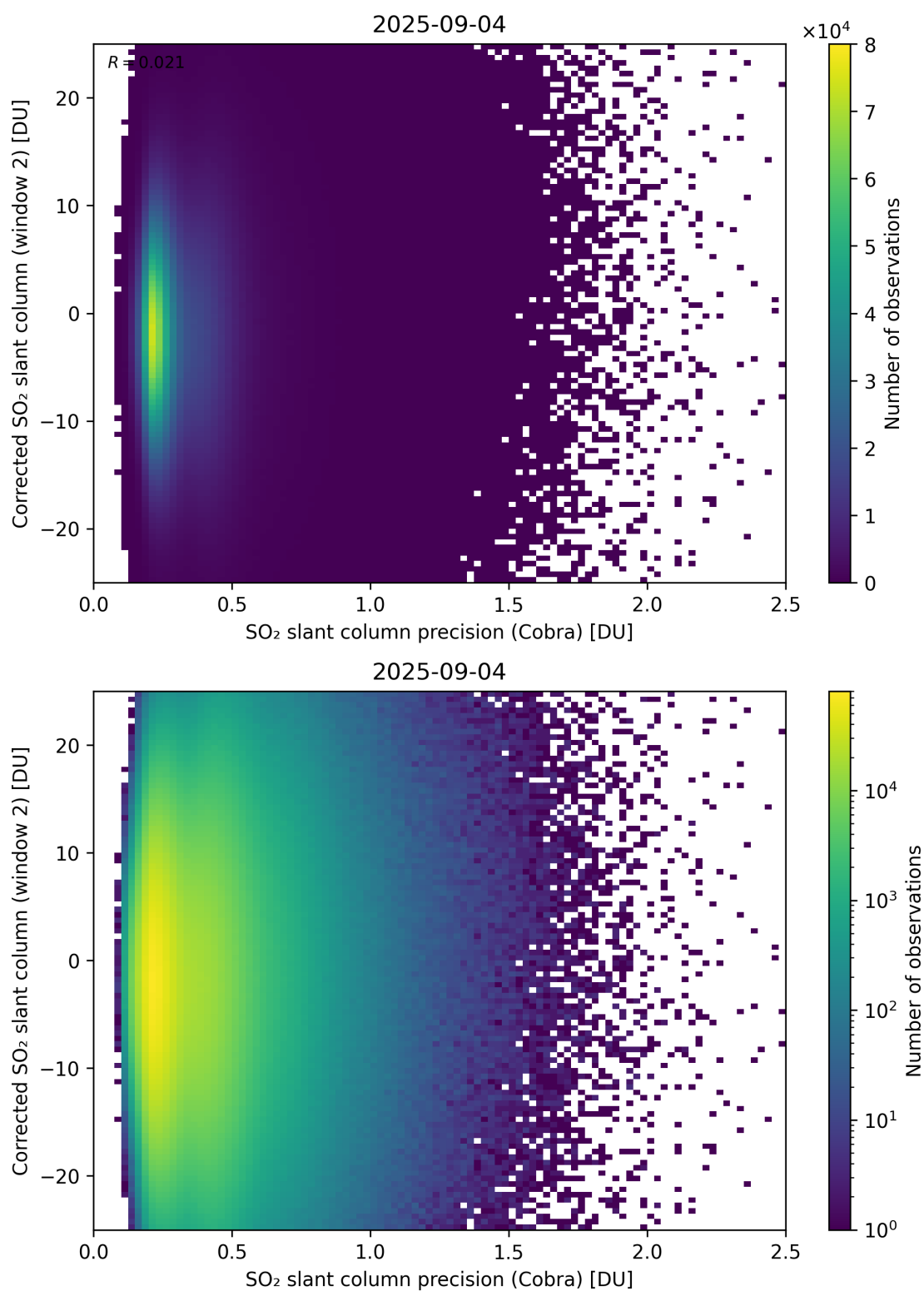
Figure 206: Scatter density plot of “SO 2 slant column precision (Cobra)” against “Corrected SO 2 slant column (window 2)” for 2025-09-04 to 2025-09-05.
