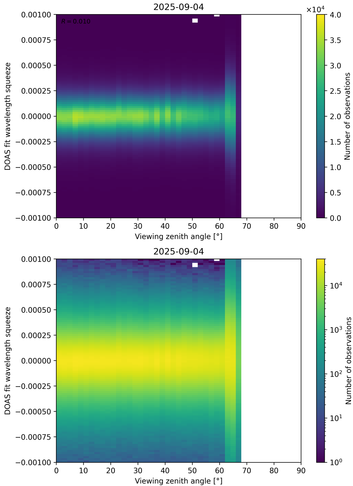
Figure 366: Scatter density plot of “Viewing zenith angle” against “DOAS fit wavelength squeeze” for 2025-09-04 to 2025-09-05.
