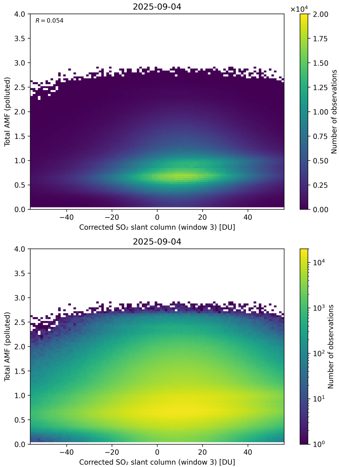
Figure 260: Scatter density plot of “Corrected SO 2 slant column (window 3)” against “Total AMF (polluted)” for 2025-09-04 to 2025-09-05.
