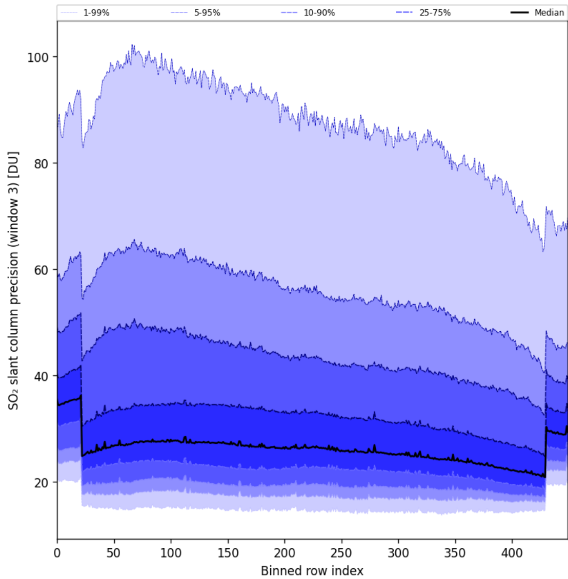
Figure 98: Along track statistics of “SO 2 slant column precision (window 3)” for 2025-09-04 to 2025-09-05
