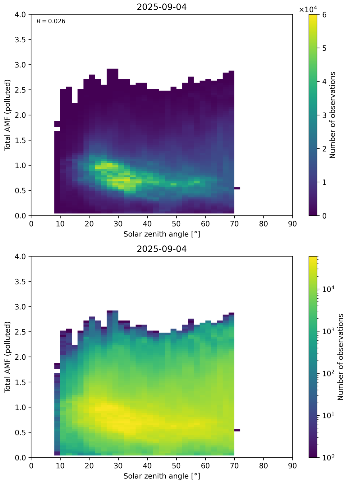
Figure 189: Scatter density plot of “Solar zenith angle” against “Total AMF (polluted)” for 2025-09-04 to 2025-09-05.
