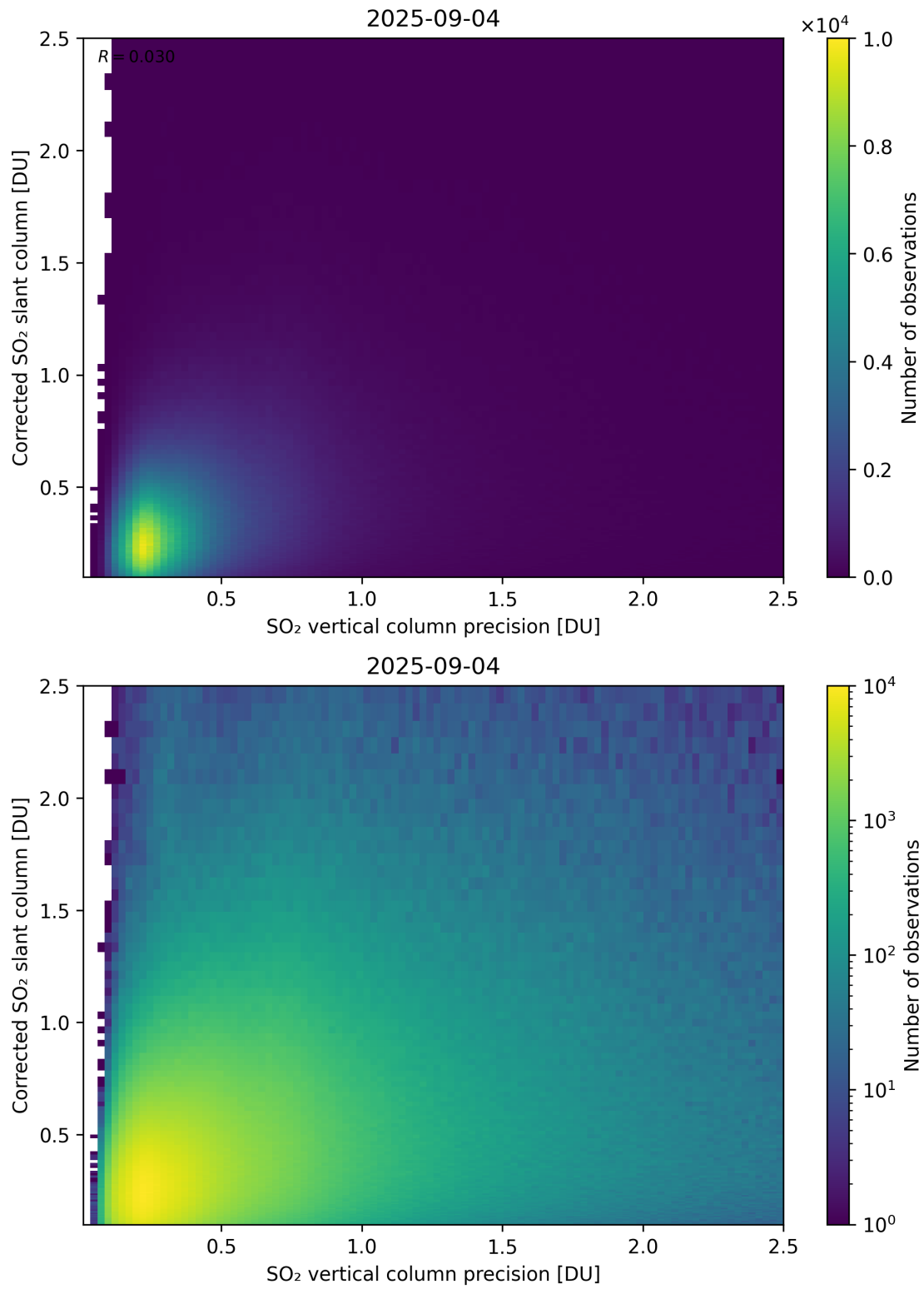
Figure 338: Scatter density plot of “SO 2 vertical column precision” against “Corrected SO 2 slant column” for 2025-09-04 to 2025-09-05.
