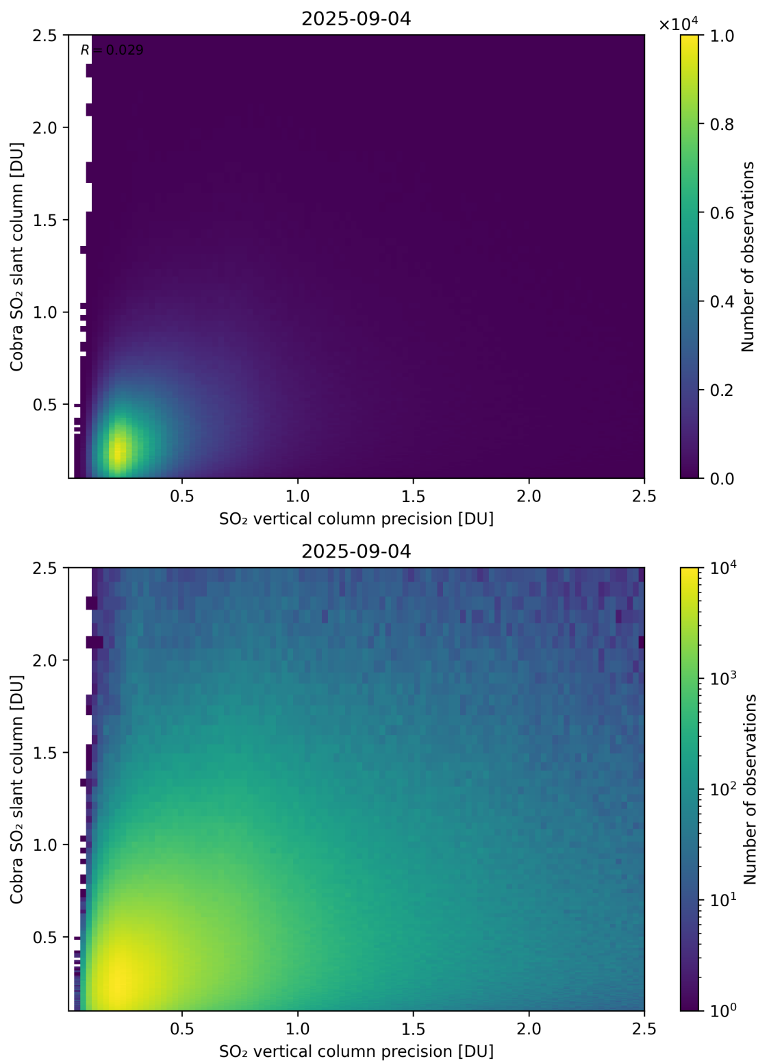
Figure 336: Scatter density plot of “SO 2 vertical column precision” against “Cobra SO 2 slant column” for 2025-09-04 to 2025-09-05.
