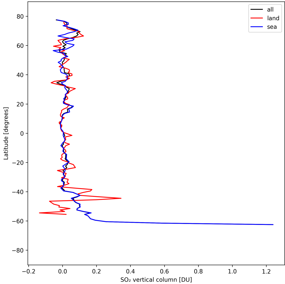
Figure 32: Zonal average of “SO 2 vertical column” for 2025-09-04 to 2025-09-05.
