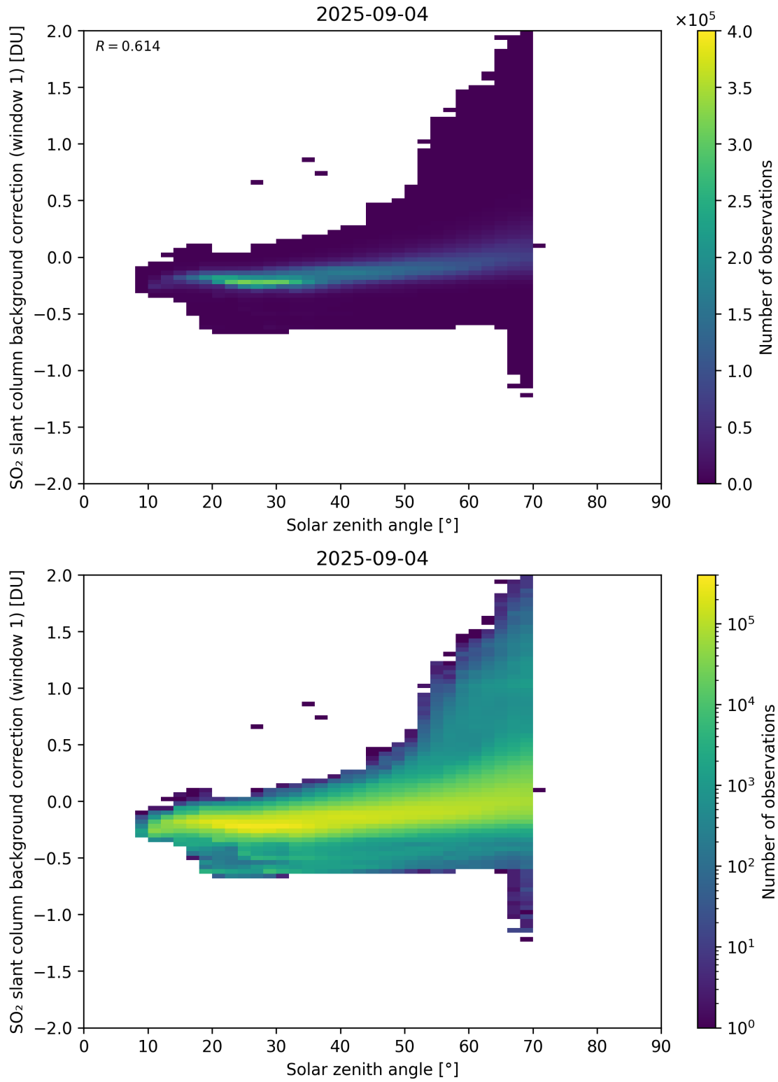
Figure 171: Scatter density plot of “Solar zenith angle” against “SO 2 slant column background correction (window 1)” for 2025-09-04 to 2025-09-05.
