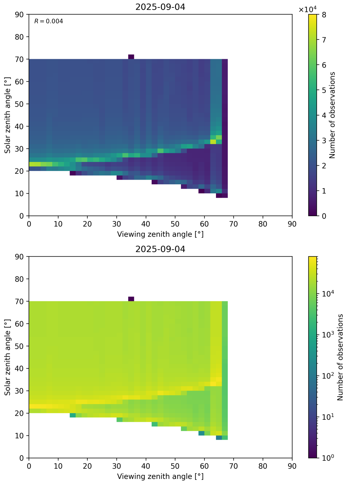
Figure 369: Scatter density plot of “Viewing zenith angle” against “Solar zenith angle” for 2025-09-04 to 2025-09-05.
