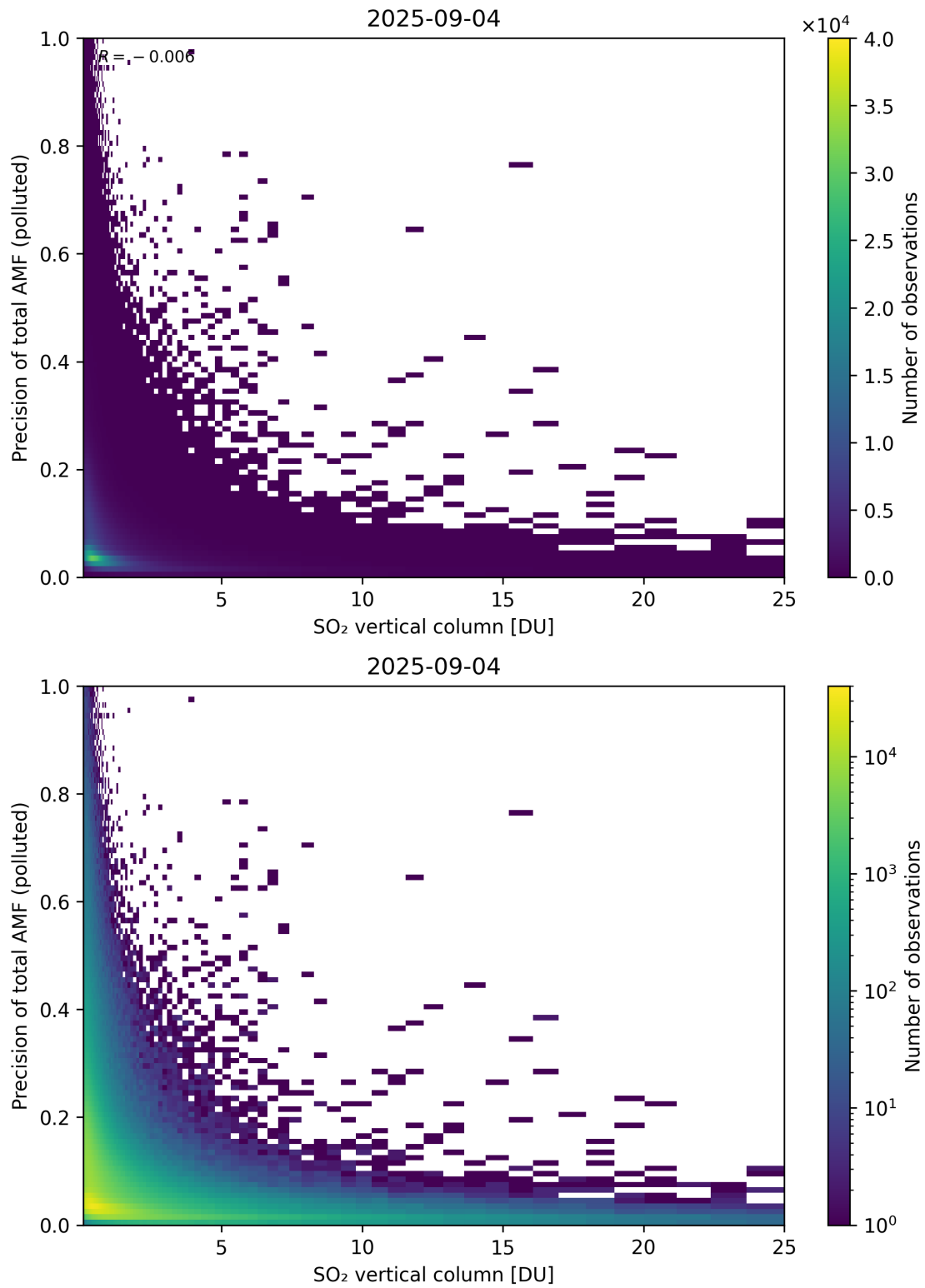
Figure 360: Scatter density plot of “SO 2 vertical column” against “Precision of total AMF (polluted)” for 2025-09-04 to 2025-09-05.
