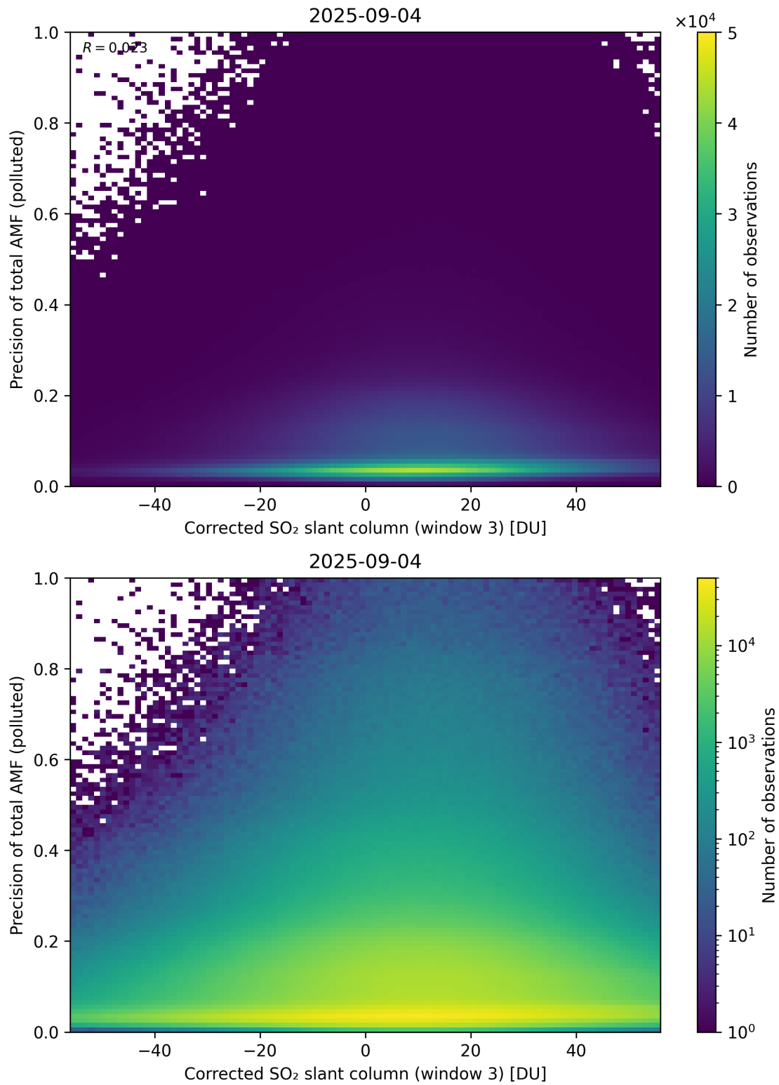
Figure 261: Scatter density plot of “Corrected SO 2 slant column (window 3)” against “Precision of total AMF (polluted)” for 2025-09-04 to 2025-09-05.
