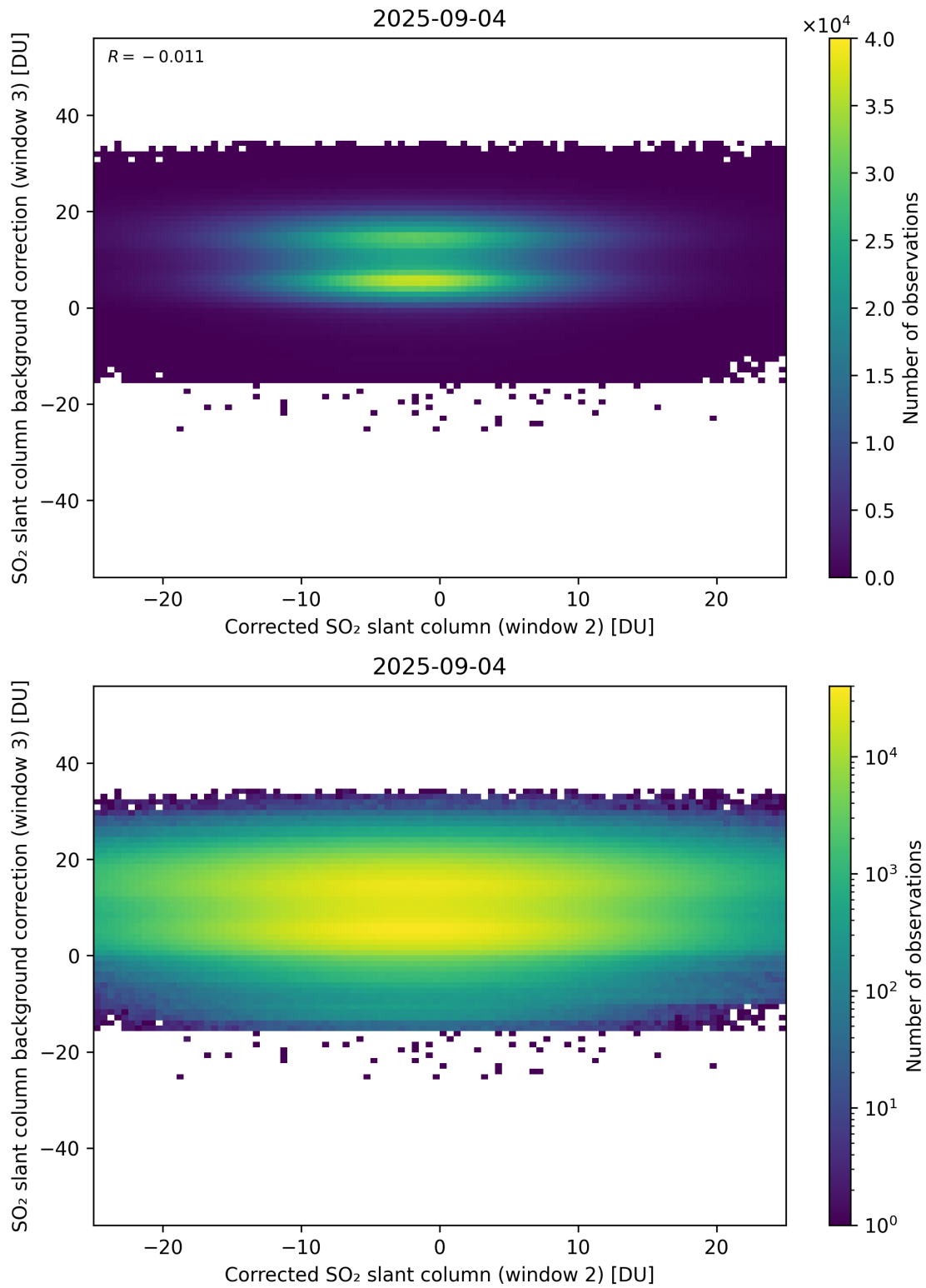
Figure 245: Scatter density plot of “Corrected SO 2 slant column (window 2)” against “SO 2 slant column background correction (window 3)” for 2025-09-04 to 2025-09-05.
