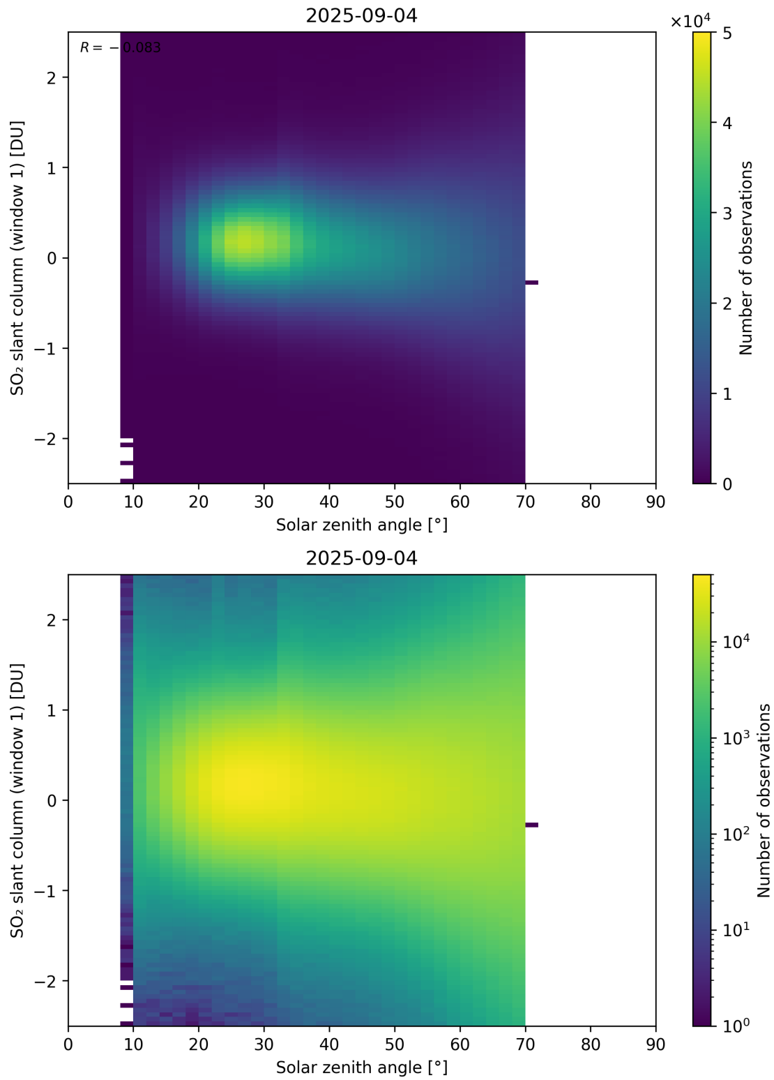
Figure 184: Scatter density plot of “Solar zenith angle” against “SO 2 slant column (window 1)” for 2025-09-04 to 2025-09-05.
