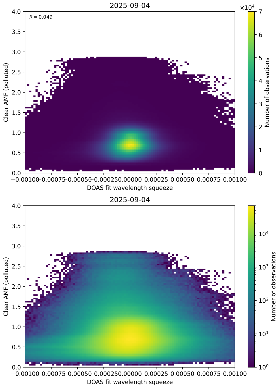
Figure 144: Scatter density plot of “DOAS fit wavelength squeeze” against “Clear AMF (polluted)” for 2025-09-04 to 2025-09-05.
