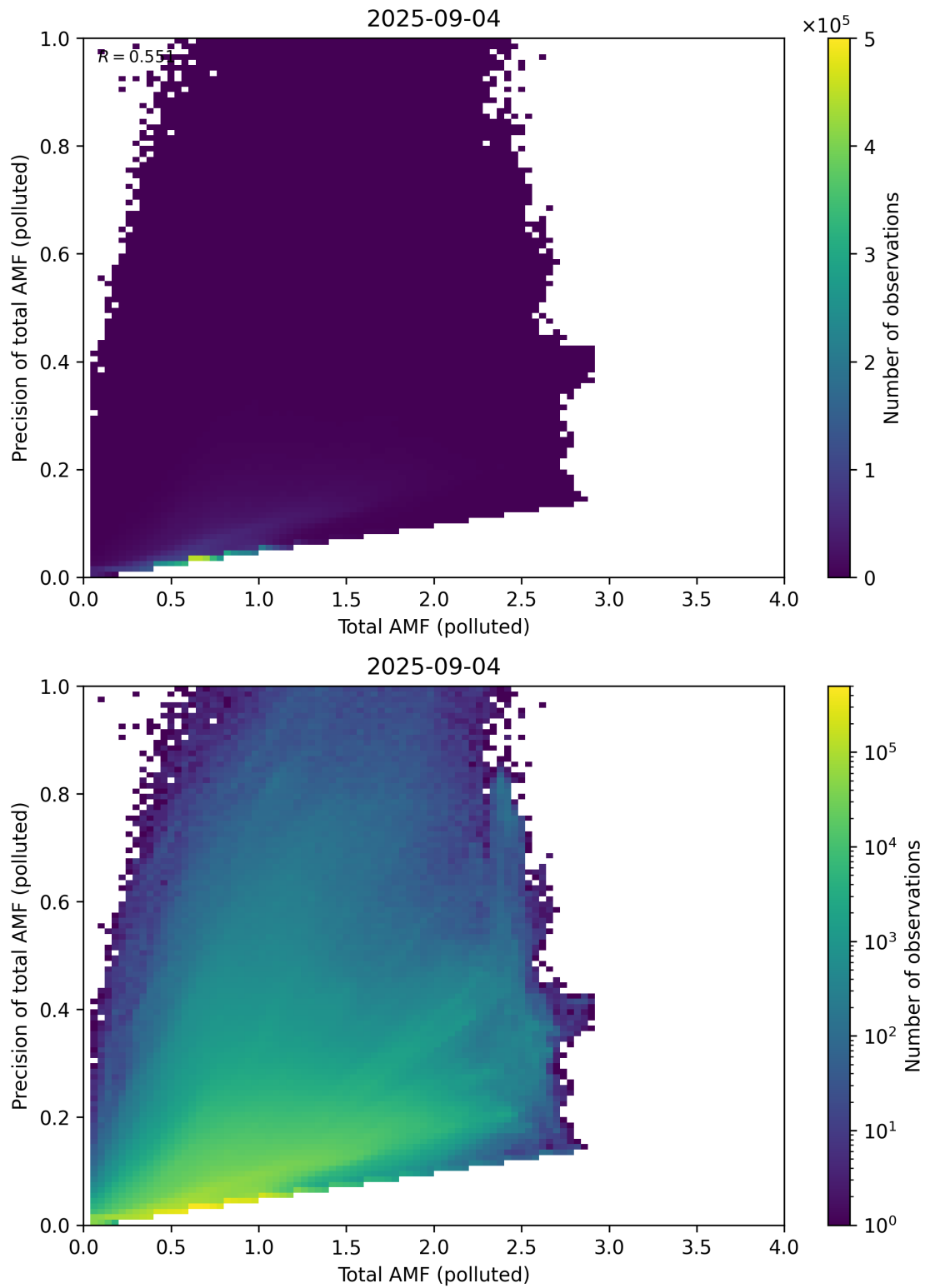
Figure 322: Scatter density plot of “Total AMF (polluted)” against “Precision of total AMF (polluted)” for 2025-09-04 to 2025-09-05.
