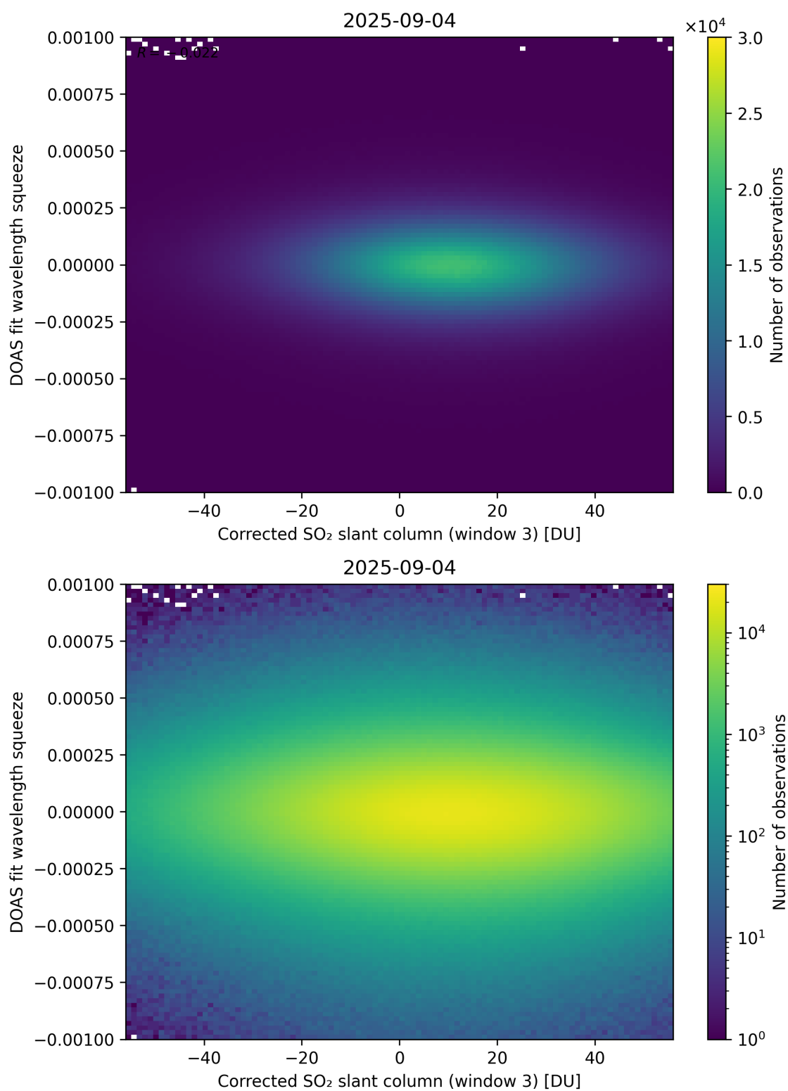
Figure 257: Scatter density plot of “Corrected SO 2 slant column (window 3)” against “DOAS fit wavelength squeeze” for 2025-09-04 to 2025-09-05.
