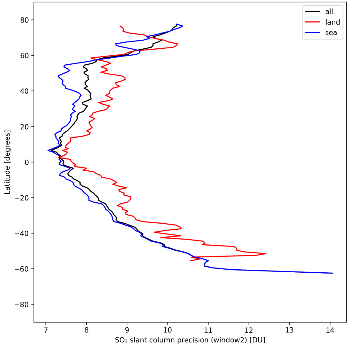
Figure 42: Zonal average of “SO 2 slant column precision (window2)” for 2025-09-04 to 2025-09-05.
