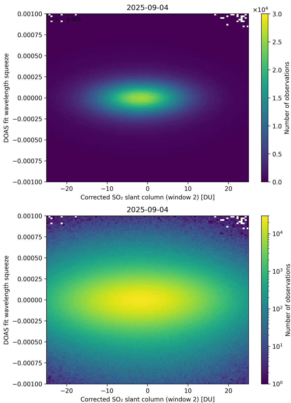
Figure 247: Scatter density plot of “Corrected SO 2 slant column (window 2)” against “DOAS fit wavelength squeeze” for 2025-09-04 to 2025-09-05.
