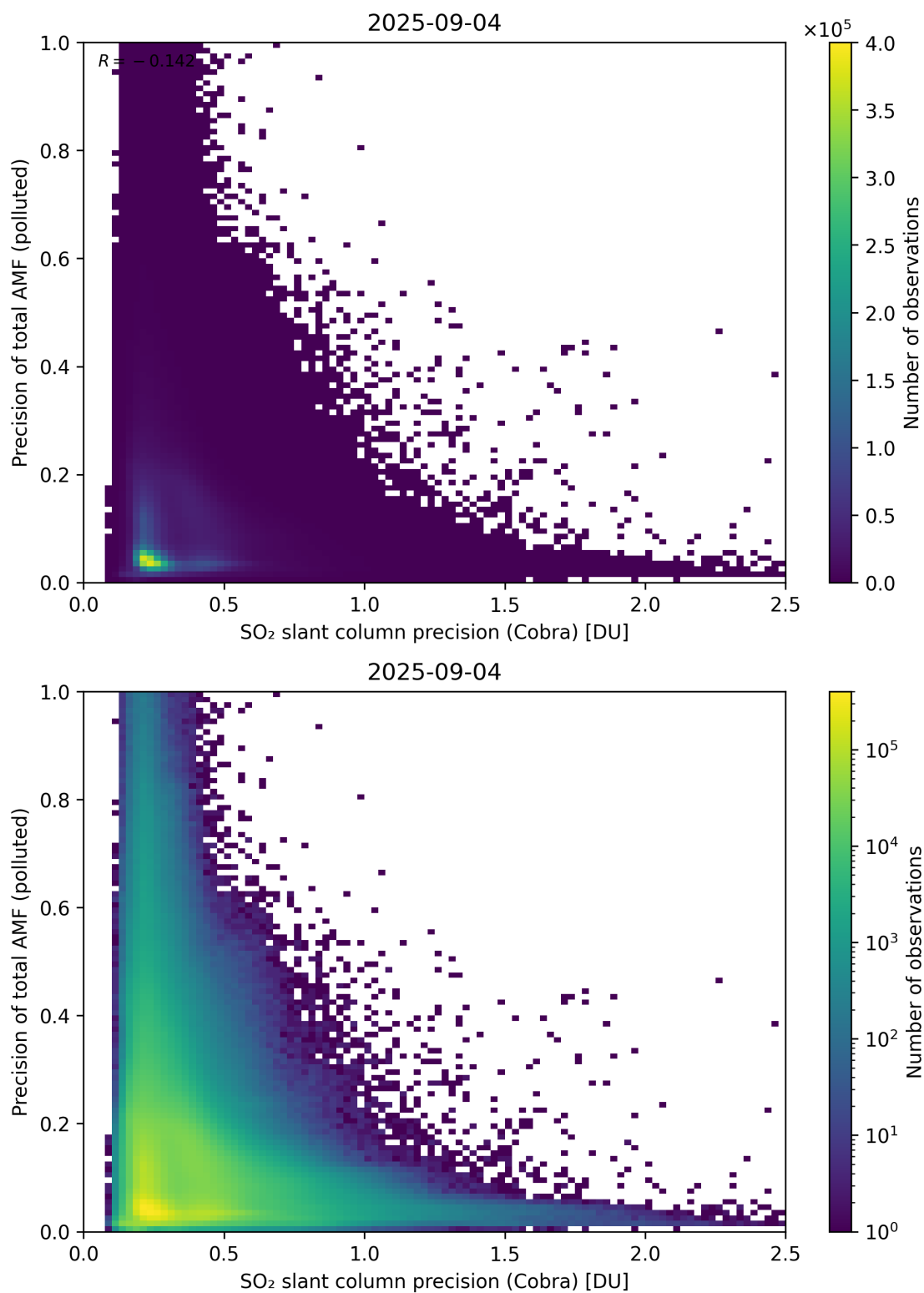
Figure 214: Scatter density plot of “SO 2 slant column precision (Cobra)” against “Precision of total AMF (polluted)” for 2025-09-04 to 2025-09-05.
