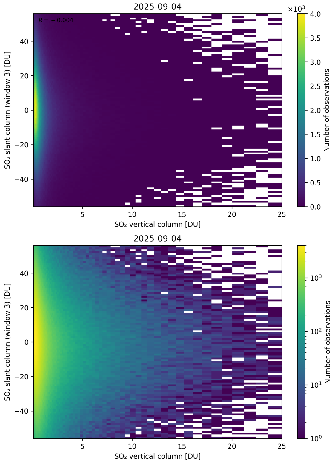
Figure 357: Scatter density plot of “SO 2 vertical column” against “SO 2 slant column (window 3)” for 2025-09-04 to 2025-09-05.
