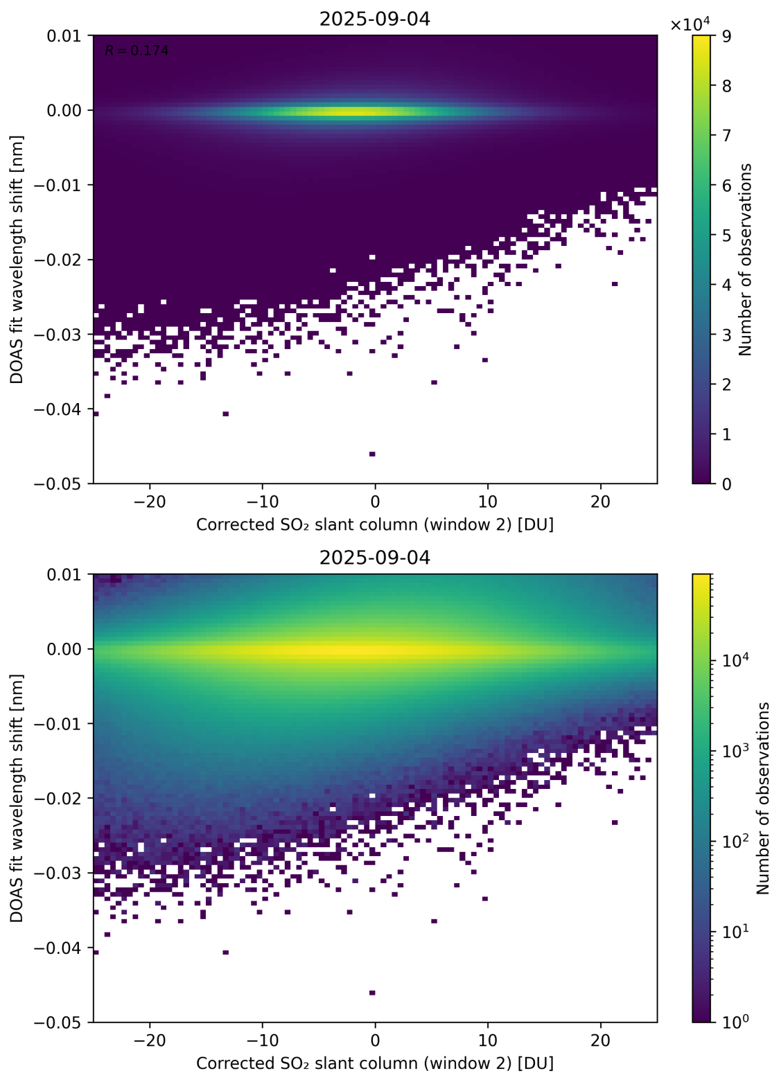
Figure 246: Scatter density plot of “Corrected SO 2 slant column (window 2)” against “DOAS fit wavelength shift” for 2025-09-04 to 2025-09-05.
