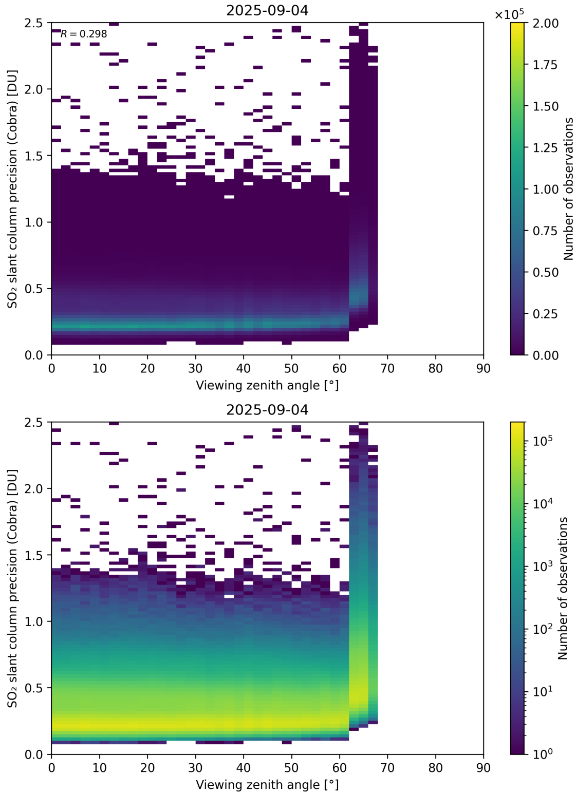
Figure 372: Scatter density plot of “Viewing zenith angle” against “SO 2 slant column precision (Cobra)” for 2025-09-04 to 2025-09-05.
