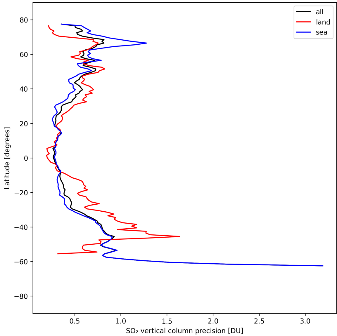
Figure 33: Zonal average of “SO 2 vertical column precision” for 2025-09-04 to 2025-09-05.
