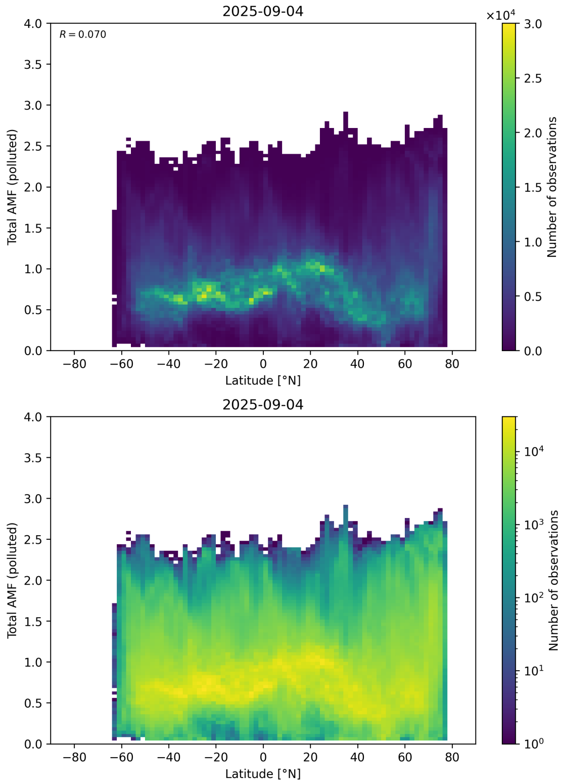
Figure 167: Scatter density plot of “Latitude” against “Total AMF (polluted)” for 2025-09-04 to 2025-09-05.
