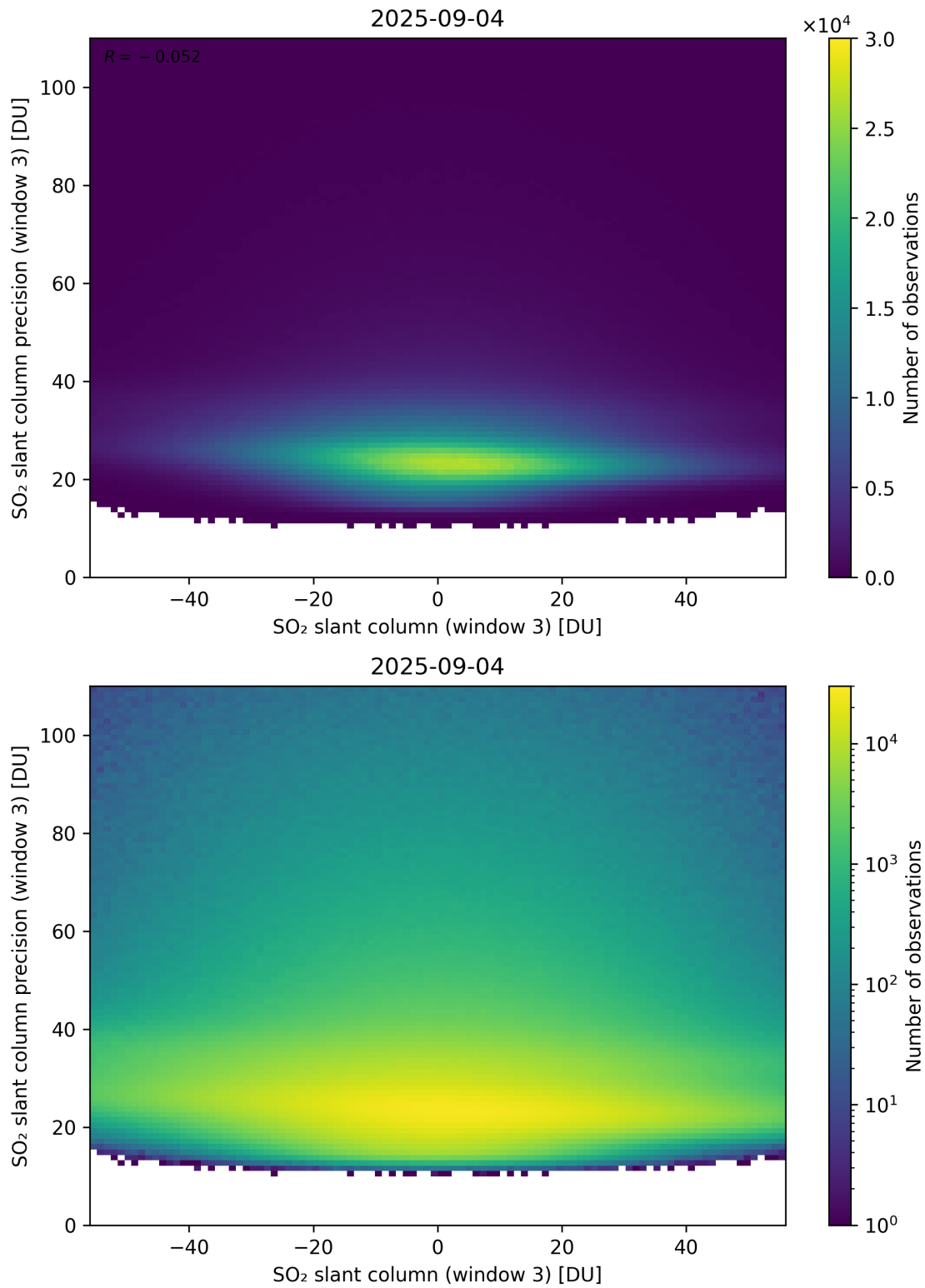
Figure 317: Scatter density plot of “SO 2 slant column (window 3)” against “SO 2 slant column precision (window 3)” for 2025-09-04 to 2025-09-05.
