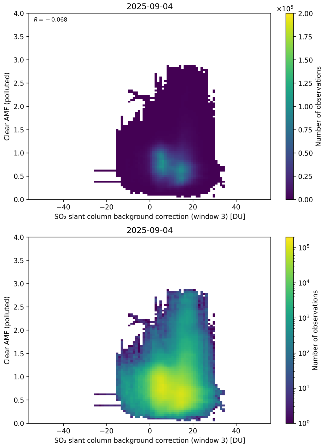
Figure 135: Scatter density plot of “SO 2 slant column background correction (window 3)” against “Clear AMF (polluted)” for 2025-09-04 to 2025-09-05.
