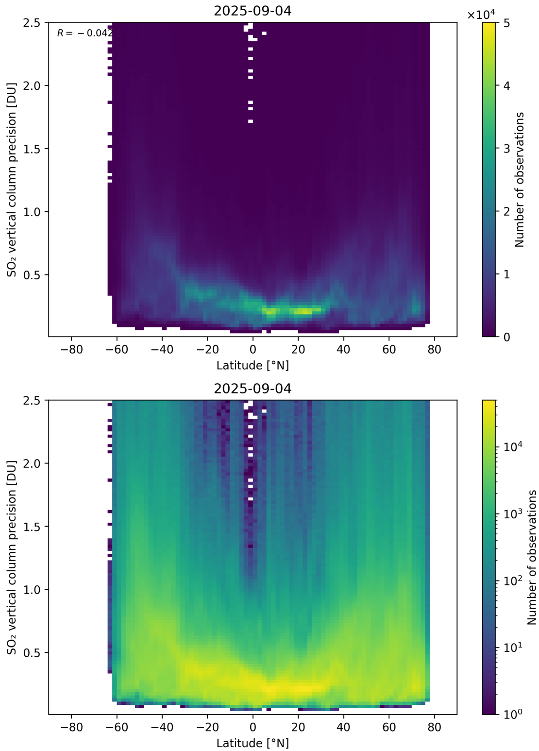
Figure 170: Scatter density plot of “Latitude” against “SO 2 vertical column precision” for 2025-09-04 to 2025-09-05.
