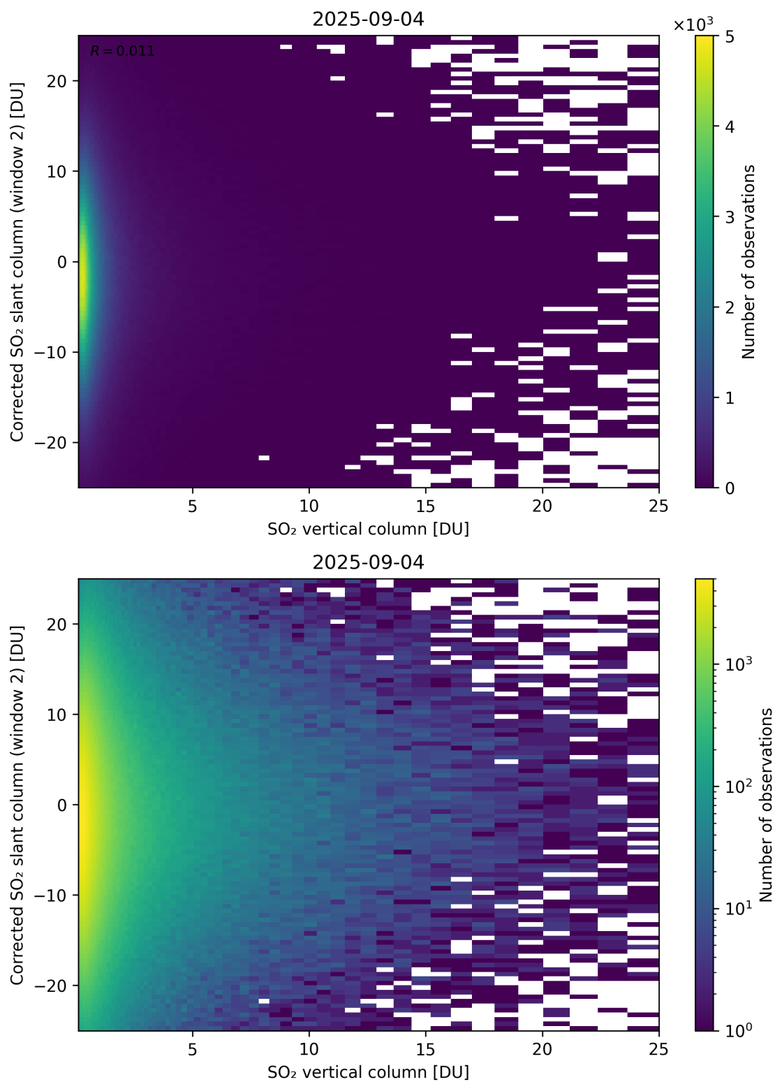
Figure 352: Scatter density plot of “SO 2 vertical column” against “Corrected SO 2 slant column (window 2)” for 2025-09-04 to 2025-09-05.
