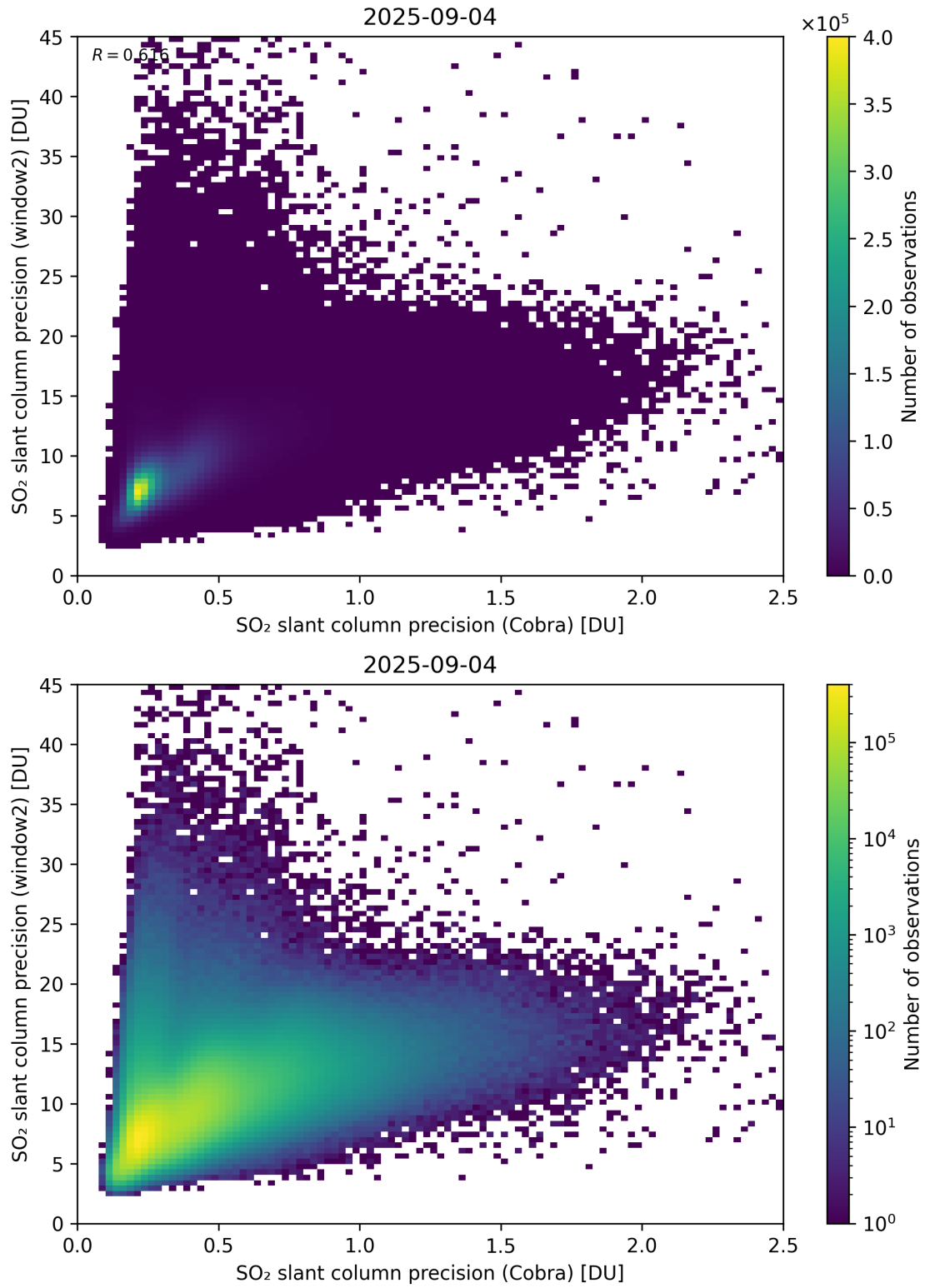
Figure 210: Scatter density plot of “SO 2 slant column precision (Cobra)” against “SO 2 slant column precision (window2)” for 2025-09-04 to 2025-09-05.
