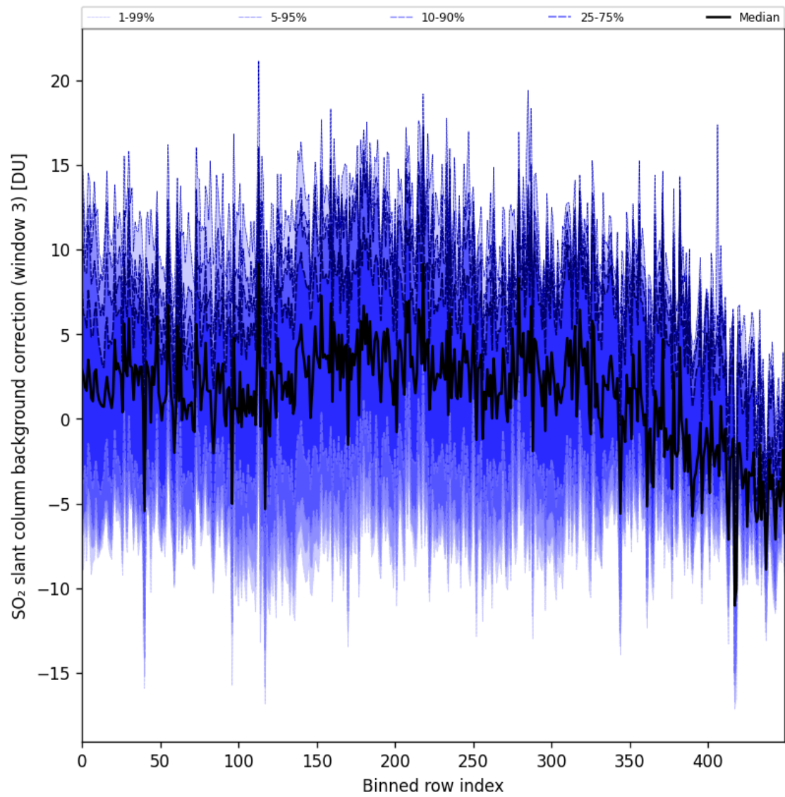
Figure 100: Along track statistics of “SO 2 slant column background correction (window 3)” for 2025-09-06 to 2025-09-08
