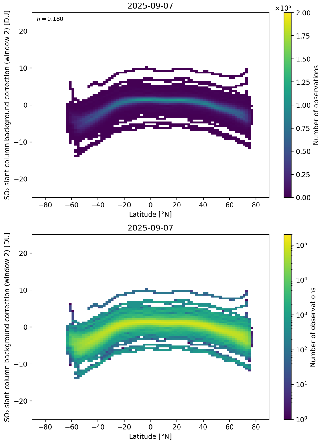
Figure 151: Scatter density plot of “Latitude” against “SO 2 slant column background correction (window 2)” for 2025-09-06 to 2025-09-08.
