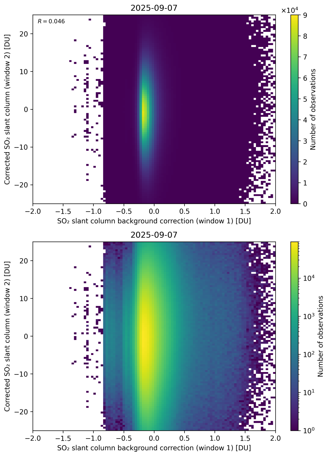
Figure 115: Scatter density plot of “SO 2 slant column background correction (window 1)” against “Corrected SO 2 slant column (window 2)” for 2025-09-06 to 2025-09-08.
