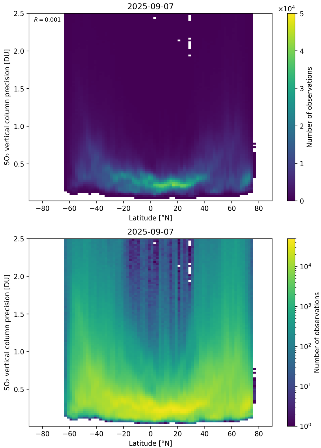
Figure 170: Scatter density plot of “Latitude” against “SO 2 vertical column precision” for 2025-09-06 to 2025-09-08.
