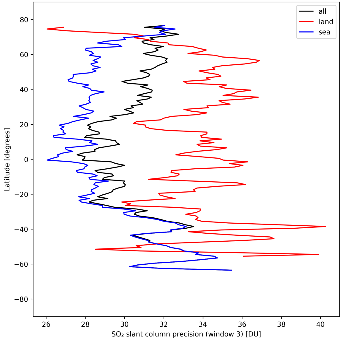
Figure 46: Zonal average of “SO 2 slant column precision (window 3)” for 2025-09-06 to 2025-09-08.
