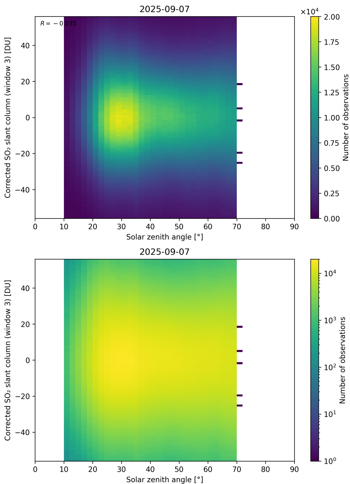
Figure 183: Scatter density plot of “Solar zenith angle” against “Corrected SO 2 slant column (window 3)” for 2025-09-06 to 2025-09-08.
