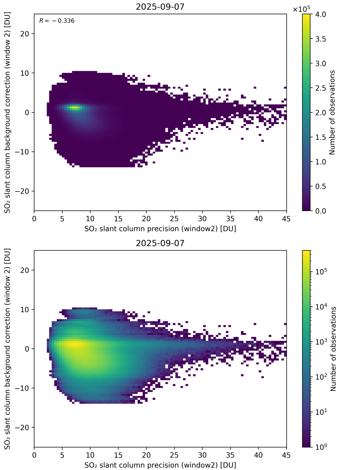
Figure 291: Scatter density plot of “SO 2 slant column precision (window2)” against “SO 2 slant column background correction (window 2)” for 2025-09-06 to 2025-09-08.
