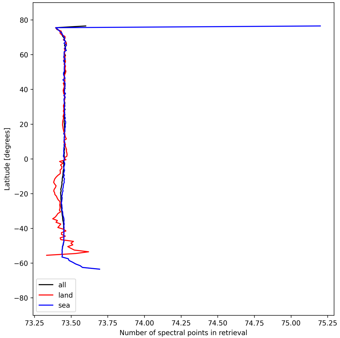
Figure 56: Zonal average of “Number of spectral points in retrieval” for 2025-09-06 to 2025-09-08.
