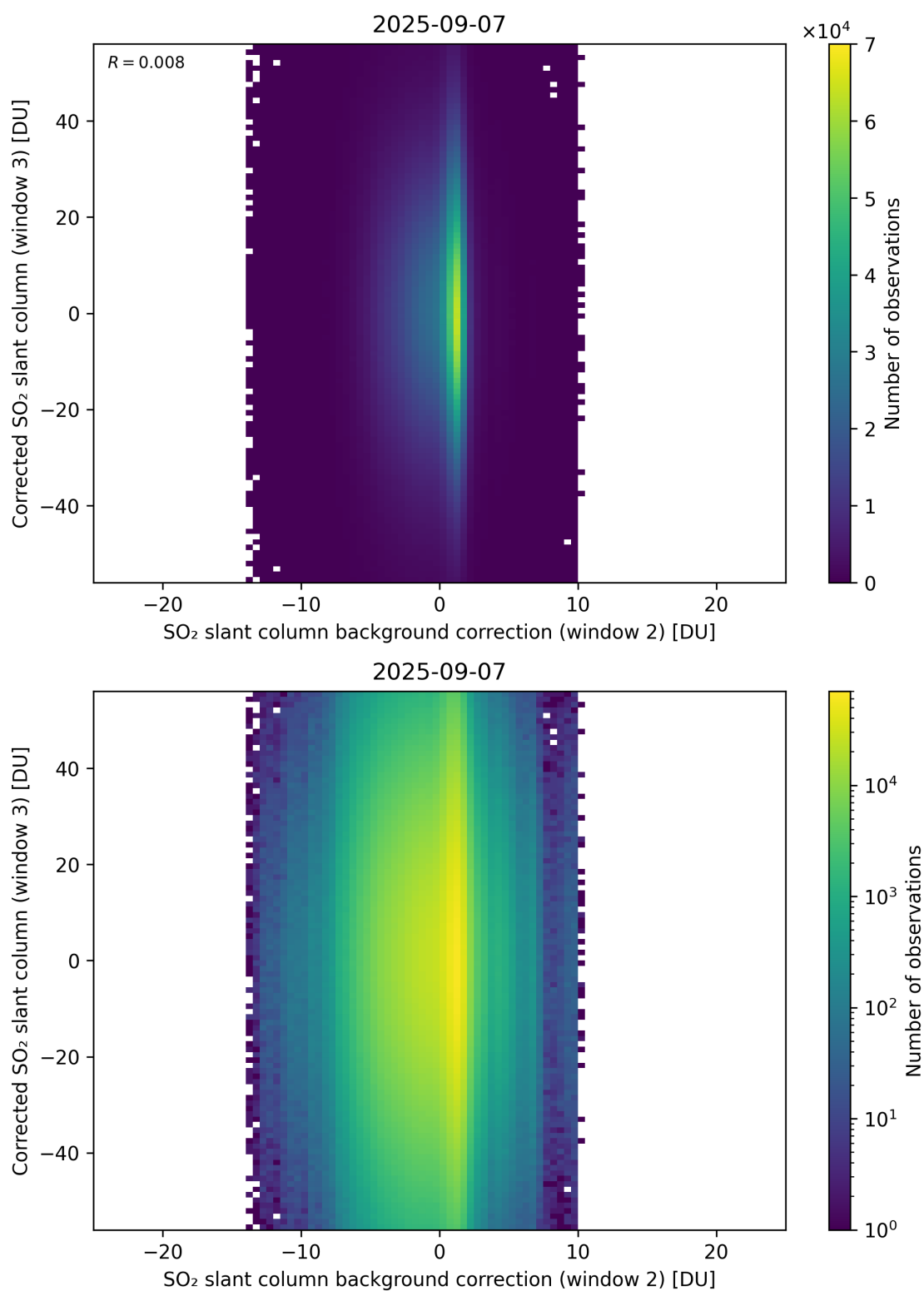
Figure 127: Scatter density plot of “SO 2 slant column background correction (window 2)” against “Corrected SO 2 slant column (window 3)” for 2025-09-06 to 2025-09-08.
