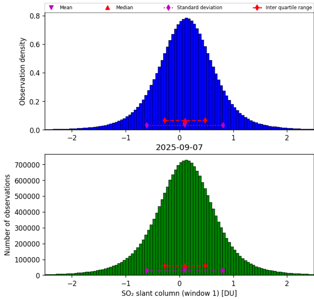
Figure 63: Histogram of “SO 2 slant column (window 1)” for 2025-09-06 to 2025-09-08
