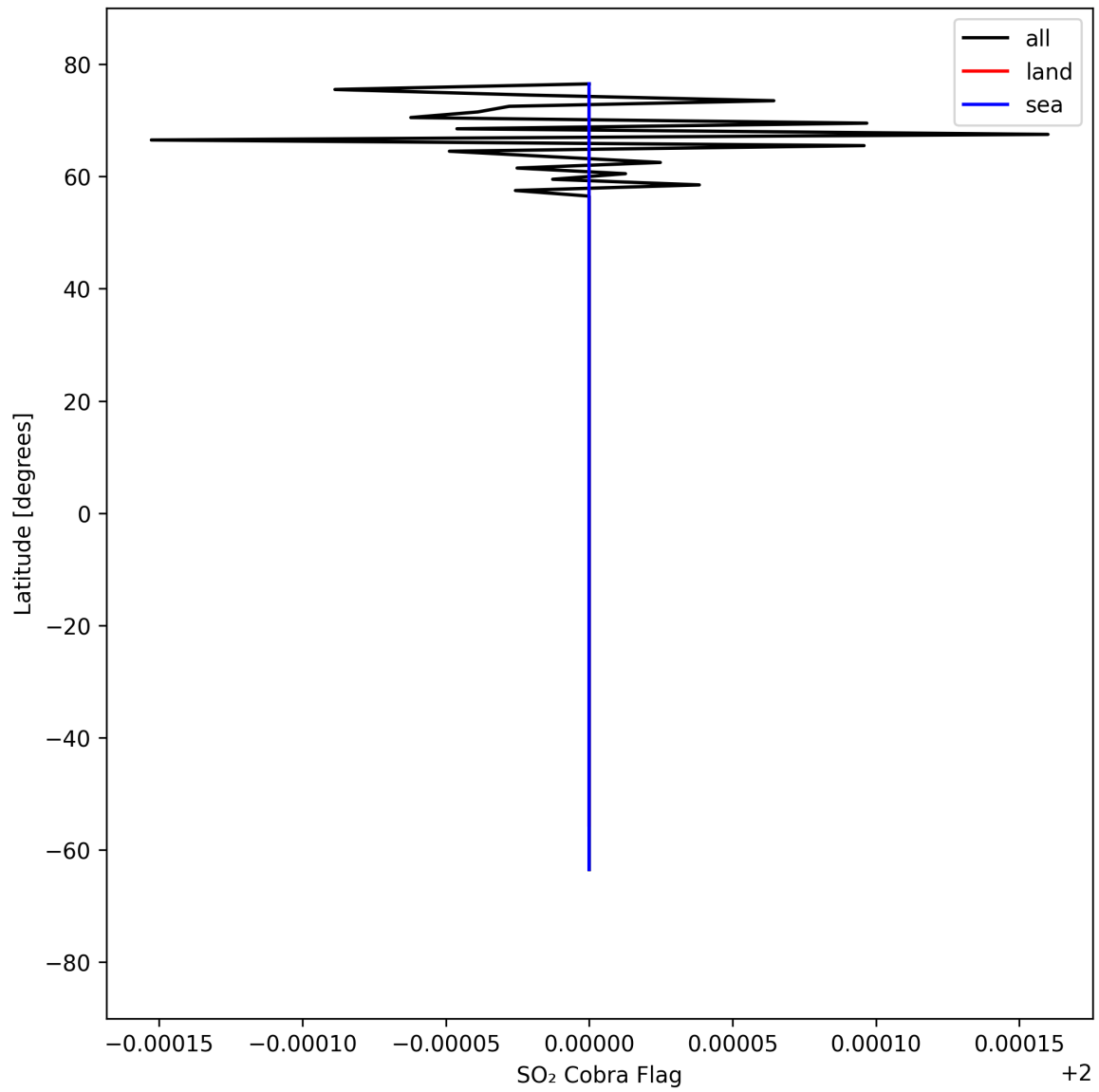
Figure 49: Zonal average of "SO 2 Cobra Flag" for 2025-09-06 to 2025-09-08.
