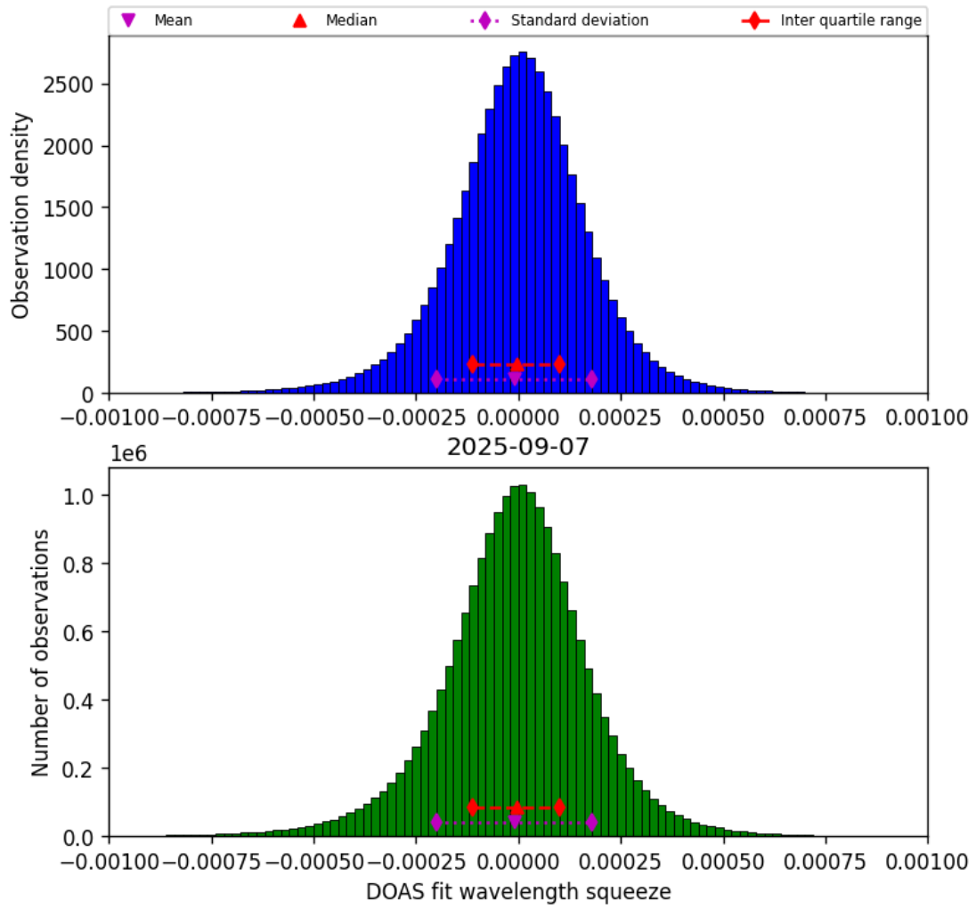
Figure 77: Histogram of “DOAS fit wavelength squeeze” for 2025-09-06 to 2025-09-08
