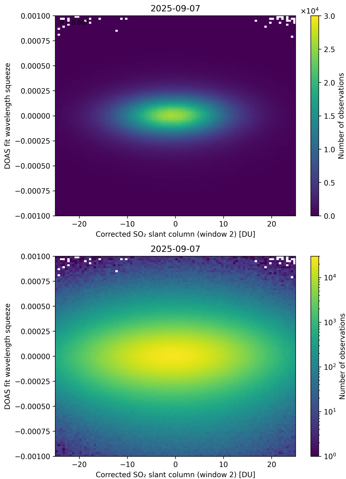
Figure 247: Scatter density plot of “Corrected SO 2 slant column (window 2)” against “DOAS fit wavelength squeeze” for 2025-09-06 to 2025-09-08.
