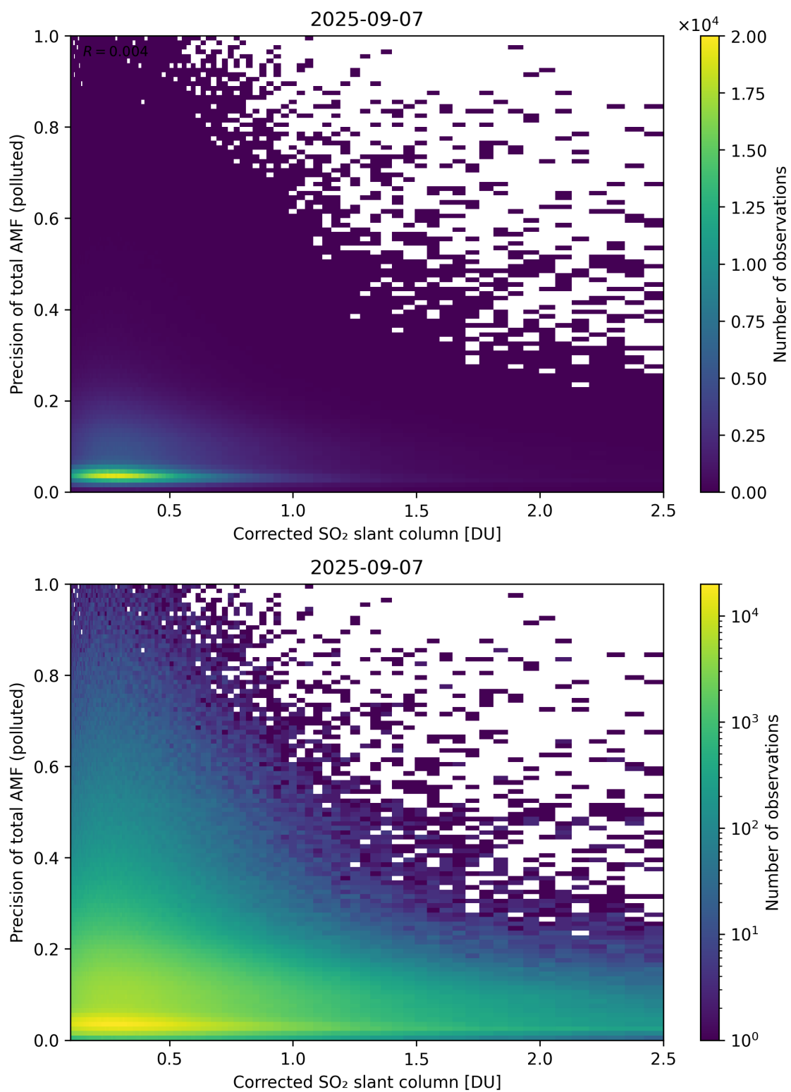
Figure 243: Scatter density plot of “Corrected SO 2 slant column” against “Precision of total AMF (polluted)” for 2025-09-06 to 2025-09-08.
