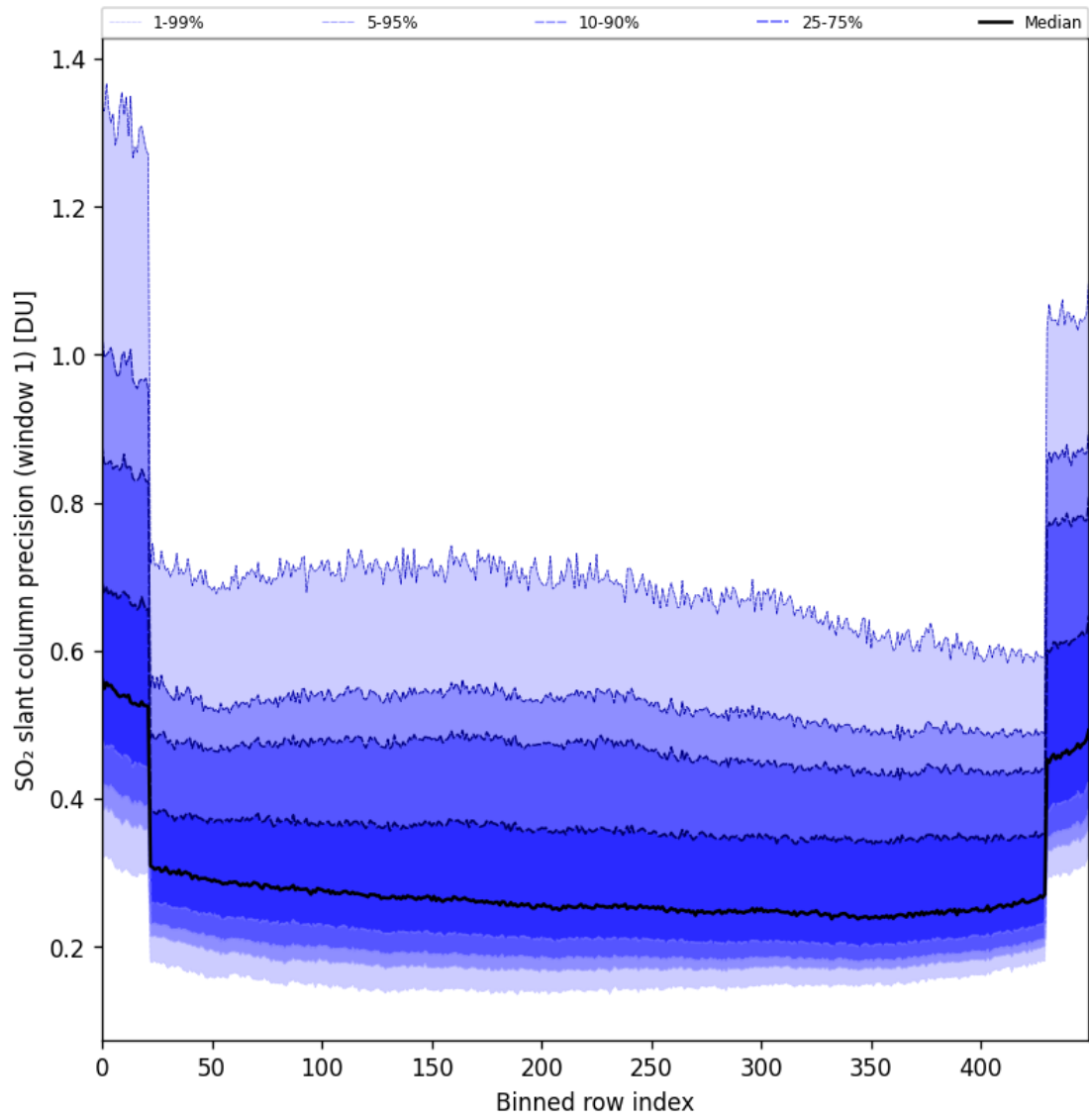
Figure 90: Along track statistics of “SO 2 slant column precision (window 1)” for 2025-09-06 to 2025-09-08
