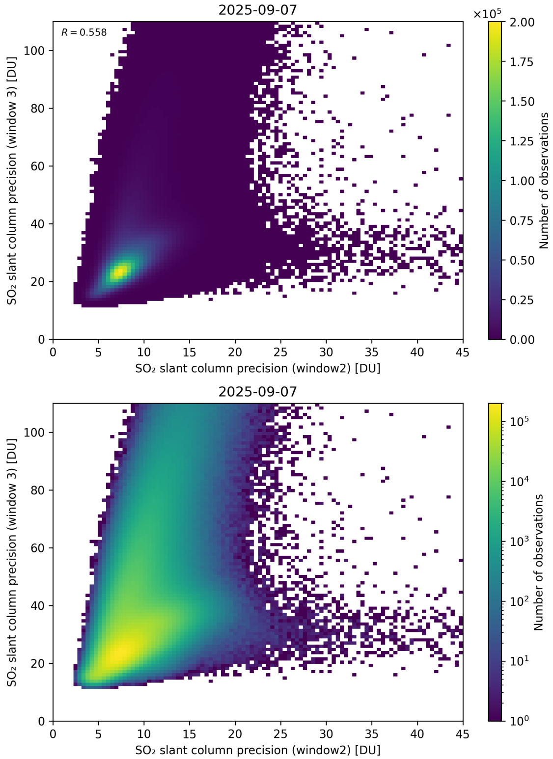
Figure 300: Scatter density plot of “SO 2 slant column precision (window2)” against “SO 2 slant column precision (window 3)” for 2025-09-06 to 2025-09-08.
