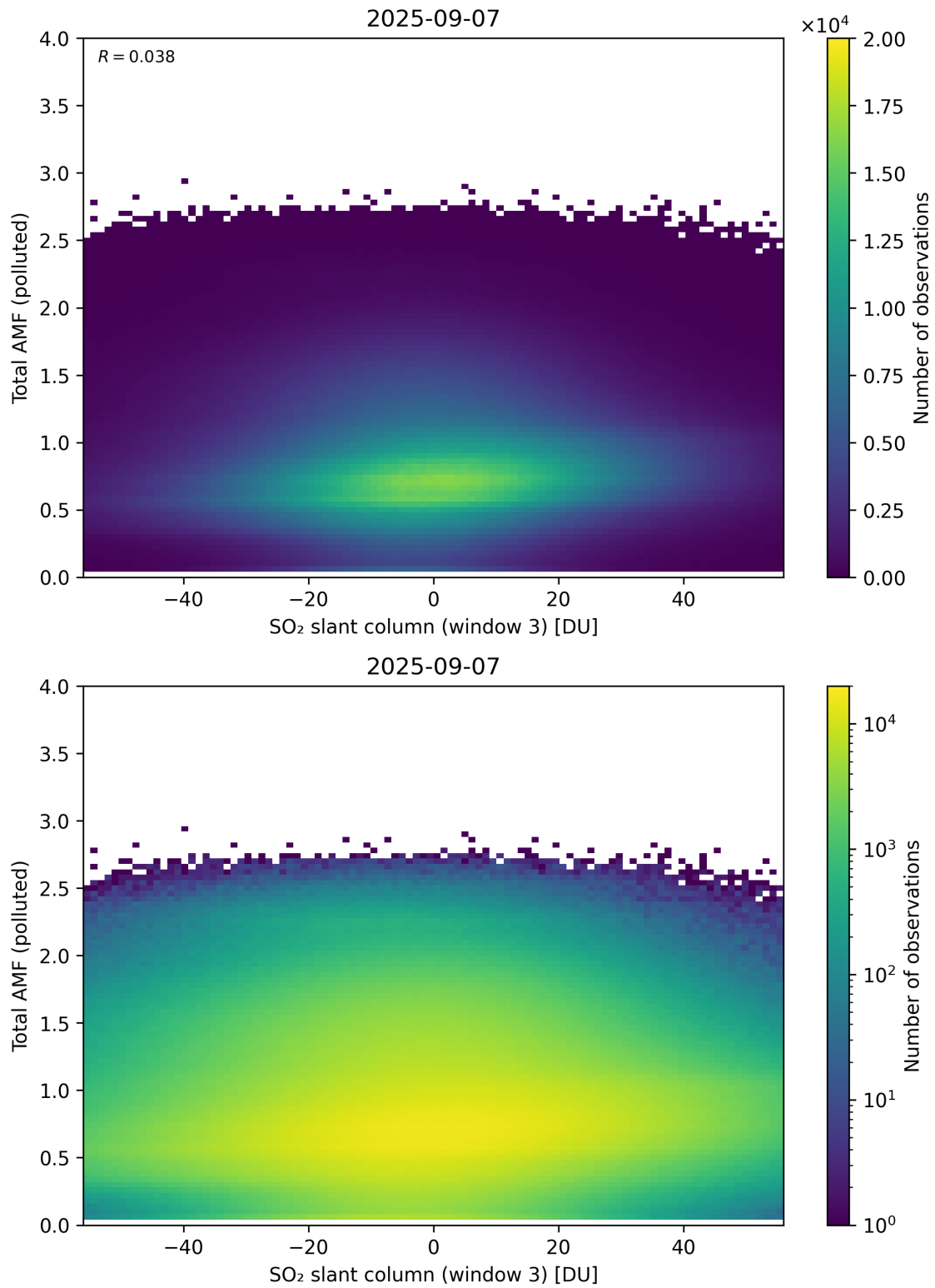
Figure 318: Scatter density plot of “SO 2 slant column (window 3)” against “Total AMF (polluted)” for 2025-09-06 to 2025-09-08.
