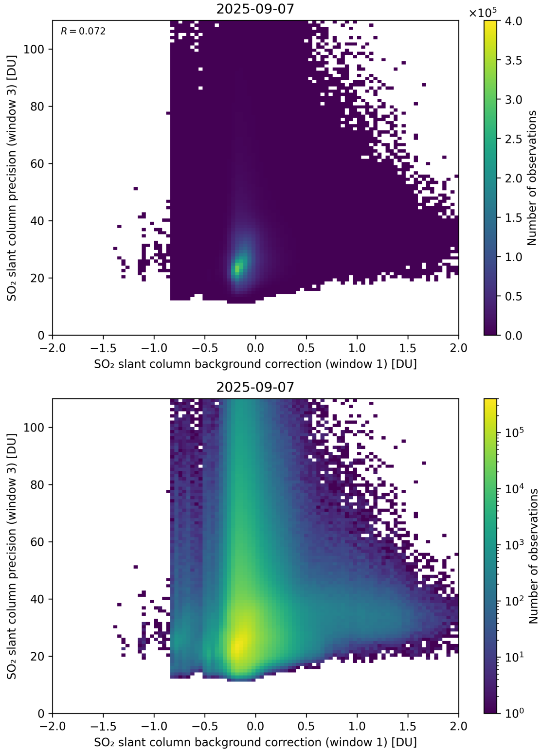
Figure 119: Scatter density plot of “SO 2 slant column background correction (window 1)” against “SO 2 slant column precision (window 3)” for 2025-09-06 to 2025-09-08.
