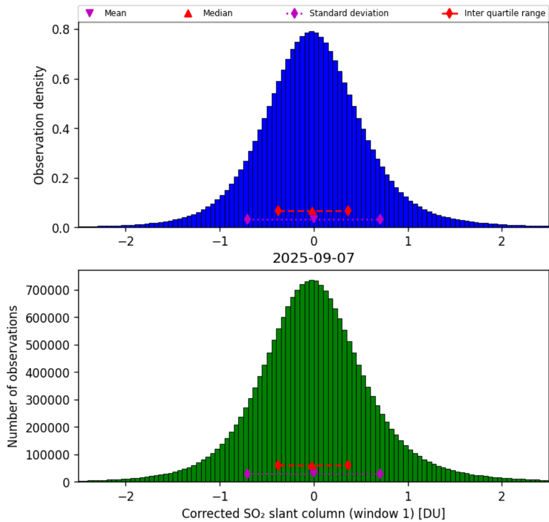
Figure 65: Histogram of “Corrected SO 2 slant column (window 1)” for 2025-09-06 to 2025-09-08
