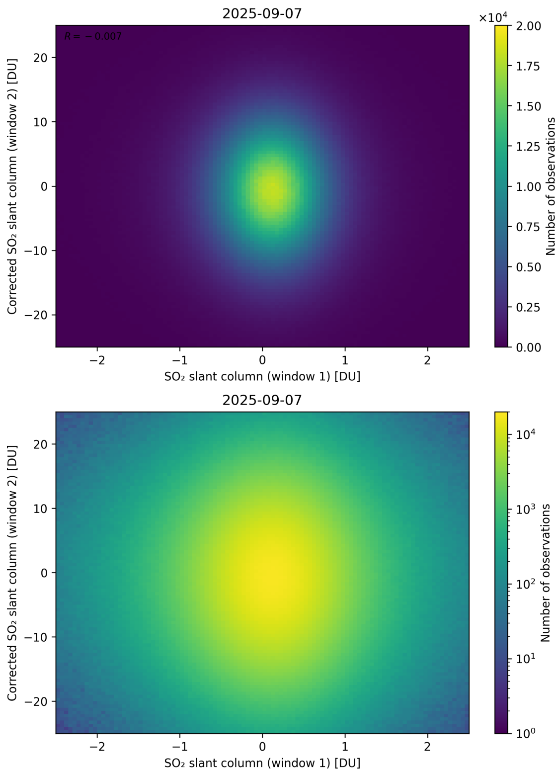
Figure 283: Scatter density plot of “SO 2 slant column (window 1)” against “Corrected SO 2 slant column (window 2)” for 2025-09-06 to 2025-09-08.
