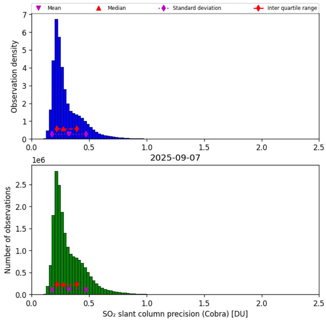
Figure 62: Histogram of “SO 2 slant column precision (Cobra)” for 2025-09-06 to 2025-09-08
