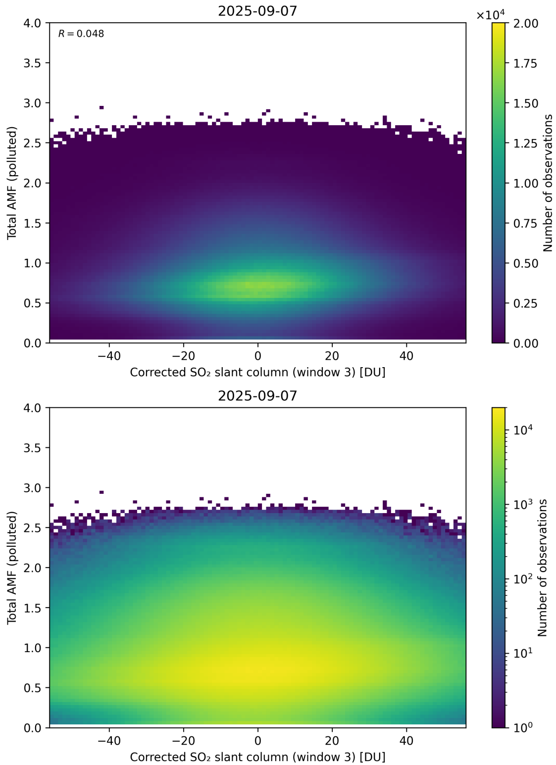
Figure 260: Scatter density plot of “Corrected SO 2 slant column (window 3)” against “Total AMF (polluted)” for 2025-09-06 to 2025-09-08.
