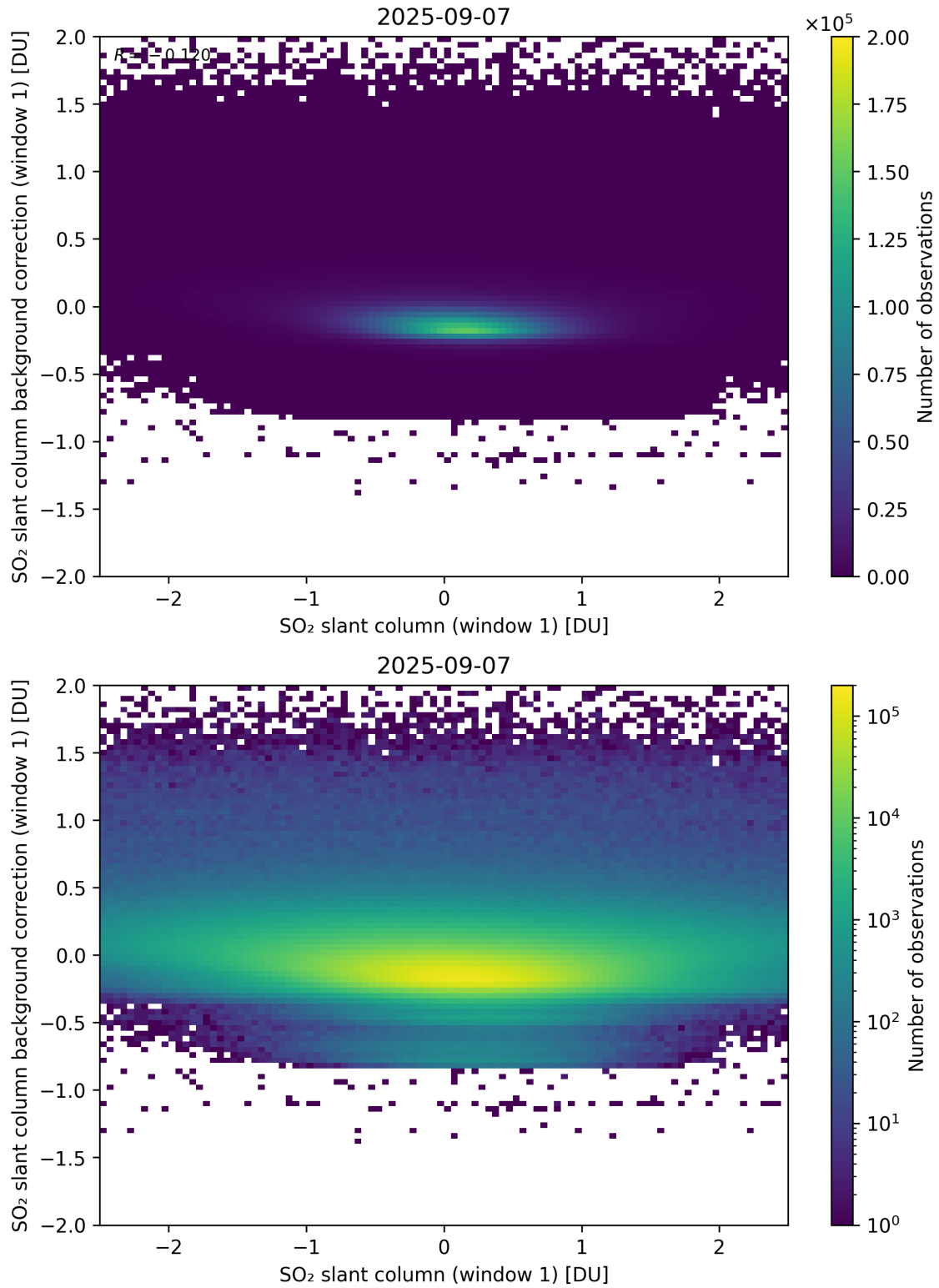
Figure 262: Scatter density plot of “SO 2 slant column (window 1)” against “SO 2 slant column background correction (window 1)” for 2025-09-06 to 2025-09-08.
