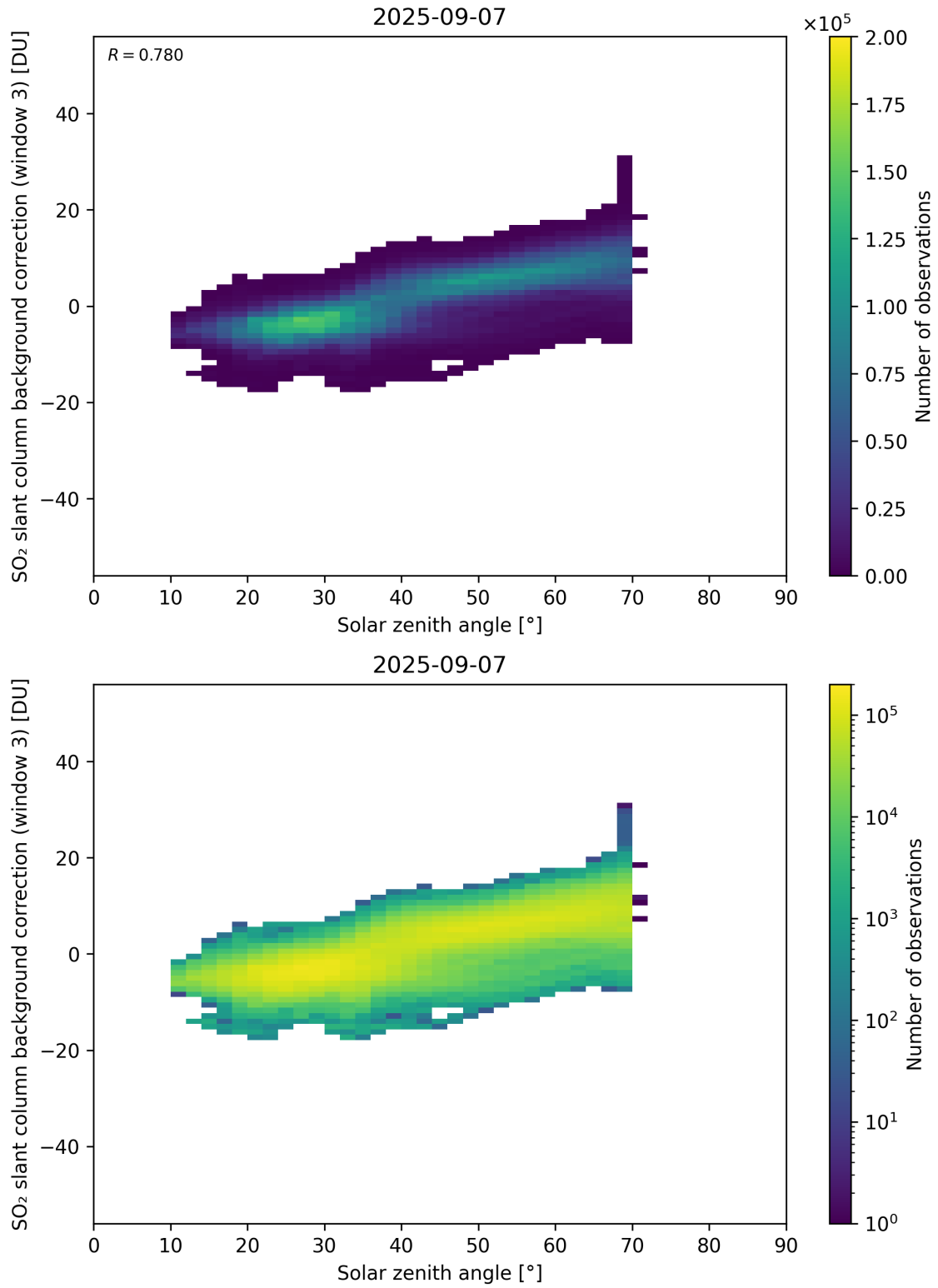
Figure 173: Scatter density plot of “Solar zenith angle” against “SO 2 slant column background correction (window 3)” for 2025-09-06 to 2025-09-08.
