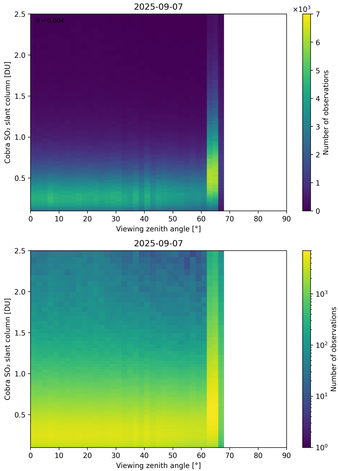
Figure 371: Scatter density plot of “Viewing zenith angle” against “Cobra SO 2 slant column” for 2025-09-06 to 2025-09-08.
