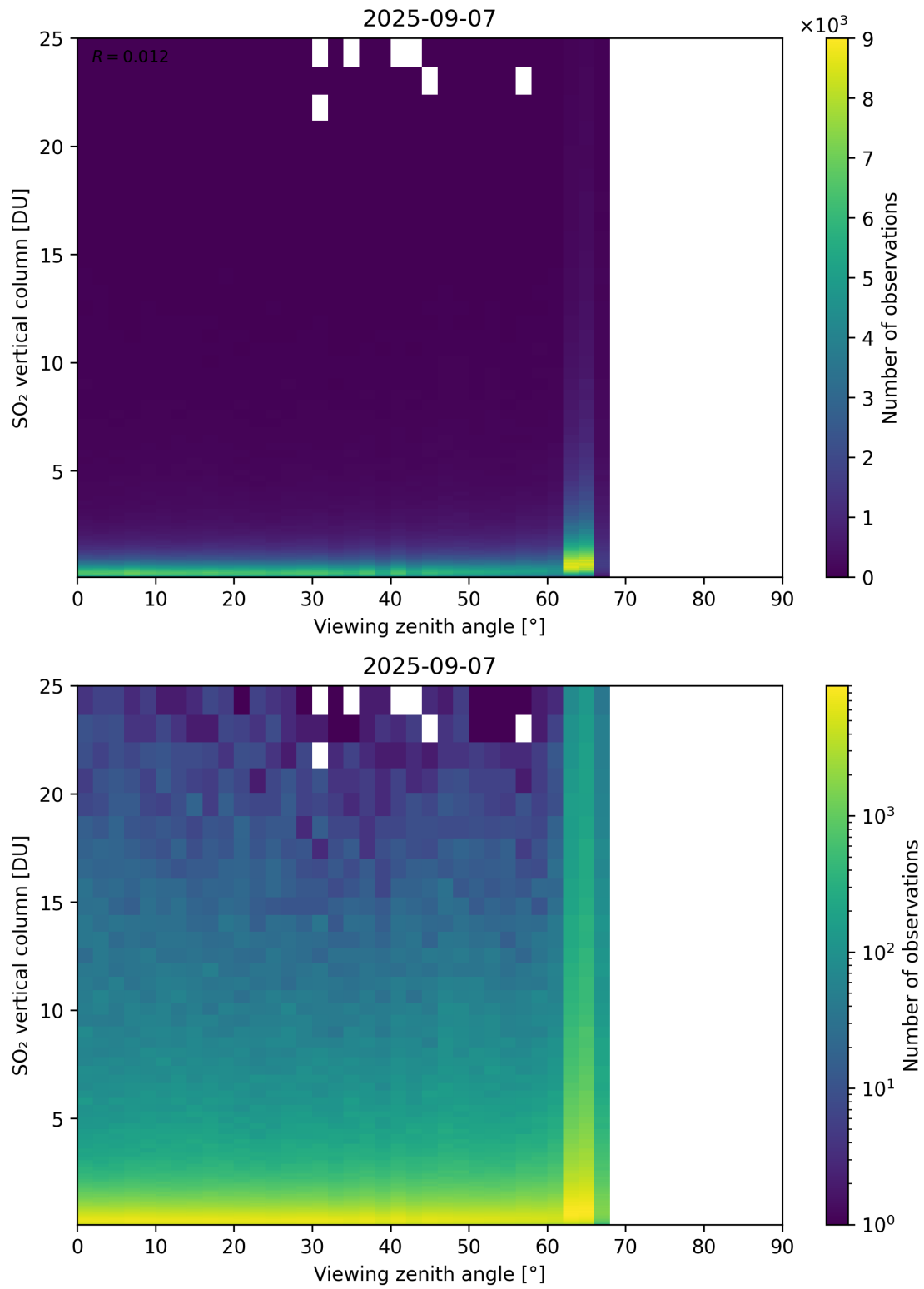
Figure 383: Scatter density plot of “Viewing zenith angle” against “SO 2 vertical column” for 2025-09-06 to 2025-09-08.
