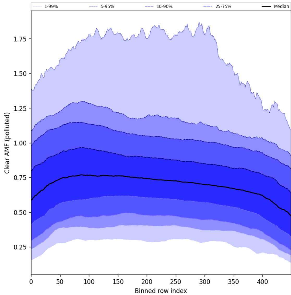
Figure 107: Along track statistics of “Clear AMF (polluted)” for 2025-09-06 to 2025-09-08
