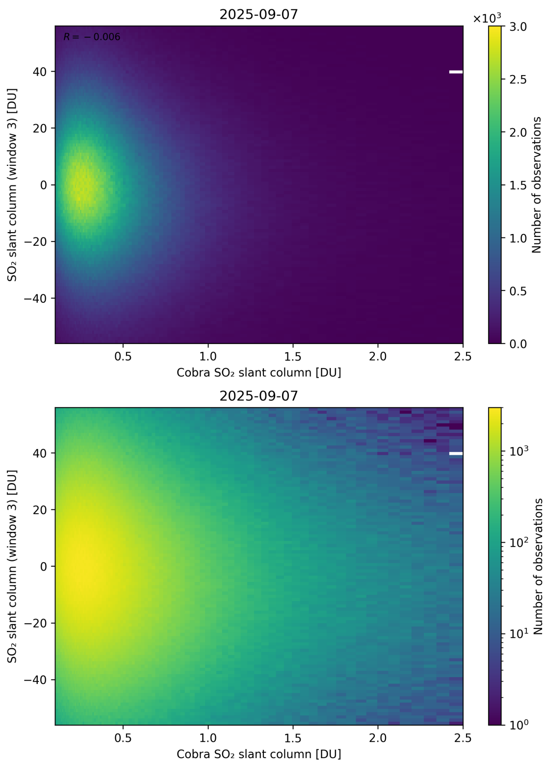
Figure 222: Scatter density plot of “Cobra SO 2 slant column” against “SO 2 slant column (window 3)” for 2025-09-06 to 2025-09-08.
