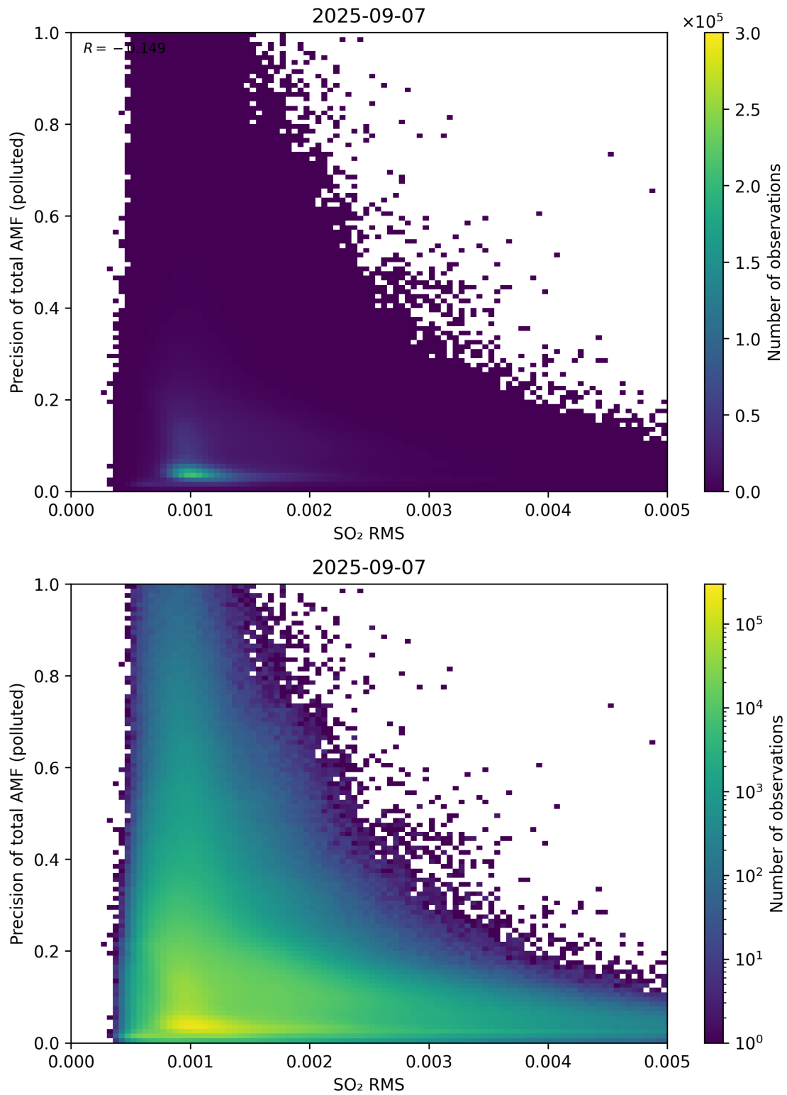
Figure 149: Scatter density plot of “SO 2 RMS” against “Precision of total AMF (polluted)” for 2025-09-06 to 2025-09-08.
