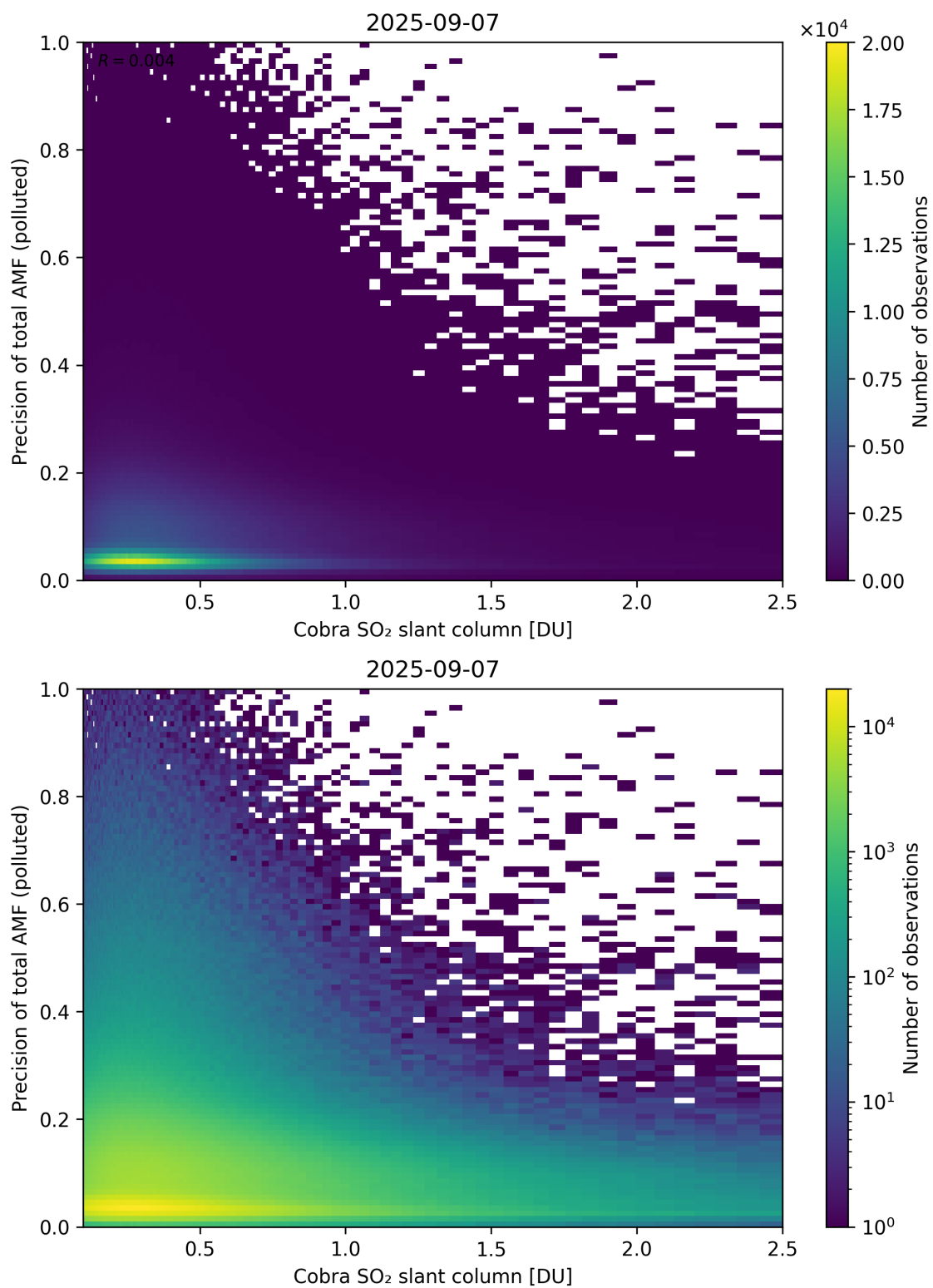
Figure 225: Scatter density plot of “Cobra SO 2 slant column” against “Precision of total AMF (polluted)” for 2025-09-06 to 2025-09-08.
