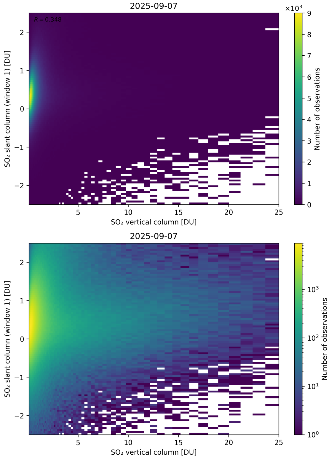
Figure 354: Scatter density plot of “SO 2 vertical column” against “SO 2 slant column (window 1)” for 2025-09-06 to 2025-09-08.
