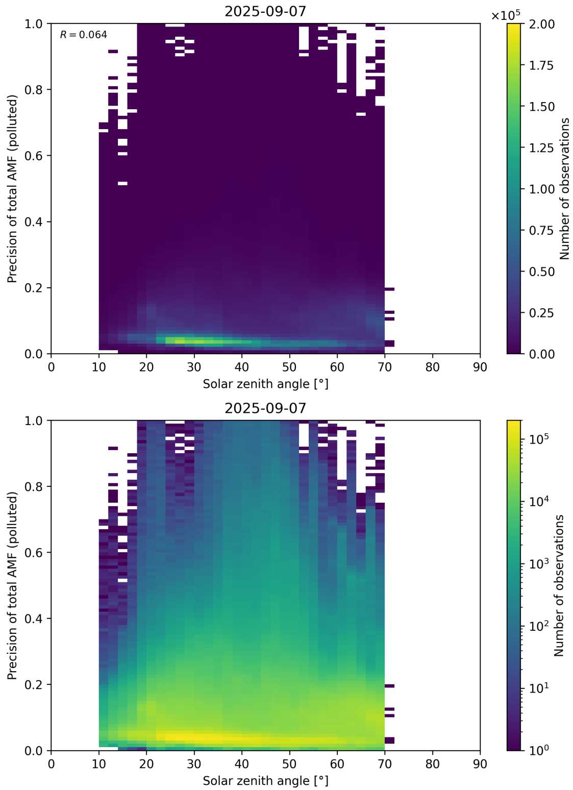
Figure 190: Scatter density plot of “Solar zenith angle” against “Precision of total AMF (polluted)” for 2025-09-06 to 2025-09-08.
