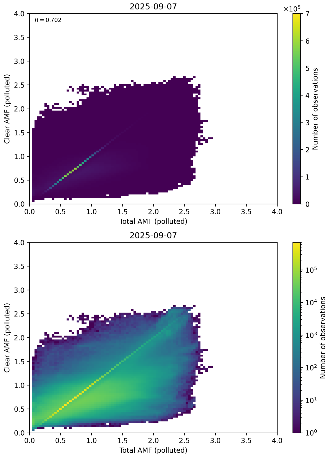
Figure 321: Scatter density plot of “Total AMF (polluted)” against “Clear AMF (polluted)” for 2025-09-06 to 2025-09-08.
