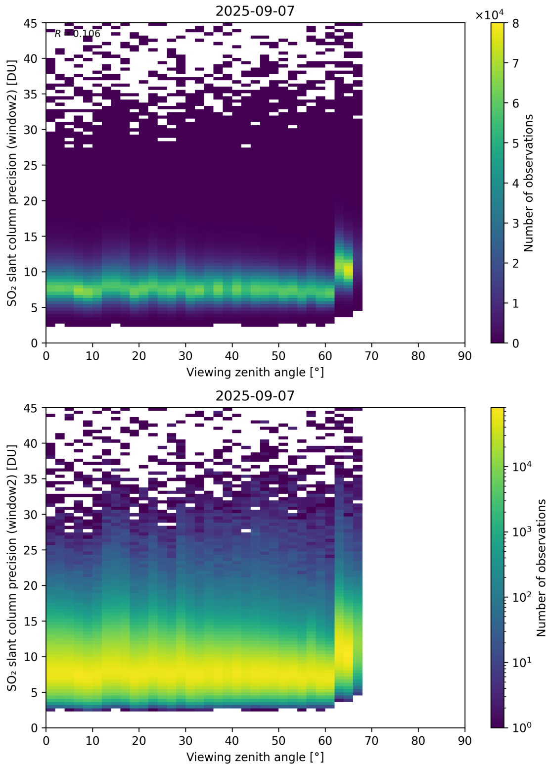
Figure 378: Scatter density plot of “Viewing zenith angle” against “SO 2 slant column precision (window2)” for 2025-09-06 to 2025-09-08.
