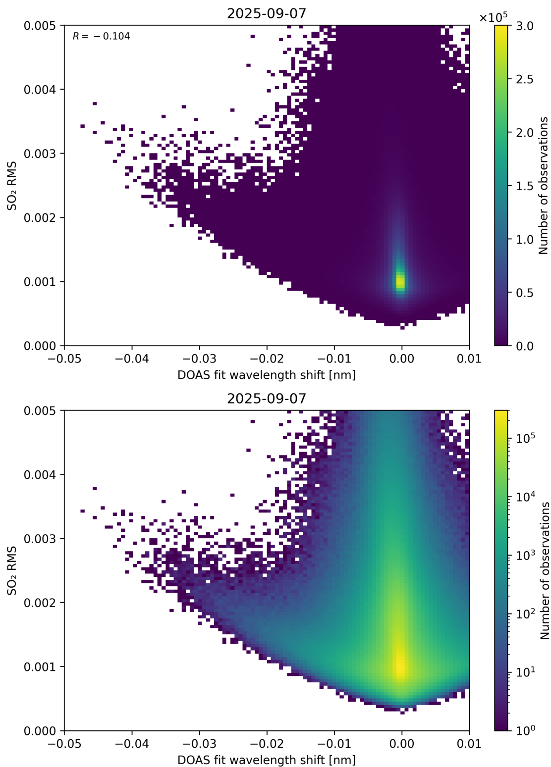
Figure 139: Scatter density plot of “DOAS fit wavelength shift” against “SO 2 RMS” for 2025-09-06 to 2025-09-08.
