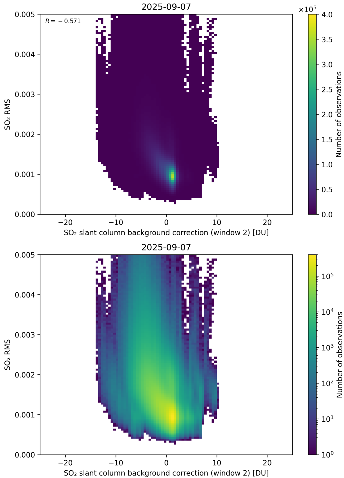
Figure 125: Scatter density plot of “SO 2 slant column background correction (window 2)” against “SO 2 RMS” for 2025-09-06 to 2025-09-08.
