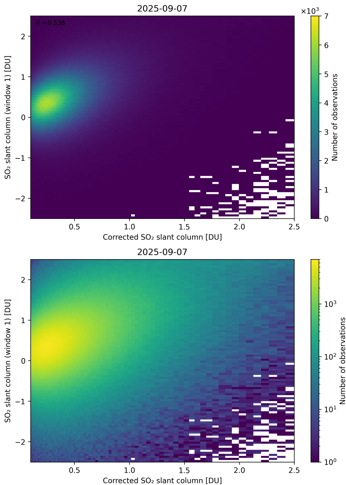
Figure 237: Scatter density plot of “Corrected SO 2 slant column” against “SO 2 slant column (window 1)” for 2025-09-06 to 2025-09-08.
