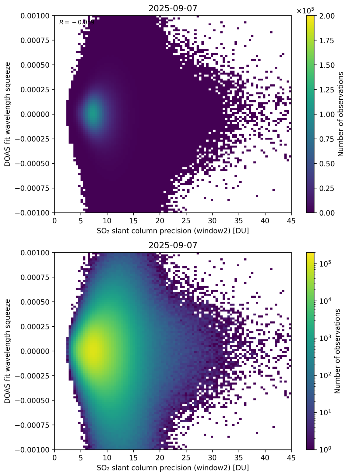
Figure 294: Scatter density plot of “SO 2 slant column precision (window2)” against “DOAS fit wavelength squeeze” for 2025-09-06 to 2025-09-08.
