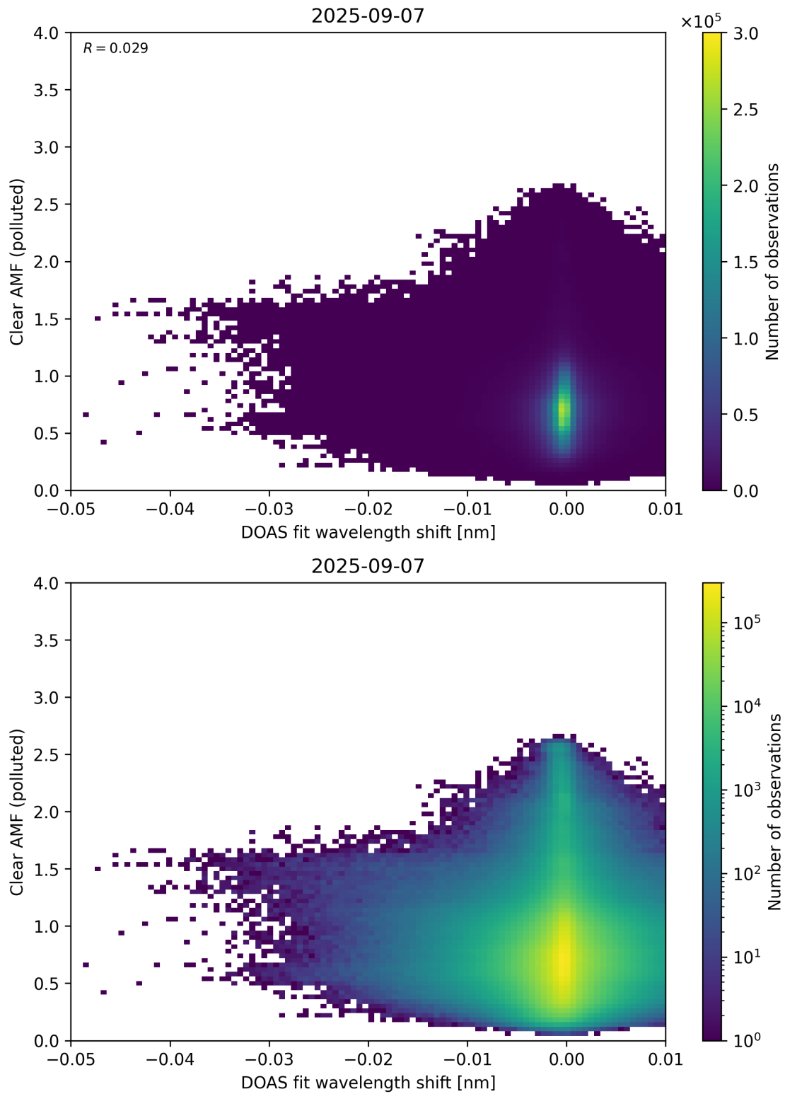
Figure 140: Scatter density plot of “DOAS fit wavelength shift” against “Clear AMF (polluted)” for 2025-09-06 to 2025-09-08.
