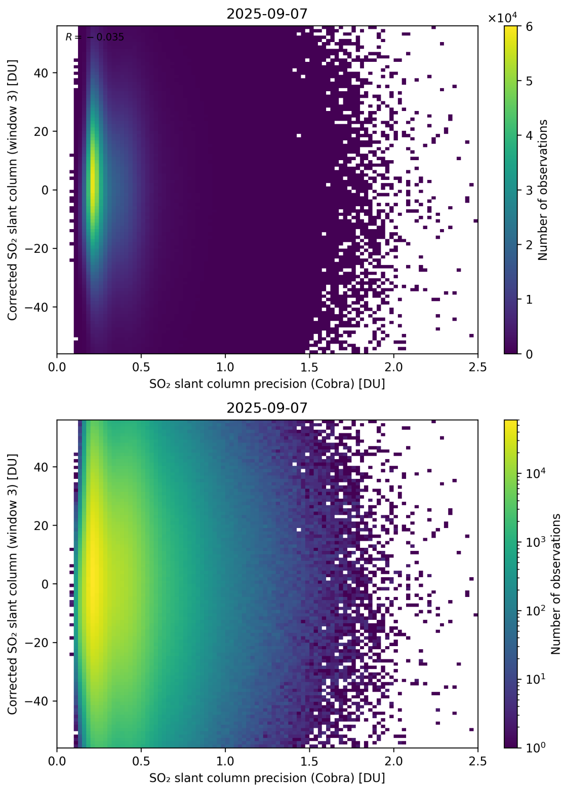
Figure 207: Scatter density plot of “SO 2 slant column precision (Cobra)” against “Corrected SO 2 slant column (window 3)” for 2025-09-06 to 2025-09-08.
