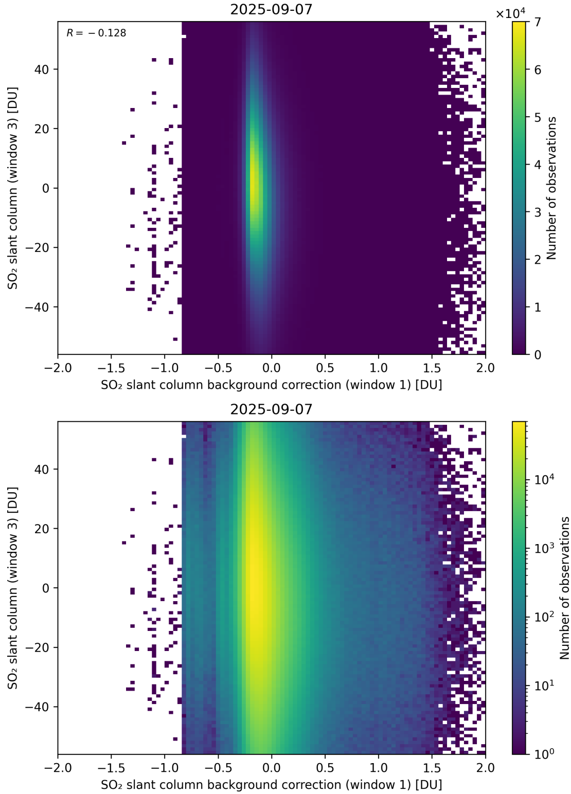
Figure 118: Scatter density plot of “SO 2 slant column background correction (window 1)” against “SO 2 slant column (window 3)” for 2025-09-06 to 2025-09-08.
