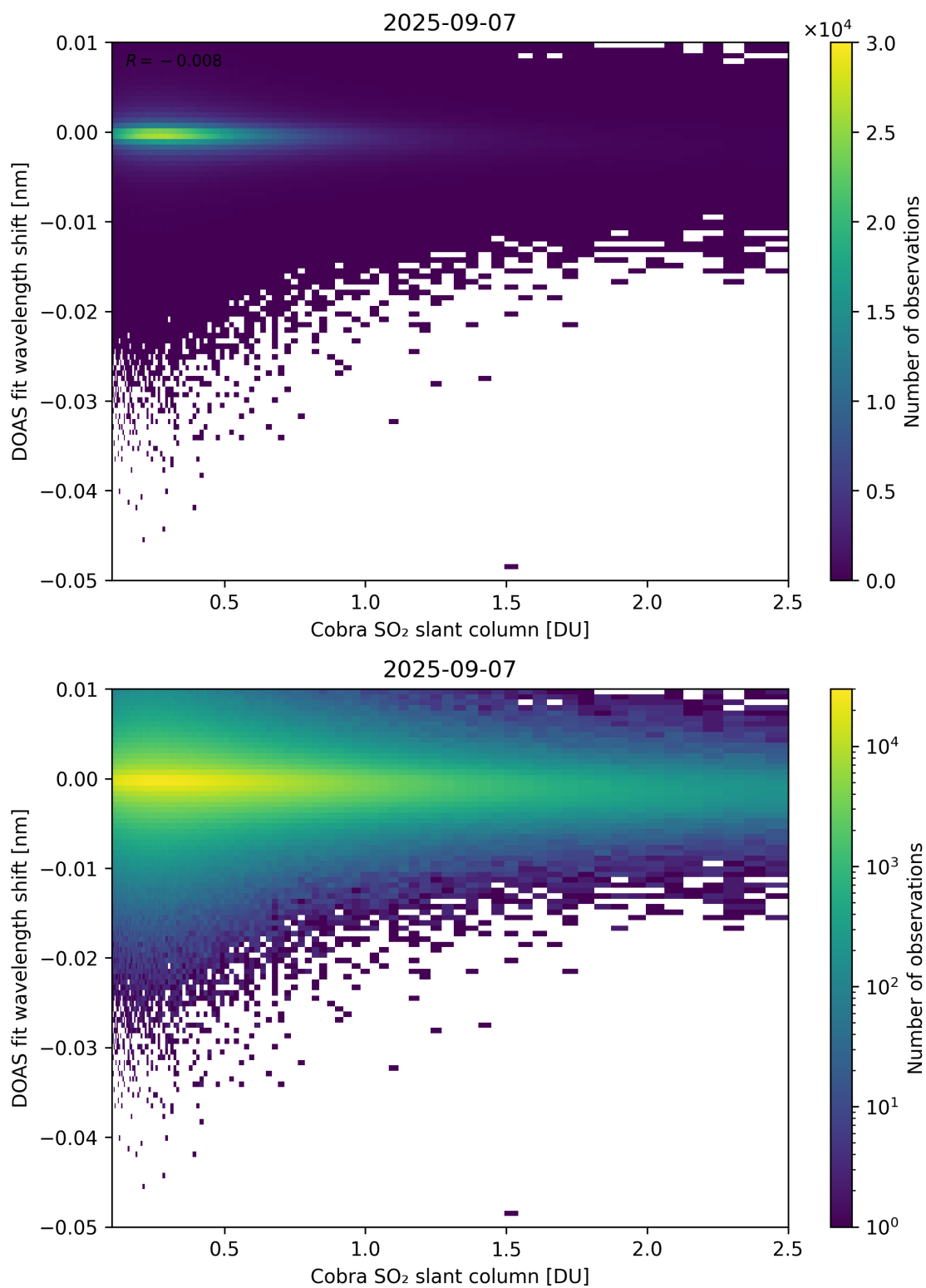
Figure 196: Scatter density plot of “Cobra SO 2 slant column” against “DOAS fit wavelength shift” for 2025-09-06 to 2025-09-08.
