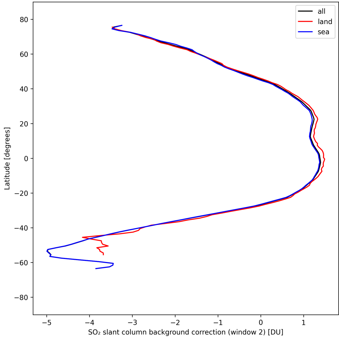
Figure 44: Zonal average of “SO 2 slant column background correction (window 2)” for 2025-09-06 to 2025-09-08.
