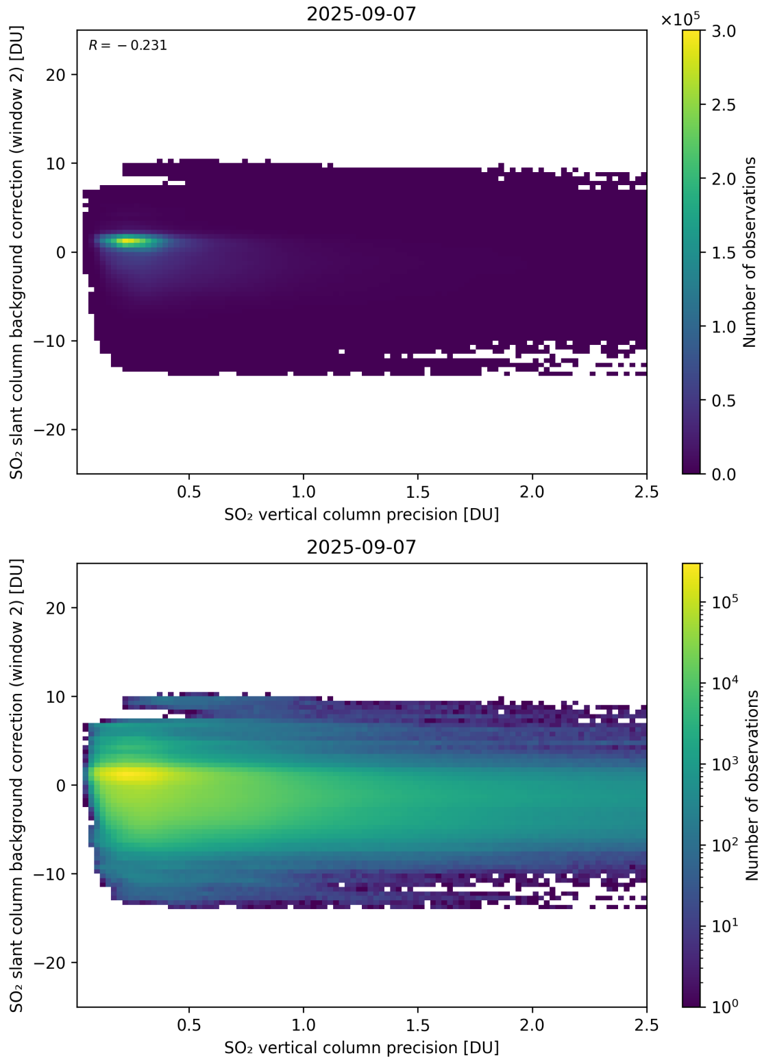
Figure 330: Scatter density plot of “SO 2 vertical column precision” against “SO 2 slant column background correction (window 2)” for 2025-09-06 to 2025-09-08.
