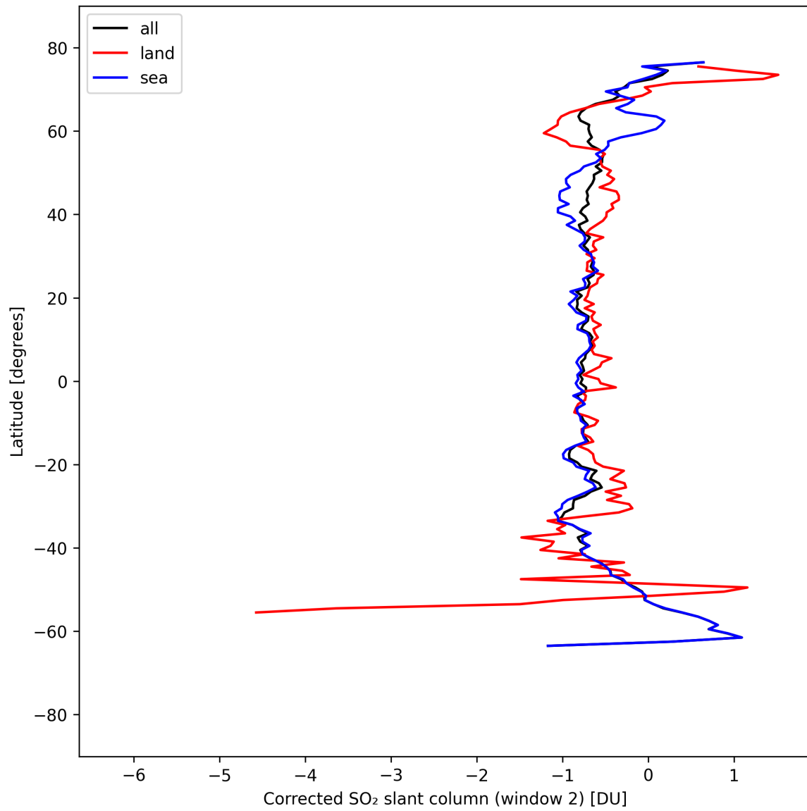
Figure 43: Zonal average of “Corrected SO 2 slant column (window 2)” for 2025-09-06 to 2025-09-08.
