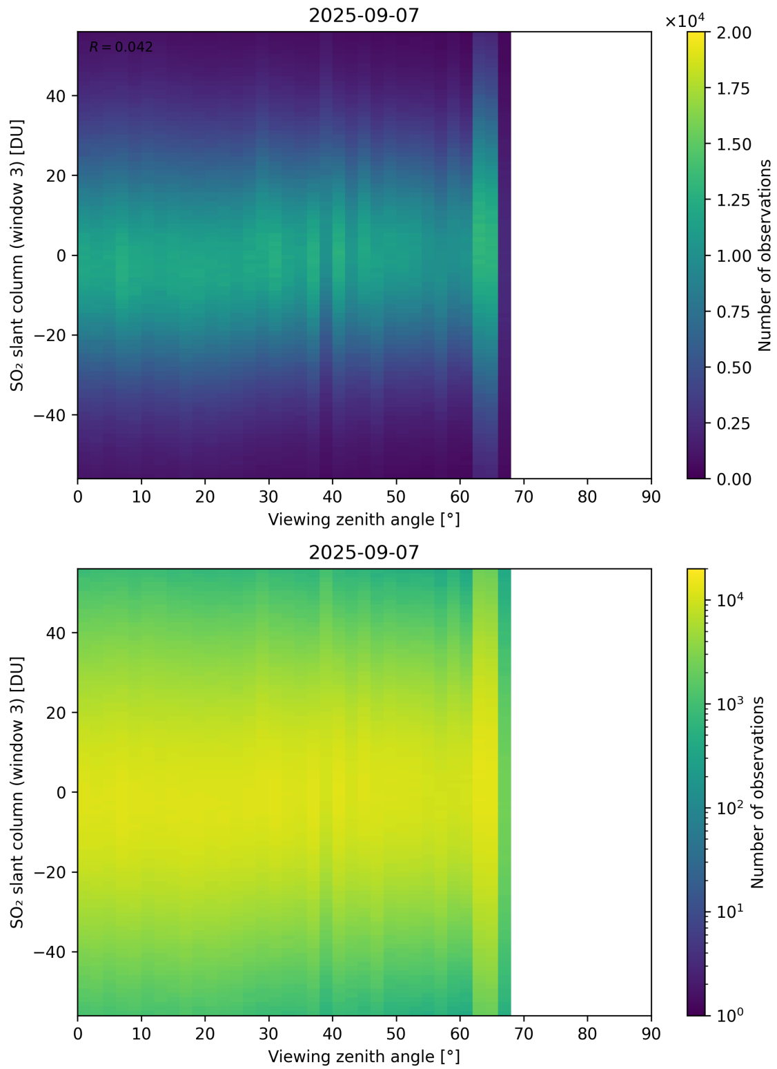
Figure 379: Scatter density plot of “Viewing zenith angle” against “SO 2 slant column (window 3)” for 2025-09-06 to 2025-09-08.
