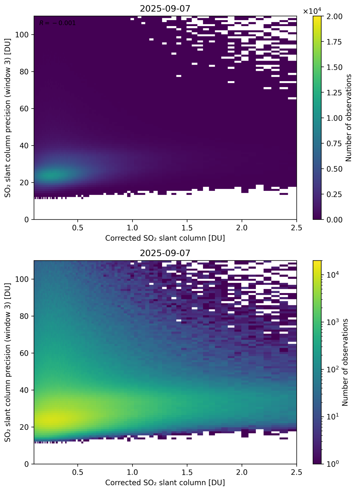
Figure 241: Scatter density plot of “Corrected SO 2 slant column” against “SO 2 slant column precision (window 3)” for 2025-09-06 to 2025-09-08.
