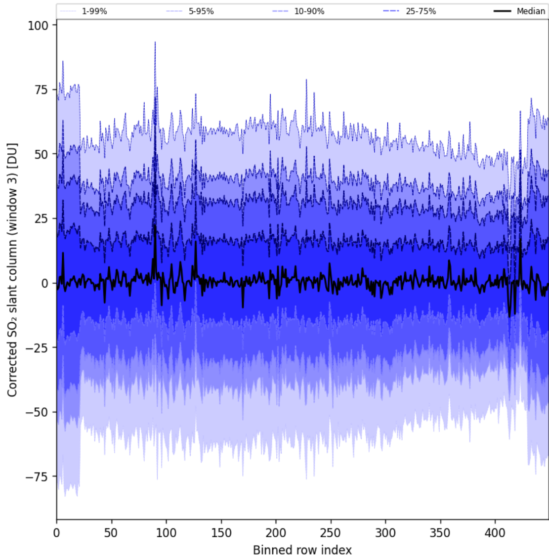
Figure 99: Along track statistics of “Corrected SO 2 slant column (window 3)” for 2025-09-06 to 2025-09-08
