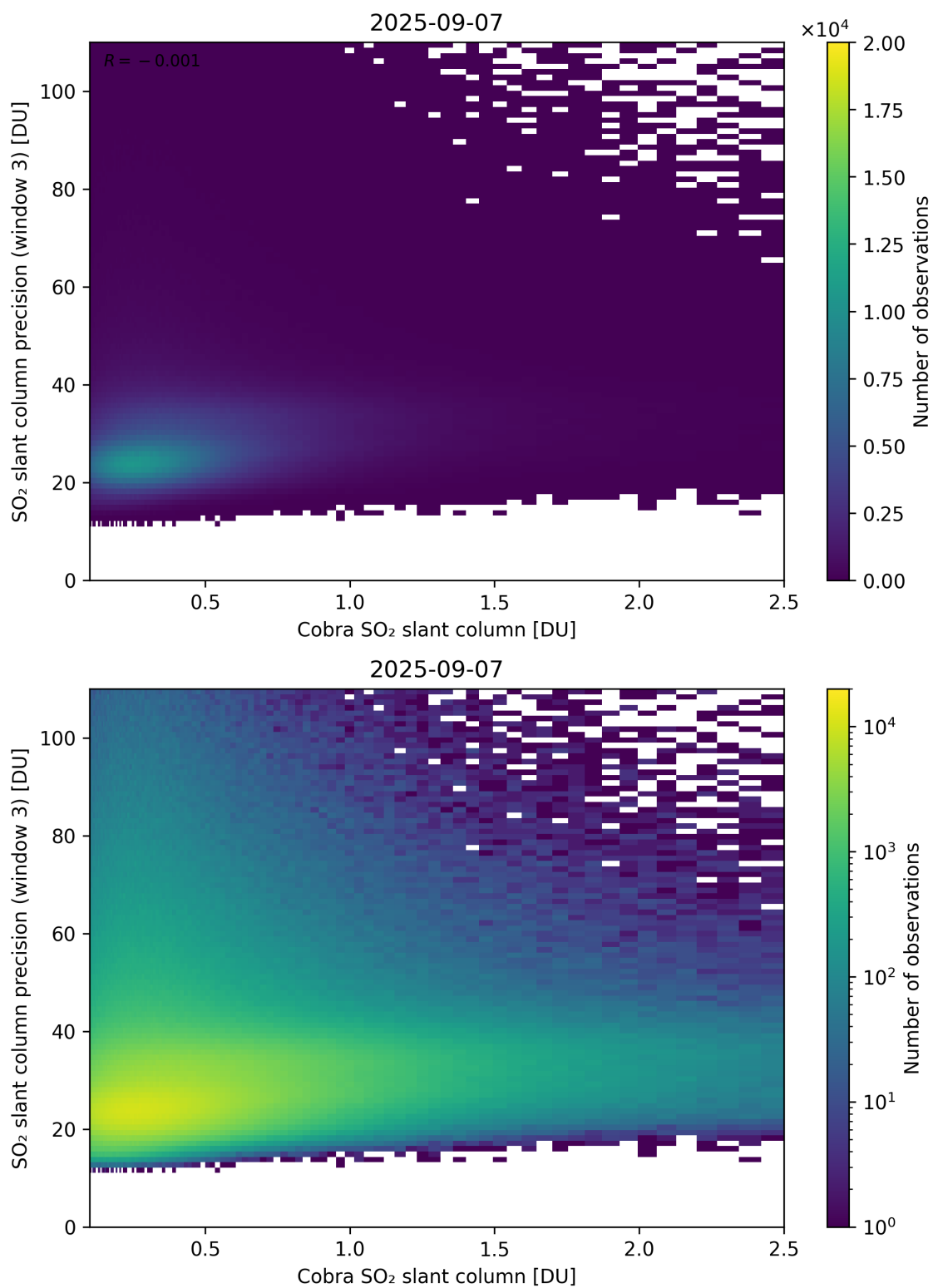
Figure 223: Scatter density plot of “Cobra SO 2 slant column” against “SO 2 slant column precision (window 3)” for 2025-09-06 to 2025-09-08.
