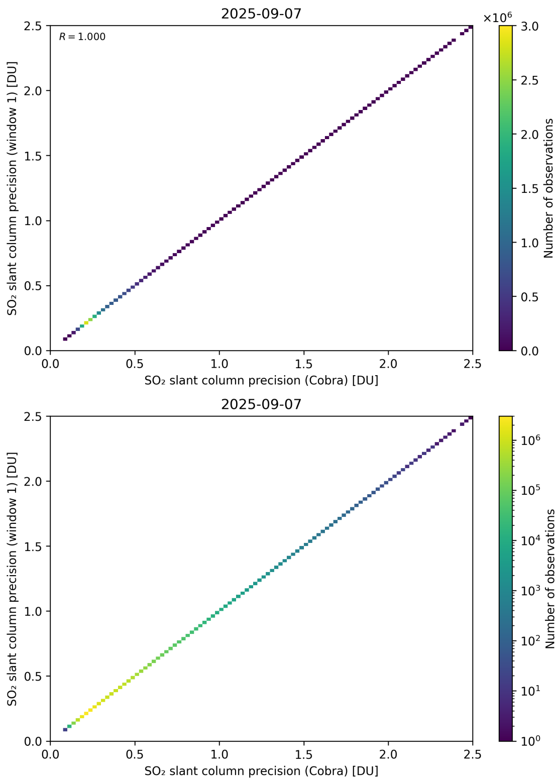
Figure 209: Scatter density plot of “SO 2 slant column precision (Cobra)” against “SO 2 slant column precision (window 1)” for 2025-09-06 to 2025-09-08.
