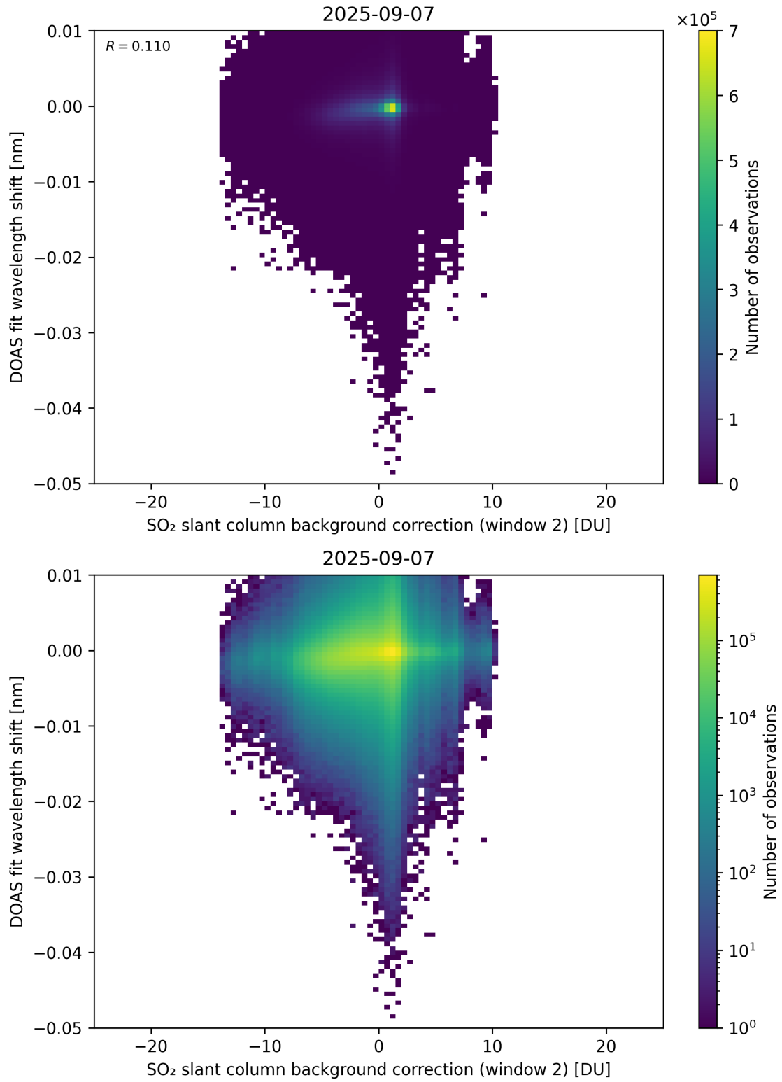
Figure 123: Scatter density plot of “SO 2 slant column background correction (window 2)” against “DOAS fit wavelength shift” for 2025-09-06 to 2025-09-08.
