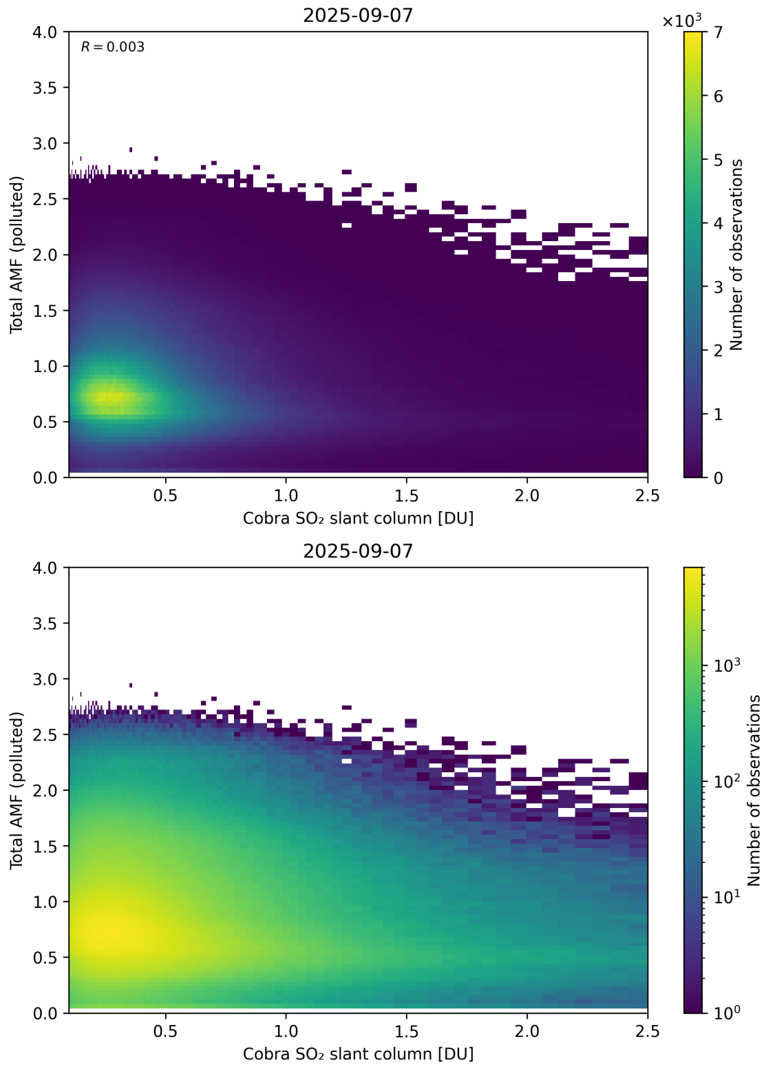
Figure 224: Scatter density plot of “Cobra SO 2 slant column” against “Total AMF (polluted)” for 2025-09-06 to 2025-09-08.
