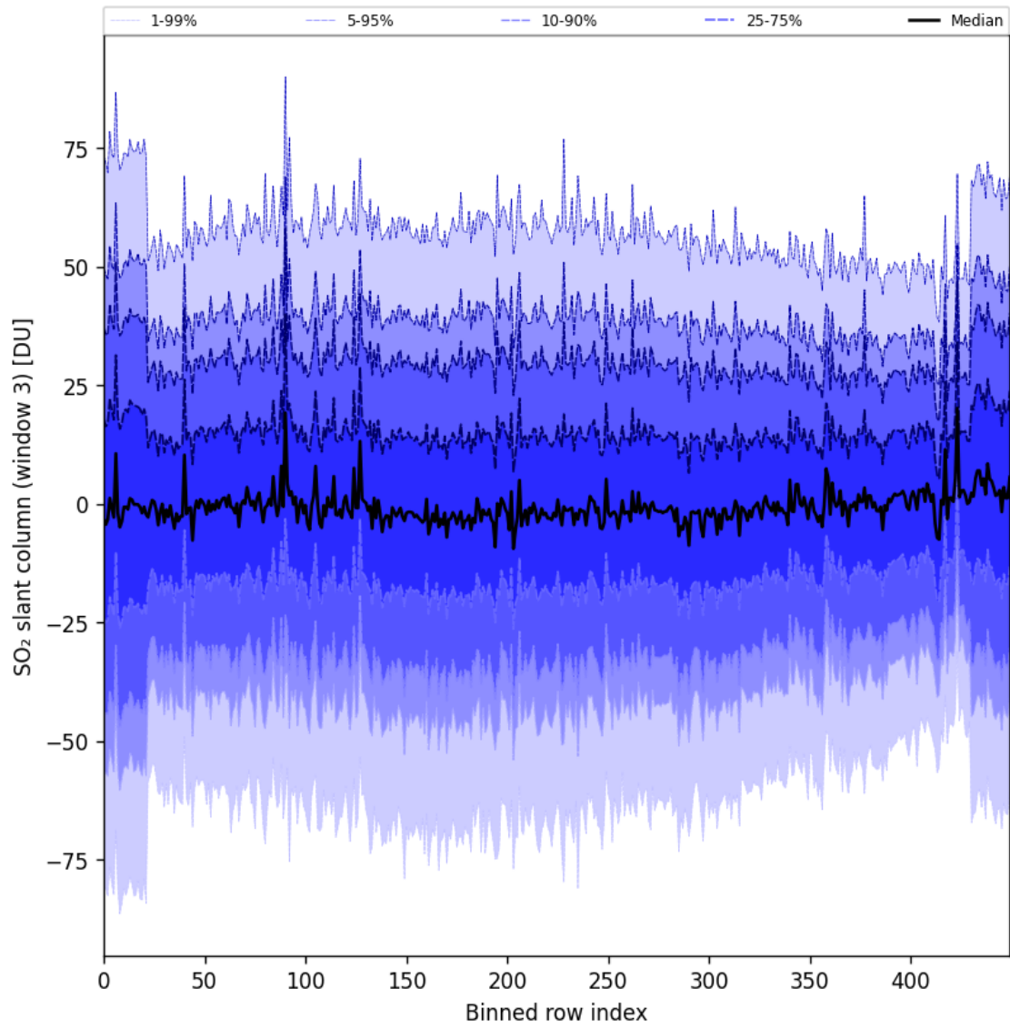
Figure 97: Along track statistics of “SO 2 slant column (window 3)” for 2025-09-06 to 2025-09-08
