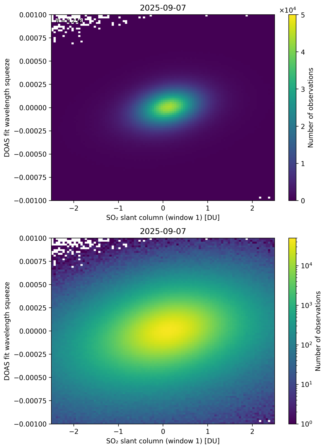
Figure 266: Scatter density plot of “SO 2 slant column (window 1)” against “DOAS fit wavelength squeeze” for 2025-09-06 to 2025-09-08.
