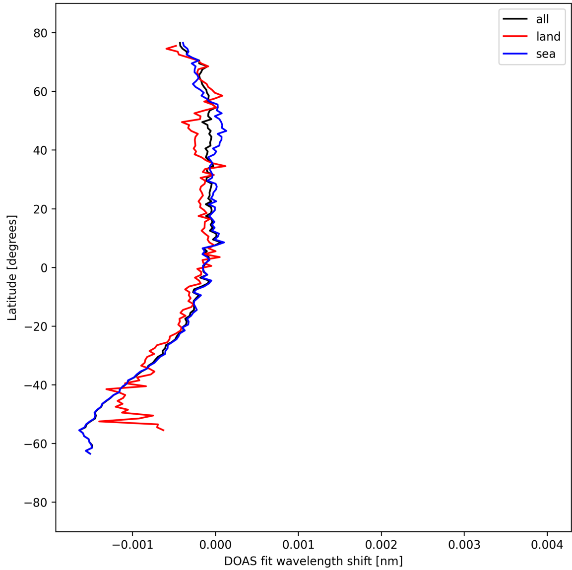
Figure 50: Zonal average of “DOAS fit wavelength shift” for 2025-09-06 to 2025-09-08.
