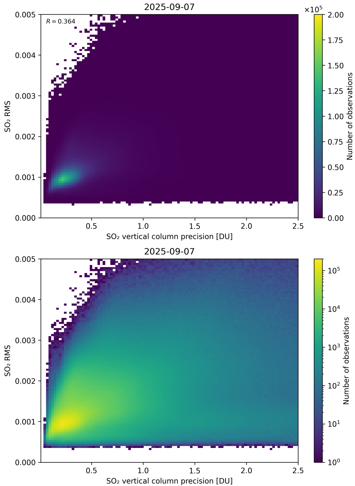
Figure 334: Scatter density plot of “SO 2 vertical column precision” against “SO 2 RMS” for 2025-09-06 to 2025-09-08.
