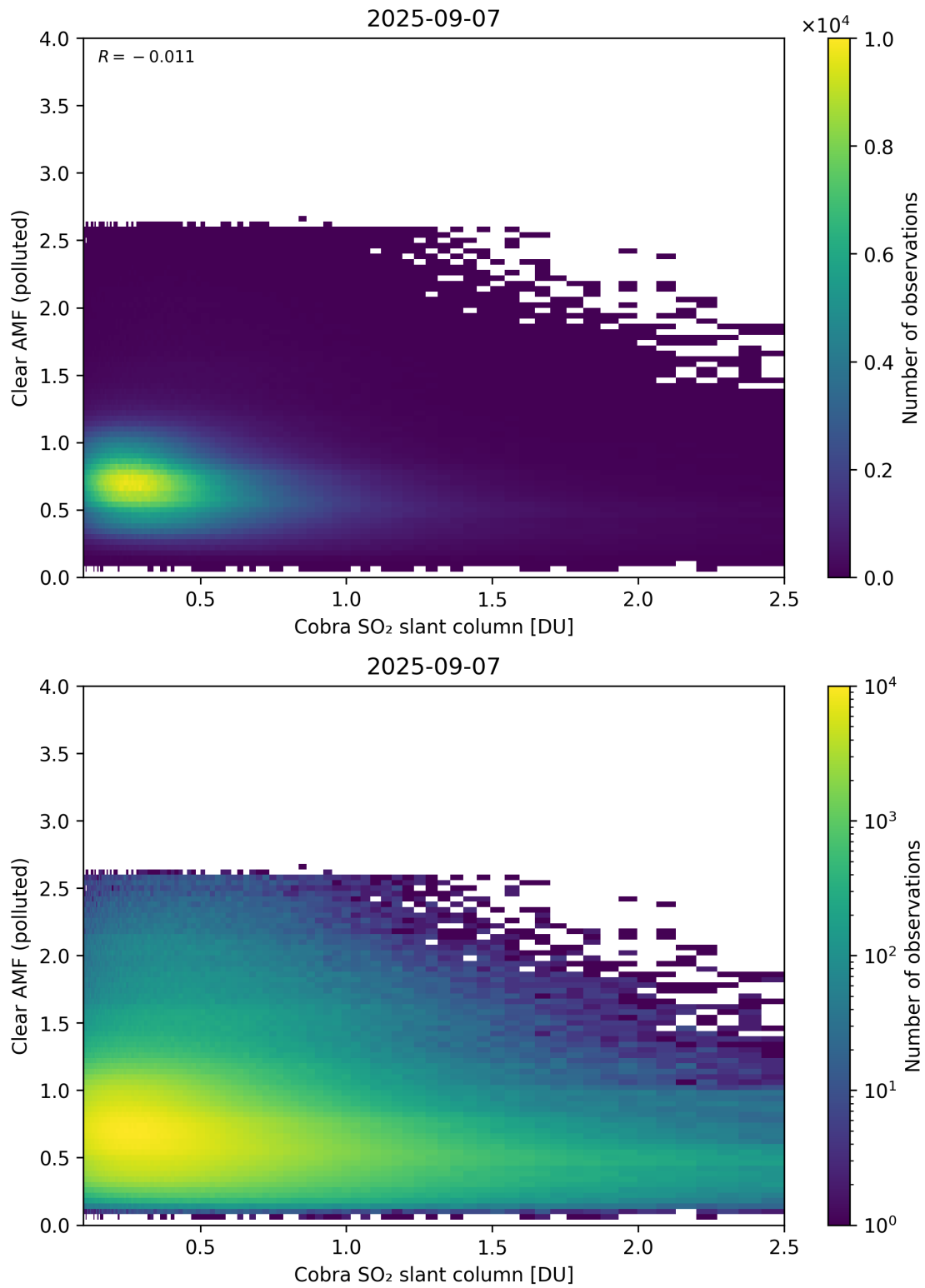
Figure 215: Scatter density plot of “Cobra SO 2 slant column” against “Clear AMF (polluted)” for 2025-09-06 to 2025-09-08.
