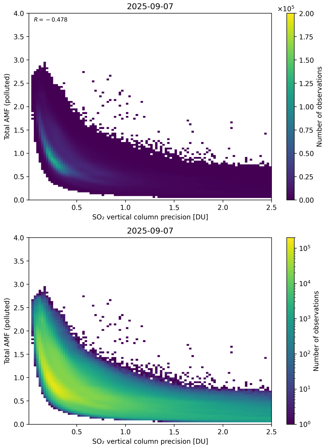
Figure 346: Scatter density plot of “SO 2 vertical column precision” against “Total AMF (polluted)” for 2025-09-06 to 2025-09-08.
