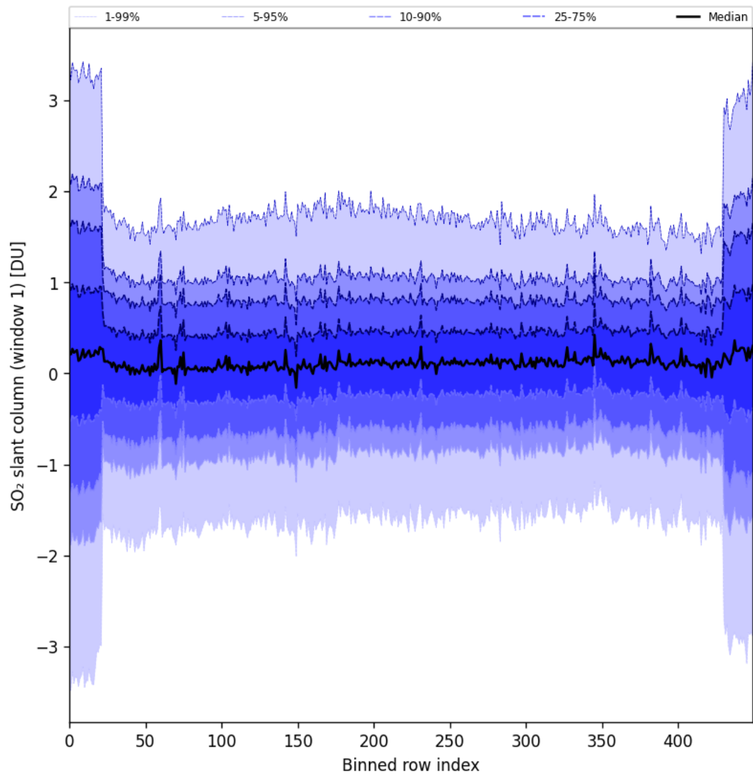
Figure 89: Along track statistics of “SO 2 slant column (window 1)” for 2025-09-06 to 2025-09-08
