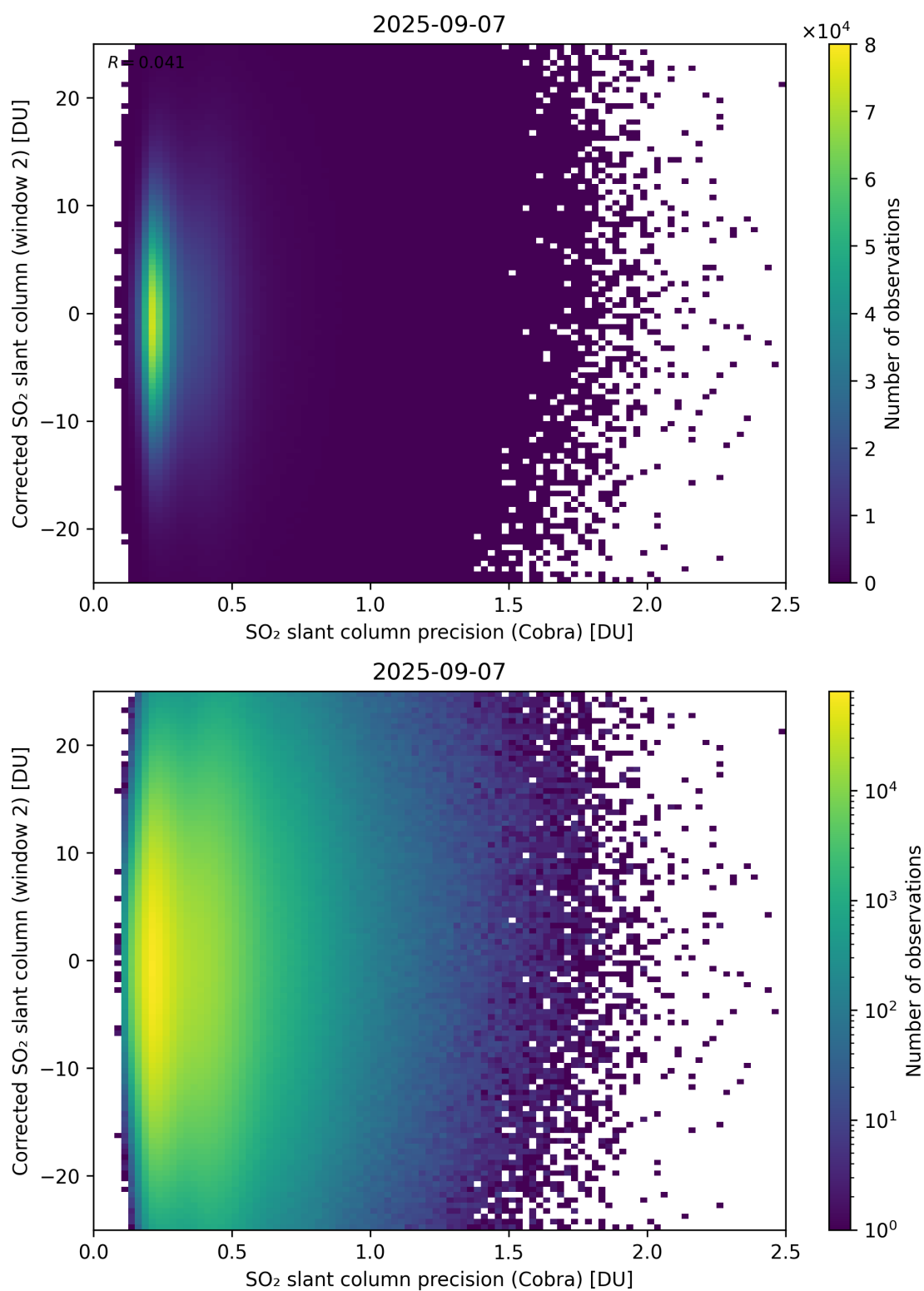
Figure 206: Scatter density plot of “SO 2 slant column precision (Cobra)” against “Corrected SO 2 slant column (window 2)” for 2025-09-06 to 2025-09-08.
