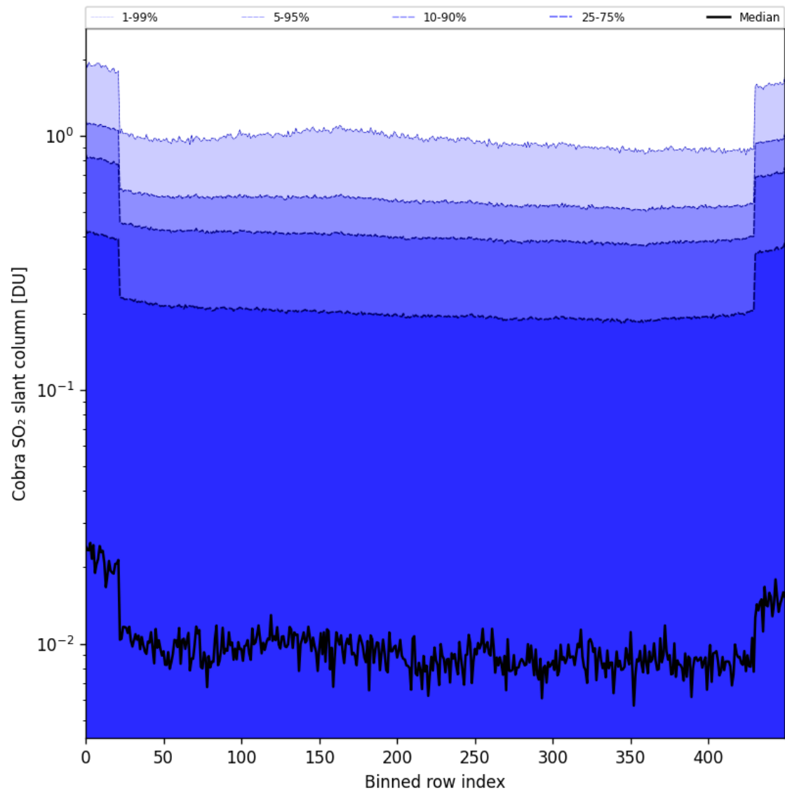
Figure 87: Along track statistics of "Cobra SO 2 slant column" for 2025-09-06 to 2025-09-08
