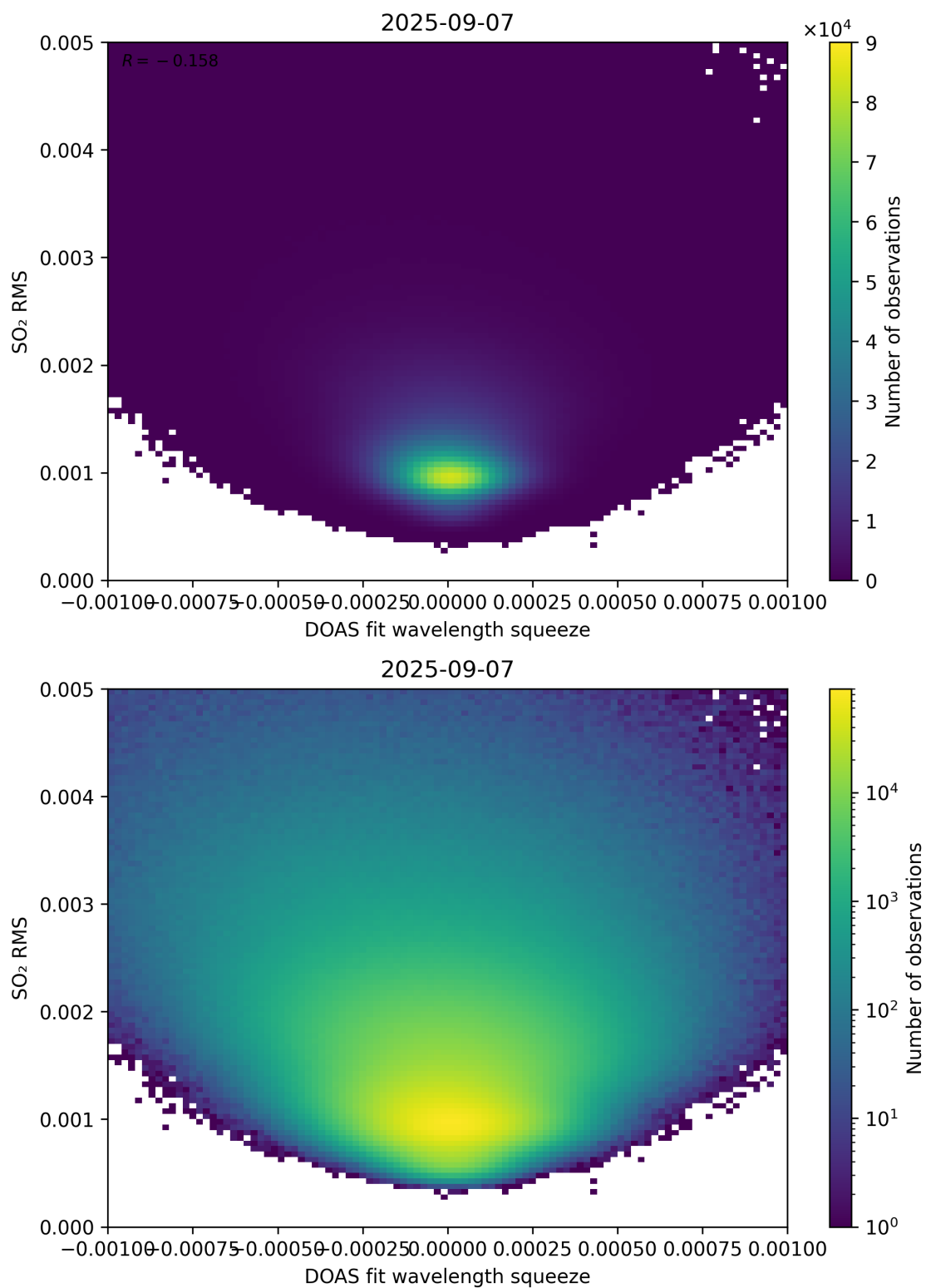
Figure 143: Scatter density plot of “DOAS fit wavelength squeeze” against “SO 2 RMS” for 2025-09-06 to 2025-09-08.
