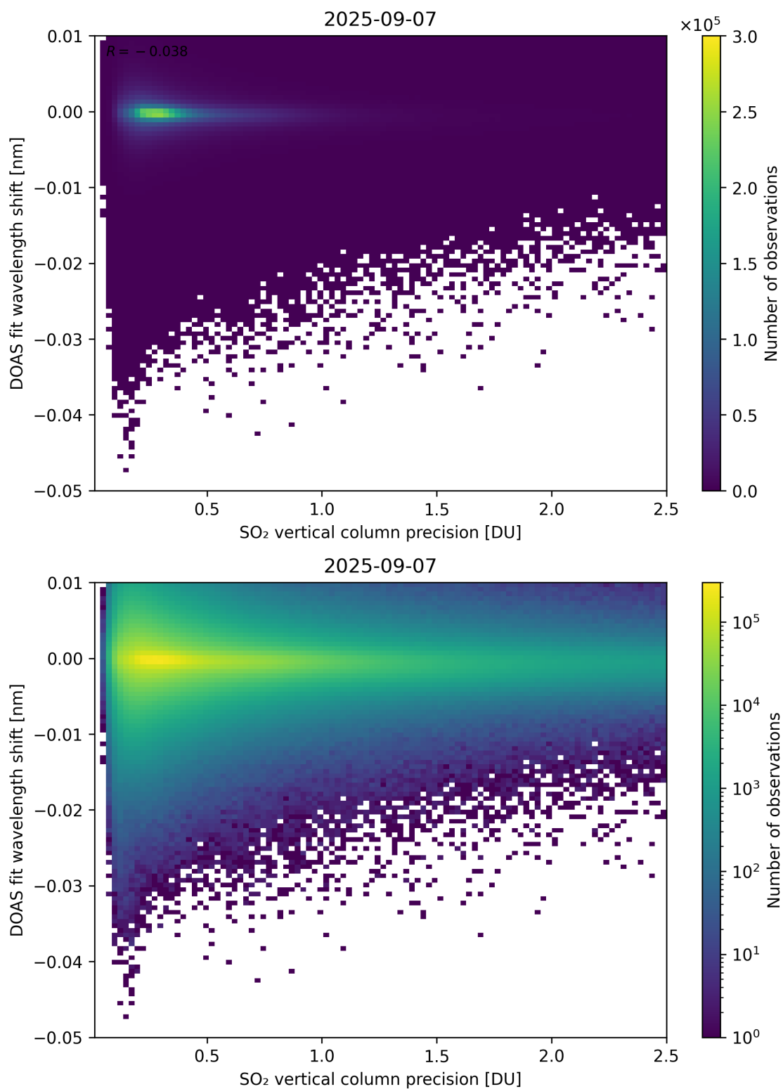
Figure 332: Scatter density plot of “SO 2 vertical column precision” against “DOAS fit wavelength shift” for 2025-09-06 to 2025-09-08.
