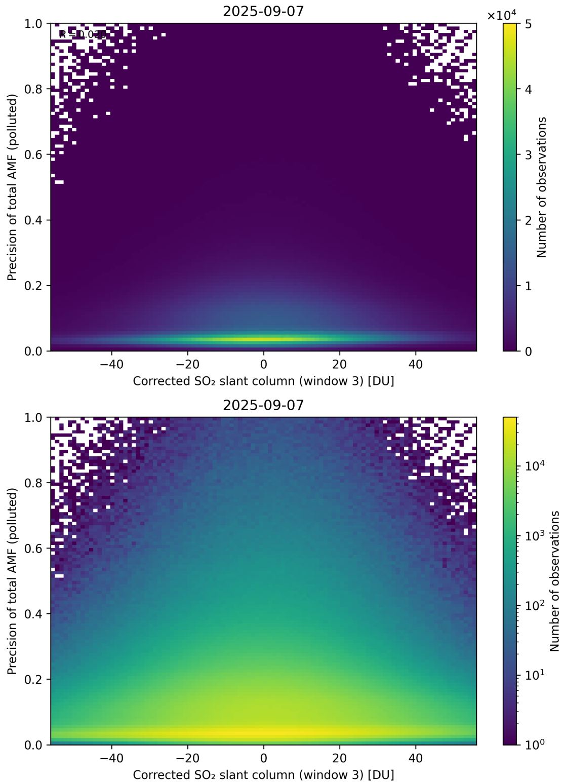
Figure 261: Scatter density plot of “Corrected SO 2 slant column (window 3)” against “Precision of total AMF (polluted)” for 2025-09-06 to 2025-09-08.
