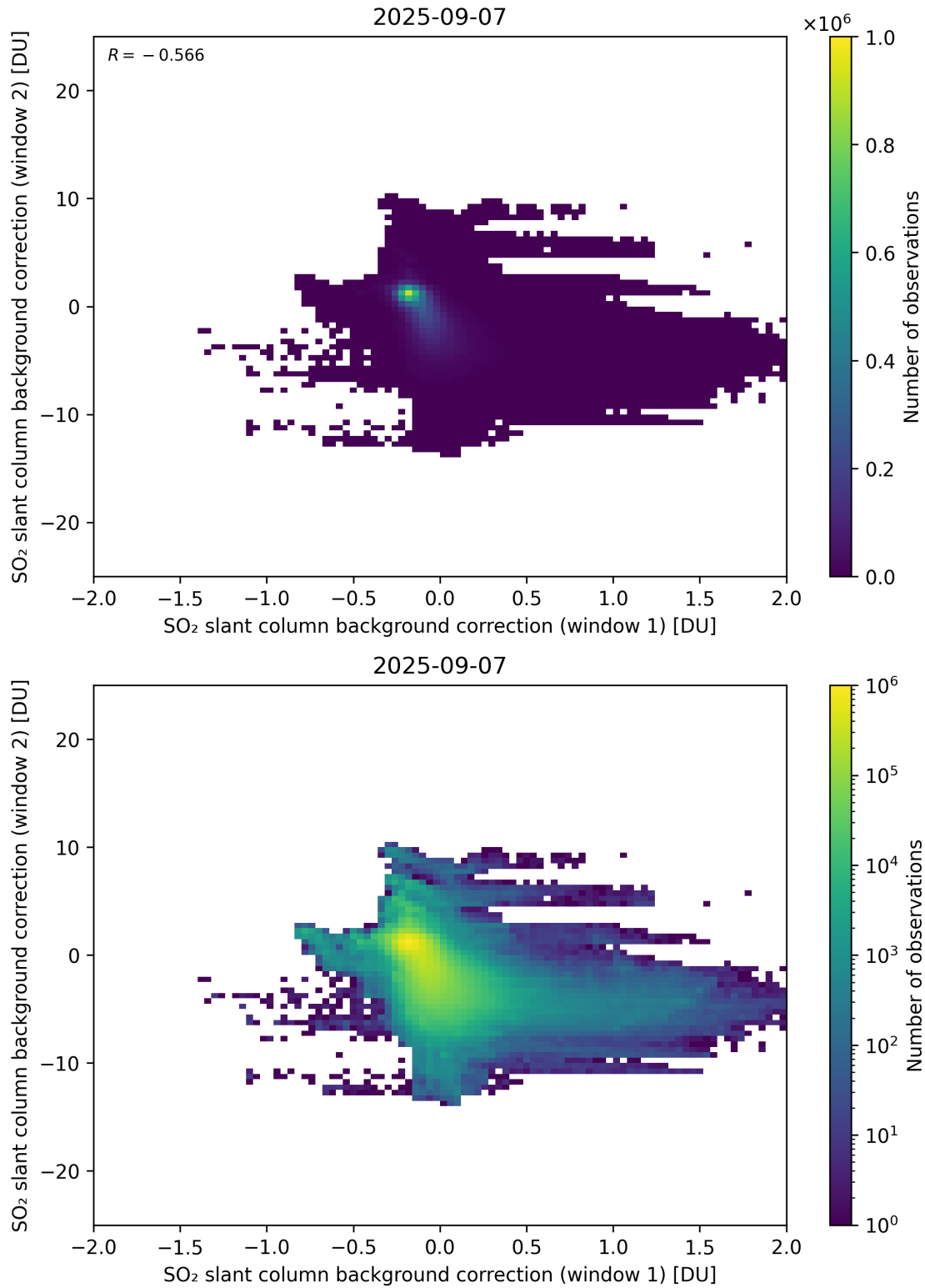
Figure 109: Scatter density plot of “SO 2 slant column background correction (window 1)” against “SO 2 slant column background correction (window 2)” for 2025-09-06 to 2025-09-08.
