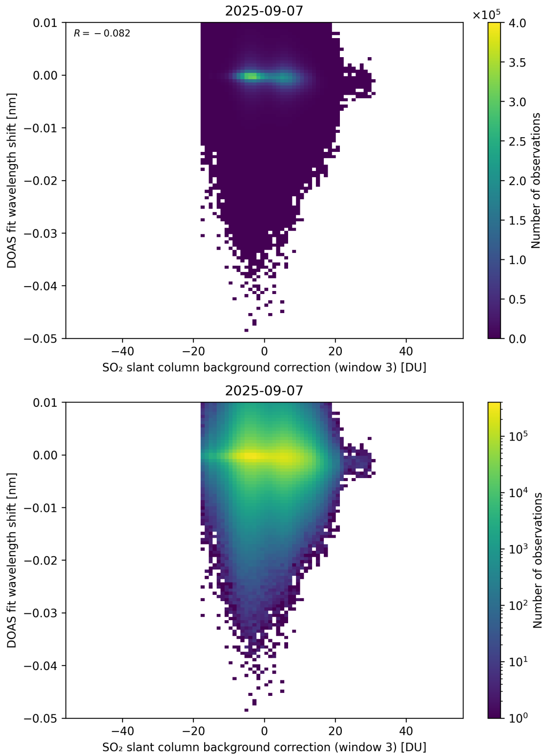
Figure 132: Scatter density plot of “SO 2 slant column background correction (window 3)” against “DOAS fit wavelength shift” for 2025-09-06 to 2025-09-08.
