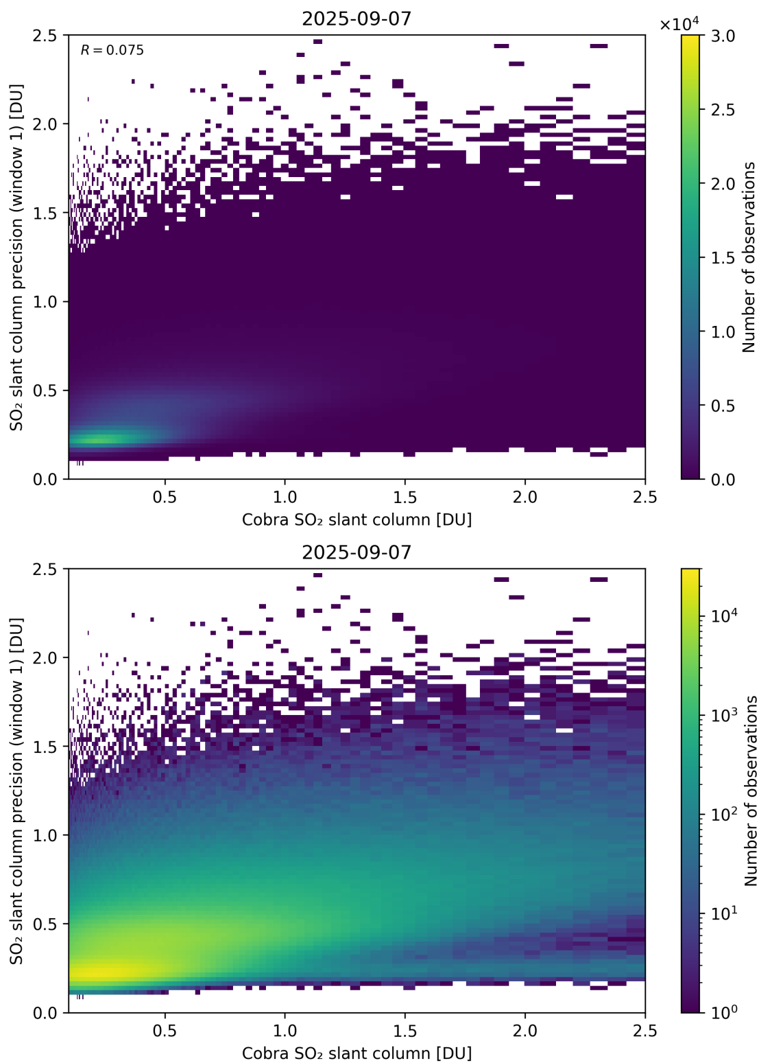
Figure 220: Scatter density plot of “Cobra SO 2 slant column” against “SO 2 slant column precision (window 1)” for 2025-09-06 to 2025-09-08.
