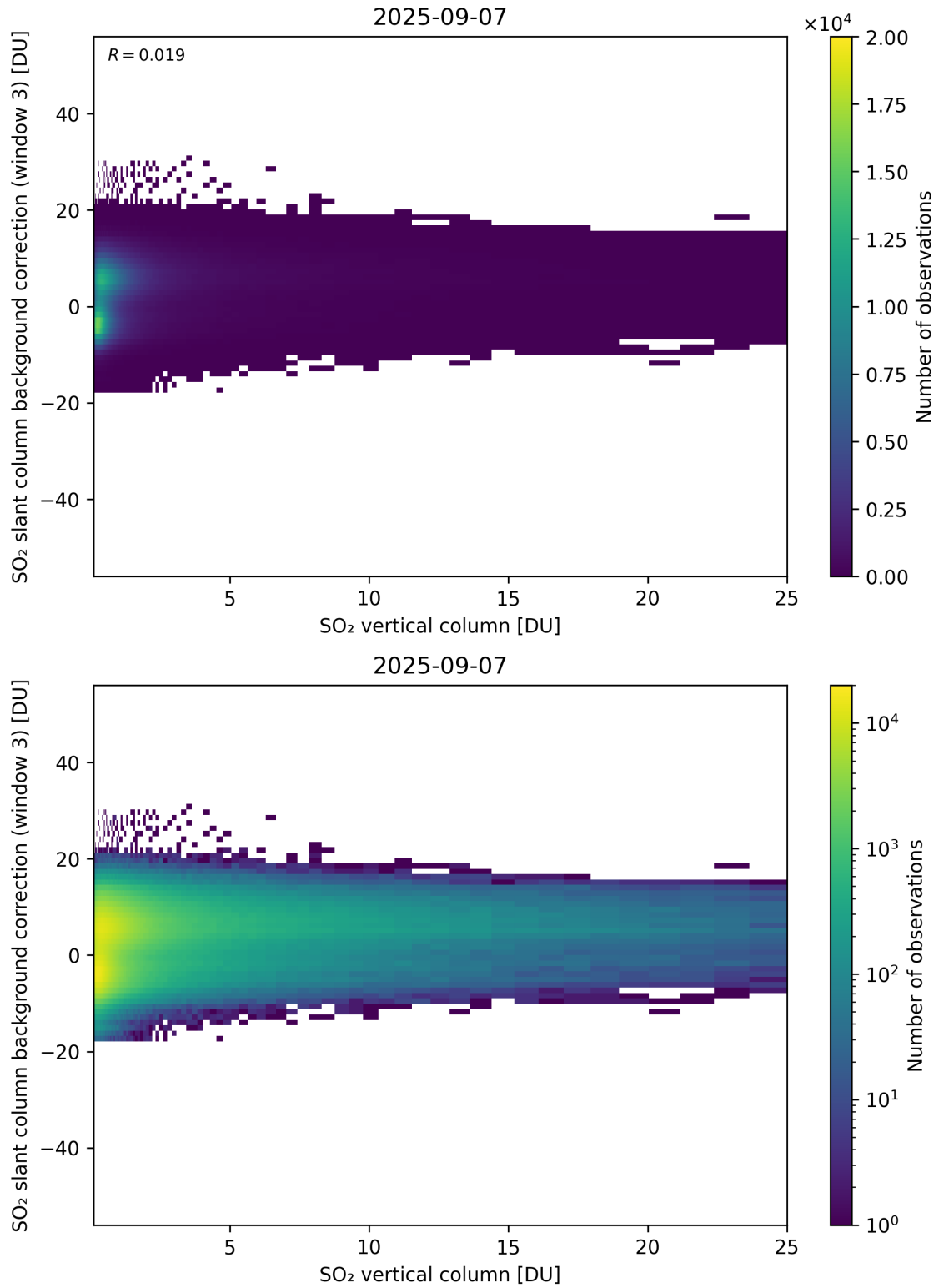
Figure 325: Scatter density plot of “SO 2 vertical column” against “SO 2 slant column background correction (window 3)” for 2025-09-06 to 2025-09-08.
