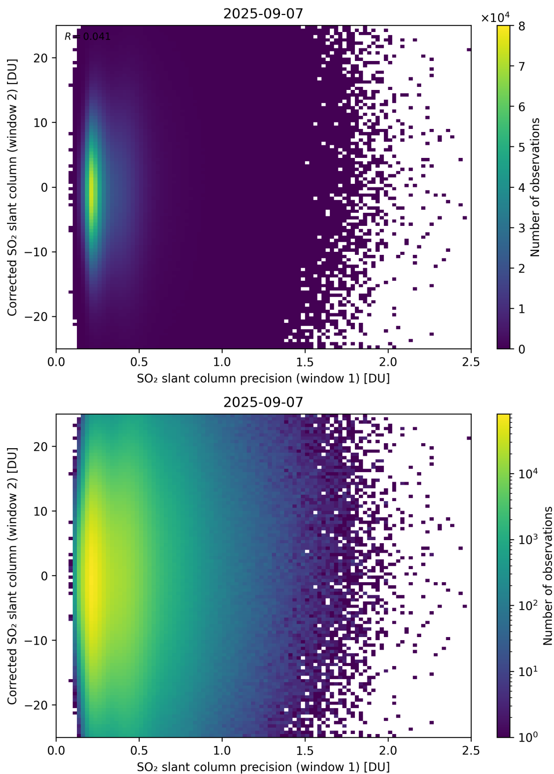
Figure 275: Scatter density plot of “SO 2 slant column precision (window 1)” against “Corrected SO 2 slant column (window 2)” for 2025-09-06 to 2025-09-08.
