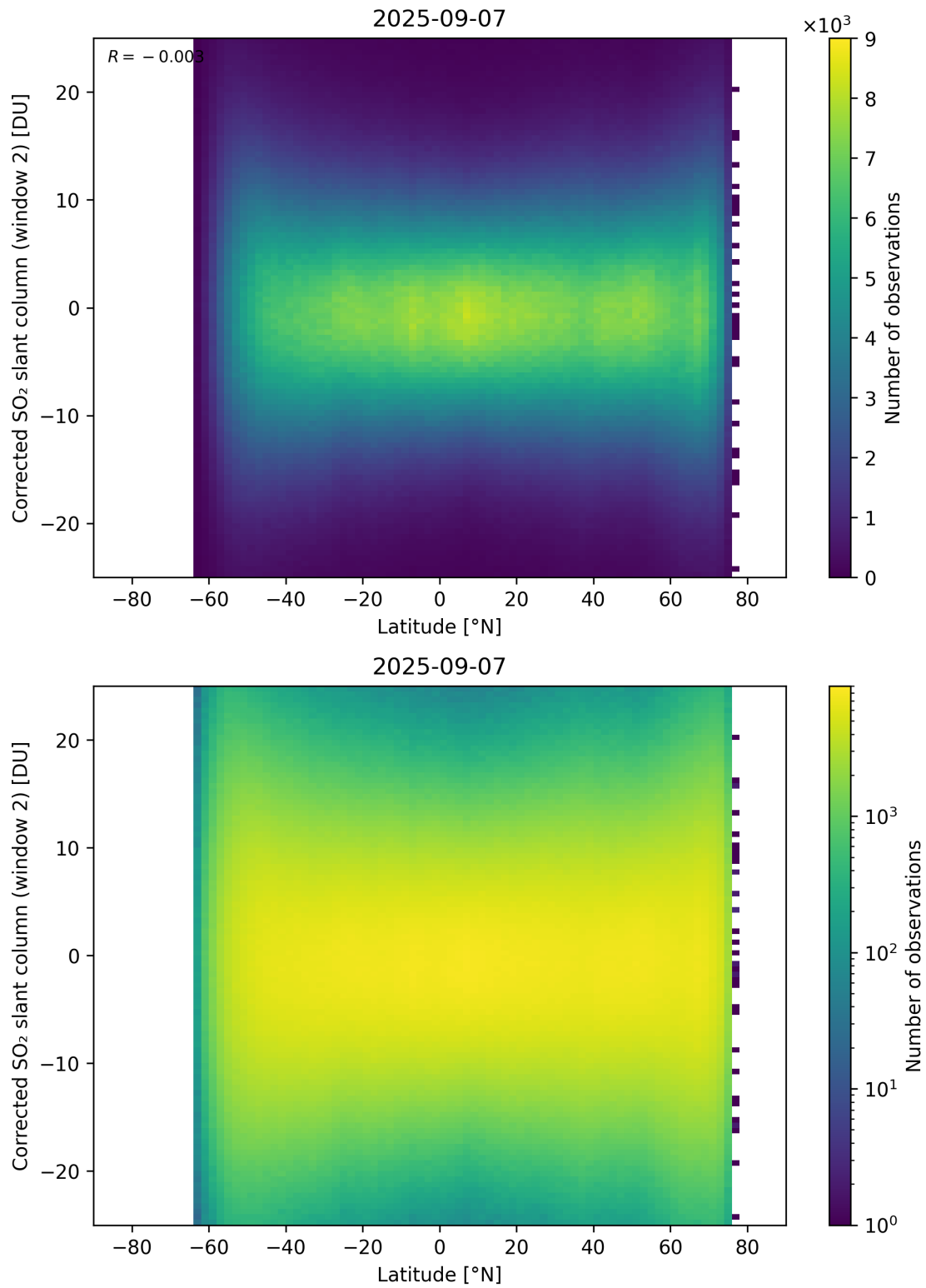
Figure 160: Scatter density plot of “Latitude” against “Corrected SO 2 slant column (window 2)” for 2025-09-06 to 2025-09-08.
