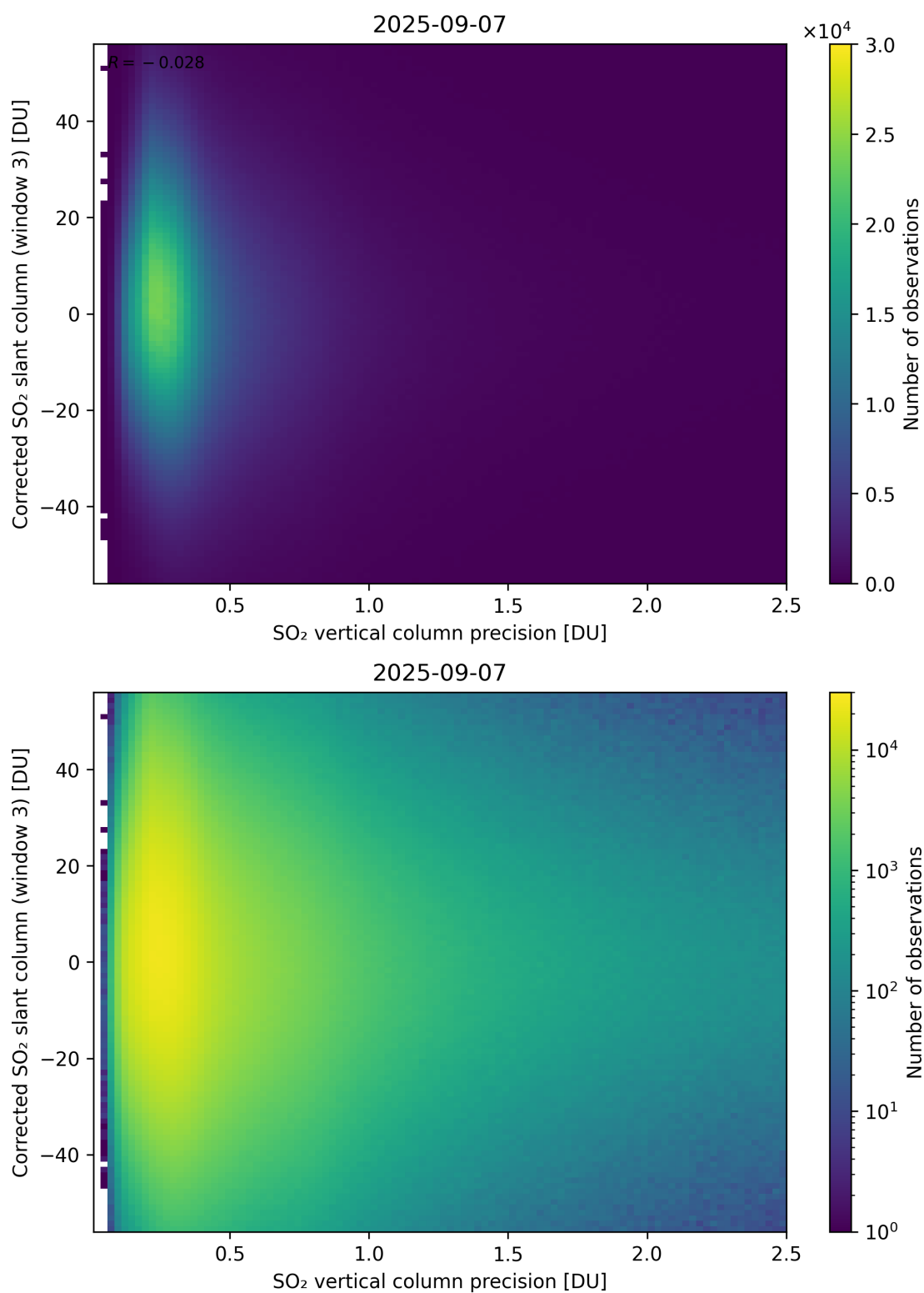
Figure 340: Scatter density plot of “SO 2 vertical column precision” against “Corrected SO 2 slant column (window 3)” for 2025-09-06 to 2025-09-08.
