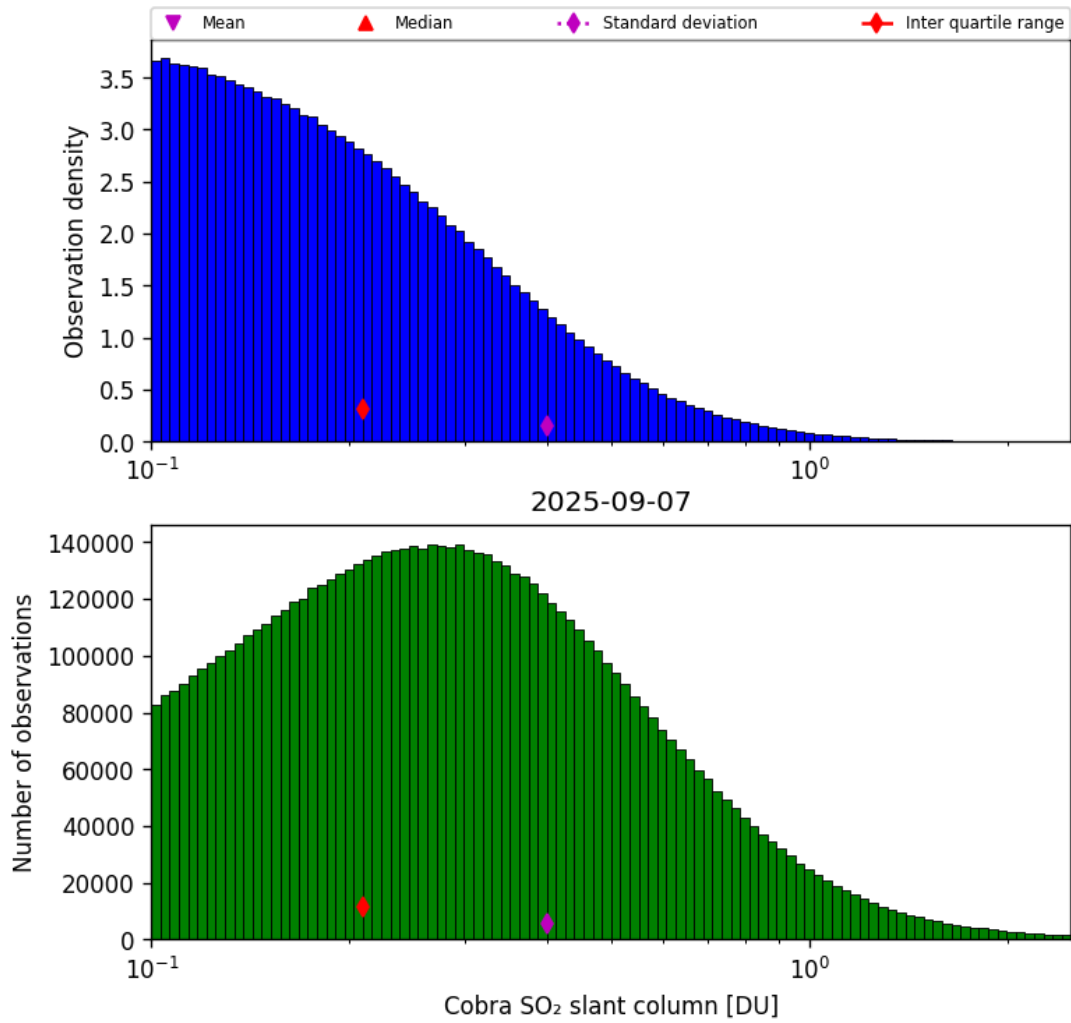
Figure 61: Histogram of “Cobra SO 2 slant column” for 2025-09-06 to 2025-09-08
