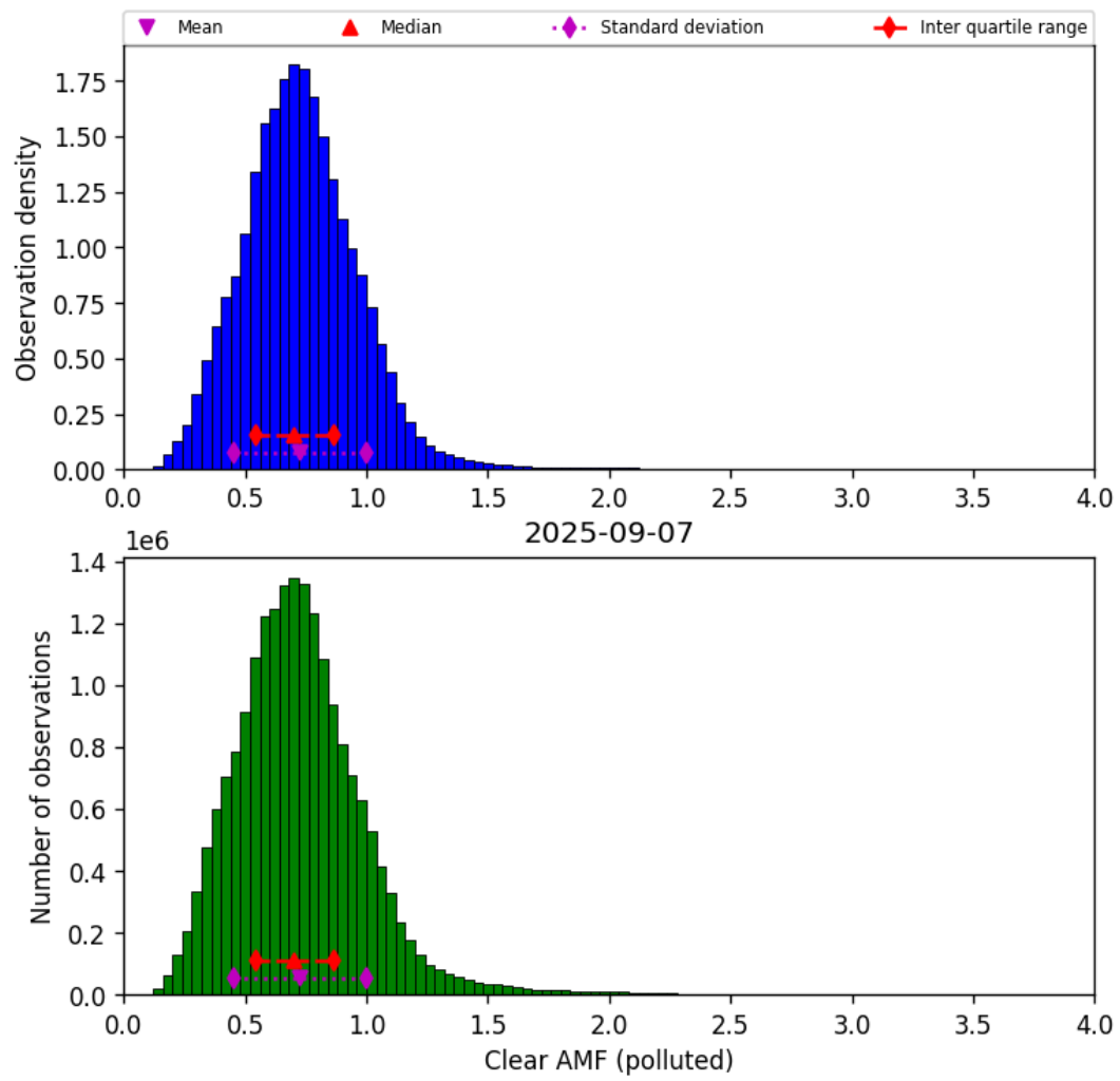
Figure 81: Histogram of “Clear AMF (polluted)” for 2025-09-06 to 2025-09-08
