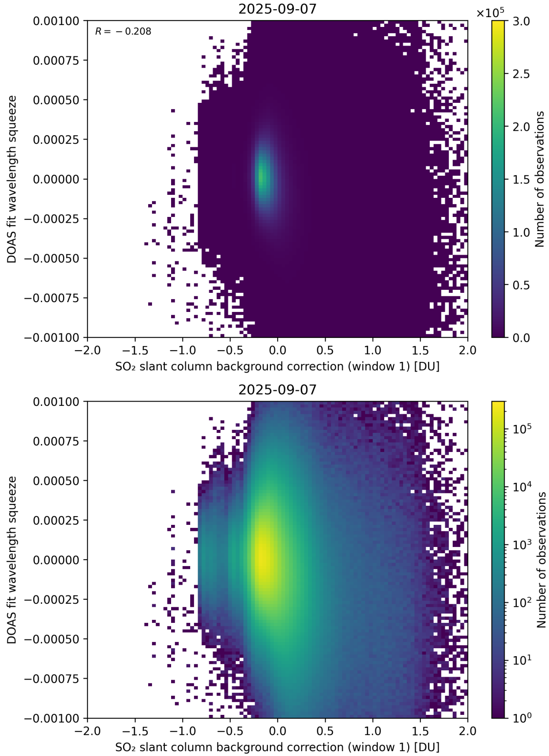
Figure 112: Scatter density plot of “SO 2 slant column background correction (window 1)” against “DOAS fit wavelength squeeze” for 2025-09-06 to 2025-09-08.
