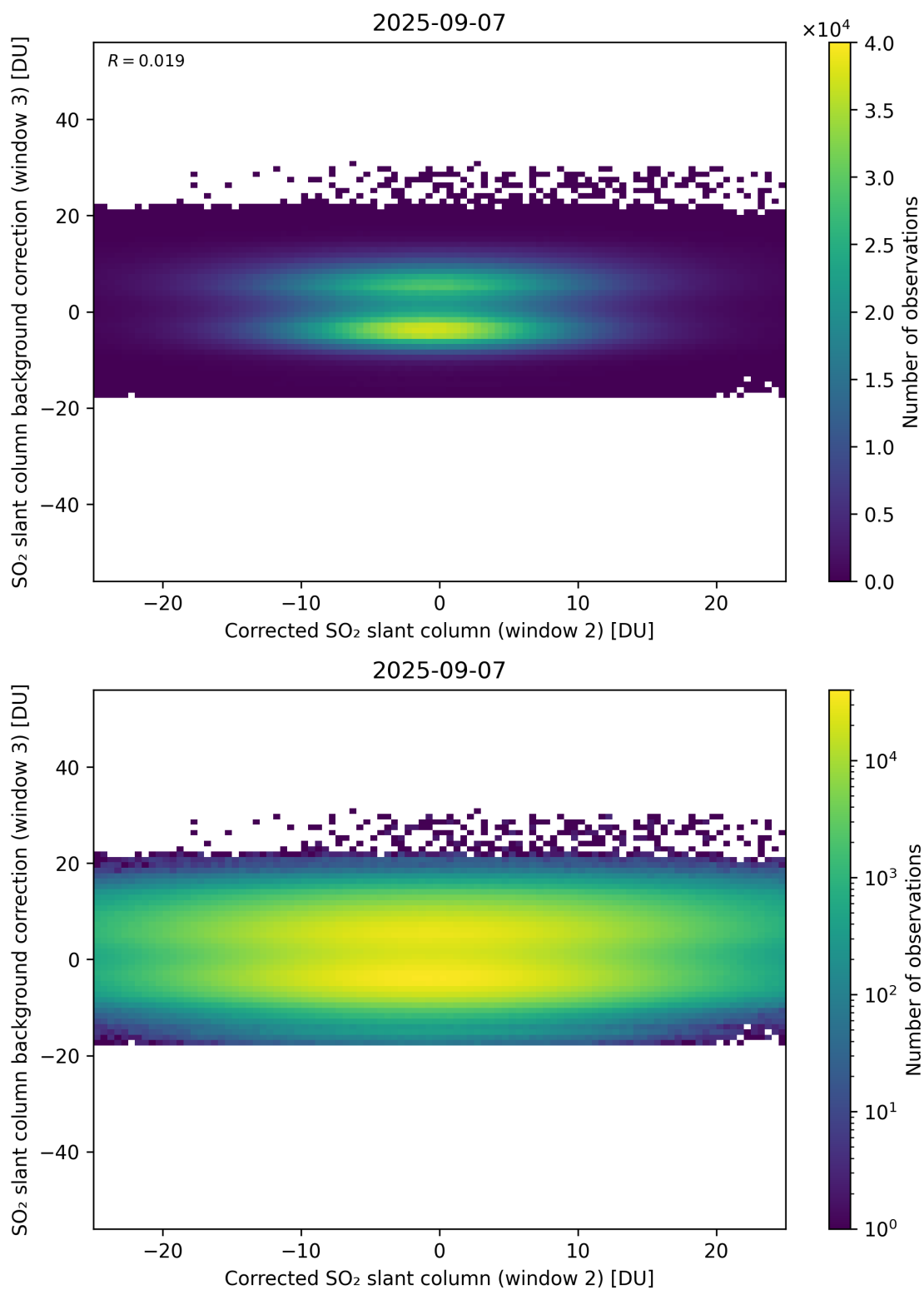
Figure 245: Scatter density plot of “Corrected SO 2 slant column (window 2)” against “SO 2 slant column background correction (window 3)” for 2025-09-06 to 2025-09-08.
