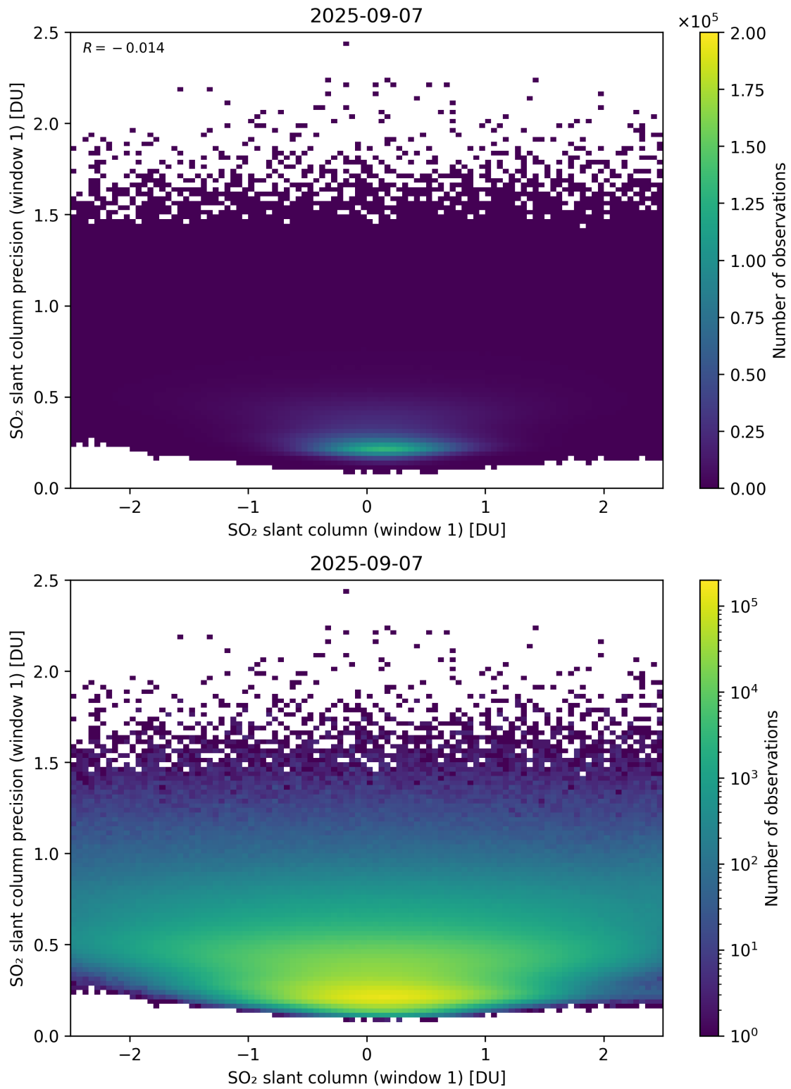
Figure 285: Scatter density plot of “SO 2 slant column (window 1)” against “SO 2 slant column precision (window 1)” for 2025-09-06 to 2025-09-08.
