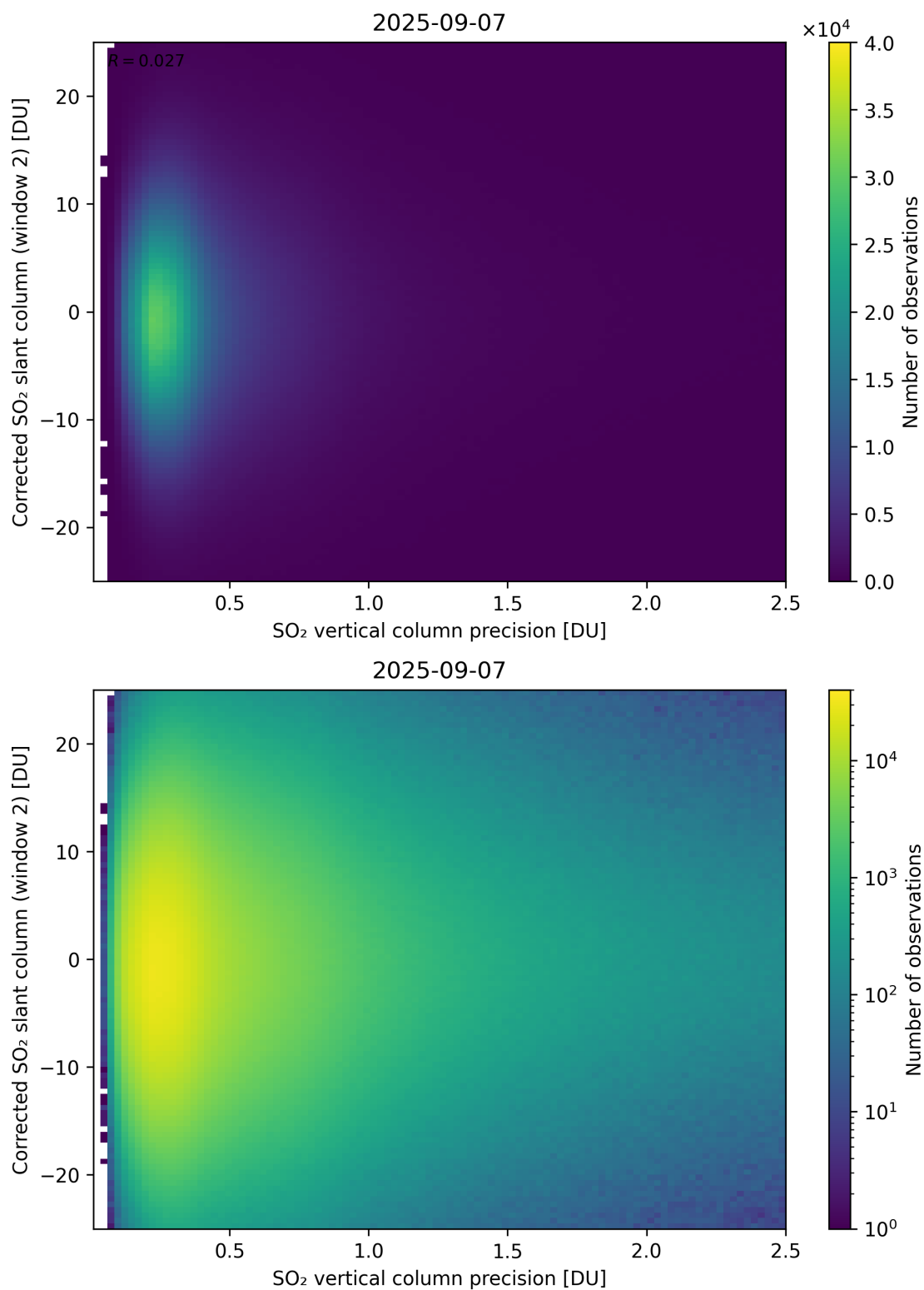
Figure 339: Scatter density plot of “SO 2 vertical column precision” against “Corrected SO 2 slant column (window 2)” for 2025-09-06 to 2025-09-08.
