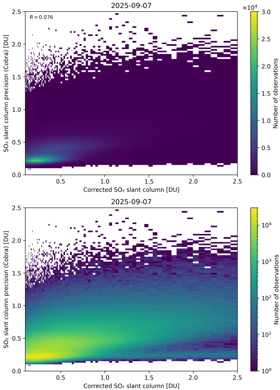
Figure 234: Scatter density plot of “Corrected SO 2 slant column” against “SO 2 slant column precision (Cobra)” for 2025-09-06 to 2025-09-08.
