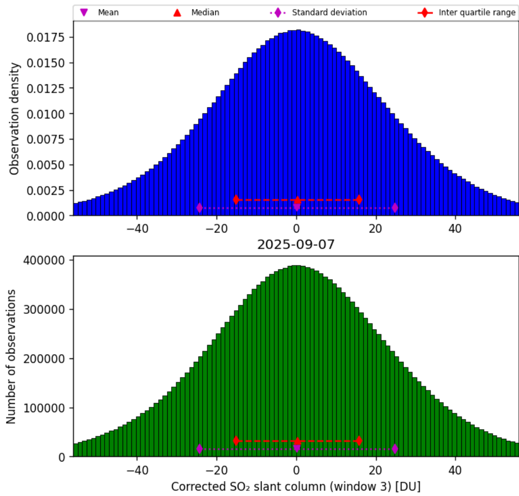
Figure 73: Histogram of “Corrected SO 2 slant column (window 3)” for 2025-09-06 to 2025-09-08
