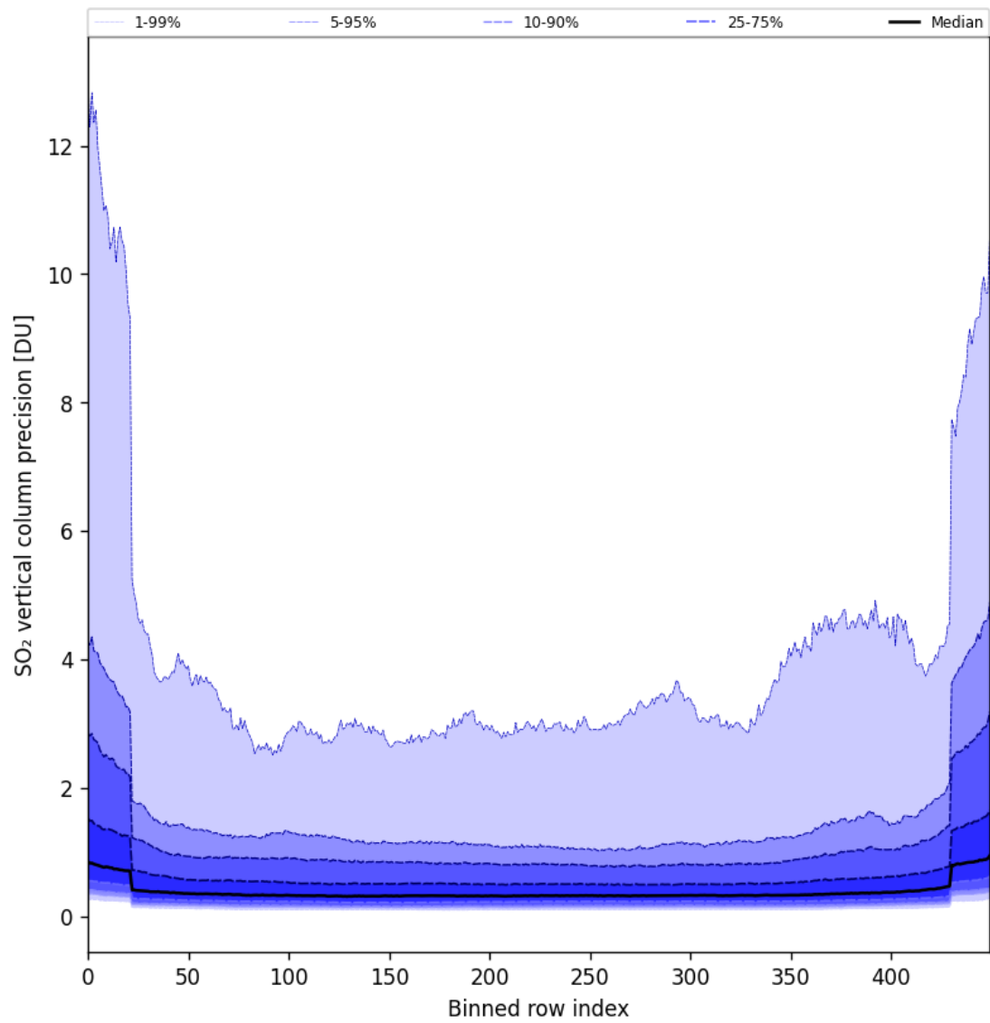
Figure 85: Along track statistics of “SO 2 vertical column precision” for 2025-09-06 to 2025-09-08
