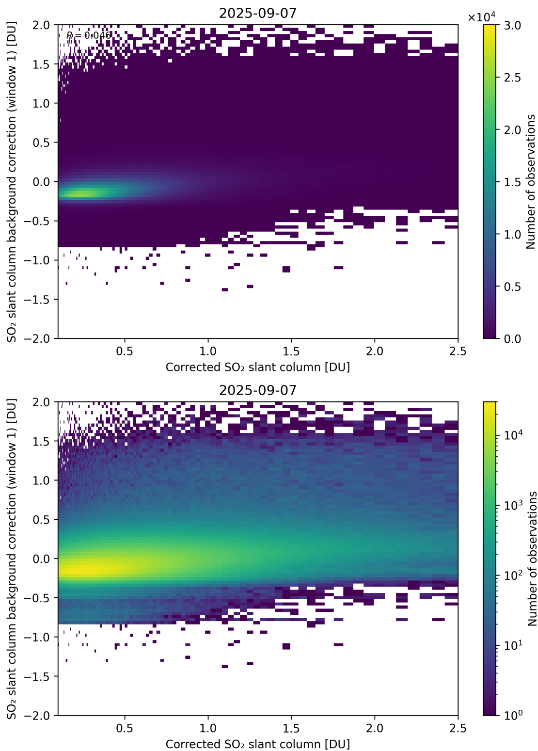
Figure 226: Scatter density plot of “Corrected SO 2 slant column” against “SO 2 slant column background correction (window 1)” for 2025-09-06 to 2025-09-08.
