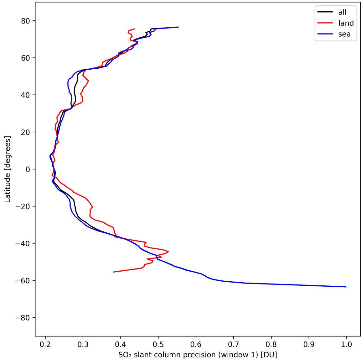
Figure 38: Zonal average of “SO 2 slant column precision (window 1)” for 2025-09-06 to 2025-09-08.
