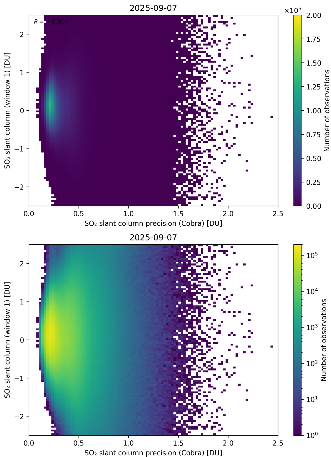
Figure 208: Scatter density plot of “SO 2 slant column precision (Cobra)” against “SO 2 slant column (window 1)” for 2025-09-06 to 2025-09-08.
