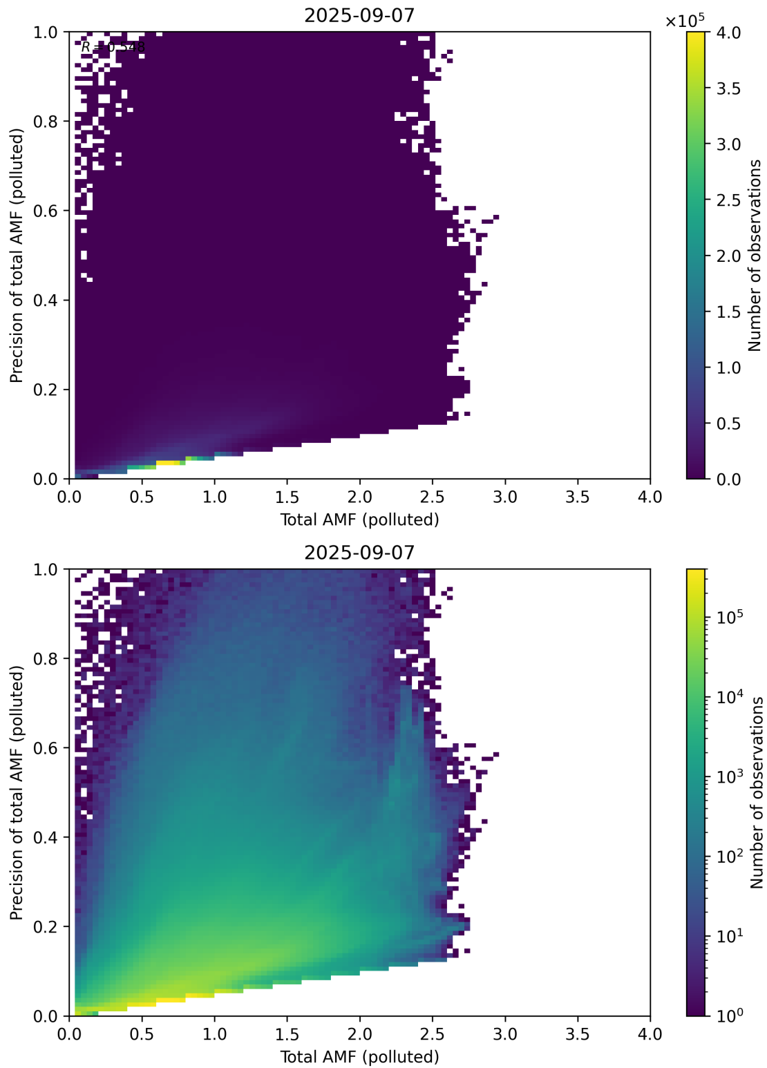
Figure 322: Scatter density plot of “Total AMF (polluted)” against “Precision of total AMF (polluted)” for 2025-09-06 to 2025-09-08.
