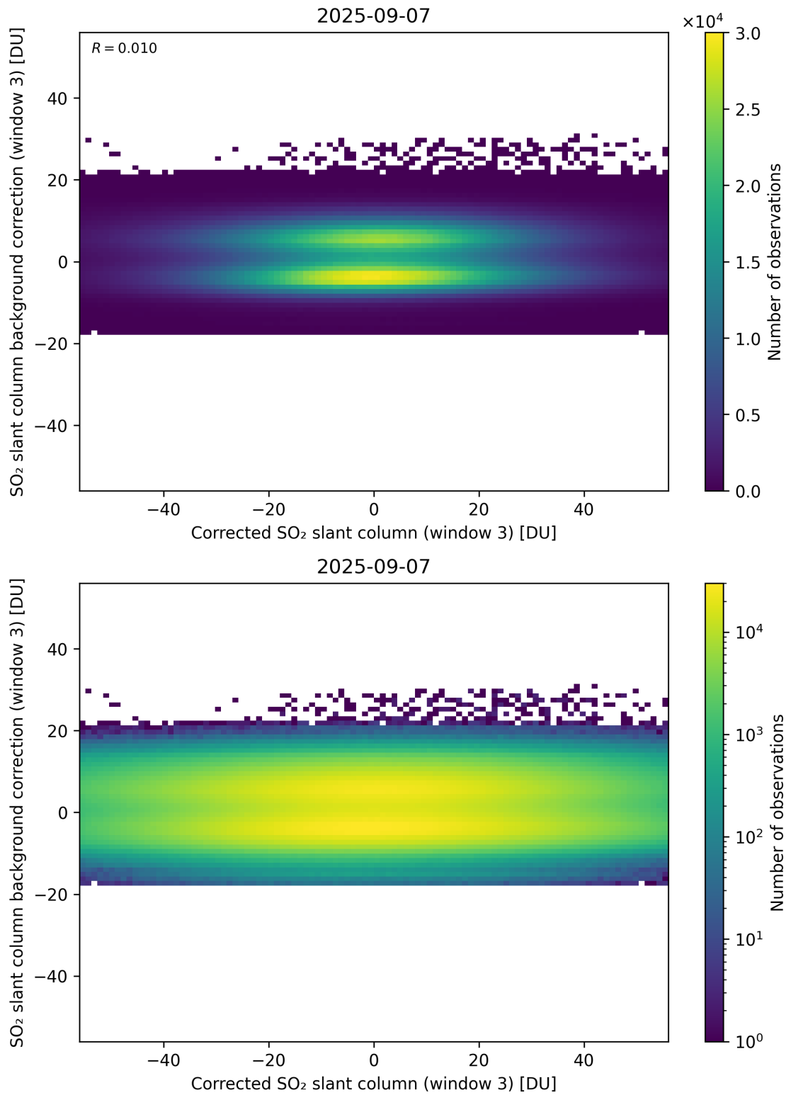
Figure 255: Scatter density plot of “Corrected SO 2 slant column (window 3)” against “SO 2 slant column background correction (window 3)” for 2025-09-06 to 2025-09-08.
