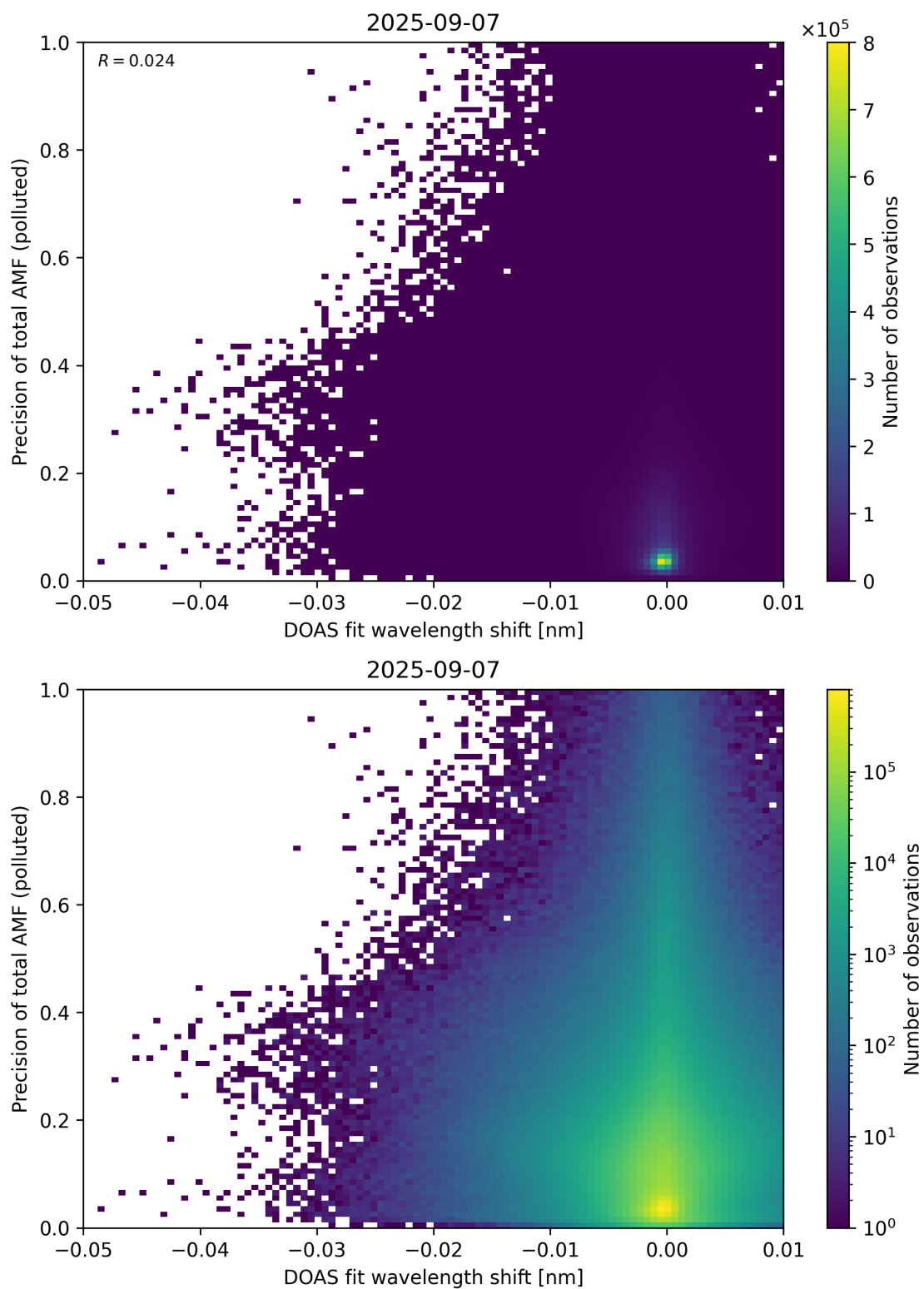
Figure 142: Scatter density plot of “DOAS fit wavelength shift” against “Precision of total AMF (polluted)” for 2025-09-06 to 2025-09-08.
