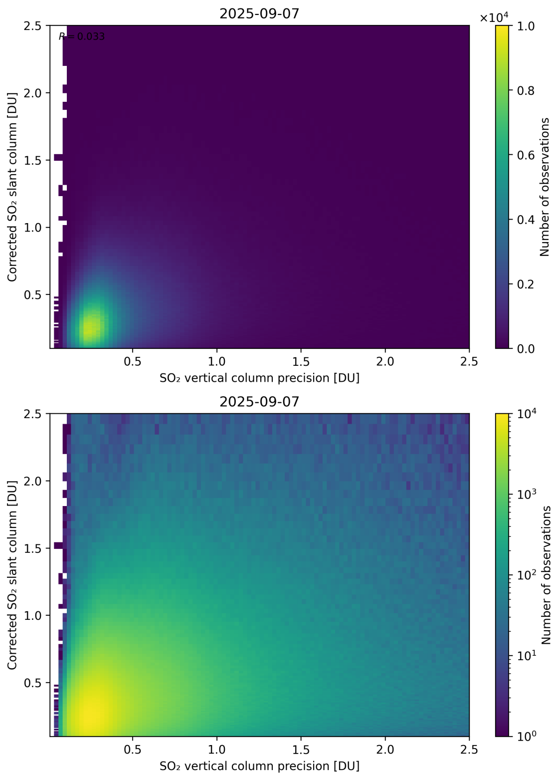
Figure 338: Scatter density plot of “SO 2 vertical column precision” against “Corrected SO 2 slant column” for 2025-09-06 to 2025-09-08.
