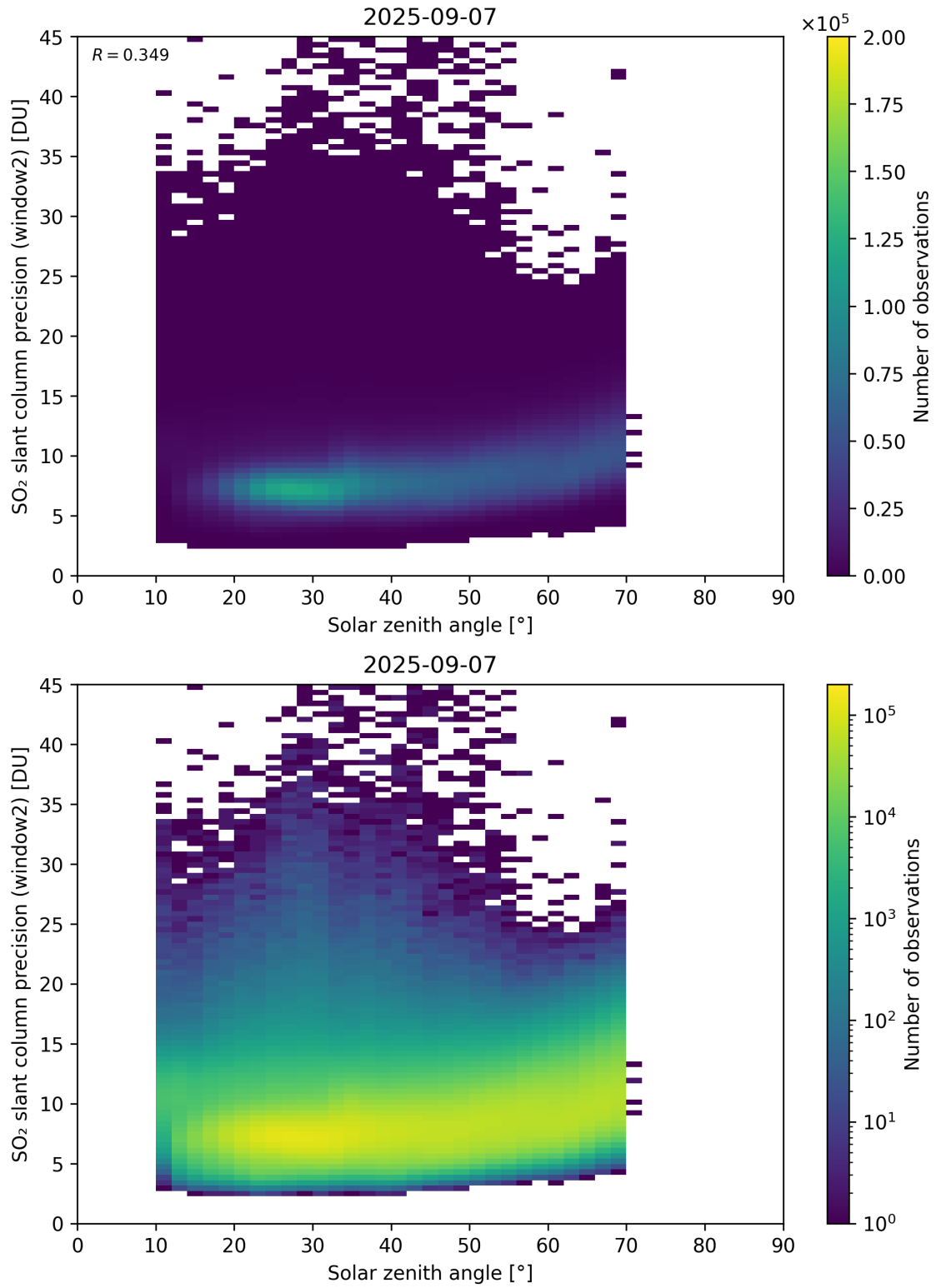
Figure 186: Scatter density plot of “Solar zenith angle” against “SO 2 slant column precision (window2)” for 2025-09-06 to 2025-09-08.
