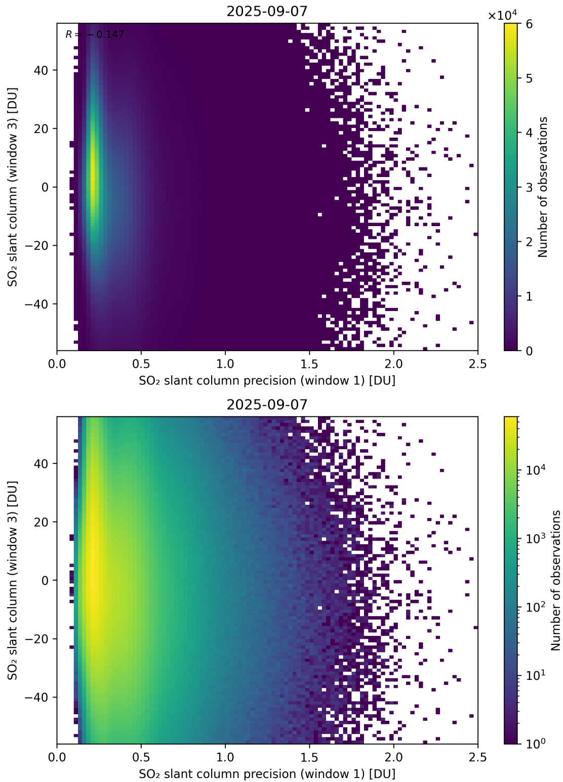
Figure 278: Scatter density plot of “SO 2 slant column precision (window 1)” against “SO 2 slant column (window 3)” for 2025-09-06 to 2025-09-08.
