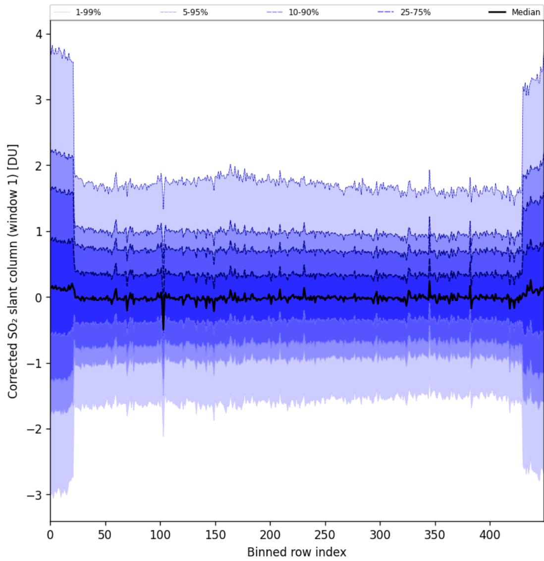
Figure 91: Along track statistics of “Corrected SO 2 slant column (window 1)” for 2025-09-06 to 2025-09-08
