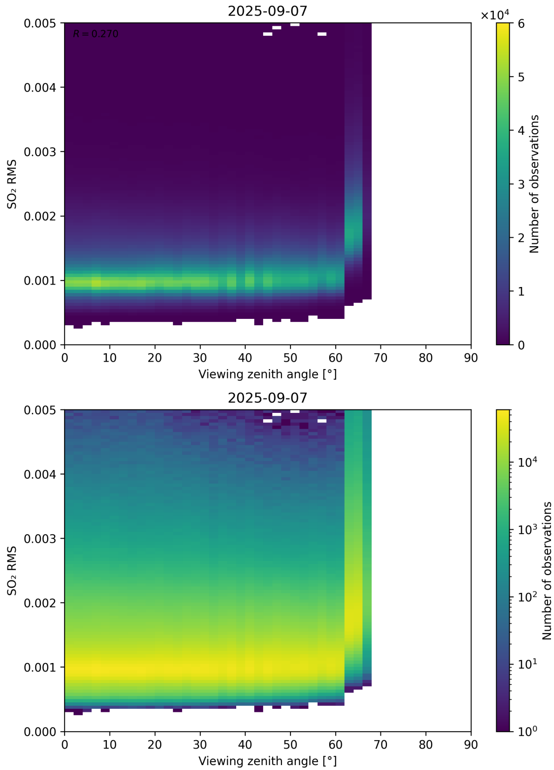
Figure 367: Scatter density plot of “Viewing zenith angle” against “SO 2 RMS” for 2025-09-06 to 2025-09-08.
