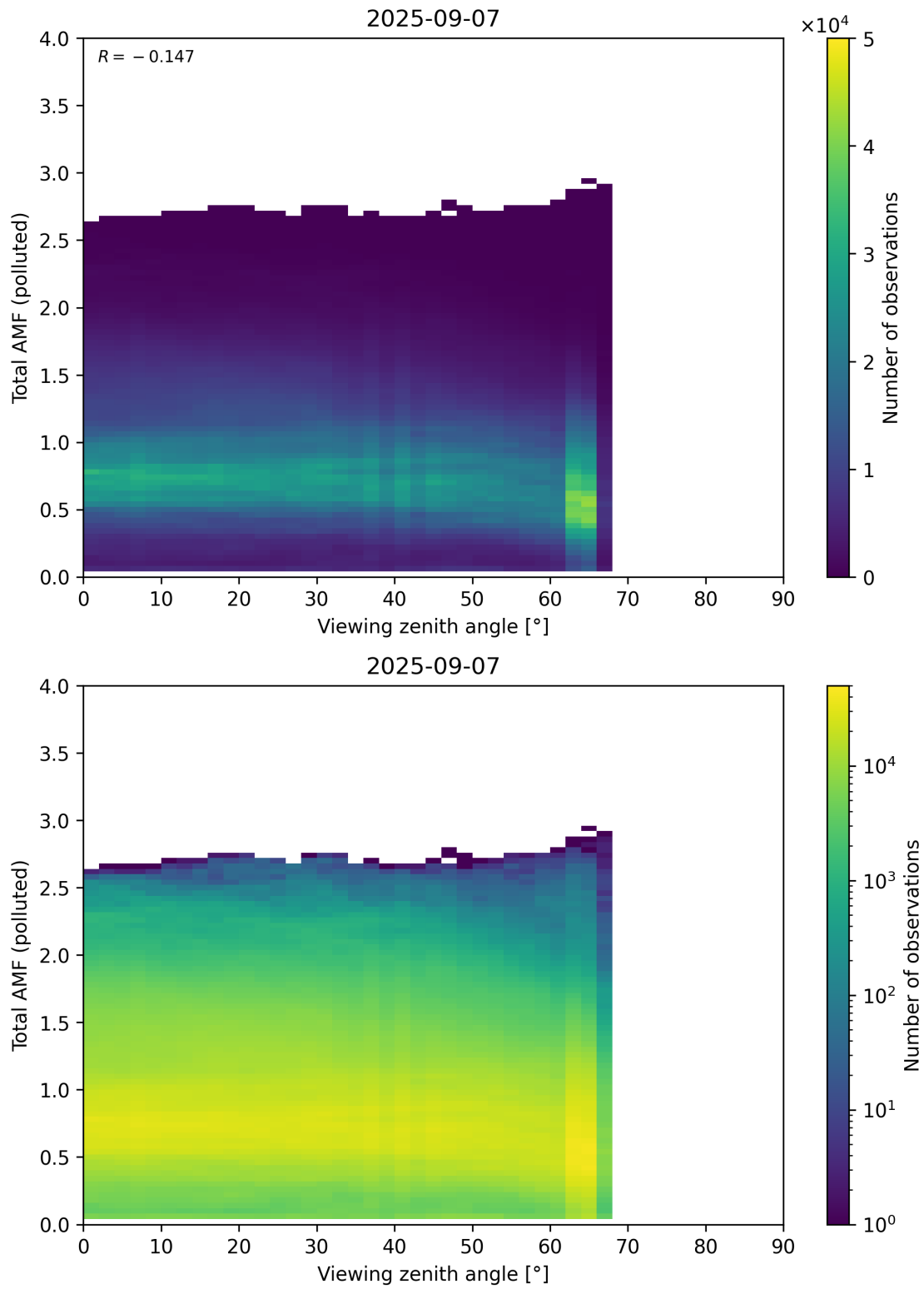
Figure 381: Scatter density plot of “Viewing zenith angle” against “Total AMF (polluted)” for 2025-09-06 to 2025-09-08.
