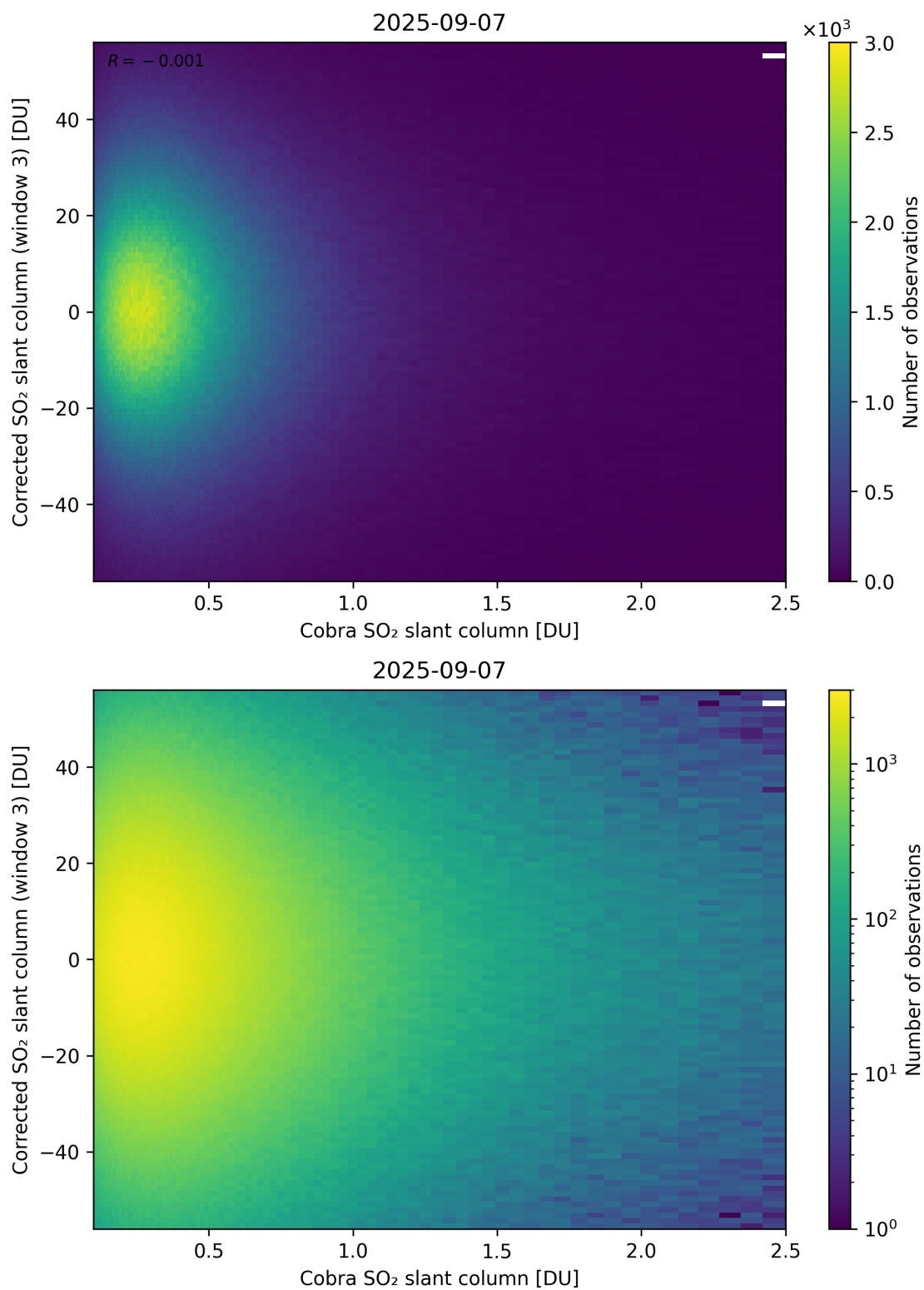
Figure 218: Scatter density plot of “Cobra SO 2 slant column” against “Corrected SO 2 slant column (window 3)” for 2025-09-06 to 2025-09-08.
