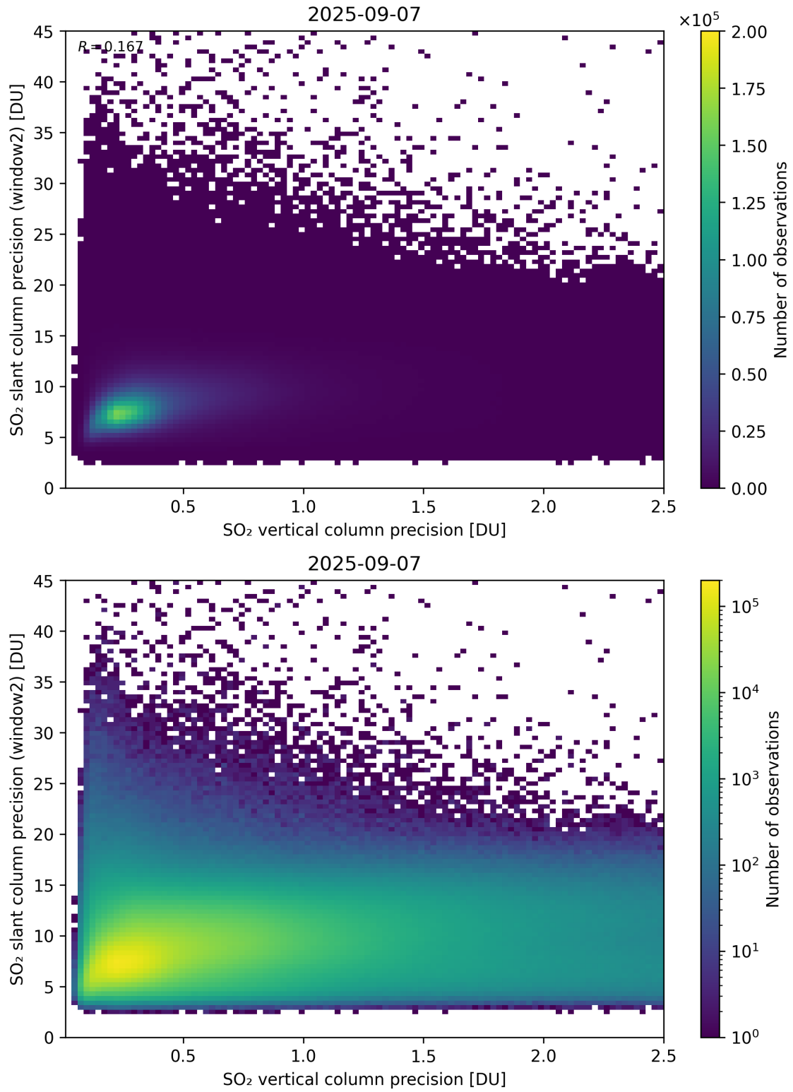
Figure 343: Scatter density plot of “SO 2 vertical column precision” against “SO 2 slant column precision (window2)” for 2025-09-06 to 2025-09-08.
