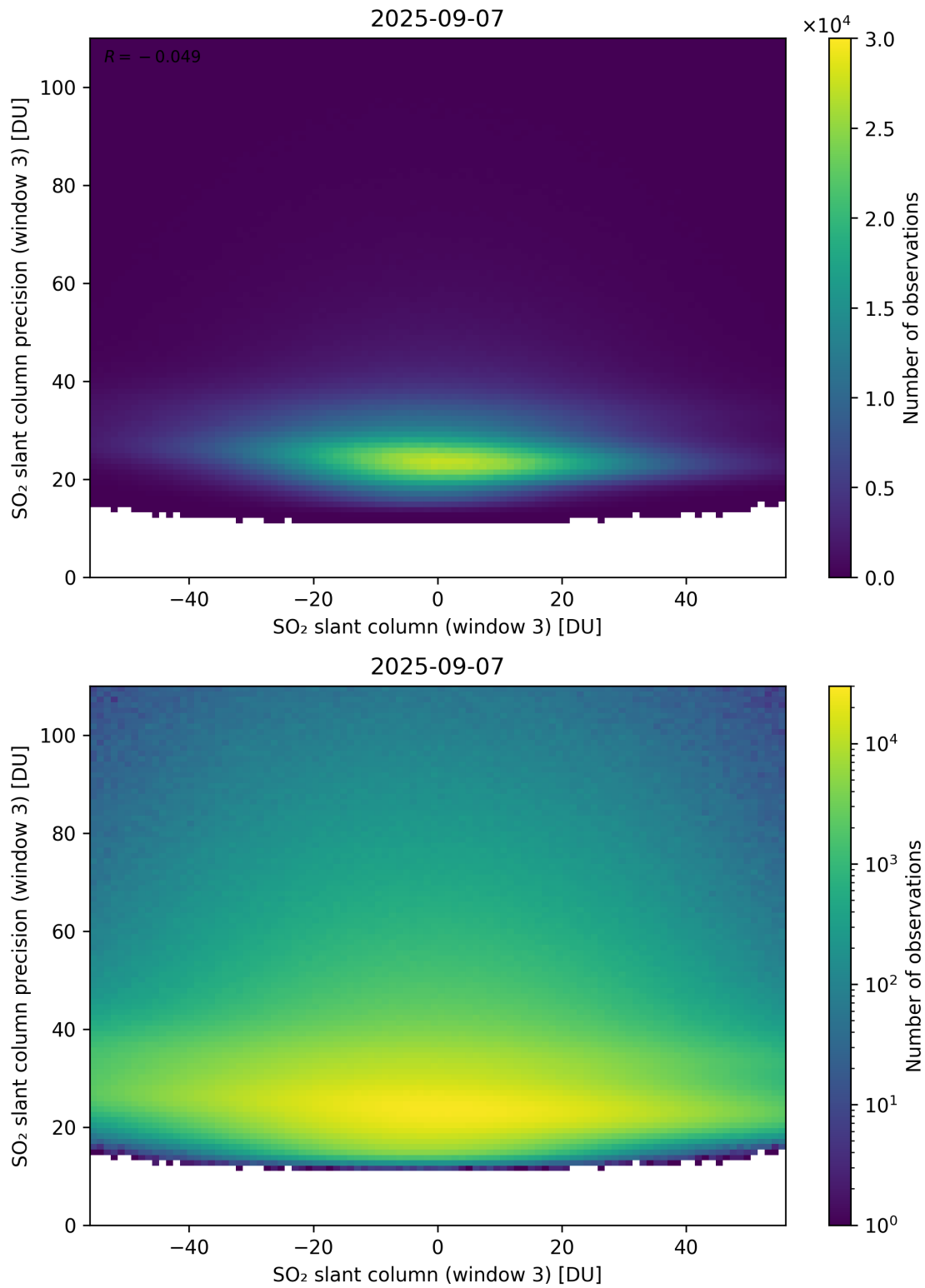
Figure 317: Scatter density plot of “SO 2 slant column (window 3)” against “SO 2 slant column precision (window 3)” for 2025-09-06 to 2025-09-08.
