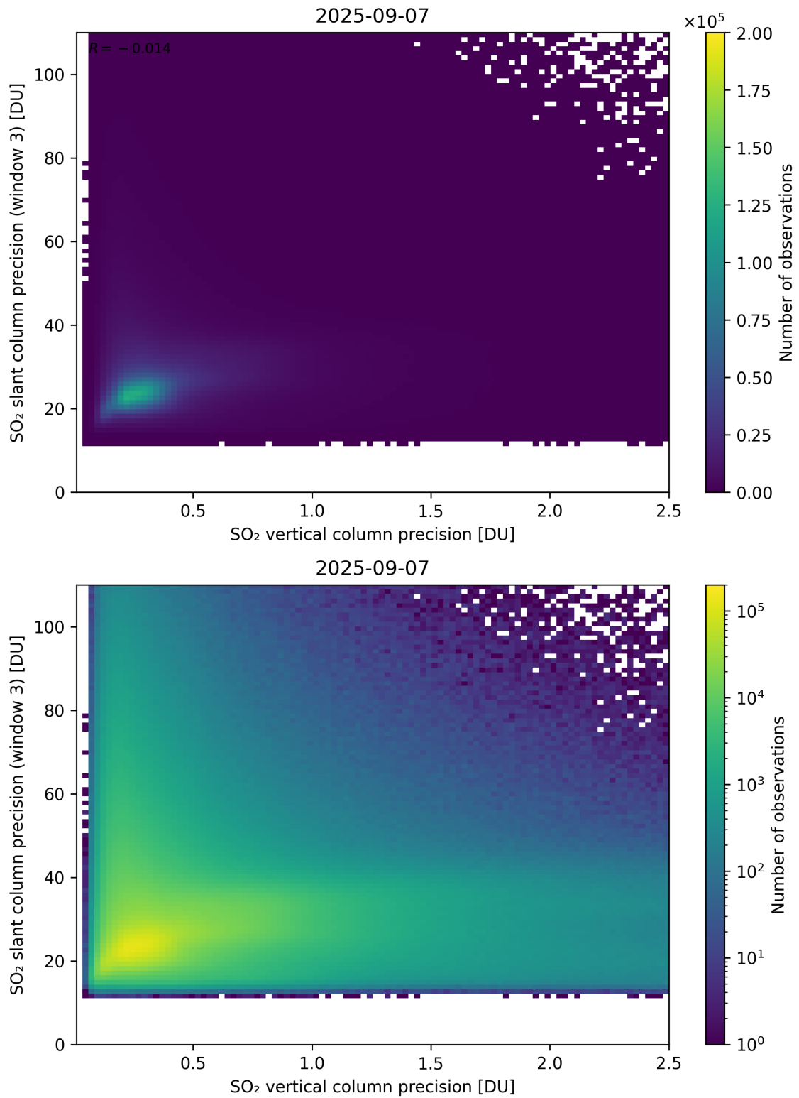
Figure 345: Scatter density plot of “SO 2 vertical column precision” against “SO 2 slant column precision (window 3)” for 2025-09-06 to 2025-09-08.
