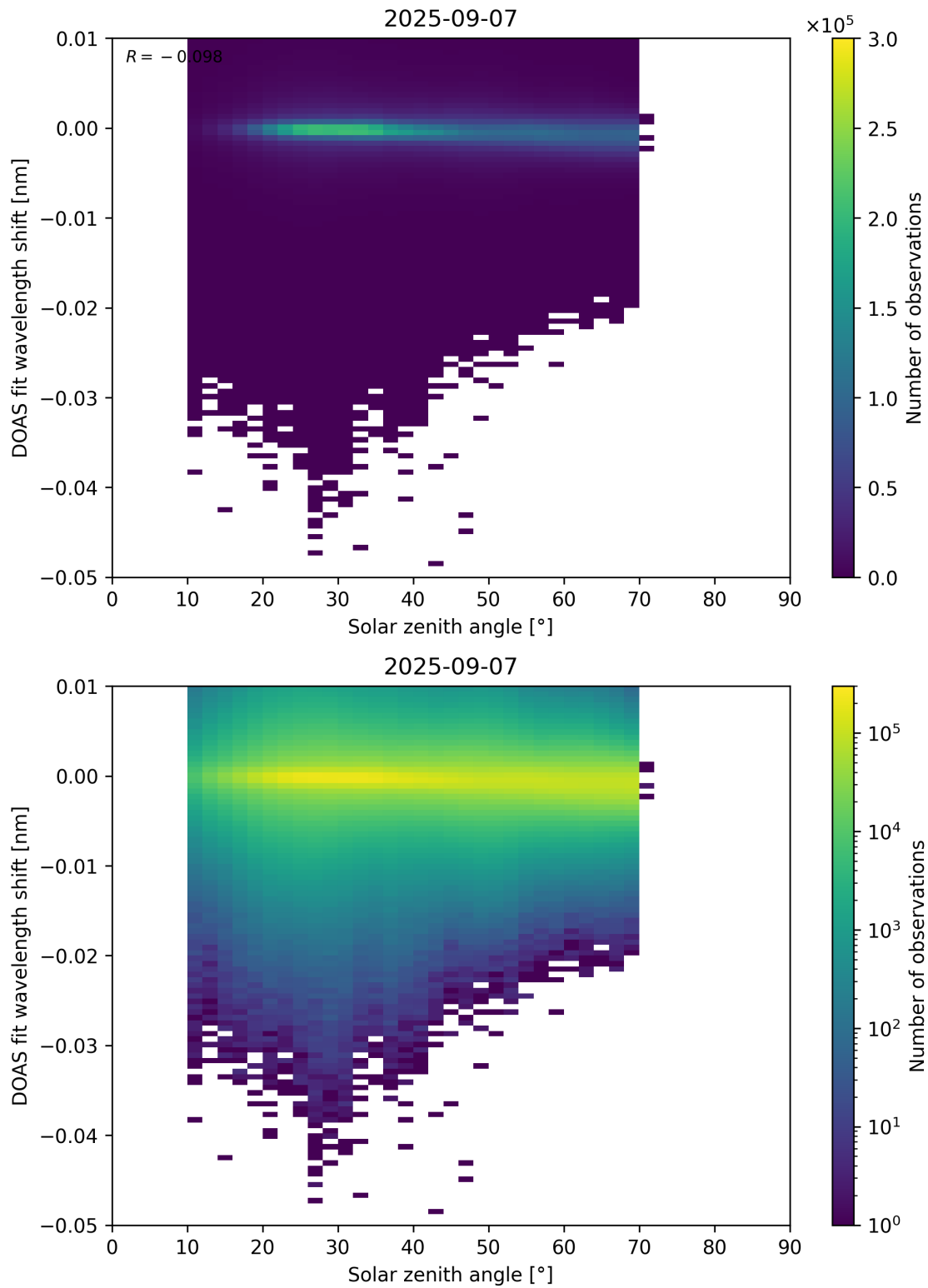
Figure 174: Scatter density plot of “Solar zenith angle” against “DOAS fit wavelength shift” for 2025-09-06 to 2025-09-08.
