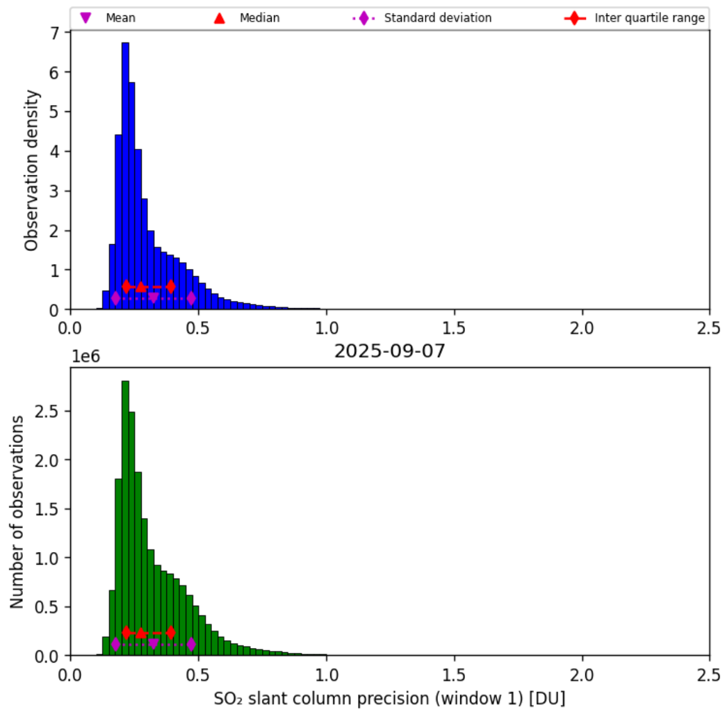
Figure 64: Histogram of “SO 2 slant column precision (window 1)” for 2025-09-06 to 2025-09-08
