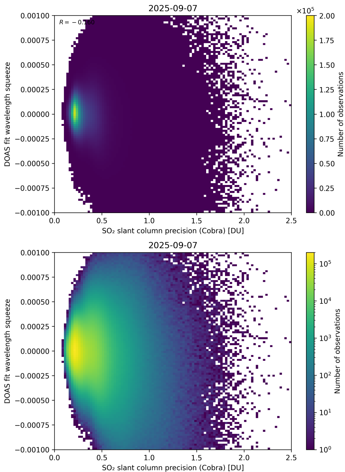
Figure 203: Scatter density plot of “SO 2 slant column precision (Cobra)” against “DOAS fit wavelength squeeze” for 2025-09-06 to 2025-09-08.
