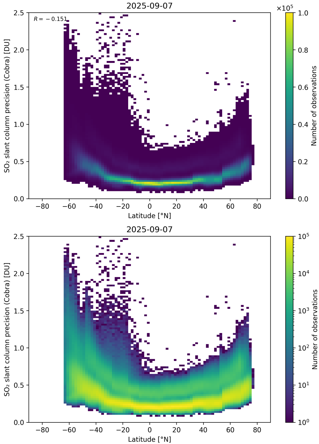
Figure 158: Scatter density plot of “Latitude” against “SO 2 slant column precision (Cobra)” for 2025-09-06 to 2025-09-08.
