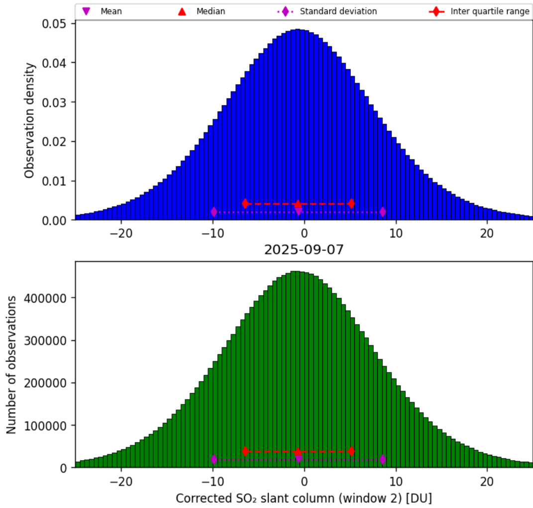
Figure 69: Histogram of “Corrected SO 2 slant column (window 2)” for 2025-09-06 to 2025-09-08
