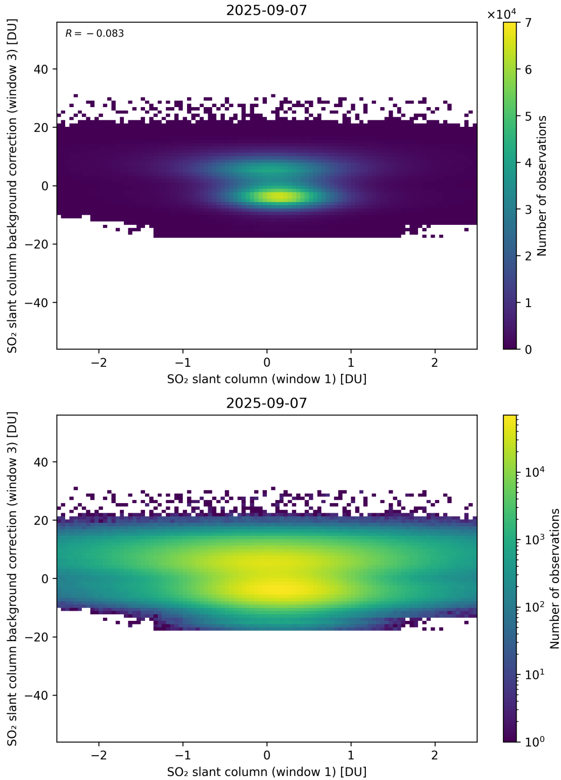
Figure 264: Scatter density plot of “SO 2 slant column (window 1)” against “SO 2 slant column background correction (window 3)” for 2025-09-06 to 2025-09-08.
