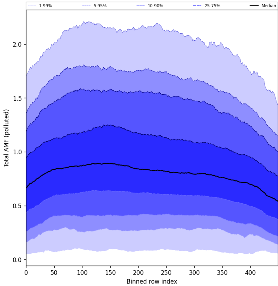
Figure 105: Along track statistics of “Total AMF (polluted)” for 2025-09-06 to 2025-09-08
