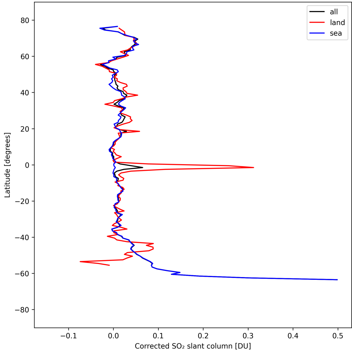
Figure 34: Zonal average of “Corrected SO 2 slant column” for 2025-09-06 to 2025-09-08.
