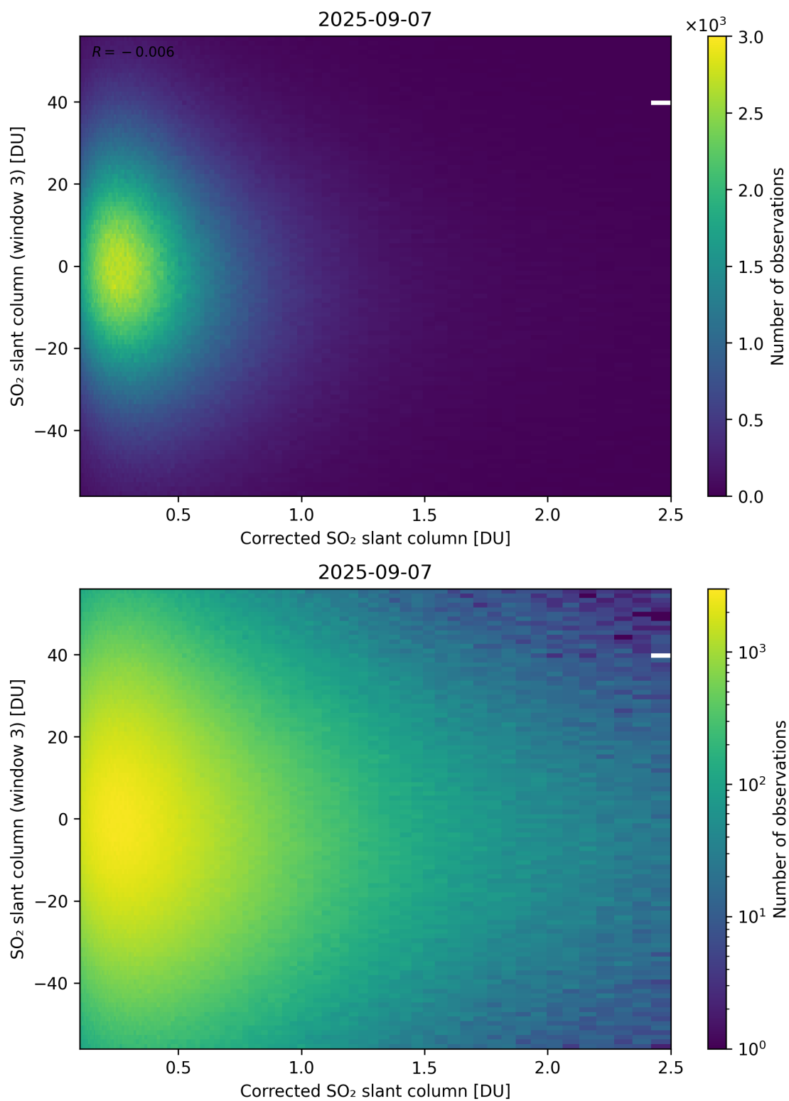
Figure 240: Scatter density plot of “Corrected SO 2 slant column” against “SO 2 slant column (window 3)” for 2025-09-06 to 2025-09-08.
