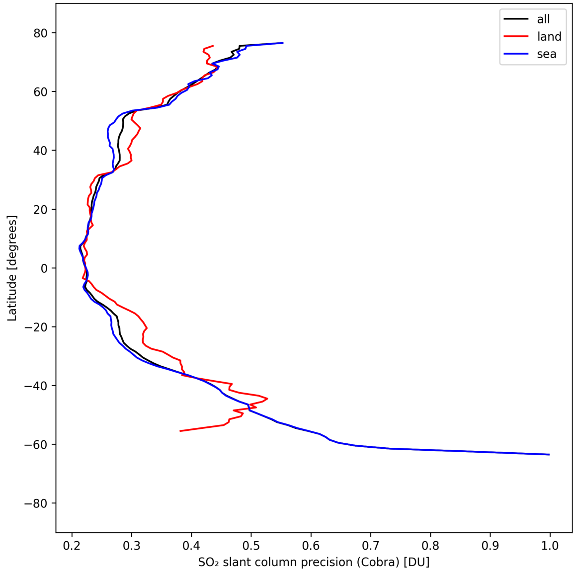
Figure 36: Zonal average of “SO 2 slant column precision (Cobra)” for 2025-09-06 to 2025-09-08.
