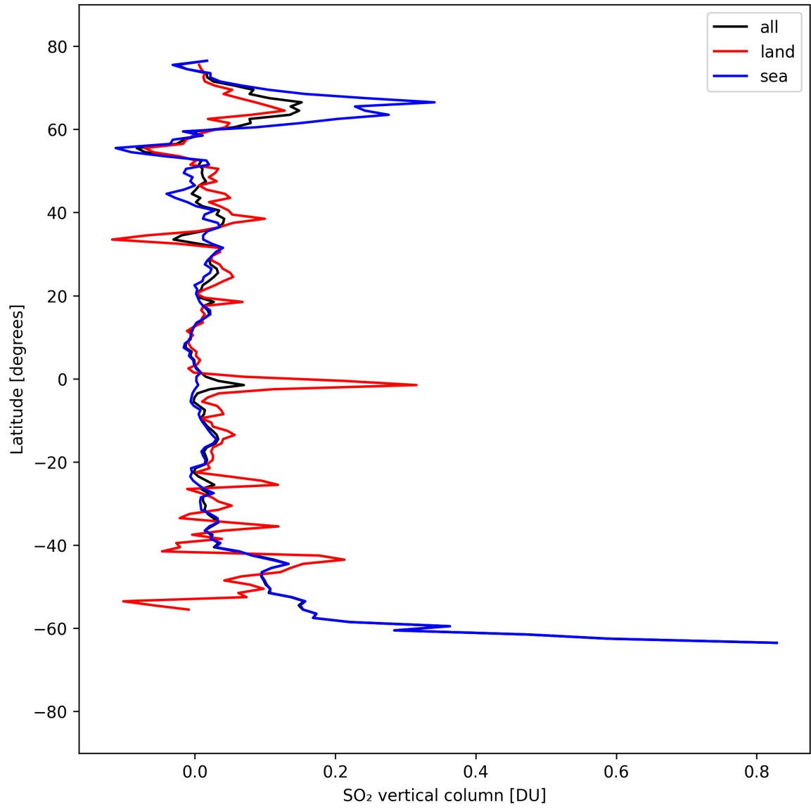
Figure 32: Zonal average of “SO 2 vertical column” for 2025-09-06 to 2025-09-08.
