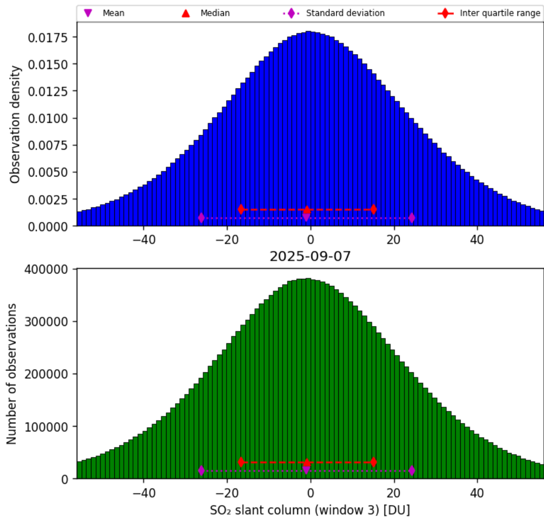
Figure 71: Histogram of “SO 2 slant column (window 3)” for 2025-09-06 to 2025-09-08
