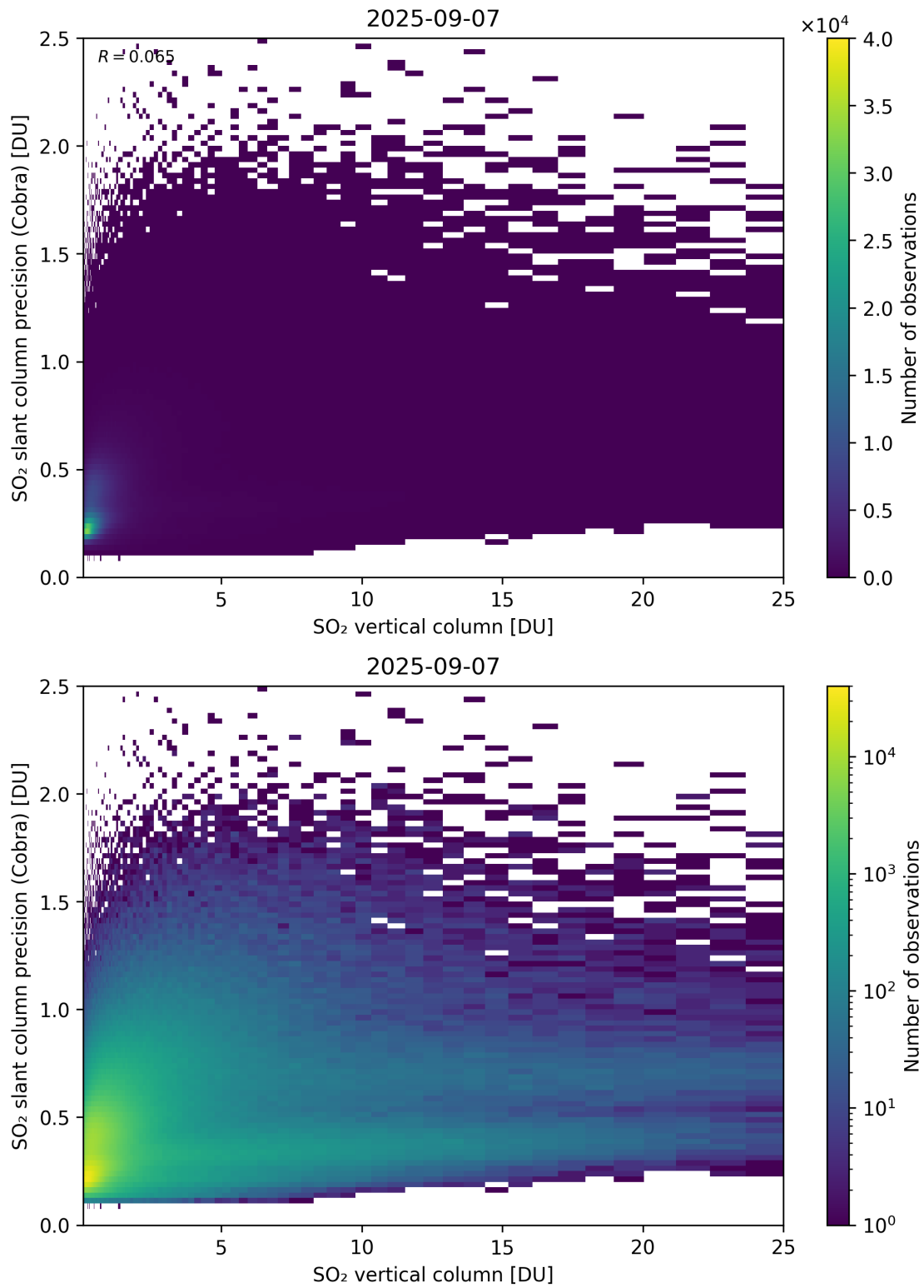
Figure 350: Scatter density plot of “SO 2 vertical column” against “SO 2 slant column precision (Cobra)” for 2025-09-06 to 2025-09-08.
