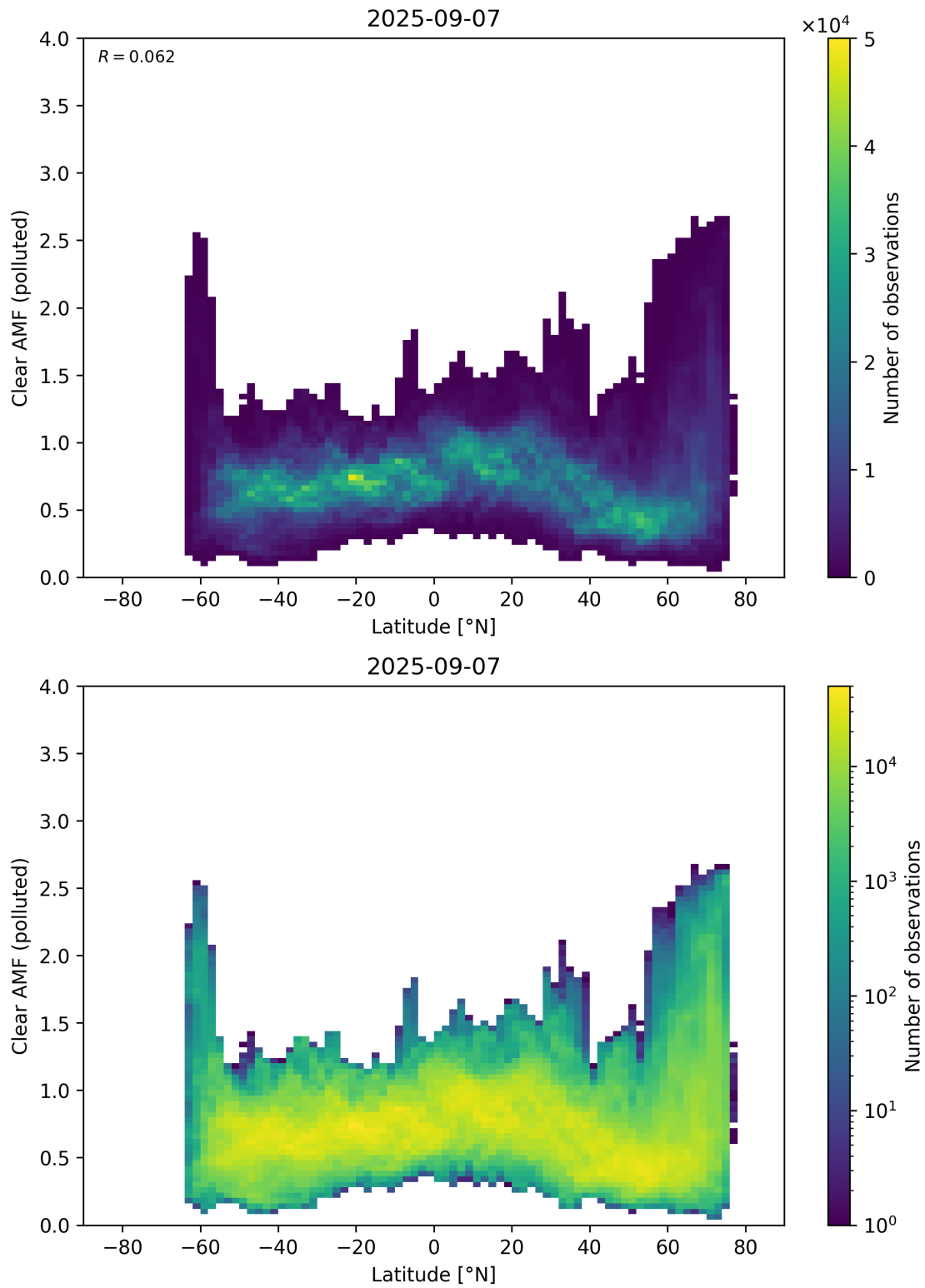
Figure 156: Scatter density plot of “Latitude” against “Clear AMF (polluted)” for 2025-09-06 to 2025-09-08.
