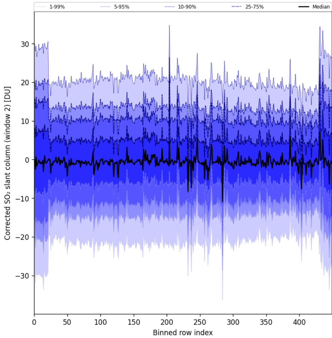
Figure 95: Along track statistics of “Corrected SO 2 slant column (window 2)” for 2025-09-06 to 2025-09-08
