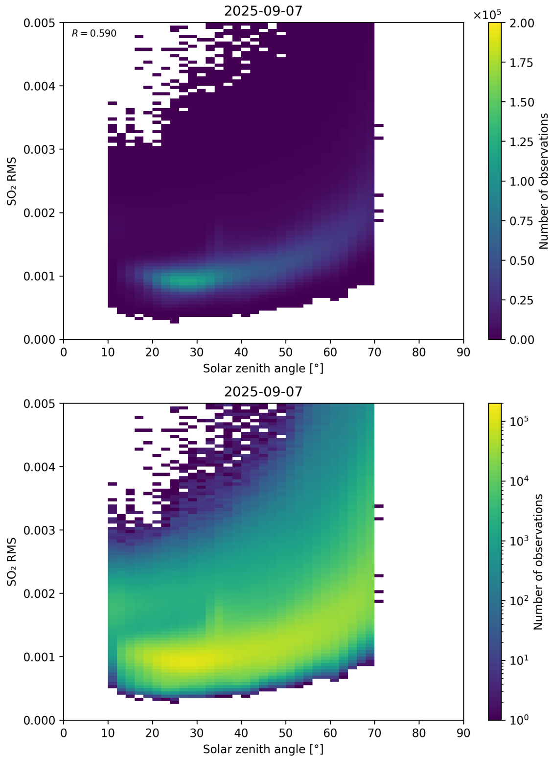
Figure 176: Scatter density plot of “Solar zenith angle” against “SO 2 RMS” for 2025-09-06 to 2025-09-08.
