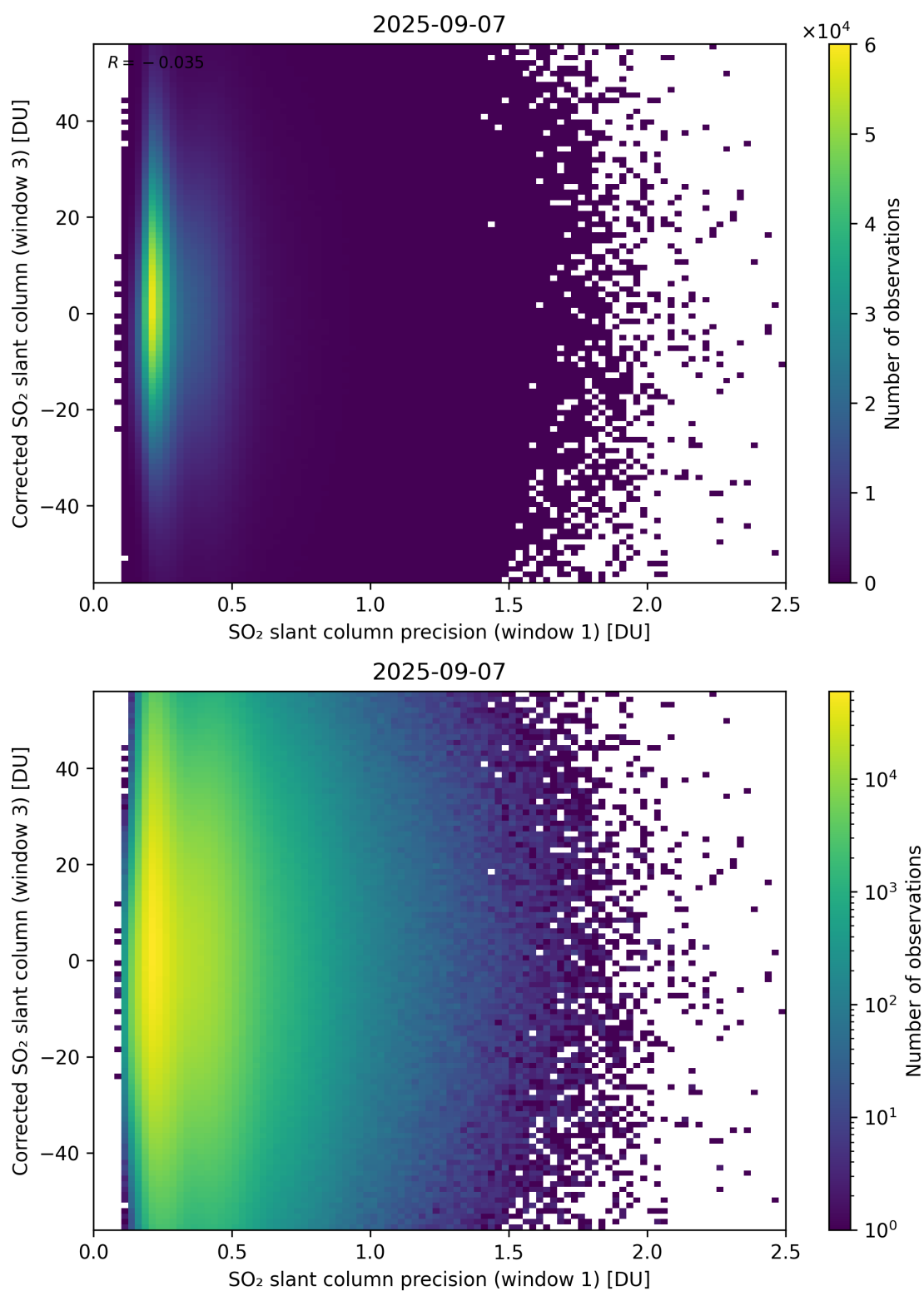
Figure 276: Scatter density plot of “SO 2 slant column precision (window 1)” against “Corrected SO 2 slant column (window 3)” for 2025-09-06 to 2025-09-08.
