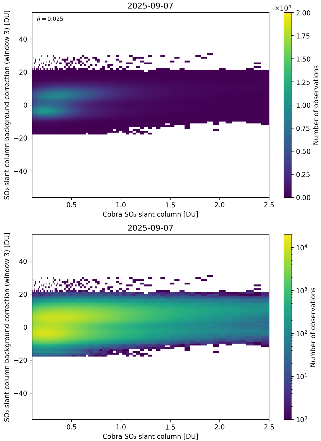
Figure 195: Scatter density plot of “Cobra SO 2 slant column” against “SO 2 slant column background correction (window 3)” for 2025-09-06 to 2025-09-08.
