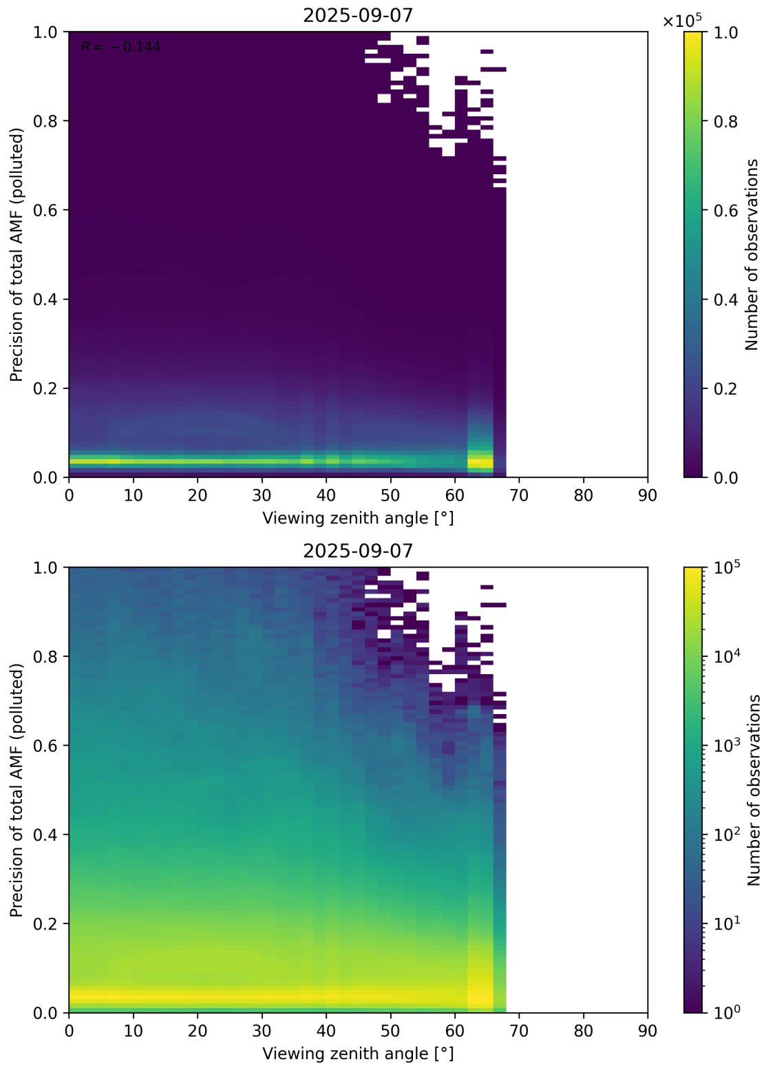
Figure 382: Scatter density plot of “Viewing zenith angle” against “Precision of total AMF (polluted)” for 2025-09-06 to 2025-09-08.
