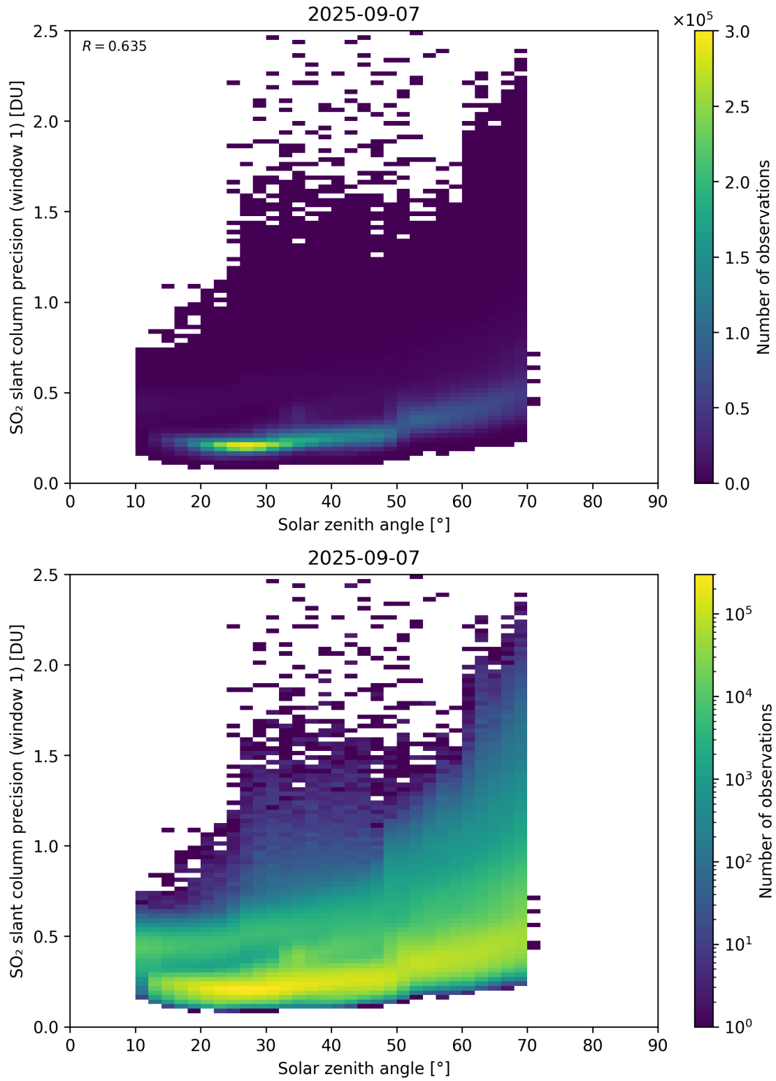
Figure 185: Scatter density plot of “Solar zenith angle” against “SO 2 slant column precision (window 1)” for 2025-09-06 to 2025-09-08.
