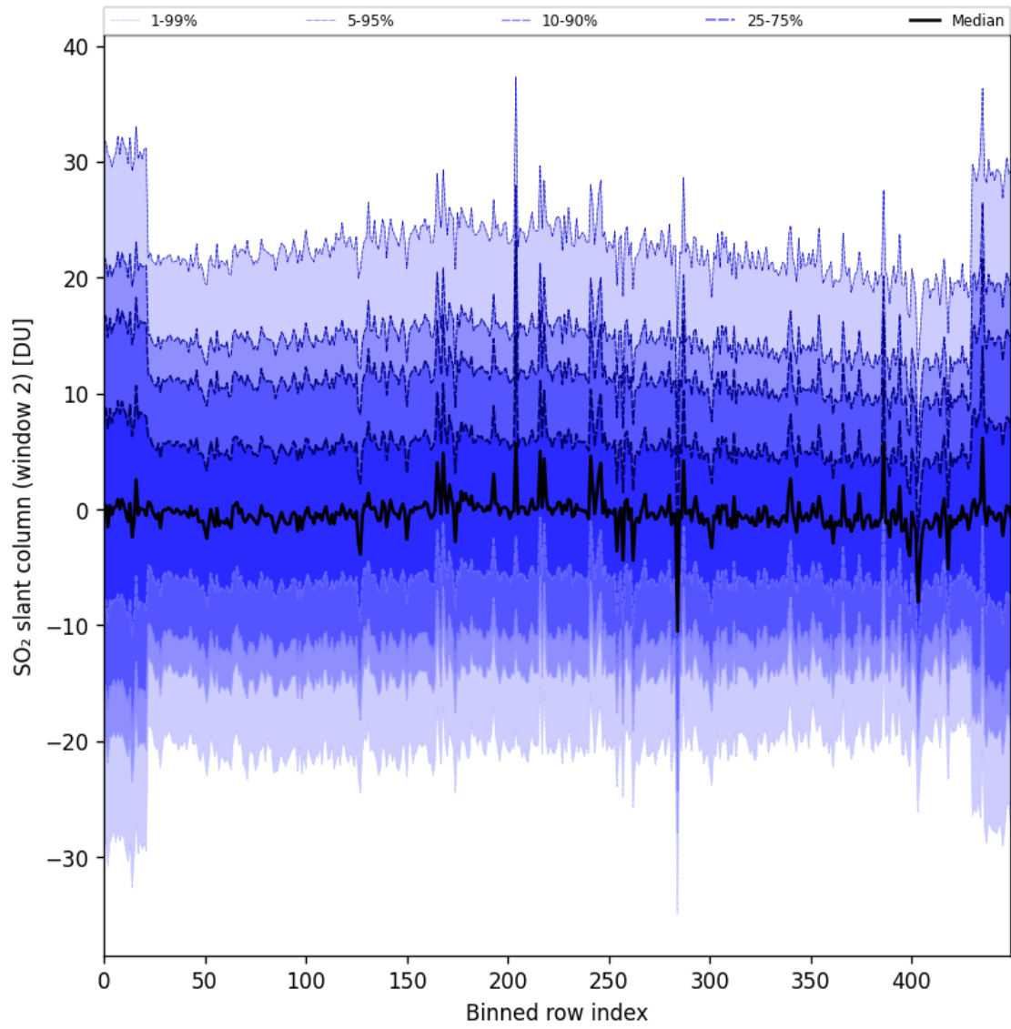
Figure 93: Along track statistics of “SO 2 slant column (window 2)” for 2025-09-06 to 2025-09-08
