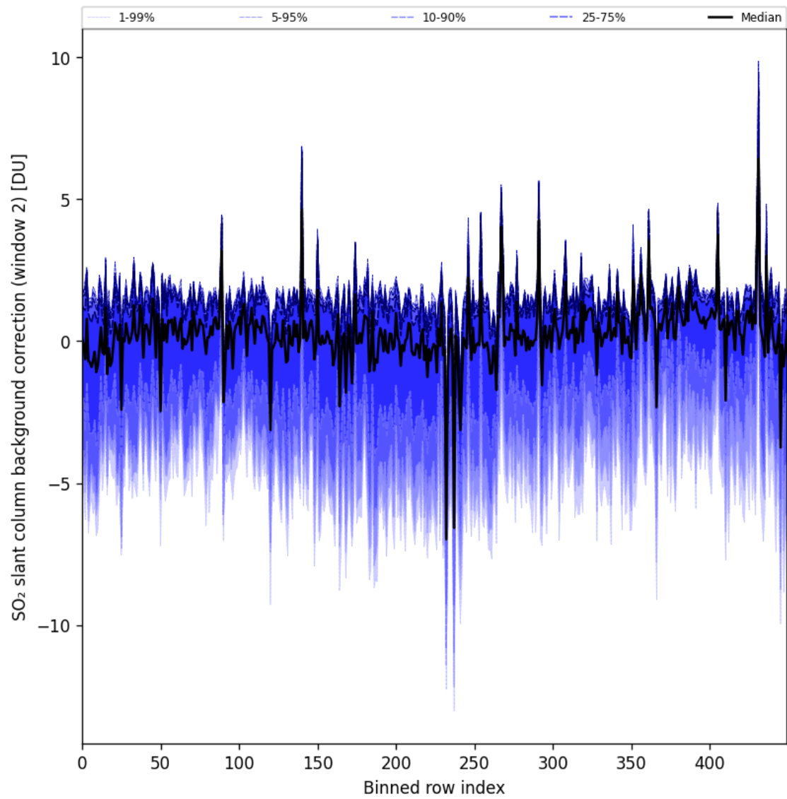
Figure 96: Along track statistics of “SO 2 slant column background correction (window 2)” for 2025-09-06 to 2025-09-08
