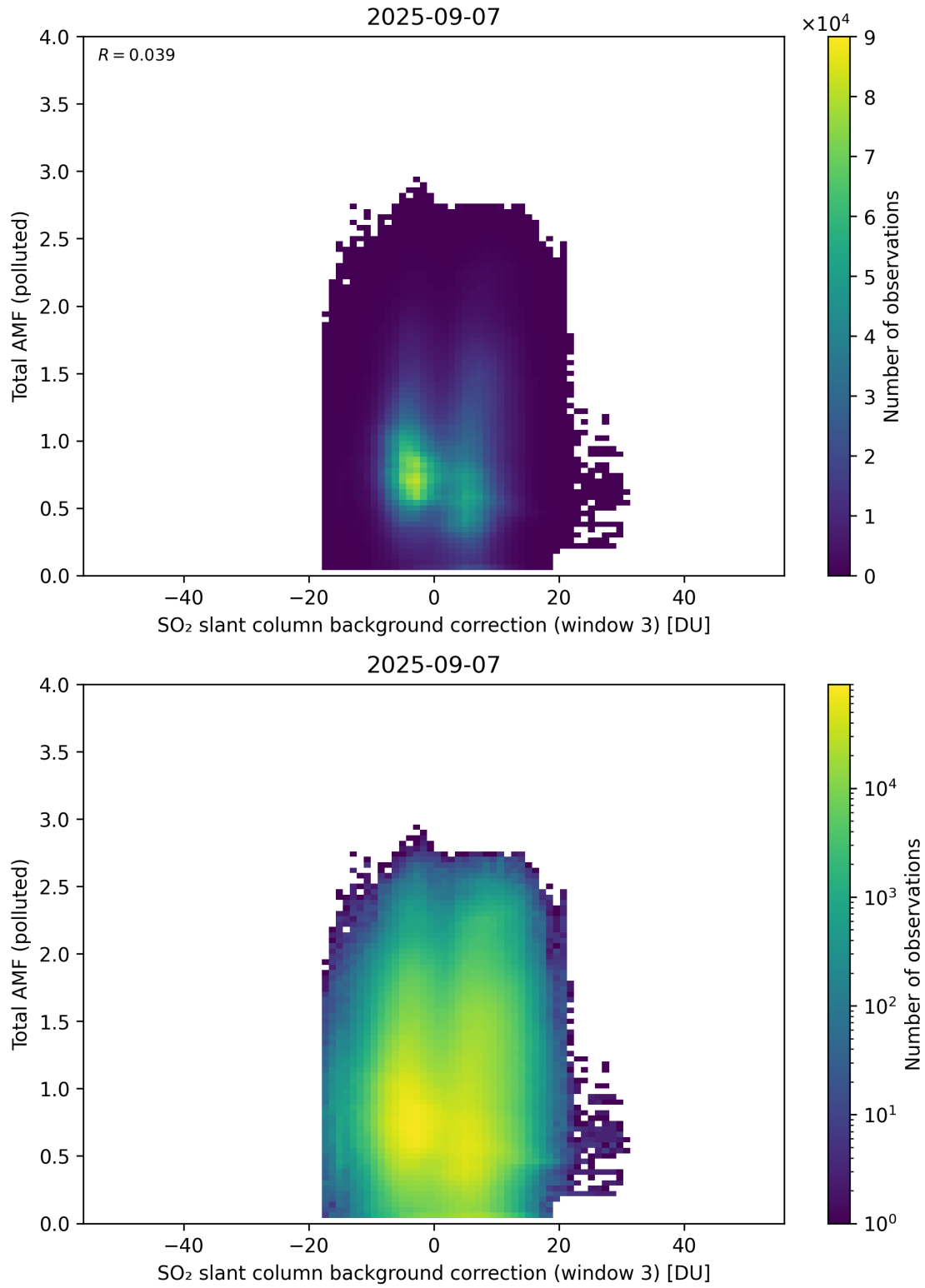
Figure 136: Scatter density plot of “SO 2 slant column background correction (window 3)” against “Total AMF (polluted)” for 2025-09-06 to 2025-09-08.
