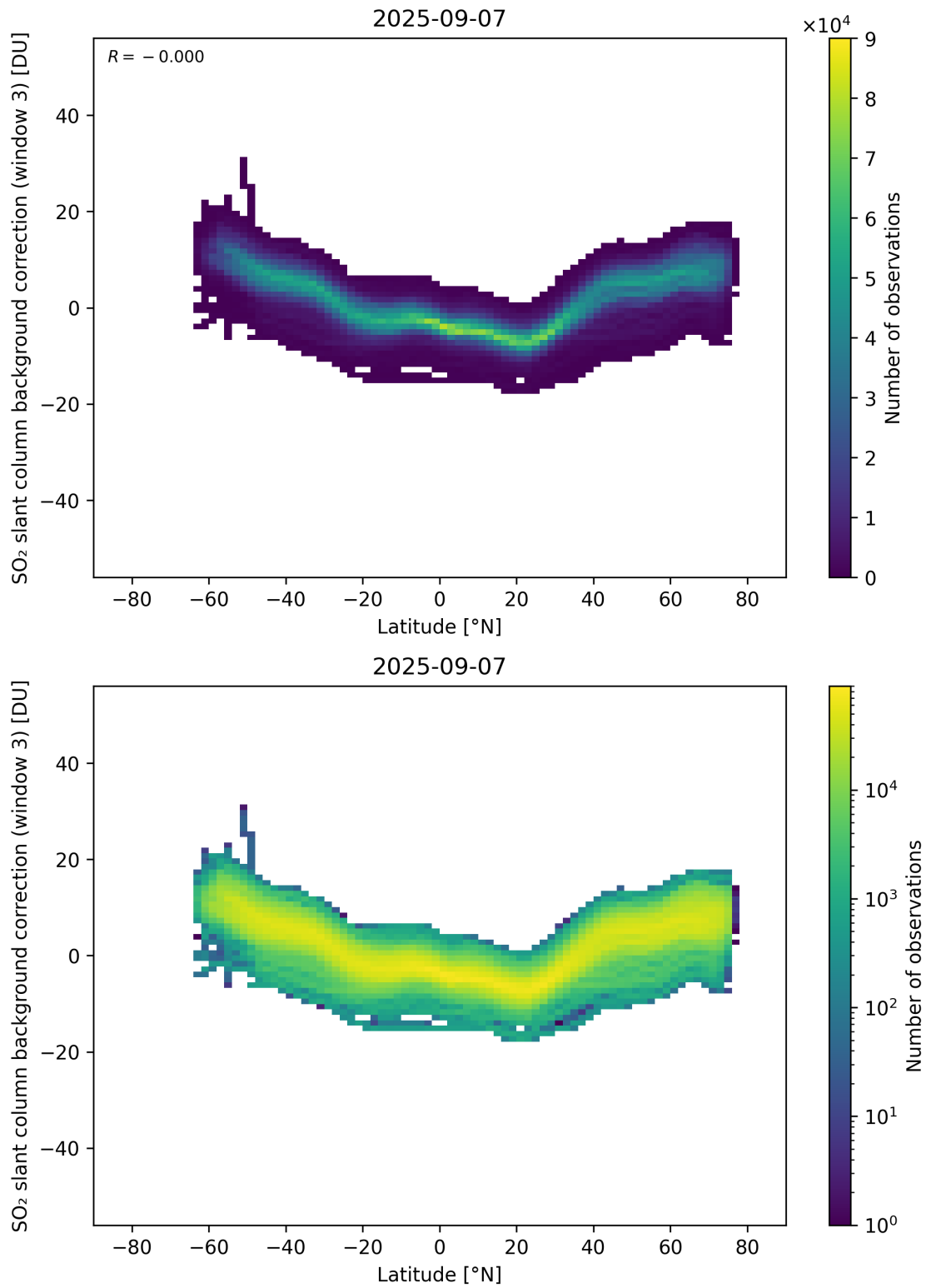
Figure 152: Scatter density plot of “Latitude” against “SO 2 slant column background correction (window 3)” for 2025-09-06 to 2025-09-08.
