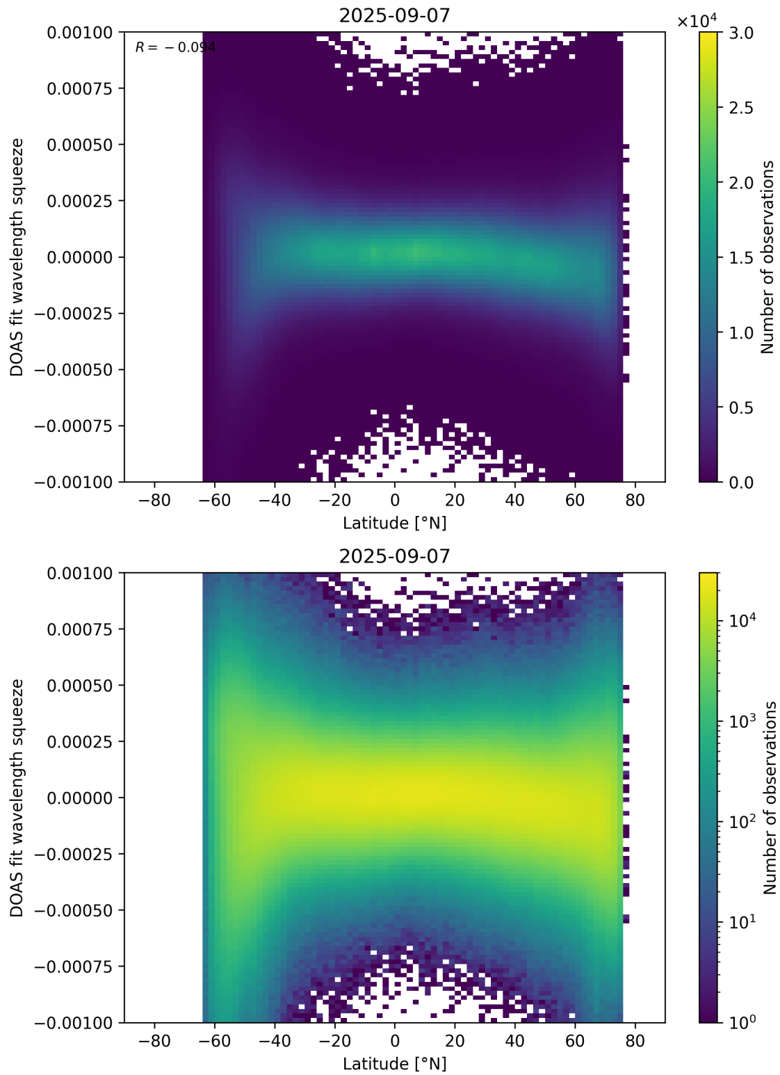
Figure 154: Scatter density plot of “Latitude” against “DOAS fit wavelength squeeze” for 2025-09-06 to 2025-09-08.
