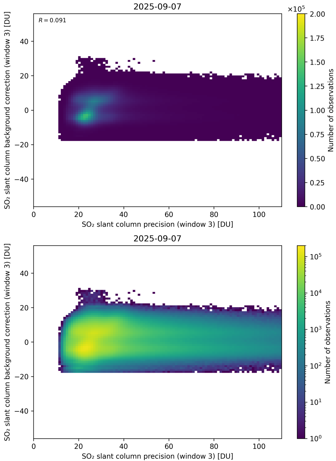
Figure 307: Scatter density plot of “SO 2 slant column precision (window 3)” against “SO 2 slant column background correction (window 3)” for 2025-09-06 to 2025-09-08.
