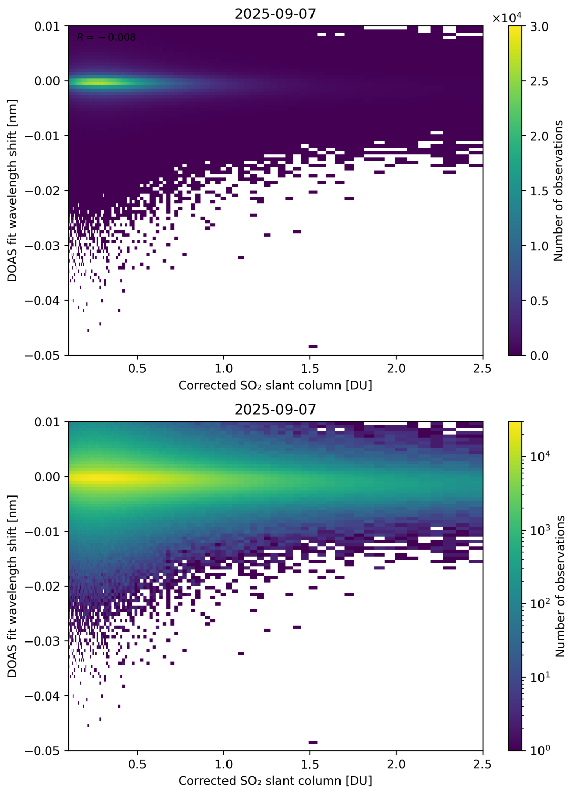
Figure 229: Scatter density plot of “Corrected SO 2 slant column” against “DOAS fit wavelength shift” for 2025-09-06 to 2025-09-08.
