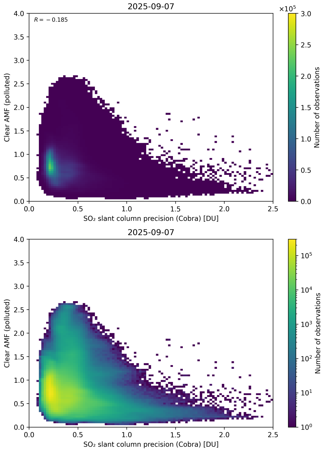
Figure 205: Scatter density plot of “SO 2 slant column precision (Cobra)” against “Clear AMF (polluted)” for 2025-09-06 to 2025-09-08.
