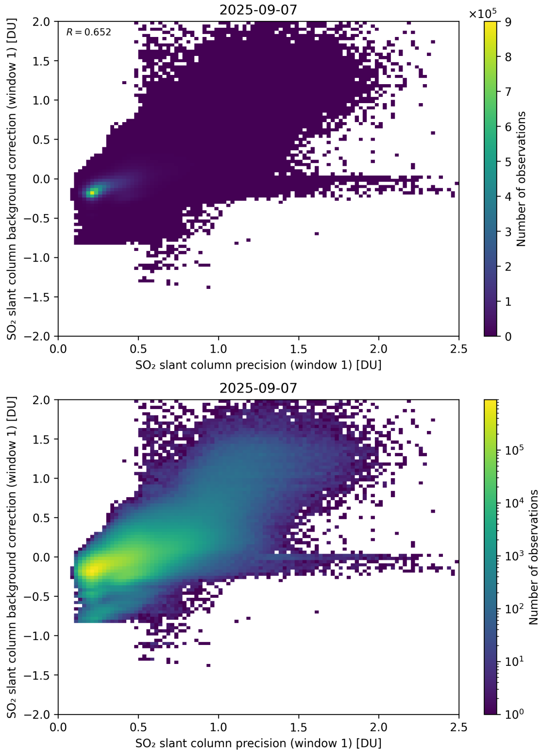
Figure 268: Scatter density plot of “SO 2 slant column precision (window 1)” against “SO 2 slant column background correction (window 1)” for 2025-09-06 to 2025-09-08.
