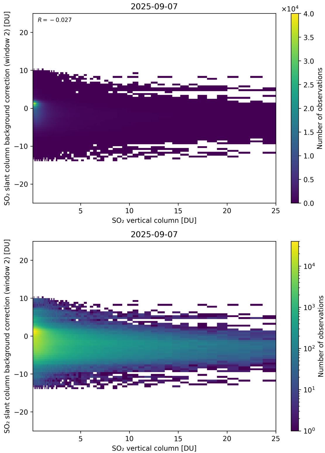
Figure 324: Scatter density plot of “SO 2 vertical column” against “SO 2 slant column background correction (window 2)” for 2025-09-06 to 2025-09-08.
