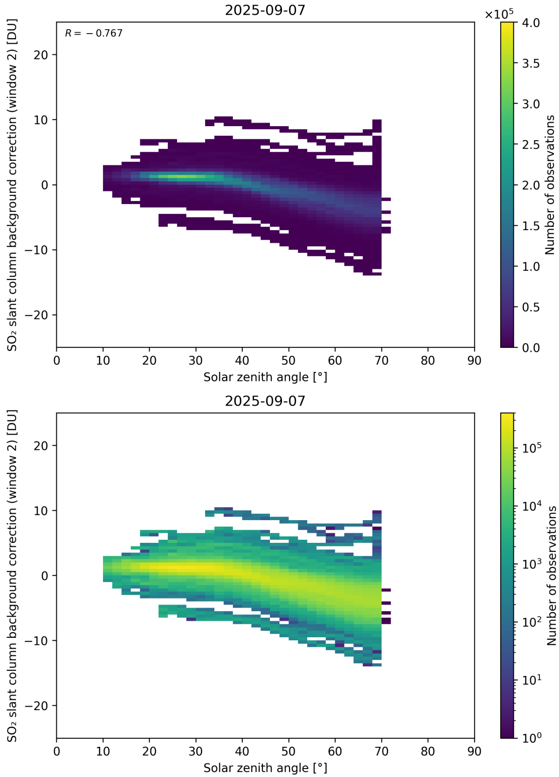
Figure 172: Scatter density plot of “Solar zenith angle” against “SO 2 slant column background correction (window 2)” for 2025-09-06 to 2025-09-08.
