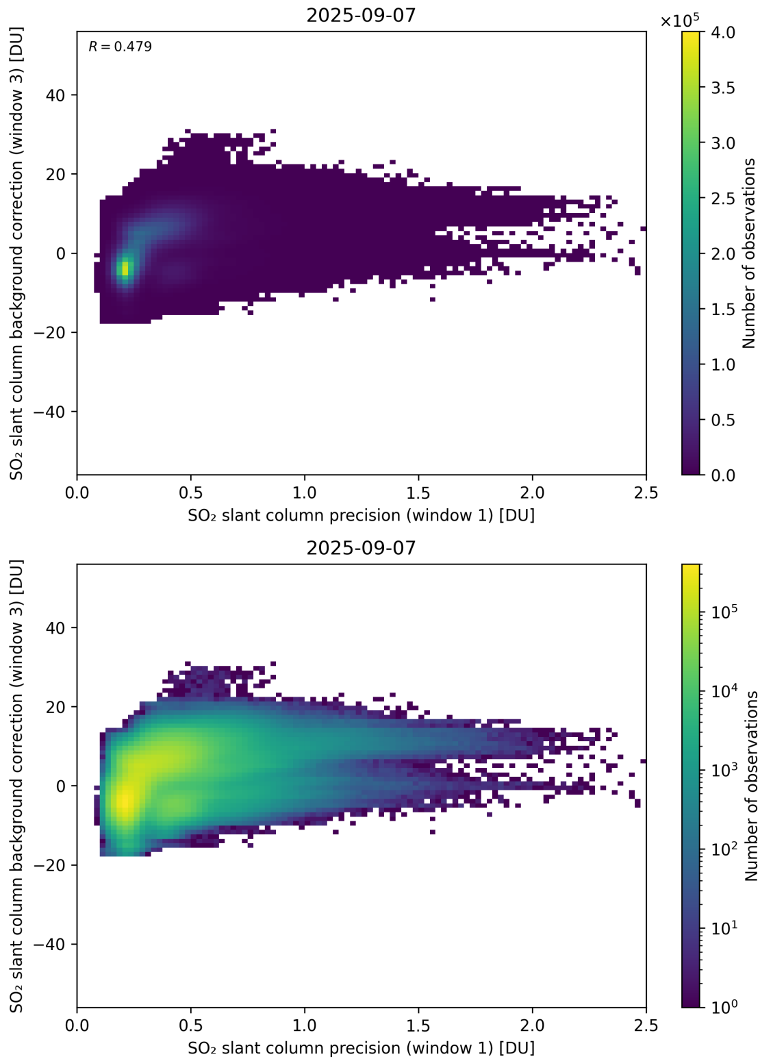
Figure 270: Scatter density plot of “SO 2 slant column precision (window 1)” against “SO 2 slant column background correction (window 3)” for 2025-09-06 to 2025-09-08.
