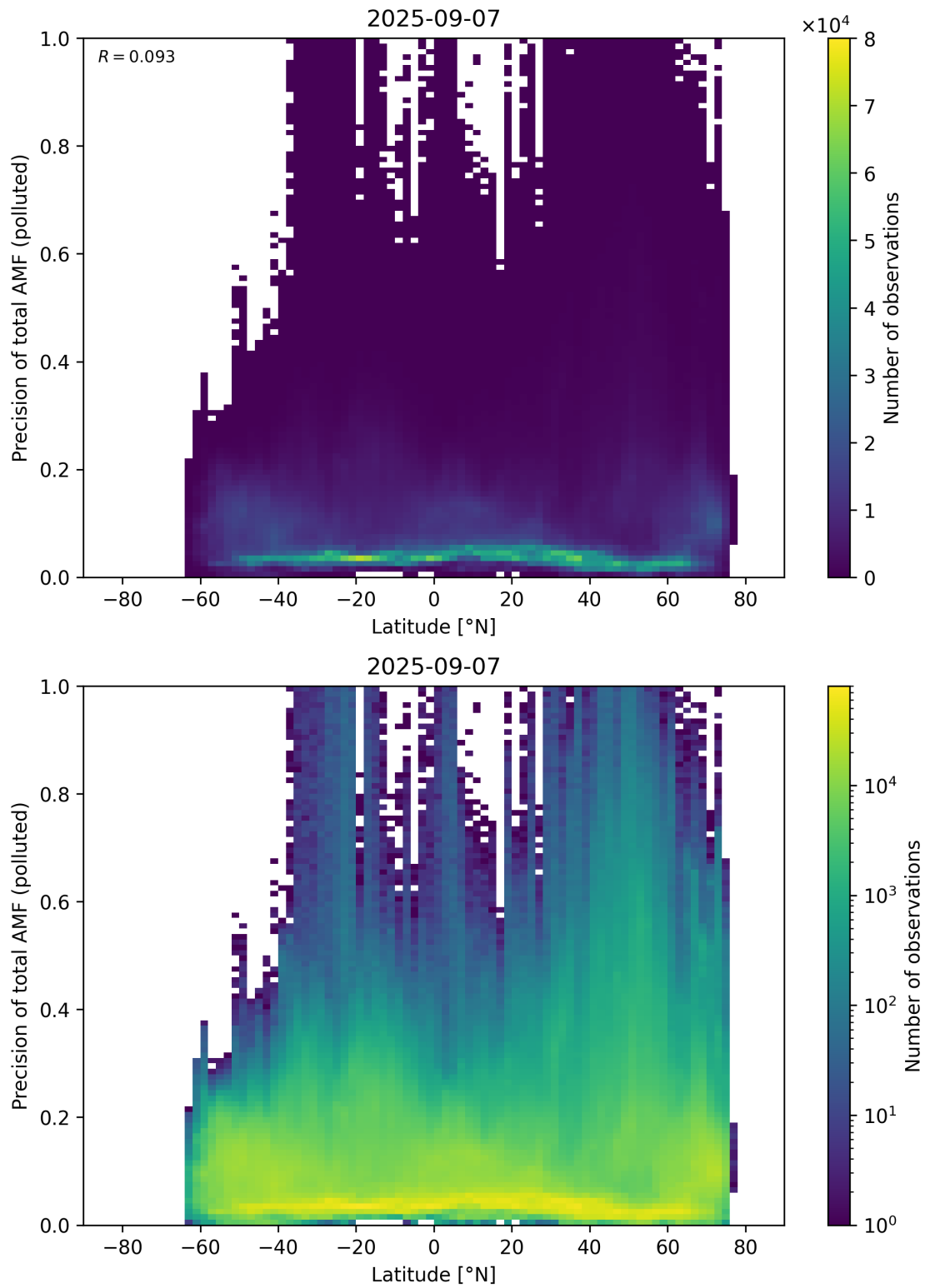
Figure 168: Scatter density plot of “Latitude” against “Precision of total AMF (polluted)” for 2025-09-06 to 2025-09-08.
