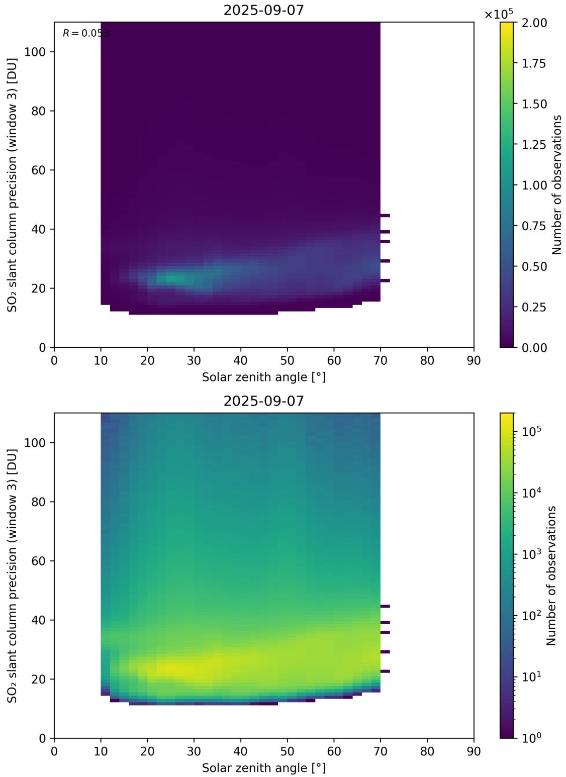
Figure 188: Scatter density plot of “Solar zenith angle” against “SO 2 slant column precision (window 3)” for 2025-09-06 to 2025-09-08.
