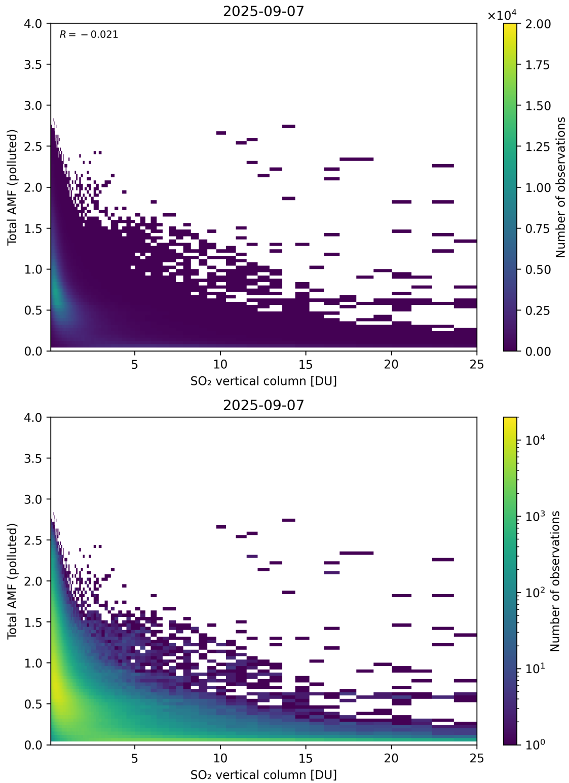
Figure 359: Scatter density plot of “SO 2 vertical column” against “Total AMF (polluted)” for 2025-09-06 to 2025-09-08.
