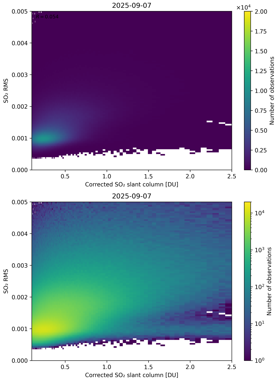
Figure 231: Scatter density plot of “Corrected SO 2 slant column” against “SO 2 RMS” for 2025-09-06 to 2025-09-08.
