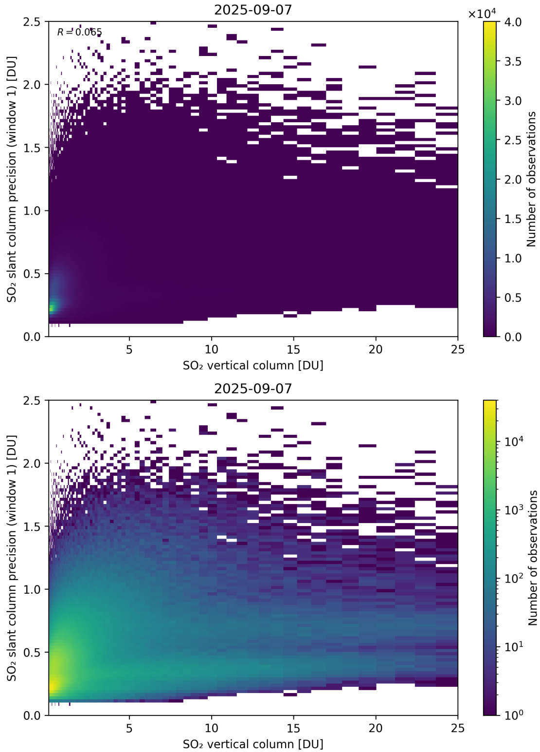
Figure 355: Scatter density plot of “SO 2 vertical column” against “SO 2 slant column precision (window 1)” for 2025-09-06 to 2025-09-08.
