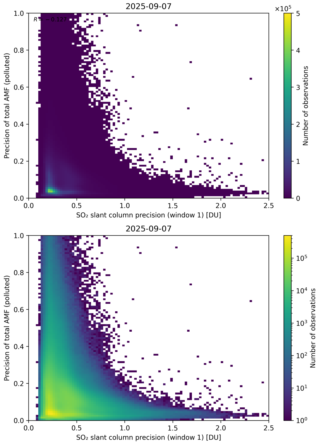
Figure 281: Scatter density plot of “SO 2 slant column precision (window 1)” against “Precision of total AMF (polluted)” for 2025-09-06 to 2025-09-08.
