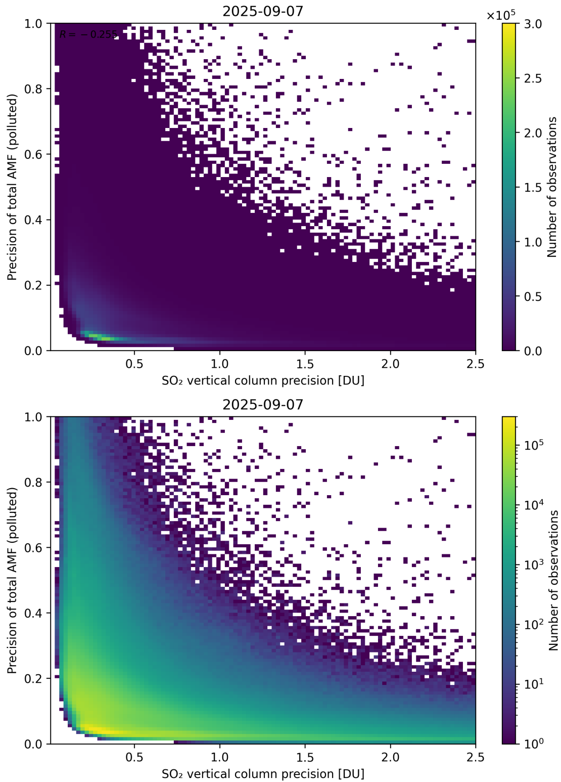
Figure 347: Scatter density plot of “SO 2 vertical column precision” against “Precision of total AMF (polluted)” for 2025-09-06 to 2025-09-08.
