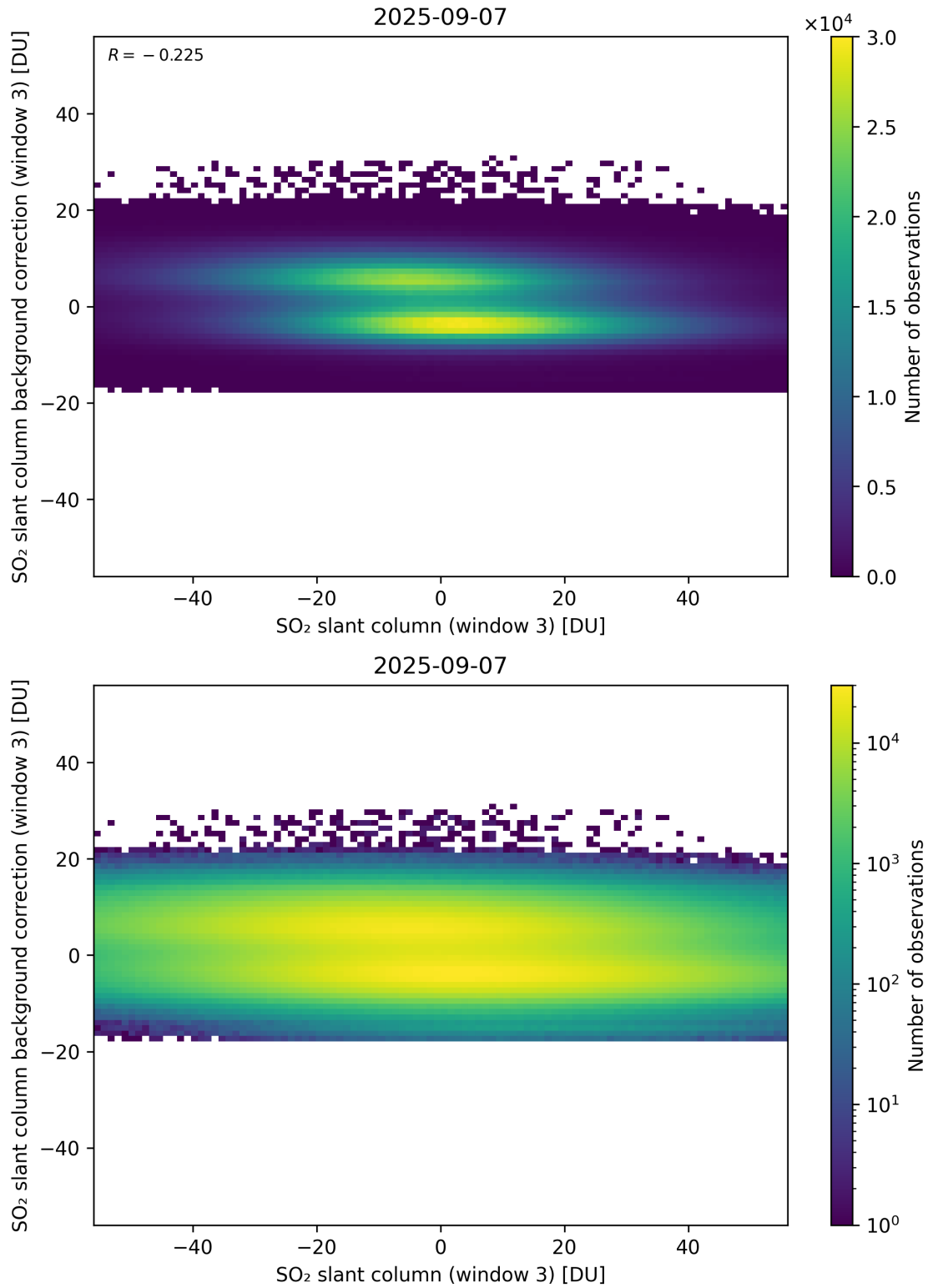
Figure 303: Scatter density plot of “SO 2 slant column (window 3)” against “SO 2 slant column background correction (window 3)” for 2025-09-06 to 2025-09-08.
