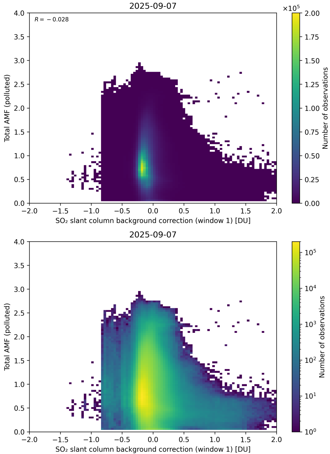
Figure 120: Scatter density plot of “SO 2 slant column background correction (window 1)” against “Total AMF (polluted)” for 2025-09-06 to 2025-09-08.
