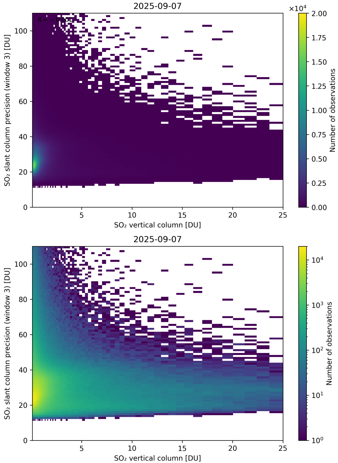
Figure 358: Scatter density plot of “SO 2 vertical column” against “SO 2 slant column precision (window 3)” for 2025-09-06 to 2025-09-08.
