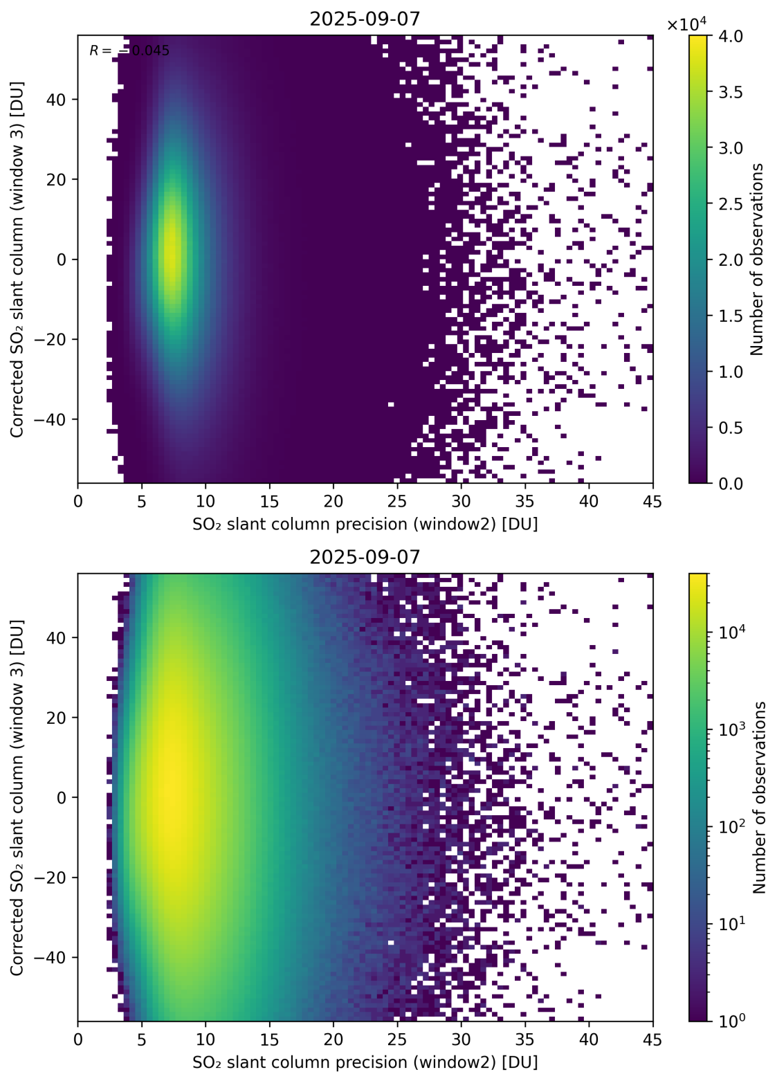
Figure 298: Scatter density plot of “SO 2 slant column precision (window2)” against “Corrected SO 2 slant column (window 3)” for 2025-09-06 to 2025-09-08.
