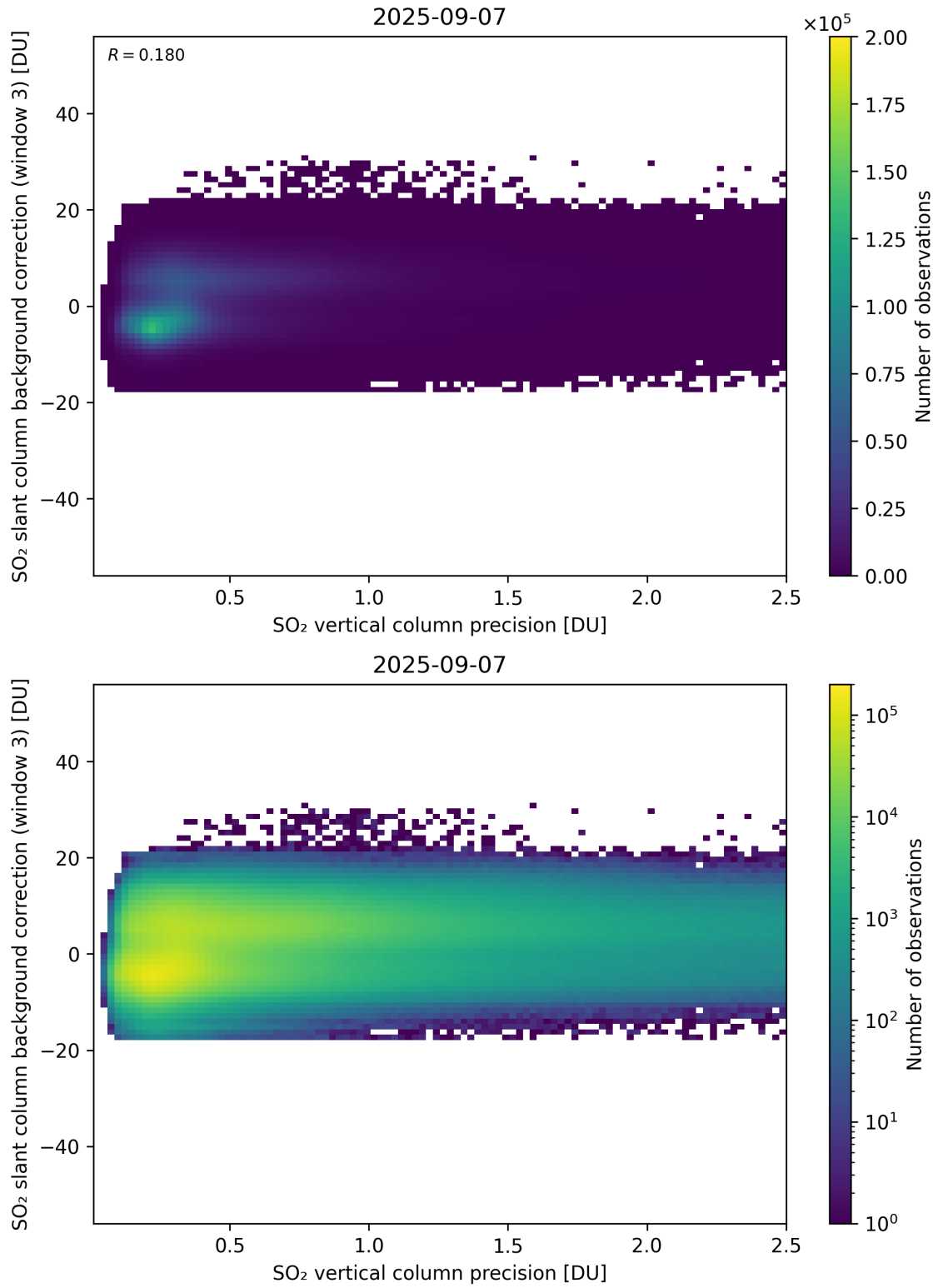
Figure 331: Scatter density plot of “SO 2 vertical column precision” against “SO 2 slant column background correction (window 3)” for 2025-09-06 to 2025-09-08.
