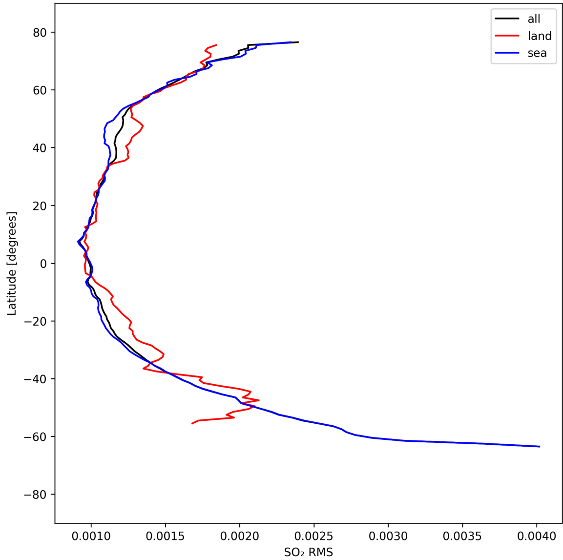
Figure 52: Zonal average of “SO 2 RMS” for 2025-09-06 to 2025-09-08.
