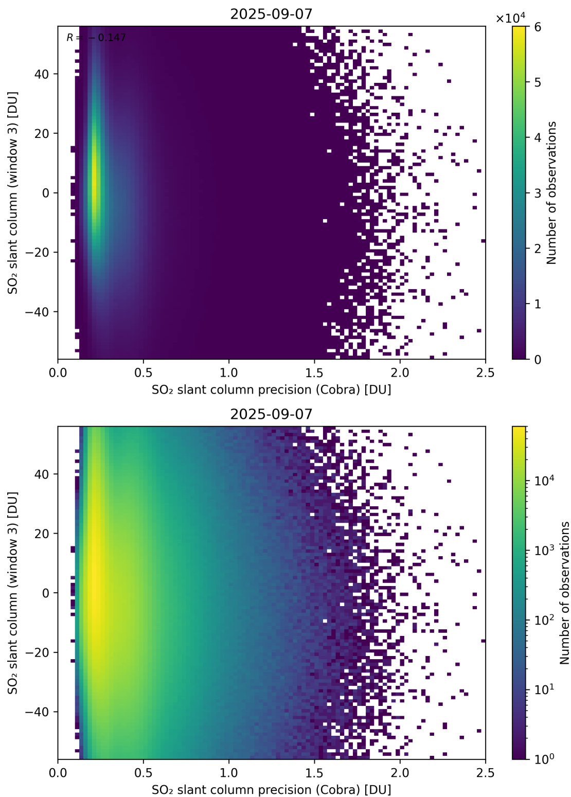
Figure 211: Scatter density plot of “SO 2 slant column precision (Cobra)” against “SO 2 slant column (window 3)” for 2025-09-06 to 2025-09-08.
