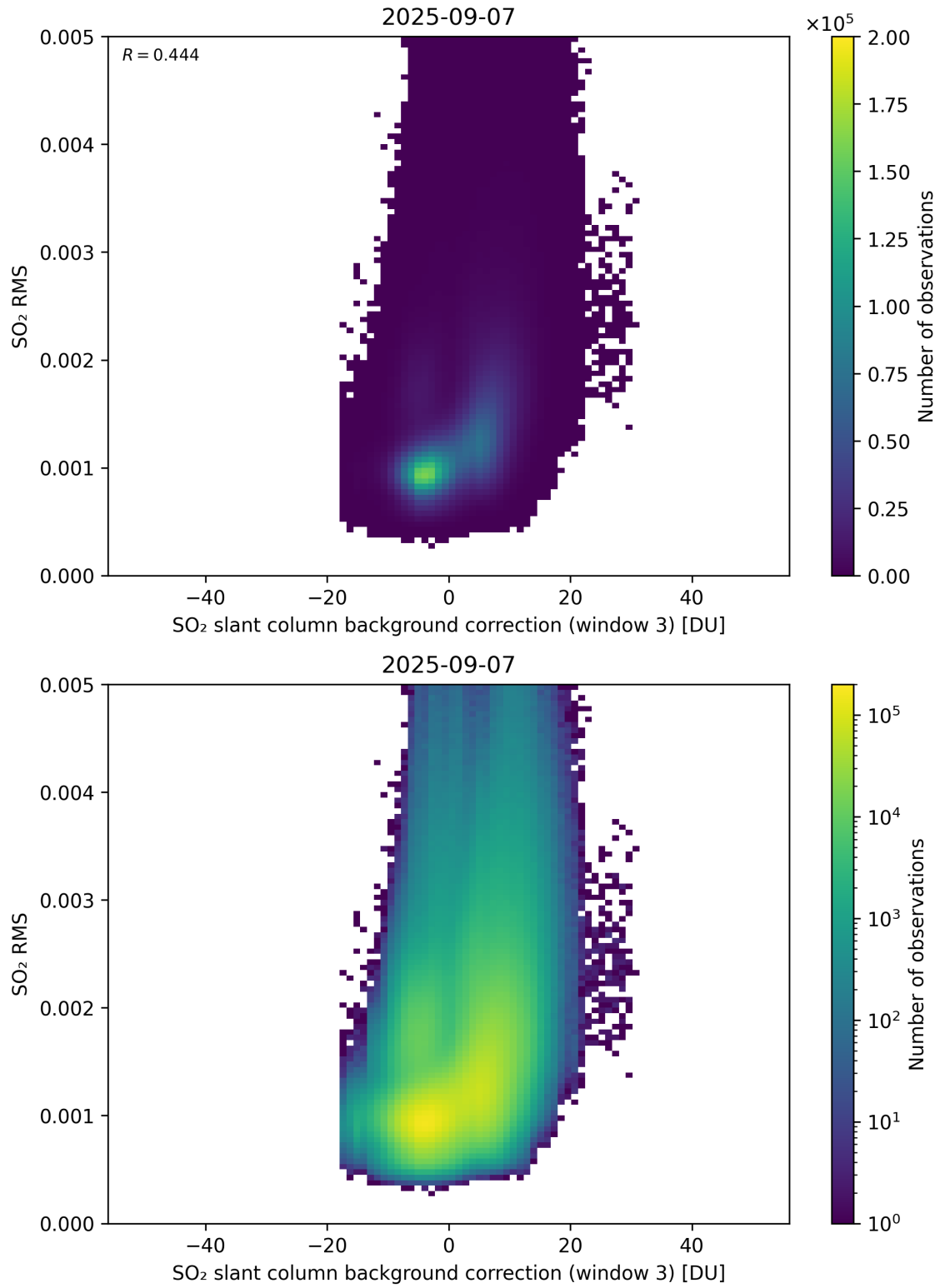
Figure 134: Scatter density plot of “SO 2 slant column background correction (window 3)” against “SO 2 RMS” for 2025-09-06 to 2025-09-08.
