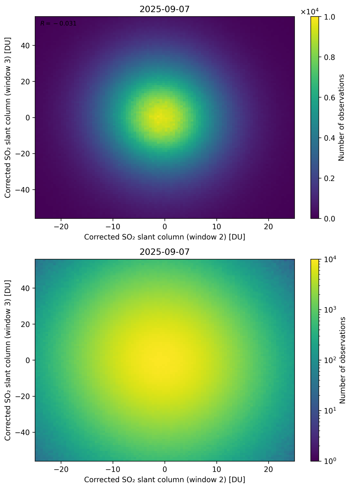
Figure 250: Scatter density plot of “Corrected SO 2 slant column (window 2)” against “Corrected SO 2 slant column (window 3)” for 2025-09-06 to 2025-09-08.
