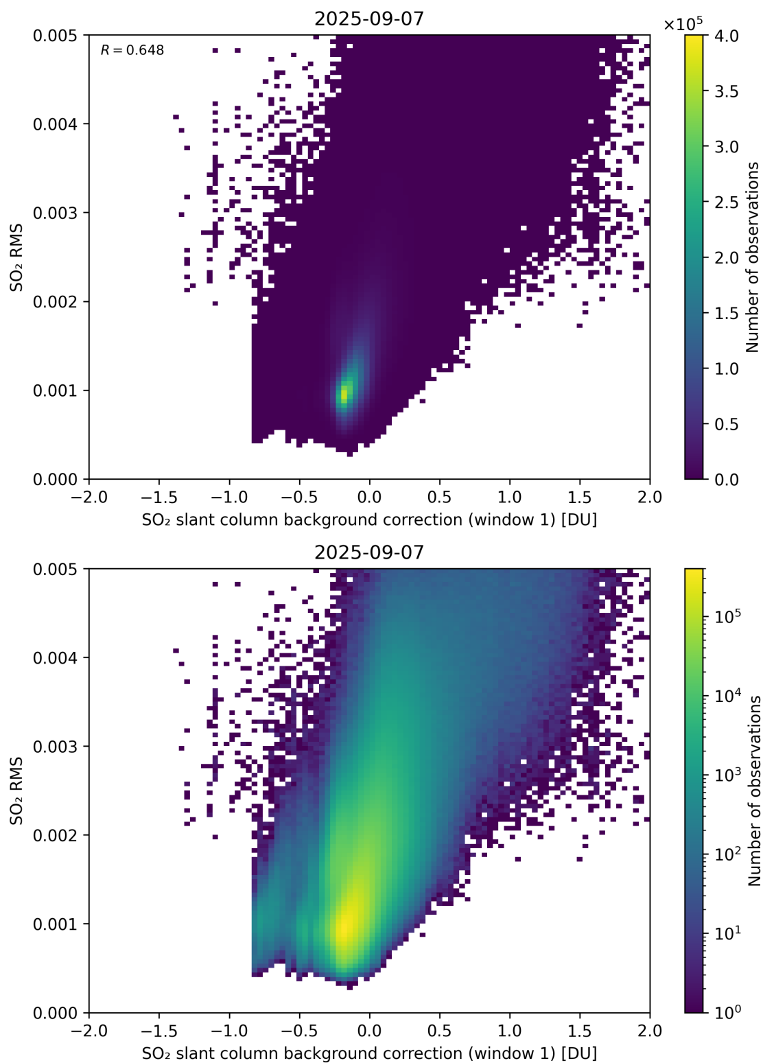
Figure 113: Scatter density plot of “SO 2 slant column background correction (window 1)” against “SO 2 RMS” for 2025-09-06 to 2025-09-08.
