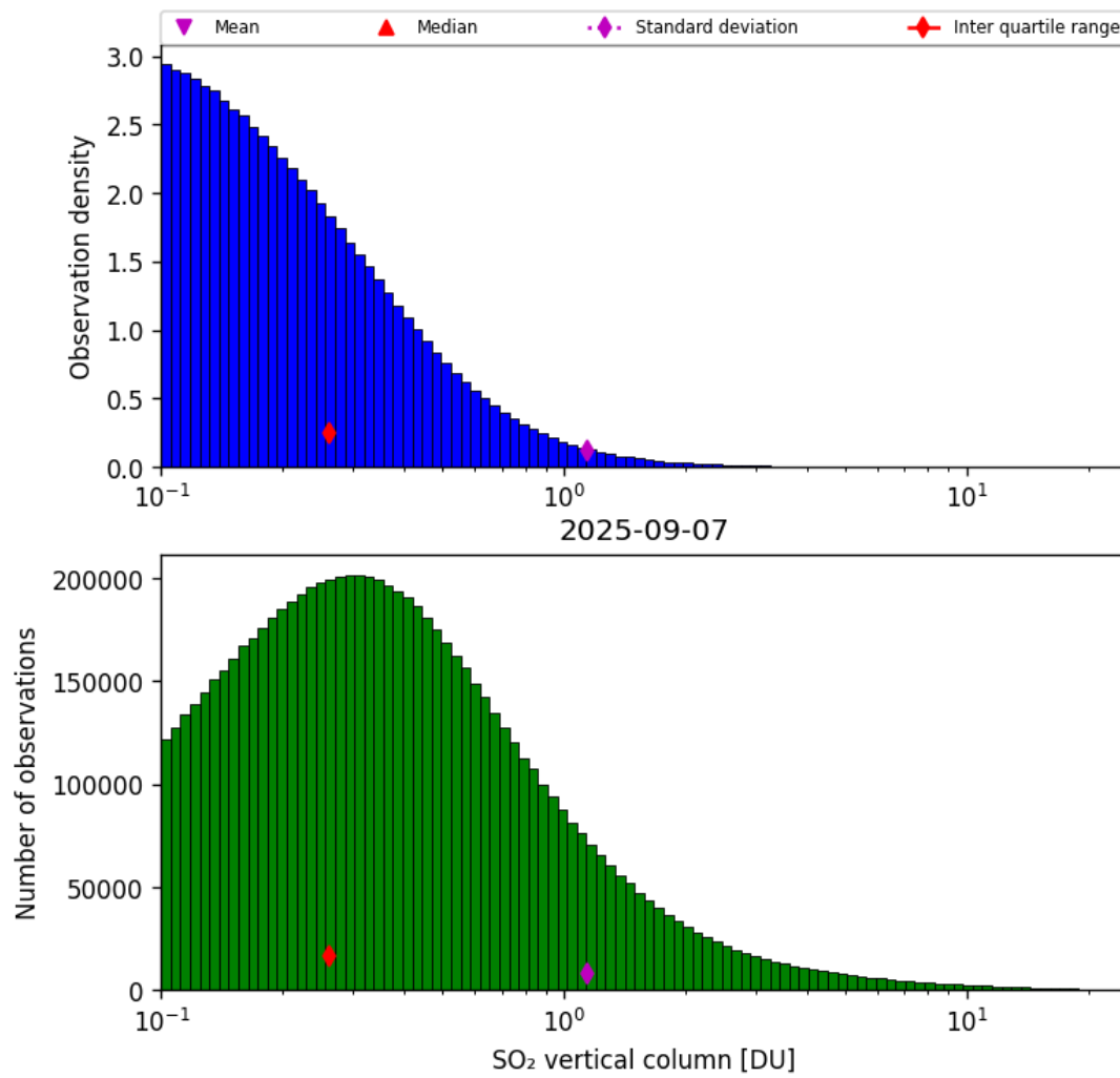
Figure 58: Histogram of “SO 2 vertical column” for 2025-09-06 to 2025-09-08
