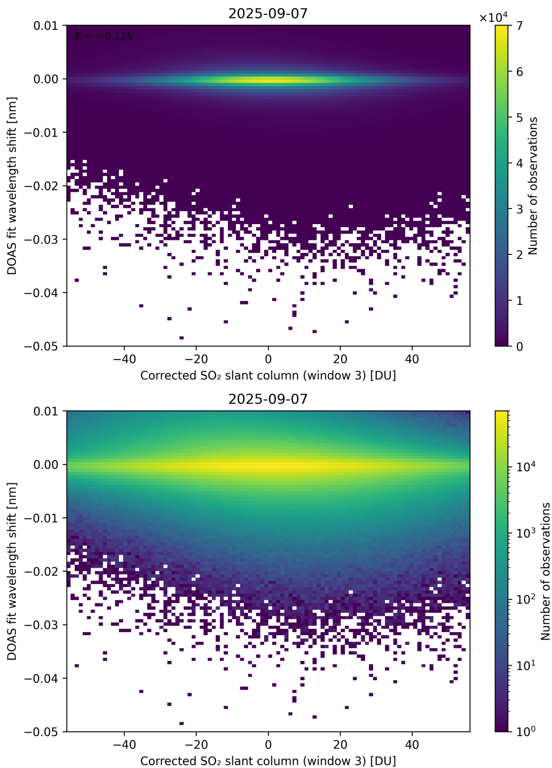
Figure 256: Scatter density plot of “Corrected SO 2 slant column (window 3)” against “DOAS fit wavelength shift” for 2025-09-06 to 2025-09-08.
