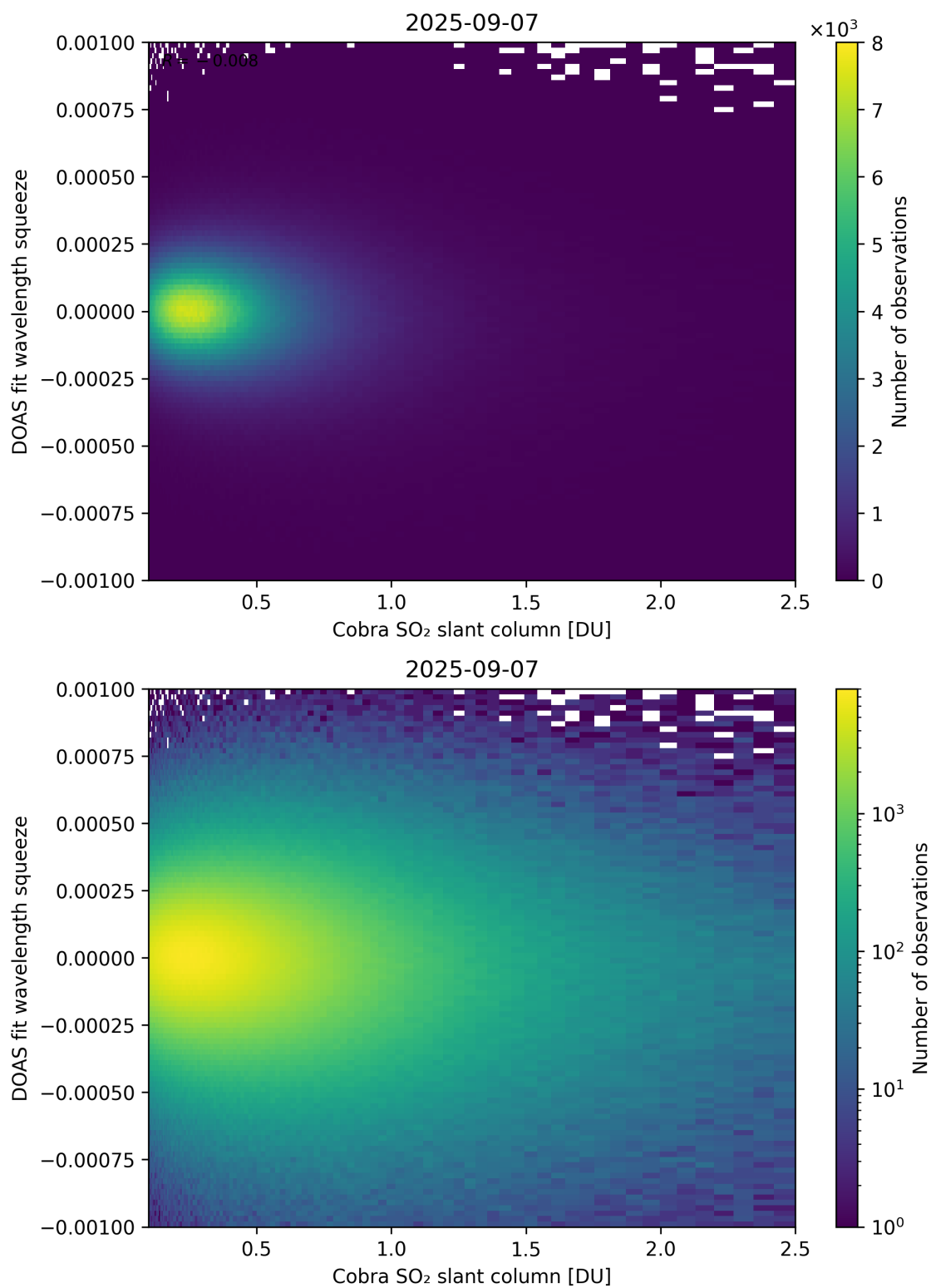
Figure 197: Scatter density plot of “Cobra SO 2 slant column” against “DOAS fit wavelength squeeze” for 2025-09-06 to 2025-09-08.
