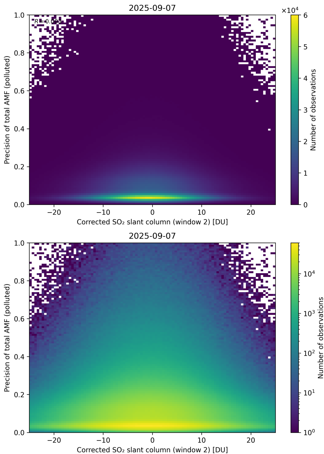
Figure 254: Scatter density plot of “Corrected SO 2 slant column (window 2)” against “Precision of total AMF (polluted)” for 2025-09-06 to 2025-09-08.
