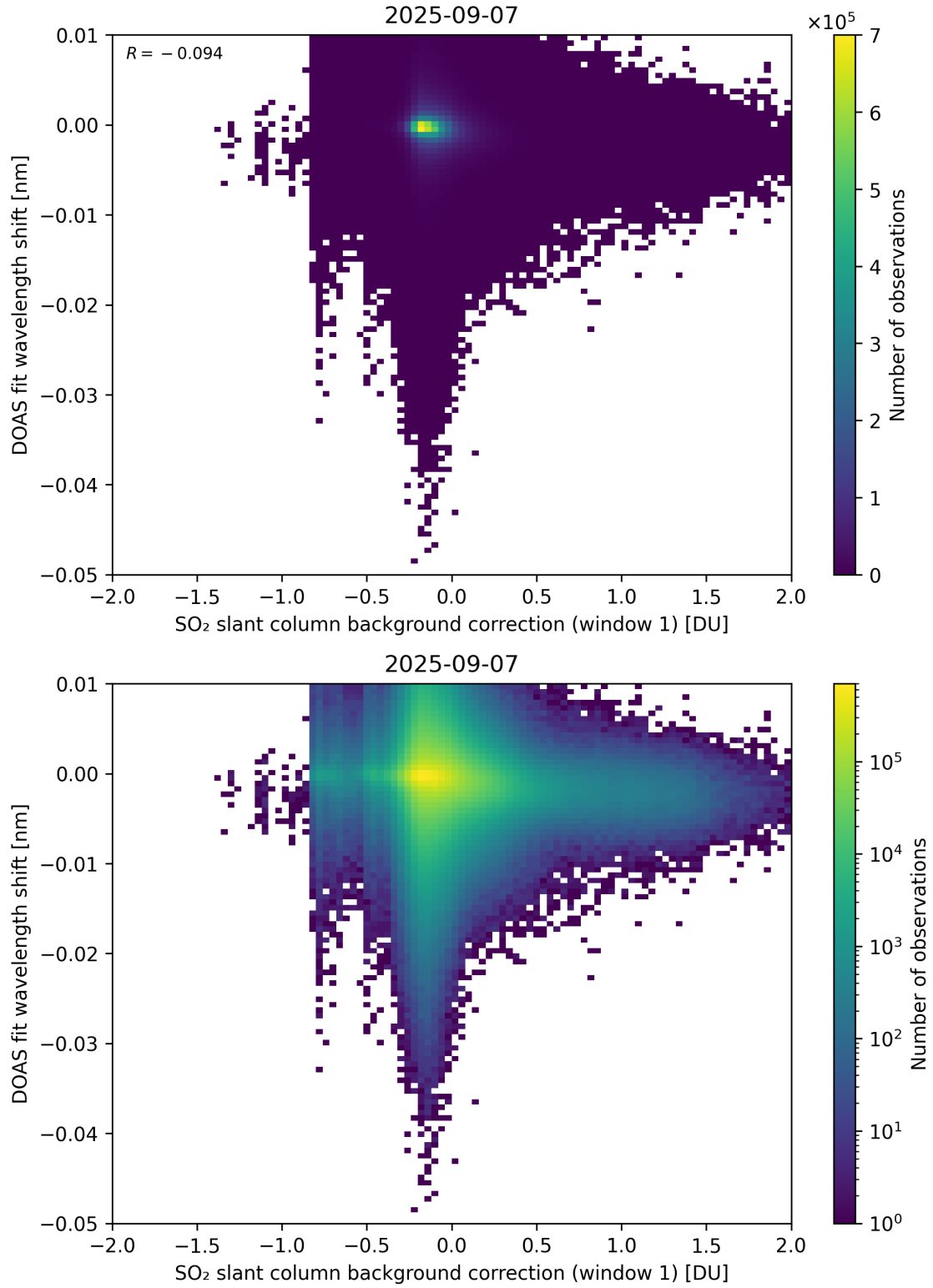
Figure 111: Scatter density plot of “SO 2 slant column background correction (window 1)” against “DOAS fit wavelength shift” for 2025-09-06 to 2025-09-08.
