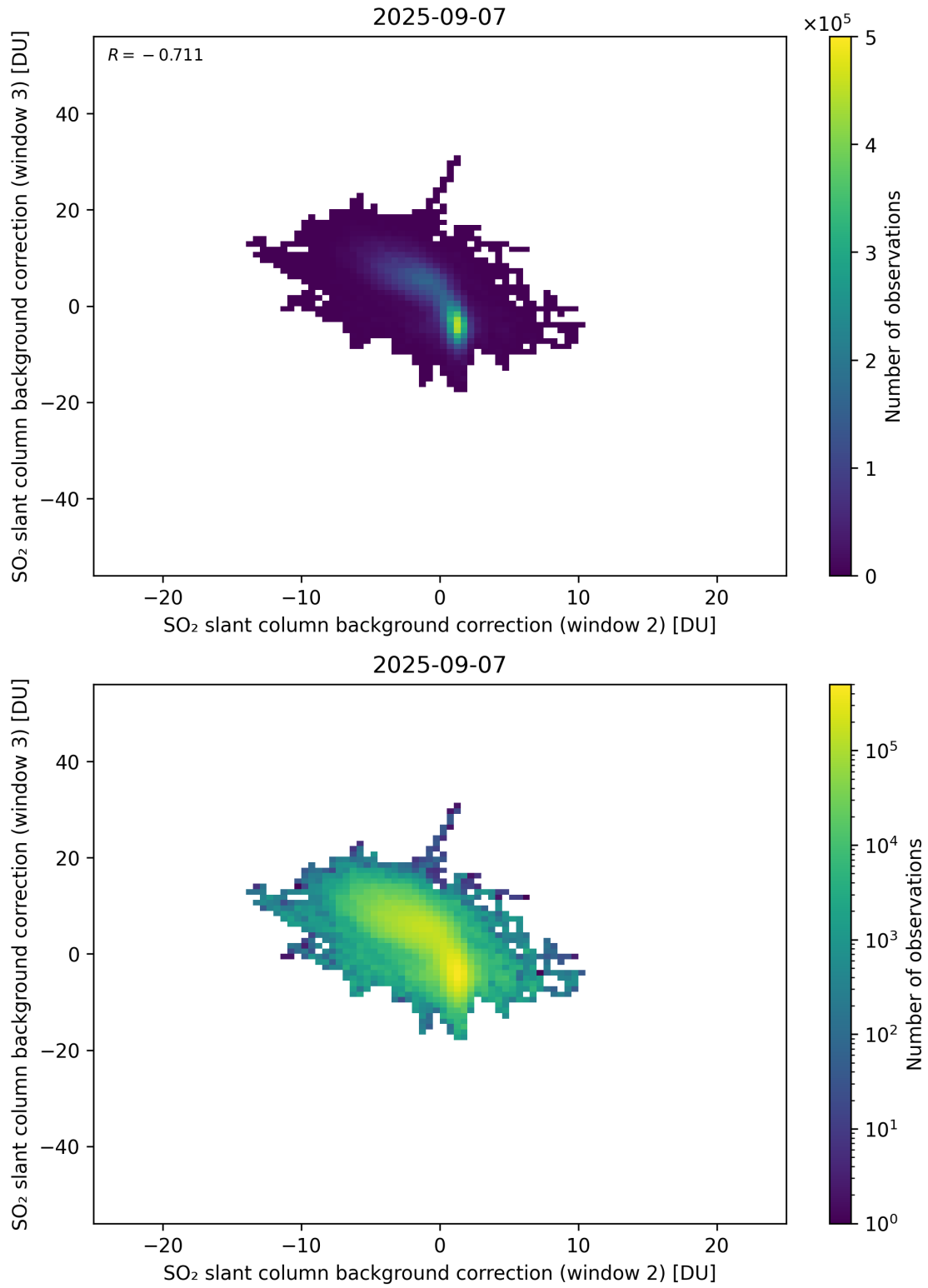
Figure 122: Scatter density plot of “SO 2 slant column background correction (window 2)” against “SO 2 slant column background correction (window 3)” for 2025-09-06 to 2025-09-08.
