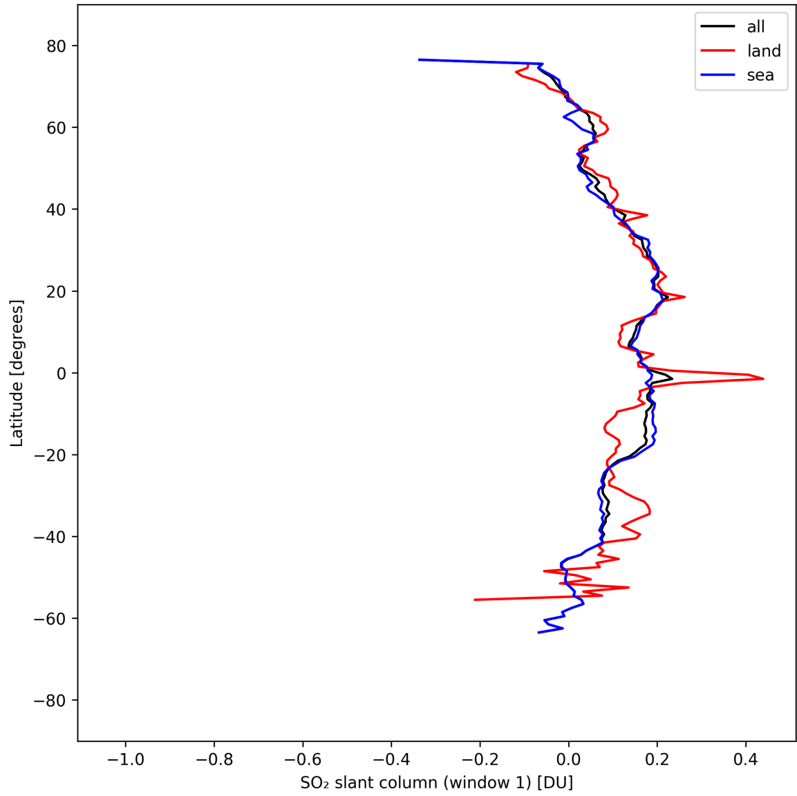
Figure 37: Zonal average of “SO 2 slant column (window 1)” for 2025-09-06 to 2025-09-08.
