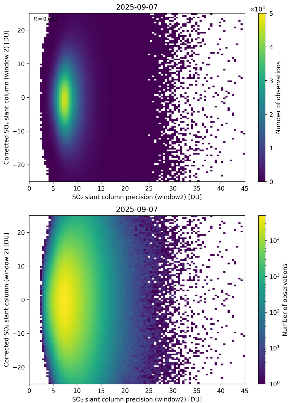
Figure 297: Scatter density plot of “SO 2 slant column precision (window2)” against “Corrected SO 2 slant column (window 2)” for 2025-09-06 to 2025-09-08.
