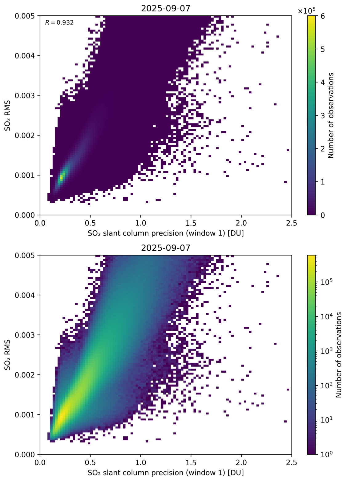
Figure 273: Scatter density plot of “SO 2 slant column precision (window 1)” against “SO 2 RMS” for 2025-09-06 to 2025-09-08.
