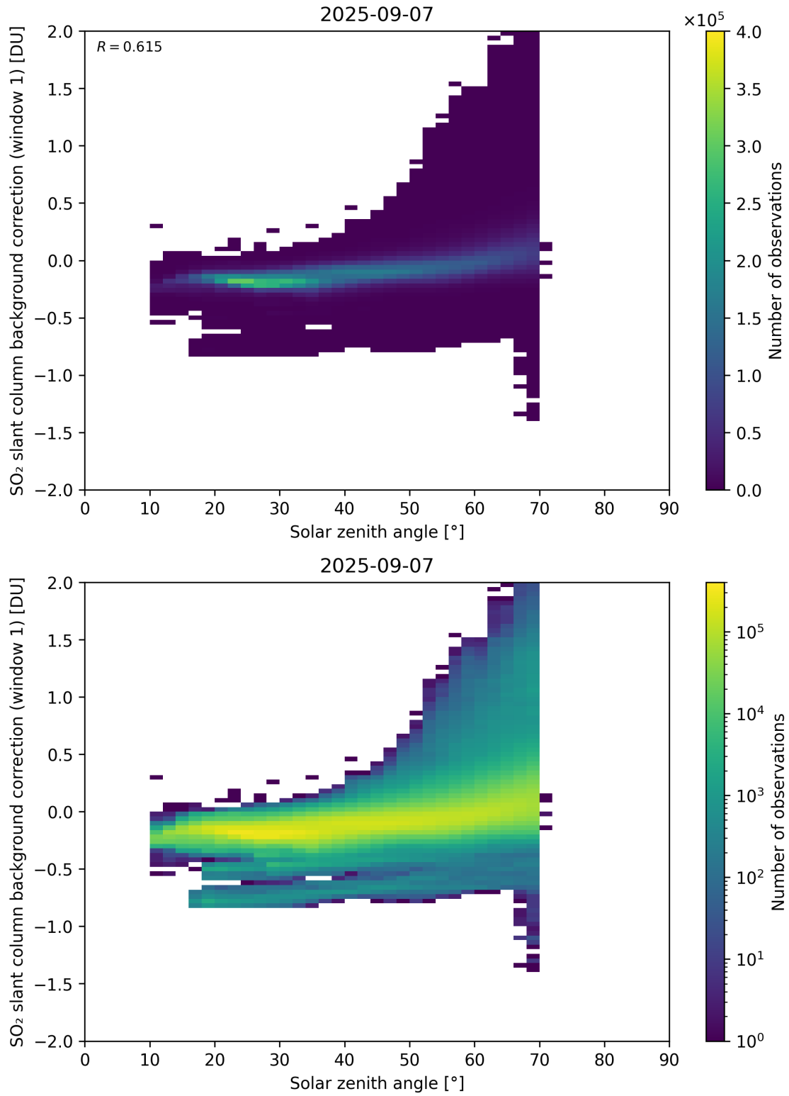
Figure 171: Scatter density plot of “Solar zenith angle” against “SO 2 slant column background correction (window 1)” for 2025-09-06 to 2025-09-08.
