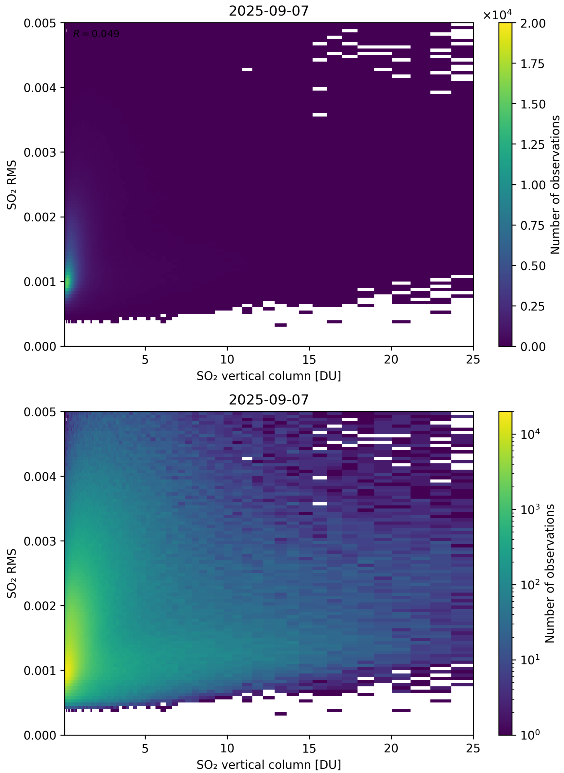
Figure 328: Scatter density plot of “SO 2 vertical column” against “SO 2 RMS” for 2025-09-06 to 2025-09-08.
