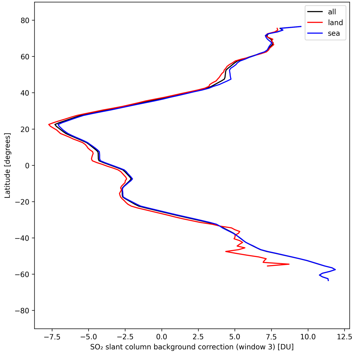
Figure 48: Zonal average of “SO 2 slant column background correction (window 3)” for 2025-09-06 to 2025-09-08.
