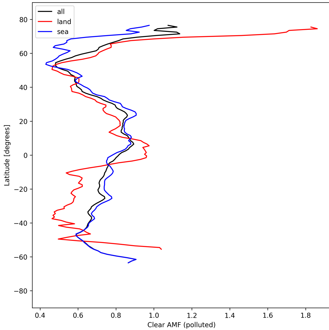
Figure 55: Zonal average of “Clear AMF (polluted)” for 2025-09-06 to 2025-09-08.
