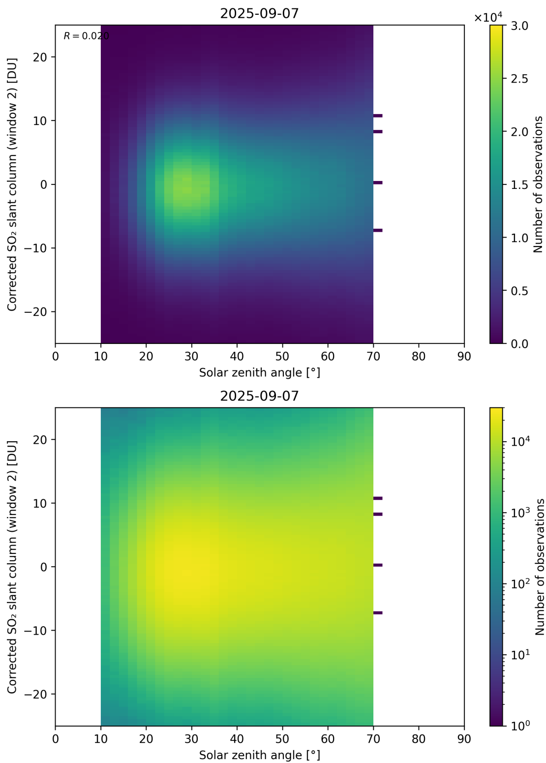
Figure 182: Scatter density plot of “Solar zenith angle” against “Corrected SO 2 slant column (window 2)” for 2025-09-06 to 2025-09-08.
