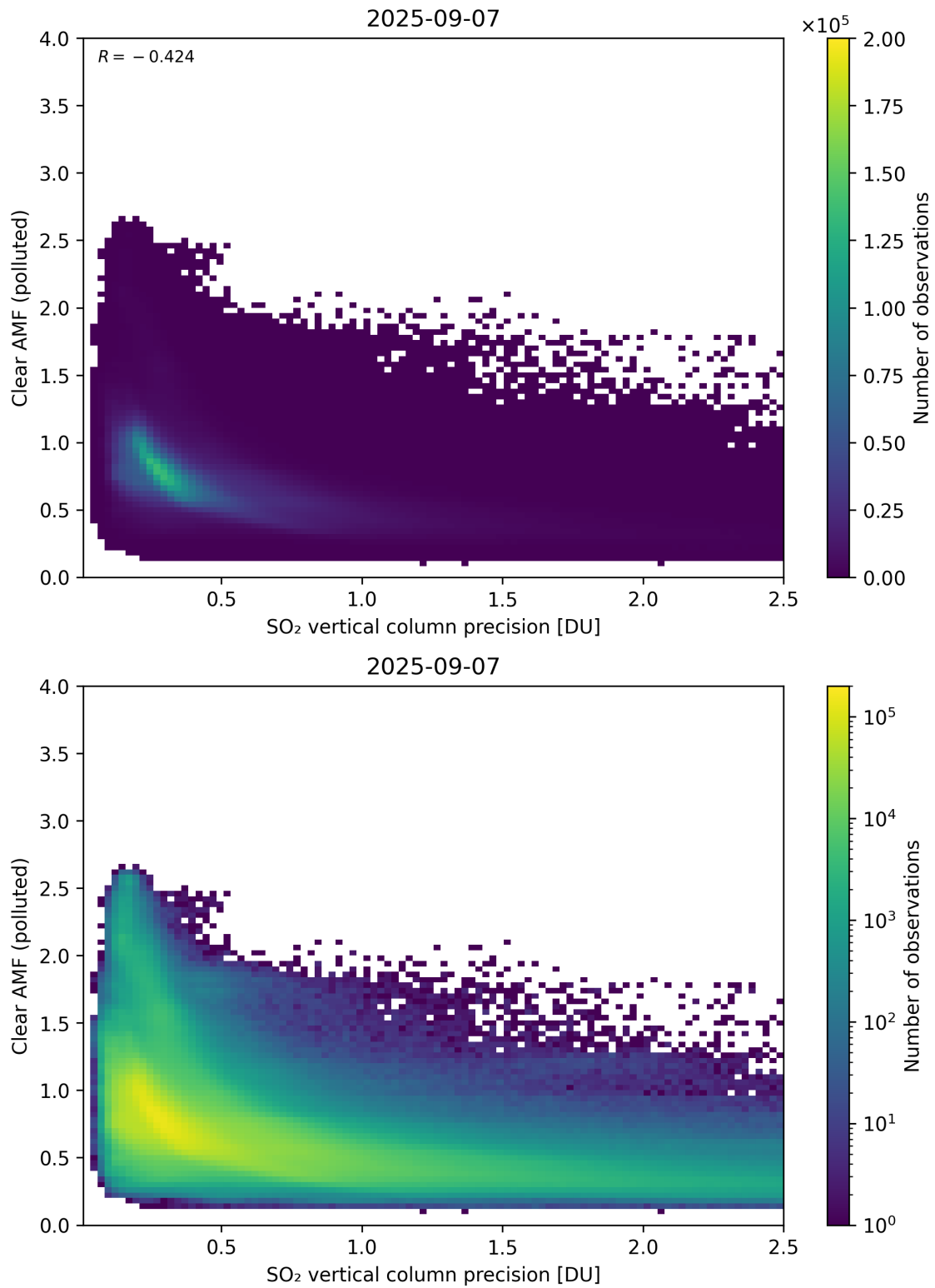
Figure 335: Scatter density plot of “SO 2 vertical column precision” against “Clear AMF (polluted)” for 2025-09-06 to 2025-09-08.
