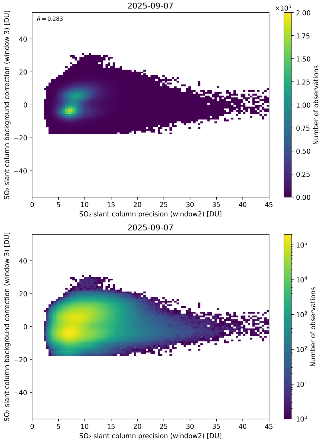
Figure 292: Scatter density plot of “SO 2 slant column precision (window2)” against “SO 2 slant column background correction (window 3)” for 2025-09-06 to 2025-09-08.
