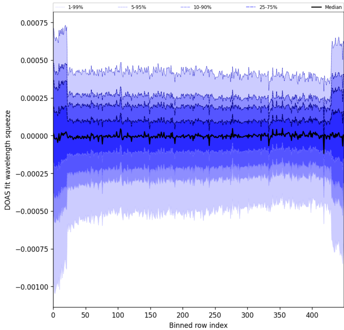
Figure 103: Along track statistics of “DOAS fit wavelength squeeze” for 2025-09-06 to 2025-09-08
