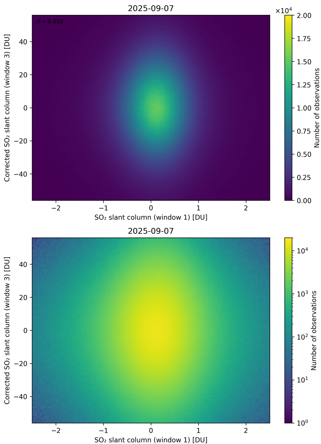
Figure 284: Scatter density plot of “SO 2 slant column (window 1)” against “Corrected SO 2 slant column (window 3)” for 2025-09-06 to 2025-09-08.
