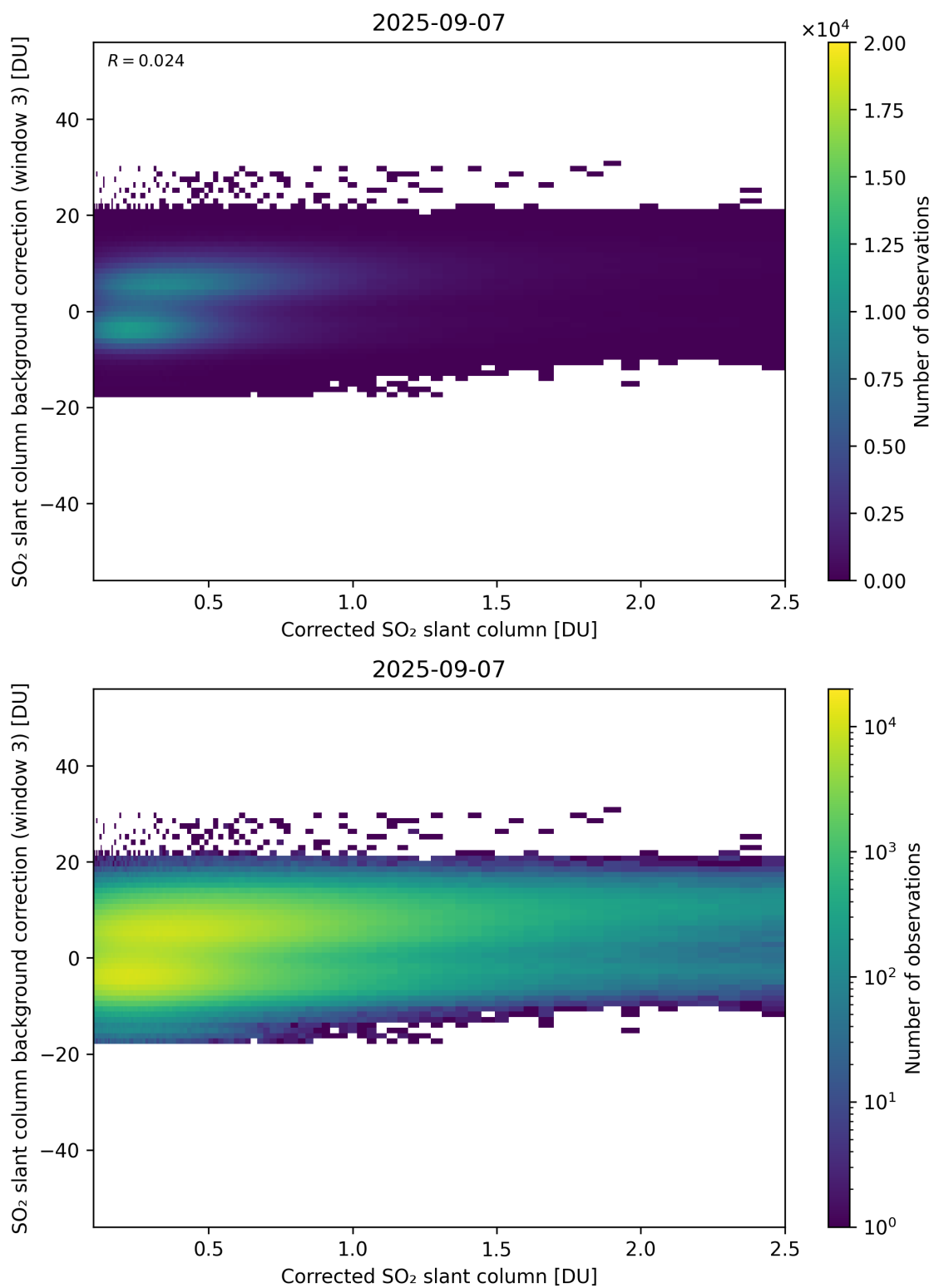
Figure 228: Scatter density plot of “Corrected SO 2 slant column” against “SO 2 slant column background correction (window 3)” for 2025-09-06 to 2025-09-08.
