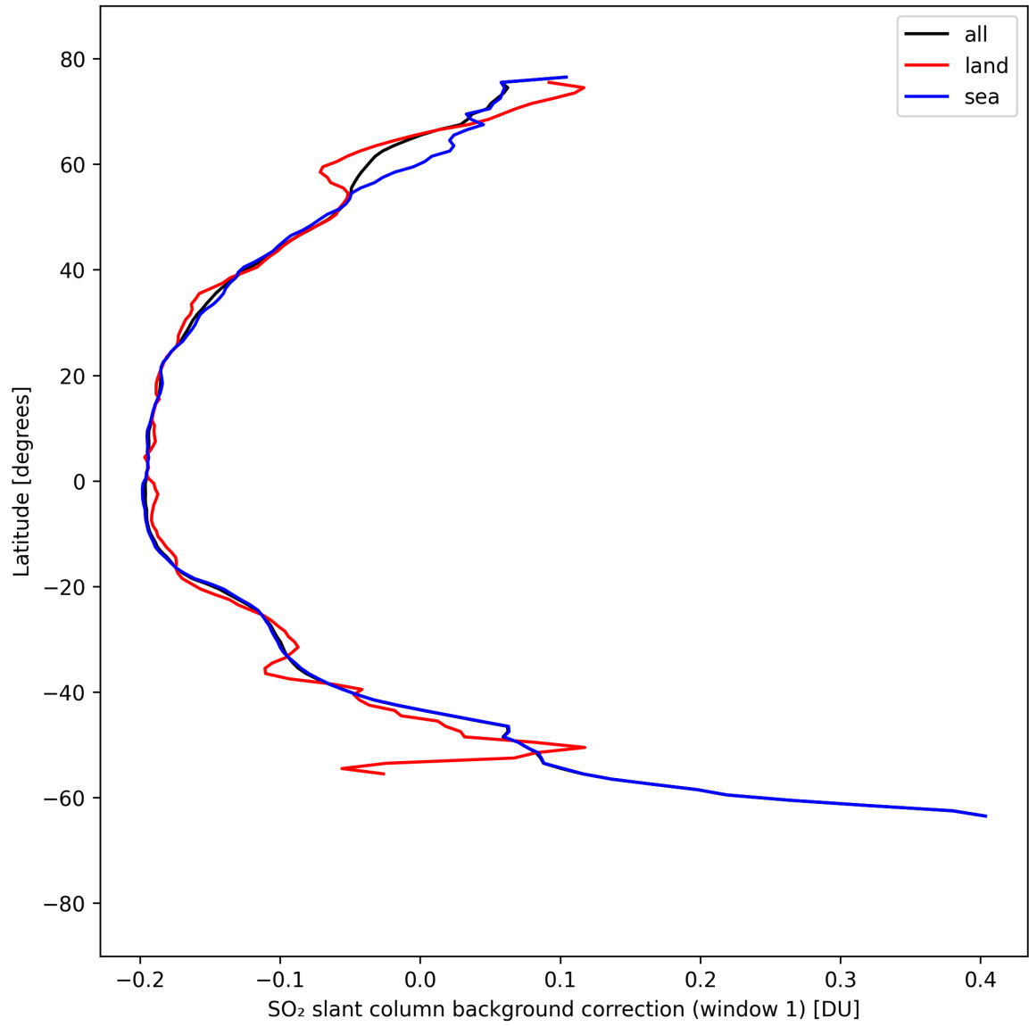
Figure 40: Zonal average of “SO 2 slant column background correction (window 1)” for 2025-09-06 to 2025-09-08.
