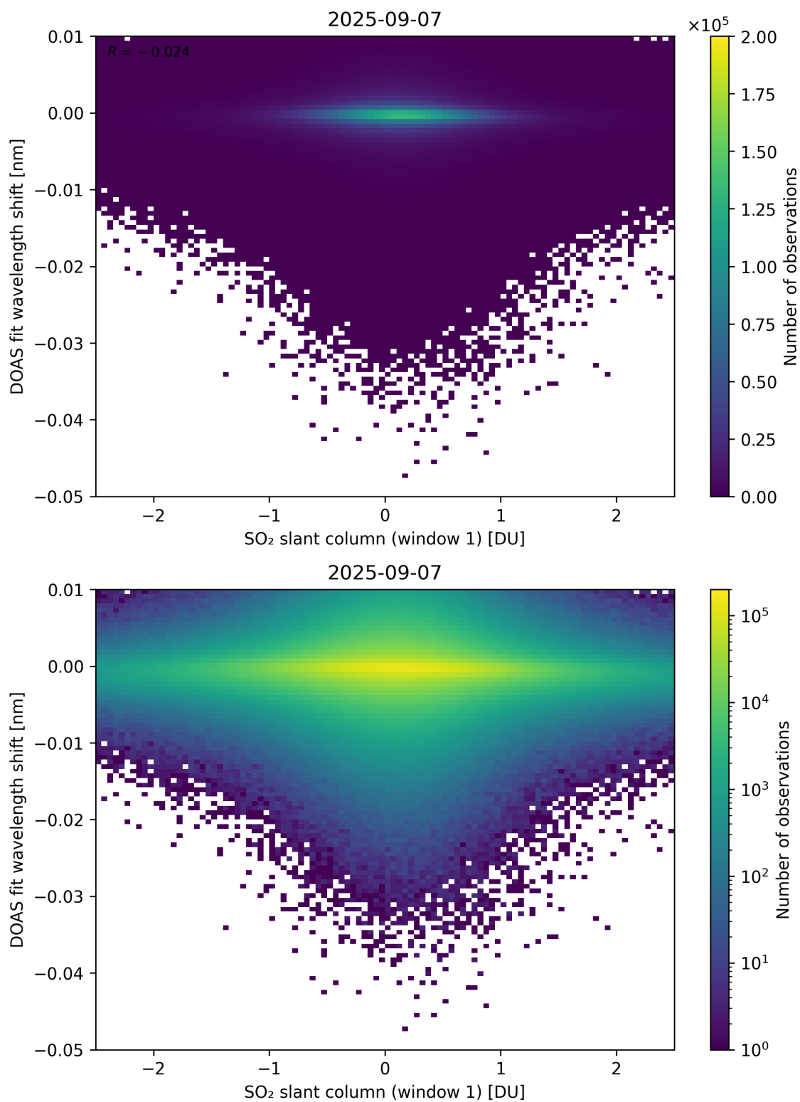
Figure 265: Scatter density plot of “SO 2 slant column (window 1)” against “DOAS fit wavelength shift” for 2025-09-06 to 2025-09-08.
