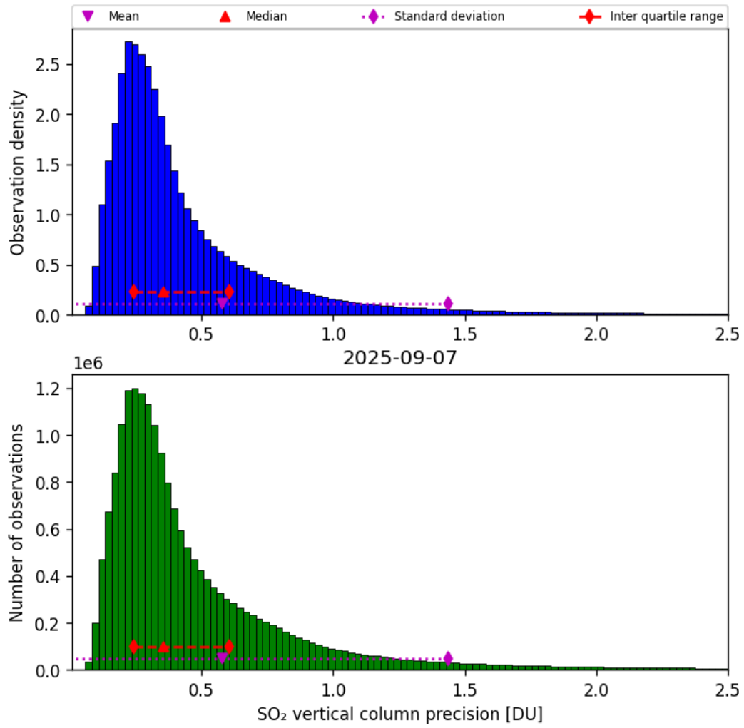
Figure 59: Histogram of “SO 2 vertical column precision” for 2025-09-06 to 2025-09-08
