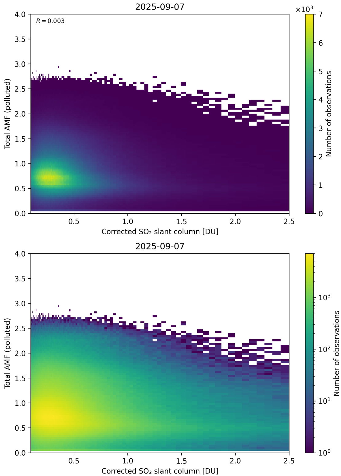
Figure 242: Scatter density plot of “Corrected SO 2 slant column” against “Total AMF (polluted)” for 2025-09-06 to 2025-09-08.
