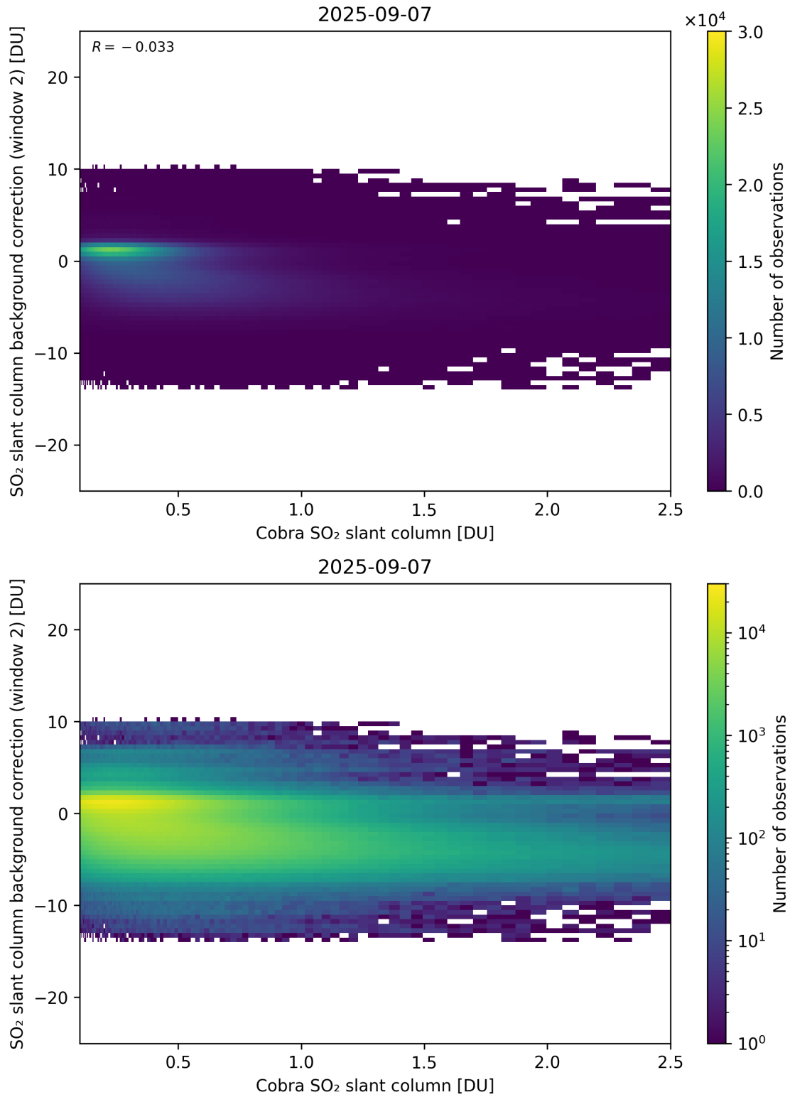
Figure 194: Scatter density plot of “Cobra SO 2 slant column” against “SO 2 slant column background correction (window 2)” for 2025-09-06 to 2025-09-08.
