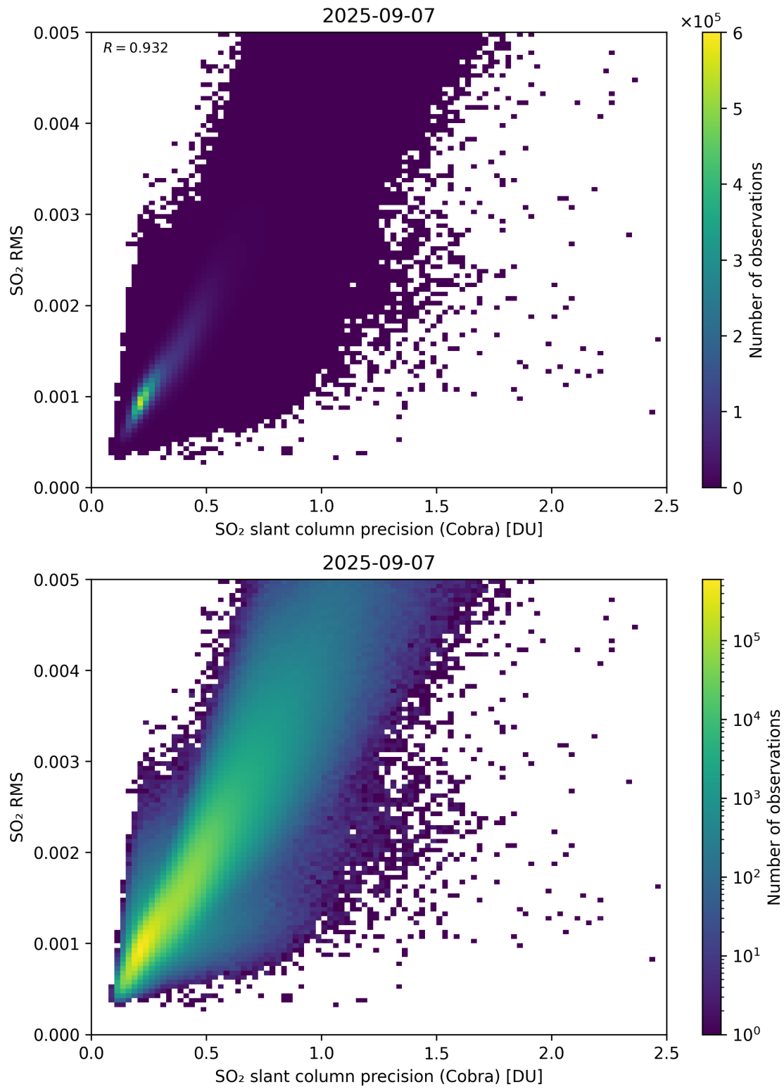
Figure 204: Scatter density plot of “SO 2 slant column precision (Cobra)” against “SO 2 RMS” for 2025-09-06 to 2025-09-08.
