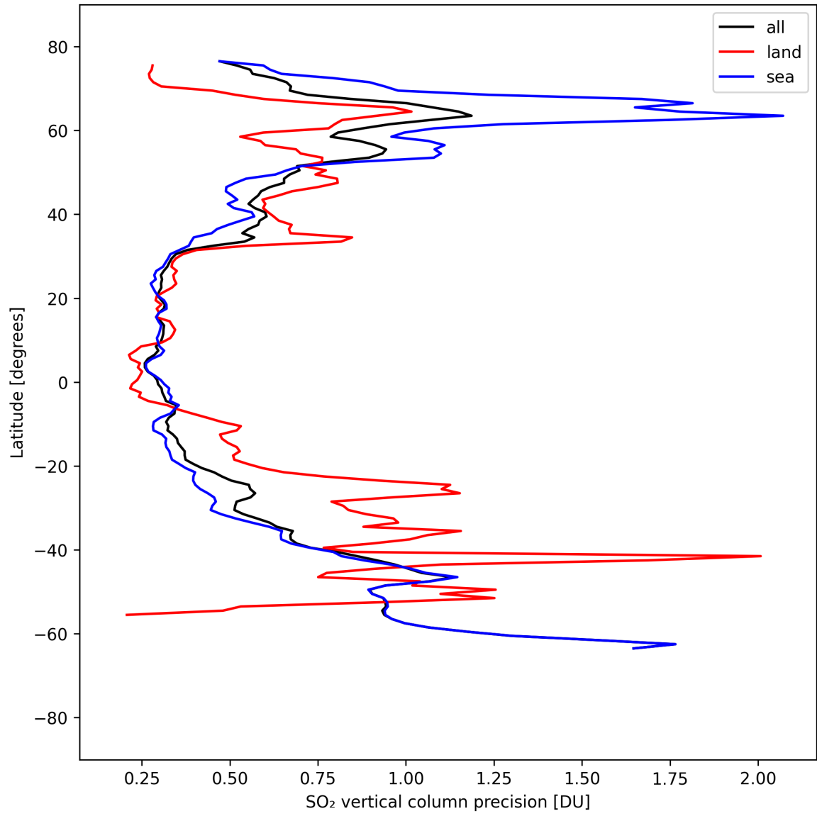
Figure 33: Zonal average of “SO 2 vertical column precision” for 2025-09-06 to 2025-09-08.
