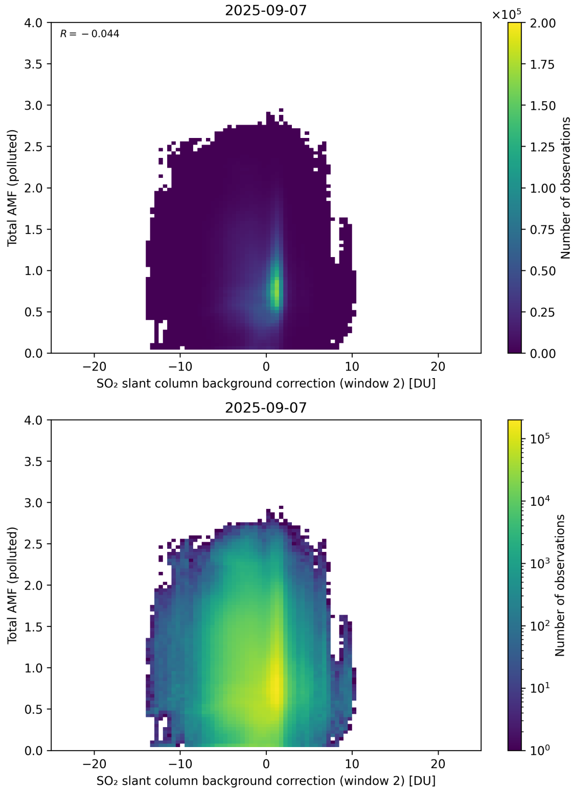
Figure 130: Scatter density plot of “SO 2 slant column background correction (window 2)” against “Total AMF (polluted)” for 2025-09-06 to 2025-09-08.
