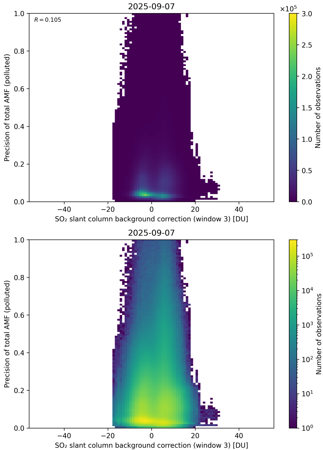
Figure 137: Scatter density plot of “SO 2 slant column background correction (window 3)” against “Precision of total AMF (polluted)” for 2025-09-06 to 2025-09-08.
