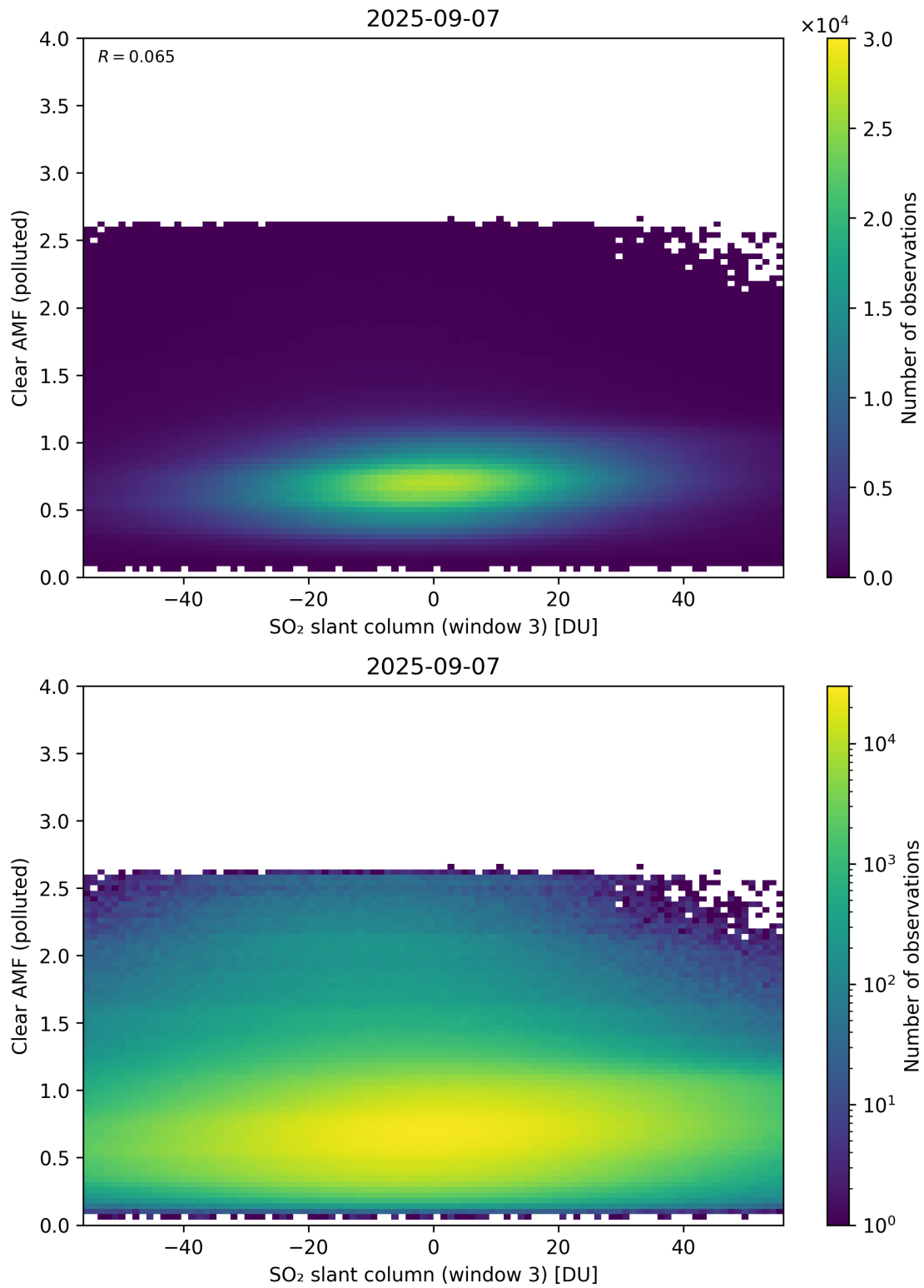
Figure 315: Scatter density plot of “SO 2 slant column (window 3)” against “Clear AMF (polluted)” for 2025-09-06 to 2025-09-08.
