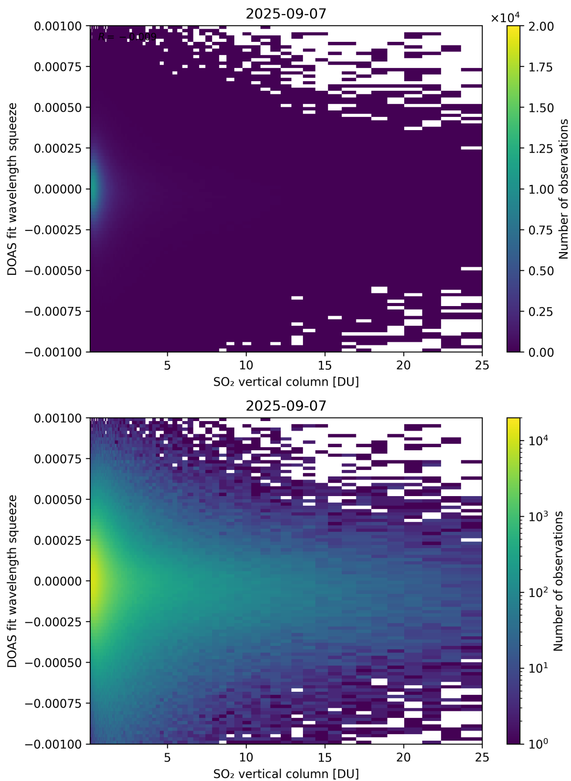
Figure 327: Scatter density plot of “SO 2 vertical column” against “DOAS fit wavelength squeeze” for 2025-09-06 to 2025-09-08.
