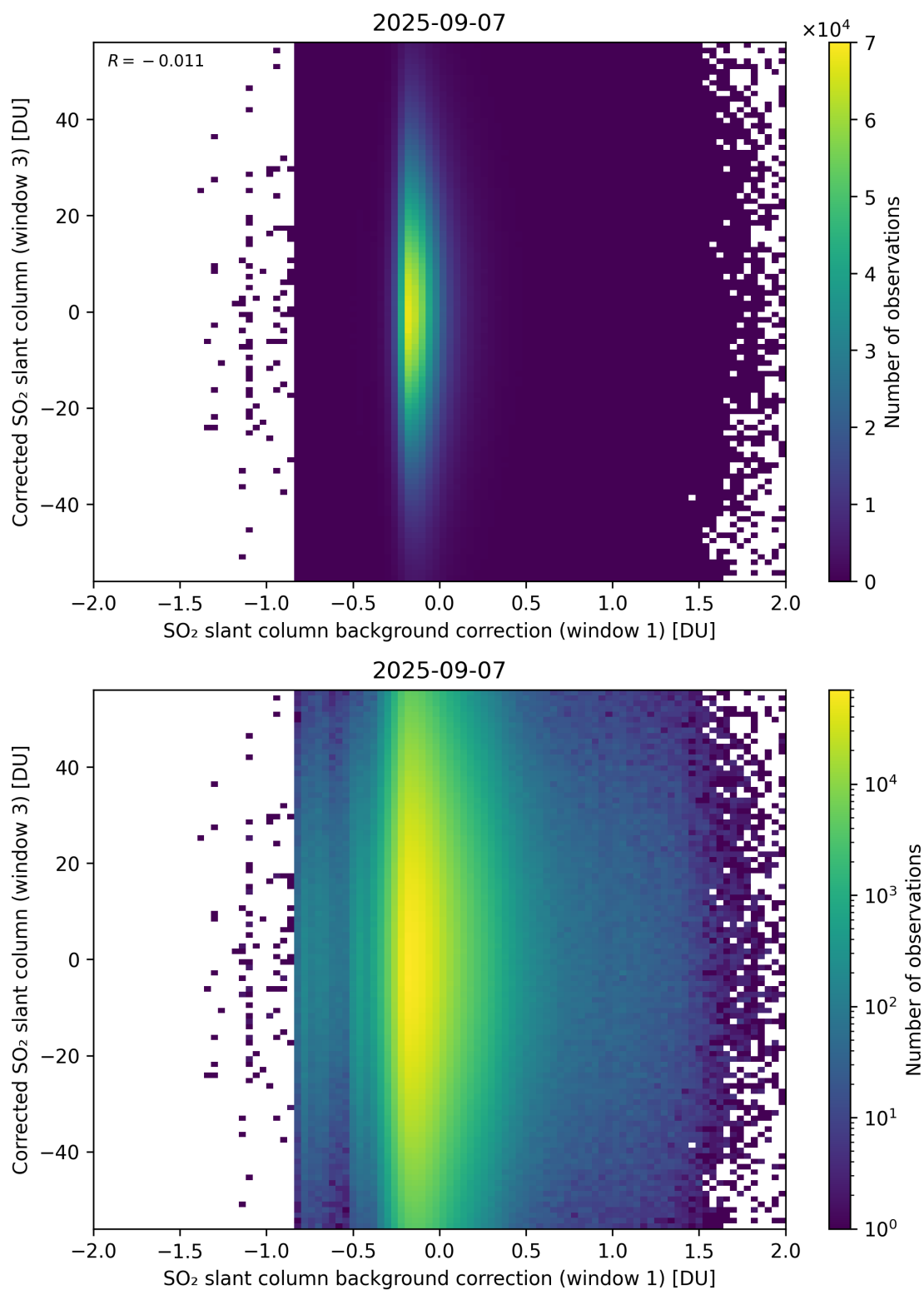
Figure 116: Scatter density plot of “SO 2 slant column background correction (window 1)” against “Corrected SO 2 slant column (window 3)” for 2025-09-06 to 2025-09-08.
