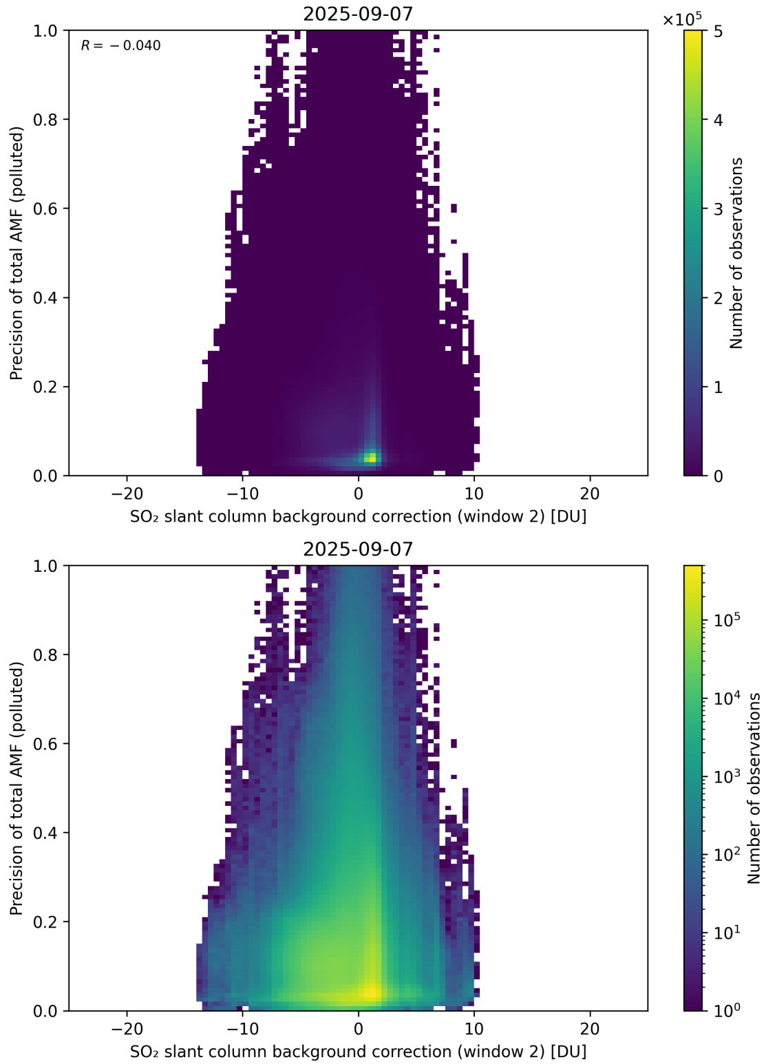
Figure 131: Scatter density plot of “SO 2 slant column background correction (window 2)” against “Precision of total AMF (polluted)” for 2025-09-06 to 2025-09-08.
