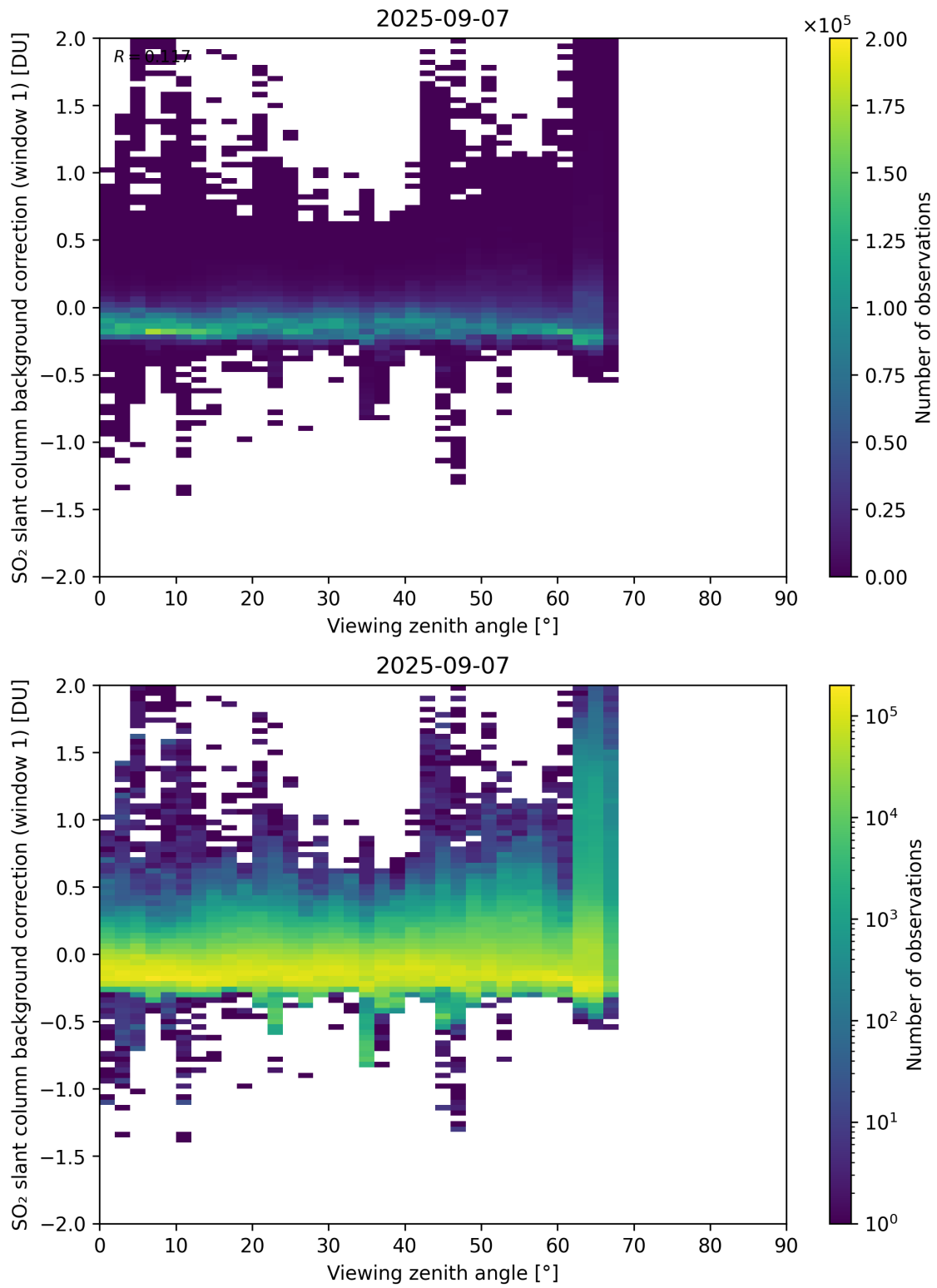
Figure 362: Scatter density plot of “Viewing zenith angle” against “SO 2 slant column background correction (window 1)” for 2025-09-06 to 2025-09-08.
