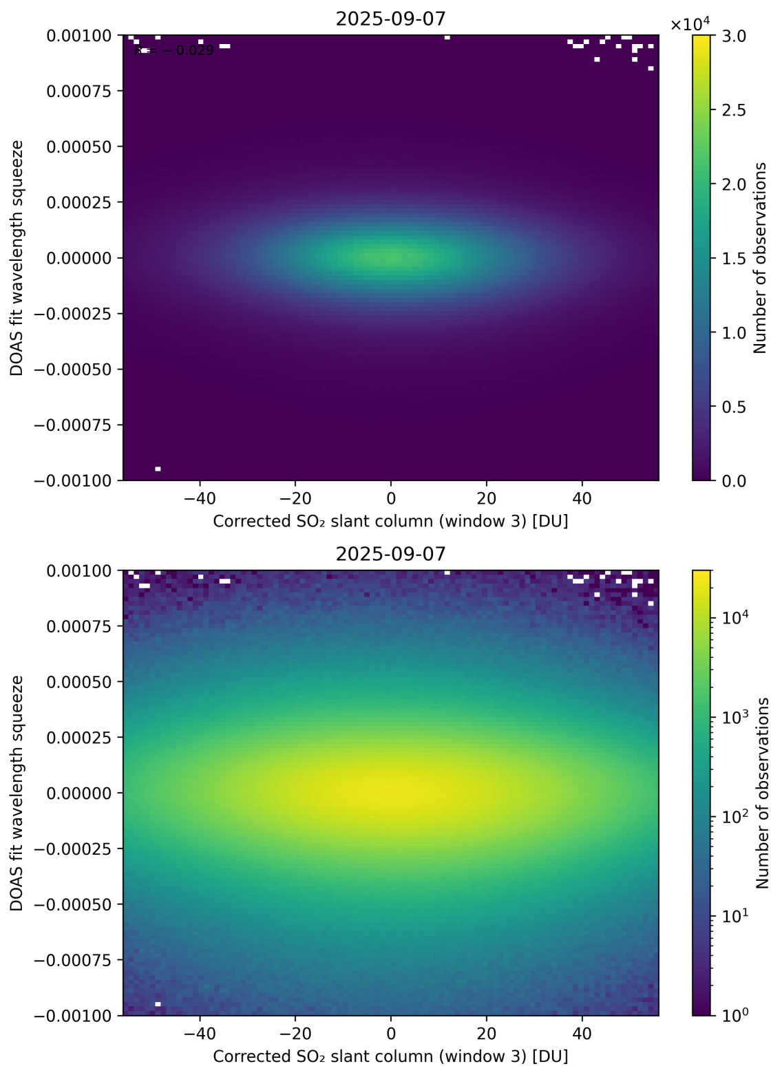
Figure 257: Scatter density plot of “Corrected SO 2 slant column (window 3)” against “DOAS fit wavelength squeeze” for 2025-09-06 to 2025-09-08.
