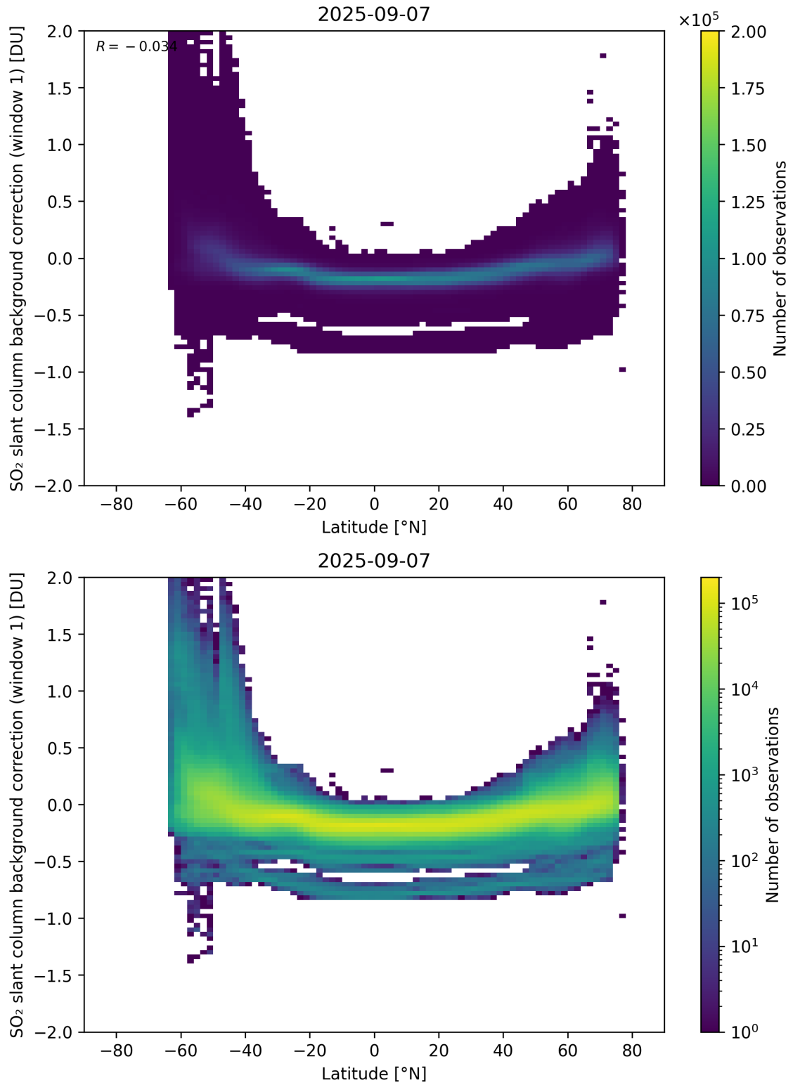
Figure 150: Scatter density plot of “Latitude” against “SO 2 slant column background correction (window 1)” for 2025-09-06 to 2025-09-08.
