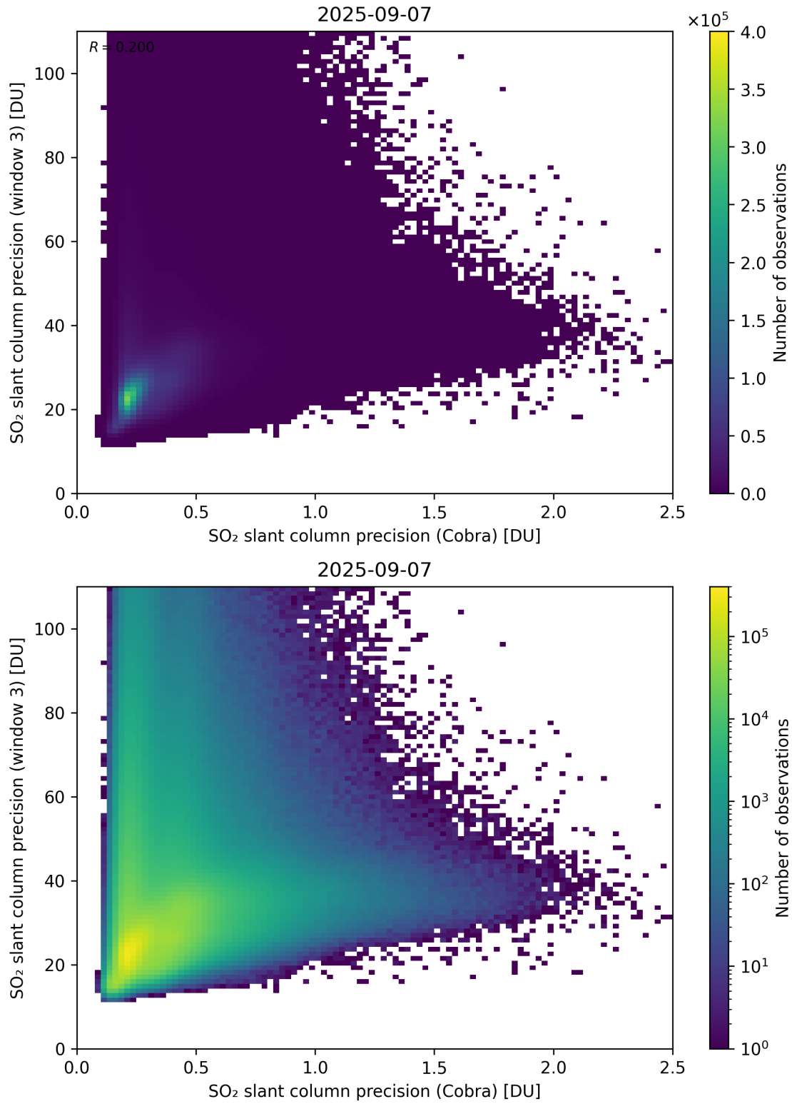
Figure 212: Scatter density plot of “SO 2 slant column precision (Cobra)” against “SO 2 slant column precision (window 3)” for 2025-09-06 to 2025-09-08.
