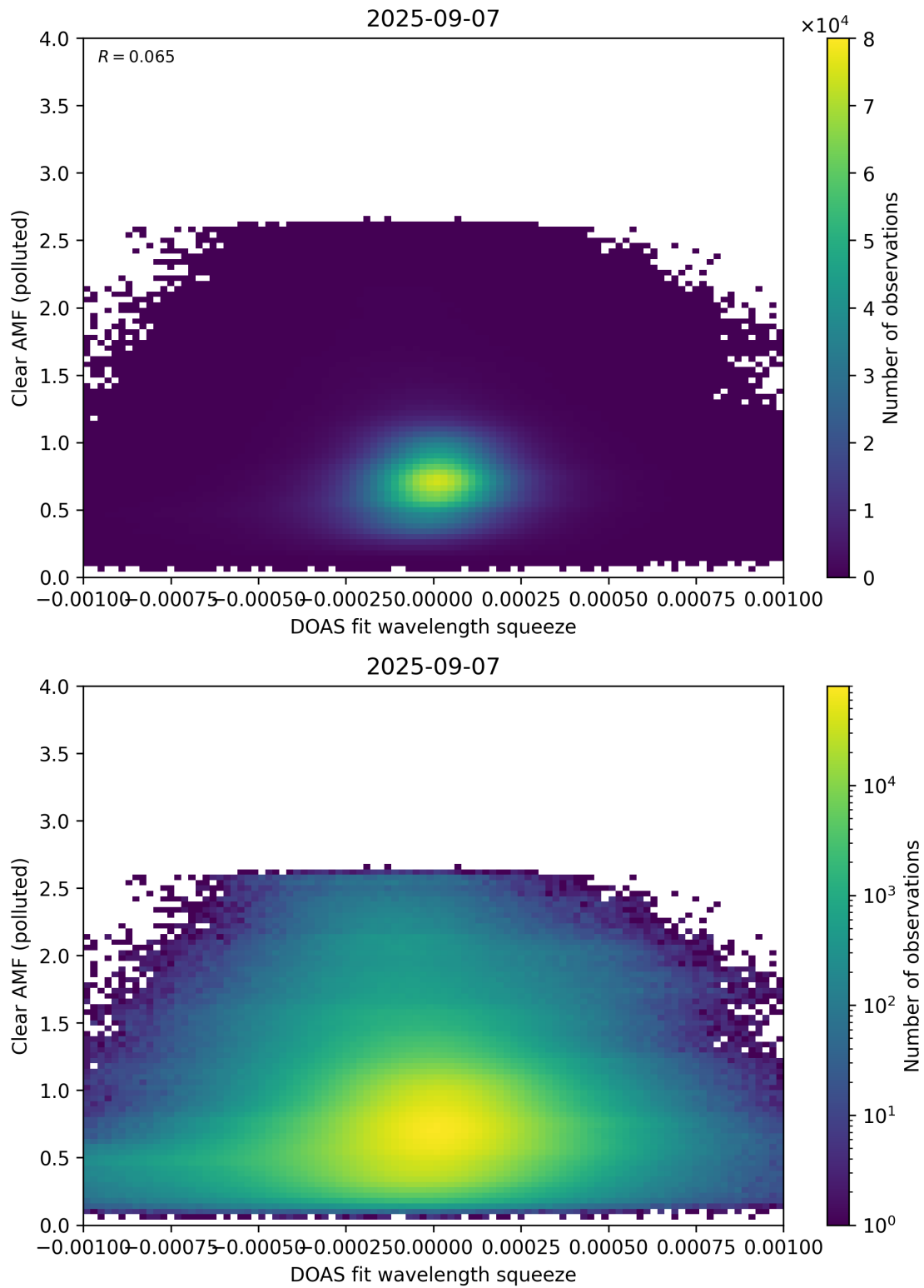
Figure 144: Scatter density plot of “DOAS fit wavelength squeeze” against “Clear AMF (polluted)” for 2025-09-06 to 2025-09-08.
