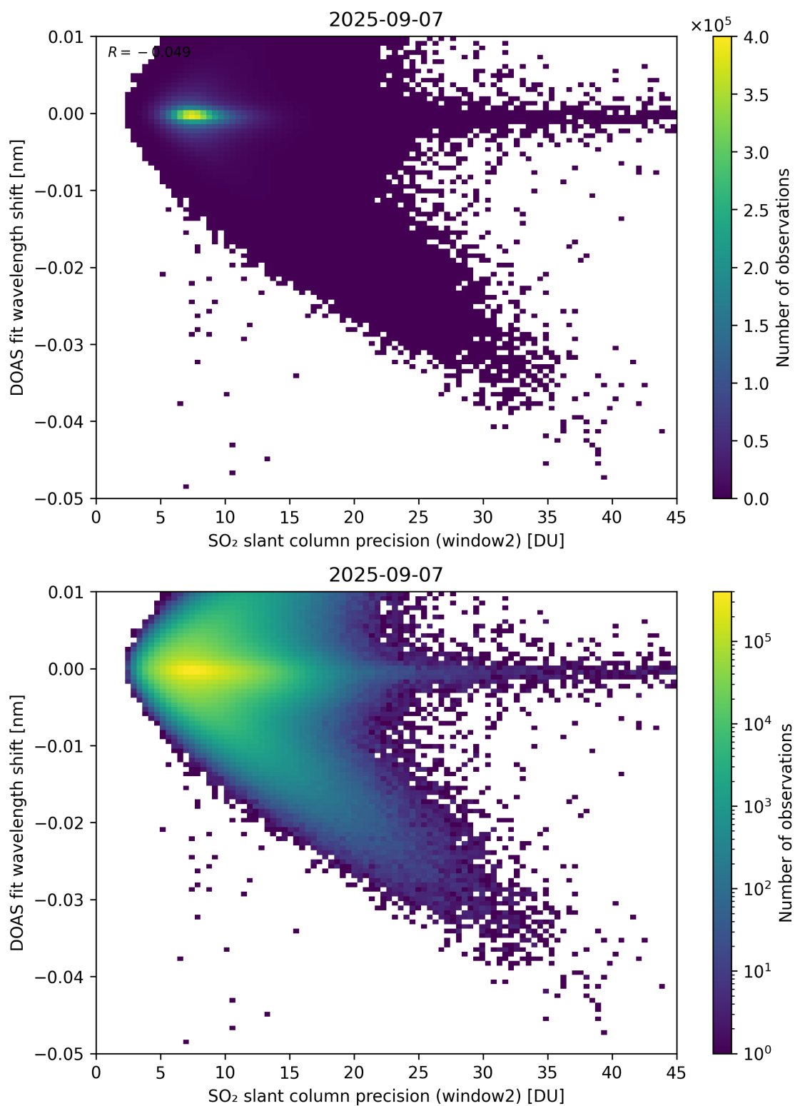
Figure 293: Scatter density plot of “SO 2 slant column precision (window2)” against “DOAS fit wavelength shift” for 2025-09-06 to 2025-09-08.
