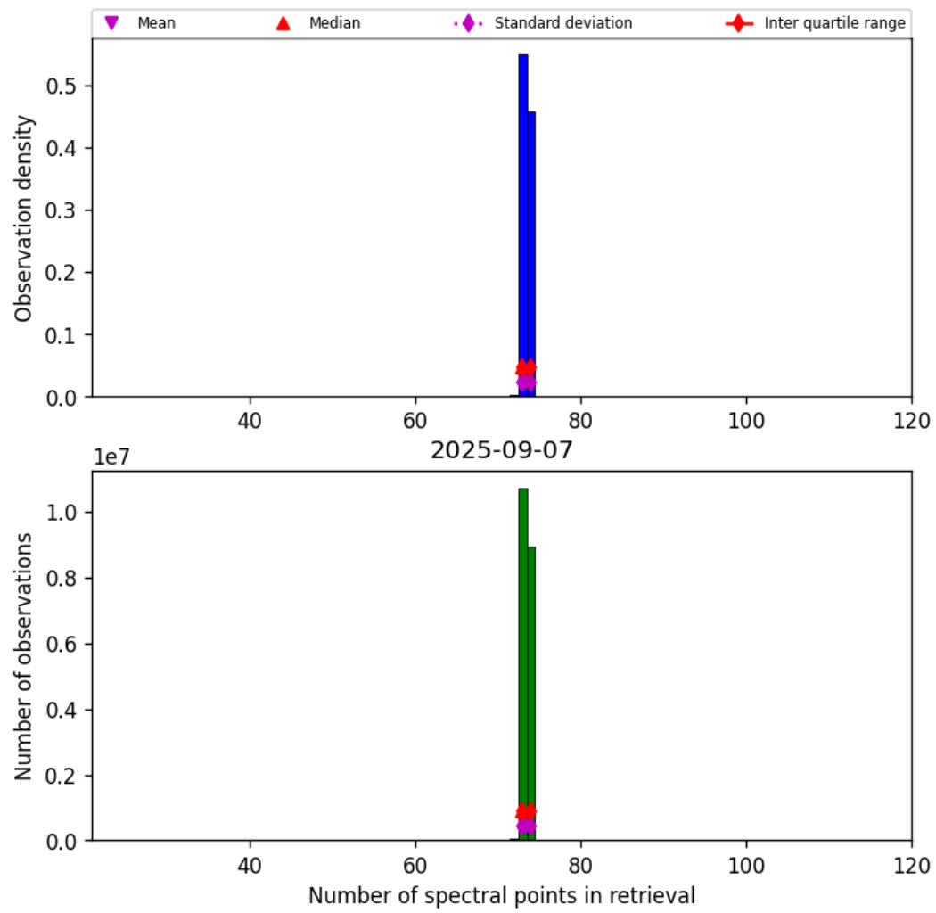
Figure 82: Histogram of “Number of spectral points in retrieval” for 2025-09-06 to 2025-09-08
