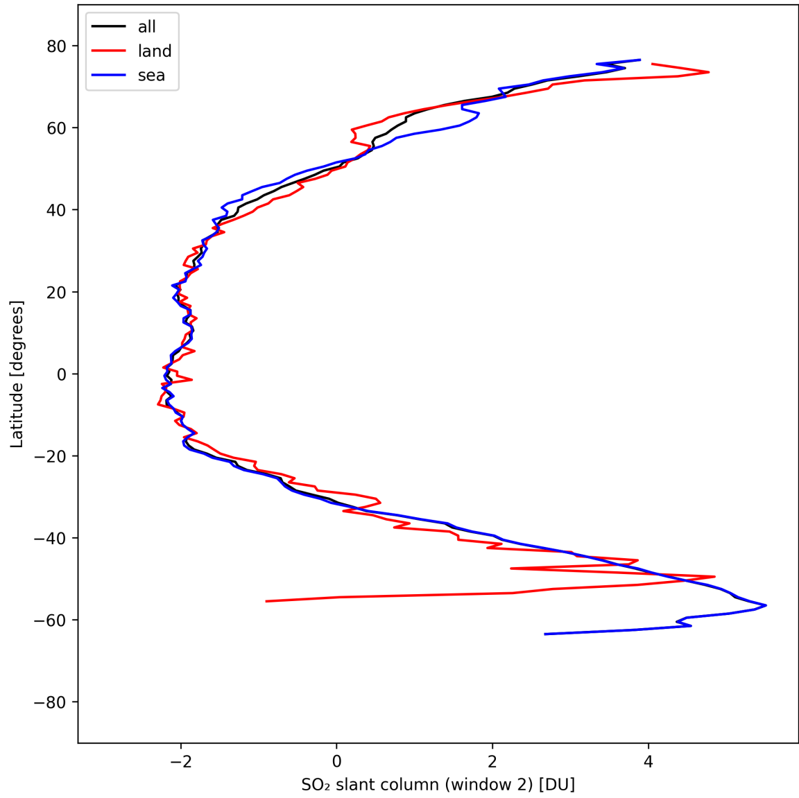
Figure 41: Zonal average of “SO 2 slant column (window 2)” for 2025-09-06 to 2025-09-08.
