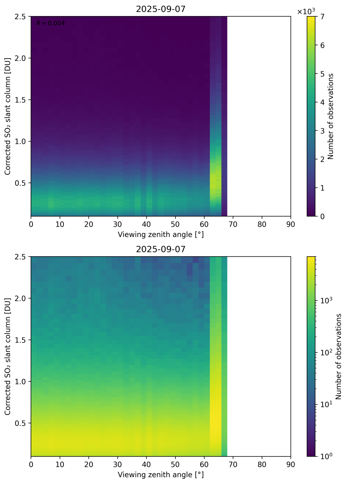
Figure 373: Scatter density plot of “Viewing zenith angle” against “Corrected SO 2 slant column” for 2025-09-06 to 2025-09-08.
