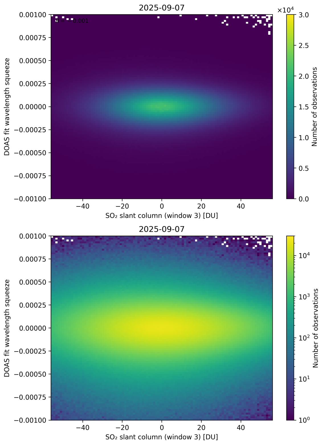
Figure 305: Scatter density plot of “SO 2 slant column (window 3)” against “DOAS fit wavelength squeeze” for 2025-09-06 to 2025-09-08.
