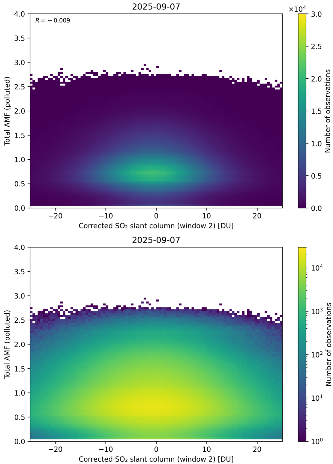
Figure 253: Scatter density plot of “Corrected SO 2 slant column (window 2)” against “Total AMF (polluted)” for 2025-09-06 to 2025-09-08.
