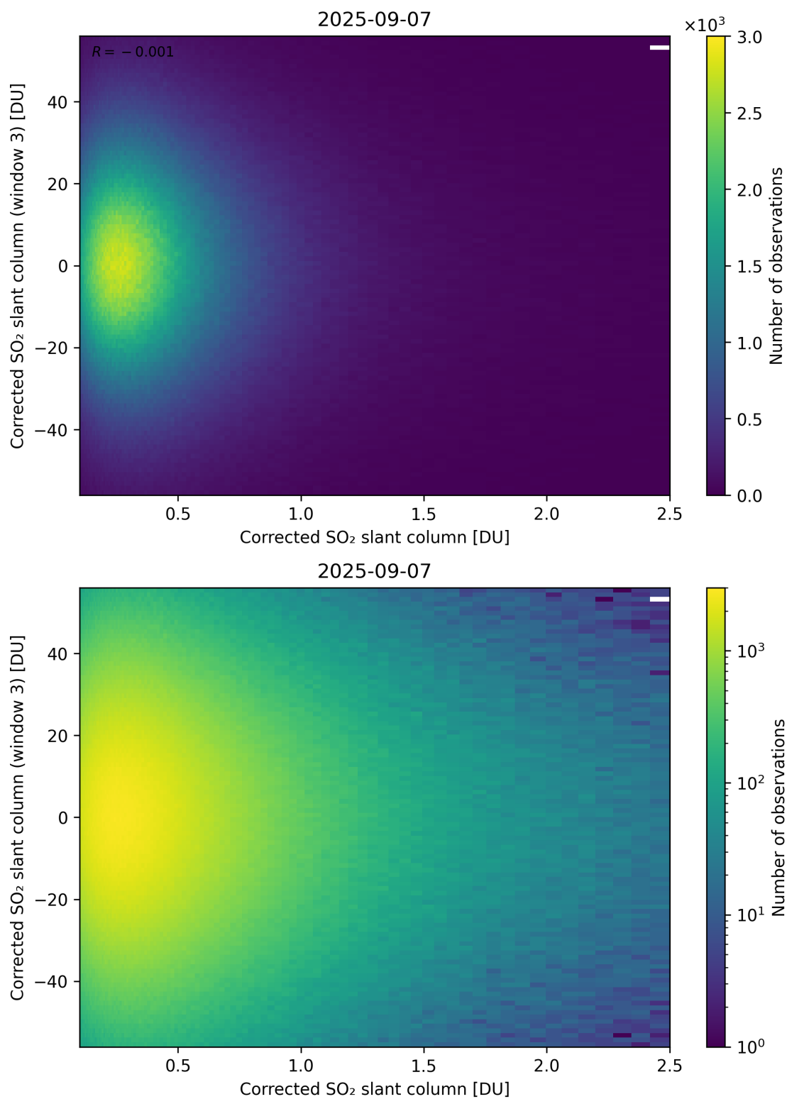
Figure 236: Scatter density plot of “Corrected SO 2 slant column” against “Corrected SO 2 slant column (window 3)” for 2025-09-06 to 2025-09-08.
