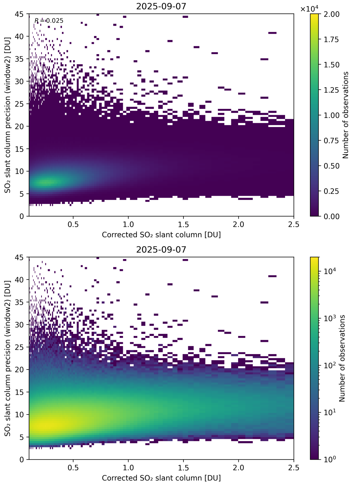
Figure 239: Scatter density plot of “Corrected SO 2 slant column” against “SO 2 slant column precision (window2)” for 2025-09-06 to 2025-09-08.
