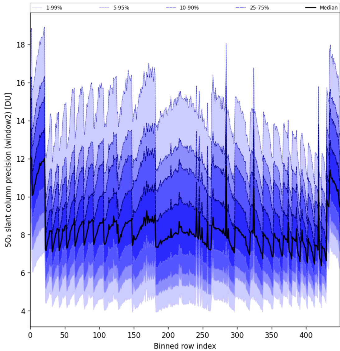
Figure 94: Along track statistics of “SO 2 slant column precision (window2)” for 2025-09-06 to 2025-09-08
