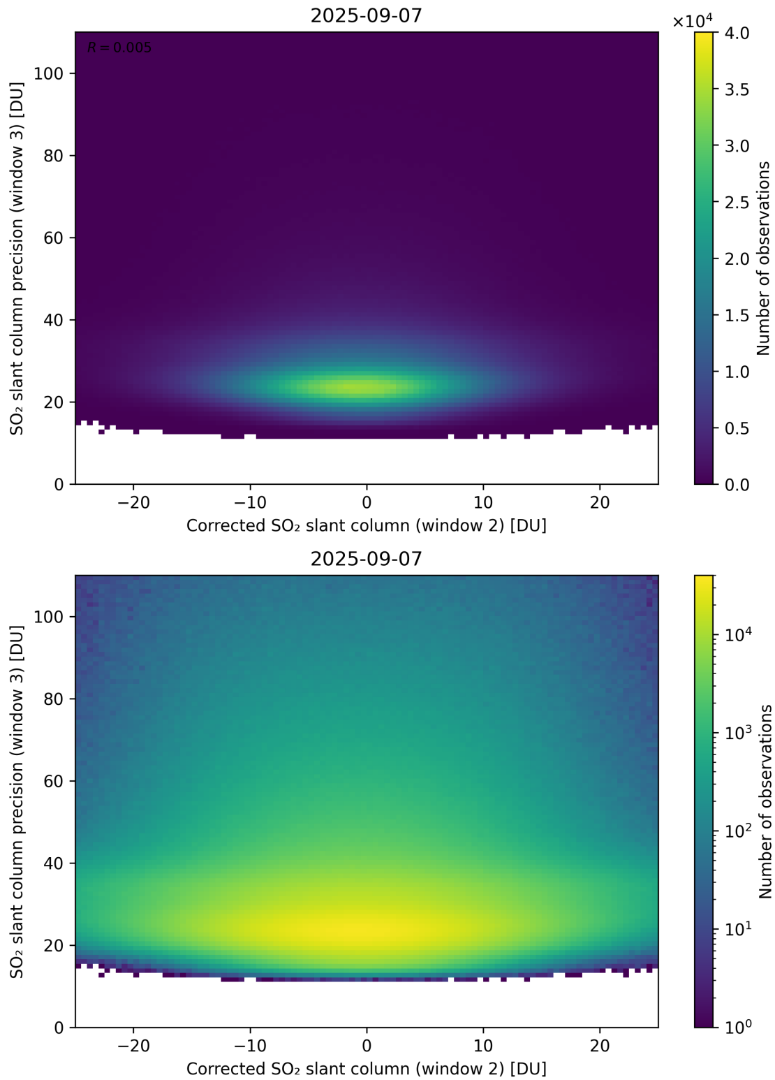
Figure 252: Scatter density plot of “Corrected SO 2 slant column (window 2)” against “SO 2 slant column precision (window 3)” for 2025-09-06 to 2025-09-08.
