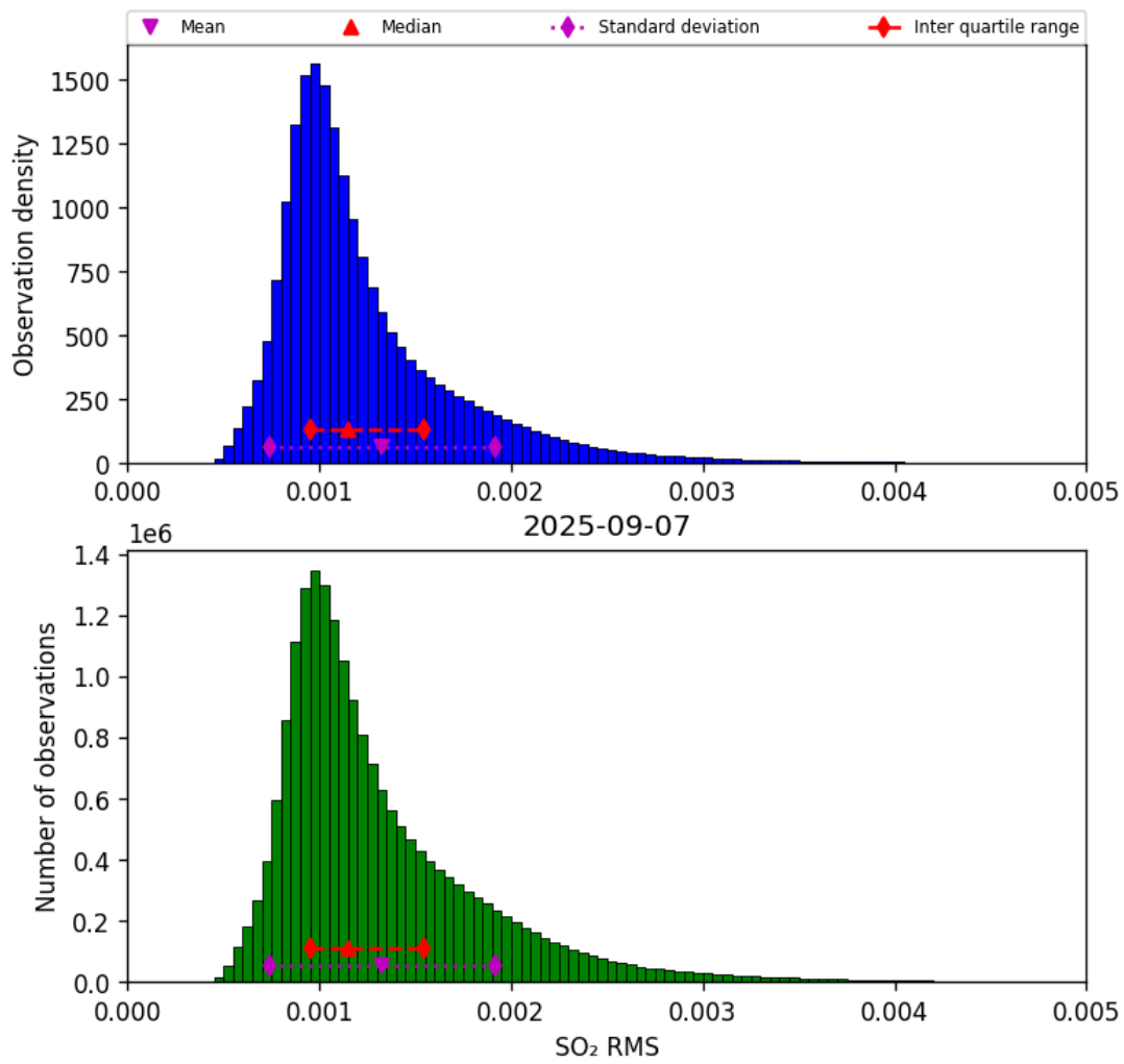
Figure 78: Histogram of “SO 2 RMS” for 2025-09-06 to 2025-09-08
