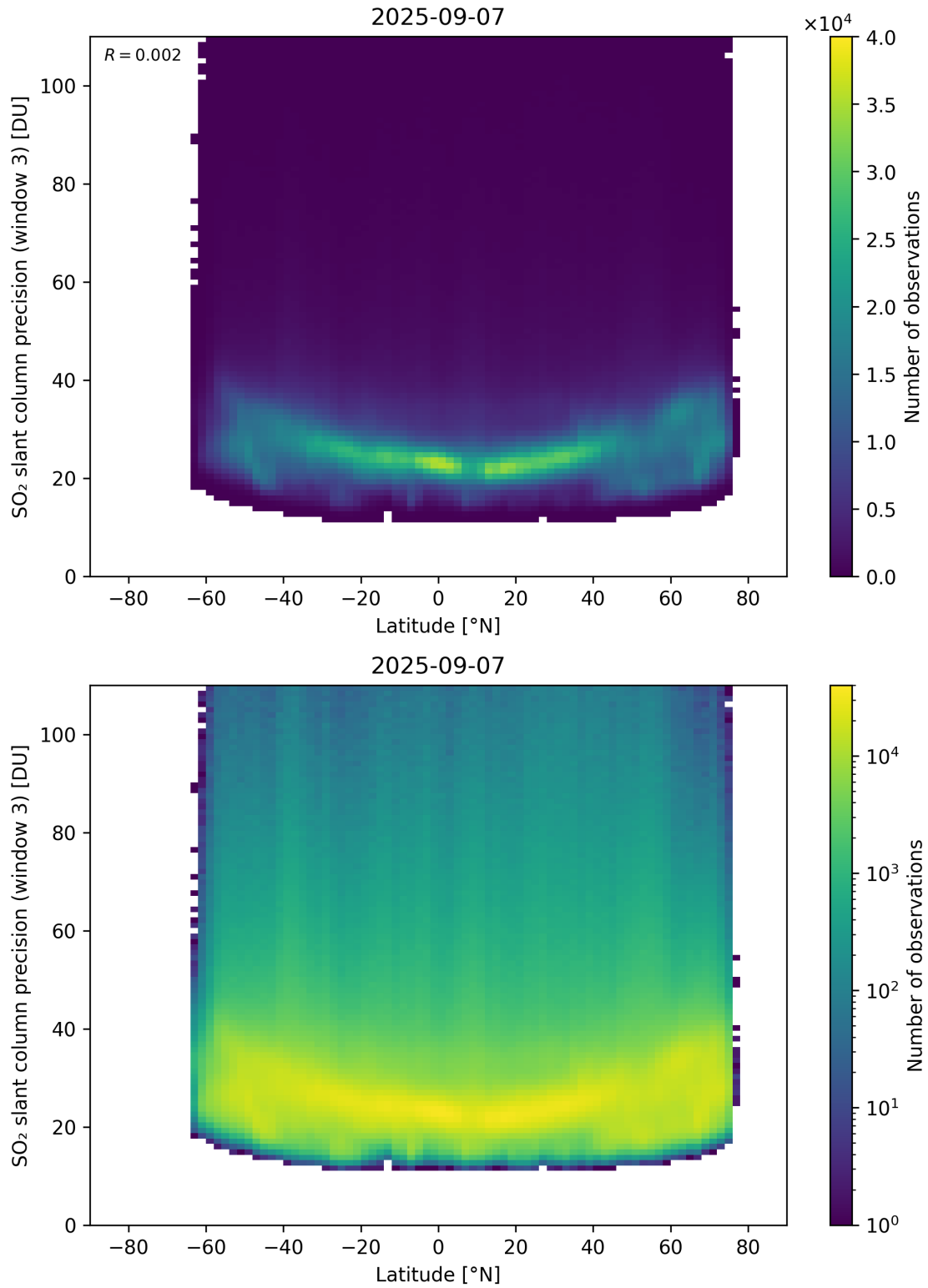
Figure 166: Scatter density plot of “Latitude” against “SO 2 slant column precision (window 3)” for 2025-09-06 to 2025-09-08.
