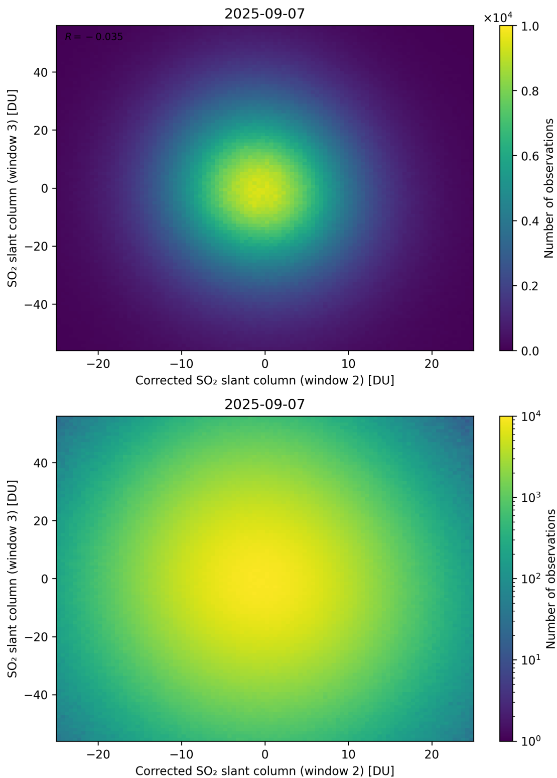
Figure 251: Scatter density plot of “Corrected SO 2 slant column (window 2)” against “SO 2 slant column (window 3)” for 2025-09-06 to 2025-09-08.
