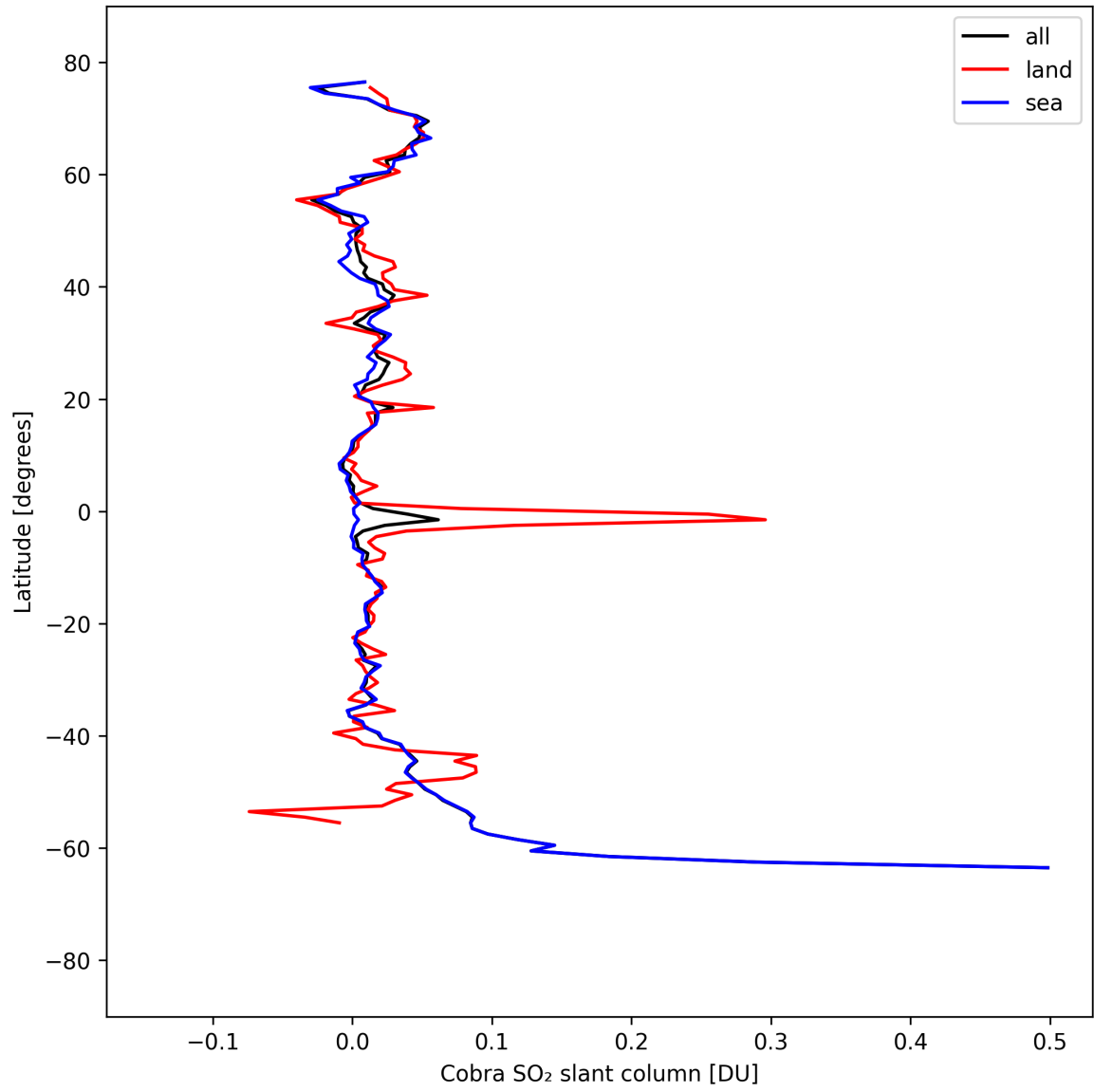
Figure 35: Zonal average of “Cobra SO 2 slant column” for 2025-09-06 to 2025-09-08.
