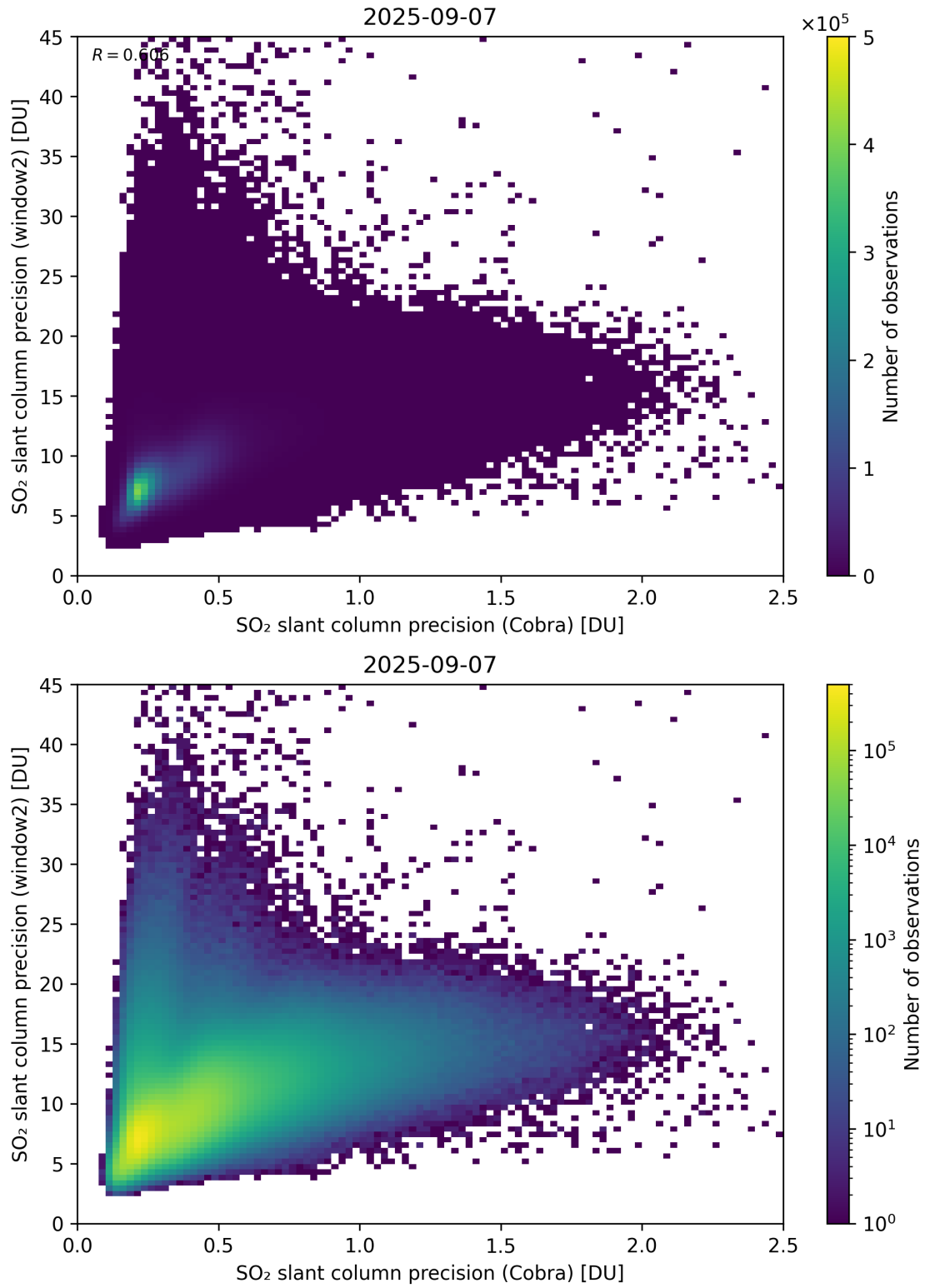
Figure 210: Scatter density plot of “SO 2 slant column precision (Cobra)” against “SO 2 slant column precision (window2)” for 2025-09-06 to 2025-09-08.
