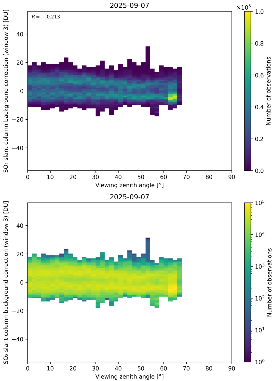
Figure 364: Scatter density plot of “Viewing zenith angle” against “SO 2 slant column background correction (window 3)” for 2025-09-06 to 2025-09-08.
