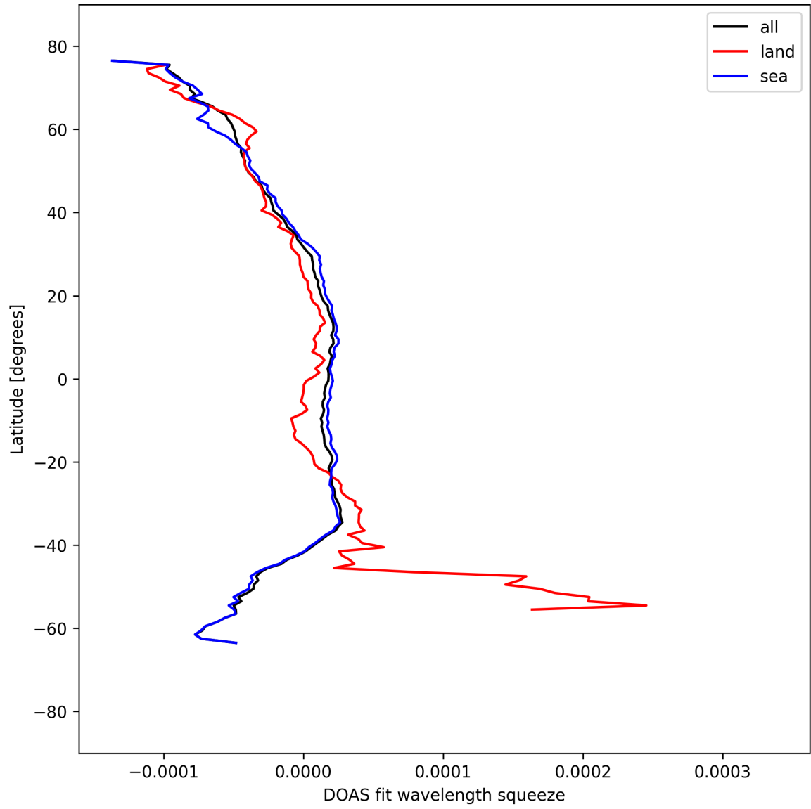
Figure 51: Zonal average of “DOAS fit wavelength squeeze” for 2025-09-06 to 2025-09-08.
