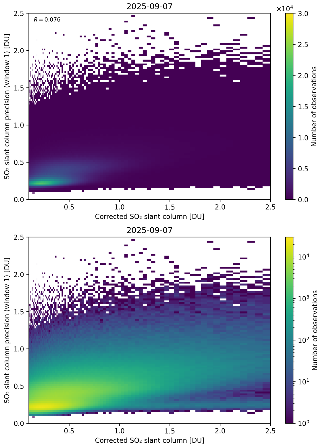
Figure 238: Scatter density plot of “Corrected SO 2 slant column” against “SO 2 slant column precision (window 1)” for 2025-09-06 to 2025-09-08.
