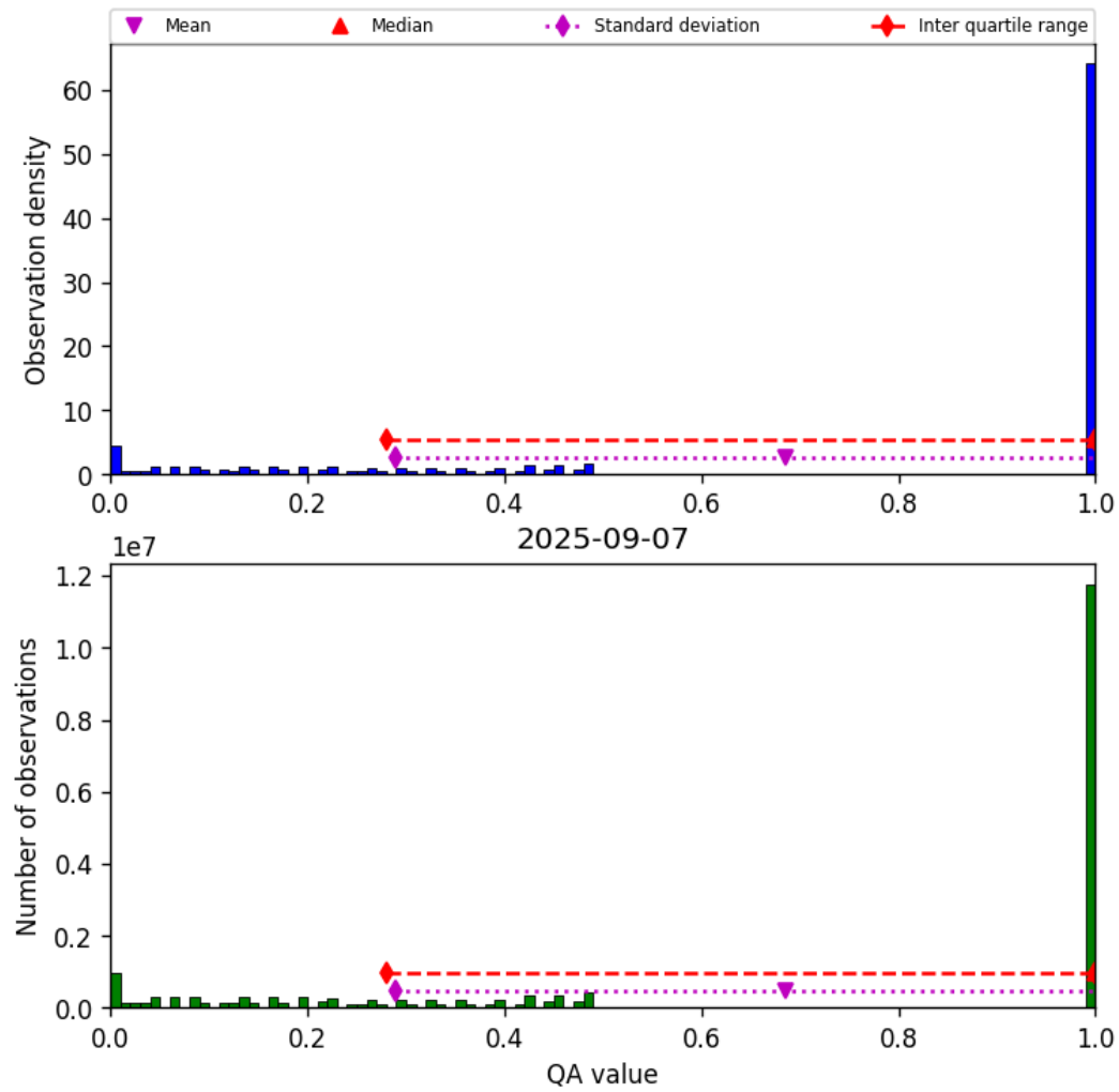
Figure 57: Histogram of “QA value” for 2025-09-06 to 2025-09-08
