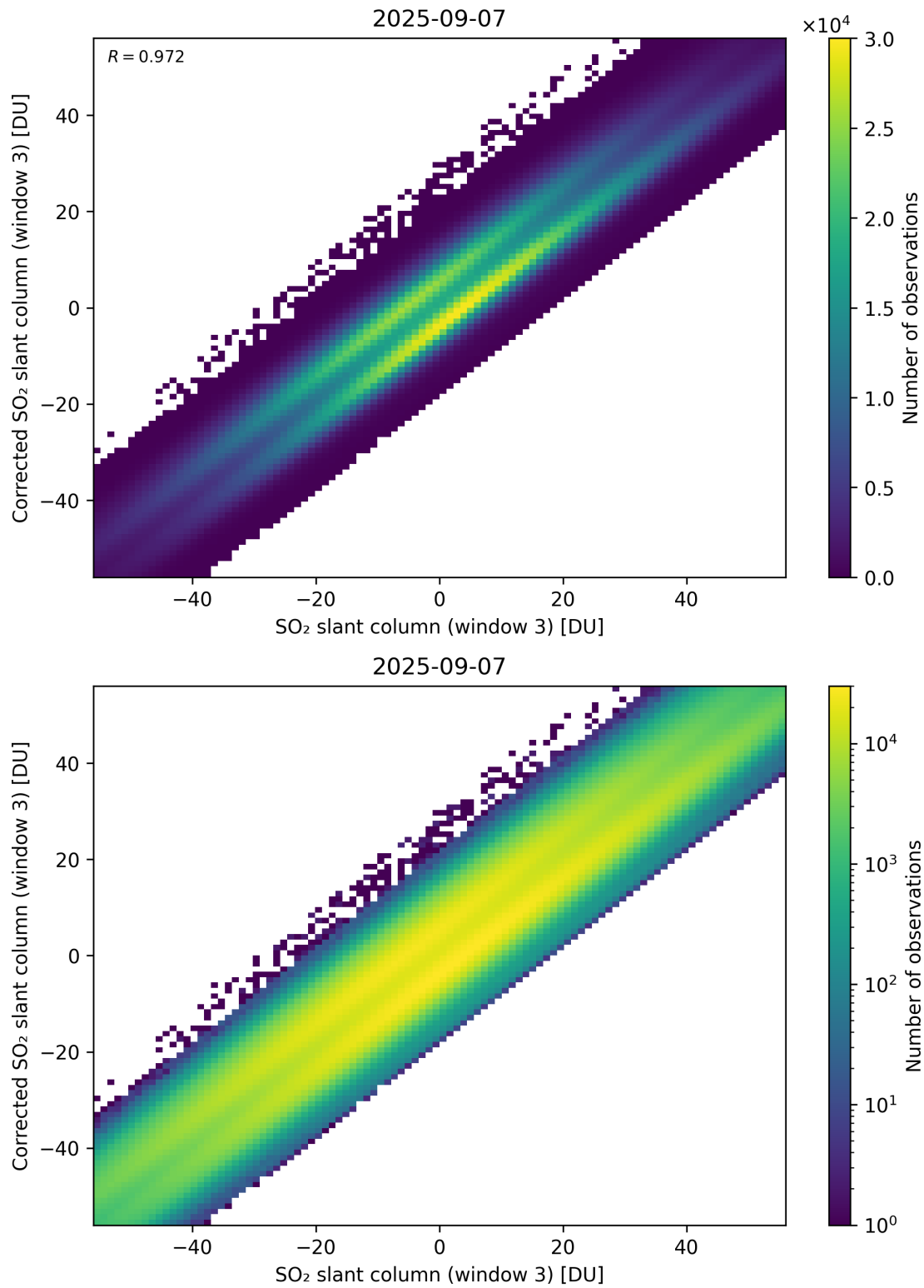
Figure 316: Scatter density plot of “SO 2 slant column (window 3)” against “Corrected SO 2 slant column (window 3)” for 2025-09-06 to 2025-09-08.
