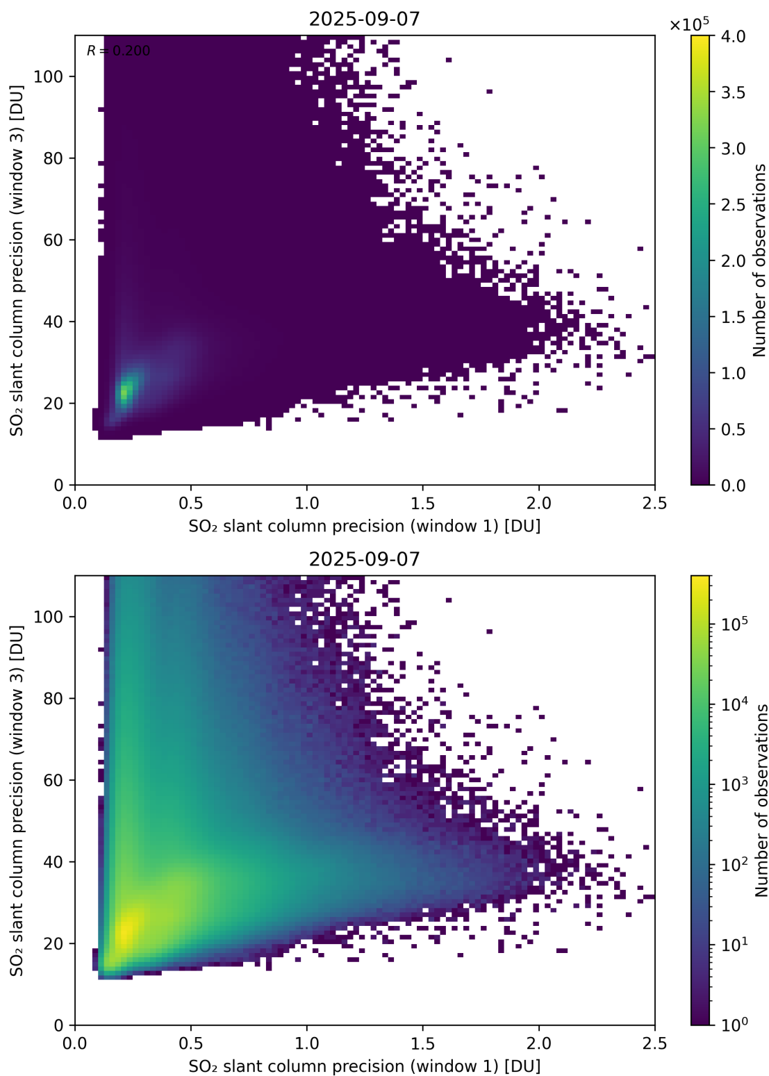
Figure 279: Scatter density plot of “SO 2 slant column precision (window 1)” against “SO 2 slant column precision (window 3)” for 2025-09-06 to 2025-09-08.
