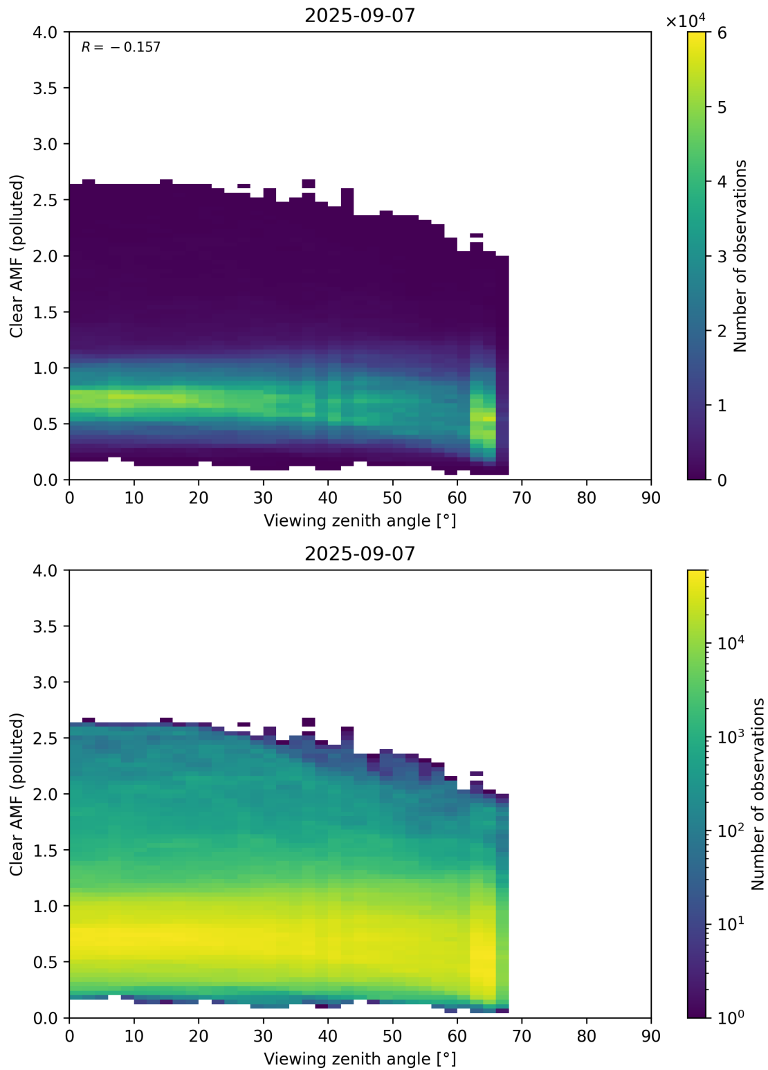
Figure 370: Scatter density plot of “Viewing zenith angle” against “Clear AMF (polluted)” for 2025-09-06 to 2025-09-08.
