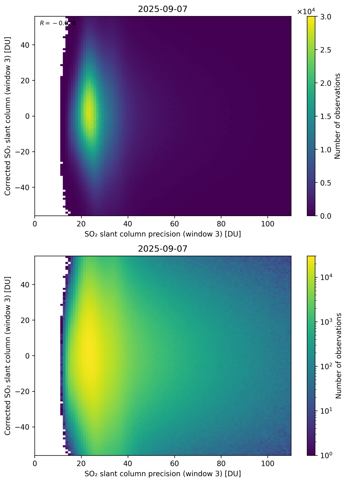
Figure 312: Scatter density plot of “SO 2 slant column precision (window 3)” against “Corrected SO 2 slant column (window 3)” for 2025-09-06 to 2025-09-08.
