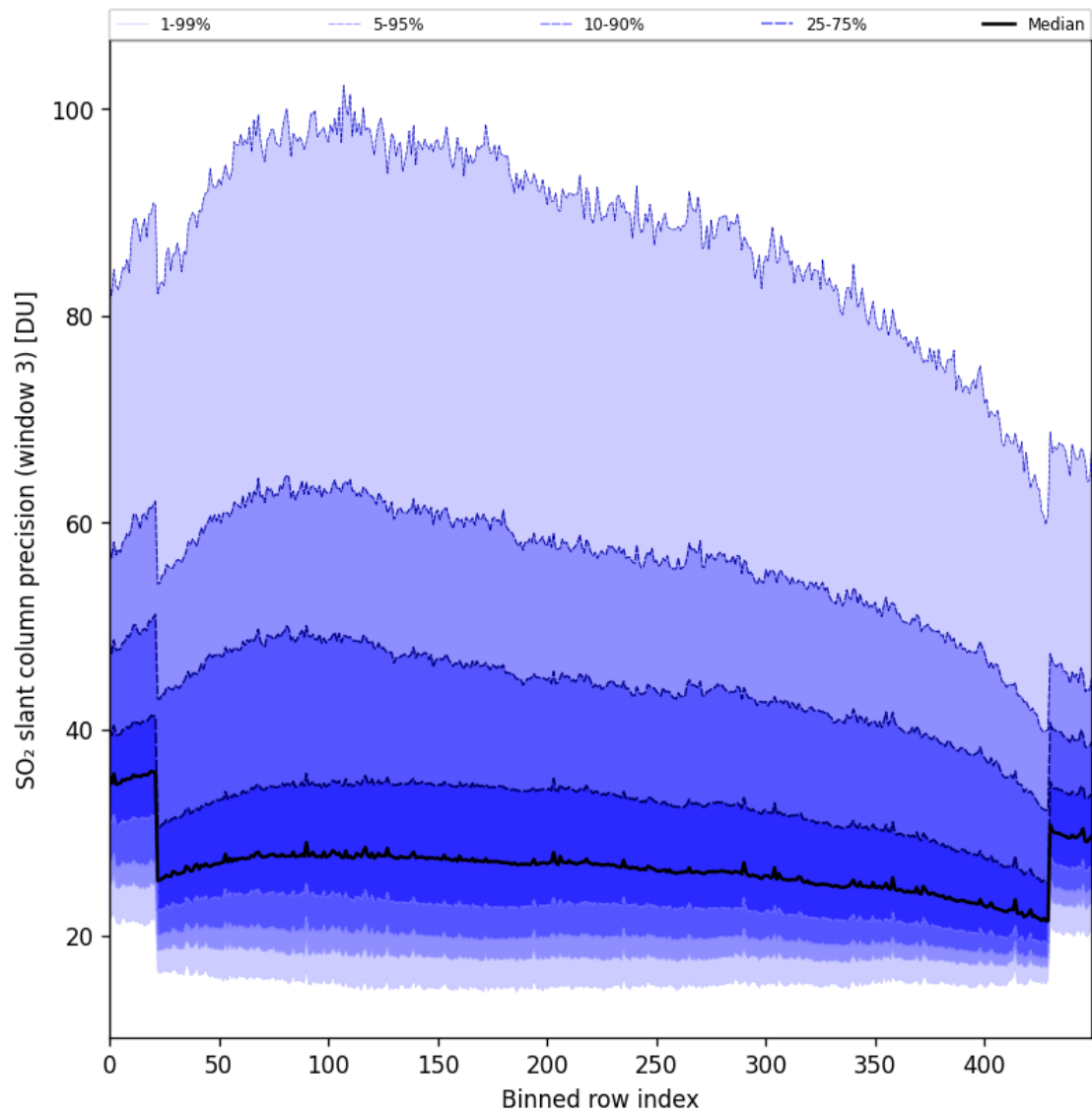
Figure 98: Along track statistics of “SO 2 slant column precision (window 3)” for 2025-09-06 to 2025-09-08
