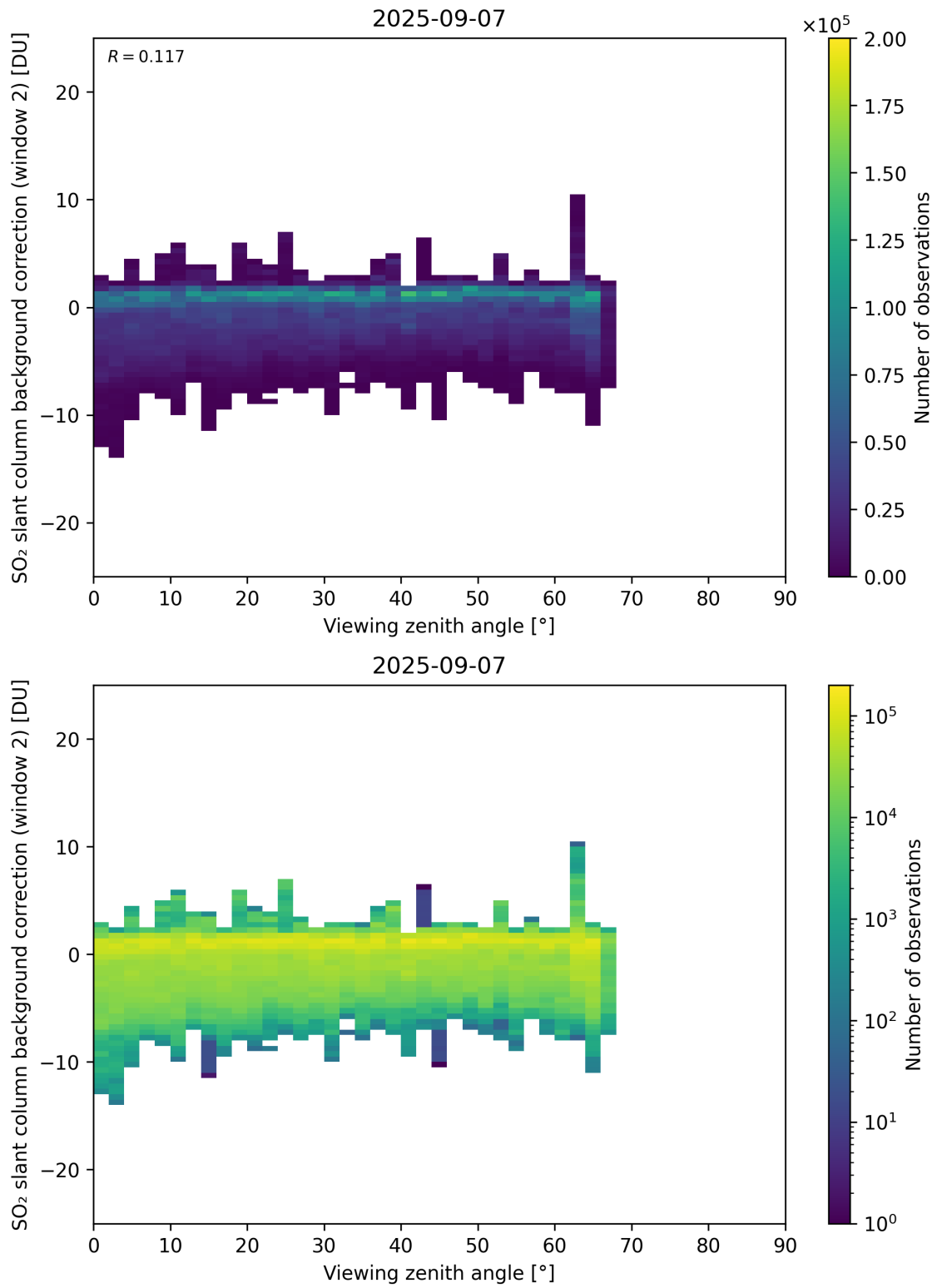
Figure 363: Scatter density plot of “Viewing zenith angle” against “SO 2 slant column background correction (window 2)” for 2025-09-06 to 2025-09-08.
