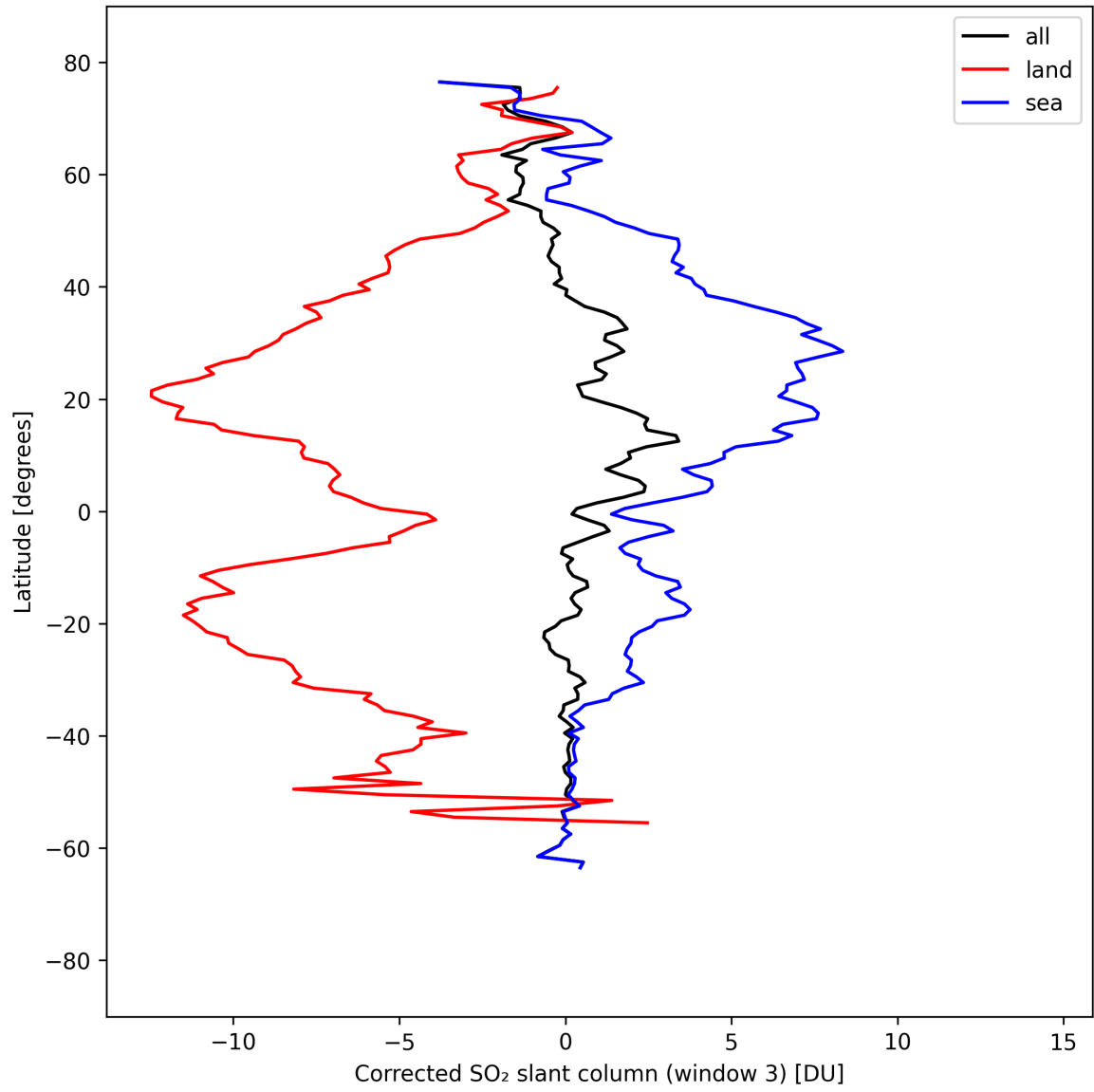
Figure 47: Zonal average of “Corrected SO 2 slant column (window 3)” for 2025-09-06 to 2025-09-08.
