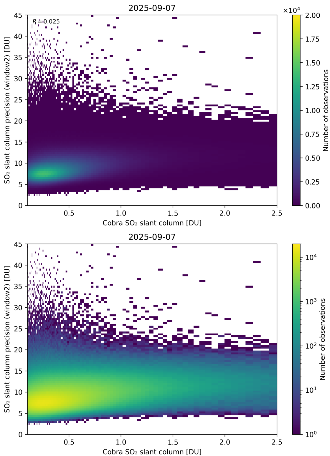
Figure 221: Scatter density plot of “Cobra SO 2 slant column” against “SO 2 slant column precision (window2)” for 2025-09-06 to 2025-09-08.
