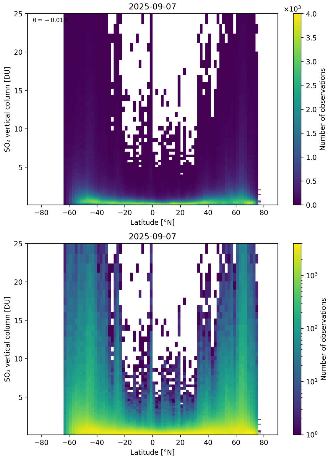
Figure 169: Scatter density plot of “Latitude” against “SO 2 vertical column” for 2025-09-06 to 2025-09-08.
