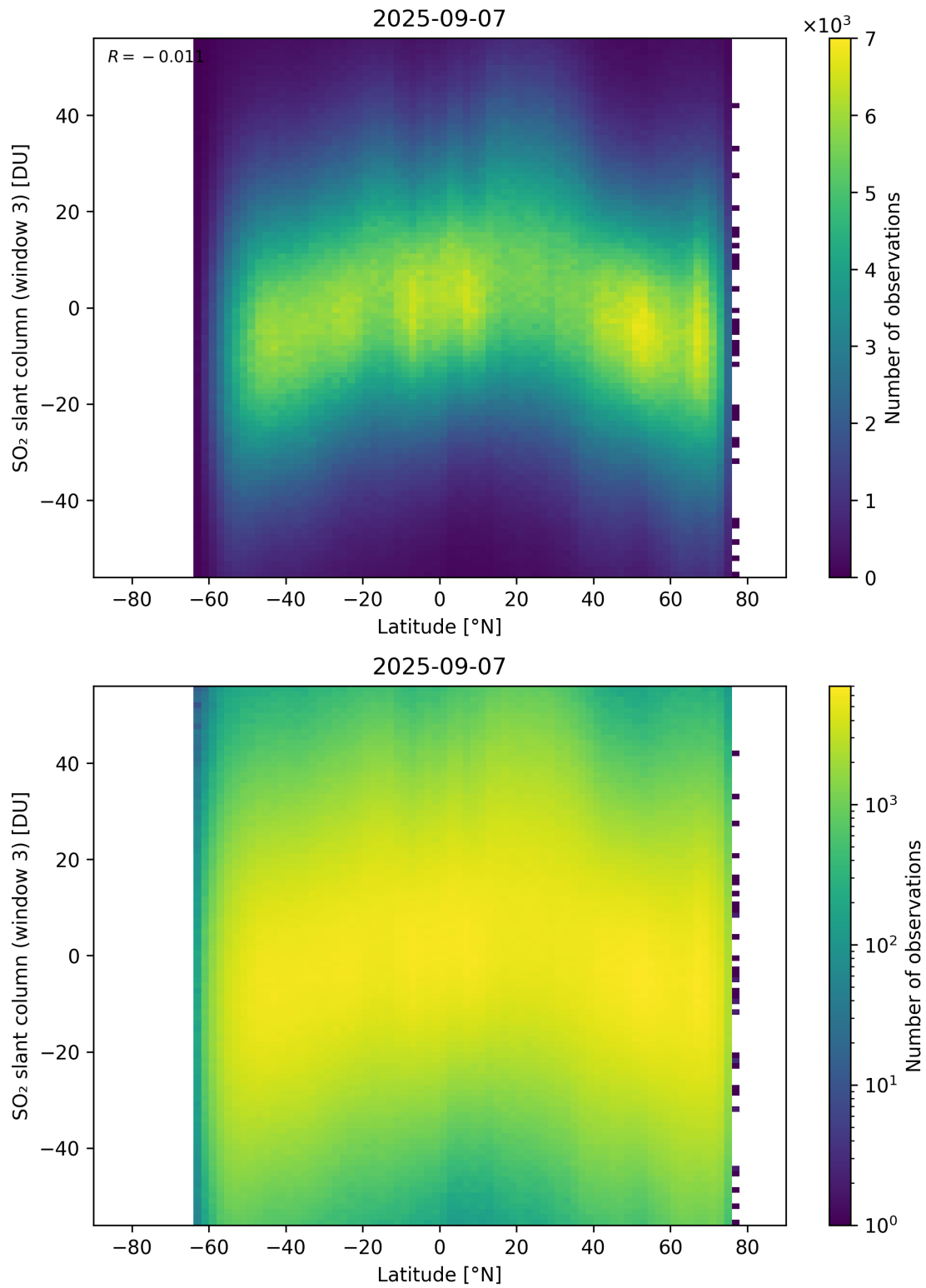
Figure 165: Scatter density plot of “Latitude” against “SO 2 slant column (window 3)” for 2025-09-06 to 2025-09-08.
