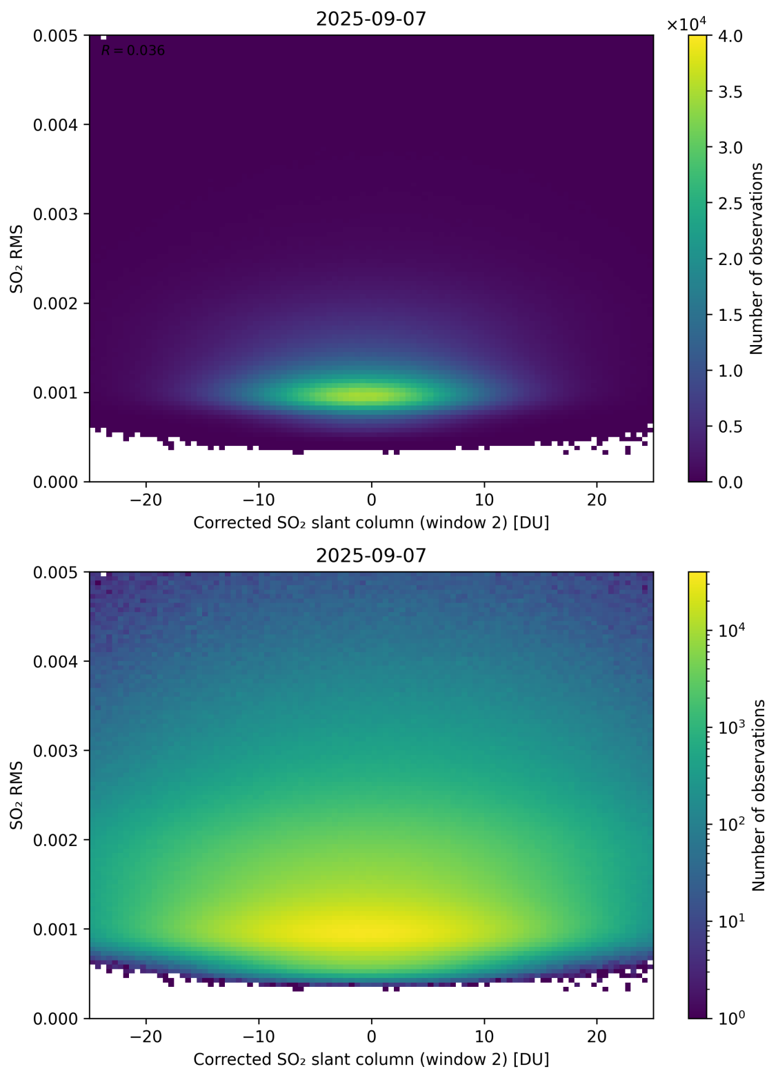
Figure 248: Scatter density plot of “Corrected SO 2 slant column (window 2)” against “SO 2 RMS” for 2025-09-06 to 2025-09-08.
