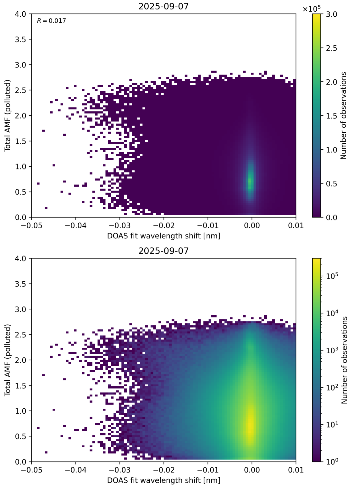
Figure 141: Scatter density plot of “DOAS fit wavelength shift” against “Total AMF (polluted)” for 2025-09-06 to 2025-09-08.
