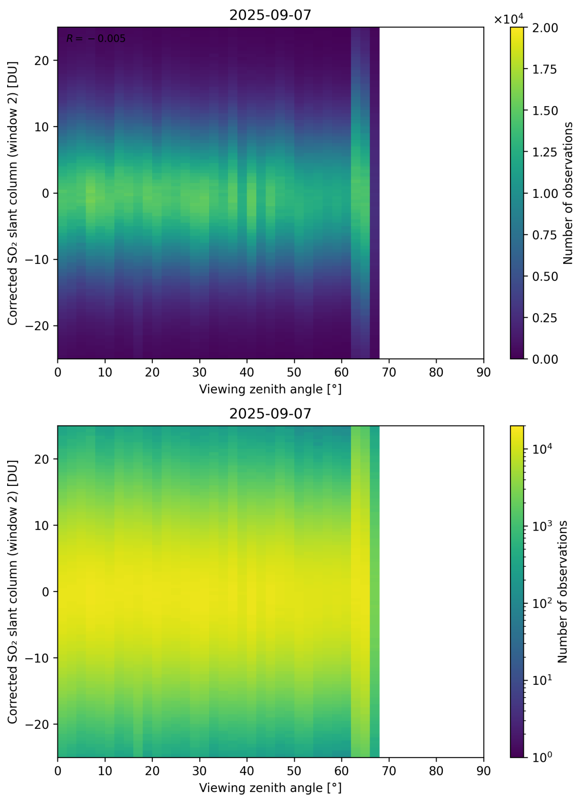
Figure 374: Scatter density plot of “Viewing zenith angle” against “Corrected SO 2 slant column (window 2)” for 2025-09-06 to 2025-09-08.
