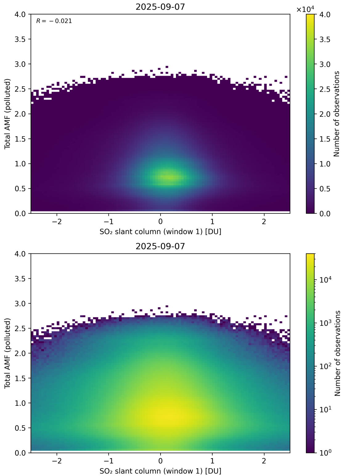
Figure 289: Scatter density plot of “SO 2 slant column (window 1)” against “Total AMF (polluted)” for 2025-09-06 to 2025-09-08.
