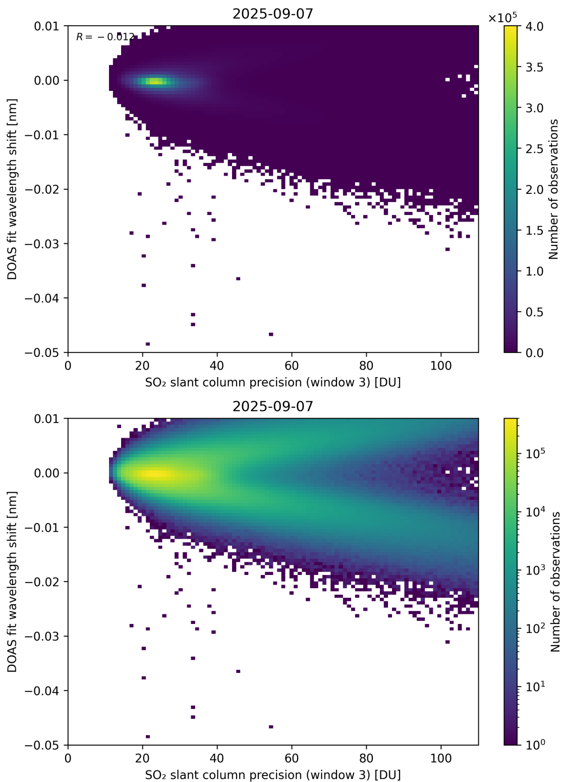
Figure 308: Scatter density plot of “SO 2 slant column precision (window 3)” against “DOAS fit wavelength shift” for 2025-09-06 to 2025-09-08.
