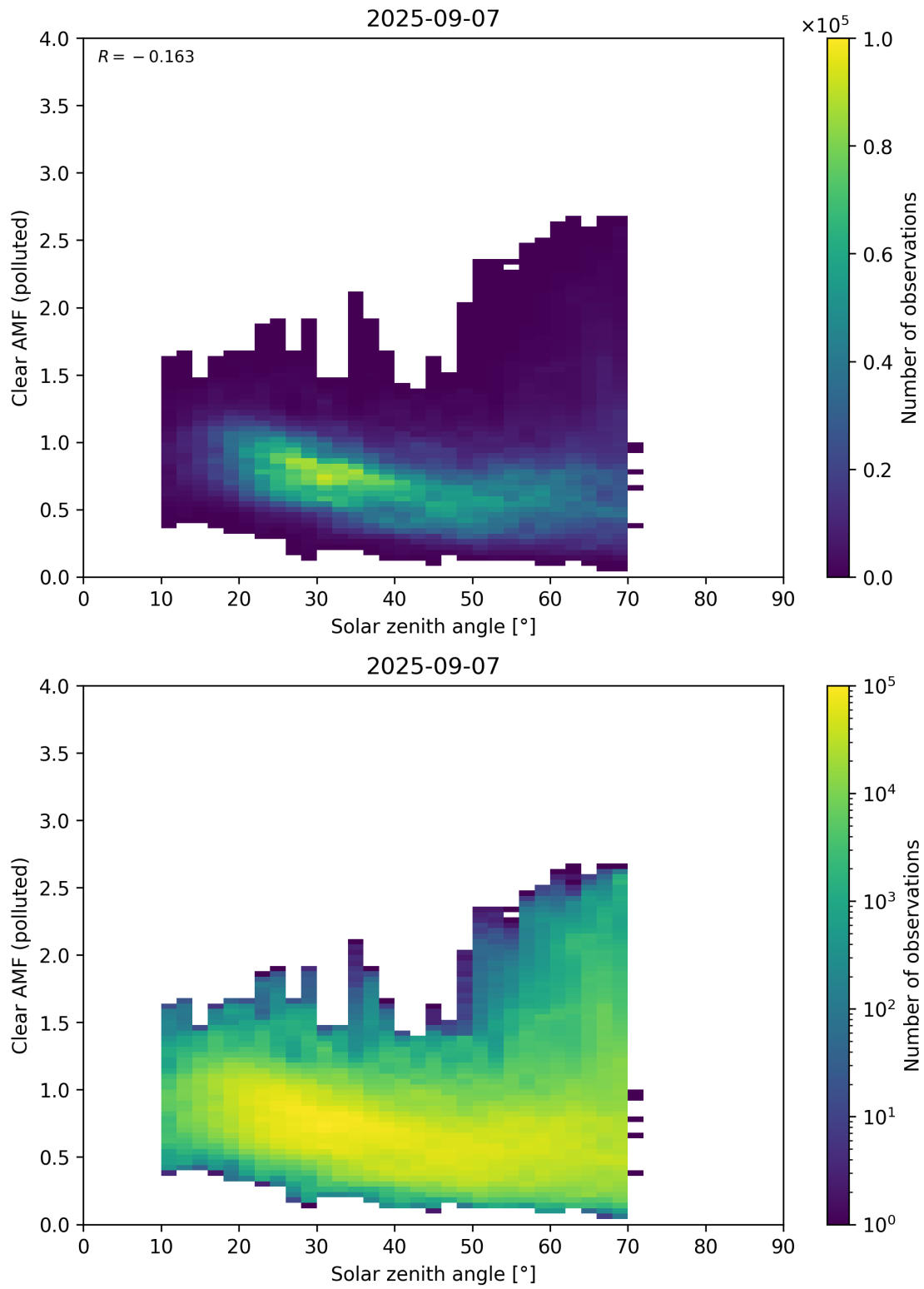
Figure 178: Scatter density plot of “Solar zenith angle” against “Clear AMF (polluted)” for 2025-09-06 to 2025-09-08.
