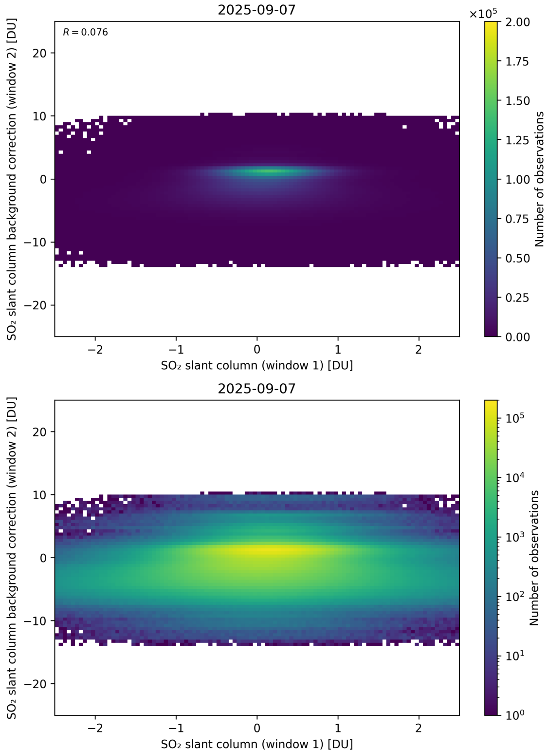
Figure 263: Scatter density plot of “SO 2 slant column (window 1)” against “SO 2 slant column background correction (window 2)” for 2025-09-06 to 2025-09-08.
