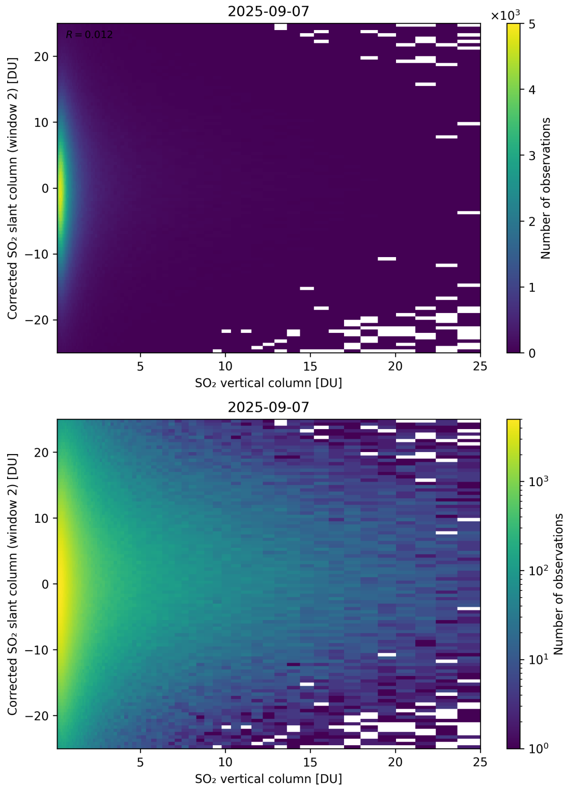
Figure 352: Scatter density plot of “SO 2 vertical column” against “Corrected SO 2 slant column (window 2)” for 2025-09-06 to 2025-09-08.
