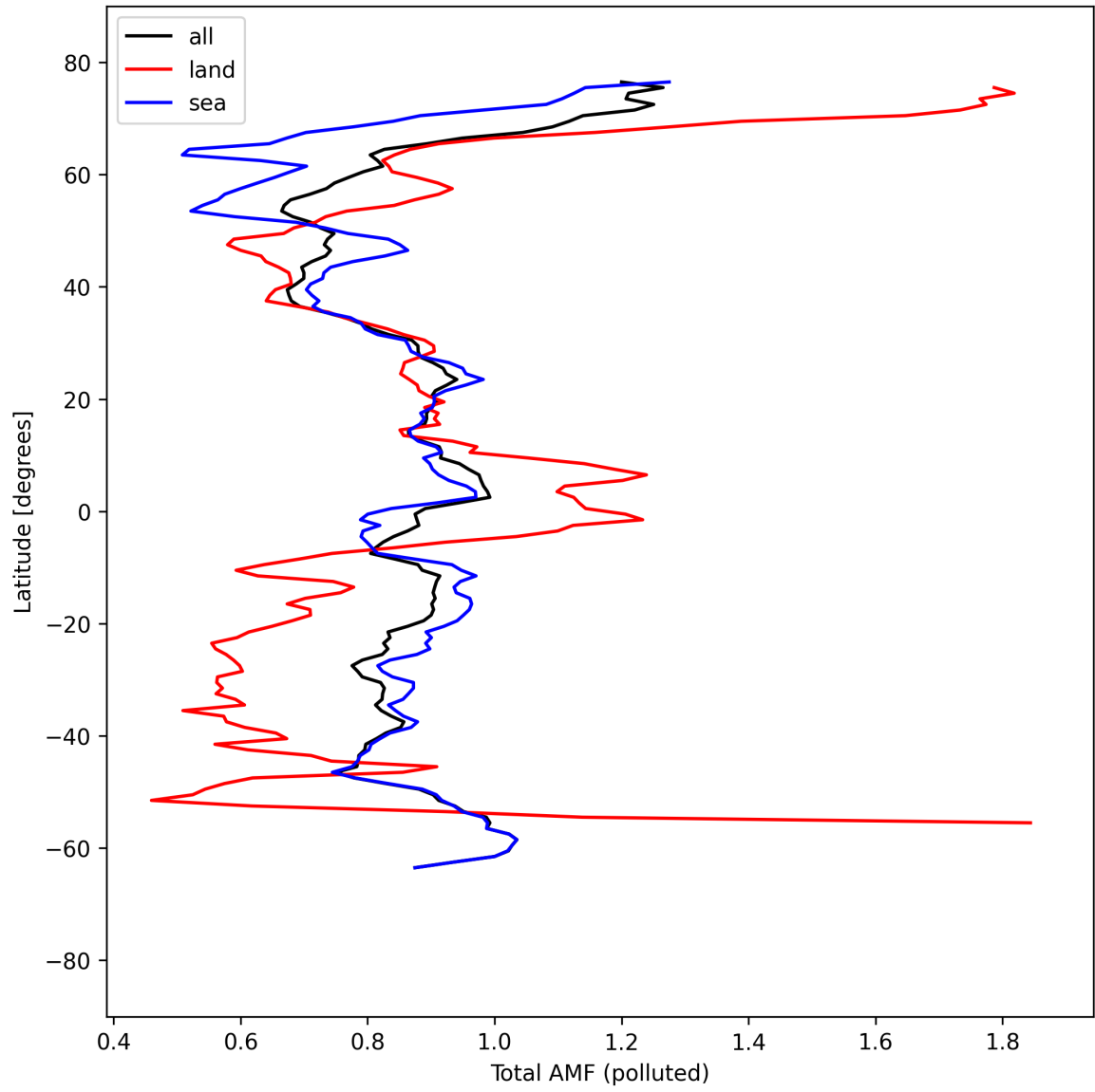
Figure 53: Zonal average of “Total AMF (polluted)” for 2025-09-06 to 2025-09-08.
