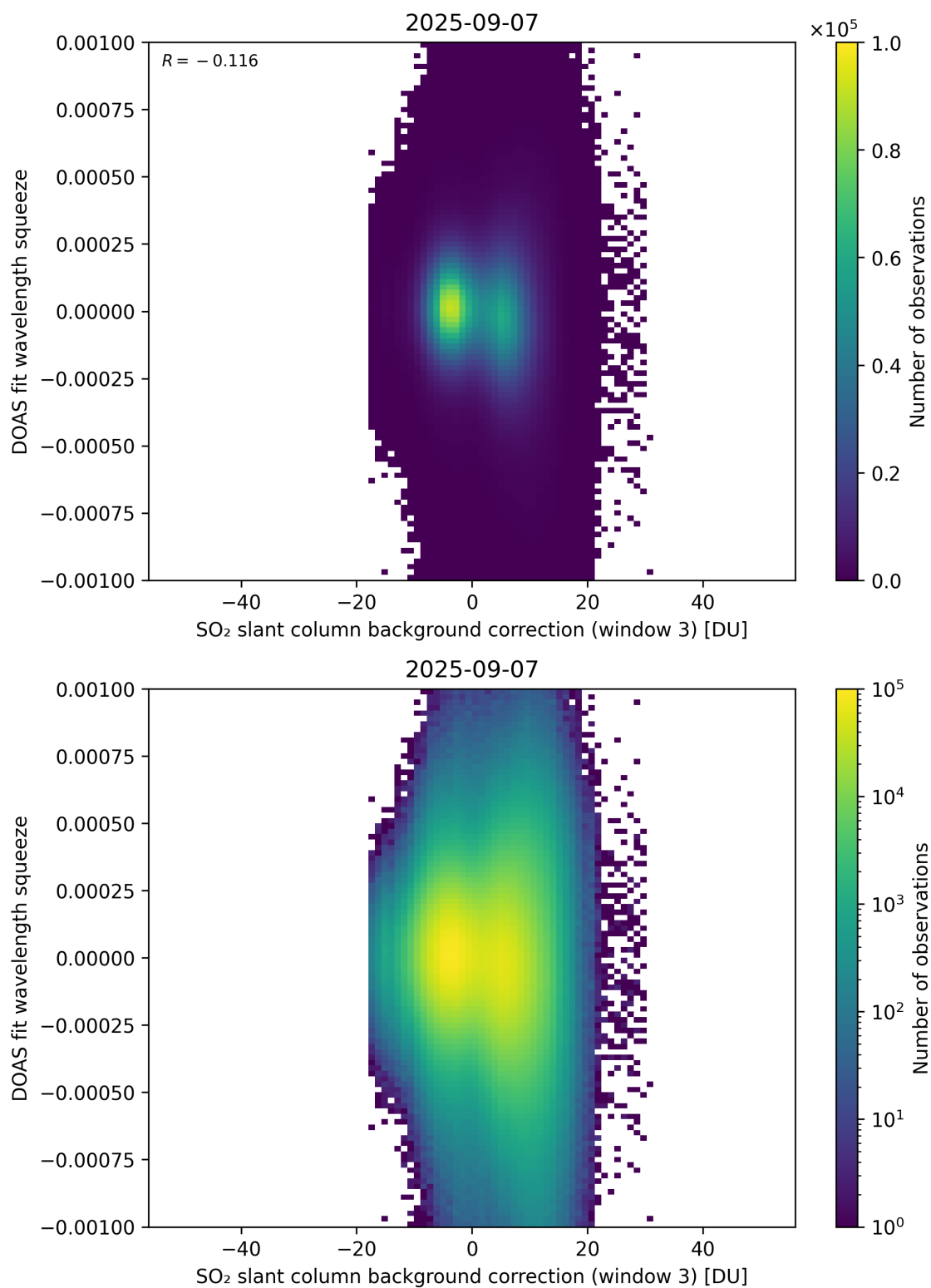
Figure 133: Scatter density plot of “SO 2 slant column background correction (window 3)” against “DOAS fit wavelength squeeze” for 2025-09-06 to 2025-09-08.
