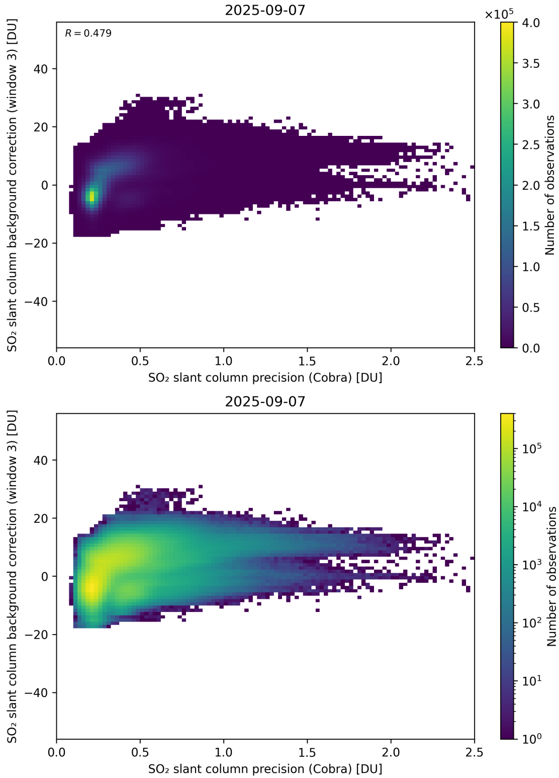
Figure 201: Scatter density plot of “SO 2 slant column precision (Cobra)” against “SO 2 slant column background correction (window 3)” for 2025-09-06 to 2025-09-08.
