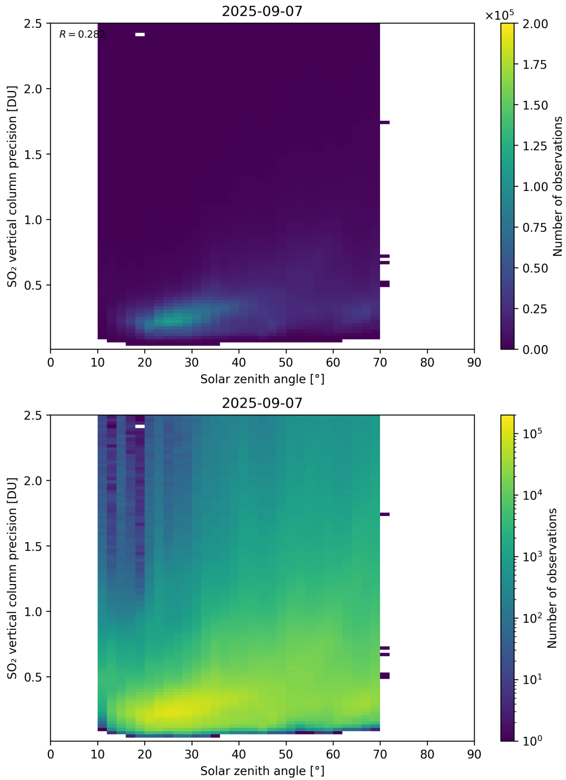
Figure 192: Scatter density plot of “Solar zenith angle” against “SO 2 vertical column precision” for 2025-09-06 to 2025-09-08.
