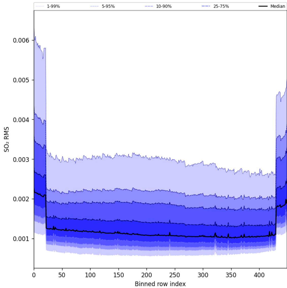
Figure 104: Along track statistics of “SO 2 RMS” for 2025-09-06 to 2025-09-08
