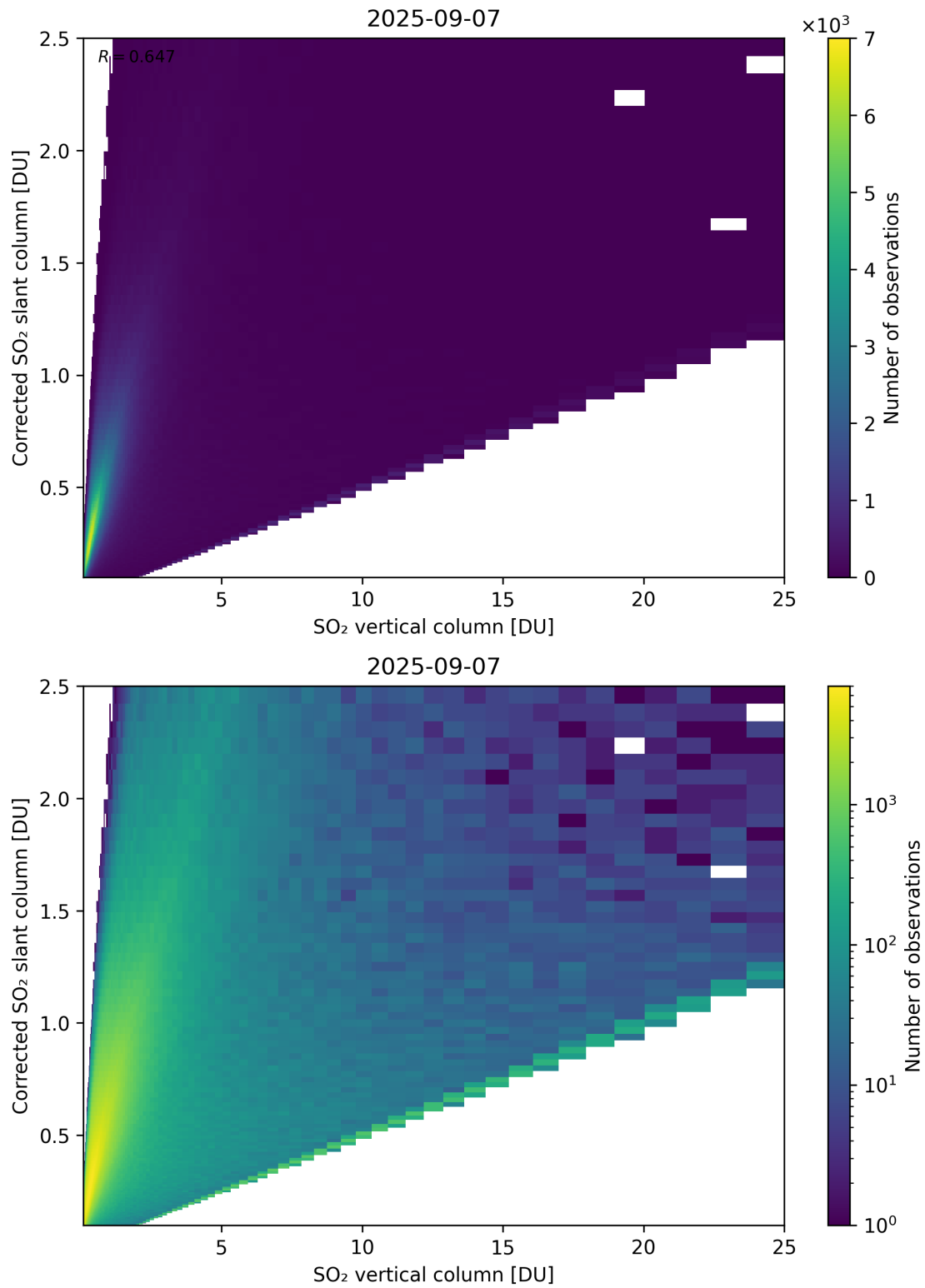
Figure 351: Scatter density plot of “SO 2 vertical column” against “Corrected SO 2 slant column” for 2025-09-06 to 2025-09-08.
