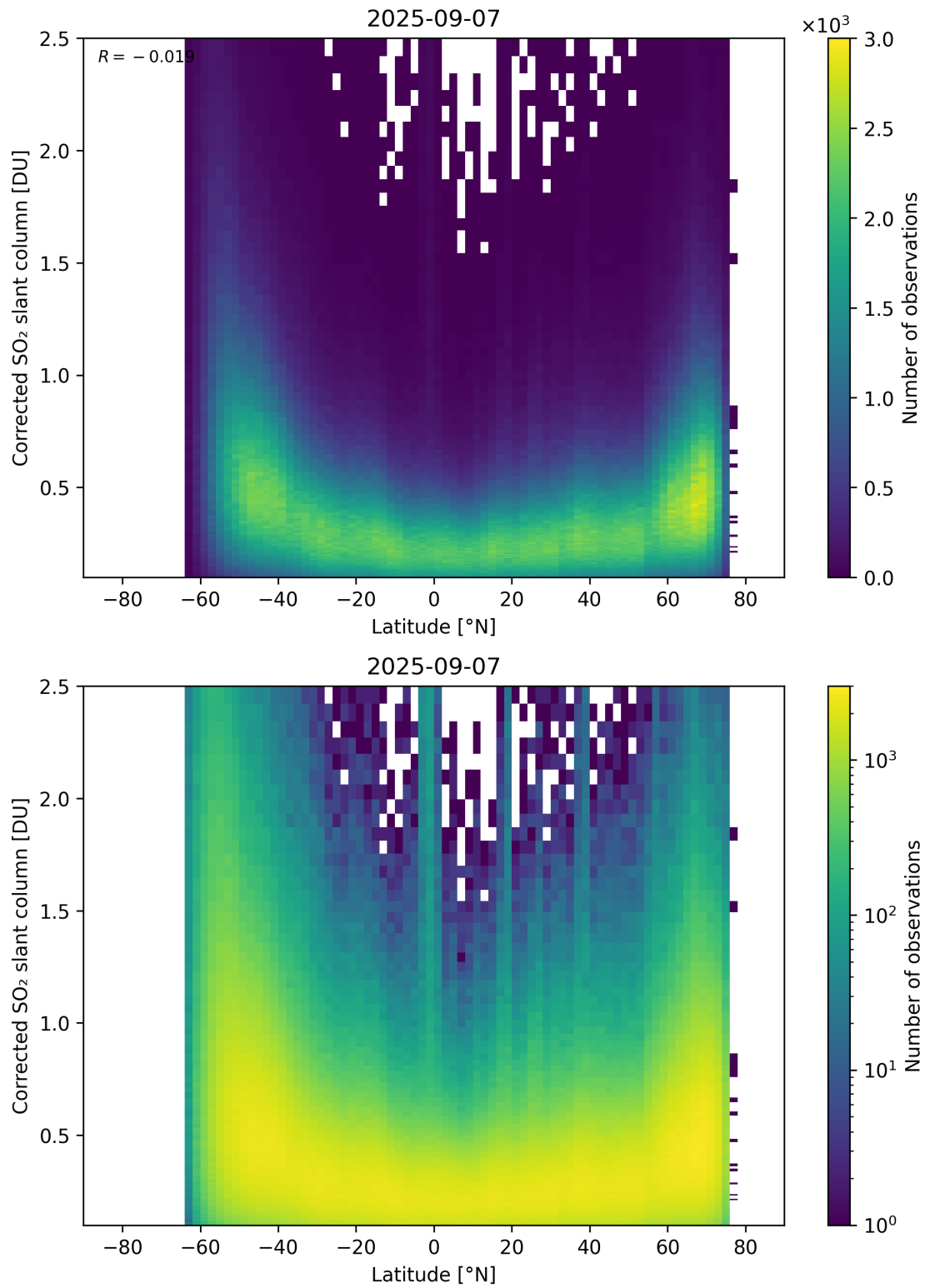
Figure 159: Scatter density plot of “Latitude” against “Corrected SO 2 slant column” for 2025-09-06 to 2025-09-08.
