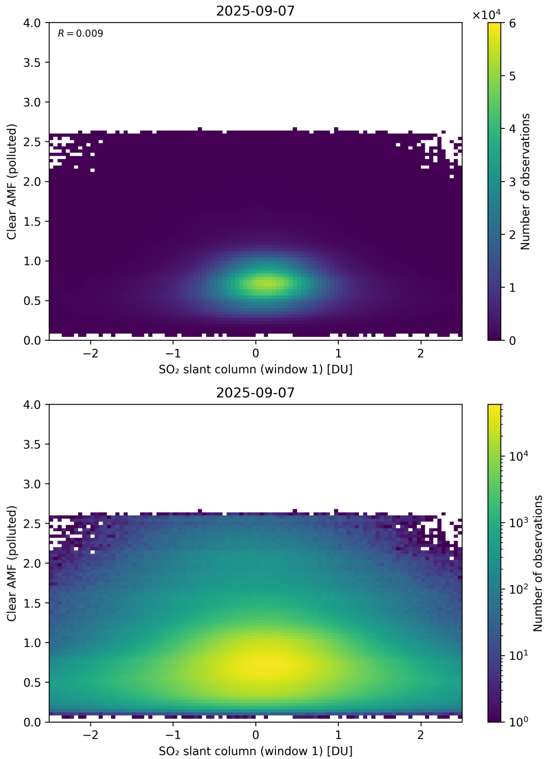
Figure 282: Scatter density plot of “SO 2 slant column (window 1)” against “Clear AMF (polluted)” for 2025-09-06 to 2025-09-08.
