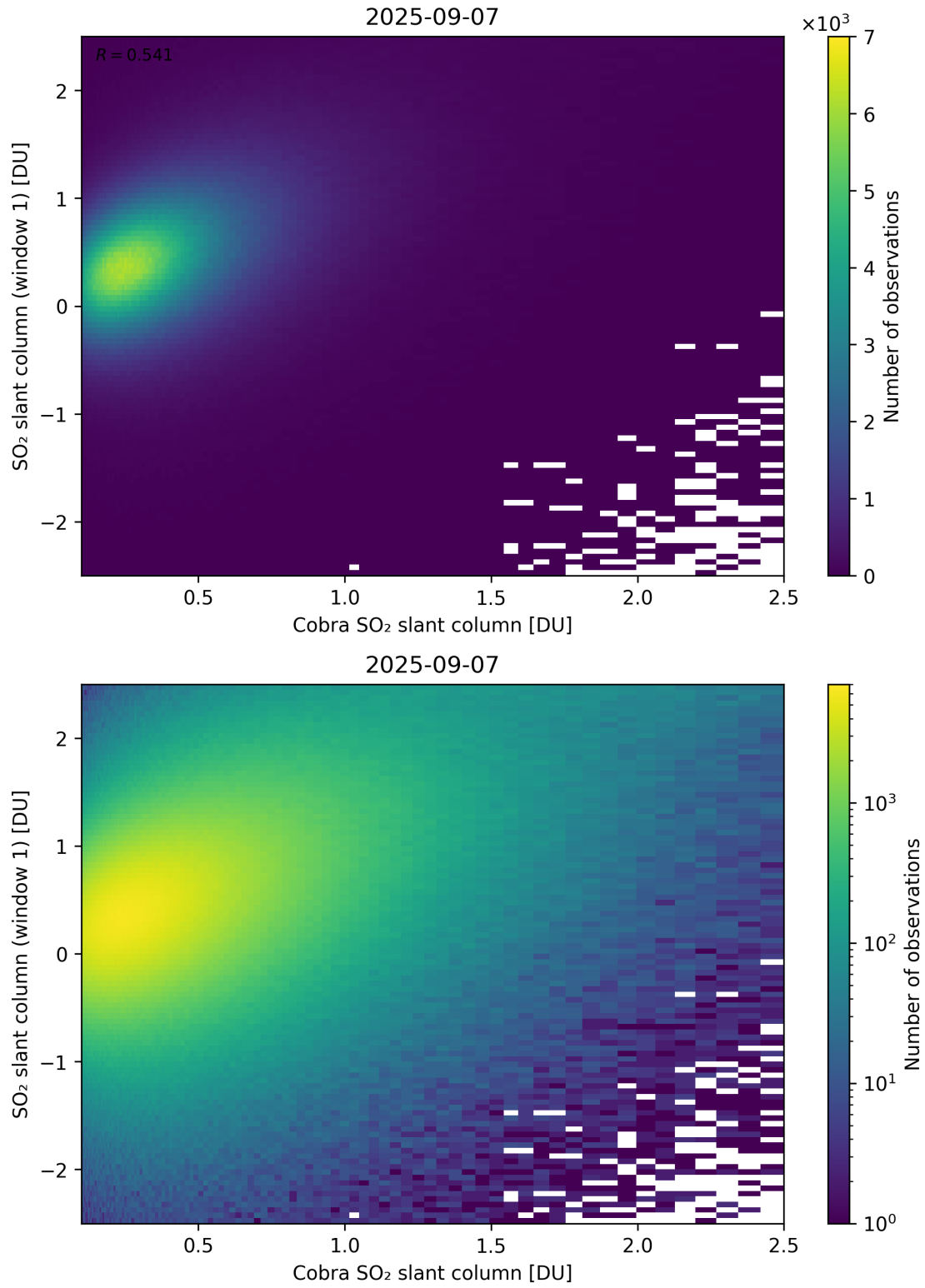
Figure 219: Scatter density plot of “Cobra SO 2 slant column” against “SO 2 slant column (window 1)” for 2025-09-06 to 2025-09-08.
