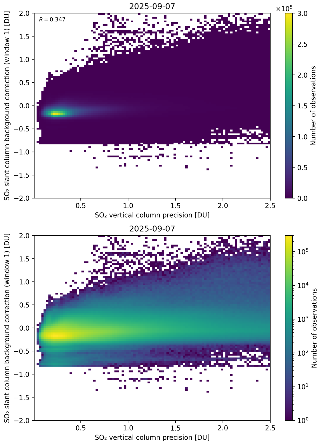
Figure 329: Scatter density plot of “SO 2 vertical column precision” against “SO 2 slant column background correction (window 1)” for 2025-09-06 to 2025-09-08.
