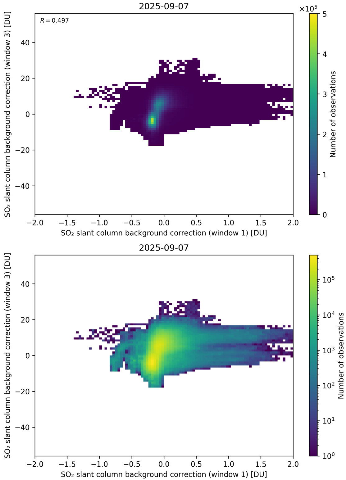
Figure 110: Scatter density plot of “SO 2 slant column background correction (window 1)” against “SO 2 slant column background correction (window 3)” for 2025-09-06 to 2025-09-08.
