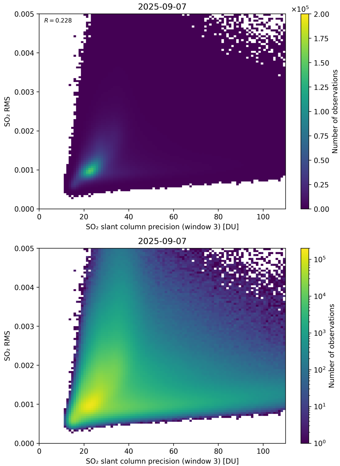
Figure 310: Scatter density plot of “SO 2 slant column precision (window 3)” against “SO 2 RMS” for 2025-09-06 to 2025-09-08.
