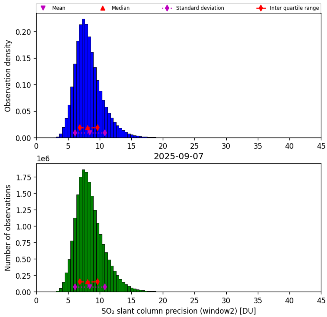
Figure 68: Histogram of “SO 2 slant column precision (window2)” for 2025-09-06 to 2025-09-08
