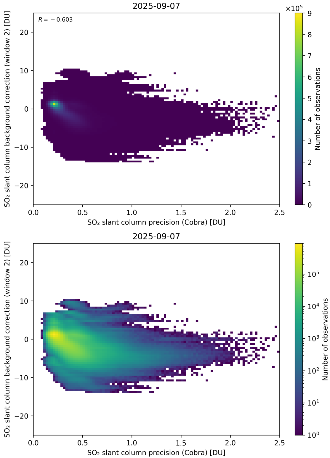
Figure 200: Scatter density plot of “SO 2 slant column precision (Cobra)” against “SO 2 slant column background correction (window 2)” for 2025-09-06 to 2025-09-08.
