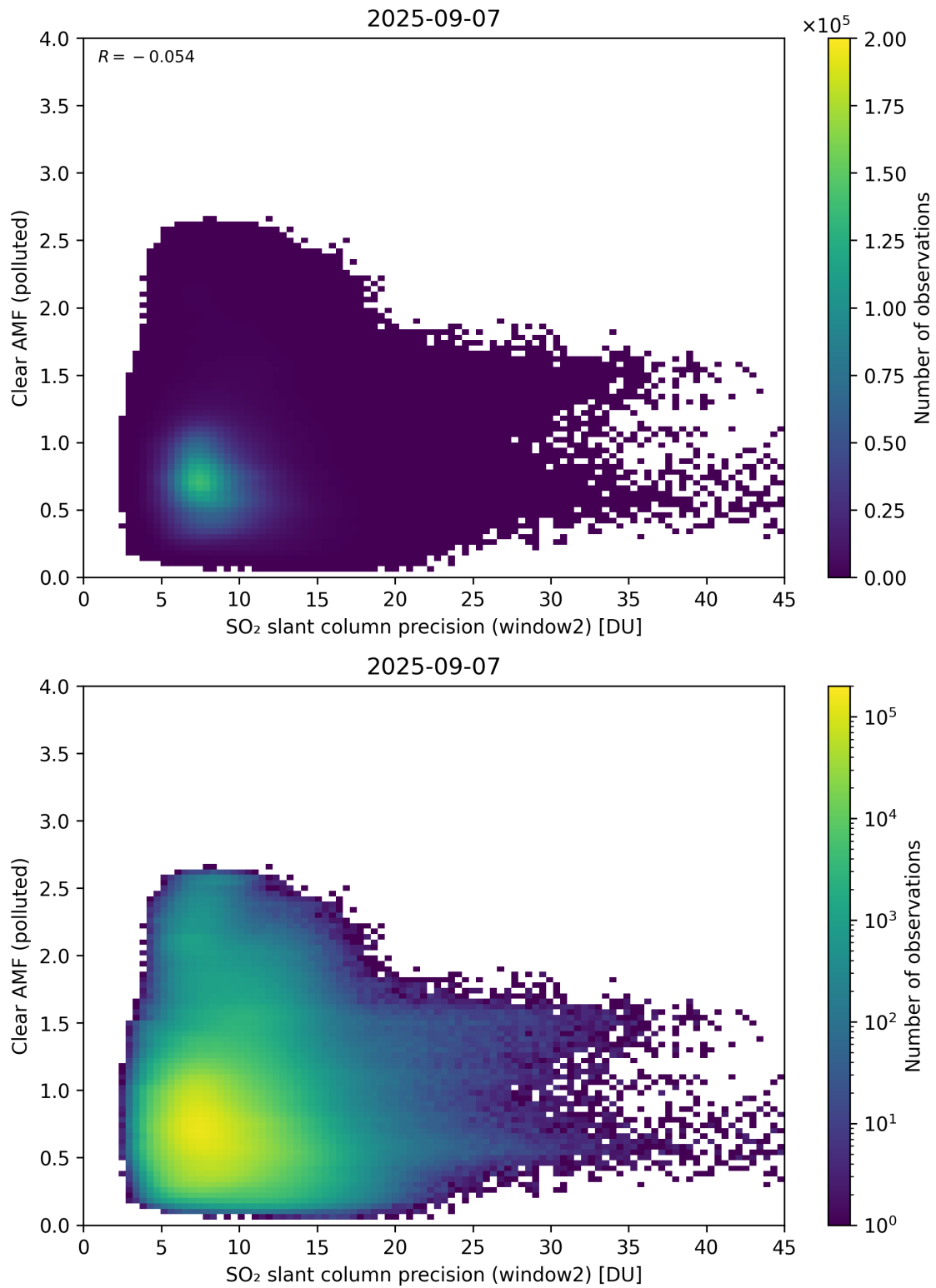
Figure 296: Scatter density plot of “SO 2 slant column precision (window2)” against “Clear AMF (polluted)” for 2025-09-06 to 2025-09-08.
