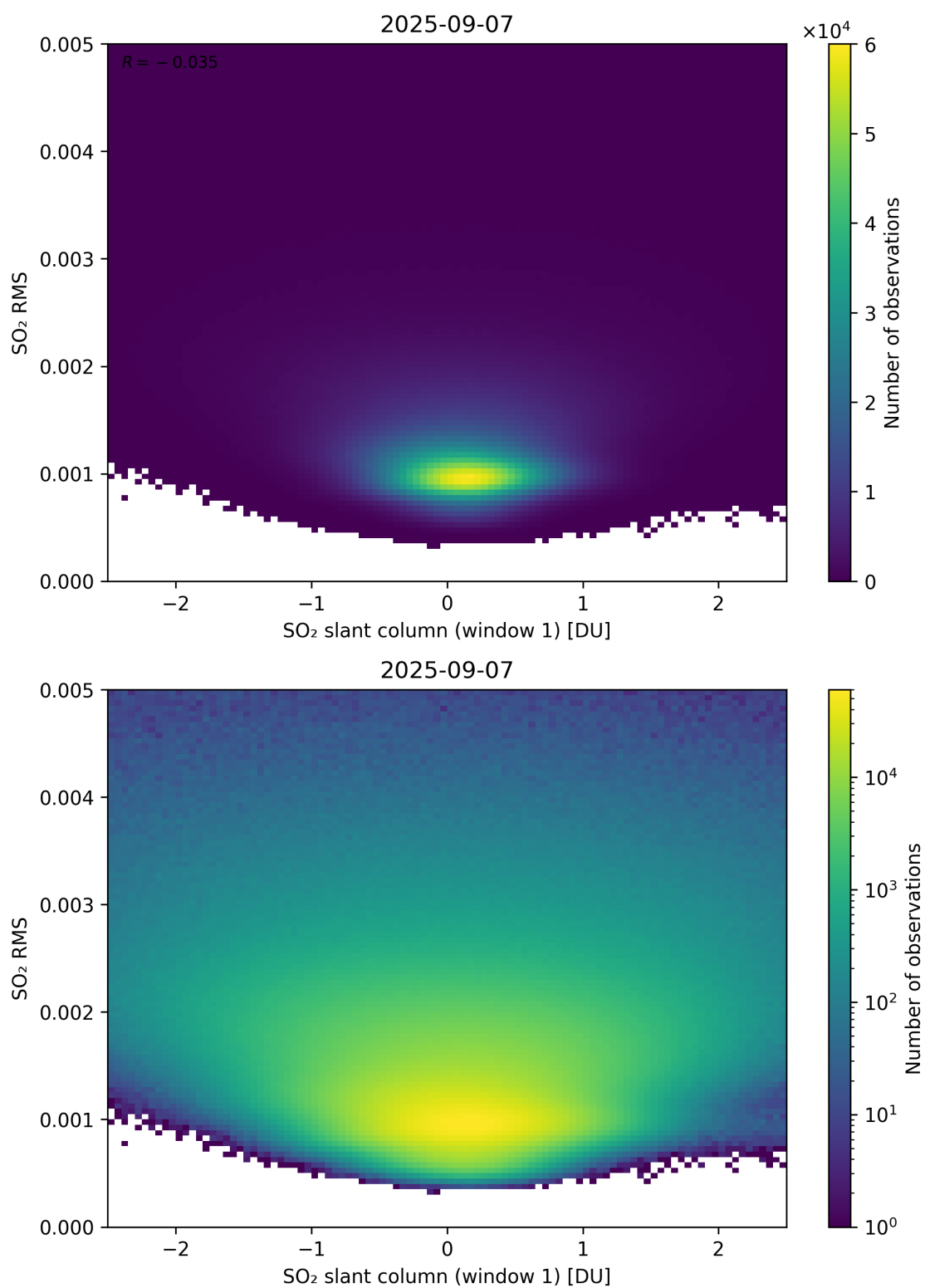
Figure 267: Scatter density plot of “SO 2 slant column (window 1)” against “SO 2 RMS” for 2025-09-06 to 2025-09-08.
