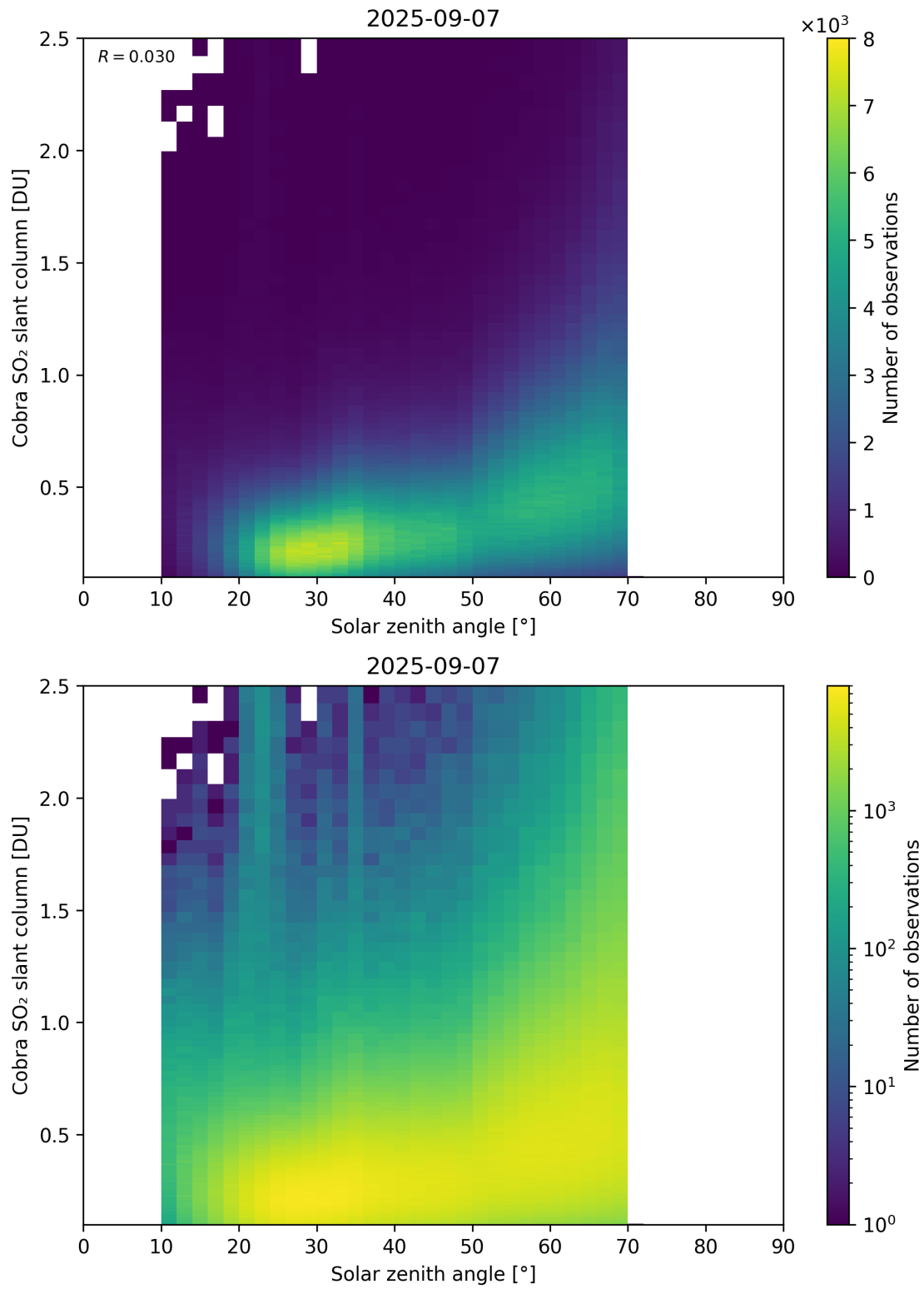
Figure 179: Scatter density plot of “Solar zenith angle” against “Cobra SO 2 slant column” for 2025-09-06 to 2025-09-08.
