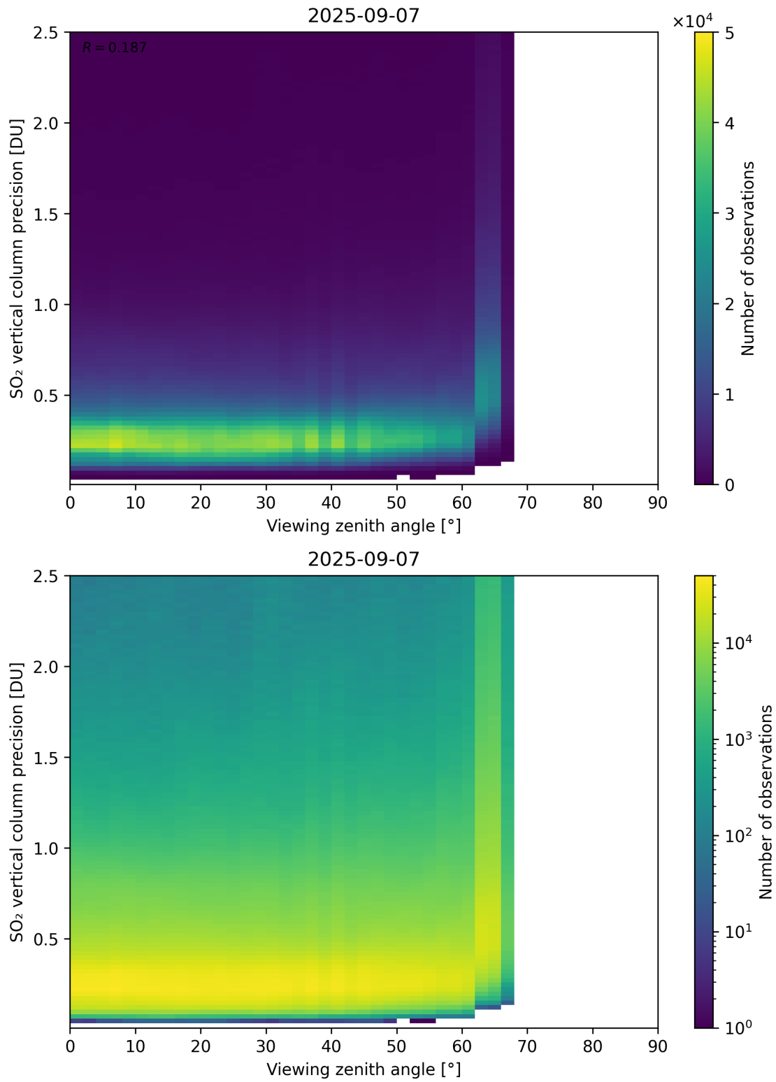
Figure 384: Scatter density plot of “Viewing zenith angle” against “SO 2 vertical column precision” for 2025-09-06 to 2025-09-08.
