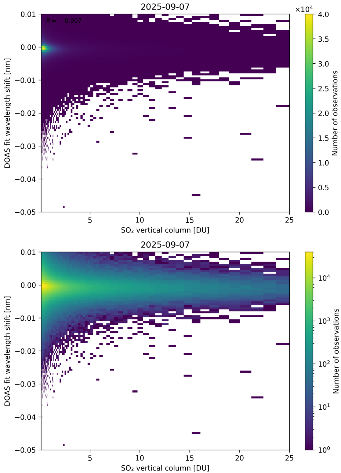
Figure 326: Scatter density plot of “SO 2 vertical column” against “DOAS fit wavelength shift” for 2025-09-06 to 2025-09-08.
