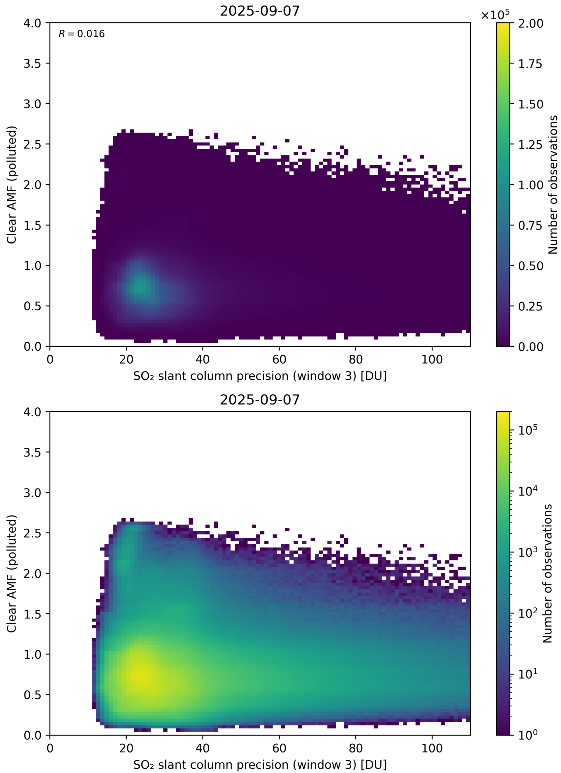
Figure 311: Scatter density plot of “SO 2 slant column precision (window 3)” against “Clear AMF (polluted)” for 2025-09-06 to 2025-09-08.
