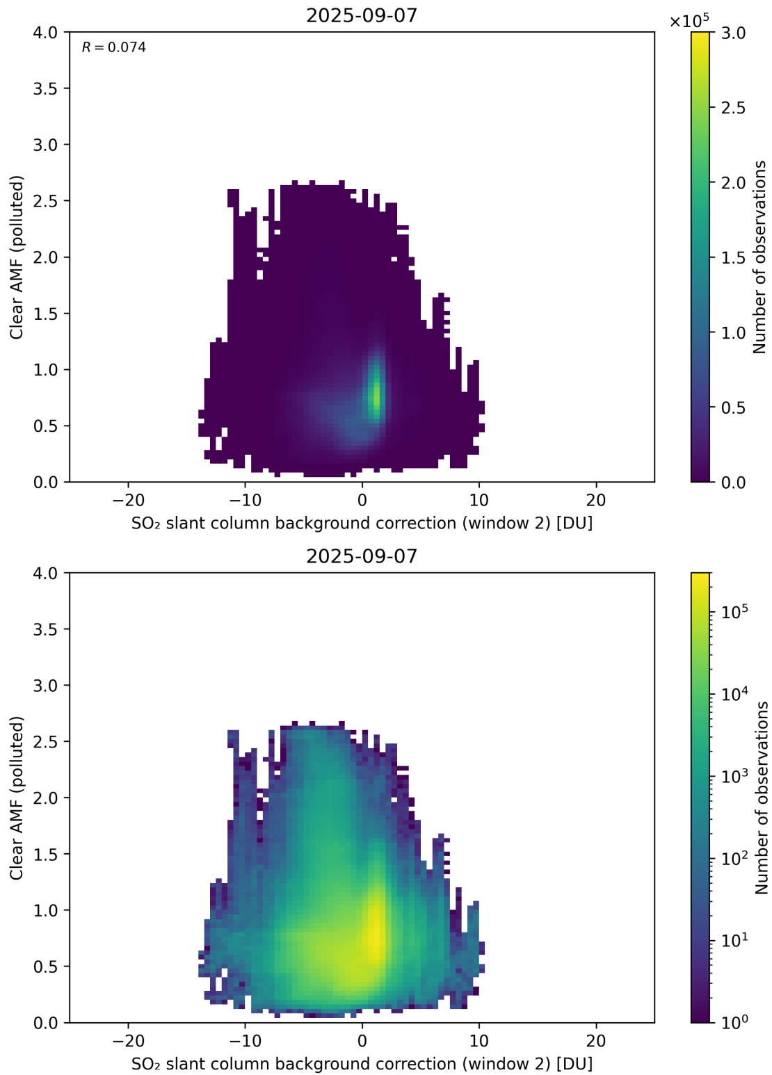
Figure 126: Scatter density plot of “SO 2 slant column background correction (window 2)” against “Clear AMF (polluted)” for 2025-09-06 to 2025-09-08.
