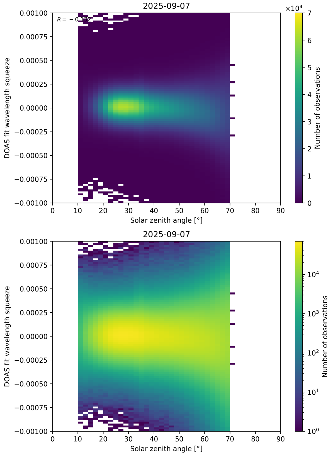
Figure 175: Scatter density plot of “Solar zenith angle” against “DOAS fit wavelength squeeze” for 2025-09-06 to 2025-09-08.
