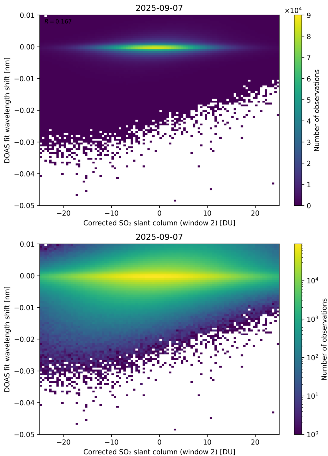
Figure 246: Scatter density plot of “Corrected SO 2 slant column (window 2)” against “DOAS fit wavelength shift” for 2025-09-06 to 2025-09-08.
