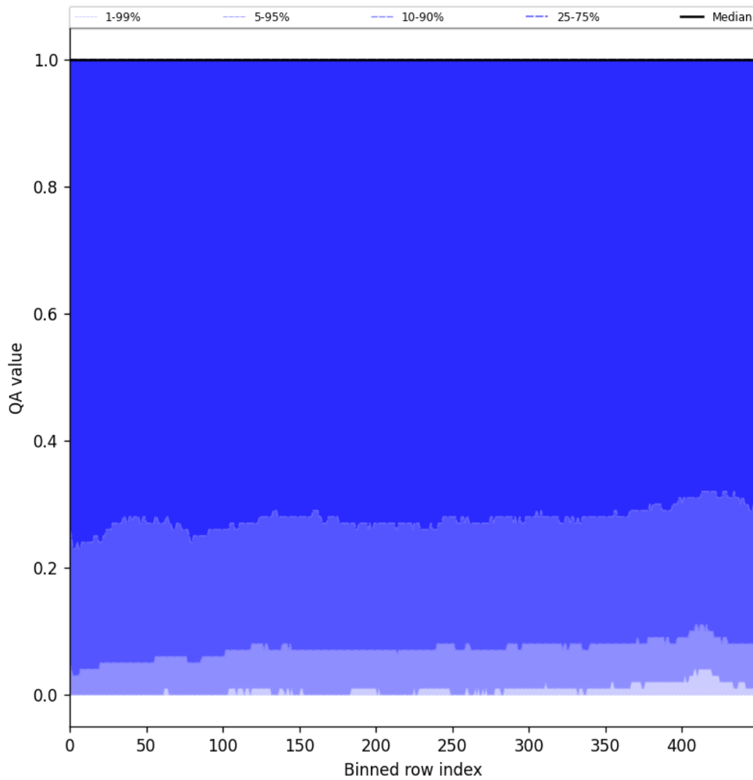
Figure 83: Along track statistics of “QA value” for 2025-09-06 to 2025-09-08
