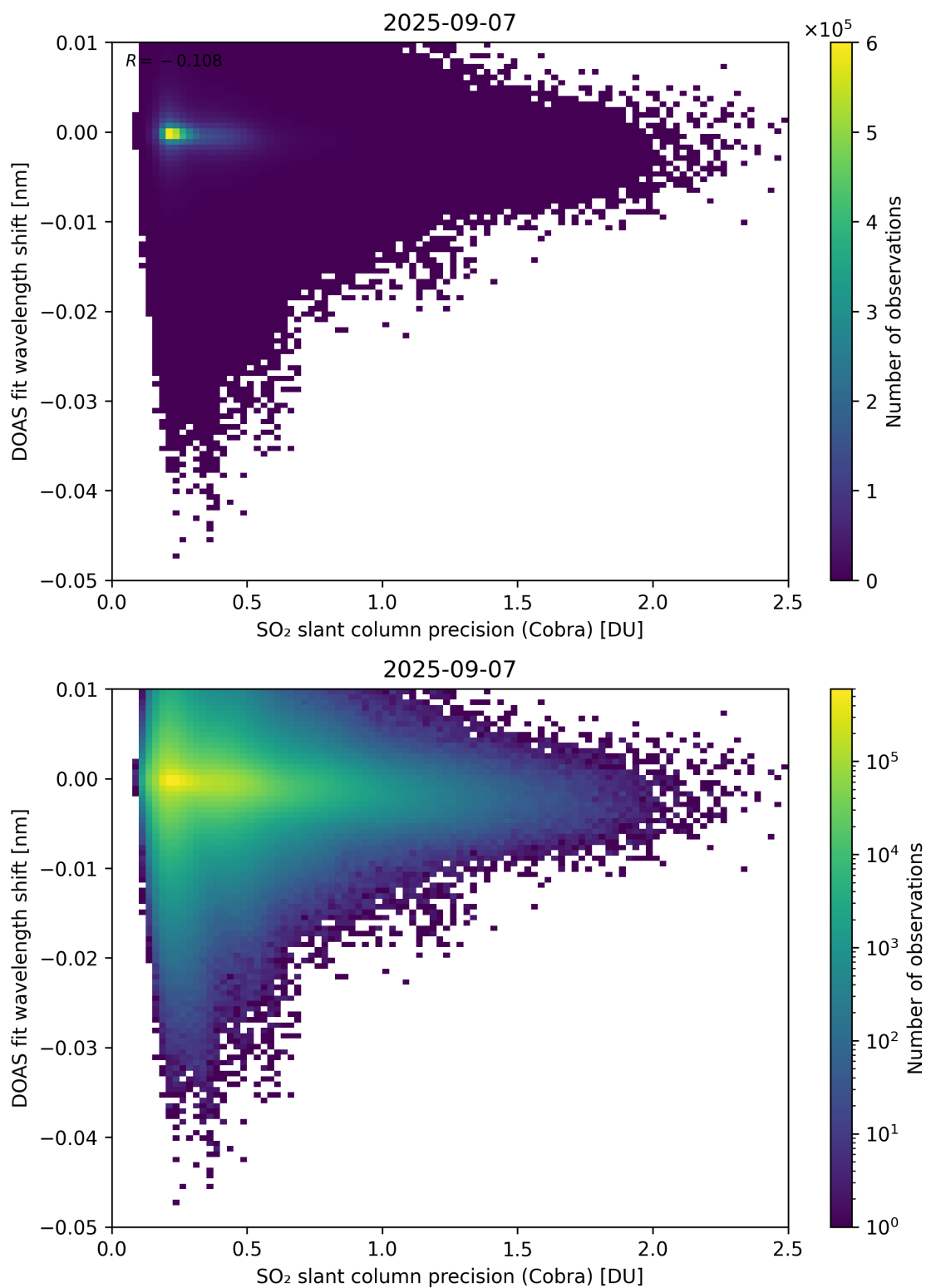
Figure 202: Scatter density plot of “SO 2 slant column precision (Cobra)” against “DOAS fit wavelength shift” for 2025-09-06 to 2025-09-08.
