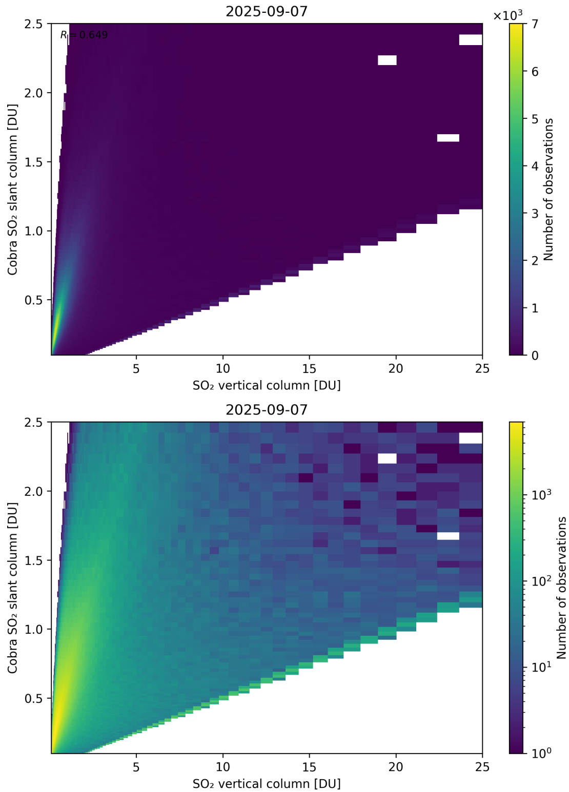
Figure 349: Scatter density plot of “SO 2 vertical column” against “Cobra SO 2 slant column” for 2025-09-06 to 2025-09-08.
