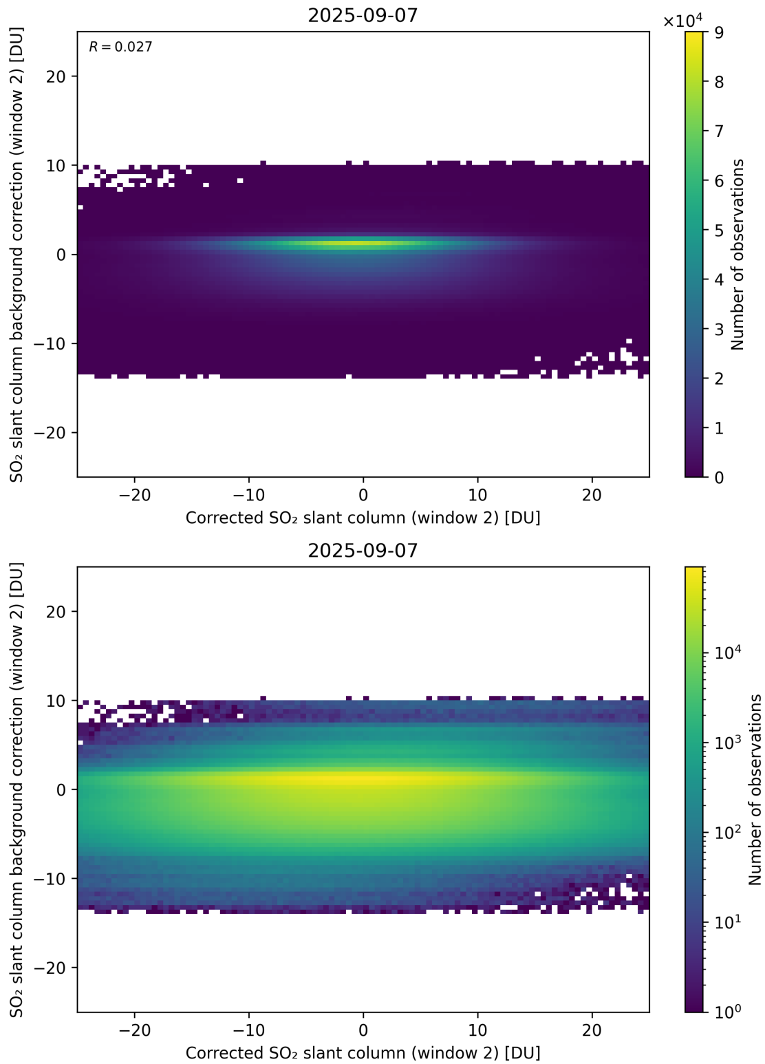
Figure 244: Scatter density plot of “Corrected SO 2 slant column (window 2)” against “SO 2 slant column background correction (window 2)” for 2025-09-06 to 2025-09-08.
