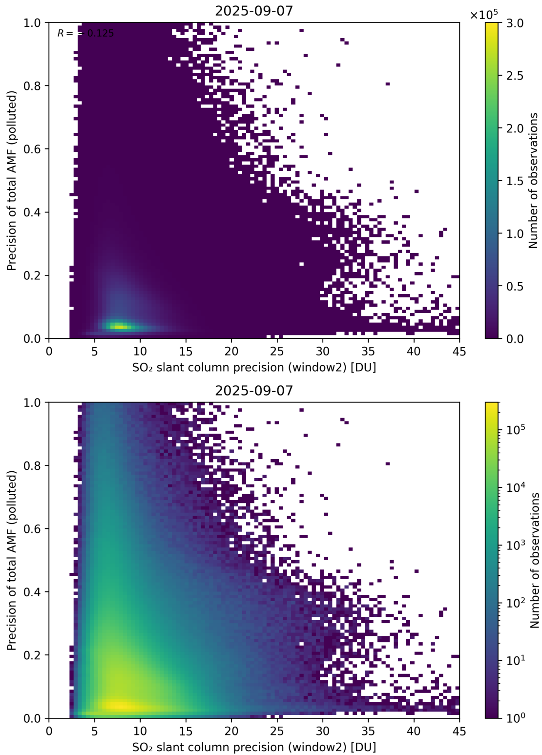
Figure 302: Scatter density plot of “SO 2 slant column precision (window2)” against “Precision of total AMF (polluted)” for 2025-09-06 to 2025-09-08.
