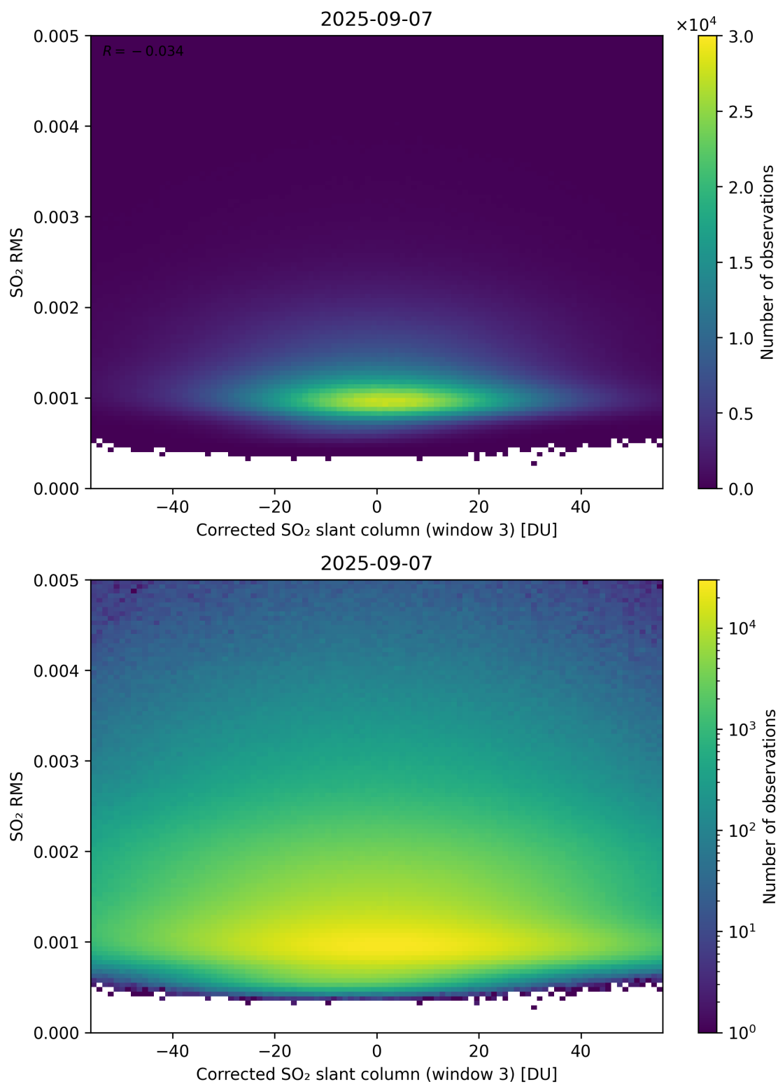
Figure 258: Scatter density plot of “Corrected SO 2 slant column (window 3)” against “SO 2 RMS” for 2025-09-06 to 2025-09-08.
