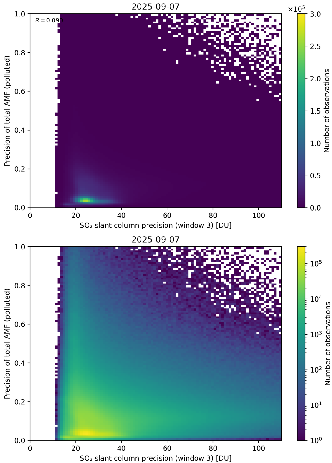
Figure 314: Scatter density plot of “SO 2 slant column precision (window 3)” against “Precision of total AMF (polluted)” for 2025-09-06 to 2025-09-08.
