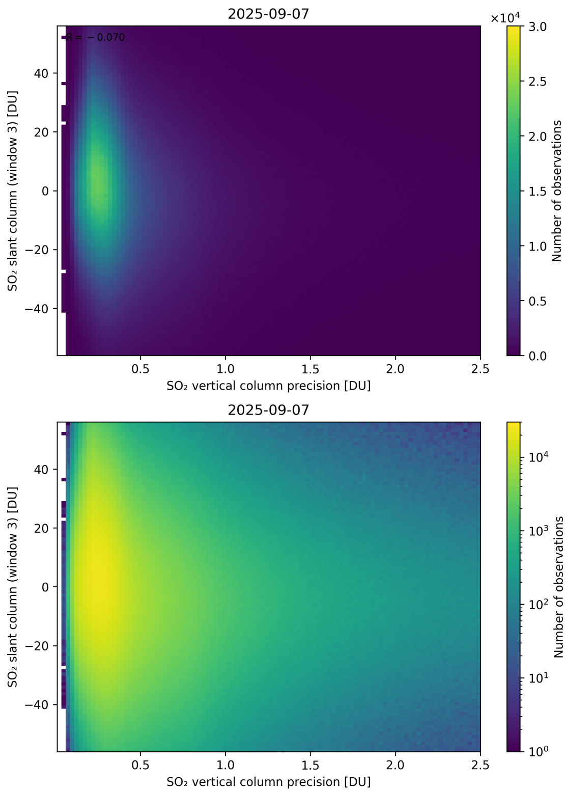
Figure 344: Scatter density plot of “SO 2 vertical column precision” against “SO 2 slant column (window 3)” for 2025-09-06 to 2025-09-08.
