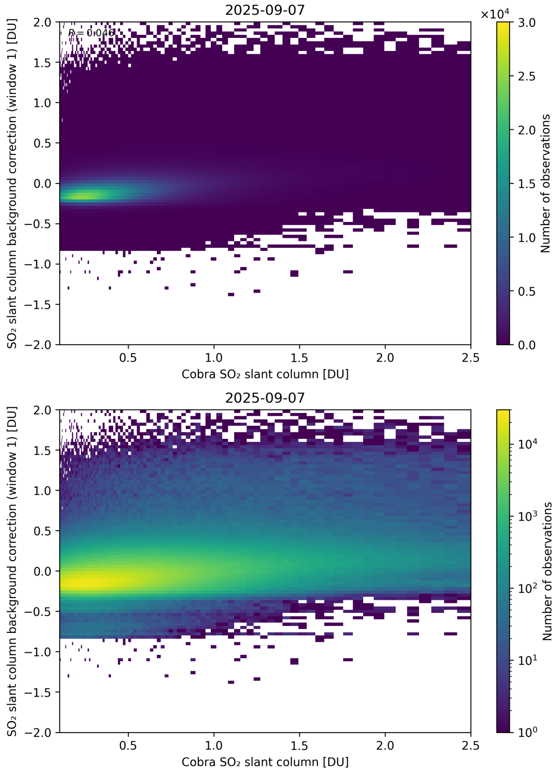
Figure 193: Scatter density plot of “Cobra SO 2 slant column” against “SO 2 slant column background correction (window 1)” for 2025-09-06 to 2025-09-08.
