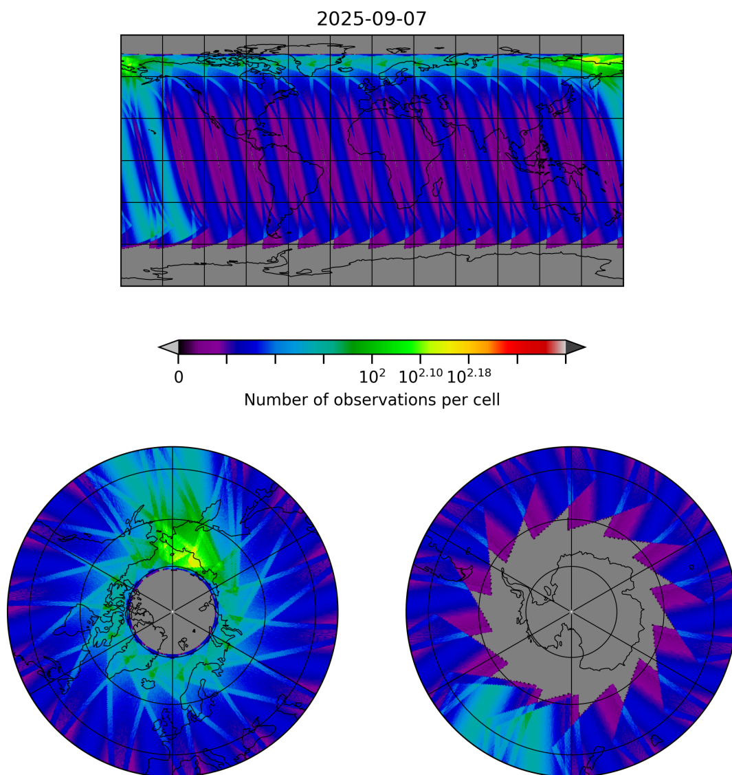
Figure 30: Map of the number of observations for 2025-09-06 to 2025-09-08
