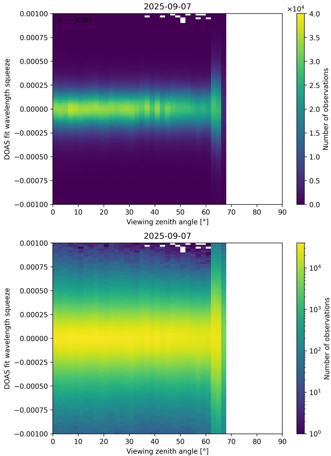
Figure 366: Scatter density plot of “Viewing zenith angle” against “DOAS fit wavelength squeeze” for 2025-09-06 to 2025-09-08.
