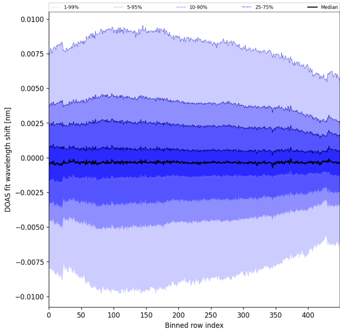
Figure 102: Along track statistics of “DOAS fit wavelength shift” for 2025-09-06 to 2025-09-08
