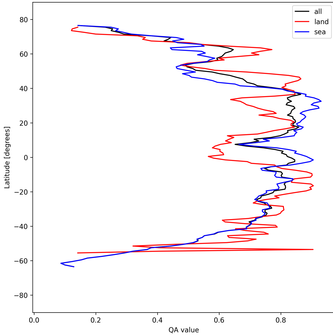
Figure 31: Zonal average of “QA value” for 2025-09-06 to 2025-09-08.
