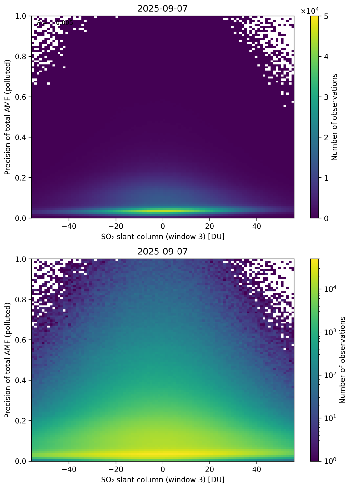
Figure 319: Scatter density plot of “SO 2 slant column (window 3)” against “Precision of total AMF (polluted)” for 2025-09-06 to 2025-09-08.
