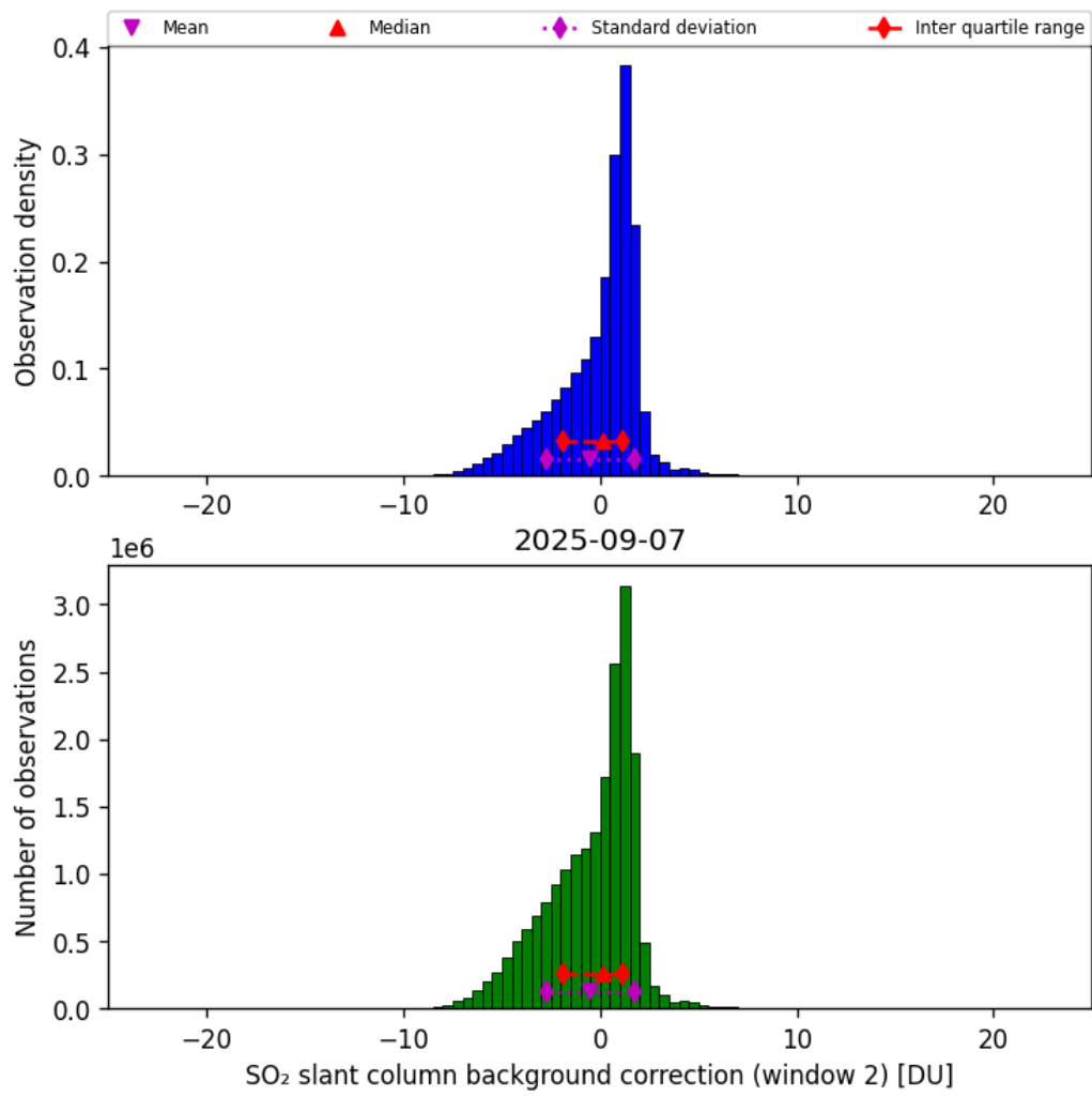
Figure 70: Histogram of “SO 2 slant column background correction (window 2)” for 2025-09-06 to 2025-09-08
