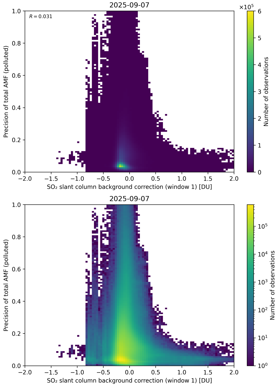
Figure 121: Scatter density plot of “SO 2 slant column background correction (window 1)” against “Precision of total AMF (polluted)” for 2025-09-06 to 2025-09-08.
