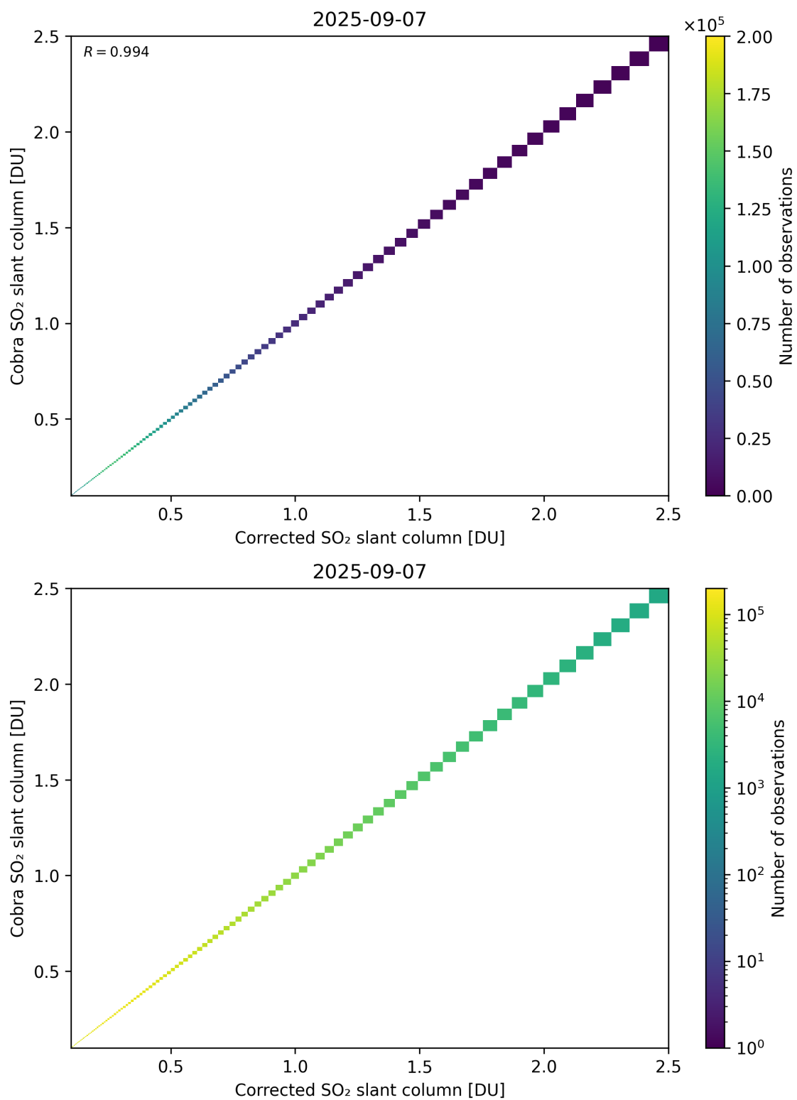
Figure 233: Scatter density plot of “Corrected SO 2 slant column” against “Cobra SO 2 slant column” for 2025-09-06 to 2025-09-08.
