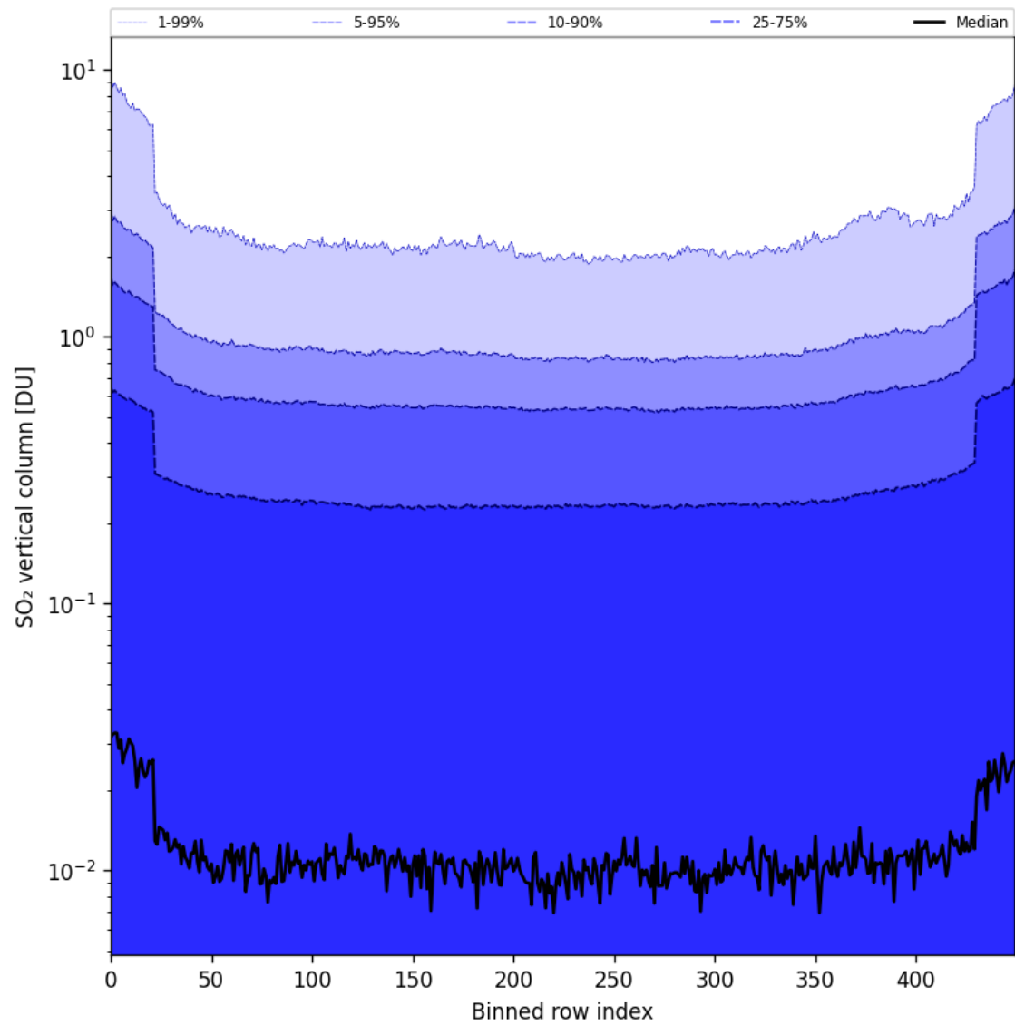
Figure 84: Along track statistics of “SO 2 vertical column” for 2025-09-06 to 2025-09-08
