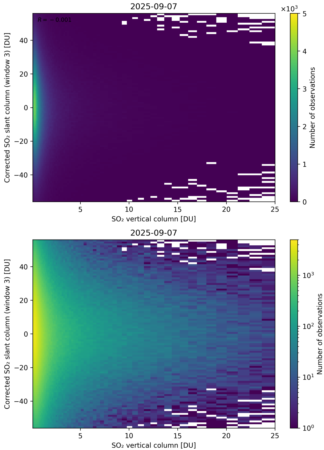
Figure 353: Scatter density plot of “SO 2 vertical column” against “Corrected SO 2 slant column (window 3)” for 2025-09-06 to 2025-09-08.
