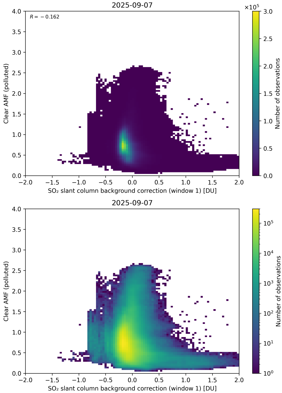
Figure 114: Scatter density plot of “SO 2 slant column background correction (window 1)” against “Clear AMF (polluted)” for 2025-09-06 to 2025-09-08.
