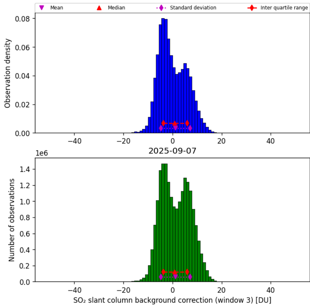
Figure 74: Histogram of “SO 2 slant column background correction (window 3)” for 2025-09-06 to 2025-09-08
