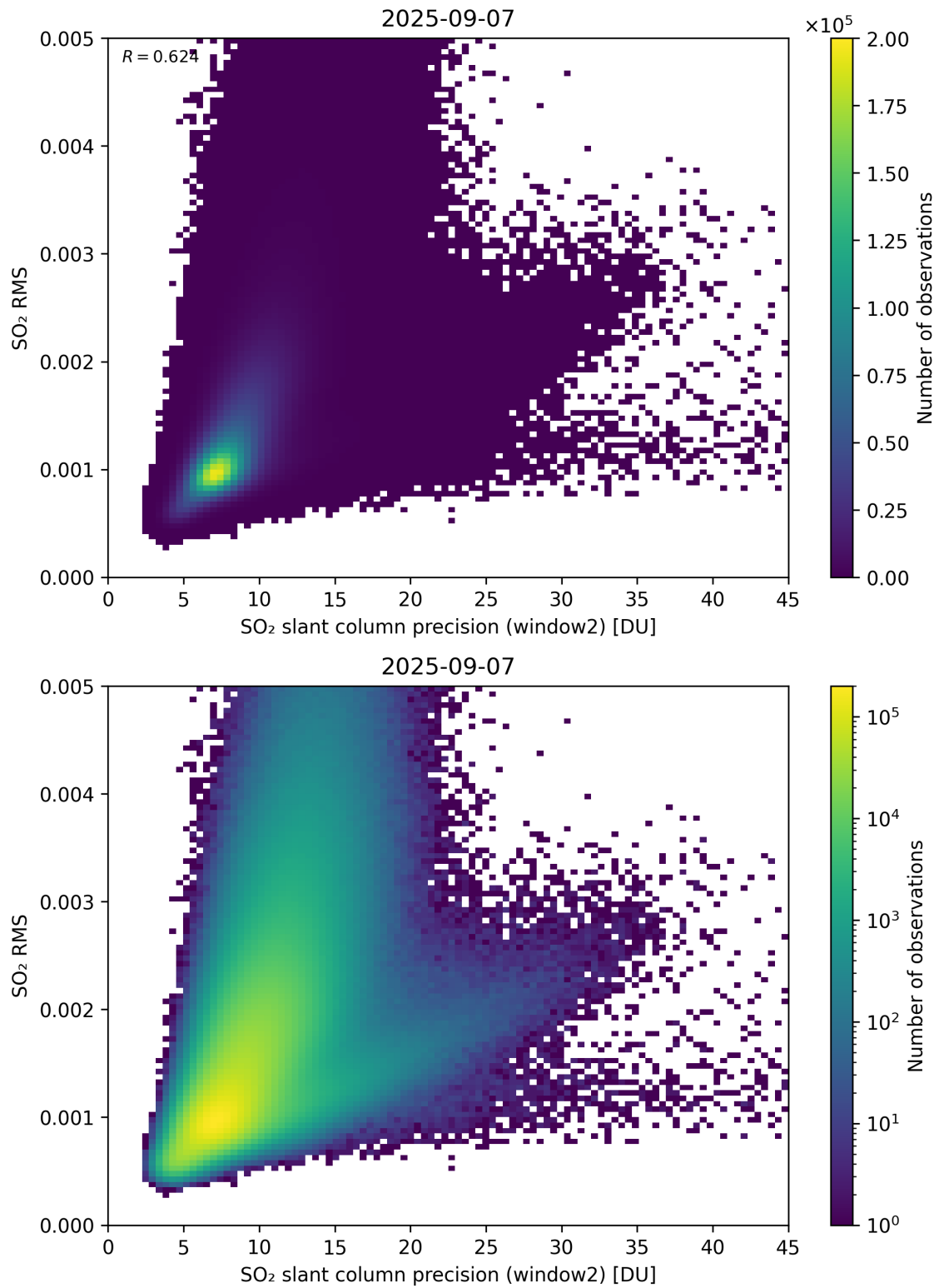
Figure 295: Scatter density plot of “SO 2 slant column precision (window2)” against “SO 2 RMS” for 2025-09-06 to 2025-09-08.
