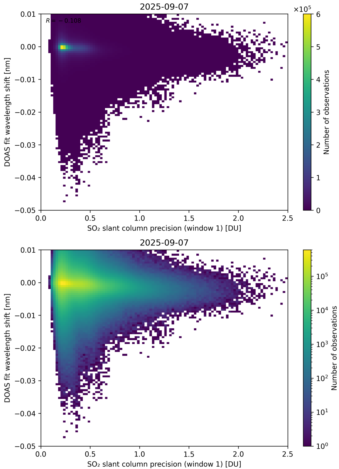
Figure 271: Scatter density plot of “SO 2 slant column precision (window 1)” against “DOAS fit wavelength shift” for 2025-09-06 to 2025-09-08.
