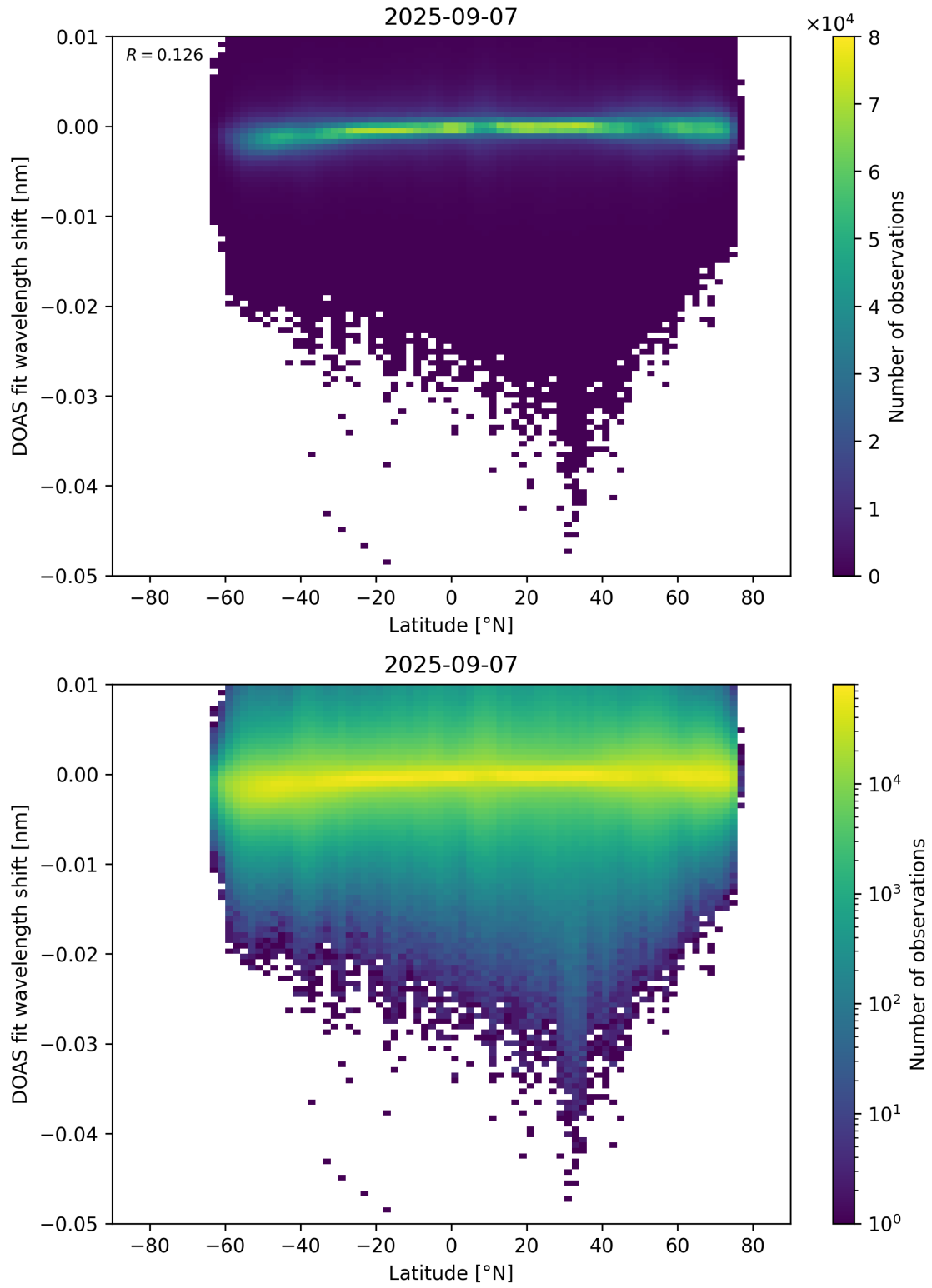
Figure 153: Scatter density plot of “Latitude” against “DOAS fit wavelength shift” for 2025-09-06 to 2025-09-08.
