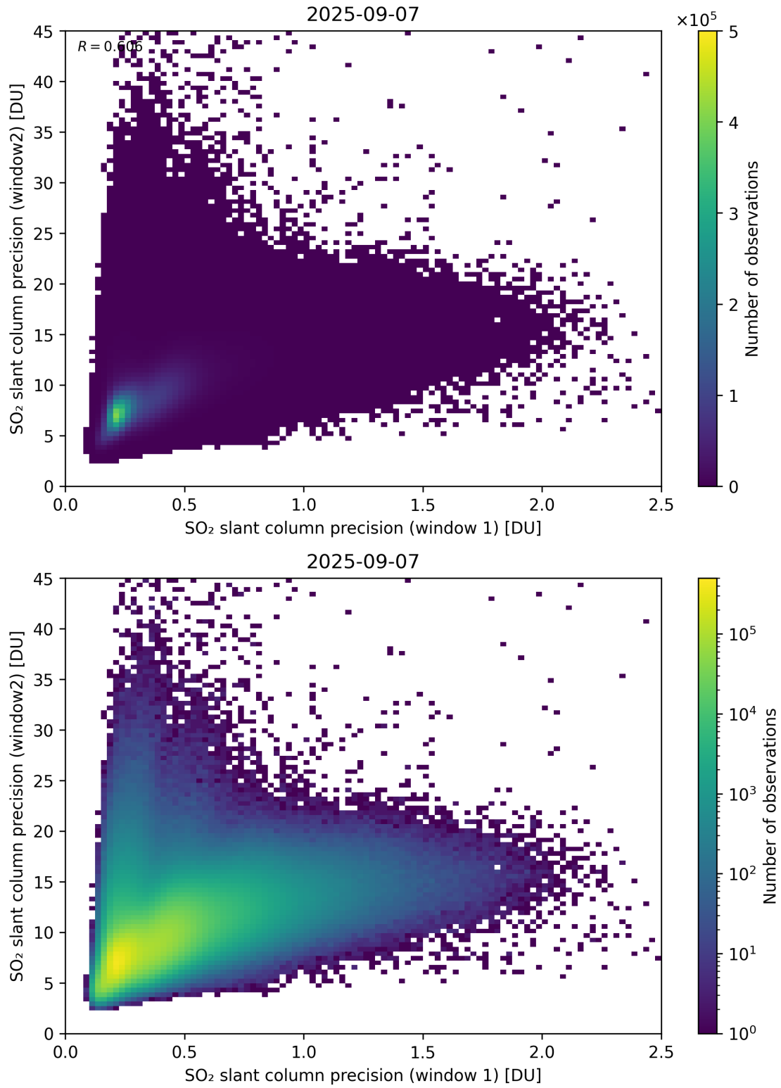
Figure 277: Scatter density plot of “SO 2 slant column precision (window 1)” against “SO 2 slant column precision (window2)” for 2025-09-06 to 2025-09-08.
