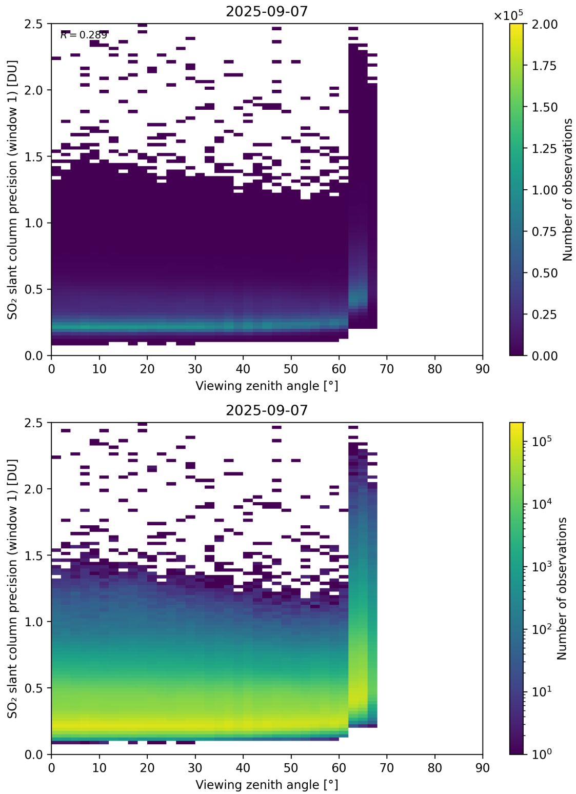
Figure 377: Scatter density plot of “Viewing zenith angle” against “SO 2 slant column precision (window 1)” for 2025-09-06 to 2025-09-08.
