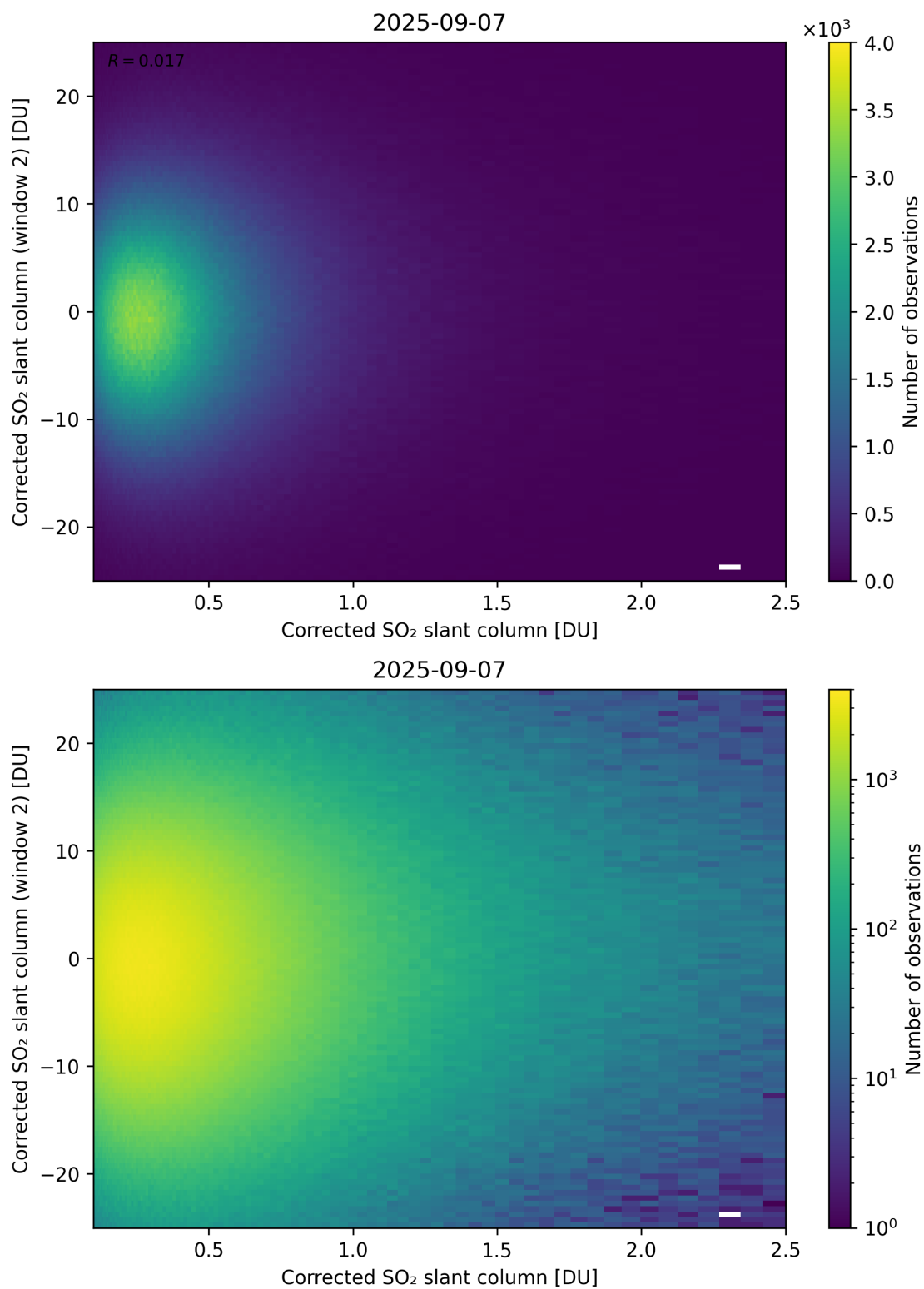
Figure 235: Scatter density plot of “Corrected SO 2 slant column” against “Corrected SO 2 slant column (window 2)” for 2025-09-06 to 2025-09-08.
