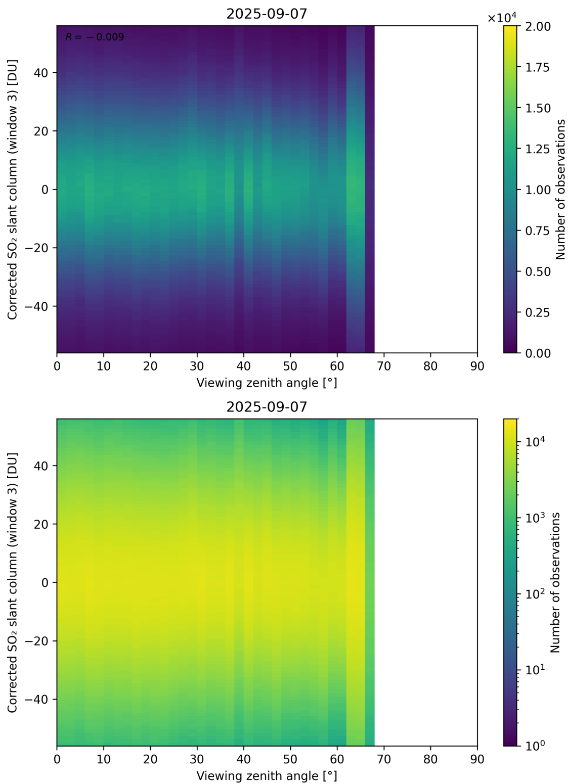
Figure 375: Scatter density plot of “Viewing zenith angle” against “Corrected SO 2 slant column (window 3)” for 2025-09-06 to 2025-09-08.
