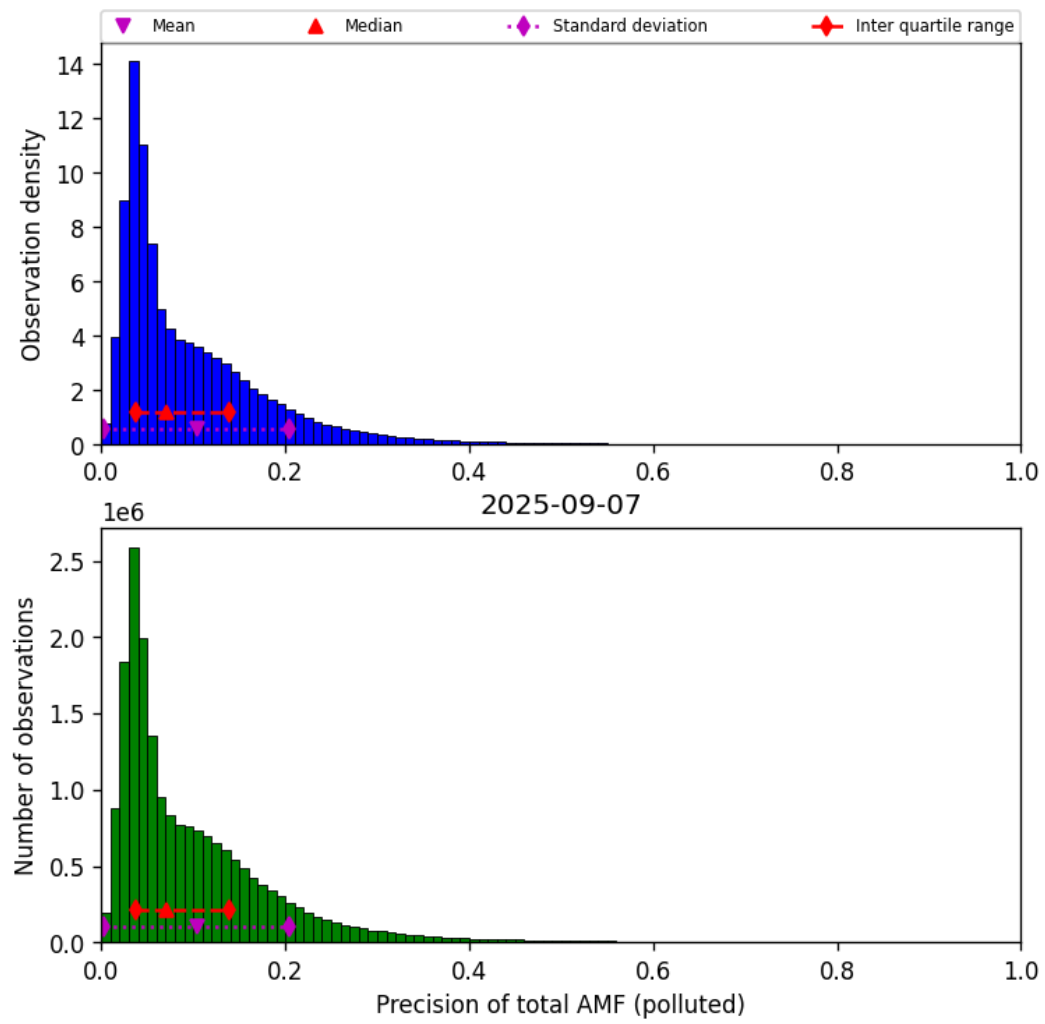
Figure 80: Histogram of “Precision of total AMF (polluted)” for 2025-09-06 to 2025-09-08
