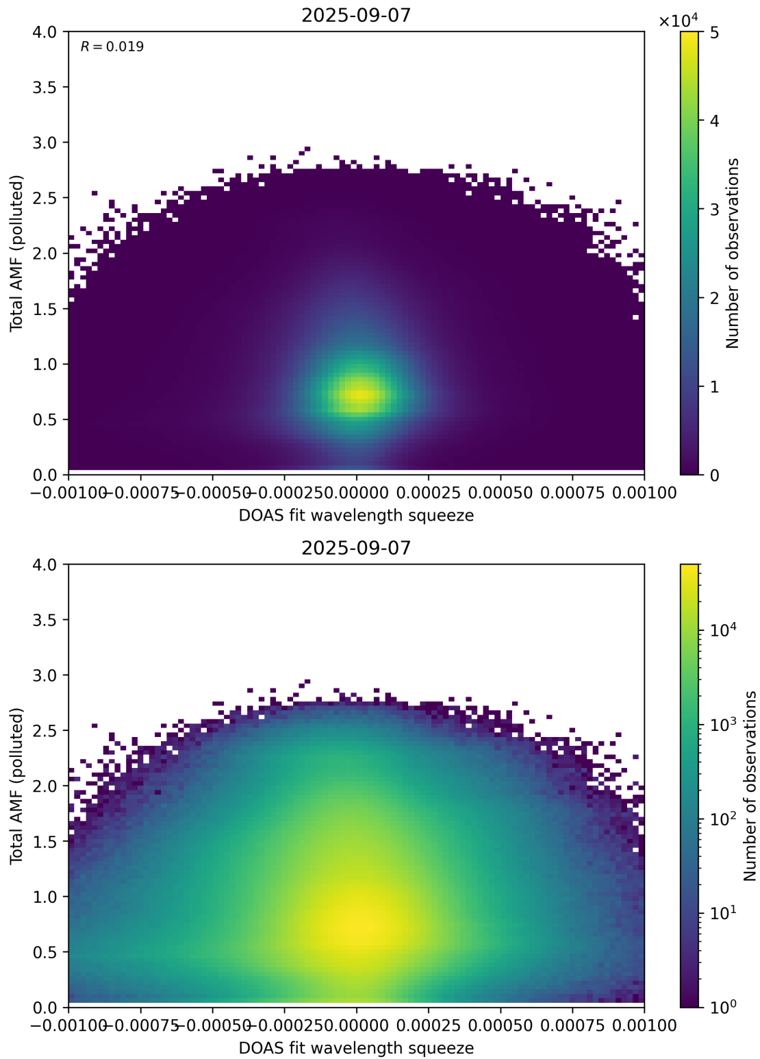
Figure 145: Scatter density plot of “DOAS fit wavelength squeeze” against “Total AMF (polluted)” for 2025-09-06 to 2025-09-08.
