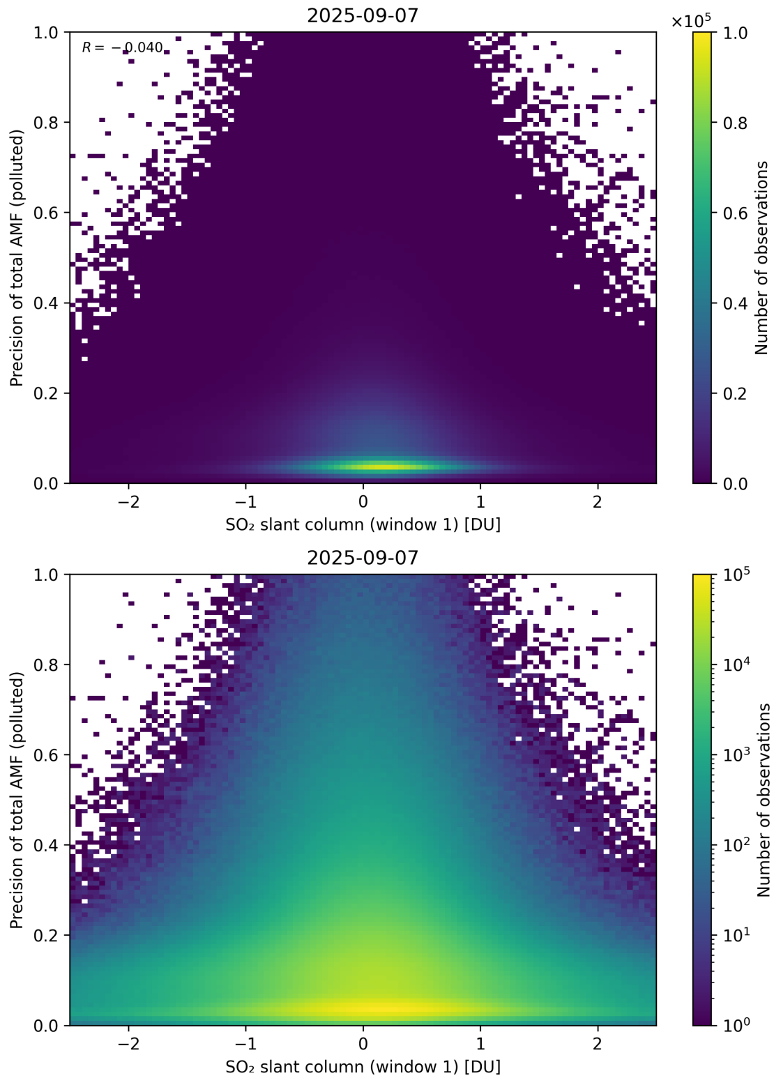
Figure 290: Scatter density plot of “SO 2 slant column (window 1)” against “Precision of total AMF (polluted)” for 2025-09-06 to 2025-09-08.
