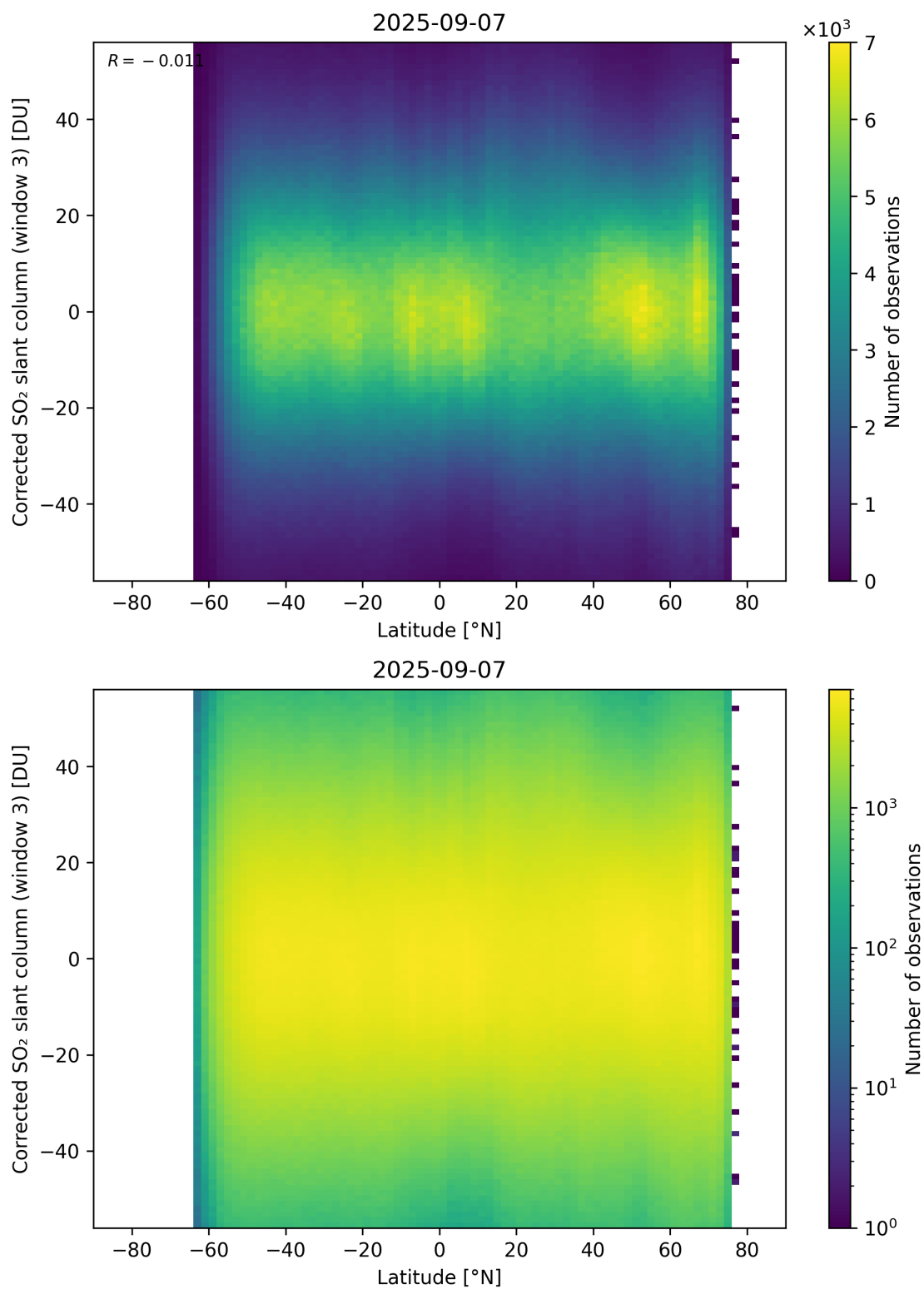
Figure 161: Scatter density plot of “Latitude” against “Corrected SO 2 slant column (window 3)” for 2025-09-06 to 2025-09-08.
