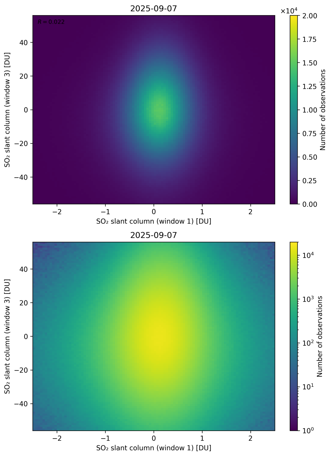
Figure 287: Scatter density plot of “SO 2 slant column (window 1)” against “SO 2 slant column (window 3)” for 2025-09-06 to 2025-09-08.
