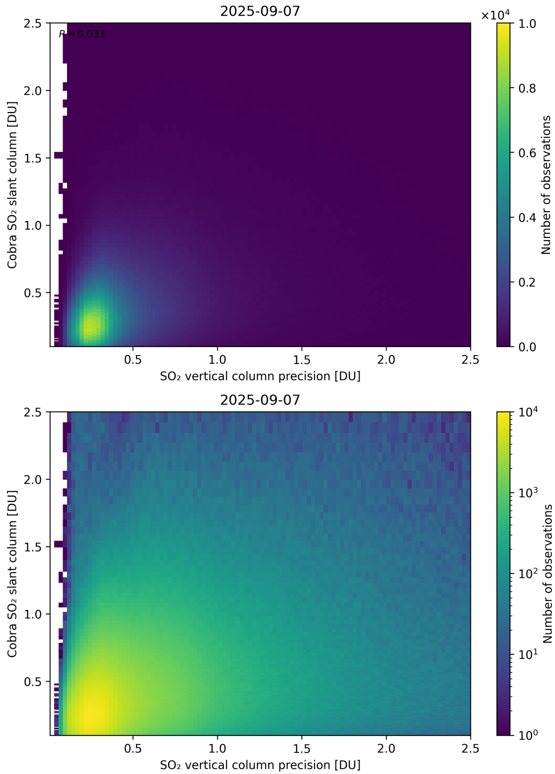
Figure 336: Scatter density plot of “SO 2 vertical column precision” against “Cobra SO 2 slant column” for 2025-09-06 to 2025-09-08.
