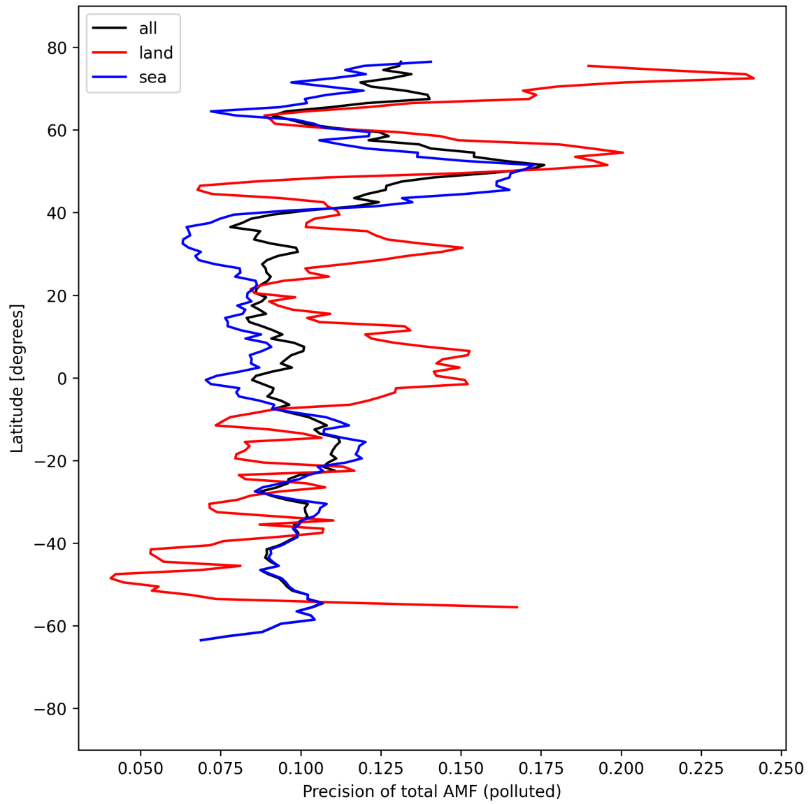
Figure 54: Zonal average of “Precision of total AMF (polluted)” for 2025-09-06 to 2025-09-08.
