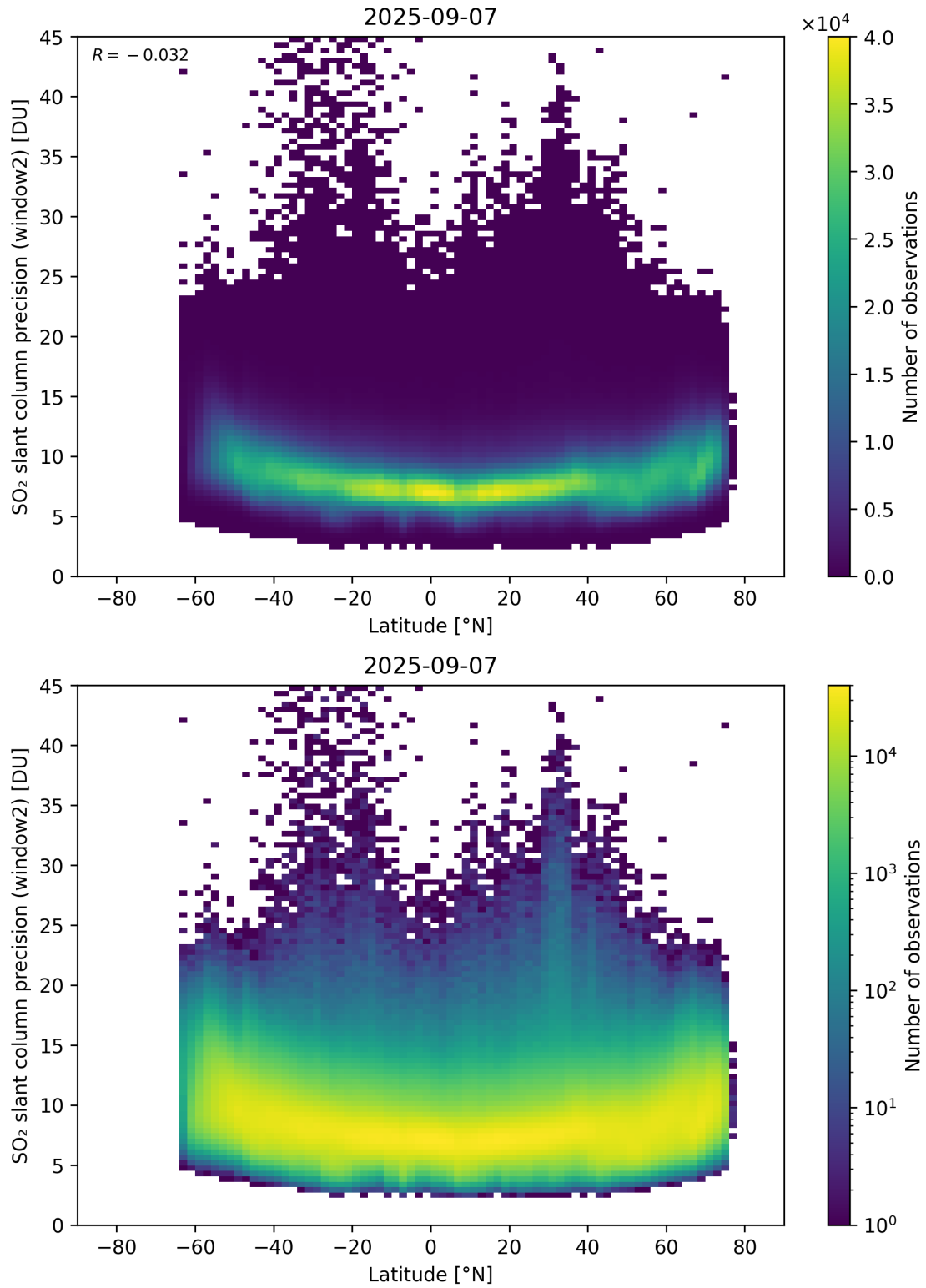
Figure 164: Scatter density plot of “Latitude” against “SO 2 slant column precision (window2)” for 2025-09-06 to 2025-09-08.
