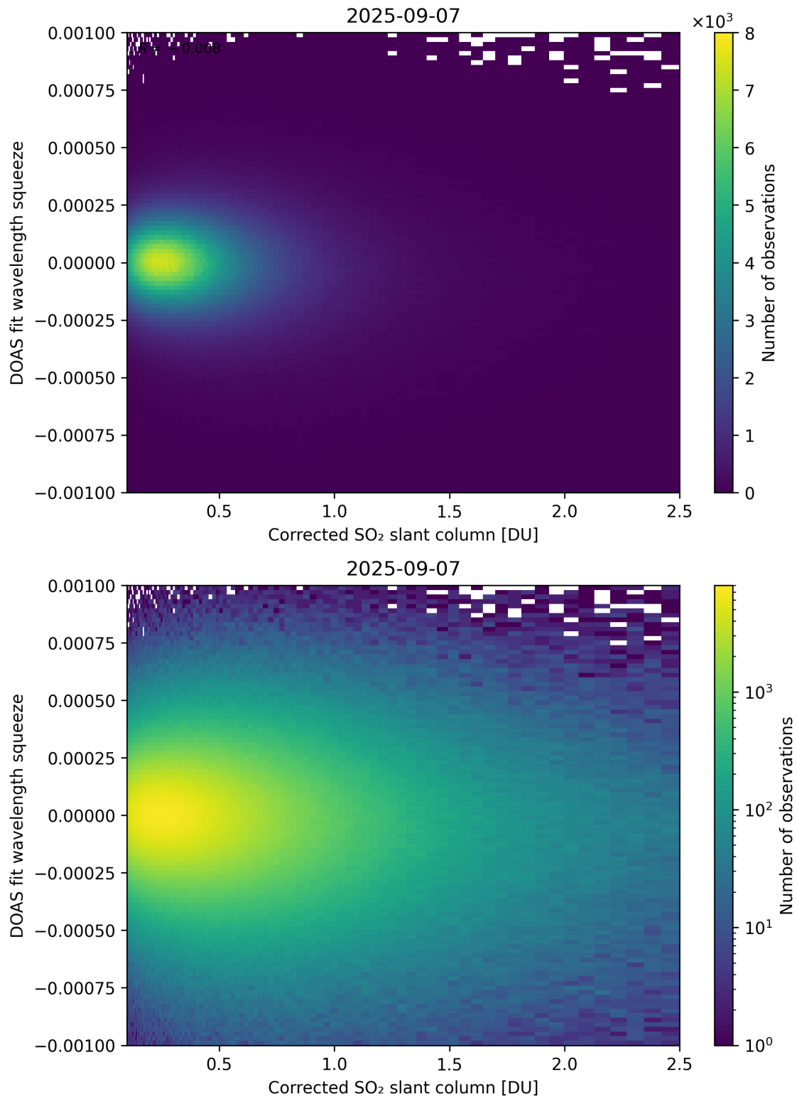
Figure 230: Scatter density plot of "Corrected SO 2 slant column" against "DOAS fit wavelength squeeze" for 2025-09-06 to 2025-09-08.
