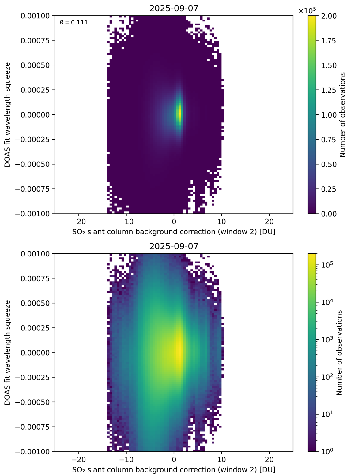
Figure 124: Scatter density plot of “SO 2 slant column background correction (window 2)” against “DOAS fit wavelength squeeze” for 2025-09-06 to 2025-09-08.
