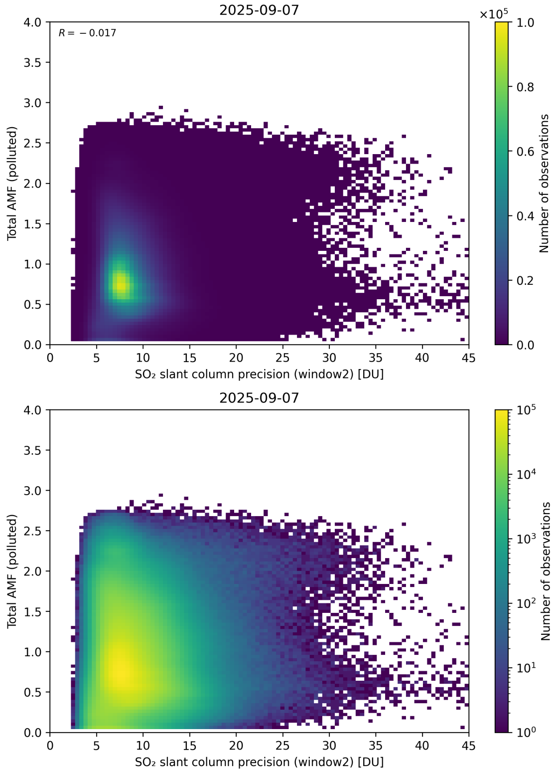
Figure 301: Scatter density plot of “SO 2 slant column precision (window2)” against “Total AMF (polluted)” for 2025-09-06 to 2025-09-08.
