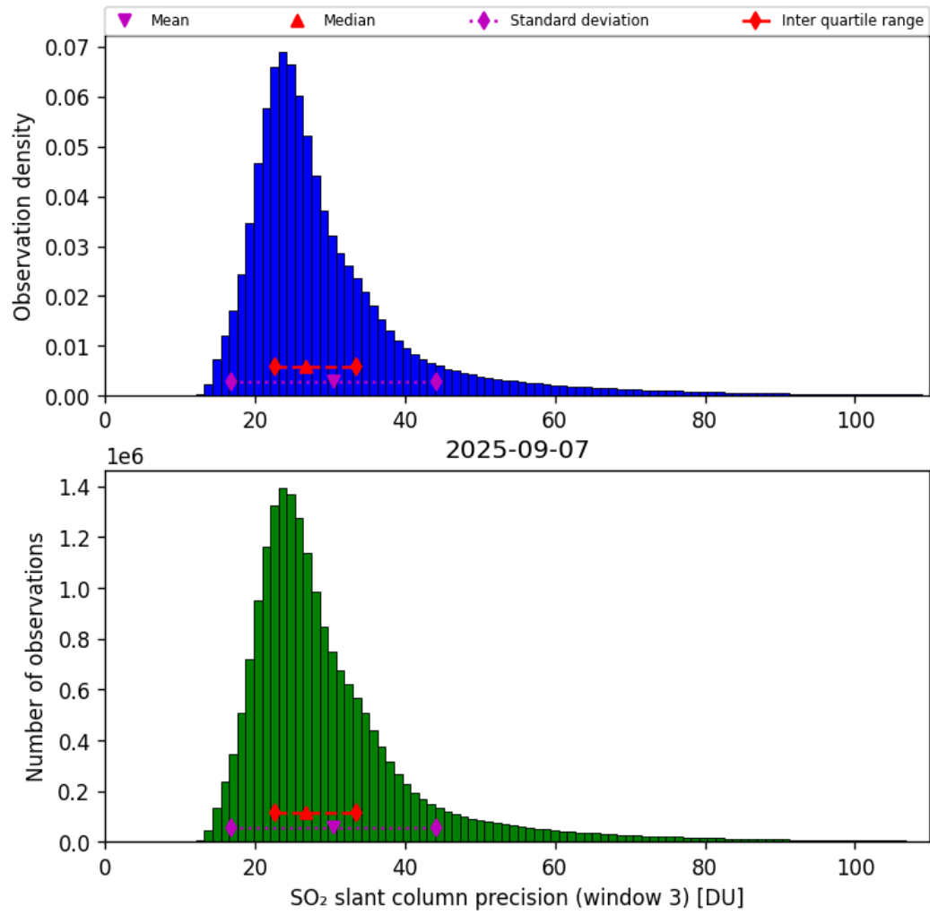
Figure 72: Histogram of “SO 2 slant column precision (window 3)” for 2025-09-06 to 2025-09-08
