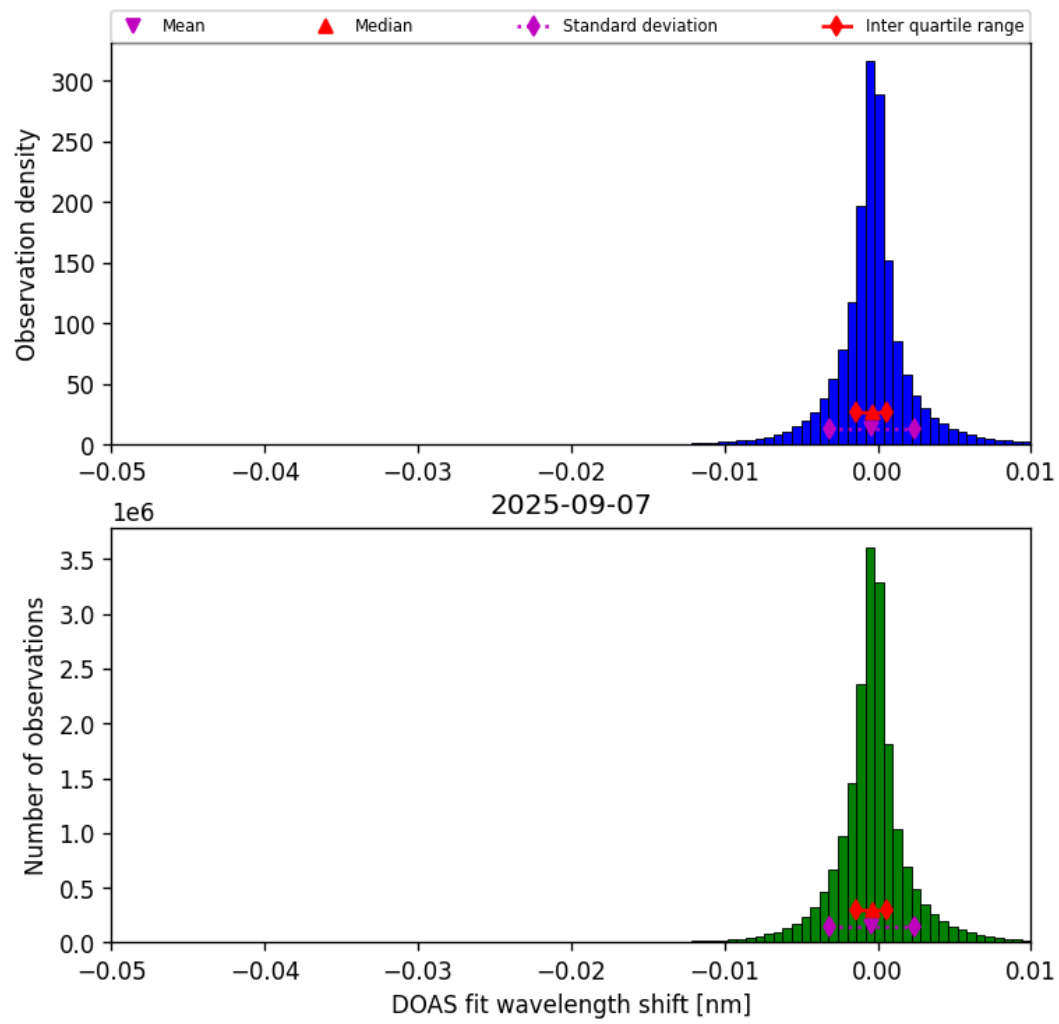
Figure 76: Histogram of “DOAS fit wavelength shift” for 2025-09-06 to 2025-09-08
