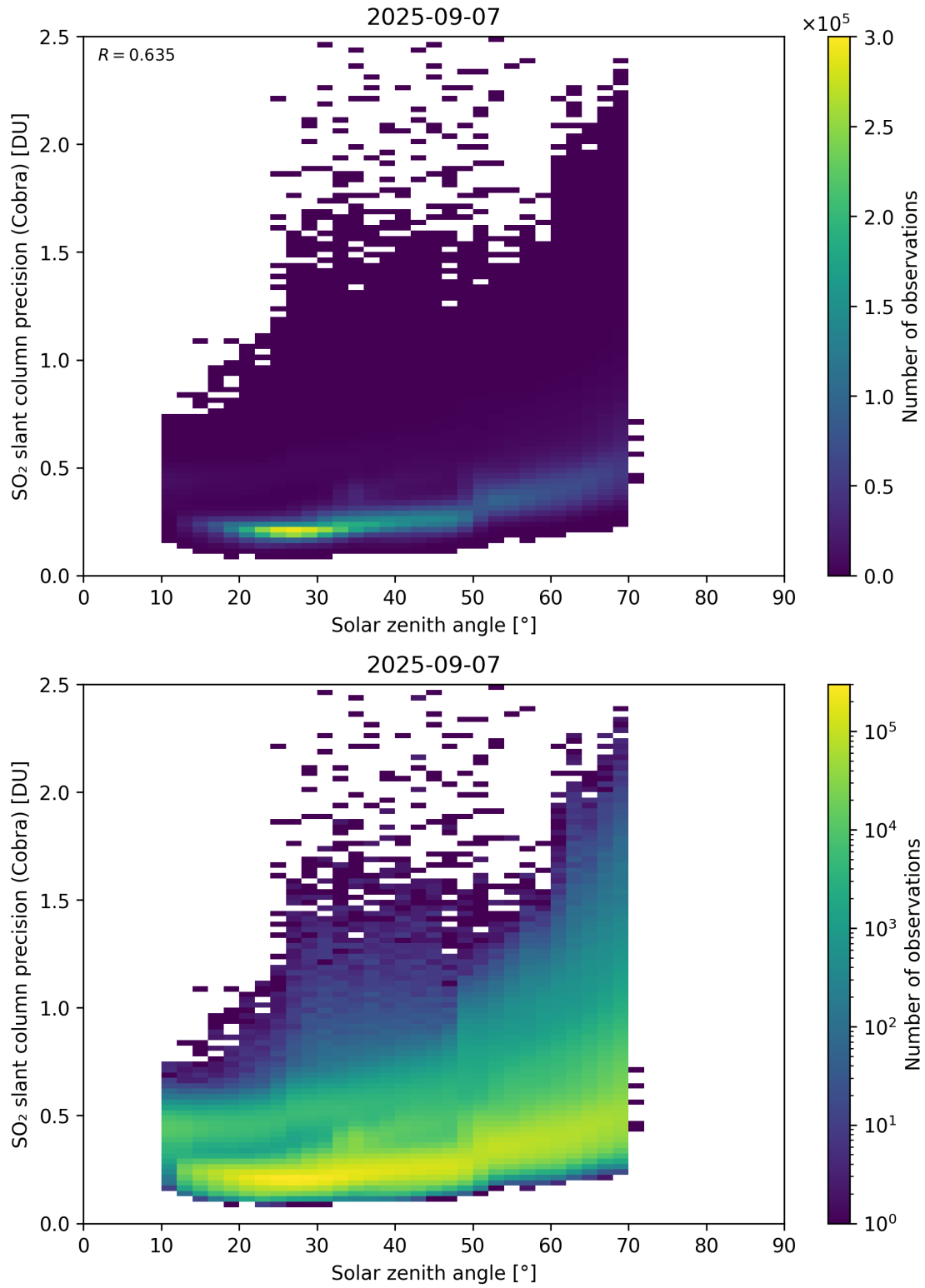
Figure 180: Scatter density plot of “Solar zenith angle” against “SO 2 slant column precision (Cobra)” for 2025-09-06 to 2025-09-08.
