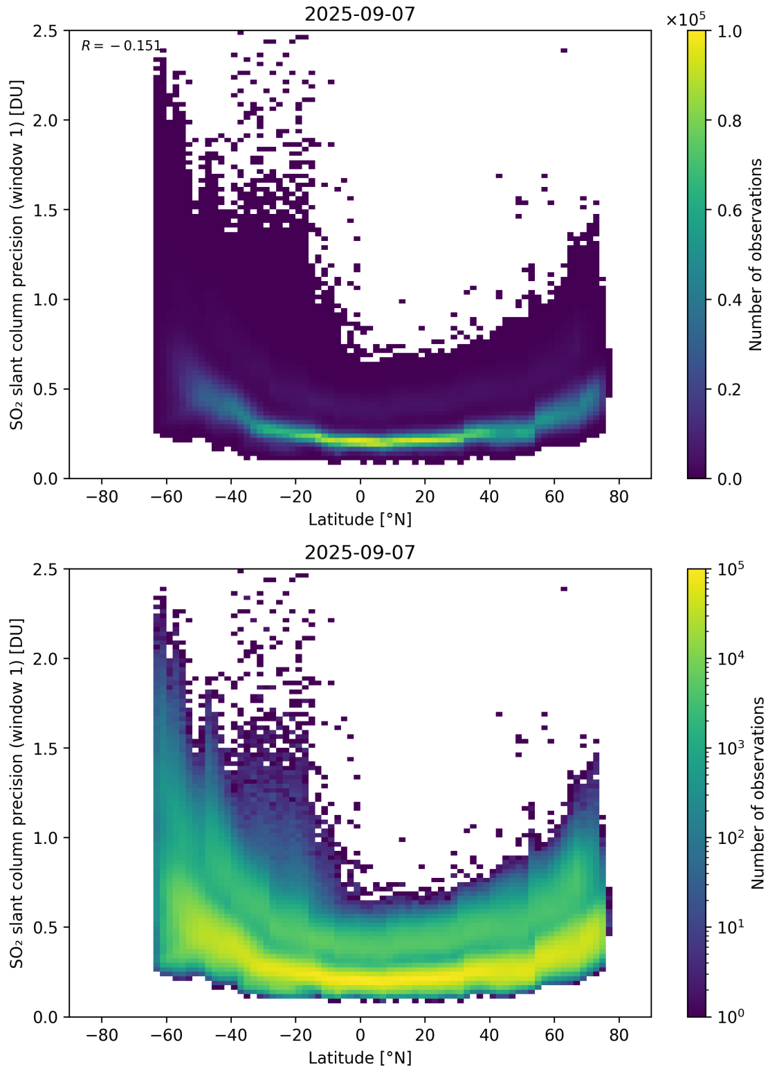
Figure 163: Scatter density plot of “Latitude” against “SO 2 slant column precision (window 1)” for 2025-09-06 to 2025-09-08.
