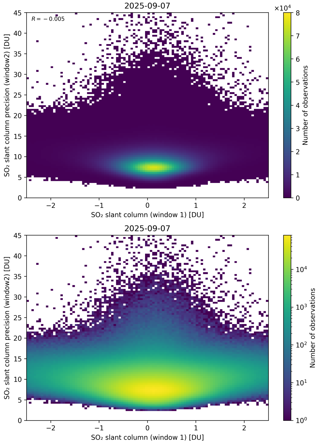
Figure 286: Scatter density plot of “SO 2 slant column (window 1)” against “SO 2 slant column precision (window2)” for 2025-09-06 to 2025-09-08.
