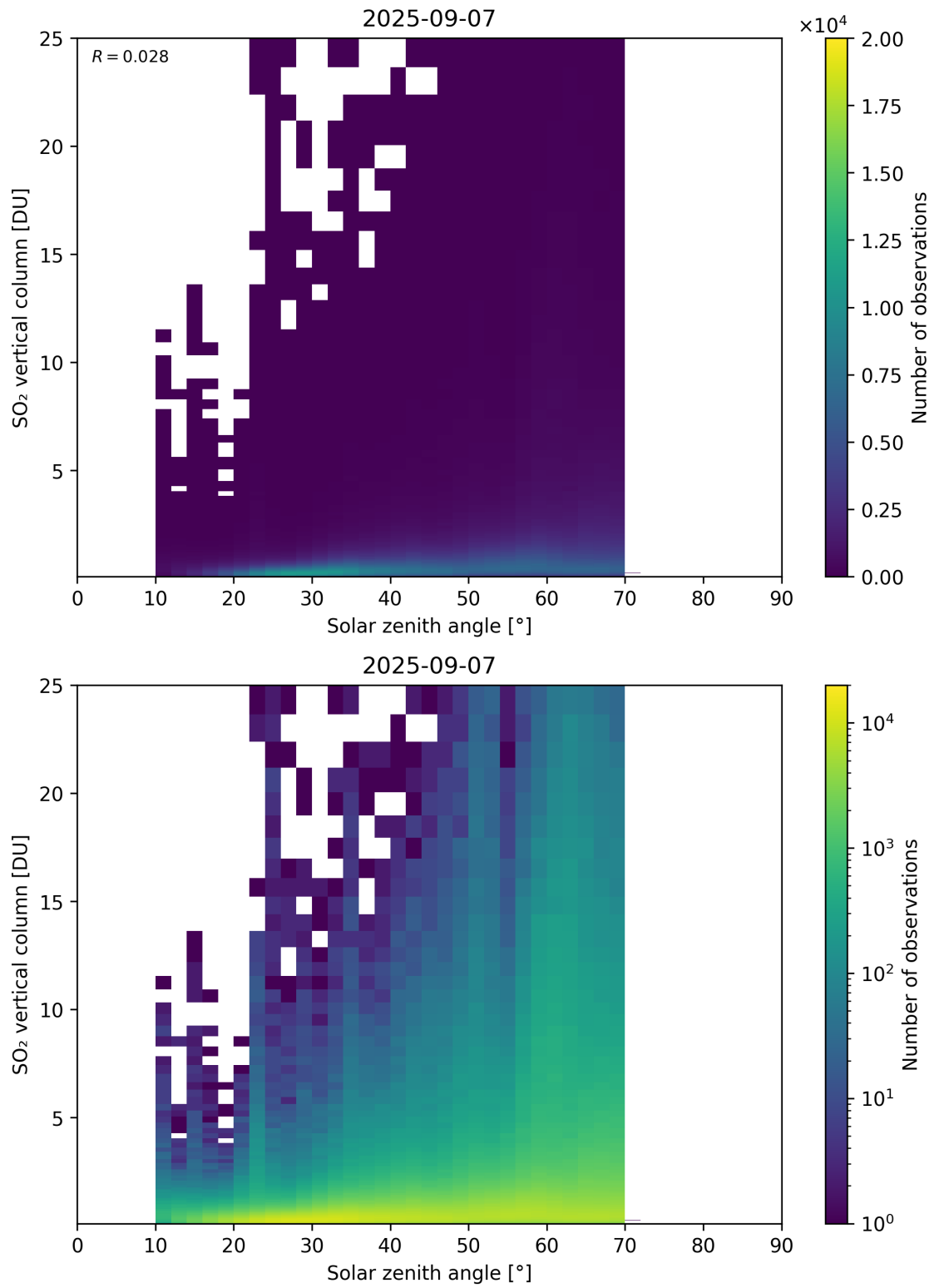
Figure 191: Scatter density plot of “Solar zenith angle” against “SO 2 vertical column” for 2025-09-06 to 2025-09-08.
