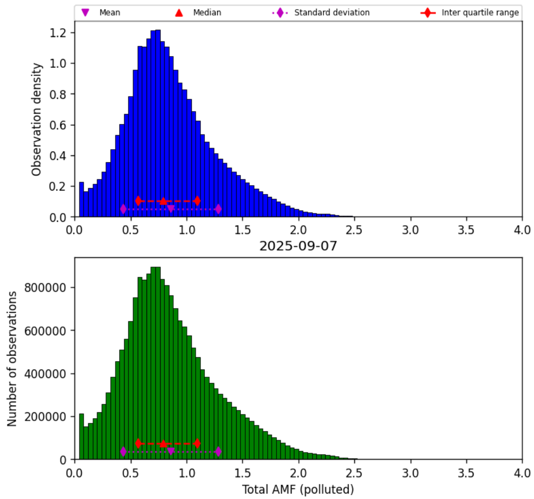
Figure 79: Histogram of “Total AMF (polluted)” for 2025-09-06 to 2025-09-08
