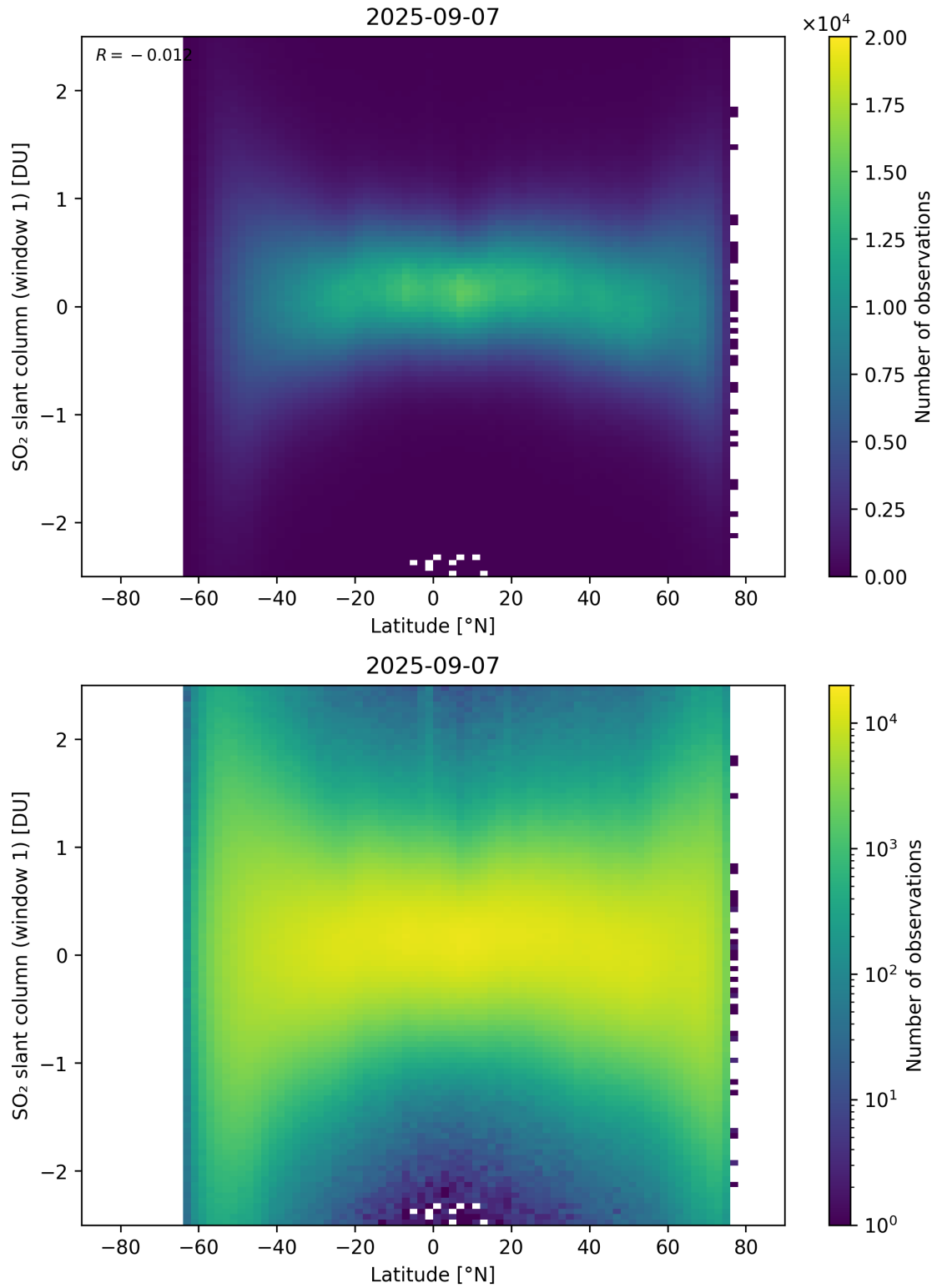
Figure 162: Scatter density plot of “Latitude” against “SO 2 slant column (window 1)” for 2025-09-06 to 2025-09-08.
