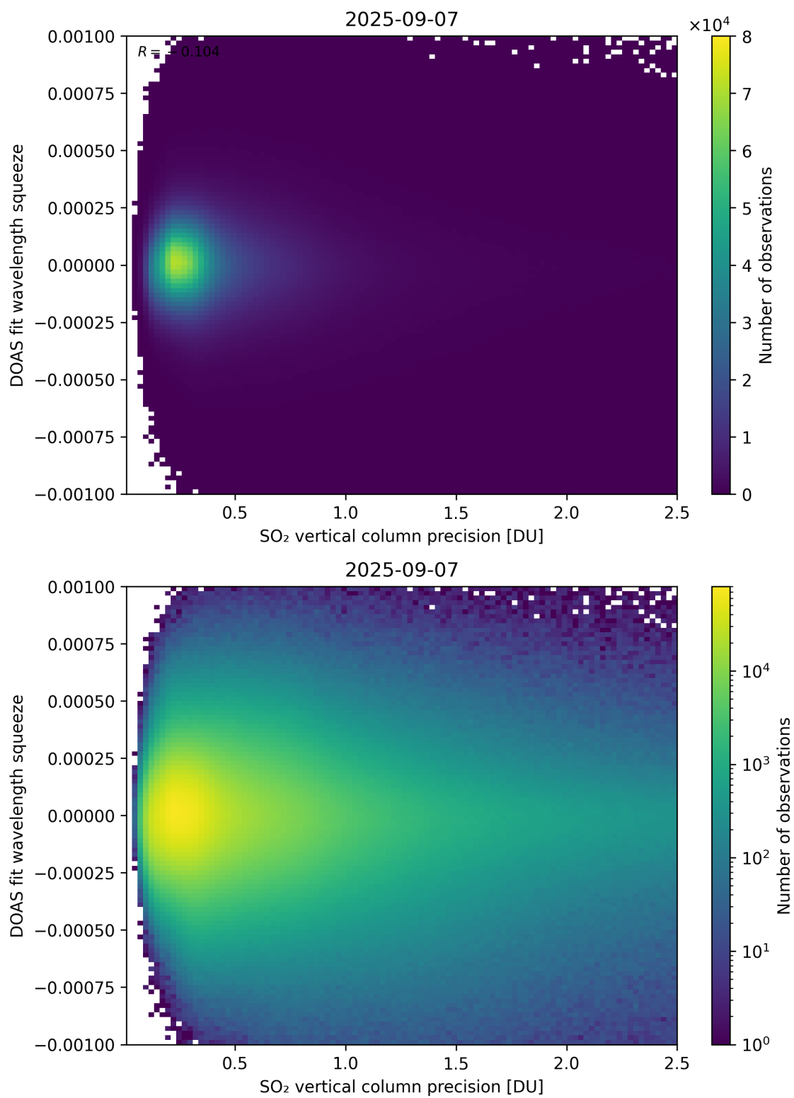
Figure 333: Scatter density plot of “SO 2 vertical column precision” against “DOAS fit wavelength squeeze” for 2025-09-06 to 2025-09-08.
