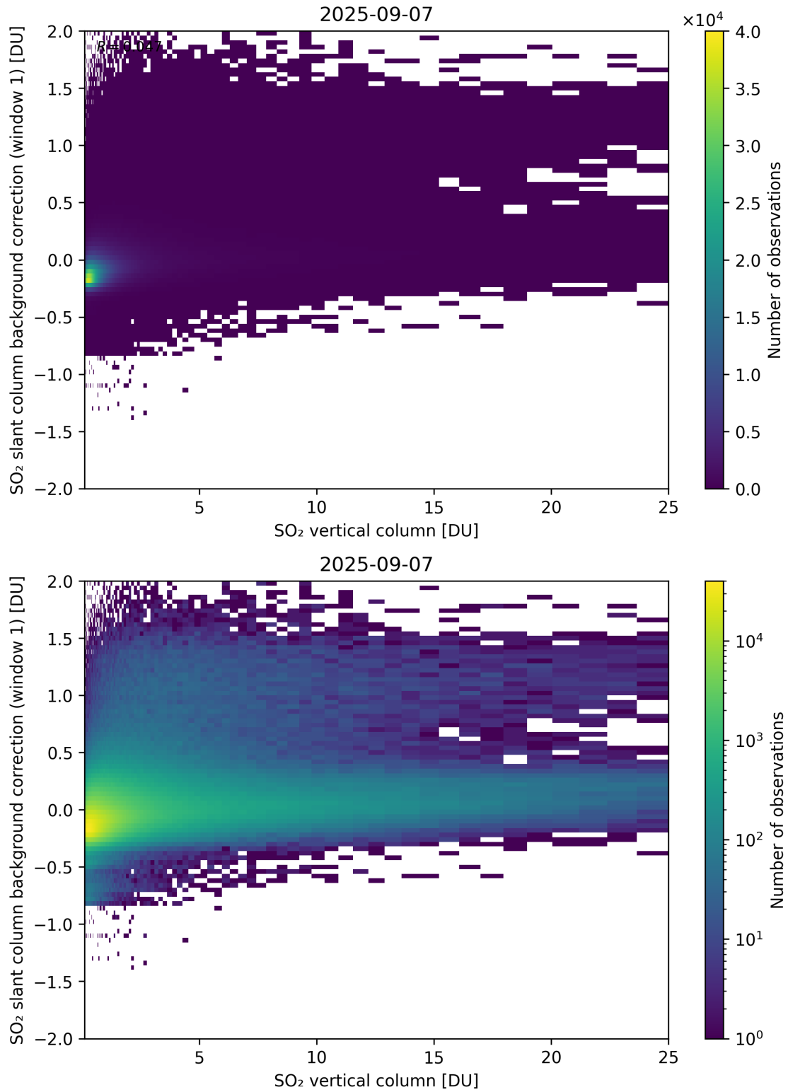
Figure 323: Scatter density plot of “SO 2 vertical column” against “SO 2 slant column background correction (window 1)” for 2025-09-06 to 2025-09-08.
