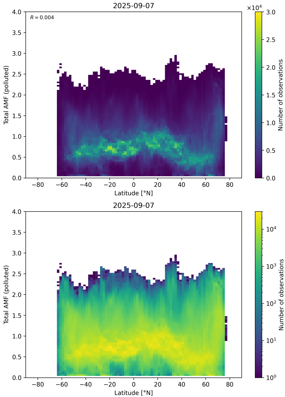
Figure 167: Scatter density plot of “Latitude” against “Total AMF (polluted)” for 2025-09-06 to 2025-09-08.
