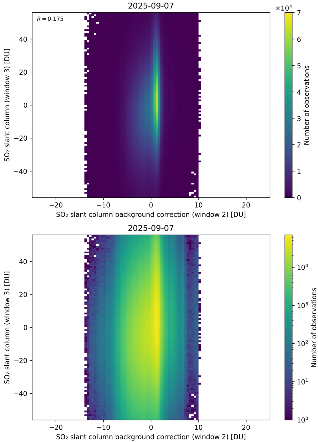
Figure 128: Scatter density plot of “SO 2 slant column background correction (window 2)” against “SO 2 slant column (window 3)” for 2025-09-06 to 2025-09-08.
