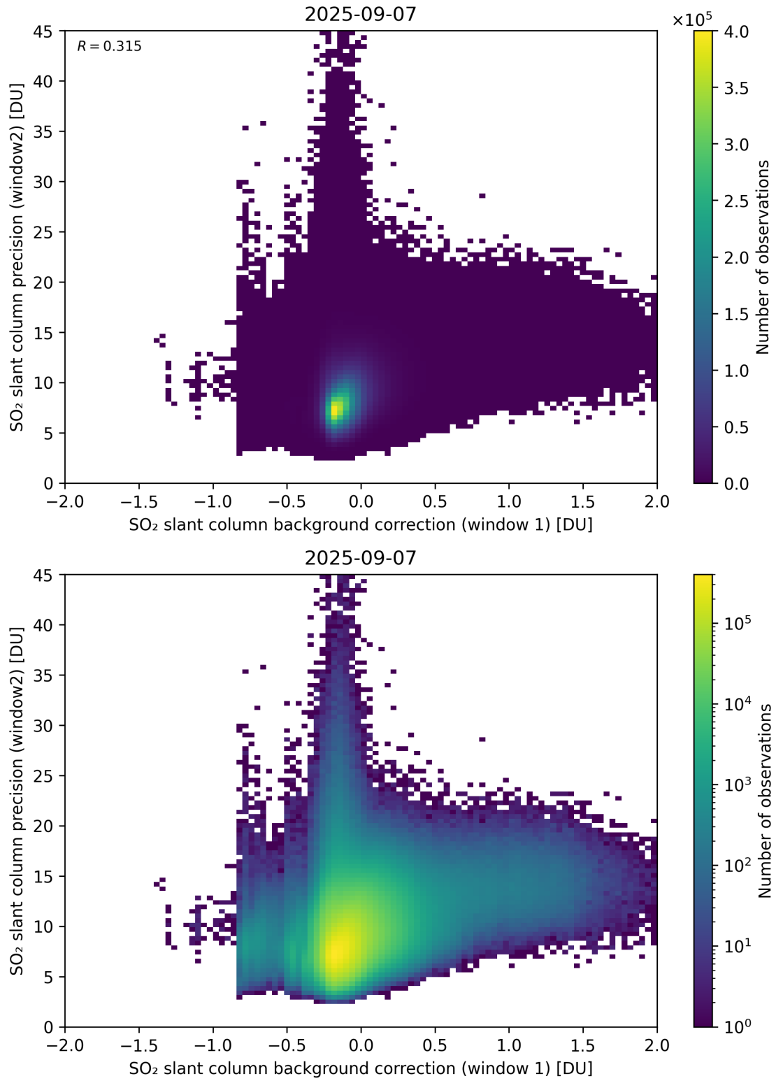
Figure 117: Scatter density plot of “SO 2 slant column background correction (window 1)” against “SO 2 slant column precision (window2)” for 2025-09-06 to 2025-09-08.
