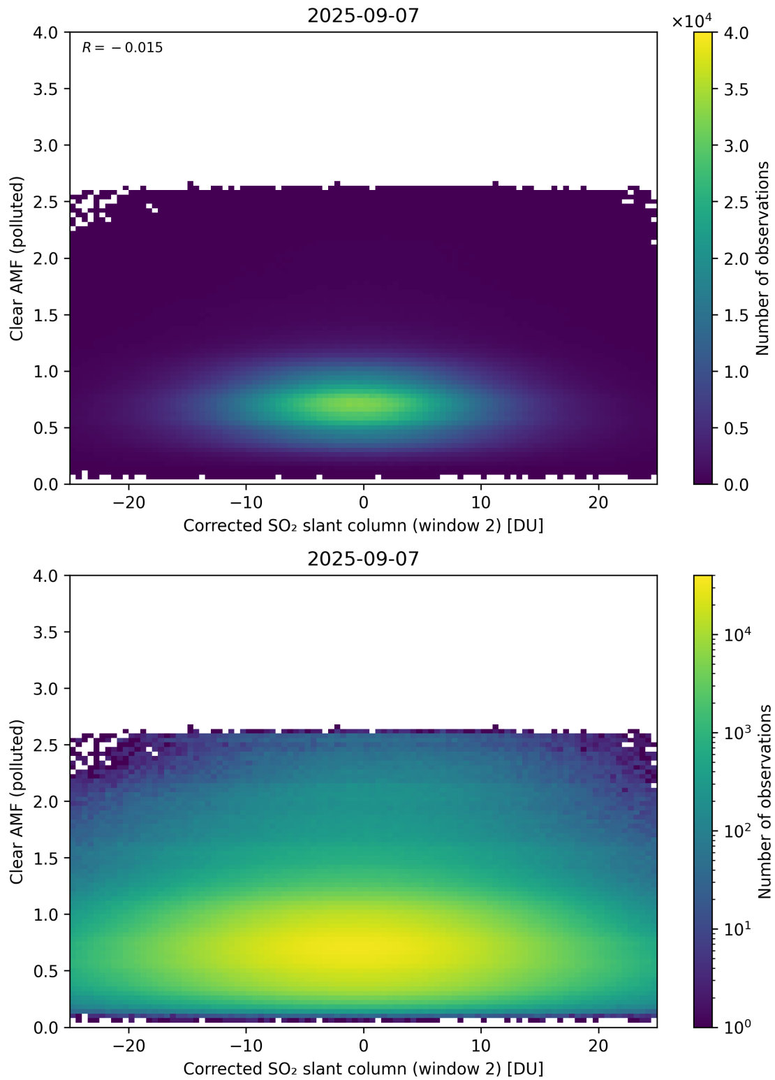
Figure 249: Scatter density plot of “Corrected SO 2 slant column (window 2)” against “Clear AMF (polluted)” for 2025-09-06 to 2025-09-08.
