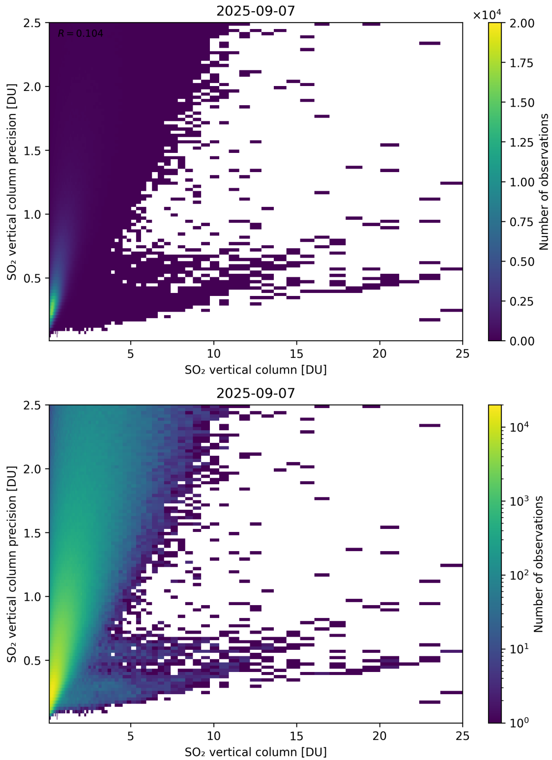
Figure 361: Scatter density plot of “SO 2 vertical column” against “SO 2 vertical column precision” for 2025-09-06 to 2025-09-08.
