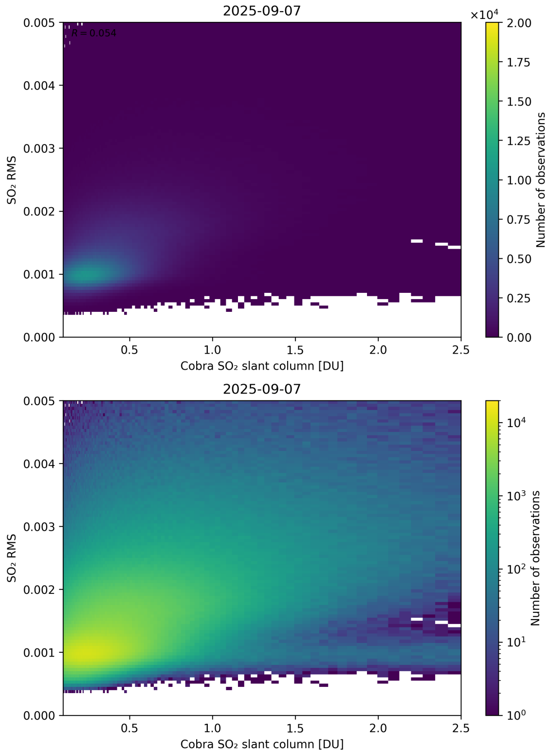
Figure 198: Scatter density plot of “Cobra SO 2 slant column” against “SO 2 RMS” for 2025-09-06 to 2025-09-08.
