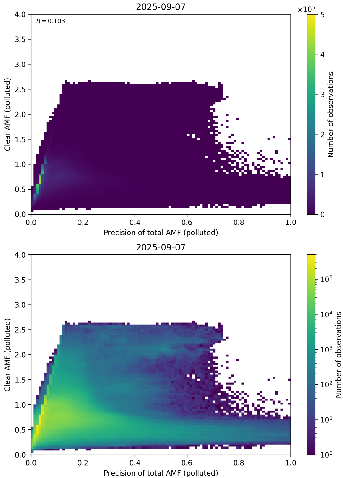
Figure 320: Scatter density plot of “Precision of total AMF (polluted)” against “Clear AMF (polluted)” for 2025-09-06 to 2025-09-08.
