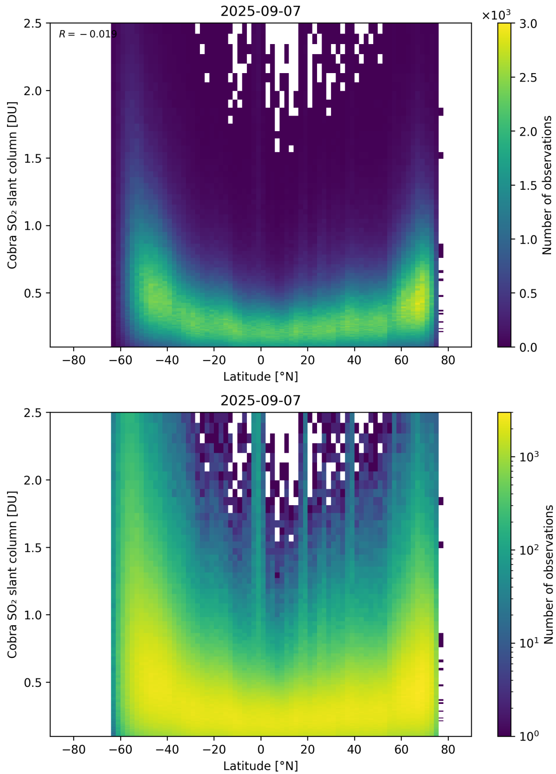
Figure 157: Scatter density plot of “Latitude” against “Cobra SO 2 slant column” for 2025-09-06 to 2025-09-08.
