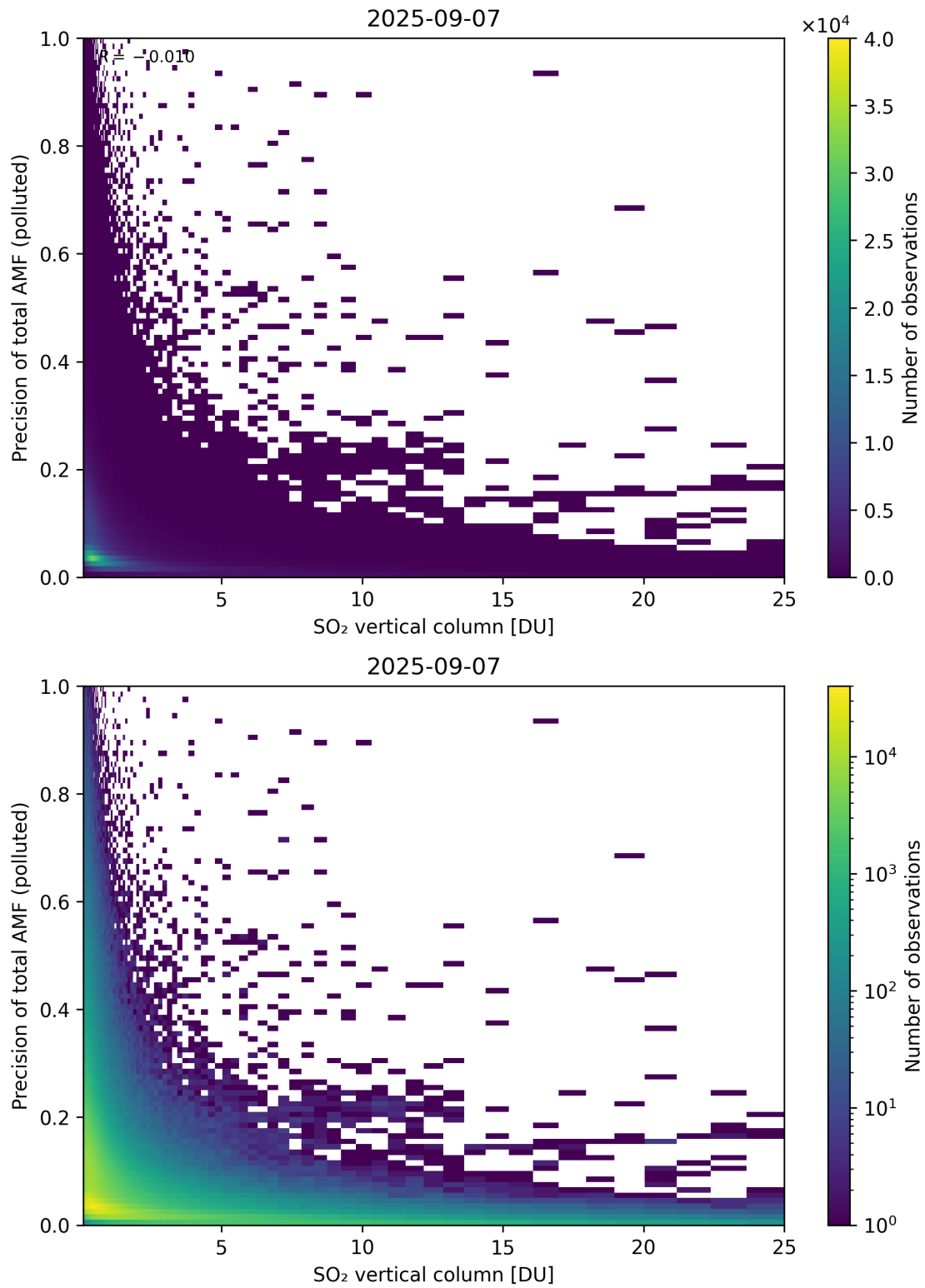
Figure 360: Scatter density plot of “SO 2 vertical column” against “Precision of total AMF (polluted)” for 2025-09-06 to 2025-09-08.
