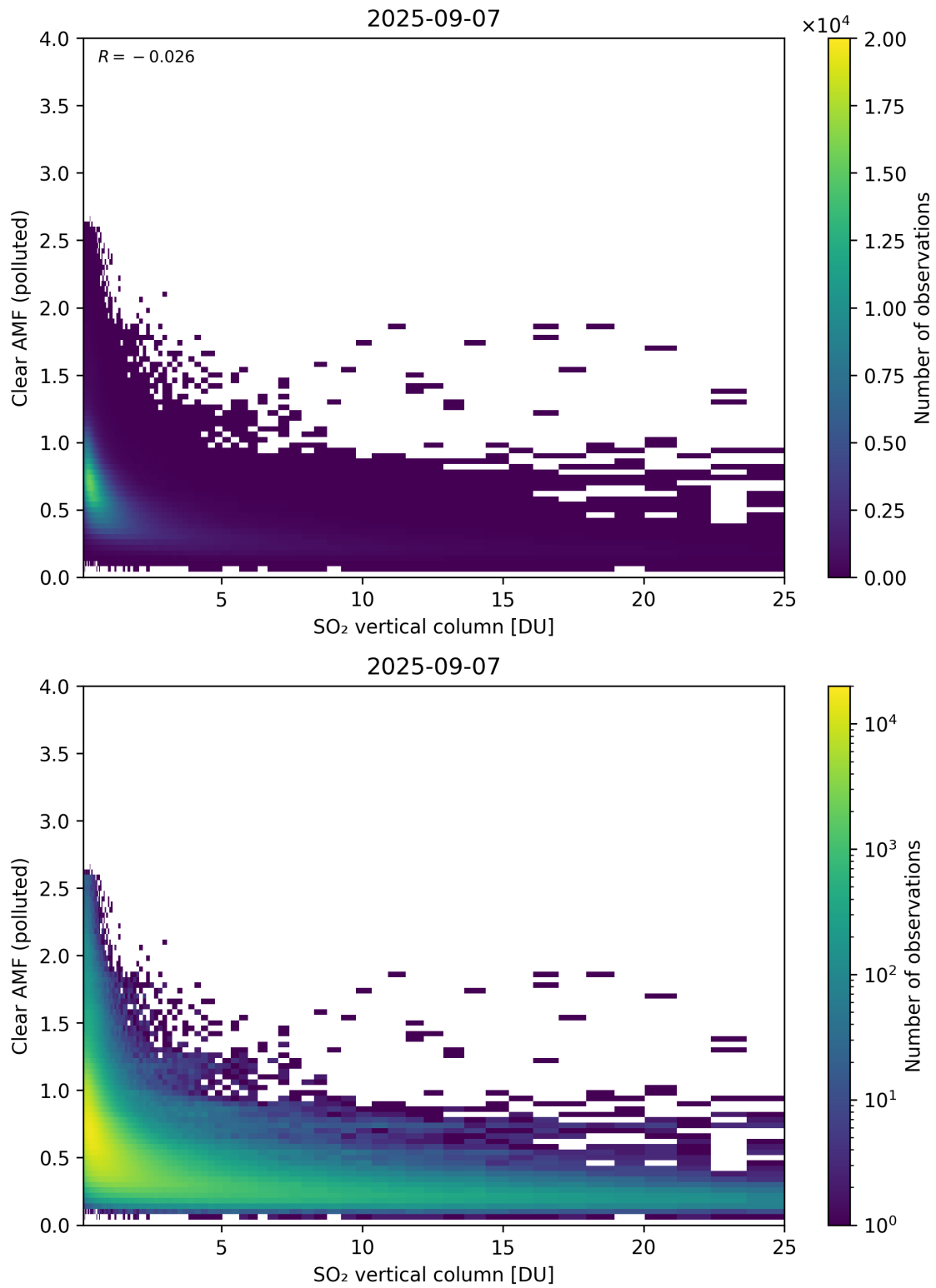
Figure 348: Scatter density plot of “SO 2 vertical column” against “Clear AMF (polluted)” for 2025-09-06 to 2025-09-08.
