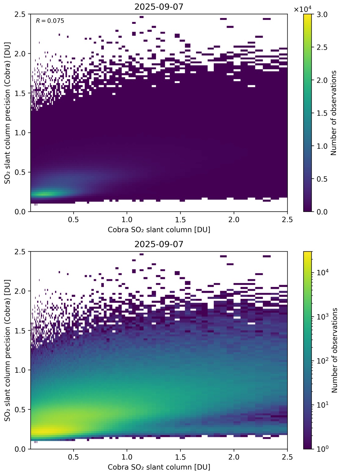
Figure 216: Scatter density plot of “Cobra SO 2 slant column” against “SO 2 slant column precision (Cobra)” for 2025-09-06 to 2025-09-08.
