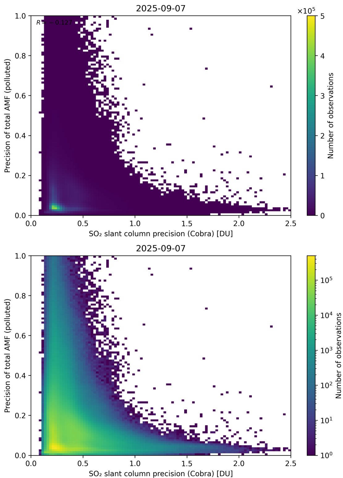
Figure 214: Scatter density plot of “SO 2 slant column precision (Cobra)” against “Precision of total AMF (polluted)” for 2025-09-06 to 2025-09-08.
