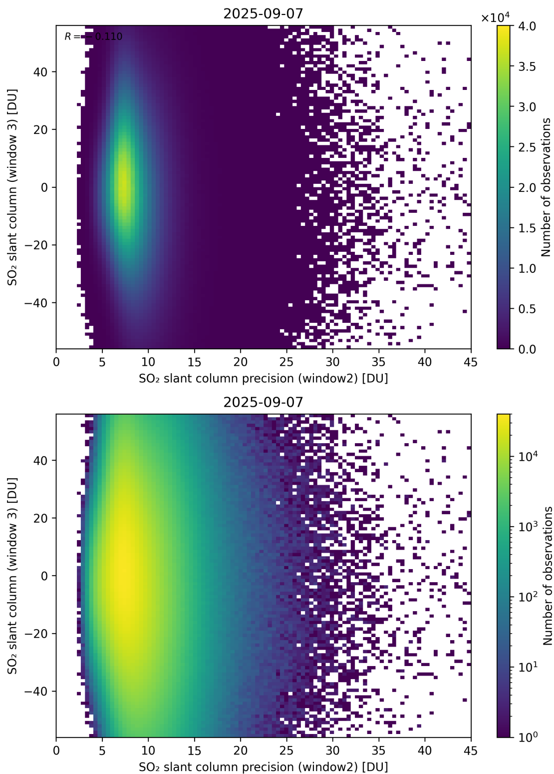
Figure 299: Scatter density plot of “SO 2 slant column precision (window2)” against “SO 2 slant column (window 3)” for 2025-09-06 to 2025-09-08.
