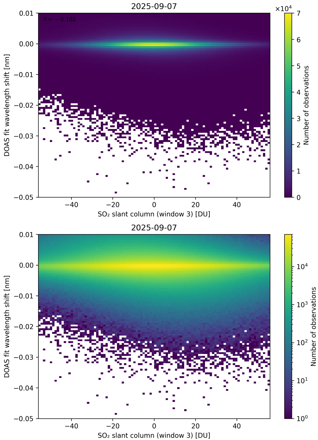
Figure 304: Scatter density plot of “SO 2 slant column (window 3)” against “DOAS fit wavelength shift” for 2025-09-06 to 2025-09-08.
