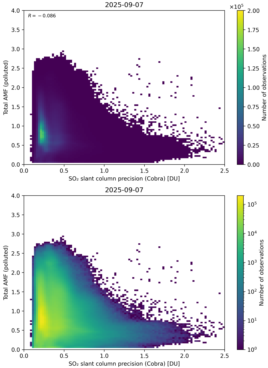
Figure 213: Scatter density plot of “SO 2 slant column precision (Cobra)” against “Total AMF (polluted)” for 2025-09-06 to 2025-09-08.
