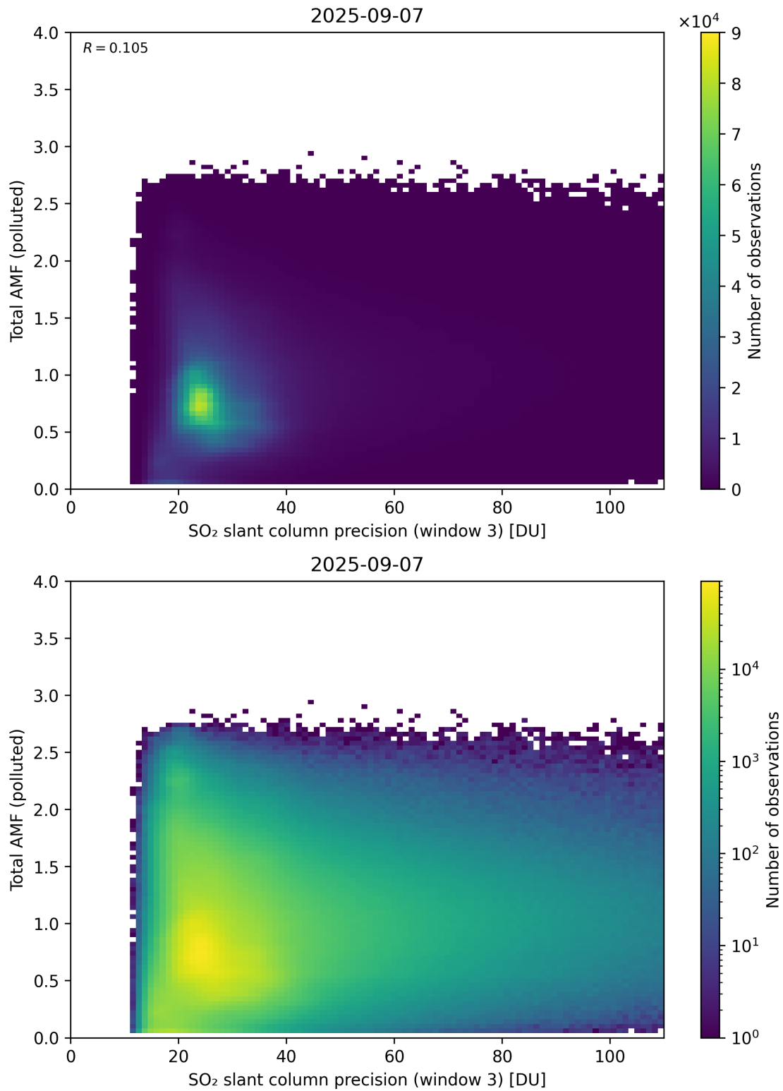
Figure 313: Scatter density plot of “SO 2 slant column precision (window 3)” against “Total AMF (polluted)” for 2025-09-06 to 2025-09-08.
