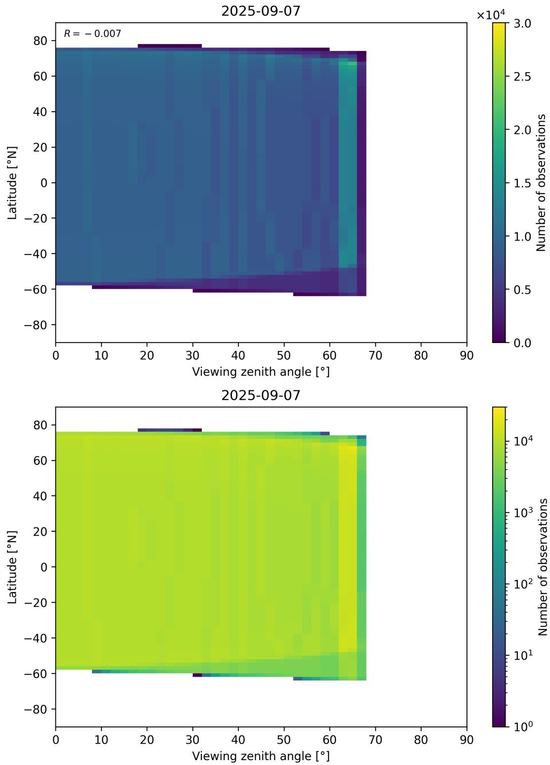
Figure 368: Scatter density plot of “Viewing zenith angle” against “Latitude” for 2025-09-06 to 2025-09-08.
