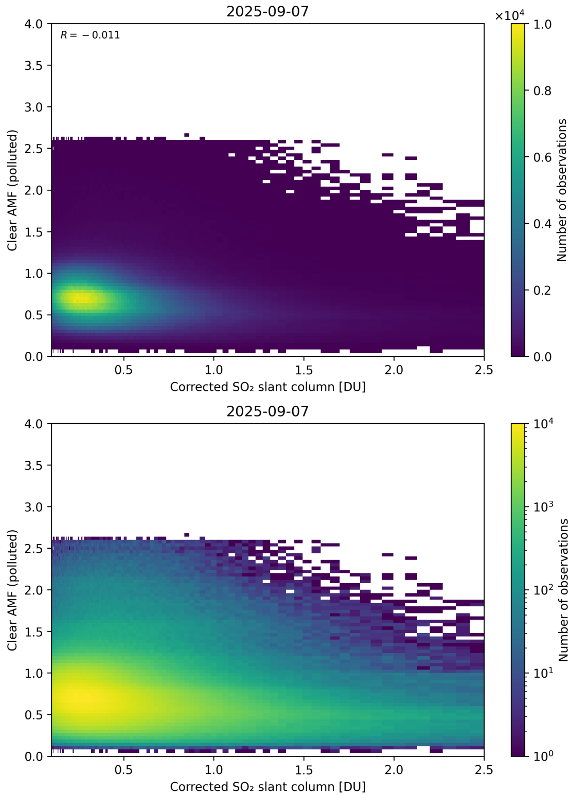
Figure 232: Scatter density plot of “Corrected SO 2 slant column” against “Clear AMF (polluted)” for 2025-09-06 to 2025-09-08.
