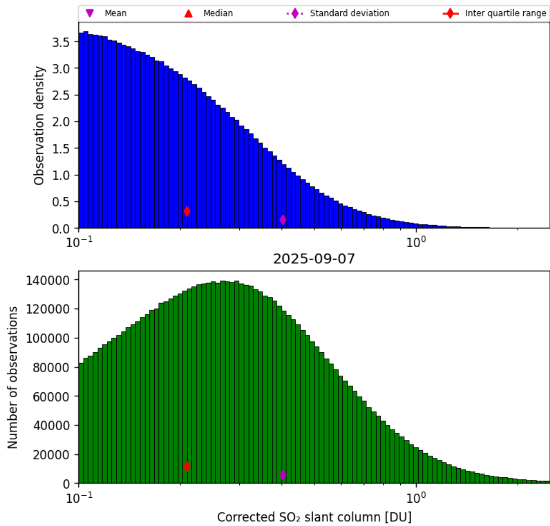
Figure 60: Histogram of "Corrected SO 2 slant column" for 2025-09-06 to 2025-09-08
