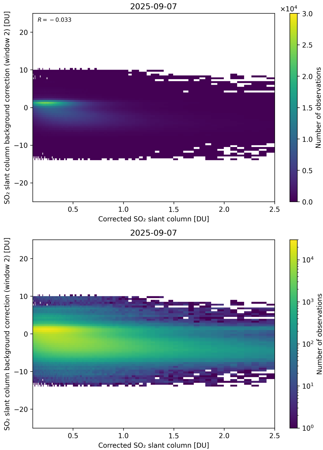
Figure 227: Scatter density plot of “Corrected SO 2 slant column” against “SO 2 slant column background correction (window 2)” for 2025-09-06 to 2025-09-08.
