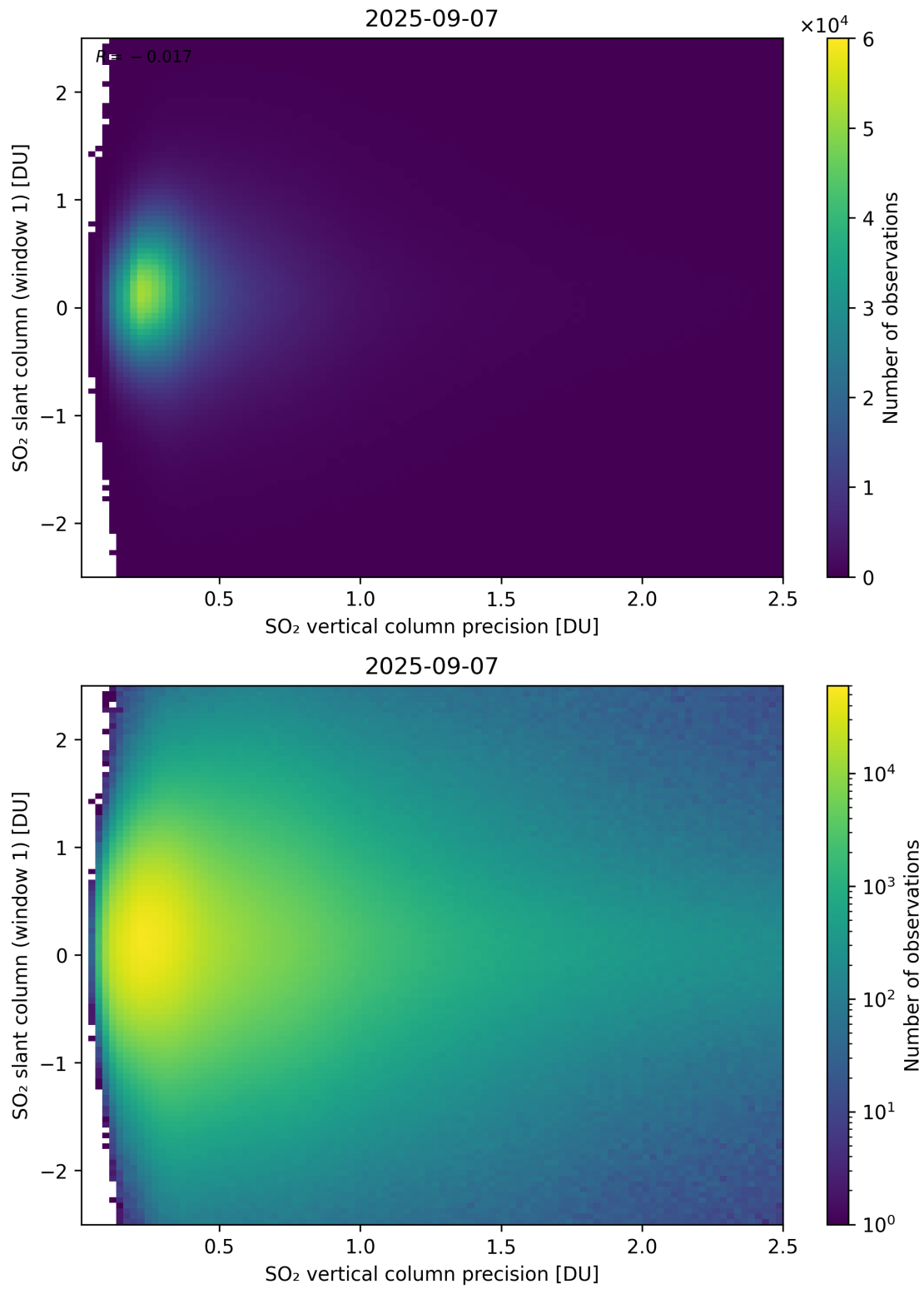
Figure 341: Scatter density plot of “SO 2 vertical column precision” against “SO 2 slant column (window 1)” for 2025-09-06 to 2025-09-08.
