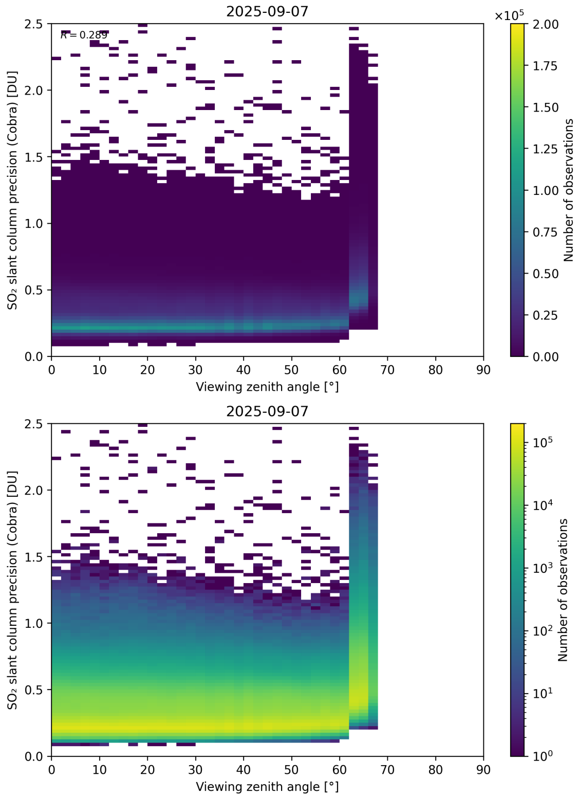
Figure 372: Scatter density plot of “Viewing zenith angle” against “SO 2 slant column precision (Cobra)” for 2025-09-06 to 2025-09-08.
