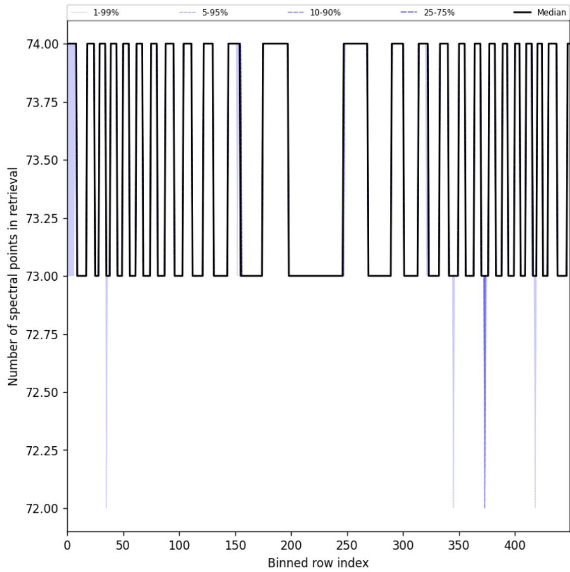
Figure 108: Along track statistics of “Number of spectral points in retrieval” for 2025-09-06 to 2025-09-08
