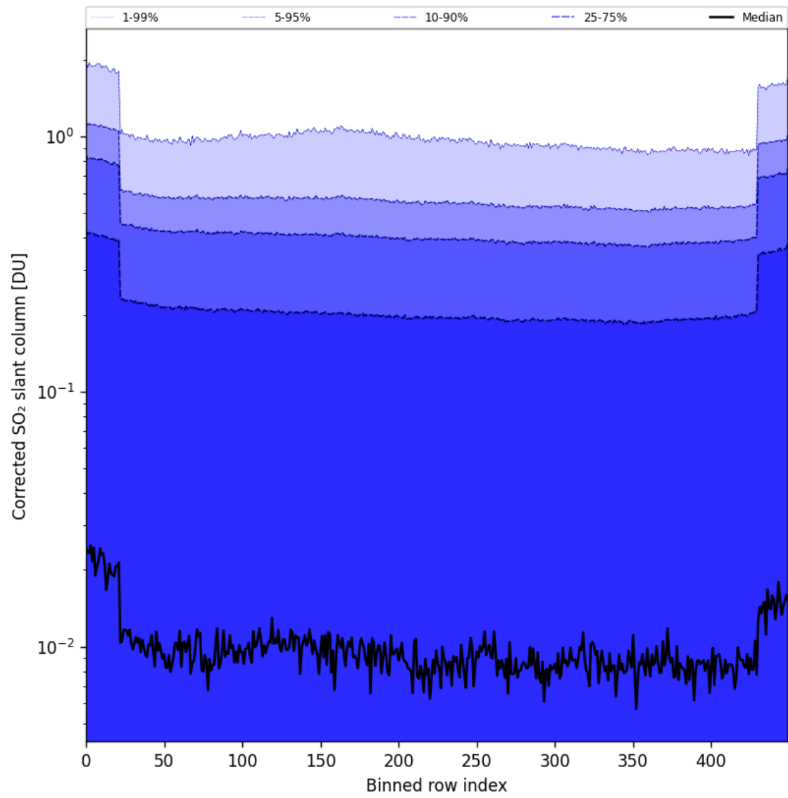
Figure 86: Along track statistics of “Corrected SO 2 slant column” for 2025-09-06 to 2025-09-08
