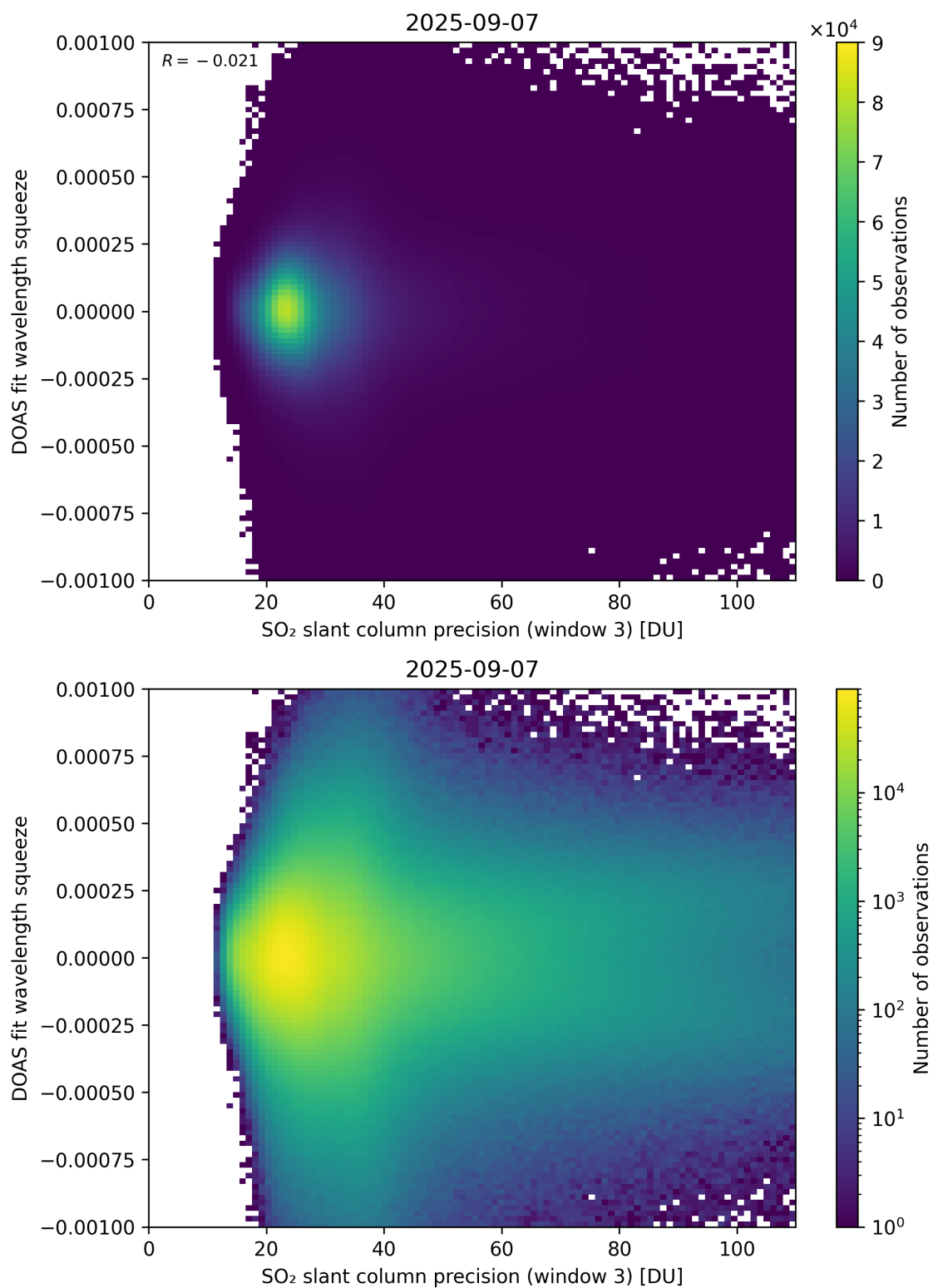
Figure 309: Scatter density plot of “SO 2 slant column precision (window 3)” against “DOAS fit wavelength squeeze” for 2025-09-06 to 2025-09-08.
