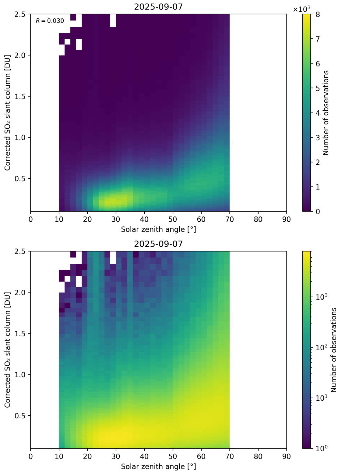
Figure 181: Scatter density plot of “Solar zenith angle” against “Corrected SO 2 slant column” for 2025-09-06 to 2025-09-08.
