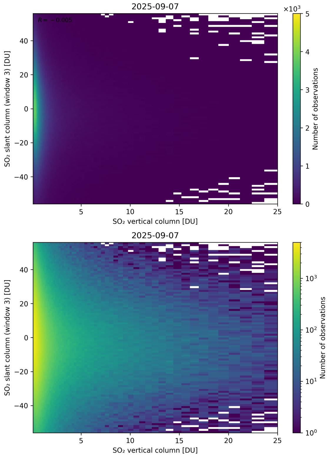
Figure 357: Scatter density plot of “SO 2 vertical column” against “SO 2 slant column (window 3)” for 2025-09-06 to 2025-09-08.
