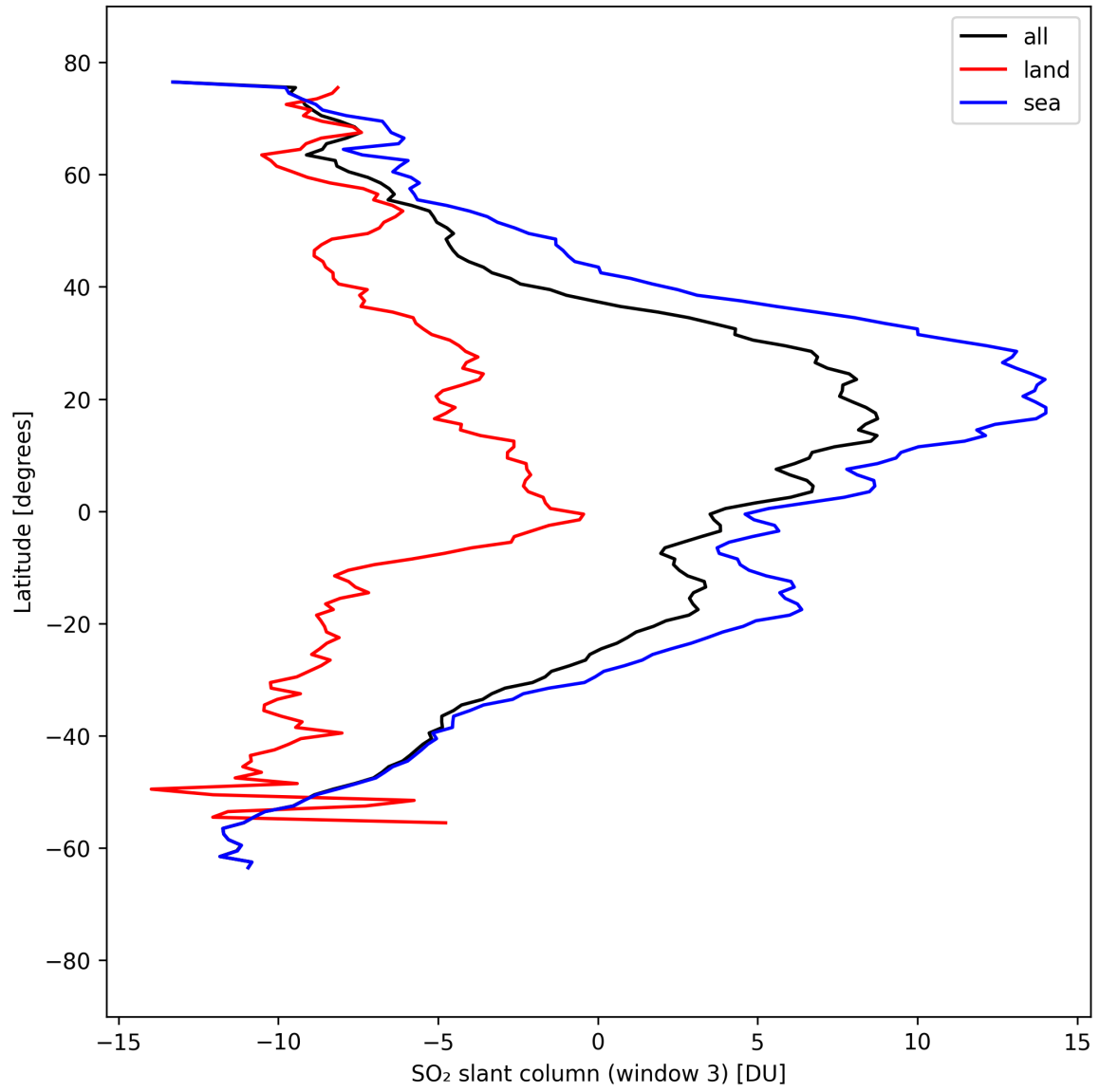
Figure 45: Zonal average of “SO 2 slant column (window 3)” for 2025-09-06 to 2025-09-08.
