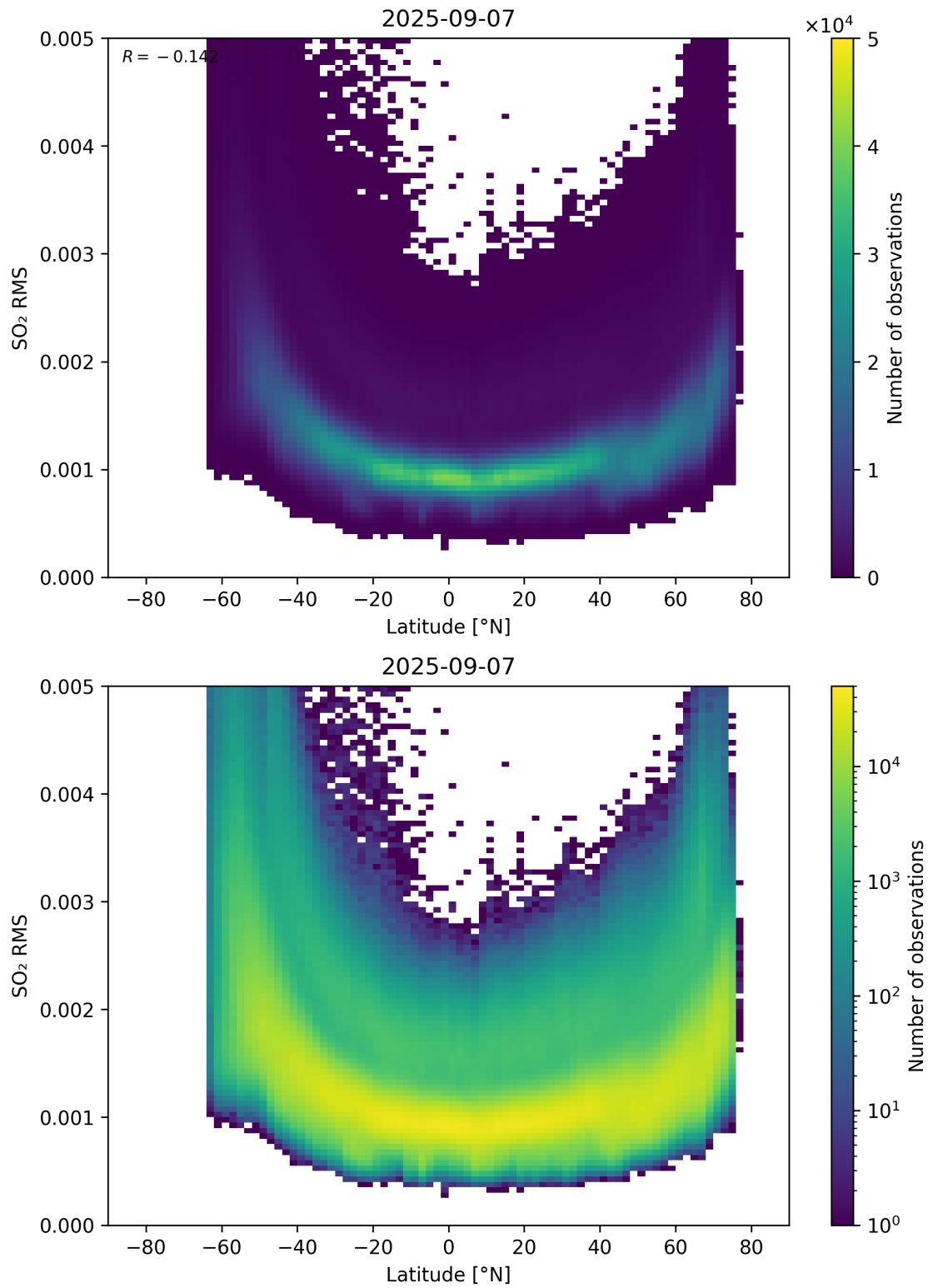
Figure 155: Scatter density plot of “Latitude” against “SO 2 RMS” for 2025-09-06 to 2025-09-08.
