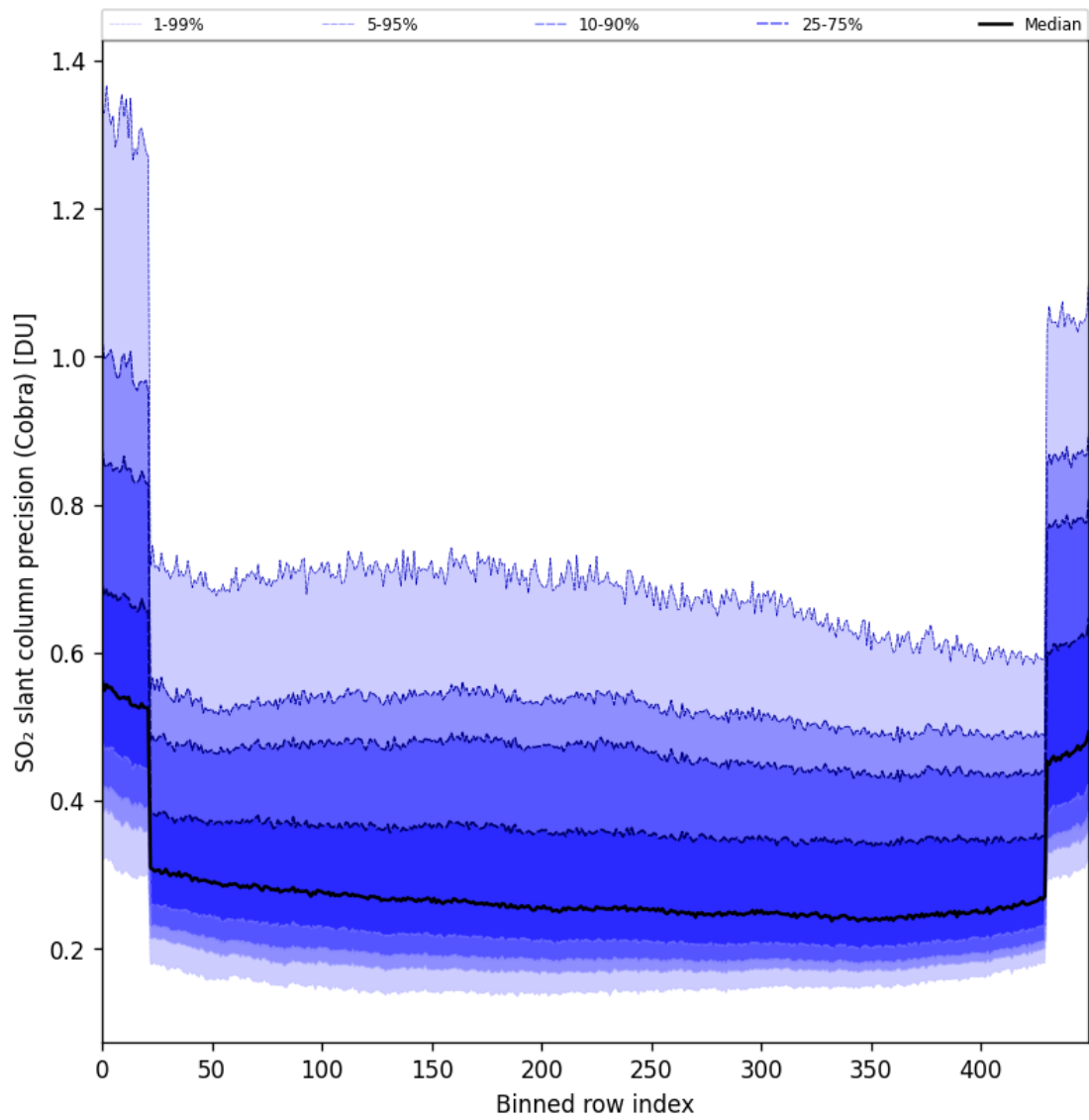
Figure 88: Along track statistics of “SO 2 slant column precision (Cobra)” for 2025-09-06 to 2025-09-08
