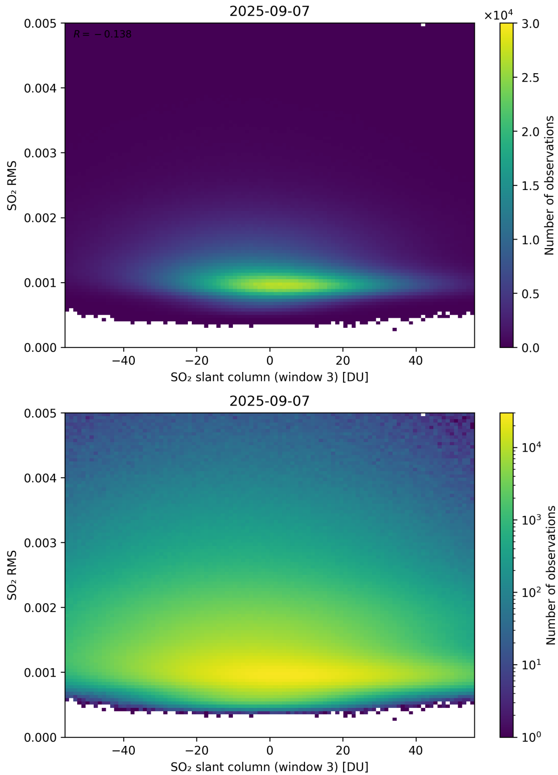
Figure 306: Scatter density plot of “SO 2 slant column (window 3)” against “SO 2 RMS” for 2025-09-06 to 2025-09-08.
