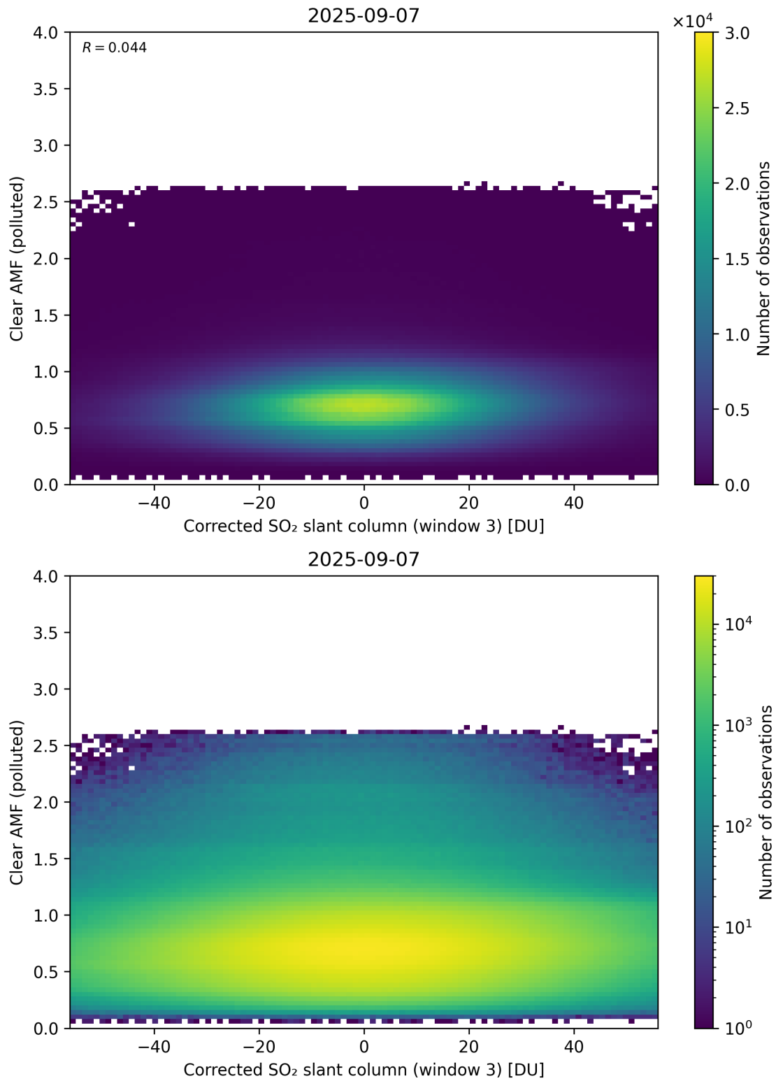
Figure 259: Scatter density plot of “Corrected SO 2 slant column (window 3)” against “Clear AMF (polluted)” for 2025-09-06 to 2025-09-08.
