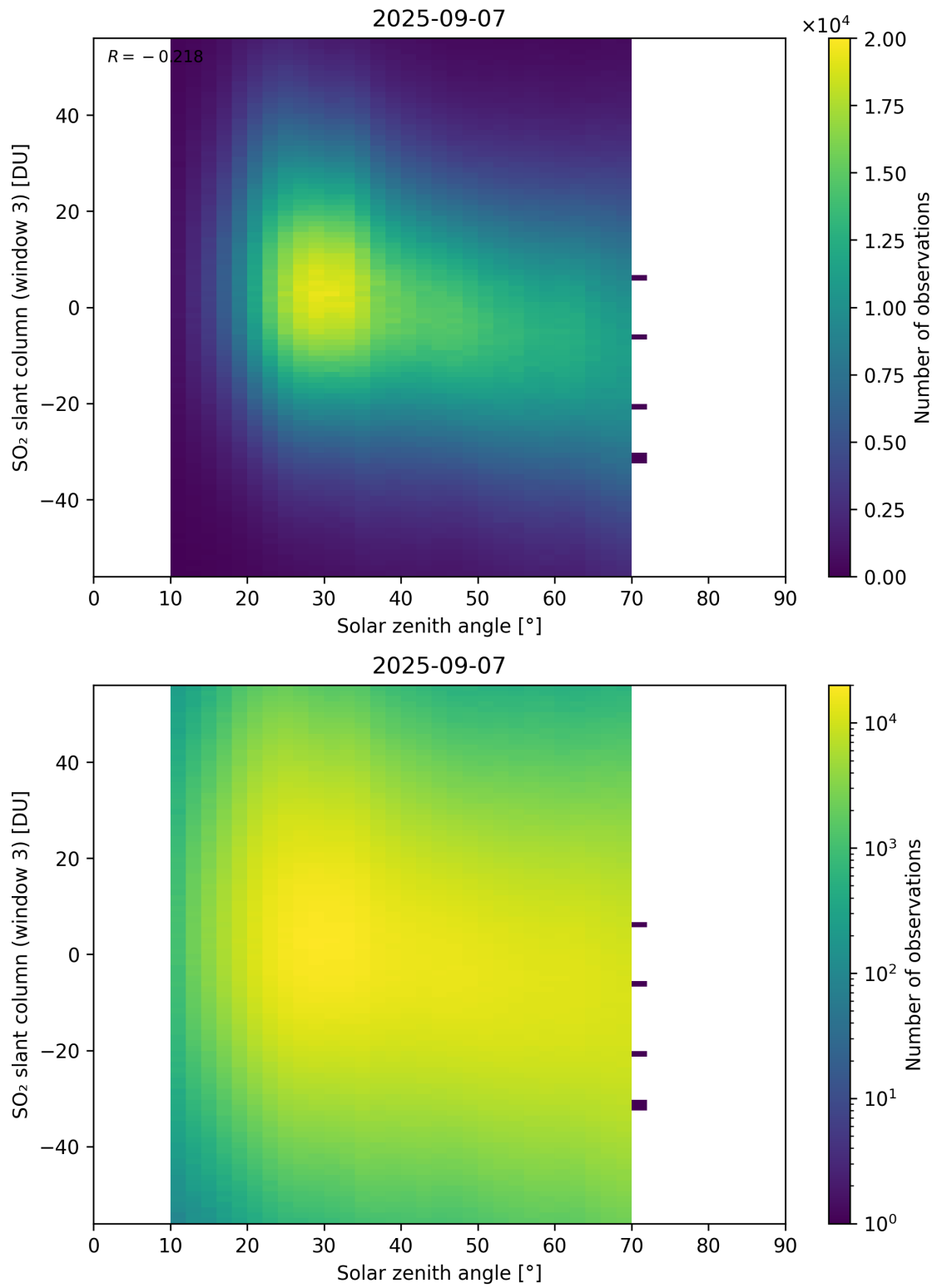
Figure 187: Scatter density plot of “Solar zenith angle” against “SO 2 slant column (window 3)” for 2025-09-06 to 2025-09-08.
