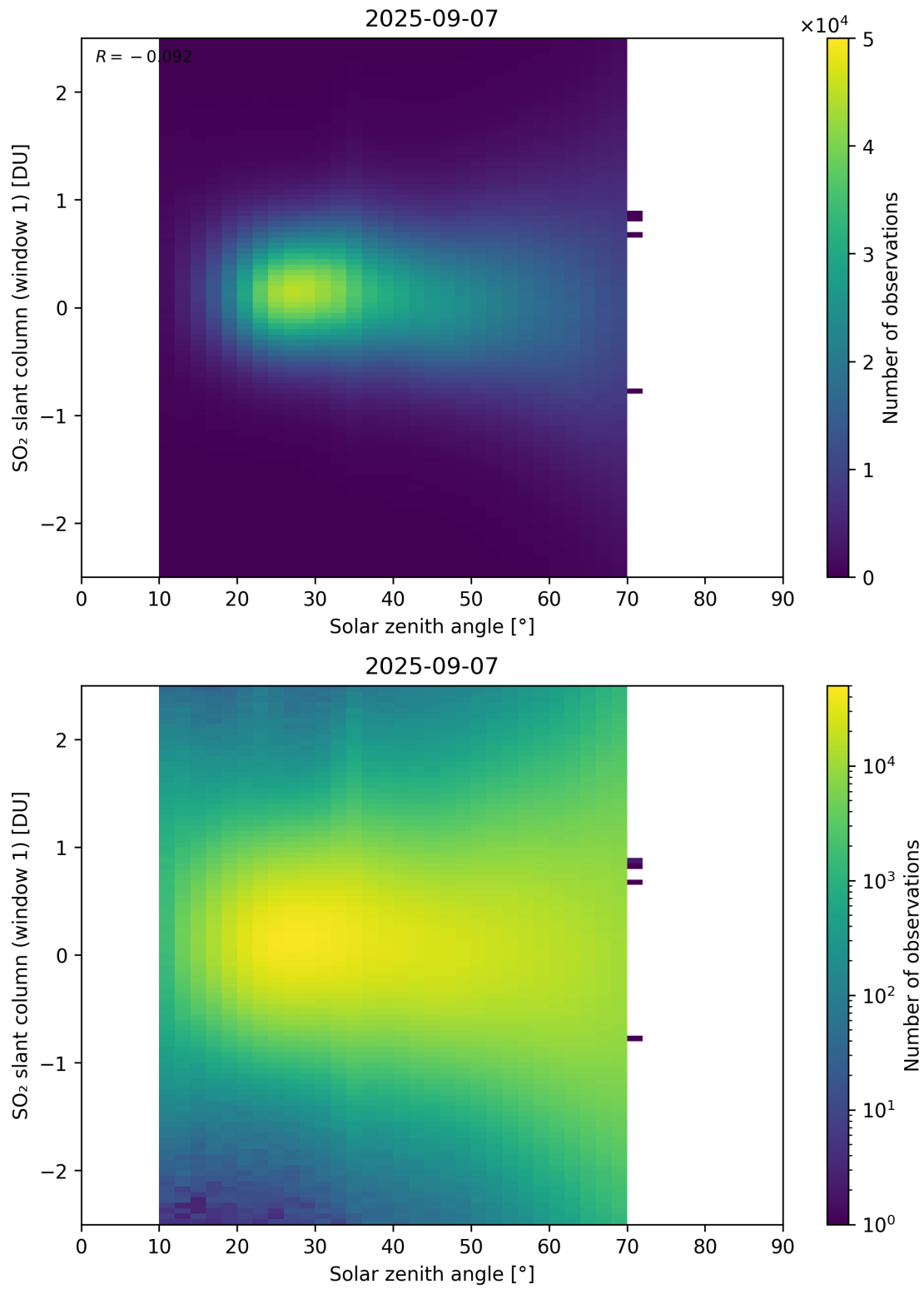
Figure 184: Scatter density plot of “Solar zenith angle” against “SO 2 slant column (window 1)” for 2025-09-06 to 2025-09-08.
