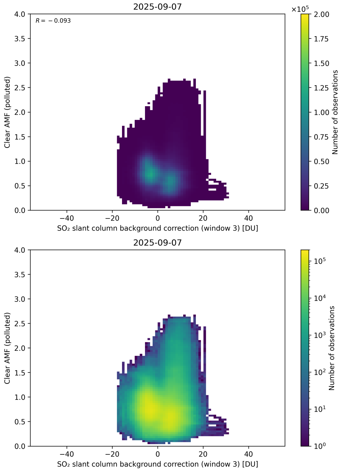
Figure 135: Scatter density plot of “SO 2 slant column background correction (window 3)” against “Clear AMF (polluted)” for 2025-09-06 to 2025-09-08.
