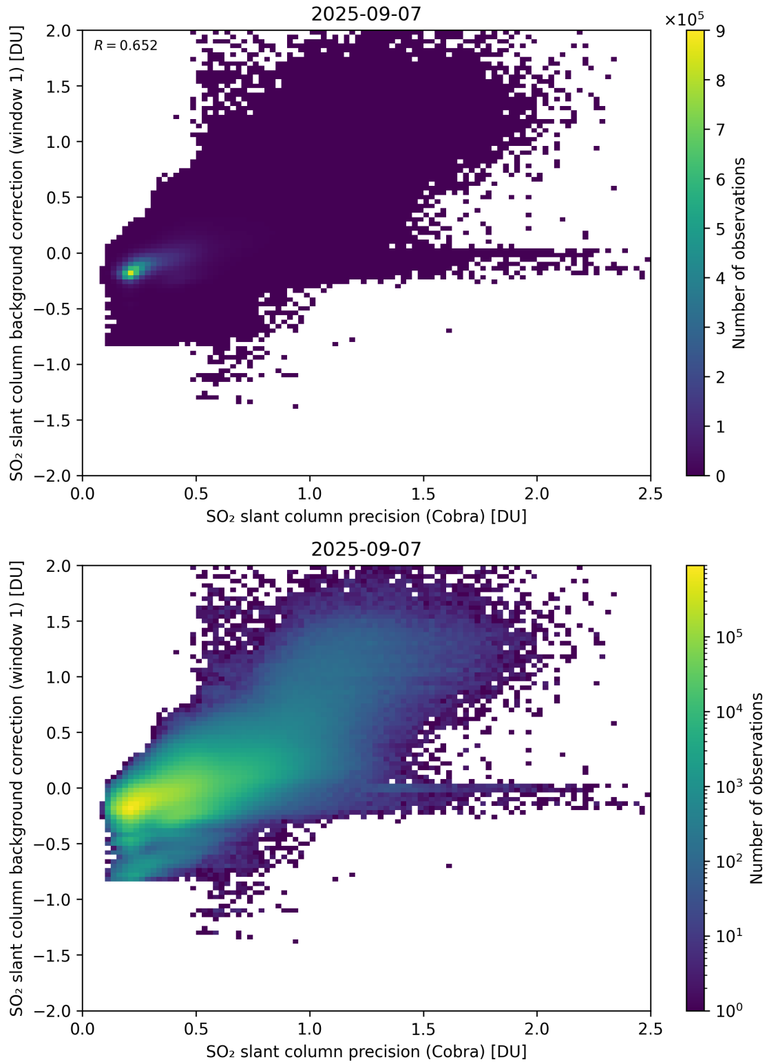
Figure 199: Scatter density plot of “SO 2 slant column precision (Cobra)” against “SO 2 slant column background correction (window 1)” for 2025-09-06 to 2025-09-08.
