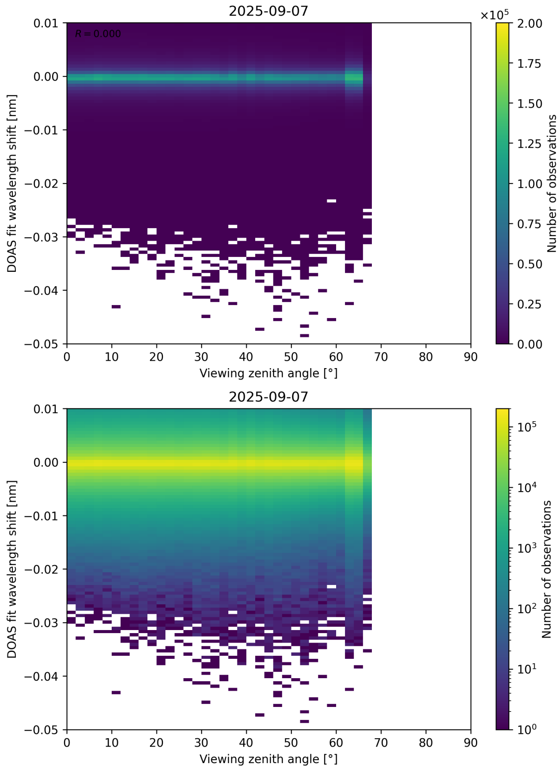
Figure 365: Scatter density plot of “Viewing zenith angle” against “DOAS fit wavelength shift” for 2025-09-06 to 2025-09-08.
