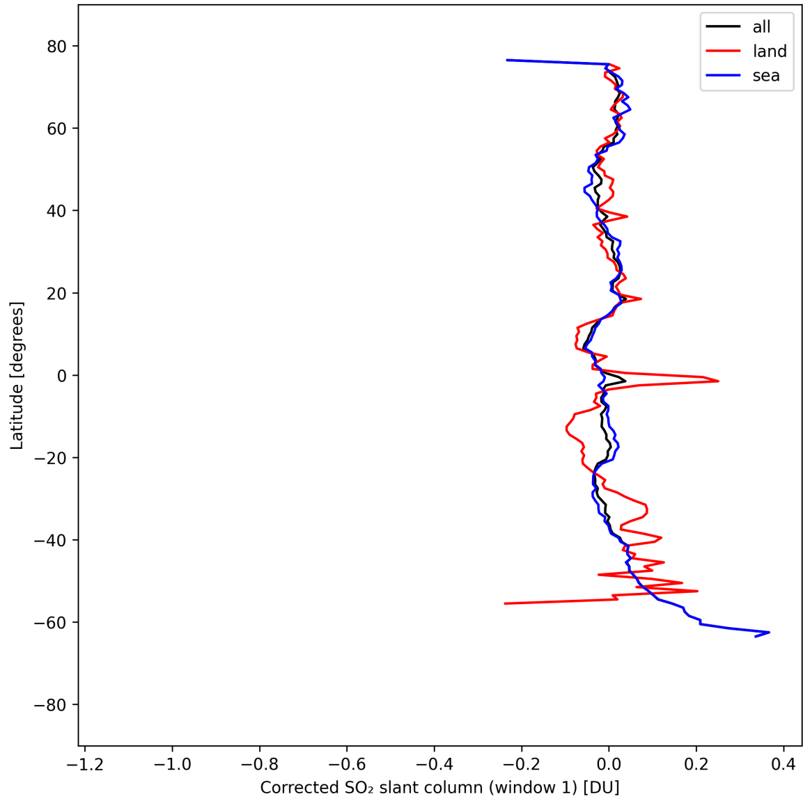
Figure 39: Zonal average of “Corrected SO 2 slant column (window 1)” for 2025-09-06 to 2025-09-08.
