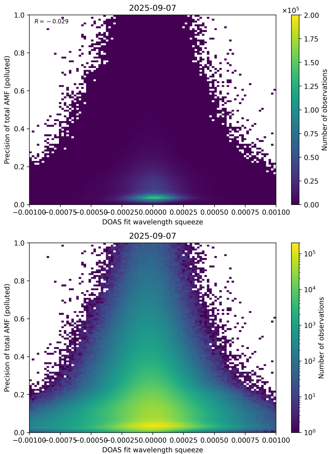
Figure 146: Scatter density plot of “DOAS fit wavelength squeeze” against “Precision of total AMF (polluted)” for 2025-09-06 to 2025-09-08.
