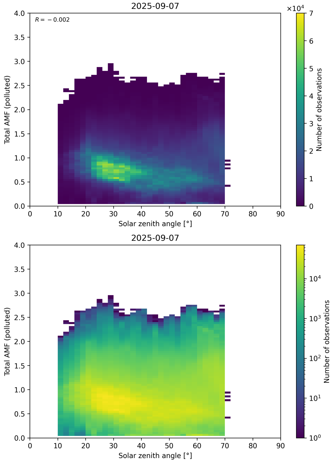
Figure 189: Scatter density plot of “Solar zenith angle” against “Total AMF (polluted)” for 2025-09-06 to 2025-09-08.
