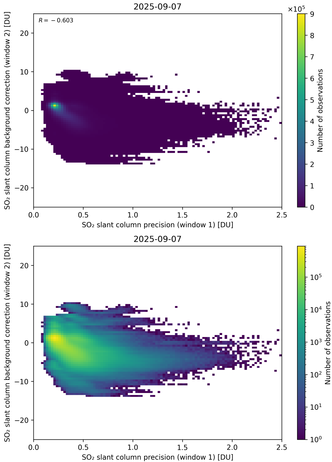
Figure 269: Scatter density plot of “SO 2 slant column precision (window 1)” against “SO 2 slant column background correction (window 2)” for 2025-09-06 to 2025-09-08.
