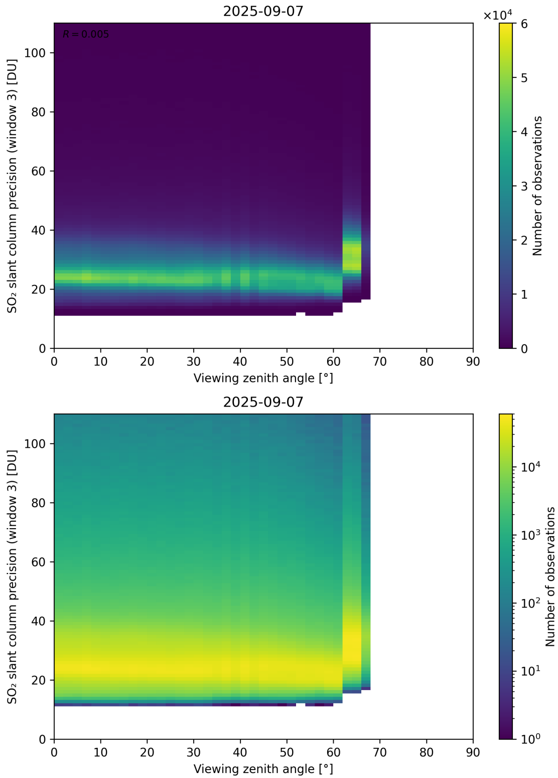
Figure 380: Scatter density plot of “Viewing zenith angle” against “SO 2 slant column precision (window 3)” for 2025-09-06 to 2025-09-08.
