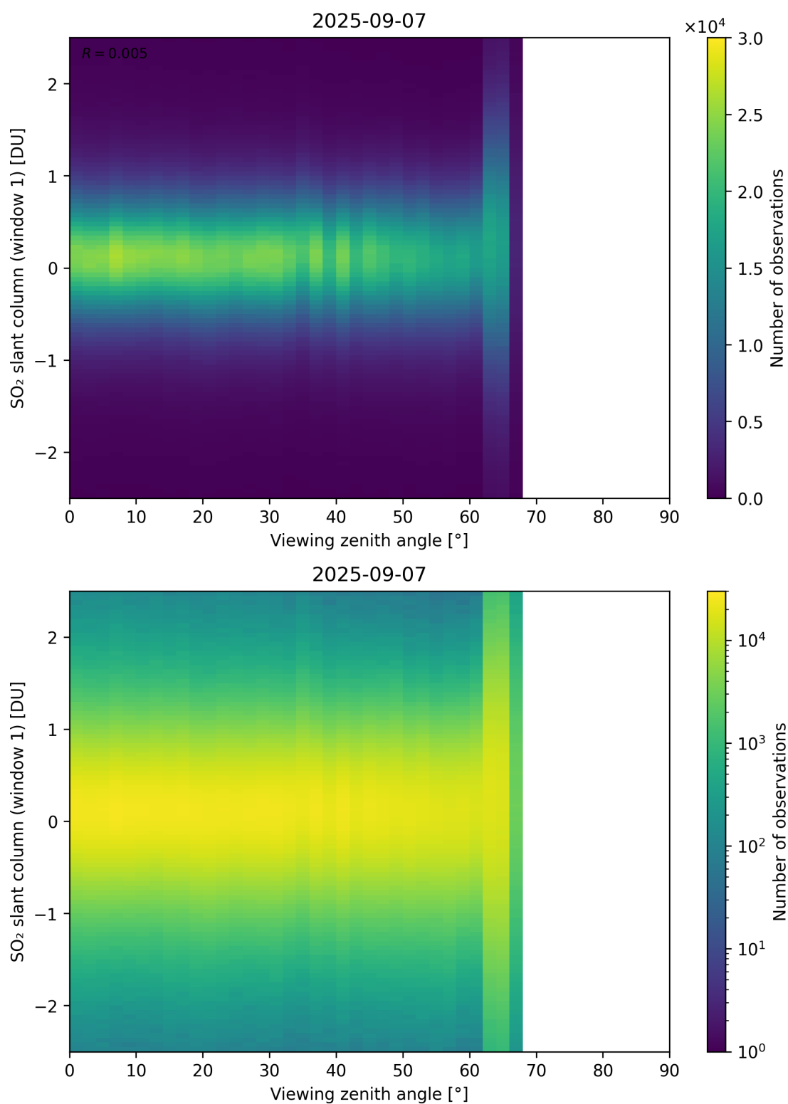
Figure 376: Scatter density plot of “Viewing zenith angle” against “SO 2 slant column (window 1)” for 2025-09-06 to 2025-09-08.
