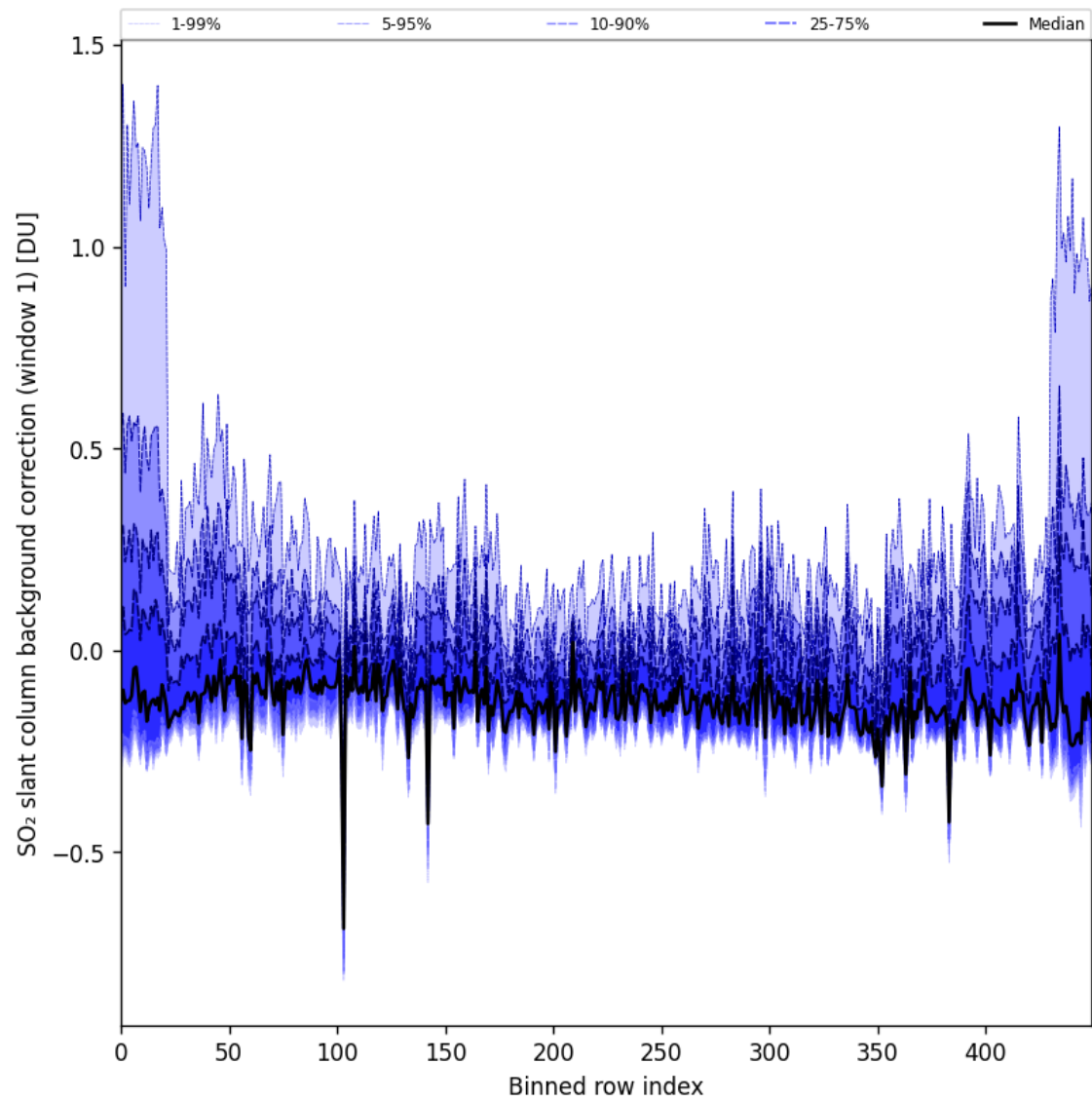
Figure 92: Along track statistics of “SO 2 slant column background correction (window 1)” for 2025-09-06 to 2025-09-08
