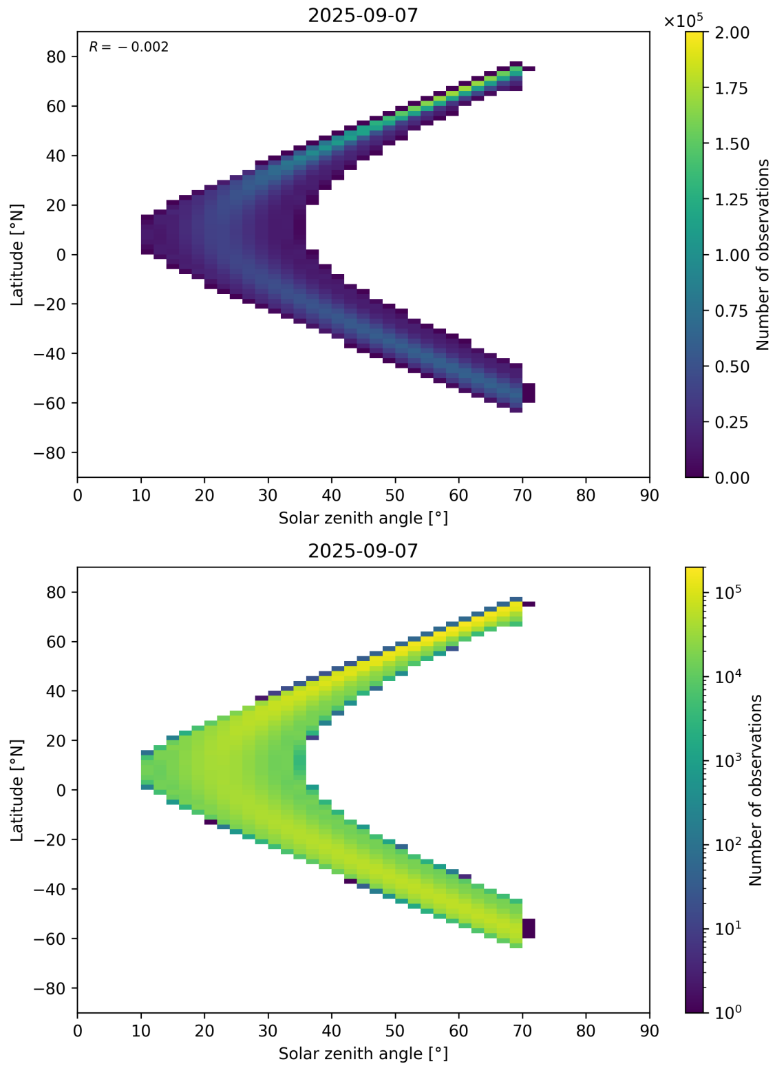
Figure 177: Scatter density plot of “Solar zenith angle” against “Latitude” for 2025-09-06 to 2025-09-08.
