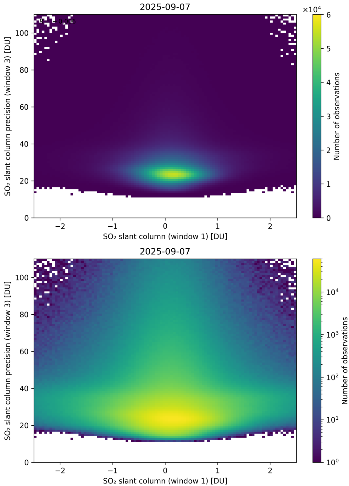
Figure 288: Scatter density plot of “SO 2 slant column (window 1)” against “SO 2 slant column precision (window 3)” for 2025-09-06 to 2025-09-08.
