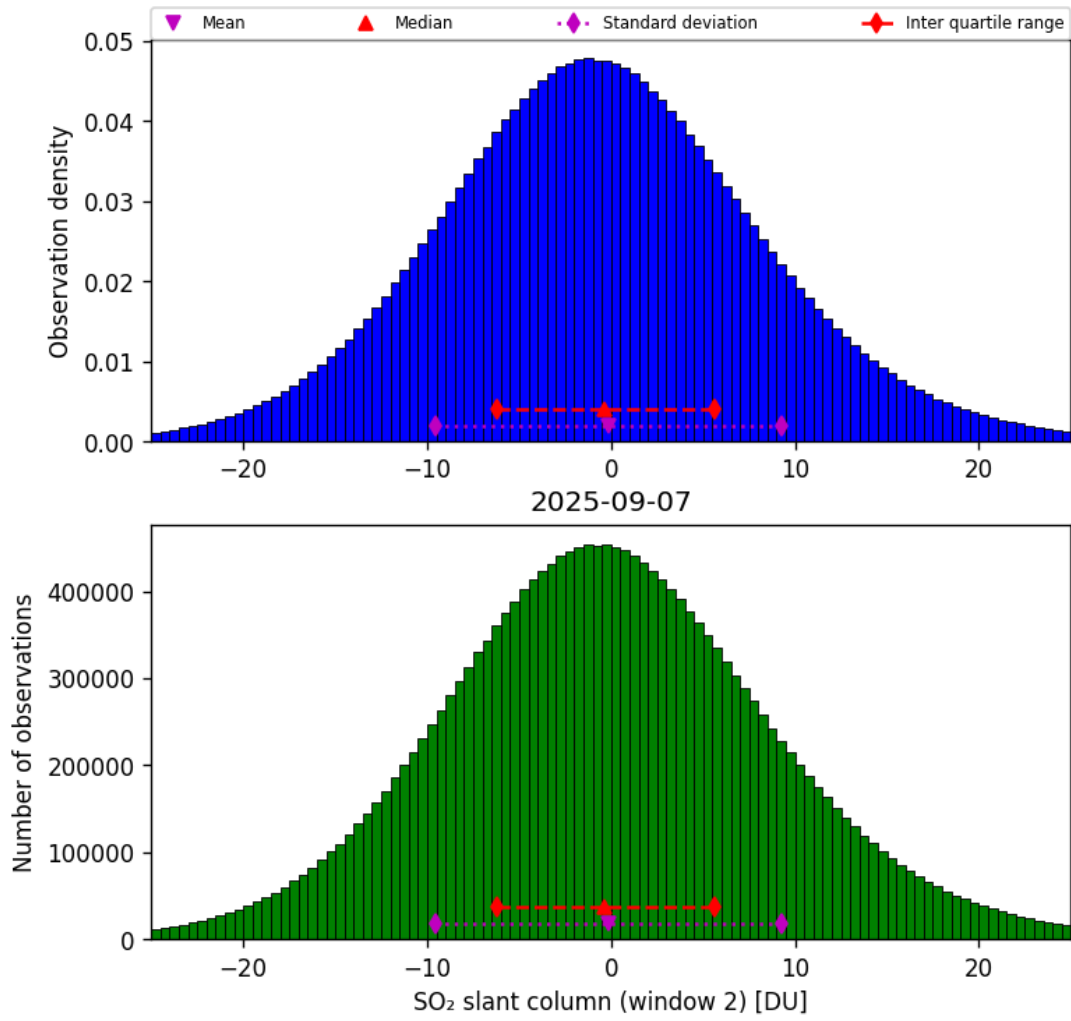
Figure 67: Histogram of “SO 2 slant column (window 2)” for 2025-09-06 to 2025-09-08
