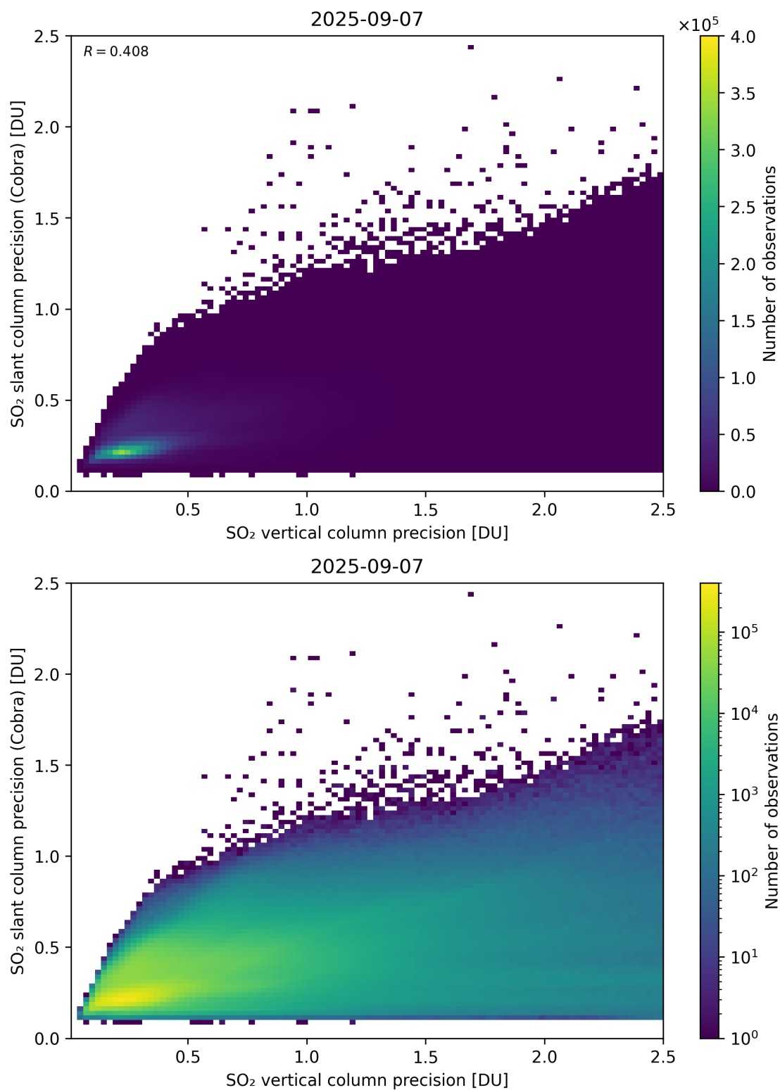
Figure 337: Scatter density plot of “SO 2 vertical column precision” against “SO 2 slant column precision (Cobra)” for 2025-09-06 to 2025-09-08.
