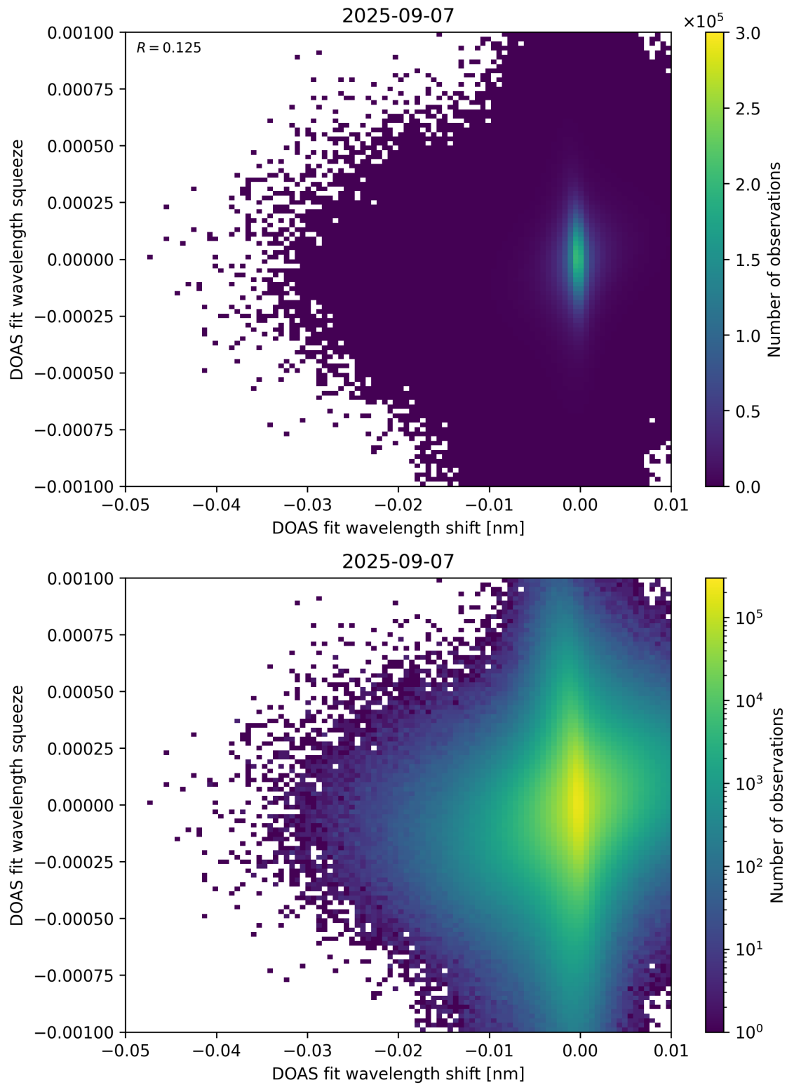
Figure 138: Scatter density plot of “DOAS fit wavelength shift” against “DOAS fit wavelength squeeze” for 2025-09-06 to 2025-09-08.
