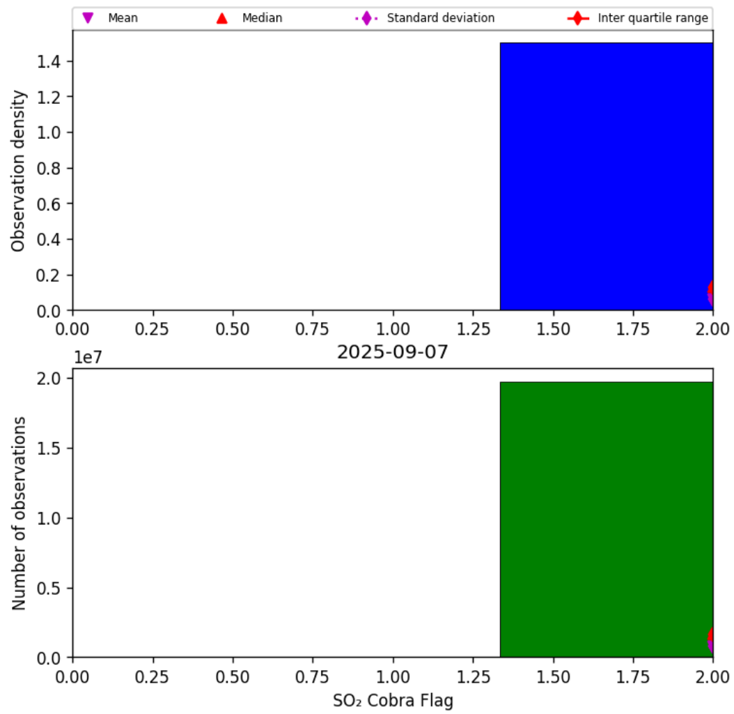
Figure 75: Histogram of “SO 2 Cobra Flag” for 2025-09-06 to 2025-09-08
