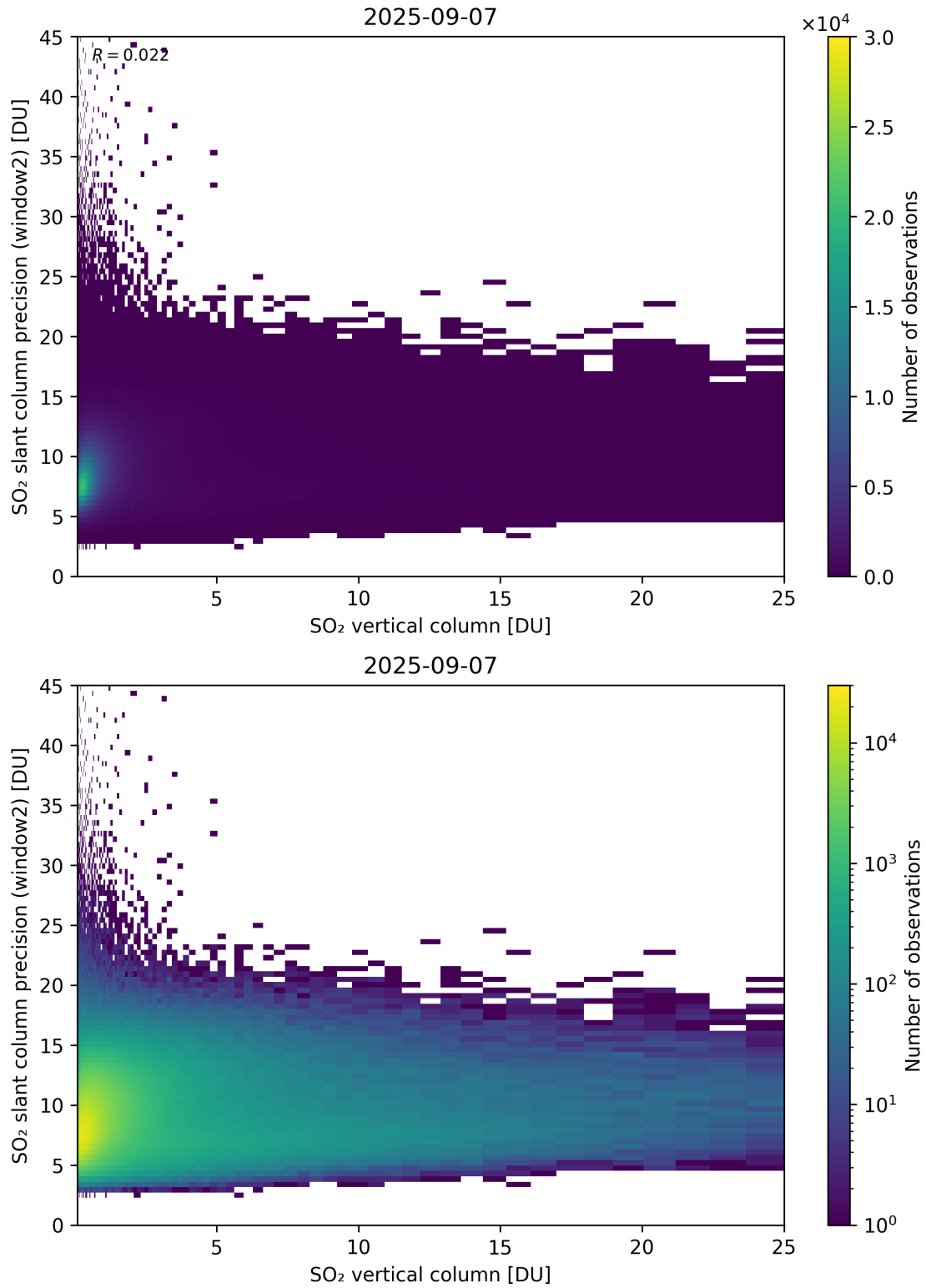
Figure 356: Scatter density plot of “SO 2 vertical column” against “SO 2 slant column precision (window2)” for 2025-09-06 to 2025-09-08.
