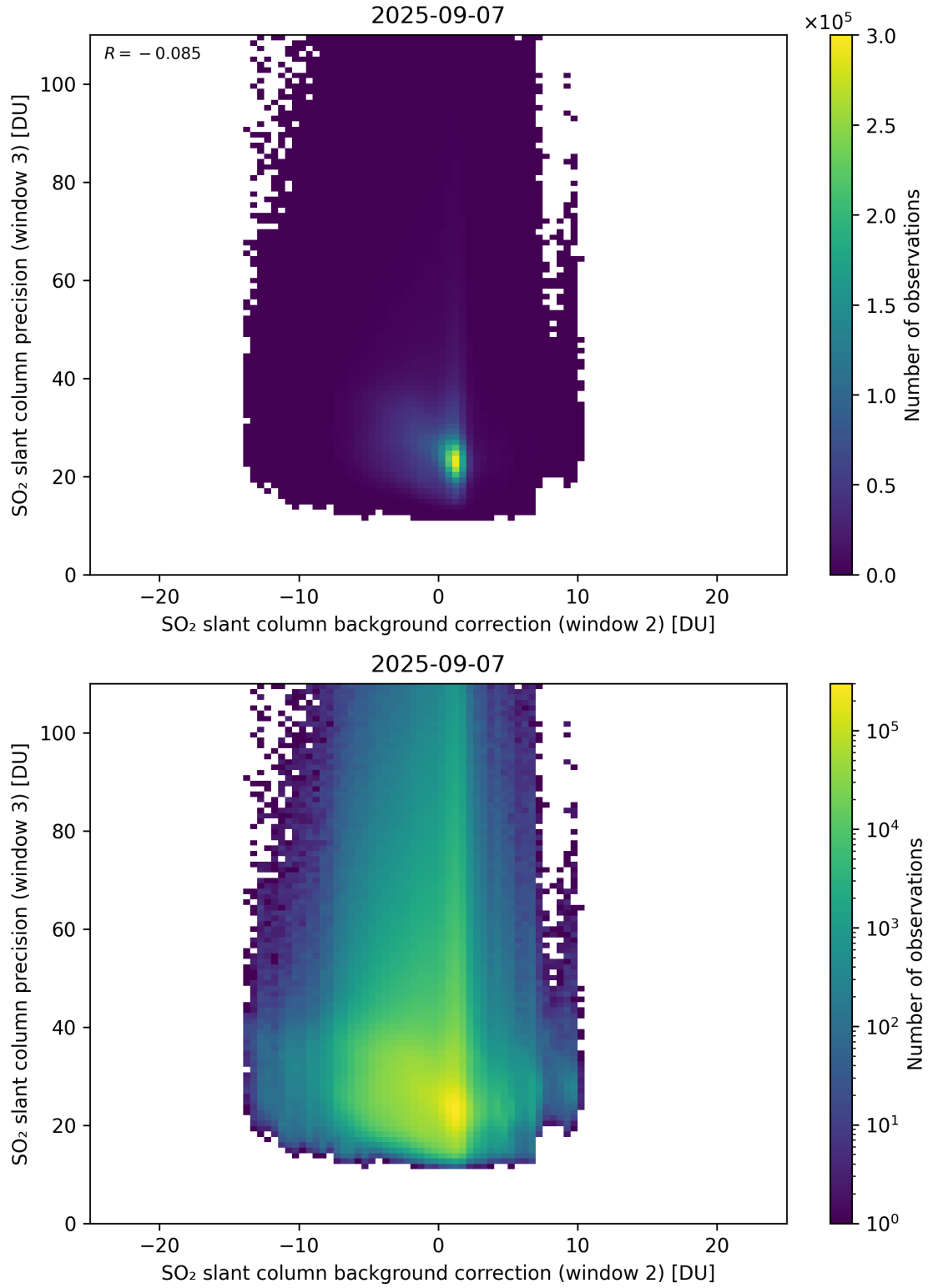
Figure 129: Scatter density plot of “SO 2 slant column background correction (window 2)” against “SO 2 slant column precision (window 3)” for 2025-09-06 to 2025-09-08.
