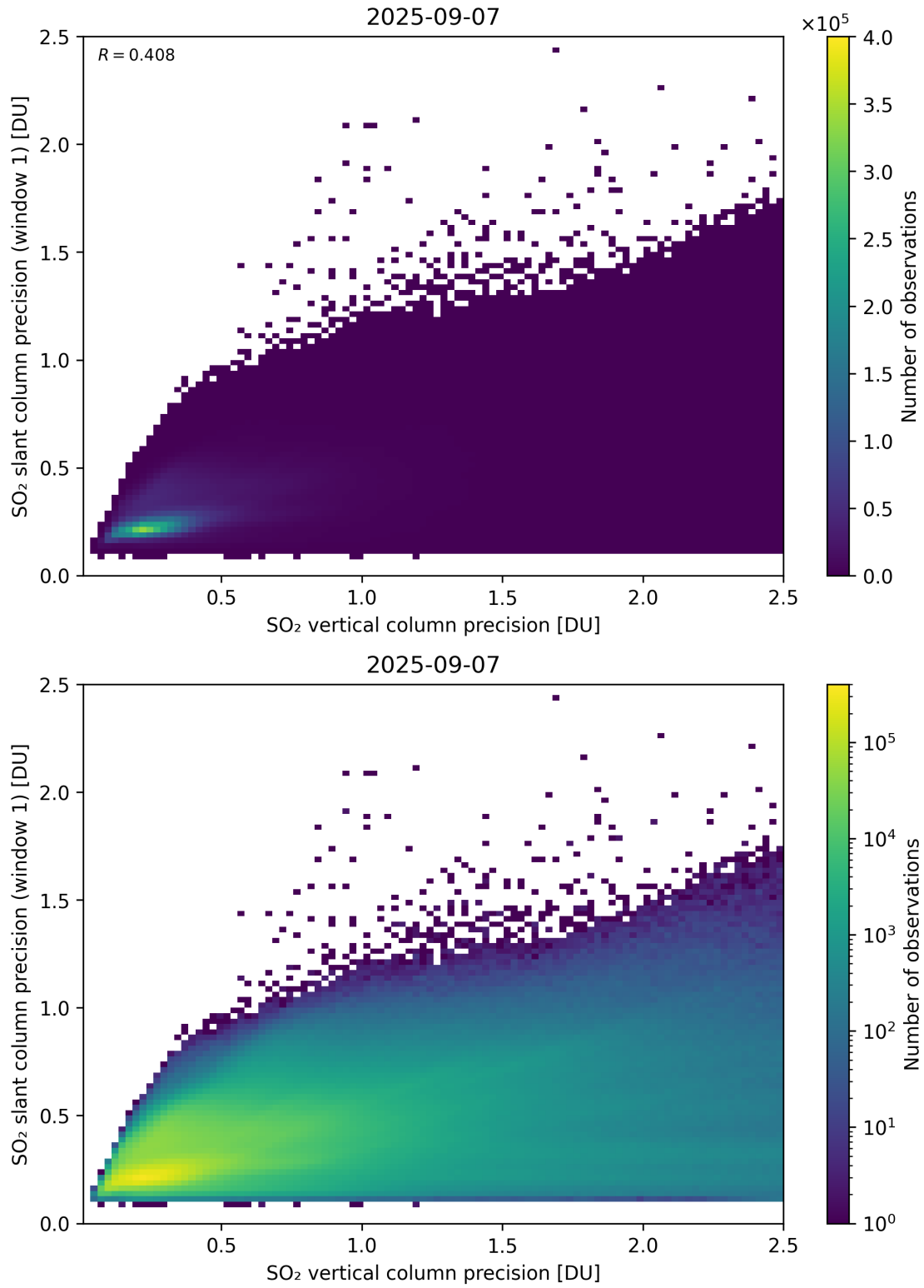
Figure 342: Scatter density plot of “SO 2 vertical column precision” against “SO 2 slant column precision (window 1)” for 2025-09-06 to 2025-09-08.
