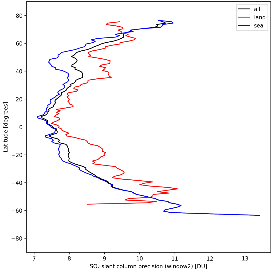
Figure 42: Zonal average of “SO 2 slant column precision (window2)” for 2025-09-06 to 2025-09-08.
