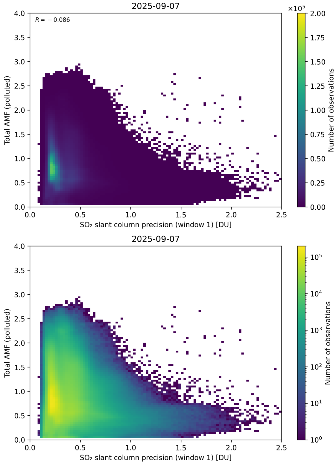
Figure 280: Scatter density plot of “SO 2 slant column precision (window 1)” against “Total AMF (polluted)” for 2025-09-06 to 2025-09-08.
