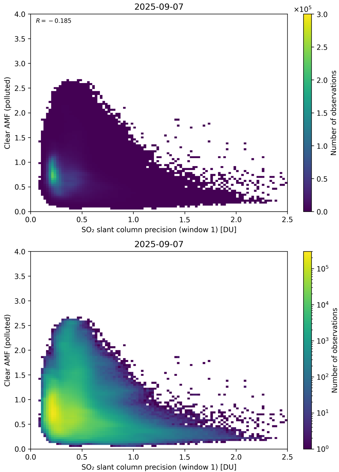
Figure 274: Scatter density plot of “SO 2 slant column precision (window 1)” against “Clear AMF (polluted)” for 2025-09-06 to 2025-09-08.
