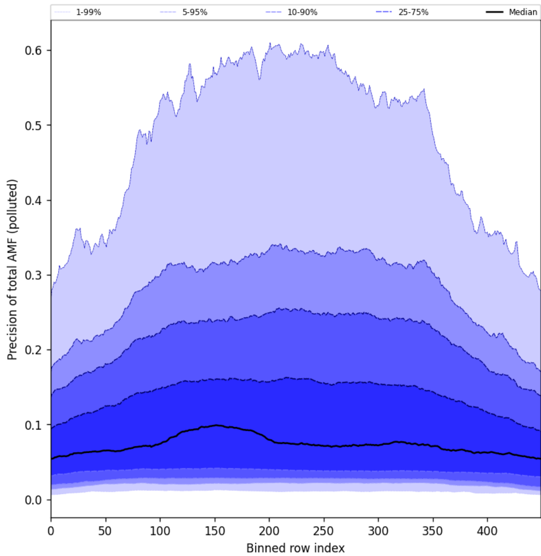
Figure 106: Along track statistics of “Precision of total AMF (polluted)” for 2025-09-06 to 2025-09-08
