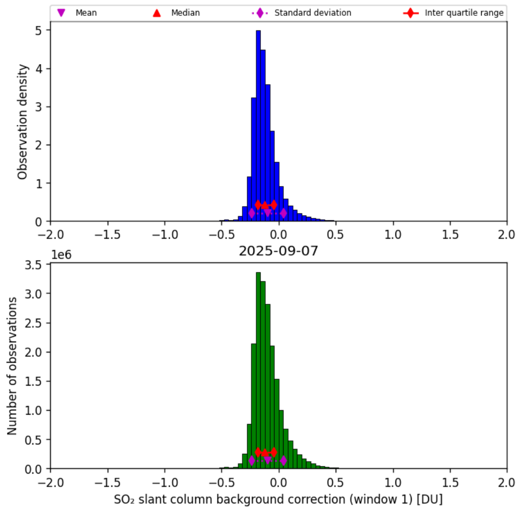
Figure 66: Histogram of “SO 2 slant column background correction (window 1)” for 2025-09-06 to 2025-09-08
