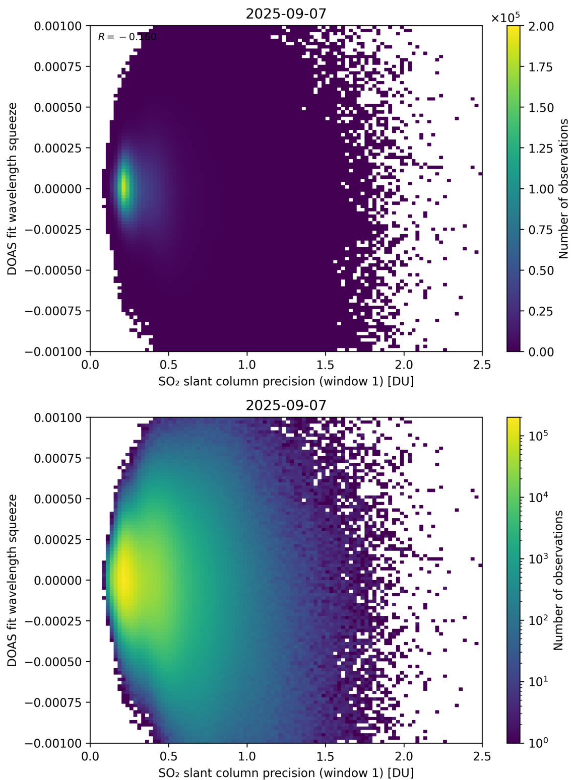
Figure 272: Scatter density plot of “SO 2 slant column precision (window 1)” against “DOAS fit wavelength squeeze” for 2025-09-06 to 2025-09-08.
