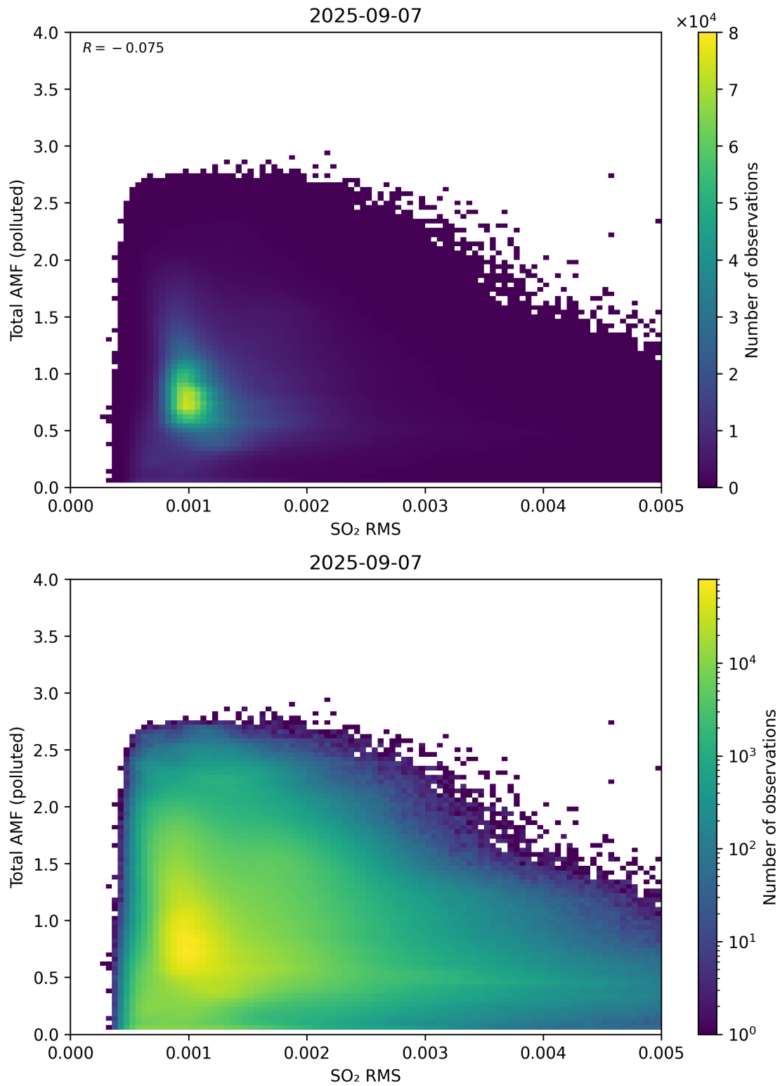
Figure 148: Scatter density plot of “SO 2 RMS” against “Total AMF (polluted)” for 2025-09-06 to 2025-09-08.
