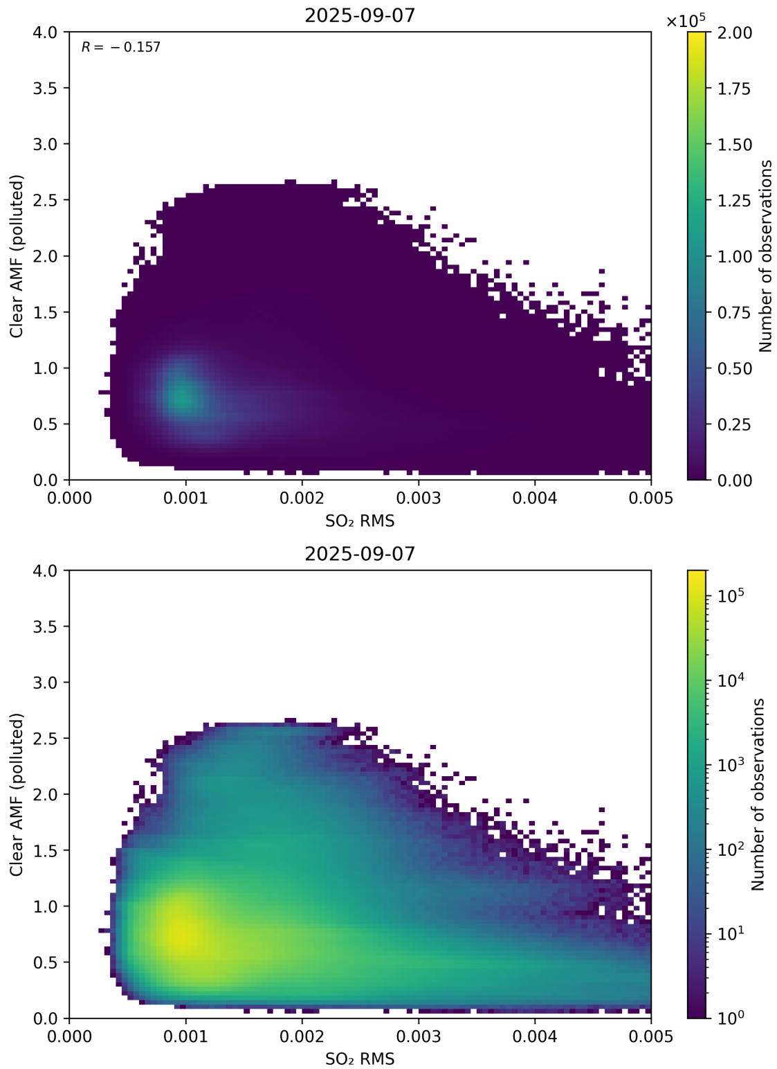
Figure 147: Scatter density plot of “SO 2 RMS” against “Clear AMF (polluted)” for 2025-09-06 to 2025-09-08.
