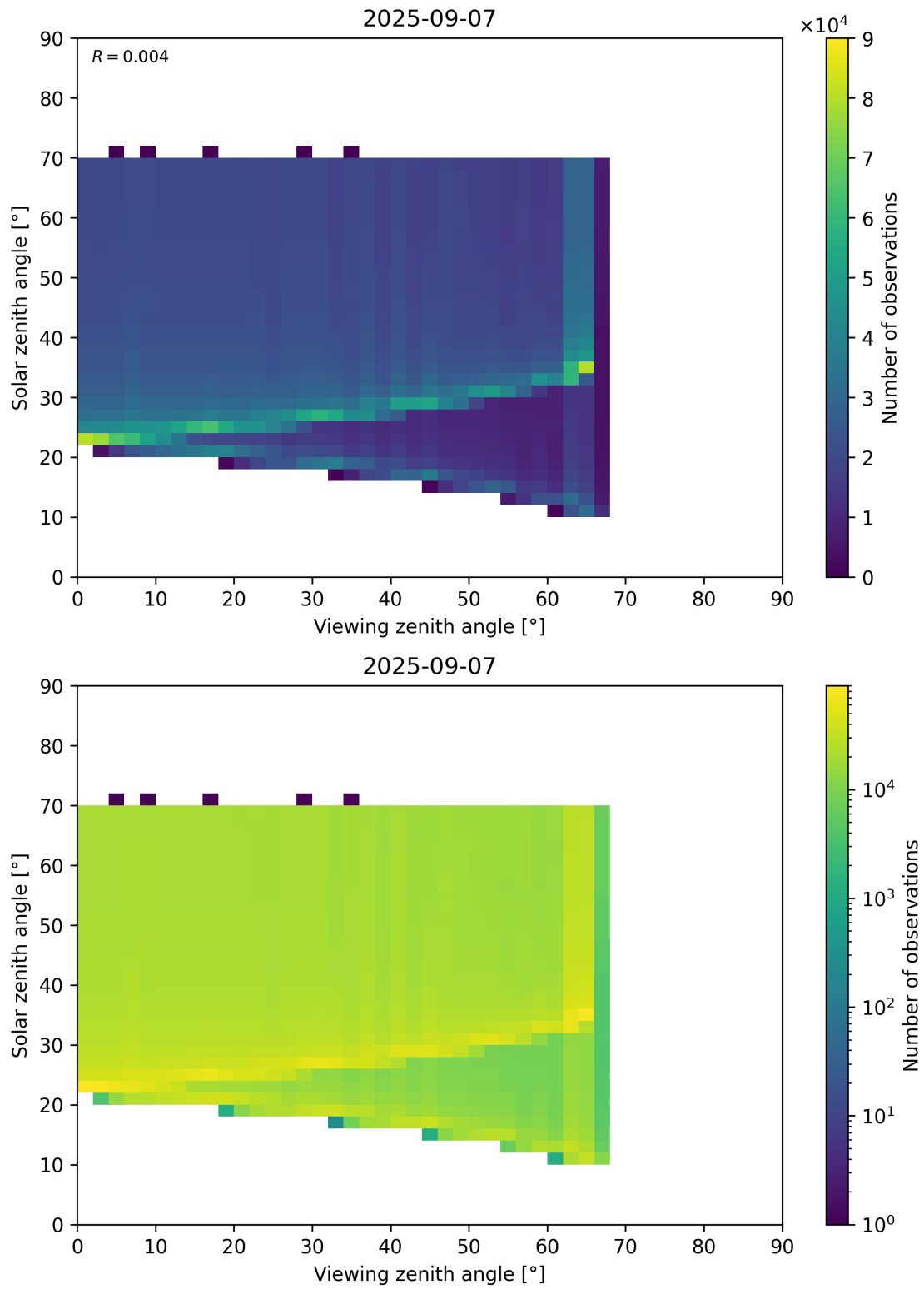
Figure 369: Scatter density plot of “Viewing zenith angle” against “Solar zenith angle” for 2025-09-06 to 2025-09-08.
