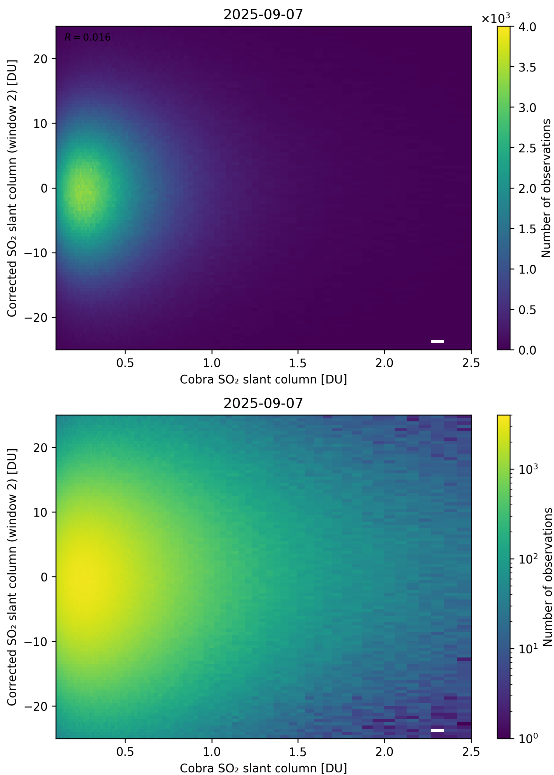
Figure 217: Scatter density plot of “Cobra SO 2 slant column” against “Corrected SO 2 slant column (window 2)” for 2025-09-06 to 2025-09-08.
