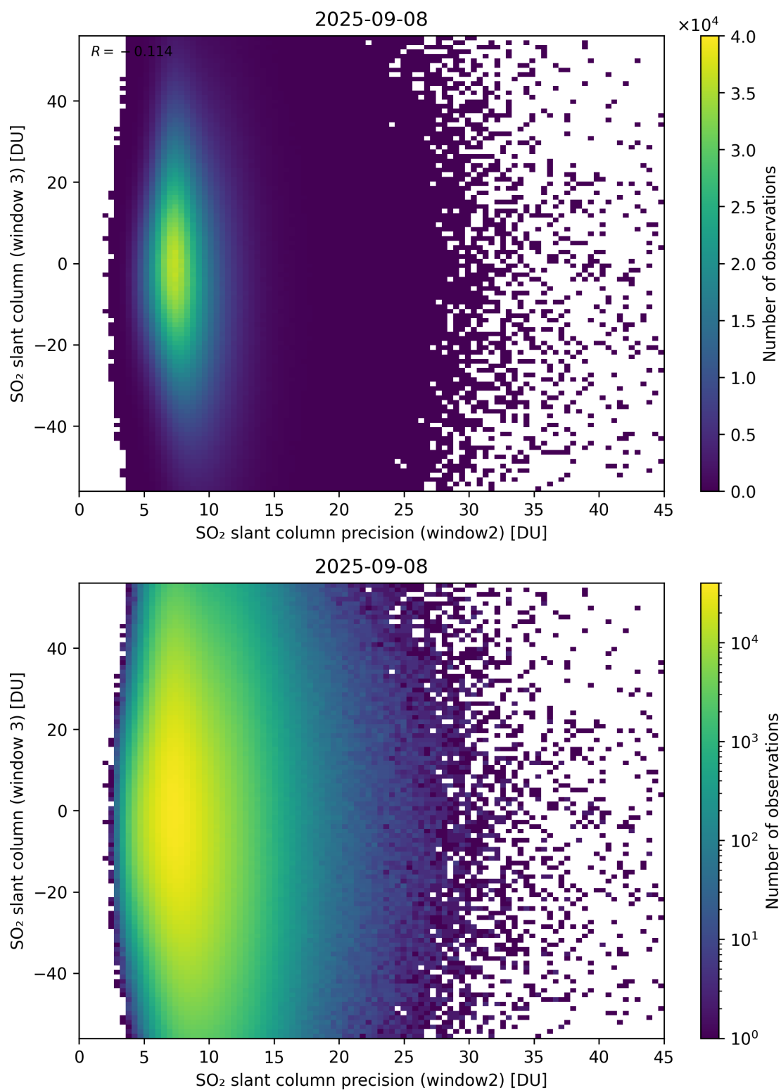
Figure 299: Scatter density plot of “SO 2 slant column precision (window2)” against “SO 2 slant column (window 3)” for 2025-09-07 to 2025-09-09.
