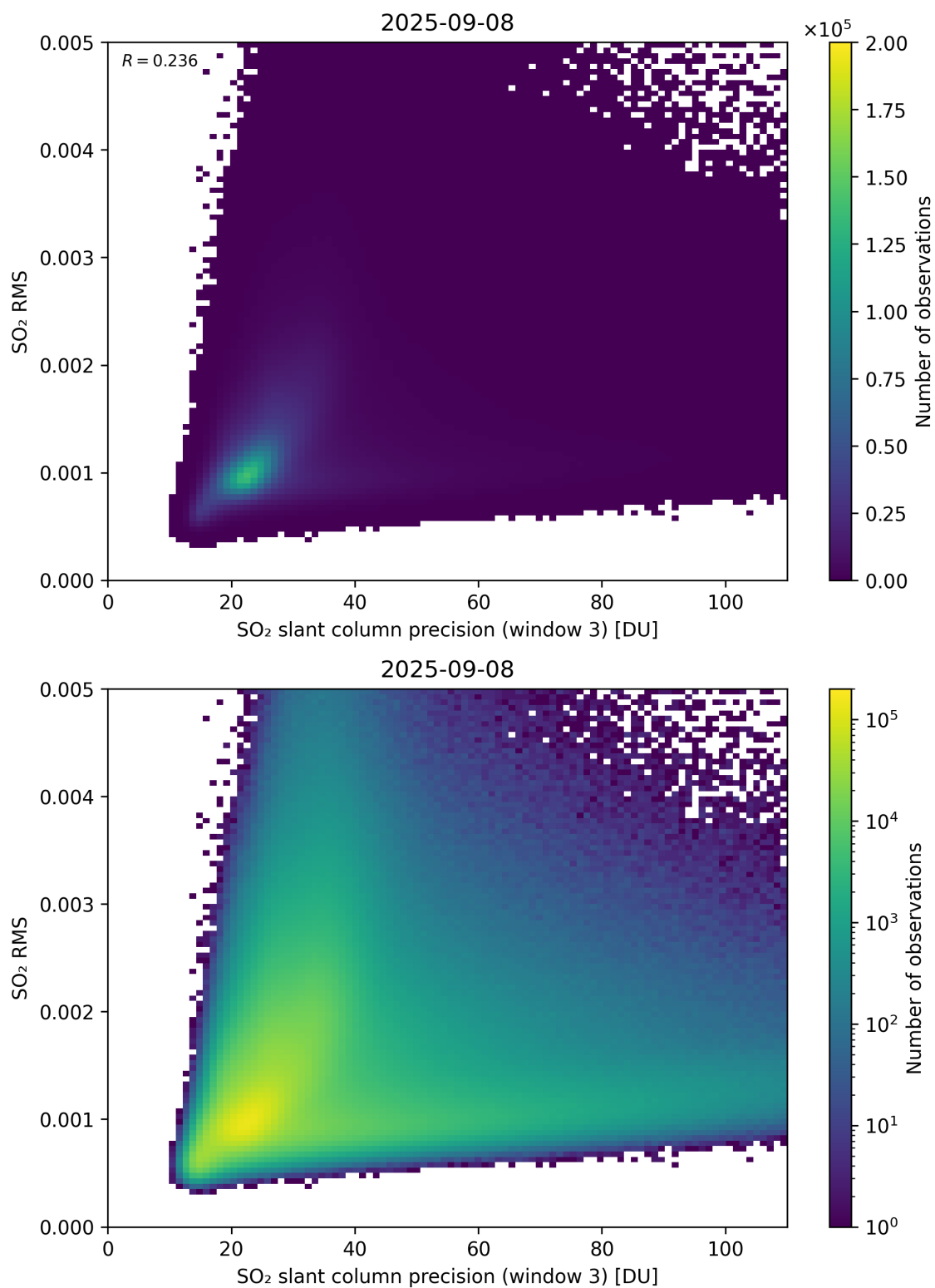
Figure 310: Scatter density plot of “SO 2 slant column precision (window 3)” against “SO 2 RMS” for 2025-09-07 to 2025-09-09.
