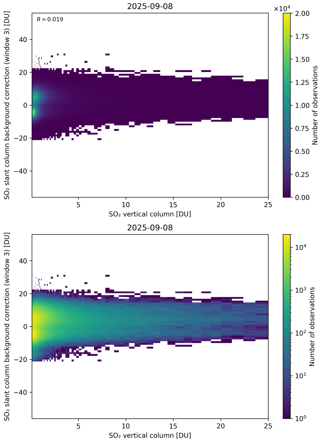
Figure 325: Scatter density plot of “SO 2 vertical column” against “SO 2 slant column background correction (window 3)” for 2025-09-07 to 2025-09-09.
