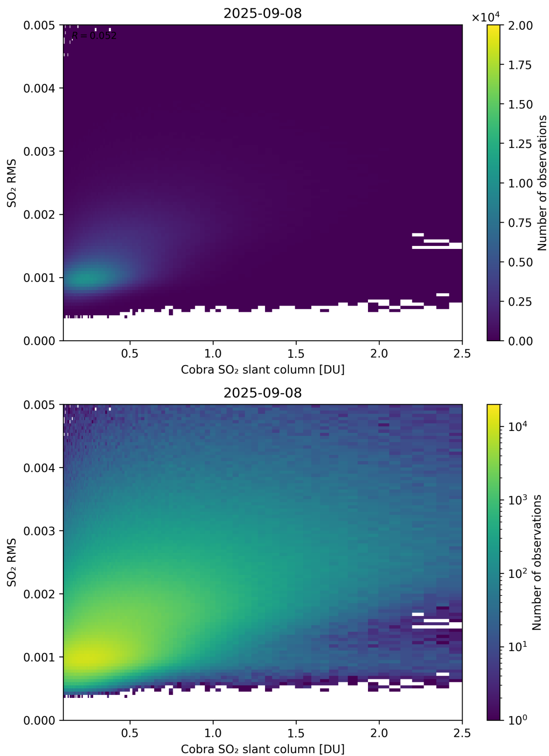
Figure 198: Scatter density plot of “Cobra SO 2 slant column” against “SO 2 RMS” for 2025-09-07 to 2025-09-09.
