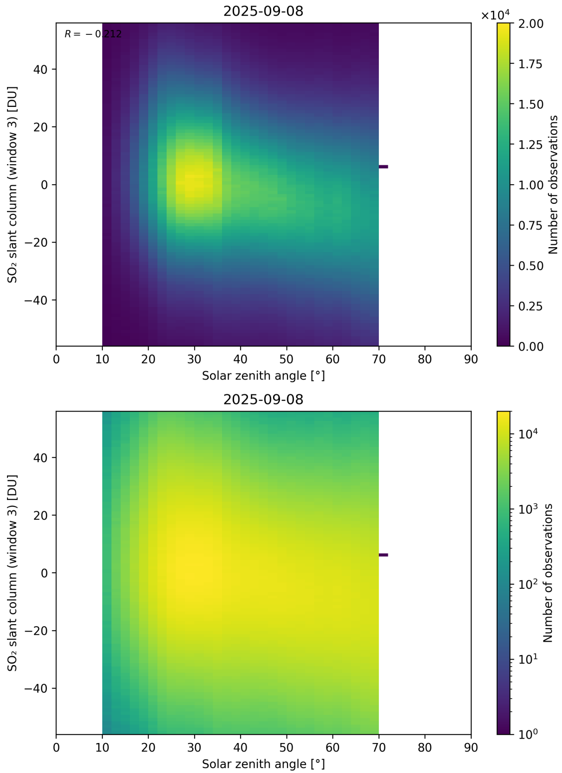
Figure 187: Scatter density plot of “Solar zenith angle” against “SO 2 slant column (window 3)” for 2025-09-07 to 2025-09-09.
