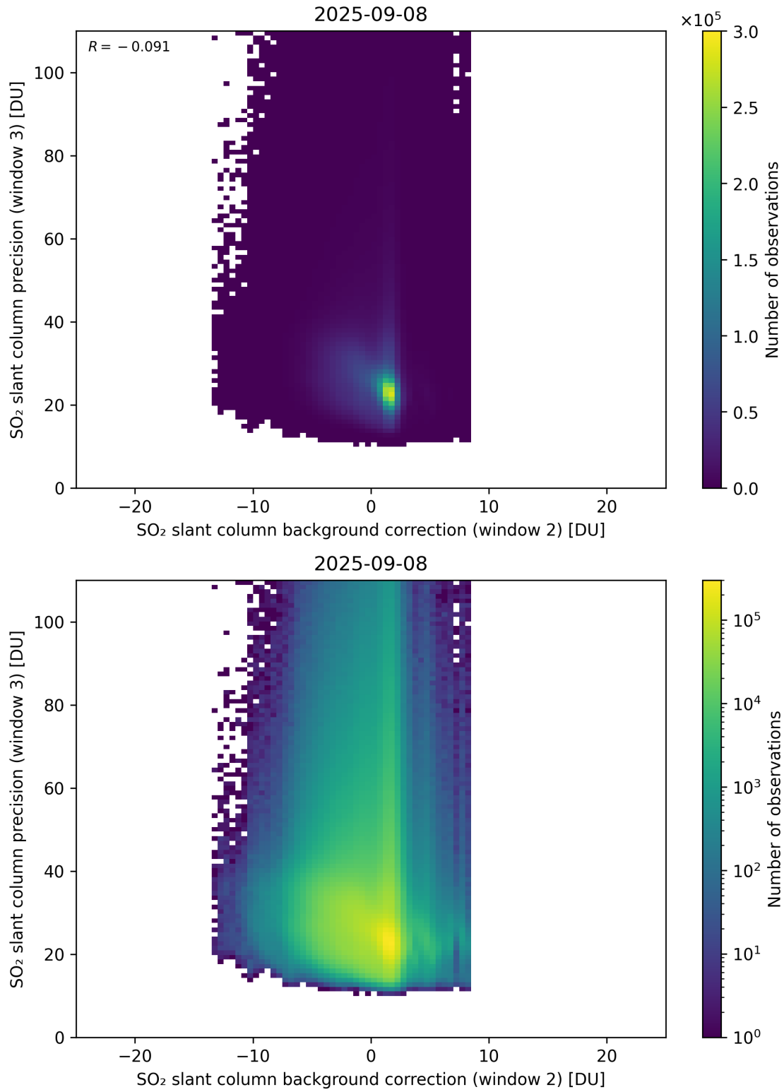
Figure 129: Scatter density plot of “SO 2 slant column background correction (window 2)” against “SO 2 slant column precision (window 3)” for 2025-09-07 to 2025-09-09.
