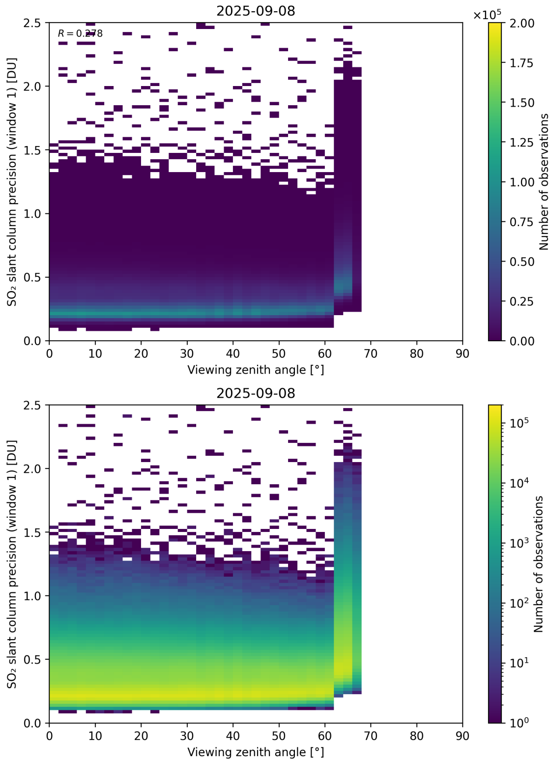
Figure 377: Scatter density plot of “Viewing zenith angle” against “SO 2 slant column precision (window 1)” for 2025-09-07 to 2025-09-09.
