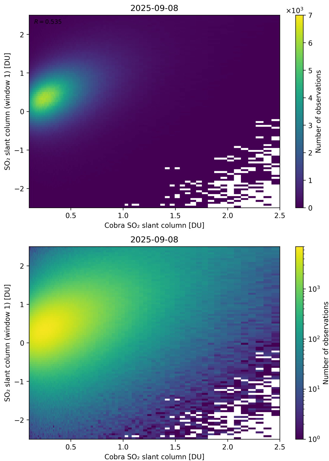
Figure 219: Scatter density plot of “Cobra SO 2 slant column” against “SO 2 slant column (window 1)” for 2025-09-07 to 2025-09-09.
