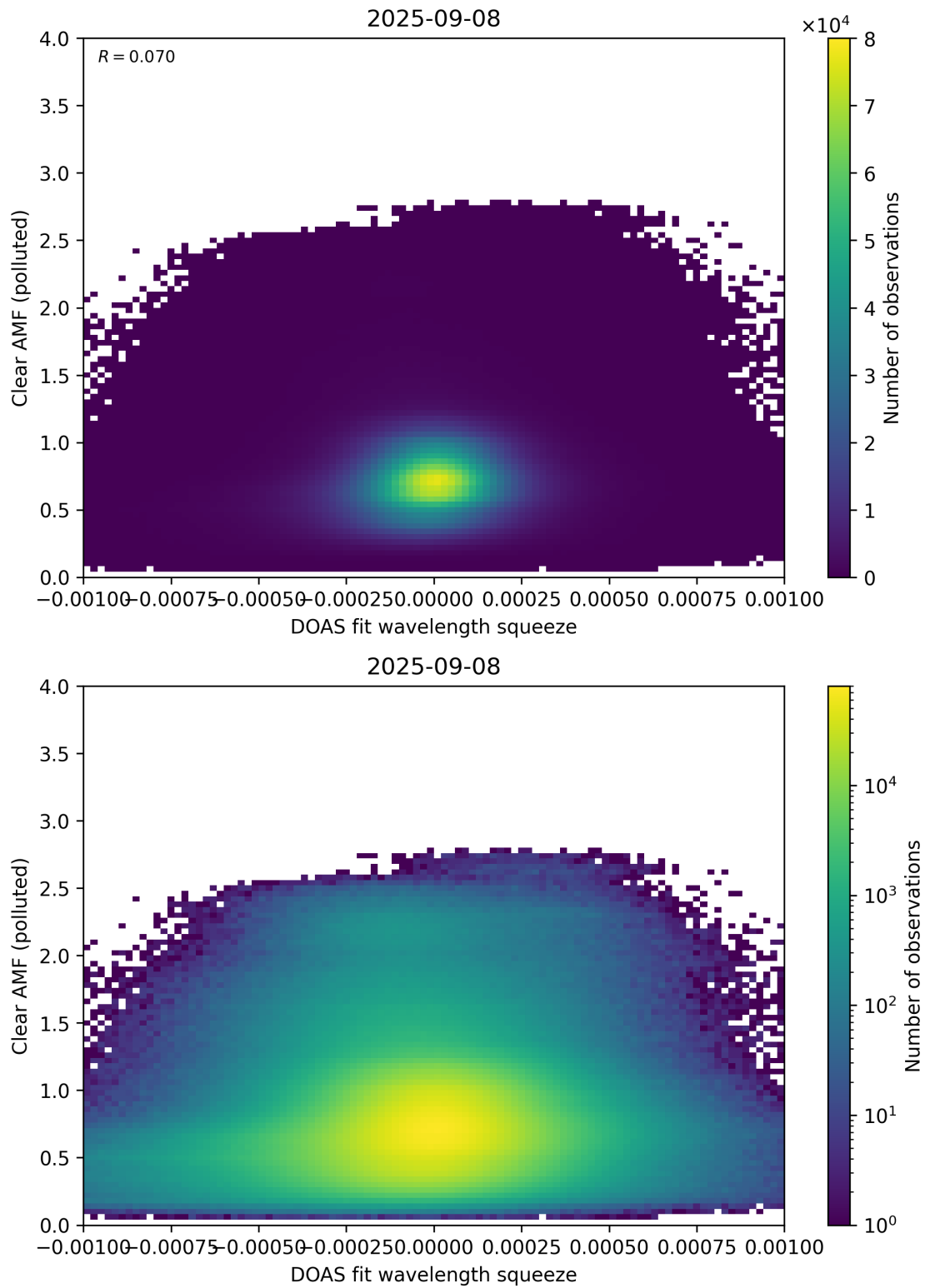
Figure 144: Scatter density plot of “DOAS fit wavelength squeeze” against “Clear AMF (polluted)” for 2025-09-07 to 2025-09-09.
