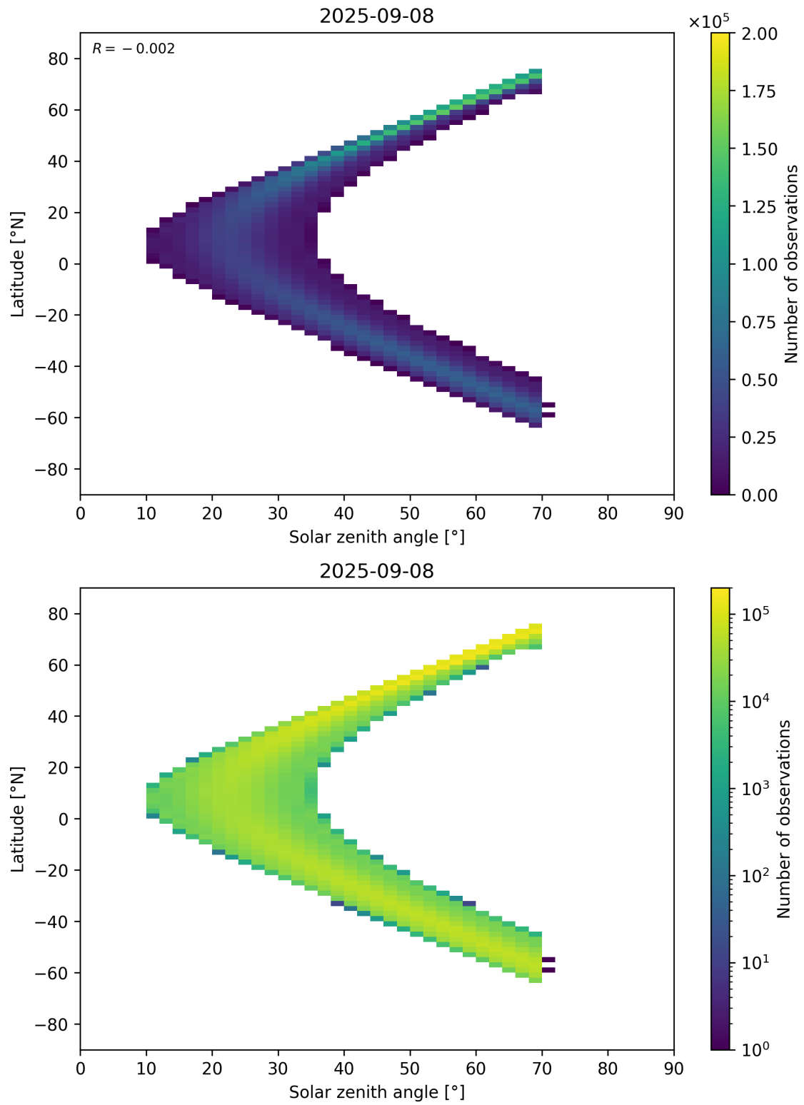
Figure 177: Scatter density plot of “Solar zenith angle” against “Latitude” for 2025-09-07 to 2025-09-09.
