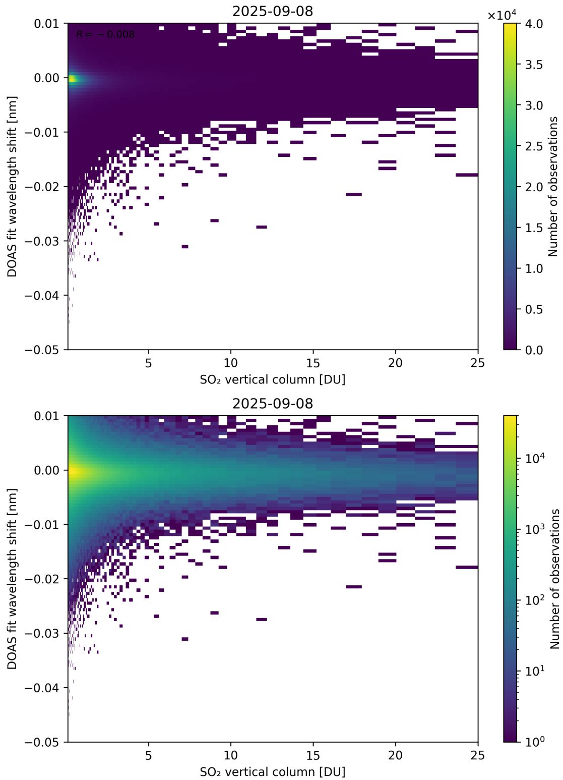
Figure 326: Scatter density plot of “SO 2 vertical column” against “DOAS fit wavelength shift” for 2025-09-07 to 2025-09-09.
