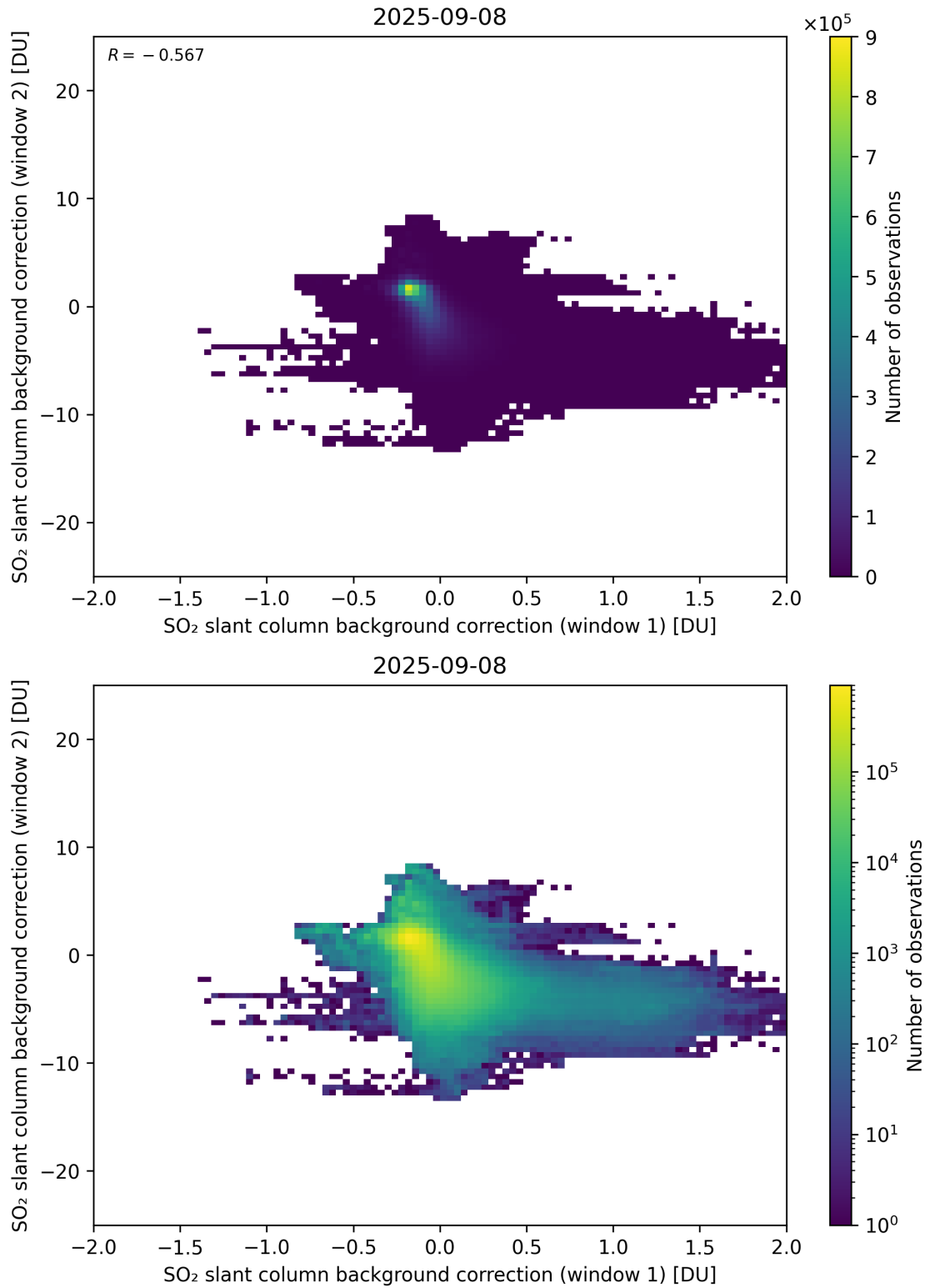
Figure 109: Scatter density plot of “SO 2 slant column background correction (window 1)” against “SO 2 slant column background correction (window 2)” for 2025-09-07 to 2025-09-09.
