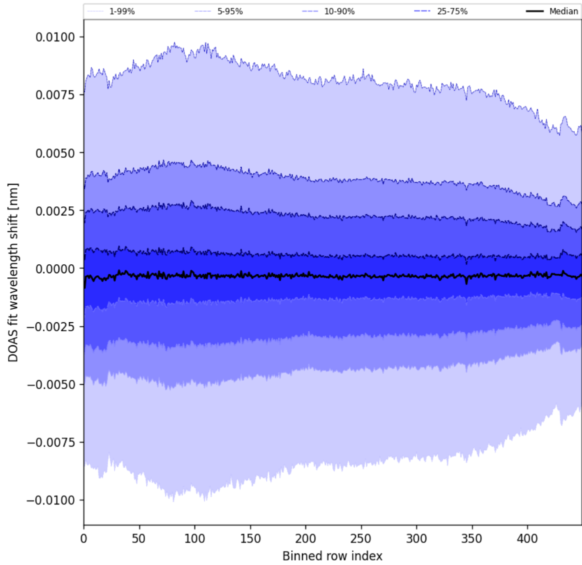
Figure 102: Along track statistics of “DOAS fit wavelength shift” for 2025-09-07 to 2025-09-09
