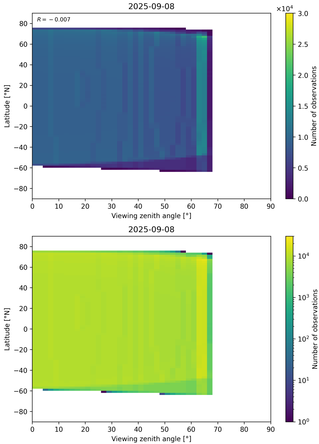
Figure 368: Scatter density plot of “Viewing zenith angle” against “Latitude” for 2025-09-07 to 2025-09-09.
