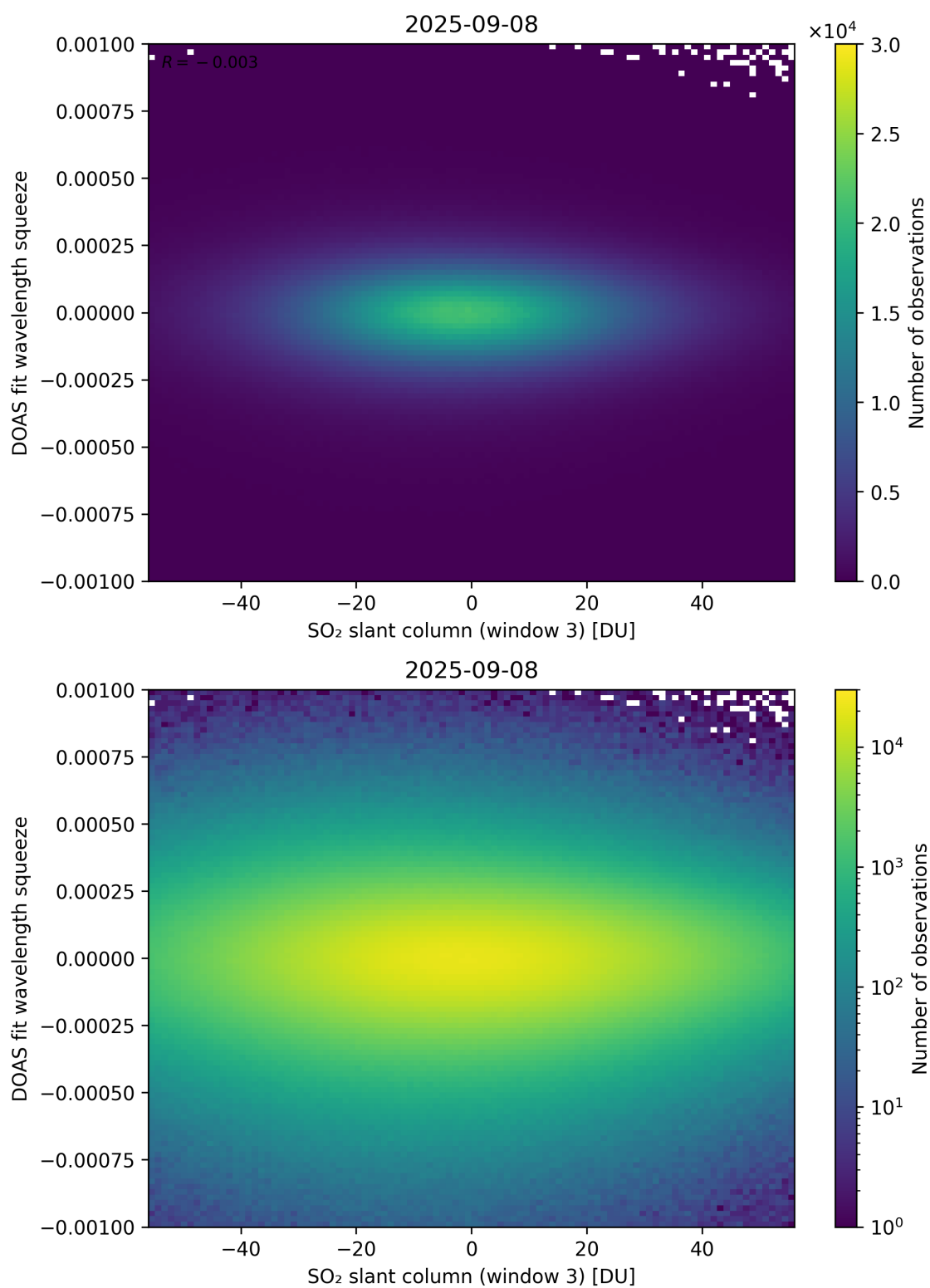
Figure 305: Scatter density plot of “SO 2 slant column (window 3)” against “DOAS fit wavelength squeeze” for 2025-09-07 to 2025-09-09.
