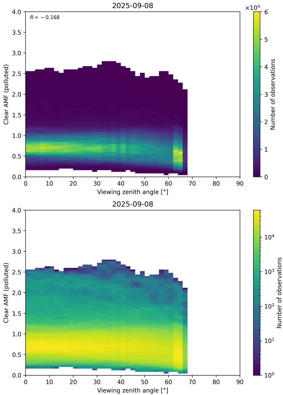
Figure 370: Scatter density plot of “Viewing zenith angle” against “Clear AMF (polluted)” for 2025-09-07 to 2025-09-09.
