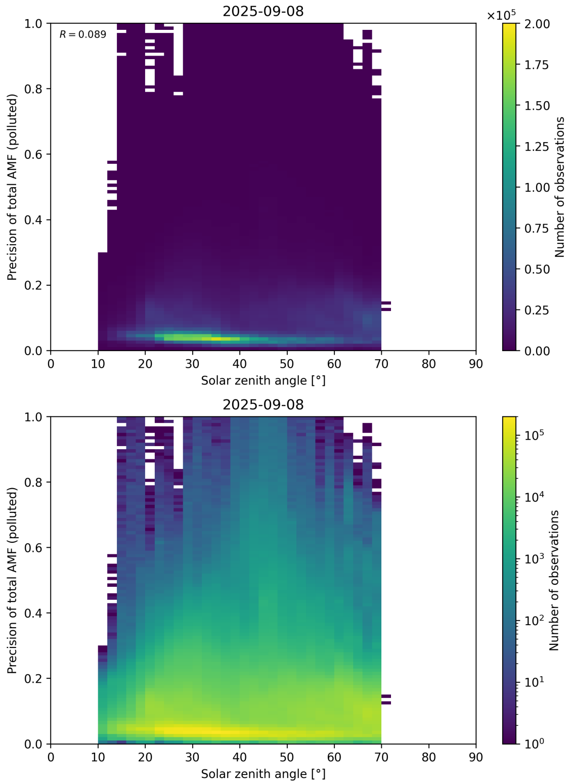
Figure 190: Scatter density plot of “Solar zenith angle” against “Precision of total AMF (polluted)” for 2025-09-07 to 2025-09-09.
