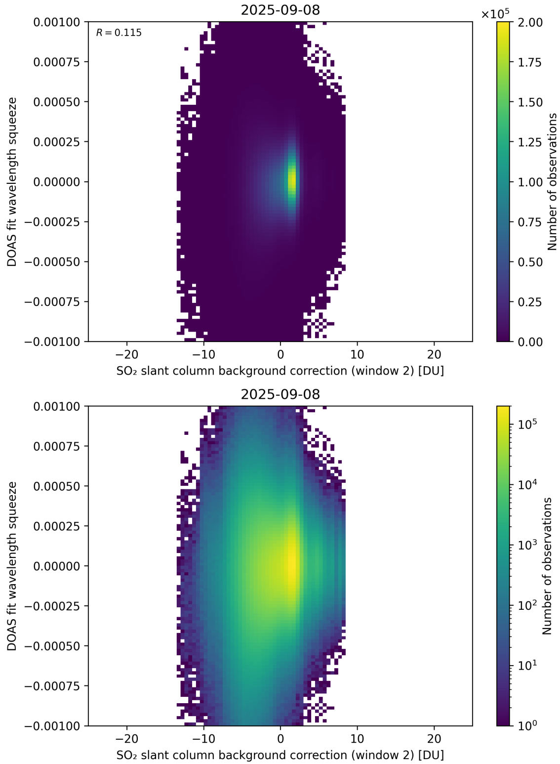
Figure 124: Scatter density plot of “SO 2 slant column background correction (window 2)” against “DOAS fit wavelength squeeze” for 2025-09-07 to 2025-09-09.
