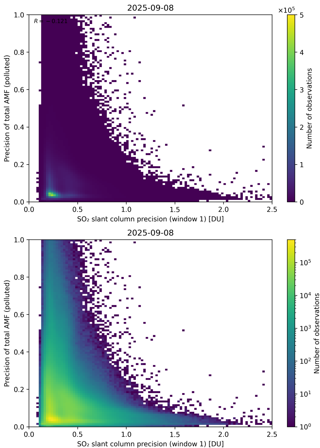
Figure 281: Scatter density plot of “SO 2 slant column precision (window 1)” against “Precision of total AMF (polluted)” for 2025-09-07 to 2025-09-09.
