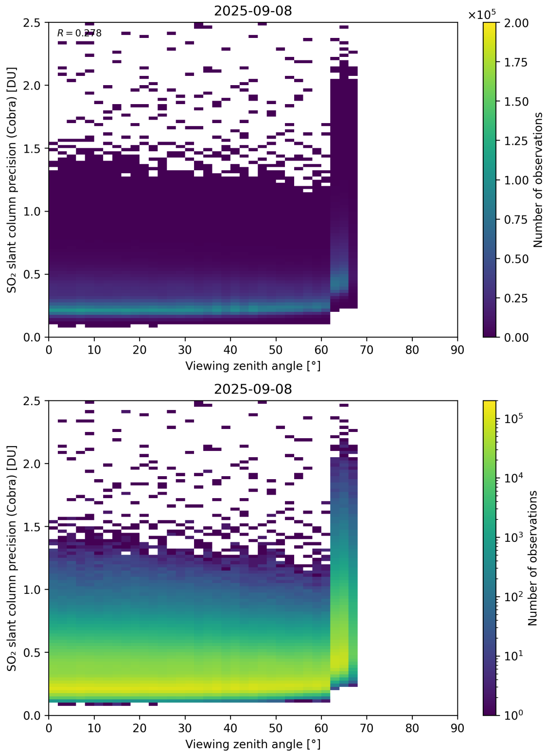
Figure 372: Scatter density plot of “Viewing zenith angle” against “SO 2 slant column precision (Cobra)” for 2025-09-07 to 2025-09-09.
