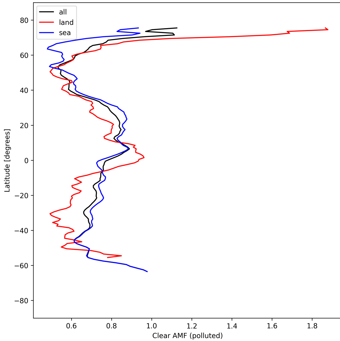
Figure 55: Zonal average of “Clear AMF (polluted)” for 2025-09-07 to 2025-09-09.
