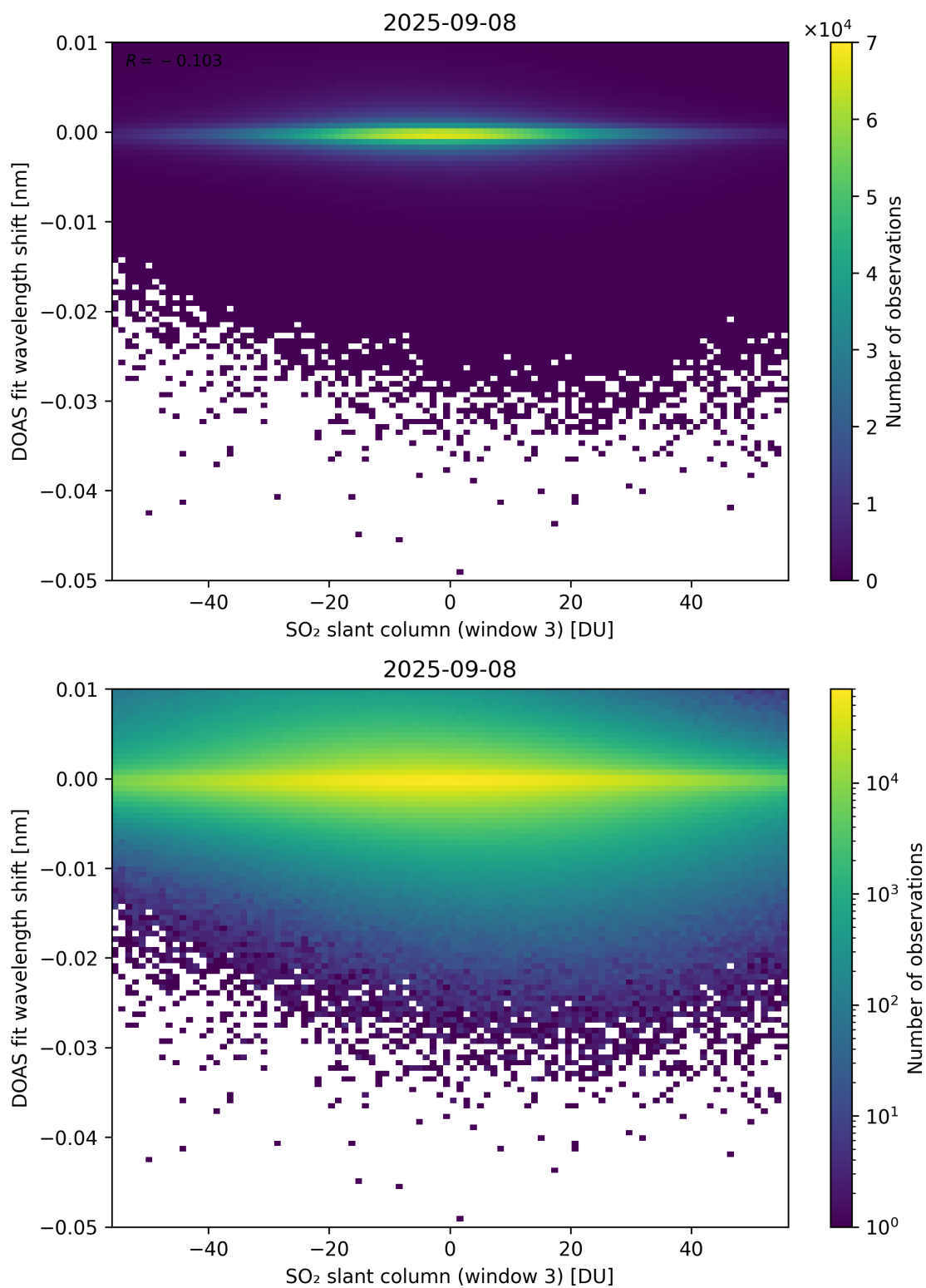
Figure 304: Scatter density plot of “SO 2 slant column (window 3)” against “DOAS fit wavelength shift” for 2025-09-07 to 2025-09-09.
