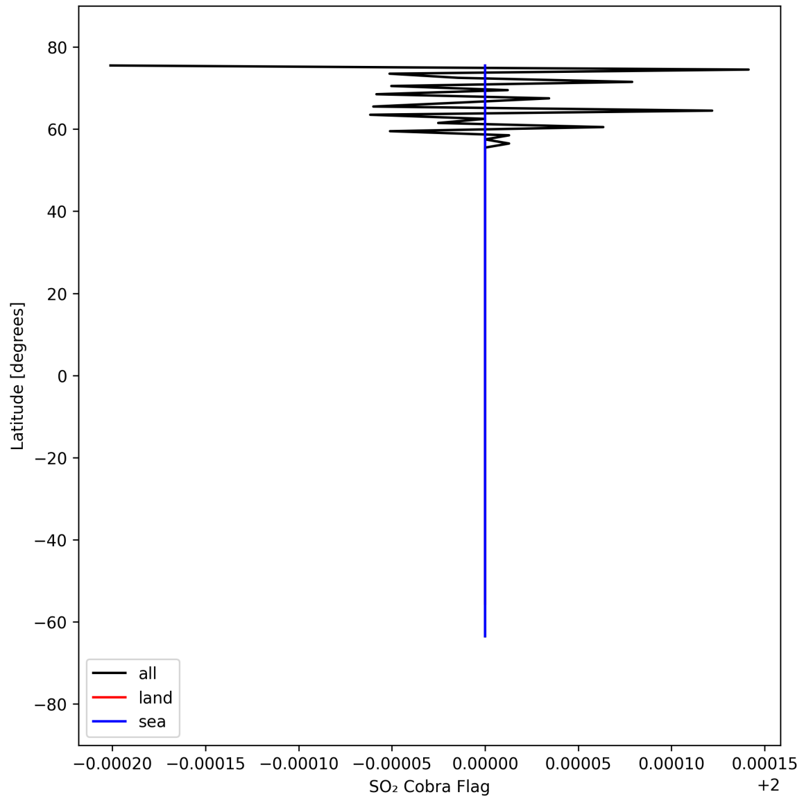
Figure 49: Zonal average of “SO 2 Cobra Flag” for 2025-09-07 to 2025-09-09.
