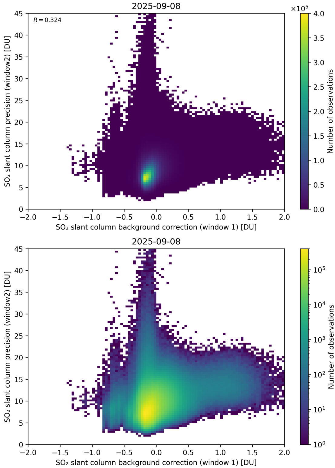
Figure 117: Scatter density plot of “SO 2 slant column background correction (window 1)” against “SO 2 slant column precision (window2)” for 2025-09-07 to 2025-09-09.
