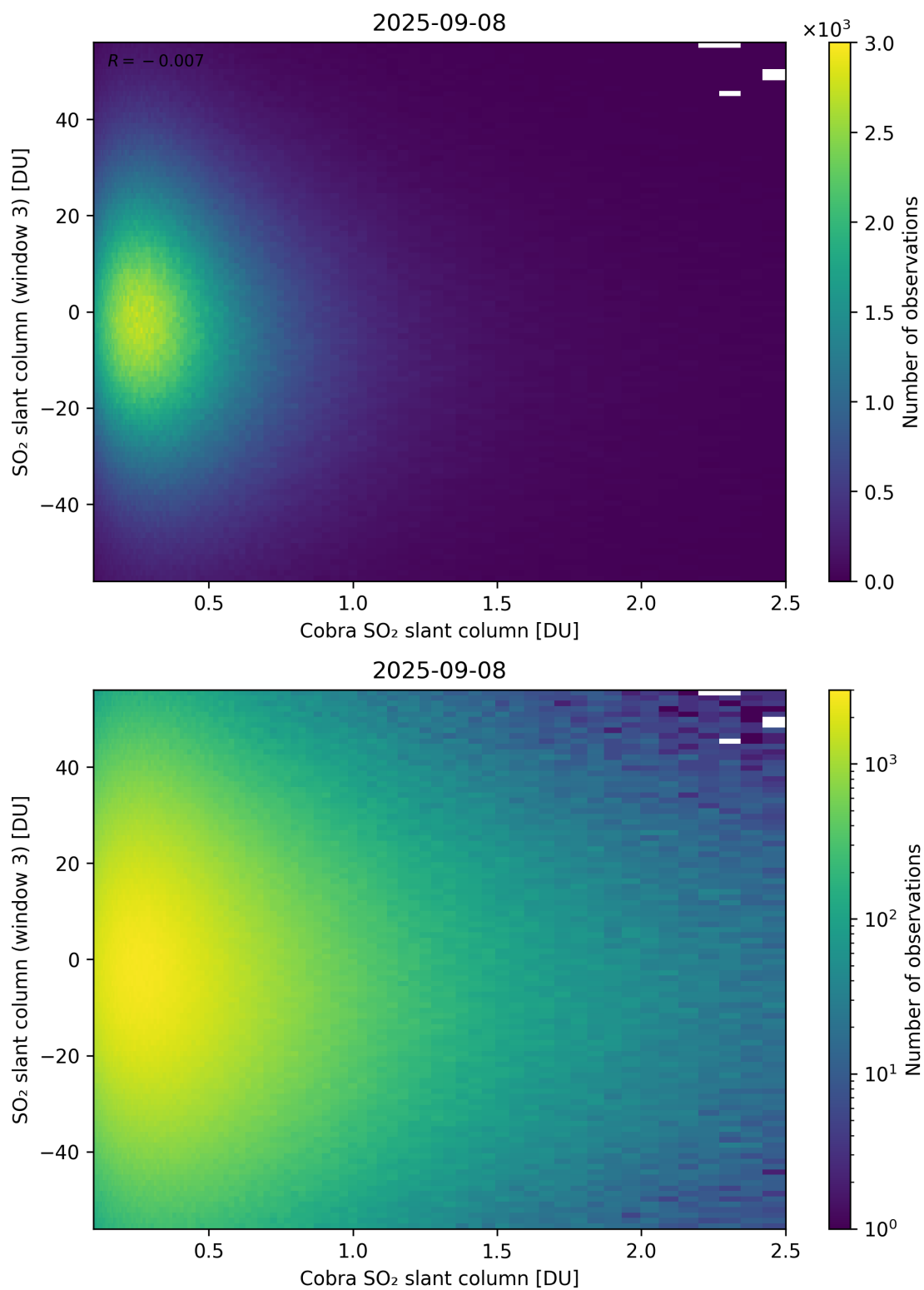
Figure 222: Scatter density plot of “Cobra SO 2 slant column” against “SO 2 slant column (window 3)” for 2025-09-07 to 2025-09-09.
