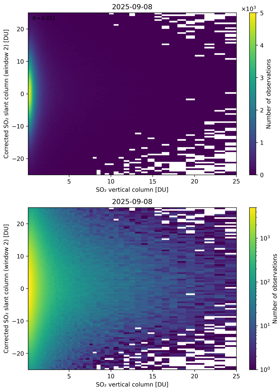
Figure 352: Scatter density plot of “SO 2 vertical column” against “Corrected SO 2 slant column (window 2)” for 2025-09-07 to 2025-09-09.
