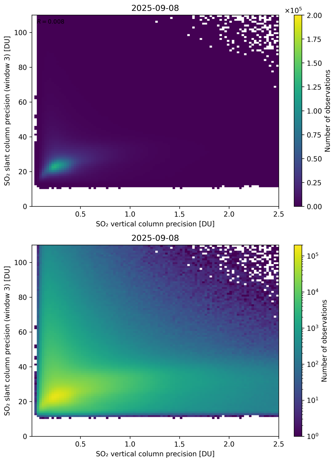
Figure 345: Scatter density plot of “SO 2 vertical column precision” against “SO 2 slant column precision (window 3)” for 2025-09-07 to 2025-09-09.
