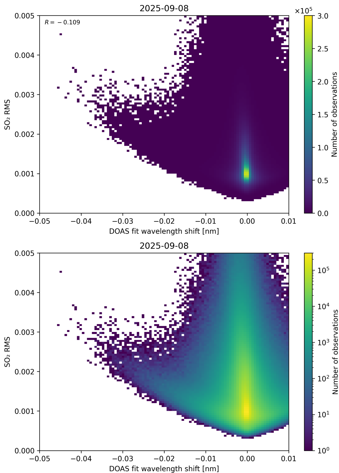
Figure 139: Scatter density plot of “DOAS fit wavelength shift” against “SO 2 RMS” for 2025-09-07 to 2025-09-09.
