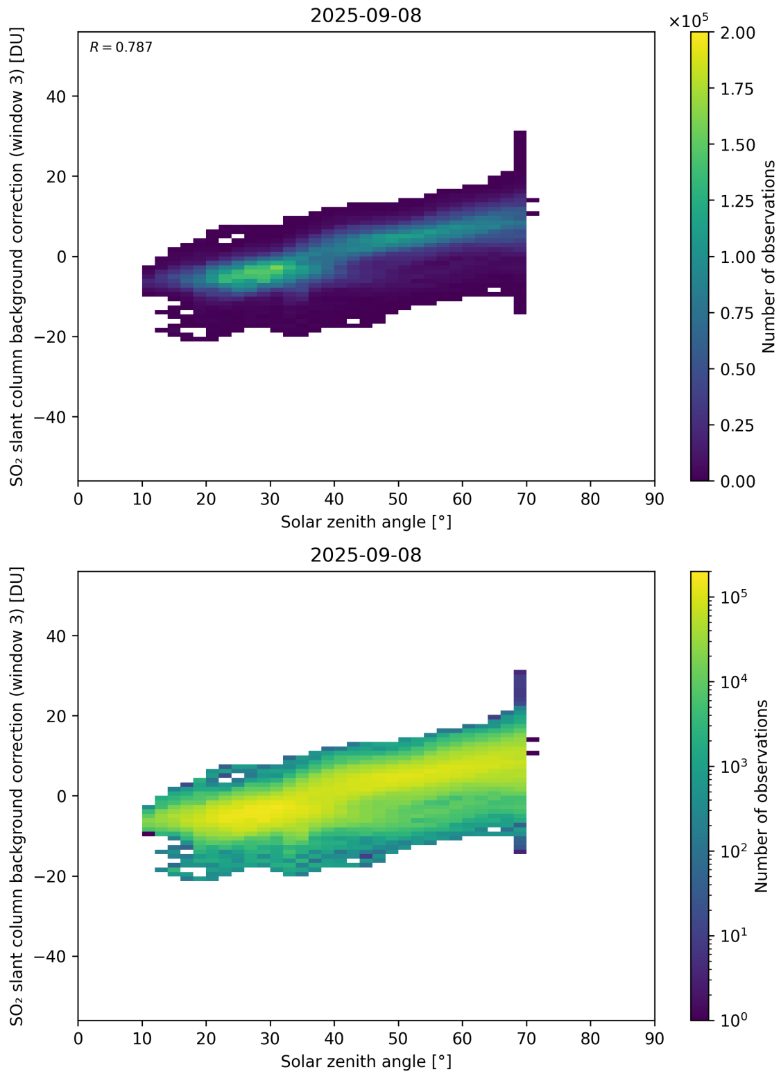
Figure 173: Scatter density plot of “Solar zenith angle” against “SO 2 slant column background correction (window 3)” for 2025-09-07 to 2025-09-09.
