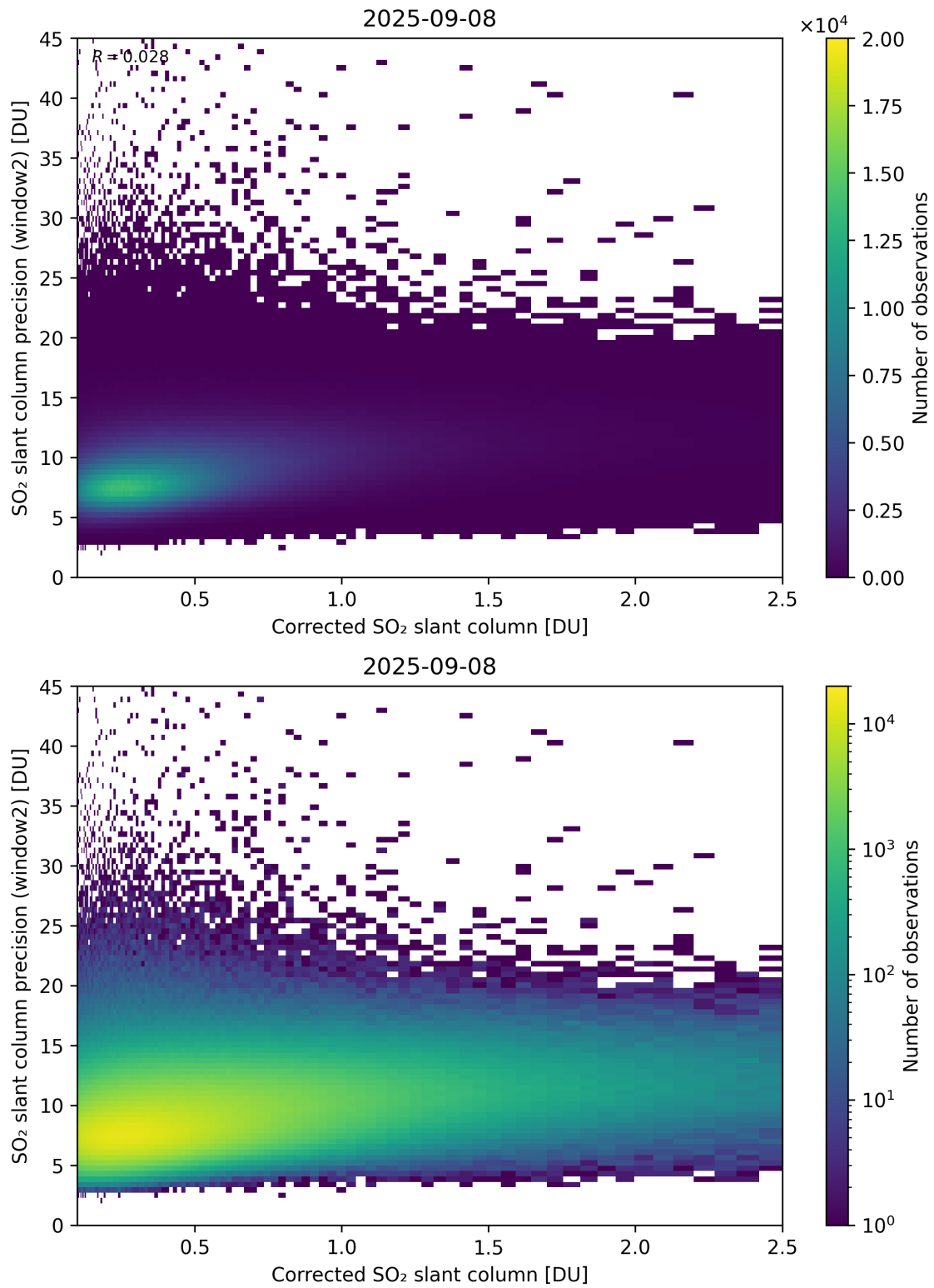
Figure 239: Scatter density plot of “Corrected SO 2 slant column” against “SO 2 slant column precision (window2)” for 2025-09-07 to 2025-09-09.
