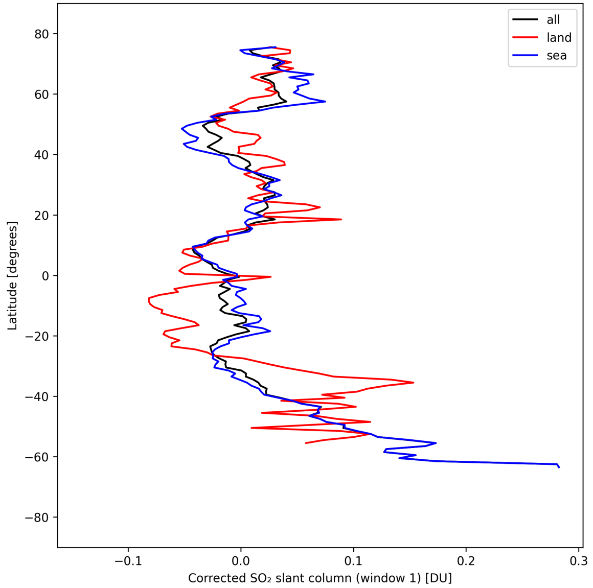
Figure 39: Zonal average of “Corrected SO 2 slant column (window 1)” for 2025-09-07 to 2025-09-09.
