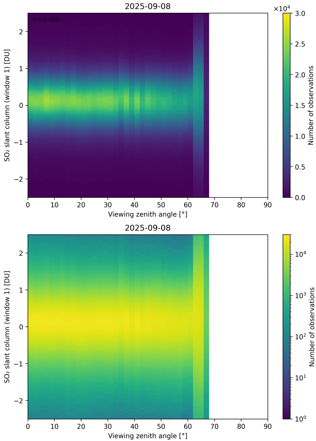
Figure 376: Scatter density plot of “Viewing zenith angle” against “SO 2 slant column (window 1)” for 2025-09-07 to 2025-09-09.
