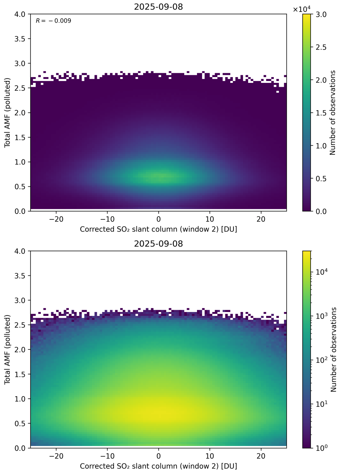
Figure 253: Scatter density plot of “Corrected SO 2 slant column (window 2)” against “Total AMF (polluted)” for 2025-09-07 to 2025-09-09.
