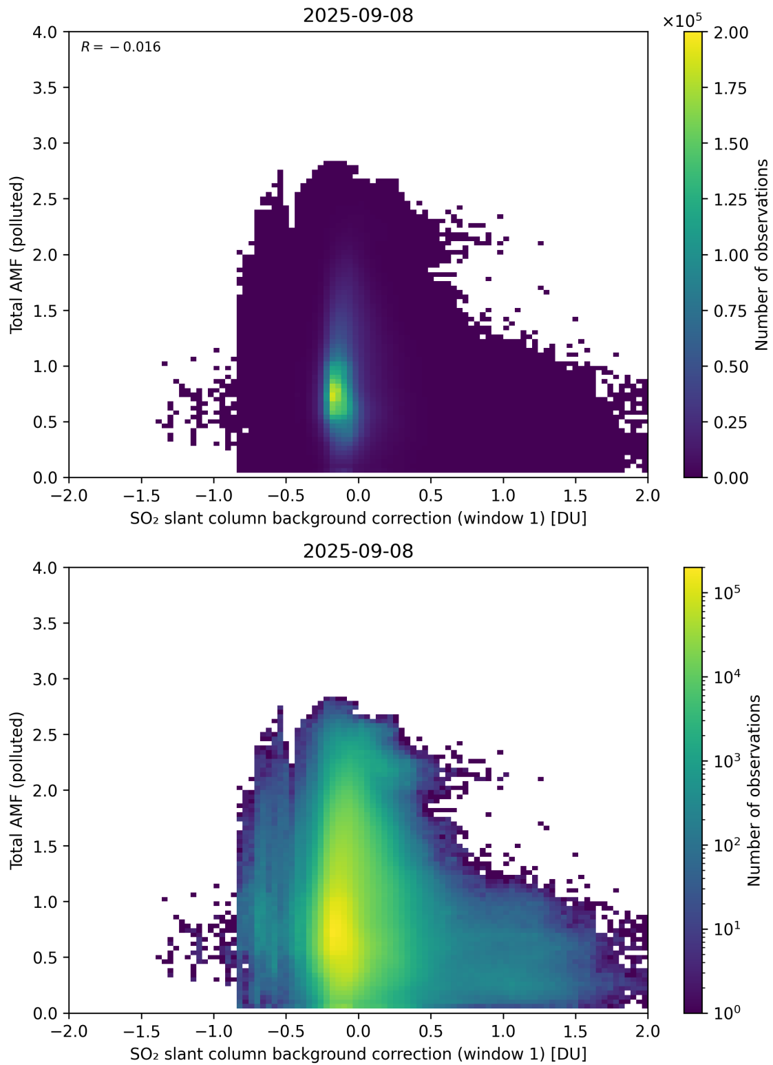
Figure 120: Scatter density plot of “SO 2 slant column background correction (window 1)” against “Total AMF (polluted)” for 2025-09-07 to 2025-09-09.
