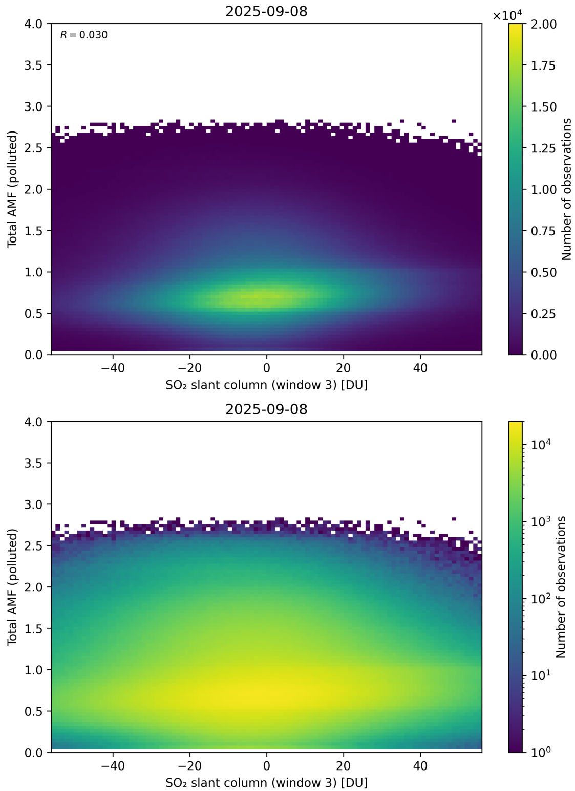
Figure 318: Scatter density plot of “SO 2 slant column (window 3)” against “Total AMF (polluted)” for 2025-09-07 to 2025-09-09.
