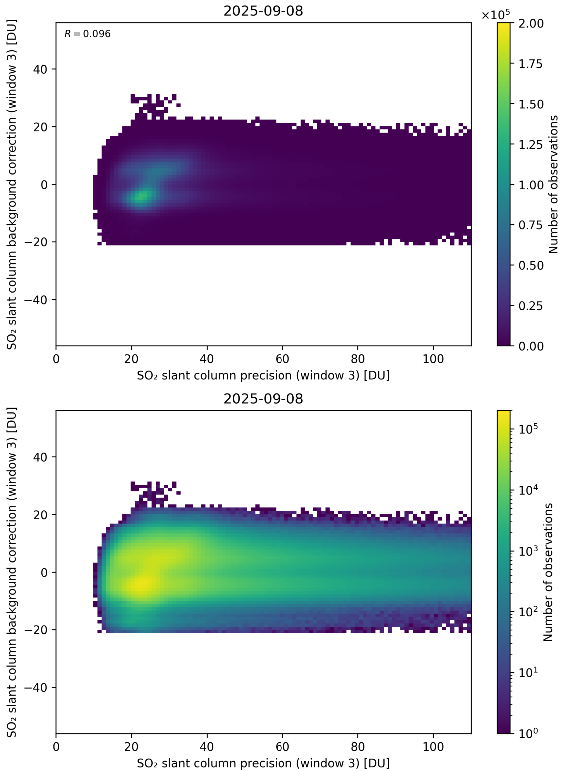
Figure 307: Scatter density plot of “SO 2 slant column precision (window 3)” against “SO 2 slant column background correction (window 3)” for 2025-09-07 to 2025-09-09.
