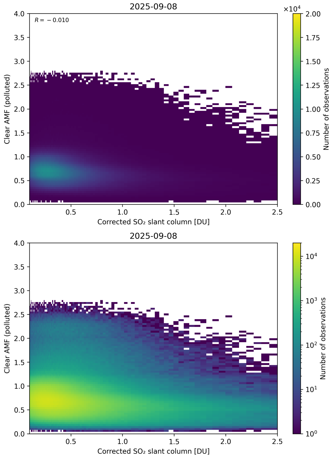
Figure 232: Scatter density plot of “Corrected SO 2 slant column” against “Clear AMF (polluted)” for 2025-09-07 to 2025-09-09.
