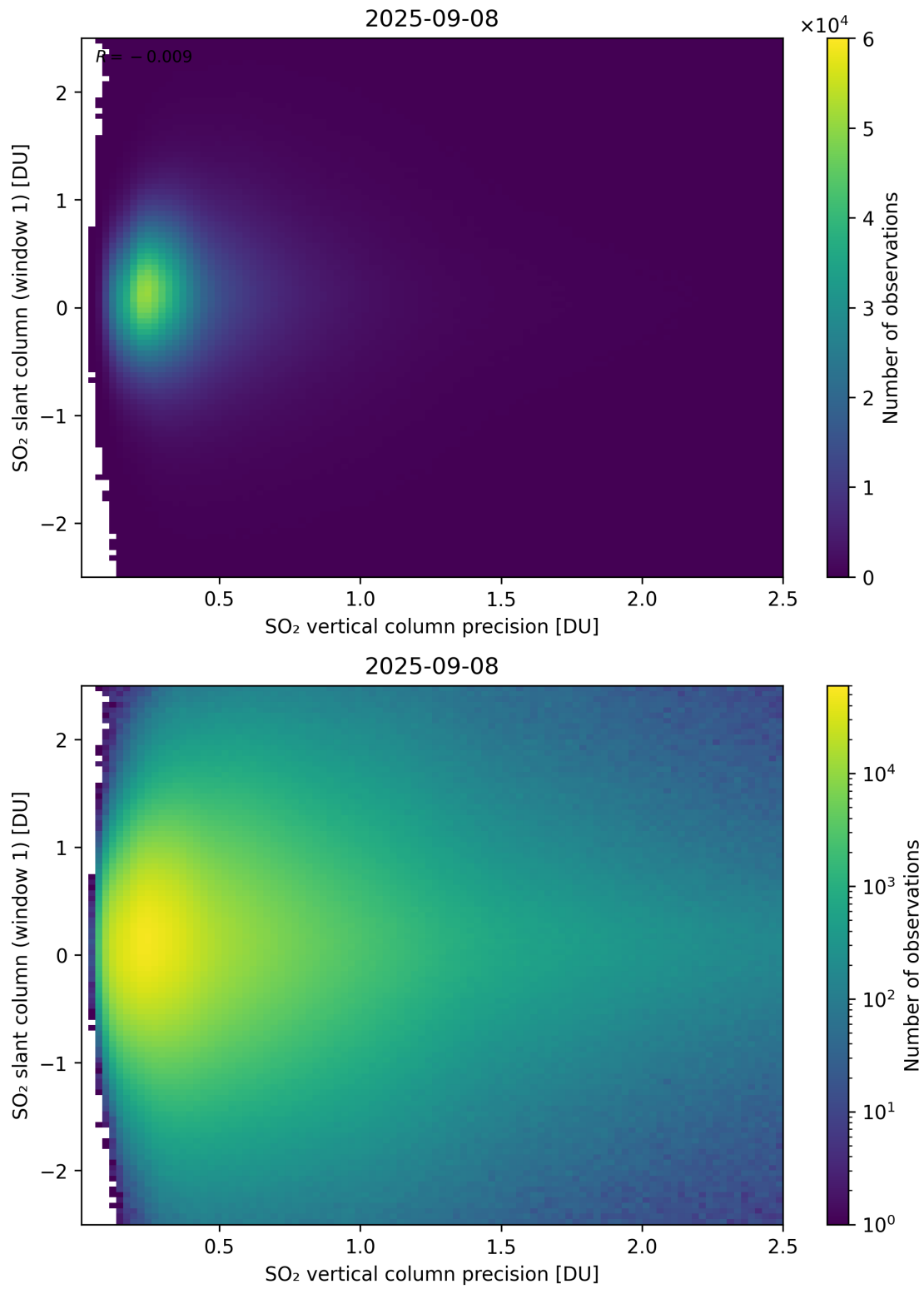
Figure 341: Scatter density plot of “SO 2 vertical column precision” against “SO 2 slant column (window 1)” for 2025-09-07 to 2025-09-09.
