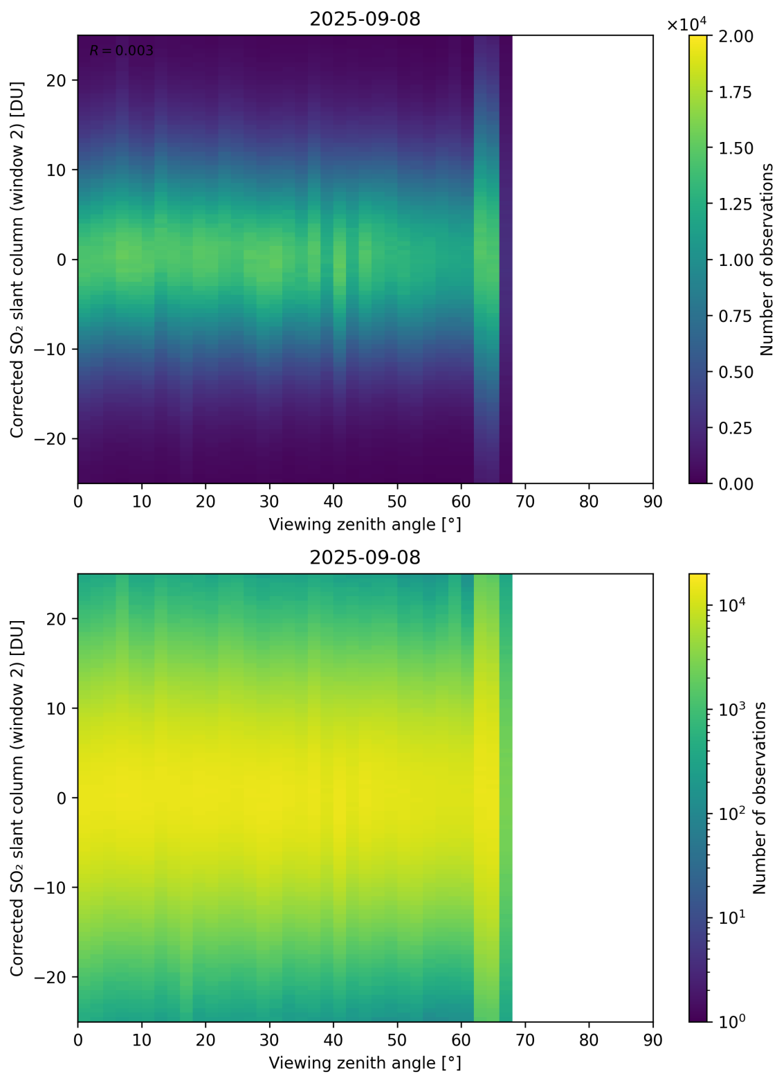
Figure 374: Scatter density plot of “Viewing zenith angle” against “Corrected SO 2 slant column (window 2)” for 2025-09-07 to 2025-09-09.
