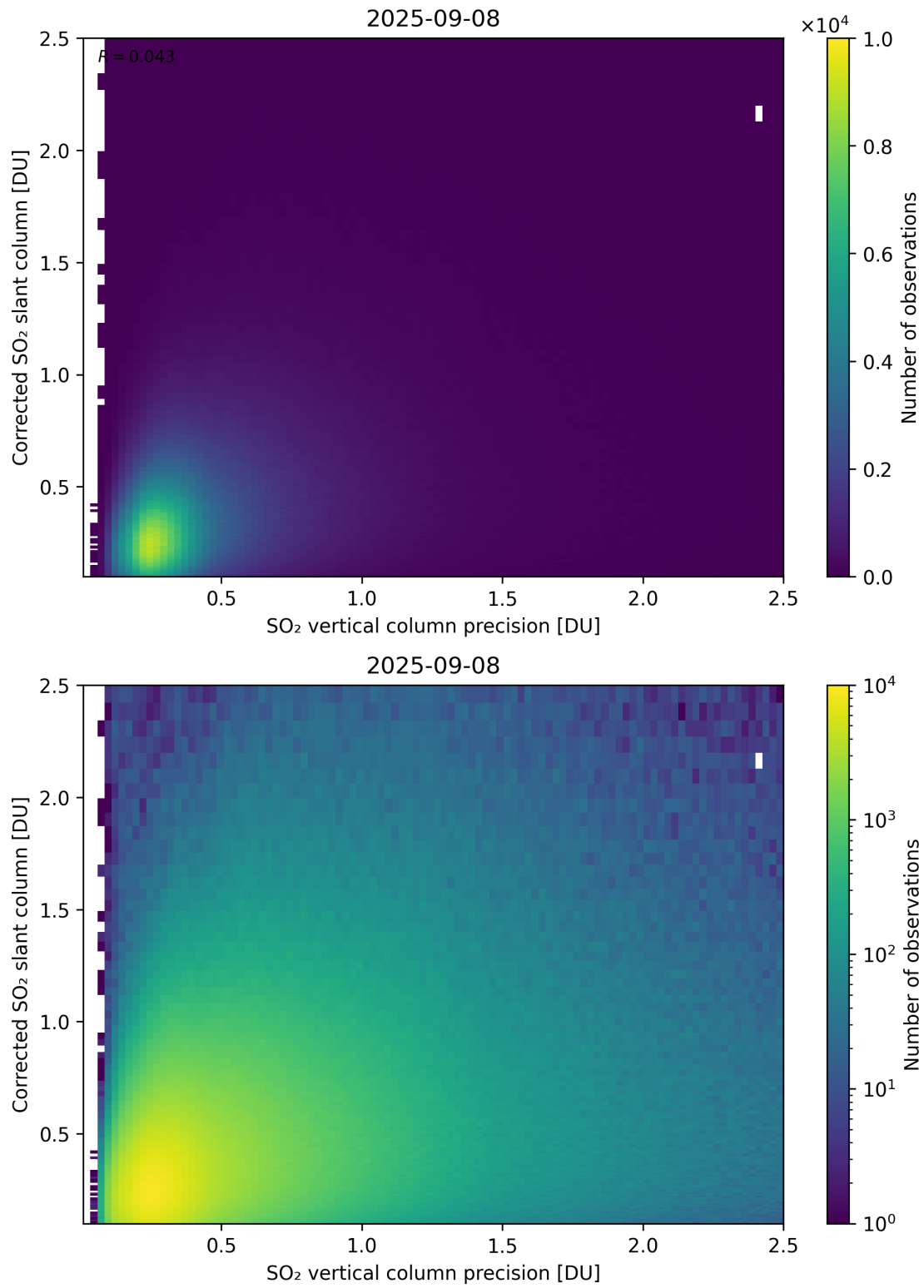
Figure 338: Scatter density plot of “SO 2 vertical column precision” against “Corrected SO 2 slant column” for 2025-09-07 to 2025-09-09.
