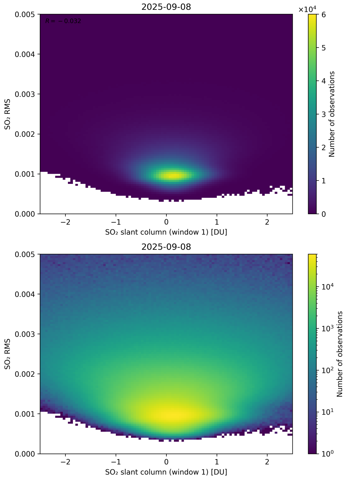
Figure 267: Scatter density plot of “SO 2 slant column (window 1)” against “SO 2 RMS” for 2025-09-07 to 2025-09-09.
