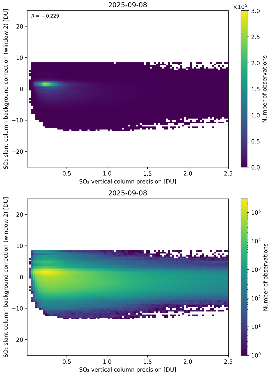
Figure 330: Scatter density plot of “SO 2 vertical column precision” against “SO 2 slant column background correction (window 2)” for 2025-09-07 to 2025-09-09.
