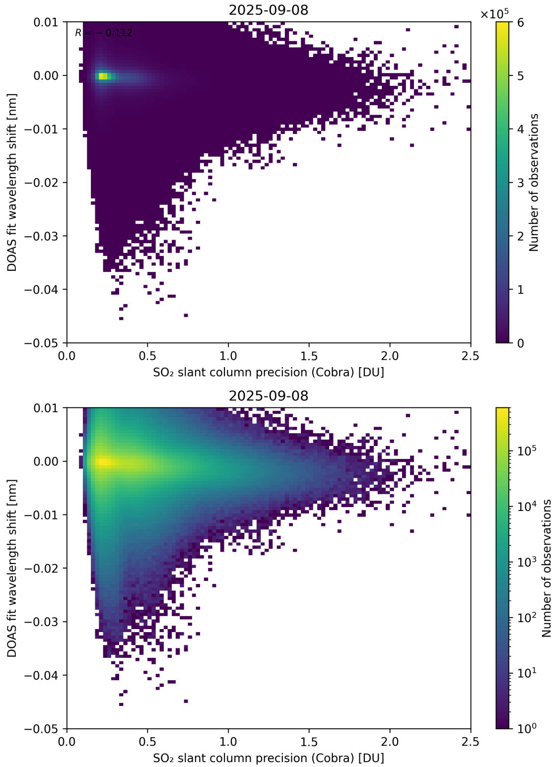
Figure 202: Scatter density plot of “SO 2 slant column precision (Cobra)” against “DOAS fit wavelength shift” for 2025-09-07 to 2025-09-09.
