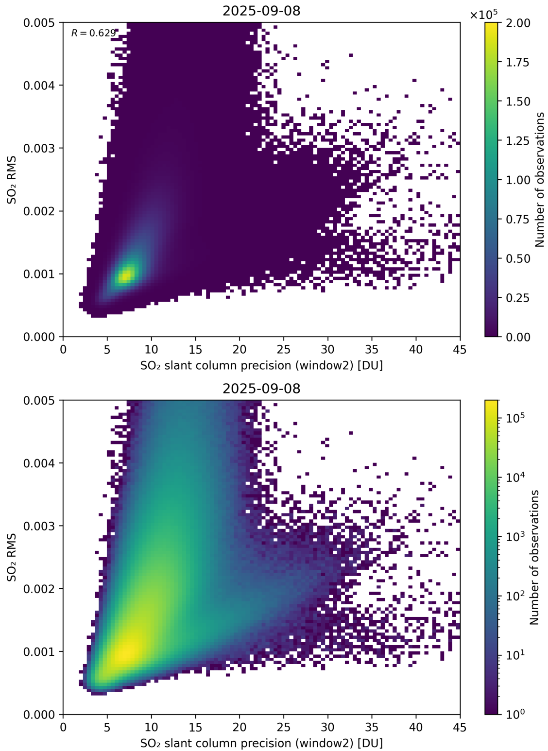
Figure 295: Scatter density plot of “SO 2 slant column precision (window2)” against “SO 2 RMS” for 2025-09-07 to 2025-09-09.
