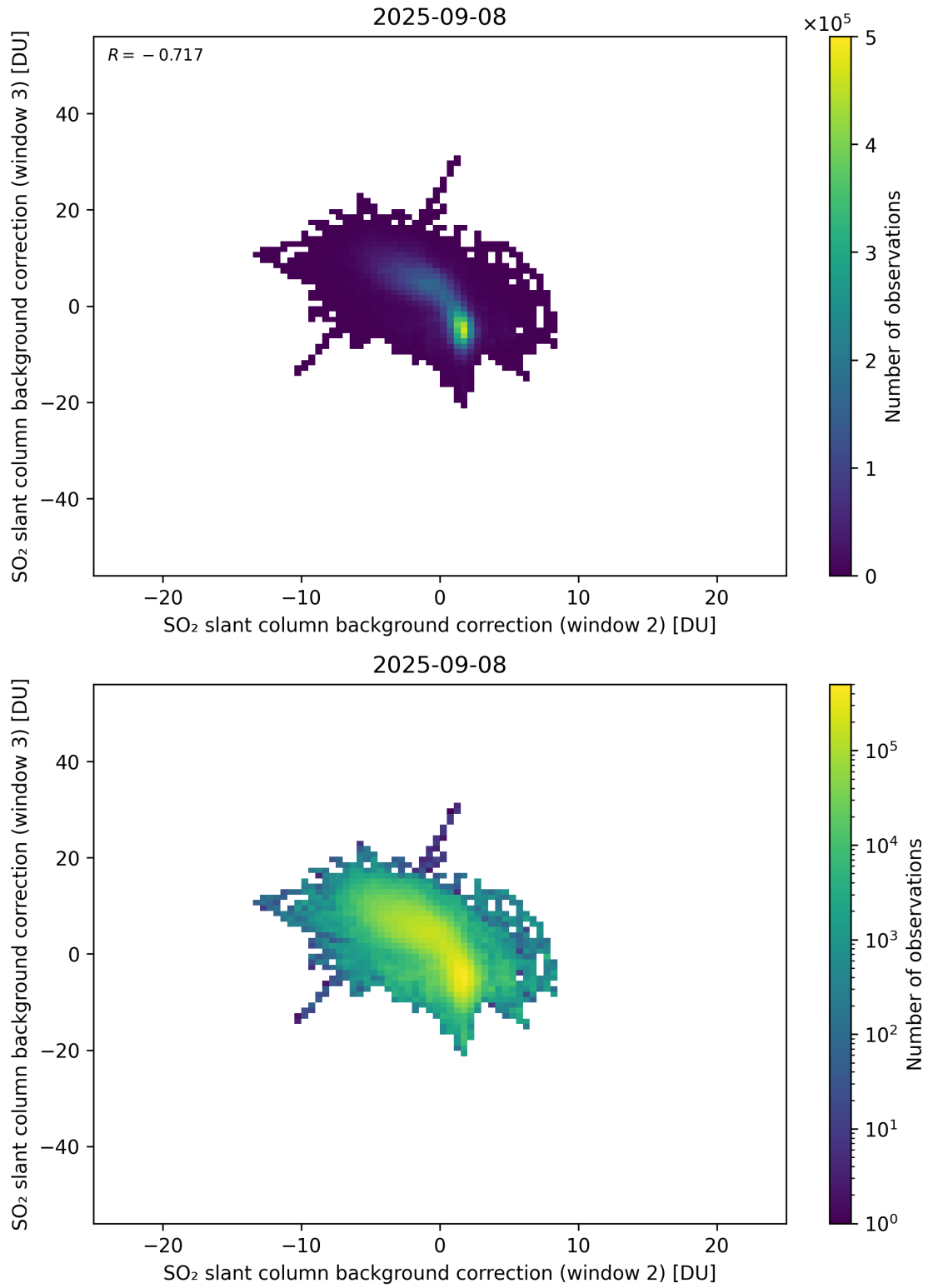
Figure 122: Scatter density plot of “SO 2 slant column background correction (window 2)” against “SO 2 slant column background correction (window 3)” for 2025-09-07 to 2025-09-09.
