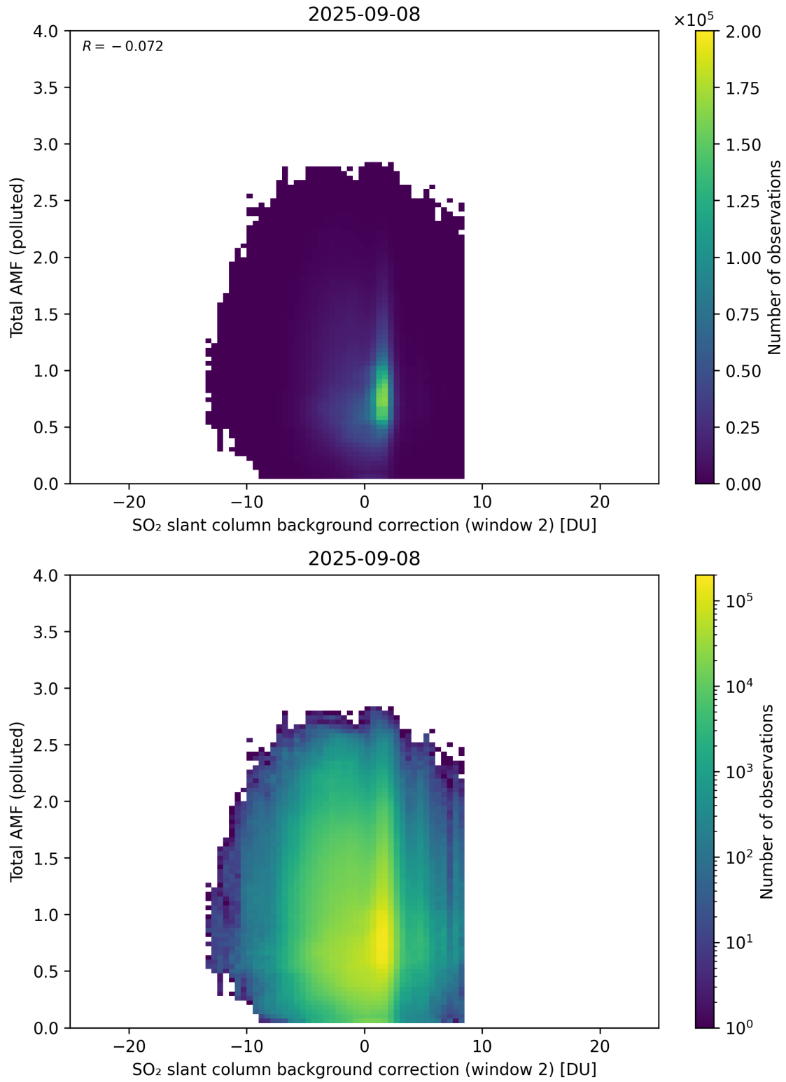
Figure 130: Scatter density plot of “SO 2 slant column background correction (window 2)” against “Total AMF (polluted)” for 2025-09-07 to 2025-09-09.
