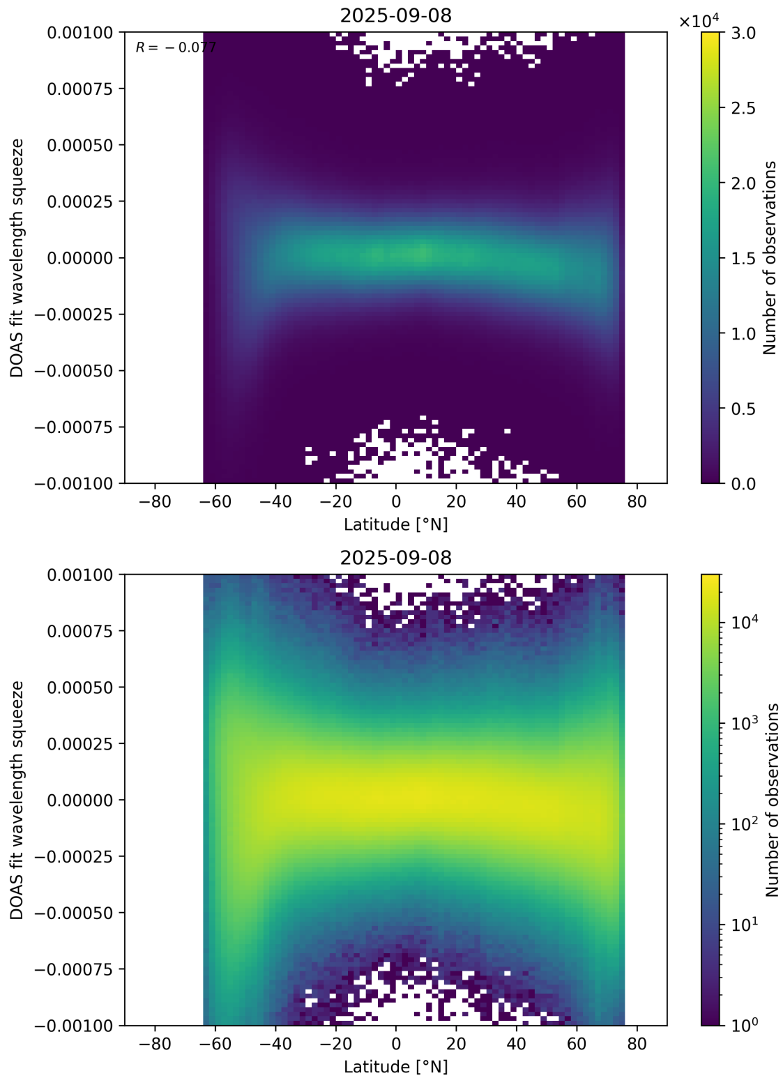
Figure 154: Scatter density plot of “Latitude” against “DOAS fit wavelength squeeze” for 2025-09-07 to 2025-09-09.
