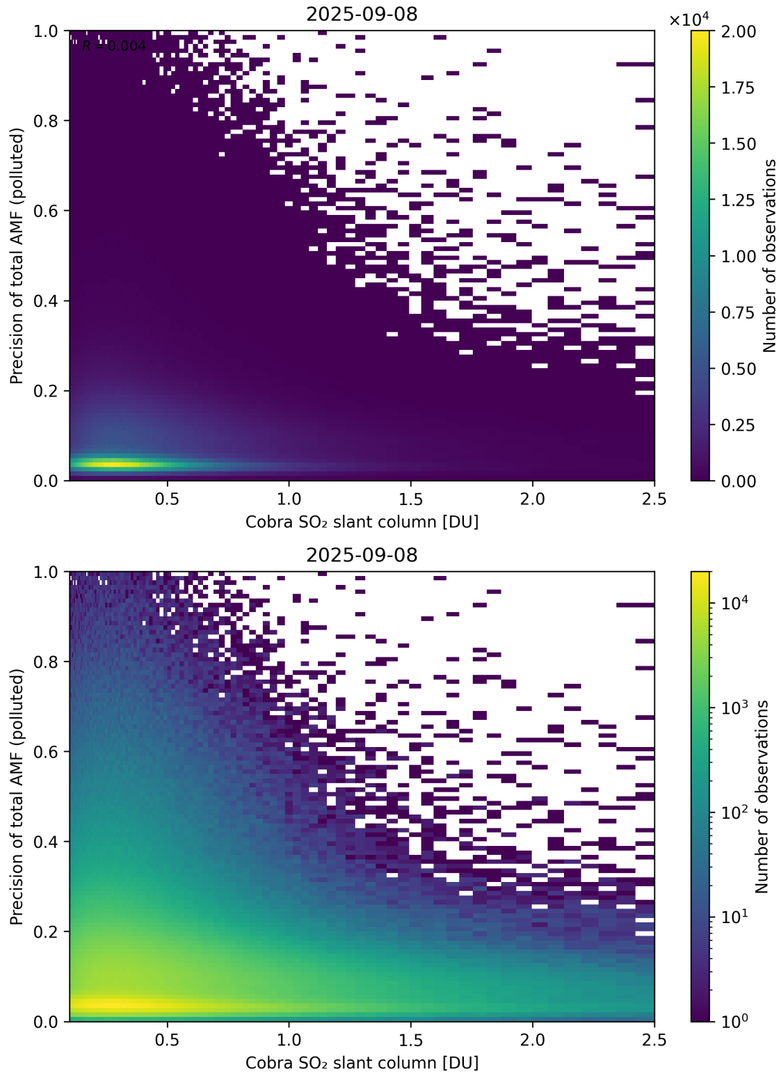
Figure 225: Scatter density plot of “Cobra SO 2 slant column” against “Precision of total AMF (polluted)” for 2025-09-07 to 2025-09-09.
