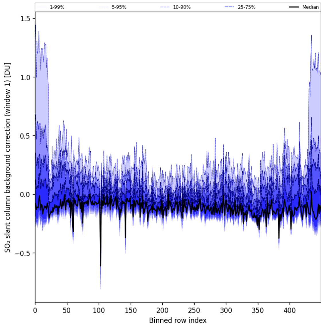
Figure 92: Along track statistics of “SO 2 slant column background correction (window 1)” for 2025-09-07 to 2025-09-09
