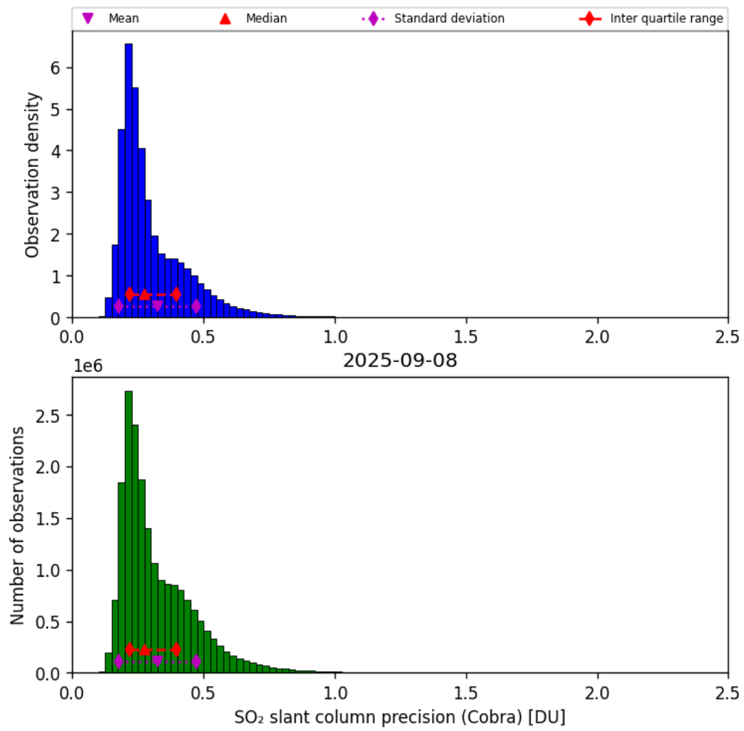
Figure 62: Histogram of “SO 2 slant column precision (Cobra)” for 2025-09-07 to 2025-09-09
