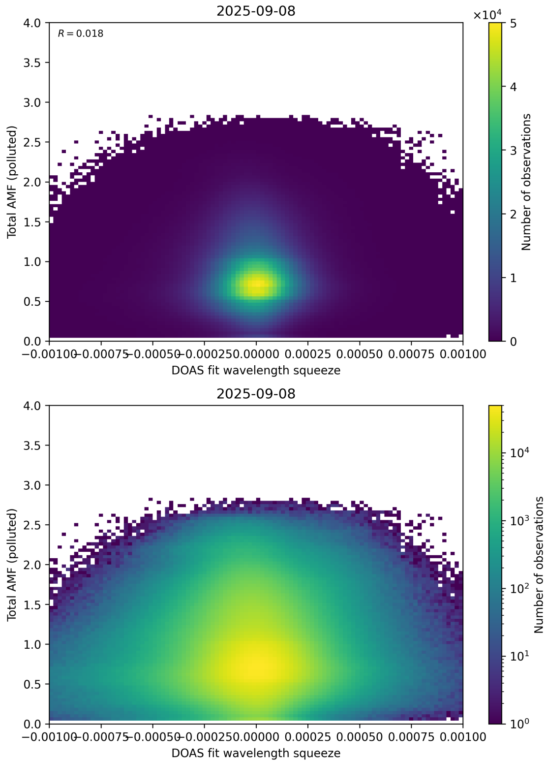
Figure 145: Scatter density plot of “DOAS fit wavelength squeeze” against “Total AMF (polluted)” for 2025-09-07 to 2025-09-09.
