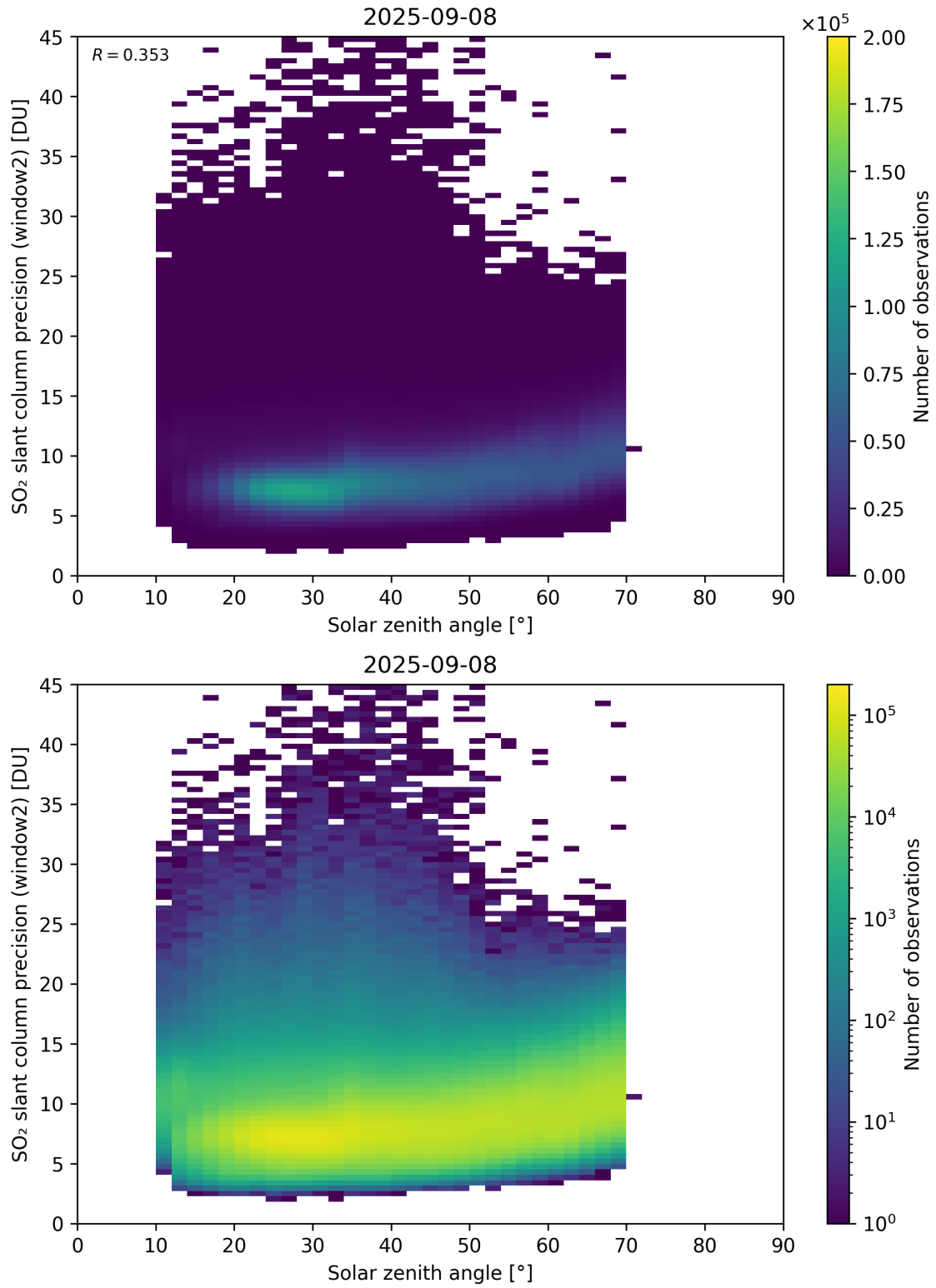
Figure 186: Scatter density plot of “Solar zenith angle” against “SO 2 slant column precision (window2)” for 2025-09-07 to 2025-09-09.
