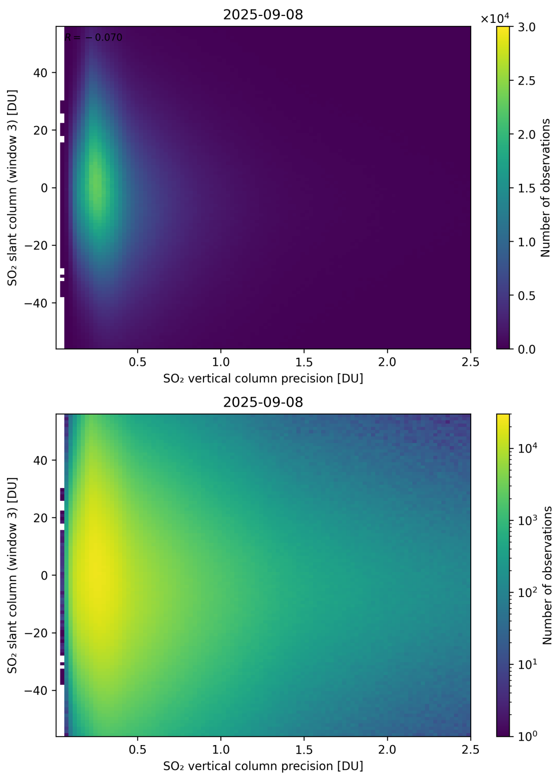
Figure 344: Scatter density plot of “SO 2 vertical column precision” against “SO 2 slant column (window 3)” for 2025-09-07 to 2025-09-09.
