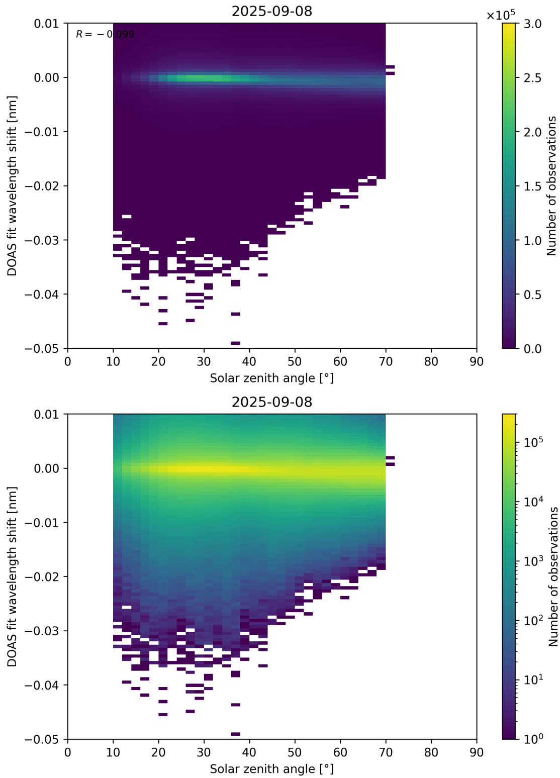
Figure 174: Scatter density plot of “Solar zenith angle” against “DOAS fit wavelength shift” for 2025-09-07 to 2025-09-09.
