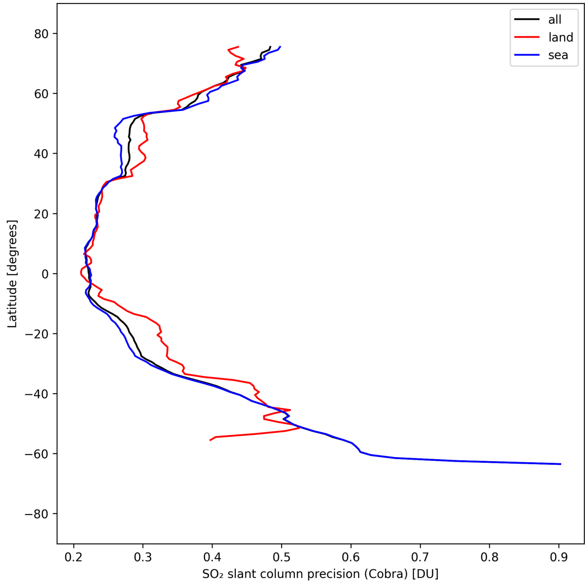
Figure 36: Zonal average of “SO 2 slant column precision (Cobra)” for 2025-09-07 to 2025-09-09.
