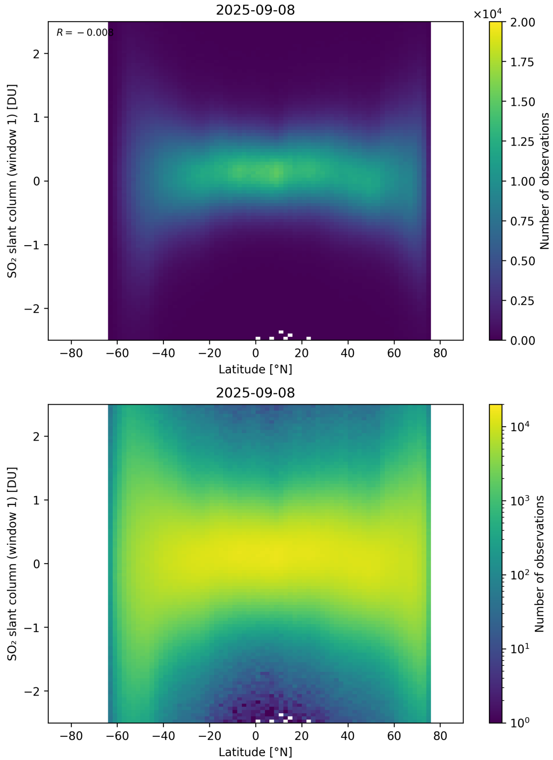
Figure 162: Scatter density plot of “Latitude” against “SO 2 slant column (window 1)” for 2025-09-07 to 2025-09-09.
