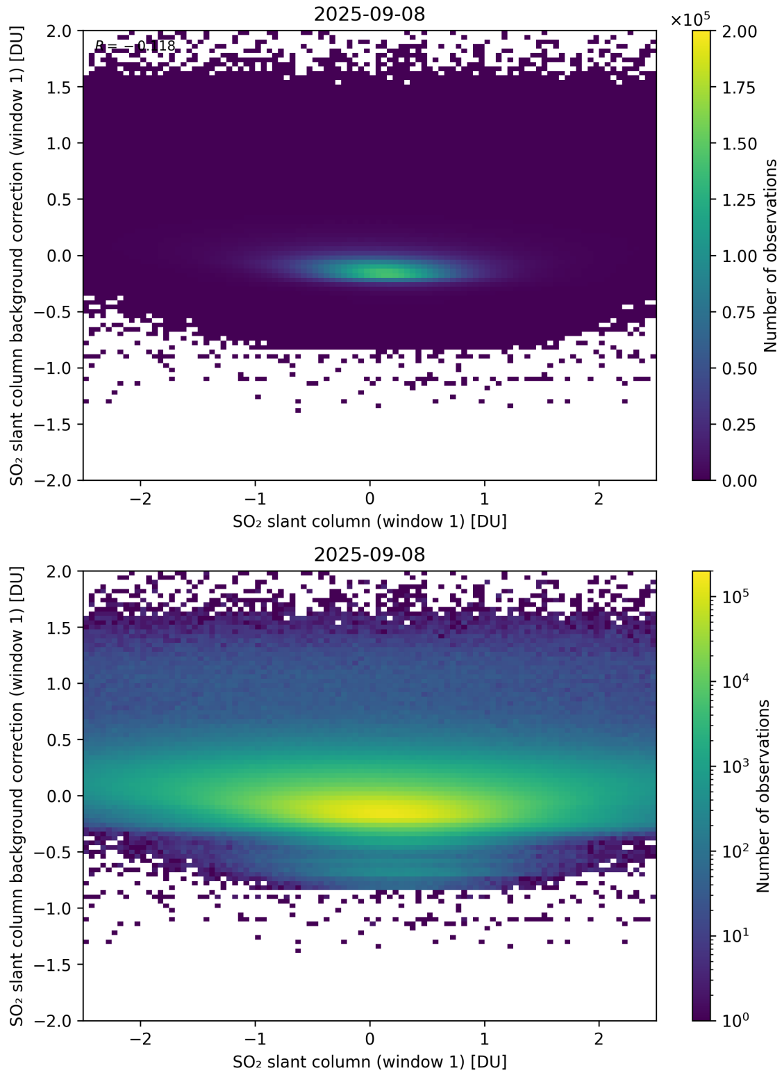
Figure 262: Scatter density plot of “SO 2 slant column (window 1)” against “SO 2 slant column background correction (window 1)” for 2025-09-07 to 2025-09-09.
