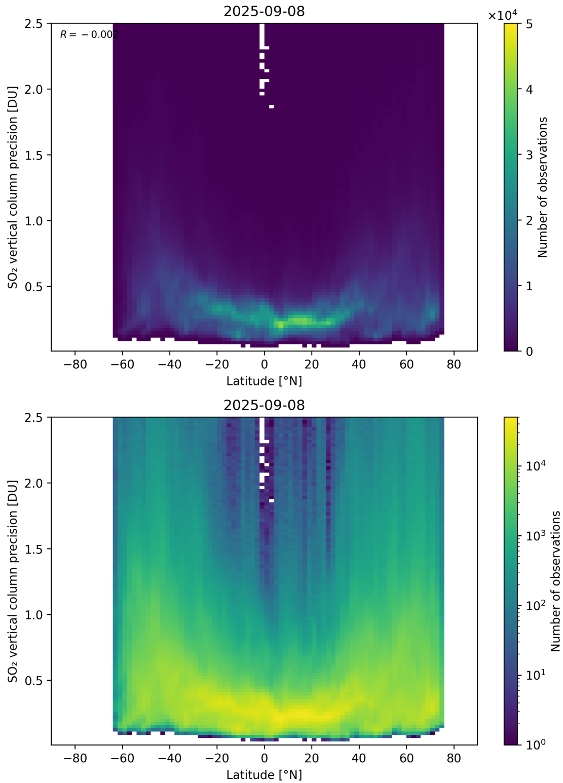
Figure 170: Scatter density plot of “Latitude” against “SO 2 vertical column precision” for 2025-09-07 to 2025-09-09.
