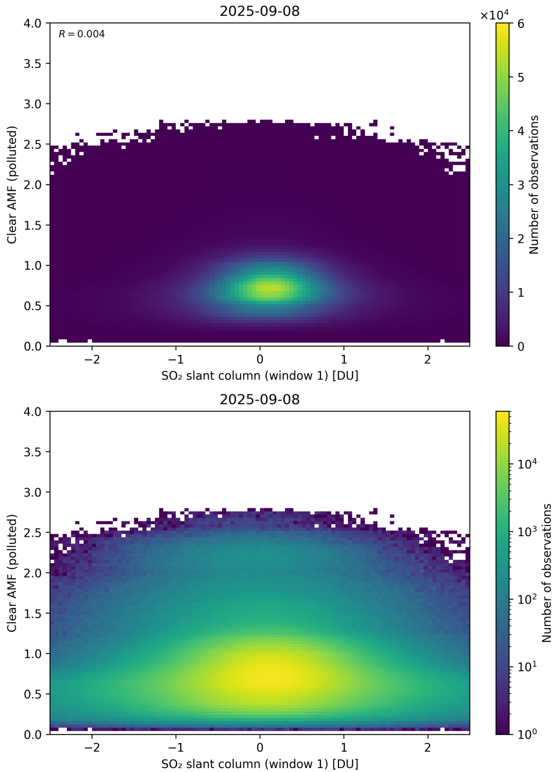
Figure 282: Scatter density plot of “SO 2 slant column (window 1)” against “Clear AMF (polluted)” for 2025-09-07 to 2025-09-09.
