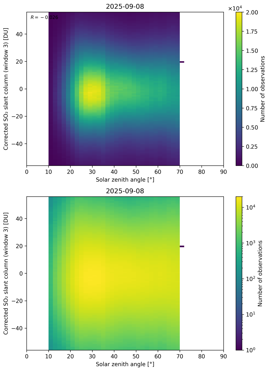
Figure 183: Scatter density plot of “Solar zenith angle” against “Corrected SO 2 slant column (window 3)” for 2025-09-07 to 2025-09-09.
