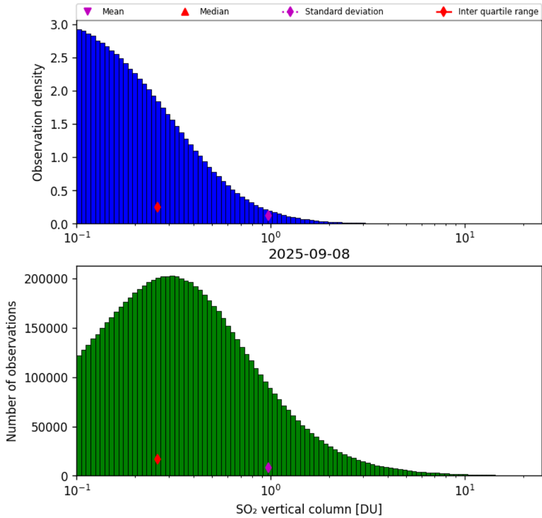
Figure 58: Histogram of “SO 2 vertical column” for 2025-09-07 to 2025-09-09
