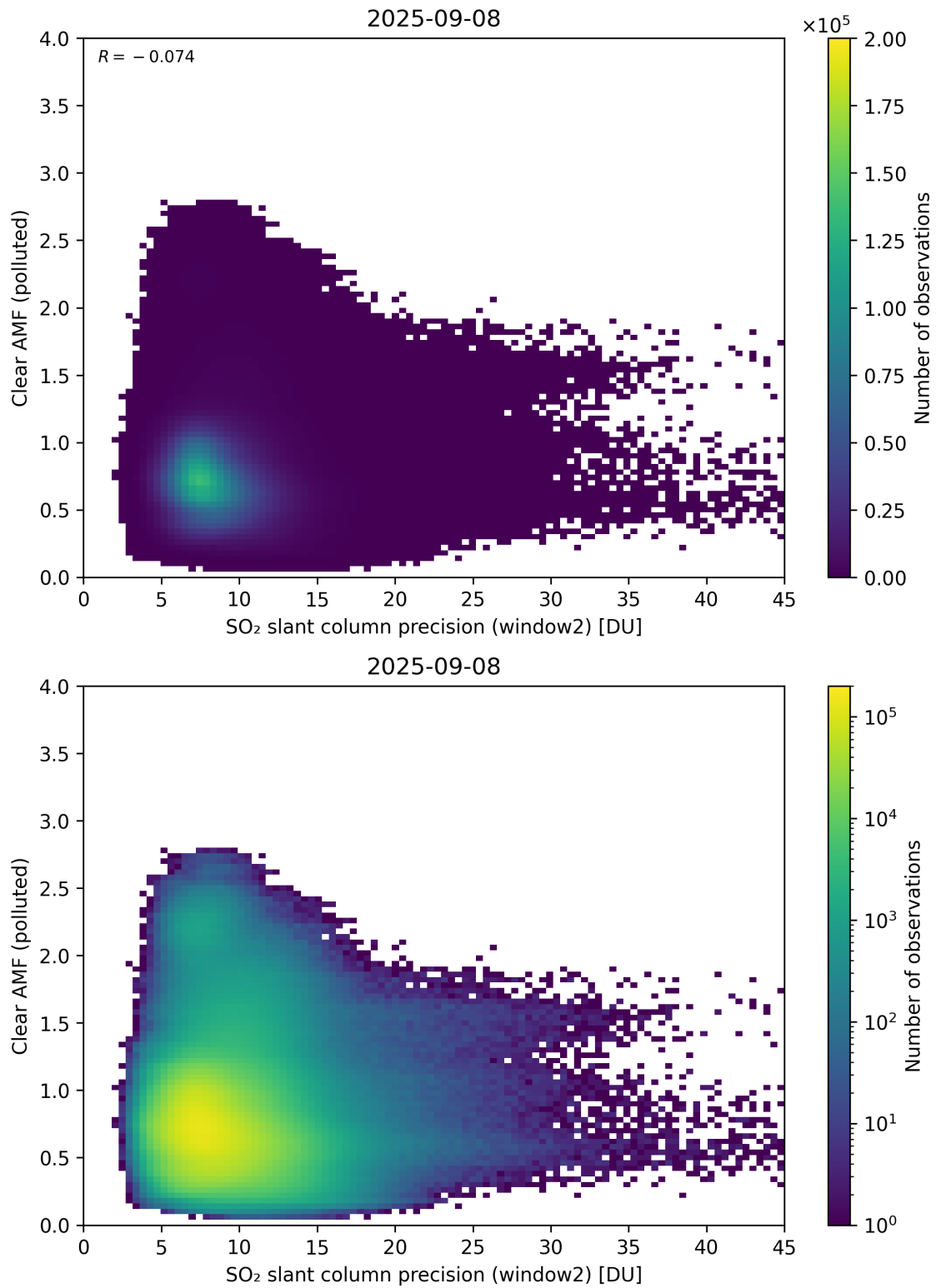
Figure 296: Scatter density plot of “SO 2 slant column precision (window2)” against “Clear AMF (polluted)” for 2025-09-07 to 2025-09-09.
