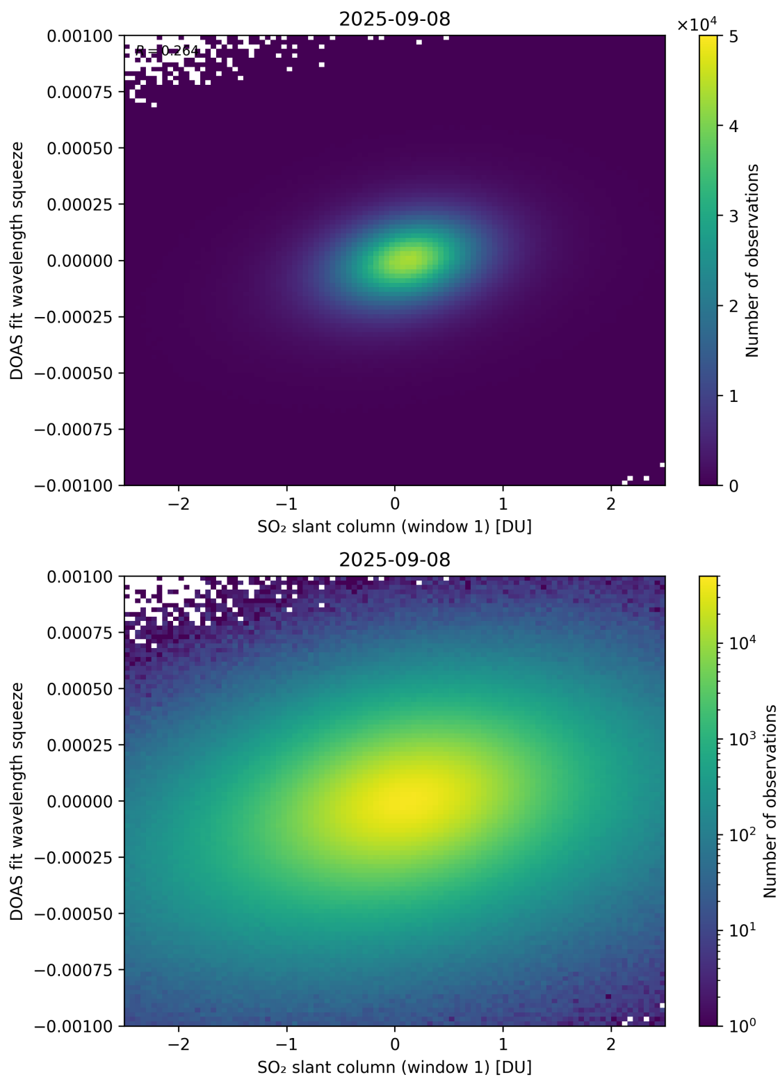
Figure 266: Scatter density plot of “SO 2 slant column (window 1)” against “DOAS fit wavelength squeeze” for 2025-09-07 to 2025-09-09.
