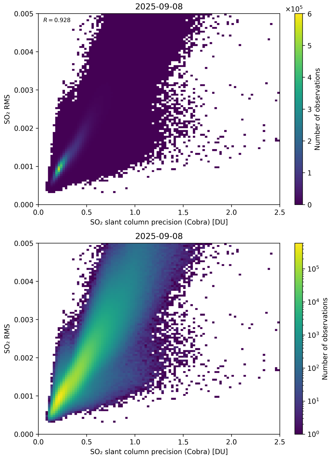
Figure 204: Scatter density plot of “SO 2 slant column precision (Cobra)” against “SO 2 RMS” for 2025-09-07 to 2025-09-09.
