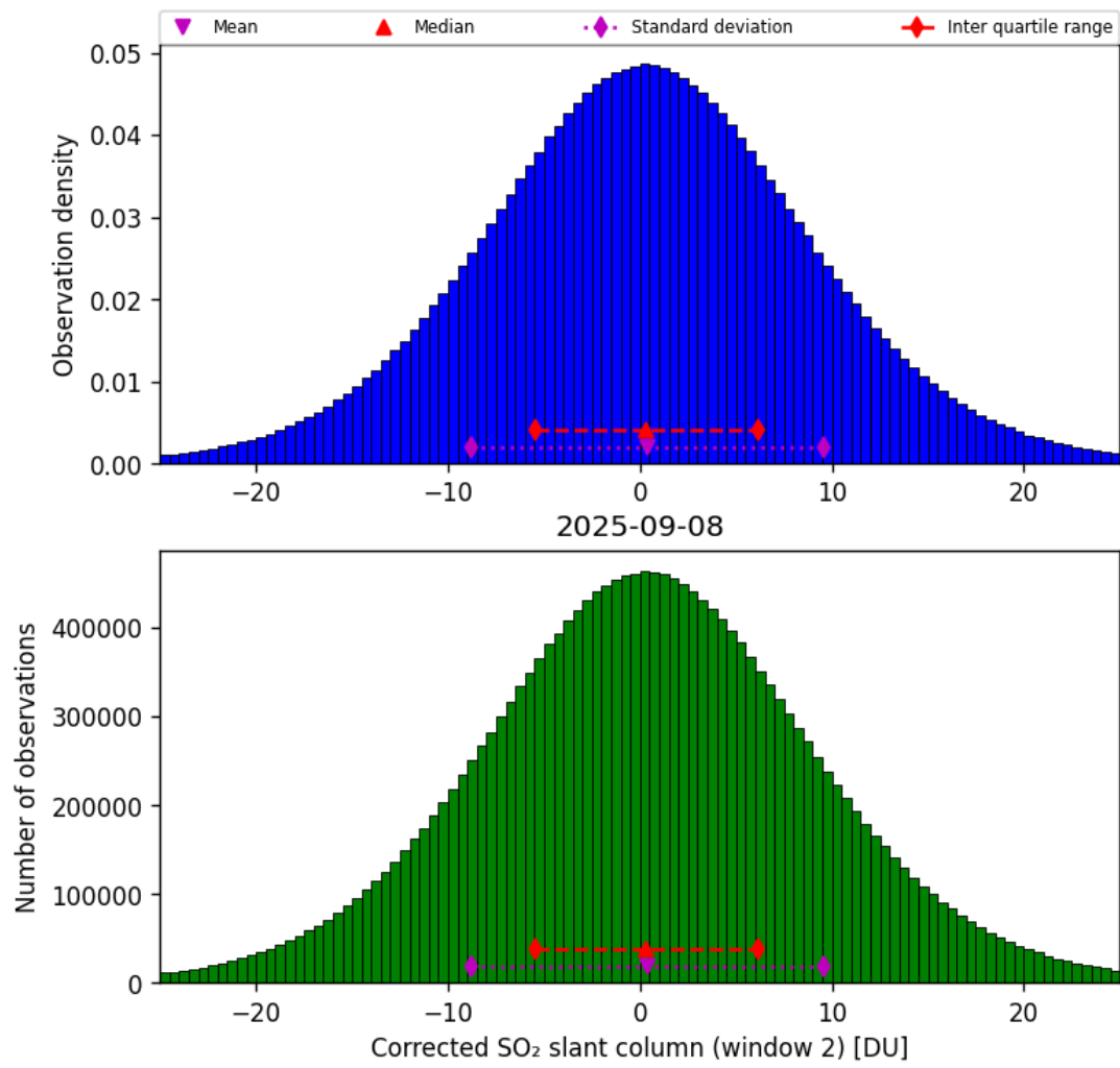
Figure 69: Histogram of “Corrected SO 2 slant column (window 2)” for 2025-09-07 to 2025-09-09
