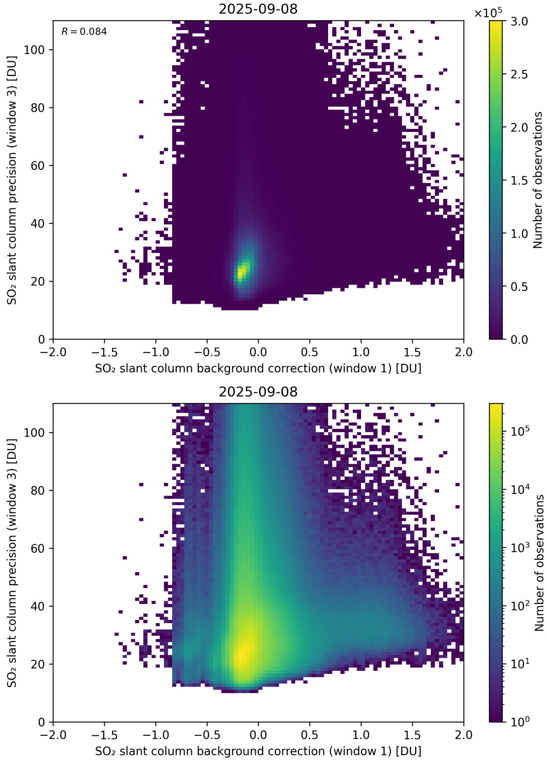
Figure 119: Scatter density plot of “SO 2 slant column background correction (window 1)” against “SO 2 slant column precision (window 3)” for 2025-09-07 to 2025-09-09.
