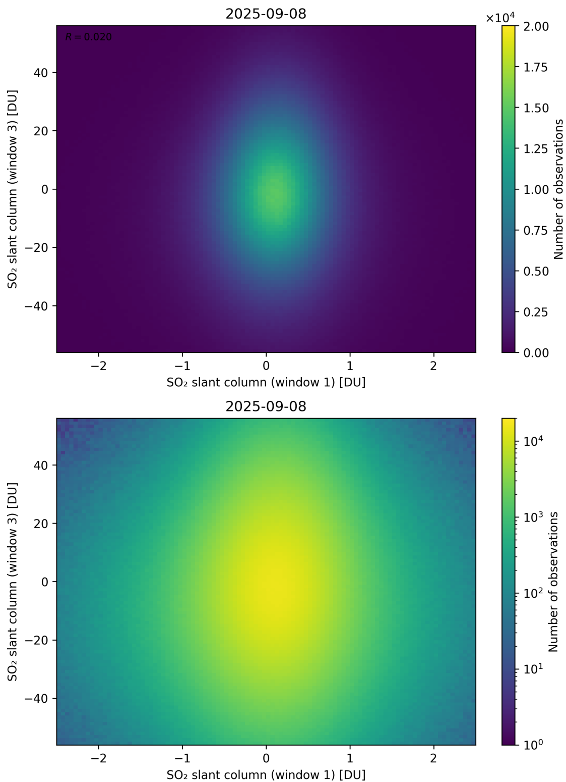
Figure 287: Scatter density plot of “SO 2 slant column (window 1)” against “SO 2 slant column (window 3)” for 2025-09-07 to 2025-09-09.
