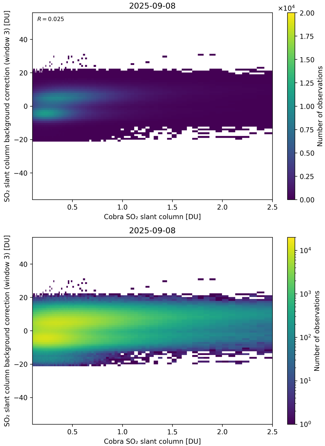
Figure 195: Scatter density plot of “Cobra SO 2 slant column” against “SO 2 slant column background correction (window 3)” for 2025-09-07 to 2025-09-09.
