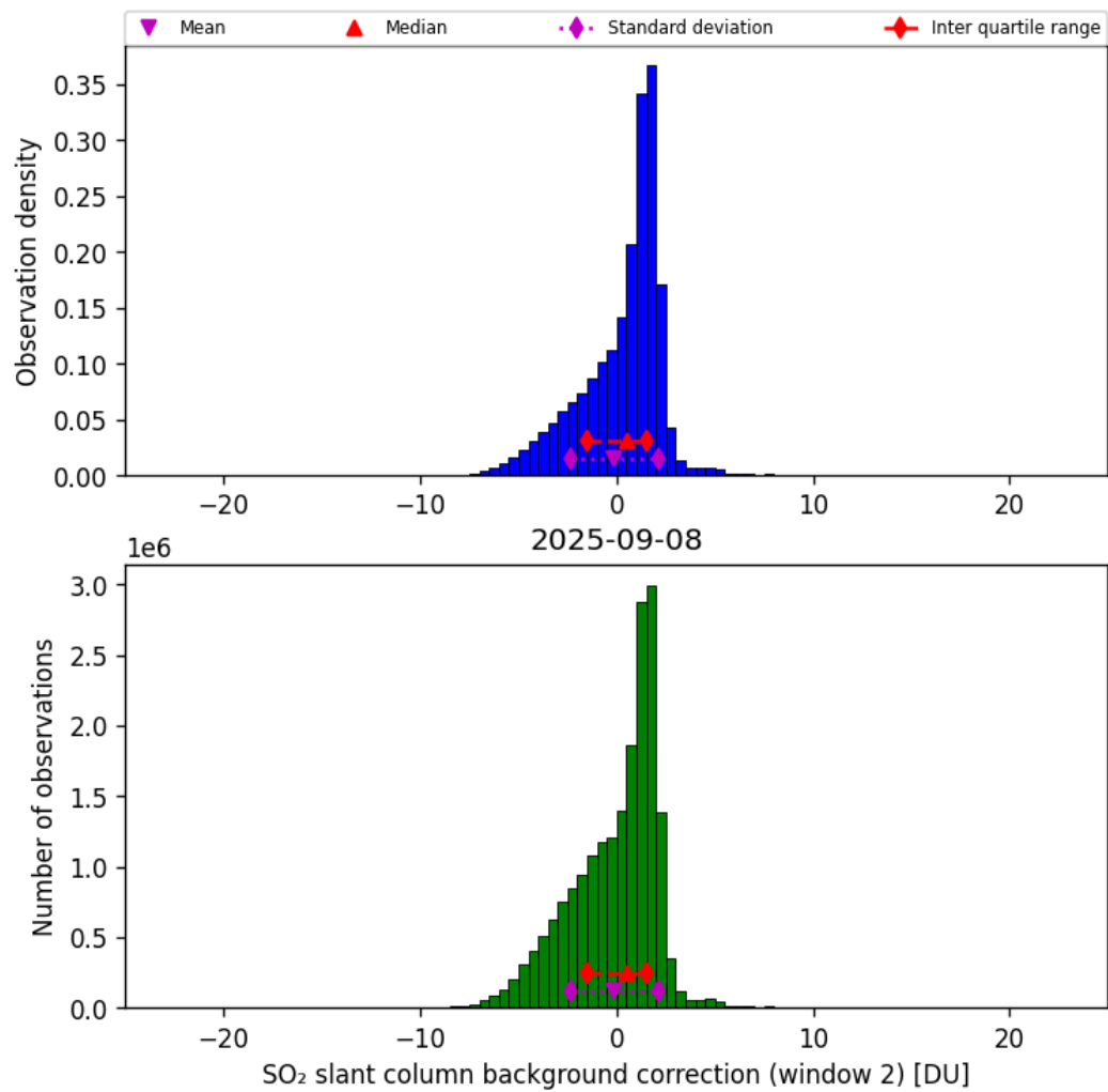
Figure 70: Histogram of “SO 2 slant column background correction (window 2)” for 2025-09-07 to 2025-09-09
