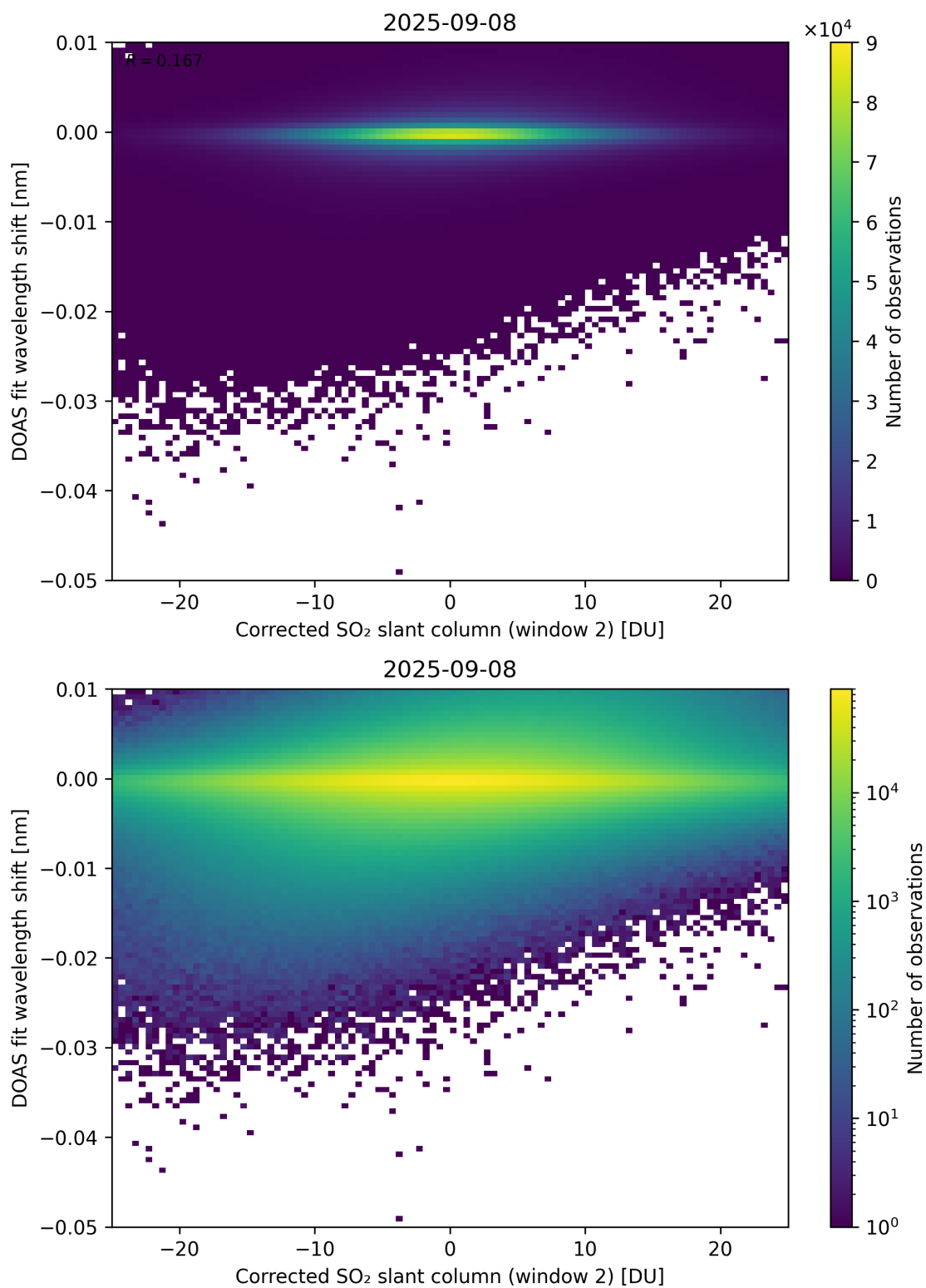
Figure 246: Scatter density plot of “Corrected SO 2 slant column (window 2)” against “DOAS fit wavelength shift” for 2025-09-07 to 2025-09-09.
