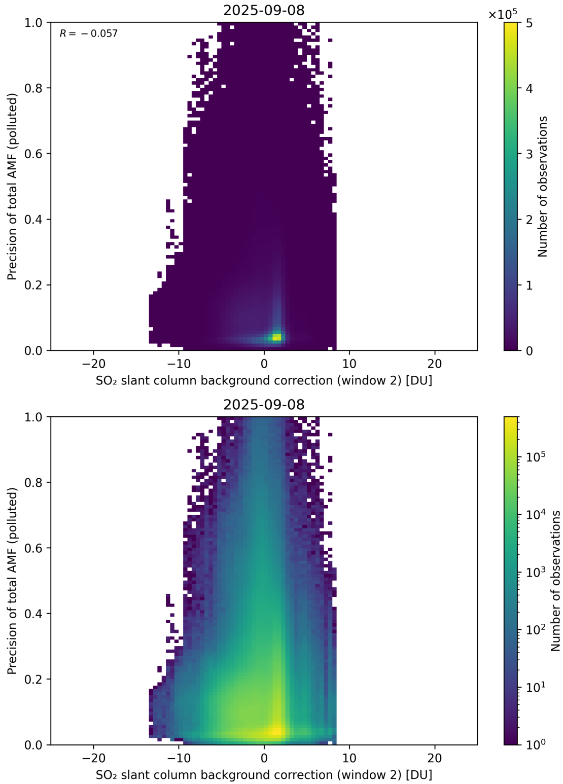
Figure 131: Scatter density plot of “SO 2 slant column background correction (window 2)” against “Precision of total AMF (polluted)” for 2025-09-07 to 2025-09-09.
