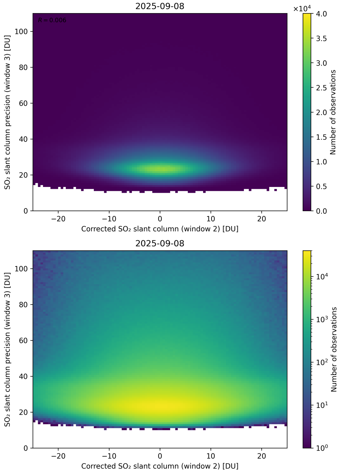
Figure 252: Scatter density plot of “Corrected SO 2 slant column (window 2)” against “SO 2 slant column precision (window 3)” for 2025-09-07 to 2025-09-09.
