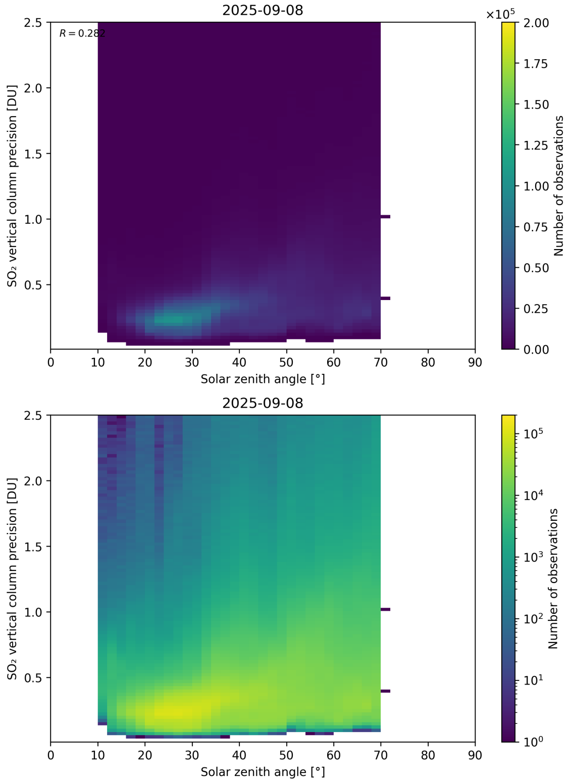
Figure 192: Scatter density plot of “Solar zenith angle” against “SO 2 vertical column precision” for 2025-09-07 to 2025-09-09.
