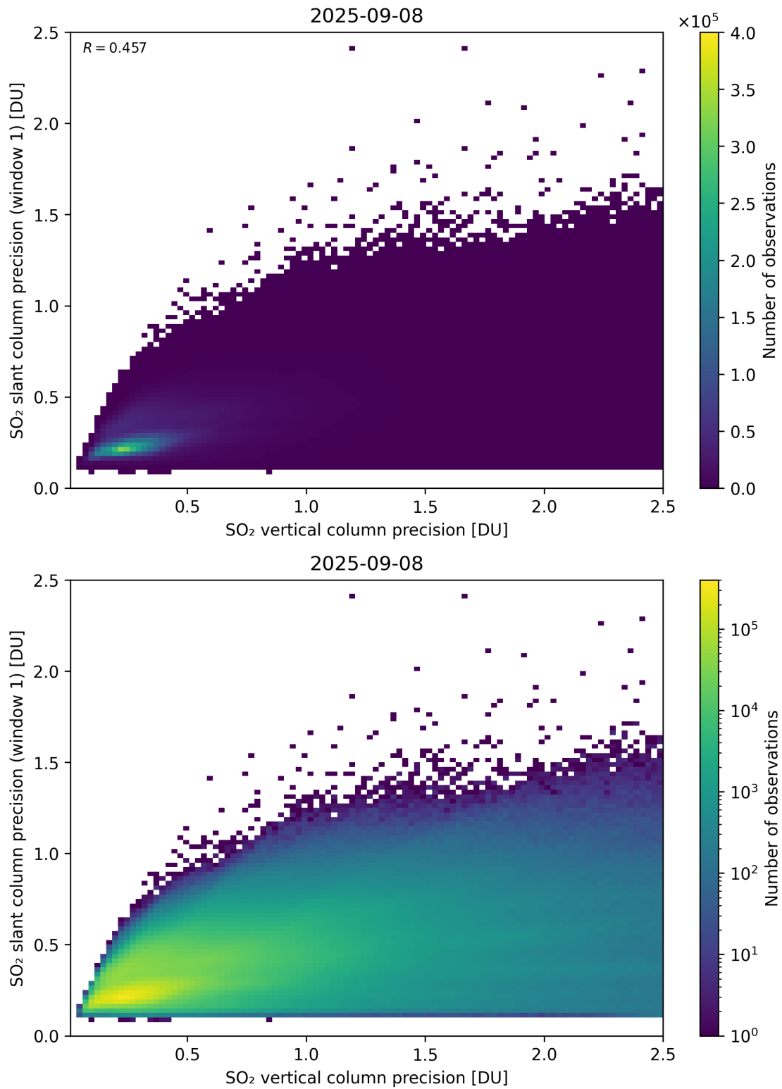
Figure 342: Scatter density plot of “SO 2 vertical column precision” against “SO 2 slant column precision (window 1)” for 2025-09-07 to 2025-09-09.
