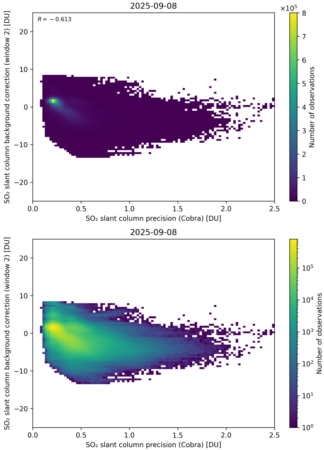
Figure 200: Scatter density plot of “SO 2 slant column precision (Cobra)” against “SO 2 slant column background correction (window 2)” for 2025-09-07 to 2025-09-09.
