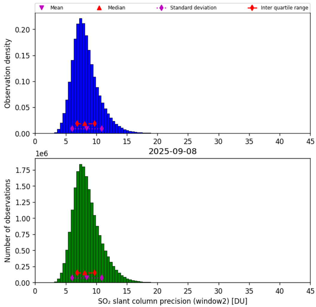
Figure 68: Histogram of “SO 2 slant column precision (window2)” for 2025-09-07 to 2025-09-09
