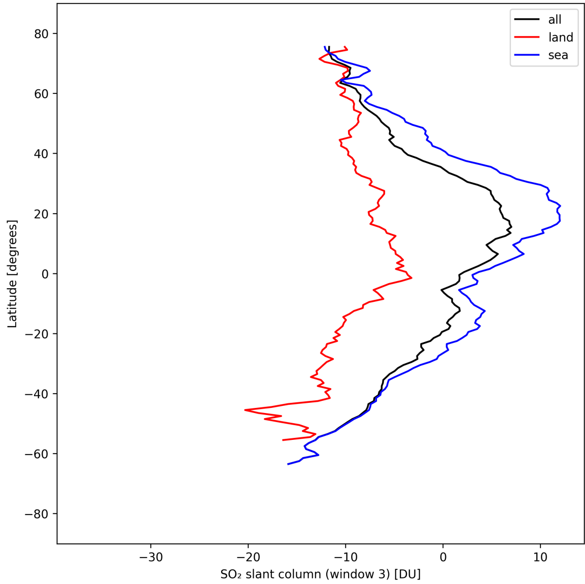
Figure 45: Zonal average of “SO 2 slant column (window 3)” for 2025-09-07 to 2025-09-09.
