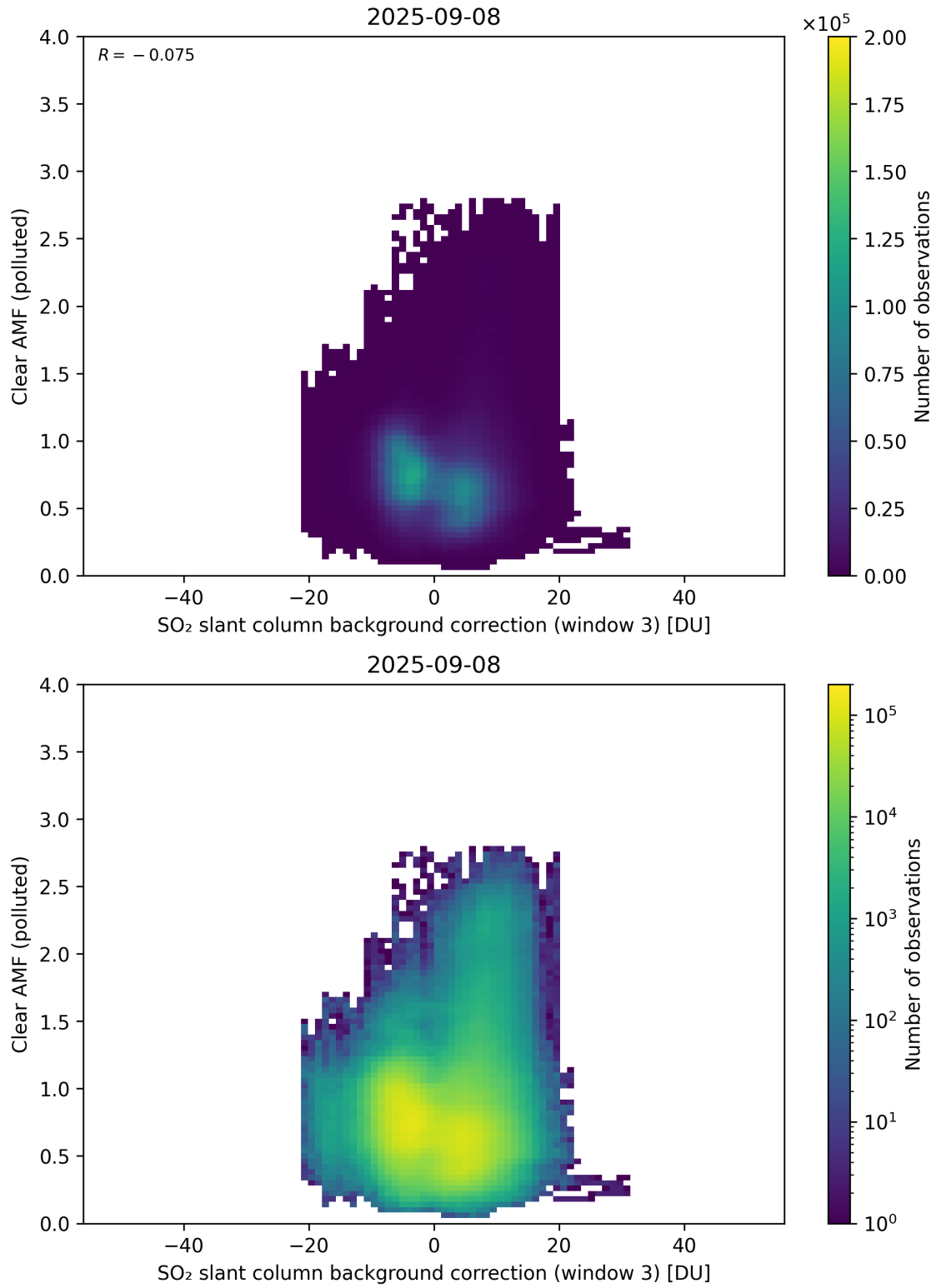
Figure 135: Scatter density plot of “SO 2 slant column background correction (window 3)” against “Clear AMF (polluted)” for 2025-09-07 to 2025-09-09.
