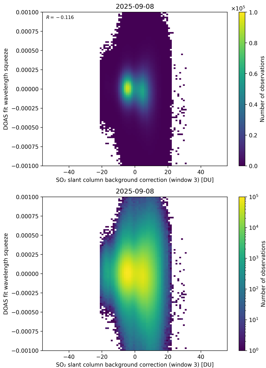
Figure 133: Scatter density plot of “SO 2 slant column background correction (window 3)” against “DOAS fit wavelength squeeze” for 2025-09-07 to 2025-09-09.
