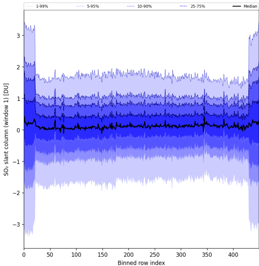
Figure 89: Along track statistics of “SO 2 slant column (window 1)” for 2025-09-07 to 2025-09-09
