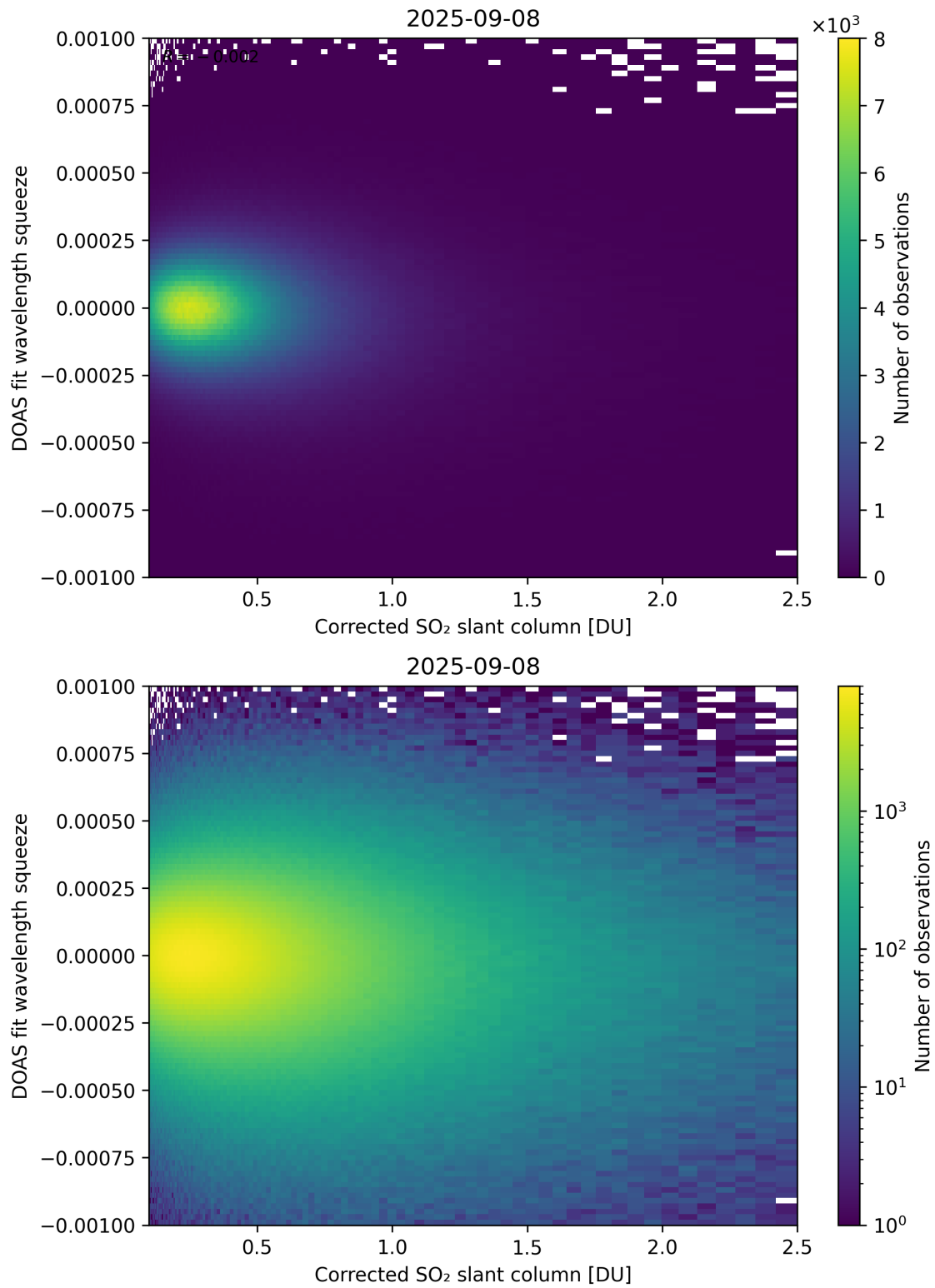
Figure 230: Scatter density plot of "Corrected SO 2 slant column" against "DOAS fit wavelength squeeze" for 2025-09-07 to 2025-09-09.
