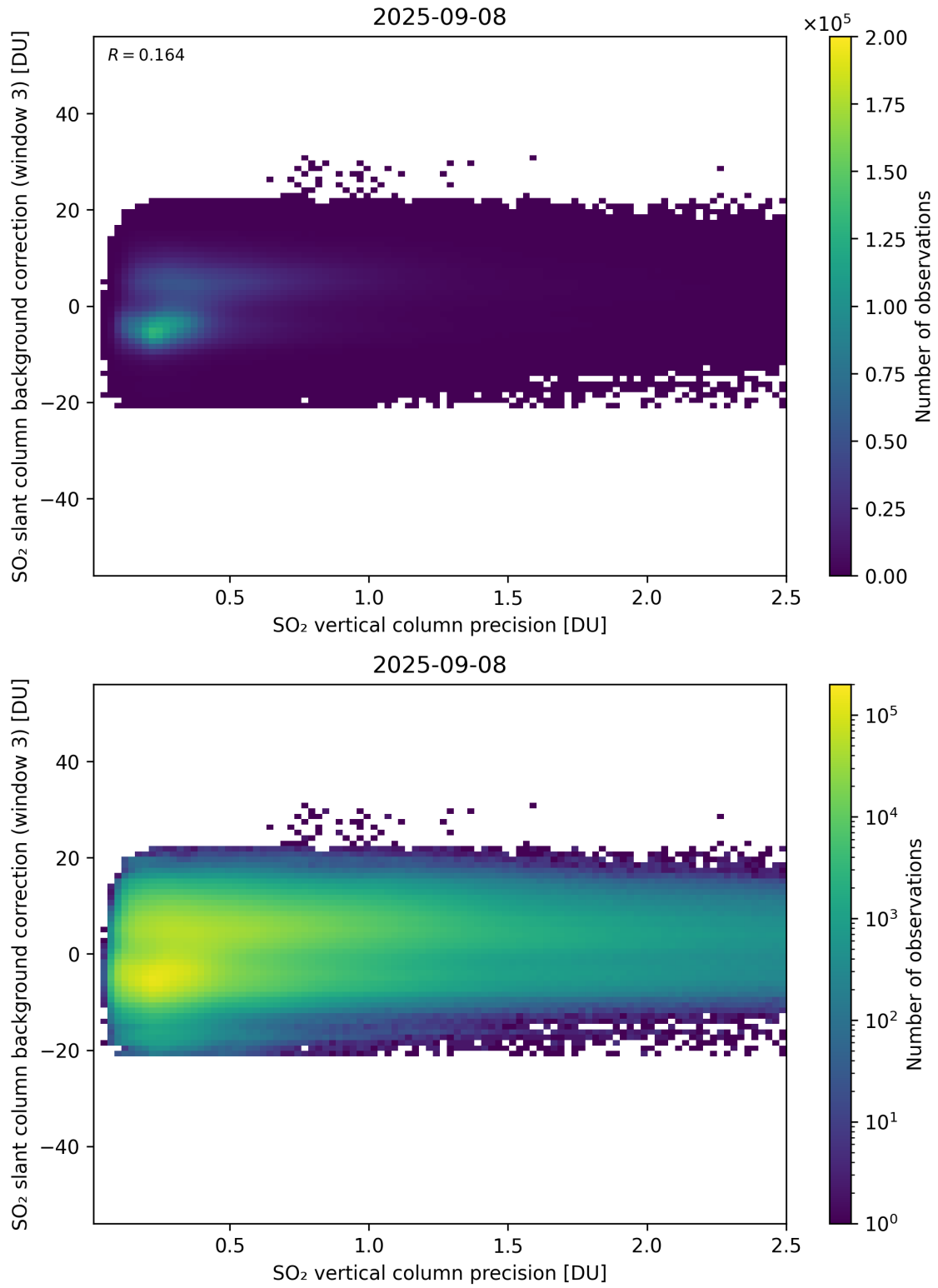
Figure 331: Scatter density plot of “SO 2 vertical column precision” against “SO 2 slant column background correction (window 3)” for 2025-09-07 to 2025-09-09.
