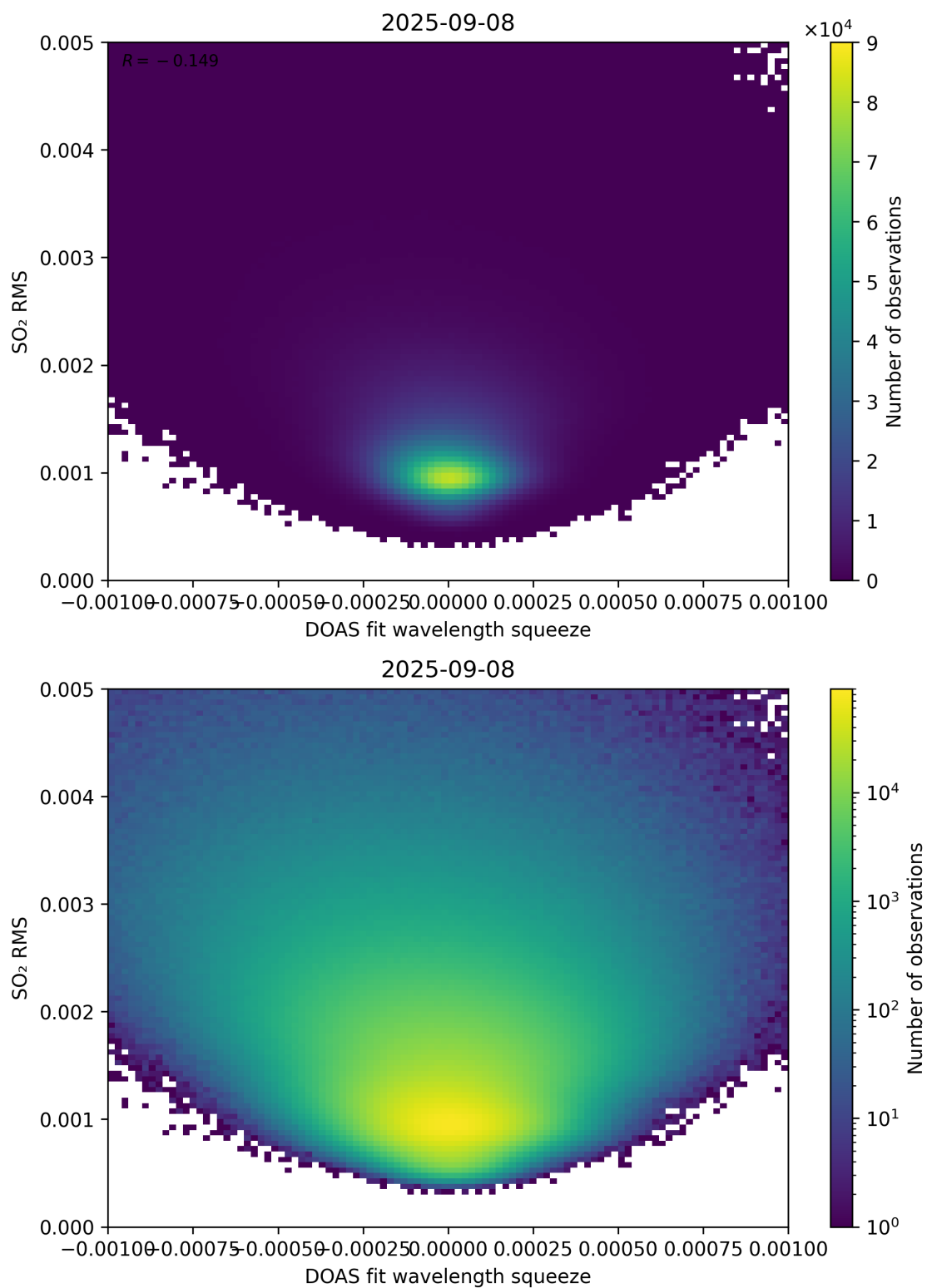
Figure 143: Scatter density plot of “DOAS fit wavelength squeeze” against “SO 2 RMS” for 2025-09-07 to 2025-09-09.
