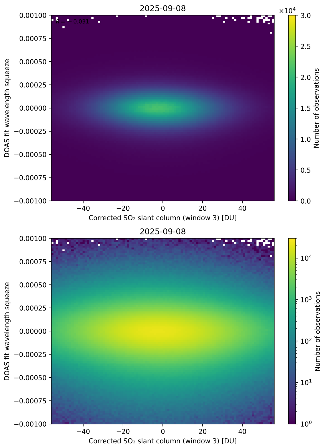
Figure 257: Scatter density plot of “Corrected SO 2 slant column (window 3)” against “DOAS fit wavelength squeeze” for 2025-09-07 to 2025-09-09.
