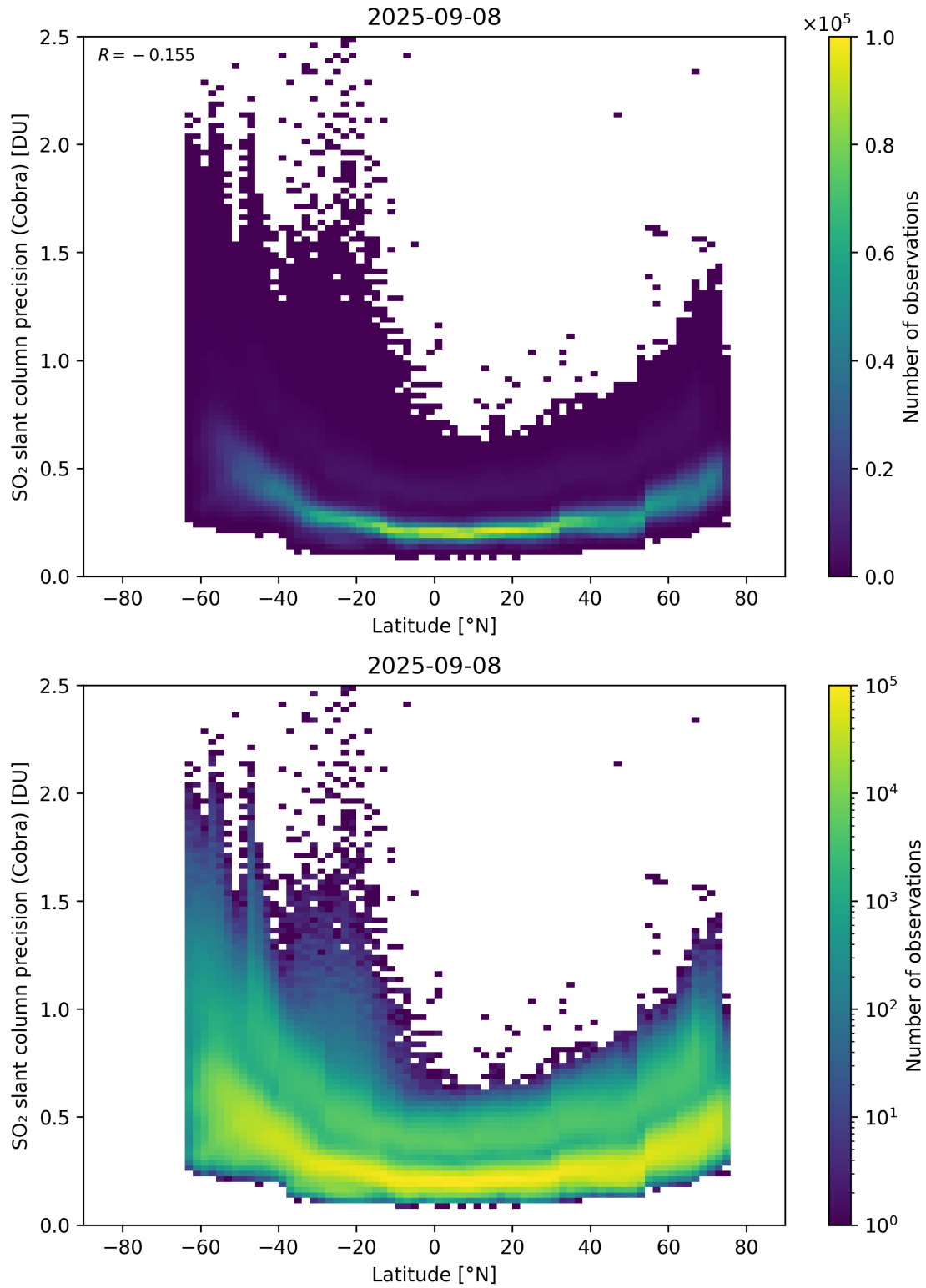
Figure 158: Scatter density plot of “Latitude” against “SO 2 slant column precision (Cobra)” for 2025-09-07 to 2025-09-09.
