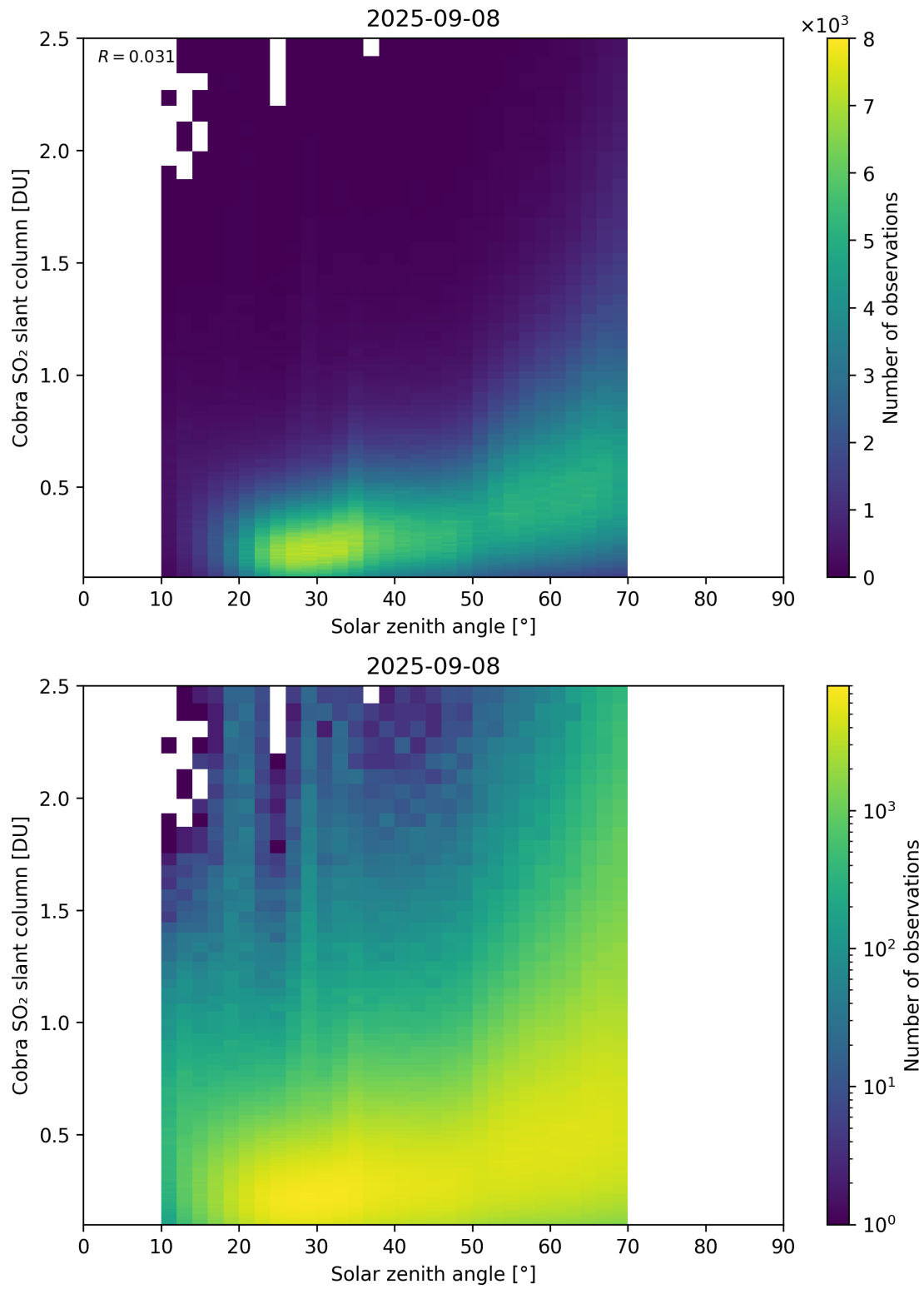
Figure 179: Scatter density plot of “Solar zenith angle” against “Cobra SO 2 slant column” for 2025-09-07 to 2025-09-09.
