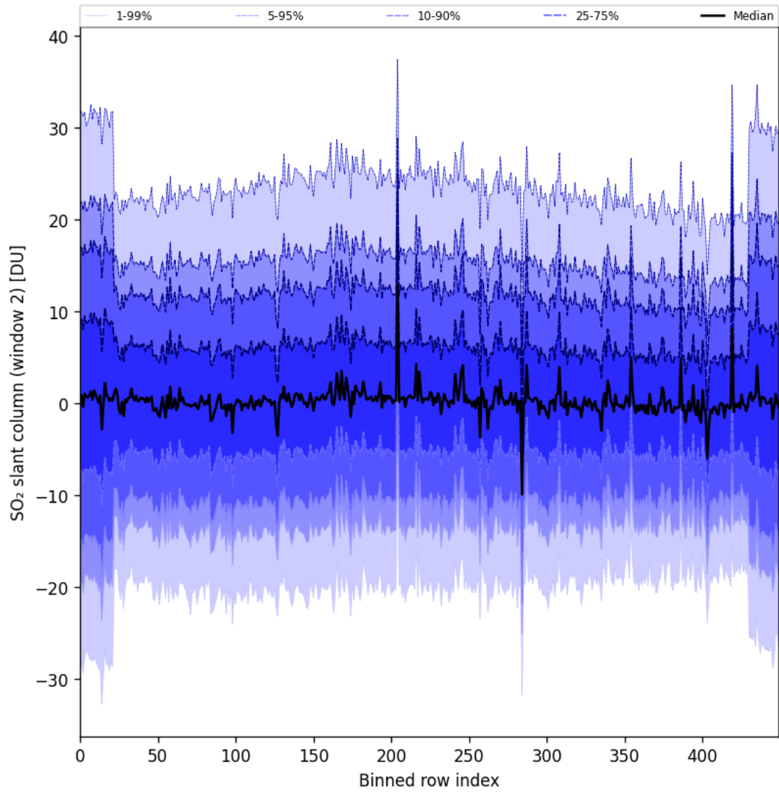
Figure 93: Along track statistics of “SO 2 slant column (window 2)” for 2025-09-07 to 2025-09-09
