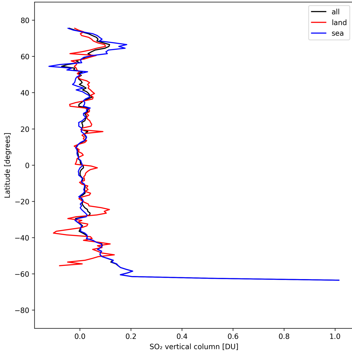
Figure 32: Zonal average of “SO 2 vertical column” for 2025-09-07 to 2025-09-09.
