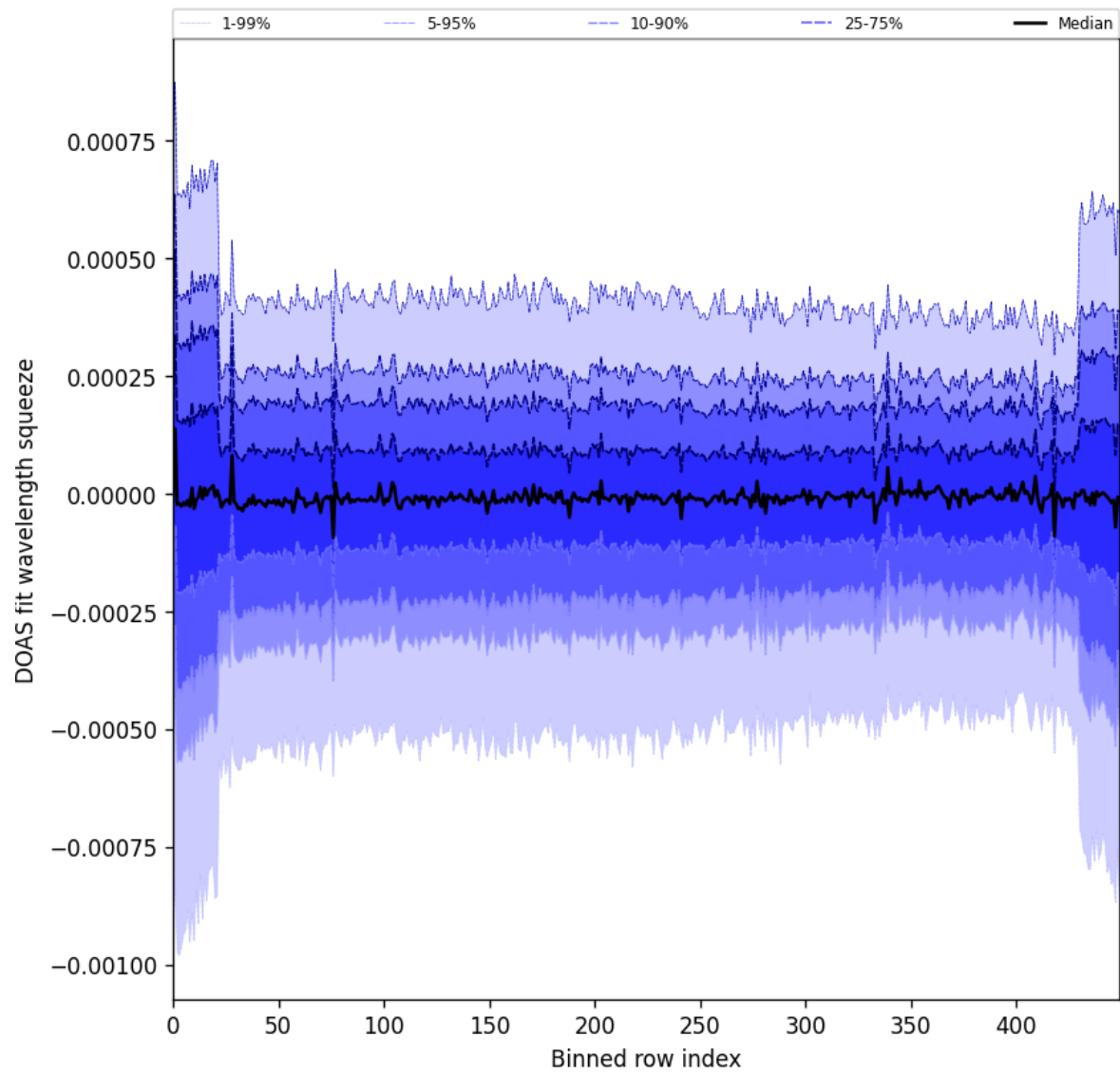
Figure 103: Along track statistics of “DOAS fit wavelength squeeze” for 2025-09-07 to 2025-09-09
