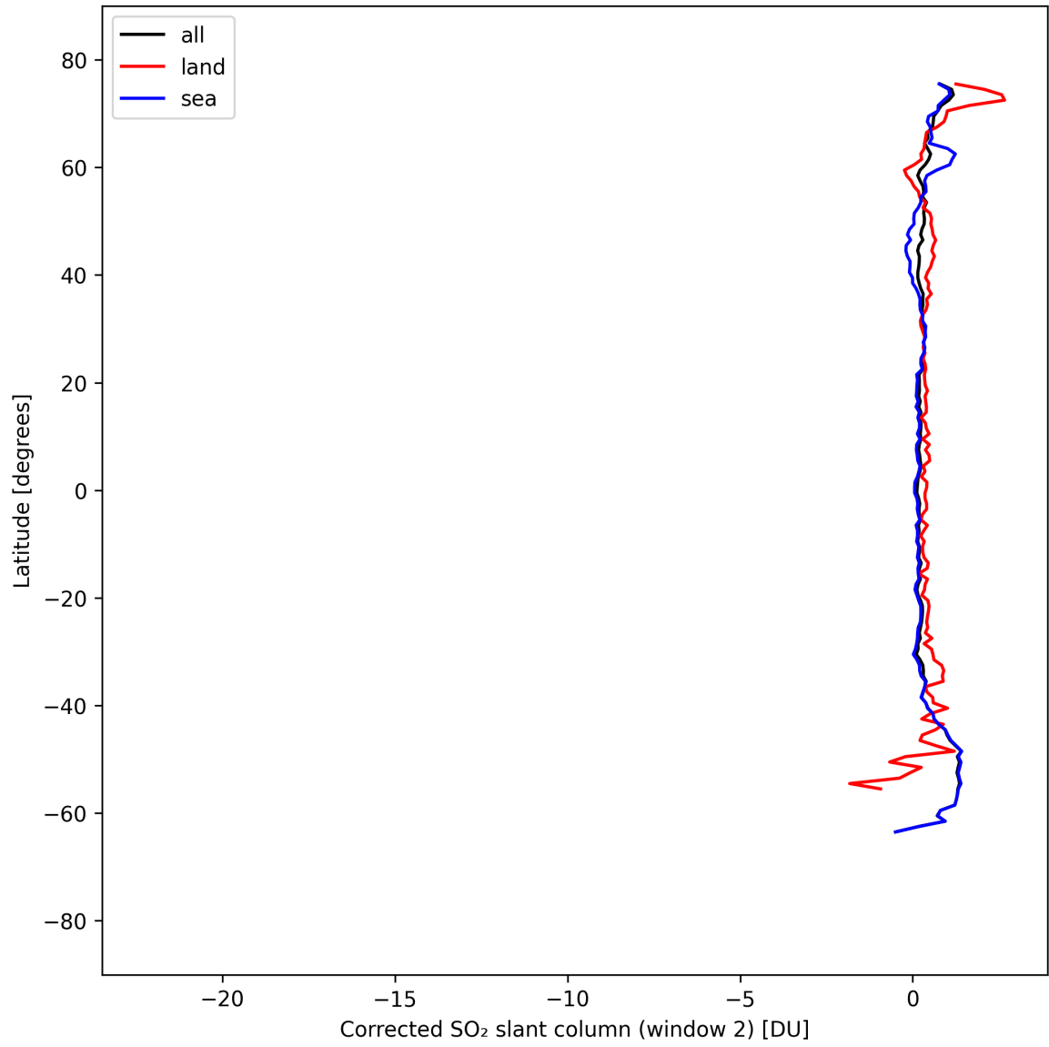
Figure 43: Zonal average of “Corrected SO 2 slant column (window 2)” for 2025-09-07 to 2025-09-09.
