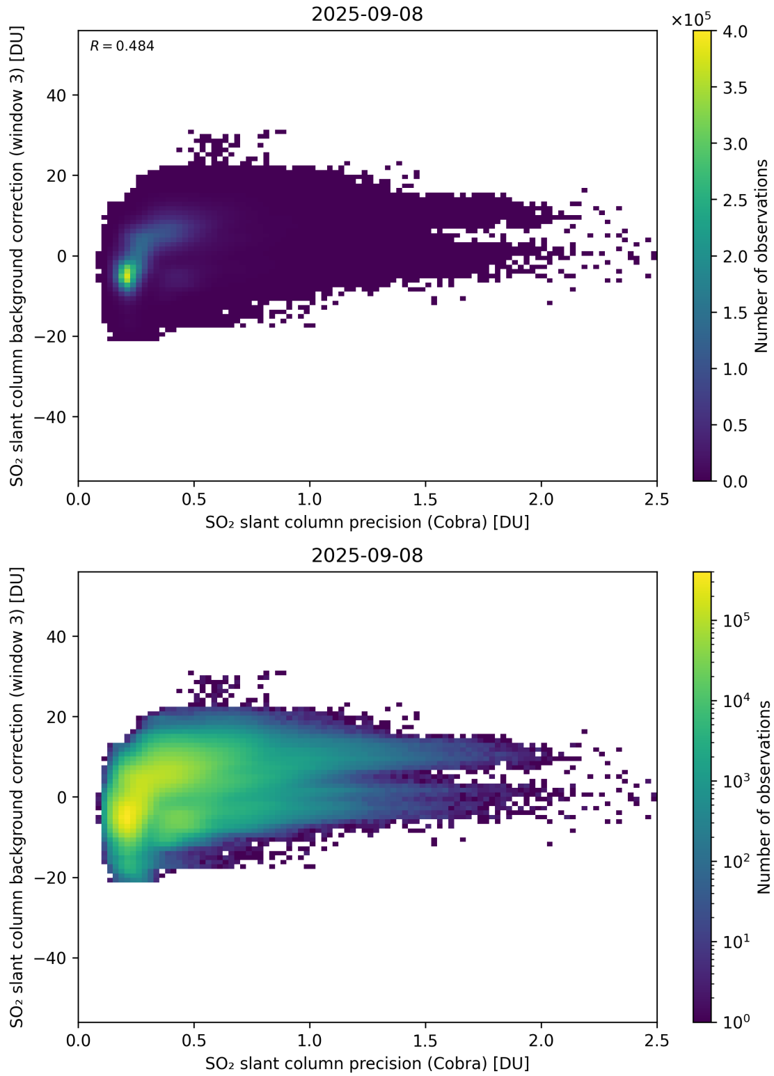
Figure 201: Scatter density plot of “SO 2 slant column precision (Cobra)” against “SO 2 slant column background correction (window 3)” for 2025-09-07 to 2025-09-09.
