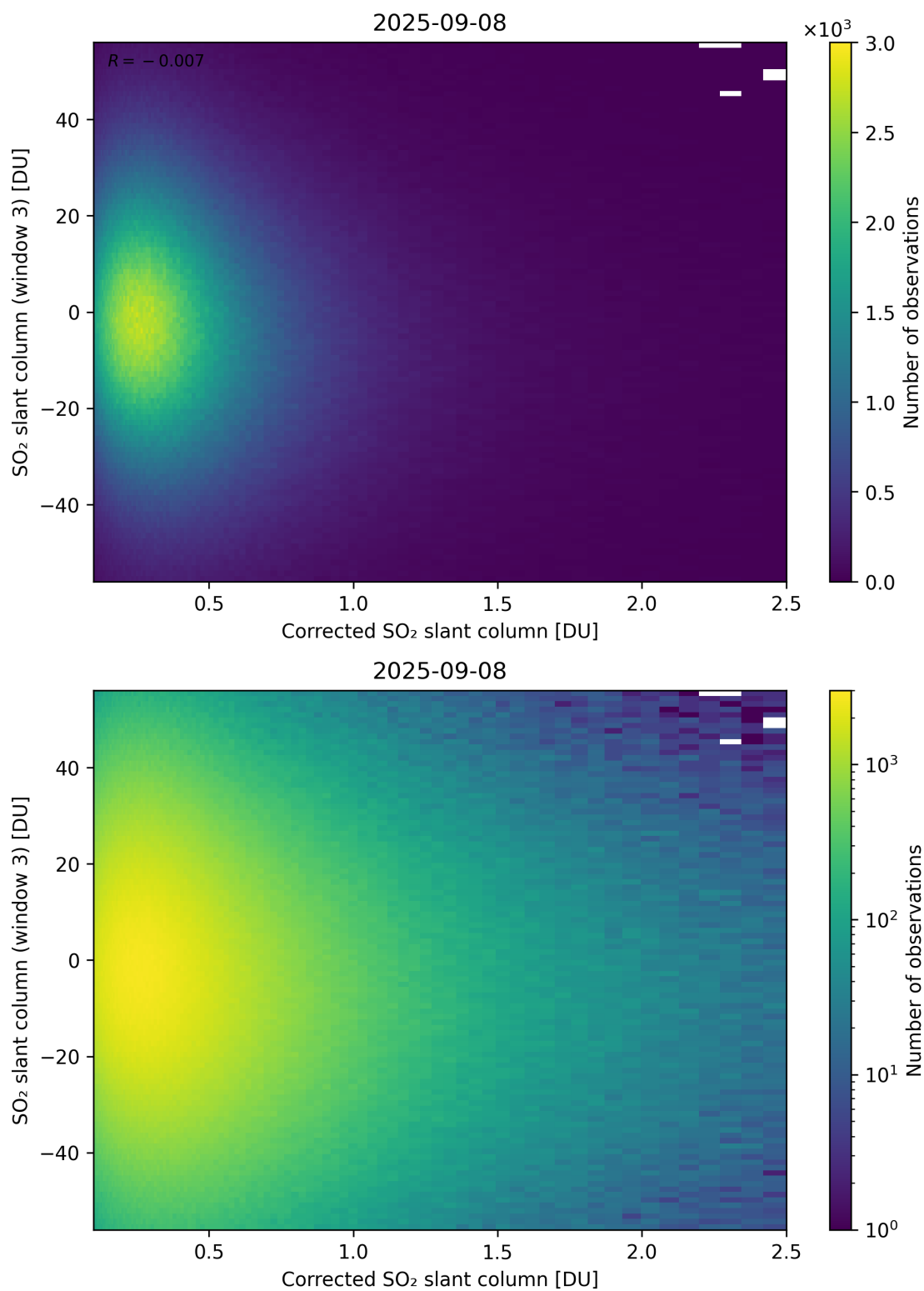
Figure 240: Scatter density plot of “Corrected SO 2 slant column” against “SO 2 slant column (window 3)” for 2025-09-07 to 2025-09-09.
