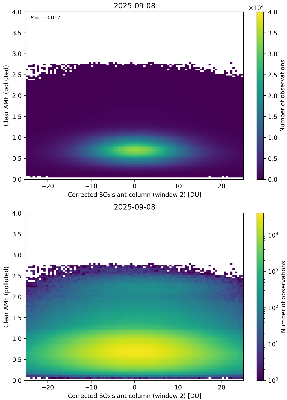
Figure 249: Scatter density plot of “Corrected SO 2 slant column (window 2)” against “Clear AMF (polluted)” for 2025-09-07 to 2025-09-09.
