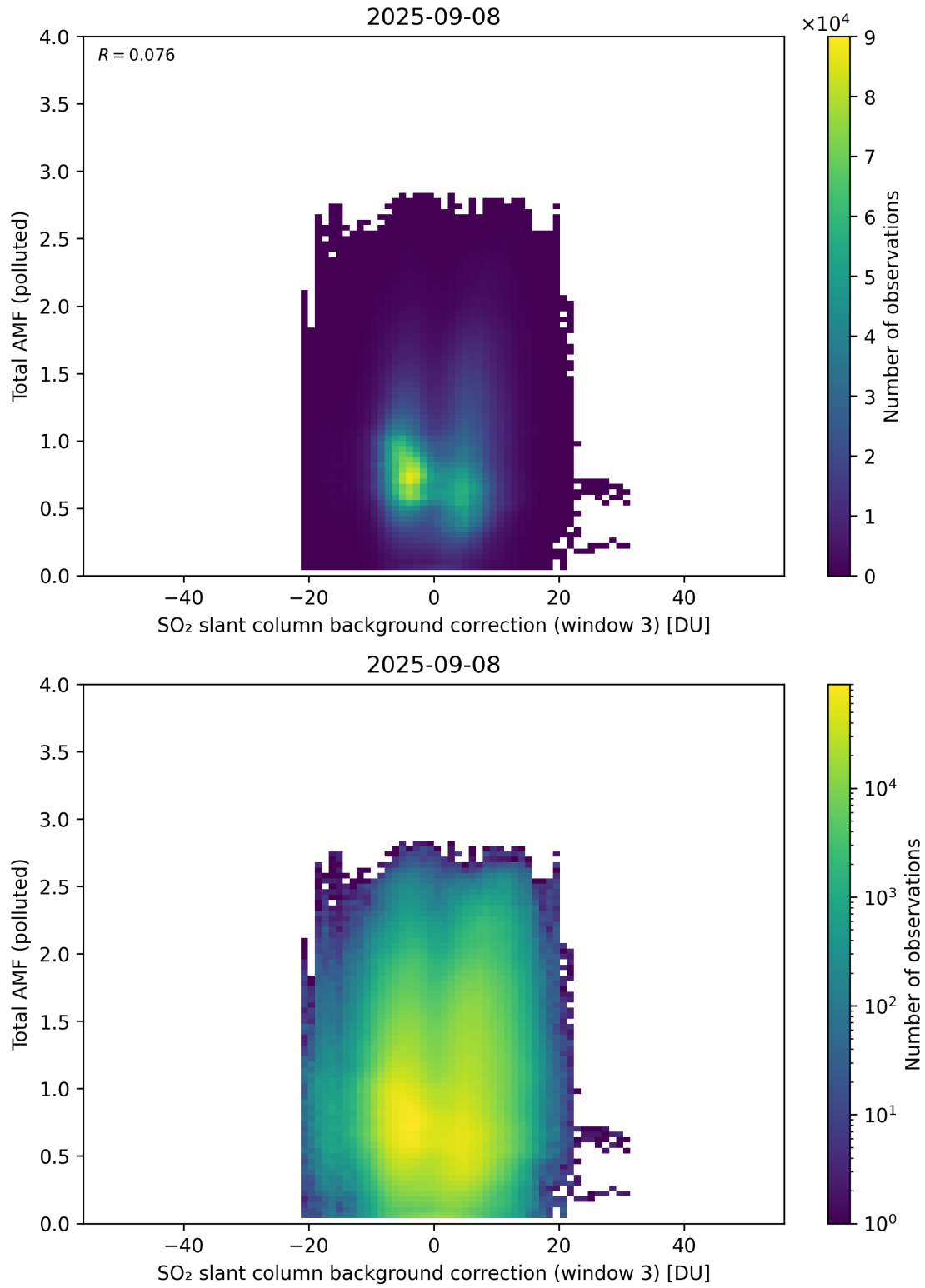
Figure 136: Scatter density plot of “SO 2 slant column background correction (window 3)” against “Total AMF (polluted)” for 2025-09-07 to 2025-09-09.
