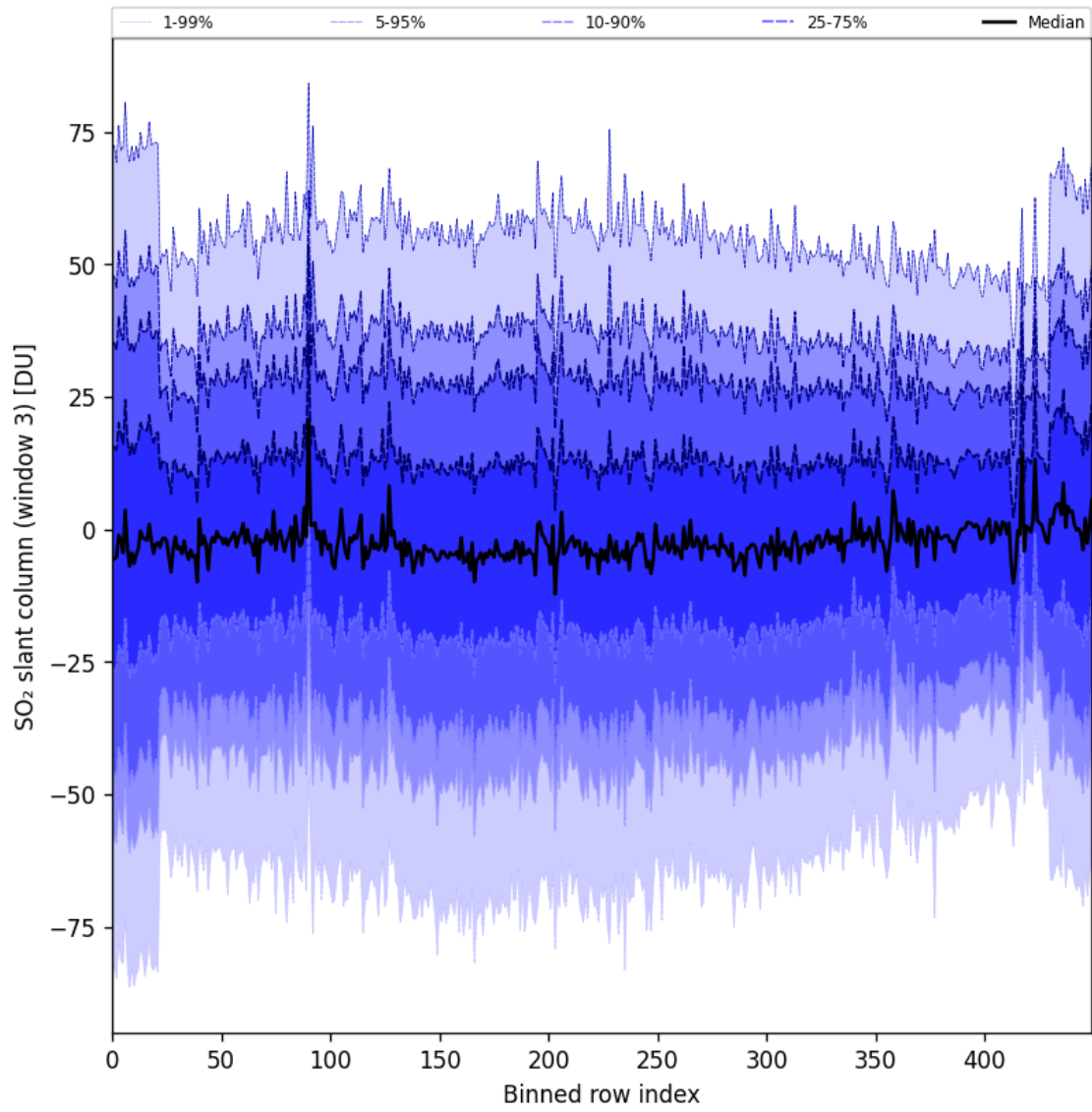
Figure 97: Along track statistics of “SO 2 slant column (window 3)” for 2025-09-07 to 2025-09-09
