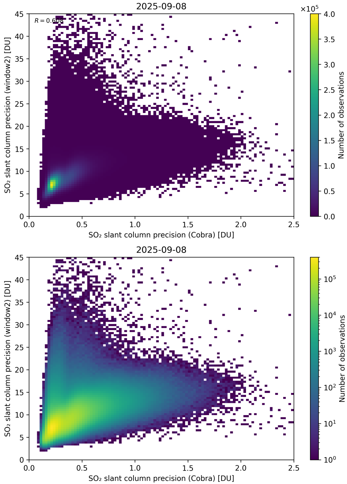
Figure 210: Scatter density plot of “SO 2 slant column precision (Cobra)” against “SO 2 slant column precision (window2)” for 2025-09-07 to 2025-09-09.
