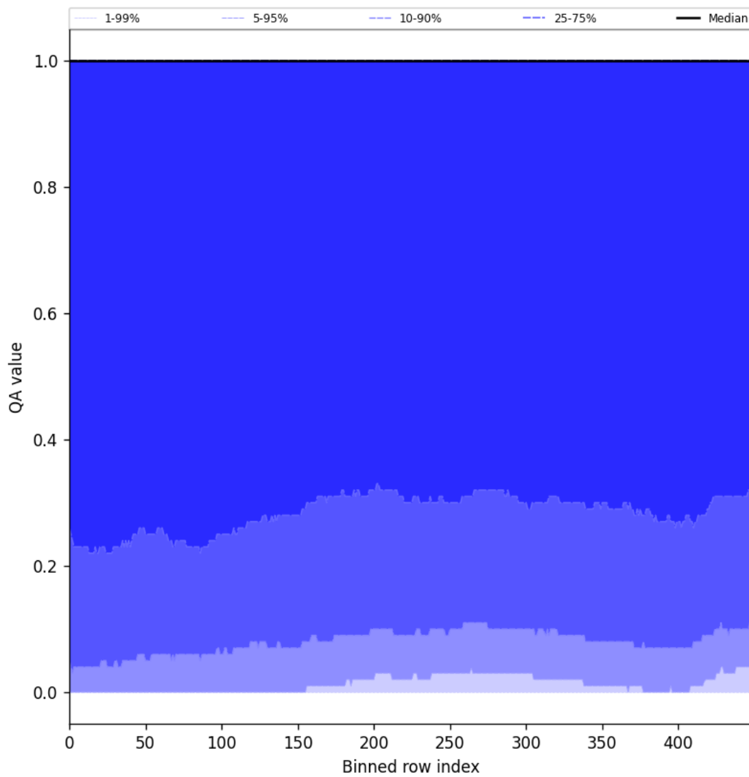
Figure 83: Along track statistics of “QA value” for 2025-09-07 to 2025-09-09
