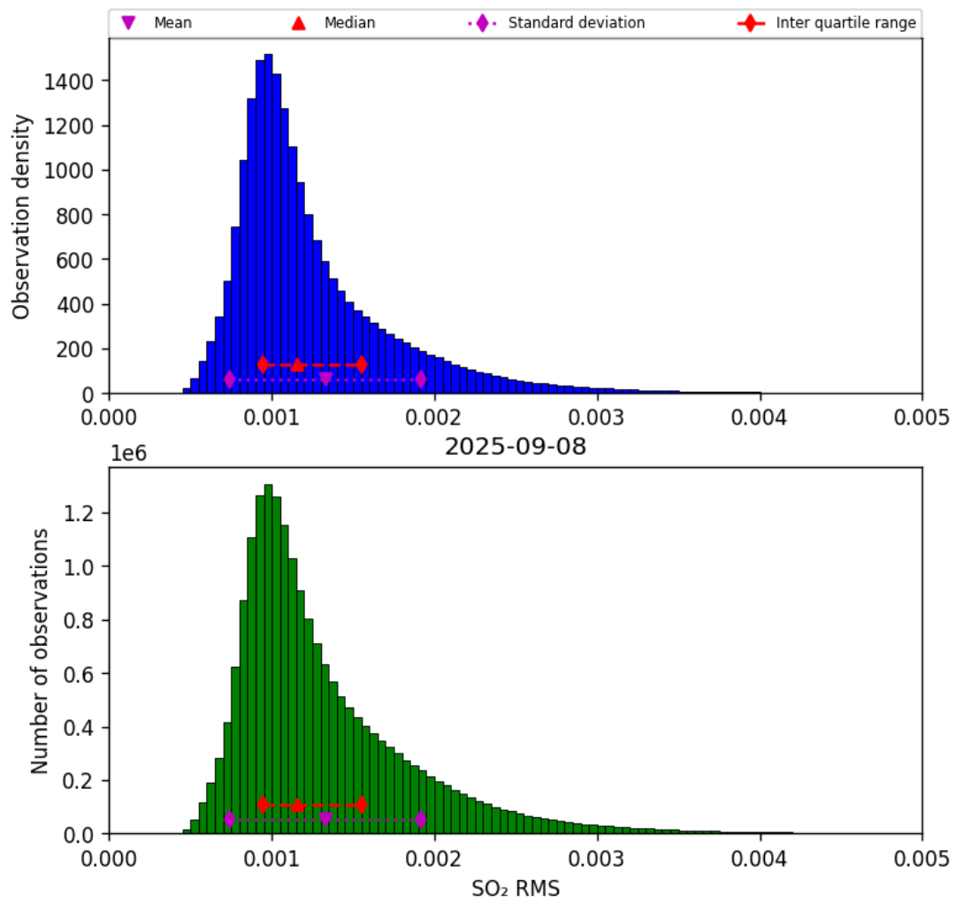
Figure 78: Histogram of “SO 2 RMS” for 2025-09-07 to 2025-09-09
