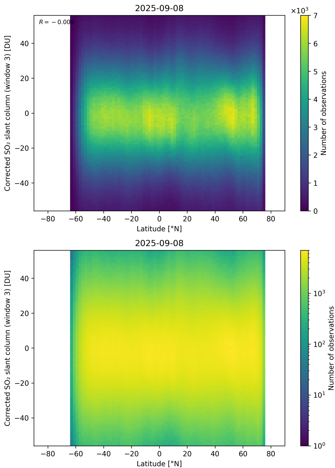
Figure 161: Scatter density plot of “Latitude” against “Corrected SO 2 slant column (window 3)” for 2025-09-07 to 2025-09-09.
