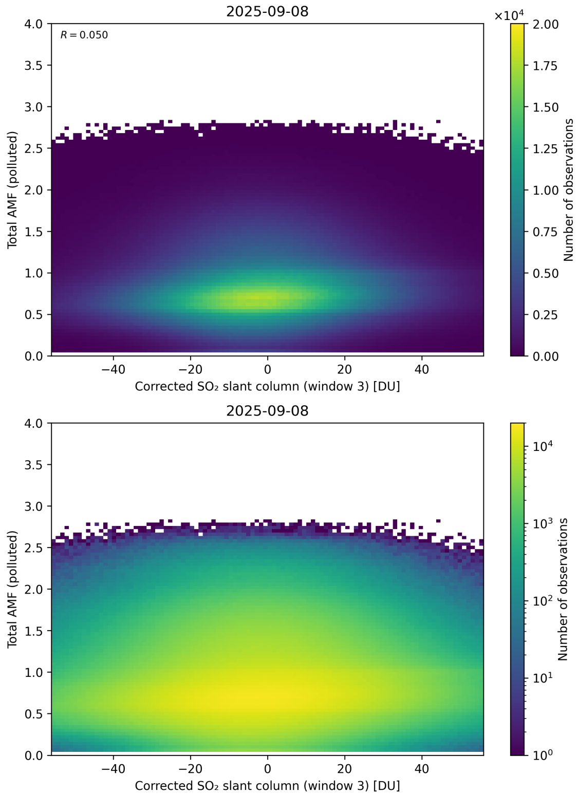
Figure 260: Scatter density plot of “Corrected SO 2 slant column (window 3)” against “Total AMF (polluted)” for 2025-09-07 to 2025-09-09.
