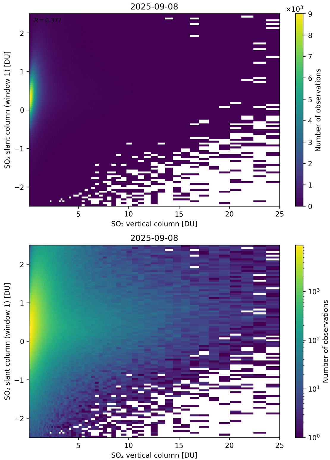
Figure 354: Scatter density plot of “SO 2 vertical column” against “SO 2 slant column (window 1)” for 2025-09-07 to 2025-09-09.
