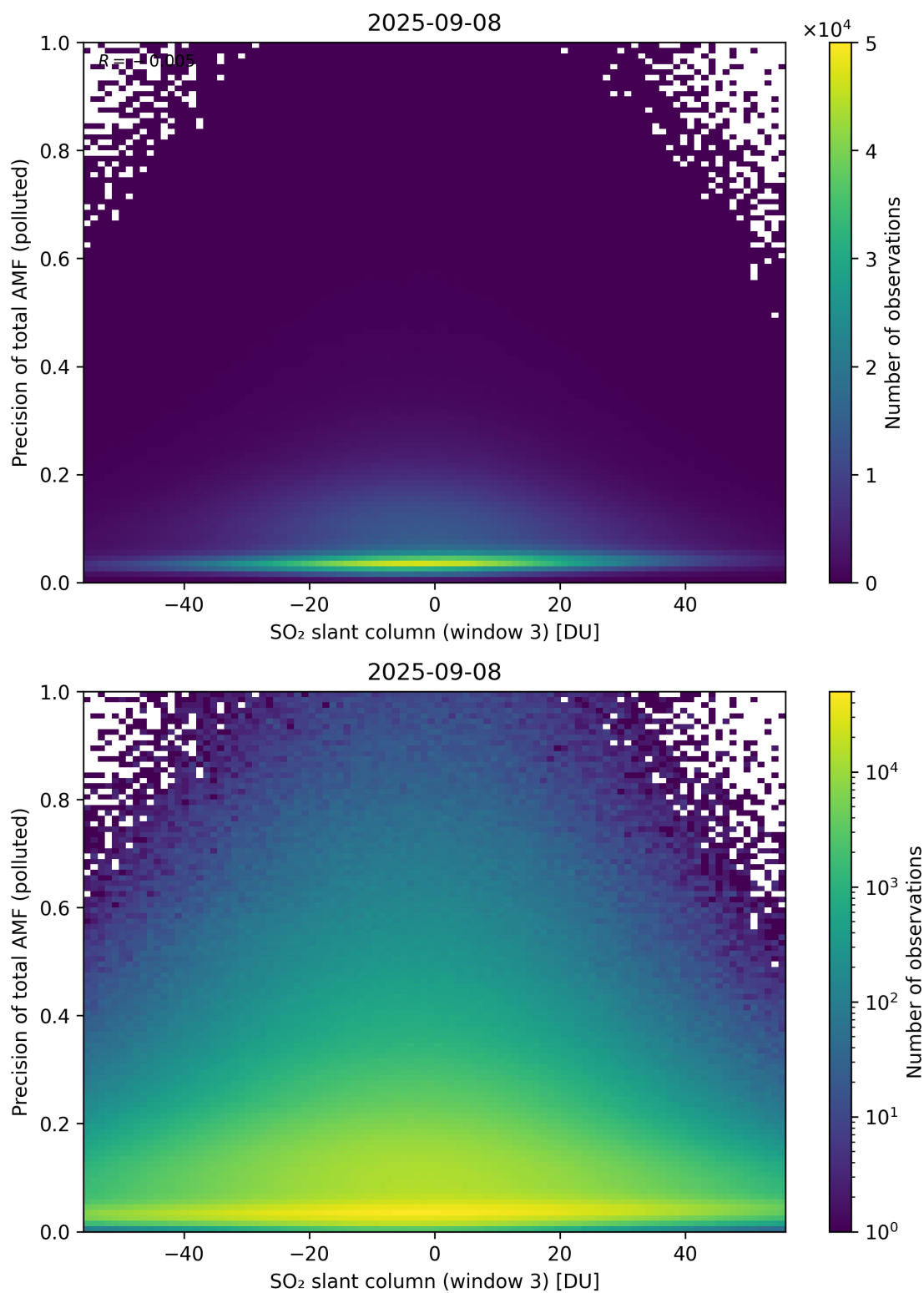
Figure 319: Scatter density plot of “SO 2 slant column (window 3)” against “Precision of total AMF (polluted)” for 2025-09-07 to 2025-09-09.
