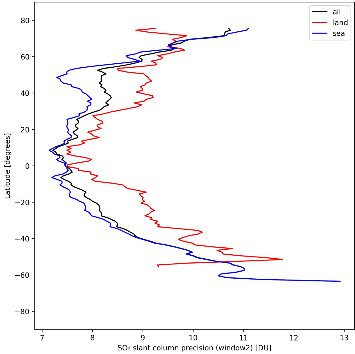
Figure 42: Zonal average of “SO 2 slant column precision (window2)” for 2025-09-07 to 2025-09-09.
