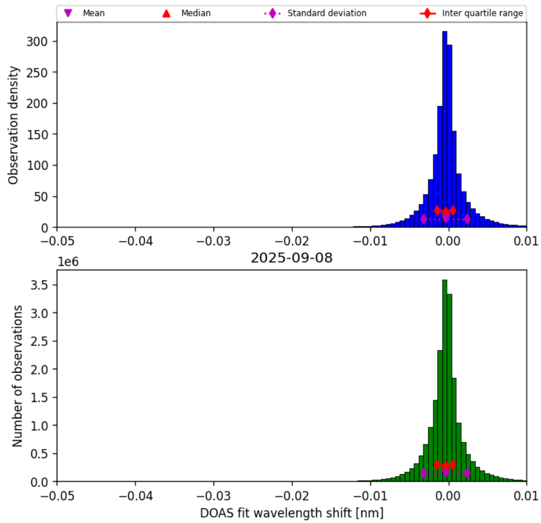
Figure 76: Histogram of “DOAS fit wavelength shift” for 2025-09-07 to 2025-09-09
