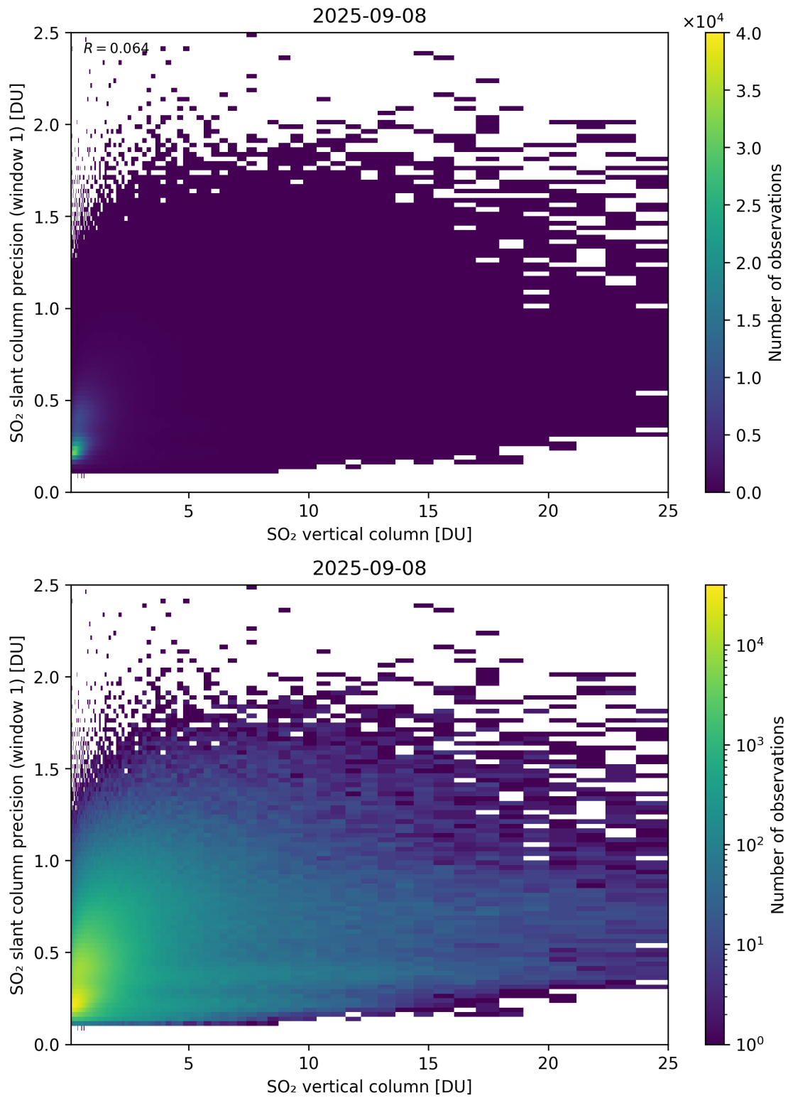
Figure 355: Scatter density plot of “SO 2 vertical column” against “SO 2 slant column precision (window 1)” for 2025-09-07 to 2025-09-09.
