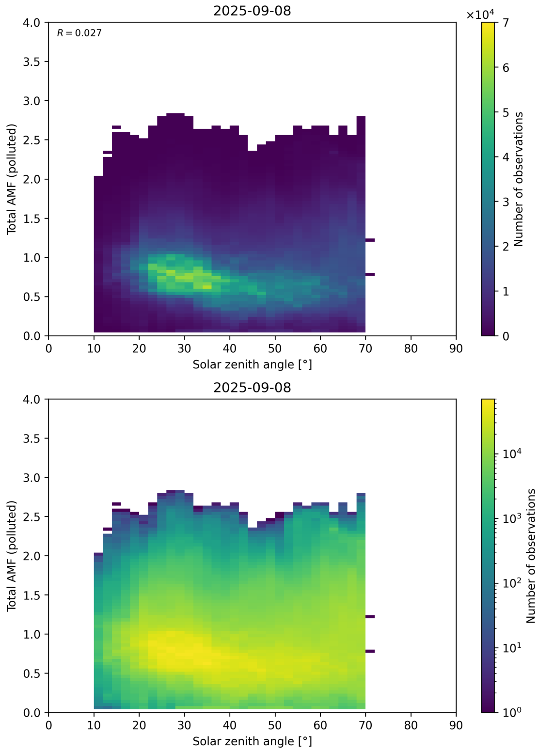
Figure 189: Scatter density plot of “Solar zenith angle” against “Total AMF (polluted)” for 2025-09-07 to 2025-09-09.
