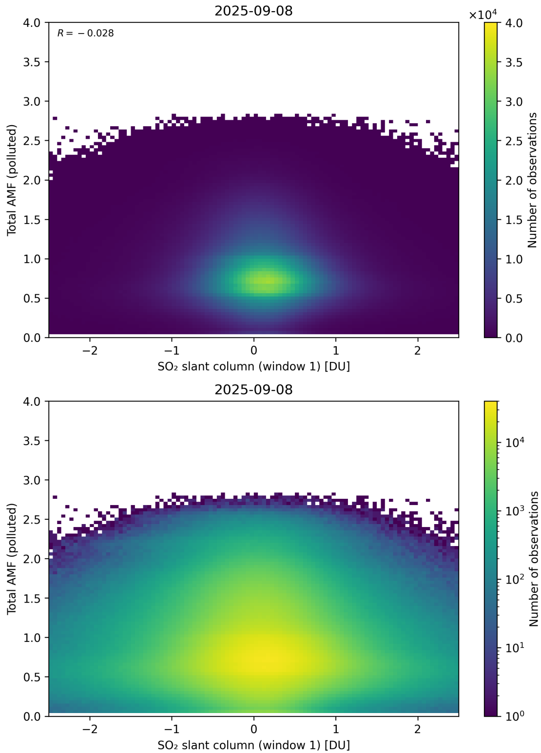
Figure 289: Scatter density plot of “SO 2 slant column (window 1)” against “Total AMF (polluted)” for 2025-09-07 to 2025-09-09.
