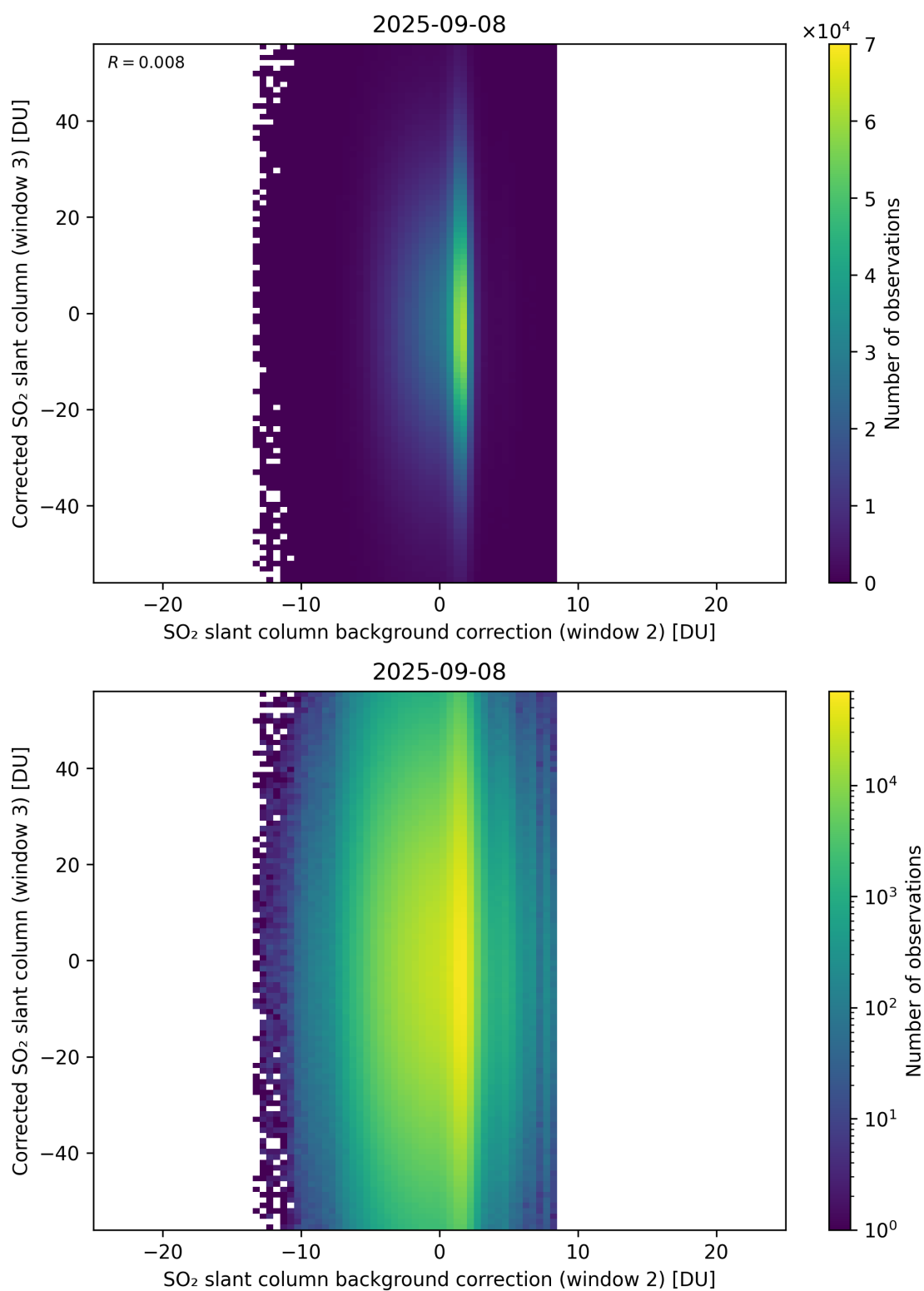
Figure 127: Scatter density plot of “SO 2 slant column background correction (window 2)” against “Corrected SO 2 slant column (window 3)” for 2025-09-07 to 2025-09-09.
