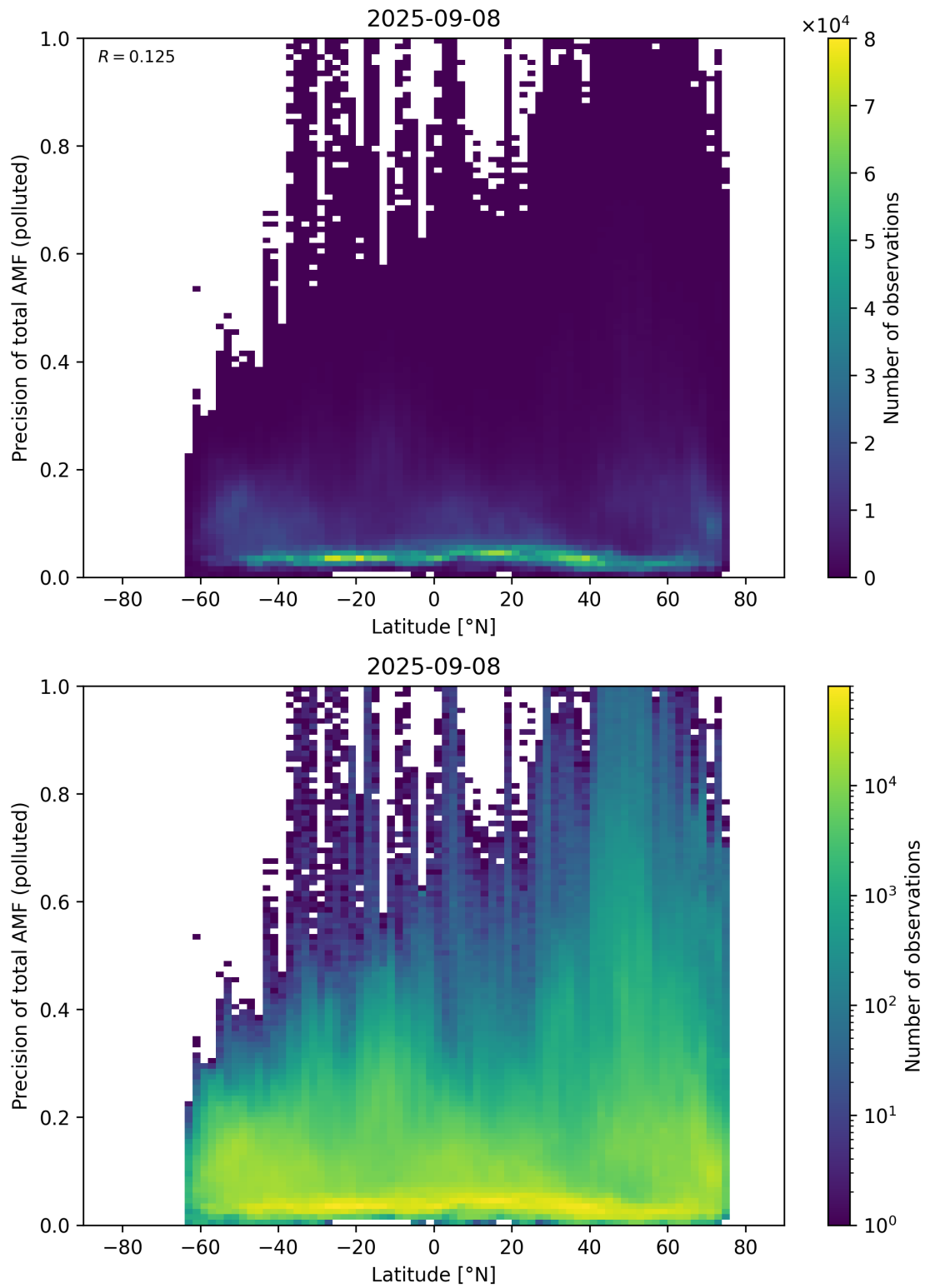
Figure 168: Scatter density plot of “Latitude” against “Precision of total AMF (polluted)” for 2025-09-07 to 2025-09-09.
