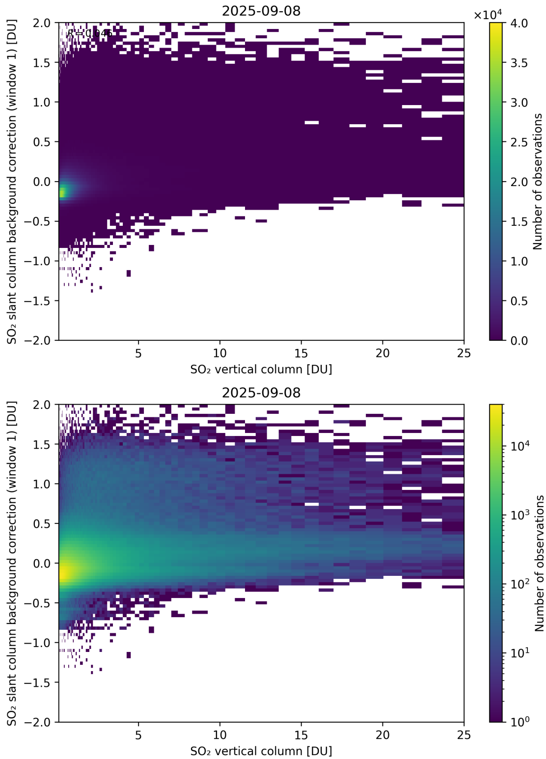
Figure 323: Scatter density plot of “SO 2 vertical column” against “SO 2 slant column background correction (window 1)” for 2025-09-07 to 2025-09-09.
