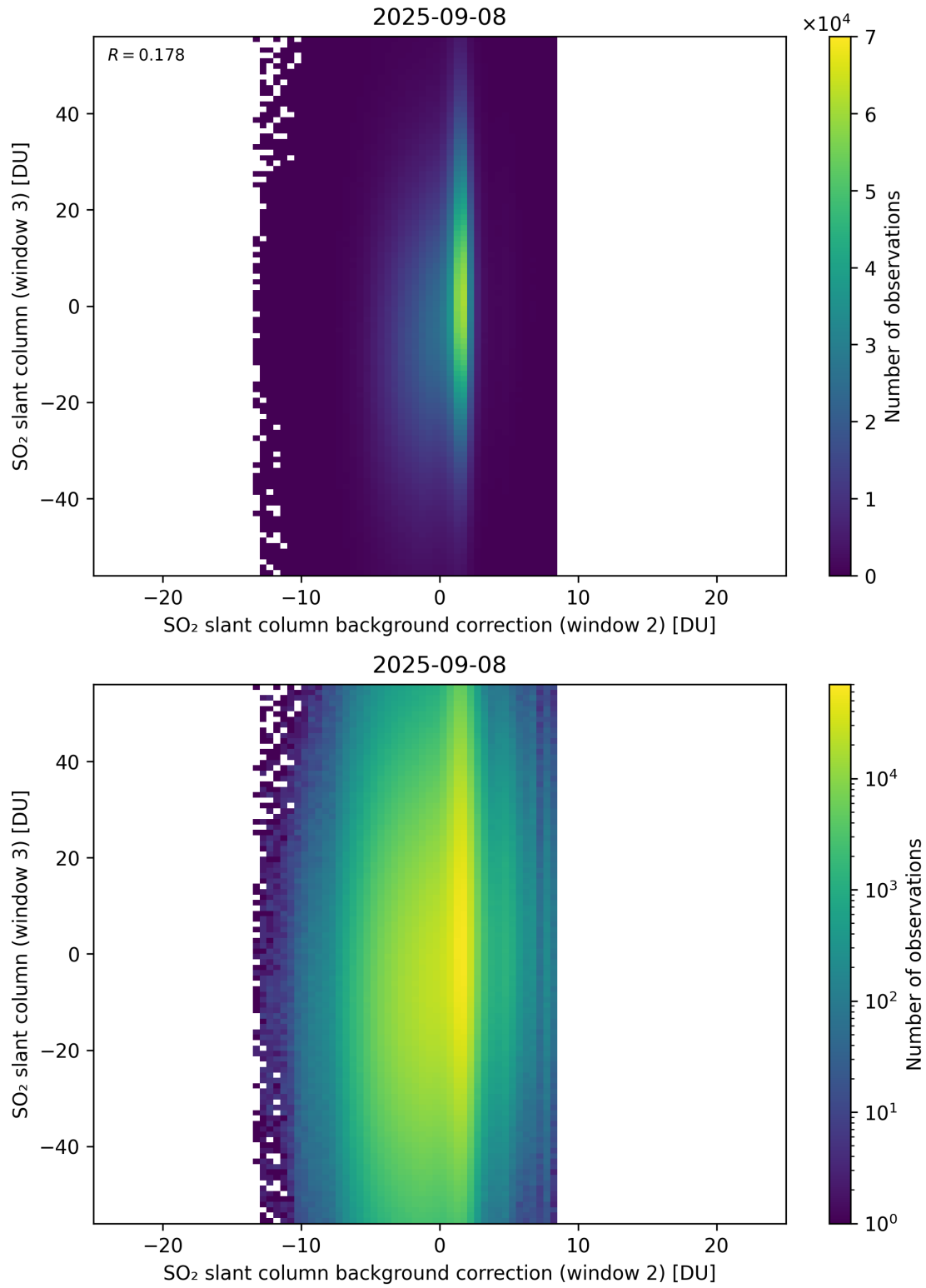
Figure 128: Scatter density plot of “SO 2 slant column background correction (window 2)” against “SO 2 slant column (window 3)” for 2025-09-07 to 2025-09-09.
