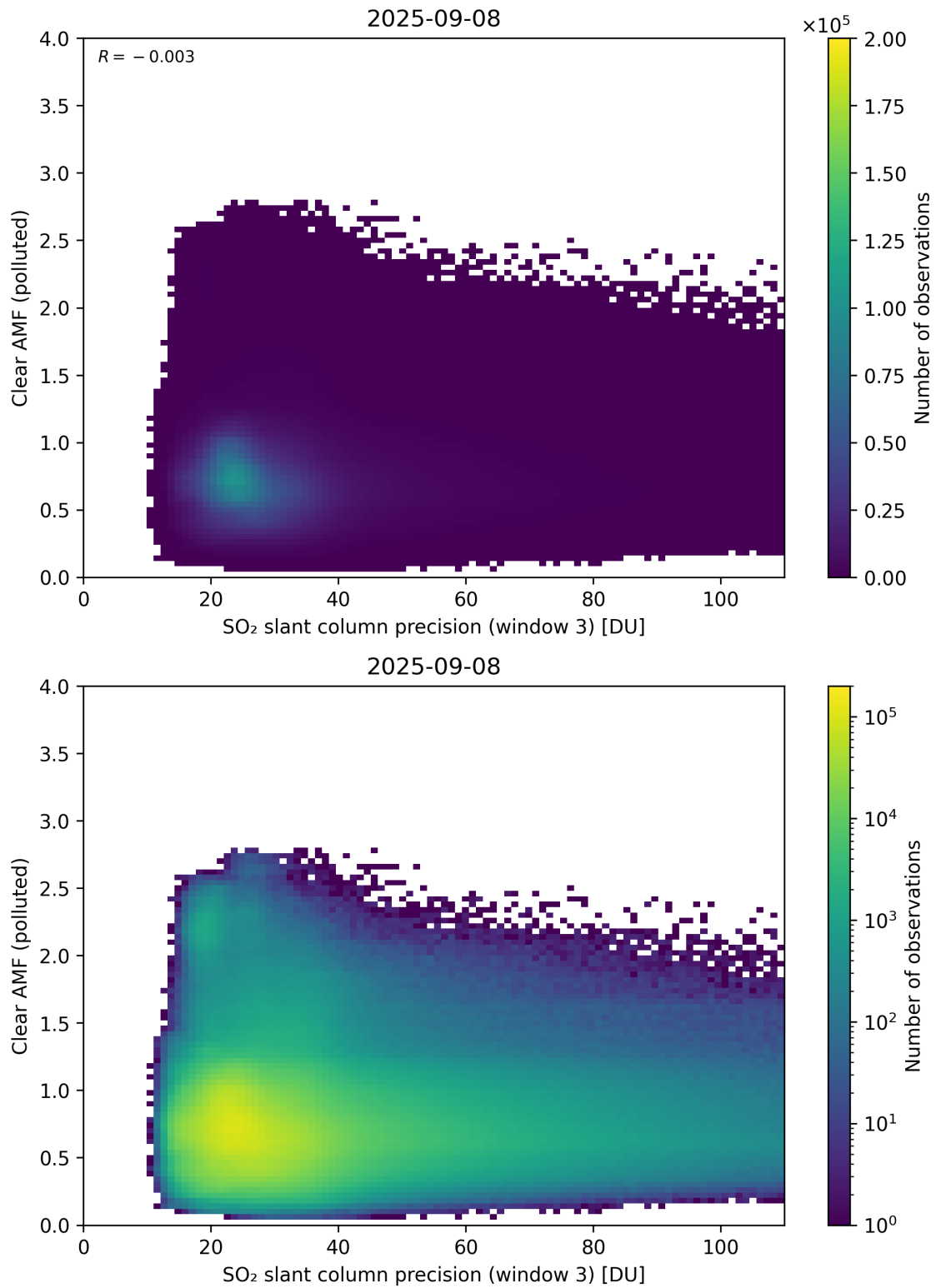
Figure 311: Scatter density plot of “SO 2 slant column precision (window 3)” against “Clear AMF (polluted)” for 2025-09-07 to 2025-09-09.
