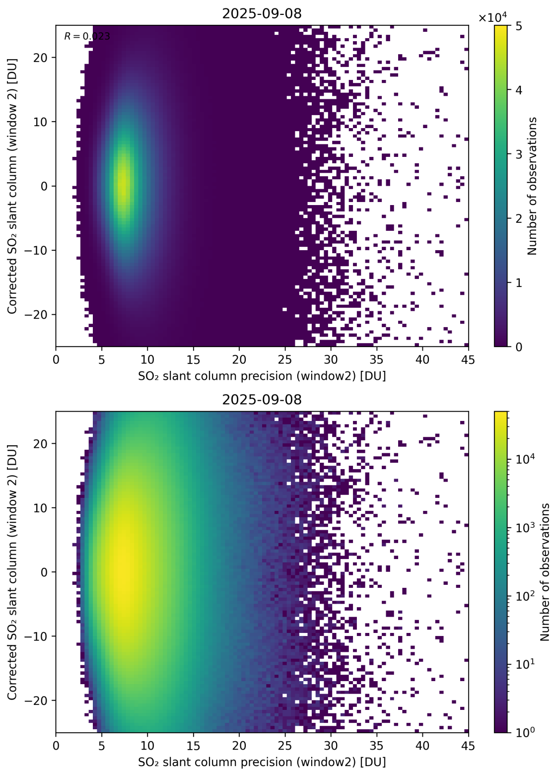
Figure 297: Scatter density plot of “SO 2 slant column precision (window2)” against “Corrected SO 2 slant column (window 2)” for 2025-09-07 to 2025-09-09.
