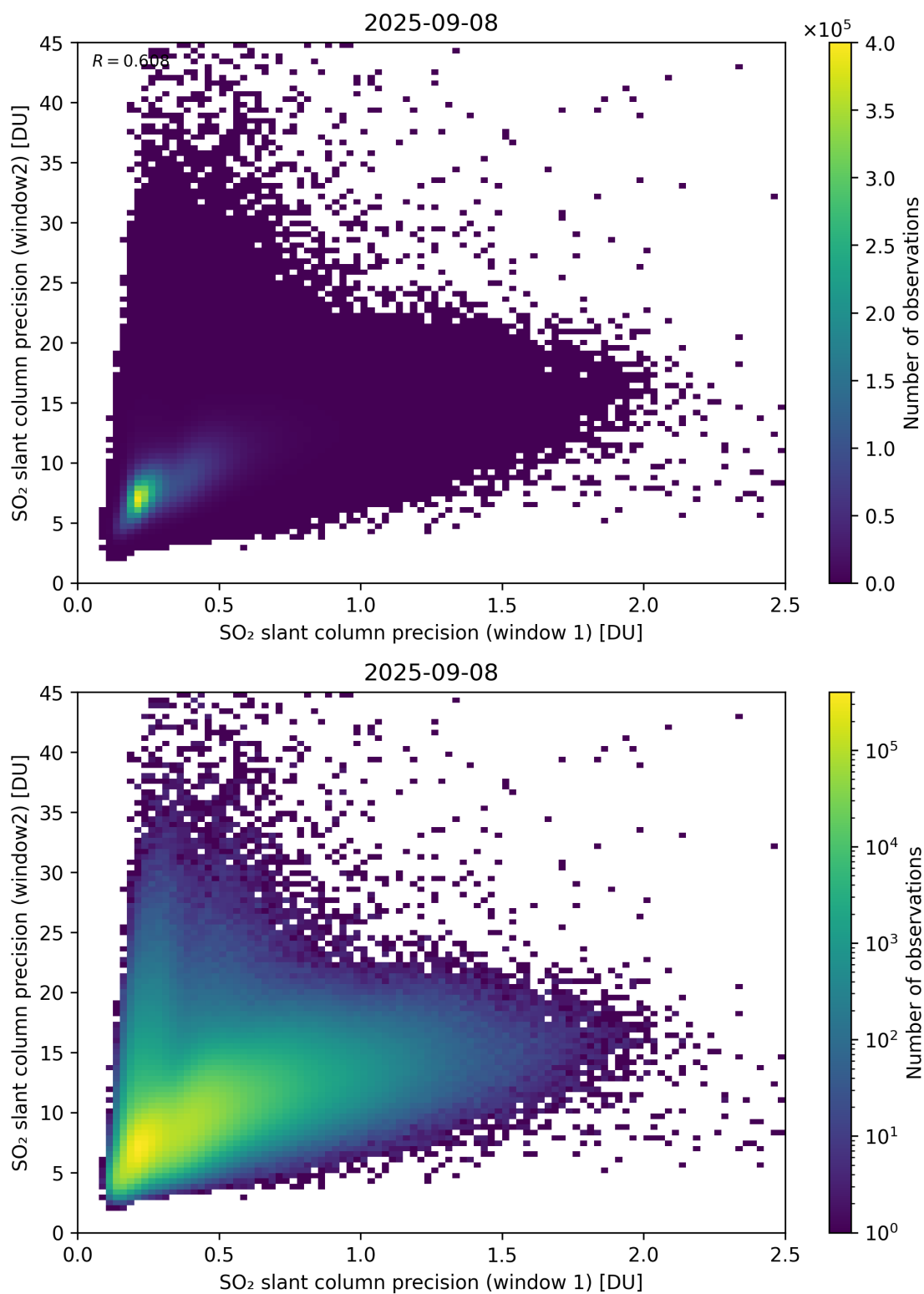
Figure 277: Scatter density plot of “SO 2 slant column precision (window 1)” against “SO 2 slant column precision (window2)” for 2025-09-07 to 2025-09-09.
