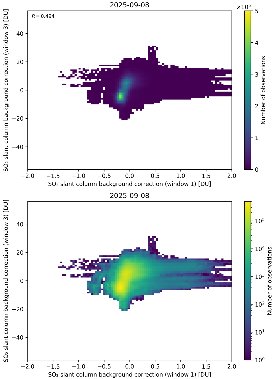
Figure 110: Scatter density plot of “SO 2 slant column background correction (window 1)” against “SO 2 slant column background correction (window 3)” for 2025-09-07 to 2025-09-09.
