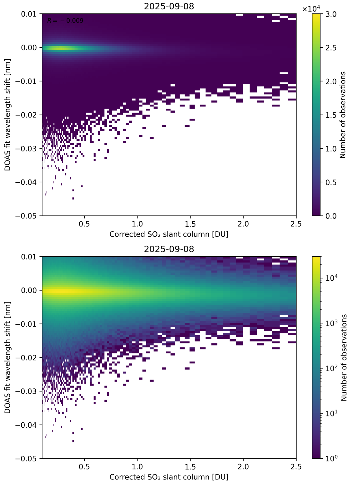
Figure 229: Scatter density plot of “Corrected SO 2 slant column” against “DOAS fit wavelength shift” for 2025-09-07 to 2025-09-09.
