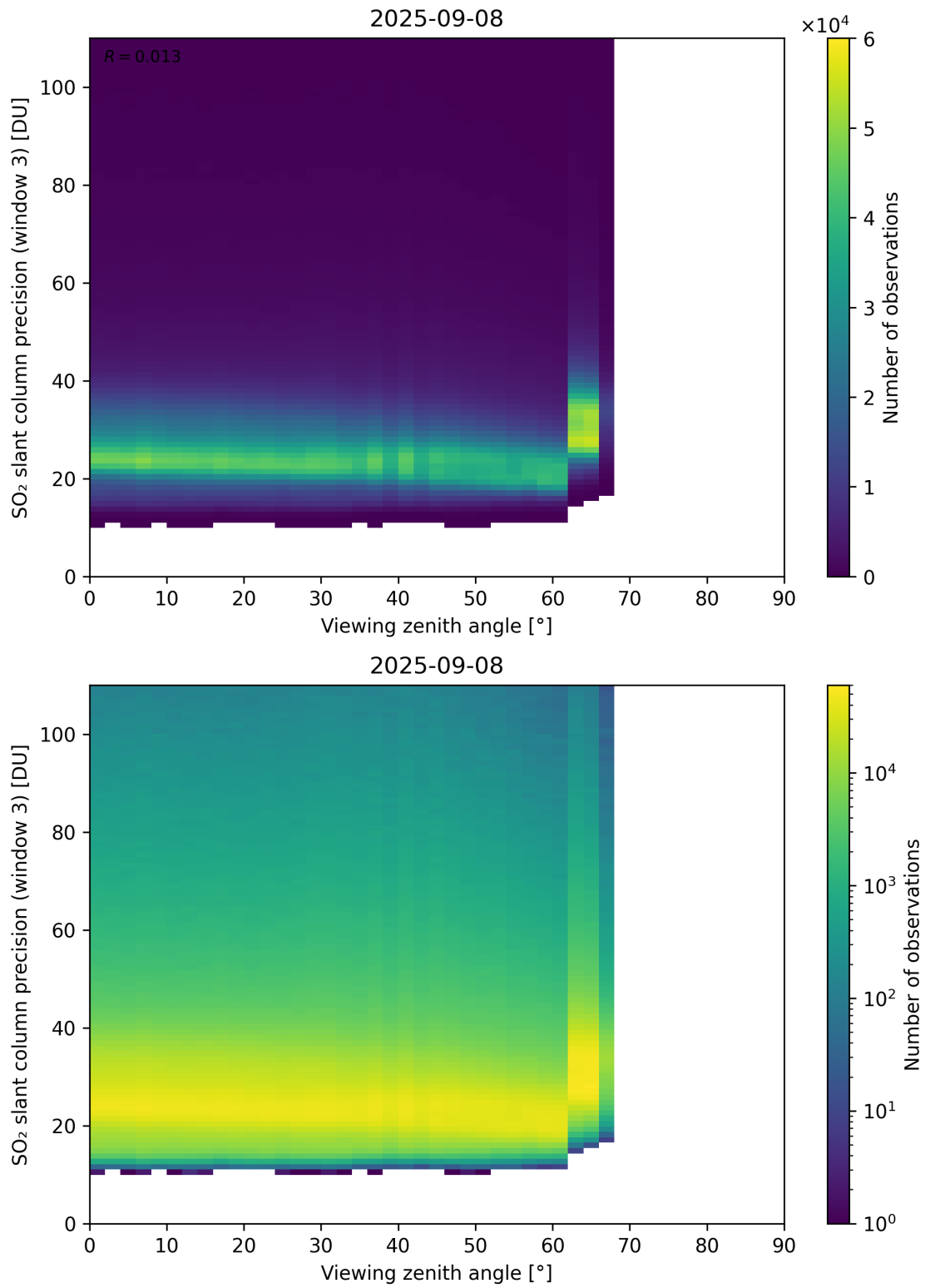
Figure 380: Scatter density plot of “Viewing zenith angle” against “SO 2 slant column precision (window 3)” for 2025-09-07 to 2025-09-09.
