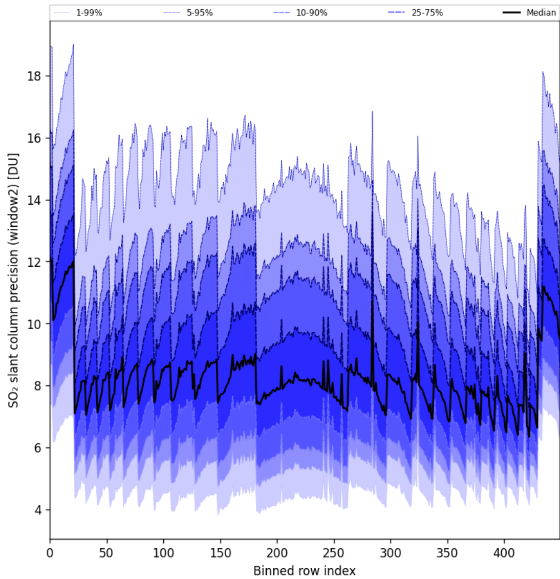
Figure 94: Along track statistics of “SO 2 slant column precision (window2)” for 2025-09-07 to 2025-09-09
