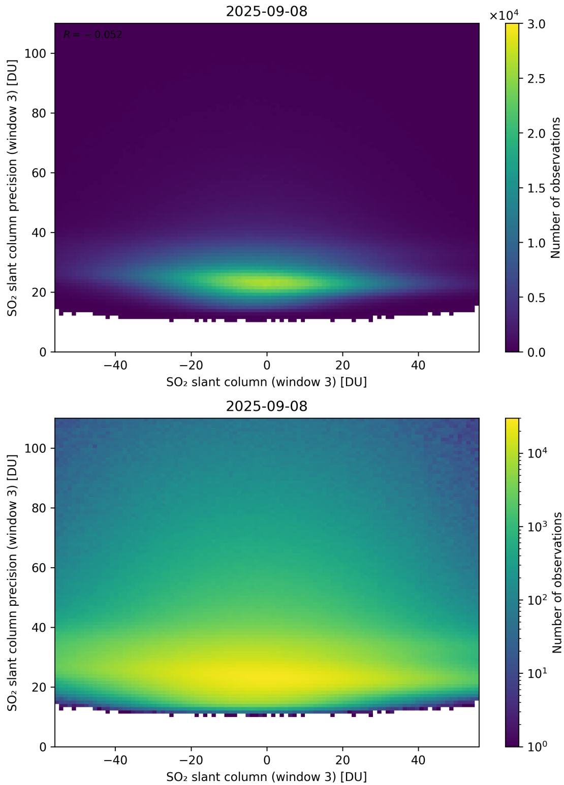
Figure 317: Scatter density plot of “SO 2 slant column (window 3)” against “SO 2 slant column precision (window 3)” for 2025-09-07 to 2025-09-09.
