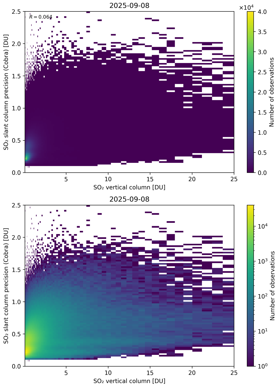
Figure 350: Scatter density plot of “SO 2 vertical column” against “SO 2 slant column precision (Cobra)” for 2025-09-07 to 2025-09-09.
