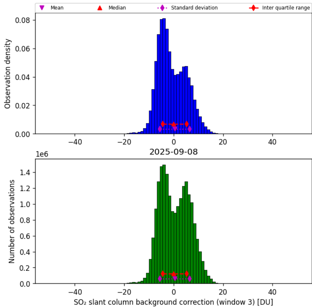
Figure 74: Histogram of “SO 2 slant column background correction (window 3)” for 2025-09-07 to 2025-09-09
