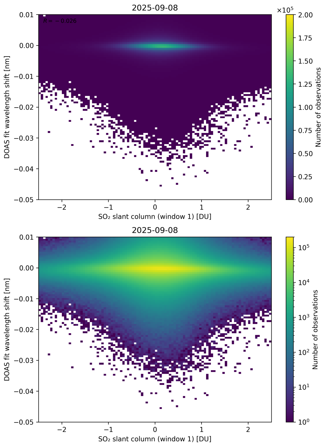
Figure 265: Scatter density plot of “SO 2 slant column (window 1)” against “DOAS fit wavelength shift” for 2025-09-07 to 2025-09-09.
