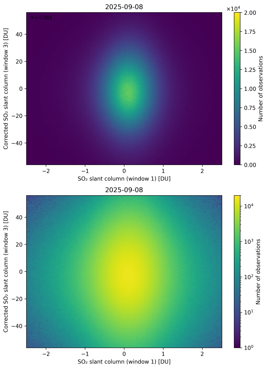
Figure 284: Scatter density plot of “SO 2 slant column (window 1)” against “Corrected SO 2 slant column (window 3)” for 2025-09-07 to 2025-09-09.
