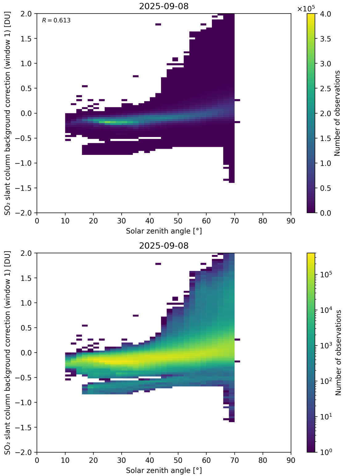
Figure 171: Scatter density plot of “Solar zenith angle” against “SO 2 slant column background correction (window 1)” for 2025-09-07 to 2025-09-09.
