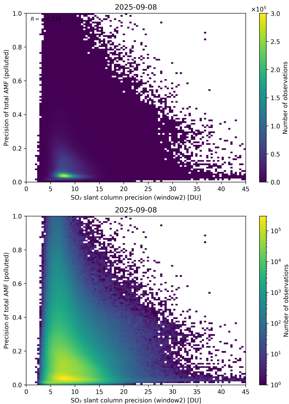
Figure 302: Scatter density plot of “SO 2 slant column precision (window2)” against “Precision of total AMF (polluted)” for 2025-09-07 to 2025-09-09.
