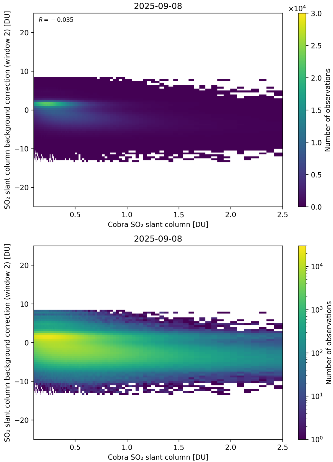
Figure 194: Scatter density plot of “Cobra SO 2 slant column” against “SO 2 slant column background correction (window 2)” for 2025-09-07 to 2025-09-09.
