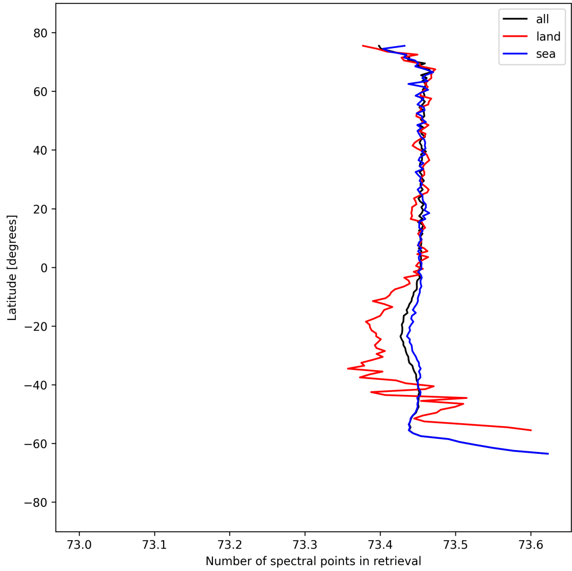
Figure 56: Zonal average of “Number of spectral points in retrieval” for 2025-09-07 to 2025-09-09.
