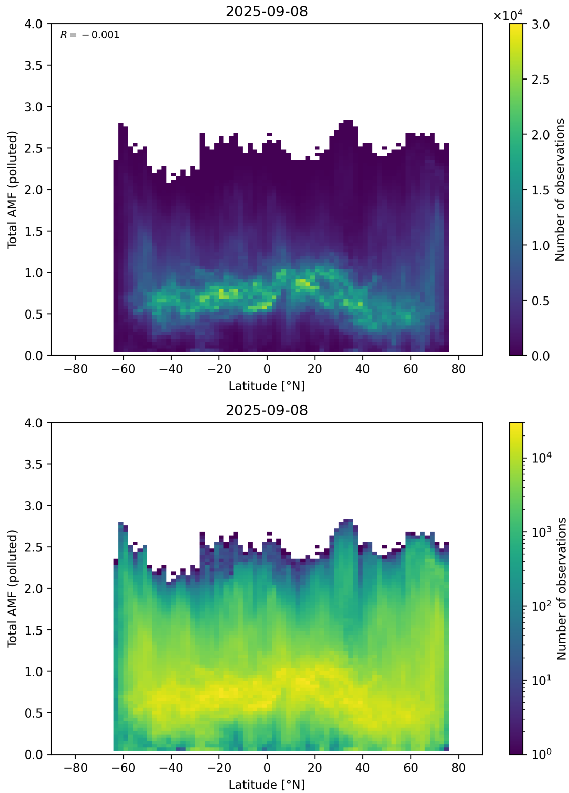
Figure 167: Scatter density plot of “Latitude” against “Total AMF (polluted)” for 2025-09-07 to 2025-09-09.
