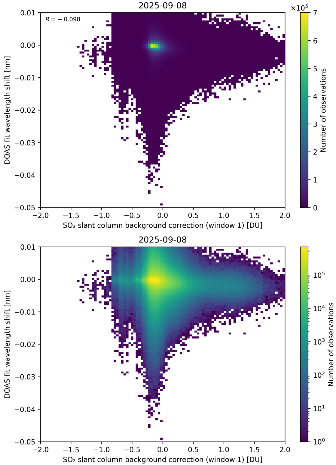
Figure 111: Scatter density plot of “SO 2 slant column background correction (window 1)” against “DOAS fit wavelength shift” for 2025-09-07 to 2025-09-09.
