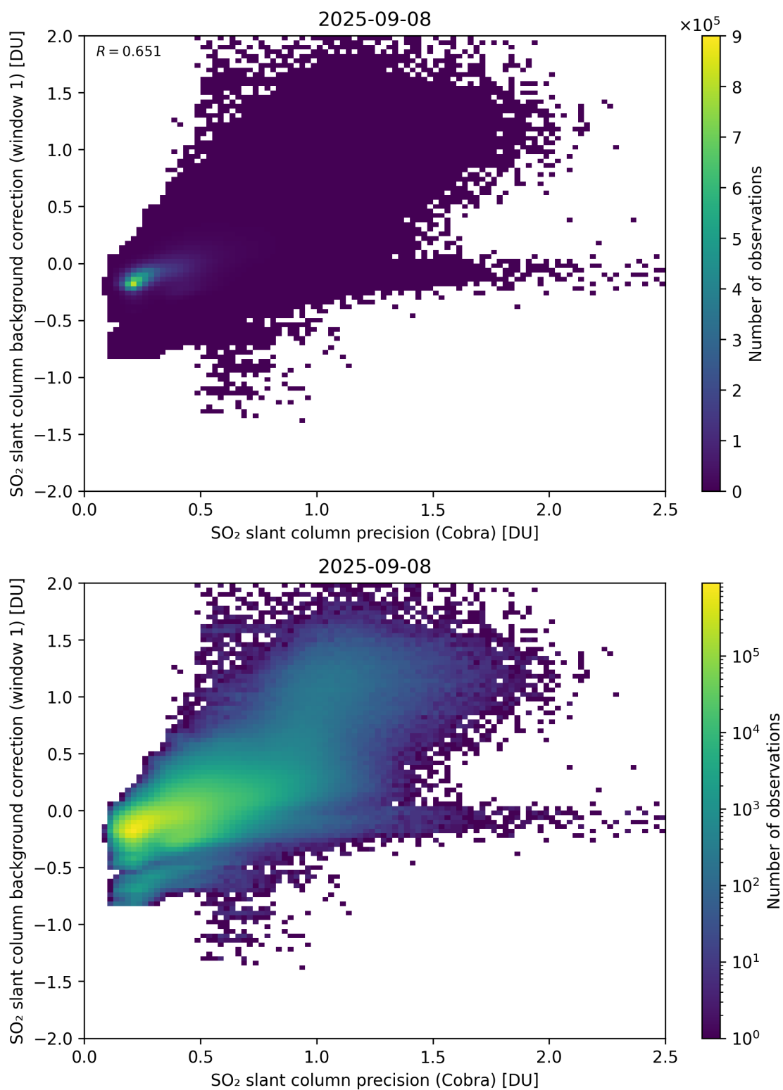
Figure 199: Scatter density plot of “SO 2 slant column precision (Cobra)” against “SO 2 slant column background correction (window 1)” for 2025-09-07 to 2025-09-09.
