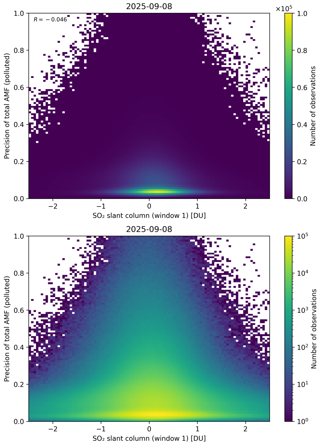
Figure 290: Scatter density plot of “SO 2 slant column (window 1)” against “Precision of total AMF (polluted)” for 2025-09-07 to 2025-09-09.
