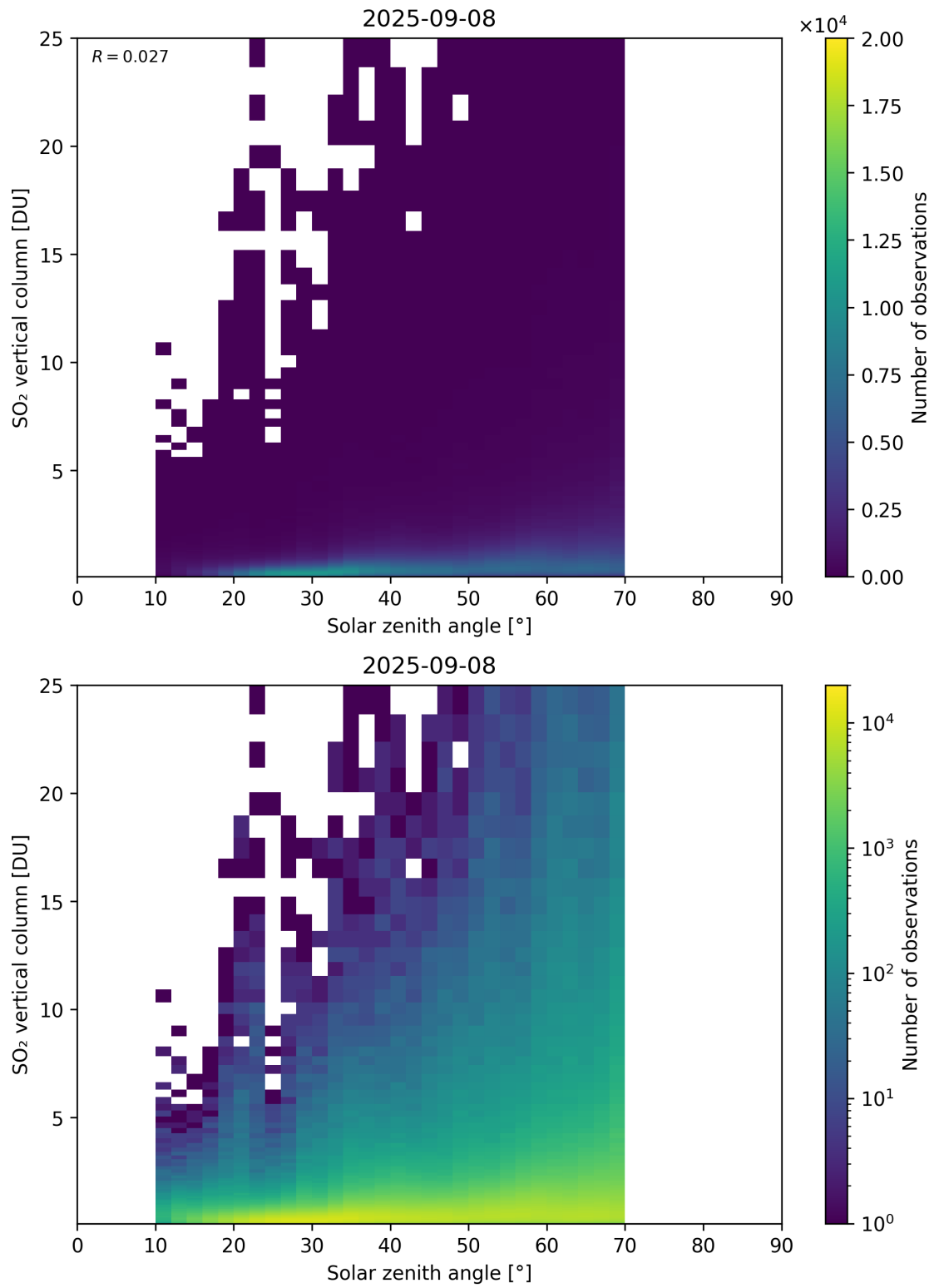
Figure 191: Scatter density plot of “Solar zenith angle” against “SO 2 vertical column” for 2025-09-07 to 2025-09-09.
