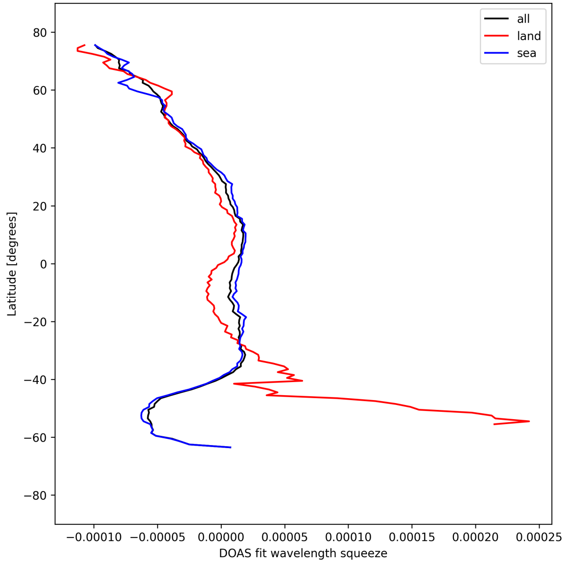
Figure 51: Zonal average of “DOAS fit wavelength squeeze” for 2025-09-07 to 2025-09-09.
