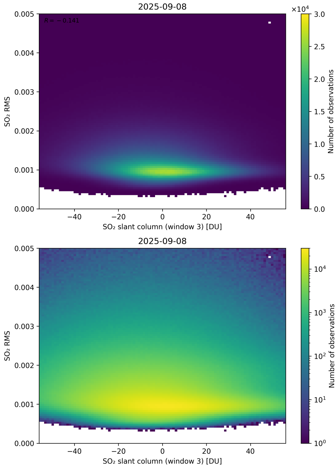
Figure 306: Scatter density plot of “SO 2 slant column (window 3)” against “SO 2 RMS” for 2025-09-07 to 2025-09-09.
