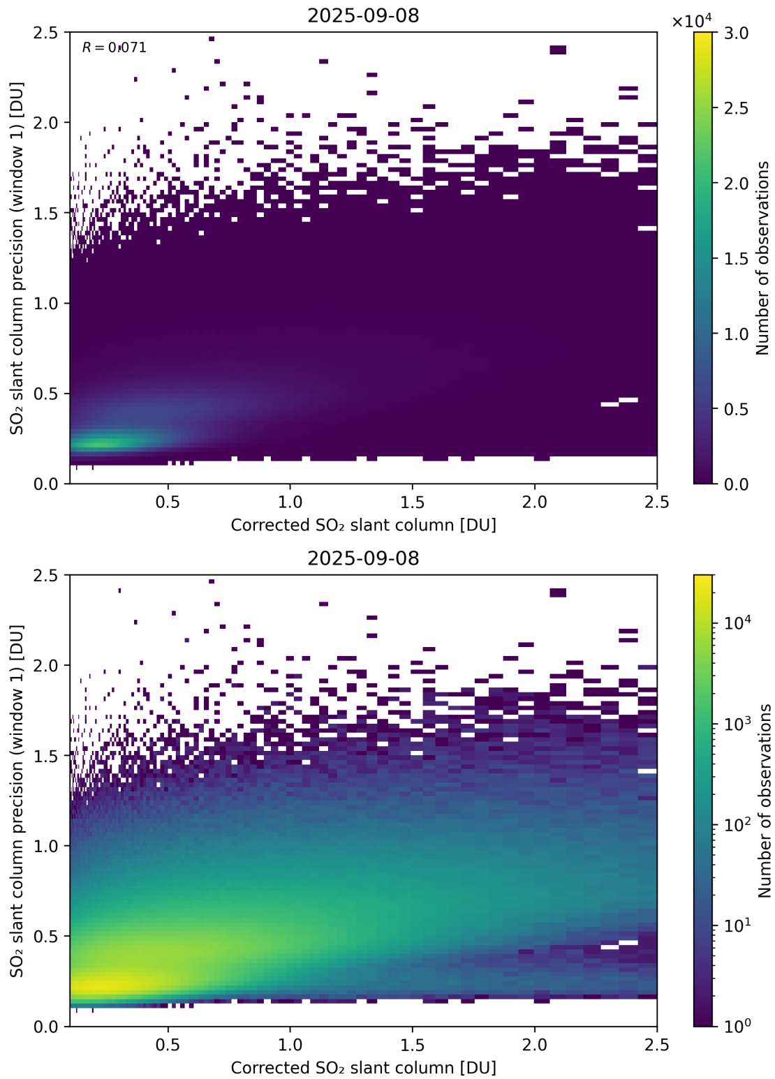
Figure 238: Scatter density plot of “Corrected SO 2 slant column” against “SO 2 slant column precision (window 1)” for 2025-09-07 to 2025-09-09.
