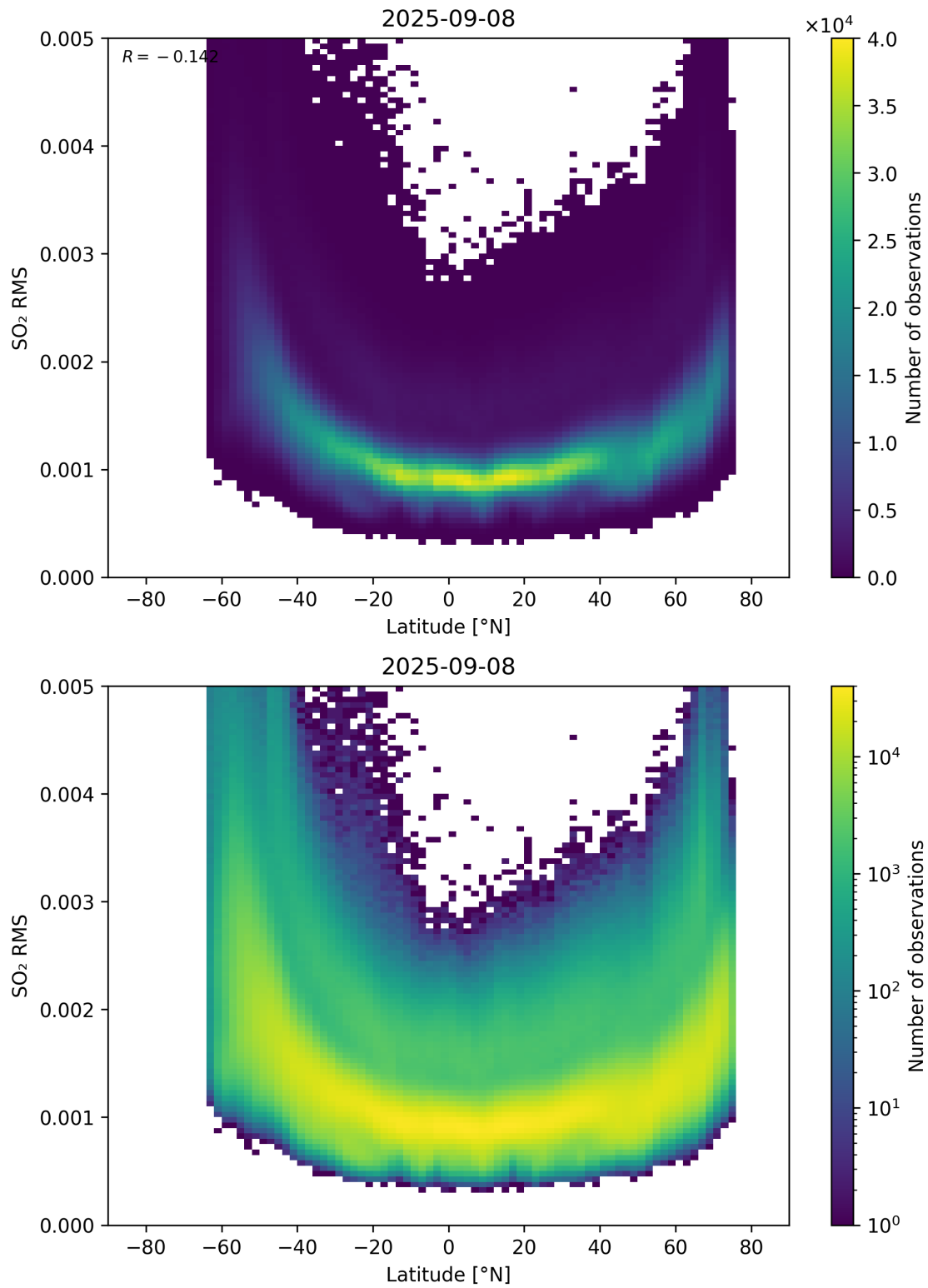
Figure 155: Scatter density plot of “Latitude” against “SO 2 RMS” for 2025-09-07 to 2025-09-09.
