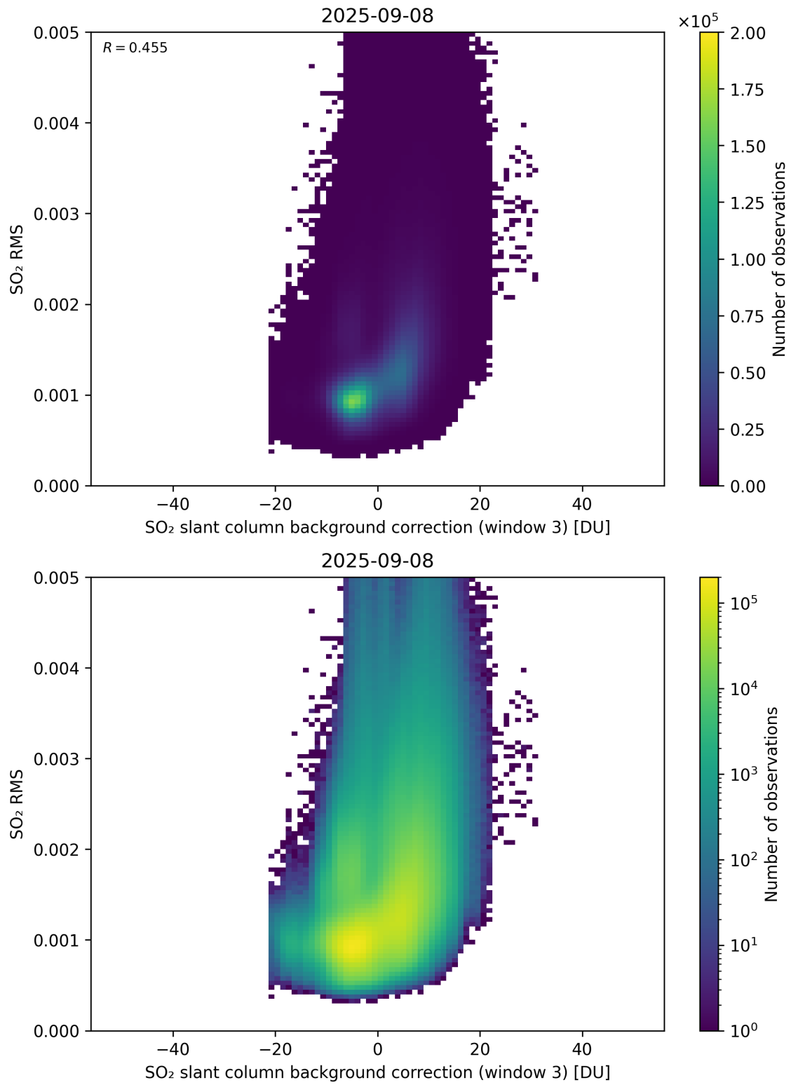
Figure 134: Scatter density plot of “SO 2 slant column background correction (window 3)” against “SO 2 RMS” for 2025-09-07 to 2025-09-09.
