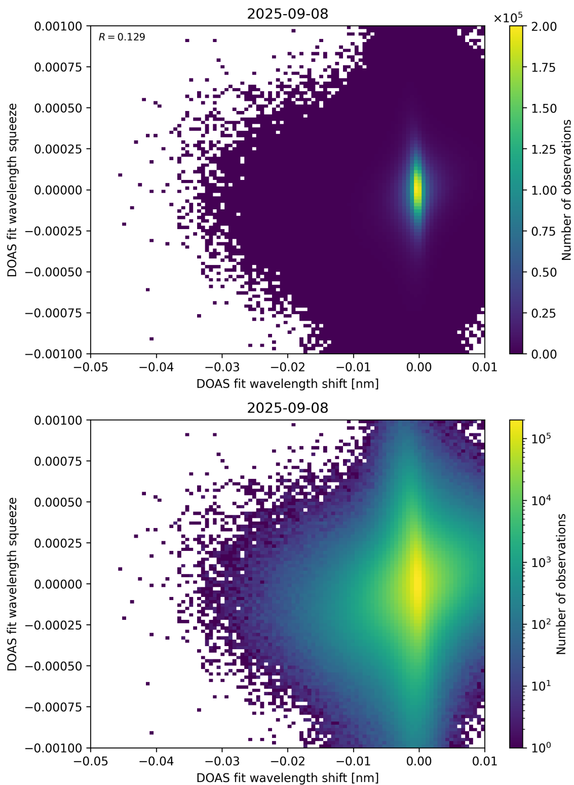
Figure 138: Scatter density plot of “DOAS fit wavelength shift” against “DOAS fit wavelength squeeze” for 2025-09-07 to 2025-09-09.
