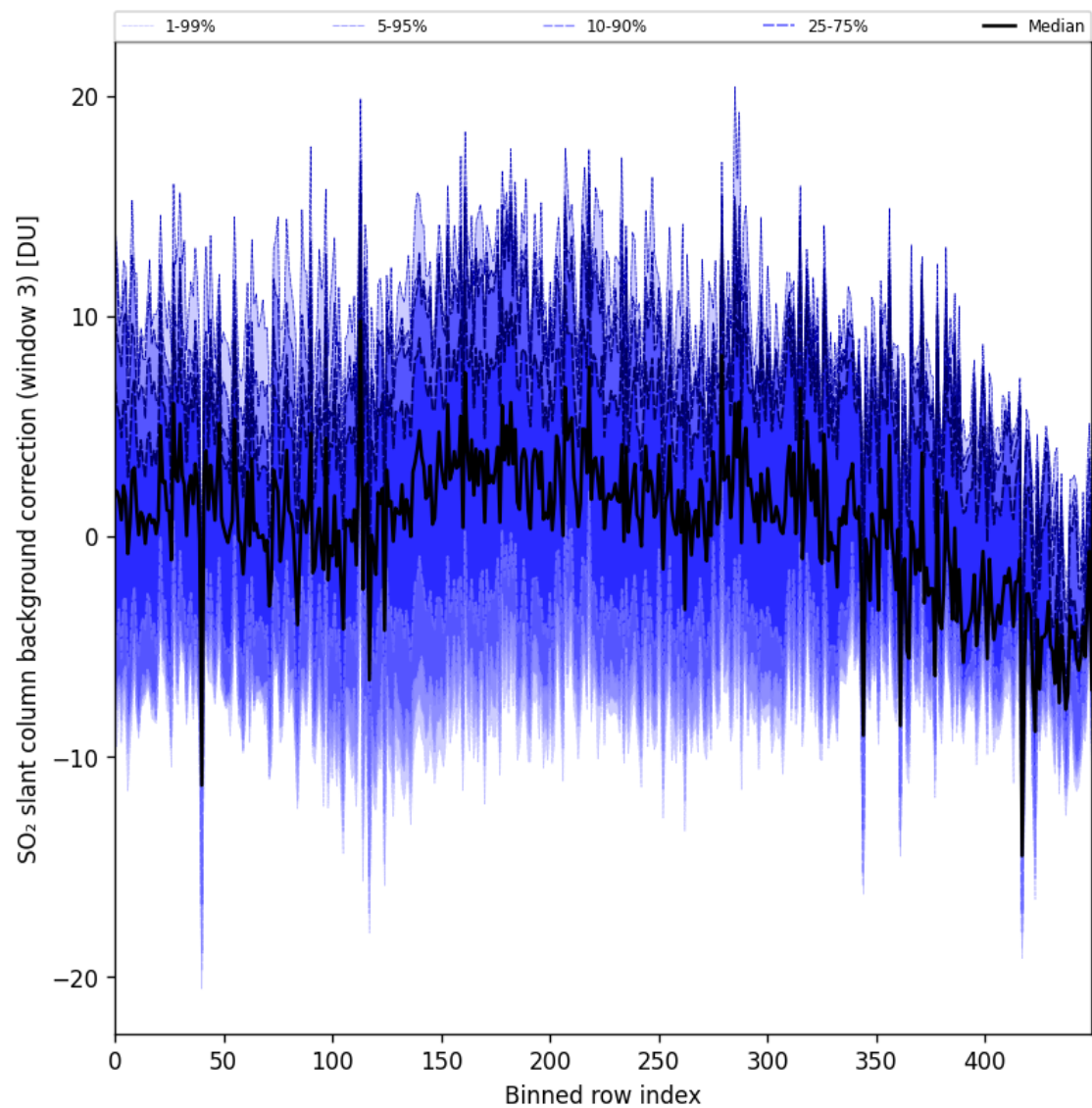
Figure 100: Along track statistics of “SO 2 slant column background correction (window 3)” for 2025-09-07 to 2025-09-09
