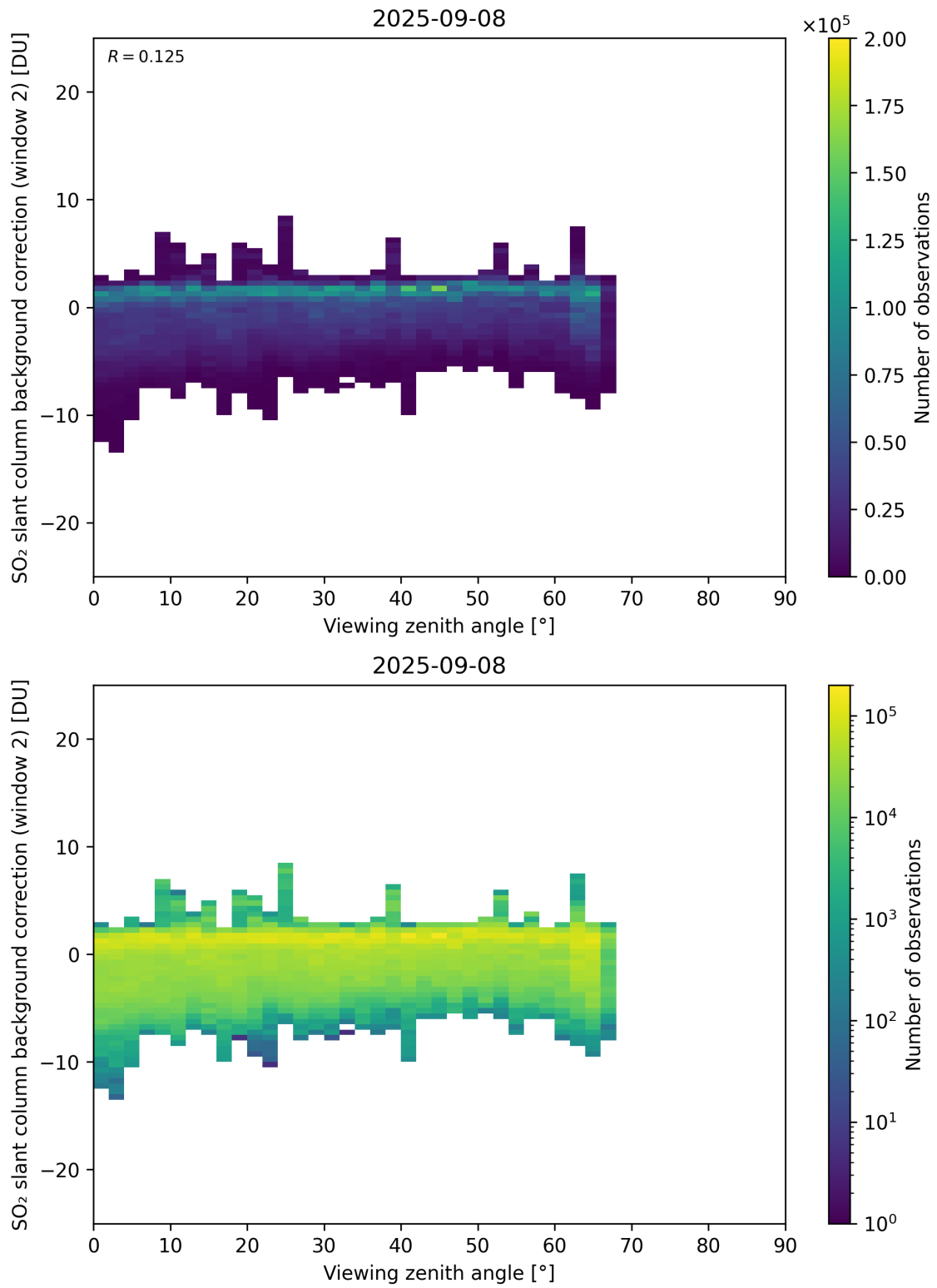
Figure 363: Scatter density plot of “Viewing zenith angle” against “SO 2 slant column background correction (window 2)” for 2025-09-07 to 2025-09-09.
