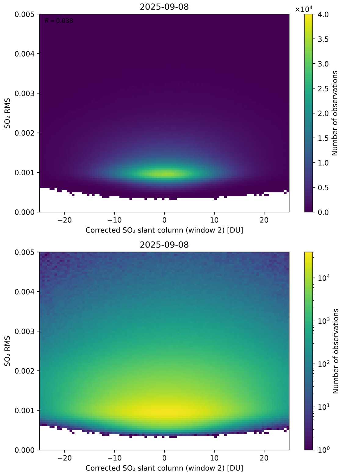
Figure 248: Scatter density plot of “Corrected SO 2 slant column (window 2)” against “SO 2 RMS” for 2025-09-07 to 2025-09-09.
