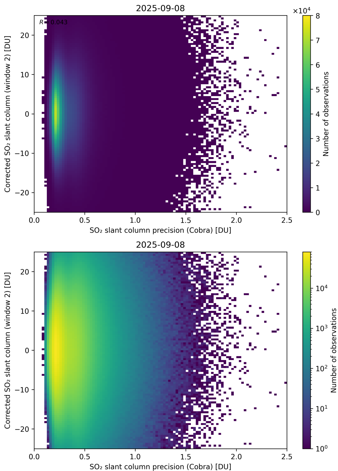
Figure 206: Scatter density plot of “SO 2 slant column precision (Cobra)” against “Corrected SO 2 slant column (window 2)” for 2025-09-07 to 2025-09-09.
