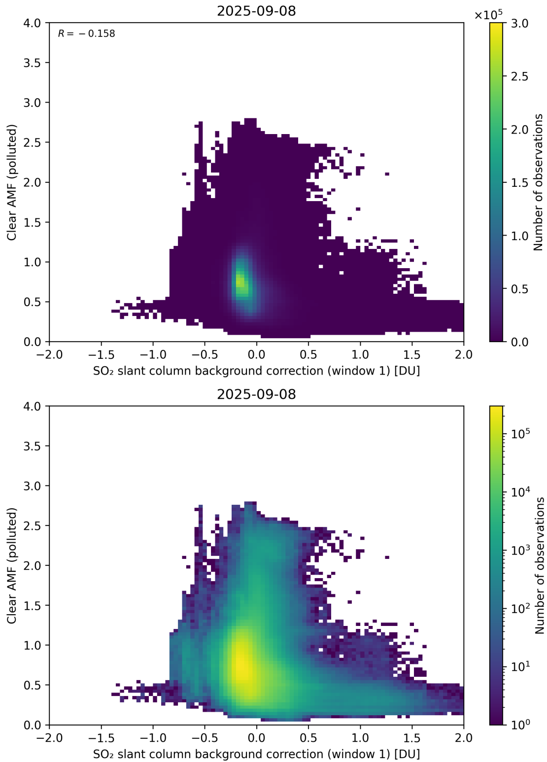
Figure 114: Scatter density plot of “SO 2 slant column background correction (window 1)” against “Clear AMF (polluted)” for 2025-09-07 to 2025-09-09.
