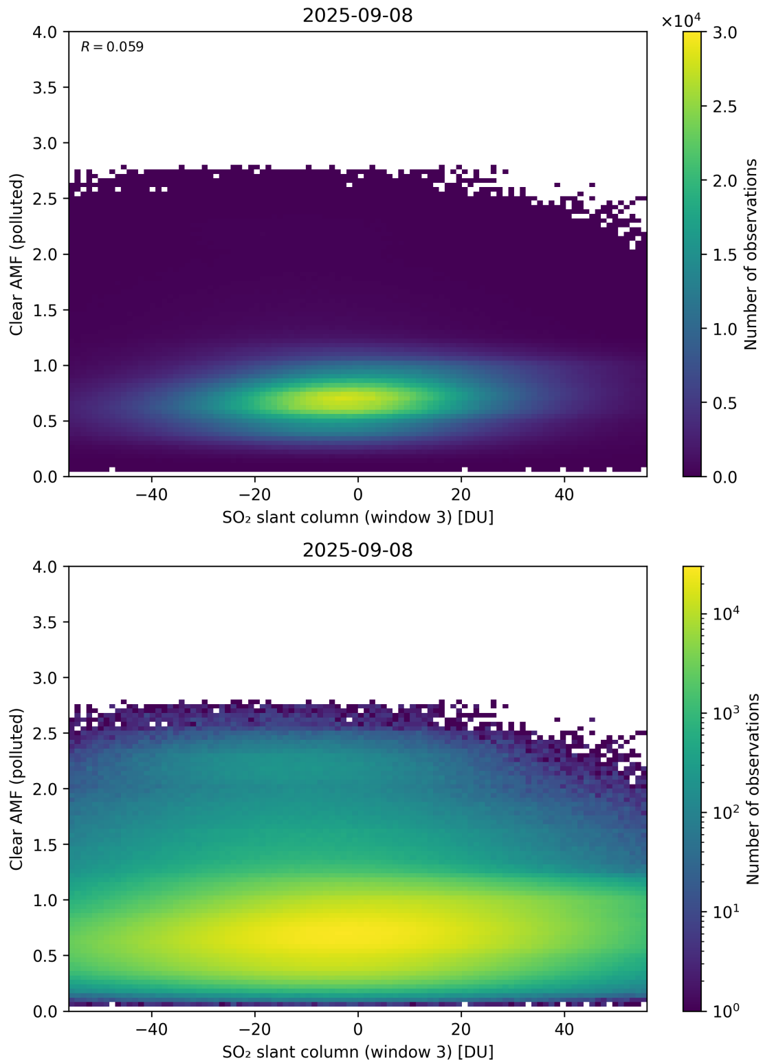
Figure 315: Scatter density plot of “SO 2 slant column (window 3)” against “Clear AMF (polluted)” for 2025-09-07 to 2025-09-09.
