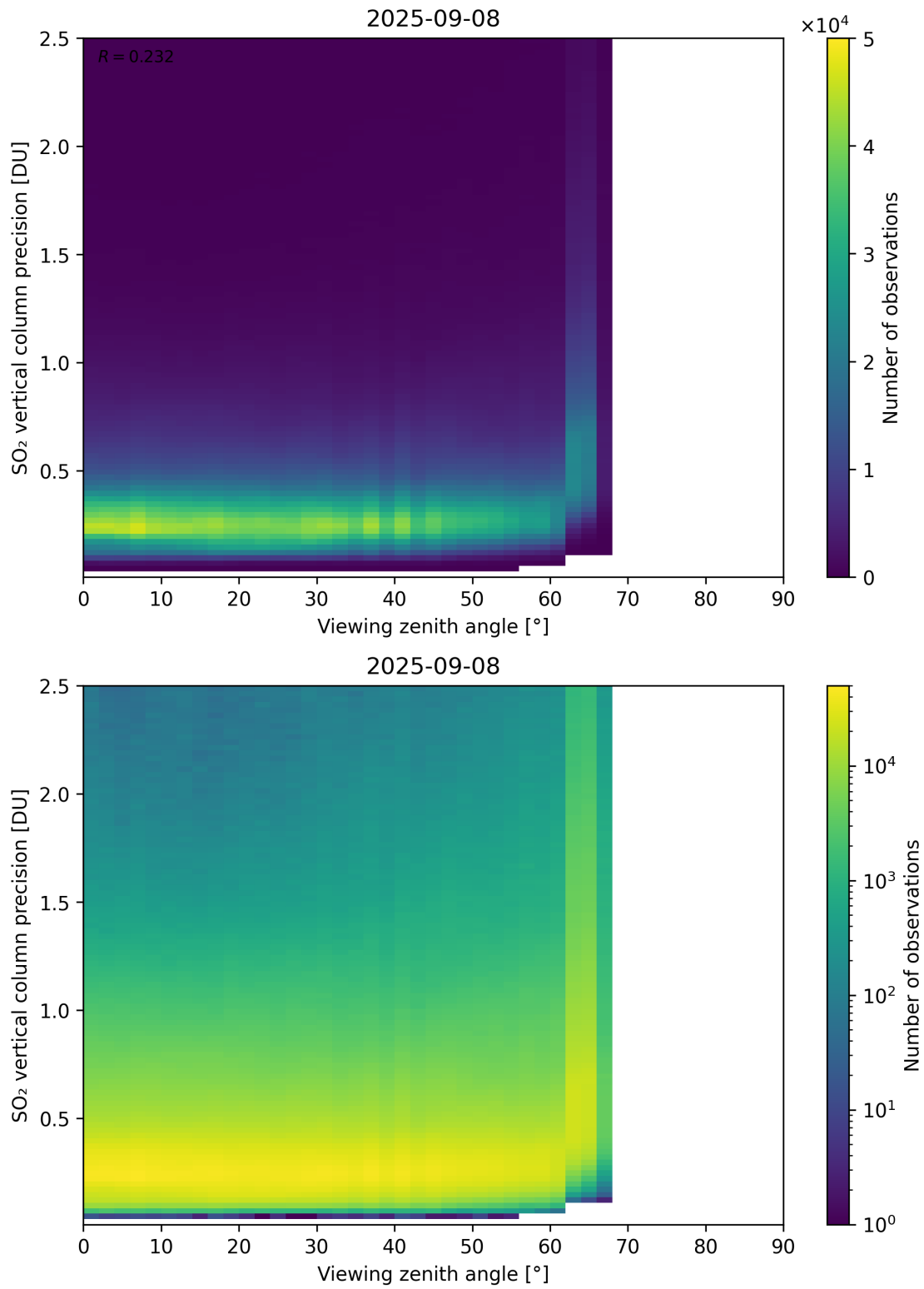
Figure 384: Scatter density plot of “Viewing zenith angle” against “SO 2 vertical column precision” for 2025-09-07 to 2025-09-09.
