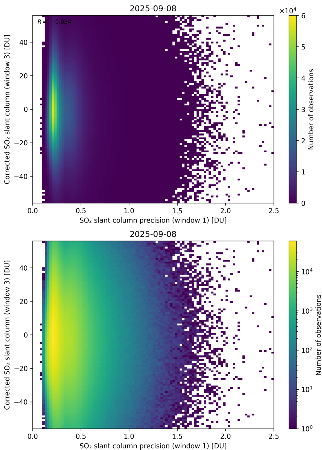
Figure 276: Scatter density plot of “SO 2 slant column precision (window 1)” against “Corrected SO 2 slant column (window 3)” for 2025-09-07 to 2025-09-09.
