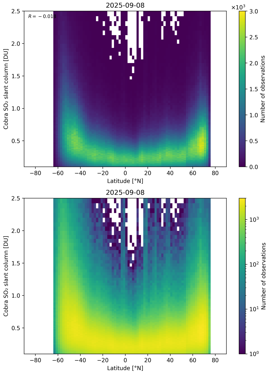
Figure 157: Scatter density plot of “Latitude” against “Cobra SO 2 slant column” for 2025-09-07 to 2025-09-09.
