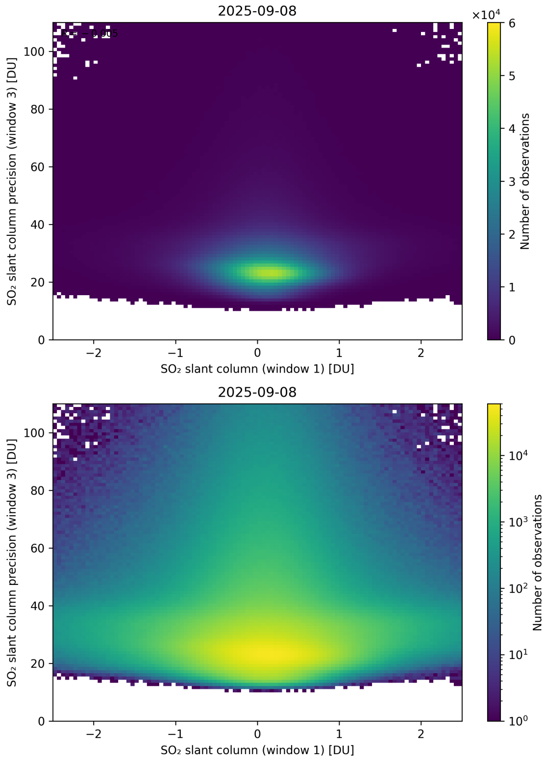
Figure 288: Scatter density plot of “SO 2 slant column (window 1)” against “SO 2 slant column precision (window 3)” for 2025-09-07 to 2025-09-09.
