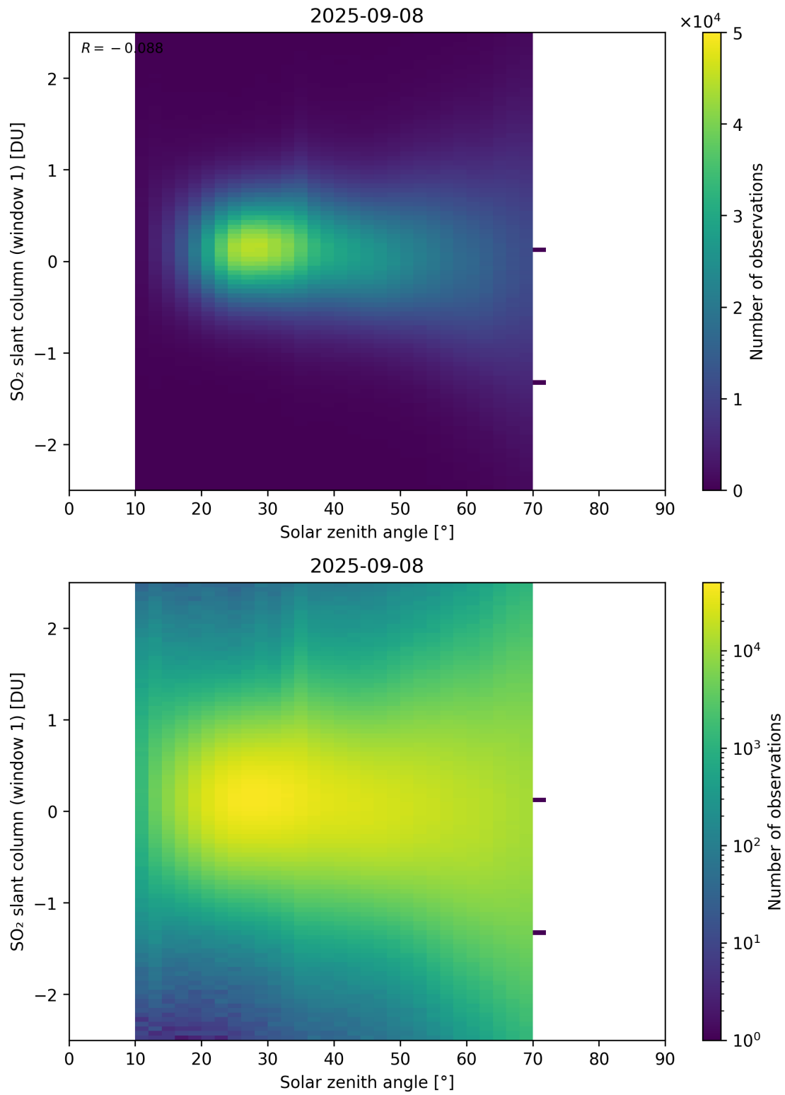
Figure 184: Scatter density plot of “Solar zenith angle” against “SO 2 slant column (window 1)” for 2025-09-07 to 2025-09-09.
