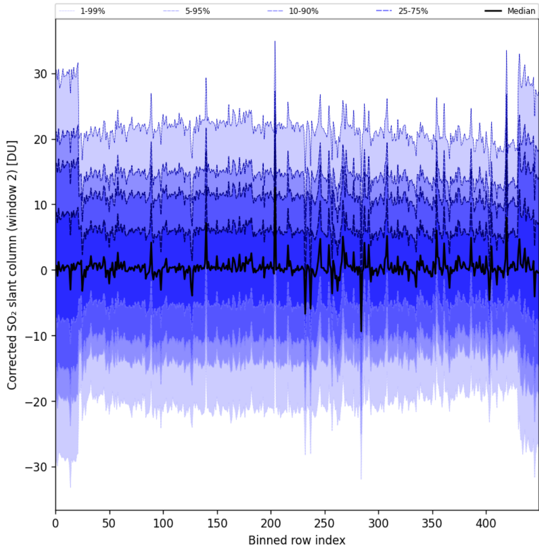
Figure 95: Along track statistics of “Corrected SO 2 slant column (window 2)” for 2025-09-07 to 2025-09-09
