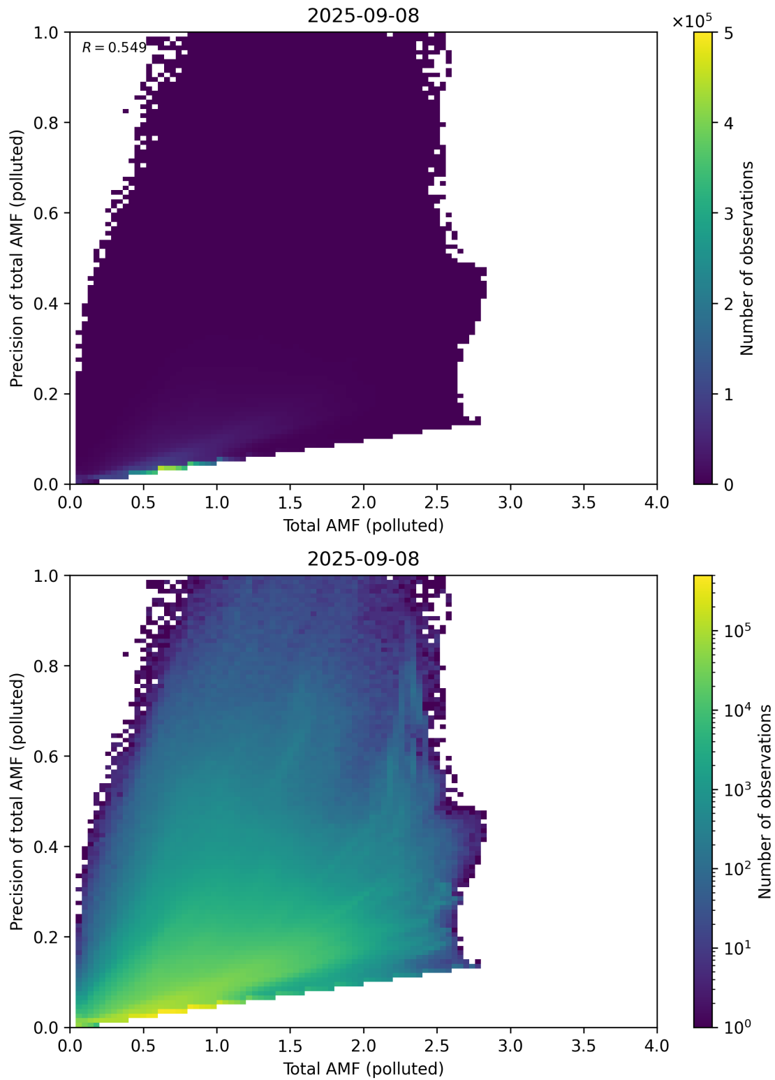
Figure 322: Scatter density plot of “Total AMF (polluted)” against “Precision of total AMF (polluted)” for 2025-09-07 to 2025-09-09.
