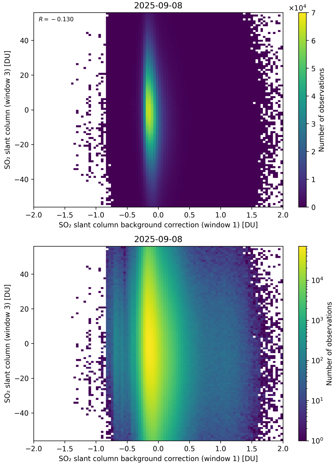
Figure 118: Scatter density plot of “SO 2 slant column background correction (window 1)” against “SO 2 slant column (window 3)” for 2025-09-07 to 2025-09-09.
