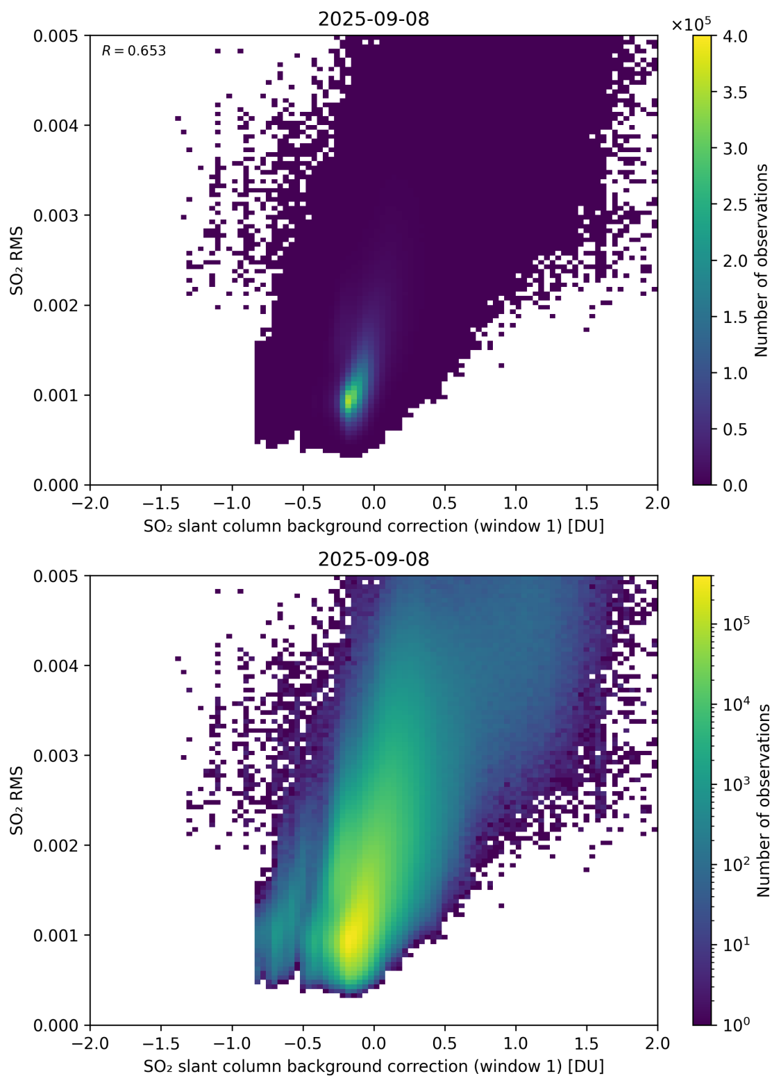
Figure 113: Scatter density plot of “SO 2 slant column background correction (window 1)” against “SO 2 RMS” for 2025-09-07 to 2025-09-09.
