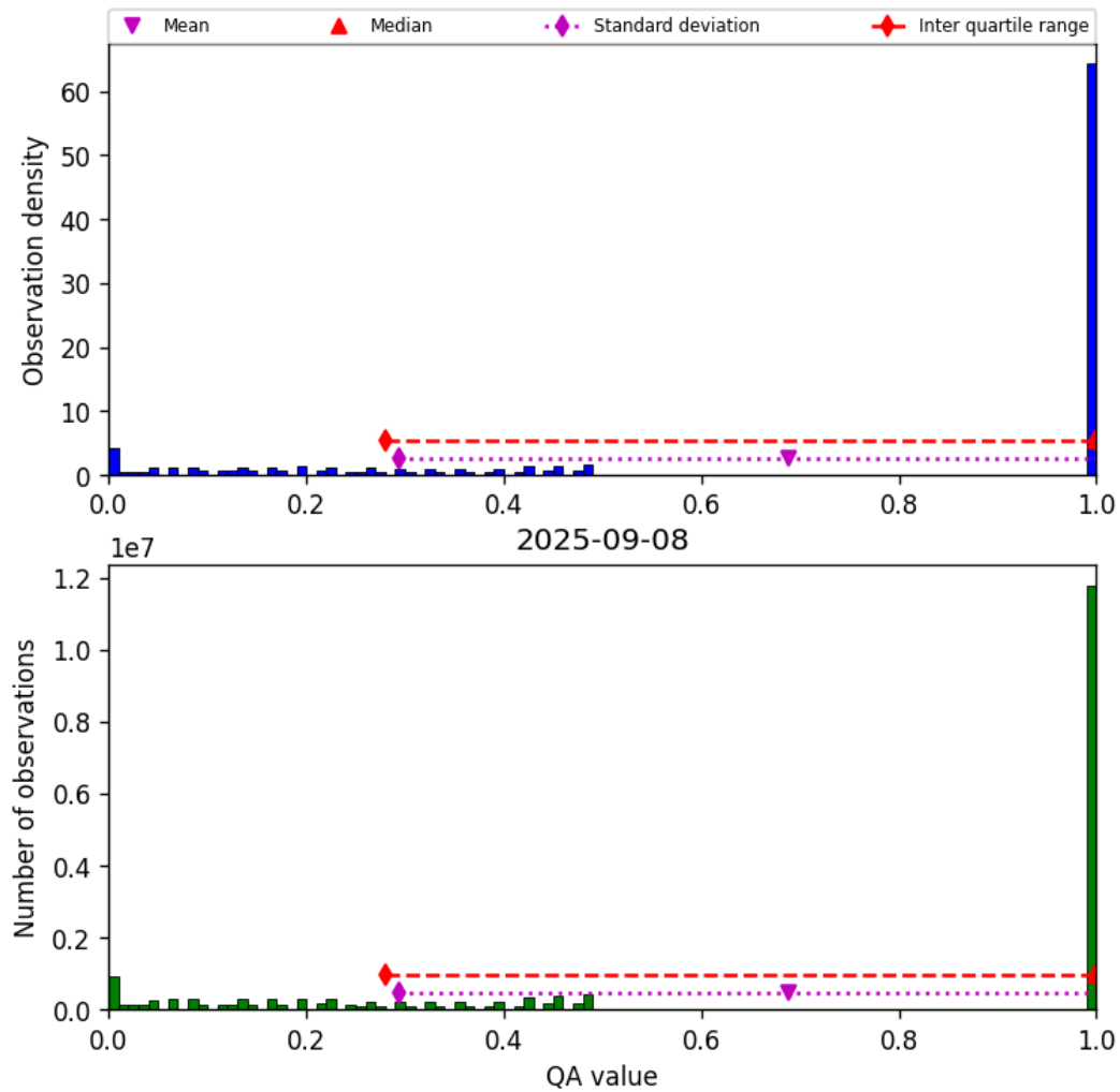
Figure 57: Histogram of “QA value” for 2025-09-07 to 2025-09-09
