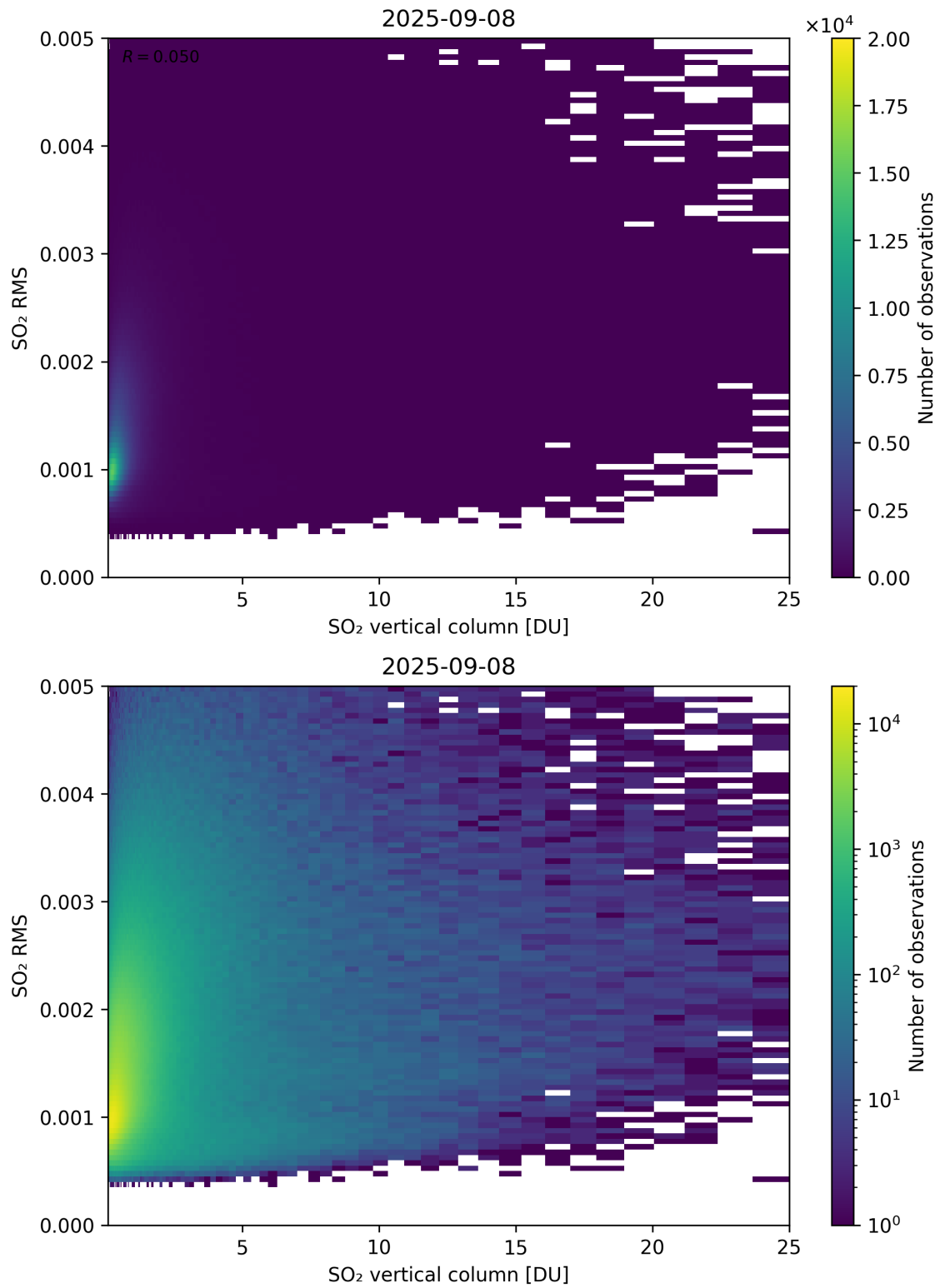
Figure 328: Scatter density plot of “SO 2 vertical column” against “SO 2 RMS” for 2025-09-07 to 2025-09-09.
