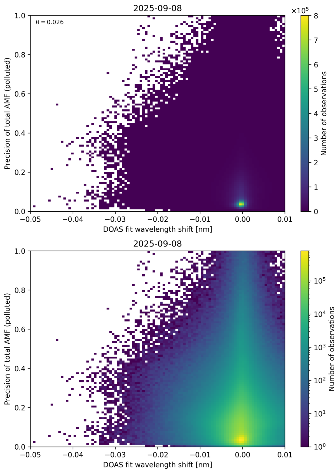
Figure 142: Scatter density plot of “DOAS fit wavelength shift” against “Precision of total AMF (polluted)” for 2025-09-07 to 2025-09-09.
