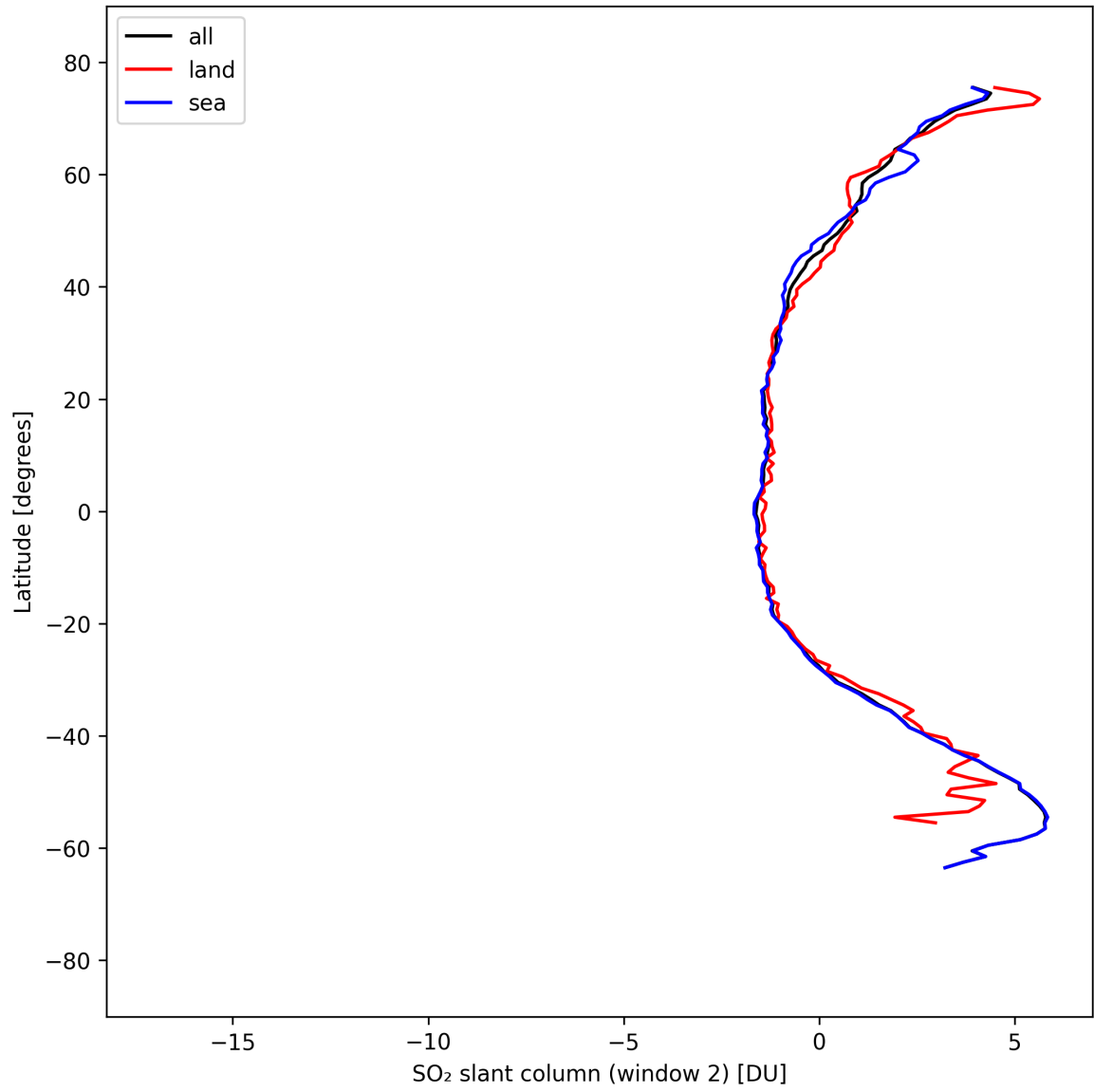
Figure 41: Zonal average of “SO 2 slant column (window 2)” for 2025-09-07 to 2025-09-09.
