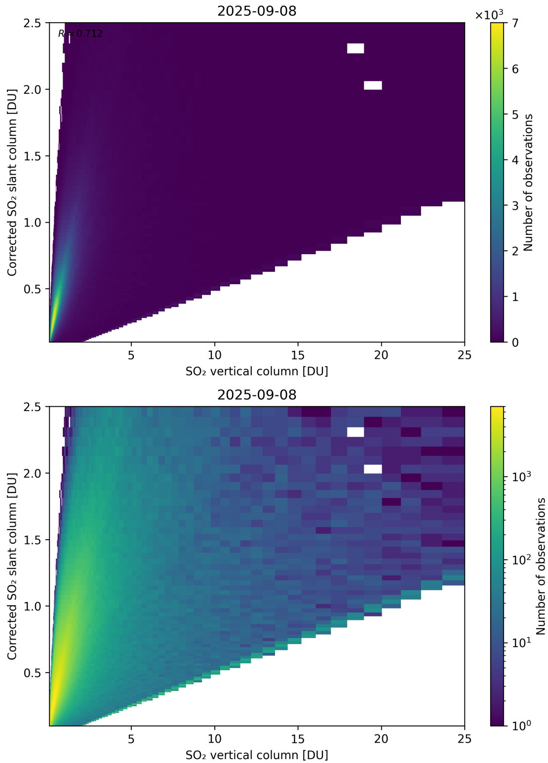
Figure 351: Scatter density plot of “SO 2 vertical column” against “Corrected SO 2 slant column” for 2025-09-07 to 2025-09-09.
