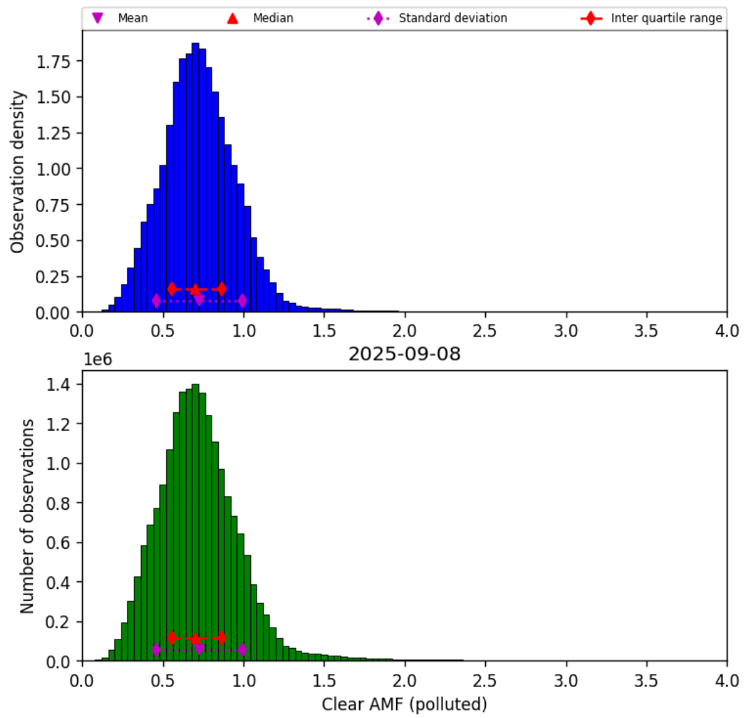
Figure 81: Histogram of “Clear AMF (polluted)” for 2025-09-07 to 2025-09-09
