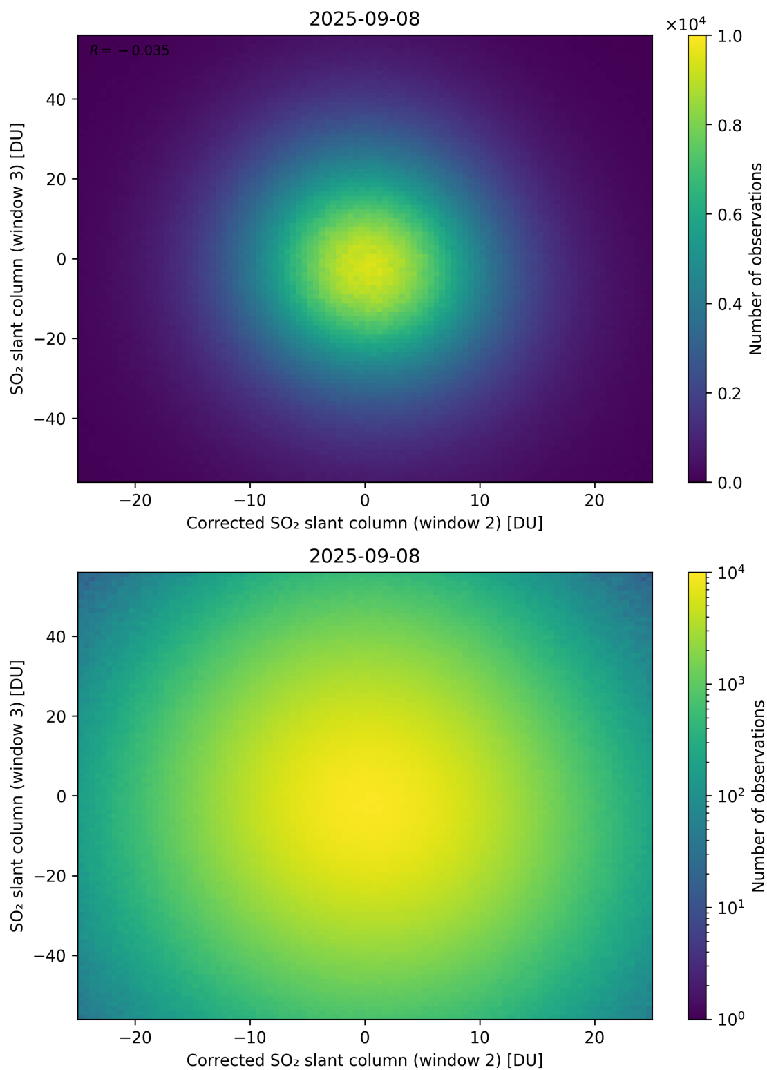
Figure 251: Scatter density plot of “Corrected SO 2 slant column (window 2)” against “SO 2 slant column (window 3)” for 2025-09-07 to 2025-09-09.
