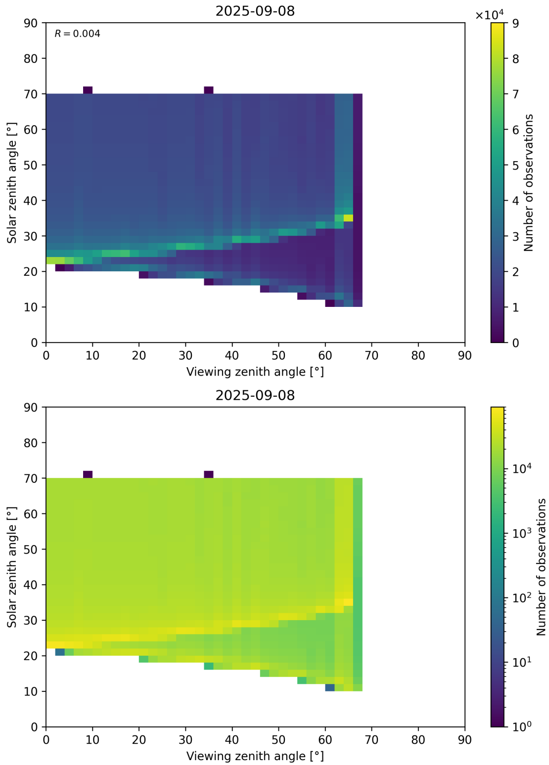
Figure 369: Scatter density plot of “Viewing zenith angle” against “Solar zenith angle” for 2025-09-07 to 2025-09-09.
