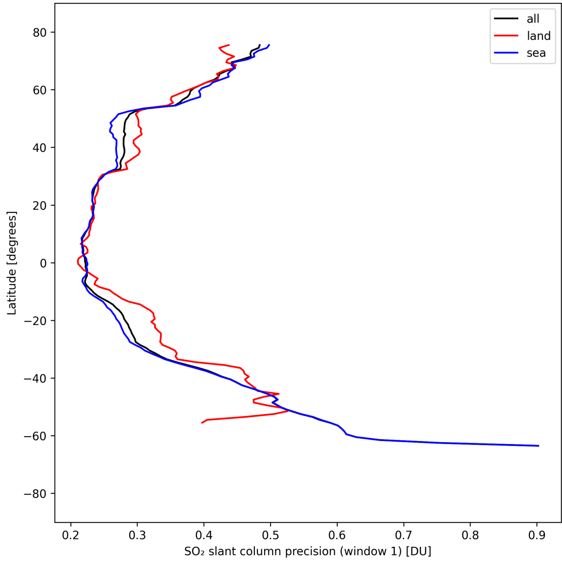
Figure 38: Zonal average of “SO 2 slant column precision (window 1)” for 2025-09-07 to 2025-09-09.
