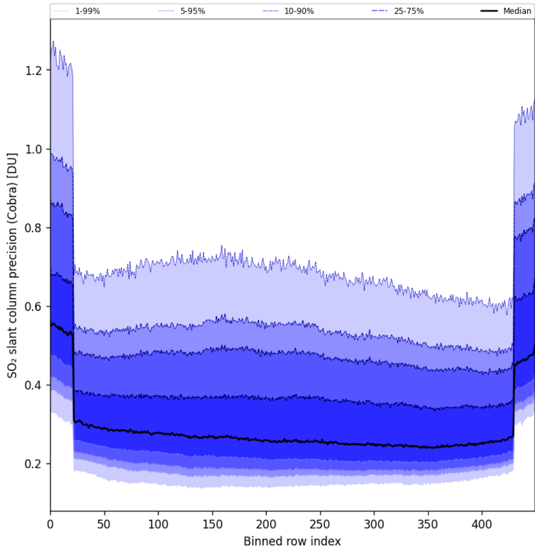
Figure 88: Along track statistics of “SO 2 slant column precision (Cobra)” for 2025-09-07 to 2025-09-09
