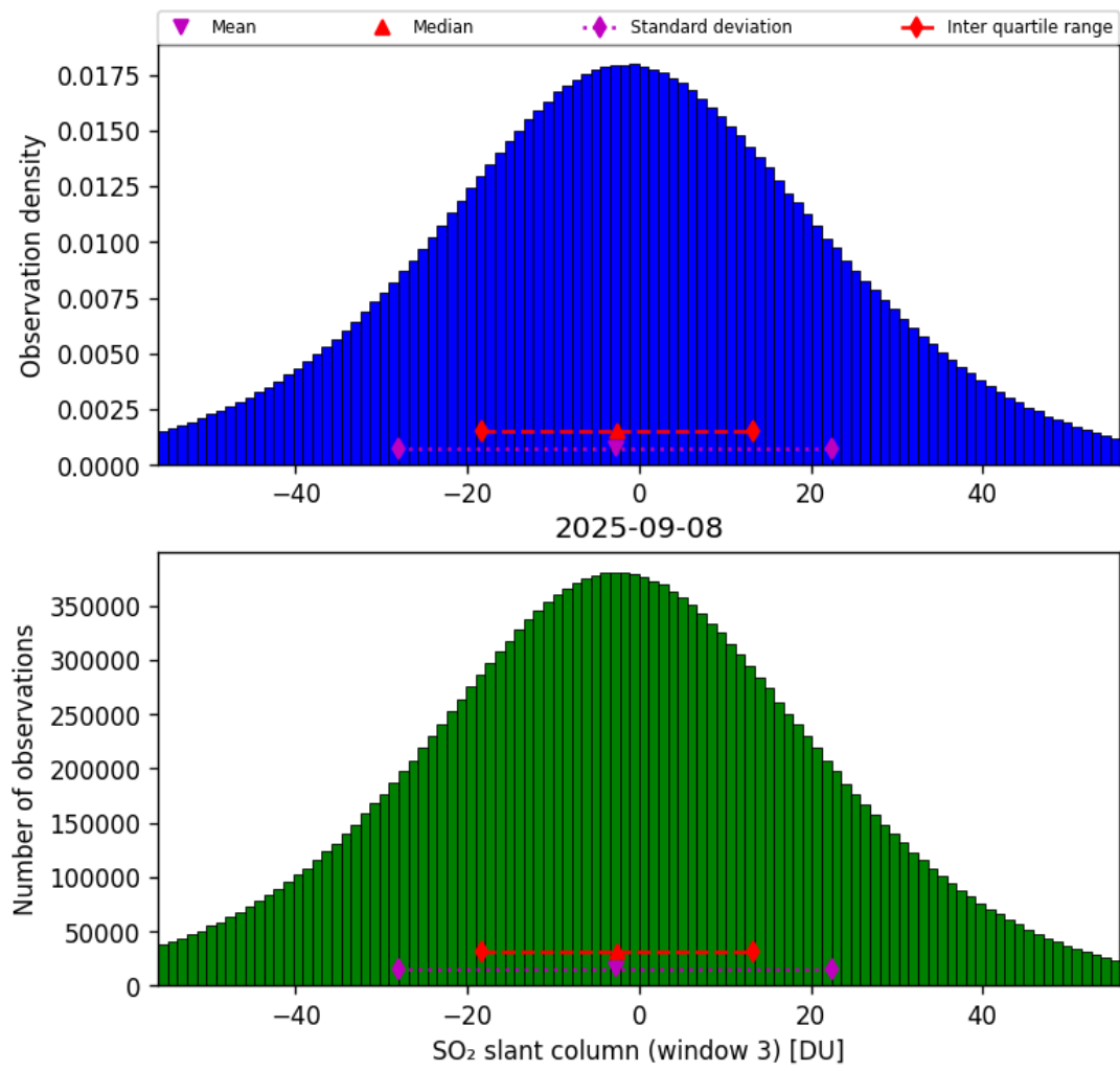
Figure 71: Histogram of “SO 2 slant column (window 3)” for 2025-09-07 to 2025-09-09
