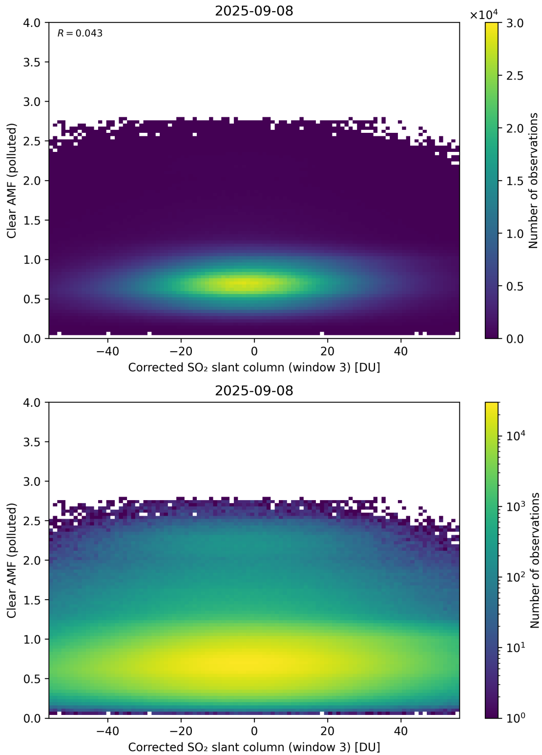
Figure 259: Scatter density plot of “Corrected SO 2 slant column (window 3)” against “Clear AMF (polluted)” for 2025-09-07 to 2025-09-09.
