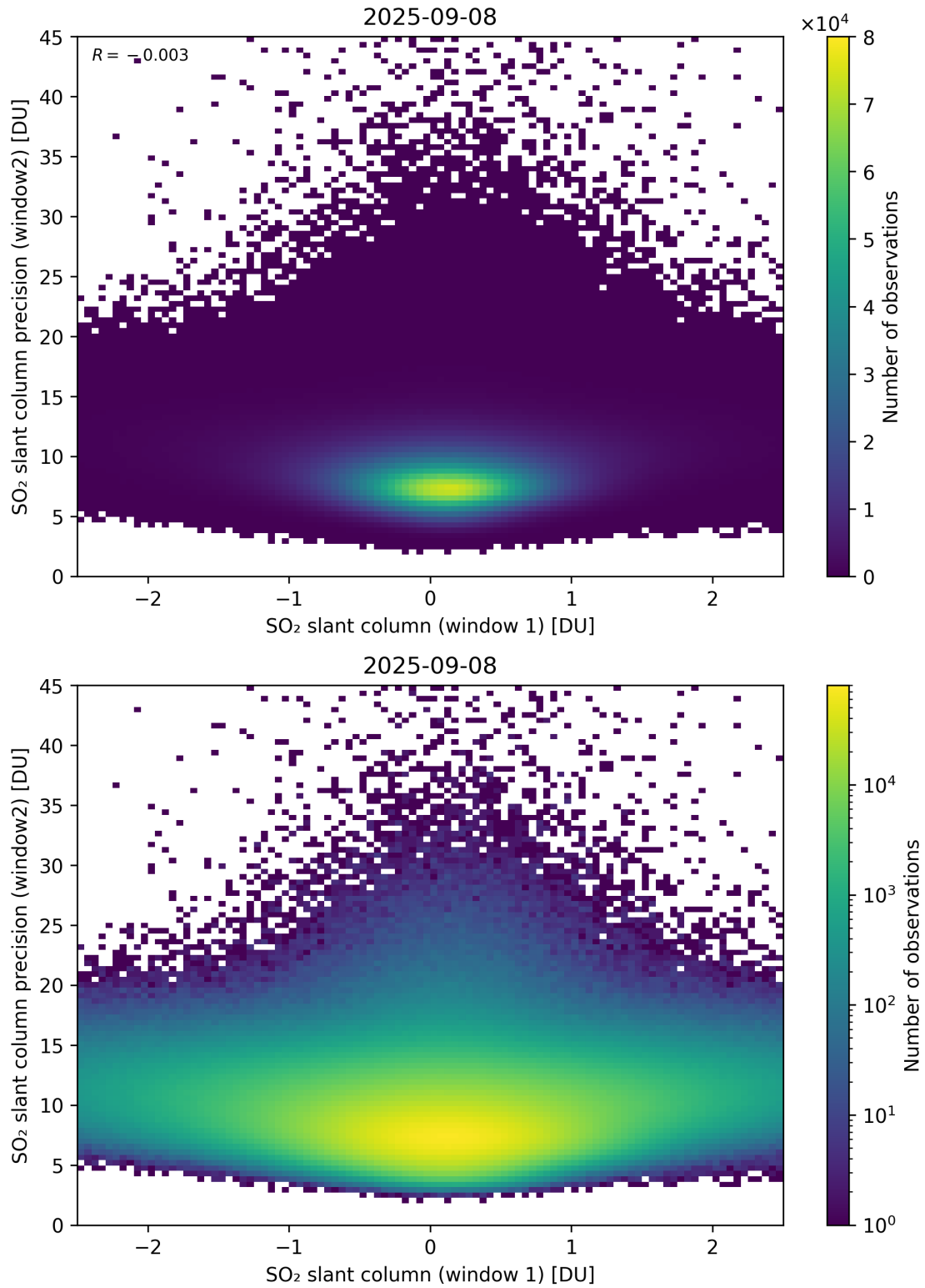
Figure 286: Scatter density plot of “SO 2 slant column (window 1)” against “SO 2 slant column precision (window2)” for 2025-09-07 to 2025-09-09.
