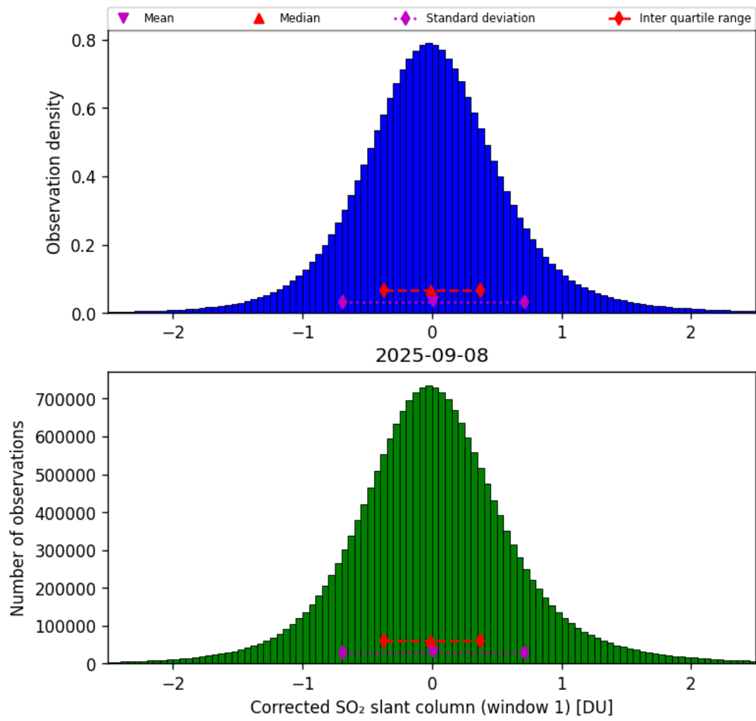
Figure 65: Histogram of “Corrected SO 2 slant column (window 1)” for 2025-09-07 to 2025-09-09
