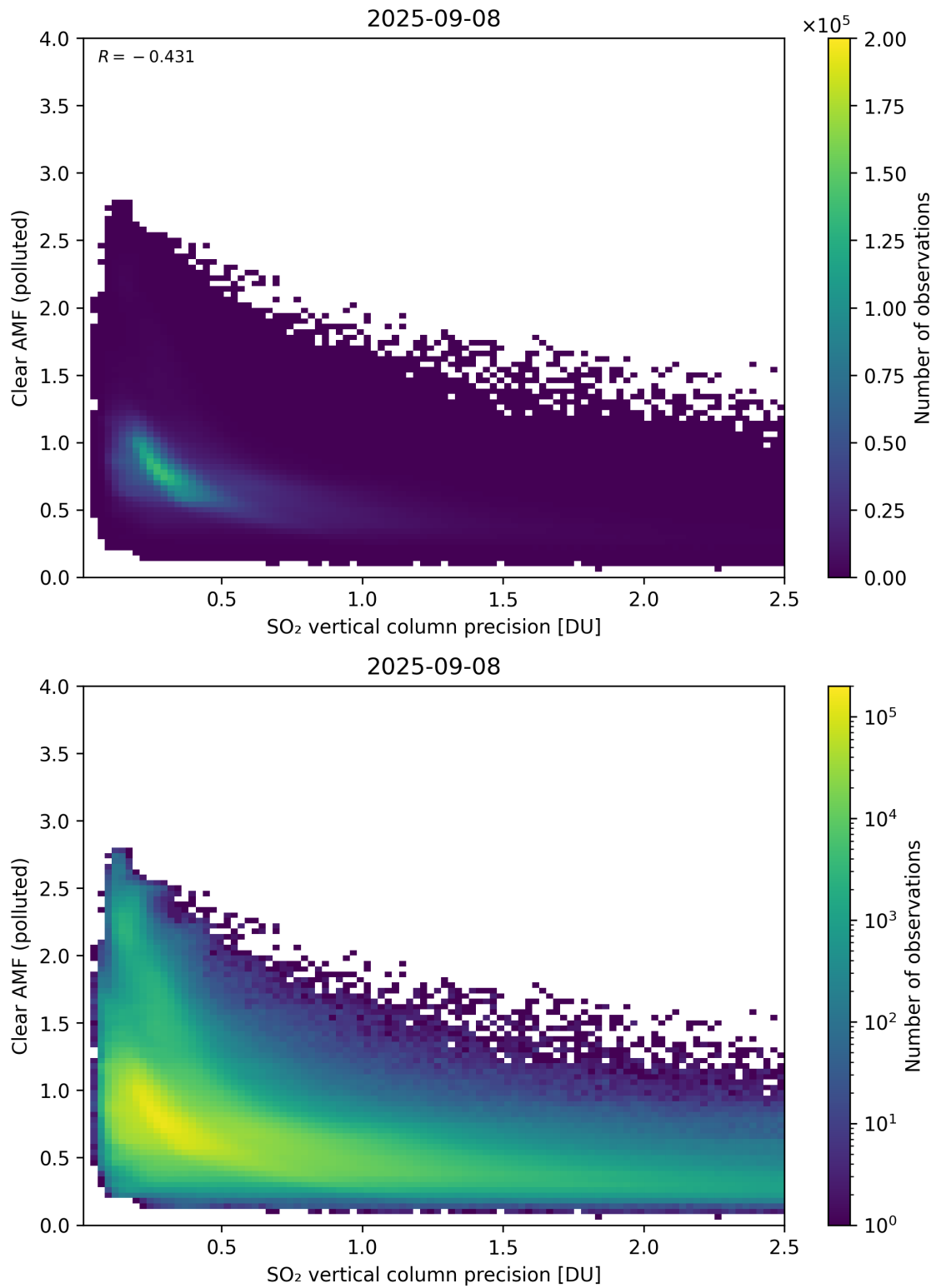
Figure 335: Scatter density plot of “SO 2 vertical column precision” against “Clear AMF (polluted)” for 2025-09-07 to 2025-09-09.
