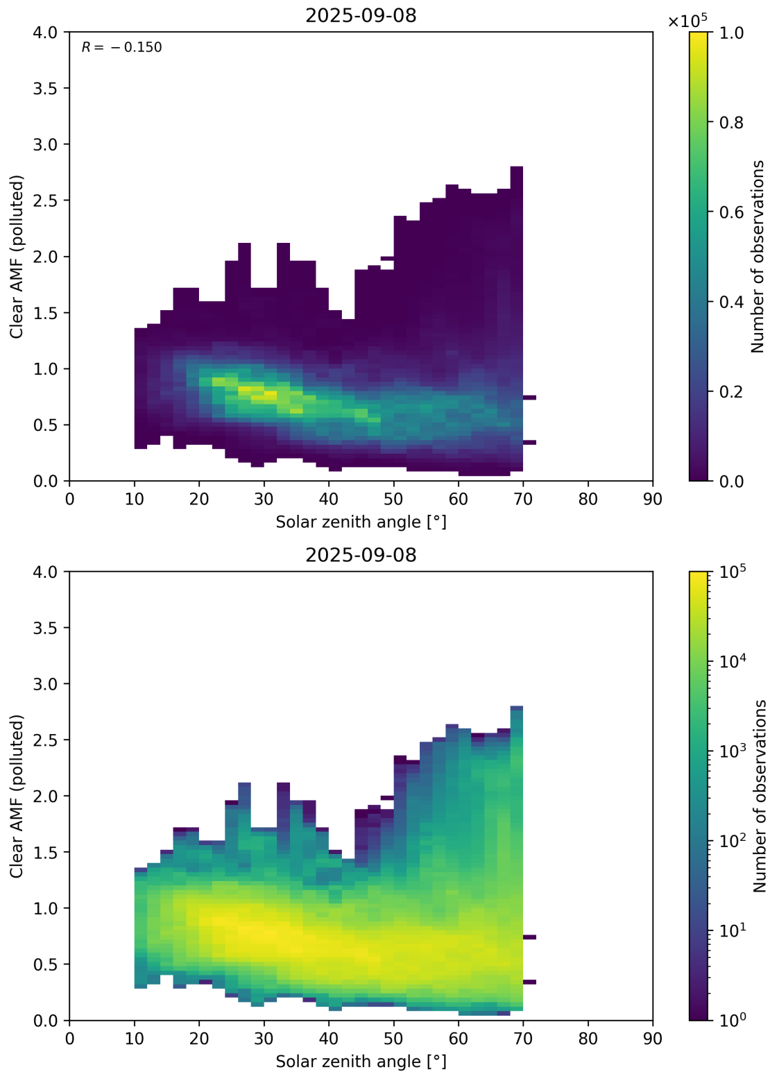
Figure 178: Scatter density plot of “Solar zenith angle” against “Clear AMF (polluted)” for 2025-09-07 to 2025-09-09.
