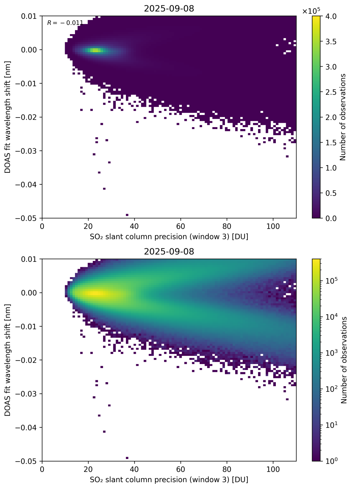
Figure 308: Scatter density plot of “SO 2 slant column precision (window 3)” against “DOAS fit wavelength shift” for 2025-09-07 to 2025-09-09.
