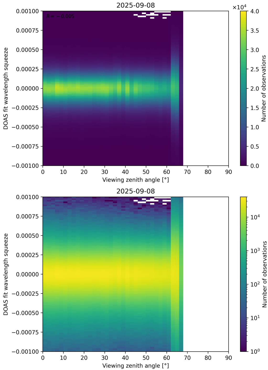
Figure 366: Scatter density plot of “Viewing zenith angle” against “DOAS fit wavelength squeeze” for 2025-09-07 to 2025-09-09.
