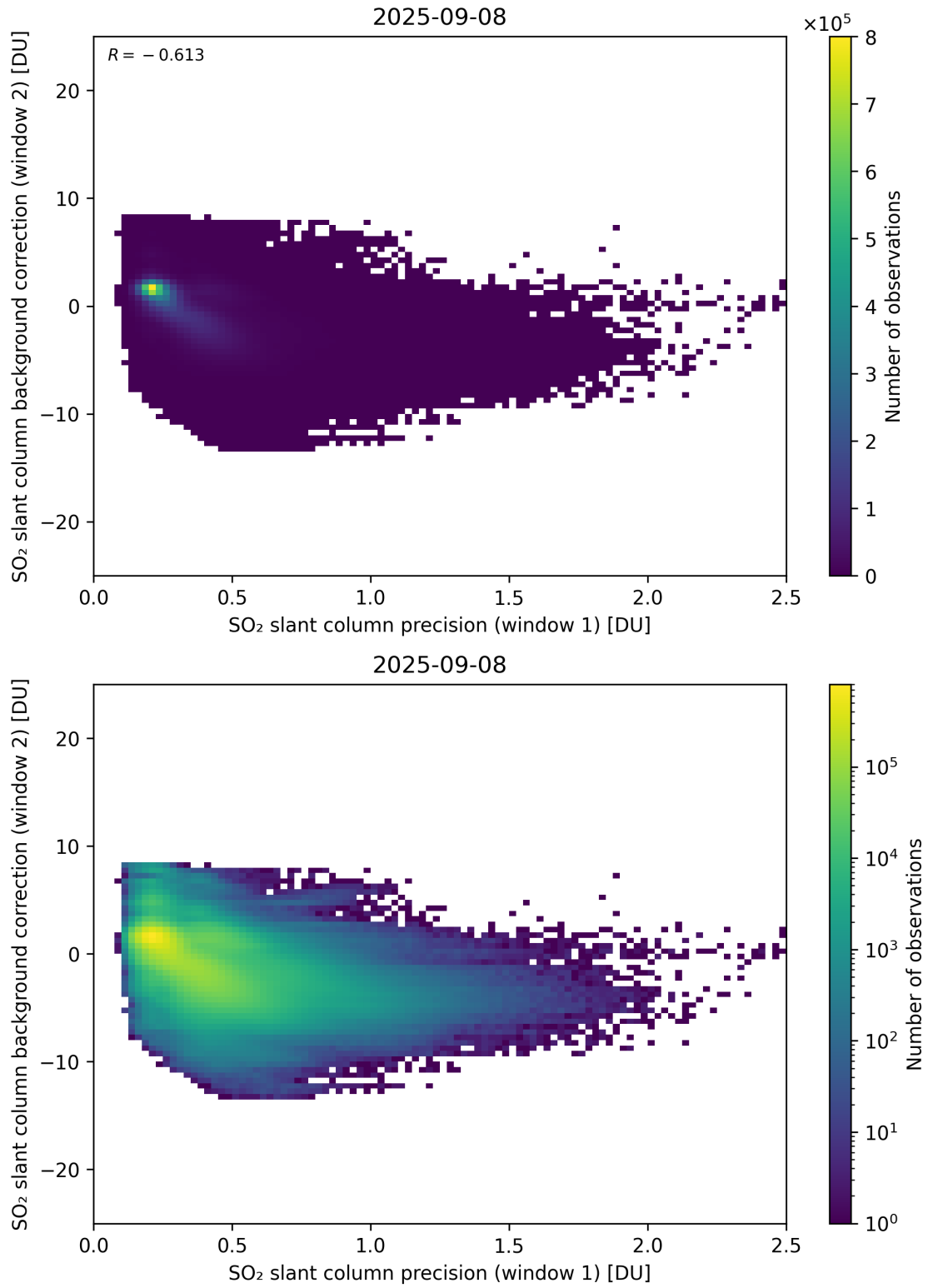
Figure 269: Scatter density plot of “SO 2 slant column precision (window 1)” against “SO 2 slant column background correction (window 2)” for 2025-09-07 to 2025-09-09.
