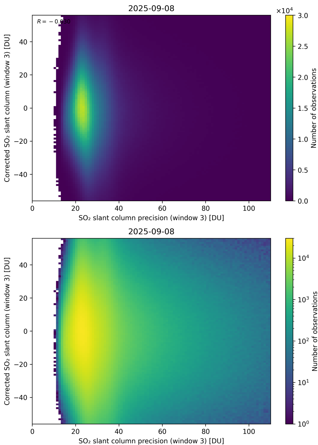
Figure 312: Scatter density plot of “SO 2 slant column precision (window 3)” against “Corrected SO 2 slant column (window 3)” for 2025-09-07 to 2025-09-09.
