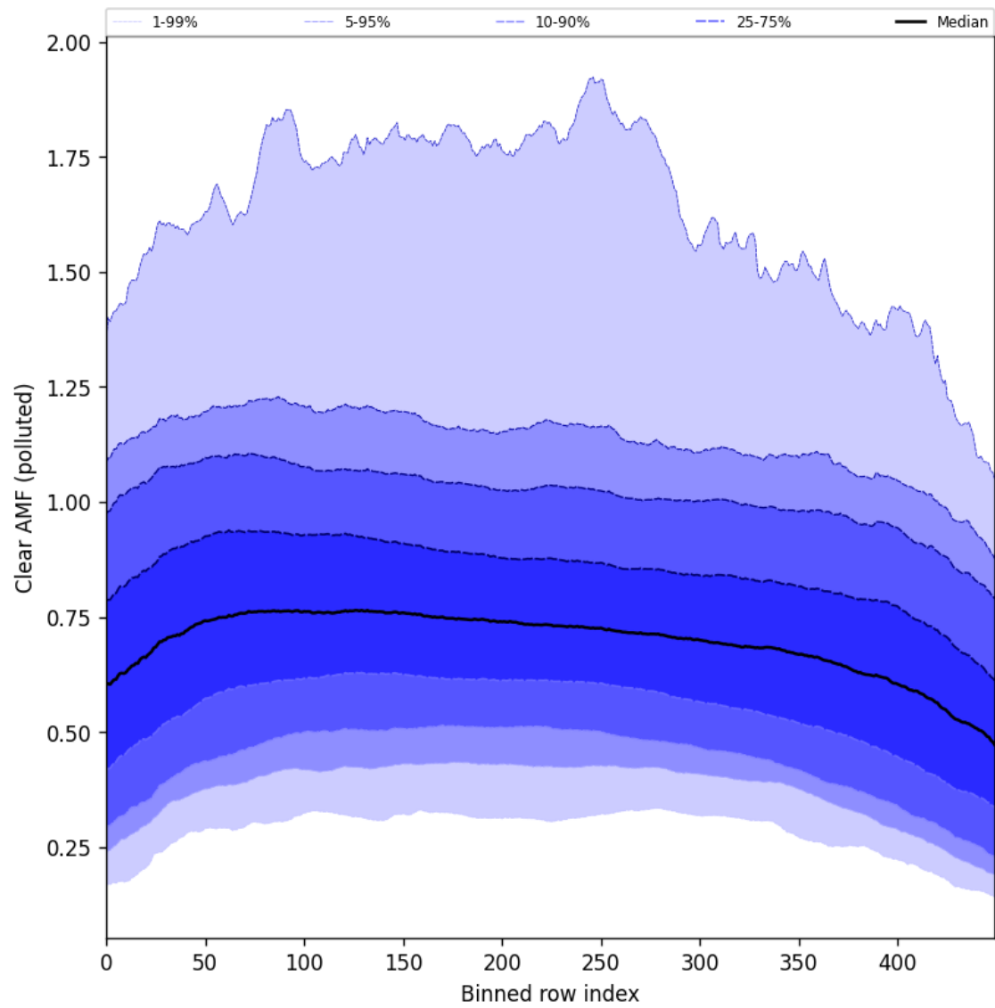
Figure 107: Along track statistics of “Clear AMF (polluted)” for 2025-09-07 to 2025-09-09
