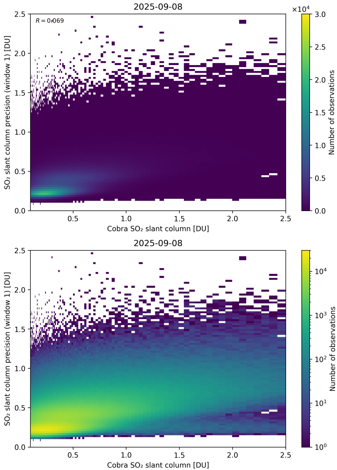
Figure 220: Scatter density plot of “Cobra SO 2 slant column” against “SO 2 slant column precision (window 1)” for 2025-09-07 to 2025-09-09.
