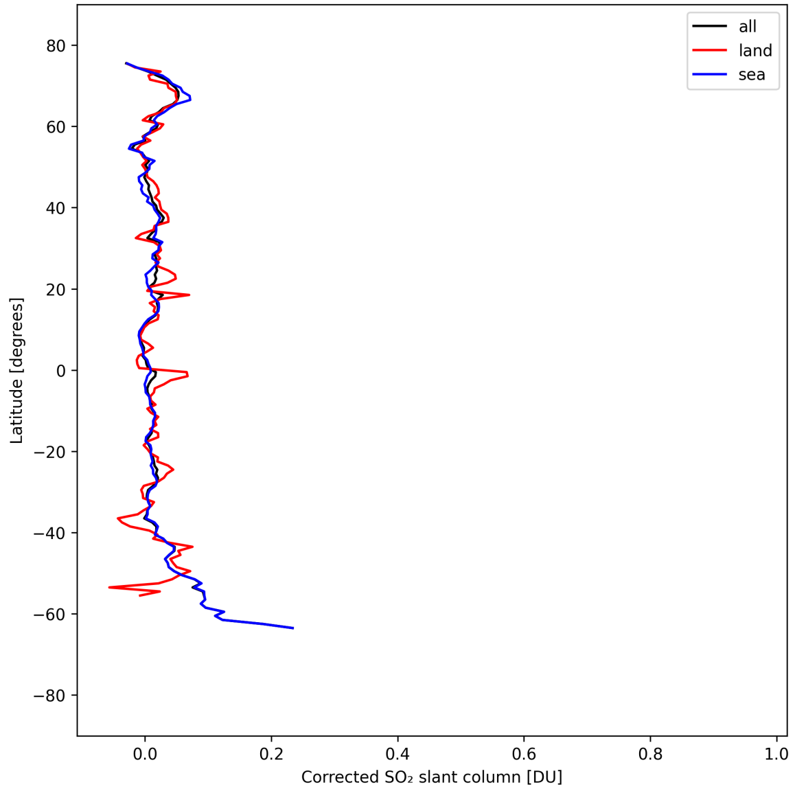
Figure 34: Zonal average of “Corrected SO 2 slant column” for 2025-09-07 to 2025-09-09.
