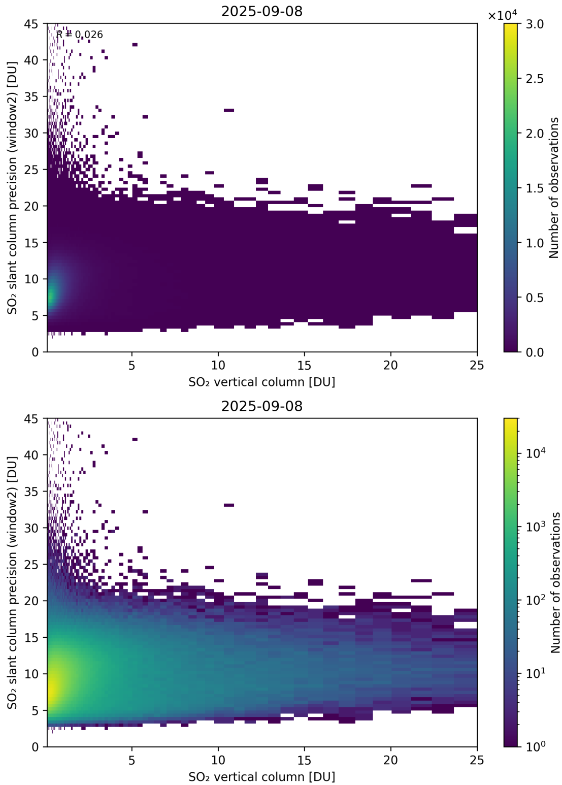
Figure 356: Scatter density plot of “SO 2 vertical column” against “SO 2 slant column precision (window2)” for 2025-09-07 to 2025-09-09.
