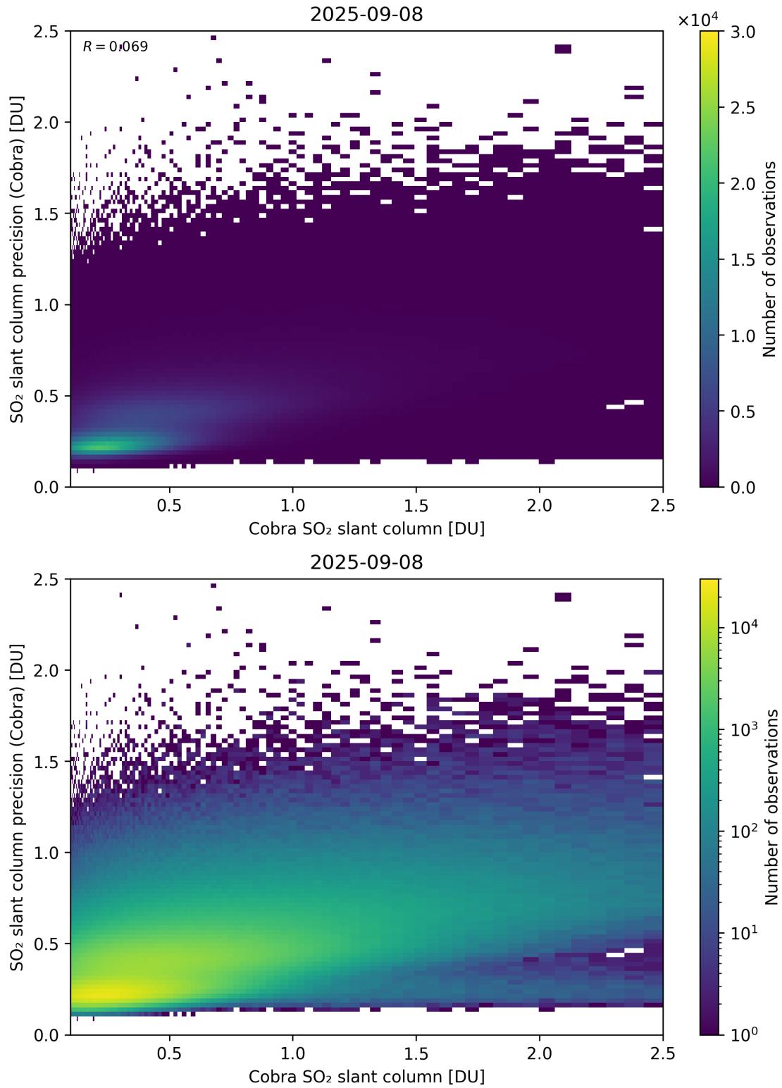
Figure 216: Scatter density plot of “Cobra SO 2 slant column” against “SO 2 slant column precision (Cobra)” for 2025-09-07 to 2025-09-09.
