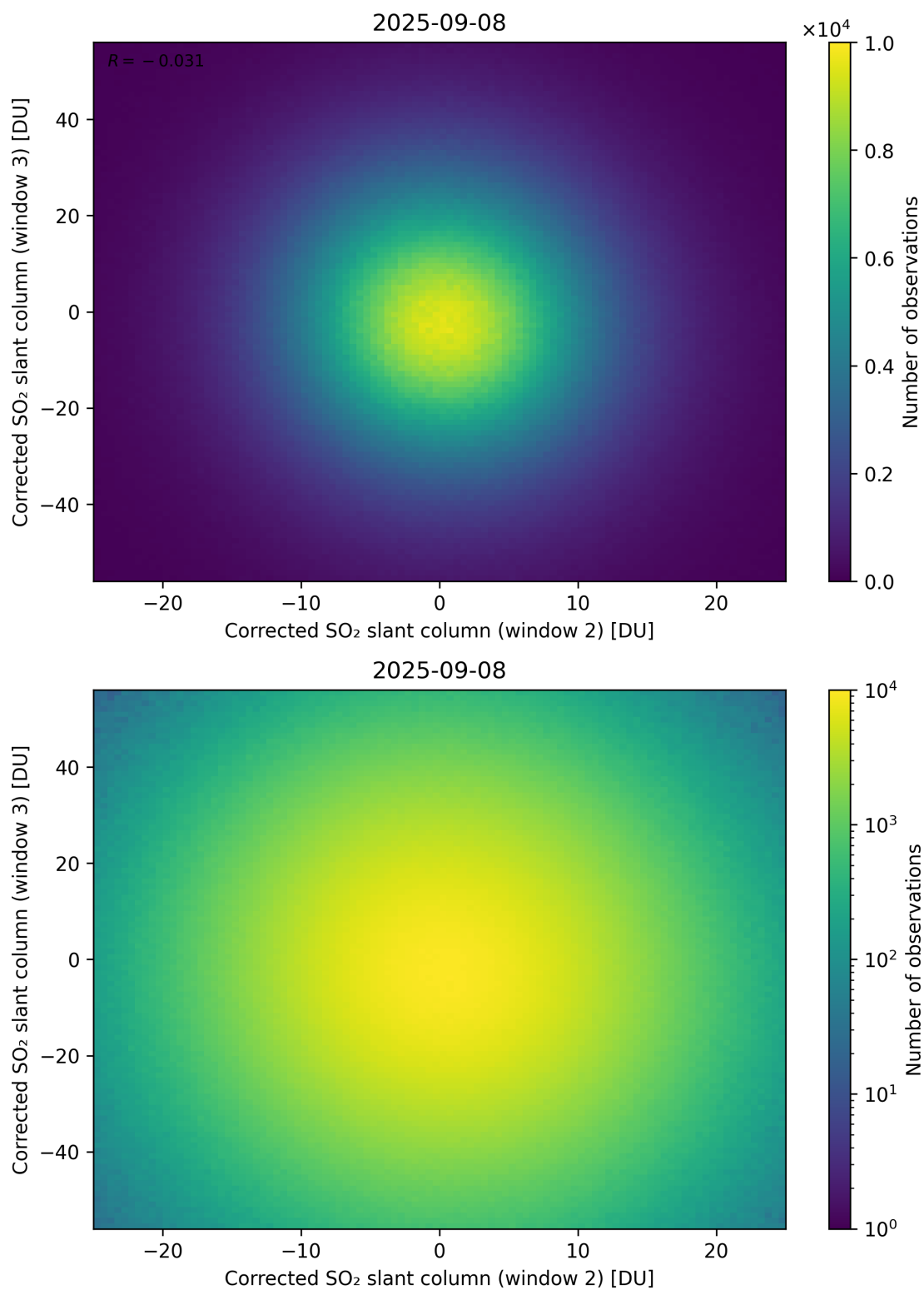
Figure 250: Scatter density plot of “Corrected SO 2 slant column (window 2)” against “Corrected SO 2 slant column (window 3)” for 2025-09-07 to 2025-09-09.
