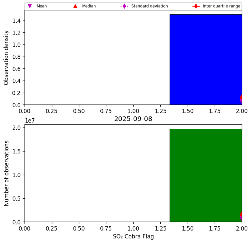
Figure 75: Histogram of “SO 2 Cobra Flag” for 2025-09-07 to 2025-09-09
