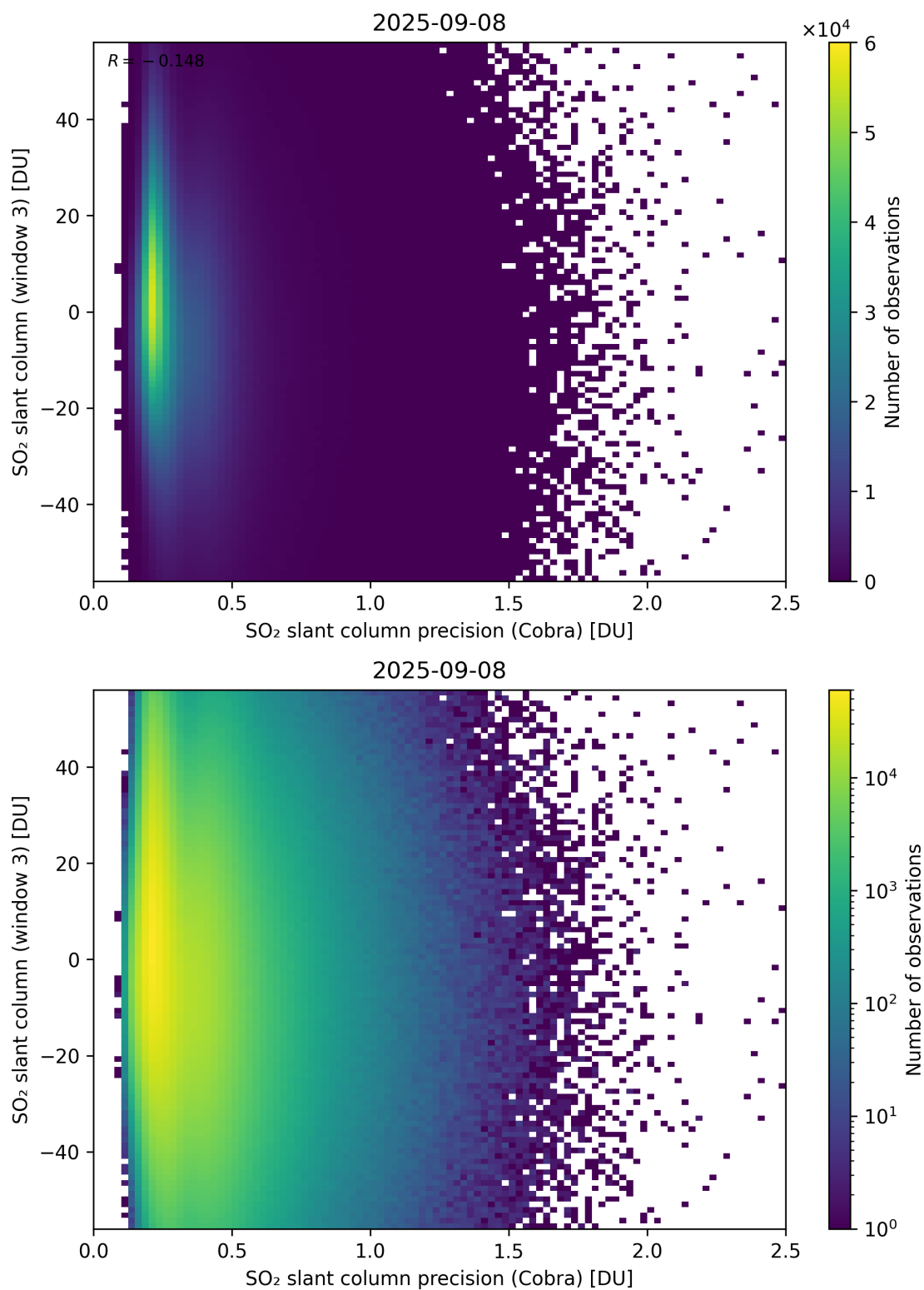
Figure 211: Scatter density plot of “SO 2 slant column precision (Cobra)” against “SO 2 slant column (window 3)” for 2025-09-07 to 2025-09-09.
