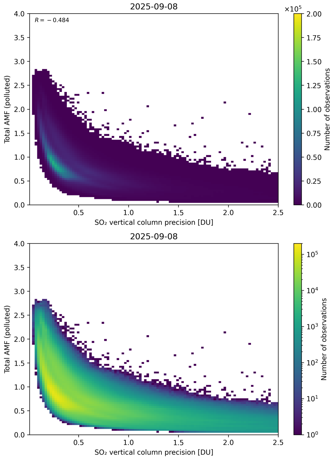
Figure 346: Scatter density plot of “SO 2 vertical column precision” against “Total AMF (polluted)” for 2025-09-07 to 2025-09-09.
