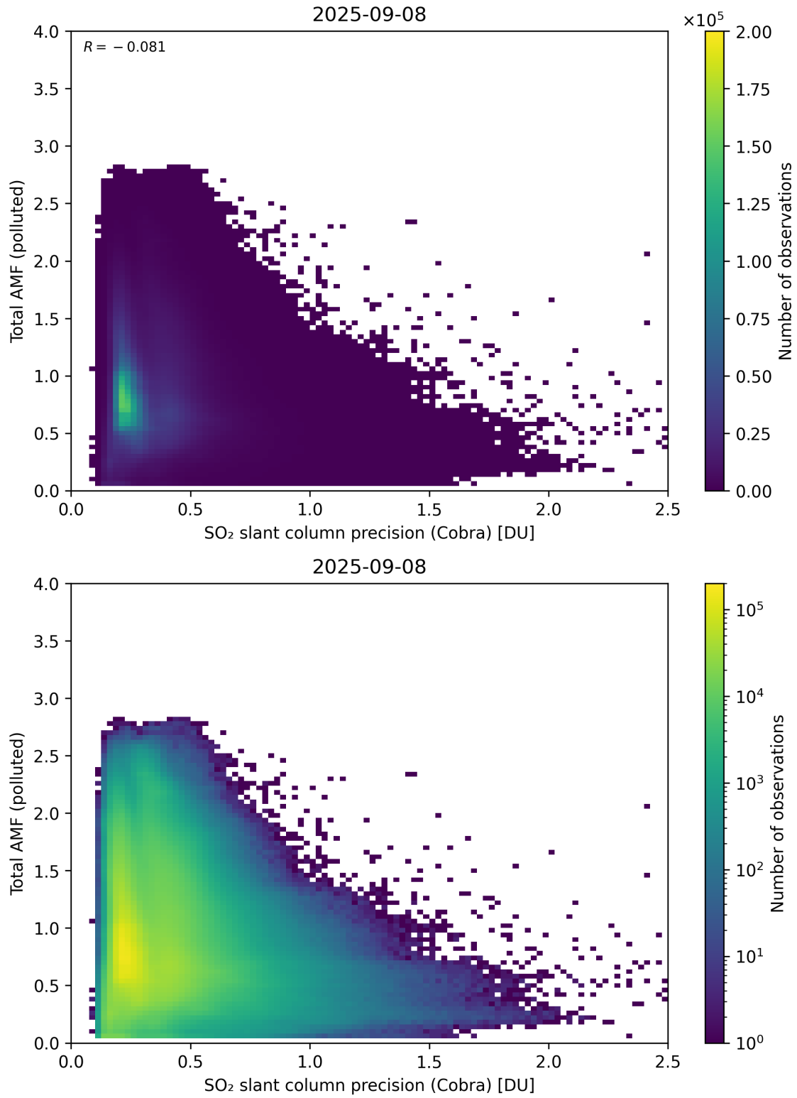
Figure 213: Scatter density plot of “SO 2 slant column precision (Cobra)” against “Total AMF (polluted)” for 2025-09-07 to 2025-09-09.
