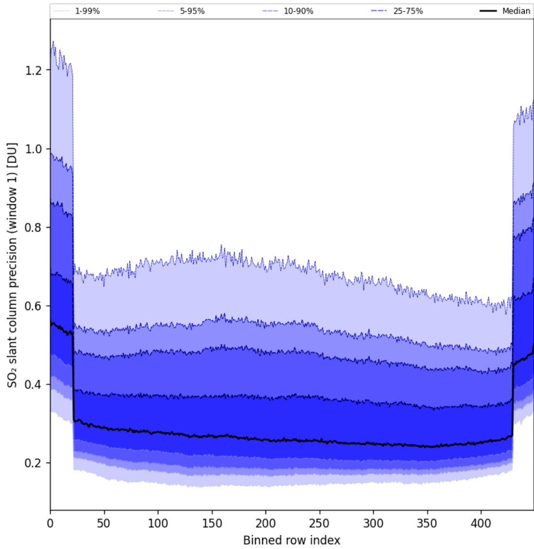
Figure 90: Along track statistics of “SO 2 slant column precision (window 1)” for 2025-09-07 to 2025-09-09
