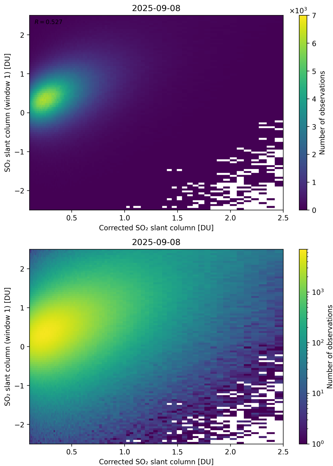
Figure 237: Scatter density plot of “Corrected SO 2 slant column” against “SO 2 slant column (window 1)” for 2025-09-07 to 2025-09-09.
