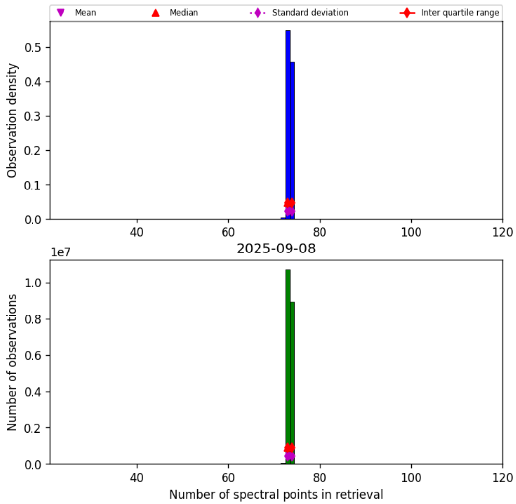
Figure 82: Histogram of “Number of spectral points in retrieval” for 2025-09-07 to 2025-09-09
