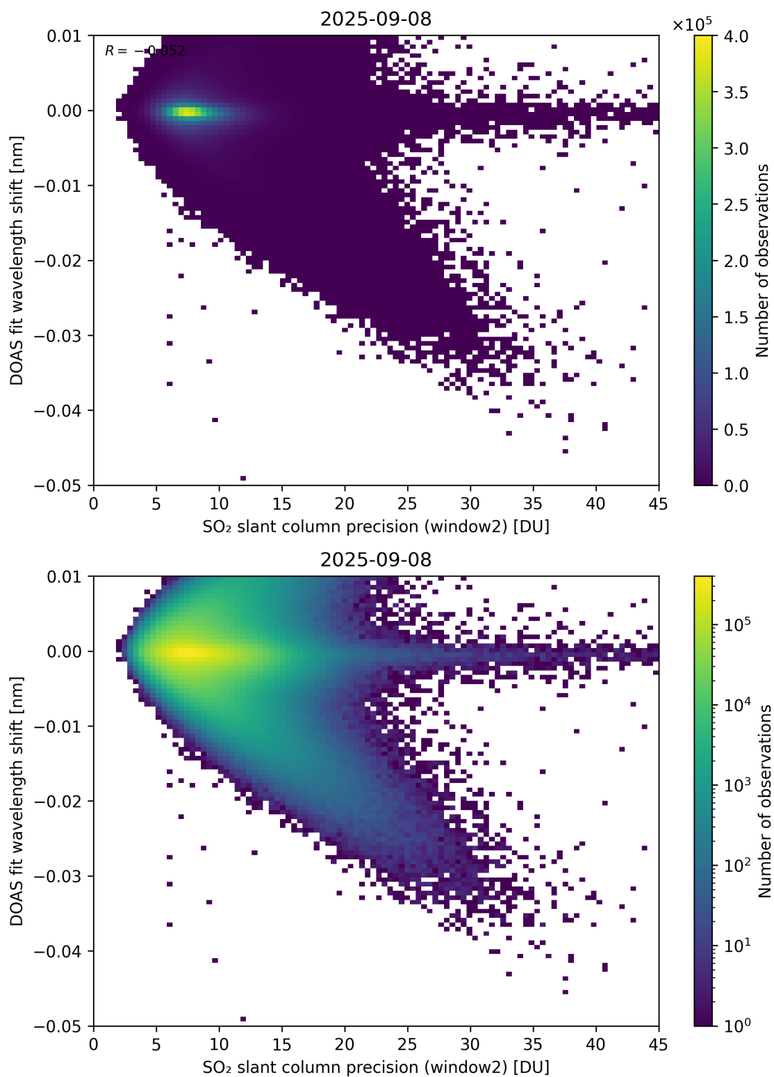
Figure 293: Scatter density plot of “SO 2 slant column precision (window2)” against “DOAS fit wavelength shift” for 2025-09-07 to 2025-09-09.
