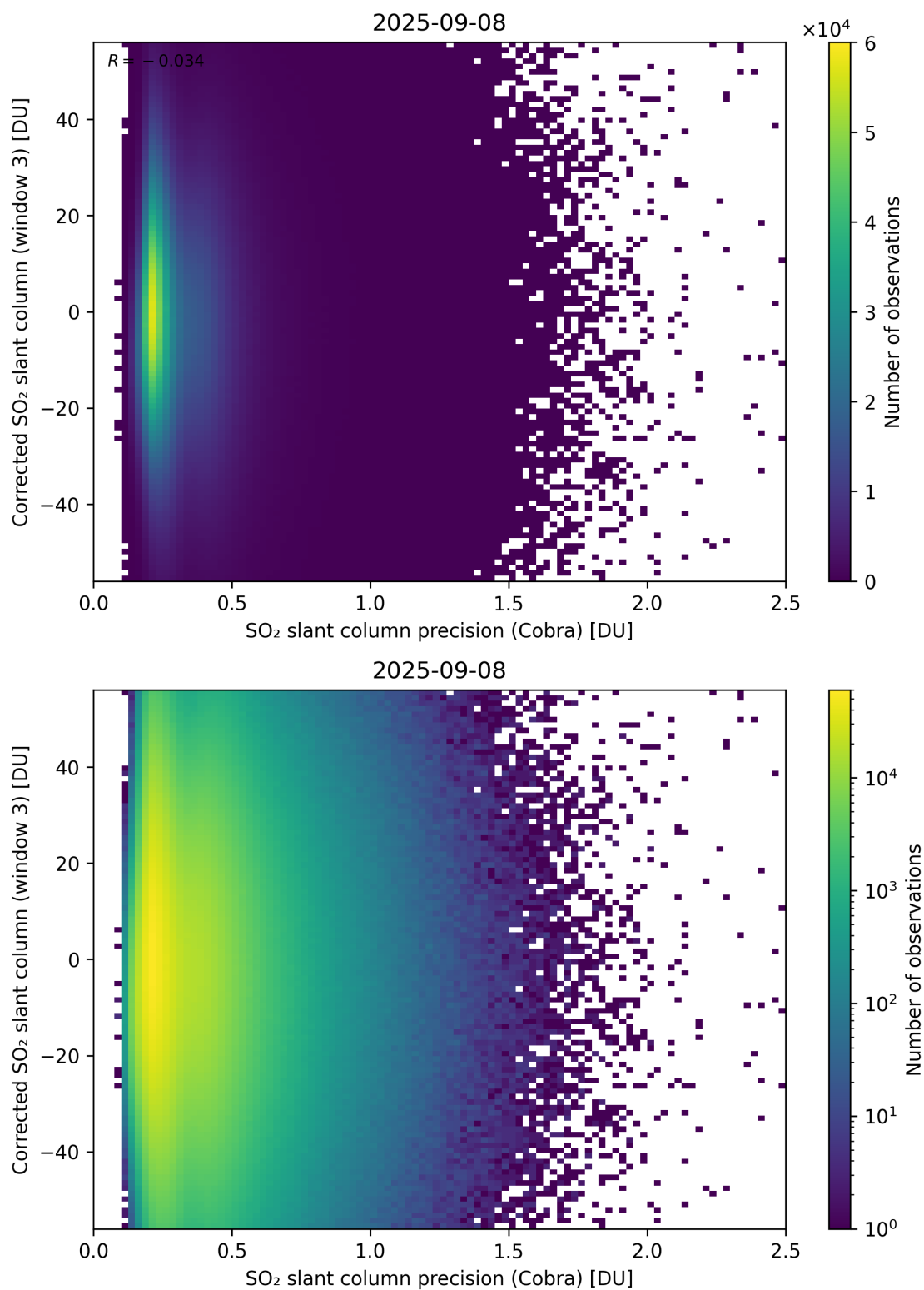
Figure 207: Scatter density plot of “SO 2 slant column precision (Cobra)” against “Corrected SO 2 slant column (window 3)” for 2025-09-07 to 2025-09-09.
