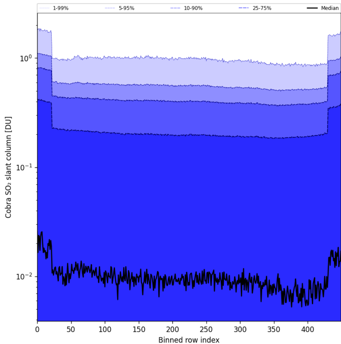
Figure 87: Along track statistics of "Cobra SO 2 slant column" for 2025-09-07 to 2025-09-09
