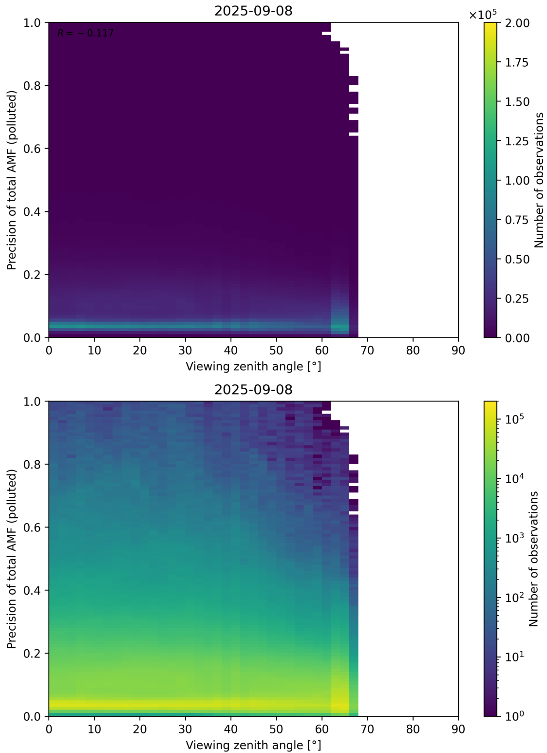
Figure 382: Scatter density plot of “Viewing zenith angle” against “Precision of total AMF (polluted)” for 2025-09-07 to 2025-09-09.
