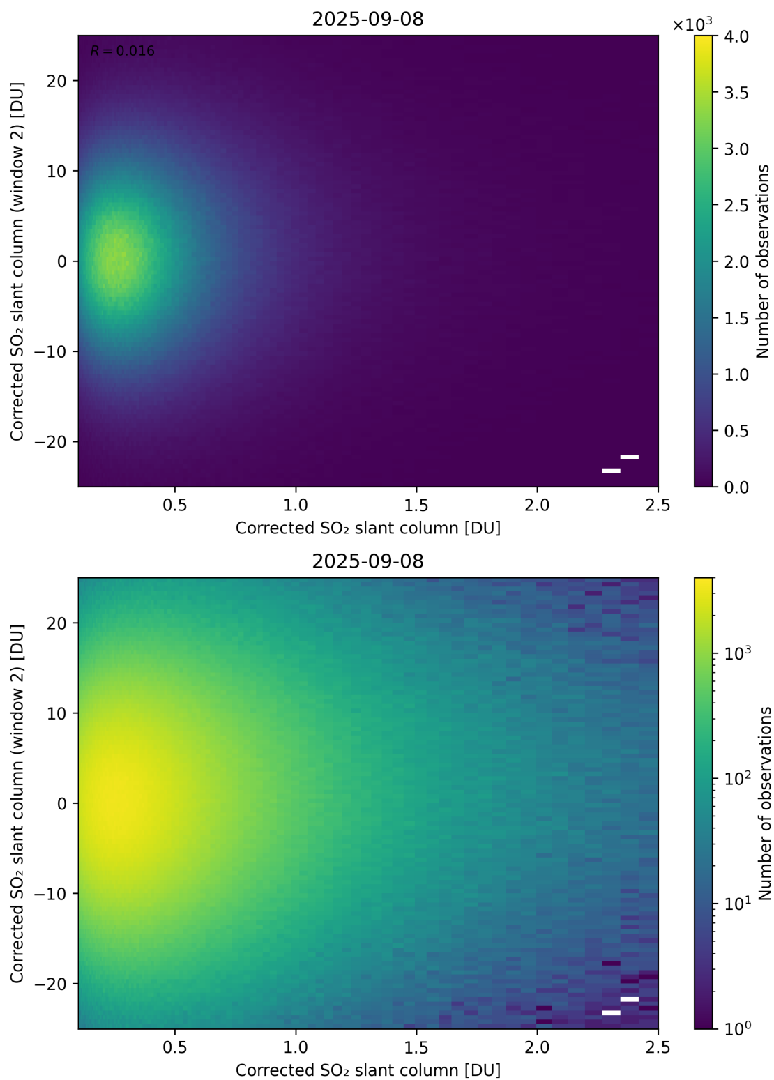
Figure 235: Scatter density plot of “Corrected SO 2 slant column” against “Corrected SO 2 slant column (window 2)” for 2025-09-07 to 2025-09-09.
