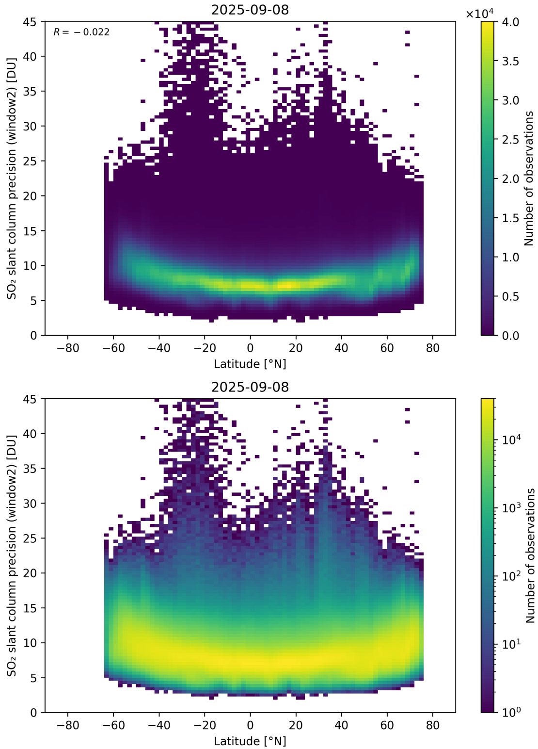
Figure 164: Scatter density plot of “Latitude” against “SO 2 slant column precision (window2)” for 2025-09-07 to 2025-09-09.
