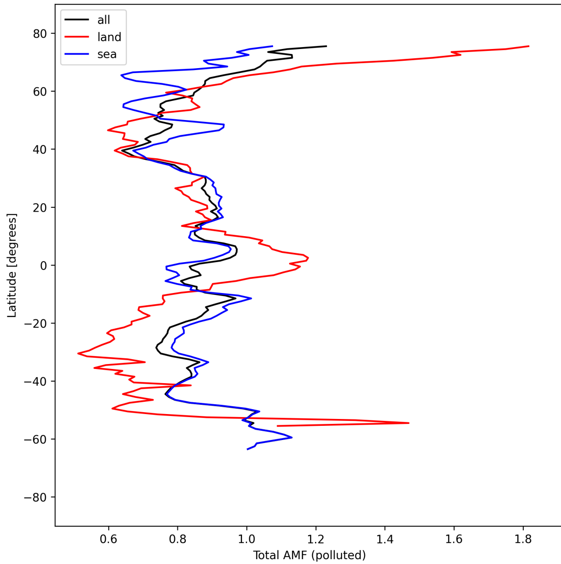
Figure 53: Zonal average of “Total AMF (polluted)” for 2025-09-07 to 2025-09-09.
