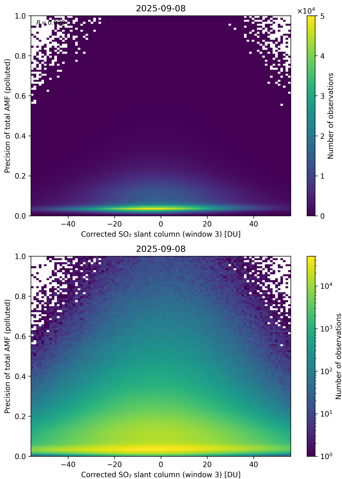
Figure 261: Scatter density plot of “Corrected SO 2 slant column (window 3)” against “Precision of total AMF (polluted)” for 2025-09-07 to 2025-09-09.
