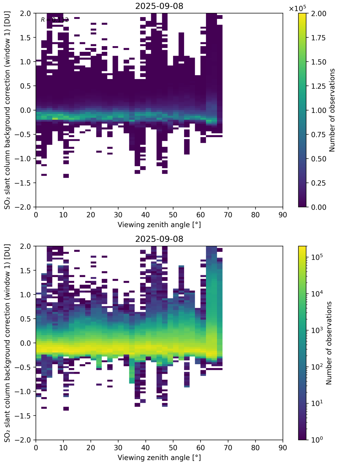
Figure 362: Scatter density plot of “Viewing zenith angle” against “SO 2 slant column background correction (window 1)” for 2025-09-07 to 2025-09-09.
