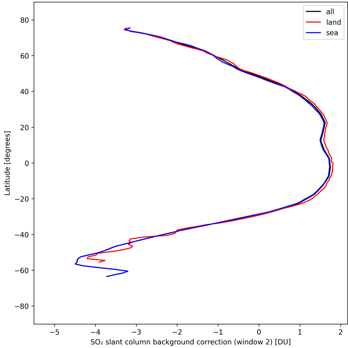
Figure 44: Zonal average of “SO 2 slant column background correction (window 2)” for 2025-09-07 to 2025-09-09.
