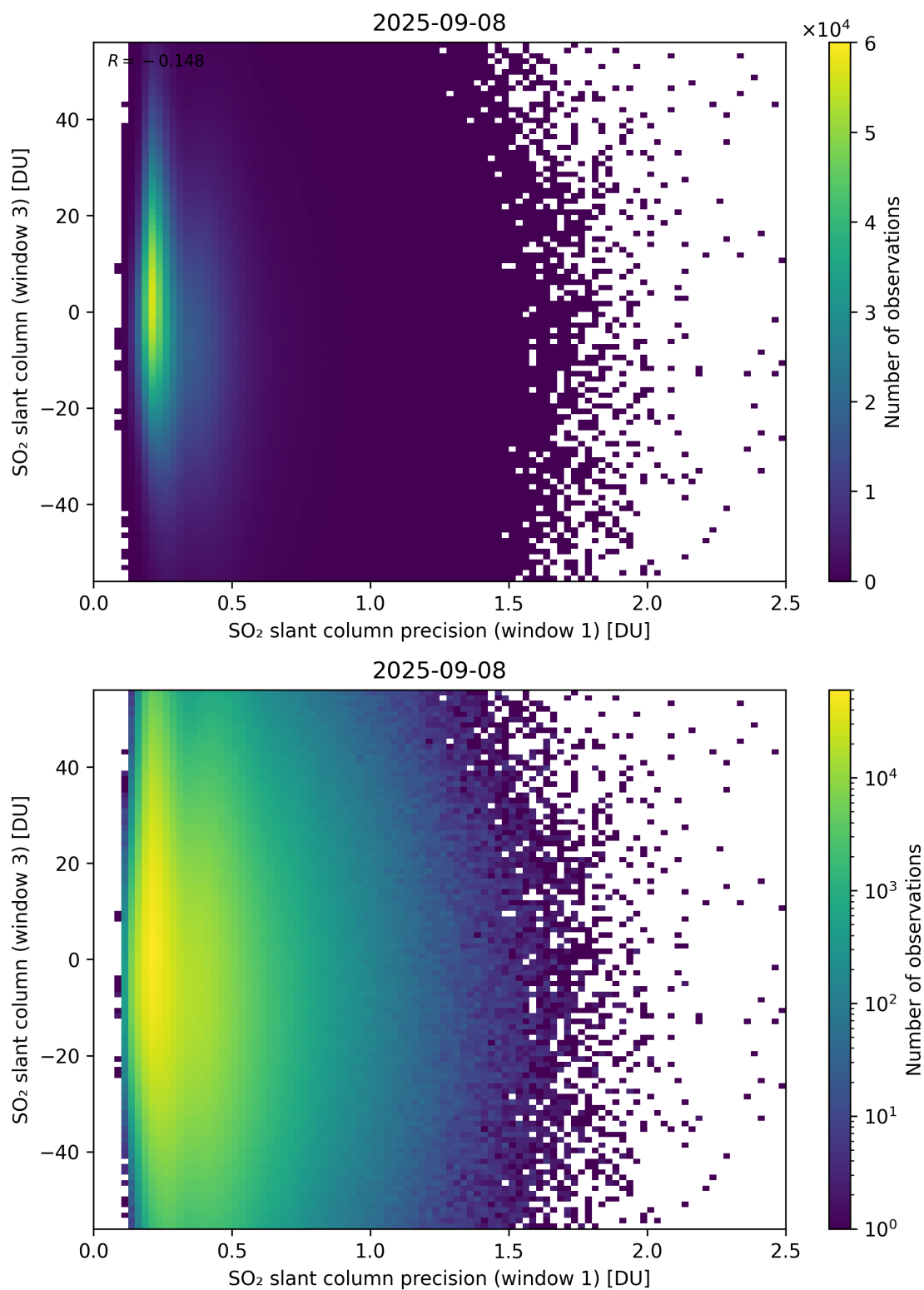
Figure 278: Scatter density plot of “SO 2 slant column precision (window 1)” against “SO 2 slant column (window 3)” for 2025-09-07 to 2025-09-09.
