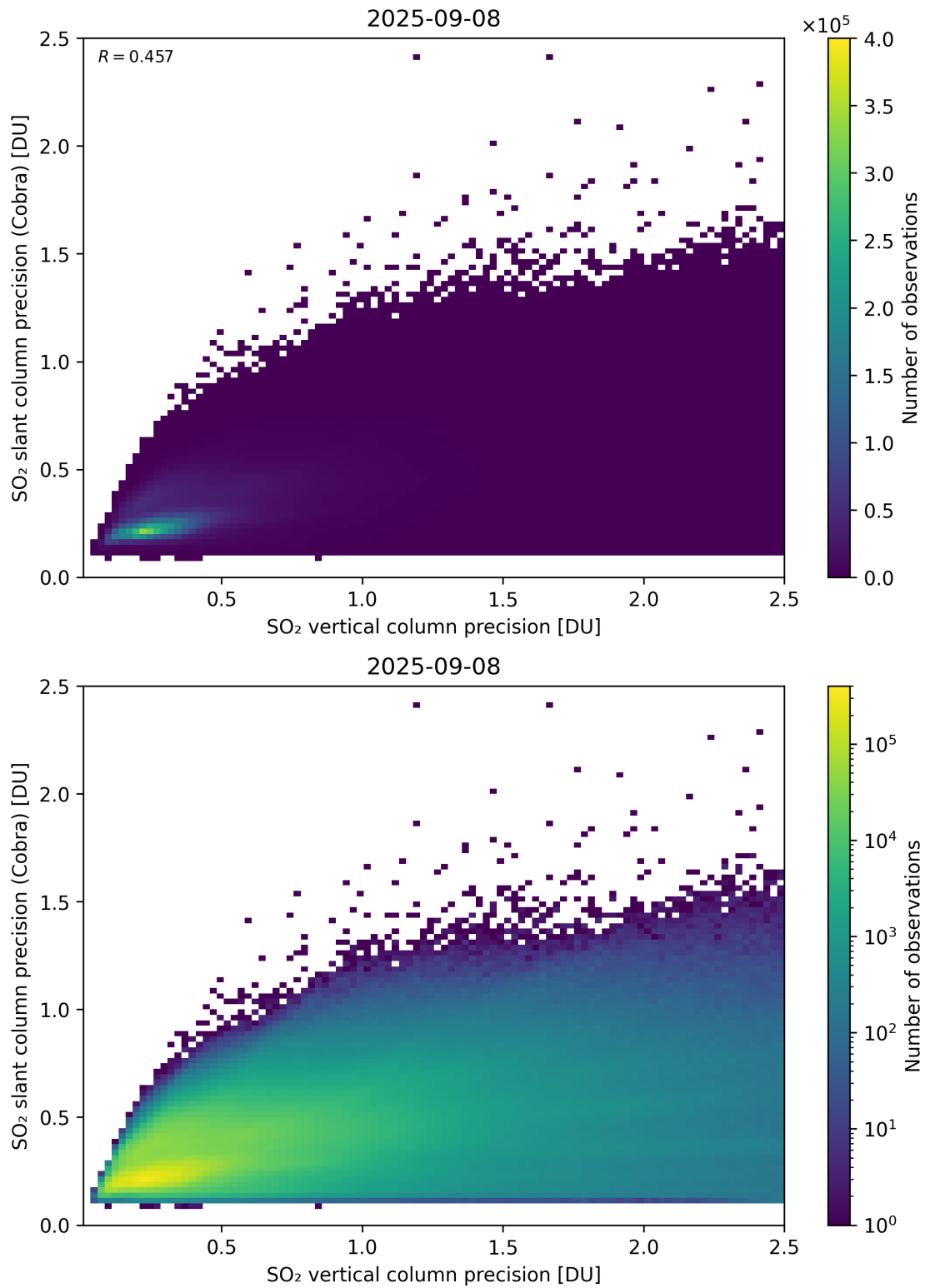
Figure 337: Scatter density plot of “SO 2 vertical column precision” against “SO 2 slant column precision (Cobra)” for 2025-09-07 to 2025-09-09.
