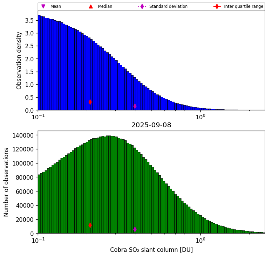
Figure 61: Histogram of “Cobra SO 2 slant column” for 2025-09-07 to 2025-09-09
