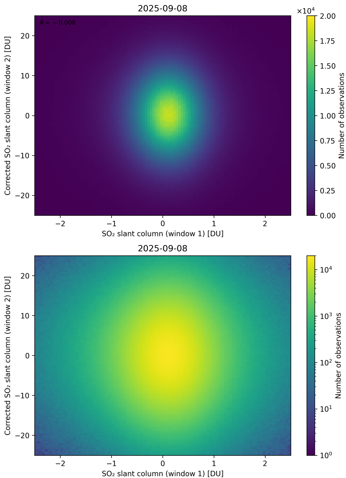
Figure 283: Scatter density plot of “SO 2 slant column (window 1)” against “Corrected SO 2 slant column (window 2)” for 2025-09-07 to 2025-09-09.
