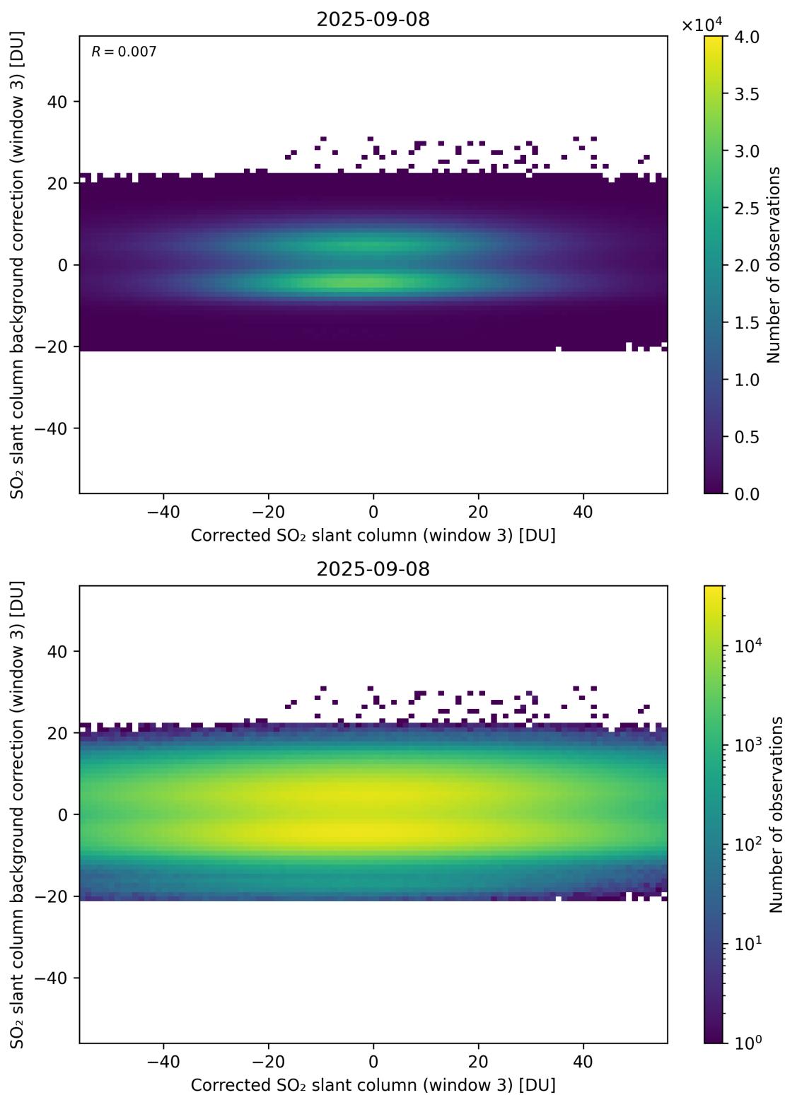
Figure 255: Scatter density plot of “Corrected SO 2 slant column (window 3)” against “SO 2 slant column background correction (window 3)” for 2025-09-07 to 2025-09-09.
