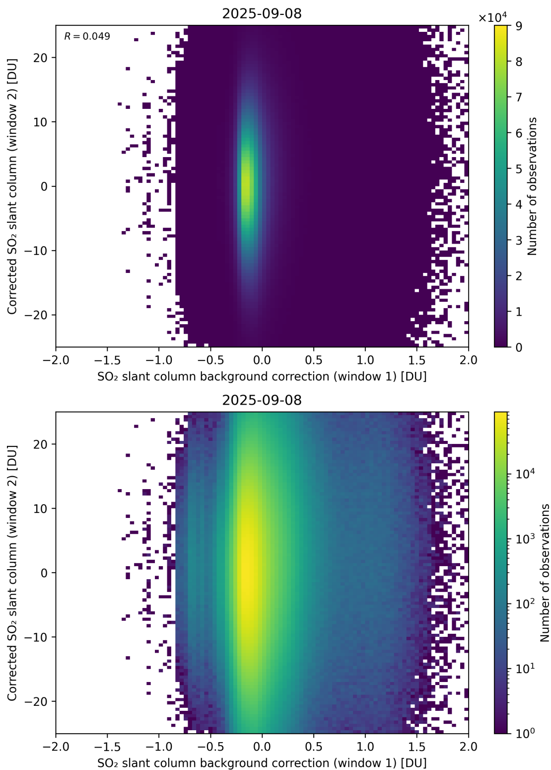
Figure 115: Scatter density plot of “SO 2 slant column background correction (window 1)” against “Corrected SO 2 slant column (window 2)” for 2025-09-07 to 2025-09-09.
