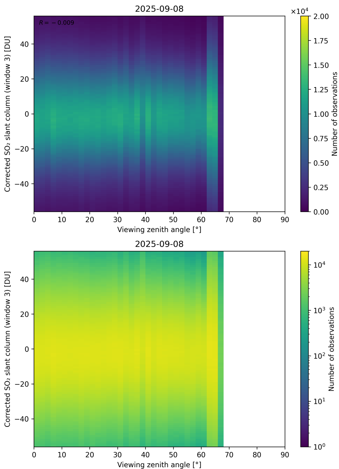
Figure 375: Scatter density plot of “Viewing zenith angle” against “Corrected SO 2 slant column (window 3)” for 2025-09-07 to 2025-09-09.
