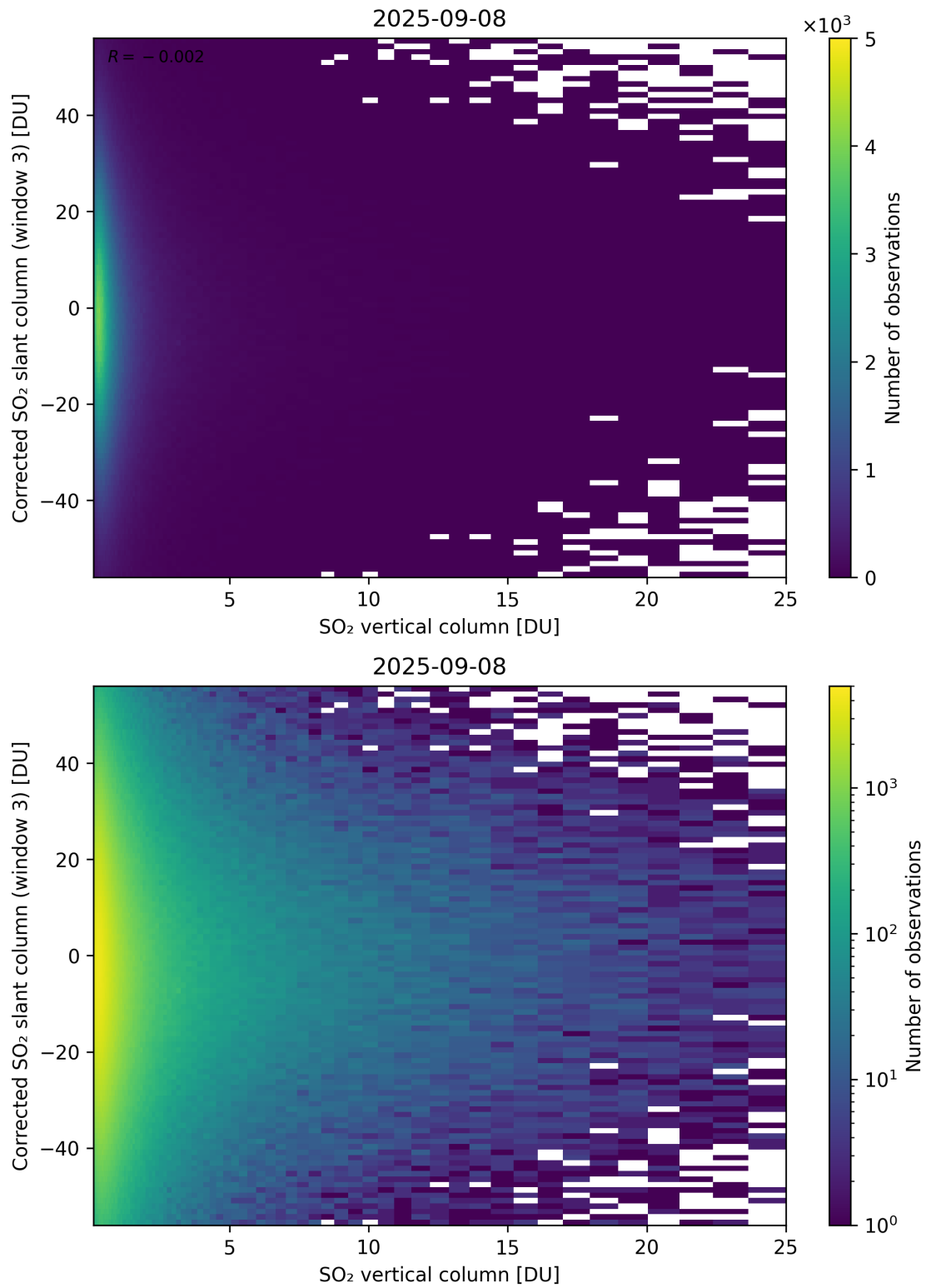
Figure 353: Scatter density plot of “SO 2 vertical column” against “Corrected SO 2 slant column (window 3)” for 2025-09-07 to 2025-09-09.
