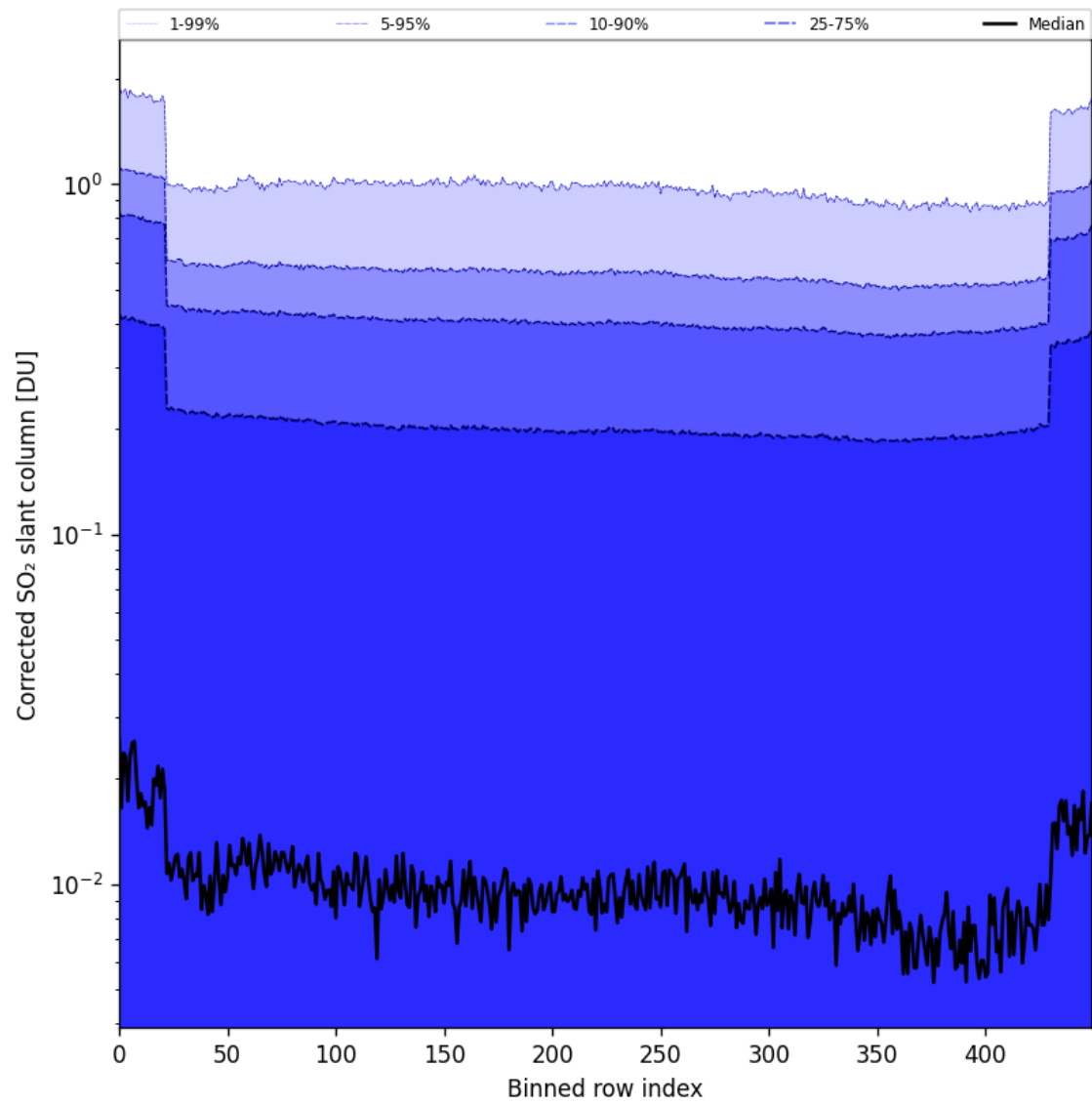
Figure 86: Along track statistics of "Corrected SO 2 slant column" for 2025-09-07 to 2025-09-09
