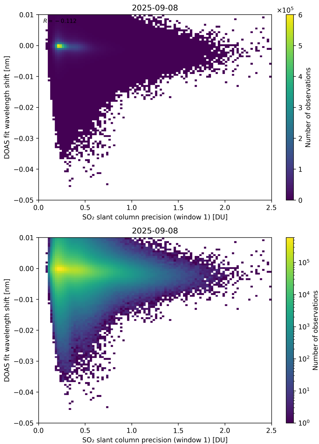
Figure 271: Scatter density plot of “SO 2 slant column precision (window 1)” against “DOAS fit wavelength shift” for 2025-09-07 to 2025-09-09.
