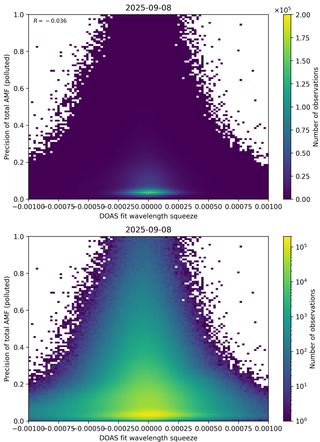
Figure 146: Scatter density plot of “DOAS fit wavelength squeeze” against “Precision of total AMF (polluted)” for 2025-09-07 to 2025-09-09.
