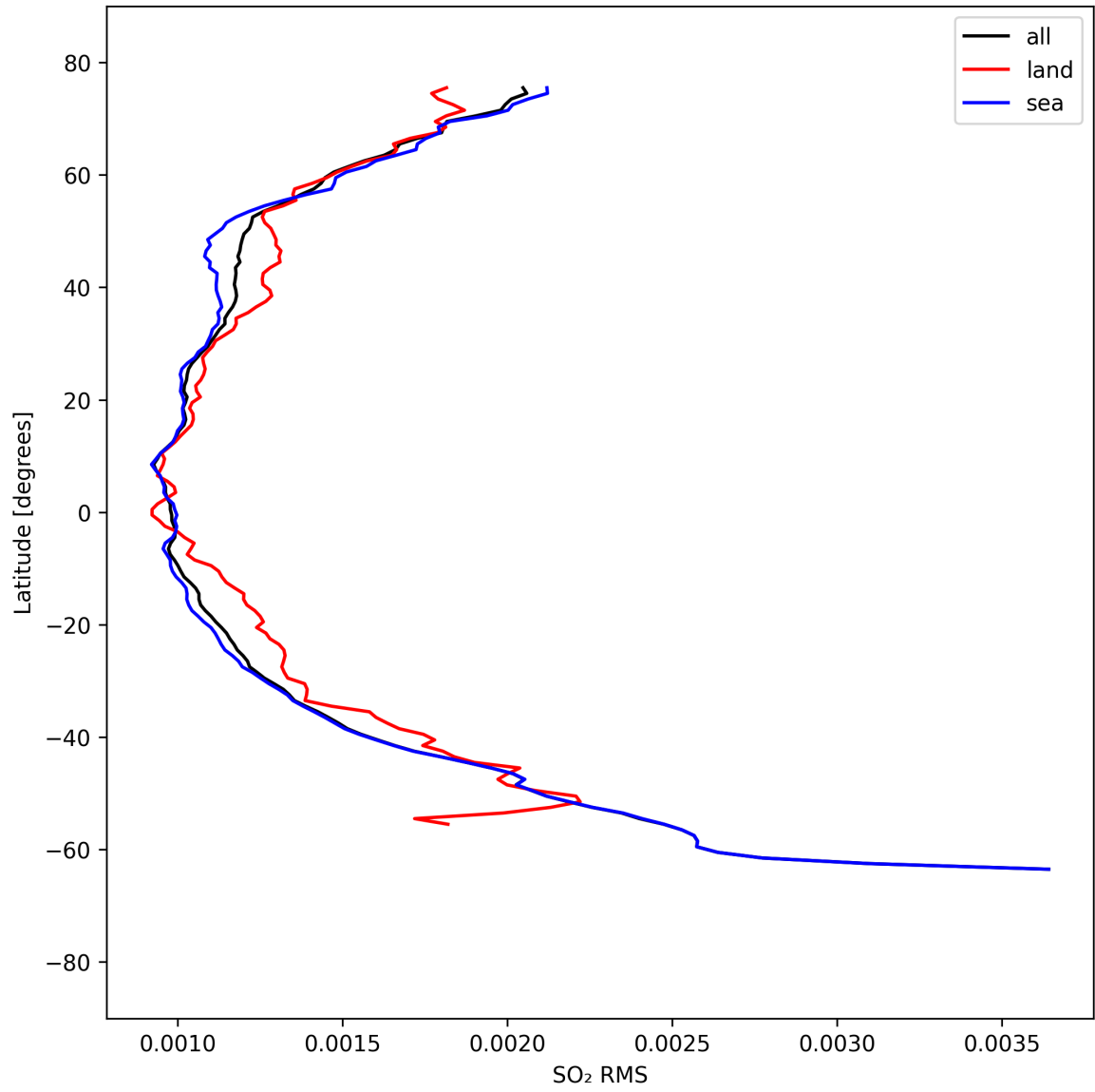
Figure 52: Zonal average of “SO 2 RMS” for 2025-09-07 to 2025-09-09.
