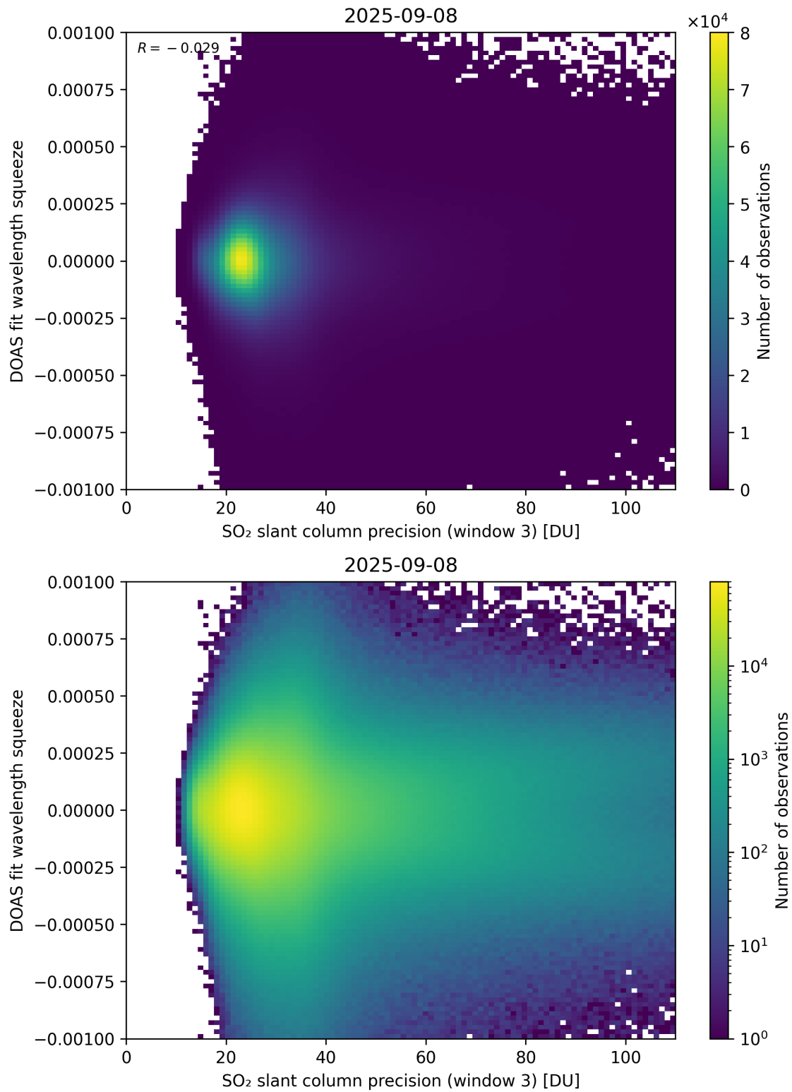
Figure 309: Scatter density plot of “SO 2 slant column precision (window 3)” against “DOAS fit wavelength squeeze” for 2025-09-07 to 2025-09-09.
