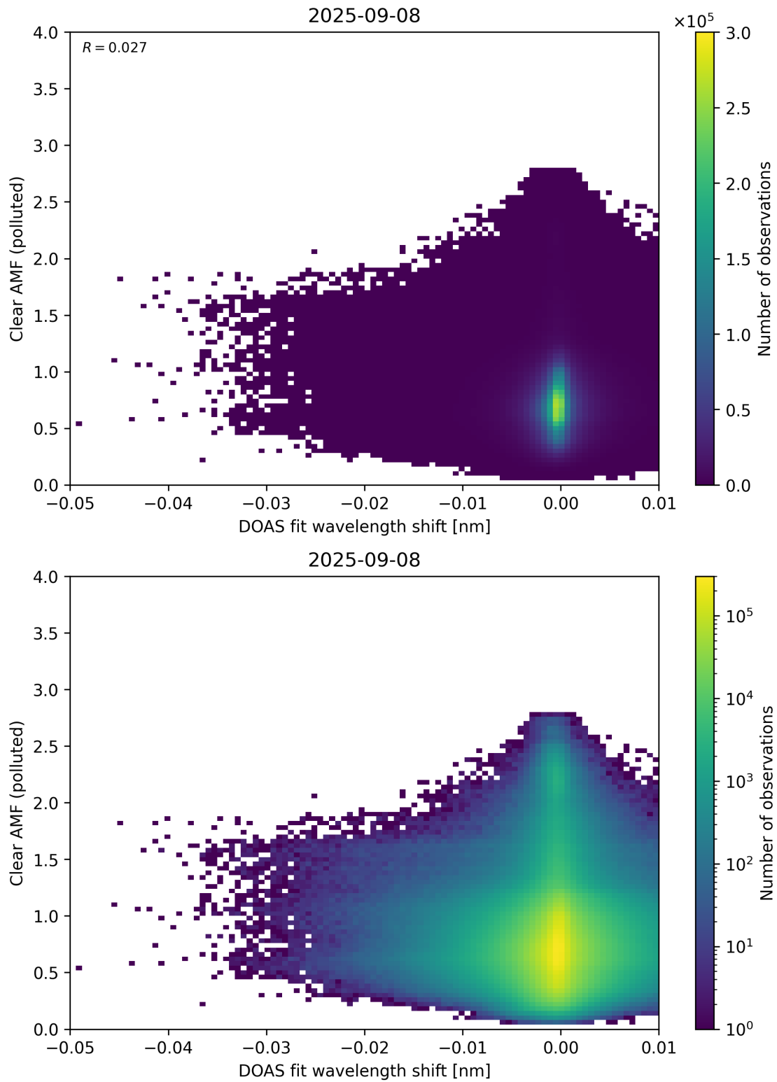
Figure 140: Scatter density plot of “DOAS fit wavelength shift” against “Clear AMF (polluted)” for 2025-09-07 to 2025-09-09.
