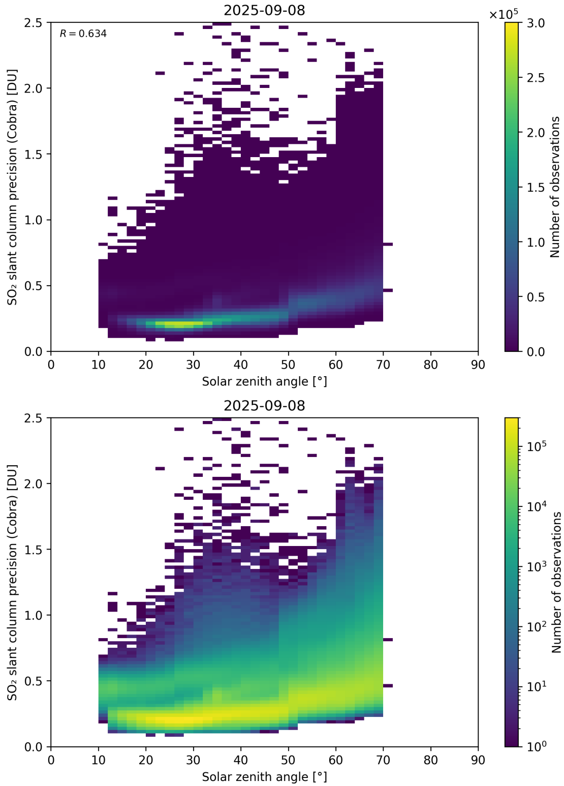
Figure 180: Scatter density plot of “Solar zenith angle” against “SO 2 slant column precision (Cobra)” for 2025-09-07 to 2025-09-09.
