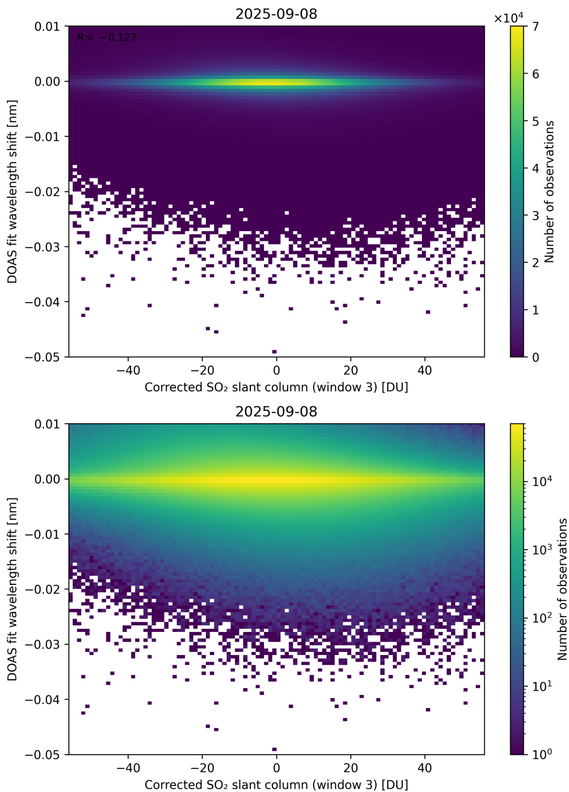
Figure 256: Scatter density plot of “Corrected SO 2 slant column (window 3)” against “DOAS fit wavelength shift” for 2025-09-07 to 2025-09-09.
