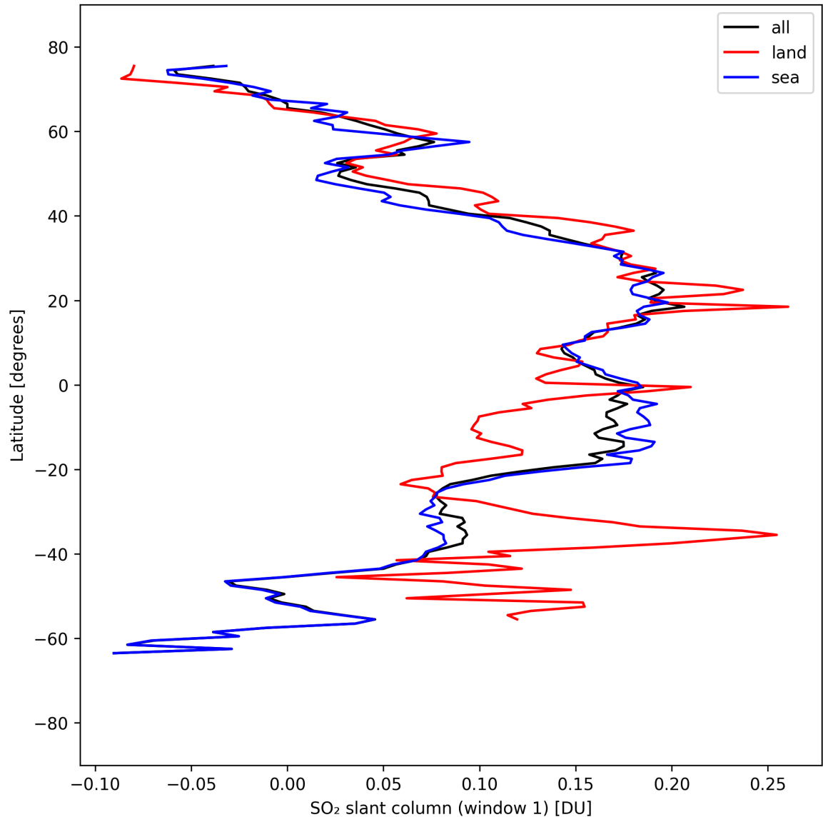
Figure 37: Zonal average of “SO 2 slant column (window 1)” for 2025-09-07 to 2025-09-09.
