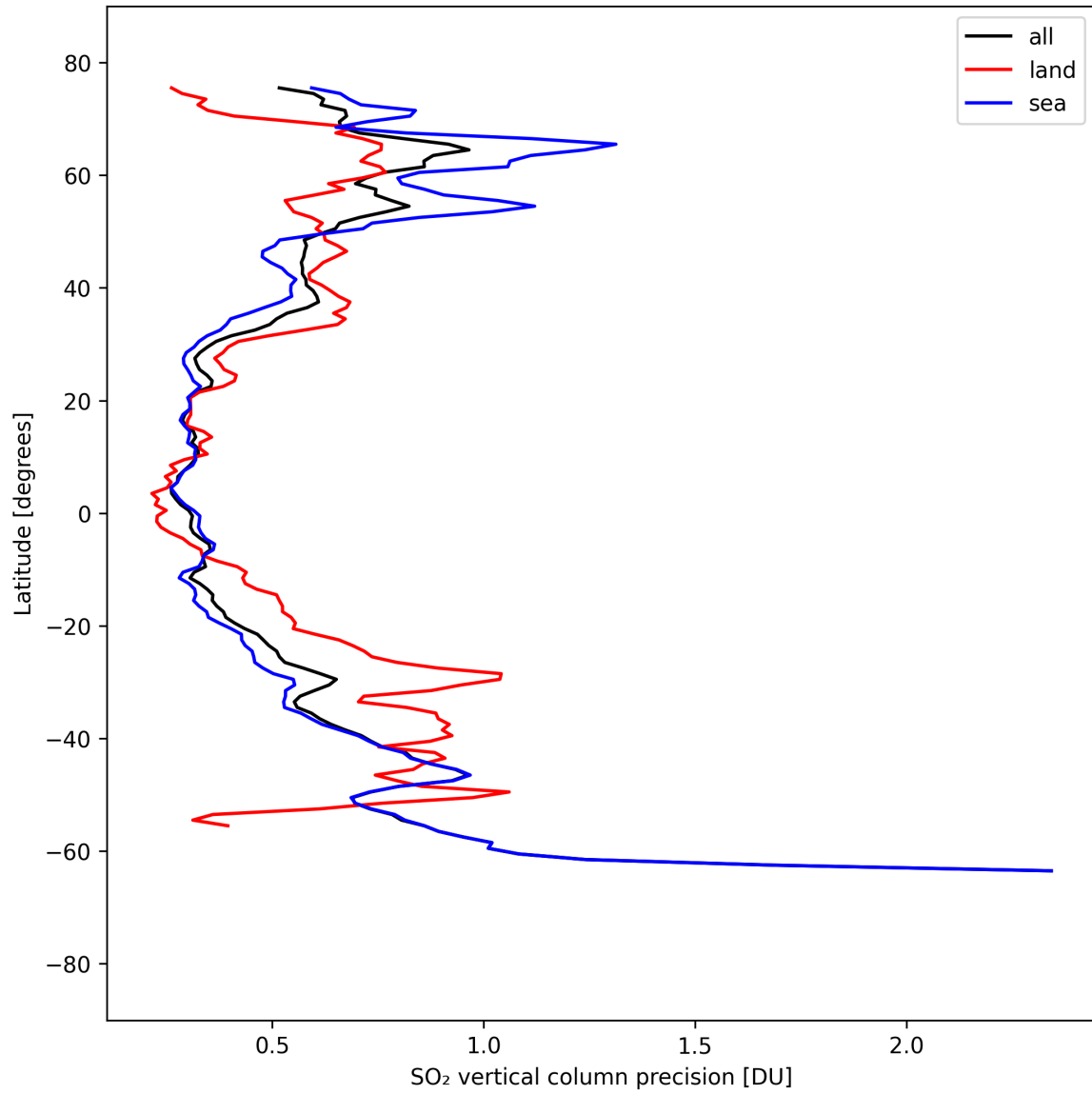
Figure 33: Zonal average of “SO 2 vertical column precision” for 2025-09-07 to 2025-09-09.
