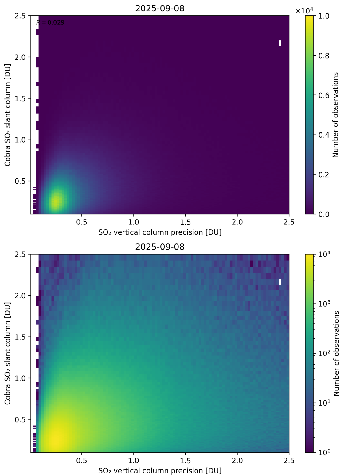
Figure 336: Scatter density plot of “SO 2 vertical column precision” against “Cobra SO 2 slant column” for 2025-09-07 to 2025-09-09.
