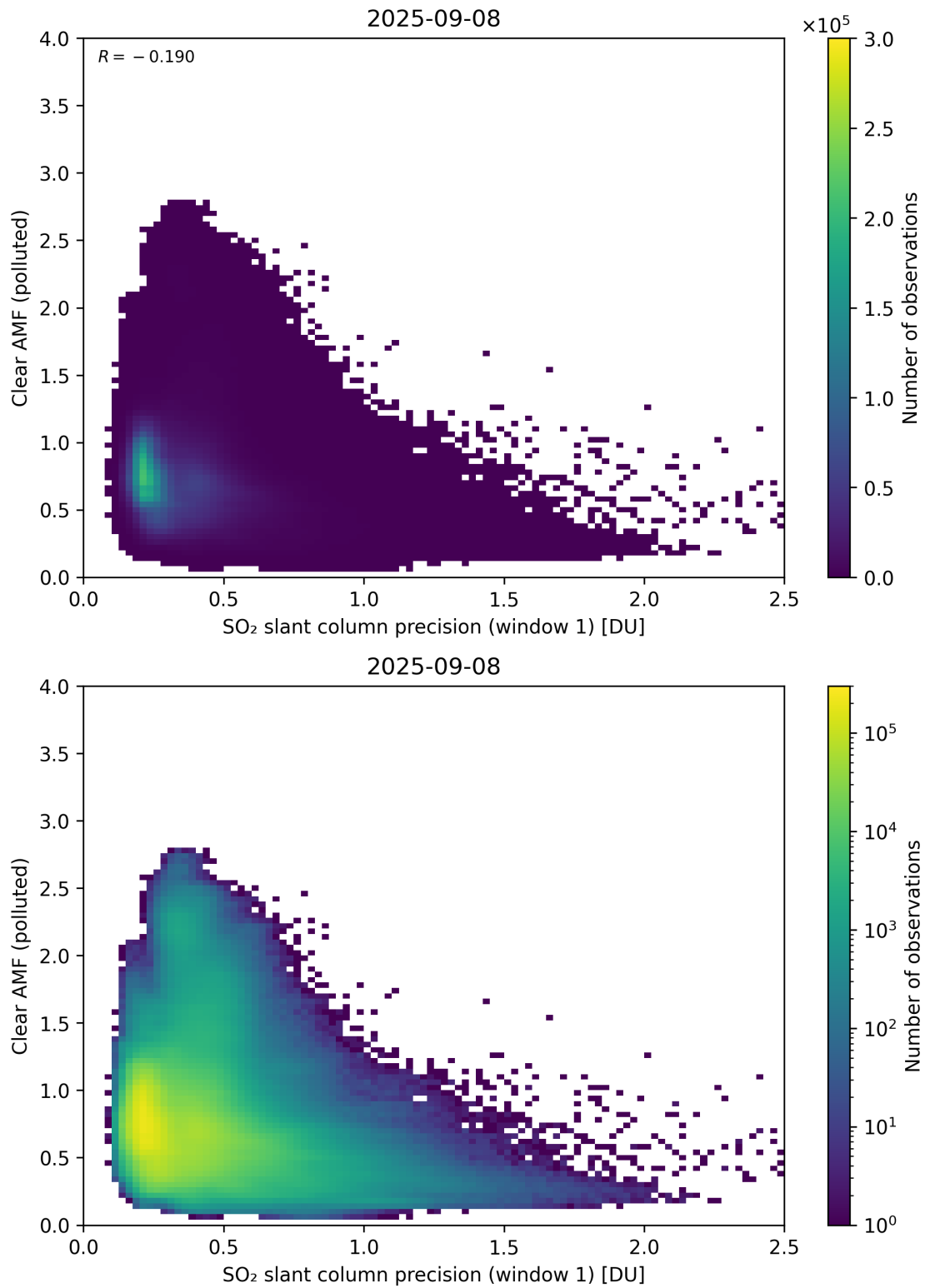
Figure 274: Scatter density plot of “SO 2 slant column precision (window 1)” against “Clear AMF (polluted)” for 2025-09-07 to 2025-09-09.
