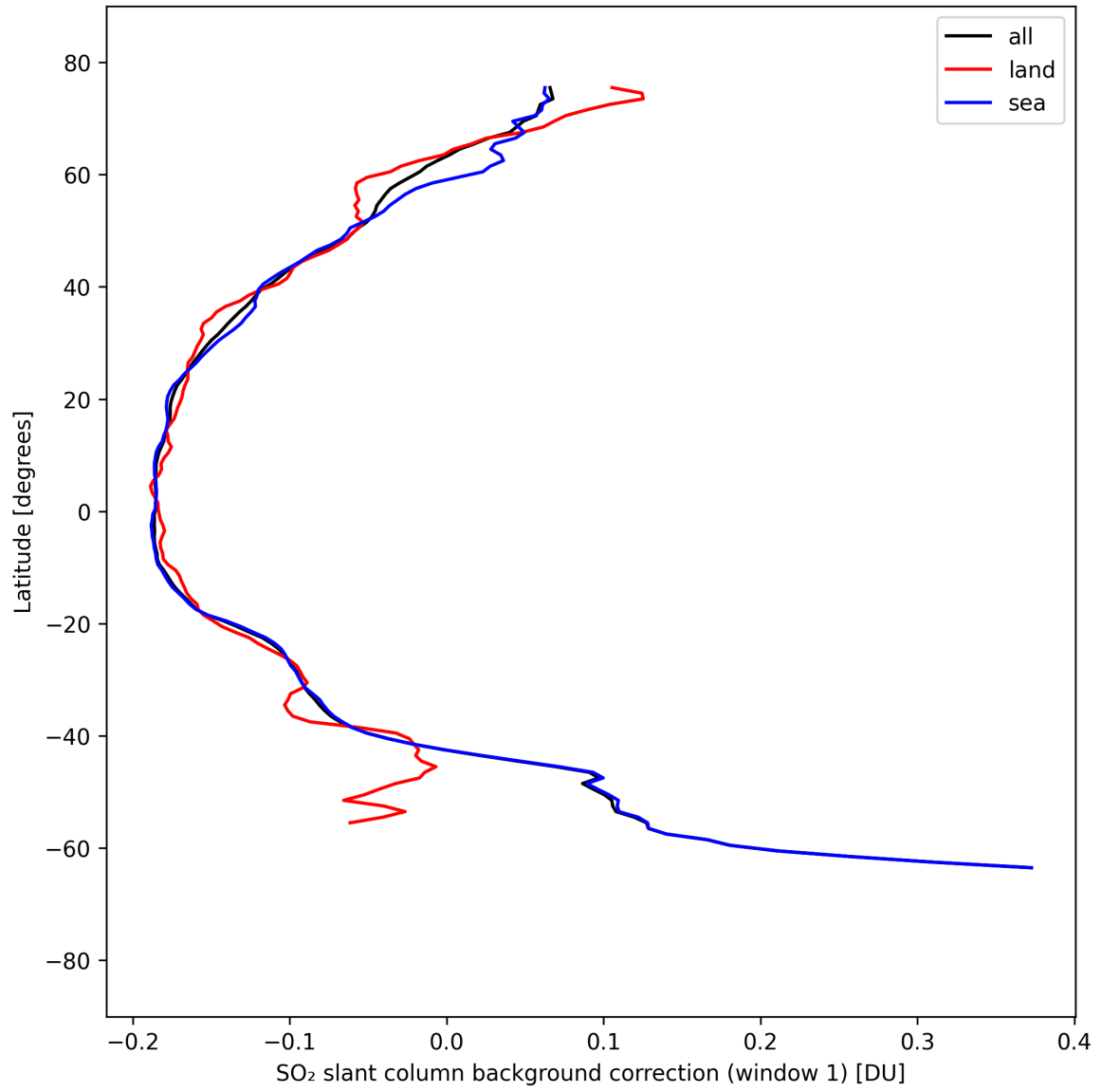
Figure 40: Zonal average of “SO 2 slant column background correction (window 1)” for 2025-09-07 to 2025-09-09.
