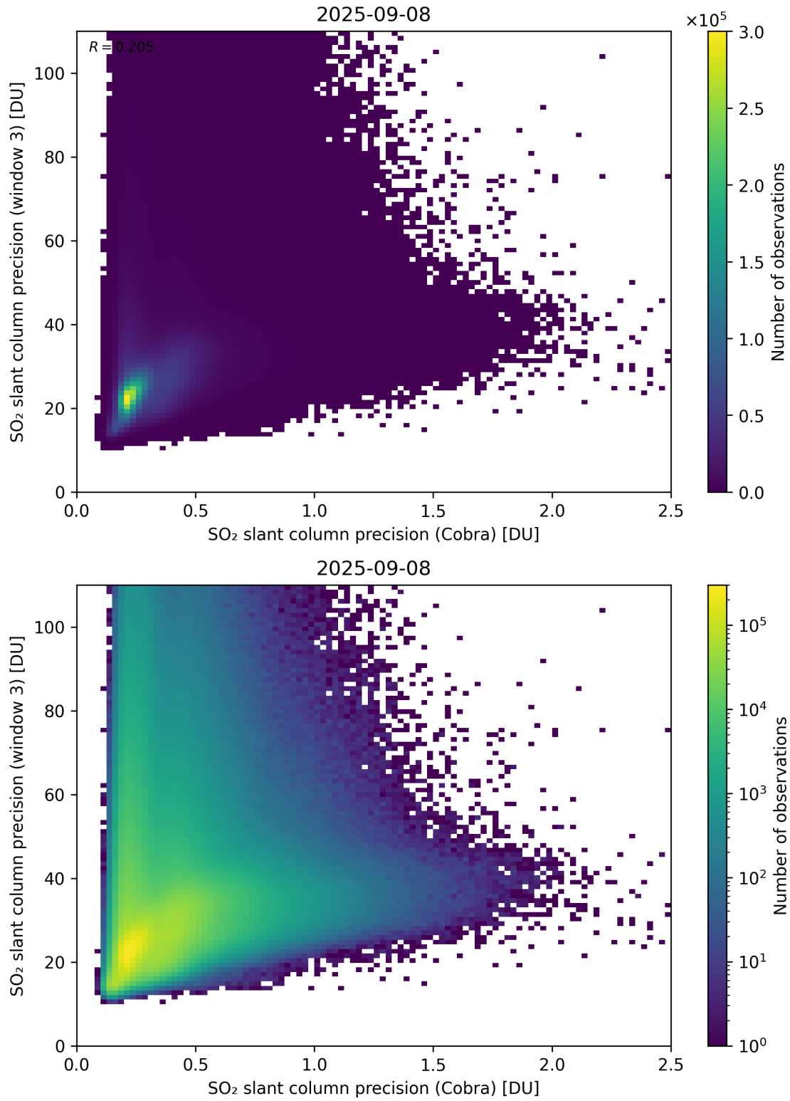
Figure 212: Scatter density plot of “SO 2 slant column precision (Cobra)” against “SO 2 slant column precision (window 3)” for 2025-09-07 to 2025-09-09.
