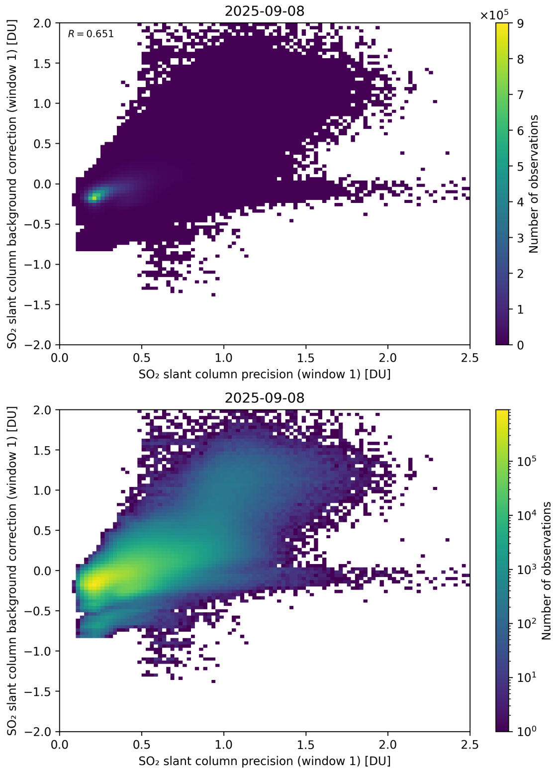
Figure 268: Scatter density plot of “SO 2 slant column precision (window 1)” against “SO 2 slant column background correction (window 1)” for 2025-09-07 to 2025-09-09.
