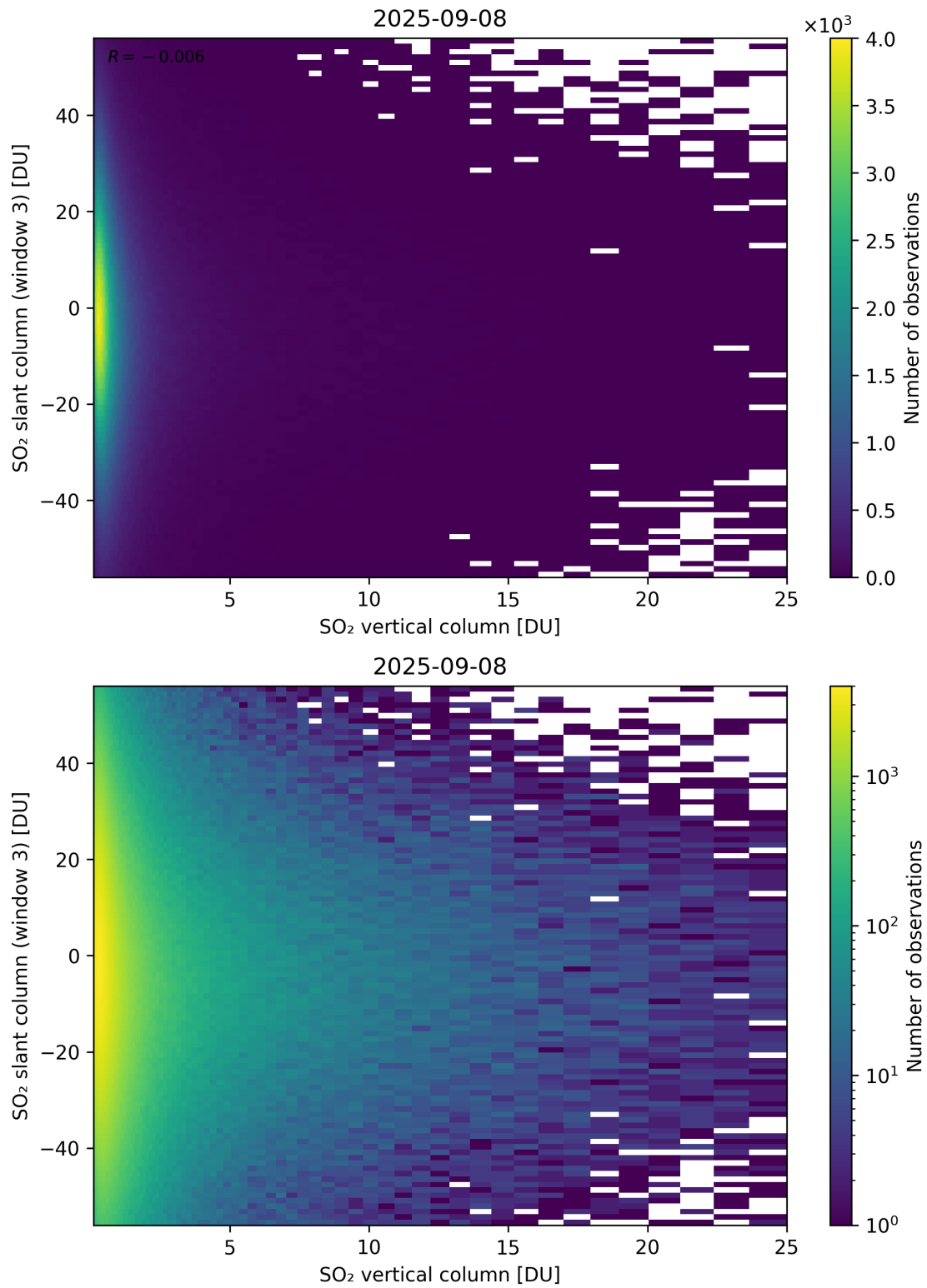
Figure 357: Scatter density plot of “SO 2 vertical column” against “SO 2 slant column (window 3)” for 2025-09-07 to 2025-09-09.
