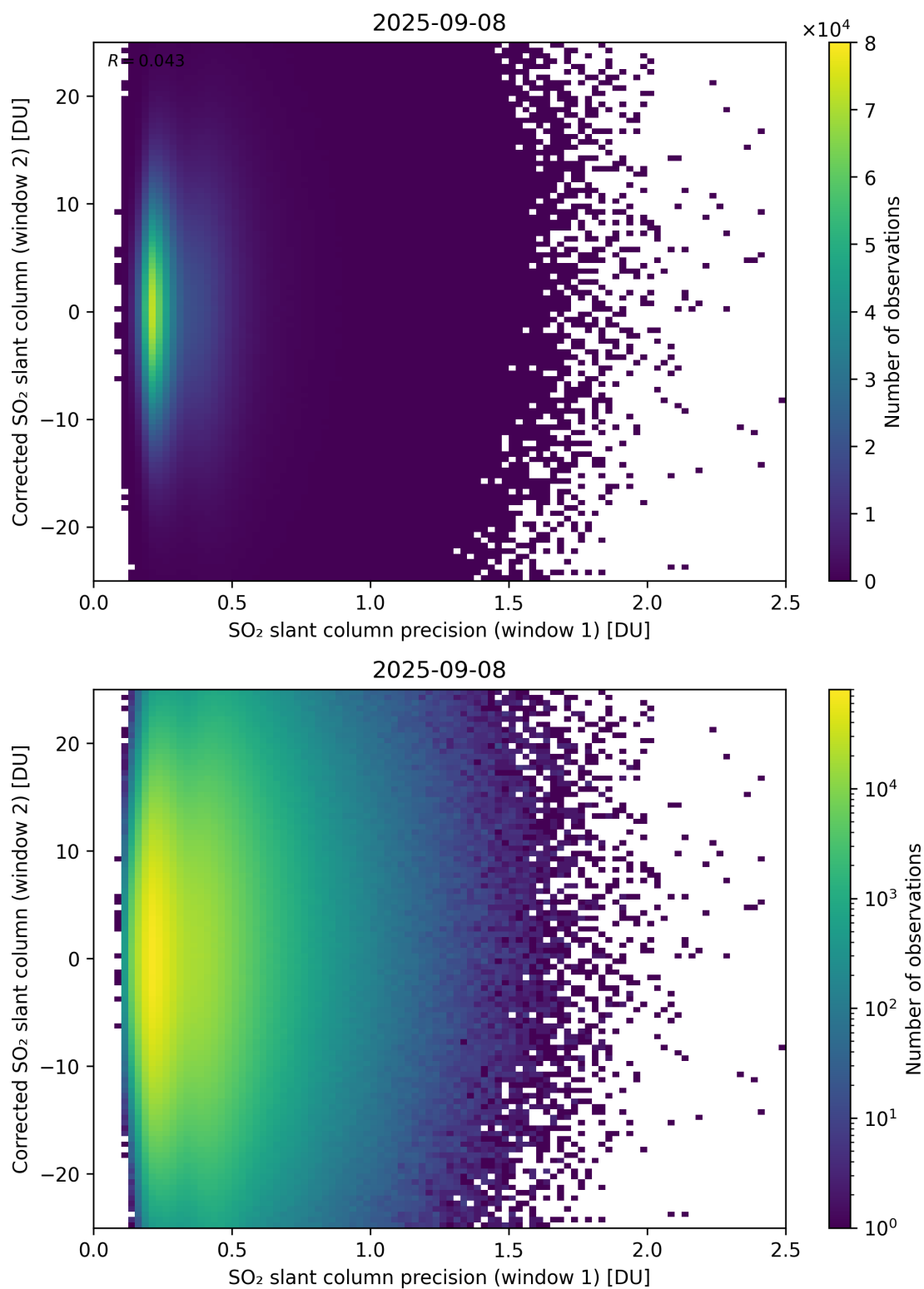
Figure 275: Scatter density plot of “SO 2 slant column precision (window 1)” against “Corrected SO 2 slant column (window 2)” for 2025-09-07 to 2025-09-09.
