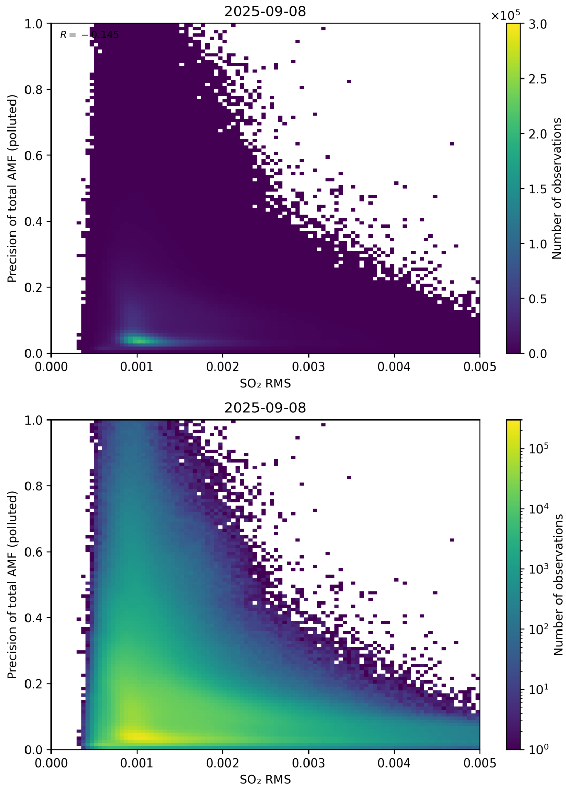
Figure 149: Scatter density plot of “SO 2 RMS” against “Precision of total AMF (polluted)” for 2025-09-07 to 2025-09-09.
