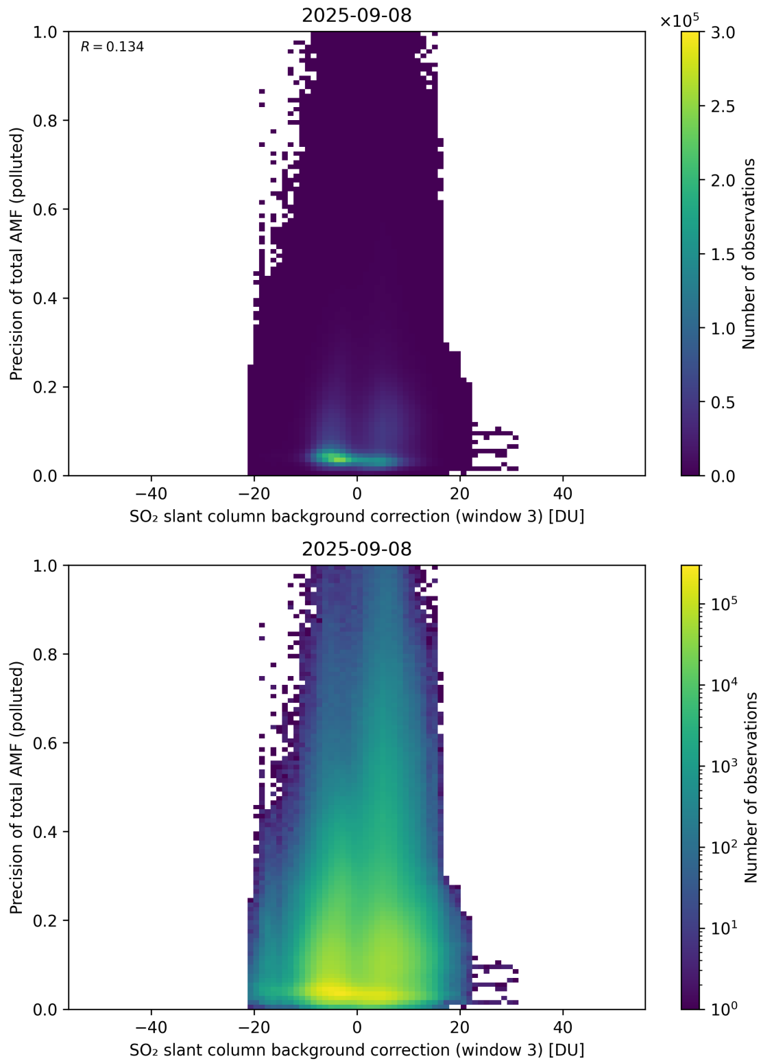
Figure 137: Scatter density plot of “SO 2 slant column background correction (window 3)” against “Precision of total AMF (polluted)” for 2025-09-07 to 2025-09-09.
