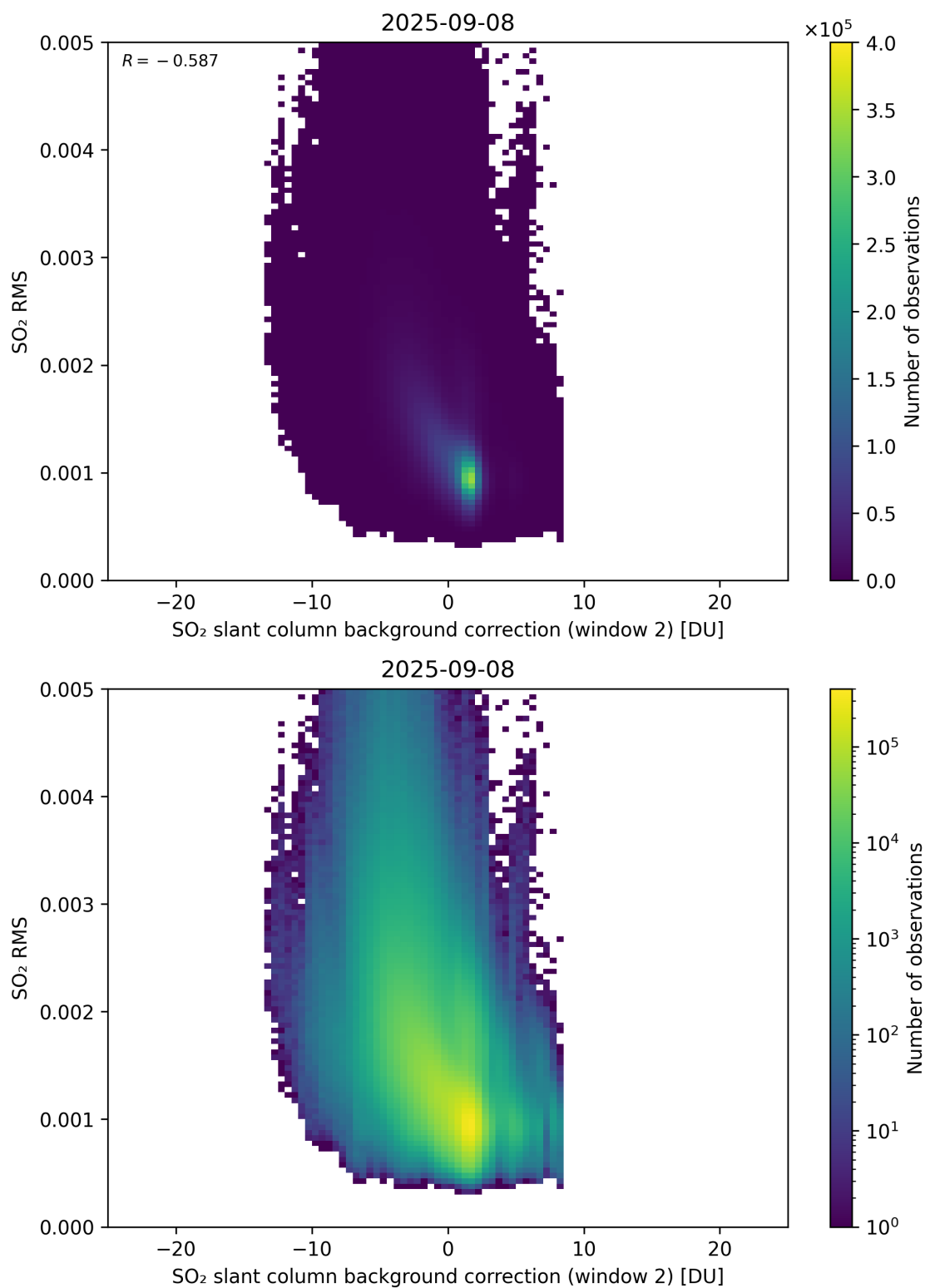
Figure 125: Scatter density plot of “SO 2 slant column background correction (window 2)” against “SO 2 RMS” for 2025-09-07 to 2025-09-09.
