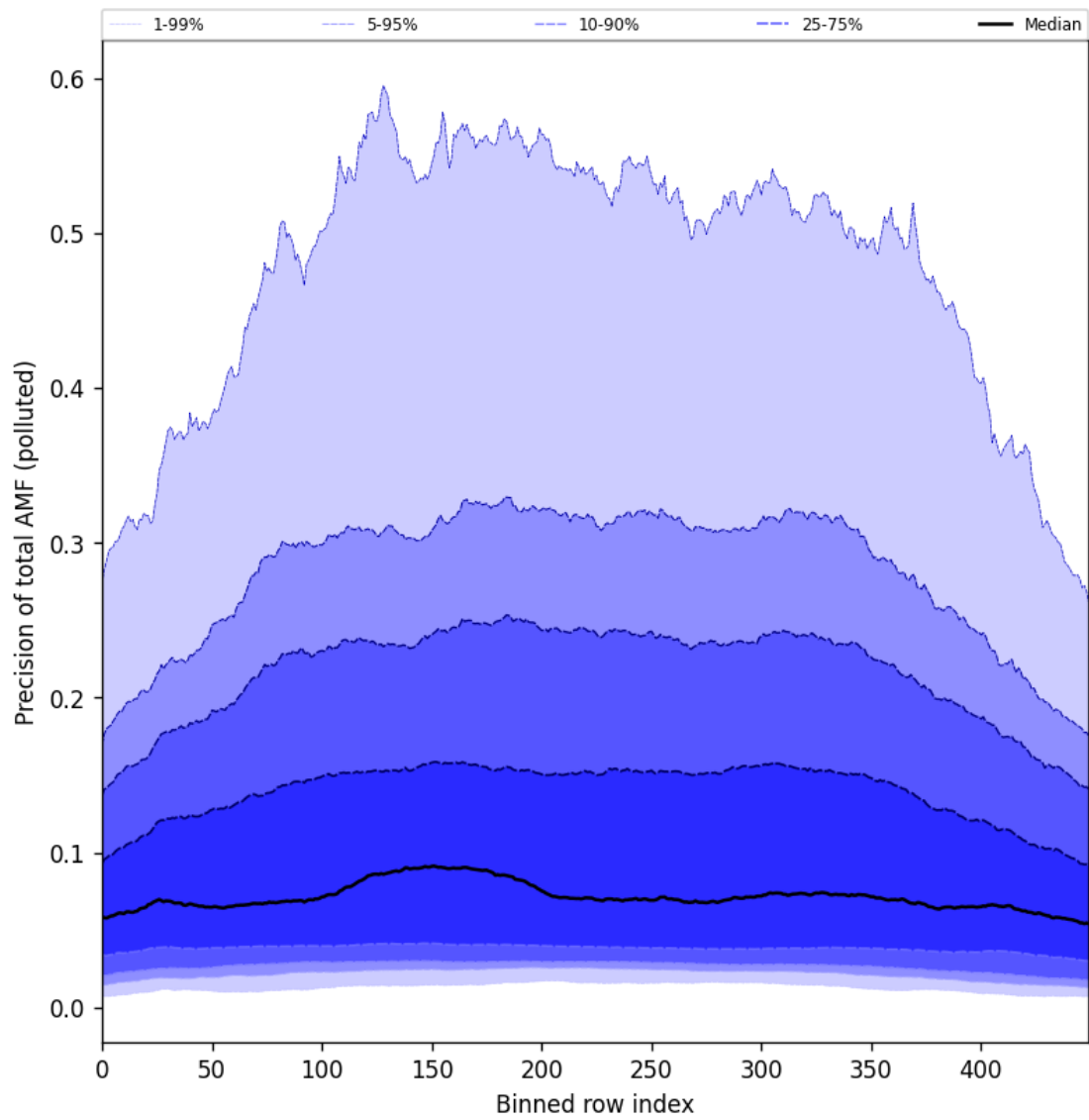
Figure 106: Along track statistics of “Precision of total AMF (polluted)” for 2025-09-07 to 2025-09-09
