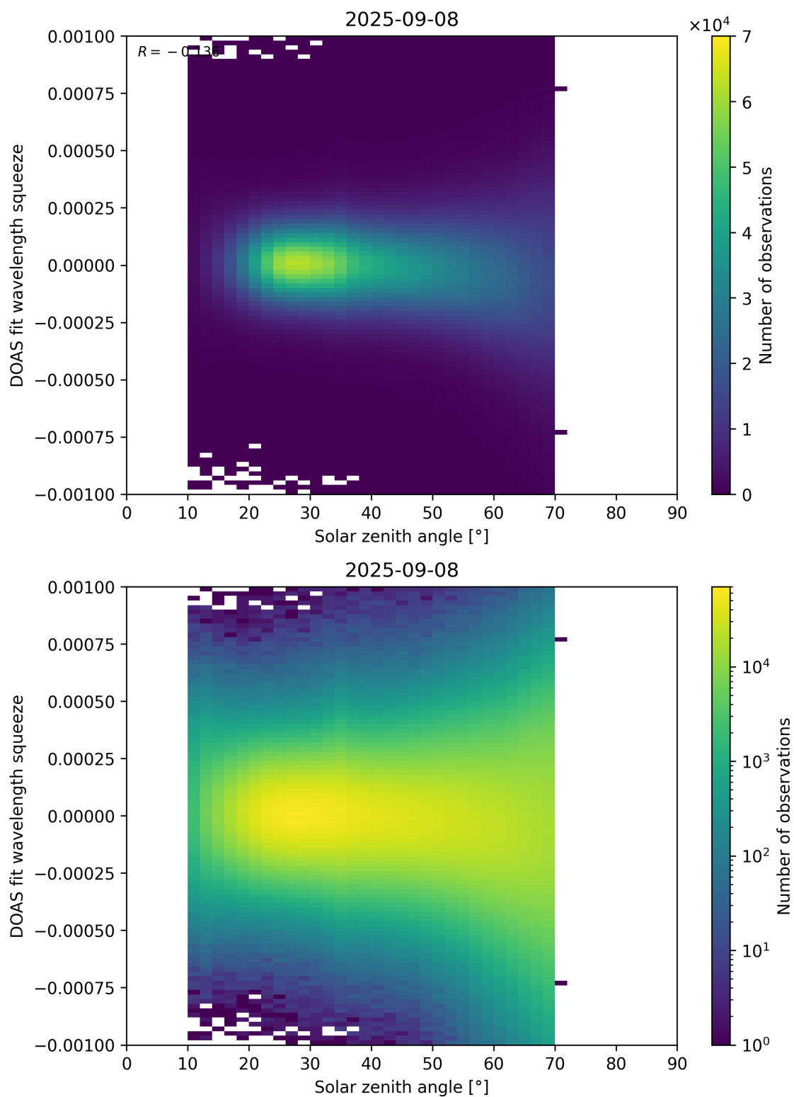
Figure 175: Scatter density plot of “Solar zenith angle” against “DOAS fit wavelength squeeze” for 2025-09-07 to 2025-09-09.
