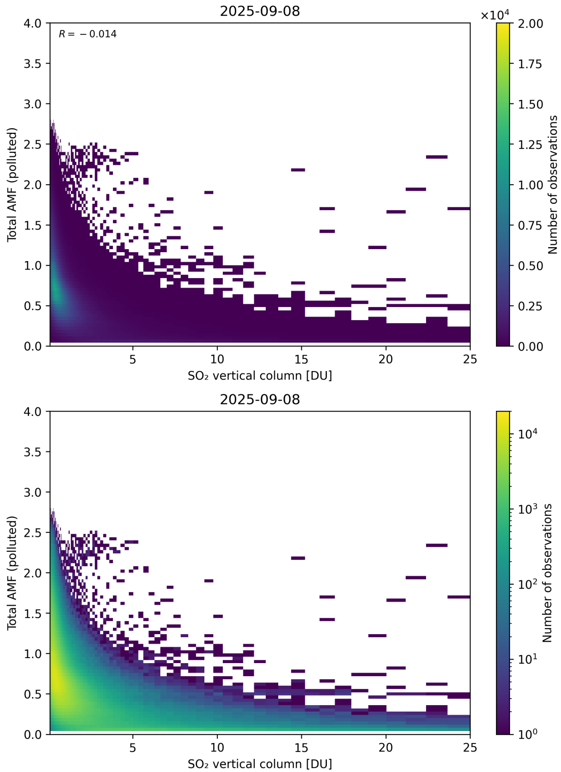
Figure 359: Scatter density plot of “SO 2 vertical column” against “Total AMF (polluted)” for 2025-09-07 to 2025-09-09.
