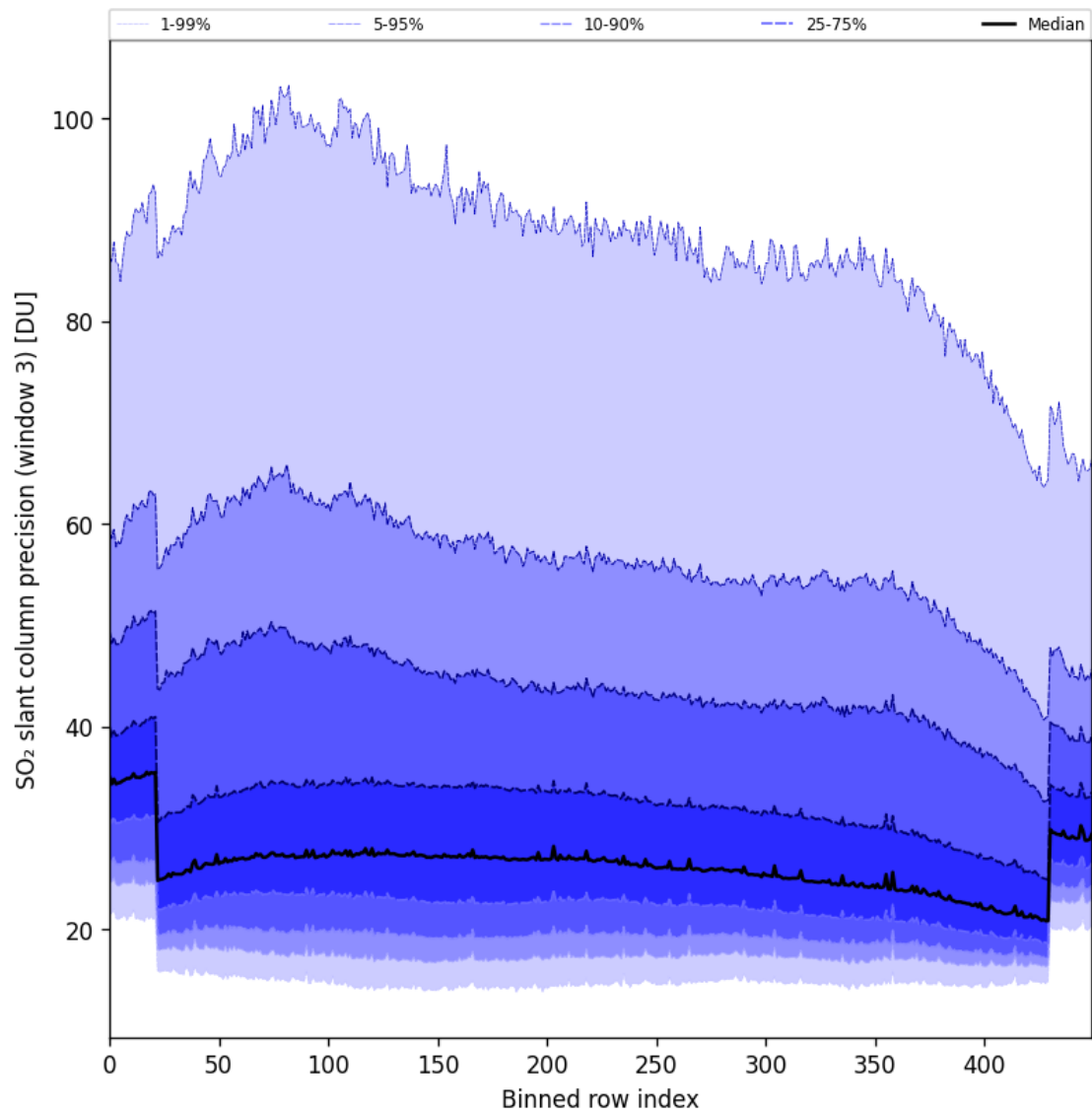
Figure 98: Along track statistics of “SO 2 slant column precision (window 3)” for 2025-09-07 to 2025-09-09
