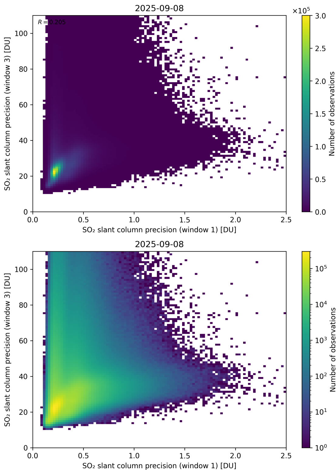
Figure 279: Scatter density plot of “SO 2 slant column precision (window 1)” against “SO 2 slant column precision (window 3)” for 2025-09-07 to 2025-09-09.
