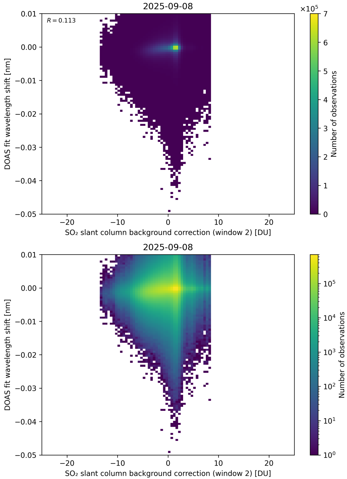
Figure 123: Scatter density plot of “SO 2 slant column background correction (window 2)” against “DOAS fit wavelength shift” for 2025-09-07 to 2025-09-09.
