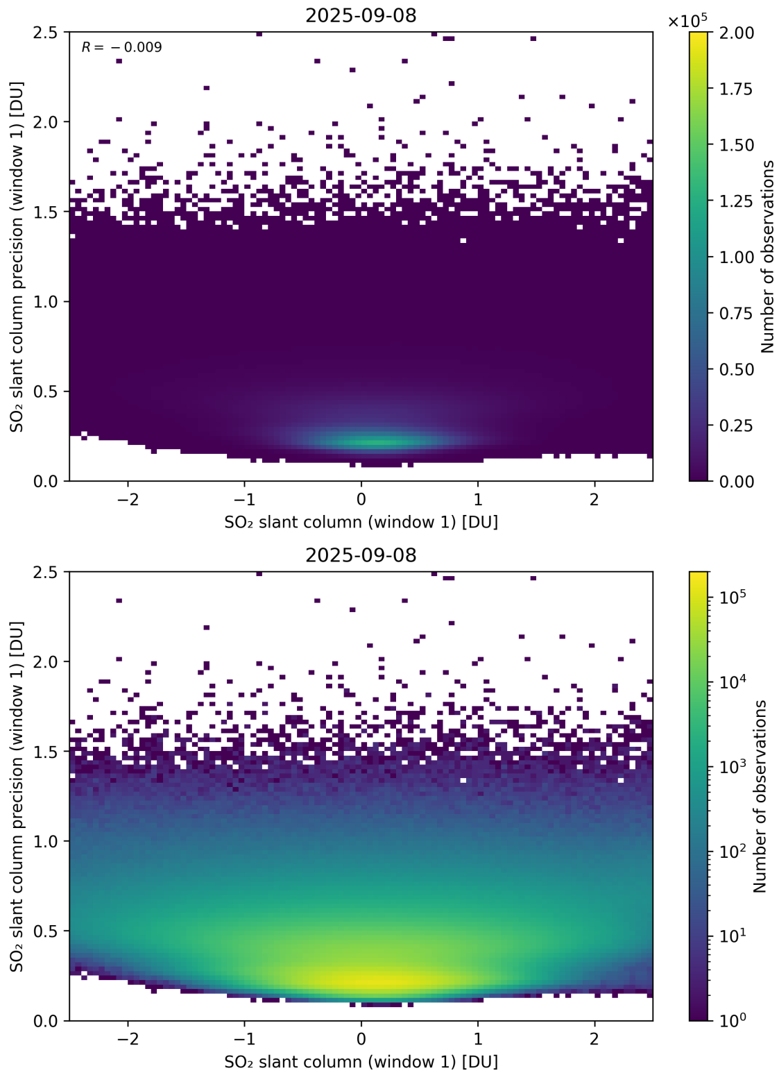
Figure 285: Scatter density plot of “SO 2 slant column (window 1)” against “SO 2 slant column precision (window 1)” for 2025-09-07 to 2025-09-09.
