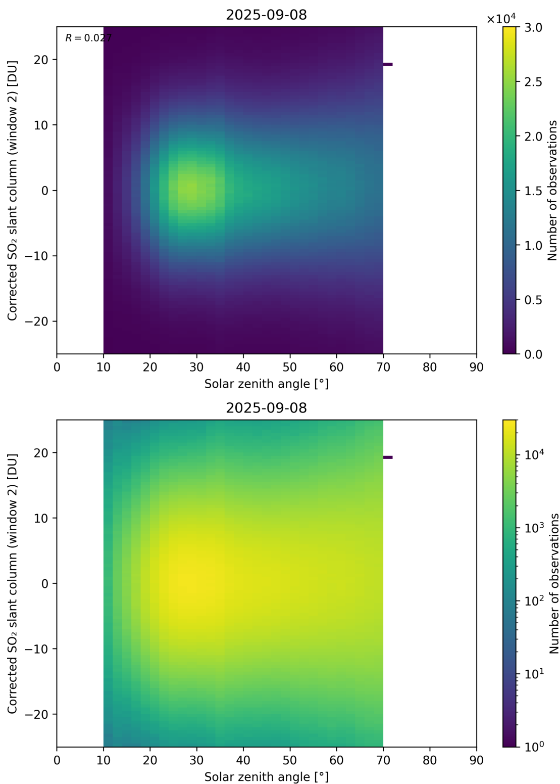
Figure 182: Scatter density plot of “Solar zenith angle” against “Corrected SO 2 slant column (window 2)” for 2025-09-07 to 2025-09-09.
