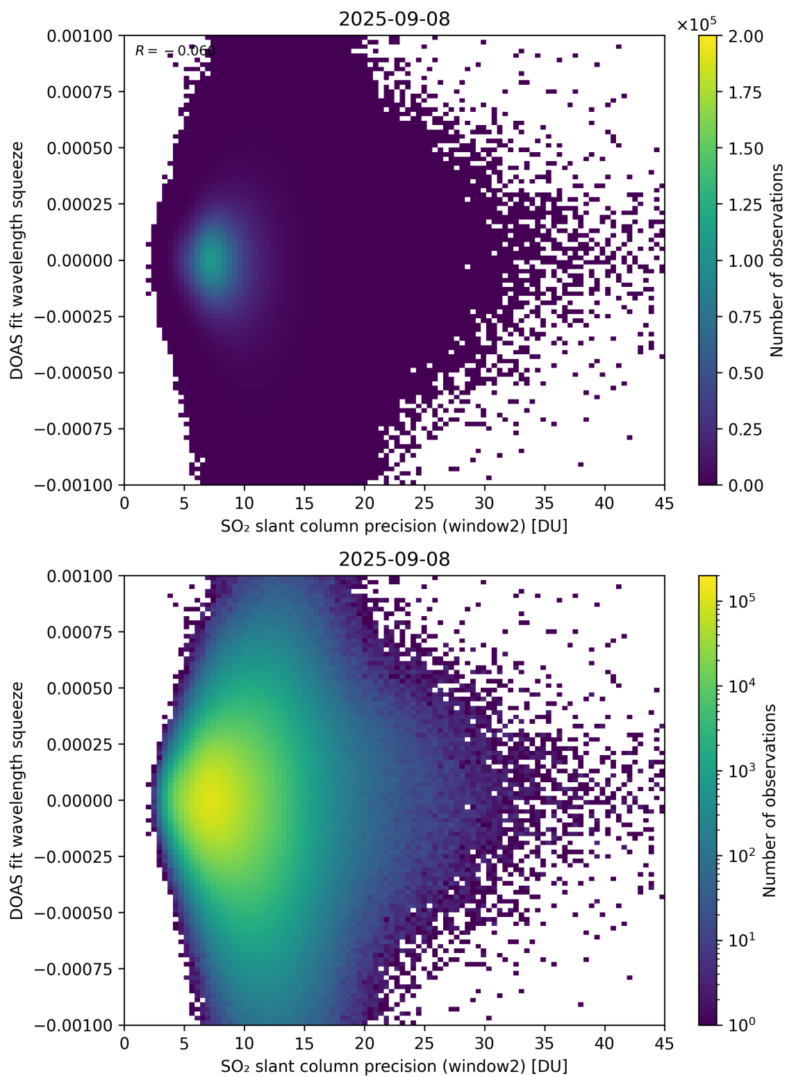
Figure 294: Scatter density plot of “SO 2 slant column precision (window2)” against “DOAS fit wavelength squeeze” for 2025-09-07 to 2025-09-09.
