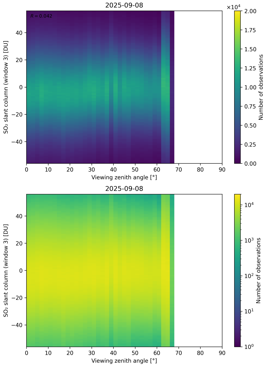
Figure 379: Scatter density plot of “Viewing zenith angle” against “SO 2 slant column (window 3)” for 2025-09-07 to 2025-09-09.
