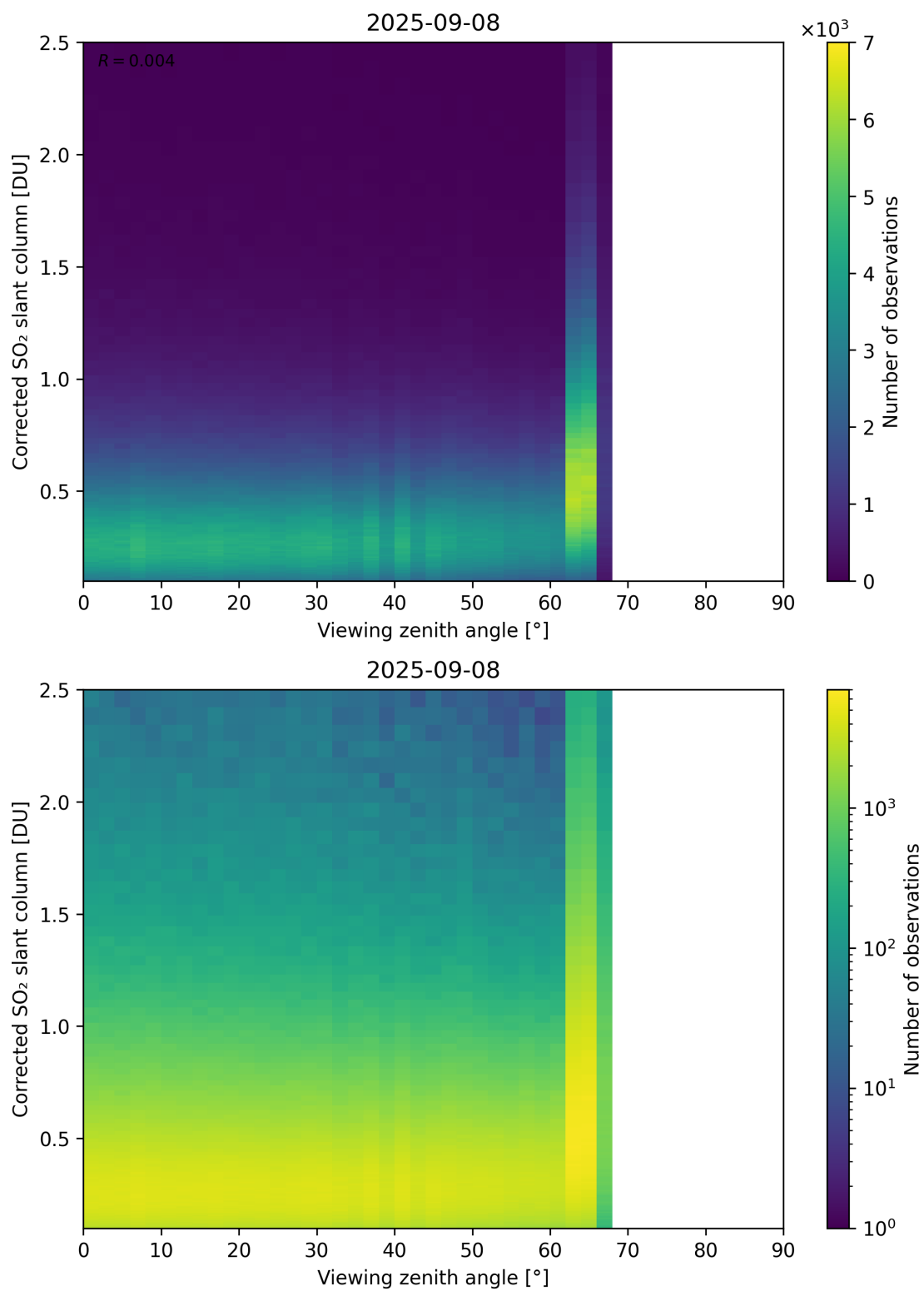
Figure 373: Scatter density plot of “Viewing zenith angle” against “Corrected SO 2 slant column” for 2025-09-07 to 2025-09-09.
