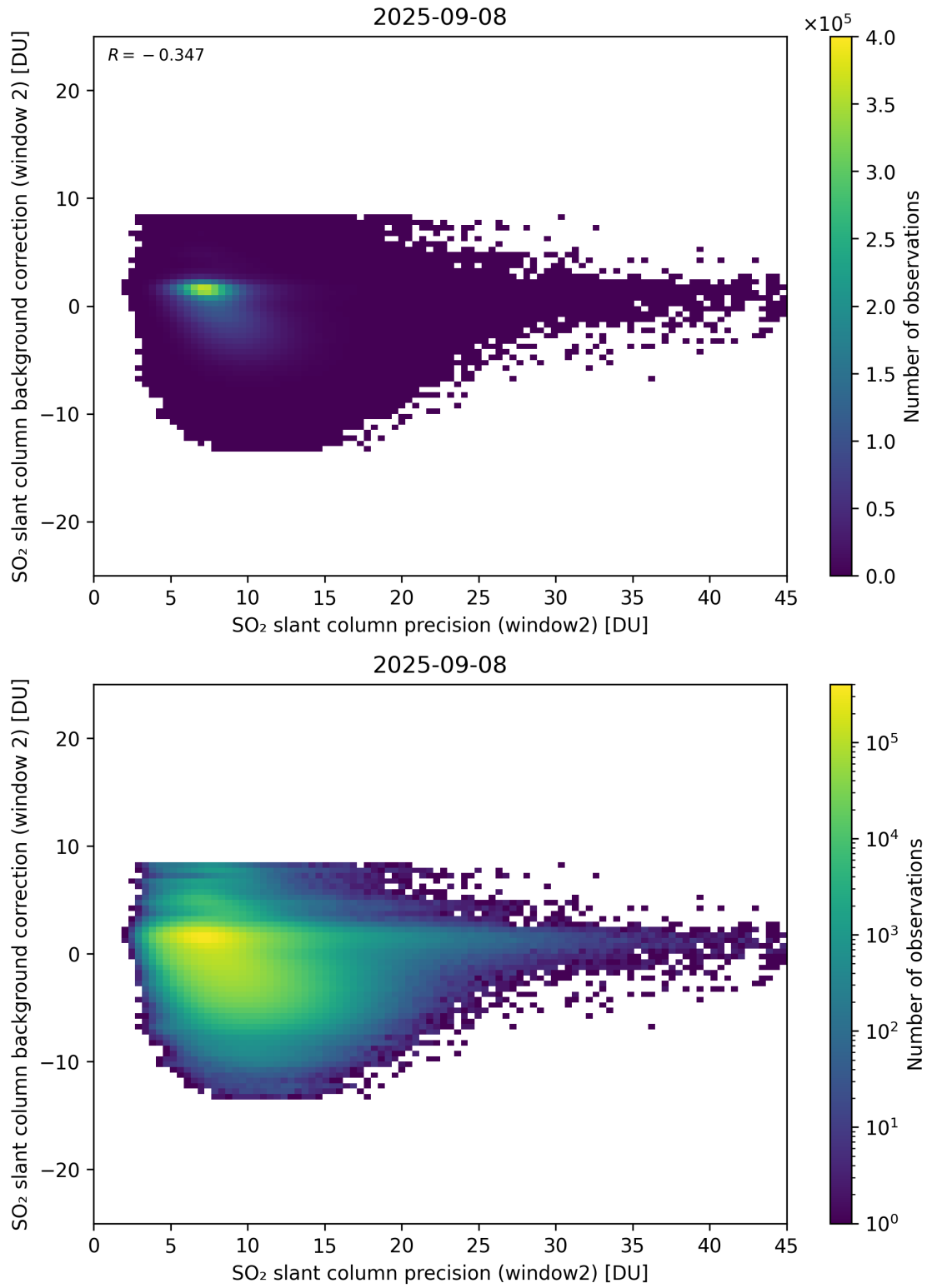
Figure 291: Scatter density plot of “SO 2 slant column precision (window2)” against “SO 2 slant column background correction (window 2)” for 2025-09-07 to 2025-09-09.
