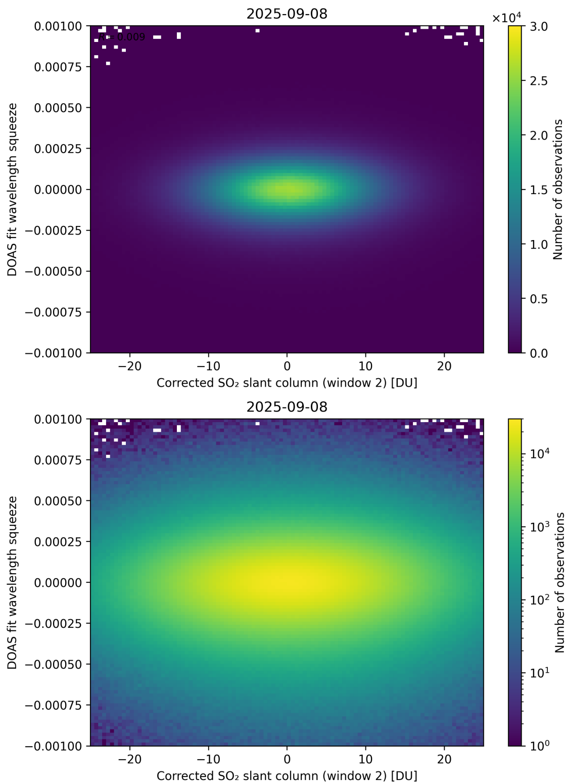
Figure 247: Scatter density plot of “Corrected SO 2 slant column (window 2)” against “DOAS fit wavelength squeeze” for 2025-09-07 to 2025-09-09.
