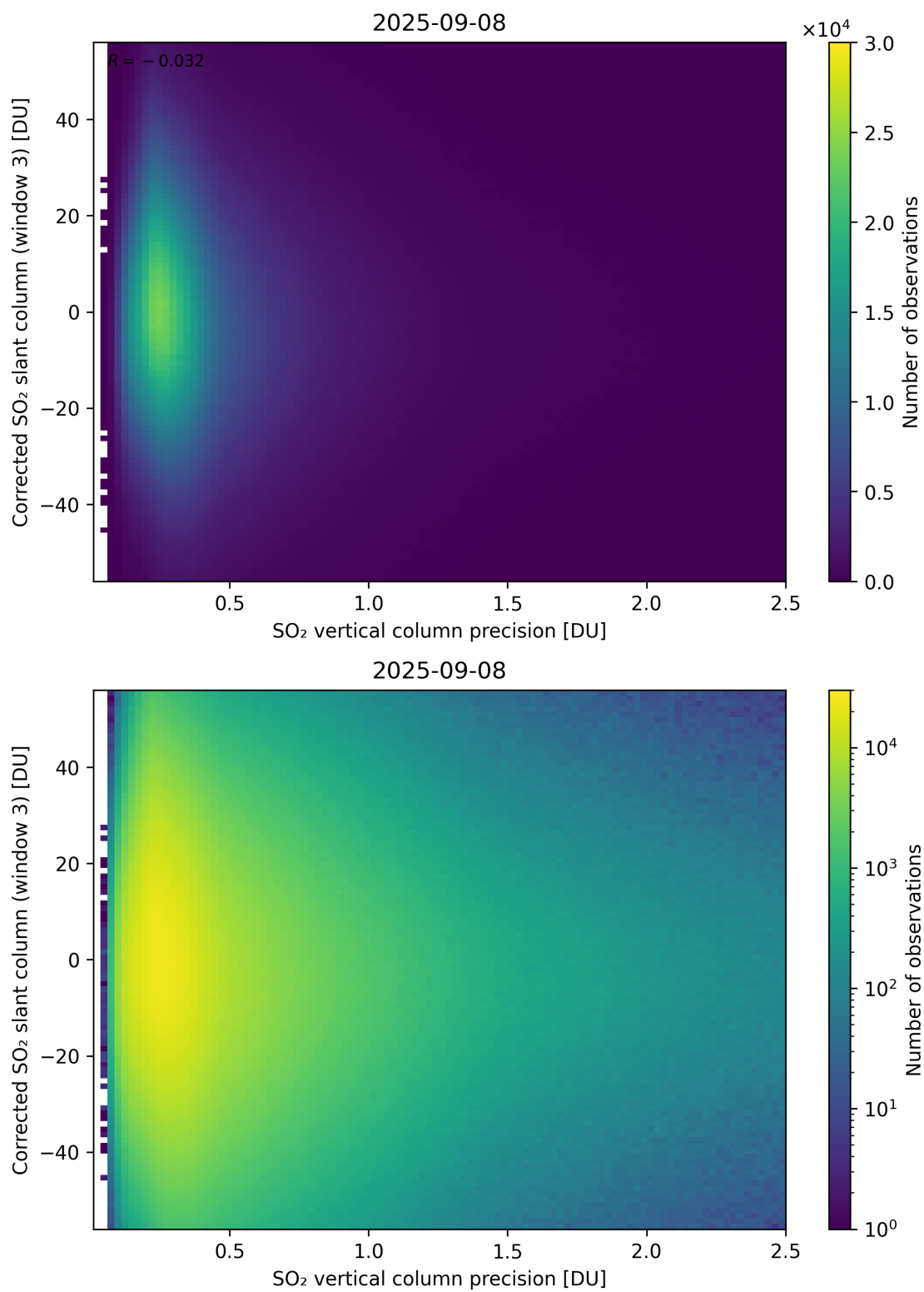
Figure 340: Scatter density plot of “SO 2 vertical column precision” against “Corrected SO 2 slant column (window 3)” for 2025-09-07 to 2025-09-09.
