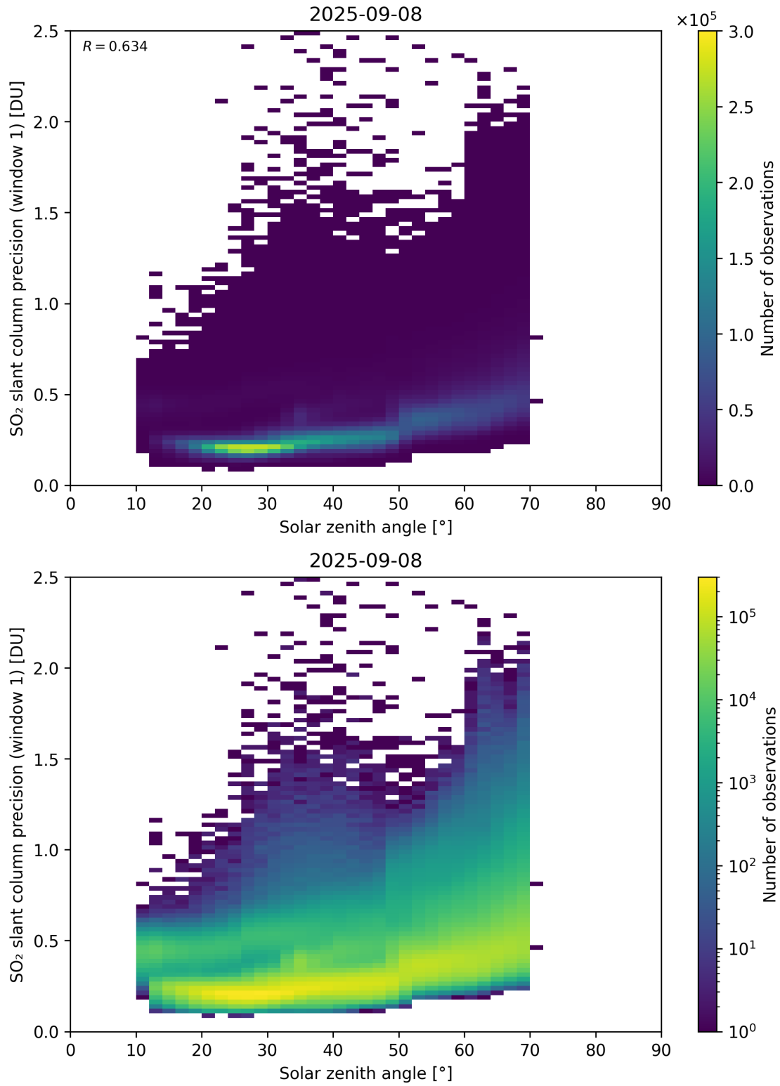
Figure 185: Scatter density plot of “Solar zenith angle” against “SO 2 slant column precision (window 1)” for 2025-09-07 to 2025-09-09.
