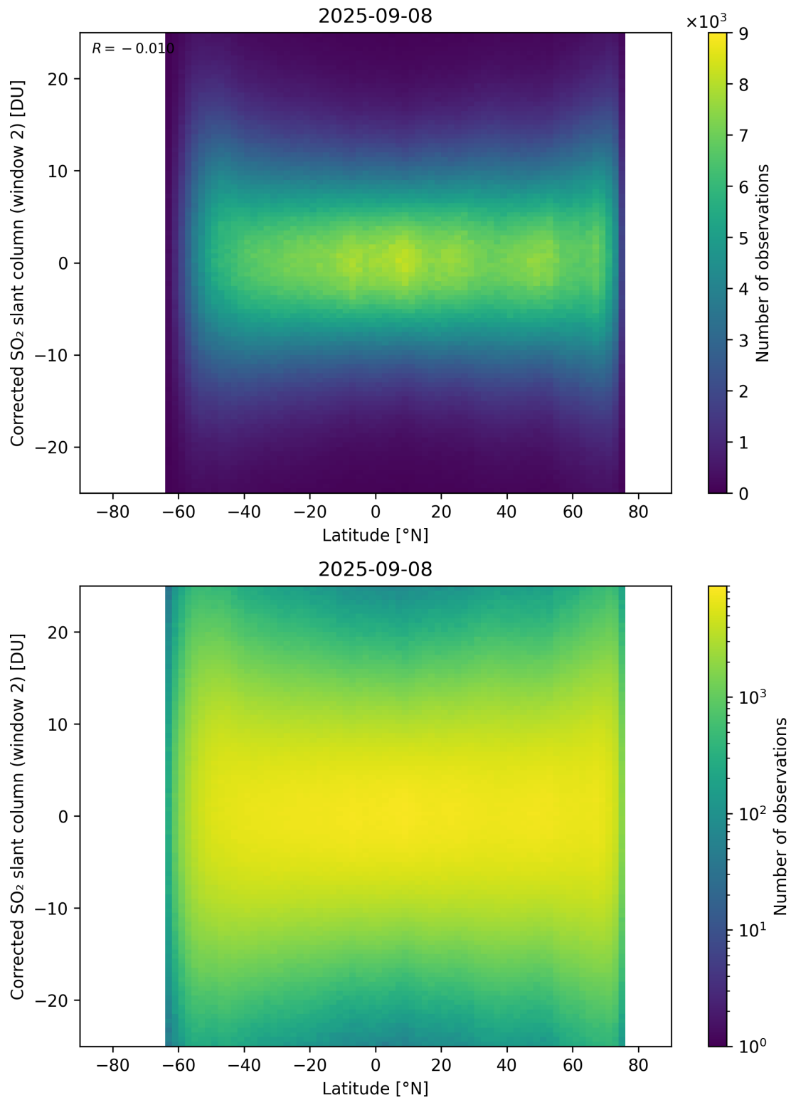
Figure 160: Scatter density plot of “Latitude” against “Corrected SO 2 slant column (window 2)” for 2025-09-07 to 2025-09-09.
