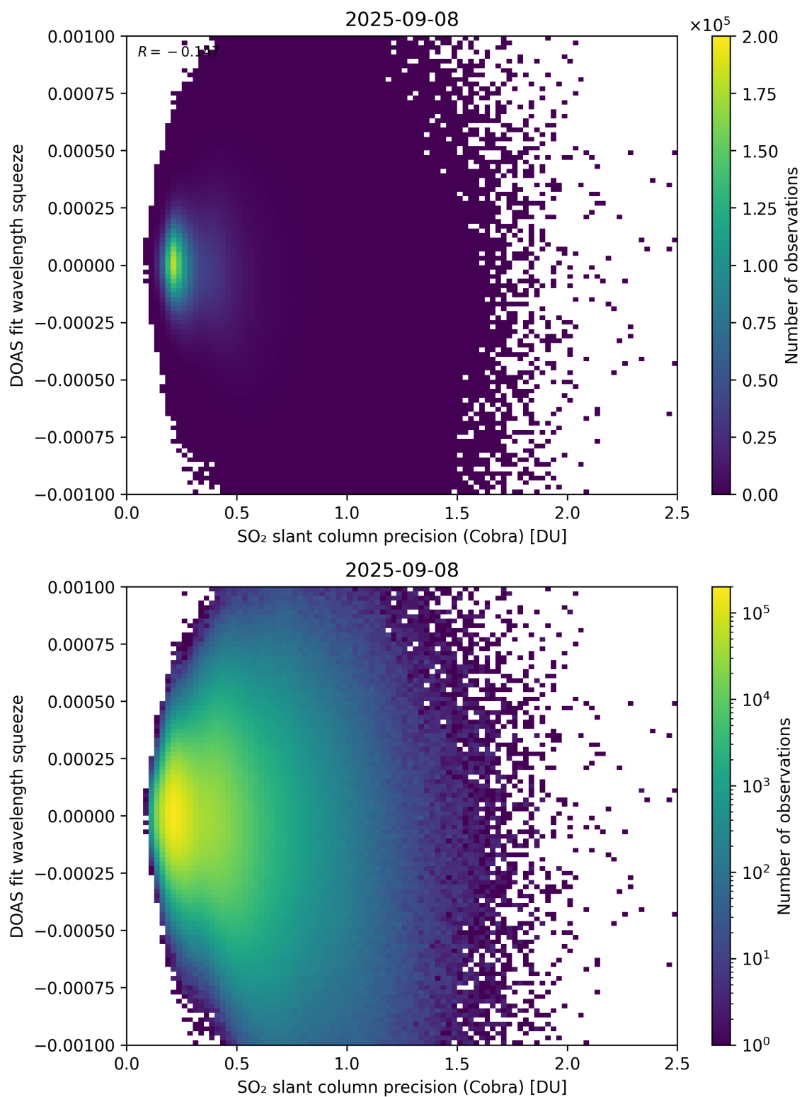
Figure 203: Scatter density plot of “SO 2 slant column precision (Cobra)” against “DOAS fit wavelength squeeze” for 2025-09-07 to 2025-09-09.
