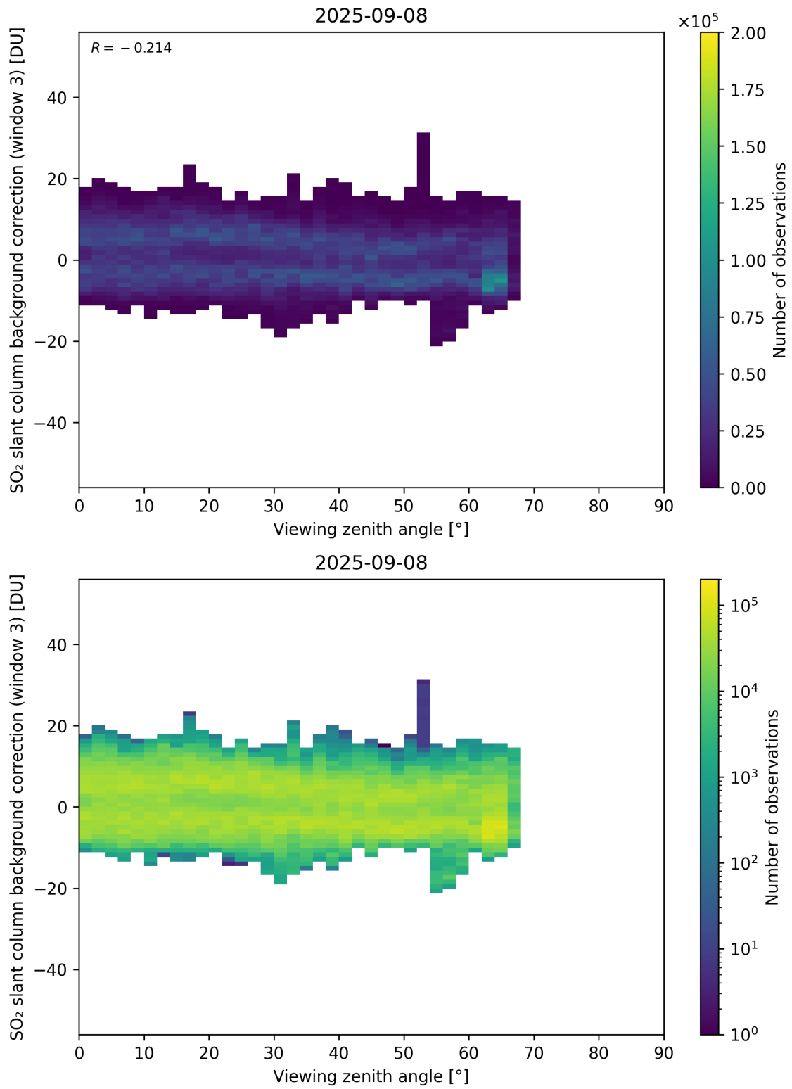
Figure 364: Scatter density plot of “Viewing zenith angle” against “SO 2 slant column background correction (window 3)” for 2025-09-07 to 2025-09-09.
