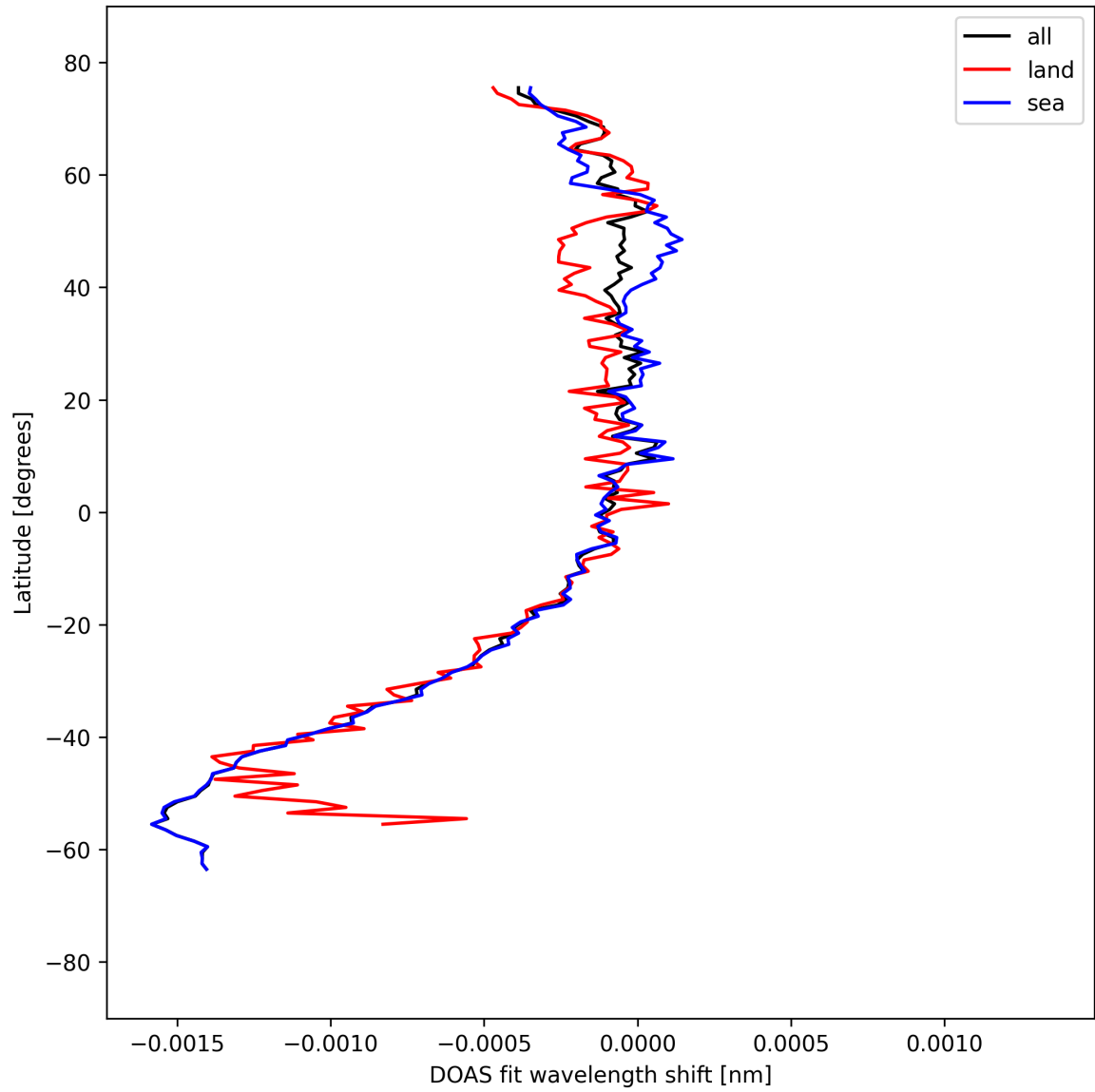
Figure 50: Zonal average of "DOAS fit wavelength shift" for 2025-09-07 to 2025-09-09.
