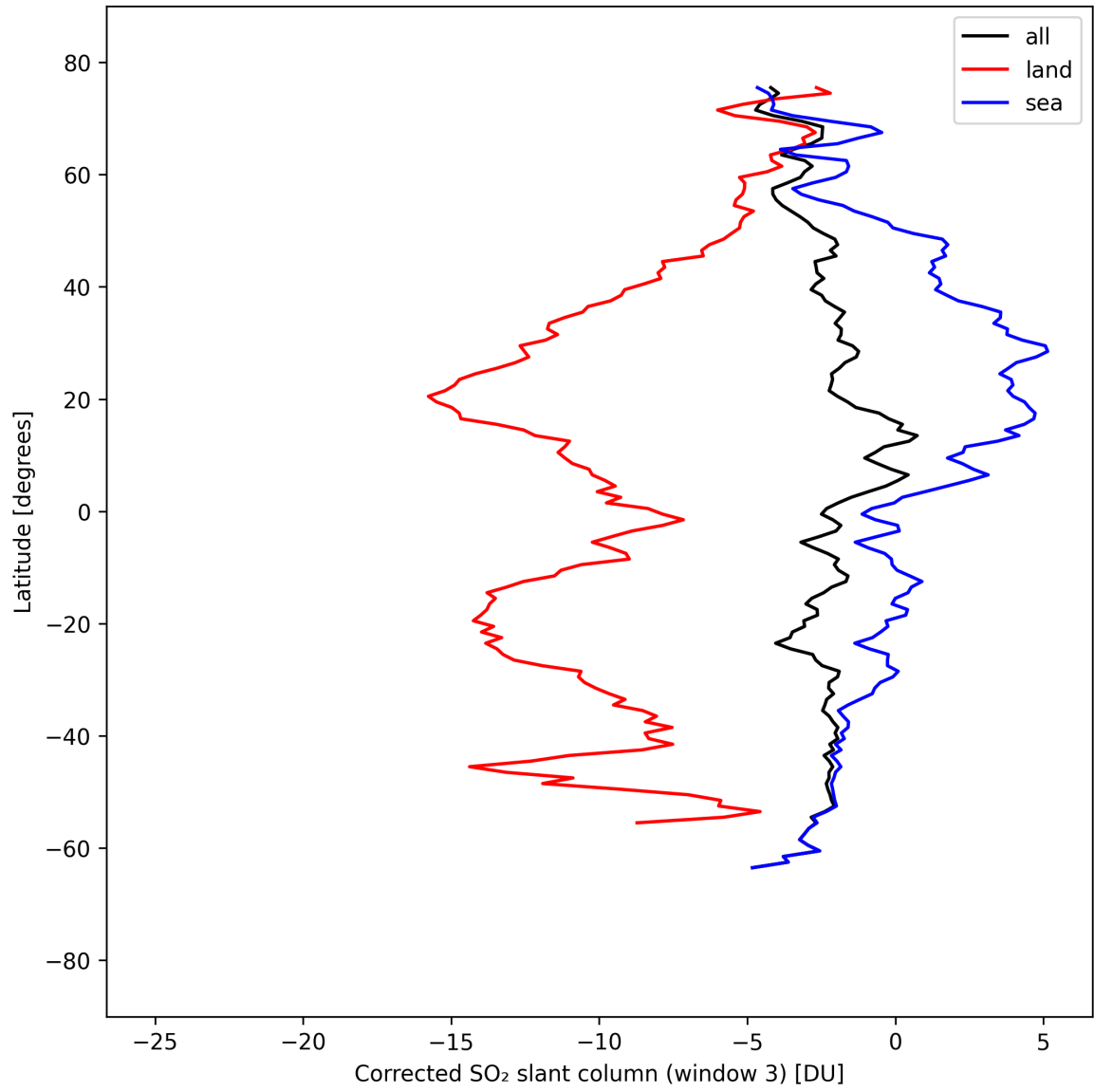
Figure 47: Zonal average of “Corrected SO 2 slant column (window 3)” for 2025-09-07 to 2025-09-09.
