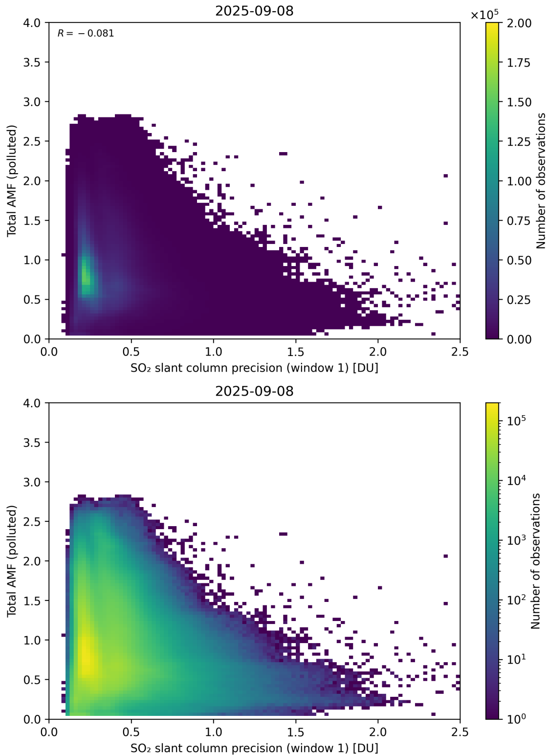
Figure 280: Scatter density plot of “SO 2 slant column precision (window 1)” against “Total AMF (polluted)” for 2025-09-07 to 2025-09-09.
