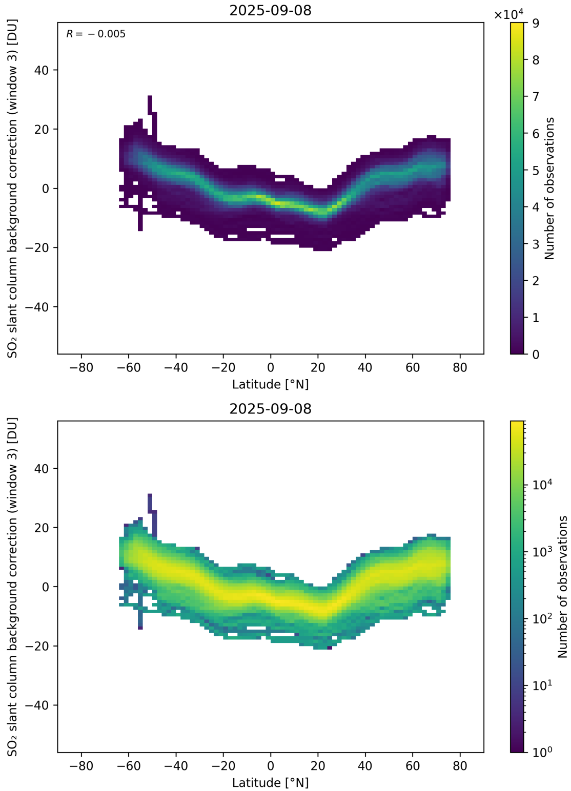
Figure 152: Scatter density plot of “Latitude” against “SO 2 slant column background correction (window 3)” for 2025-09-07 to 2025-09-09.
