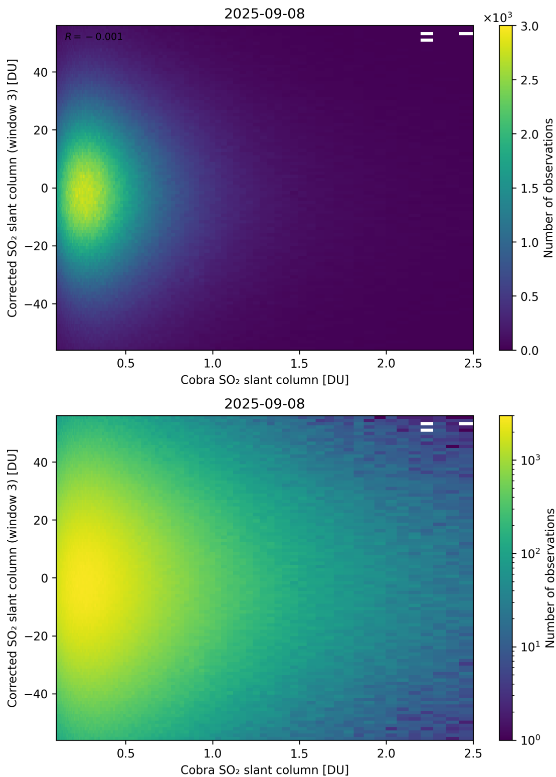
Figure 218: Scatter density plot of “Cobra SO 2 slant column” against “Corrected SO 2 slant column (window 3)” for 2025-09-07 to 2025-09-09.
