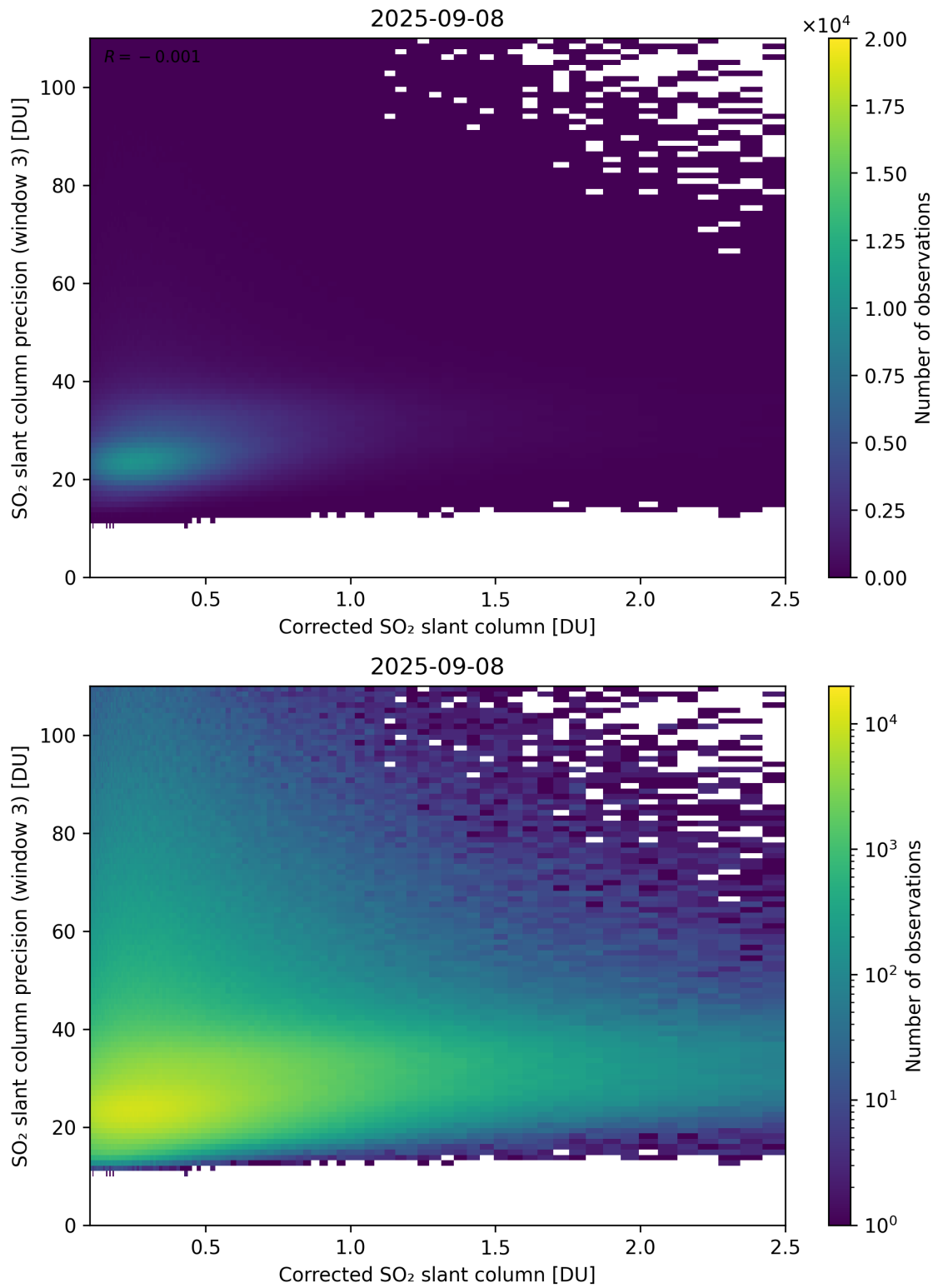
Figure 241: Scatter density plot of “Corrected SO 2 slant column” against “SO 2 slant column precision (window 3)” for 2025-09-07 to 2025-09-09.
