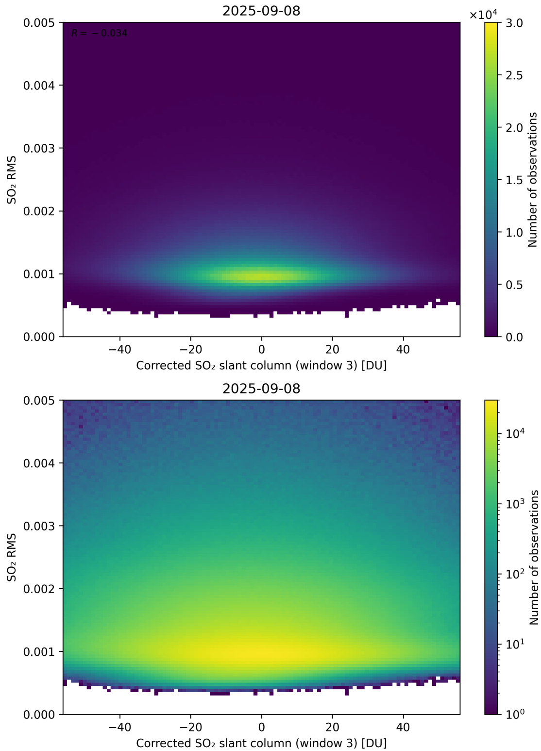
Figure 258: Scatter density plot of “Corrected SO 2 slant column (window 3)” against “SO 2 RMS” for 2025-09-07 to 2025-09-09.
