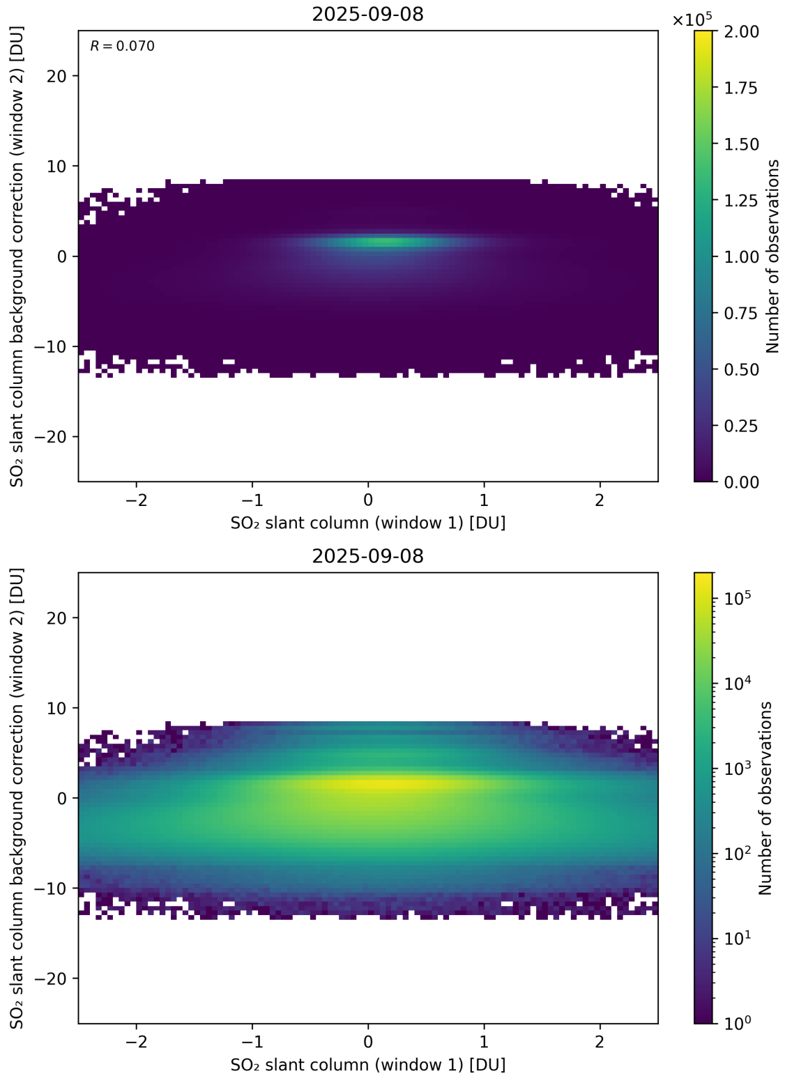
Figure 263: Scatter density plot of “SO 2 slant column (window 1)” against “SO 2 slant column background correction (window 2)” for 2025-09-07 to 2025-09-09.
