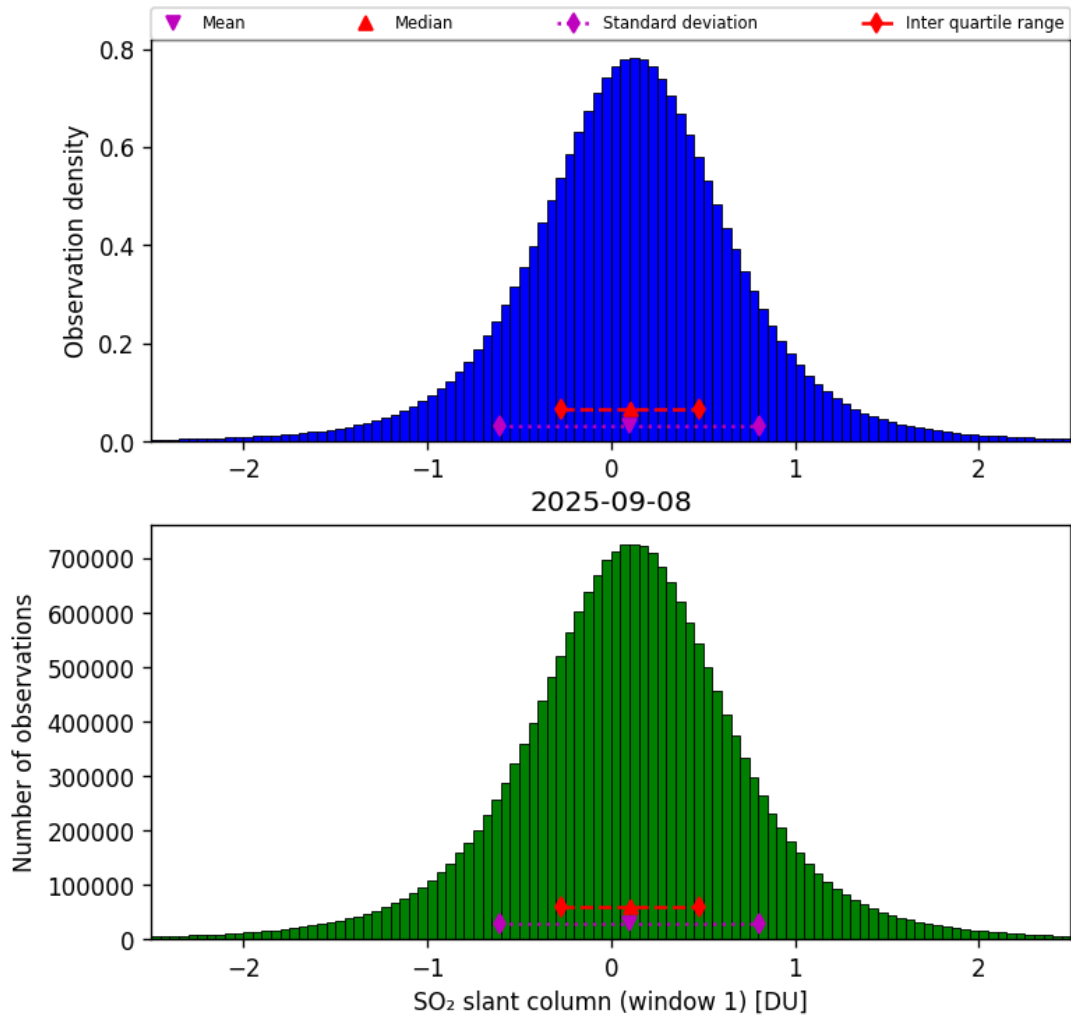
Figure 63: Histogram of “SO 2 slant column (window 1)” for 2025-09-07 to 2025-09-09
