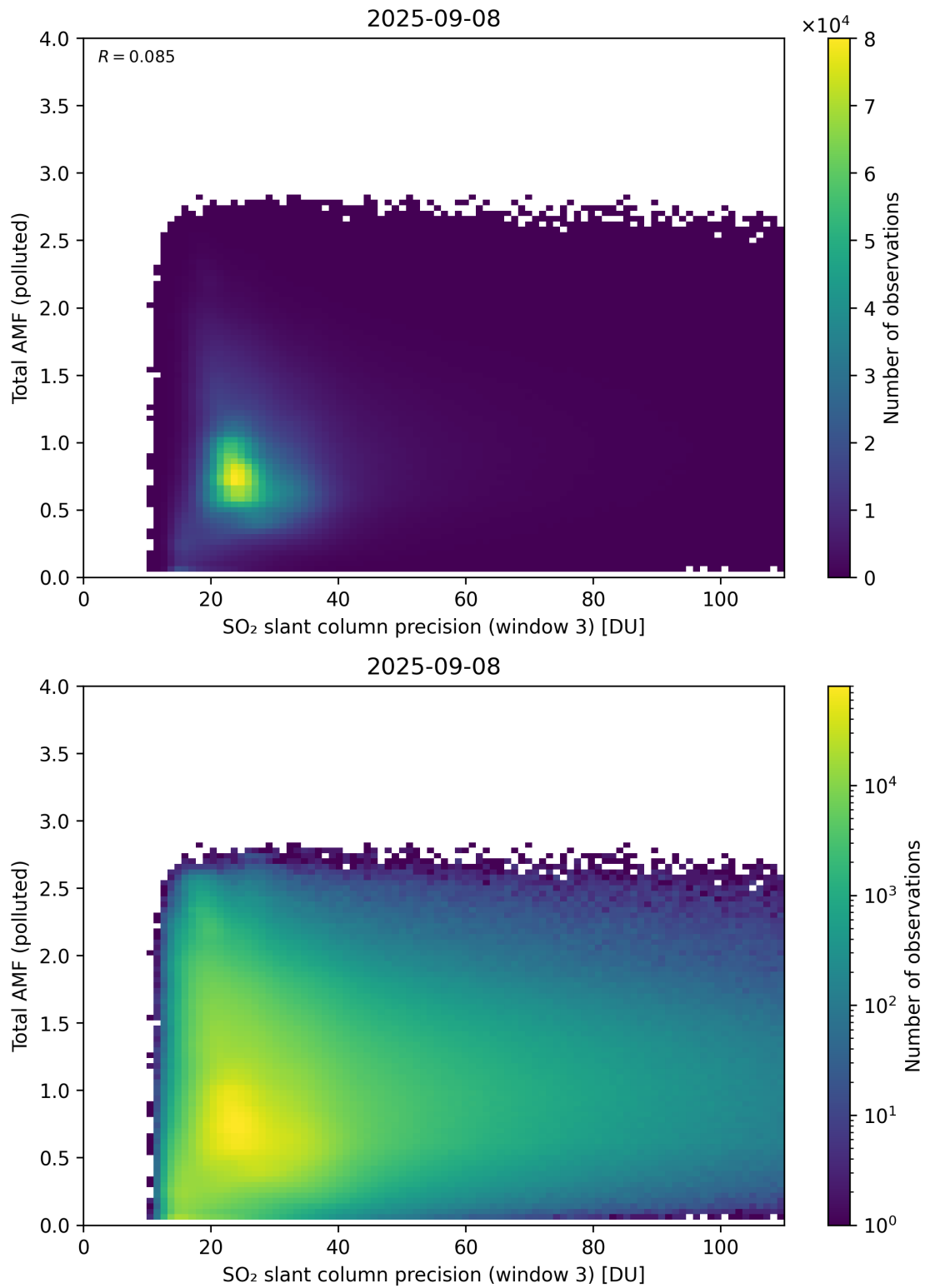
Figure 313: Scatter density plot of “SO 2 slant column precision (window 3)” against “Total AMF (polluted)” for 2025-09-07 to 2025-09-09.
