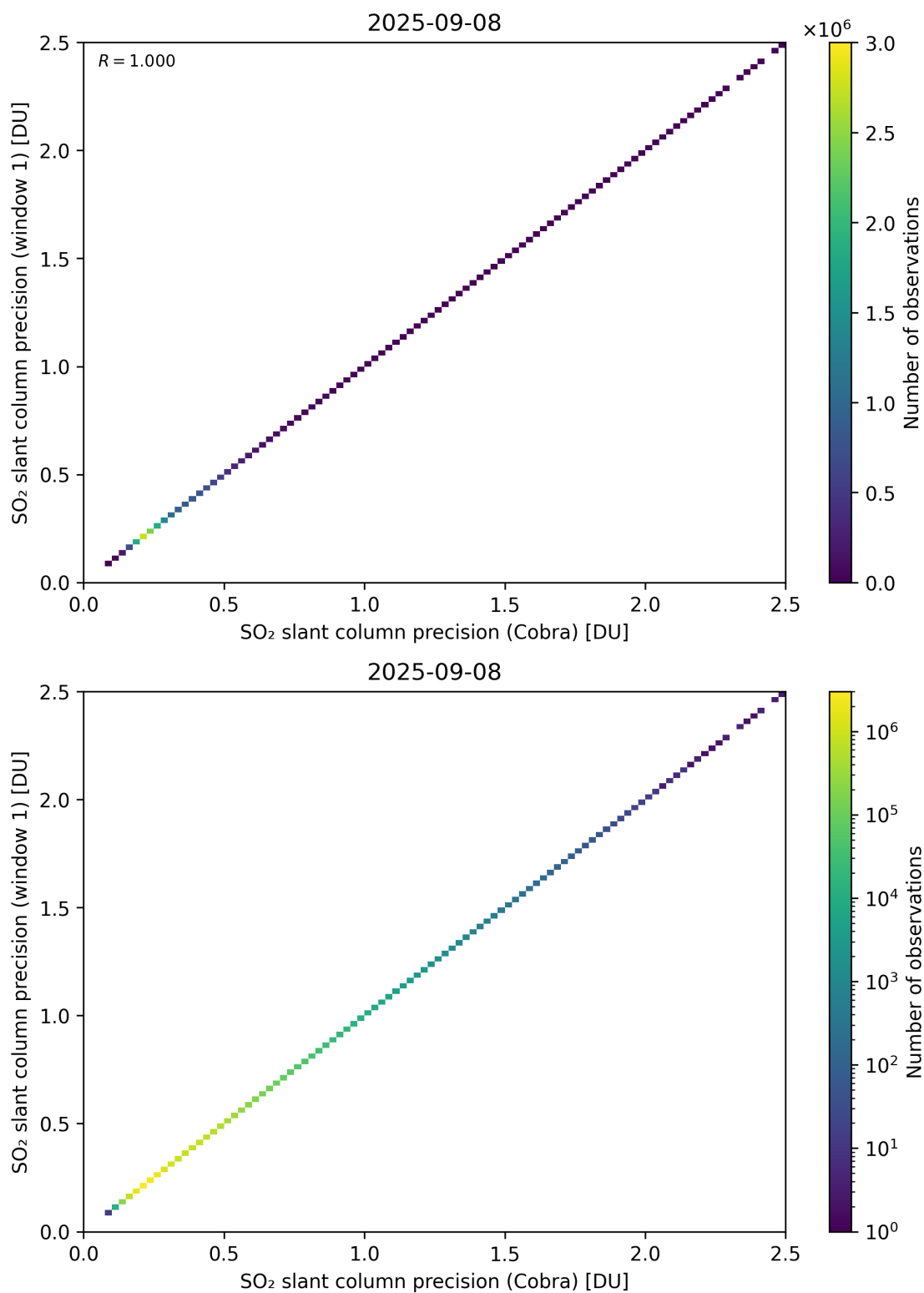
Figure 209: Scatter density plot of “SO 2 slant column precision (Cobra)” against “SO 2 slant column precision (window 1)” for 2025-09-07 to 2025-09-09.
