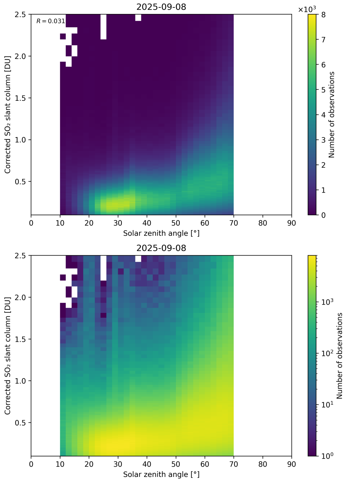
Figure 181: Scatter density plot of “Solar zenith angle” against “Corrected SO 2 slant column” for 2025-09-07 to 2025-09-09.
