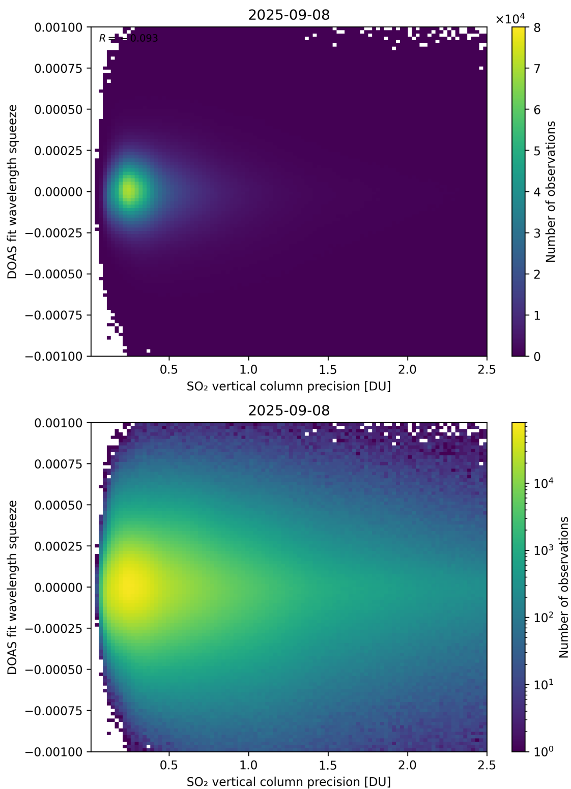
Figure 333: Scatter density plot of “SO 2 vertical column precision” against “DOAS fit wavelength squeeze” for 2025-09-07 to 2025-09-09.
