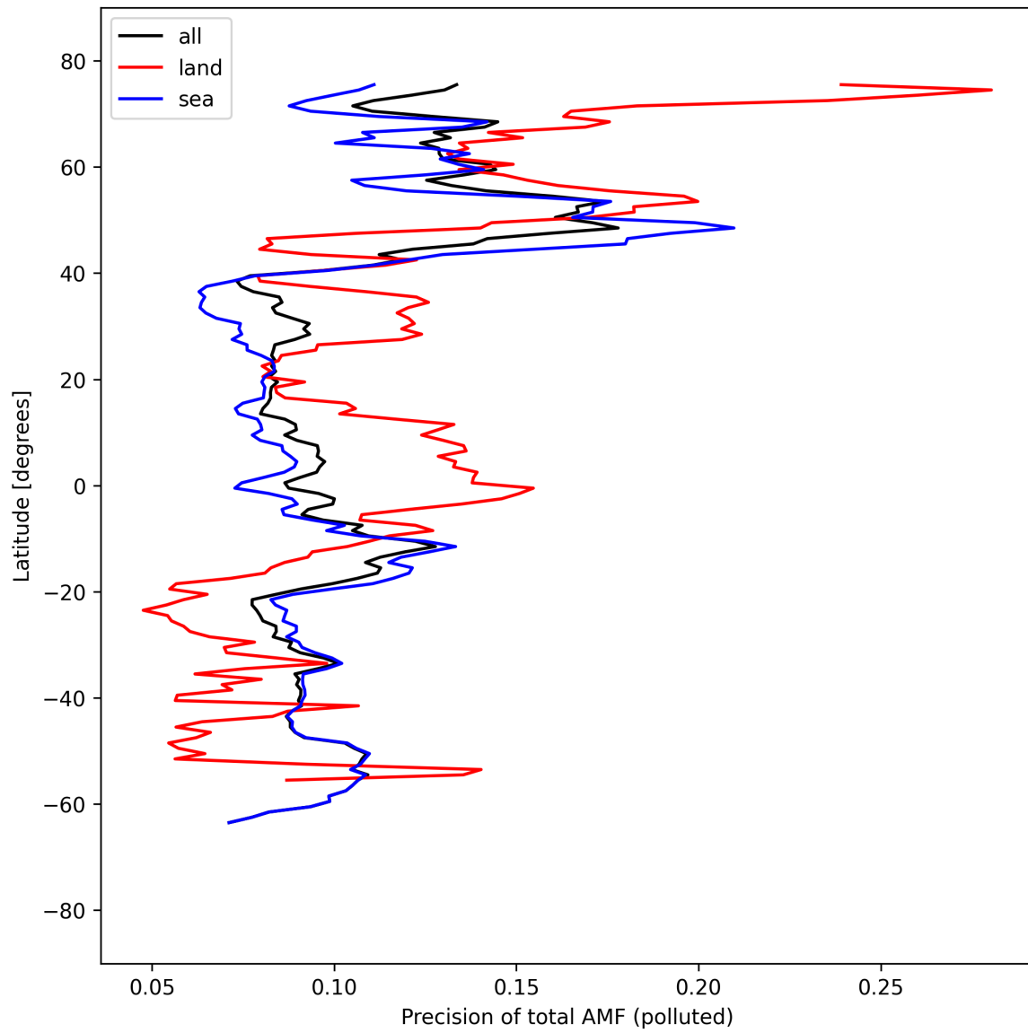
Figure 54: Zonal average of “Precision of total AMF (polluted)” for 2025-09-07 to 2025-09-09.
