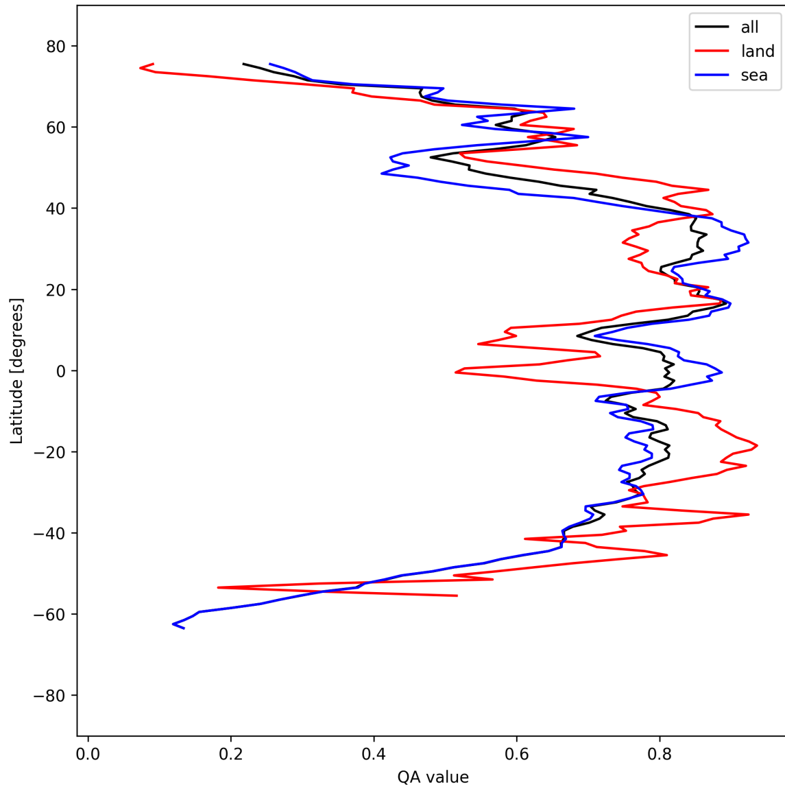
Figure 31: Zonal average of “QA value” for 2025-09-07 to 2025-09-09.
