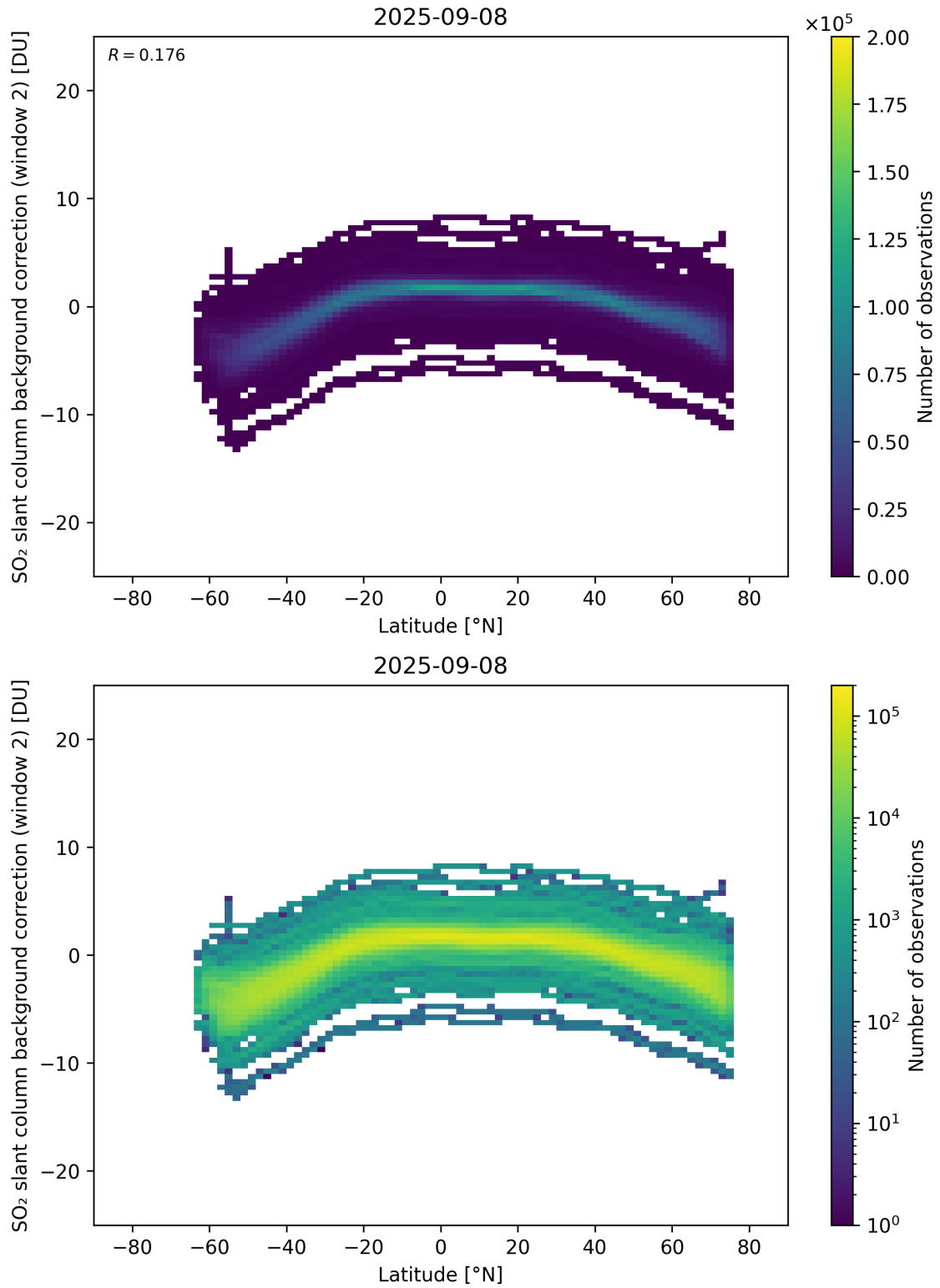
Figure 151: Scatter density plot of “Latitude” against “SO 2 slant column background correction (window 2)” for 2025-09-07 to 2025-09-09.
