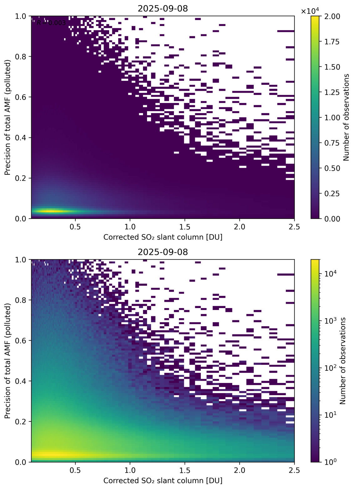
Figure 243: Scatter density plot of “Corrected SO 2 slant column” against “Precision of total AMF (polluted)” for 2025-09-07 to 2025-09-09.
