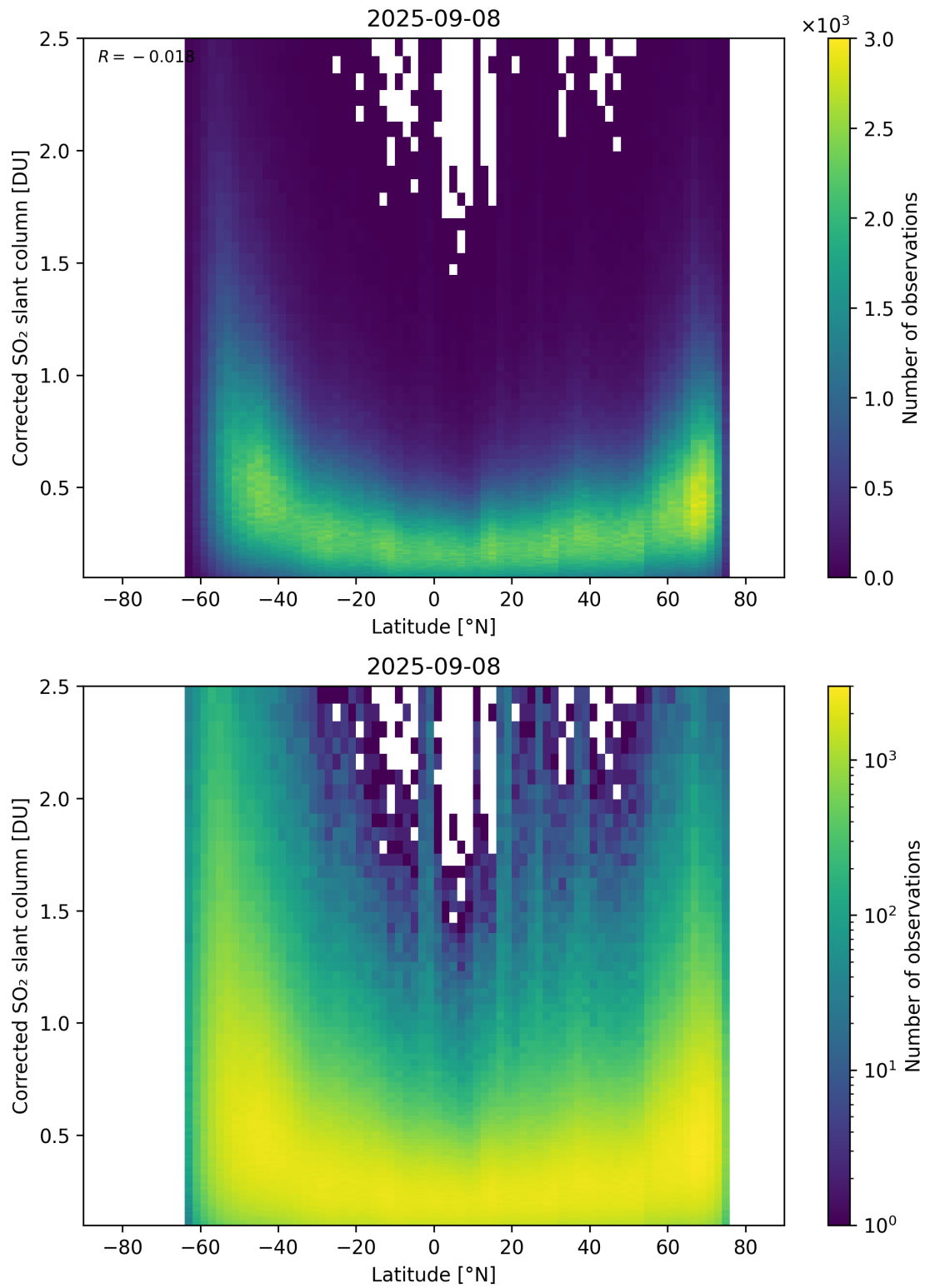
Figure 159: Scatter density plot of “Latitude” against “Corrected SO 2 slant column” for 2025-09-07 to 2025-09-09.
