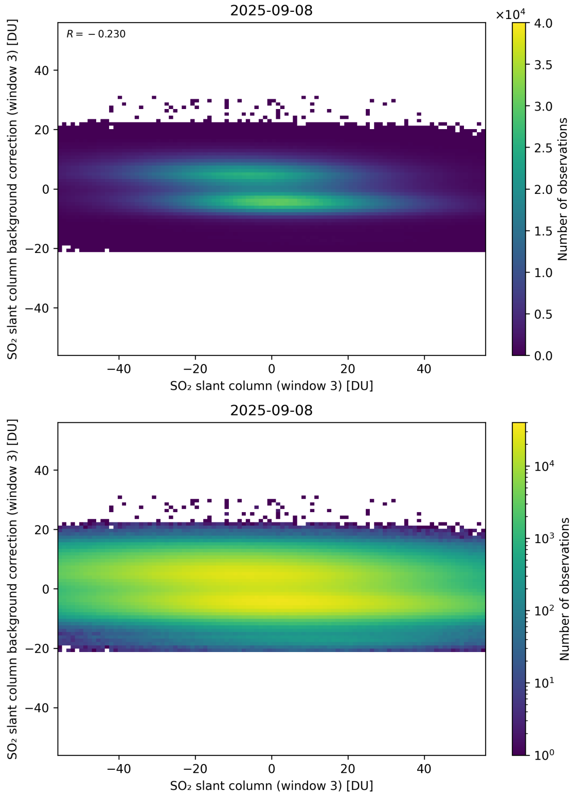
Figure 303: Scatter density plot of “SO 2 slant column (window 3)” against “SO 2 slant column background correction (window 3)” for 2025-09-07 to 2025-09-09.
