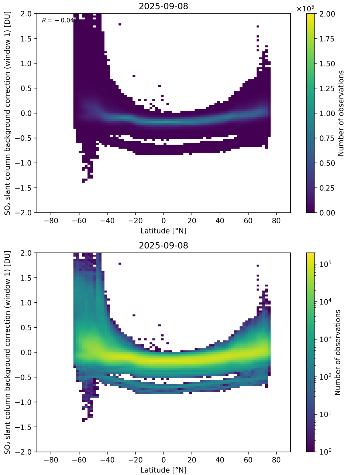
Figure 150: Scatter density plot of “Latitude” against “SO 2 slant column background correction (window 1)” for 2025-09-07 to 2025-09-09.
