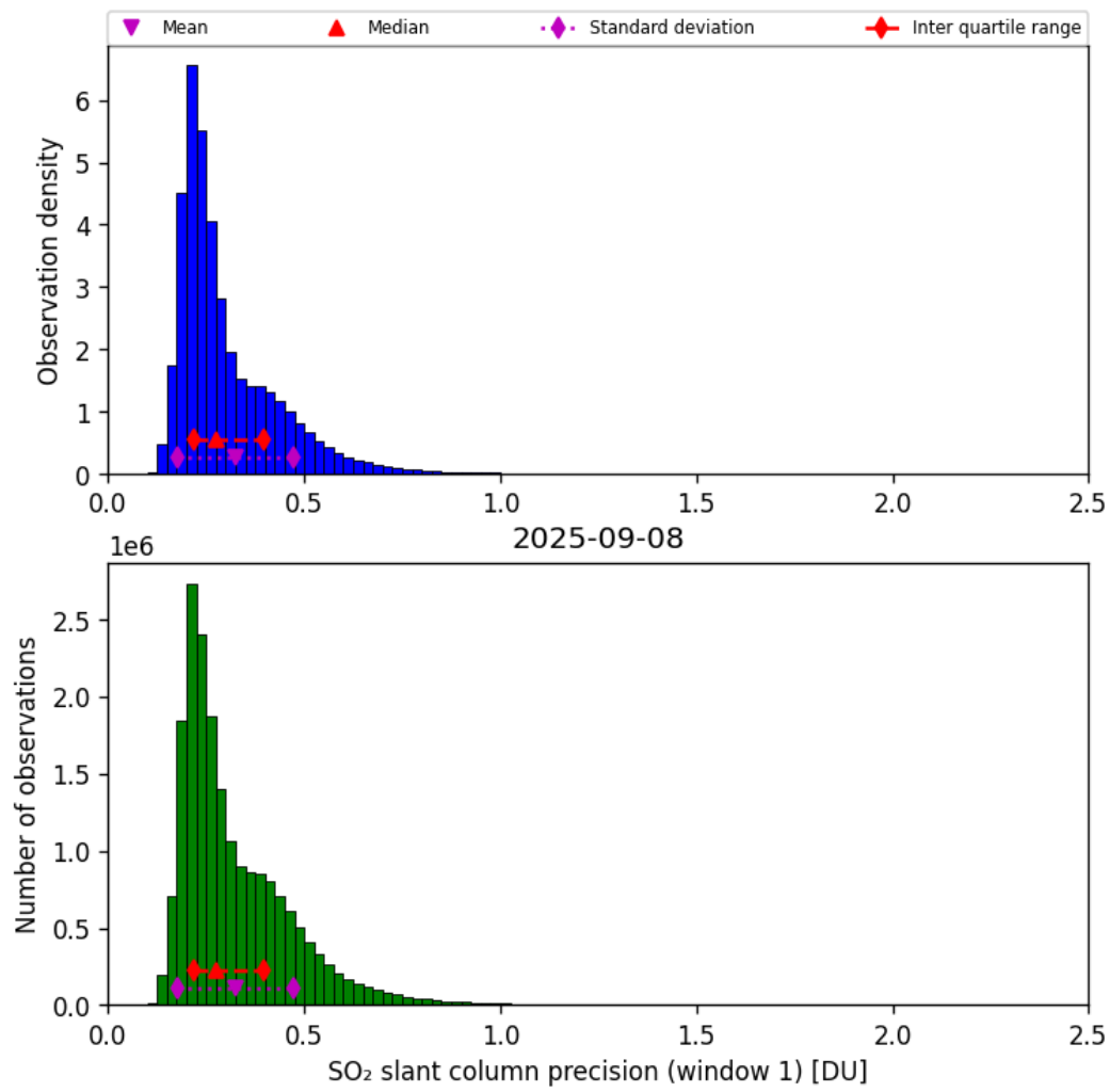
Figure 64: Histogram of “SO 2 slant column precision (window 1)” for 2025-09-07 to 2025-09-09
