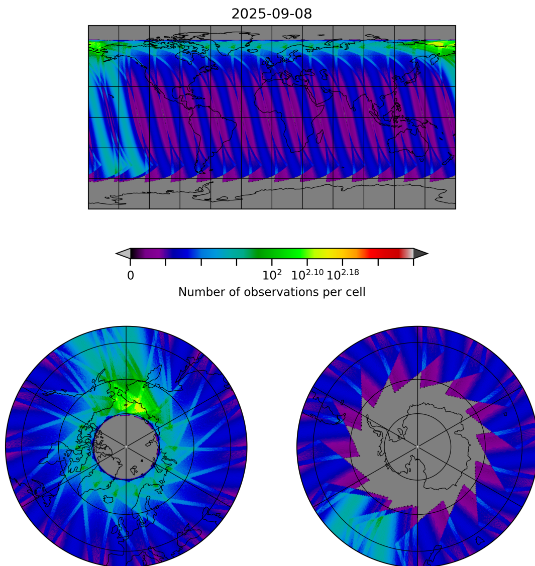
Figure 30: Map of the number of observations for 2025-09-07 to 2025-09-09
