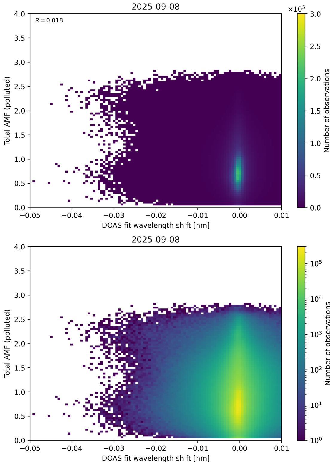
Figure 141: Scatter density plot of “DOAS fit wavelength shift” against “Total AMF (polluted)” for 2025-09-07 to 2025-09-09.
