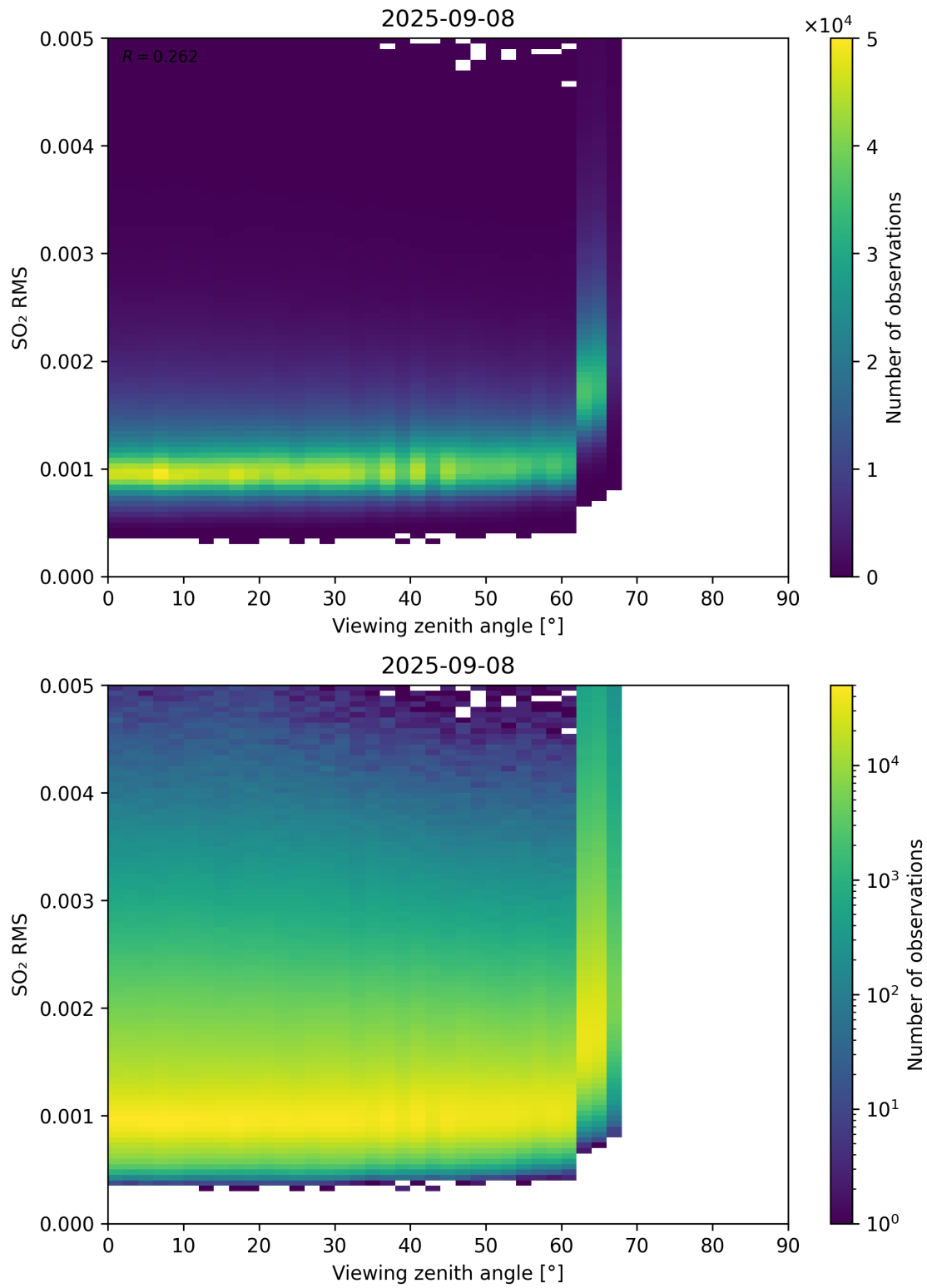
Figure 367: Scatter density plot of “Viewing zenith angle” against “SO 2 RMS” for 2025-09-07 to 2025-09-09.
