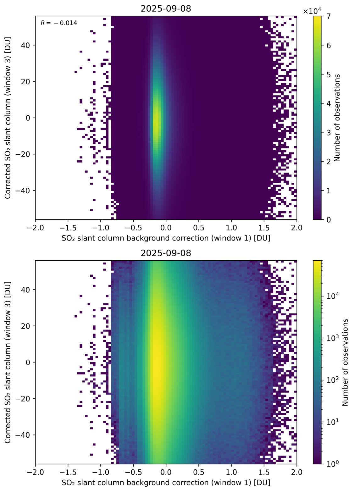
Figure 116: Scatter density plot of “SO 2 slant column background correction (window 1)” against “Corrected SO 2 slant column (window 3)” for 2025-09-07 to 2025-09-09.
