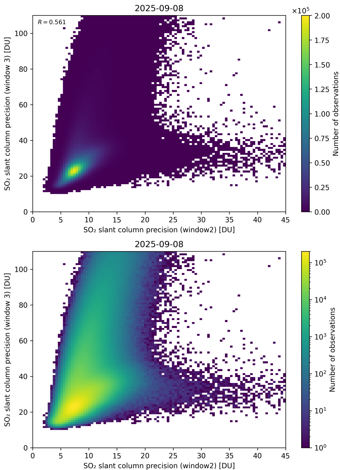
Figure 300: Scatter density plot of “SO 2 slant column precision (window2)” against “SO 2 slant column precision (window 3)” for 2025-09-07 to 2025-09-09.
