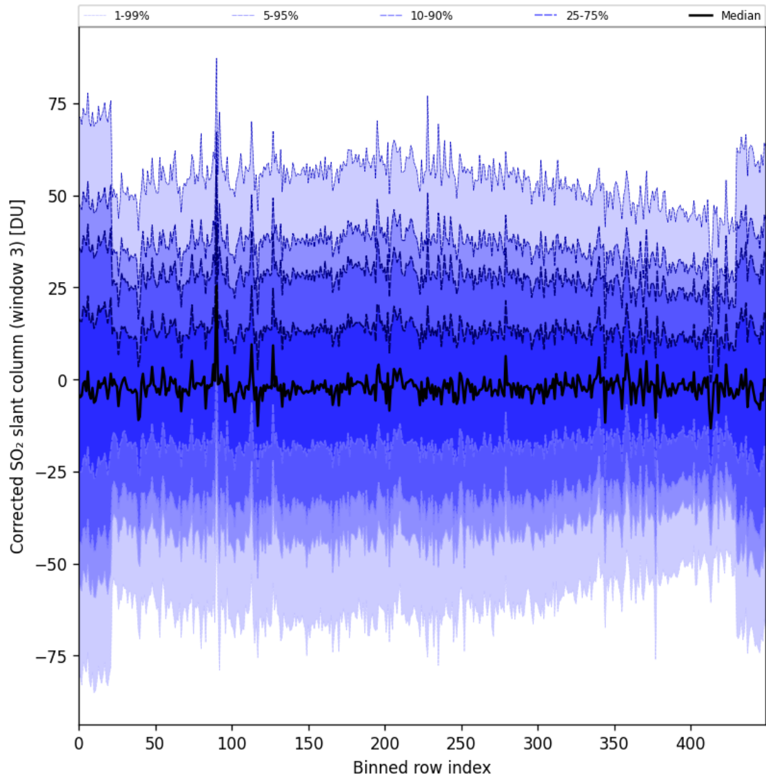
Figure 99: Along track statistics of “Corrected SO 2 slant column (window 3)” for 2025-09-07 to 2025-09-09
