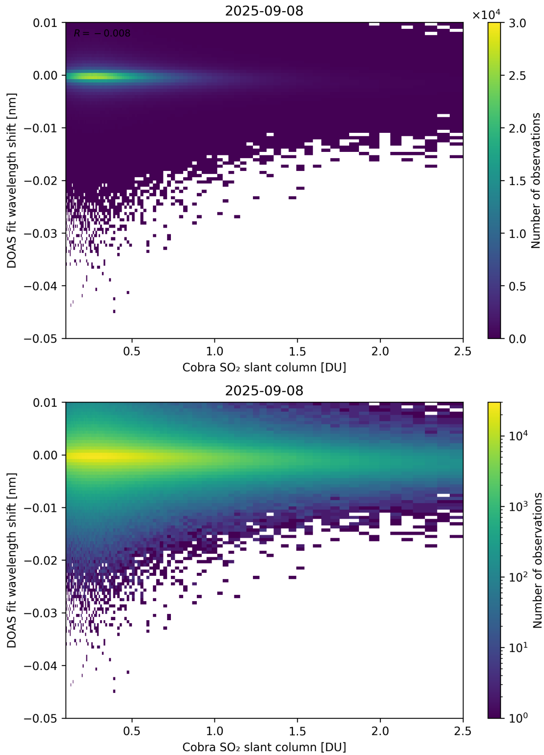
Figure 196: Scatter density plot of “Cobra SO 2 slant column” against “DOAS fit wavelength shift” for 2025-09-07 to 2025-09-09.
