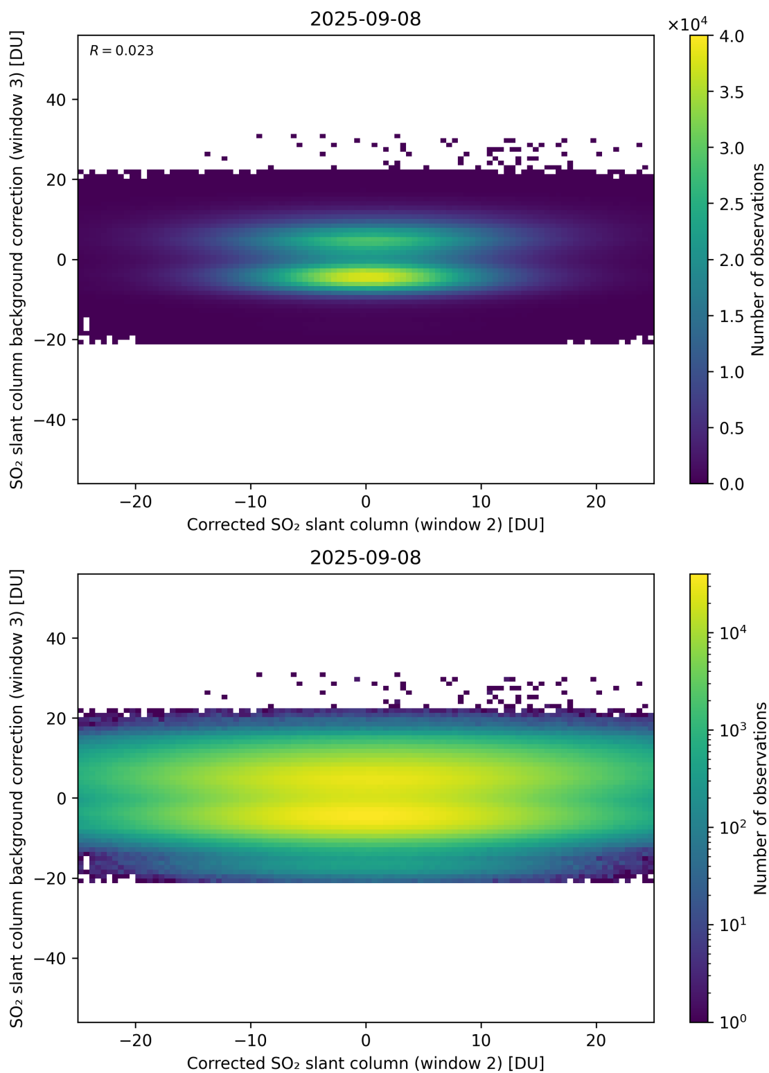
Figure 245: Scatter density plot of “Corrected SO 2 slant column (window 2)” against “SO 2 slant column background correction (window 3)” for 2025-09-07 to 2025-09-09.
