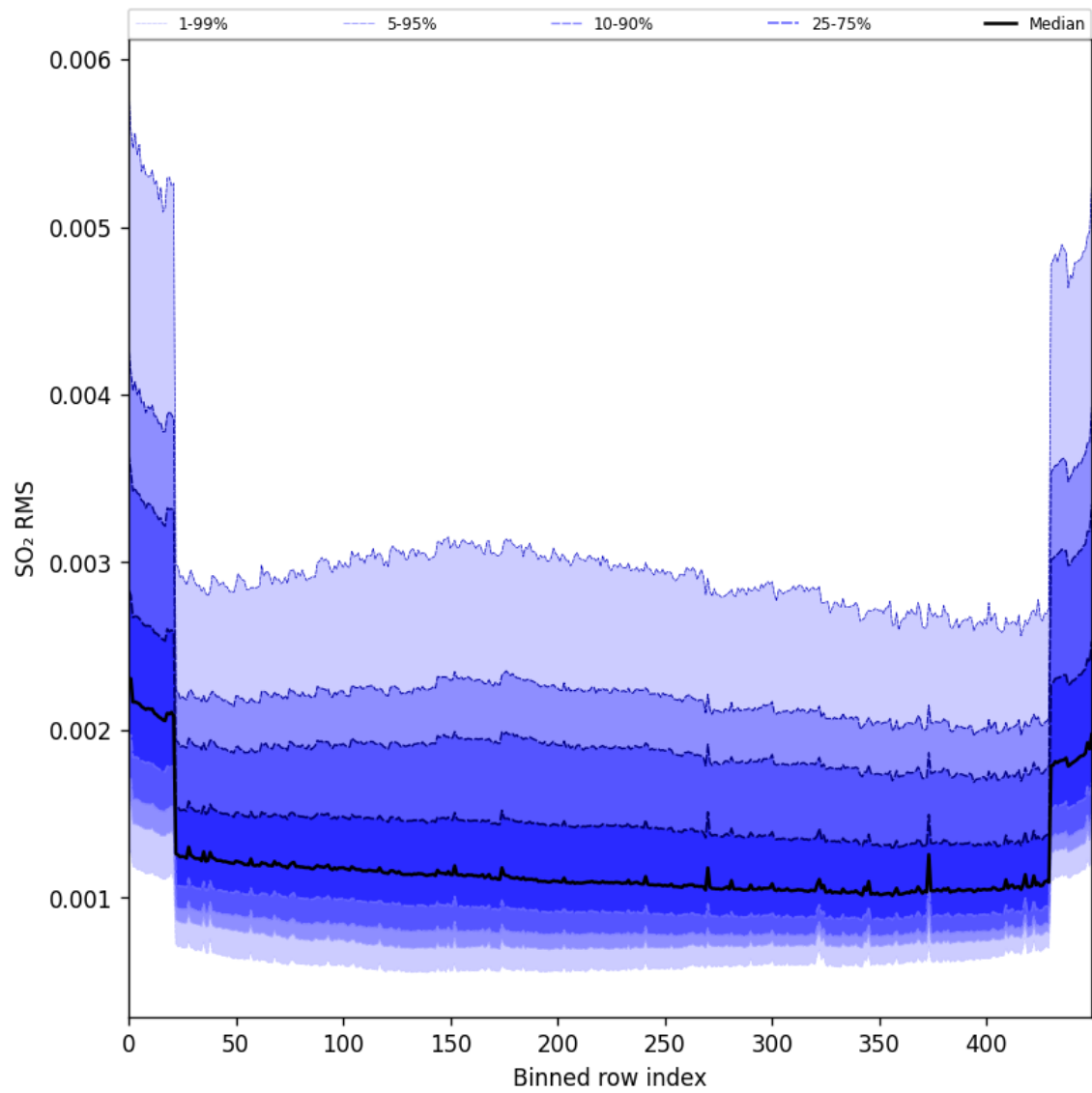
Figure 104: Along track statistics of “SO 2 RMS” for 2025-09-07 to 2025-09-09
