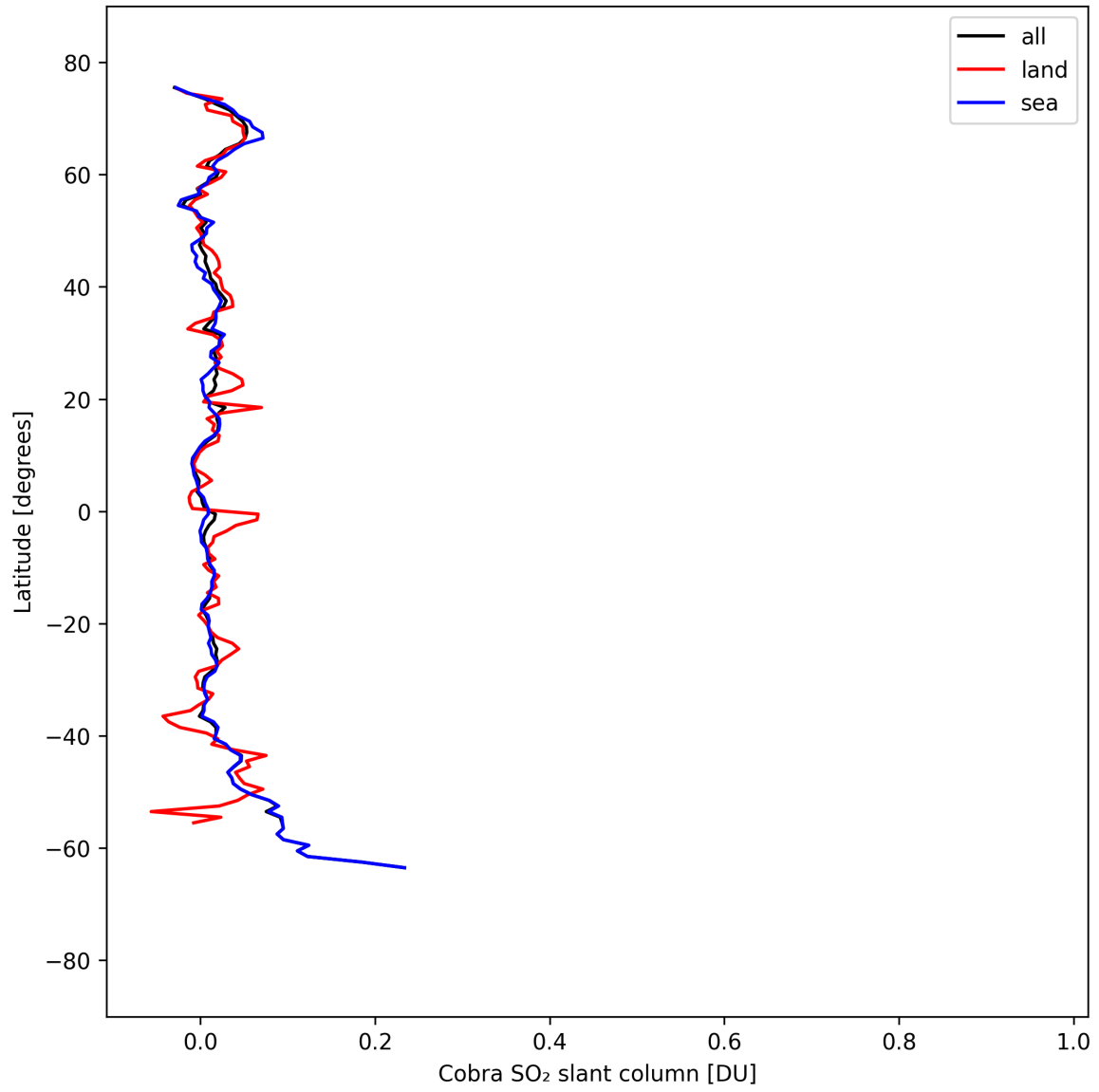
Figure 35: Zonal average of “Cobra SO 2 slant column” for 2025-09-07 to 2025-09-09.
