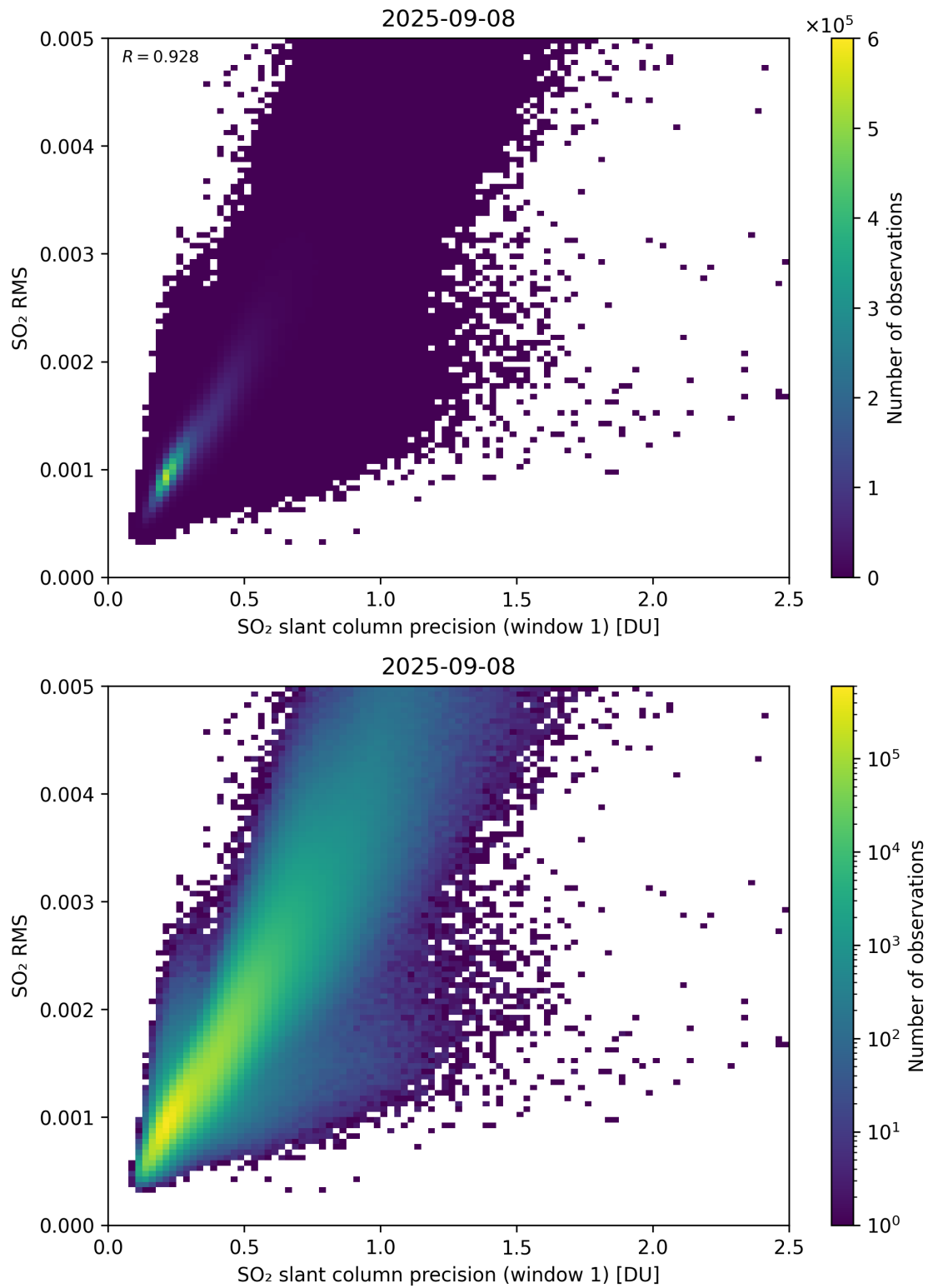
Figure 273: Scatter density plot of “SO 2 slant column precision (window 1)” against “SO 2 RMS” for 2025-09-07 to 2025-09-09.
