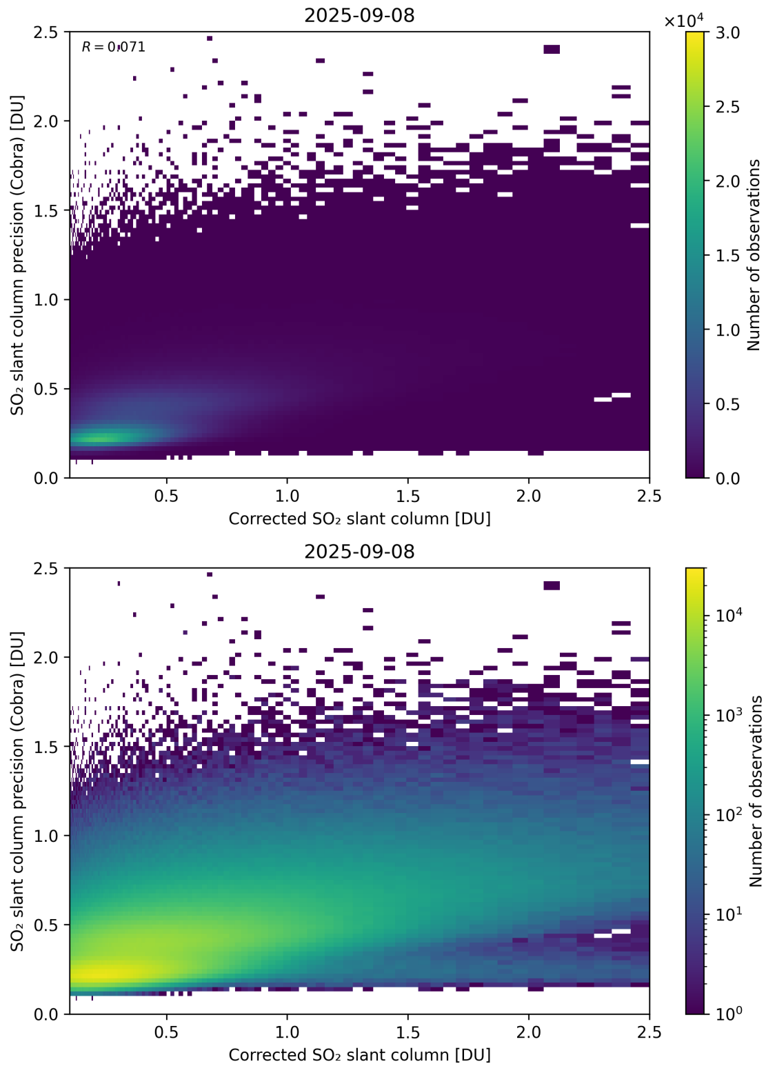
Figure 234: Scatter density plot of “Corrected SO 2 slant column” against “SO 2 slant column precision (Cobra)” for 2025-09-07 to 2025-09-09.
