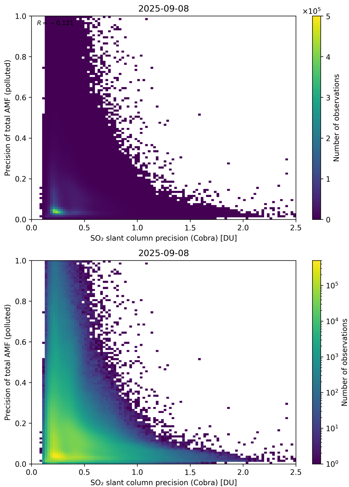
Figure 214: Scatter density plot of “SO 2 slant column precision (Cobra)” against “Precision of total AMF (polluted)” for 2025-09-07 to 2025-09-09.
