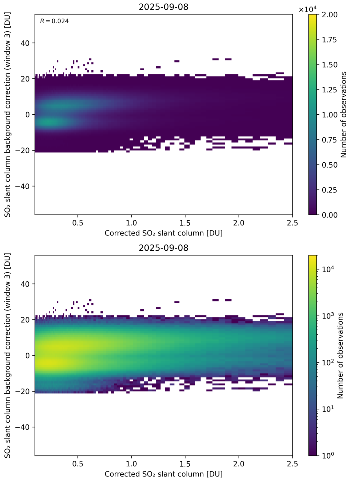
Figure 228: Scatter density plot of “Corrected SO 2 slant column” against “SO 2 slant column background correction (window 3)” for 2025-09-07 to 2025-09-09.
