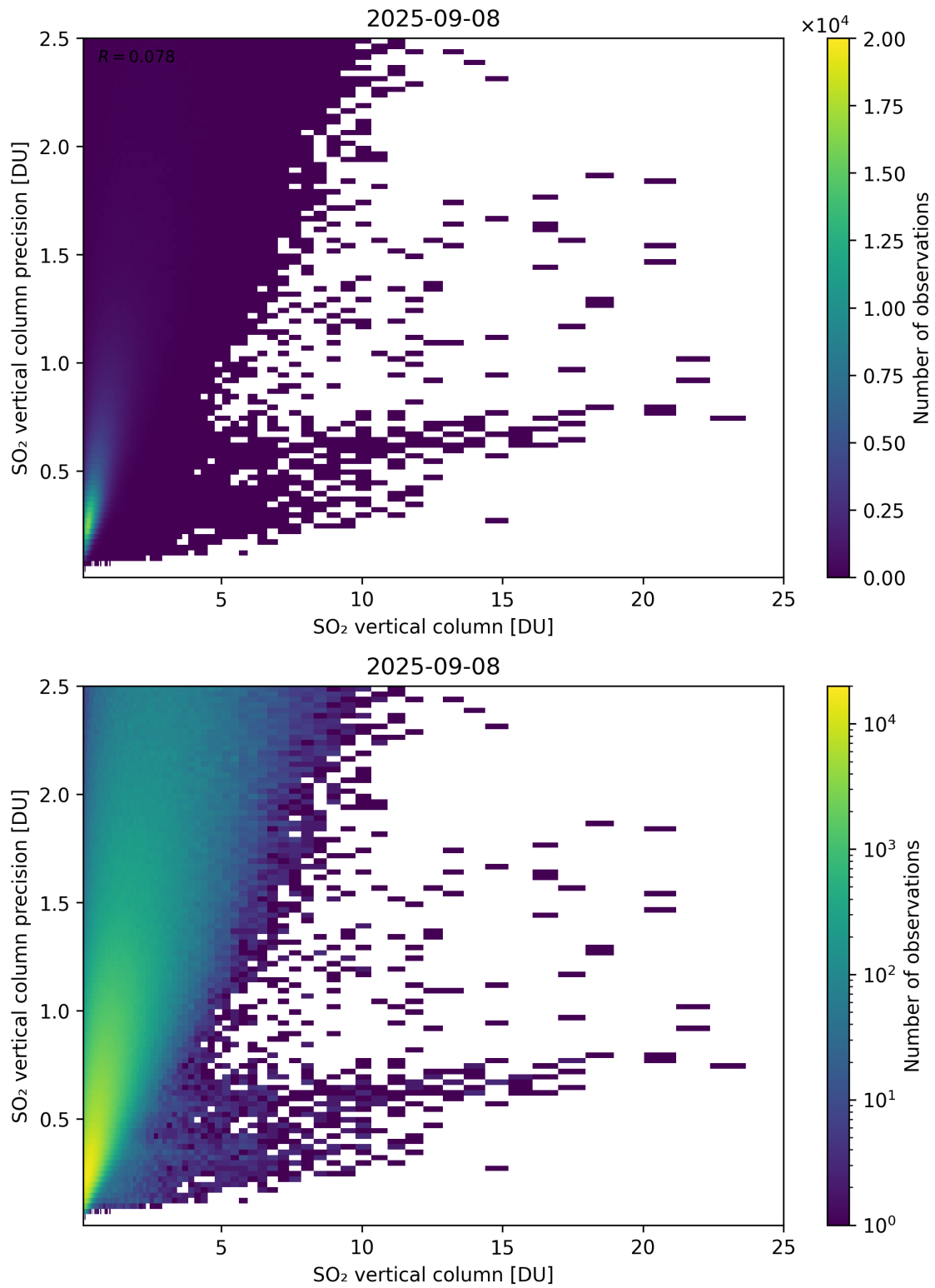
Figure 361: Scatter density plot of “SO 2 vertical column” against “SO 2 vertical column precision” for 2025-09-07 to 2025-09-09.
