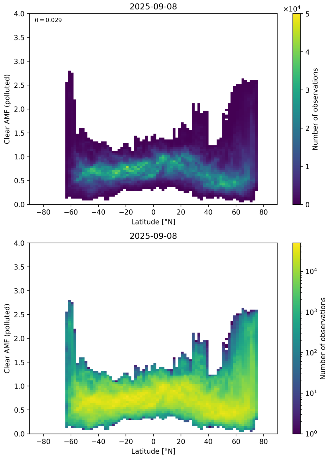
Figure 156: Scatter density plot of “Latitude” against “Clear AMF (polluted)” for 2025-09-07 to 2025-09-09.
