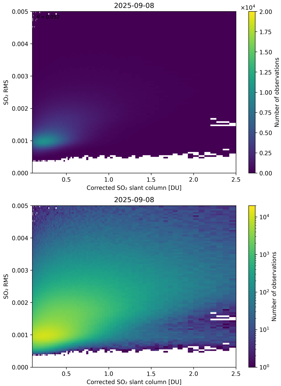
Figure 231: Scatter density plot of “Corrected SO 2 slant column” against “SO 2 RMS” for 2025-09-07 to 2025-09-09.
