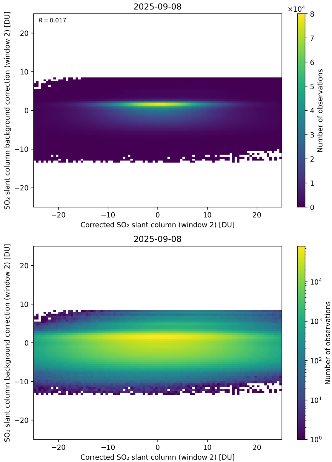
Figure 244: Scatter density plot of “Corrected SO 2 slant column (window 2)” against “SO 2 slant column background correction (window 2)” for 2025-09-07 to 2025-09-09.
