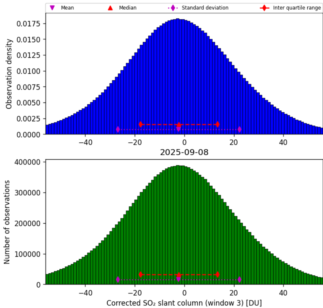
Figure 73: Histogram of “Corrected SO 2 slant column (window 3)” for 2025-09-07 to 2025-09-09
