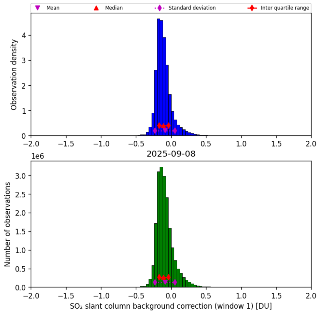
Figure 66: Histogram of “SO 2 slant column background correction (window 1)” for 2025-09-07 to 2025-09-09
