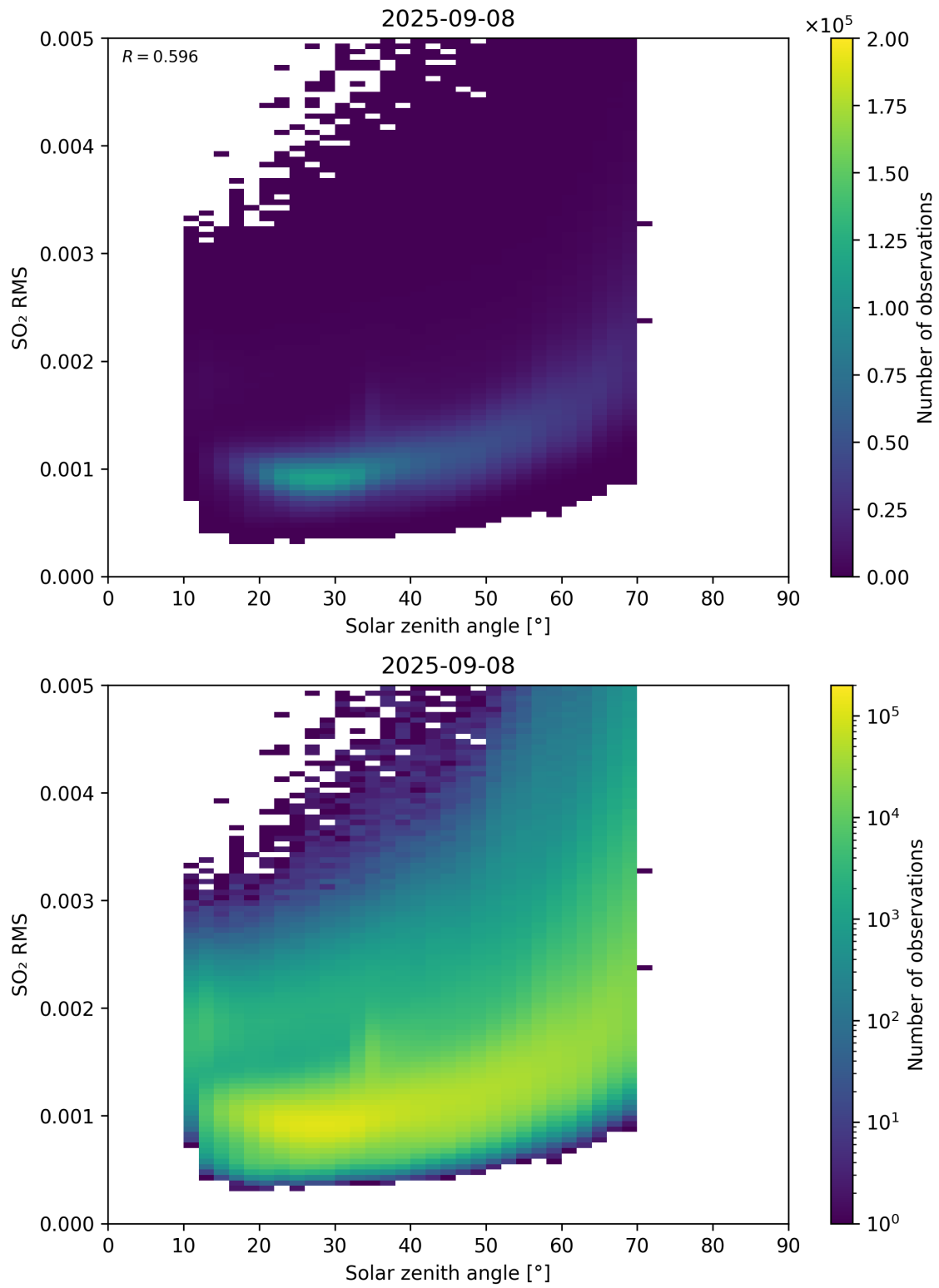
Figure 176: Scatter density plot of “Solar zenith angle” against “SO 2 RMS” for 2025-09-07 to 2025-09-09.
