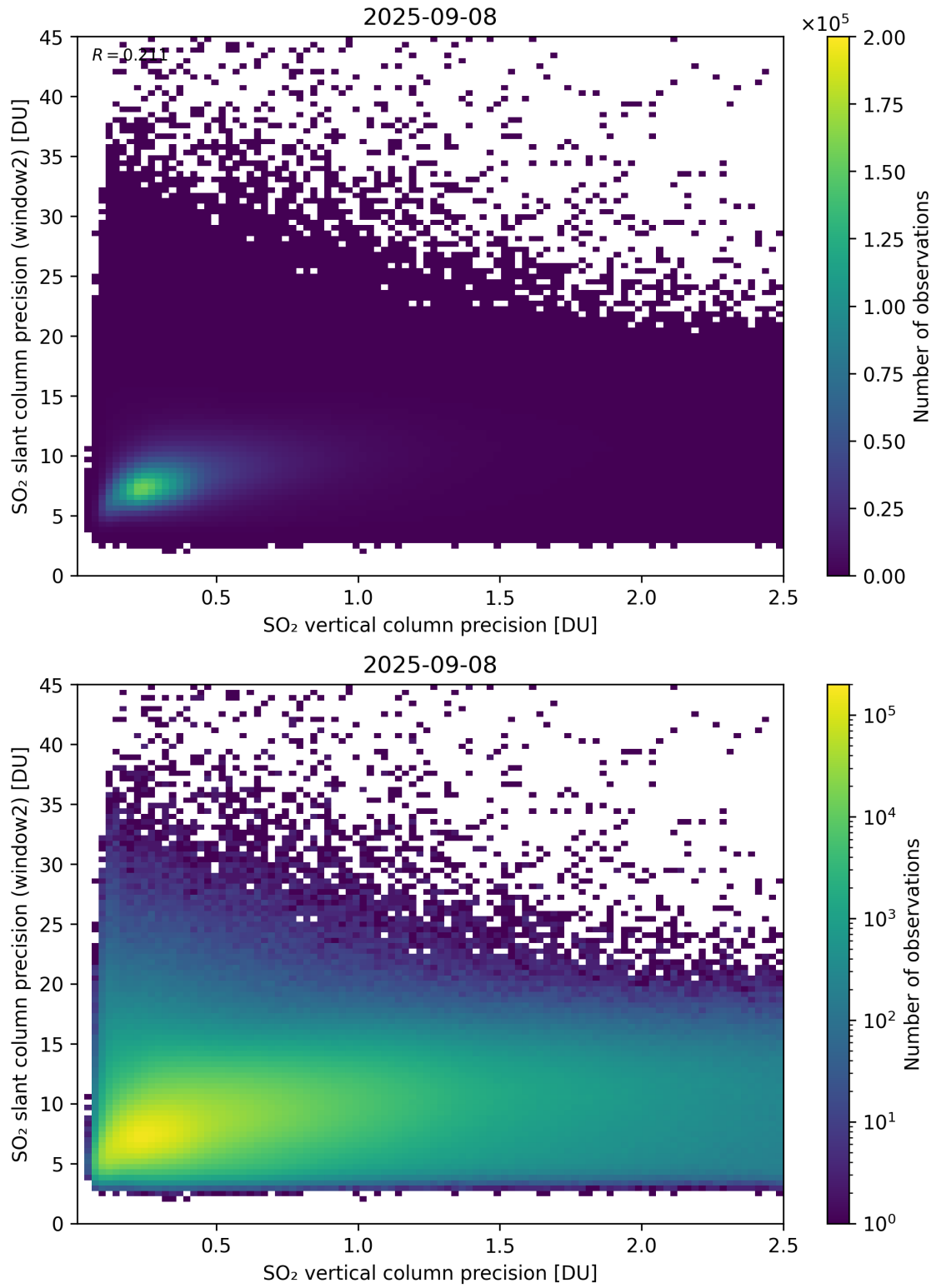
Figure 343: Scatter density plot of “SO 2 vertical column precision” against “SO 2 slant column precision (window2)” for 2025-09-07 to 2025-09-09.
