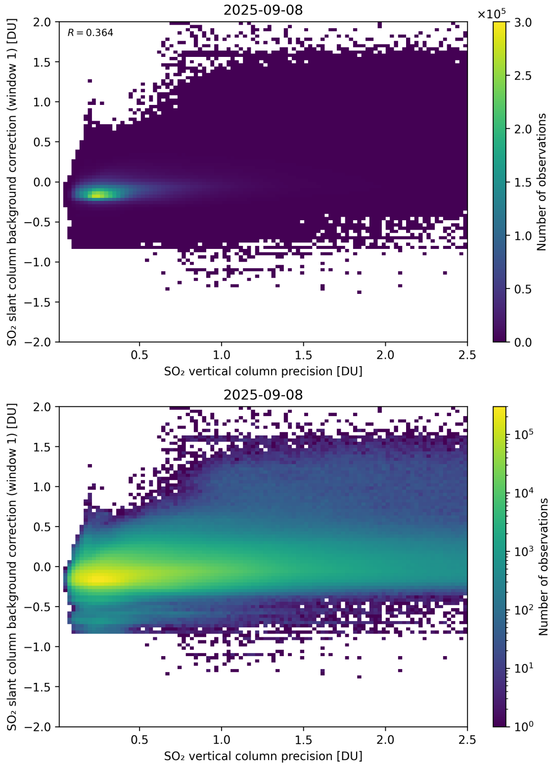
Figure 329: Scatter density plot of “SO 2 vertical column precision” against “SO 2 slant column background correction (window 1)” for 2025-09-07 to 2025-09-09.
