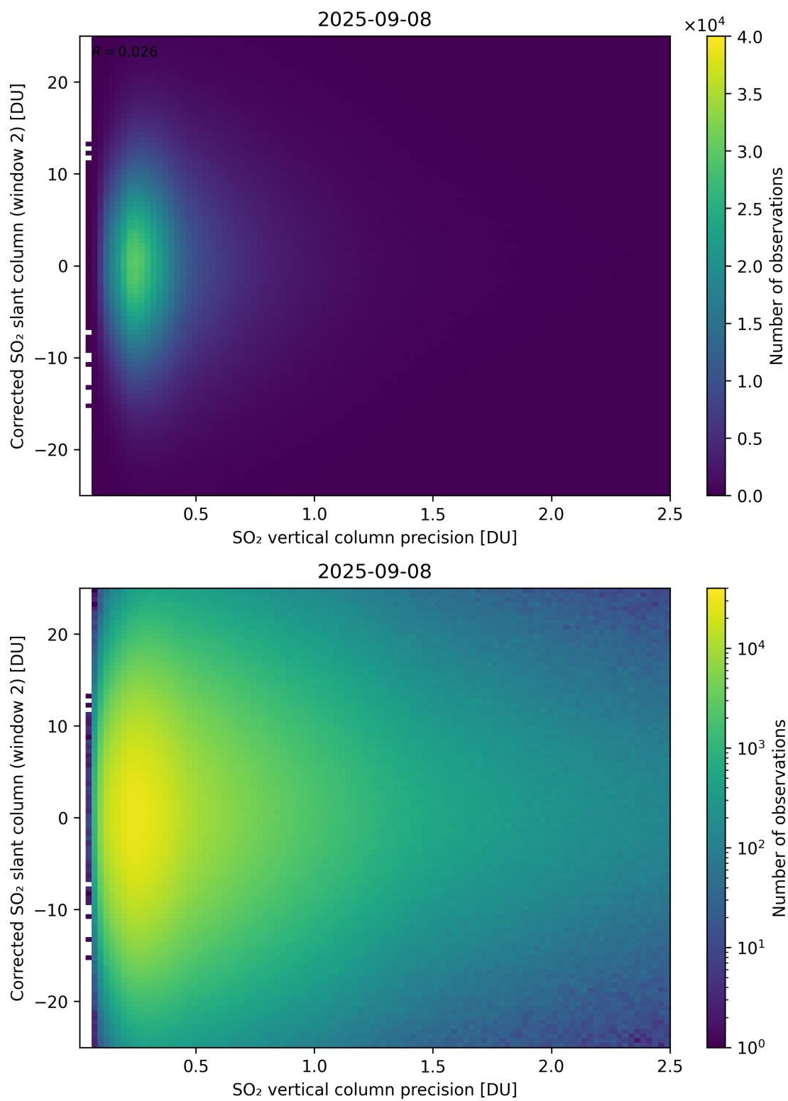
Figure 339: Scatter density plot of “SO 2 vertical column precision” against “Corrected SO 2 slant column (window 2)” for 2025-09-07 to 2025-09-09.
