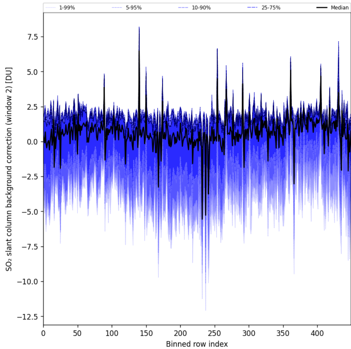
Figure 96: Along track statistics of "SO 2 slant column background correction (window 2)" for 2025-09-07 to 2025-09-09
