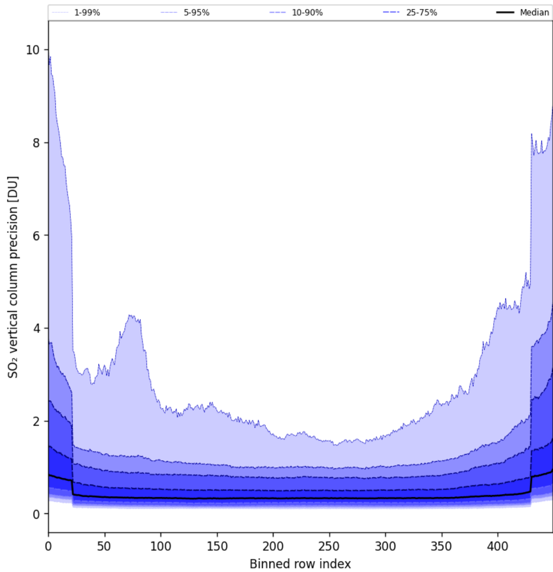
Figure 85: Along track statistics of “SO 2 vertical column precision” for 2025-09-07 to 2025-09-09
