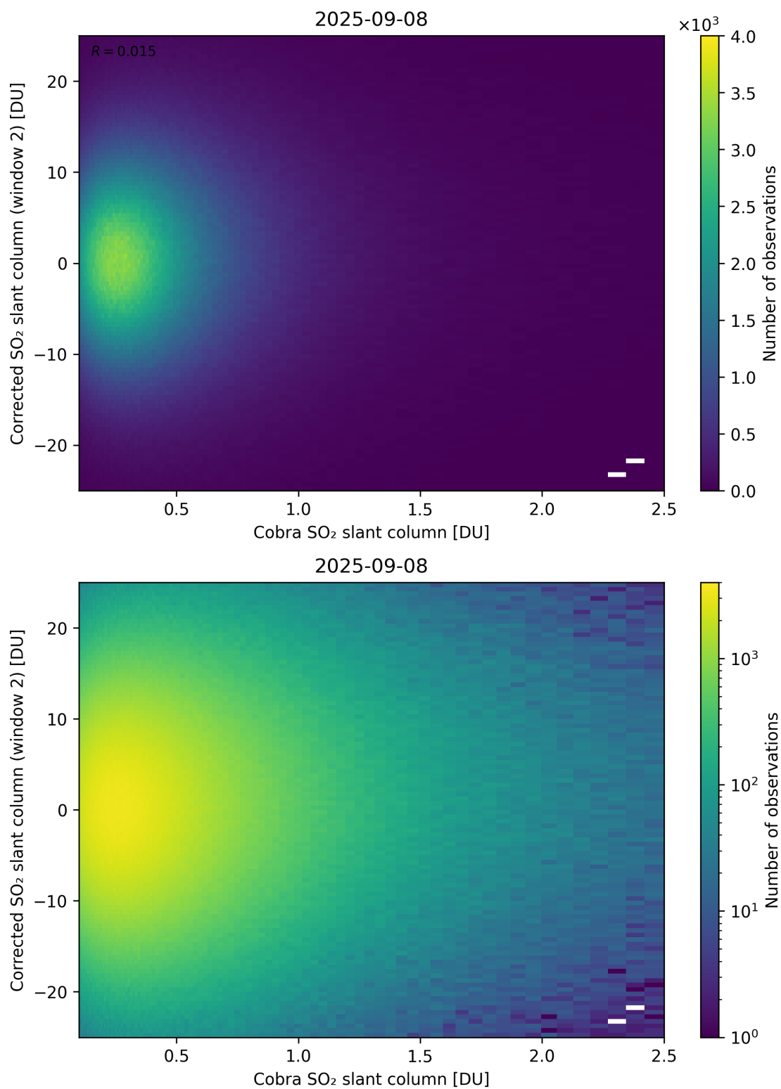
Figure 217: Scatter density plot of “Cobra SO 2 slant column” against “Corrected SO 2 slant column (window 2)” for 2025-09-07 to 2025-09-09.
