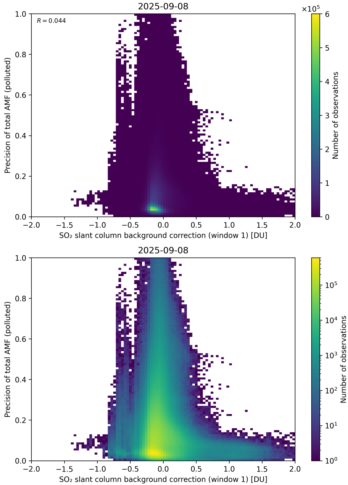
Figure 121: Scatter density plot of “SO 2 slant column background correction (window 1)” against “Precision of total AMF (polluted)” for 2025-09-07 to 2025-09-09.
