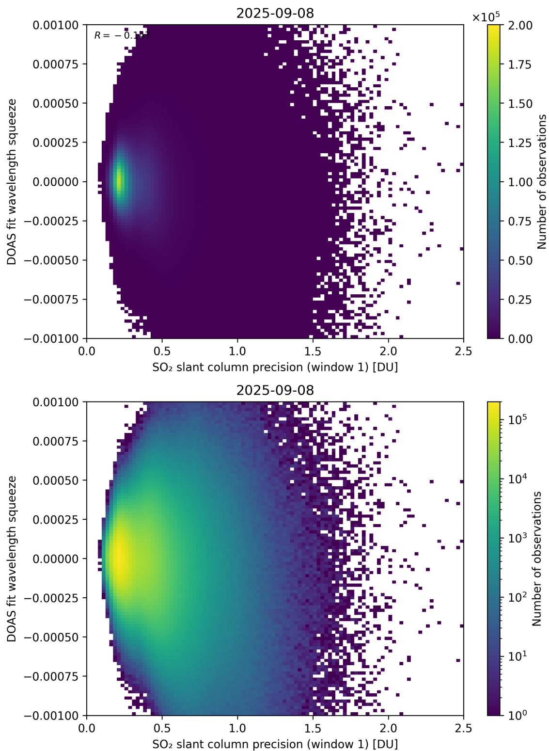
Figure 272: Scatter density plot of “SO 2 slant column precision (window 1)” against “DOAS fit wavelength squeeze” for 2025-09-07 to 2025-09-09.
