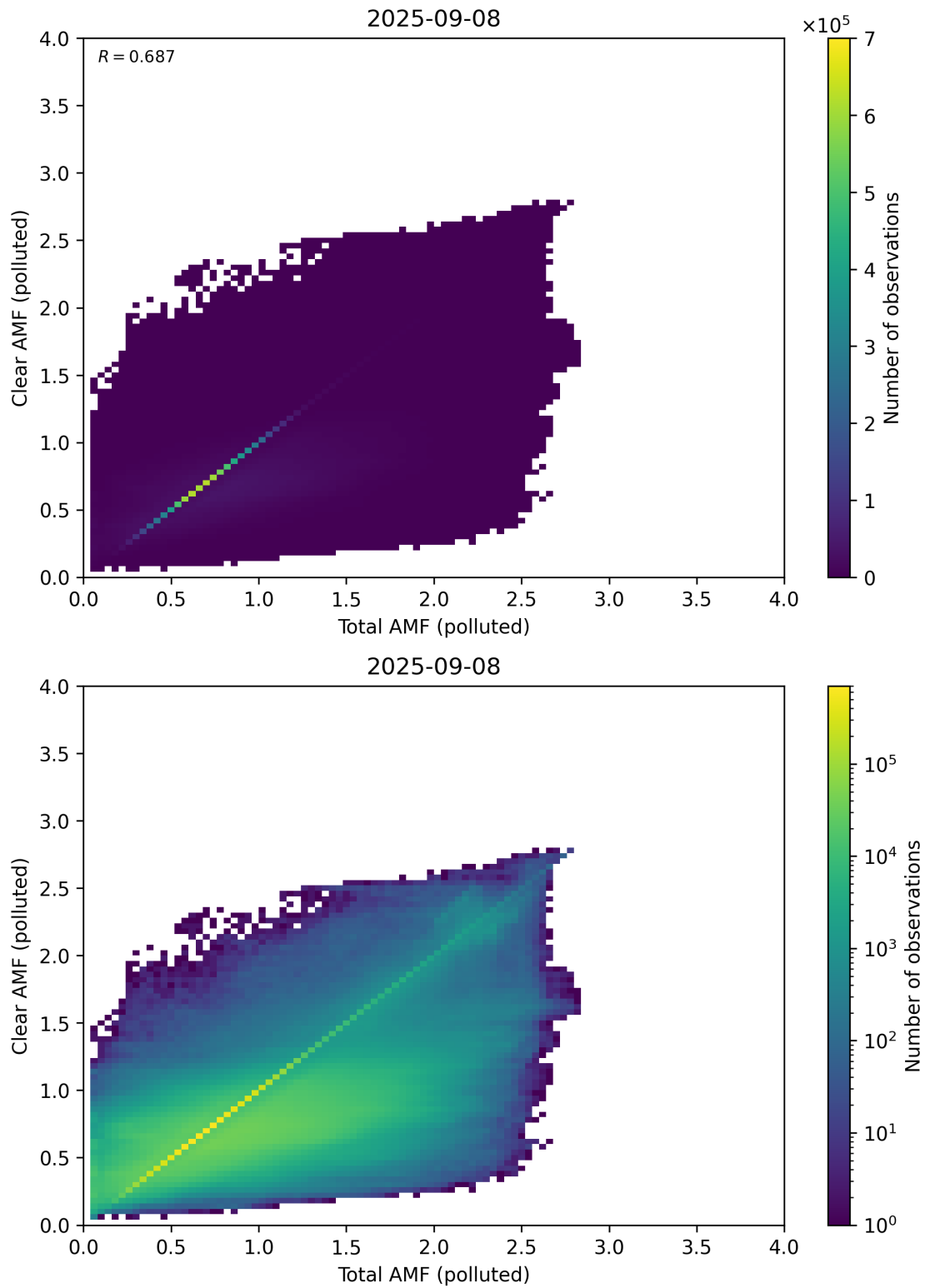
Figure 321: Scatter density plot of “Total AMF (polluted)” against “Clear AMF (polluted)” for 2025-09-07 to 2025-09-09.
