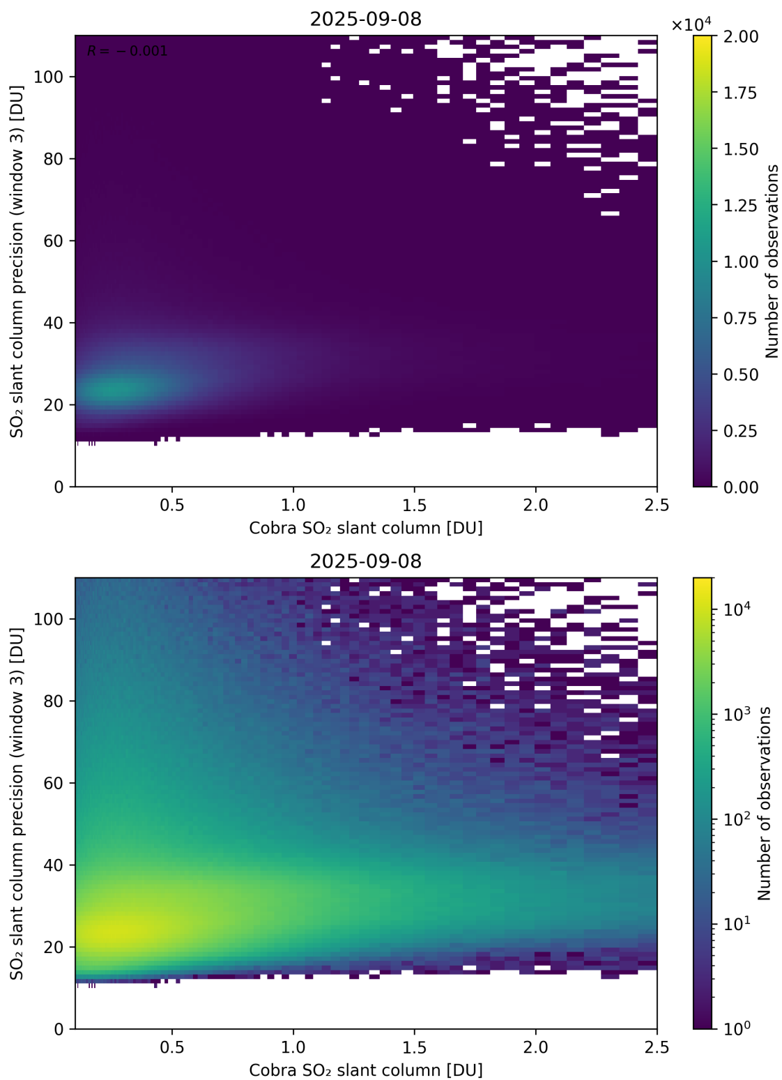
Figure 223: Scatter density plot of “Cobra SO 2 slant column” against “SO 2 slant column precision (window 3)” for 2025-09-07 to 2025-09-09.
