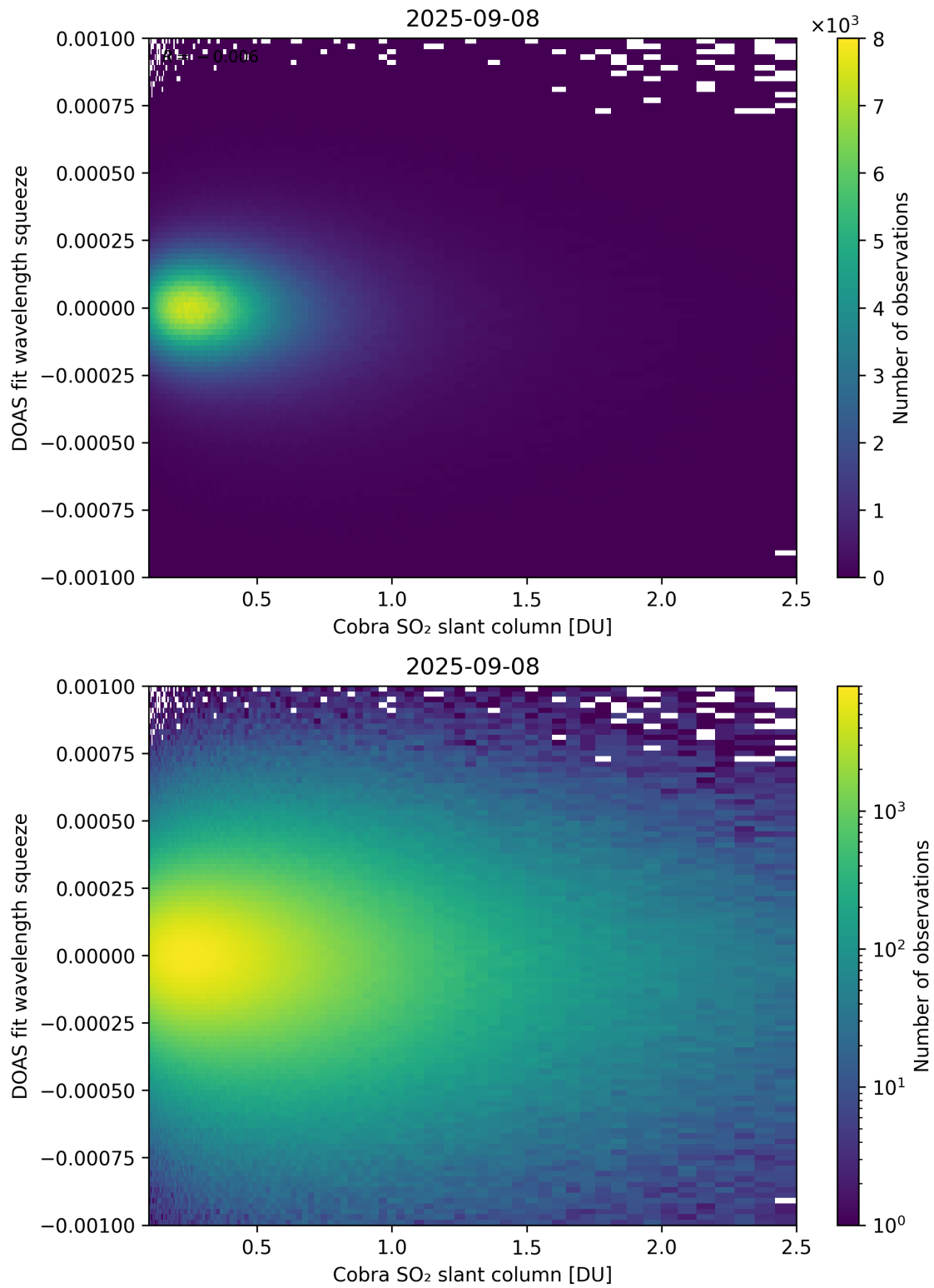
Figure 197: Scatter density plot of “Cobra SO 2 slant column” against “DOAS fit wavelength squeeze” for 2025-09-07 to 2025-09-09.
