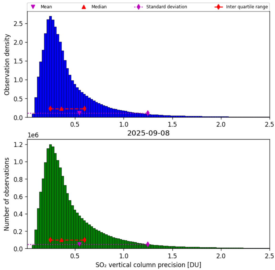
Figure 59: Histogram of “SO 2 vertical column precision” for 2025-09-07 to 2025-09-09
