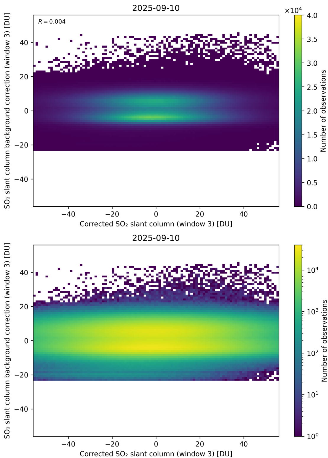
Figure 255: Scatter density plot of “Corrected SO 2 slant column (window 3)” against “SO 2 slant column background correction (window 3)” for 2025-09-10 to 2025-09-11.
