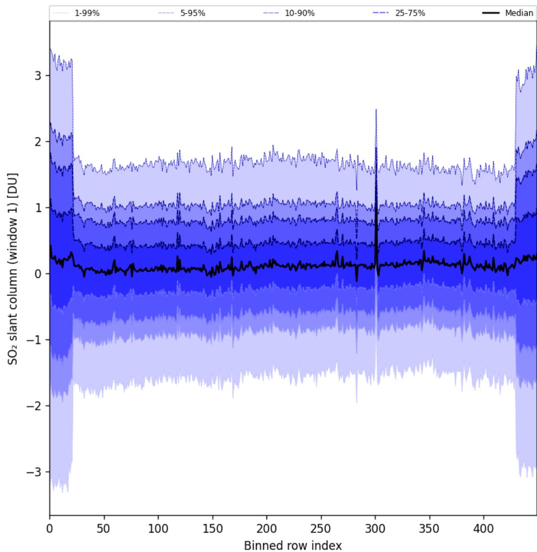
Figure 89: Along track statistics of “SO 2 slant column (window 1)” for 2025-09-10 to 2025-09-11
