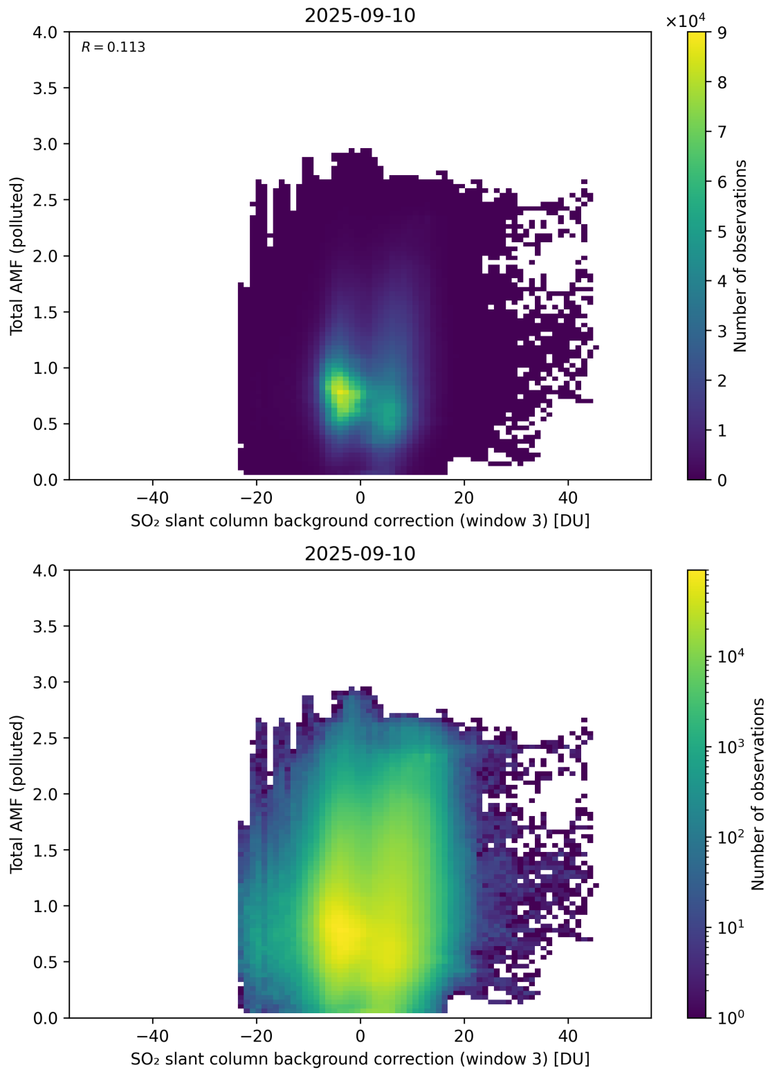
Figure 136: Scatter density plot of “SO 2 slant column background correction (window 3)” against “Total AMF (polluted)” for 2025-09-10 to 2025-09-11.
