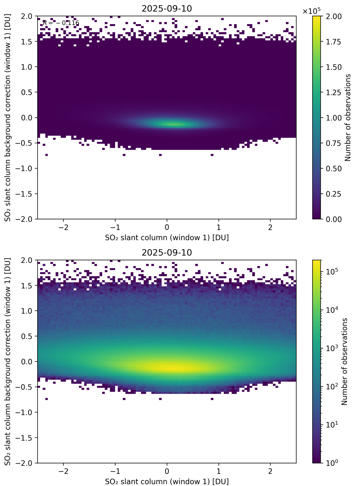
Figure 262: Scatter density plot of “SO 2 slant column (window 1)” against “SO 2 slant column background correction (window 1)” for 2025-09-10 to 2025-09-11.
