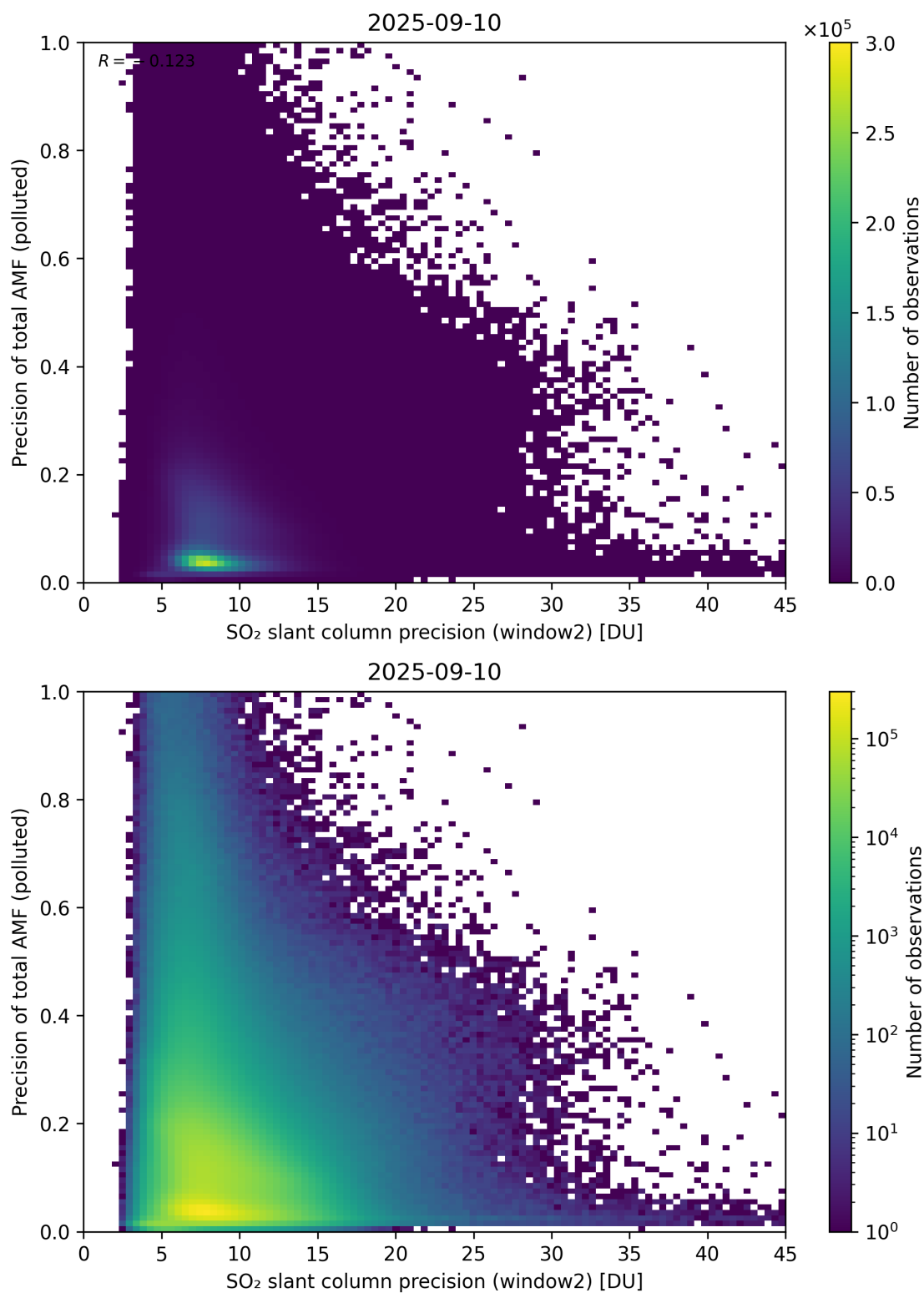
Figure 302: Scatter density plot of “SO 2 slant column precision (window2)” against “Precision of total AMF (polluted)” for 2025-09-10 to 2025-09-11.
