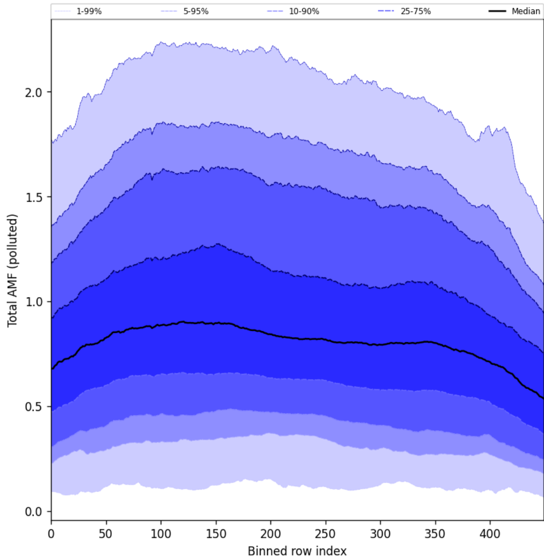
Figure 105: Along track statistics of “Total AMF (polluted)” for 2025-09-10 to 2025-09-11
