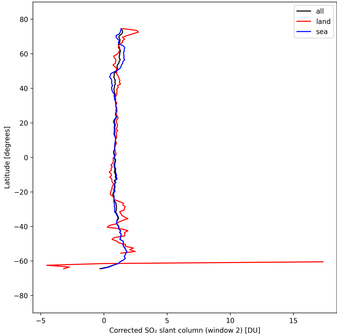
Figure 43: Zonal average of “Corrected SO 2 slant column (window 2)” for 2025-09-10 to 2025-09-11.
