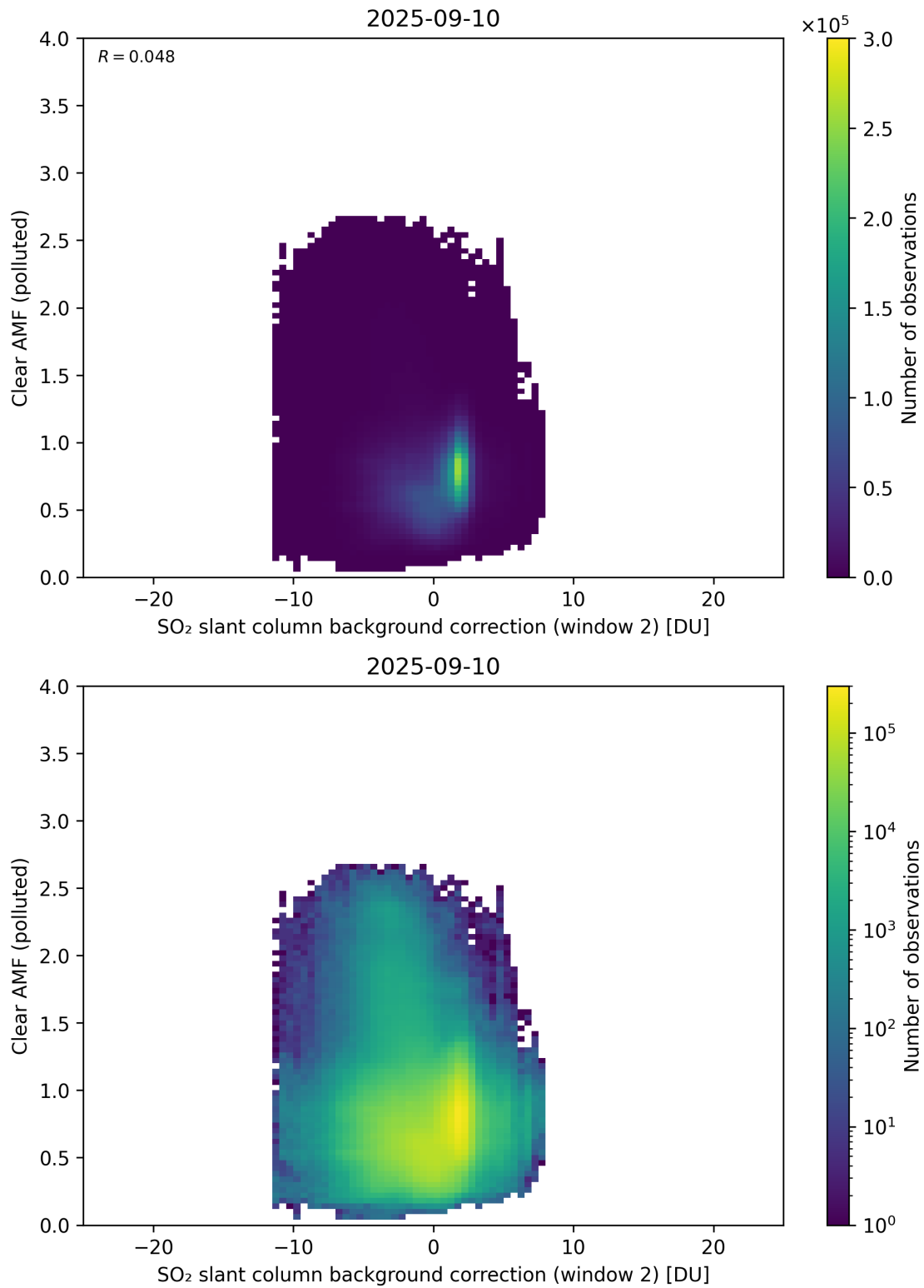
Figure 126: Scatter density plot of “SO 2 slant column background correction (window 2)” against “Clear AMF (polluted)” for 2025-09-10 to 2025-09-11.
