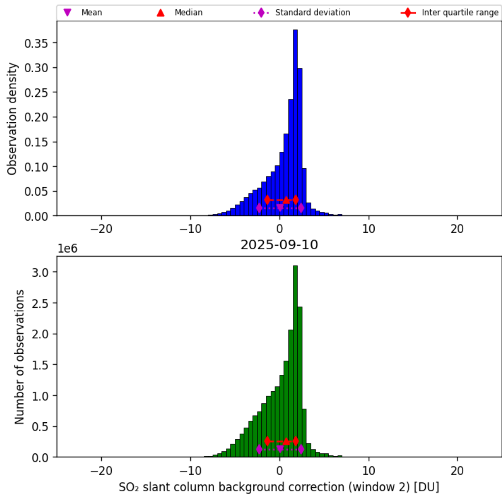
Figure 70: Histogram of “SO 2 slant column background correction (window 2)” for 2025-09-10 to 2025-09-11
