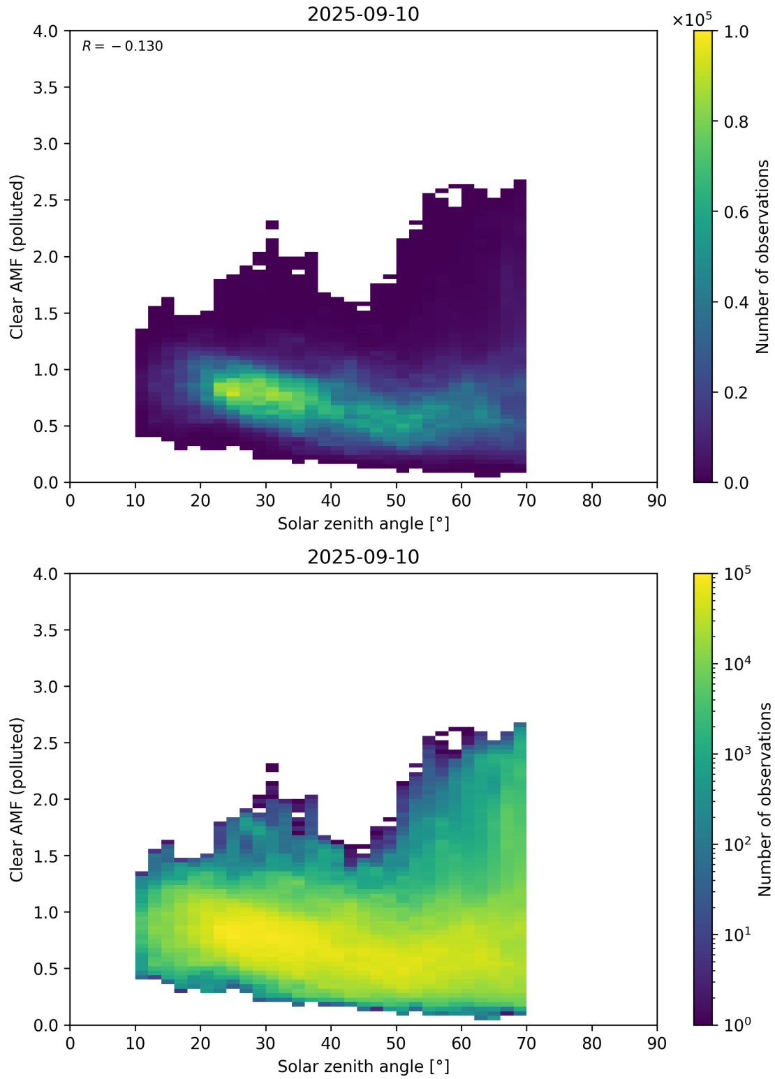
Figure 178: Scatter density plot of “Solar zenith angle” against “Clear AMF (polluted)” for 2025-09-10 to 2025-09-11.
