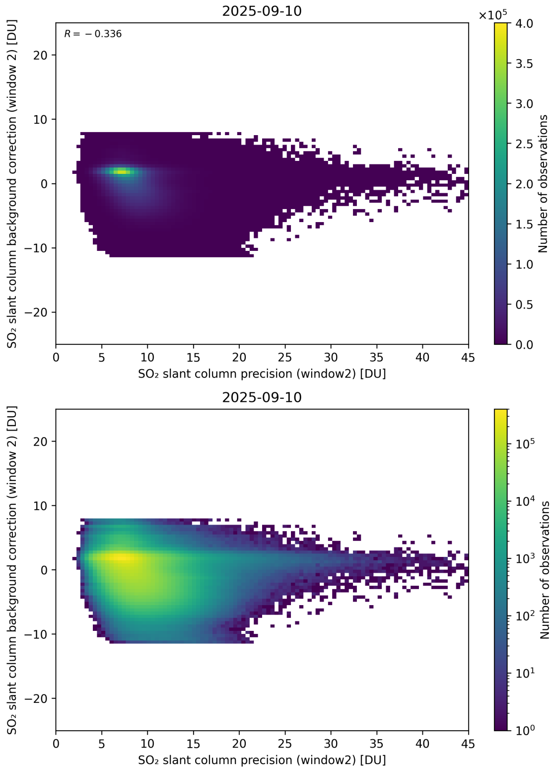
Figure 291: Scatter density plot of “SO 2 slant column precision (window2)” against “SO 2 slant column background correction (window 2)” for 2025-09-10 to 2025-09-11.
