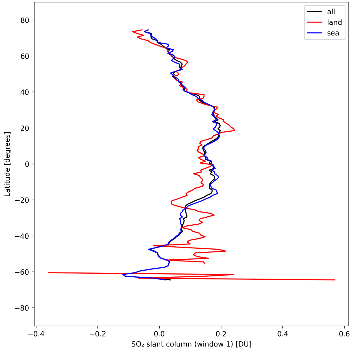
Figure 37: Zonal average of “SO 2 slant column (window 1)” for 2025-09-10 to 2025-09-11.
