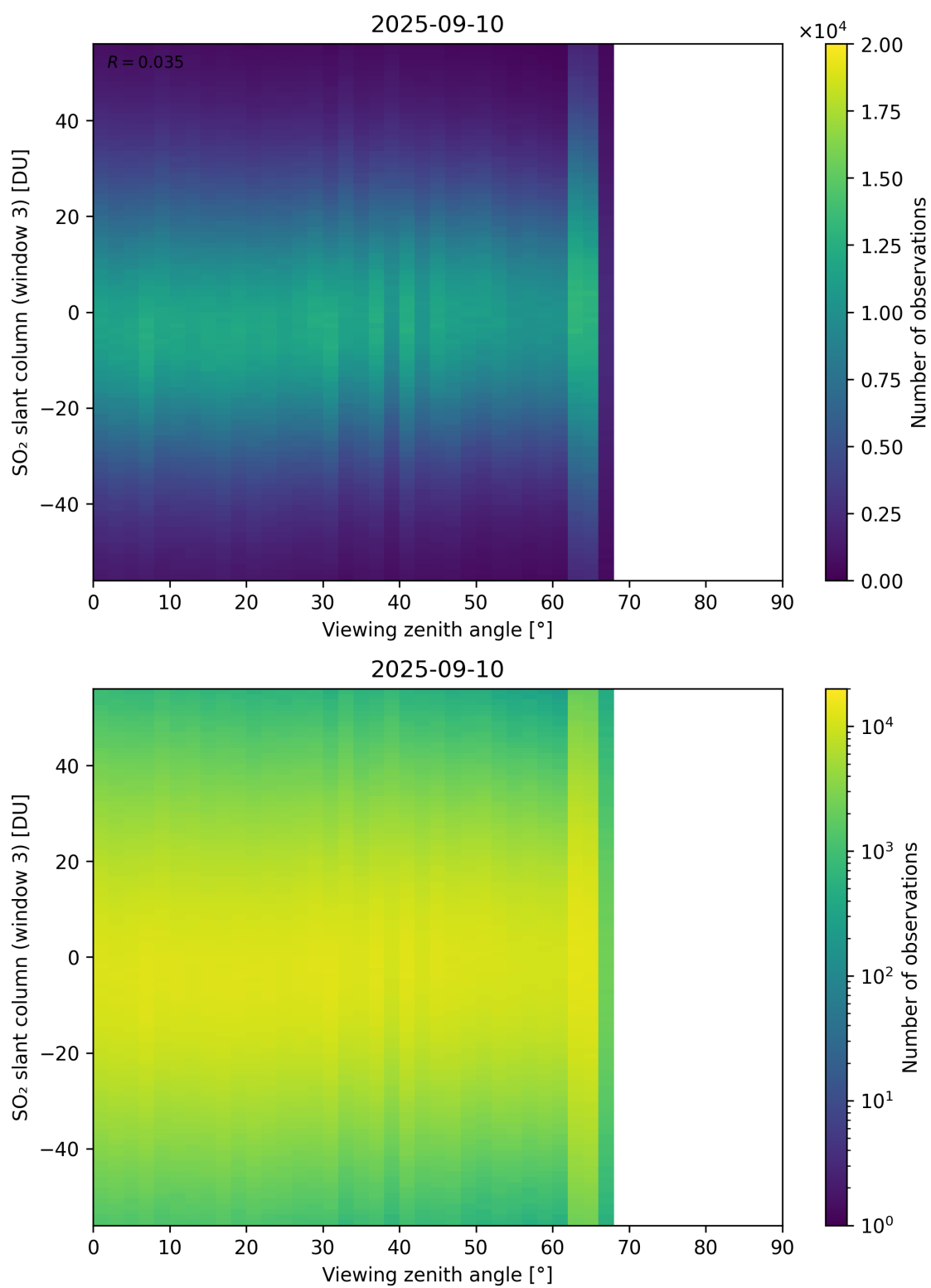
Figure 379: Scatter density plot of “Viewing zenith angle” against “SO 2 slant column (window 3)” for 2025-09-10 to 2025-09-11.
