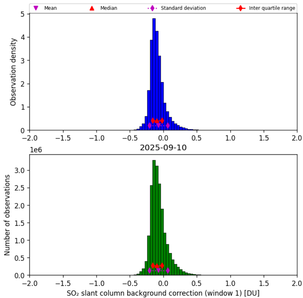
Figure 66: Histogram of “SO 2 slant column background correction (window 1)” for 2025-09-10 to 2025-09-11
