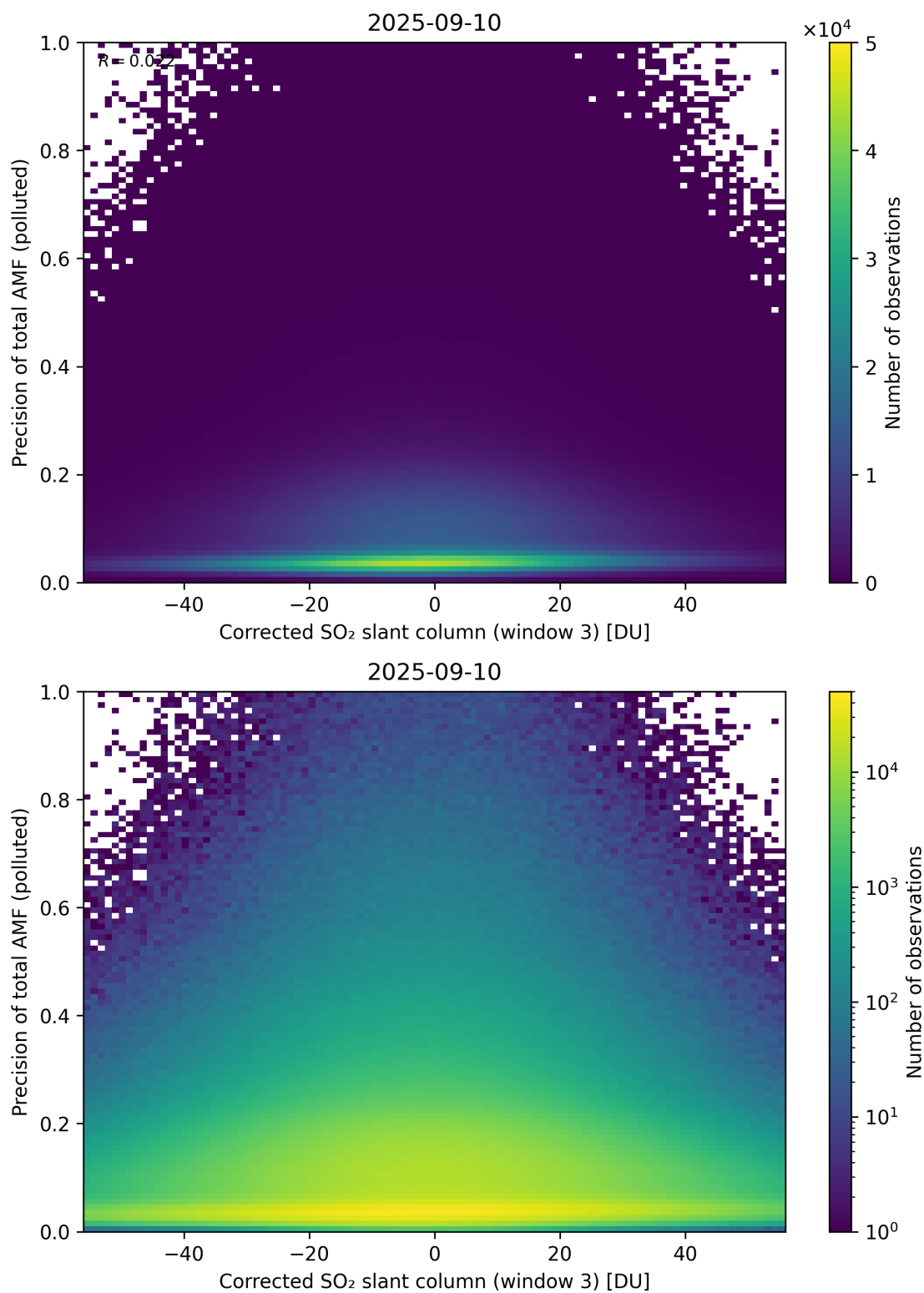
Figure 261: Scatter density plot of “Corrected SO 2 slant column (window 3)” against “Precision of total AMF (polluted)” for 2025-09-10 to 2025-09-11.
