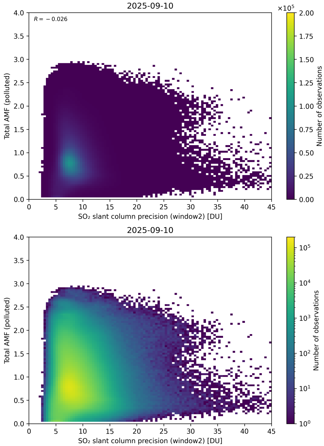
Figure 301: Scatter density plot of “SO 2 slant column precision (window2)” against “Total AMF (polluted)” for 2025-09-10 to 2025-09-11.
