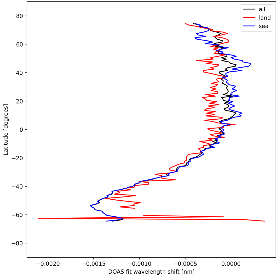
Figure 50: Zonal average of “DOAS fit wavelength shift” for 2025-09-10 to 2025-09-11.
