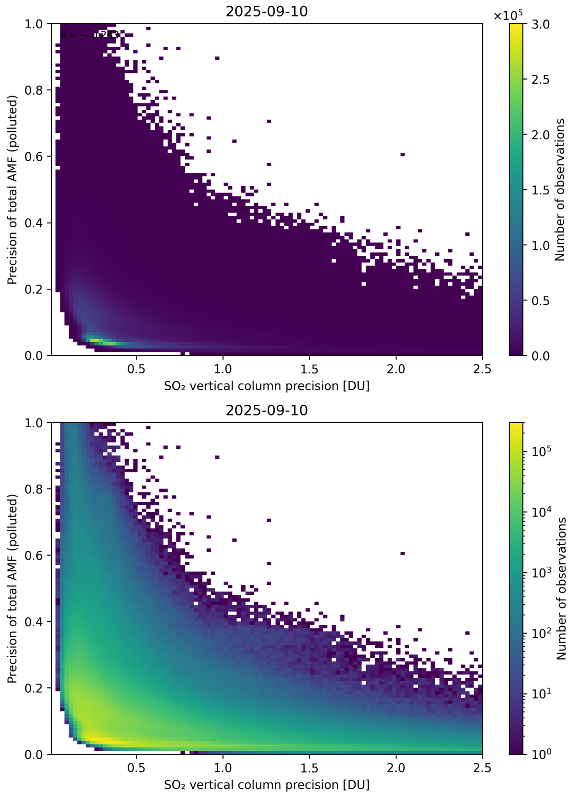
Figure 347: Scatter density plot of “SO 2 vertical column precision” against “Precision of total AMF (polluted)” for 2025-09-10 to 2025-09-11.
