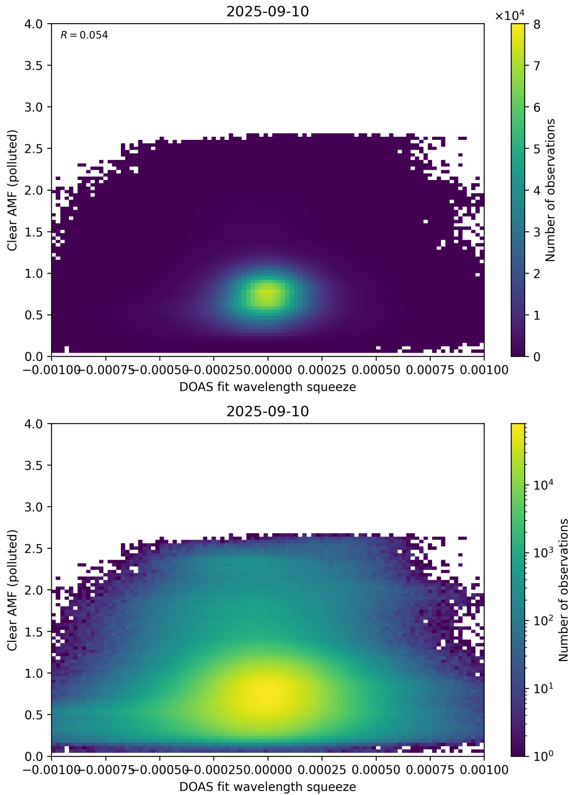
Figure 144: Scatter density plot of “DOAS fit wavelength squeeze” against “Clear AMF (polluted)” for 2025-09-10 to 2025-09-11.
