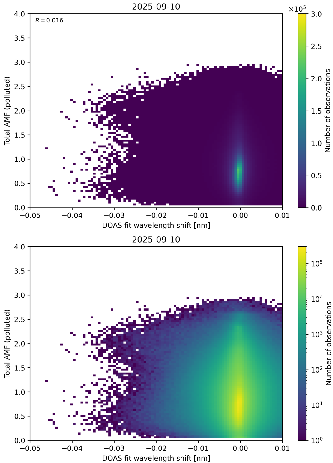
Figure 141: Scatter density plot of “DOAS fit wavelength shift” against “Total AMF (polluted)” for 2025-09-10 to 2025-09-11.
