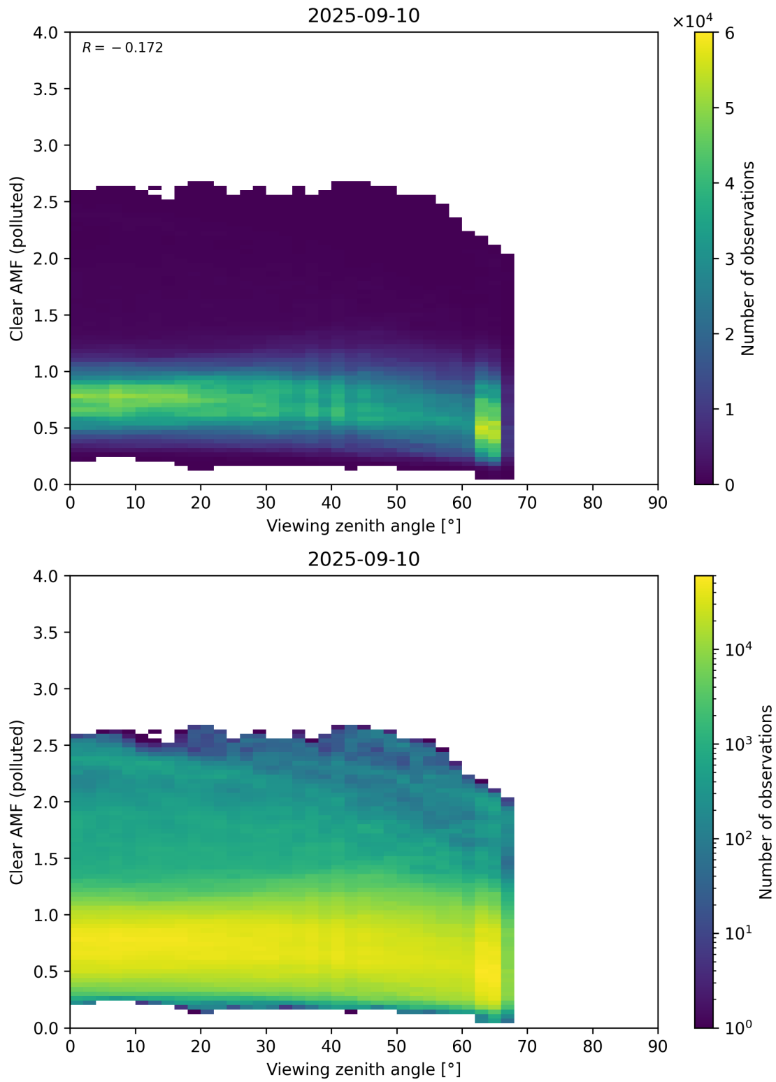
Figure 370: Scatter density plot of “Viewing zenith angle” against “Clear AMF (polluted)” for 2025-09-10 to 2025-09-11.
