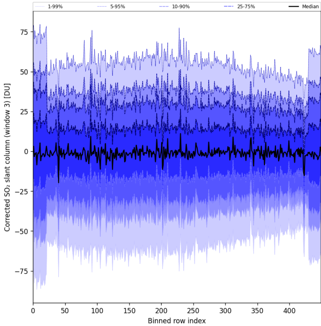
Figure 99: Along track statistics of “Corrected SO 2 slant column (window 3)” for 2025-09-10 to 2025-09-11
