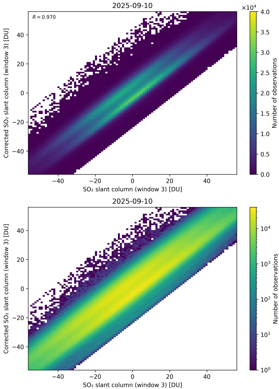
Figure 316: Scatter density plot of “SO 2 slant column (window 3)” against “Corrected SO 2 slant column (window 3)” for 2025-09-10 to 2025-09-11.
