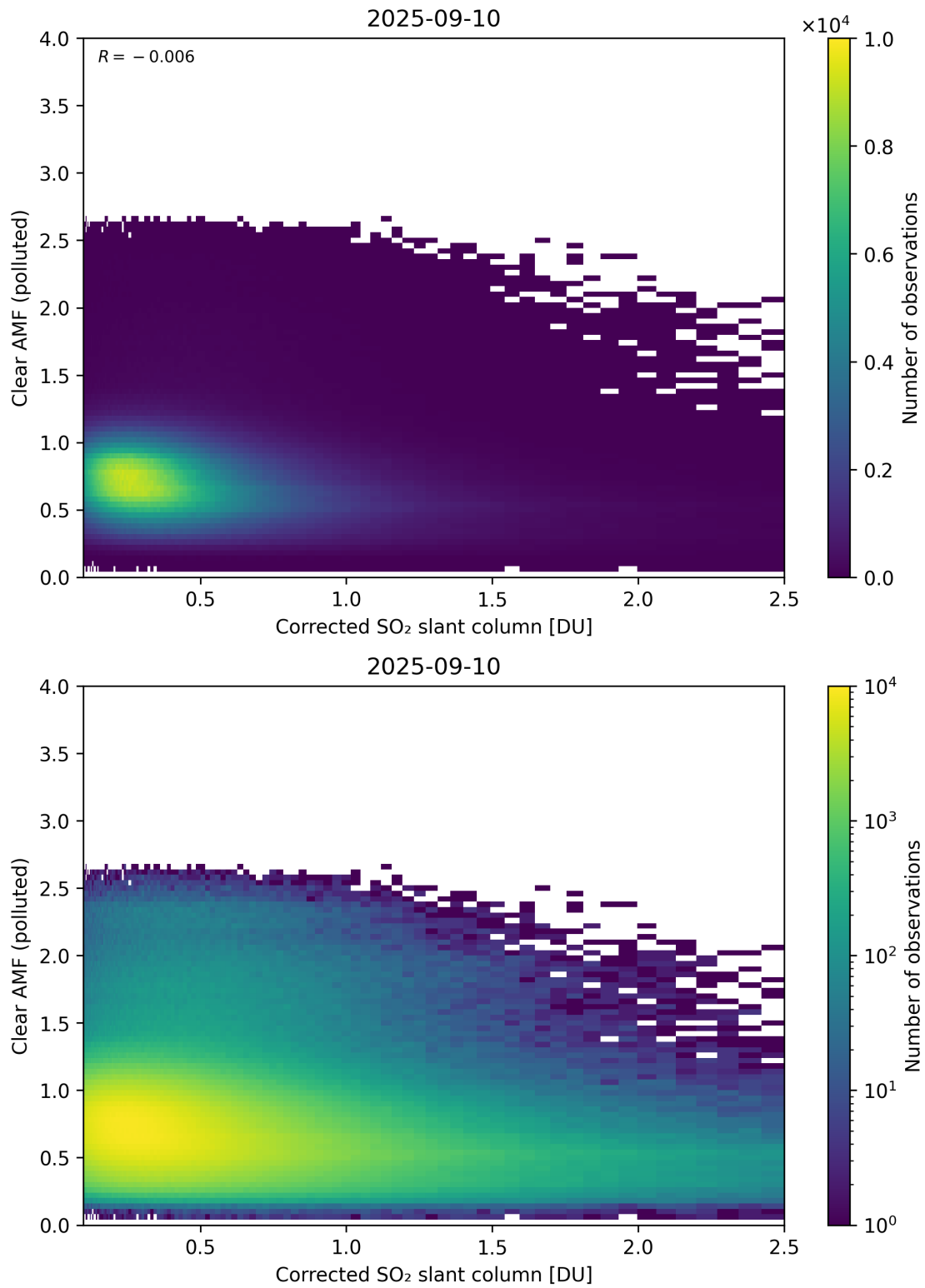
Figure 232: Scatter density plot of “Corrected SO 2 slant column” against “Clear AMF (polluted)” for 2025-09-10 to 2025-09-11.
