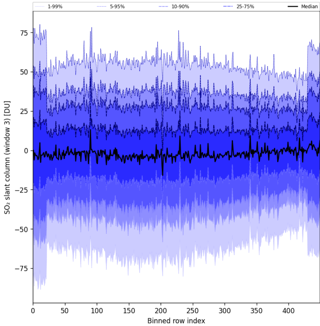
Figure 97: Along track statistics of “SO 2 slant column (window 3)” for 2025-09-10 to 2025-09-11
