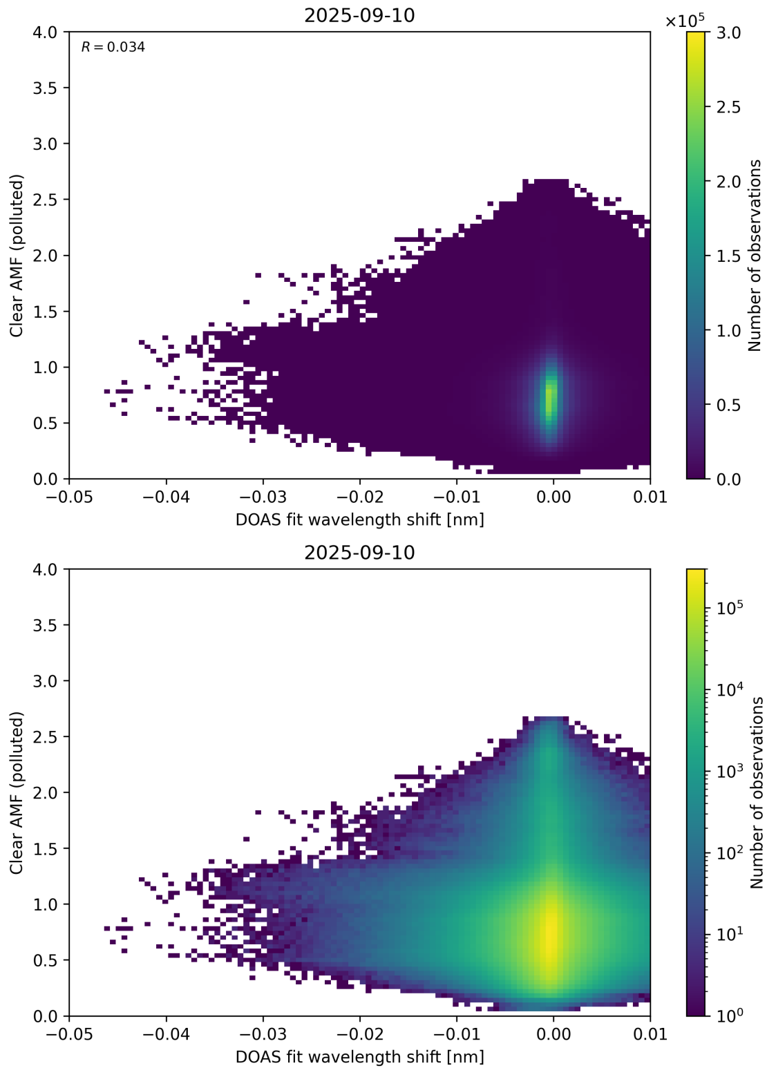
Figure 140: Scatter density plot of “DOAS fit wavelength shift” against “Clear AMF (polluted)” for 2025-09-10 to 2025-09-11.
