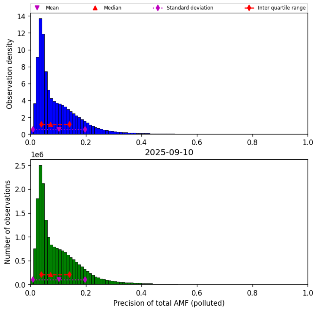
Figure 80: Histogram of “Precision of total AMF (polluted)” for 2025-09-10 to 2025-09-11
