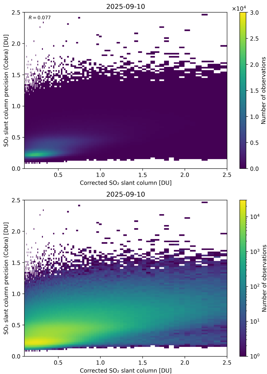
Figure 234: Scatter density plot of “Corrected SO 2 slant column” against “SO 2 slant column precision (Cobra)” for 2025-09-10 to 2025-09-11.
