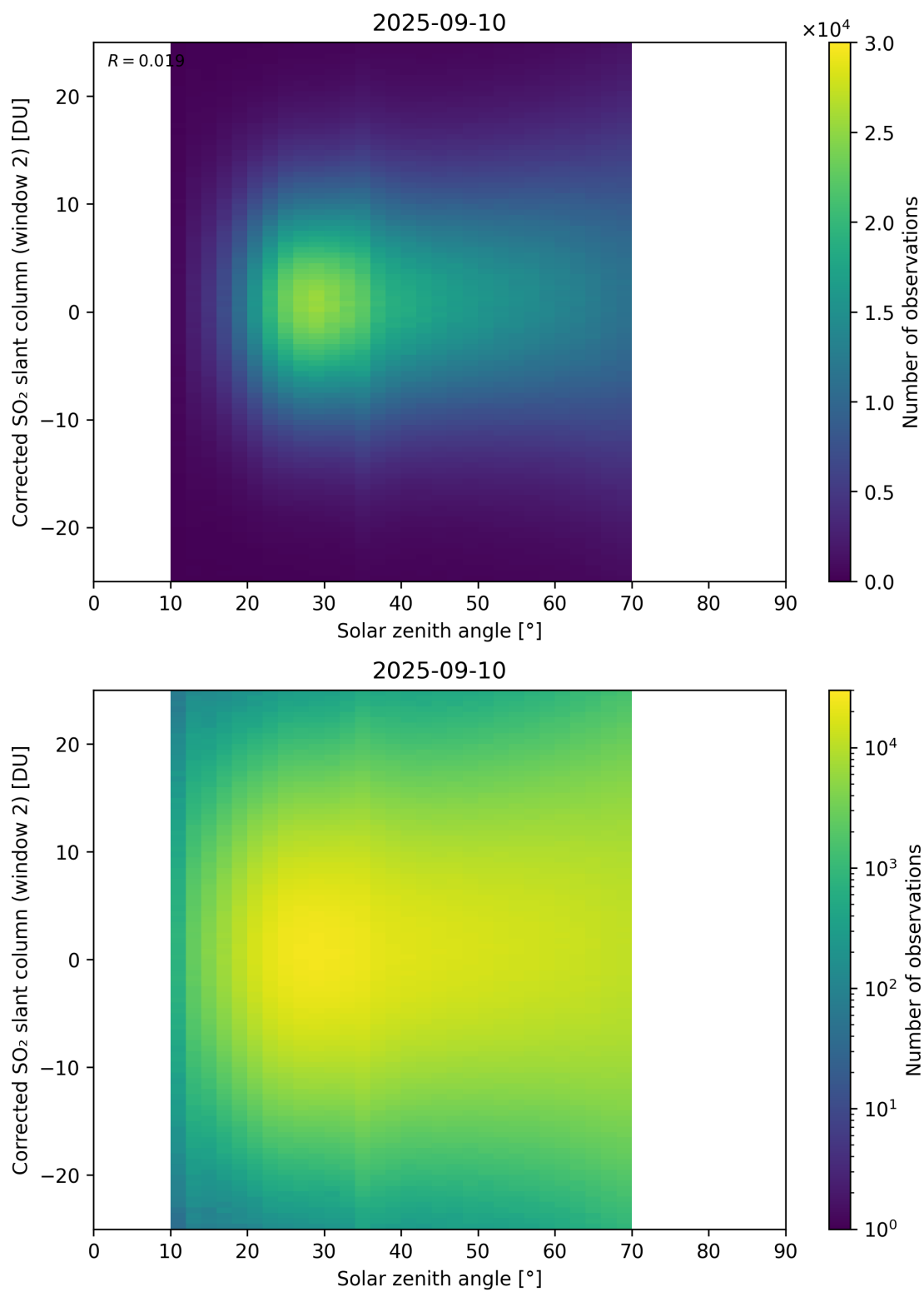
Figure 182: Scatter density plot of “Solar zenith angle” against “Corrected SO 2 slant column (window 2)” for 2025-09-10 to 2025-09-11.
