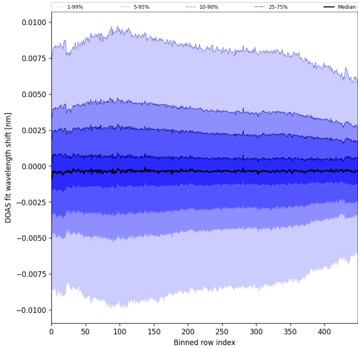
Figure 102: Along track statistics of “DOAS fit wavelength shift” for 2025-09-10 to 2025-09-11
