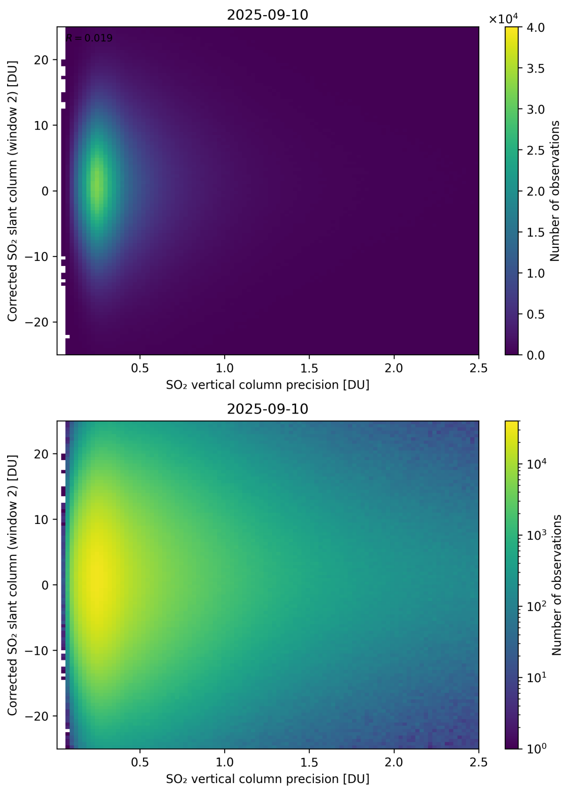
Figure 339: Scatter density plot of “SO 2 vertical column precision” against “Corrected SO 2 slant column (window 2)” for 2025-09-10 to 2025-09-11.
