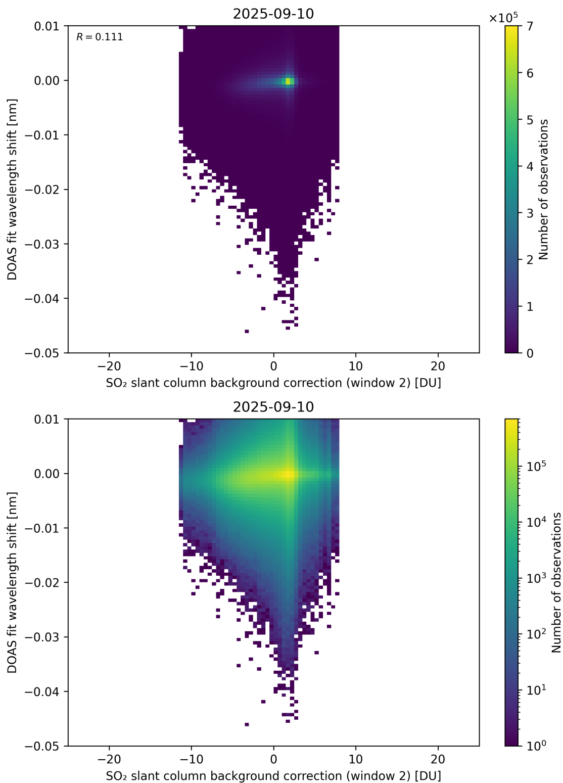
Figure 123: Scatter density plot of “SO 2 slant column background correction (window 2)” against “DOAS fit wavelength shift” for 2025-09-10 to 2025-09-11.
