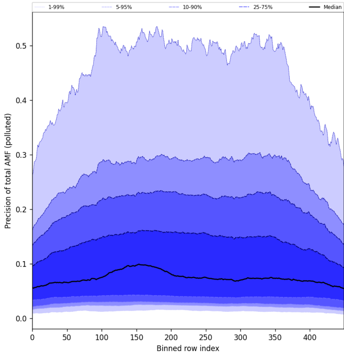
Figure 106: Along track statistics of “Precision of total AMF (polluted)” for 2025-09-10 to 2025-09-11
