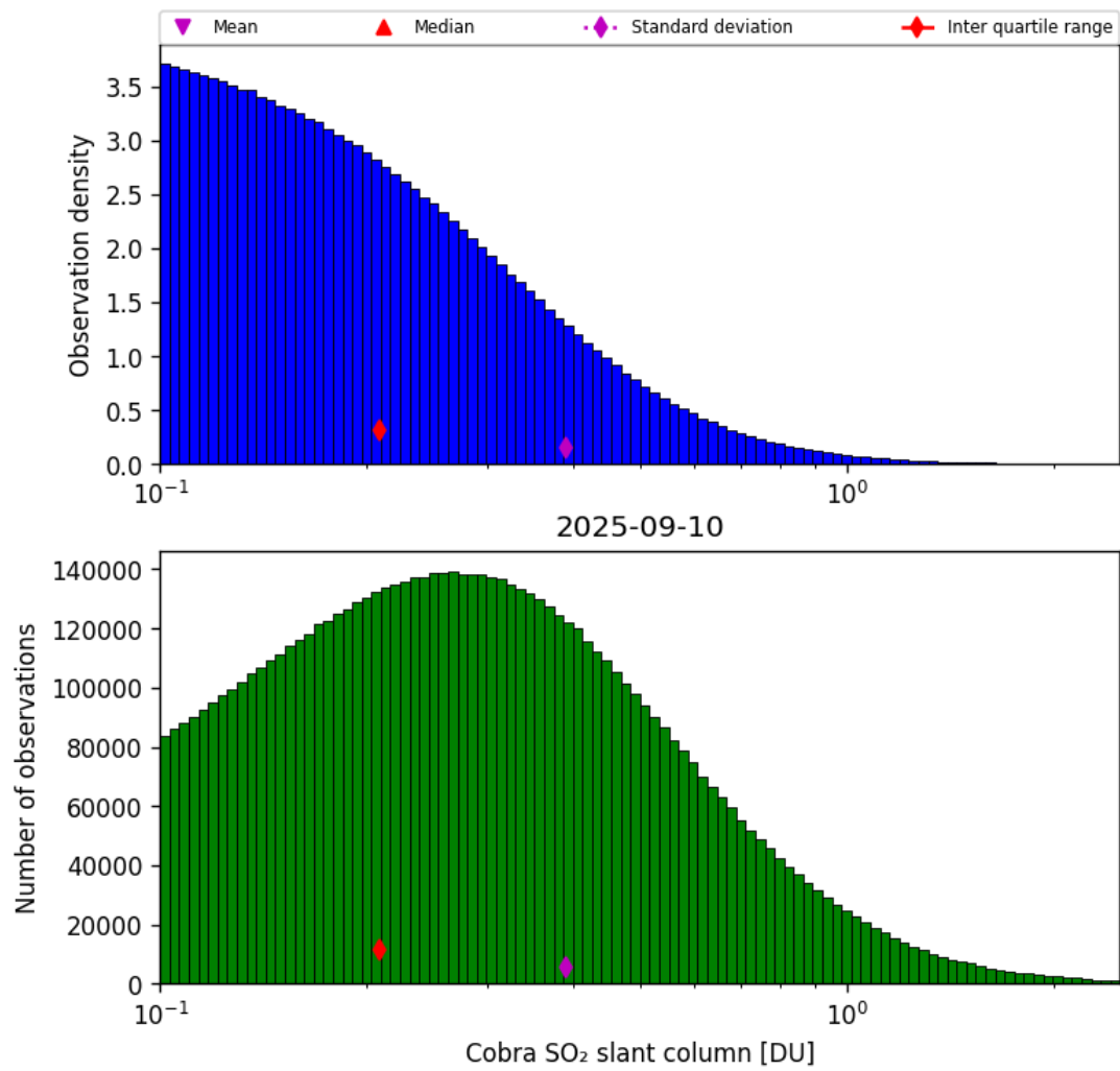
Figure 61: Histogram of “Cobra SO 2 slant column” for 2025-09-10 to 2025-09-11
