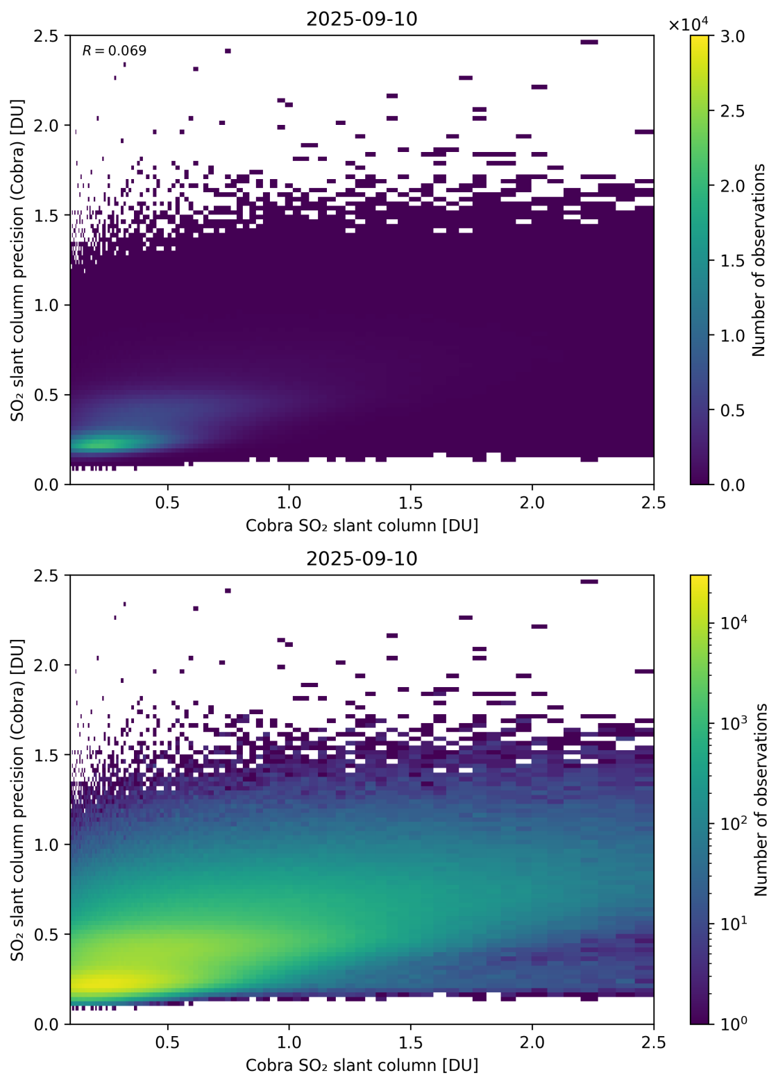
Figure 216: Scatter density plot of “Cobra SO 2 slant column” against “SO 2 slant column precision (Cobra)” for 2025-09-10 to 2025-09-11.
