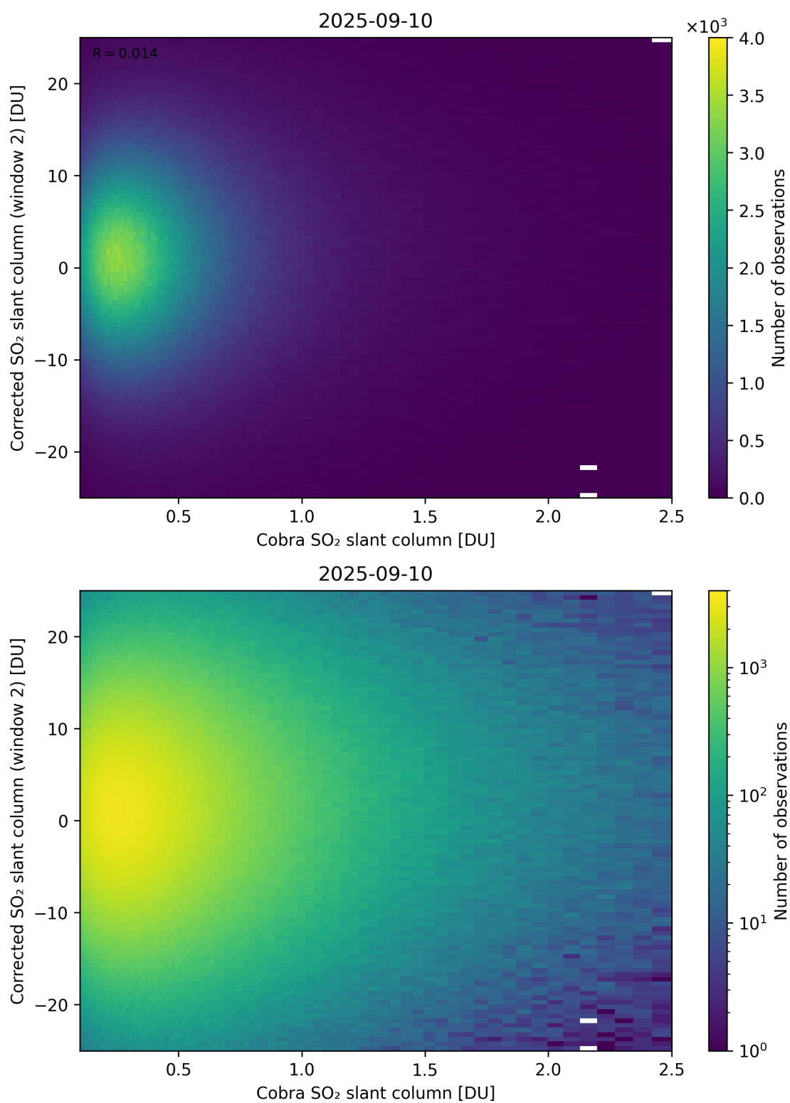
Figure 217: Scatter density plot of “Cobra SO 2 slant column” against “Corrected SO 2 slant column (window 2)” for 2025-09-10 to 2025-09-11.
