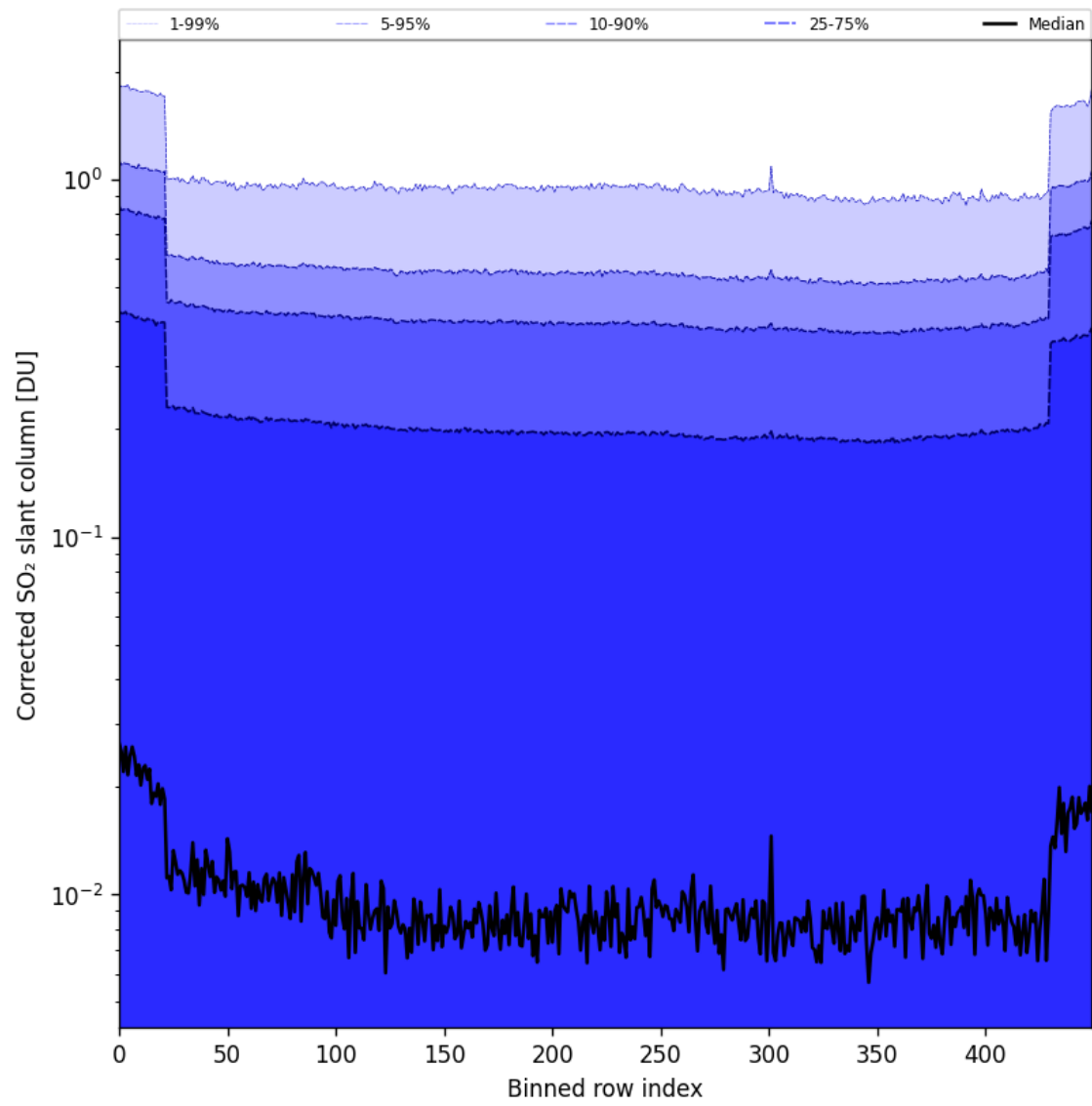
Figure 86: Along track statistics of “Corrected SO 2 slant column” for 2025-09-10 to 2025-09-11
