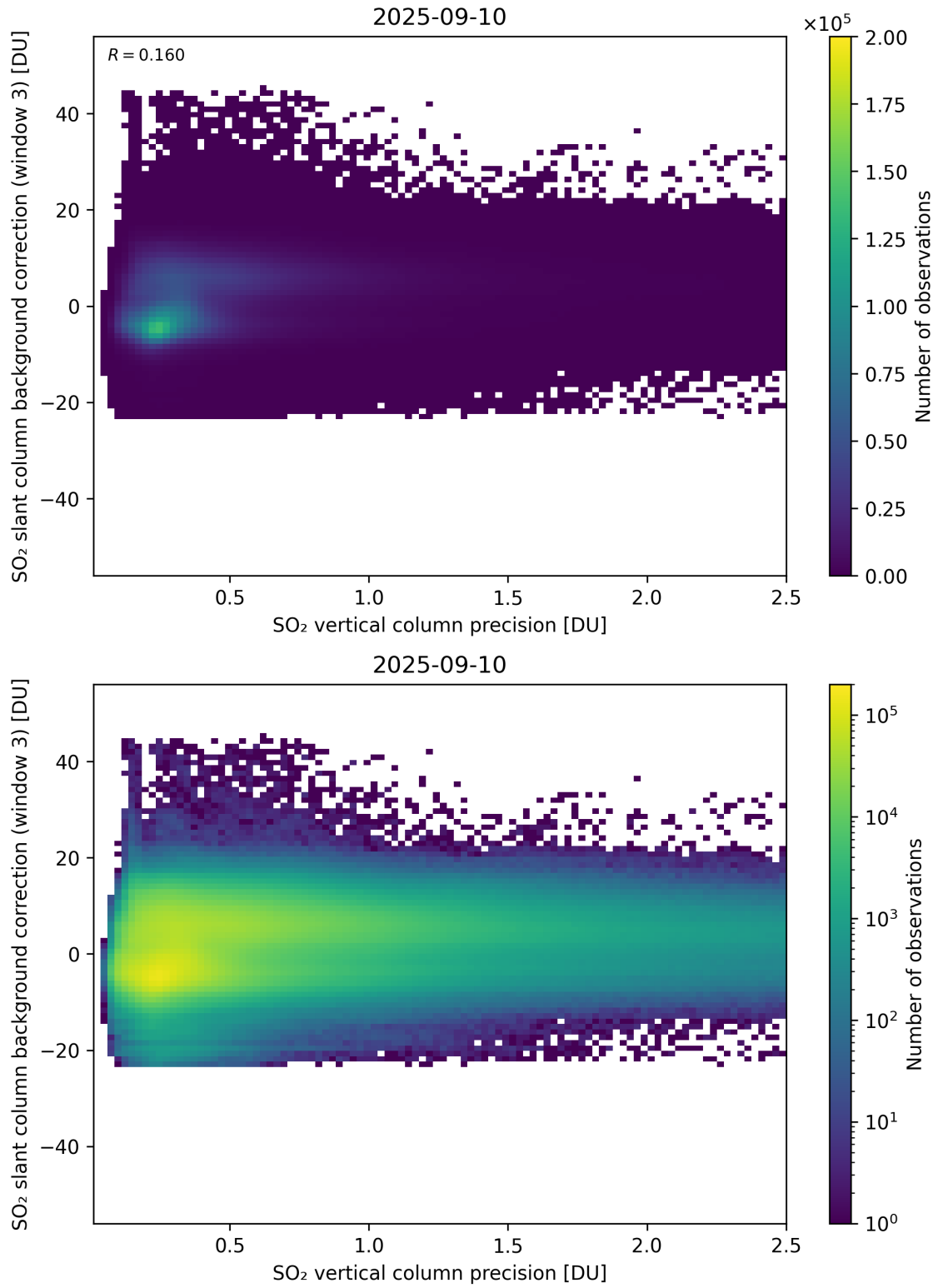
Figure 331: Scatter density plot of “SO 2 vertical column precision” against “SO 2 slant column background correction (window 3)” for 2025-09-10 to 2025-09-11.
