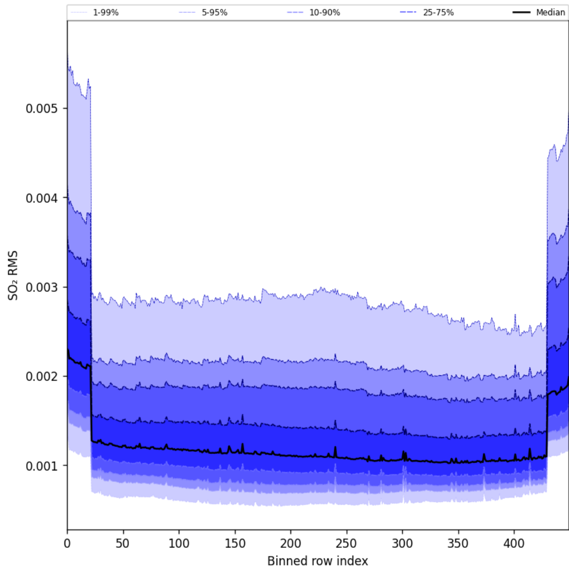
Figure 104: Along track statistics of “SO 2 RMS” for 2025-09-10 to 2025-09-11
