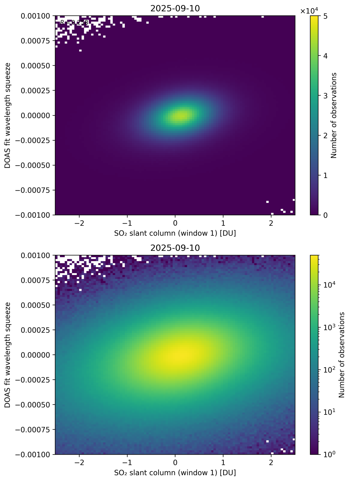
Figure 266: Scatter density plot of “SO 2 slant column (window 1)” against “DOAS fit wavelength squeeze” for 2025-09-10 to 2025-09-11.
