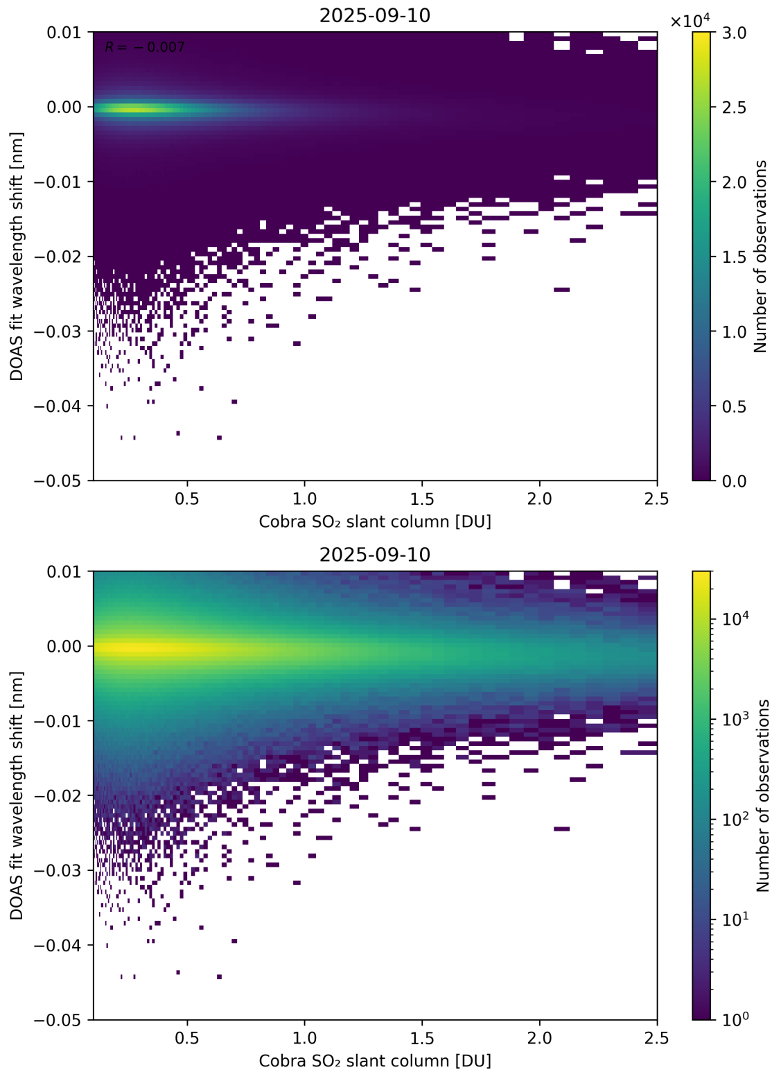
Figure 196: Scatter density plot of “Cobra SO 2 slant column” against “DOAS fit wavelength shift” for 2025-09-10 to 2025-09-11.
