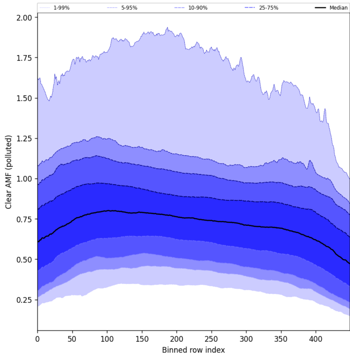
Figure 107: Along track statistics of “Clear AMF (polluted)” for 2025-09-10 to 2025-09-11
