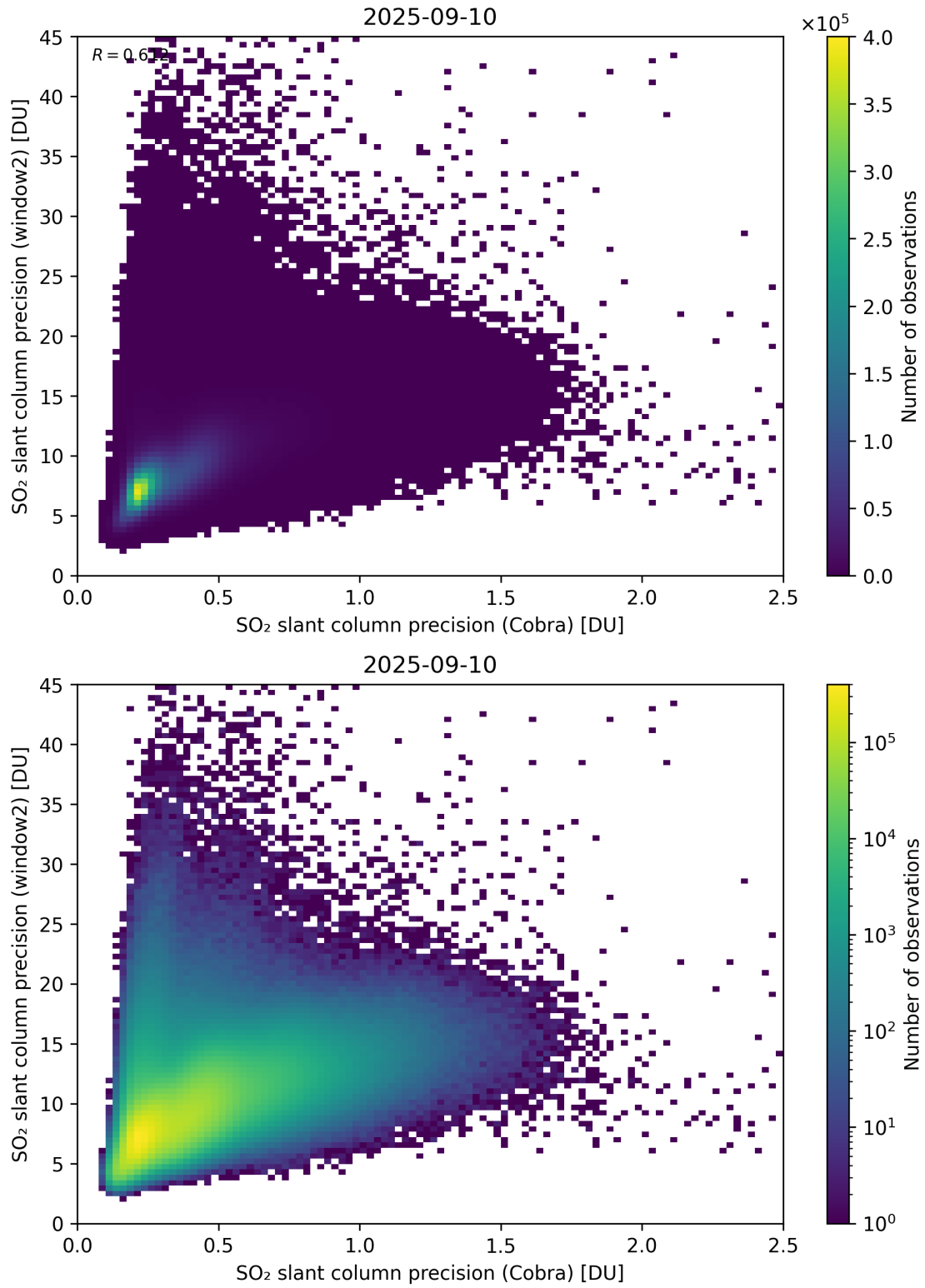
Figure 210: Scatter density plot of “SO 2 slant column precision (Cobra)” against “SO 2 slant column precision (window2)” for 2025-09-10 to 2025-09-11.
