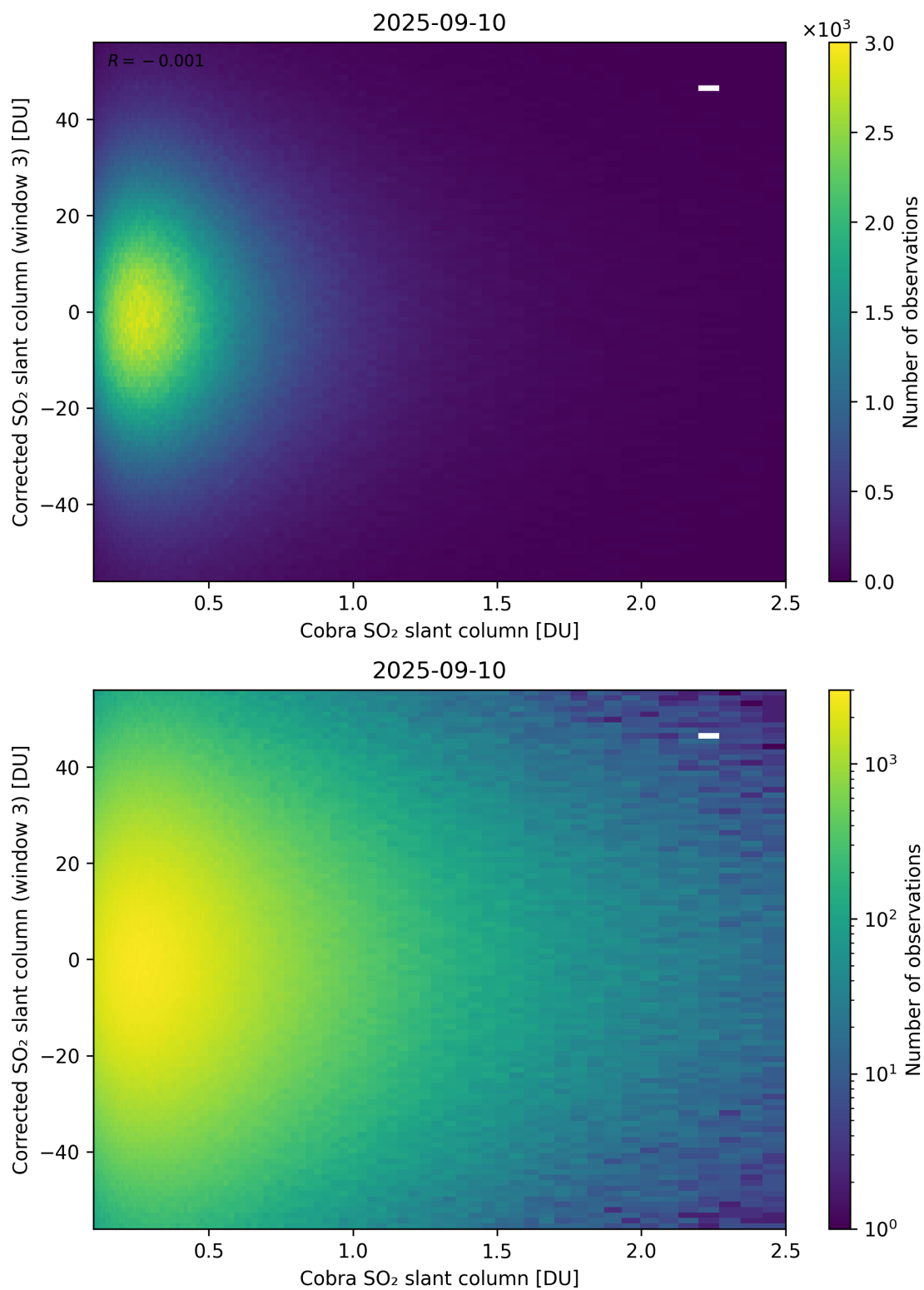
Figure 218: Scatter density plot of “Cobra SO 2 slant column” against “Corrected SO 2 slant column (window 3)” for 2025-09-10 to 2025-09-11.
