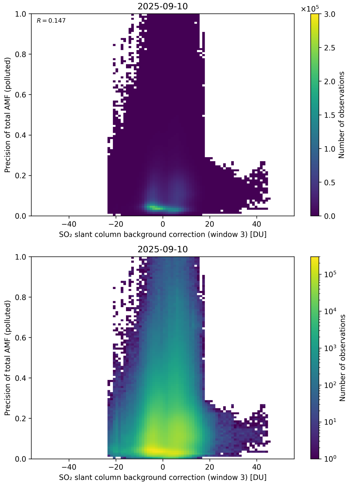
Figure 137: Scatter density plot of “SO 2 slant column background correction (window 3)” against “Precision of total AMF (polluted)” for 2025-09-10 to 2025-09-11.
