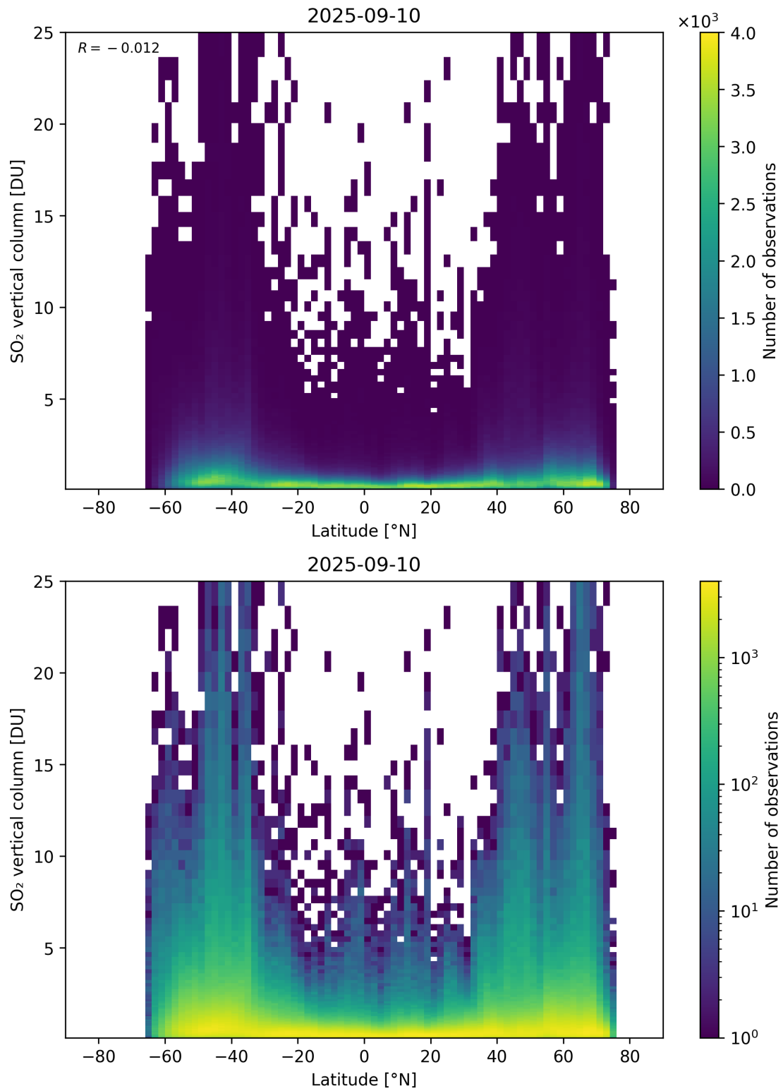
Figure 169: Scatter density plot of “Latitude” against “SO 2 vertical column” for 2025-09-10 to 2025-09-11.
