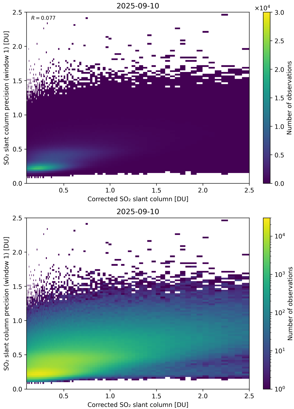
Figure 238: Scatter density plot of “Corrected SO 2 slant column” against “SO 2 slant column precision (window 1)” for 2025-09-10 to 2025-09-11.
