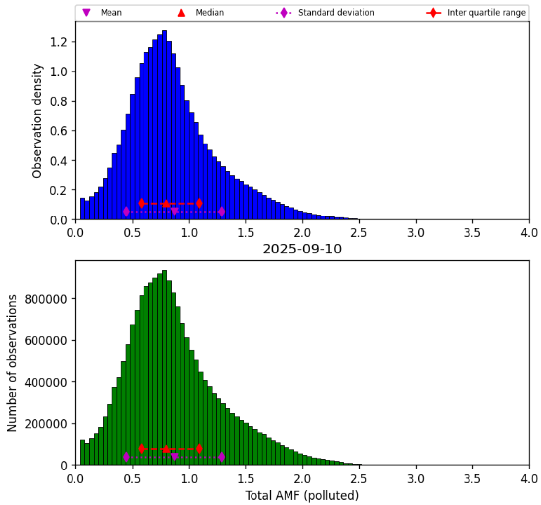
Figure 79: Histogram of “Total AMF (polluted)” for 2025-09-10 to 2025-09-11
