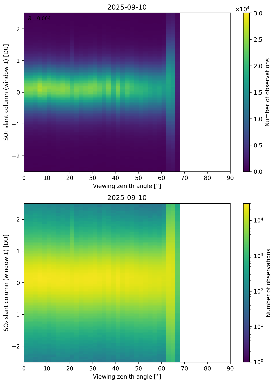
Figure 376: Scatter density plot of “Viewing zenith angle” against “SO 2 slant column (window 1)” for 2025-09-10 to 2025-09-11.
