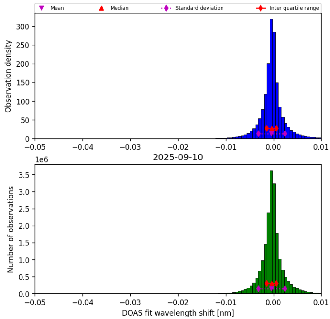
Figure 76: Histogram of “DOAS fit wavelength shift” for 2025-09-10 to 2025-09-11
