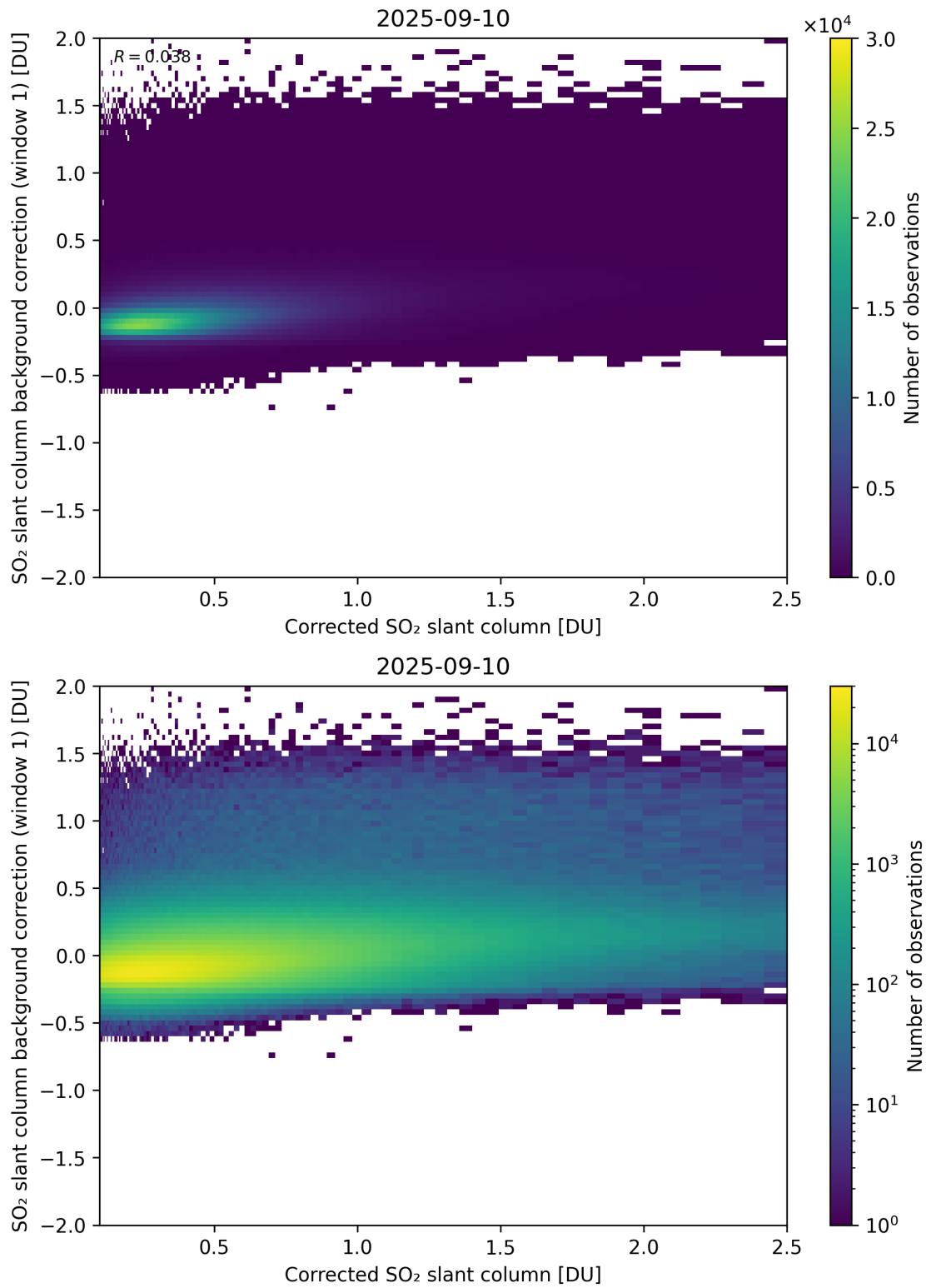
Figure 226: Scatter density plot of “Corrected SO 2 slant column” against “SO 2 slant column background correction (window 1)” for 2025-09-10 to 2025-09-11.
