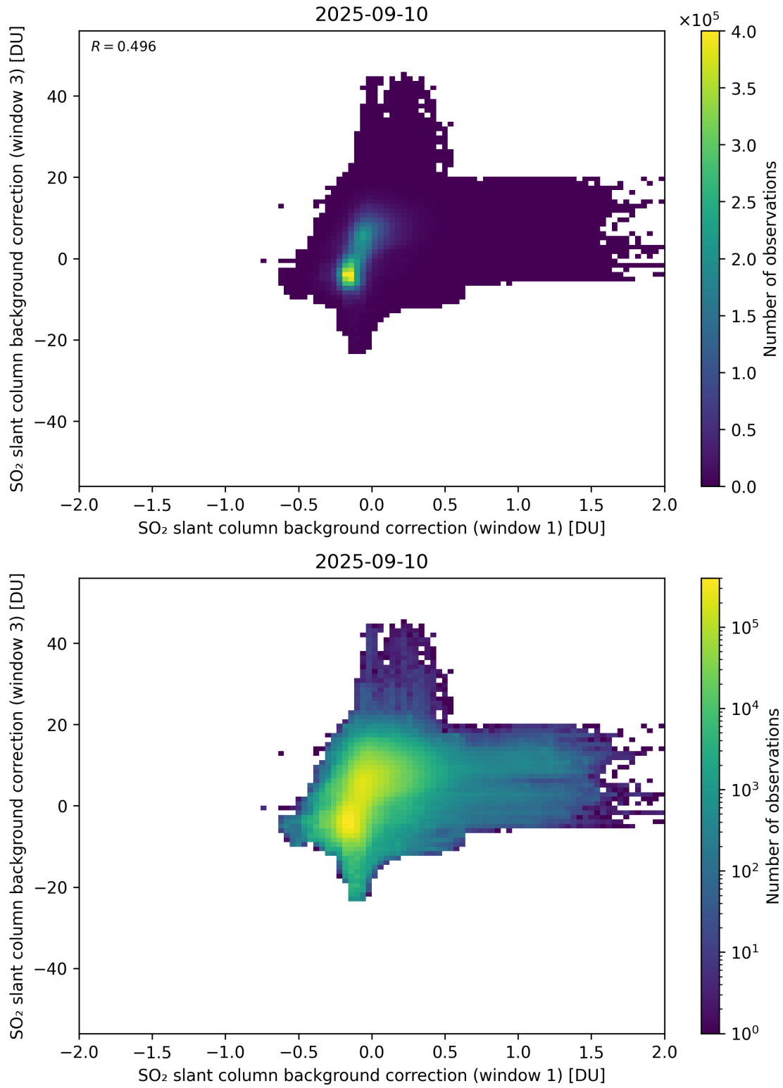
Figure 110: Scatter density plot of “SO 2 slant column background correction (window 1)” against “SO 2 slant column background correction (window 3)” for 2025-09-10 to 2025-09-11.
