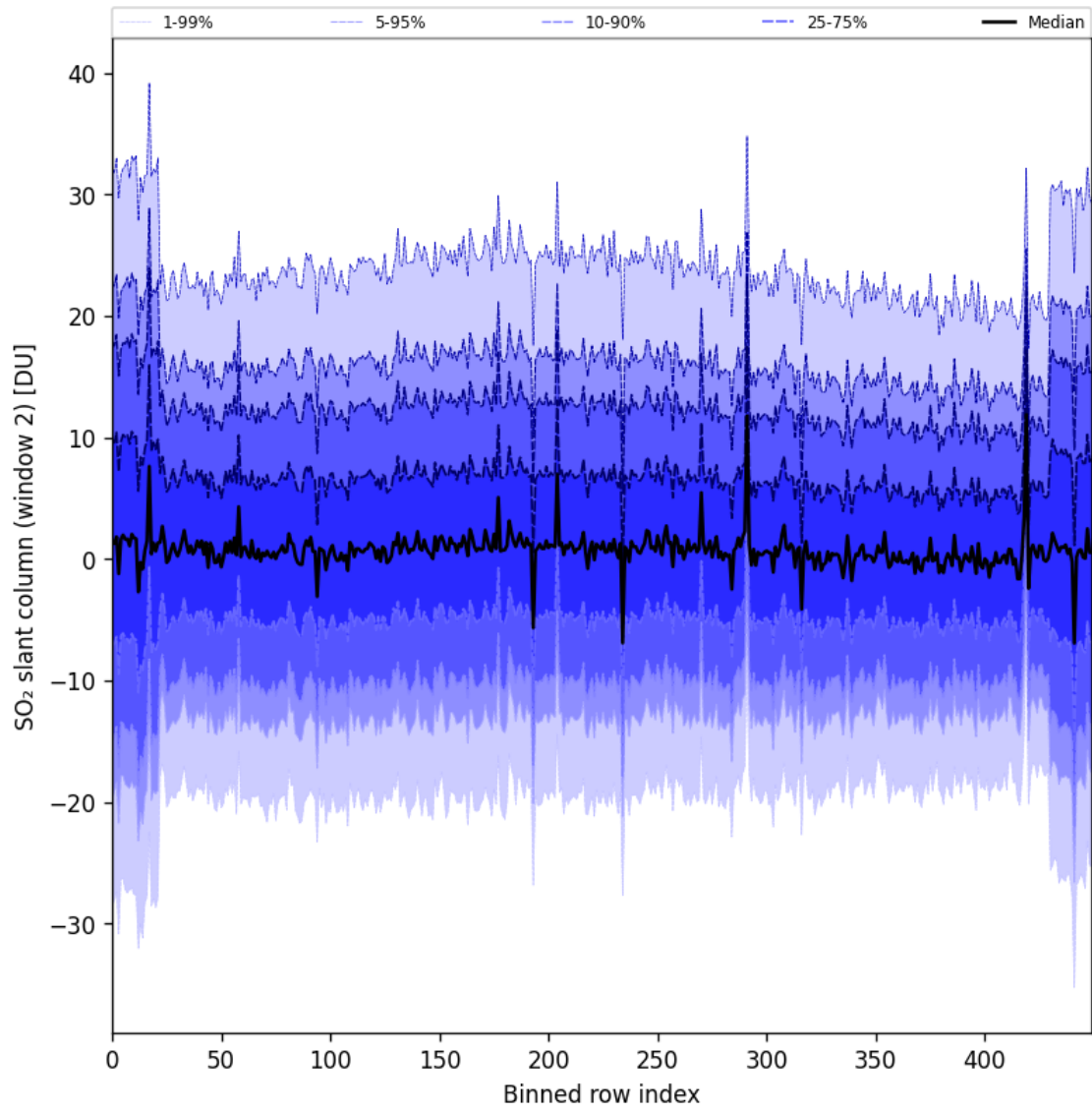
Figure 93: Along track statistics of “SO 2 slant column (window 2)” for 2025-09-10 to 2025-09-11
