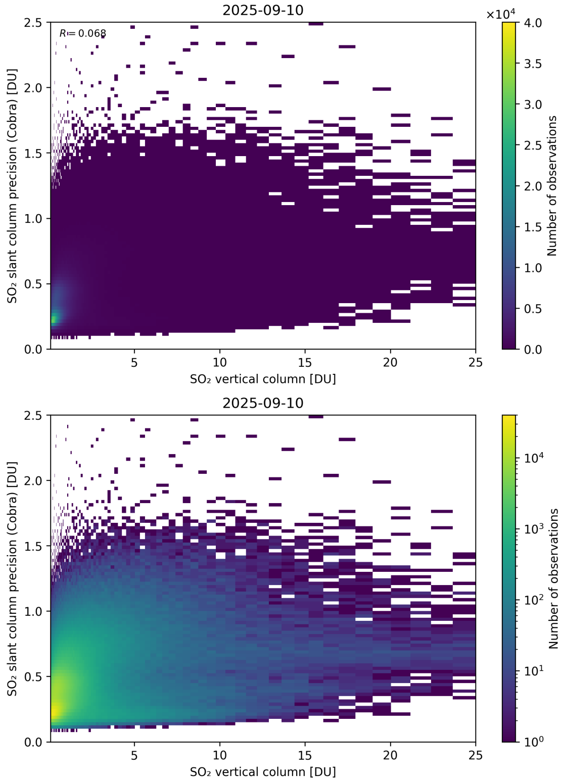
Figure 350: Scatter density plot of “SO 2 vertical column” against “SO 2 slant column precision (Cobra)” for 2025-09-10 to 2025-09-11.
