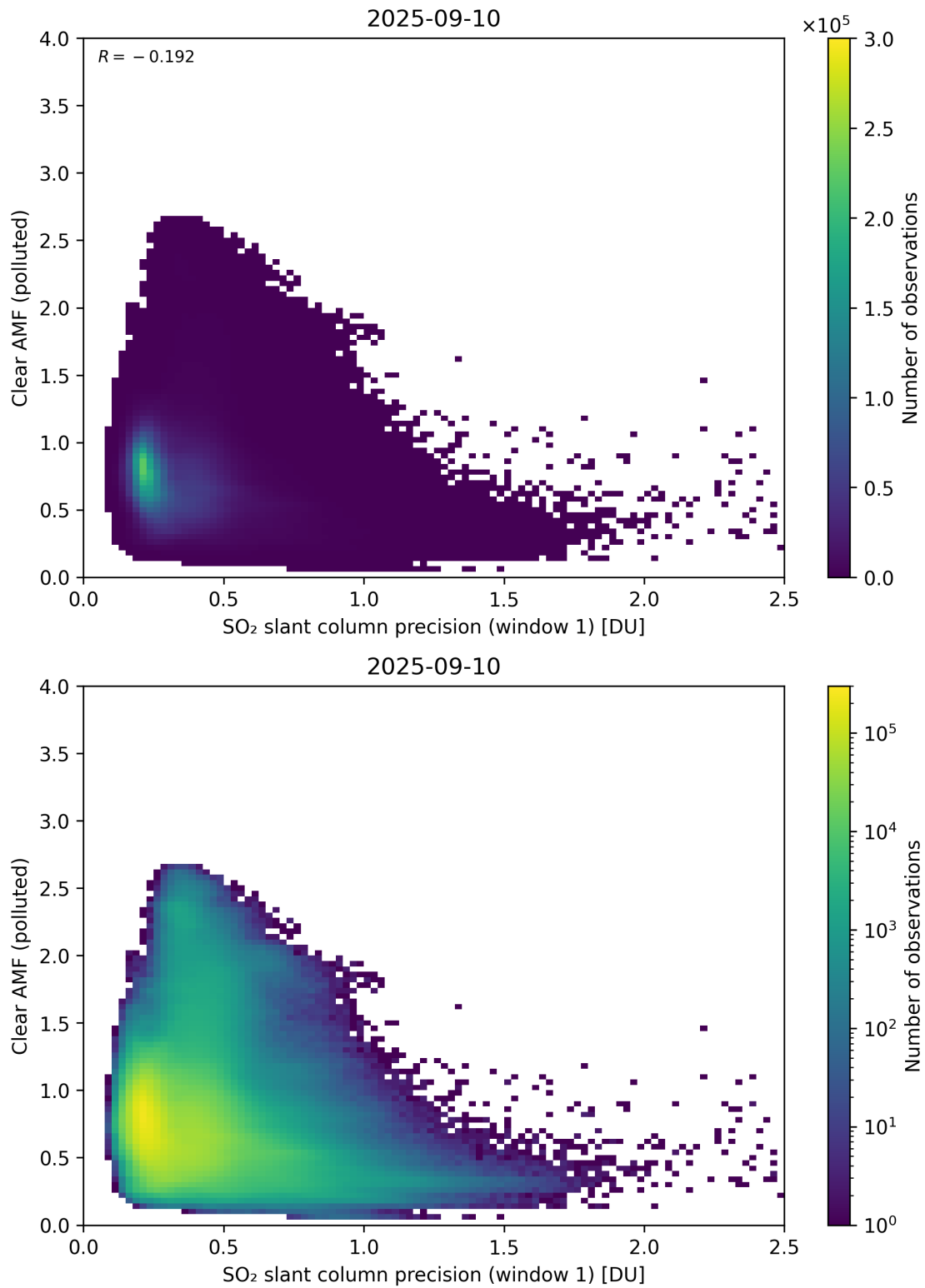
Figure 274: Scatter density plot of “SO 2 slant column precision (window 1)” against “Clear AMF (polluted)” for 2025-09-10 to 2025-09-11.
