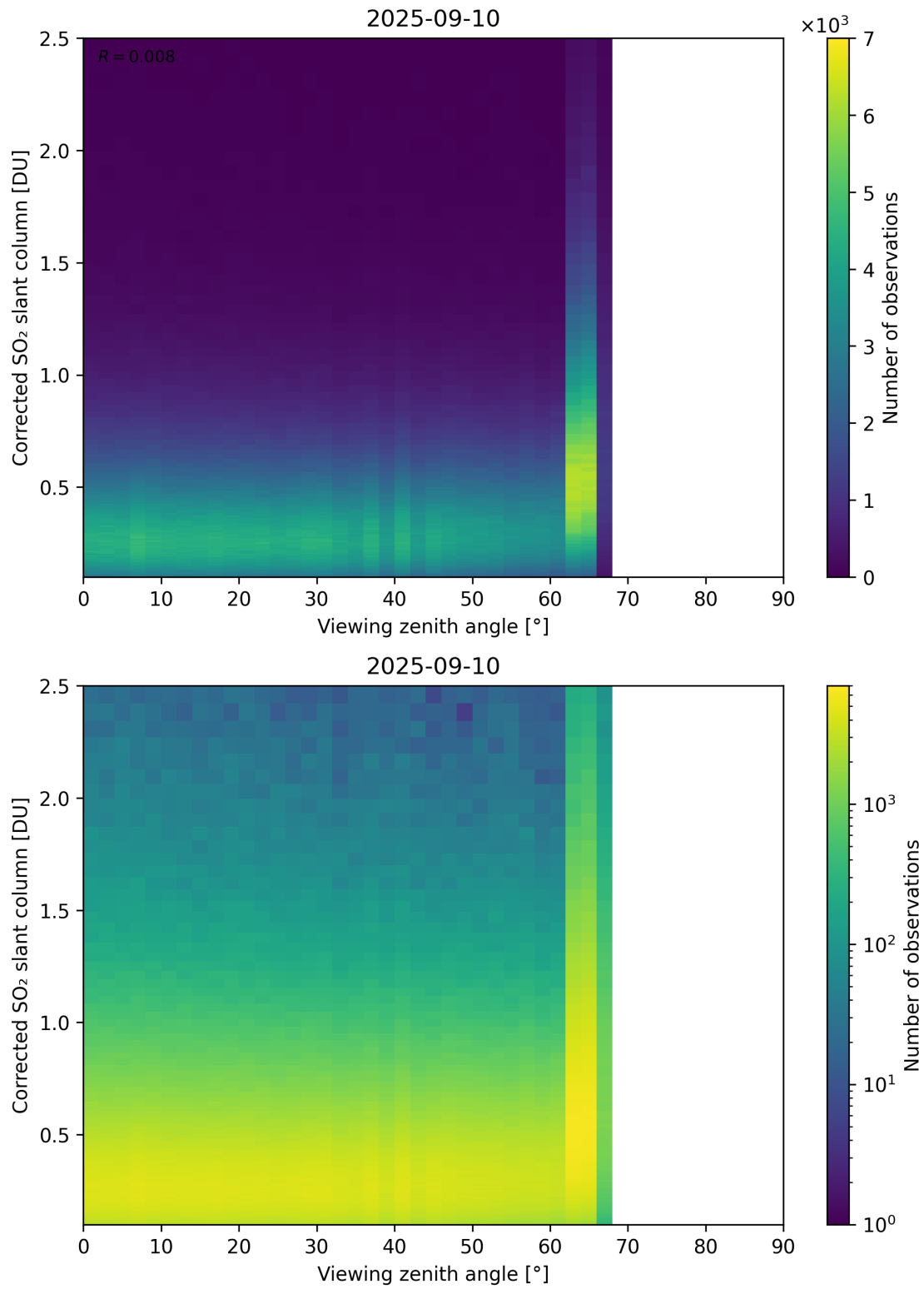
Figure 373: Scatter density plot of “Viewing zenith angle” against “Corrected SO 2 slant column” for 2025-09-10 to 2025-09-11.
