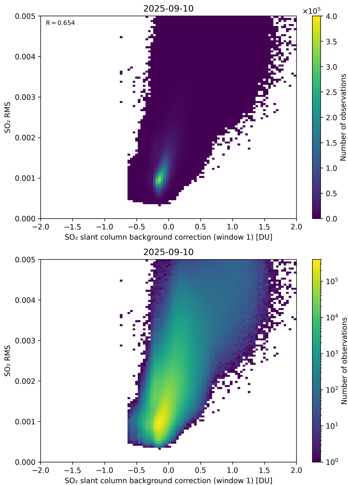
Figure 113: Scatter density plot of “SO 2 slant column background correction (window 1)” against “SO 2 RMS” for 2025-09-10 to 2025-09-11.
