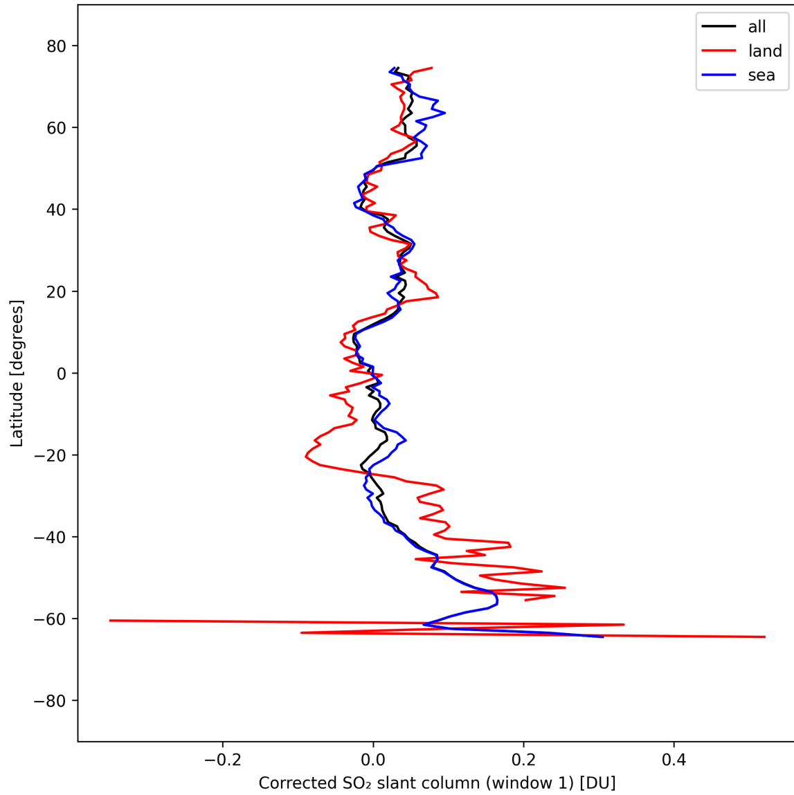
Figure 39: Zonal average of “Corrected SO 2 slant column (window 1)” for 2025-09-10 to 2025-09-11.
