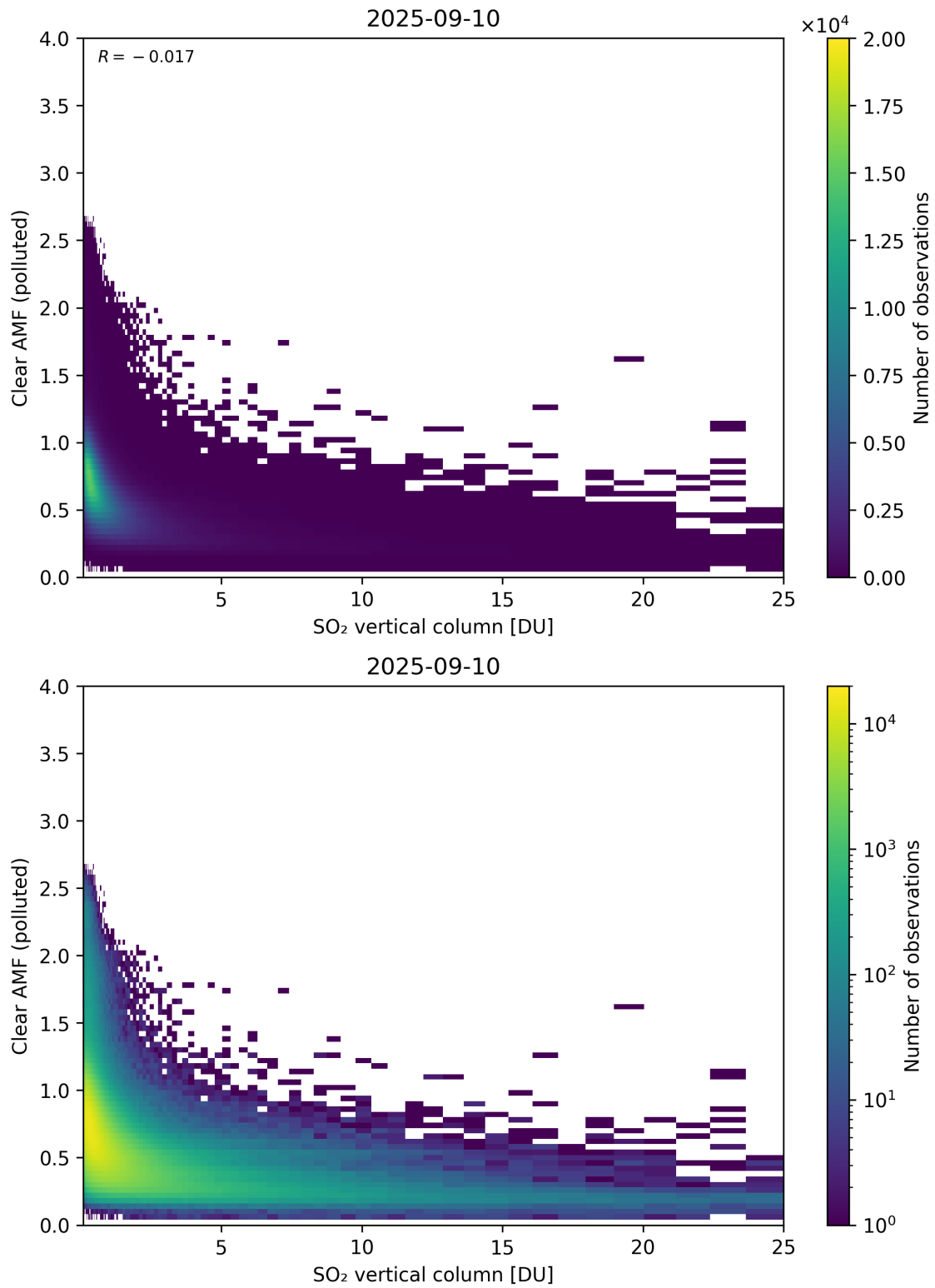
Figure 348: Scatter density plot of “SO 2 vertical column” against “Clear AMF (polluted)” for 2025-09-10 to 2025-09-11.
