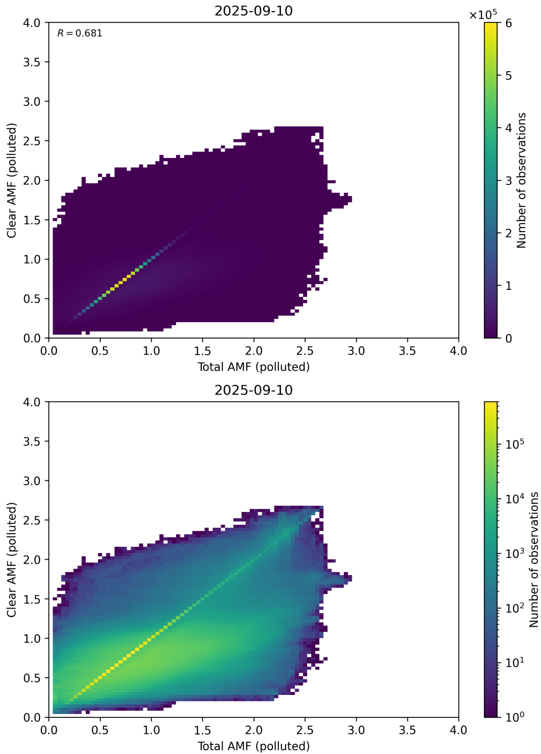
Figure 321: Scatter density plot of “Total AMF (polluted)” against “Clear AMF (polluted)” for 2025-09-10 to 2025-09-11.
