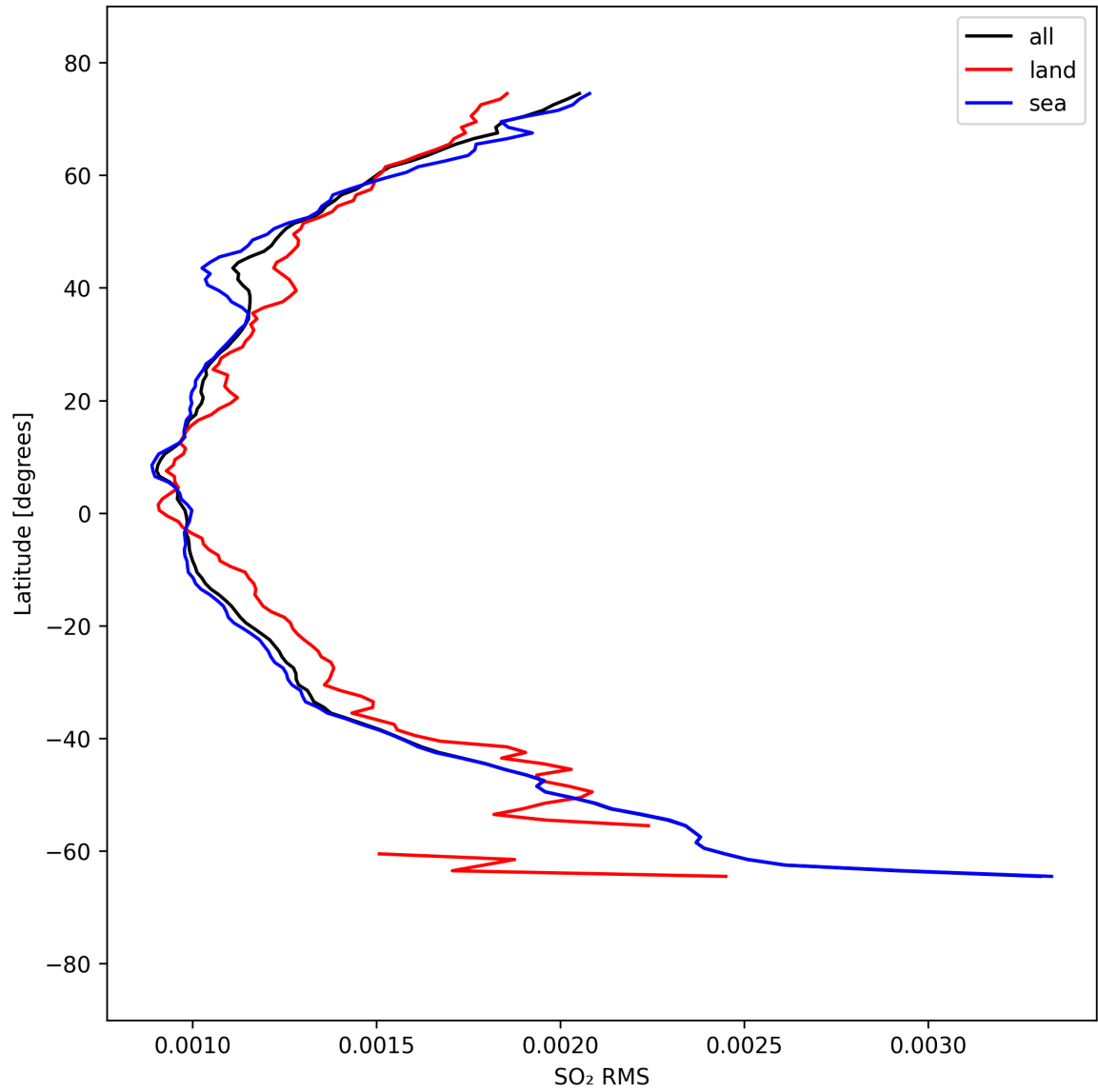
Figure 52: Zonal average of “SO 2 RMS” for 2025-09-10 to 2025-09-11.
