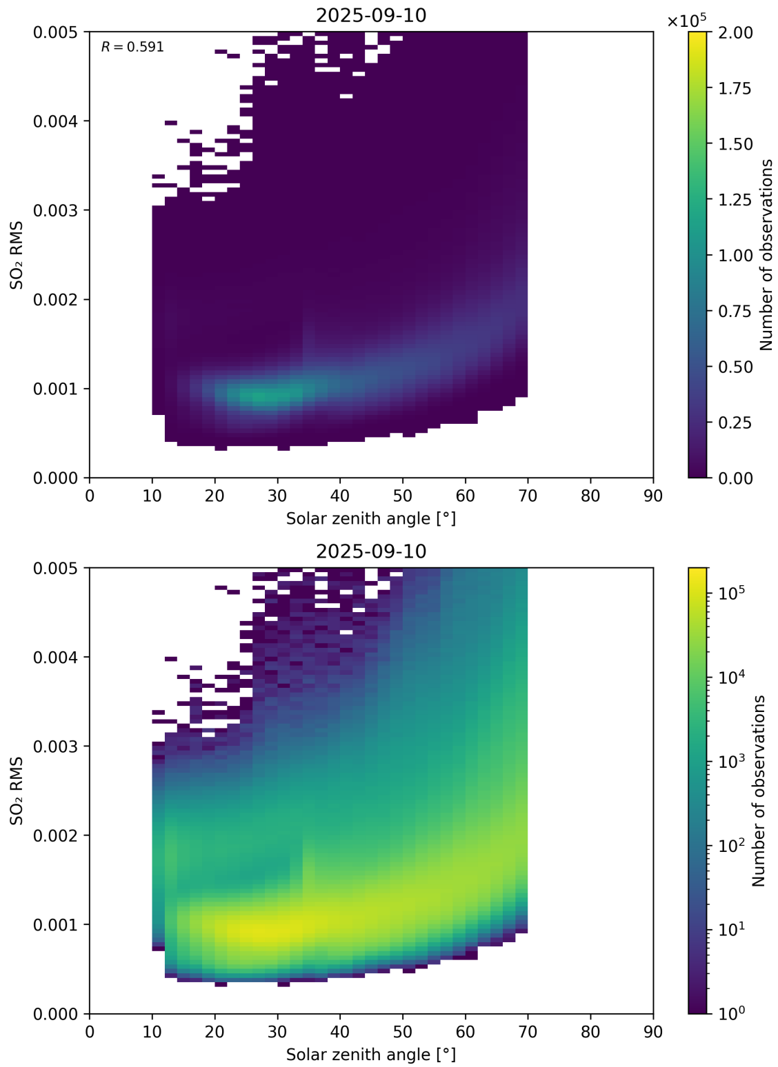
Figure 176: Scatter density plot of “Solar zenith angle” against “SO 2 RMS” for 2025-09-10 to 2025-09-11.
