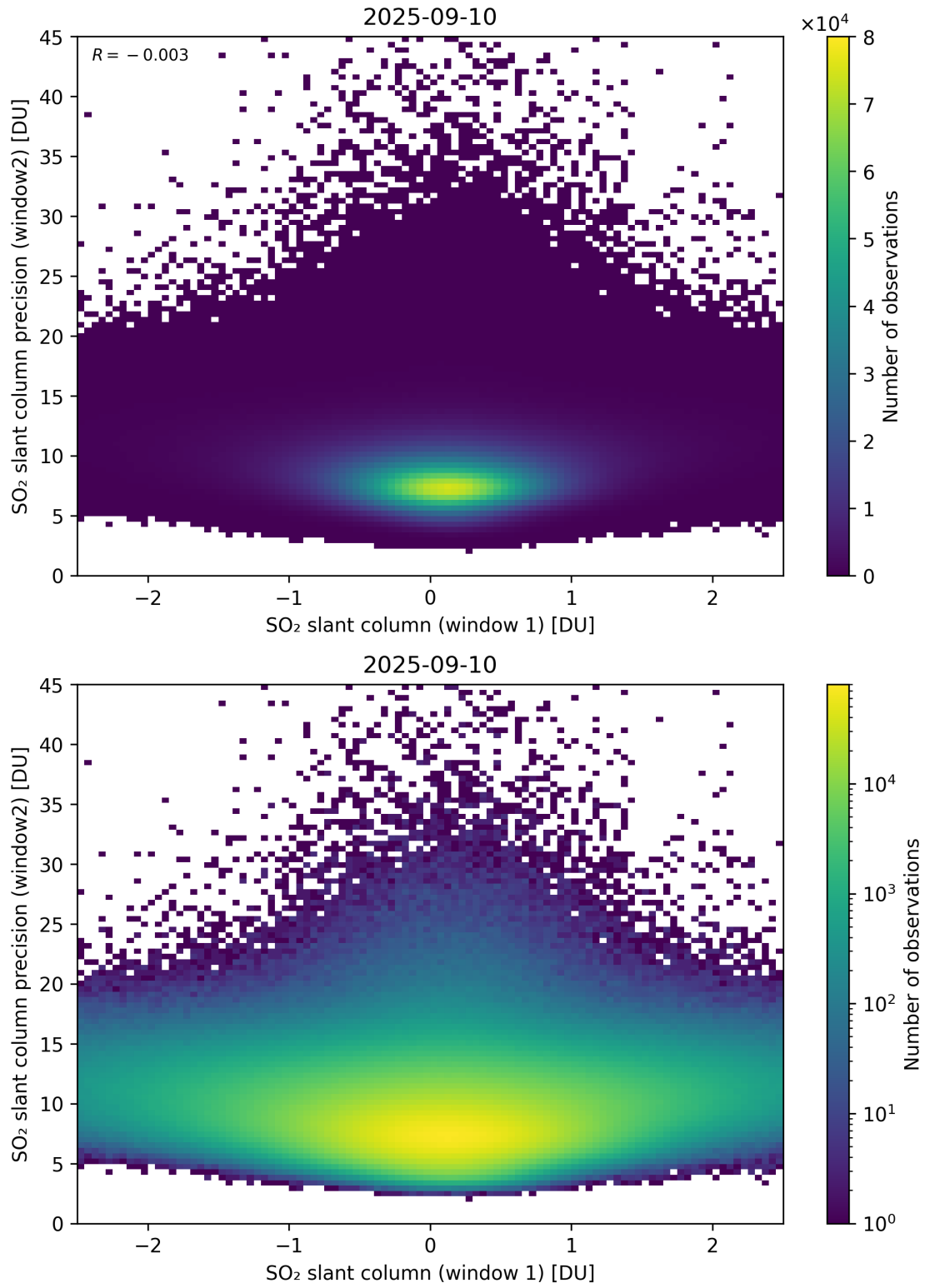
Figure 286: Scatter density plot of “SO 2 slant column (window 1)” against “SO 2 slant column precision (window2)” for 2025-09-10 to 2025-09-11.
