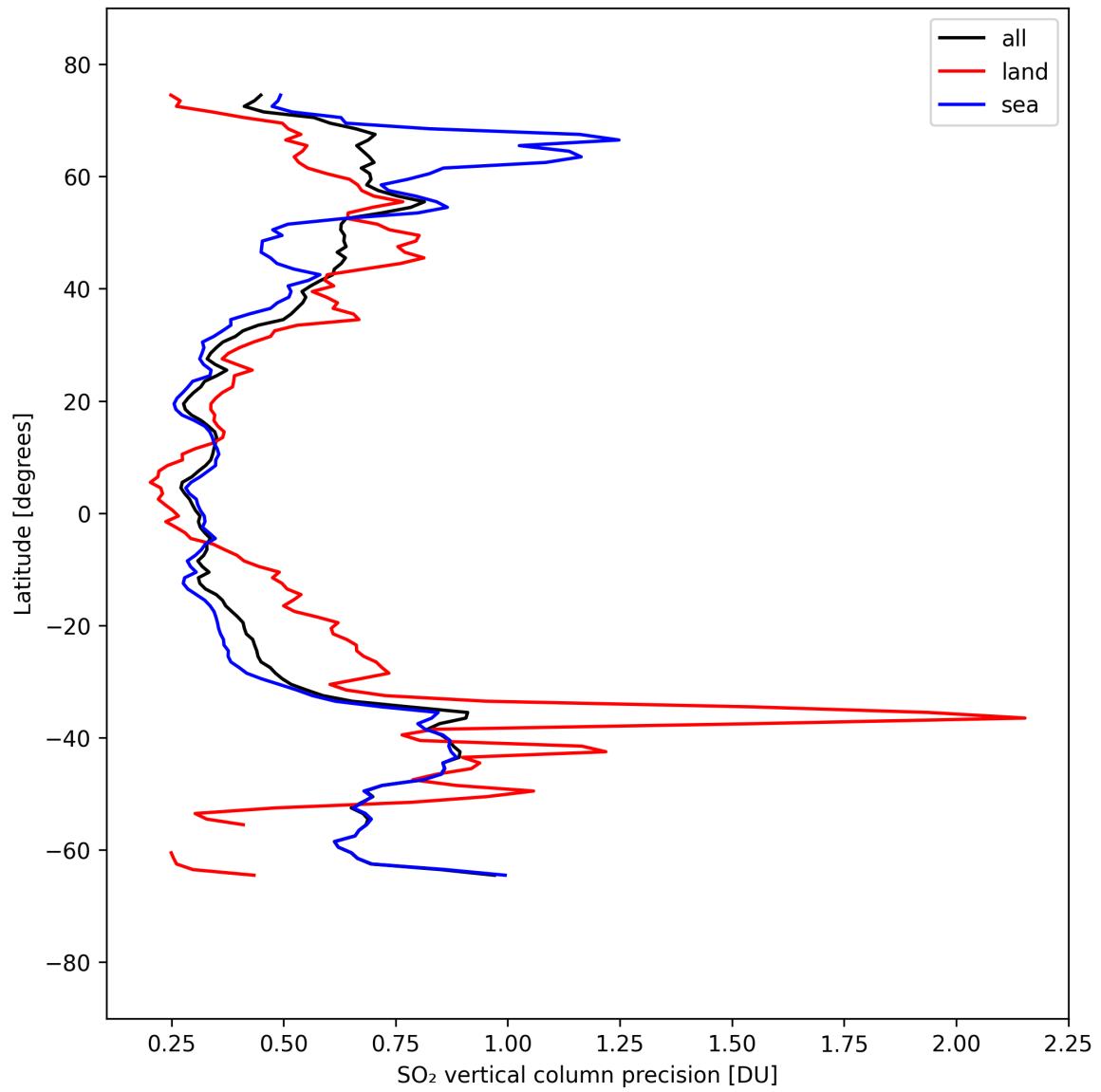
Figure 33: Zonal average of “SO 2 vertical column precision” for 2025-09-10 to 2025-09-11.
