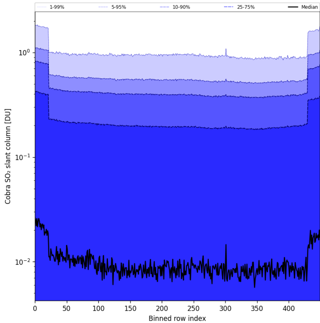
Figure 87: Along track statistics of "Cobra SO 2 slant column" for 2025-09-10 to 2025-09-11
