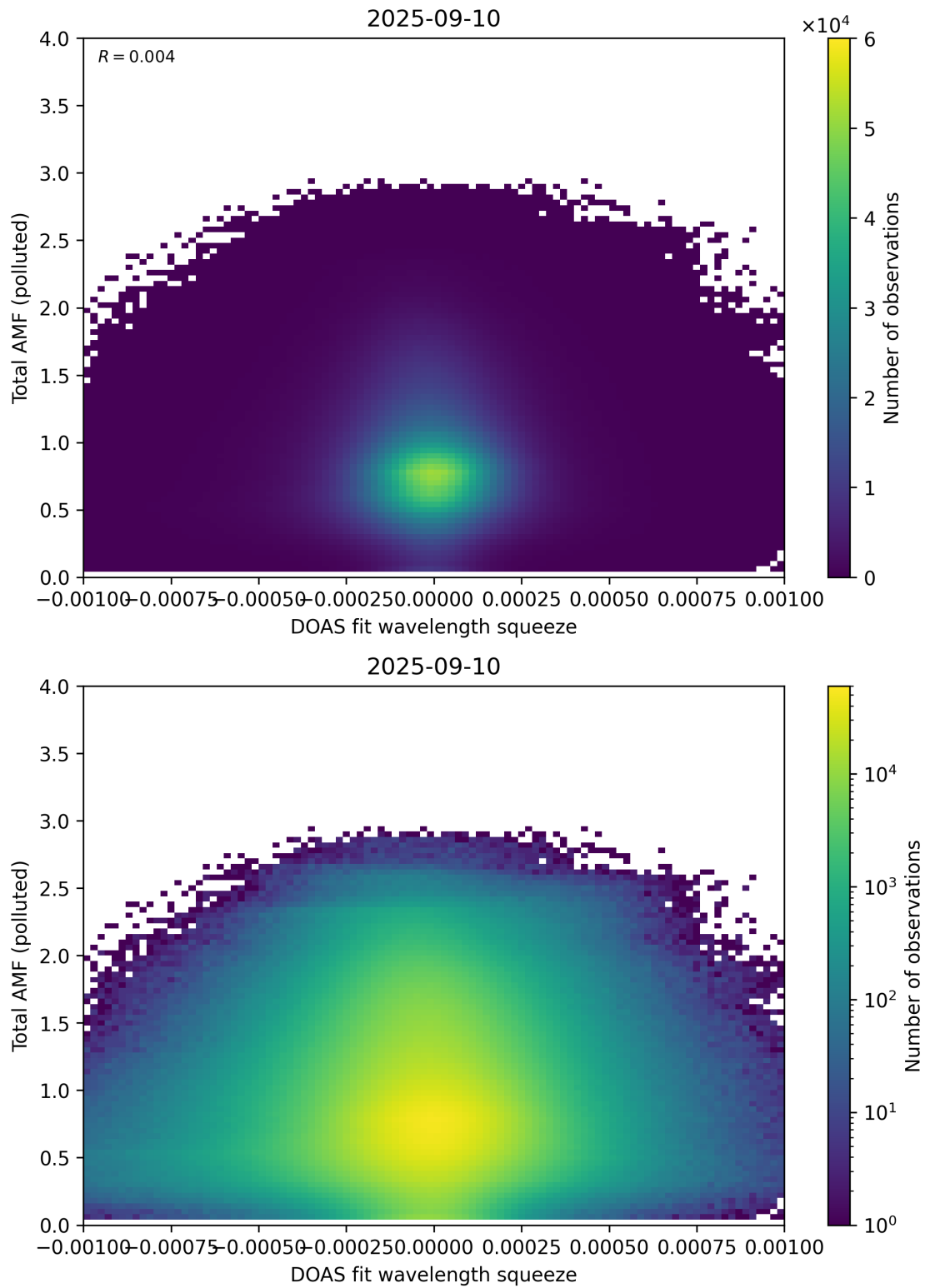
Figure 145: Scatter density plot of “DOAS fit wavelength squeeze” against “Total AMF (polluted)” for 2025-09-10 to 2025-09-11.
