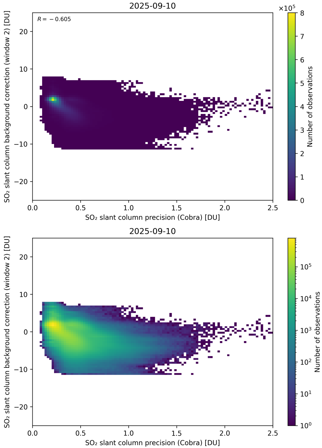
Figure 200: Scatter density plot of “SO 2 slant column precision (Cobra)” against “SO 2 slant column background correction (window 2)” for 2025-09-10 to 2025-09-11.
