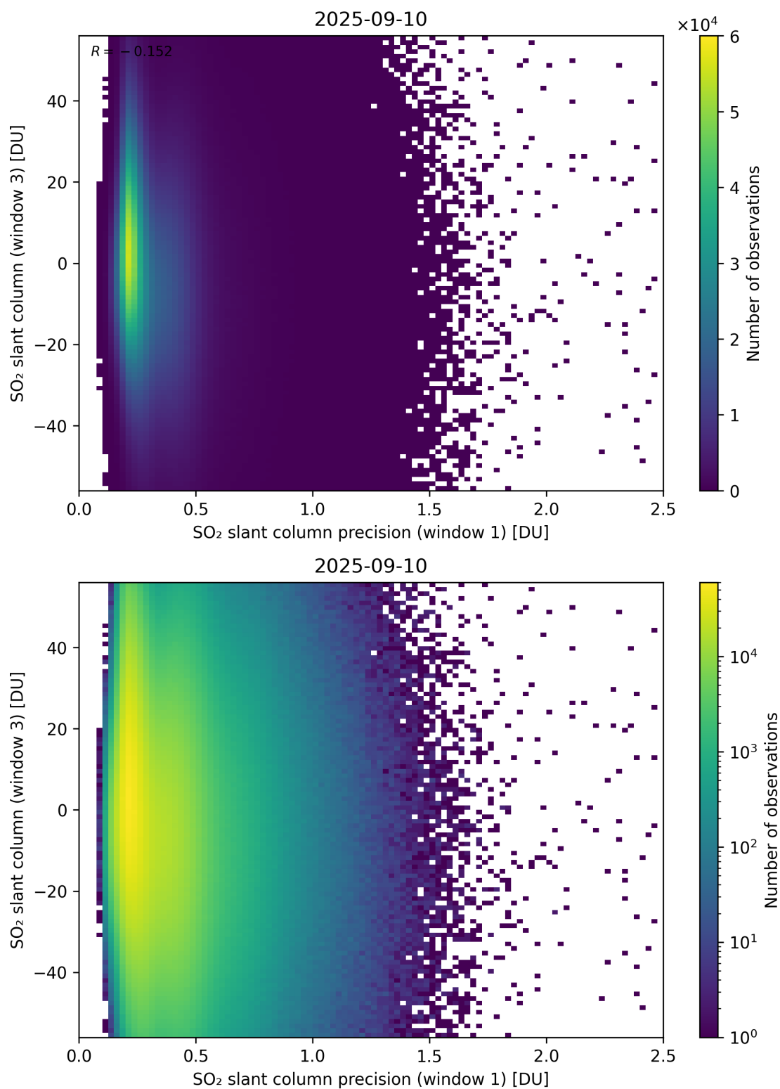
Figure 278: Scatter density plot of “SO 2 slant column precision (window 1)” against “SO 2 slant column (window 3)” for 2025-09-10 to 2025-09-11.
