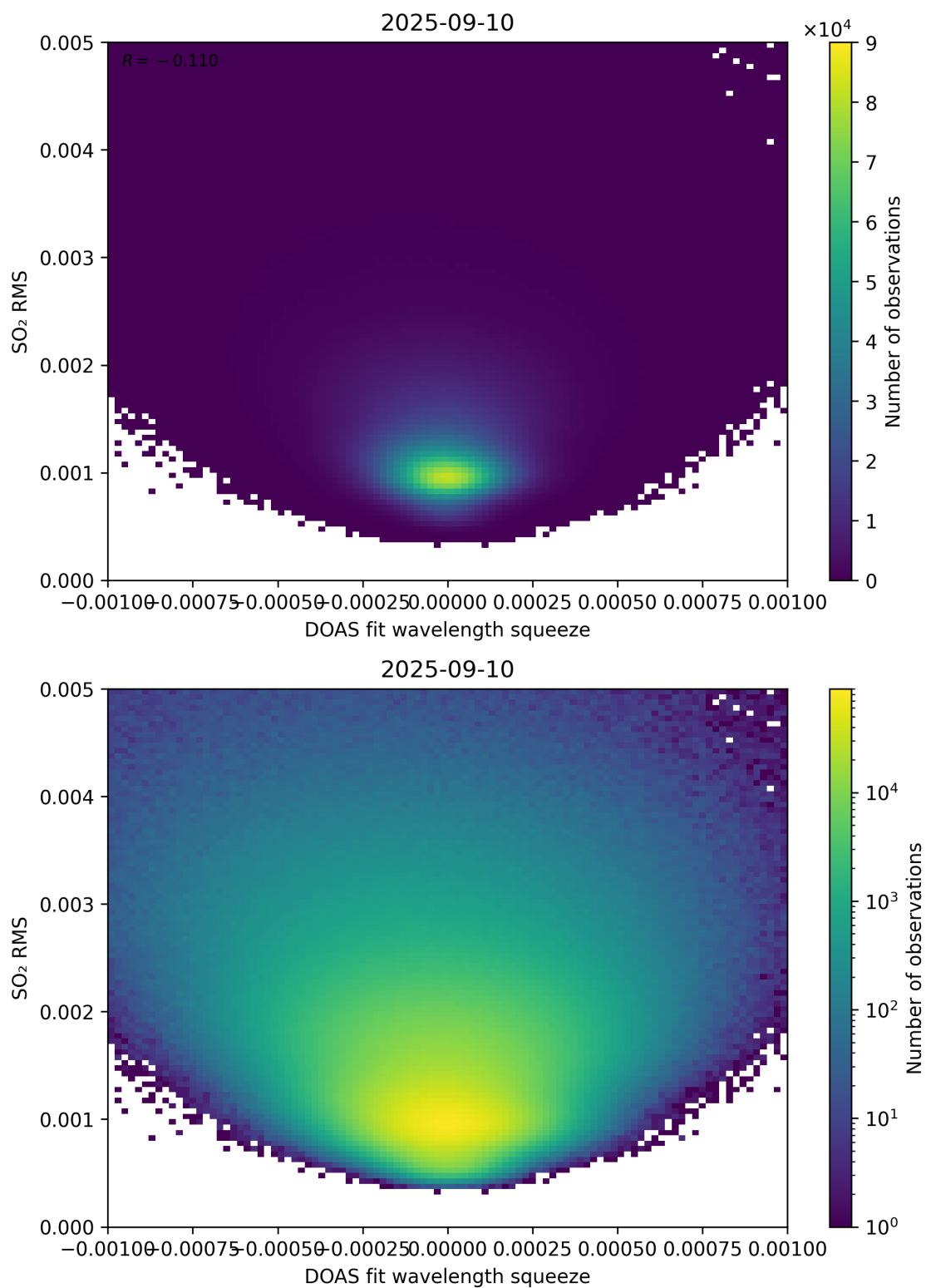
Figure 143: Scatter density plot of “DOAS fit wavelength squeeze” against “SO 2 RMS” for 2025-09-10 to 2025-09-11.
