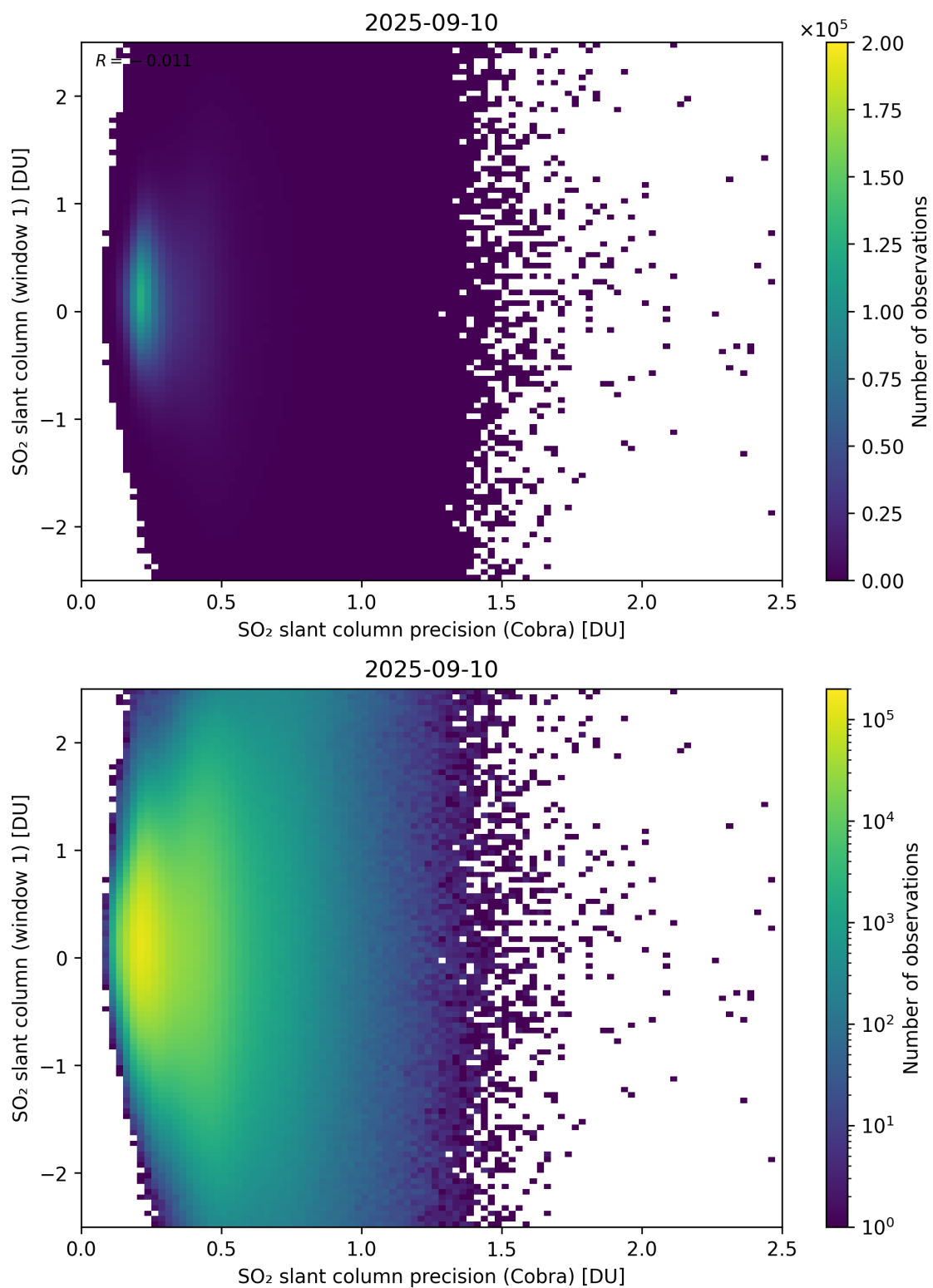
Figure 208: Scatter density plot of “SO 2 slant column precision (Cobra)” against “SO 2 slant column (window 1)” for 2025-09-10 to 2025-09-11.
