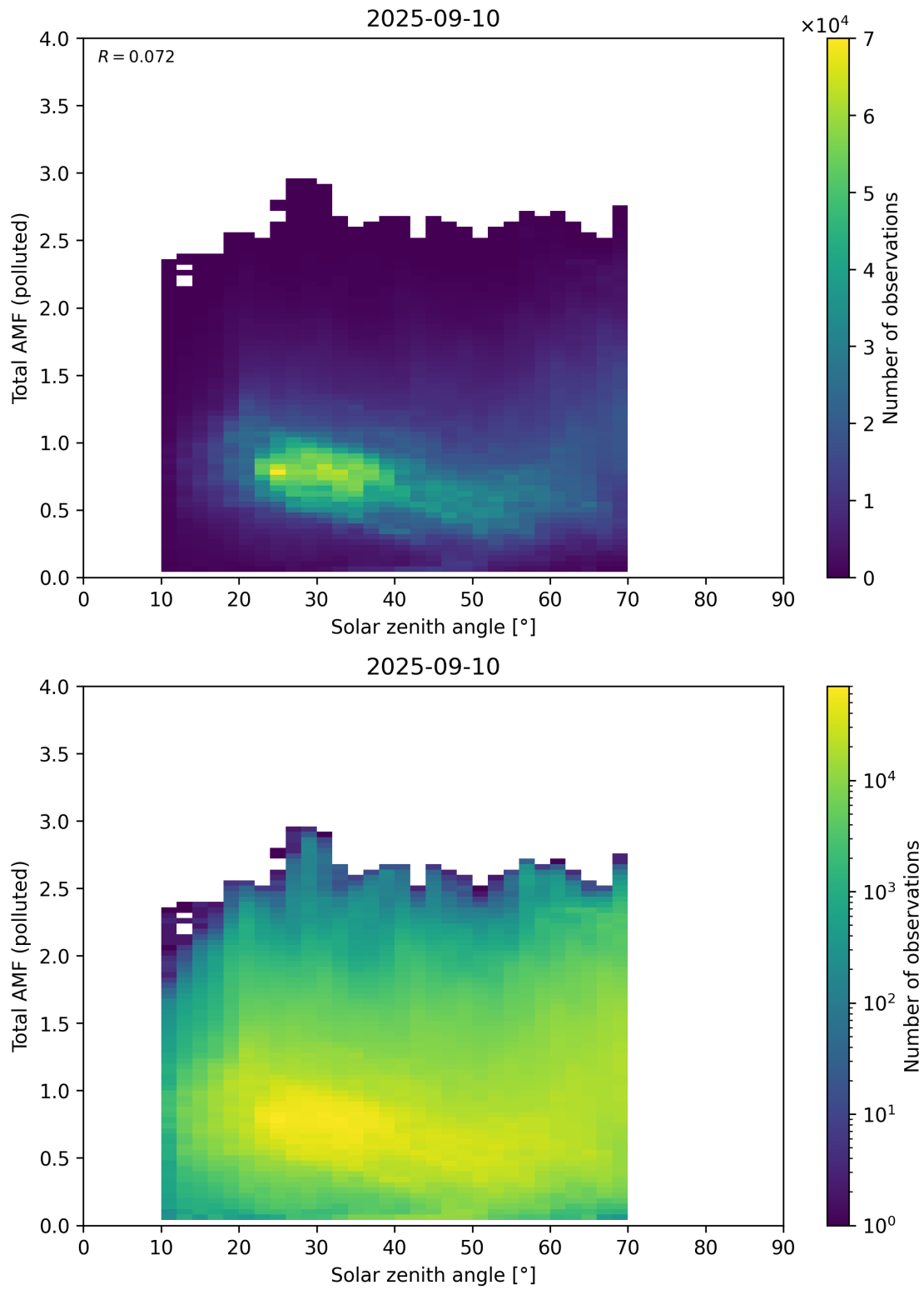
Figure 189: Scatter density plot of “Solar zenith angle” against “Total AMF (polluted)” for 2025-09-10 to 2025-09-11.
