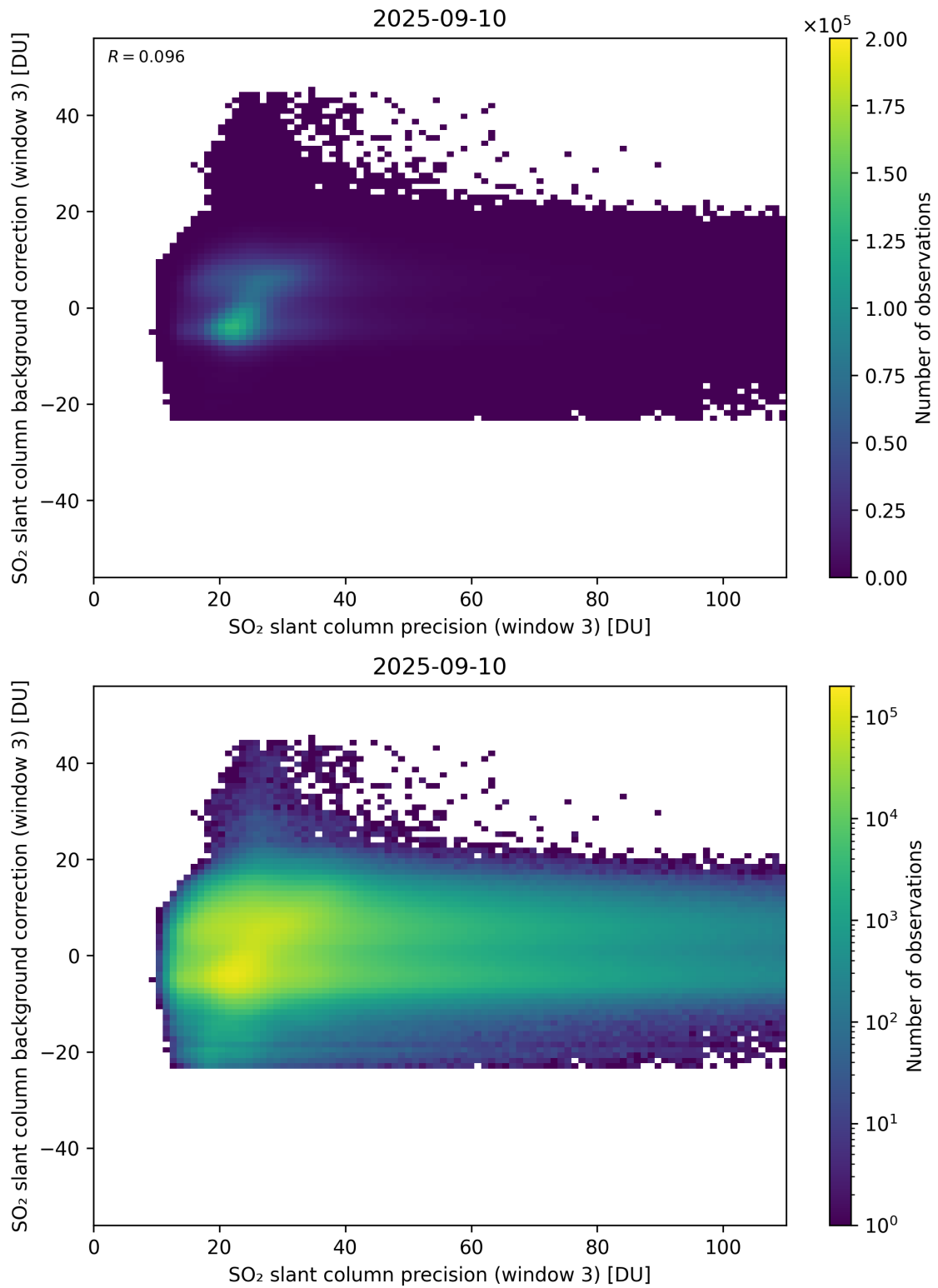
Figure 307: Scatter density plot of “SO 2 slant column precision (window 3)” against “SO 2 slant column background correction (window 3)” for 2025-09-10 to 2025-09-11.
