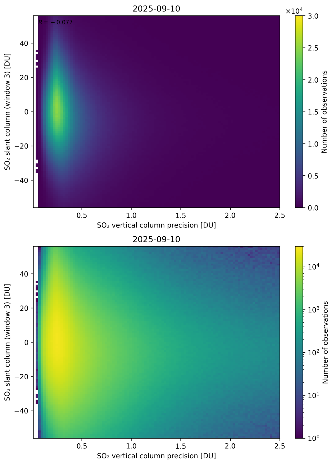
Figure 344: Scatter density plot of “SO 2 vertical column precision” against “SO 2 slant column (window 3)” for 2025-09-10 to 2025-09-11.
