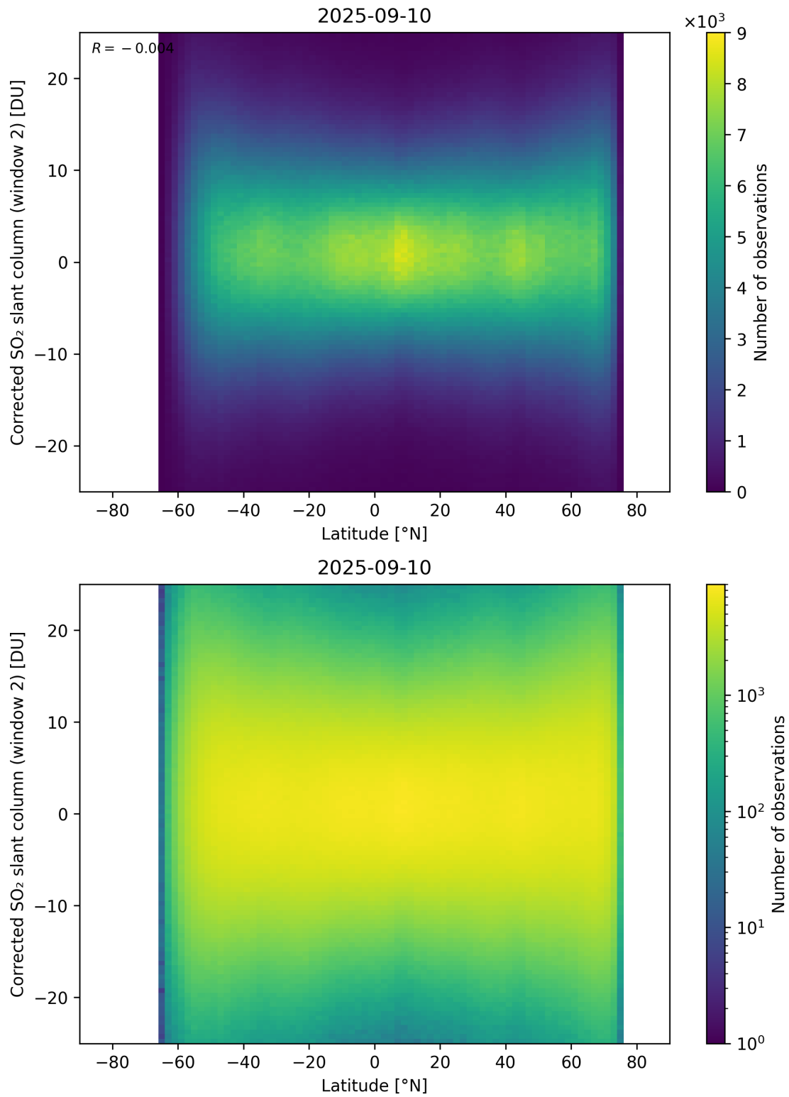
Figure 160: Scatter density plot of “Latitude” against “Corrected SO 2 slant column (window 2)” for 2025-09-10 to 2025-09-11.
