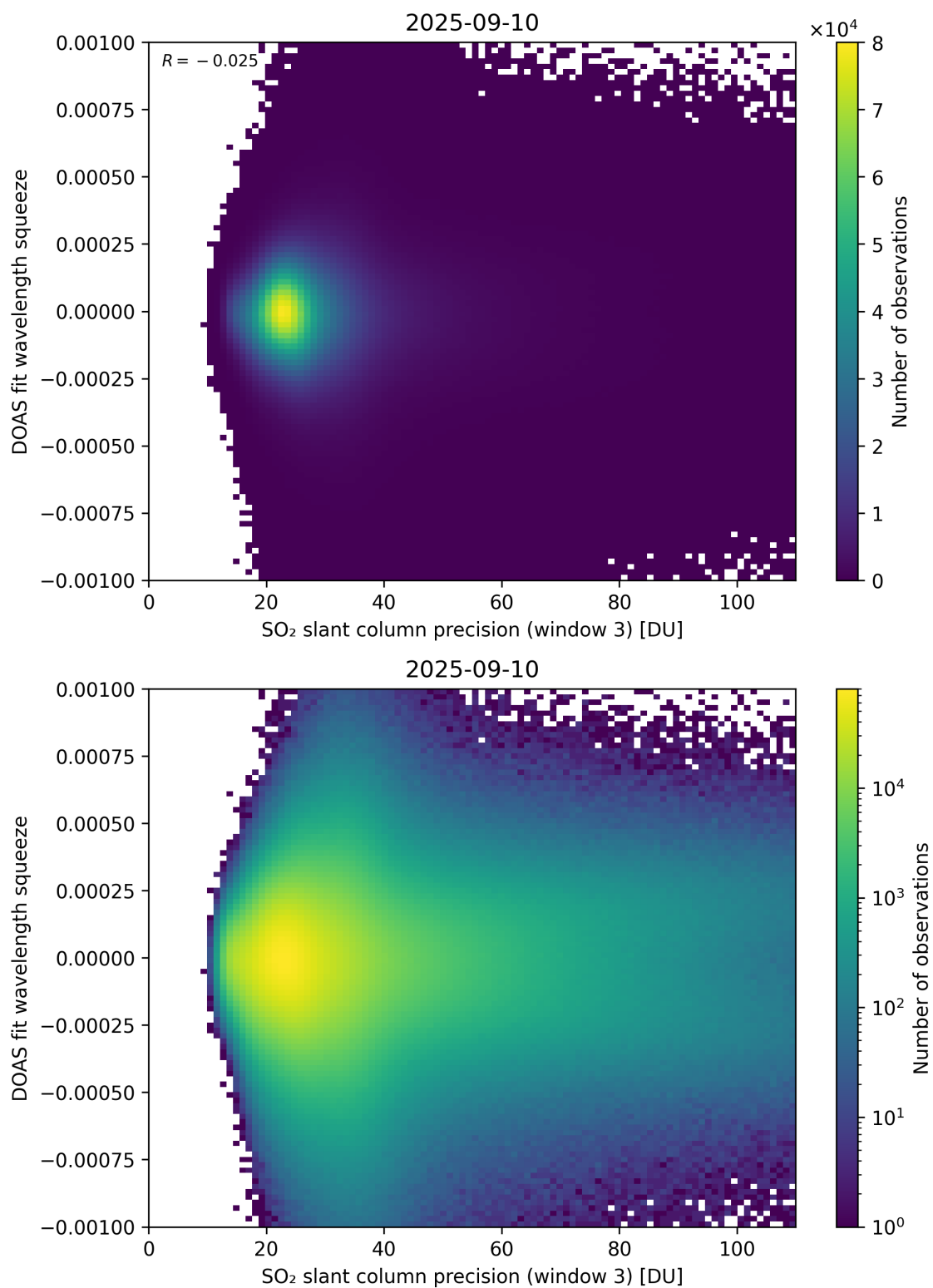
Figure 309: Scatter density plot of “SO 2 slant column precision (window 3)” against “DOAS fit wavelength squeeze” for 2025-09-10 to 2025-09-11.
