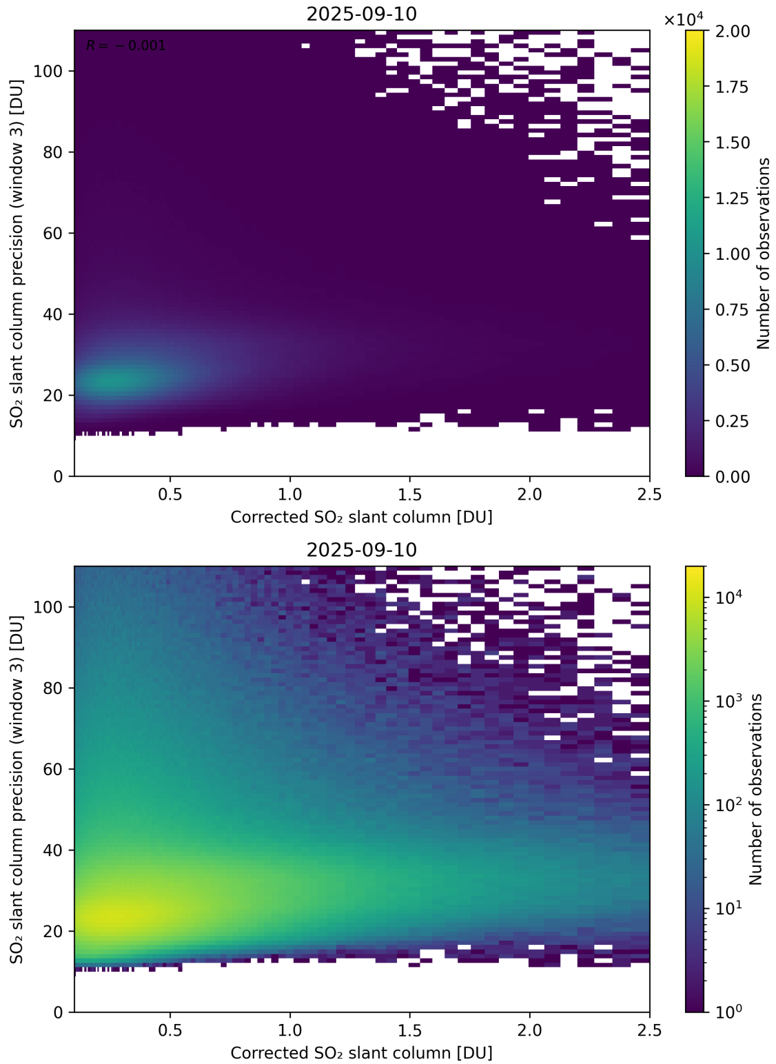
Figure 241: Scatter density plot of “Corrected SO 2 slant column” against “SO 2 slant column precision (window 3)” for 2025-09-10 to 2025-09-11.
