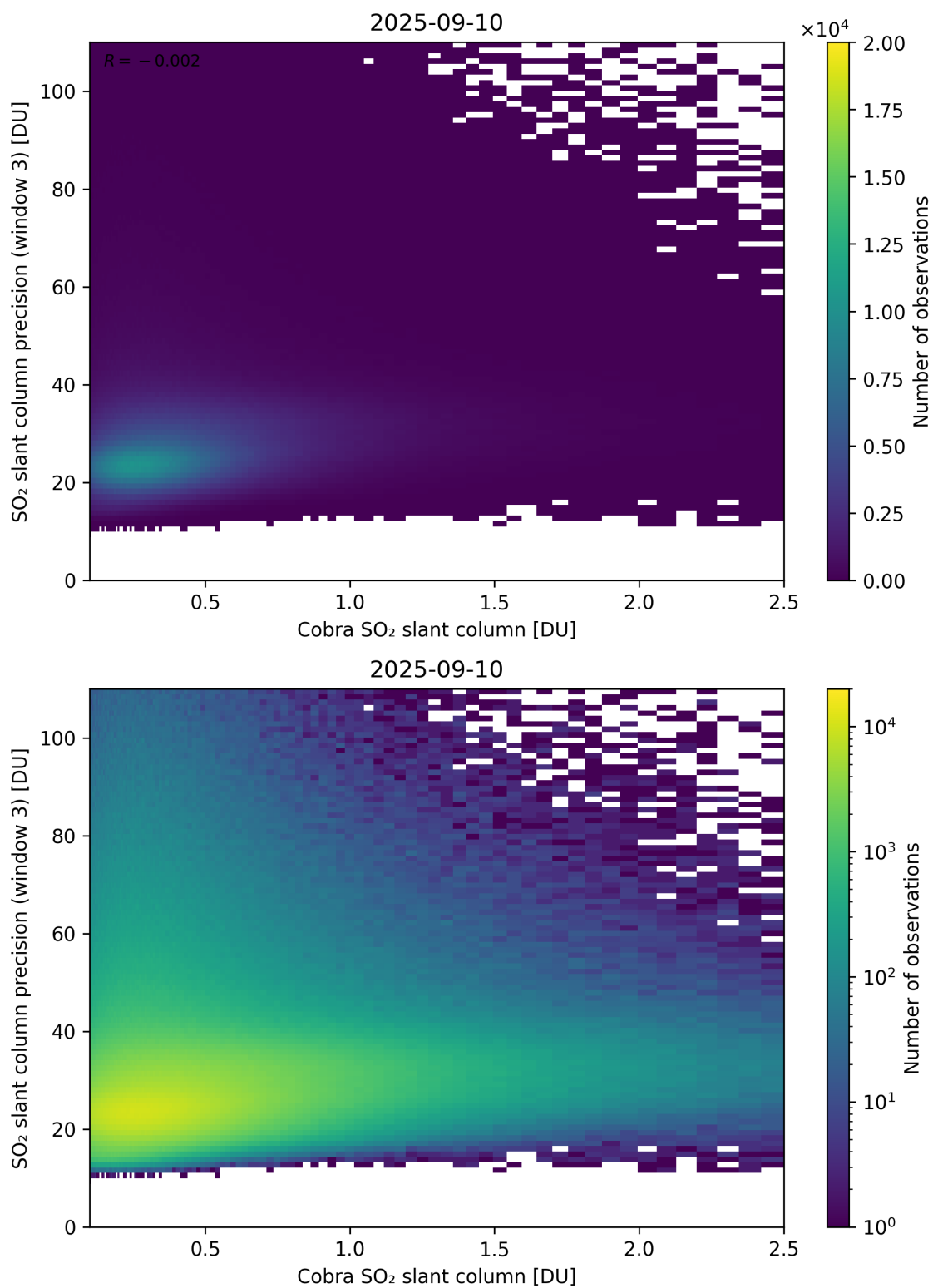
Figure 223: Scatter density plot of “Cobra SO 2 slant column” against “SO 2 slant column precision (window 3)” for 2025-09-10 to 2025-09-11.
