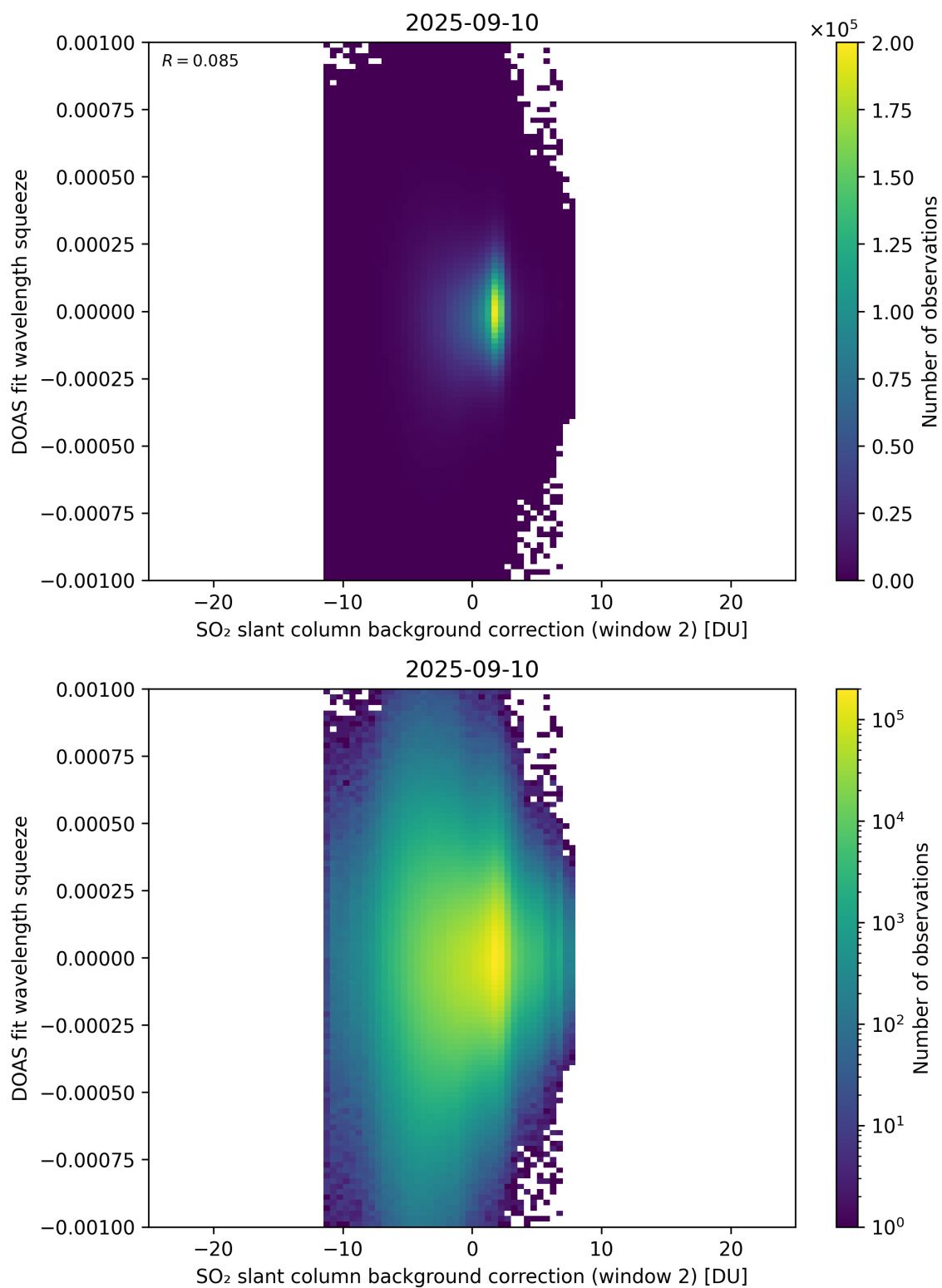
Figure 124: Scatter density plot of “SO 2 slant column background correction (window 2)” against “DOAS fit wavelength squeeze” for 2025-09-10 to 2025-09-11.
