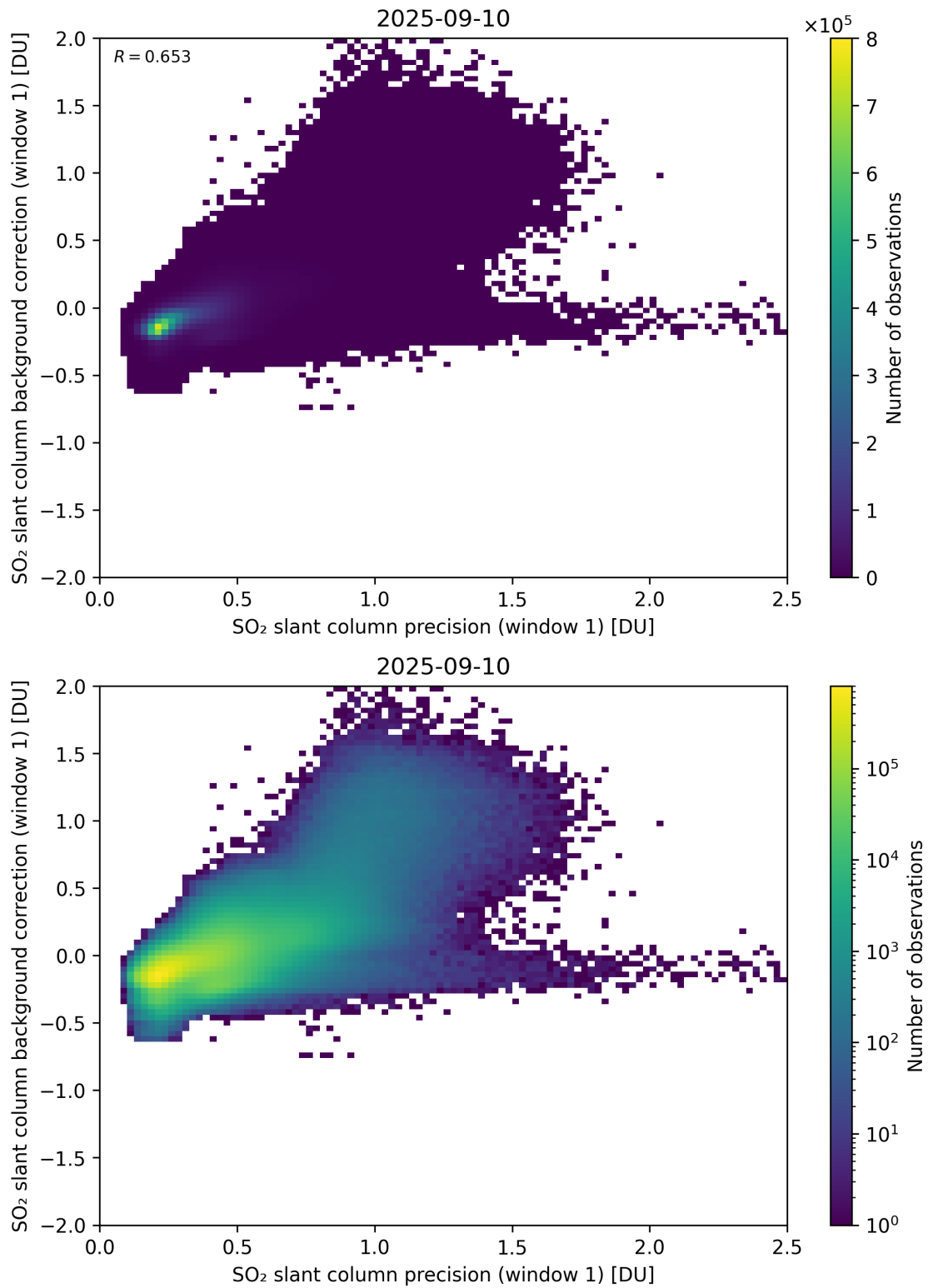
Figure 268: Scatter density plot of “SO 2 slant column precision (window 1)” against “SO 2 slant column background correction (window 1)” for 2025-09-10 to 2025-09-11.
