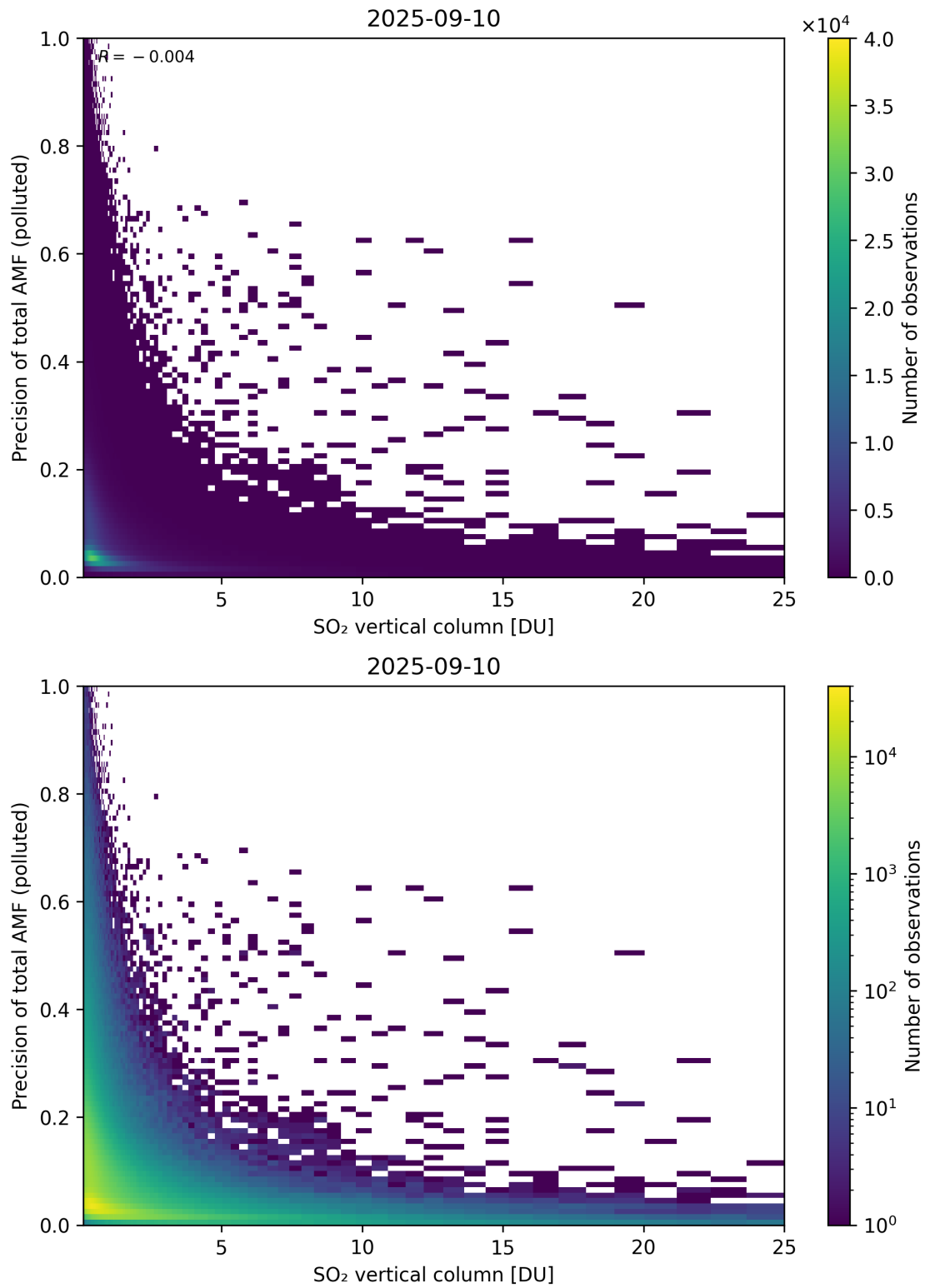
Figure 360: Scatter density plot of “SO 2 vertical column” against “Precision of total AMF (polluted)” for 2025-09-10 to 2025-09-11.
