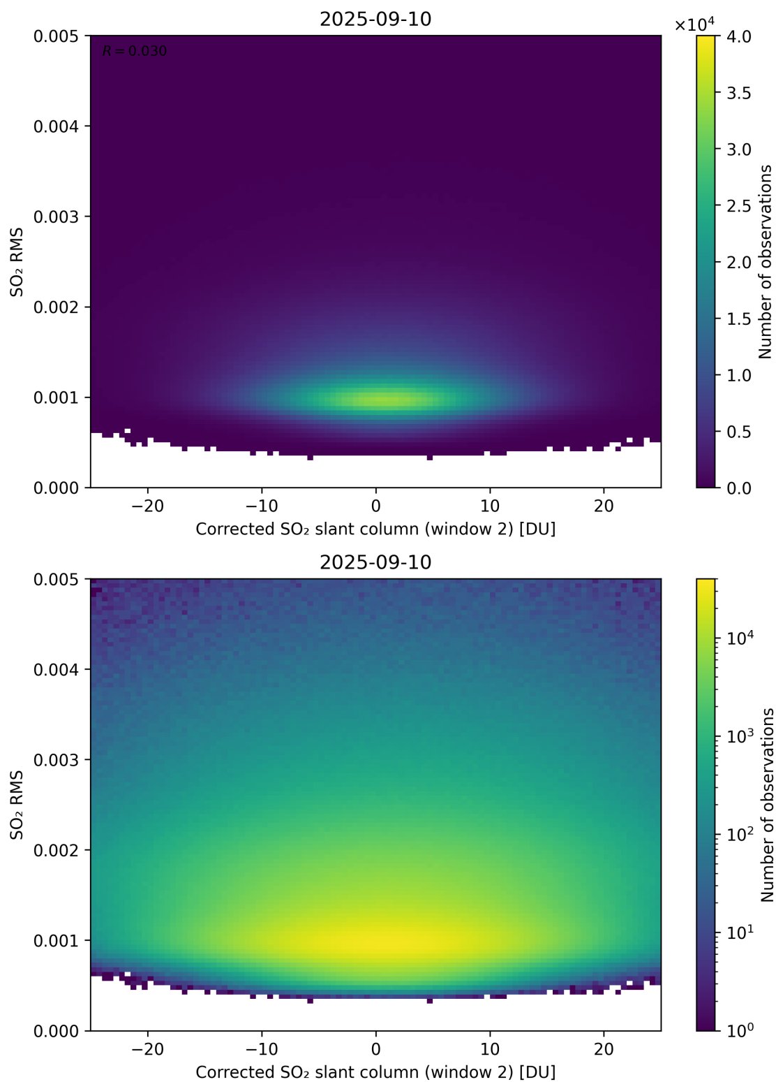
Figure 248: Scatter density plot of “Corrected SO 2 slant column (window 2)” against “SO 2 RMS” for 2025-09-10 to 2025-09-11.
