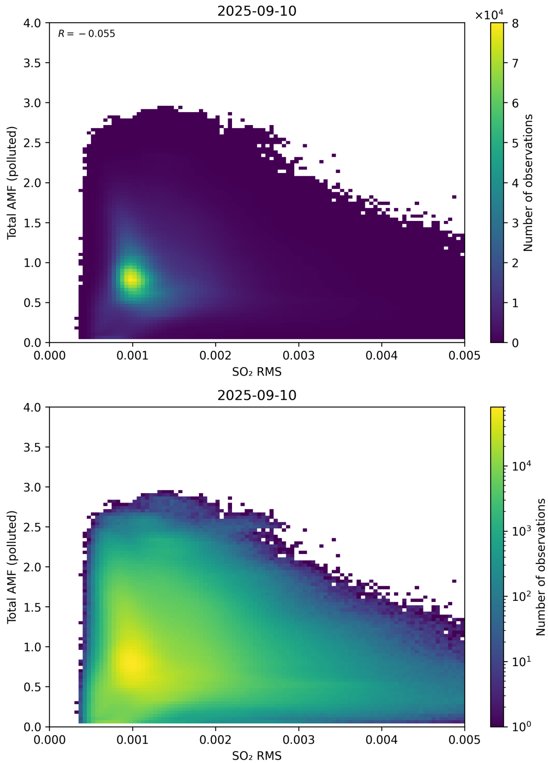
Figure 148: Scatter density plot of “SO 2 RMS” against “Total AMF (polluted)” for 2025-09-10 to 2025-09-11.
