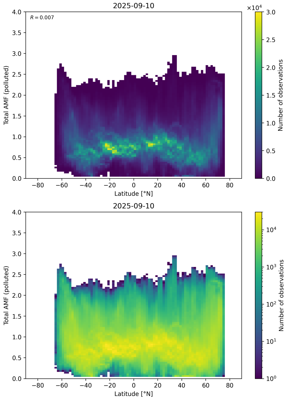
Figure 167: Scatter density plot of “Latitude” against “Total AMF (polluted)” for 2025-09-10 to 2025-09-11.
