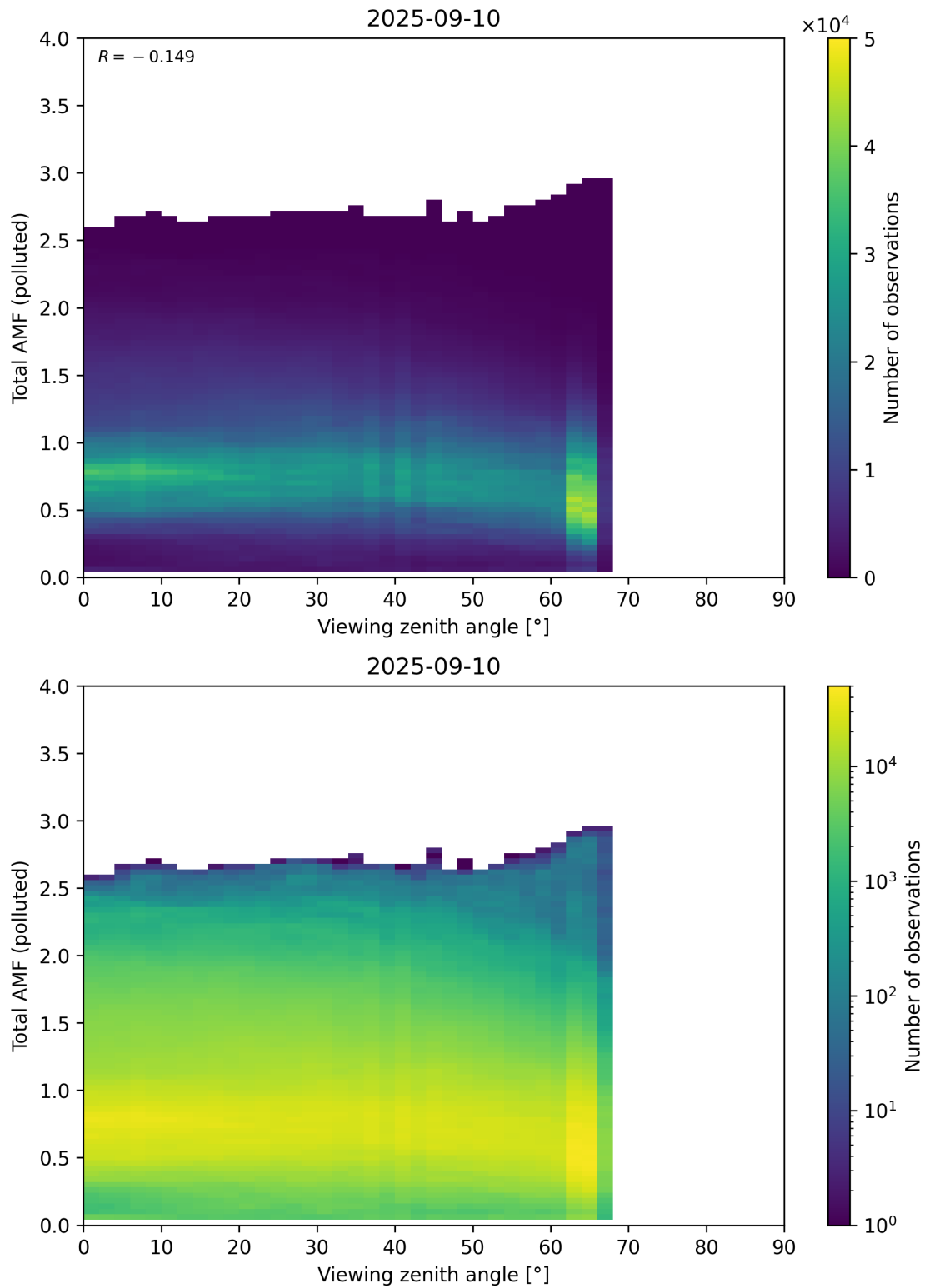
Figure 381: Scatter density plot of “Viewing zenith angle” against “Total AMF (polluted)” for 2025-09-10 to 2025-09-11.
