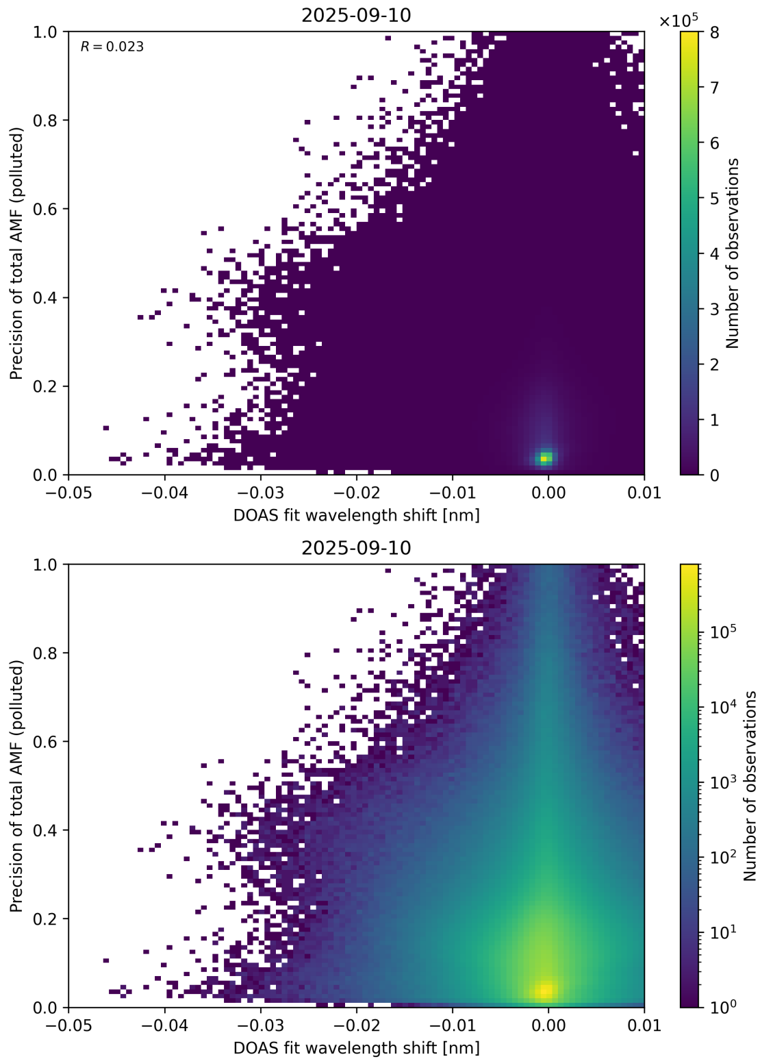
Figure 142: Scatter density plot of “DOAS fit wavelength shift” against “Precision of total AMF (polluted)” for 2025-09-10 to 2025-09-11.
