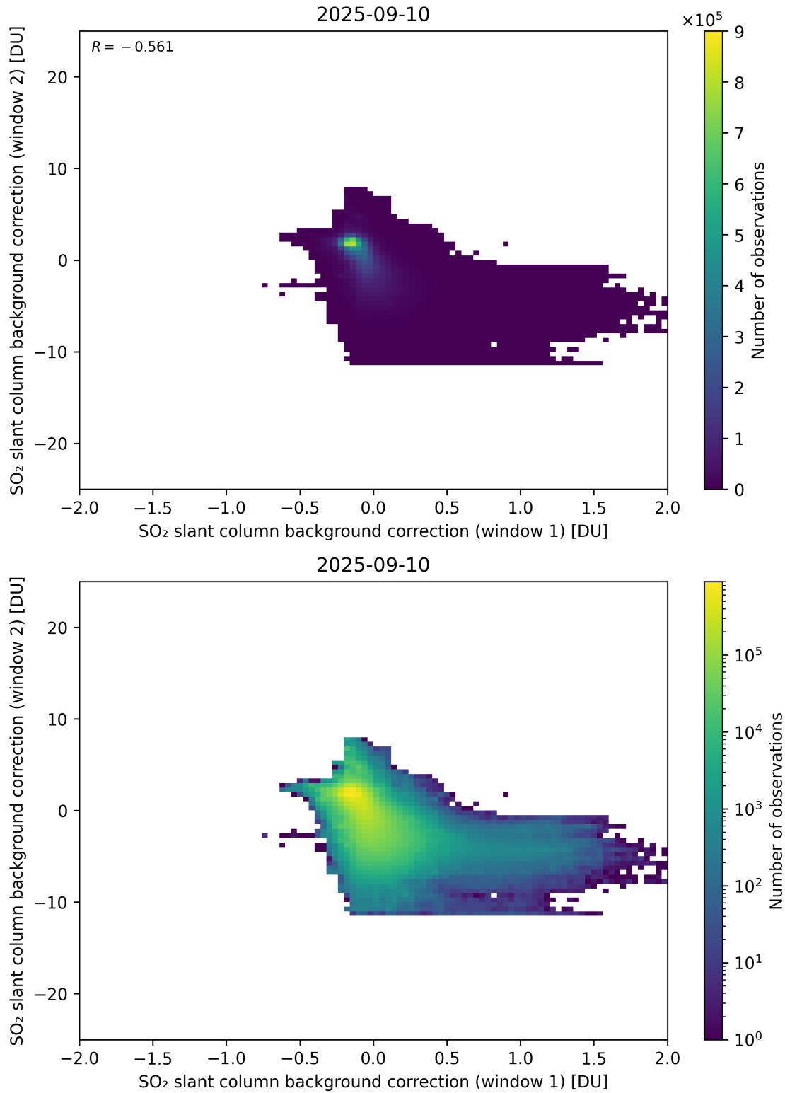
Figure 109: Scatter density plot of “SO 2 slant column background correction (window 1)” against “SO 2 slant column background correction (window 2)” for 2025-09-10 to 2025-09-11.
