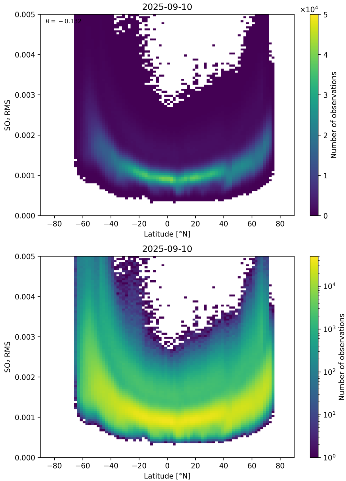
Figure 155: Scatter density plot of “Latitude” against “SO 2 RMS” for 2025-09-10 to 2025-09-11.
