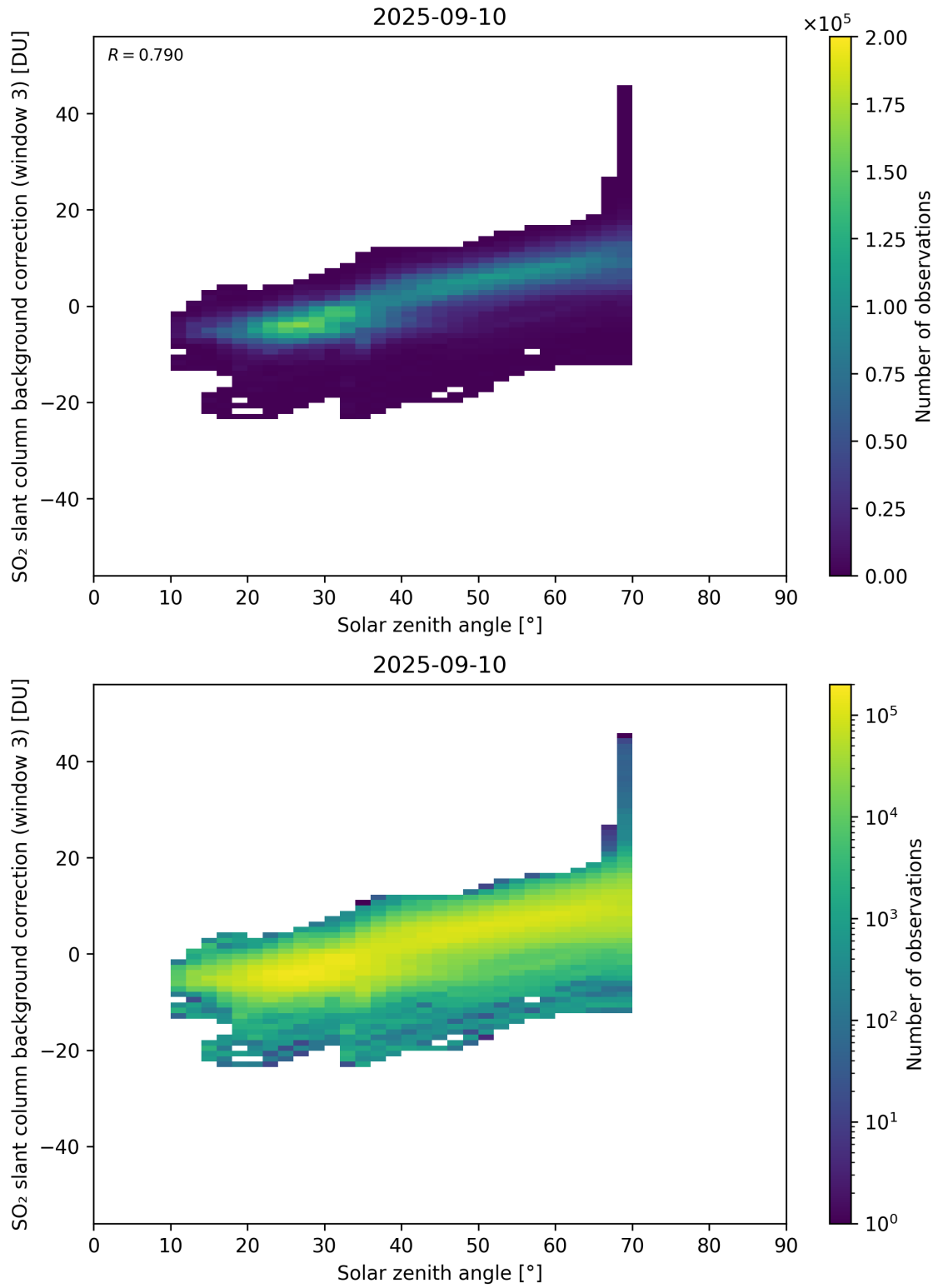
Figure 173: Scatter density plot of “Solar zenith angle” against “SO 2 slant column background correction (window 3)” for 2025-09-10 to 2025-09-11.
