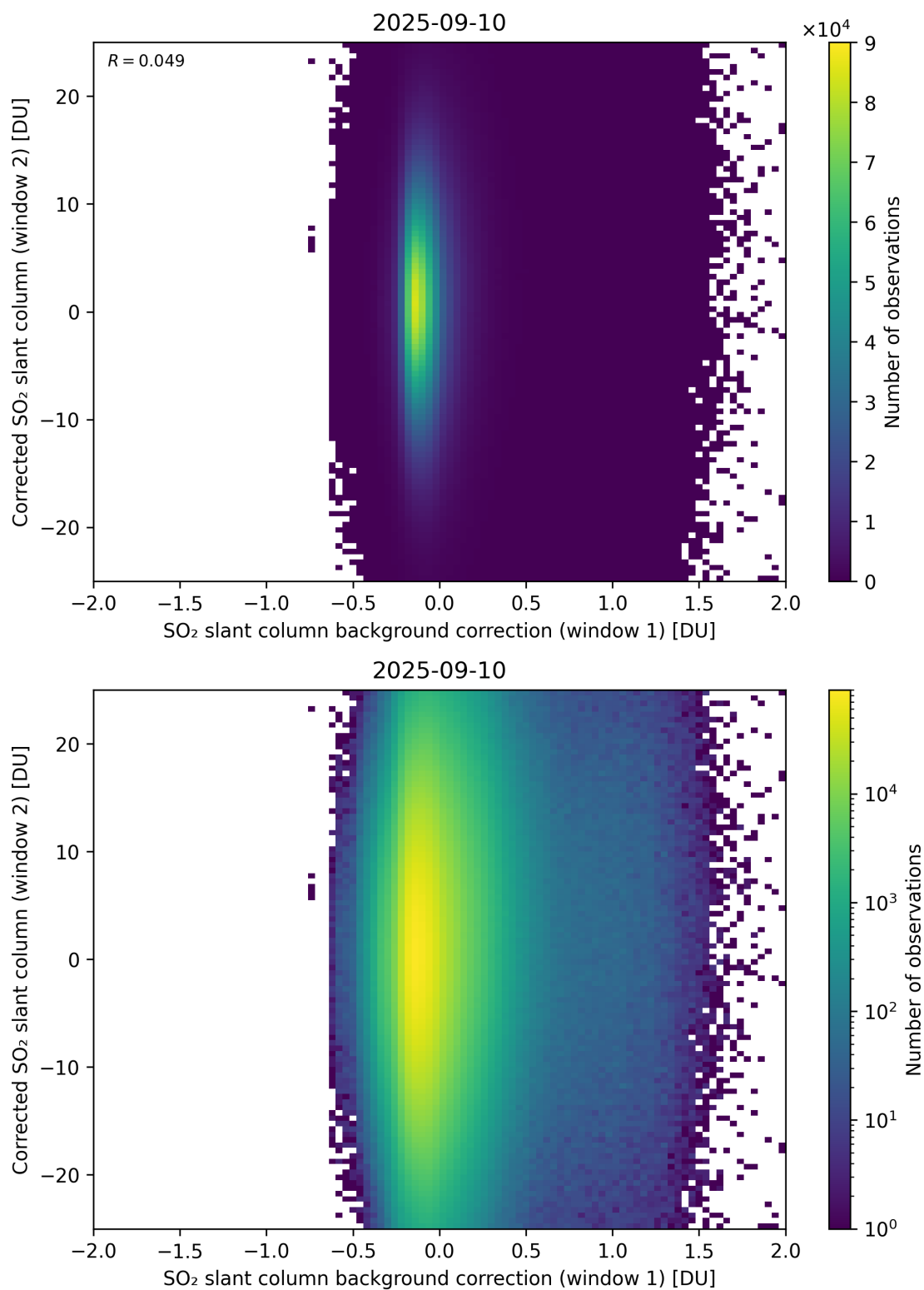
Figure 115: Scatter density plot of “SO 2 slant column background correction (window 1)” against “Corrected SO 2 slant column (window 2)” for 2025-09-10 to 2025-09-11.
