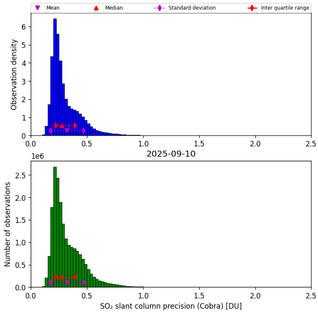
Figure 62: Histogram of “SO 2 slant column precision (Cobra)” for 2025-09-10 to 2025-09-11
