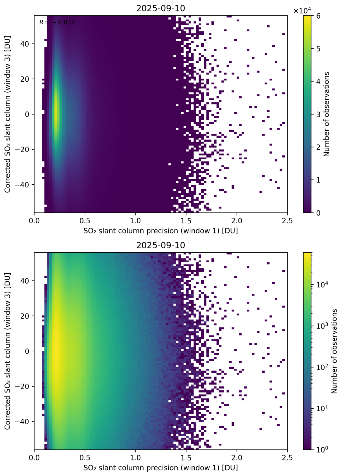
Figure 276: Scatter density plot of “SO 2 slant column precision (window 1)” against “Corrected SO 2 slant column (window 3)” for 2025-09-10 to 2025-09-11.
