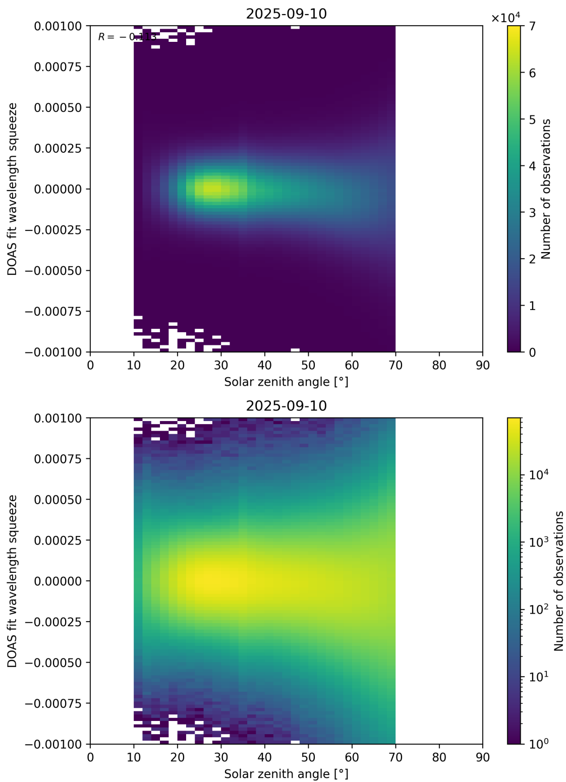
Figure 175: Scatter density plot of “Solar zenith angle” against “DOAS fit wavelength squeeze” for 2025-09-10 to 2025-09-11.
