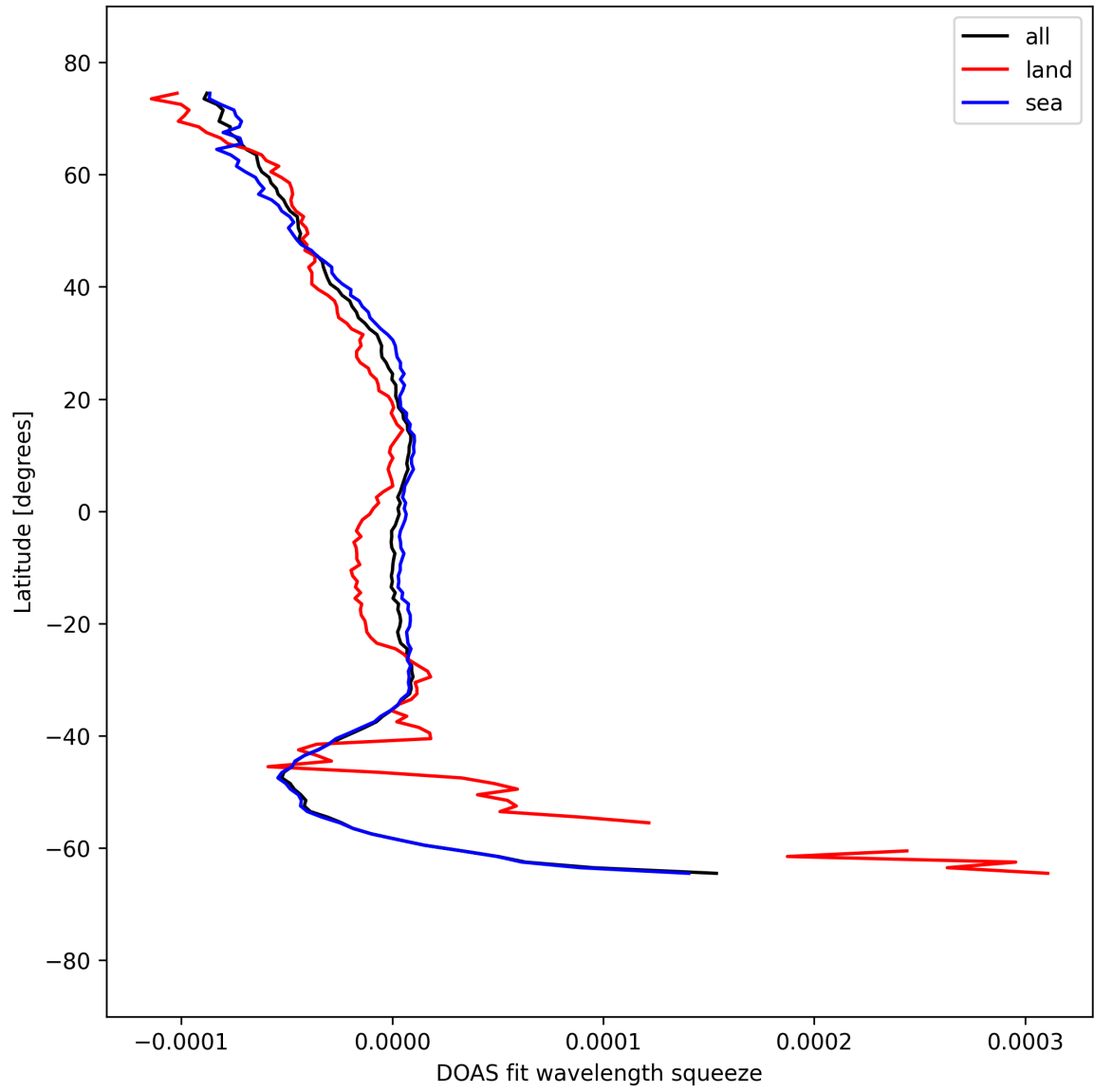
Figure 51: Zonal average of "DOAS fit wavelength squeeze" for 2025-09-10 to 2025-09-11.
