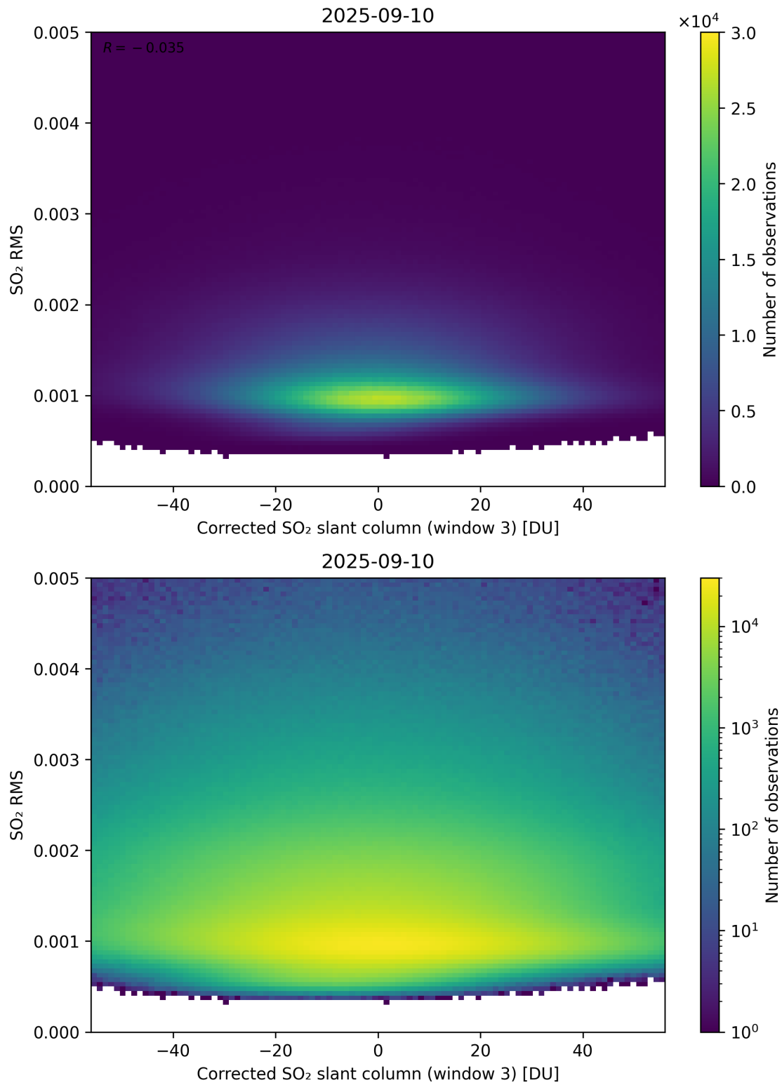
Figure 258: Scatter density plot of “Corrected SO 2 slant column (window 3)” against “SO 2 RMS” for 2025-09-10 to 2025-09-11.
