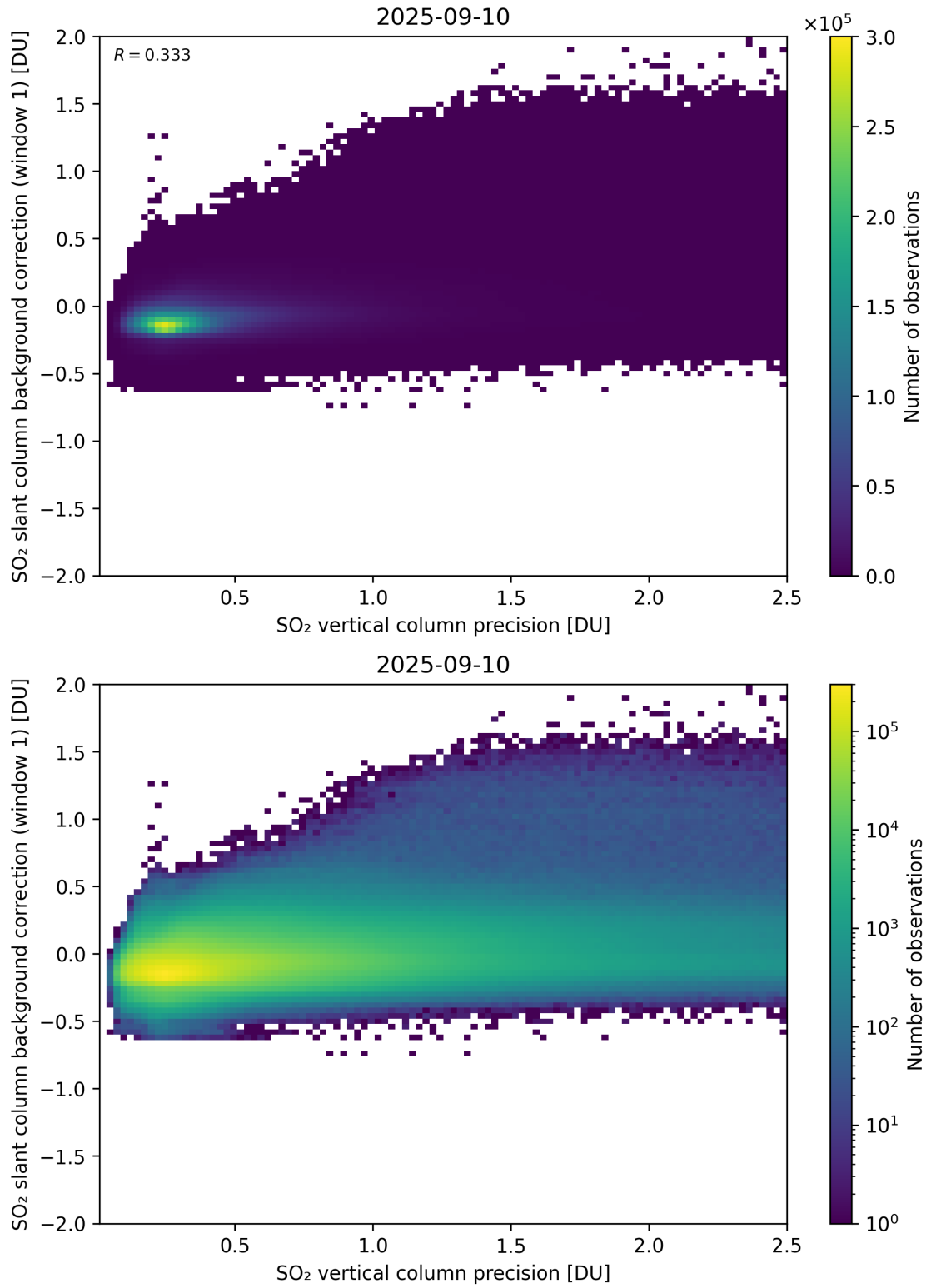
Figure 329: Scatter density plot of “SO 2 vertical column precision” against “SO 2 slant column background correction (window 1)” for 2025-09-10 to 2025-09-11.
