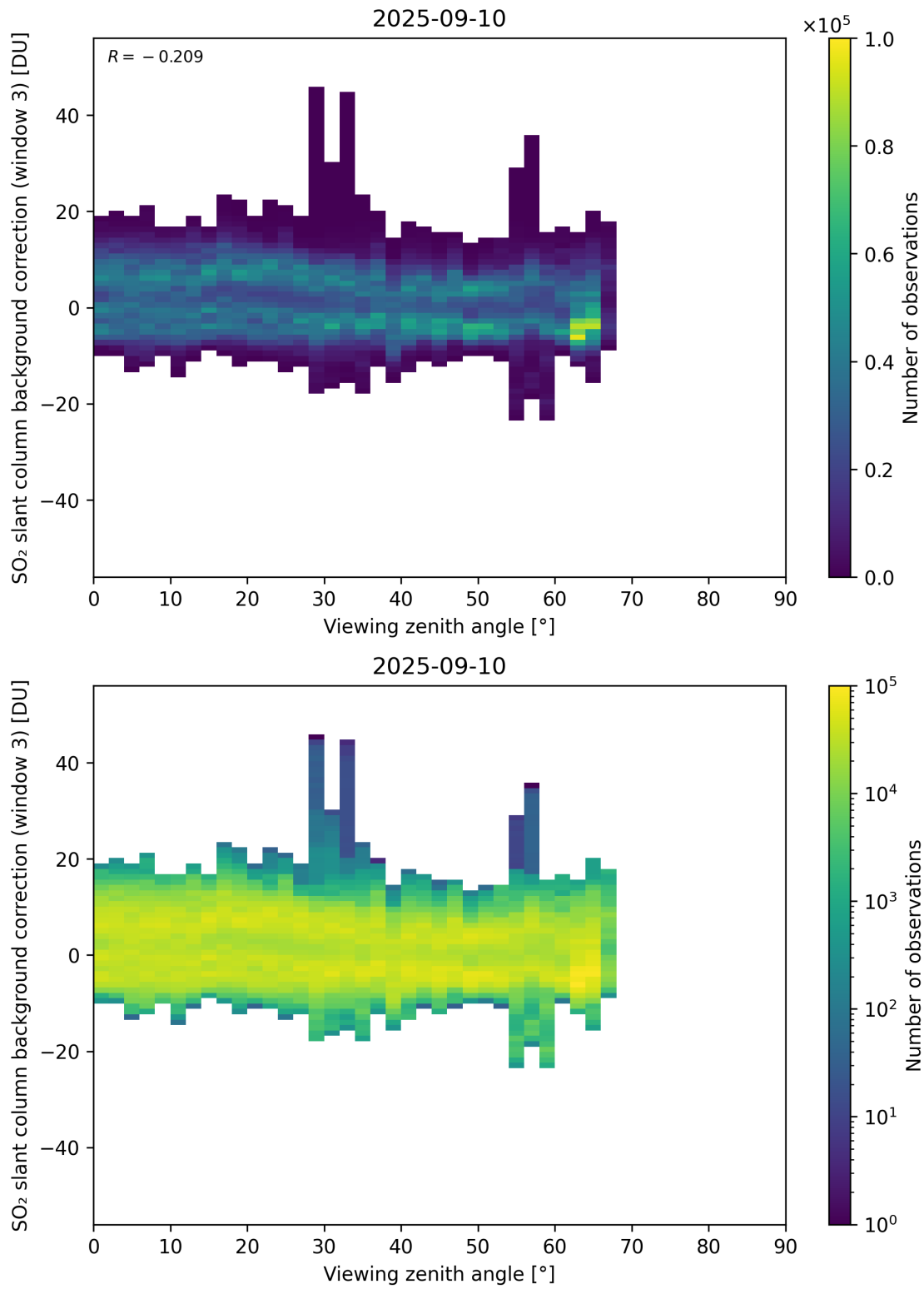
Figure 364: Scatter density plot of “Viewing zenith angle” against “SO 2 slant column background correction (window 3)” for 2025-09-10 to 2025-09-11.
