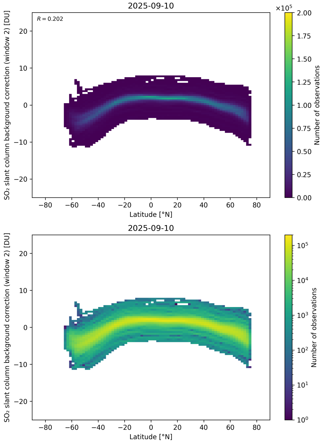
Figure 151: Scatter density plot of “Latitude” against “SO 2 slant column background correction (window 2)” for 2025-09-10 to 2025-09-11.
