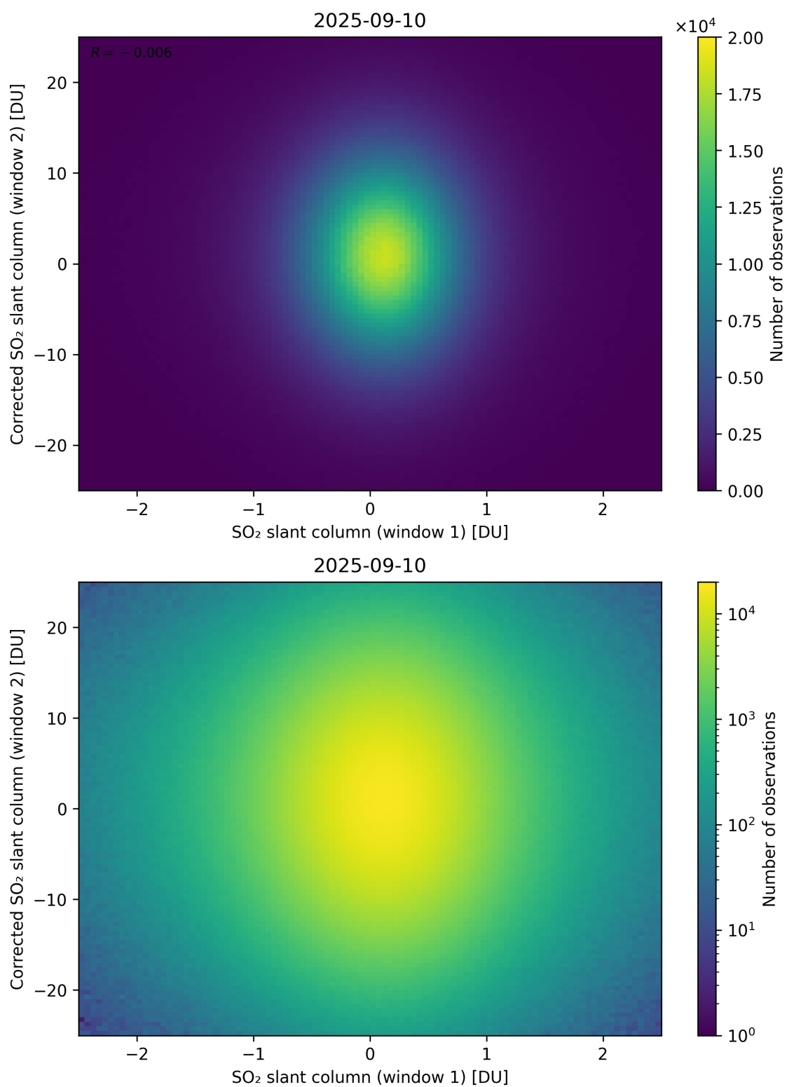
Figure 283: Scatter density plot of “SO 2 slant column (window 1)” against “Corrected SO 2 slant column (window 2)” for 2025-09-10 to 2025-09-11.
