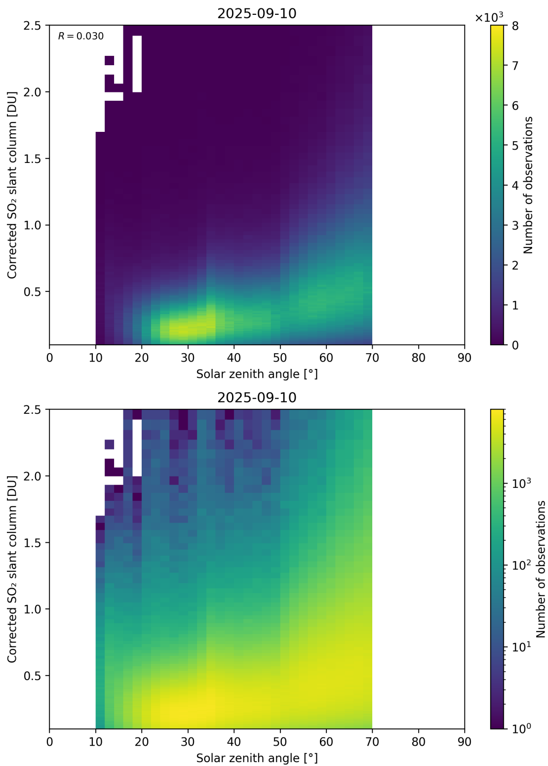
Figure 181: Scatter density plot of “Solar zenith angle” against “Corrected SO 2 slant column” for 2025-09-10 to 2025-09-11.
