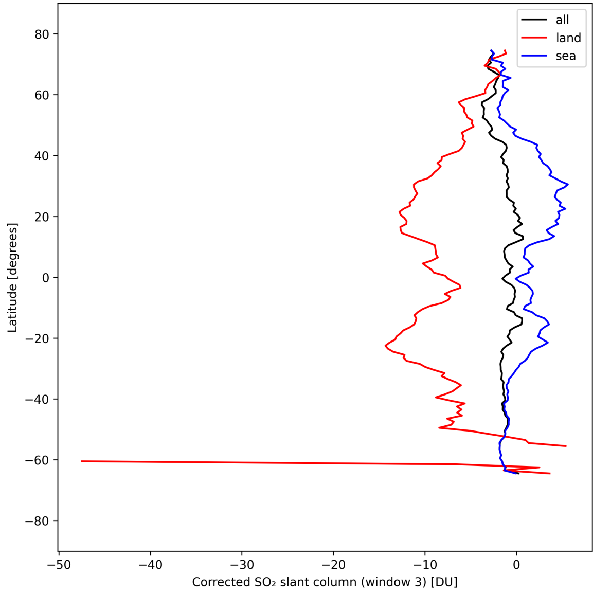
Figure 47: Zonal average of “Corrected SO 2 slant column (window 3)” for 2025-09-10 to 2025-09-11.
