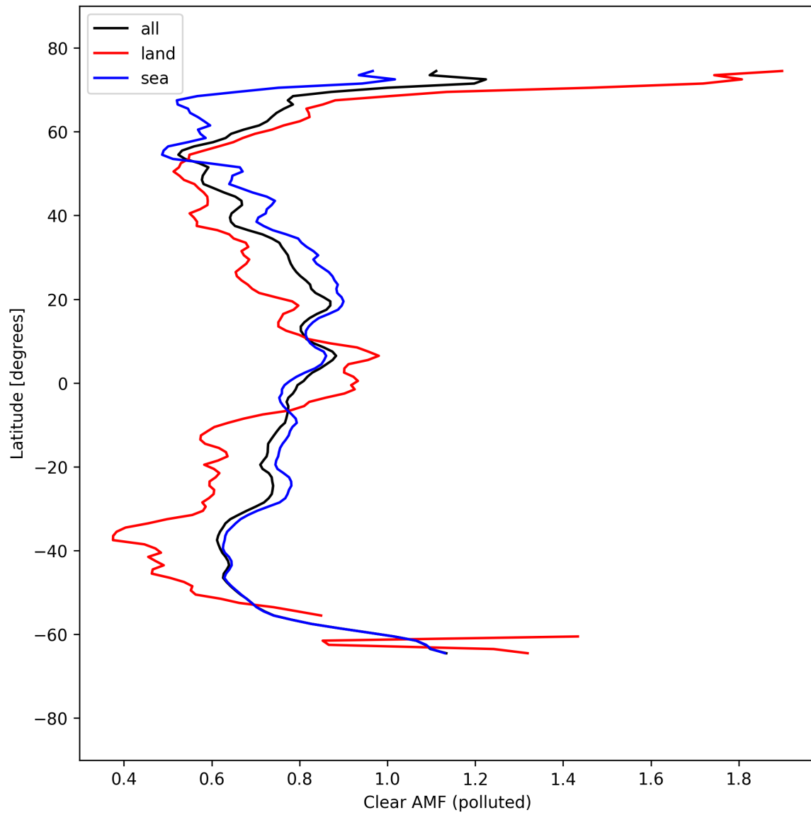
Figure 55: Zonal average of “Clear AMF (polluted)” for 2025-09-10 to 2025-09-11.
