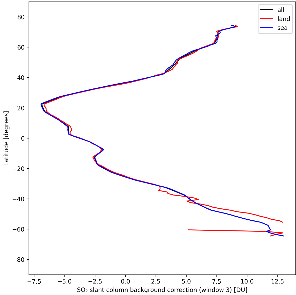
Figure 48: Zonal average of “SO 2 slant column background correction (window 3)” for 2025-09-10 to 2025-09-11.
