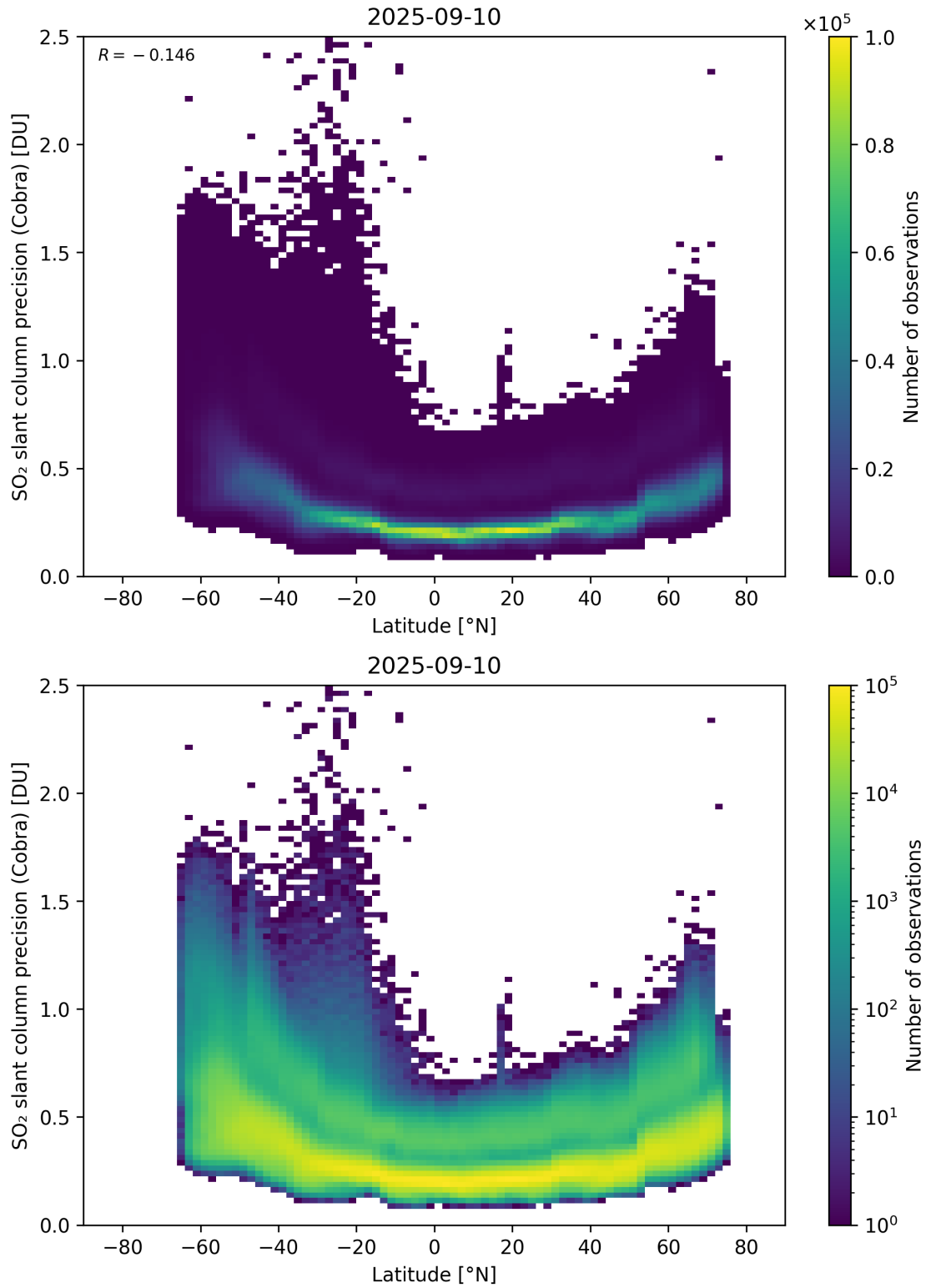
Figure 158: Scatter density plot of “Latitude” against “SO 2 slant column precision (Cobra)” for 2025-09-10 to 2025-09-11.
