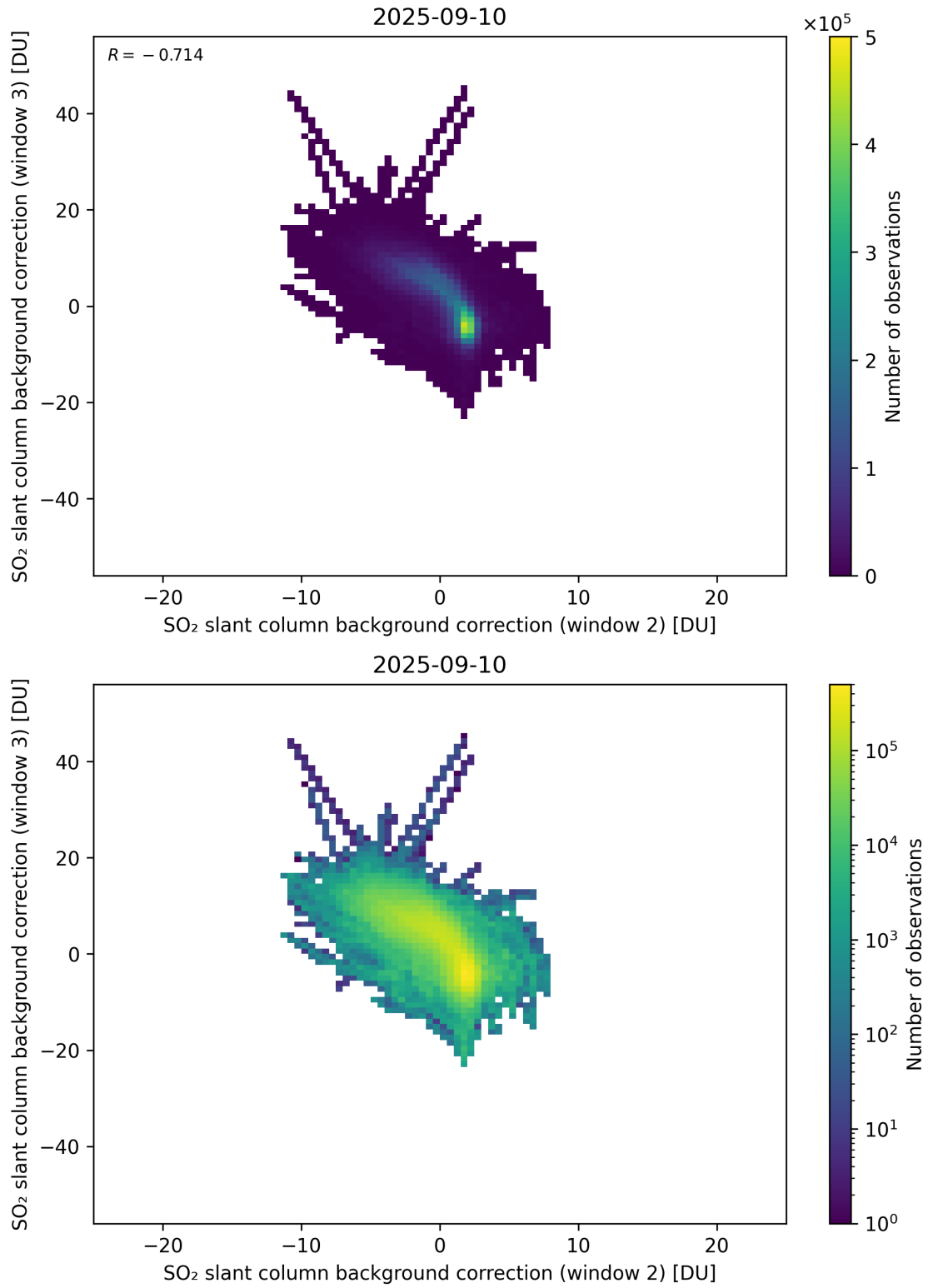
Figure 122: Scatter density plot of “SO 2 slant column background correction (window 2)” against “SO 2 slant column background correction (window 3)” for 2025-09-10 to 2025-09-11.
