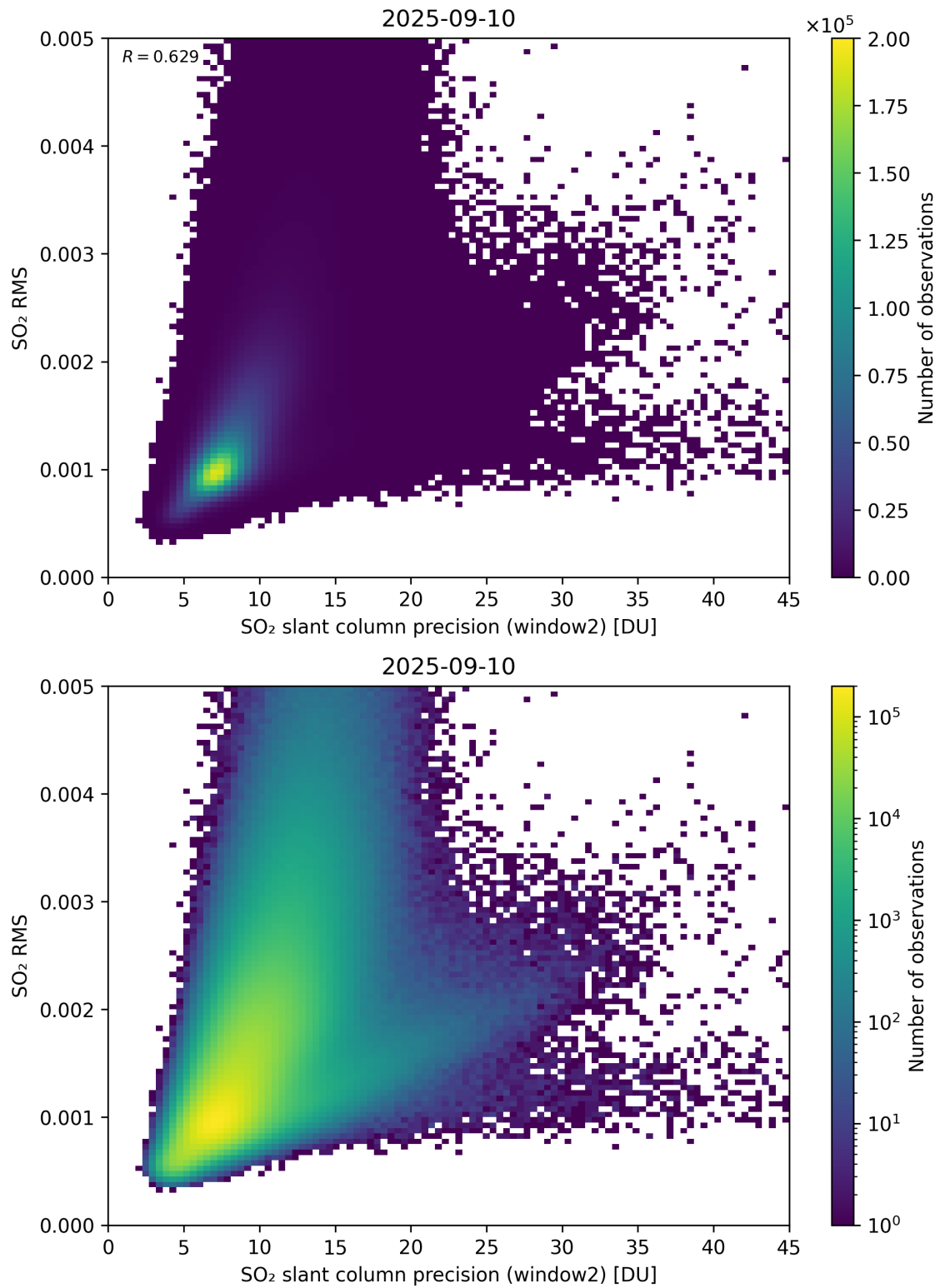
Figure 295: Scatter density plot of “SO 2 slant column precision (window2)” against “SO 2 RMS” for 2025-09-10 to 2025-09-11.
