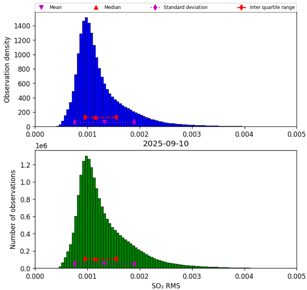
Figure 78: Histogram of “SO 2 RMS” for 2025-09-10 to 2025-09-11
