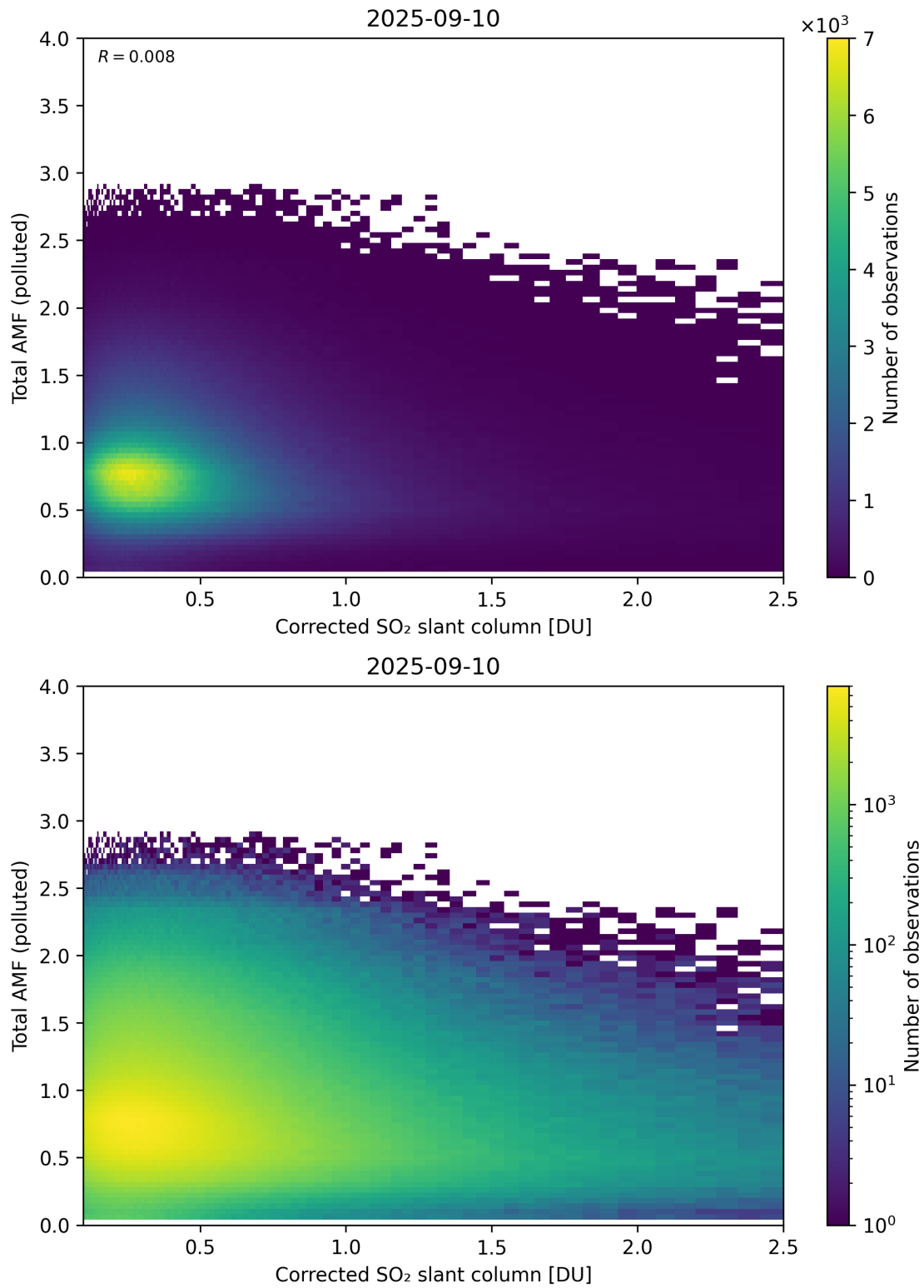
Figure 242: Scatter density plot of “Corrected SO 2 slant column” against “Total AMF (polluted)” for 2025-09-10 to 2025-09-11.
