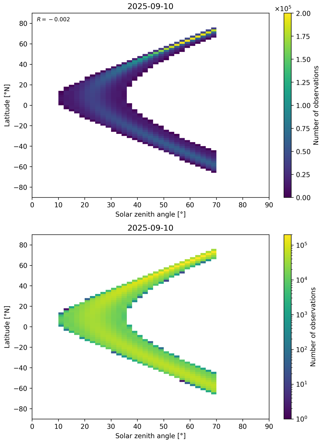
Figure 177: Scatter density plot of “Solar zenith angle” against “Latitude” for 2025-09-10 to 2025-09-11.
