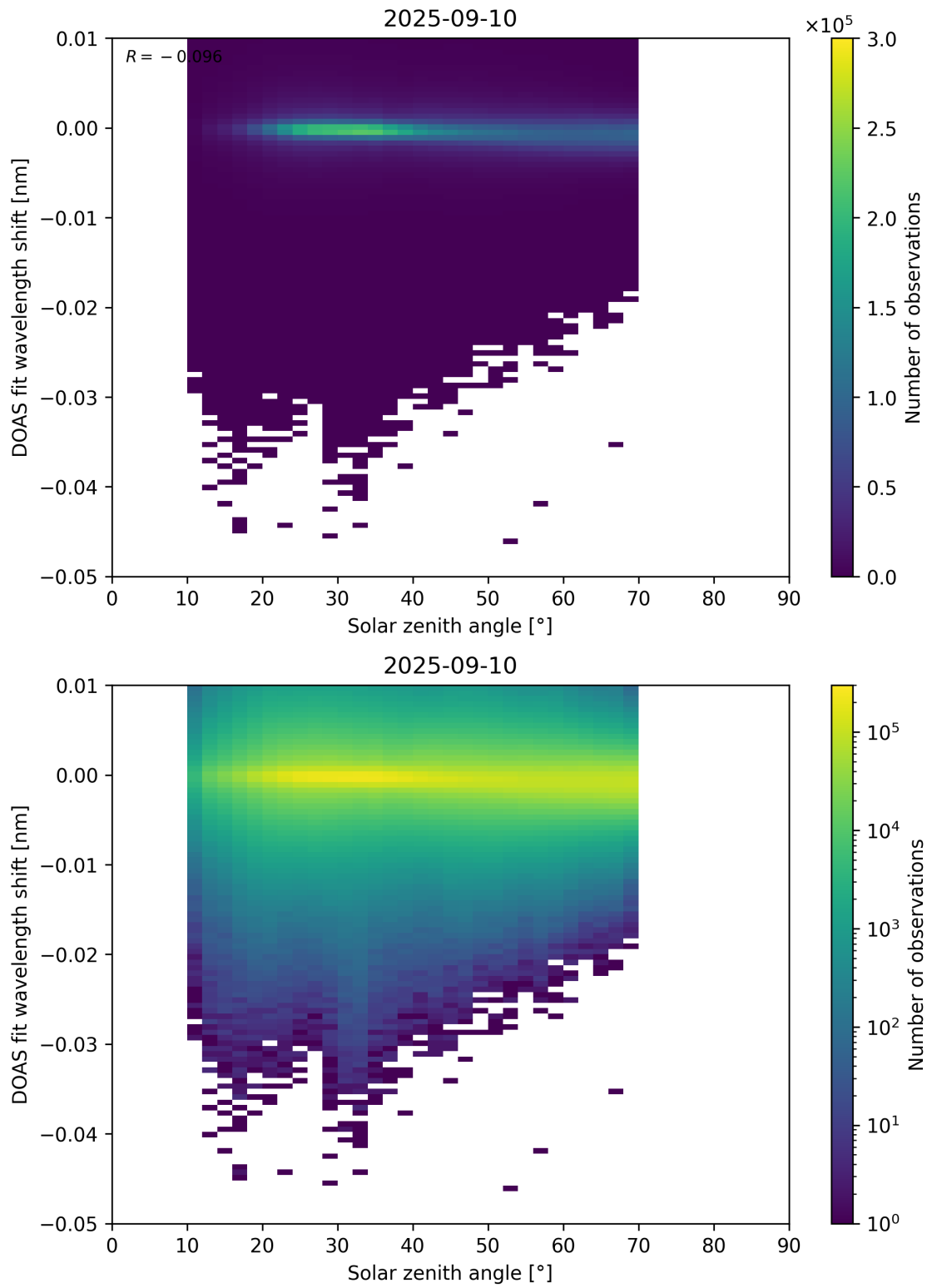
Figure 174: Scatter density plot of “Solar zenith angle” against “DOAS fit wavelength shift” for 2025-09-10 to 2025-09-11.
