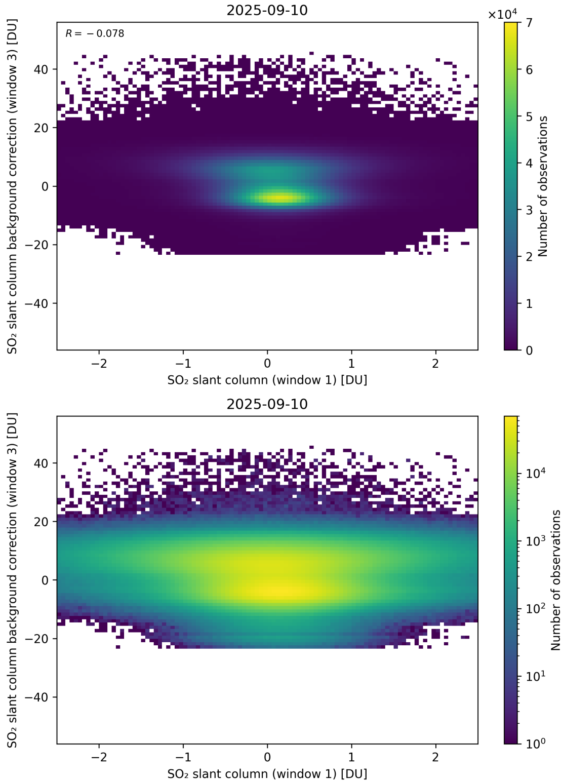
Figure 264: Scatter density plot of “SO 2 slant column (window 1)” against “SO 2 slant column background correction (window 3)” for 2025-09-10 to 2025-09-11.
