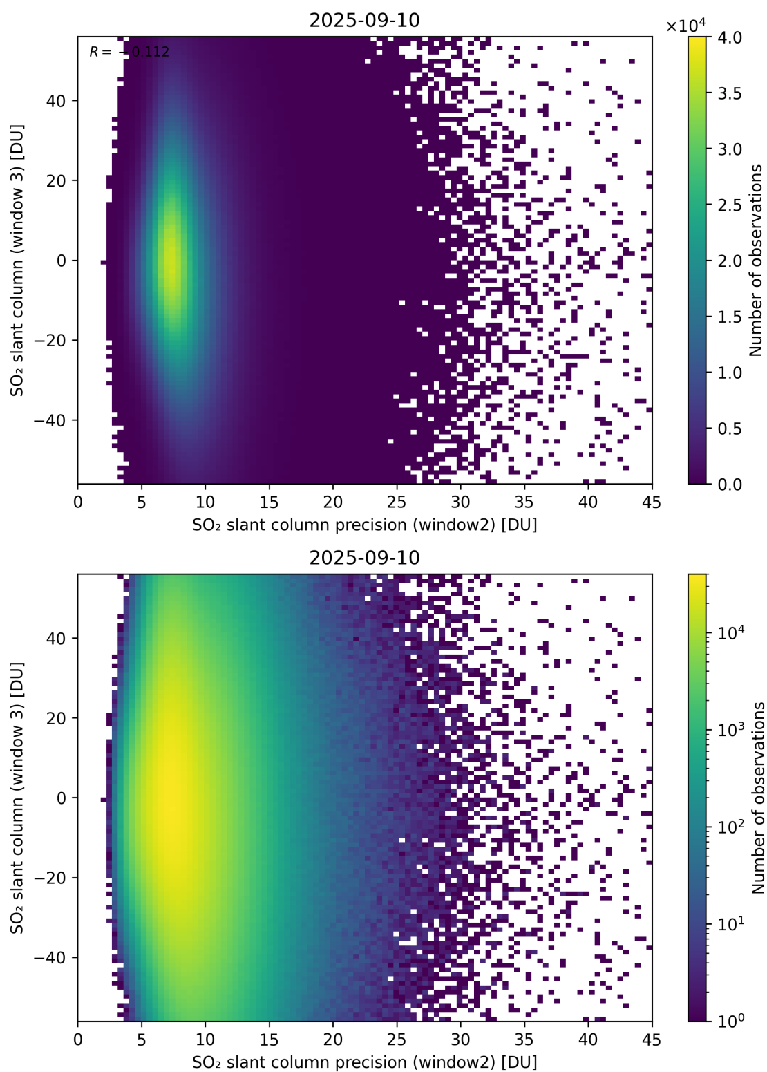
Figure 299: Scatter density plot of “SO 2 slant column precision (window2)” against “SO 2 slant column (window 3)” for 2025-09-10 to 2025-09-11.
