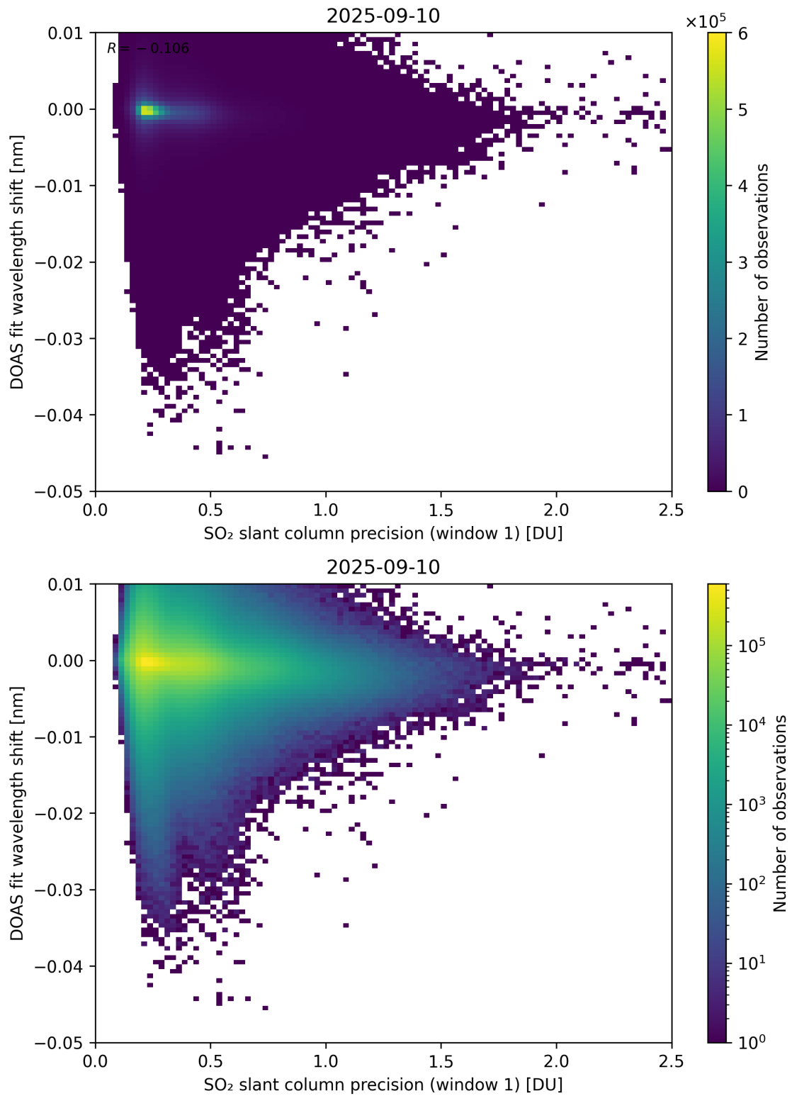
Figure 271: Scatter density plot of “SO 2 slant column precision (window 1)” against “DOAS fit wavelength shift” for 2025-09-10 to 2025-09-11.
