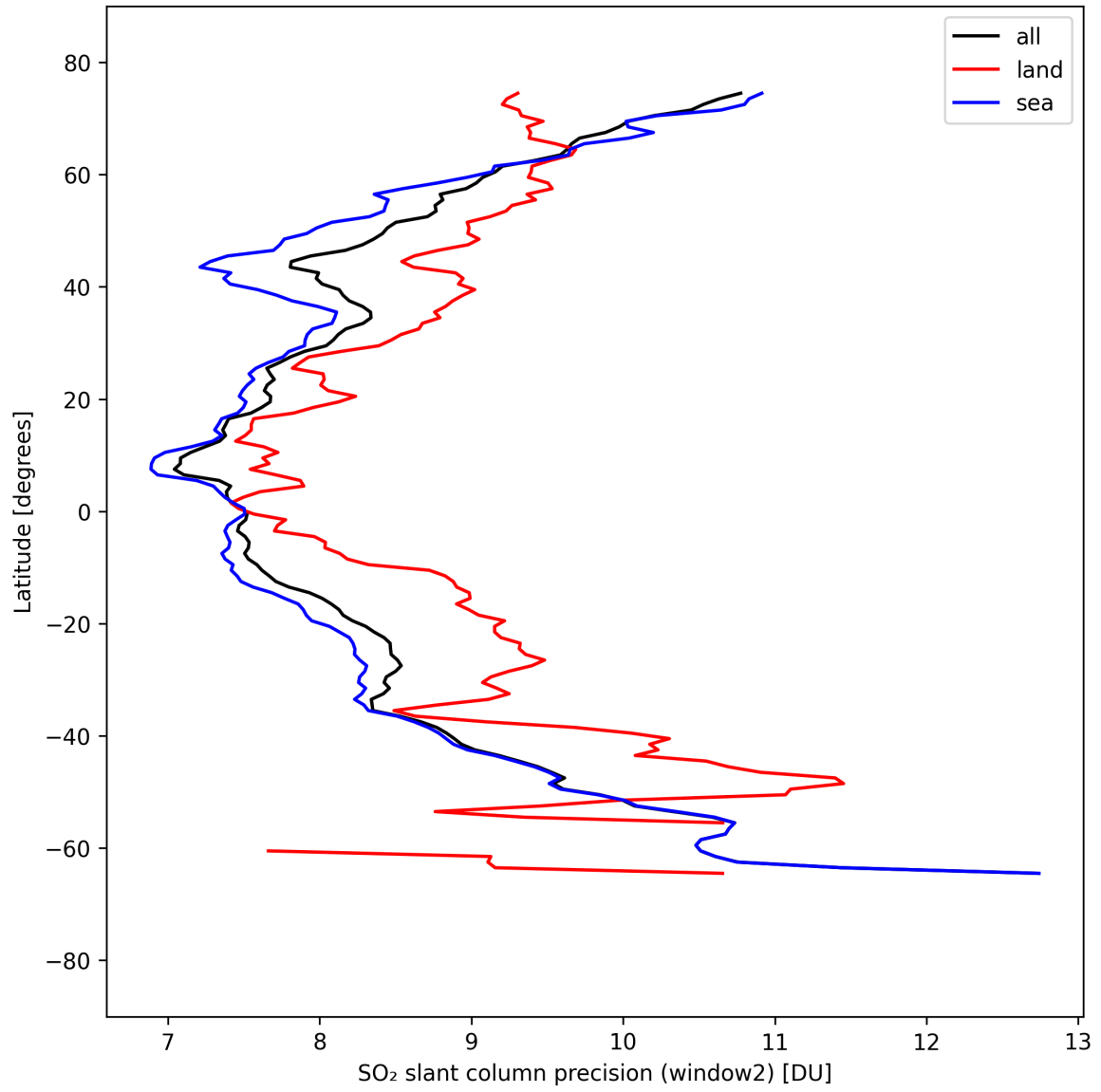
Figure 42: Zonal average of “SO 2 slant column precision (window2)” for 2025-09-10 to 2025-09-11.
