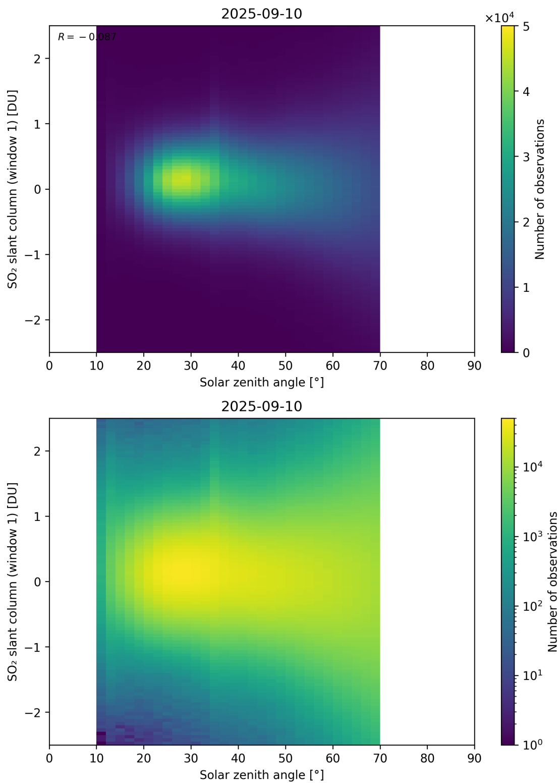
Figure 184: Scatter density plot of “Solar zenith angle” against “SO 2 slant column (window 1)” for 2025-09-10 to 2025-09-11.
