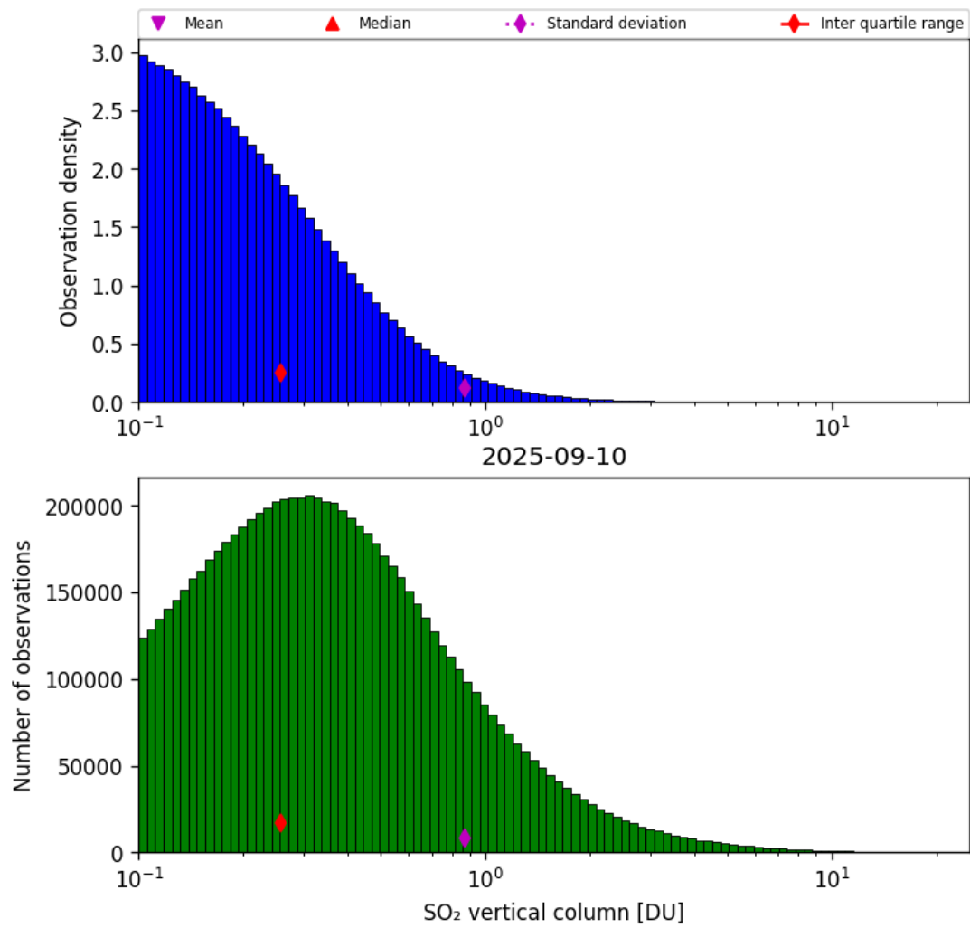
Figure 58: Histogram of “SO 2 vertical column” for 2025-09-10 to 2025-09-11
