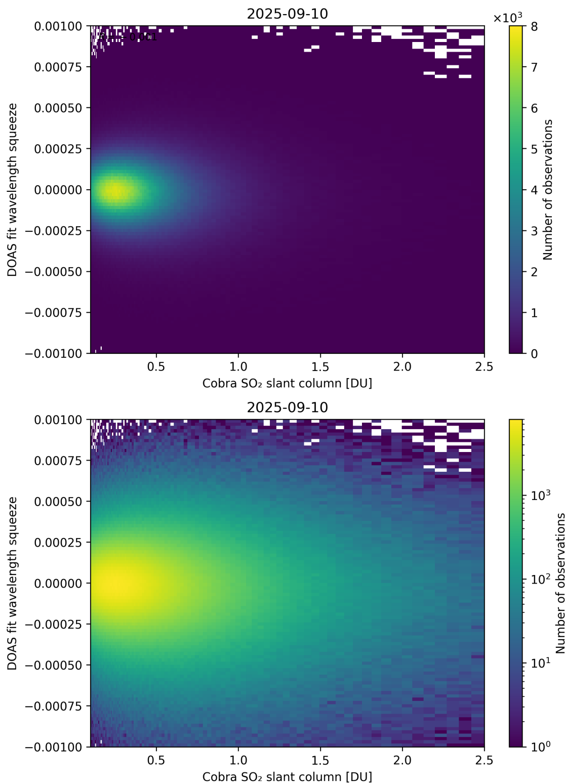
Figure 197: Scatter density plot of “Cobra SO 2 slant column” against “DOAS fit wavelength squeeze” for 2025-09-10 to 2025-09-11.
