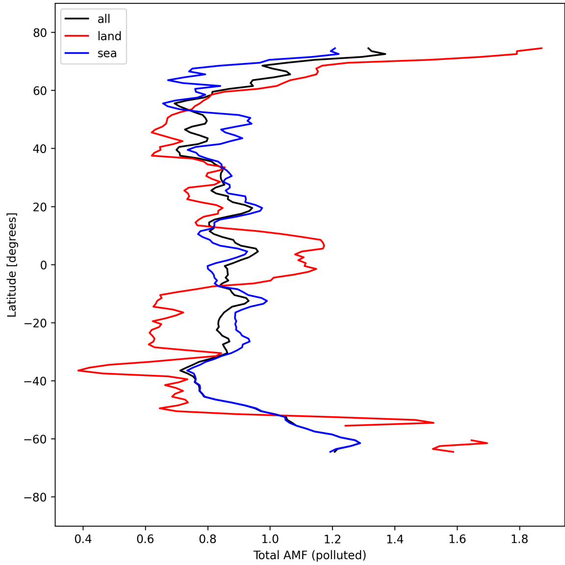
Figure 53: Zonal average of “Total AMF (polluted)” for 2025-09-10 to 2025-09-11.
