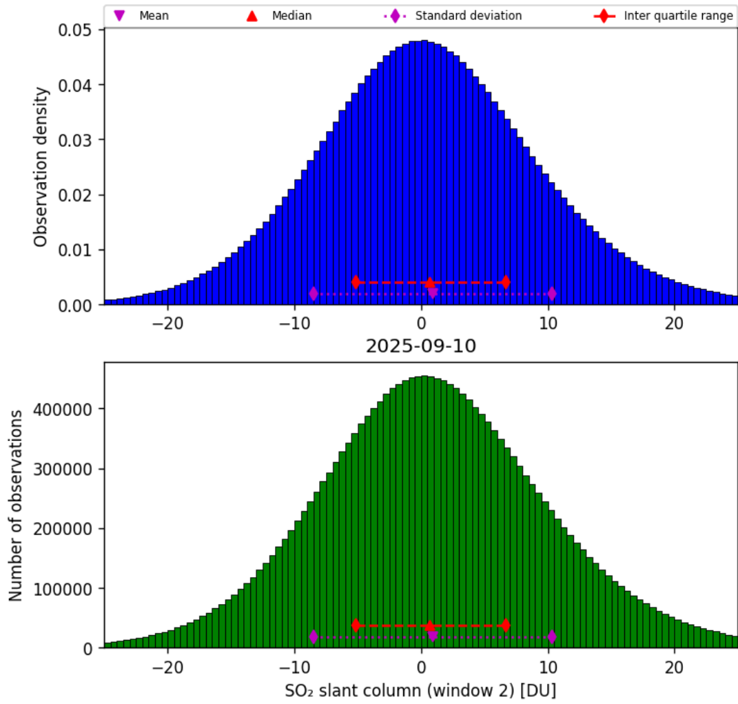
Figure 67: Histogram of “SO 2 slant column (window 2)” for 2025-09-10 to 2025-09-11
