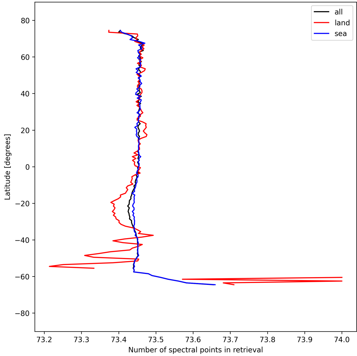
Figure 56: Zonal average of “Number of spectral points in retrieval” for 2025-09-10 to 2025-09-11.
