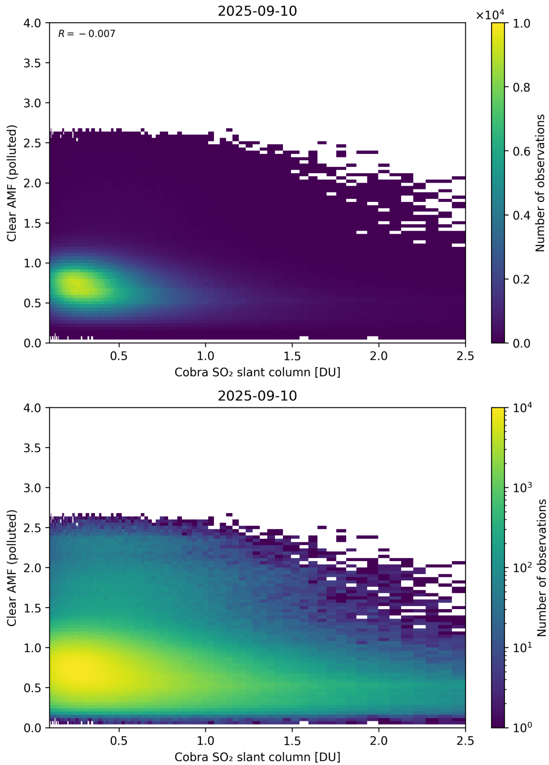
Figure 215: Scatter density plot of “Cobra SO 2 slant column” against “Clear AMF (polluted)” for 2025-09-10 to 2025-09-11.
