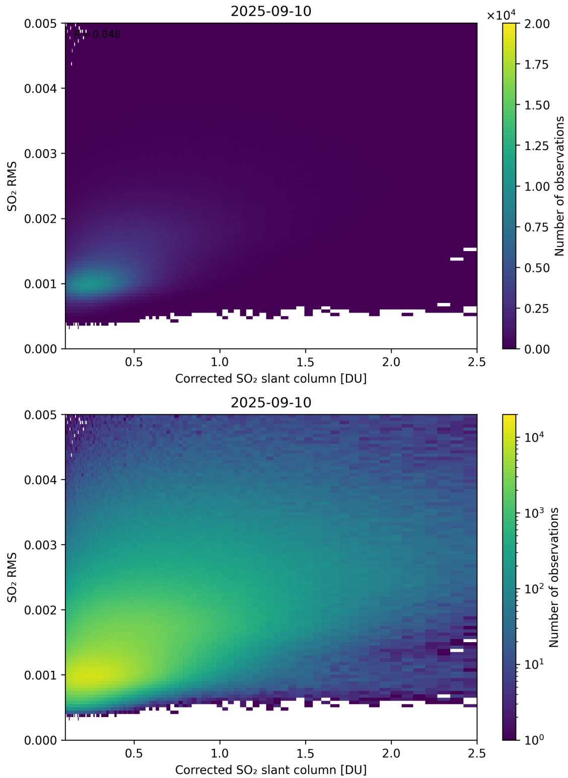
Figure 231: Scatter density plot of “Corrected SO 2 slant column” against “SO 2 RMS” for 2025-09-10 to 2025-09-11.
