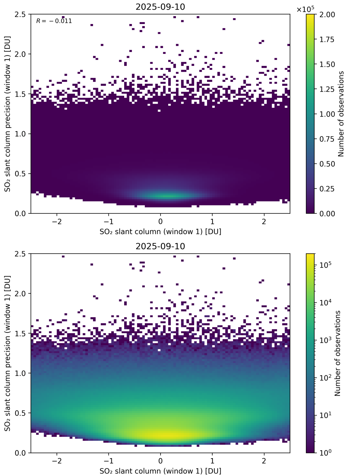
Figure 285: Scatter density plot of “SO 2 slant column (window 1)” against “SO 2 slant column precision (window 1)” for 2025-09-10 to 2025-09-11.
