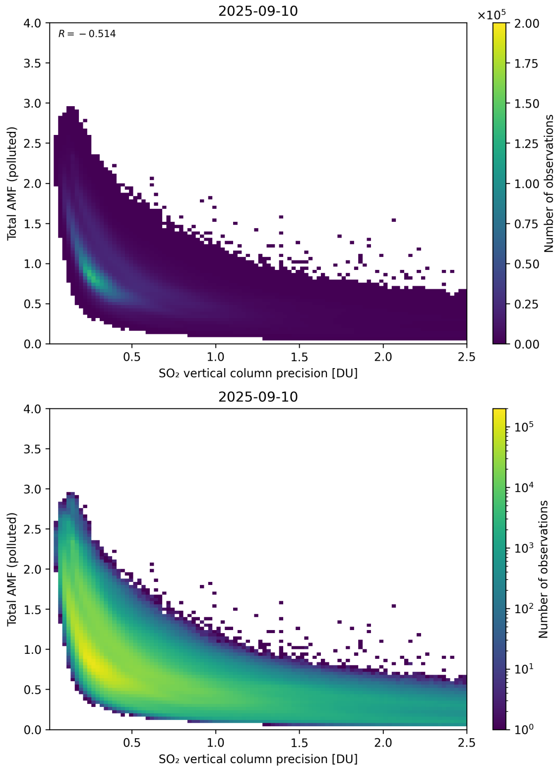
Figure 346: Scatter density plot of “SO 2 vertical column precision” against “Total AMF (polluted)” for 2025-09-10 to 2025-09-11.
