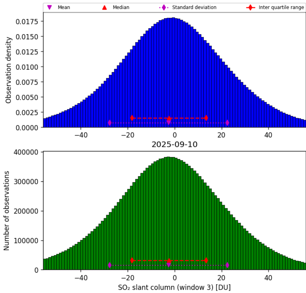
Figure 71: Histogram of “SO 2 slant column (window 3)” for 2025-09-10 to 2025-09-11
