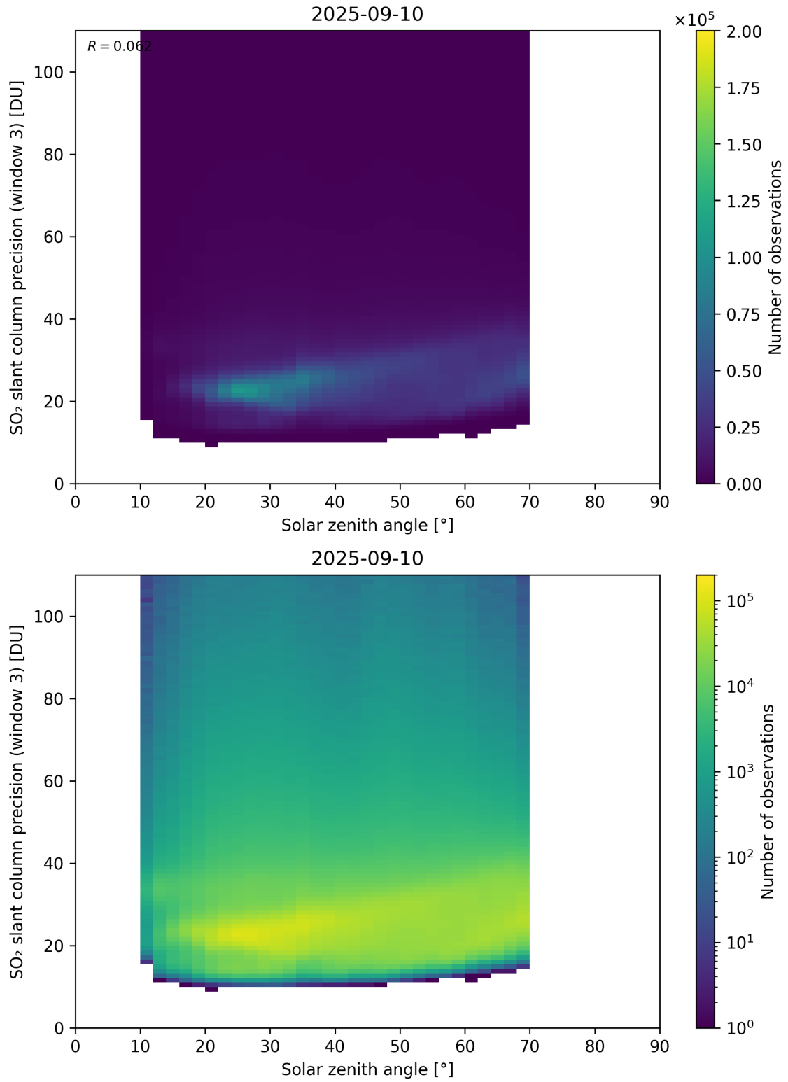
Figure 188: Scatter density plot of “Solar zenith angle” against “SO 2 slant column precision (window 3)” for 2025-09-10 to 2025-09-11.
