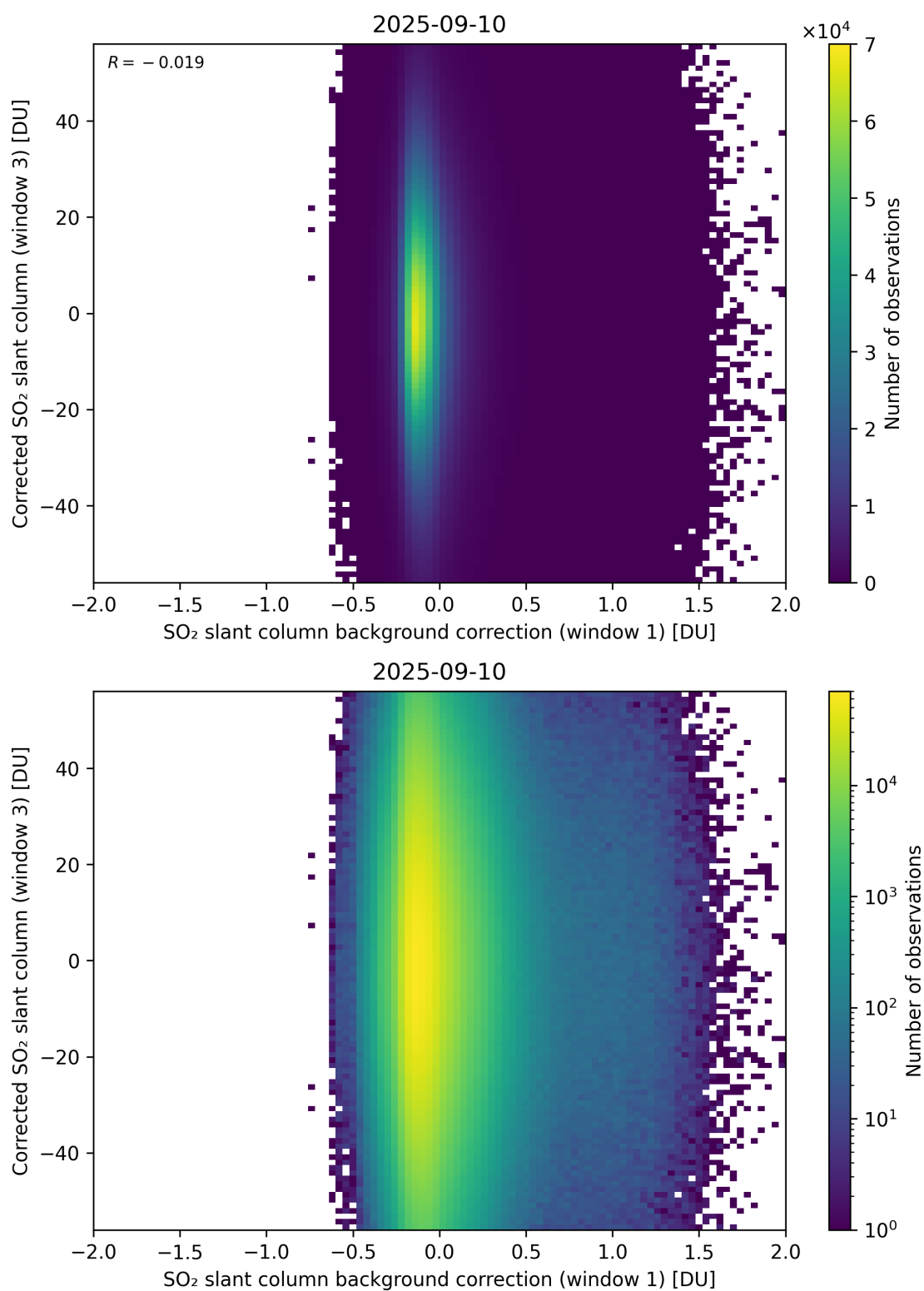
Figure 116: Scatter density plot of “SO 2 slant column background correction (window 1)” against “Corrected SO 2 slant column (window 3)” for 2025-09-10 to 2025-09-11.
