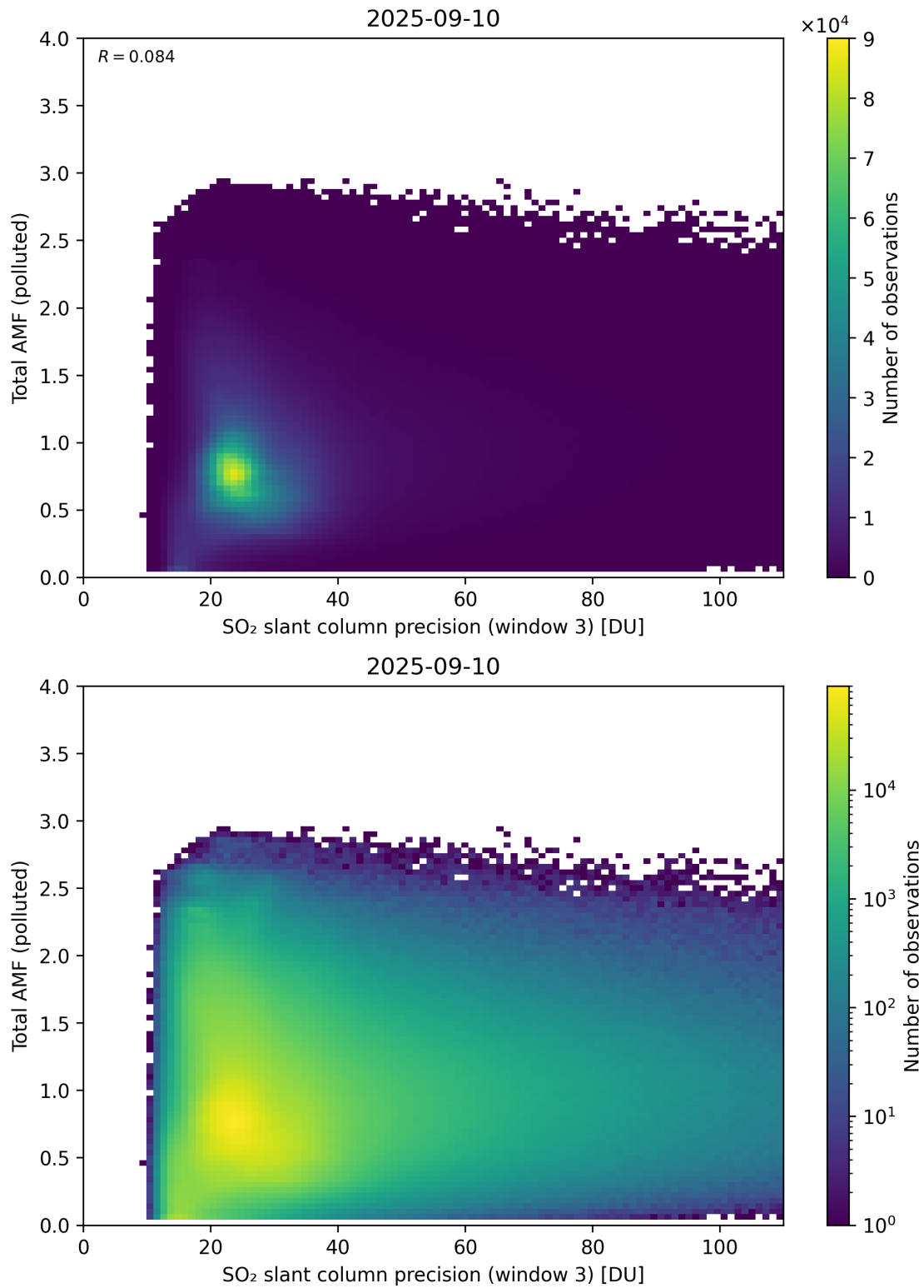
Figure 313: Scatter density plot of “SO 2 slant column precision (window 3)” against “Total AMF (polluted)” for 2025-09-10 to 2025-09-11.
