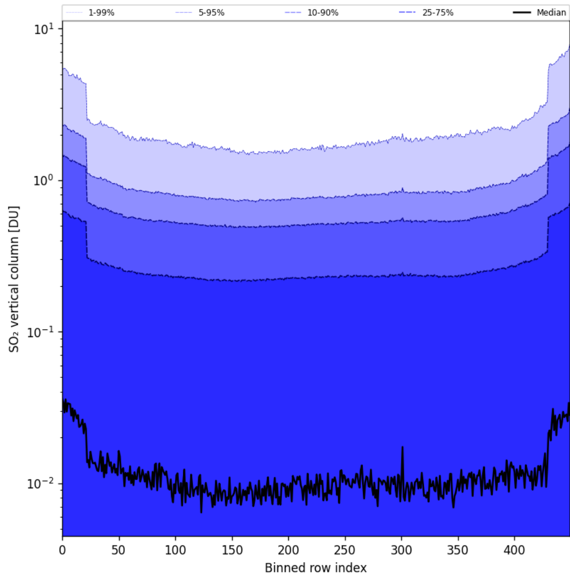
Figure 84: Along track statistics of “SO 2 vertical column” for 2025-09-10 to 2025-09-11
