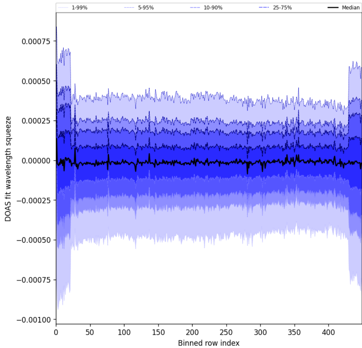
Figure 103: Along track statistics of “DOAS fit wavelength squeeze” for 2025-09-10 to 2025-09-11
