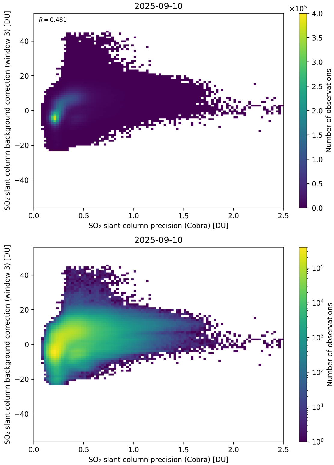
Figure 201: Scatter density plot of “SO 2 slant column precision (Cobra)” against “SO 2 slant column background correction (window 3)” for 2025-09-10 to 2025-09-11.
