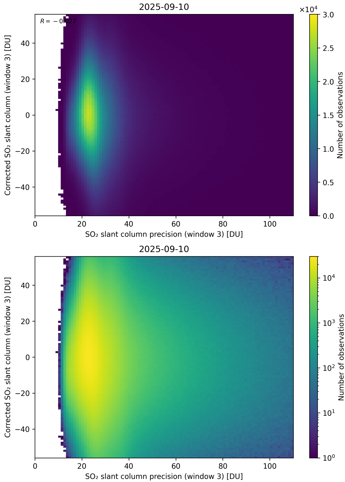
Figure 312: Scatter density plot of “SO 2 slant column precision (window 3)” against “Corrected SO 2 slant column (window 3)” for 2025-09-10 to 2025-09-11.
