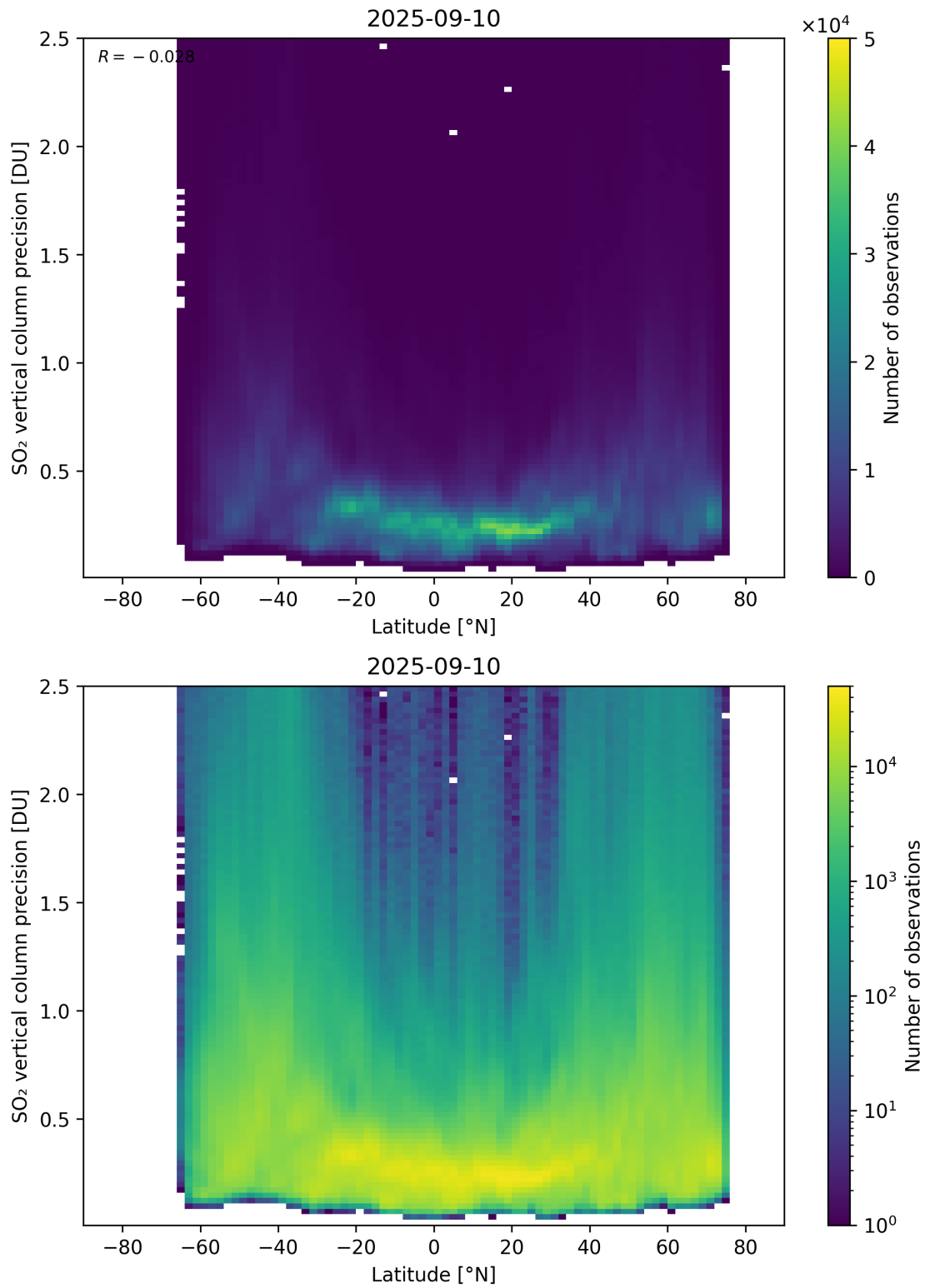
Figure 170: Scatter density plot of “Latitude” against “SO 2 vertical column precision” for 2025-09-10 to 2025-09-11.
