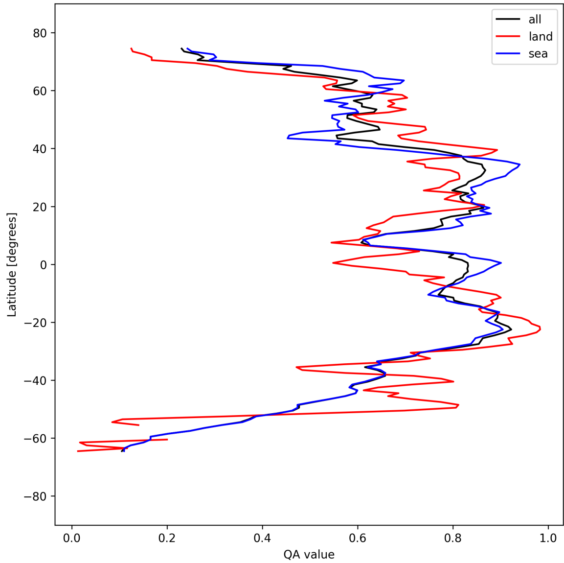
Figure 31: Zonal average of “QA value” for 2025-09-10 to 2025-09-11.
