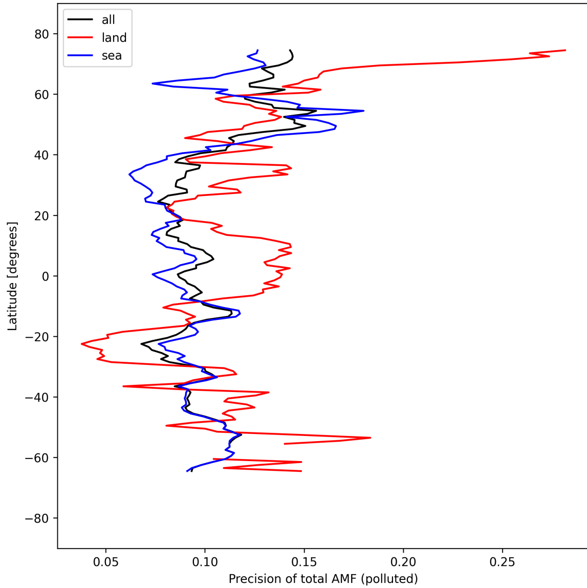
Figure 54: Zonal average of “Precision of total AMF (polluted)” for 2025-09-10 to 2025-09-11.
