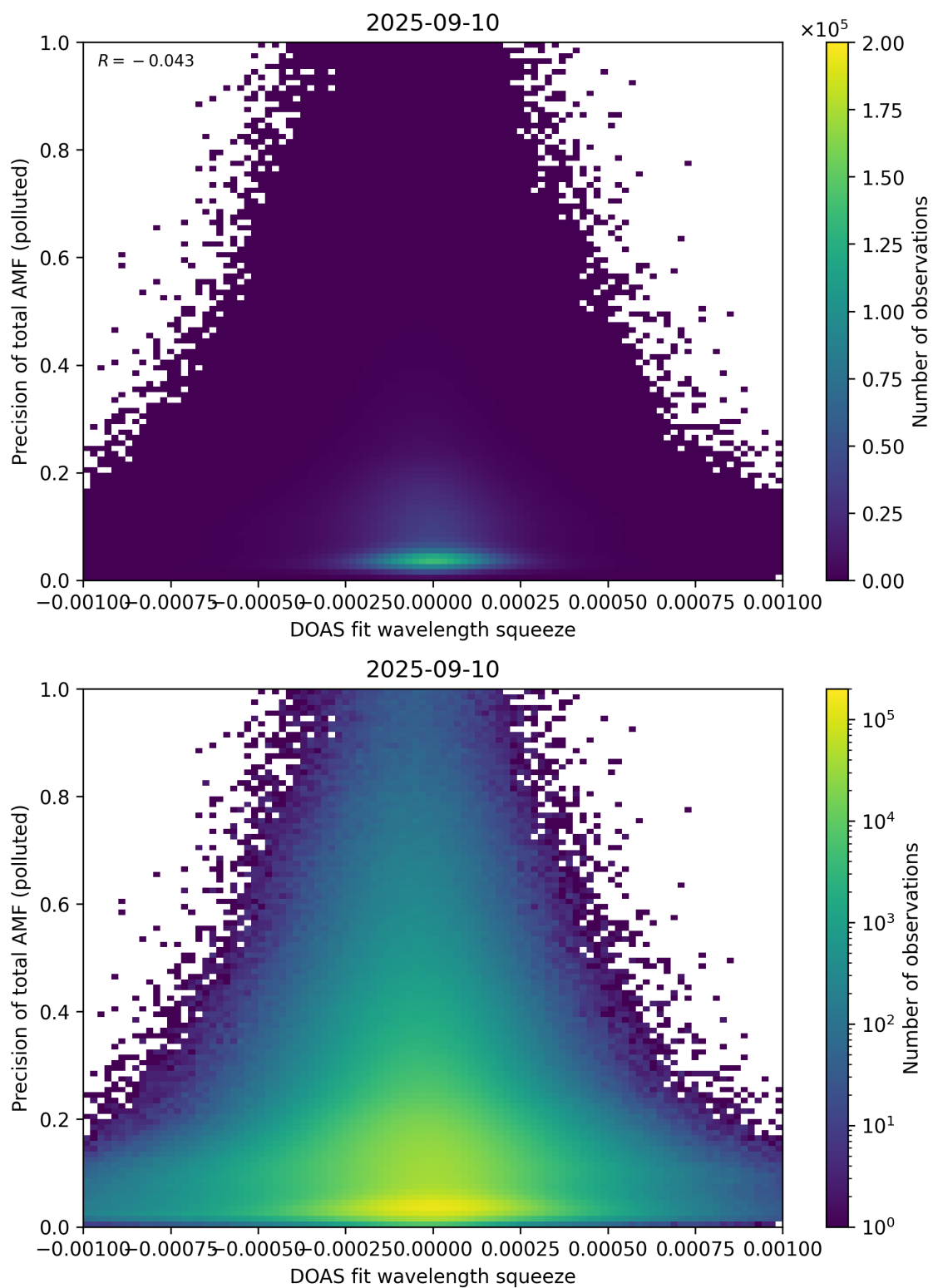
Figure 146: Scatter density plot of “DOAS fit wavelength squeeze” against “Precision of total AMF (polluted)” for 2025-09-10 to 2025-09-11.
