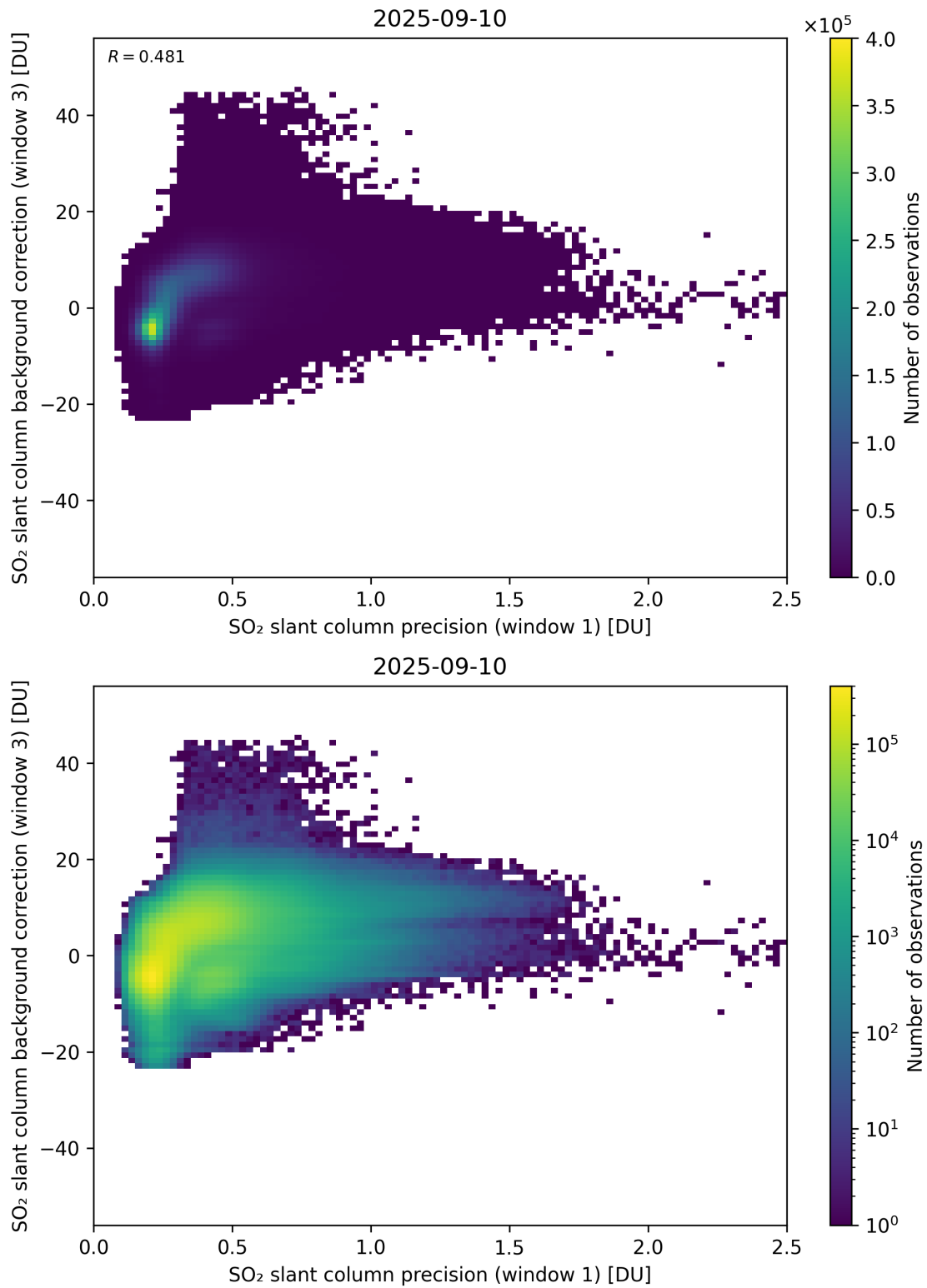
Figure 270: Scatter density plot of “SO 2 slant column precision (window 1)” against “SO 2 slant column background correction (window 3)” for 2025-09-10 to 2025-09-11.
