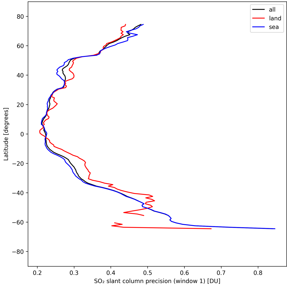
Figure 38: Zonal average of “SO 2 slant column precision (window 1)” for 2025-09-10 to 2025-09-11.
