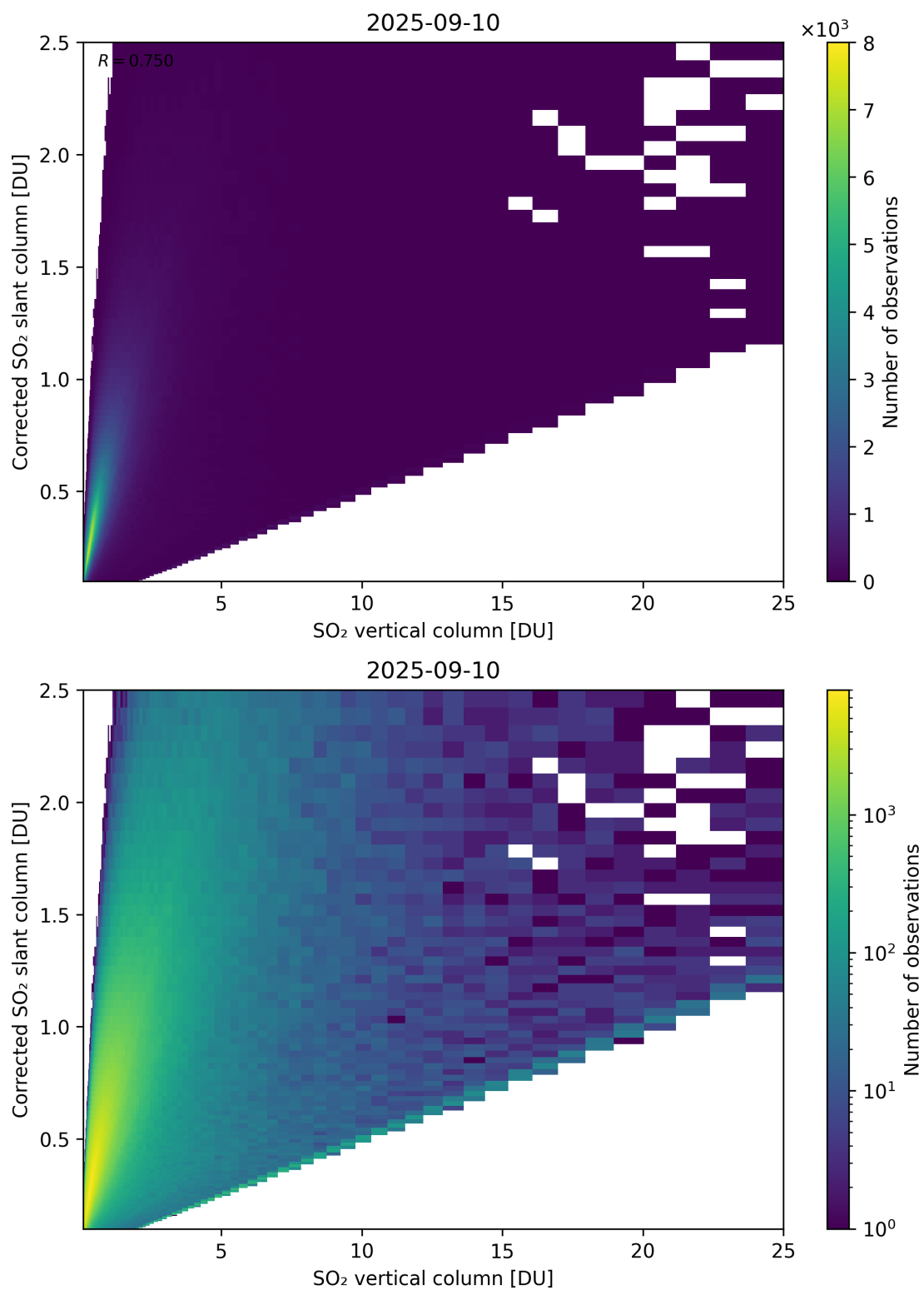
Figure 351: Scatter density plot of “SO 2 vertical column” against “Corrected SO 2 slant column” for 2025-09-10 to 2025-09-11.
