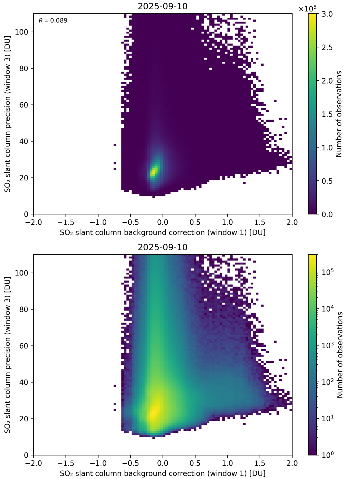
Figure 119: Scatter density plot of “SO 2 slant column background correction (window 1)” against “SO 2 slant column precision (window 3)” for 2025-09-10 to 2025-09-11.
