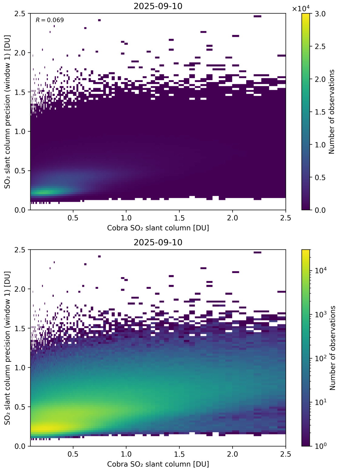
Figure 220: Scatter density plot of “Cobra SO 2 slant column” against “SO 2 slant column precision (window 1)” for 2025-09-10 to 2025-09-11.
