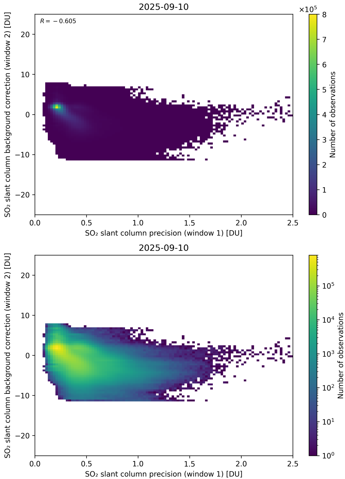
Figure 269: Scatter density plot of “SO 2 slant column precision (window 1)” against “SO 2 slant column background correction (window 2)” for 2025-09-10 to 2025-09-11.
