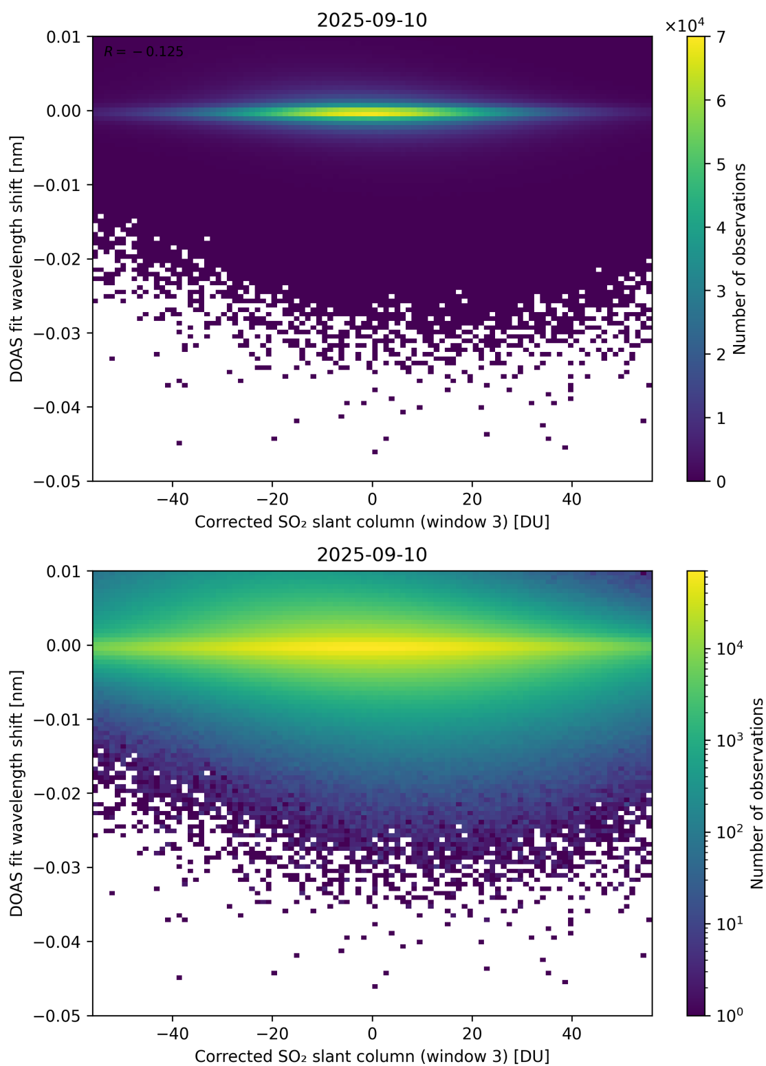
Figure 256: Scatter density plot of “Corrected SO 2 slant column (window 3)” against “DOAS fit wavelength shift” for 2025-09-10 to 2025-09-11.
