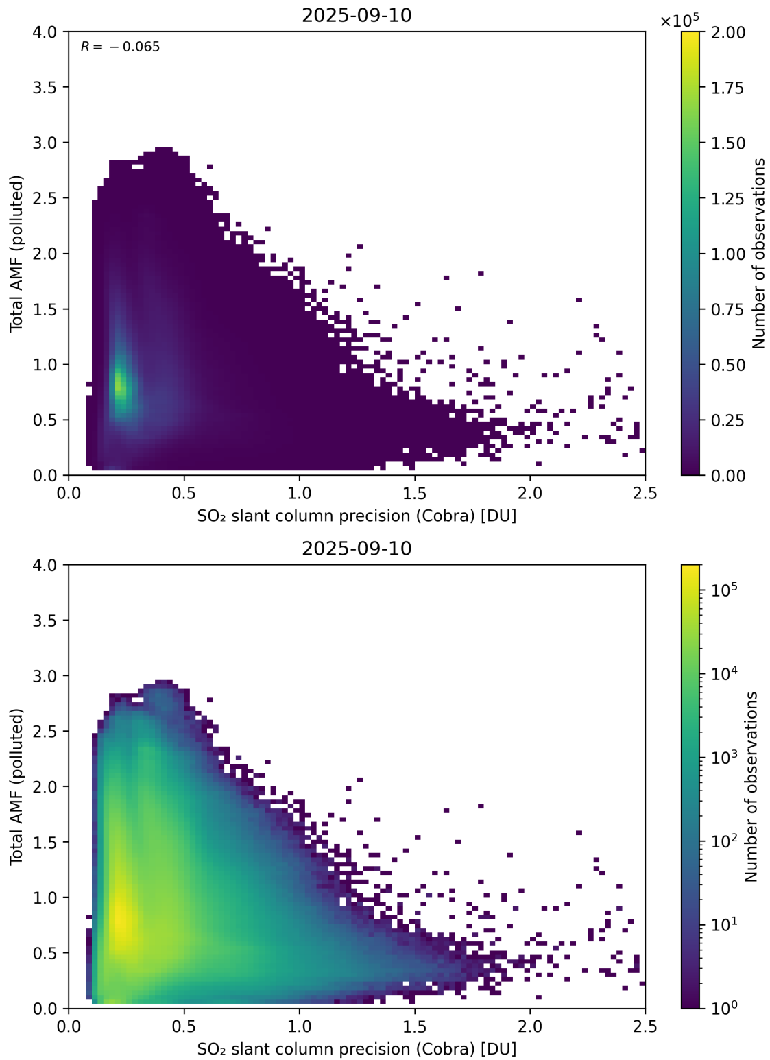
Figure 213: Scatter density plot of “SO 2 slant column precision (Cobra)” against “Total AMF (polluted)” for 2025-09-10 to 2025-09-11.
