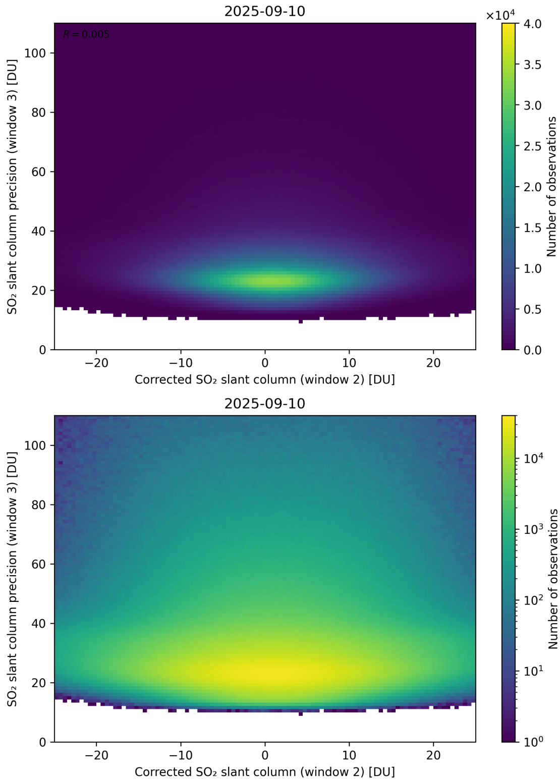
Figure 252: Scatter density plot of “Corrected SO 2 slant column (window 2)” against “SO 2 slant column precision (window 3)” for 2025-09-10 to 2025-09-11.
