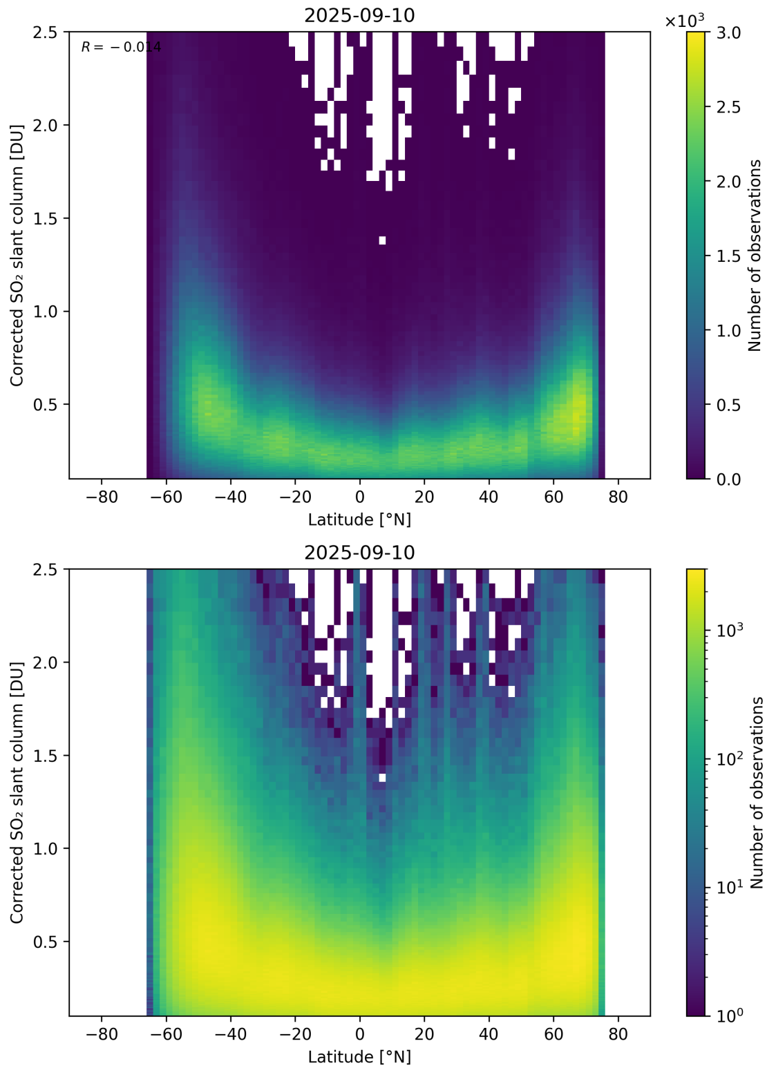
Figure 159: Scatter density plot of “Latitude” against “Corrected SO 2 slant column” for 2025-09-10 to 2025-09-11.
