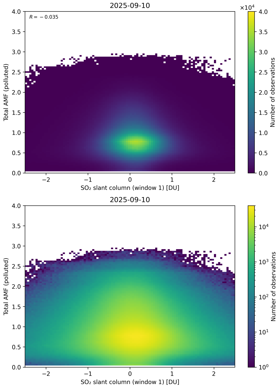
Figure 289: Scatter density plot of “SO 2 slant column (window 1)” against “Total AMF (polluted)” for 2025-09-10 to 2025-09-11.
