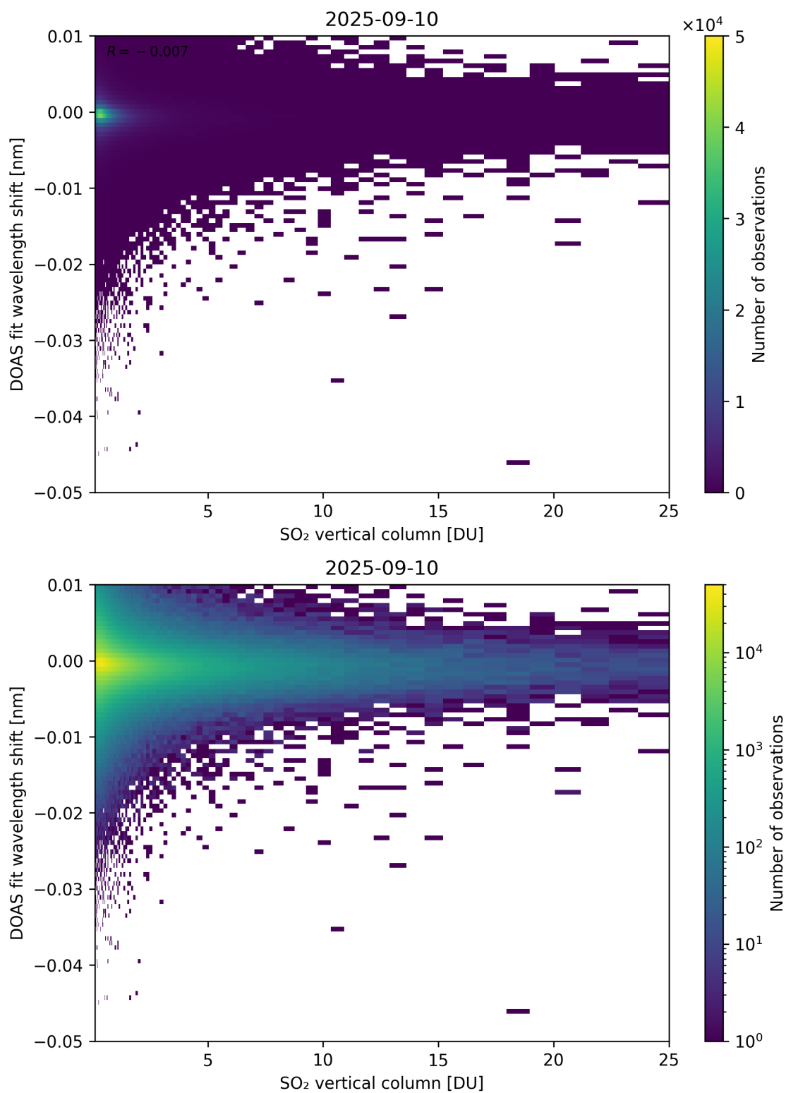
Figure 326: Scatter density plot of “SO 2 vertical column” against “DOAS fit wavelength shift” for 2025-09-10 to 2025-09-11.
