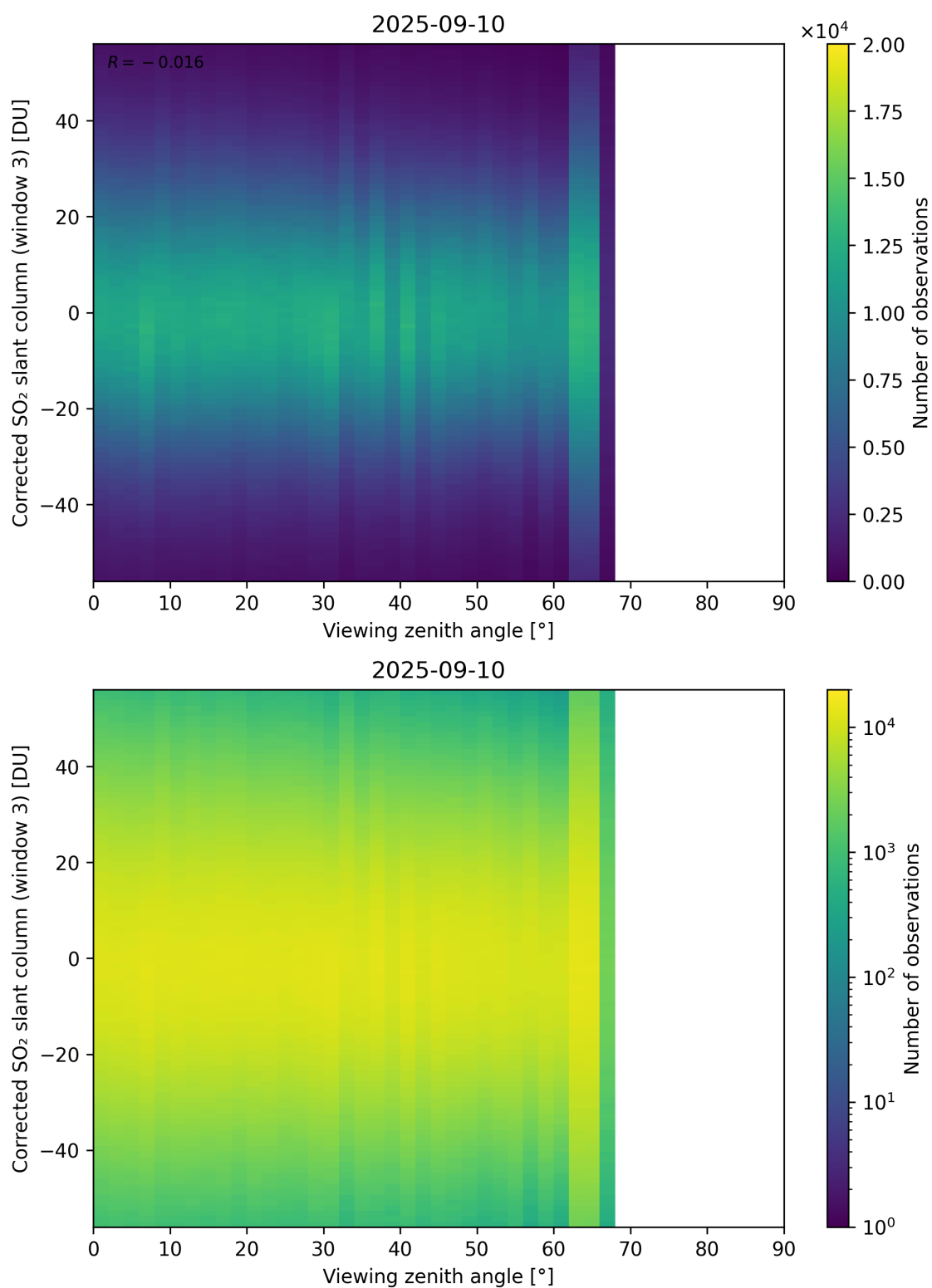
Figure 375: Scatter density plot of “Viewing zenith angle” against “Corrected SO 2 slant column (window 3)” for 2025-09-10 to 2025-09-11.
