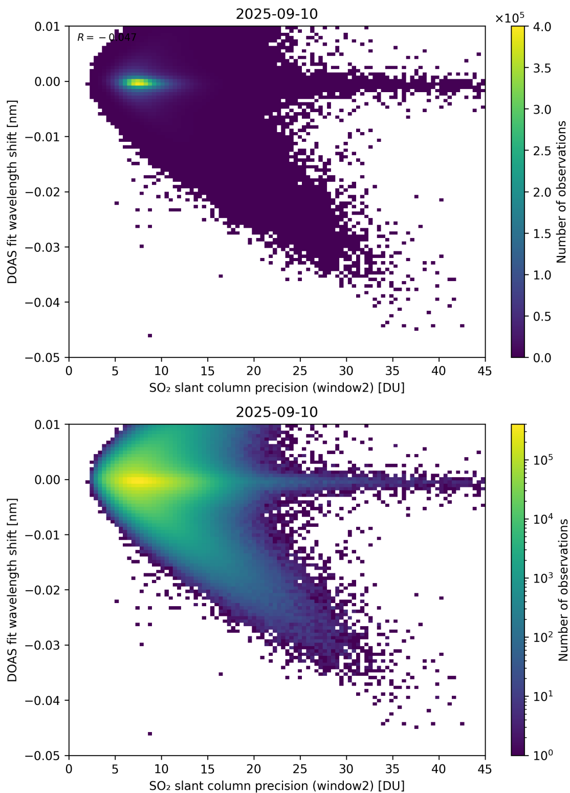
Figure 293: Scatter density plot of “SO 2 slant column precision (window2)” against “DOAS fit wavelength shift” for 2025-09-10 to 2025-09-11.
