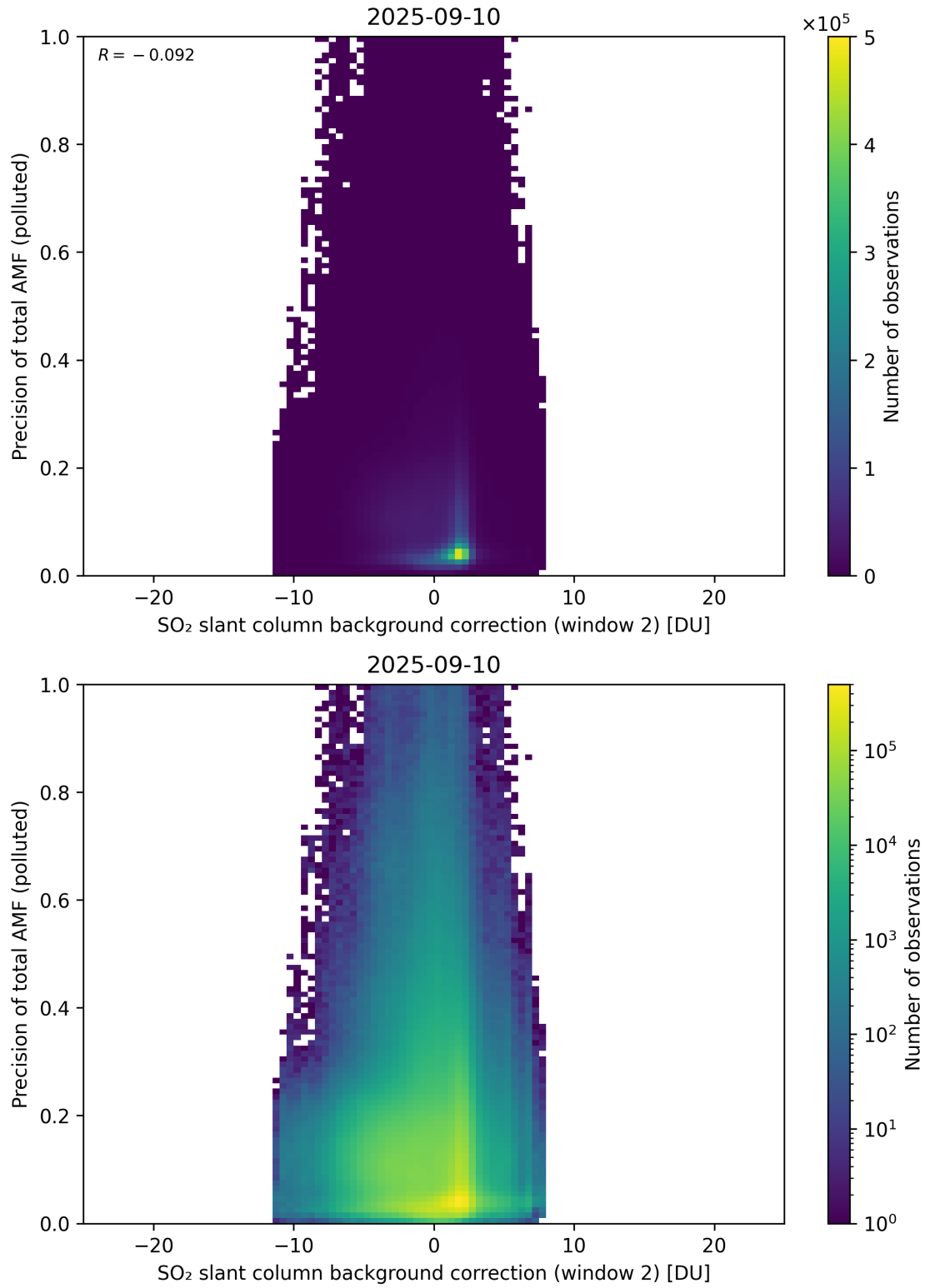
Figure 131: Scatter density plot of “SO 2 slant column background correction (window 2)” against “Precision of total AMF (polluted)” for 2025-09-10 to 2025-09-11.
