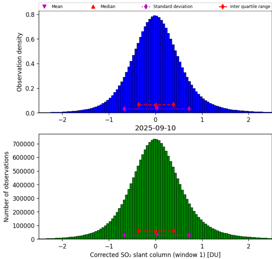
Figure 65: Histogram of “Corrected SO 2 slant column (window 1)” for 2025-09-10 to 2025-09-11
