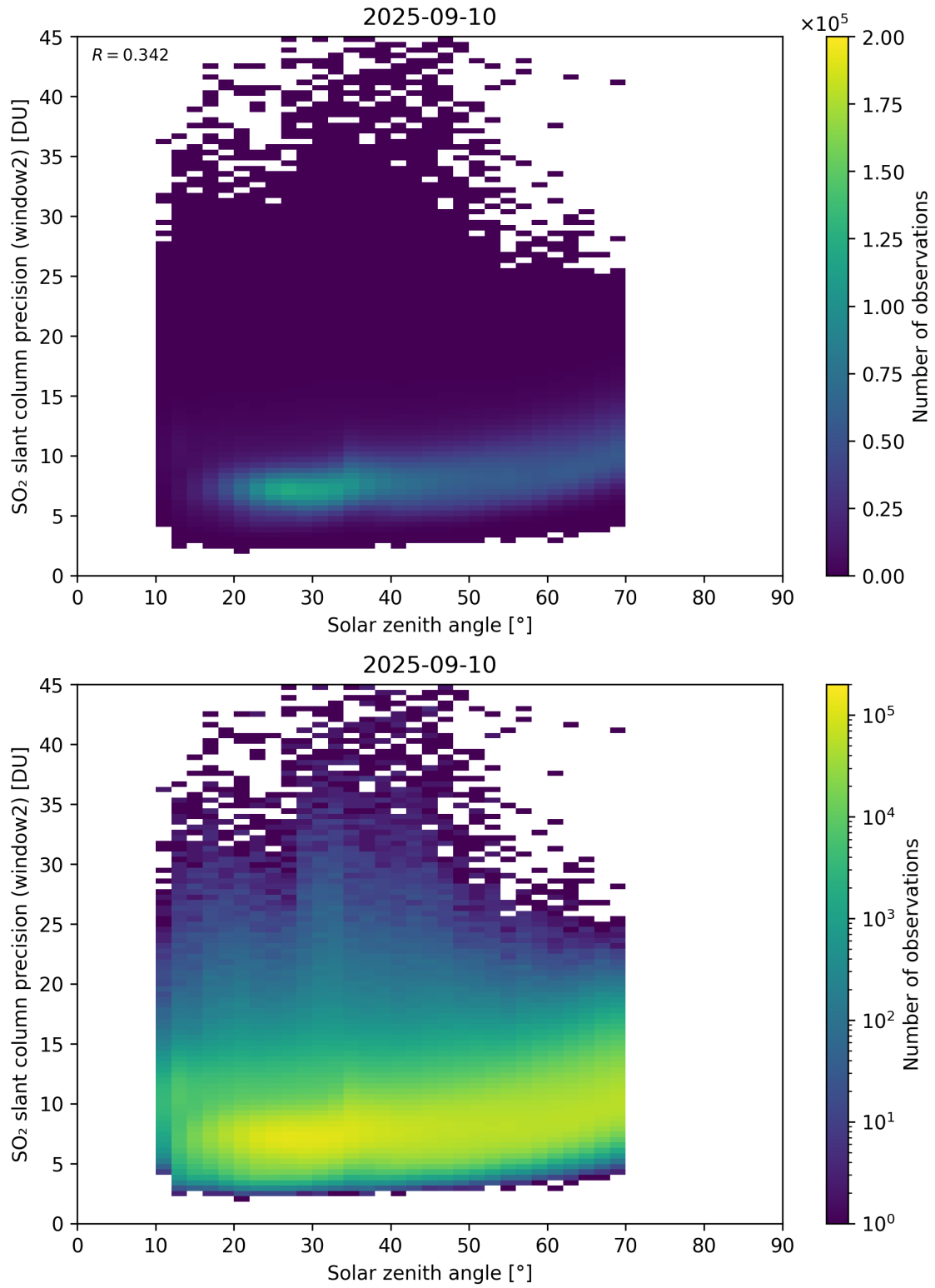
Figure 186: Scatter density plot of “Solar zenith angle” against “SO 2 slant column precision (window2)” for 2025-09-10 to 2025-09-11.
