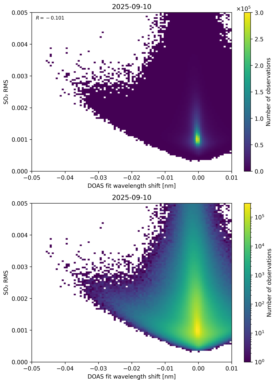
Figure 139: Scatter density plot of “DOAS fit wavelength shift” against “SO 2 RMS” for 2025-09-10 to 2025-09-11.
