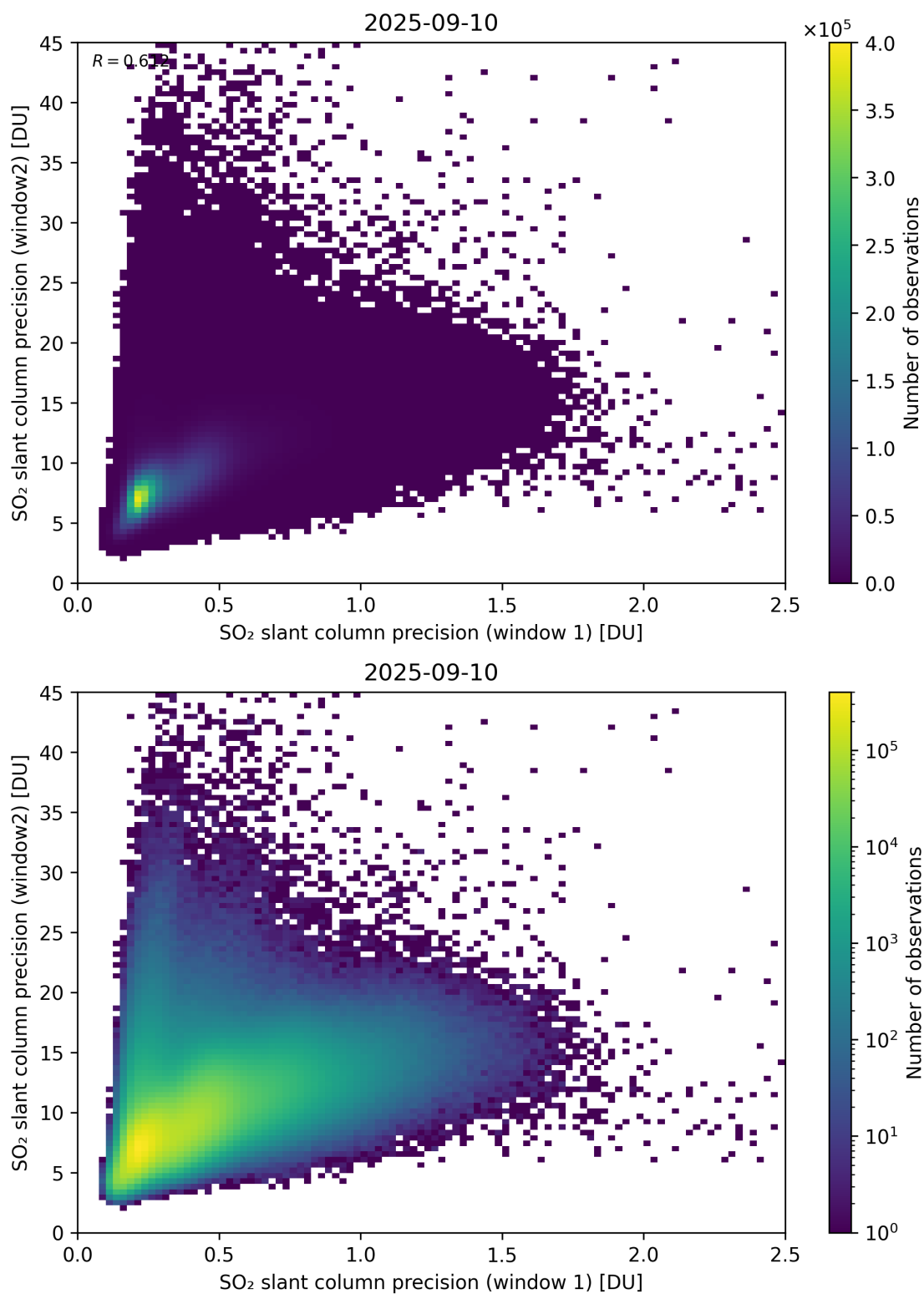
Figure 277: Scatter density plot of “SO 2 slant column precision (window 1)” against “SO 2 slant column precision (window2)” for 2025-09-10 to 2025-09-11.
