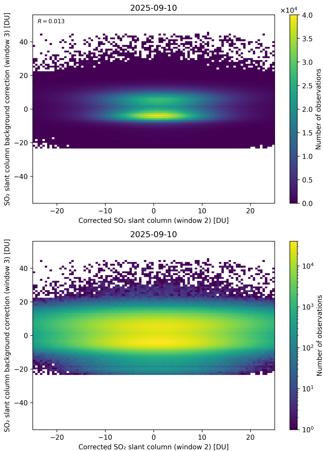
Figure 245: Scatter density plot of “Corrected SO 2 slant column (window 2)” against “SO 2 slant column background correction (window 3)” for 2025-09-10 to 2025-09-11.
