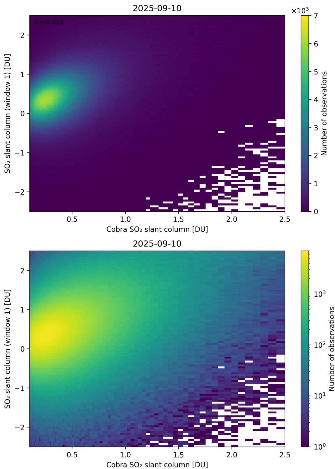
Figure 219: Scatter density plot of “Cobra SO 2 slant column” against “SO 2 slant column (window 1)” for 2025-09-10 to 2025-09-11.
