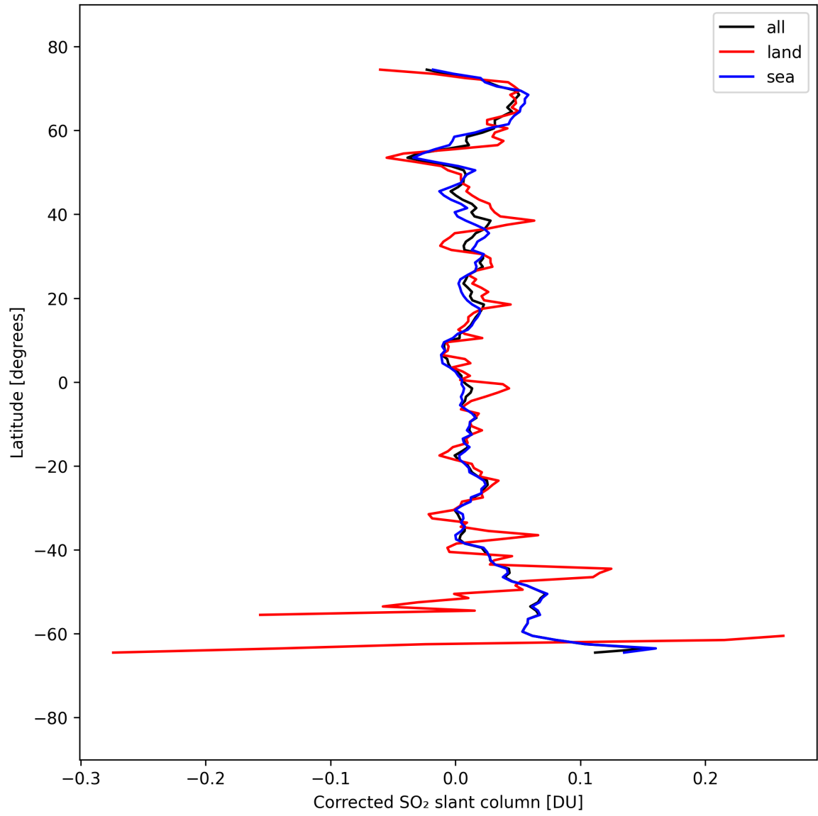
Figure 34: Zonal average of "Corrected SO 2 slant column" for 2025-09-10 to 2025-09-11.
