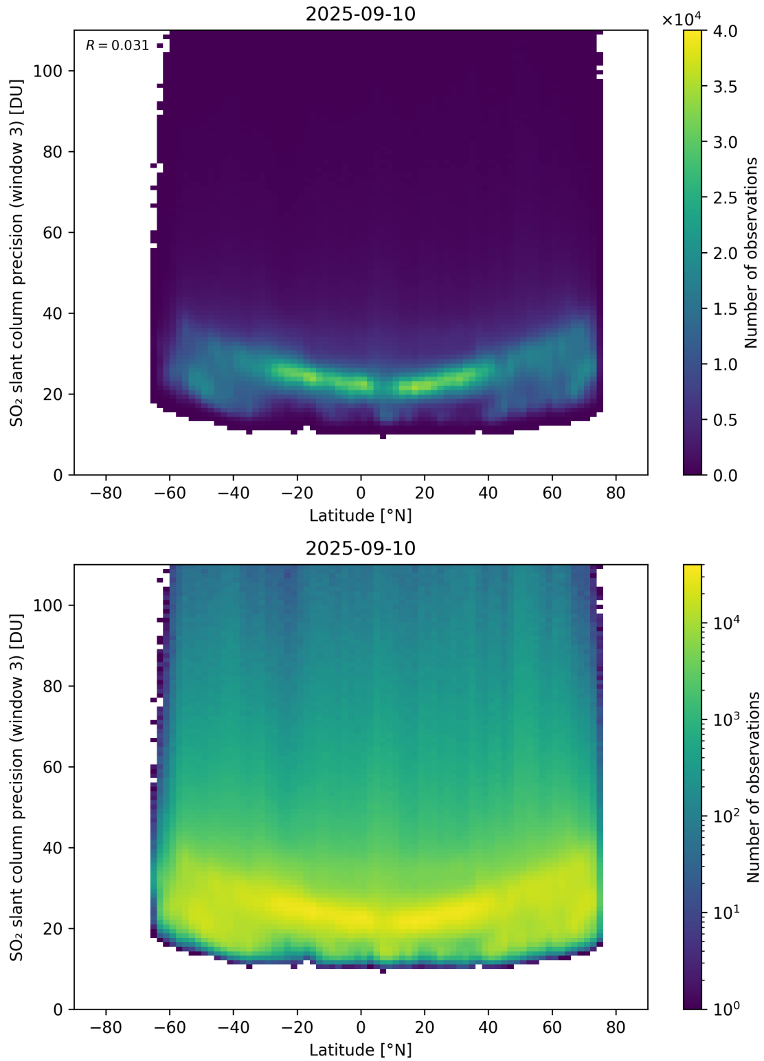
Figure 166: Scatter density plot of “Latitude” against “SO 2 slant column precision (window 3)” for 2025-09-10 to 2025-09-11.
