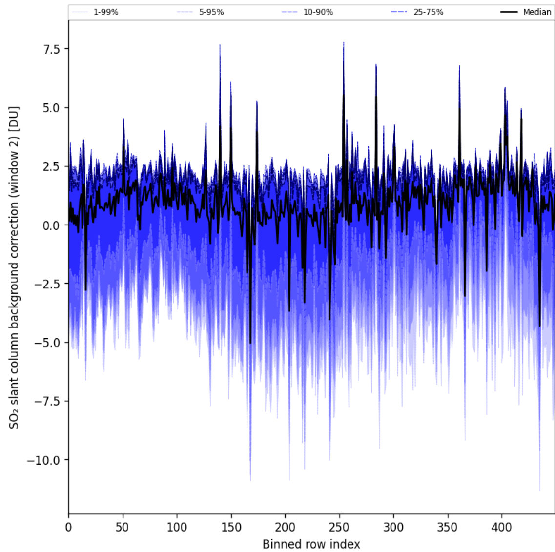
Figure 96: Along track statistics of “SO 2 slant column background correction (window 2)” for 2025-09-10 to 2025-09-11
