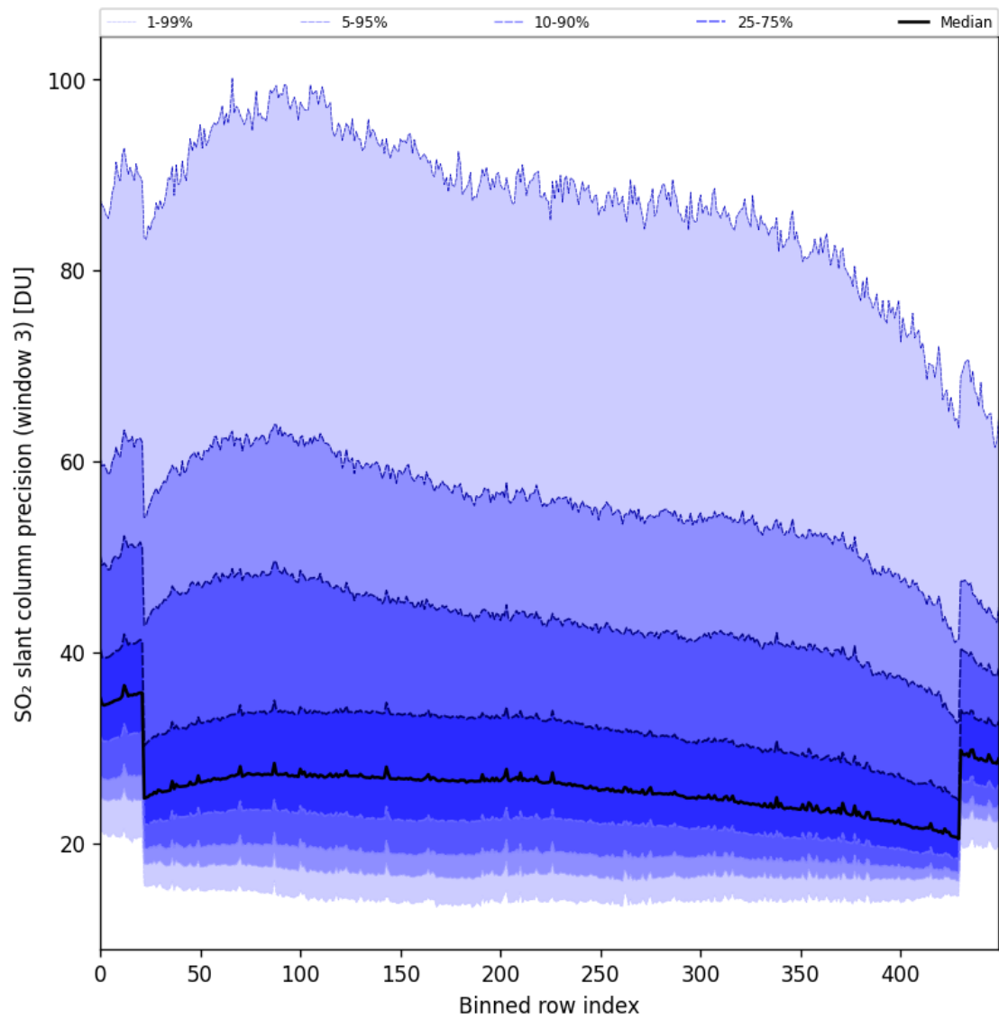
Figure 98: Along track statistics of “SO 2 slant column precision (window 3)” for 2025-09-10 to 2025-09-11
