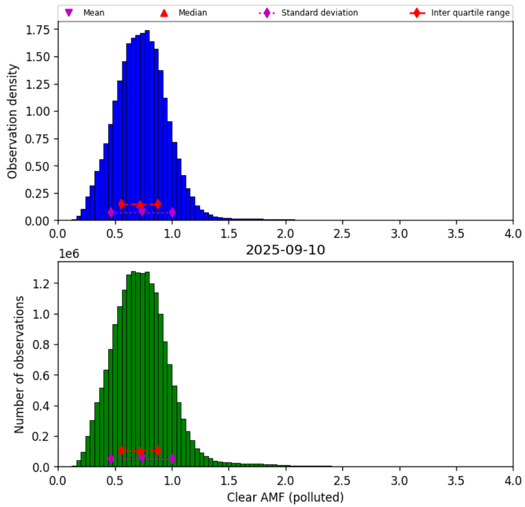
Figure 81: Histogram of “Clear AMF (polluted)” for 2025-09-10 to 2025-09-11
