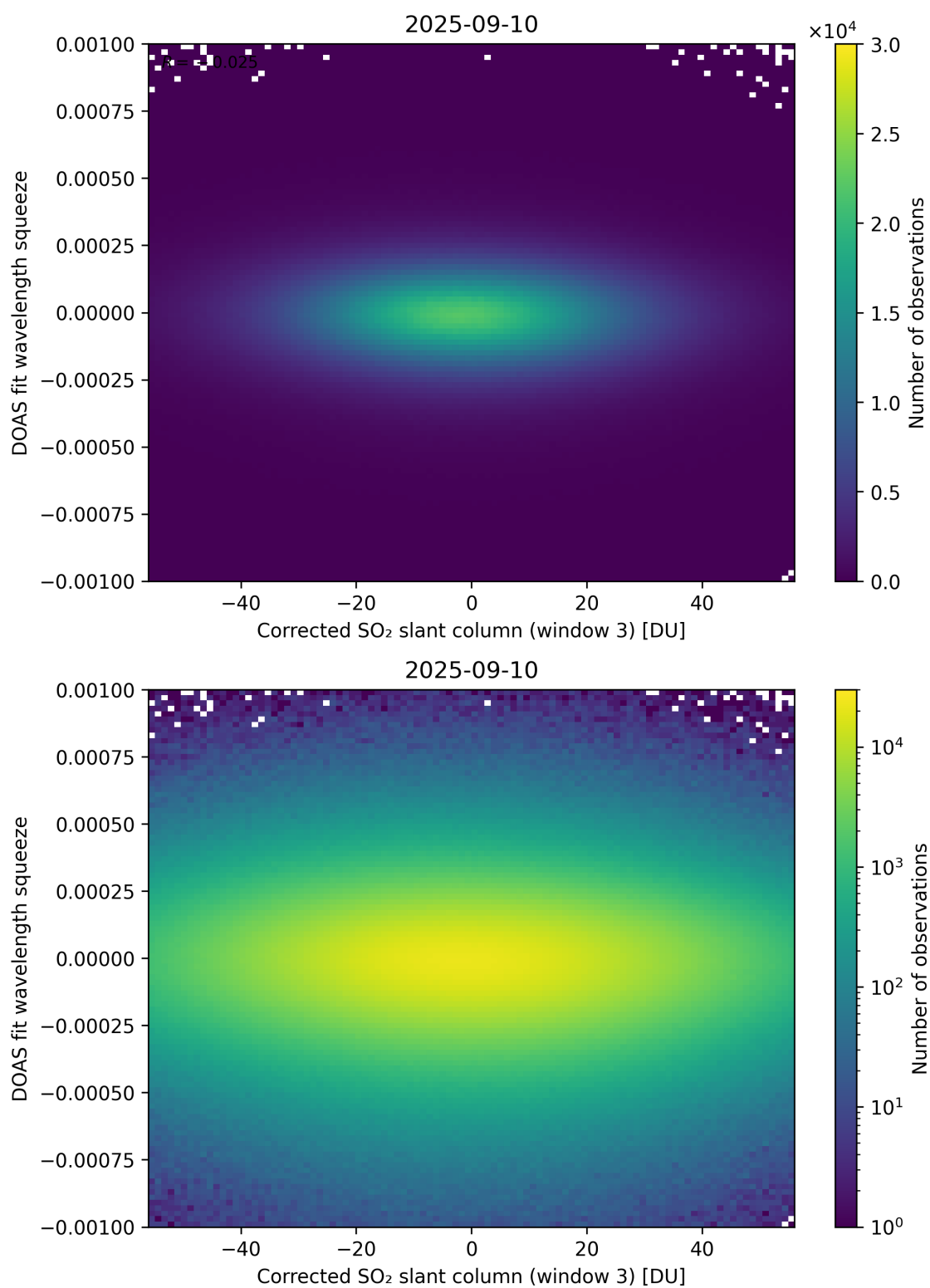
Figure 257: Scatter density plot of “Corrected SO 2 slant column (window 3)” against “DOAS fit wavelength squeeze” for 2025-09-10 to 2025-09-11.
