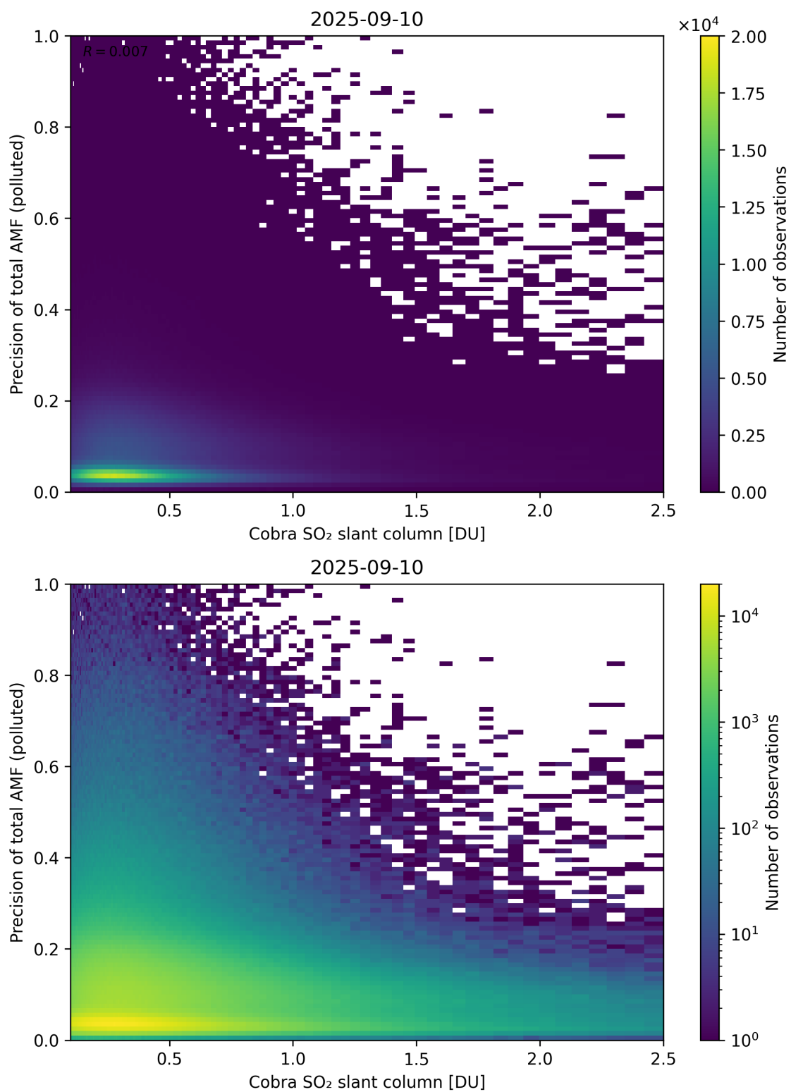
Figure 225: Scatter density plot of “Cobra SO 2 slant column” against “Precision of total AMF (polluted)” for 2025-09-10 to 2025-09-11.
