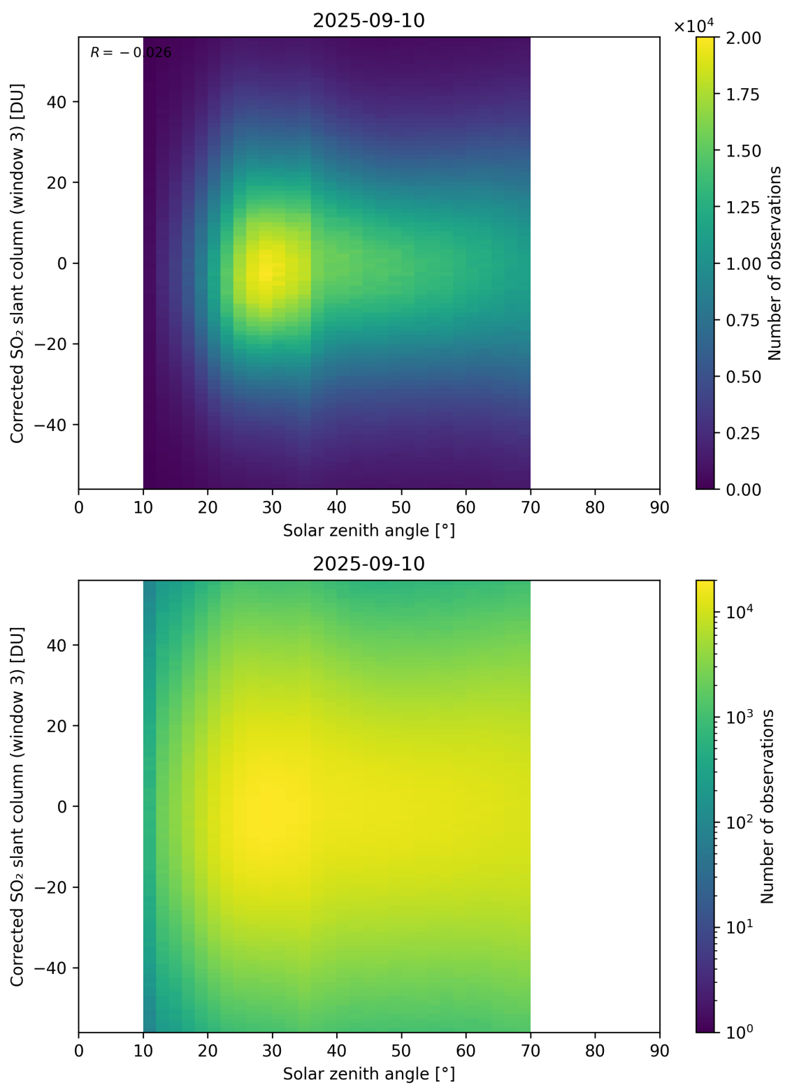
Figure 183: Scatter density plot of “Solar zenith angle” against “Corrected SO 2 slant column (window 3)” for 2025-09-10 to 2025-09-11.
