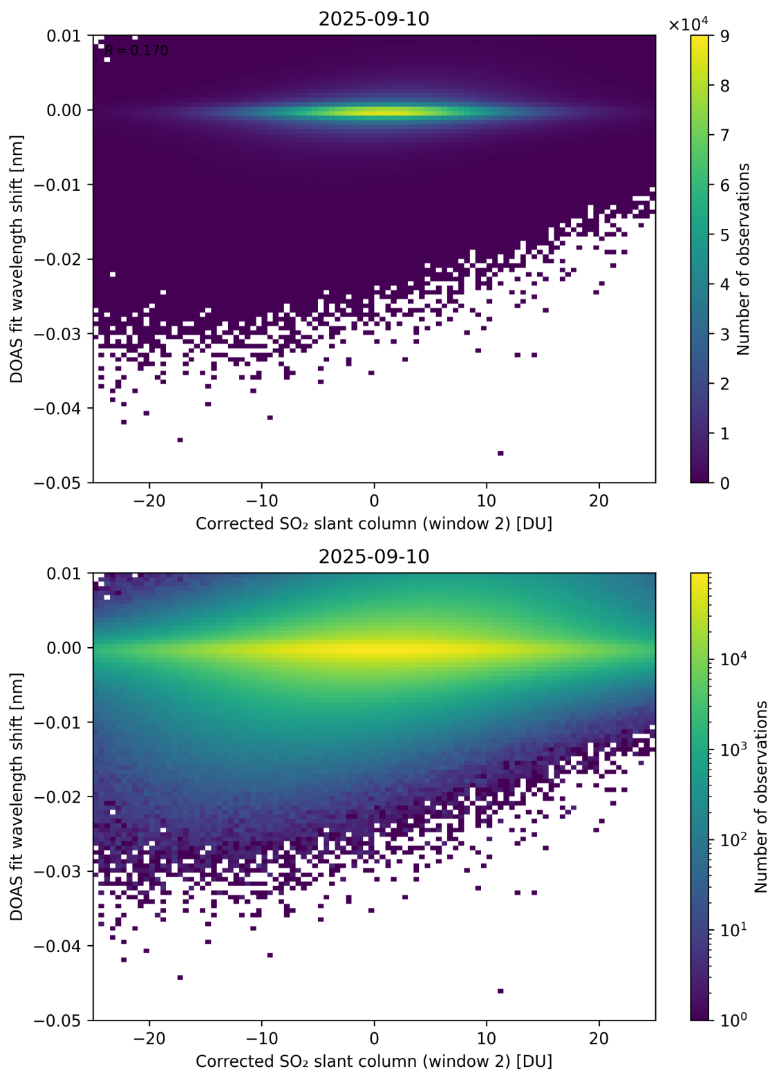
Figure 246: Scatter density plot of “Corrected SO 2 slant column (window 2)” against “DOAS fit wavelength shift” for 2025-09-10 to 2025-09-11.
