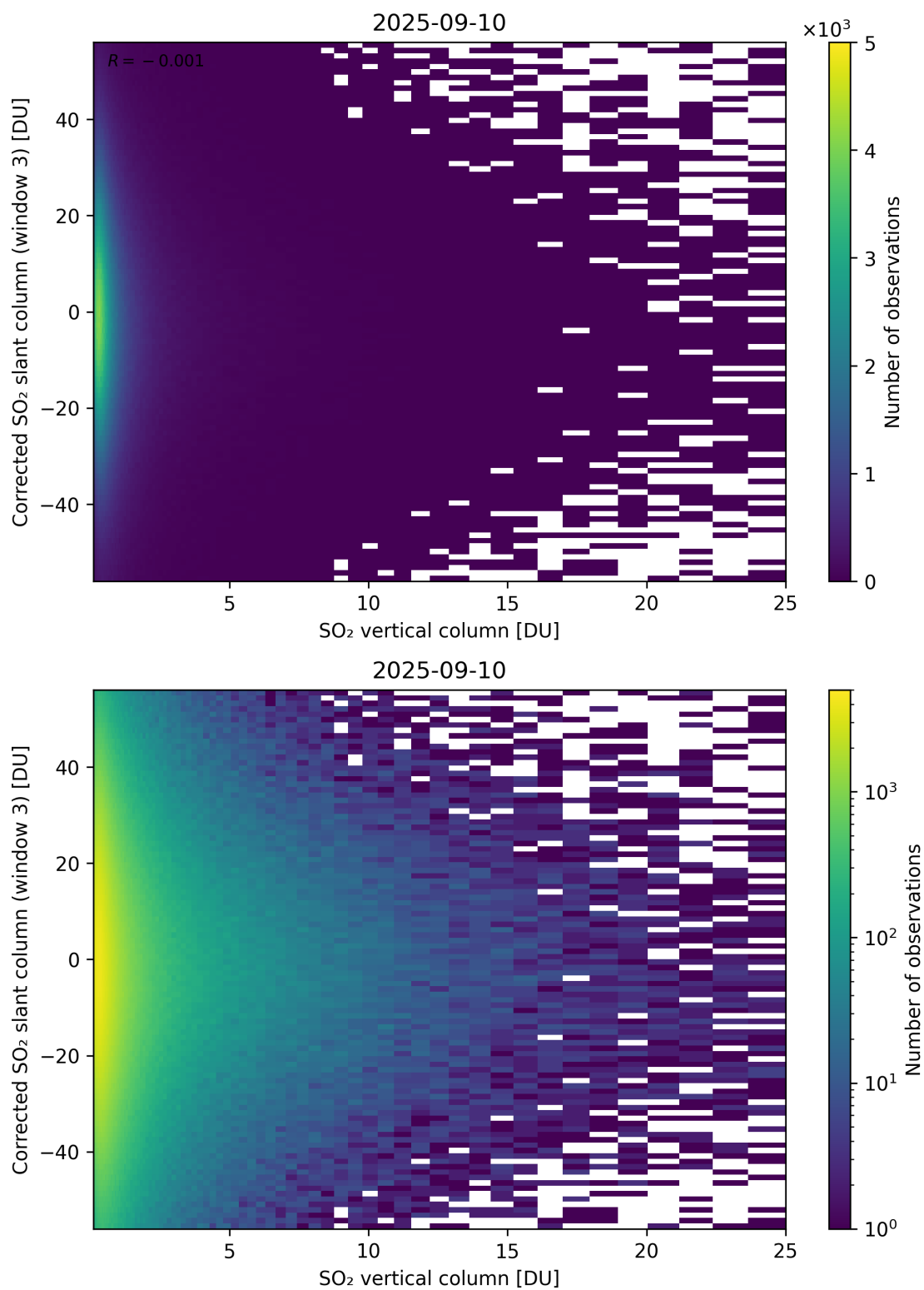
Figure 353: Scatter density plot of “SO 2 vertical column” against “Corrected SO 2 slant column (window 3)” for 2025-09-10 to 2025-09-11.
