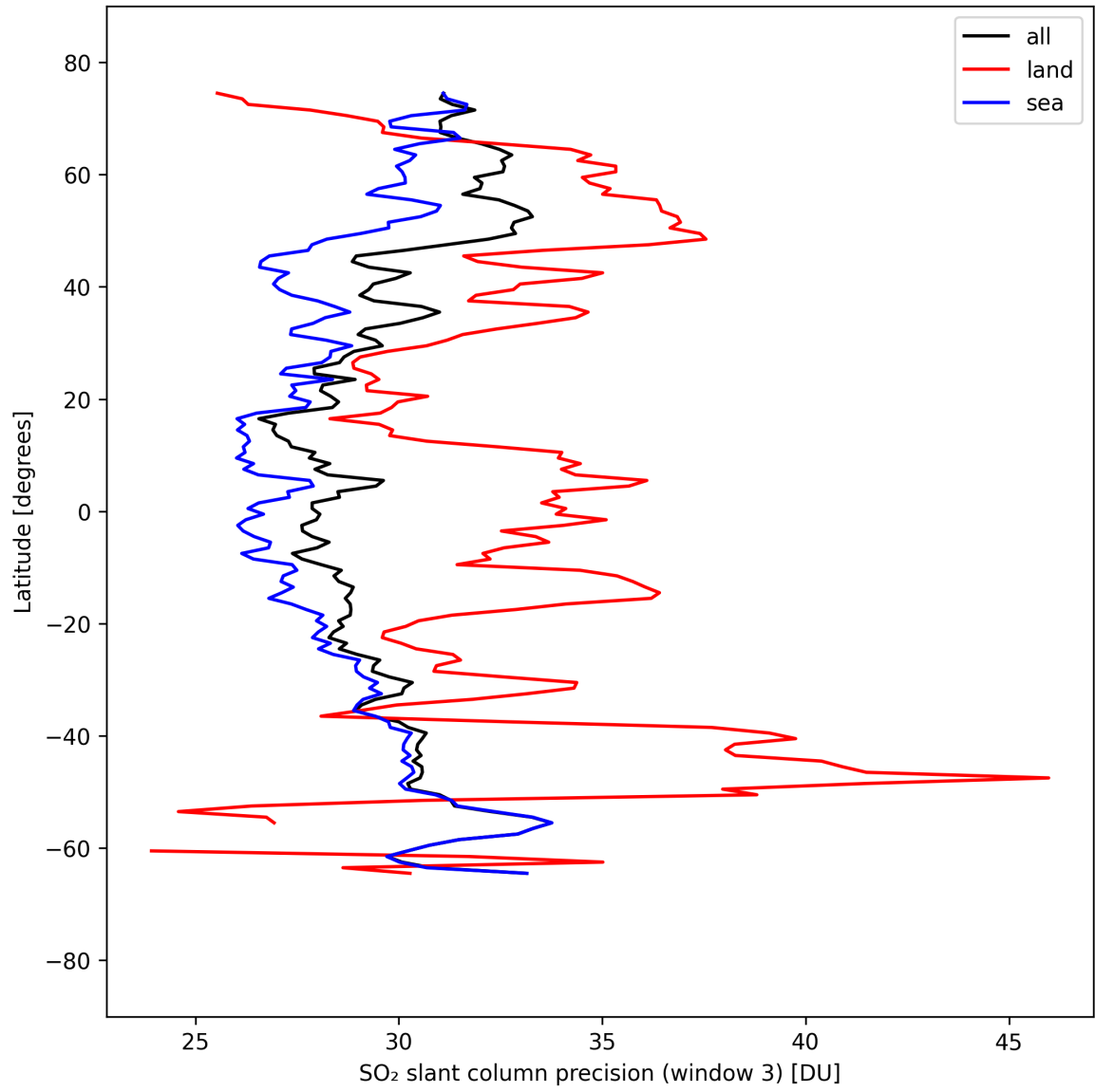
Figure 46: Zonal average of “SO 2 slant column precision (window 3)” for 2025-09-10 to 2025-09-11.
