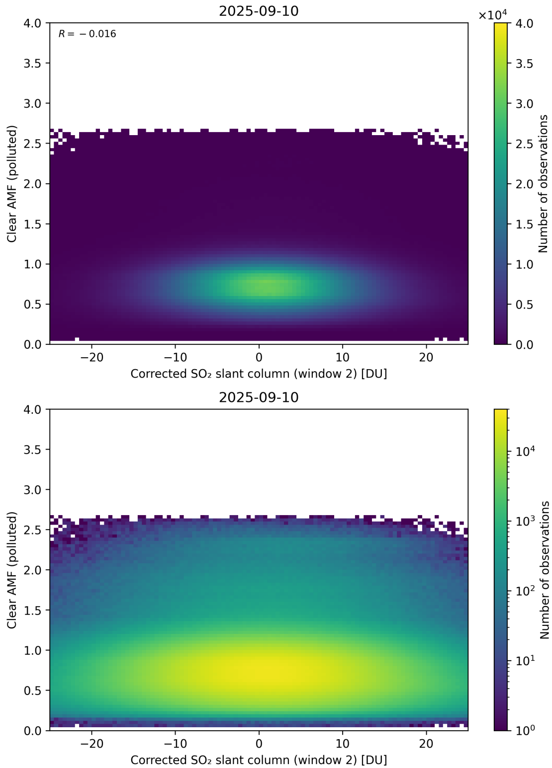
Figure 249: Scatter density plot of “Corrected SO 2 slant column (window 2)” against “Clear AMF (polluted)” for 2025-09-10 to 2025-09-11.
