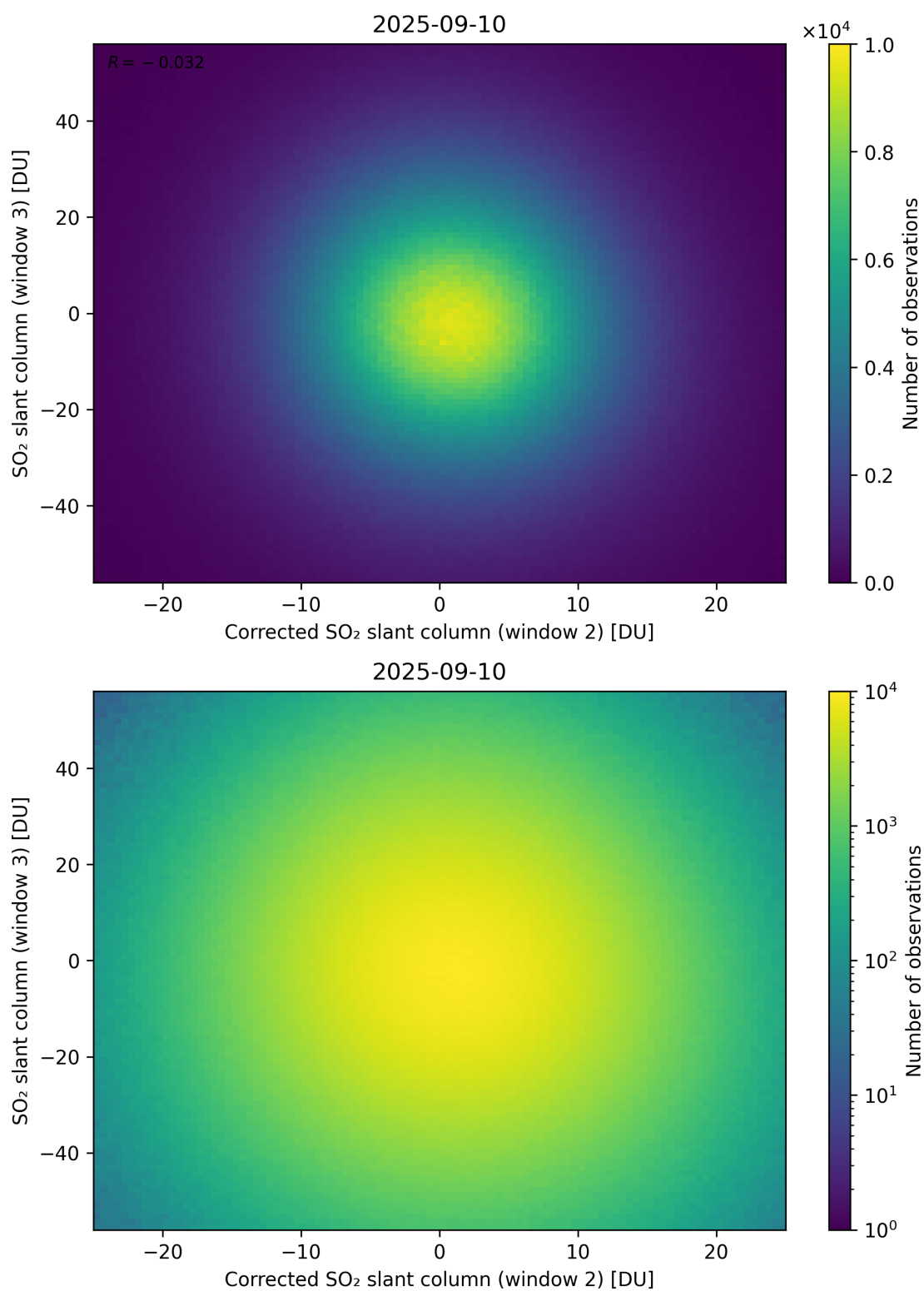
Figure 251: Scatter density plot of “Corrected SO 2 slant column (window 2)” against “SO 2 slant column (window 3)” for 2025-09-10 to 2025-09-11.
