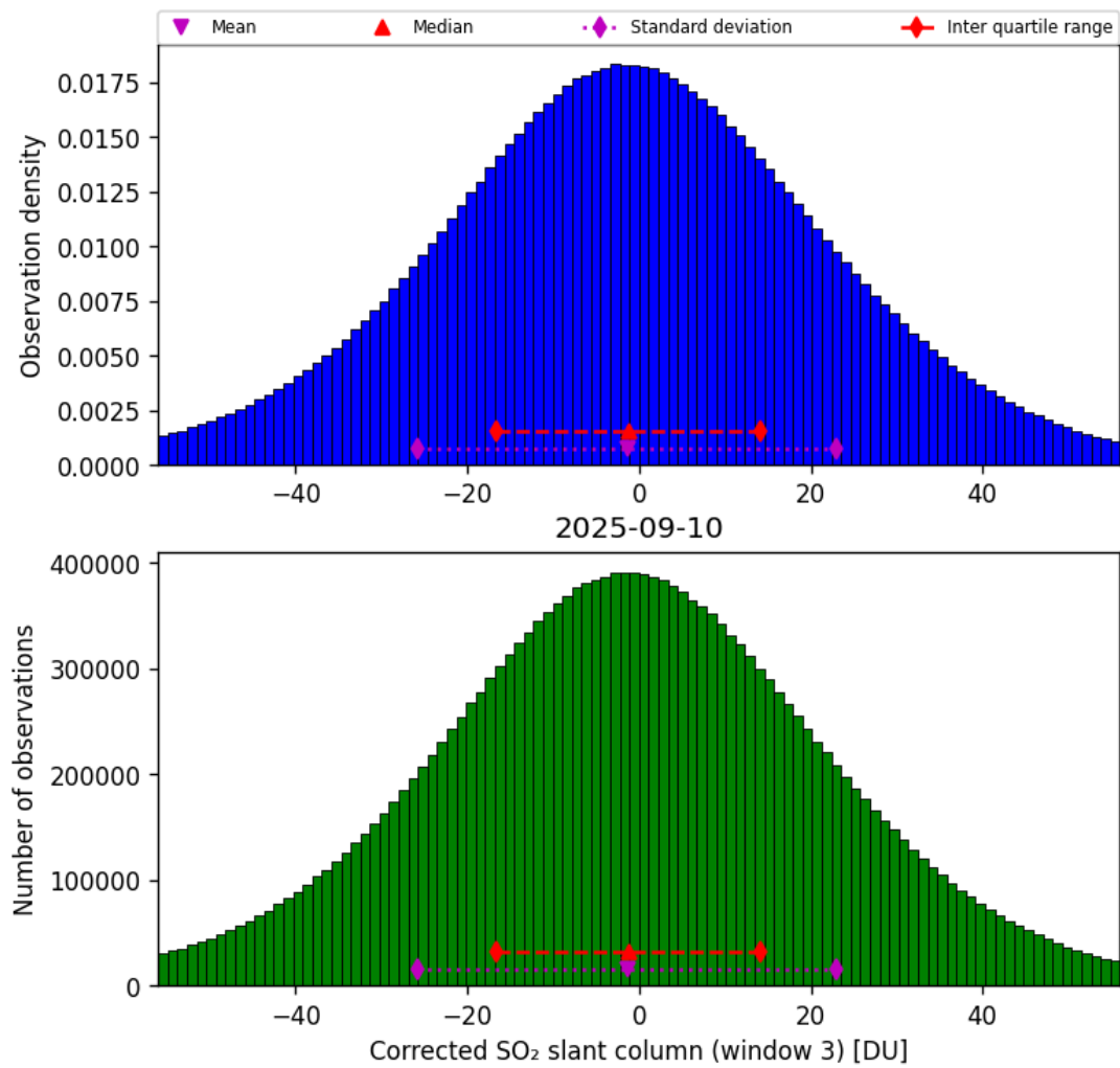
Figure 73: Histogram of “Corrected SO 2 slant column (window 3)” for 2025-09-10 to 2025-09-11
