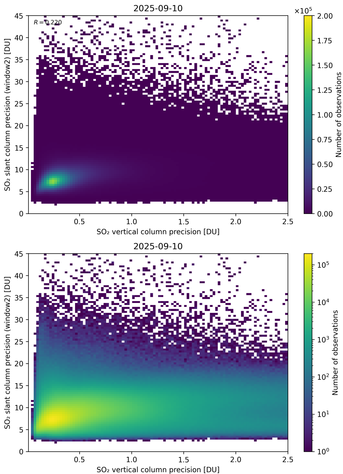
Figure 343: Scatter density plot of “SO 2 vertical column precision” against “SO 2 slant column precision (window2)” for 2025-09-10 to 2025-09-11.
