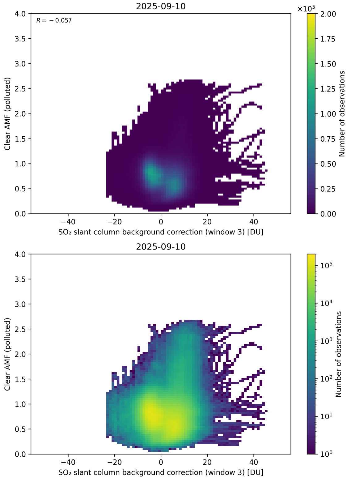
Figure 135: Scatter density plot of “SO 2 slant column background correction (window 3)” against “Clear AMF (polluted)” for 2025-09-10 to 2025-09-11.
