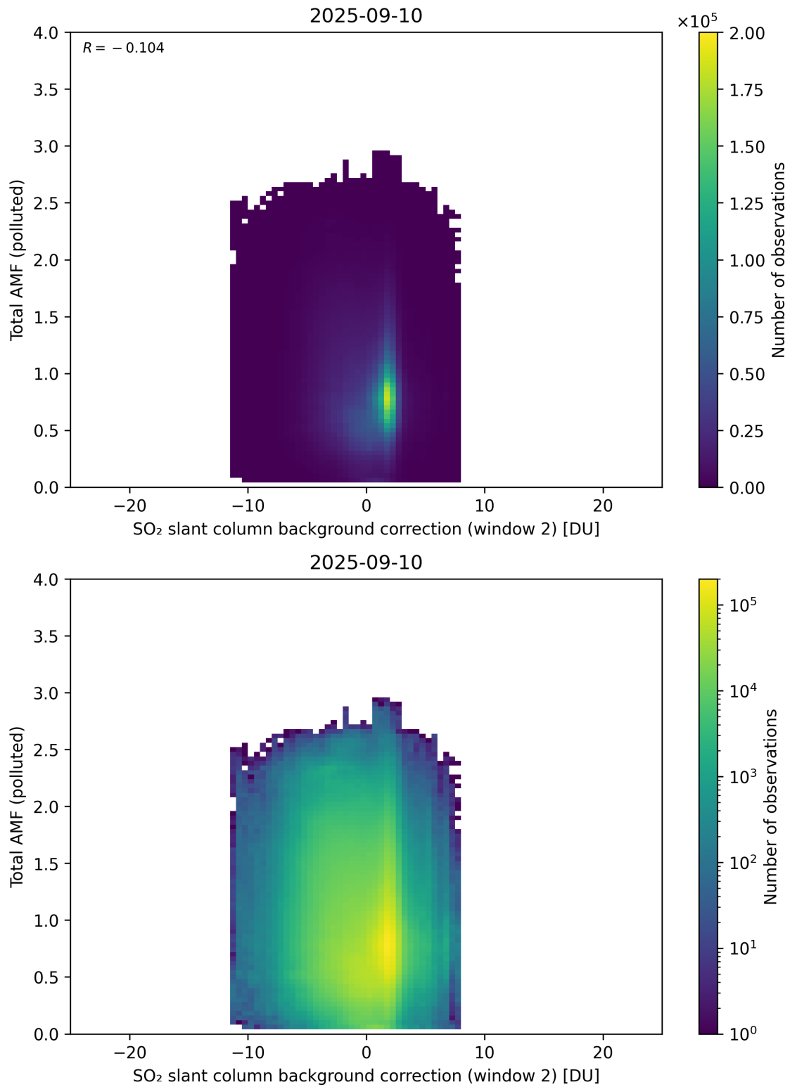
Figure 130: Scatter density plot of “SO 2 slant column background correction (window 2)” against “Total AMF (polluted)” for 2025-09-10 to 2025-09-11.
