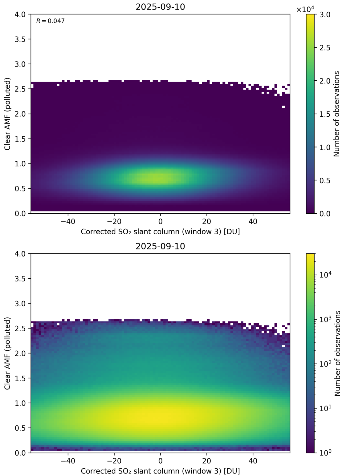
Figure 259: Scatter density plot of “Corrected SO 2 slant column (window 3)” against “Clear AMF (polluted)” for 2025-09-10 to 2025-09-11.
