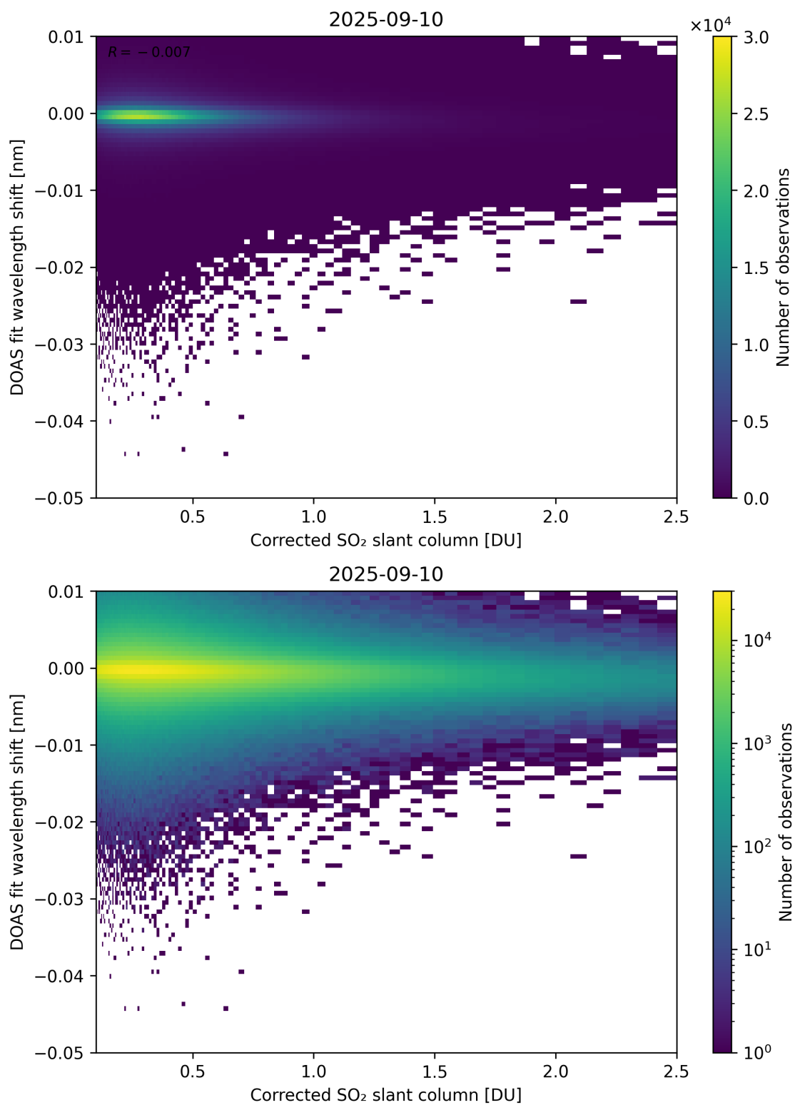
Figure 229: Scatter density plot of “Corrected SO 2 slant column” against “DOAS fit wavelength shift” for 2025-09-10 to 2025-09-11.
