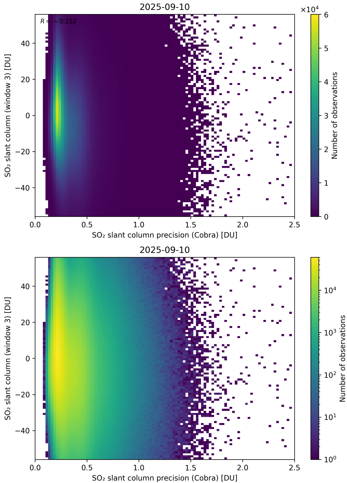
Figure 211: Scatter density plot of “SO 2 slant column precision (Cobra)” against “SO 2 slant column (window 3)” for 2025-09-10 to 2025-09-11.
