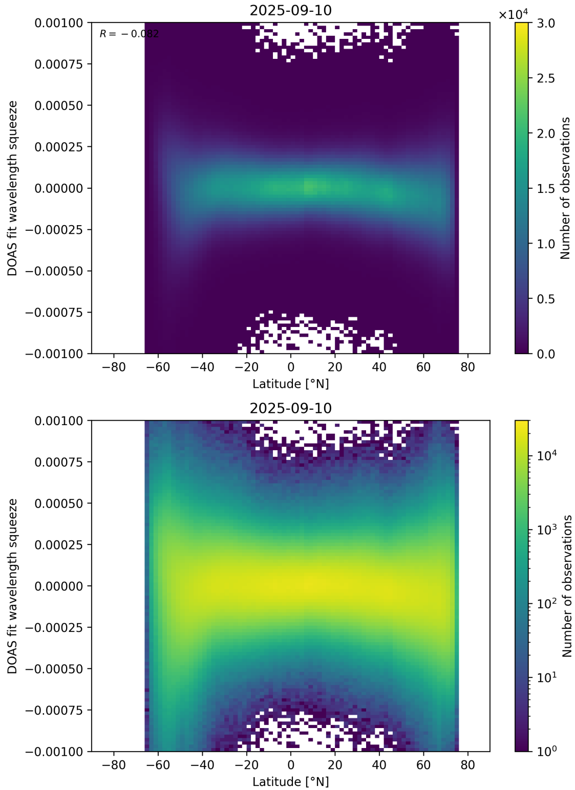
Figure 154: Scatter density plot of “Latitude” against “DOAS fit wavelength squeeze” for 2025-09-10 to 2025-09-11.
