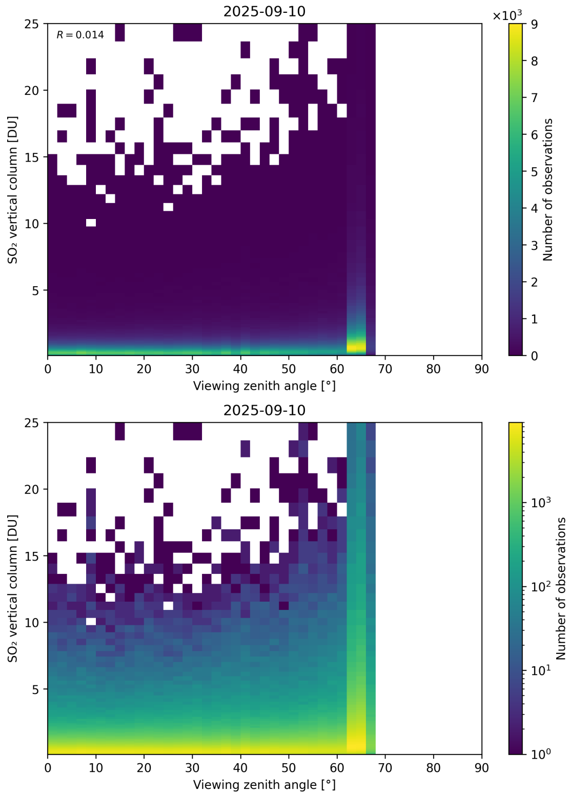
Figure 383: Scatter density plot of “Viewing zenith angle” against “SO 2 vertical column” for 2025-09-10 to 2025-09-11.
