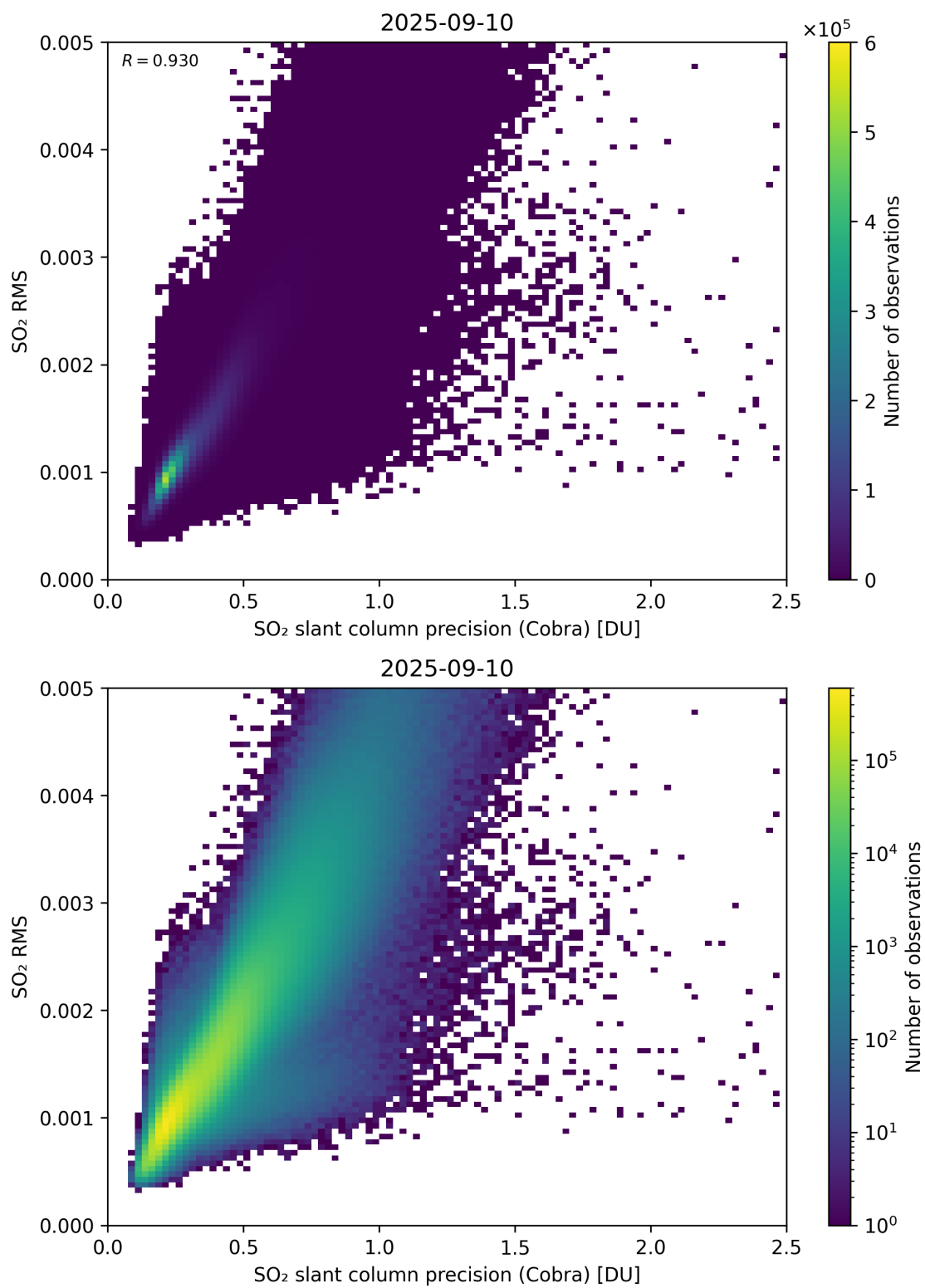
Figure 204: Scatter density plot of “SO 2 slant column precision (Cobra)” against “SO 2 RMS” for 2025-09-10 to 2025-09-11.
