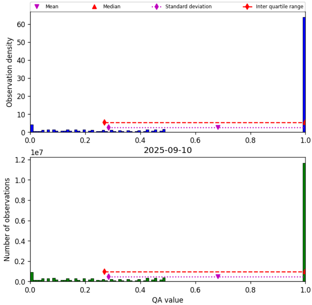
Figure 57: Histogram of “QA value” for 2025-09-10 to 2025-09-11
