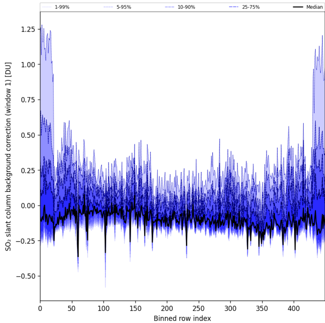
Figure 92: Along track statistics of “SO 2 slant column background correction (window 1)” for 2025-09-10 to 2025-09-11
