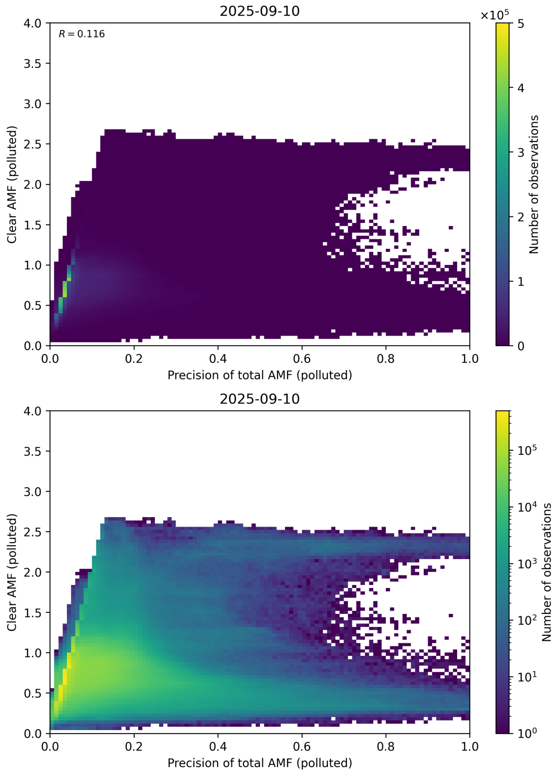
Figure 320: Scatter density plot of “Precision of total AMF (polluted)” against “Clear AMF (polluted)” for 2025-09-10 to 2025-09-11.
