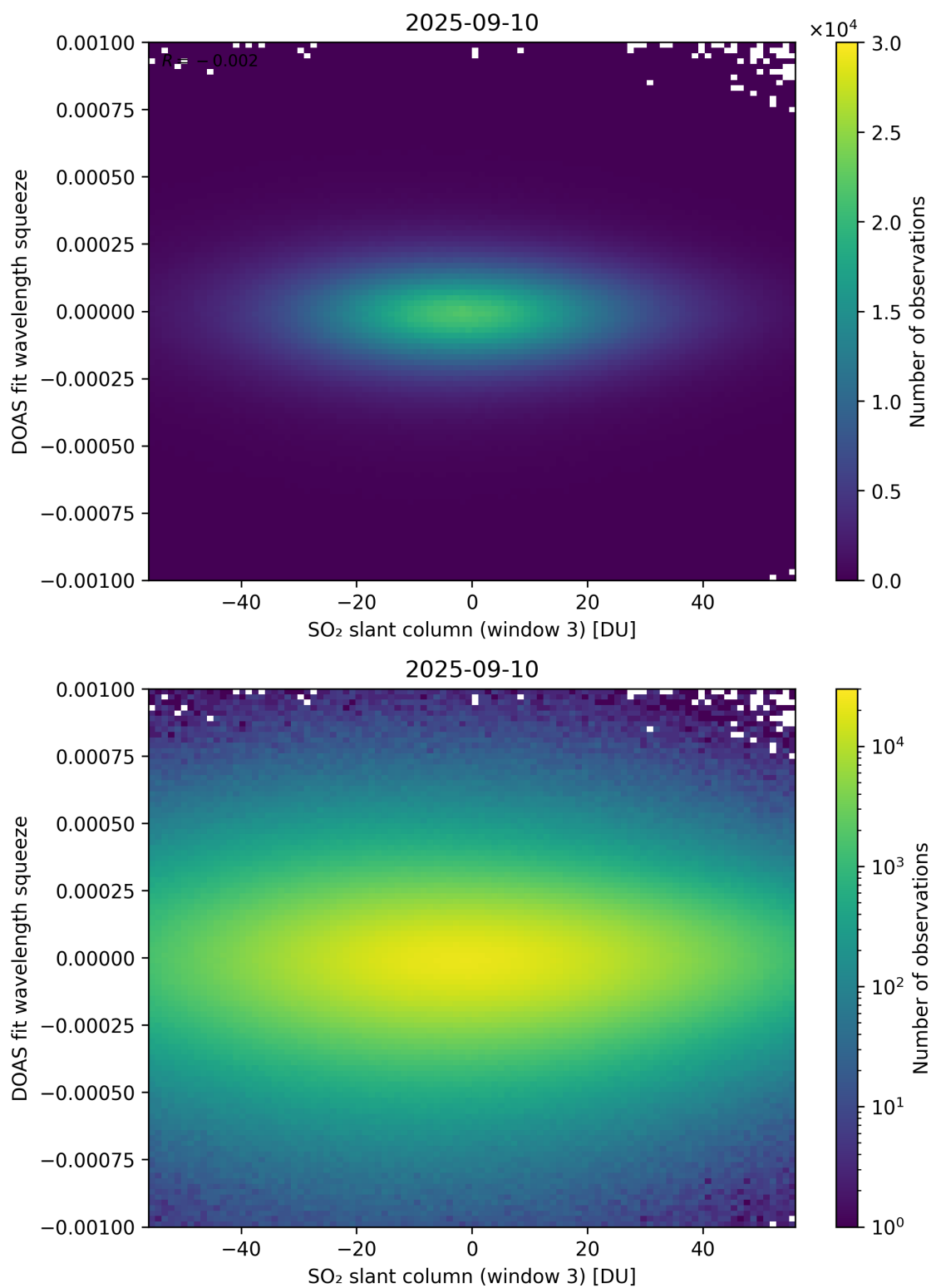
Figure 305: Scatter density plot of “SO 2 slant column (window 3)” against “DOAS fit wavelength squeeze” for 2025-09-10 to 2025-09-11.
