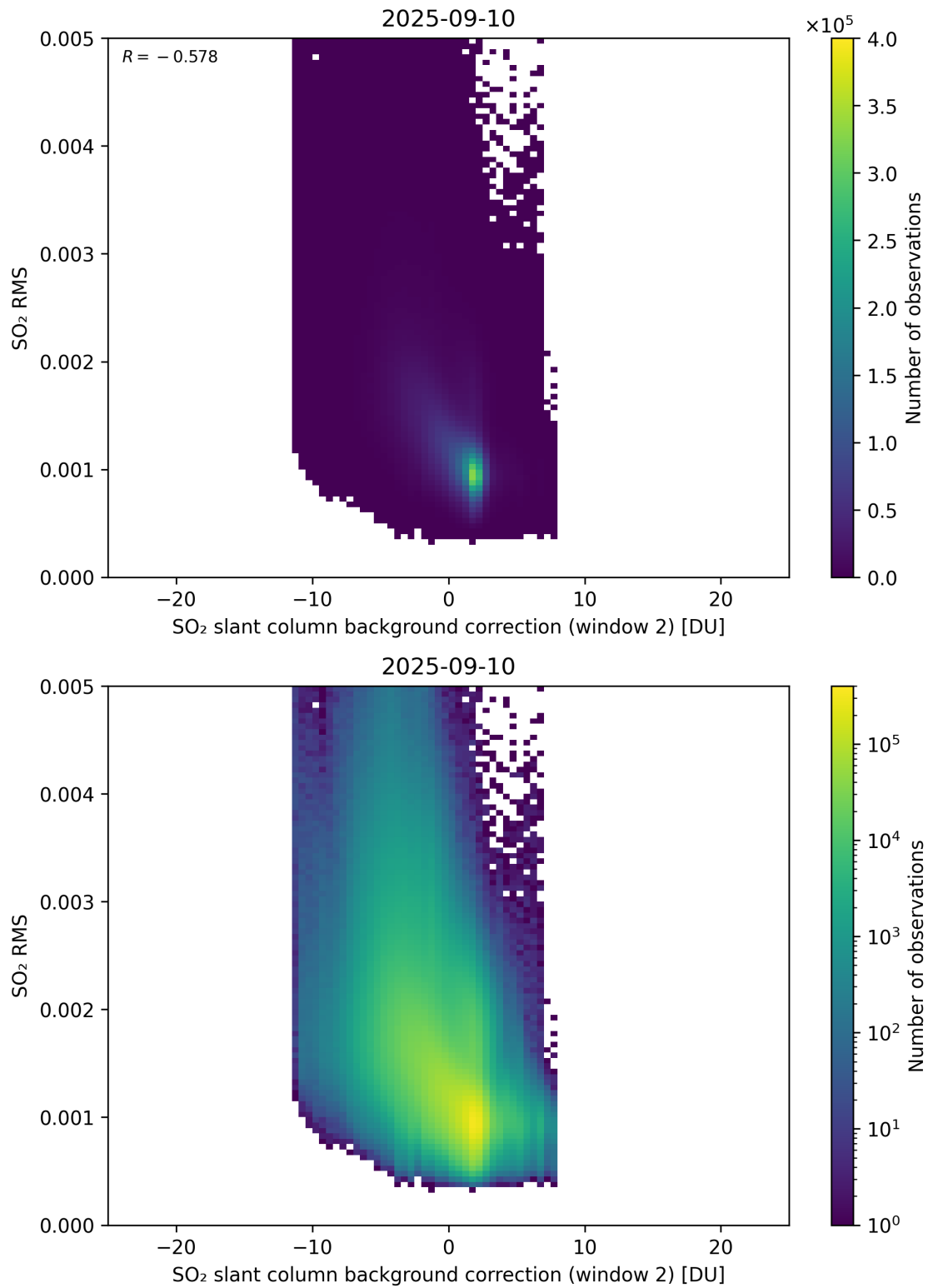
Figure 125: Scatter density plot of “SO 2 slant column background correction (window 2)” against “SO 2 RMS” for 2025-09-10 to 2025-09-11.
