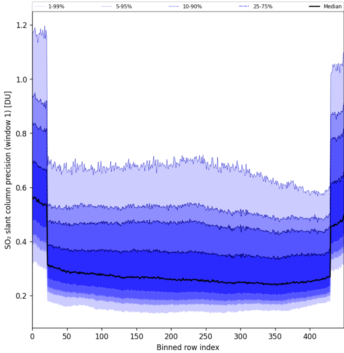
Figure 90: Along track statistics of “SO 2 slant column precision (window 1)” for 2025-09-10 to 2025-09-11
