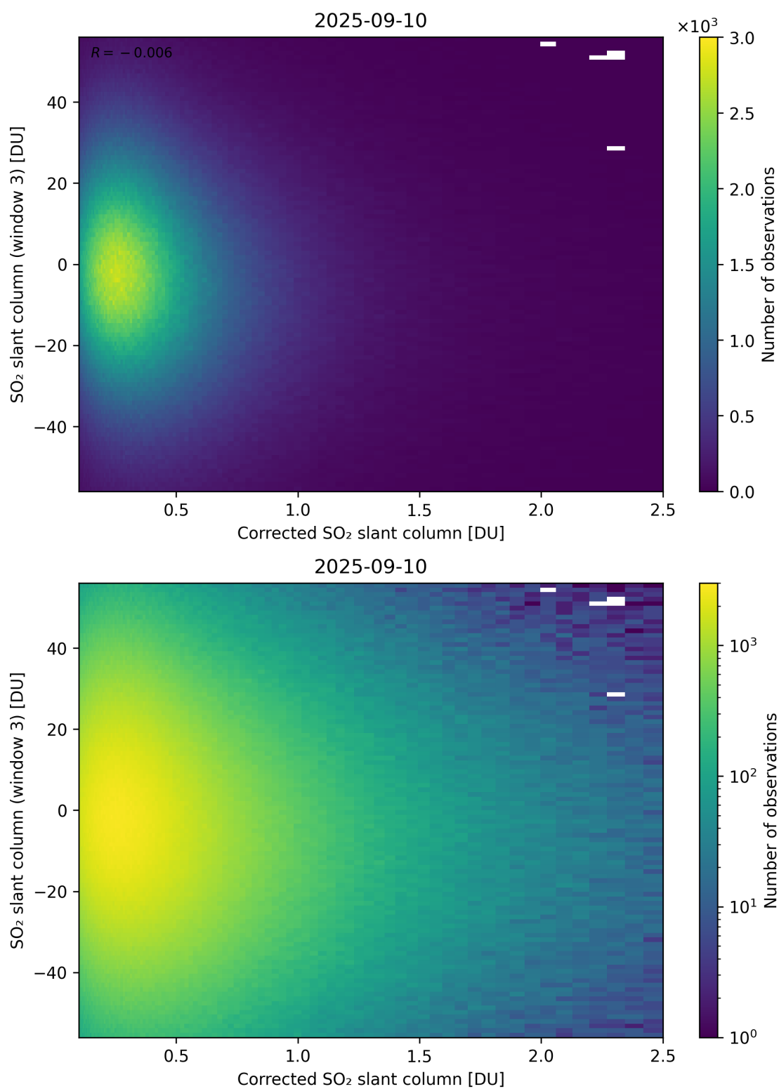
Figure 240: Scatter density plot of “Corrected SO 2 slant column” against “SO 2 slant column (window 3)” for 2025-09-10 to 2025-09-11.
