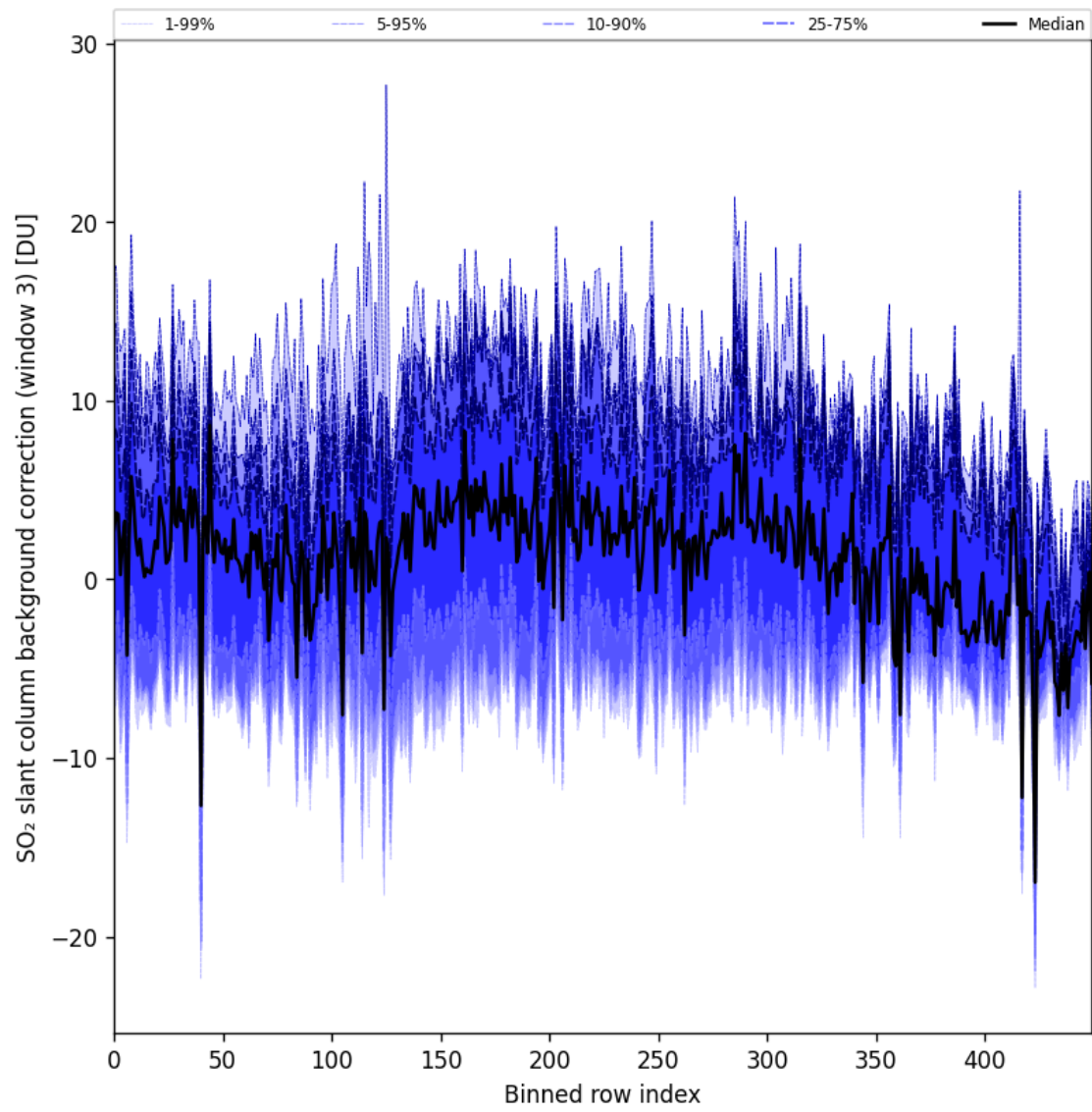
Figure 100: Along track statistics of “SO 2 slant column background correction (window 3)” for 2025-09-10 to 2025-09-11
