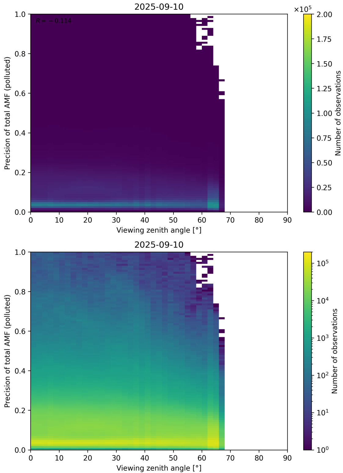
Figure 382: Scatter density plot of “Viewing zenith angle” against “Precision of total AMF (polluted)” for 2025-09-10 to 2025-09-11.
