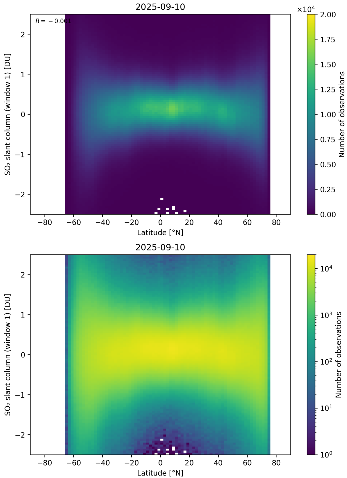
Figure 162: Scatter density plot of “Latitude” against “SO 2 slant column (window 1)” for 2025-09-10 to 2025-09-11.
