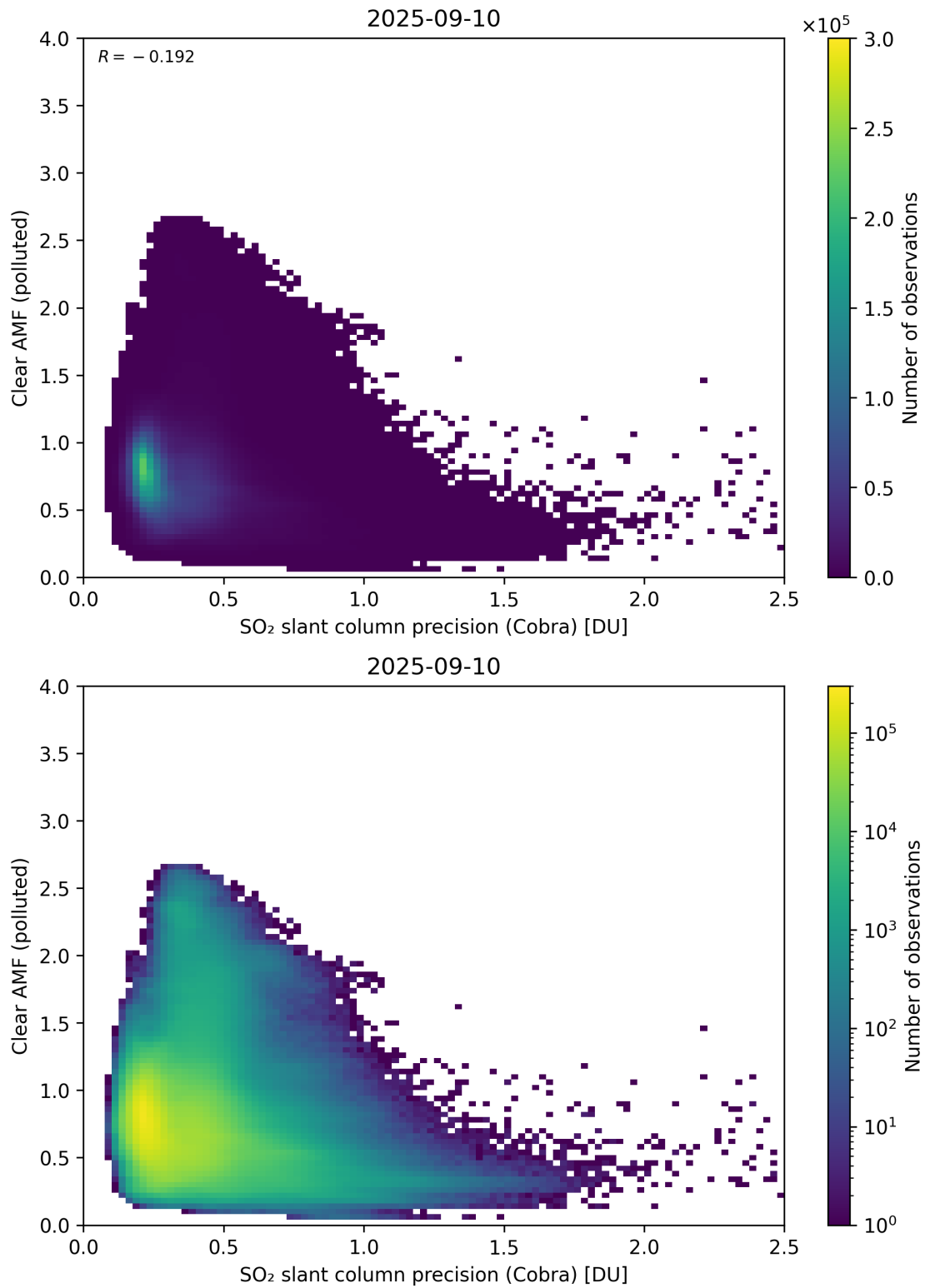
Figure 205: Scatter density plot of “SO 2 slant column precision (Cobra)” against “Clear AMF (polluted)” for 2025-09-10 to 2025-09-11.
