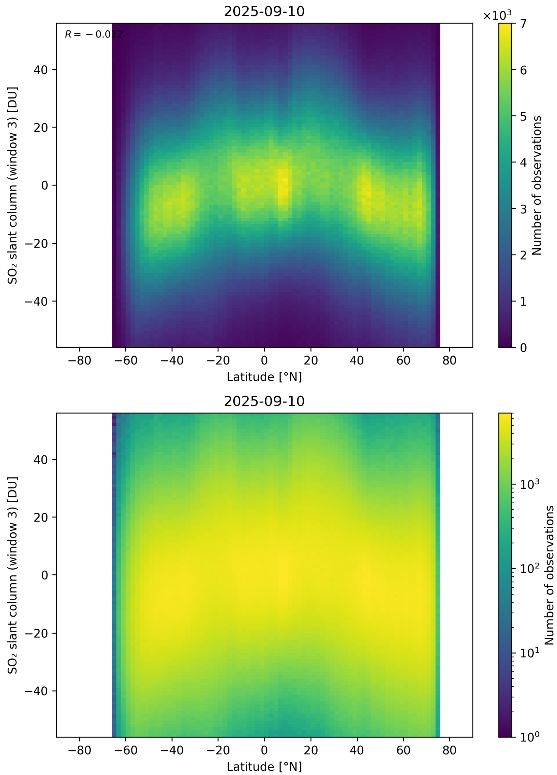
Figure 165: Scatter density plot of “Latitude” against “SO 2 slant column (window 3)” for 2025-09-10 to 2025-09-11.
