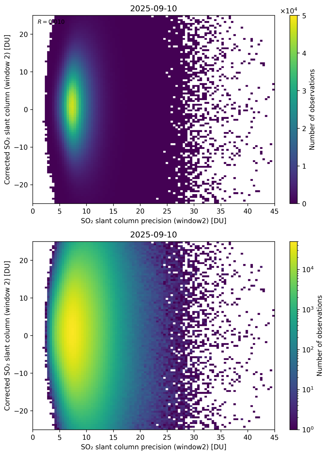
Figure 297: Scatter density plot of “SO 2 slant column precision (window2)” against “Corrected SO 2 slant column (window 2)” for 2025-09-10 to 2025-09-11.
