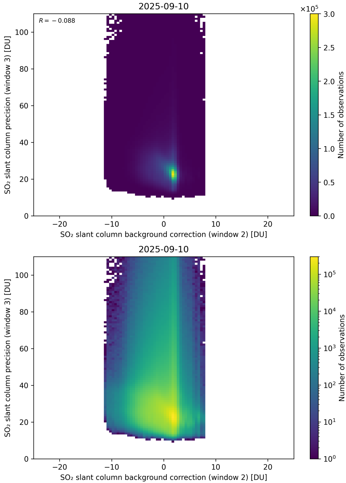
Figure 129: Scatter density plot of “SO 2 slant column background correction (window 2)” against “SO 2 slant column precision (window 3)” for 2025-09-10 to 2025-09-11.
