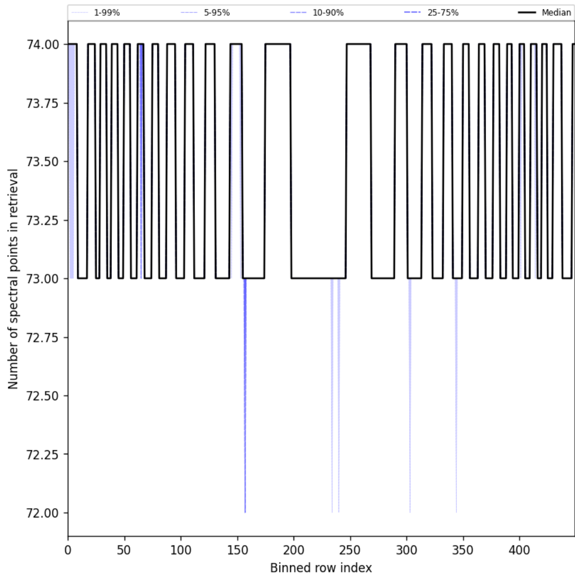
Figure 108: Along track statistics of “Number of spectral points in retrieval” for 2025-09-10 to 2025-09-11
