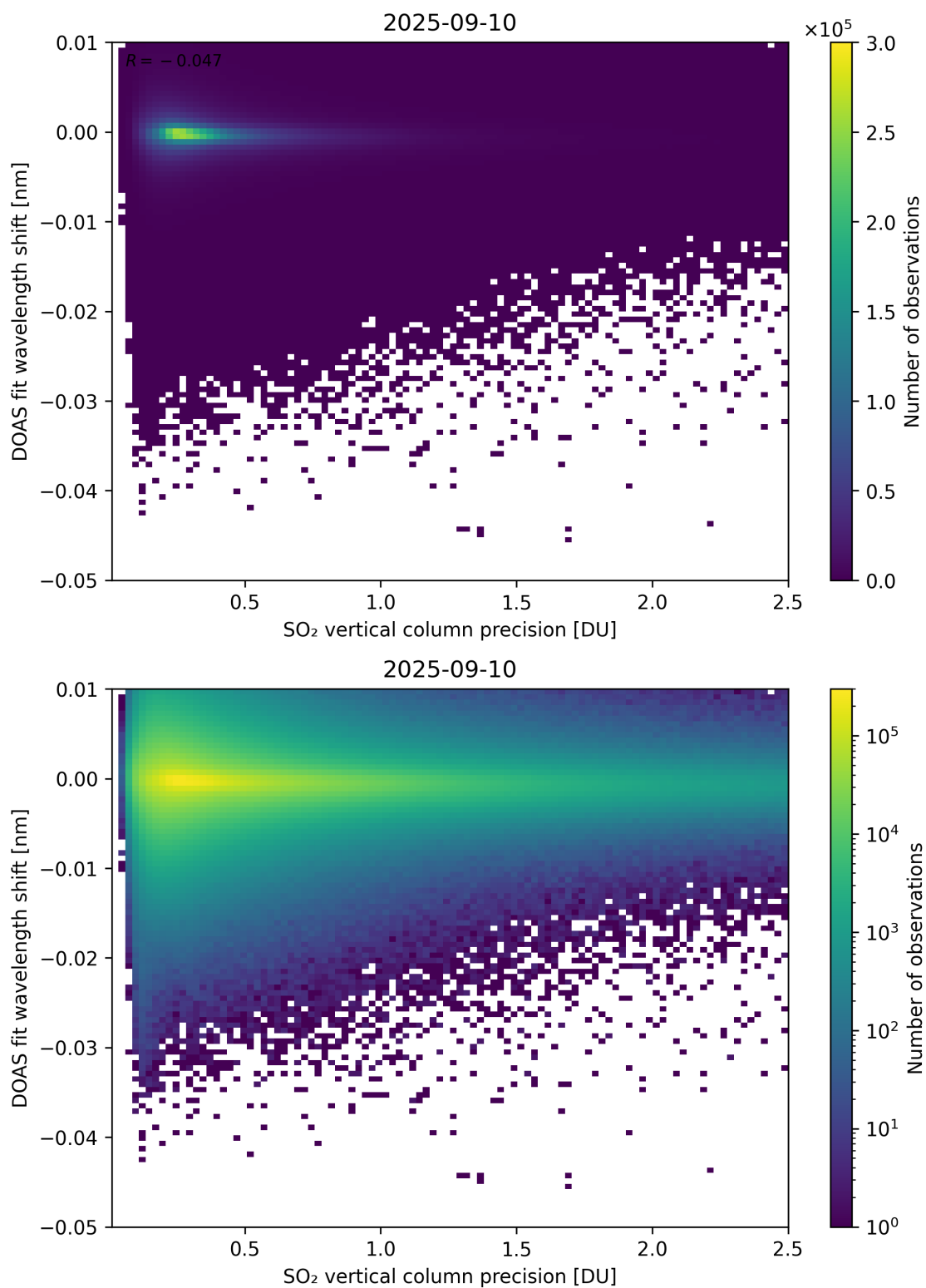
Figure 332: Scatter density plot of “SO 2 vertical column precision” against “DOAS fit wavelength shift” for 2025-09-10 to 2025-09-11.
