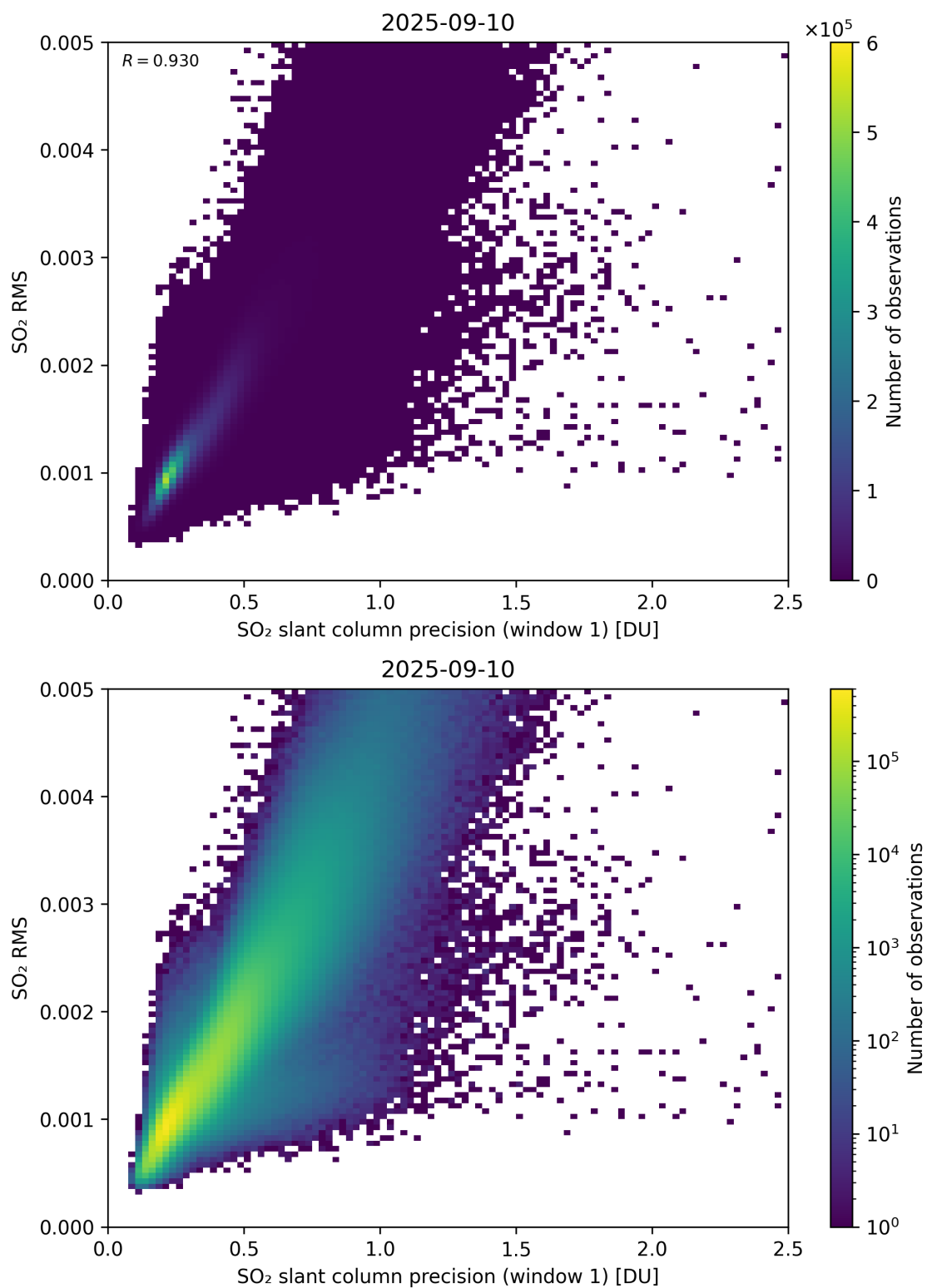
Figure 273: Scatter density plot of “SO 2 slant column precision (window 1)” against “SO 2 RMS” for 2025-09-10 to 2025-09-11.
