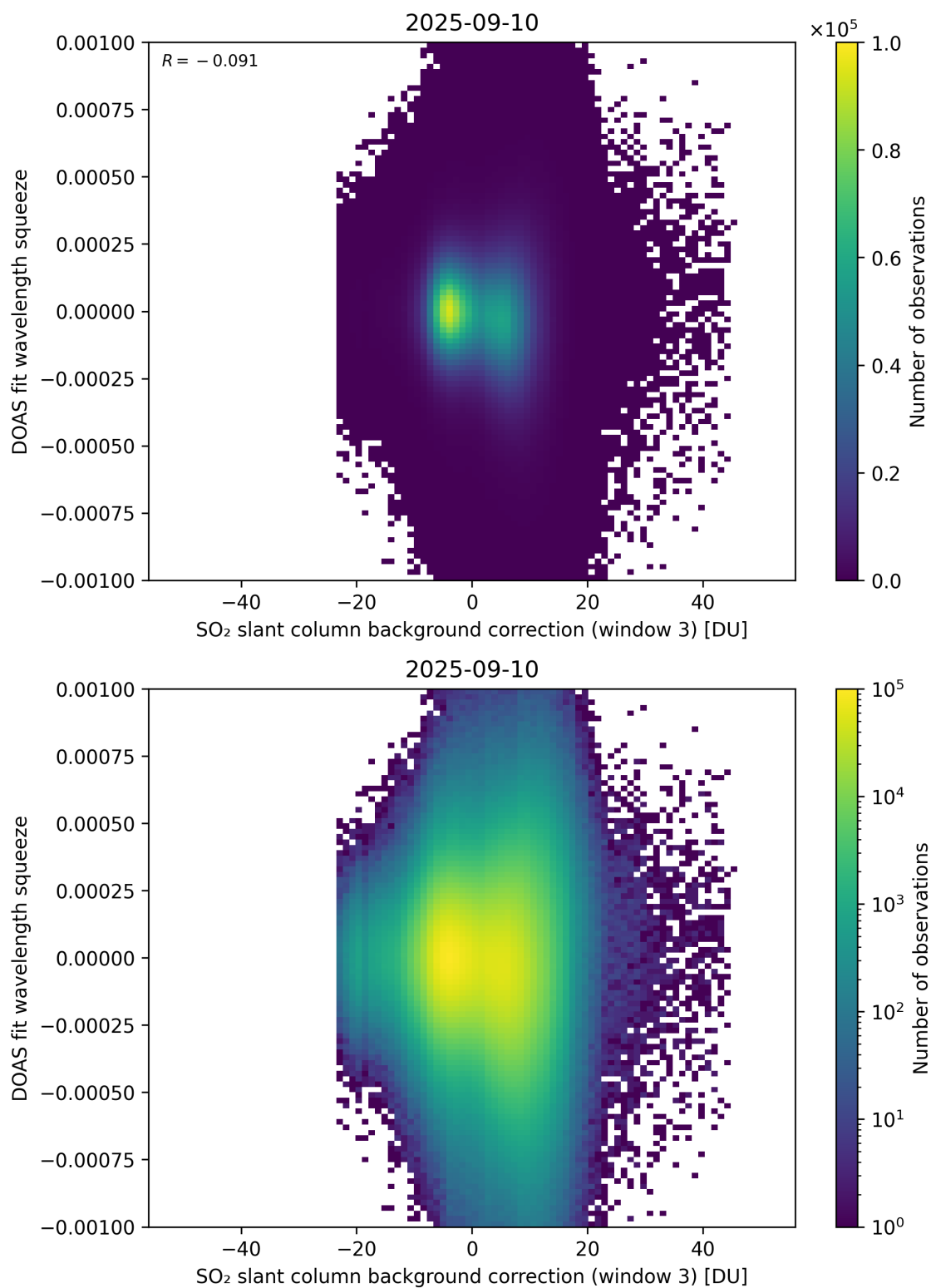
Figure 133: Scatter density plot of “SO 2 slant column background correction (window 3)” against “DOAS fit wavelength squeeze” for 2025-09-10 to 2025-09-11.
