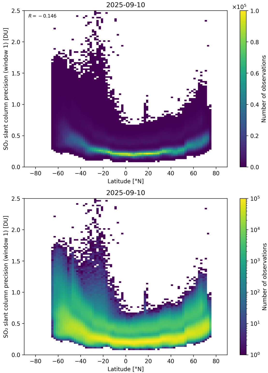
Figure 163: Scatter density plot of “Latitude” against “SO 2 slant column precision (window 1)” for 2025-09-10 to 2025-09-11.
