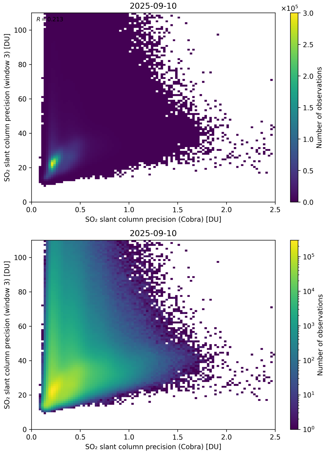
Figure 212: Scatter density plot of “SO 2 slant column precision (Cobra)” against “SO 2 slant column precision (window 3)” for 2025-09-10 to 2025-09-11.
