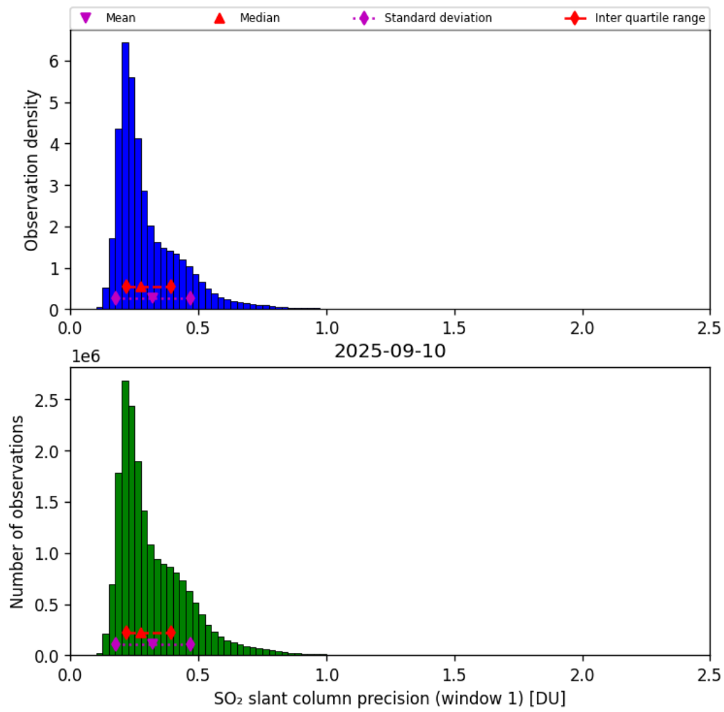
Figure 64: Histogram of “SO 2 slant column precision (window 1)” for 2025-09-10 to 2025-09-11
