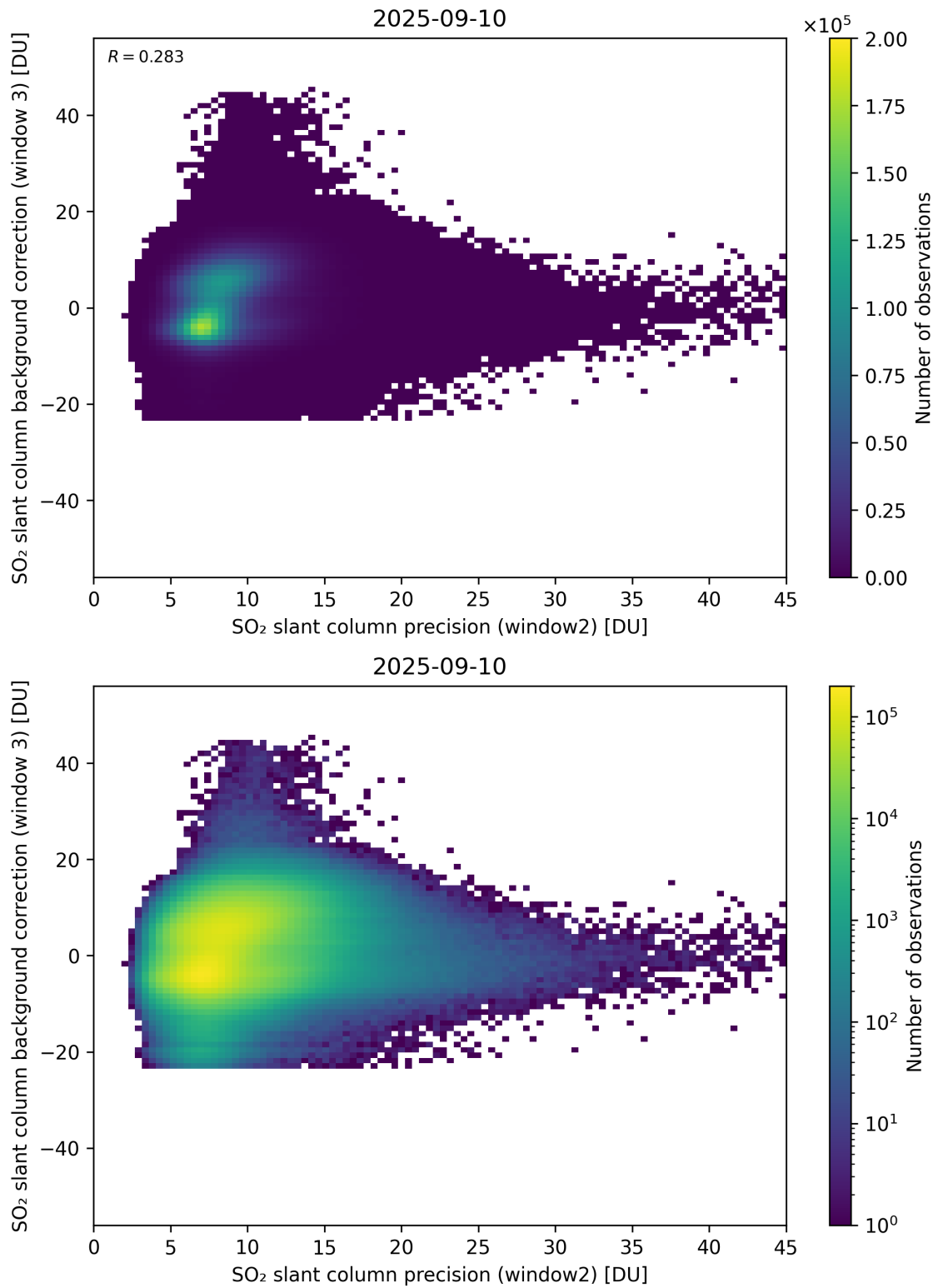
Figure 292: Scatter density plot of “SO 2 slant column precision (window2)” against “SO 2 slant column background correction (window 3)” for 2025-09-10 to 2025-09-11.
