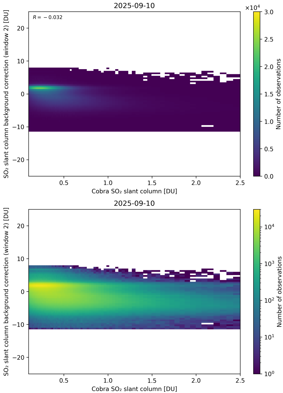
Figure 194: Scatter density plot of “Cobra SO 2 slant column” against “SO 2 slant column background correction (window 2)” for 2025-09-10 to 2025-09-11.
