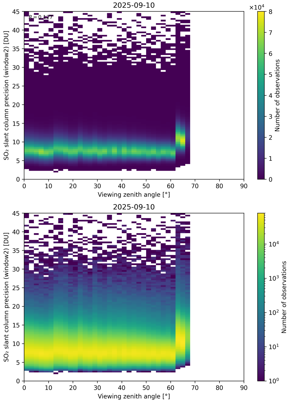
Figure 378: Scatter density plot of “Viewing zenith angle” against “SO 2 slant column precision (window2)” for 2025-09-10 to 2025-09-11.
