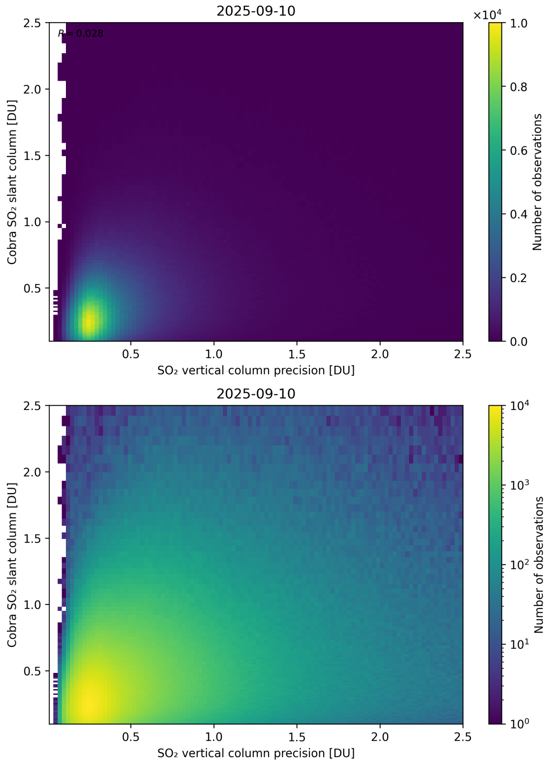
Figure 336: Scatter density plot of “SO 2 vertical column precision” against “Cobra SO 2 slant column” for 2025-09-10 to 2025-09-11.
