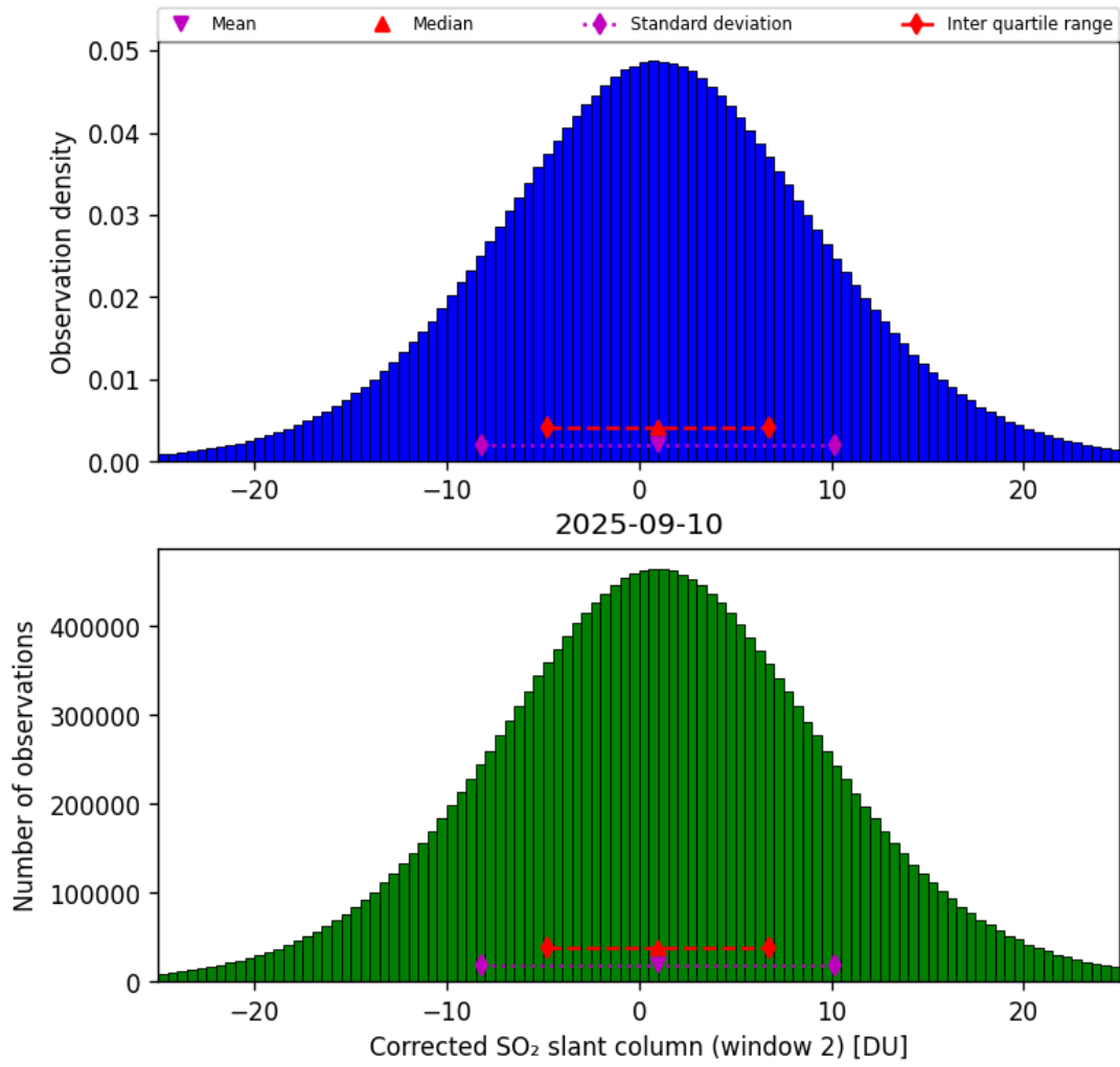
Figure 69: Histogram of “Corrected SO 2 slant column (window 2)” for 2025-09-10 to 2025-09-11
