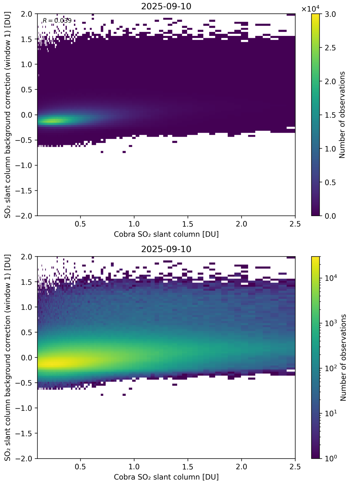
Figure 193: Scatter density plot of “Cobra SO 2 slant column” against “SO 2 slant column background correction (window 1)” for 2025-09-10 to 2025-09-11.
