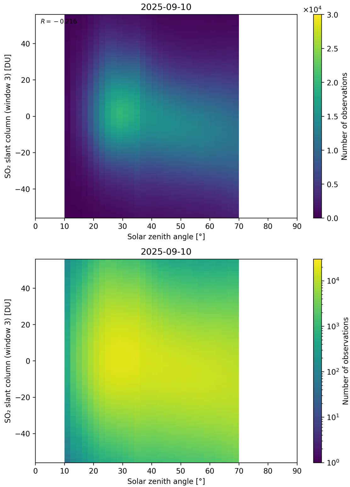
Figure 187: Scatter density plot of “Solar zenith angle” against “SO 2 slant column (window 3)” for 2025-09-10 to 2025-09-11.
