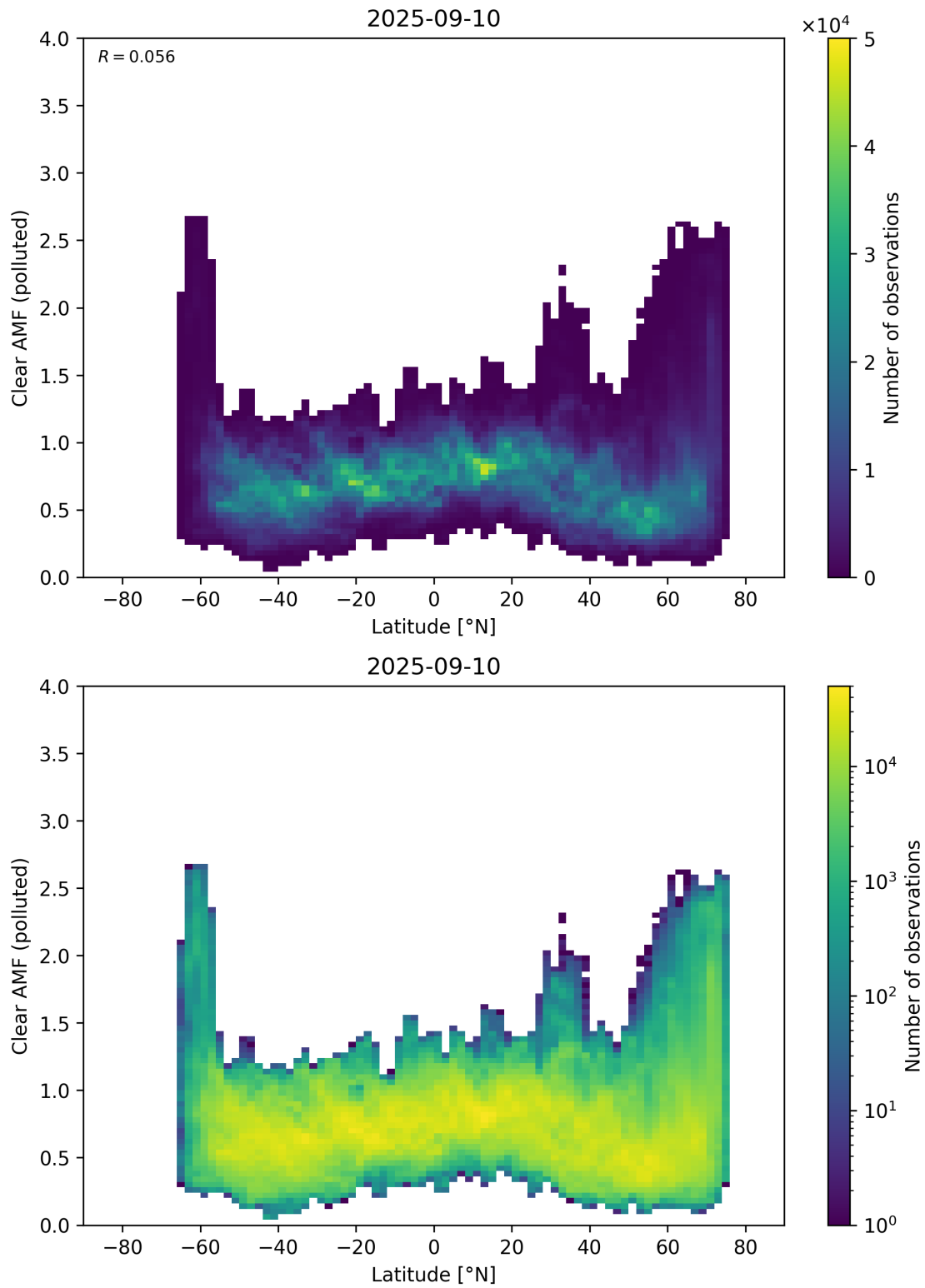
Figure 156: Scatter density plot of “Latitude” against “Clear AMF (polluted)” for 2025-09-10 to 2025-09-11.
