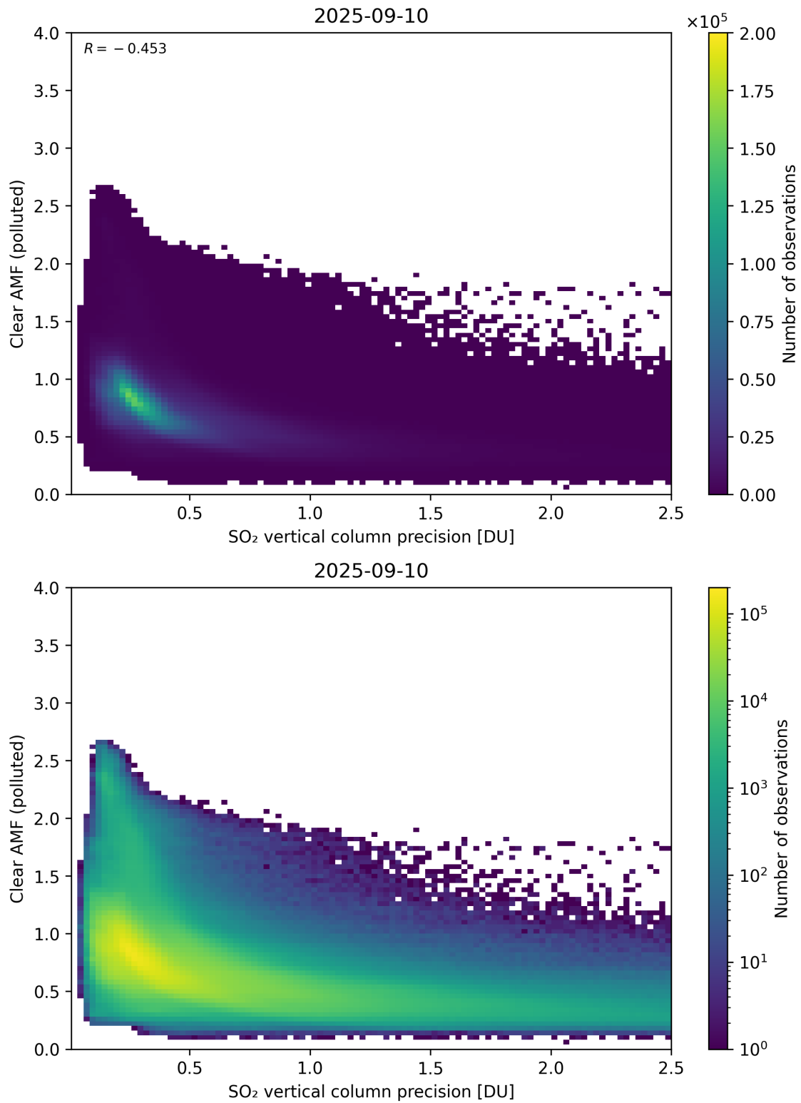
Figure 335: Scatter density plot of “SO 2 vertical column precision” against “Clear AMF (polluted)” for 2025-09-10 to 2025-09-11.
