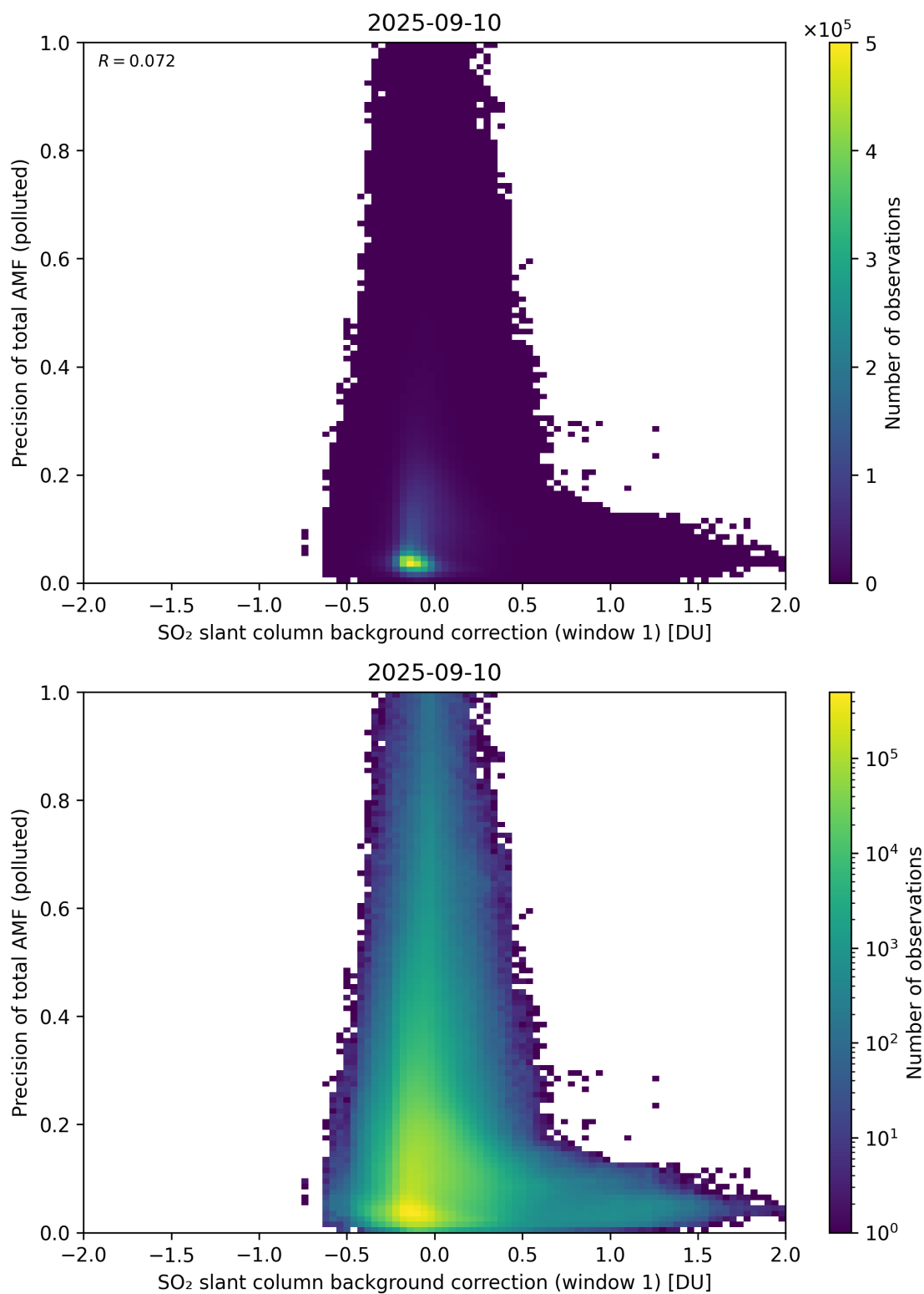
Figure 121: Scatter density plot of “SO 2 slant column background correction (window 1)” against “Precision of total AMF (polluted)” for 2025-09-10 to 2025-09-11.
