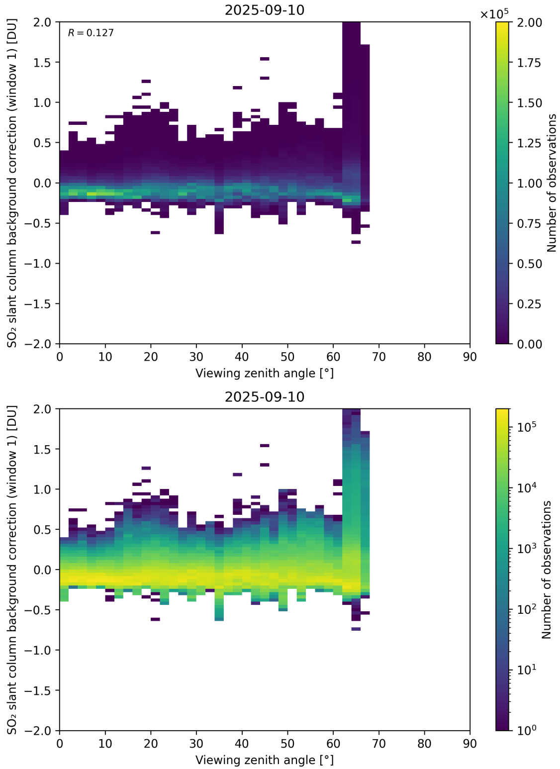
Figure 362: Scatter density plot of “Viewing zenith angle” against “SO 2 slant column background correction (window 1)” for 2025-09-10 to 2025-09-11.
