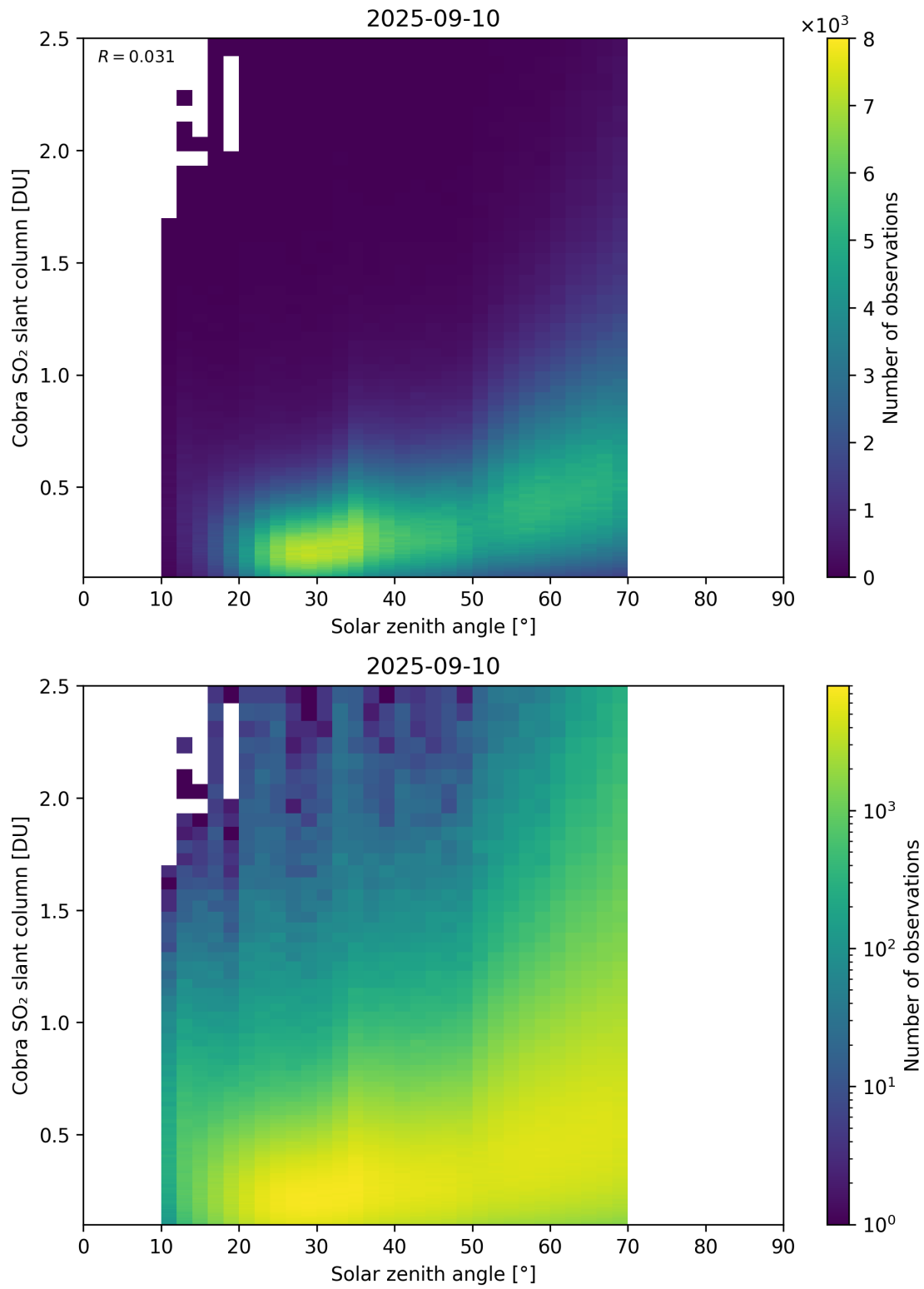
Figure 179: Scatter density plot of “Solar zenith angle” against “Cobra SO 2 slant column” for 2025-09-10 to 2025-09-11.
