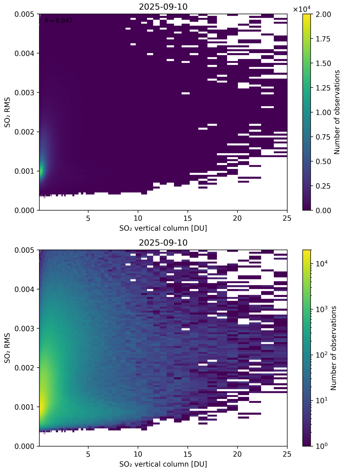
Figure 328: Scatter density plot of “SO 2 vertical column” against “SO 2 RMS” for 2025-09-10 to 2025-09-11.
