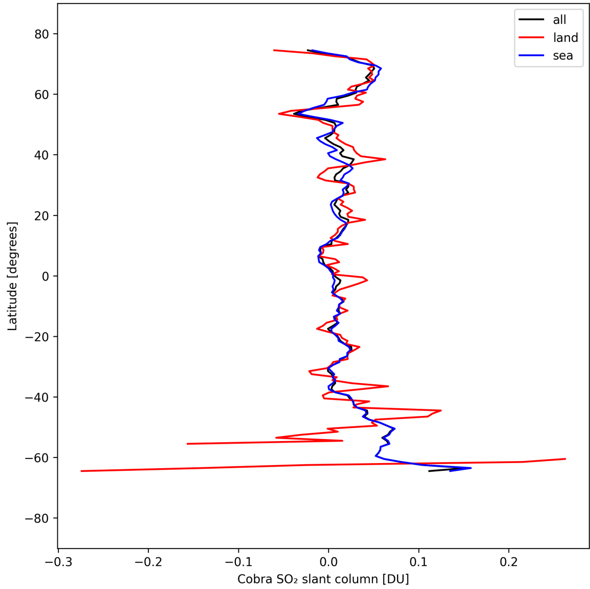
Figure 35: Zonal average of “Cobra SO 2 slant column” for 2025-09-10 to 2025-09-11.
