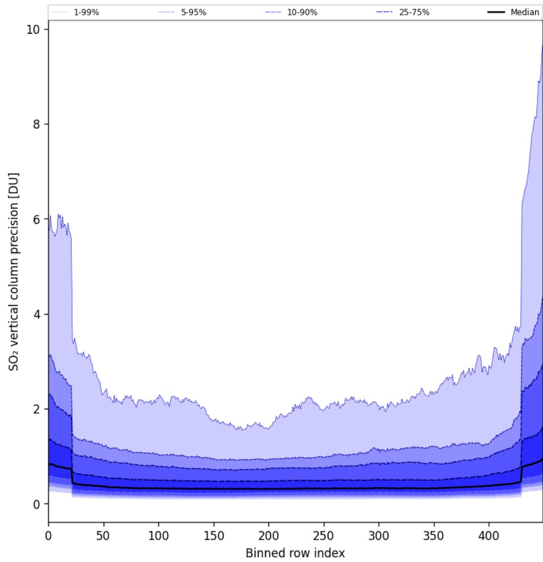
Figure 85: Along track statistics of “SO 2 vertical column precision” for 2025-09-10 to 2025-09-11
