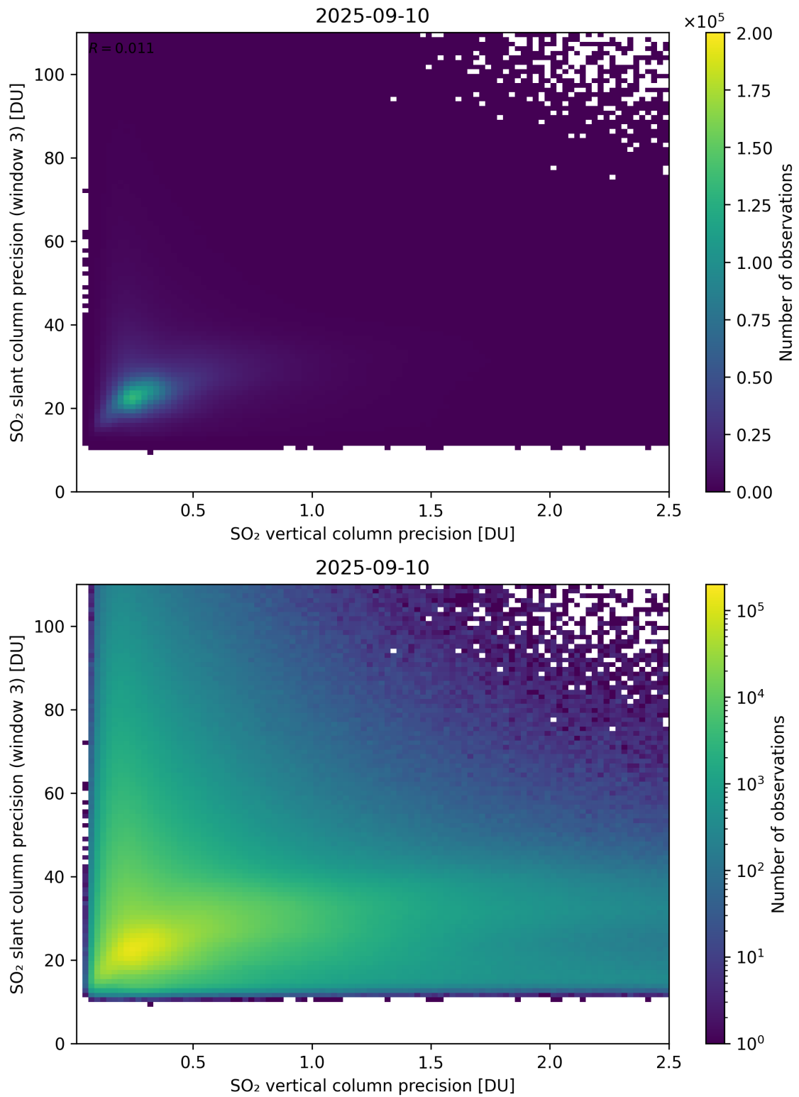
Figure 345: Scatter density plot of “SO 2 vertical column precision” against “SO 2 slant column precision (window 3)” for 2025-09-10 to 2025-09-11.
