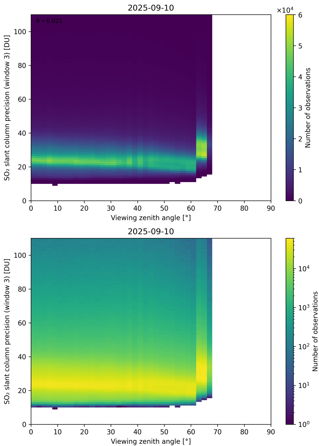
Figure 380: Scatter density plot of “Viewing zenith angle” against “SO 2 slant column precision (window 3)” for 2025-09-10 to 2025-09-11.
