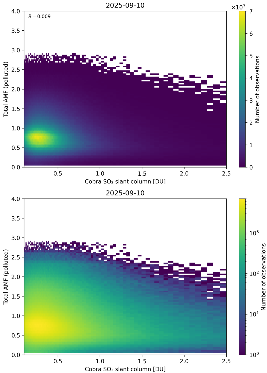
Figure 224: Scatter density plot of “Cobra SO 2 slant column” against “Total AMF (polluted)” for 2025-09-10 to 2025-09-11.
