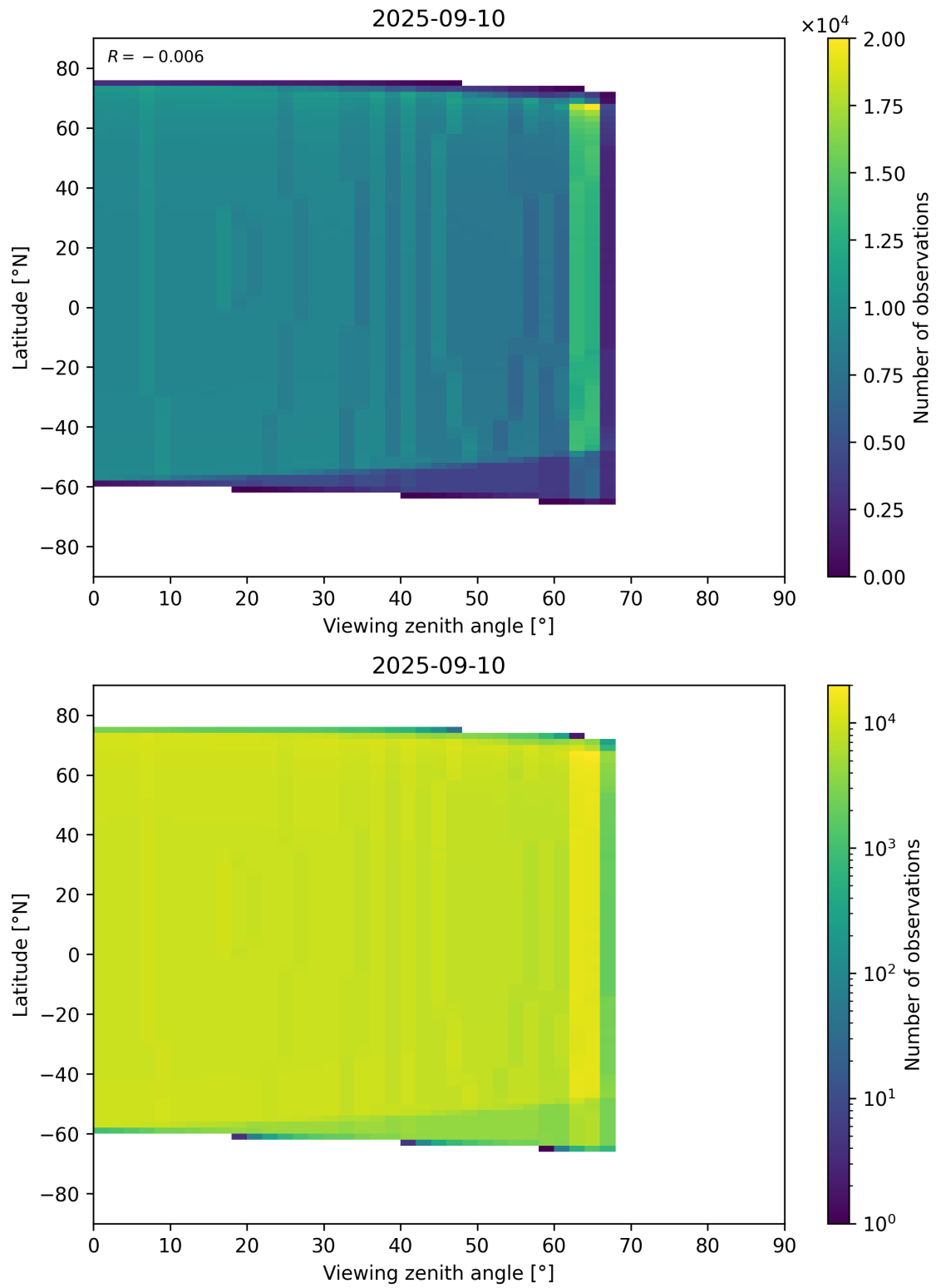
Figure 368: Scatter density plot of “Viewing zenith angle” against “Latitude” for 2025-09-10 to 2025-09-11.
