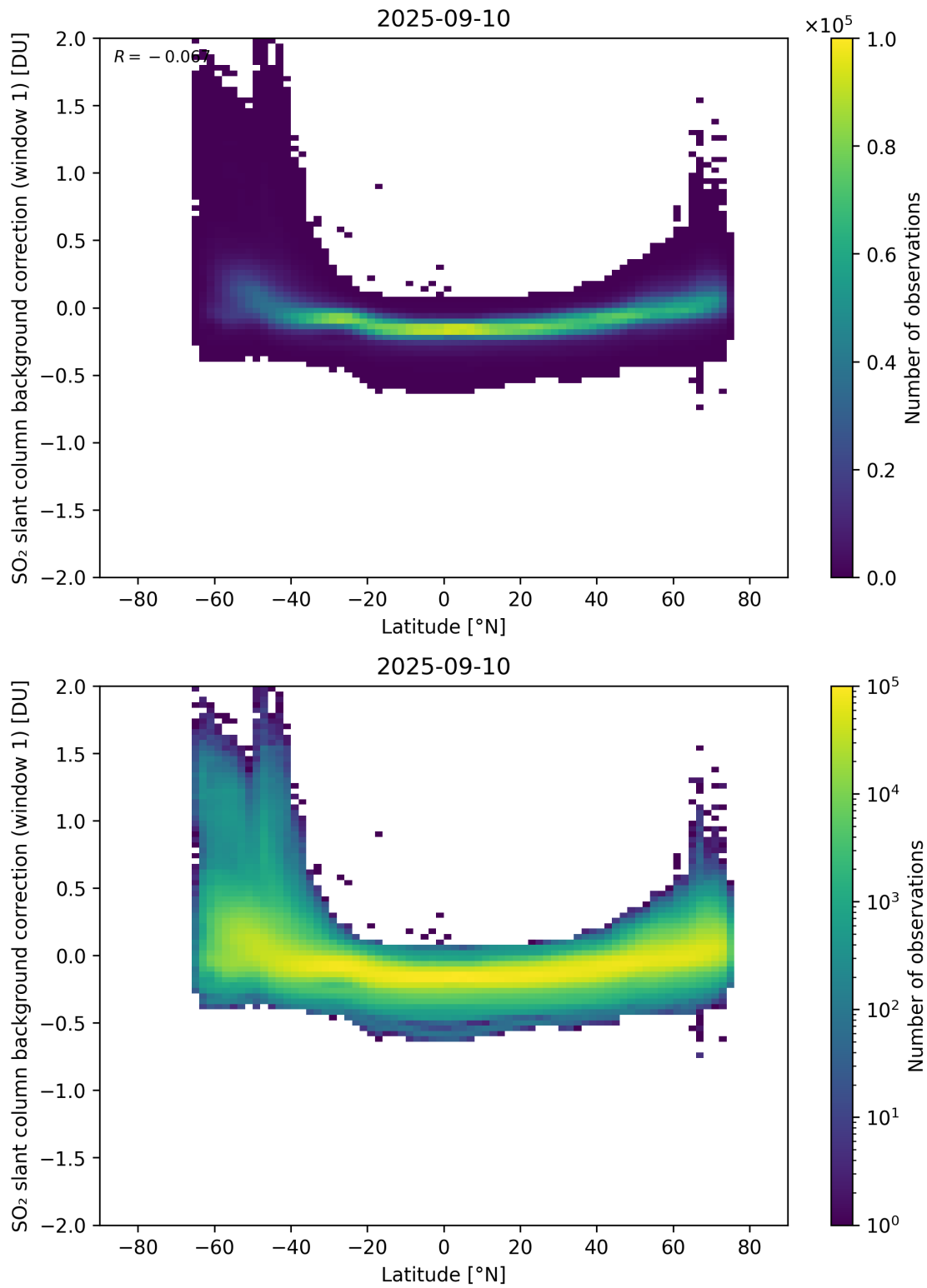
Figure 150: Scatter density plot of “Latitude” against “SO 2 slant column background correction (window 1)” for 2025-09-10 to 2025-09-11.
