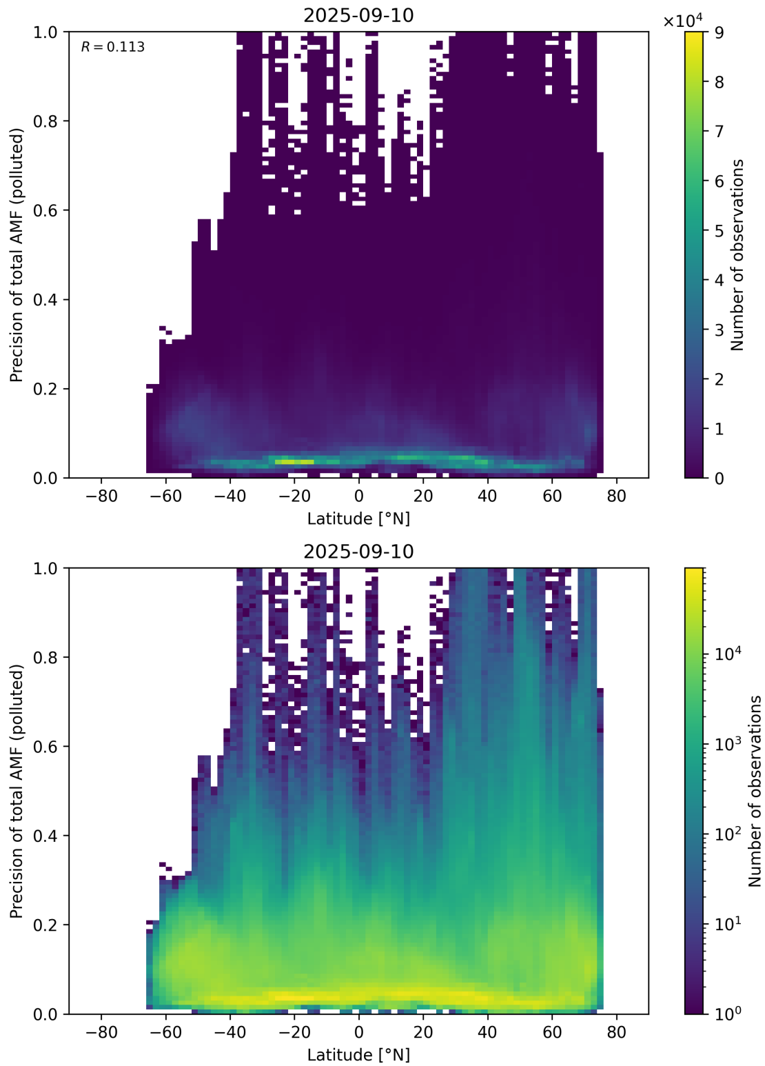
Figure 168: Scatter density plot of “Latitude” against “Precision of total AMF (polluted)” for 2025-09-10 to 2025-09-11.
