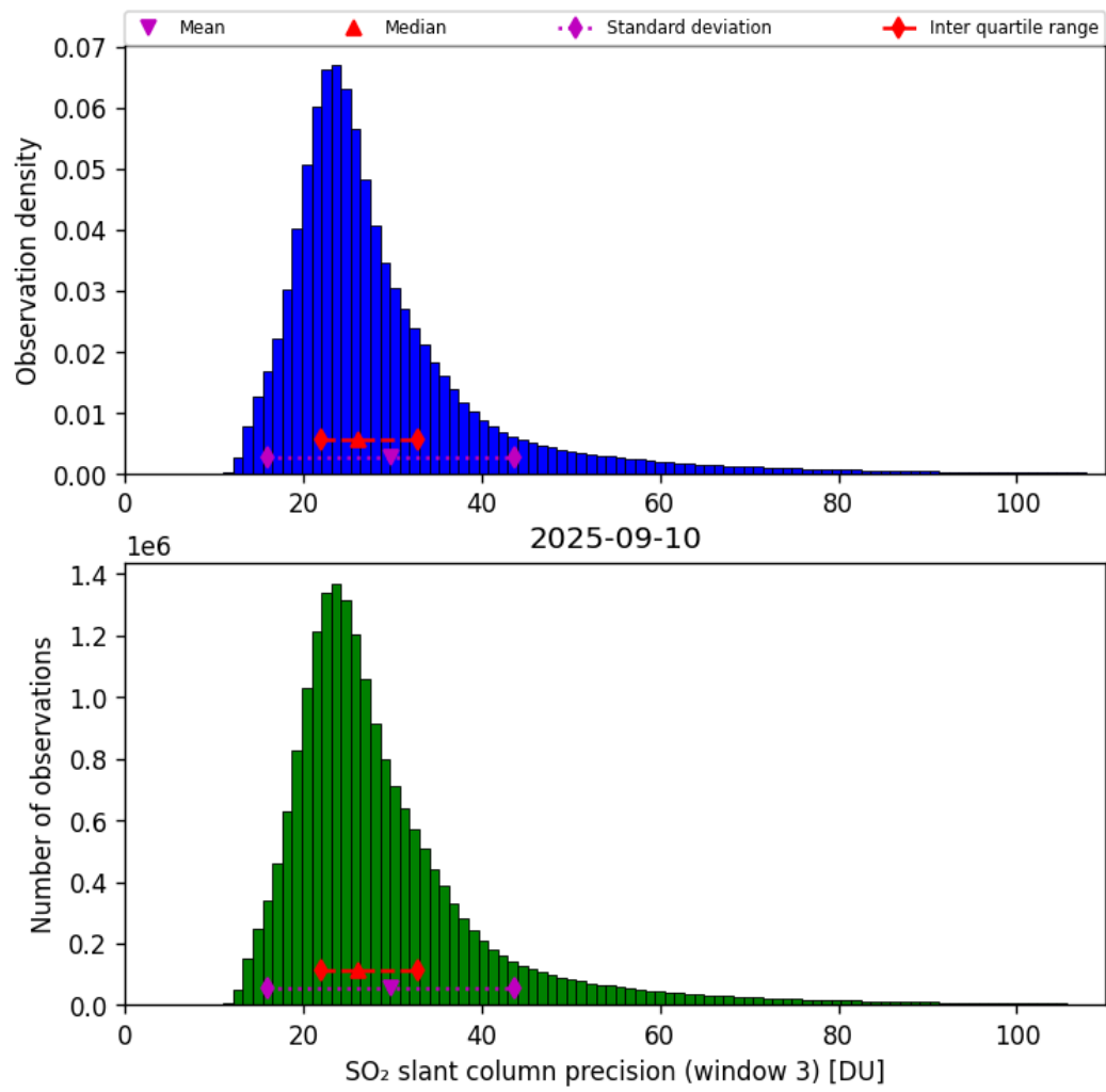
Figure 72: Histogram of “SO 2 slant column precision (window 3)” for 2025-09-10 to 2025-09-11
