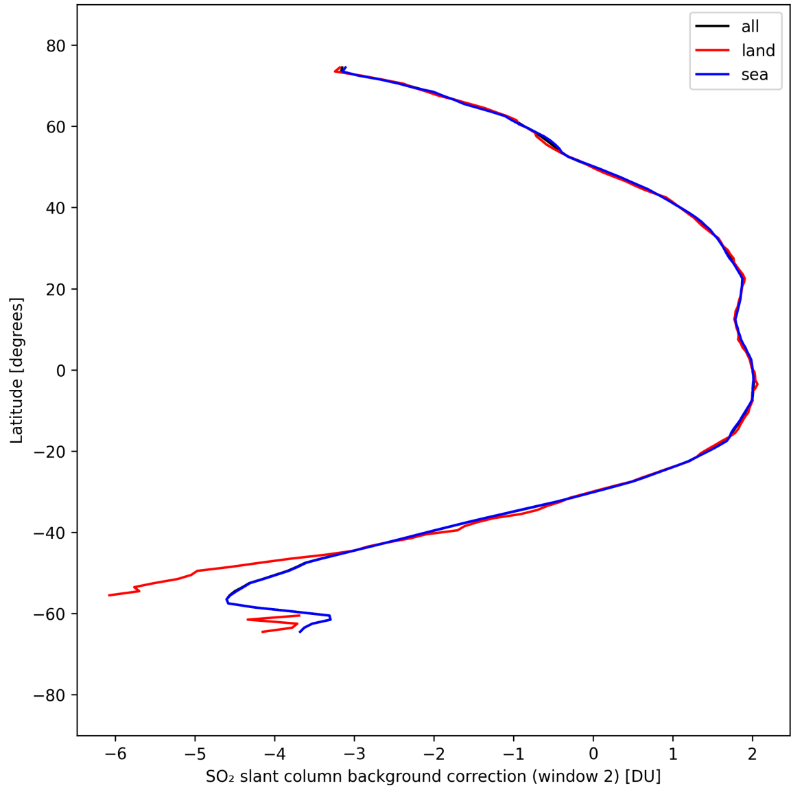
Figure 44: Zonal average of “SO 2 slant column background correction (window 2)” for 2025-09-10 to 2025-09-11.
