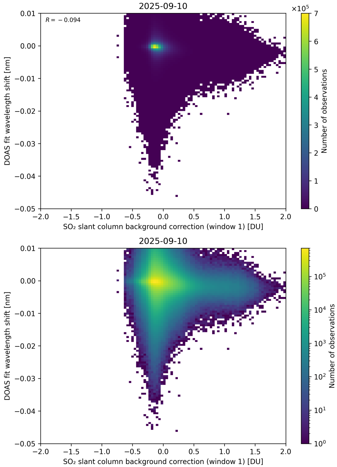
Figure 111: Scatter density plot of “SO 2 slant column background correction (window 1)” against “DOAS fit wavelength shift” for 2025-09-10 to 2025-09-11.
