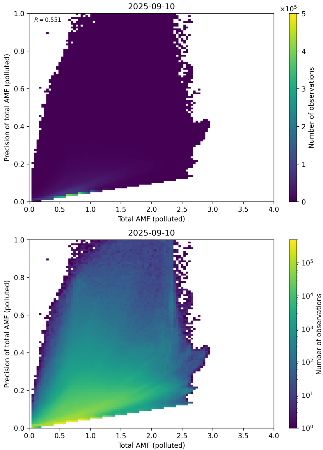
Figure 322: Scatter density plot of “Total AMF (polluted)” against “Precision of total AMF (polluted)” for 2025-09-10 to 2025-09-11.
