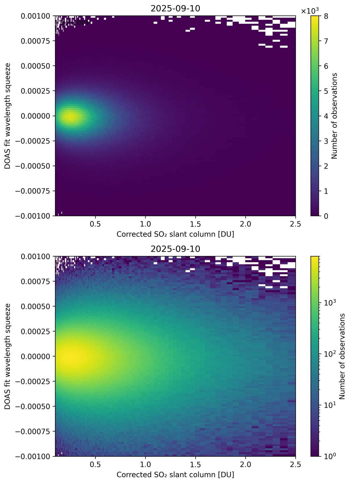
Figure 230: Scatter density plot of “Corrected SO 2 slant column” against “DOAS fit wavelength squeeze” for 2025-09-10 to 2025-09-11.
