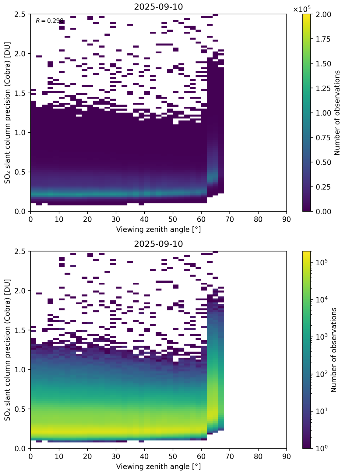
Figure 372: Scatter density plot of “Viewing zenith angle” against “SO 2 slant column precision (Cobra)” for 2025-09-10 to 2025-09-11.
