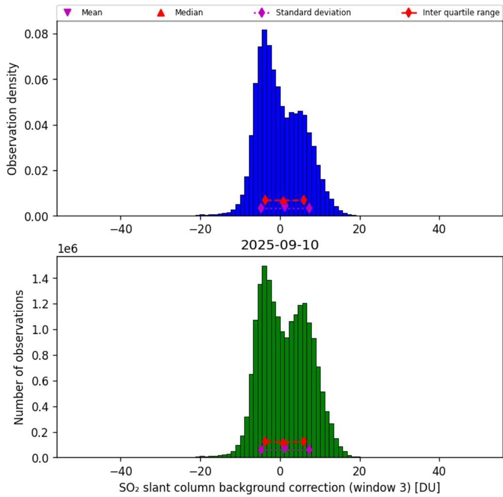
Figure 74: Histogram of “SO 2 slant column background correction (window 3)” for 2025-09-10 to 2025-09-11
