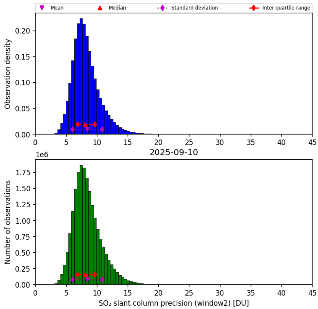
Figure 68: Histogram of “SO 2 slant column precision (window2)” for 2025-09-10 to 2025-09-11
