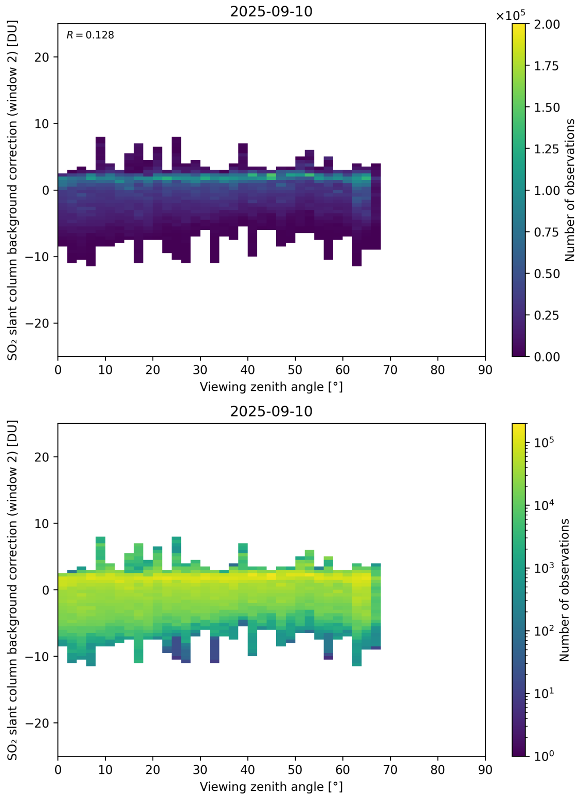
Figure 363: Scatter density plot of “Viewing zenith angle” against “SO 2 slant column background correction (window 2)” for 2025-09-10 to 2025-09-11.
