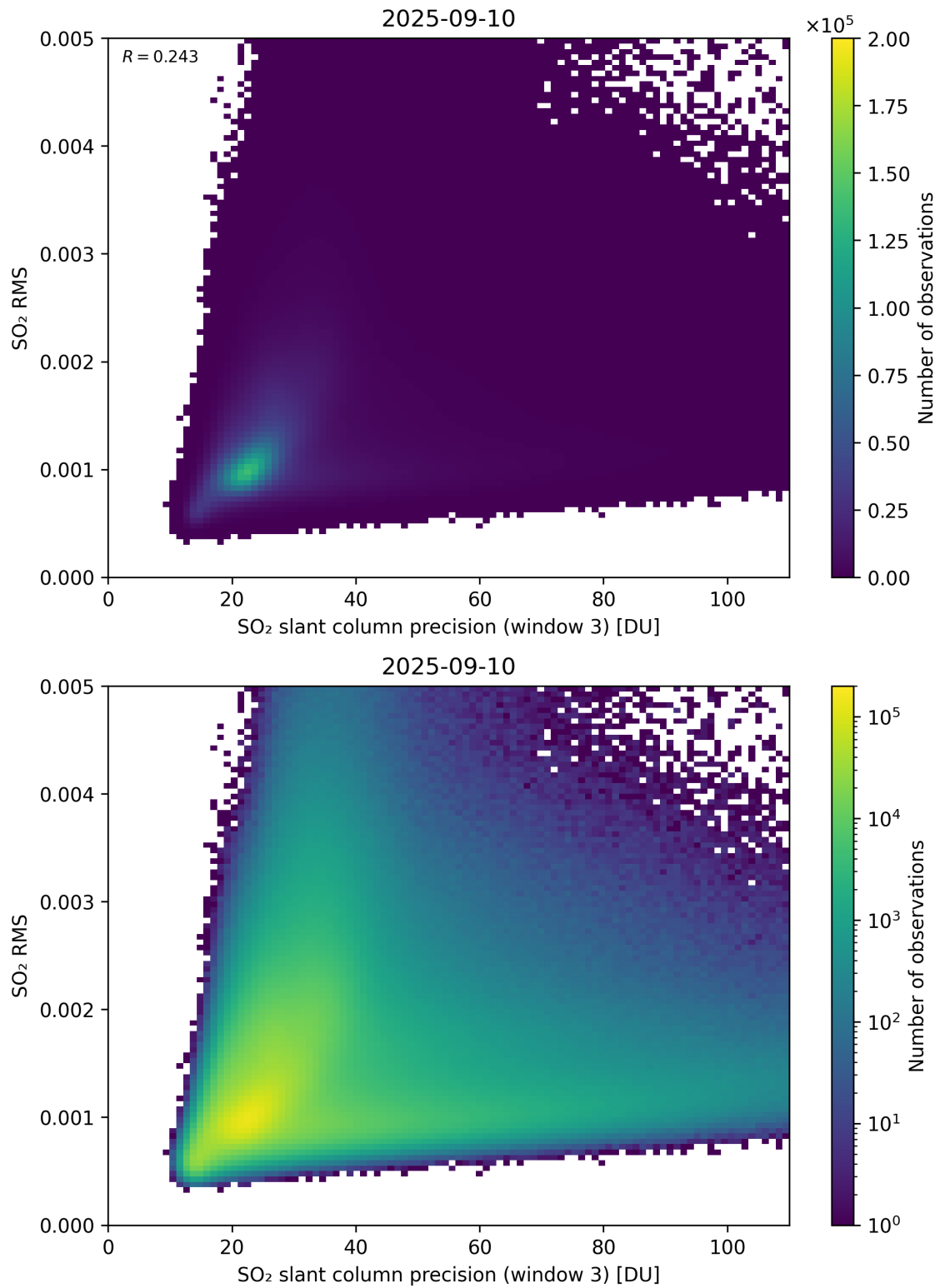
Figure 310: Scatter density plot of “SO 2 slant column precision (window 3)” against “SO 2 RMS” for 2025-09-10 to 2025-09-11.
