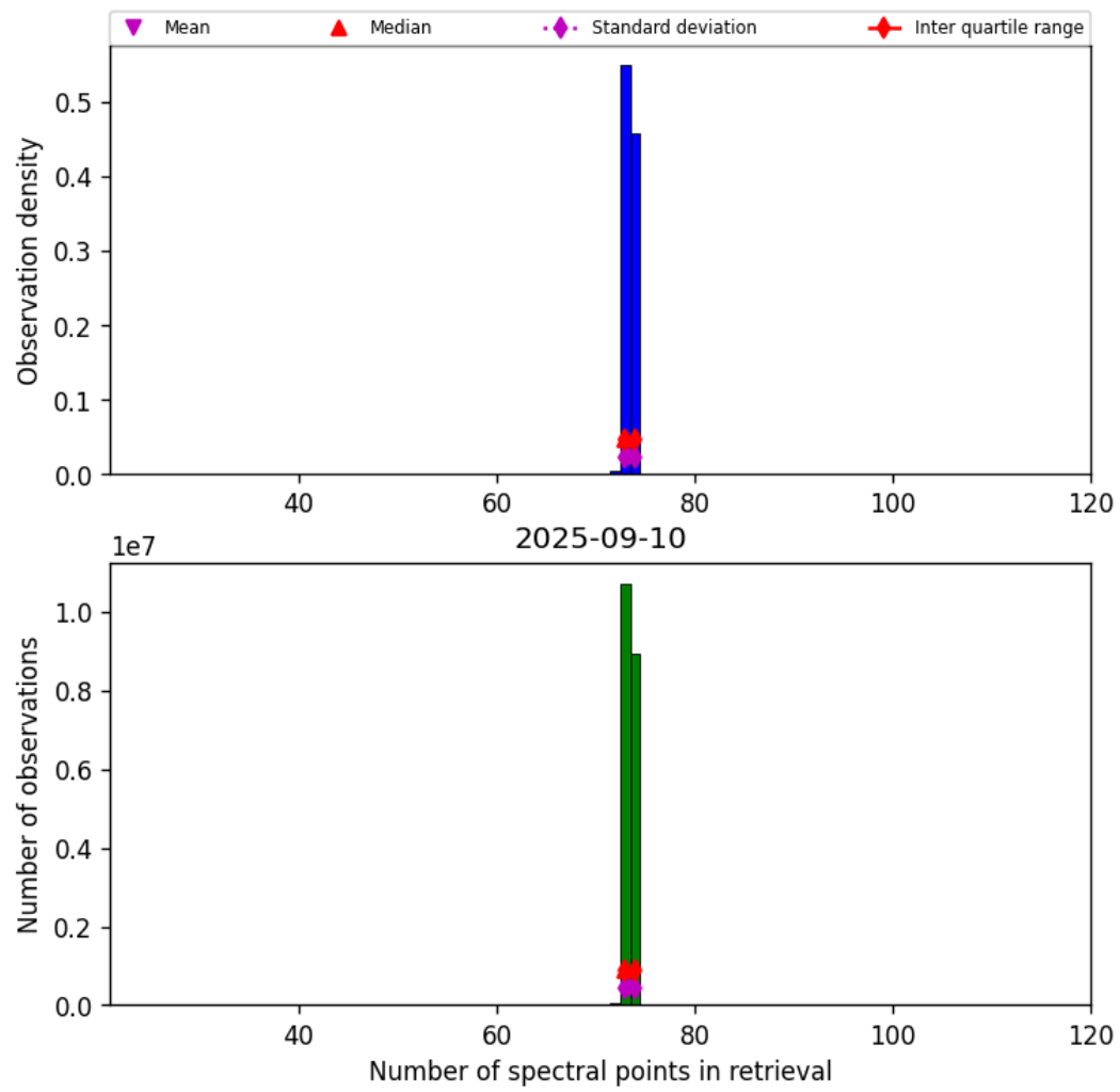
Figure 82: Histogram of "Number of spectral points in retrieval" for 2025-09-10 to 2025-09-11
