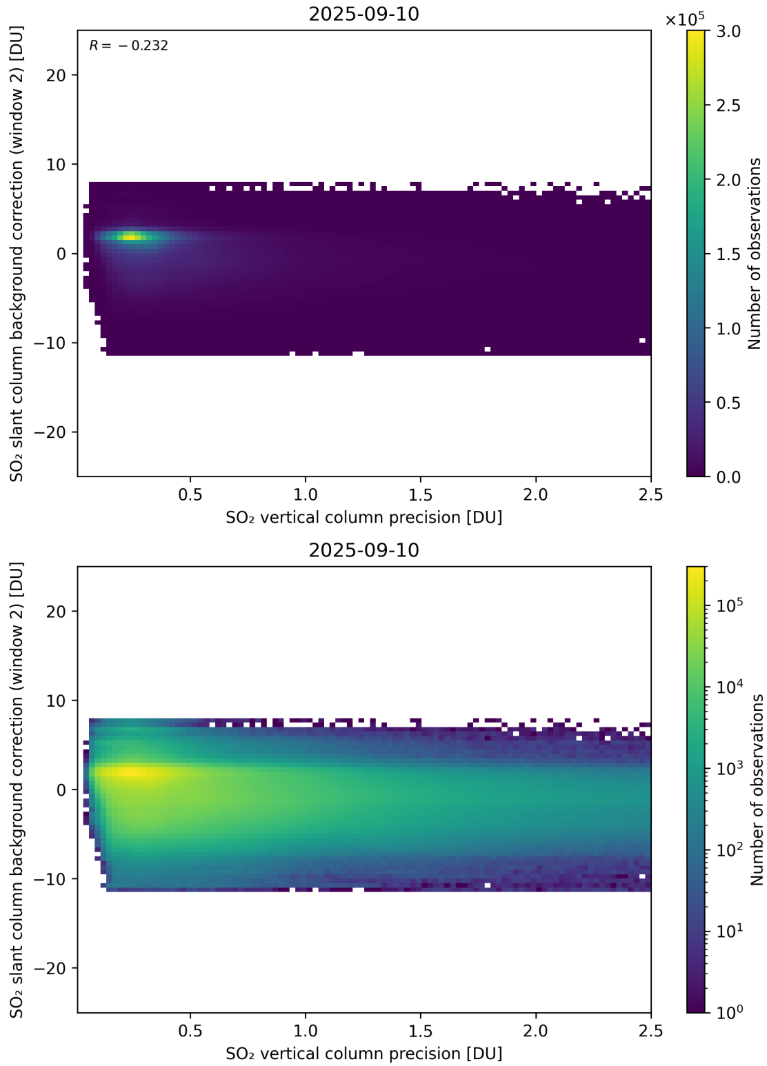
Figure 330: Scatter density plot of “SO 2 vertical column precision” against “SO 2 slant column background correction (window 2)” for 2025-09-10 to 2025-09-11.
