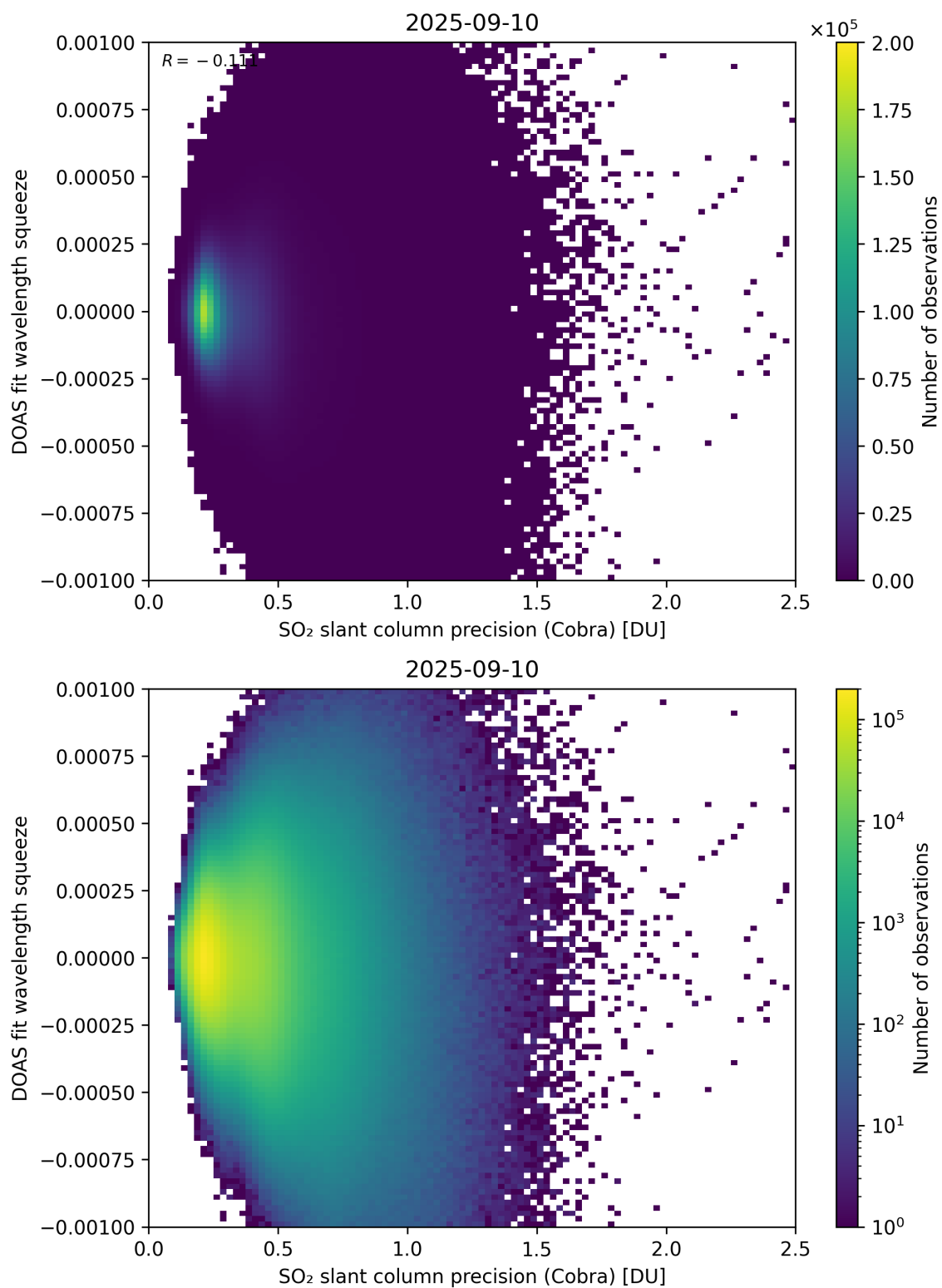
Figure 203: Scatter density plot of “SO 2 slant column precision (Cobra)” against “DOAS fit wavelength squeeze” for 2025-09-10 to 2025-09-11.
