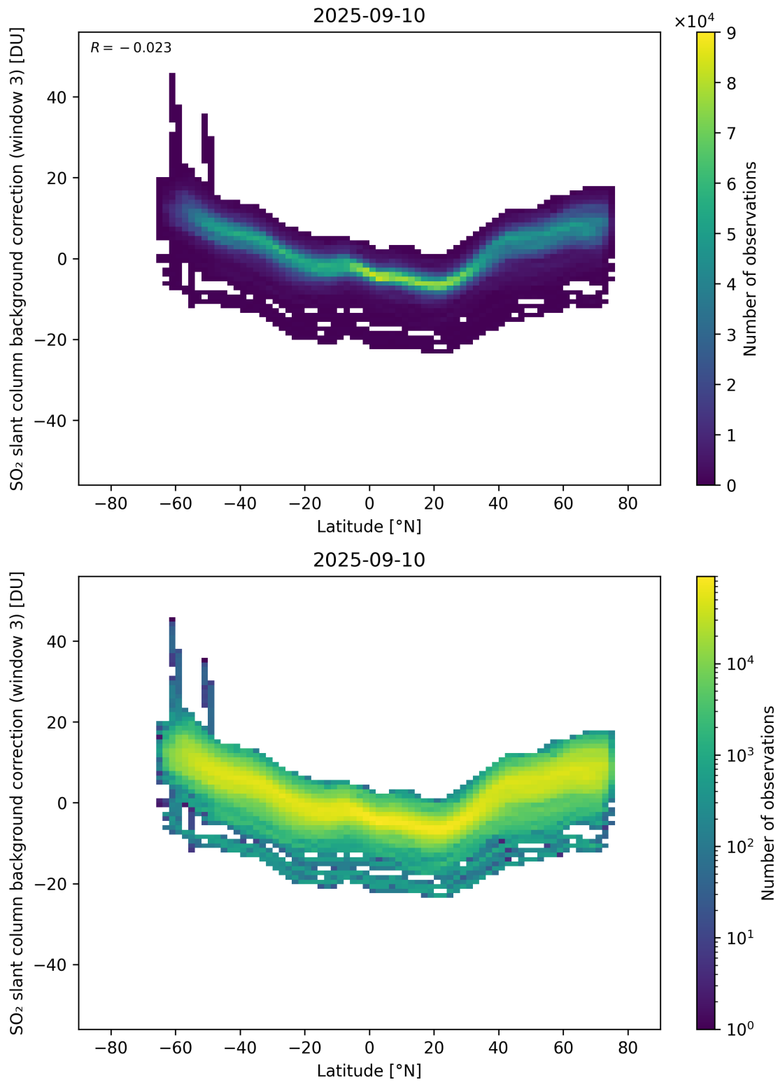
Figure 152: Scatter density plot of “Latitude” against “SO 2 slant column background correction (window 3)” for 2025-09-10 to 2025-09-11.
