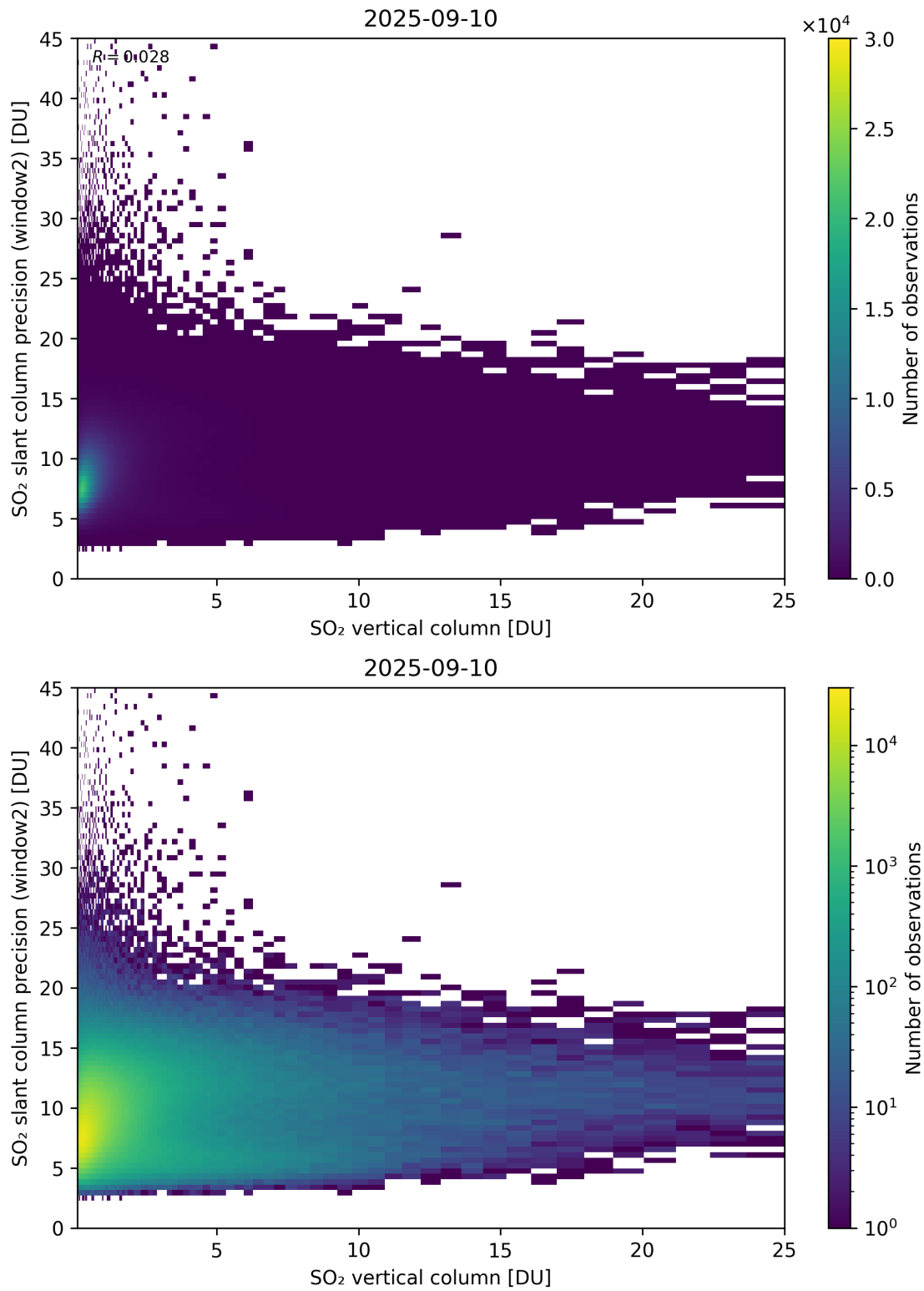
Figure 356: Scatter density plot of “SO 2 vertical column” against “SO 2 slant column precision (window2)” for 2025-09-10 to 2025-09-11.
