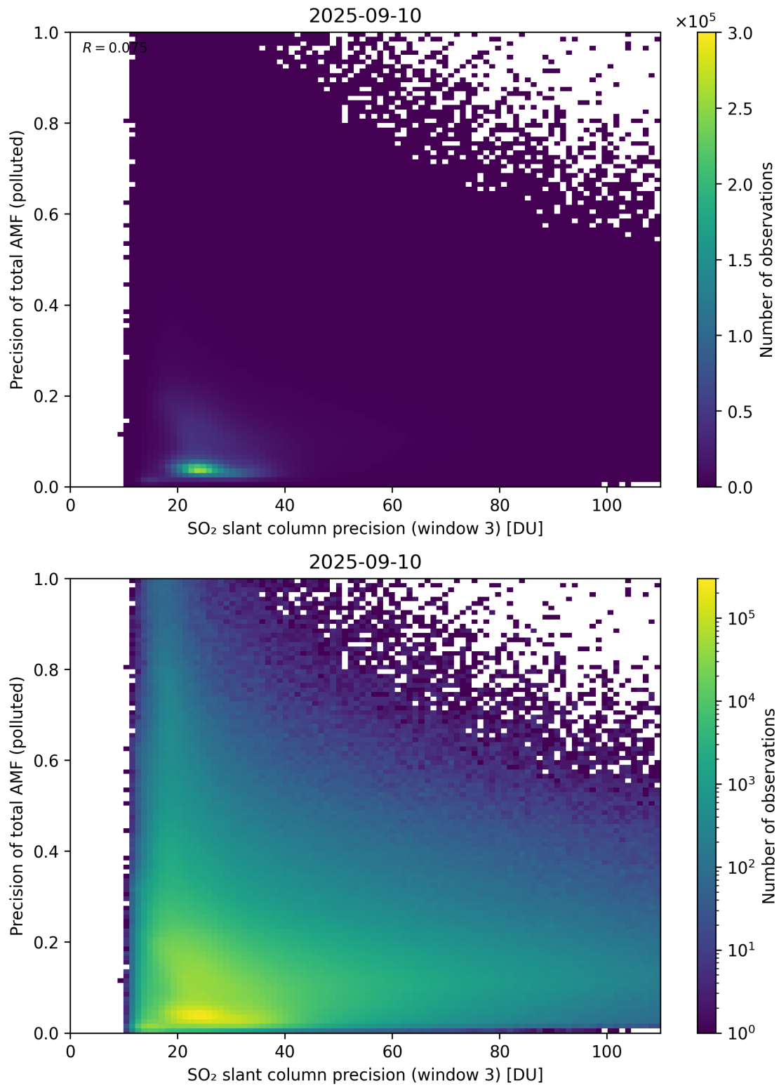
Figure 314: Scatter density plot of “SO 2 slant column precision (window 3)” against “Precision of total AMF (polluted)” for 2025-09-10 to 2025-09-11.
