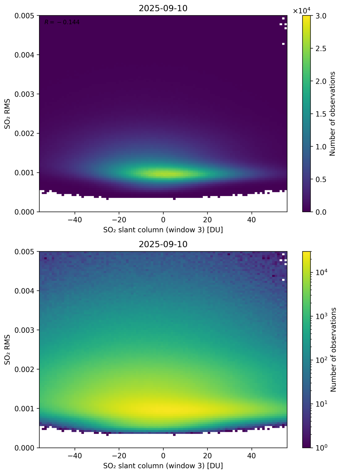
Figure 306: Scatter density plot of “SO 2 slant column (window 3)” against “SO 2 RMS” for 2025-09-10 to 2025-09-11.
