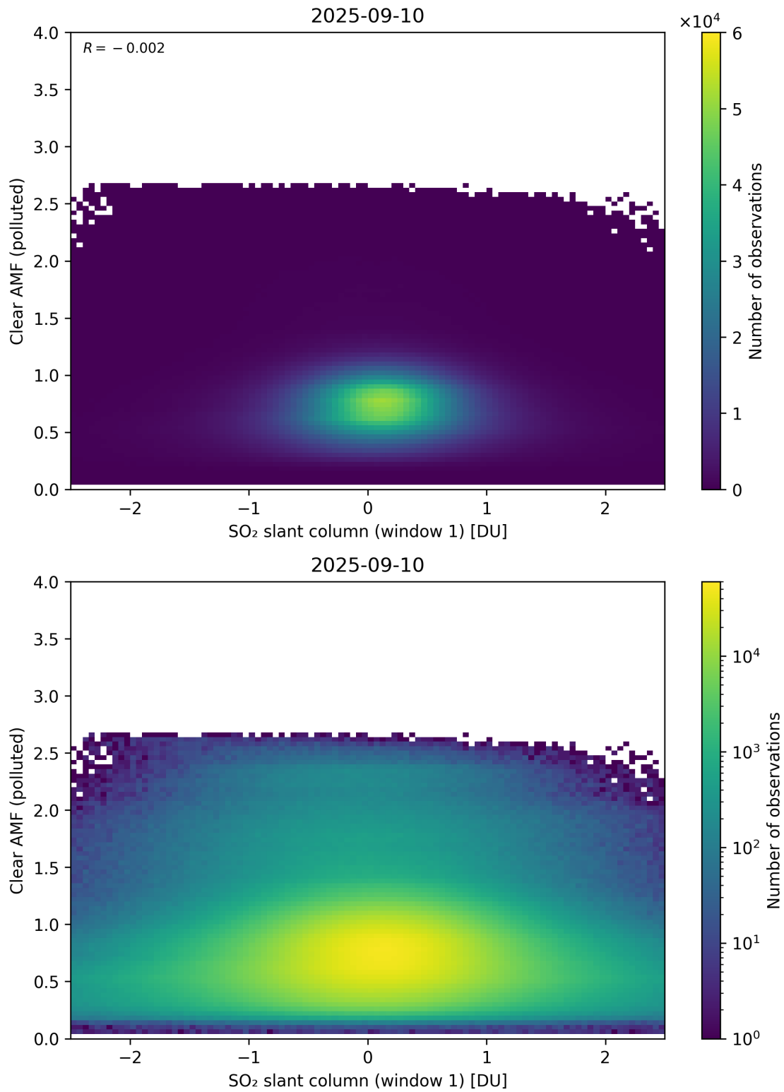
Figure 282: Scatter density plot of “SO 2 slant column (window 1)” against “Clear AMF (polluted)” for 2025-09-10 to 2025-09-11.
