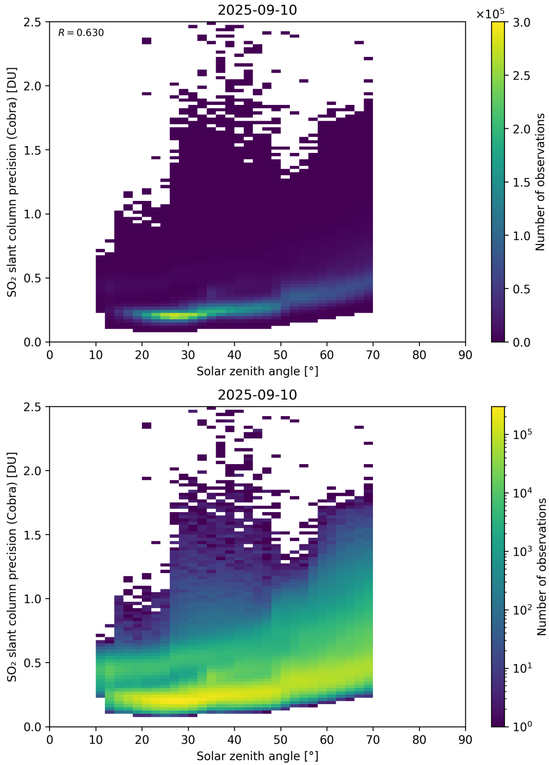
Figure 180: Scatter density plot of “Solar zenith angle” against “SO 2 slant column precision (Cobra)” for 2025-09-10 to 2025-09-11.
