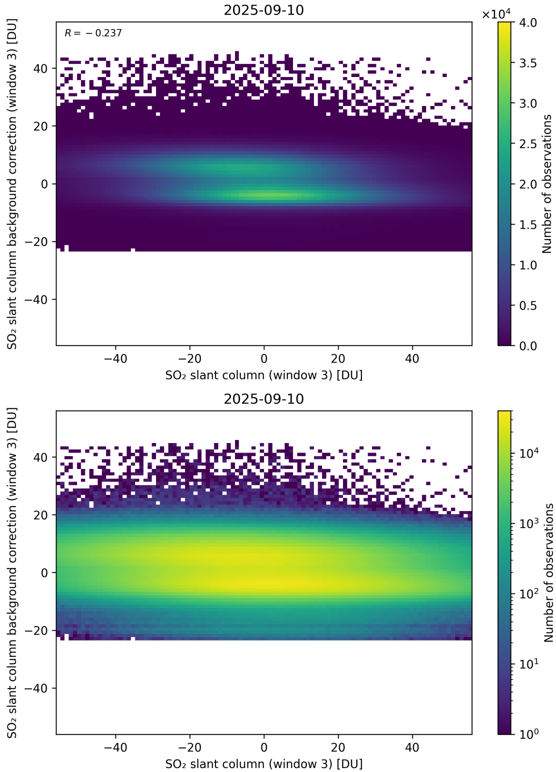
Figure 303: Scatter density plot of “SO 2 slant column (window 3)” against “SO 2 slant column background correction (window 3)” for 2025-09-10 to 2025-09-11.
