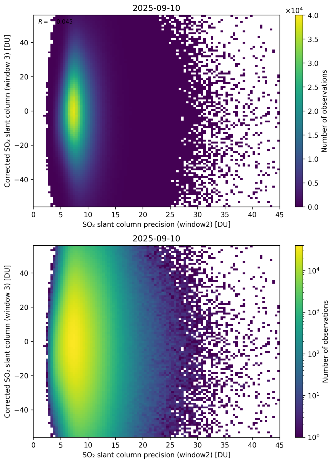
Figure 298: Scatter density plot of “SO 2 slant column precision (window2)” against “Corrected SO 2 slant column (window 3)” for 2025-09-10 to 2025-09-11.
