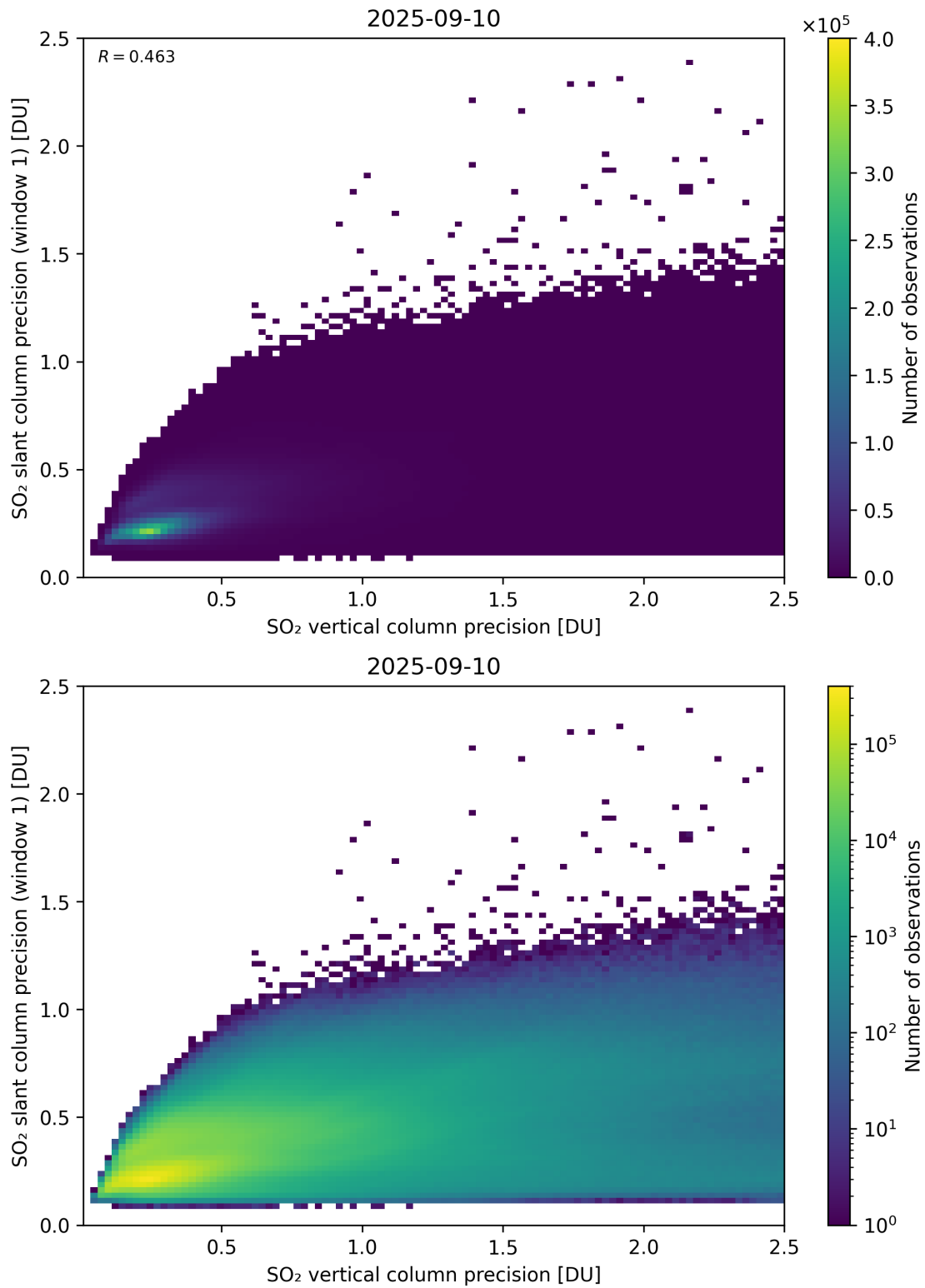
Figure 342: Scatter density plot of “SO 2 vertical column precision” against “SO 2 slant column precision (window 1)” for 2025-09-10 to 2025-09-11.
