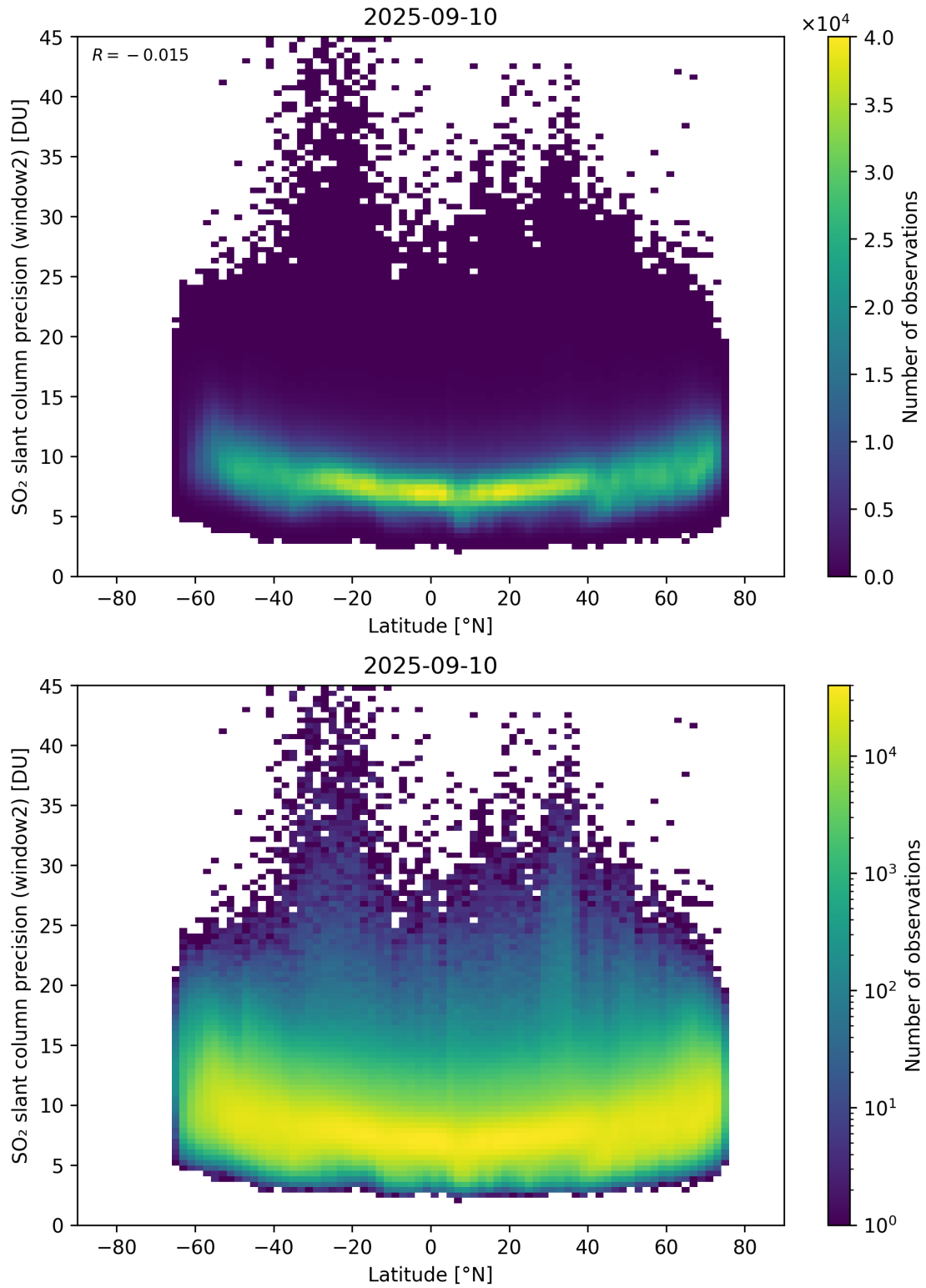
Figure 164: Scatter density plot of “Latitude” against “SO 2 slant column precision (window2)” for 2025-09-10 to 2025-09-11.
