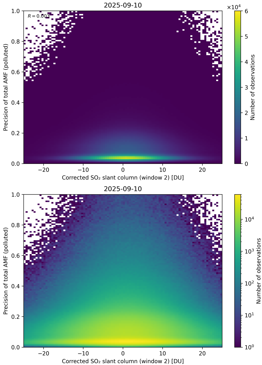
Figure 254: Scatter density plot of “Corrected SO 2 slant column (window 2)” against “Precision of total AMF (polluted)” for 2025-09-10 to 2025-09-11.
