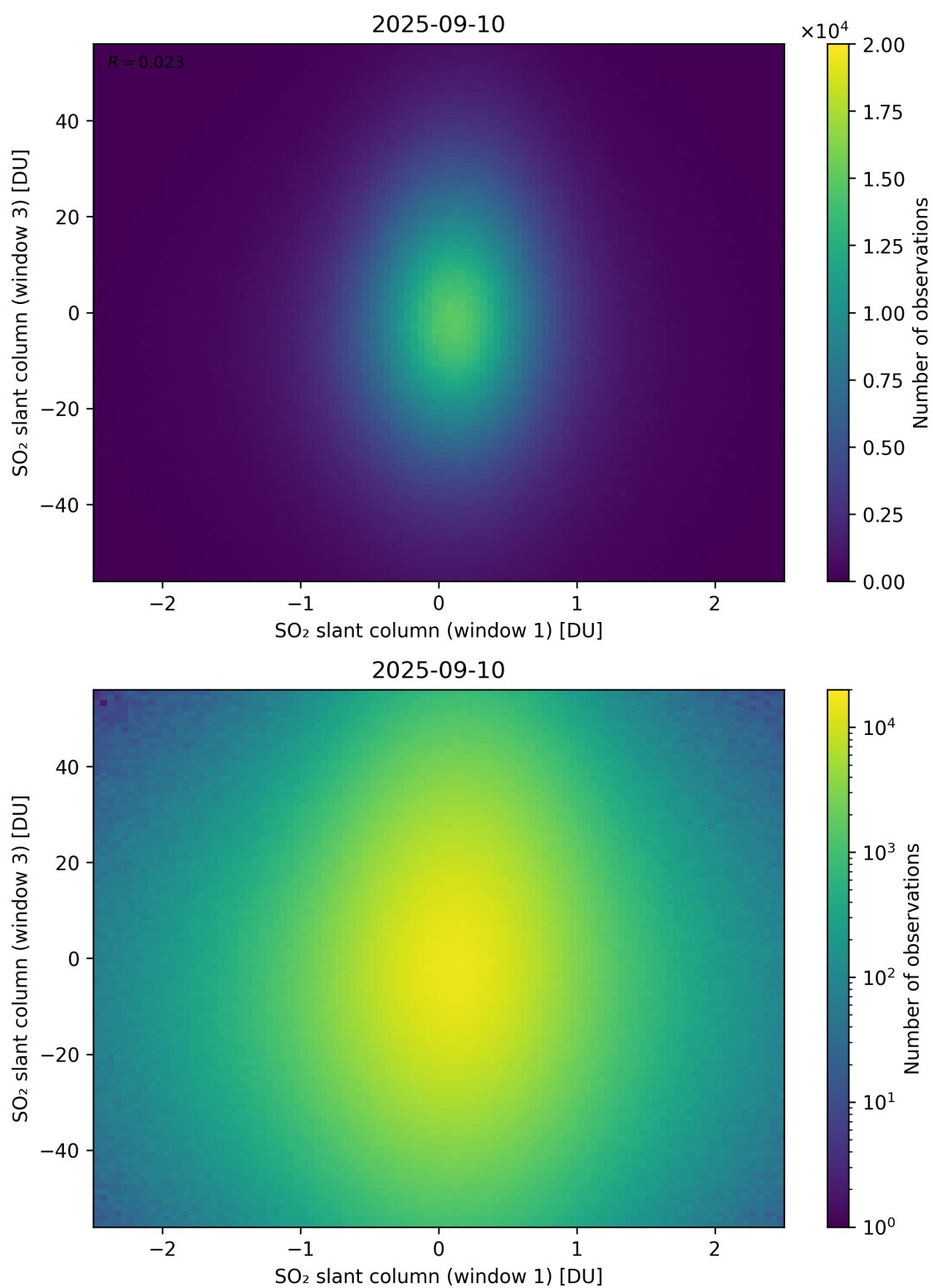
Figure 287: Scatter density plot of “SO 2 slant column (window 1)” against “SO 2 slant column (window 3)” for 2025-09-10 to 2025-09-11.
