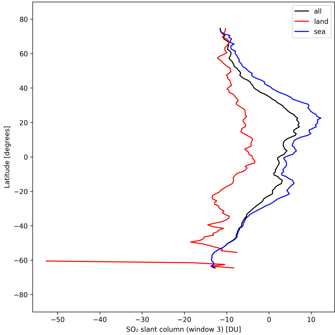
Figure 45: Zonal average of “SO 2 slant column (window 3)” for 2025-09-10 to 2025-09-11.
