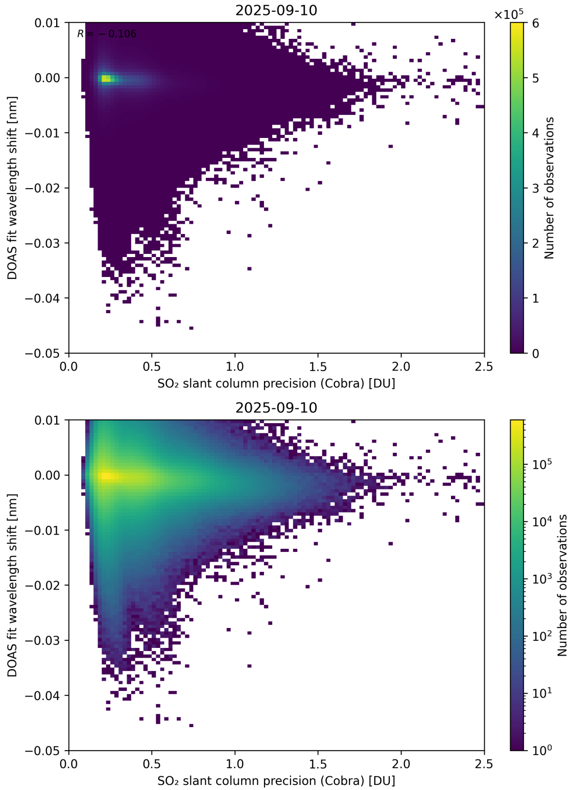
Figure 202: Scatter density plot of “SO 2 slant column precision (Cobra)” against “DOAS fit wavelength shift” for 2025-09-10 to 2025-09-11.
