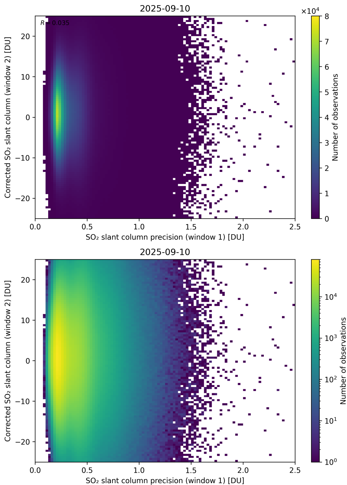
Figure 275: Scatter density plot of “SO 2 slant column precision (window 1)” against “Corrected SO 2 slant column (window 2)” for 2025-09-10 to 2025-09-11.
