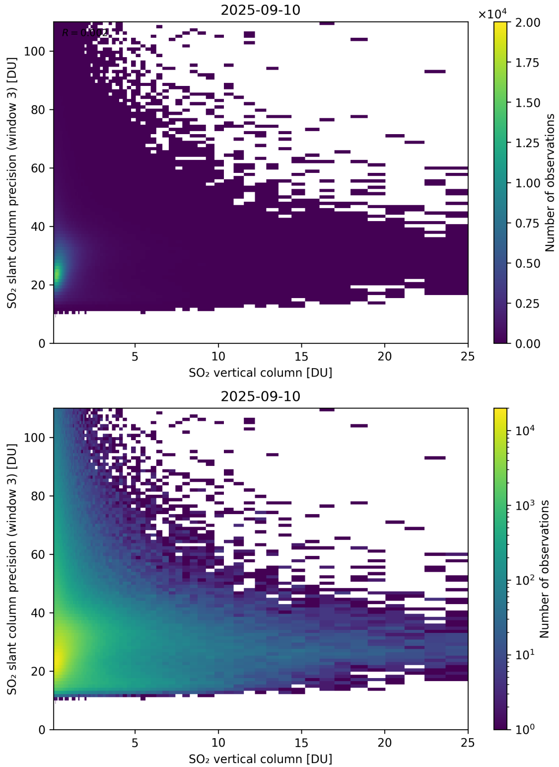
Figure 358: Scatter density plot of “SO 2 vertical column” against “SO 2 slant column precision (window 3)” for 2025-09-10 to 2025-09-11.
