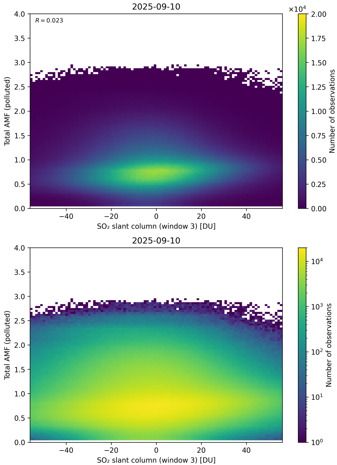
Figure 318: Scatter density plot of “SO 2 slant column (window 3)” against “Total AMF (polluted)” for 2025-09-10 to 2025-09-11.
