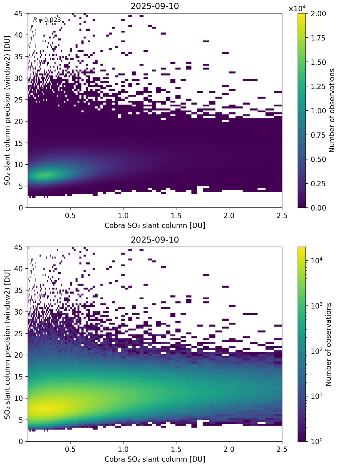
Figure 221: Scatter density plot of “Cobra SO 2 slant column” against “SO 2 slant column precision (window2)” for 2025-09-10 to 2025-09-11.
