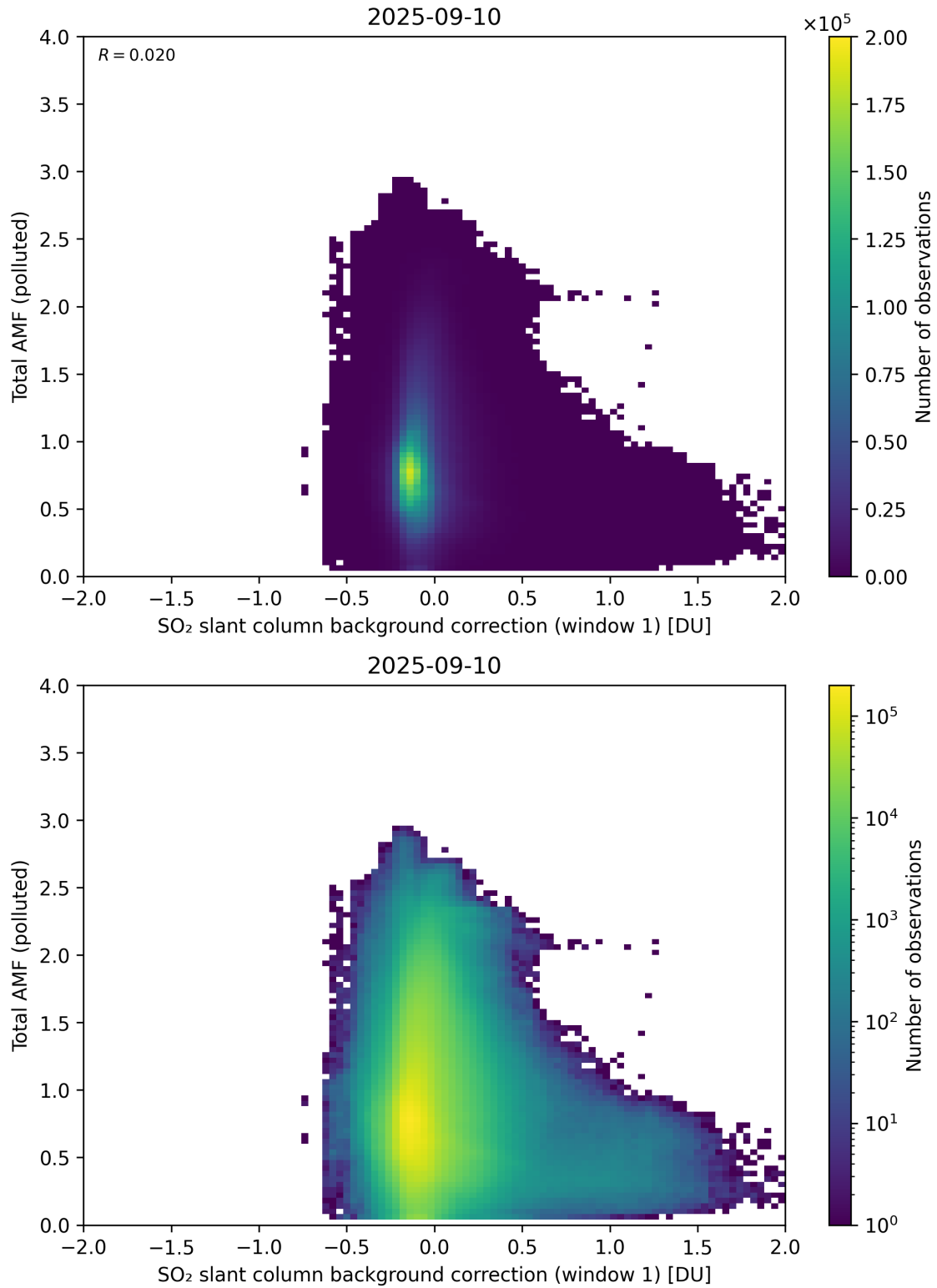
Figure 120: Scatter density plot of “SO 2 slant column background correction (window 1)” against “Total AMF (polluted)” for 2025-09-10 to 2025-09-11.
