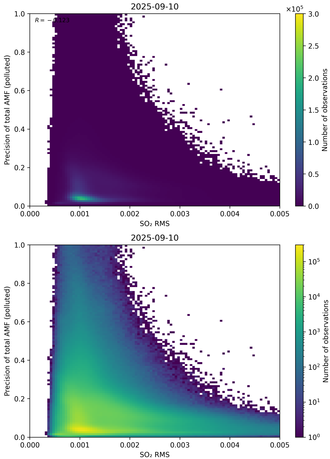
Figure 149: Scatter density plot of “SO 2 RMS” against “Precision of total AMF (polluted)” for 2025-09-10 to 2025-09-11.
