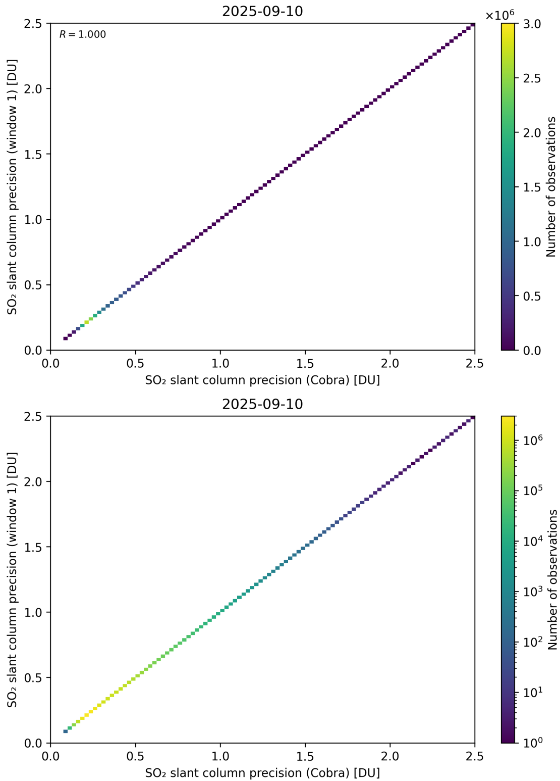
Figure 209: Scatter density plot of “SO 2 slant column precision (Cobra)” against “SO 2 slant column precision (window 1)” for 2025-09-10 to 2025-09-11.
