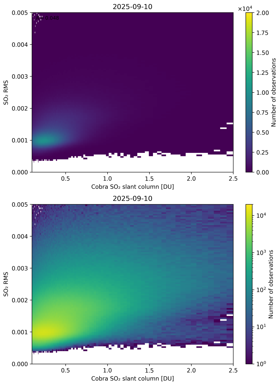
Figure 198: Scatter density plot of “Cobra SO 2 slant column” against “SO 2 RMS” for 2025-09-10 to 2025-09-11.
