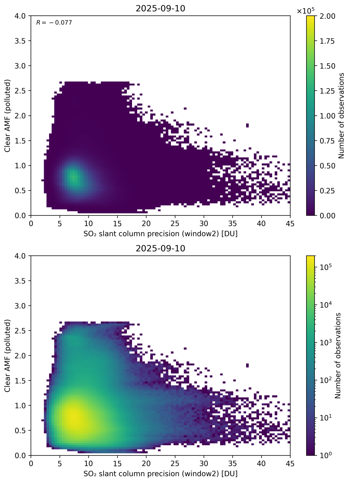
Figure 296: Scatter density plot of “SO 2 slant column precision (window2)” against “Clear AMF (polluted)” for 2025-09-10 to 2025-09-11.
