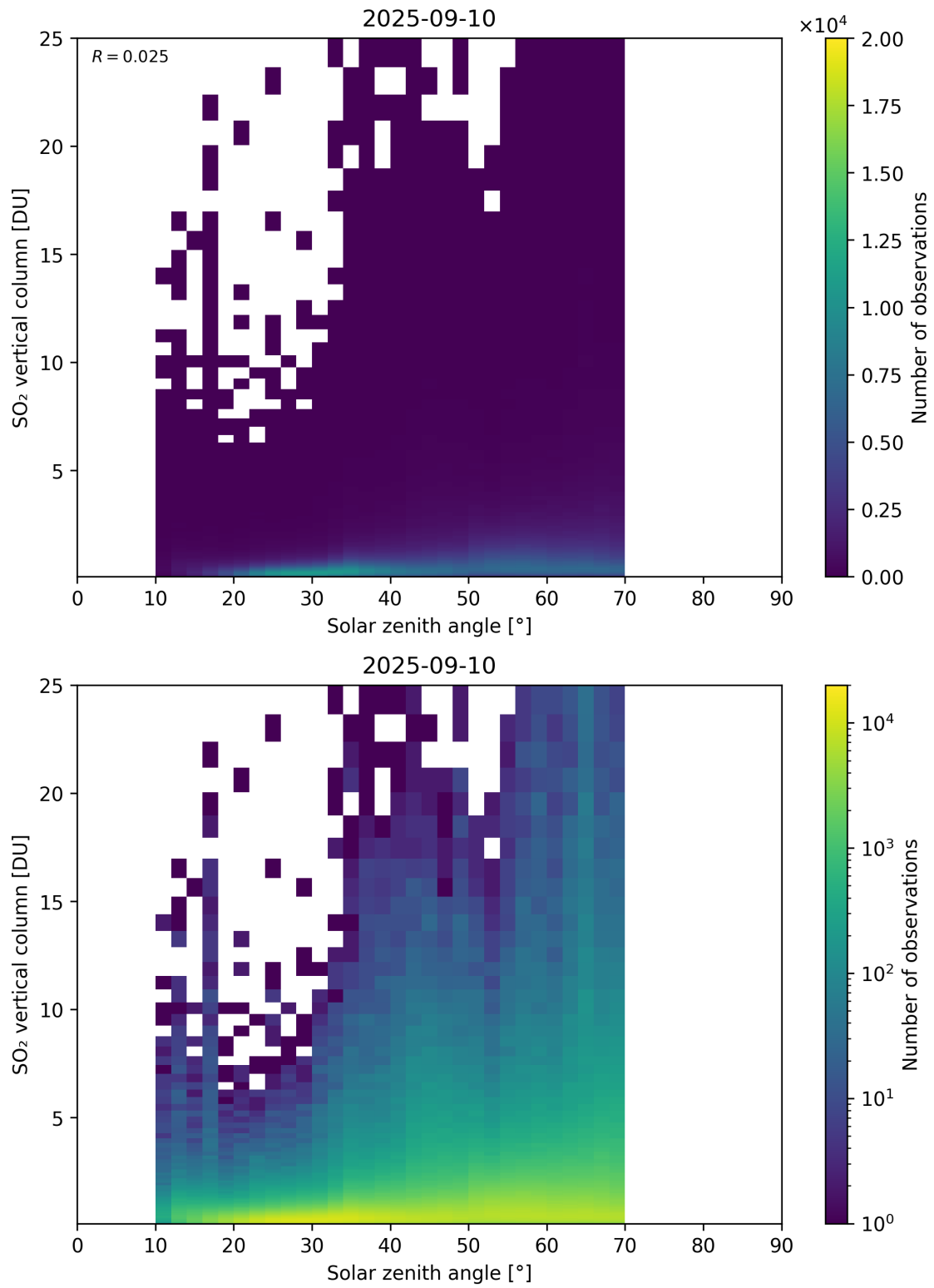
Figure 191: Scatter density plot of “Solar zenith angle” against “SO 2 vertical column” for 2025-09-10 to 2025-09-11.
