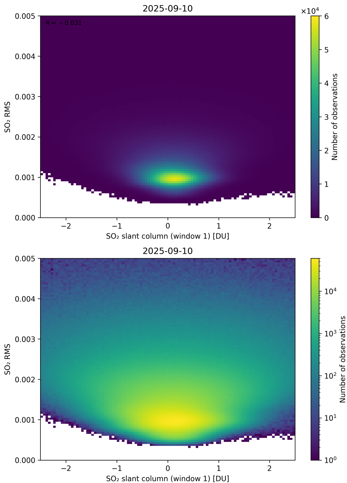
Figure 267: Scatter density plot of “SO 2 slant column (window 1)” against “SO 2 RMS” for 2025-09-10 to 2025-09-11.
