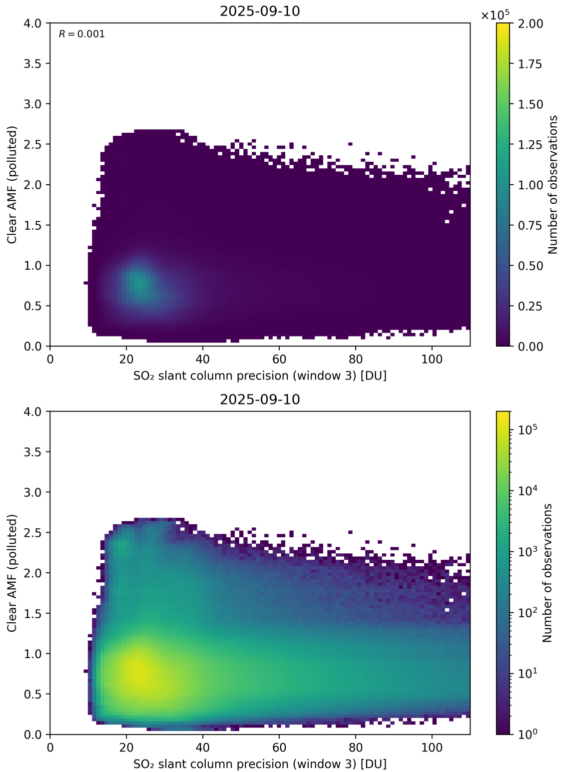
Figure 311: Scatter density plot of “SO 2 slant column precision (window 3)” against “Clear AMF (polluted)” for 2025-09-10 to 2025-09-11.
