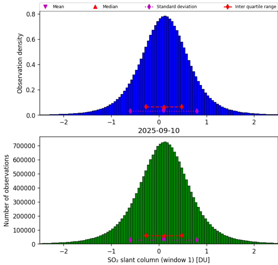
Figure 63: Histogram of “SO 2 slant column (window 1)” for 2025-09-10 to 2025-09-11
