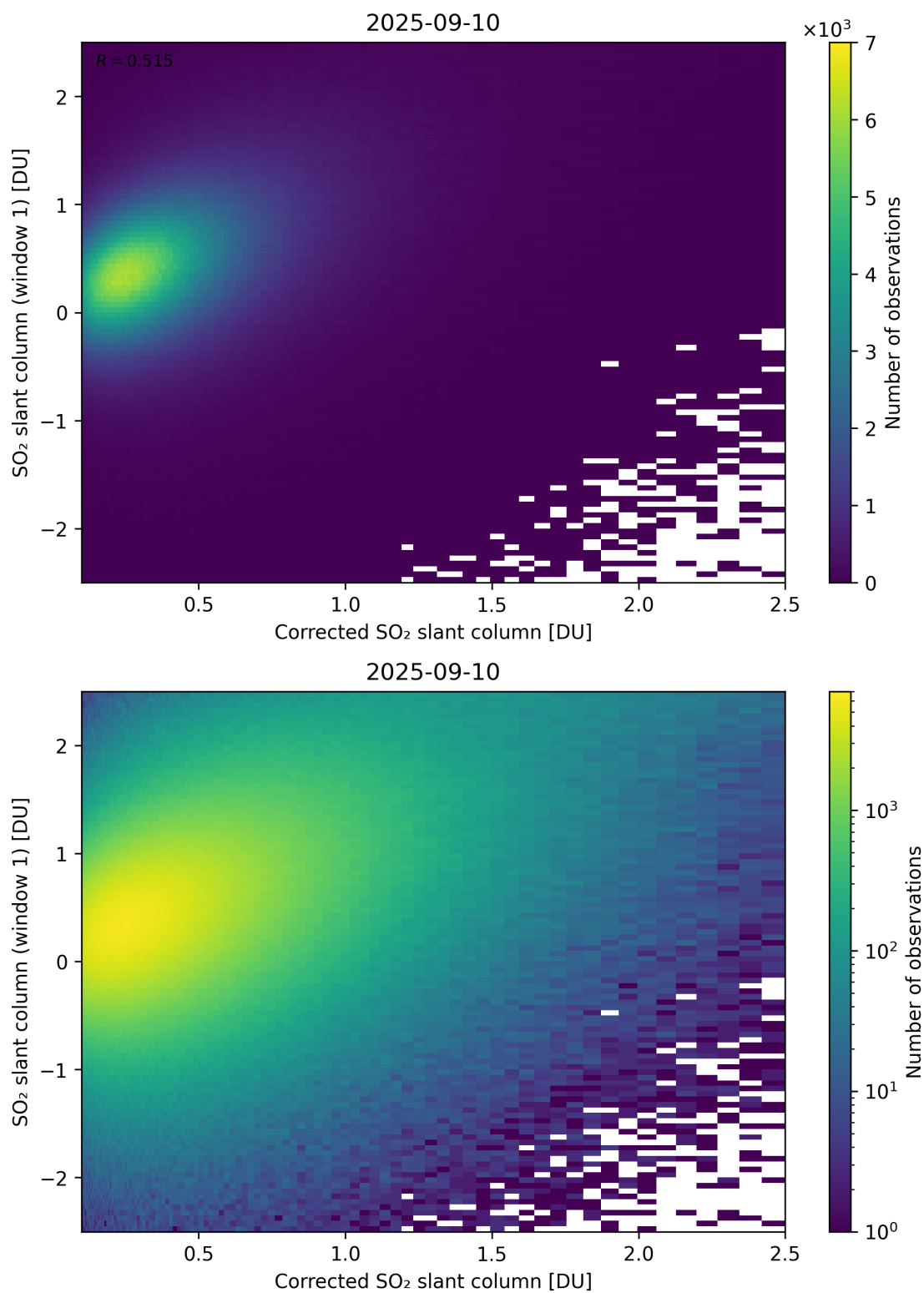
Figure 237: Scatter density plot of “Corrected SO 2 slant column” against “SO 2 slant column (window 1)” for 2025-09-10 to 2025-09-11.
