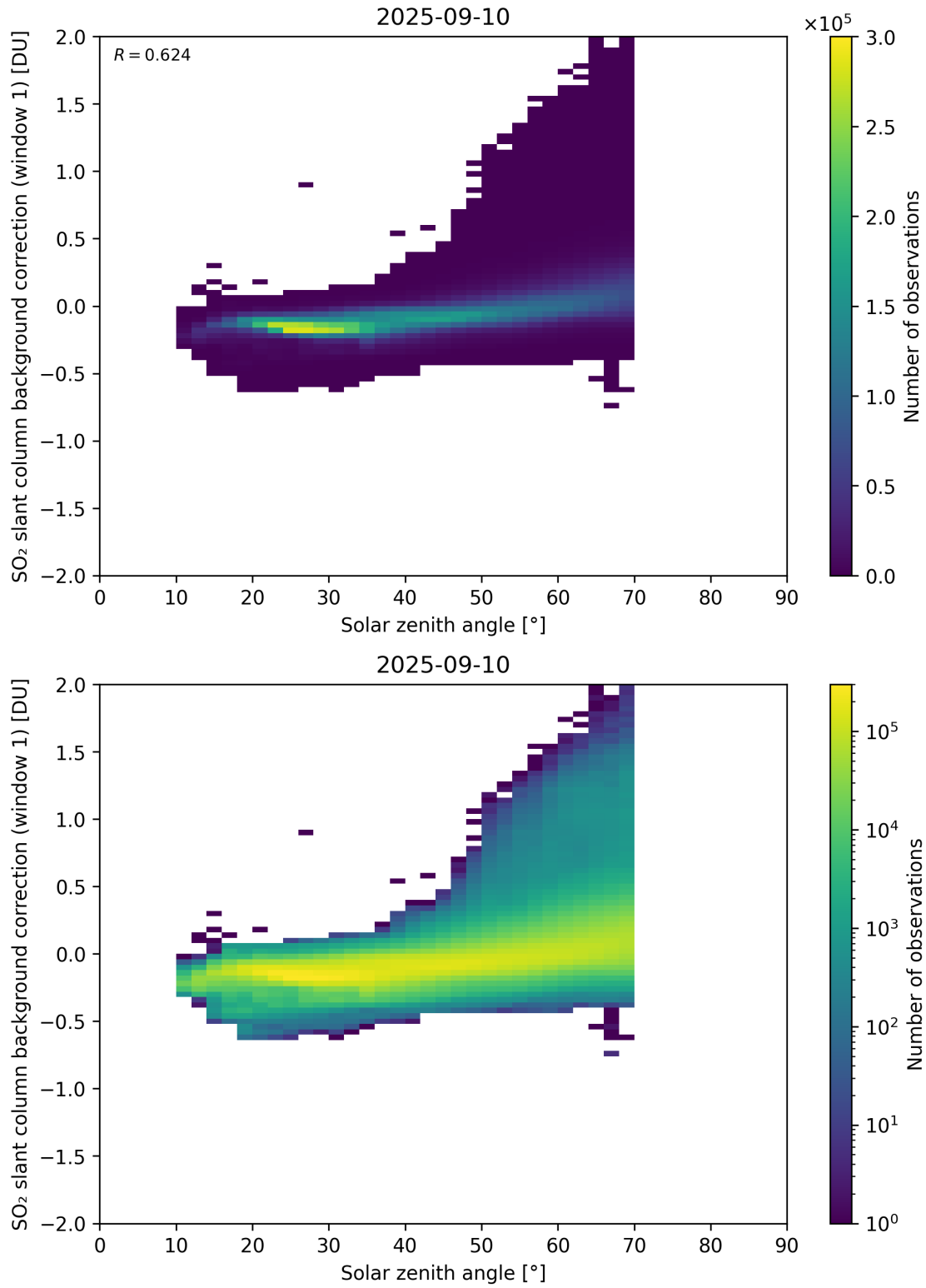
Figure 171: Scatter density plot of “Solar zenith angle” against “SO 2 slant column background correction (window 1)” for 2025-09-10 to 2025-09-11.
