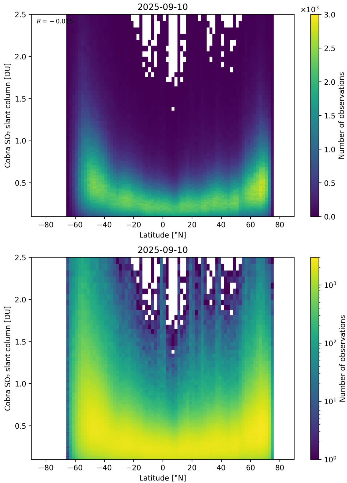
Figure 157: Scatter density plot of “Latitude” against “Cobra SO 2 slant column” for 2025-09-10 to 2025-09-11.
