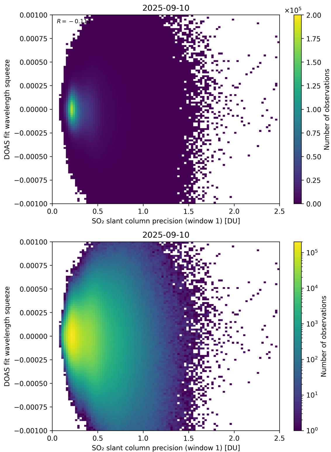
Figure 272: Scatter density plot of “SO 2 slant column precision (window 1)” against “DOAS fit wavelength squeeze” for 2025-09-10 to 2025-09-11.
