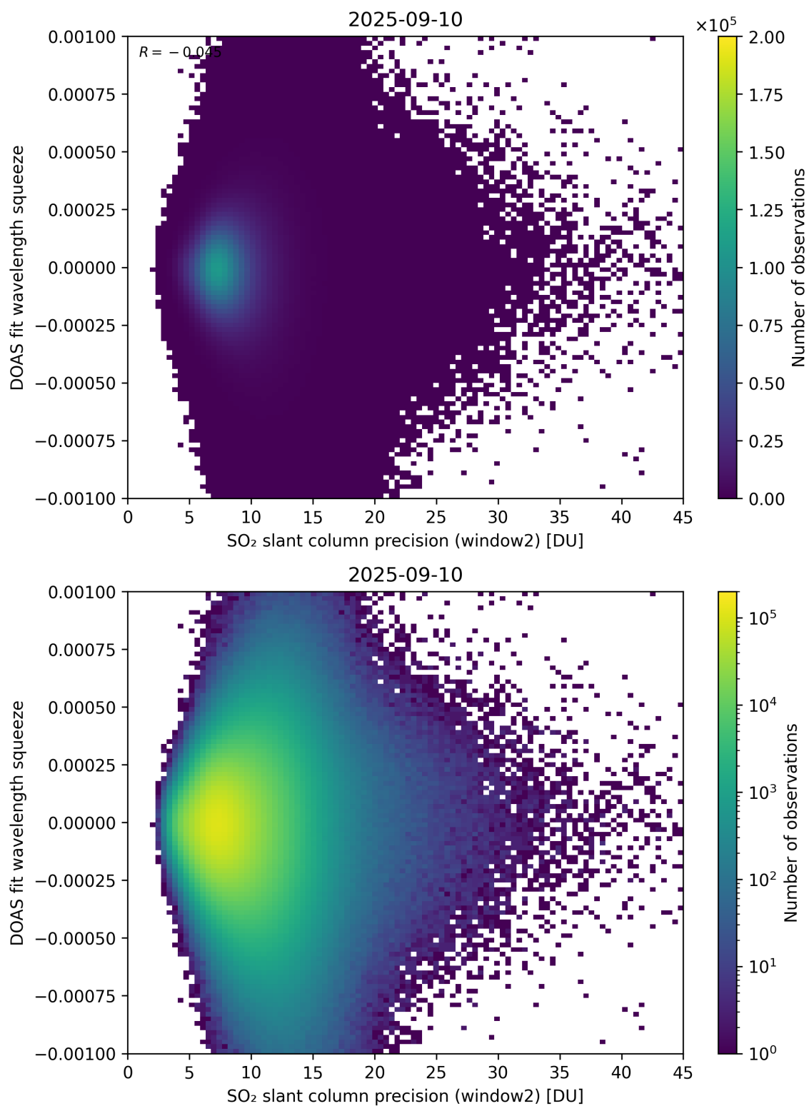
Figure 294: Scatter density plot of “SO 2 slant column precision (window2)” against “DOAS fit wavelength squeeze” for 2025-09-10 to 2025-09-11.
