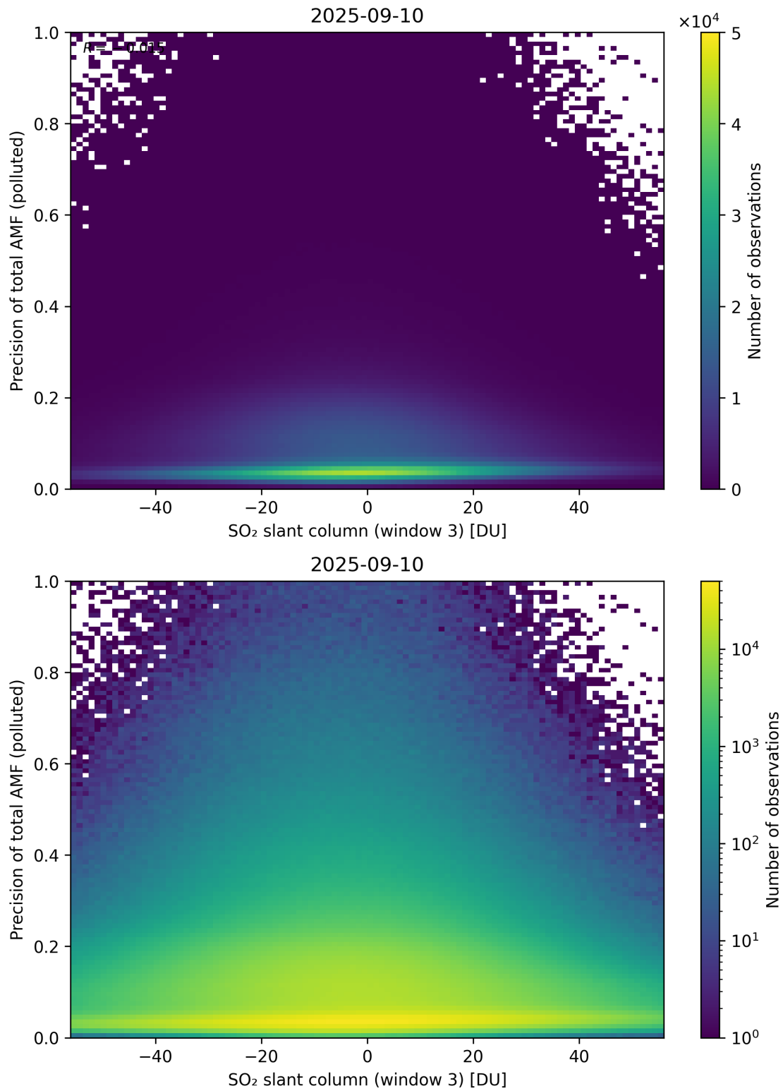
Figure 319: Scatter density plot of “SO 2 slant column (window 3)” against “Precision of total AMF (polluted)” for 2025-09-10 to 2025-09-11.
