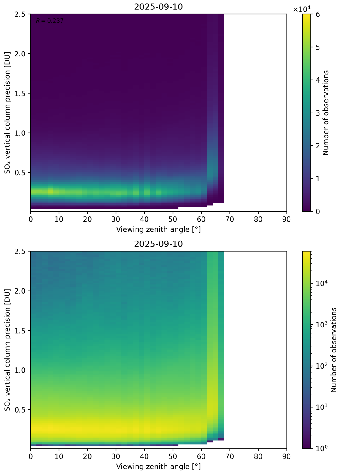
Figure 384: Scatter density plot of “Viewing zenith angle” against “SO 2 vertical column precision” for 2025-09-10 to 2025-09-11.
