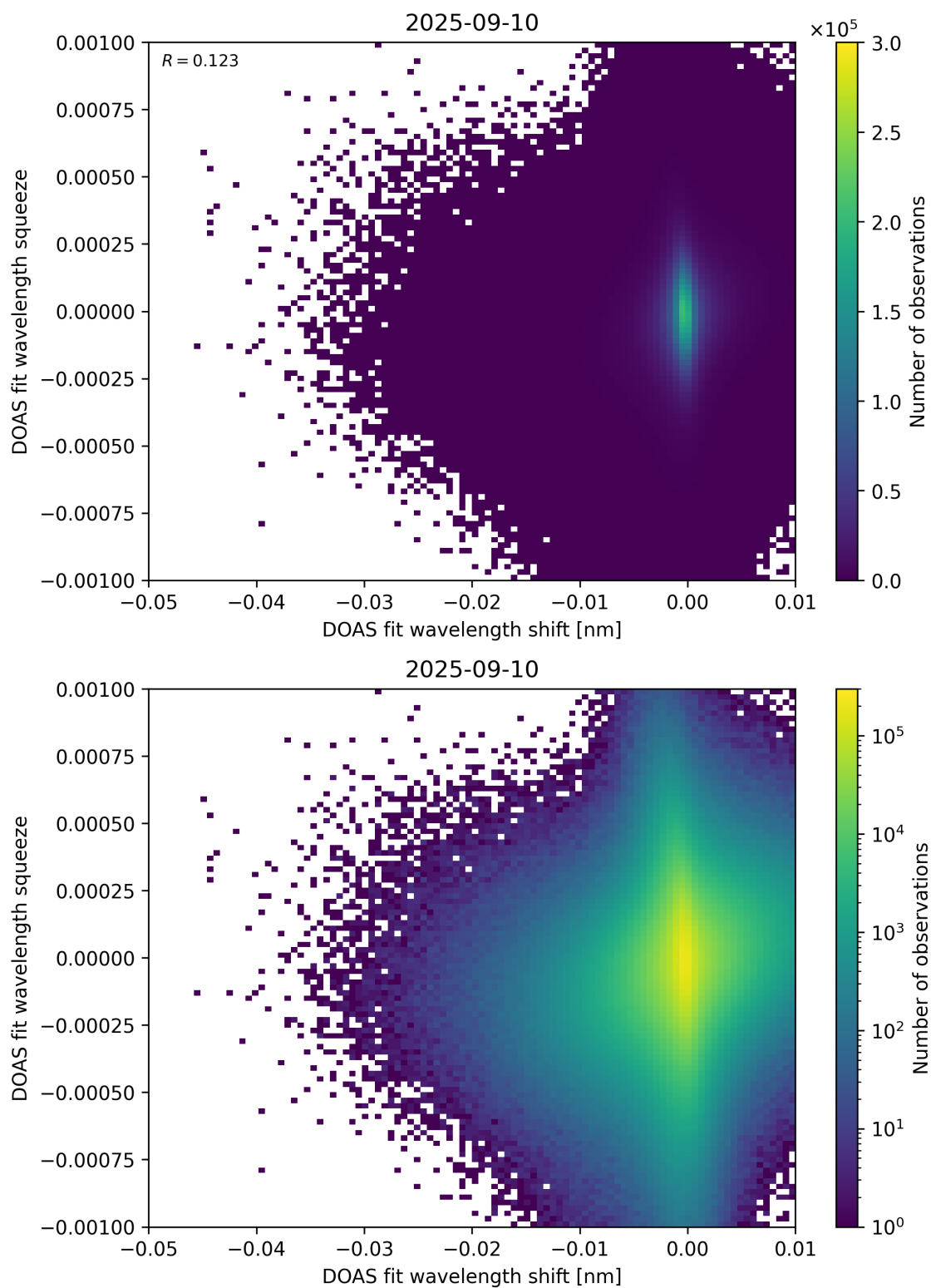
Figure 138: Scatter density plot of “DOAS fit wavelength shift” against “DOAS fit wavelength squeeze” for 2025-09-10 to 2025-09-11.
