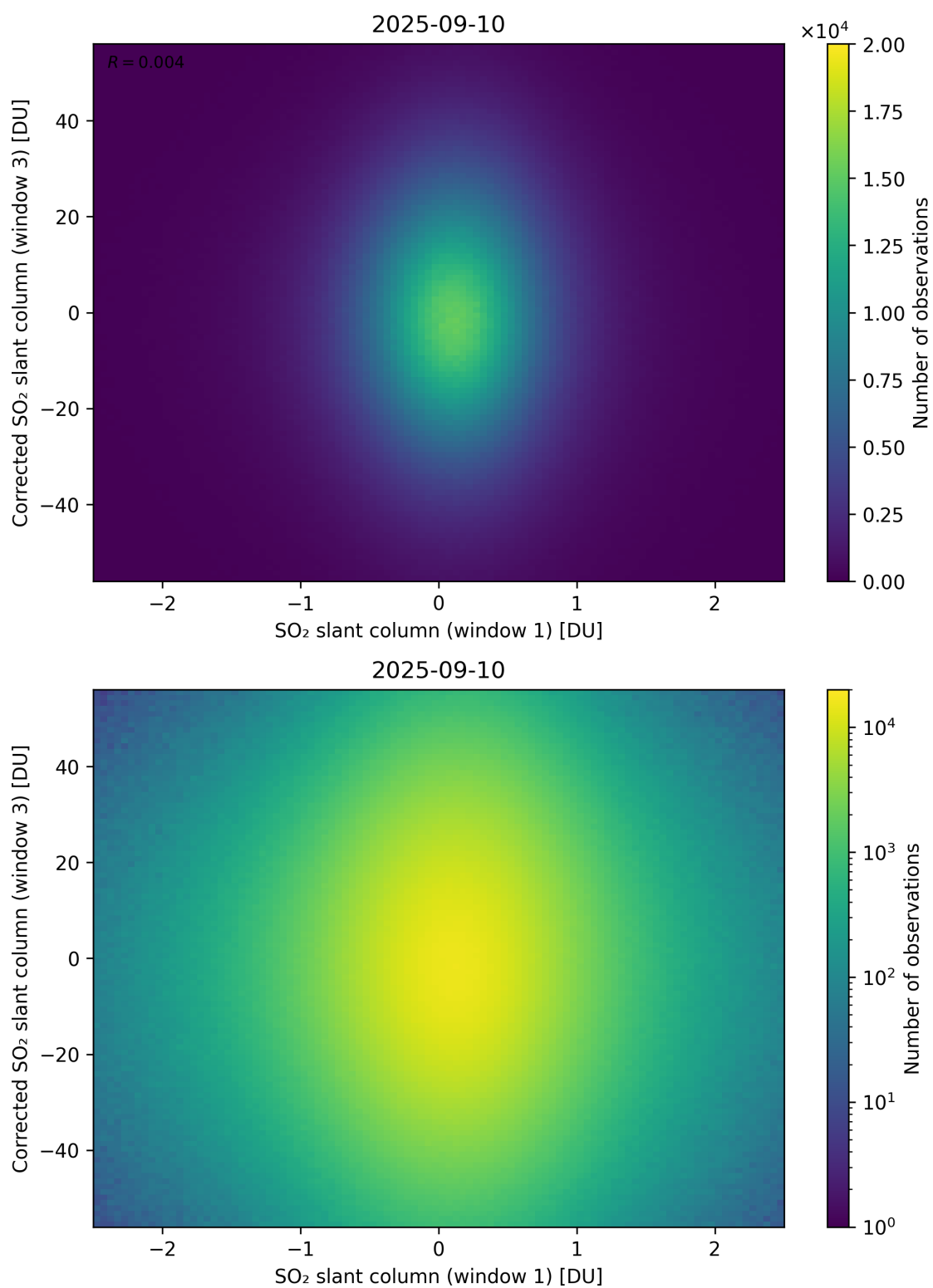
Figure 284: Scatter density plot of “SO 2 slant column (window 1)” against “Corrected SO 2 slant column (window 3)” for 2025-09-10 to 2025-09-11.
