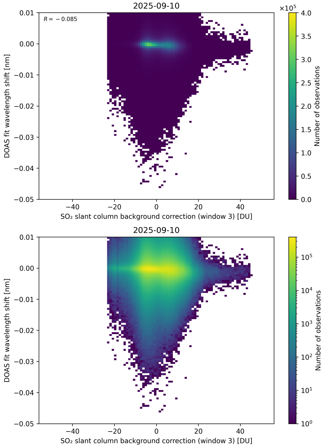
Figure 132: Scatter density plot of “SO 2 slant column background correction (window 3)” against “DOAS fit wavelength shift” for 2025-09-10 to 2025-09-11.
