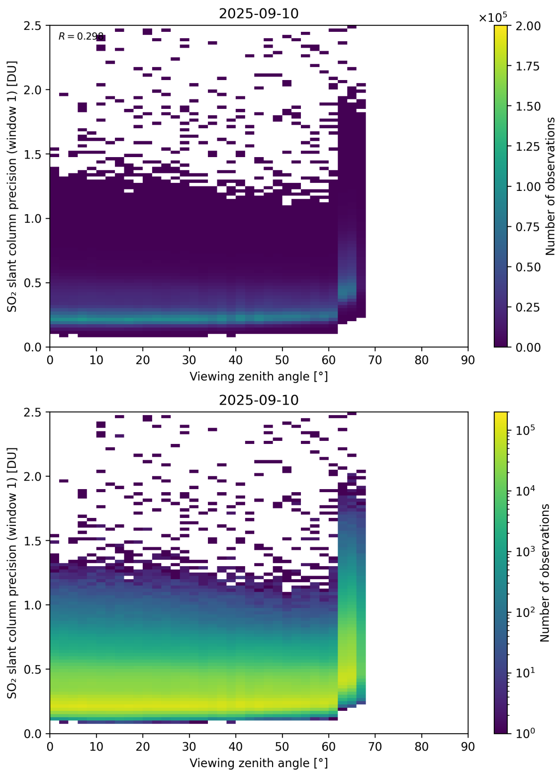
Figure 377: Scatter density plot of “Viewing zenith angle” against “SO 2 slant column precision (window 1)” for 2025-09-10 to 2025-09-11.
