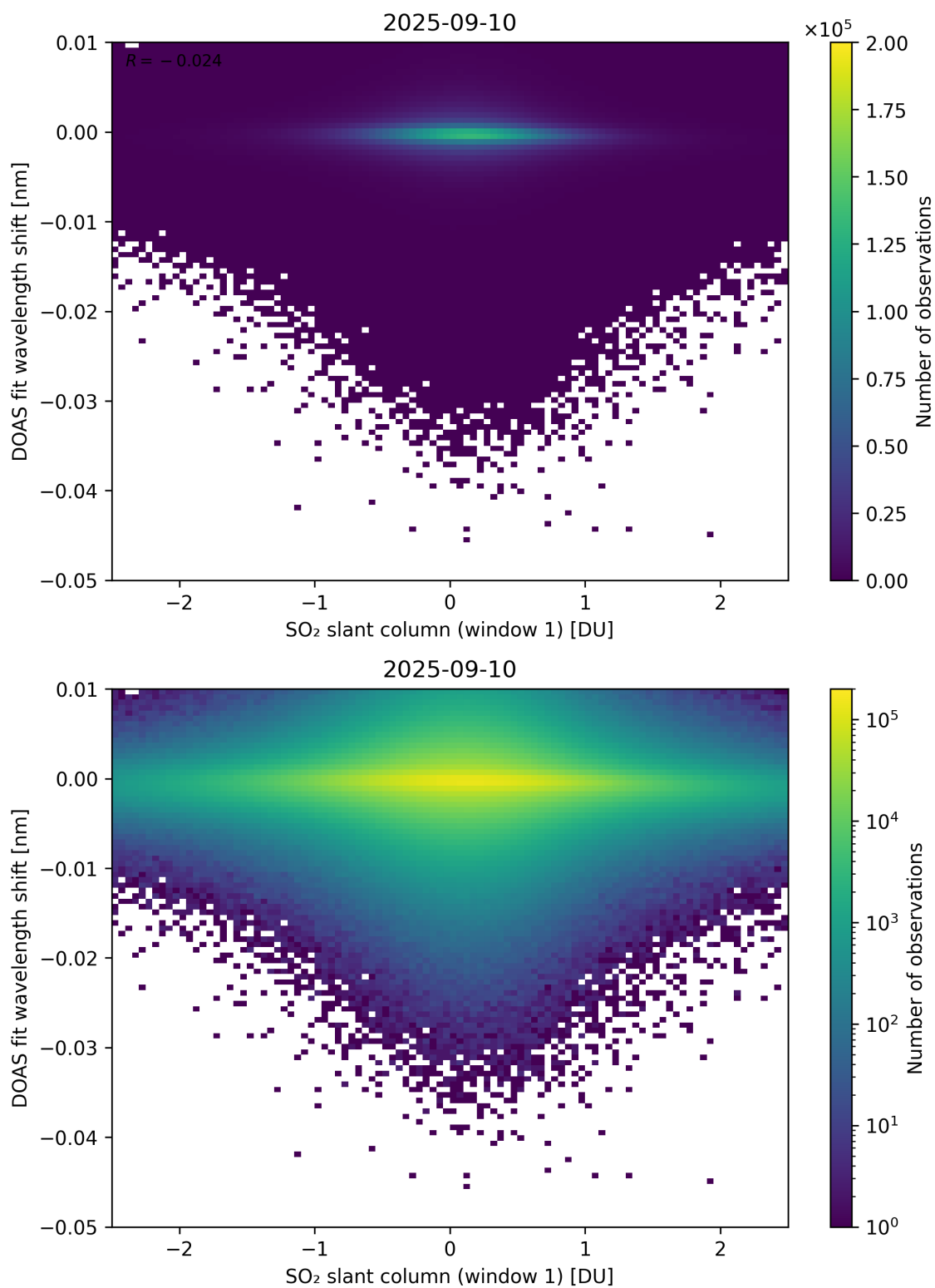
Figure 265: Scatter density plot of “SO 2 slant column (window 1)” against “DOAS fit wavelength shift” for 2025-09-10 to 2025-09-11.
