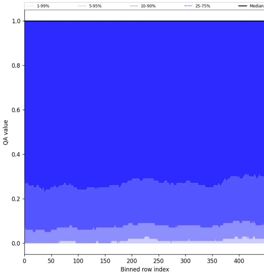
Figure 83: Along track statistics of “QA value” for 2025-09-10 to 2025-09-11
