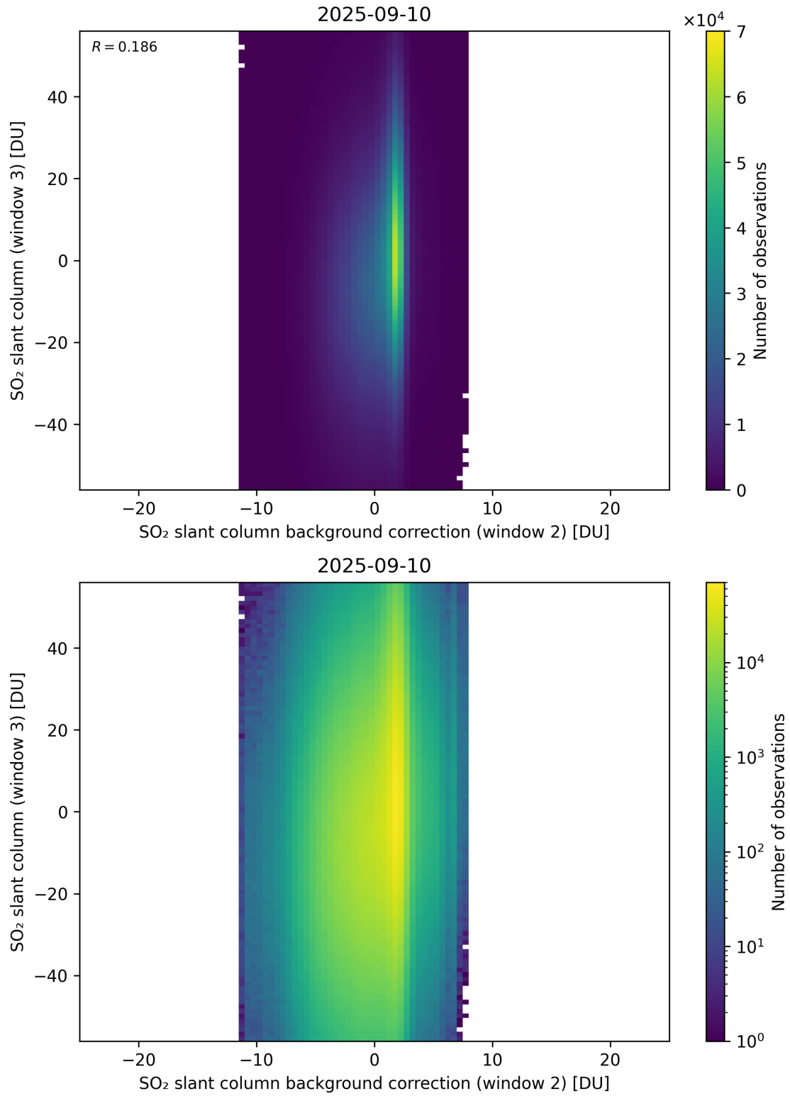
Figure 128: Scatter density plot of “SO 2 slant column background correction (window 2)” against “SO 2 slant column (window 3)” for 2025-09-10 to 2025-09-11.
