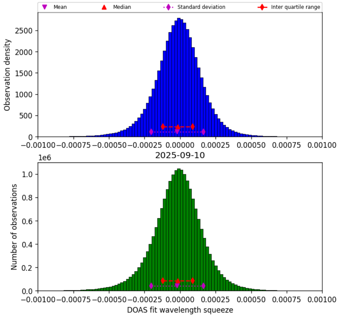
Figure 77: Histogram of “DOAS fit wavelength squeeze” for 2025-09-10 to 2025-09-11
