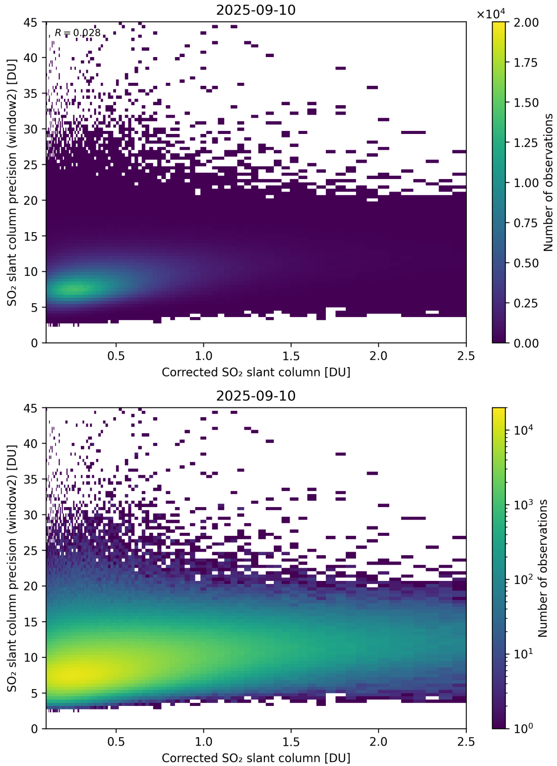
Figure 239: Scatter density plot of “Corrected SO 2 slant column” against “SO 2 slant column precision (window2)” for 2025-09-10 to 2025-09-11.
