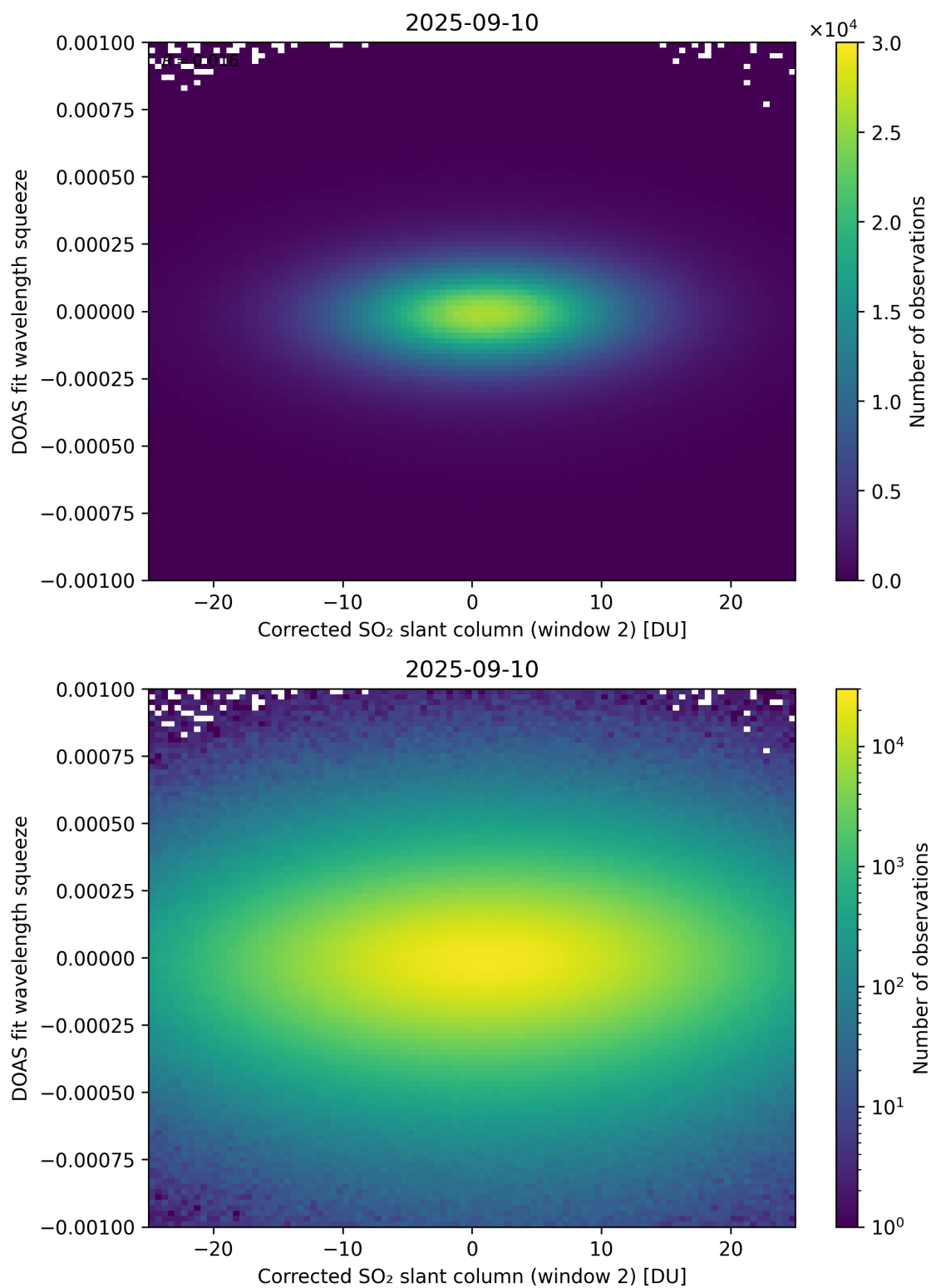
Figure 247: Scatter density plot of “Corrected SO 2 slant column (window 2)” against “DOAS fit wavelength squeeze” for 2025-09-10 to 2025-09-11.
