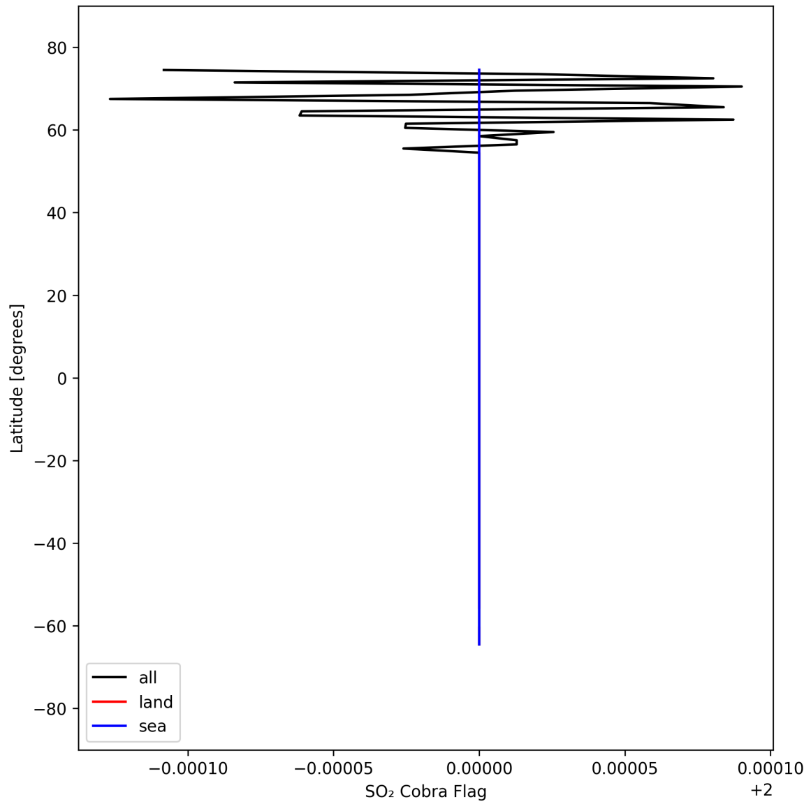
Figure 49: Zonal average of "SO 2 Cobra Flag" for 2025-09-10 to 2025-09-11.
