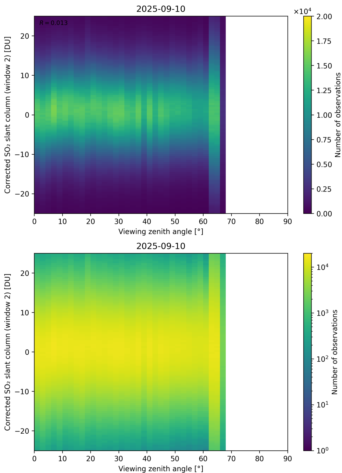
Figure 374: Scatter density plot of “Viewing zenith angle” against “Corrected SO 2 slant column (window 2)” for 2025-09-10 to 2025-09-11.
