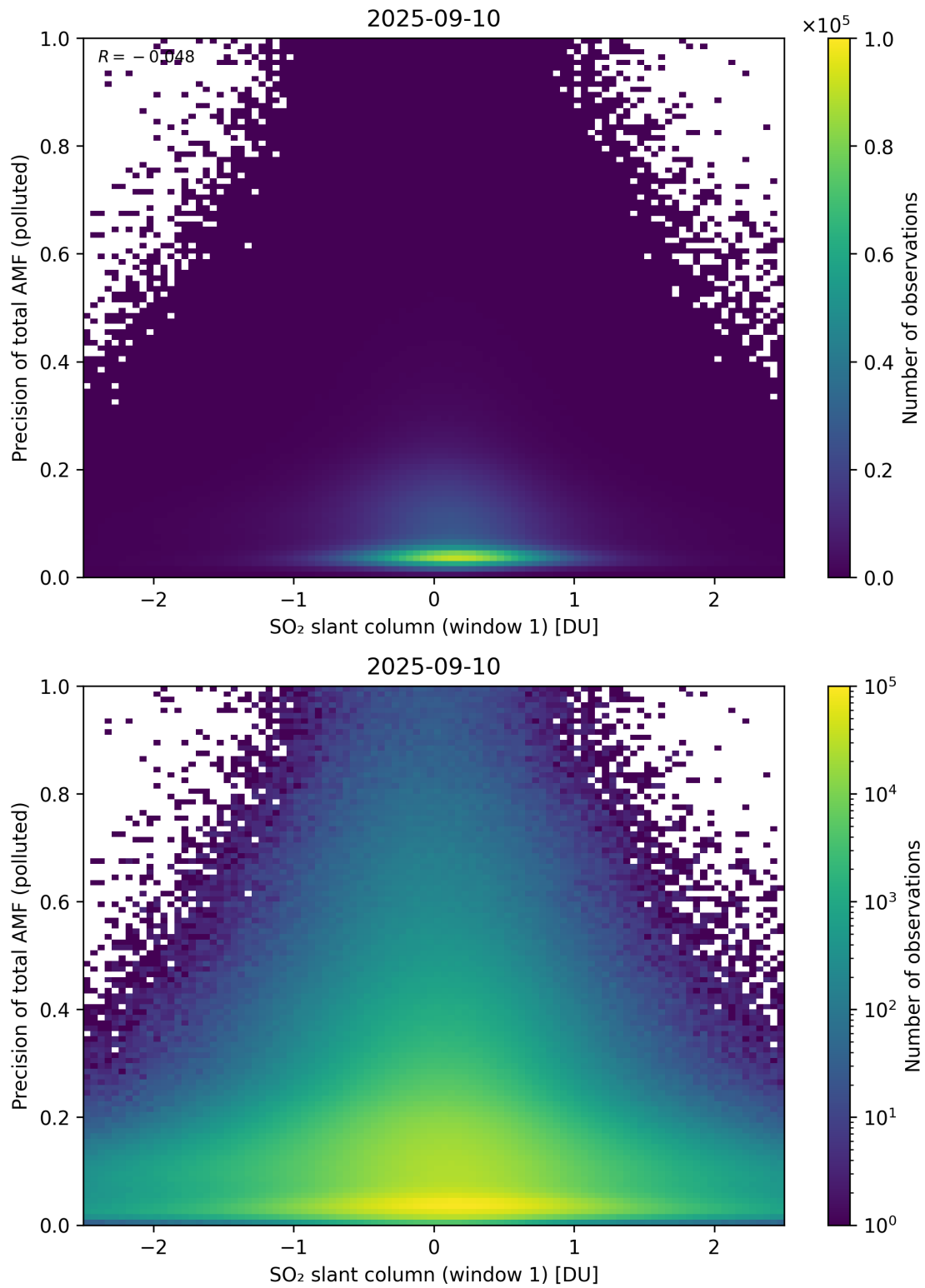
Figure 290: Scatter density plot of “SO 2 slant column (window 1)” against “Precision of total AMF (polluted)” for 2025-09-10 to 2025-09-11.
