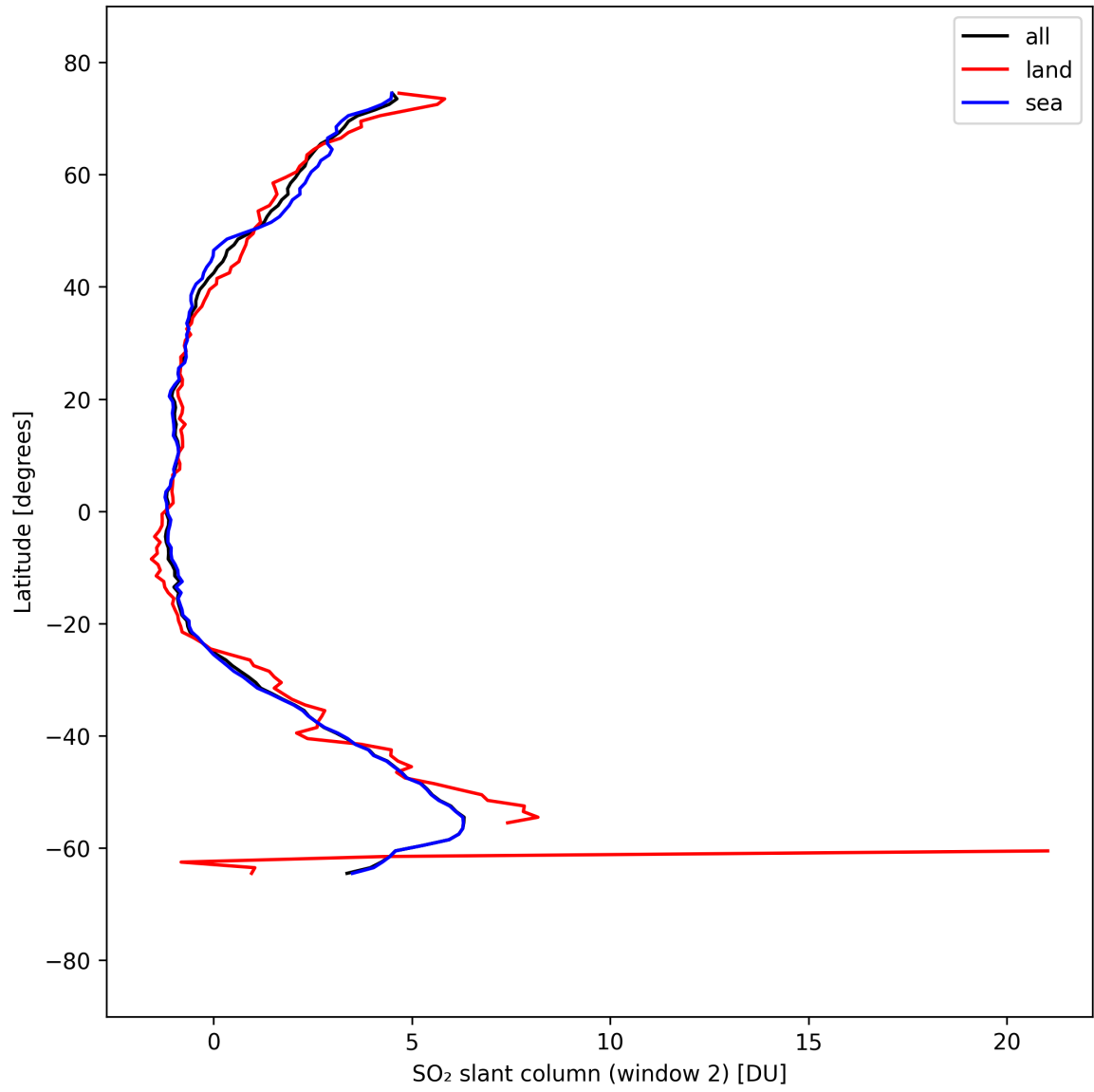
Figure 41: Zonal average of “SO 2 slant column (window 2)” for 2025-09-10 to 2025-09-11.
