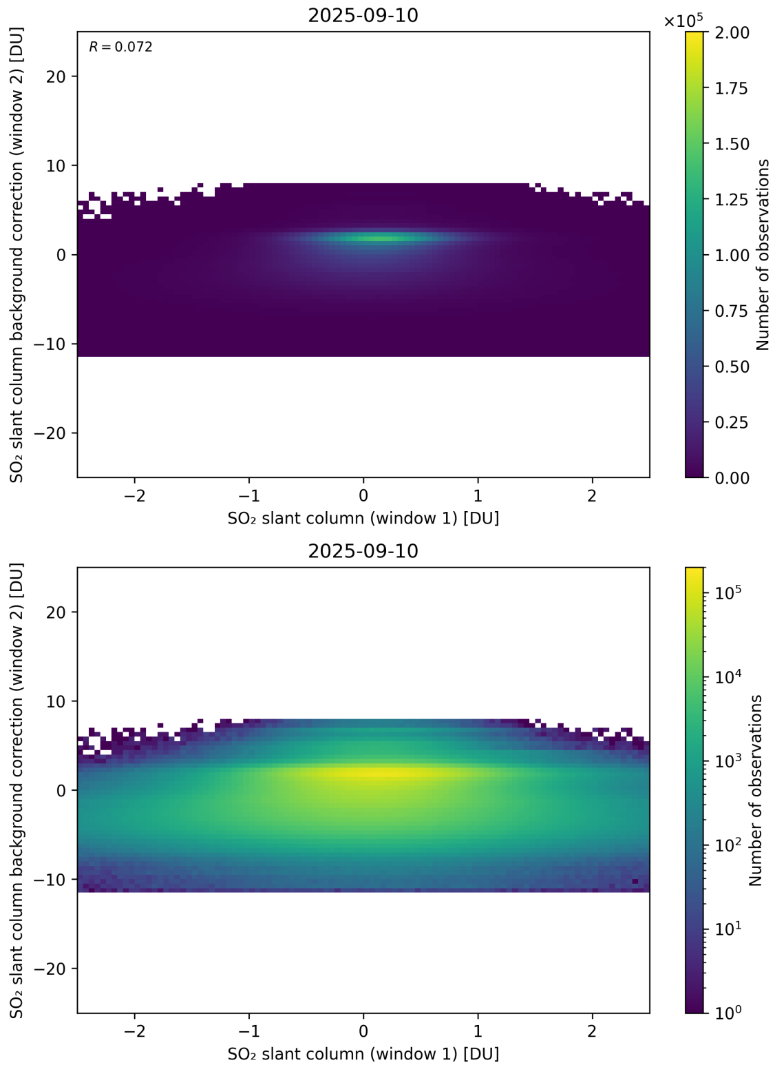
Figure 263: Scatter density plot of “SO 2 slant column (window 1)” against “SO 2 slant column background correction (window 2)” for 2025-09-10 to 2025-09-11.
