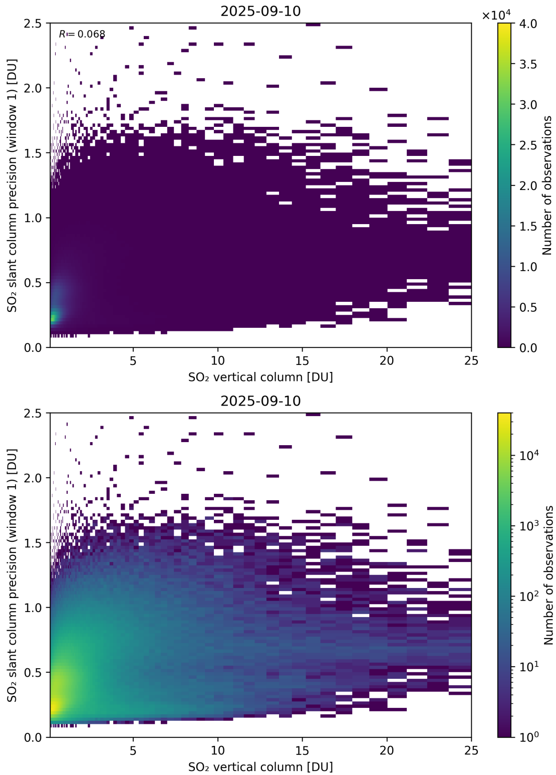
Figure 355: Scatter density plot of “SO 2 vertical column” against “SO 2 slant column precision (window 1)” for 2025-09-10 to 2025-09-11.
