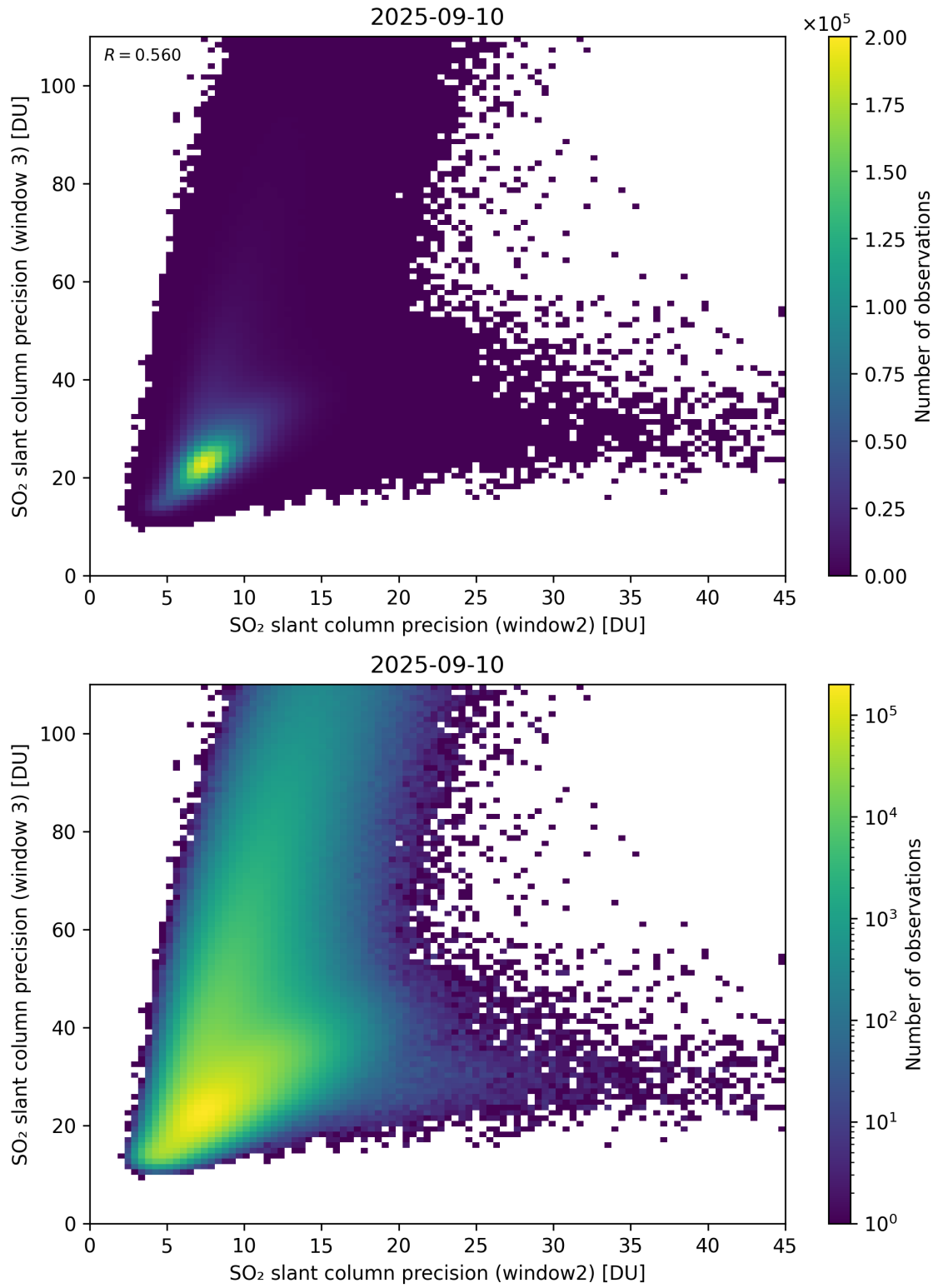
Figure 300: Scatter density plot of “SO 2 slant column precision (window2)” against “SO 2 slant column precision (window 3)” for 2025-09-10 to 2025-09-11.
