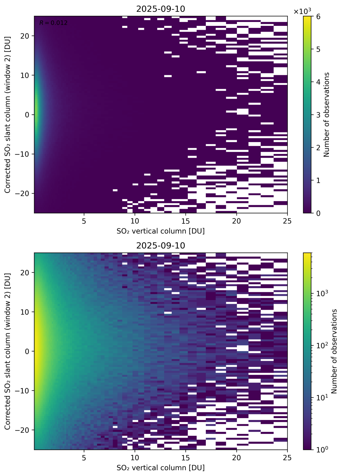
Figure 352: Scatter density plot of “SO 2 vertical column” against “Corrected SO 2 slant column (window 2)” for 2025-09-10 to 2025-09-11.
