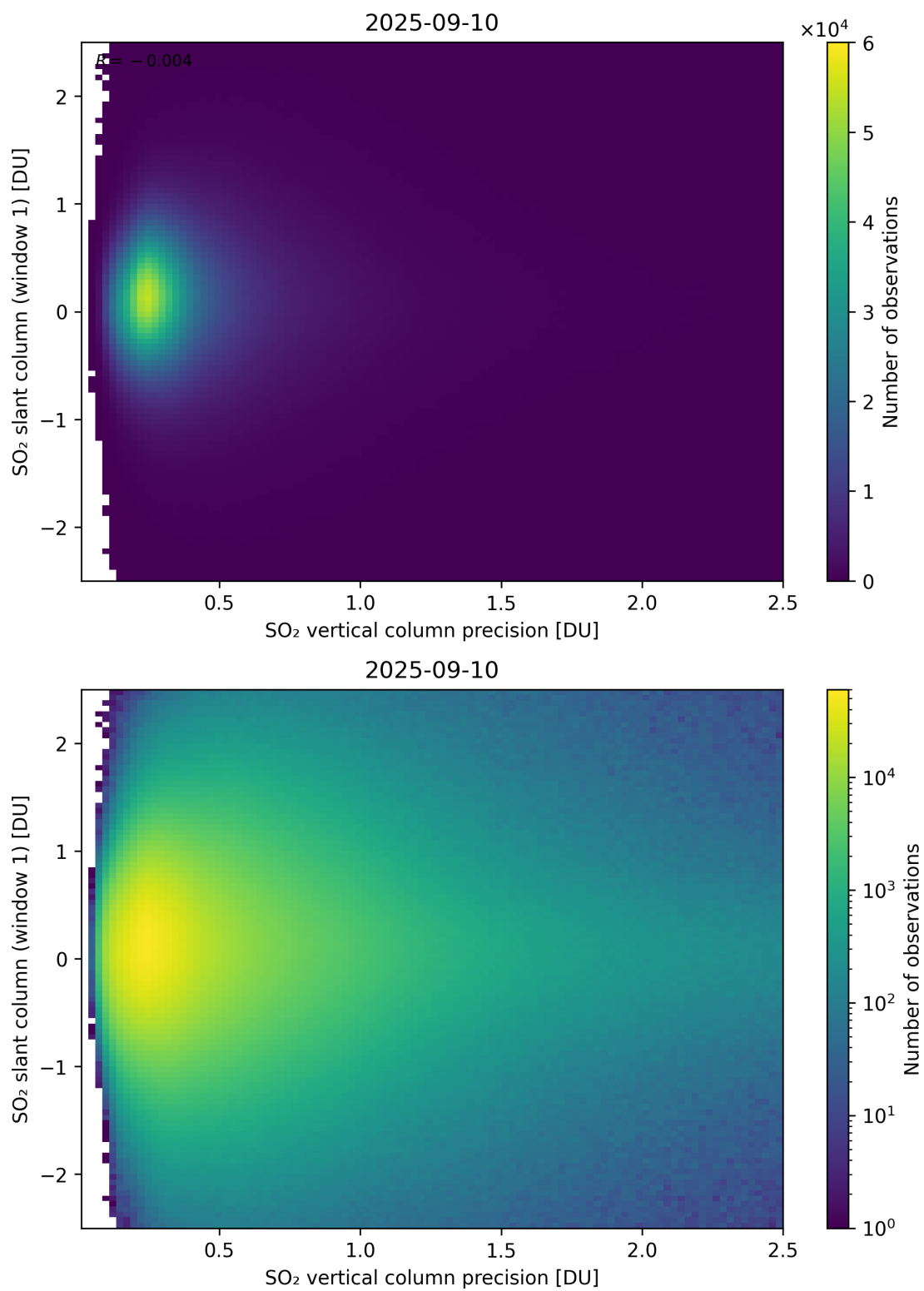
Figure 341: Scatter density plot of “SO 2 vertical column precision” against “SO 2 slant column (window 1)” for 2025-09-10 to 2025-09-11.
