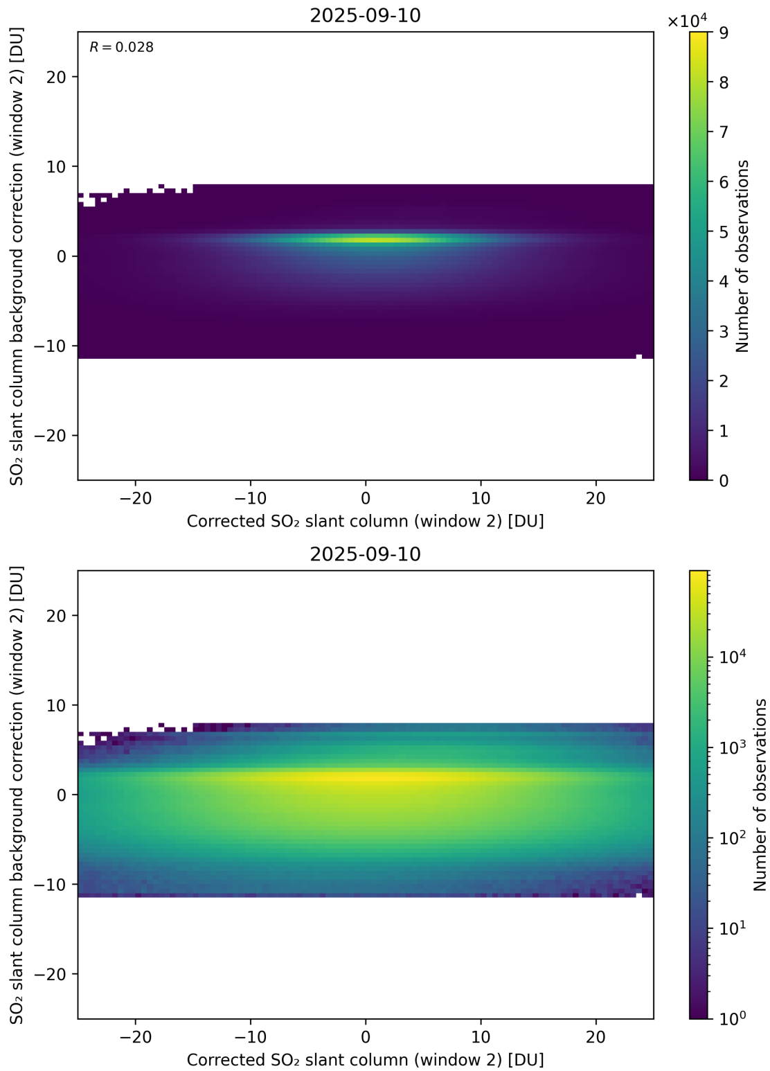
Figure 244: Scatter density plot of “Corrected SO 2 slant column (window 2)” against “SO 2 slant column background correction (window 2)” for 2025-09-10 to 2025-09-11.
