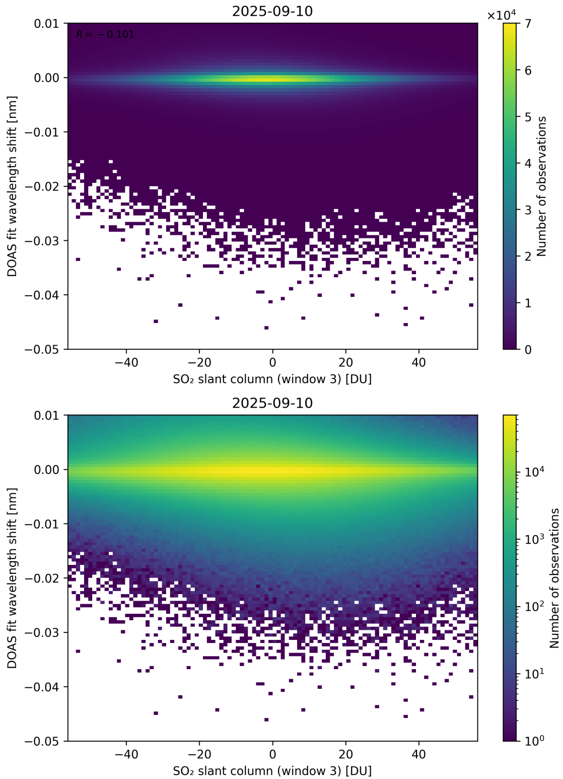
Figure 304: Scatter density plot of “SO 2 slant column (window 3)” against “DOAS fit wavelength shift” for 2025-09-10 to 2025-09-11.
