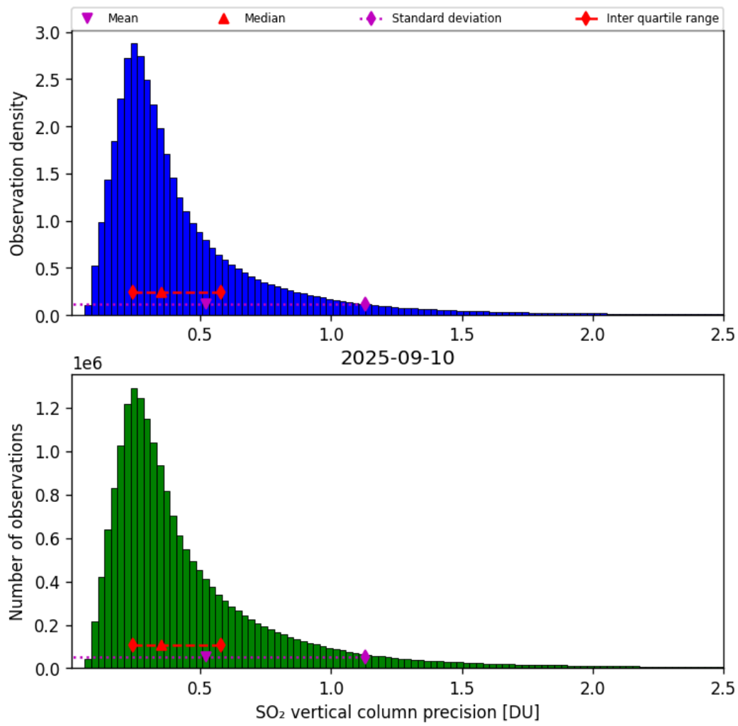
Figure 59: Histogram of “SO 2 vertical column precision” for 2025-09-10 to 2025-09-11
