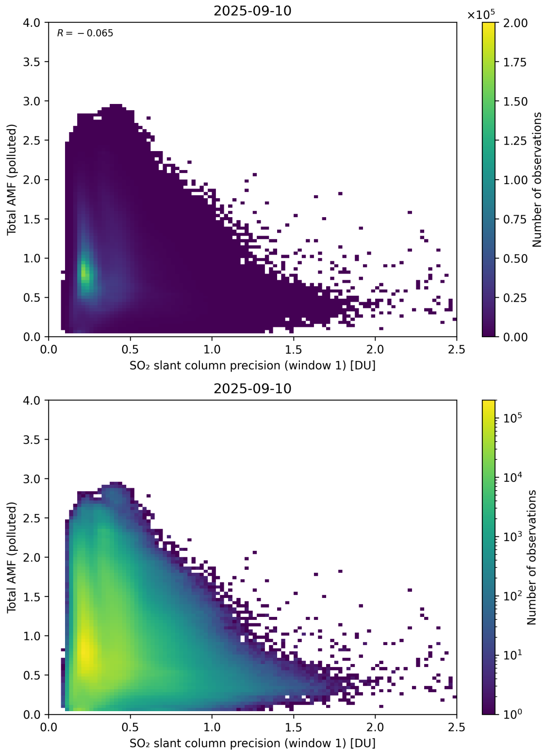
Figure 280: Scatter density plot of “SO 2 slant column precision (window 1)” against “Total AMF (polluted)” for 2025-09-10 to 2025-09-11.
