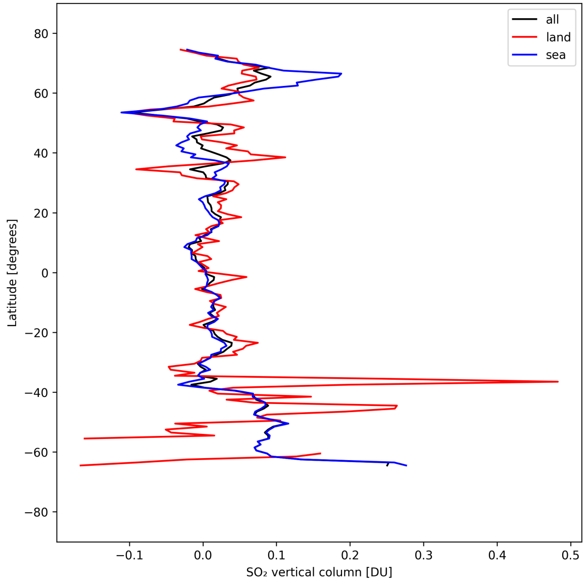
Figure 32: Zonal average of “SO 2 vertical column” for 2025-09-10 to 2025-09-11.
