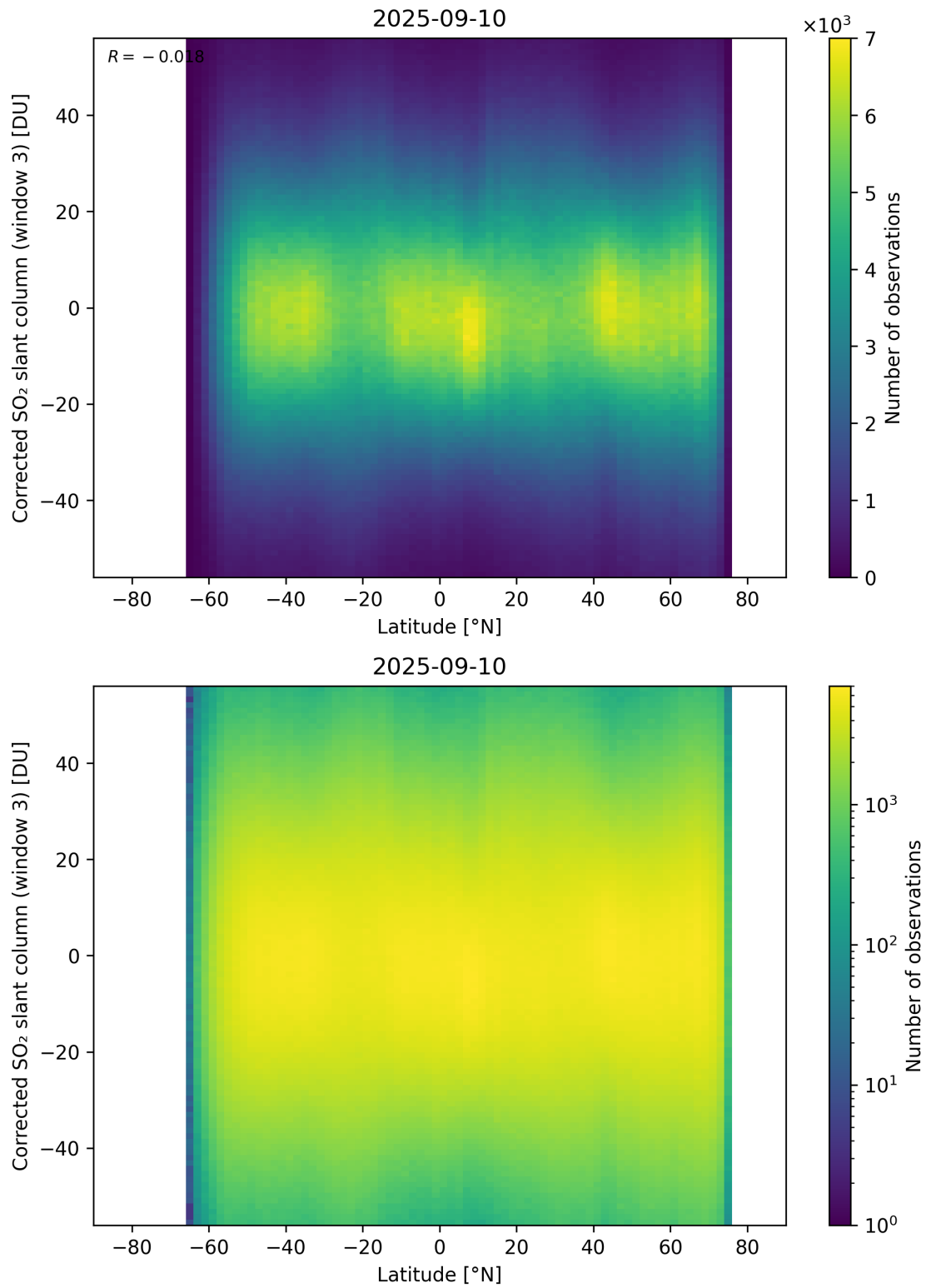
Figure 161: Scatter density plot of “Latitude” against “Corrected SO 2 slant column (window 3)” for 2025-09-10 to 2025-09-11.
