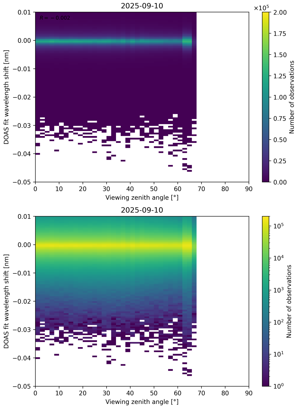
Figure 365: Scatter density plot of “Viewing zenith angle” against “DOAS fit wavelength shift” for 2025-09-10 to 2025-09-11.
