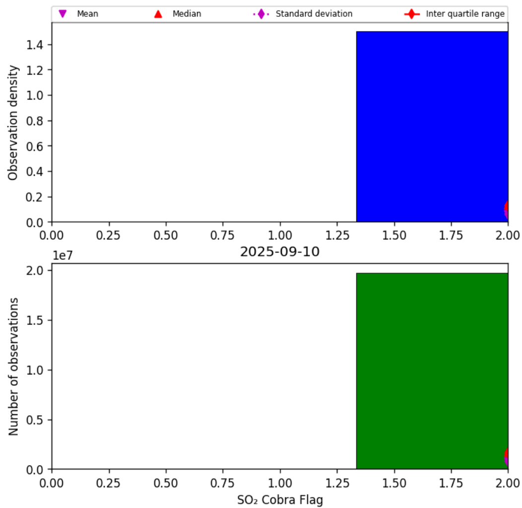
Figure 75: Histogram of “SO 2 Cobra Flag” for 2025-09-10 to 2025-09-11
