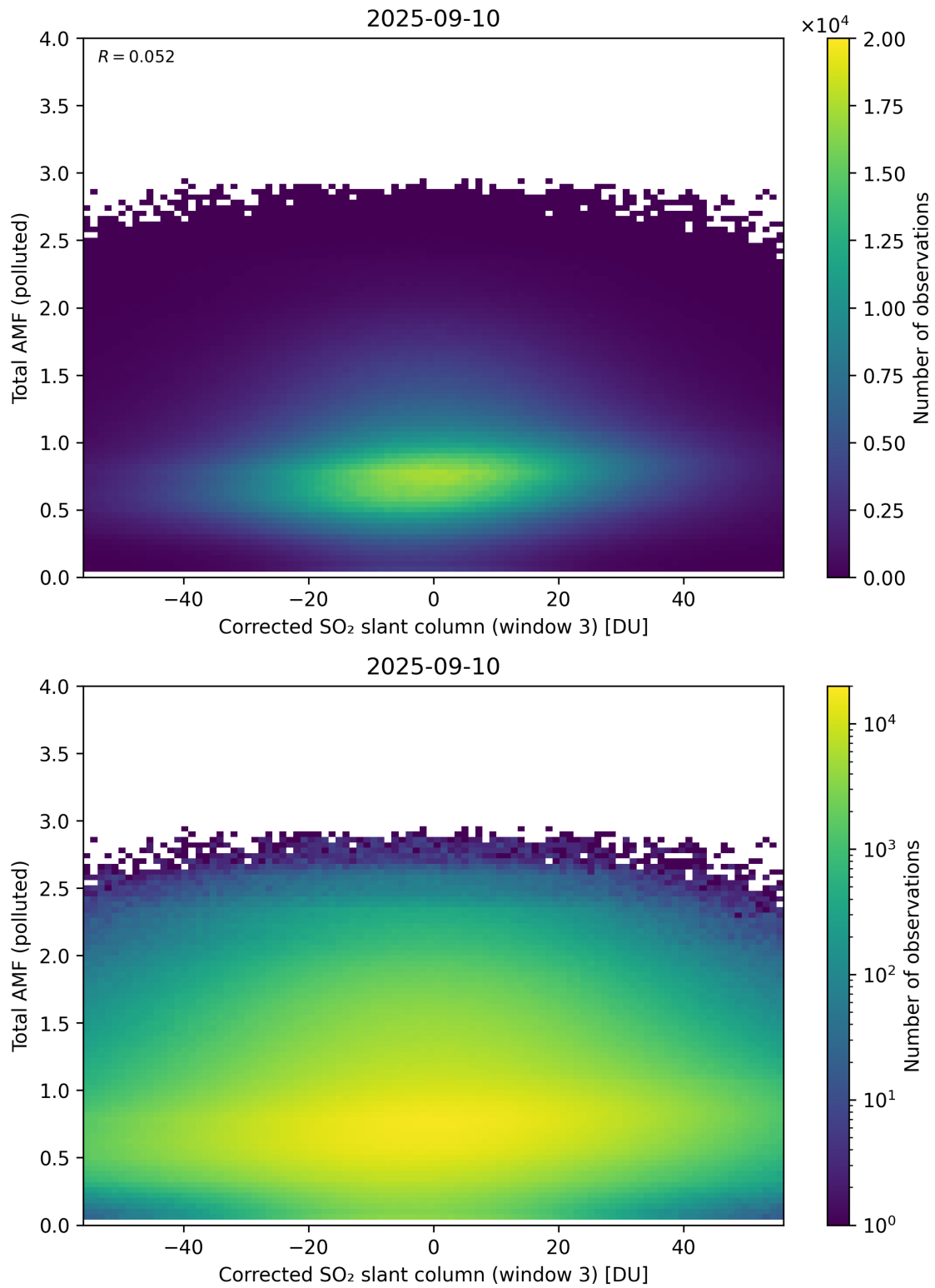
Figure 260: Scatter density plot of “Corrected SO 2 slant column (window 3)” against “Total AMF (polluted)” for 2025-09-10 to 2025-09-11.
