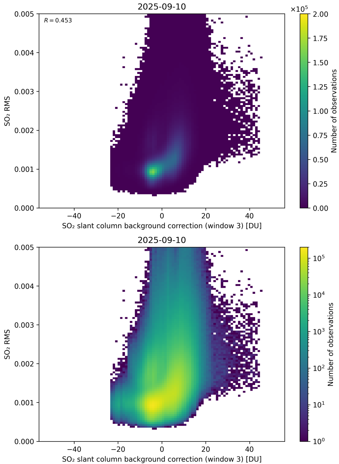
Figure 134: Scatter density plot of “SO 2 slant column background correction (window 3)” against “SO 2 RMS” for 2025-09-10 to 2025-09-11.
