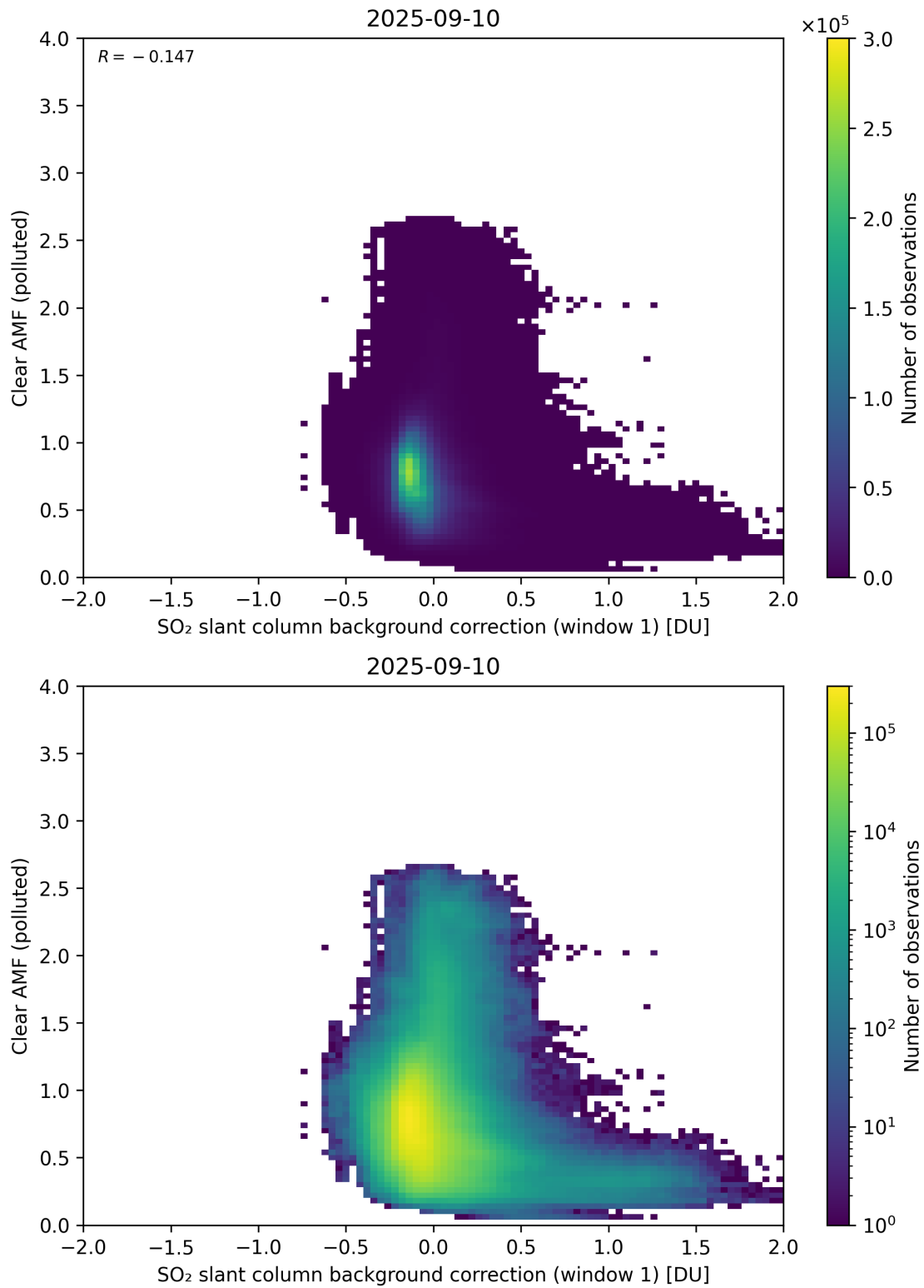
Figure 114: Scatter density plot of “SO 2 slant column background correction (window 1)” against “Clear AMF (polluted)” for 2025-09-10 to 2025-09-11.
