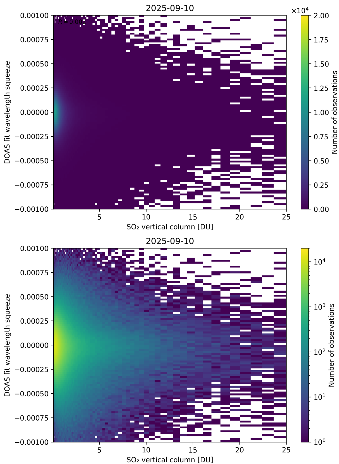
Figure 327: Scatter density plot of “SO 2 vertical column” against “DOAS fit wavelength squeeze” for 2025-09-10 to 2025-09-11.
