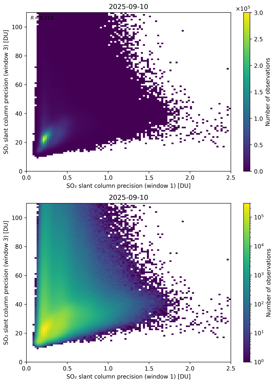
Figure 279: Scatter density plot of “SO 2 slant column precision (window 1)” against “SO 2 slant column precision (window 3)” for 2025-09-10 to 2025-09-11.
