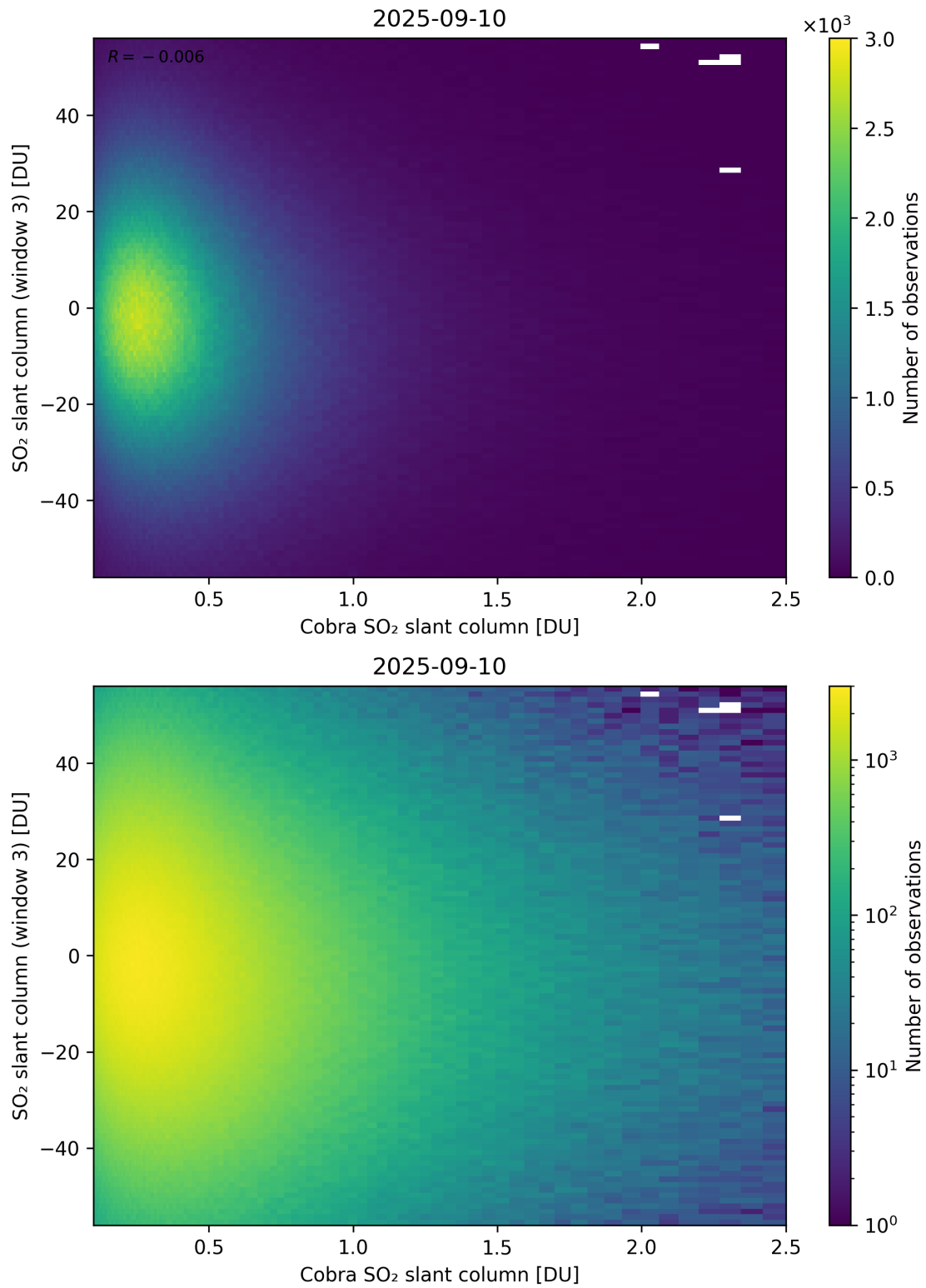
Figure 222: Scatter density plot of “Cobra SO 2 slant column” against “SO 2 slant column (window 3)” for 2025-09-10 to 2025-09-11.
