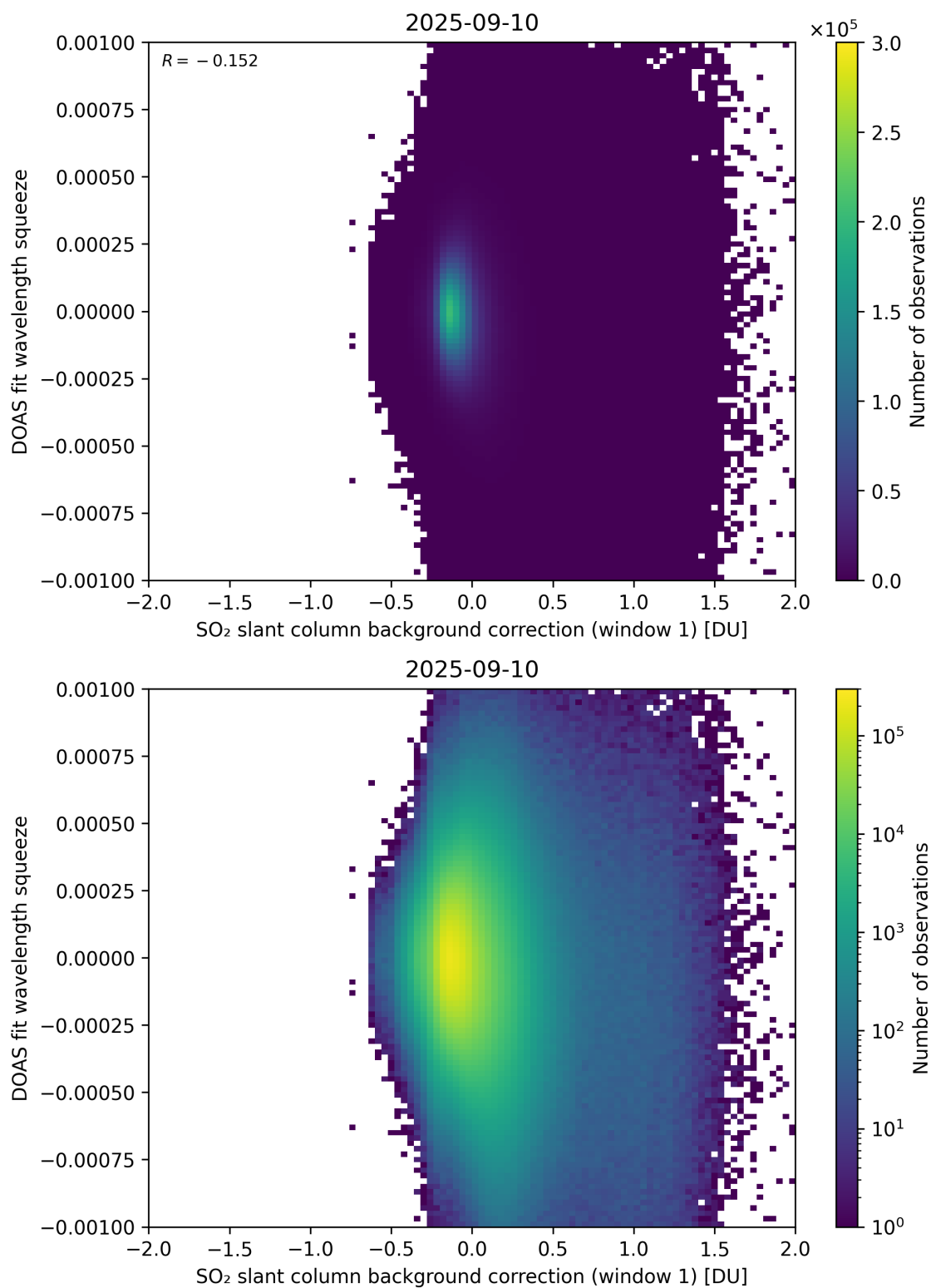
Figure 112: Scatter density plot of “SO 2 slant column background correction (window 1)” against “DOAS fit wavelength squeeze” for 2025-09-10 to 2025-09-11.
