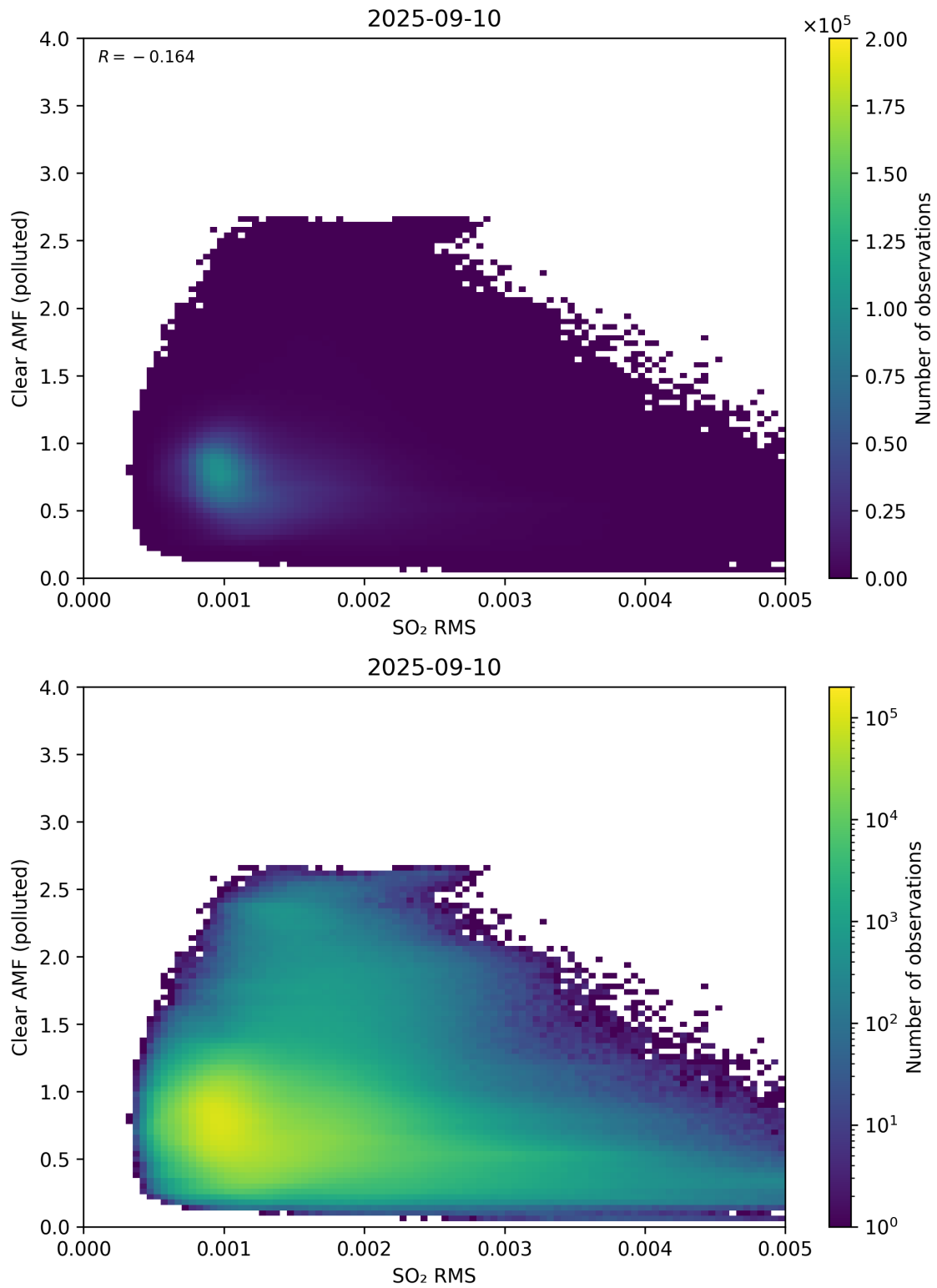
Figure 147: Scatter density plot of “SO 2 RMS” against “Clear AMF (polluted)” for 2025-09-10 to 2025-09-11.
