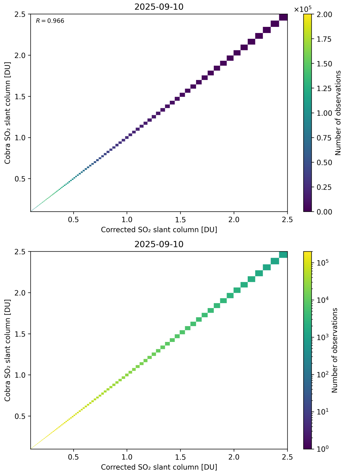
Figure 233: Scatter density plot of “Corrected SO 2 slant column” against “Cobra SO 2 slant column” for 2025-09-10 to 2025-09-11.
