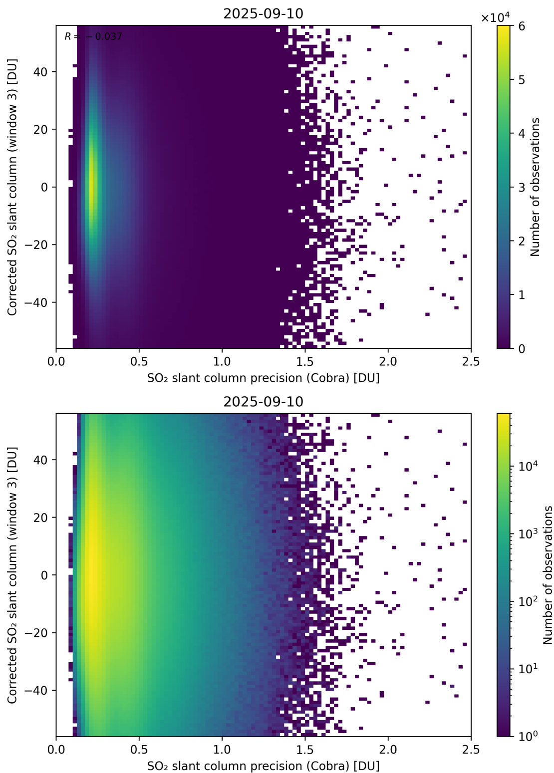
Figure 207: Scatter density plot of “SO 2 slant column precision (Cobra)” against “Corrected SO 2 slant column (window 3)” for 2025-09-10 to 2025-09-11.
