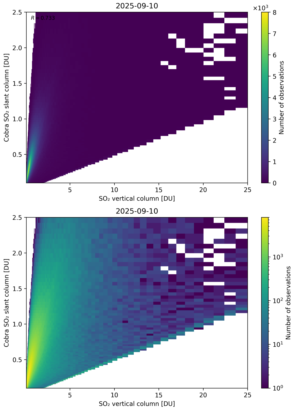
Figure 349: Scatter density plot of “SO 2 vertical column” against “Cobra SO 2 slant column” for 2025-09-10 to 2025-09-11.
