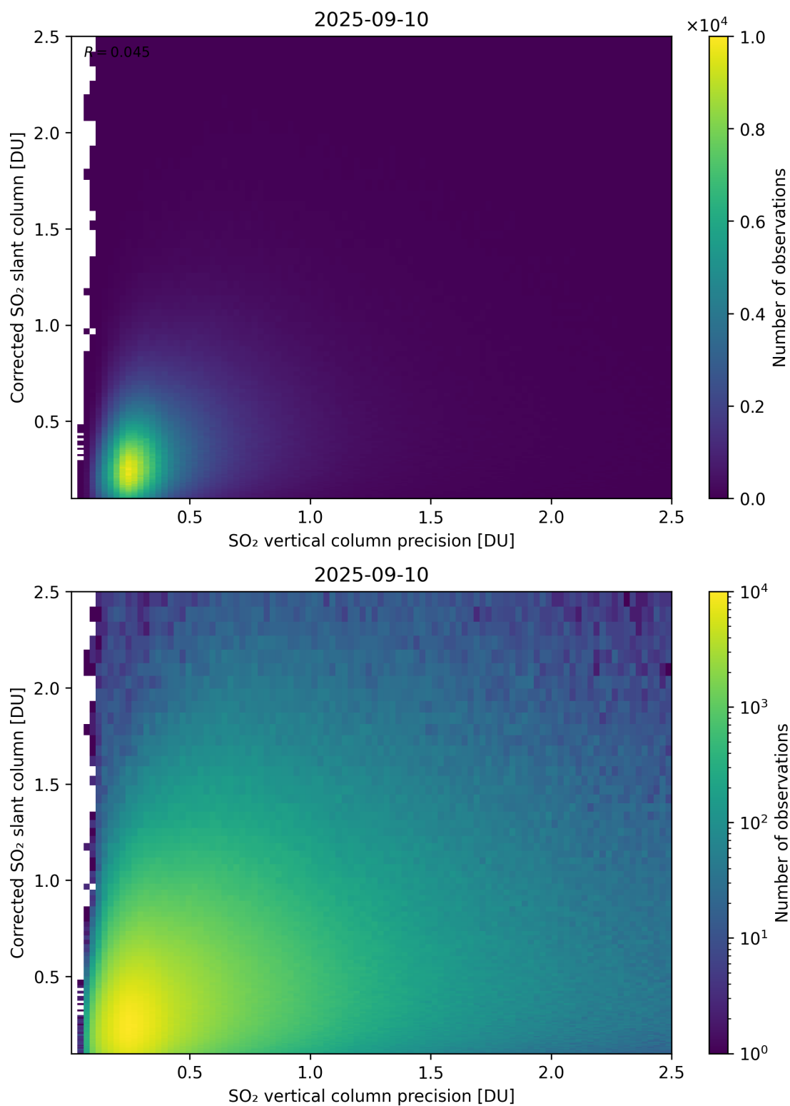
Figure 338: Scatter density plot of “SO 2 vertical column precision” against “Corrected SO 2 slant column” for 2025-09-10 to 2025-09-11.
