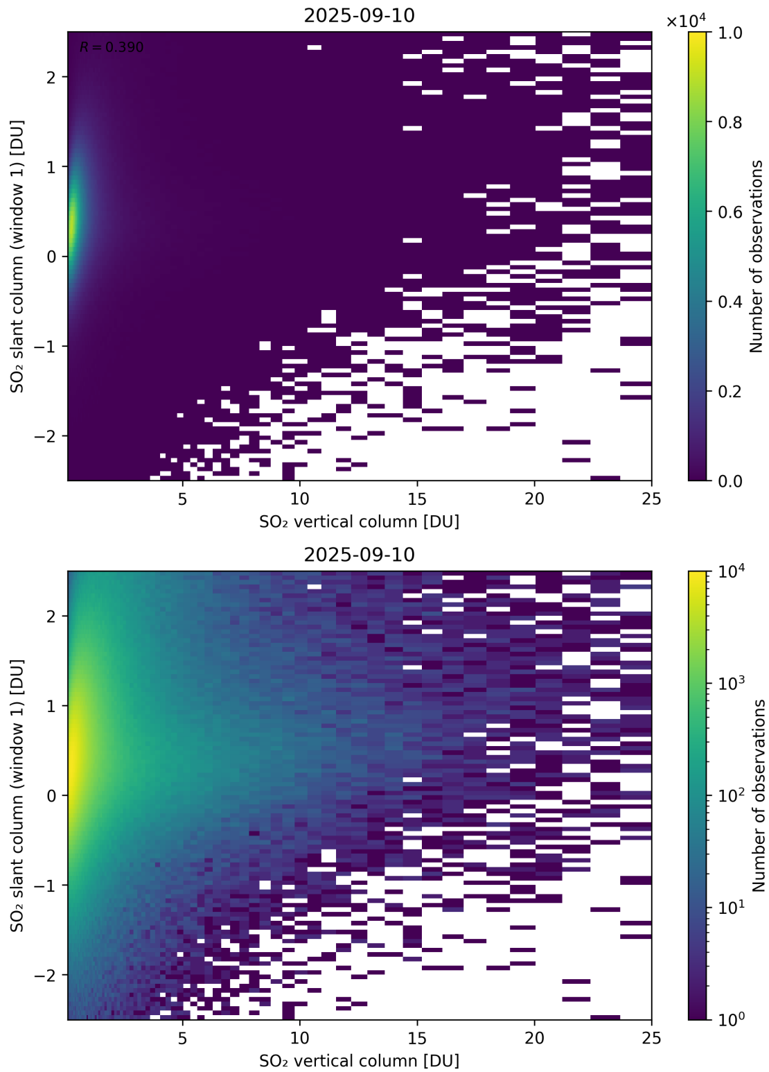
Figure 354: Scatter density plot of “SO 2 vertical column” against “SO 2 slant column (window 1)” for 2025-09-10 to 2025-09-11.
