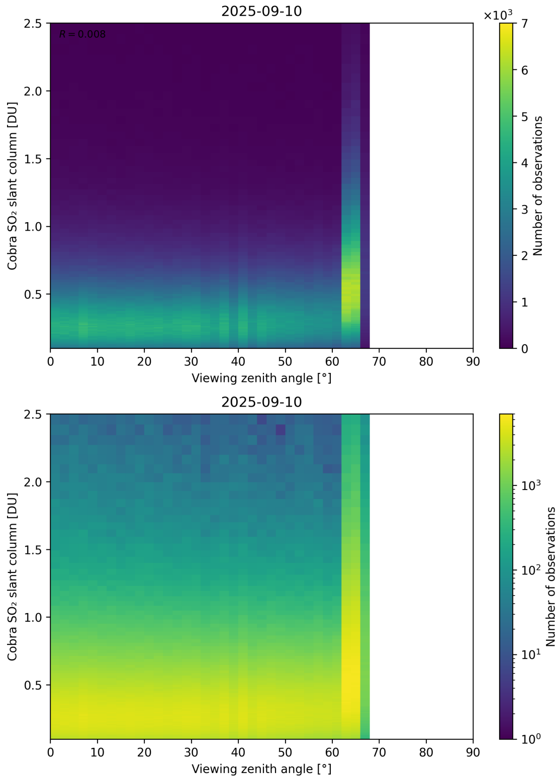
Figure 371: Scatter density plot of “Viewing zenith angle” against “Cobra SO 2 slant column” for 2025-09-10 to 2025-09-11.
