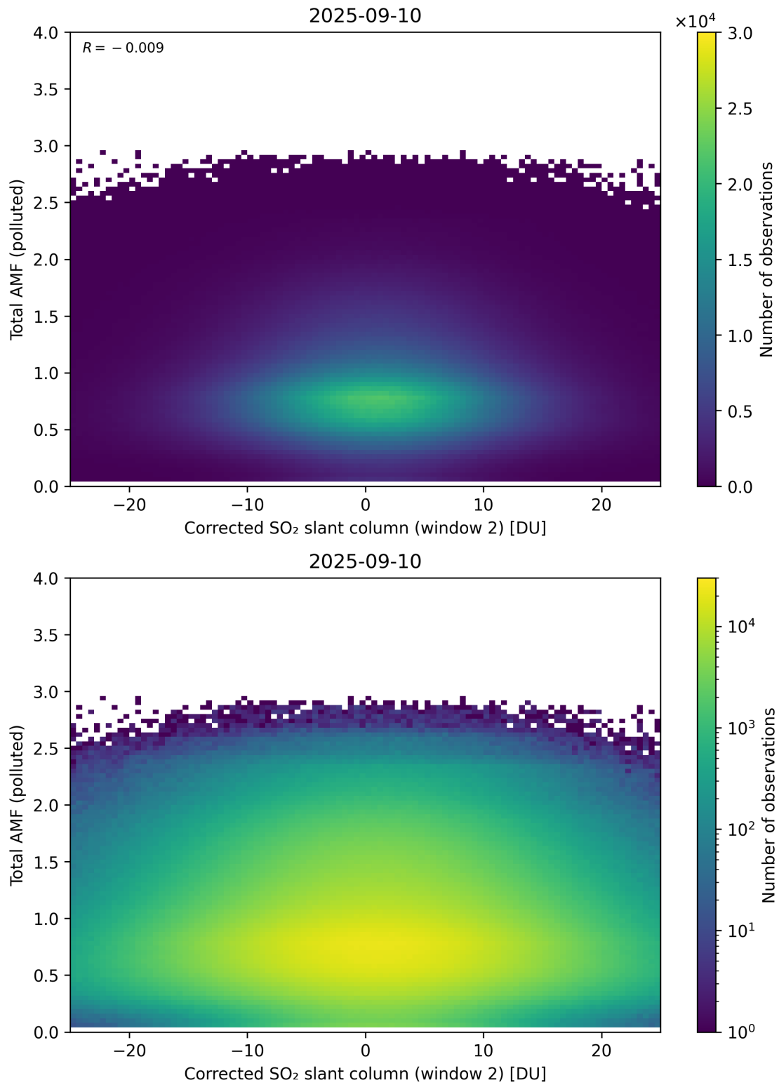
Figure 253: Scatter density plot of “Corrected SO 2 slant column (window 2)” against “Total AMF (polluted)” for 2025-09-10 to 2025-09-11.
