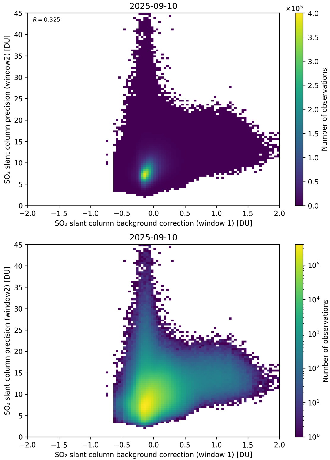
Figure 117: Scatter density plot of “SO 2 slant column background correction (window 1)” against “SO 2 slant column precision (window2)” for 2025-09-10 to 2025-09-11.
