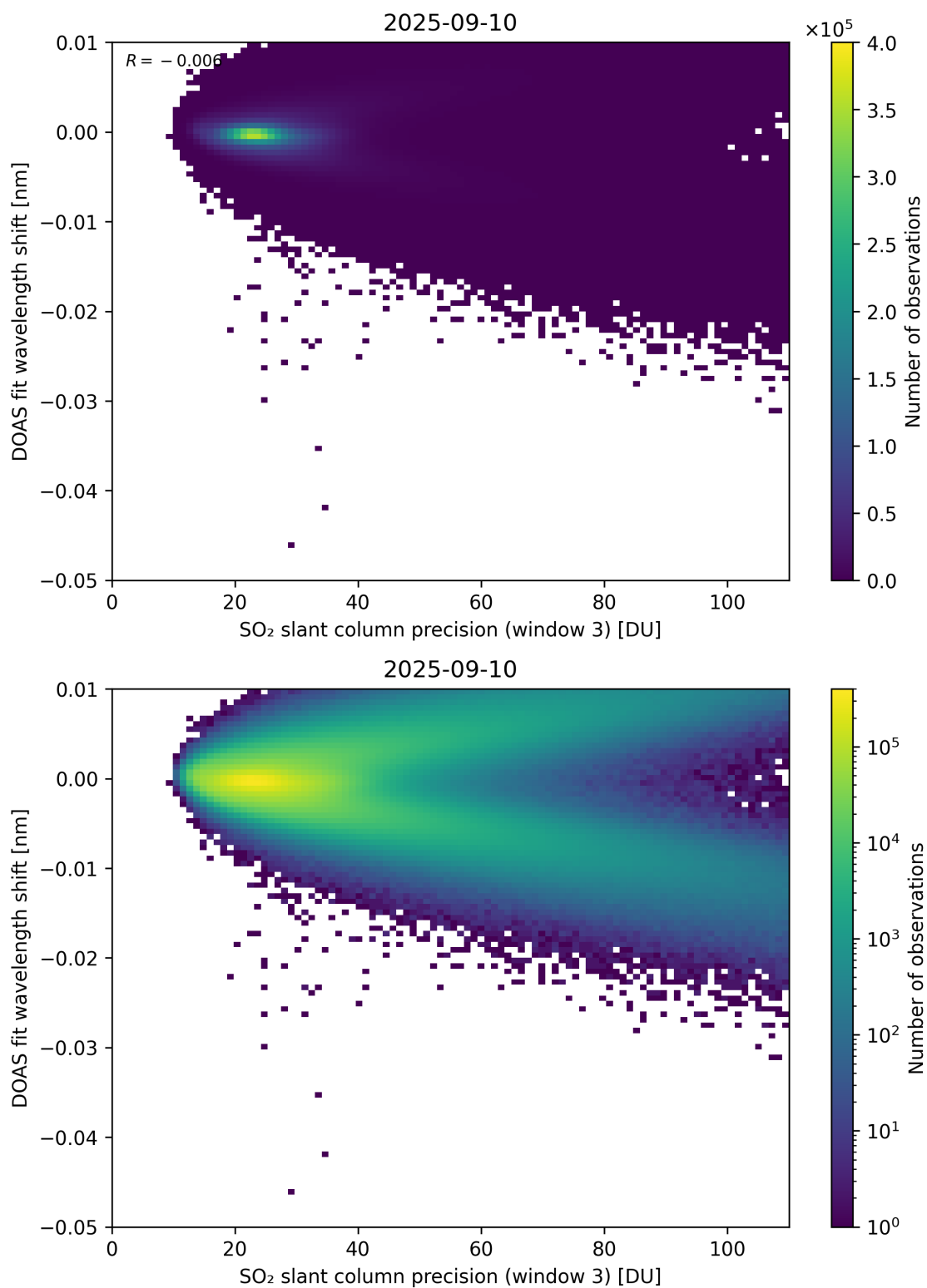
Figure 308: Scatter density plot of “SO 2 slant column precision (window 3)” against “DOAS fit wavelength shift” for 2025-09-10 to 2025-09-11.
