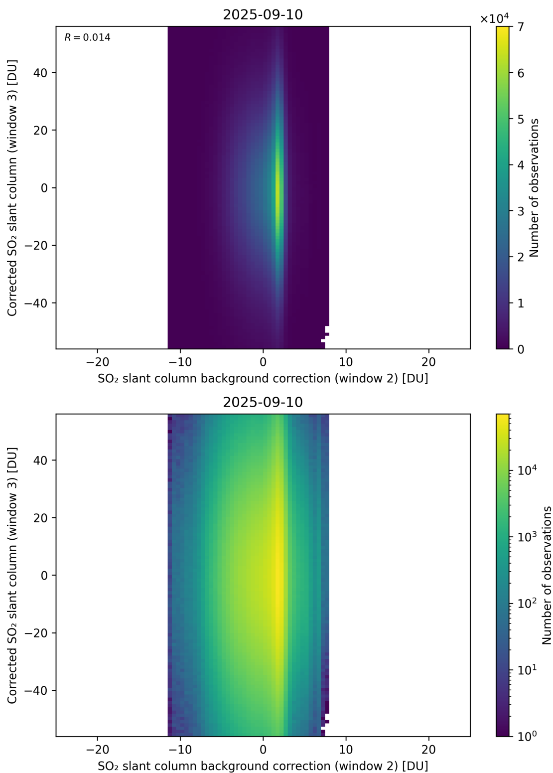
Figure 127: Scatter density plot of “SO 2 slant column background correction (window 2)” against “Corrected SO 2 slant column (window 3)” for 2025-09-10 to 2025-09-11.
