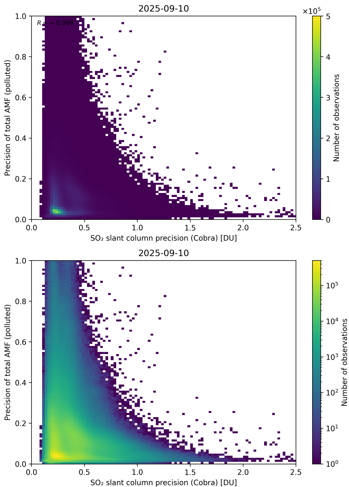
Figure 214: Scatter density plot of “SO 2 slant column precision (Cobra)” against “Precision of total AMF (polluted)” for 2025-09-10 to 2025-09-11.
