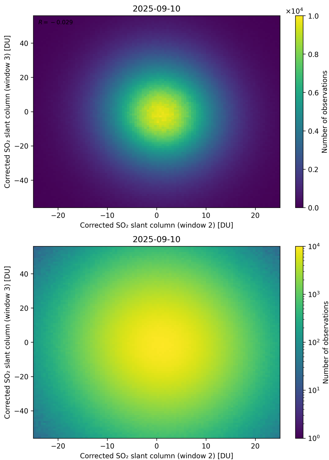
Figure 250: Scatter density plot of “Corrected SO 2 slant column (window 2)” against “Corrected SO 2 slant column (window 3)” for 2025-09-10 to 2025-09-11.
