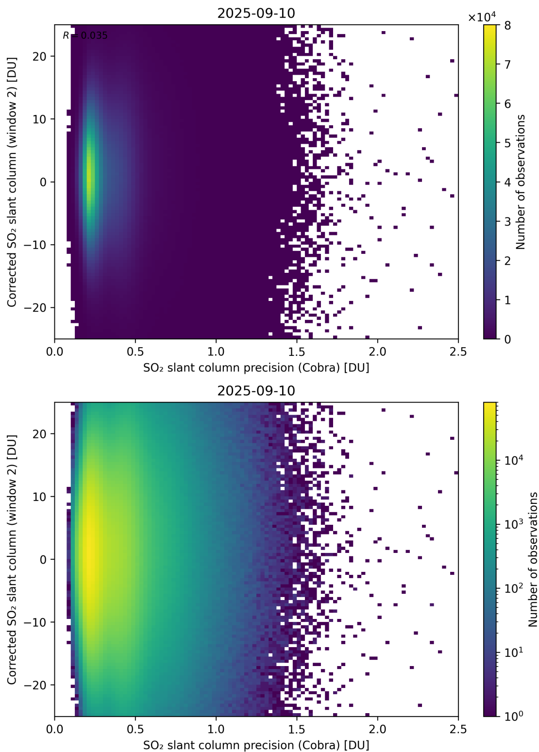
Figure 206: Scatter density plot of “SO 2 slant column precision (Cobra)” against “Corrected SO 2 slant column (window 2)” for 2025-09-10 to 2025-09-11.
