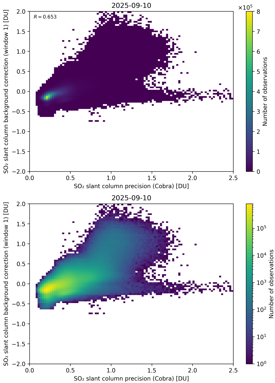
Figure 199: Scatter density plot of “SO 2 slant column precision (Cobra)” against “SO 2 slant column background correction (window 1)” for 2025-09-10 to 2025-09-11.
