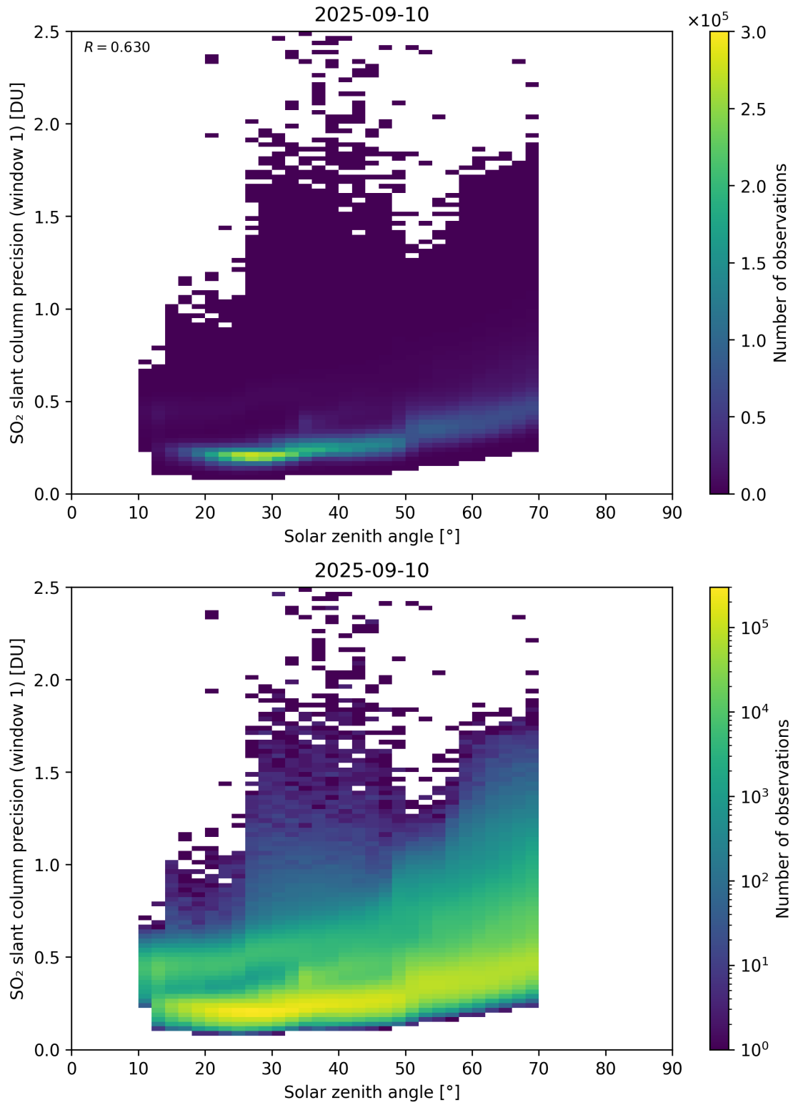
Figure 185: Scatter density plot of “Solar zenith angle” against “SO 2 slant column precision (window 1)” for 2025-09-10 to 2025-09-11.
