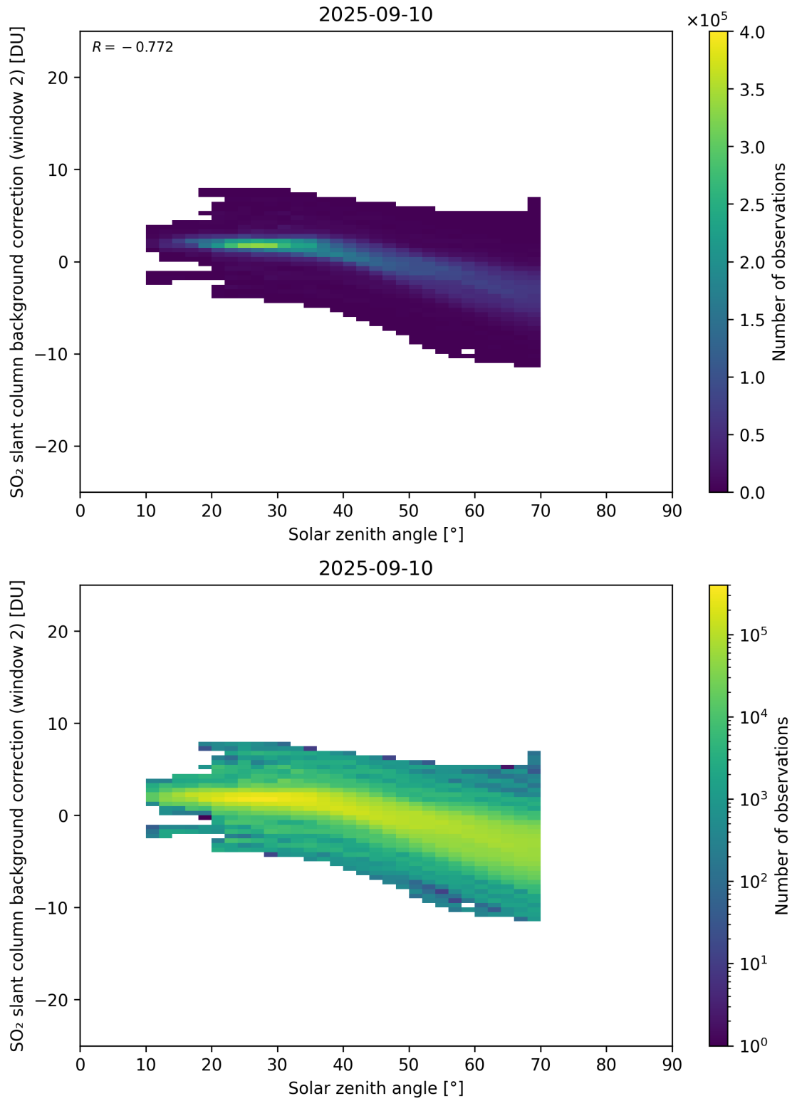
Figure 172: Scatter density plot of “Solar zenith angle” against “SO 2 slant column background correction (window 2)” for 2025-09-10 to 2025-09-11.
