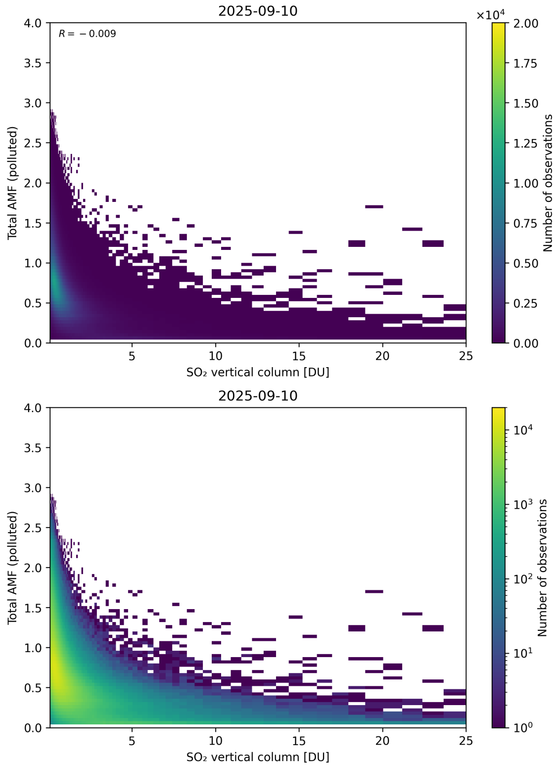
Figure 359: Scatter density plot of “SO 2 vertical column” against “Total AMF (polluted)” for 2025-09-10 to 2025-09-11.
