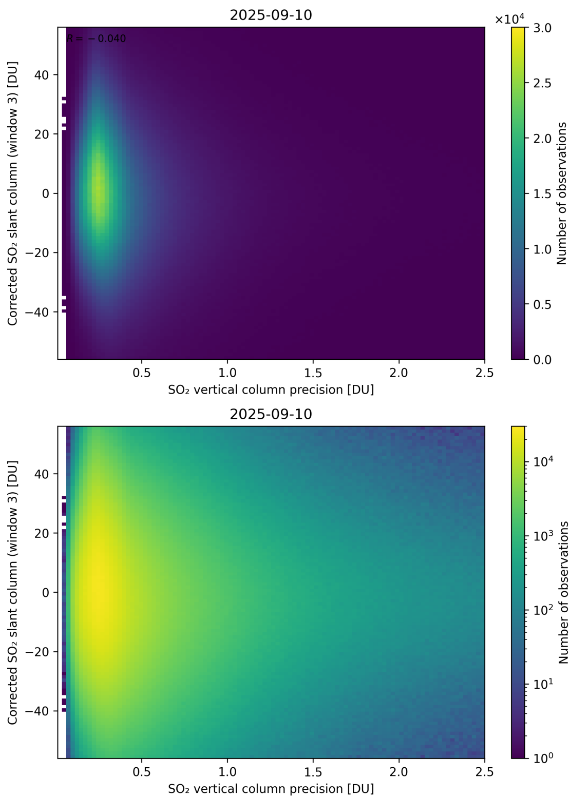
Figure 340: Scatter density plot of “SO 2 vertical column precision” against “Corrected SO 2 slant column (window 3)” for 2025-09-10 to 2025-09-11.
