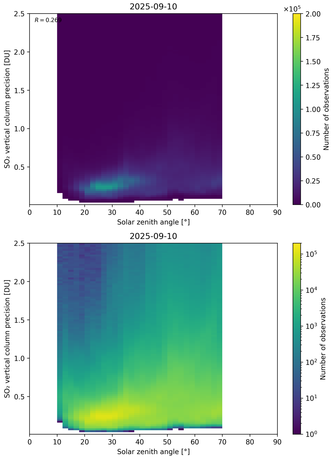
Figure 192: Scatter density plot of “Solar zenith angle” against “SO 2 vertical column precision” for 2025-09-10 to 2025-09-11.
