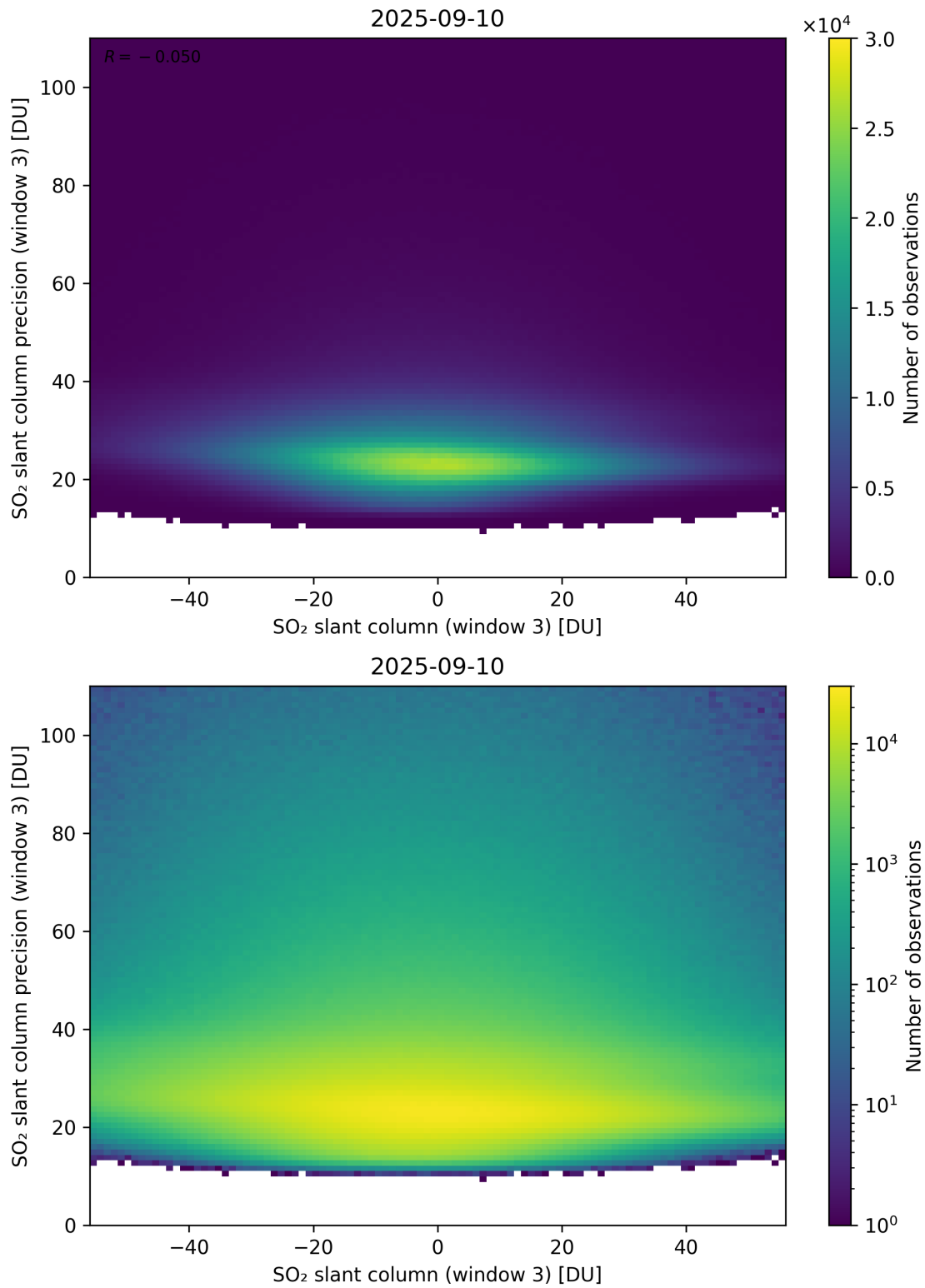
Figure 317: Scatter density plot of “SO 2 slant column (window 3)” against “SO 2 slant column precision (window 3)” for 2025-09-10 to 2025-09-11.
