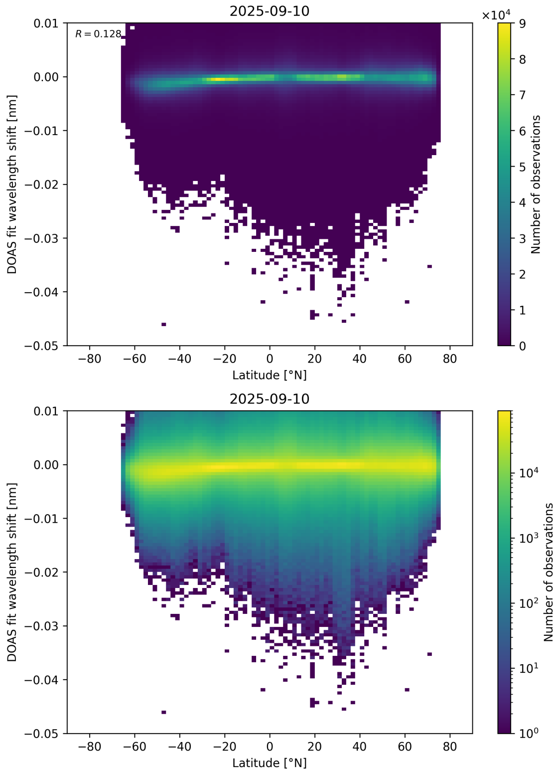
Figure 153: Scatter density plot of “Latitude” against “DOAS fit wavelength shift” for 2025-09-10 to 2025-09-11.
