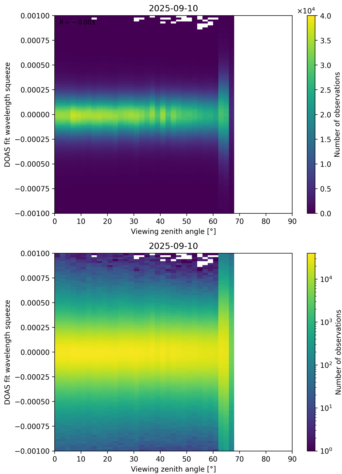
Figure 366: Scatter density plot of “Viewing zenith angle” against “DOAS fit wavelength squeeze” for 2025-09-10 to 2025-09-11.
