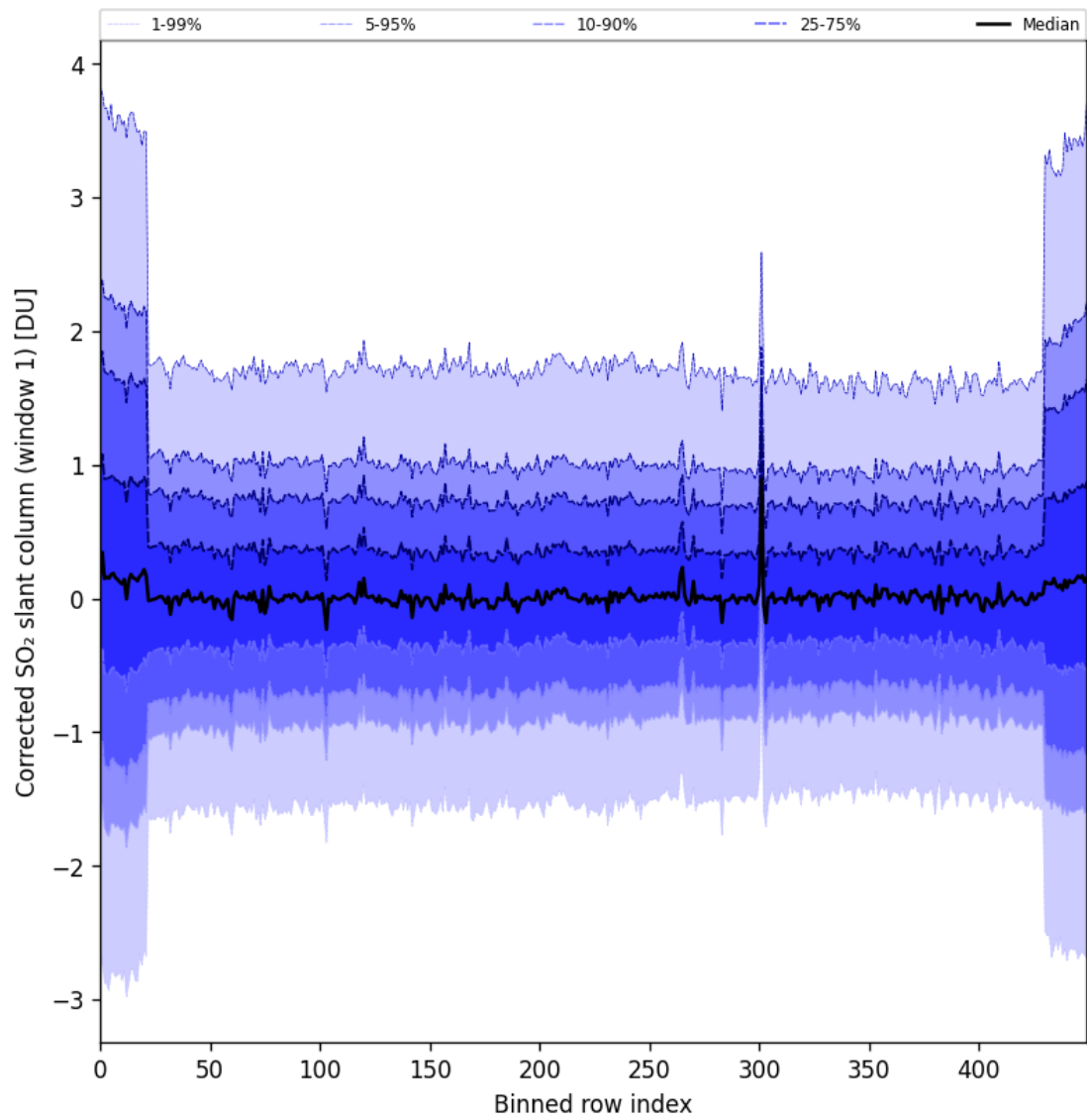
Figure 91: Along track statistics of “Corrected SO 2 slant column (window 1)” for 2025-09-10 to 2025-09-11
