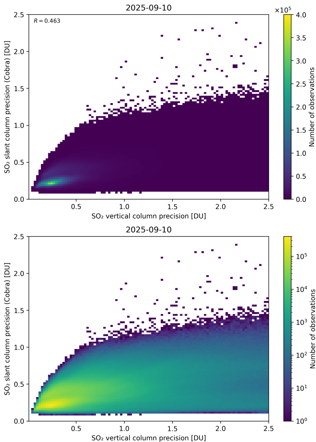
Figure 337: Scatter density plot of “SO 2 vertical column precision” against “SO 2 slant column precision (Cobra)” for 2025-09-10 to 2025-09-11.
