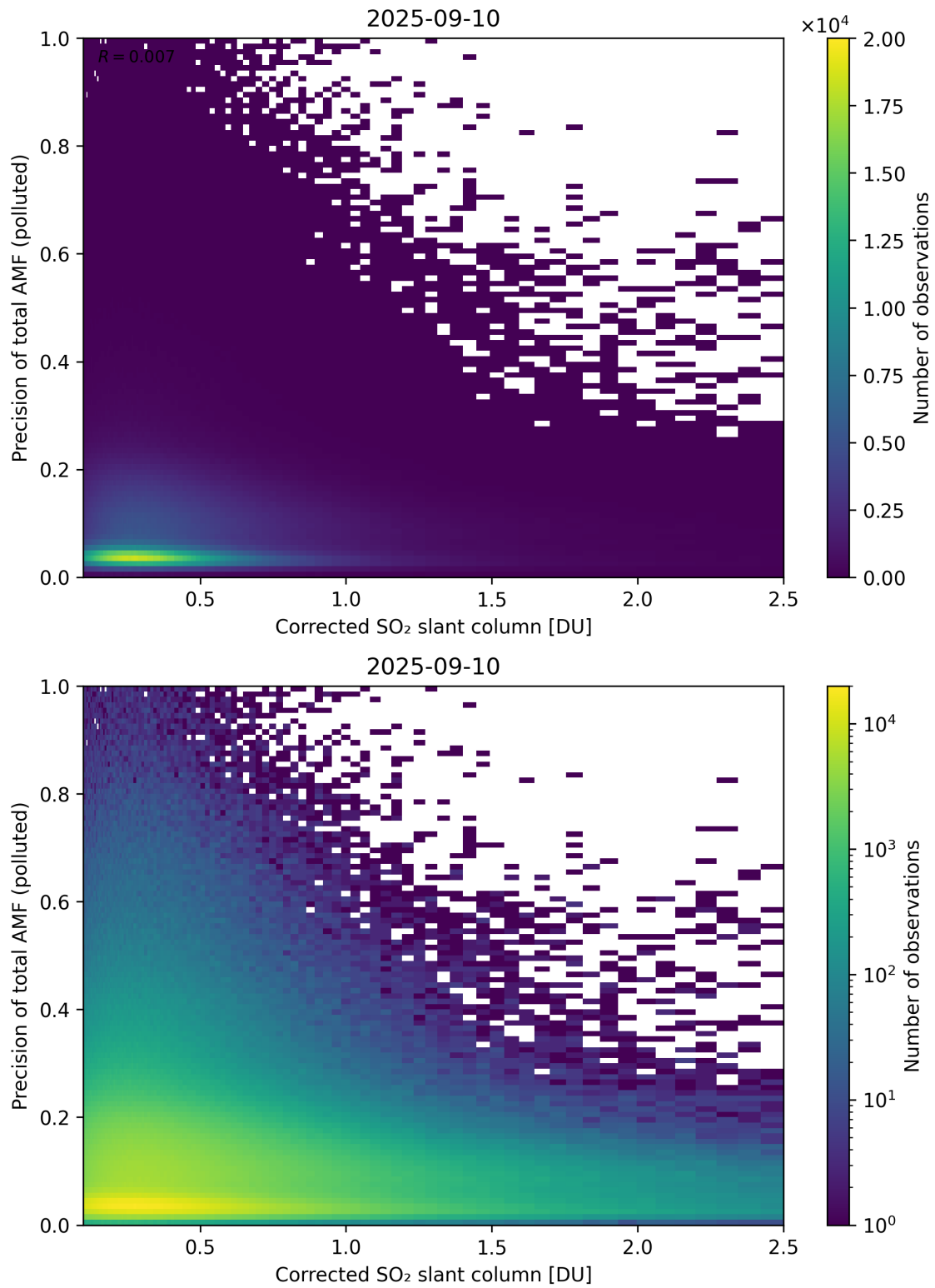
Figure 243: Scatter density plot of “Corrected SO 2 slant column” against “Precision of total AMF (polluted)” for 2025-09-10 to 2025-09-11.
