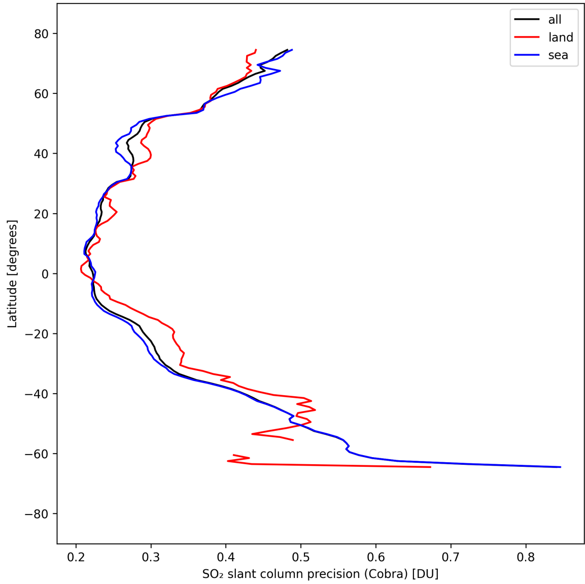
Figure 36: Zonal average of “SO 2 slant column precision (Cobra)” for 2025-09-10 to 2025-09-11.
