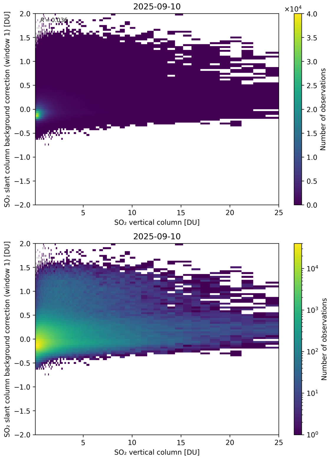
Figure 323: Scatter density plot of “SO 2 vertical column” against “SO 2 slant column background correction (window 1)” for 2025-09-10 to 2025-09-11.
