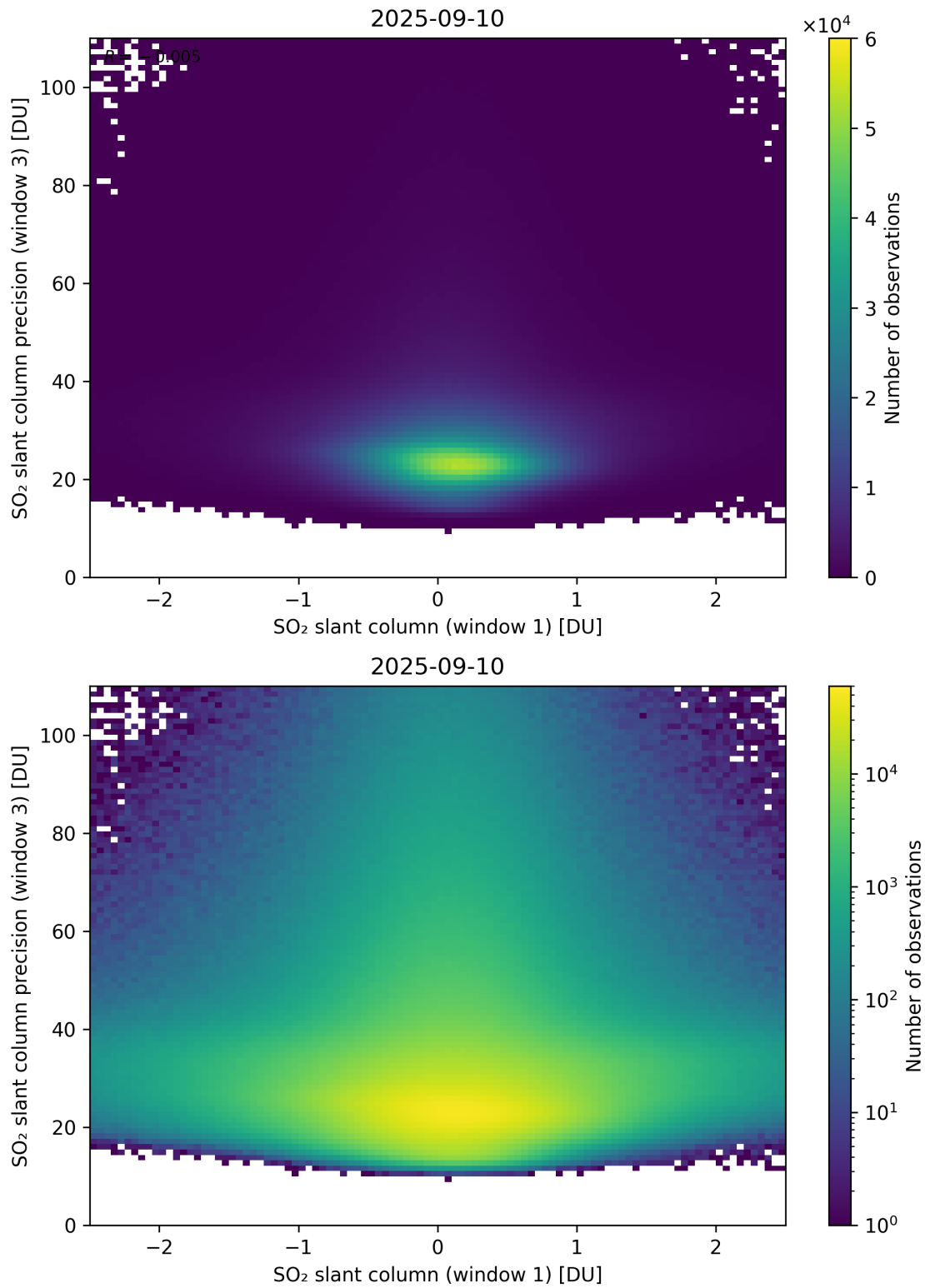
Figure 288: Scatter density plot of “SO 2 slant column (window 1)” against “SO 2 slant column precision (window 3)” for 2025-09-10 to 2025-09-11.
