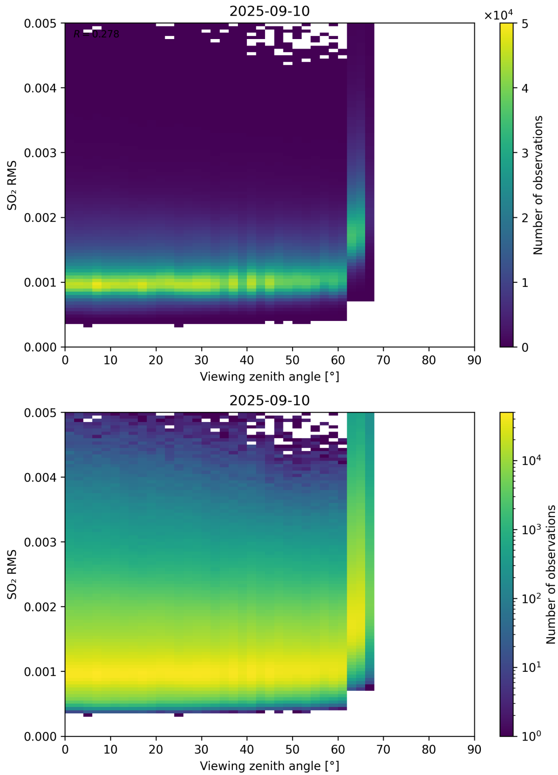
Figure 367: Scatter density plot of “Viewing zenith angle” against “SO 2 RMS” for 2025-09-10 to 2025-09-11.
