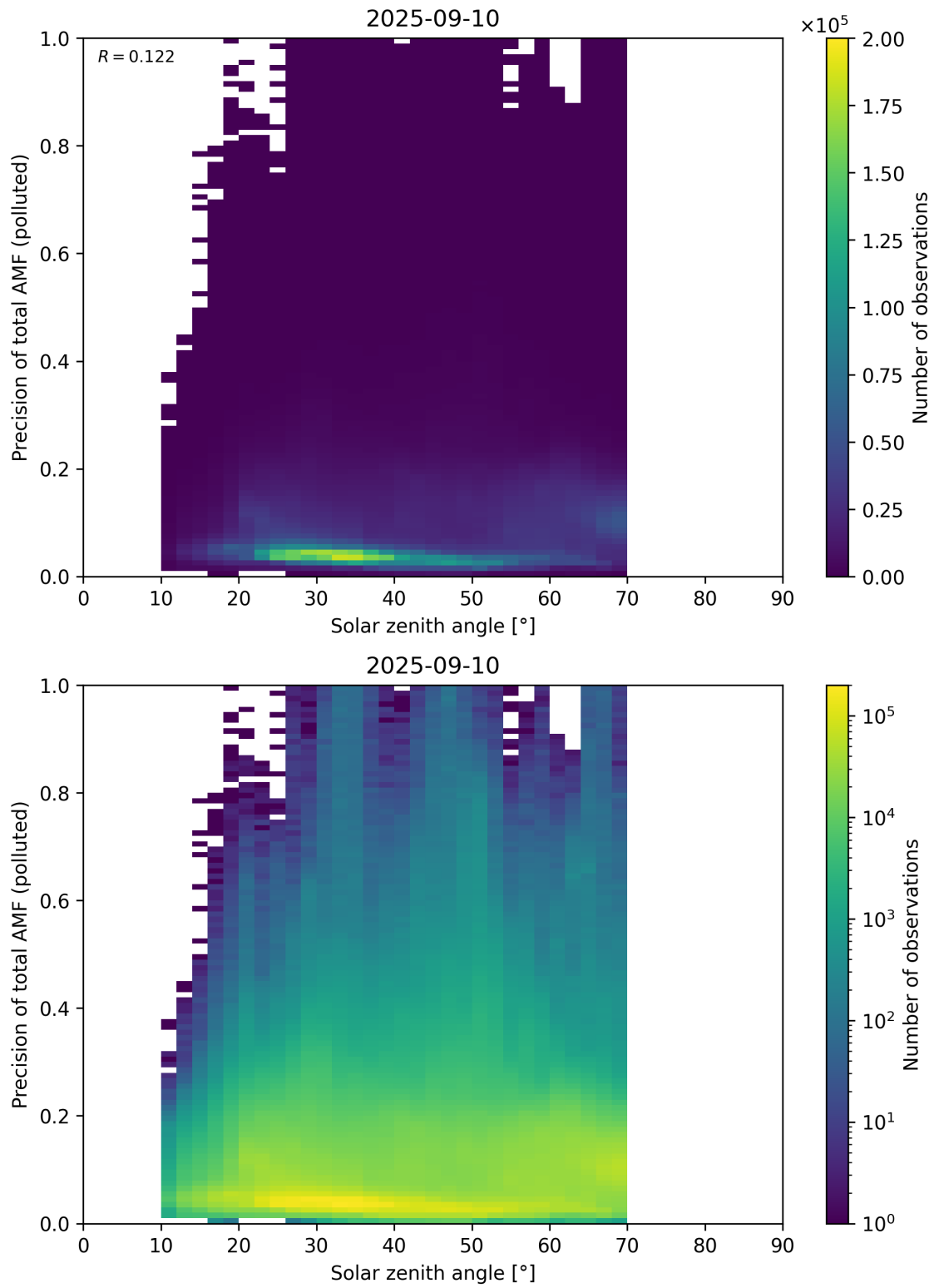
Figure 190: Scatter density plot of “Solar zenith angle” against “Precision of total AMF (polluted)” for 2025-09-10 to 2025-09-11.
