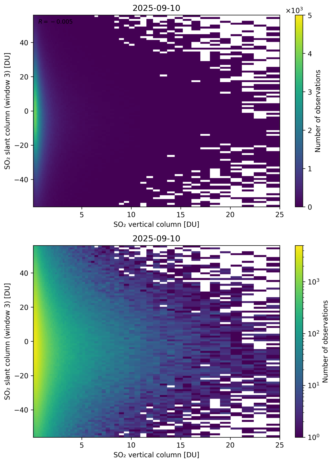
Figure 357: Scatter density plot of “SO 2 vertical column” against “SO 2 slant column (window 3)” for 2025-09-10 to 2025-09-11.
