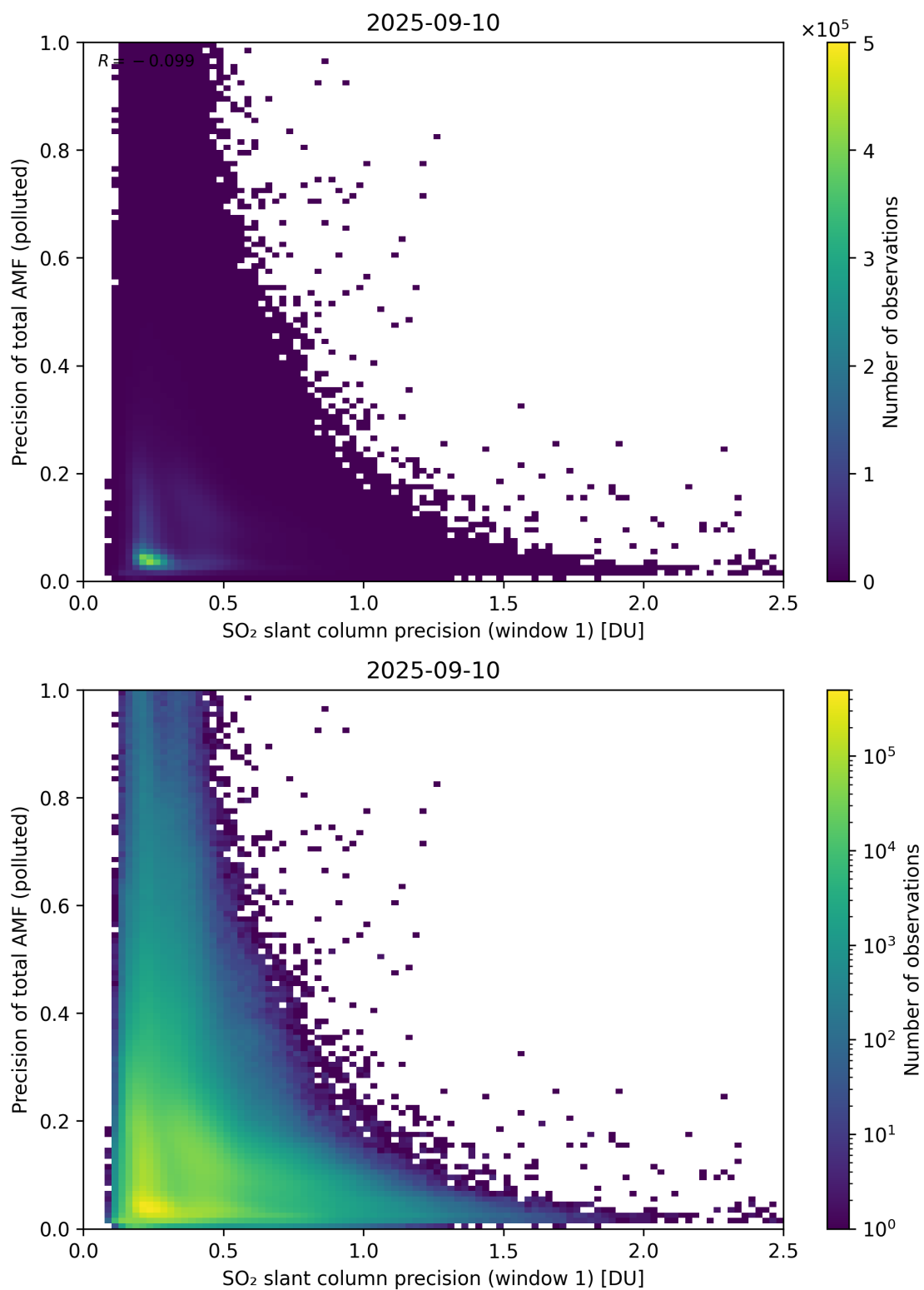
Figure 281: Scatter density plot of “SO 2 slant column precision (window 1)” against “Precision of total AMF (polluted)” for 2025-09-10 to 2025-09-11.
