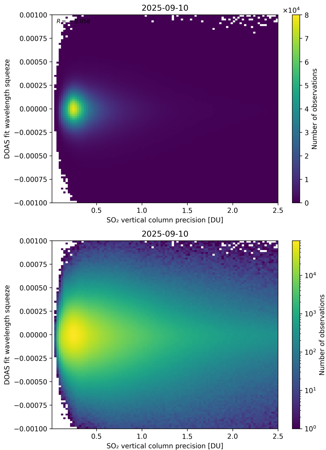
Figure 333: Scatter density plot of “SO 2 vertical column precision” against “DOAS fit wavelength squeeze” for 2025-09-10 to 2025-09-11.
