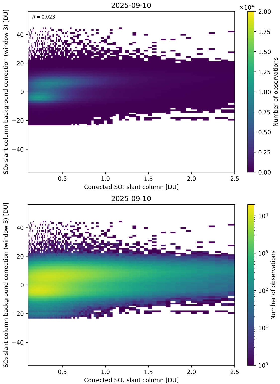
Figure 228: Scatter density plot of “Corrected SO 2 slant column” against “SO 2 slant column background correction (window 3)” for 2025-09-10 to 2025-09-11.
