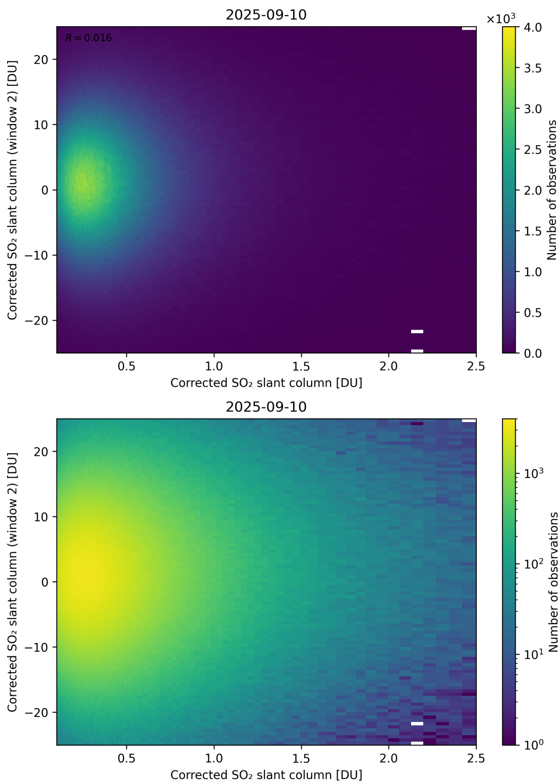
Figure 235: Scatter density plot of “Corrected SO 2 slant column” against “Corrected SO 2 slant column (window 2)” for 2025-09-10 to 2025-09-11.
