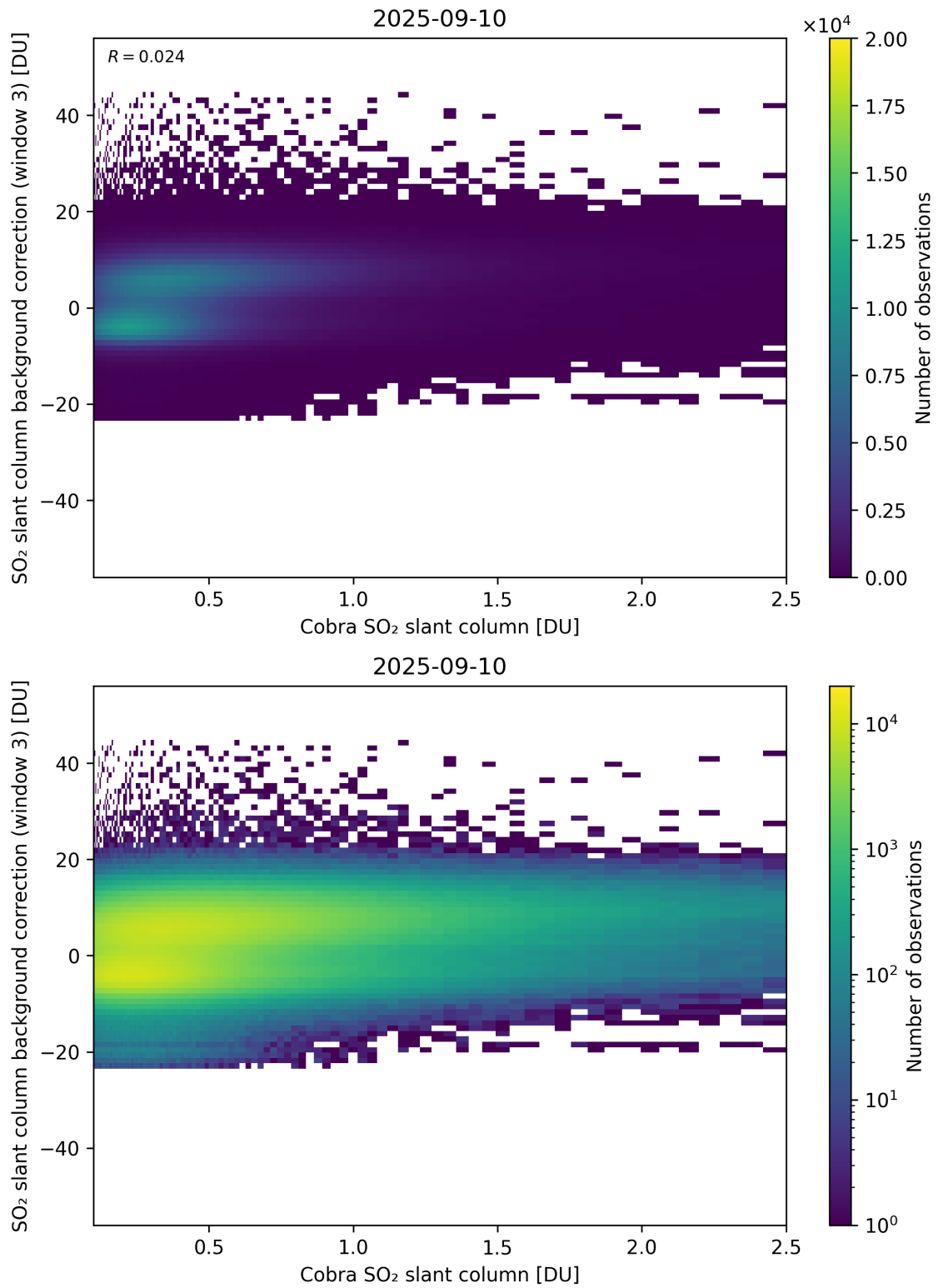
Figure 195: Scatter density plot of “Cobra SO 2 slant column” against “SO 2 slant column background correction (window 3)” for 2025-09-10 to 2025-09-11.
