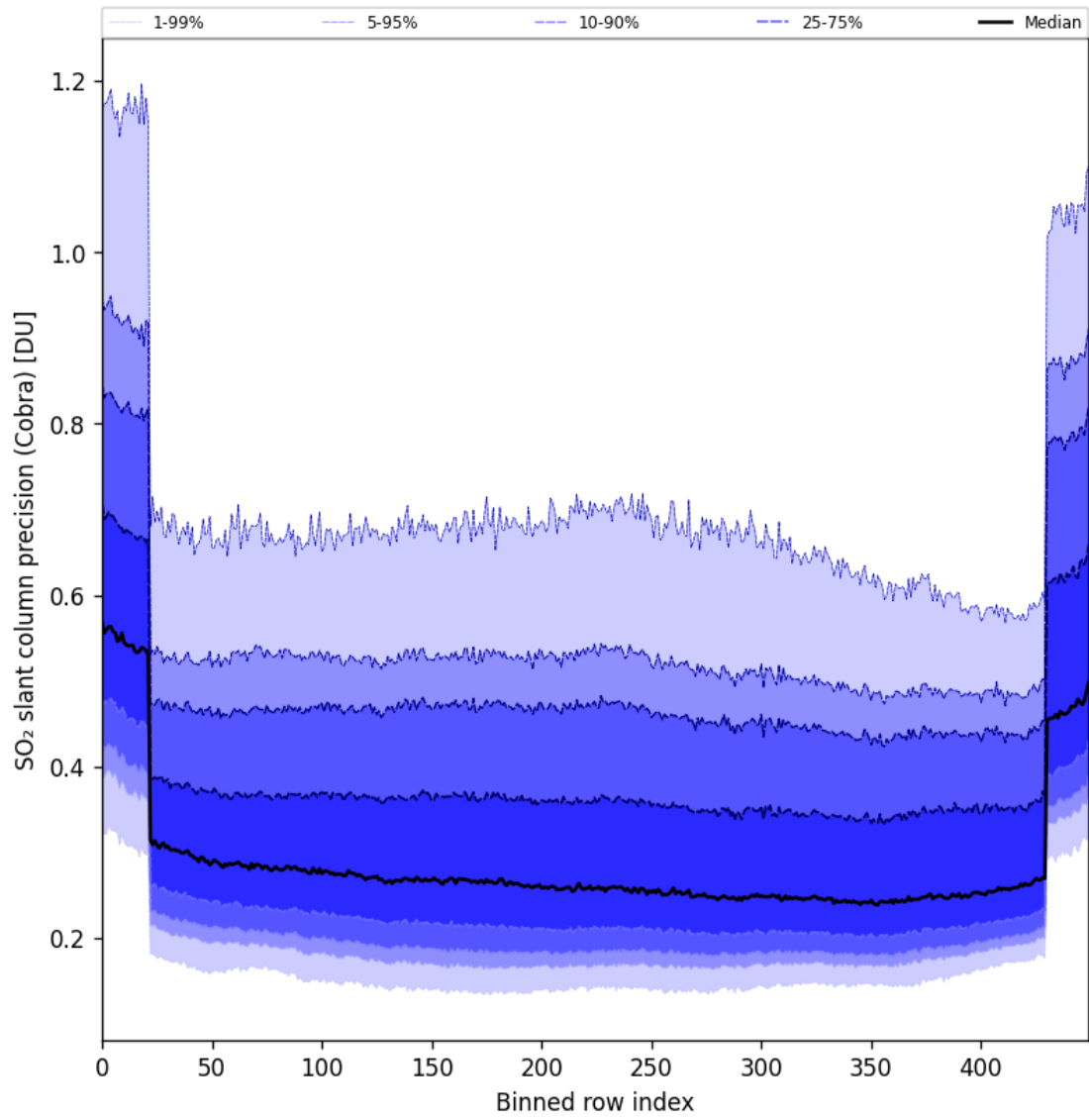
Figure 88: Along track statistics of “SO 2 slant column precision (Cobra)” for 2025-09-10 to 2025-09-11
