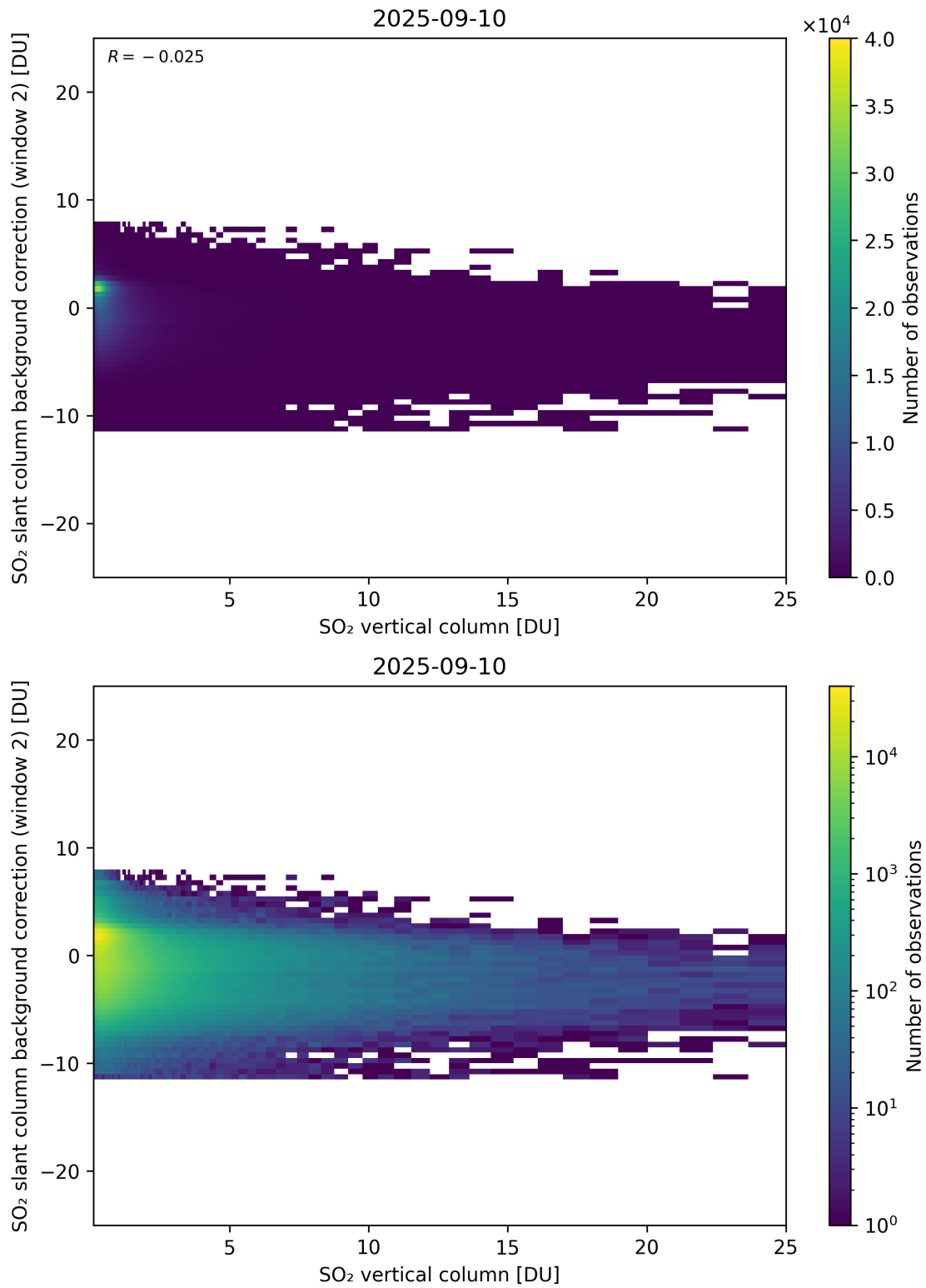
Figure 324: Scatter density plot of “SO 2 vertical column” against “SO 2 slant column background correction (window 2)” for 2025-09-10 to 2025-09-11.
