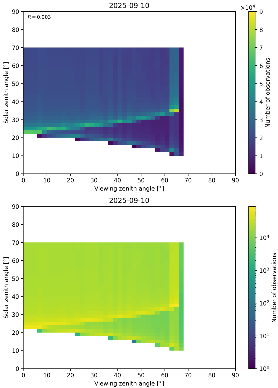
Figure 369: Scatter density plot of “Viewing zenith angle” against “Solar zenith angle” for 2025-09-10 to 2025-09-11.
