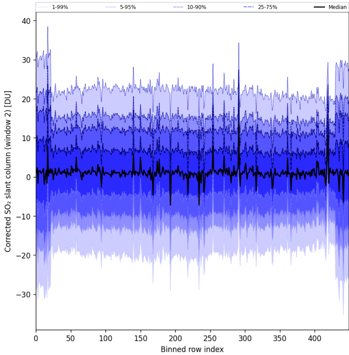
Figure 95: Along track statistics of “Corrected SO 2 slant column (window 2)” for 2025-09-10 to 2025-09-11
