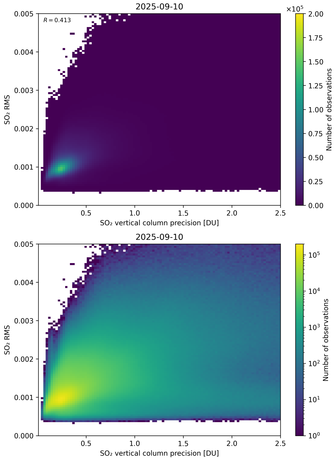
Figure 334: Scatter density plot of “SO 2 vertical column precision” against “SO 2 RMS” for 2025-09-10 to 2025-09-11.
