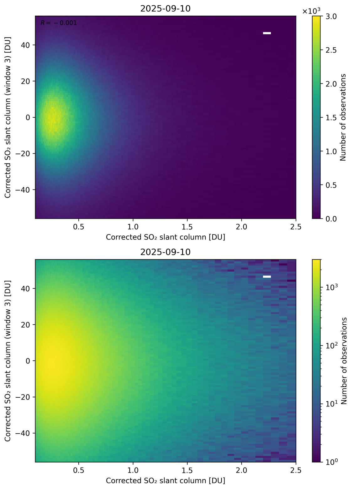
Figure 236: Scatter density plot of “Corrected SO 2 slant column” against “Corrected SO 2 slant column (window 3)” for 2025-09-10 to 2025-09-11.
