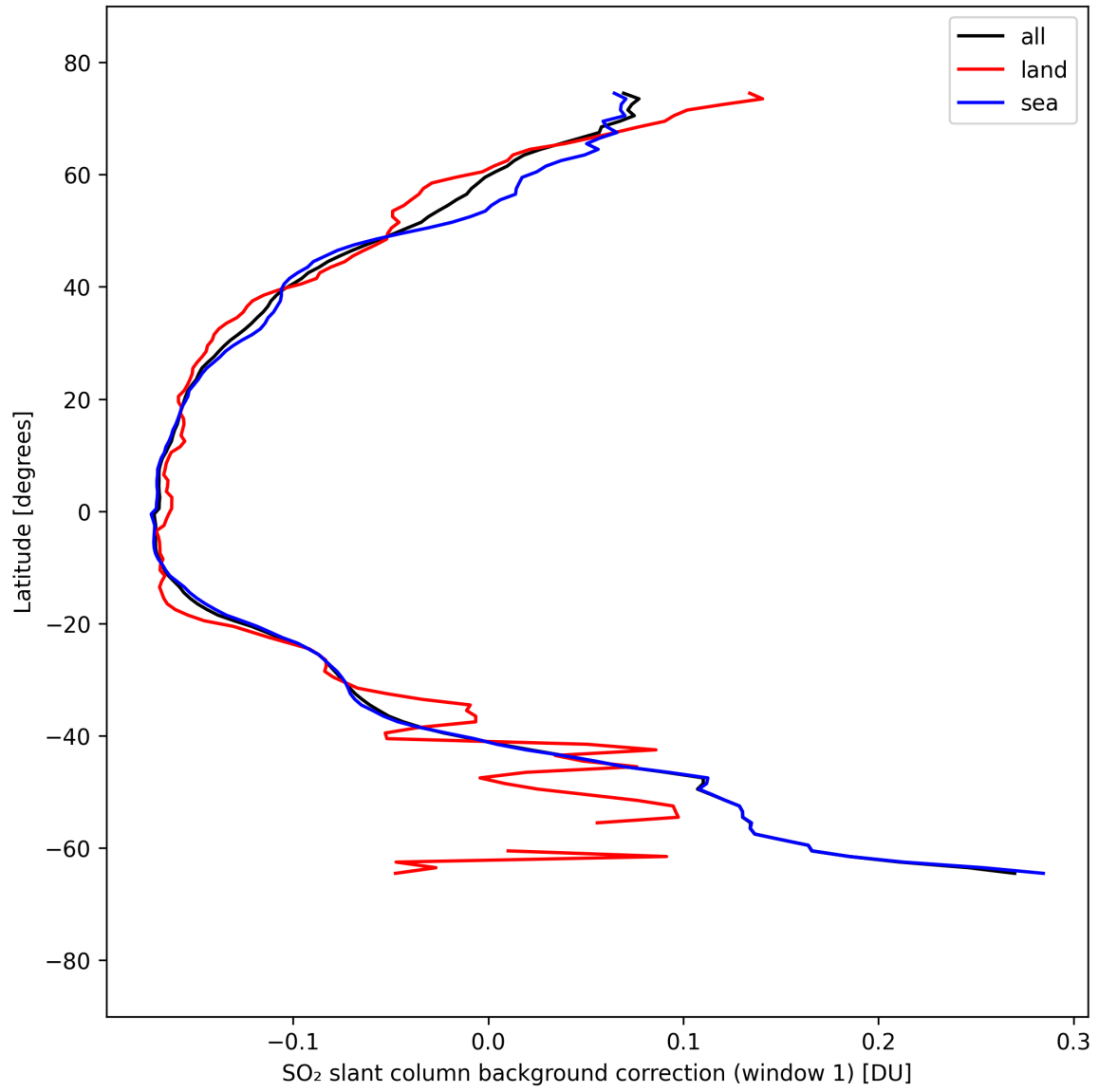
Figure 40: Zonal average of “SO 2 slant column background correction (window 1)” for 2025-09-10 to 2025-09-11.
