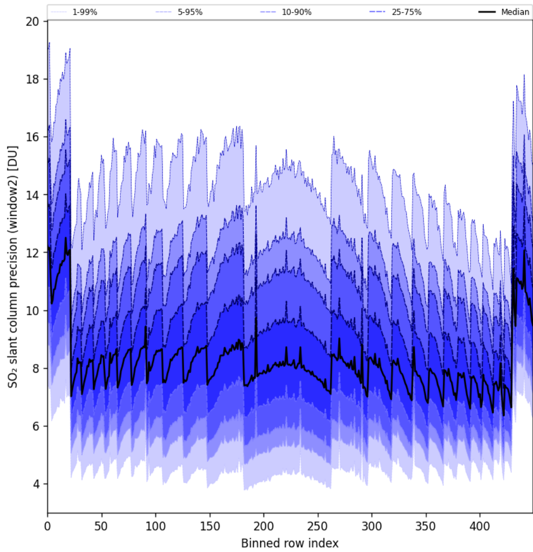
Figure 94: Along track statistics of “SO 2 slant column precision (window2)” for 2025-09-10 to 2025-09-11
