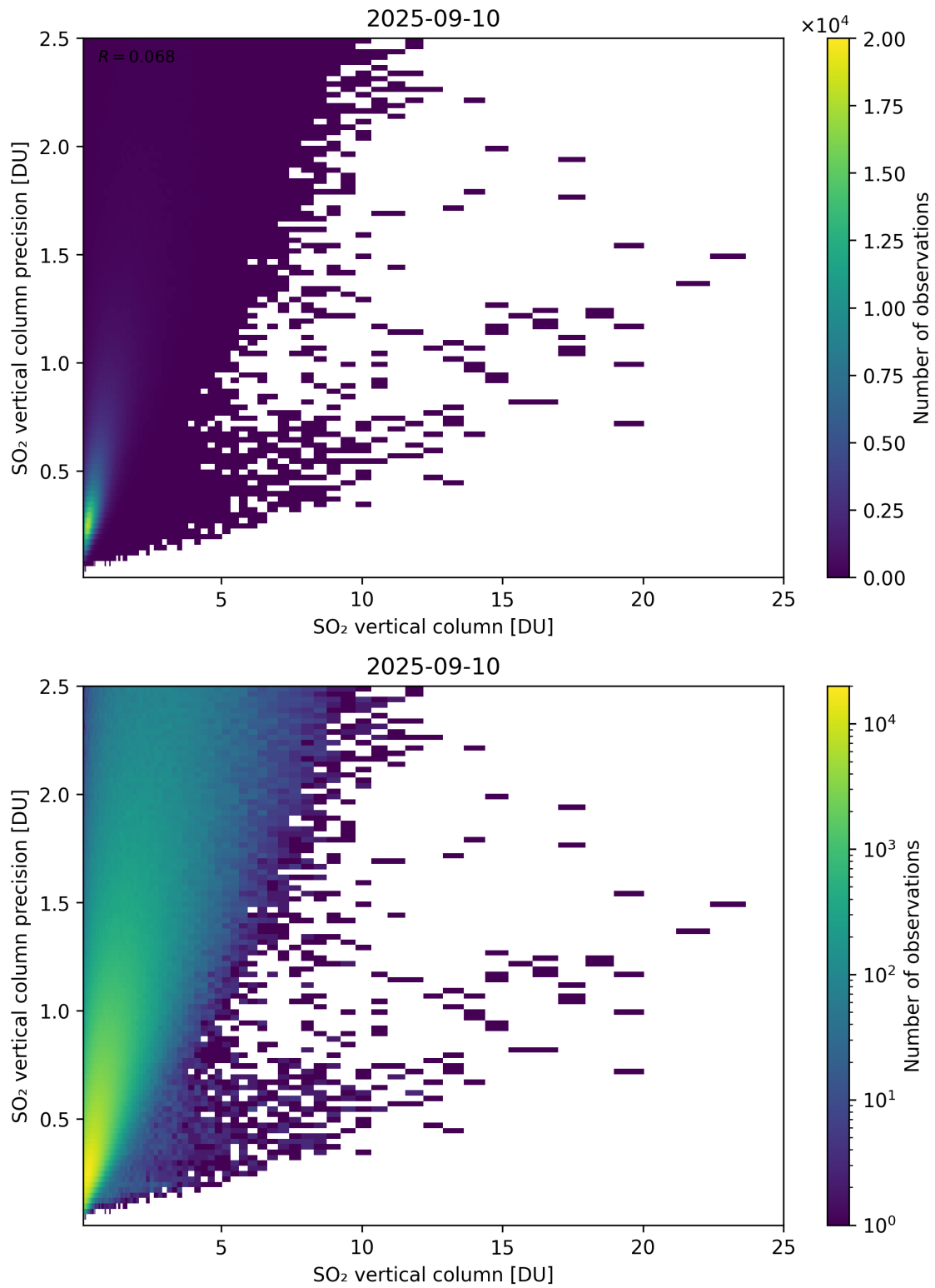
Figure 361: Scatter density plot of “SO 2 vertical column” against “SO 2 vertical column precision” for 2025-09-10 to 2025-09-11.
