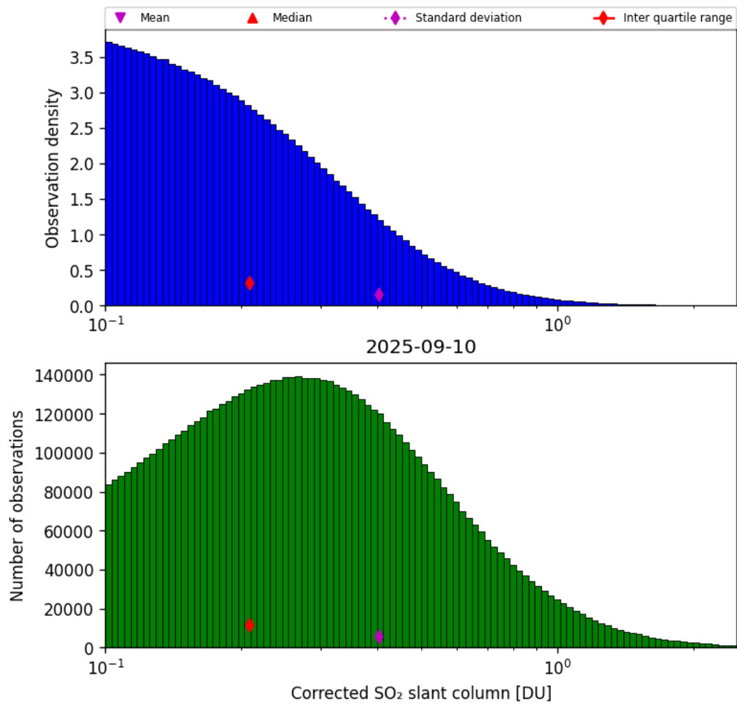
Figure 60: Histogram of “Corrected SO 2 slant column” for 2025-09-10 to 2025-09-11
