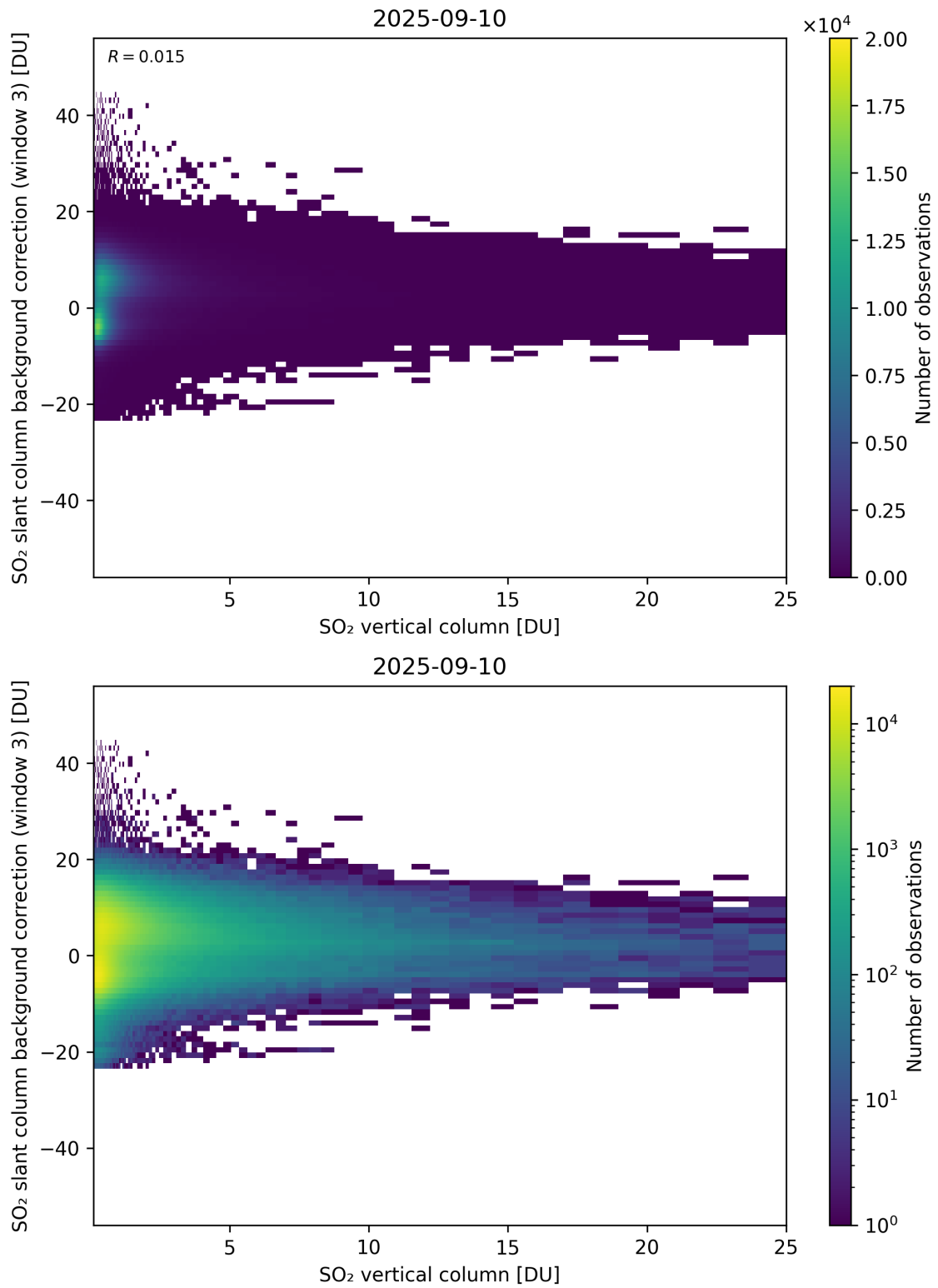
Figure 325: Scatter density plot of “SO 2 vertical column” against “SO 2 slant column background correction (window 3)” for 2025-09-10 to 2025-09-11.
