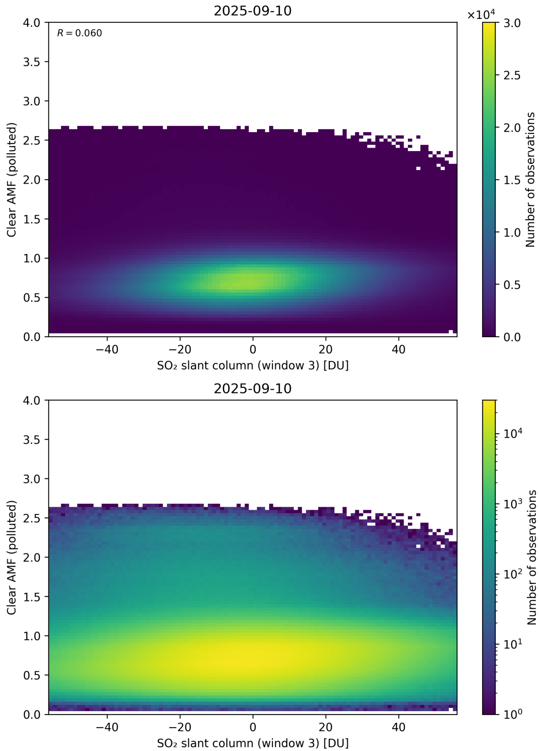
Figure 315: Scatter density plot of “SO 2 slant column (window 3)” against “Clear AMF (polluted)” for 2025-09-10 to 2025-09-11.
