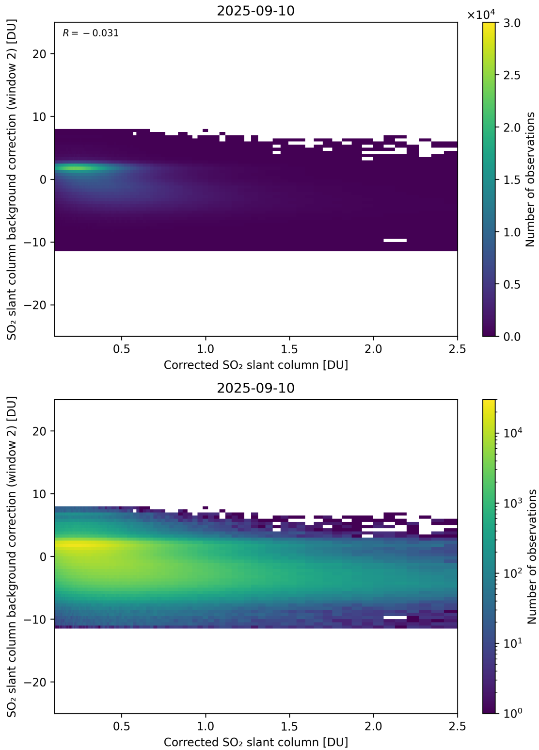
Figure 227: Scatter density plot of “Corrected SO 2 slant column” against “SO 2 slant column background correction (window 2)” for 2025-09-10 to 2025-09-11.
