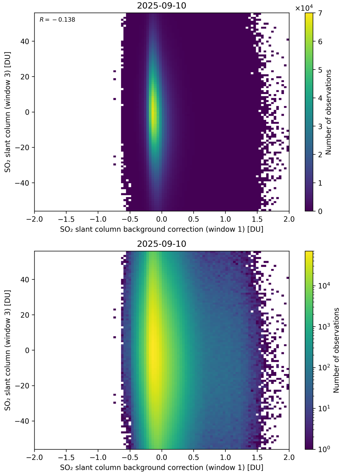
Figure 118: Scatter density plot of “SO 2 slant column background correction (window 1)” against “SO 2 slant column (window 3)” for 2025-09-10 to 2025-09-11.
