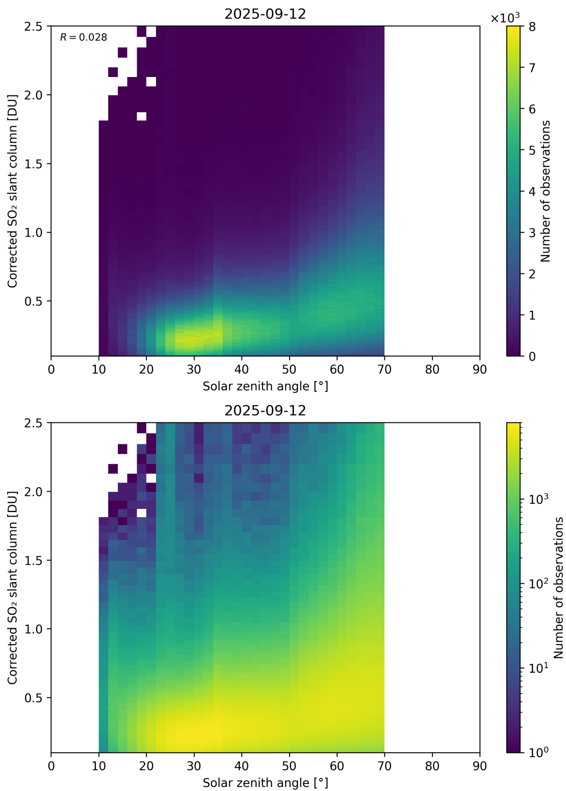
Figure 181: Scatter density plot of “Solar zenith angle” against “Corrected SO 2 slant column” for 2025-09-11 to 2025-09-13.
