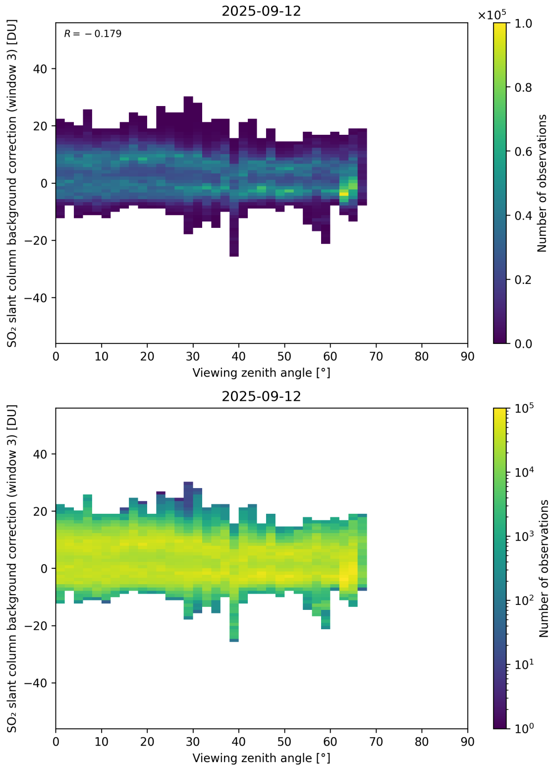
Figure 364: Scatter density plot of “Viewing zenith angle” against “SO 2 slant column background correction (window 3)” for 2025-09-11 to 2025-09-13.
