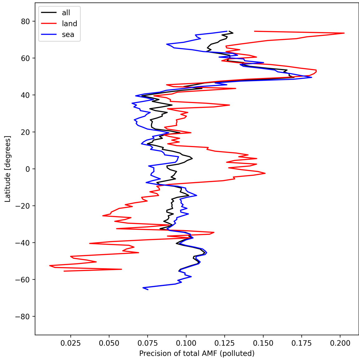
Figure 54: Zonal average of “Precision of total AMF (polluted)” for 2025-09-11 to 2025-09-13.
