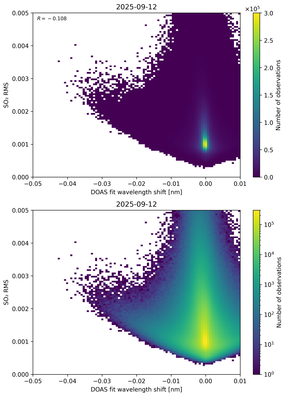
Figure 139: Scatter density plot of “DOAS fit wavelength shift” against “SO 2 RMS” for 2025-09-11 to 2025-09-13.
