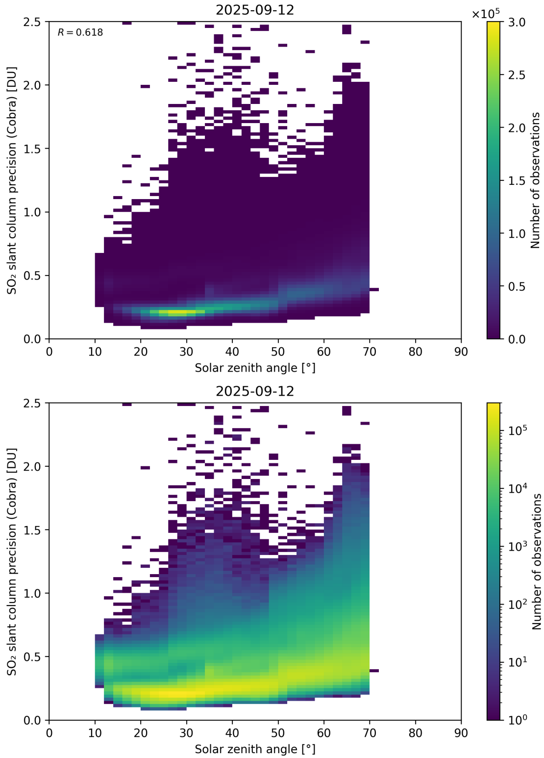
Figure 180: Scatter density plot of “Solar zenith angle” against “SO 2 slant column precision (Cobra)” for 2025-09-11 to 2025-09-13.
