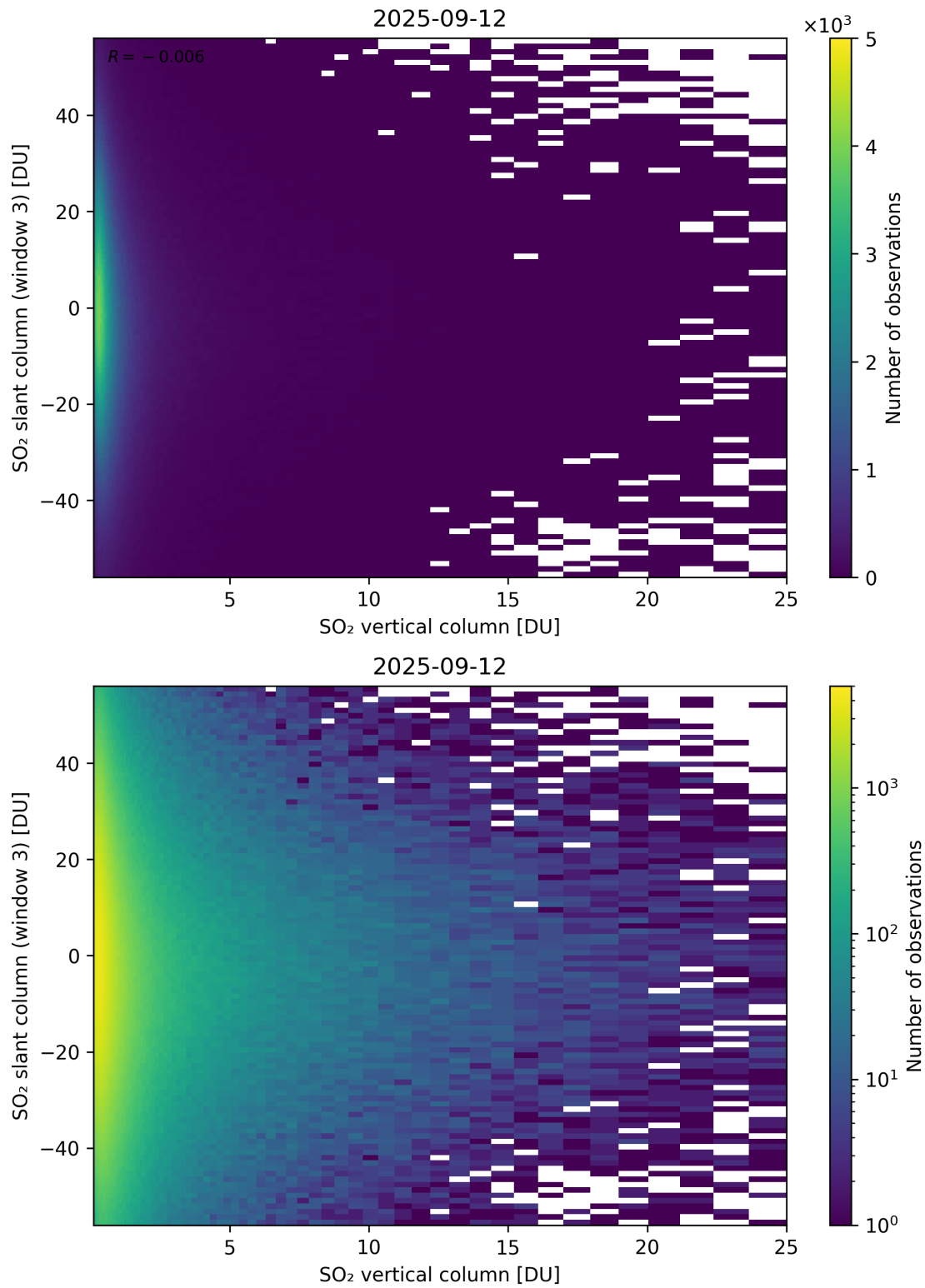
Figure 357: Scatter density plot of “SO 2 vertical column” against “SO 2 slant column (window 3)” for 2025-09-11 to 2025-09-13.
