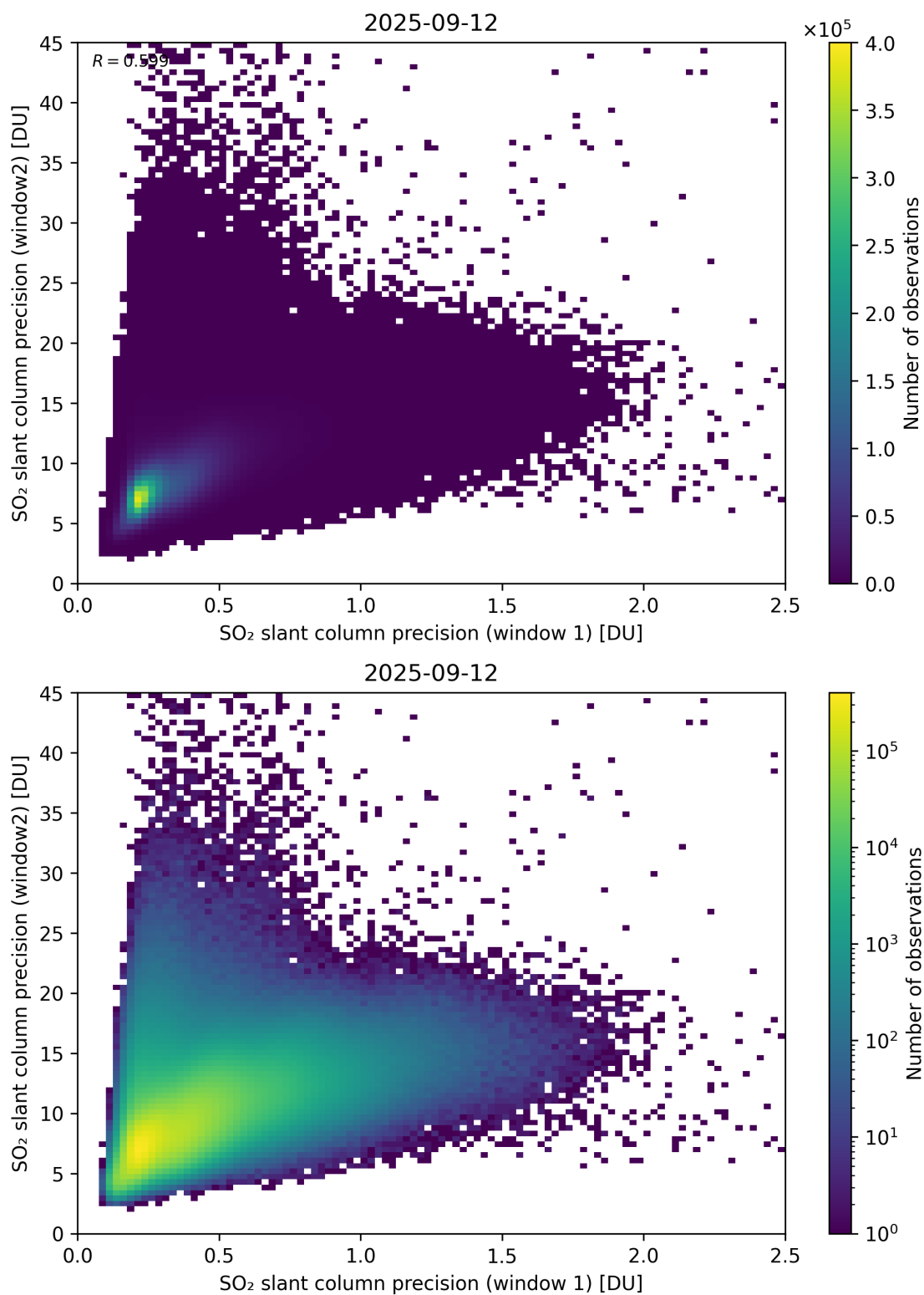
Figure 277: Scatter density plot of “SO 2 slant column precision (window 1)” against “SO 2 slant column precision (window2)” for 2025-09-11 to 2025-09-13.
