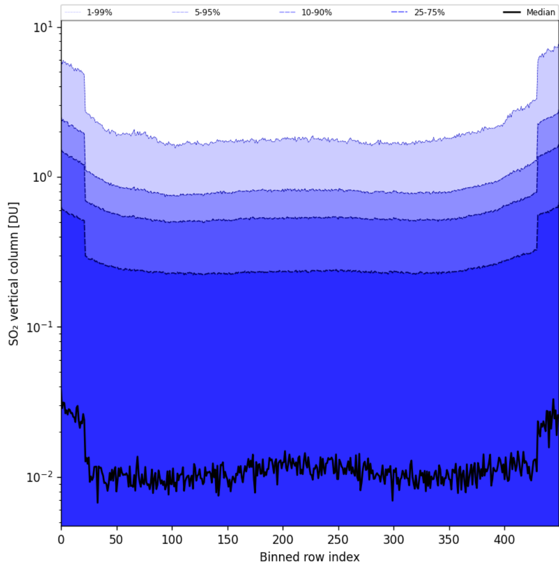
Figure 84: Along track statistics of “SO 2 vertical column” for 2025-09-11 to 2025-09-13
