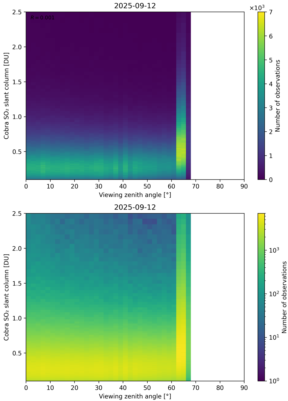
Figure 371: Scatter density plot of “Viewing zenith angle” against “Cobra SO 2 slant column” for 2025-09-11 to 2025-09-13.
