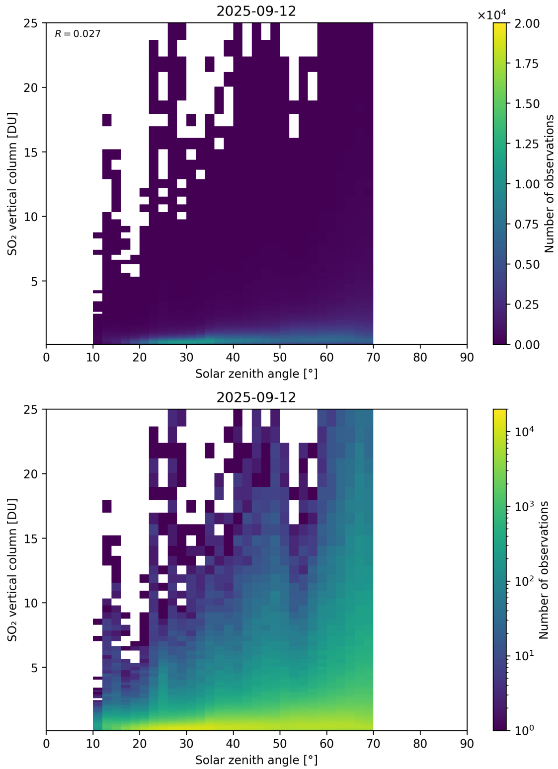
Figure 191: Scatter density plot of “Solar zenith angle” against “SO 2 vertical column” for 2025-09-11 to 2025-09-13.
