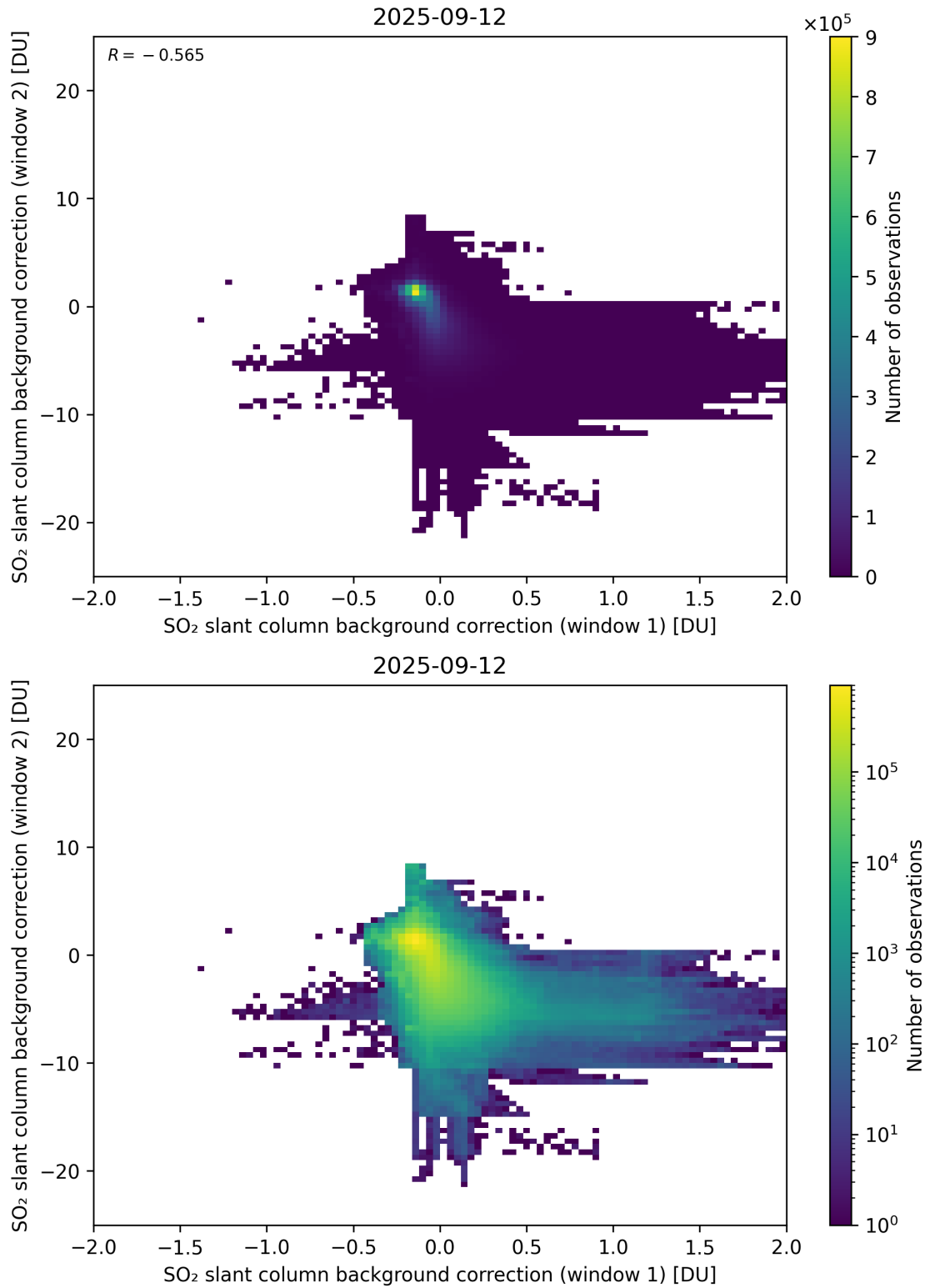
Figure 109: Scatter density plot of “SO 2 slant column background correction (window 1)” against “SO 2 slant column background correction (window 2)” for 2025-09-11 to 2025-09-13.
