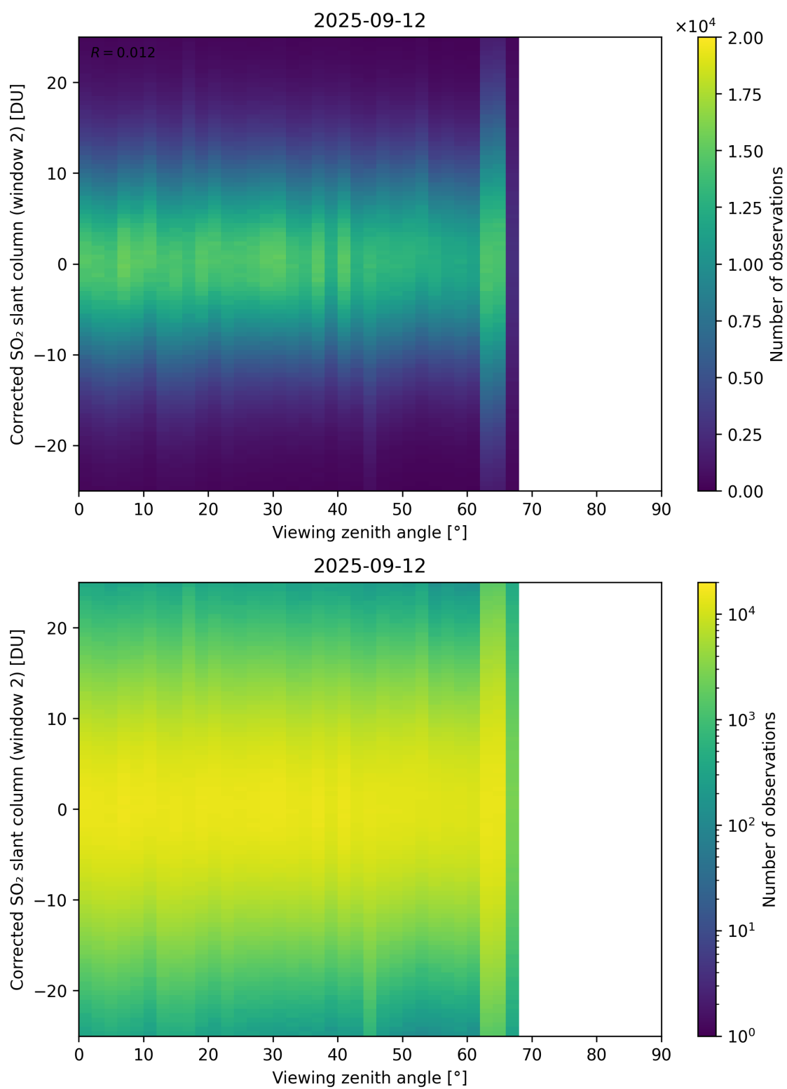
Figure 374: Scatter density plot of “Viewing zenith angle” against “Corrected SO 2 slant column (window 2)” for 2025-09-11 to 2025-09-13.
