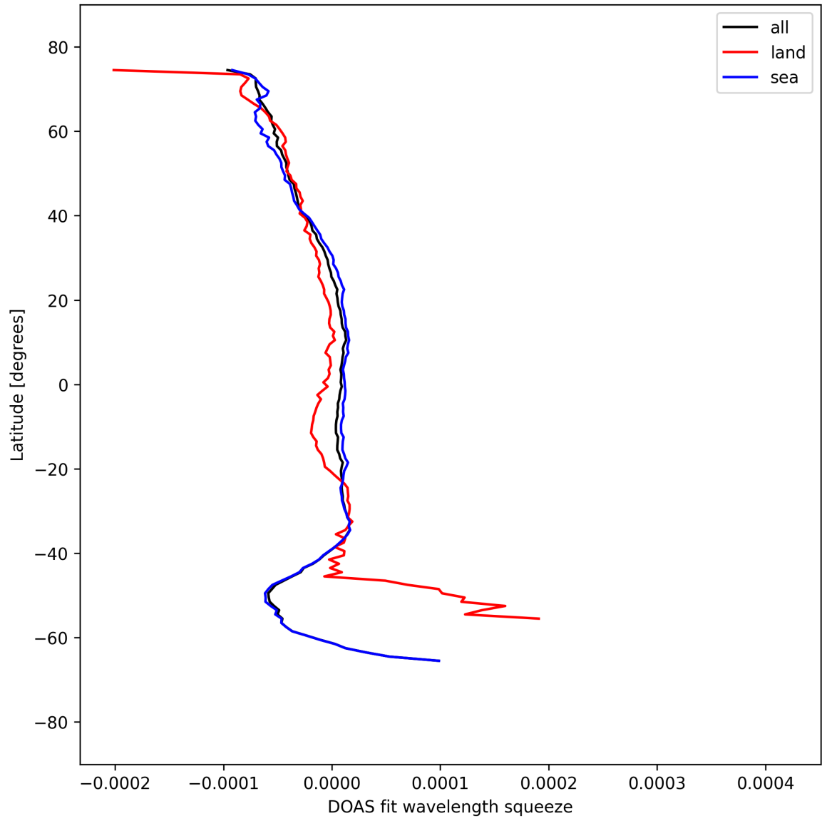
Figure 51: Zonal average of “DOAS fit wavelength squeeze” for 2025-09-11 to 2025-09-13.
