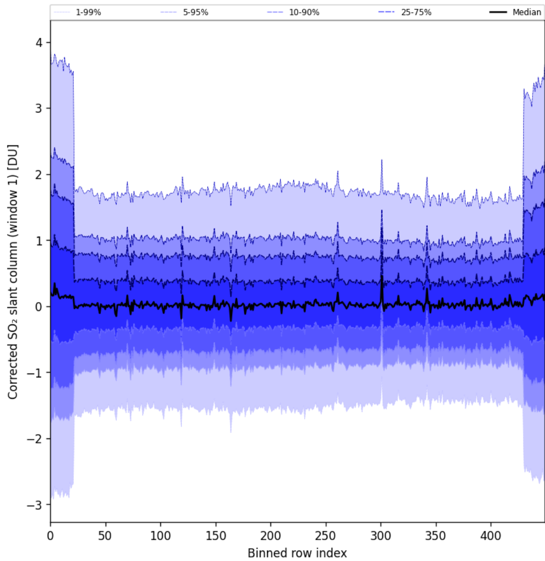
Figure 91: Along track statistics of “Corrected SO 2 slant column (window 1)” for 2025-09-11 to 2025-09-13
