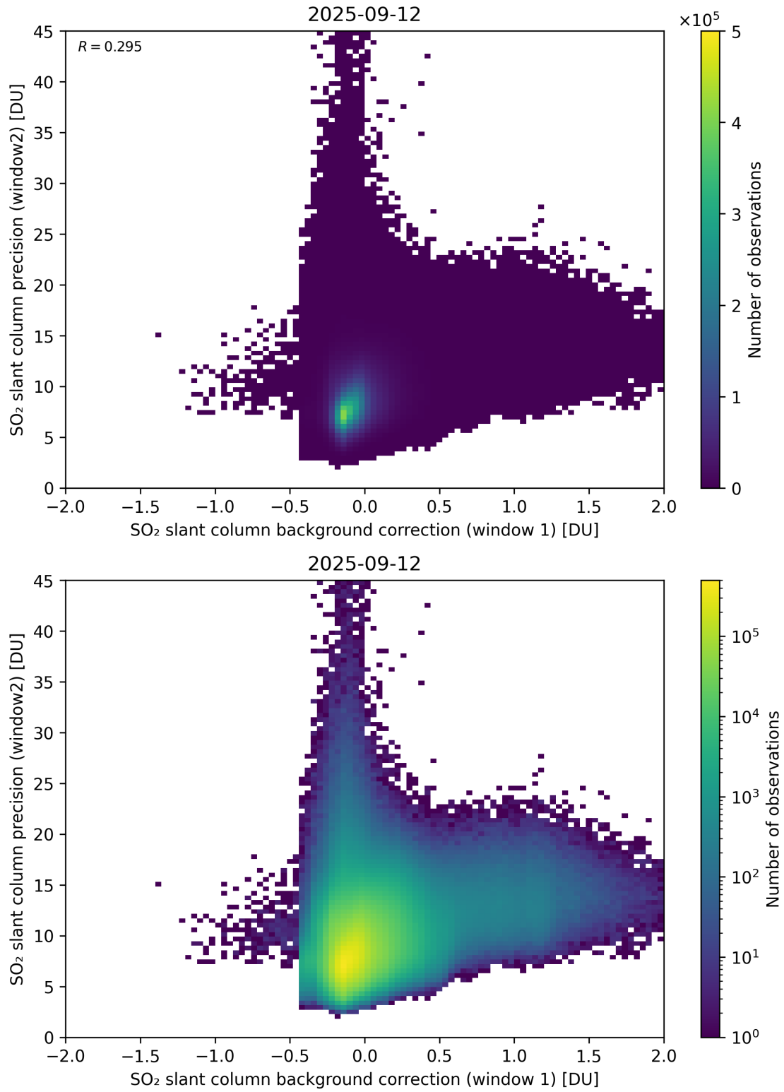
Figure 117: Scatter density plot of “SO 2 slant column background correction (window 1)” against “SO 2 slant column precision (window2)” for 2025-09-11 to 2025-09-13.
