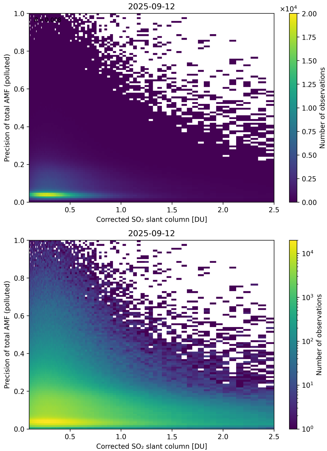
Figure 243: Scatter density plot of “Corrected SO 2 slant column” against “Precision of total AMF (polluted)” for 2025-09-11 to 2025-09-13.
