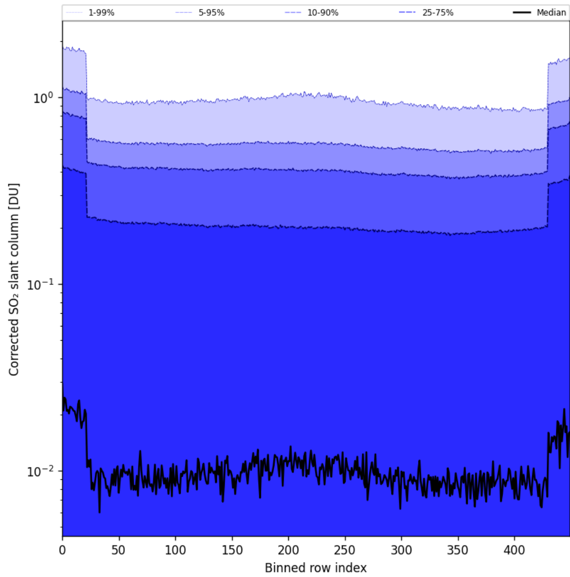
Figure 86: Along track statistics of “Corrected SO 2 slant column” for 2025-09-11 to 2025-09-13
