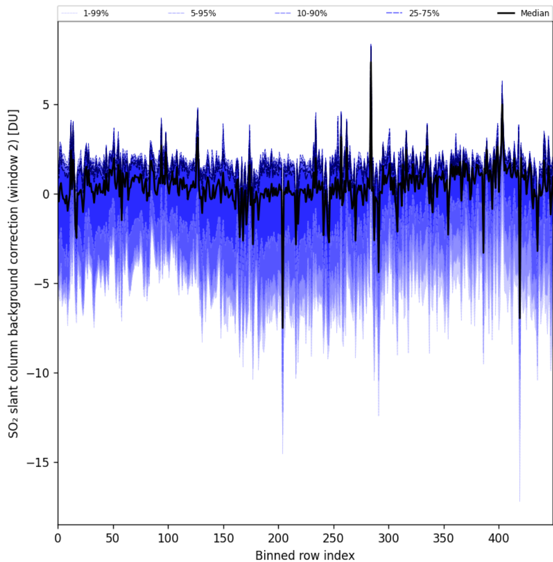
Figure 96: Along track statistics of “SO 2 slant column background correction (window 2)” for 2025-09-11 to 2025-09-13
