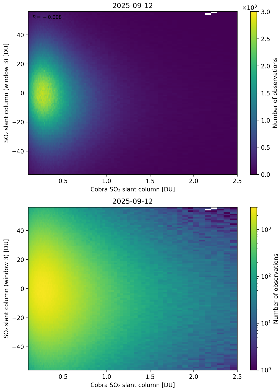
Figure 222: Scatter density plot of “Cobra SO 2 slant column” against “SO 2 slant column (window 3)” for 2025-09-11 to 2025-09-13.
