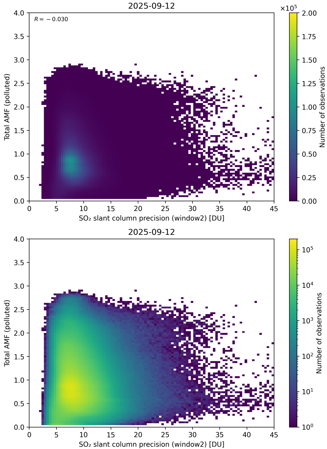
Figure 301: Scatter density plot of “SO 2 slant column precision (window2)” against “Total AMF (polluted)” for 2025-09-11 to 2025-09-13.
