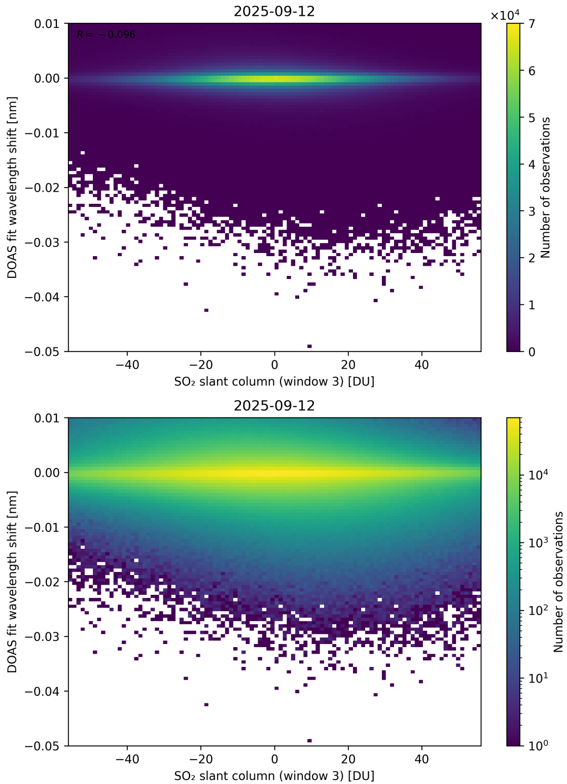
Figure 304: Scatter density plot of “SO 2 slant column (window 3)” against “DOAS fit wavelength shift” for 2025-09-11 to 2025-09-13.
