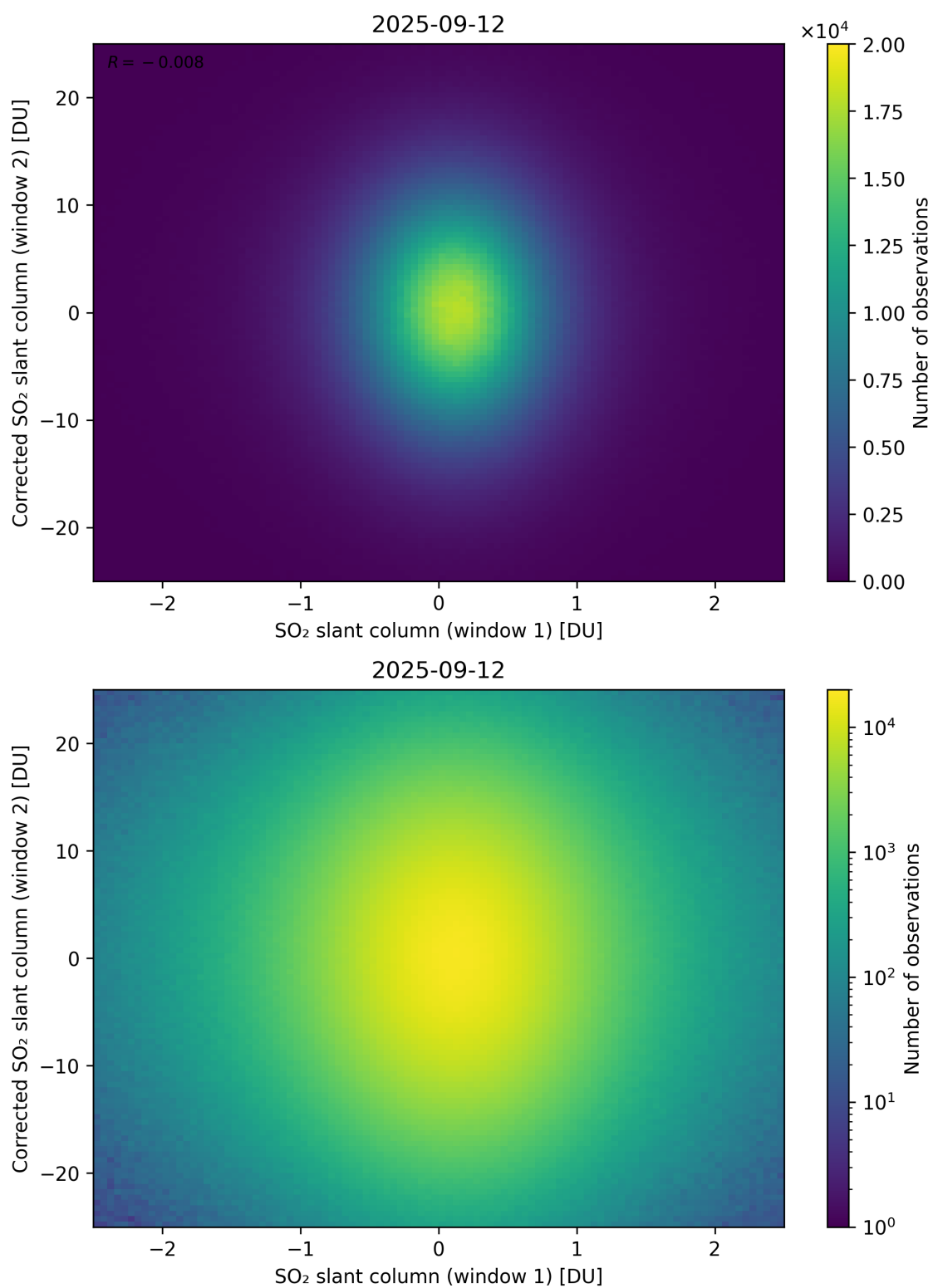
Figure 283: Scatter density plot of “SO 2 slant column (window 1)” against “Corrected SO 2 slant column (window 2)” for 2025-09-11 to 2025-09-13.
