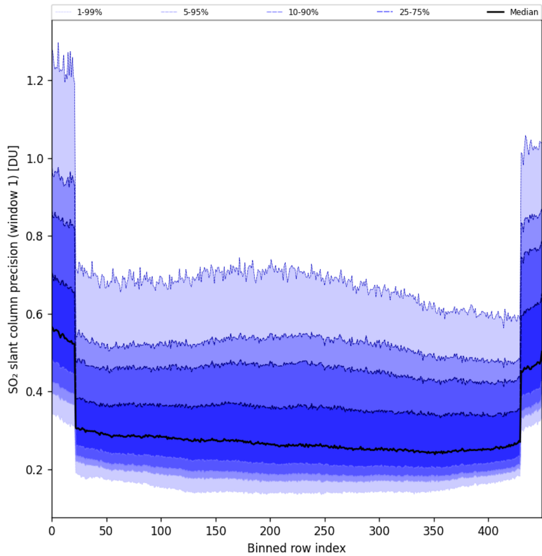
Figure 90: Along track statistics of “SO 2 slant column precision (window 1)” for 2025-09-11 to 2025-09-13
