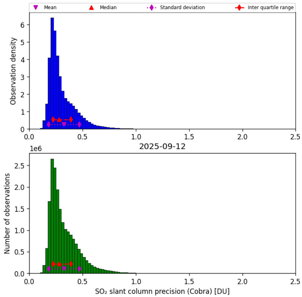
Figure 62: Histogram of “SO 2 slant column precision (Cobra)” for 2025-09-11 to 2025-09-13
