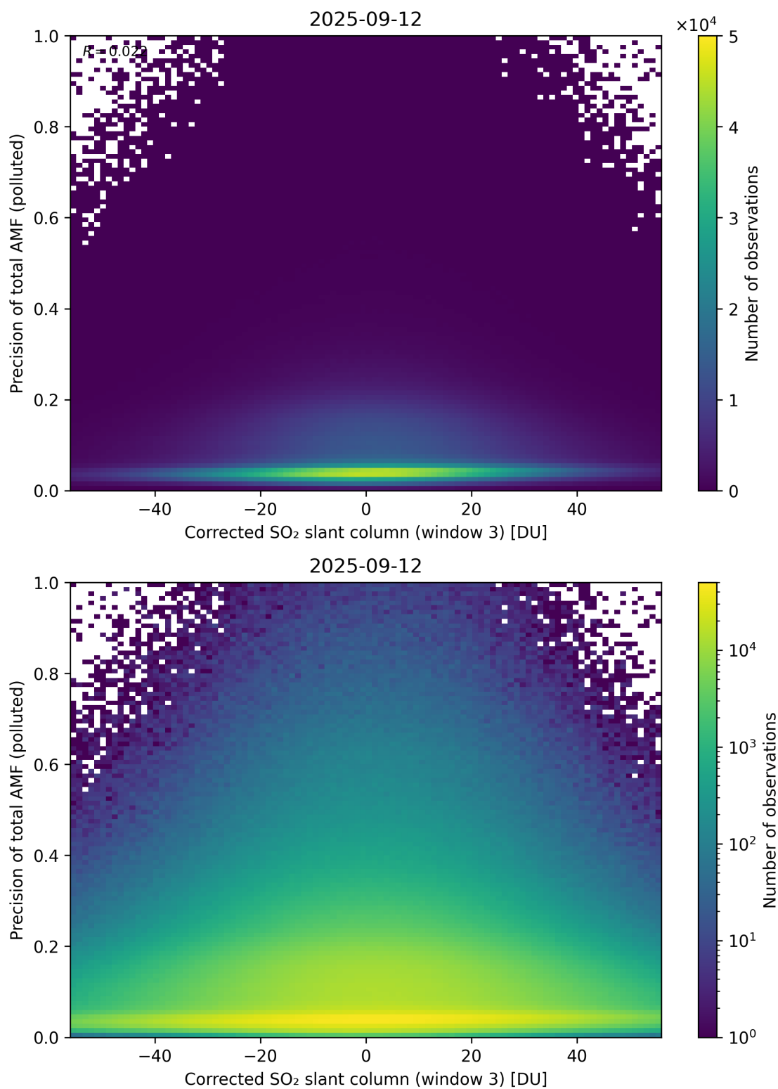
Figure 261: Scatter density plot of “Corrected SO 2 slant column (window 3)” against “Precision of total AMF (polluted)” for 2025-09-11 to 2025-09-13.
