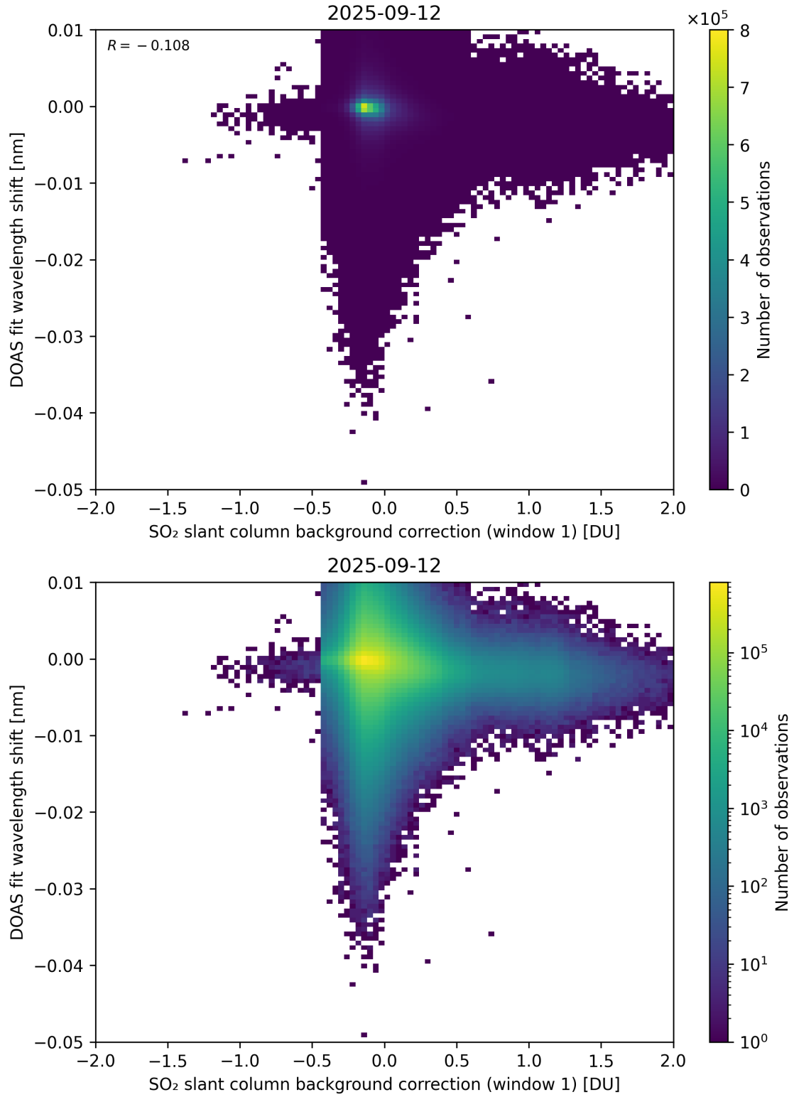
Figure 111: Scatter density plot of “SO 2 slant column background correction (window 1)” against “DOAS fit wavelength shift” for 2025-09-11 to 2025-09-13.
