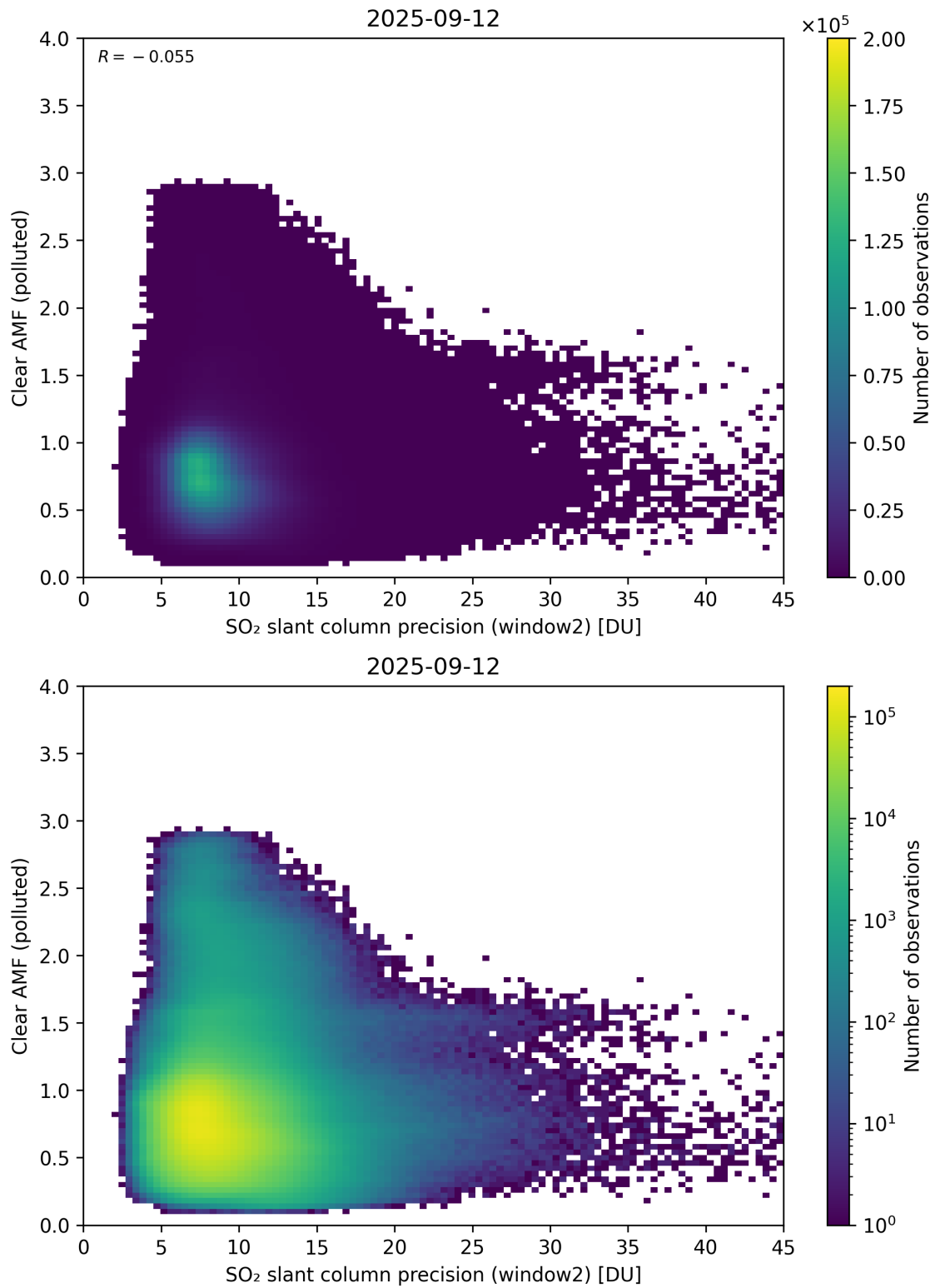
Figure 296: Scatter density plot of “SO 2 slant column precision (window2)” against “Clear AMF (polluted)” for 2025-09-11 to 2025-09-13.
