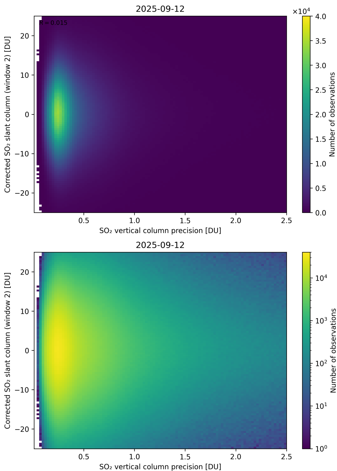
Figure 339: Scatter density plot of “SO 2 vertical column precision” against “Corrected SO 2 slant column (window 2)” for 2025-09-11 to 2025-09-13.
