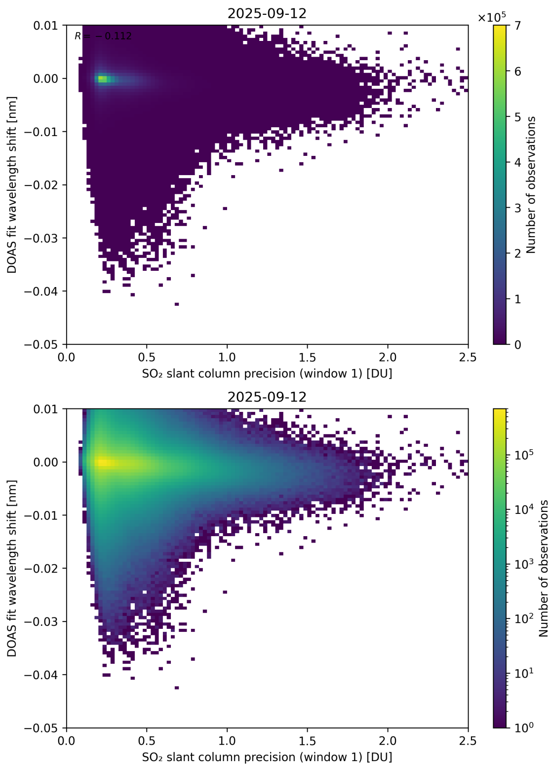
Figure 271: Scatter density plot of “SO 2 slant column precision (window 1)” against “DOAS fit wavelength shift” for 2025-09-11 to 2025-09-13.
