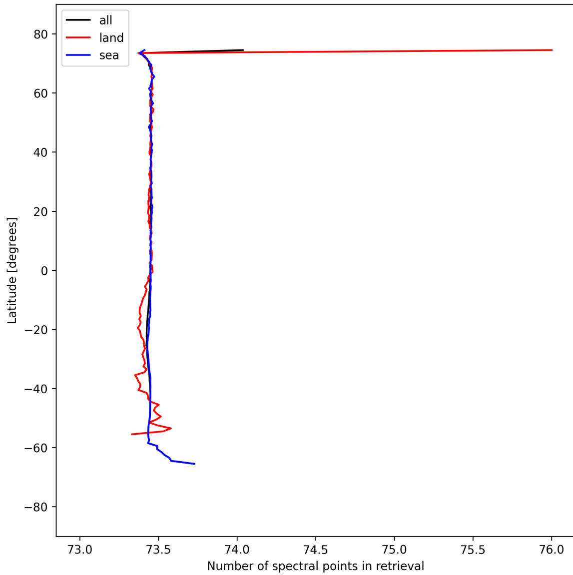
Figure 56: Zonal average of “Number of spectral points in retrieval” for 2025-09-11 to 2025-09-13.
