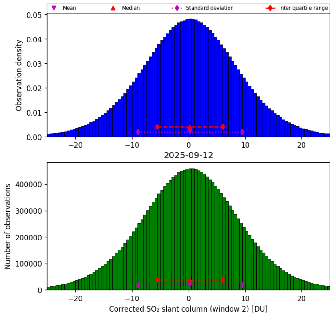
Figure 69: Histogram of “Corrected SO 2 slant column (window 2)” for 2025-09-11 to 2025-09-13
