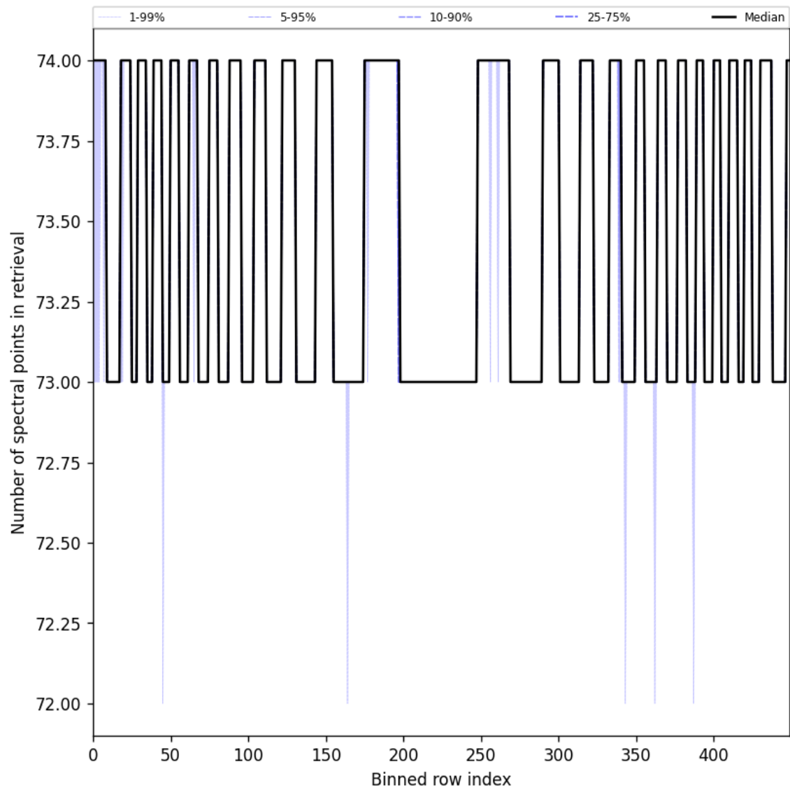
Figure 108: Along track statistics of “Number of spectral points in retrieval” for 2025-09-11 to 2025-09-13
