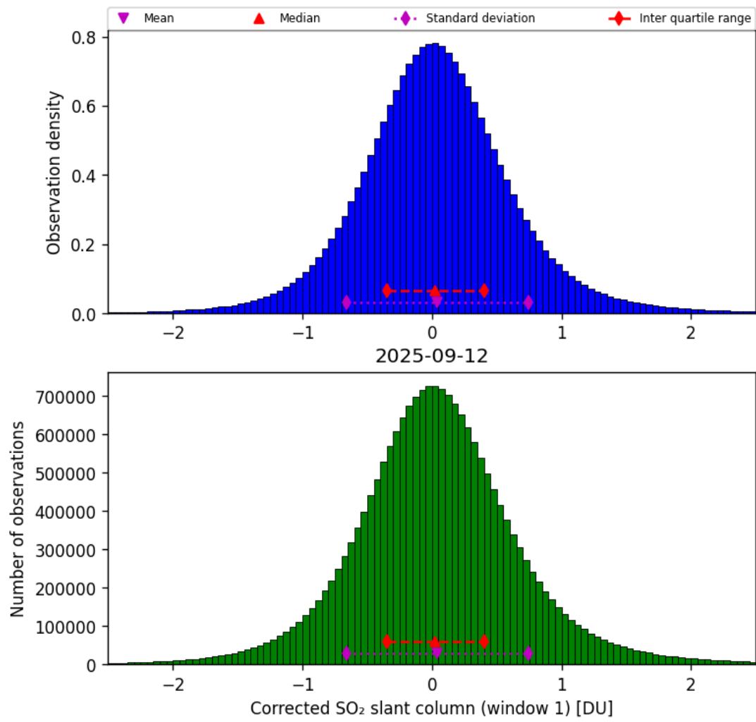
Figure 65: Histogram of “Corrected SO 2 slant column (window 1)” for 2025-09-11 to 2025-09-13
