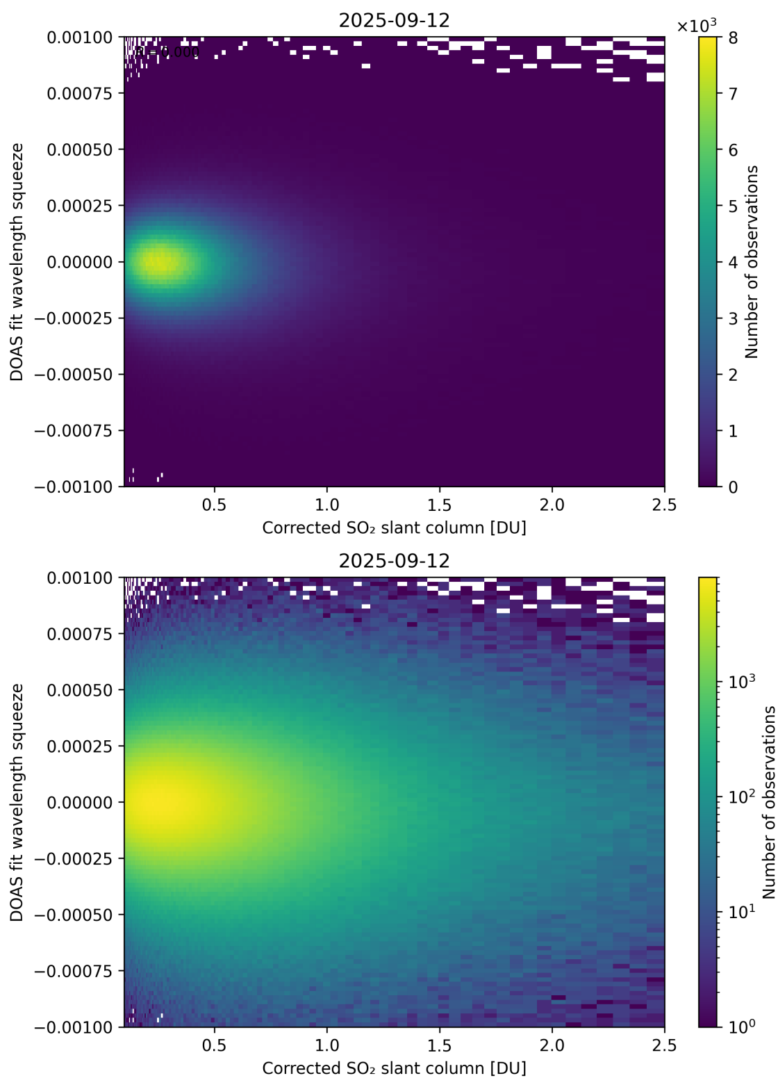
Figure 230: Scatter density plot of "Corrected SO 2 slant column" against "DOAS fit wavelength squeeze" for 2025-09-11 to 2025-09-13.
