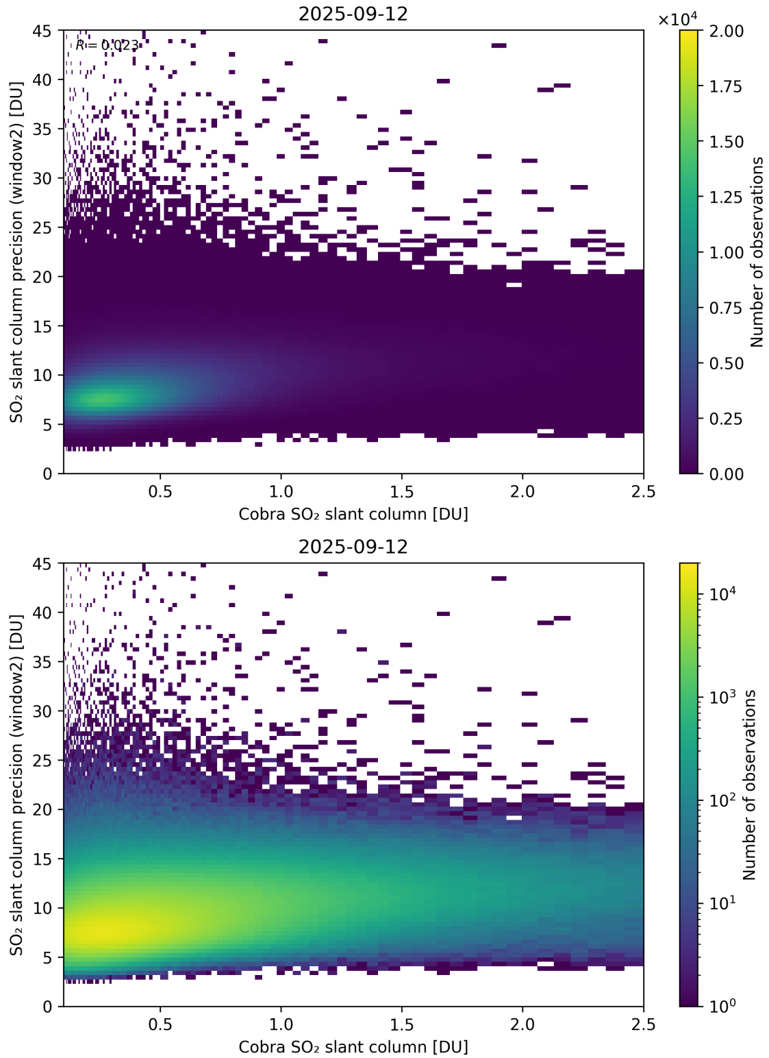
Figure 221: Scatter density plot of “Cobra SO 2 slant column” against “SO 2 slant column precision (window2)” for 2025-09-11 to 2025-09-13.
