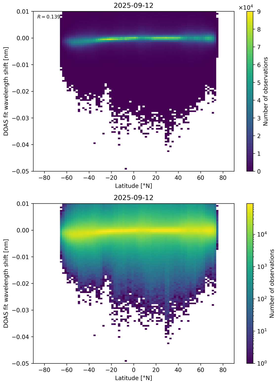
Figure 153: Scatter density plot of “Latitude” against “DOAS fit wavelength shift” for 2025-09-11 to 2025-09-13.
