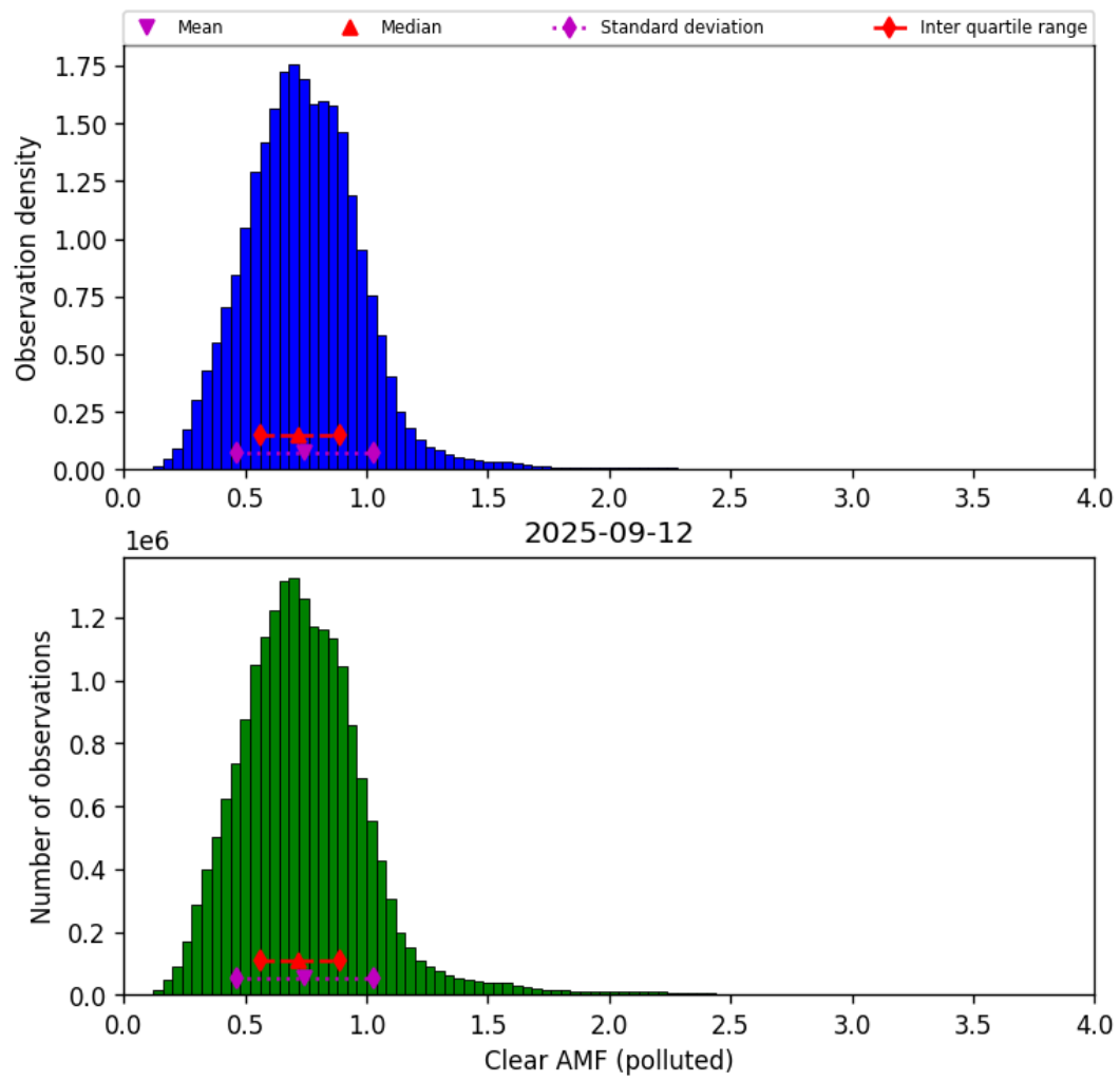
Figure 81: Histogram of “Clear AMF (polluted)” for 2025-09-11 to 2025-09-13
