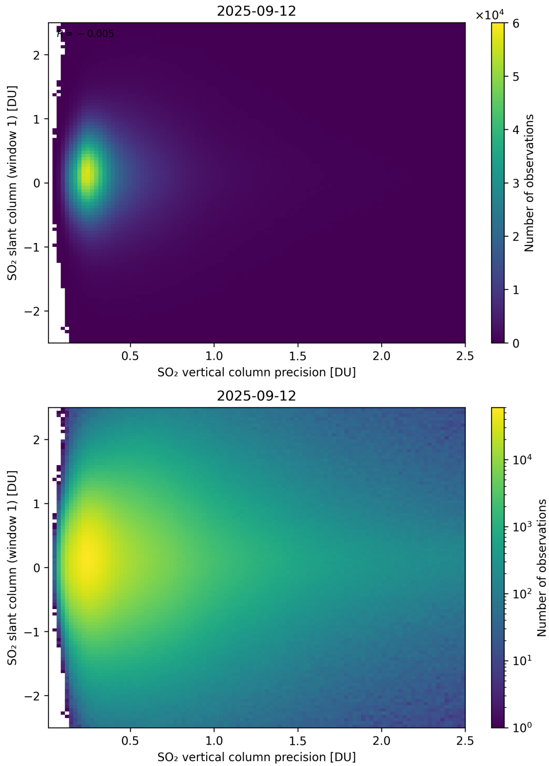
Figure 341: Scatter density plot of “SO 2 vertical column precision” against “SO 2 slant column (window 1)” for 2025-09-11 to 2025-09-13.
