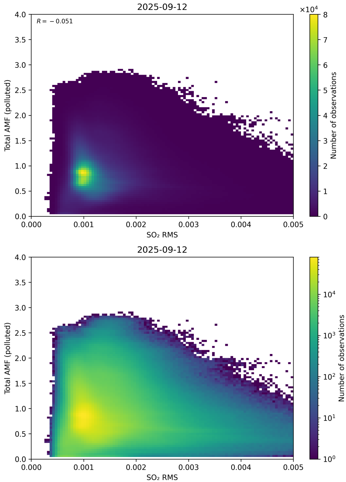
Figure 148: Scatter density plot of “SO 2 RMS” against “Total AMF (polluted)” for 2025-09-11 to 2025-09-13.
