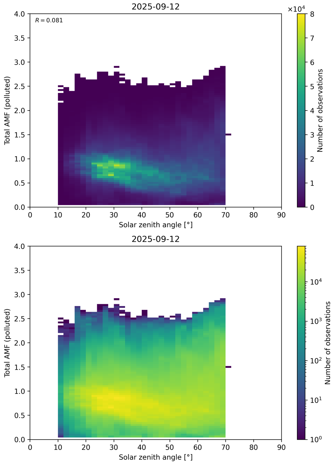
Figure 189: Scatter density plot of “Solar zenith angle” against “Total AMF (polluted)” for 2025-09-11 to 2025-09-13.
