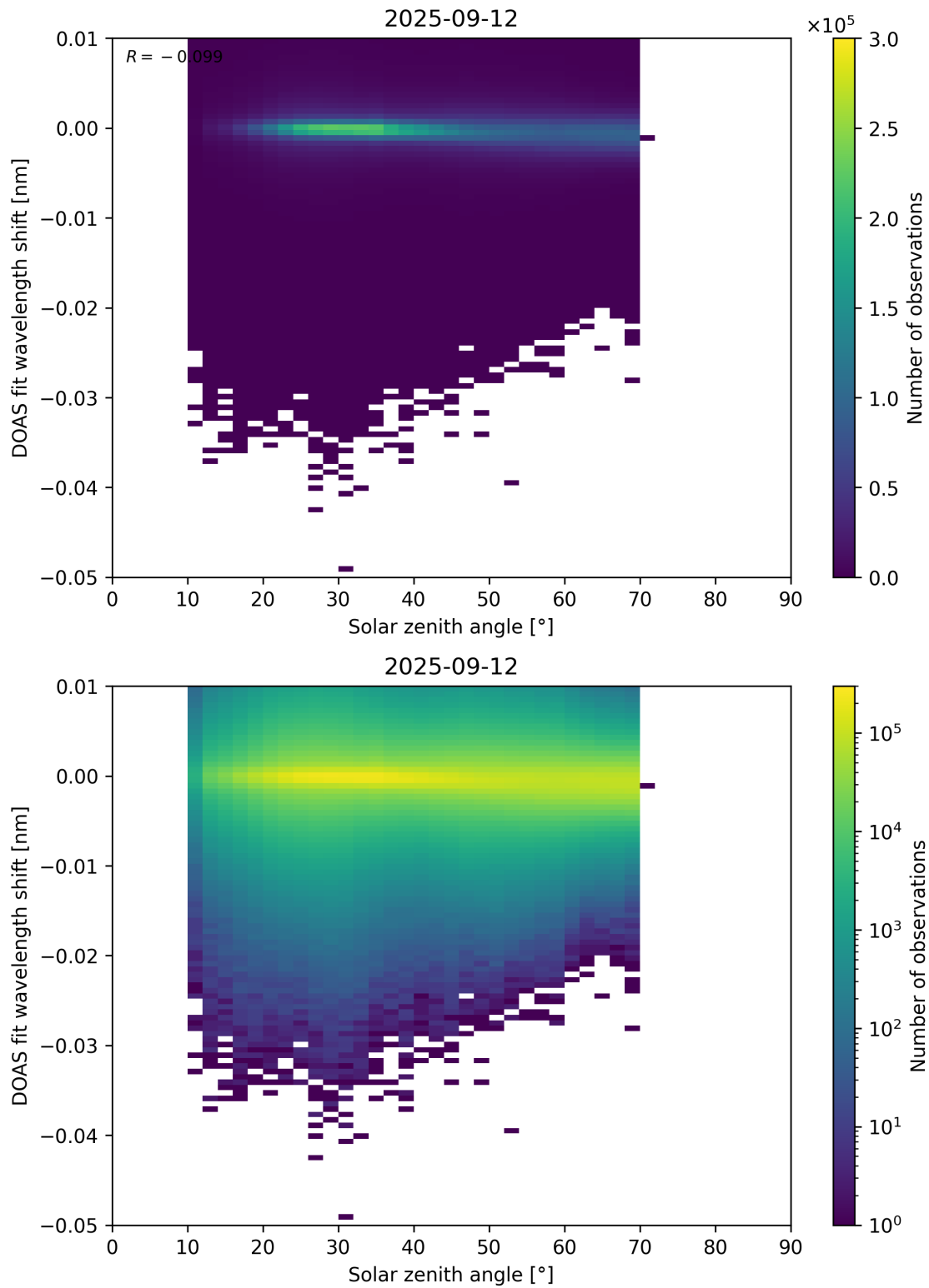
Figure 174: Scatter density plot of “Solar zenith angle” against “DOAS fit wavelength shift” for 2025-09-11 to 2025-09-13.
