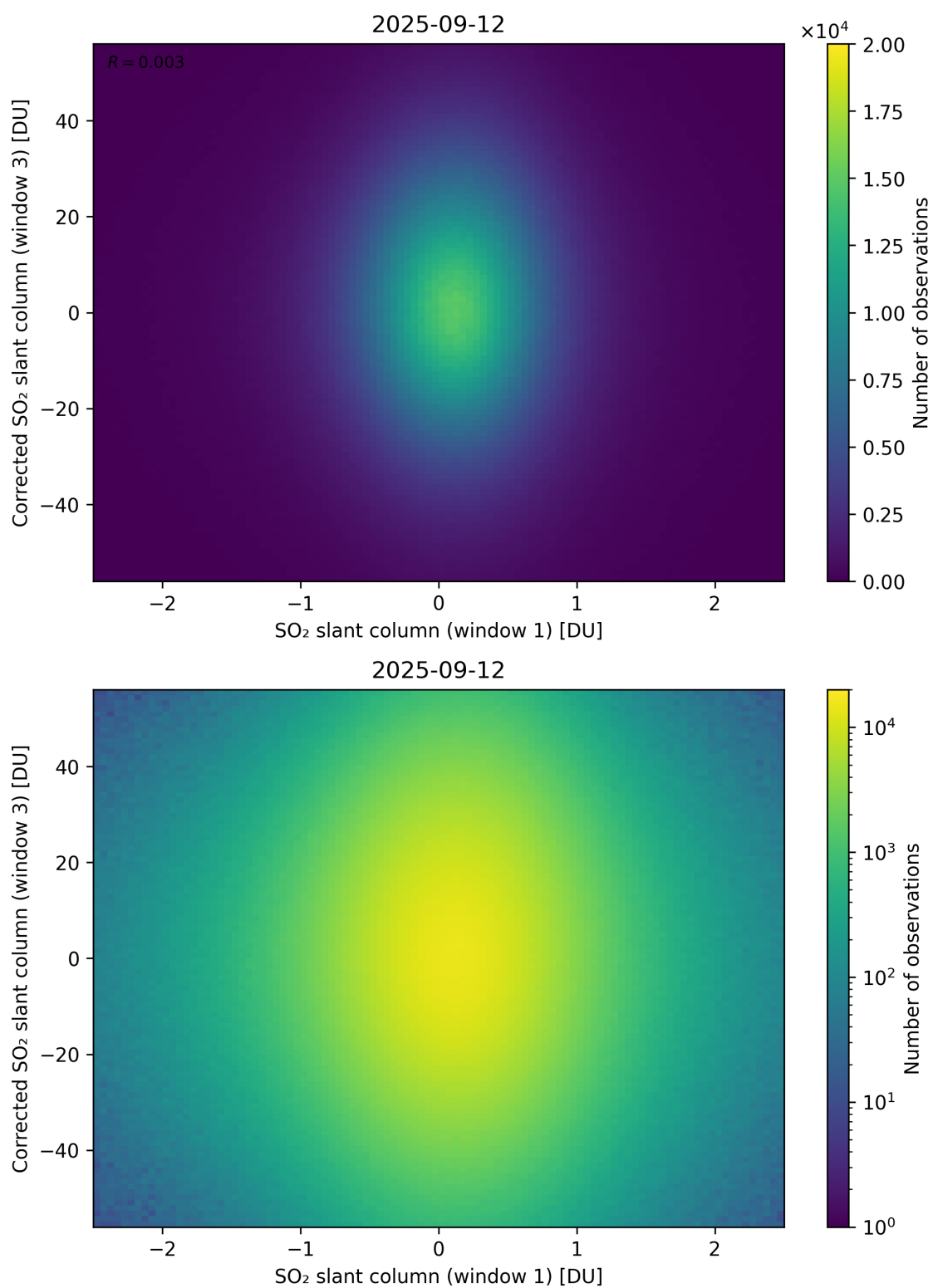
Figure 284: Scatter density plot of “SO 2 slant column (window 1)” against “Corrected SO 2 slant column (window 3)” for 2025-09-11 to 2025-09-13.
