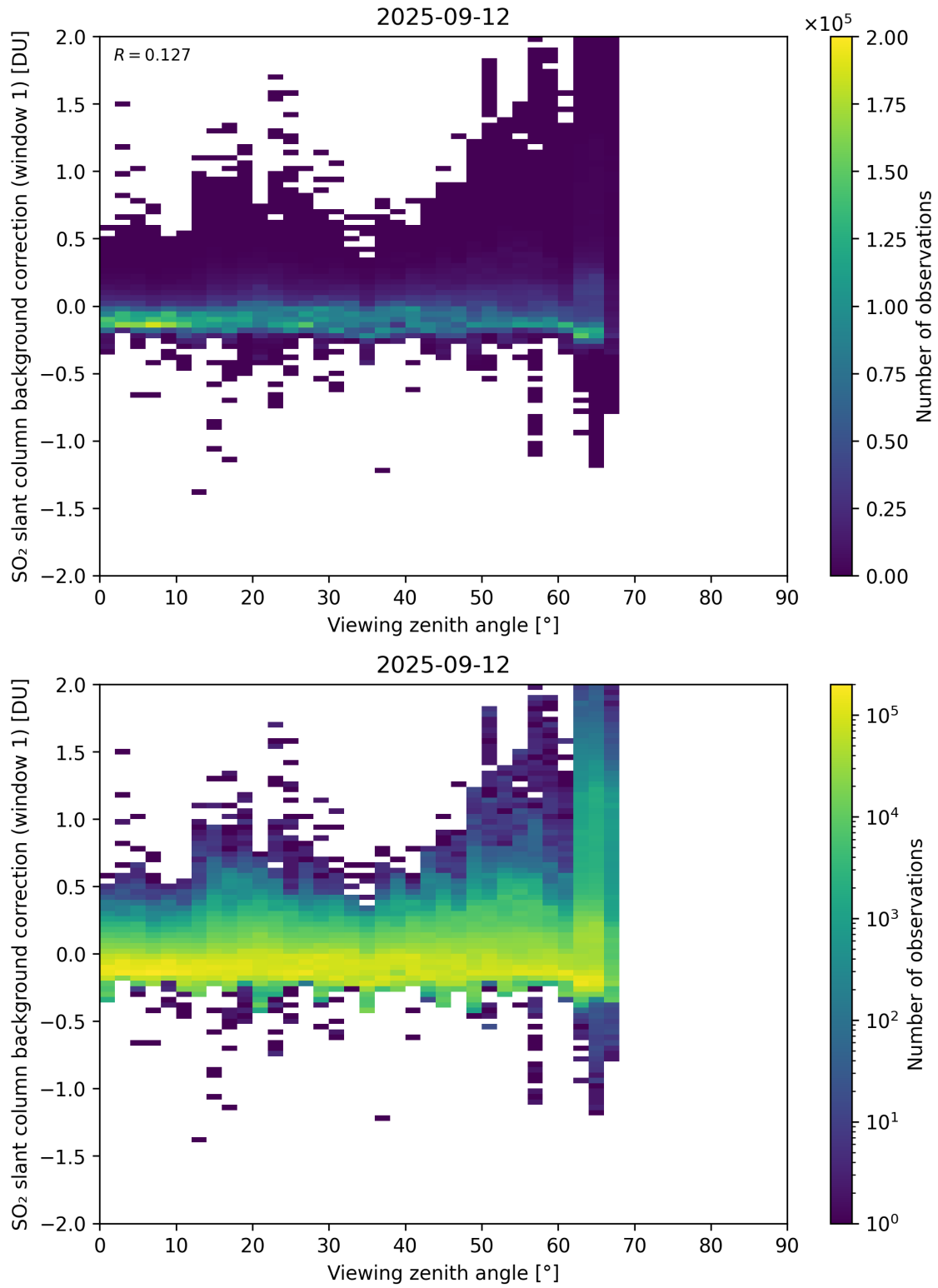
Figure 362: Scatter density plot of “Viewing zenith angle” against “SO 2 slant column background correction (window 1)” for 2025-09-11 to 2025-09-13.
