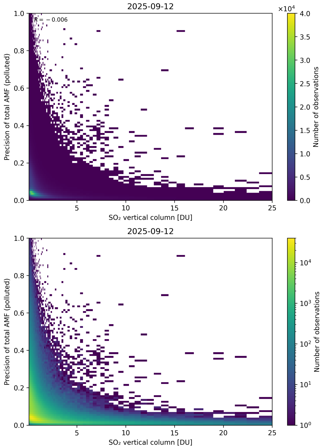
Figure 360: Scatter density plot of “SO 2 vertical column” against “Precision of total AMF (polluted)” for 2025-09-11 to 2025-09-13.
