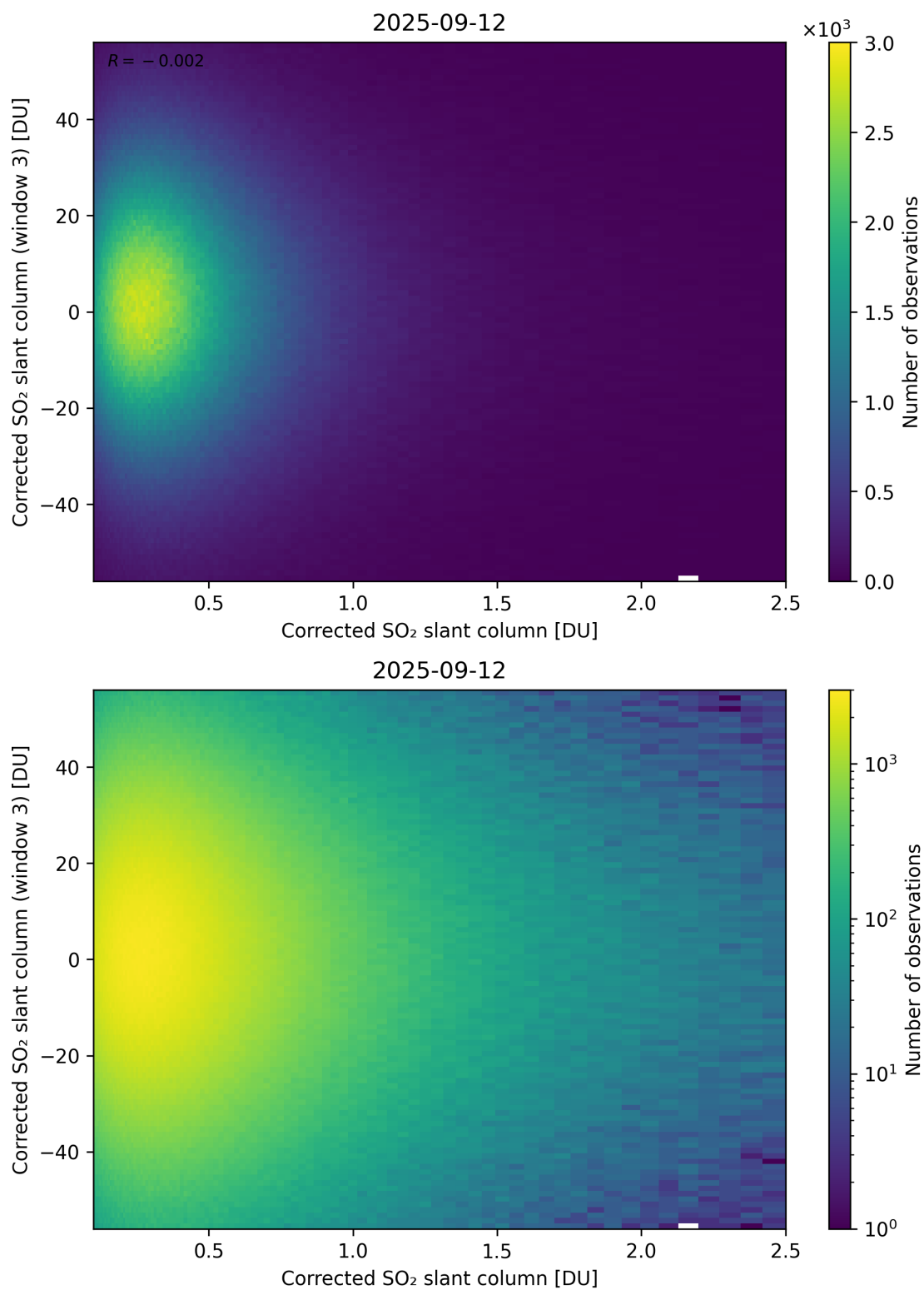
Figure 236: Scatter density plot of “Corrected SO 2 slant column” against “Corrected SO 2 slant column (window 3)” for 2025-09-11 to 2025-09-13.
