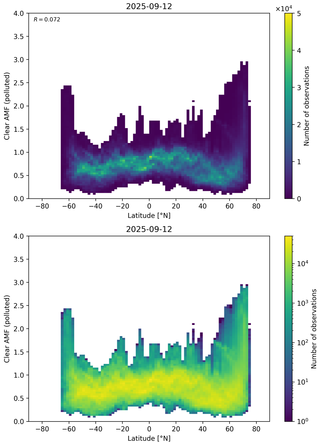
Figure 156: Scatter density plot of “Latitude” against “Clear AMF (polluted)” for 2025-09-11 to 2025-09-13.
