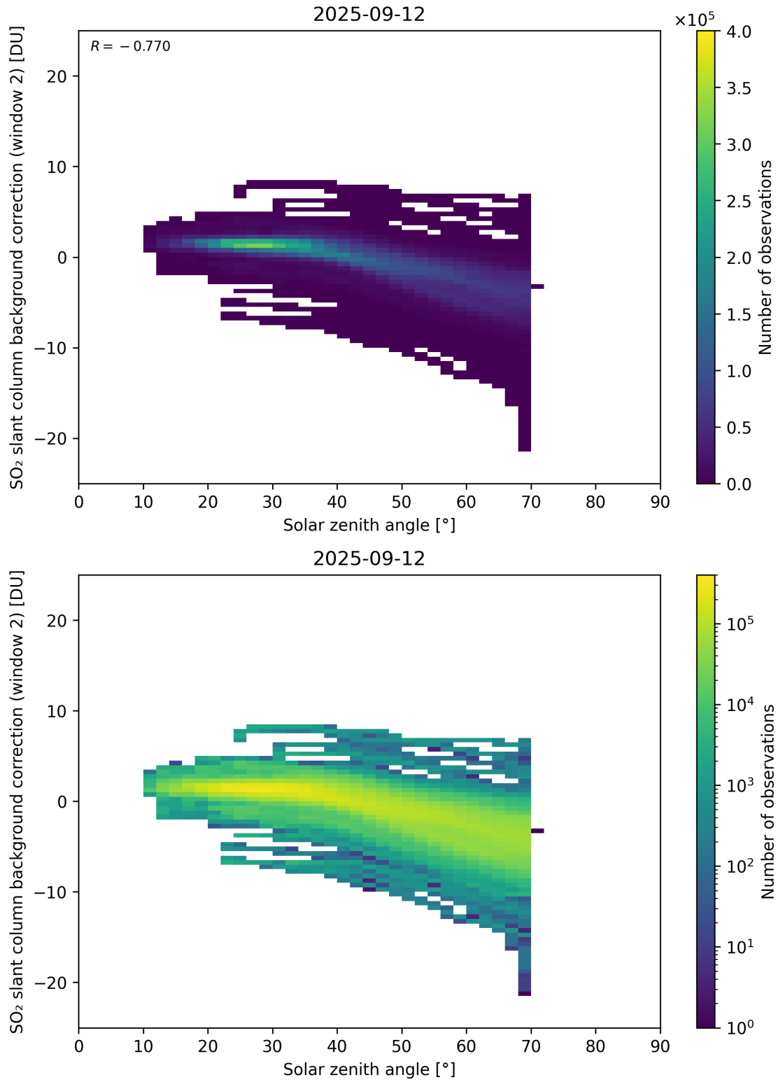
Figure 172: Scatter density plot of “Solar zenith angle” against “SO 2 slant column background correction (window 2)” for 2025-09-11 to 2025-09-13.
