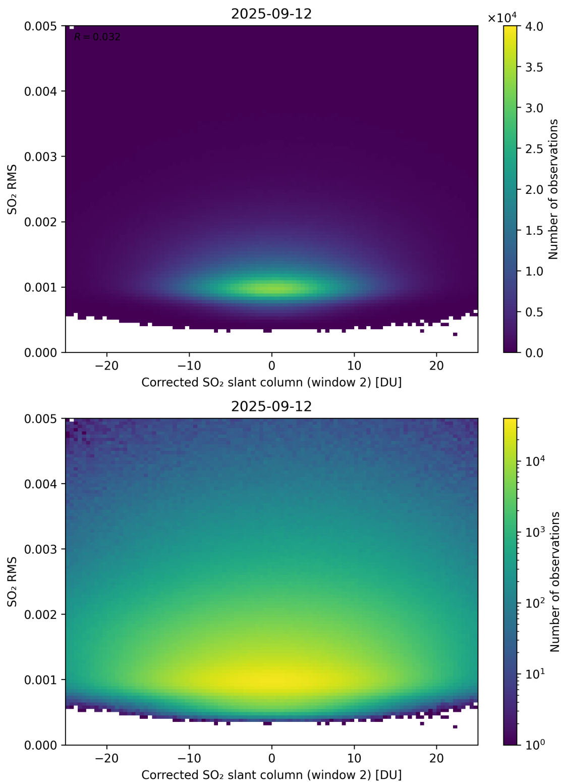
Figure 248: Scatter density plot of “Corrected SO 2 slant column (window 2)” against “SO 2 RMS” for 2025-09-11 to 2025-09-13.
