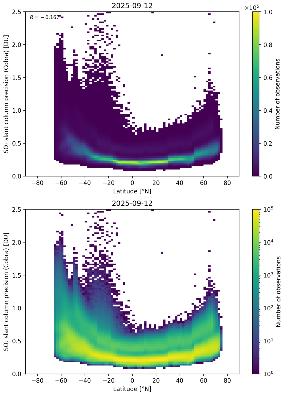
Figure 158: Scatter density plot of “Latitude” against “SO 2 slant column precision (Cobra)” for 2025-09-11 to 2025-09-13.
