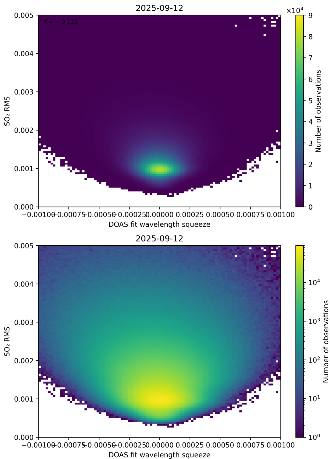
Figure 143: Scatter density plot of “DOAS fit wavelength squeeze” against “SO 2 RMS” for 2025-09-11 to 2025-09-13.
