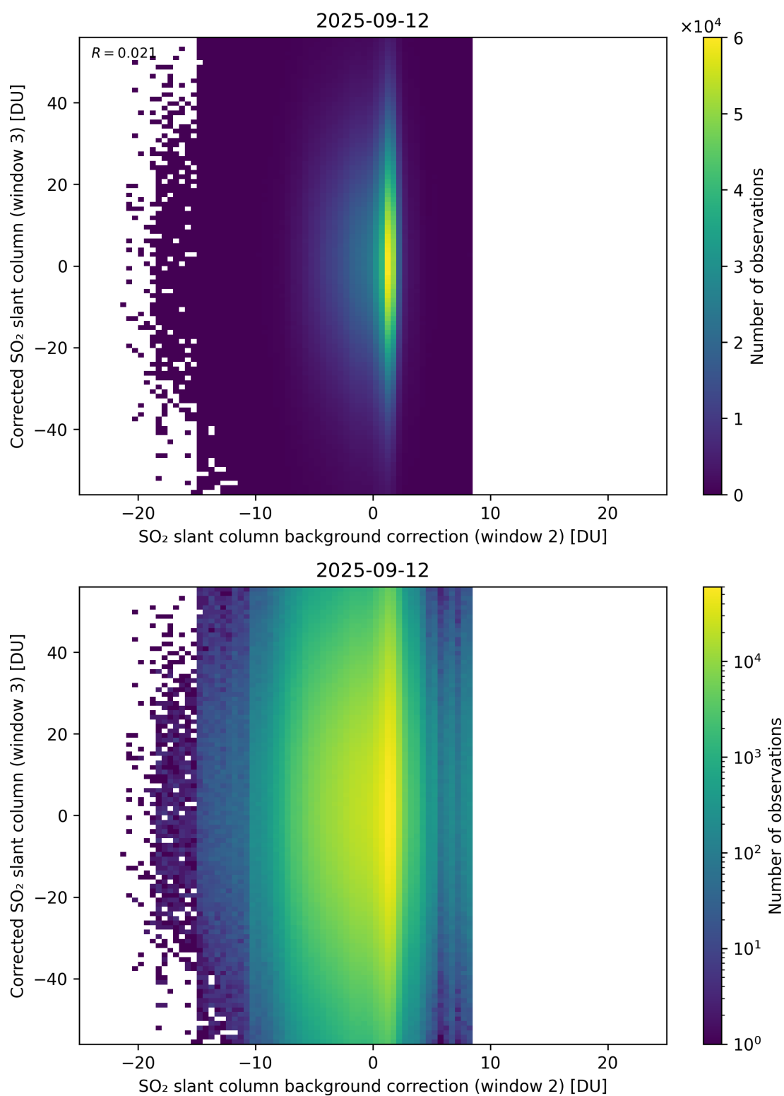
Figure 127: Scatter density plot of “SO 2 slant column background correction (window 2)” against “Corrected SO 2 slant column (window 3)” for 2025-09-11 to 2025-09-13.
