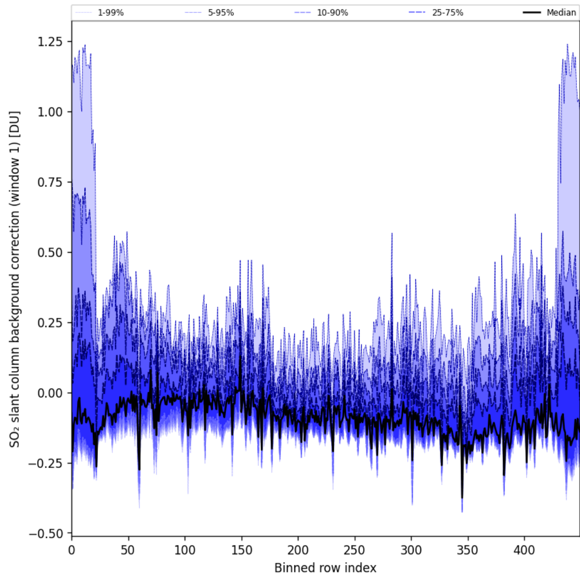
Figure 92: Along track statistics of “SO 2 slant column background correction (window 1)” for 2025-09-11 to 2025-09-13
