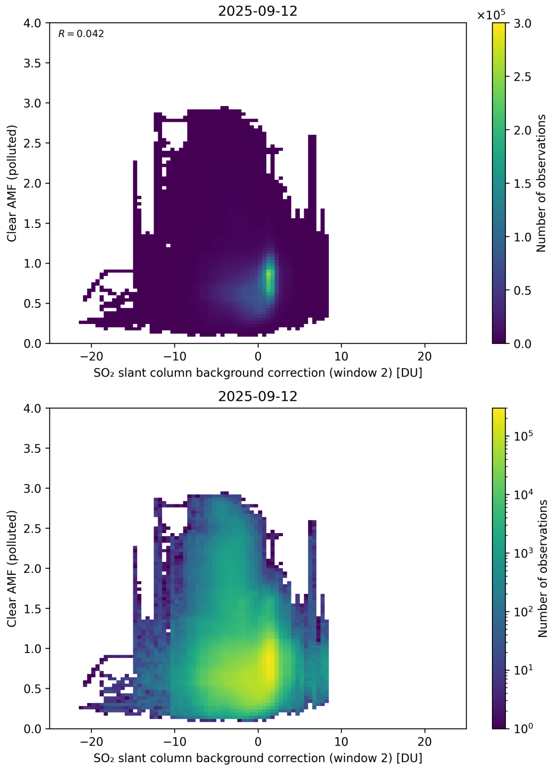
Figure 126: Scatter density plot of “SO 2 slant column background correction (window 2)” against “Clear AMF (polluted)” for 2025-09-11 to 2025-09-13.
