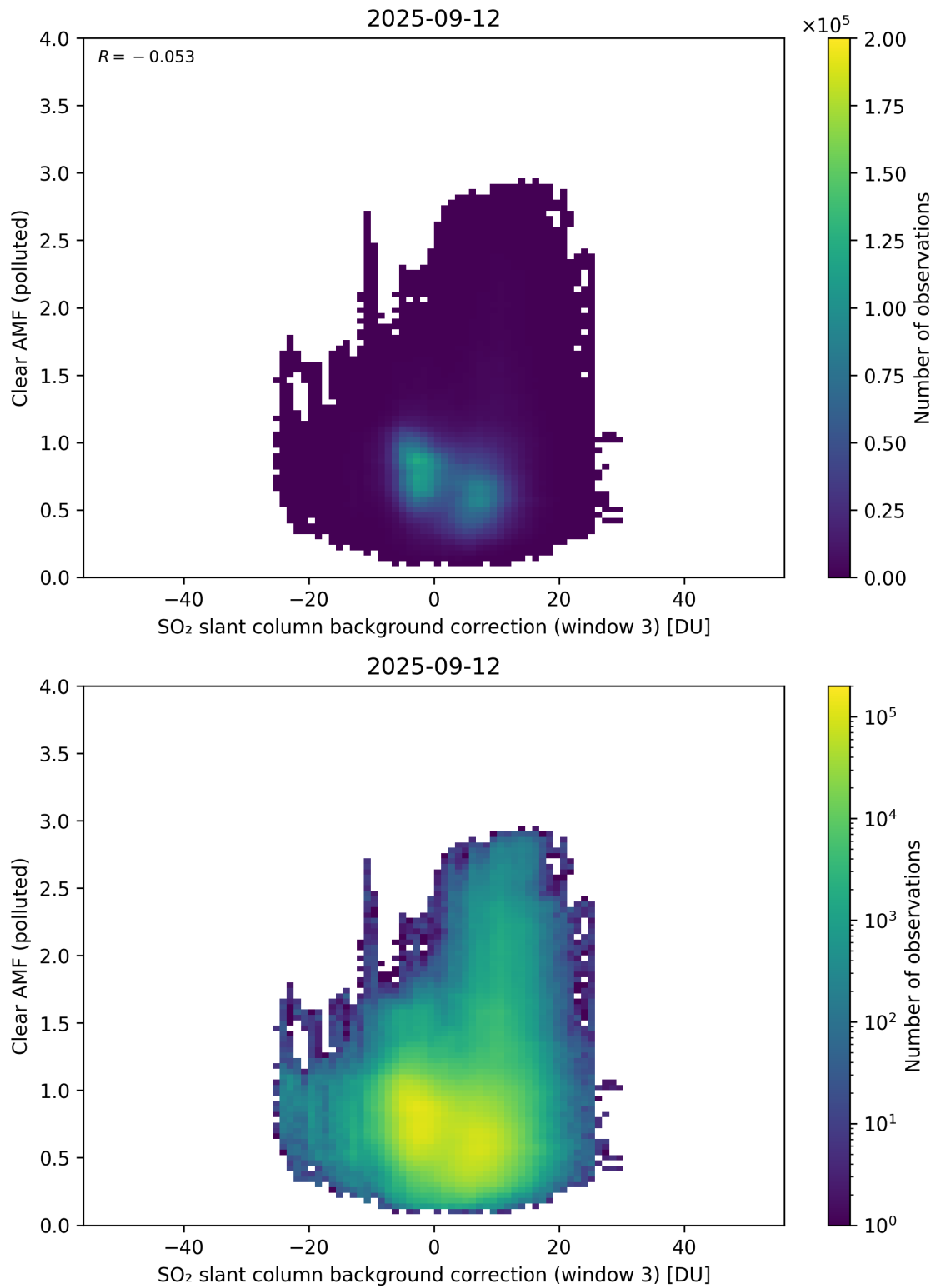
Figure 135: Scatter density plot of “SO 2 slant column background correction (window 3)” against “Clear AMF (polluted)” for 2025-09-11 to 2025-09-13.
