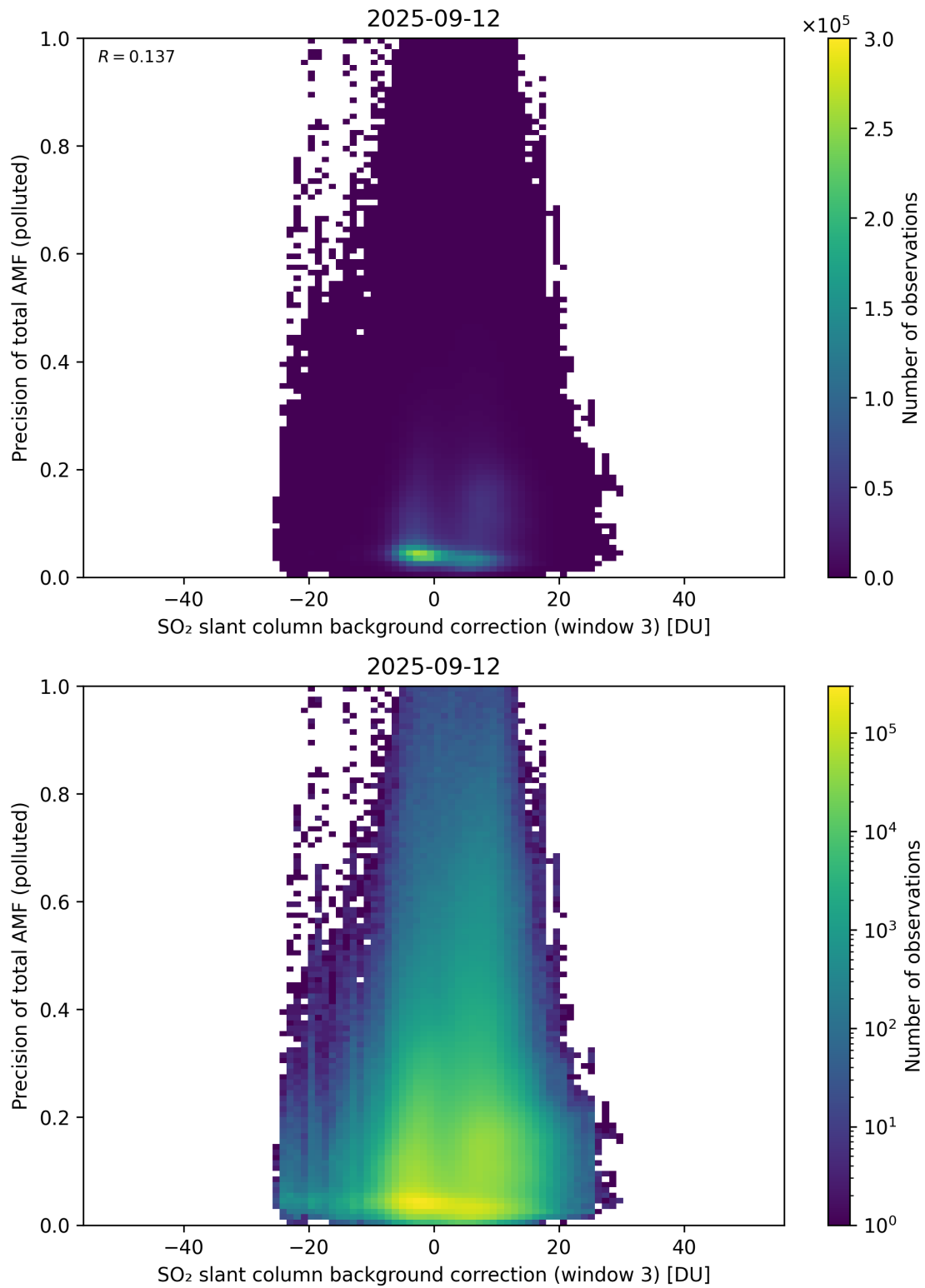
Figure 137: Scatter density plot of “SO 2 slant column background correction (window 3)” against “Precision of total AMF (polluted)” for 2025-09-11 to 2025-09-13.
