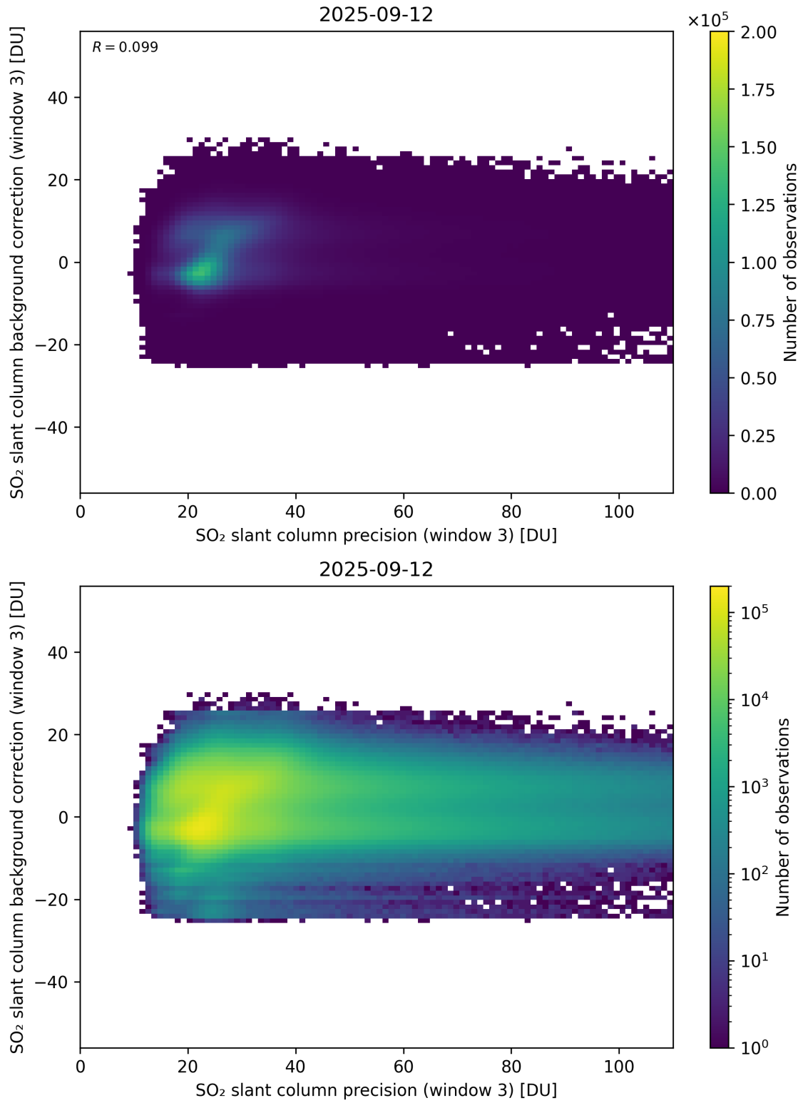
Figure 307: Scatter density plot of “SO 2 slant column precision (window 3)” against “SO 2 slant column background correction (window 3)” for 2025-09-11 to 2025-09-13.
