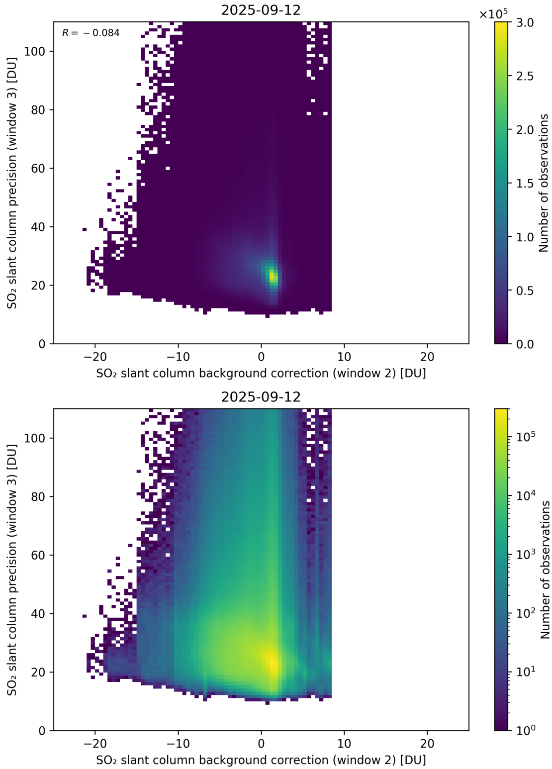
Figure 129: Scatter density plot of “SO 2 slant column background correction (window 2)” against “SO 2 slant column precision (window 3)” for 2025-09-11 to 2025-09-13.
