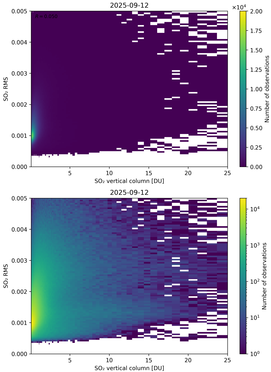
Figure 328: Scatter density plot of “SO 2 vertical column” against “SO 2 RMS” for 2025-09-11 to 2025-09-13.
