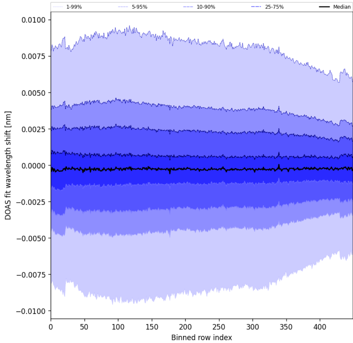
Figure 102: Along track statistics of “DOAS fit wavelength shift” for 2025-09-11 to 2025-09-13
