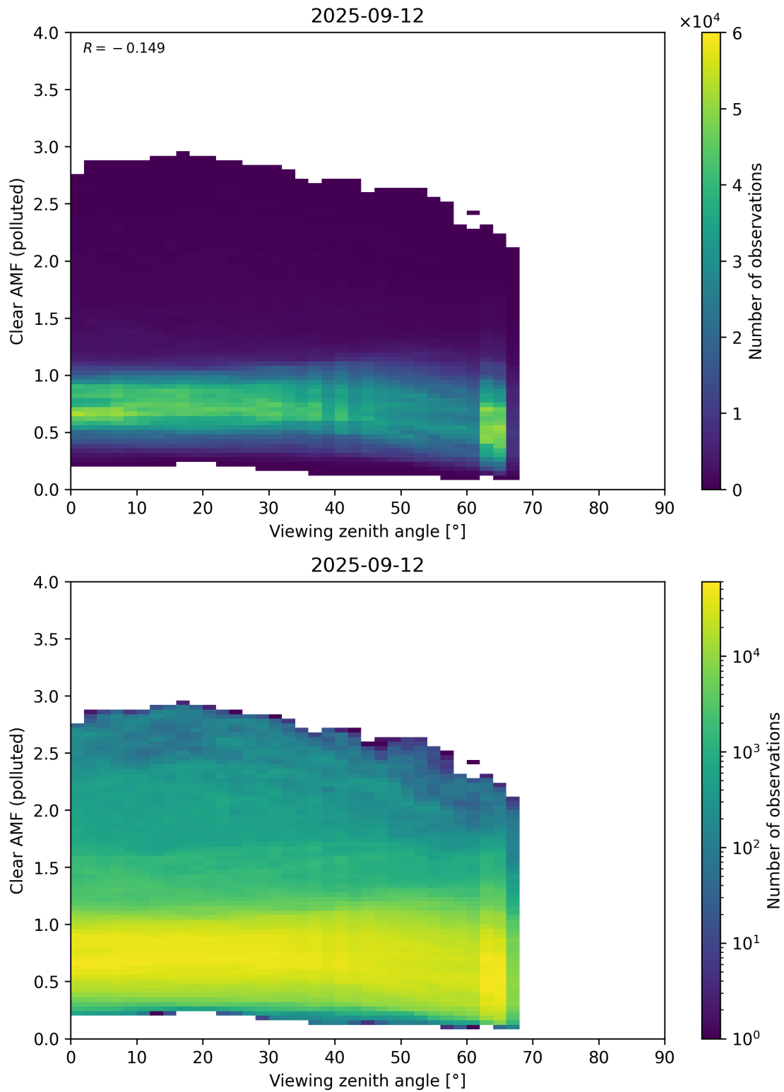
Figure 370: Scatter density plot of “Viewing zenith angle” against “Clear AMF (polluted)” for 2025-09-11 to 2025-09-13.
