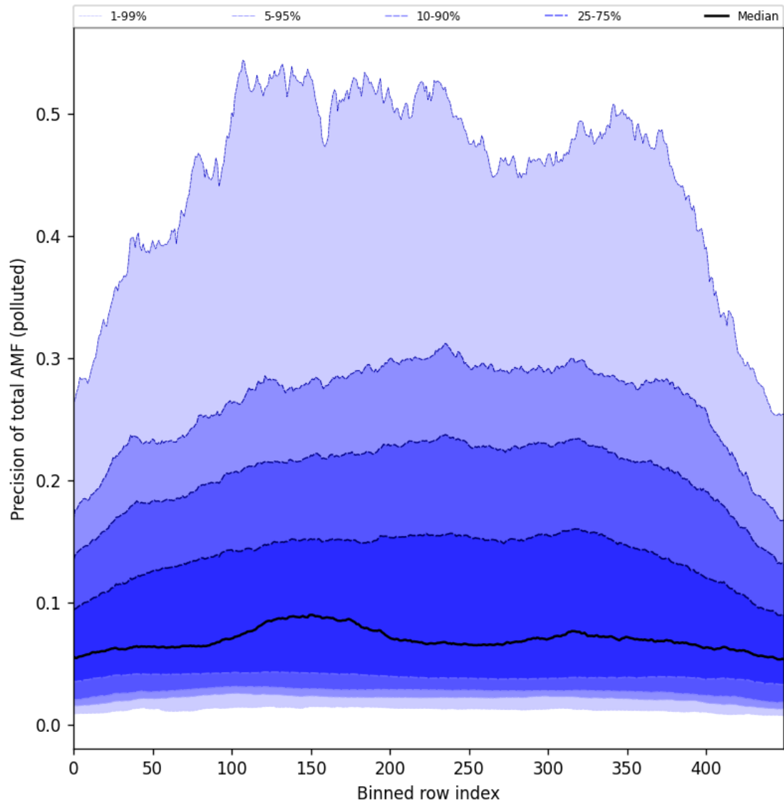
Figure 106: Along track statistics of “Precision of total AMF (polluted)” for 2025-09-11 to 2025-09-13
