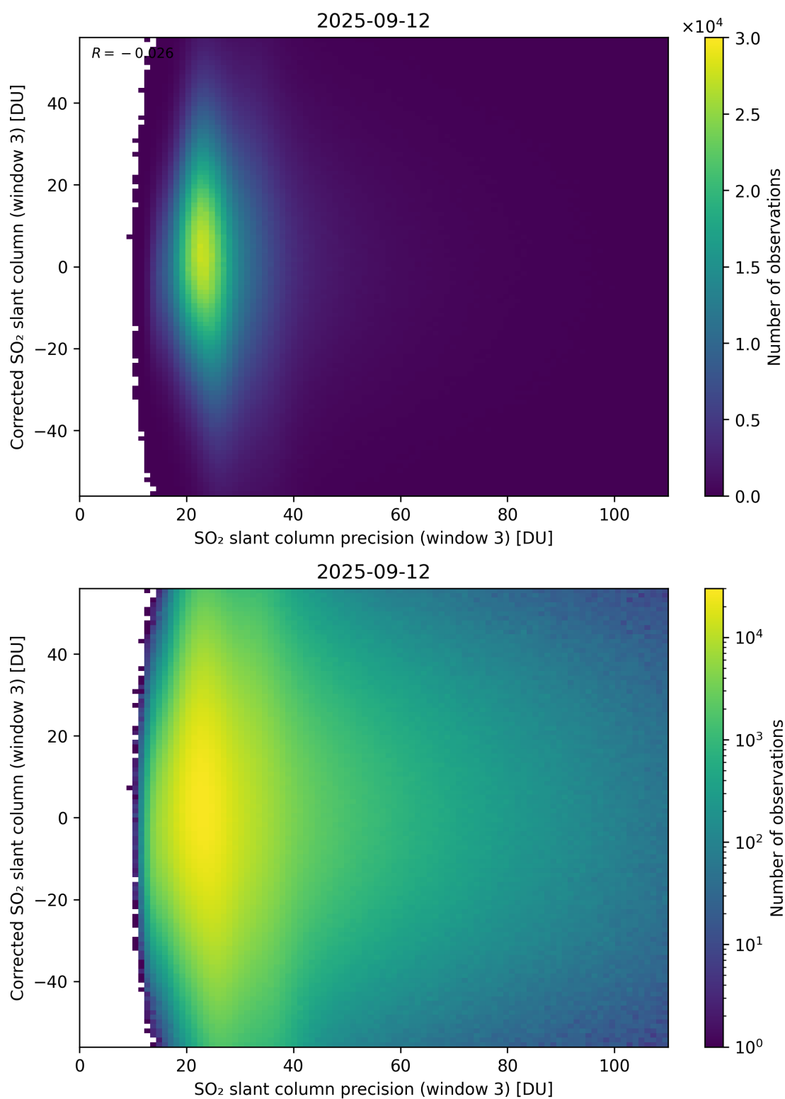
Figure 312: Scatter density plot of “SO 2 slant column precision (window 3)” against “Corrected SO 2 slant column (window 3)” for 2025-09-11 to 2025-09-13.
