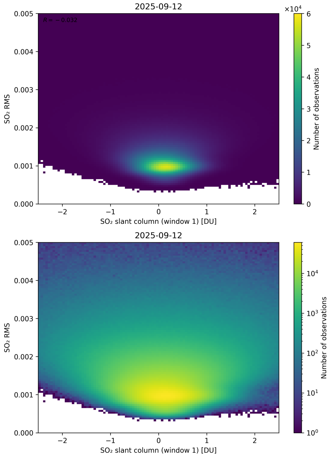
Figure 267: Scatter density plot of “SO 2 slant column (window 1)” against “SO 2 RMS” for 2025-09-11 to 2025-09-13.
