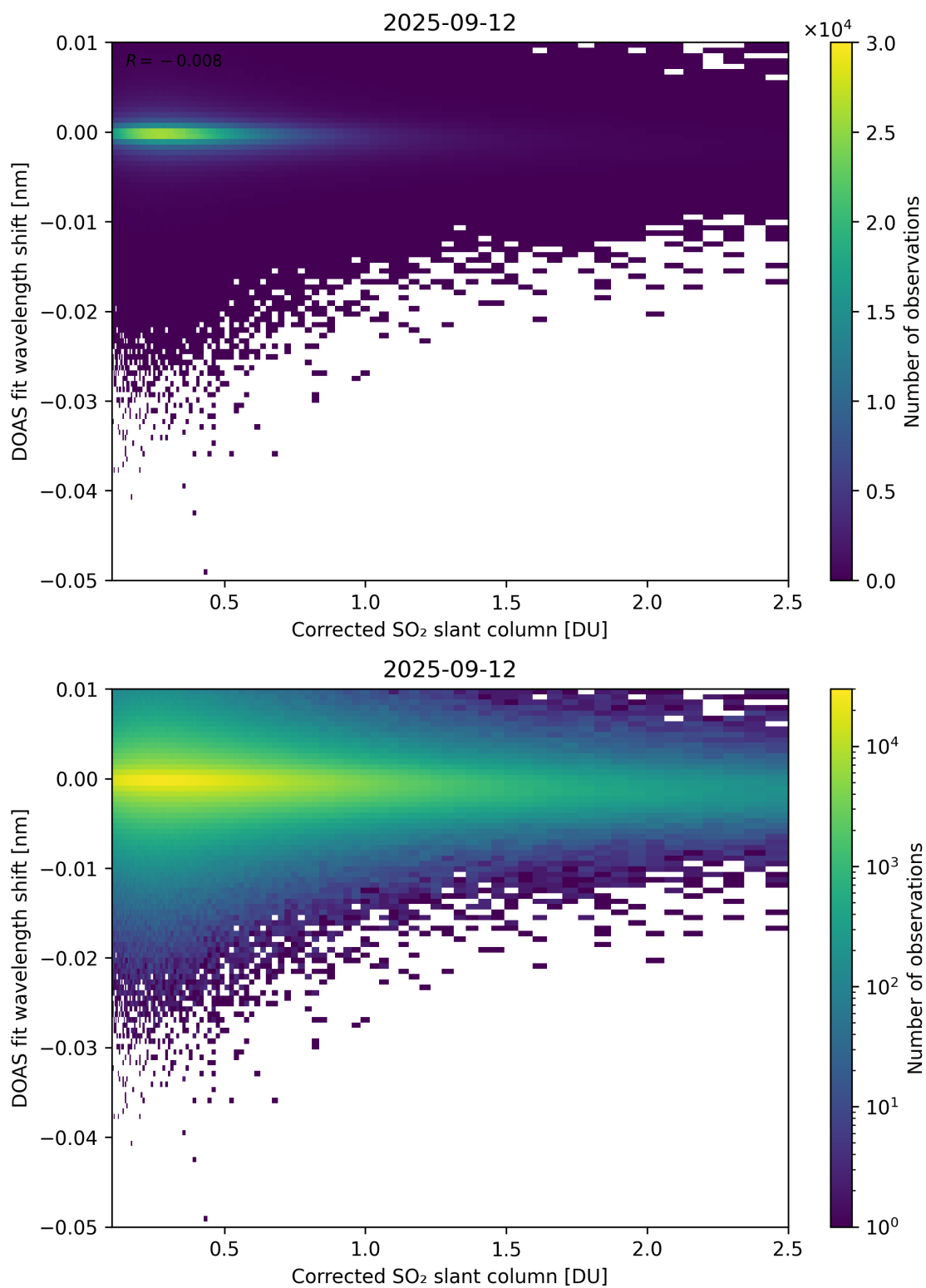
Figure 229: Scatter density plot of “Corrected SO 2 slant column” against “DOAS fit wavelength shift” for 2025-09-11 to 2025-09-13.
