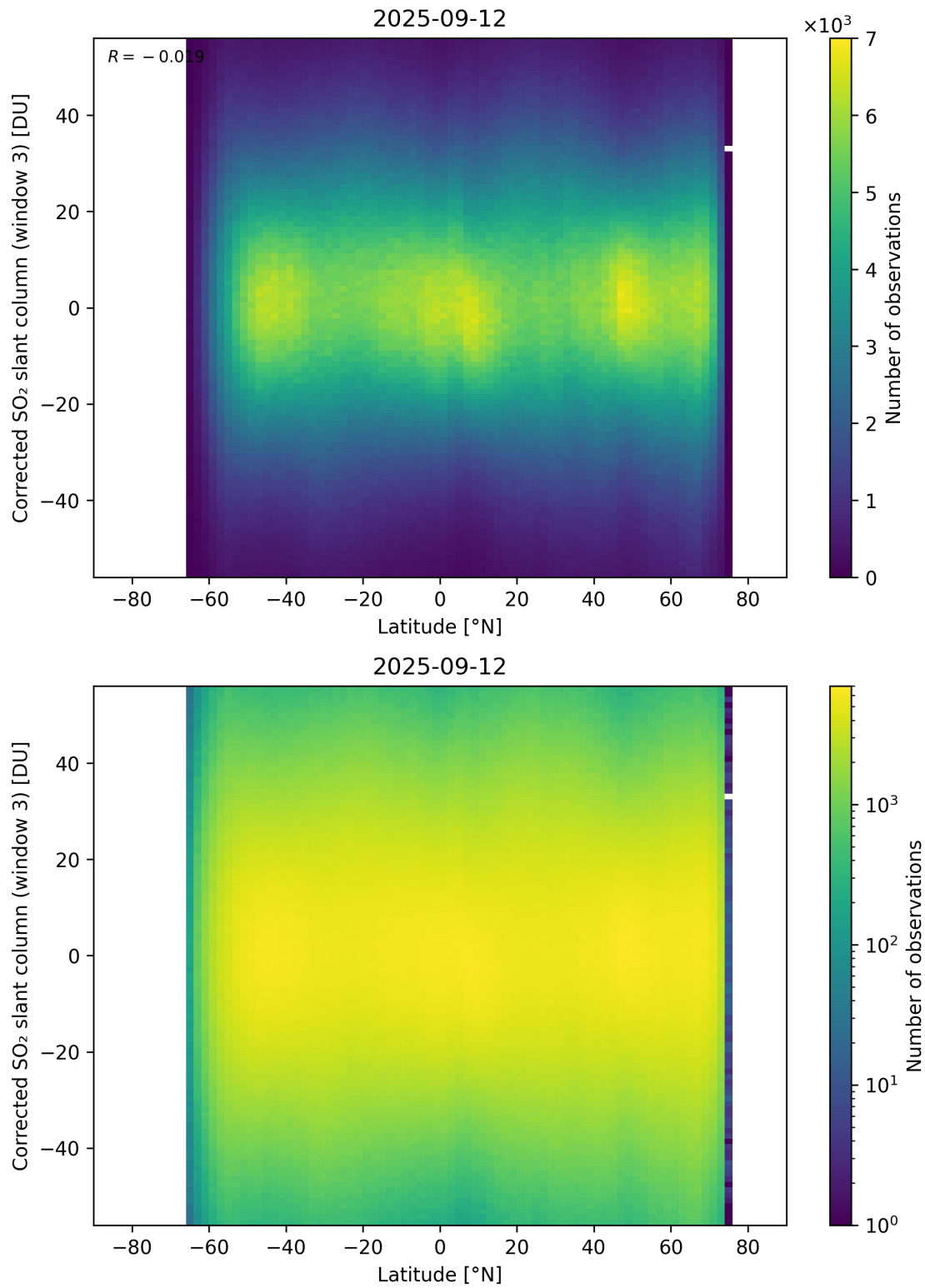
Figure 161: Scatter density plot of “Latitude” against “Corrected SO 2 slant column (window 3)” for 2025-09-11 to 2025-09-13.
