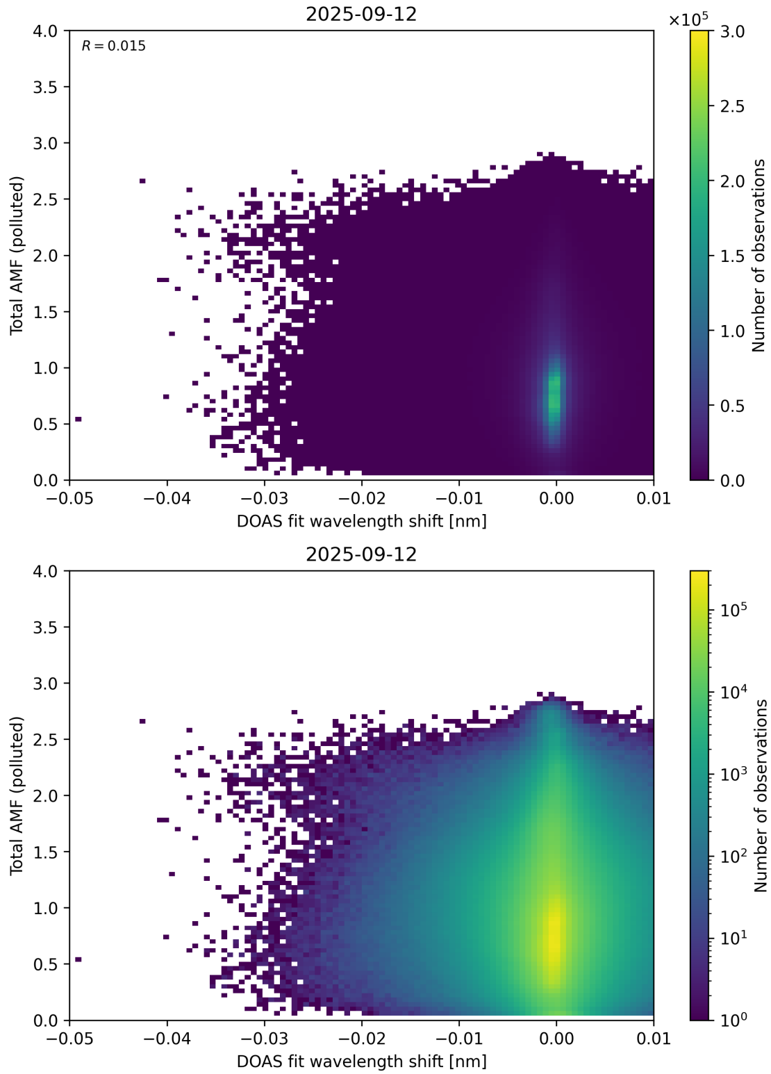
Figure 141: Scatter density plot of “DOAS fit wavelength shift” against “Total AMF (polluted)” for 2025-09-11 to 2025-09-13.
