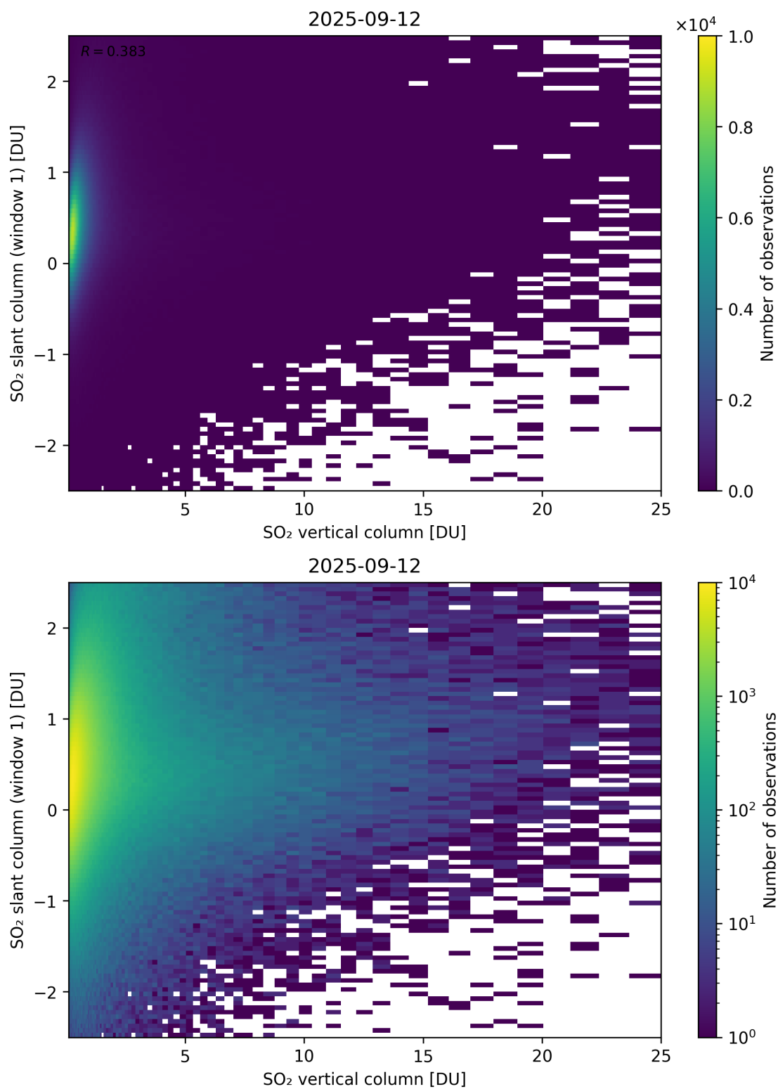
Figure 354: Scatter density plot of “SO 2 vertical column” against “SO 2 slant column (window 1)” for 2025-09-11 to 2025-09-13.
