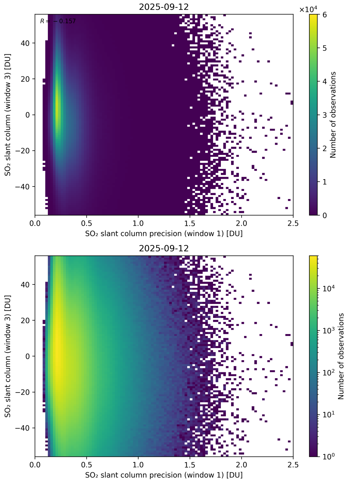
Figure 278: Scatter density plot of “SO 2 slant column precision (window 1)” against “SO 2 slant column (window 3)” for 2025-09-11 to 2025-09-13.
