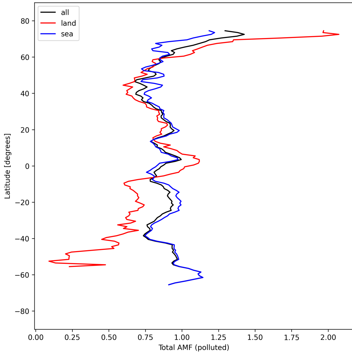
Figure 53: Zonal average of “Total AMF (polluted)” for 2025-09-11 to 2025-09-13.
