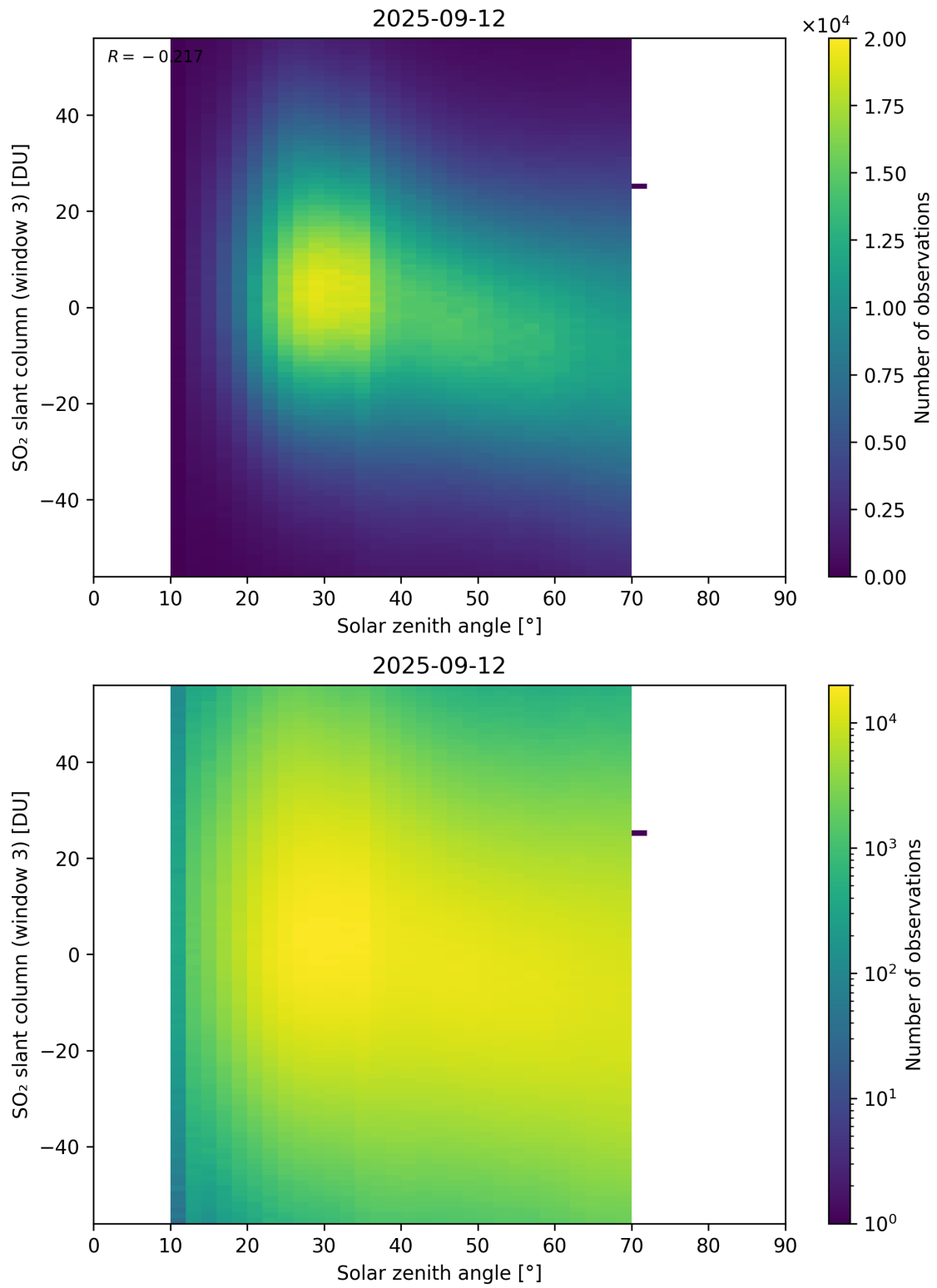
Figure 187: Scatter density plot of “Solar zenith angle” against “SO 2 slant column (window 3)” for 2025-09-11 to 2025-09-13.
