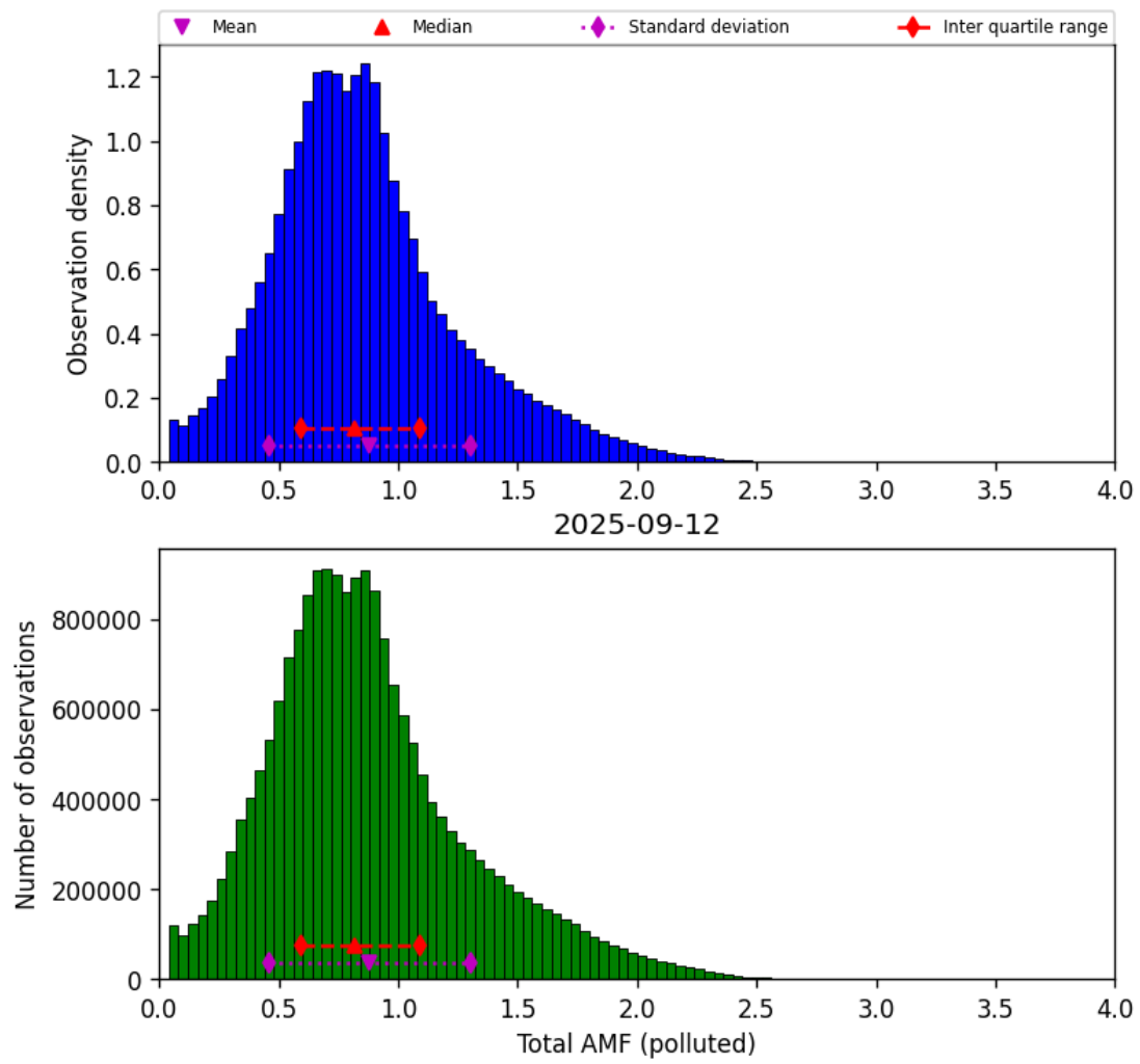
Figure 79: Histogram of “Total AMF (polluted)” for 2025-09-11 to 2025-09-13
