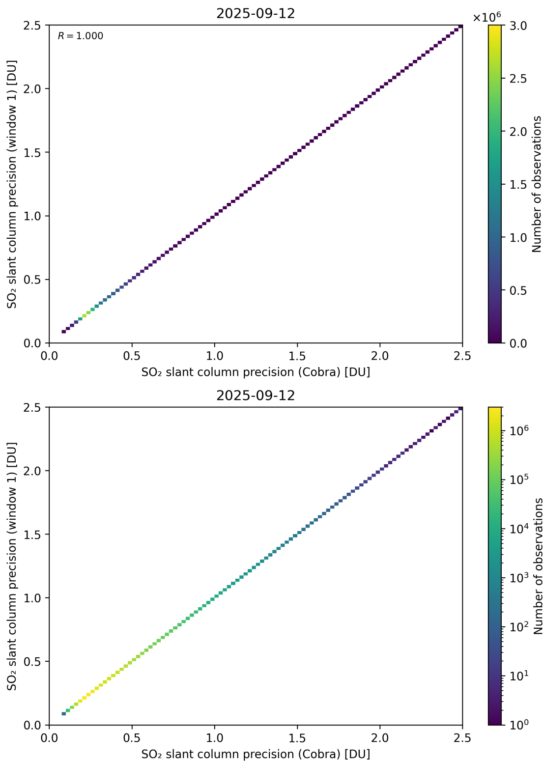
Figure 209: Scatter density plot of “SO 2 slant column precision (Cobra)” against “SO 2 slant column precision (window 1)” for 2025-09-11 to 2025-09-13.
