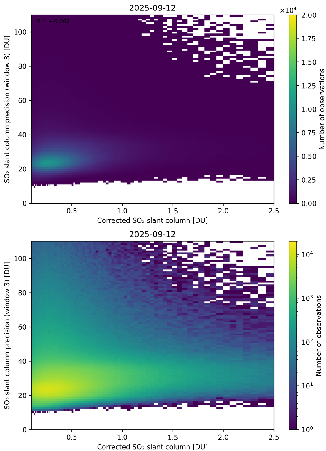
Figure 241: Scatter density plot of “Corrected SO 2 slant column” against “SO 2 slant column precision (window 3)” for 2025-09-11 to 2025-09-13.
