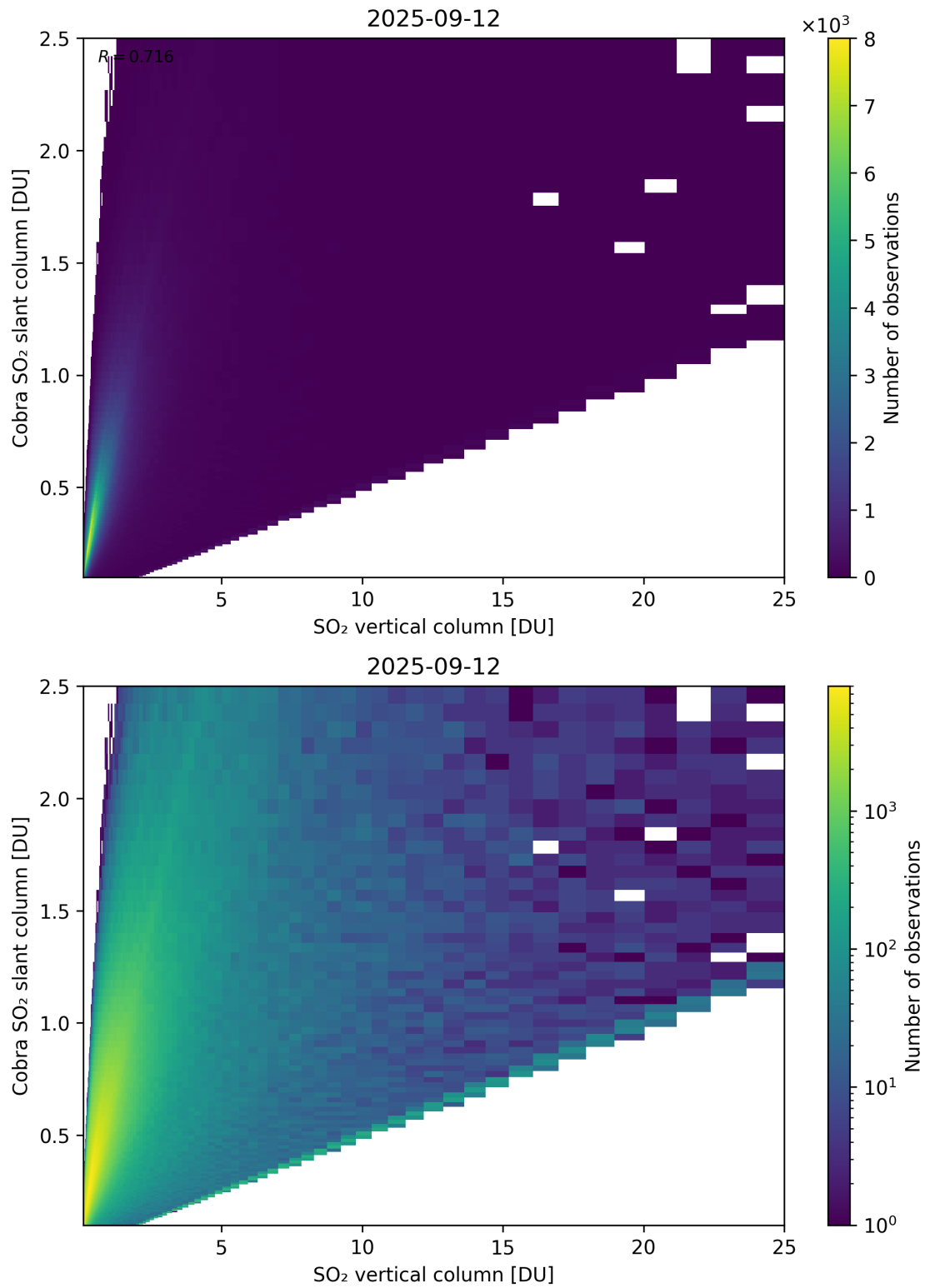
Figure 349: Scatter density plot of “SO 2 vertical column” against “Cobra SO 2 slant column” for 2025-09-11 to 2025-09-13.
