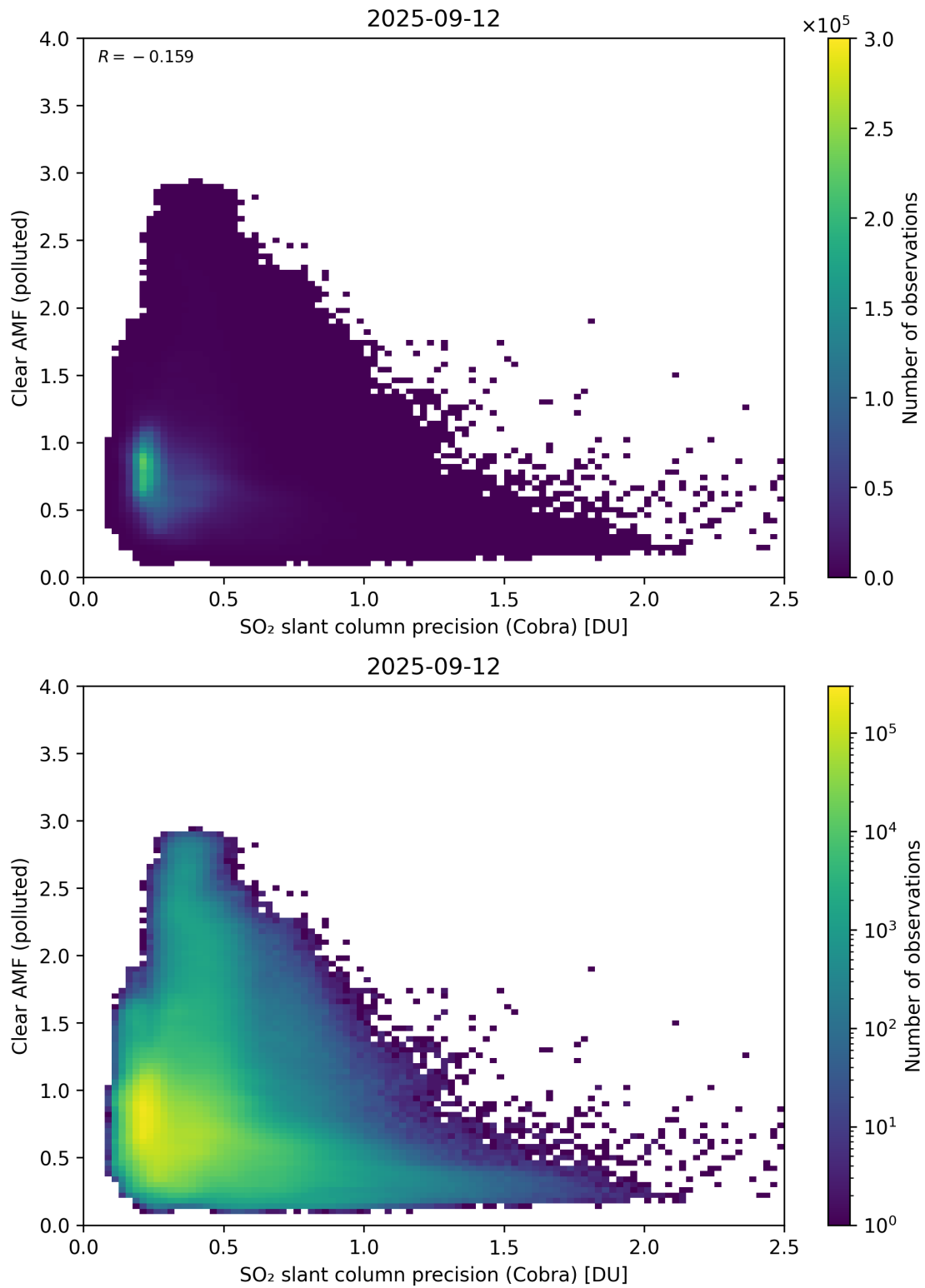
Figure 205: Scatter density plot of “SO 2 slant column precision (Cobra)” against “Clear AMF (polluted)” for 2025-09-11 to 2025-09-13.
