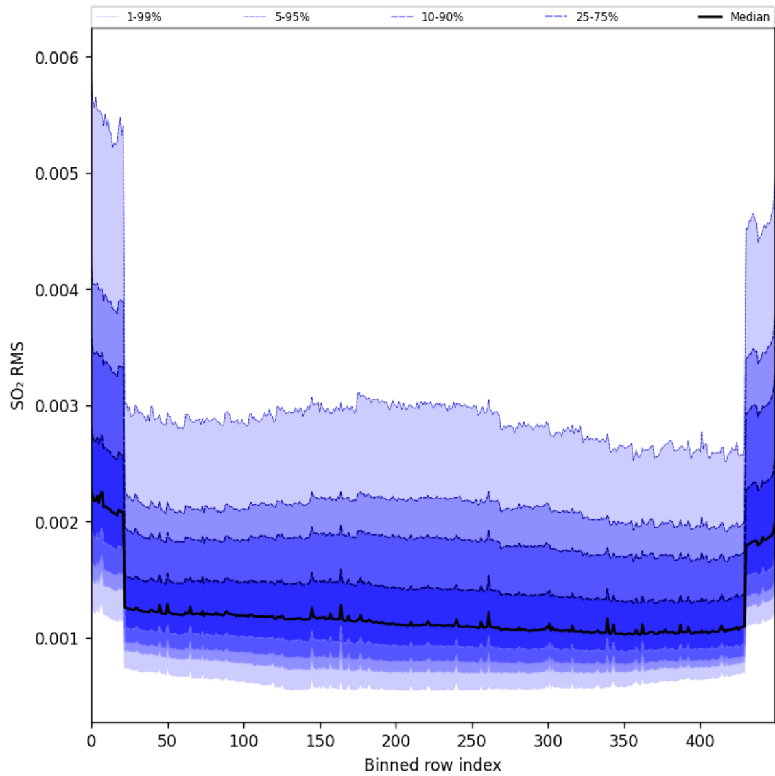
Figure 104: Along track statistics of “SO 2 RMS” for 2025-09-11 to 2025-09-13
