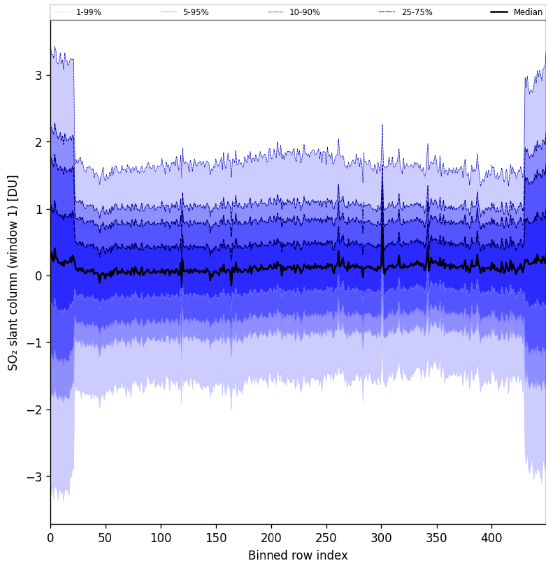
Figure 89: Along track statistics of “SO 2 slant column (window 1)” for 2025-09-11 to 2025-09-13
