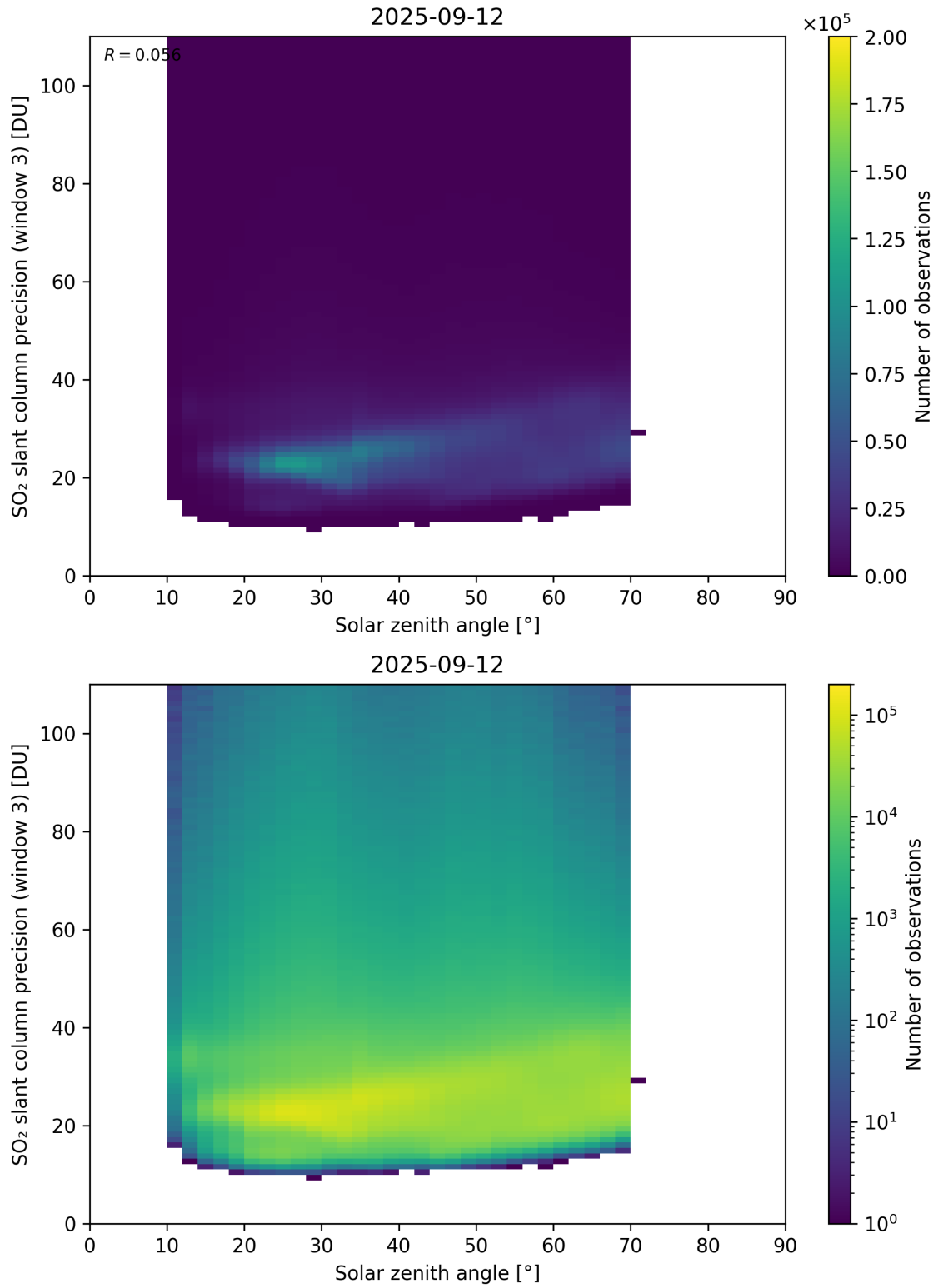
Figure 188: Scatter density plot of “Solar zenith angle” against “SO 2 slant column precision (window 3)” for 2025-09-11 to 2025-09-13.
