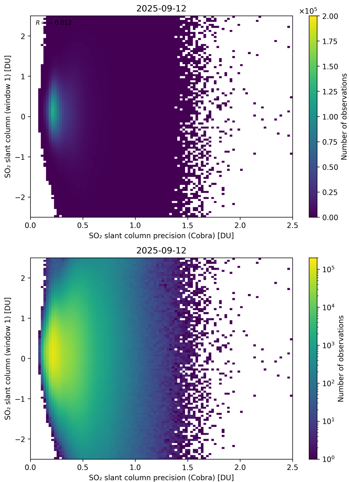
Figure 208: Scatter density plot of “SO 2 slant column precision (Cobra)” against “SO 2 slant column (window 1)” for 2025-09-11 to 2025-09-13.
