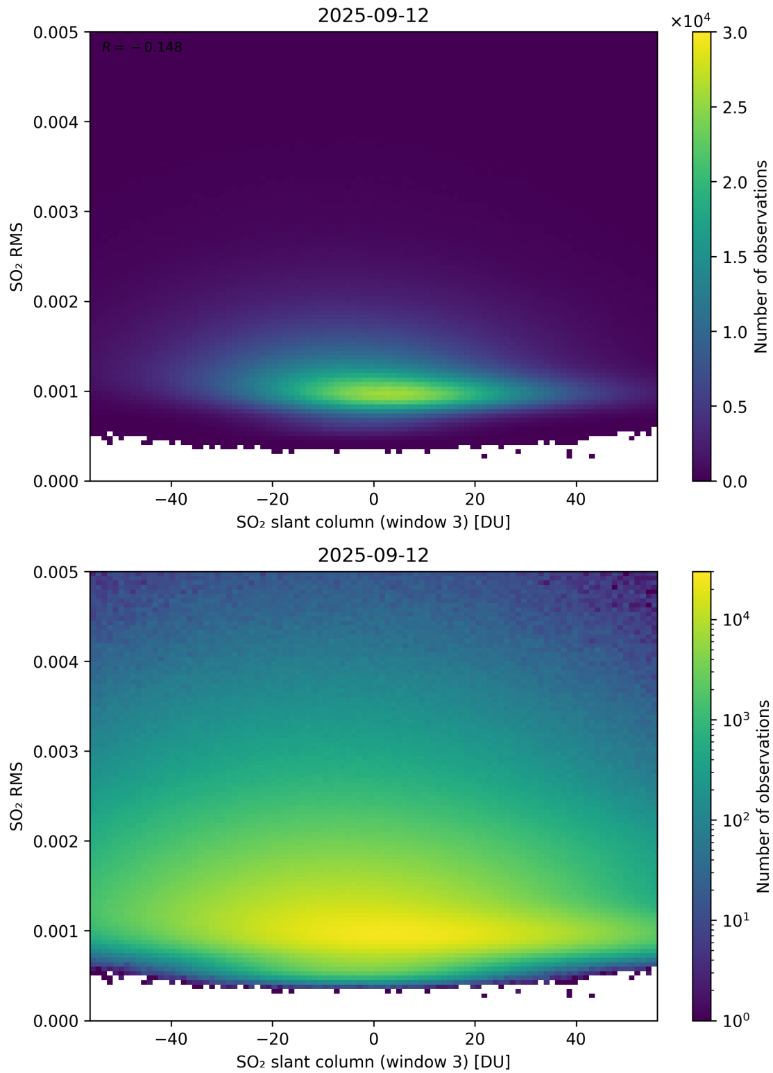
Figure 306: Scatter density plot of “SO 2 slant column (window 3)” against “SO 2 RMS” for 2025-09-11 to 2025-09-13.
