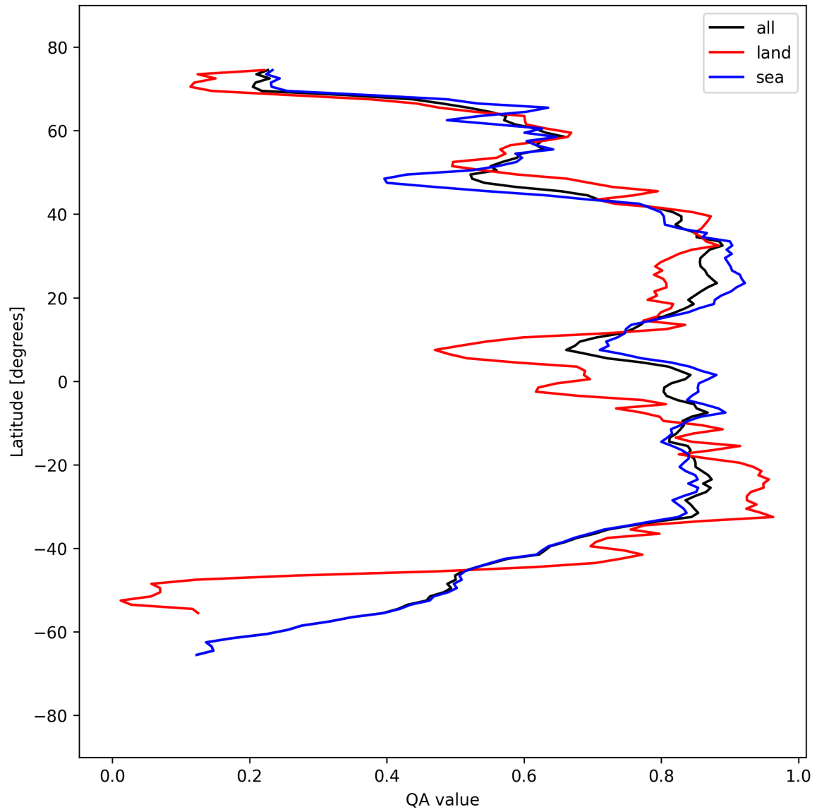
Figure 31: Zonal average of “QA value” for 2025-09-11 to 2025-09-13.
