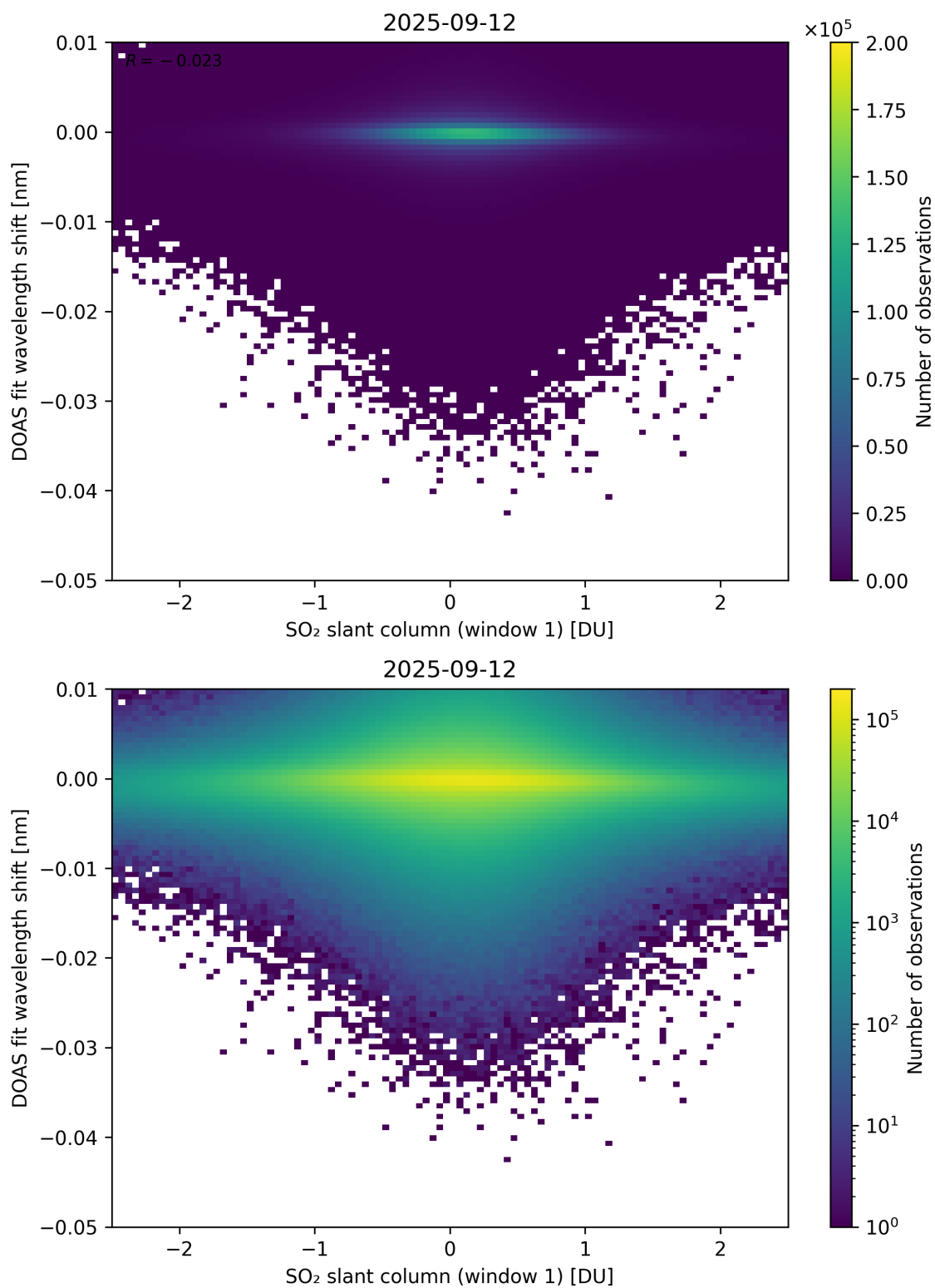
Figure 265: Scatter density plot of “SO 2 slant column (window 1)” against “DOAS fit wavelength shift” for 2025-09-11 to 2025-09-13.
