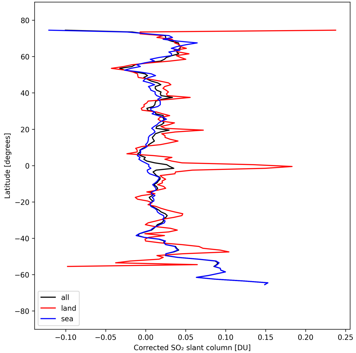
Figure 34: Zonal average of “Corrected SO 2 slant column” for 2025-09-11 to 2025-09-13.
