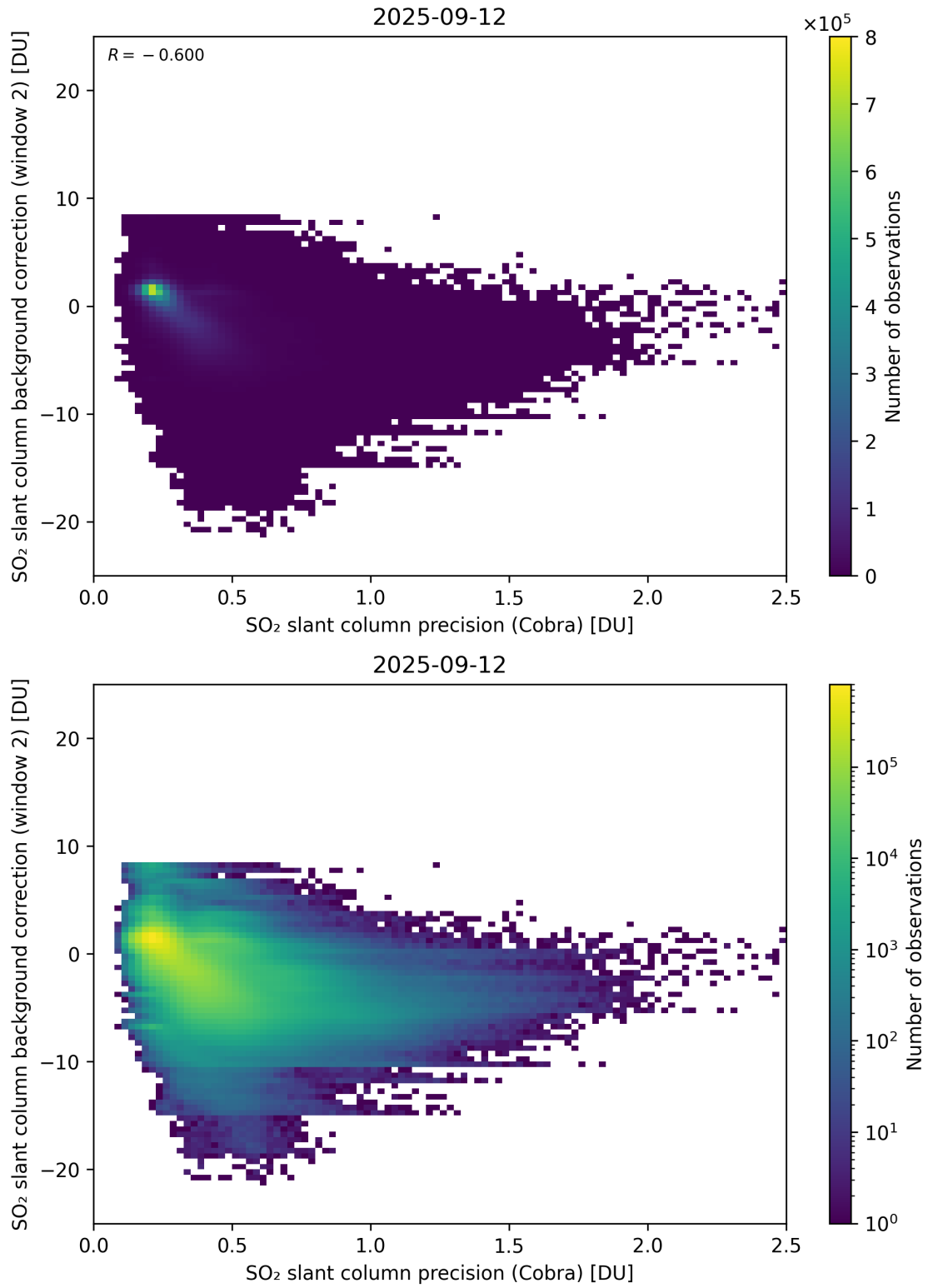
Figure 200: Scatter density plot of “SO 2 slant column precision (Cobra)” against “SO 2 slant column background correction (window 2)” for 2025-09-11 to 2025-09-13.
