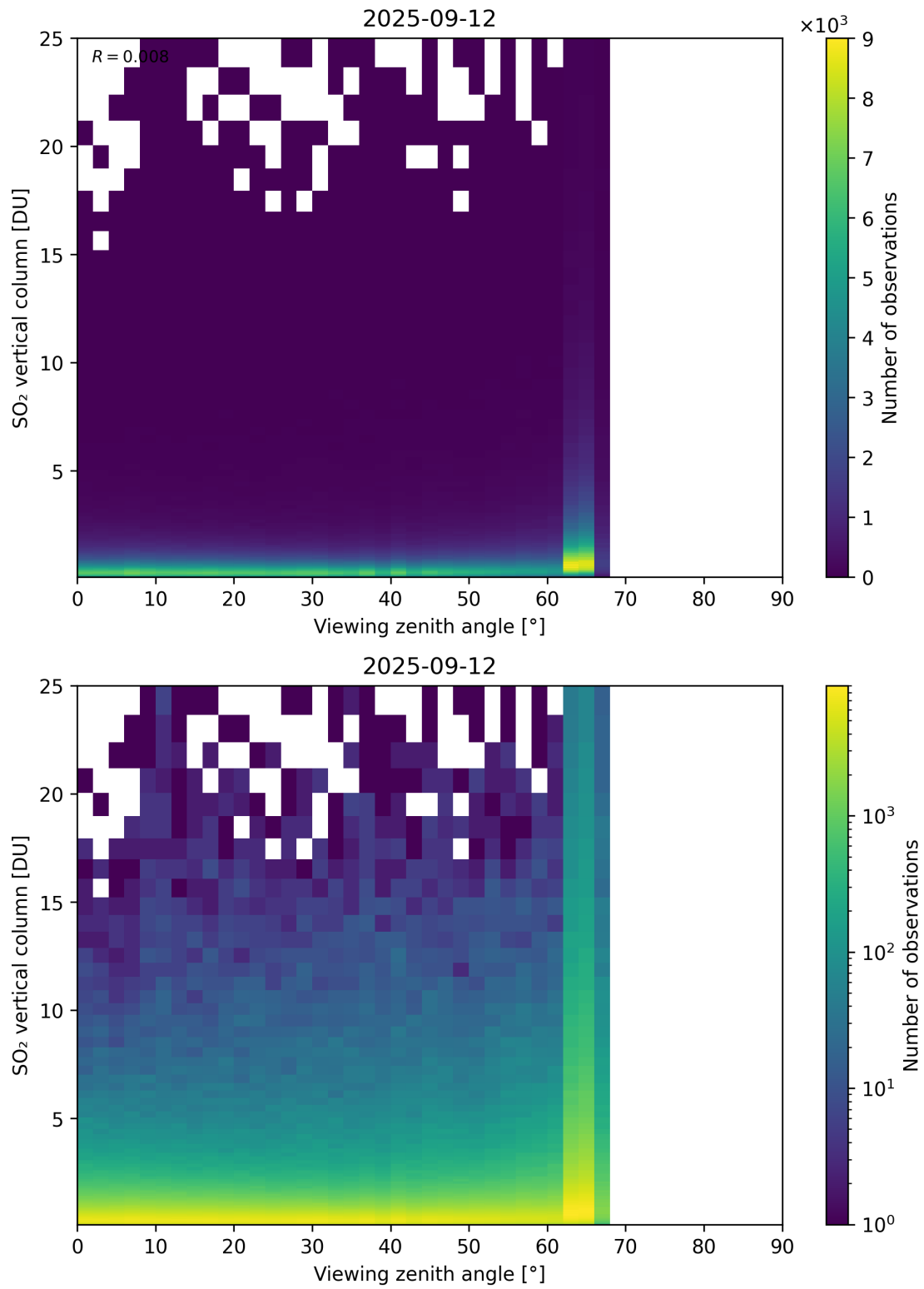
Figure 383: Scatter density plot of “Viewing zenith angle” against “SO 2 vertical column” for 2025-09-11 to 2025-09-13.
