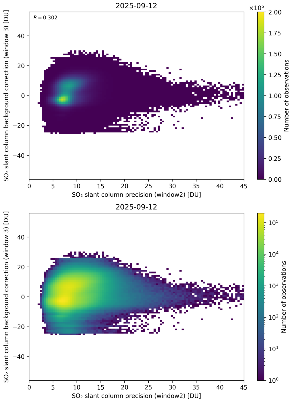
Figure 292: Scatter density plot of “SO 2 slant column precision (window2)” against “SO 2 slant column background correction (window 3)” for 2025-09-11 to 2025-09-13.
