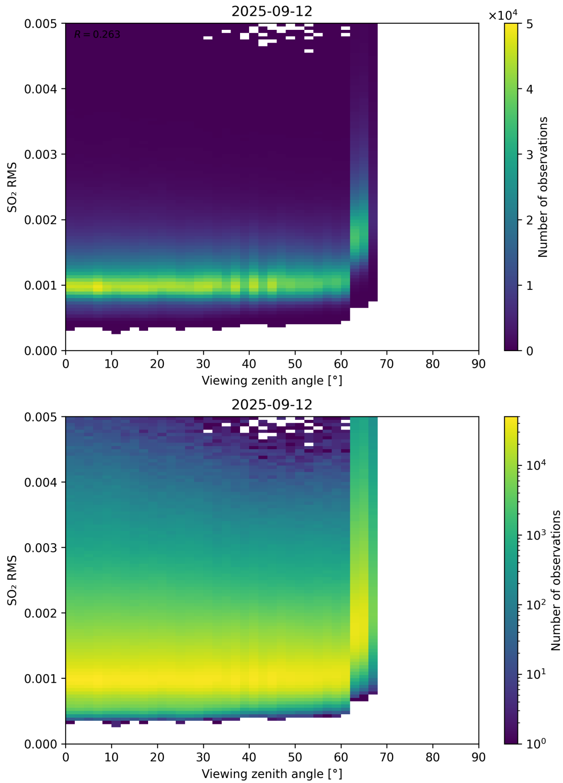
Figure 367: Scatter density plot of “Viewing zenith angle” against “SO 2 RMS” for 2025-09-11 to 2025-09-13.
