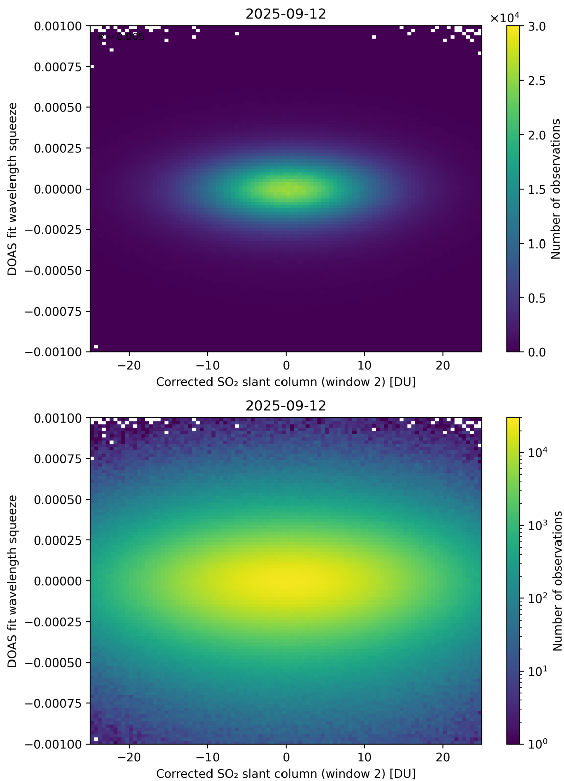
Figure 247: Scatter density plot of “Corrected SO 2 slant column (window 2)” against “DOAS fit wavelength squeeze” for 2025-09-11 to 2025-09-13.
