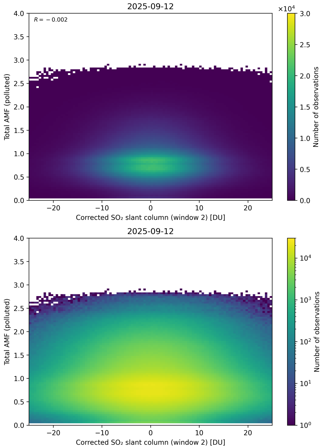
Figure 253: Scatter density plot of “Corrected SO 2 slant column (window 2)” against “Total AMF (polluted)” for 2025-09-11 to 2025-09-13.
