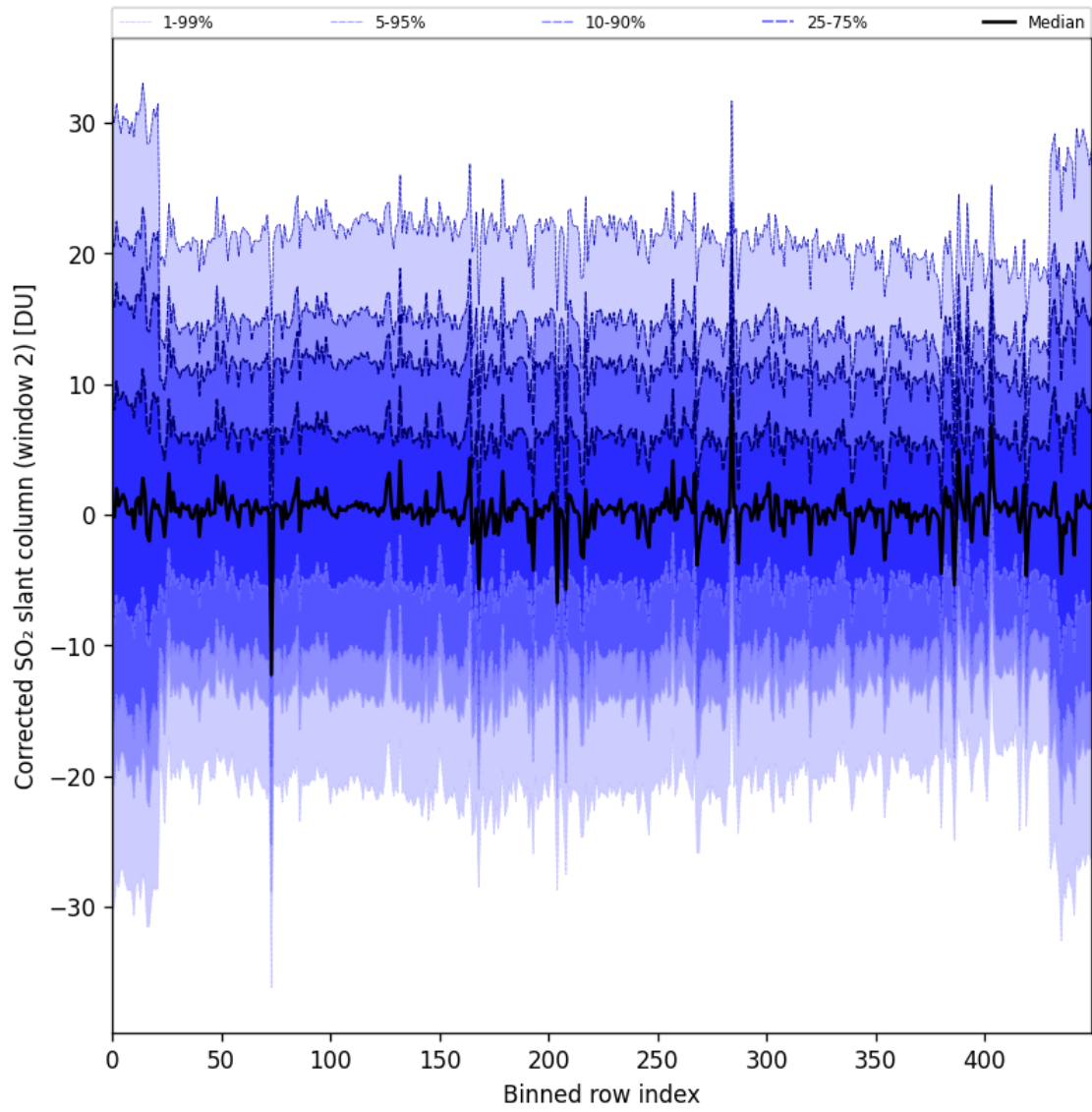
Figure 95: Along track statistics of “Corrected SO 2 slant column (window 2)” for 2025-09-11 to 2025-09-13
