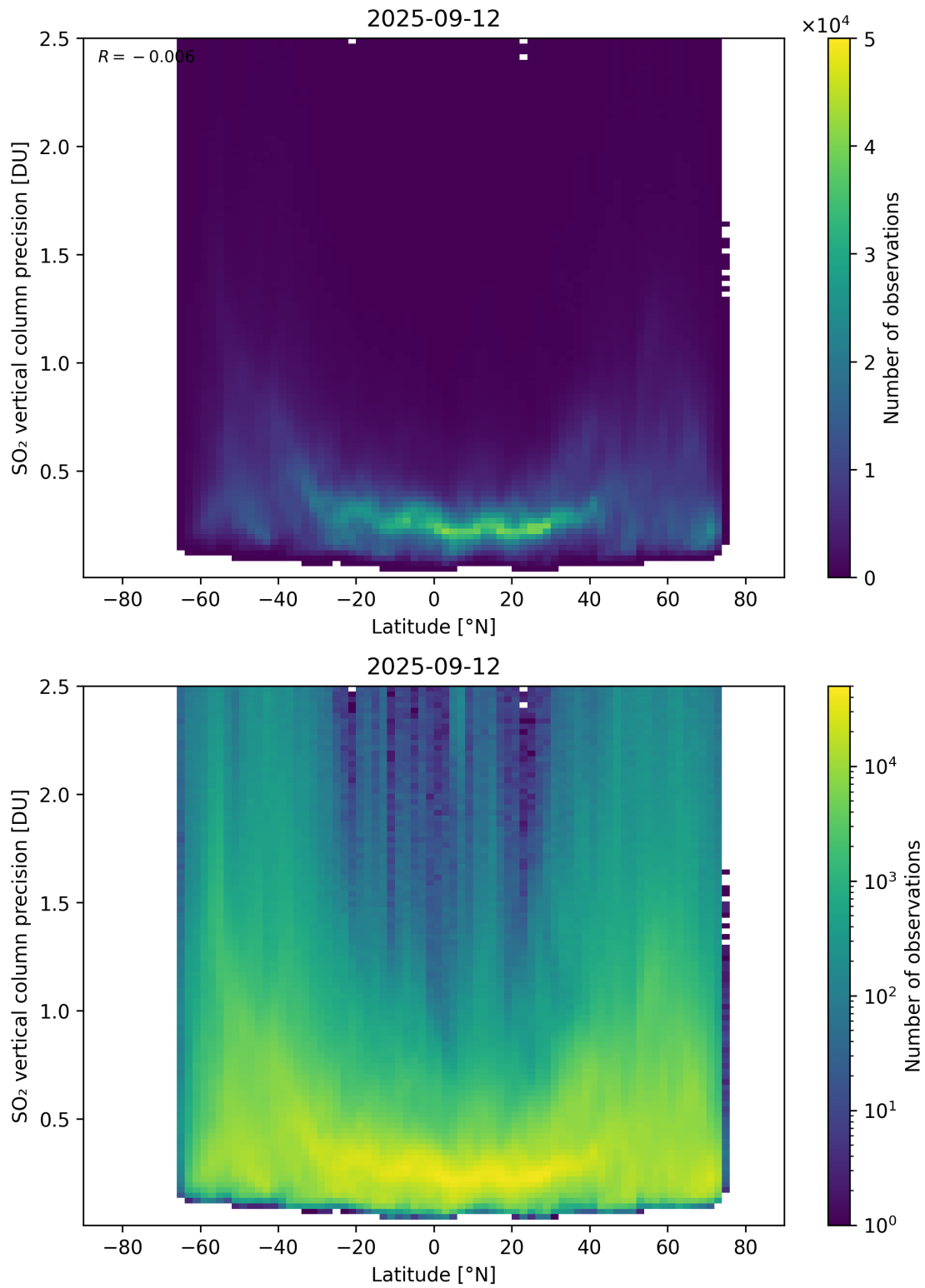
Figure 170: Scatter density plot of “Latitude” against “SO 2 vertical column precision” for 2025-09-11 to 2025-09-13.
