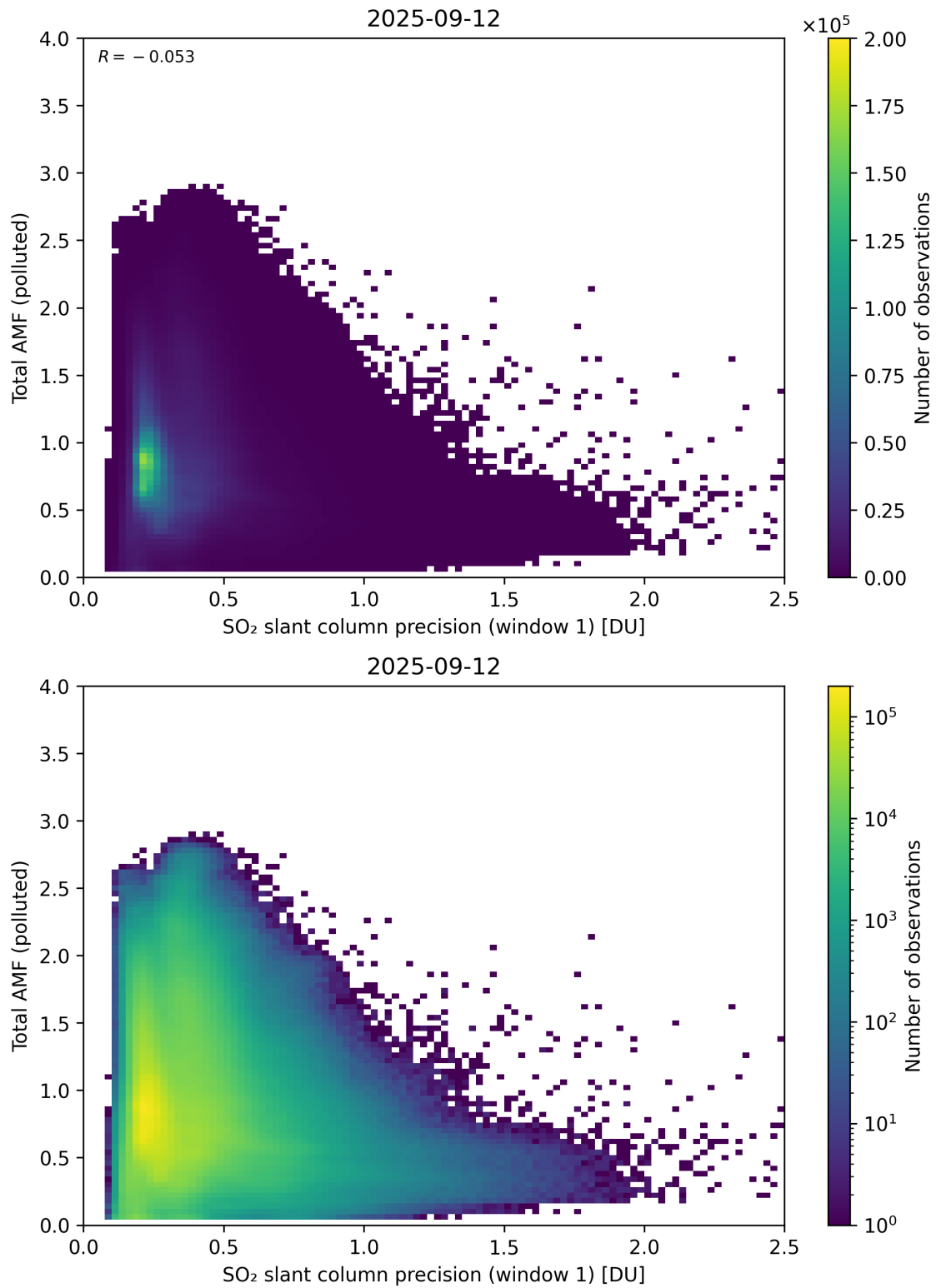
Figure 280: Scatter density plot of “SO 2 slant column precision (window 1)” against “Total AMF (polluted)” for 2025-09-11 to 2025-09-13.
