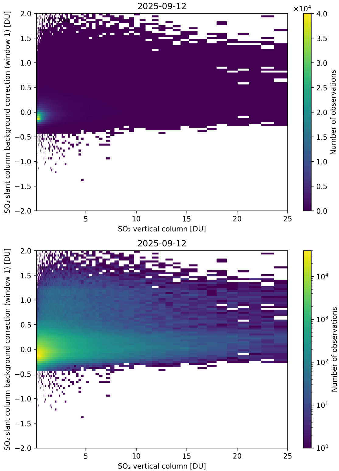
Figure 323: Scatter density plot of “SO 2 vertical column” against “SO 2 slant column background correction (window 1)” for 2025-09-11 to 2025-09-13.
