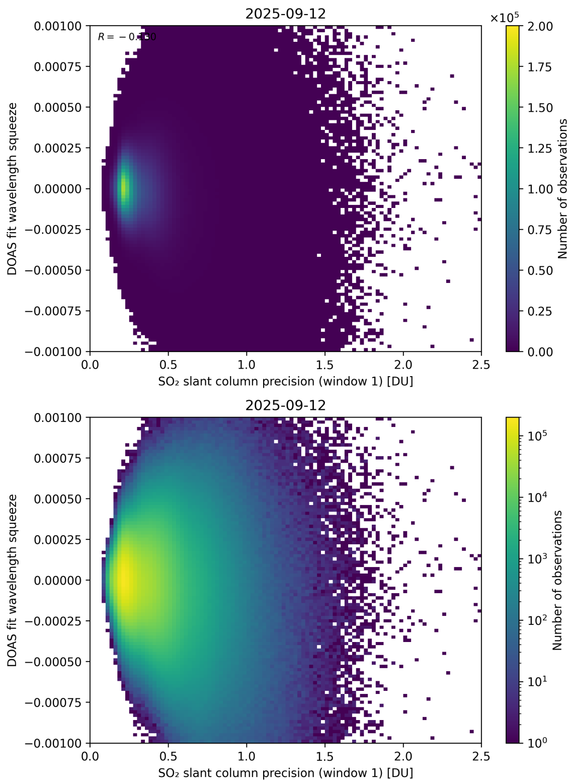
Figure 272: Scatter density plot of “SO 2 slant column precision (window 1)” against “DOAS fit wavelength squeeze” for 2025-09-11 to 2025-09-13.
