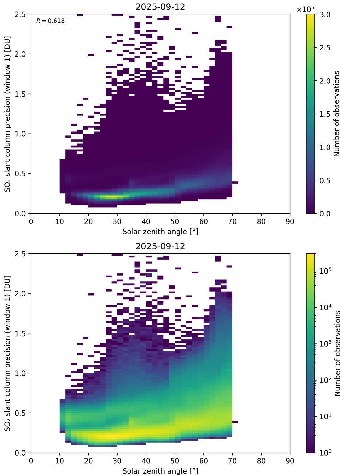
Figure 185: Scatter density plot of “Solar zenith angle” against “SO 2 slant column precision (window 1)” for 2025-09-11 to 2025-09-13.
