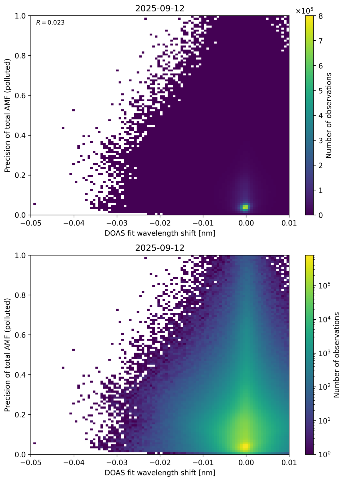
Figure 142: Scatter density plot of “DOAS fit wavelength shift” against “Precision of total AMF (polluted)” for 2025-09-11 to 2025-09-13.
