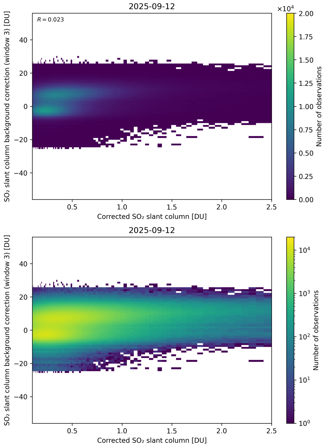
Figure 228: Scatter density plot of “Corrected SO 2 slant column” against “SO 2 slant column background correction (window 3)” for 2025-09-11 to 2025-09-13.
