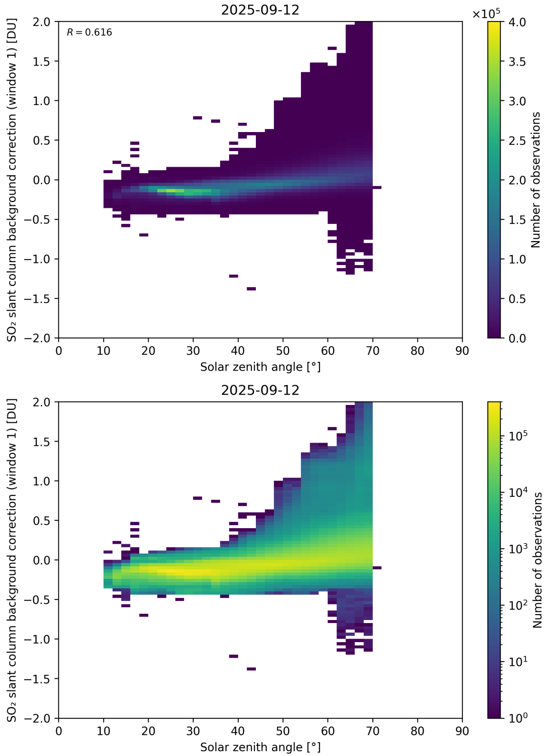
Figure 171: Scatter density plot of “Solar zenith angle” against “SO 2 slant column background correction (window 1)” for 2025-09-11 to 2025-09-13.
