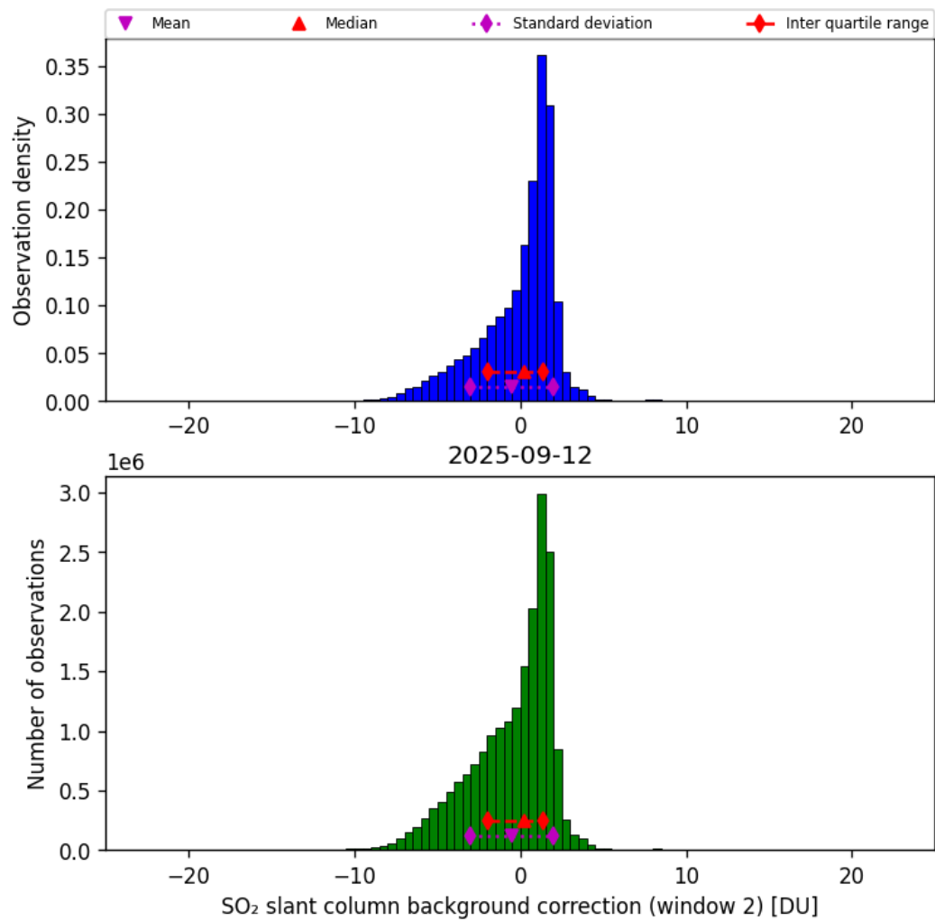
Figure 70: Histogram of “SO 2 slant column background correction (window 2)” for 2025-09-11 to 2025-09-13
