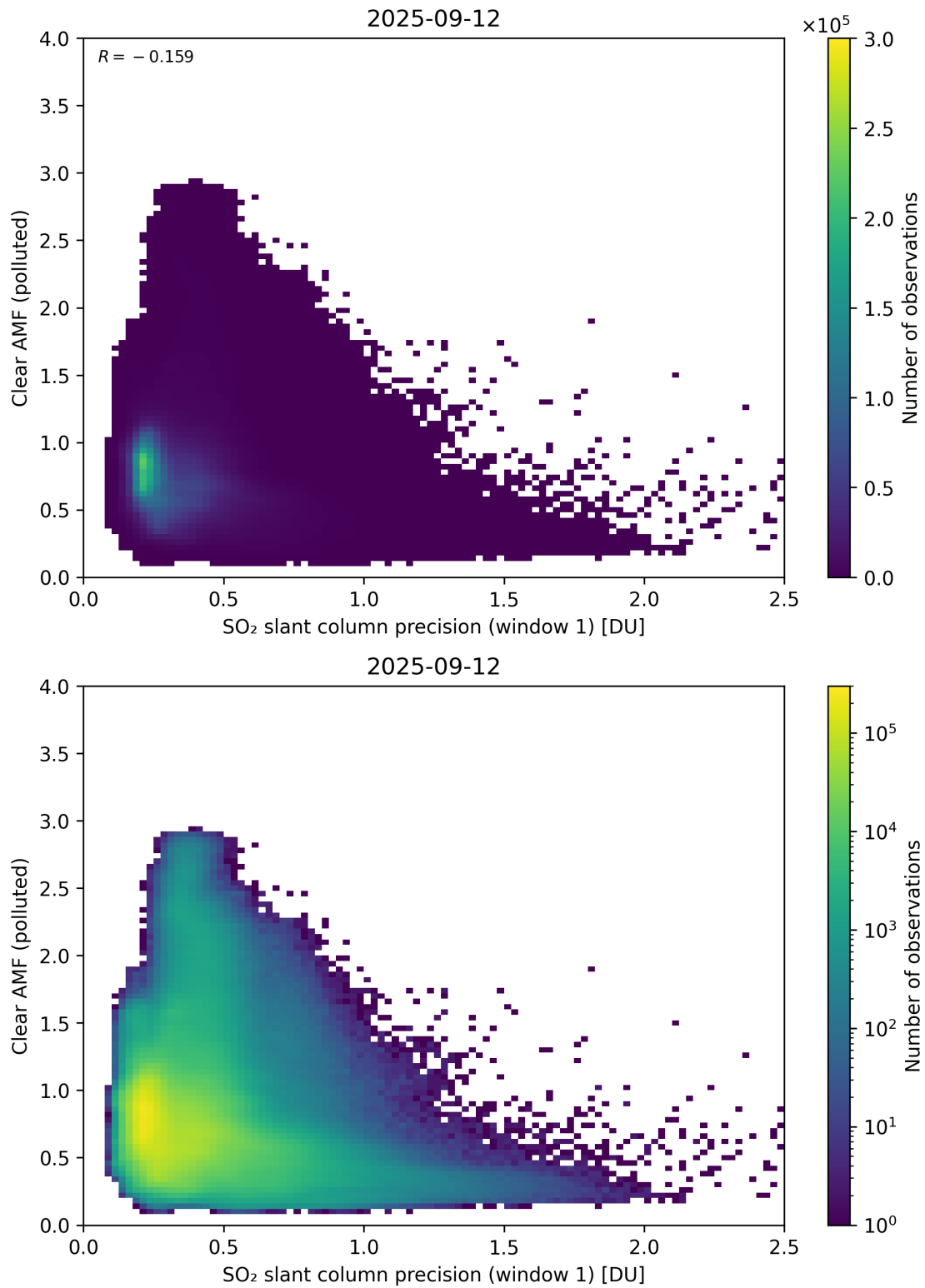
Figure 274: Scatter density plot of “SO 2 slant column precision (window 1)” against “Clear AMF (polluted)” for 2025-09-11 to 2025-09-13.
