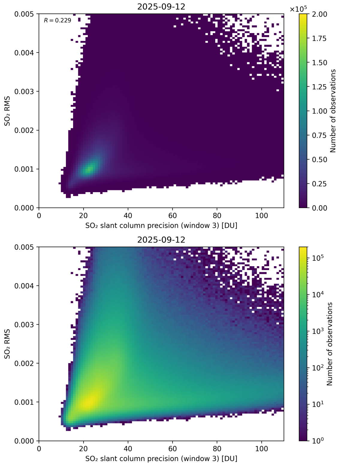
Figure 310: Scatter density plot of “SO 2 slant column precision (window 3)” against “SO 2 RMS” for 2025-09-11 to 2025-09-13.
