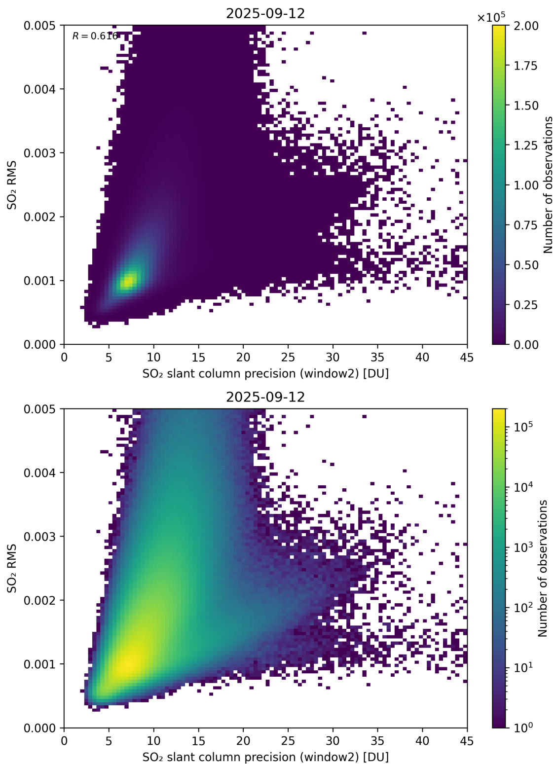
Figure 295: Scatter density plot of “SO 2 slant column precision (window2)” against “SO 2 RMS” for 2025-09-11 to 2025-09-13.
