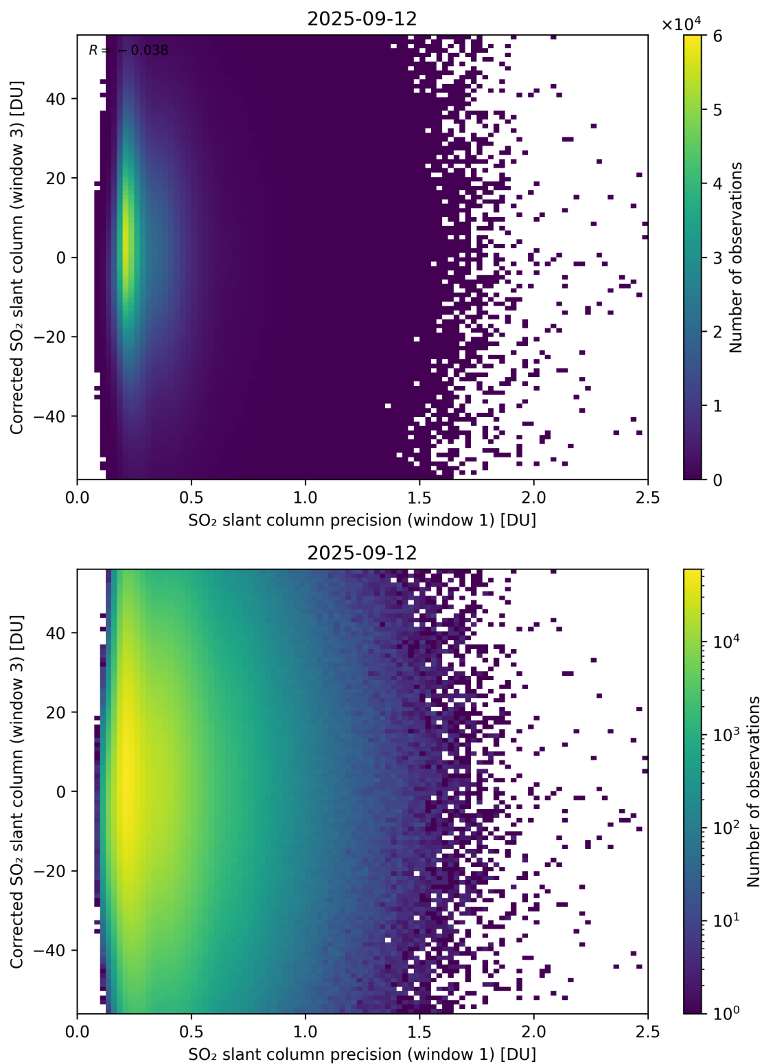
Figure 276: Scatter density plot of “SO 2 slant column precision (window 1)” against “Corrected SO 2 slant column (window 3)” for 2025-09-11 to 2025-09-13.
