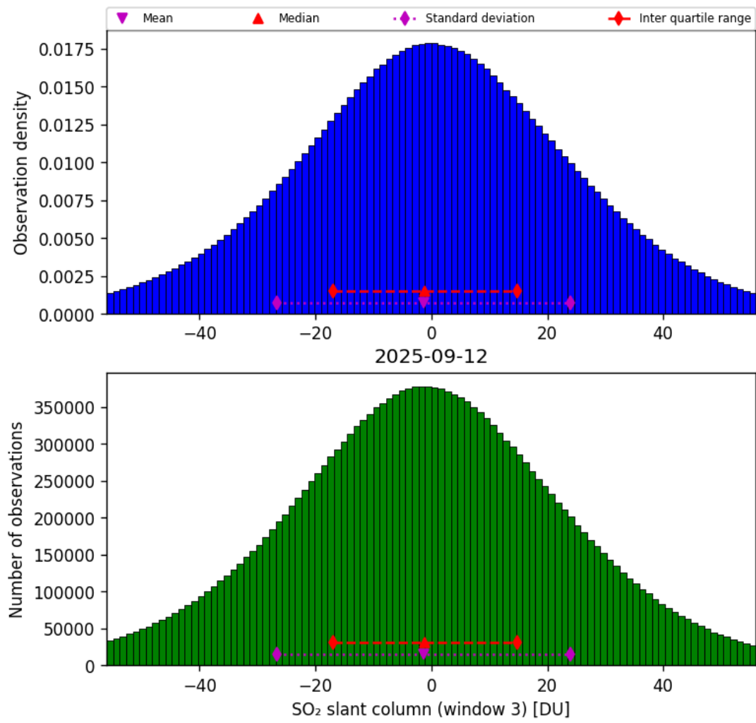
Figure 71: Histogram of “SO 2 slant column (window 3)” for 2025-09-11 to 2025-09-13
