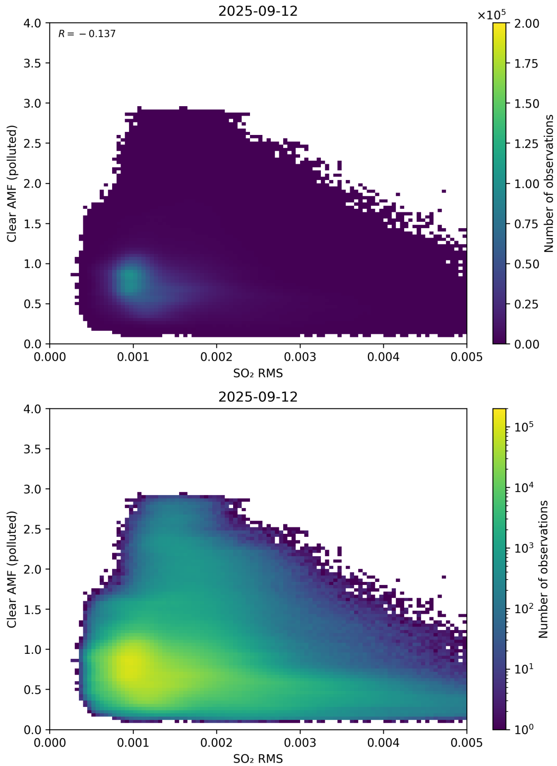
Figure 147: Scatter density plot of “SO 2 RMS” against “Clear AMF (polluted)” for 2025-09-11 to 2025-09-13.
