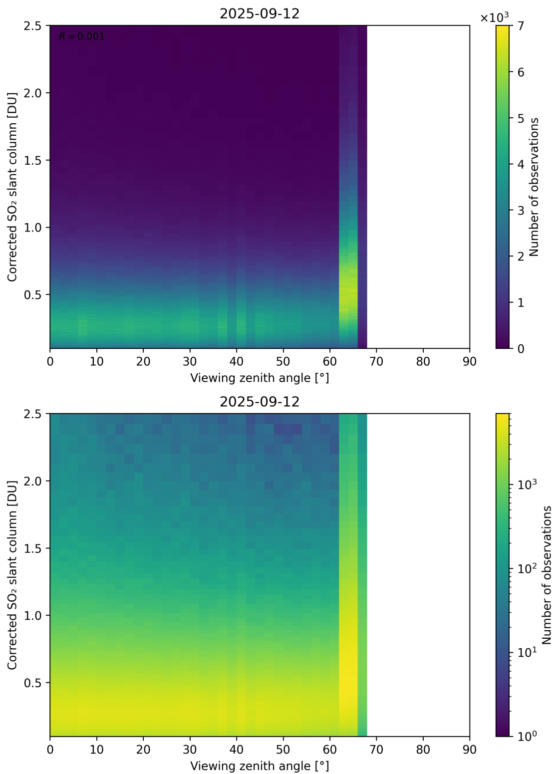
Figure 373: Scatter density plot of “Viewing zenith angle” against “Corrected SO 2 slant column” for 2025-09-11 to 2025-09-13.
