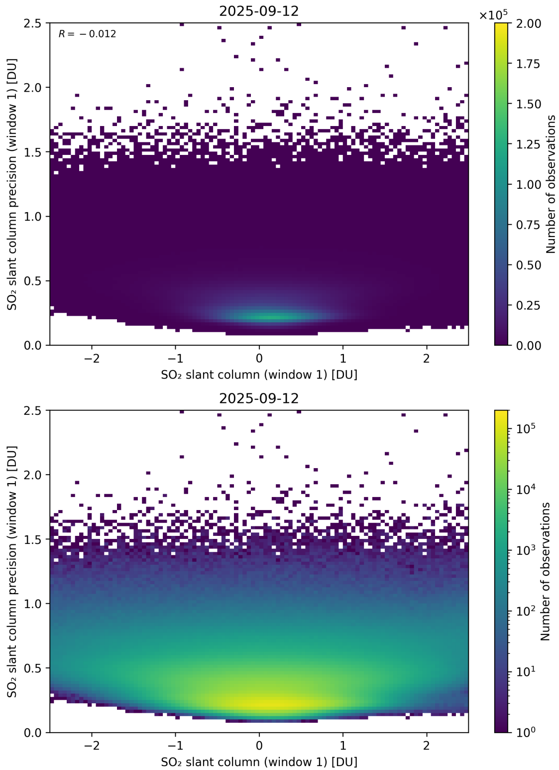
Figure 285: Scatter density plot of “SO 2 slant column (window 1)” against “SO 2 slant column precision (window 1)” for 2025-09-11 to 2025-09-13.
