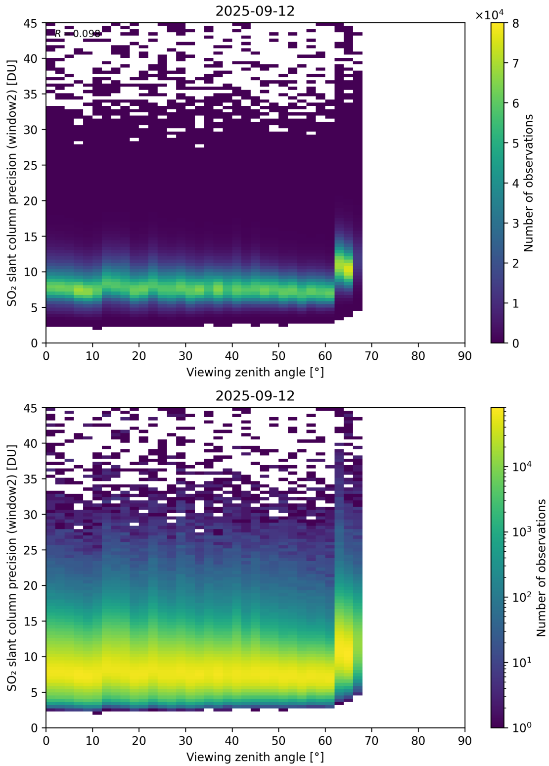
Figure 378: Scatter density plot of “Viewing zenith angle” against “SO 2 slant column precision (window2)” for 2025-09-11 to 2025-09-13.
