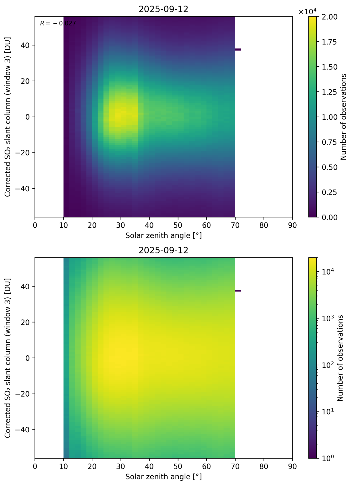
Figure 183: Scatter density plot of “Solar zenith angle” against “Corrected SO 2 slant column (window 3)” for 2025-09-11 to 2025-09-13.
