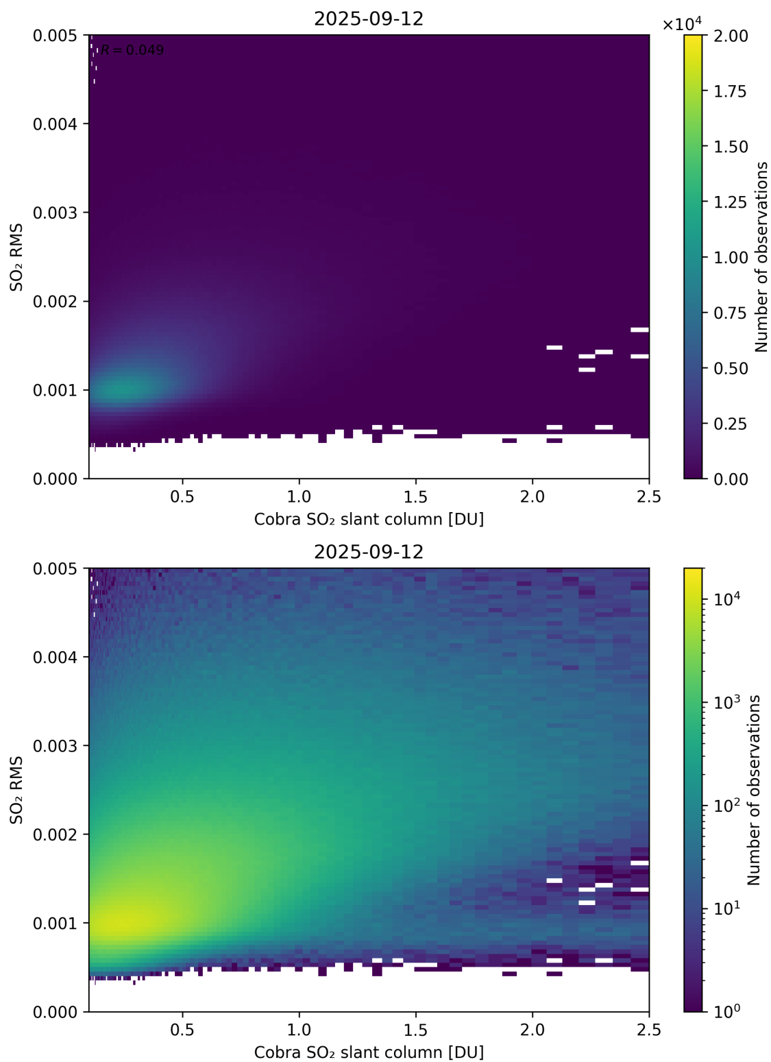
Figure 198: Scatter density plot of “Cobra SO 2 slant column” against “SO 2 RMS” for 2025-09-11 to 2025-09-13.
