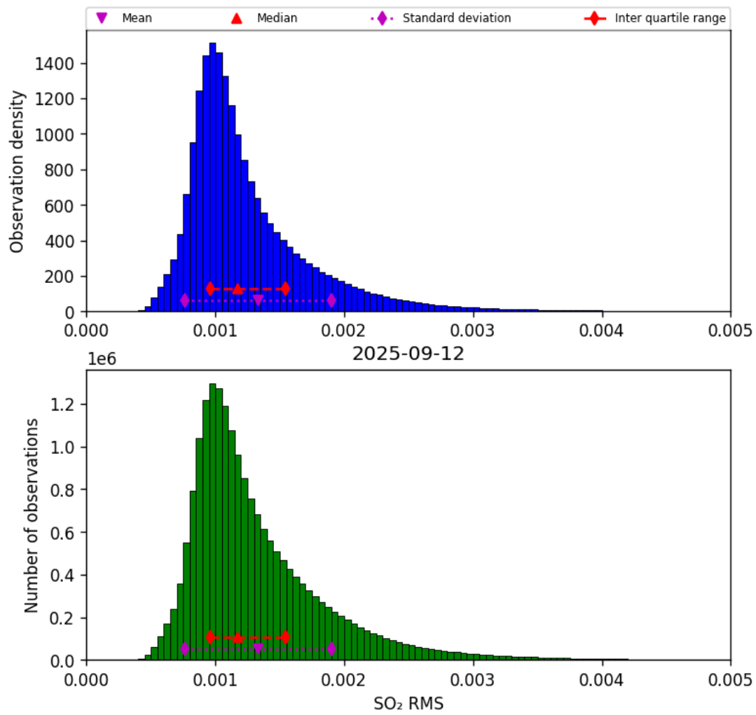
Figure 78: Histogram of “SO 2 RMS” for 2025-09-11 to 2025-09-13
