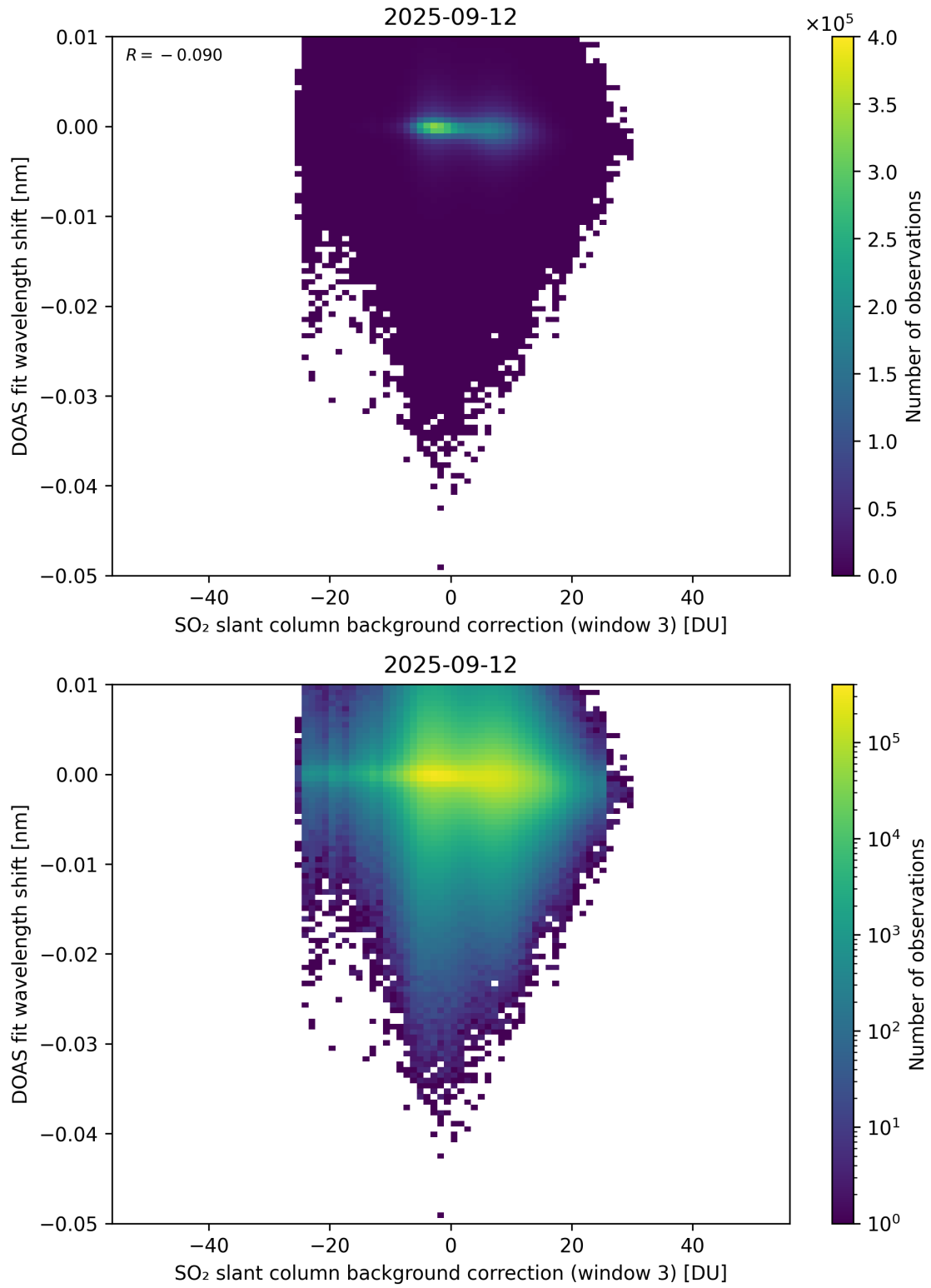
Figure 132: Scatter density plot of “SO 2 slant column background correction (window 3)” against “DOAS fit wavelength shift” for 2025-09-11 to 2025-09-13.
