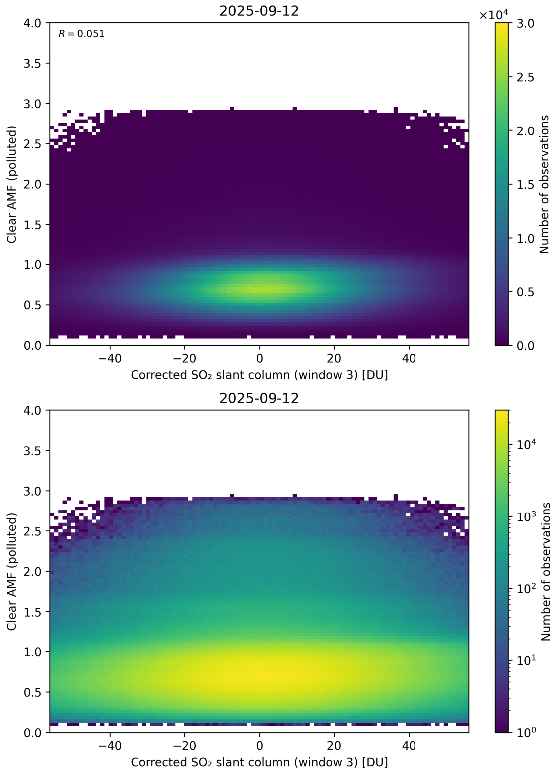
Figure 259: Scatter density plot of “Corrected SO 2 slant column (window 3)” against “Clear AMF (polluted)” for 2025-09-11 to 2025-09-13.
