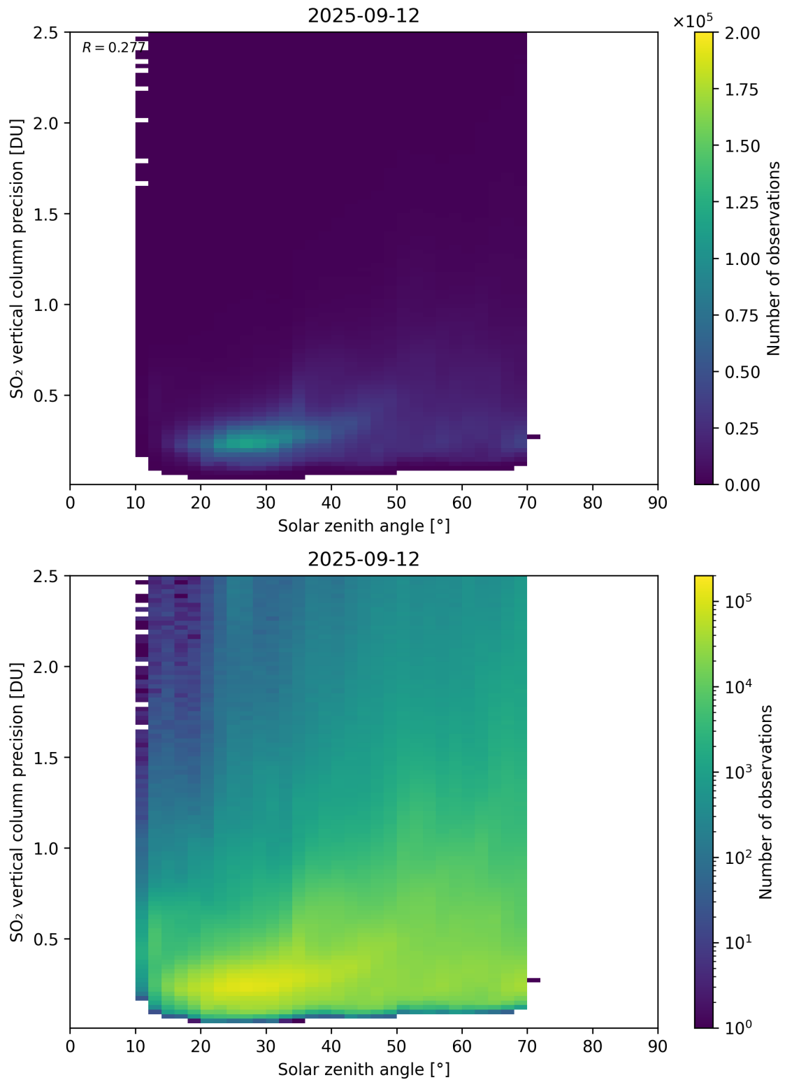
Figure 192: Scatter density plot of “Solar zenith angle” against “SO 2 vertical column precision” for 2025-09-11 to 2025-09-13.
