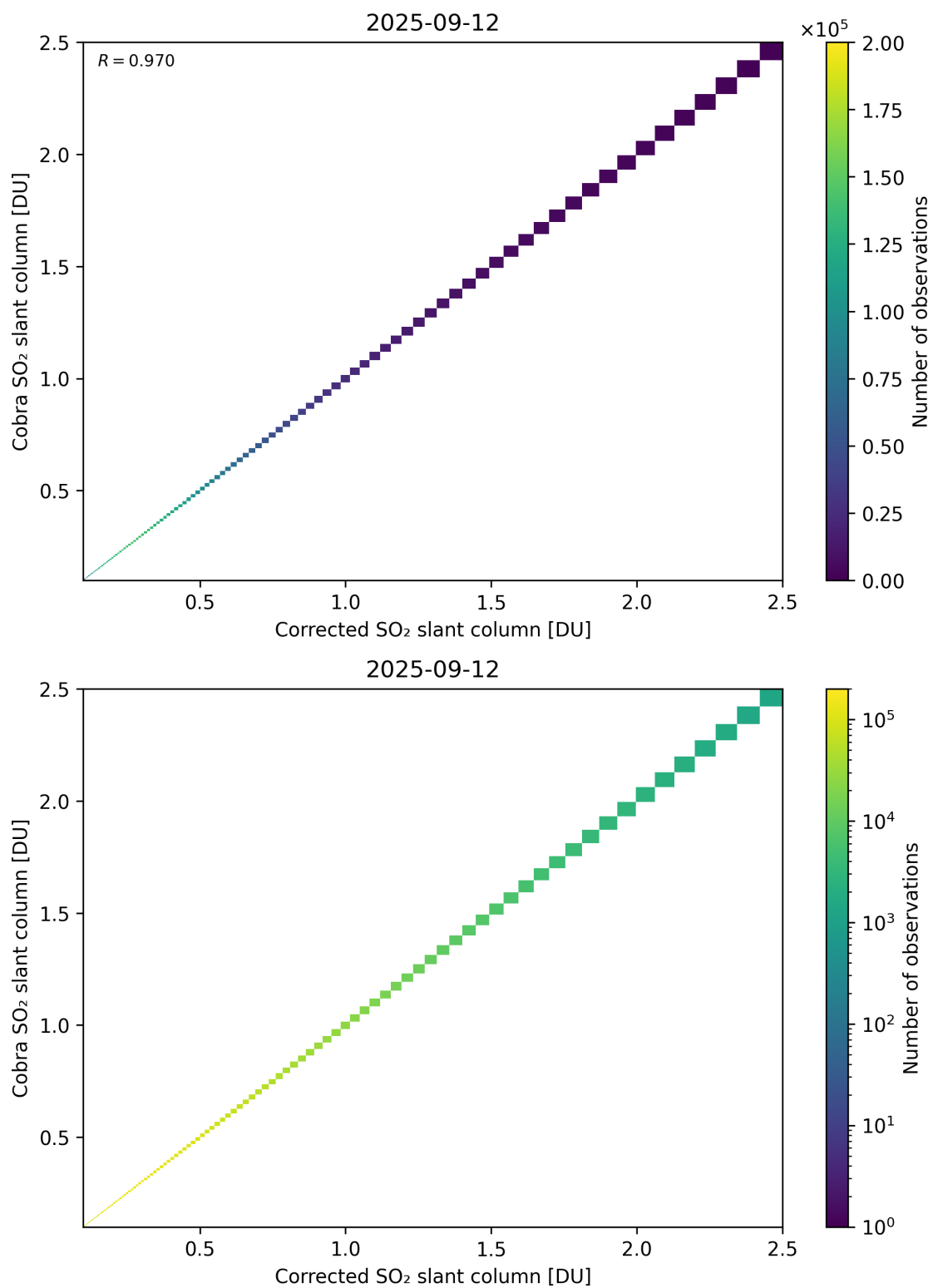
Figure 233: Scatter density plot of “Corrected SO 2 slant column” against “Cobra SO 2 slant column” for 2025-09-11 to 2025-09-13.
