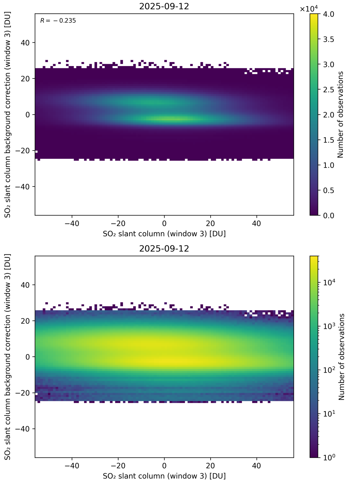
Figure 303: Scatter density plot of “SO 2 slant column (window 3)” against “SO 2 slant column background correction (window 3)” for 2025-09-11 to 2025-09-13.
