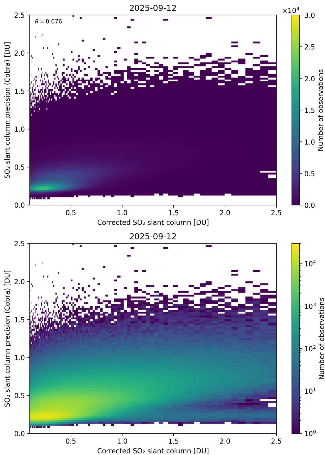
Figure 234: Scatter density plot of “Corrected SO 2 slant column” against “SO 2 slant column precision (Cobra)” for 2025-09-11 to 2025-09-13.
