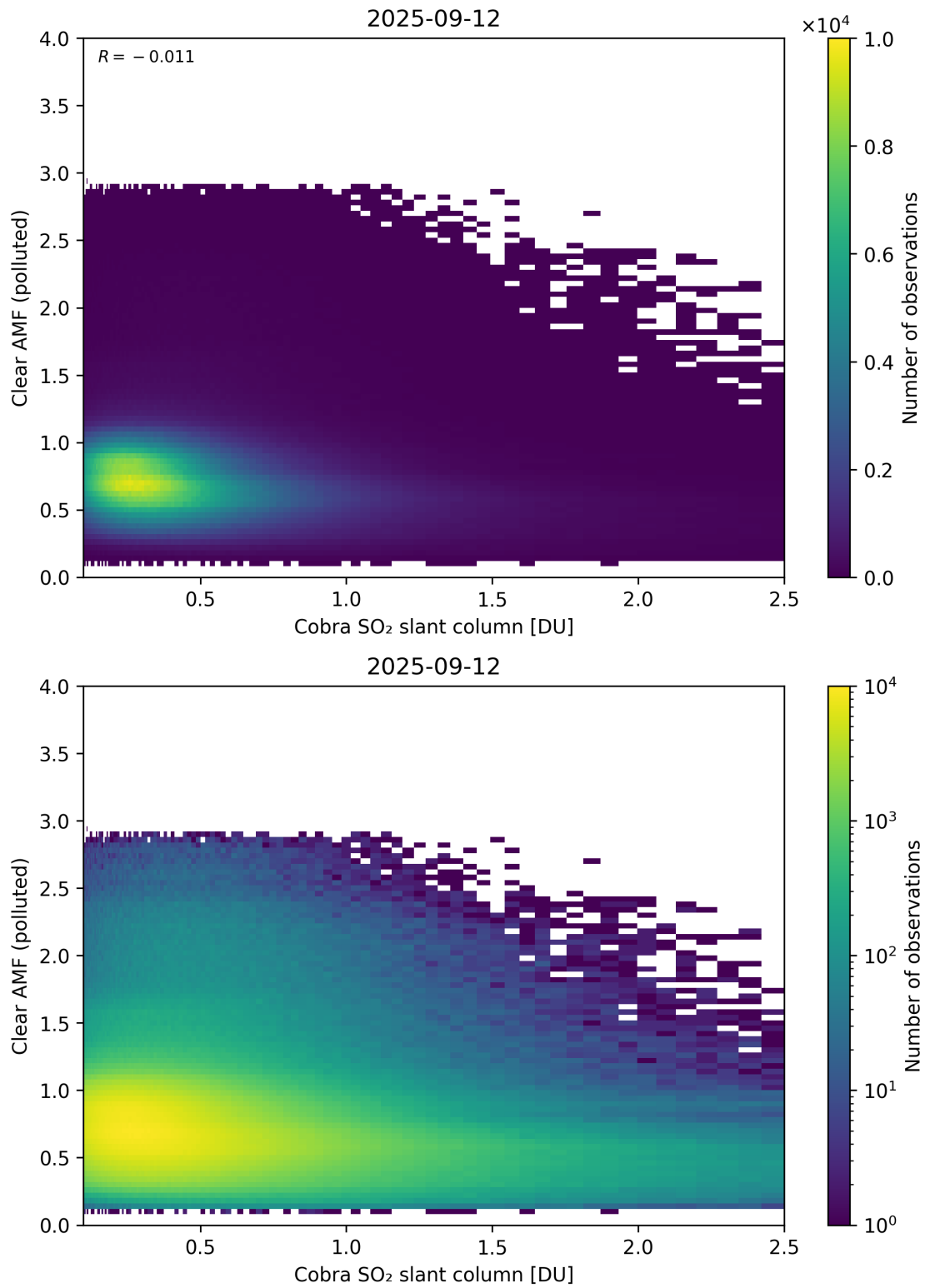
Figure 215: Scatter density plot of “Cobra SO 2 slant column” against “Clear AMF (polluted)” for 2025-09-11 to 2025-09-13.
