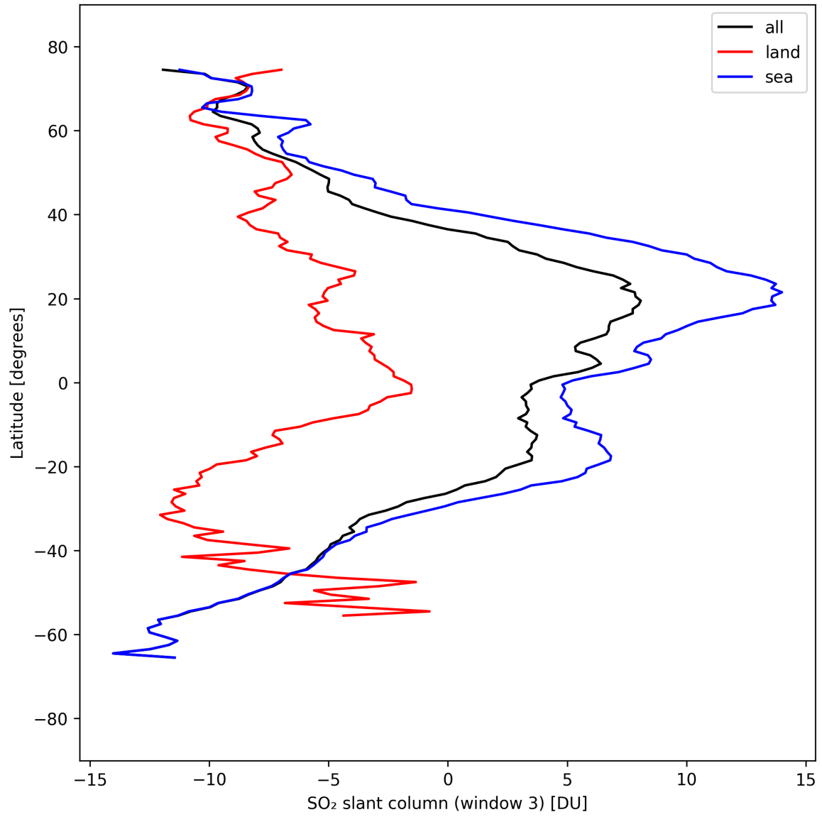
Figure 45: Zonal average of “SO 2 slant column (window 3)” for 2025-09-11 to 2025-09-13.
