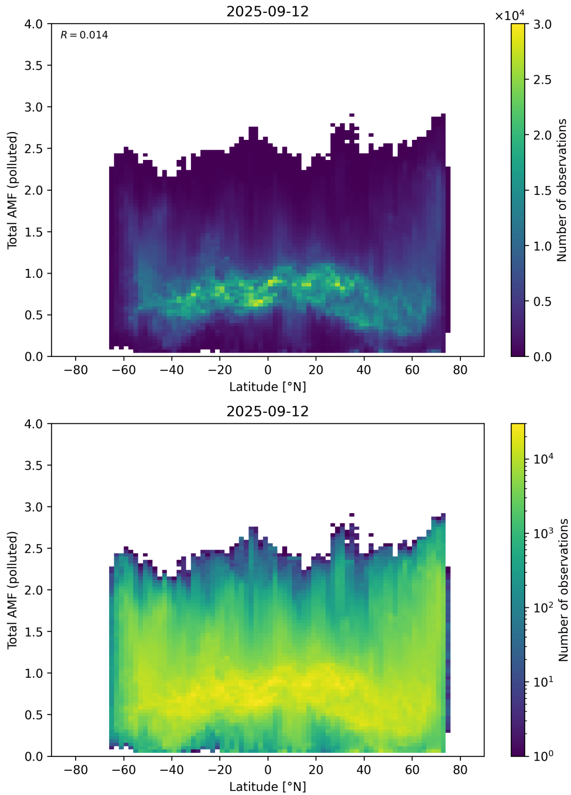
Figure 167: Scatter density plot of “Latitude” against “Total AMF (polluted)” for 2025-09-11 to 2025-09-13.
