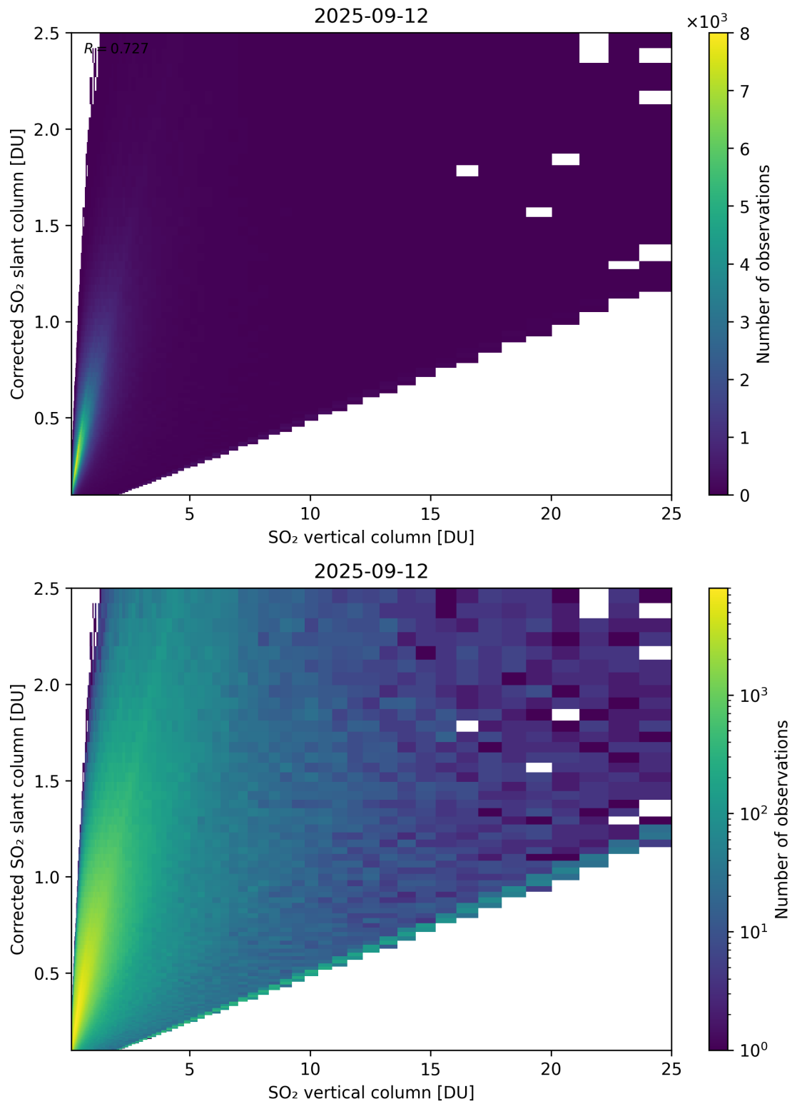
Figure 351: Scatter density plot of “SO 2 vertical column” against “Corrected SO 2 slant column” for 2025-09-11 to 2025-09-13.
