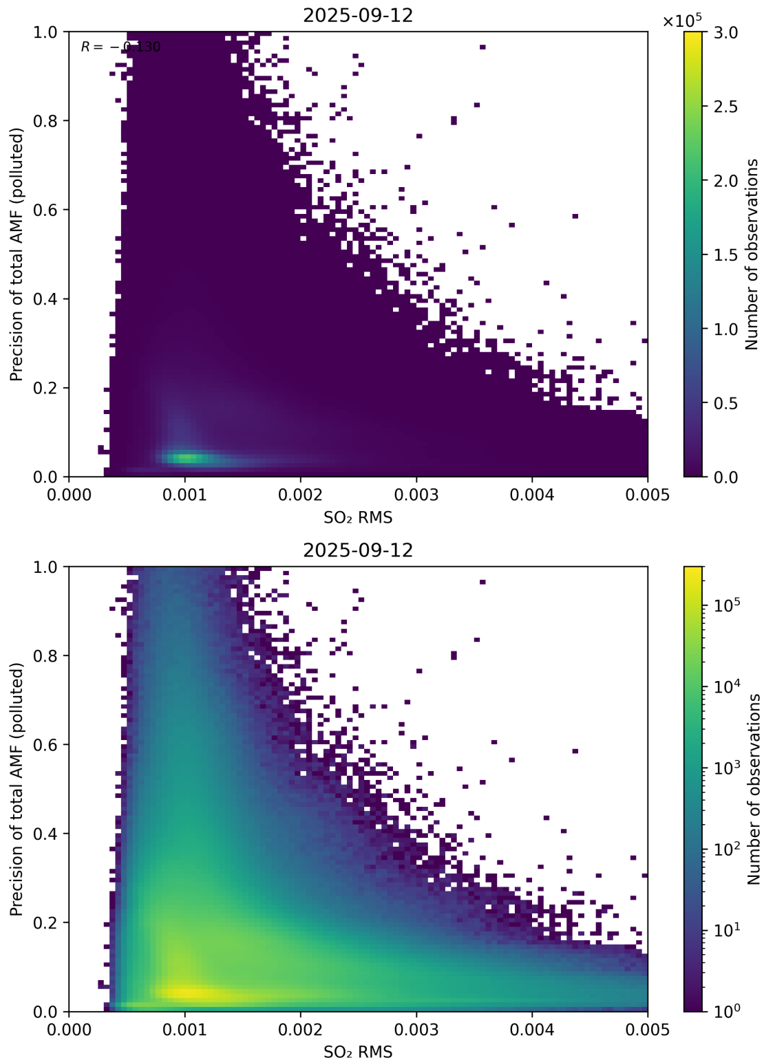
Figure 149: Scatter density plot of “SO 2 RMS” against “Precision of total AMF (polluted)” for 2025-09-11 to 2025-09-13.
