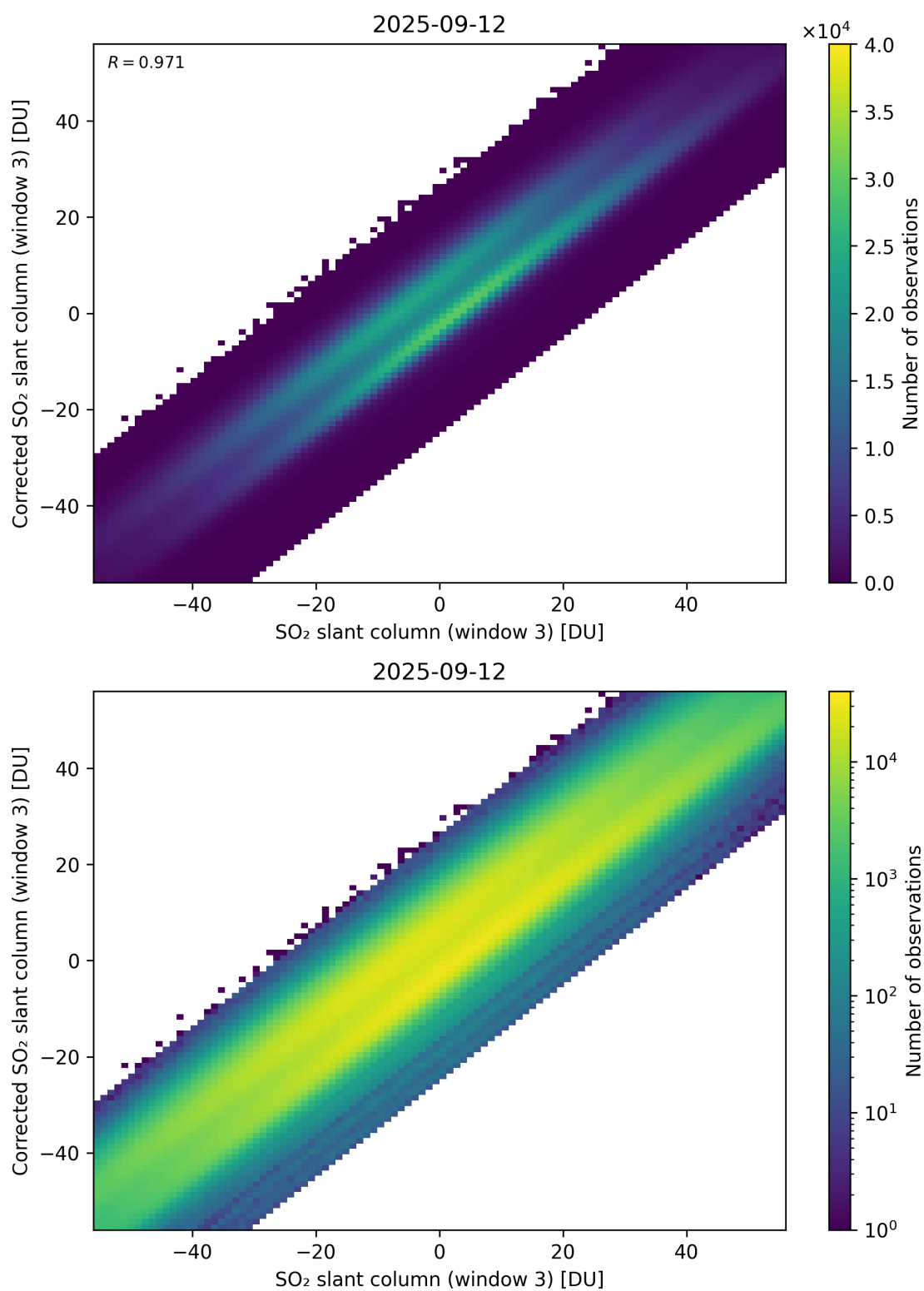
Figure 316: Scatter density plot of “SO 2 slant column (window 3)” against “Corrected SO 2 slant column (window 3)” for 2025-09-11 to 2025-09-13.
