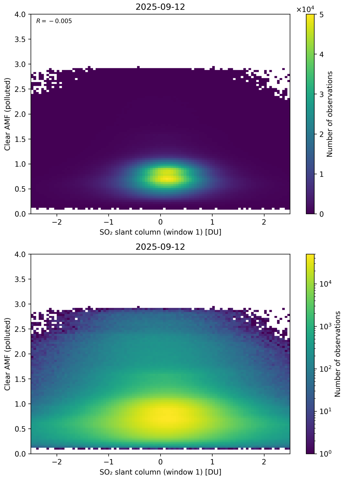
Figure 282: Scatter density plot of “SO 2 slant column (window 1)” against “Clear AMF (polluted)” for 2025-09-11 to 2025-09-13.
