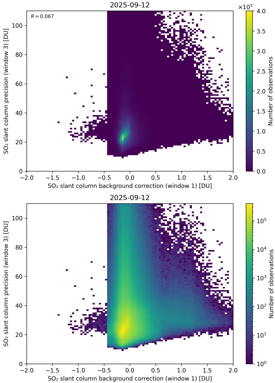
Figure 119: Scatter density plot of “SO 2 slant column background correction (window 1)” against “SO 2 slant column precision (window 3)” for 2025-09-11 to 2025-09-13.
