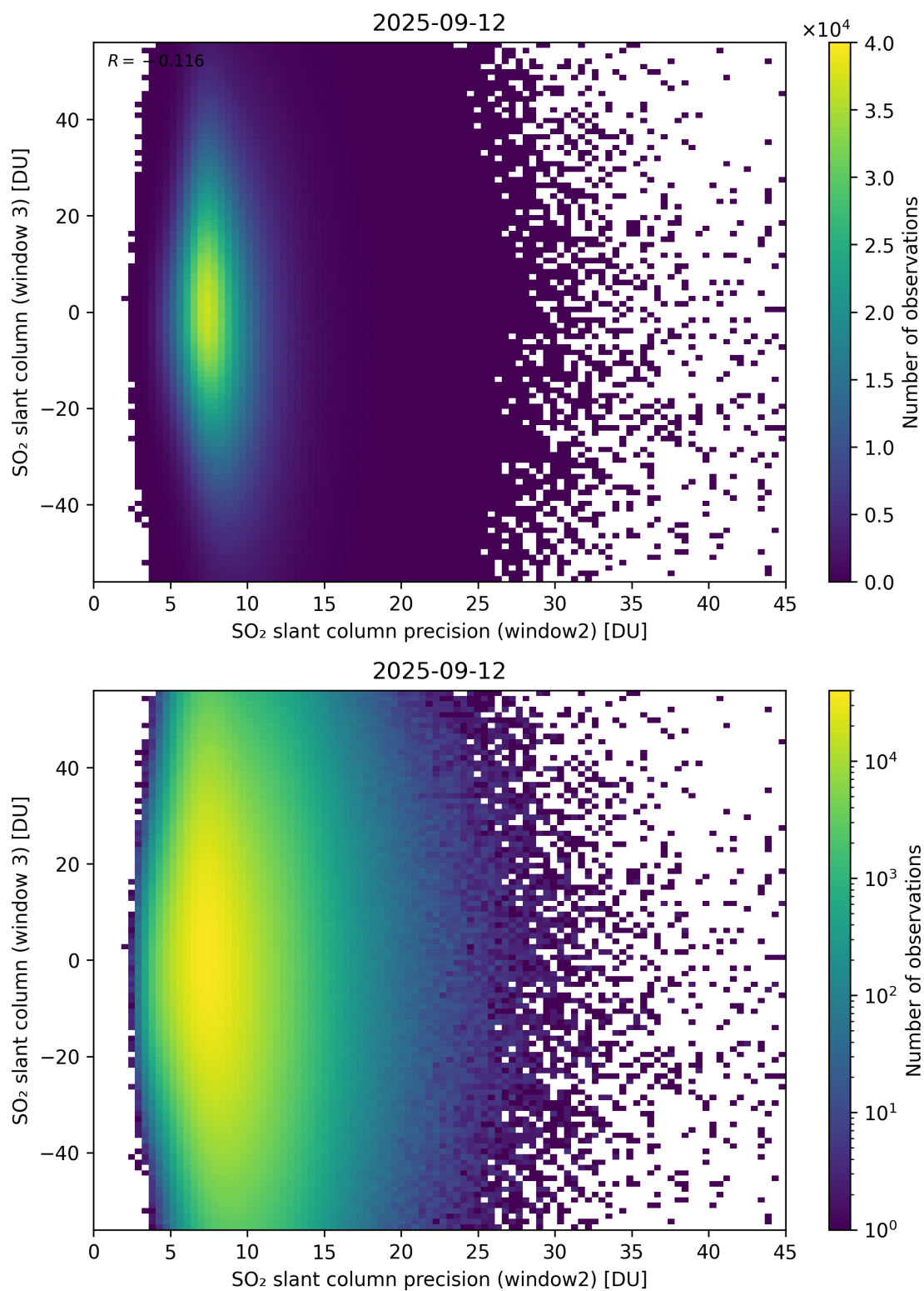
Figure 299: Scatter density plot of “SO 2 slant column precision (window2)” against “SO 2 slant column (window 3)” for 2025-09-11 to 2025-09-13.
