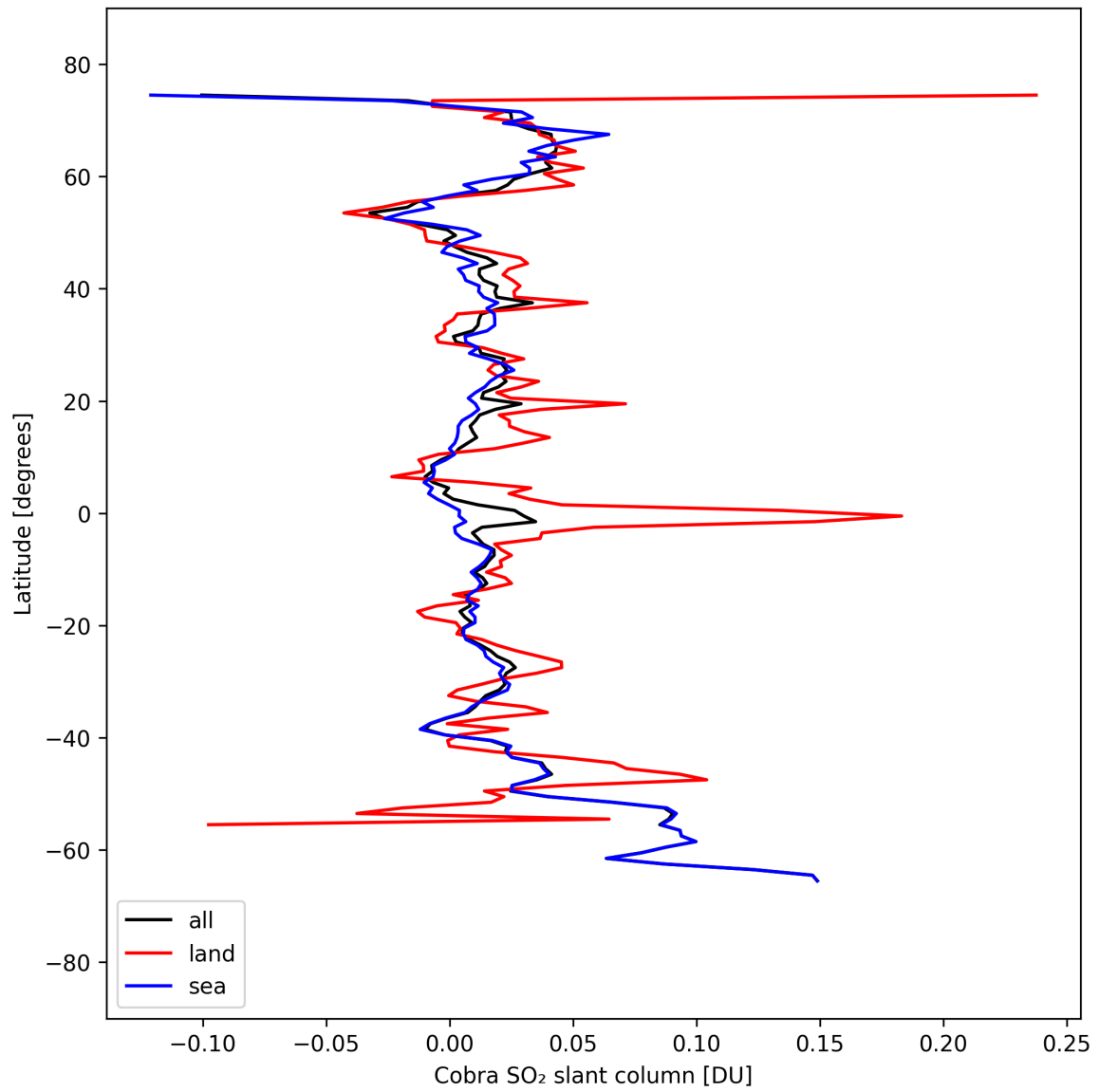
Figure 35: Zonal average of “Cobra SO 2 slant column” for 2025-09-11 to 2025-09-13.
