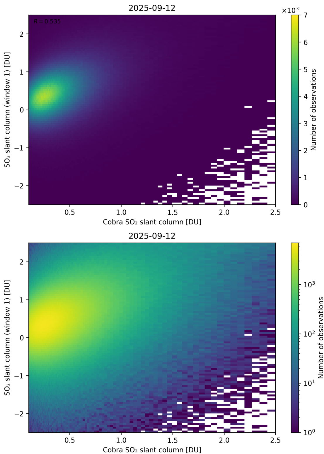
Figure 219: Scatter density plot of “Cobra SO 2 slant column” against “SO 2 slant column (window 1)” for 2025-09-11 to 2025-09-13.
