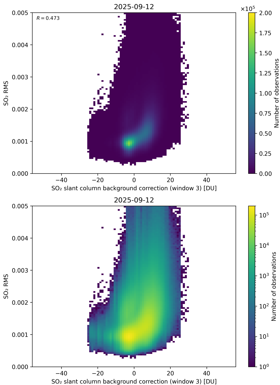
Figure 134: Scatter density plot of “SO 2 slant column background correction (window 3)” against “SO 2 RMS” for 2025-09-11 to 2025-09-13.
