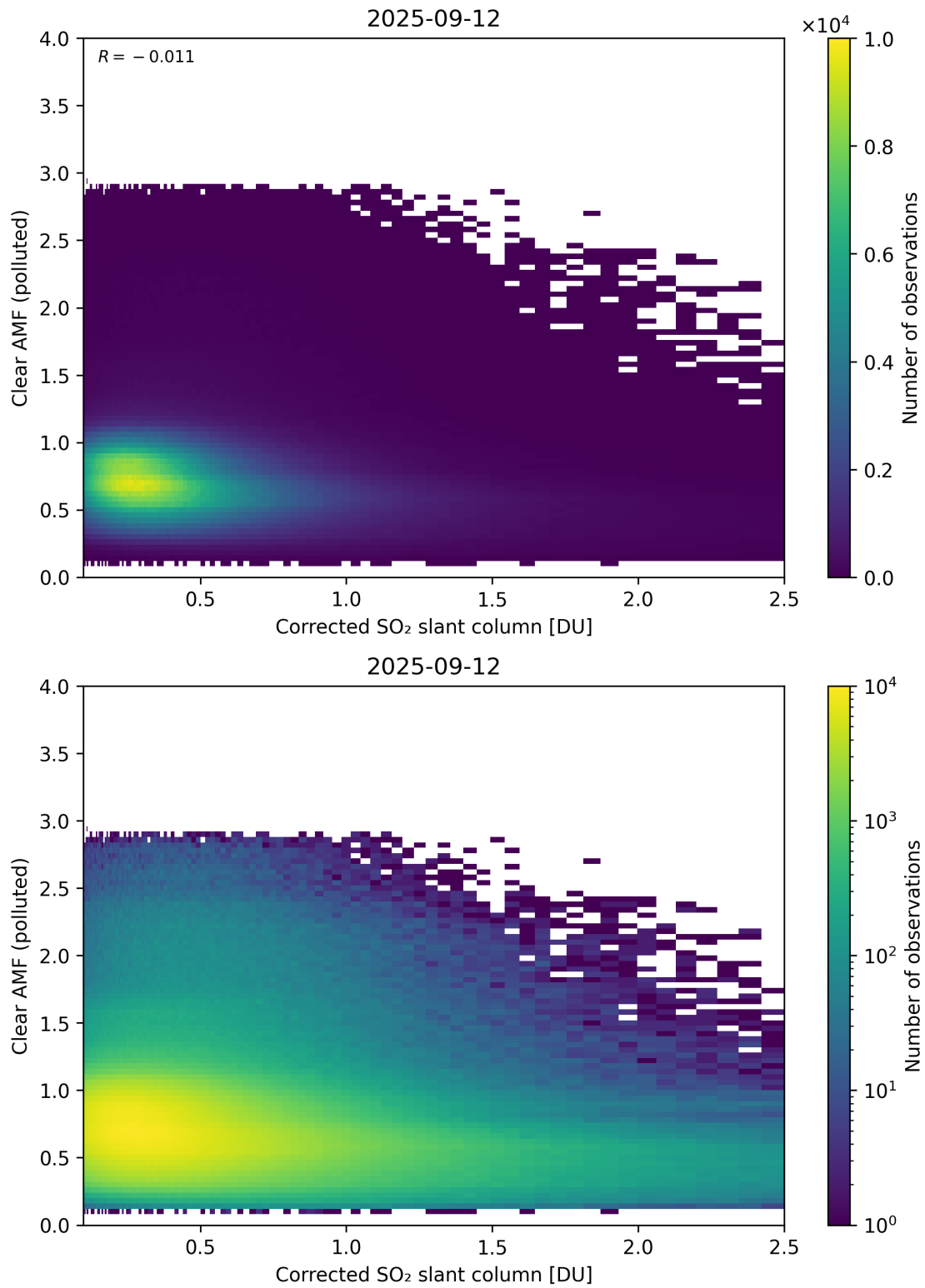
Figure 232: Scatter density plot of “Corrected SO 2 slant column” against “Clear AMF (polluted)” for 2025-09-11 to 2025-09-13.
