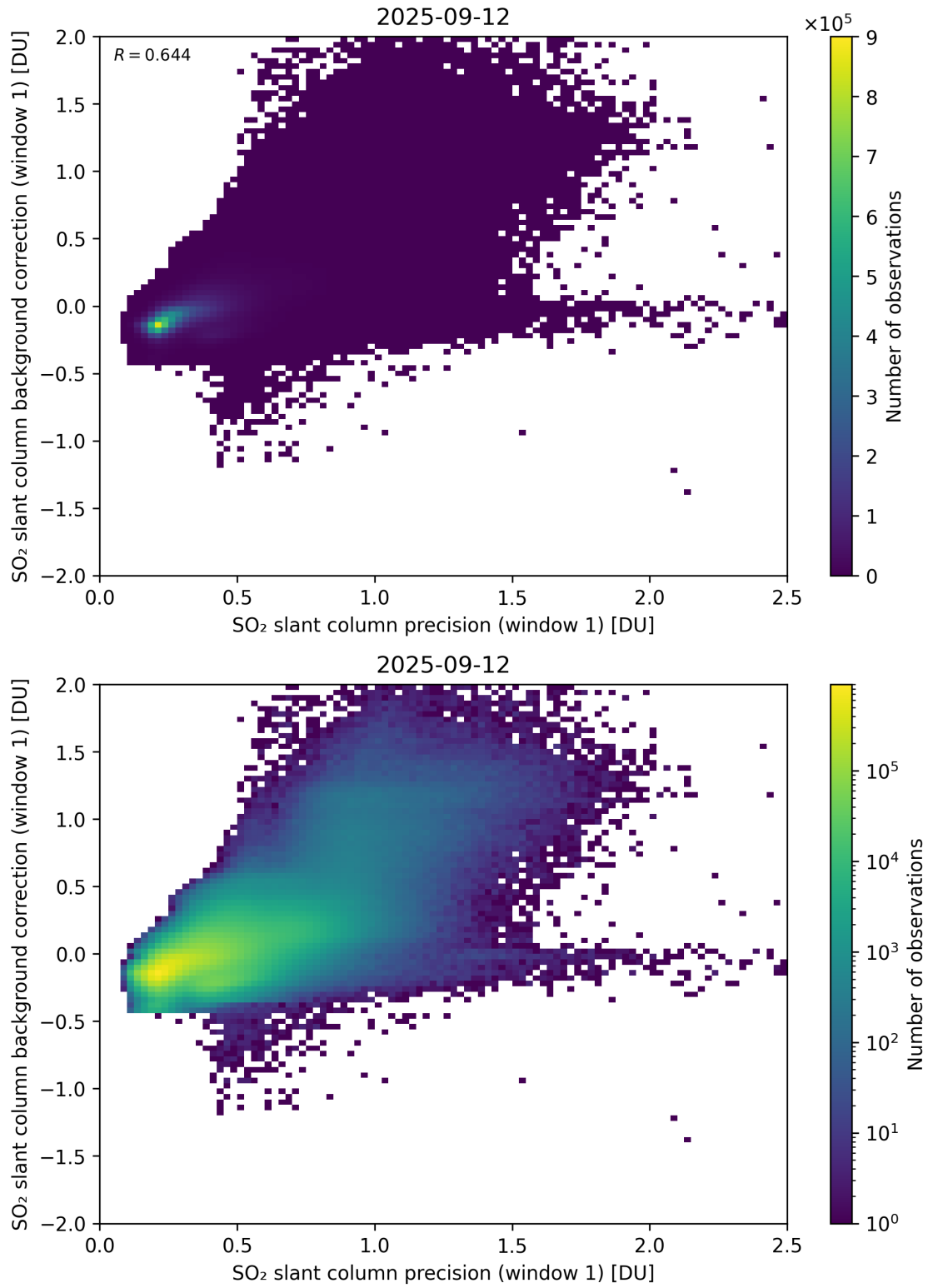
Figure 268: Scatter density plot of “SO 2 slant column precision (window 1)” against “SO 2 slant column background correction (window 1)” for 2025-09-11 to 2025-09-13.
