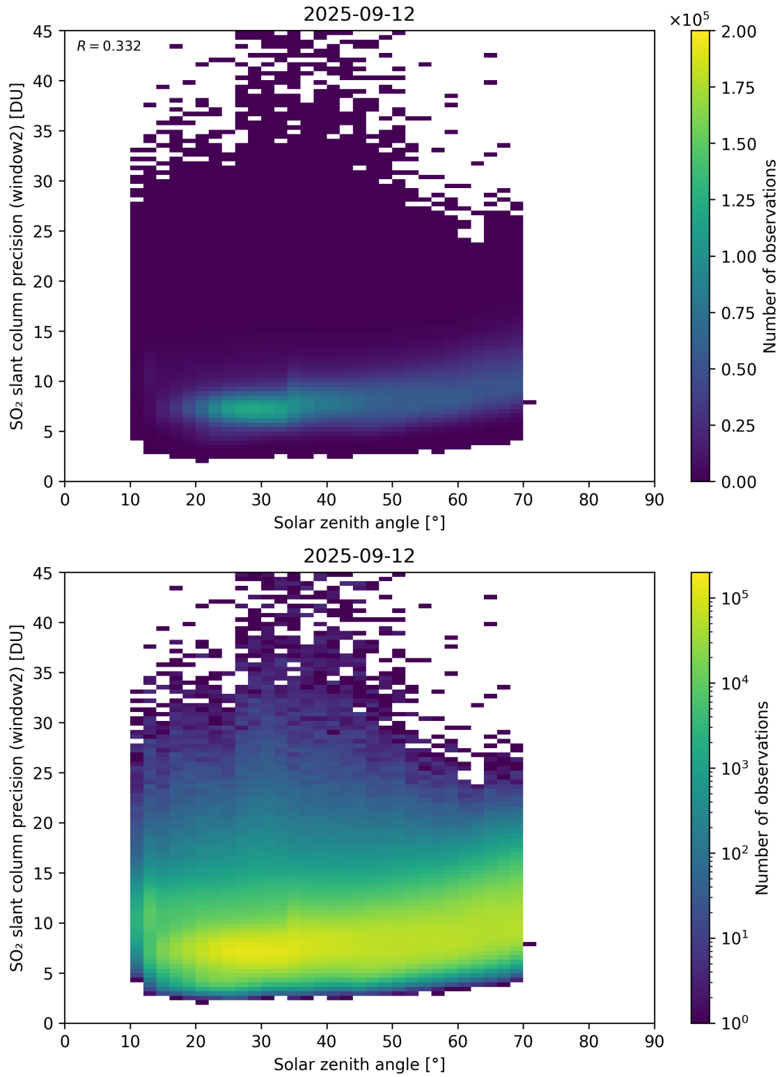
Figure 186: Scatter density plot of “Solar zenith angle” against “SO 2 slant column precision (window2)” for 2025-09-11 to 2025-09-13.
