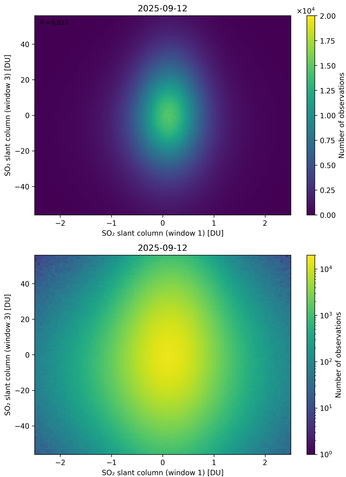
Figure 287: Scatter density plot of “SO 2 slant column (window 1)” against “SO 2 slant column (window 3)” for 2025-09-11 to 2025-09-13.
