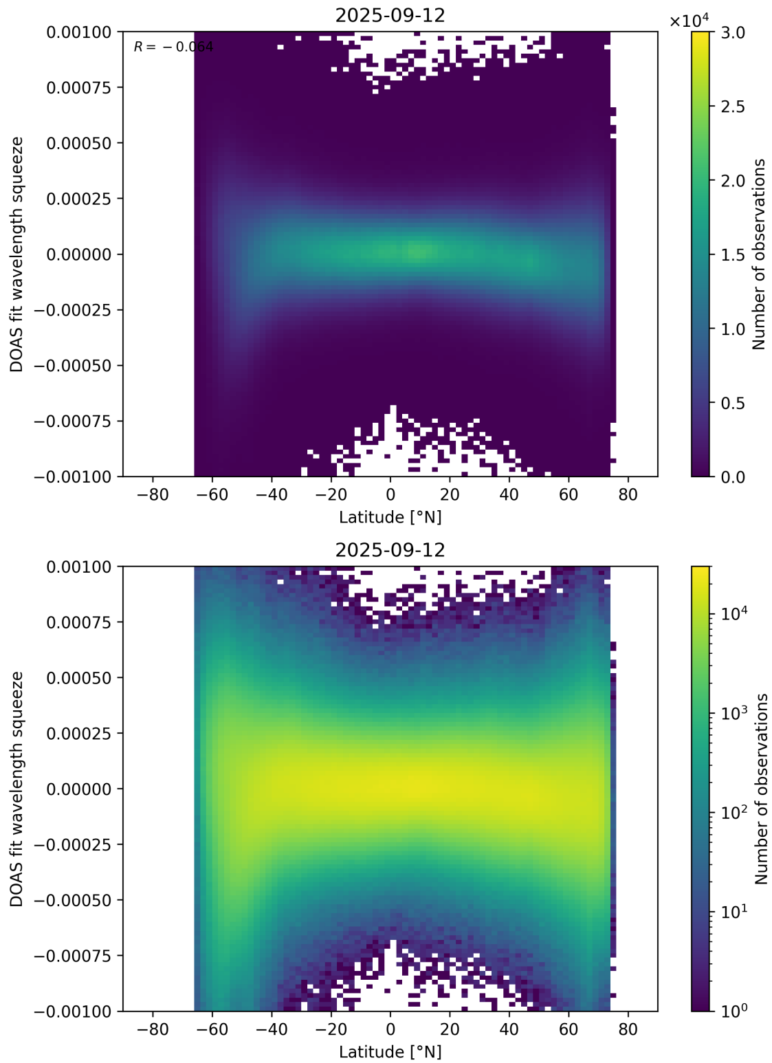
Figure 154: Scatter density plot of “Latitude” against “DOAS fit wavelength squeeze” for 2025-09-11 to 2025-09-13.
