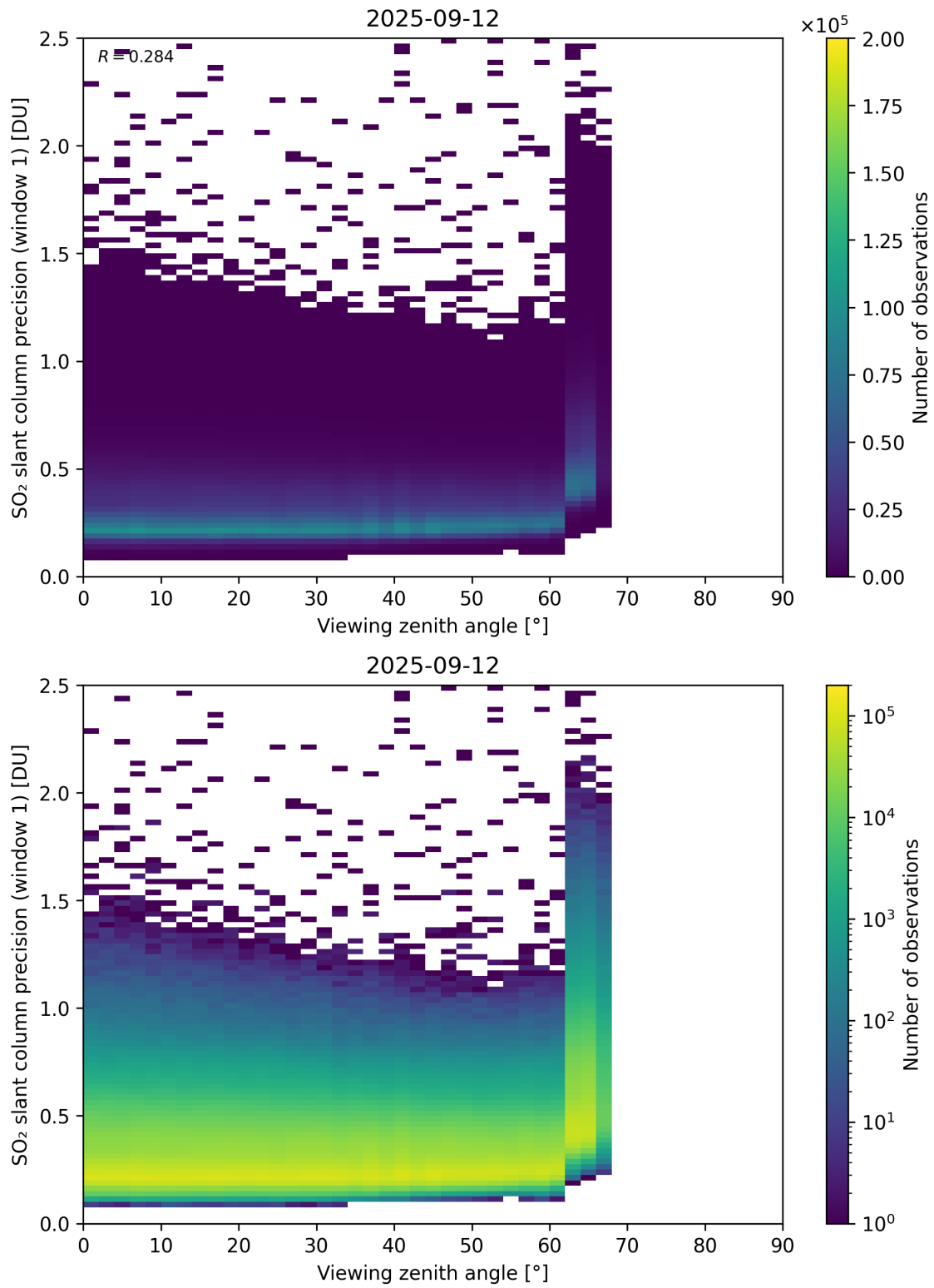
Figure 377: Scatter density plot of “Viewing zenith angle” against “SO 2 slant column precision (window 1)” for 2025-09-11 to 2025-09-13.
