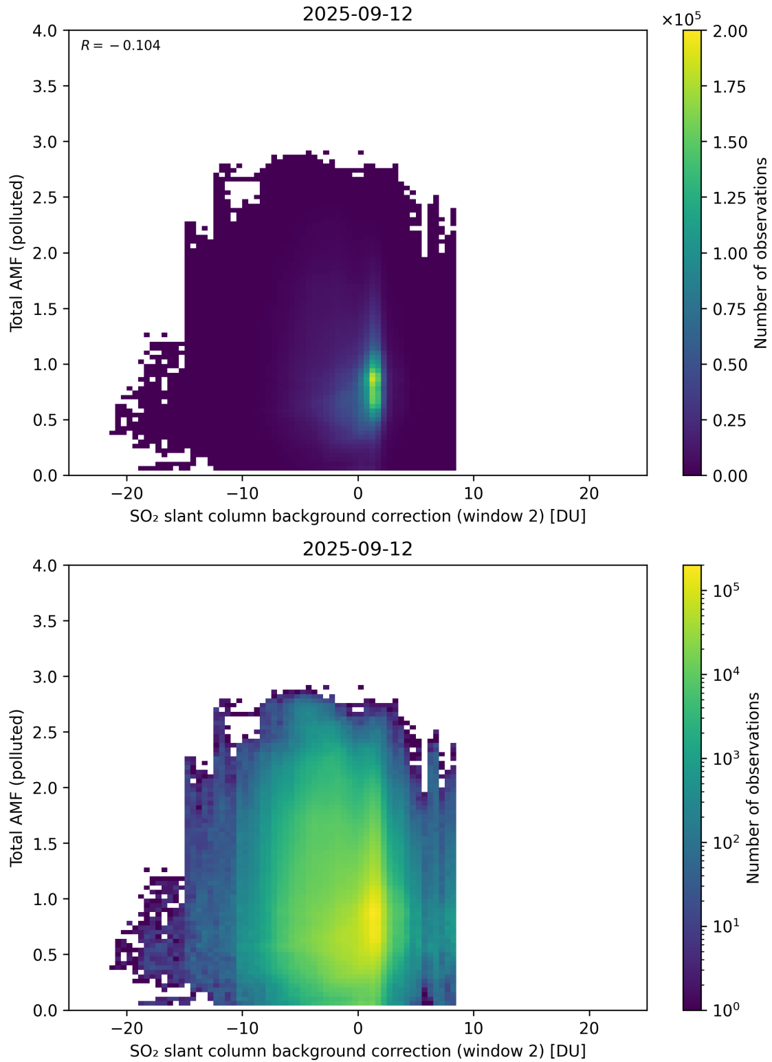
Figure 130: Scatter density plot of “SO 2 slant column background correction (window 2)” against “Total AMF (polluted)” for 2025-09-11 to 2025-09-13.
