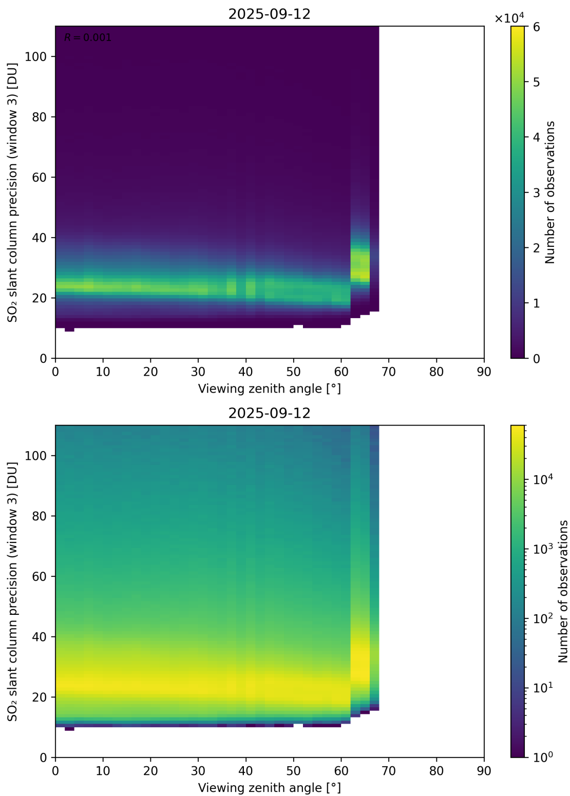
Figure 380: Scatter density plot of “Viewing zenith angle” against “SO 2 slant column precision (window 3)” for 2025-09-11 to 2025-09-13.
