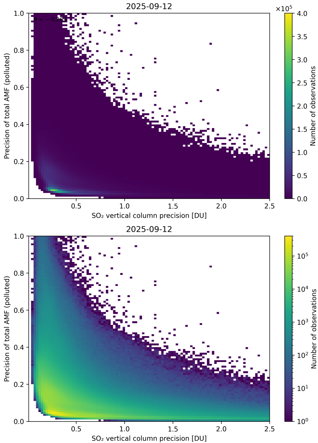
Figure 347: Scatter density plot of “SO 2 vertical column precision” against “Precision of total AMF (polluted)” for 2025-09-11 to 2025-09-13.
