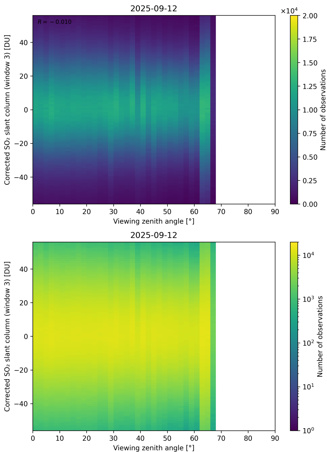
Figure 375: Scatter density plot of “Viewing zenith angle” against “Corrected SO 2 slant column (window 3)” for 2025-09-11 to 2025-09-13.
