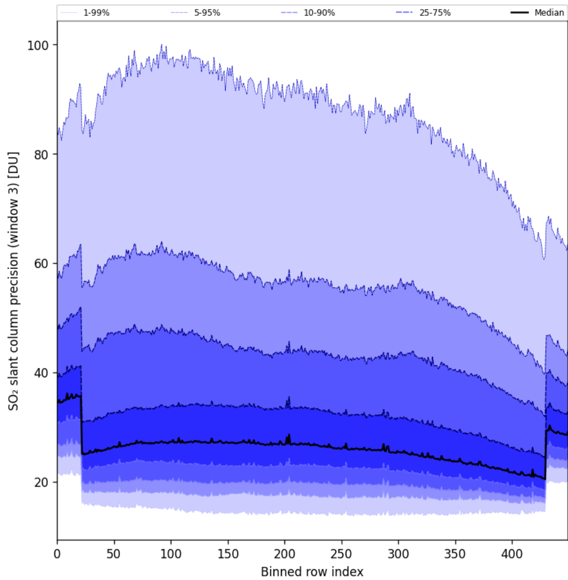
Figure 98: Along track statistics of “SO 2 slant column precision (window 3)” for 2025-09-11 to 2025-09-13
