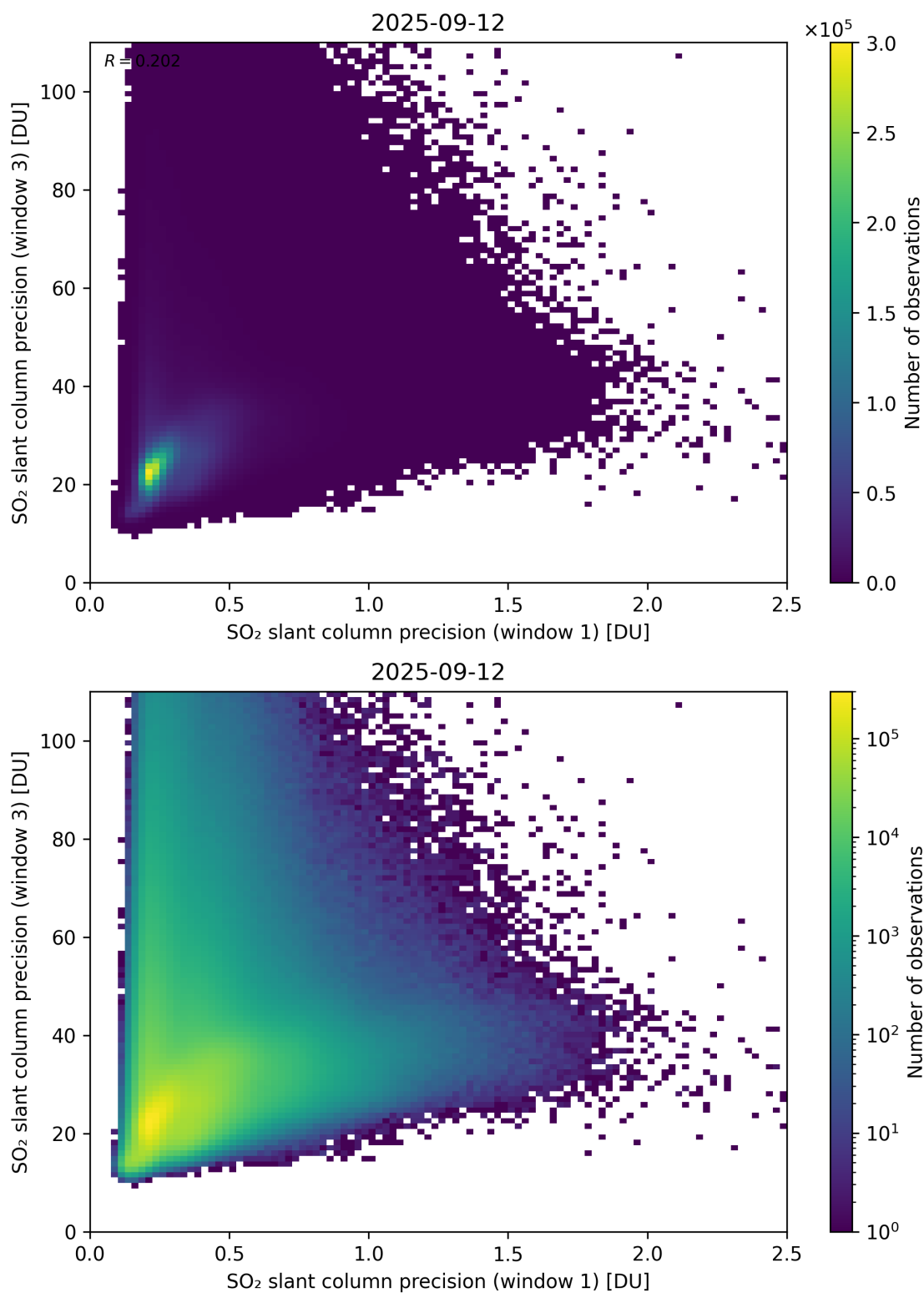
Figure 279: Scatter density plot of “SO 2 slant column precision (window 1)” against “SO 2 slant column precision (window 3)” for 2025-09-11 to 2025-09-13.
