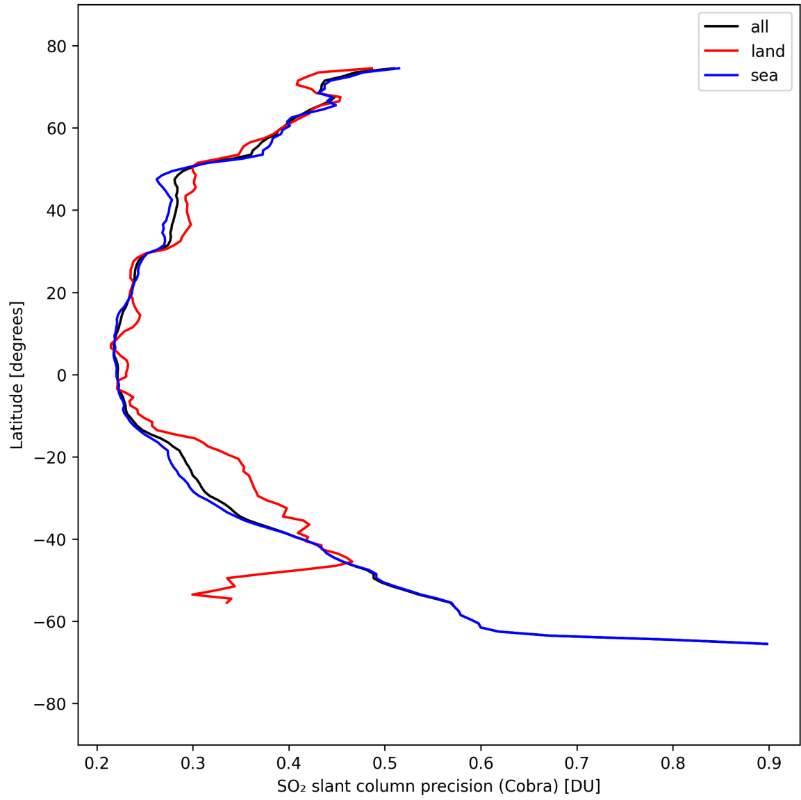
Figure 36: Zonal average of “SO 2 slant column precision (Cobra)” for 2025-09-11 to 2025-09-13.
