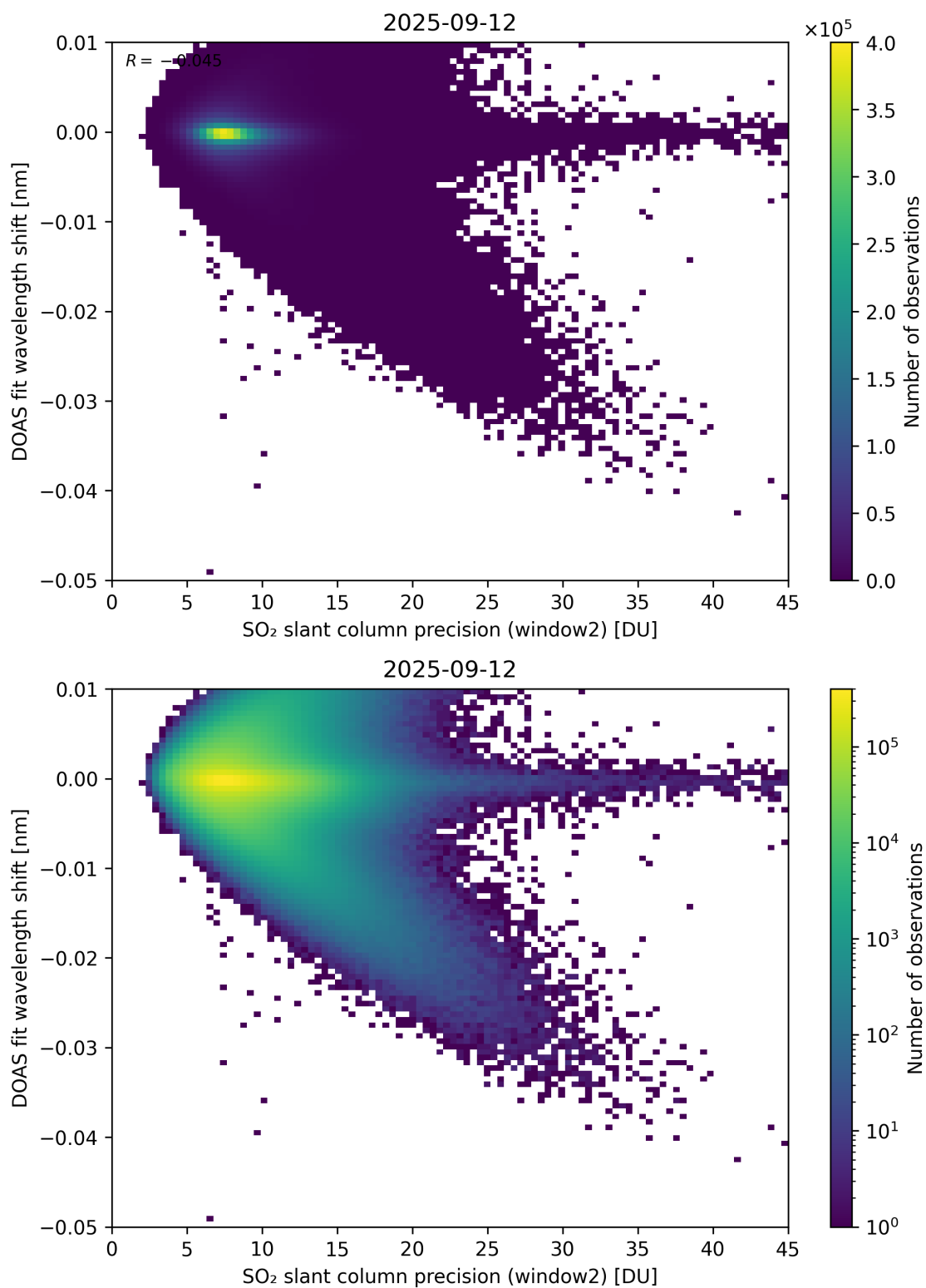
Figure 293: Scatter density plot of “SO 2 slant column precision (window2)” against “DOAS fit wavelength shift” for 2025-09-11 to 2025-09-13.
