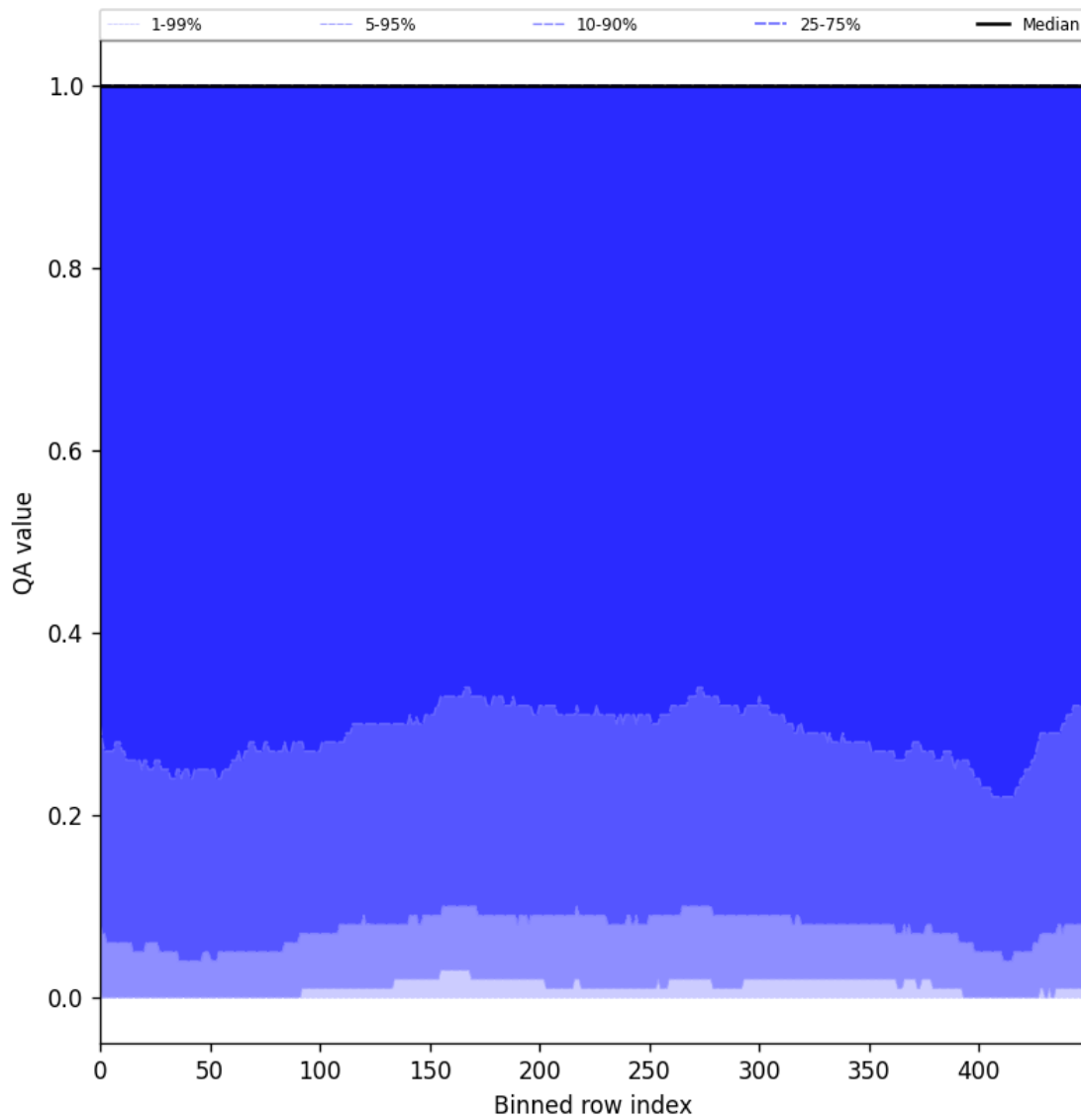
Figure 83: Along track statistics of “QA value” for 2025-09-11 to 2025-09-13
