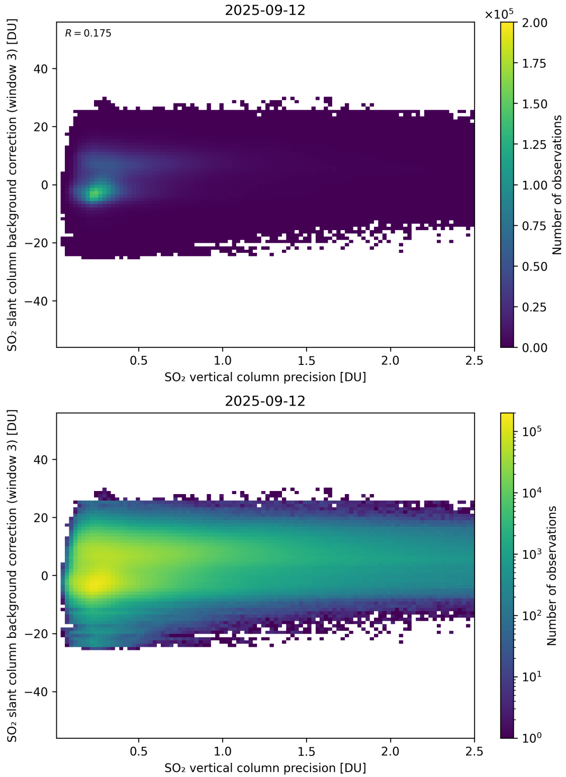
Figure 331: Scatter density plot of “SO 2 vertical column precision” against “SO 2 slant column background correction (window 3)” for 2025-09-11 to 2025-09-13.
