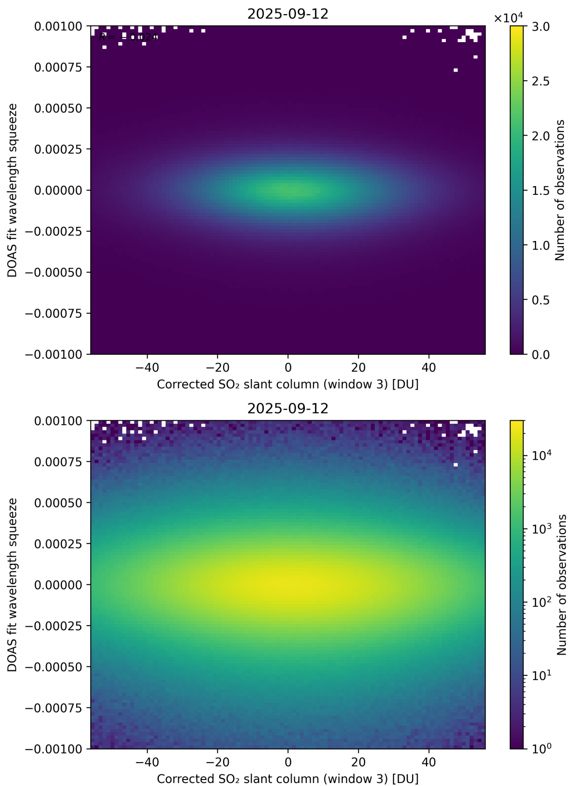
Figure 257: Scatter density plot of “Corrected SO 2 slant column (window 3)” against “DOAS fit wavelength squeeze” for 2025-09-11 to 2025-09-13.
