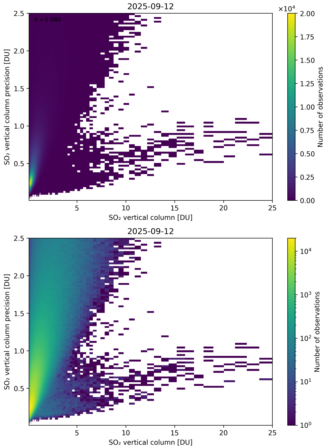
Figure 361: Scatter density plot of “SO 2 vertical column” against “SO 2 vertical column precision” for 2025-09-11 to 2025-09-13.
