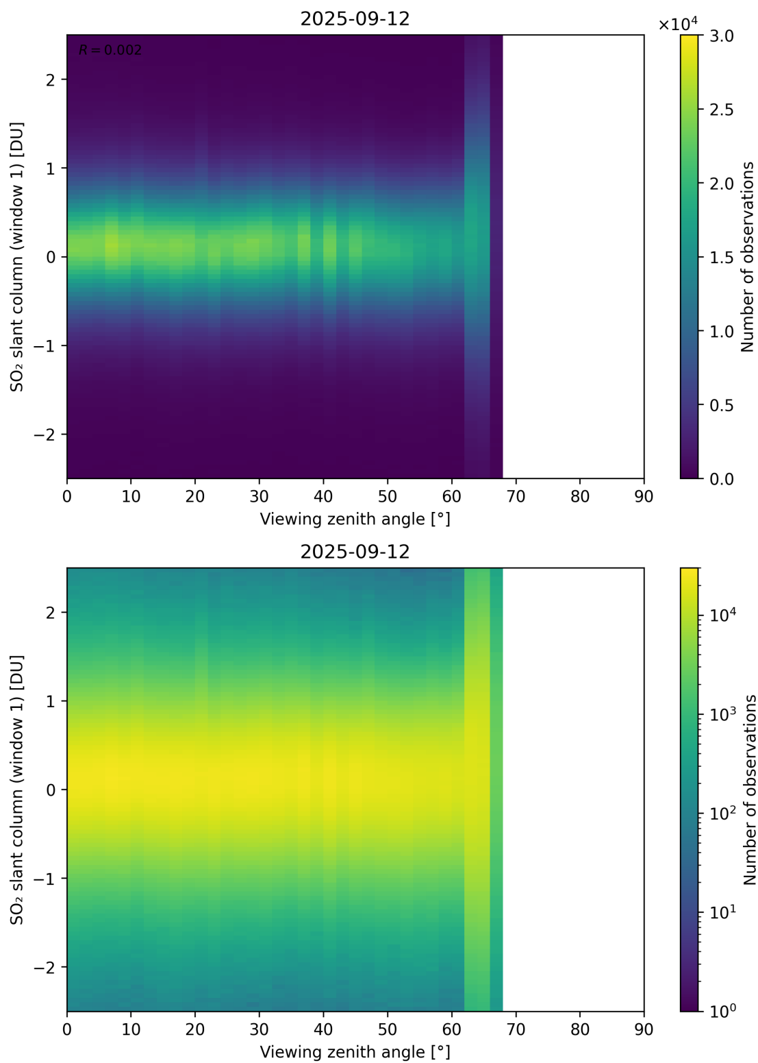
Figure 376: Scatter density plot of “Viewing zenith angle” against “SO 2 slant column (window 1)” for 2025-09-11 to 2025-09-13.
