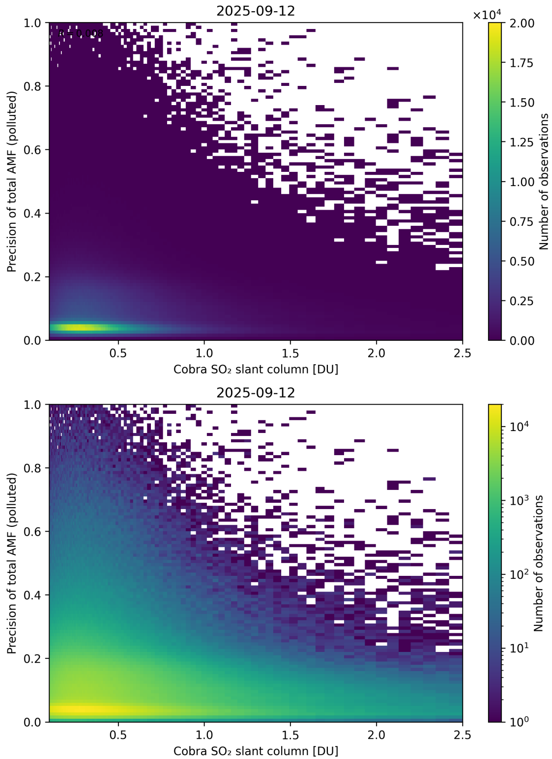
Figure 225: Scatter density plot of “Cobra SO 2 slant column” against “Precision of total AMF (polluted)” for 2025-09-11 to 2025-09-13.
