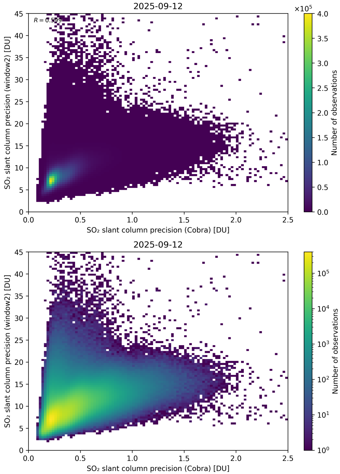
Figure 210: Scatter density plot of “SO 2 slant column precision (Cobra)” against “SO 2 slant column precision (window2)” for 2025-09-11 to 2025-09-13.
