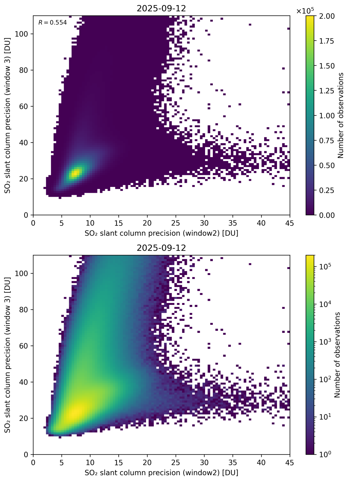
Figure 300: Scatter density plot of “SO 2 slant column precision (window2)” against “SO 2 slant column precision (window 3)” for 2025-09-11 to 2025-09-13.
