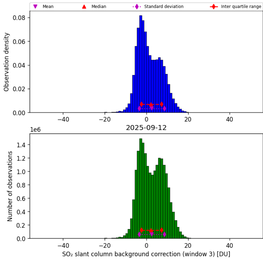
Figure 74: Histogram of “SO 2 slant column background correction (window 3)” for 2025-09-11 to 2025-09-13
