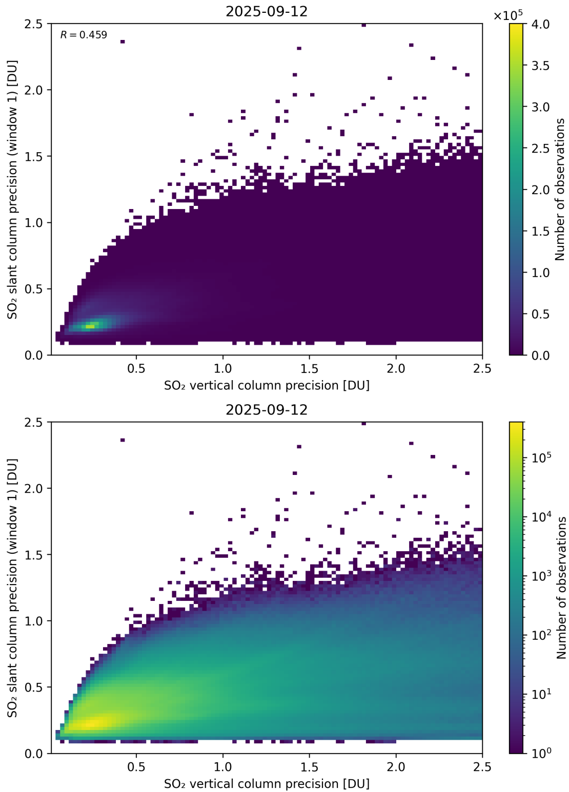
Figure 342: Scatter density plot of “SO 2 vertical column precision” against “SO 2 slant column precision (window 1)” for 2025-09-11 to 2025-09-13.
