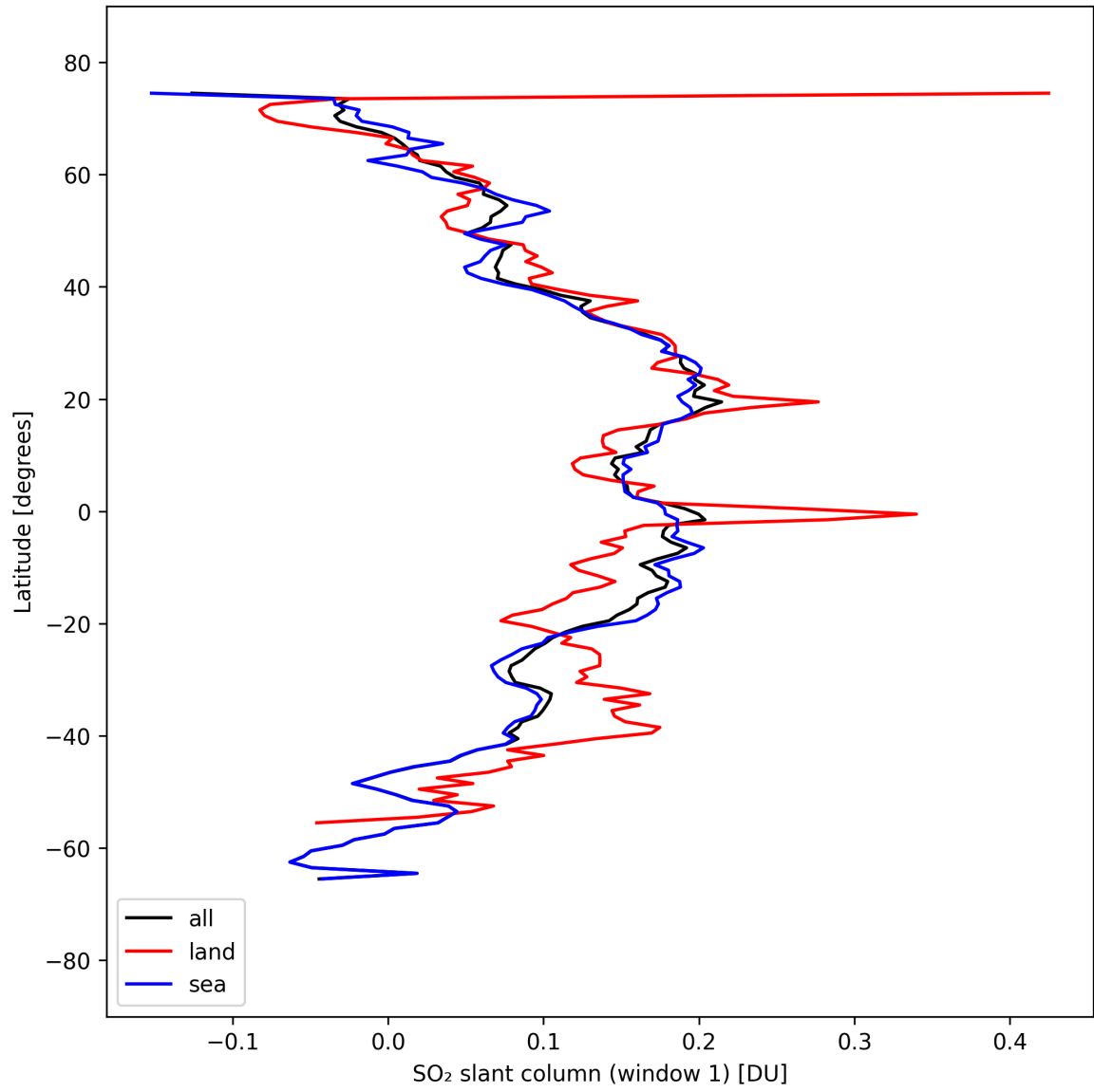
Figure 37: Zonal average of “SO 2 slant column (window 1)” for 2025-09-11 to 2025-09-13.
