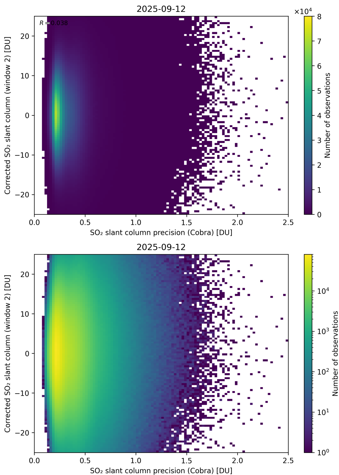
Figure 206: Scatter density plot of “SO 2 slant column precision (Cobra)” against “Corrected SO 2 slant column (window 2)” for 2025-09-11 to 2025-09-13.
