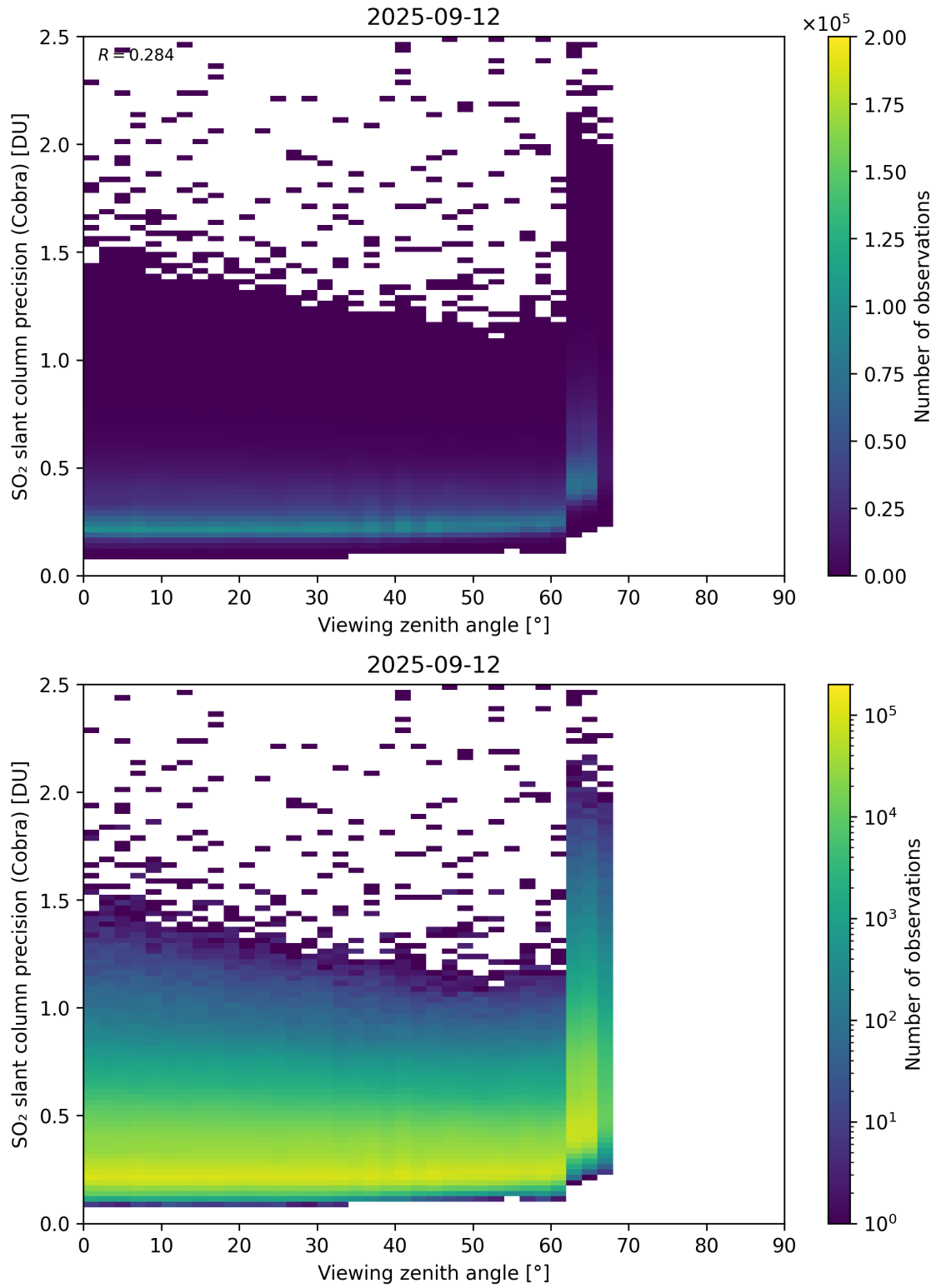
Figure 372: Scatter density plot of “Viewing zenith angle” against “SO 2 slant column precision (Cobra)” for 2025-09-11 to 2025-09-13.
