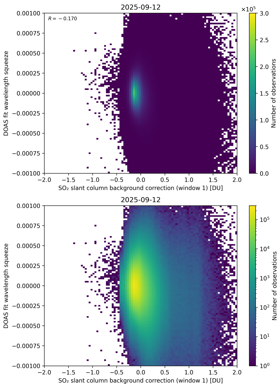
Figure 112: Scatter density plot of “SO 2 slant column background correction (window 1)” against “DOAS fit wavelength squeeze” for 2025-09-11 to 2025-09-13.
