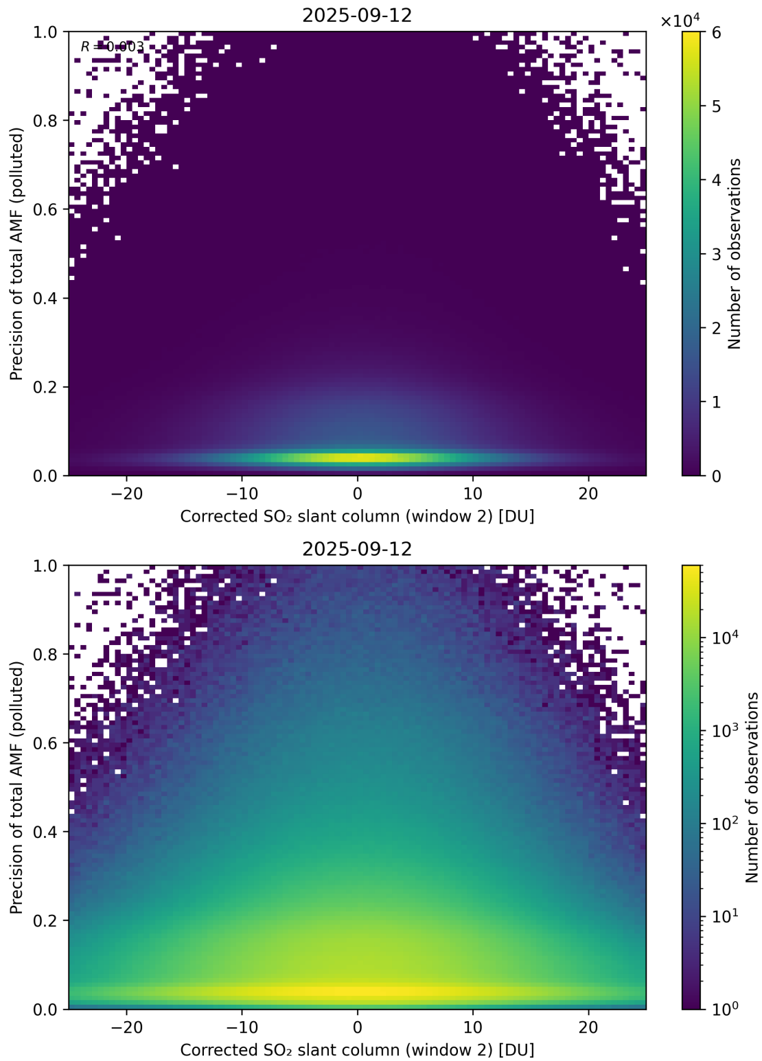
Figure 254: Scatter density plot of “Corrected SO 2 slant column (window 2)” against “Precision of total AMF (polluted)” for 2025-09-11 to 2025-09-13.
