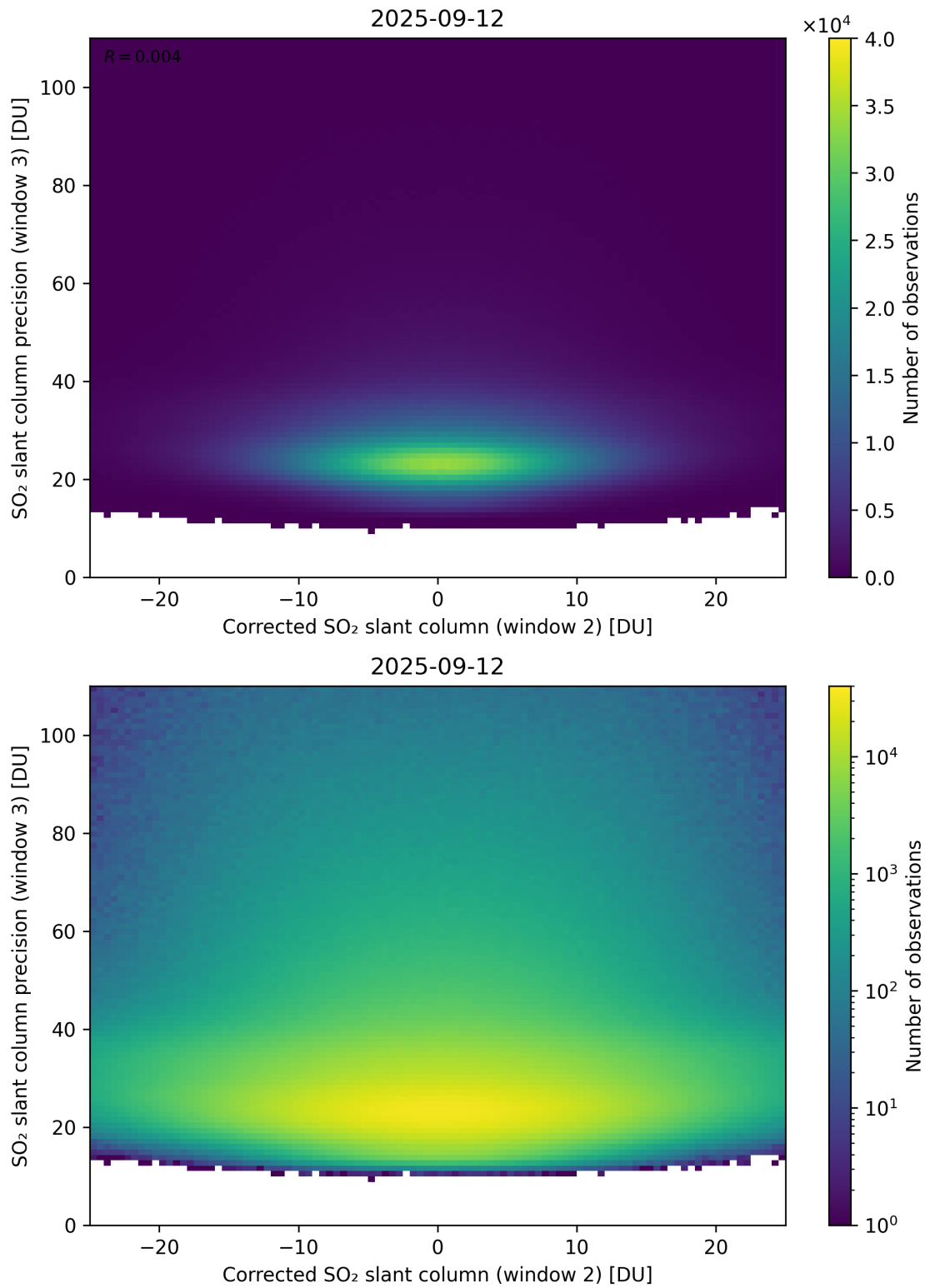
Figure 252: Scatter density plot of “Corrected SO 2 slant column (window 2)” against “SO 2 slant column precision (window 3)” for 2025-09-11 to 2025-09-13.
