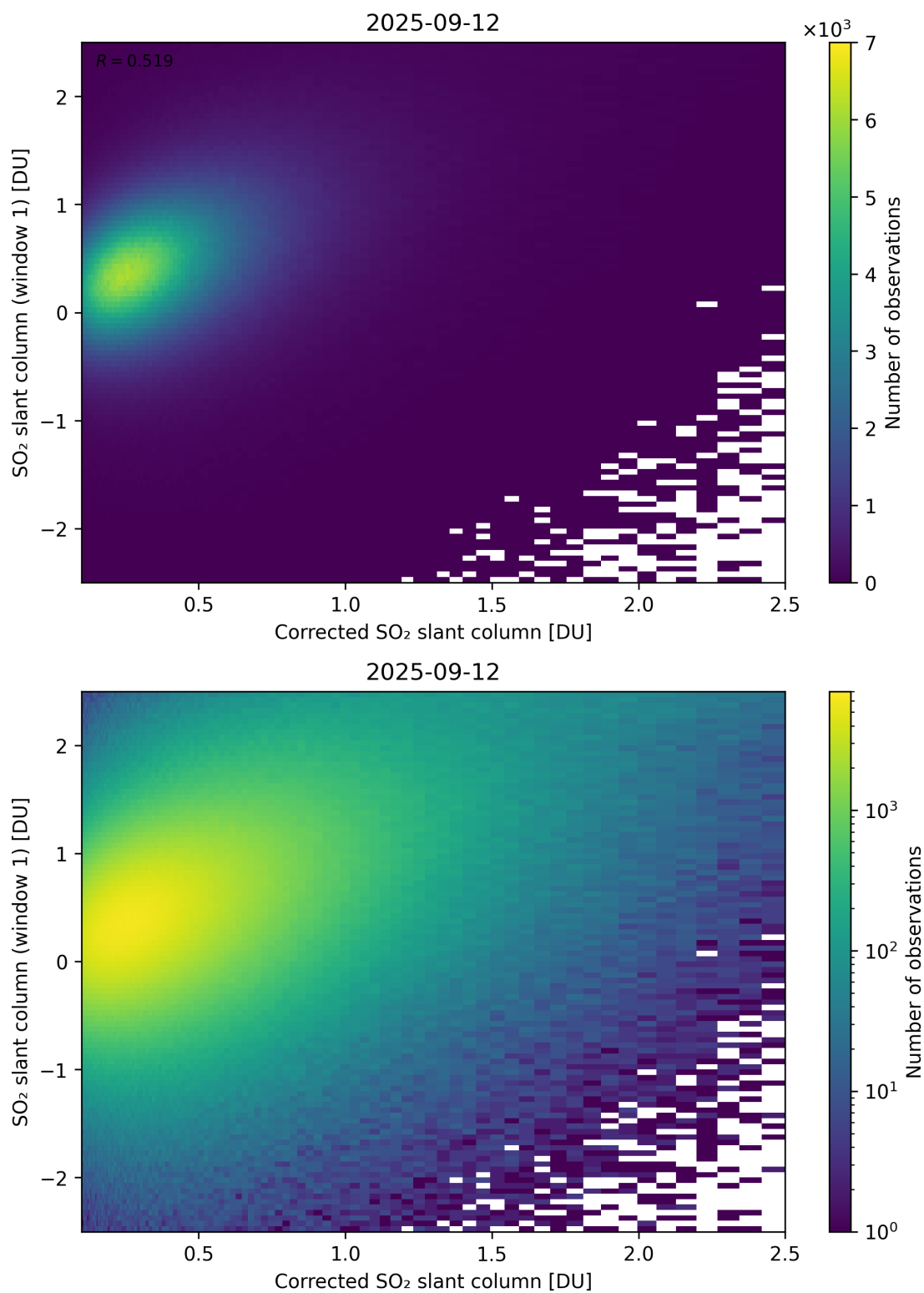
Figure 237: Scatter density plot of “Corrected SO 2 slant column” against “SO 2 slant column (window 1)” for 2025-09-11 to 2025-09-13.
