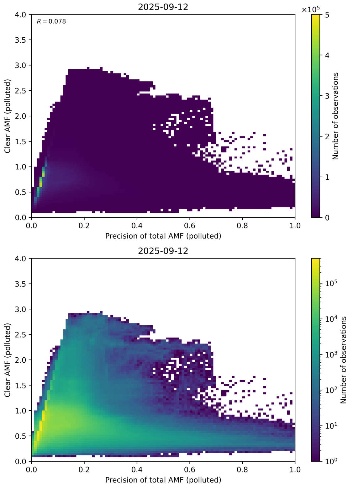
Figure 320: Scatter density plot of “Precision of total AMF (polluted)” against “Clear AMF (polluted)” for 2025-09-11 to 2025-09-13.
