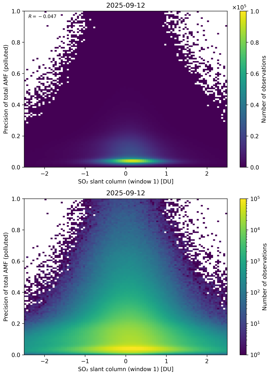
Figure 290: Scatter density plot of “SO 2 slant column (window 1)” against “Precision of total AMF (polluted)” for 2025-09-11 to 2025-09-13.
