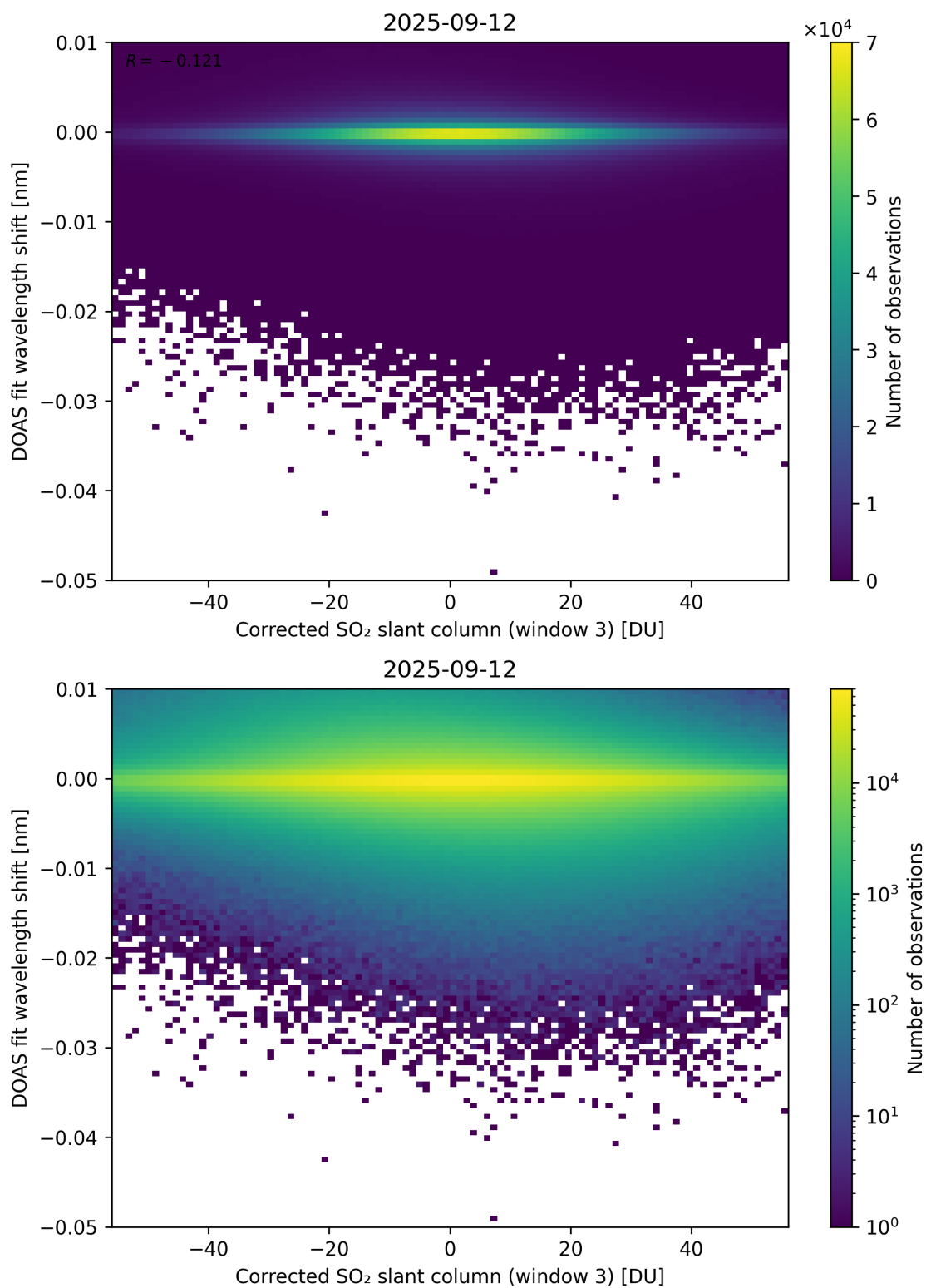
Figure 256: Scatter density plot of “Corrected SO 2 slant column (window 3)” against “DOAS fit wavelength shift” for 2025-09-11 to 2025-09-13.
