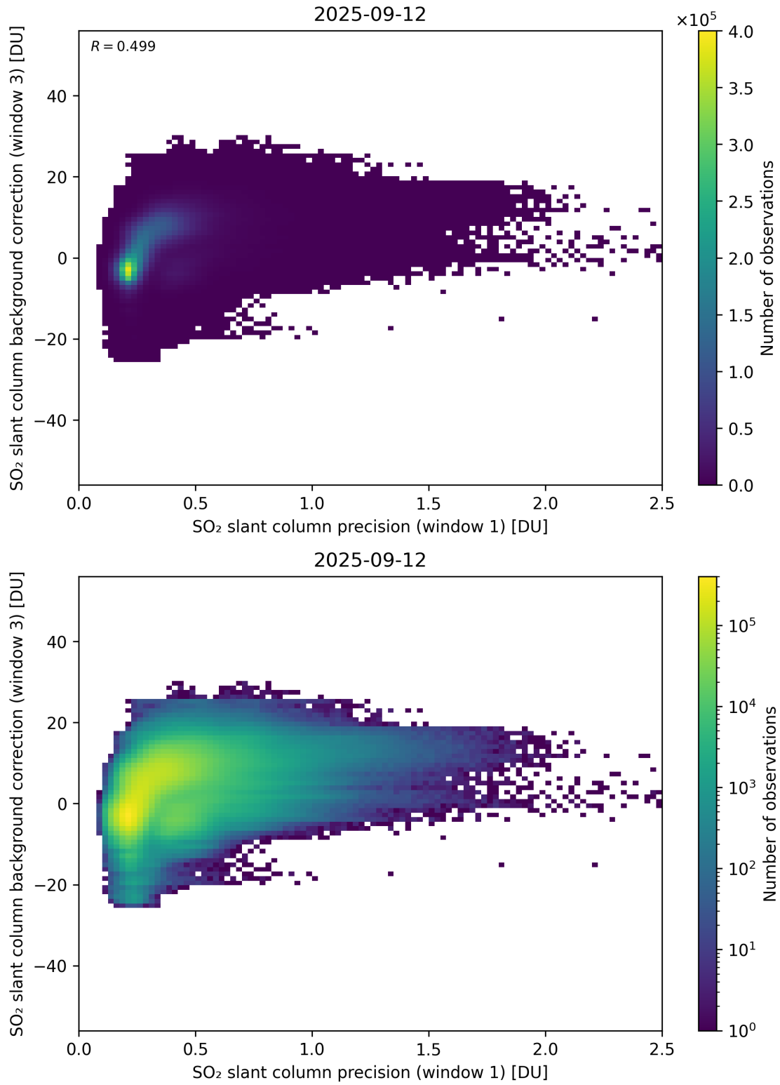
Figure 270: Scatter density plot of “SO 2 slant column precision (window 1)” against “SO 2 slant column background correction (window 3)” for 2025-09-11 to 2025-09-13.
