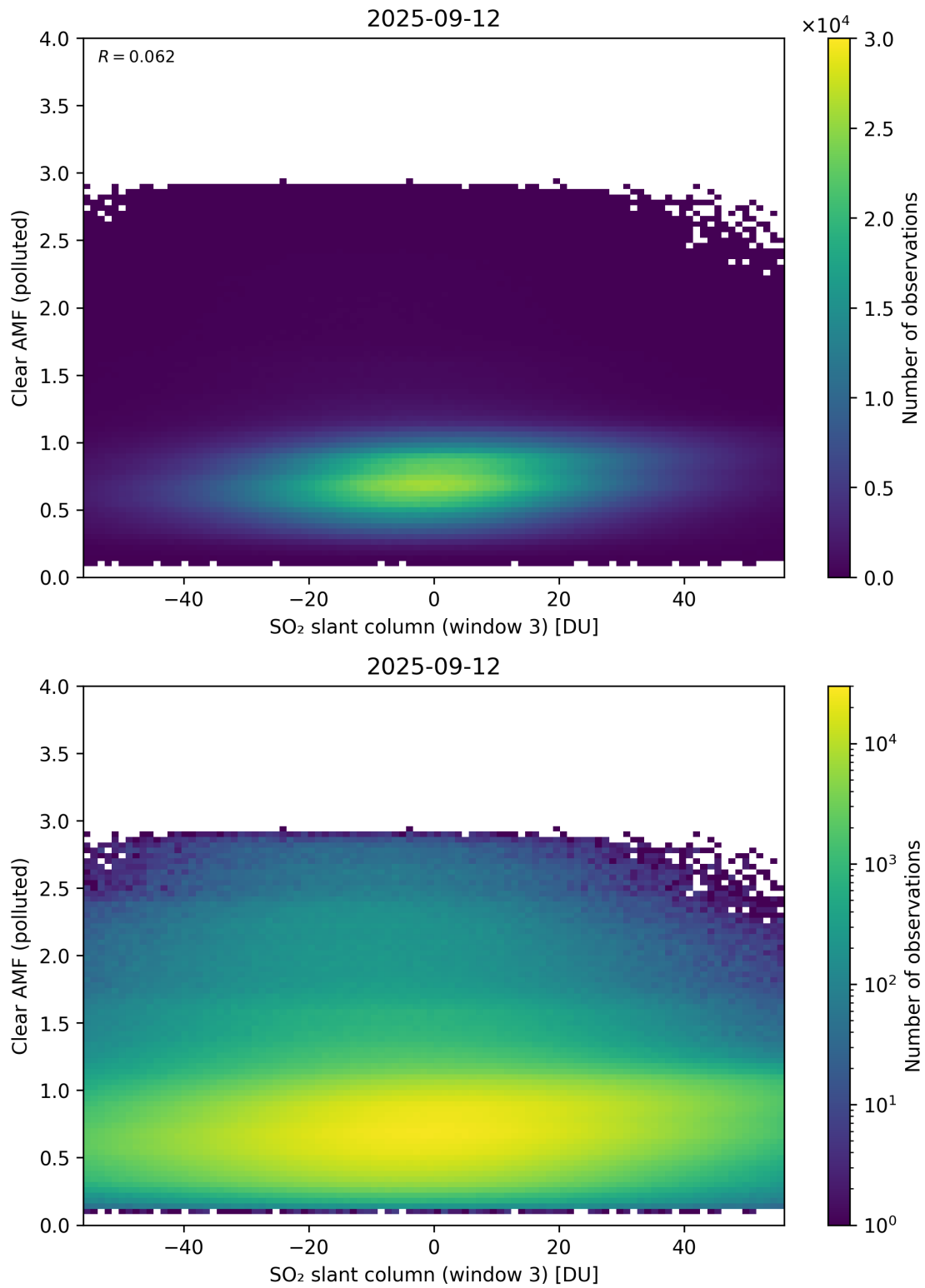
Figure 315: Scatter density plot of “SO 2 slant column (window 3)” against “Clear AMF (polluted)” for 2025-09-11 to 2025-09-13.
