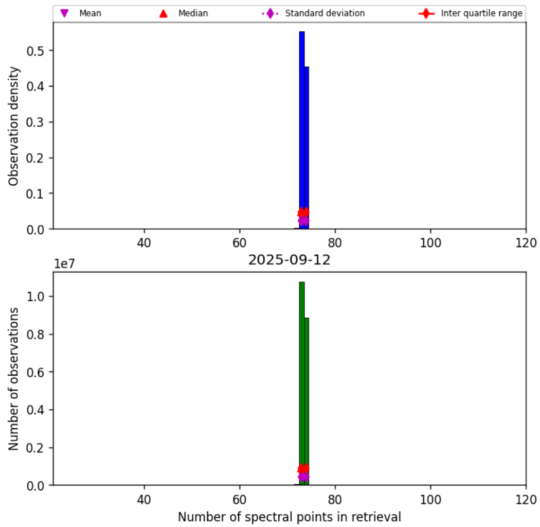
Figure 82: Histogram of “Number of spectral points in retrieval” for 2025-09-11 to 2025-09-13
