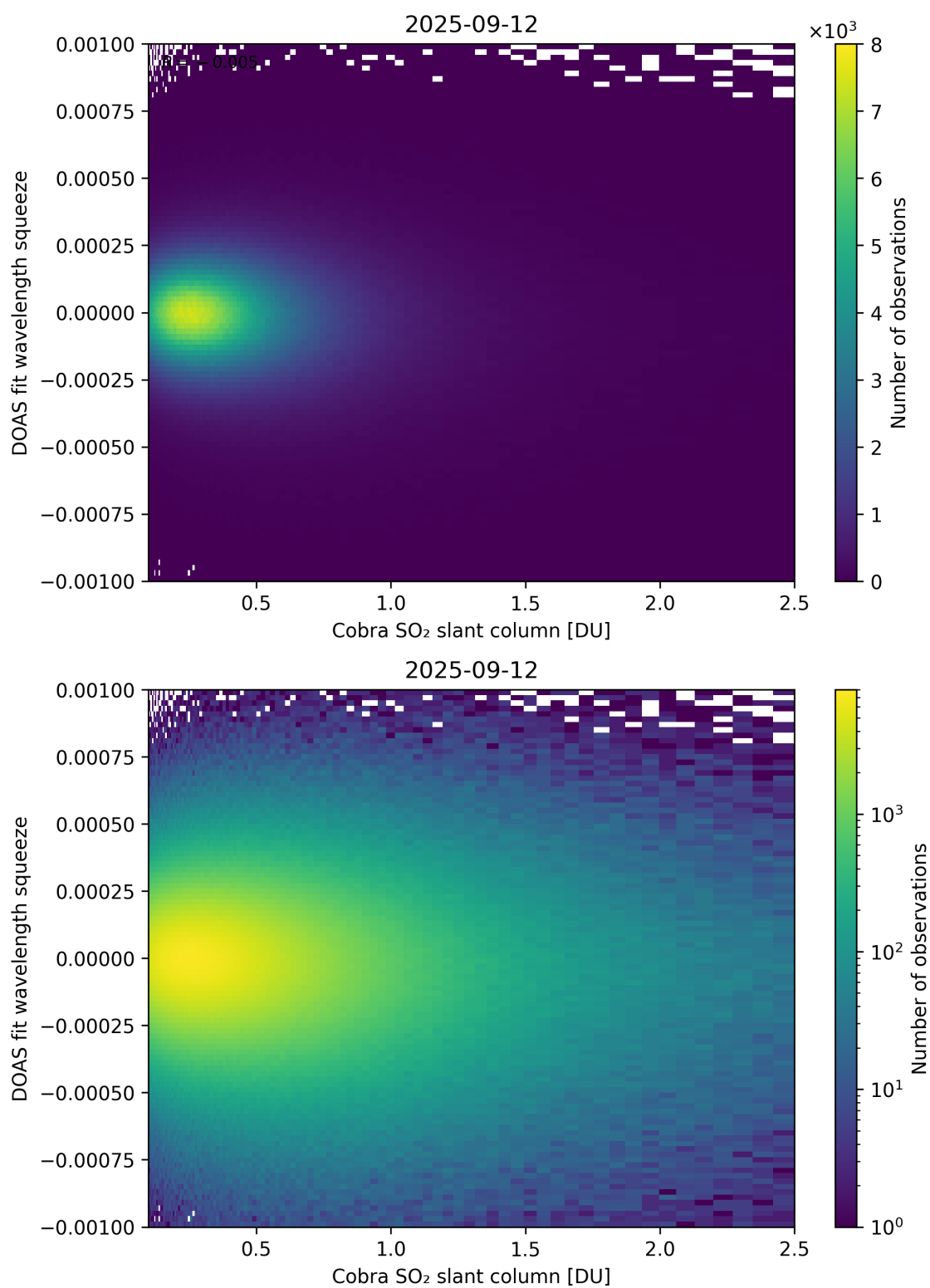
Figure 197: Scatter density plot of “Cobra SO 2 slant column” against “DOAS fit wavelength squeeze” for 2025-09-11 to 2025-09-13.
