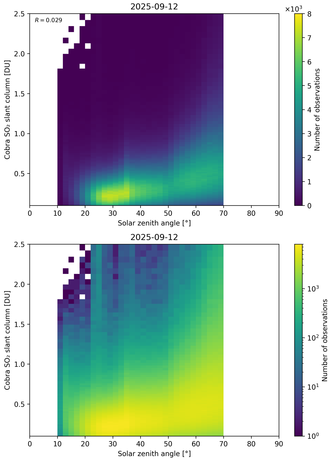
Figure 179: Scatter density plot of “Solar zenith angle” against “Cobra SO 2 slant column” for 2025-09-11 to 2025-09-13.
