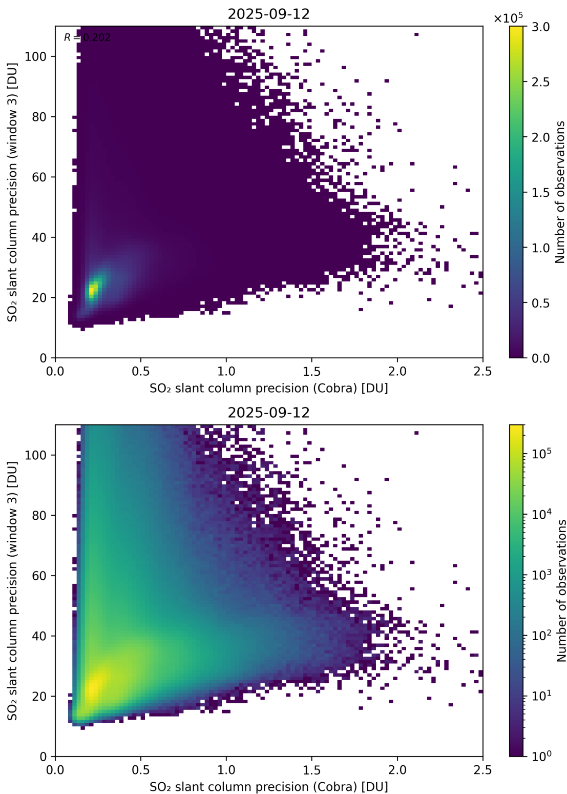
Figure 212: Scatter density plot of “SO 2 slant column precision (Cobra)” against “SO 2 slant column precision (window 3)” for 2025-09-11 to 2025-09-13.
