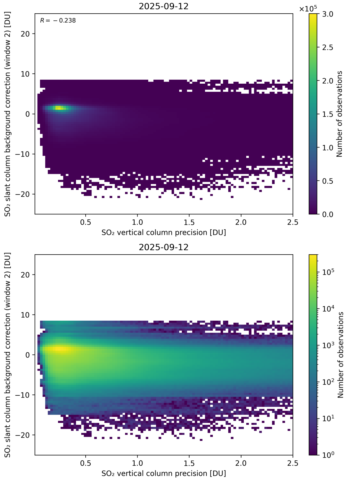
Figure 330: Scatter density plot of “SO 2 vertical column precision” against “SO 2 slant column background correction (window 2)” for 2025-09-11 to 2025-09-13.
