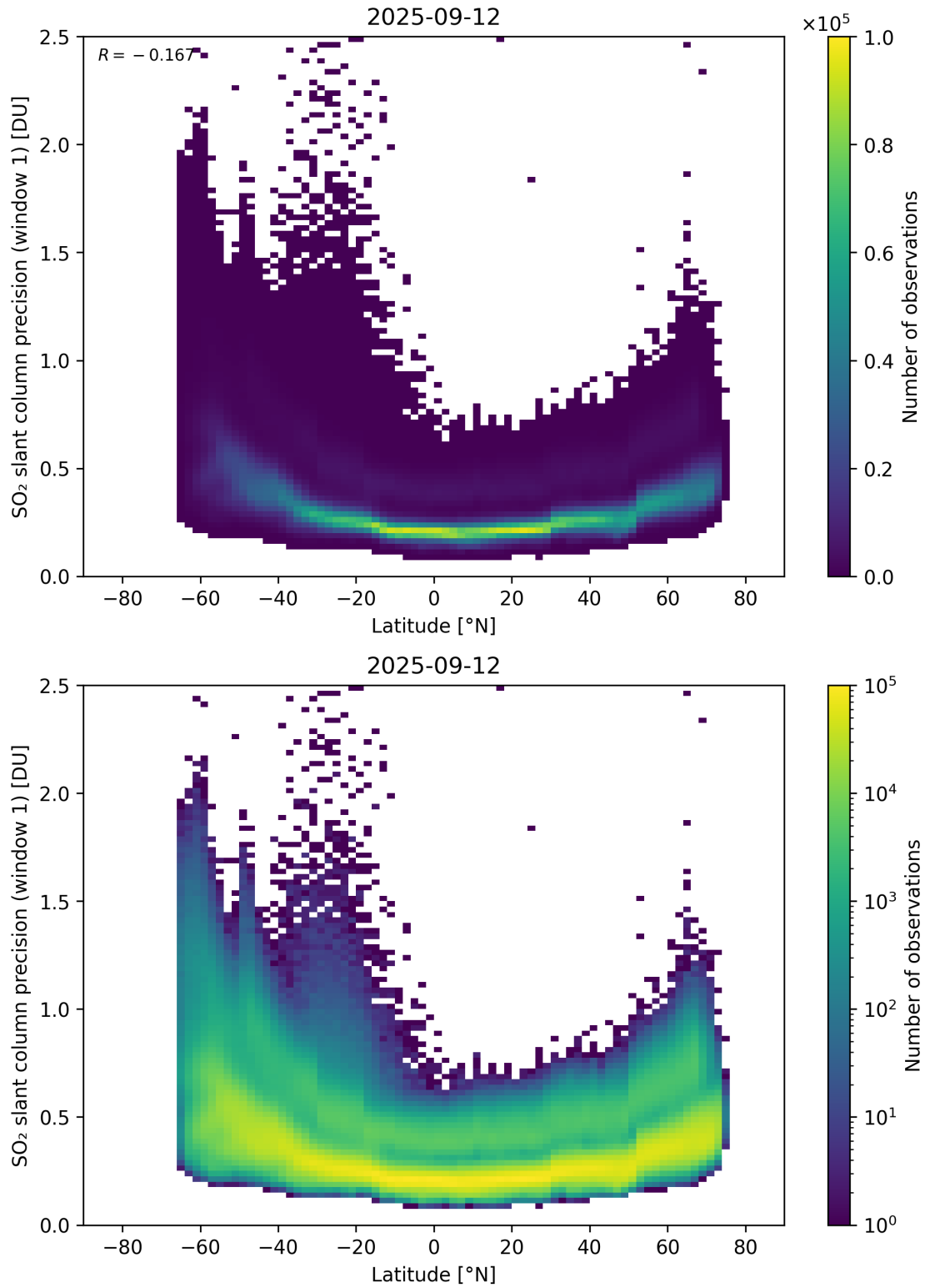
Figure 163: Scatter density plot of “Latitude” against “SO 2 slant column precision (window 1)” for 2025-09-11 to 2025-09-13.
