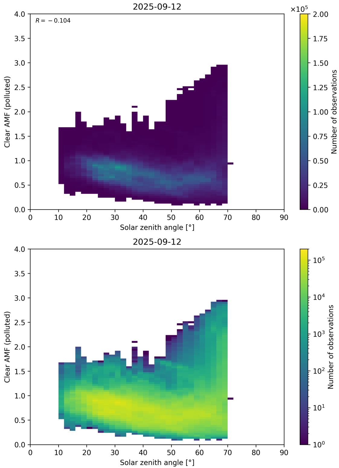
Figure 178: Scatter density plot of “Solar zenith angle” against “Clear AMF (polluted)” for 2025-09-11 to 2025-09-13.
