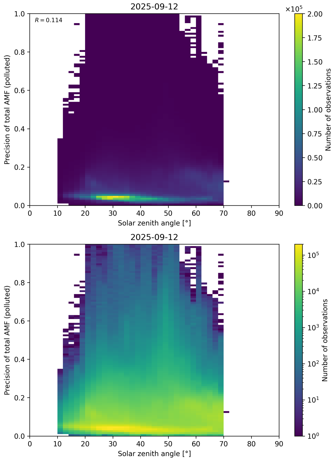
Figure 190: Scatter density plot of “Solar zenith angle” against “Precision of total AMF (polluted)” for 2025-09-11 to 2025-09-13.
