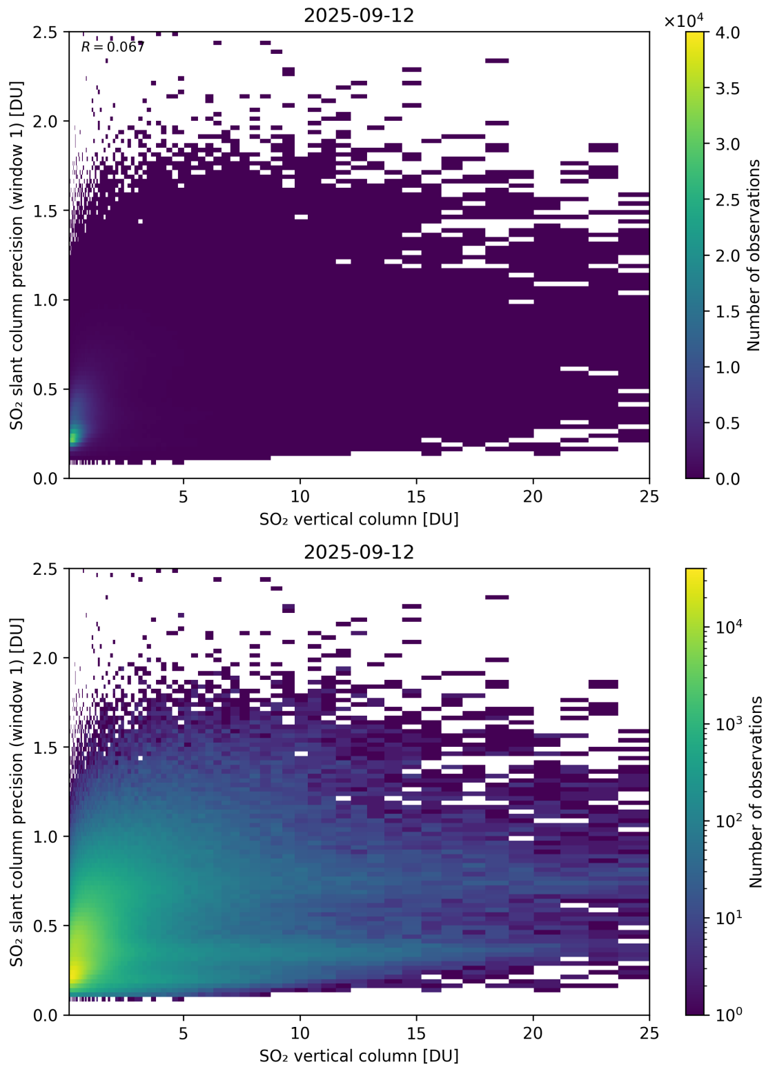
Figure 355: Scatter density plot of “SO 2 vertical column” against “SO 2 slant column precision (window 1)” for 2025-09-11 to 2025-09-13.
