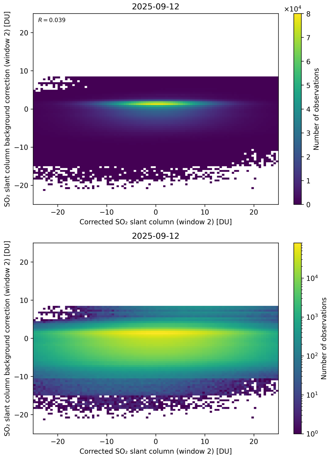
Figure 244: Scatter density plot of “Corrected SO 2 slant column (window 2)” against “SO 2 slant column background correction (window 2)” for 2025-09-11 to 2025-09-13.
