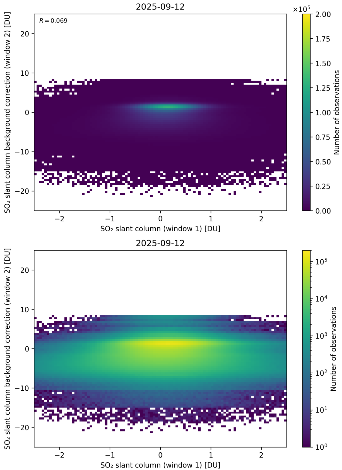
Figure 263: Scatter density plot of “SO 2 slant column (window 1)” against “SO 2 slant column background correction (window 2)” for 2025-09-11 to 2025-09-13.
