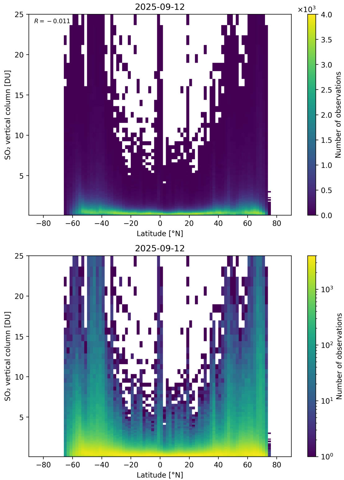
Figure 169: Scatter density plot of “Latitude” against “SO 2 vertical column” for 2025-09-11 to 2025-09-13.
