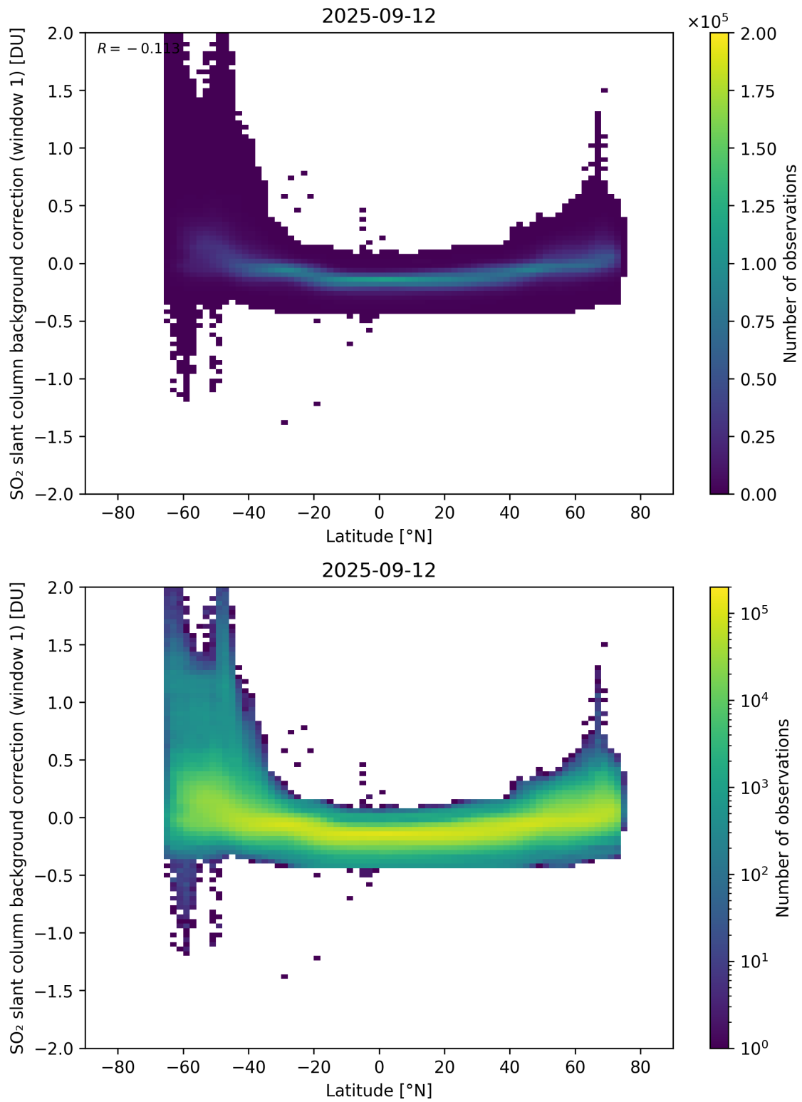
Figure 150: Scatter density plot of “Latitude” against “SO 2 slant column background correction (window 1)” for 2025-09-11 to 2025-09-13.
