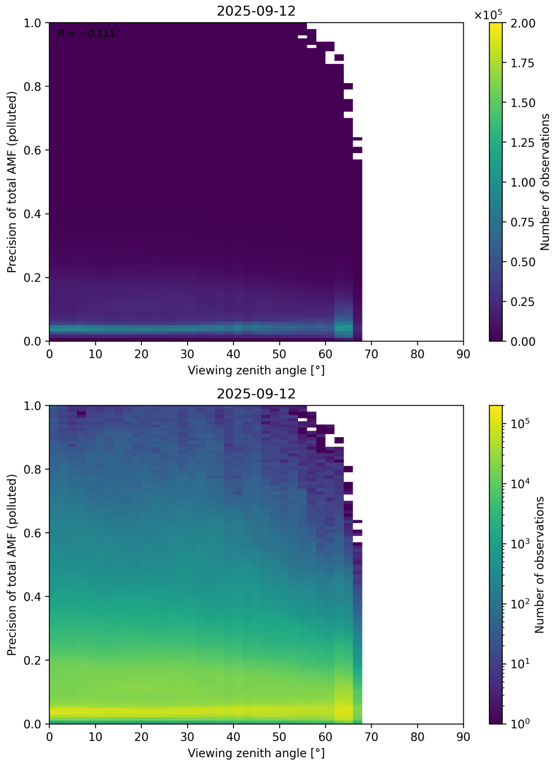
Figure 382: Scatter density plot of “Viewing zenith angle” against “Precision of total AMF (polluted)” for 2025-09-11 to 2025-09-13.
