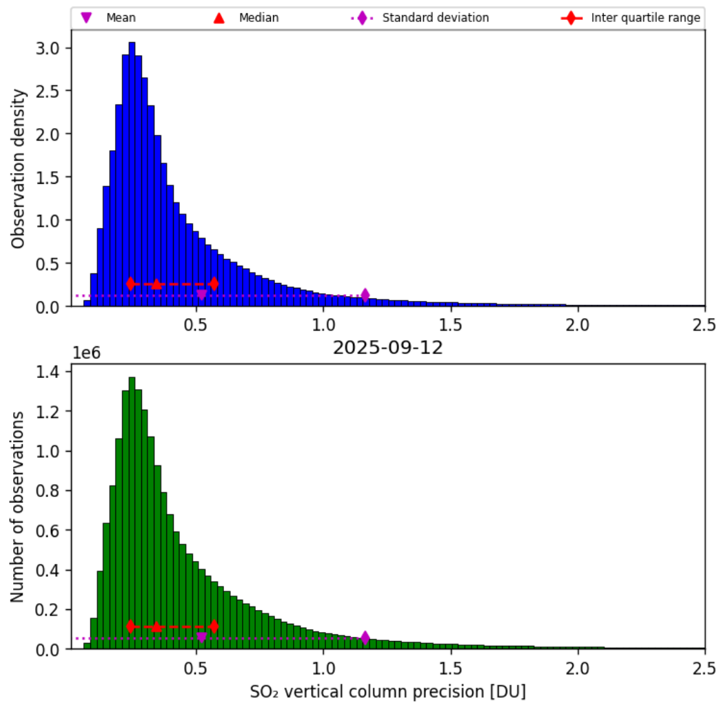
Figure 59: Histogram of “SO 2 vertical column precision” for 2025-09-11 to 2025-09-13
