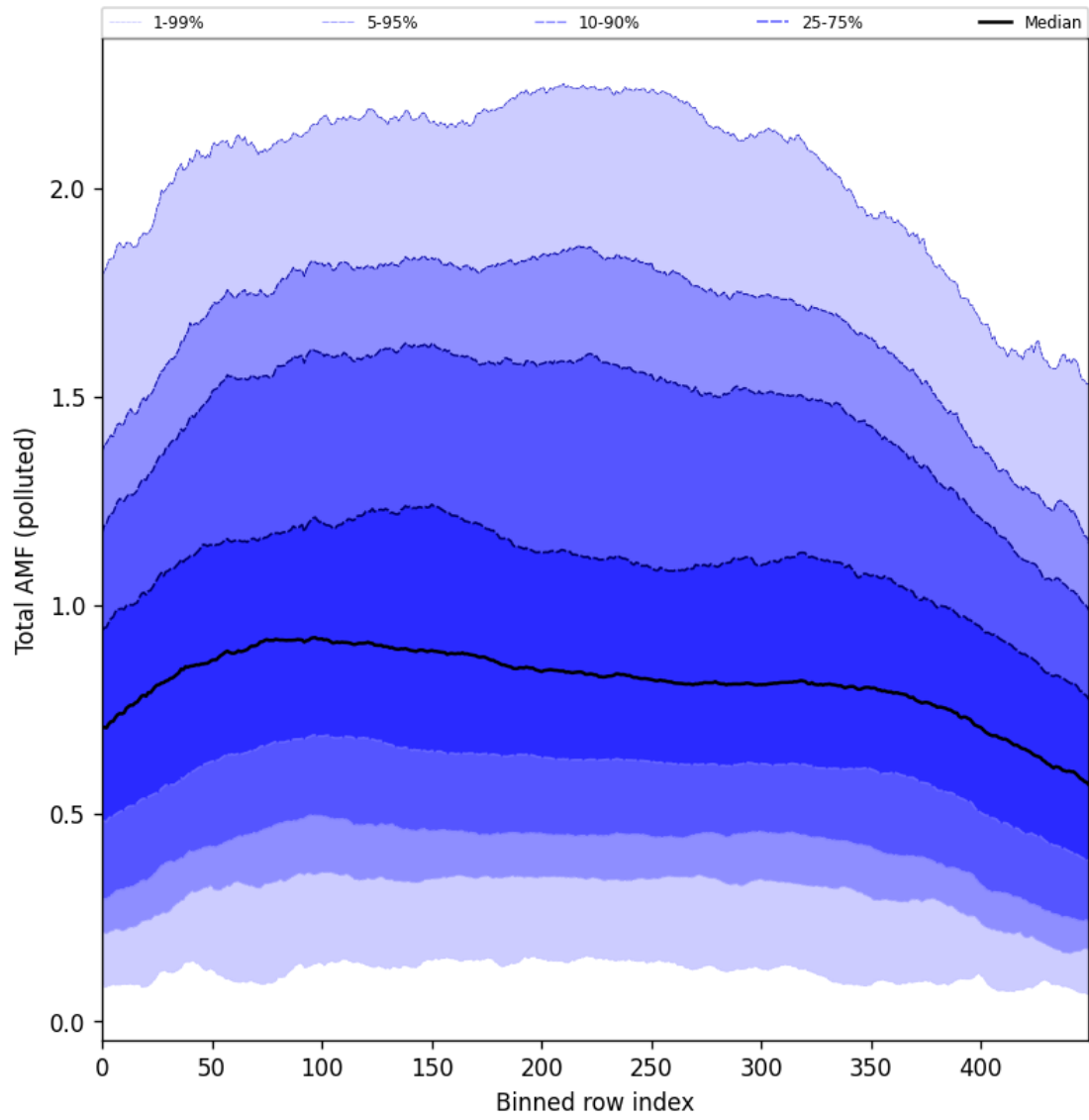
Figure 105: Along track statistics of “Total AMF (polluted)” for 2025-09-11 to 2025-09-13
