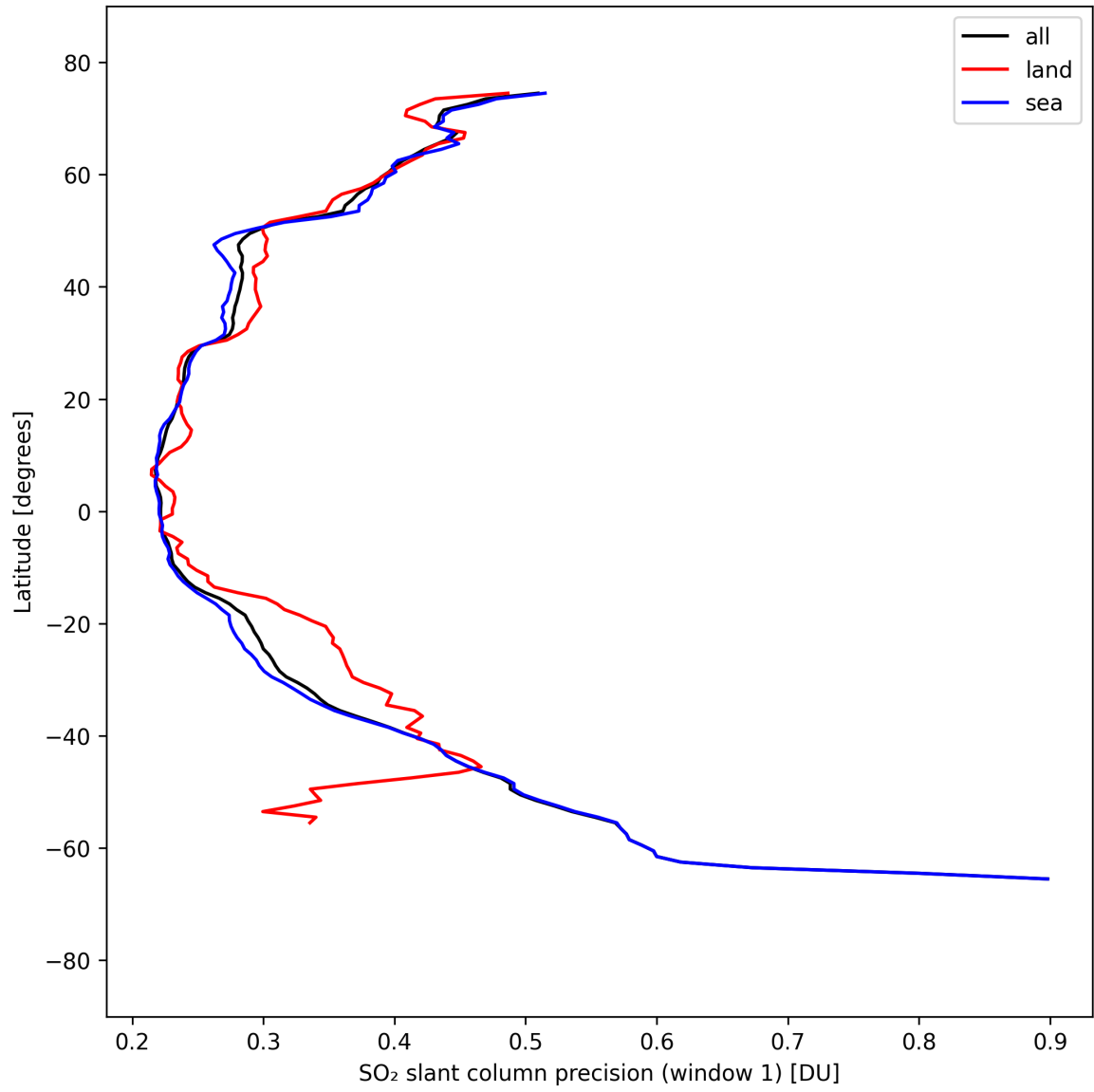
Figure 38: Zonal average of “SO 2 slant column precision (window 1)” for 2025-09-11 to 2025-09-13.
