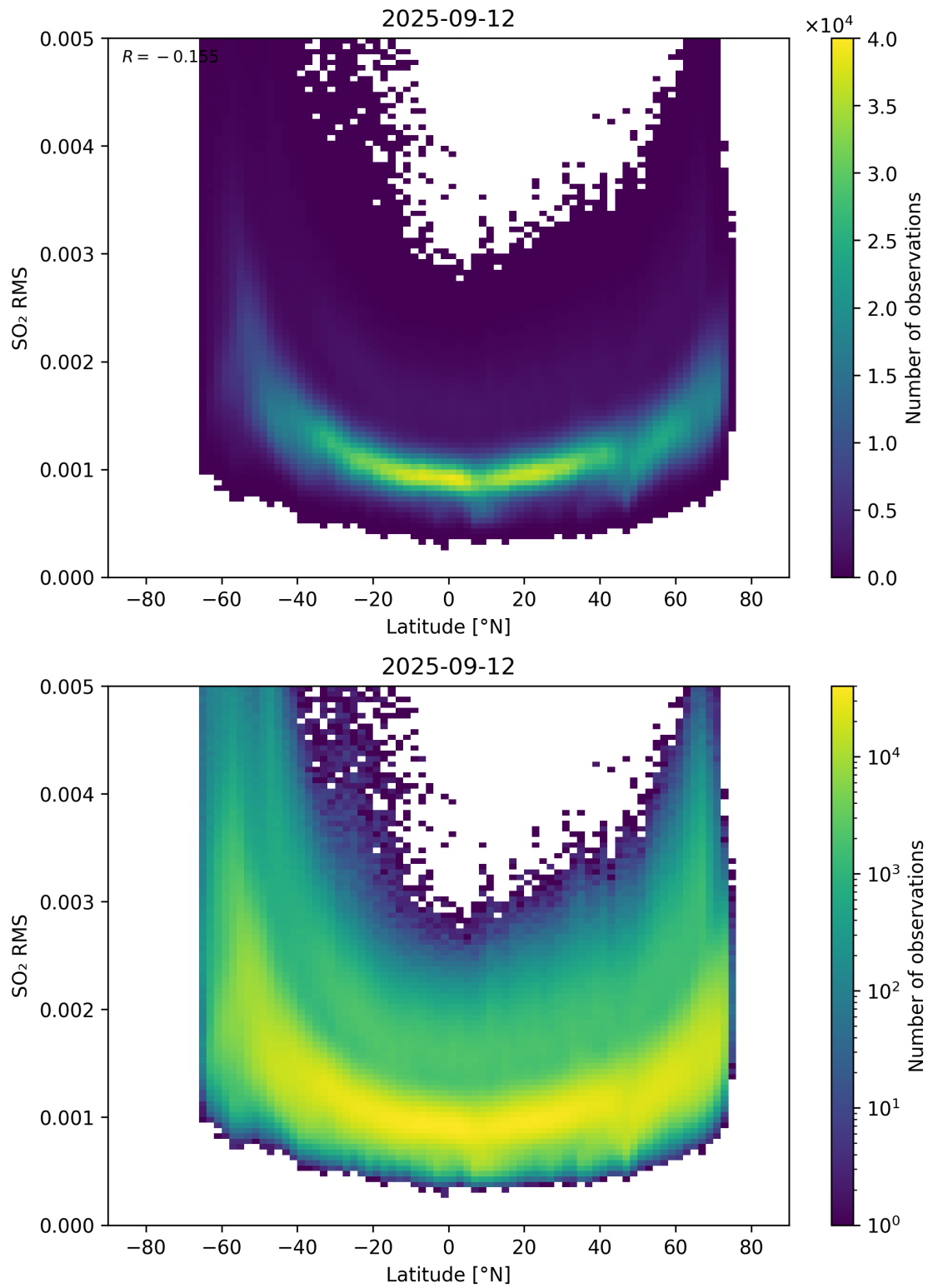
Figure 155: Scatter density plot of “Latitude” against “SO 2 RMS” for 2025-09-11 to 2025-09-13.
