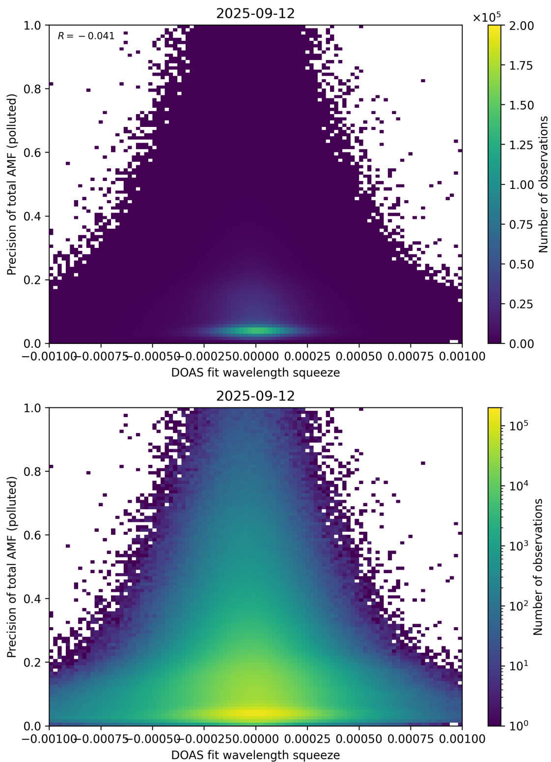
Figure 146: Scatter density plot of “DOAS fit wavelength squeeze” against “Precision of total AMF (polluted)” for 2025-09-11 to 2025-09-13.
