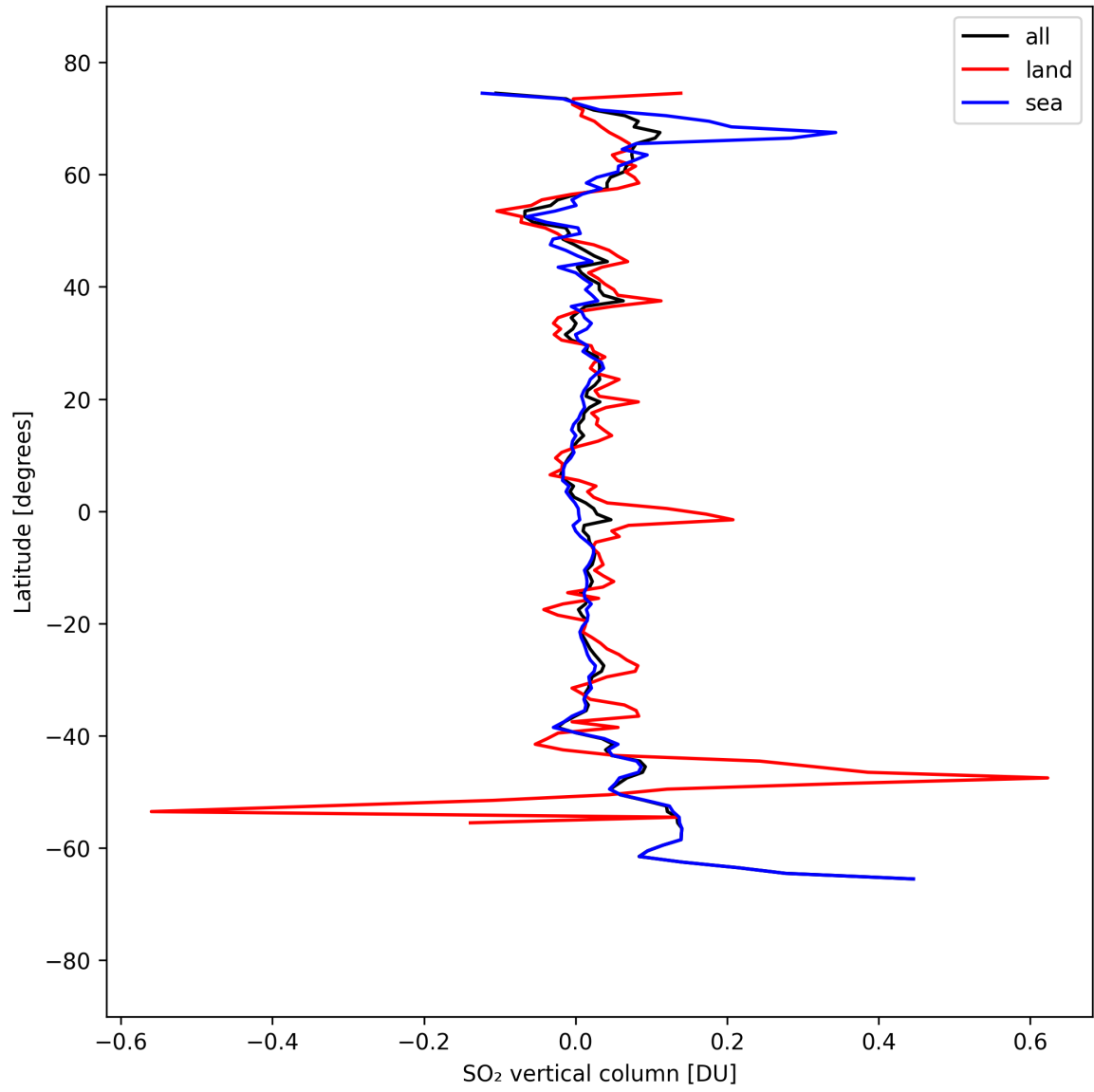
Figure 32: Zonal average of “SO 2 vertical column” for 2025-09-11 to 2025-09-13.
