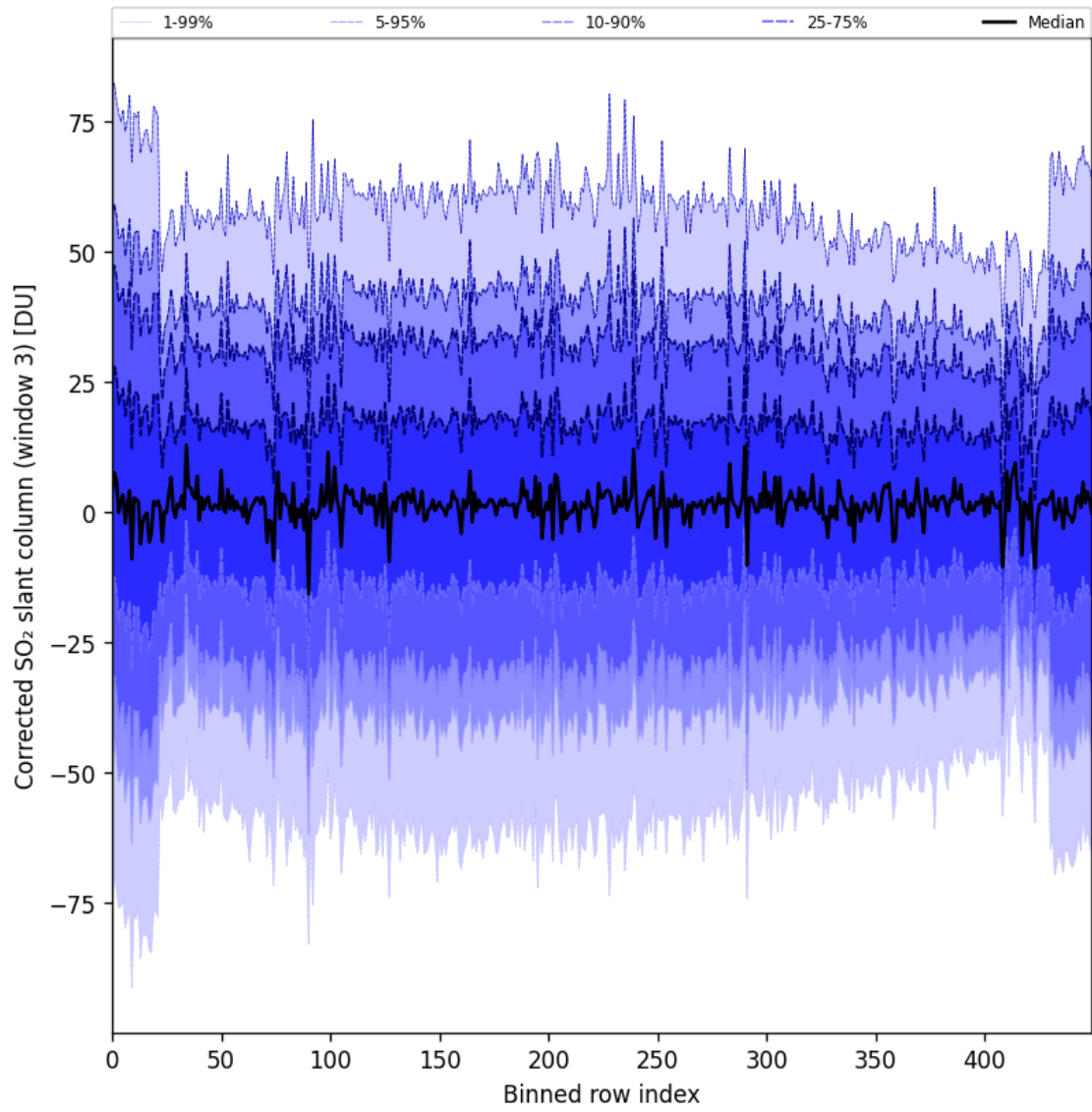
Figure 99: Along track statistics of “Corrected SO 2 slant column (window 3)” for 2025-09-11 to 2025-09-13
