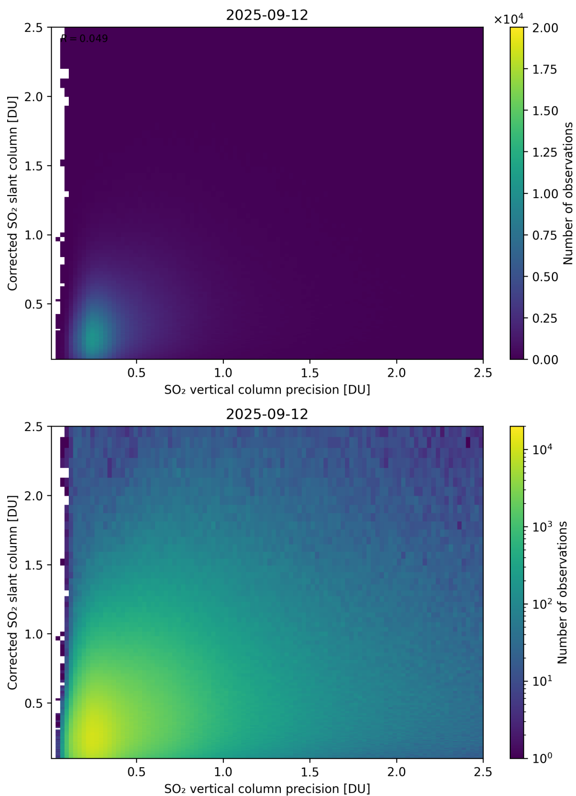
Figure 338: Scatter density plot of “SO 2 vertical column precision” against “Corrected SO 2 slant column” for 2025-09-11 to 2025-09-13.
