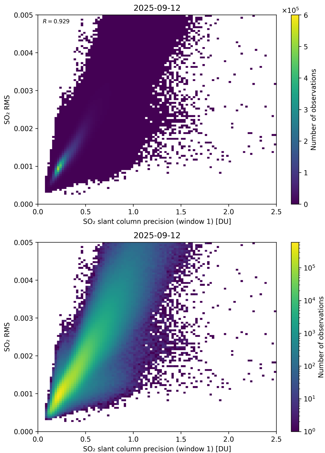
Figure 273: Scatter density plot of “SO 2 slant column precision (window 1)” against “SO 2 RMS” for 2025-09-11 to 2025-09-13.
