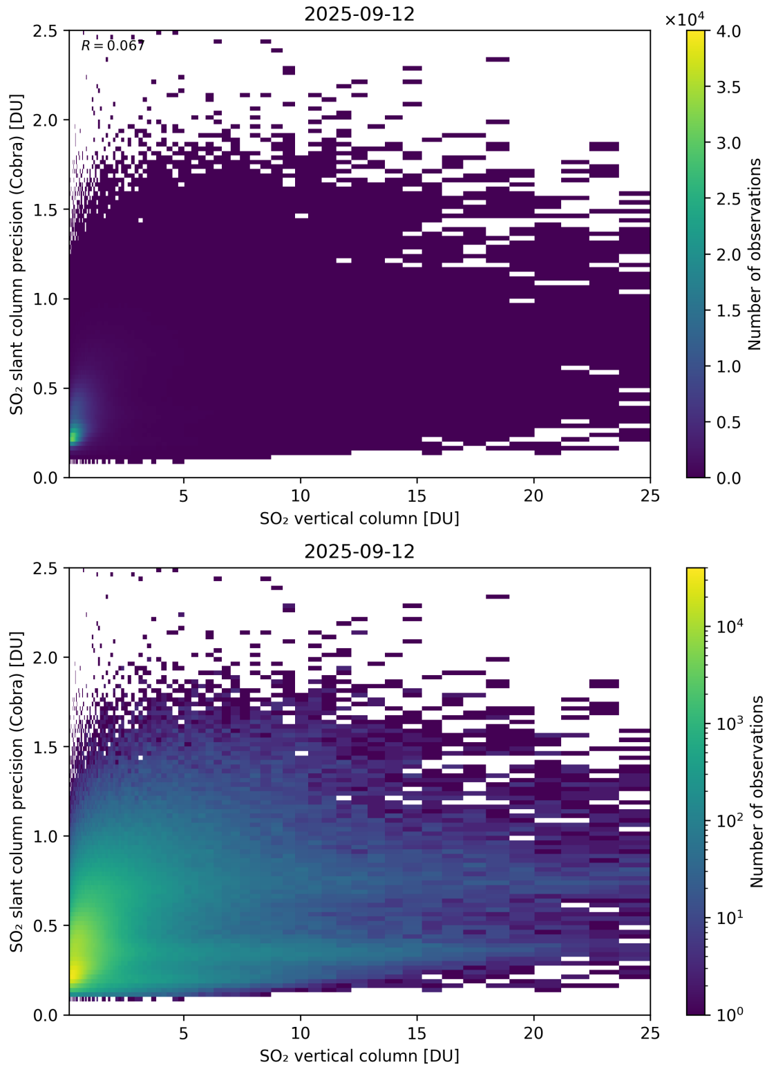
Figure 350: Scatter density plot of “SO 2 vertical column” against “SO 2 slant column precision (Cobra)” for 2025-09-11 to 2025-09-13.
