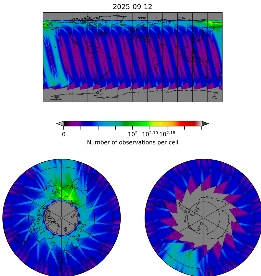
Figure 30: Map of the number of observations for 2025-09-11 to 2025-09-13
