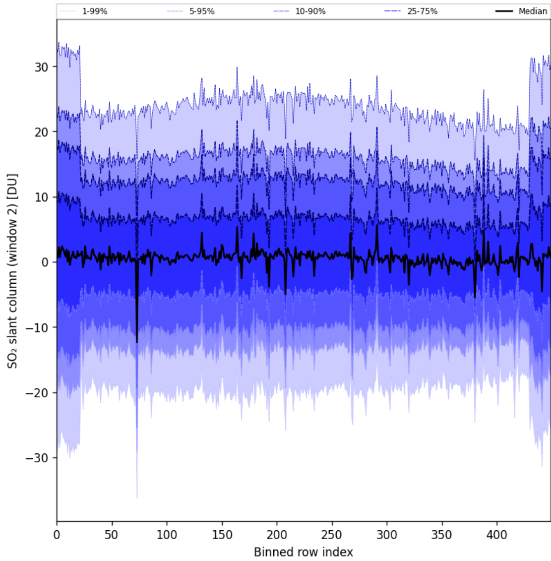
Figure 93: Along track statistics of “SO 2 slant column (window 2)” for 2025-09-11 to 2025-09-13
