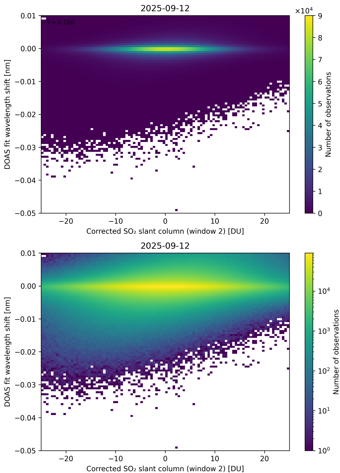
Figure 246: Scatter density plot of “Corrected SO 2 slant column (window 2)” against “DOAS fit wavelength shift” for 2025-09-11 to 2025-09-13.
