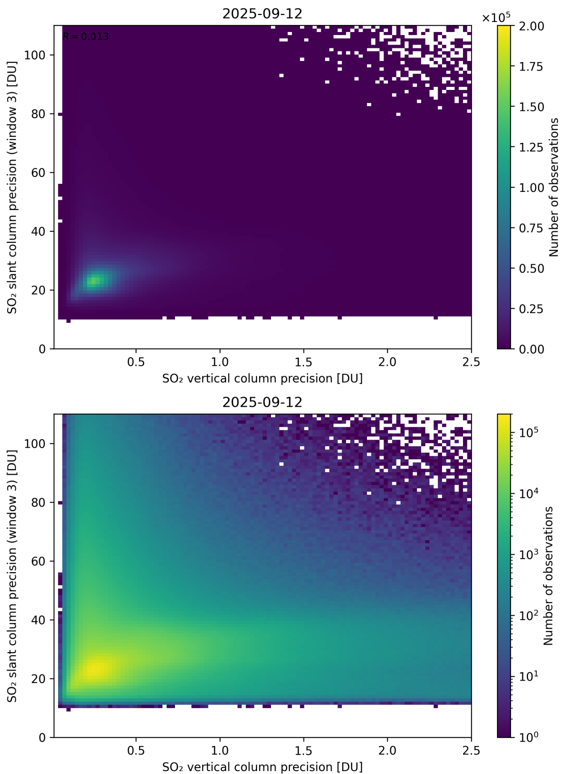
Figure 345: Scatter density plot of “SO 2 vertical column precision” against “SO 2 slant column precision (window 3)” for 2025-09-11 to 2025-09-13.
