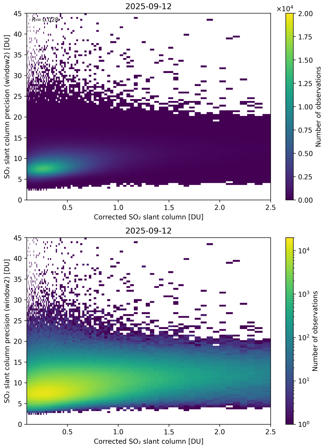
Figure 239: Scatter density plot of “Corrected SO 2 slant column” against “SO 2 slant column precision (window2)” for 2025-09-11 to 2025-09-13.
