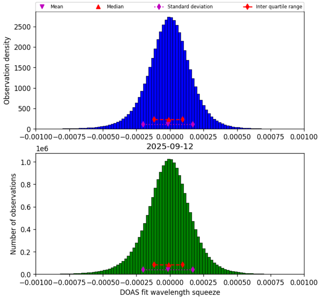
Figure 77: Histogram of “DOAS fit wavelength squeeze” for 2025-09-11 to 2025-09-13
