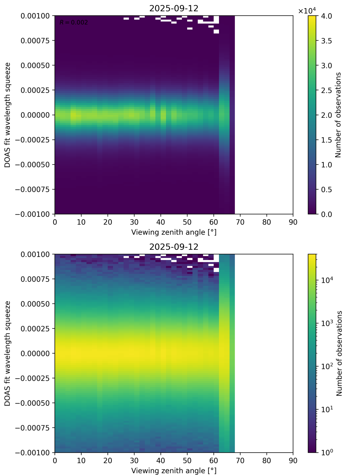
Figure 366: Scatter density plot of “Viewing zenith angle” against “DOAS fit wavelength squeeze” for 2025-09-11 to 2025-09-13.
