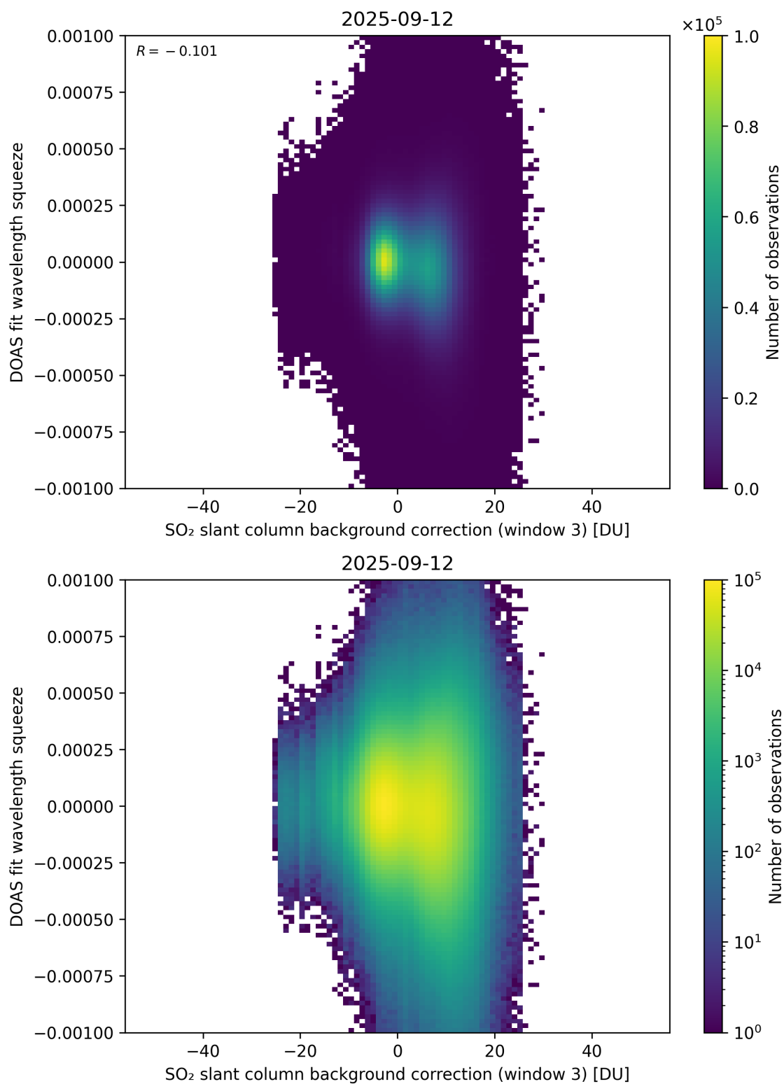
Figure 133: Scatter density plot of “SO 2 slant column background correction (window 3)” against “DOAS fit wavelength squeeze” for 2025-09-11 to 2025-09-13.
