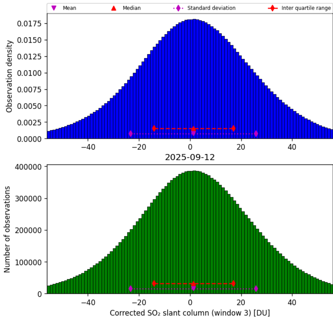
Figure 73: Histogram of “Corrected SO 2 slant column (window 3)” for 2025-09-11 to 2025-09-13
