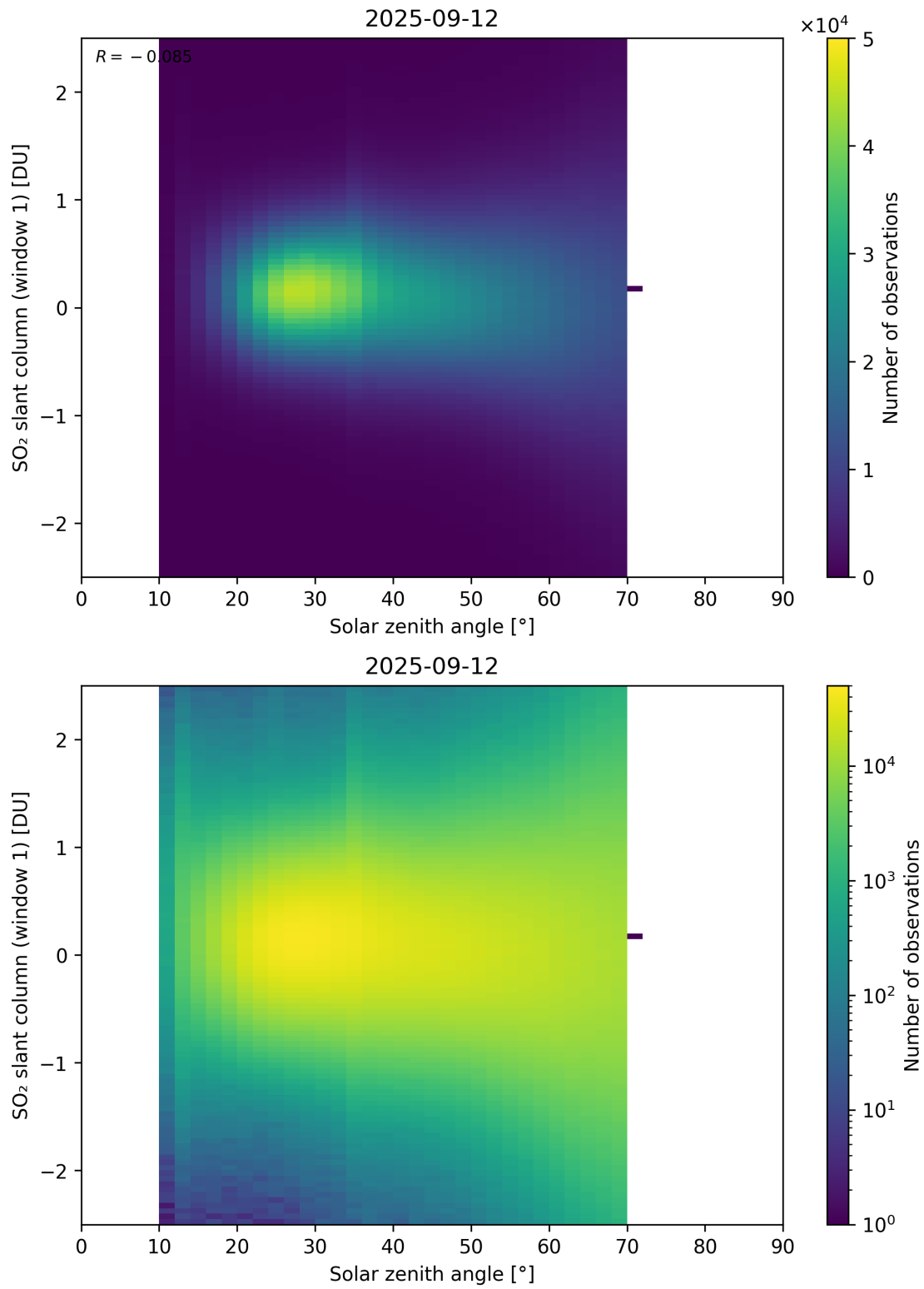
Figure 184: Scatter density plot of “Solar zenith angle” against “SO 2 slant column (window 1)” for 2025-09-11 to 2025-09-13.
