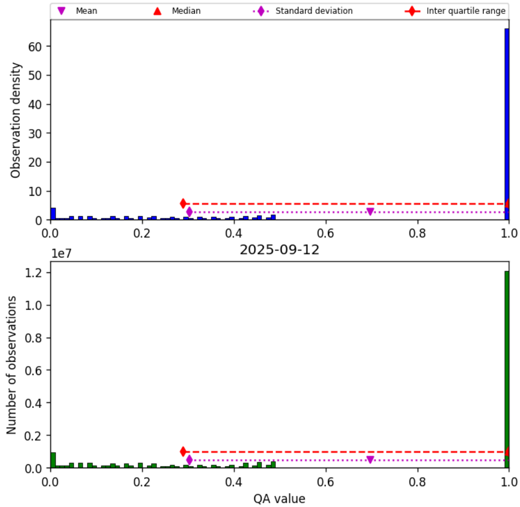
Figure 57: Histogram of “QA value” for 2025-09-11 to 2025-09-13
