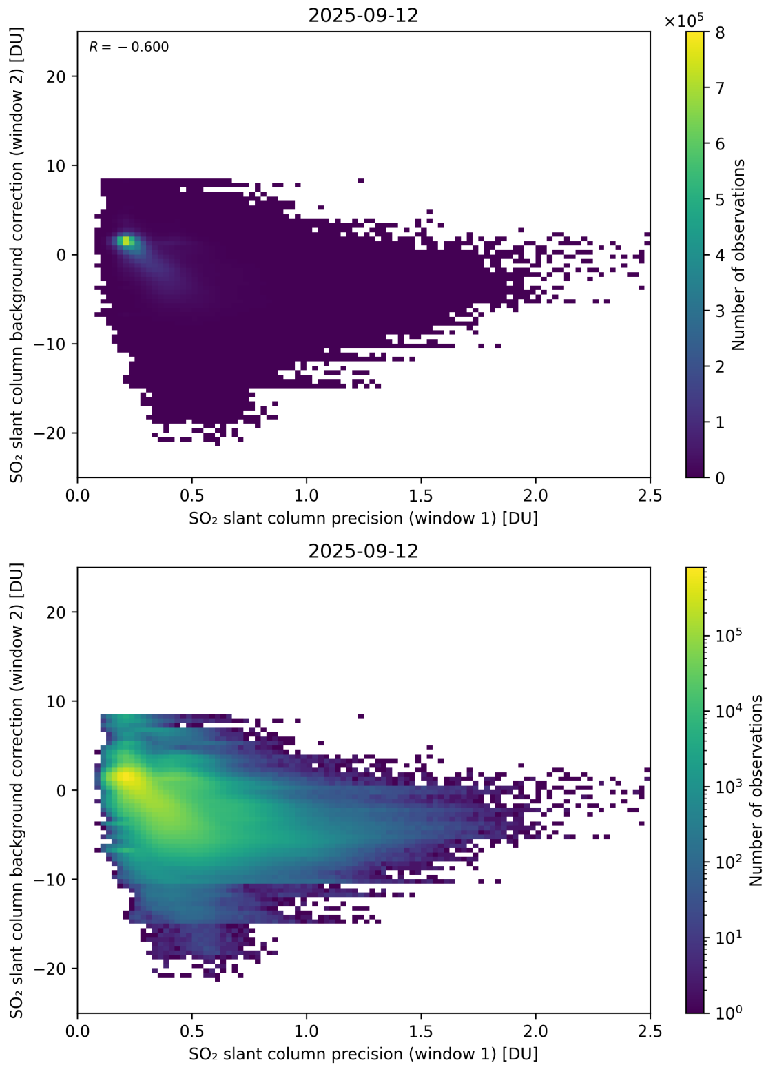
Figure 269: Scatter density plot of “SO 2 slant column precision (window 1)” against “SO 2 slant column background correction (window 2)” for 2025-09-11 to 2025-09-13.
