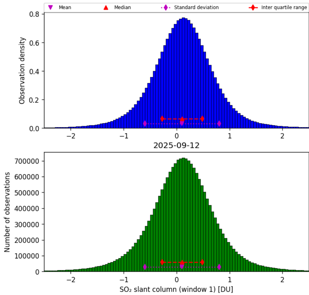
Figure 63: Histogram of “SO 2 slant column (window 1)” for 2025-09-11 to 2025-09-13
