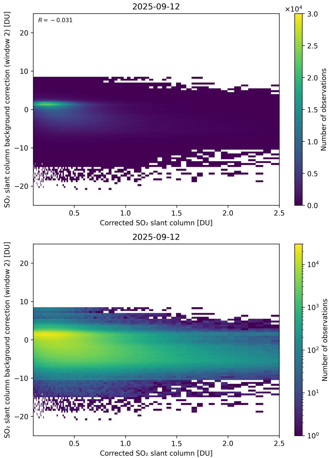
Figure 227: Scatter density plot of “Corrected SO 2 slant column” against “SO 2 slant column background correction (window 2)” for 2025-09-11 to 2025-09-13.
