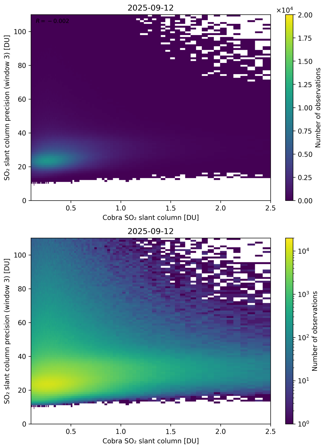
Figure 223: Scatter density plot of “Cobra SO 2 slant column” against “SO 2 slant column precision (window 3)” for 2025-09-11 to 2025-09-13.
