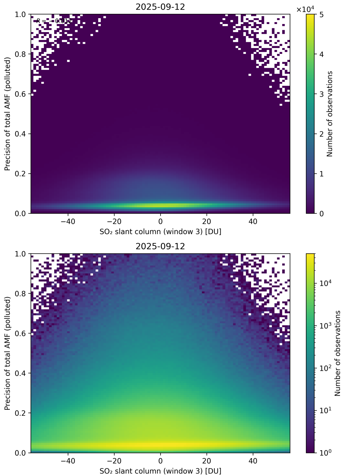
Figure 319: Scatter density plot of “SO 2 slant column (window 3)” against “Precision of total AMF (polluted)” for 2025-09-11 to 2025-09-13.
