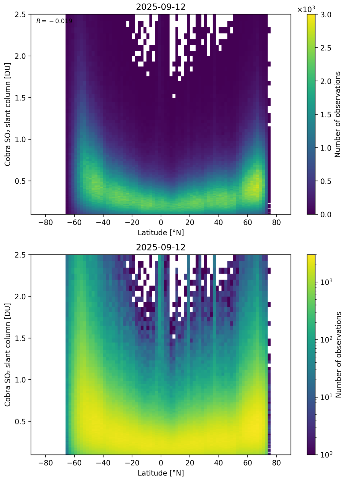
Figure 157: Scatter density plot of “Latitude” against “Cobra SO 2 slant column” for 2025-09-11 to 2025-09-13.
