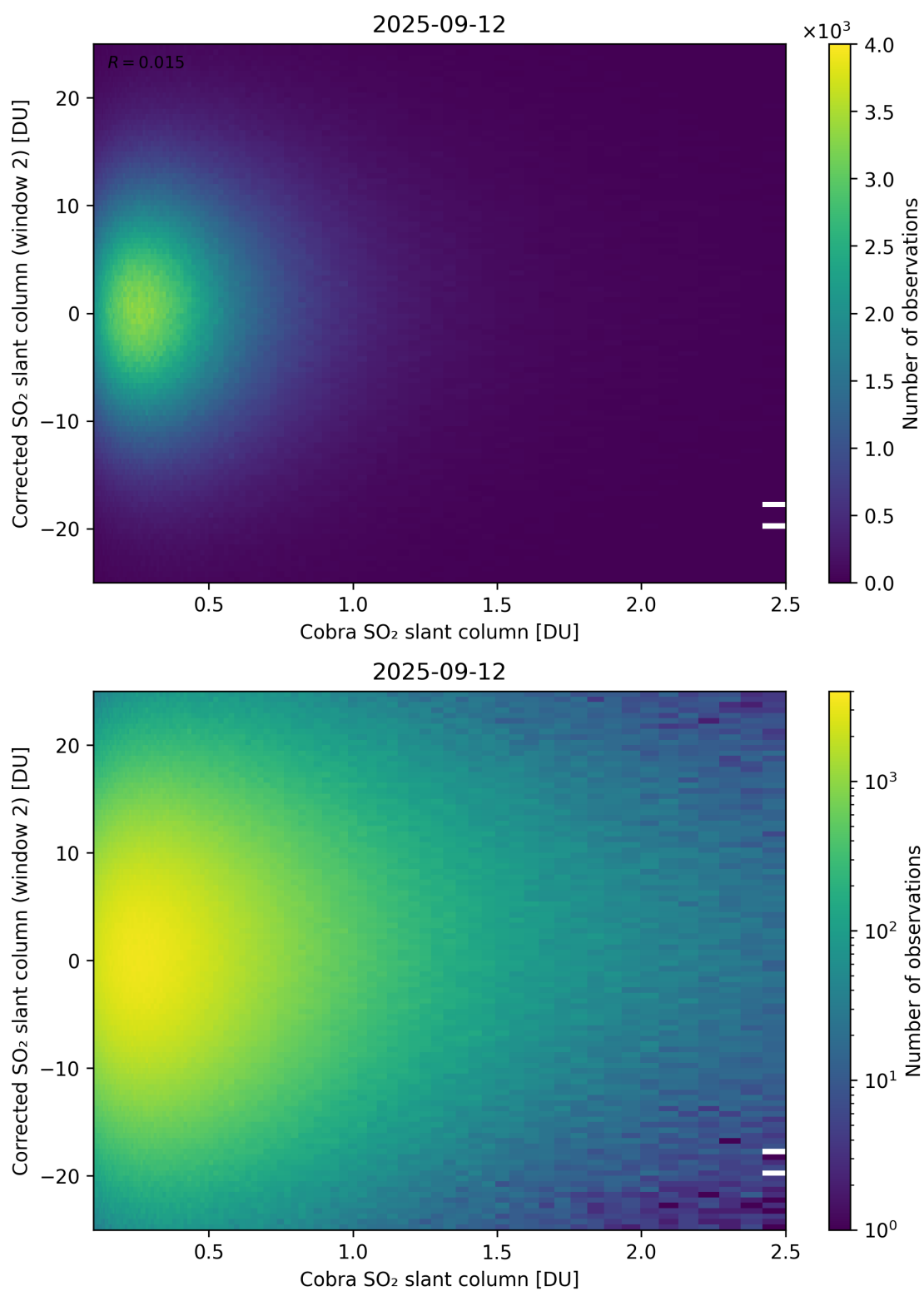
Figure 217: Scatter density plot of “Cobra SO 2 slant column” against “Corrected SO 2 slant column (window 2)” for 2025-09-11 to 2025-09-13.
