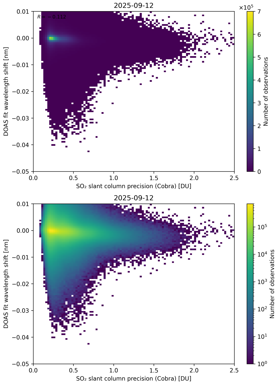
Figure 202: Scatter density plot of “SO 2 slant column precision (Cobra)” against “DOAS fit wavelength shift” for 2025-09-11 to 2025-09-13.
