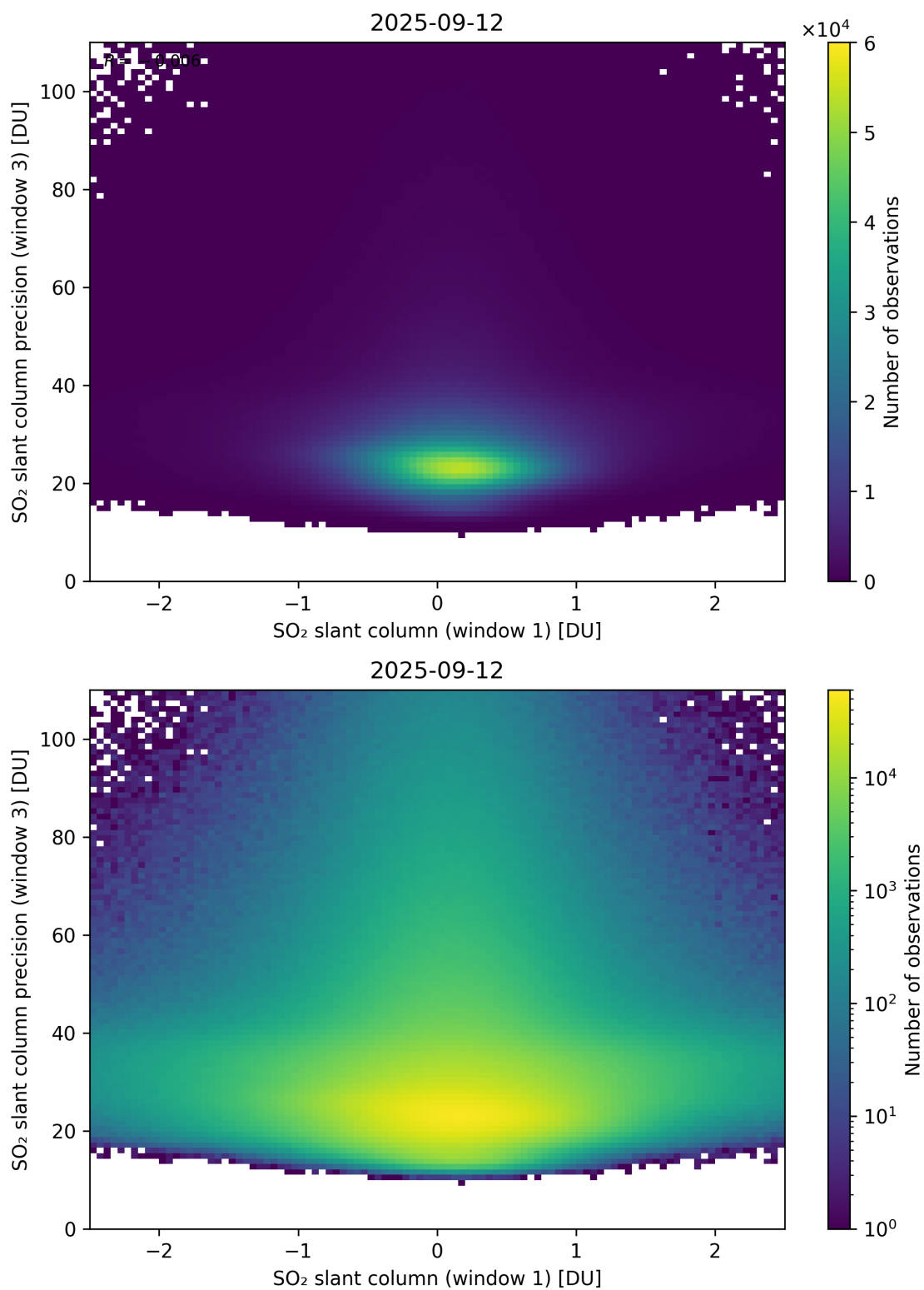
Figure 288: Scatter density plot of “SO 2 slant column (window 1)” against “SO 2 slant column precision (window 3)” for 2025-09-11 to 2025-09-13.
