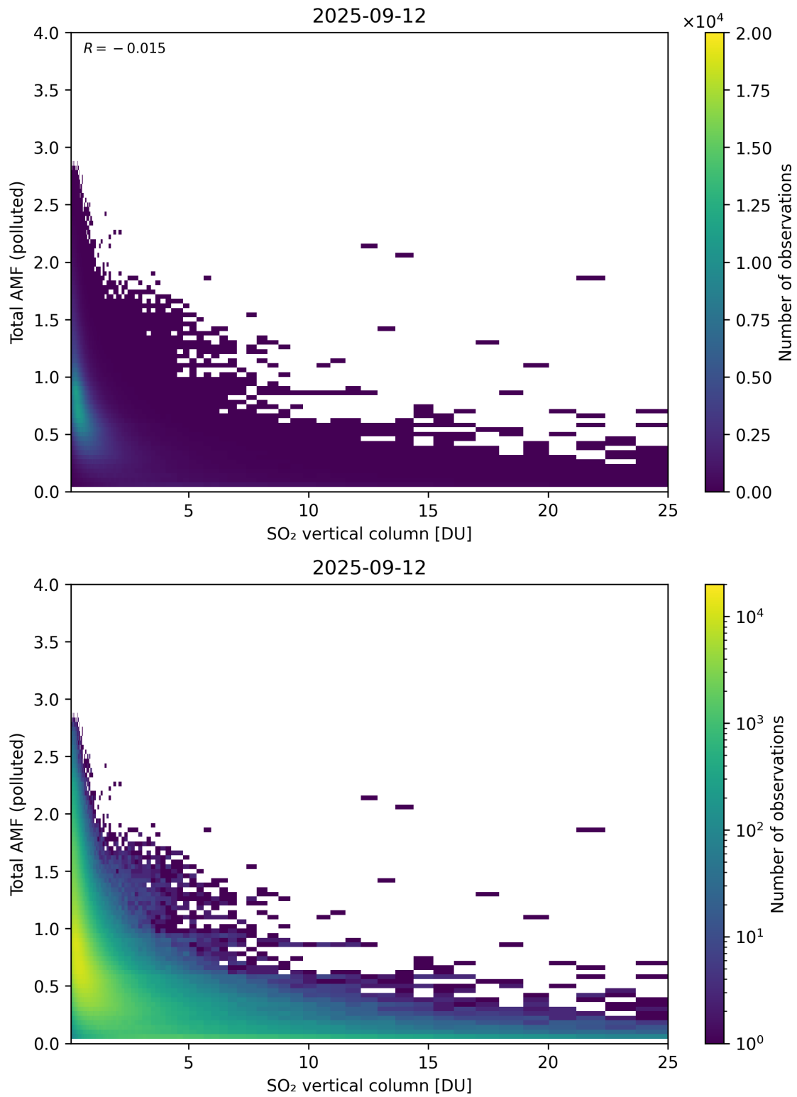
Figure 359: Scatter density plot of “SO 2 vertical column” against “Total AMF (polluted)” for 2025-09-11 to 2025-09-13.
