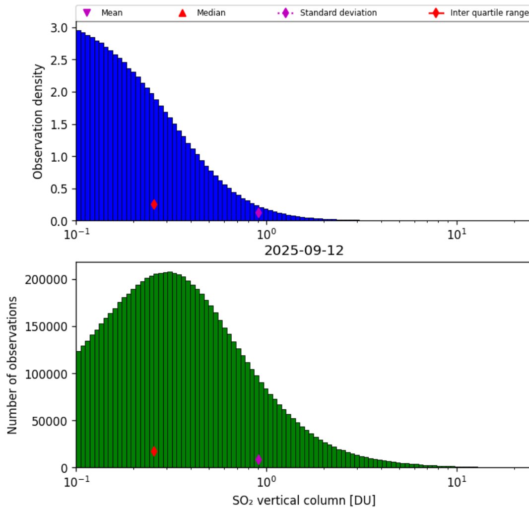
Figure 58: Histogram of “SO 2 vertical column” for 2025-09-11 to 2025-09-13
