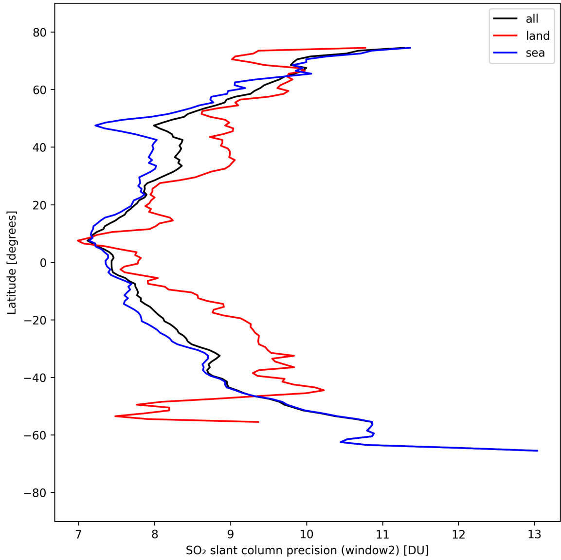
Figure 42: Zonal average of “SO 2 slant column precision (window2)” for 2025-09-11 to 2025-09-13.
