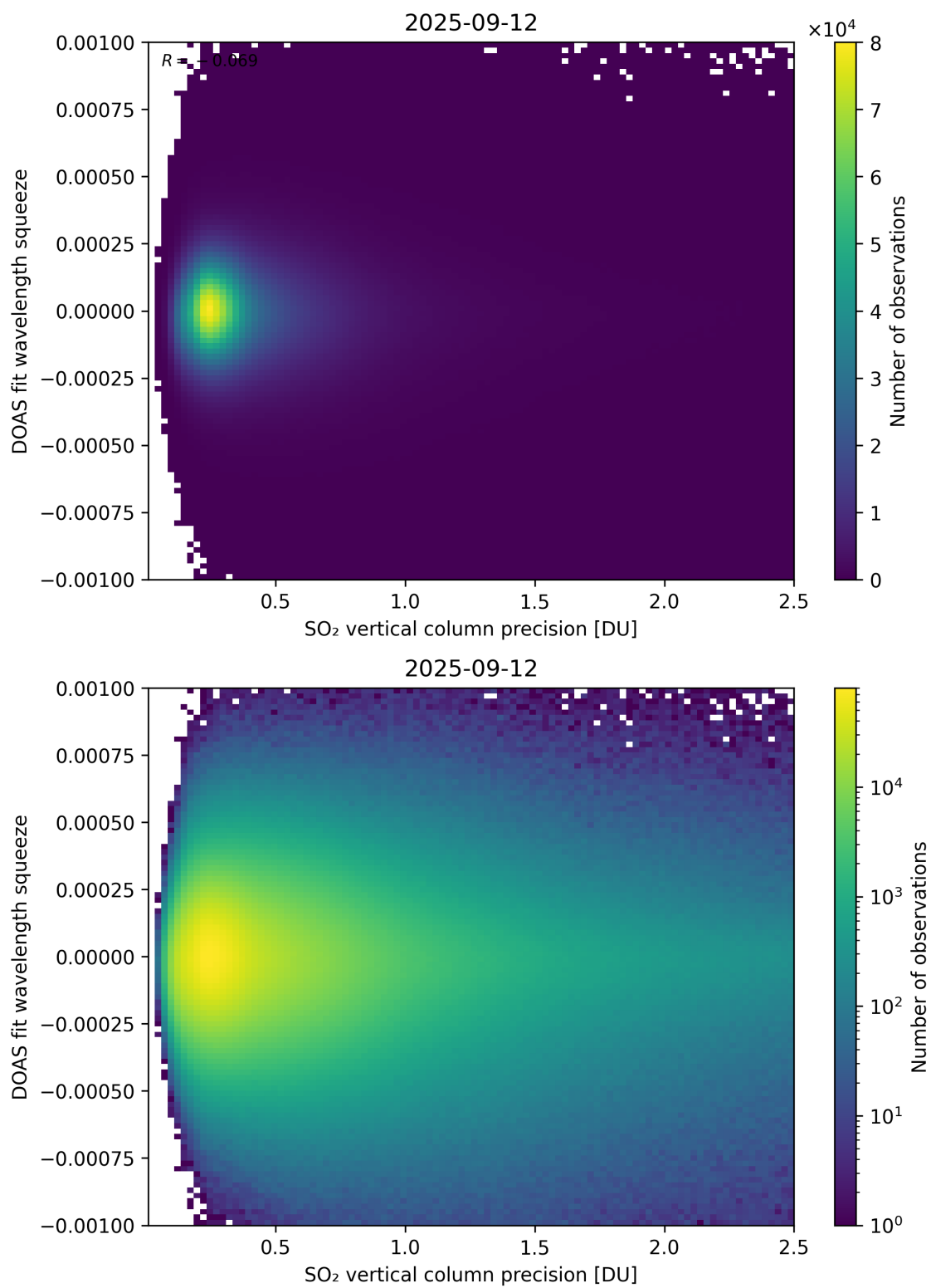
Figure 333: Scatter density plot of “SO 2 vertical column precision” against “DOAS fit wavelength squeeze” for 2025-09-11 to 2025-09-13.
