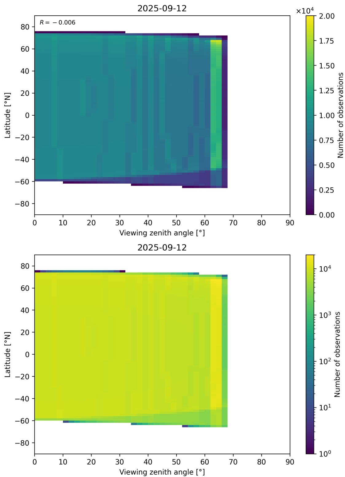
Figure 368: Scatter density plot of “Viewing zenith angle” against “Latitude” for 2025-09-11 to 2025-09-13.
