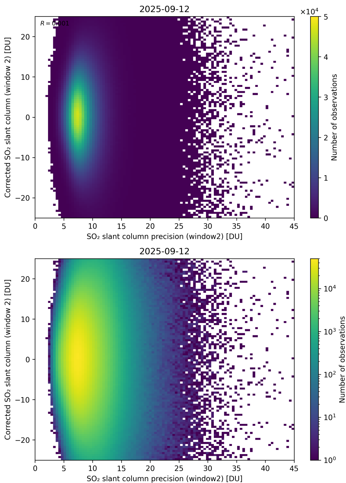
Figure 297: Scatter density plot of “SO 2 slant column precision (window2)” against “Corrected SO 2 slant column (window 2)” for 2025-09-11 to 2025-09-13.
