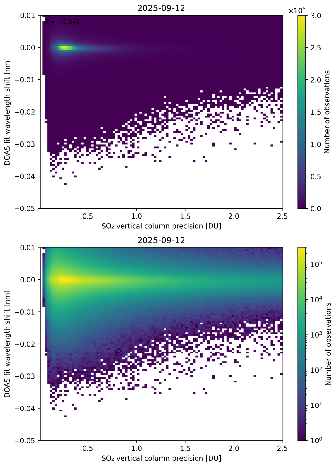
Figure 332: Scatter density plot of “SO 2 vertical column precision” against “DOAS fit wavelength shift” for 2025-09-11 to 2025-09-13.
