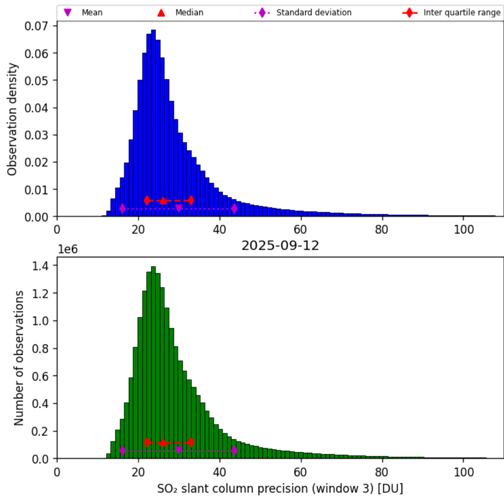
Figure 72: Histogram of “SO 2 slant column precision (window 3)” for 2025-09-11 to 2025-09-13
