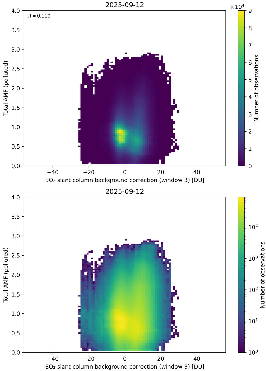
Figure 136: Scatter density plot of “SO 2 slant column background correction (window 3)” against “Total AMF (polluted)” for 2025-09-11 to 2025-09-13.
