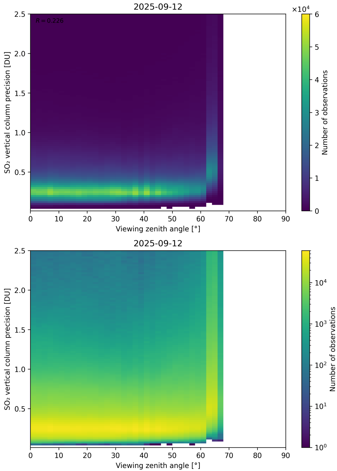
Figure 384: Scatter density plot of “Viewing zenith angle” against “SO 2 vertical column precision” for 2025-09-11 to 2025-09-13.
