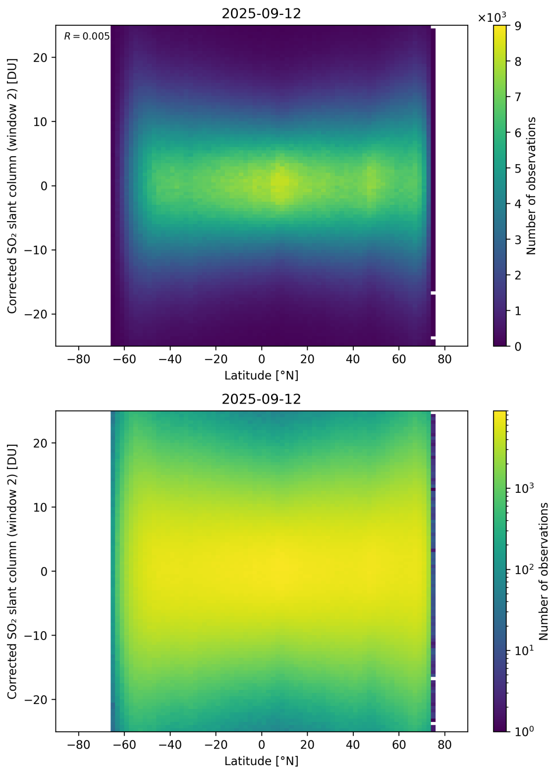
Figure 160: Scatter density plot of “Latitude” against “Corrected SO 2 slant column (window 2)” for 2025-09-11 to 2025-09-13.
