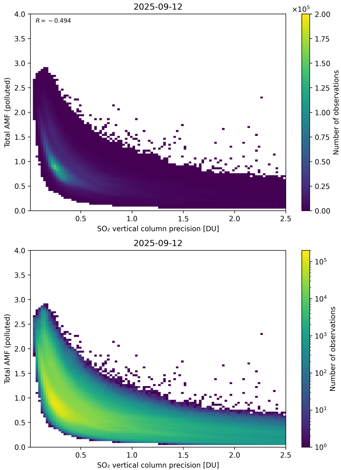
Figure 346: Scatter density plot of “SO 2 vertical column precision” against “Total AMF (polluted)” for 2025-09-11 to 2025-09-13.
