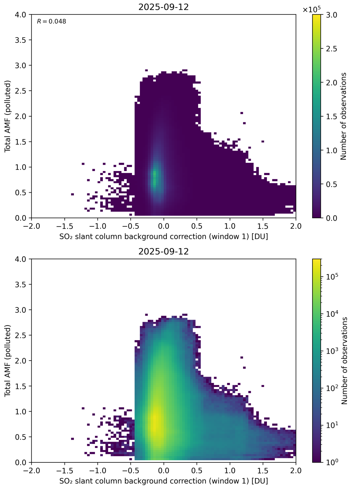
Figure 120: Scatter density plot of “SO 2 slant column background correction (window 1)” against “Total AMF (polluted)” for 2025-09-11 to 2025-09-13.
