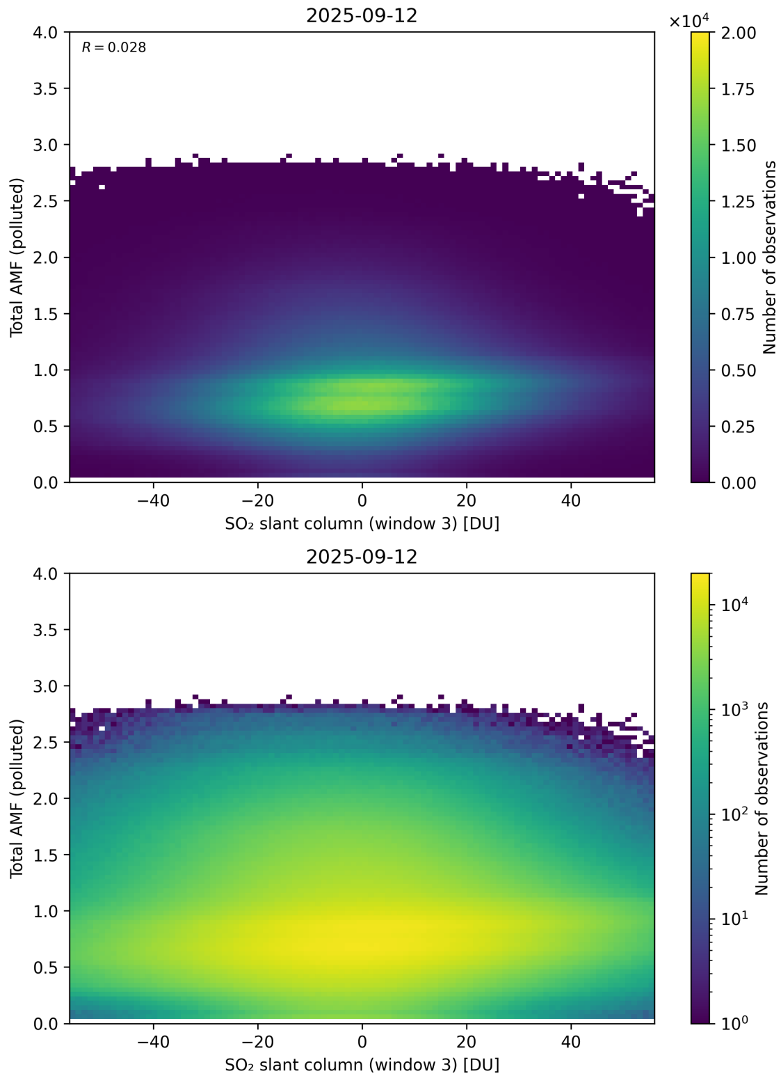
Figure 318: Scatter density plot of “SO 2 slant column (window 3)” against “Total AMF (polluted)” for 2025-09-11 to 2025-09-13.
