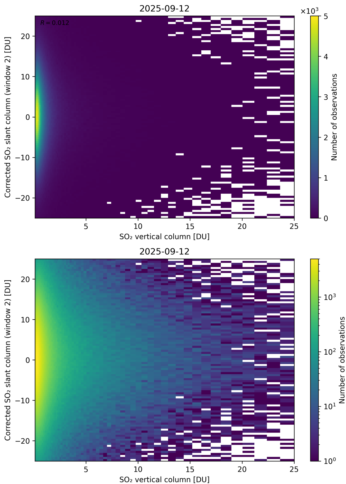
Figure 352: Scatter density plot of “SO 2 vertical column” against “Corrected SO 2 slant column (window 2)” for 2025-09-11 to 2025-09-13.
