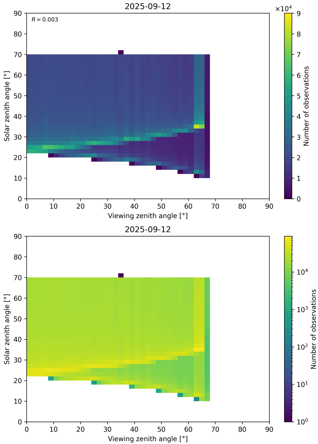
Figure 369: Scatter density plot of “Viewing zenith angle” against “Solar zenith angle” for 2025-09-11 to 2025-09-13.
