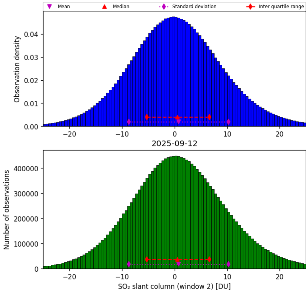
Figure 67: Histogram of “SO 2 slant column (window 2)” for 2025-09-11 to 2025-09-13
