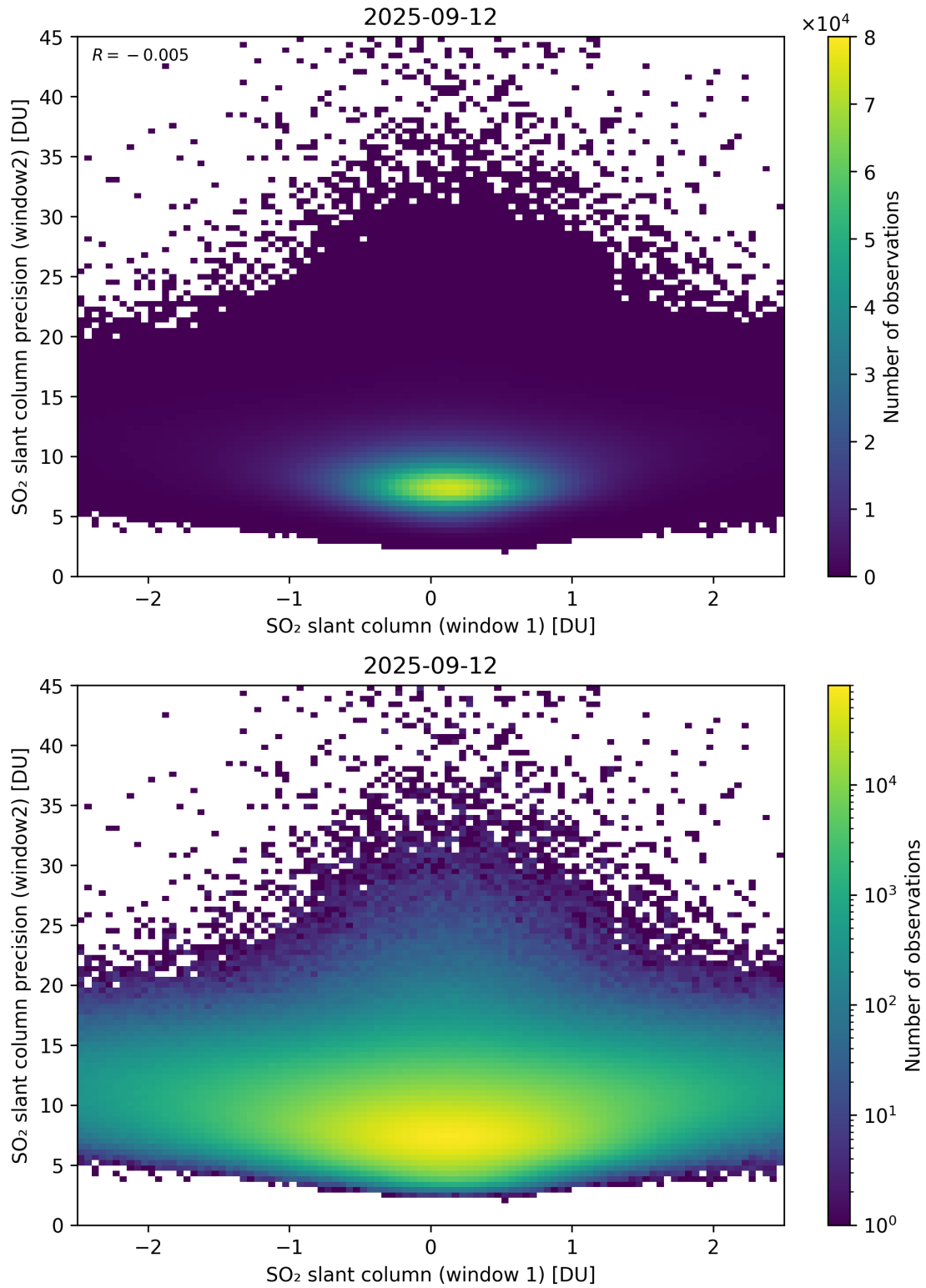
Figure 286: Scatter density plot of “SO 2 slant column (window 1)” against “SO 2 slant column precision (window2)” for 2025-09-11 to 2025-09-13.
