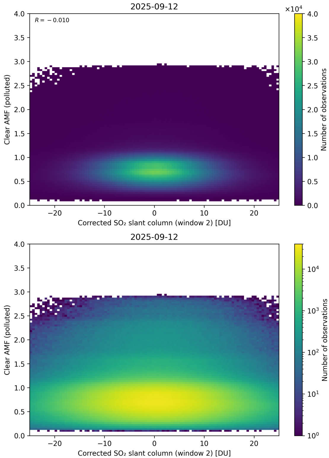
Figure 249: Scatter density plot of “Corrected SO 2 slant column (window 2)” against “Clear AMF (polluted)” for 2025-09-11 to 2025-09-13.
