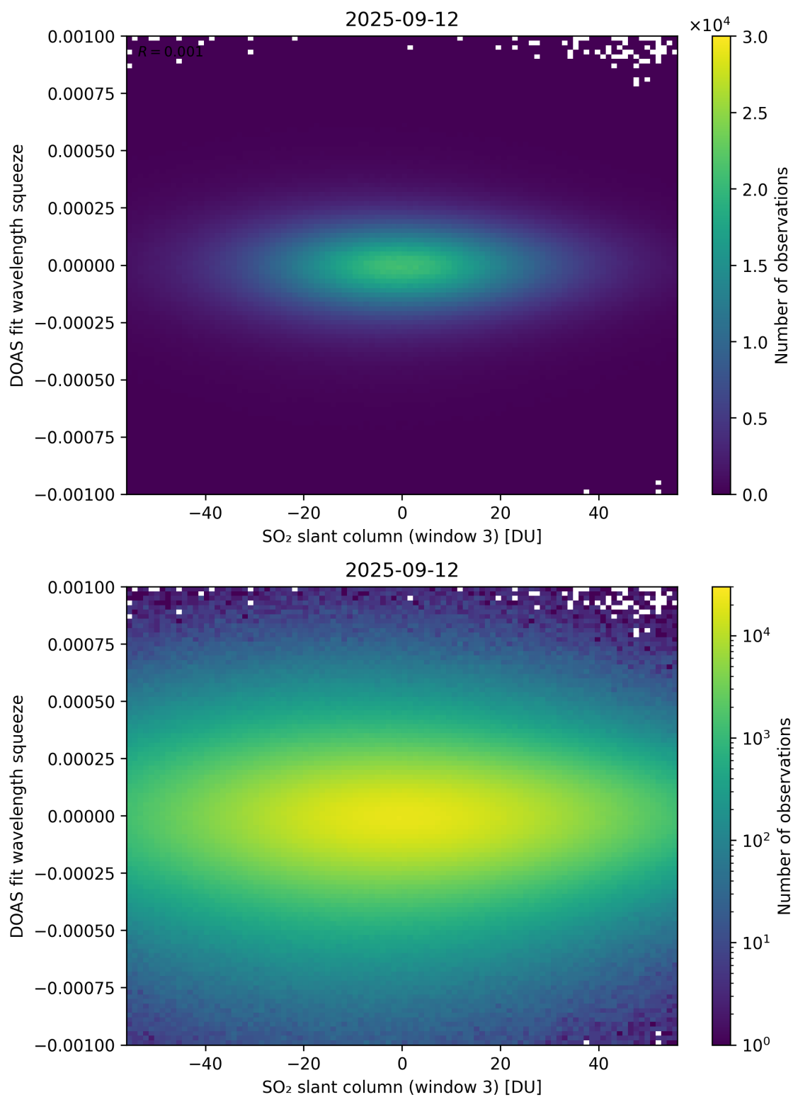
Figure 305: Scatter density plot of “SO 2 slant column (window 3)” against “DOAS fit wavelength squeeze” for 2025-09-11 to 2025-09-13.
