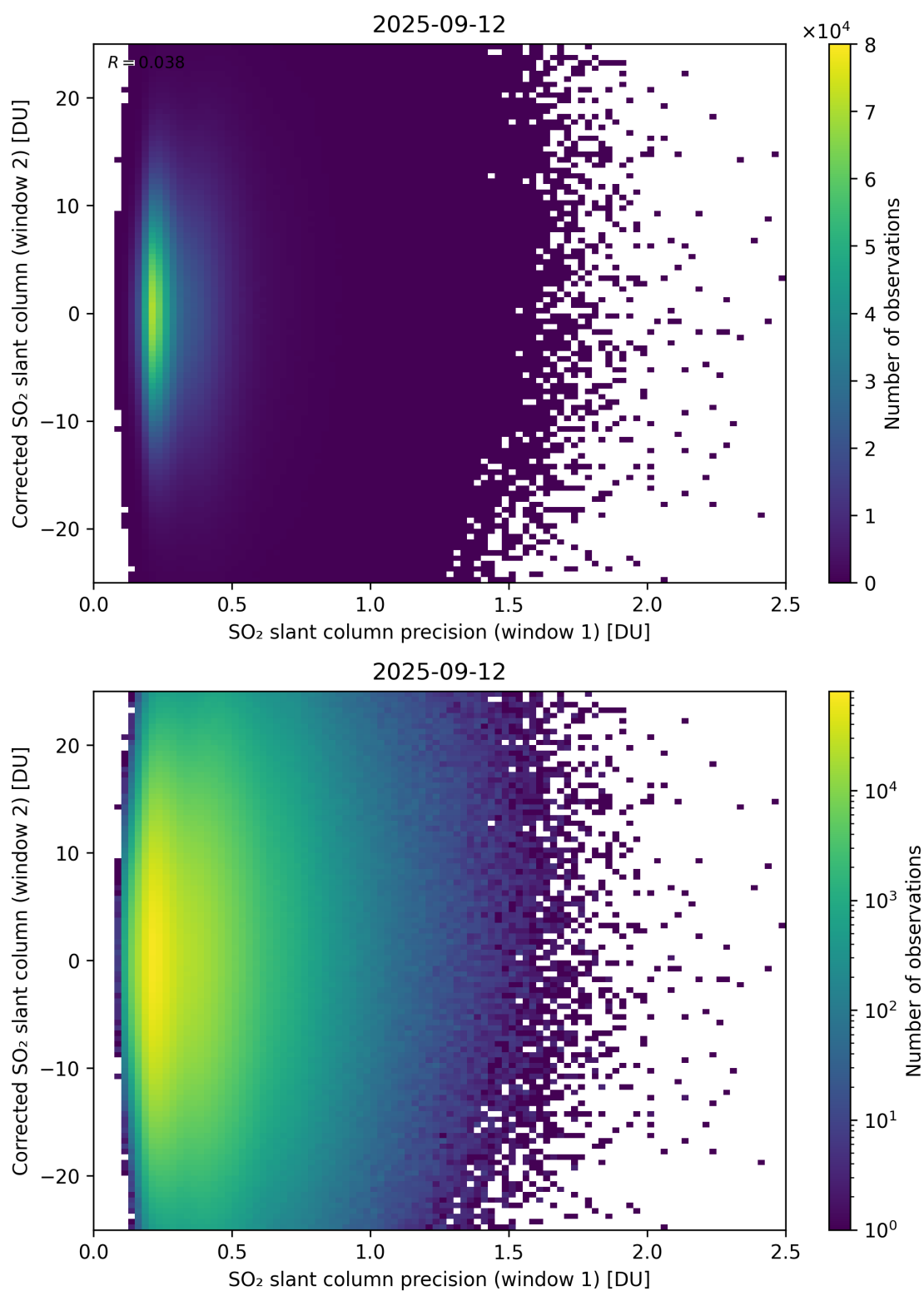
Figure 275: Scatter density plot of “SO 2 slant column precision (window 1)” against “Corrected SO 2 slant column (window 2)” for 2025-09-11 to 2025-09-13.
