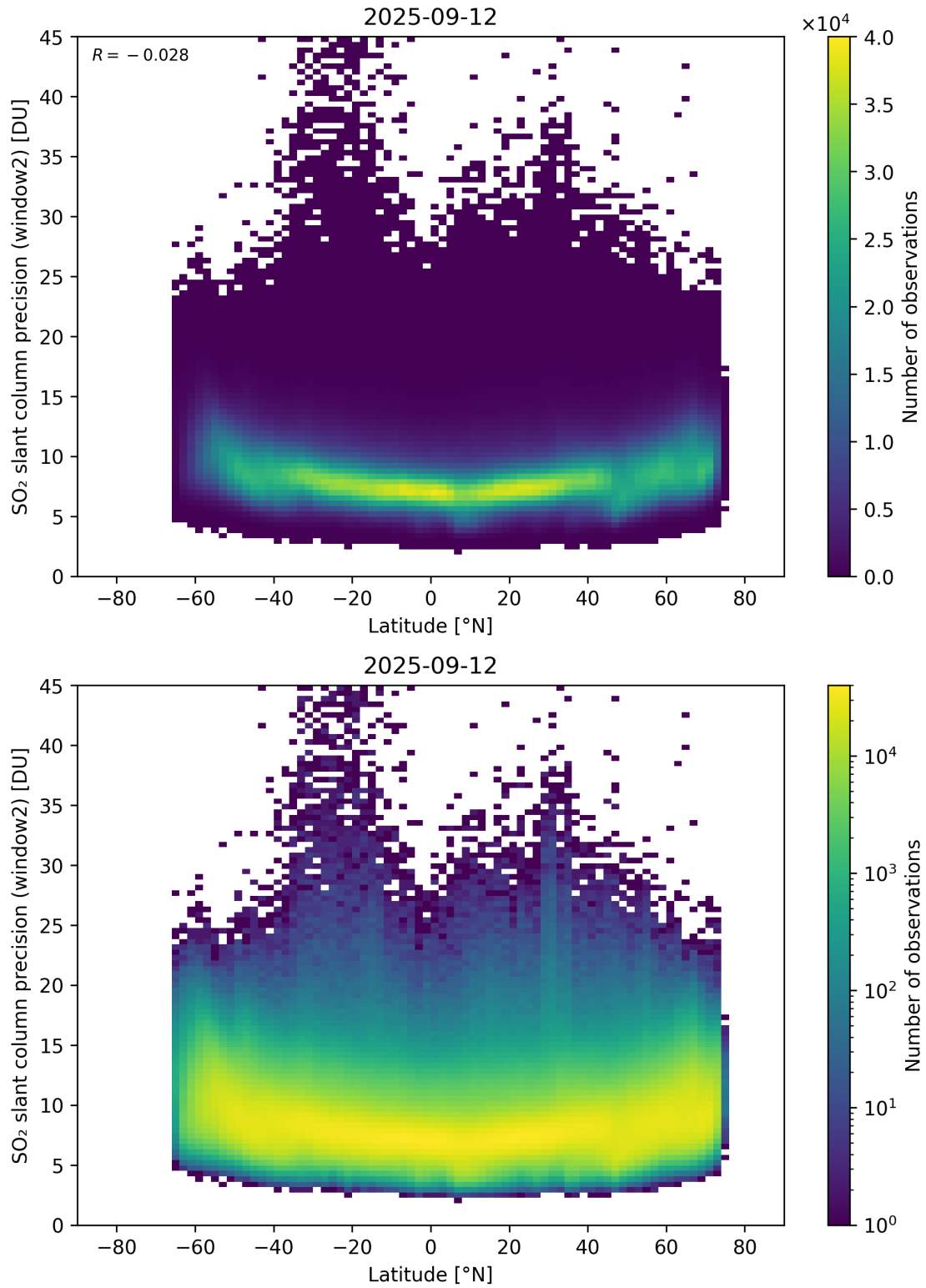
Figure 164: Scatter density plot of “Latitude” against “SO 2 slant column precision (window2)” for 2025-09-11 to 2025-09-13.
