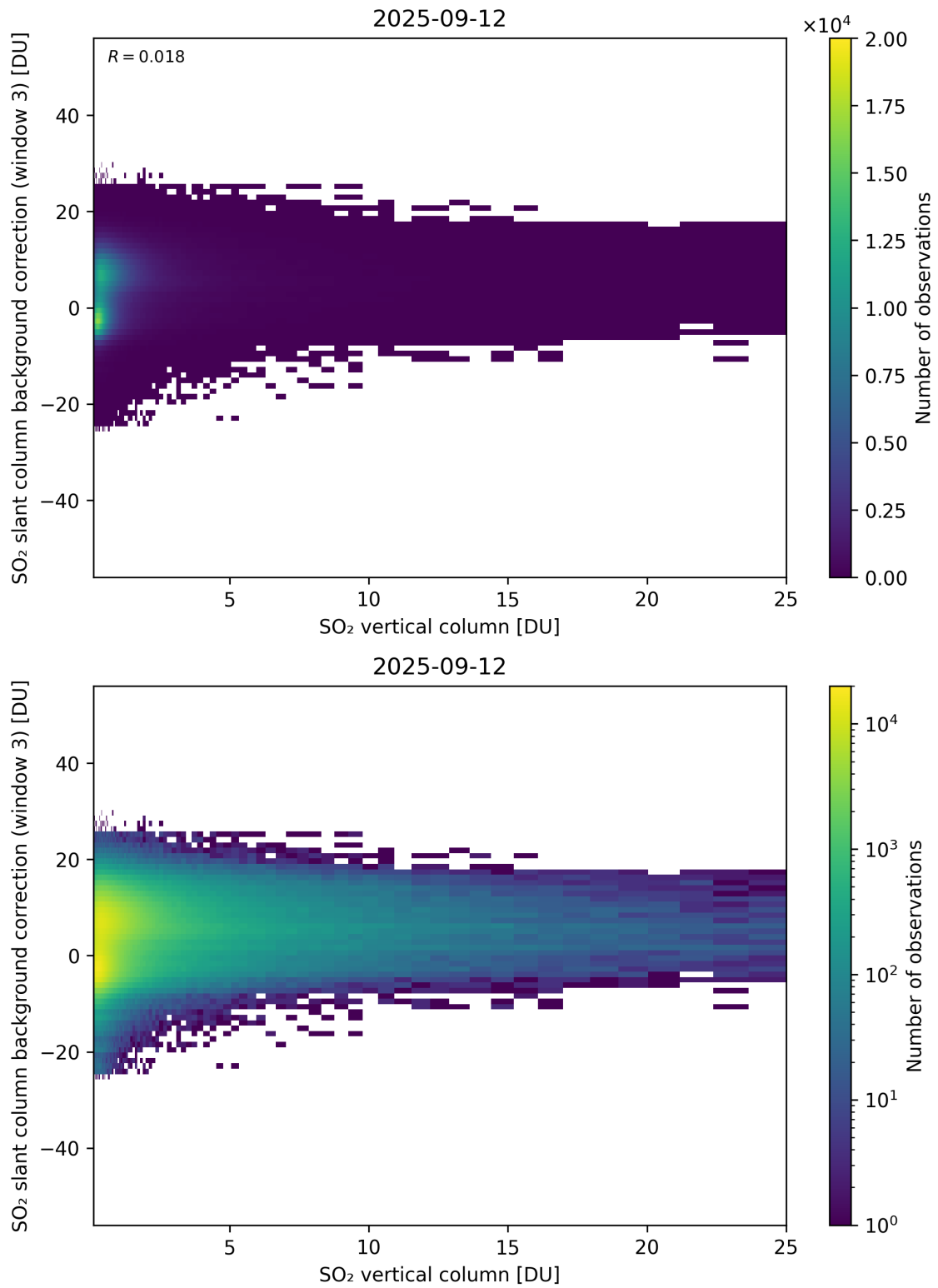
Figure 325: Scatter density plot of “SO 2 vertical column” against “SO 2 slant column background correction (window 3)” for 2025-09-11 to 2025-09-13.
