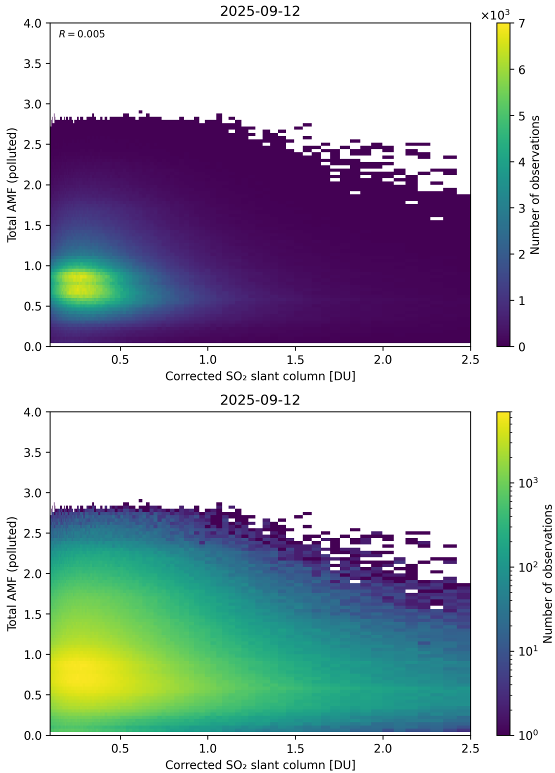
Figure 242: Scatter density plot of “Corrected SO 2 slant column” against “Total AMF (polluted)” for 2025-09-11 to 2025-09-13.
