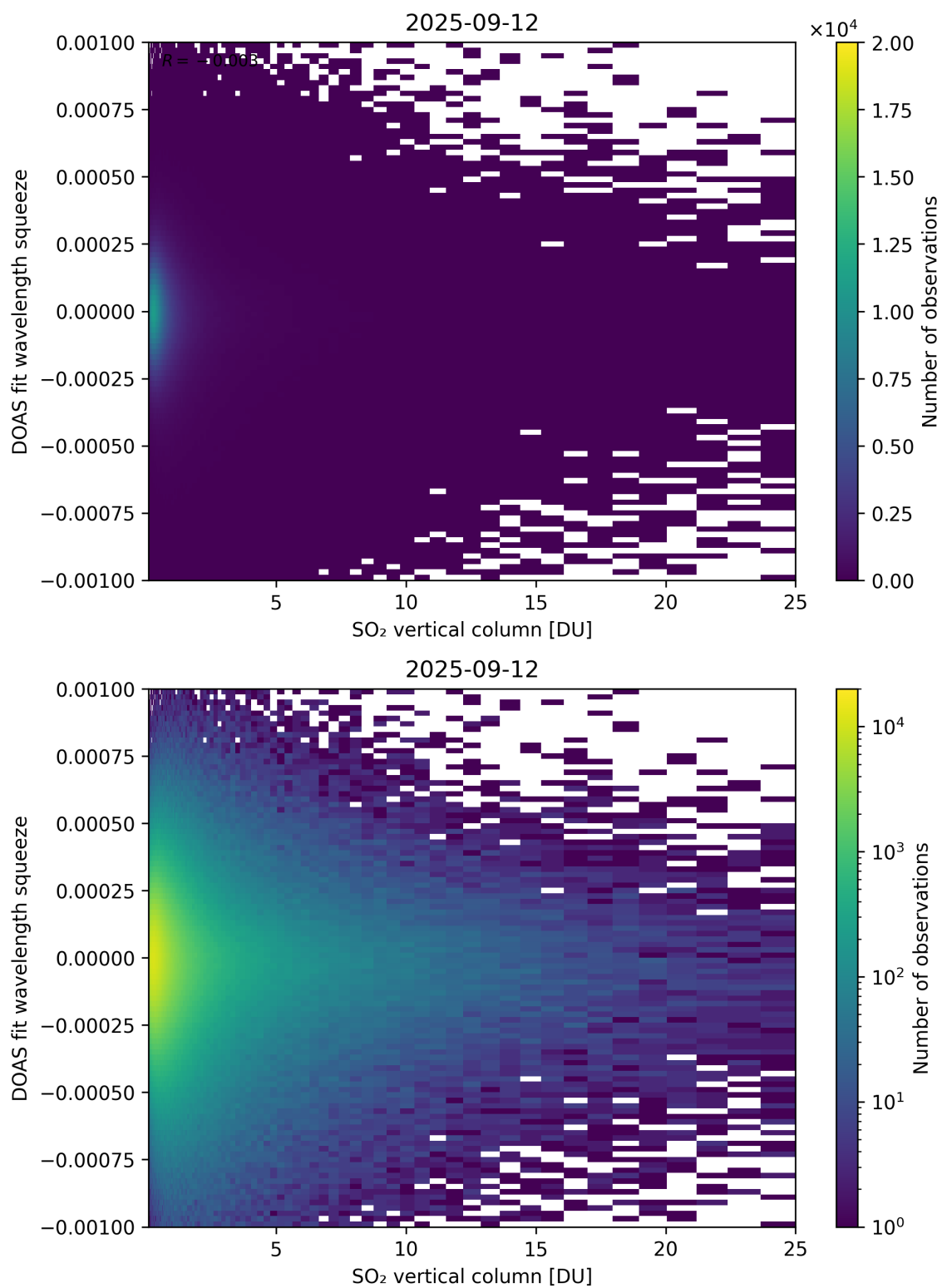
Figure 327: Scatter density plot of “SO 2 vertical column” against “DOAS fit wavelength squeeze” for 2025-09-11 to 2025-09-13.
