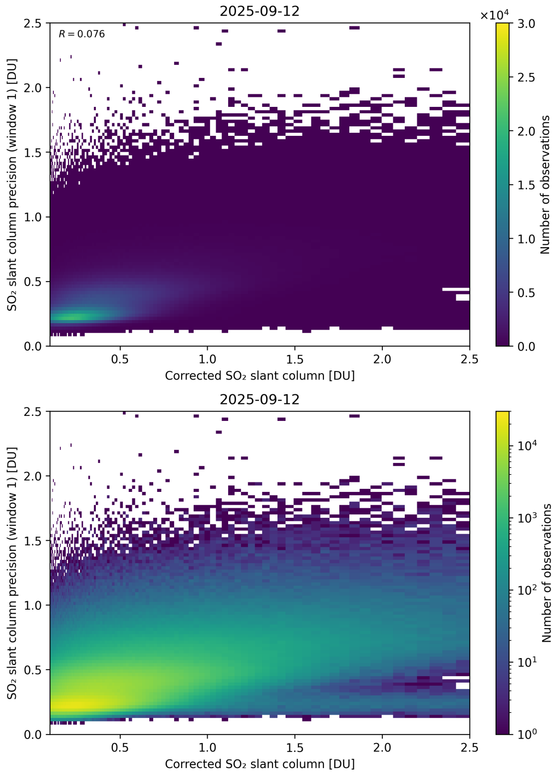
Figure 238: Scatter density plot of “Corrected SO 2 slant column” against “SO 2 slant column precision (window 1)” for 2025-09-11 to 2025-09-13.
