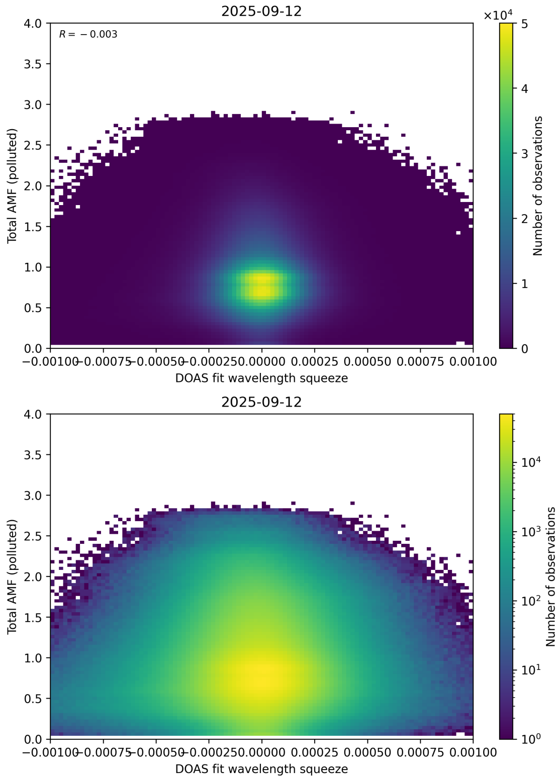
Figure 145: Scatter density plot of “DOAS fit wavelength squeeze” against “Total AMF (polluted)” for 2025-09-11 to 2025-09-13.
