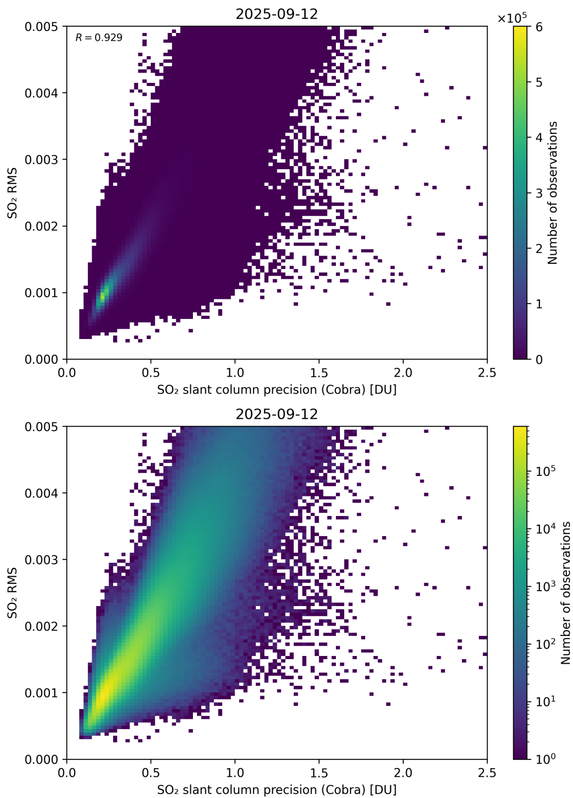
Figure 204: Scatter density plot of “SO 2 slant column precision (Cobra)” against “SO 2 RMS” for 2025-09-11 to 2025-09-13.
