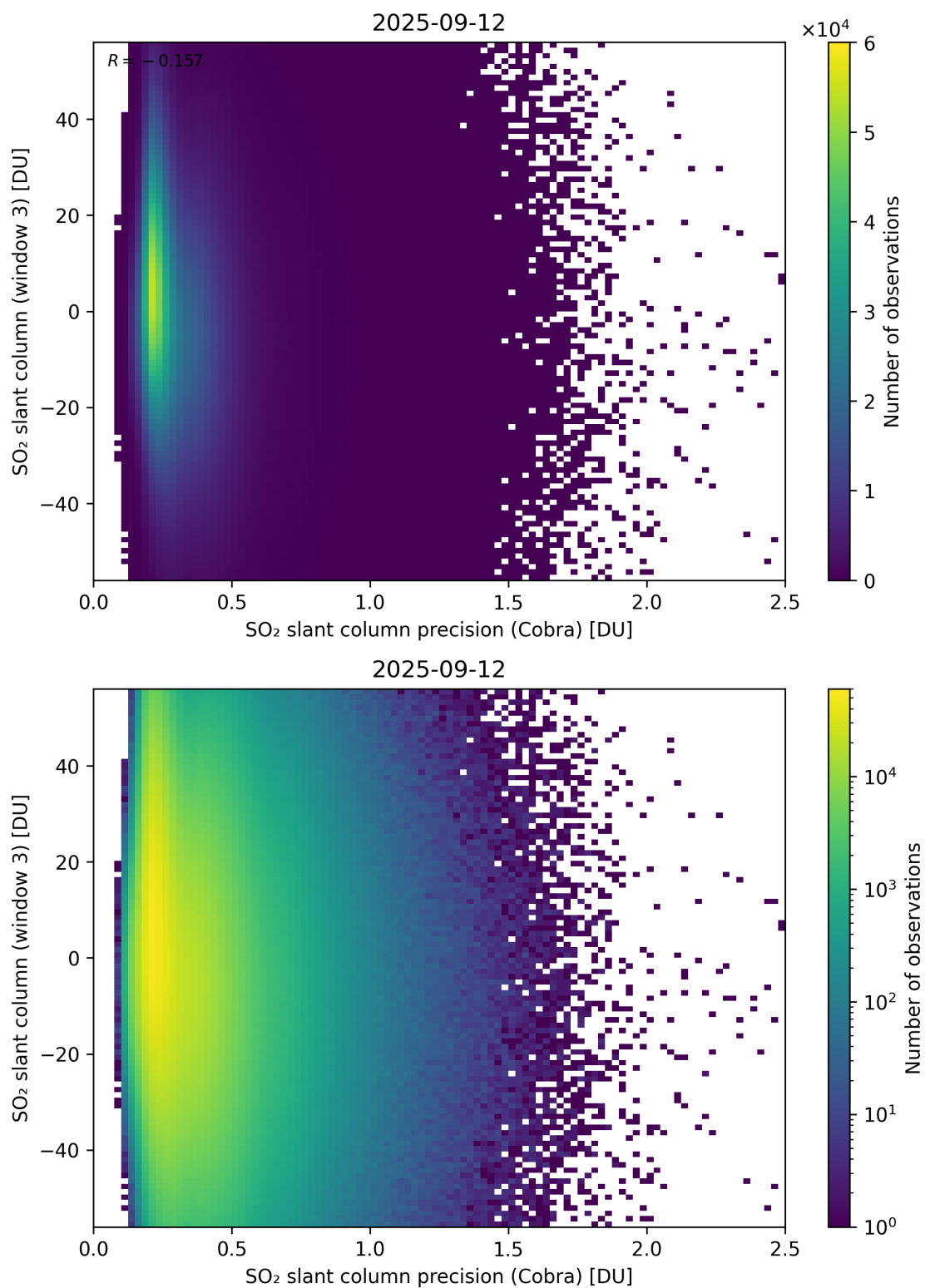
Figure 211: Scatter density plot of “SO 2 slant column precision (Cobra)” against “SO 2 slant column (window 3)” for 2025-09-11 to 2025-09-13.
