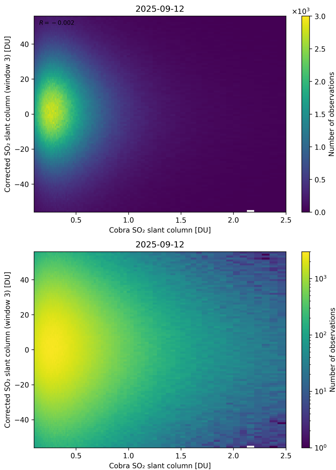
Figure 218: Scatter density plot of “Cobra SO 2 slant column” against “Corrected SO 2 slant column (window 3)” for 2025-09-11 to 2025-09-13.
