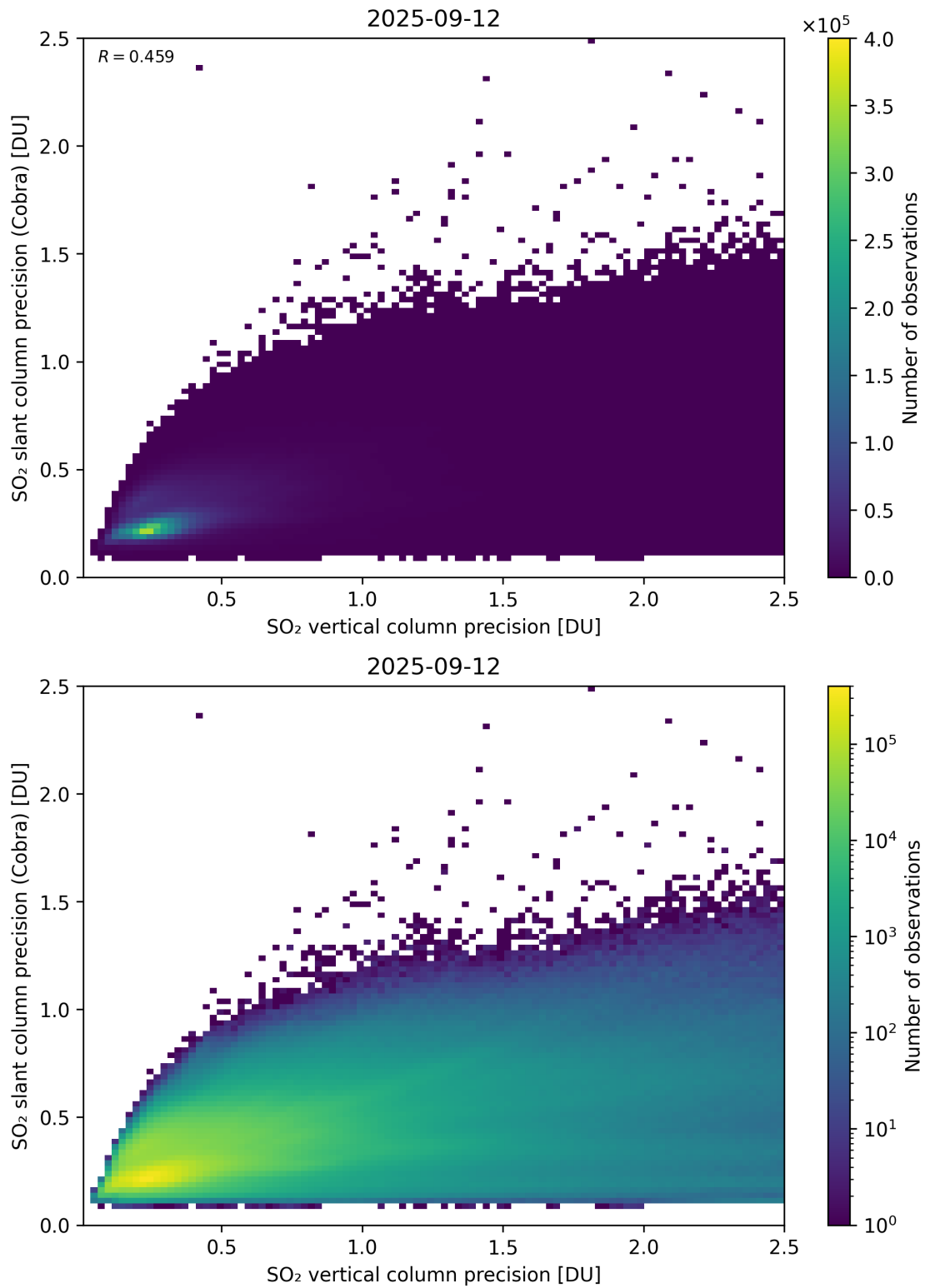
Figure 337: Scatter density plot of “SO 2 vertical column precision” against “SO 2 slant column precision (Cobra)” for 2025-09-11 to 2025-09-13.
