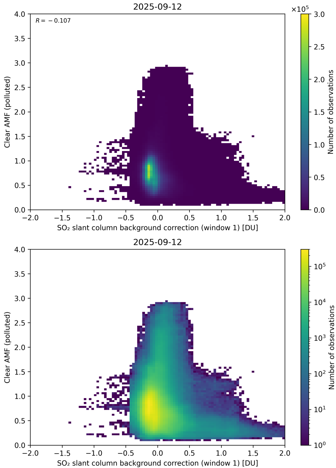
Figure 114: Scatter density plot of “SO 2 slant column background correction (window 1)” against “Clear AMF (polluted)” for 2025-09-11 to 2025-09-13.
