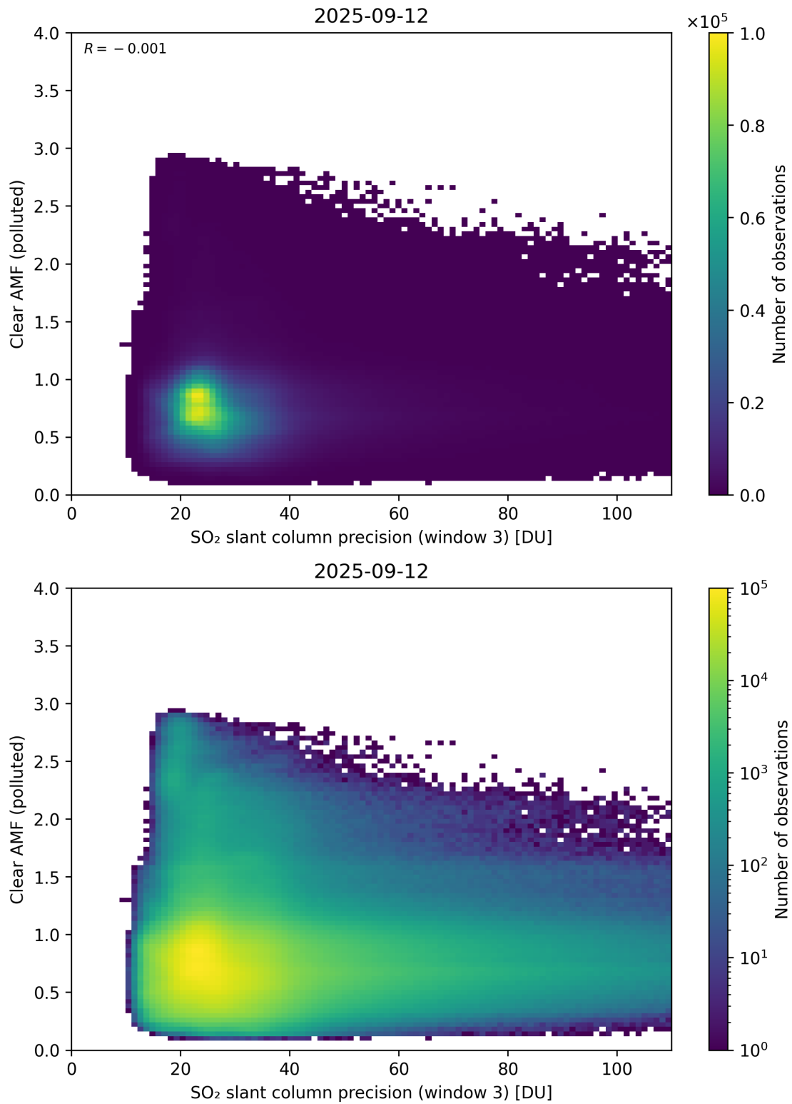
Figure 311: Scatter density plot of “SO 2 slant column precision (window 3)” against “Clear AMF (polluted)” for 2025-09-11 to 2025-09-13.
