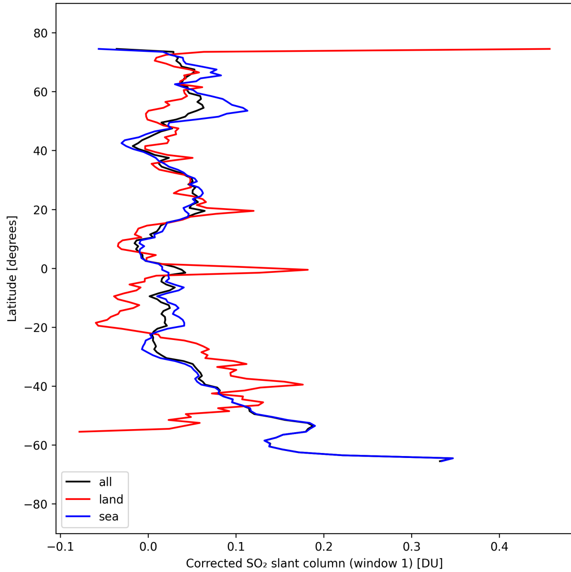
Figure 39: Zonal average of “Corrected SO 2 slant column (window 1)” for 2025-09-11 to 2025-09-13.
