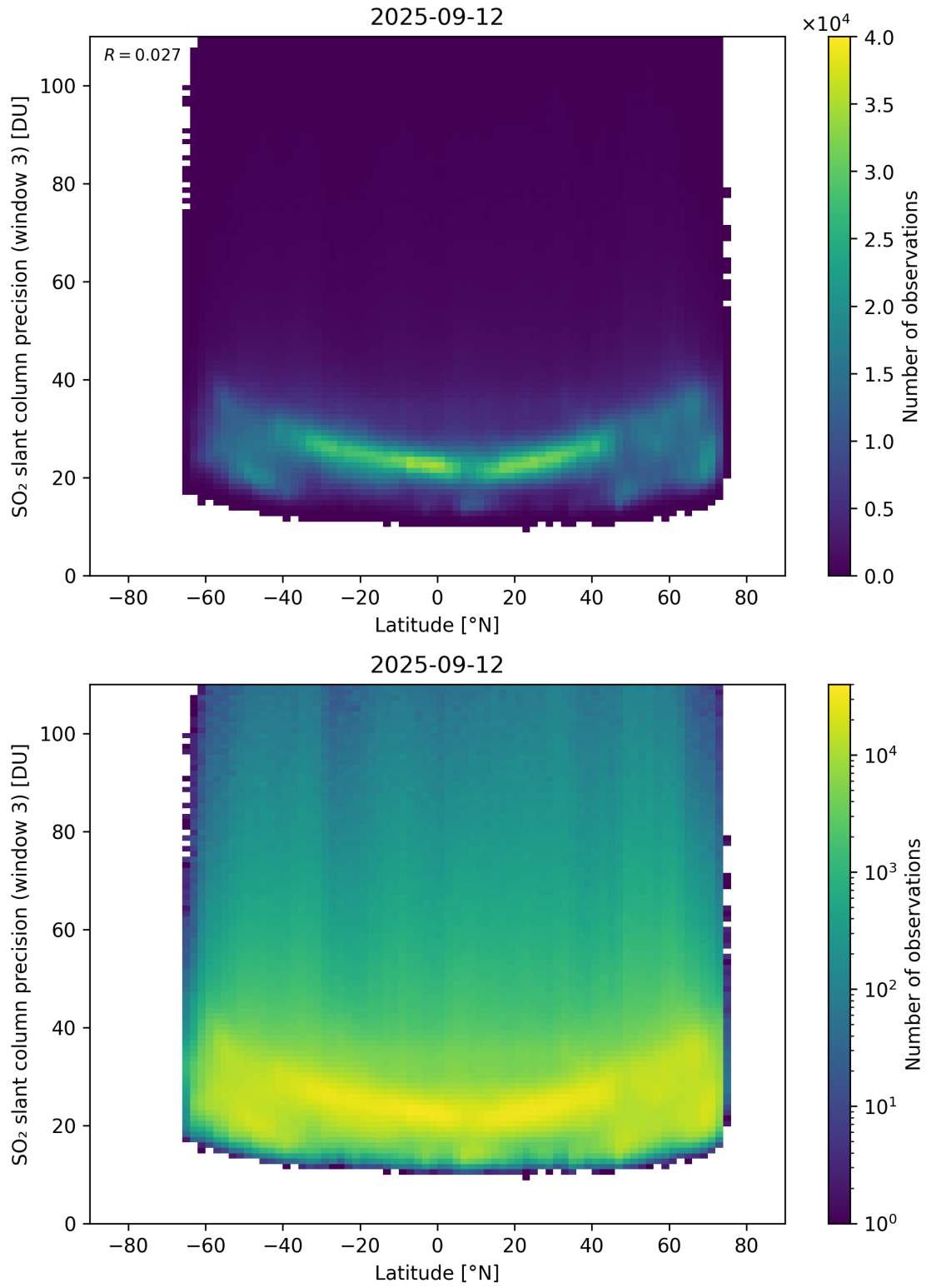
Figure 166: Scatter density plot of “Latitude” against “SO 2 slant column precision (window 3)” for 2025-09-11 to 2025-09-13.
