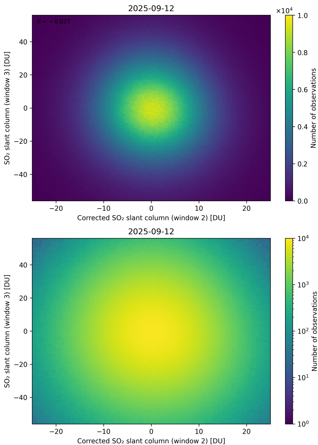
Figure 251: Scatter density plot of “Corrected SO 2 slant column (window 2)” against “SO 2 slant column (window 3)” for 2025-09-11 to 2025-09-13.
