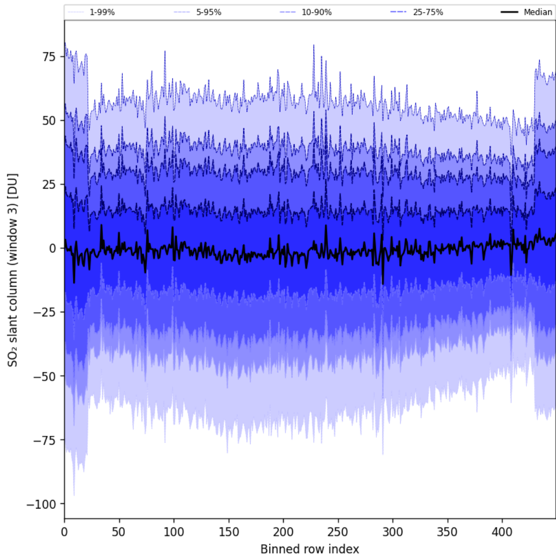
Figure 97: Along track statistics of “SO 2 slant column (window 3)” for 2025-09-11 to 2025-09-13
