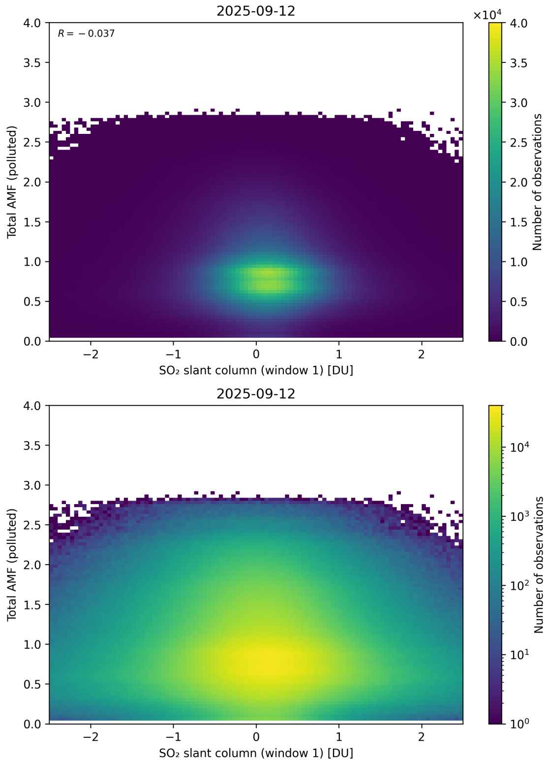
Figure 289: Scatter density plot of “SO 2 slant column (window 1)” against “Total AMF (polluted)” for 2025-09-11 to 2025-09-13.
