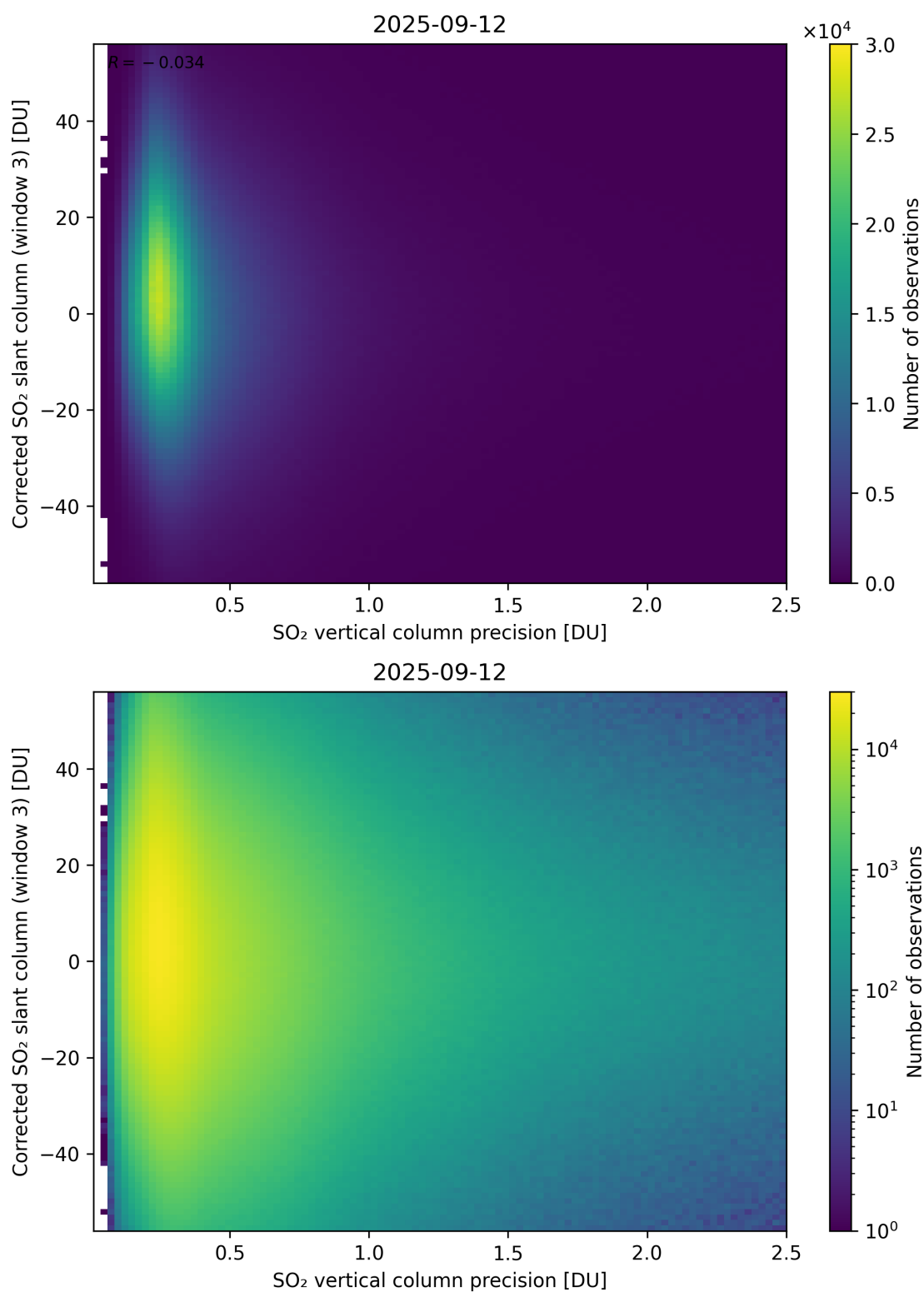
Figure 340: Scatter density plot of “SO 2 vertical column precision” against “Corrected SO 2 slant column (window 3)” for 2025-09-11 to 2025-09-13.
