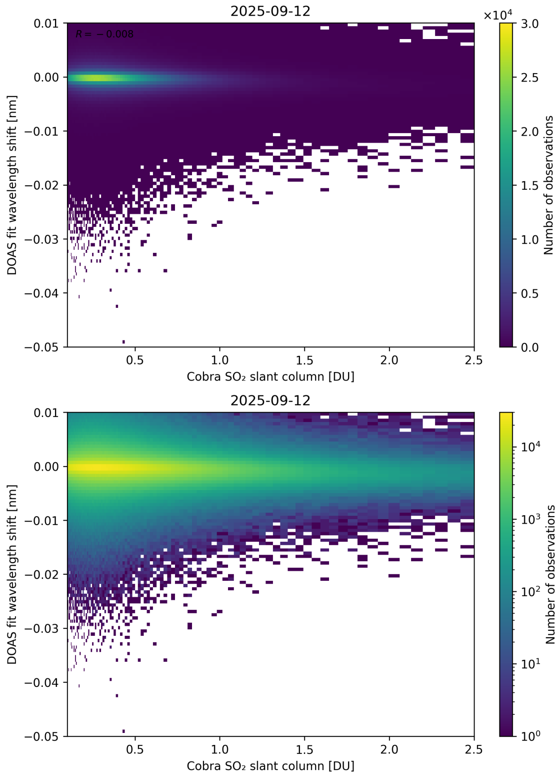
Figure 196: Scatter density plot of “Cobra SO 2 slant column” against “DOAS fit wavelength shift” for 2025-09-11 to 2025-09-13.
