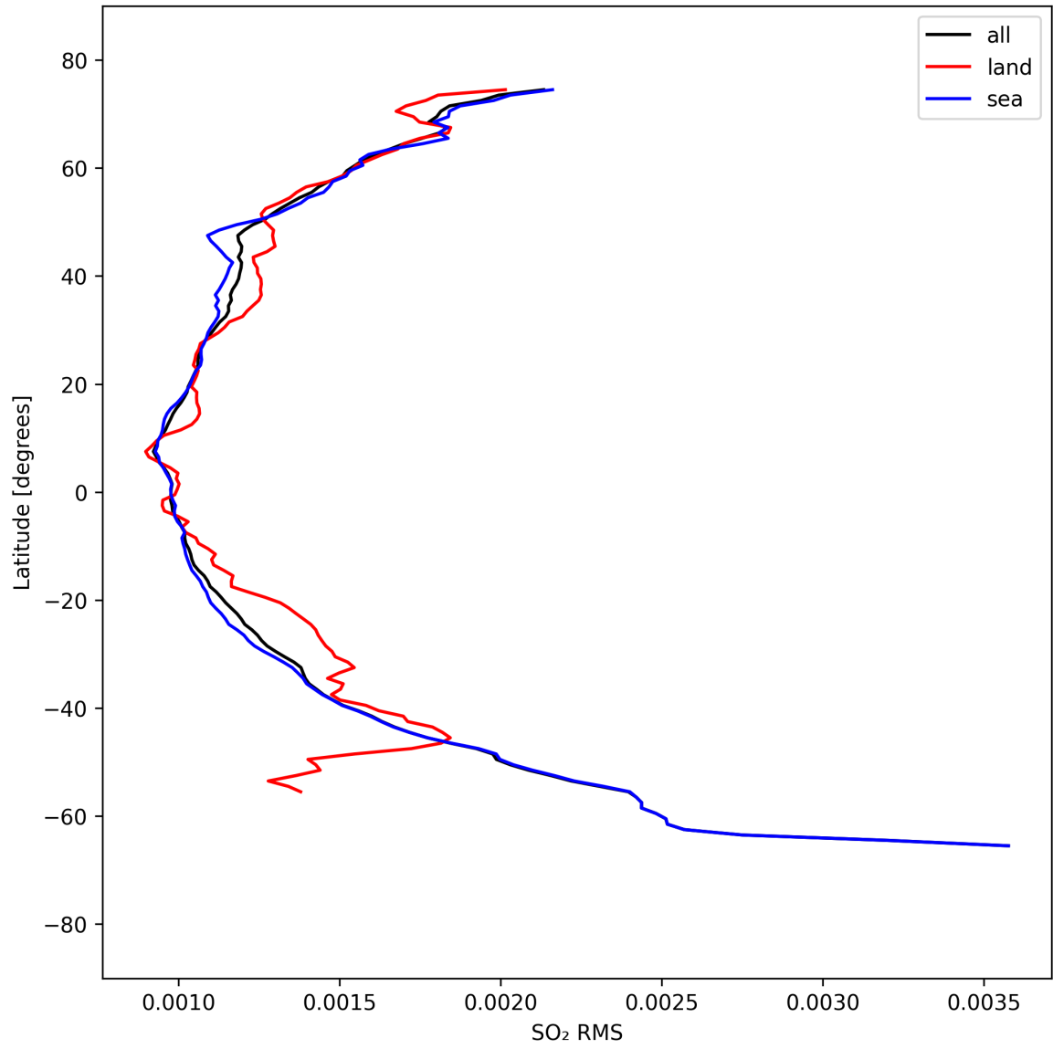
Figure 52: Zonal average of “SO 2 RMS” for 2025-09-11 to 2025-09-13.
