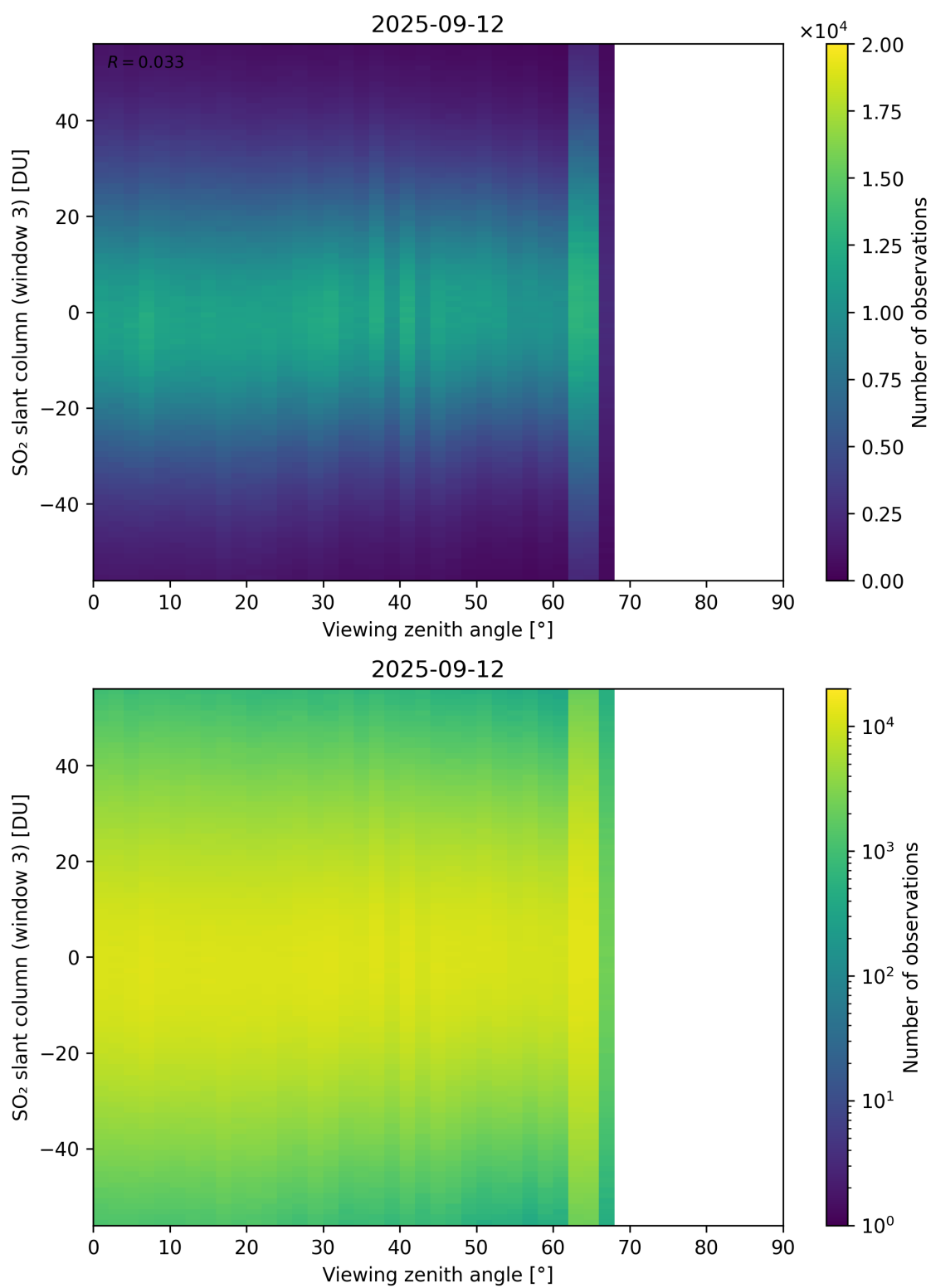
Figure 379: Scatter density plot of “Viewing zenith angle” against “SO 2 slant column (window 3)” for 2025-09-11 to 2025-09-13.
