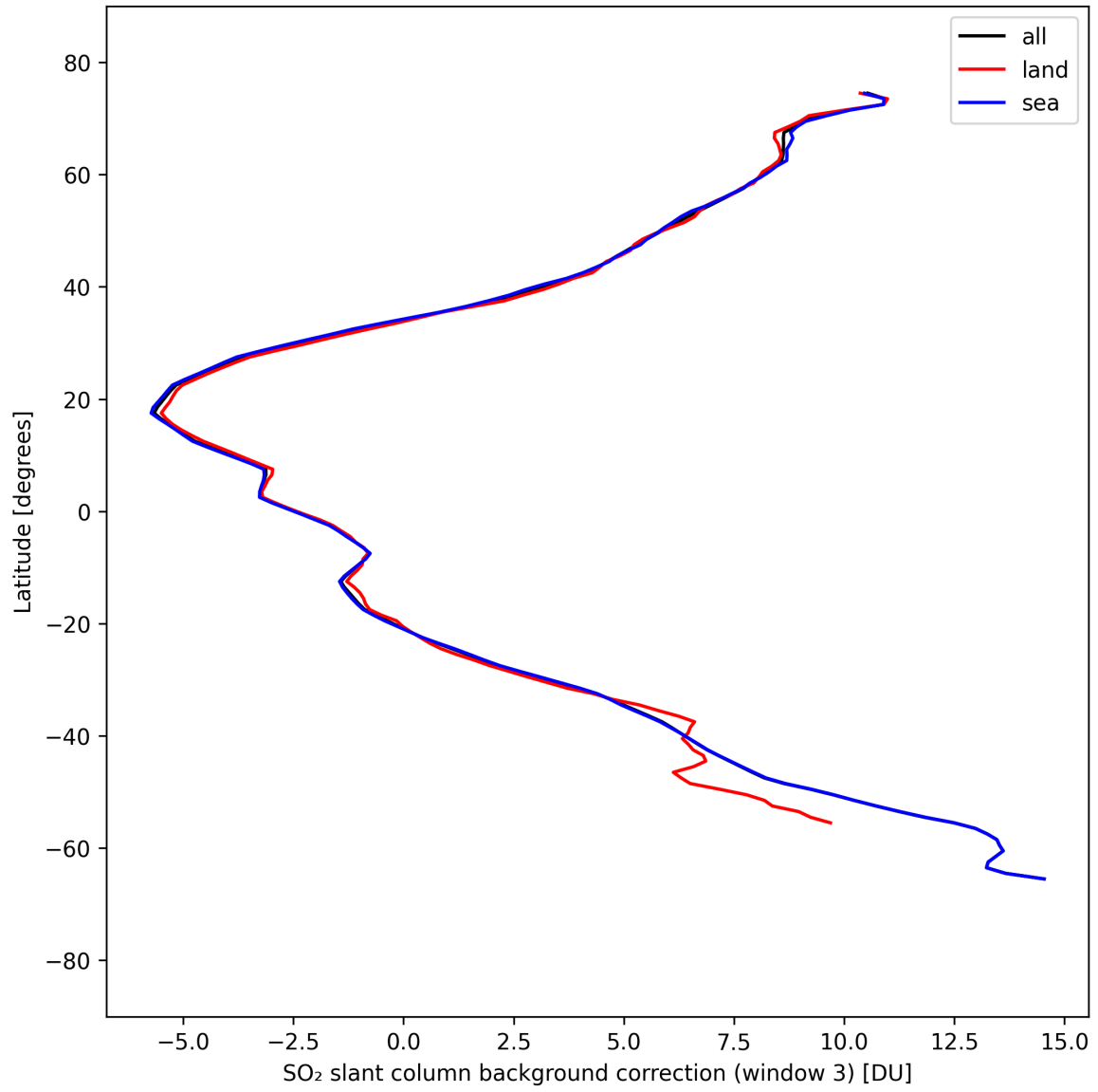
Figure 48: Zonal average of “SO 2 slant column background correction (window 3)” for 2025-09-11 to 2025-09-13.
