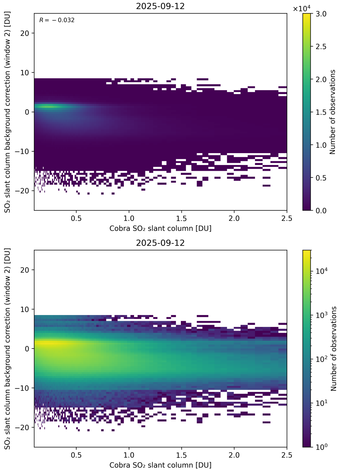
Figure 194: Scatter density plot of “Cobra SO 2 slant column” against “SO 2 slant column background correction (window 2)” for 2025-09-11 to 2025-09-13.
