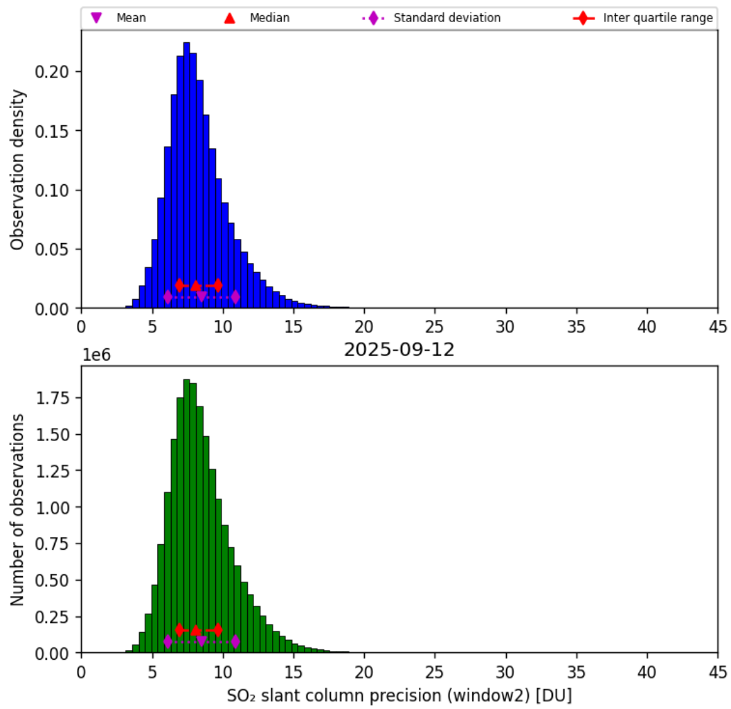
Figure 68: Histogram of “SO 2 slant column precision (window2)” for 2025-09-11 to 2025-09-13
