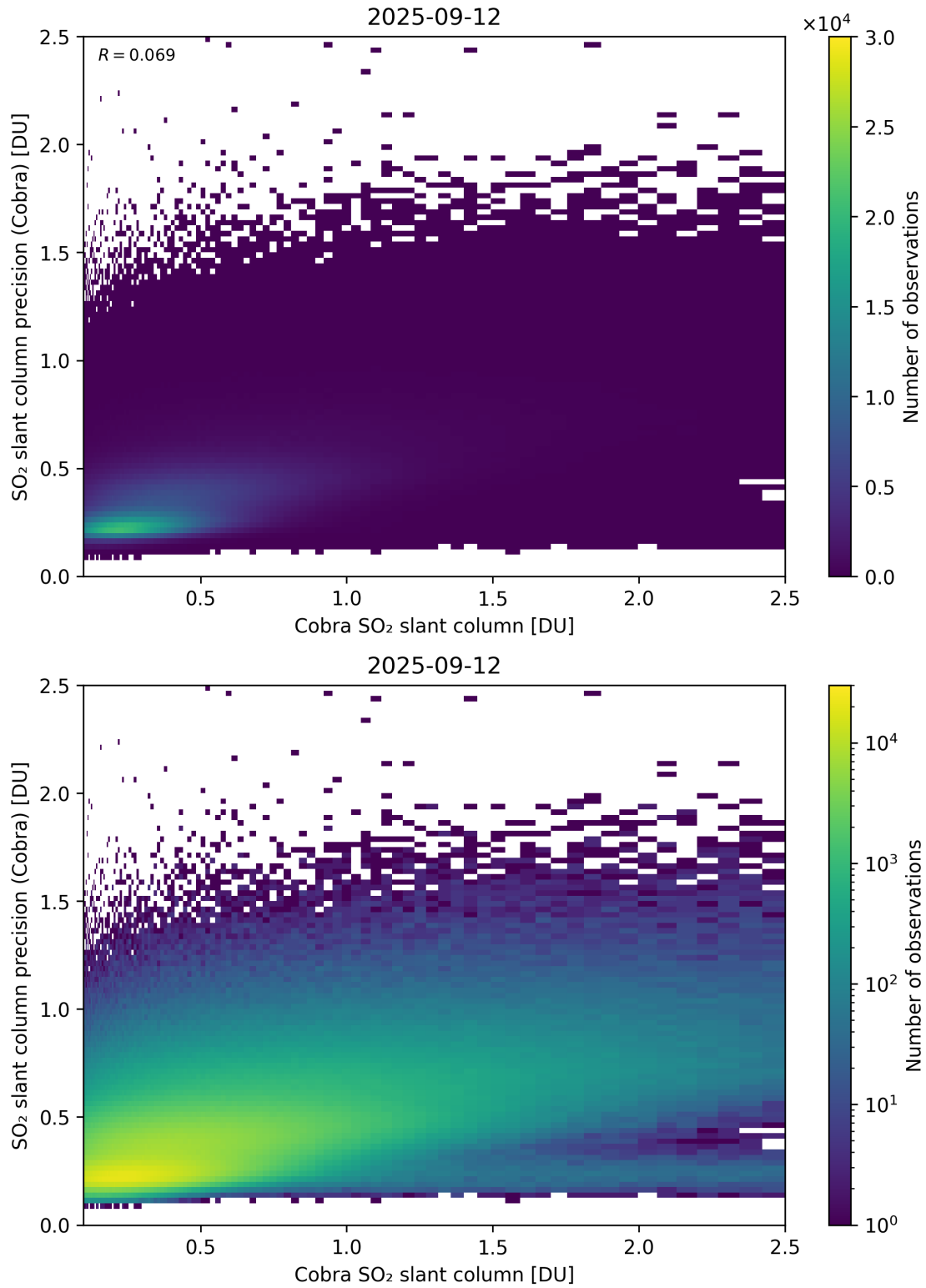
Figure 216: Scatter density plot of “Cobra SO 2 slant column” against “SO 2 slant column precision (Cobra)” for 2025-09-11 to 2025-09-13.
