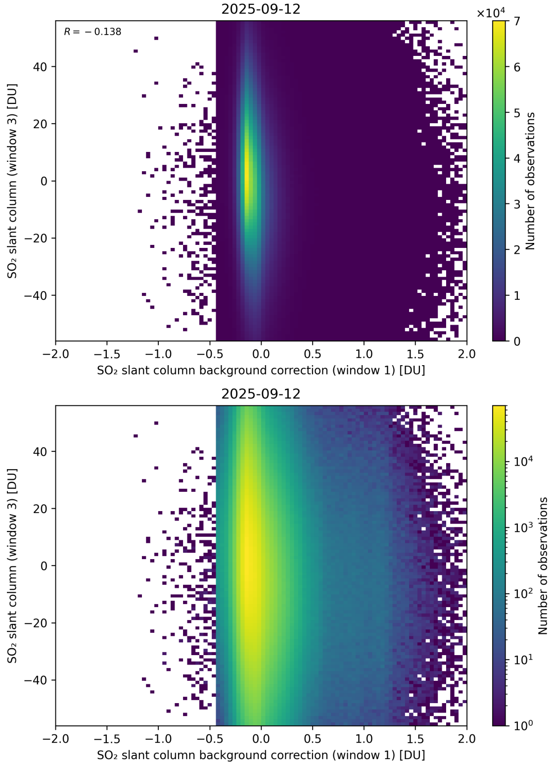
Figure 118: Scatter density plot of “SO 2 slant column background correction (window 1)” against “SO 2 slant column (window 3)” for 2025-09-11 to 2025-09-13.
