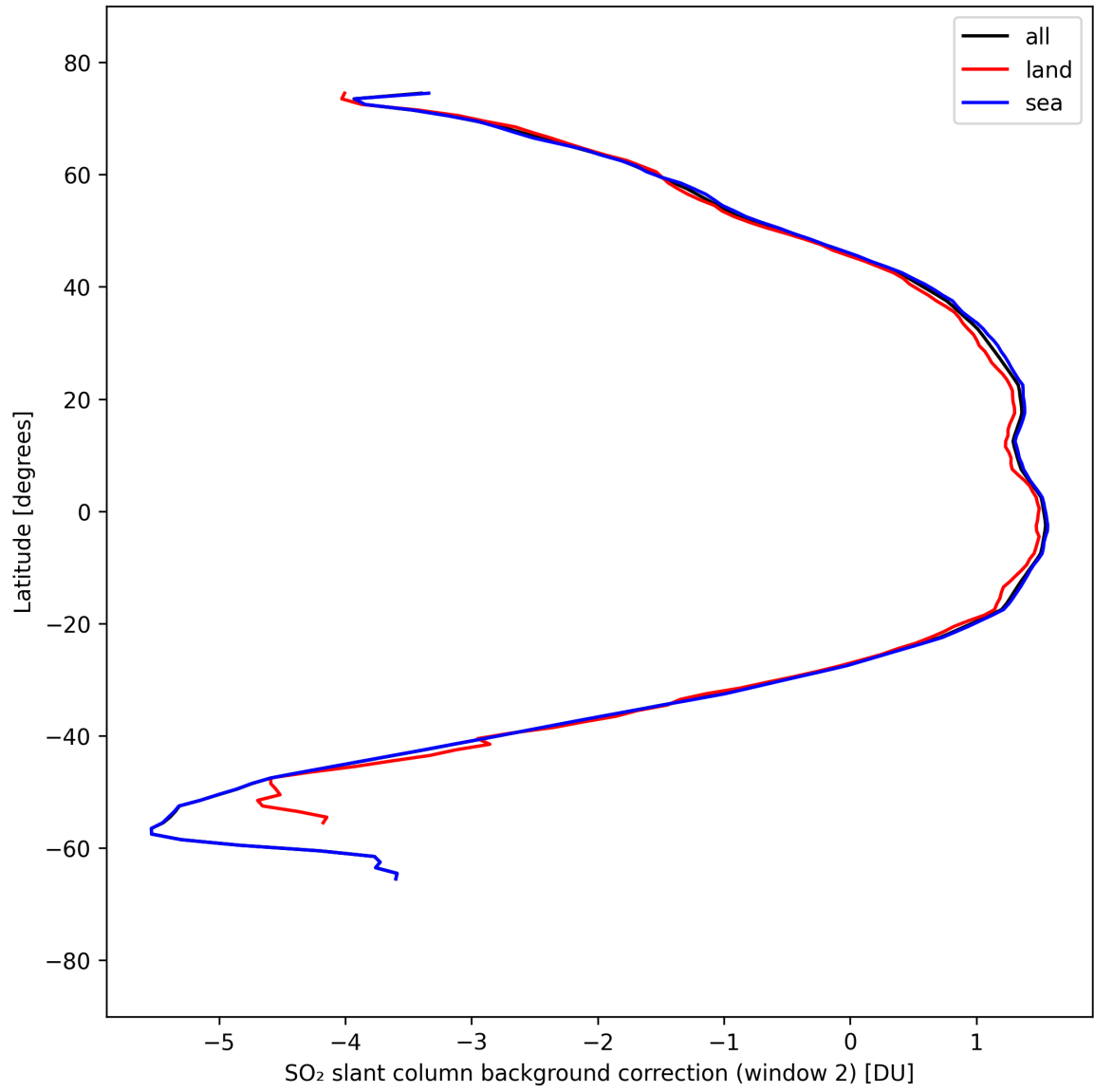
Figure 44: Zonal average of “SO 2 slant column background correction (window 2)” for 2025-09-11 to 2025-09-13.
