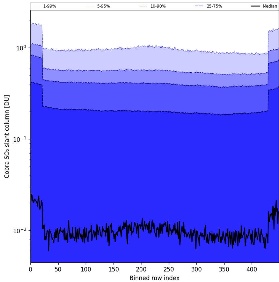
Figure 87: Along track statistics of “Cobra SO 2 slant column” for 2025-09-11 to 2025-09-13
