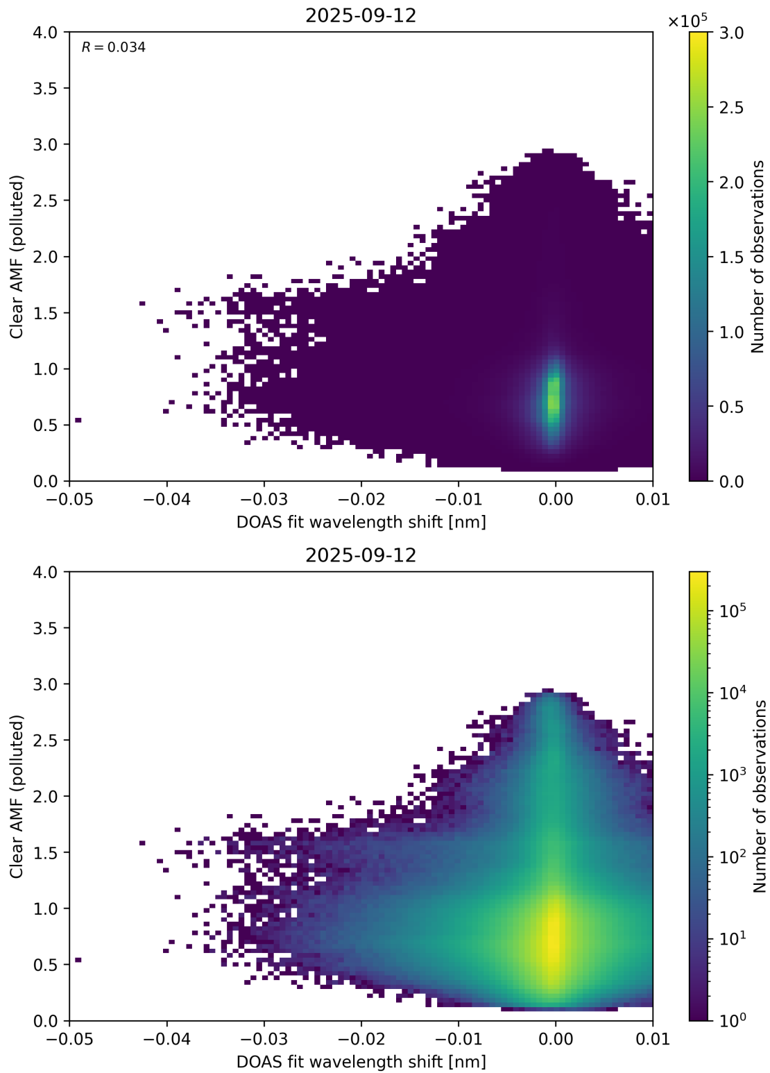
Figure 140: Scatter density plot of “DOAS fit wavelength shift” against “Clear AMF (polluted)” for 2025-09-11 to 2025-09-13.
