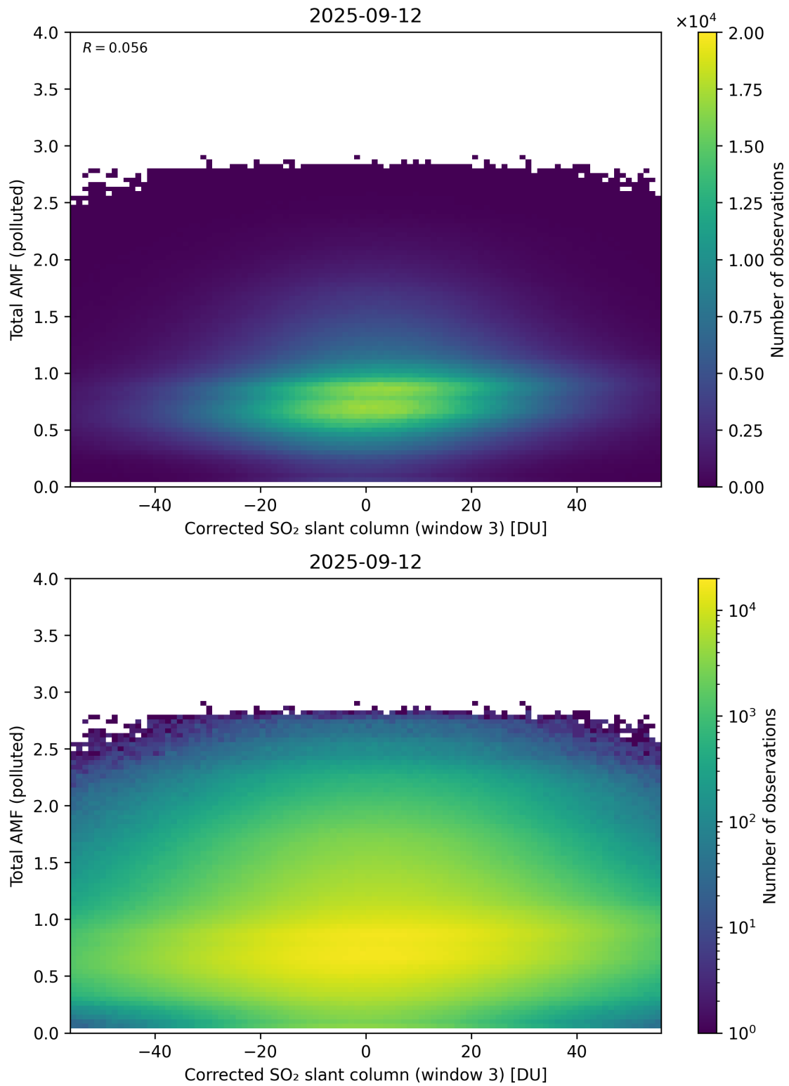
Figure 260: Scatter density plot of “Corrected SO 2 slant column (window 3)” against “Total AMF (polluted)” for 2025-09-11 to 2025-09-13.
