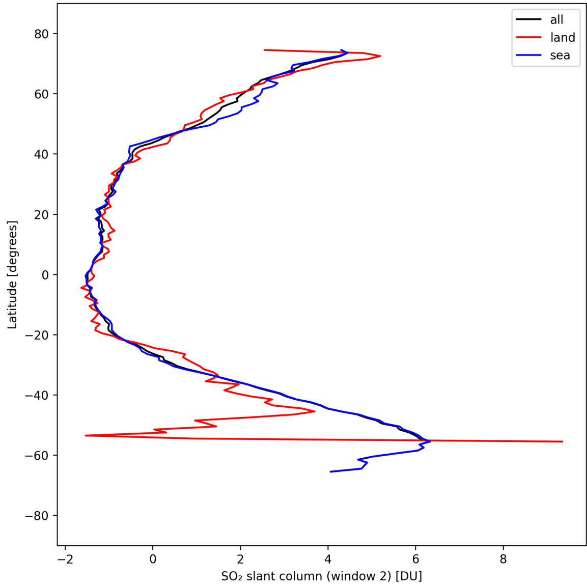
Figure 41: Zonal average of “SO 2 slant column (window 2)” for 2025-09-11 to 2025-09-13.
