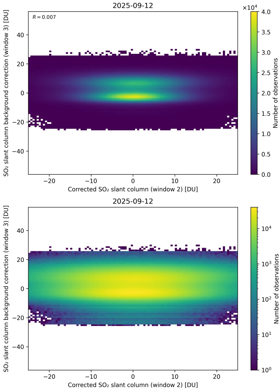
Figure 245: Scatter density plot of “Corrected SO 2 slant column (window 2)” against “SO 2 slant column background correction (window 3)” for 2025-09-11 to 2025-09-13.
