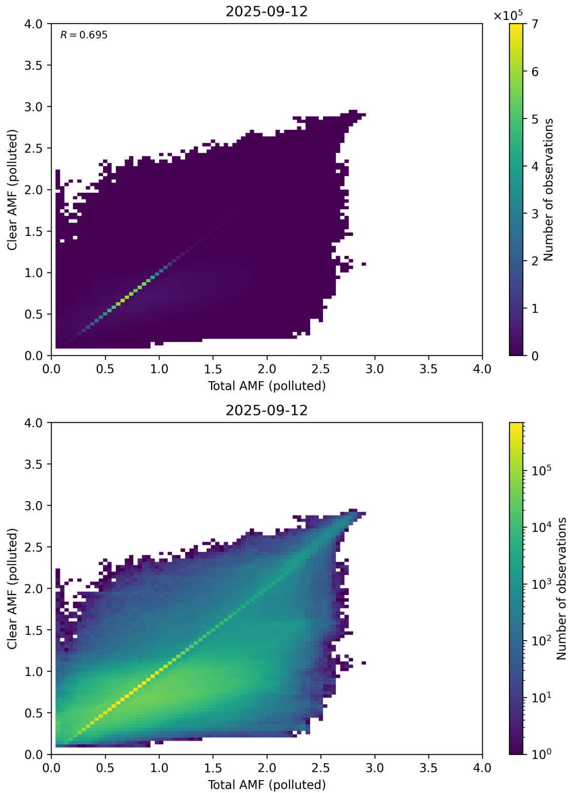
Figure 321: Scatter density plot of “Total AMF (polluted)” against “Clear AMF (polluted)” for 2025-09-11 to 2025-09-13.
