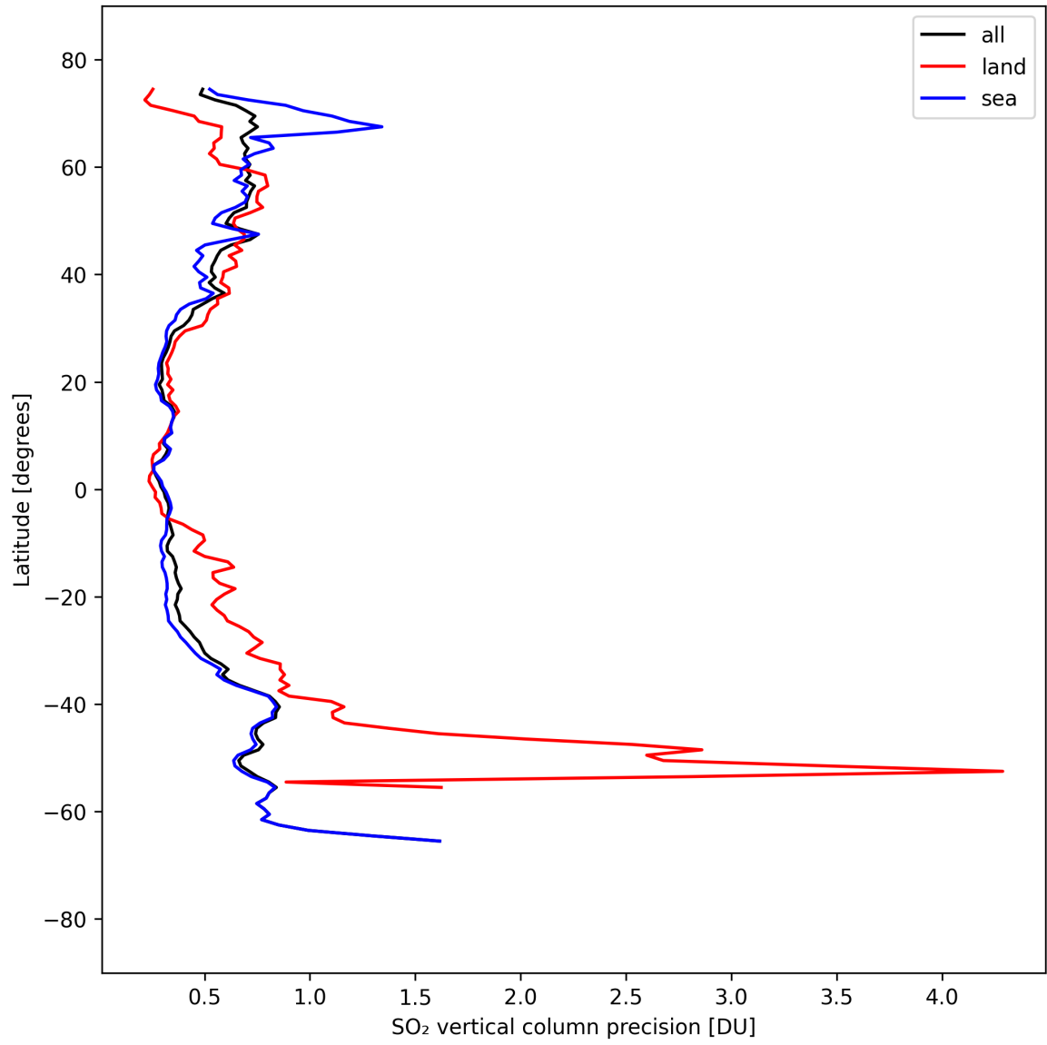
Figure 33: Zonal average of “SO 2 vertical column precision” for 2025-09-11 to 2025-09-13.
