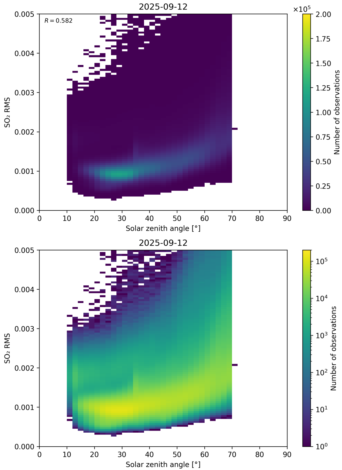
Figure 176: Scatter density plot of “Solar zenith angle” against “SO 2 RMS” for 2025-09-11 to 2025-09-13.
