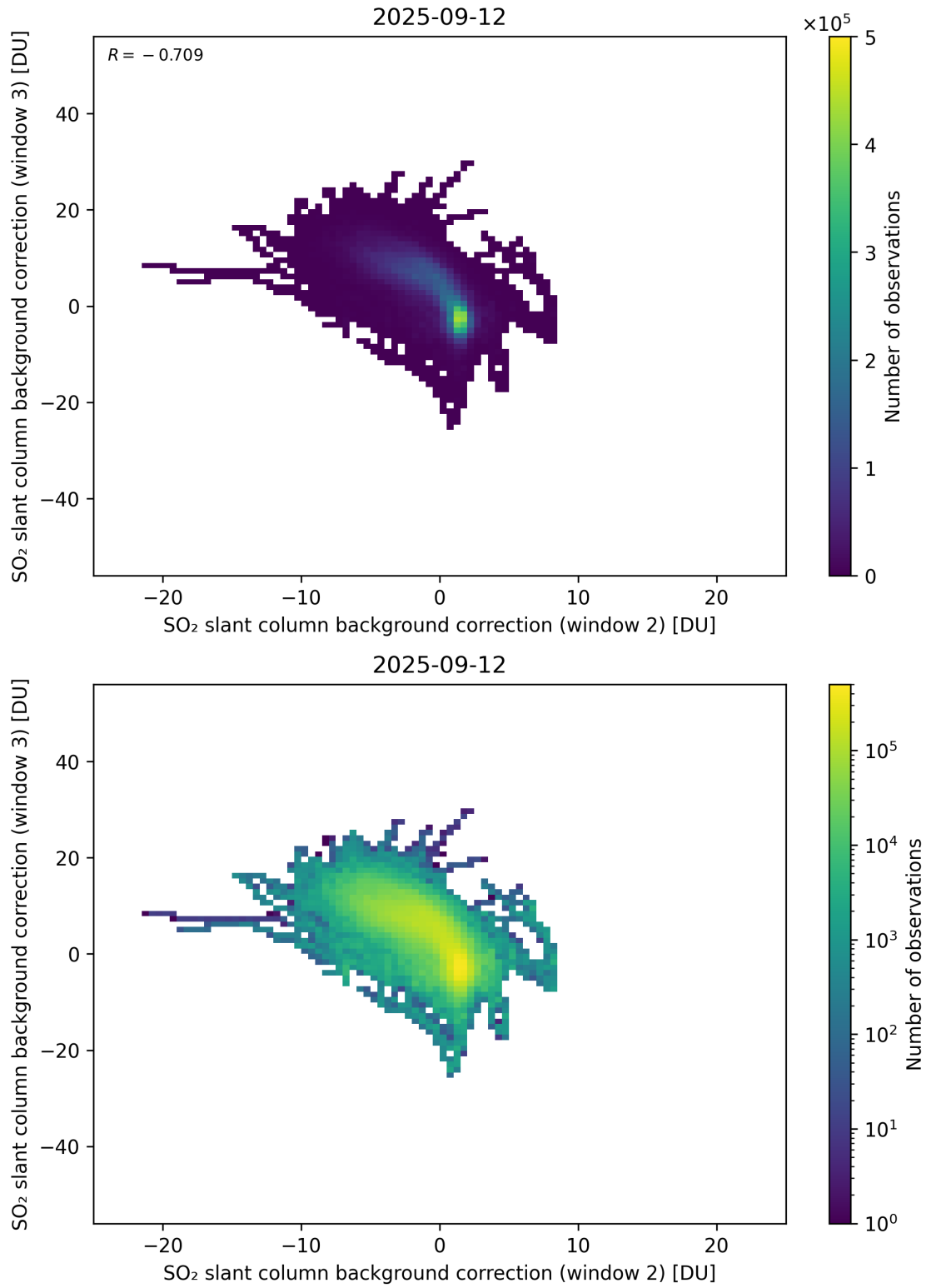
Figure 122: Scatter density plot of “SO 2 slant column background correction (window 2)” against “SO 2 slant column background correction (window 3)” for 2025-09-11 to 2025-09-13.
