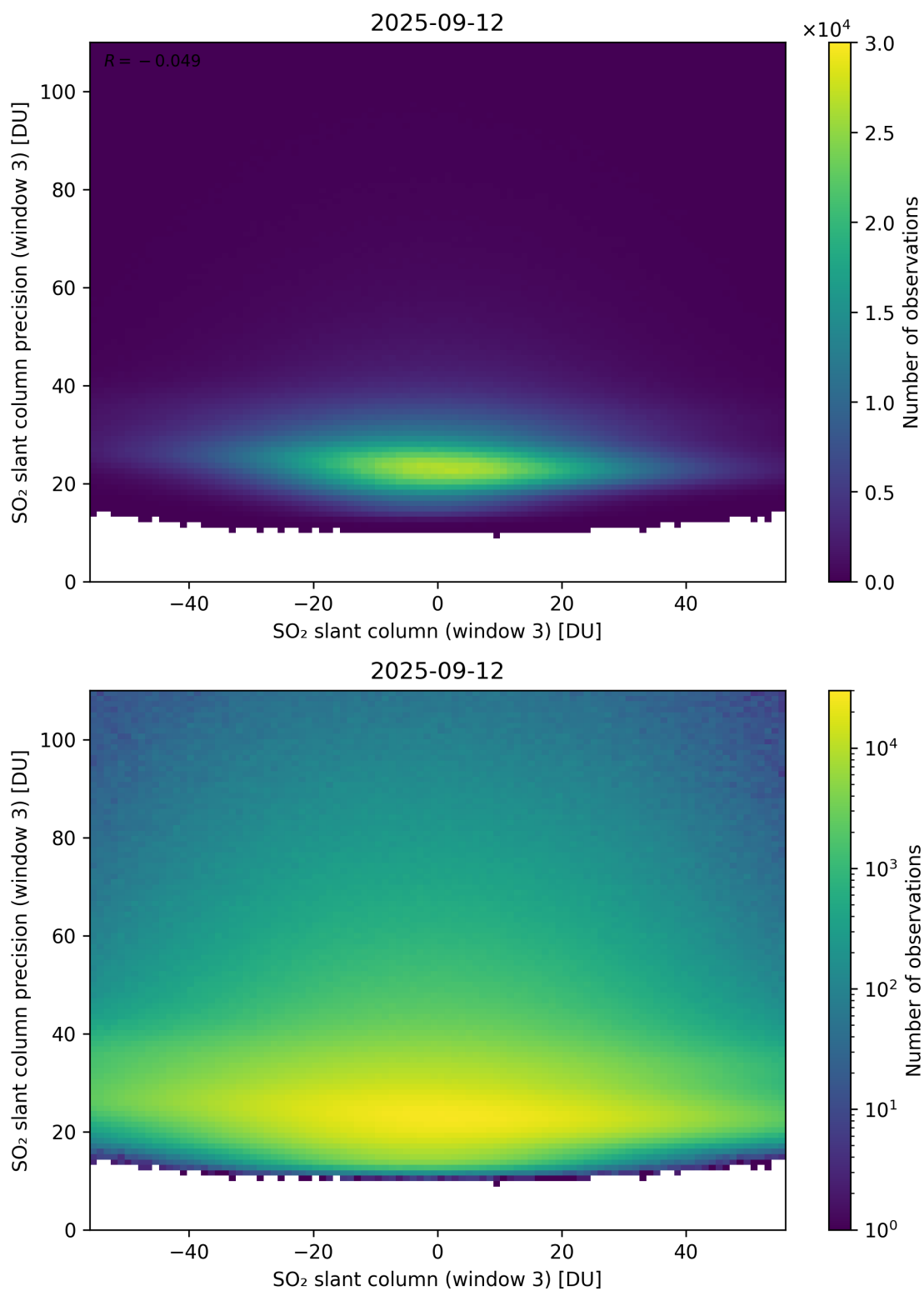
Figure 317: Scatter density plot of “SO 2 slant column (window 3)” against “SO 2 slant column precision (window 3)” for 2025-09-11 to 2025-09-13.
