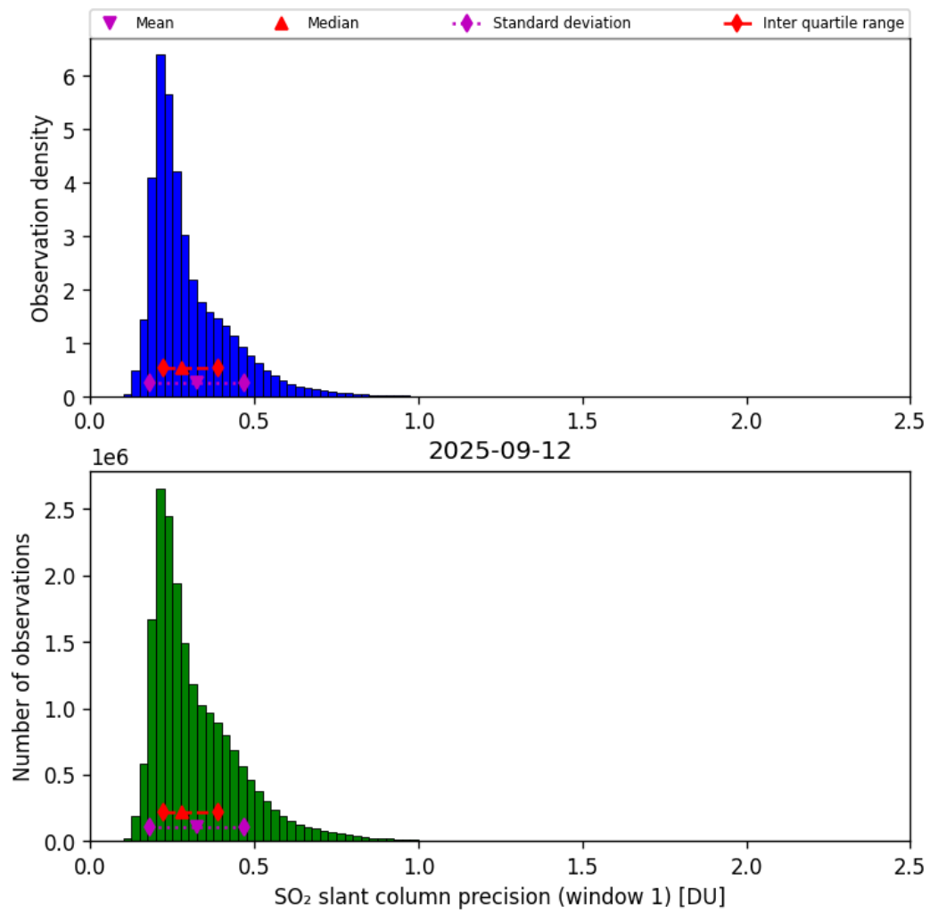
Figure 64: Histogram of “SO 2 slant column precision (window 1)” for 2025-09-11 to 2025-09-13
