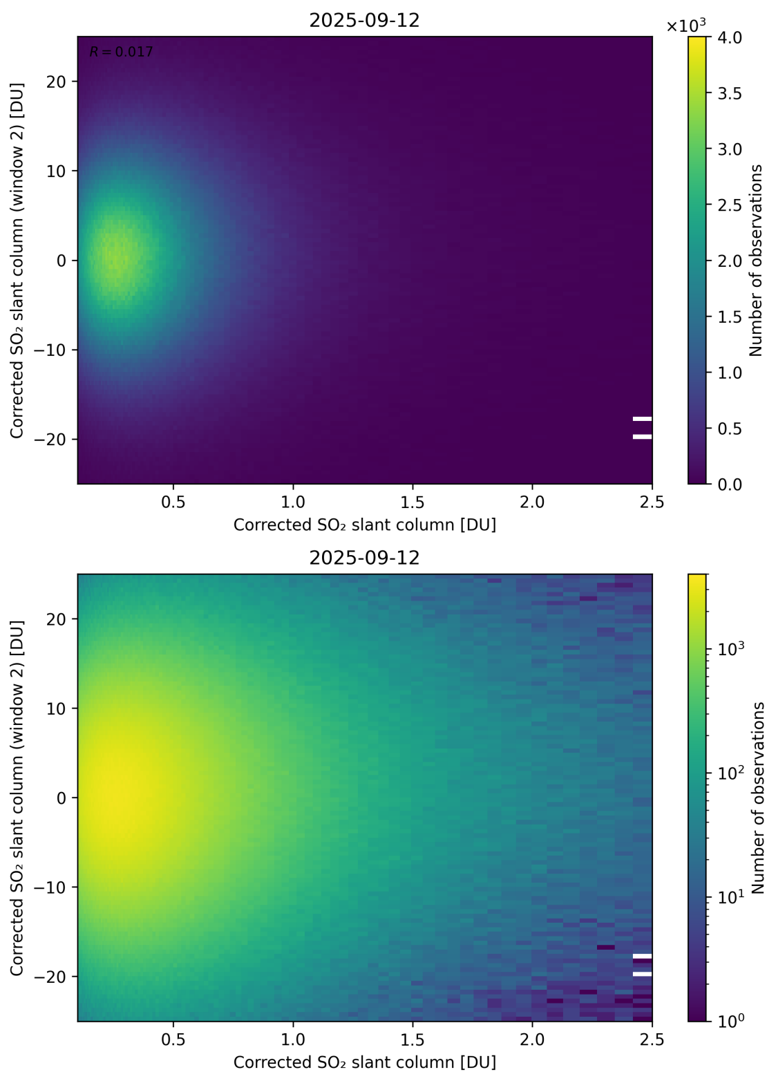
Figure 235: Scatter density plot of “Corrected SO 2 slant column” against “Corrected SO 2 slant column (window 2)” for 2025-09-11 to 2025-09-13.
