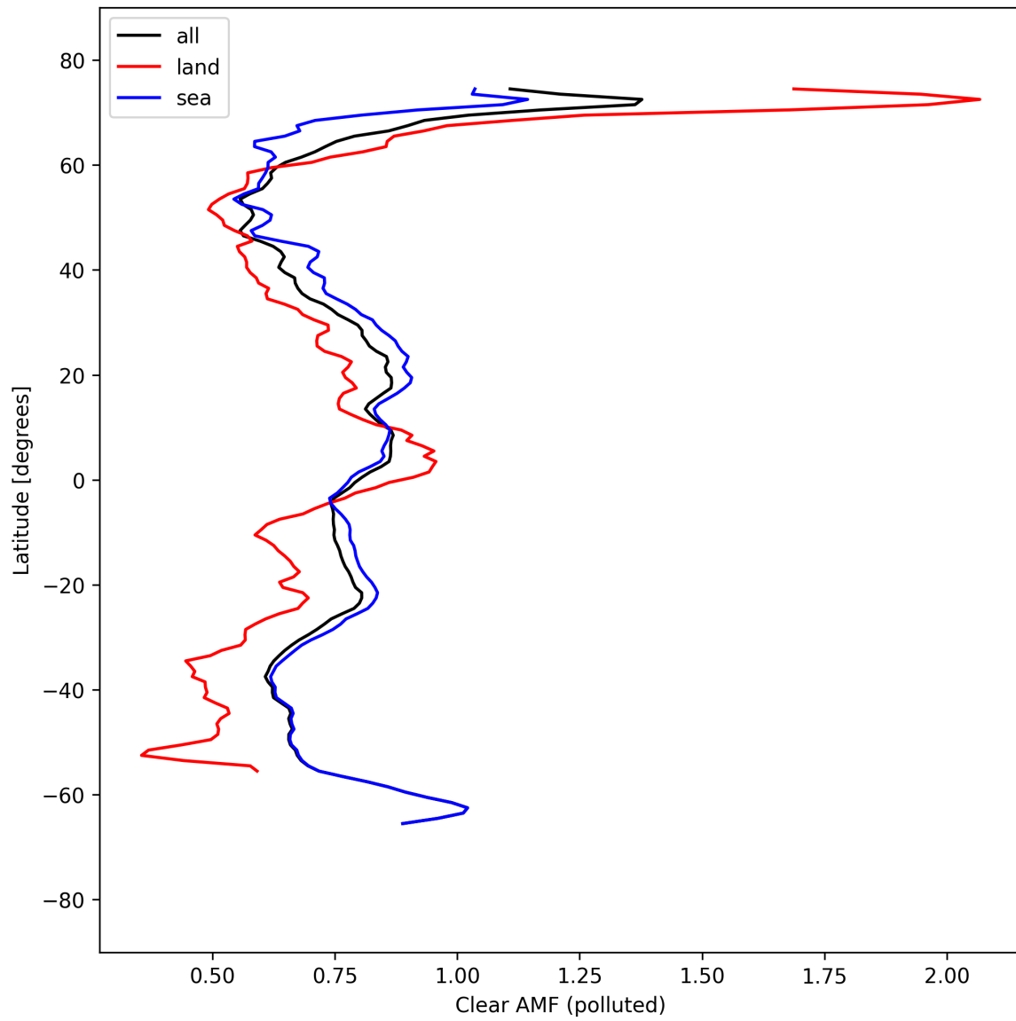
Figure 55: Zonal average of “Clear AMF (polluted)” for 2025-09-11 to 2025-09-13.
