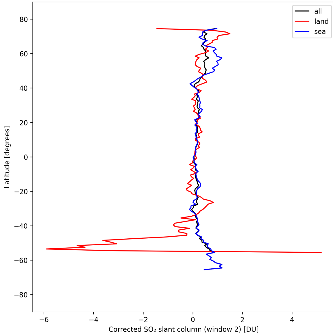
Figure 43: Zonal average of “Corrected SO 2 slant column (window 2)” for 2025-09-11 to 2025-09-13.
