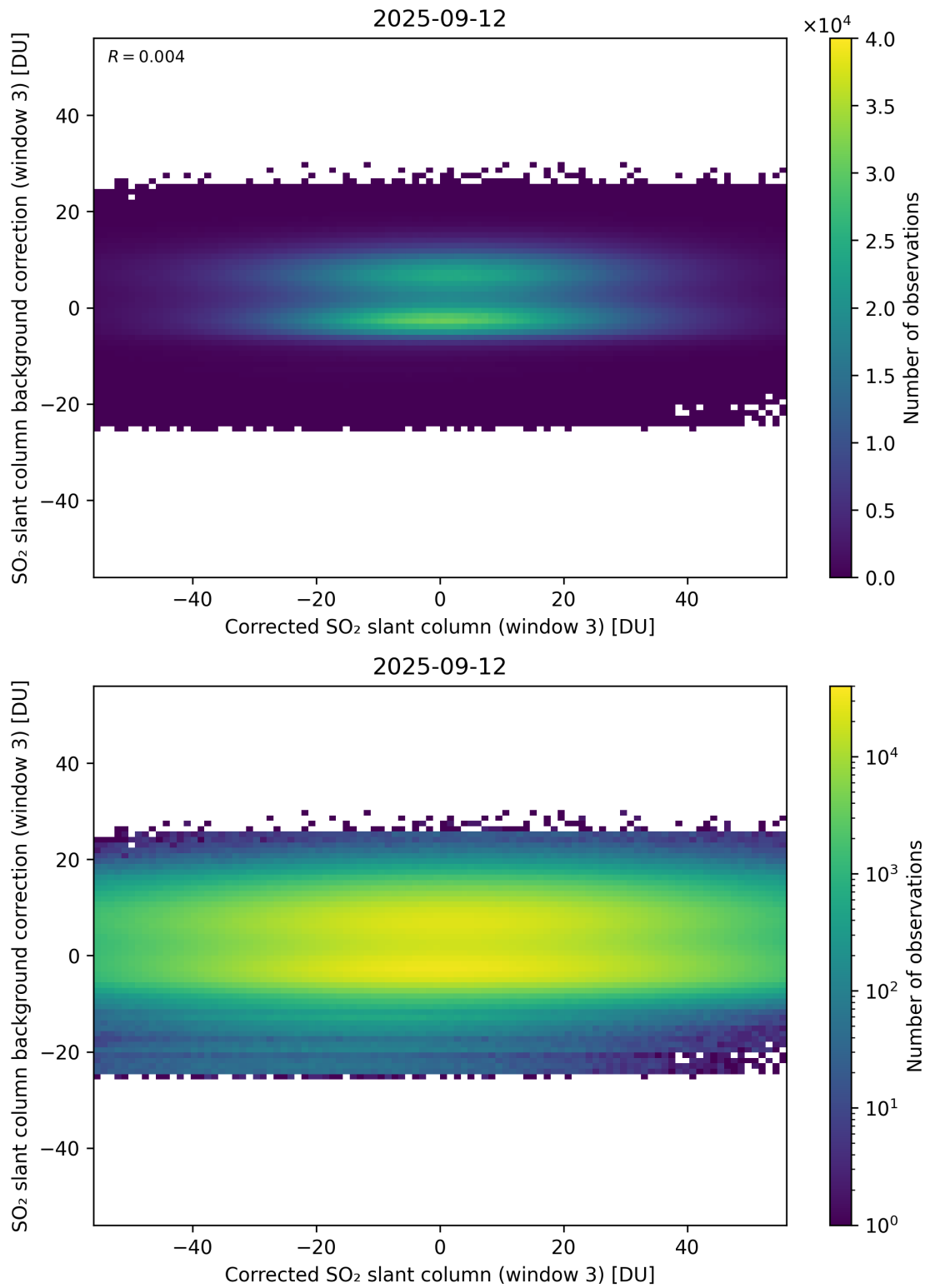
Figure 255: Scatter density plot of “Corrected SO 2 slant column (window 3)” against “SO 2 slant column background correction (window 3)” for 2025-09-11 to 2025-09-13.
