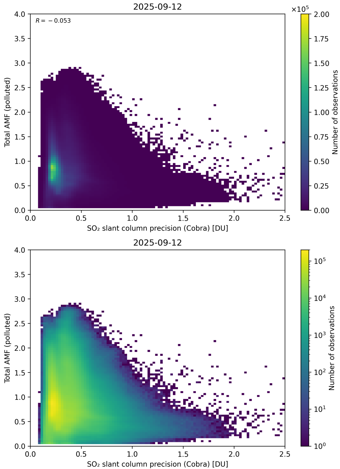
Figure 213: Scatter density plot of “SO 2 slant column precision (Cobra)” against “Total AMF (polluted)” for 2025-09-11 to 2025-09-13.
