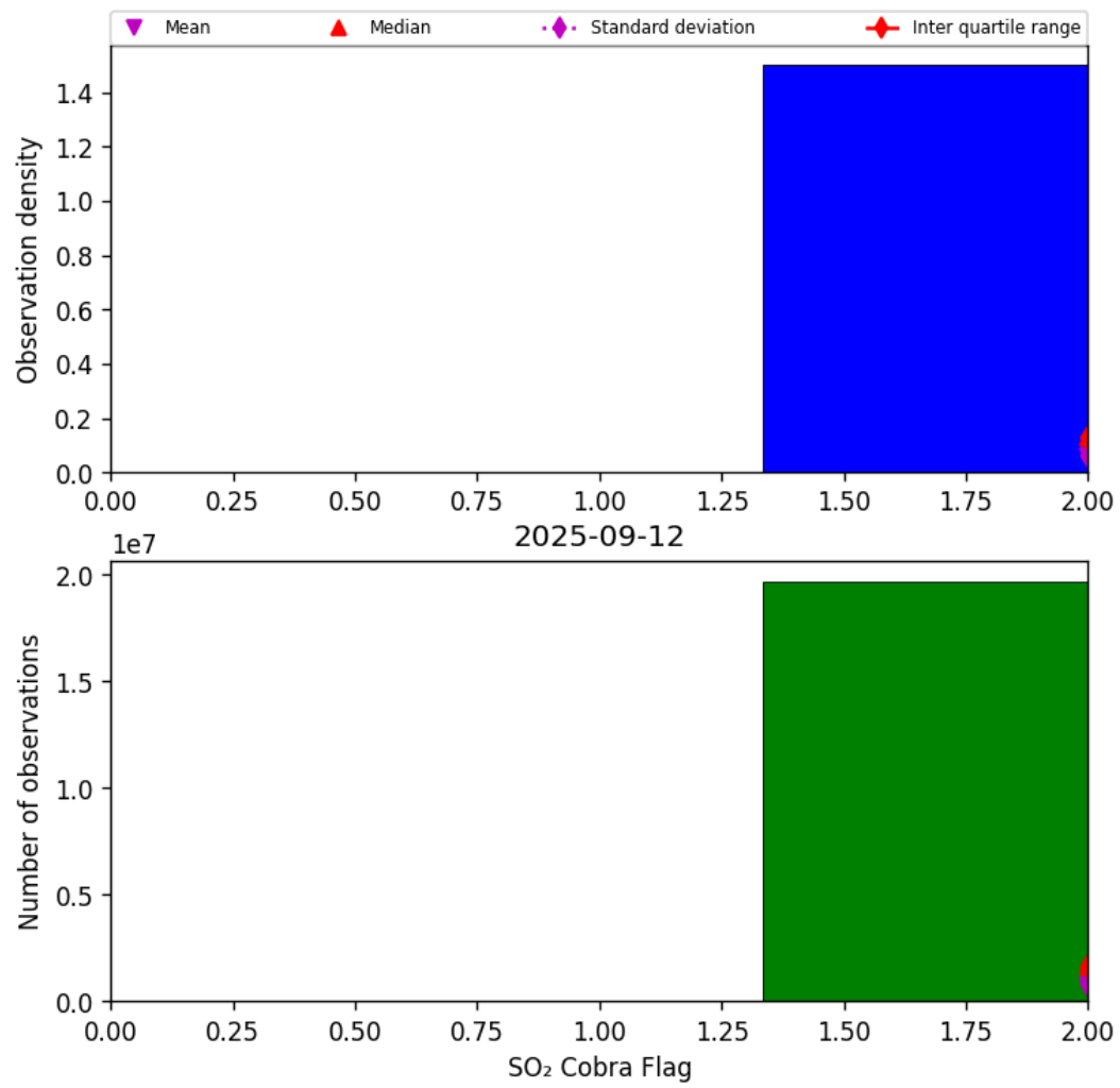
Figure 75: Histogram of “SO 2 Cobra Flag” for 2025-09-11 to 2025-09-13
