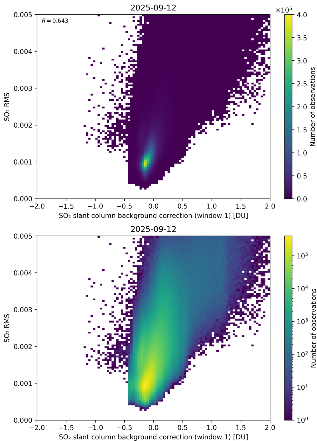
Figure 113: Scatter density plot of “SO 2 slant column background correction (window 1)” against “SO 2 RMS” for 2025-09-11 to 2025-09-13.
