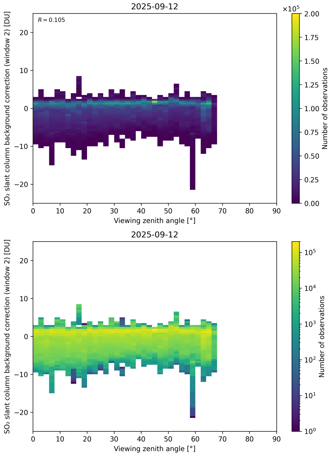
Figure 363: Scatter density plot of “Viewing zenith angle” against “SO 2 slant column background correction (window 2)” for 2025-09-11 to 2025-09-13.
