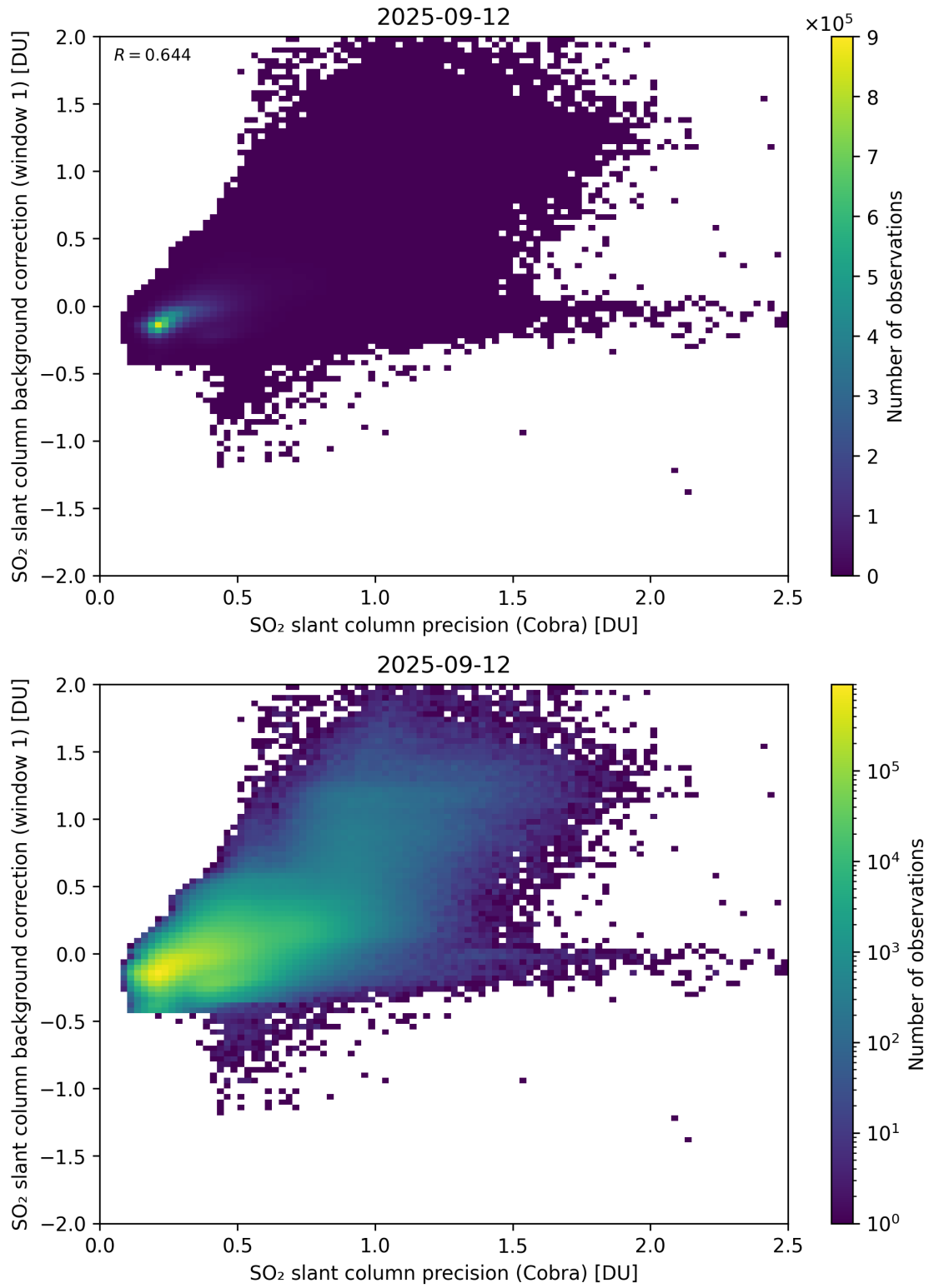
Figure 199: Scatter density plot of “SO 2 slant column precision (Cobra)” against “SO 2 slant column background correction (window 1)” for 2025-09-11 to 2025-09-13.
