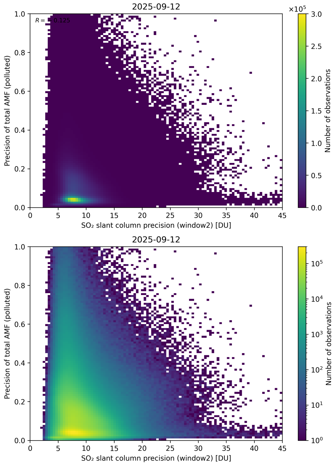
Figure 302: Scatter density plot of “SO 2 slant column precision (window2)” against “Precision of total AMF (polluted)” for 2025-09-11 to 2025-09-13.
