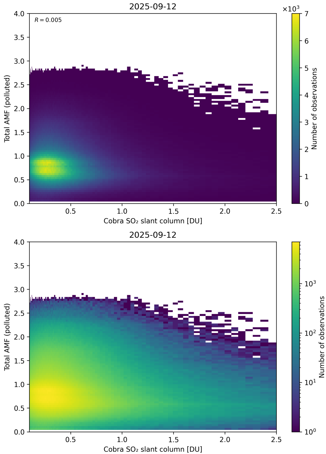
Figure 224: Scatter density plot of “Cobra SO 2 slant column” against “Total AMF (polluted)” for 2025-09-11 to 2025-09-13.
