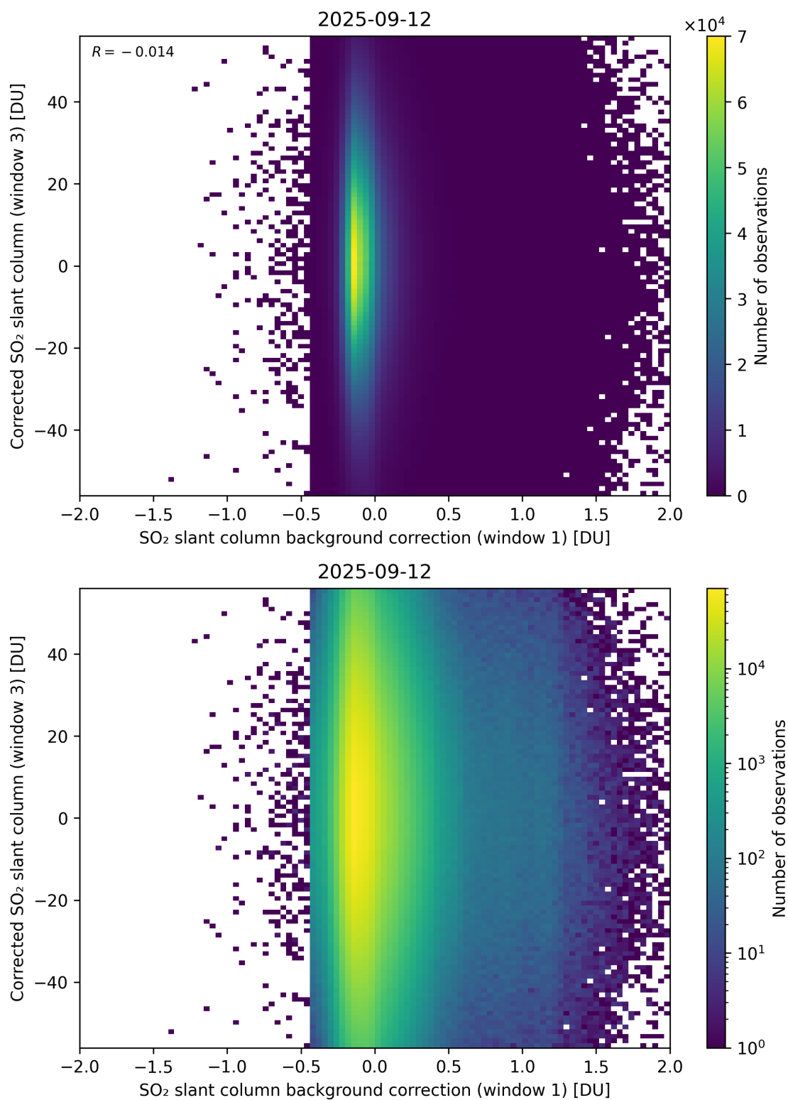
Figure 116: Scatter density plot of “SO 2 slant column background correction (window 1)” against “Corrected SO 2 slant column (window 3)” for 2025-09-11 to 2025-09-13.
