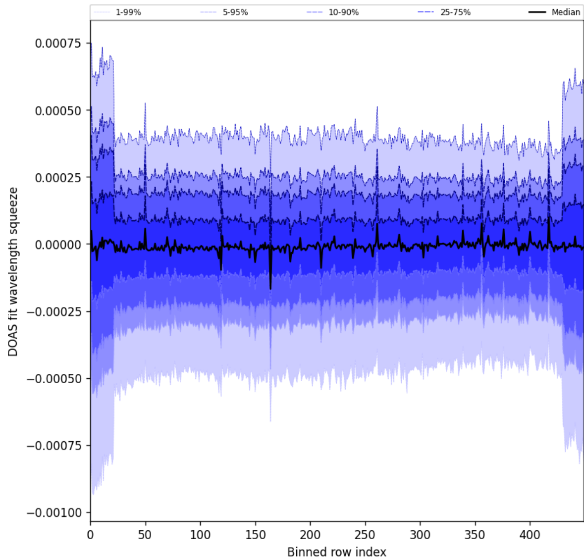
Figure 103: Along track statistics of “DOAS fit wavelength squeeze” for 2025-09-11 to 2025-09-13
