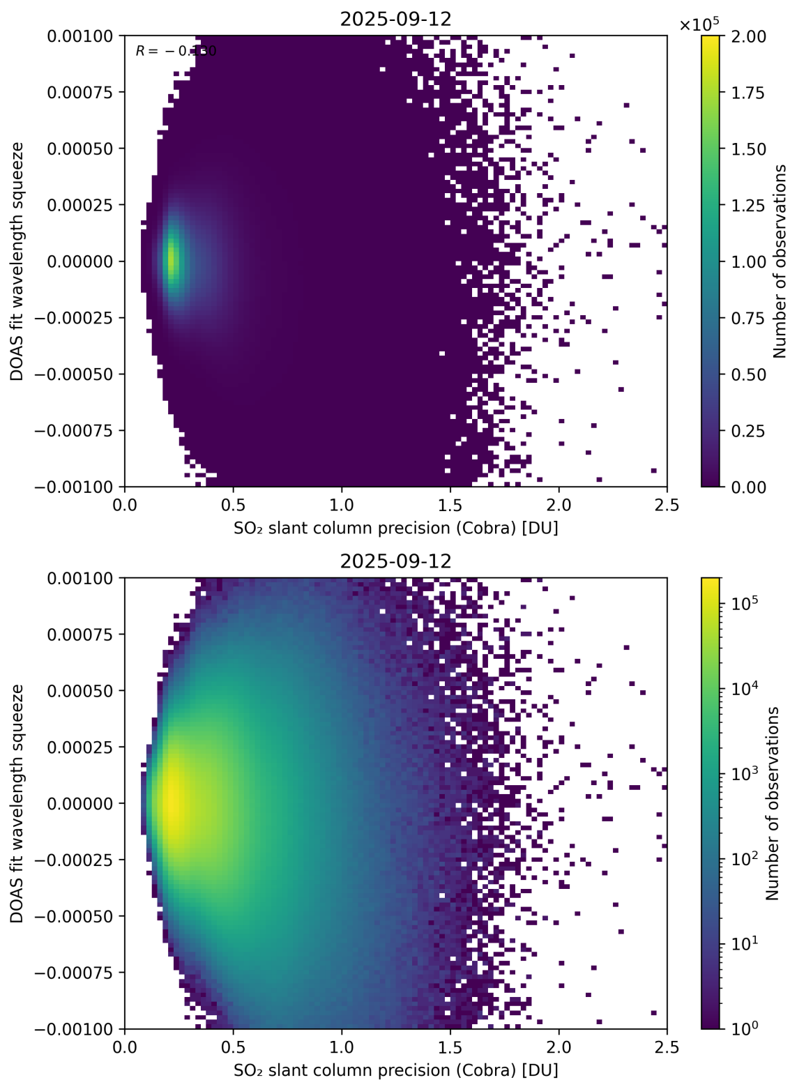
Figure 203: Scatter density plot of “SO 2 slant column precision (Cobra)” against “DOAS fit wavelength squeeze” for 2025-09-11 to 2025-09-13.
