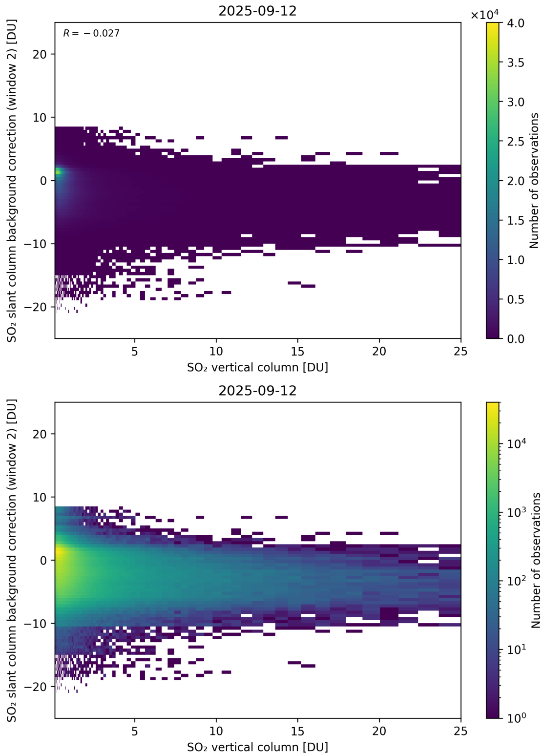
Figure 324: Scatter density plot of “SO 2 vertical column” against “SO 2 slant column background correction (window 2)” for 2025-09-11 to 2025-09-13.
