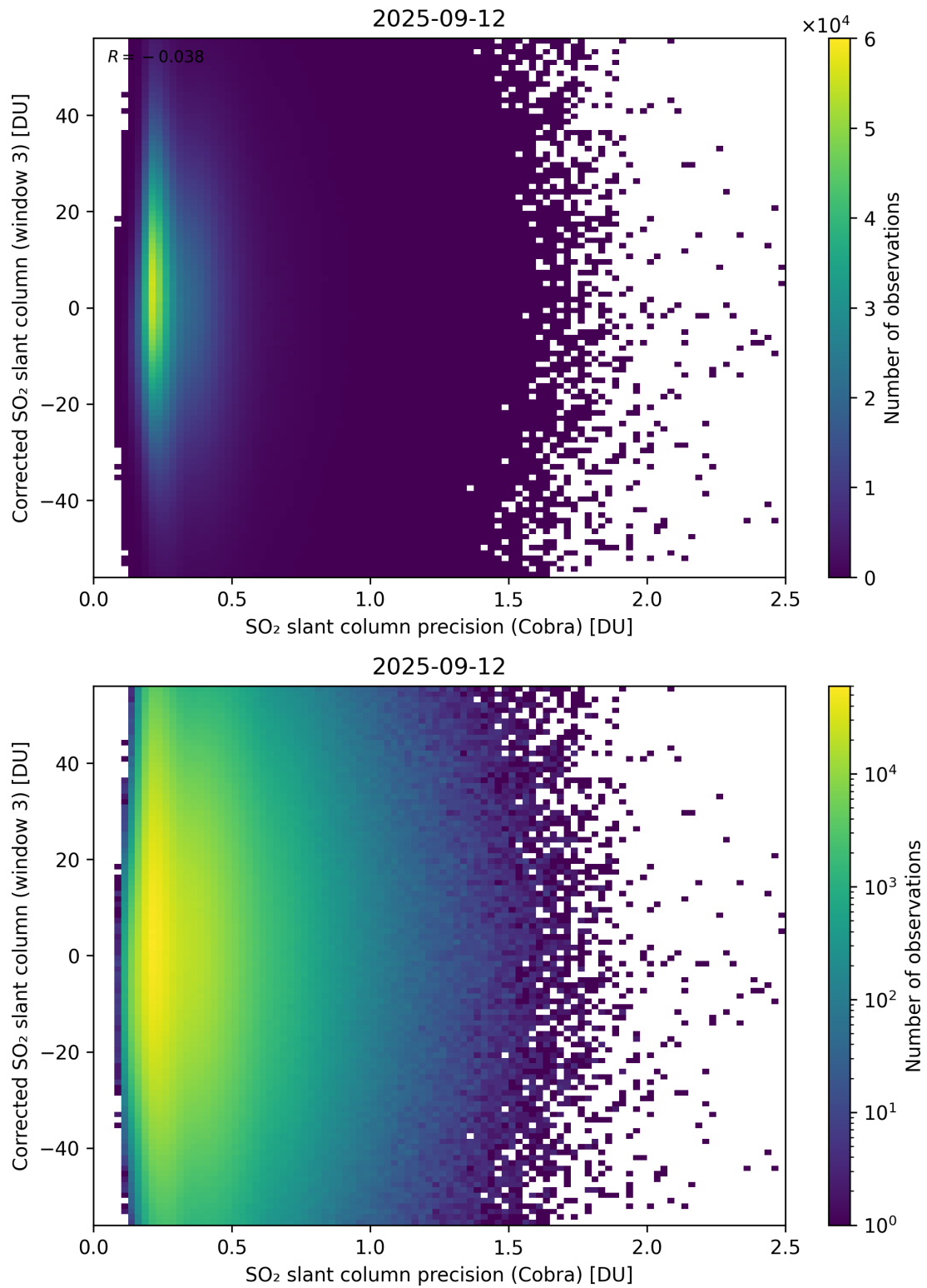
Figure 207: Scatter density plot of “SO 2 slant column precision (Cobra)” against “Corrected SO 2 slant column (window 3)” for 2025-09-11 to 2025-09-13.
