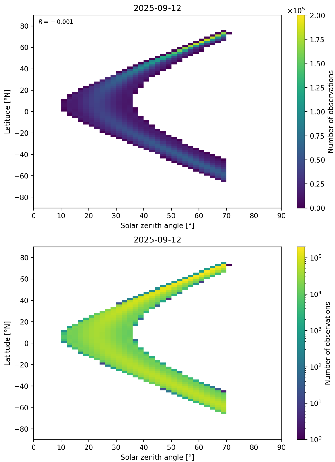
Figure 177: Scatter density plot of “Solar zenith angle” against “Latitude” for 2025-09-11 to 2025-09-13.
