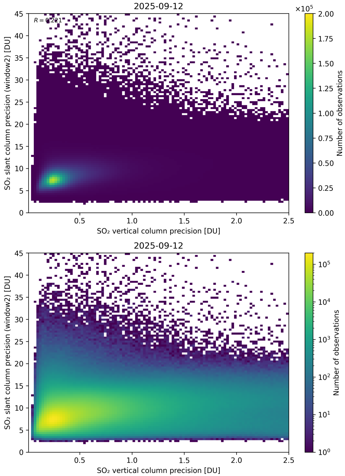
Figure 343: Scatter density plot of “SO 2 vertical column precision” against “SO 2 slant column precision (window2)” for 2025-09-11 to 2025-09-13.
