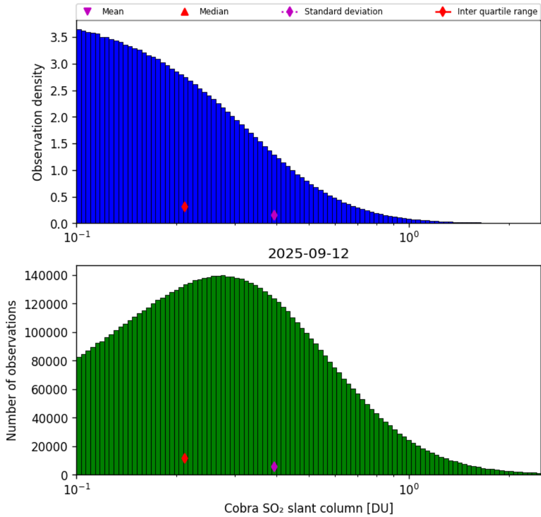
Figure 61: Histogram of “Cobra SO 2 slant column” for 2025-09-11 to 2025-09-13
