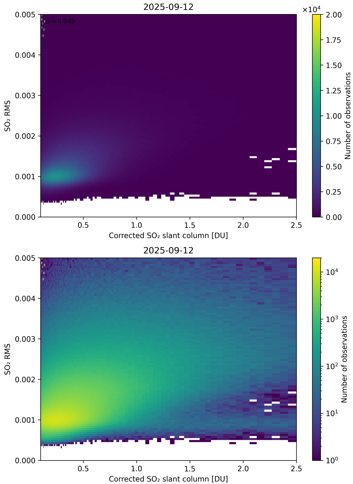
Figure 231: Scatter density plot of “Corrected SO 2 slant column” against “SO 2 RMS” for 2025-09-11 to 2025-09-13.
