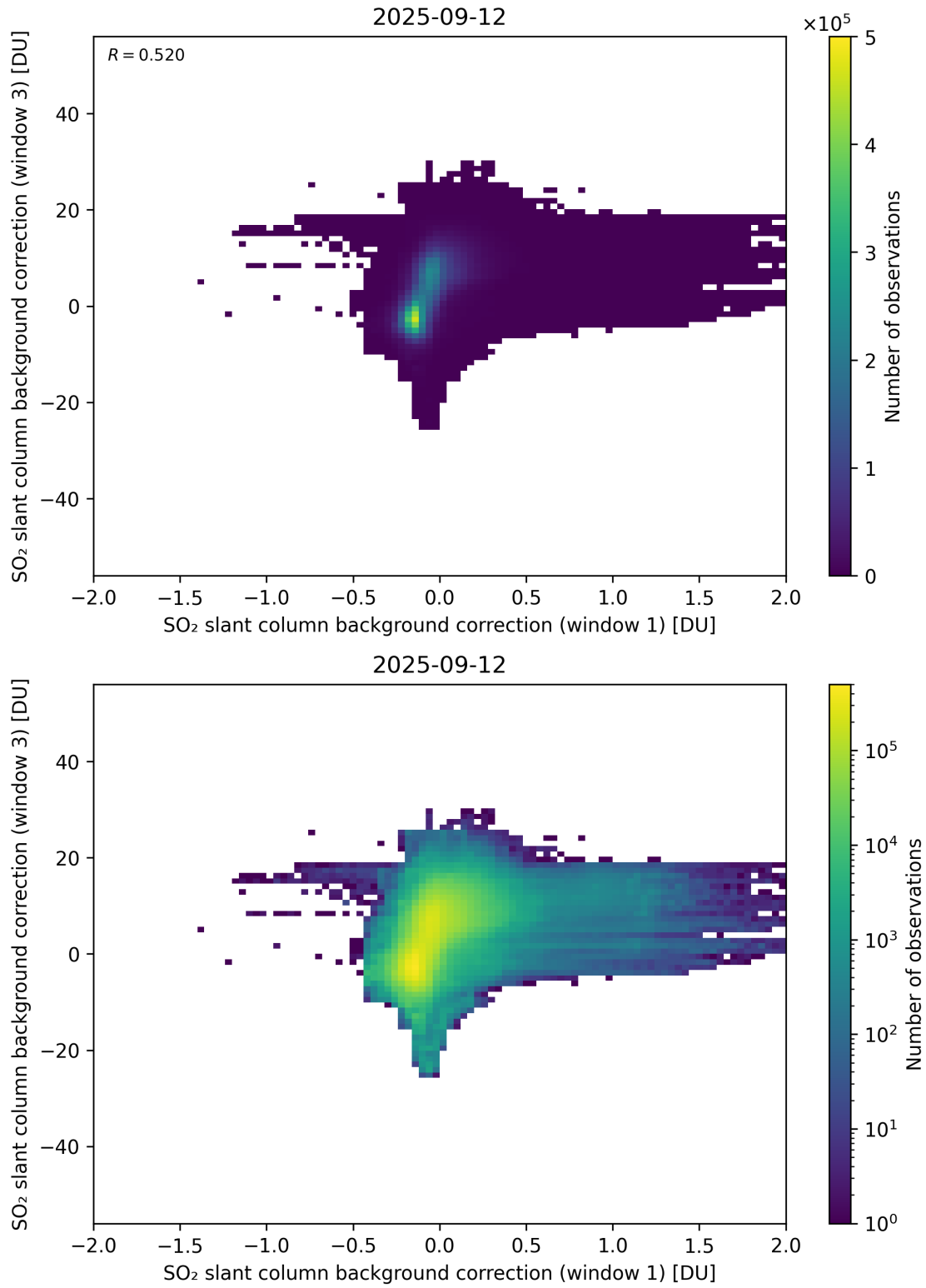
Figure 110: Scatter density plot of “SO 2 slant column background correction (window 1)” against “SO 2 slant column background correction (window 3)” for 2025-09-11 to 2025-09-13.
