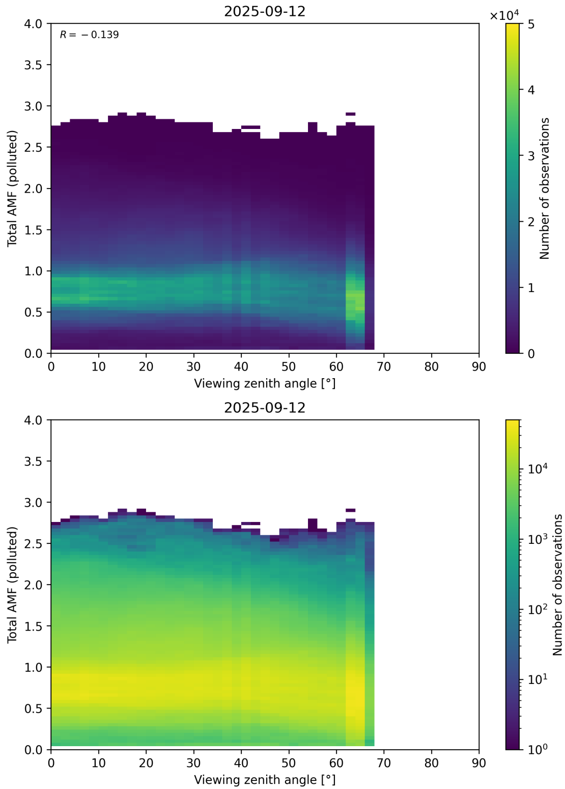
Figure 381: Scatter density plot of “Viewing zenith angle” against “Total AMF (polluted)” for 2025-09-11 to 2025-09-13.
