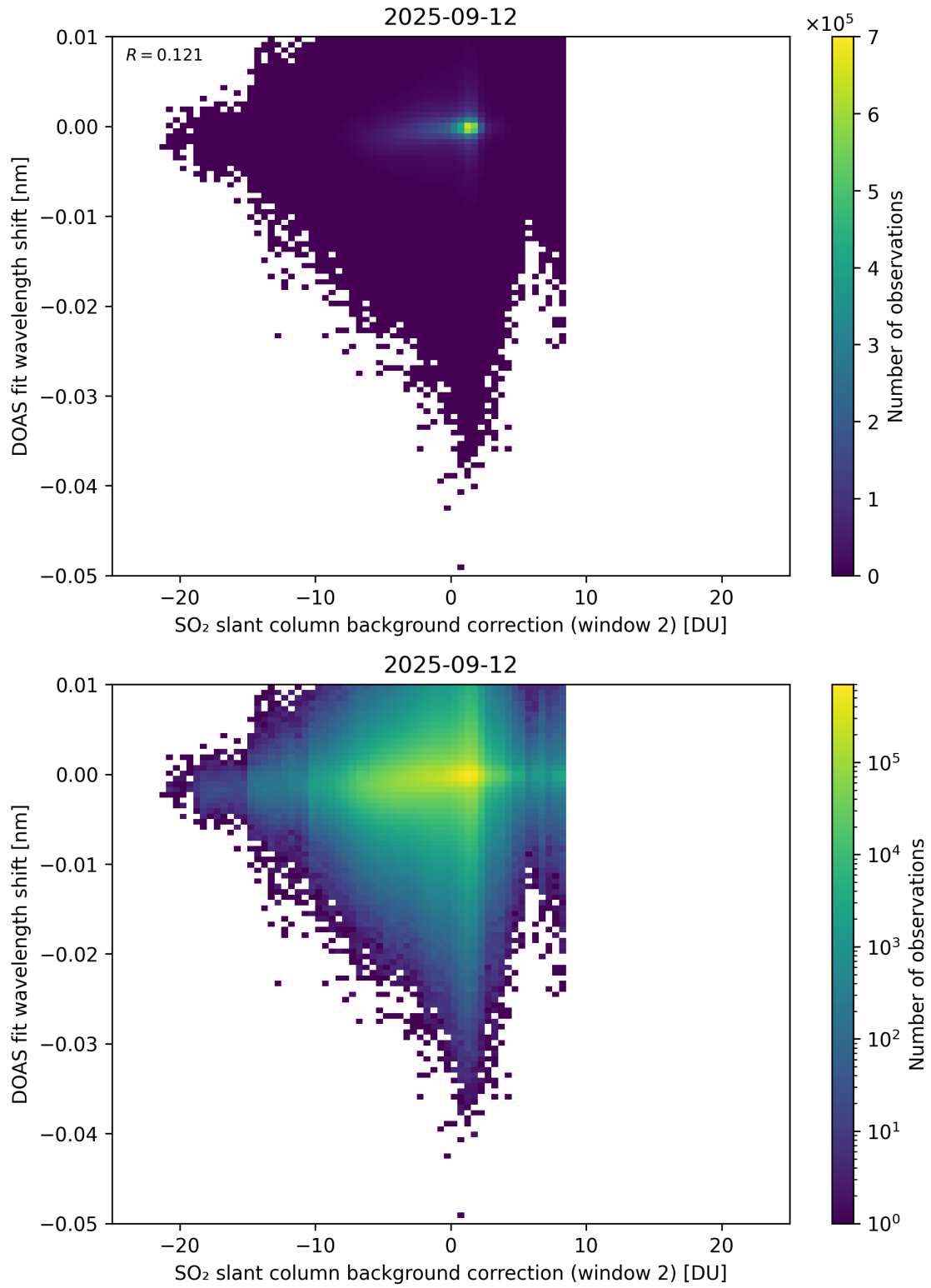
Figure 123: Scatter density plot of “SO 2 slant column background correction (window 2)” against “DOAS fit wavelength shift” for 2025-09-11 to 2025-09-13.
