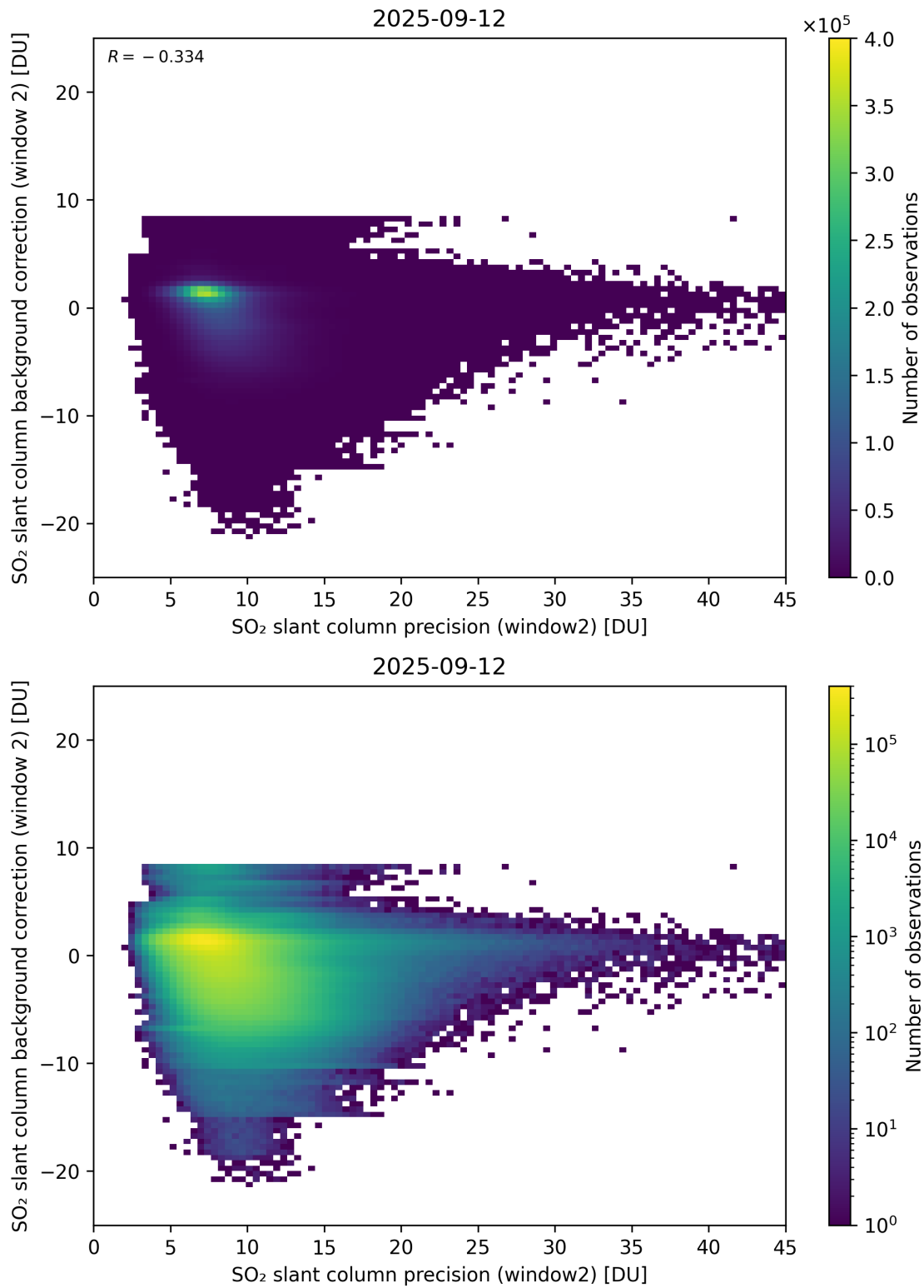
Figure 291: Scatter density plot of “SO 2 slant column precision (window2)” against “SO 2 slant column background correction (window 2)” for 2025-09-11 to 2025-09-13.
