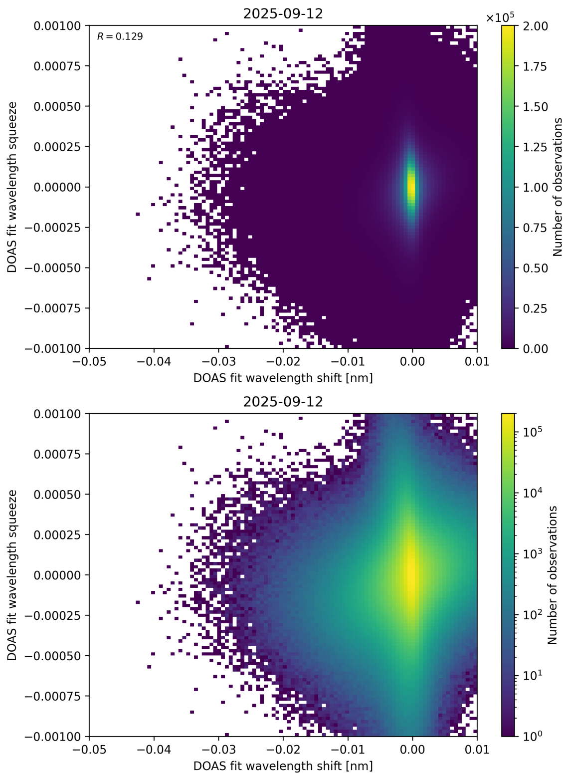
Figure 138: Scatter density plot of “DOAS fit wavelength shift” against “DOAS fit wavelength squeeze” for 2025-09-11 to 2025-09-13.
