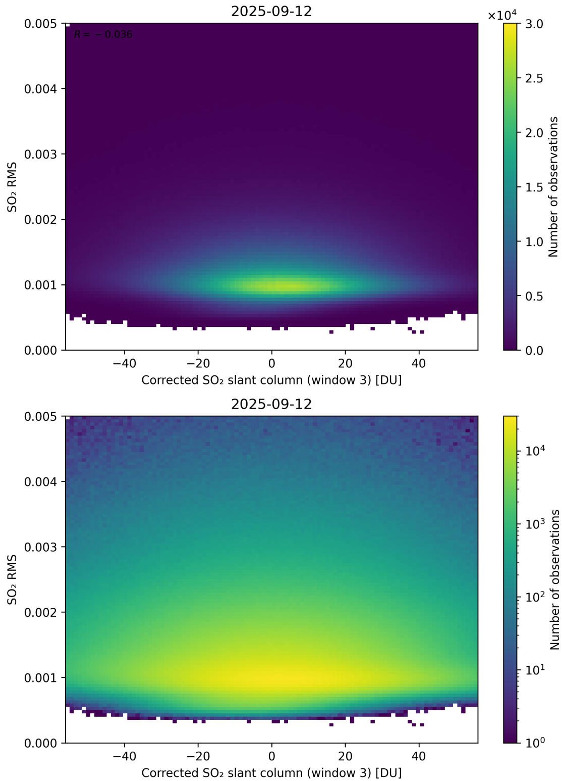
Figure 258: Scatter density plot of “Corrected SO 2 slant column (window 3)” against “SO 2 RMS” for 2025-09-11 to 2025-09-13.
