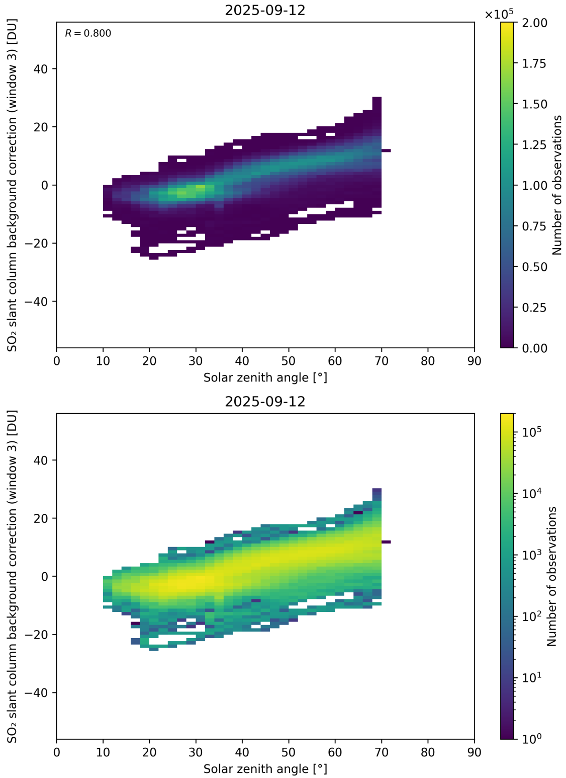
Figure 173: Scatter density plot of “Solar zenith angle” against “SO 2 slant column background correction (window 3)” for 2025-09-11 to 2025-09-13.
