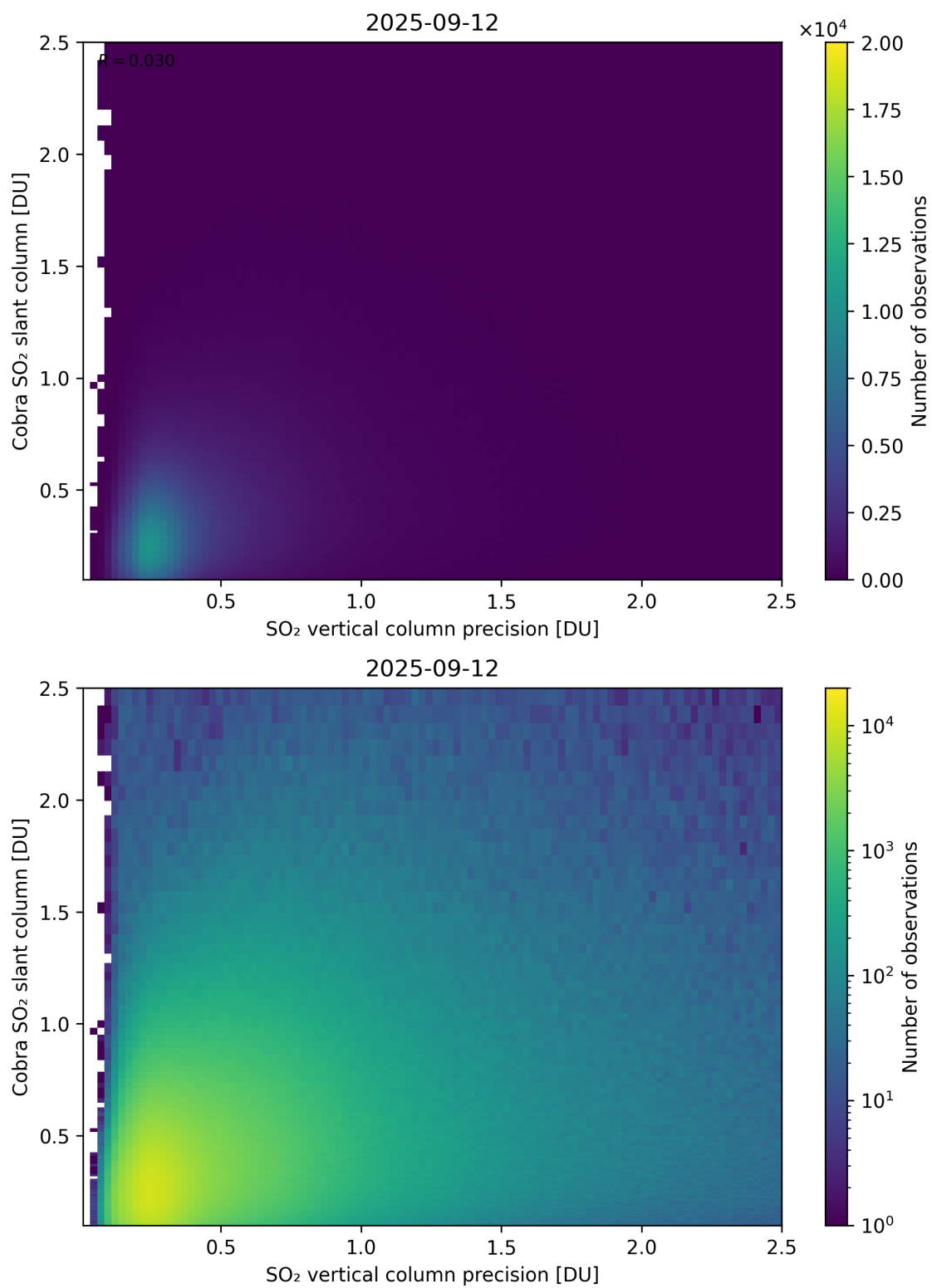
Figure 336: Scatter density plot of “SO 2 vertical column precision” against “Cobra SO 2 slant column” for 2025-09-11 to 2025-09-13.
