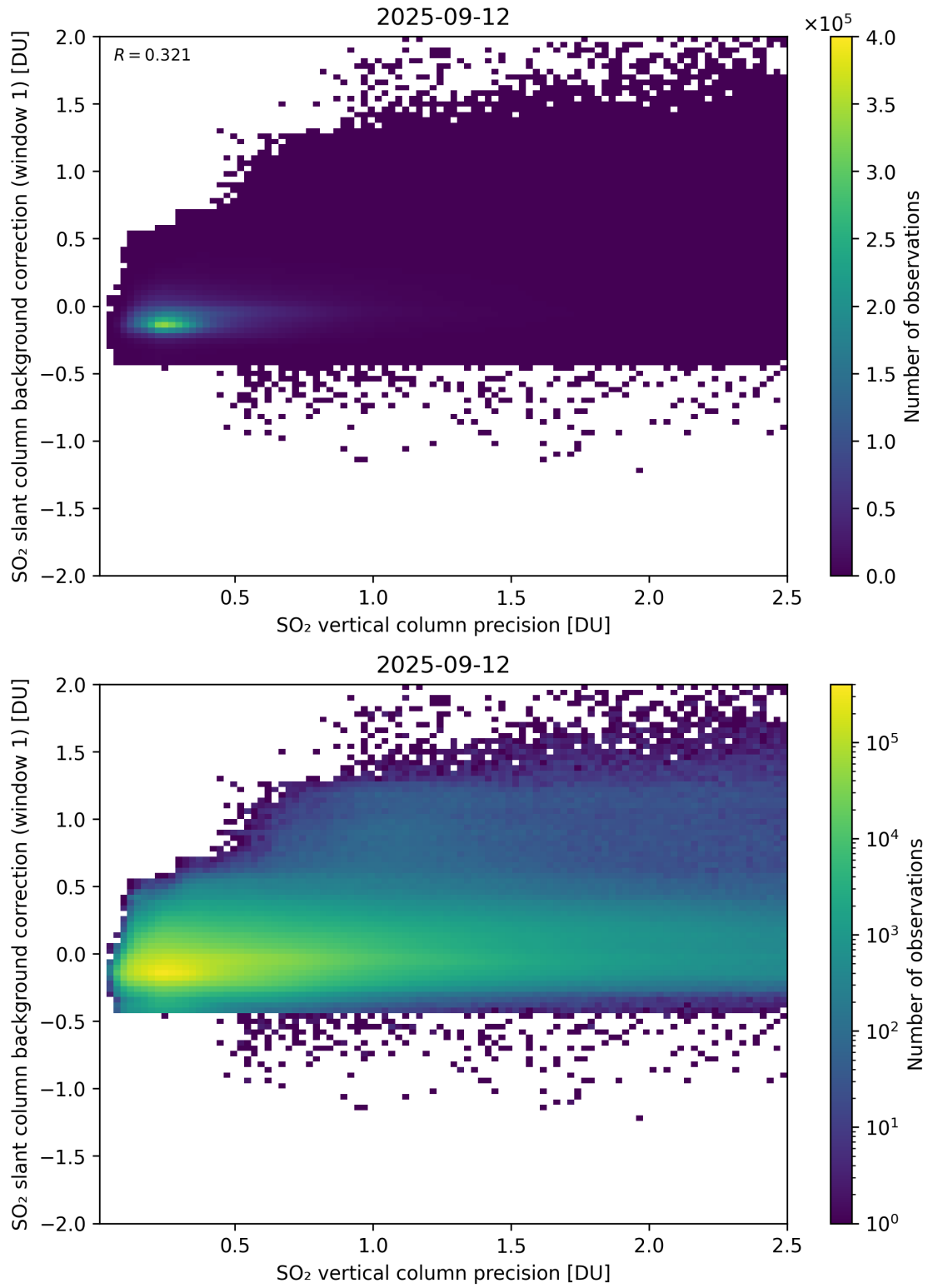
Figure 329: Scatter density plot of “SO 2 vertical column precision” against “SO 2 slant column background correction (window 1)” for 2025-09-11 to 2025-09-13.
