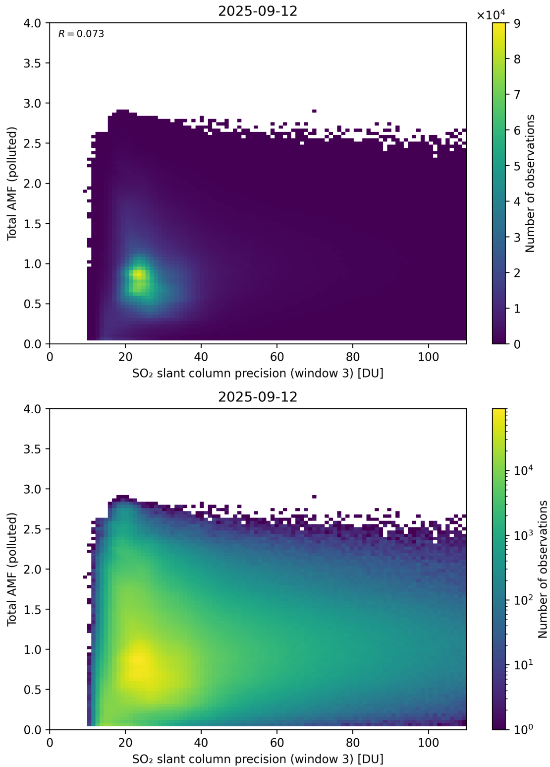
Figure 313: Scatter density plot of “SO 2 slant column precision (window 3)” against “Total AMF (polluted)” for 2025-09-11 to 2025-09-13.
