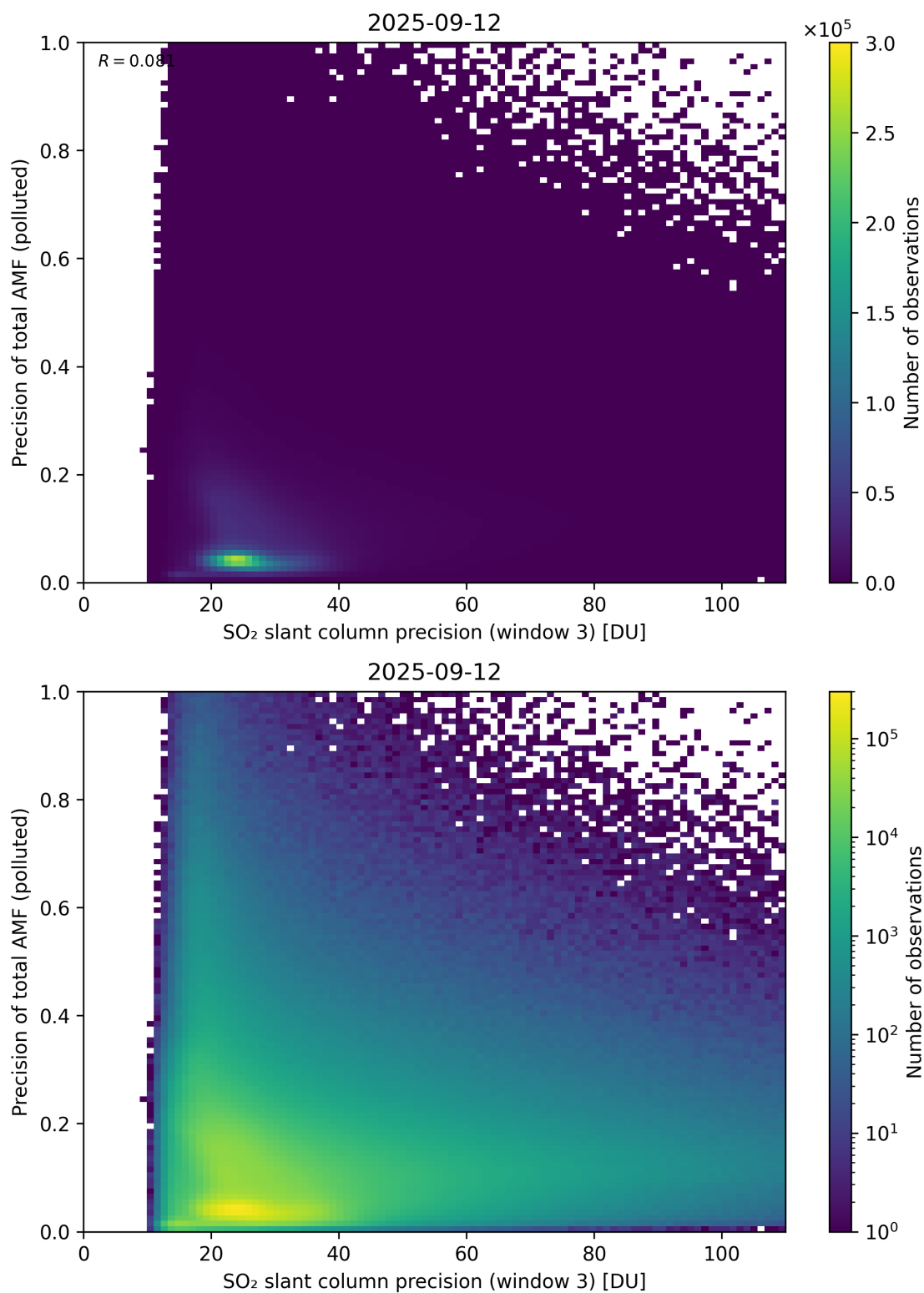
Figure 314: Scatter density plot of “SO 2 slant column precision (window 3)” against “Precision of total AMF (polluted)” for 2025-09-11 to 2025-09-13.
