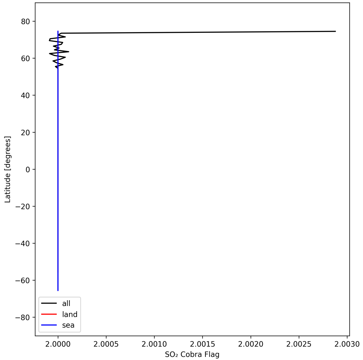
Figure 49: Zonal average of “SO 2 Cobra Flag” for 2025-09-11 to 2025-09-13.
