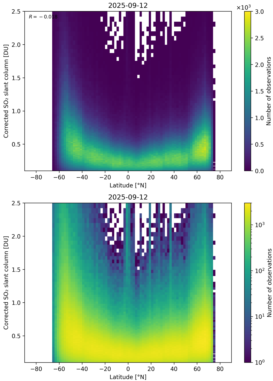
Figure 159: Scatter density plot of “Latitude” against “Corrected SO 2 slant column” for 2025-09-11 to 2025-09-13.
