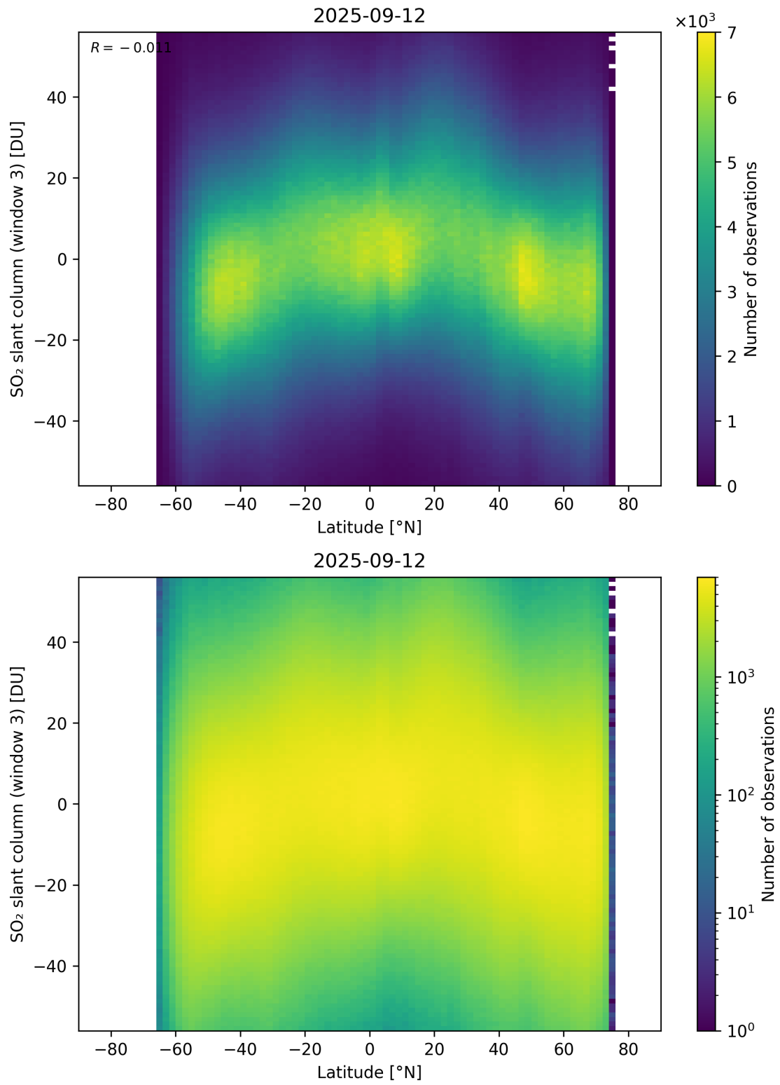
Figure 165: Scatter density plot of “Latitude” against “SO 2 slant column (window 3)” for 2025-09-11 to 2025-09-13.
