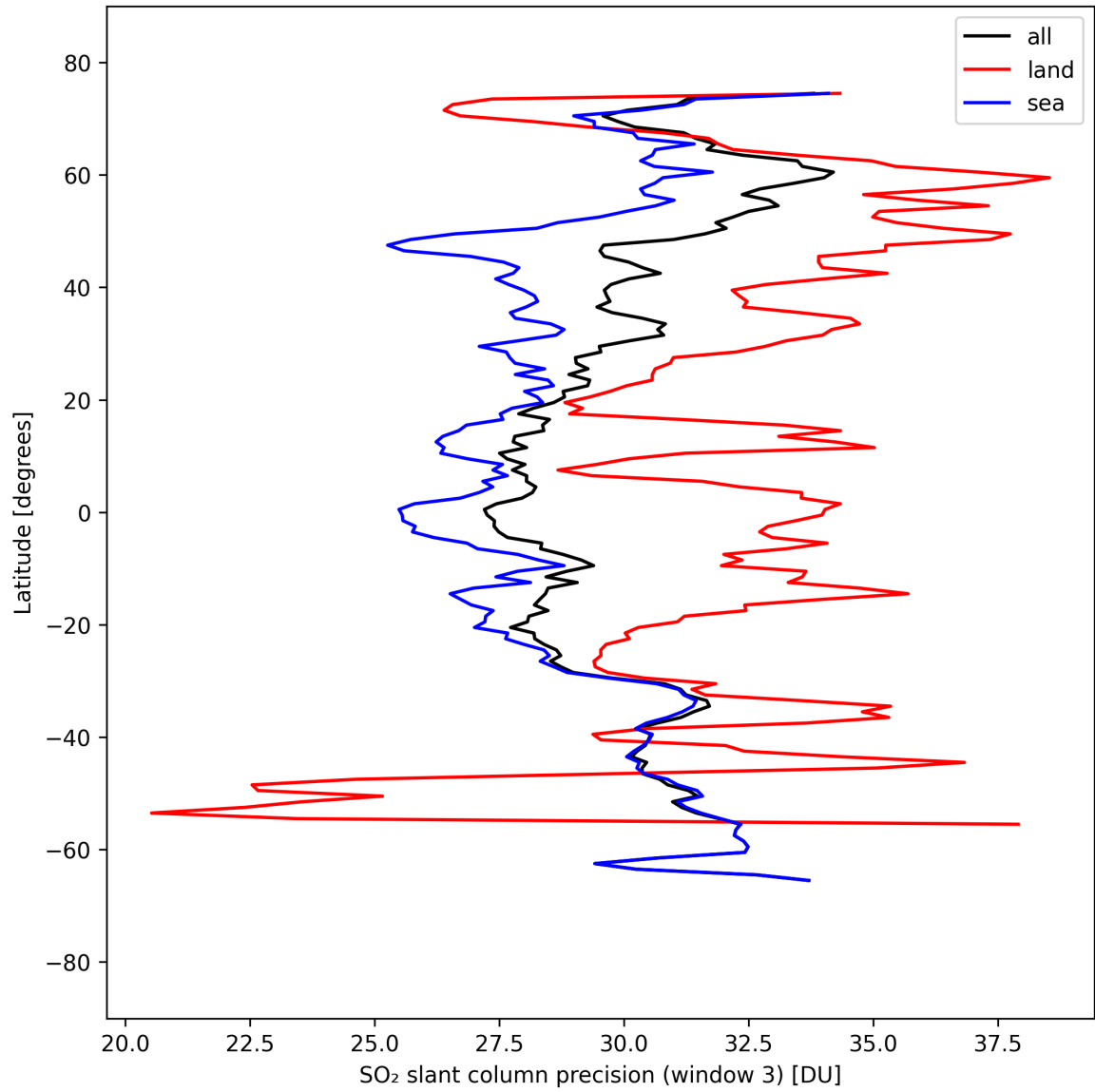
Figure 46: Zonal average of “SO 2 slant column precision (window 3)” for 2025-09-11 to 2025-09-13.
