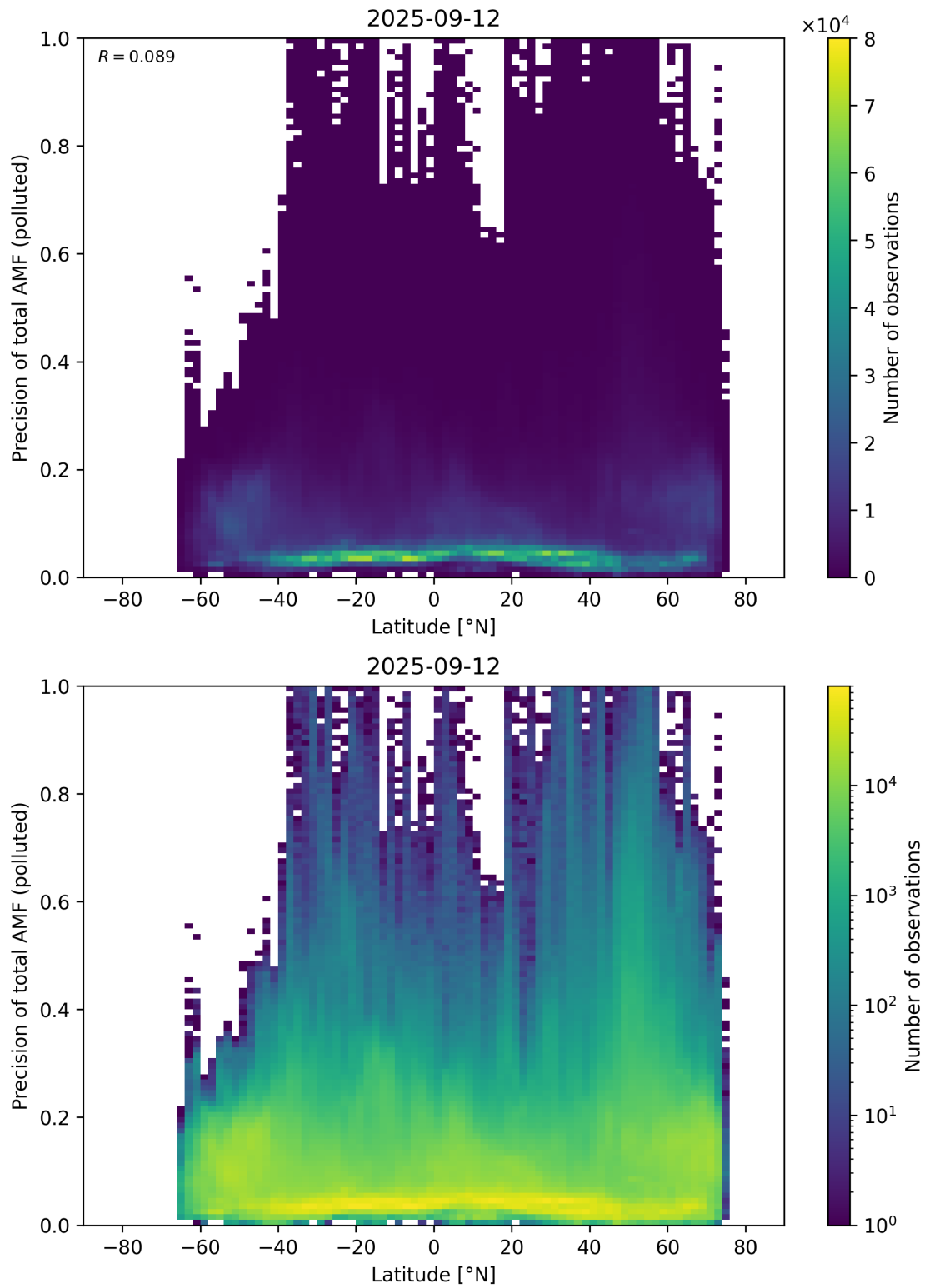
Figure 168: Scatter density plot of “Latitude” against “Precision of total AMF (polluted)” for 2025-09-11 to 2025-09-13.
