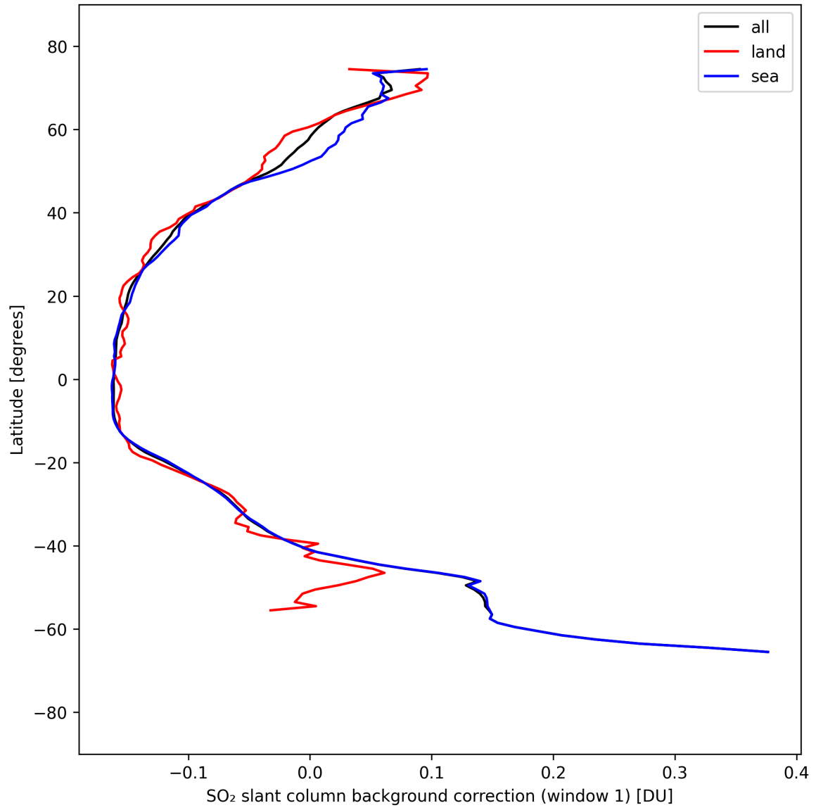
Figure 40: Zonal average of “SO 2 slant column background correction (window 1)” for 2025-09-11 to 2025-09-13.
