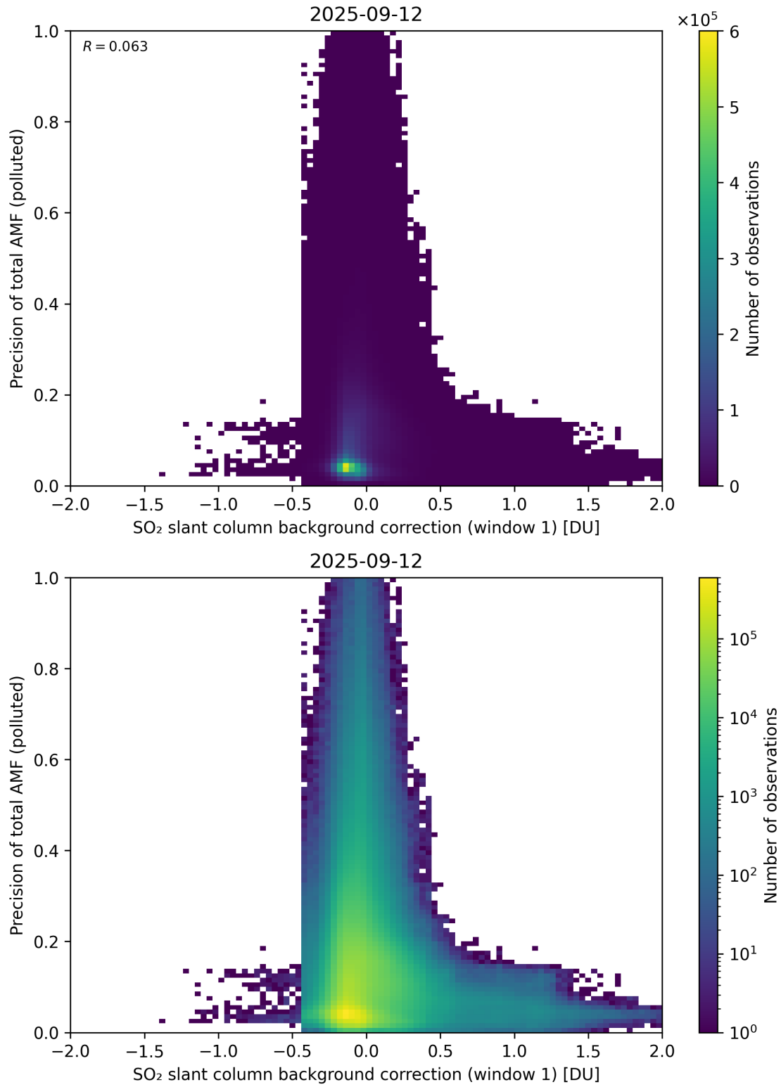
Figure 121: Scatter density plot of “SO 2 slant column background correction (window 1)” against “Precision of total AMF (polluted)” for 2025-09-11 to 2025-09-13.
