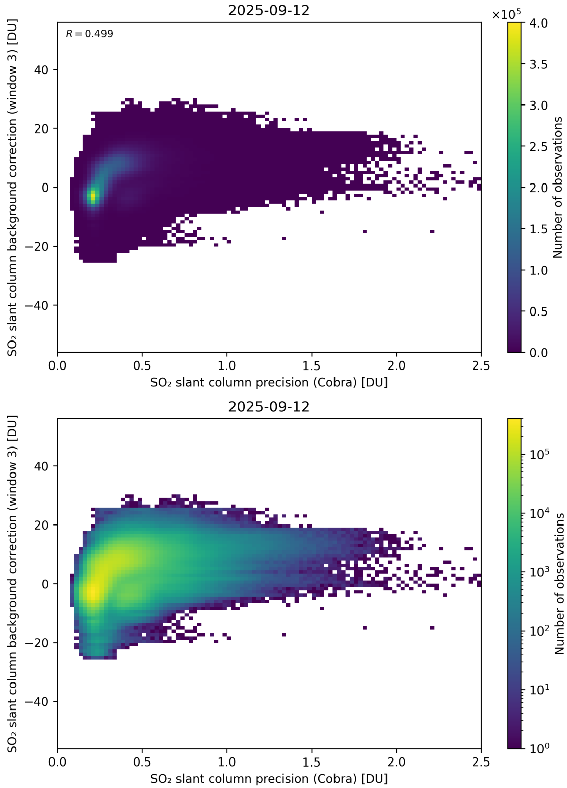
Figure 201: Scatter density plot of “SO 2 slant column precision (Cobra)” against “SO 2 slant column background correction (window 3)” for 2025-09-11 to 2025-09-13.
