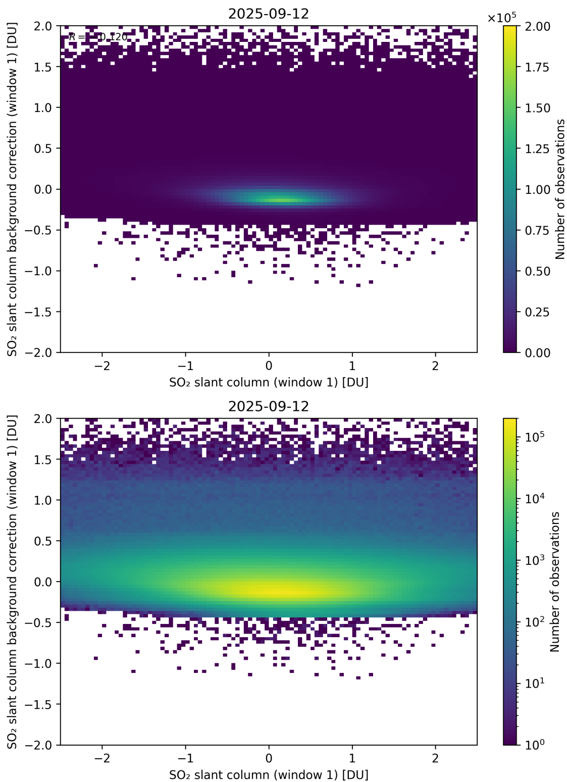
Figure 262: Scatter density plot of “SO 2 slant column (window 1)” against “SO 2 slant column background correction (window 1)” for 2025-09-11 to 2025-09-13.
