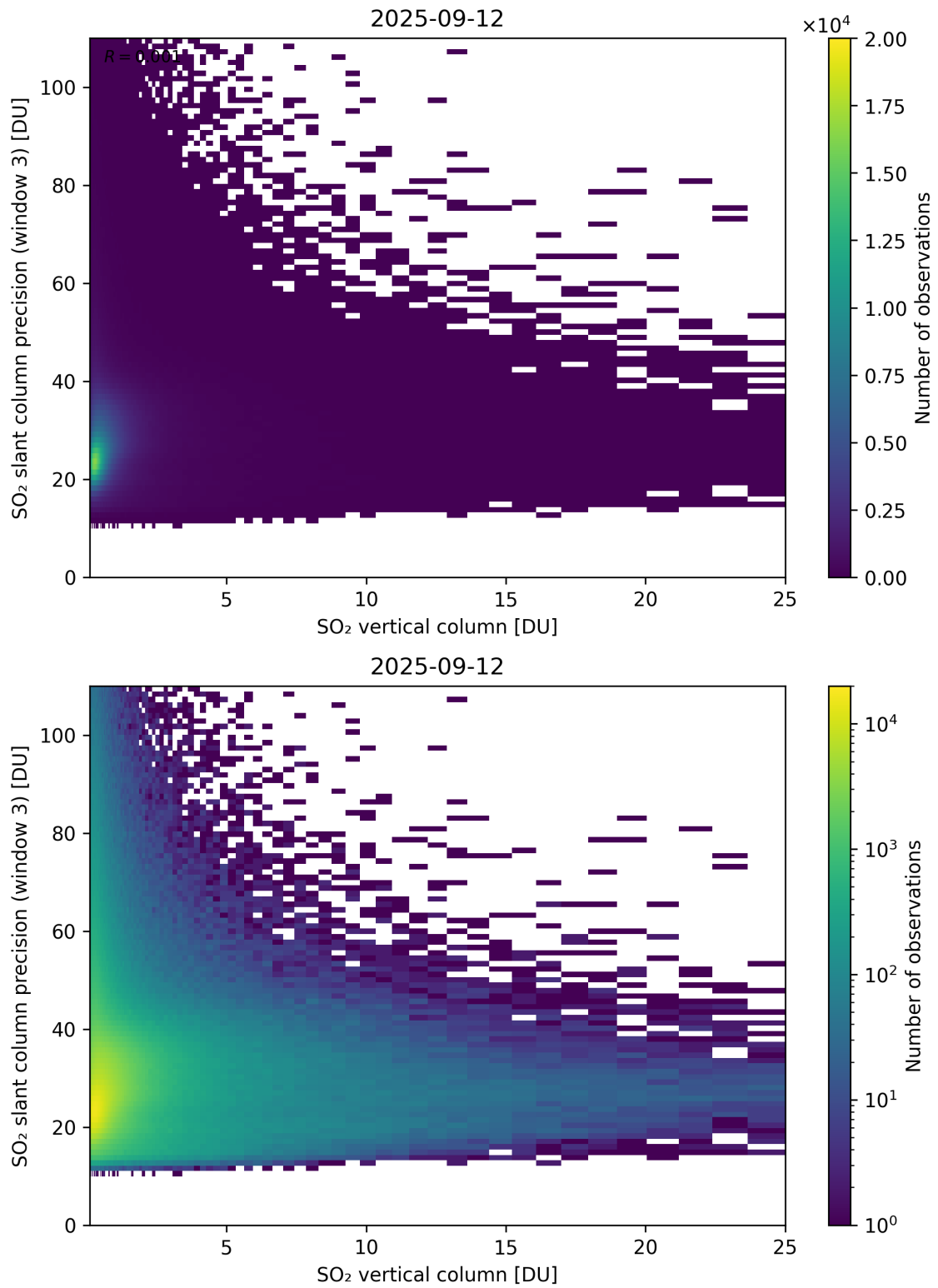
Figure 358: Scatter density plot of “SO 2 vertical column” against “SO 2 slant column precision (window 3)” for 2025-09-11 to 2025-09-13.
