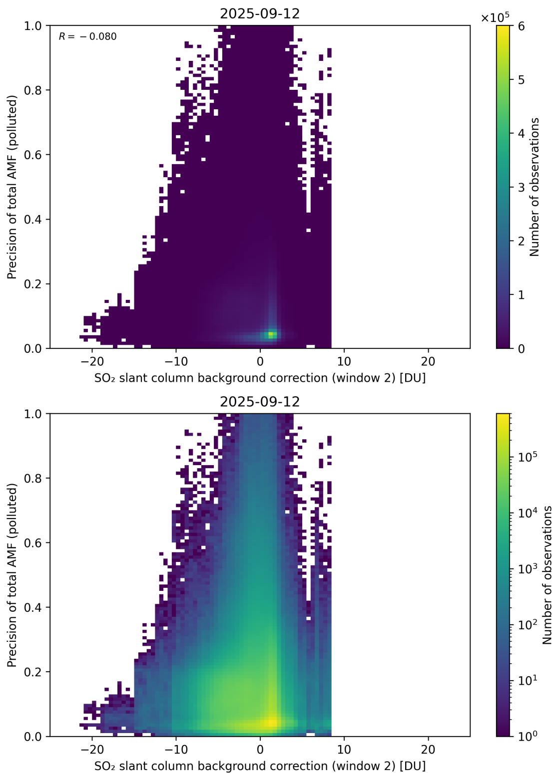
Figure 131: Scatter density plot of “SO 2 slant column background correction (window 2)” against “Precision of total AMF (polluted)” for 2025-09-11 to 2025-09-13.
