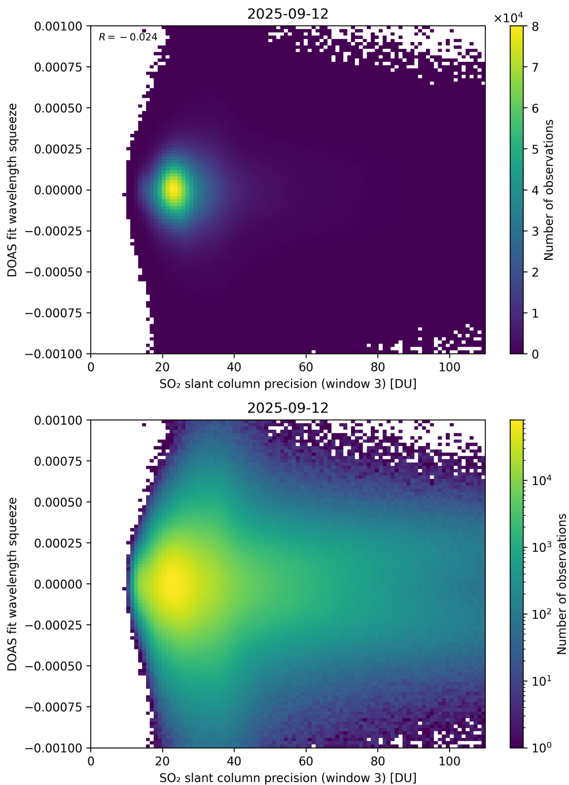
Figure 309: Scatter density plot of “SO 2 slant column precision (window 3)” against “DOAS fit wavelength squeeze” for 2025-09-11 to 2025-09-13.
