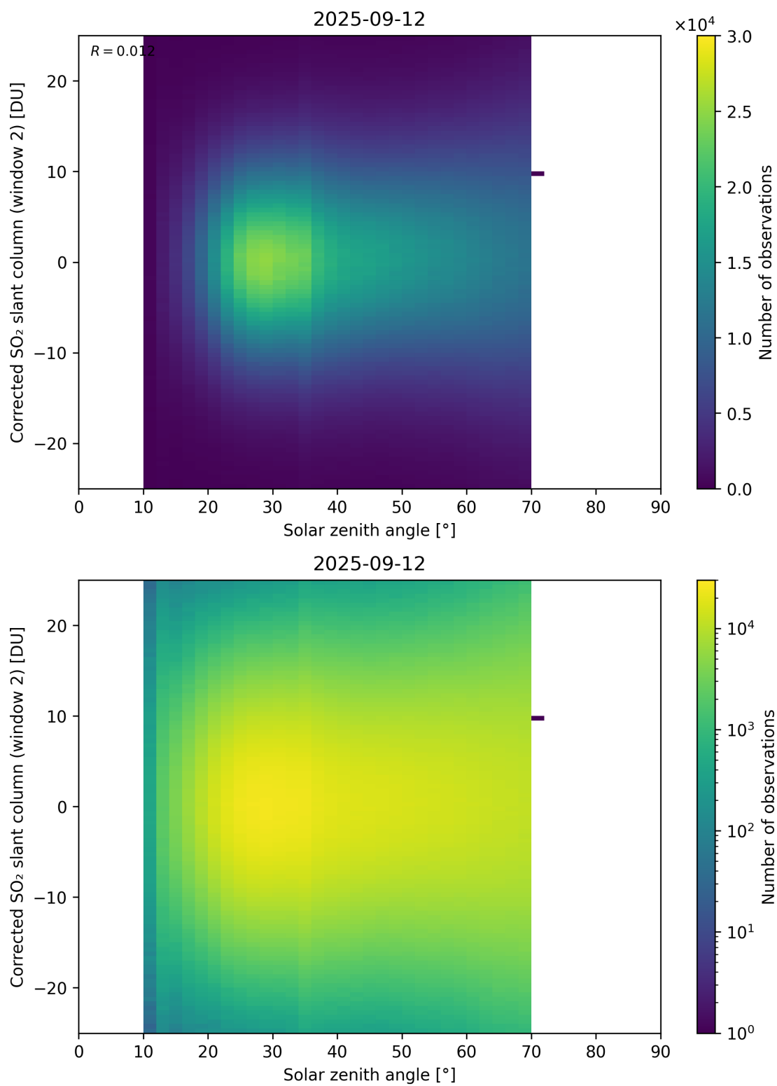
Figure 182: Scatter density plot of “Solar zenith angle” against “Corrected SO 2 slant column (window 2)” for 2025-09-11 to 2025-09-13.
