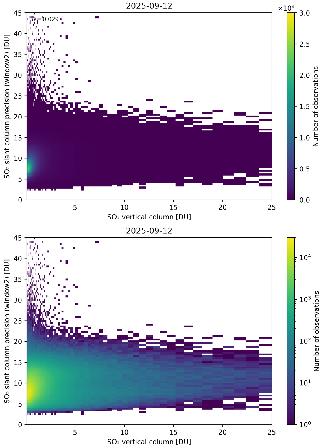
Figure 356: Scatter density plot of “SO 2 vertical column” against “SO 2 slant column precision (window2)” for 2025-09-11 to 2025-09-13.
