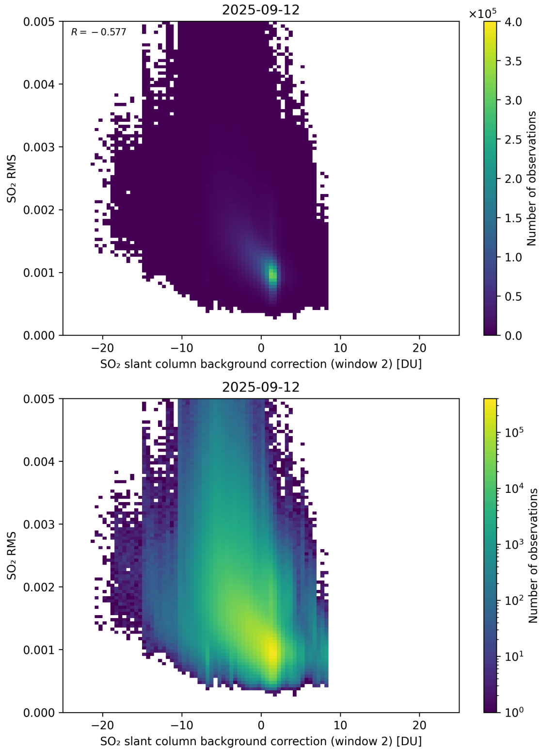
Figure 125: Scatter density plot of “SO 2 slant column background correction (window 2)” against “SO 2 RMS” for 2025-09-11 to 2025-09-13.
