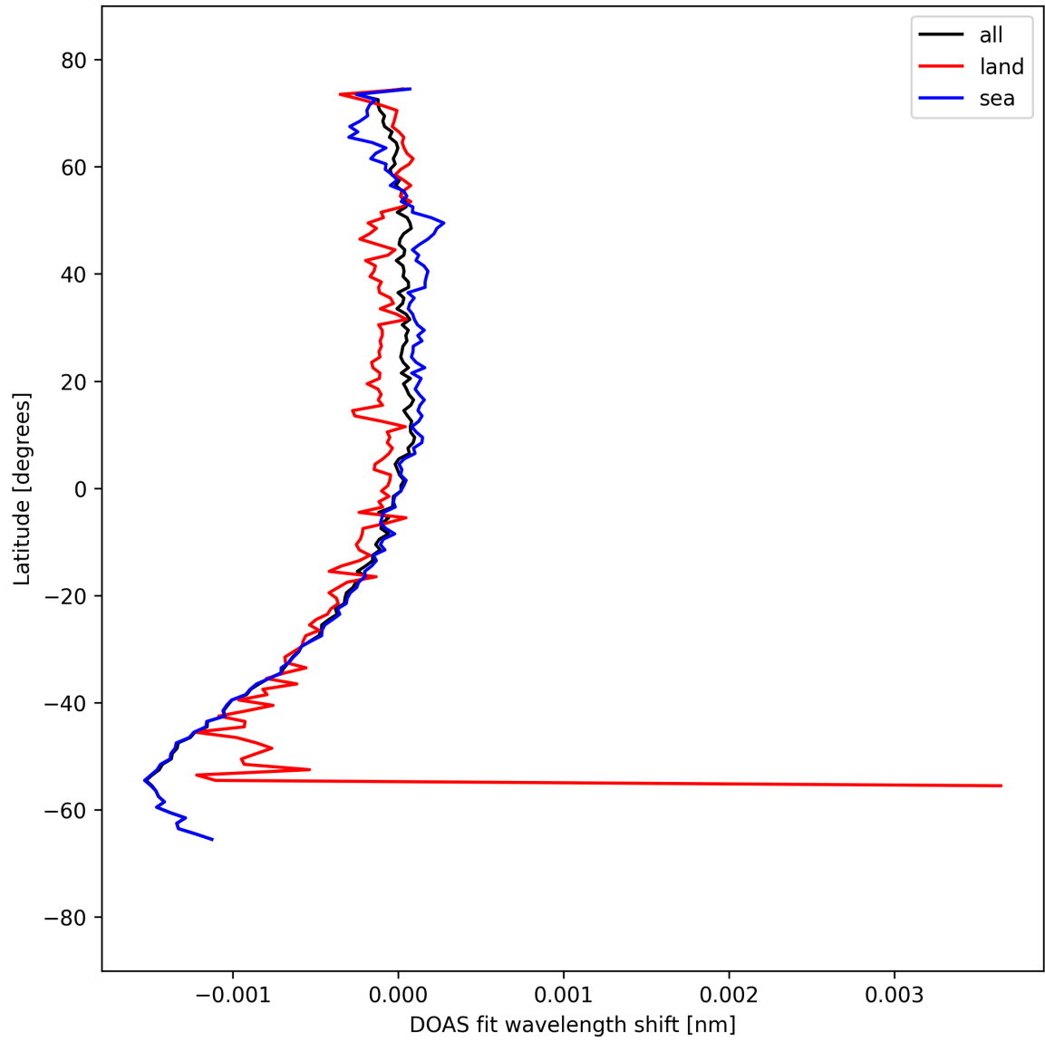
Figure 50: Zonal average of “DOAS fit wavelength shift” for 2025-09-11 to 2025-09-13.
