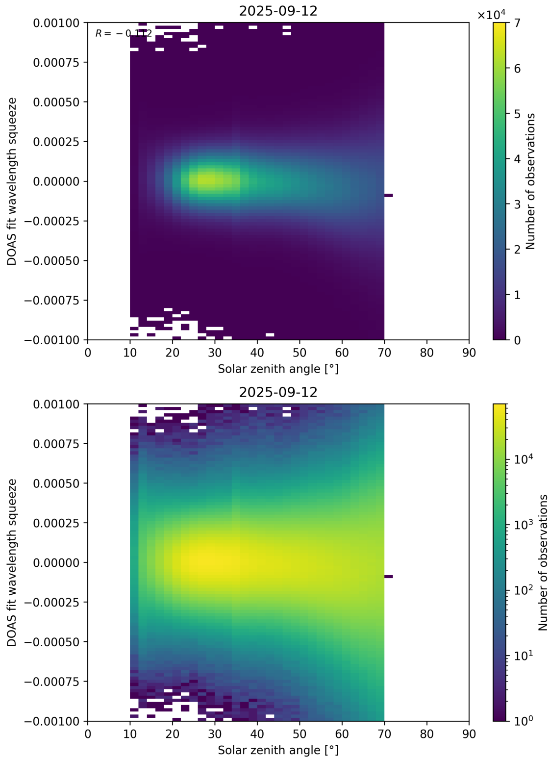
Figure 175: Scatter density plot of “Solar zenith angle” against “DOAS fit wavelength squeeze” for 2025-09-11 to 2025-09-13.
