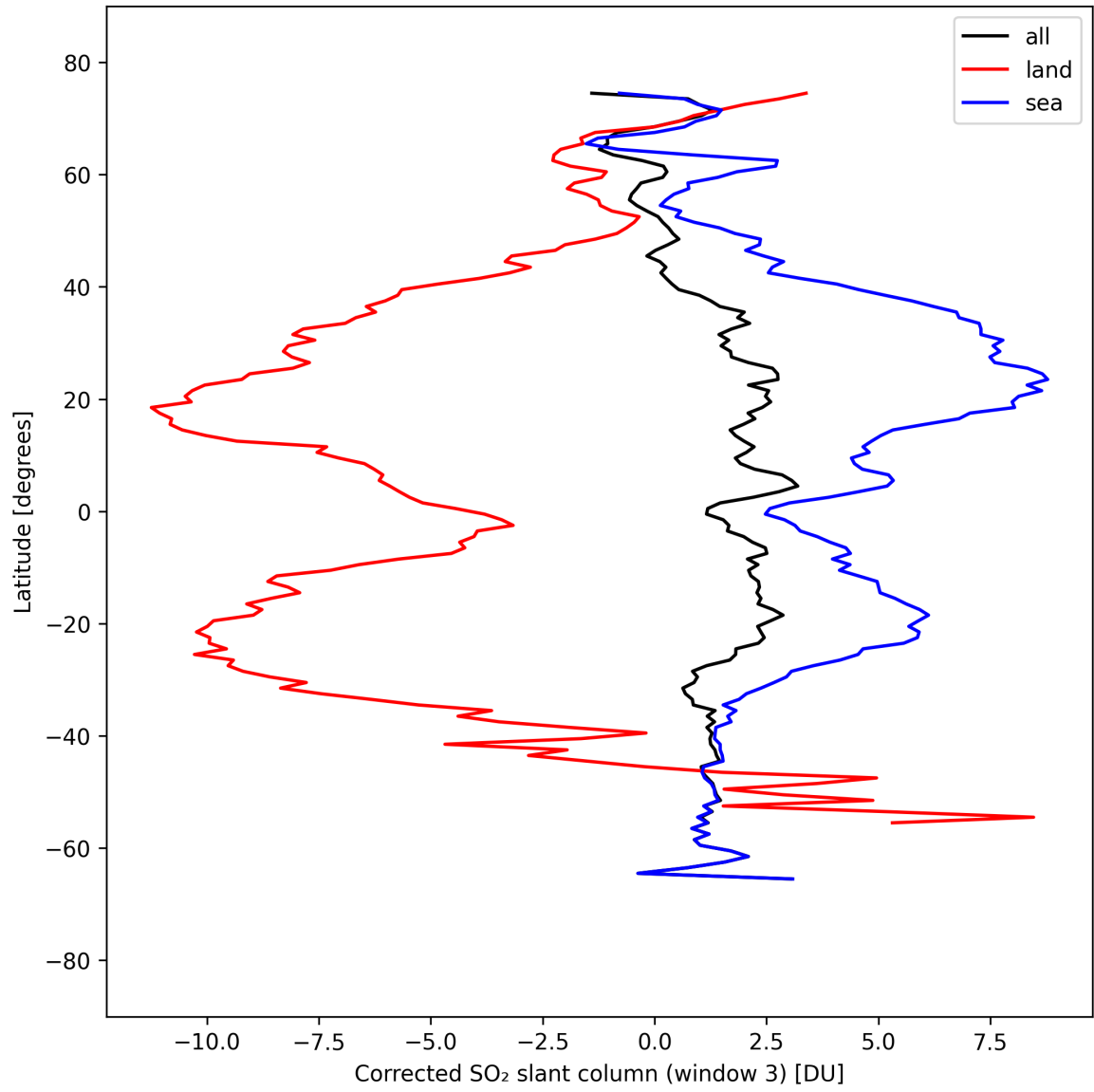
Figure 47: Zonal average of “Corrected SO 2 slant column (window 3)” for 2025-09-11 to 2025-09-13.
