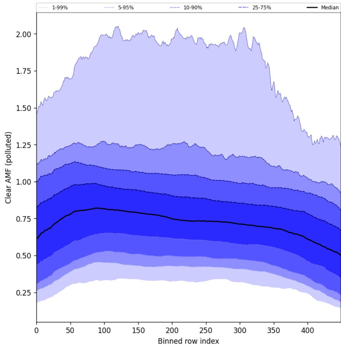
Figure 107: Along track statistics of “Clear AMF (polluted)” for 2025-09-11 to 2025-09-13
