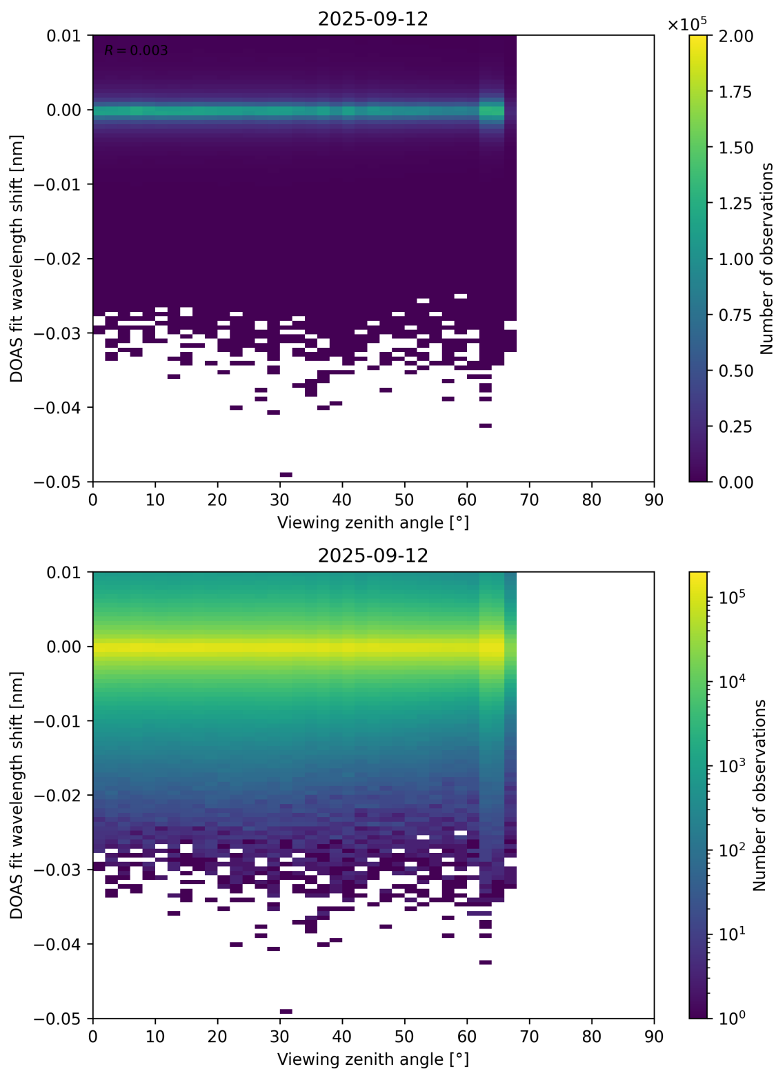
Figure 365: Scatter density plot of “Viewing zenith angle” against “DOAS fit wavelength shift” for 2025-09-11 to 2025-09-13.
