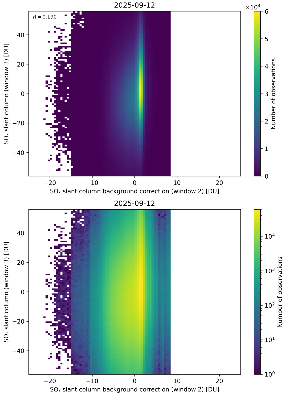
Figure 128: Scatter density plot of “SO 2 slant column background correction (window 2)” against “SO 2 slant column (window 3)” for 2025-09-11 to 2025-09-13.
