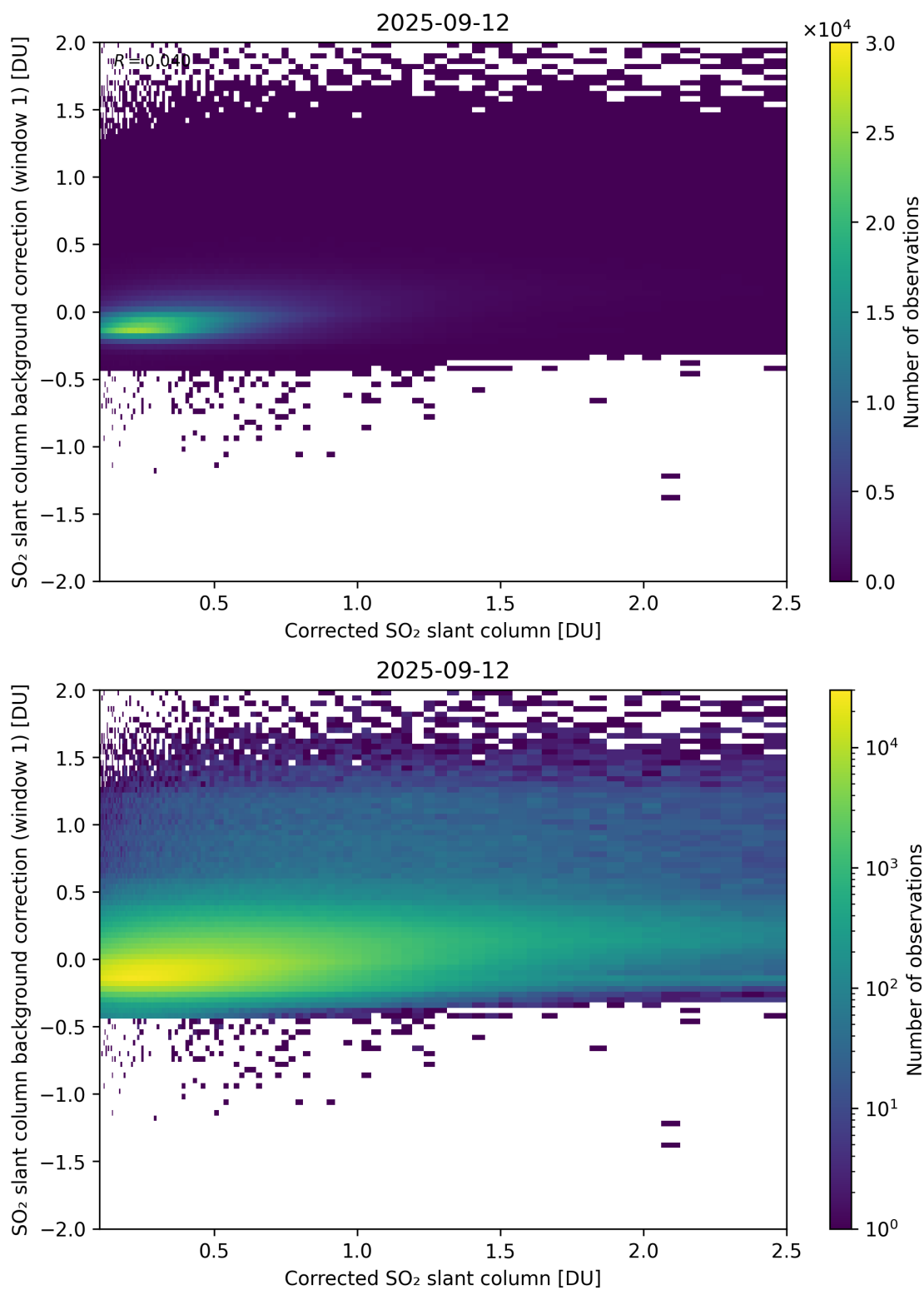
Figure 226: Scatter density plot of “Corrected SO 2 slant column” against “SO 2 slant column background correction (window 1)” for 2025-09-11 to 2025-09-13.
