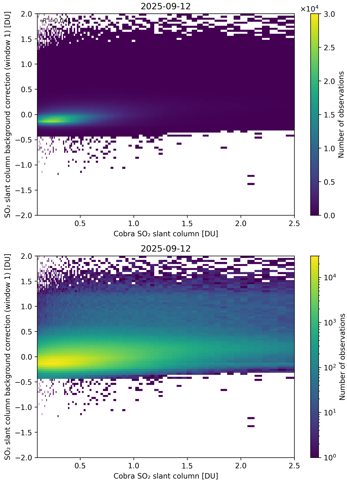
Figure 193: Scatter density plot of “Cobra SO 2 slant column” against “SO 2 slant column background correction (window 1)” for 2025-09-11 to 2025-09-13.
