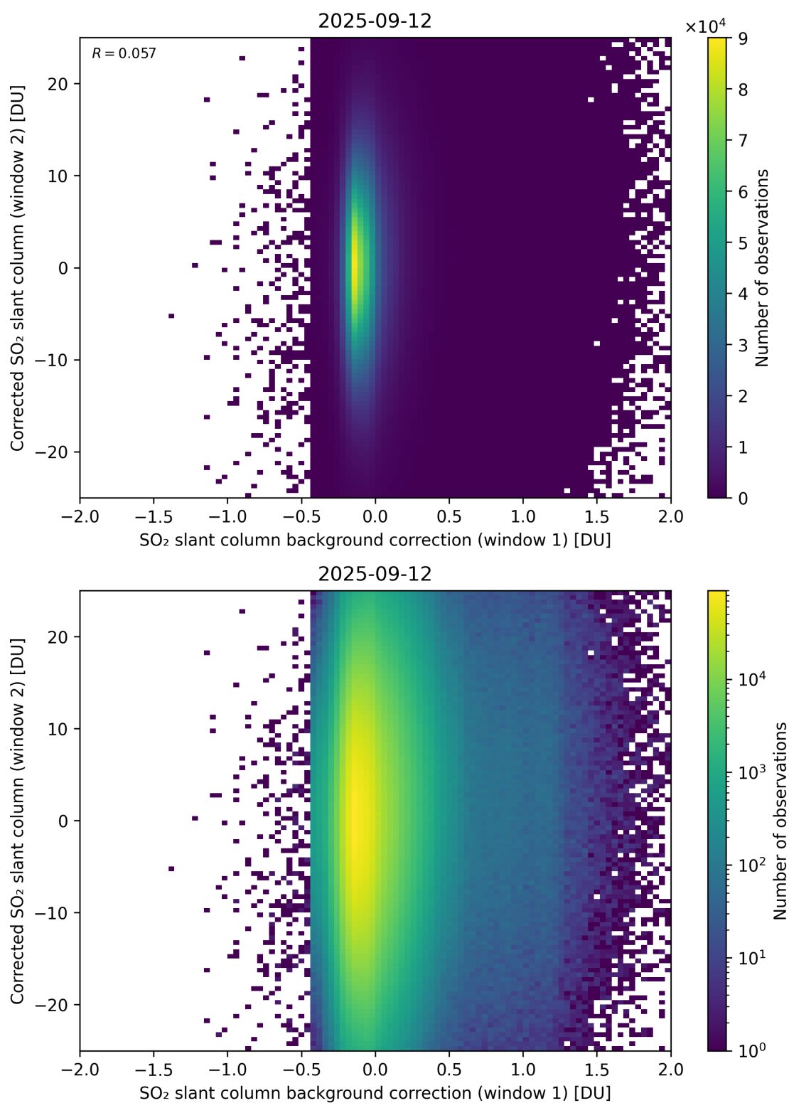
Figure 115: Scatter density plot of “SO 2 slant column background correction (window 1)” against “Corrected SO 2 slant column (window 2)” for 2025-09-11 to 2025-09-13.
