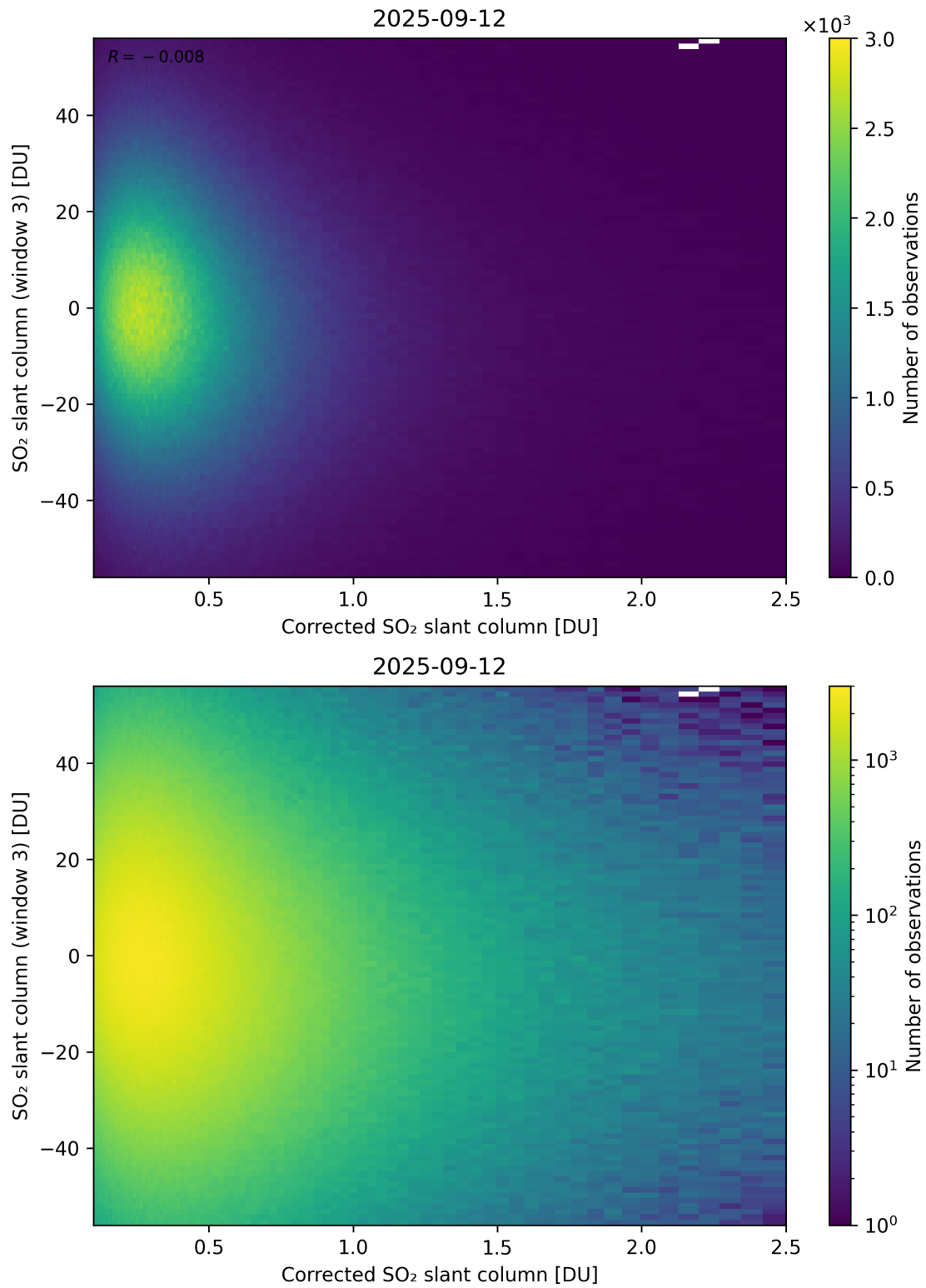
Figure 240: Scatter density plot of “Corrected SO 2 slant column” against “SO 2 slant column (window 3)” for 2025-09-11 to 2025-09-13.
