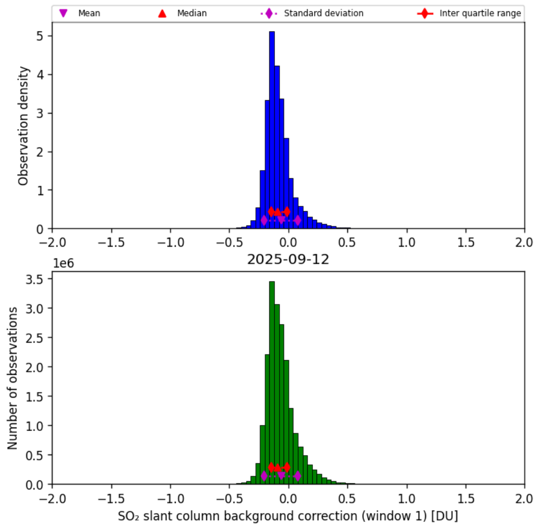
Figure 66: Histogram of “SO 2 slant column background correction (window 1)” for 2025-09-11 to 2025-09-13
