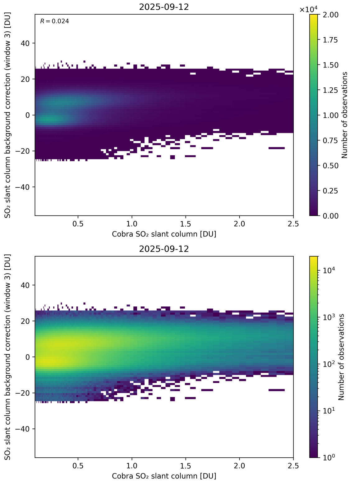
Figure 195: Scatter density plot of “Cobra SO 2 slant column” against “SO 2 slant column background correction (window 3)” for 2025-09-11 to 2025-09-13.
