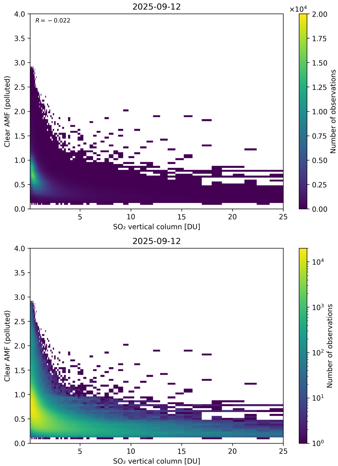
Figure 348: Scatter density plot of “SO 2 vertical column” against “Clear AMF (polluted)” for 2025-09-11 to 2025-09-13.
