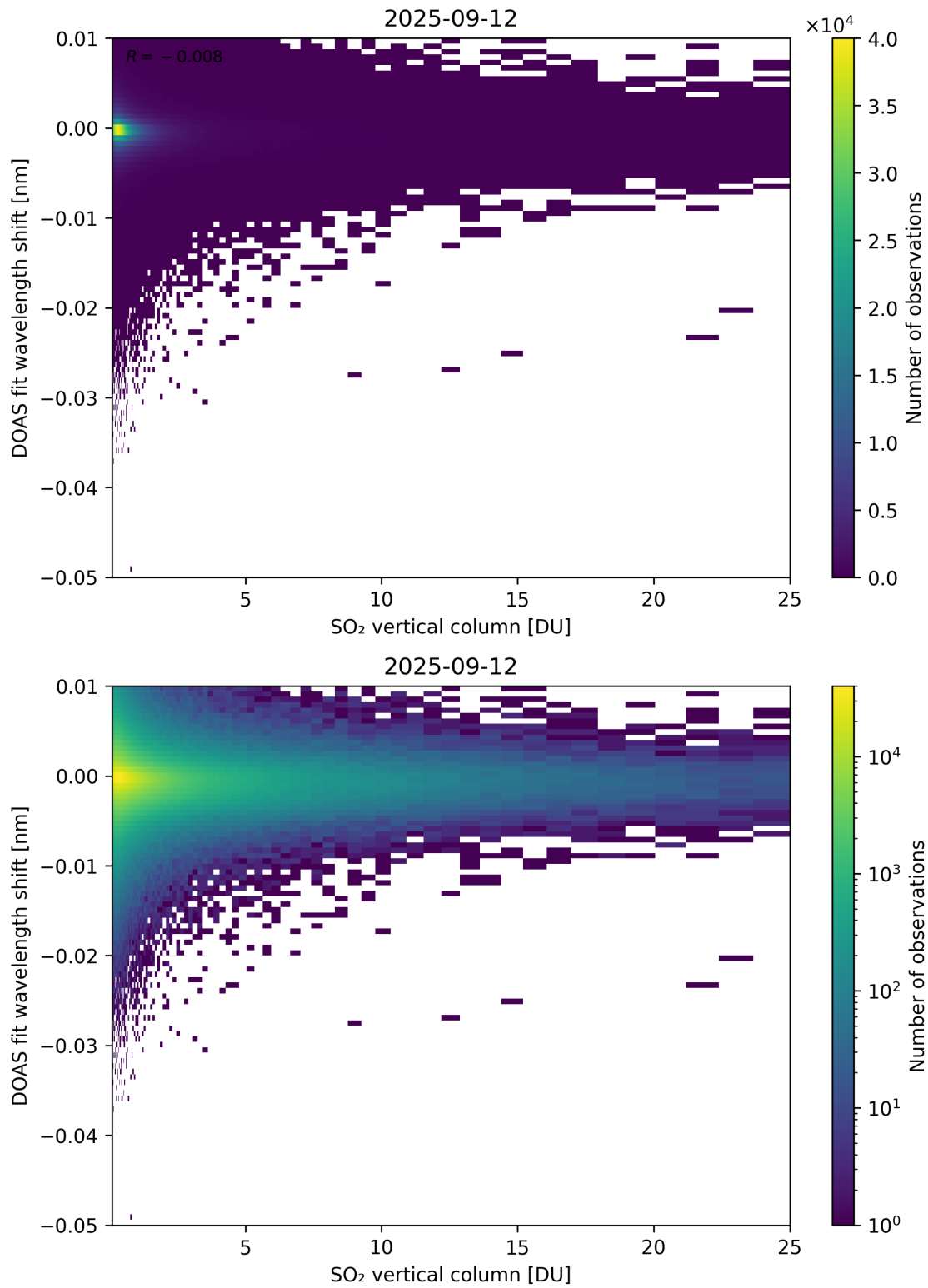
Figure 326: Scatter density plot of “SO 2 vertical column” against “DOAS fit wavelength shift” for 2025-09-11 to 2025-09-13.
