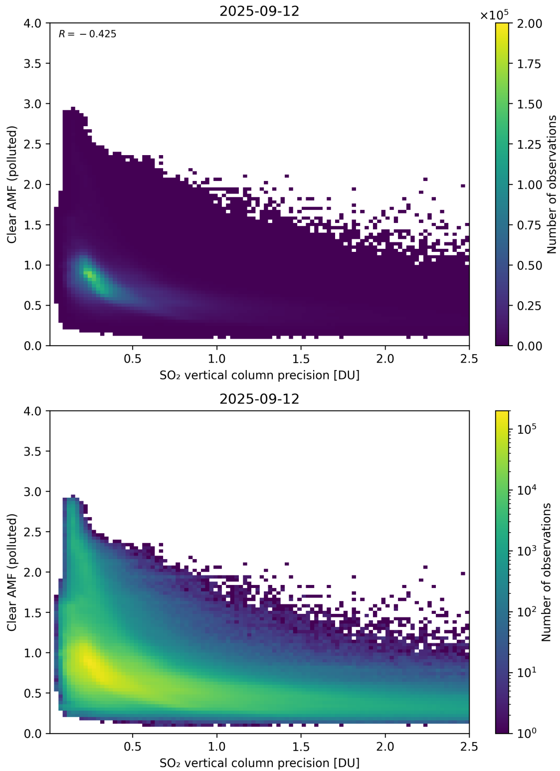
Figure 335: Scatter density plot of “SO 2 vertical column precision” against “Clear AMF (polluted)” for 2025-09-11 to 2025-09-13.
