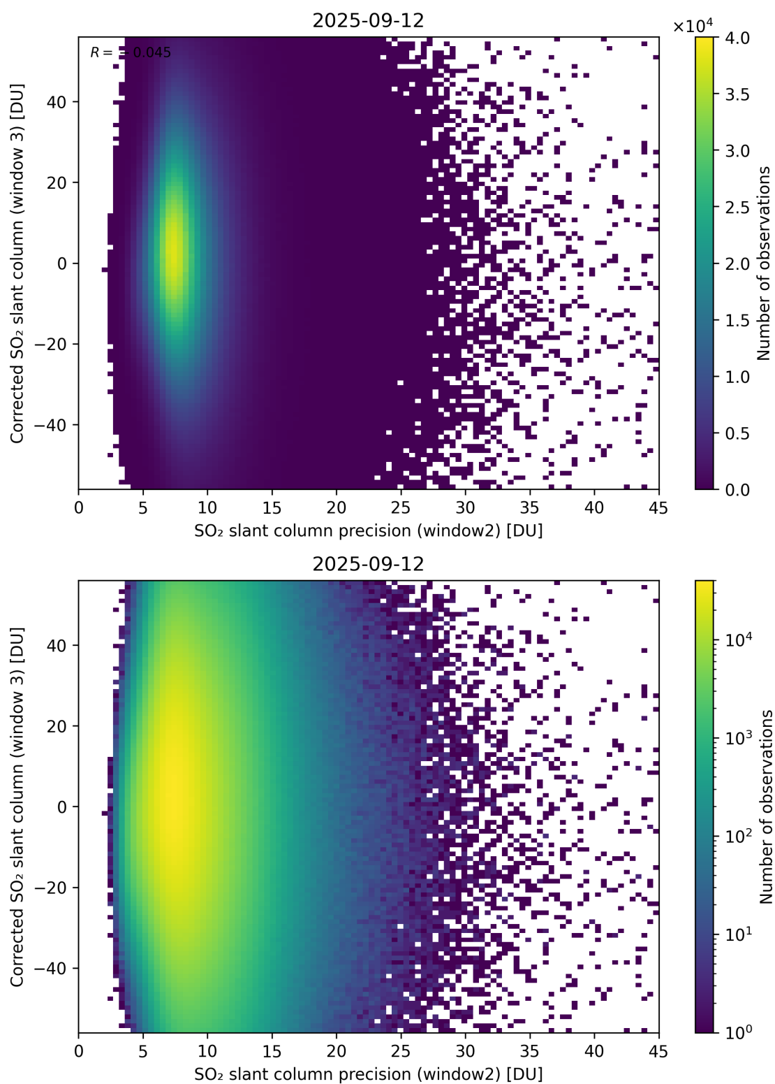
Figure 298: Scatter density plot of “SO 2 slant column precision (window2)” against “Corrected SO 2 slant column (window 3)” for 2025-09-11 to 2025-09-13.
