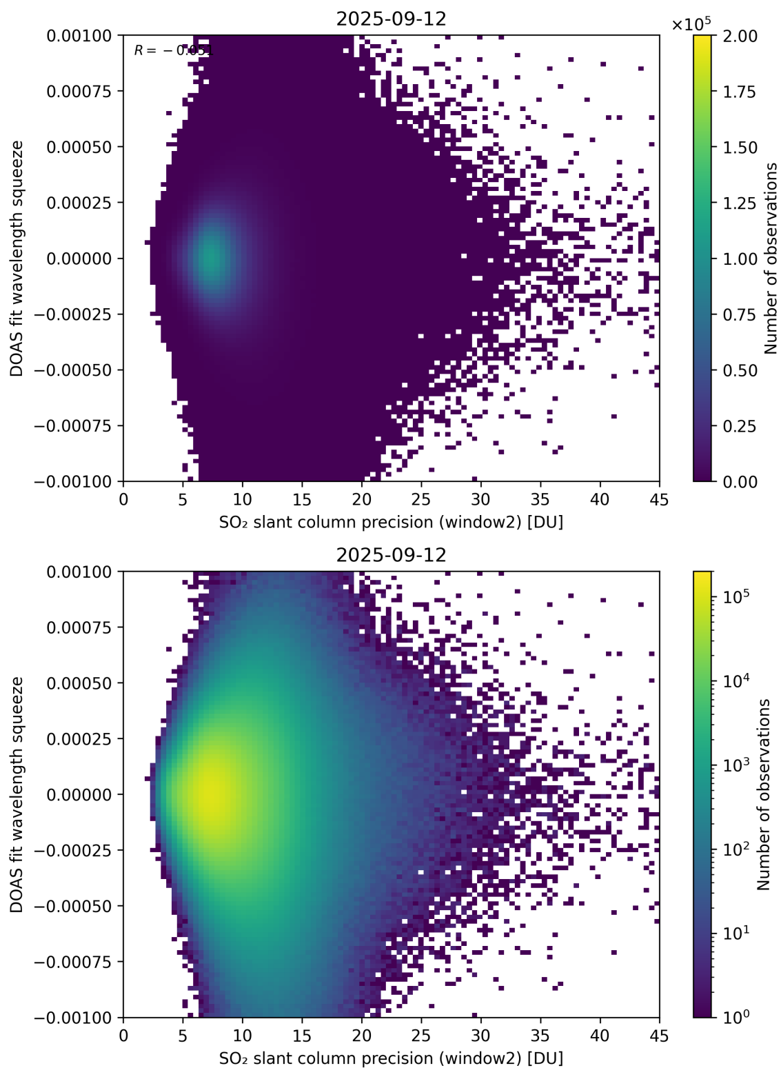
Figure 294: Scatter density plot of “SO 2 slant column precision (window2)” against “DOAS fit wavelength squeeze” for 2025-09-11 to 2025-09-13.
