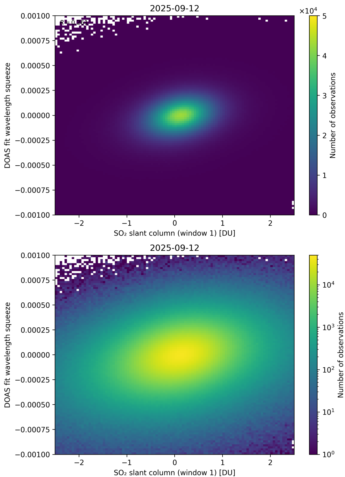
Figure 266: Scatter density plot of “SO 2 slant column (window 1)” against “DOAS fit wavelength squeeze” for 2025-09-11 to 2025-09-13.
