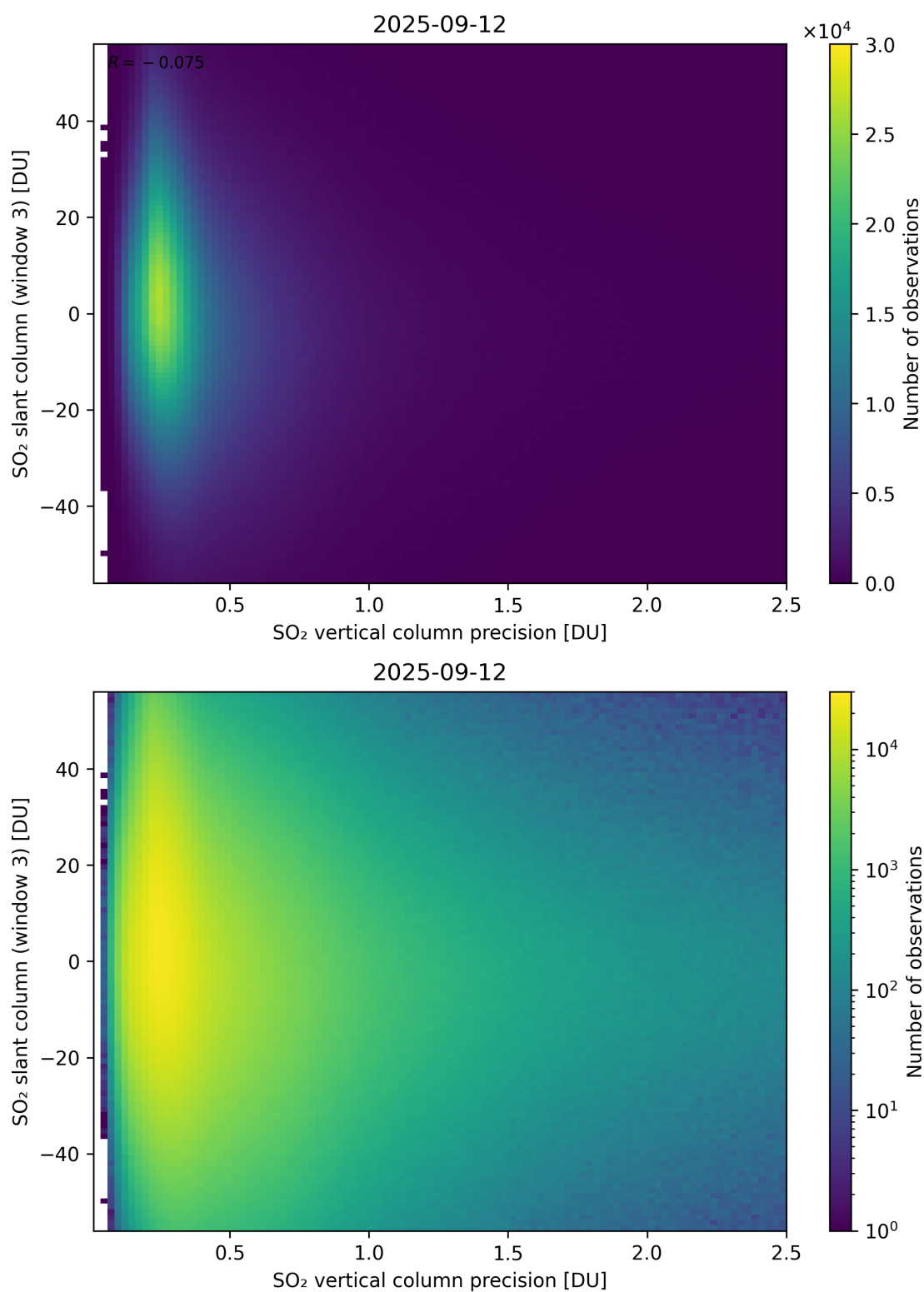
Figure 344: Scatter density plot of “SO 2 vertical column precision” against “SO 2 slant column (window 3)” for 2025-09-11 to 2025-09-13.
