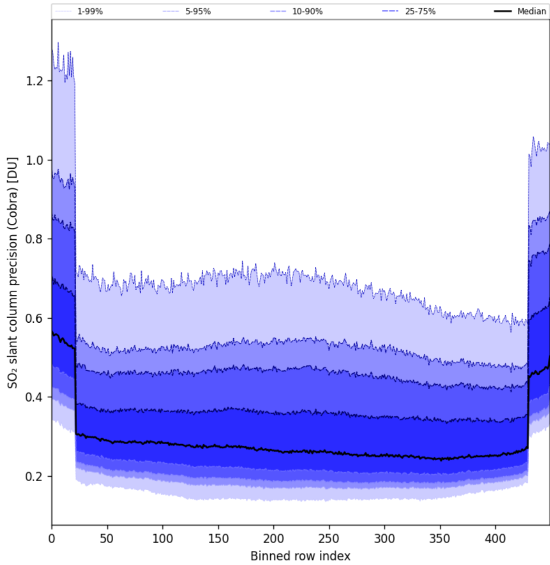
Figure 88: Along track statistics of "SO 2 slant column precision (Cobra)" for 2025-09-11 to 2025-09-13
