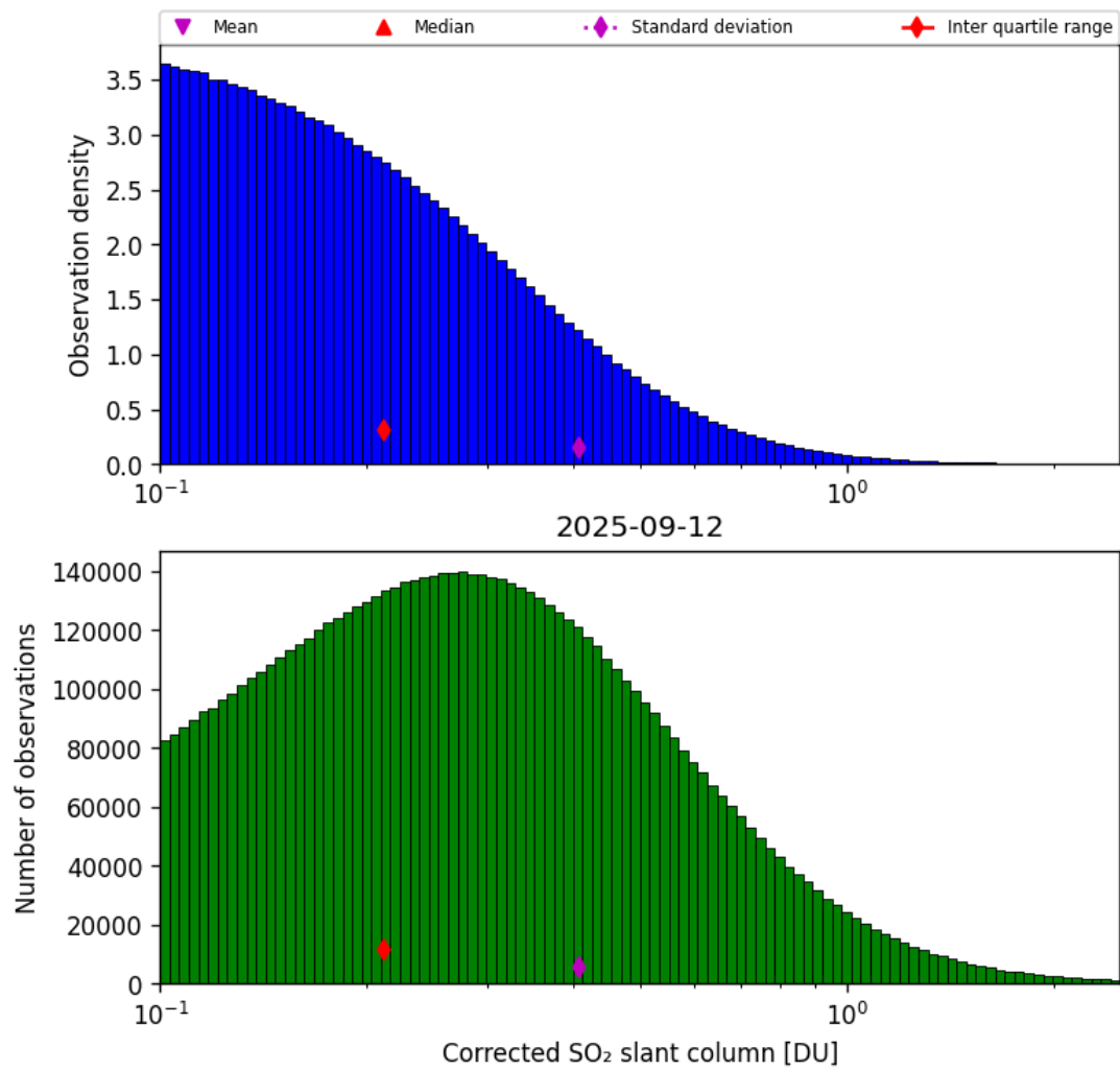
Figure 60: Histogram of "Corrected SO 2 slant column" for 2025-09-11 to 2025-09-13
