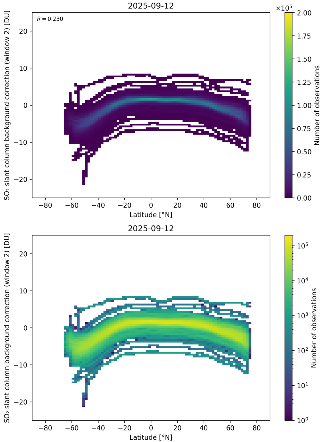
Figure 151: Scatter density plot of “Latitude” against “SO 2 slant column background correction (window 2)” for 2025-09-11 to 2025-09-13.
