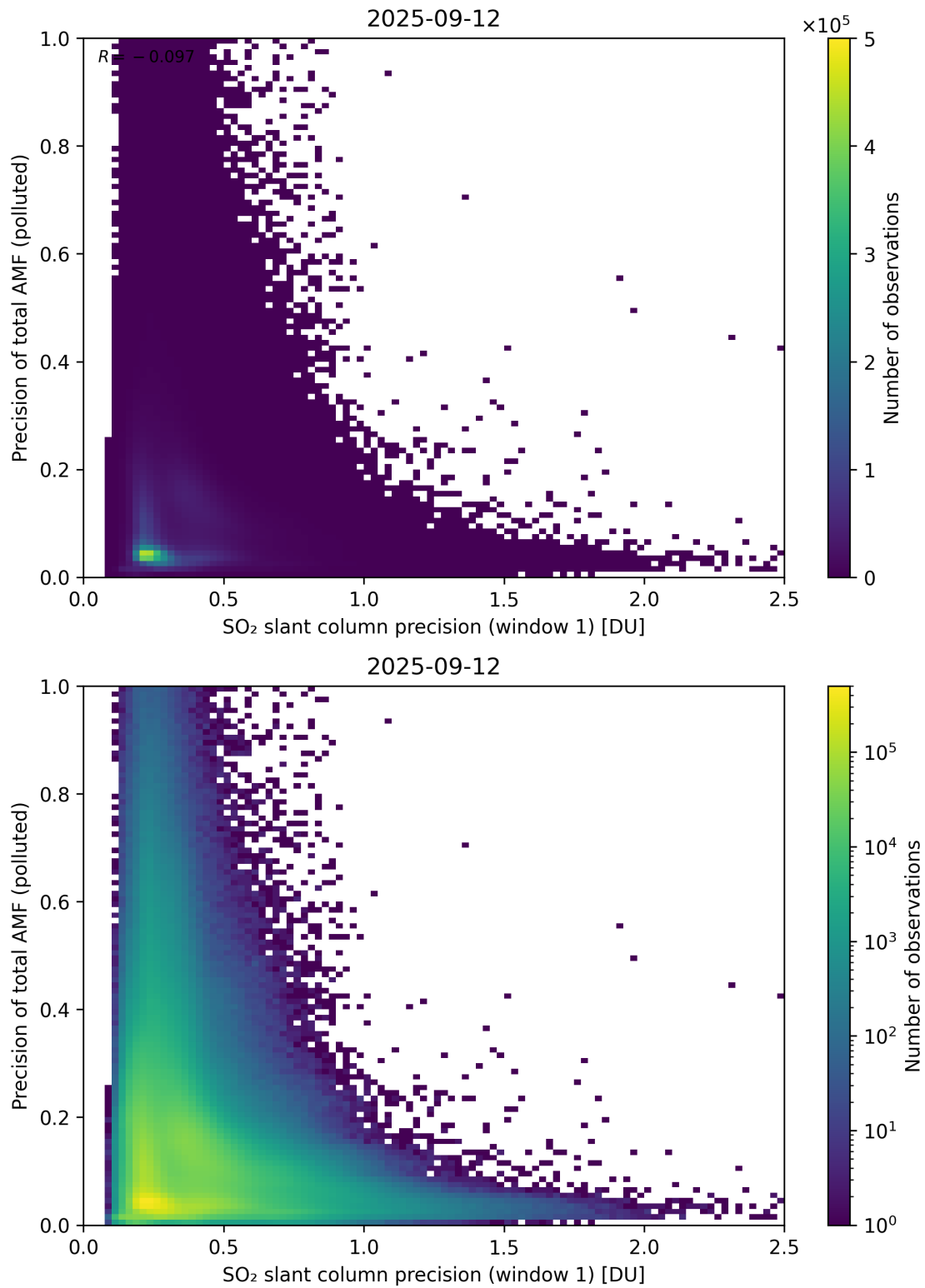
Figure 281: Scatter density plot of “SO 2 slant column precision (window 1)” against “Precision of total AMF (polluted)” for 2025-09-11 to 2025-09-13.
