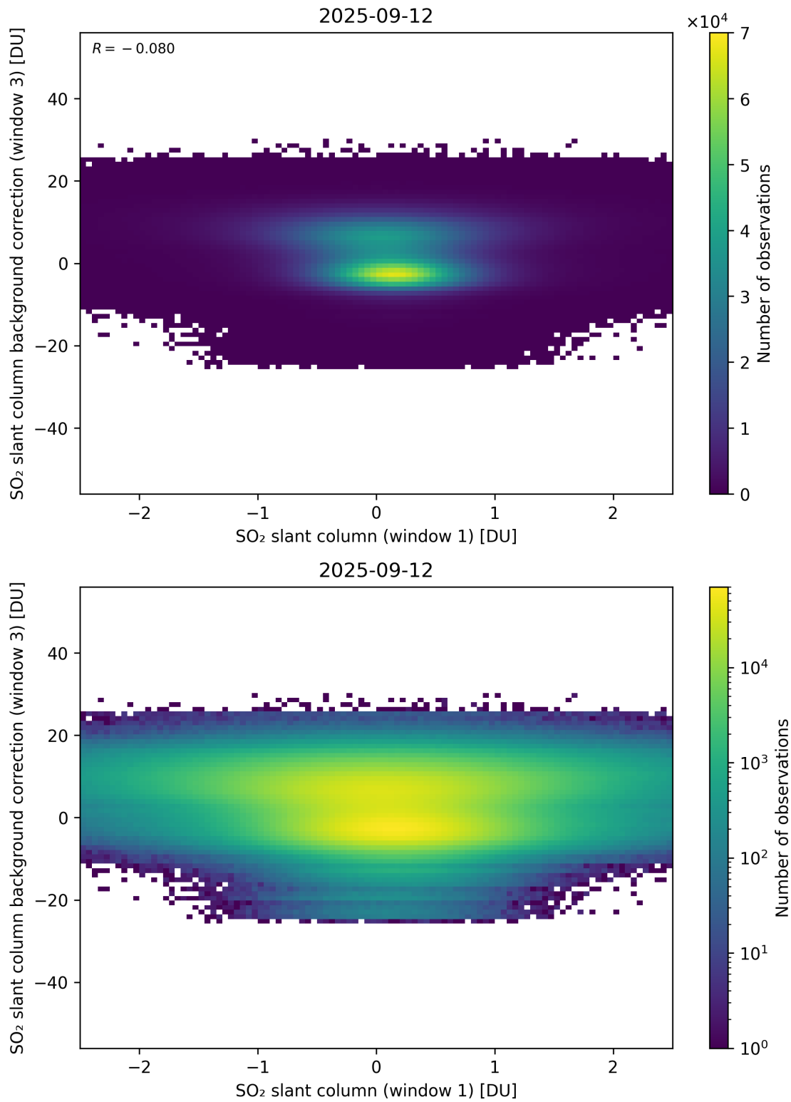
Figure 264: Scatter density plot of “SO 2 slant column (window 1)” against “SO 2 slant column background correction (window 3)” for 2025-09-11 to 2025-09-13.
