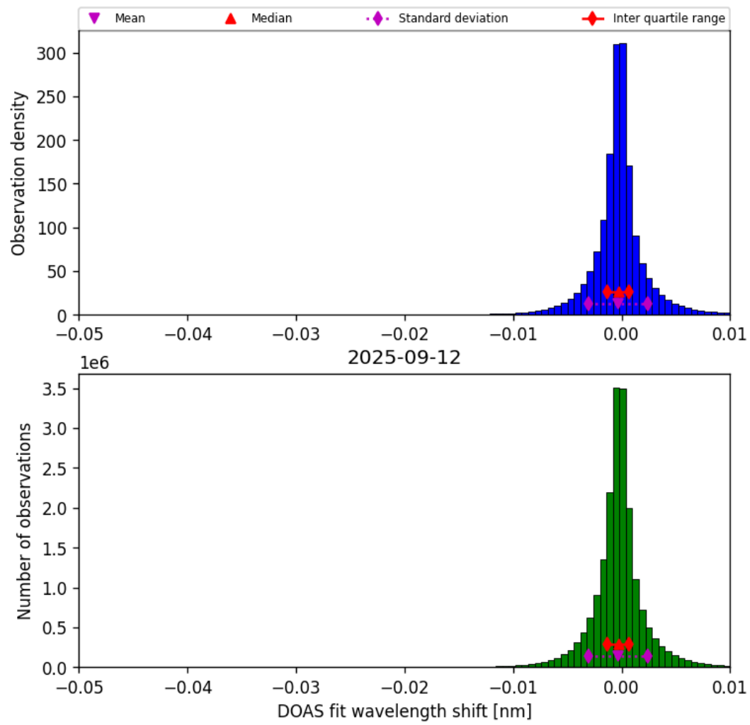
Figure 76: Histogram of “DOAS fit wavelength shift” for 2025-09-11 to 2025-09-13
