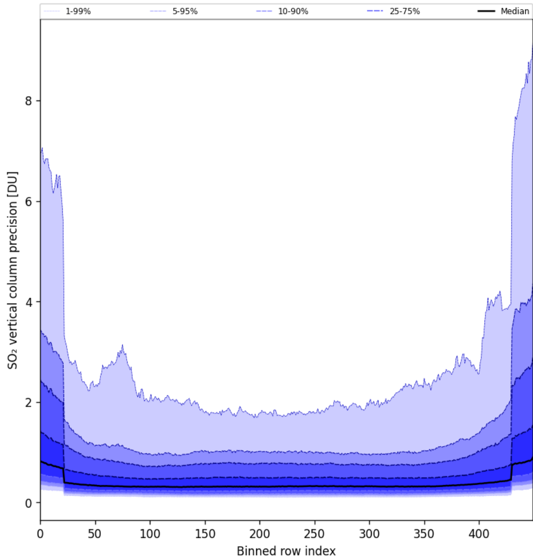
Figure 85: Along track statistics of “SO 2 vertical column precision” for 2025-09-11 to 2025-09-13
