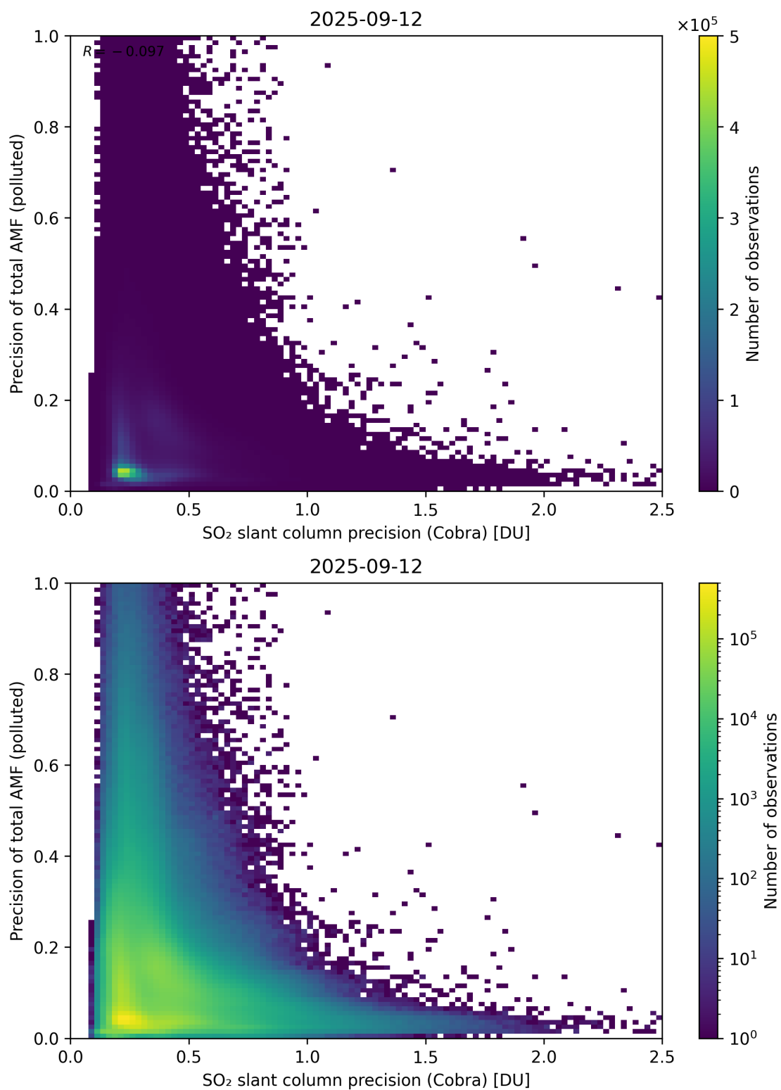
Figure 214: Scatter density plot of “SO 2 slant column precision (Cobra)” against “Precision of total AMF (polluted)” for 2025-09-11 to 2025-09-13.
