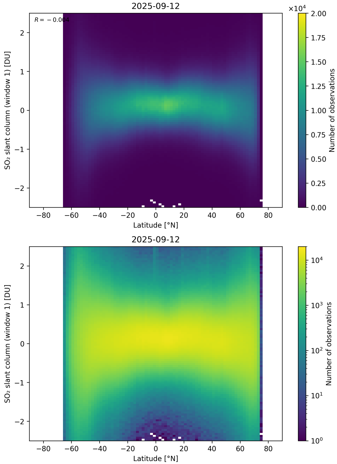
Figure 162: Scatter density plot of “Latitude” against “SO 2 slant column (window 1)” for 2025-09-11 to 2025-09-13.
