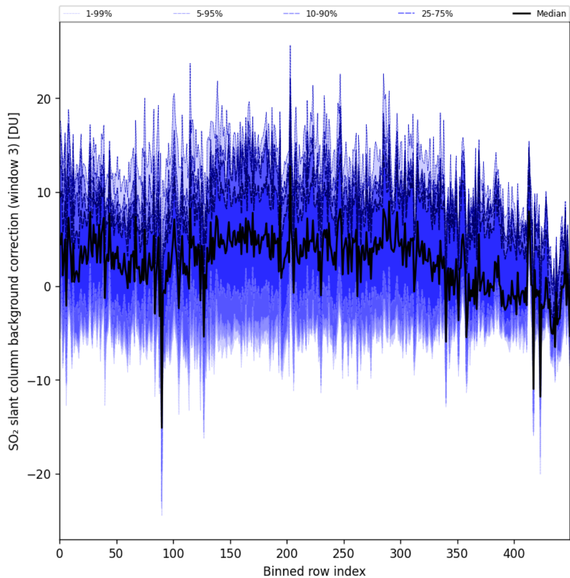
Figure 100: Along track statistics of “SO 2 slant column background correction (window 3)” for 2025-09-11 to 2025-09-13
