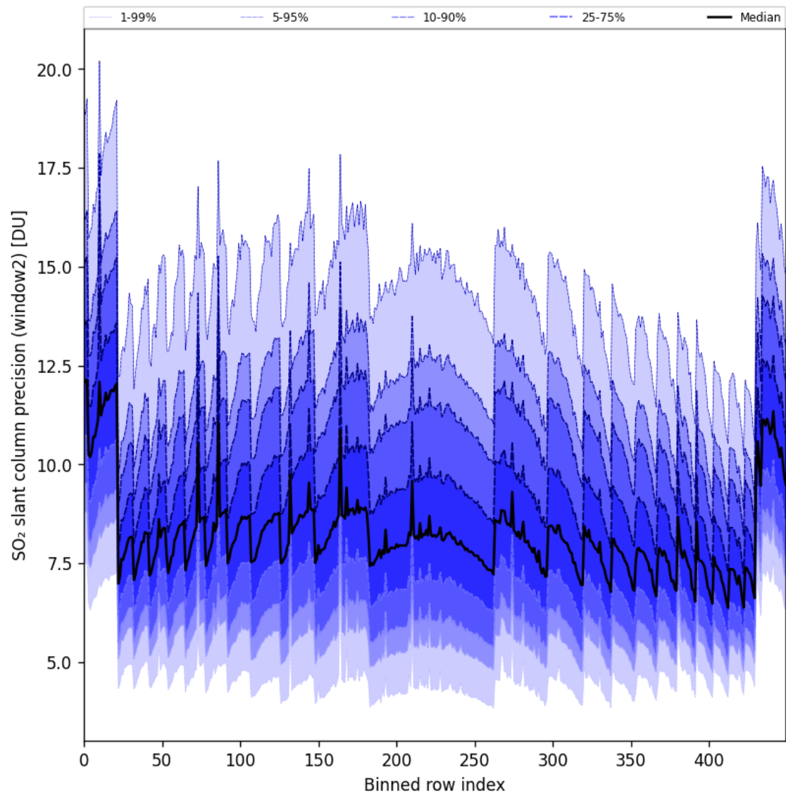
Figure 94: Along track statistics of “SO 2 slant column precision (window2)” for 2025-09-11 to 2025-09-13
