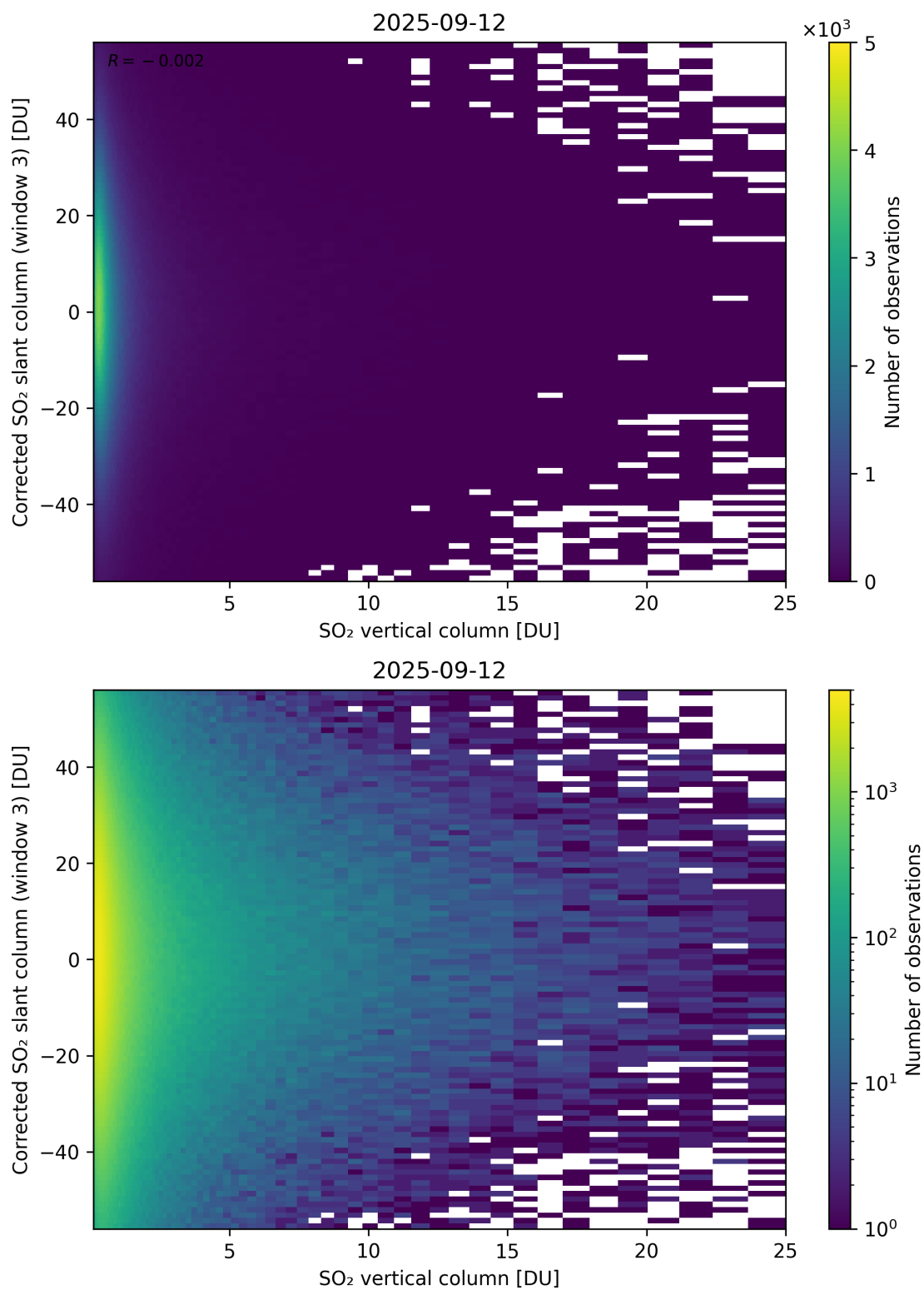
Figure 353: Scatter density plot of “SO 2 vertical column” against “Corrected SO 2 slant column (window 3)” for 2025-09-11 to 2025-09-13.
