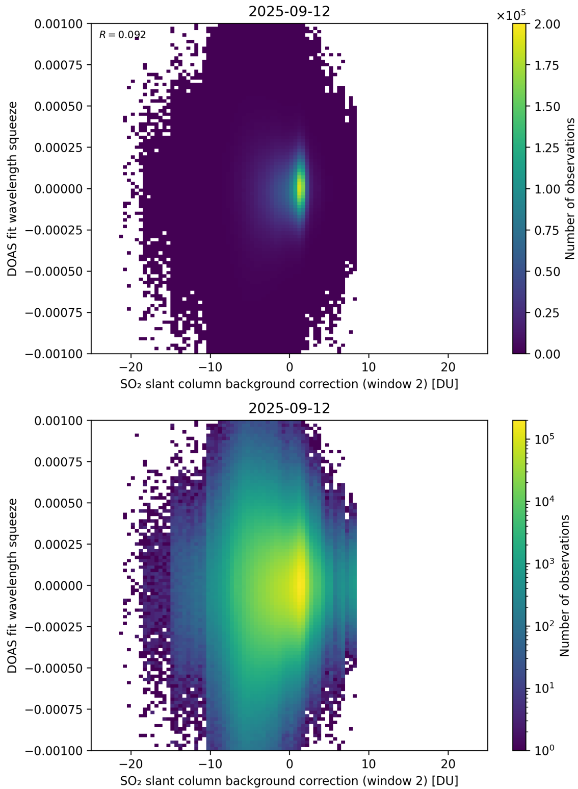
Figure 124: Scatter density plot of “SO 2 slant column background correction (window 2)” against “DOAS fit wavelength squeeze” for 2025-09-11 to 2025-09-13.
