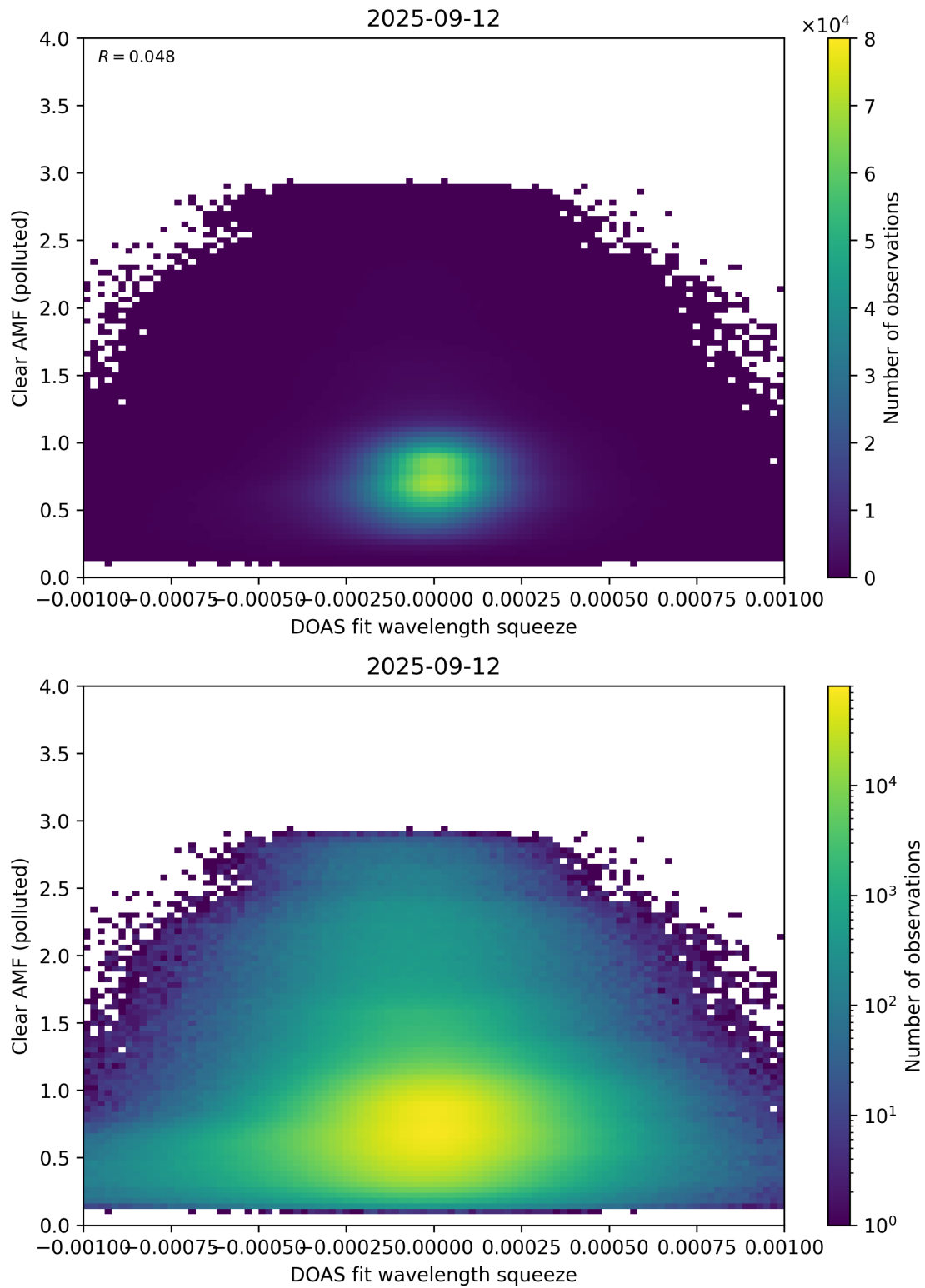
Figure 144: Scatter density plot of “DOAS fit wavelength squeeze” against “Clear AMF (polluted)” for 2025-09-11 to 2025-09-13.
