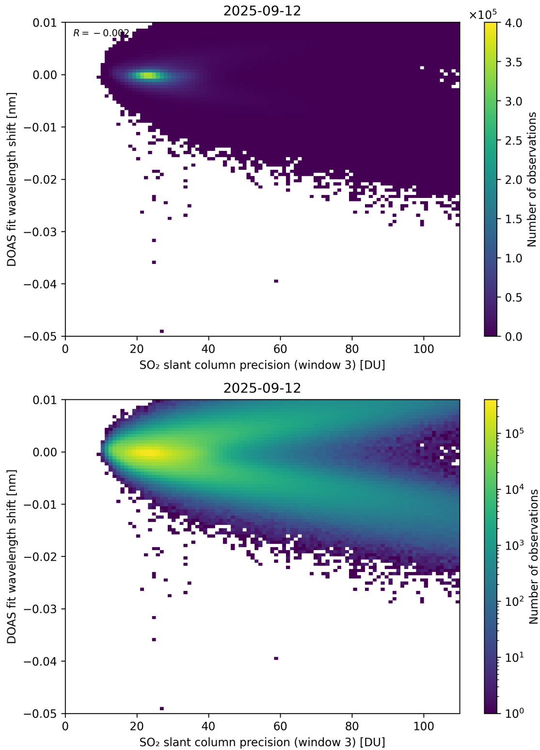
Figure 308: Scatter density plot of “SO 2 slant column precision (window 3)” against “DOAS fit wavelength shift” for 2025-09-11 to 2025-09-13.
