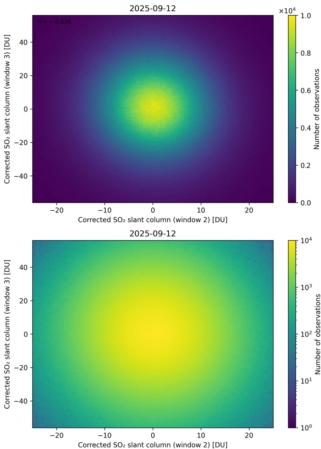
Figure 250: Scatter density plot of “Corrected SO 2 slant column (window 2)” against “Corrected SO 2 slant column (window 3)” for 2025-09-11 to 2025-09-13.
