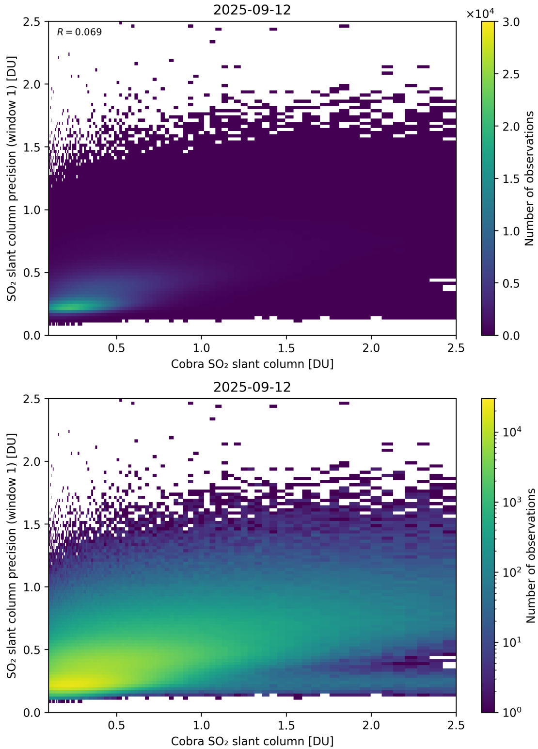
Figure 220: Scatter density plot of “Cobra SO 2 slant column” against “SO 2 slant column precision (window 1)” for 2025-09-11 to 2025-09-13.
