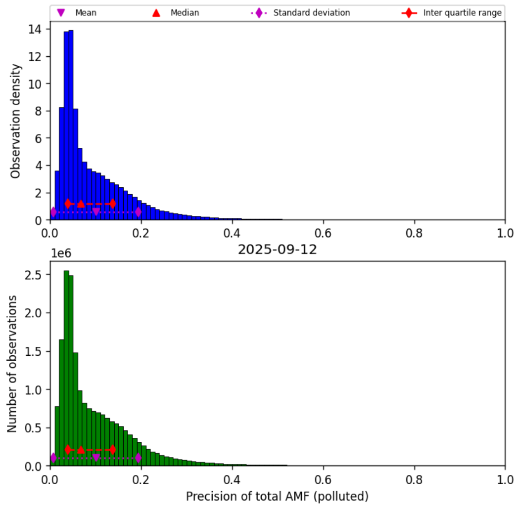
Figure 80: Histogram of “Precision of total AMF (polluted)” for 2025-09-11 to 2025-09-13
