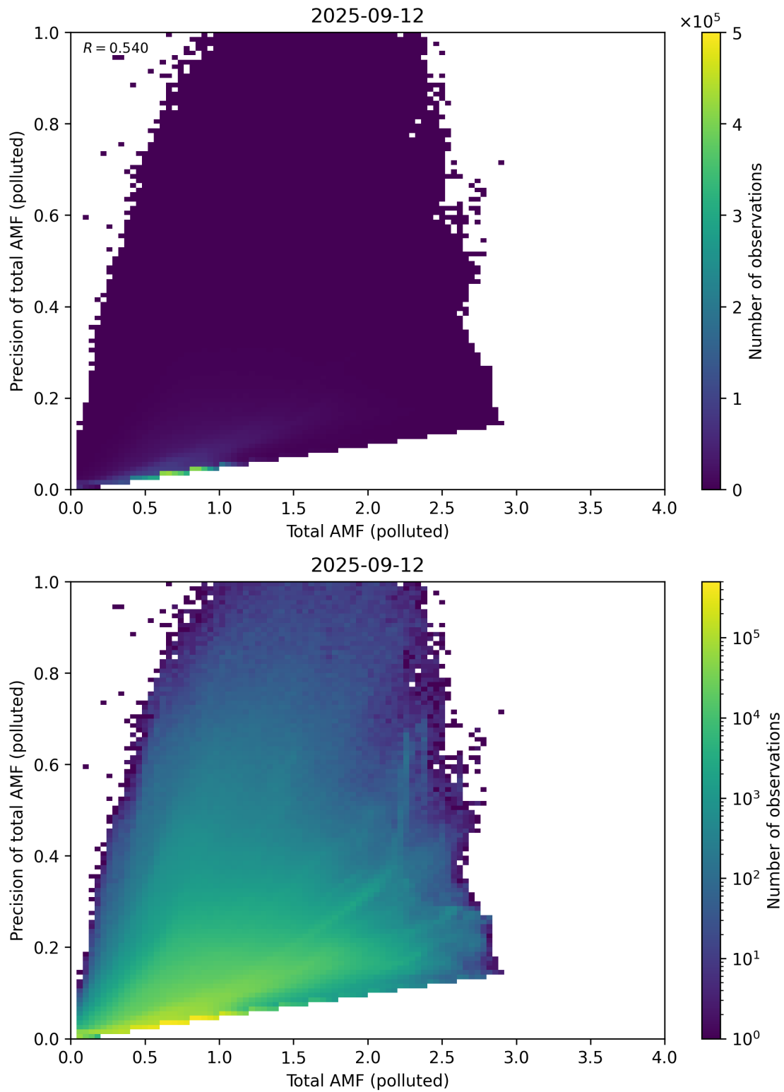
Figure 322: Scatter density plot of “Total AMF (polluted)” against “Precision of total AMF (polluted)” for 2025-09-11 to 2025-09-13.
