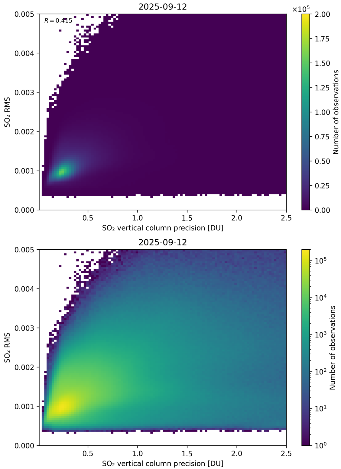
Figure 334: Scatter density plot of “SO 2 vertical column precision” against “SO 2 RMS” for 2025-09-11 to 2025-09-13.
