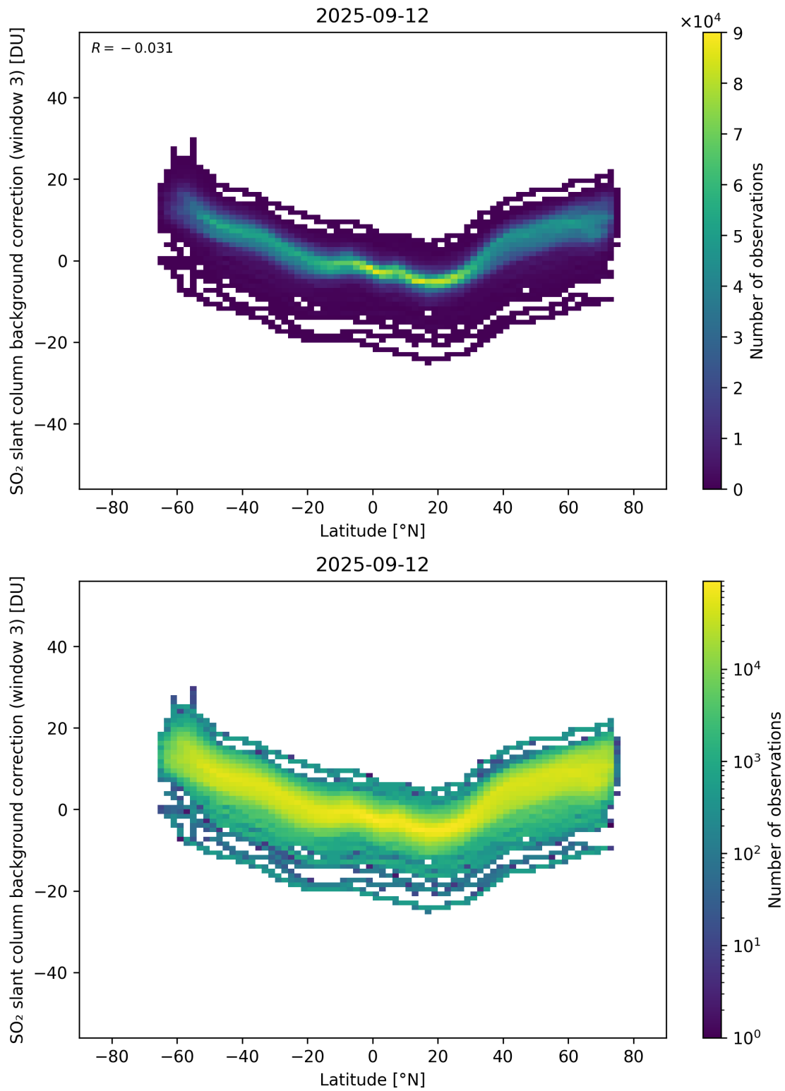
Figure 152: Scatter density plot of “Latitude” against “SO 2 slant column background correction (window 3)” for 2025-09-11 to 2025-09-13.
