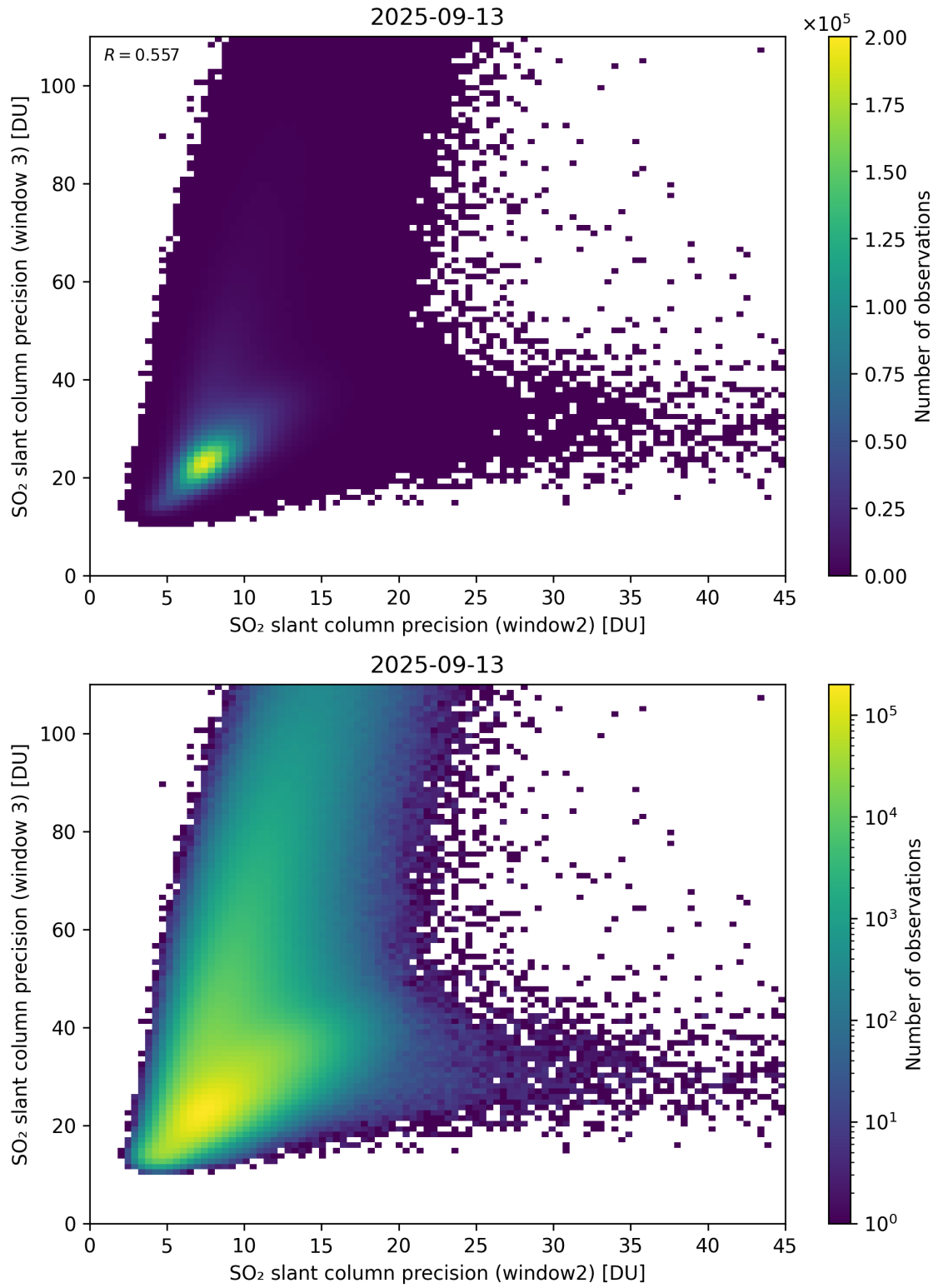
Figure 300: Scatter density plot of “SO 2 slant column precision (window2)” against “SO 2 slant column precision (window 3)” for 2025-09-12 to 2025-09-14.
