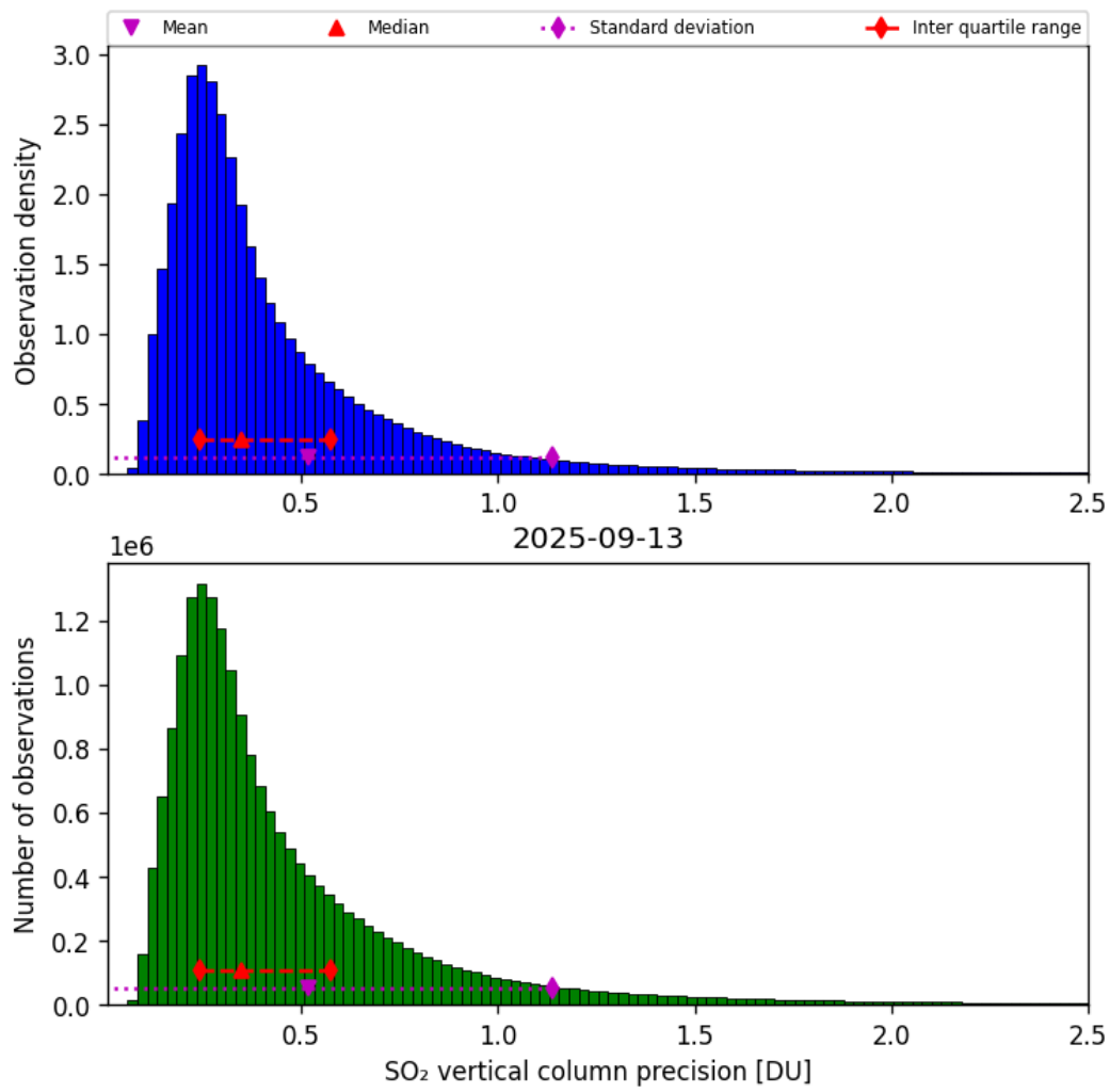
Figure 59: Histogram of “SO 2 vertical column precision” for 2025-09-12 to 2025-09-14
