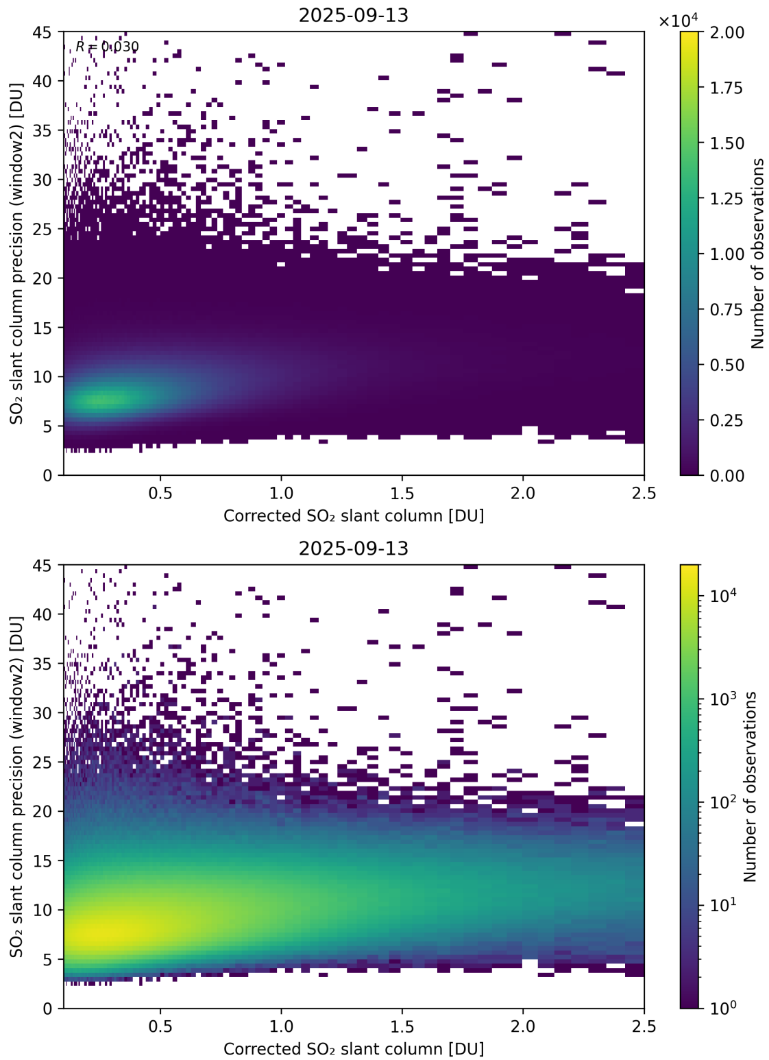
Figure 239: Scatter density plot of “Corrected SO 2 slant column” against “SO 2 slant column precision (window2)” for 2025-09-12 to 2025-09-14.
