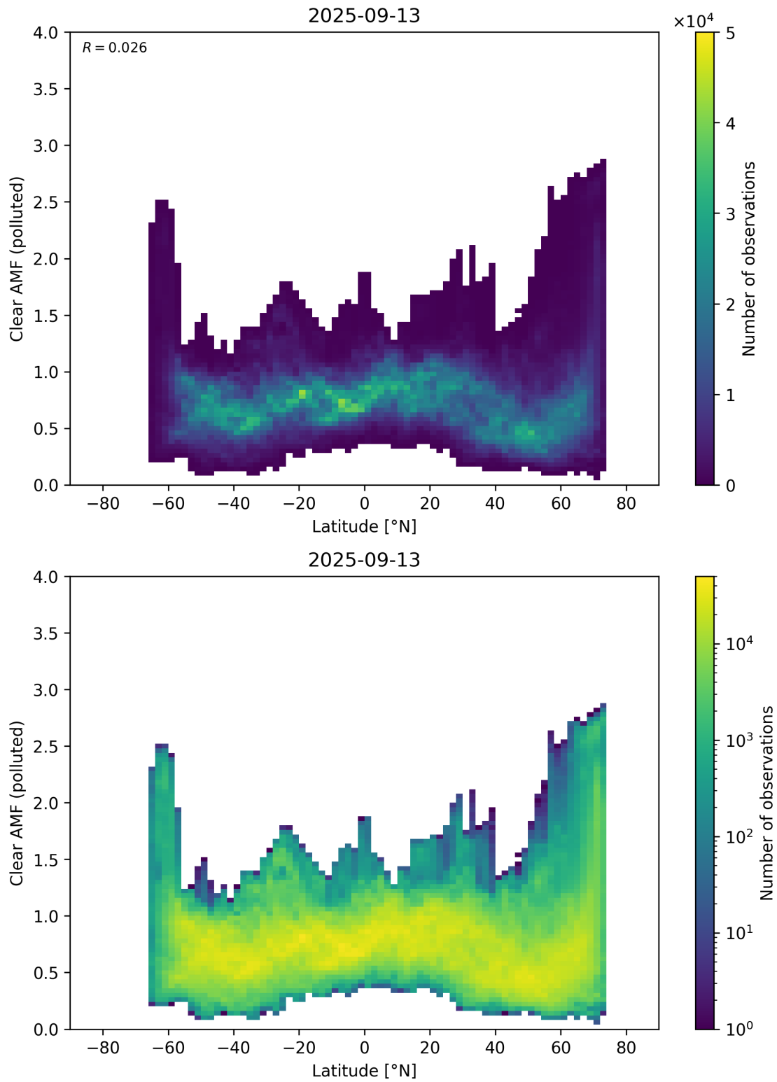
Figure 156: Scatter density plot of “Latitude” against “Clear AMF (polluted)” for 2025-09-12 to 2025-09-14.
