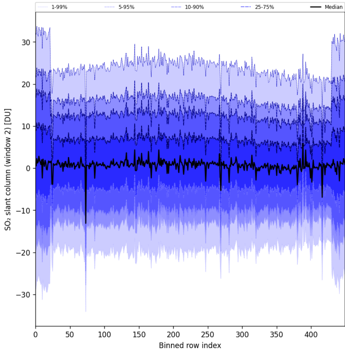
Figure 93: Along track statistics of “SO 2 slant column (window 2)” for 2025-09-12 to 2025-09-14
