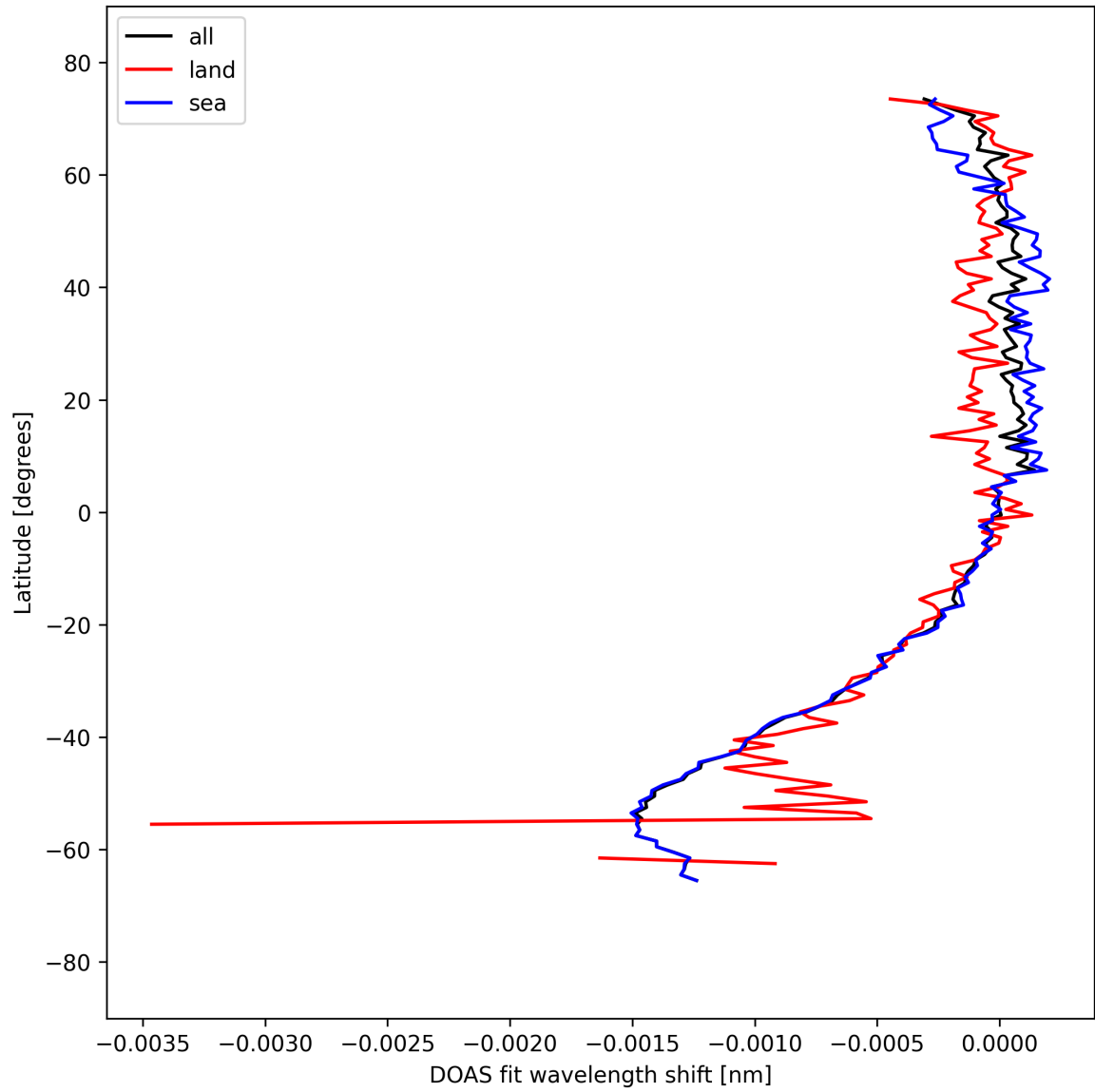
Figure 50: Zonal average of “DOAS fit wavelength shift” for 2025-09-12 to 2025-09-14.
