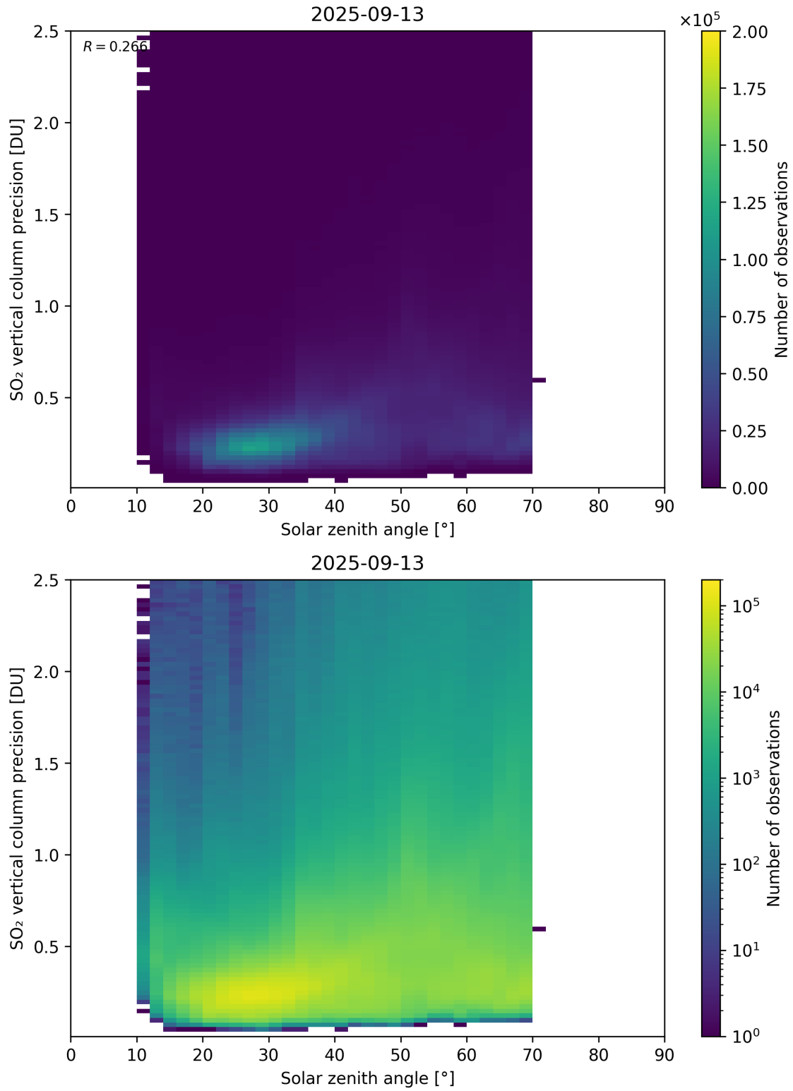
Figure 192: Scatter density plot of “Solar zenith angle” against “SO 2 vertical column precision” for 2025-09-12 to 2025-09-14.
