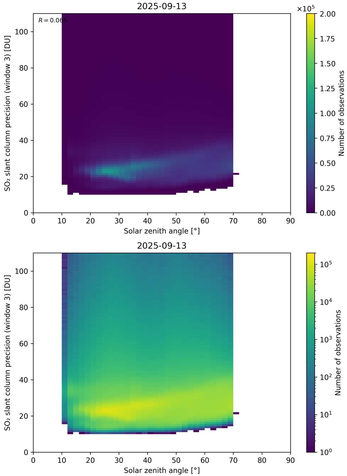
Figure 188: Scatter density plot of “Solar zenith angle” against “SO 2 slant column precision (window 3)” for 2025-09-12 to 2025-09-14.
