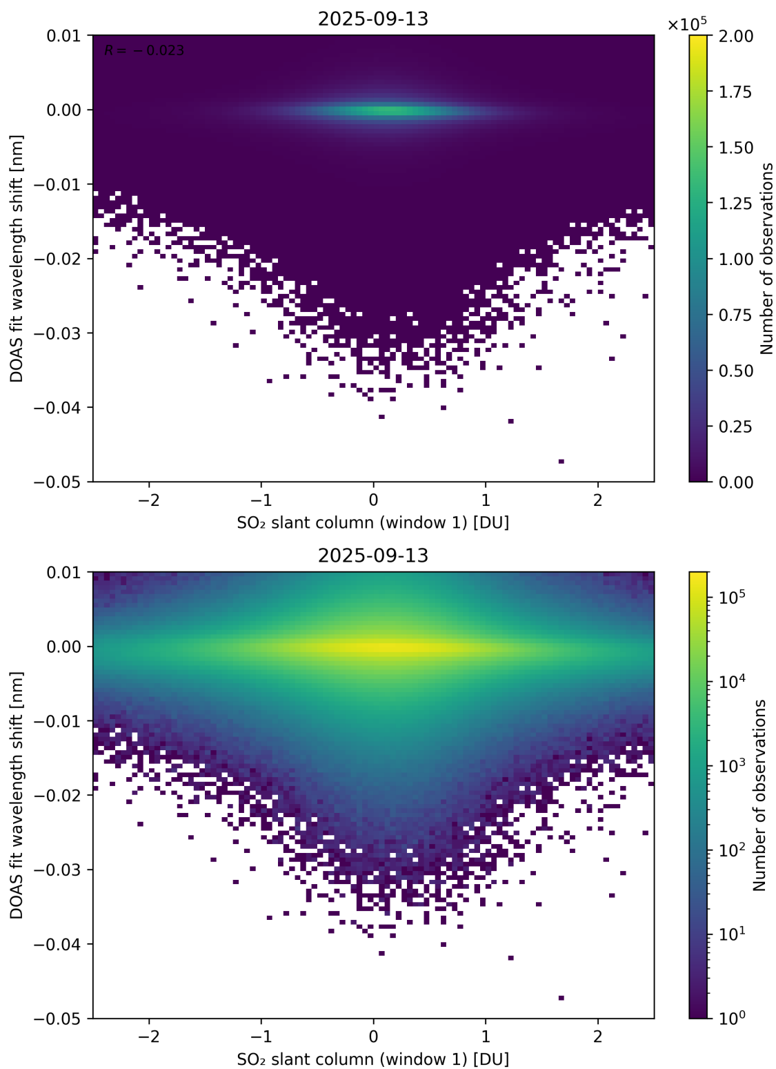
Figure 265: Scatter density plot of “SO 2 slant column (window 1)” against “DOAS fit wavelength shift” for 2025-09-12 to 2025-09-14.
