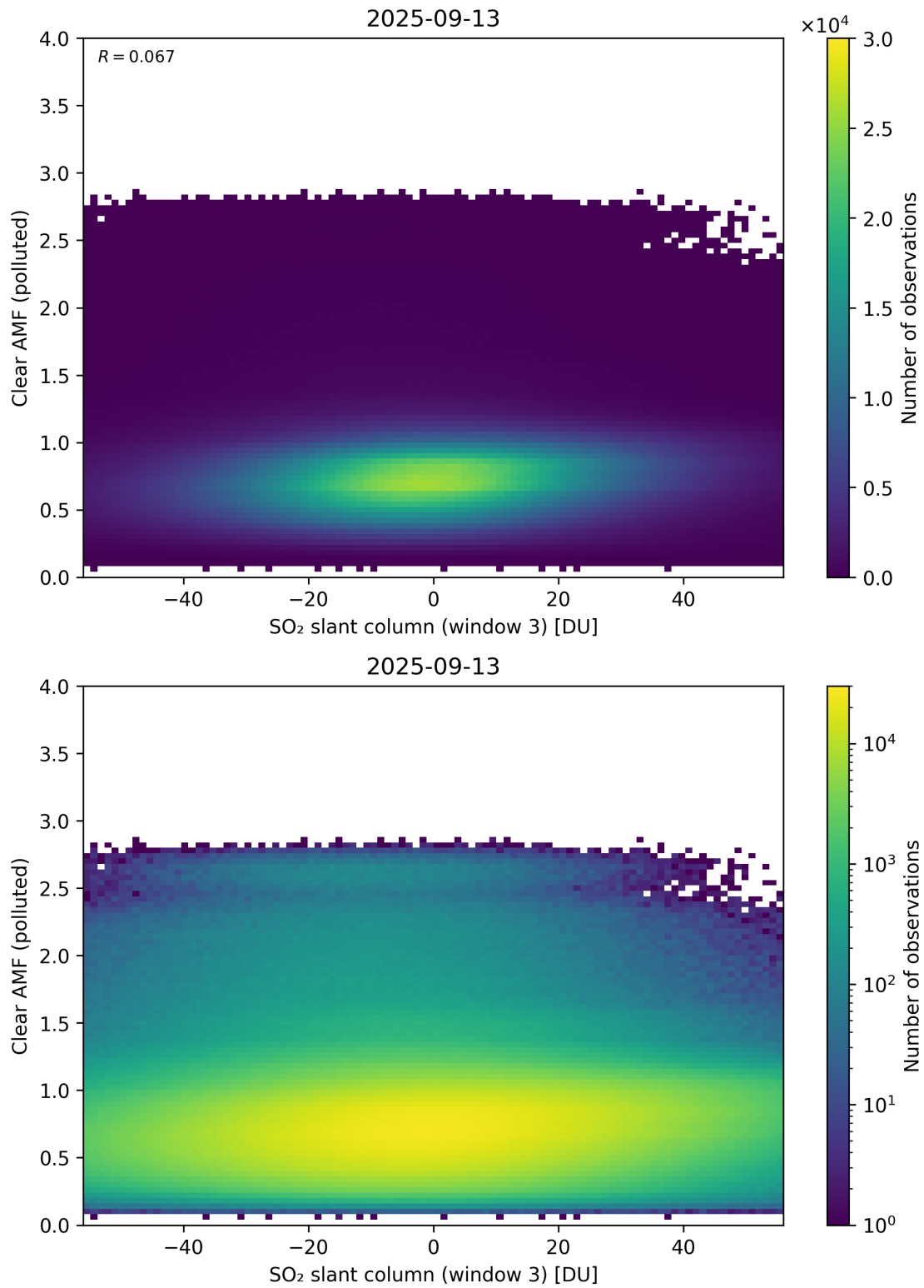
Figure 315: Scatter density plot of “SO 2 slant column (window 3)” against “Clear AMF (polluted)” for 2025-09-12 to 2025-09-14.
