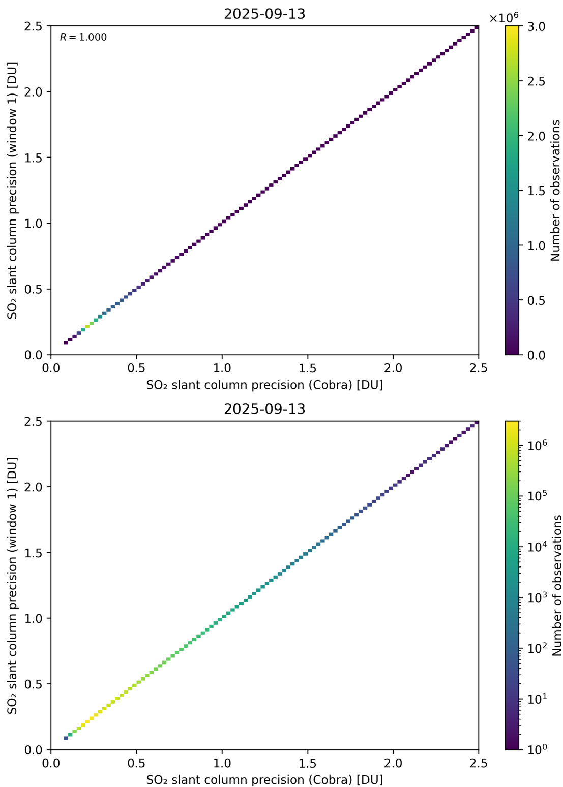
Figure 209: Scatter density plot of “SO 2 slant column precision (Cobra)” against “SO 2 slant column precision (window 1)” for 2025-09-12 to 2025-09-14.
