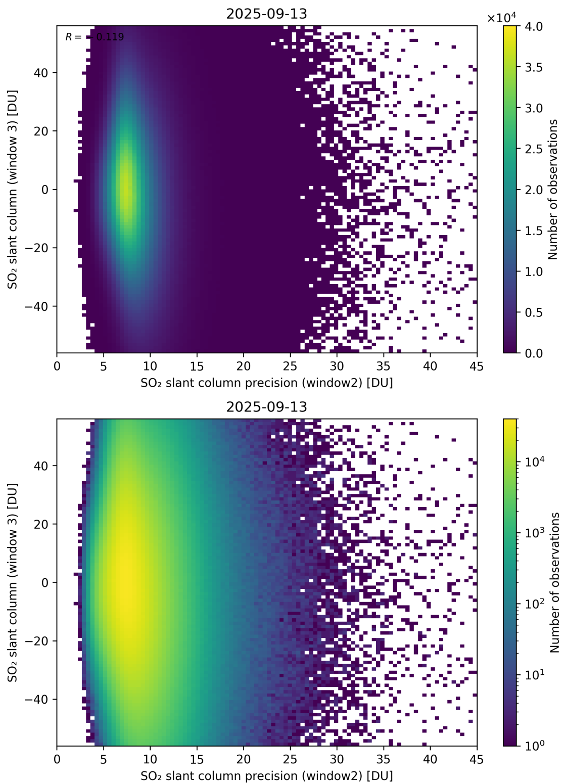
Figure 299: Scatter density plot of “SO 2 slant column precision (window2)” against “SO 2 slant column (window 3)” for 2025-09-12 to 2025-09-14.
