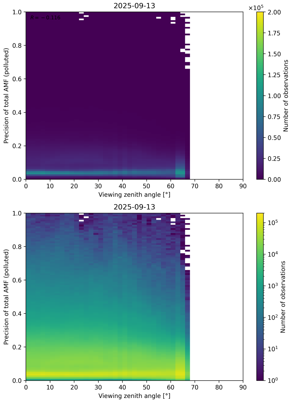
Figure 382: Scatter density plot of “Viewing zenith angle” against “Precision of total AMF (polluted)” for 2025-09-12 to 2025-09-14.
