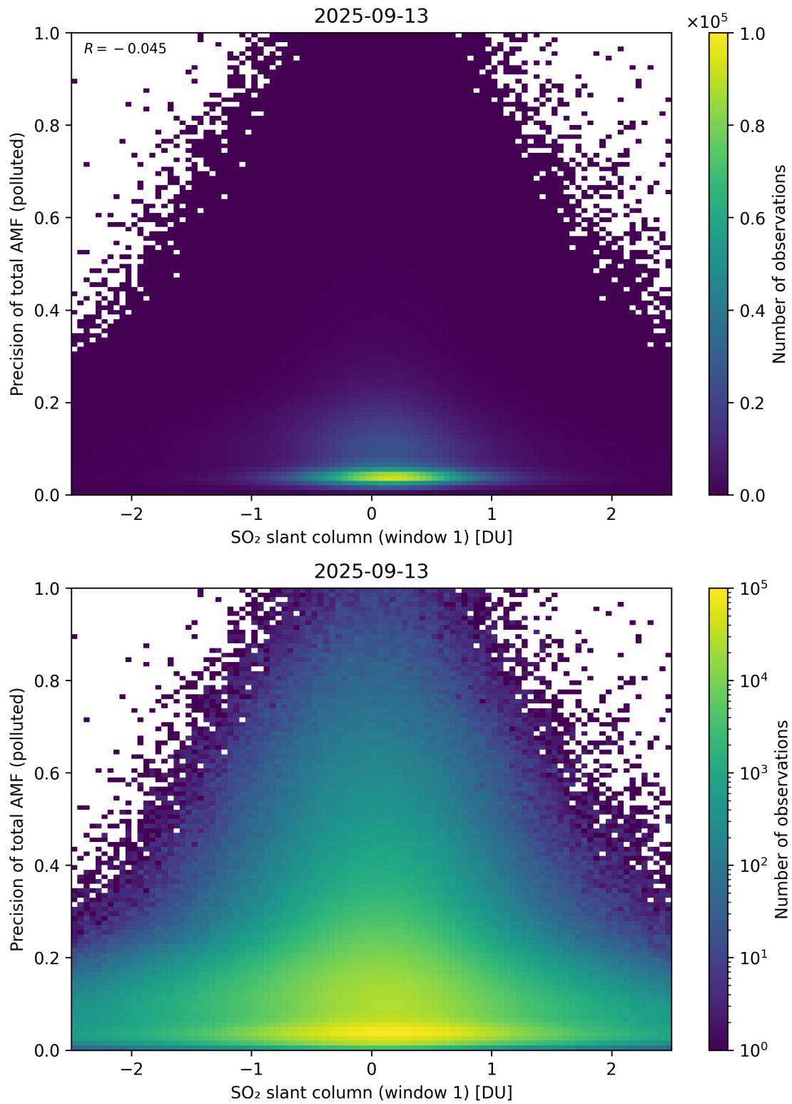
Figure 290: Scatter density plot of “SO 2 slant column (window 1)” against “Precision of total AMF (polluted)” for 2025-09-12 to 2025-09-14.
