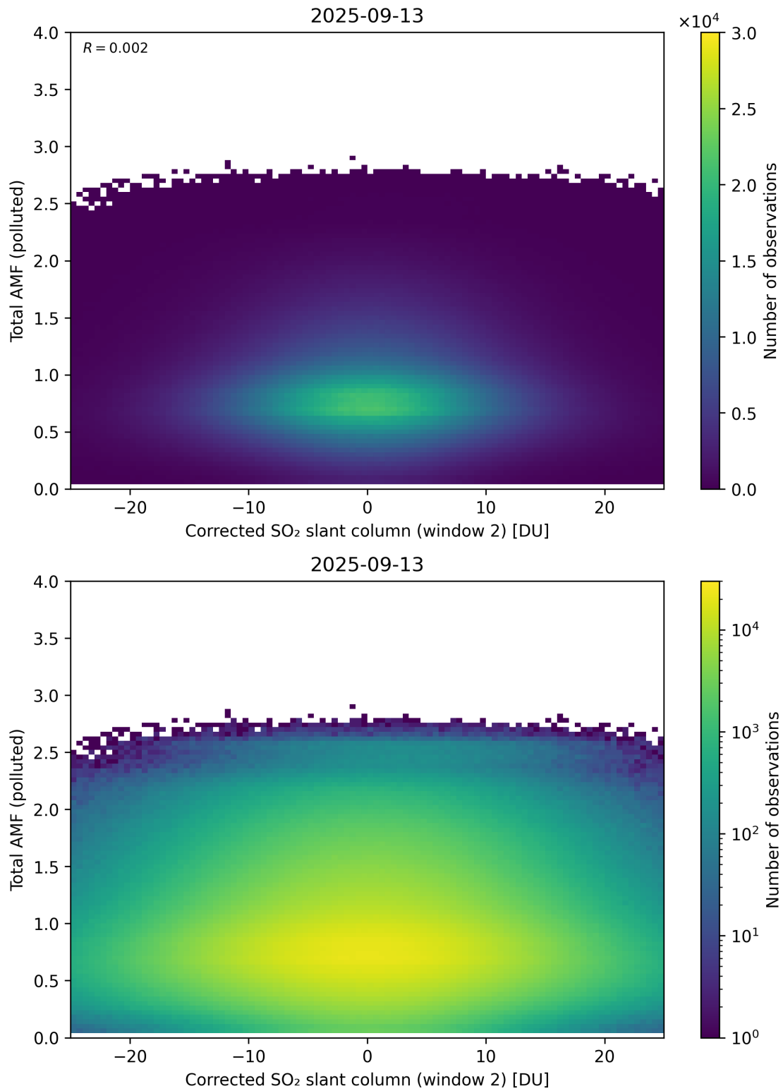
Figure 253: Scatter density plot of “Corrected SO 2 slant column (window 2)” against “Total AMF (polluted)” for 2025-09-12 to 2025-09-14.
