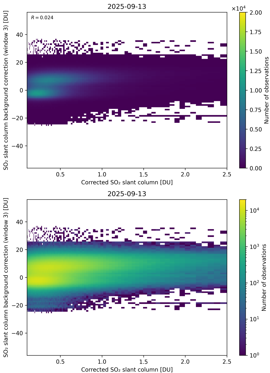
Figure 228: Scatter density plot of “Corrected SO 2 slant column” against “SO 2 slant column background correction (window 3)” for 2025-09-12 to 2025-09-14.
