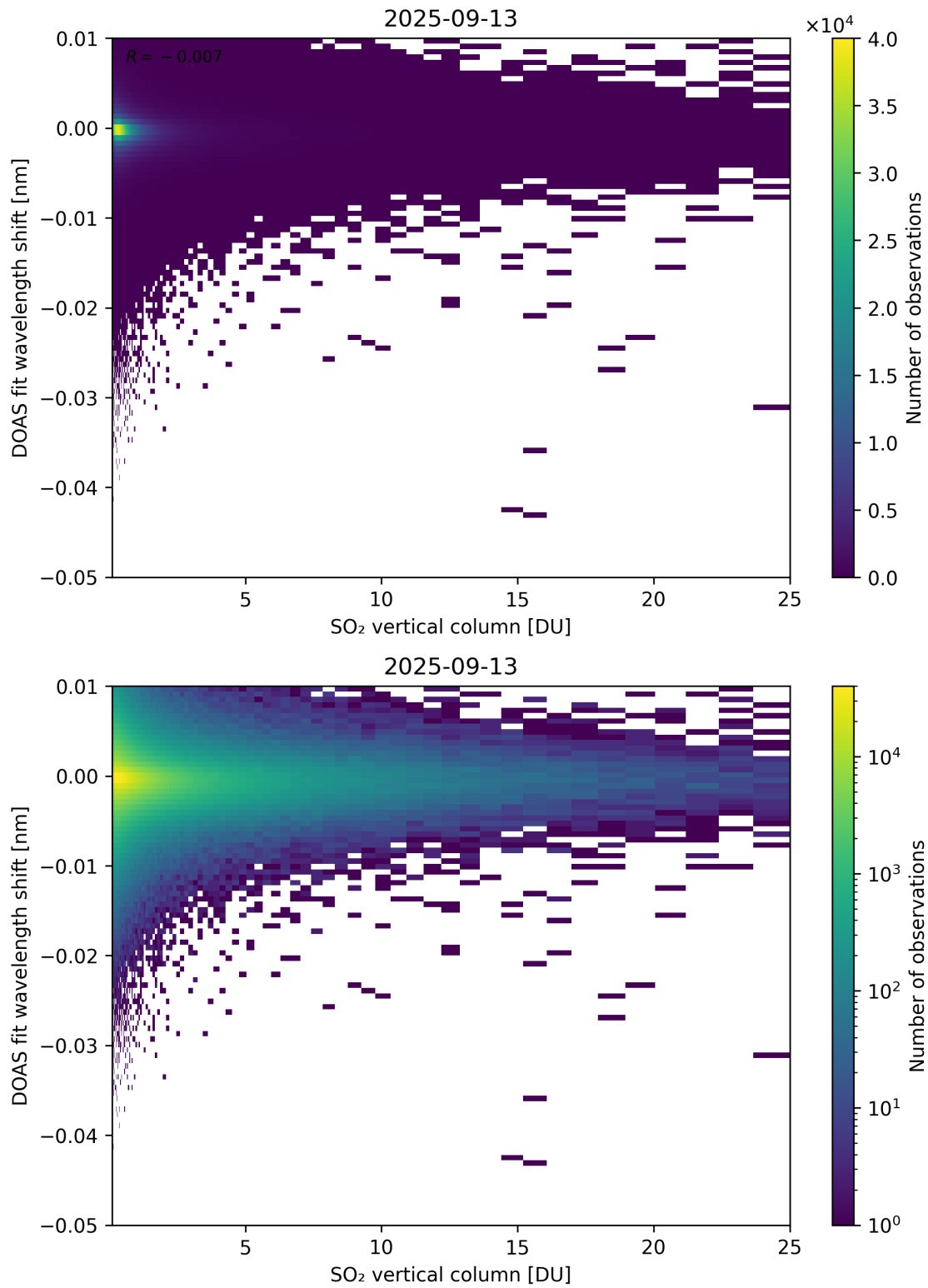
Figure 326: Scatter density plot of “SO 2 vertical column” against “DOAS fit wavelength shift” for 2025-09-12 to 2025-09-14.
