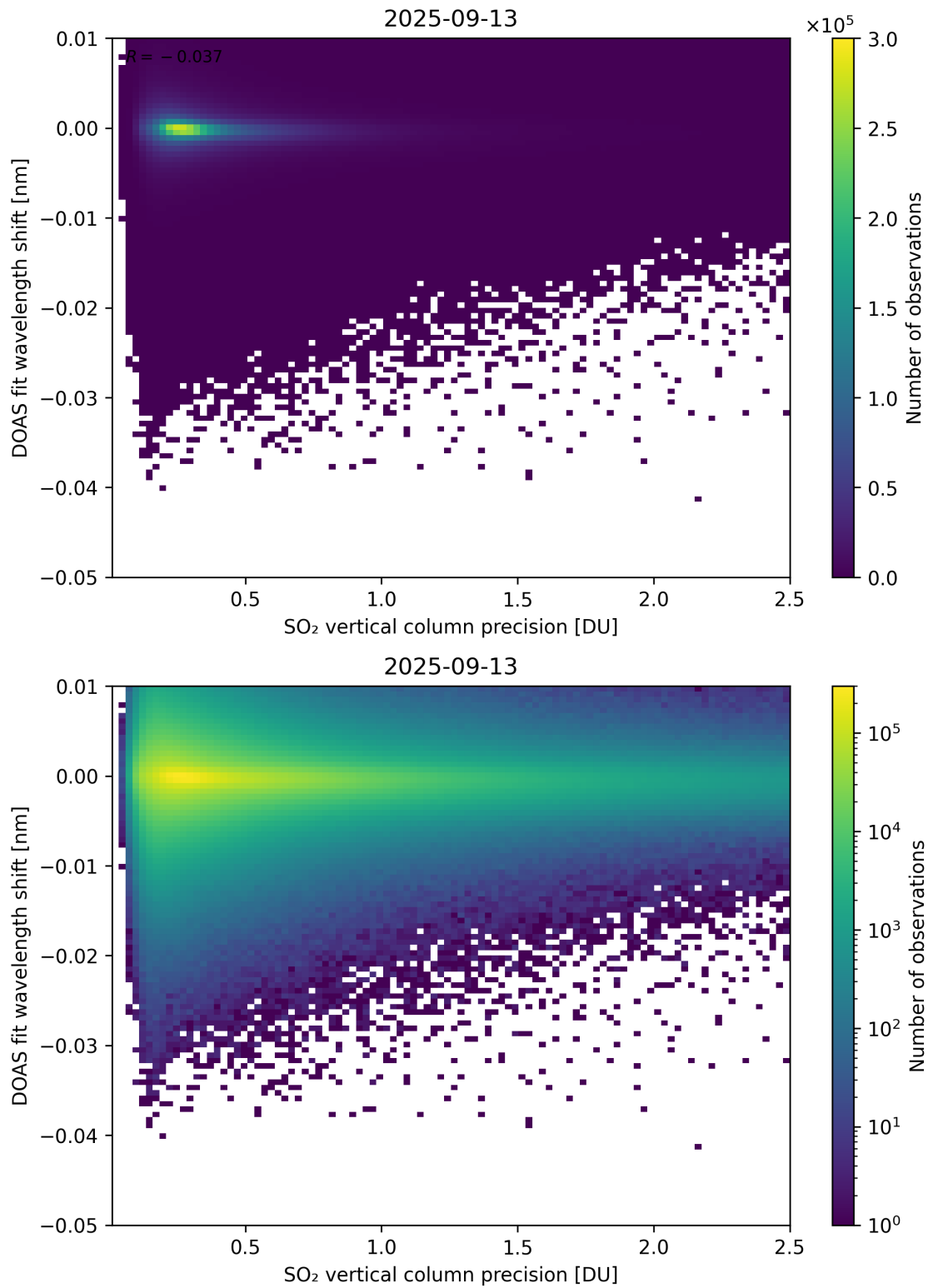
Figure 332: Scatter density plot of “SO 2 vertical column precision” against “DOAS fit wavelength shift” for 2025-09-12 to 2025-09-14.
