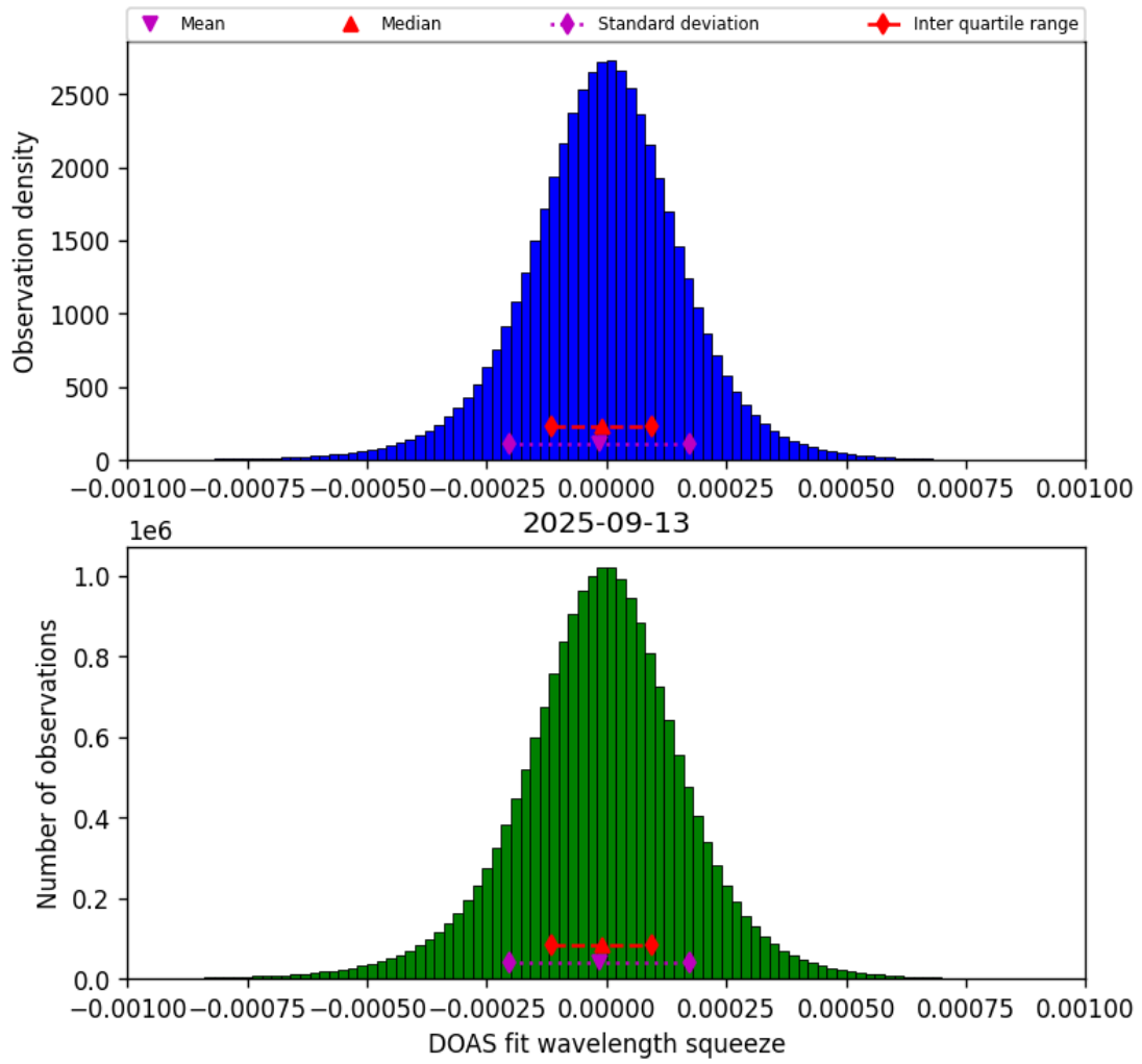
Figure 77: Histogram of “DOAS fit wavelength squeeze” for 2025-09-12 to 2025-09-14
