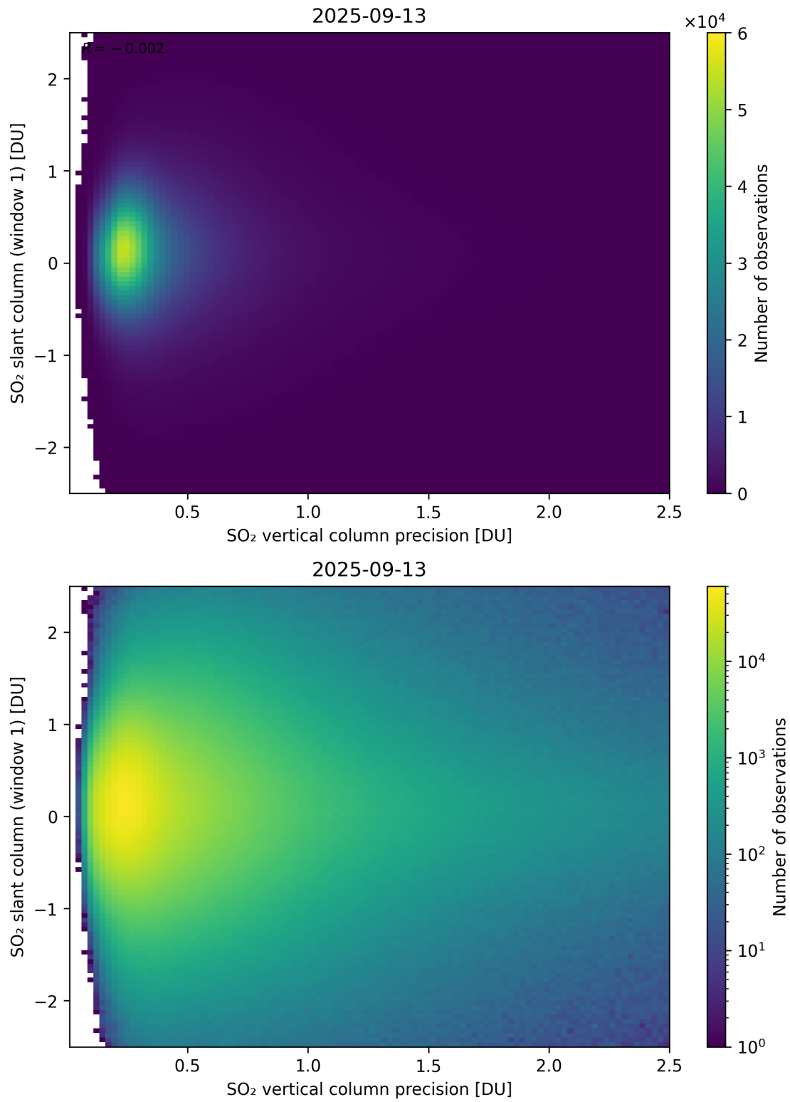
Figure 341: Scatter density plot of “SO 2 vertical column precision” against “SO 2 slant column (window 1)” for 2025-09-12 to 2025-09-14.
