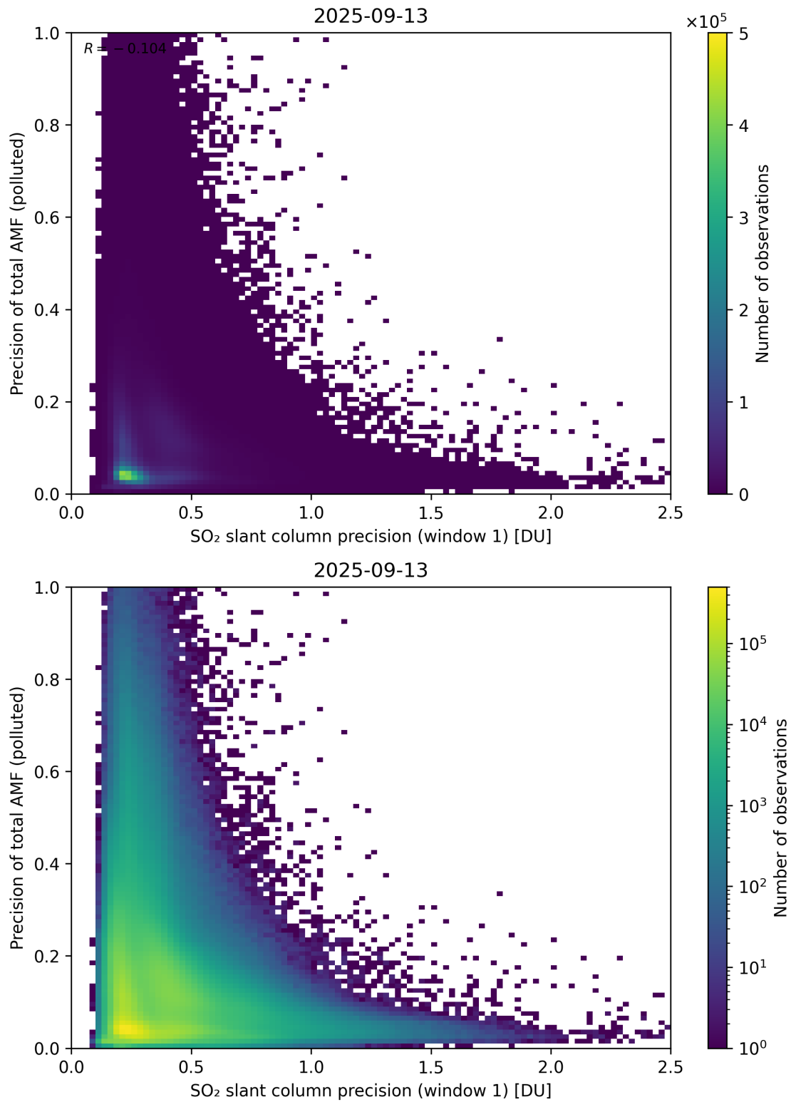
Figure 281: Scatter density plot of “SO 2 slant column precision (window 1)” against “Precision of total AMF (polluted)” for 2025-09-12 to 2025-09-14.
