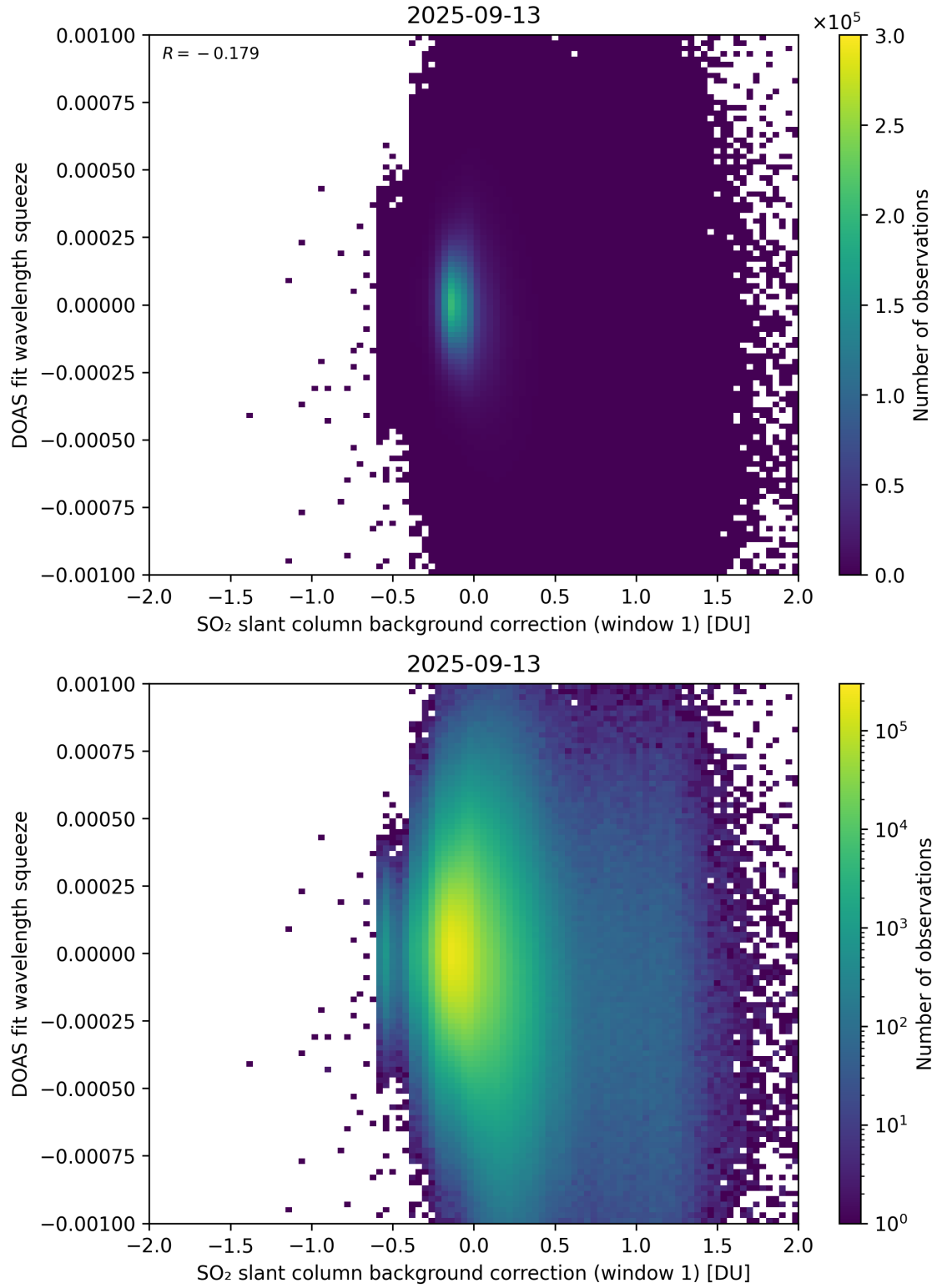
Figure 112: Scatter density plot of “SO 2 slant column background correction (window 1)” against “DOAS fit wavelength squeeze” for 2025-09-12 to 2025-09-14.
