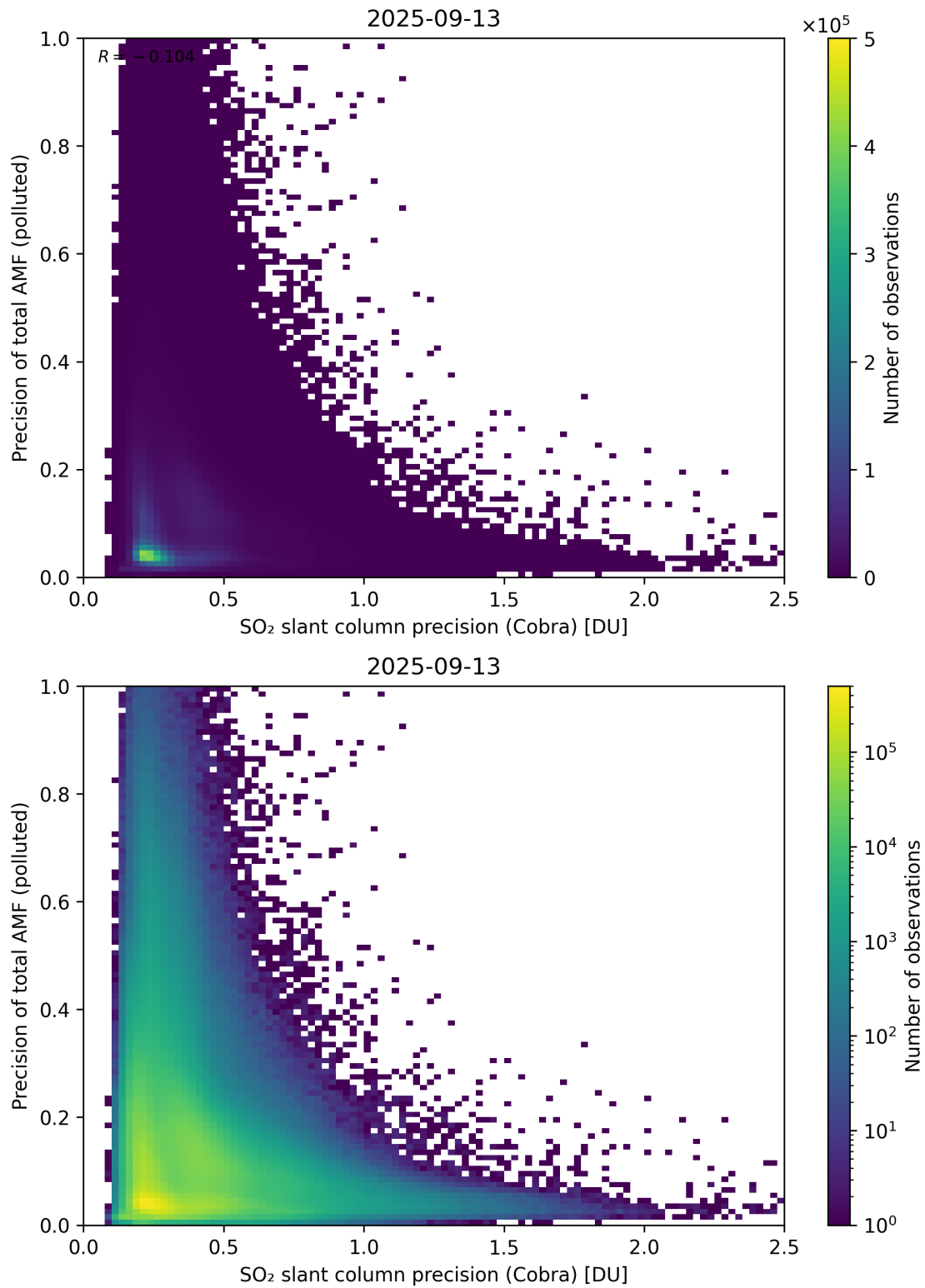
Figure 214: Scatter density plot of “SO 2 slant column precision (Cobra)” against “Precision of total AMF (polluted)” for 2025-09-12 to 2025-09-14.
