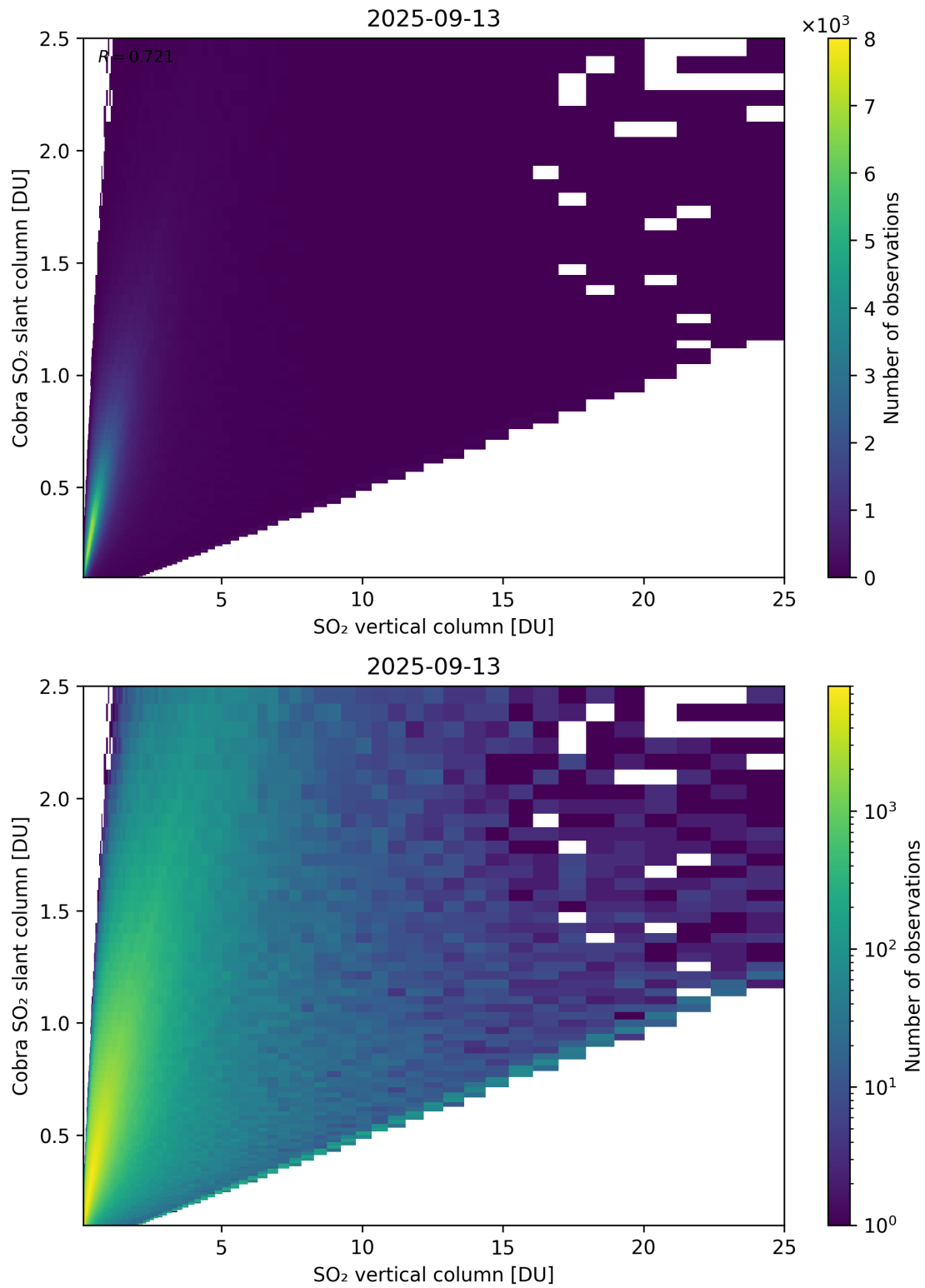
Figure 349: Scatter density plot of “SO 2 vertical column” against “Cobra SO 2 slant column” for 2025-09-12 to 2025-09-14.
