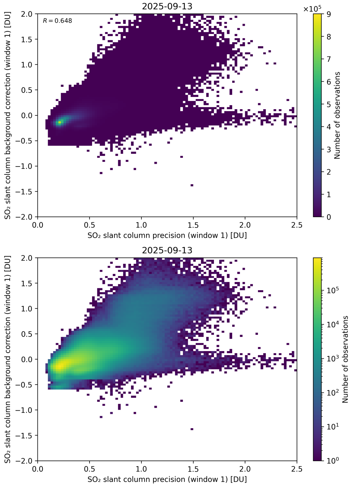
Figure 268: Scatter density plot of “SO 2 slant column precision (window 1)” against “SO 2 slant column background correction (window 1)” for 2025-09-12 to 2025-09-14.
