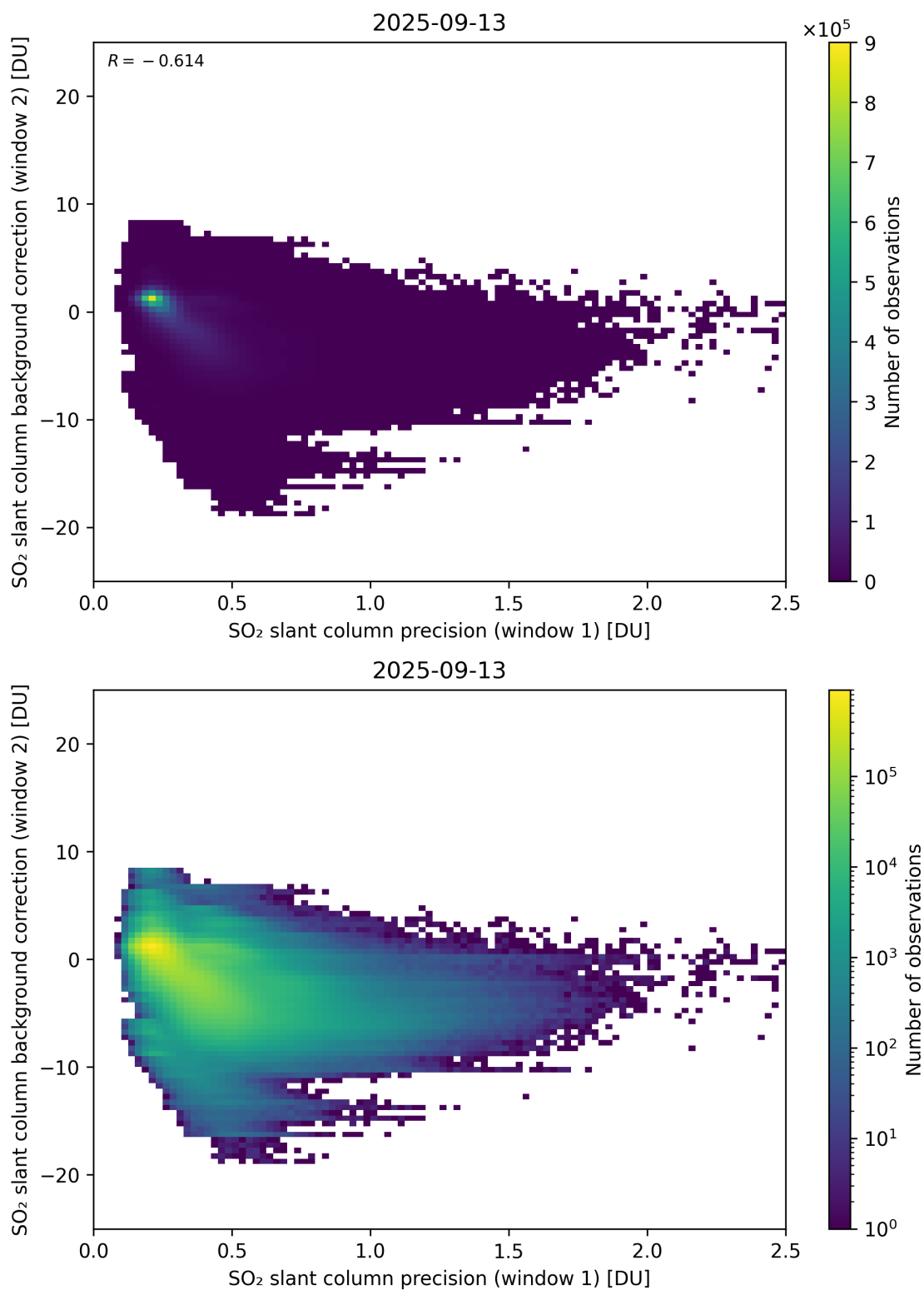
Figure 269: Scatter density plot of “SO 2 slant column precision (window 1)” against “SO 2 slant column background correction (window 2)” for 2025-09-12 to 2025-09-14.
