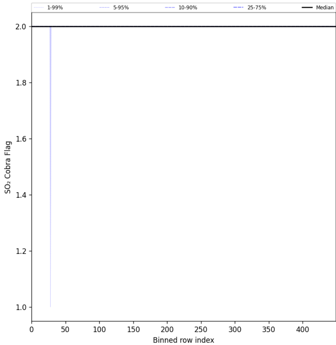
Figure 101: Along track statistics of “SO 2 Cobra Flag” for 2025-09-12 to 2025-09-14
