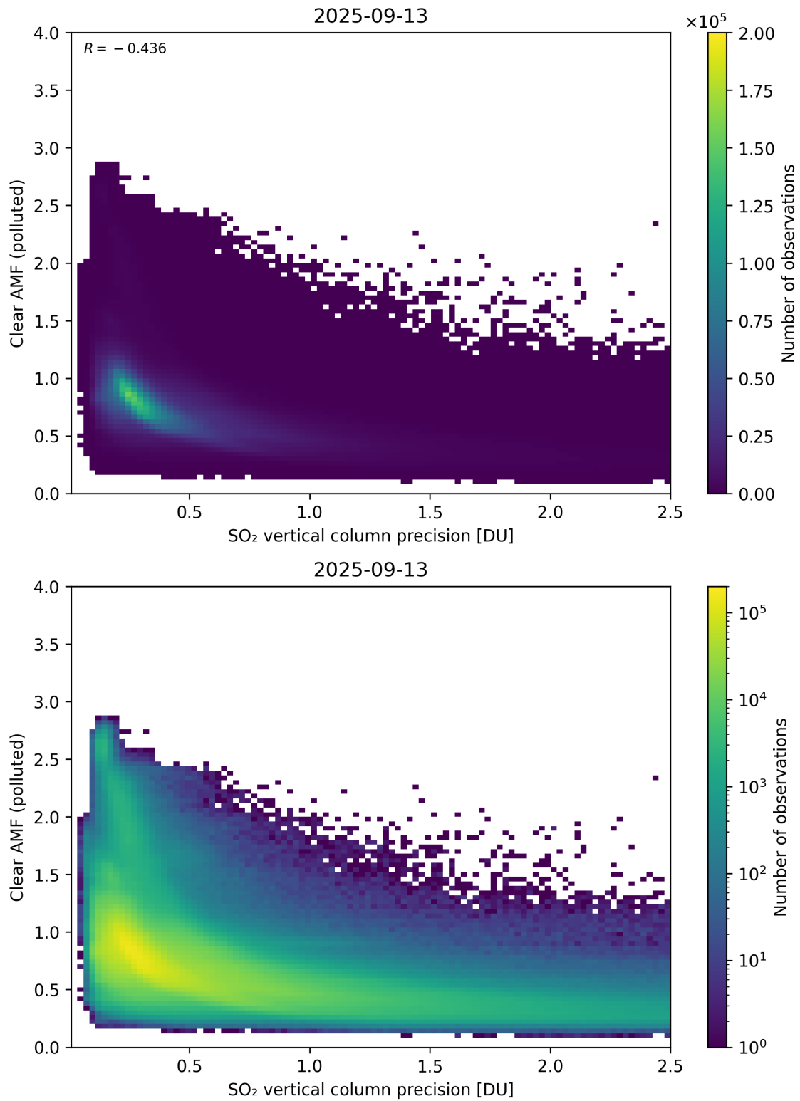
Figure 335: Scatter density plot of “SO 2 vertical column precision” against “Clear AMF (polluted)” for 2025-09-12 to 2025-09-14.
