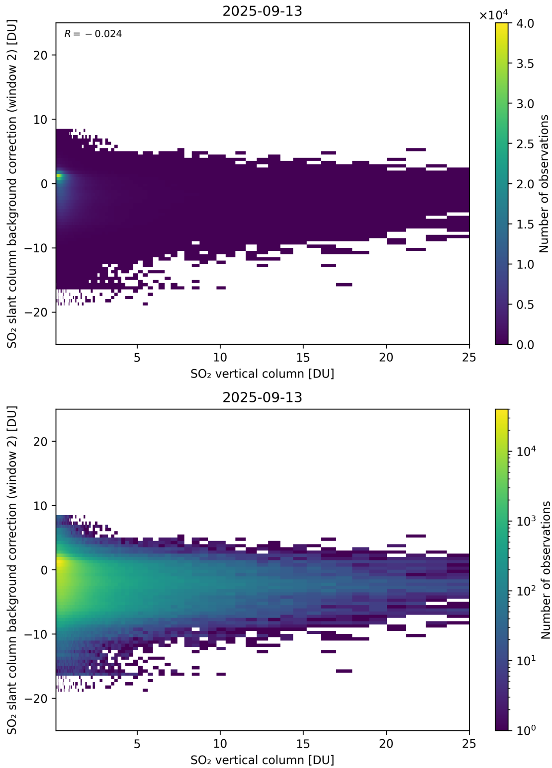
Figure 324: Scatter density plot of “SO 2 vertical column” against “SO 2 slant column background correction (window 2)” for 2025-09-12 to 2025-09-14.
