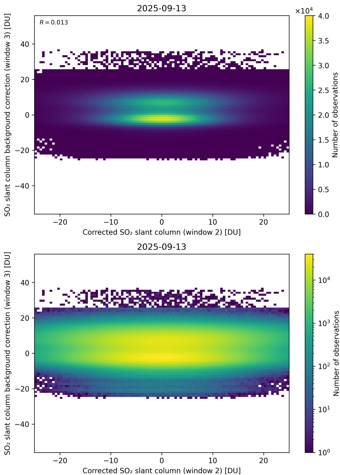
Figure 245: Scatter density plot of “Corrected SO 2 slant column (window 2)” against “SO 2 slant column background correction (window 3)” for 2025-09-12 to 2025-09-14.
