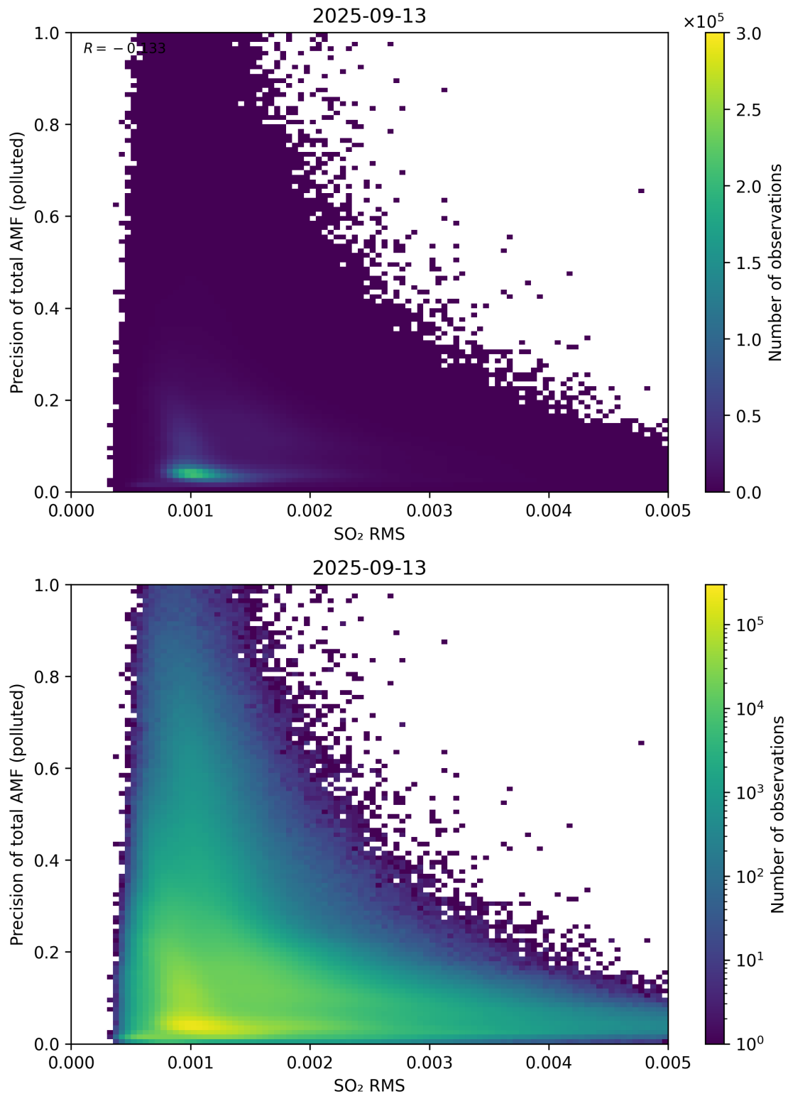
Figure 149: Scatter density plot of “SO 2 RMS” against “Precision of total AMF (polluted)” for 2025-09-12 to 2025-09-14.
