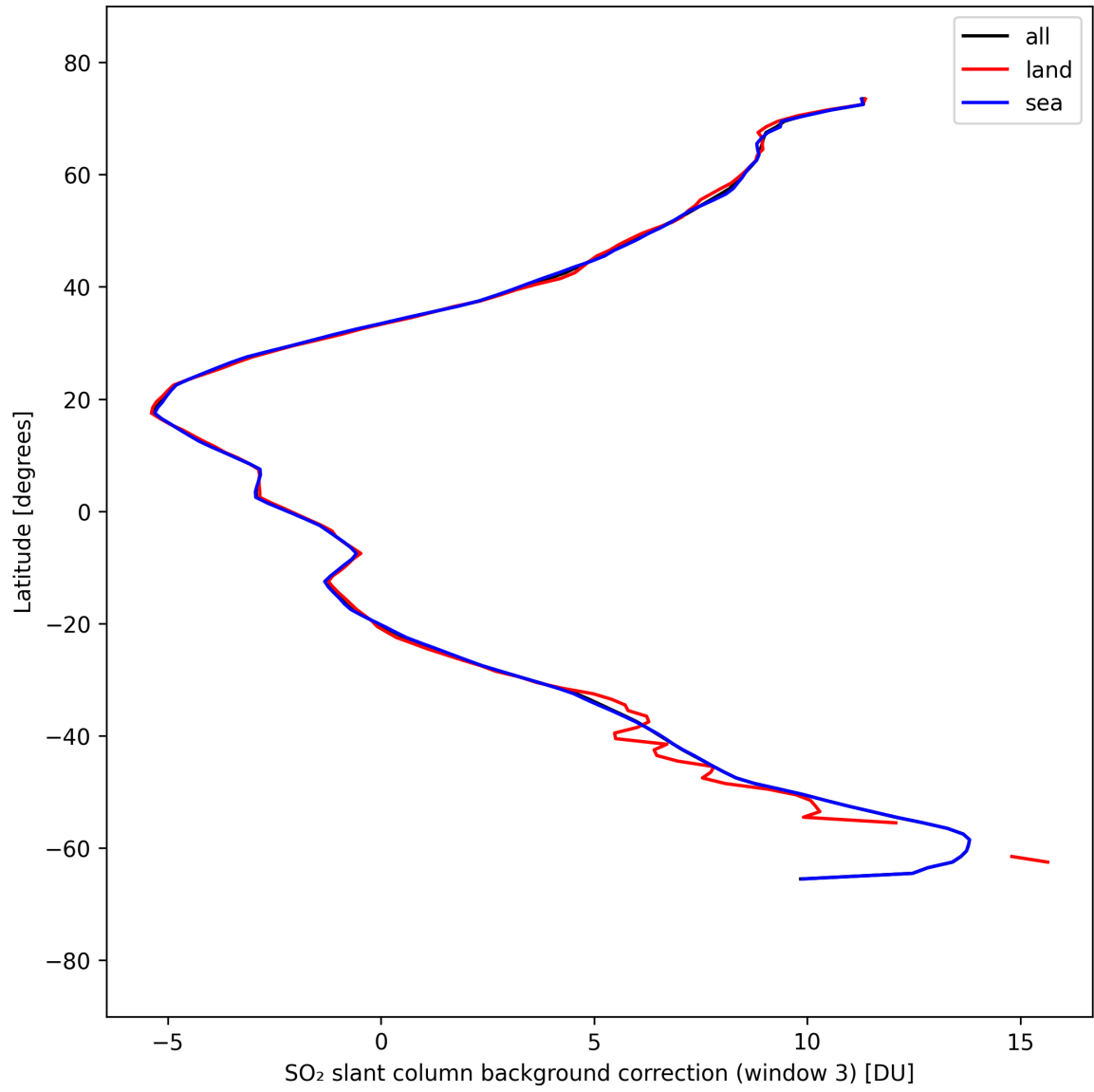
Figure 48: Zonal average of “SO 2 slant column background correction (window 3)” for 2025-09-12 to 2025-09-14.
