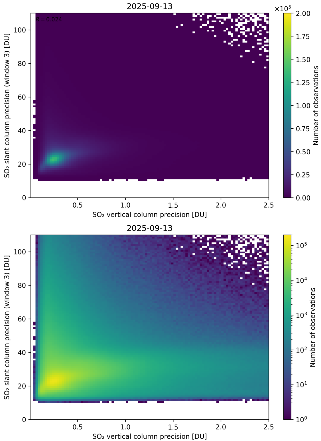
Figure 345: Scatter density plot of “SO 2 vertical column precision” against “SO 2 slant column precision (window 3)” for 2025-09-12 to 2025-09-14.
