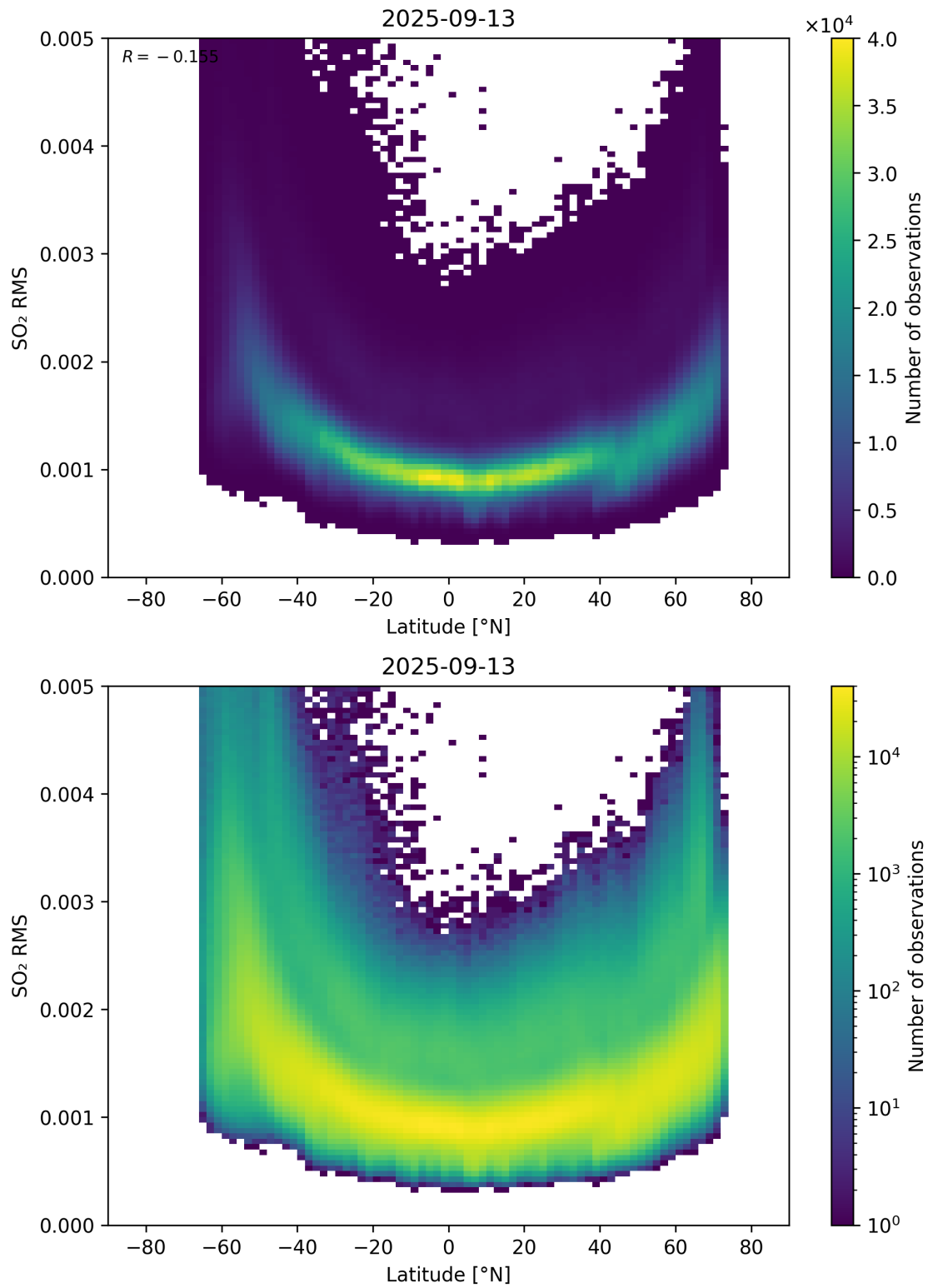
Figure 155: Scatter density plot of “Latitude” against “SO 2 RMS” for 2025-09-12 to 2025-09-14.
