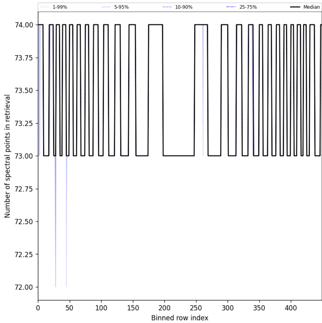
Figure 108: Along track statistics of “Number of spectral points in retrieval” for 2025-09-12 to 2025-09-14
