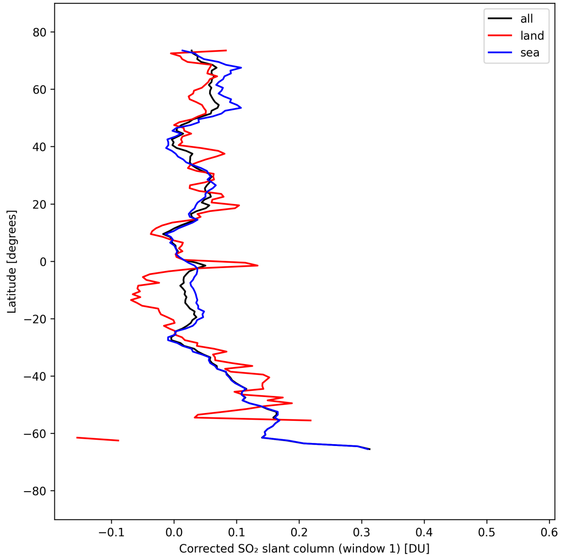
Figure 39: Zonal average of “Corrected SO 2 slant column (window 1)” for 2025-09-12 to 2025-09-14.
