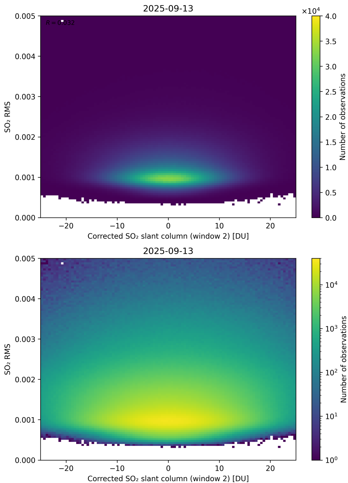
Figure 248: Scatter density plot of “Corrected SO 2 slant column (window 2)” against “SO 2 RMS” for 2025-09-12 to 2025-09-14.
