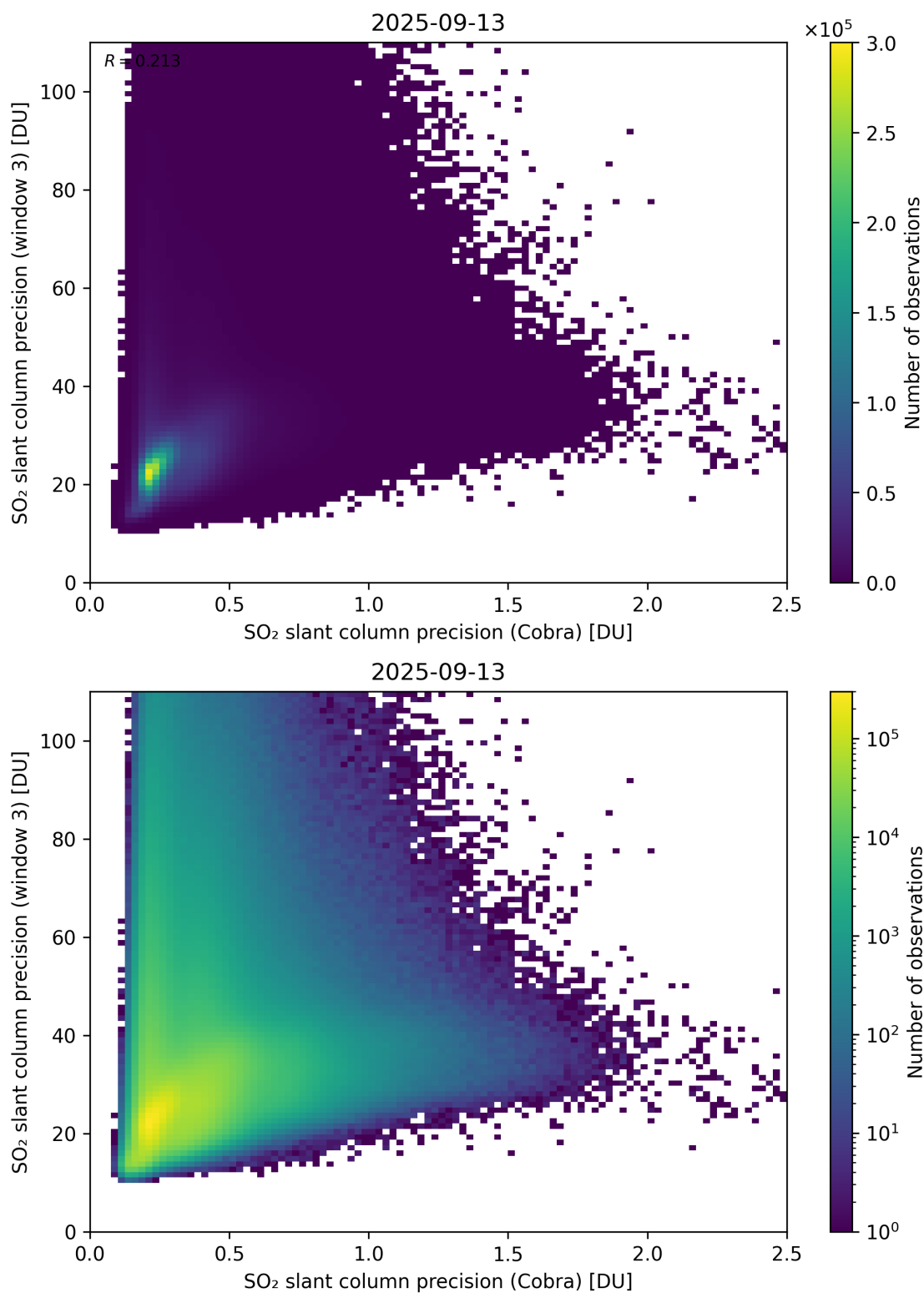
Figure 212: Scatter density plot of “SO 2 slant column precision (Cobra)” against “SO 2 slant column precision (window 3)” for 2025-09-12 to 2025-09-14.
