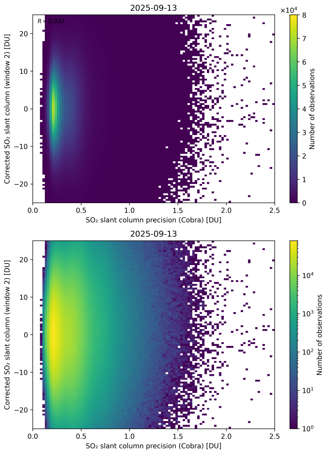
Figure 206: Scatter density plot of “SO 2 slant column precision (Cobra)” against “Corrected SO 2 slant column (window 2)” for 2025-09-12 to 2025-09-14.
