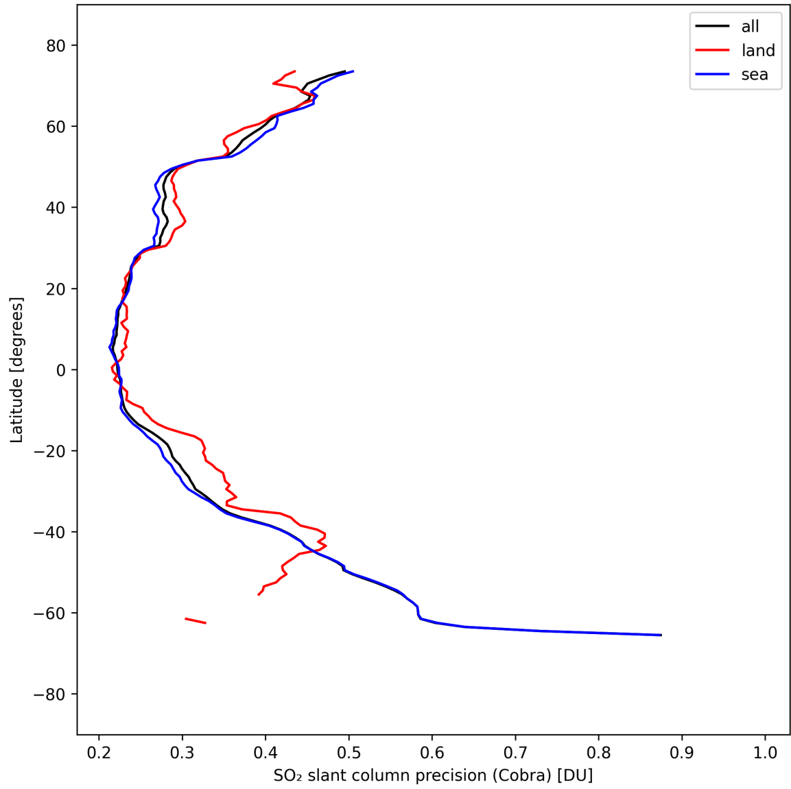
Figure 36: Zonal average of “SO 2 slant column precision (Cobra)” for 2025-09-12 to 2025-09-14.
