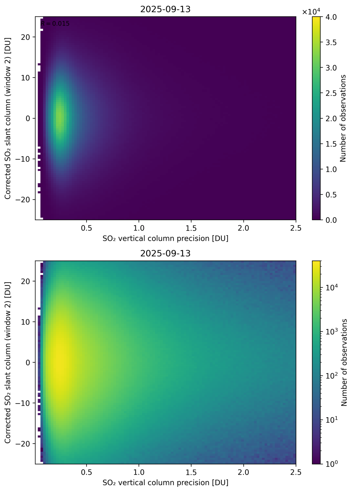
Figure 339: Scatter density plot of “SO 2 vertical column precision” against “Corrected SO 2 slant column (window 2)” for 2025-09-12 to 2025-09-14.
