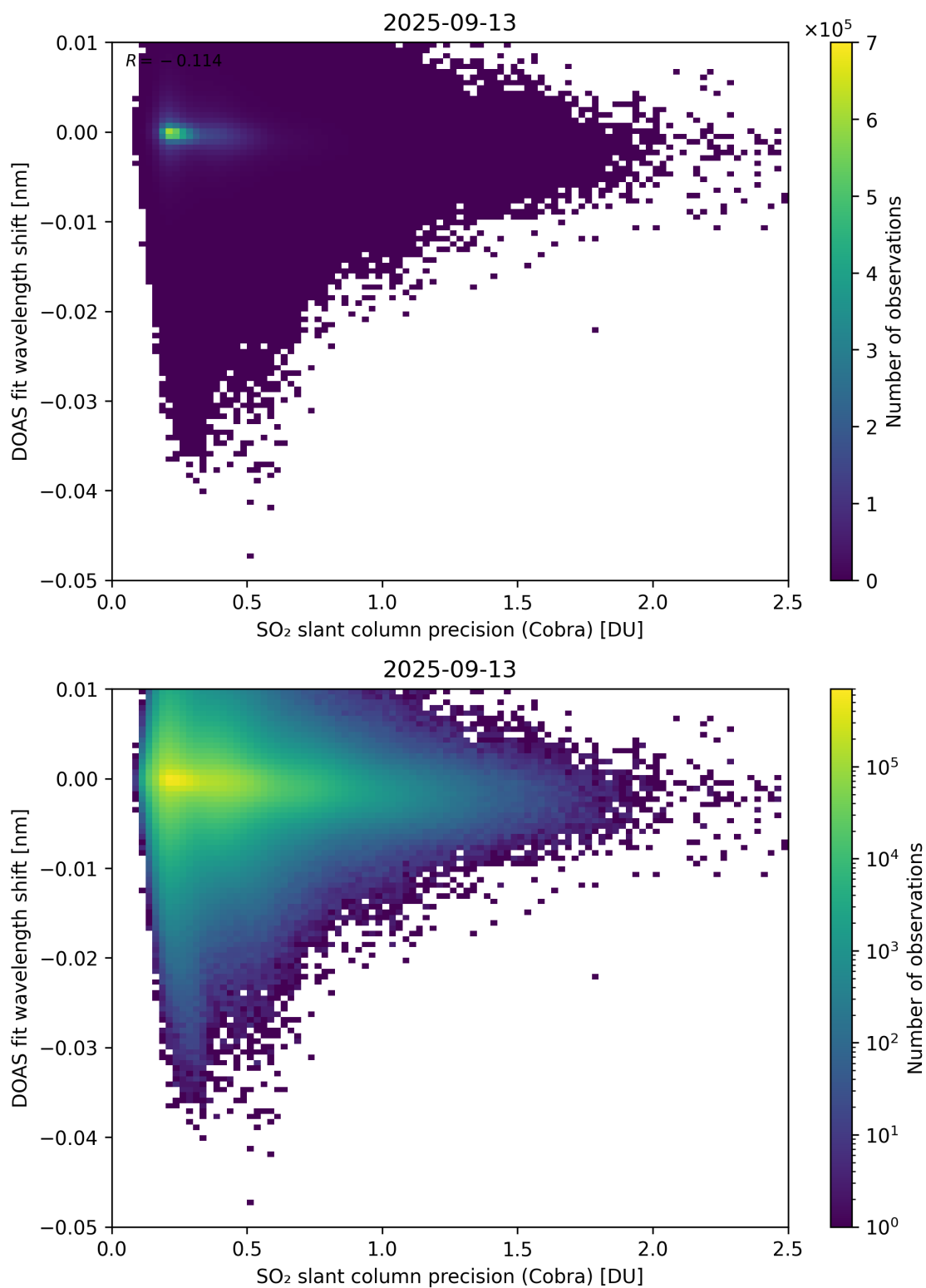
Figure 202: Scatter density plot of “SO 2 slant column precision (Cobra)” against “DOAS fit wavelength shift” for 2025-09-12 to 2025-09-14.
