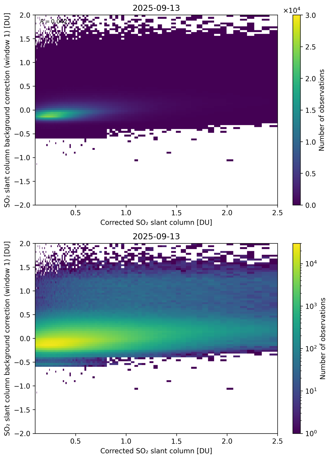
Figure 226: Scatter density plot of “Corrected SO 2 slant column” against “SO 2 slant column background correction (window 1)” for 2025-09-12 to 2025-09-14.
