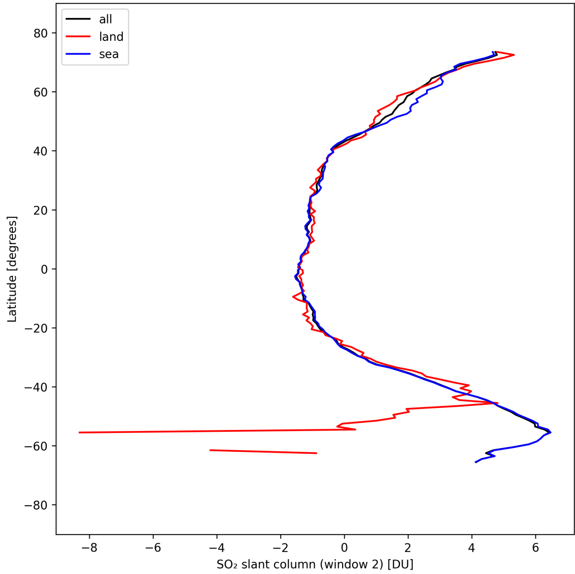
Figure 41: Zonal average of “SO 2 slant column (window 2)” for 2025-09-12 to 2025-09-14.
