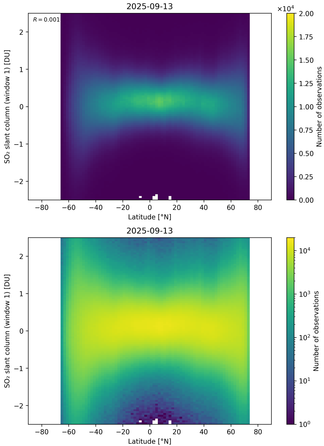
Figure 162: Scatter density plot of “Latitude” against “SO 2 slant column (window 1)” for 2025-09-12 to 2025-09-14.
