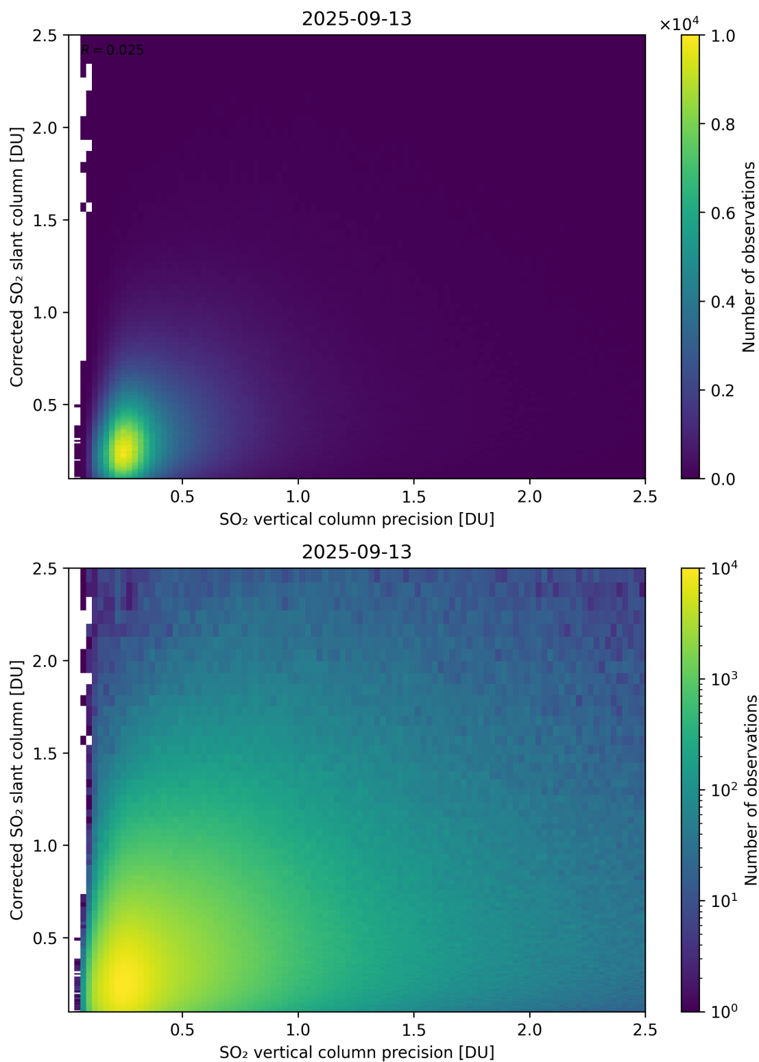
Figure 338: Scatter density plot of “SO 2 vertical column precision” against “Corrected SO 2 slant column” for 2025-09-12 to 2025-09-14.
