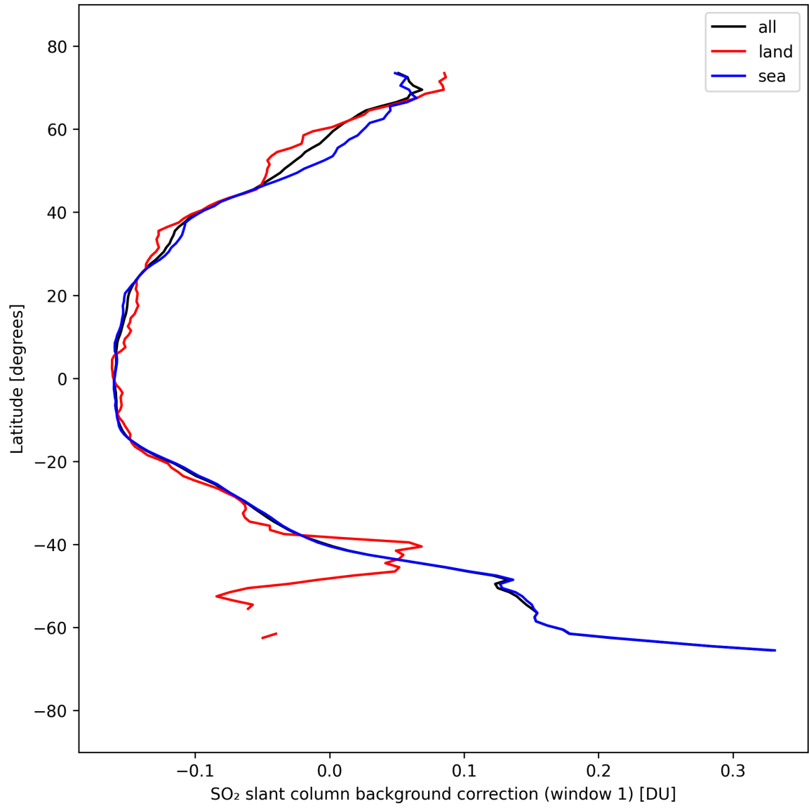
Figure 40: Zonal average of “SO 2 slant column background correction (window 1)” for 2025-09-12 to 2025-09-14.
