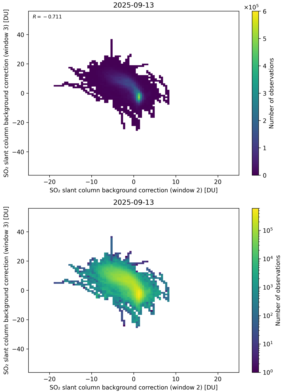
Figure 122: Scatter density plot of “SO 2 slant column background correction (window 2)” against “SO 2 slant column background correction (window 3)” for 2025-09-12 to 2025-09-14.
