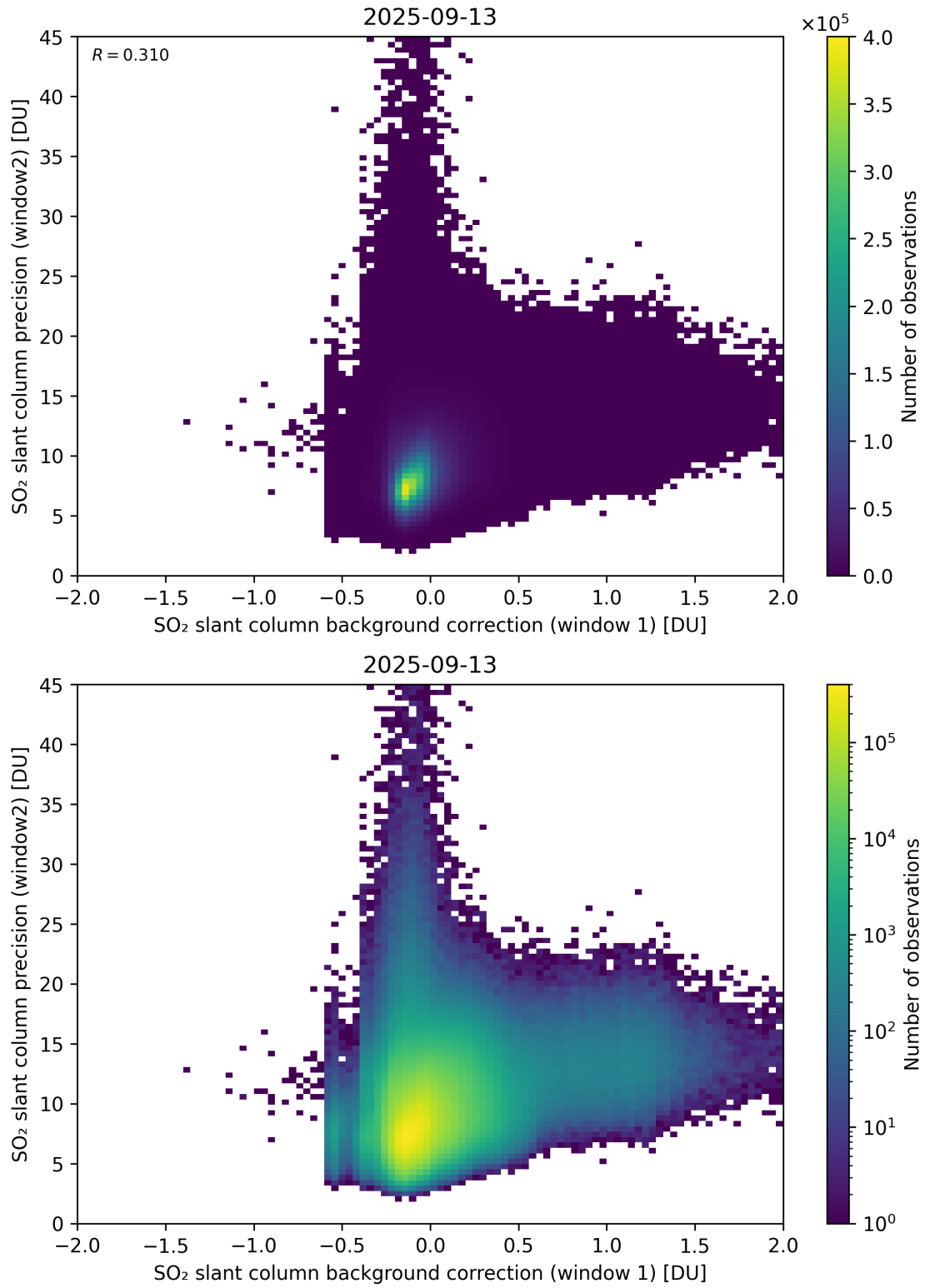
Figure 117: Scatter density plot of “SO 2 slant column background correction (window 1)” against “SO 2 slant column precision (window2)” for 2025-09-12 to 2025-09-14.
