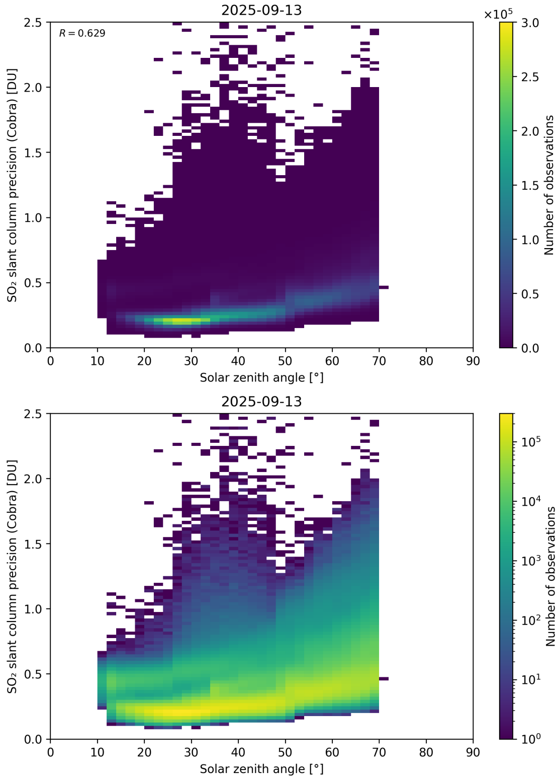
Figure 180: Scatter density plot of “Solar zenith angle” against “SO 2 slant column precision (Cobra)” for 2025-09-12 to 2025-09-14.
