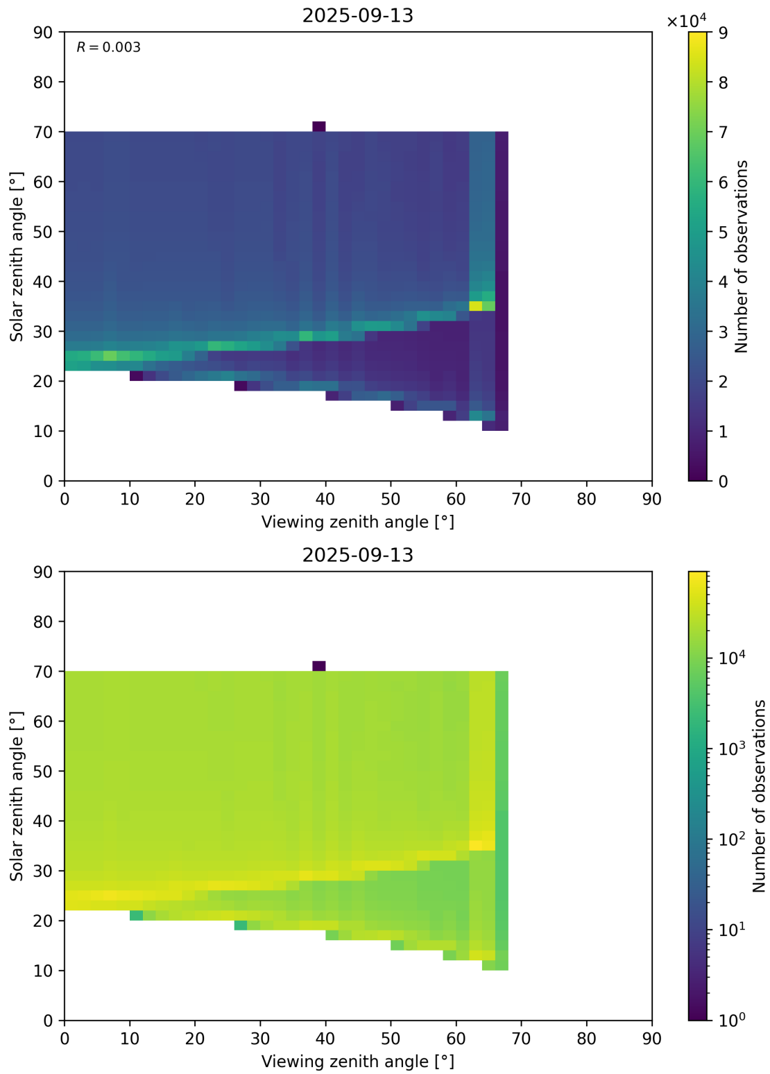
Figure 369: Scatter density plot of “Viewing zenith angle” against “Solar zenith angle” for 2025-09-12 to 2025-09-14.
