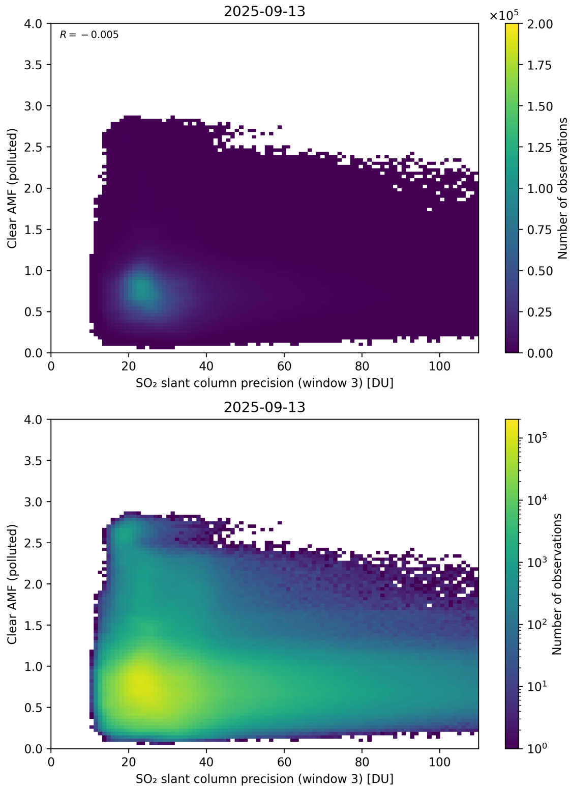
Figure 311: Scatter density plot of “SO 2 slant column precision (window 3)” against “Clear AMF (polluted)” for 2025-09-12 to 2025-09-14.
