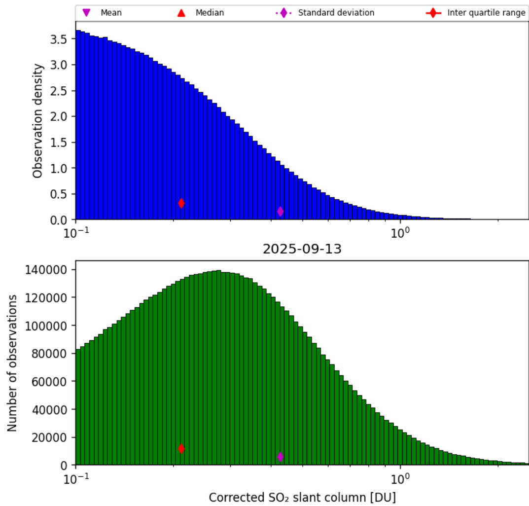
Figure 60: Histogram of "Corrected SO 2 slant column" for 2025-09-12 to 2025-09-14
