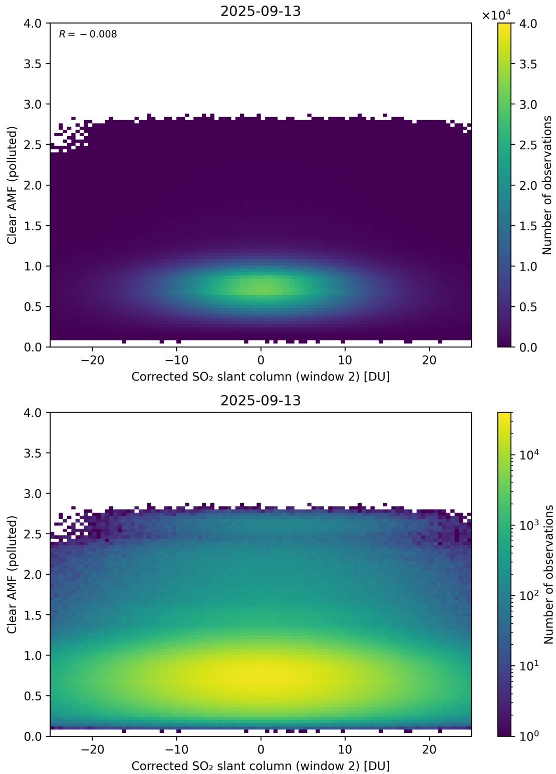
Figure 249: Scatter density plot of “Corrected SO 2 slant column (window 2)” against “Clear AMF (polluted)” for 2025-09-12 to 2025-09-14.
