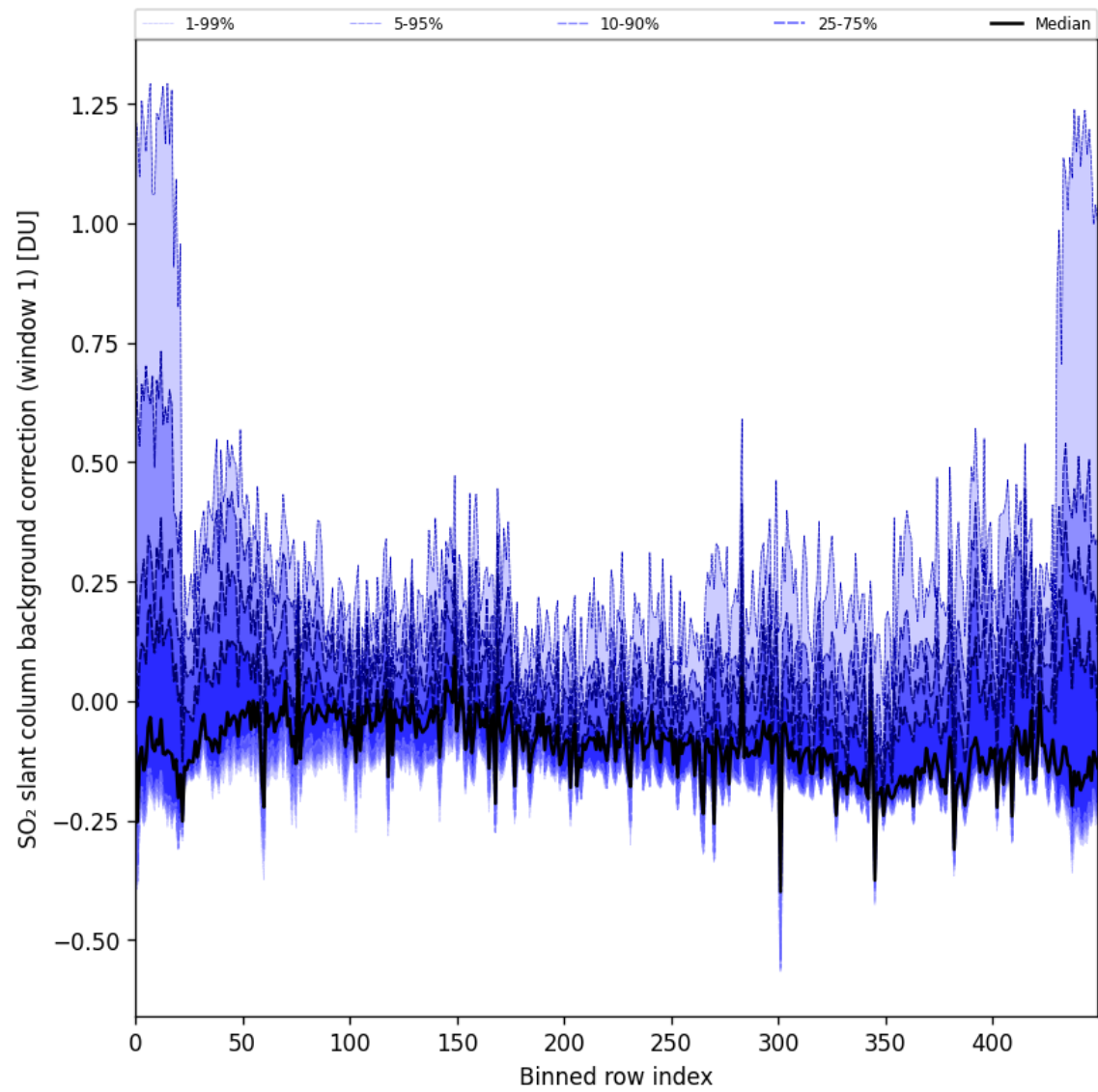
Figure 92: Along track statistics of “SO 2 slant column background correction (window 1)” for 2025-09-12 to 2025-09-14
