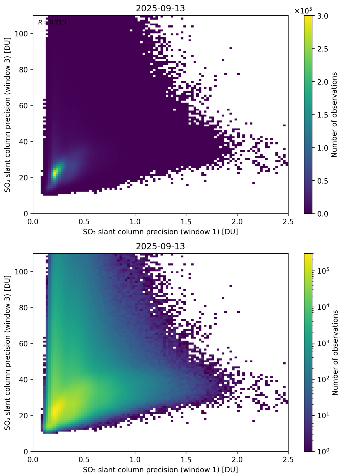
Figure 279: Scatter density plot of “SO 2 slant column precision (window 1)” against “SO 2 slant column precision (window 3)” for 2025-09-12 to 2025-09-14.
