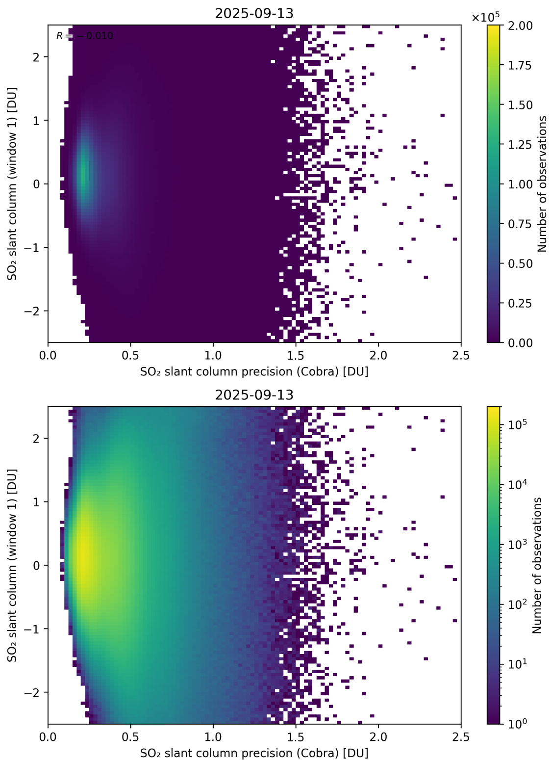
Figure 208: Scatter density plot of “SO 2 slant column precision (Cobra)” against “SO 2 slant column (window 1)” for 2025-09-12 to 2025-09-14.
