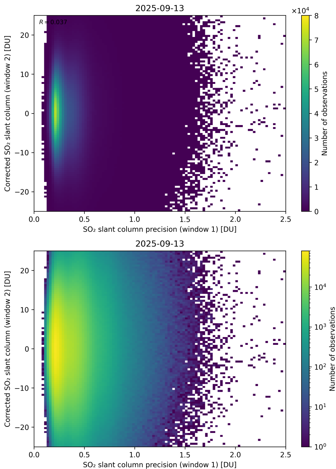
Figure 275: Scatter density plot of “SO 2 slant column precision (window 1)” against “Corrected SO 2 slant column (window 2)” for 2025-09-12 to 2025-09-14.
