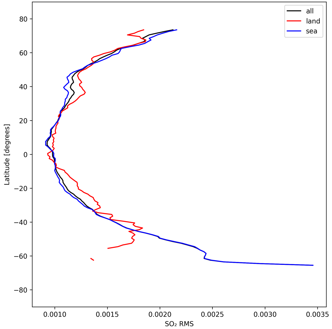
Figure 52: Zonal average of “ \text{SO}_2 RMS” for 2025-09-12 to 2025-09-14.
