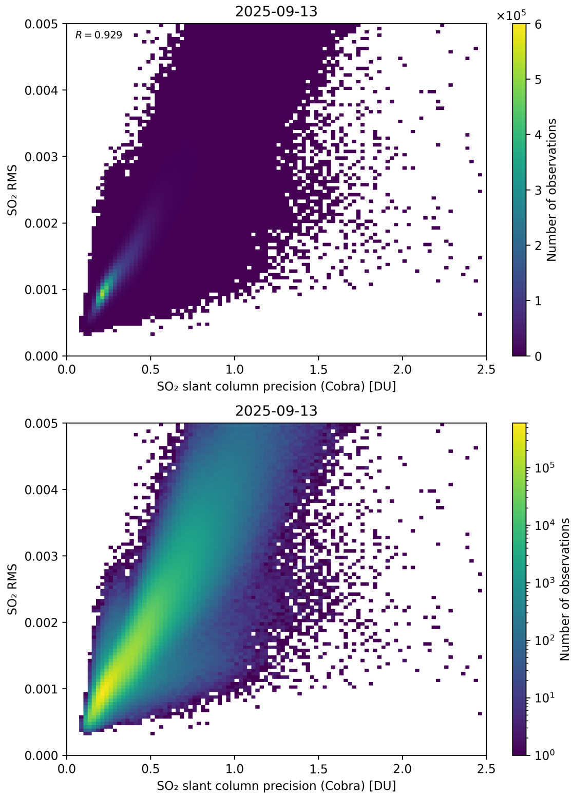
Figure 204: Scatter density plot of “SO 2 slant column precision (Cobra)” against “SO 2 RMS” for 2025-09-12 to 2025-09-14.
