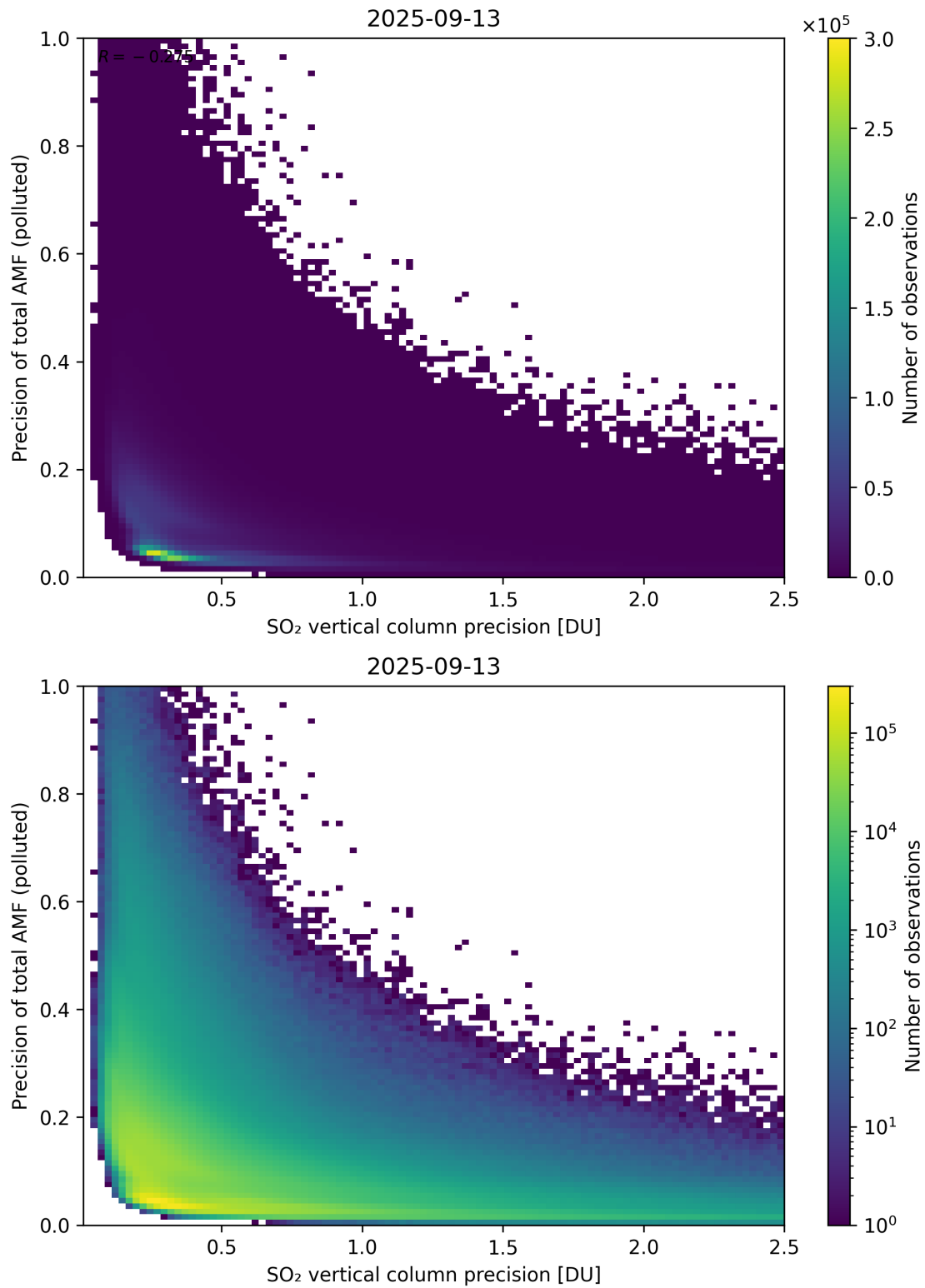
Figure 347: Scatter density plot of “SO 2 vertical column precision” against “Precision of total AMF (polluted)” for 2025-09-12 to 2025-09-14.
