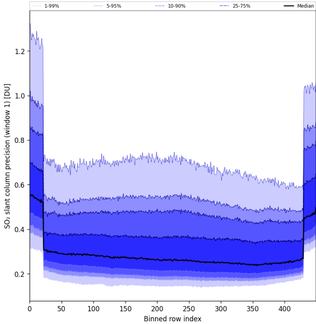
Figure 90: Along track statistics of “SO 2 slant column precision (window 1)” for 2025-09-12 to 2025-09-14
