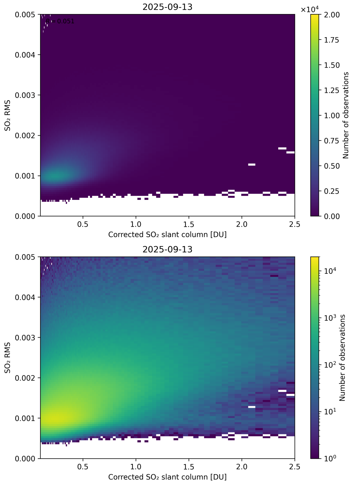
Figure 231: Scatter density plot of “Corrected SO 2 slant column” against “SO 2 RMS” for 2025-09-12 to 2025-09-14.
