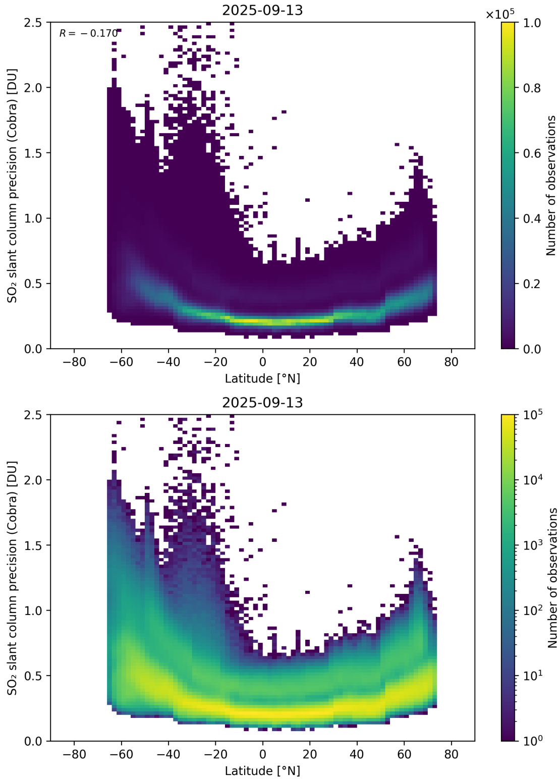
Figure 158: Scatter density plot of “Latitude” against “SO 2 slant column precision (Cobra)” for 2025-09-12 to 2025-09-14.
