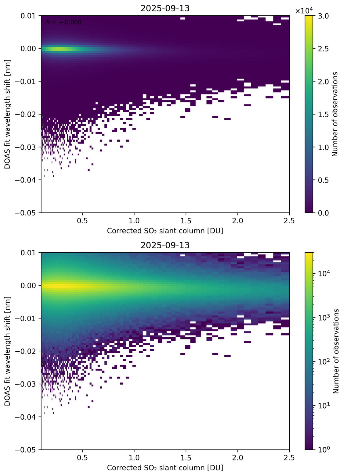
Figure 229: Scatter density plot of “Corrected SO 2 slant column” against “DOAS fit wavelength shift” for 2025-09-12 to 2025-09-14.
