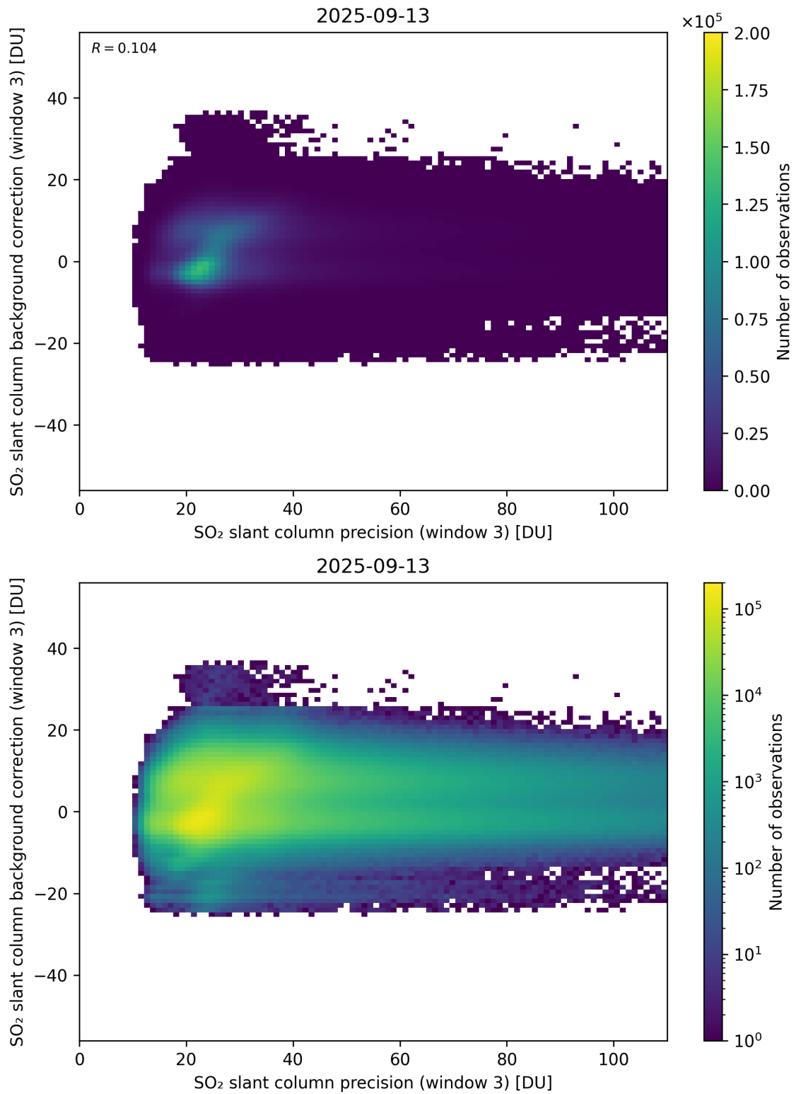
Figure 307: Scatter density plot of “SO 2 slant column precision (window 3)” against “SO 2 slant column background correction (window 3)” for 2025-09-12 to 2025-09-14.
