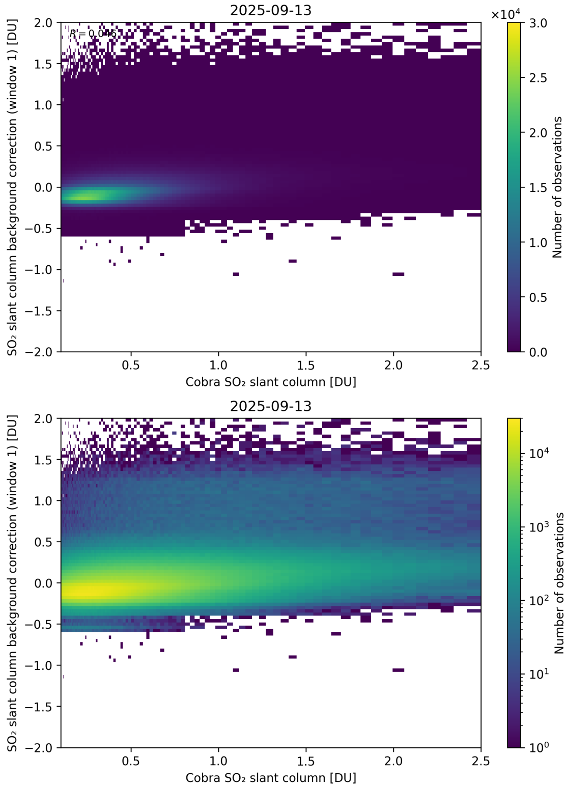
Figure 193: Scatter density plot of “Cobra SO 2 slant column” against “SO 2 slant column background correction (window 1)” for 2025-09-12 to 2025-09-14.
