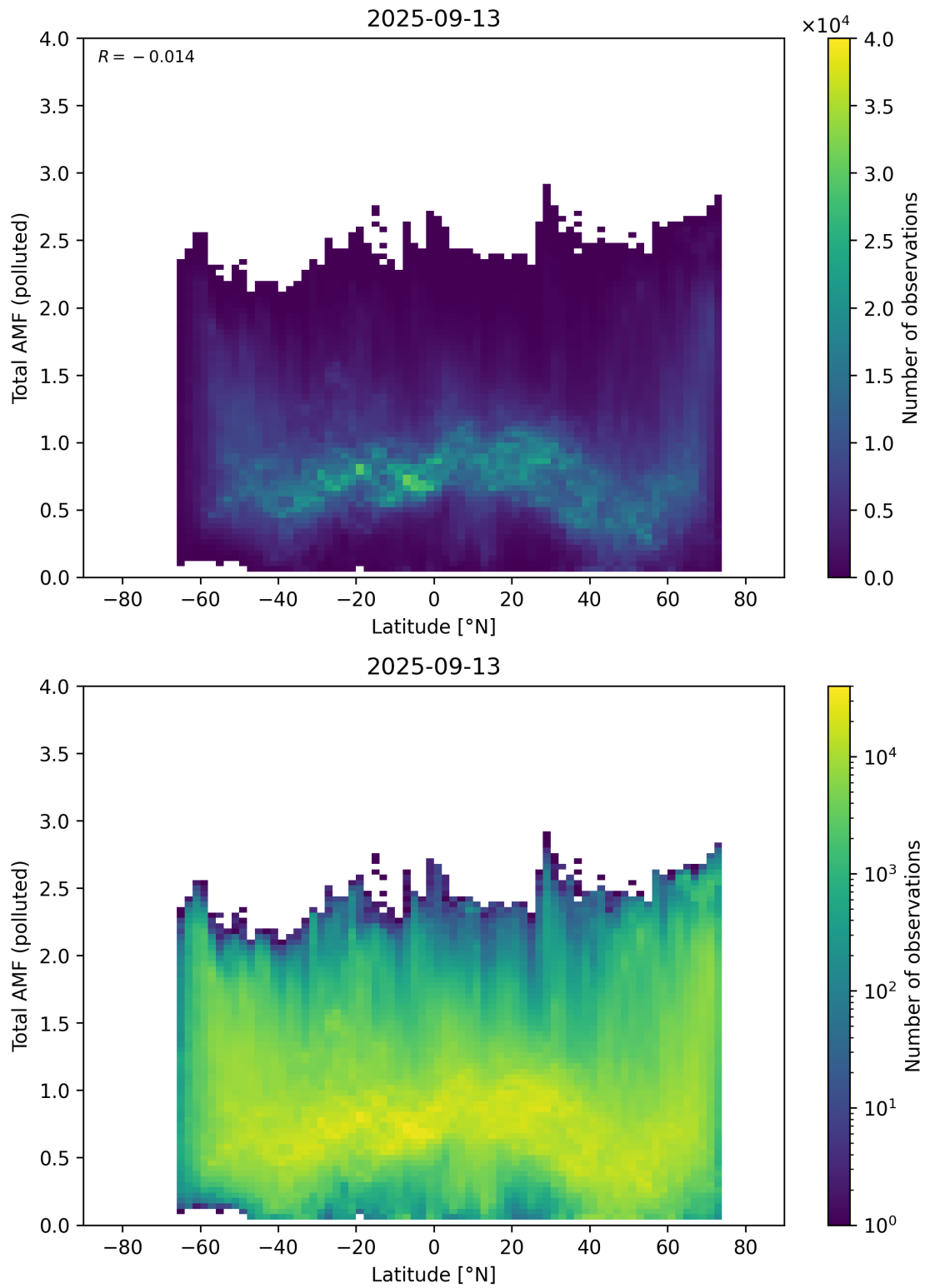
Figure 167: Scatter density plot of “Latitude” against “Total AMF (polluted)” for 2025-09-12 to 2025-09-14.
