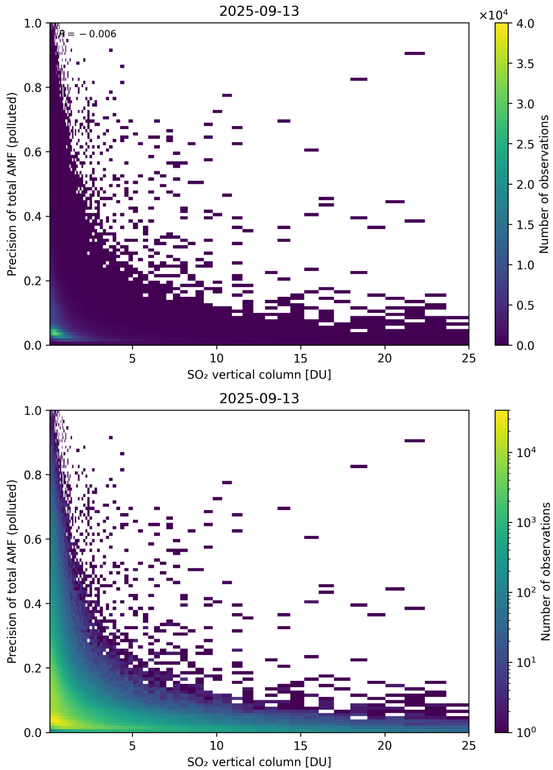
Figure 360: Scatter density plot of “SO 2 vertical column” against “Precision of total AMF (polluted)” for 2025-09-12 to 2025-09-14.
