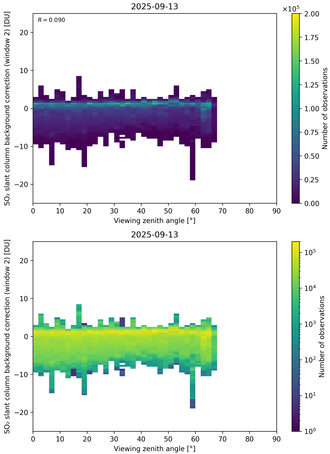
Figure 363: Scatter density plot of “Viewing zenith angle” against “SO 2 slant column background correction (window 2)” for 2025-09-12 to 2025-09-14.
