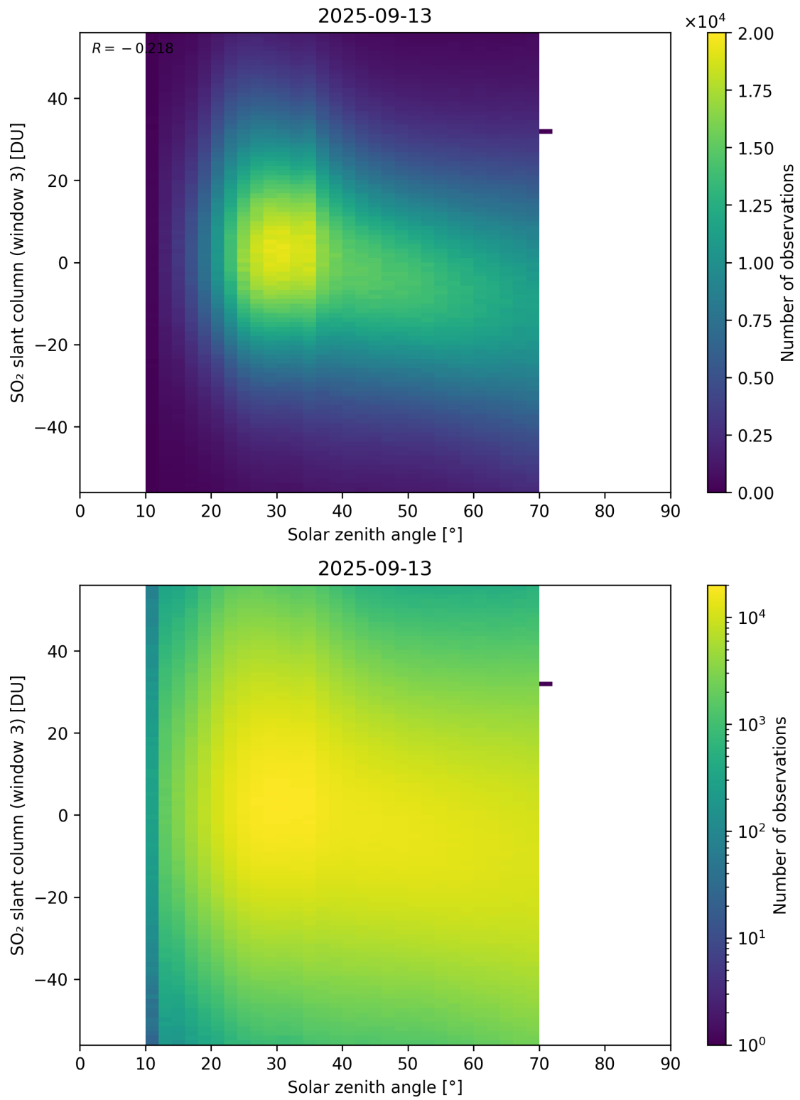
Figure 187: Scatter density plot of “Solar zenith angle” against “SO 2 slant column (window 3)” for 2025-09-12 to 2025-09-14.
