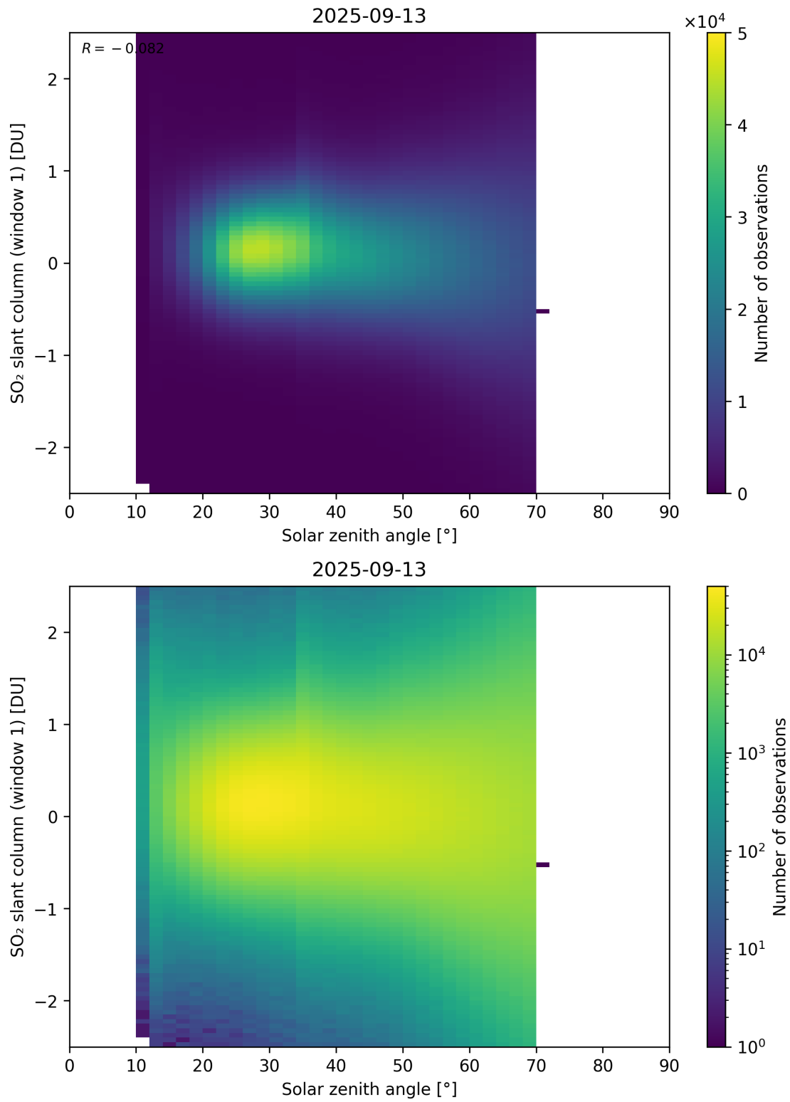
Figure 184: Scatter density plot of “Solar zenith angle” against “SO 2 slant column (window 1)” for 2025-09-12 to 2025-09-14.
