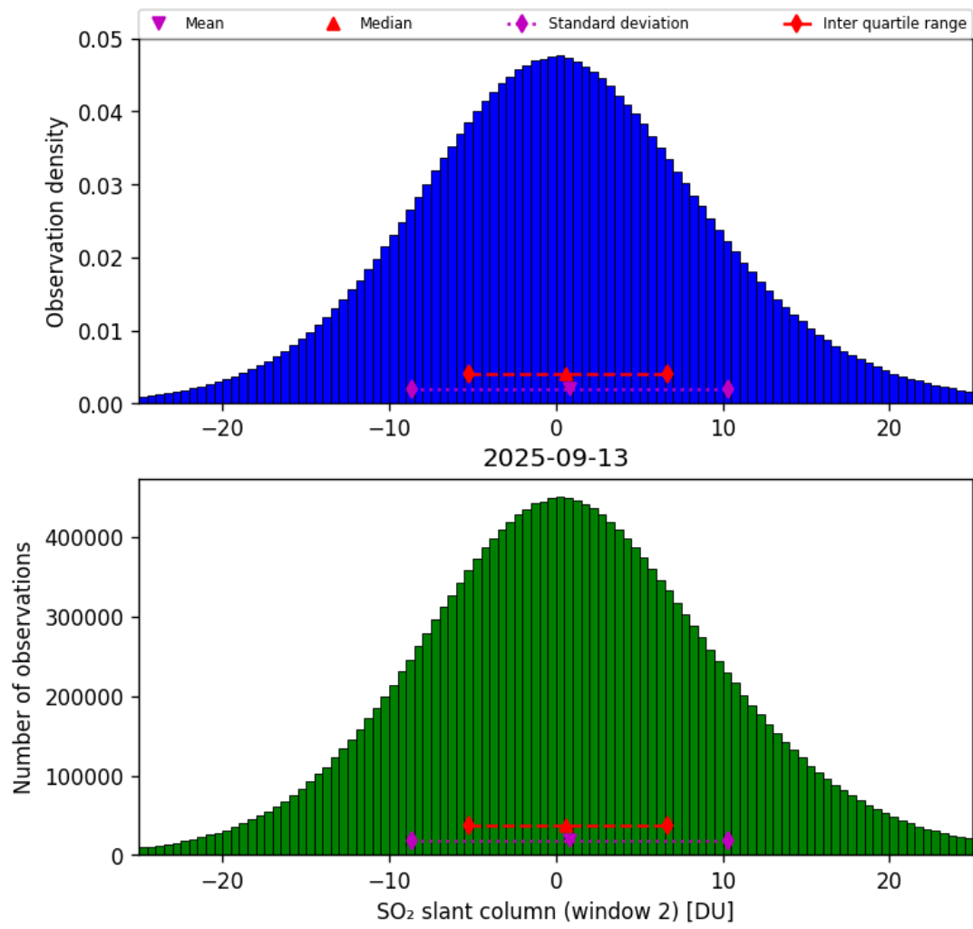
Figure 67: Histogram of “SO 2 slant column (window 2)” for 2025-09-12 to 2025-09-14
