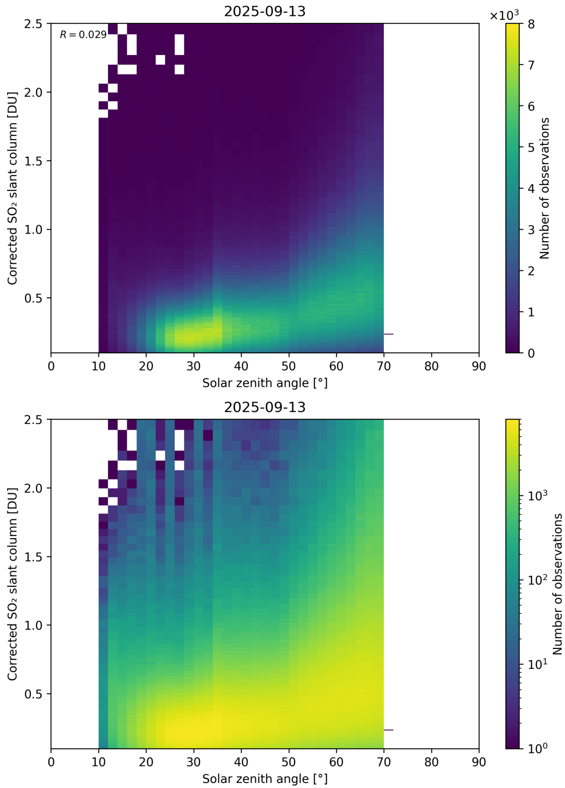
Figure 181: Scatter density plot of “Solar zenith angle” against “Corrected SO 2 slant column” for 2025-09-12 to 2025-09-14.
