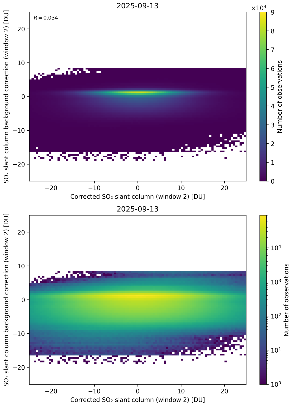
Figure 244: Scatter density plot of “Corrected SO 2 slant column (window 2)” against “SO 2 slant column background correction (window 2)” for 2025-09-12 to 2025-09-14.
