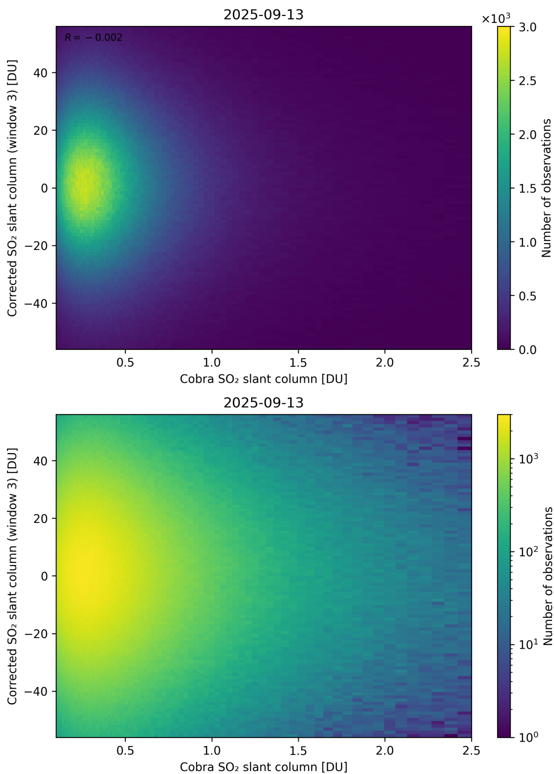
Figure 218: Scatter density plot of “Cobra SO 2 slant column” against “Corrected SO 2 slant column (window 3)” for 2025-09-12 to 2025-09-14.
