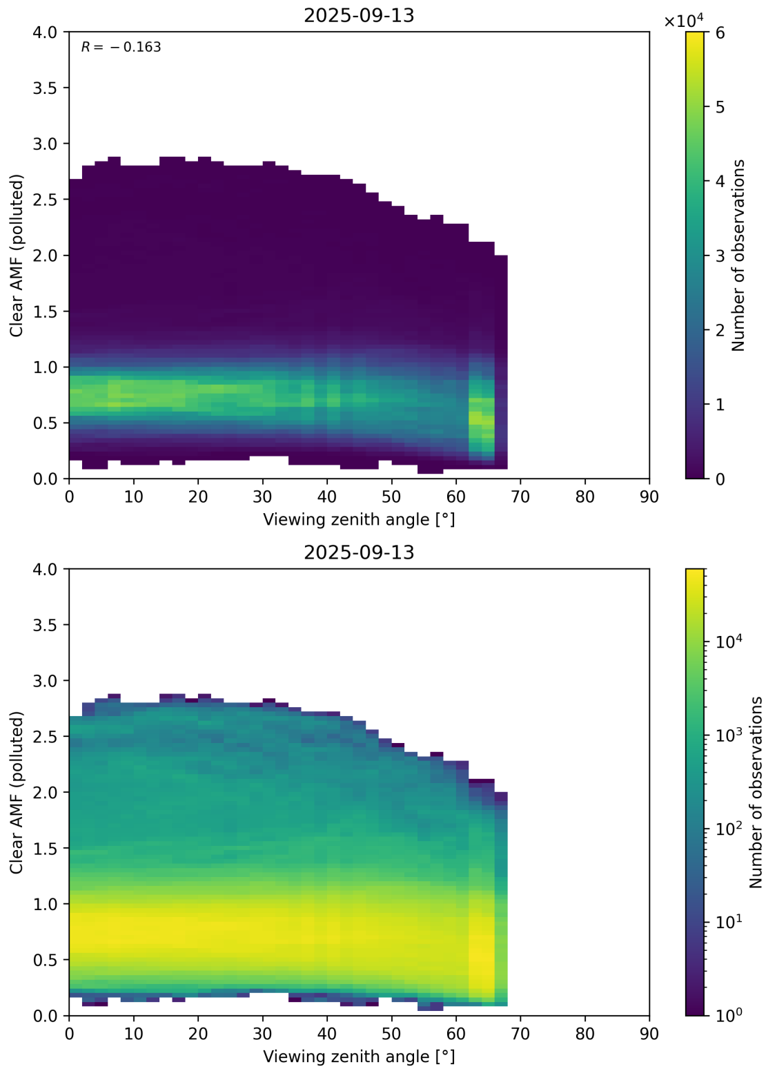
Figure 370: Scatter density plot of “Viewing zenith angle” against “Clear AMF (polluted)” for 2025-09-12 to 2025-09-14.
