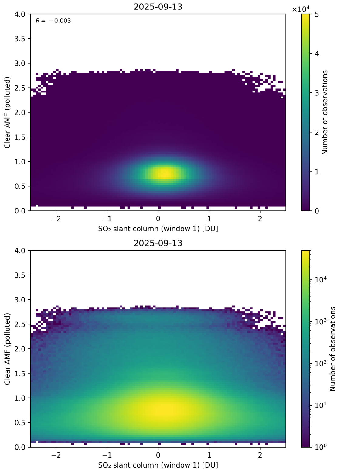
Figure 282: Scatter density plot of “SO 2 slant column (window 1)” against “Clear AMF (polluted)” for 2025-09-12 to 2025-09-14.
