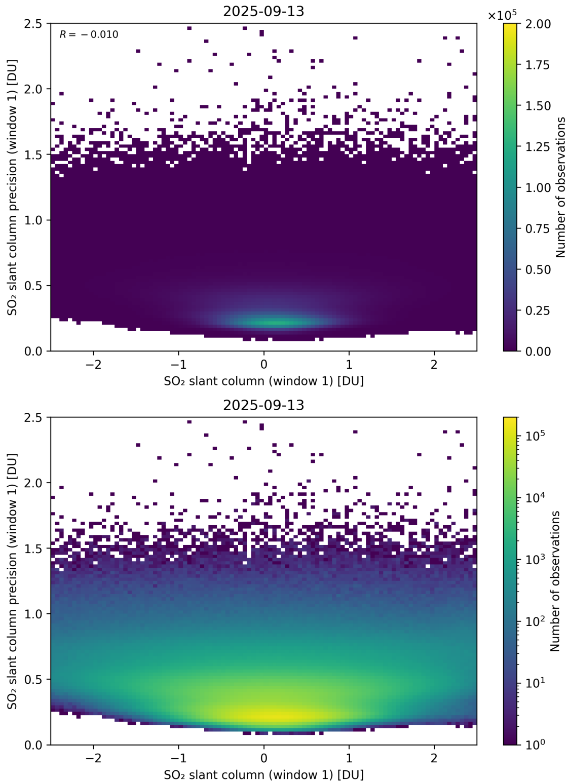
Figure 285: Scatter density plot of “SO 2 slant column (window 1)” against “SO 2 slant column precision (window 1)” for 2025-09-12 to 2025-09-14.
