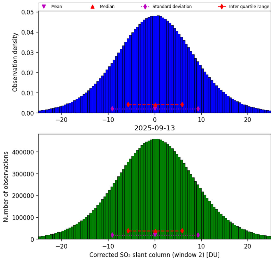
Figure 69: Histogram of “Corrected SO 2 slant column (window 2)” for 2025-09-12 to 2025-09-14
