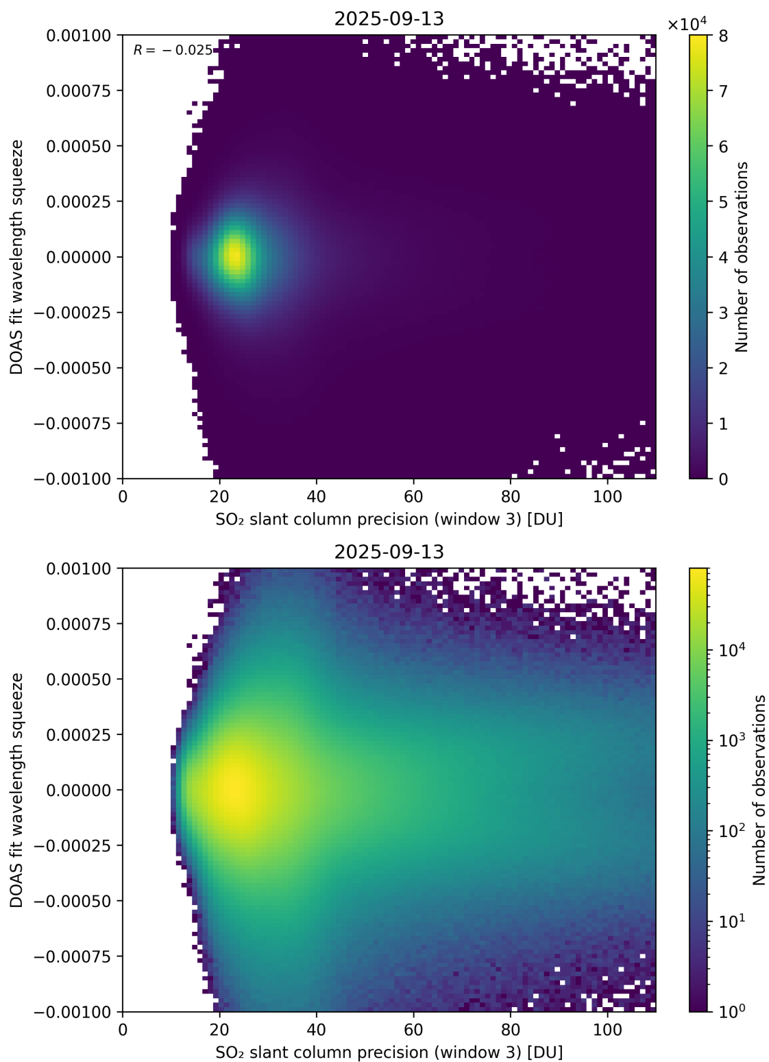
Figure 309: Scatter density plot of “SO 2 slant column precision (window 3)” against “DOAS fit wavelength squeeze” for 2025-09-12 to 2025-09-14.
