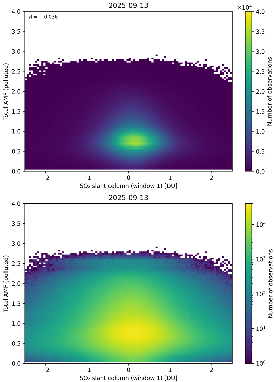
Figure 289: Scatter density plot of “SO 2 slant column (window 1)” against “Total AMF (polluted)” for 2025-09-12 to 2025-09-14.
