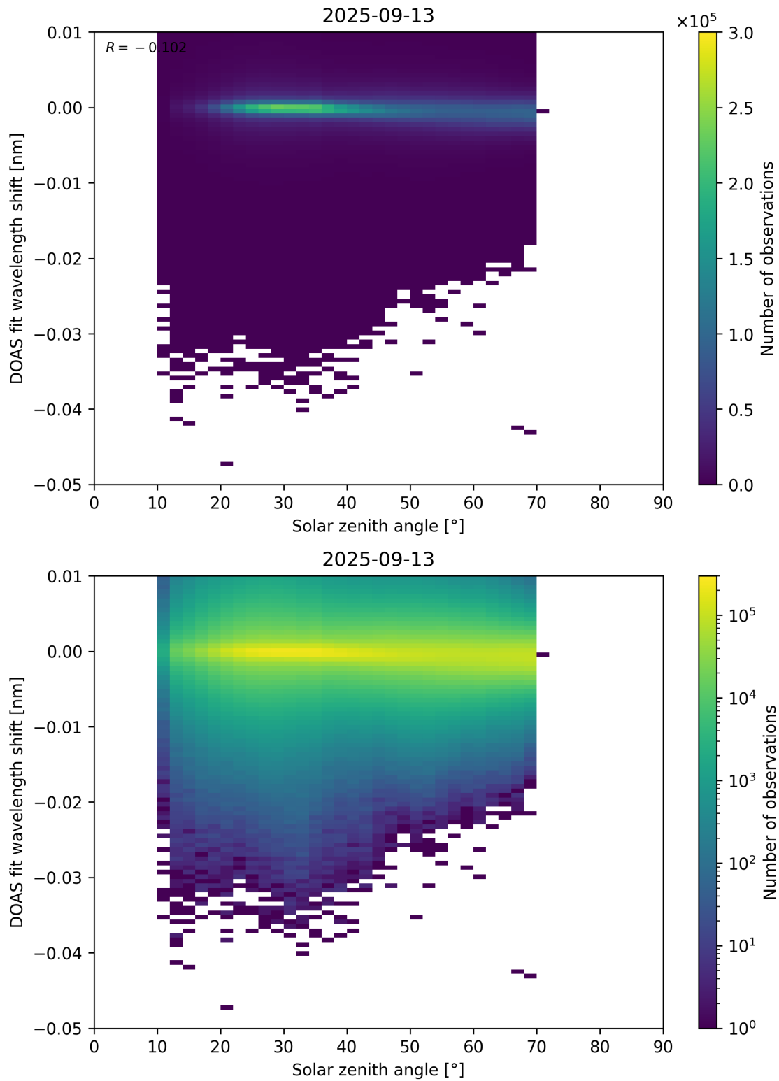
Figure 174: Scatter density plot of “Solar zenith angle” against “DOAS fit wavelength shift” for 2025-09-12 to 2025-09-14.
