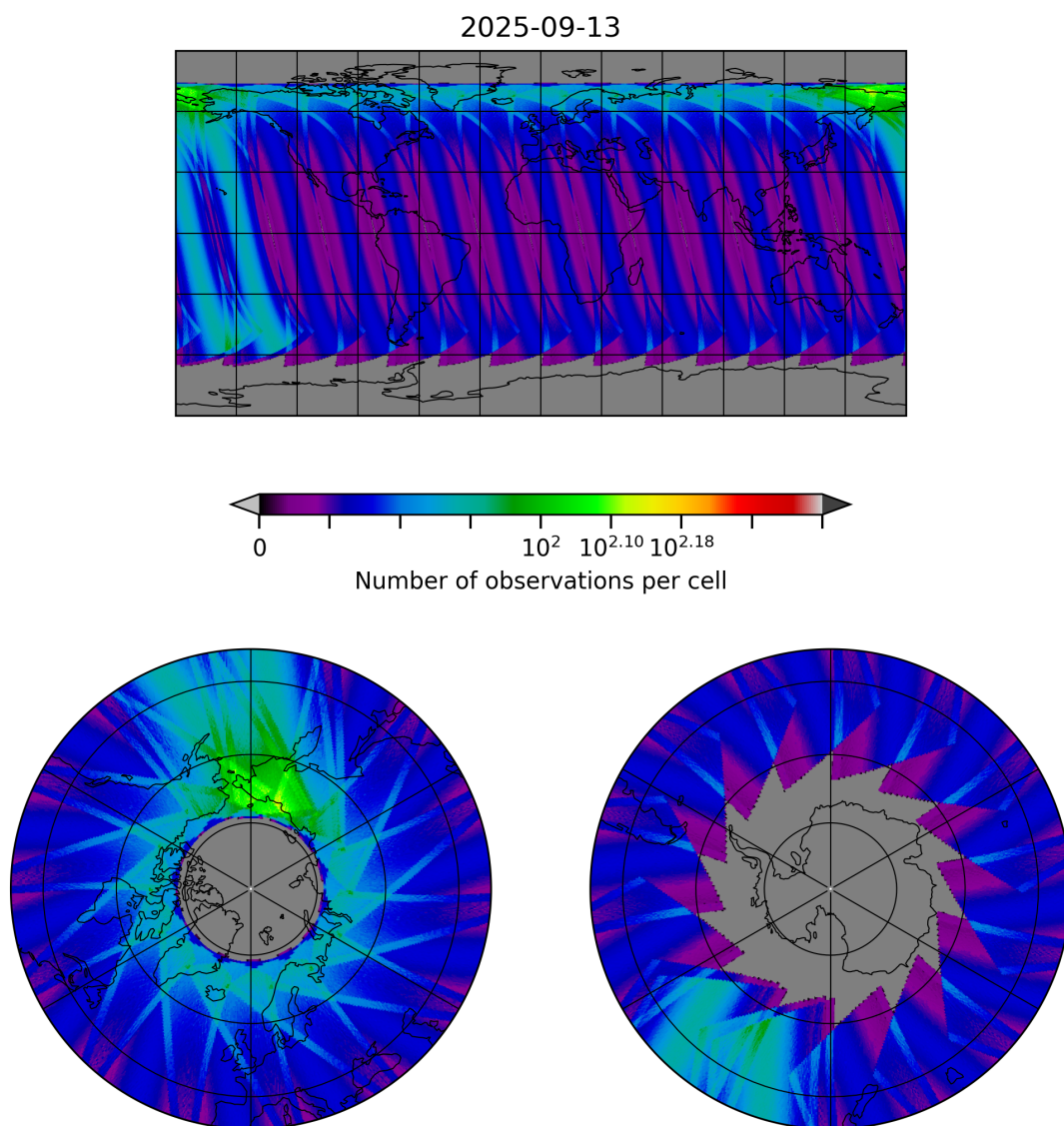
Figure 30: Map of the number of observations for 2025-09-12 to 2025-09-14
