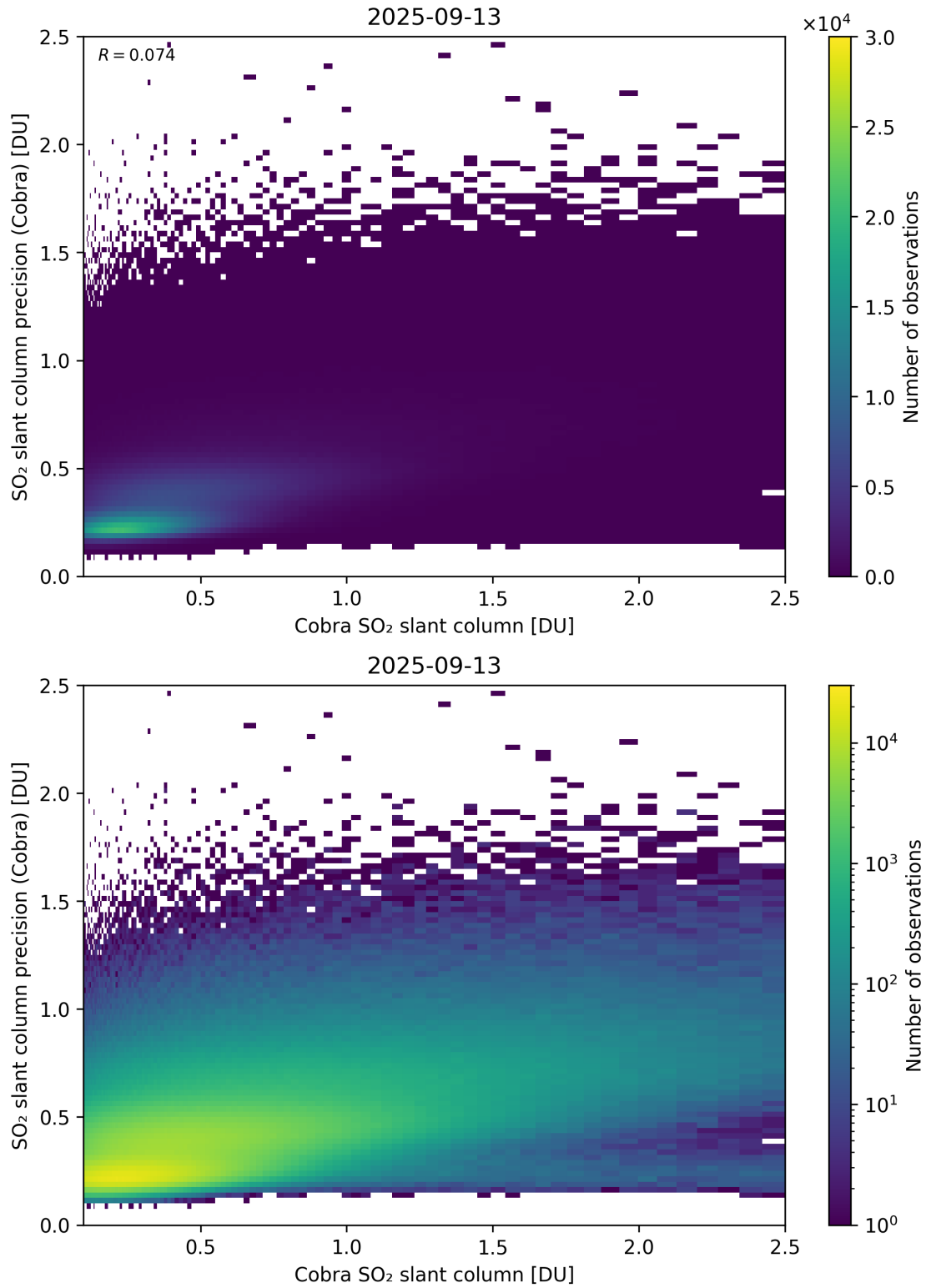
Figure 216: Scatter density plot of “Cobra SO 2 slant column” against “SO 2 slant column precision (Cobra)” for 2025-09-12 to 2025-09-14.
