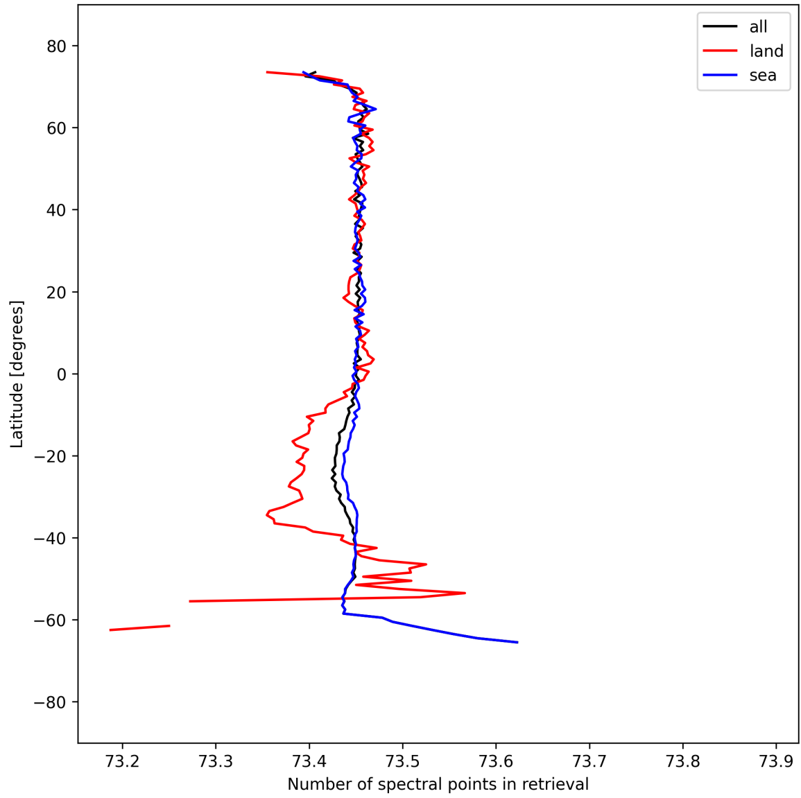
Figure 56: Zonal average of “Number of spectral points in retrieval” for 2025-09-12 to 2025-09-14.
