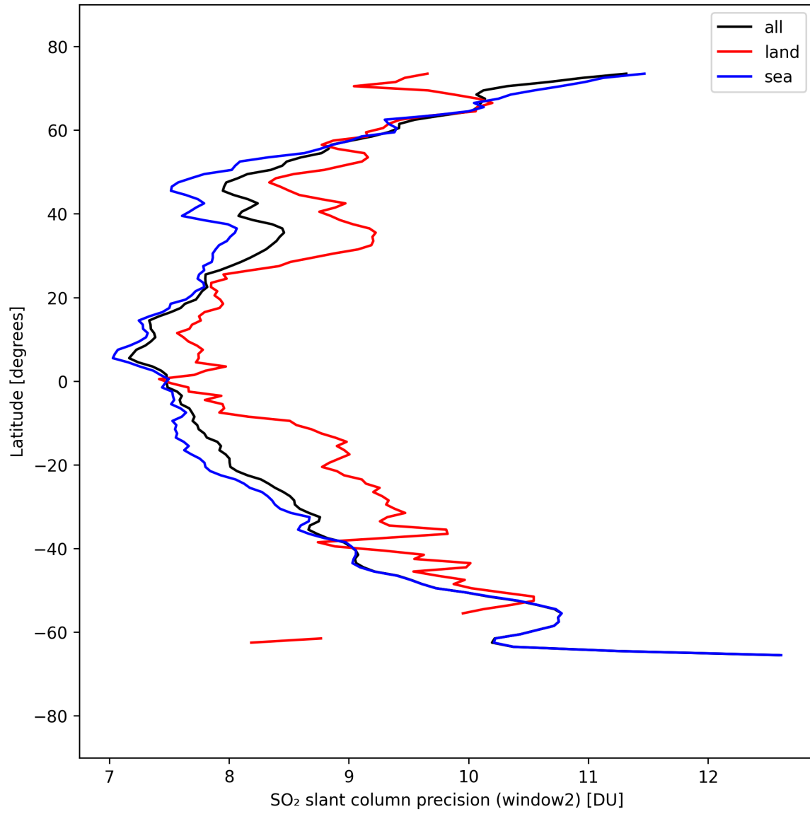
Figure 42: Zonal average of “SO 2 slant column precision (window2)” for 2025-09-12 to 2025-09-14.
