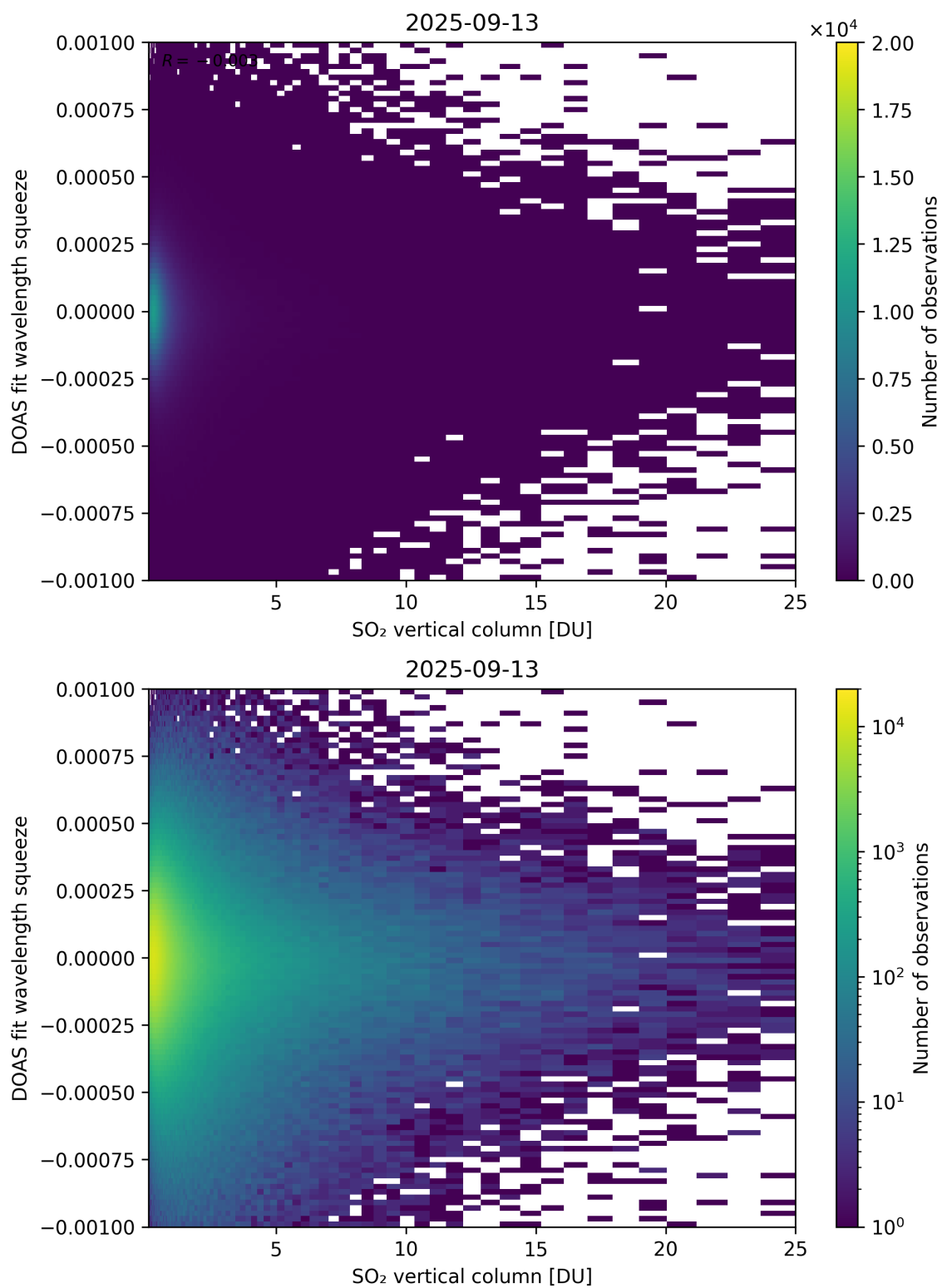
Figure 327: Scatter density plot of “SO 2 vertical column” against “DOAS fit wavelength squeeze” for 2025-09-12 to 2025-09-14.
