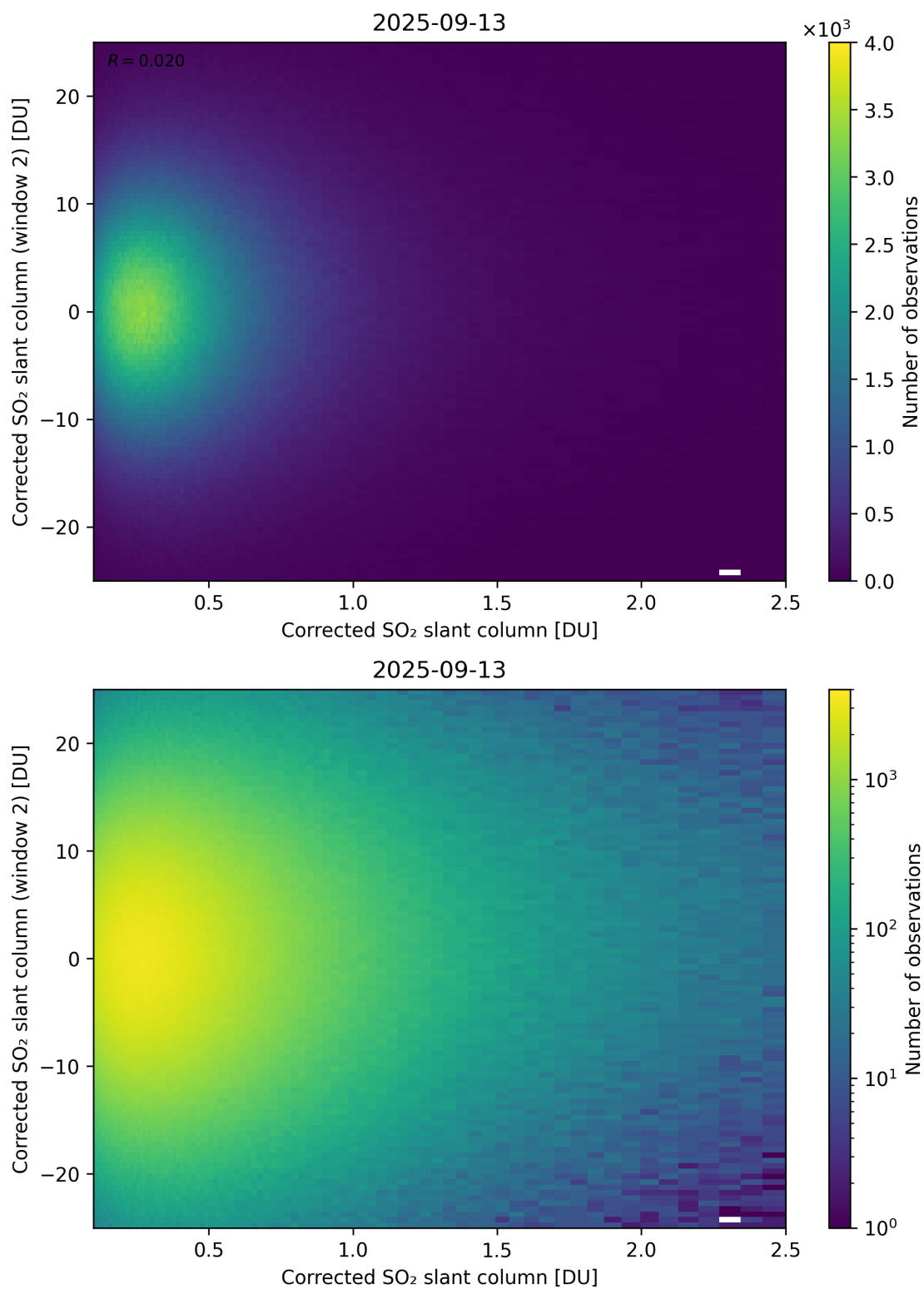
Figure 235: Scatter density plot of “Corrected SO 2 slant column” against “Corrected SO 2 slant column (window 2)” for 2025-09-12 to 2025-09-14.
