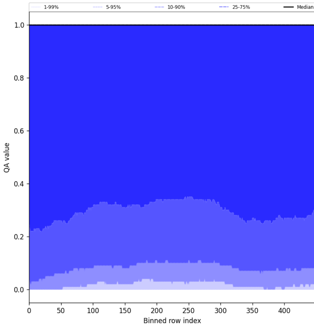
Figure 83: Along track statistics of “QA value” for 2025-09-12 to 2025-09-14
