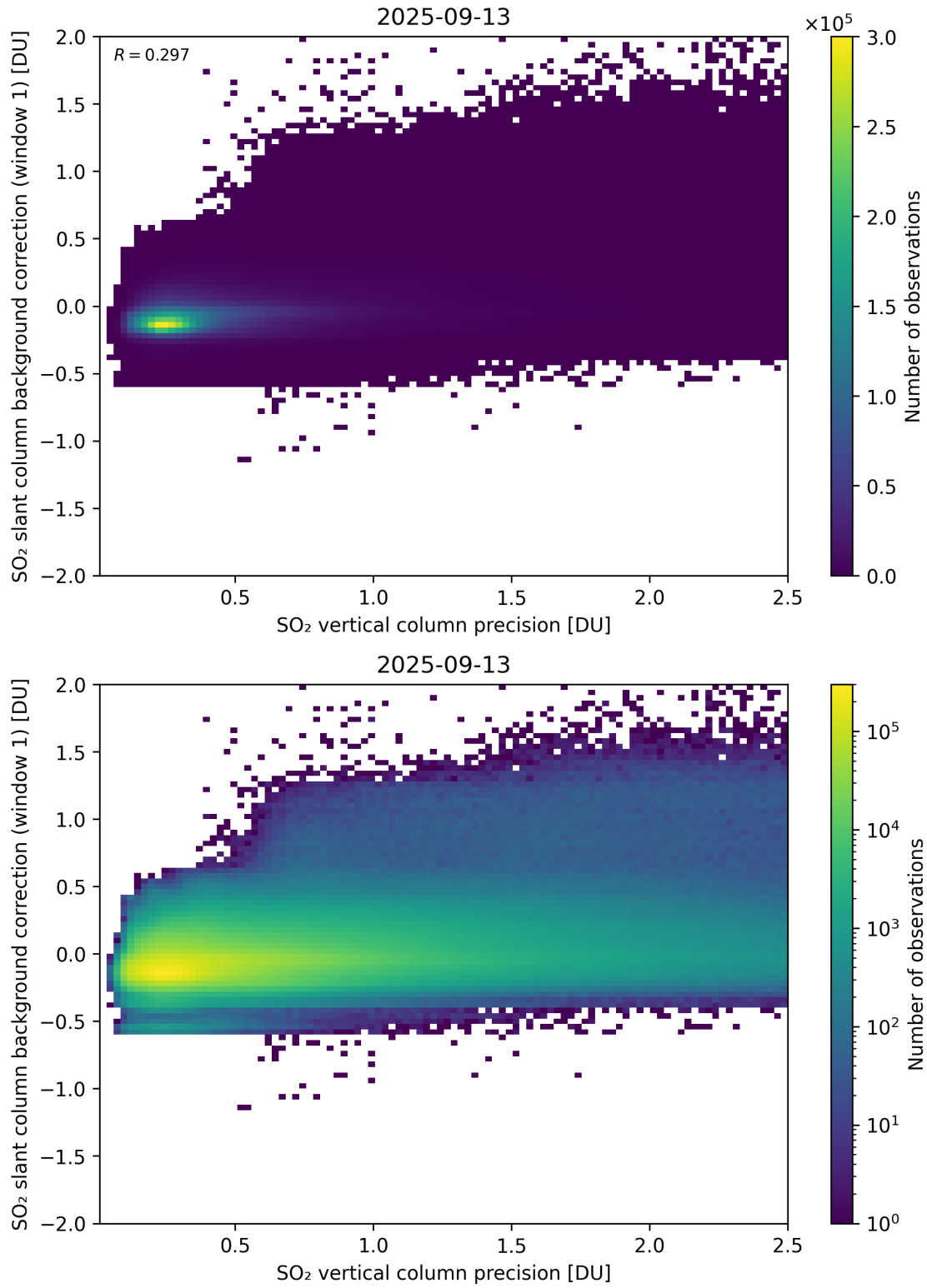
Figure 329: Scatter density plot of “SO 2 vertical column precision” against “SO 2 slant column background correction (window 1)” for 2025-09-12 to 2025-09-14.
