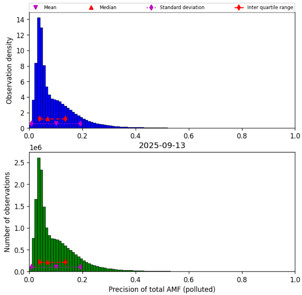
Figure 80: Histogram of “Precision of total AMF (polluted)” for 2025-09-12 to 2025-09-14
