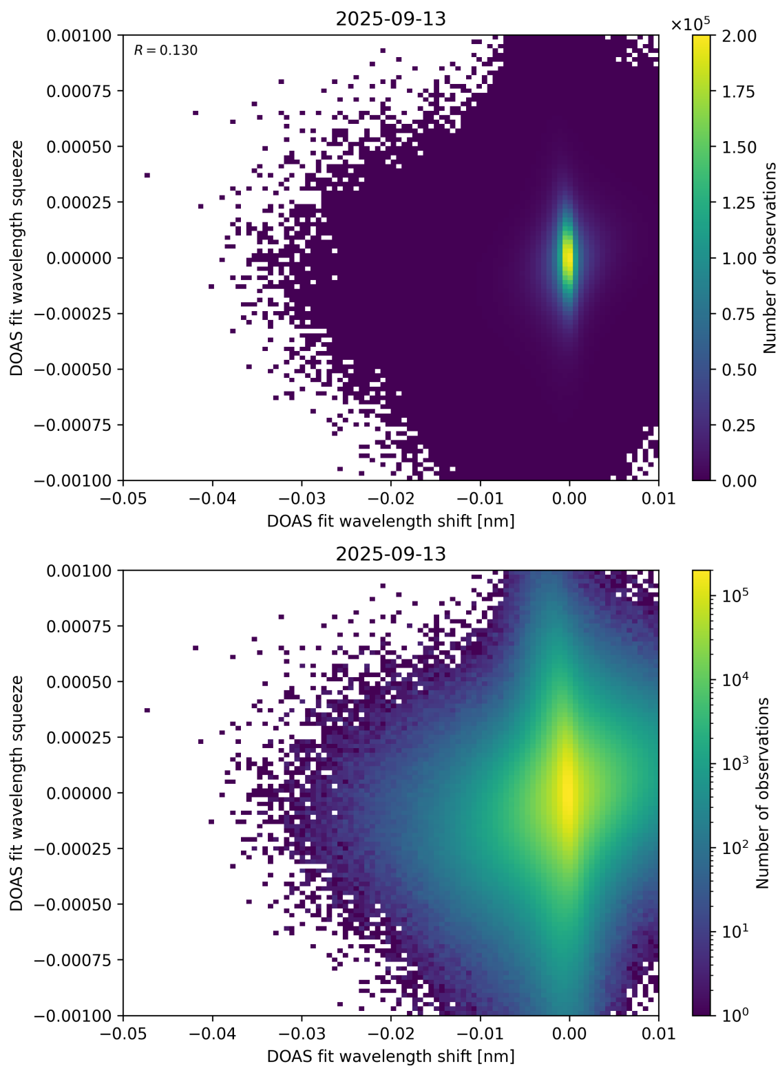
Figure 138: Scatter density plot of “DOAS fit wavelength shift” against “DOAS fit wavelength squeeze” for 2025-09-12 to 2025-09-14.
