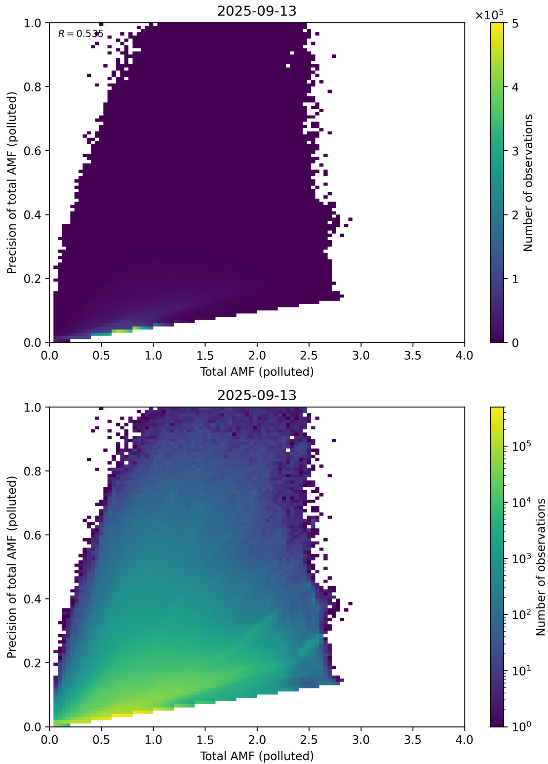
Figure 322: Scatter density plot of “Total AMF (polluted)” against “Precision of total AMF (polluted)” for 2025-09-12 to 2025-09-14.
