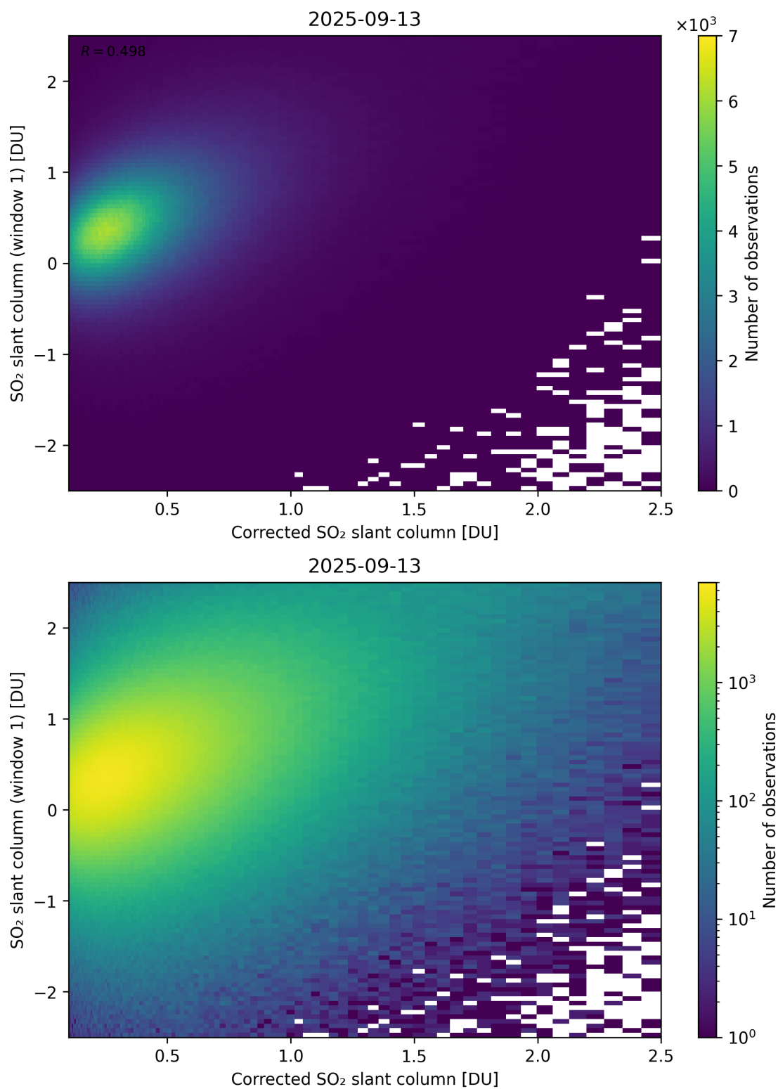
Figure 237: Scatter density plot of “Corrected SO 2 slant column” against “SO 2 slant column (window 1)” for 2025-09-12 to 2025-09-14.
