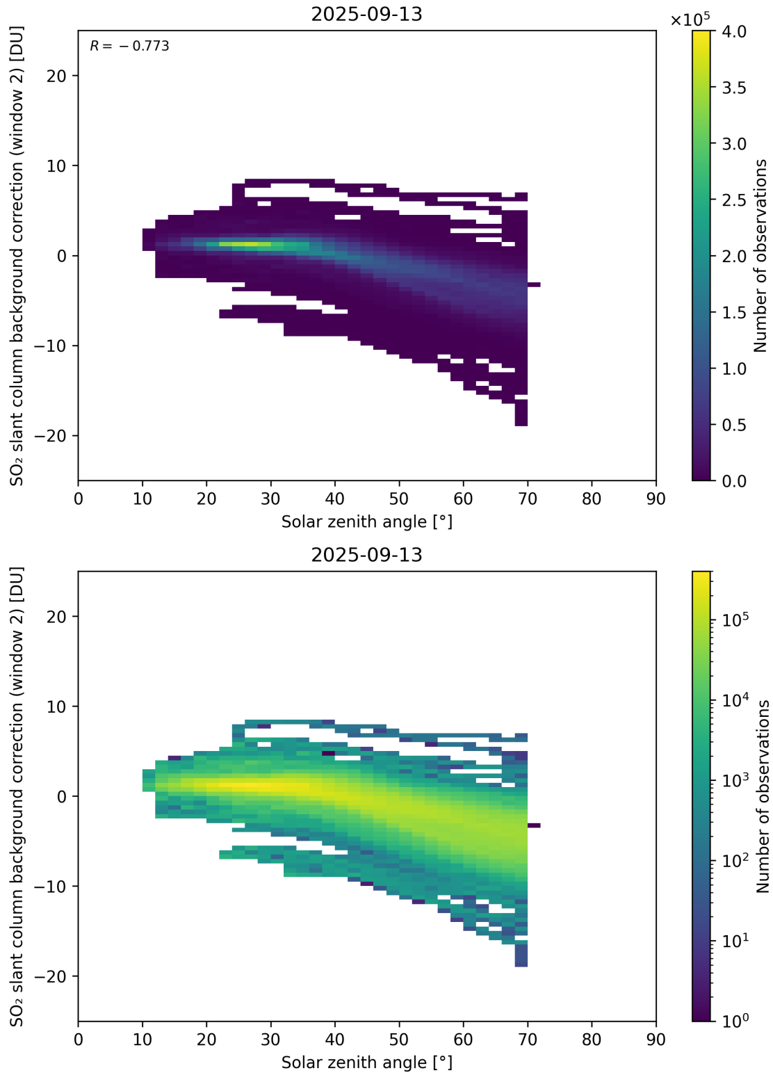
Figure 172: Scatter density plot of “Solar zenith angle” against “SO 2 slant column background correction (window 2)” for 2025-09-12 to 2025-09-14.
