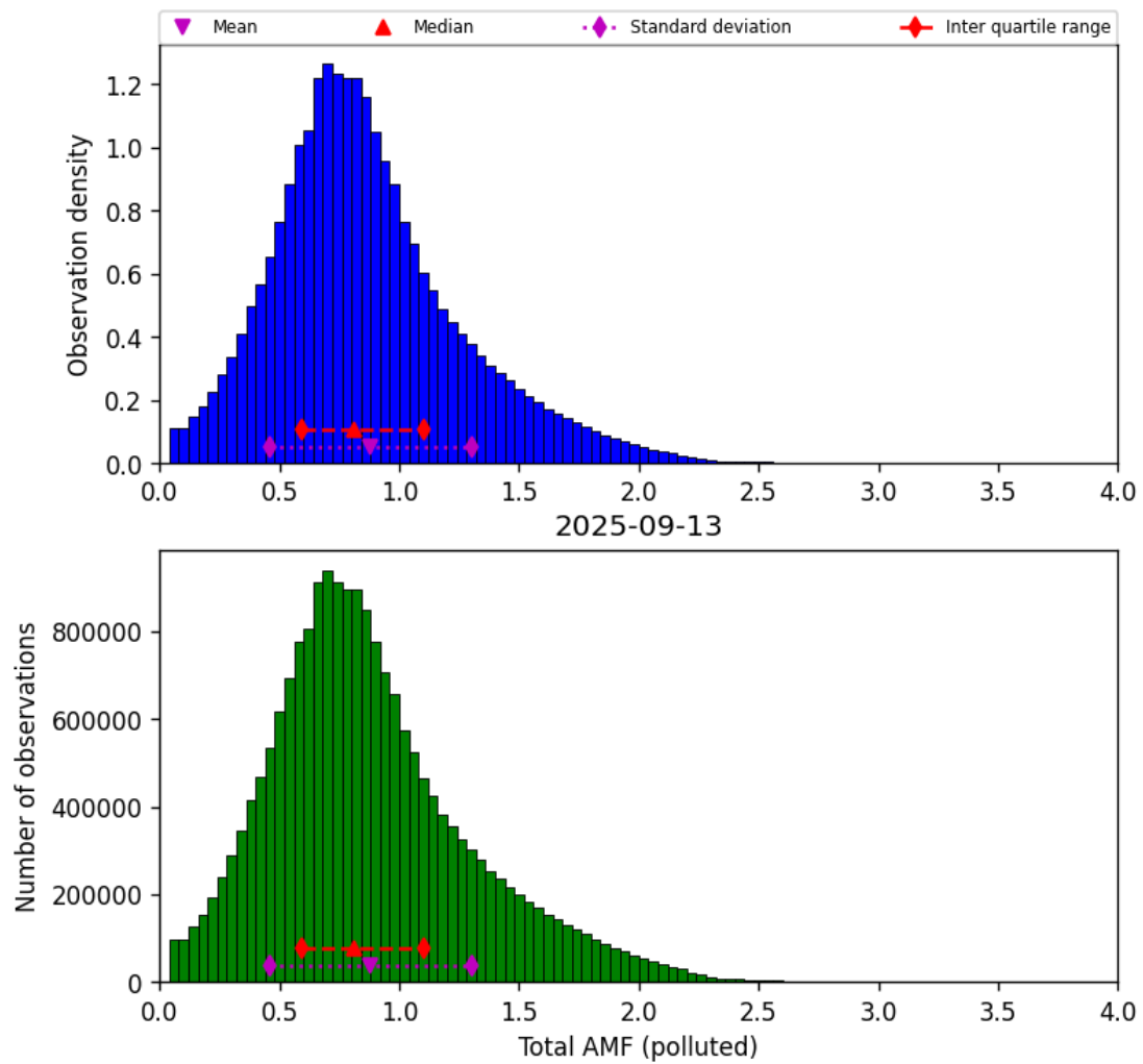
Figure 79: Histogram of “Total AMF (polluted)” for 2025-09-12 to 2025-09-14
