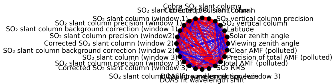
Figure 1: Map of correlation graph for 2025-09-12 to 2025-09-14.
