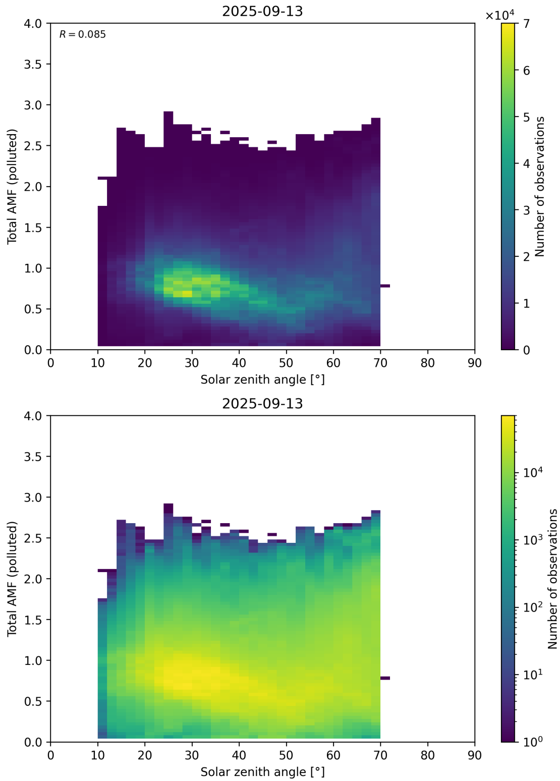
Figure 189: Scatter density plot of “Solar zenith angle” against “Total AMF (polluted)” for 2025-09-12 to 2025-09-14.
