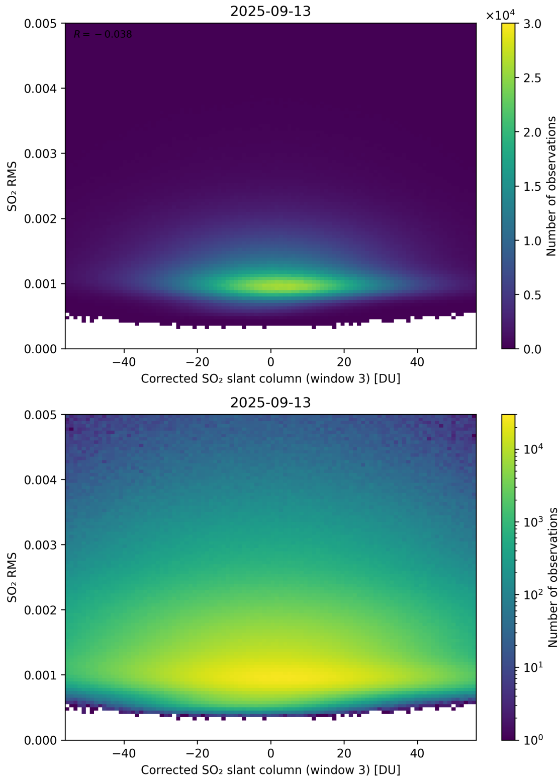
Figure 258: Scatter density plot of “Corrected SO 2 slant column (window 3)” against “SO 2 RMS” for 2025-09-12 to 2025-09-14.
