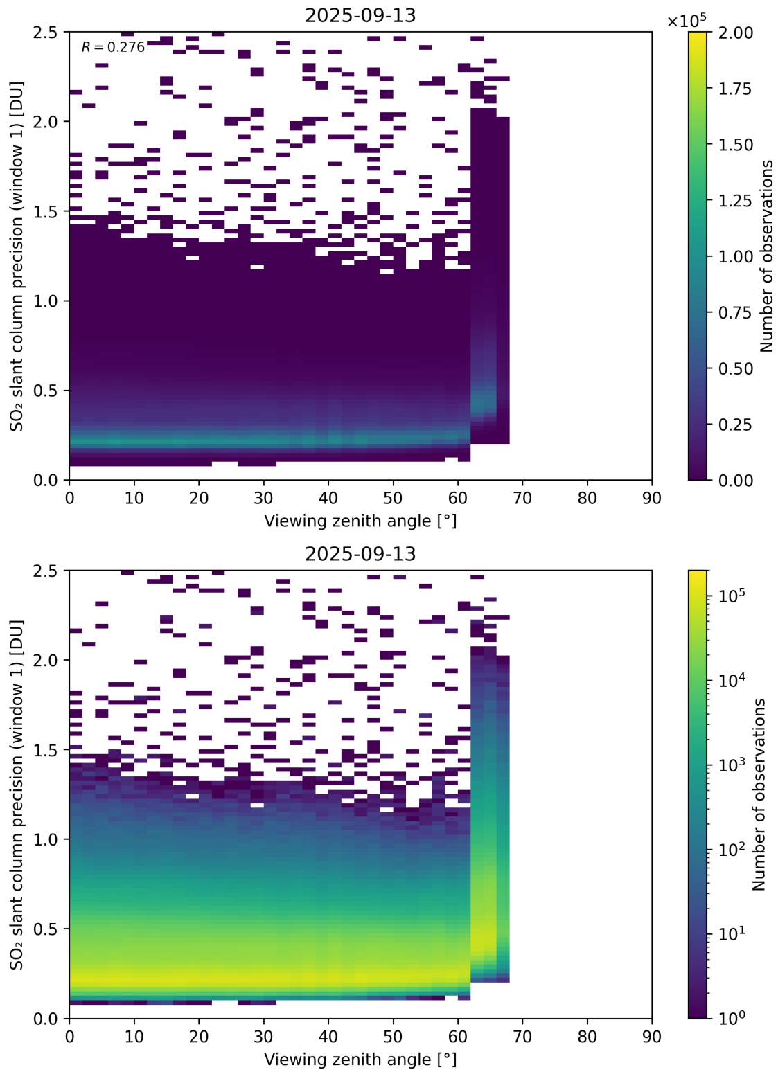
Figure 377: Scatter density plot of “Viewing zenith angle” against “SO 2 slant column precision (window 1)” for 2025-09-12 to 2025-09-14.
