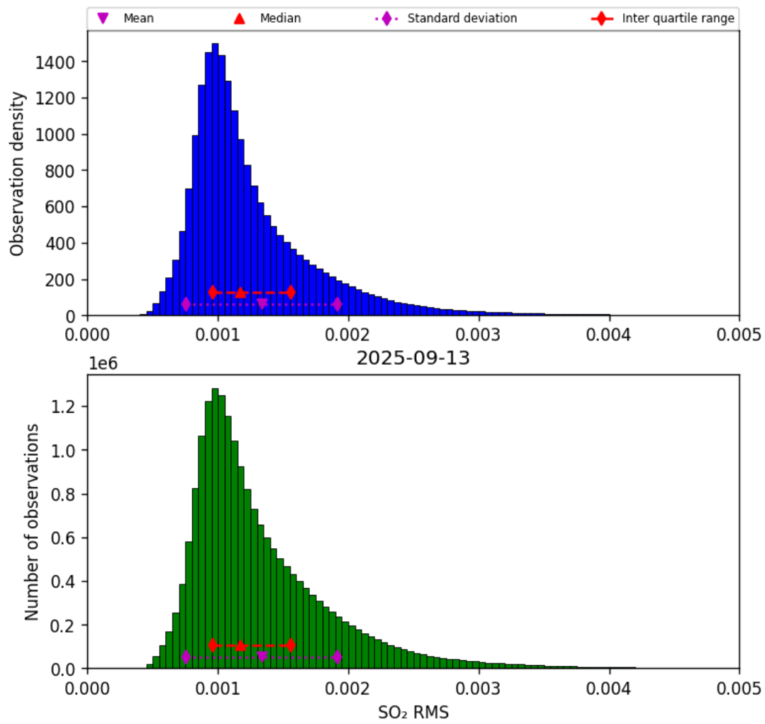
Figure 78: Histogram of “SO 2 RMS” for 2025-09-12 to 2025-09-14
