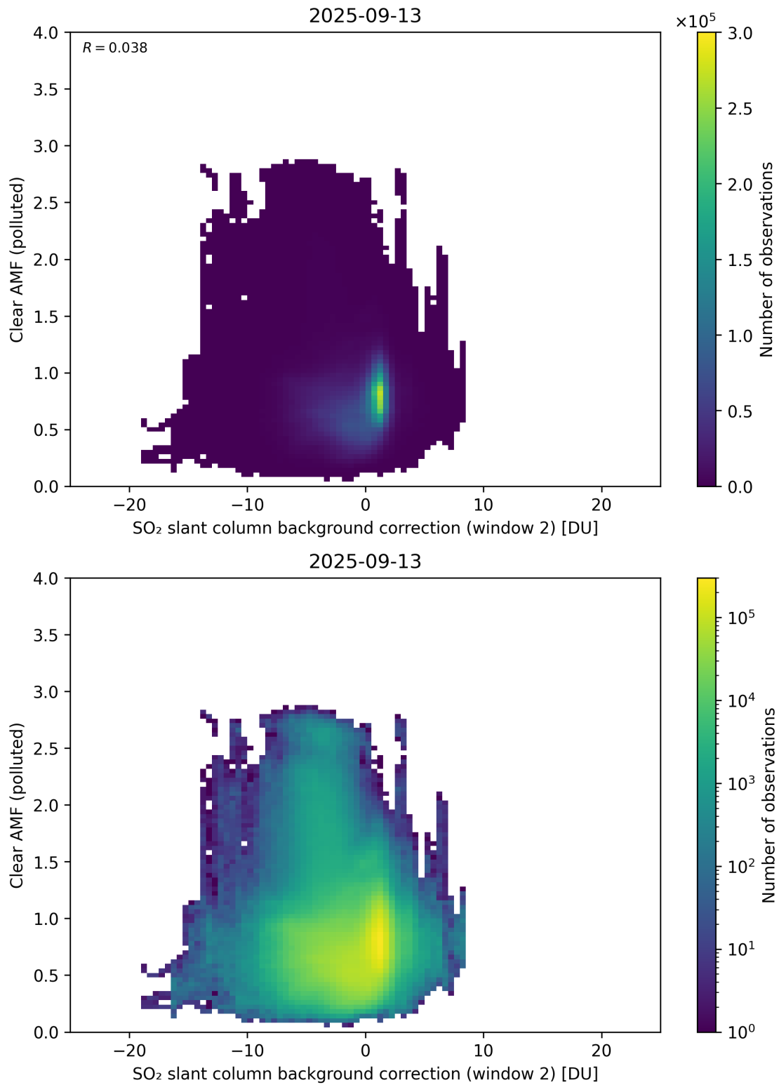
Figure 126: Scatter density plot of “SO 2 slant column background correction (window 2)” against “Clear AMF (polluted)” for 2025-09-12 to 2025-09-14.
