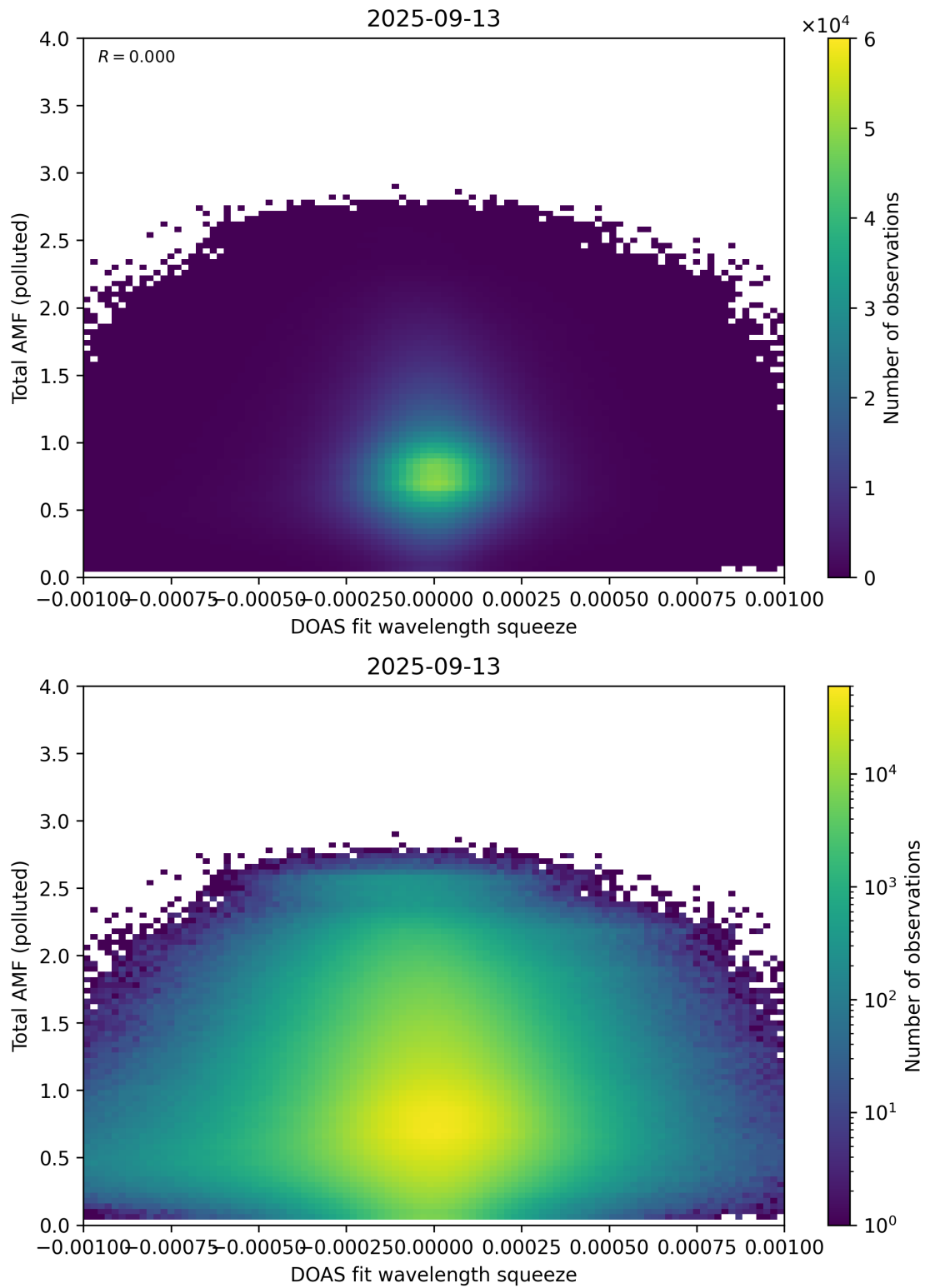
Figure 145: Scatter density plot of “DOAS fit wavelength squeeze” against “Total AMF (polluted)” for 2025-09-12 to 2025-09-14.
