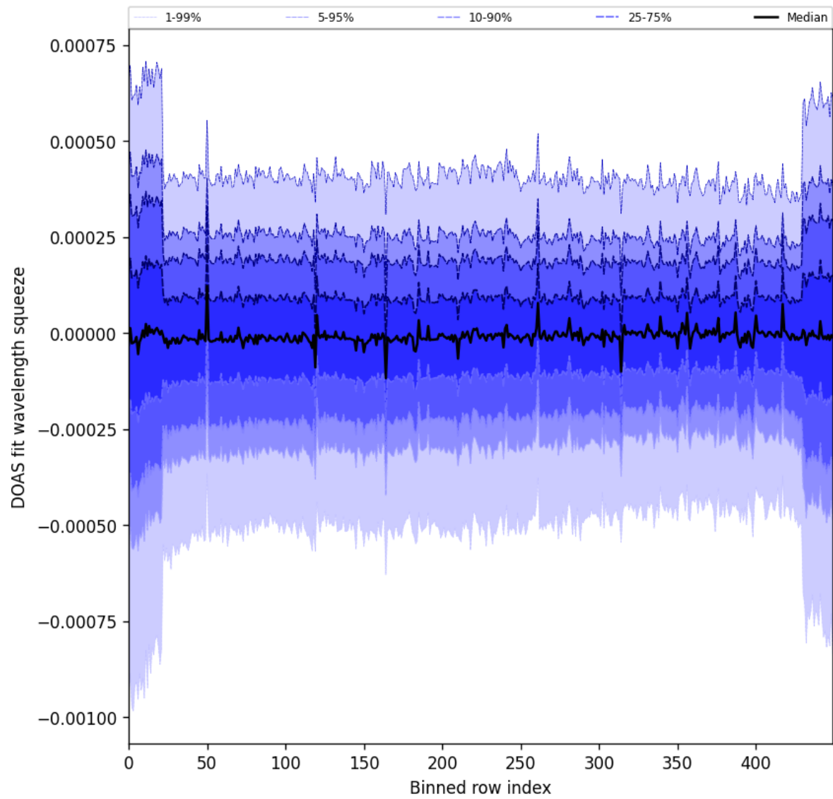
Figure 103: Along track statistics of “DOAS fit wavelength squeeze” for 2025-09-12 to 2025-09-14
