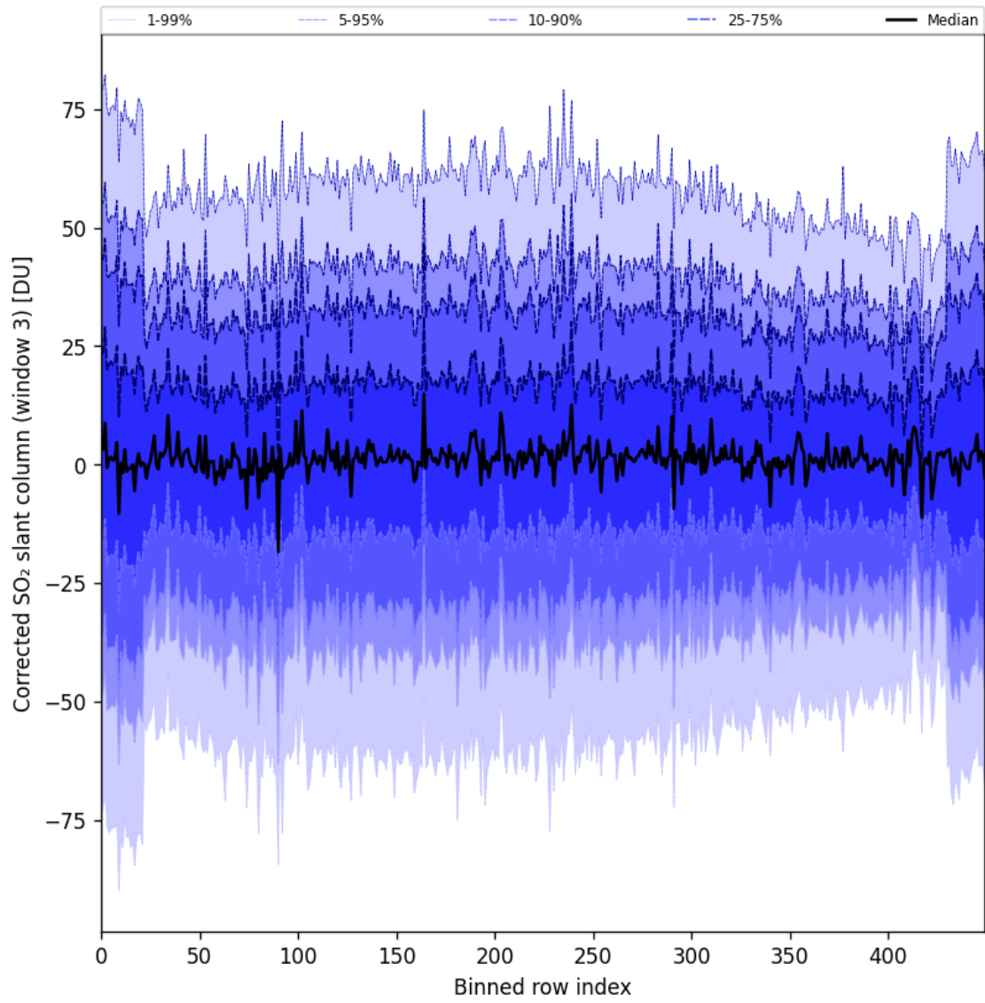
Figure 99: Along track statistics of “Corrected SO 2 slant column (window 3)” for 2025-09-12 to 2025-09-14
