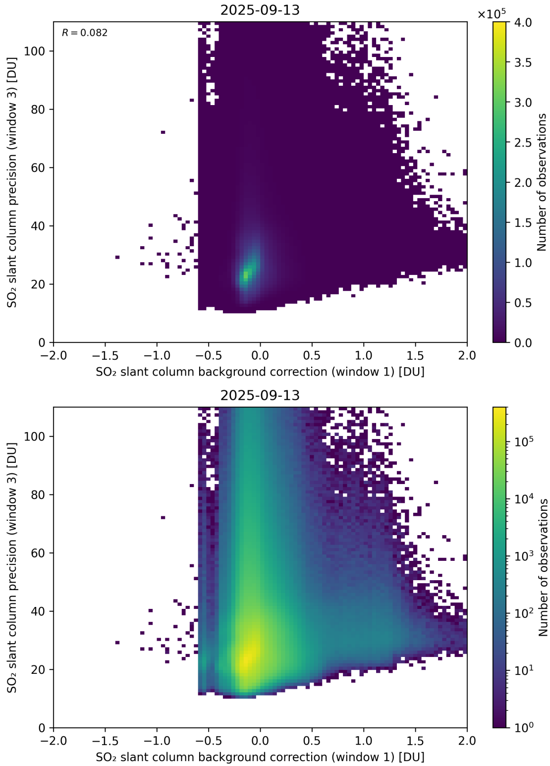
Figure 119: Scatter density plot of “SO 2 slant column background correction (window 1)” against “SO 2 slant column precision (window 3)” for 2025-09-12 to 2025-09-14.
