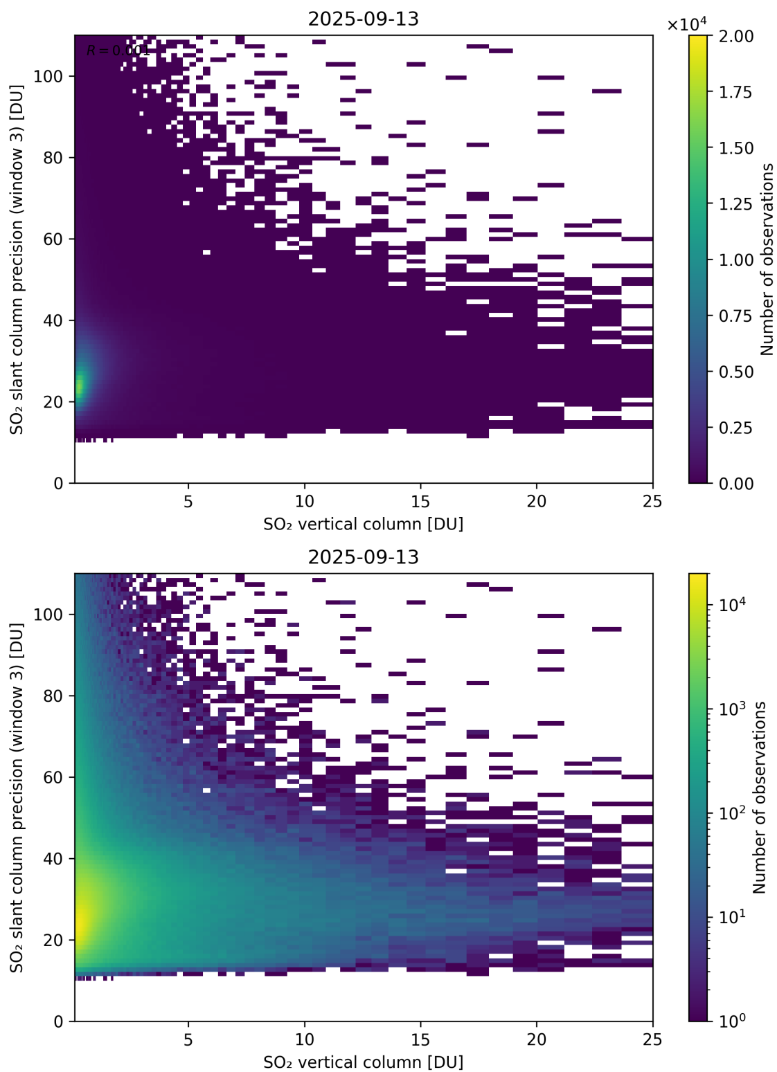
Figure 358: Scatter density plot of “SO 2 vertical column” against “SO 2 slant column precision (window 3)” for 2025-09-12 to 2025-09-14.
