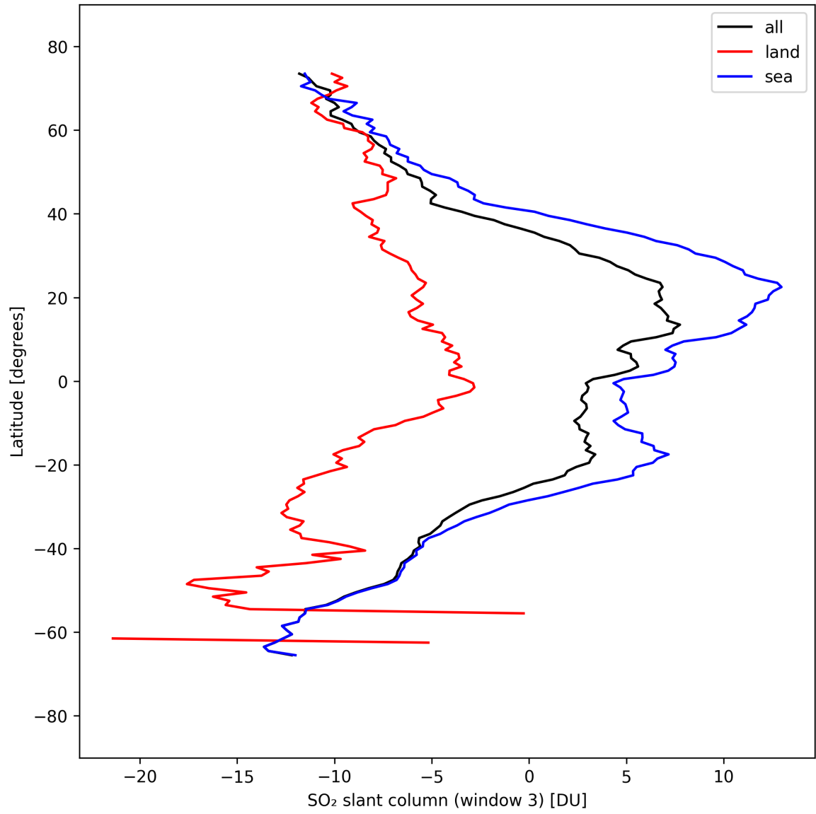
Figure 45: Zonal average of “SO 2 slant column (window 3)” for 2025-09-12 to 2025-09-14.
