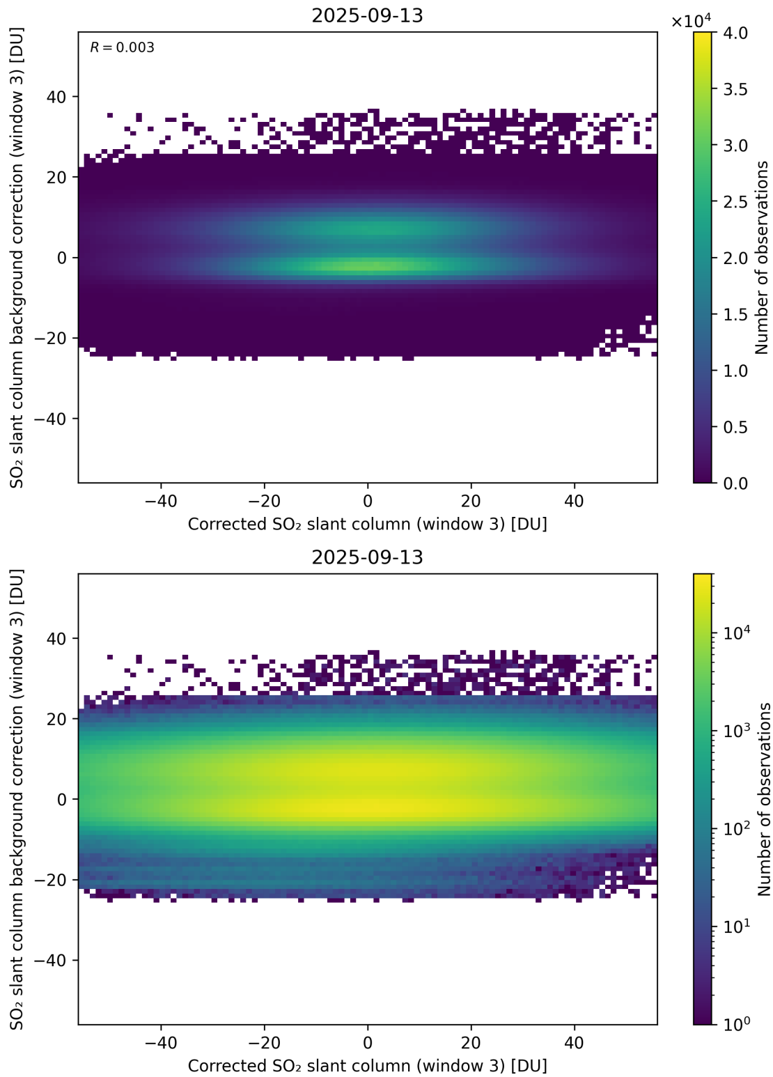
Figure 255: Scatter density plot of “Corrected SO 2 slant column (window 3)” against “SO 2 slant column background correction (window 3)” for 2025-09-12 to 2025-09-14.
