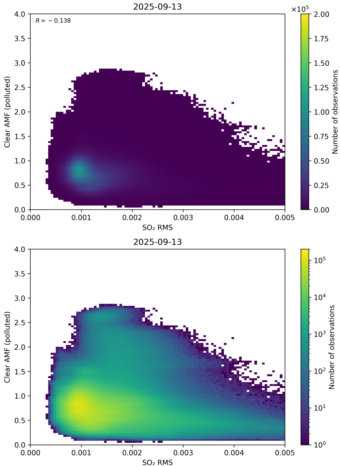
Figure 147: Scatter density plot of “SO 2 RMS” against “Clear AMF (polluted)” for 2025-09-12 to 2025-09-14.
