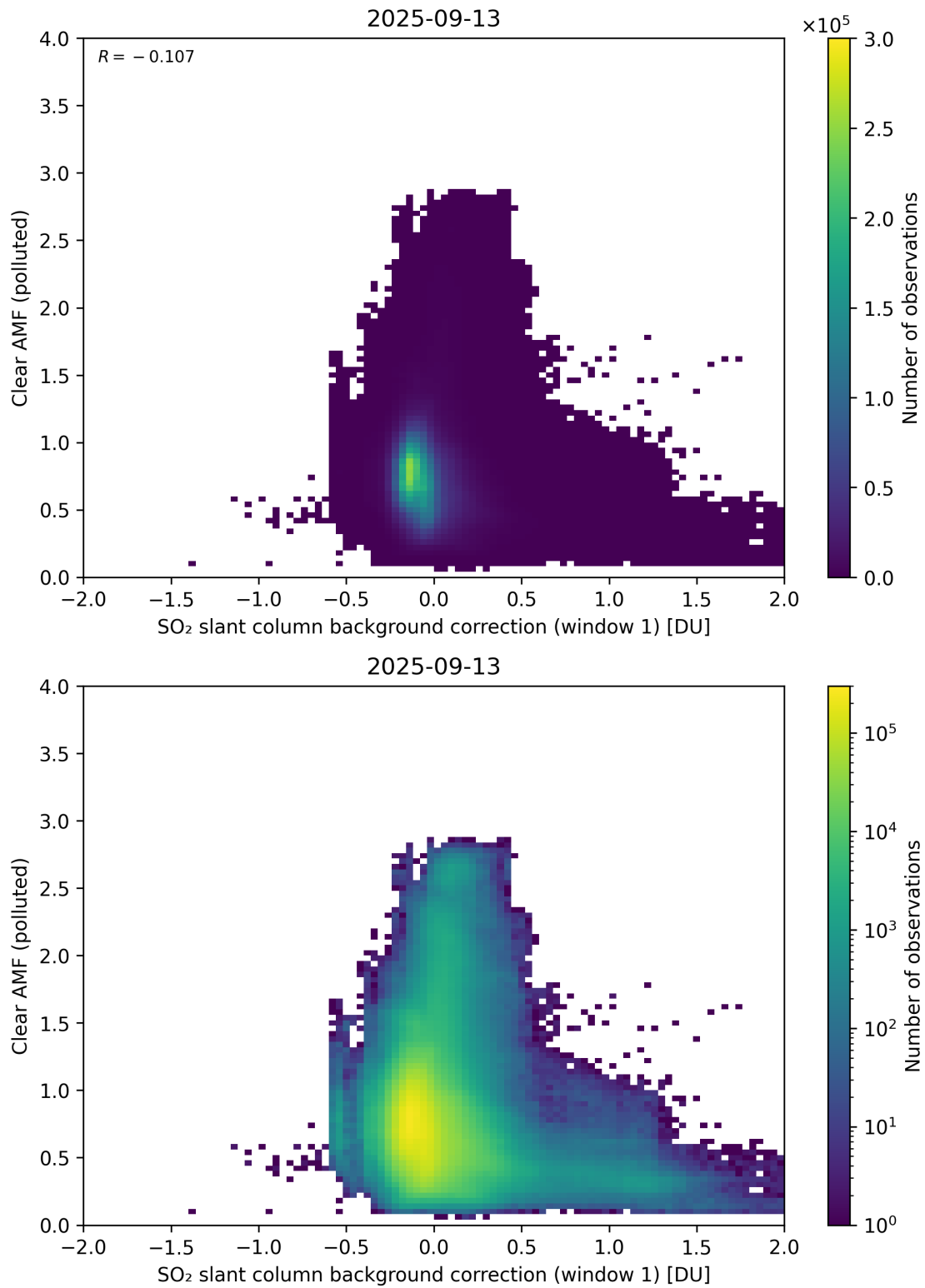
Figure 114: Scatter density plot of “SO 2 slant column background correction (window 1)” against “Clear AMF (polluted)” for 2025-09-12 to 2025-09-14.
