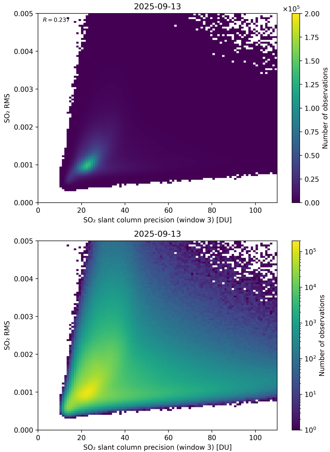
Figure 310: Scatter density plot of “SO 2 slant column precision (window 3)” against “SO 2 RMS” for 2025-09-12 to 2025-09-14.
