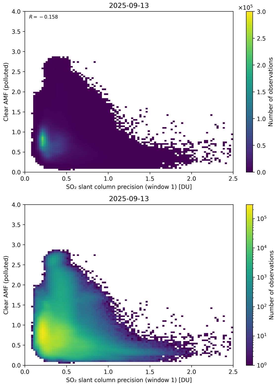
Figure 274: Scatter density plot of “SO 2 slant column precision (window 1)” against “Clear AMF (polluted)” for 2025-09-12 to 2025-09-14.
