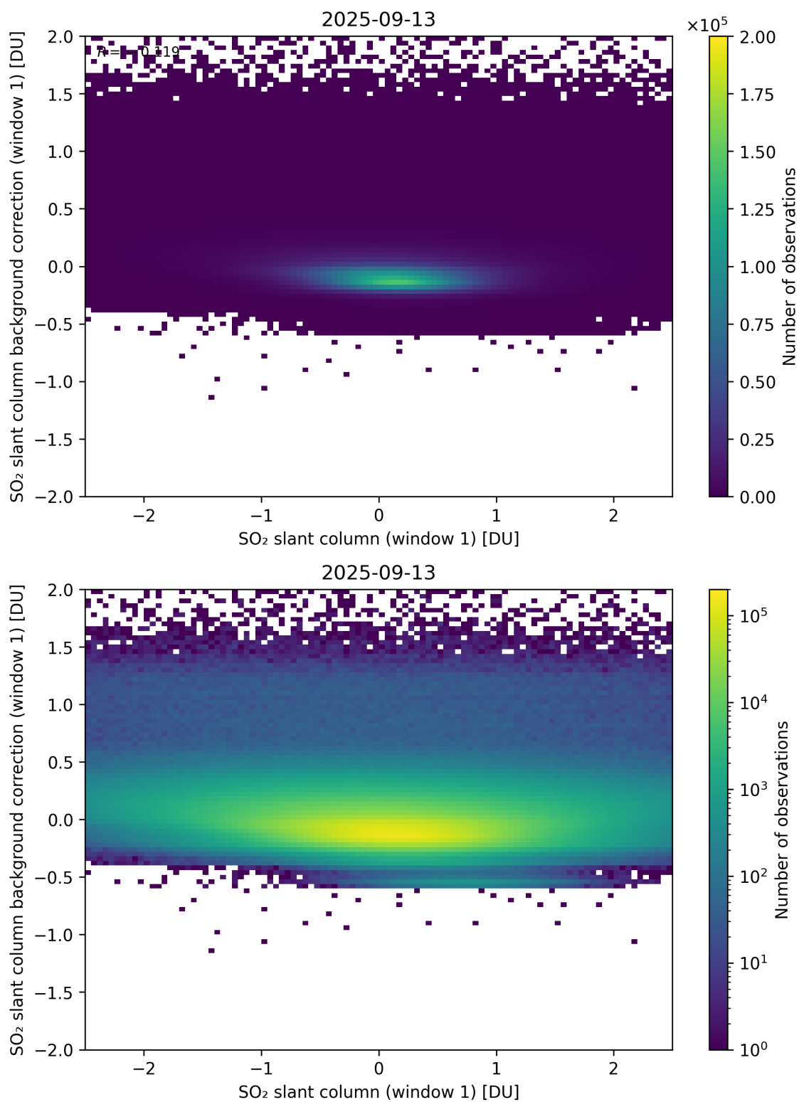
Figure 262: Scatter density plot of “SO 2 slant column (window 1)” against “SO 2 slant column background correction (window 1)” for 2025-09-12 to 2025-09-14.
