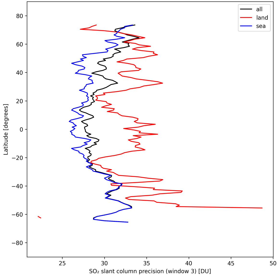
Figure 46: Zonal average of “SO 2 slant column precision (window 3)” for 2025-09-12 to 2025-09-14.
