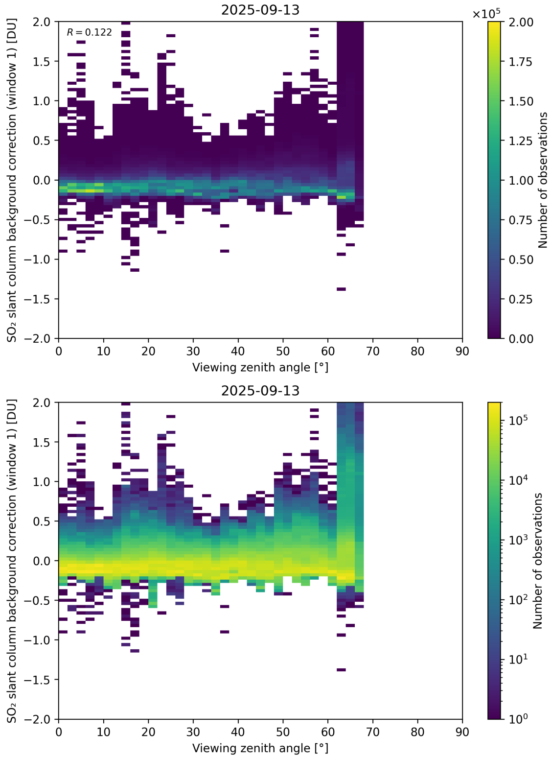
Figure 362: Scatter density plot of “Viewing zenith angle” against “SO 2 slant column background correction (window 1)” for 2025-09-12 to 2025-09-14.
