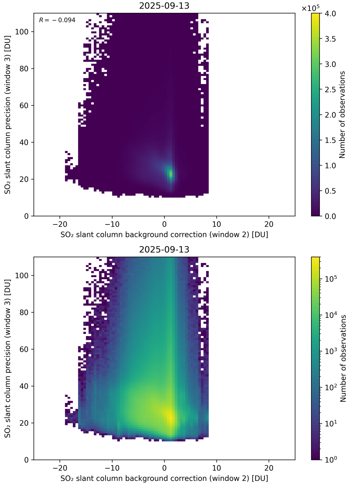
Figure 129: Scatter density plot of “SO 2 slant column background correction (window 2)” against “SO 2 slant column precision (window 3)” for 2025-09-12 to 2025-09-14.
