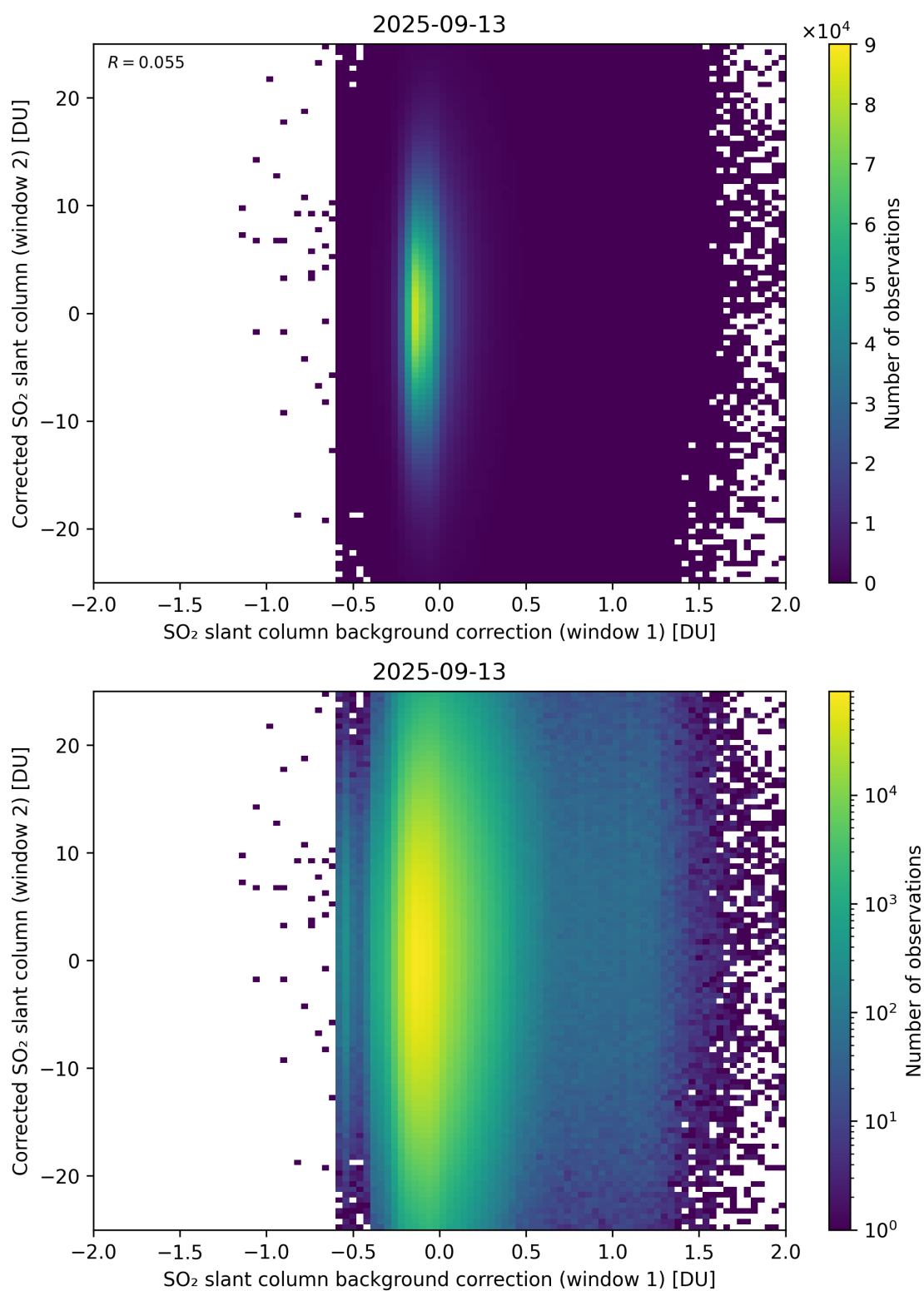
Figure 115: Scatter density plot of “SO 2 slant column background correction (window 1)” against “Corrected SO 2 slant column (window 2)” for 2025-09-12 to 2025-09-14.
