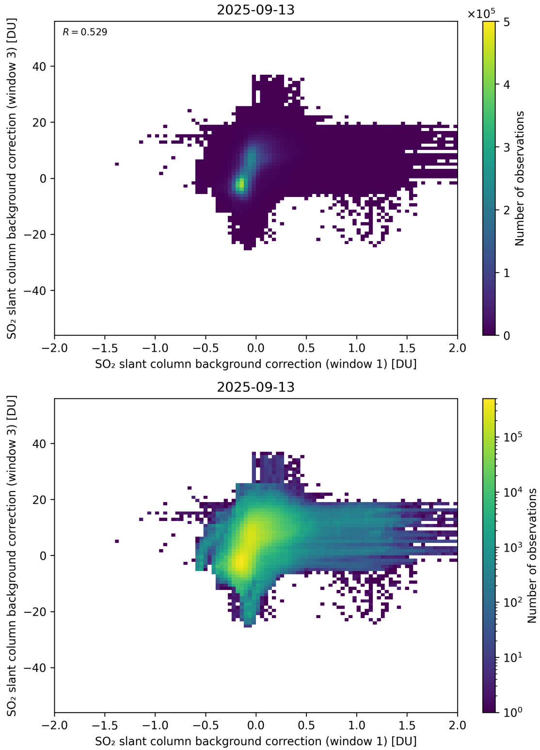
Figure 110: Scatter density plot of “SO 2 slant column background correction (window 1)” against “SO 2 slant column background correction (window 3)” for 2025-09-12 to 2025-09-14.
