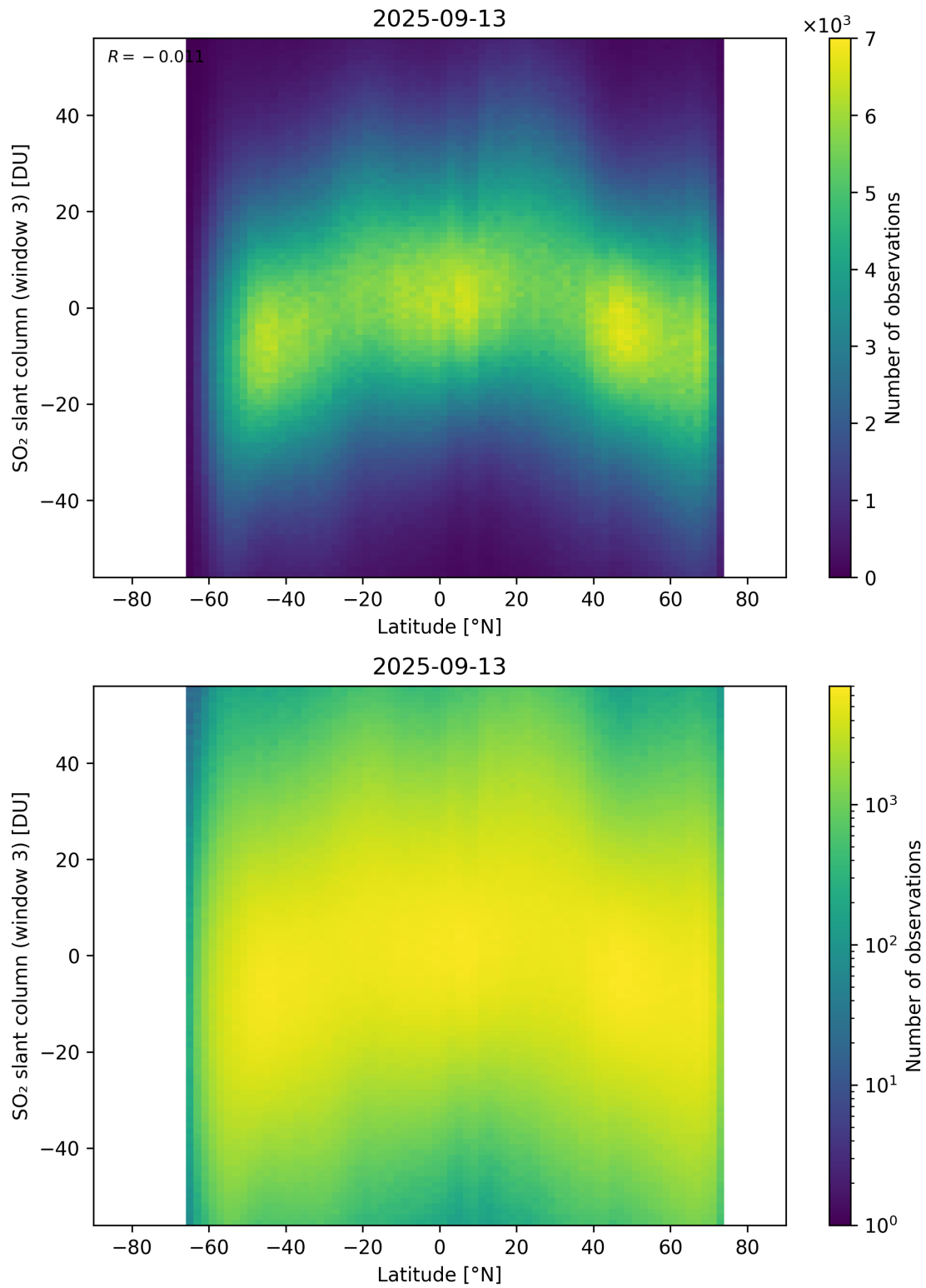
Figure 165: Scatter density plot of “Latitude” against “SO 2 slant column (window 3)” for 2025-09-12 to 2025-09-14.
