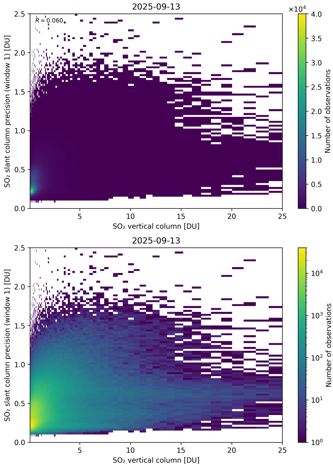
Figure 355: Scatter density plot of “SO 2 vertical column” against “SO 2 slant column precision (window 1)” for 2025-09-12 to 2025-09-14.
