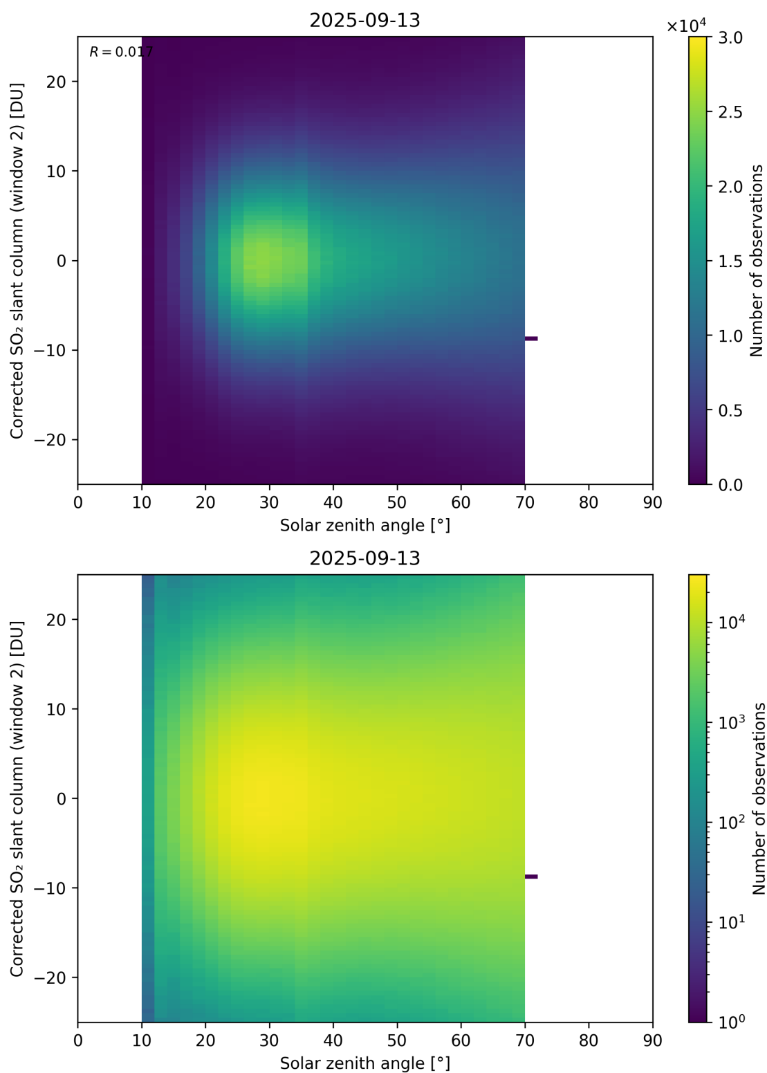
Figure 182: Scatter density plot of “Solar zenith angle” against “Corrected SO 2 slant column (window 2)” for 2025-09-12 to 2025-09-14.
