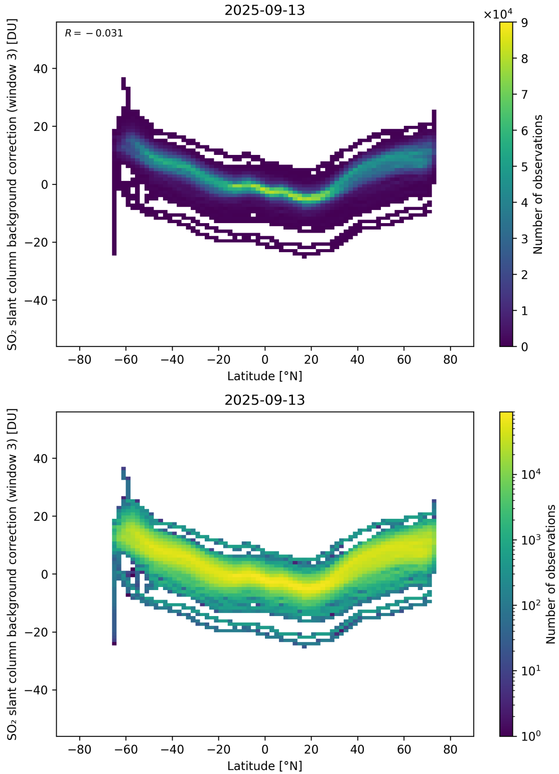
Figure 152: Scatter density plot of “Latitude” against “SO 2 slant column background correction (window 3)” for 2025-09-12 to 2025-09-14.
