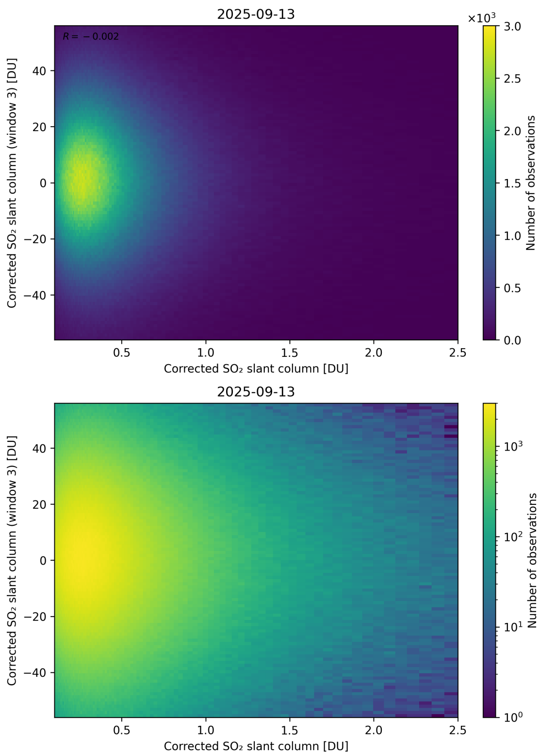
Figure 236: Scatter density plot of “Corrected SO 2 slant column” against “Corrected SO 2 slant column (window 3)” for 2025-09-12 to 2025-09-14.
