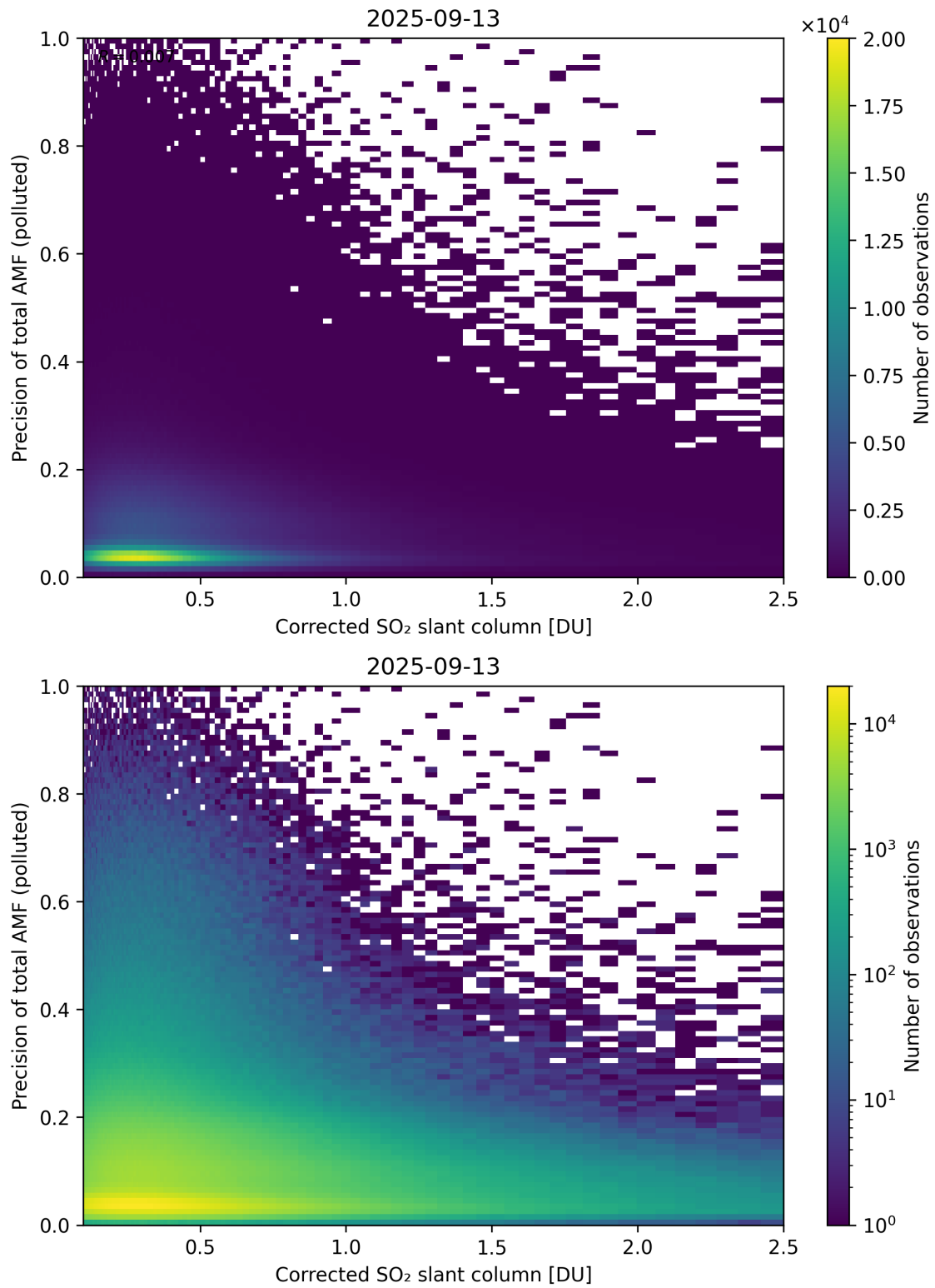
Figure 243: Scatter density plot of “Corrected SO 2 slant column” against “Precision of total AMF (polluted)” for 2025-09-12 to 2025-09-14.
