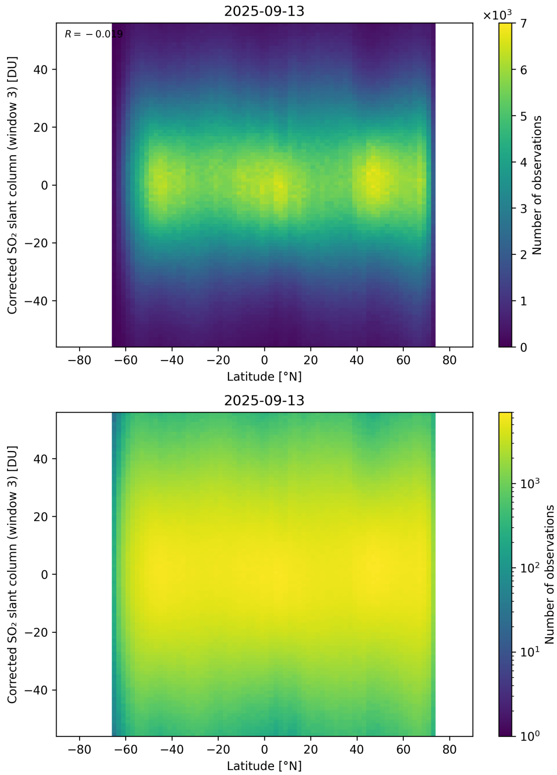
Figure 161: Scatter density plot of “Latitude” against “Corrected SO 2 slant column (window 3)” for 2025-09-12 to 2025-09-14.
