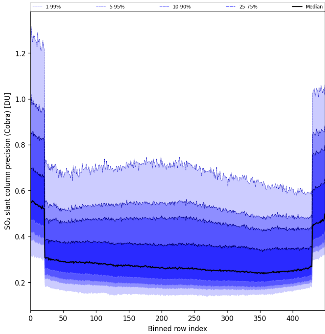
Figure 88: Along track statistics of “SO 2 slant column precision (Cobra)” for 2025-09-12 to 2025-09-14
