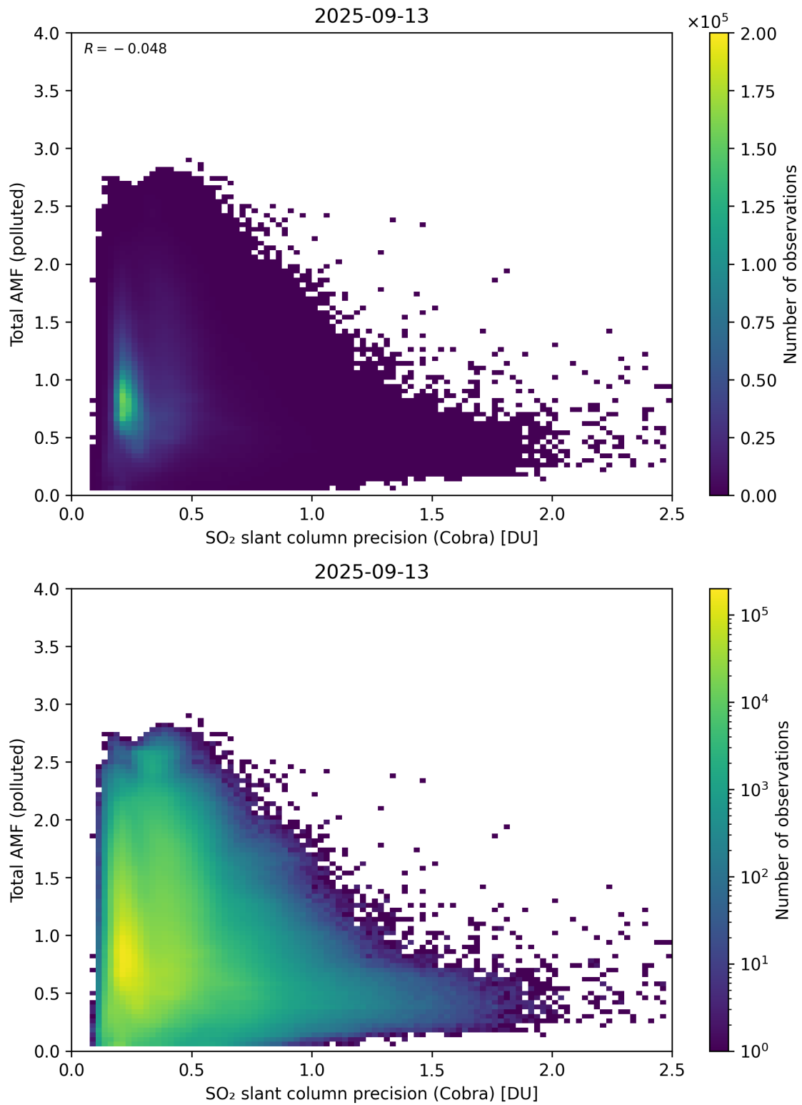
Figure 213: Scatter density plot of “SO 2 slant column precision (Cobra)” against “Total AMF (polluted)” for 2025-09-12 to 2025-09-14.
