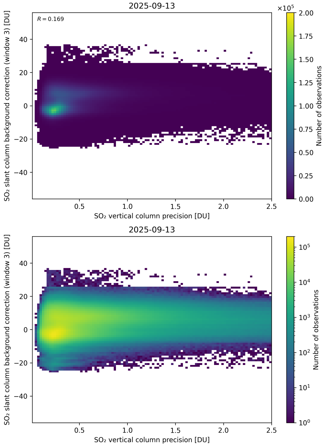
Figure 331: Scatter density plot of “SO 2 vertical column precision” against “SO 2 slant column background correction (window 3)” for 2025-09-12 to 2025-09-14.
