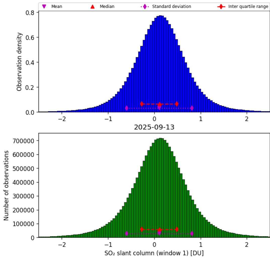
Figure 63: Histogram of “SO 2 slant column (window 1)” for 2025-09-12 to 2025-09-14
