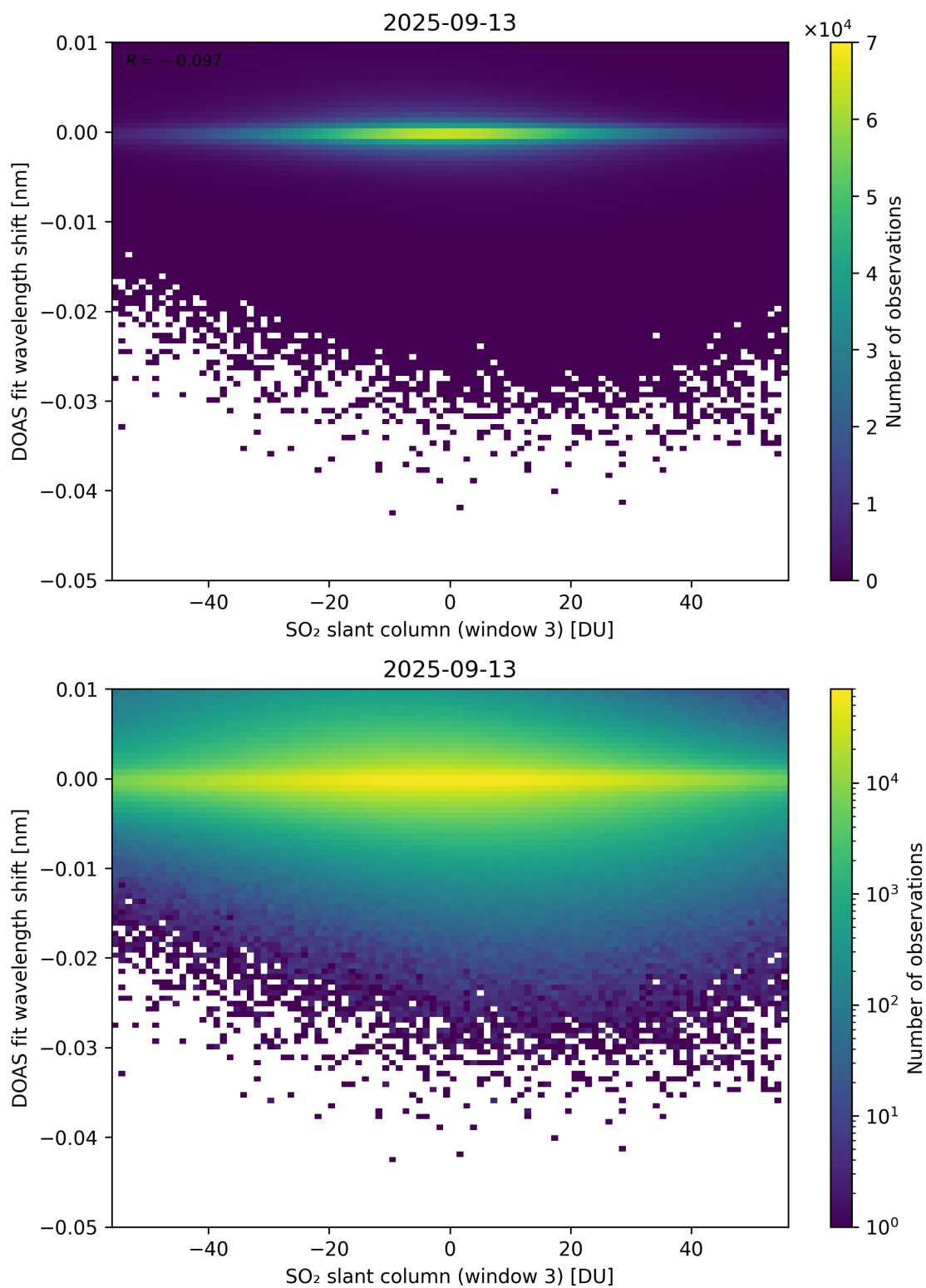
Figure 304: Scatter density plot of “SO 2 slant column (window 3)” against “DOAS fit wavelength shift” for 2025-09-12 to 2025-09-14.
