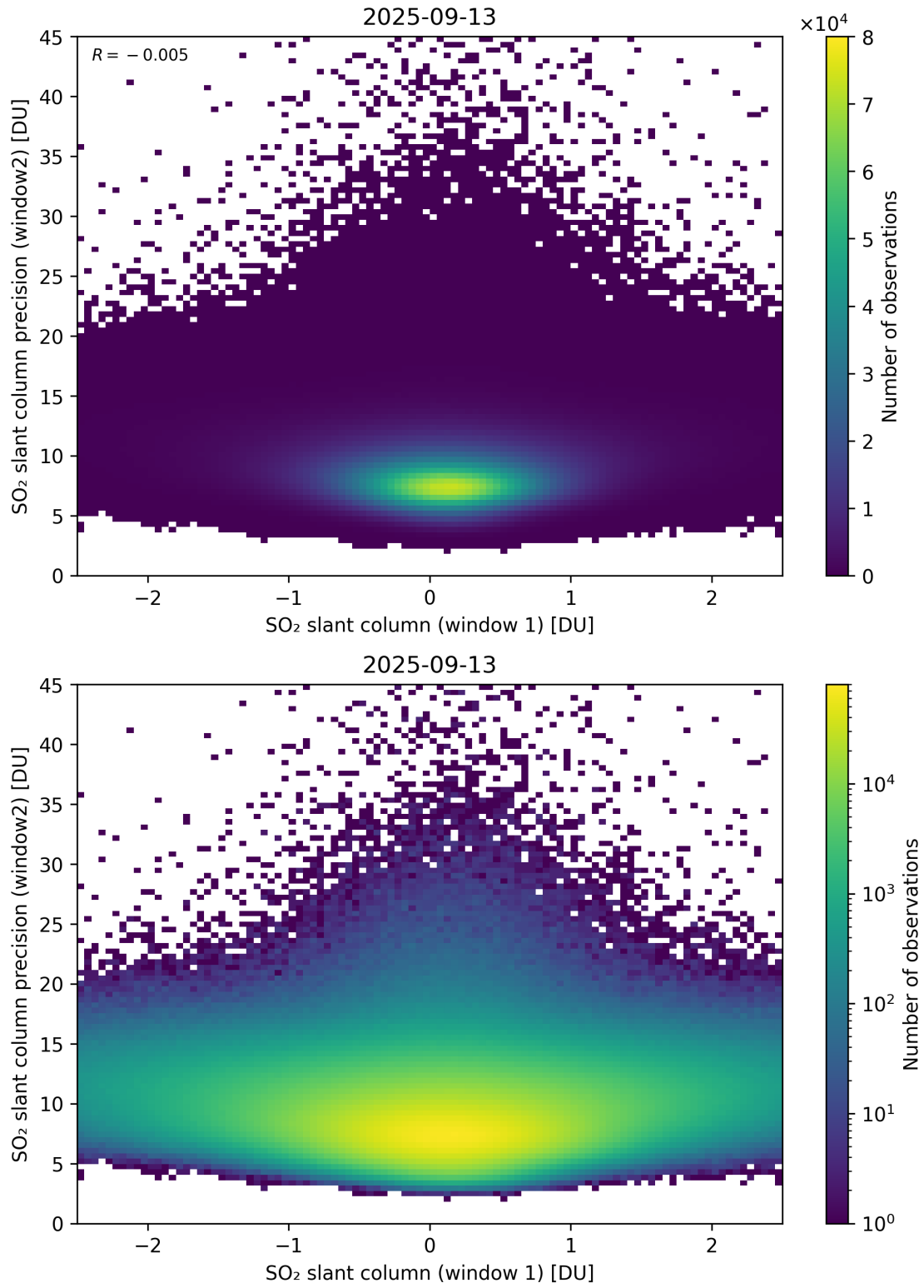
Figure 286: Scatter density plot of “SO 2 slant column (window 1)” against “SO 2 slant column precision (window2)” for 2025-09-12 to 2025-09-14.
