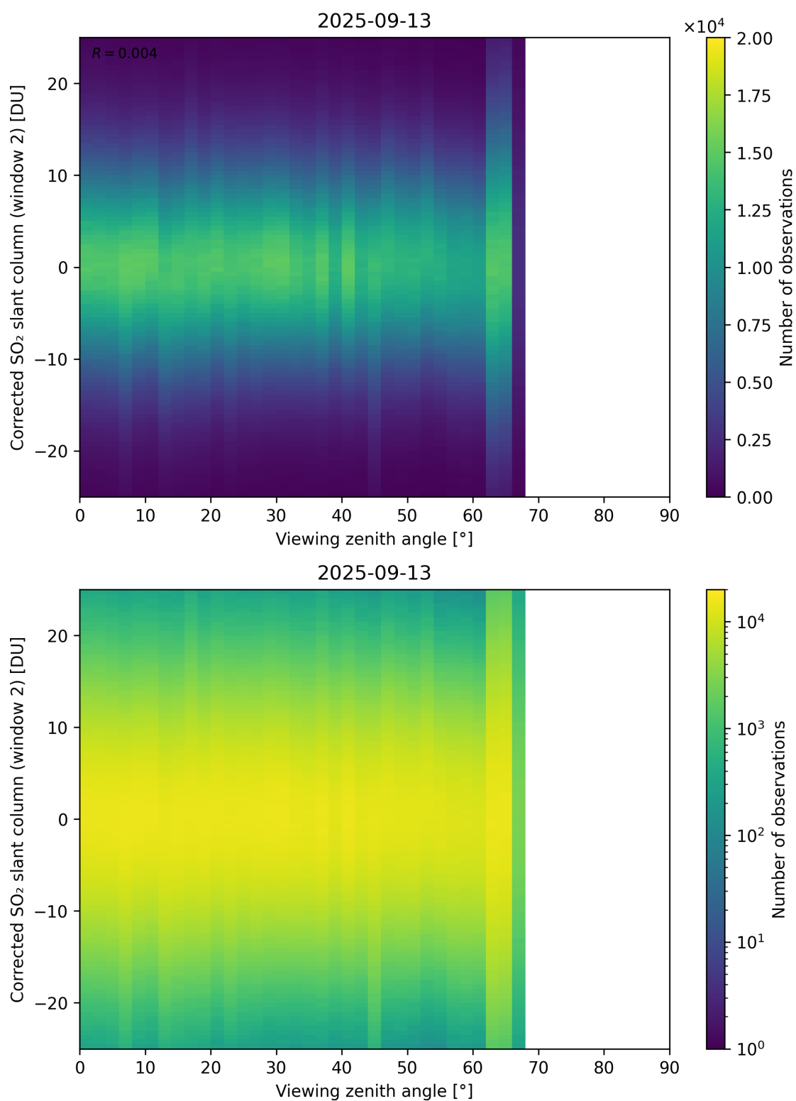
Figure 374: Scatter density plot of “Viewing zenith angle” against “Corrected SO 2 slant column (window 2)” for 2025-09-12 to 2025-09-14.
