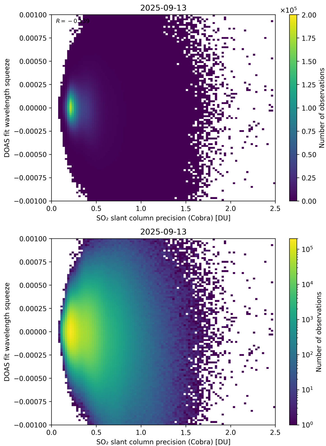
Figure 203: Scatter density plot of “SO 2 slant column precision (Cobra)” against “DOAS fit wavelength squeeze” for 2025-09-12 to 2025-09-14.
