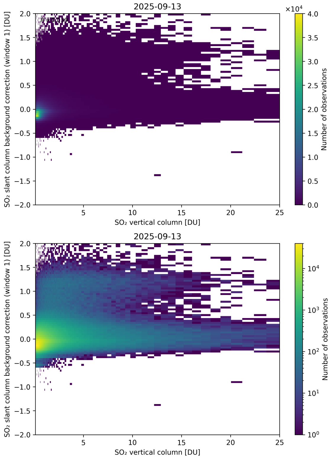
Figure 323: Scatter density plot of “SO 2 vertical column” against “SO 2 slant column background correction (window 1)” for 2025-09-12 to 2025-09-14.
