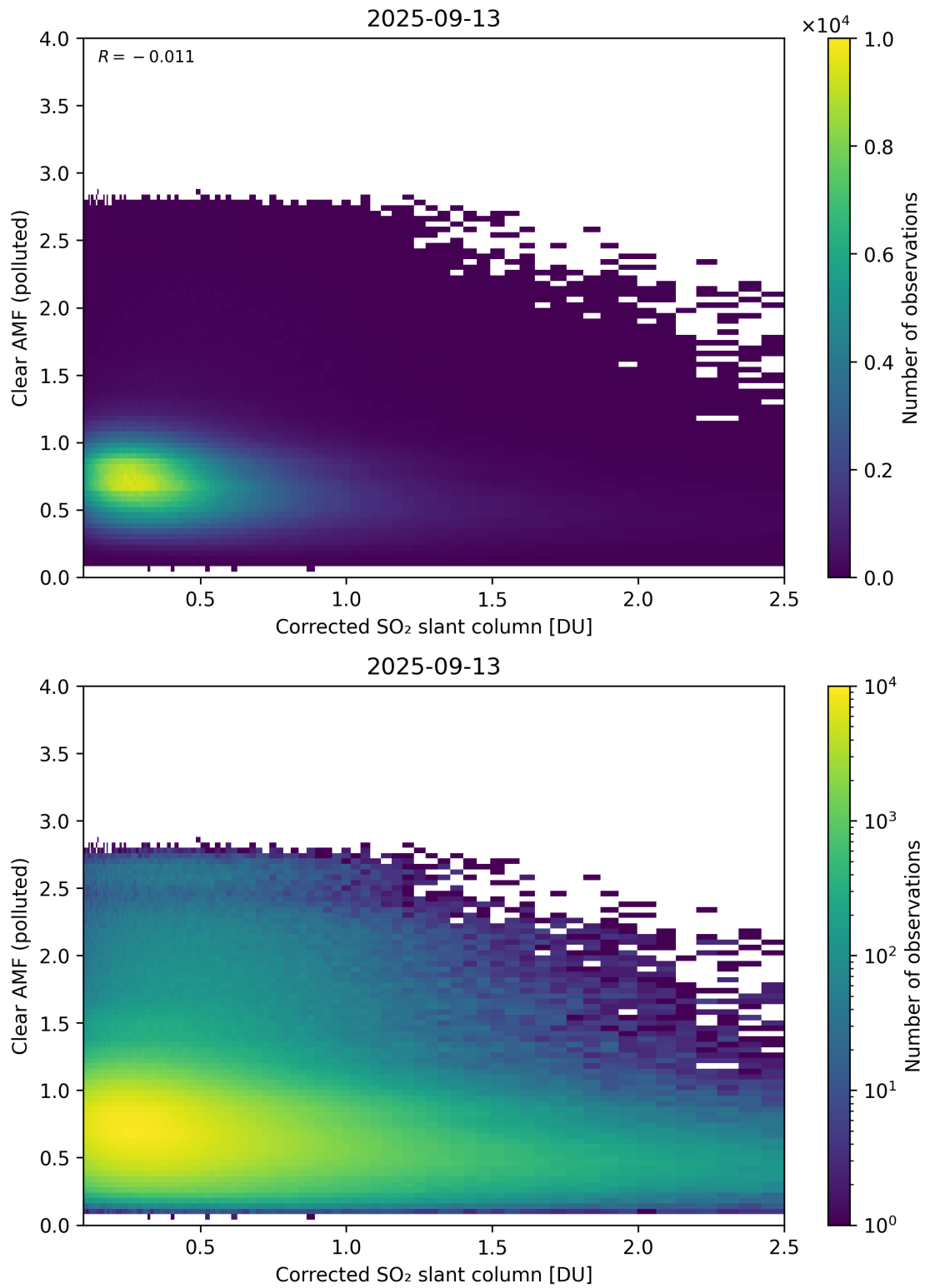
Figure 232: Scatter density plot of “Corrected SO 2 slant column” against “Clear AMF (polluted)” for 2025-09-12 to 2025-09-14.
