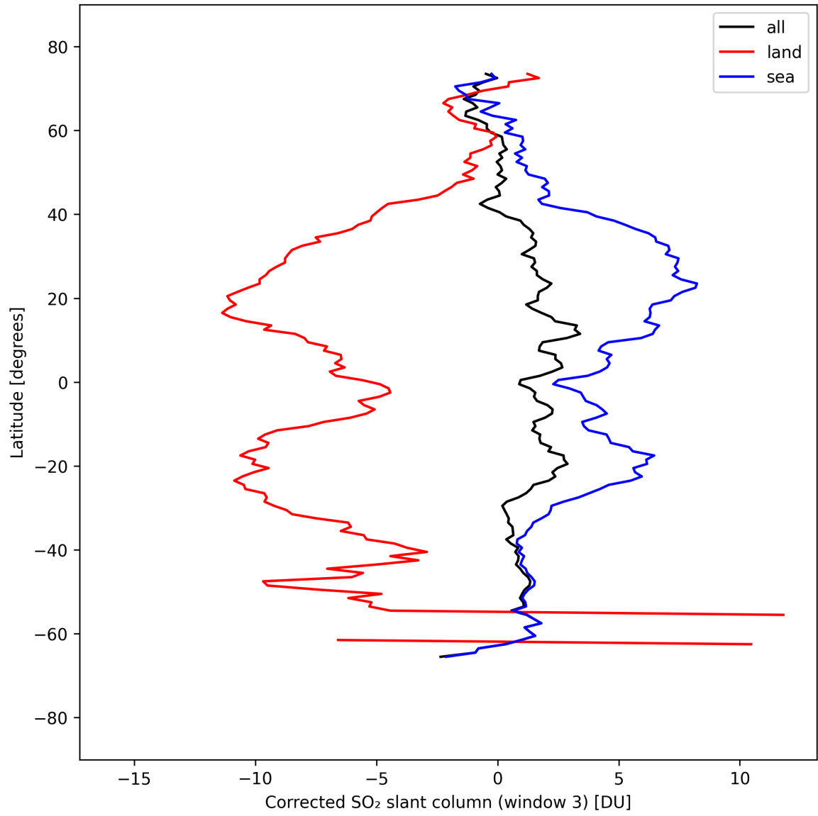
Figure 47: Zonal average of “Corrected SO 2 slant column (window 3)” for 2025-09-12 to 2025-09-14.
