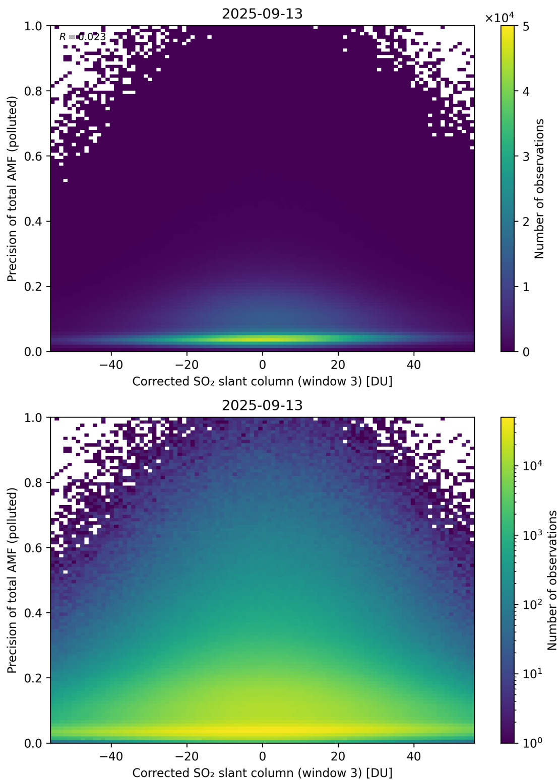
Figure 261: Scatter density plot of “Corrected SO 2 slant column (window 3)” against “Precision of total AMF (polluted)” for 2025-09-12 to 2025-09-14.
