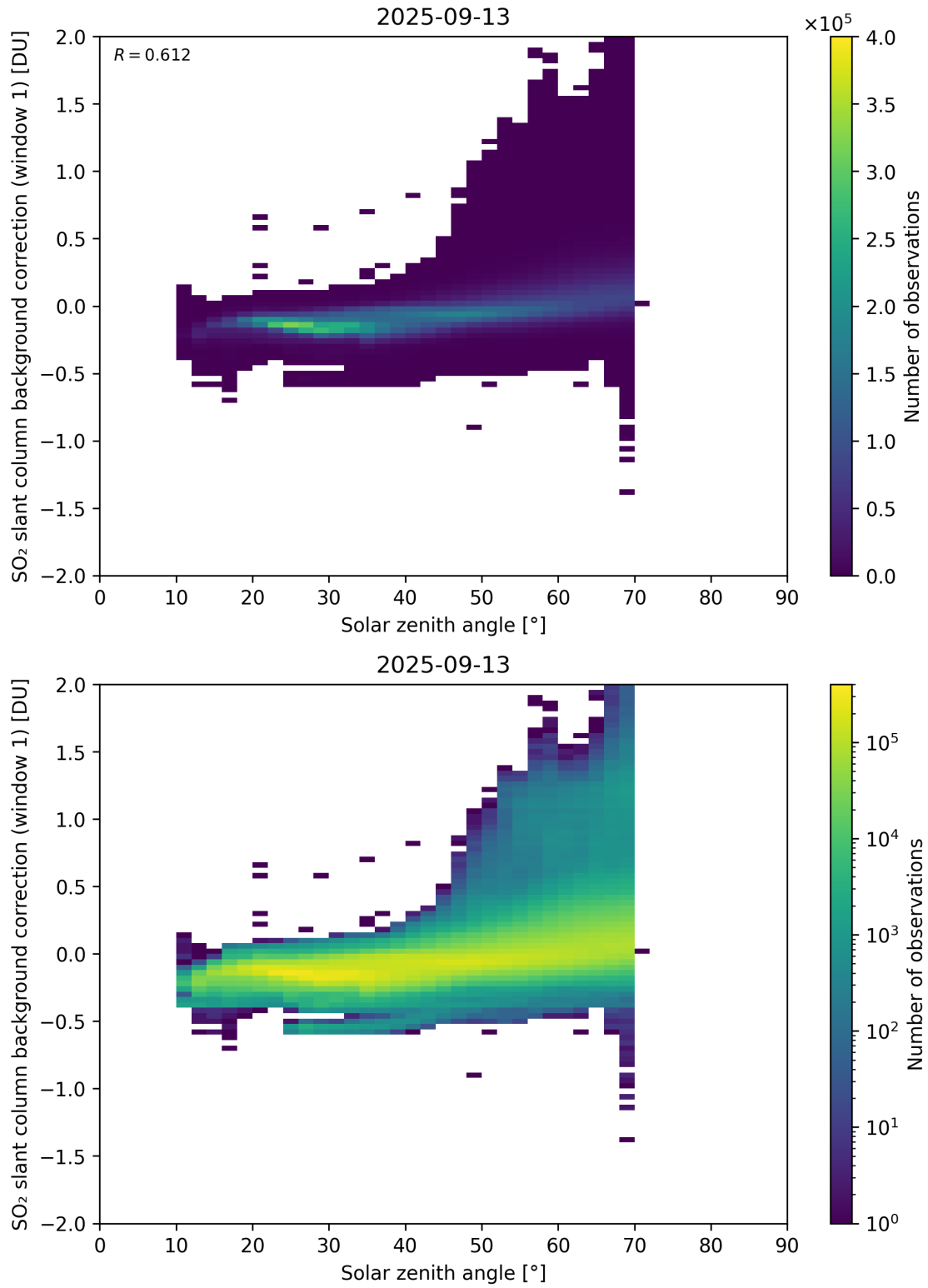
Figure 171: Scatter density plot of “Solar zenith angle” against “SO 2 slant column background correction (window 1)” for 2025-09-12 to 2025-09-14.
