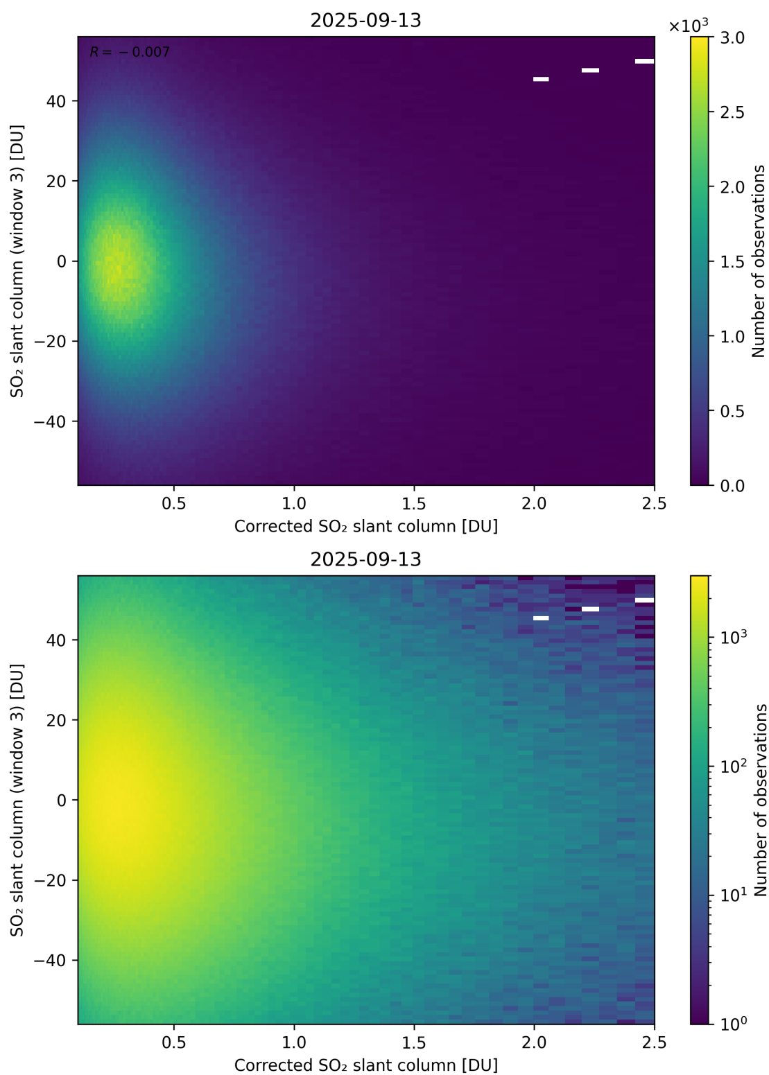
Figure 240: Scatter density plot of “Corrected SO 2 slant column” against “SO 2 slant column (window 3)” for 2025-09-12 to 2025-09-14.
