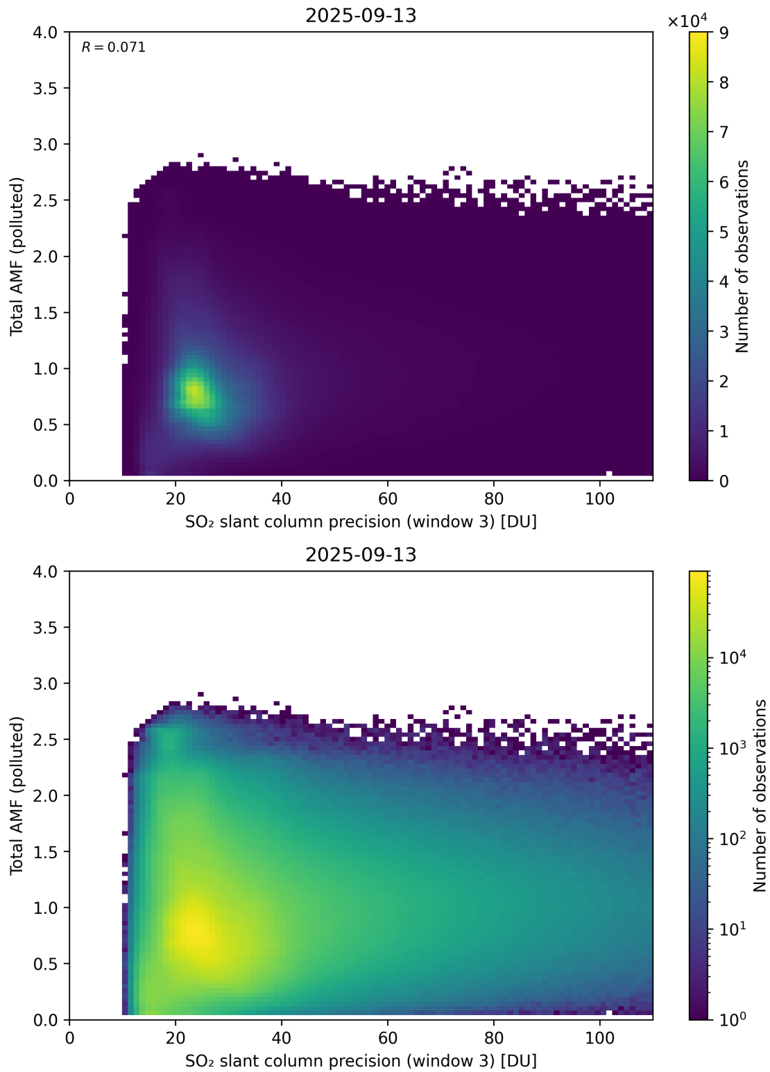
Figure 313: Scatter density plot of “SO 2 slant column precision (window 3)” against “Total AMF (polluted)” for 2025-09-12 to 2025-09-14.
