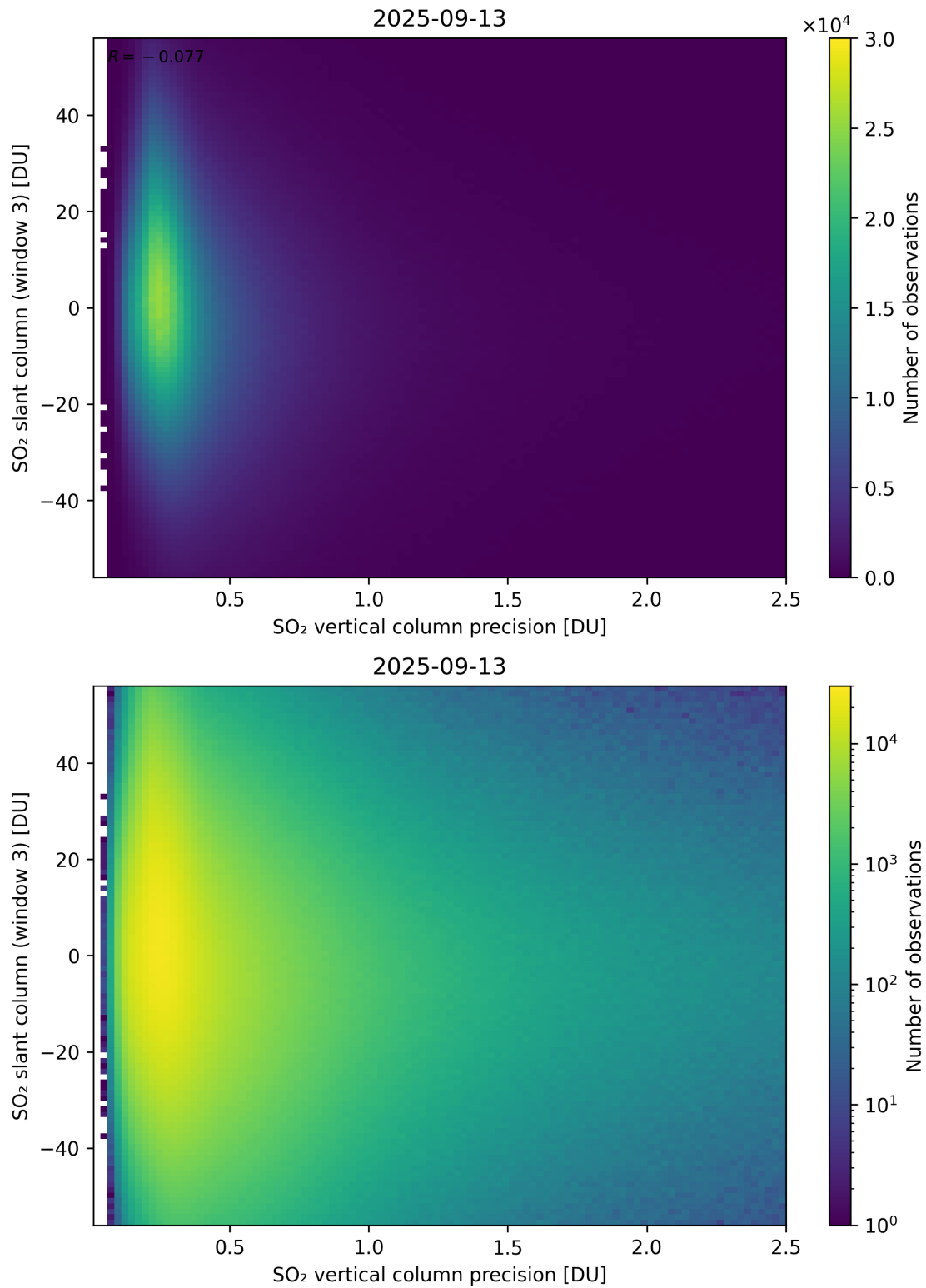
Figure 344: Scatter density plot of “SO 2 vertical column precision” against “SO 2 slant column (window 3)” for 2025-09-12 to 2025-09-14.
