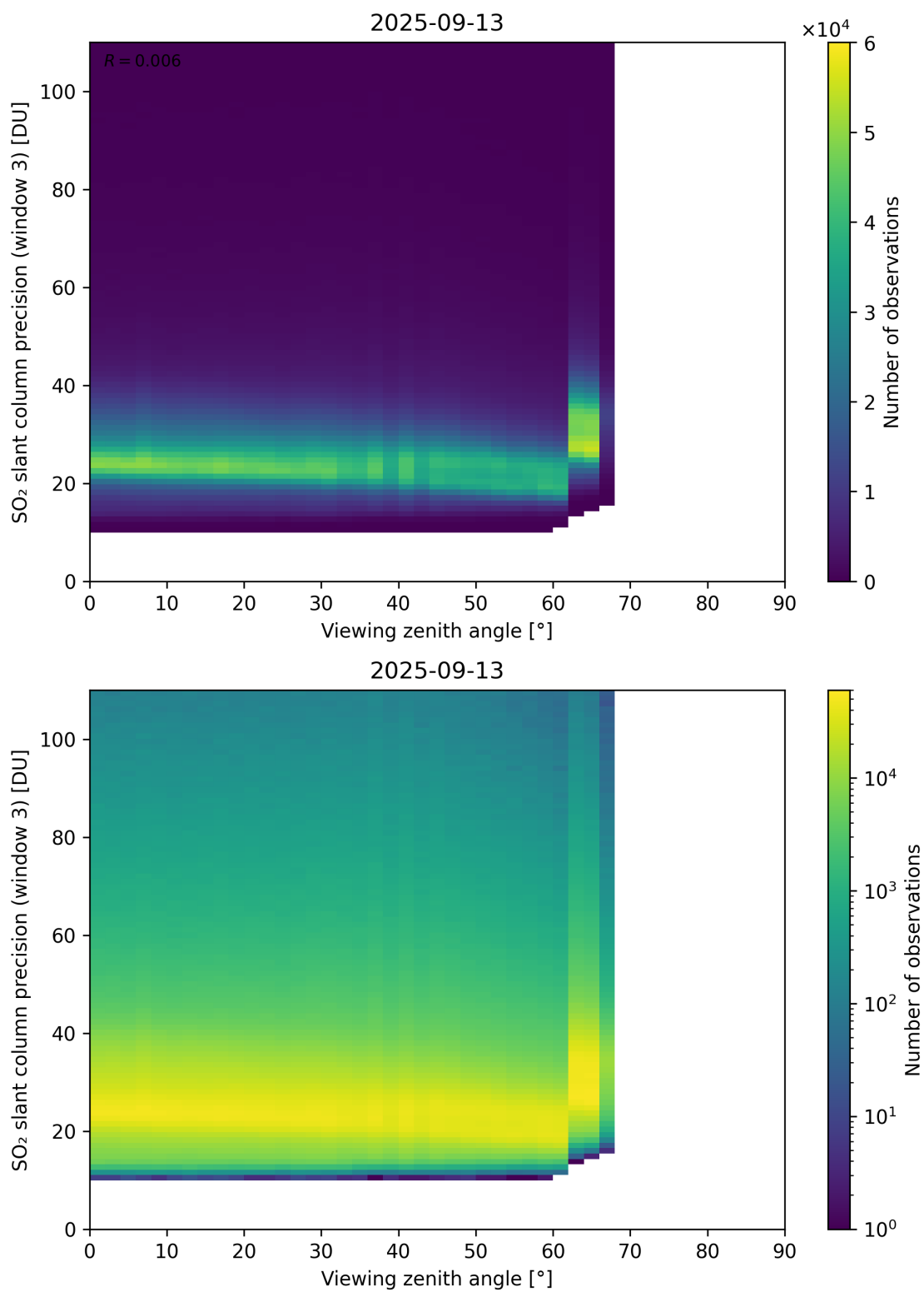
Figure 380: Scatter density plot of “Viewing zenith angle” against “SO 2 slant column precision (window 3)” for 2025-09-12 to 2025-09-14.
