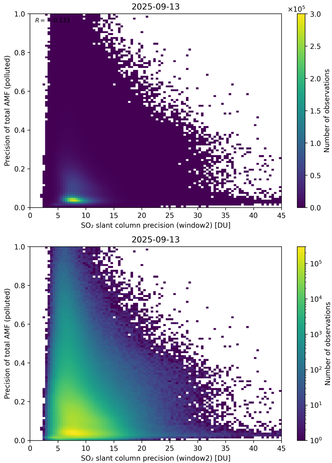
Figure 302: Scatter density plot of “SO 2 slant column precision (window2)” against “Precision of total AMF (polluted)” for 2025-09-12 to 2025-09-14.
