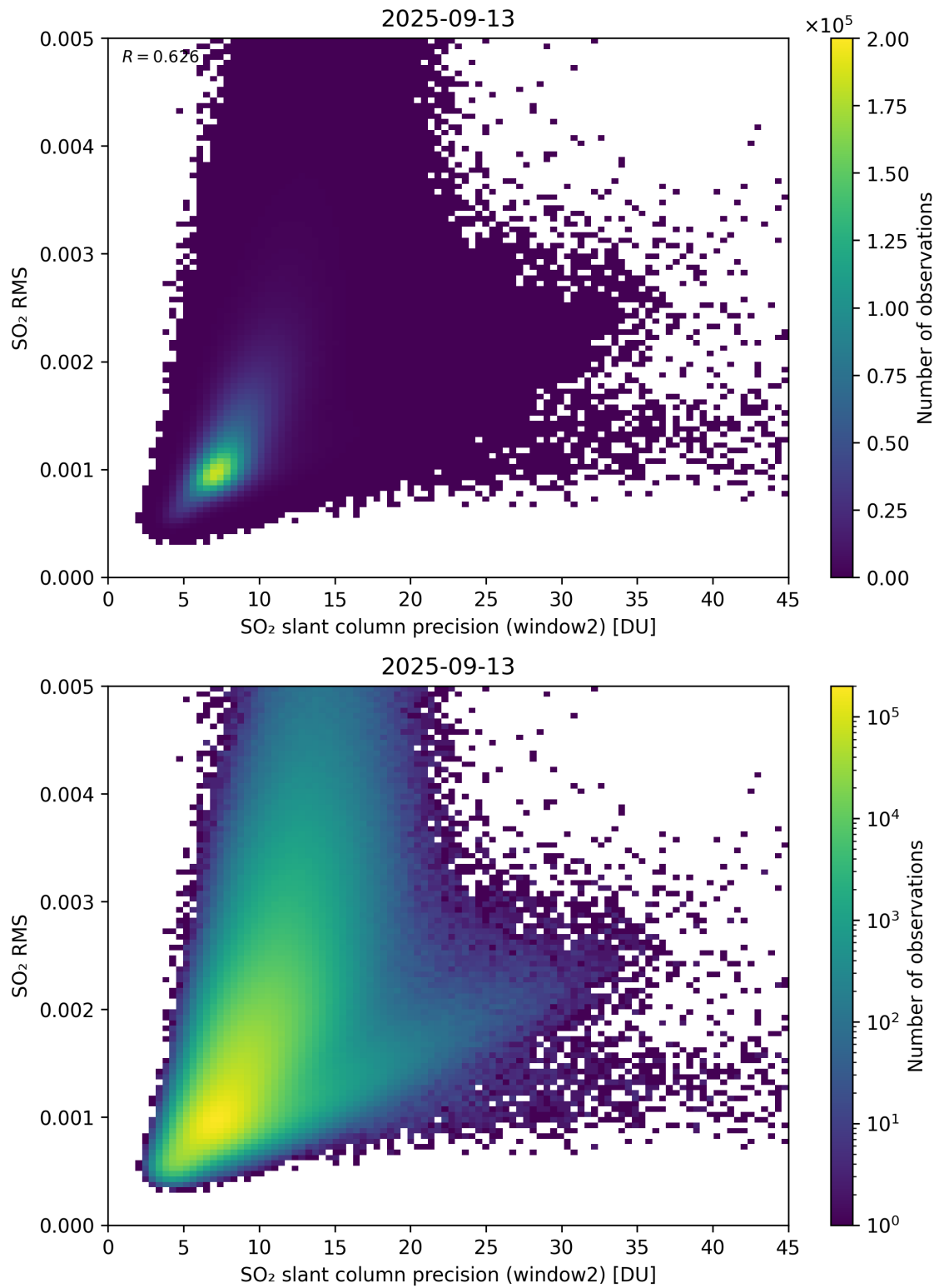
Figure 295: Scatter density plot of “SO 2 slant column precision (window2)” against “SO 2 RMS” for 2025-09-12 to 2025-09-14.
