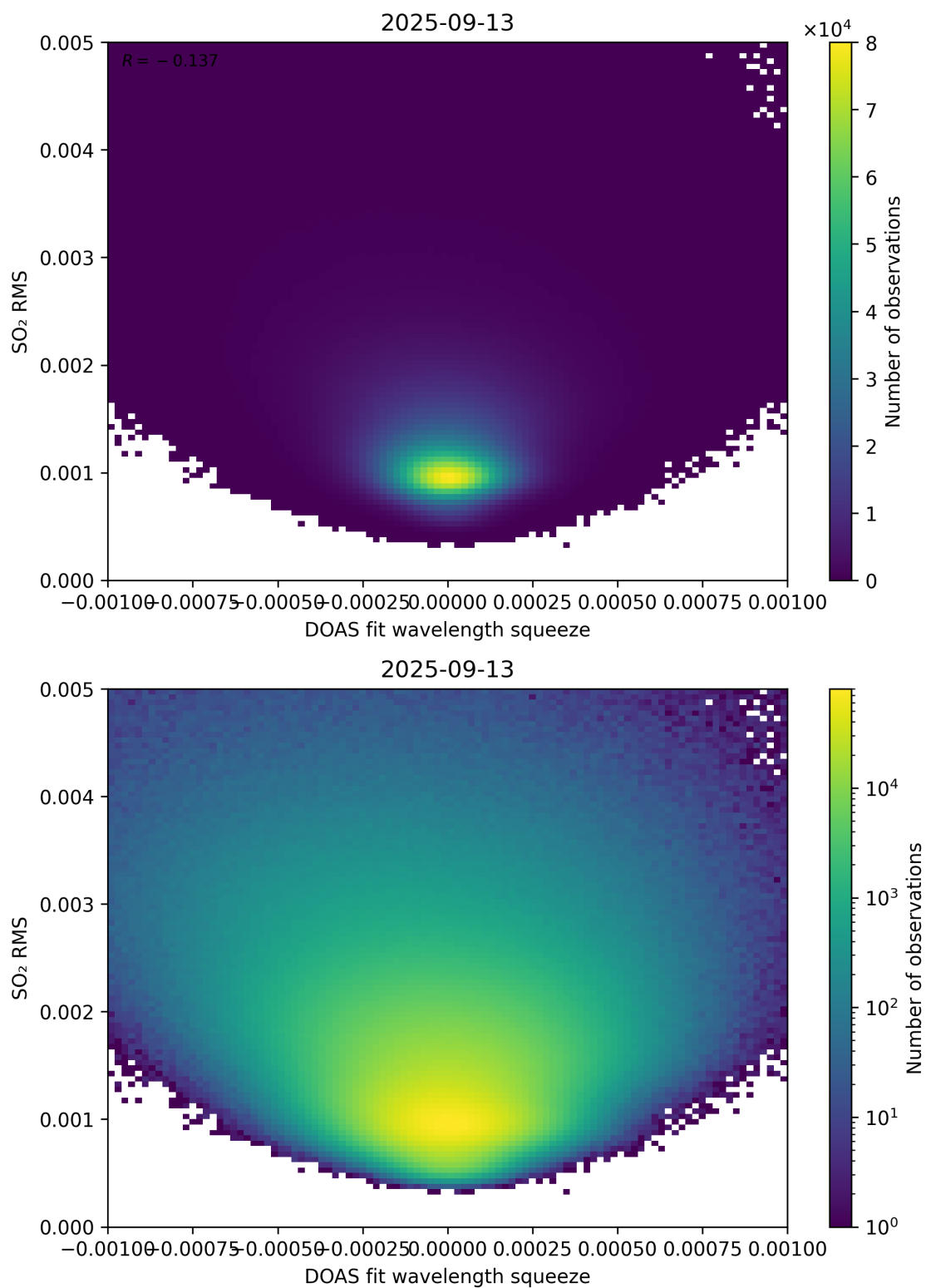
Figure 143: Scatter density plot of “DOAS fit wavelength squeeze” against “SO 2 RMS” for 2025-09-12 to 2025-09-14.
