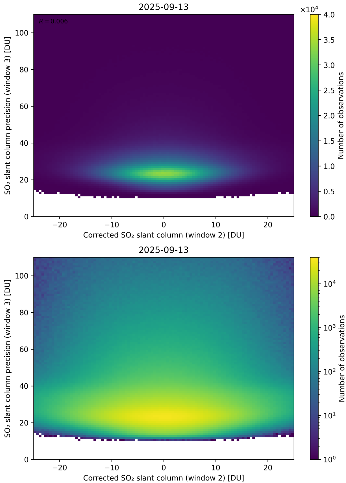
Figure 252: Scatter density plot of “Corrected SO 2 slant column (window 2)” against “SO 2 slant column precision (window 3)” for 2025-09-12 to 2025-09-14.
