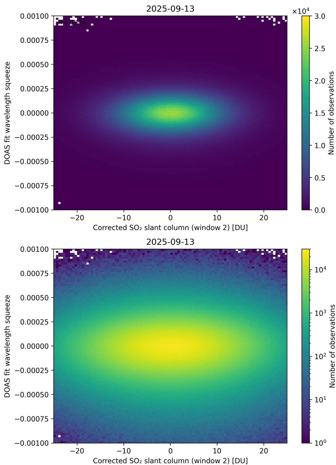
Figure 247: Scatter density plot of “Corrected SO 2 slant column (window 2)” against “DOAS fit wavelength squeeze” for 2025-09-12 to 2025-09-14.
