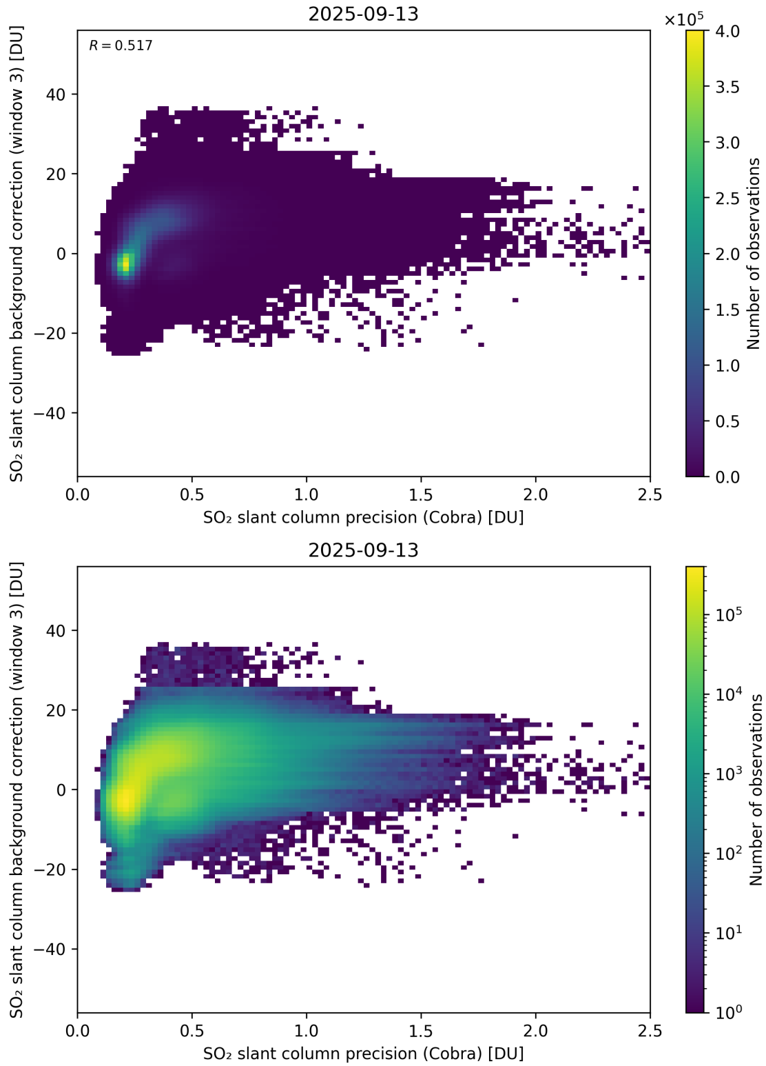
Figure 201: Scatter density plot of “SO 2 slant column precision (Cobra)” against “SO 2 slant column background correction (window 3)” for 2025-09-12 to 2025-09-14.
