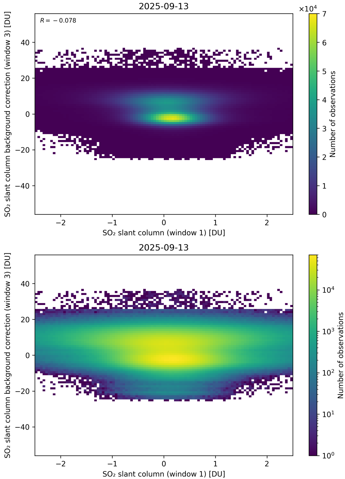
Figure 264: Scatter density plot of “SO 2 slant column (window 1)” against “SO 2 slant column background correction (window 3)” for 2025-09-12 to 2025-09-14.
