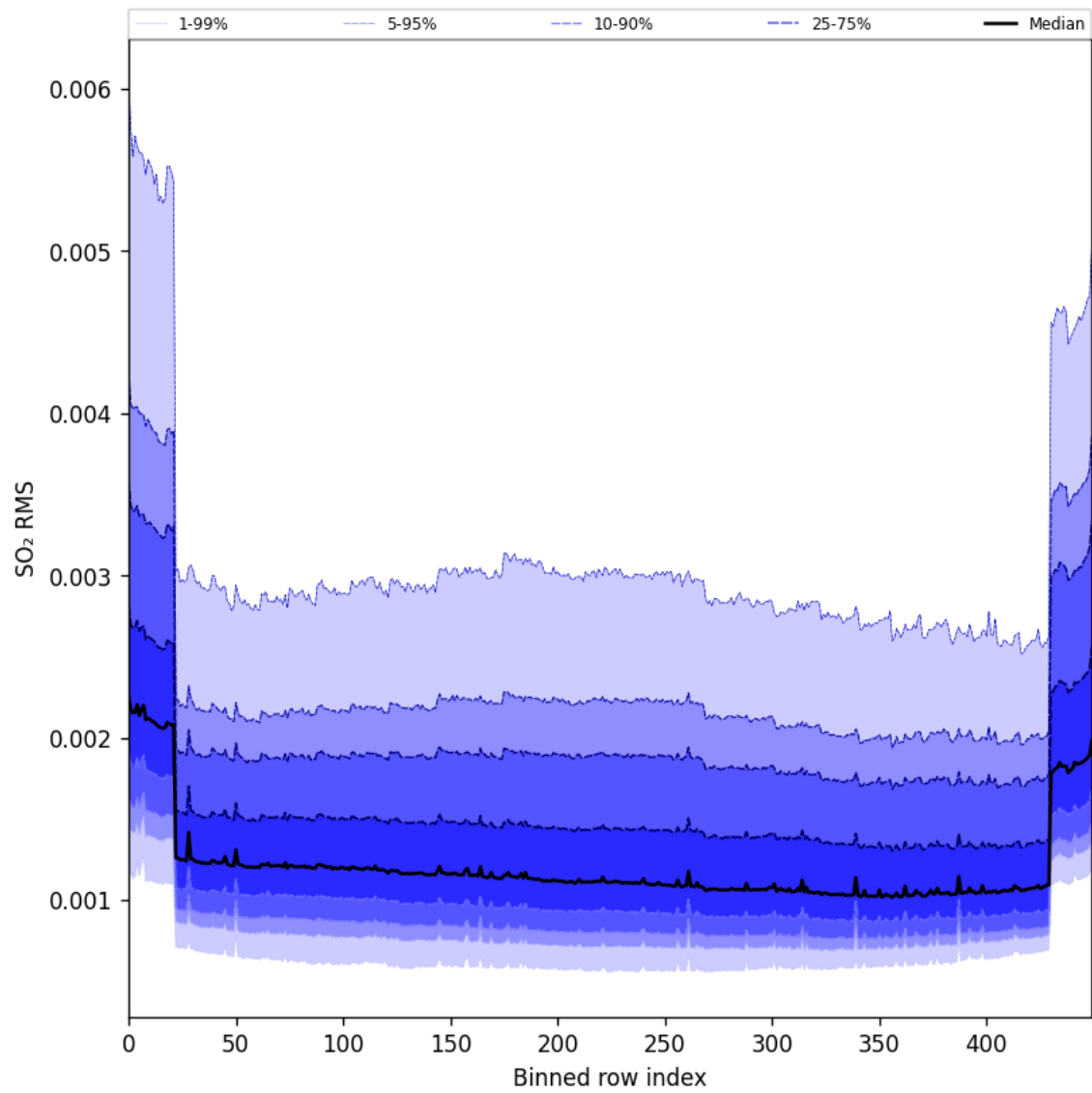
Figure 104: Along track statistics of “SO 2 RMS” for 2025-09-12 to 2025-09-14
