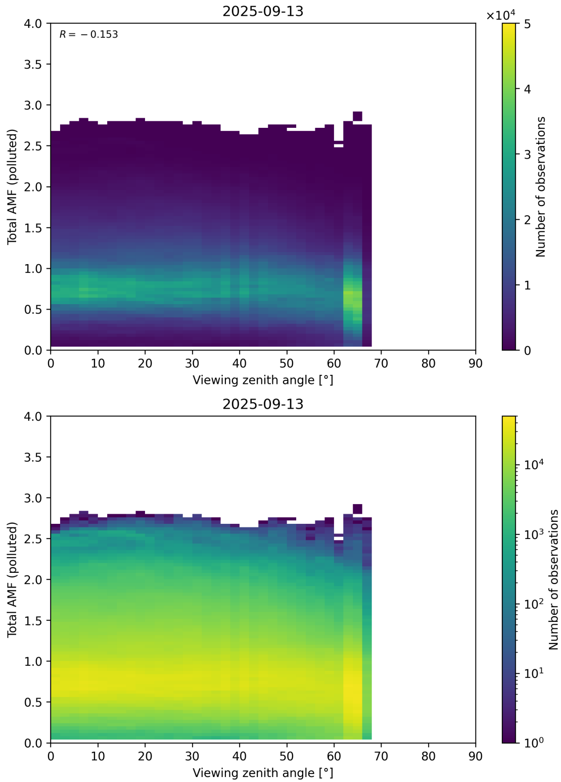
Figure 381: Scatter density plot of “Viewing zenith angle” against “Total AMF (polluted)” for 2025-09-12 to 2025-09-14.
