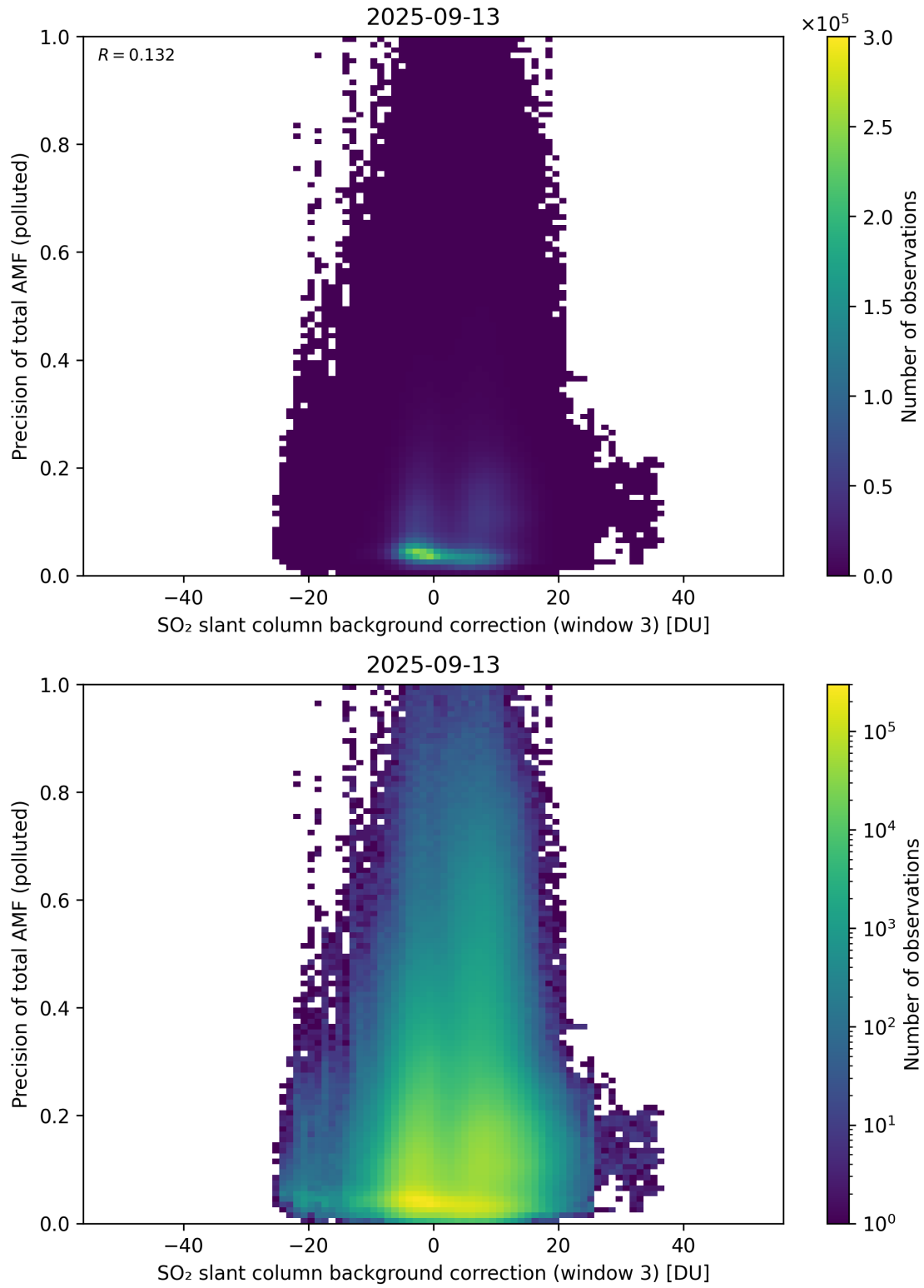
Figure 137: Scatter density plot of “SO 2 slant column background correction (window 3)” against “Precision of total AMF (polluted)” for 2025-09-12 to 2025-09-14.
