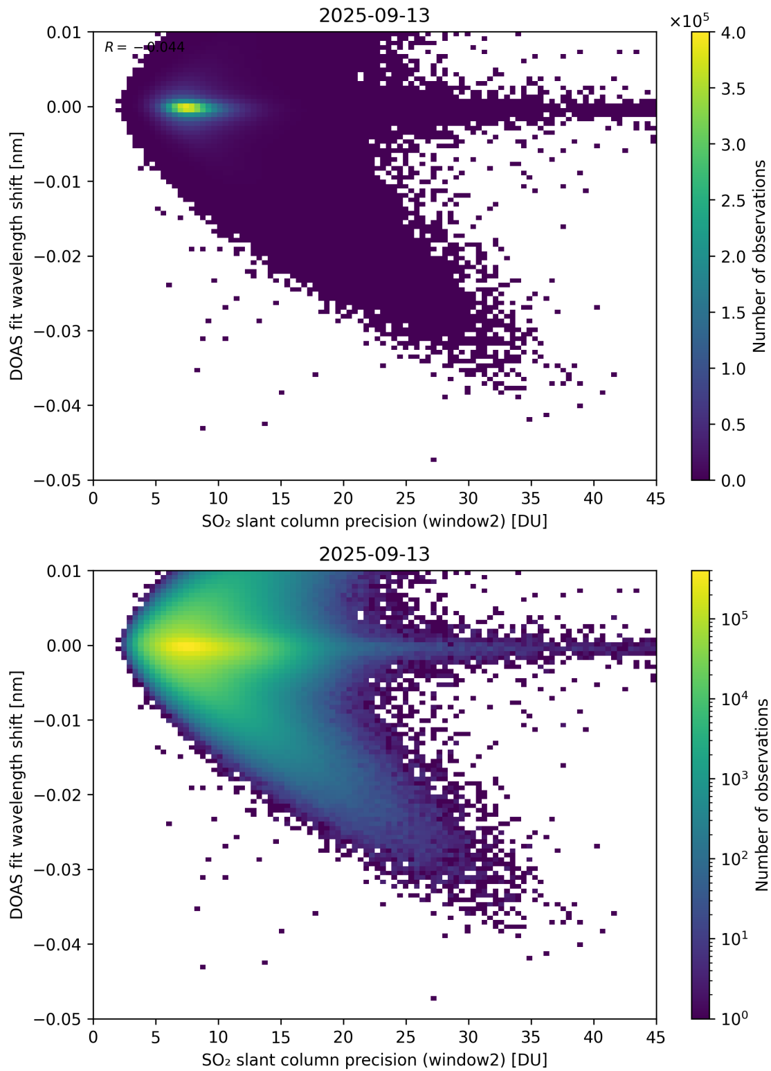
Figure 293: Scatter density plot of “SO 2 slant column precision (window2)” against “DOAS fit wavelength shift” for 2025-09-12 to 2025-09-14.
