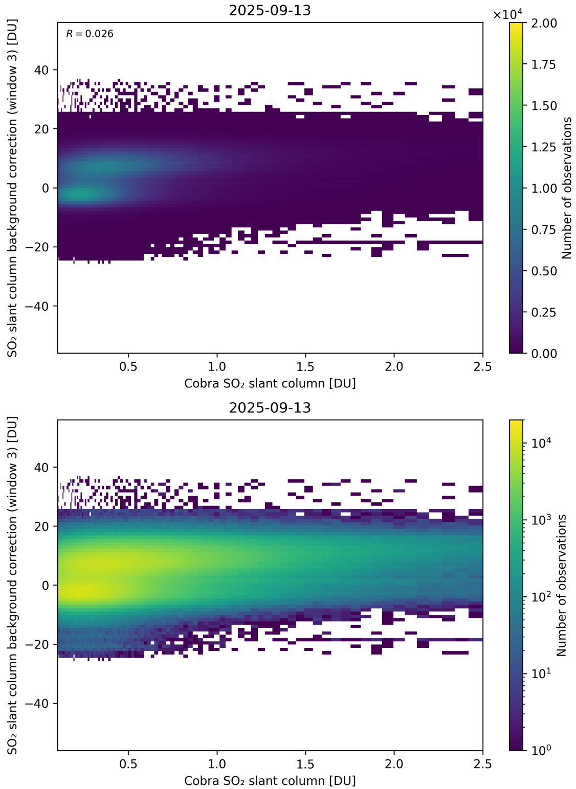
Figure 195: Scatter density plot of “Cobra SO 2 slant column” against “SO 2 slant column background correction (window 3)” for 2025-09-12 to 2025-09-14.
