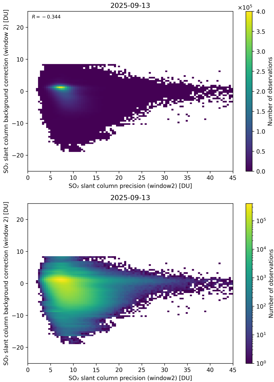
Figure 291: Scatter density plot of “SO 2 slant column precision (window2)” against “SO 2 slant column background correction (window 2)” for 2025-09-12 to 2025-09-14.
