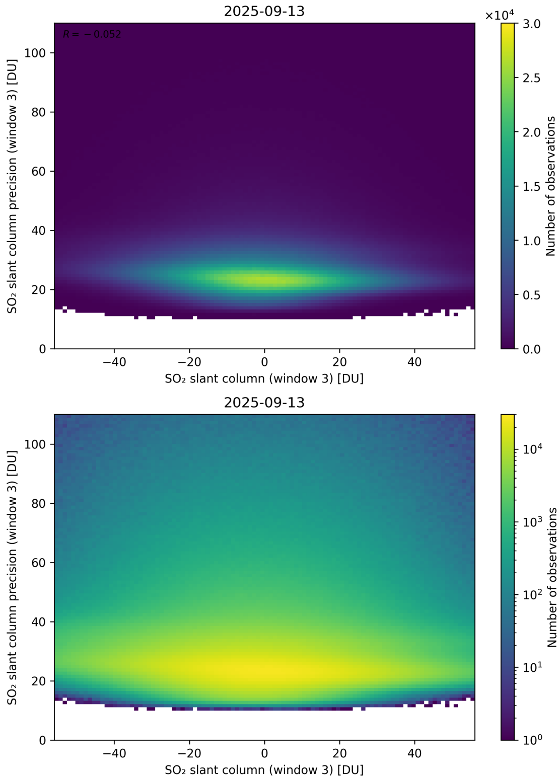
Figure 317: Scatter density plot of “SO 2 slant column (window 3)” against “SO 2 slant column precision (window 3)” for 2025-09-12 to 2025-09-14.
