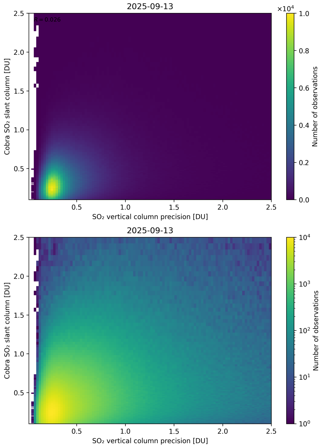
Figure 336: Scatter density plot of “SO 2 vertical column precision” against “Cobra SO 2 slant column” for 2025-09-12 to 2025-09-14.
