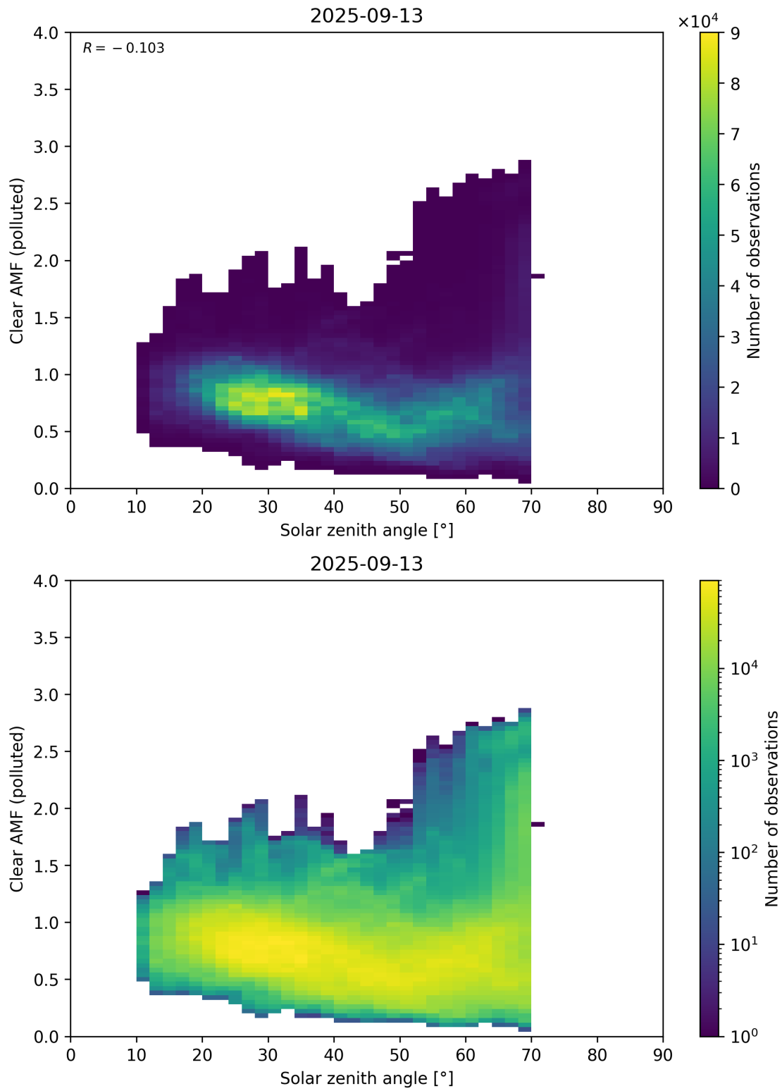
Figure 178: Scatter density plot of “Solar zenith angle” against “Clear AMF (polluted)” for 2025-09-12 to 2025-09-14.
