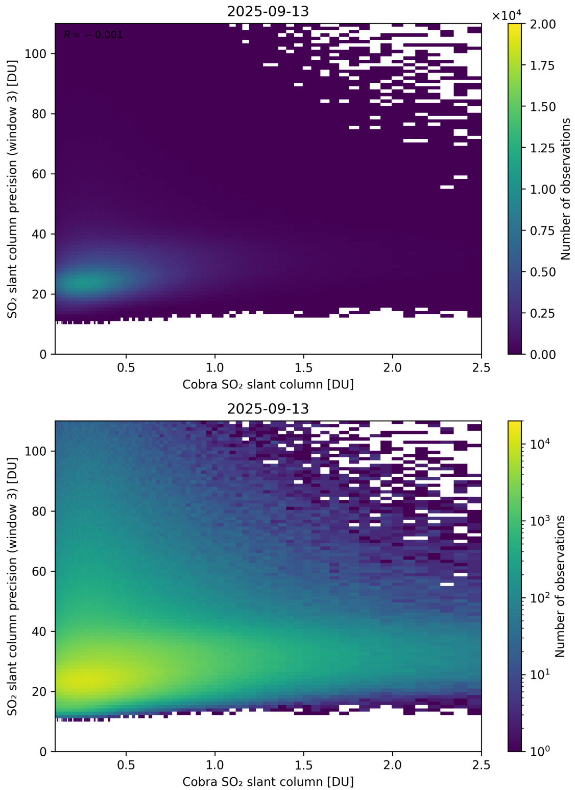
Figure 223: Scatter density plot of “Cobra SO 2 slant column” against “SO 2 slant column precision (window 3)” for 2025-09-12 to 2025-09-14.
