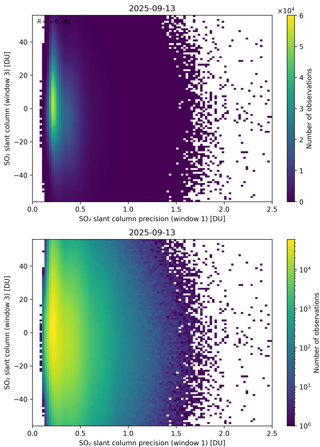
Figure 278: Scatter density plot of “SO 2 slant column precision (window 1)” against “SO 2 slant column (window 3)” for 2025-09-12 to 2025-09-14.
