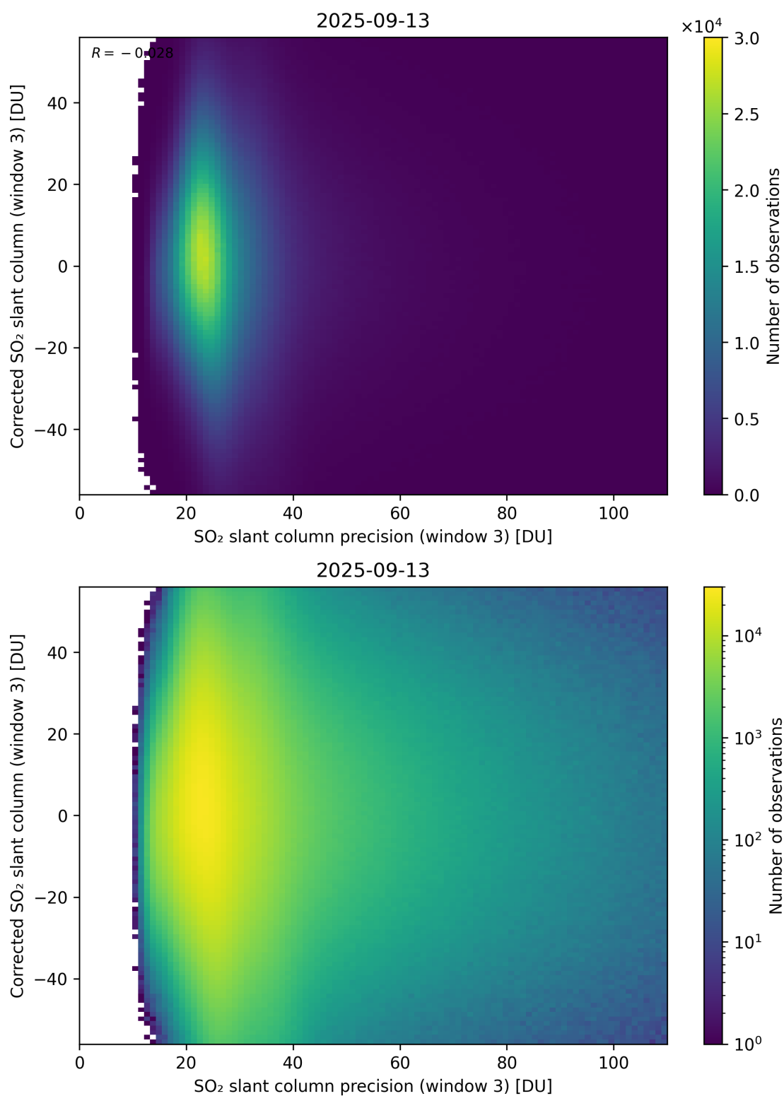
Figure 312: Scatter density plot of “SO 2 slant column precision (window 3)” against “Corrected SO 2 slant column (window 3)” for 2025-09-12 to 2025-09-14.
