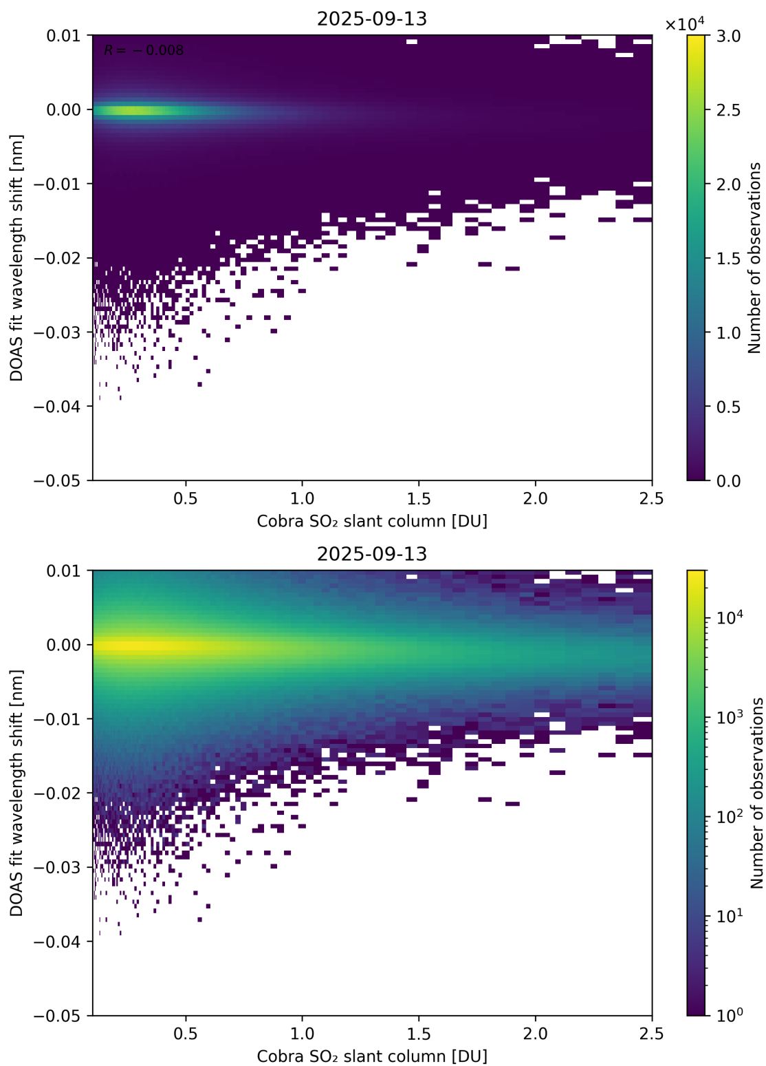
Figure 196: Scatter density plot of “Cobra SO 2 slant column” against “DOAS fit wavelength shift” for 2025-09-12 to 2025-09-14.
