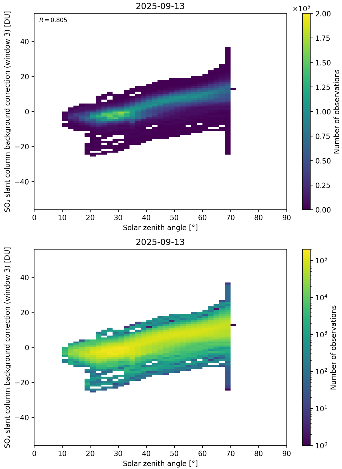
Figure 173: Scatter density plot of “Solar zenith angle” against “SO 2 slant column background correction (window 3)” for 2025-09-12 to 2025-09-14.
