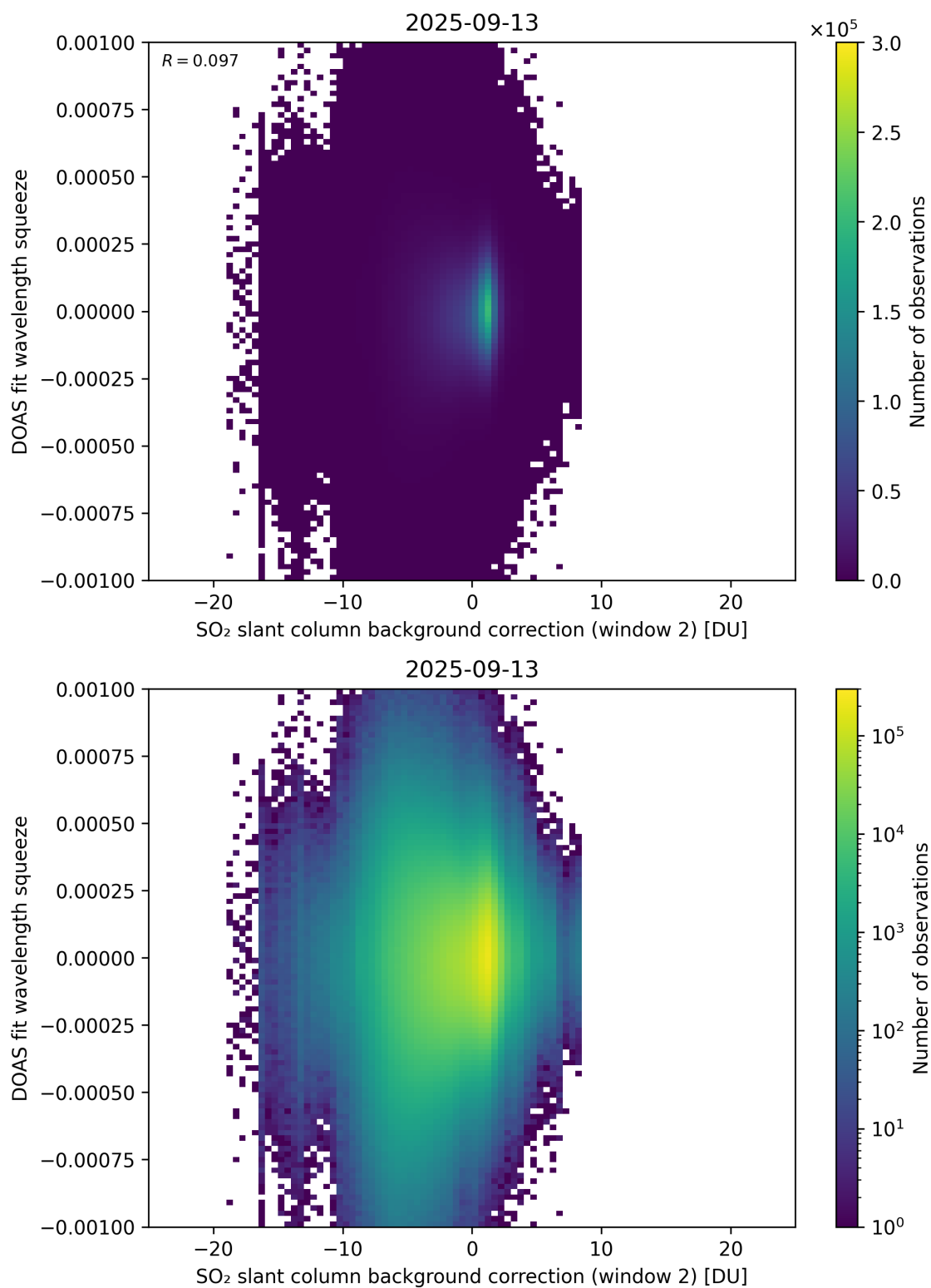
Figure 124: Scatter density plot of “SO 2 slant column background correction (window 2)” against “DOAS fit wavelength squeeze” for 2025-09-12 to 2025-09-14.
