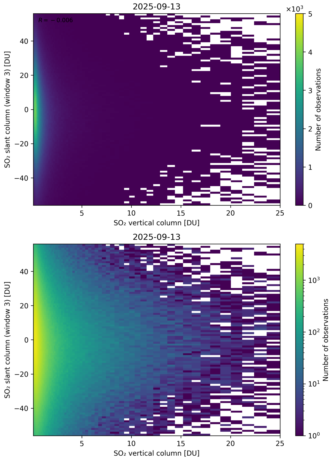
Figure 357: Scatter density plot of “SO 2 vertical column” against “SO 2 slant column (window 3)” for 2025-09-12 to 2025-09-14.
