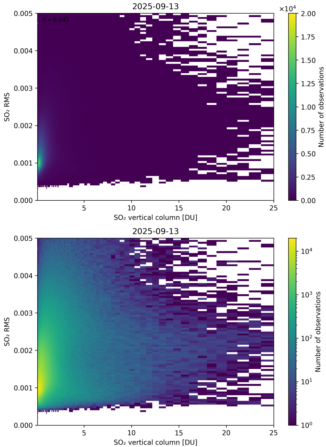
Figure 328: Scatter density plot of “SO 2 vertical column” against “SO 2 RMS” for 2025-09-12 to 2025-09-14.
