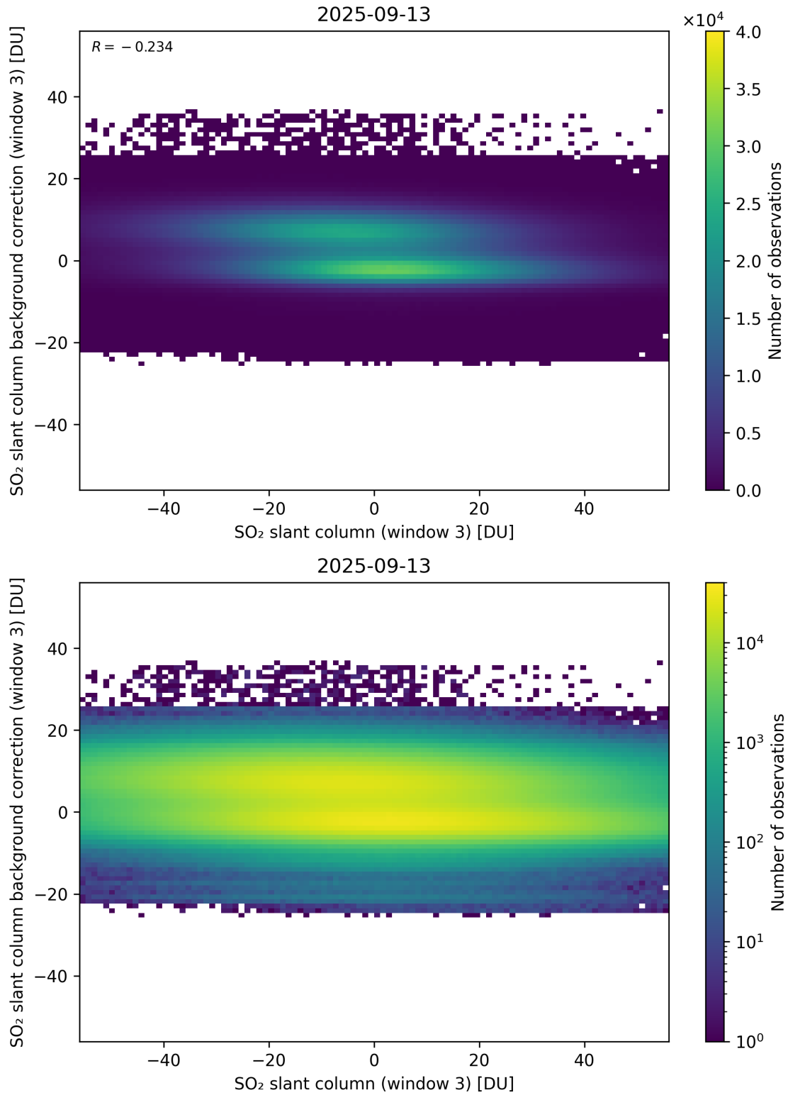
Figure 303: Scatter density plot of “SO 2 slant column (window 3)” against “SO 2 slant column background correction (window 3)” for 2025-09-12 to 2025-09-14.
