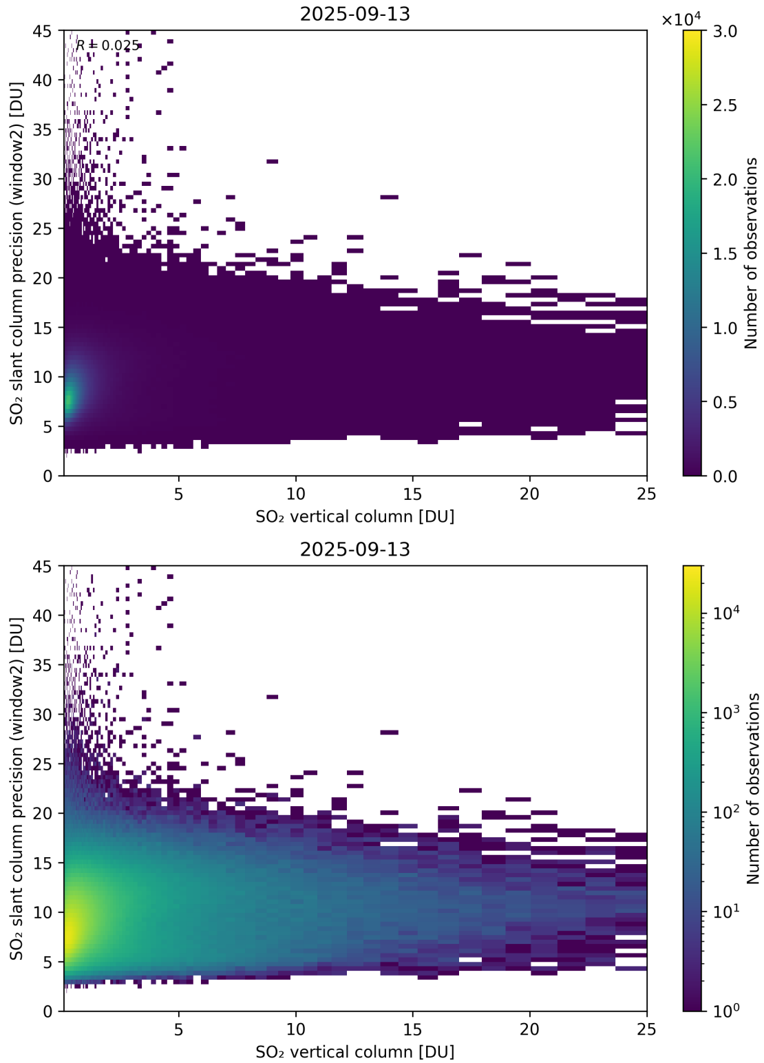
Figure 356: Scatter density plot of “SO 2 vertical column” against “SO 2 slant column precision (window2)” for 2025-09-12 to 2025-09-14.
