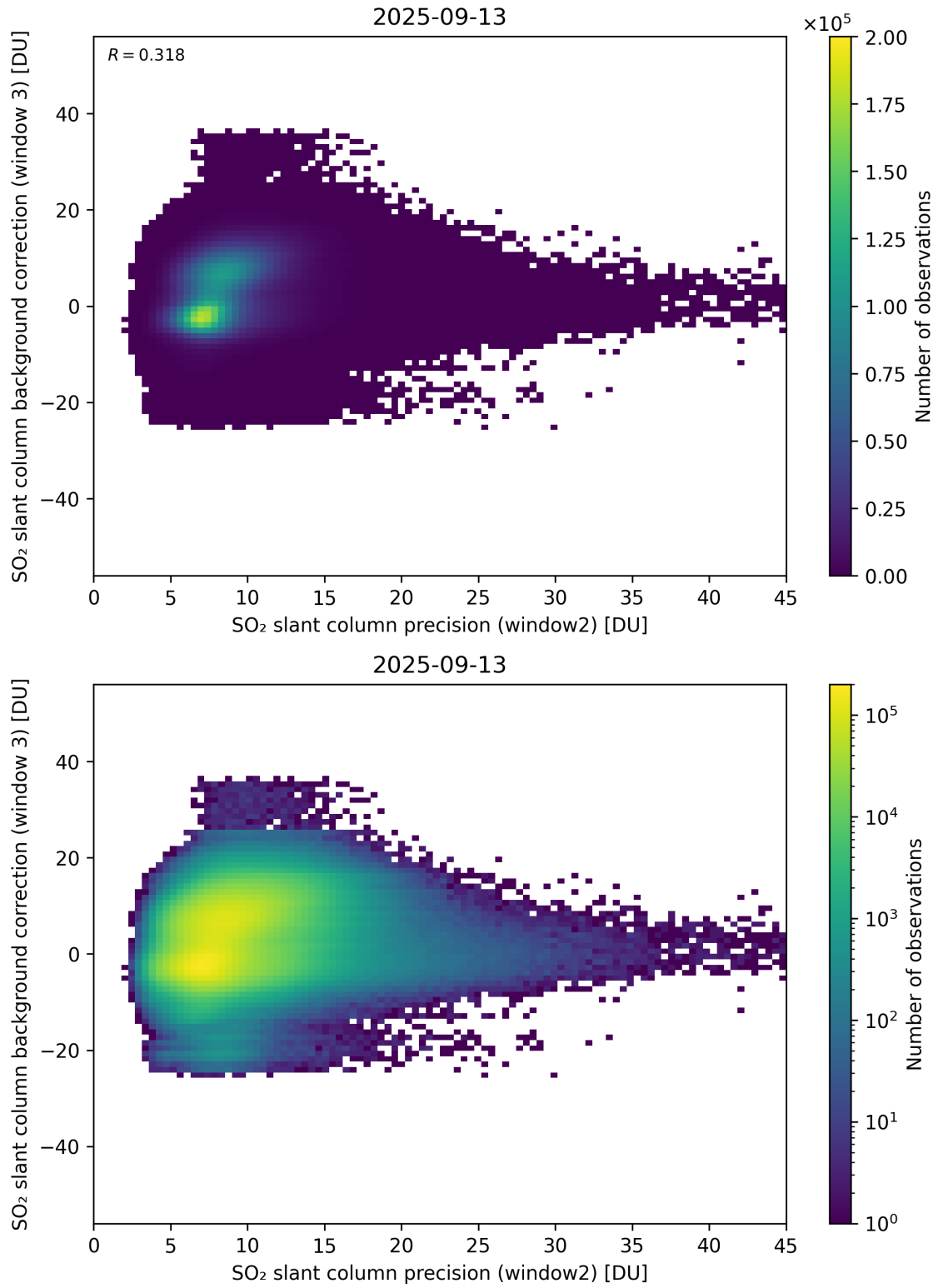
Figure 292: Scatter density plot of “SO 2 slant column precision (window2)” against “SO 2 slant column background correction (window 3)” for 2025-09-12 to 2025-09-14.
