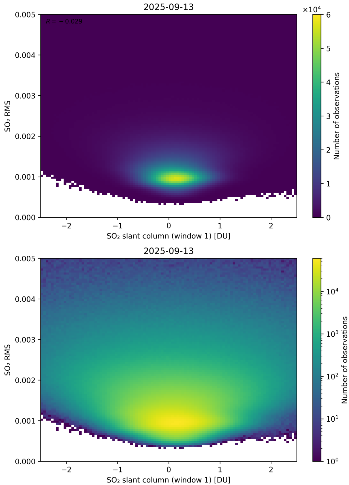
Figure 267: Scatter density plot of “SO 2 slant column (window 1)” against “SO 2 RMS” for 2025-09-12 to 2025-09-14.
