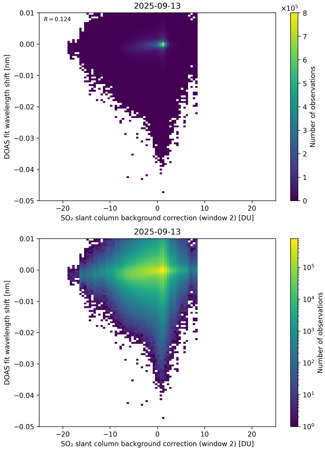
Figure 123: Scatter density plot of “SO 2 slant column background correction (window 2)” against “DOAS fit wavelength shift” for 2025-09-12 to 2025-09-14.
