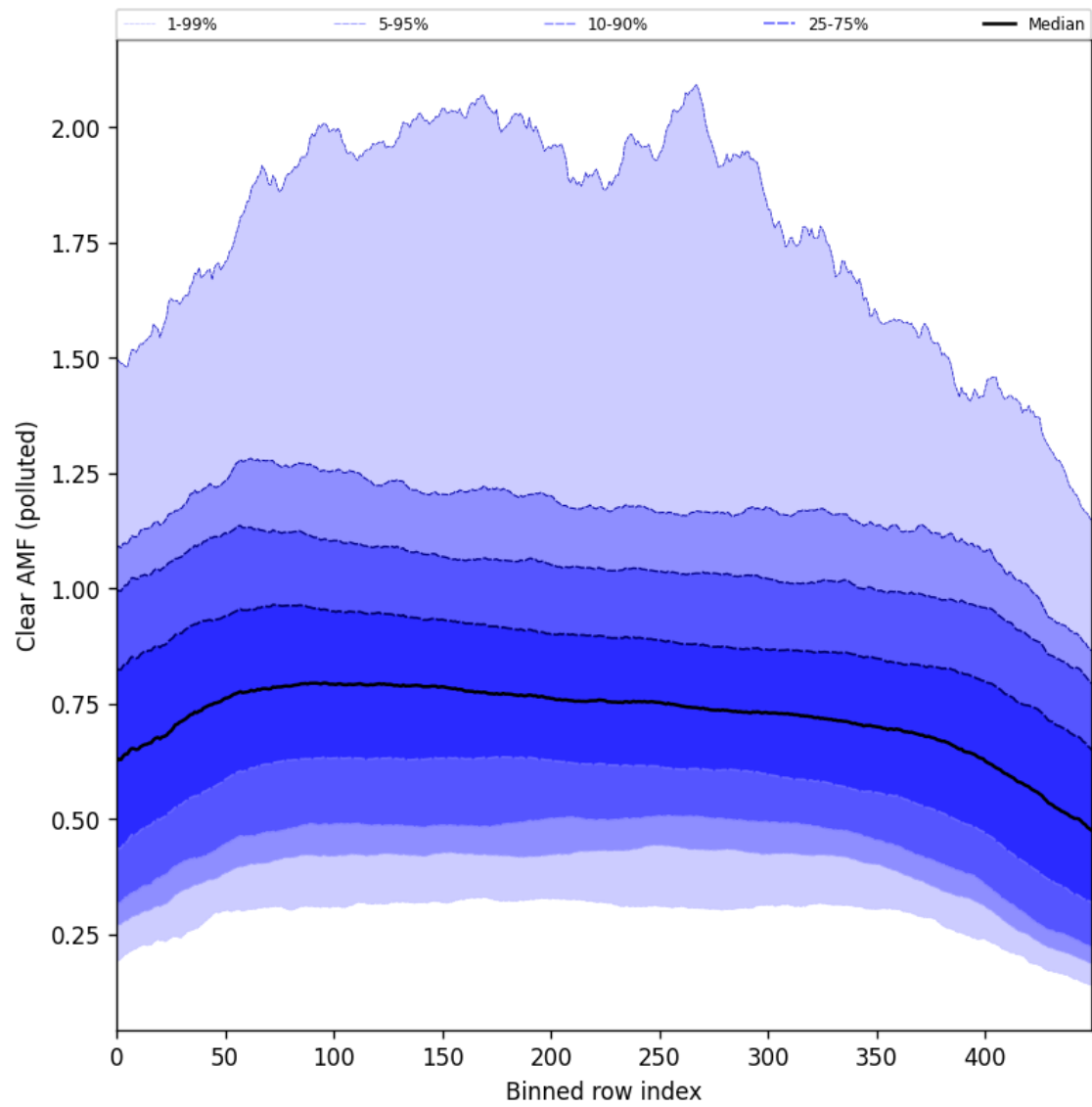
Figure 107: Along track statistics of “Clear AMF (polluted)” for 2025-09-12 to 2025-09-14
