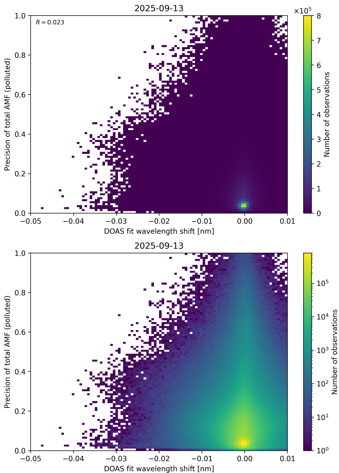
Figure 142: Scatter density plot of “DOAS fit wavelength shift” against “Precision of total AMF (polluted)” for 2025-09-12 to 2025-09-14.
