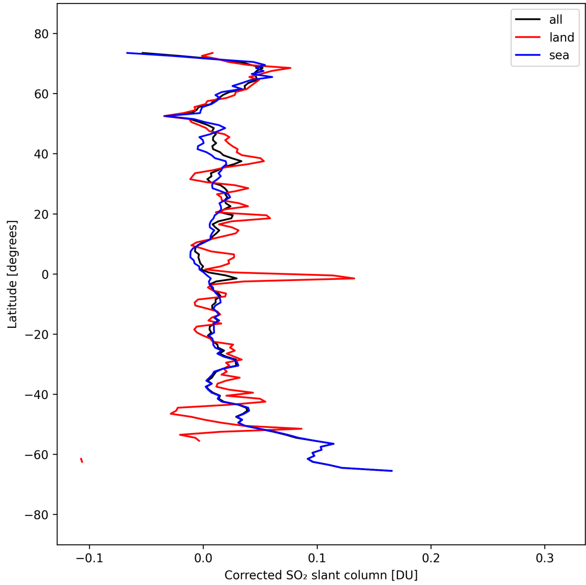
Figure 34: Zonal average of “Corrected SO 2 slant column” for 2025-09-12 to 2025-09-14.
