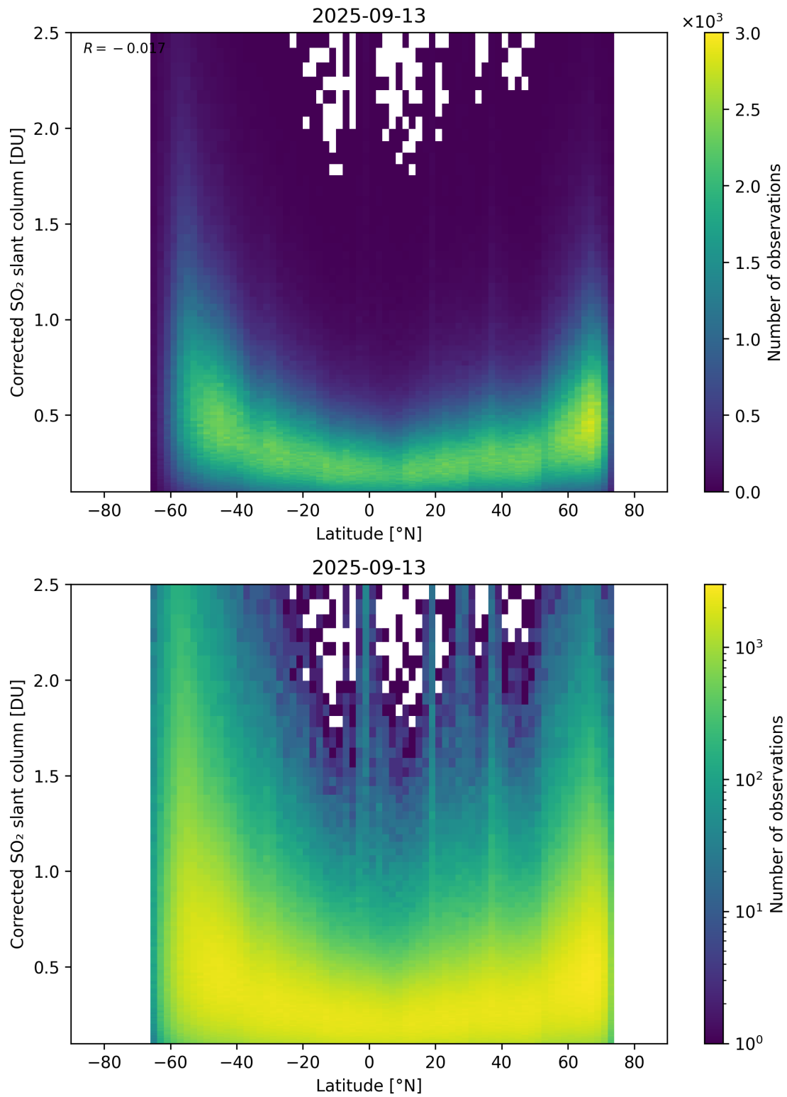
Figure 159: Scatter density plot of “Latitude” against “Corrected SO 2 slant column” for 2025-09-12 to 2025-09-14.
