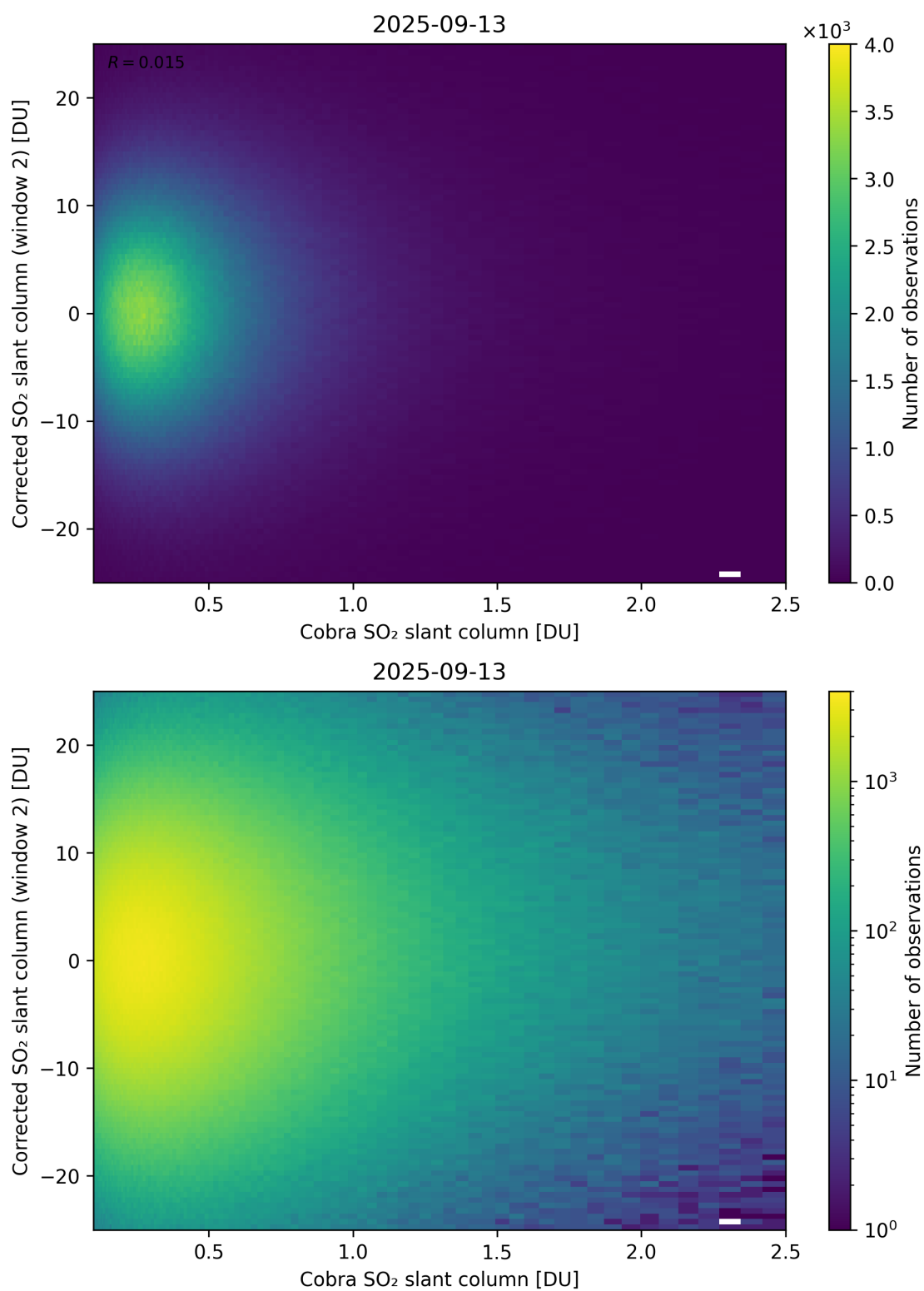
Figure 217: Scatter density plot of “Cobra SO 2 slant column” against “Corrected SO 2 slant column (window 2)” for 2025-09-12 to 2025-09-14.
