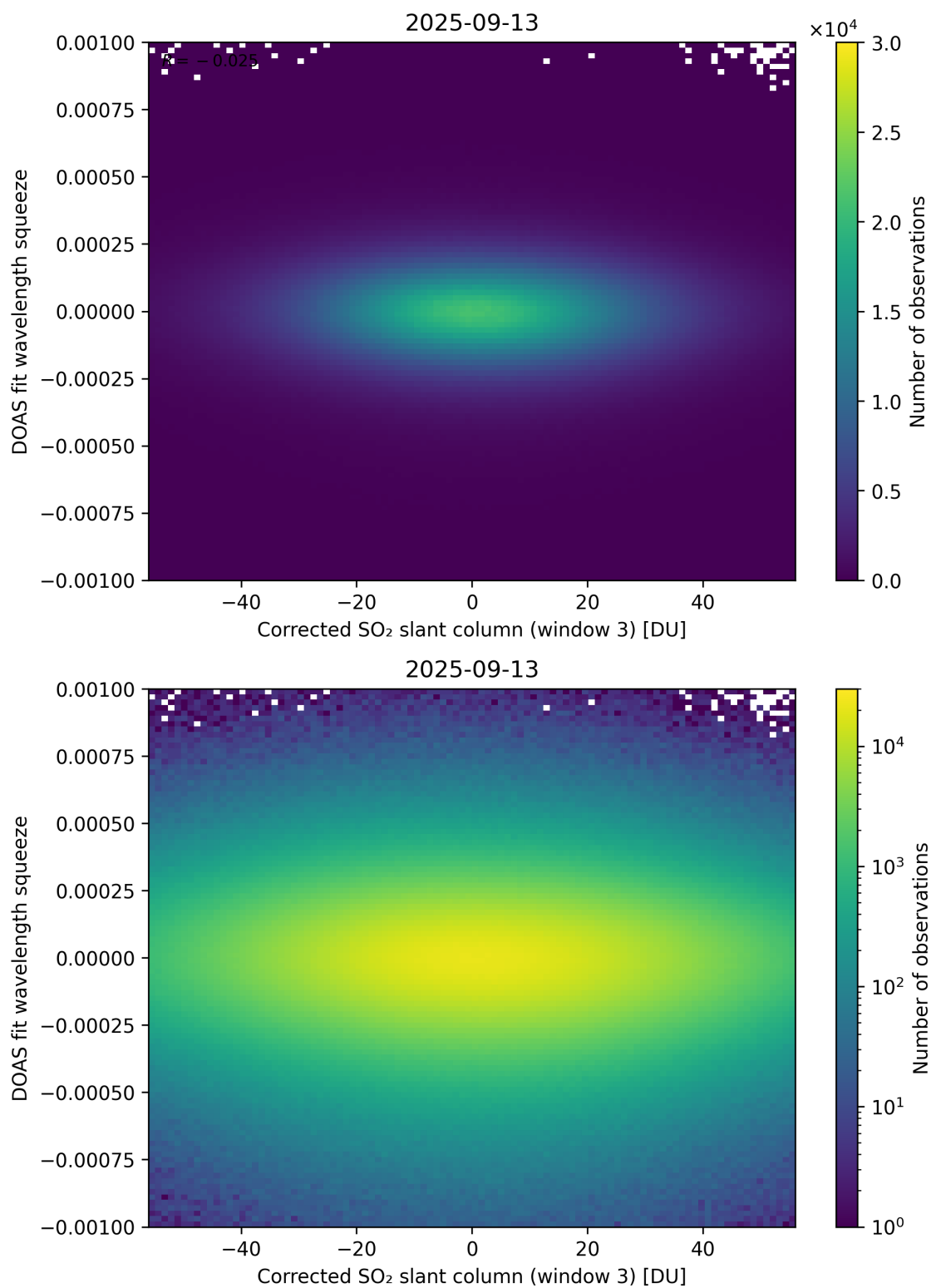
Figure 257: Scatter density plot of “Corrected SO 2 slant column (window 3)” against “DOAS fit wavelength squeeze” for 2025-09-12 to 2025-09-14.
