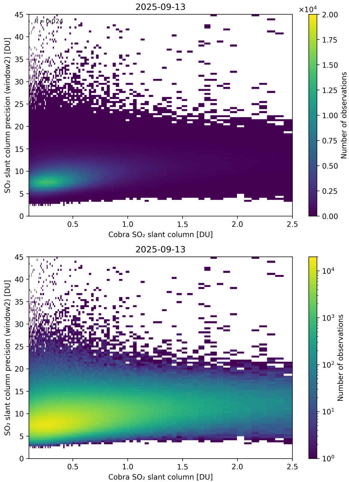
Figure 221: Scatter density plot of “Cobra SO 2 slant column” against “SO 2 slant column precision (window2)” for 2025-09-12 to 2025-09-14.
