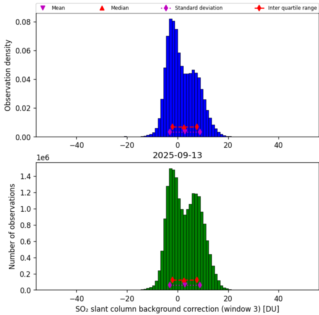
Figure 74: Histogram of “SO 2 slant column background correction (window 3)” for 2025-09-12 to 2025-09-14
