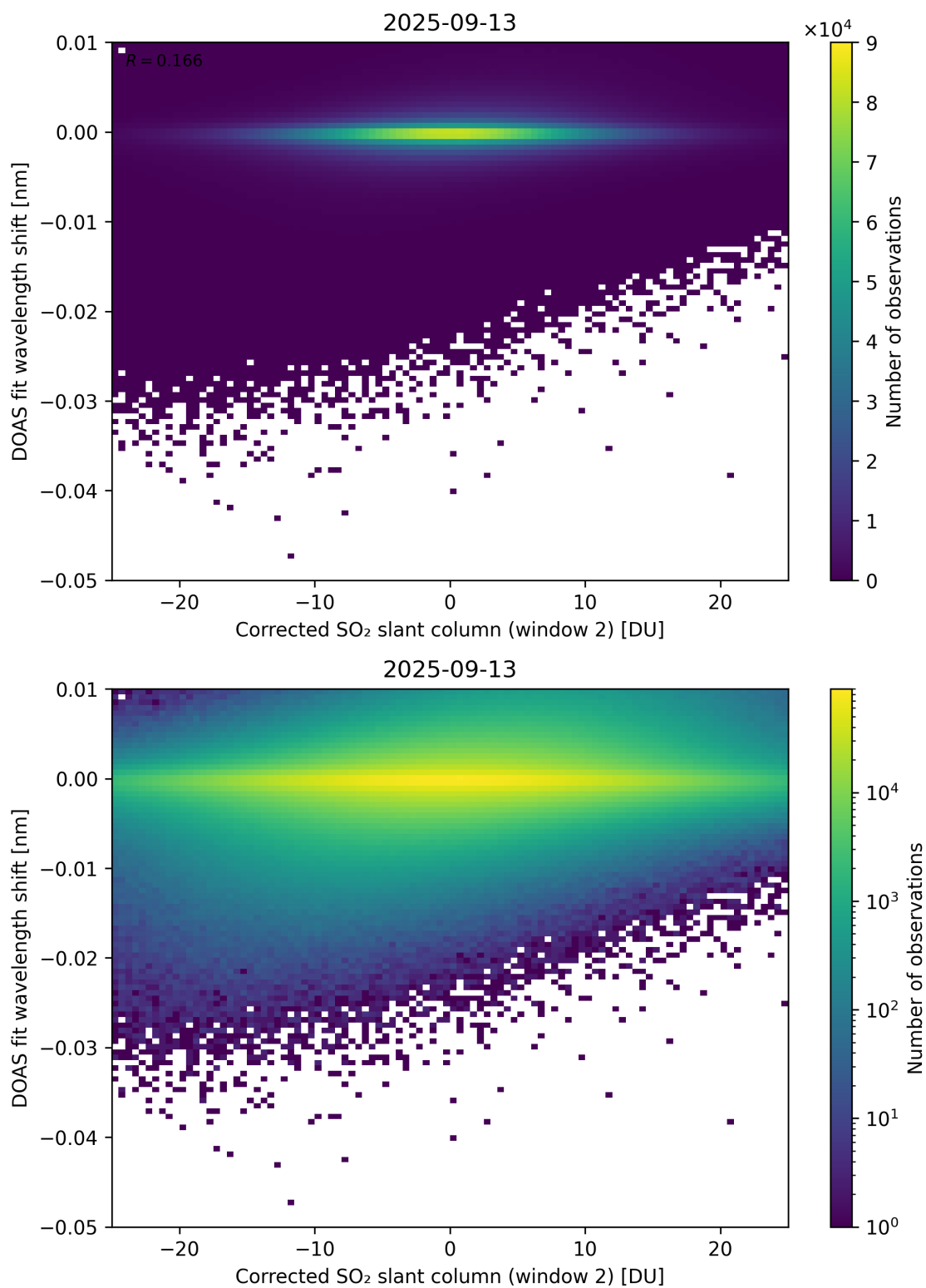
Figure 246: Scatter density plot of “Corrected SO 2 slant column (window 2)” against “DOAS fit wavelength shift” for 2025-09-12 to 2025-09-14.
