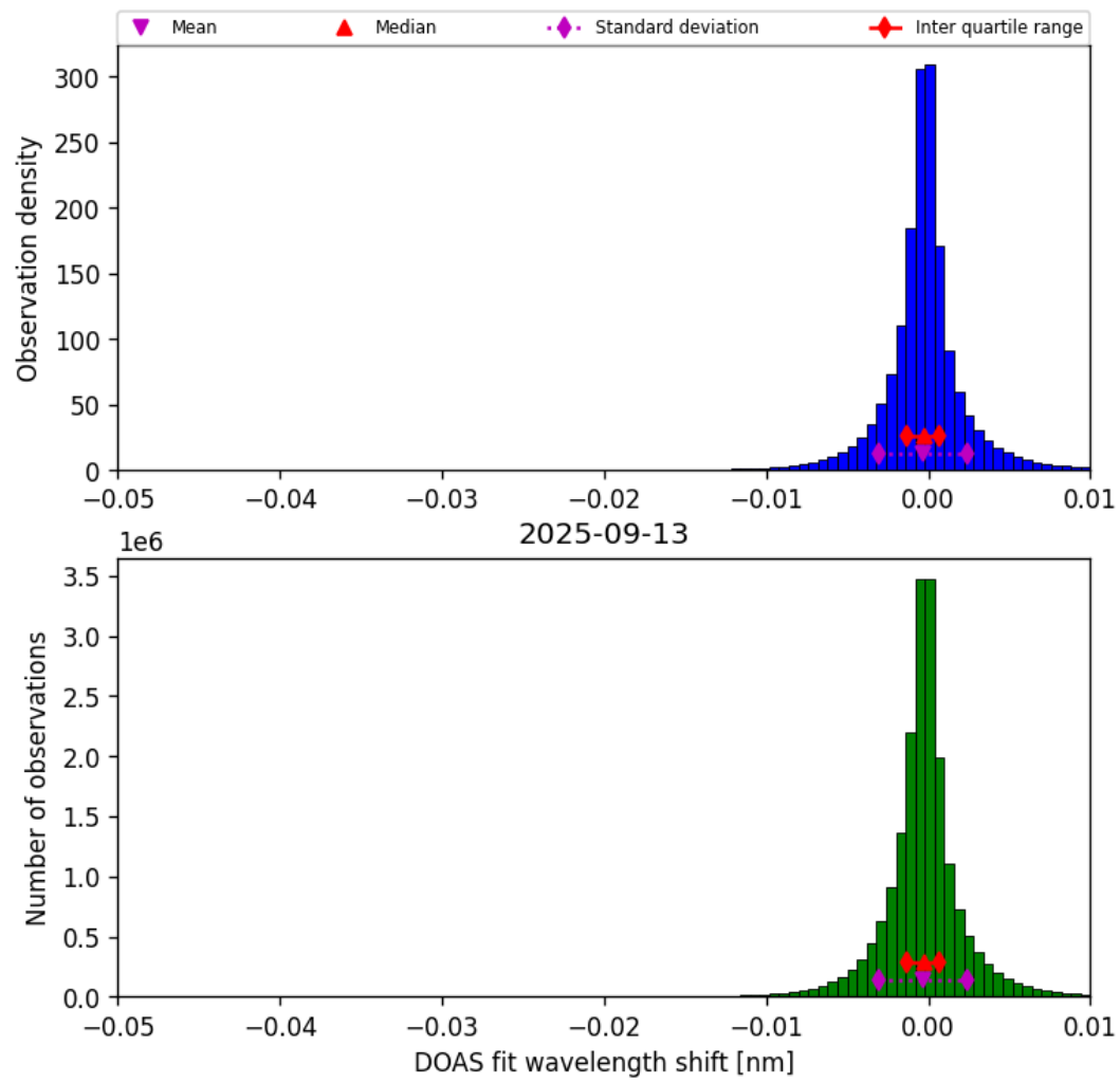
Figure 76: Histogram of “DOAS fit wavelength shift” for 2025-09-12 to 2025-09-14
