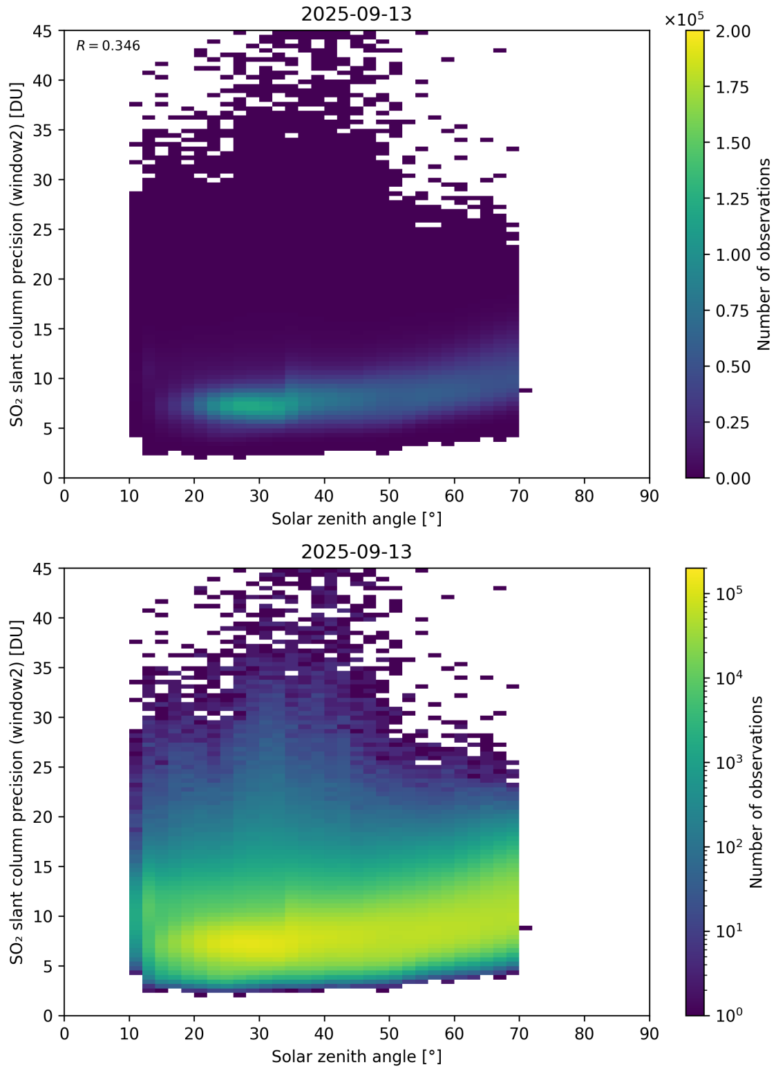
Figure 186: Scatter density plot of “Solar zenith angle” against “SO 2 slant column precision (window2)” for 2025-09-12 to 2025-09-14.
