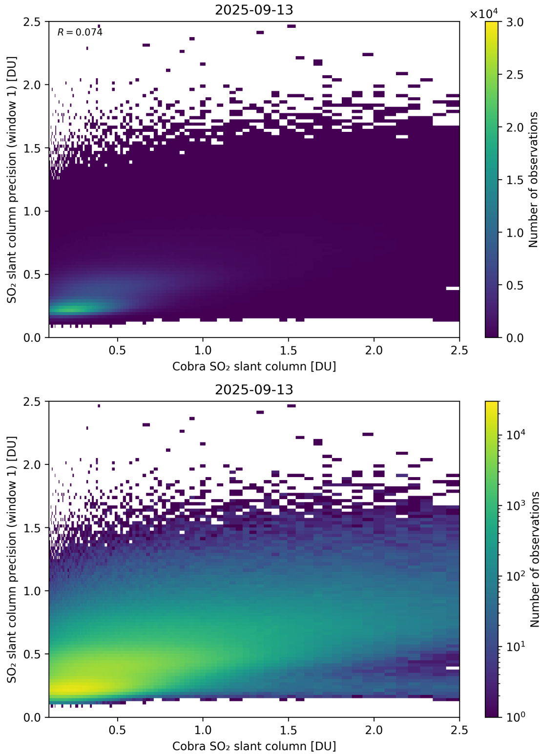
Figure 220: Scatter density plot of “Cobra SO 2 slant column” against “SO 2 slant column precision (window 1)” for 2025-09-12 to 2025-09-14.
