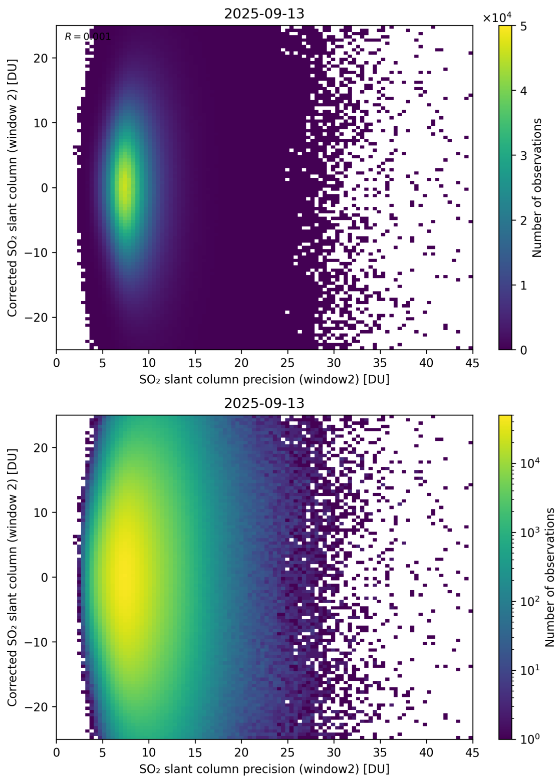
Figure 297: Scatter density plot of “SO 2 slant column precision (window2)” against “Corrected SO 2 slant column (window 2)” for 2025-09-12 to 2025-09-14.
