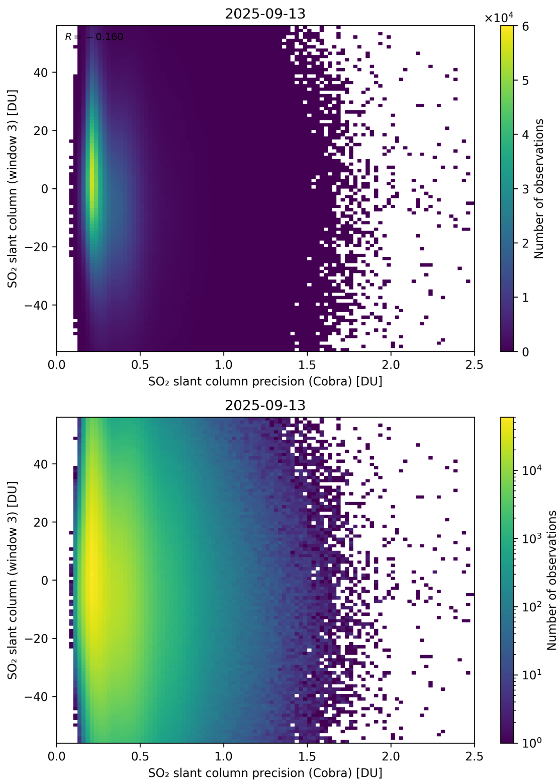
Figure 211: Scatter density plot of “SO 2 slant column precision (Cobra)” against “SO 2 slant column (window 3)” for 2025-09-12 to 2025-09-14.
