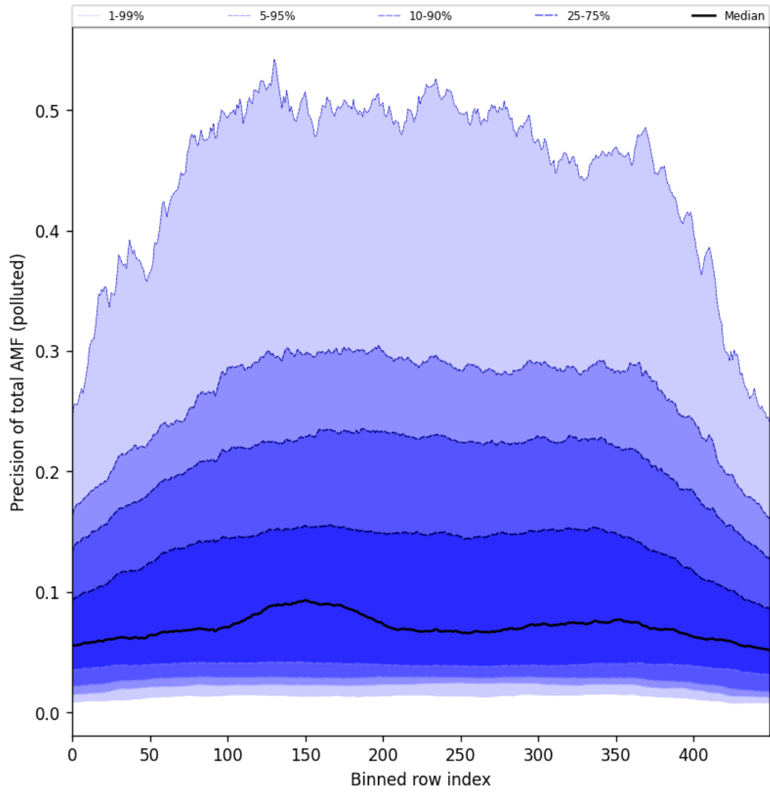
Figure 106: Along track statistics of “Precision of total AMF (polluted)” for 2025-09-12 to 2025-09-14
