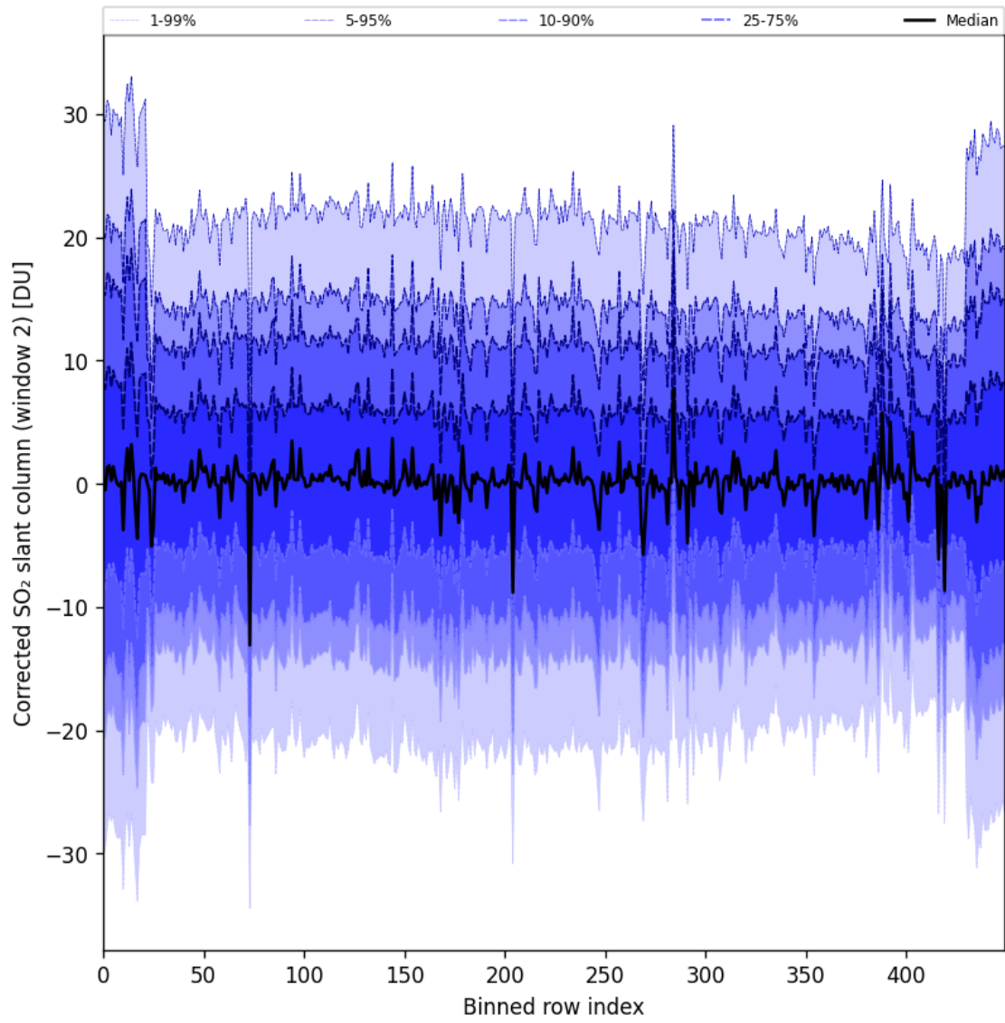
Figure 95: Along track statistics of “Corrected SO 2 slant column (window 2)” for 2025-09-12 to 2025-09-14
