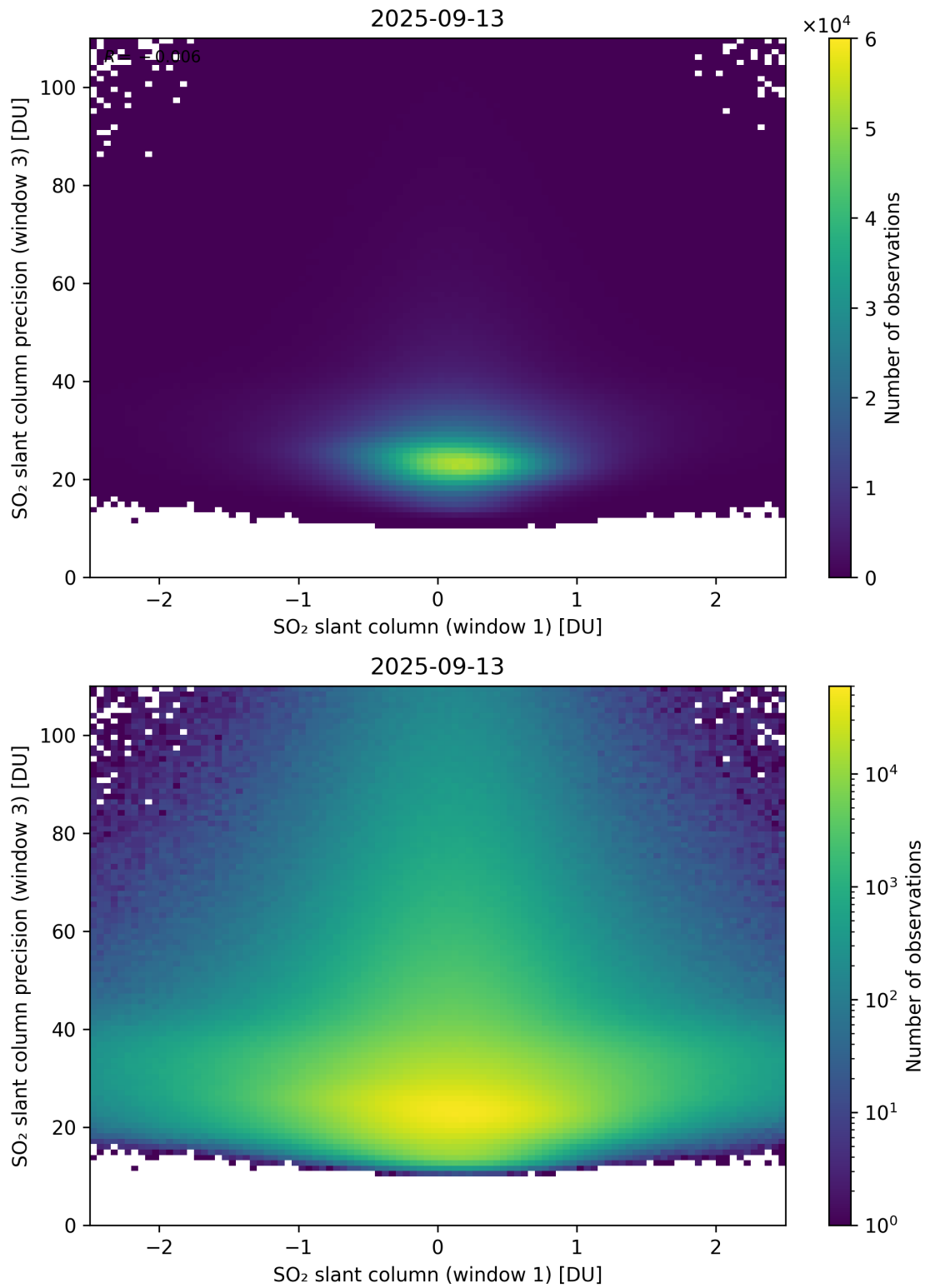
Figure 288: Scatter density plot of “SO 2 slant column (window 1)” against “SO 2 slant column precision (window 3)” for 2025-09-12 to 2025-09-14.
