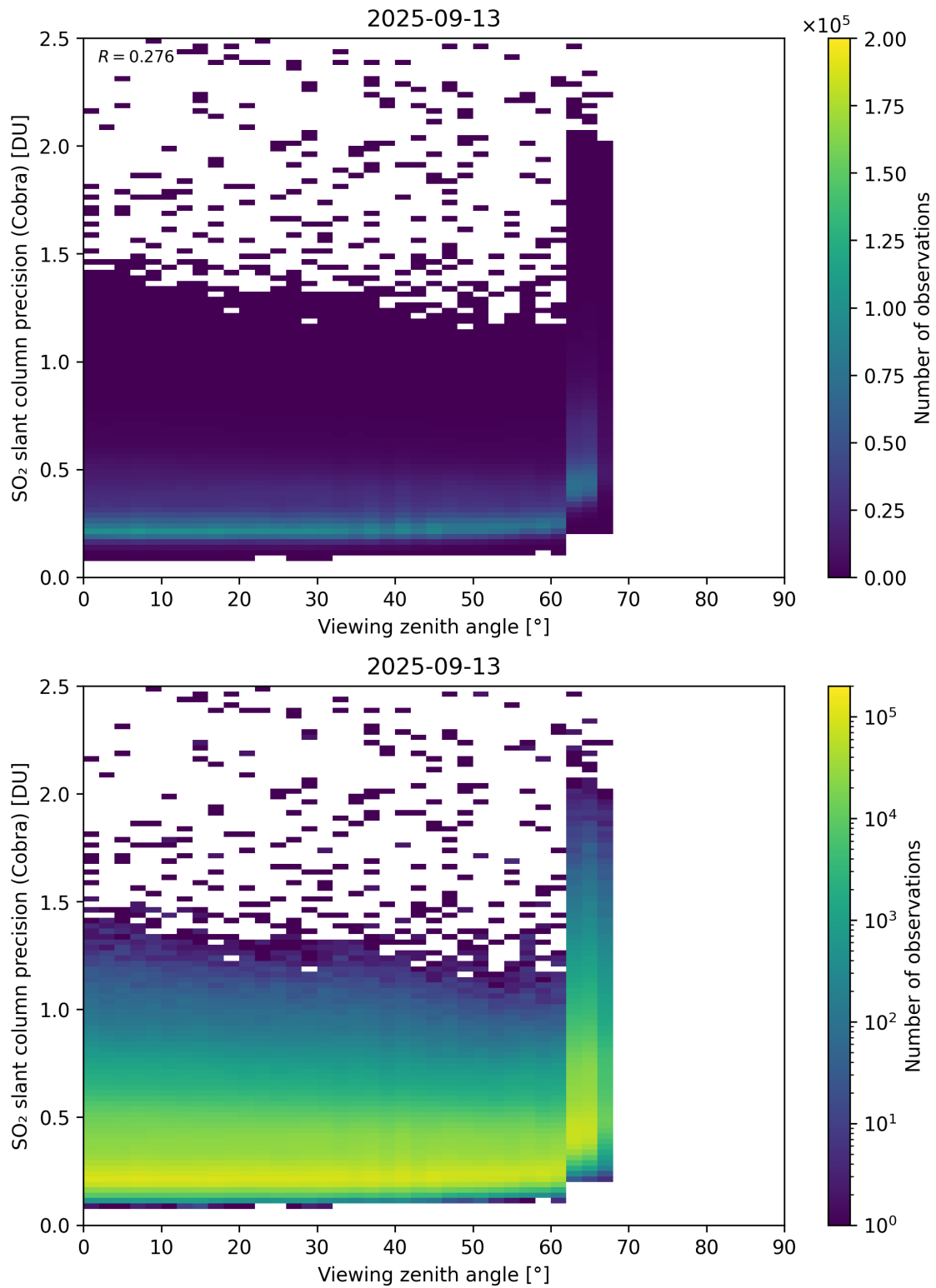
Figure 372: Scatter density plot of “Viewing zenith angle” against “SO 2 slant column precision (Cobra)” for 2025-09-12 to 2025-09-14.
