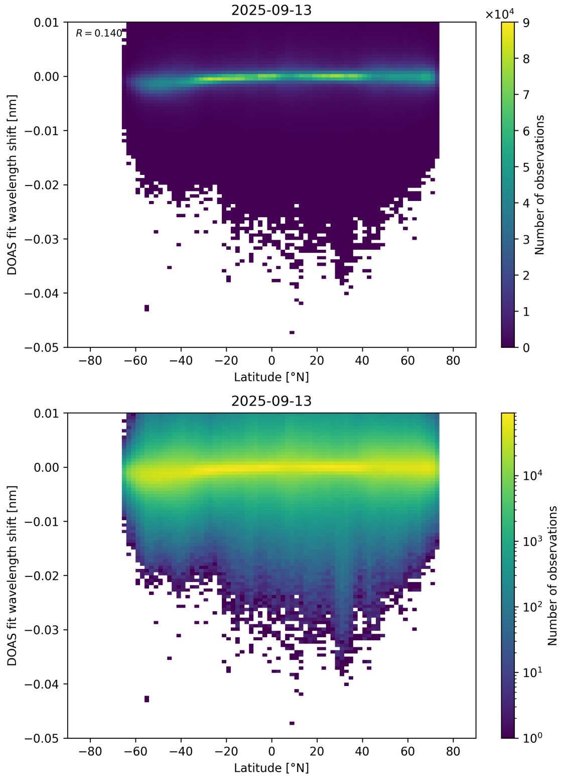
Figure 153: Scatter density plot of “Latitude” against “DOAS fit wavelength shift” for 2025-09-12 to 2025-09-14.
