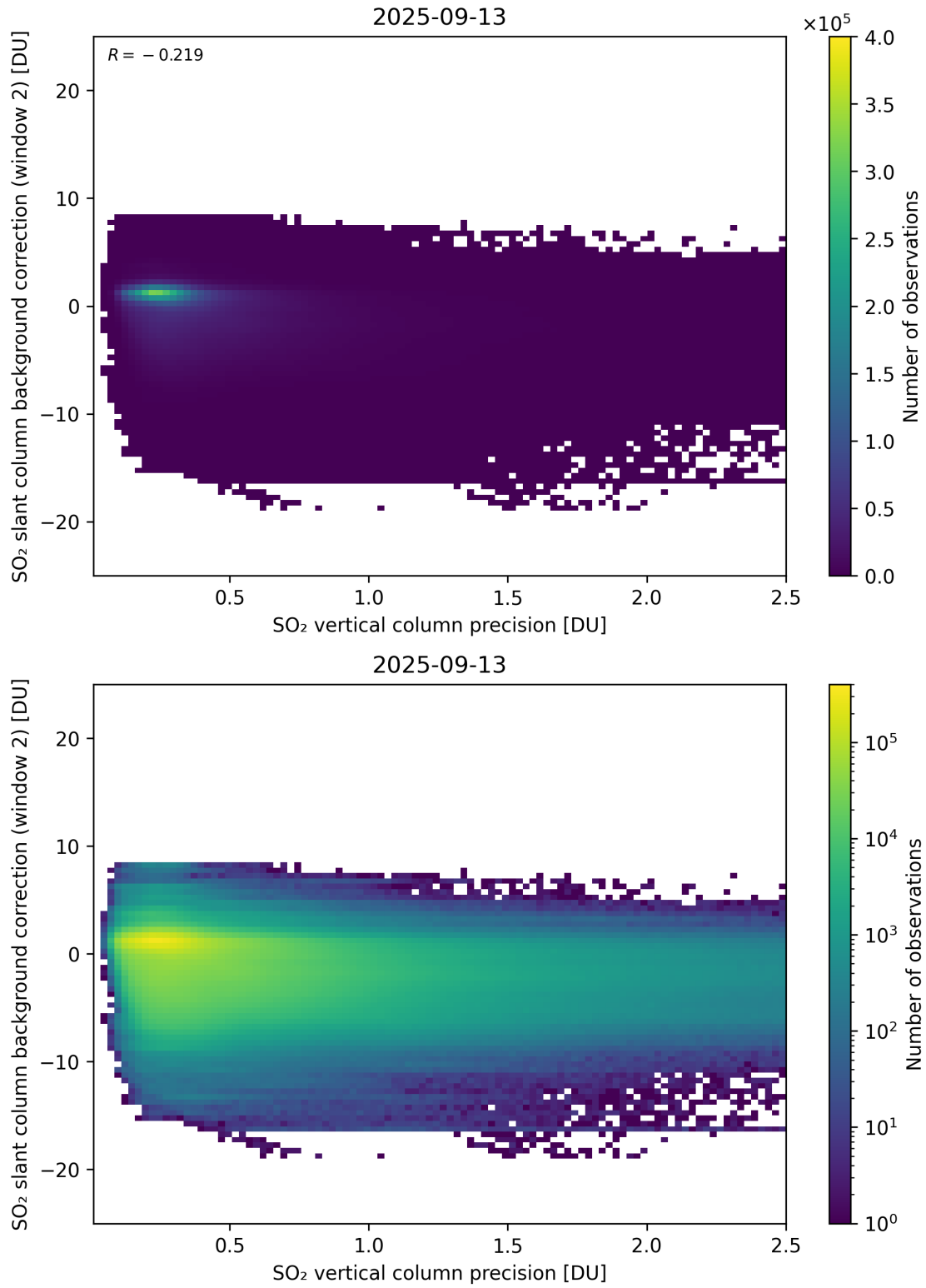
Figure 330: Scatter density plot of “SO 2 vertical column precision” against “SO 2 slant column background correction (window 2)” for 2025-09-12 to 2025-09-14.
