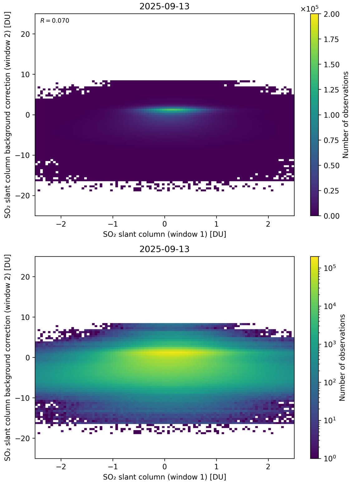
Figure 263: Scatter density plot of “SO 2 slant column (window 1)” against “SO 2 slant column background correction (window 2)” for 2025-09-12 to 2025-09-14.
