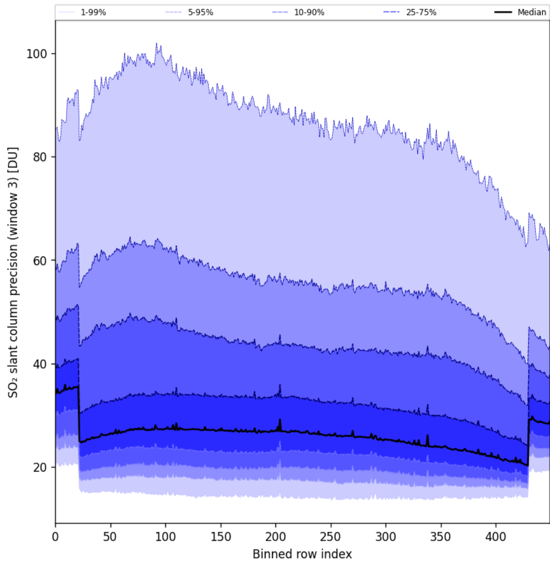
Figure 98: Along track statistics of “SO 2 slant column precision (window 3)” for 2025-09-12 to 2025-09-14
