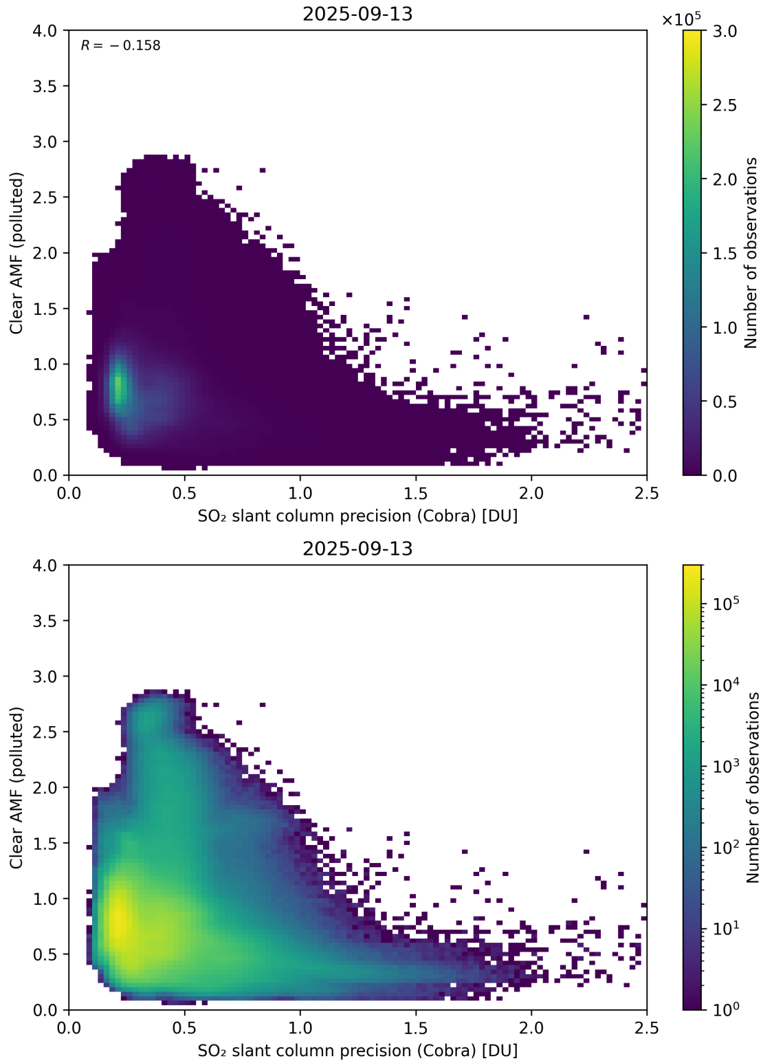
Figure 205: Scatter density plot of “SO 2 slant column precision (Cobra)” against “Clear AMF (polluted)” for 2025-09-12 to 2025-09-14.
