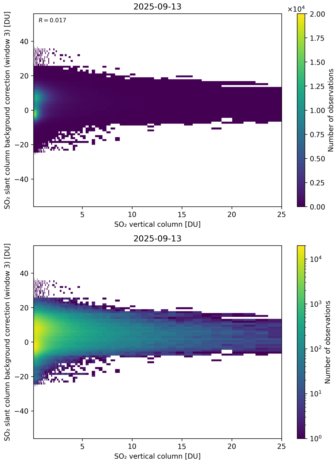
Figure 325: Scatter density plot of “SO 2 vertical column” against “SO 2 slant column background correction (window 3)” for 2025-09-12 to 2025-09-14.
