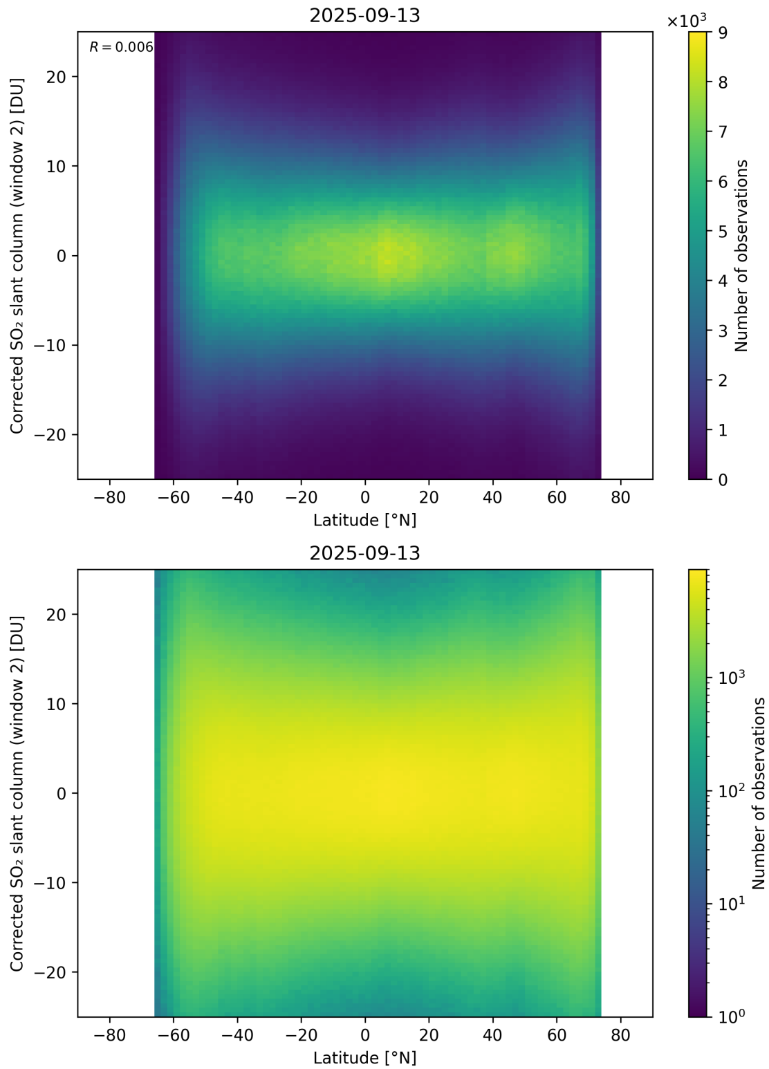
Figure 160: Scatter density plot of “Latitude” against “Corrected SO 2 slant column (window 2)” for 2025-09-12 to 2025-09-14.
