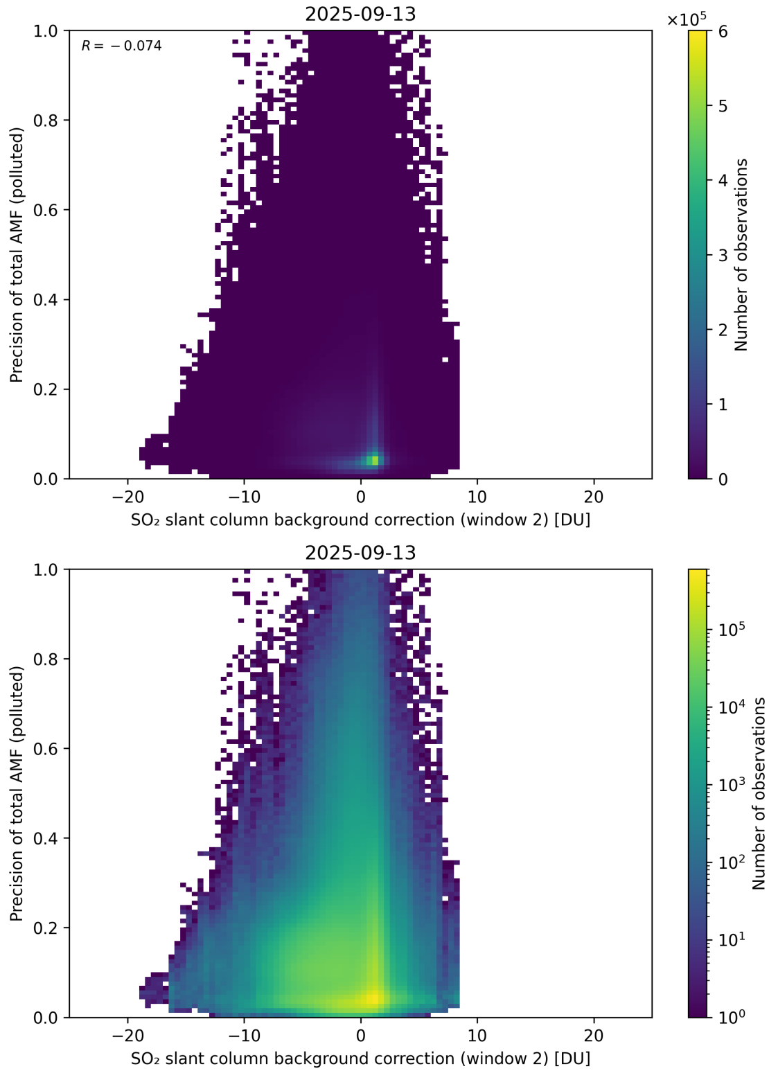
Figure 131: Scatter density plot of “SO 2 slant column background correction (window 2)” against “Precision of total AMF (polluted)” for 2025-09-12 to 2025-09-14.
