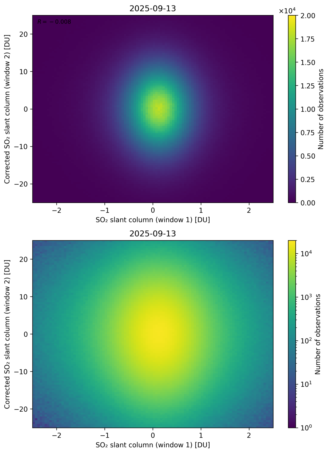
Figure 283: Scatter density plot of “SO 2 slant column (window 1)” against “Corrected SO 2 slant column (window 2)” for 2025-09-12 to 2025-09-14.
