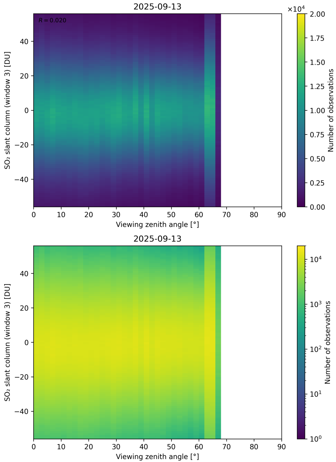
Figure 379: Scatter density plot of “Viewing zenith angle” against “SO 2 slant column (window 3)” for 2025-09-12 to 2025-09-14.
