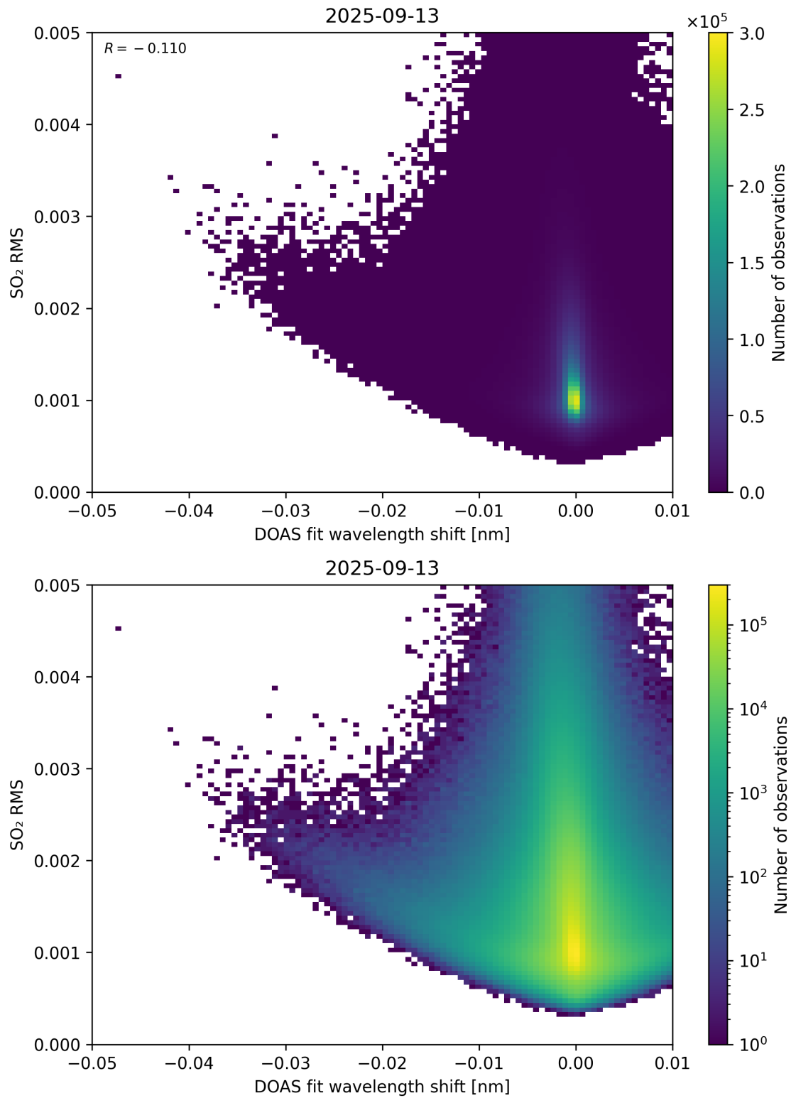
Figure 139: Scatter density plot of “DOAS fit wavelength shift” against “SO 2 RMS” for 2025-09-12 to 2025-09-14.
