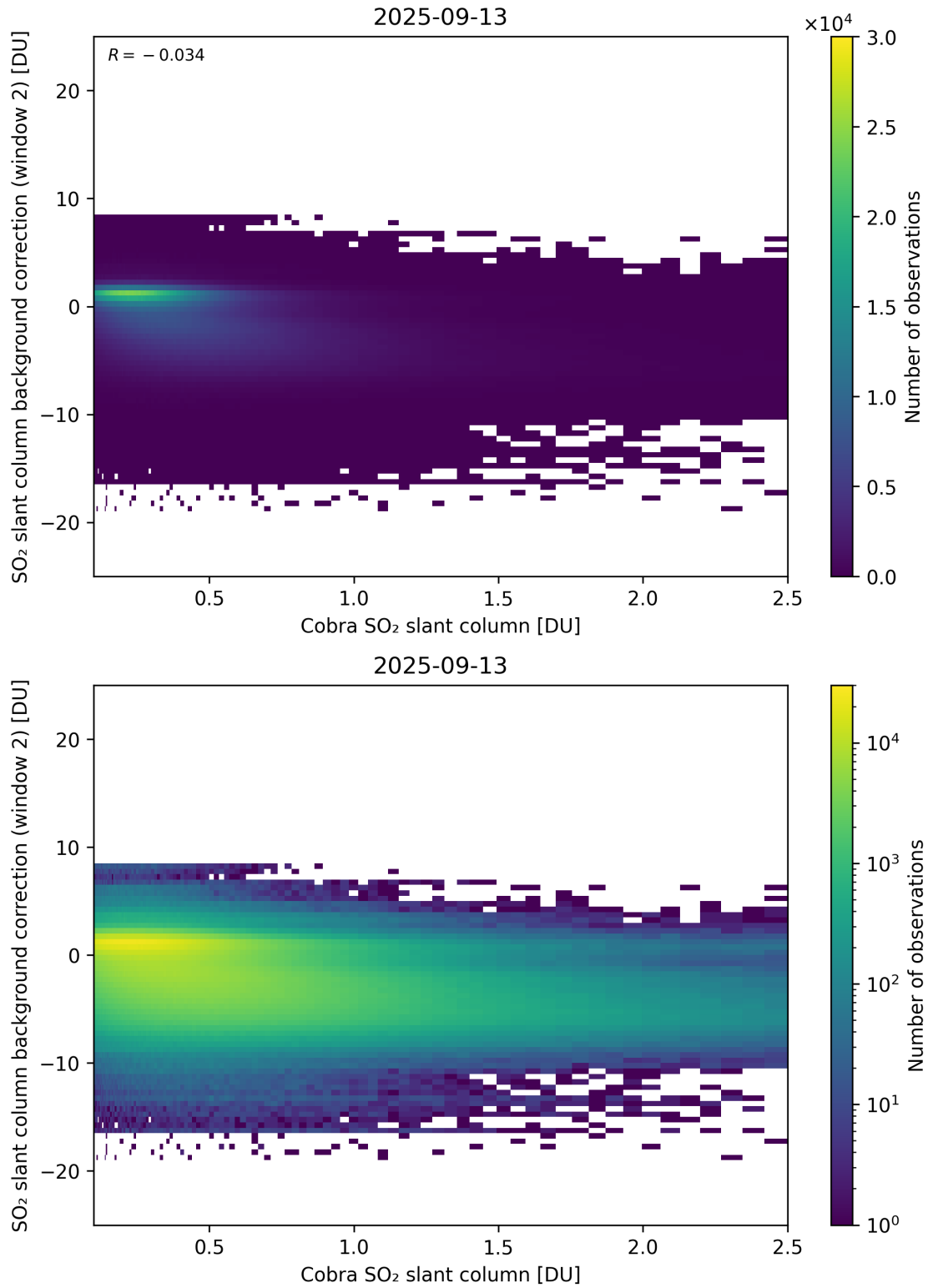
Figure 194: Scatter density plot of “Cobra SO 2 slant column” against “SO 2 slant column background correction (window 2)” for 2025-09-12 to 2025-09-14.
