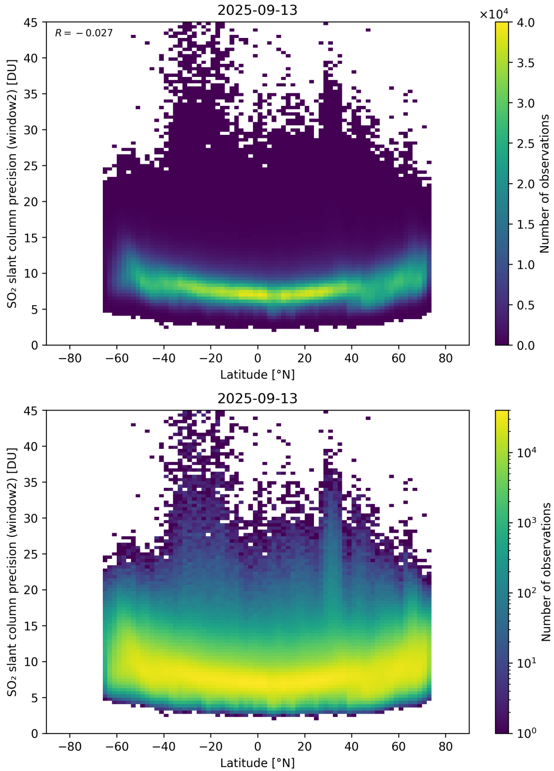
Figure 164: Scatter density plot of “Latitude” against “SO 2 slant column precision (window2)” for 2025-09-12 to 2025-09-14.
