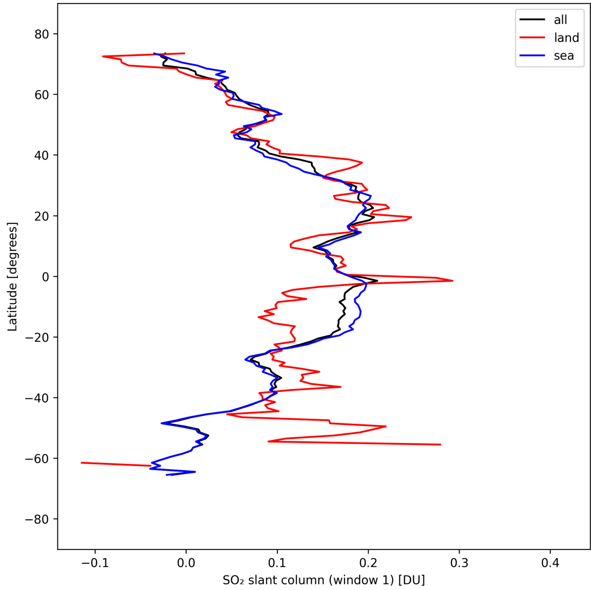
Figure 37: Zonal average of “SO 2 slant column (window 1)” for 2025-09-12 to 2025-09-14.
