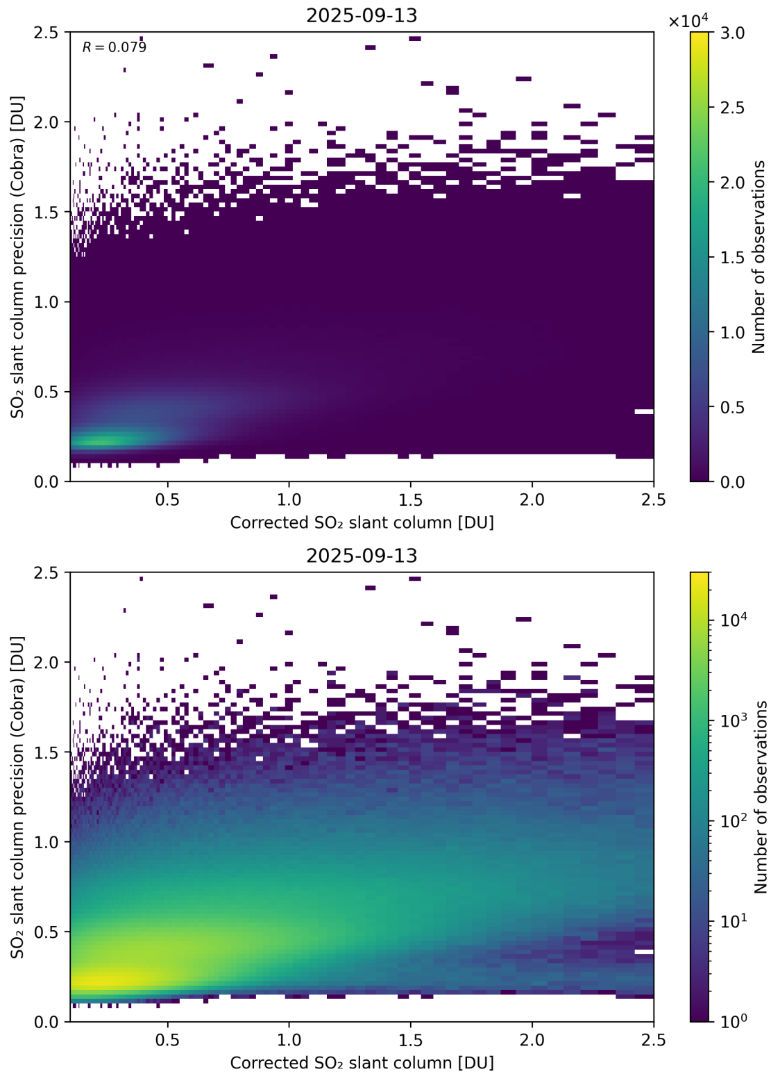
Figure 234: Scatter density plot of “Corrected SO 2 slant column” against “SO 2 slant column precision (Cobra)” for 2025-09-12 to 2025-09-14.
