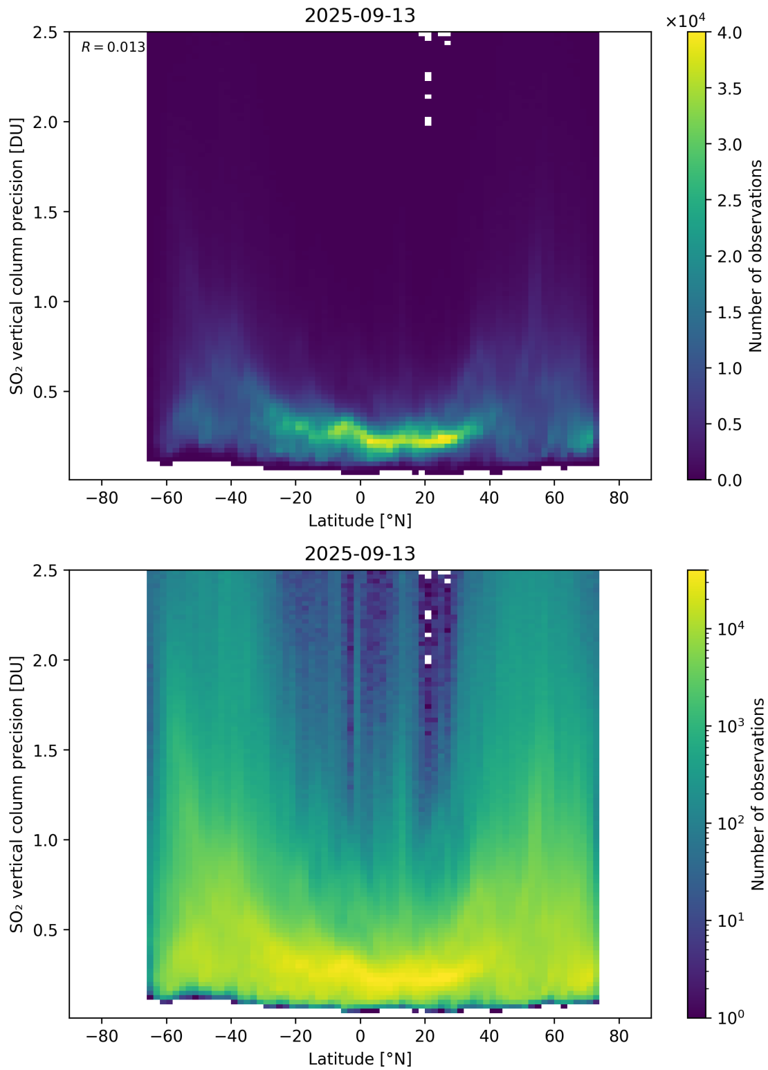
Figure 170: Scatter density plot of “Latitude” against “SO 2 vertical column precision” for 2025-09-12 to 2025-09-14.
