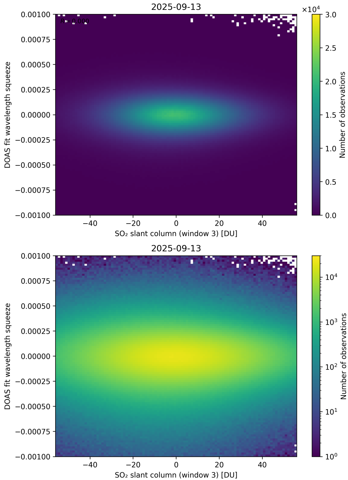
Figure 305: Scatter density plot of “SO 2 slant column (window 3)” against “DOAS fit wavelength squeeze” for 2025-09-12 to 2025-09-14.
