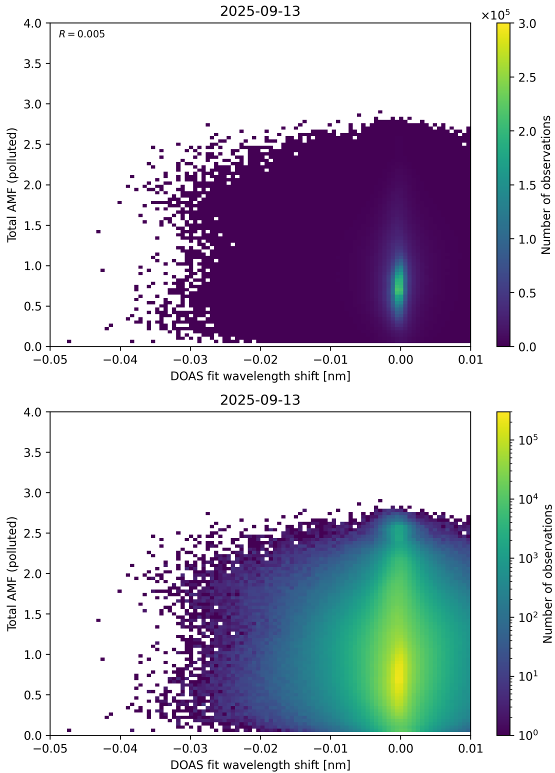
Figure 141: Scatter density plot of “DOAS fit wavelength shift” against “Total AMF (polluted)” for 2025-09-12 to 2025-09-14.
