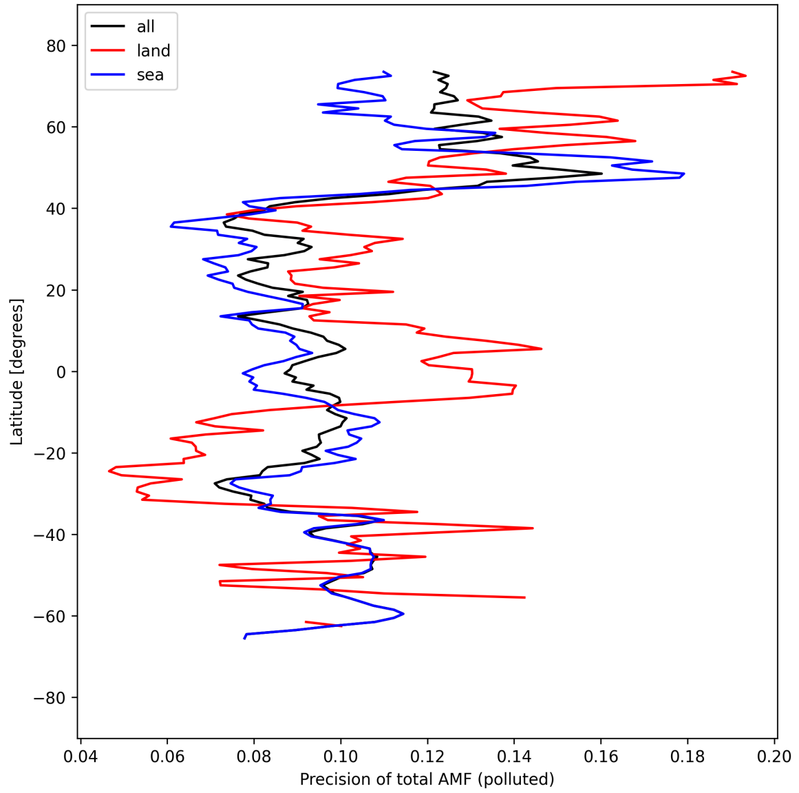
Figure 54: Zonal average of “Precision of total AMF (polluted)” for 2025-09-12 to 2025-09-14.
