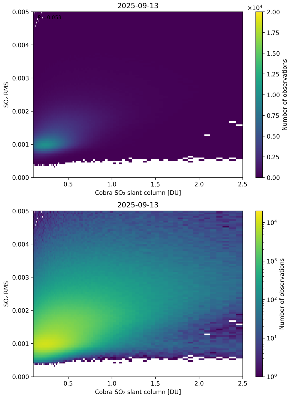
Figure 198: Scatter density plot of “Cobra SO 2 slant column” against “SO 2 RMS” for 2025-09-12 to 2025-09-14.
