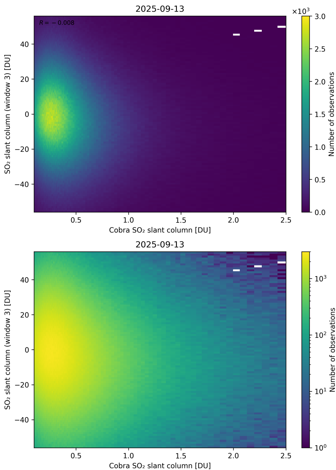
Figure 222: Scatter density plot of “Cobra SO 2 slant column” against “SO 2 slant column (window 3)” for 2025-09-12 to 2025-09-14.
