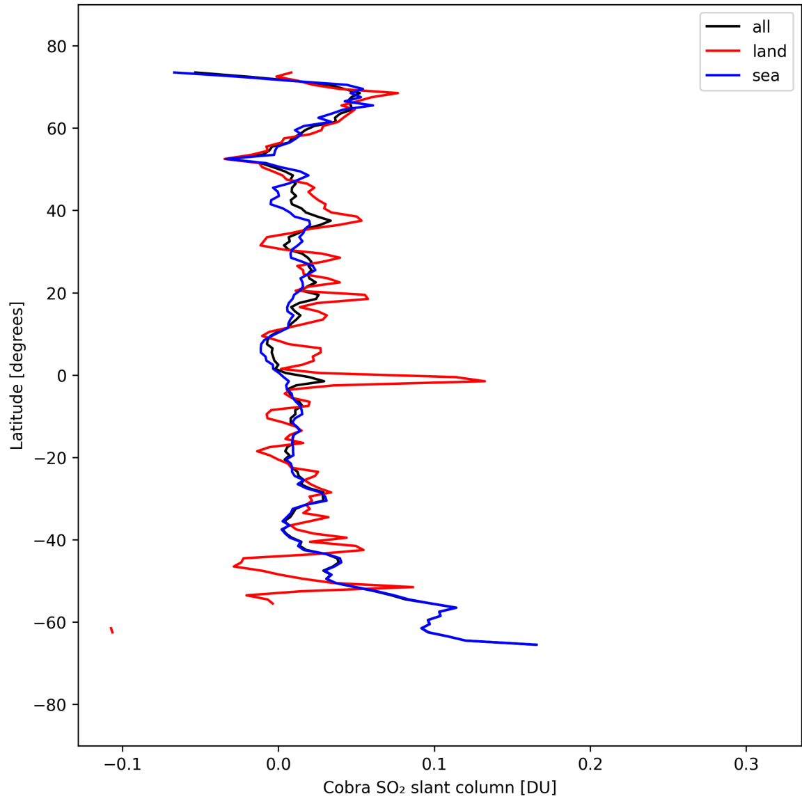
Figure 35: Zonal average of “Cobra SO 2 slant column” for 2025-09-12 to 2025-09-14.
