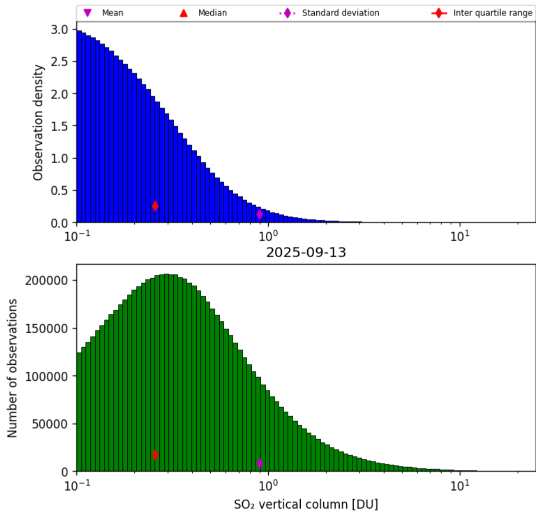
Figure 58: Histogram of “SO 2 vertical column” for 2025-09-12 to 2025-09-14
