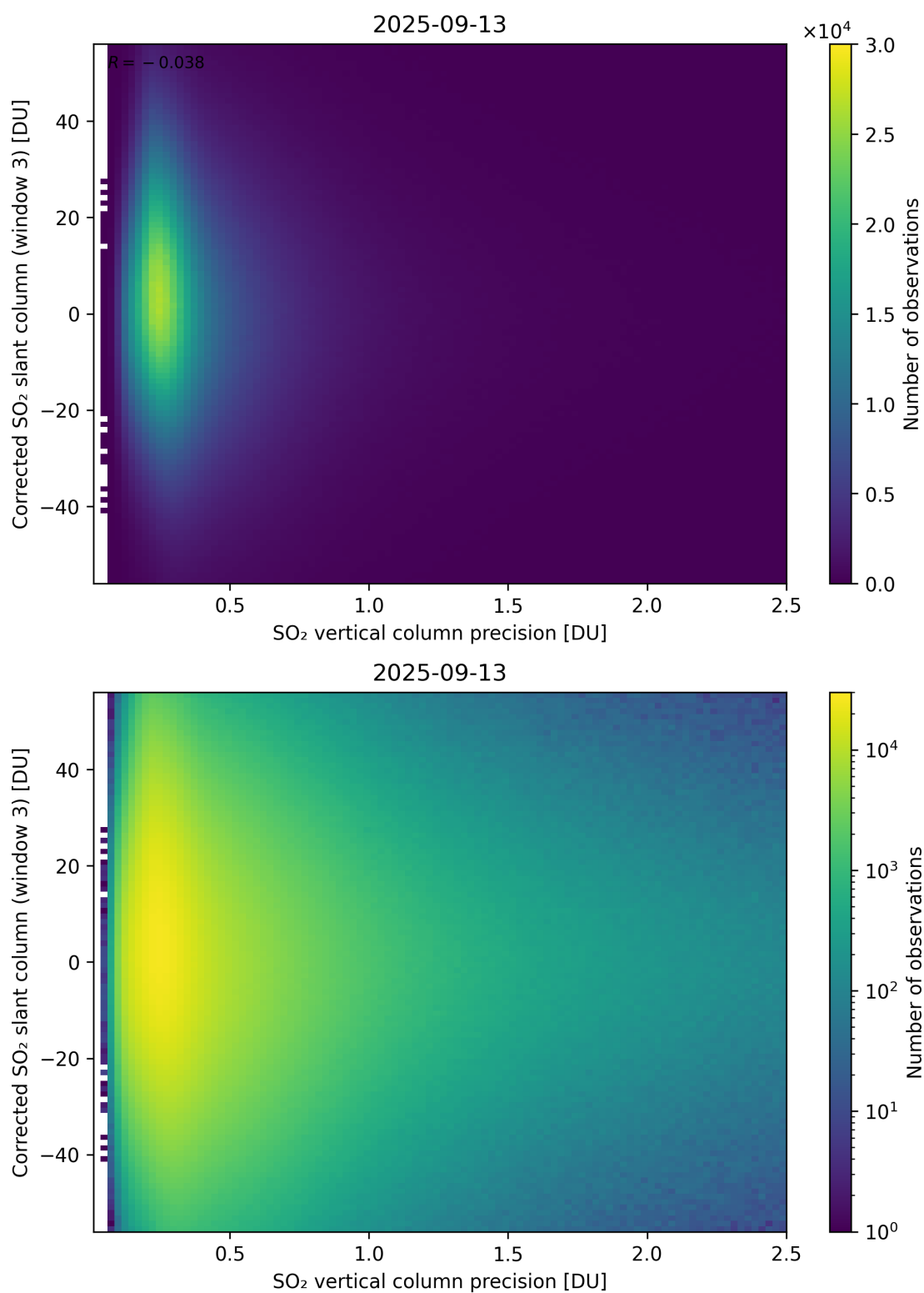
Figure 340: Scatter density plot of “SO 2 vertical column precision” against “Corrected SO 2 slant column (window 3)” for 2025-09-12 to 2025-09-14.
