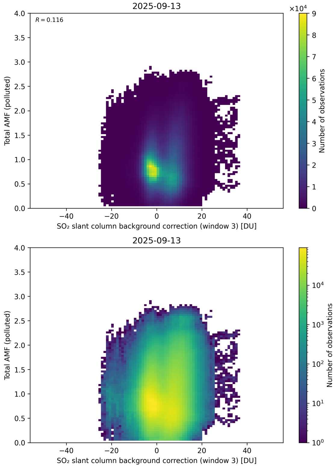
Figure 136: Scatter density plot of “SO 2 slant column background correction (window 3)” against “Total AMF (polluted)” for 2025-09-12 to 2025-09-14.
