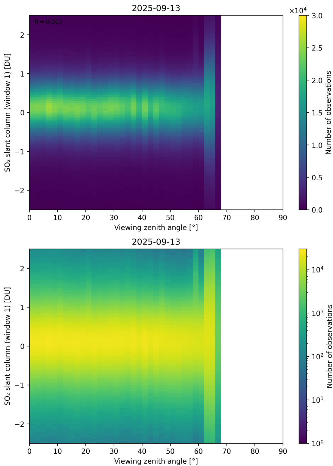
Figure 376: Scatter density plot of “Viewing zenith angle” against “SO 2 slant column (window 1)” for 2025-09-12 to 2025-09-14.
