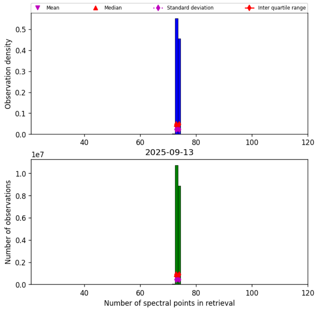
Figure 82: Histogram of “Number of spectral points in retrieval” for 2025-09-12 to 2025-09-14
