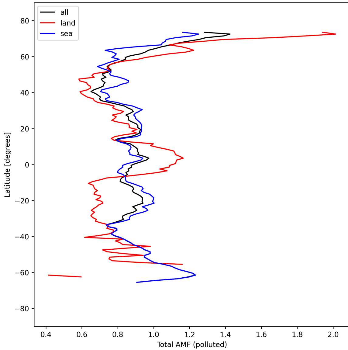
Figure 53: Zonal average of “Total AMF (polluted)” for 2025-09-12 to 2025-09-14.
