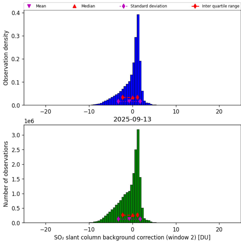
Figure 70: Histogram of “SO 2 slant column background correction (window 2)” for 2025-09-12 to 2025-09-14
