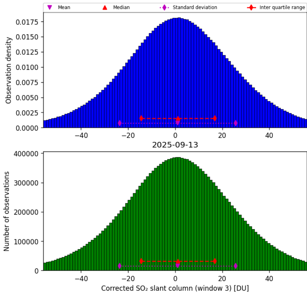
Figure 73: Histogram of “Corrected SO 2 slant column (window 3)” for 2025-09-12 to 2025-09-14
