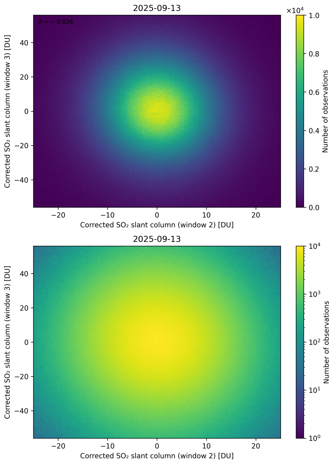
Figure 250: Scatter density plot of “Corrected SO 2 slant column (window 2)” against “Corrected SO 2 slant column (window 3)” for 2025-09-12 to 2025-09-14.
