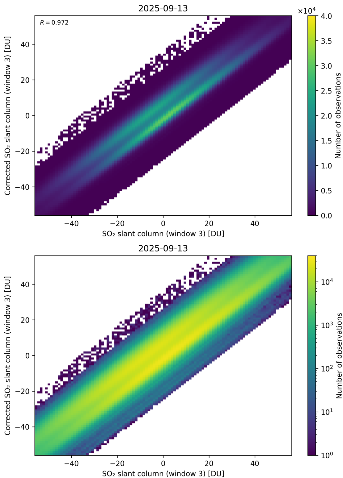
Figure 316: Scatter density plot of “SO 2 slant column (window 3)” against “Corrected SO 2 slant column (window 3)” for 2025-09-12 to 2025-09-14.
