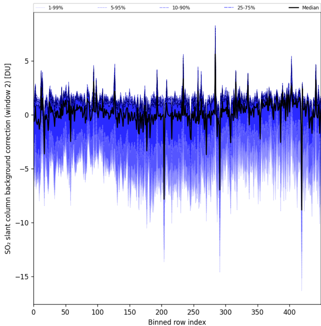
Figure 96: Along track statistics of “SO 2 slant column background correction (window 2)” for 2025-09-12 to 2025-09-14
