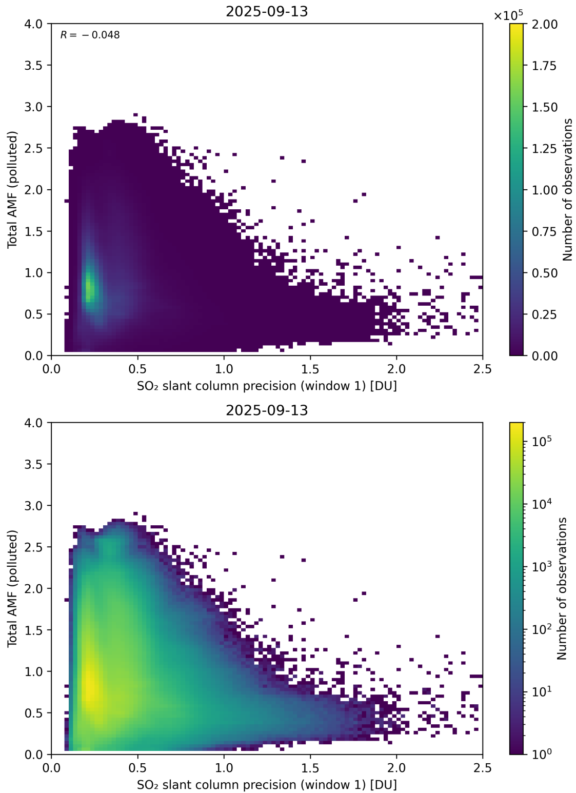
Figure 280: Scatter density plot of “SO 2 slant column precision (window 1)” against “Total AMF (polluted)” for 2025-09-12 to 2025-09-14.
