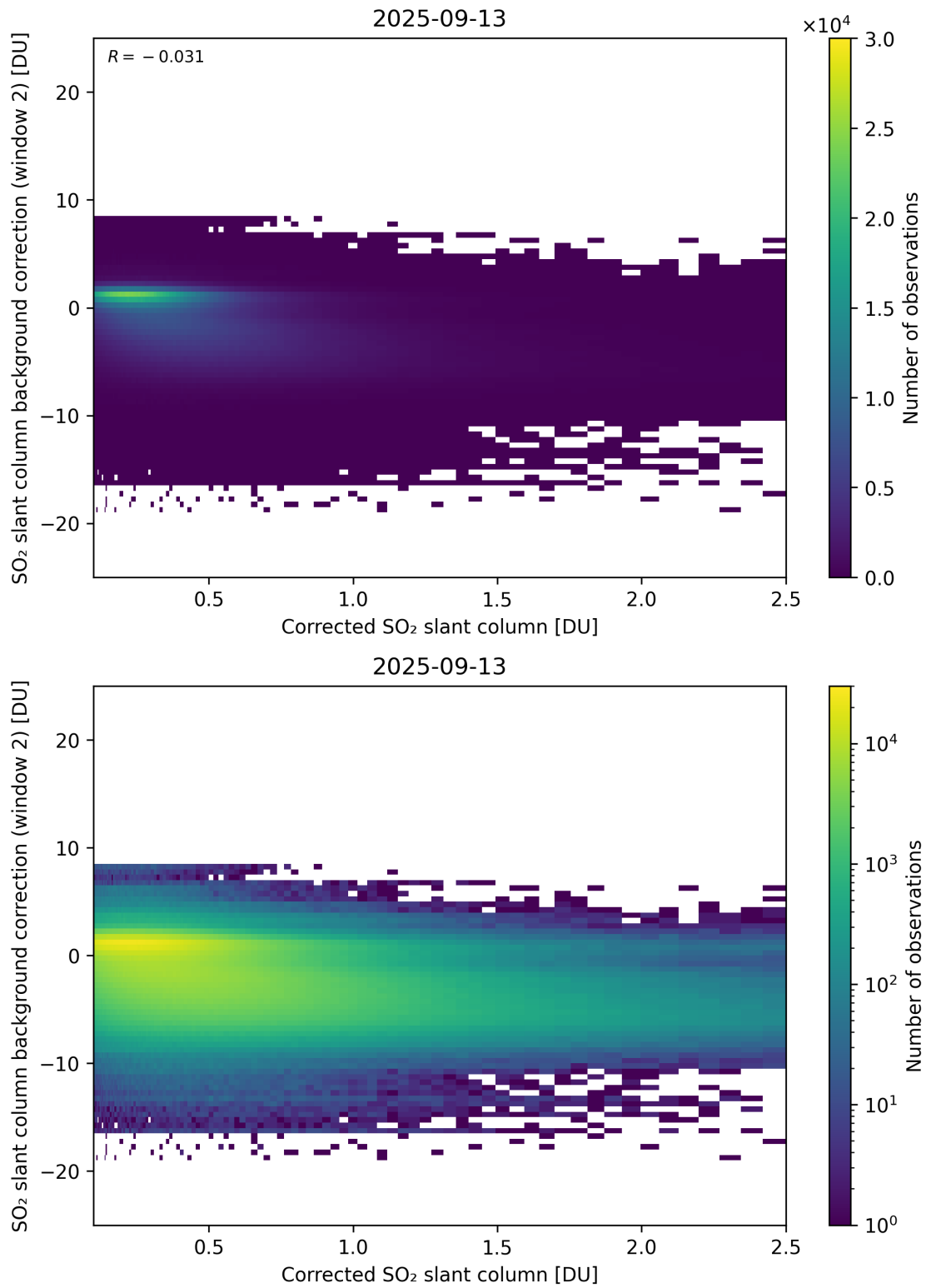
Figure 227: Scatter density plot of “Corrected SO 2 slant column” against “SO 2 slant column background correction (window 2)” for 2025-09-12 to 2025-09-14.
