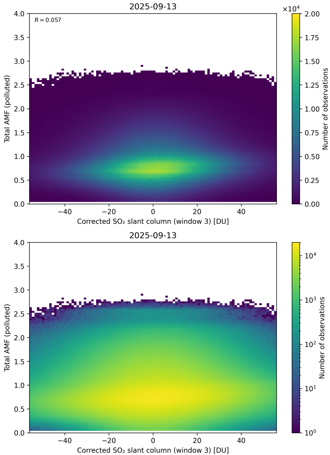
Figure 260: Scatter density plot of “Corrected SO 2 slant column (window 3)” against “Total AMF (polluted)” for 2025-09-12 to 2025-09-14.
