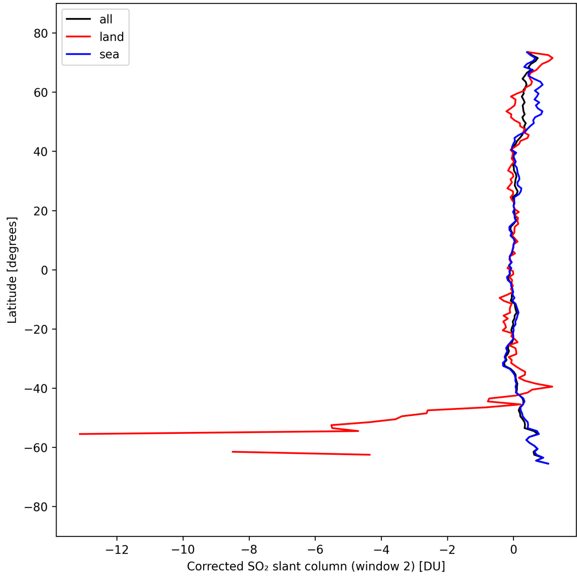
Figure 43: Zonal average of “Corrected SO 2 slant column (window 2)” for 2025-09-12 to 2025-09-14.
