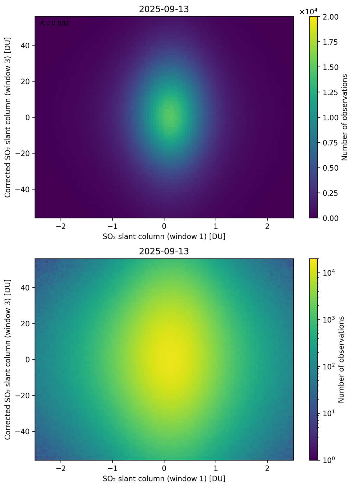
Figure 284: Scatter density plot of “SO 2 slant column (window 1)” against “Corrected SO 2 slant column (window 3)” for 2025-09-12 to 2025-09-14.
