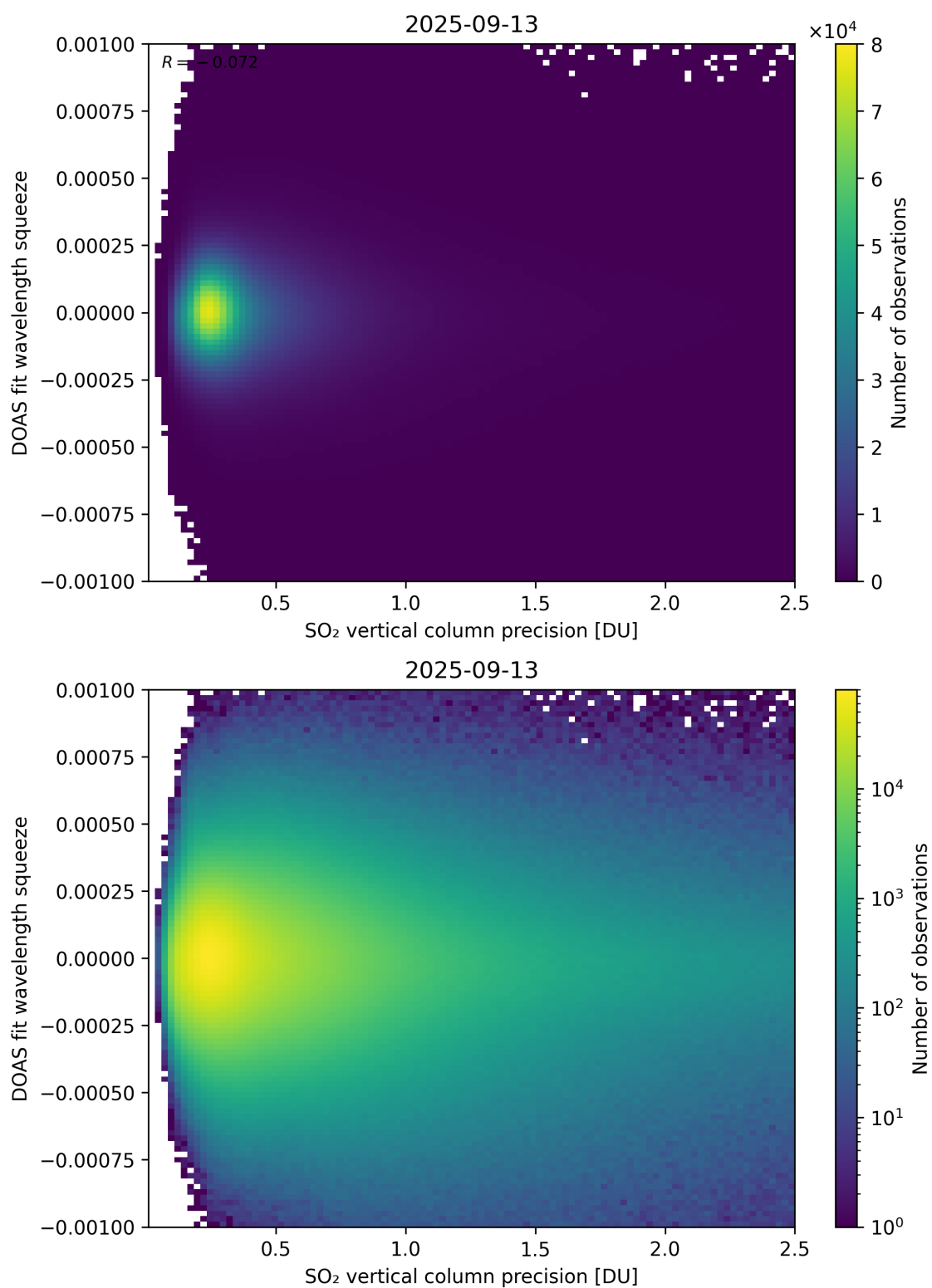
Figure 333: Scatter density plot of “SO 2 vertical column precision” against “DOAS fit wavelength squeeze” for 2025-09-12 to 2025-09-14.
