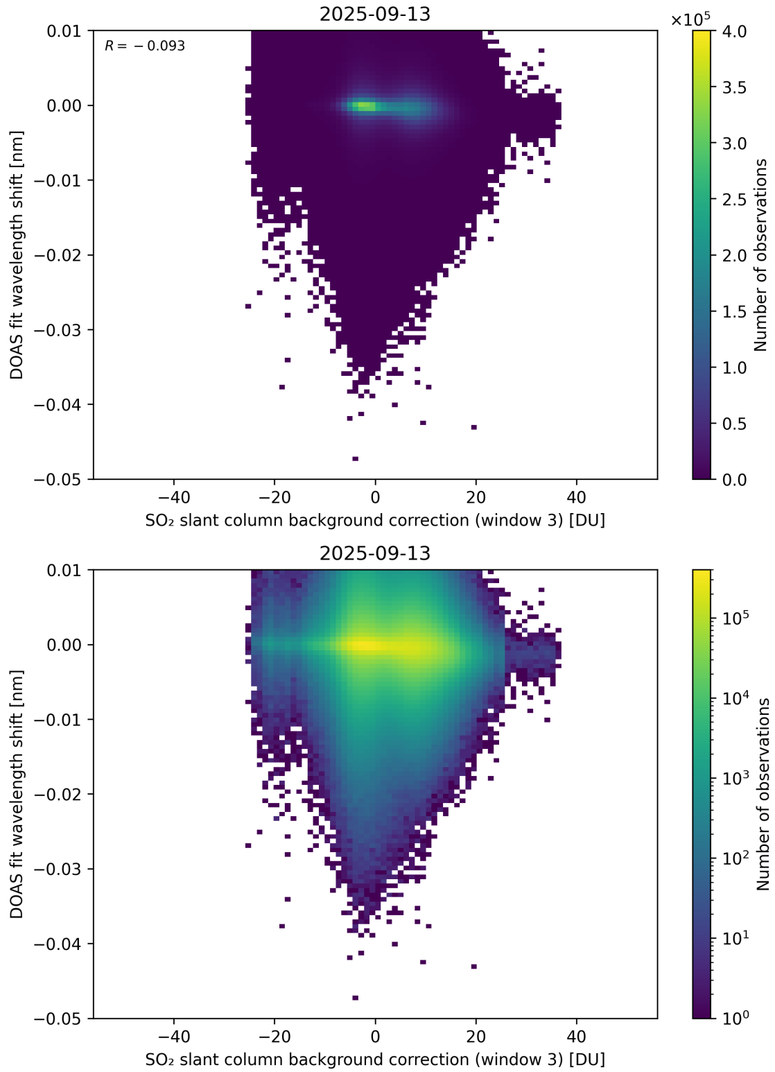
Figure 132: Scatter density plot of “SO 2 slant column background correction (window 3)” against “DOAS fit wavelength shift” for 2025-09-12 to 2025-09-14.
