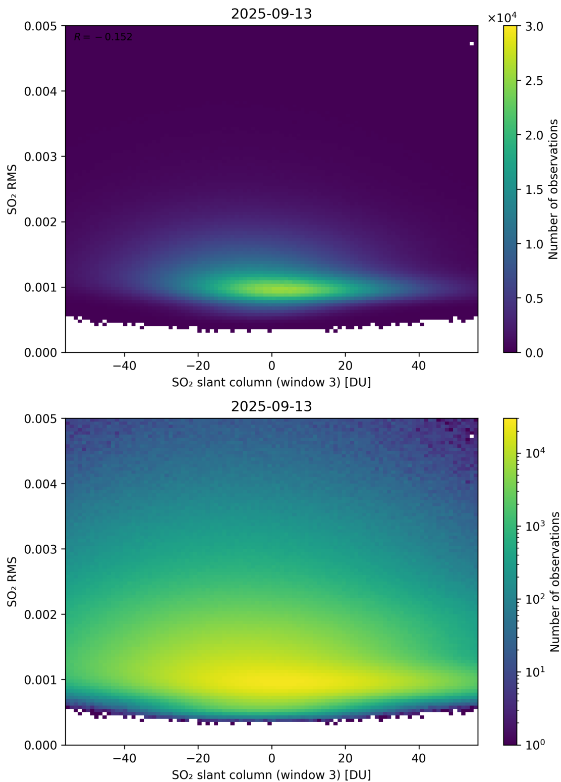
Figure 306: Scatter density plot of “SO 2 slant column (window 3)” against “SO 2 RMS” for 2025-09-12 to 2025-09-14.
