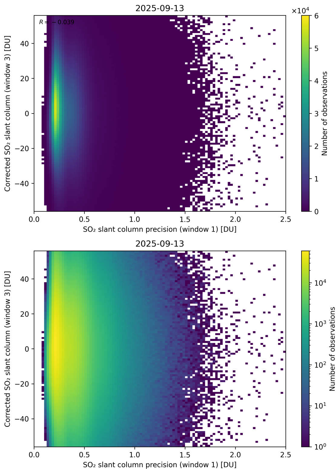
Figure 276: Scatter density plot of “SO 2 slant column precision (window 1)” against “Corrected SO 2 slant column (window 3)” for 2025-09-12 to 2025-09-14.
