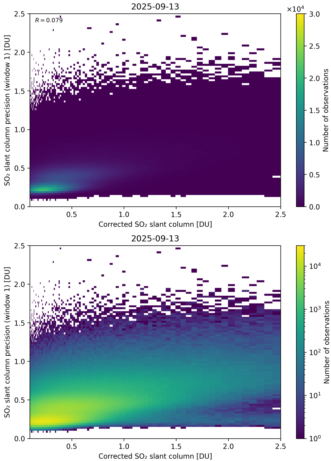
Figure 238: Scatter density plot of “Corrected SO 2 slant column” against “SO 2 slant column precision (window 1)” for 2025-09-12 to 2025-09-14.
