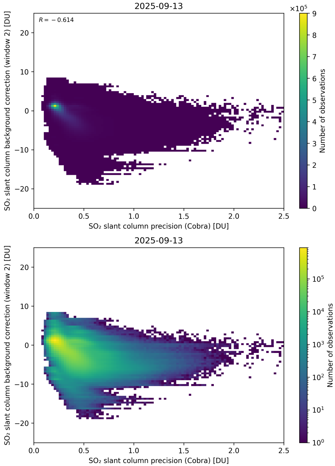
Figure 200: Scatter density plot of “SO 2 slant column precision (Cobra)” against “SO 2 slant column background correction (window 2)” for 2025-09-12 to 2025-09-14.
