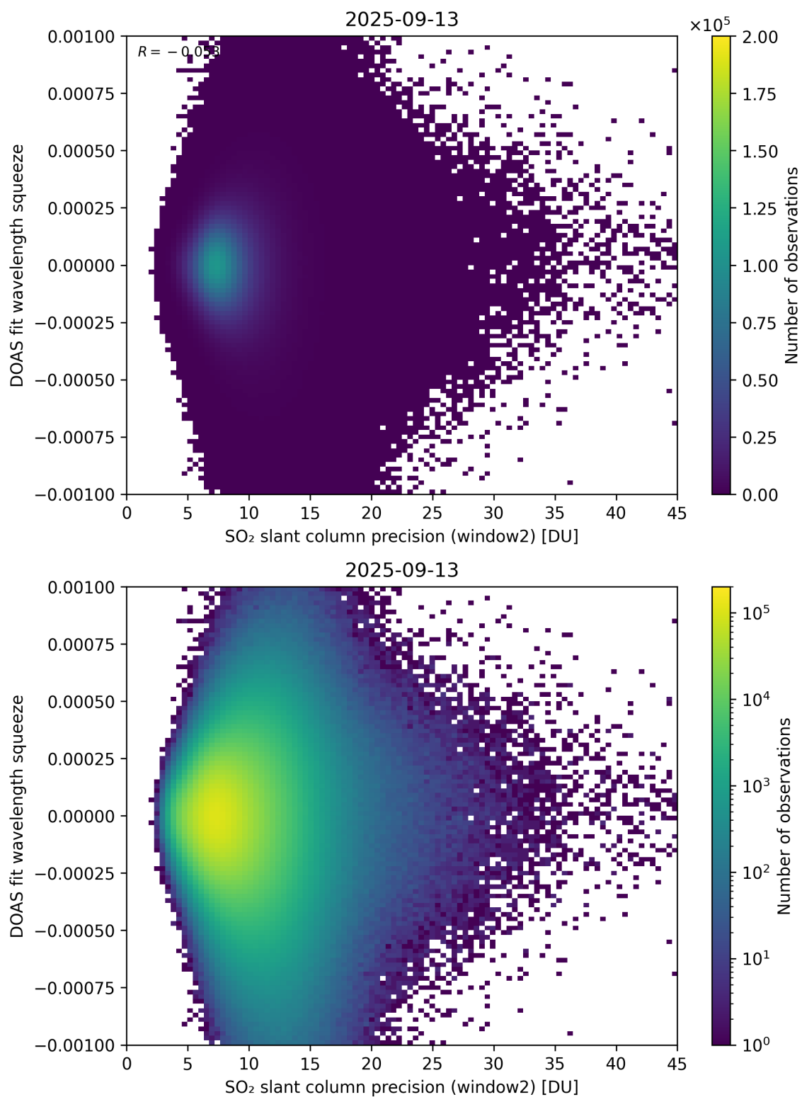
Figure 294: Scatter density plot of “SO 2 slant column precision (window2)” against “DOAS fit wavelength squeeze” for 2025-09-12 to 2025-09-14.
