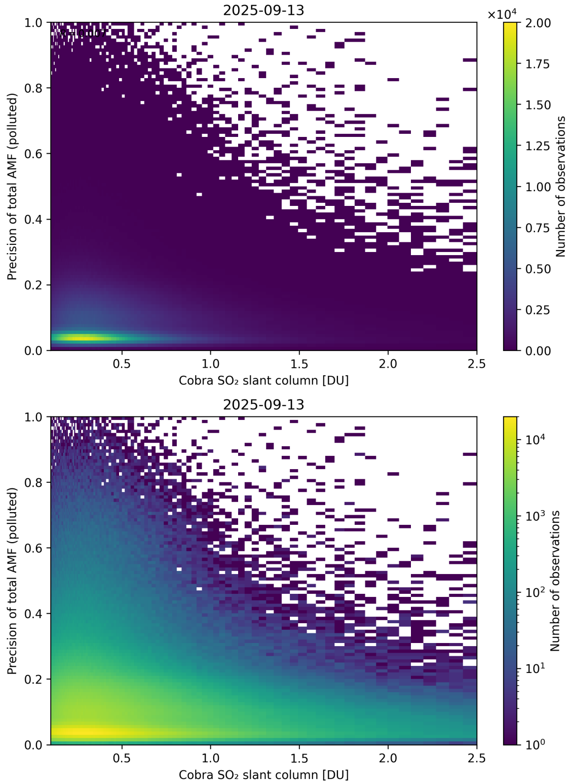
Figure 225: Scatter density plot of “Cobra SO 2 slant column” against “Precision of total AMF (polluted)” for 2025-09-12 to 2025-09-14.
