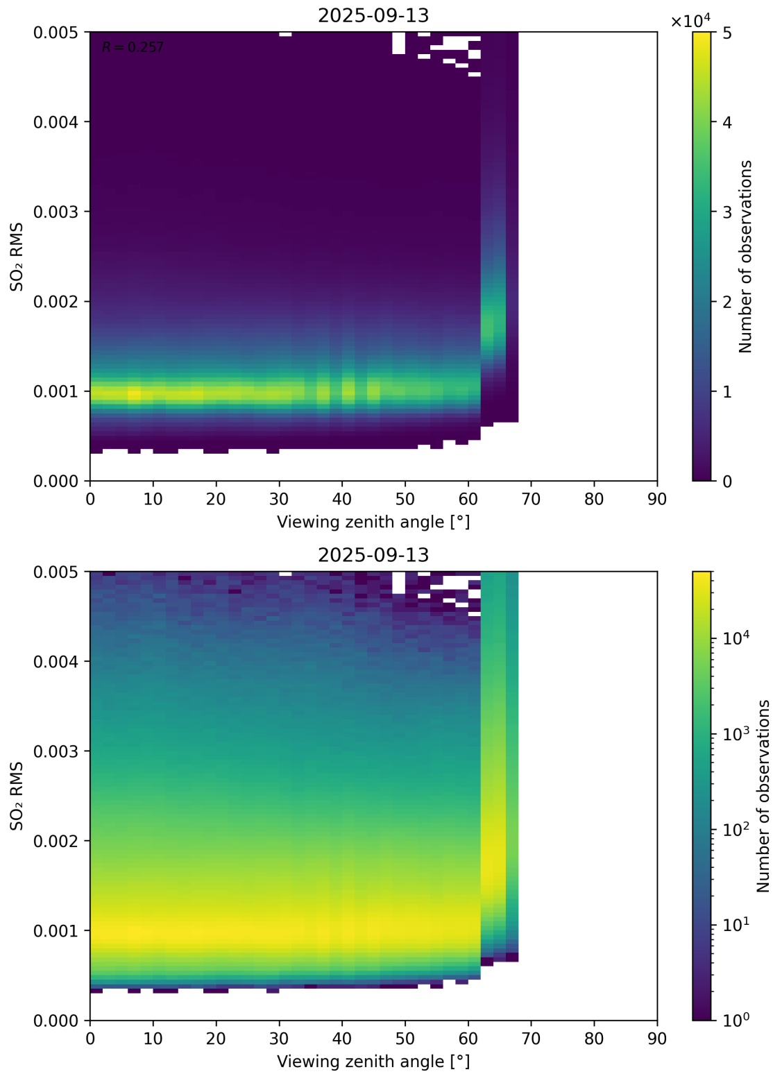
Figure 367: Scatter density plot of “Viewing zenith angle” against “SO 2 RMS” for 2025-09-12 to 2025-09-14.
