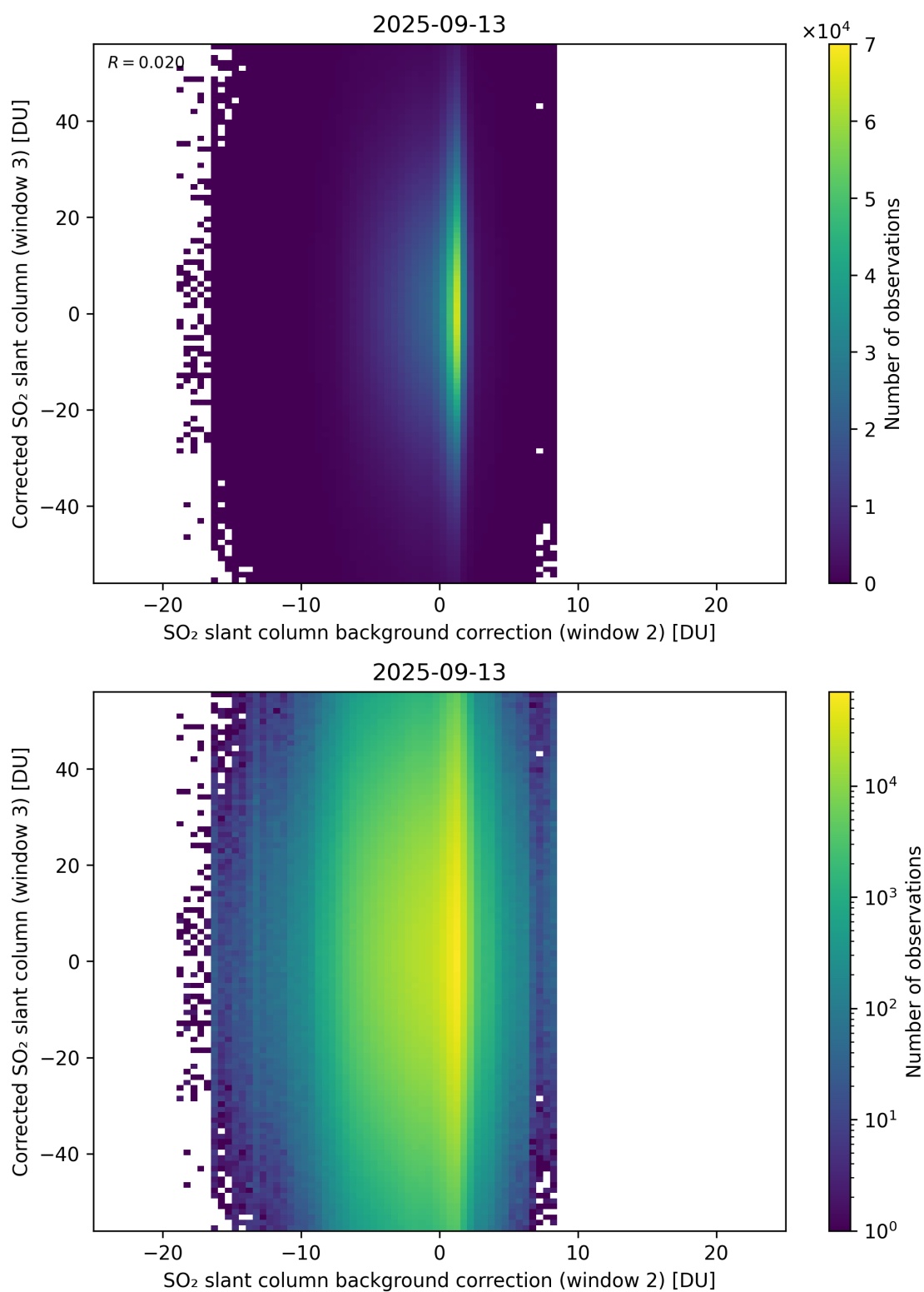
Figure 127: Scatter density plot of “SO 2 slant column background correction (window 2)” against “Corrected SO 2 slant column (window 3)” for 2025-09-12 to 2025-09-14.
