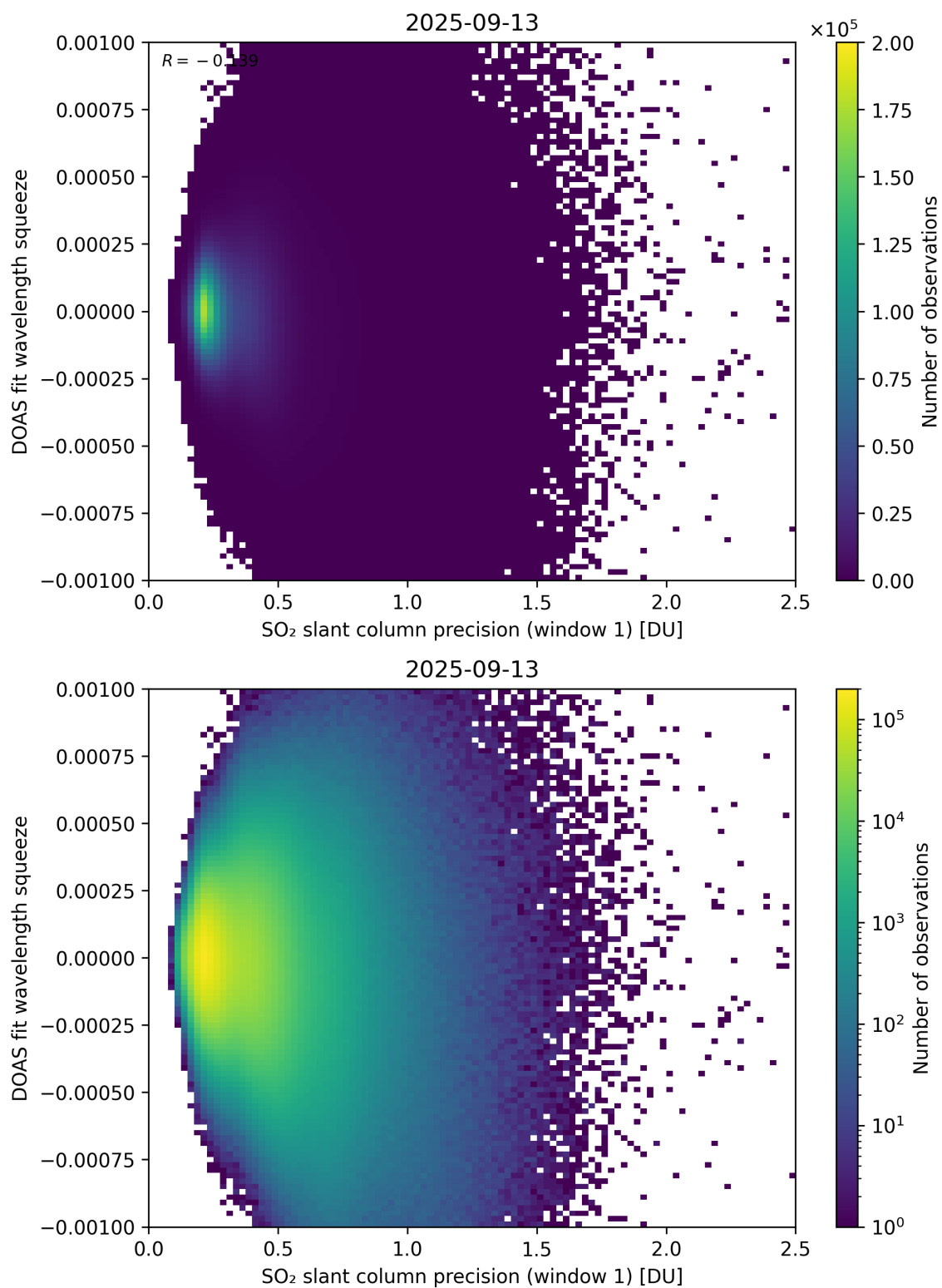
Figure 272: Scatter density plot of “SO 2 slant column precision (window 1)” against “DOAS fit wavelength squeeze” for 2025-09-12 to 2025-09-14.
