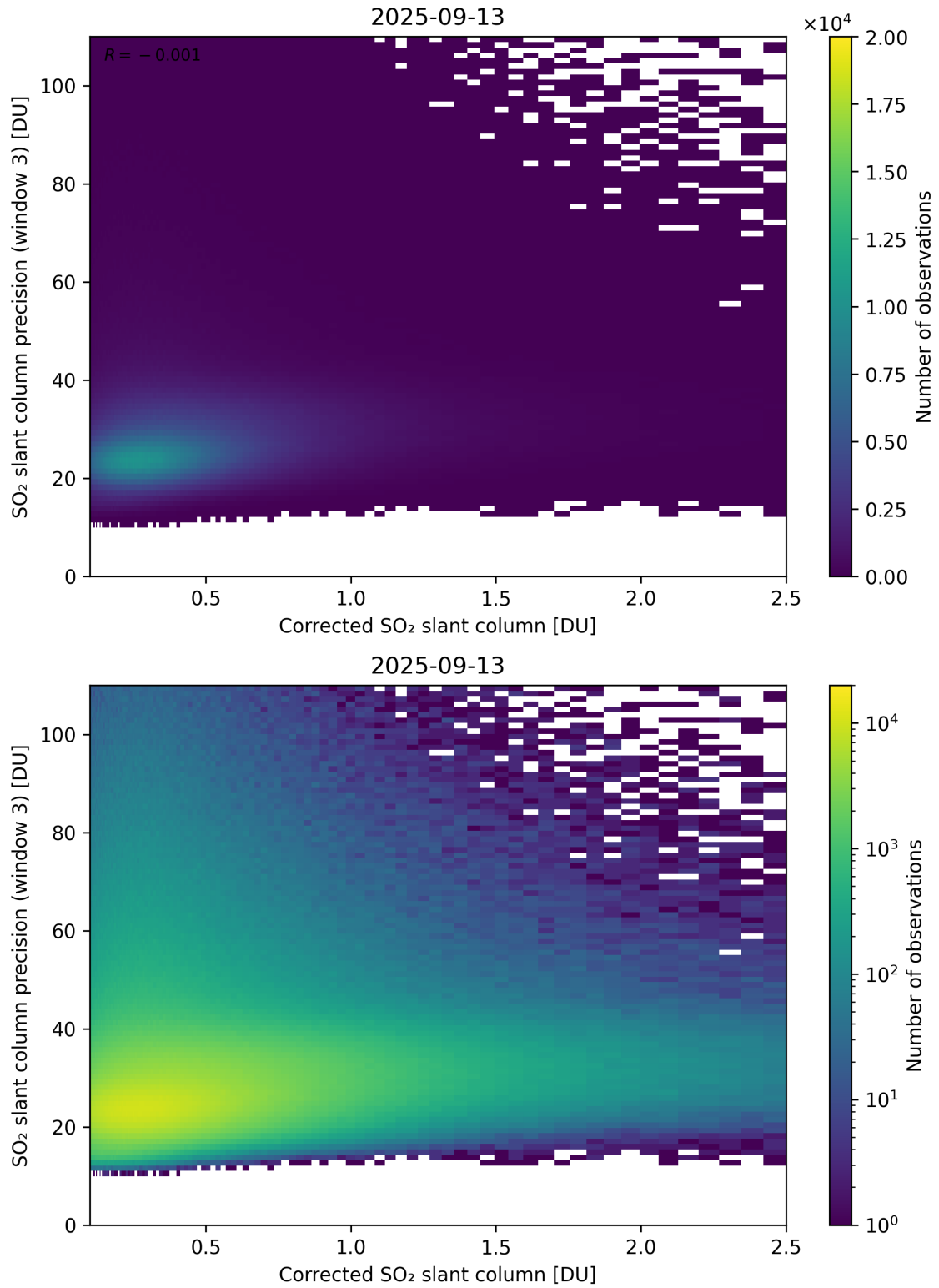
Figure 241: Scatter density plot of “Corrected SO 2 slant column” against “SO 2 slant column precision (window 3)” for 2025-09-12 to 2025-09-14.
