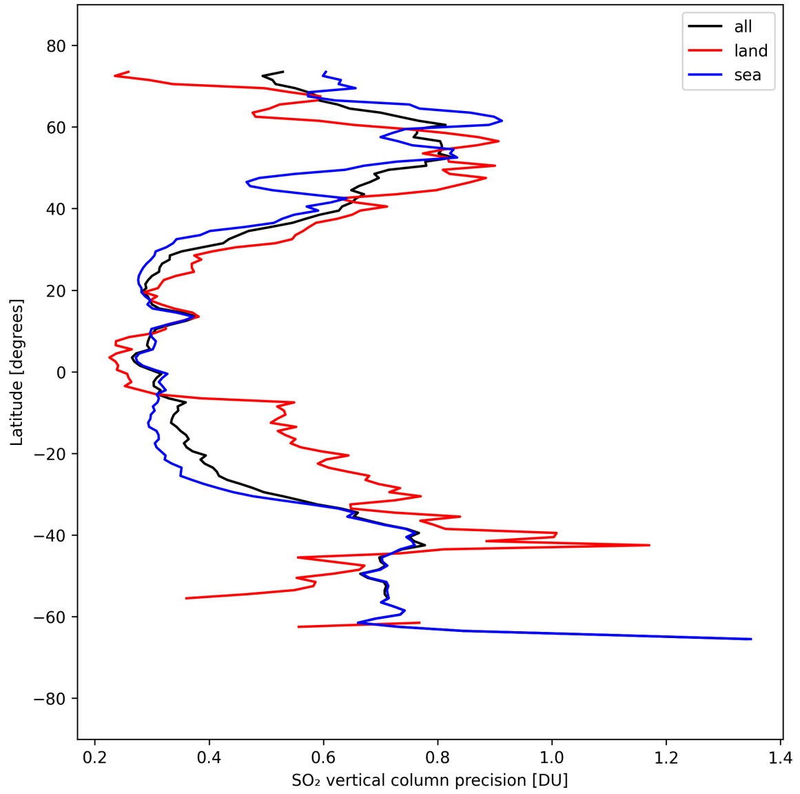
Figure 33: Zonal average of “SO 2 vertical column precision” for 2025-09-12 to 2025-09-14.
