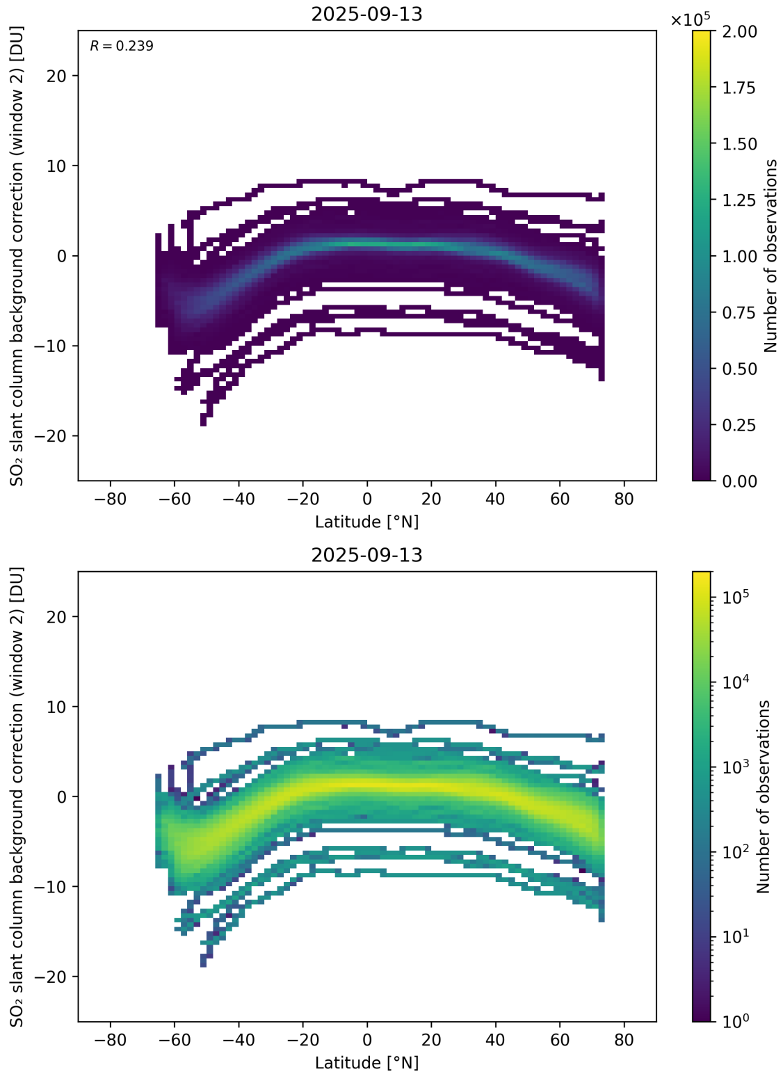
Figure 151: Scatter density plot of “Latitude” against “SO 2 slant column background correction (window 2)” for 2025-09-12 to 2025-09-14.
