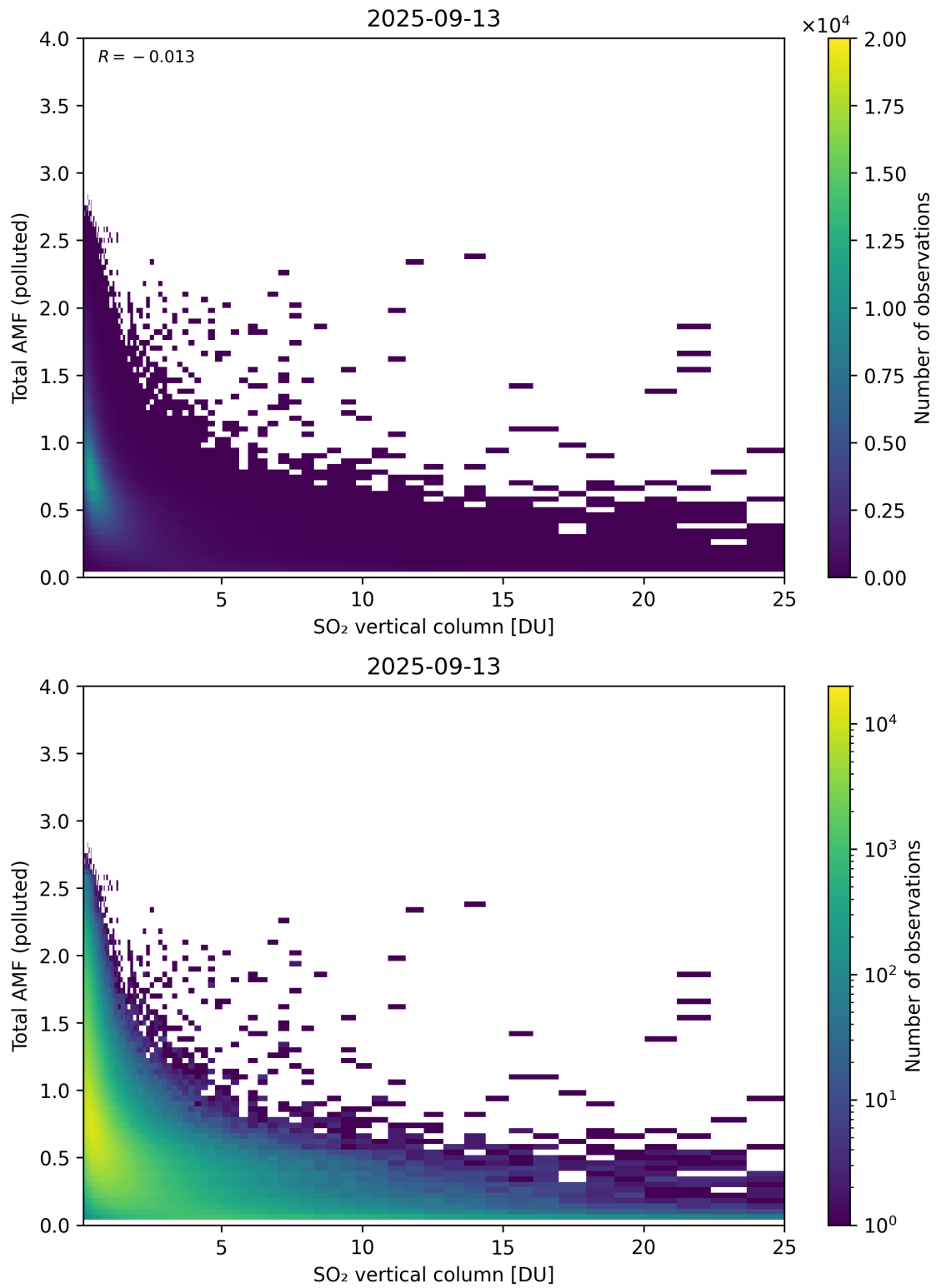
Figure 359: Scatter density plot of “SO 2 vertical column” against “Total AMF (polluted)” for 2025-09-12 to 2025-09-14.
