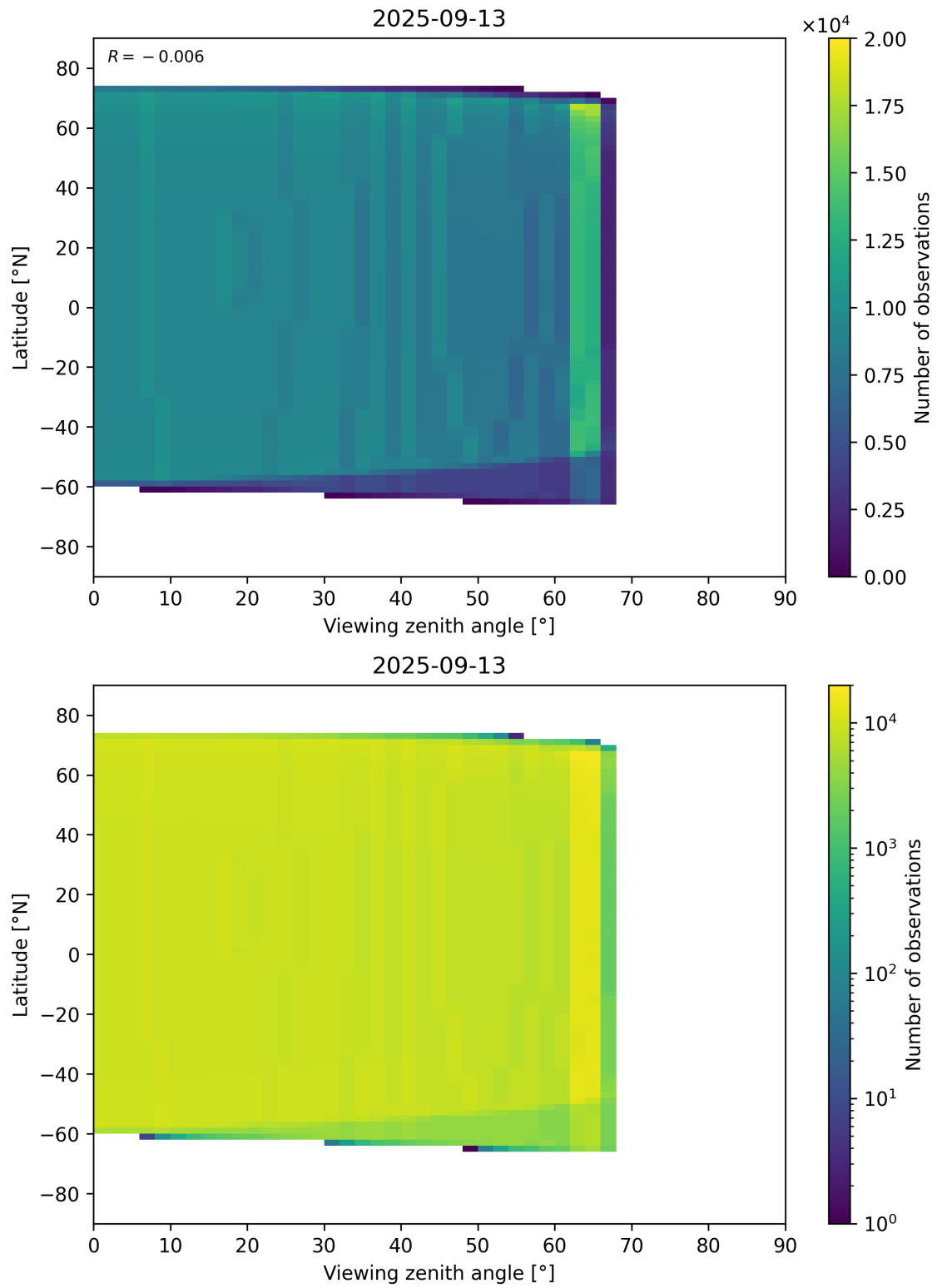
Figure 368: Scatter density plot of “Viewing zenith angle” against “Latitude” for 2025-09-12 to 2025-09-14.
