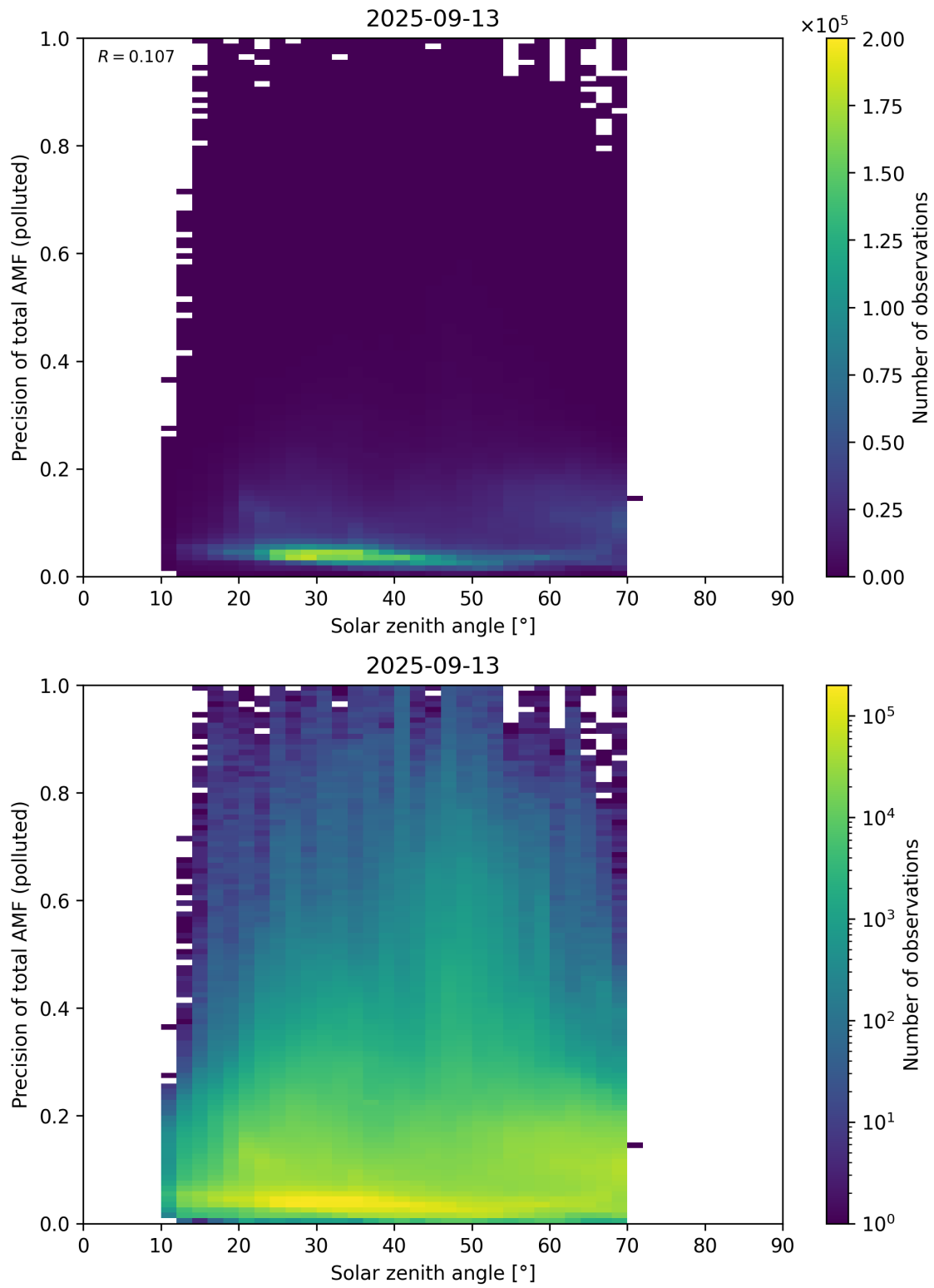
Figure 190: Scatter density plot of “Solar zenith angle” against “Precision of total AMF (polluted)” for 2025-09-12 to 2025-09-14.
