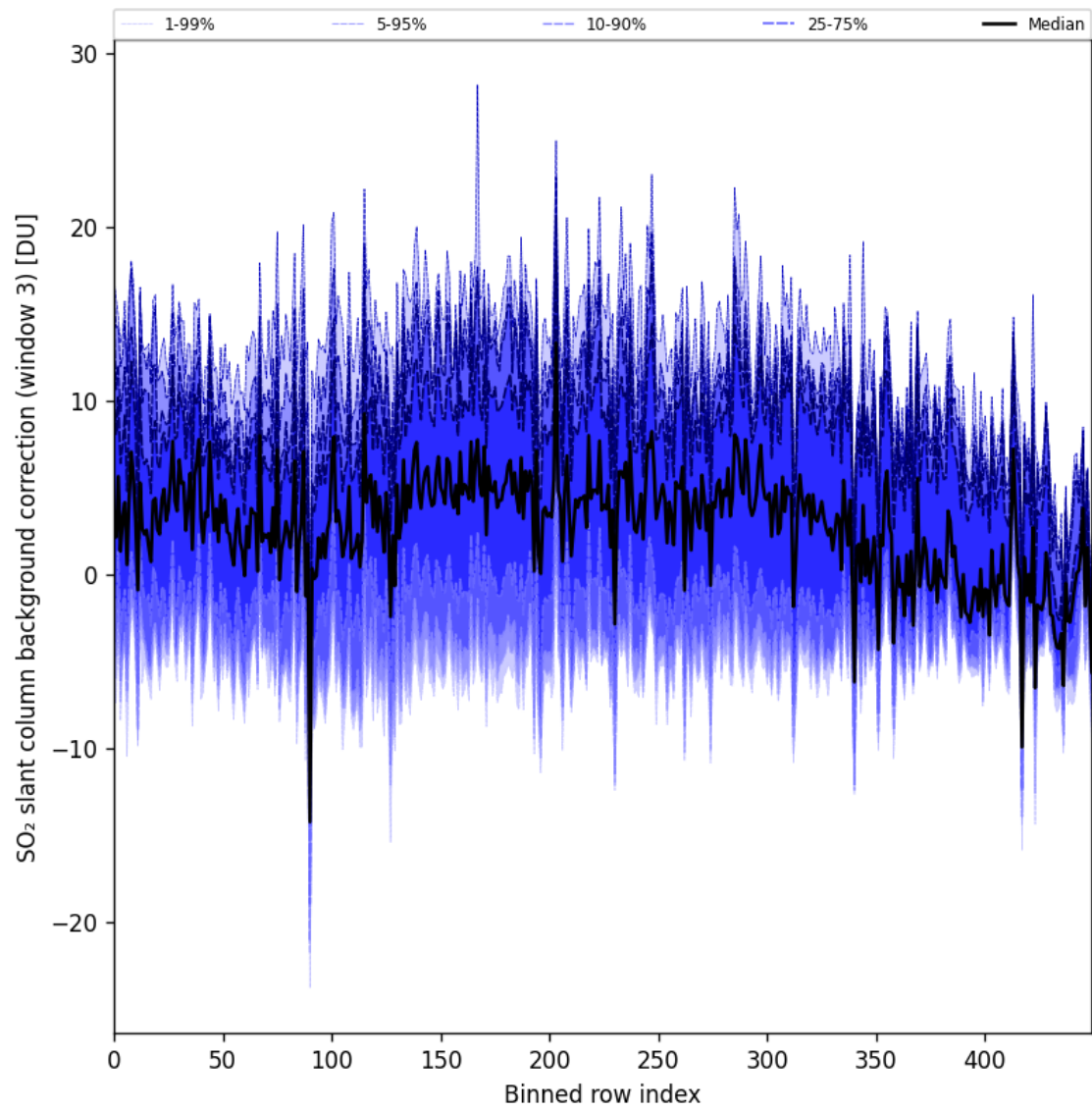
Figure 100: Along track statistics of “SO 2 slant column background correction (window 3)” for 2025-09-12 to 2025-09-14
