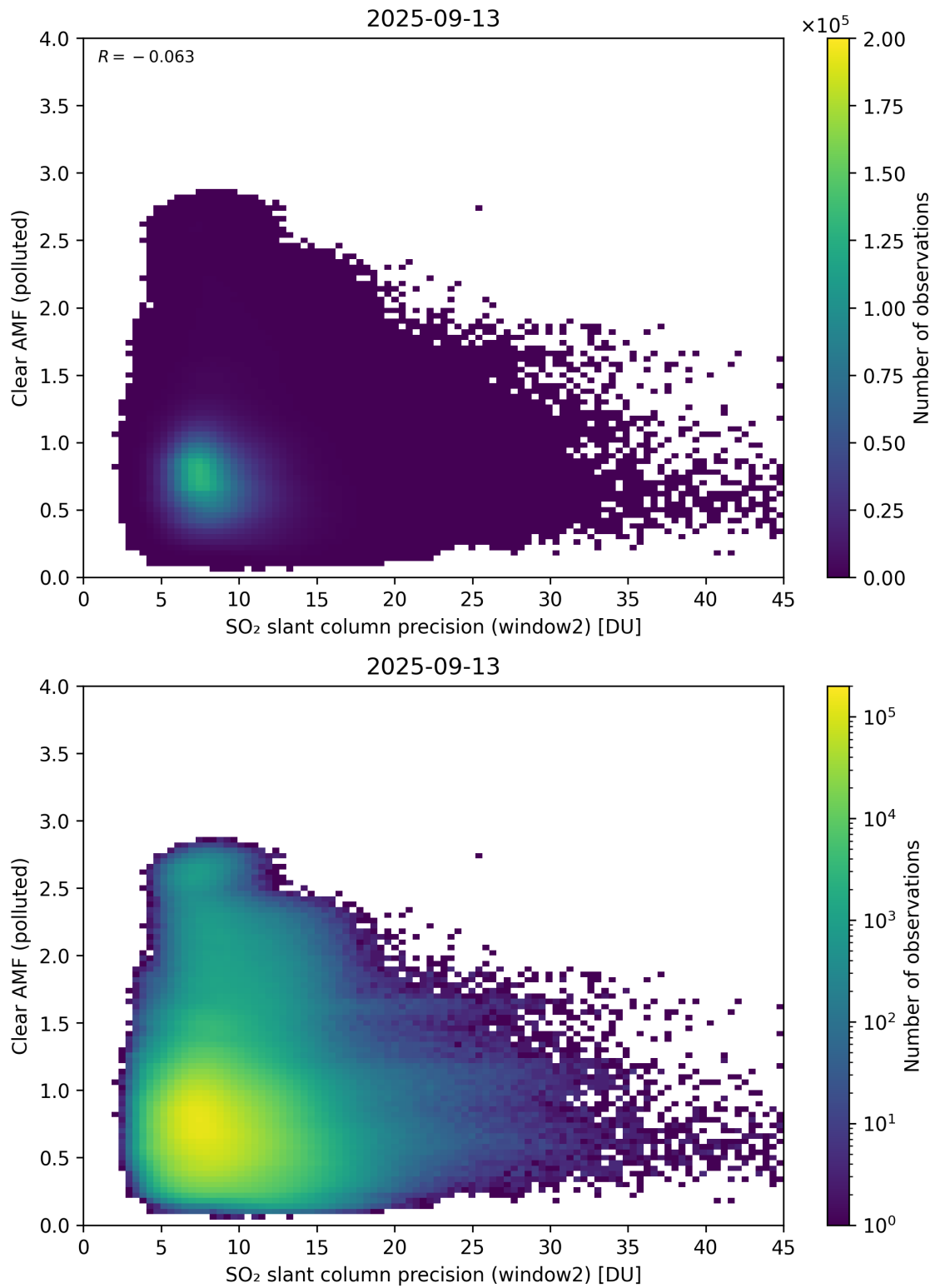
Figure 296: Scatter density plot of “SO 2 slant column precision (window2)” against “Clear AMF (polluted)” for 2025-09-12 to 2025-09-14.
