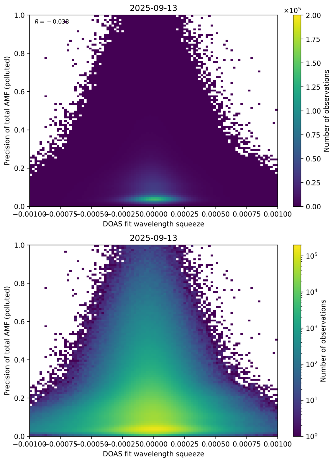
Figure 146: Scatter density plot of “DOAS fit wavelength squeeze” against “Precision of total AMF (polluted)” for 2025-09-12 to 2025-09-14.
