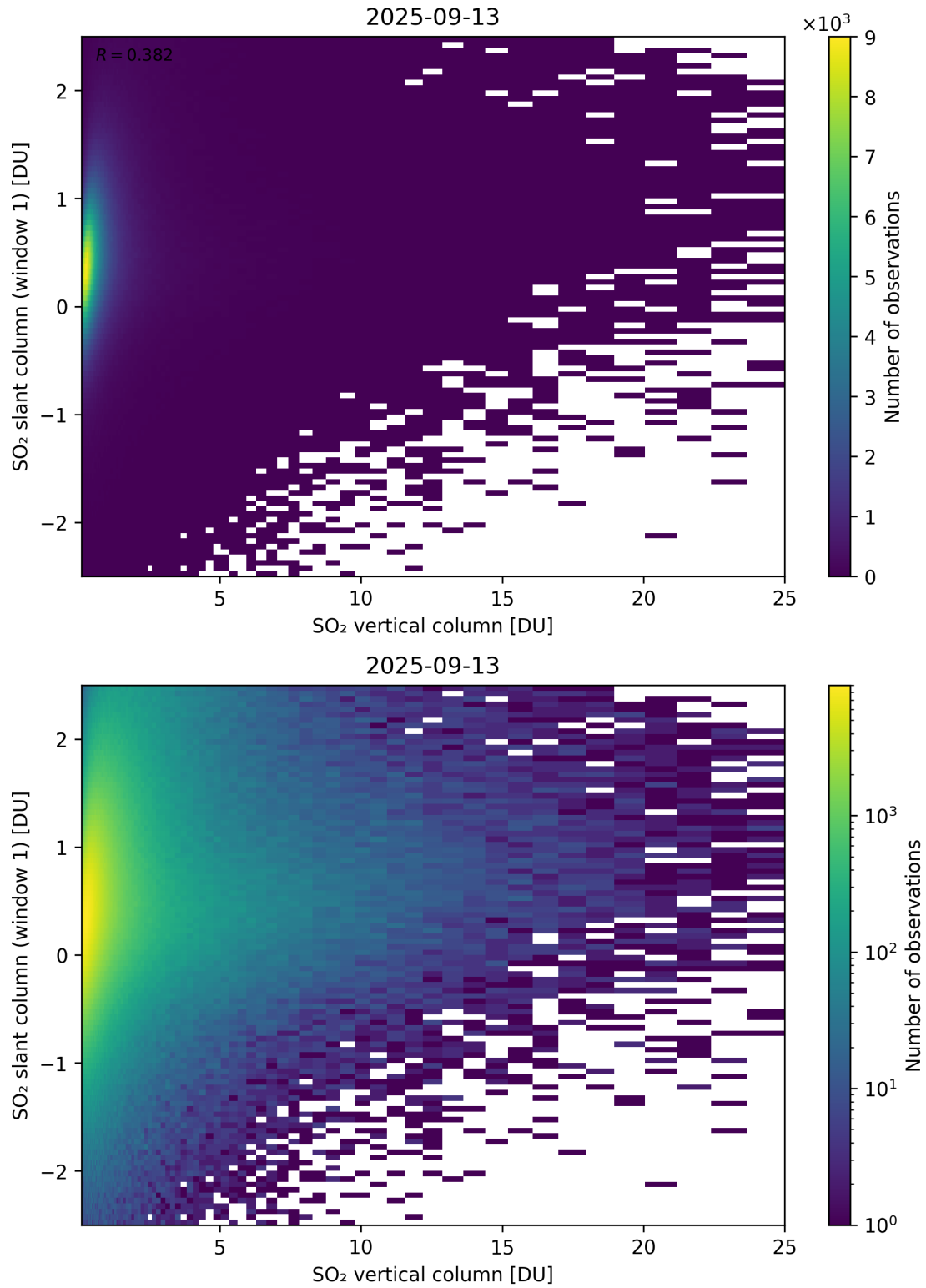
Figure 354: Scatter density plot of “SO 2 vertical column” against “SO 2 slant column (window 1)” for 2025-09-12 to 2025-09-14.
