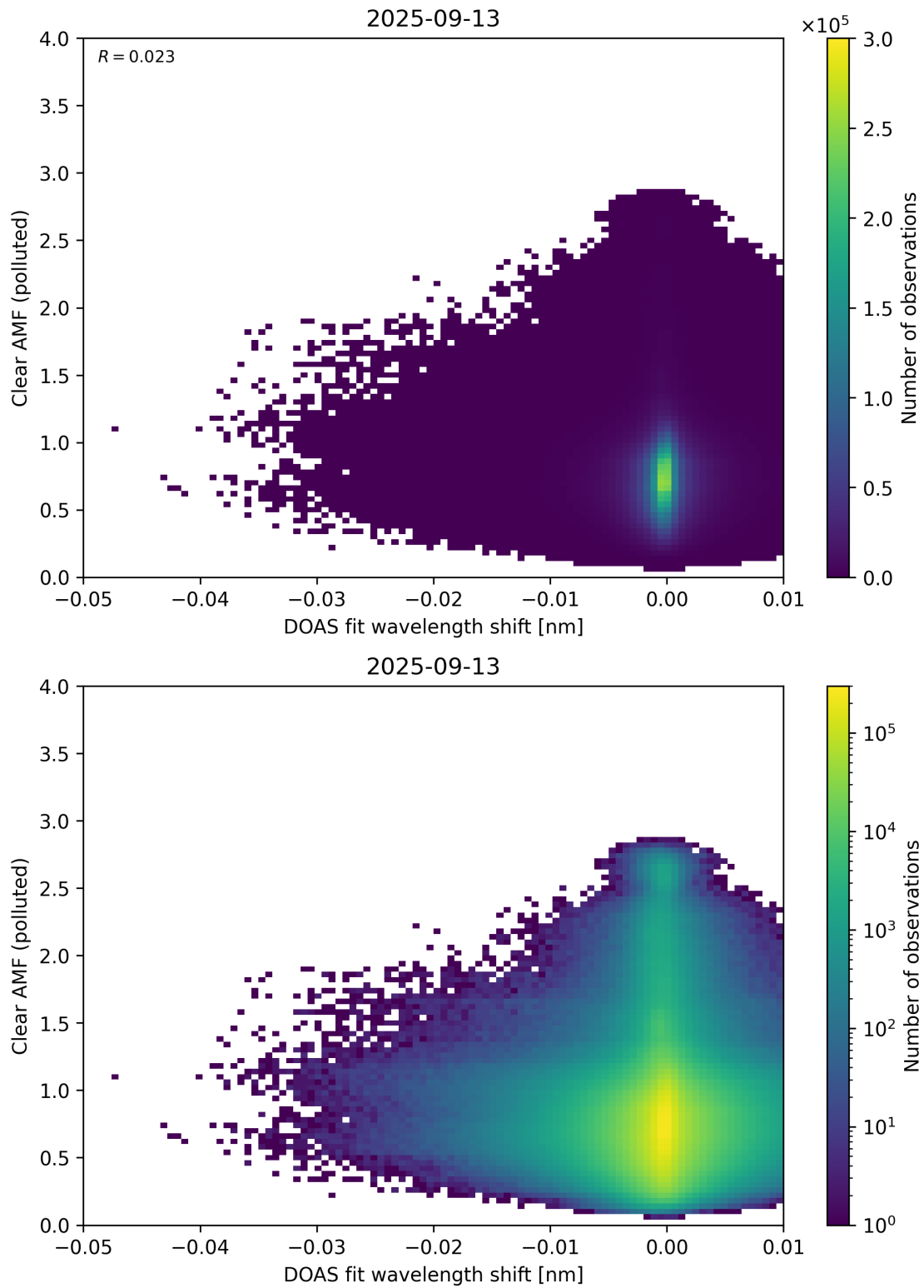
Figure 140: Scatter density plot of “DOAS fit wavelength shift” against “Clear AMF (polluted)” for 2025-09-12 to 2025-09-14.
