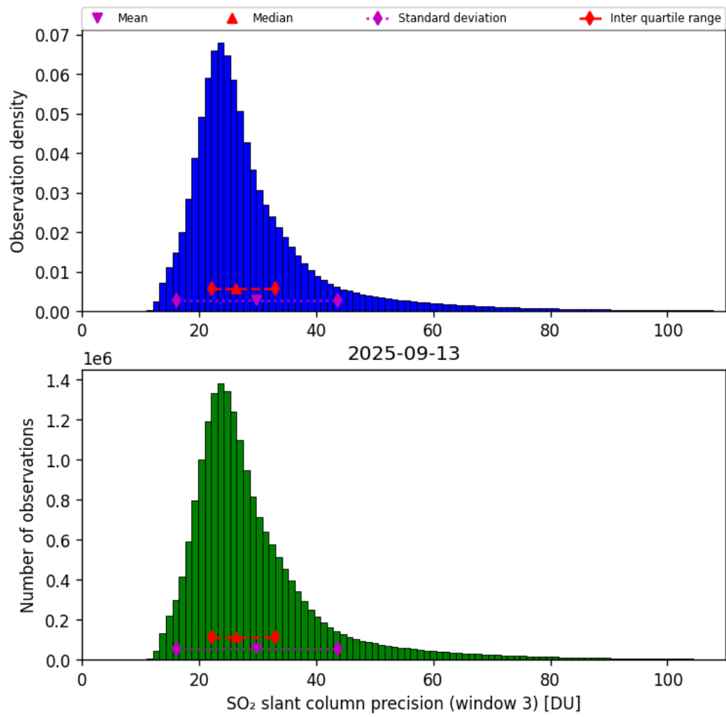
Figure 72: Histogram of “SO 2 slant column precision (window 3)” for 2025-09-12 to 2025-09-14
