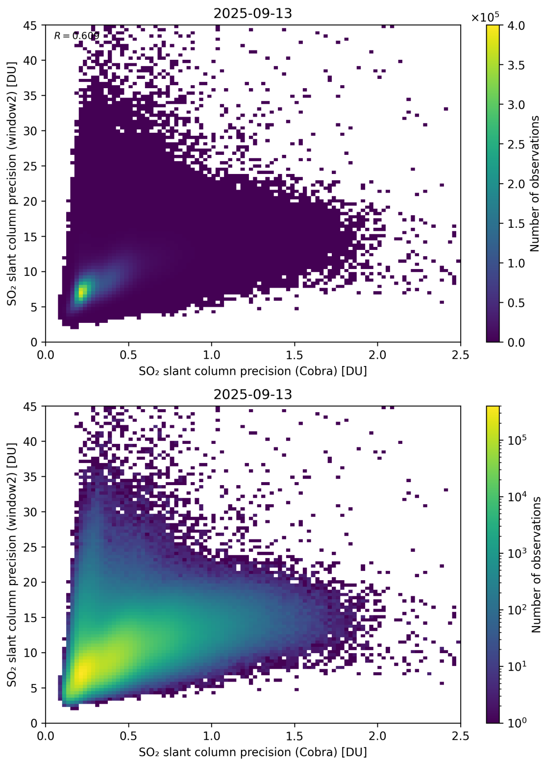
Figure 210: Scatter density plot of “SO 2 slant column precision (Cobra)” against “SO 2 slant column precision (window2)” for 2025-09-12 to 2025-09-14.
