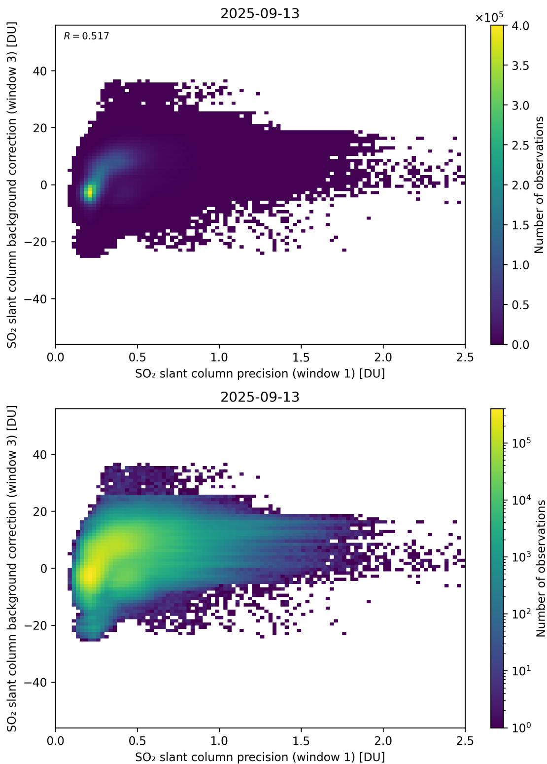
Figure 270: Scatter density plot of “SO 2 slant column precision (window 1)” against “SO 2 slant column background correction (window 3)” for 2025-09-12 to 2025-09-14.
