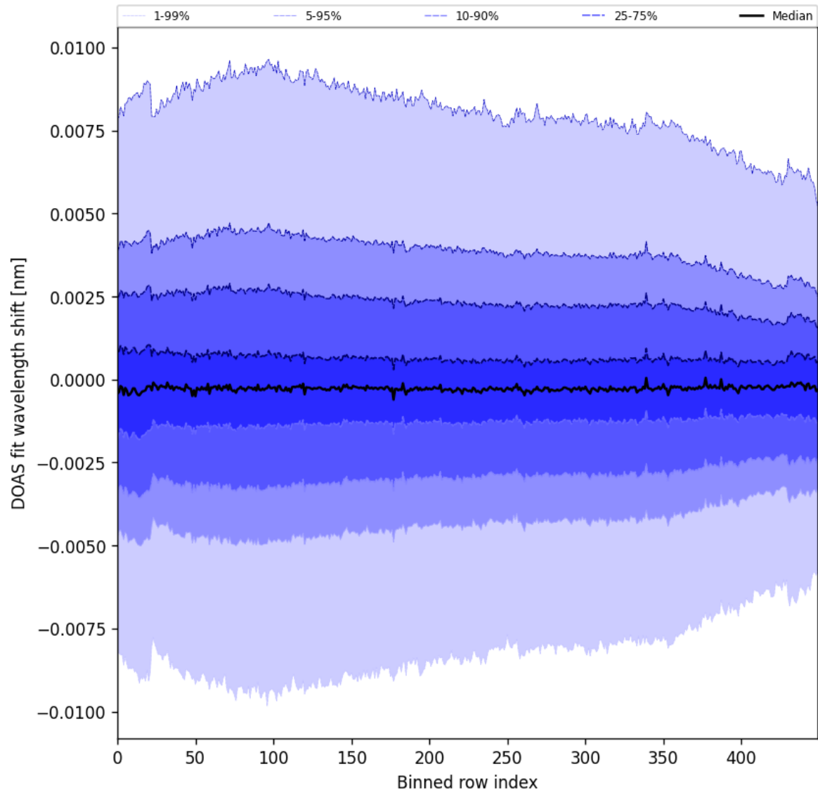
Figure 102: Along track statistics of “DOAS fit wavelength shift” for 2025-09-12 to 2025-09-14
