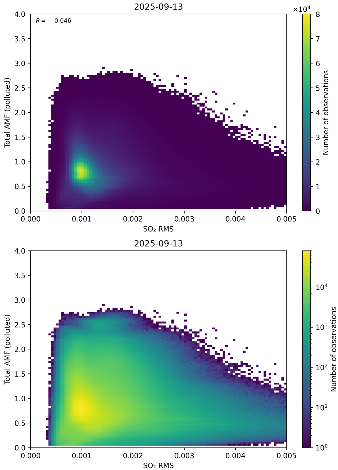
Figure 148: Scatter density plot of “SO 2 RMS” against “Total AMF (polluted)” for 2025-09-12 to 2025-09-14.
