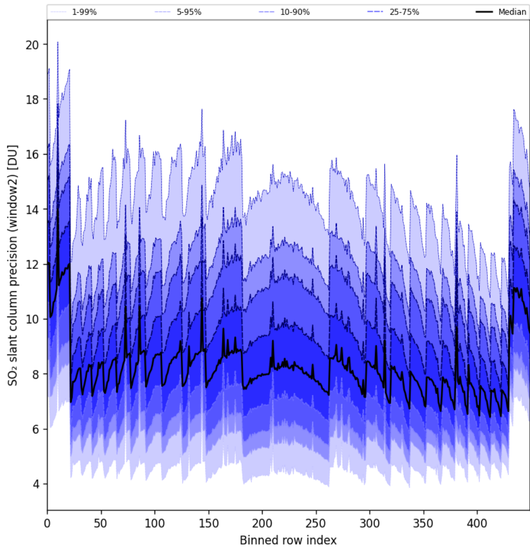
Figure 94: Along track statistics of “SO 2 slant column precision (window2)” for 2025-09-12 to 2025-09-14
