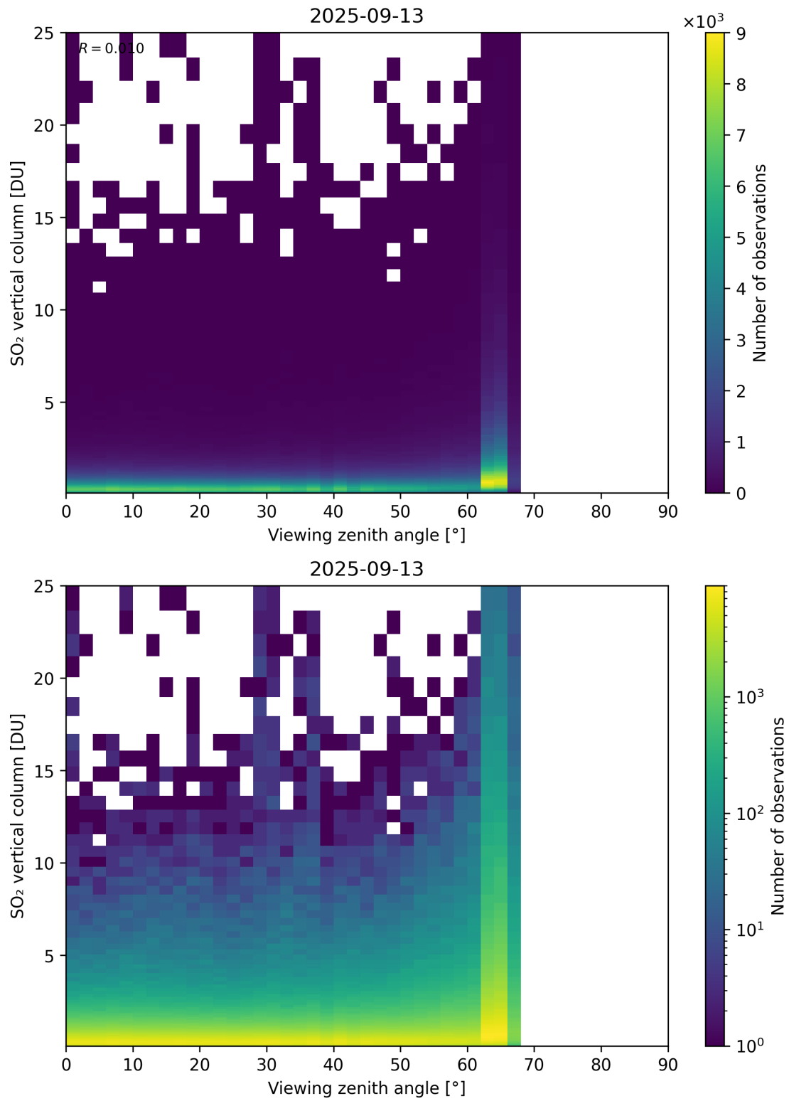
Figure 383: Scatter density plot of “Viewing zenith angle” against “SO 2 vertical column” for 2025-09-12 to 2025-09-14.
