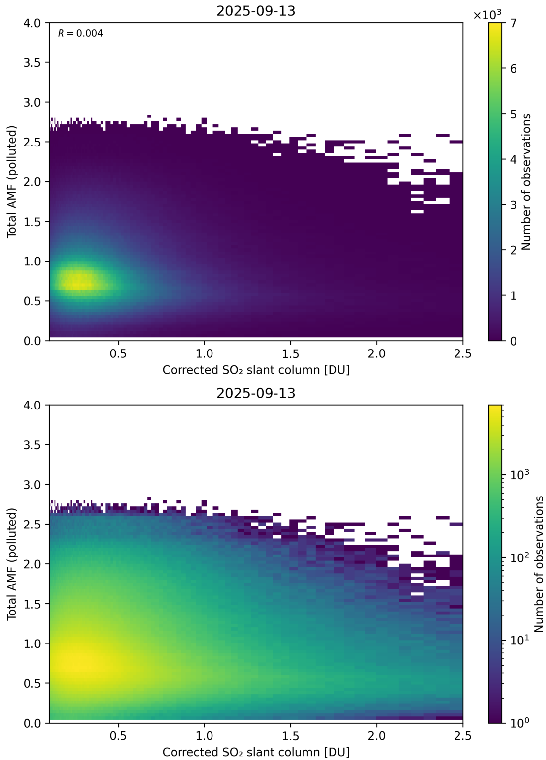
Figure 242: Scatter density plot of “Corrected SO 2 slant column” against “Total AMF (polluted)” for 2025-09-12 to 2025-09-14.
