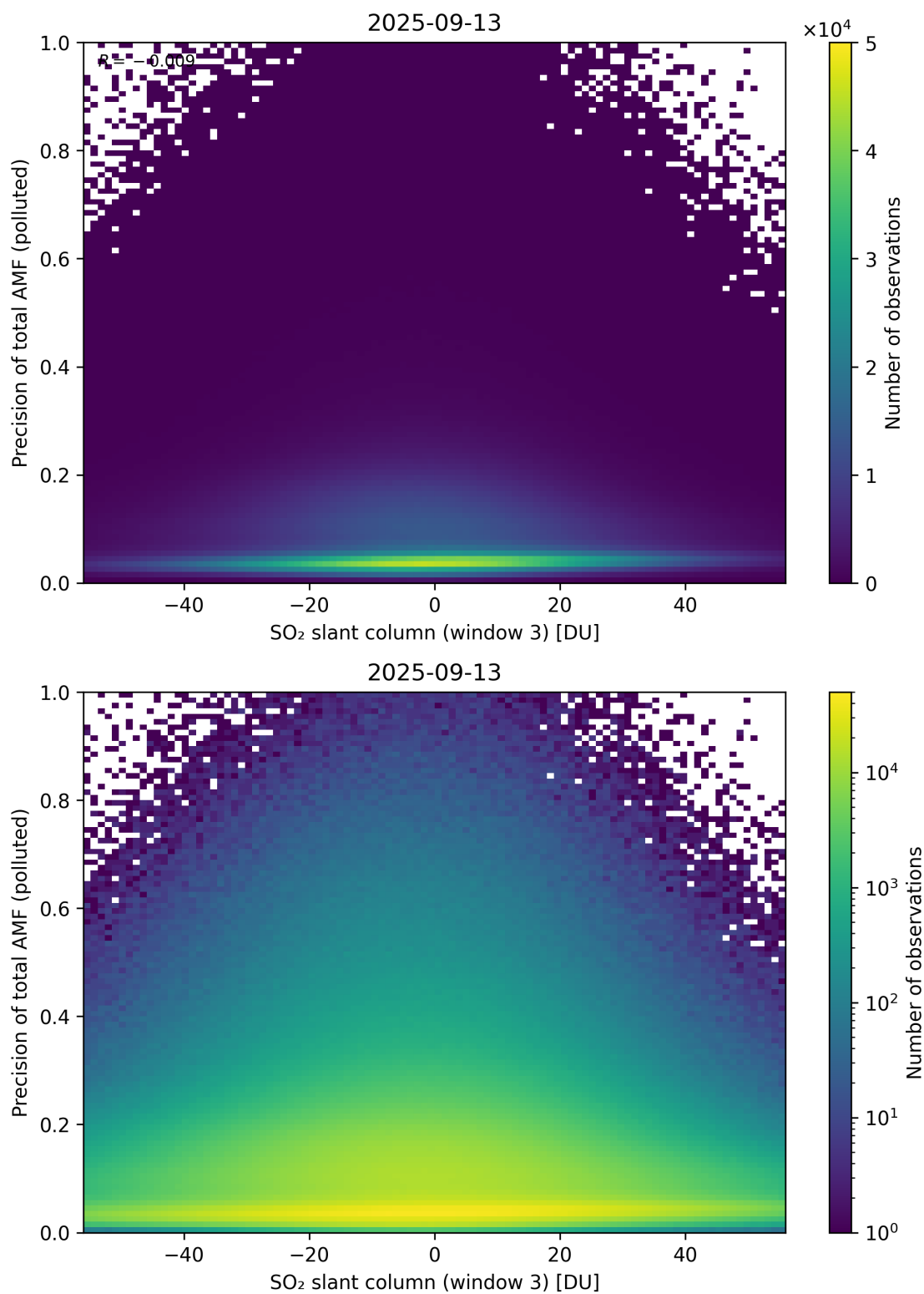
Figure 319: Scatter density plot of “SO 2 slant column (window 3)” against “Precision of total AMF (polluted)” for 2025-09-12 to 2025-09-14.
