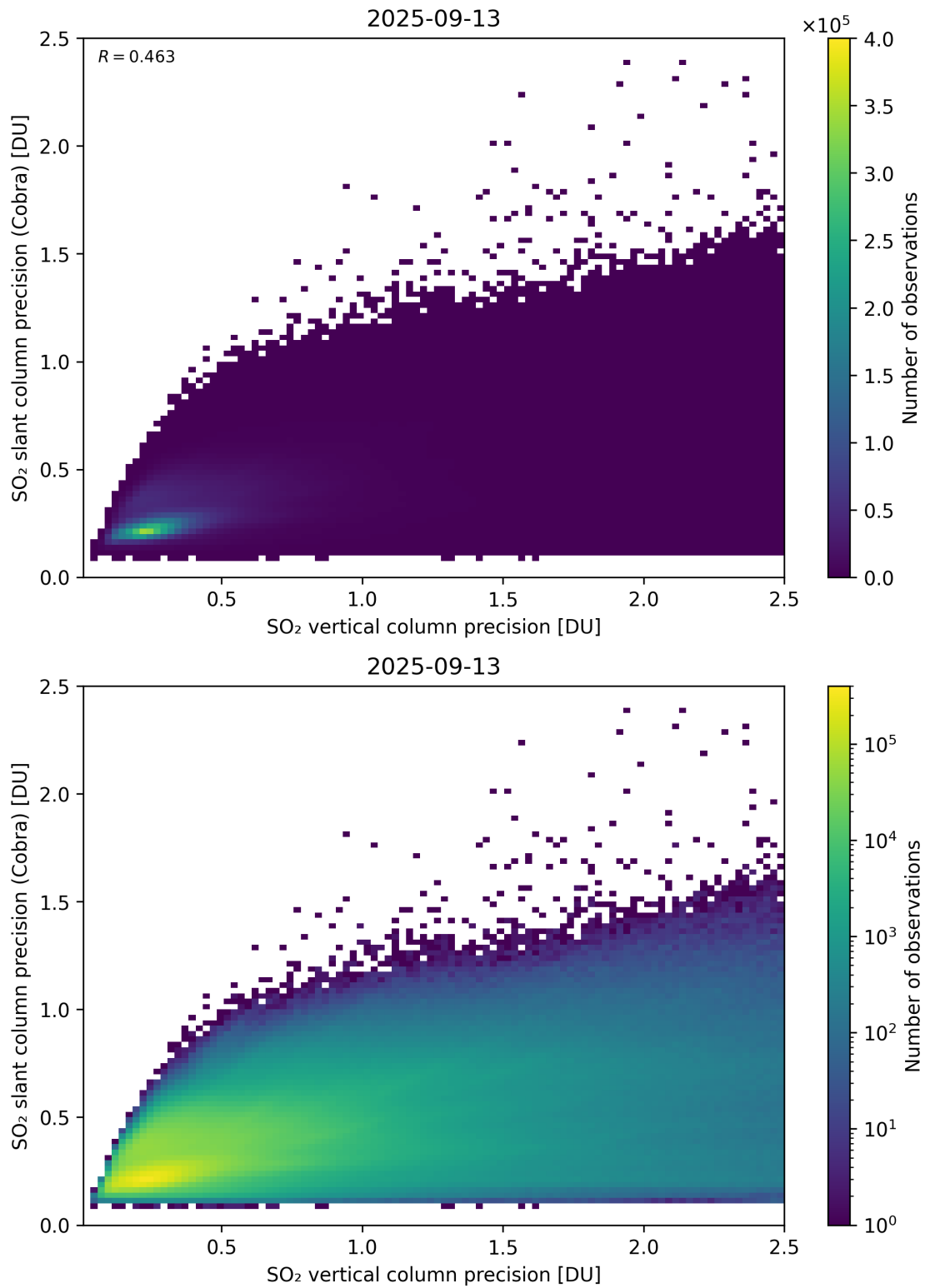
Figure 337: Scatter density plot of “SO 2 vertical column precision” against “SO 2 slant column precision (Cobra)” for 2025-09-12 to 2025-09-14.
