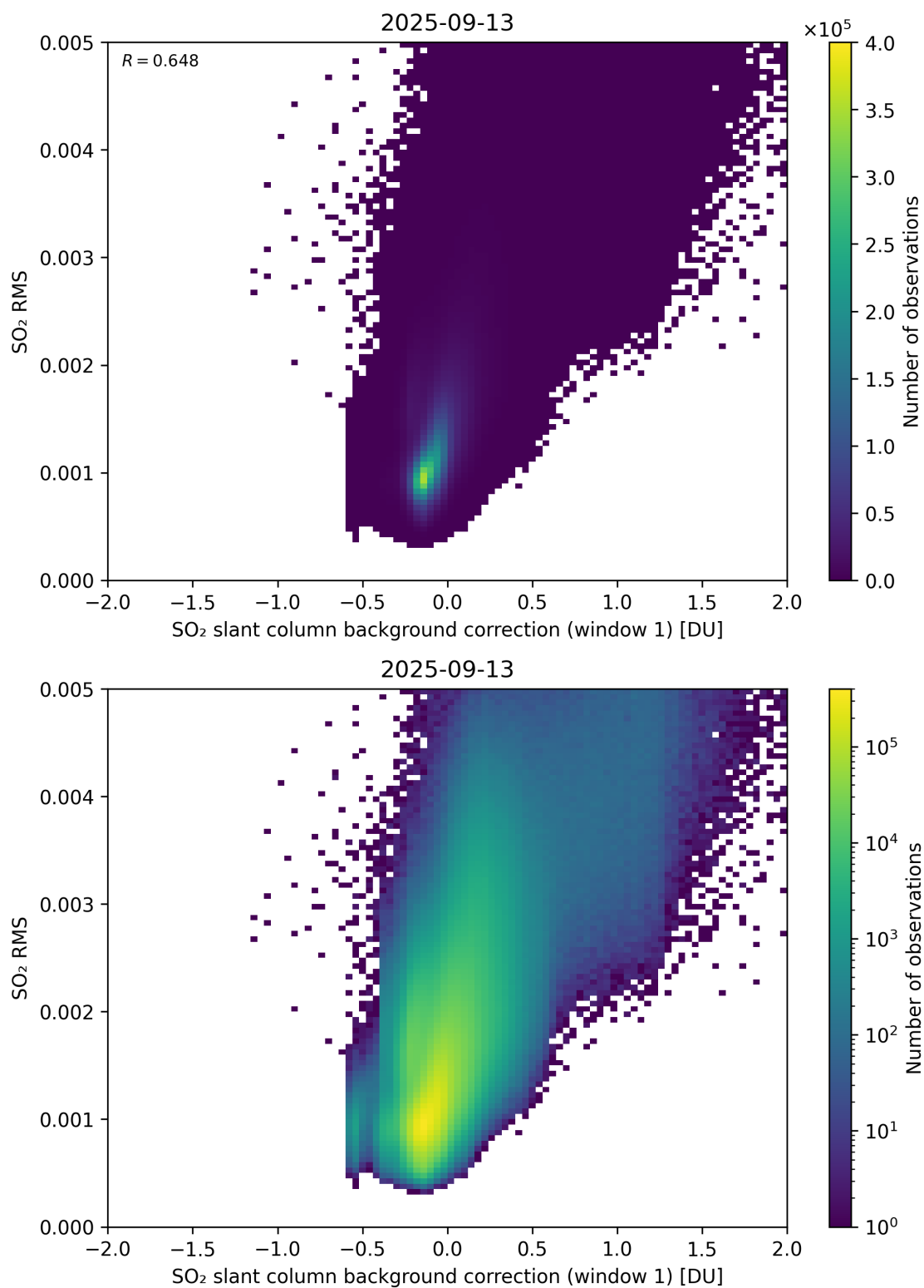
Figure 113: Scatter density plot of “SO 2 slant column background correction (window 1)” against “SO 2 RMS” for 2025-09-12 to 2025-09-14.
