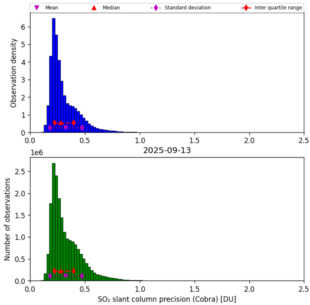
Figure 62: Histogram of “SO 2 slant column precision (Cobra)” for 2025-09-12 to 2025-09-14
