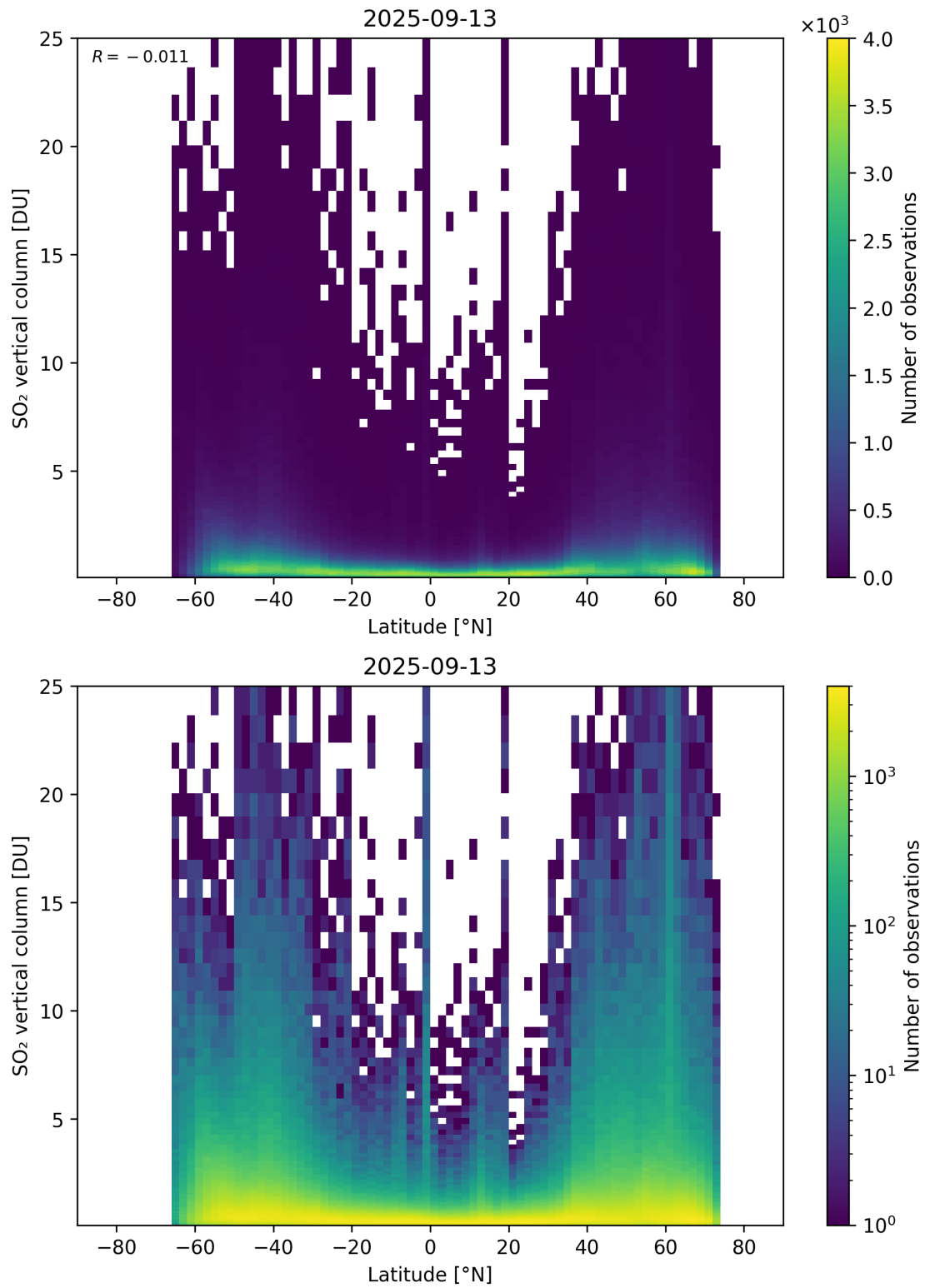
Figure 169: Scatter density plot of “Latitude” against “SO 2 vertical column” for 2025-09-12 to 2025-09-14.
