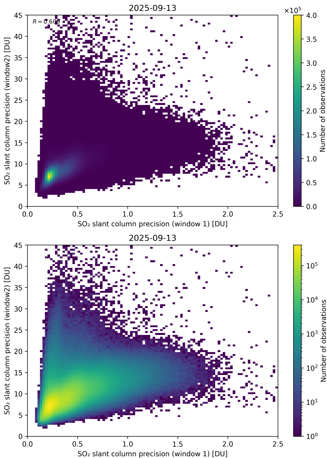
Figure 277: Scatter density plot of “SO 2 slant column precision (window 1)” against “SO 2 slant column precision (window2)” for 2025-09-12 to 2025-09-14.
