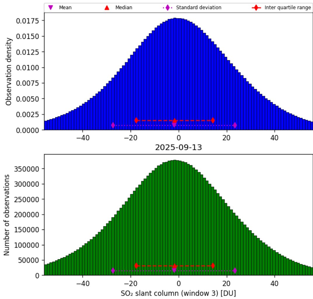
Figure 71: Histogram of “SO 2 slant column (window 3)” for 2025-09-12 to 2025-09-14
