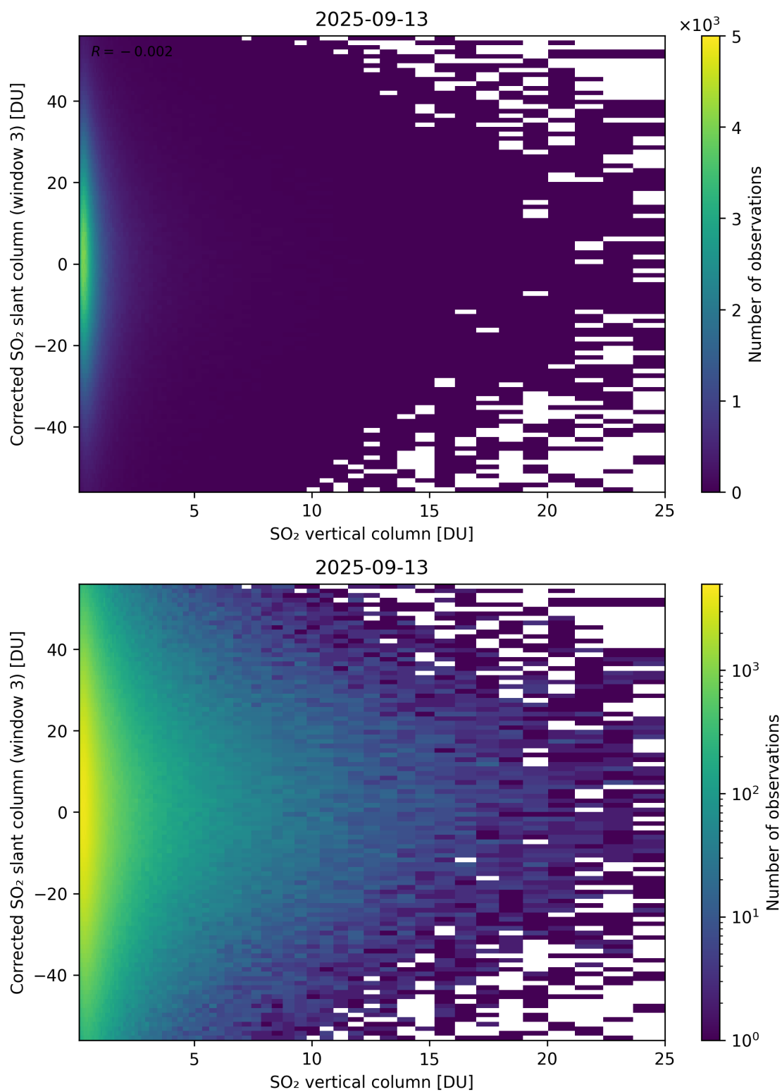
Figure 353: Scatter density plot of “SO 2 vertical column” against “Corrected SO 2 slant column (window 3)” for 2025-09-12 to 2025-09-14.
