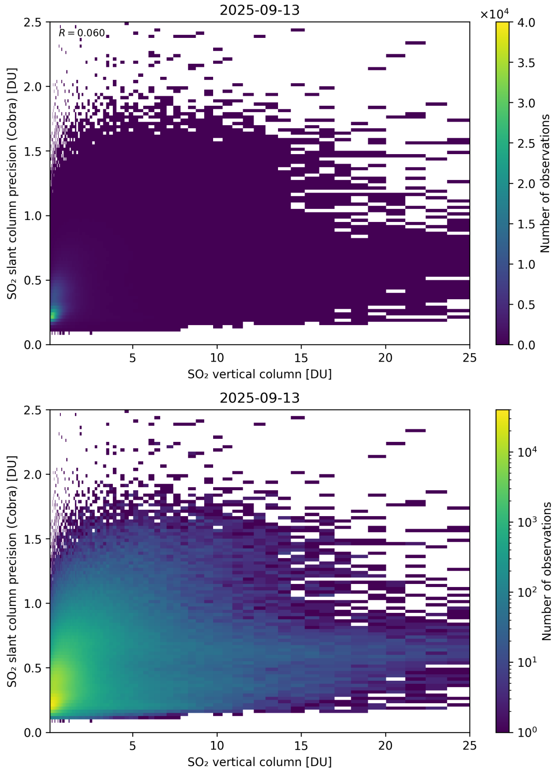
Figure 350: Scatter density plot of “SO 2 vertical column” against “SO 2 slant column precision (Cobra)” for 2025-09-12 to 2025-09-14.
