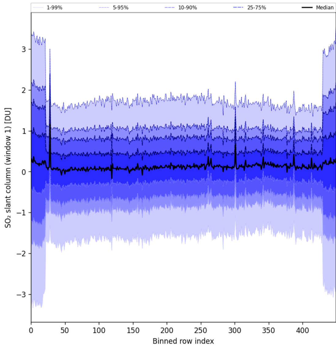
Figure 89: Along track statistics of “SO 2 slant column (window 1)” for 2025-09-12 to 2025-09-14
