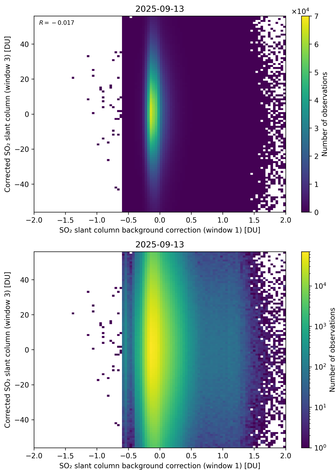
Figure 116: Scatter density plot of “SO 2 slant column background correction (window 1)” against “Corrected SO 2 slant column (window 3)” for 2025-09-12 to 2025-09-14.
