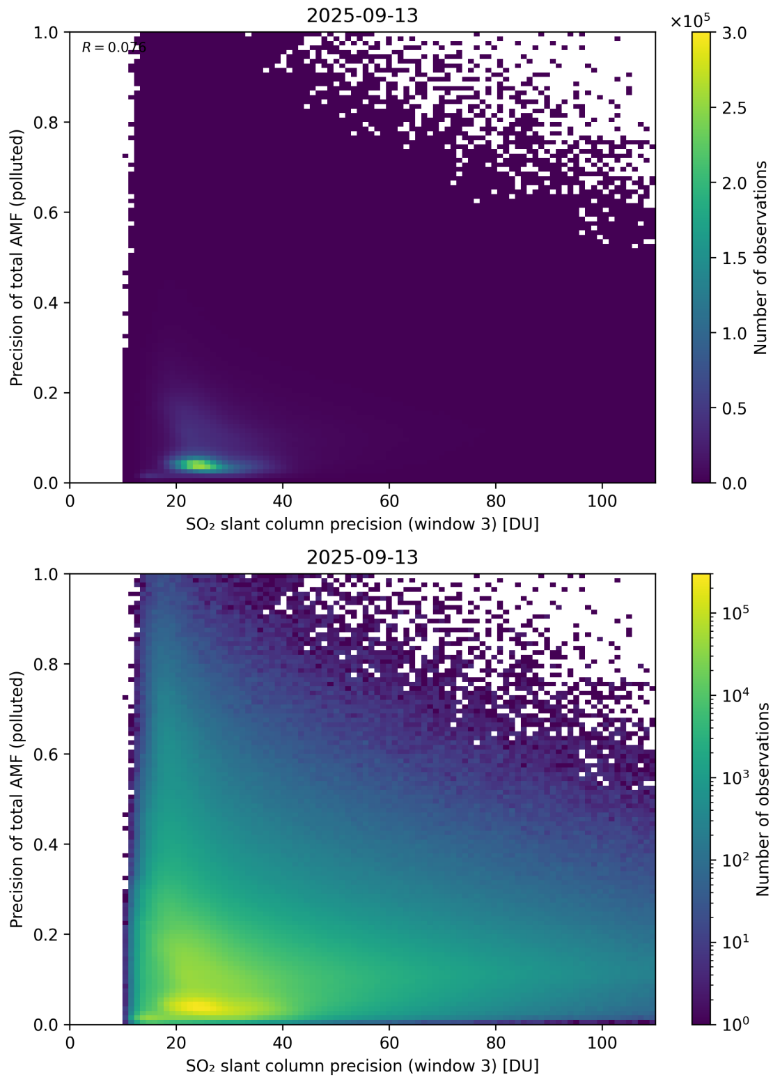
Figure 314: Scatter density plot of “SO 2 slant column precision (window 3)” against “Precision of total AMF (polluted)” for 2025-09-12 to 2025-09-14.
