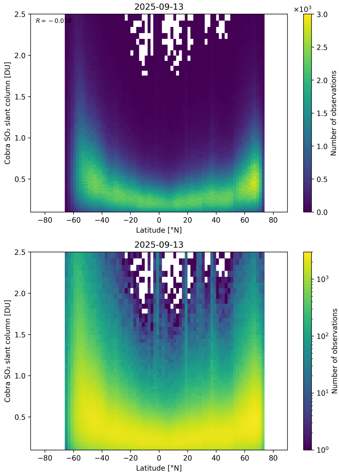
Figure 157: Scatter density plot of “Latitude” against “Cobra SO 2 slant column” for 2025-09-12 to 2025-09-14.
