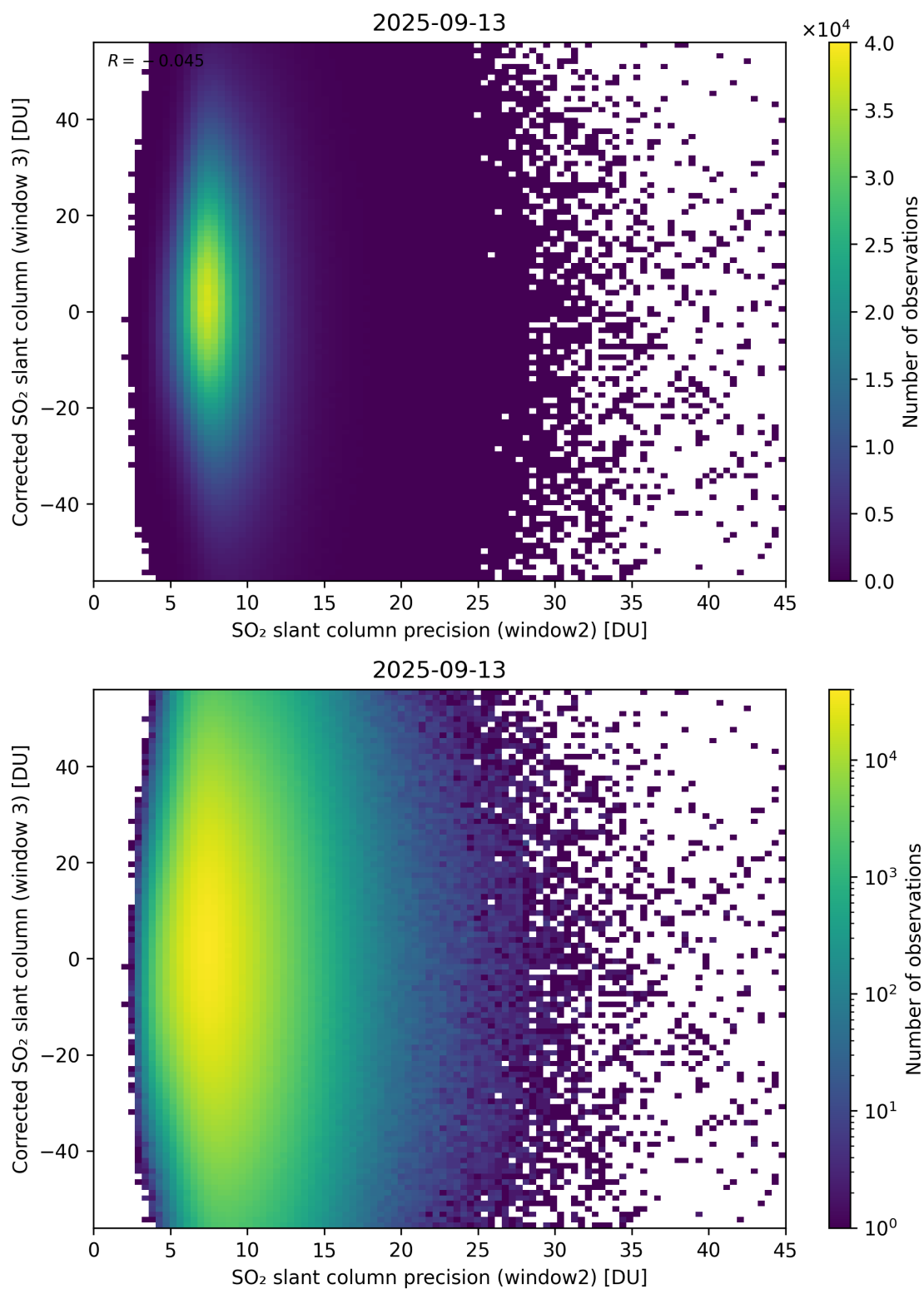
Figure 298: Scatter density plot of “SO 2 slant column precision (window2)” against “Corrected SO 2 slant column (window 3)” for 2025-09-12 to 2025-09-14.
