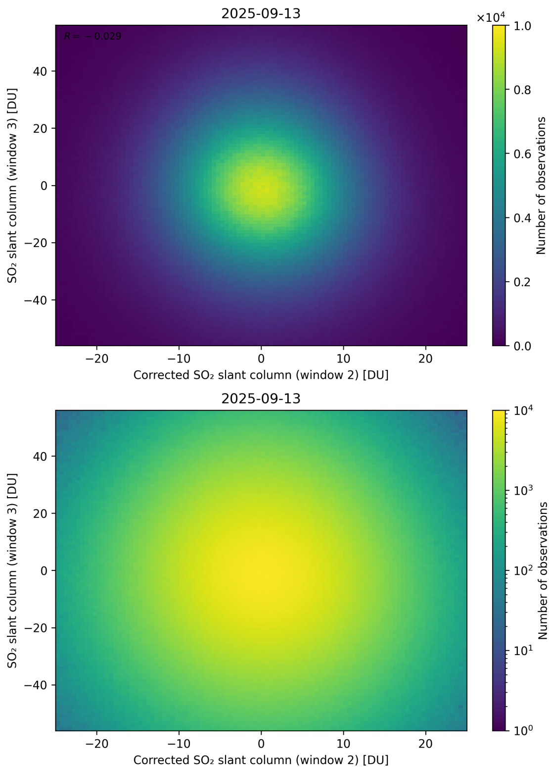
Figure 251: Scatter density plot of “Corrected SO 2 slant column (window 2)” against “SO 2 slant column (window 3)” for 2025-09-12 to 2025-09-14.
