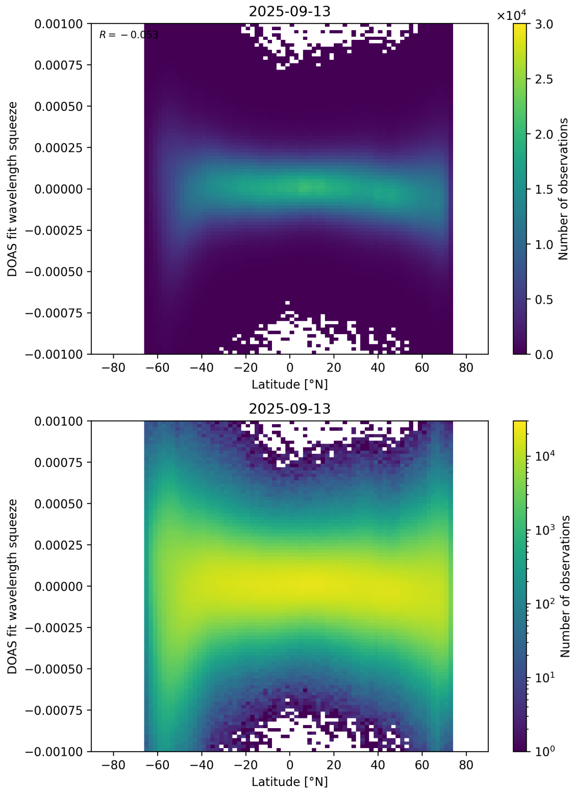
Figure 154: Scatter density plot of “Latitude” against “DOAS fit wavelength squeeze” for 2025-09-12 to 2025-09-14.
