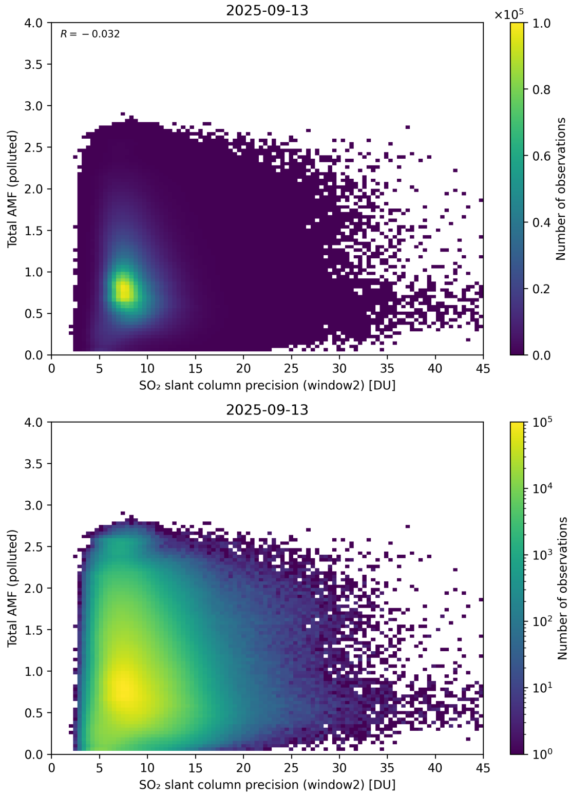
Figure 301: Scatter density plot of “SO 2 slant column precision (window2)” against “Total AMF (polluted)” for 2025-09-12 to 2025-09-14.
