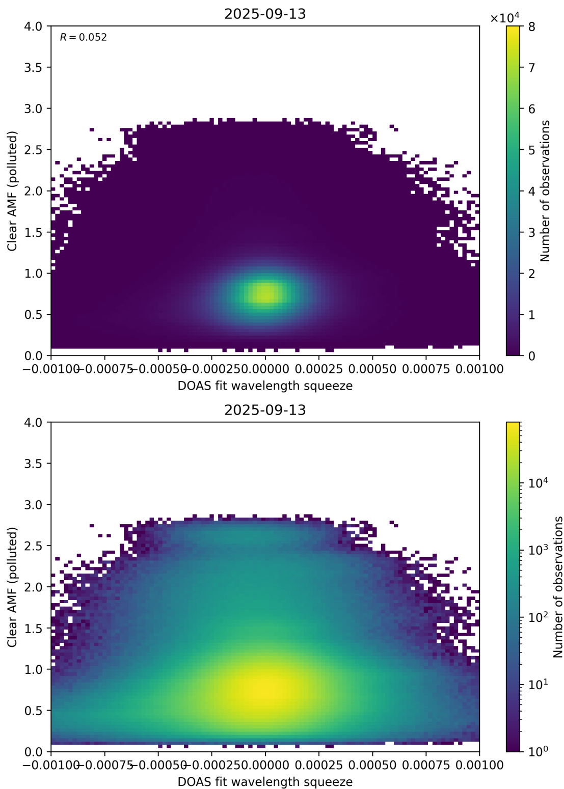
Figure 144: Scatter density plot of “DOAS fit wavelength squeeze” against “Clear AMF (polluted)” for 2025-09-12 to 2025-09-14.
