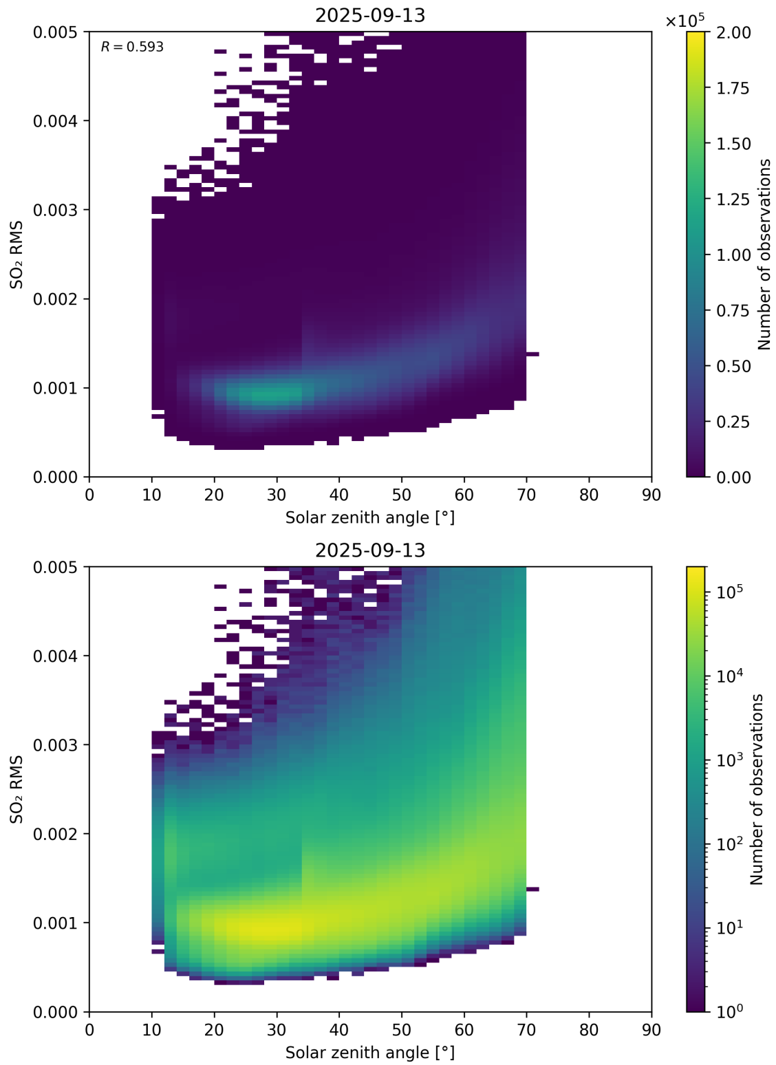
Figure 176: Scatter density plot of “Solar zenith angle” against “SO 2 RMS” for 2025-09-12 to 2025-09-14.
