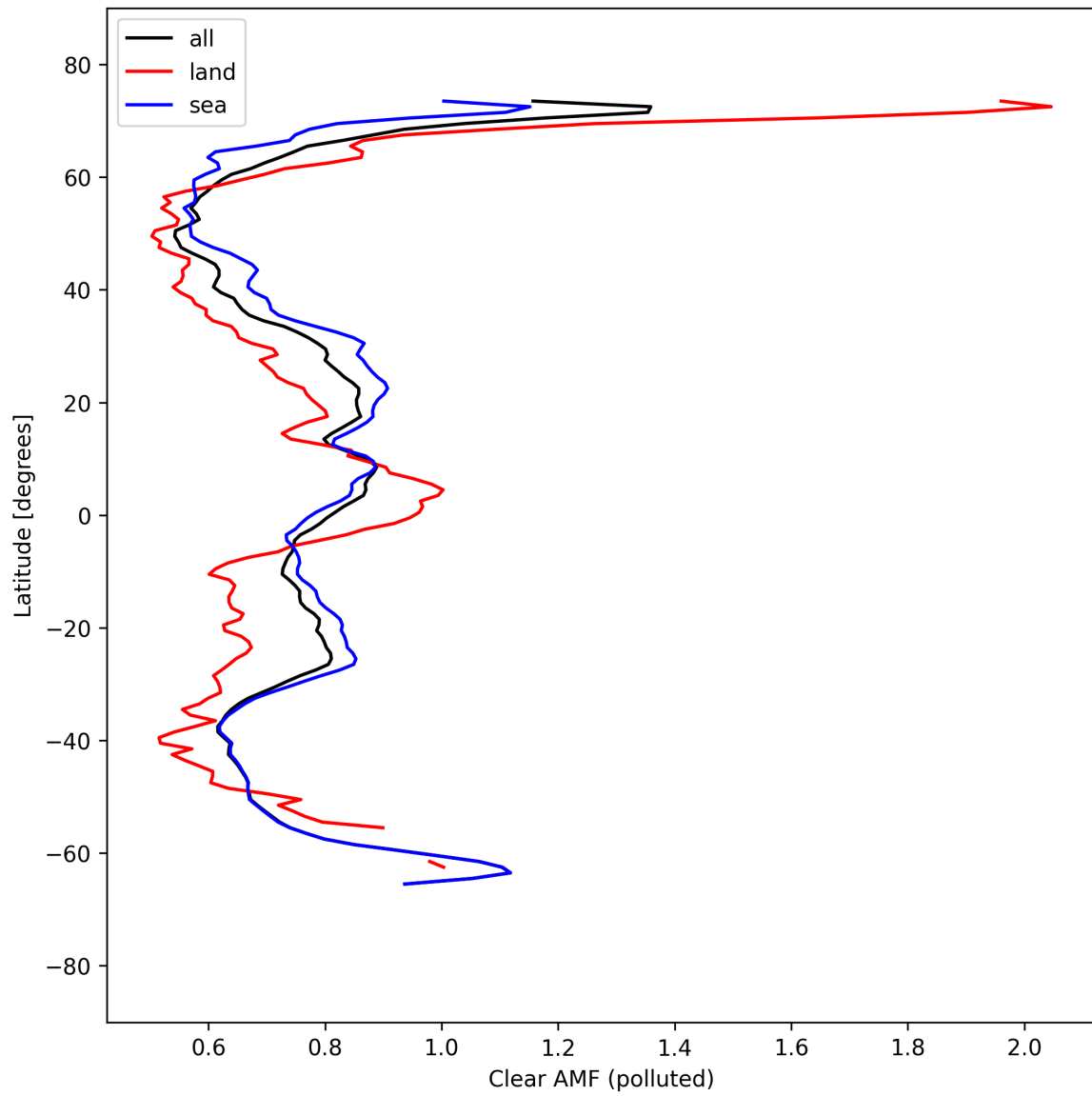
Figure 55: Zonal average of “Clear AMF (polluted)” for 2025-09-12 to 2025-09-14.
