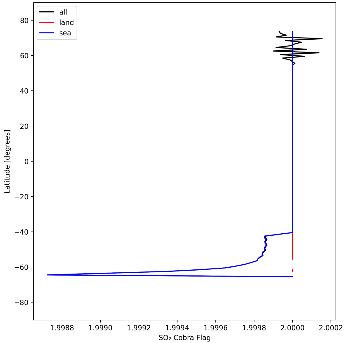
Figure 49: Zonal average of “SO 2 Cobra Flag” for 2025-09-12 to 2025-09-14.
