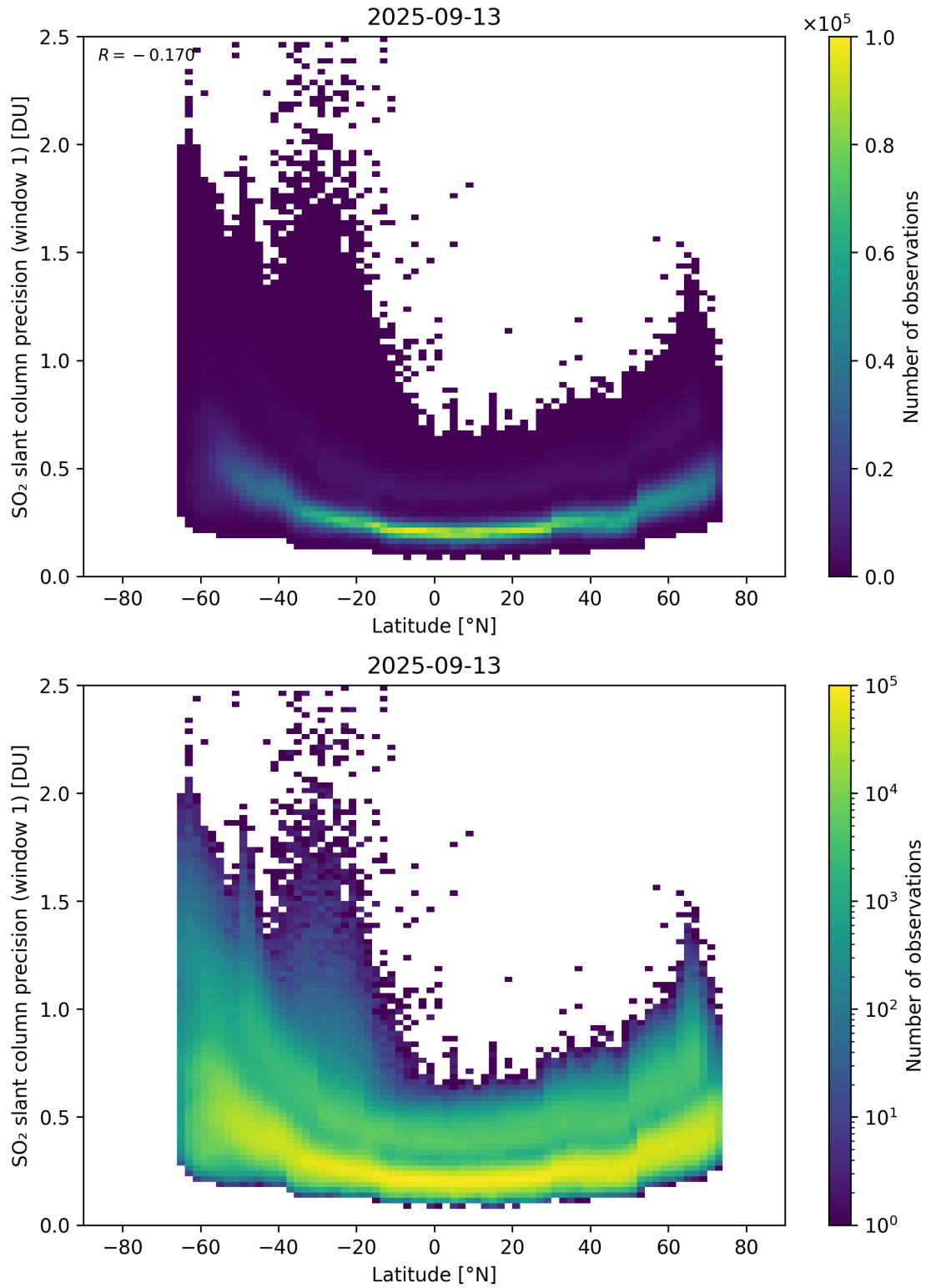
Figure 163: Scatter density plot of “Latitude” against “SO 2 slant column precision (window 1)” for 2025-09-12 to 2025-09-14.
