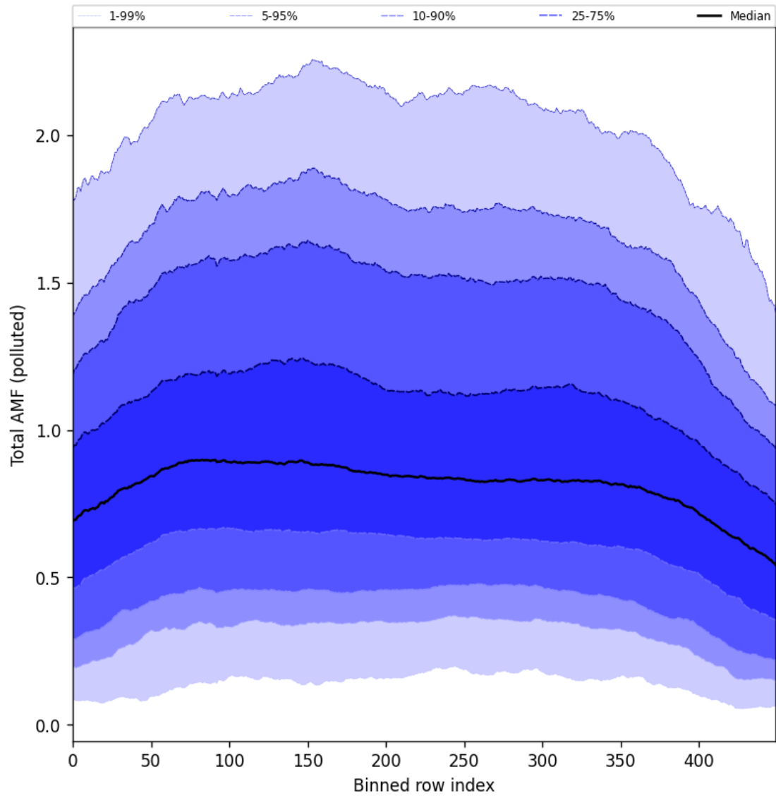
Figure 105: Along track statistics of “Total AMF (polluted)” for 2025-09-12 to 2025-09-14
