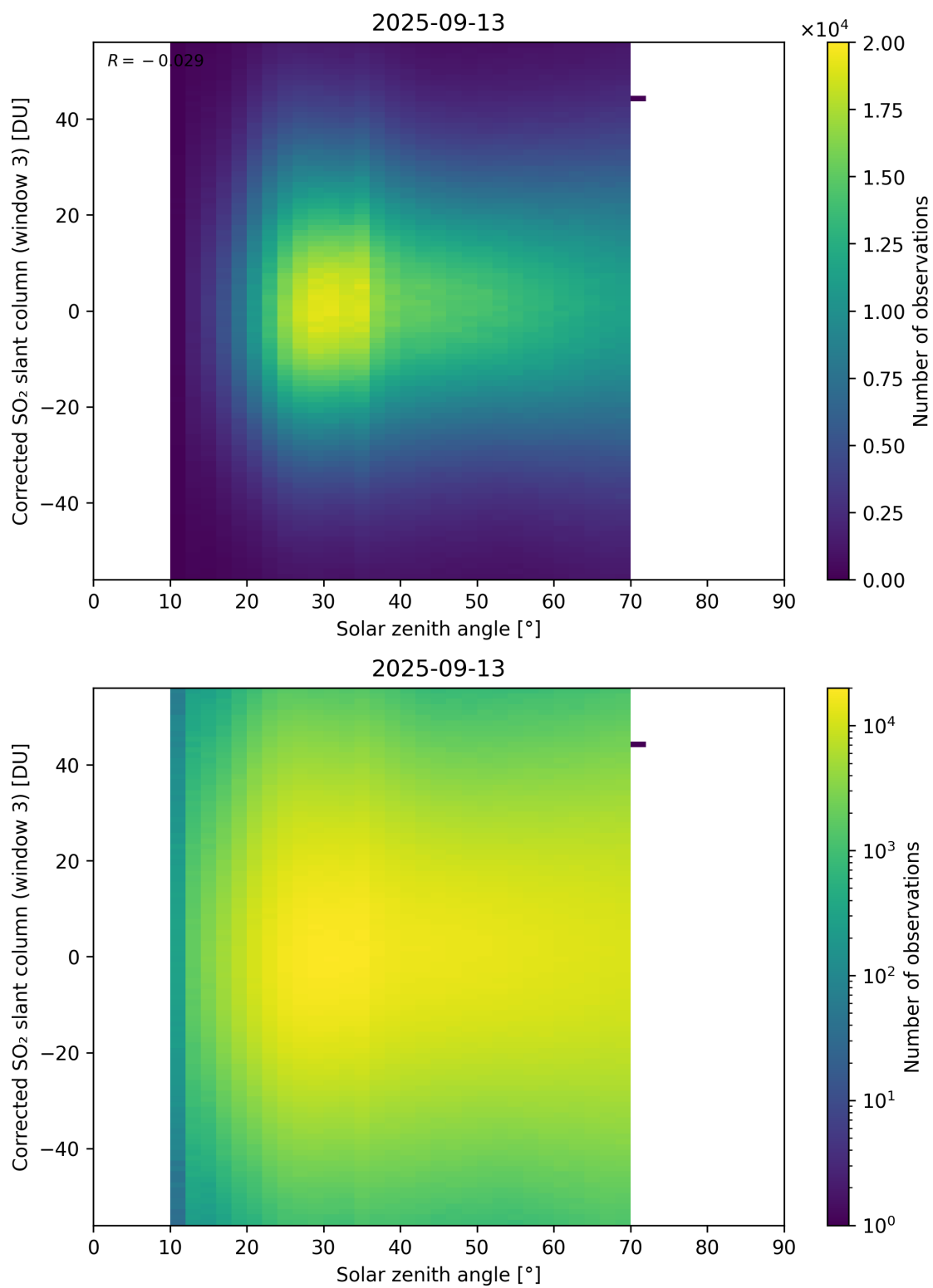
Figure 183: Scatter density plot of “Solar zenith angle” against “Corrected SO 2 slant column (window 3)” for 2025-09-12 to 2025-09-14.
