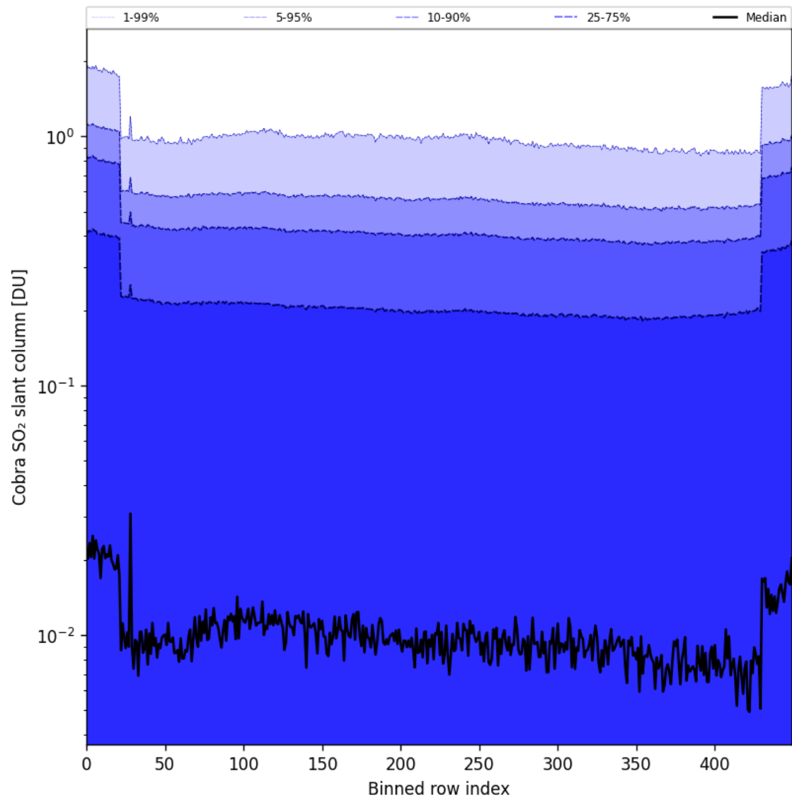
Figure 87: Along track statistics of “Cobra SO 2 slant column” for 2025-09-12 to 2025-09-14
