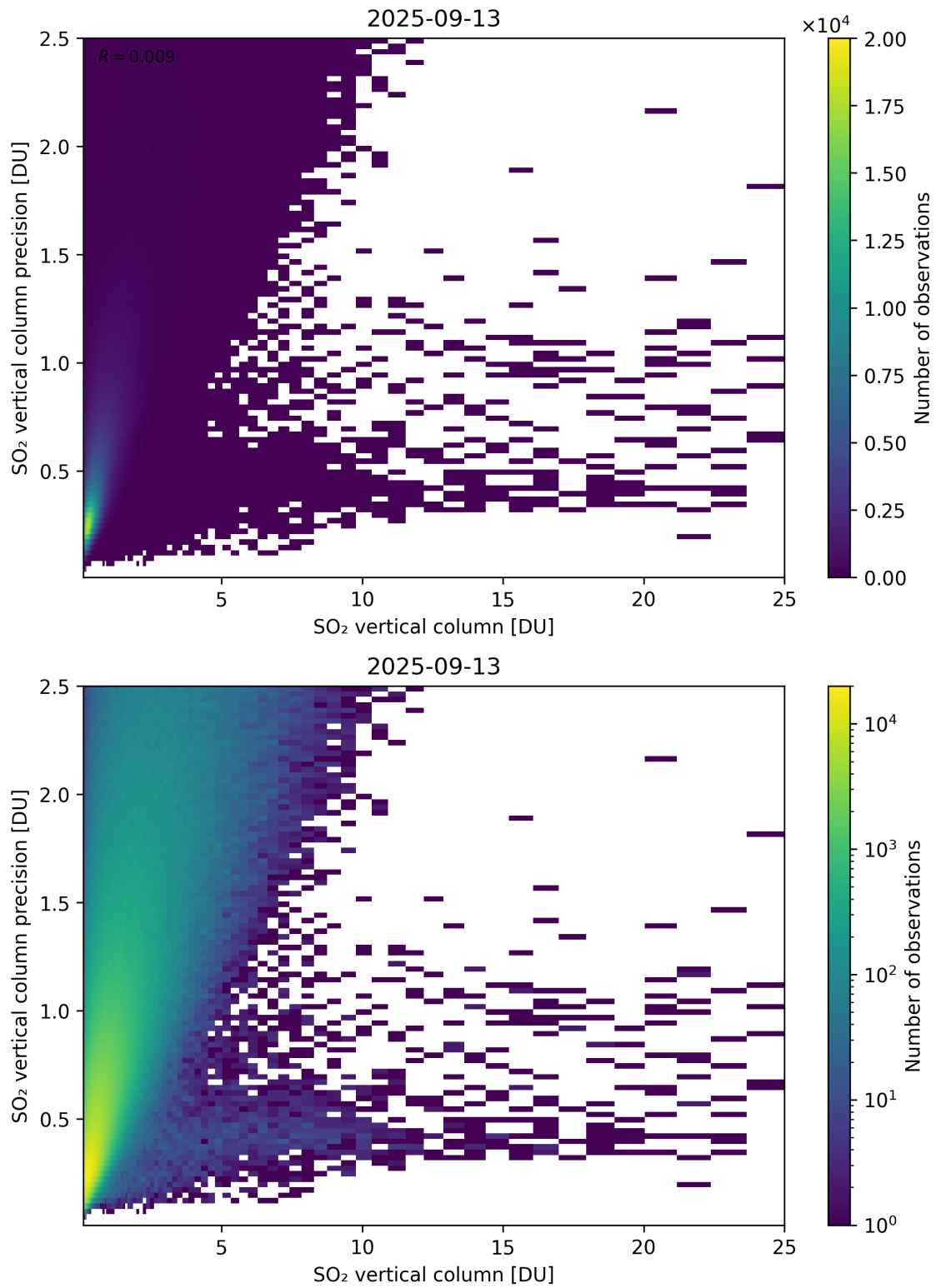
Figure 361: Scatter density plot of “SO 2 vertical column” against “SO 2 vertical column precision” for 2025-09-12 to 2025-09-14.
