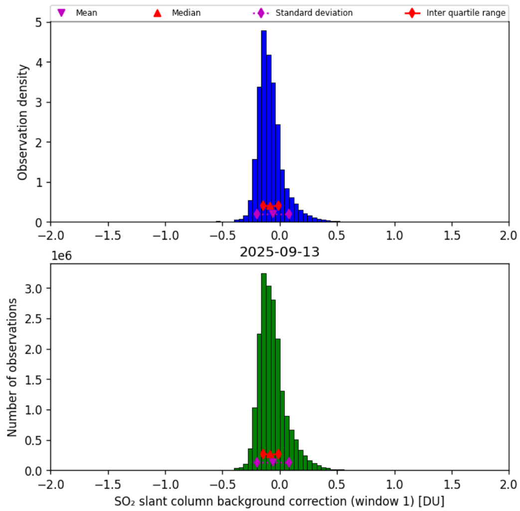
Figure 66: Histogram of “SO 2 slant column background correction (window 1)” for 2025-09-12 to 2025-09-14
