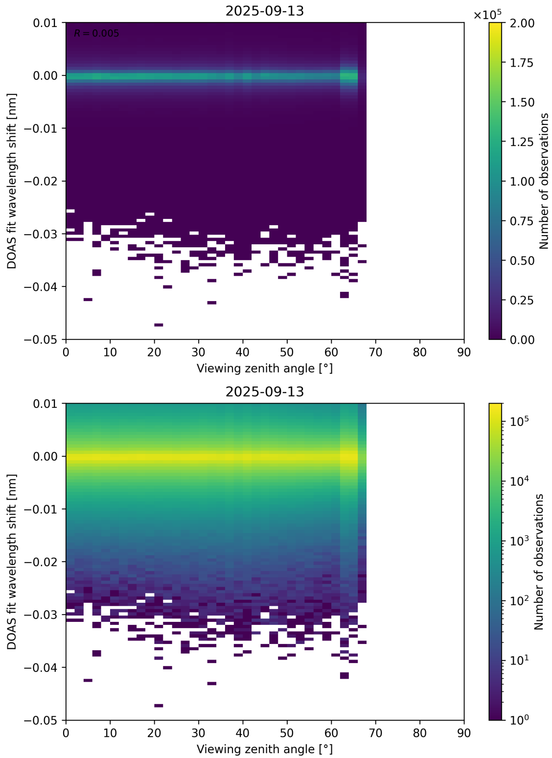
Figure 365: Scatter density plot of “Viewing zenith angle” against “DOAS fit wavelength shift” for 2025-09-12 to 2025-09-14.
