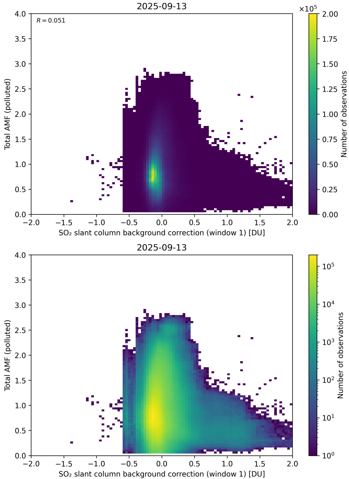
Figure 120: Scatter density plot of “SO 2 slant column background correction (window 1)” against “Total AMF (polluted)” for 2025-09-12 to 2025-09-14.
