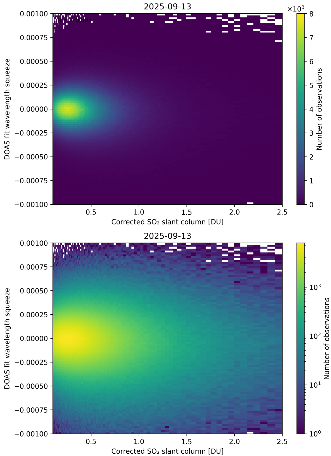
Figure 230: Scatter density plot of "Corrected SO 2 slant column" against "DOAS fit wavelength squeeze" for 2025-09-12 to 2025-09-14.
