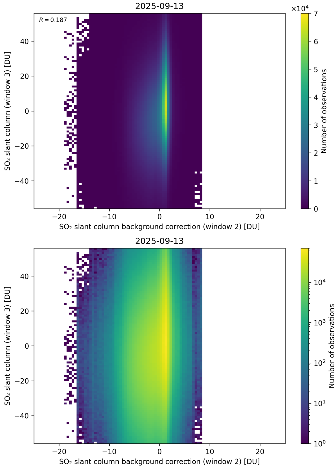
Figure 128: Scatter density plot of “SO 2 slant column background correction (window 2)” against “SO 2 slant column (window 3)” for 2025-09-12 to 2025-09-14.
