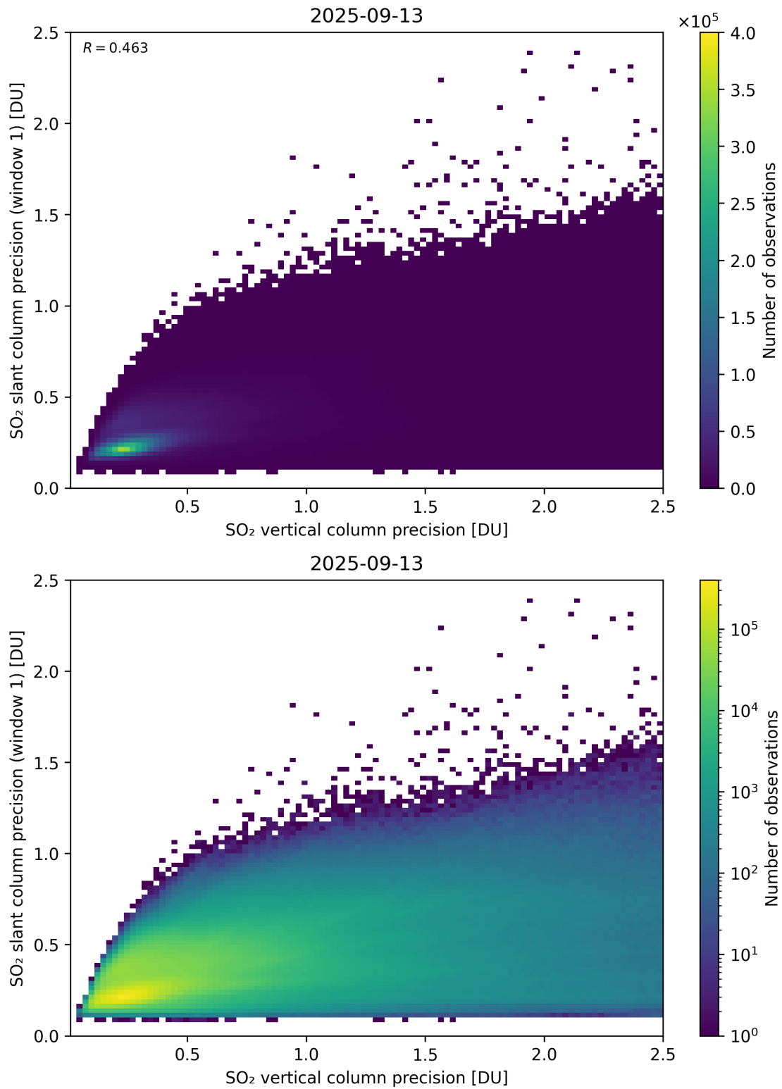
Figure 342: Scatter density plot of “SO 2 vertical column precision” against “SO 2 slant column precision (window 1)” for 2025-09-12 to 2025-09-14.
