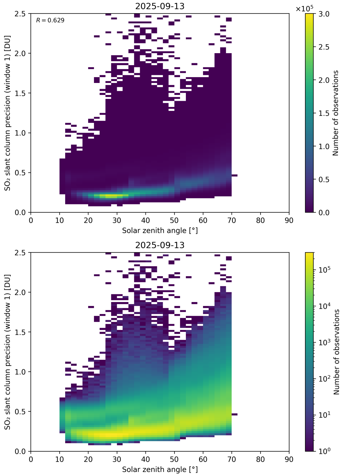
Figure 185: Scatter density plot of “Solar zenith angle” against “SO 2 slant column precision (window 1)” for 2025-09-12 to 2025-09-14.
