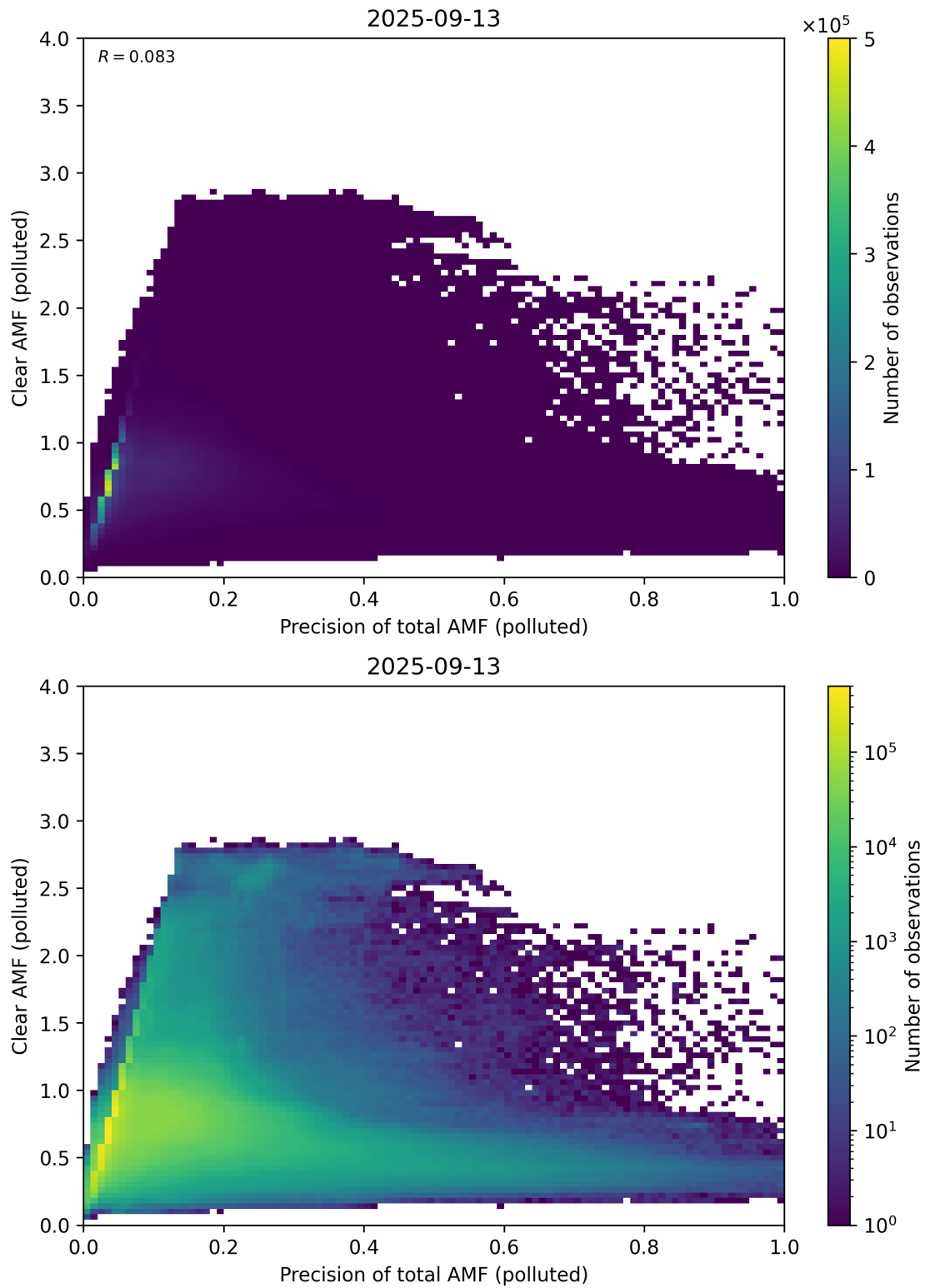
Figure 320: Scatter density plot of “Precision of total AMF (polluted)” against “Clear AMF (polluted)” for 2025-09-12 to 2025-09-14.
