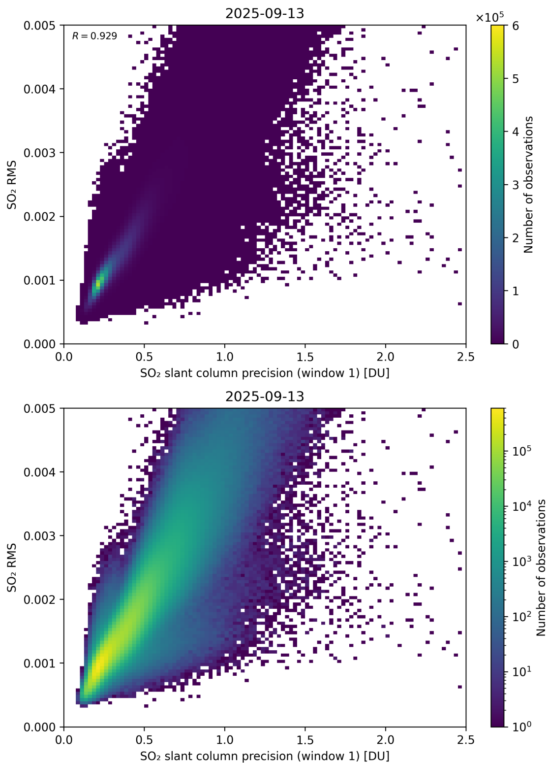
Figure 273: Scatter density plot of “SO 2 slant column precision (window 1)” against “SO 2 RMS” for 2025-09-12 to 2025-09-14.
