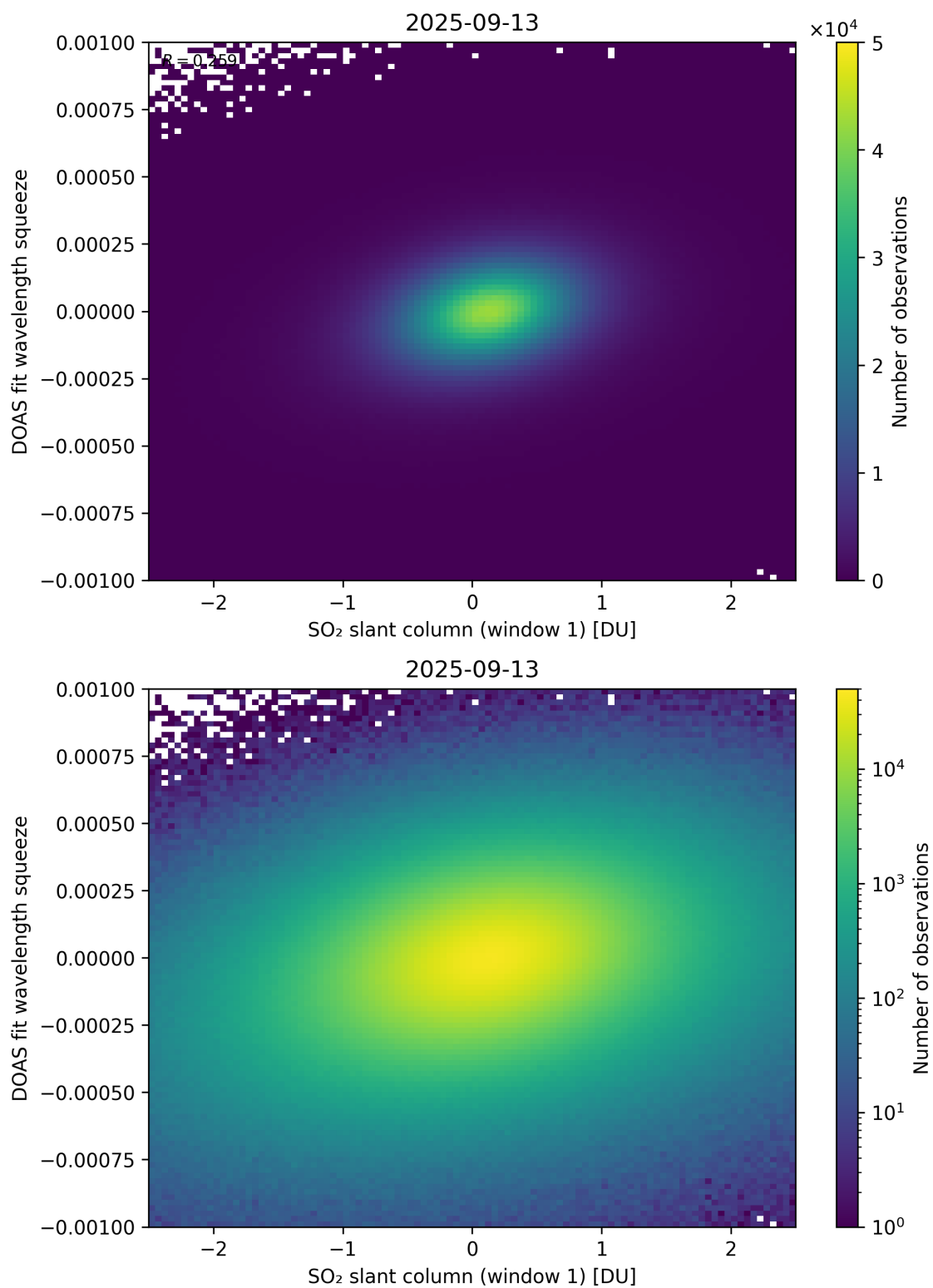
Figure 266: Scatter density plot of “SO 2 slant column (window 1)” against “DOAS fit wavelength squeeze” for 2025-09-12 to 2025-09-14.
