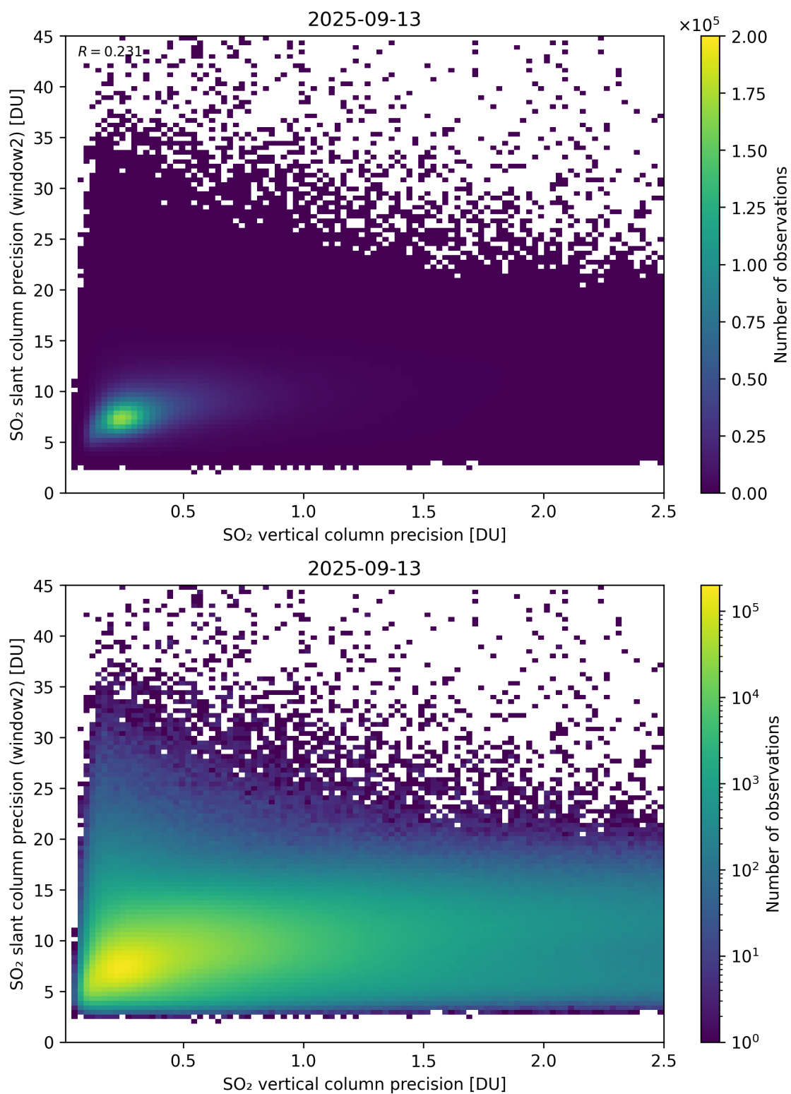
Figure 343: Scatter density plot of “SO 2 vertical column precision” against “SO 2 slant column precision (window2)” for 2025-09-12 to 2025-09-14.
