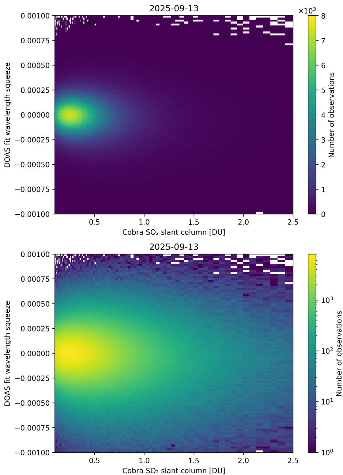
Figure 197: Scatter density plot of “Cobra SO 2 slant column” against “DOAS fit wavelength squeeze” for 2025-09-12 to 2025-09-14.
