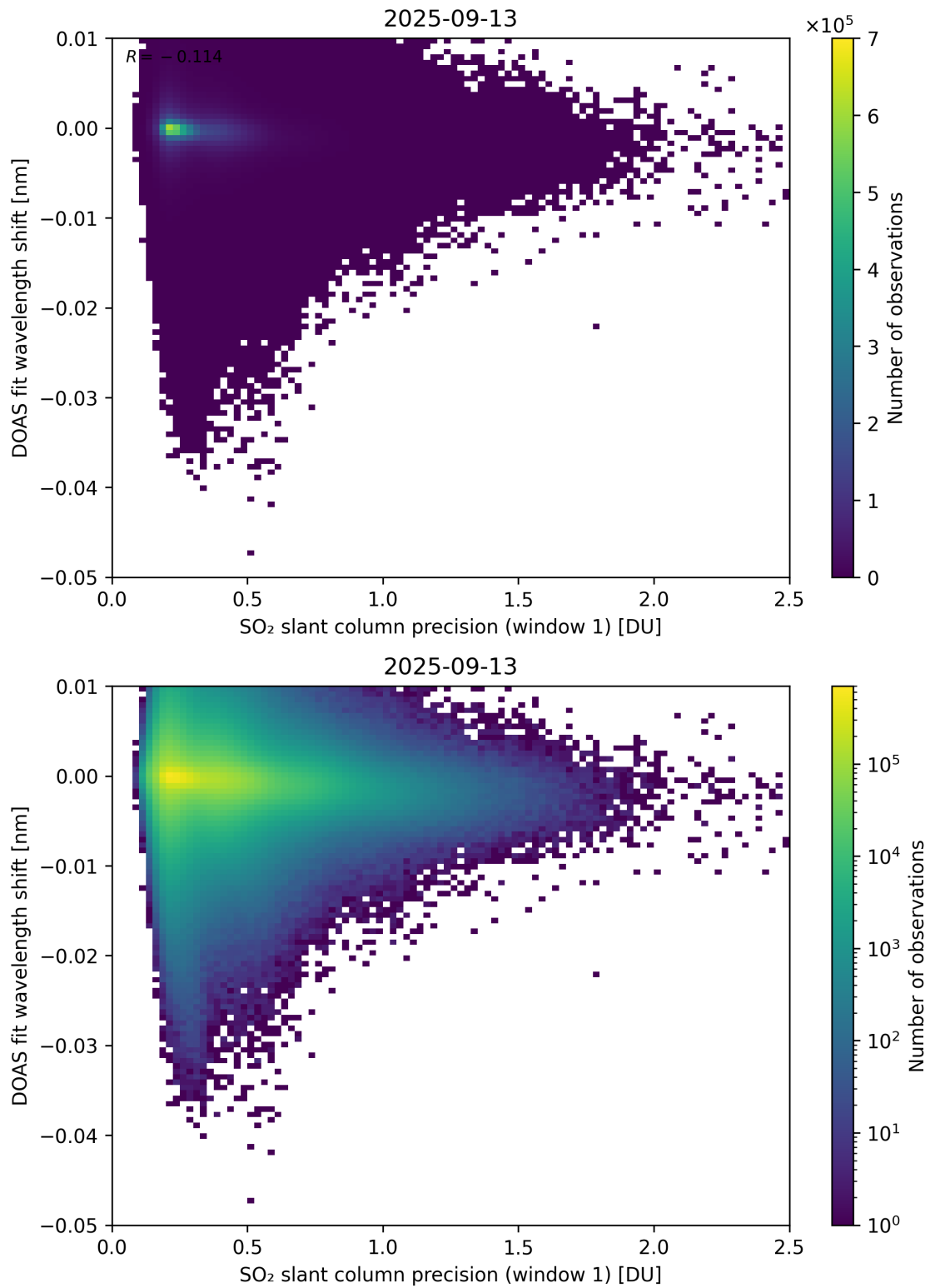
Figure 271: Scatter density plot of “SO 2 slant column precision (window 1)” against “DOAS fit wavelength shift” for 2025-09-12 to 2025-09-14.
