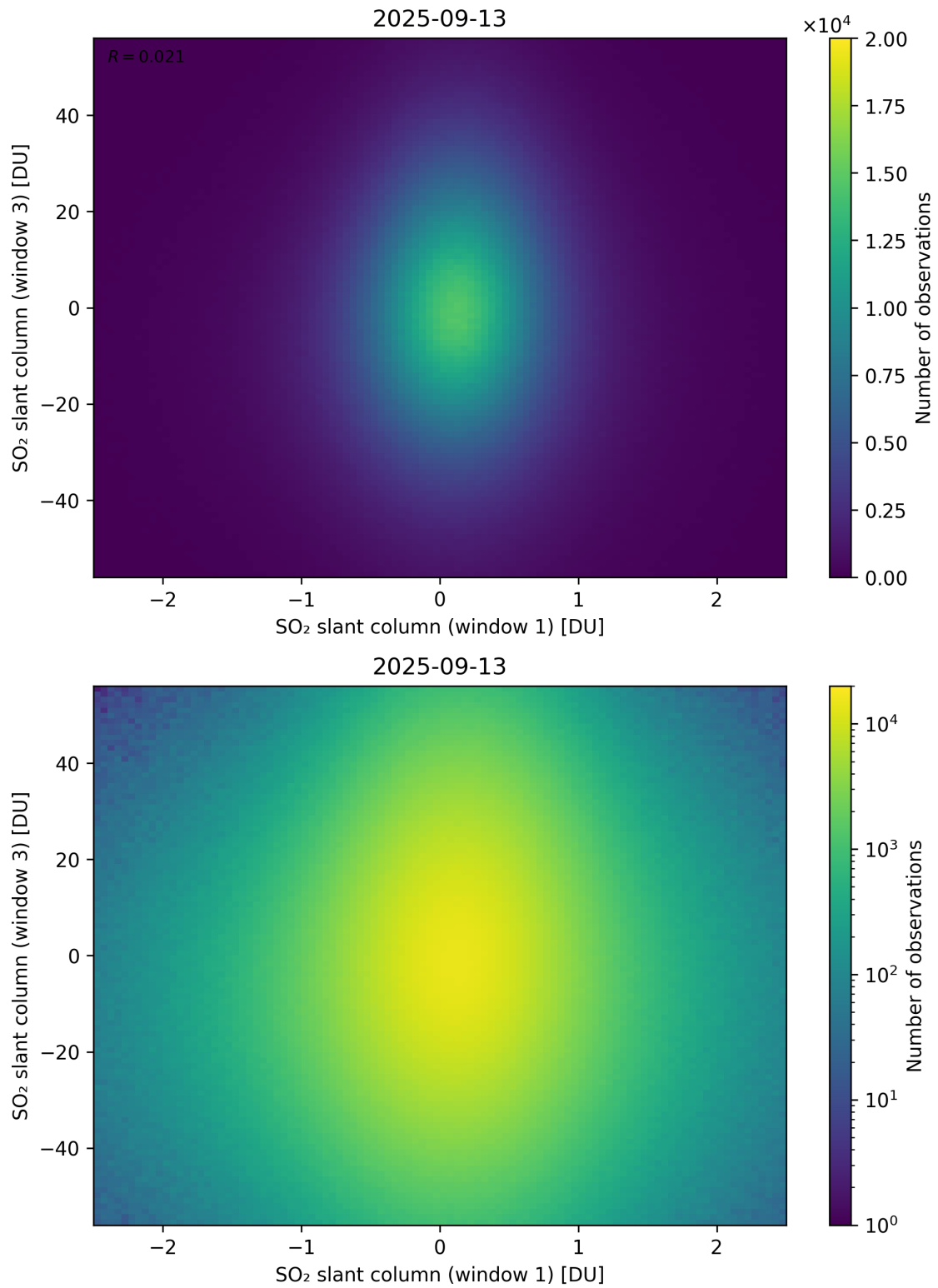
Figure 287: Scatter density plot of “SO 2 slant column (window 1)” against “SO 2 slant column (window 3)” for 2025-09-12 to 2025-09-14.
