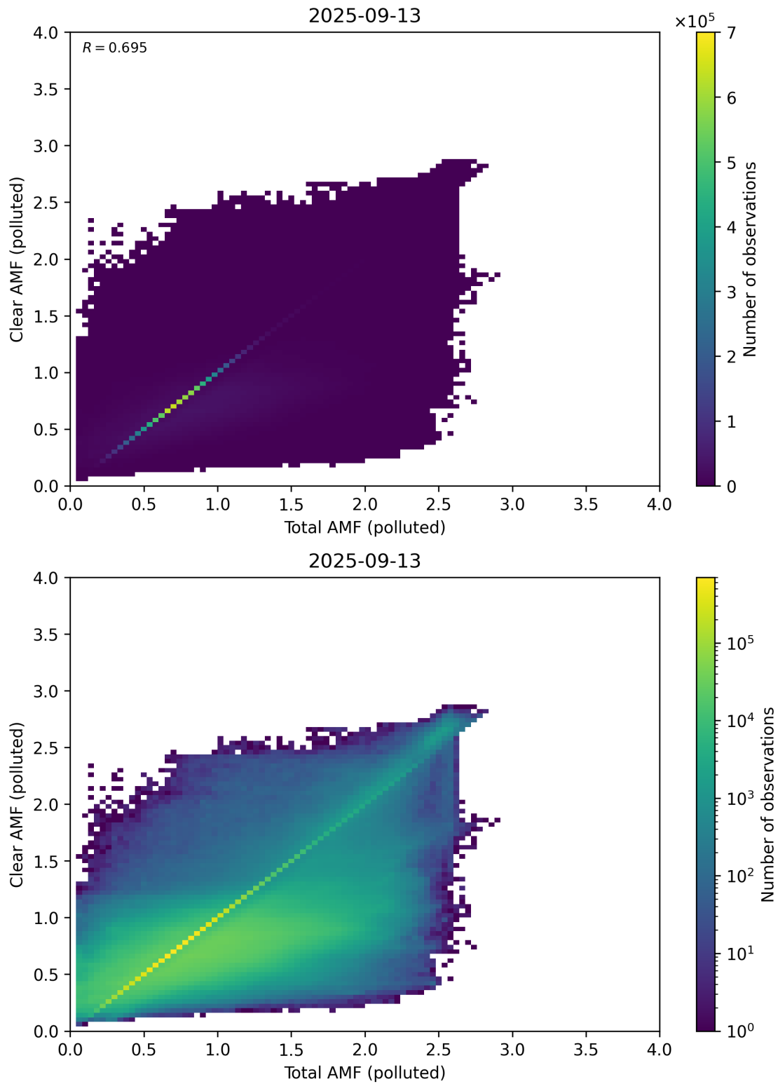
Figure 321: Scatter density plot of “Total AMF (polluted)” against “Clear AMF (polluted)” for 2025-09-12 to 2025-09-14.
