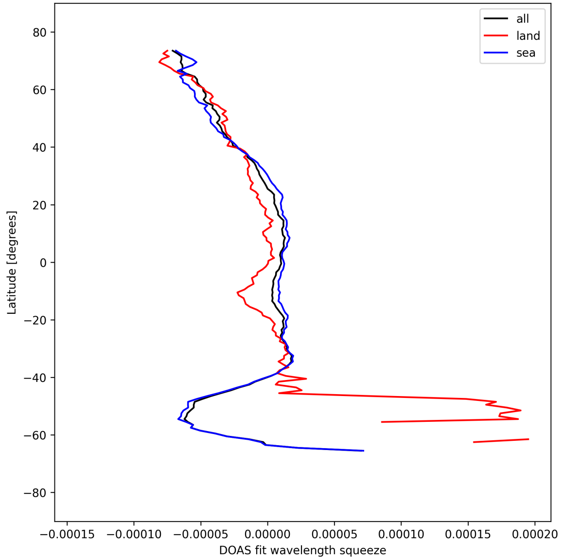
Figure 51: Zonal average of “DOAS fit wavelength squeeze” for 2025-09-12 to 2025-09-14.
