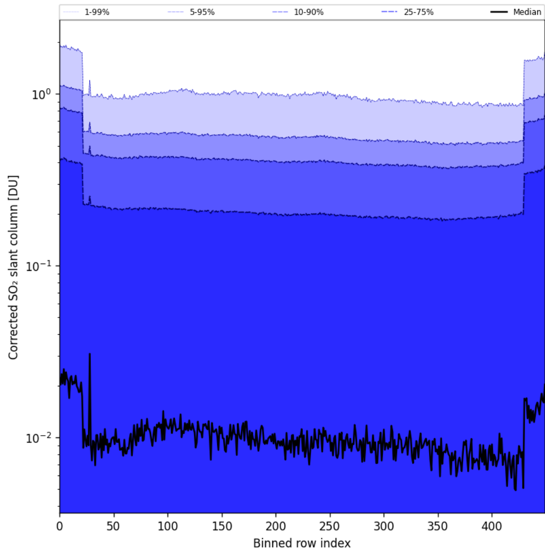
Figure 86: Along track statistics of “Corrected SO 2 slant column” for 2025-09-12 to 2025-09-14
