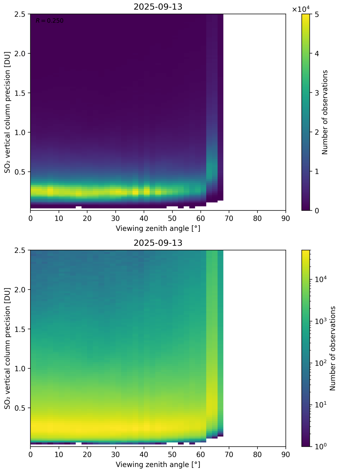
Figure 384: Scatter density plot of “Viewing zenith angle” against “SO 2 vertical column precision” for 2025-09-12 to 2025-09-14.
