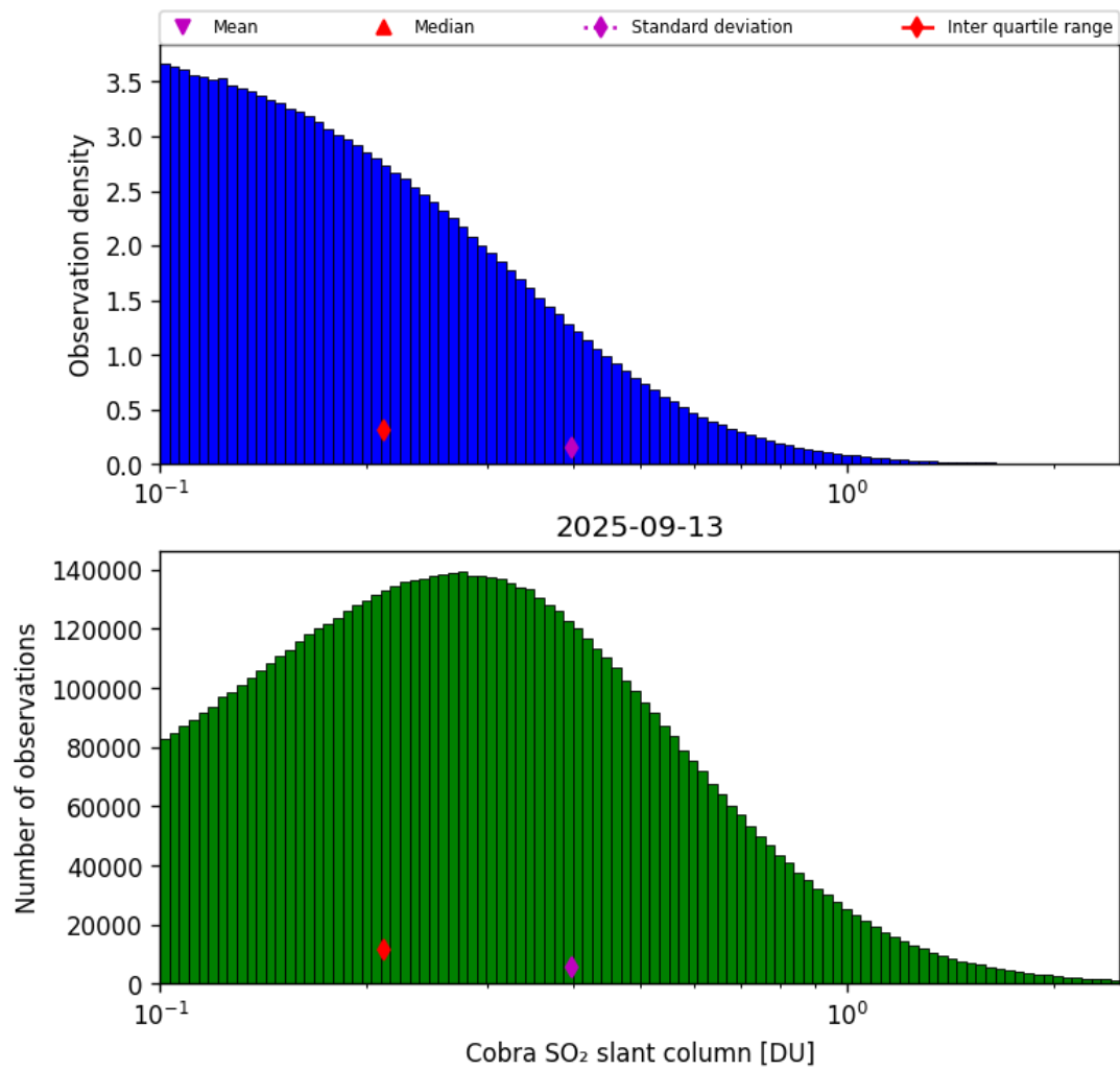
Figure 61: Histogram of “Cobra SO 2 slant column” for 2025-09-12 to 2025-09-14
