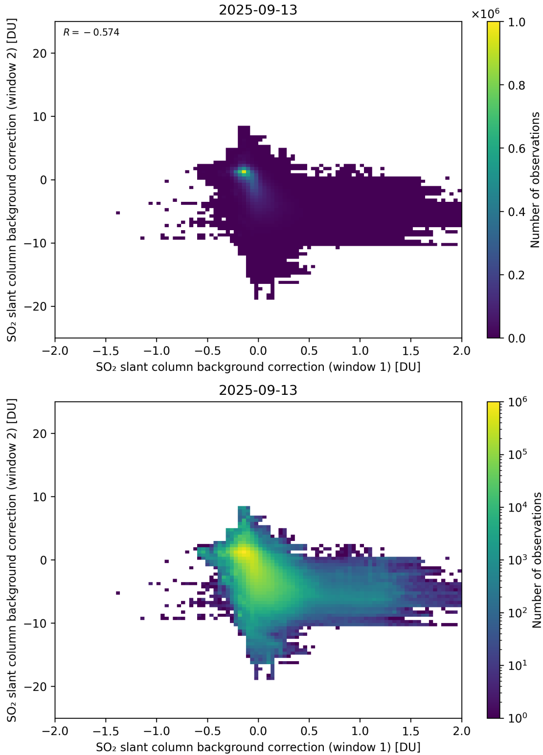
Figure 109: Scatter density plot of “SO 2 slant column background correction (window 1)” against “SO 2 slant column background correction (window 2)” for 2025-09-12 to 2025-09-14.
