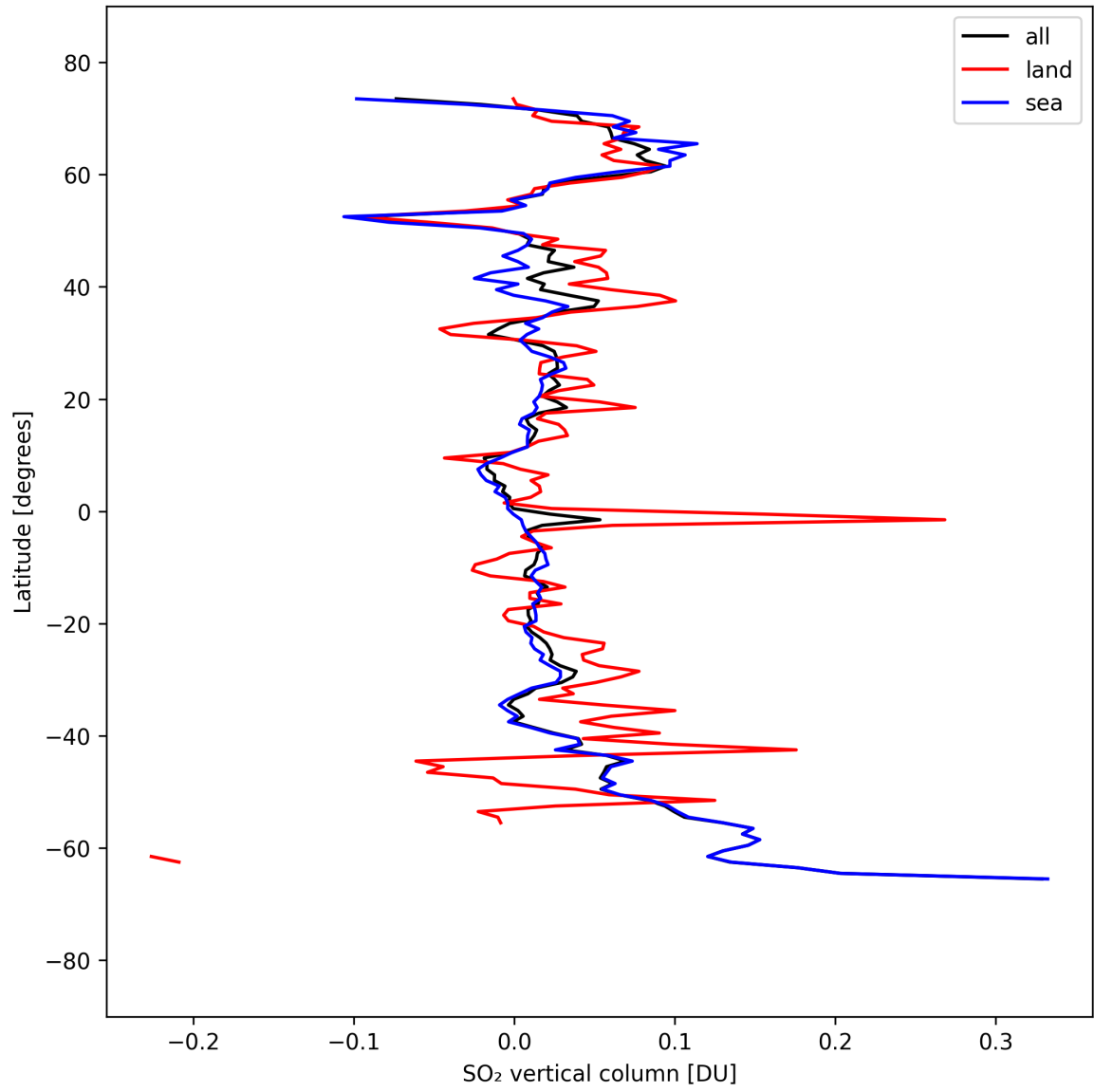
Figure 32: Zonal average of “SO 2 vertical column” for 2025-09-12 to 2025-09-14.
