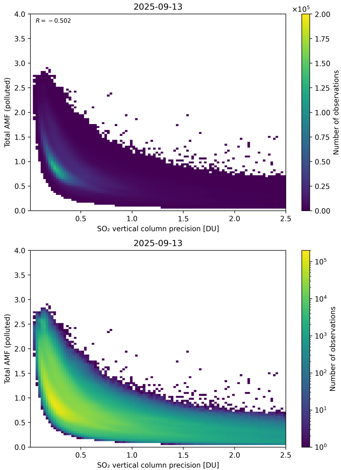
Figure 346: Scatter density plot of “SO 2 vertical column precision” against “Total AMF (polluted)” for 2025-09-12 to 2025-09-14.
