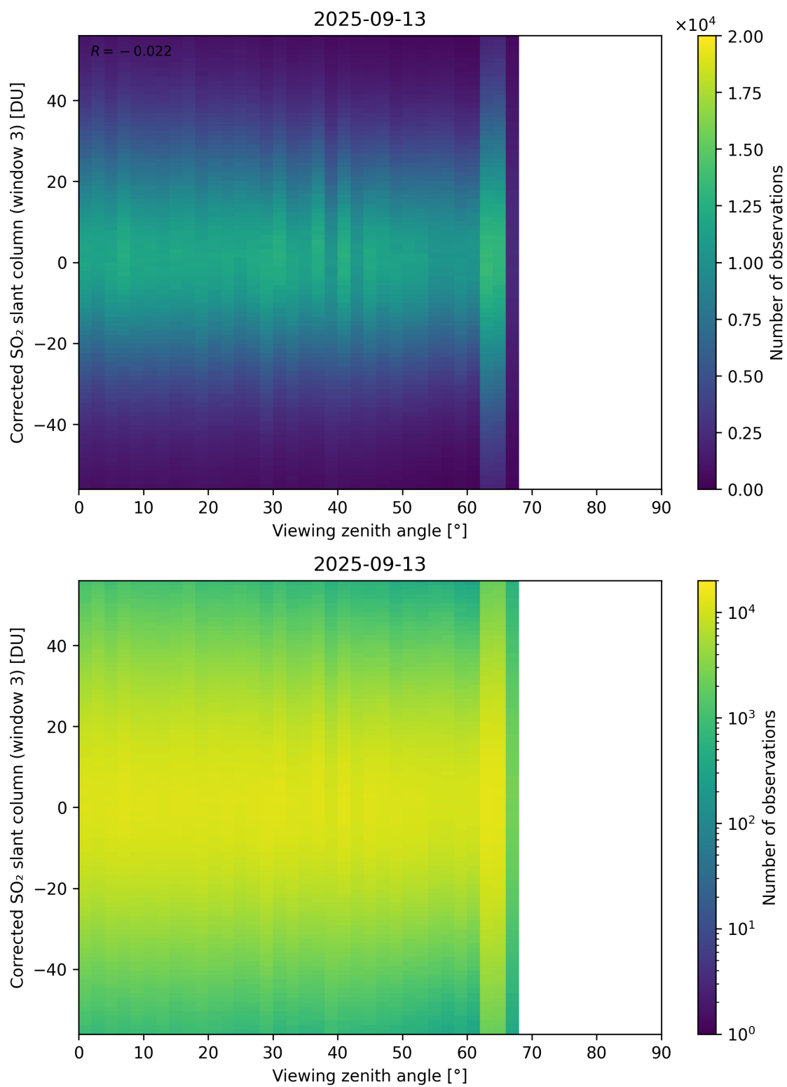
Figure 375: Scatter density plot of “Viewing zenith angle” against “Corrected SO 2 slant column (window 3)” for 2025-09-12 to 2025-09-14.
