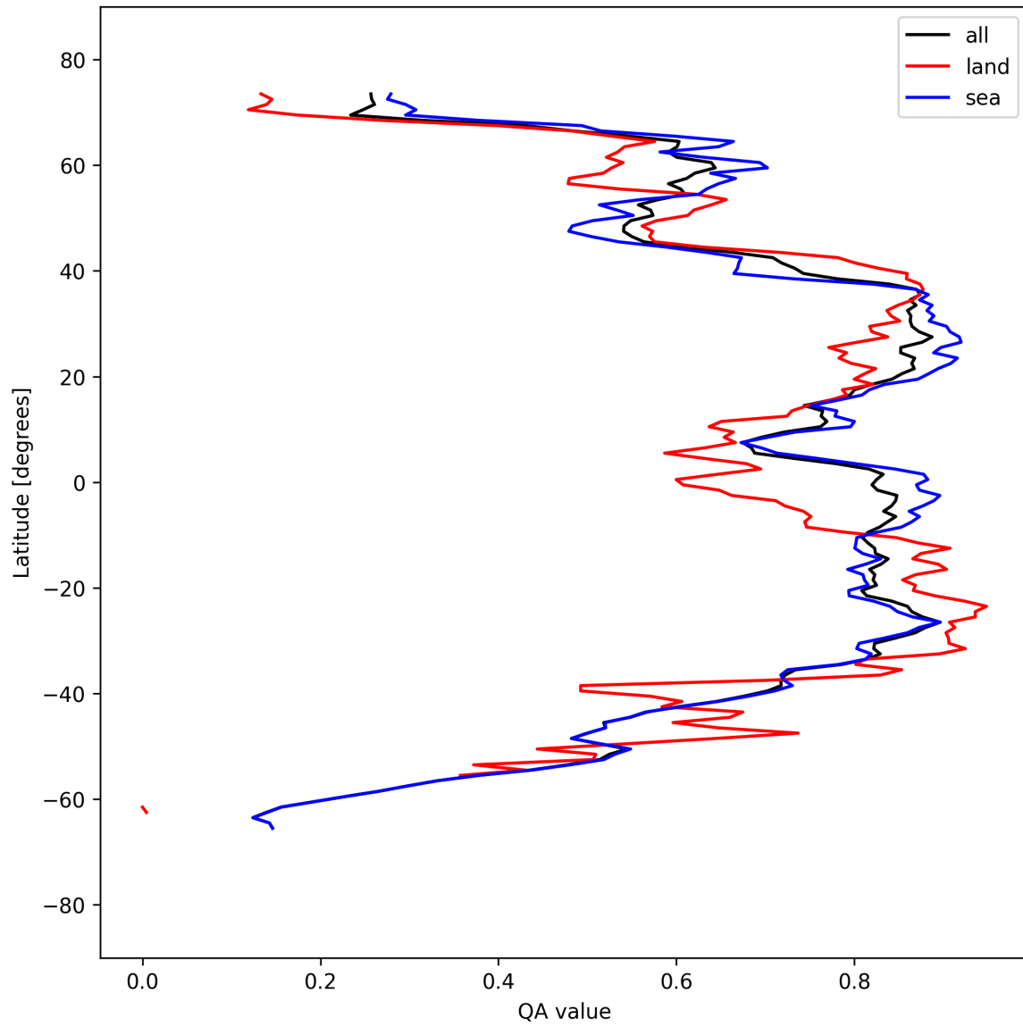
Figure 31: Zonal average of “QA value” for 2025-09-12 to 2025-09-14.
