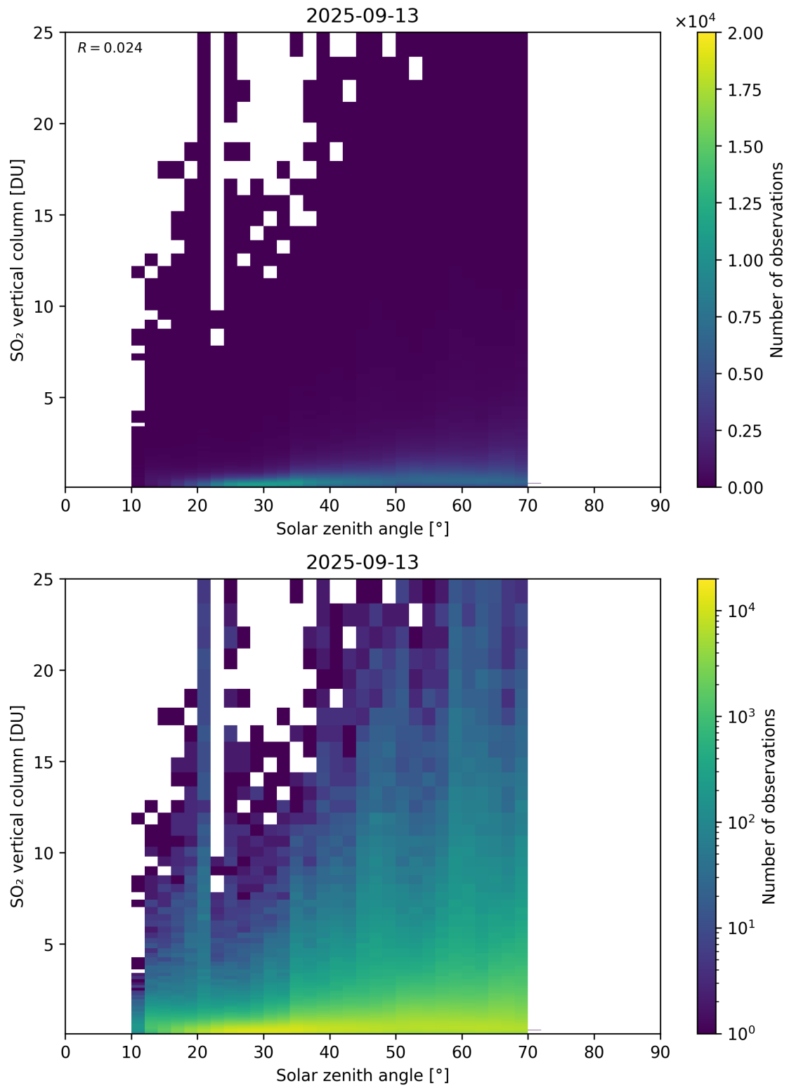
Figure 191: Scatter density plot of “Solar zenith angle” against “SO 2 vertical column” for 2025-09-12 to 2025-09-14.
