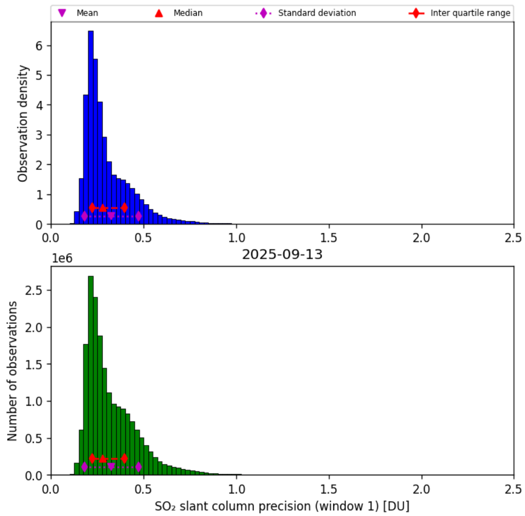
Figure 64: Histogram of “SO 2 slant column precision (window 1)” for 2025-09-12 to 2025-09-14
