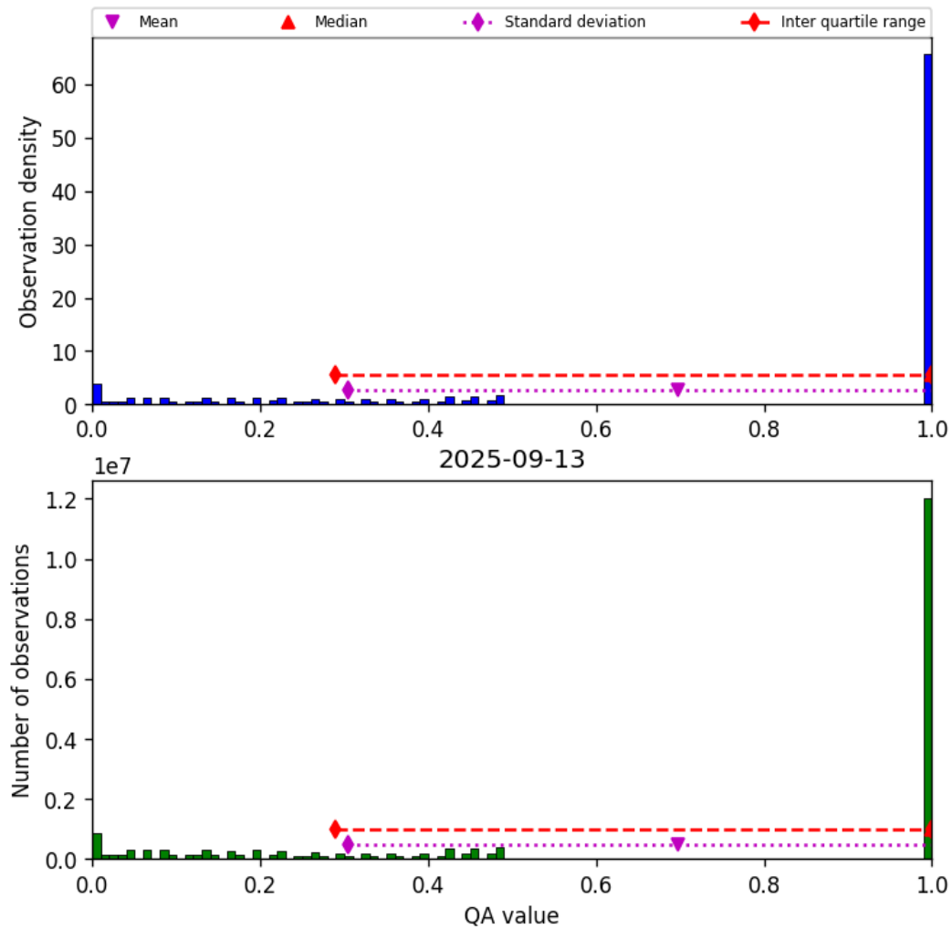
Figure 57: Histogram of “QA value” for 2025-09-12 to 2025-09-14
