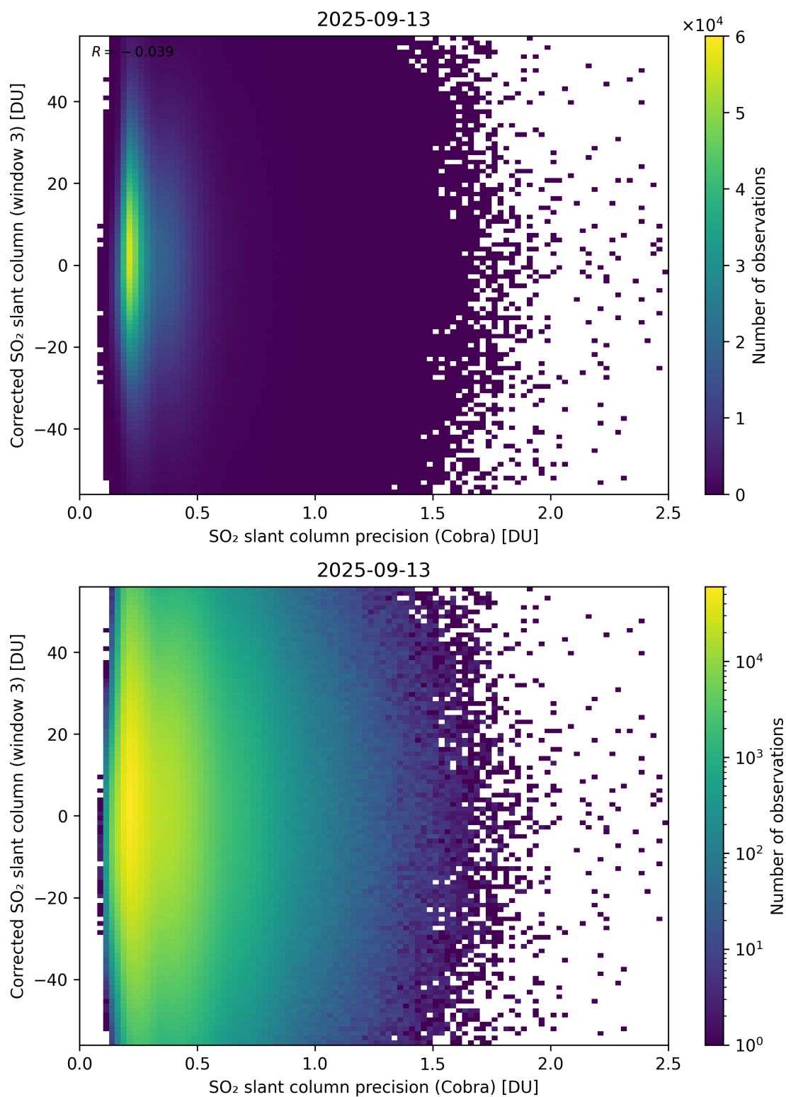
Figure 207: Scatter density plot of “SO 2 slant column precision (Cobra)” against “Corrected SO 2 slant column (window 3)” for 2025-09-12 to 2025-09-14.
