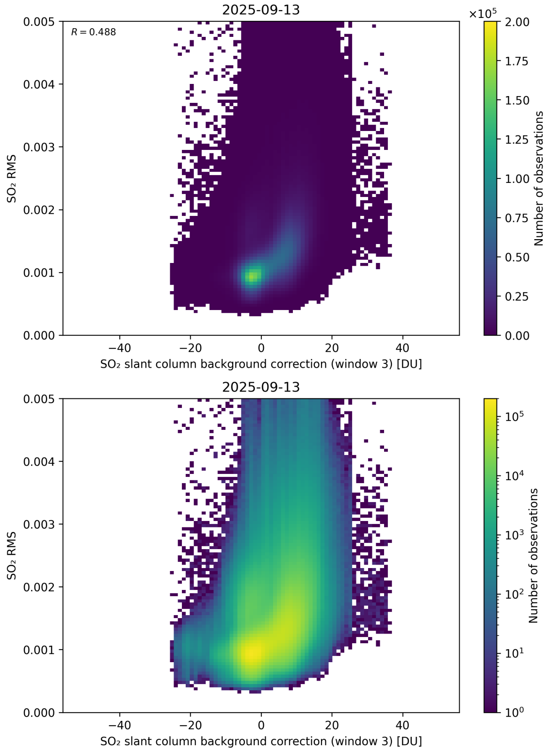
Figure 134: Scatter density plot of “SO 2 slant column background correction (window 3)” against “SO 2 RMS” for 2025-09-12 to 2025-09-14.
