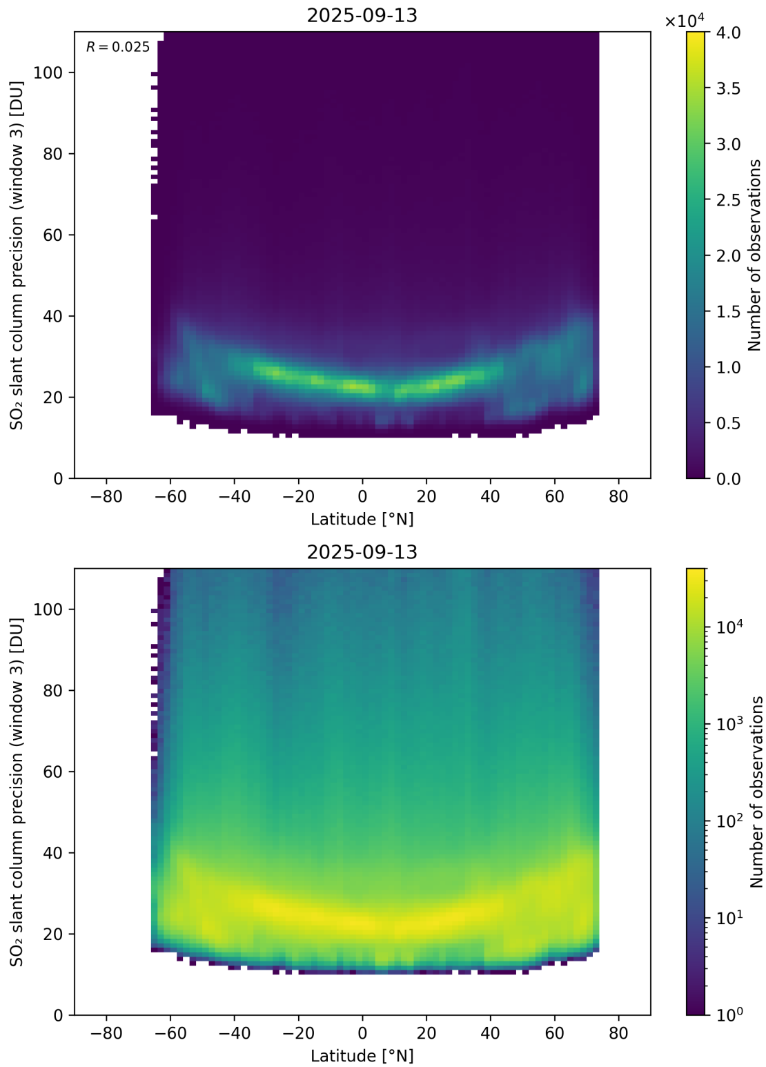
Figure 166: Scatter density plot of “Latitude” against “SO 2 slant column precision (window 3)” for 2025-09-12 to 2025-09-14.
