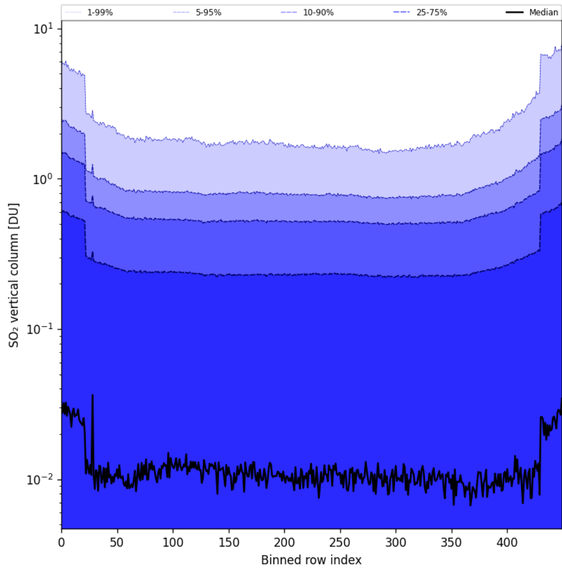
Figure 84: Along track statistics of “SO 2 vertical column” for 2025-09-12 to 2025-09-14
