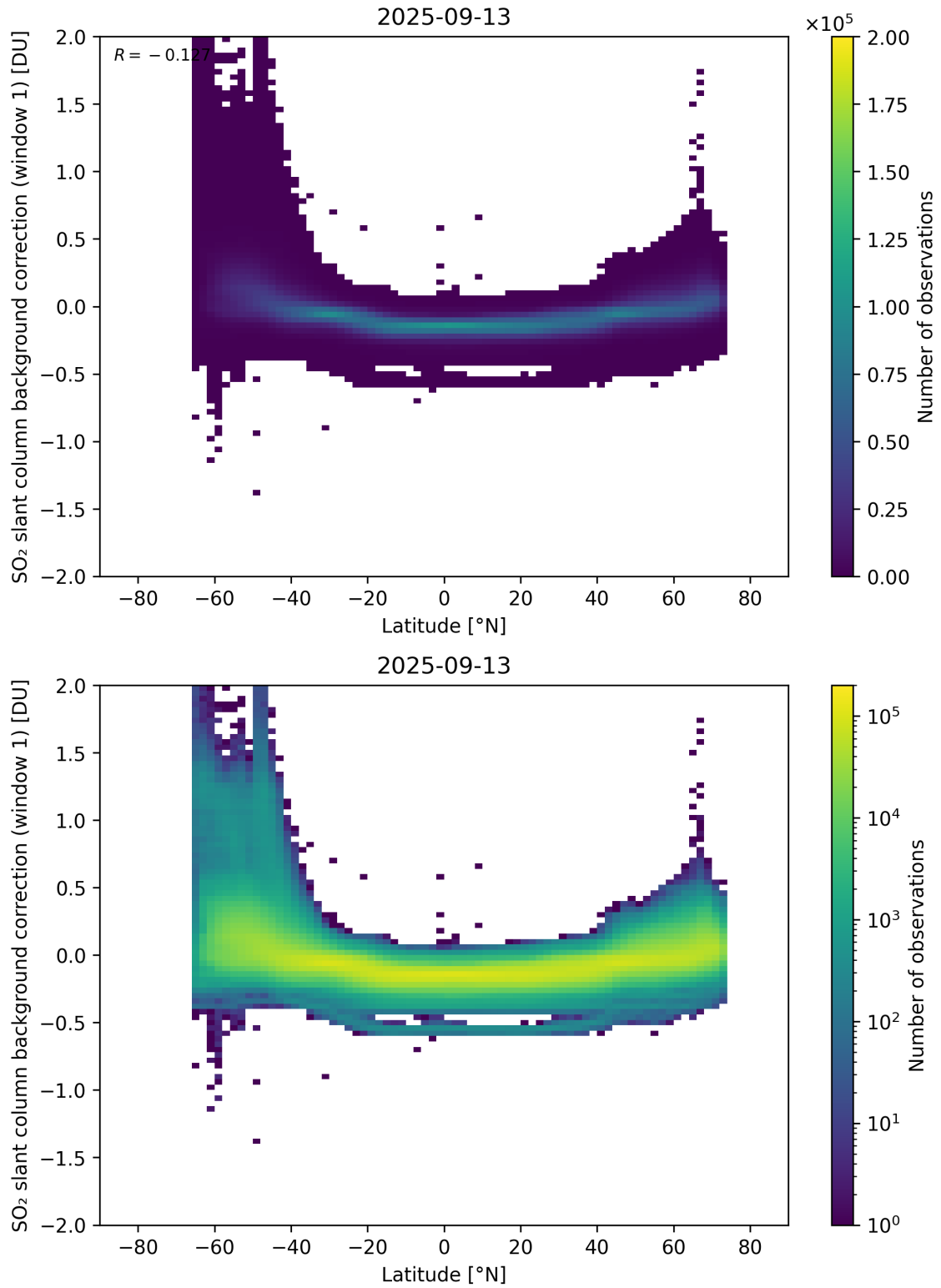
Figure 150: Scatter density plot of “Latitude” against “SO 2 slant column background correction (window 1)” for 2025-09-12 to 2025-09-14.
