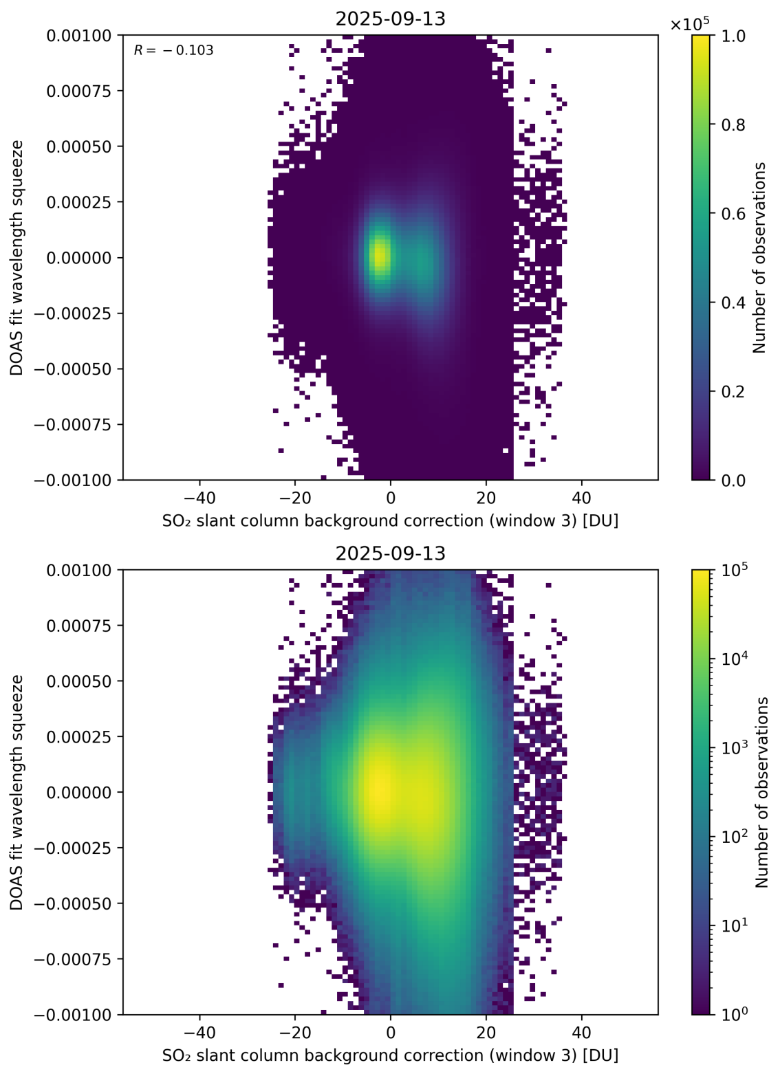
Figure 133: Scatter density plot of “SO 2 slant column background correction (window 3)” against “DOAS fit wavelength squeeze” for 2025-09-12 to 2025-09-14.
