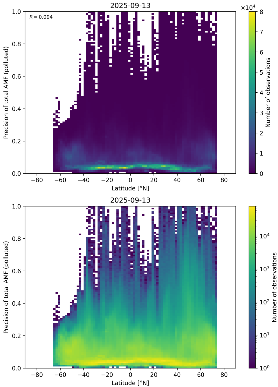
Figure 168: Scatter density plot of “Latitude” against “Precision of total AMF (polluted)” for 2025-09-12 to 2025-09-14.
