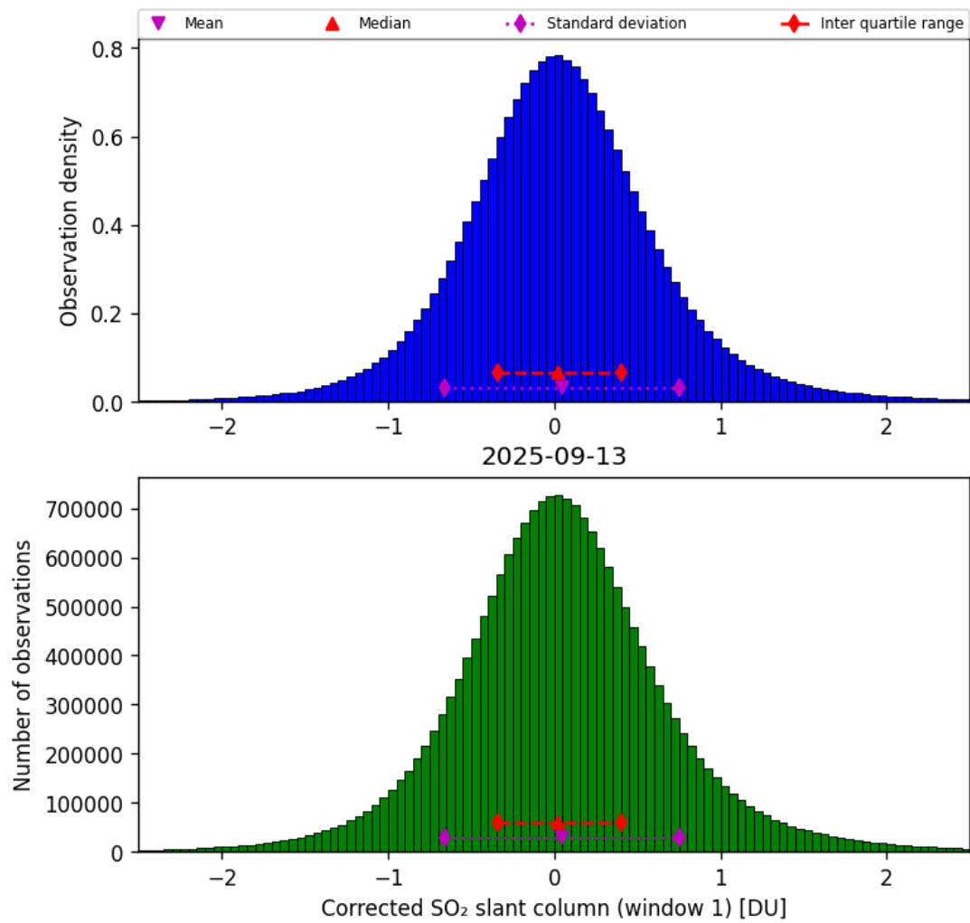
Figure 65: Histogram of “Corrected SO 2 slant column (window 1)” for 2025-09-12 to 2025-09-14
