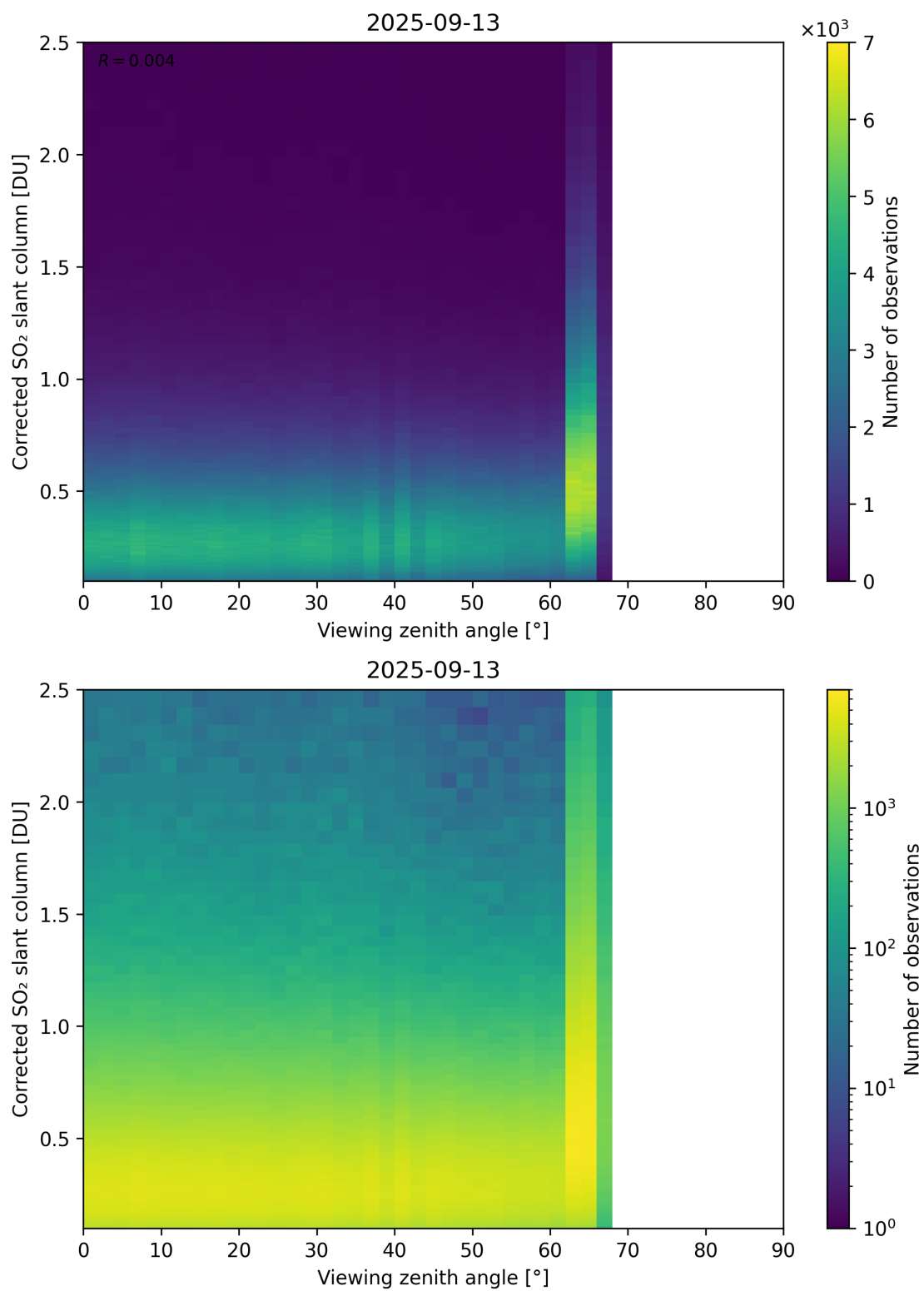
Figure 373: Scatter density plot of “Viewing zenith angle” against “Corrected SO 2 slant column” for 2025-09-12 to 2025-09-14.
