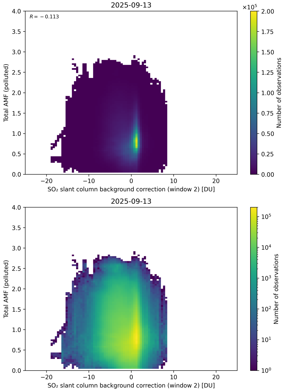
Figure 130: Scatter density plot of “SO 2 slant column background correction (window 2)” against “Total AMF (polluted)” for 2025-09-12 to 2025-09-14.
