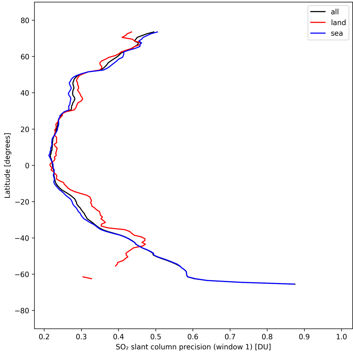
Figure 38: Zonal average of “SO 2 slant column precision (window 1)” for 2025-09-12 to 2025-09-14.
