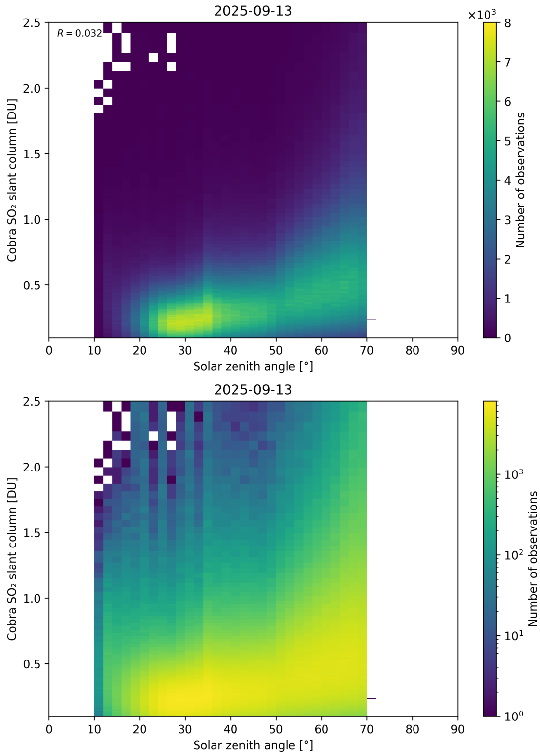
Figure 179: Scatter density plot of “Solar zenith angle” against “Cobra SO 2 slant column” for 2025-09-12 to 2025-09-14.
