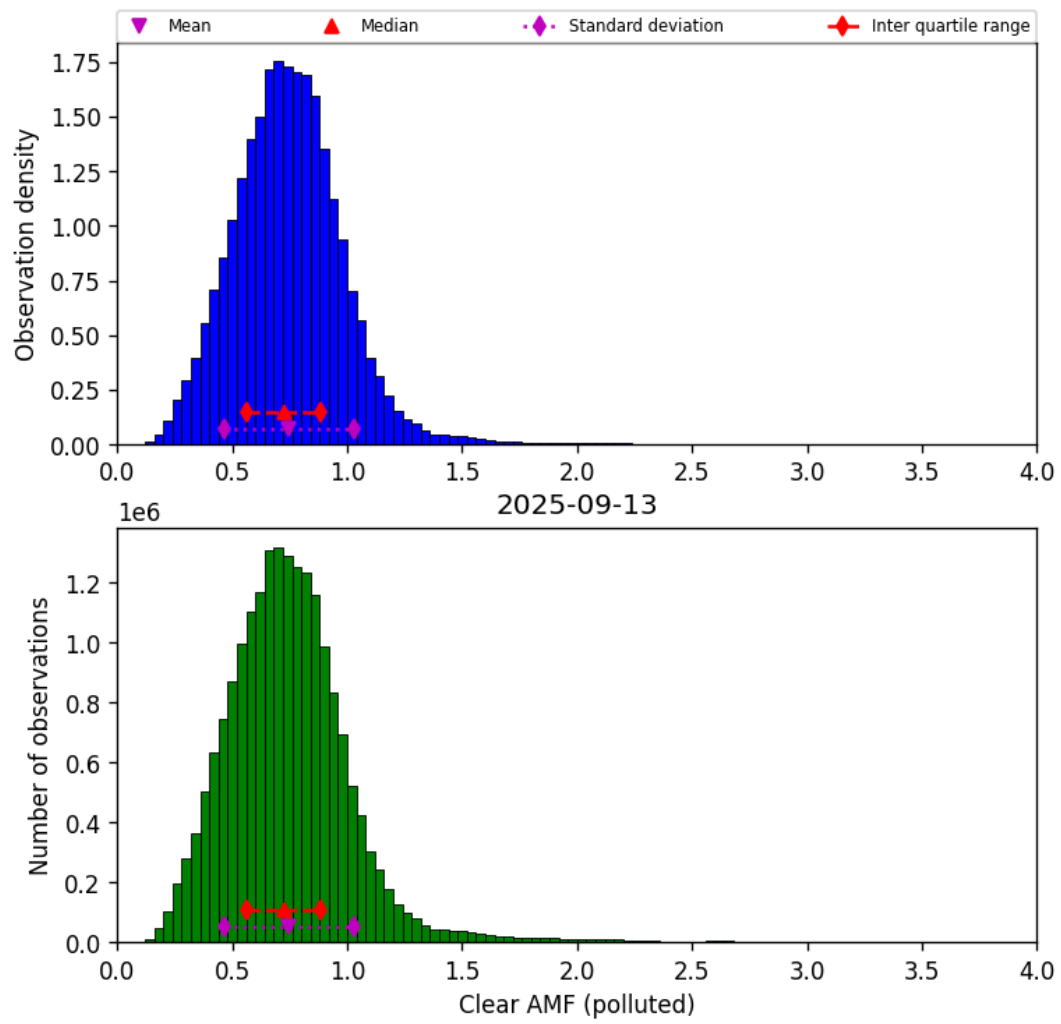
Figure 81: Histogram of “Clear AMF (polluted)” for 2025-09-12 to 2025-09-14
