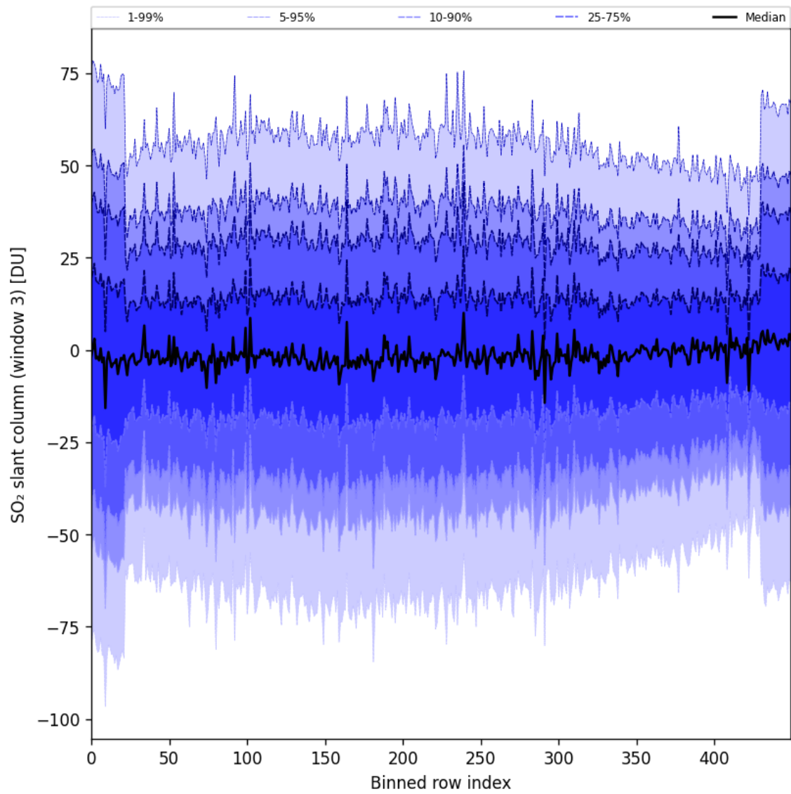
Figure 97: Along track statistics of “SO 2 slant column (window 3)” for 2025-09-12 to 2025-09-14
