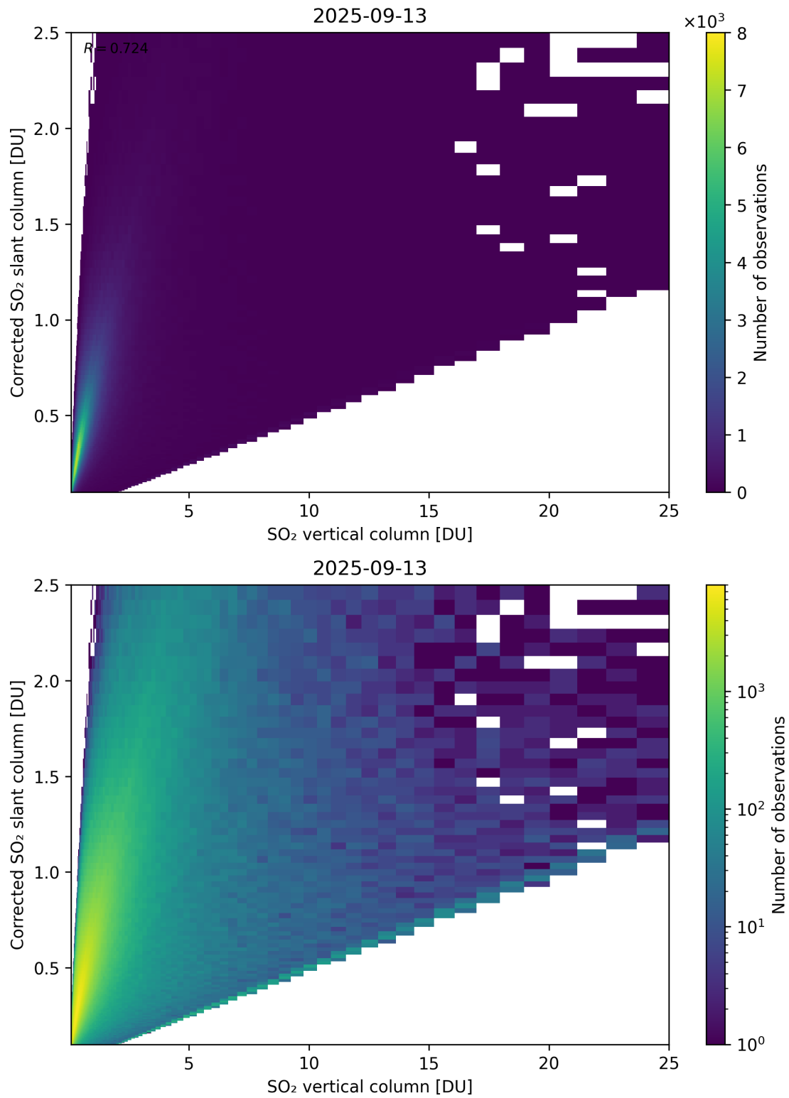
Figure 351: Scatter density plot of “SO 2 vertical column” against “Corrected SO 2 slant column” for 2025-09-12 to 2025-09-14.
