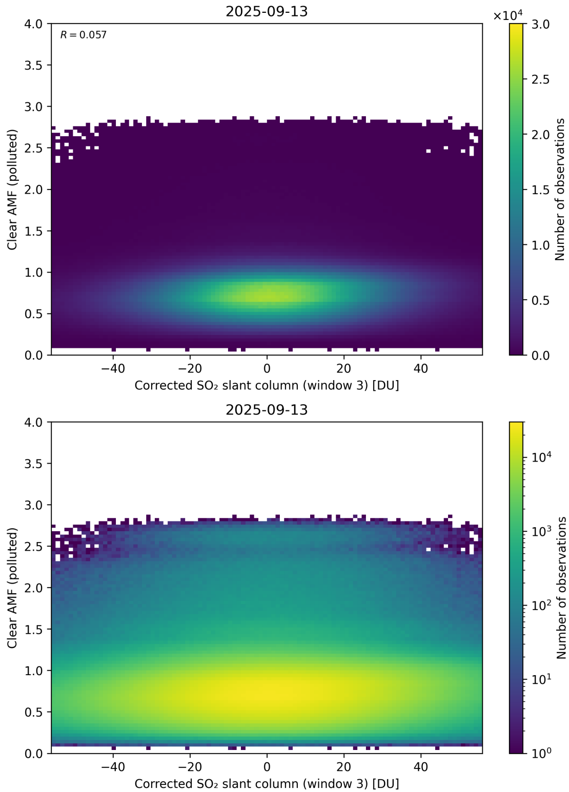
Figure 259: Scatter density plot of “Corrected SO 2 slant column (window 3)” against “Clear AMF (polluted)” for 2025-09-12 to 2025-09-14.
