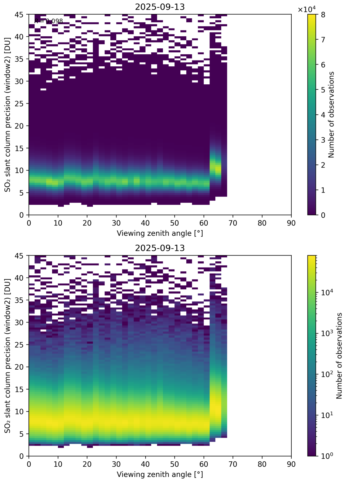
Figure 378: Scatter density plot of “Viewing zenith angle” against “SO 2 slant column precision (window2)” for 2025-09-12 to 2025-09-14.
