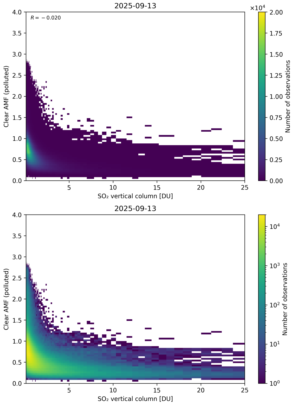
Figure 348: Scatter density plot of “SO 2 vertical column” against “Clear AMF (polluted)” for 2025-09-12 to 2025-09-14.
