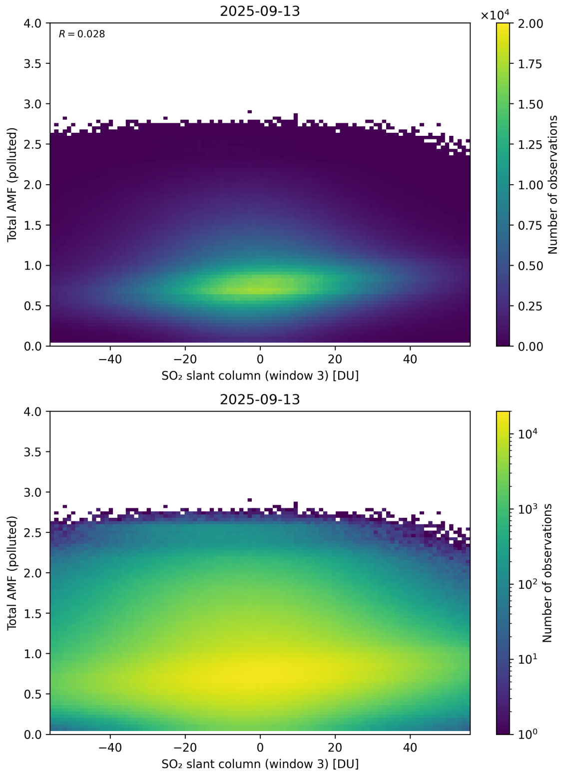
Figure 318: Scatter density plot of “SO 2 slant column (window 3)” against “Total AMF (polluted)” for 2025-09-12 to 2025-09-14.
