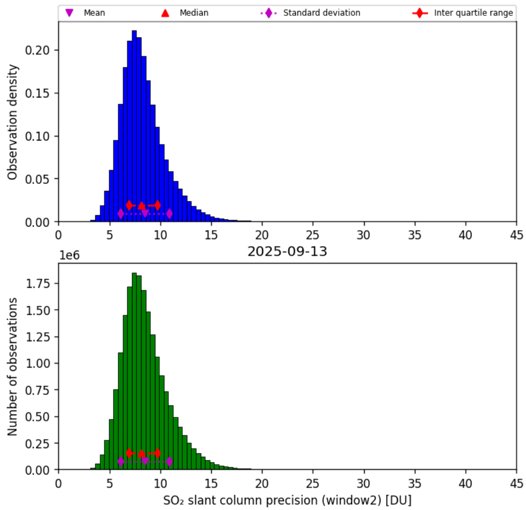
Figure 68: Histogram of “SO 2 slant column precision (window2)” for 2025-09-12 to 2025-09-14
