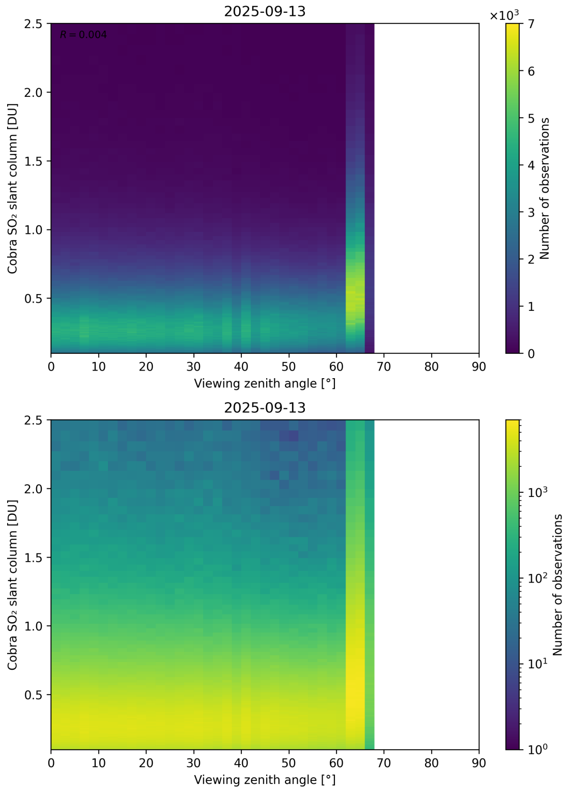
Figure 371: Scatter density plot of “Viewing zenith angle” against “Cobra SO 2 slant column” for 2025-09-12 to 2025-09-14.
