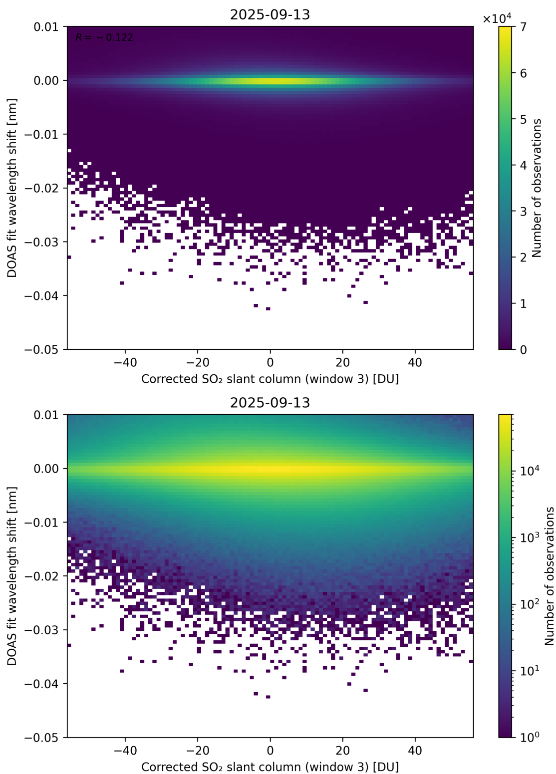
Figure 256: Scatter density plot of “Corrected SO 2 slant column (window 3)” against “DOAS fit wavelength shift” for 2025-09-12 to 2025-09-14.
