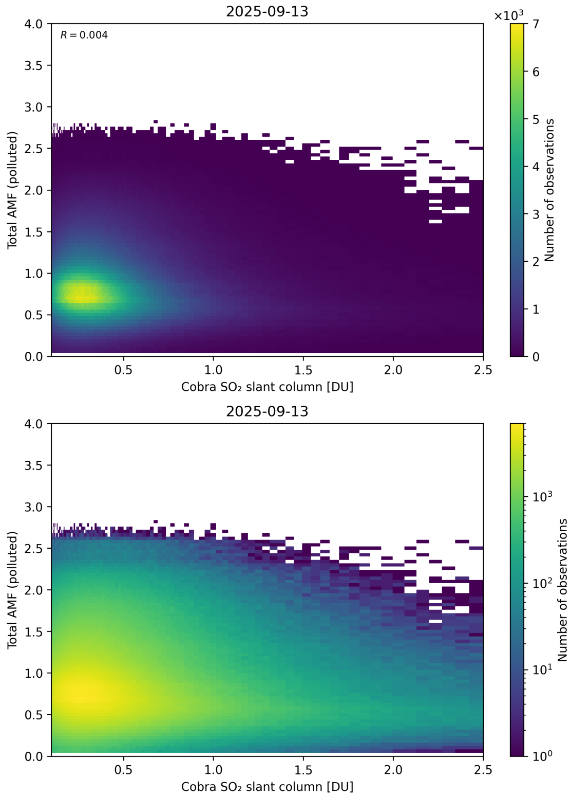
Figure 224: Scatter density plot of “Cobra SO 2 slant column” against “Total AMF (polluted)” for 2025-09-12 to 2025-09-14.
