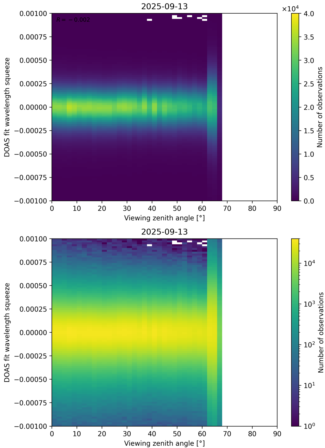
Figure 366: Scatter density plot of “Viewing zenith angle” against “DOAS fit wavelength squeeze” for 2025-09-12 to 2025-09-14.
