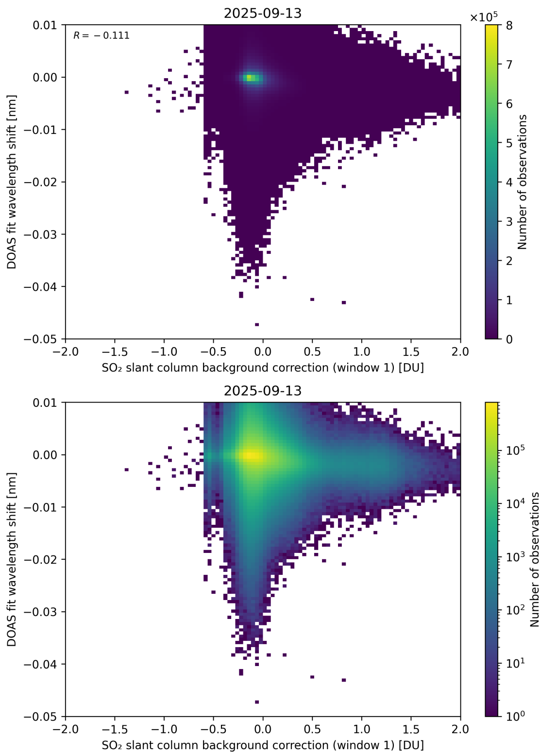
Figure 111: Scatter density plot of “SO 2 slant column background correction (window 1)” against “DOAS fit wavelength shift” for 2025-09-12 to 2025-09-14.
