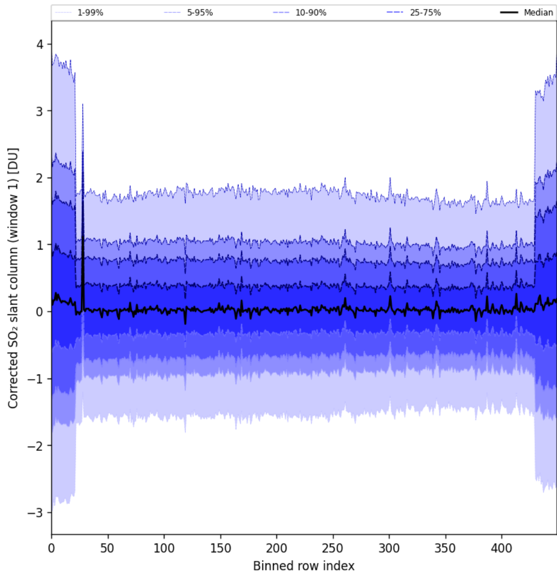
Figure 91: Along track statistics of “Corrected SO 2 slant column (window 1)” for 2025-09-12 to 2025-09-14
