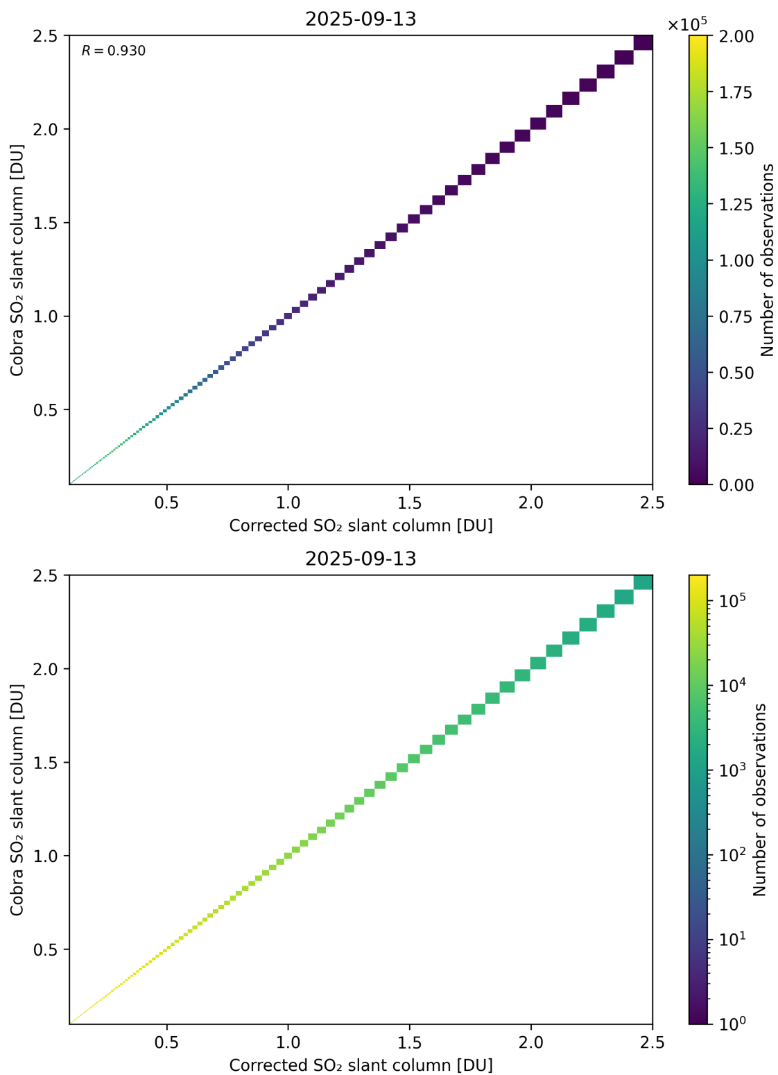
Figure 233: Scatter density plot of “Corrected SO 2 slant column” against “Cobra SO 2 slant column” for 2025-09-12 to 2025-09-14.
