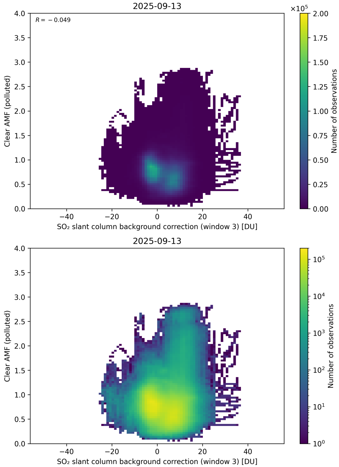
Figure 135: Scatter density plot of “SO 2 slant column background correction (window 3)” against “Clear AMF (polluted)” for 2025-09-12 to 2025-09-14.
