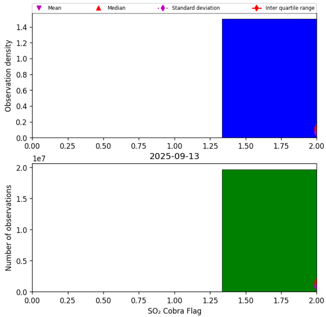
Figure 75: Histogram of “SO 2 Cobra Flag” for 2025-09-12 to 2025-09-14
