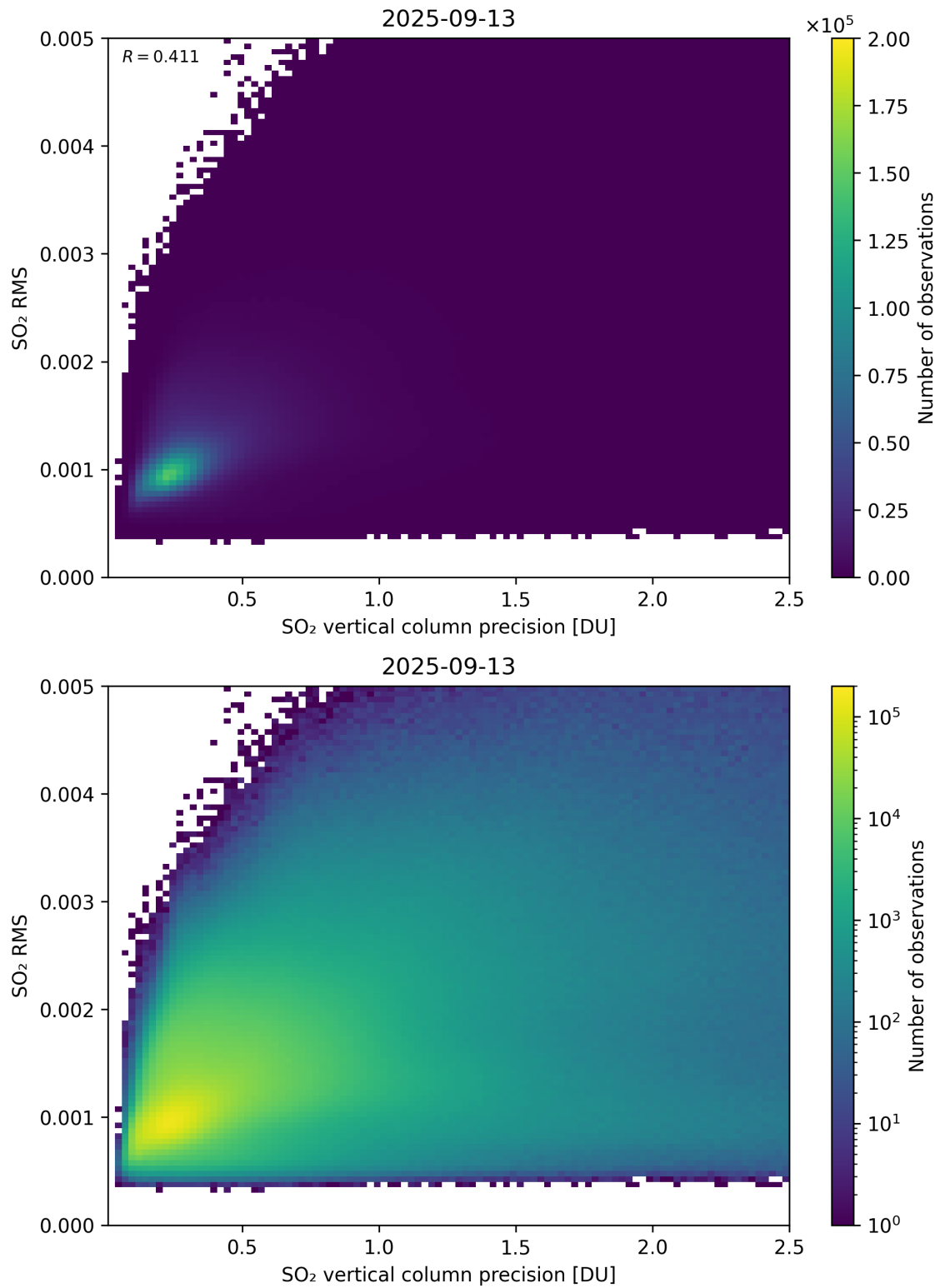
Figure 334: Scatter density plot of “SO 2 vertical column precision” against “SO 2 RMS” for 2025-09-12 to 2025-09-14.
