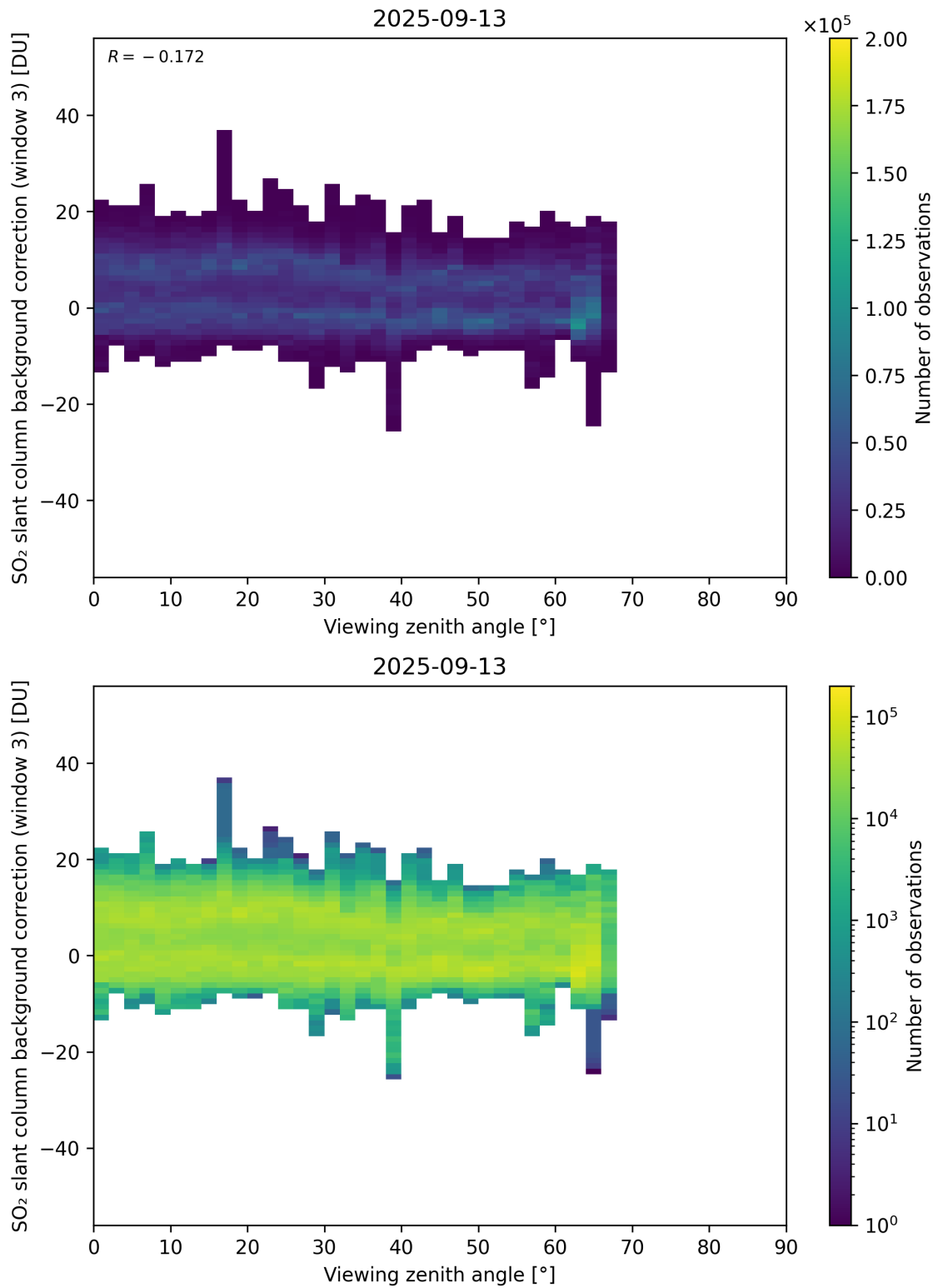
Figure 364: Scatter density plot of “Viewing zenith angle” against “SO 2 slant column background correction (window 3)” for 2025-09-12 to 2025-09-14.
