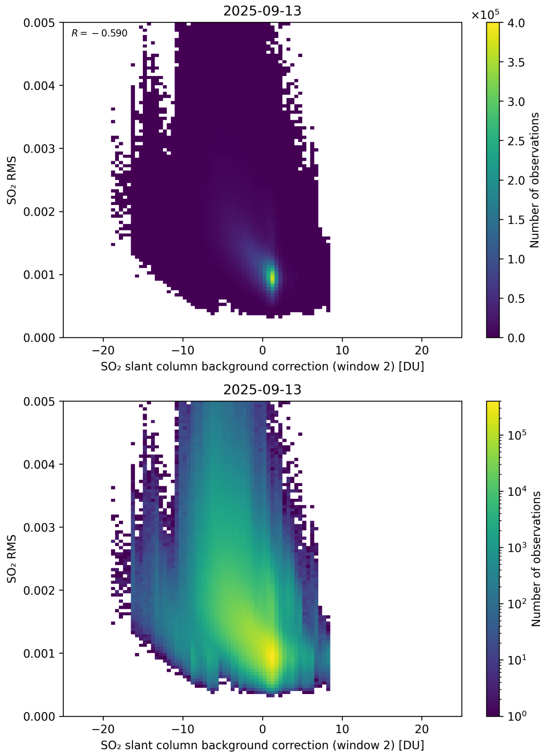
Figure 125: Scatter density plot of “SO 2 slant column background correction (window 2)” against “SO 2 RMS” for 2025-09-12 to 2025-09-14.
