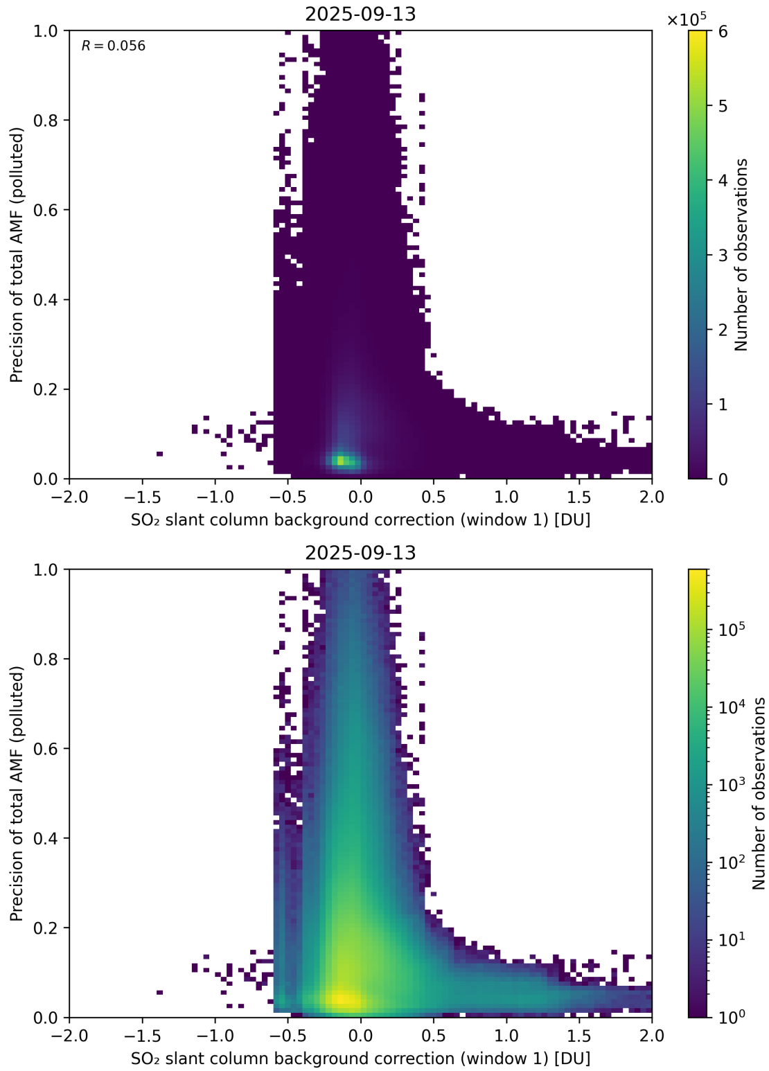
Figure 121: Scatter density plot of “SO 2 slant column background correction (window 1)” against “Precision of total AMF (polluted)” for 2025-09-12 to 2025-09-14.
