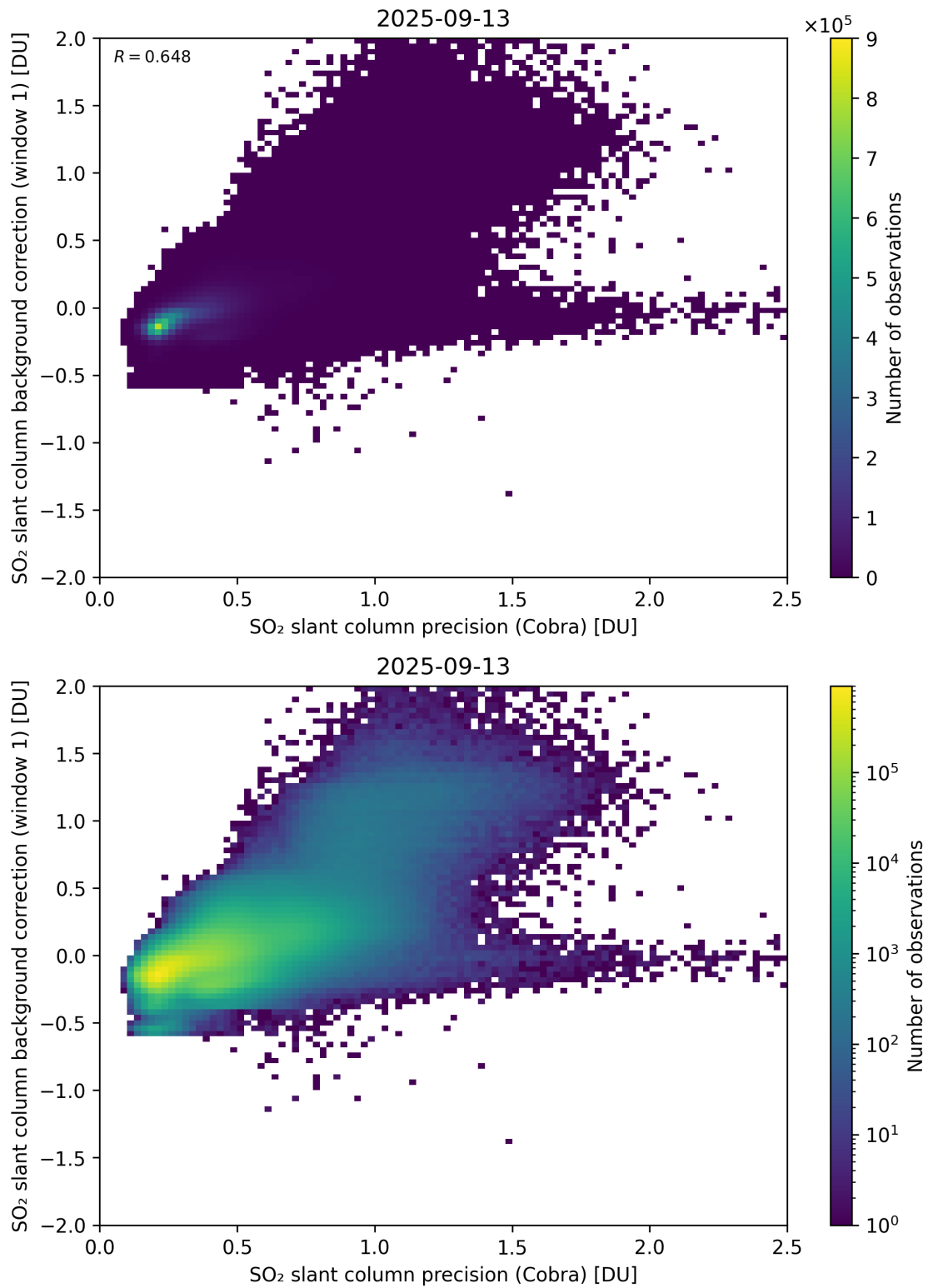
Figure 199: Scatter density plot of “SO 2 slant column precision (Cobra)” against “SO 2 slant column background correction (window 1)” for 2025-09-12 to 2025-09-14.
