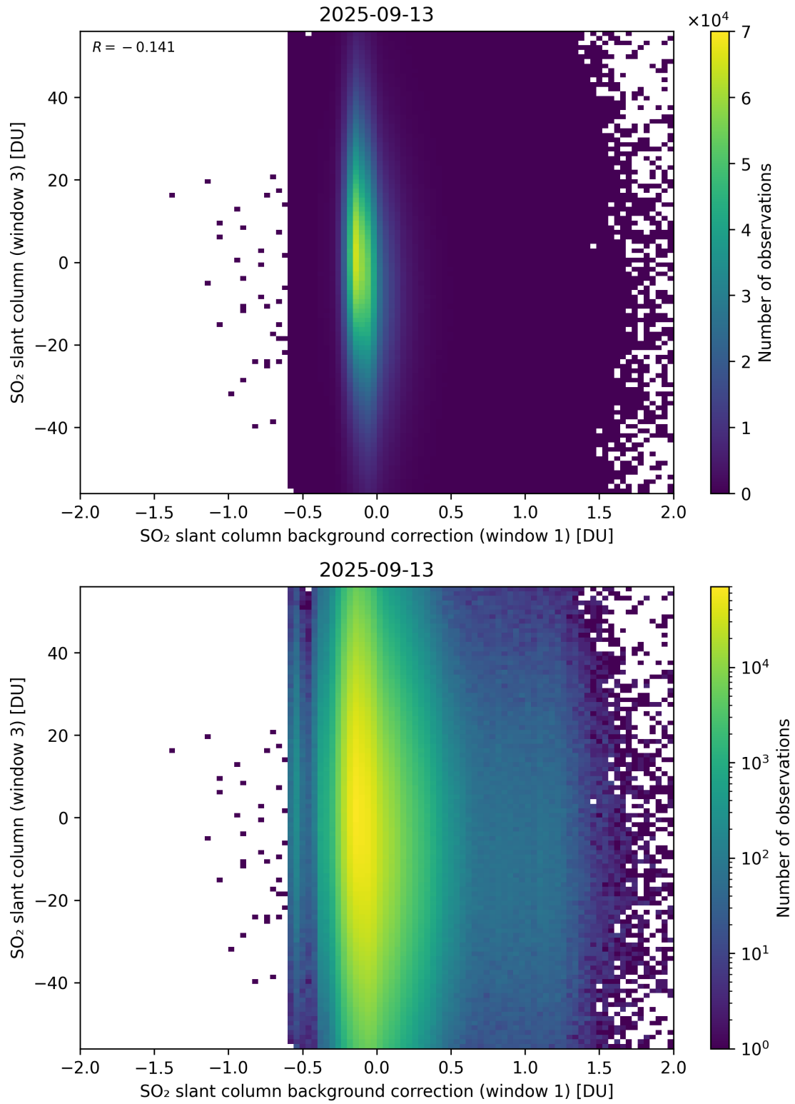
Figure 118: Scatter density plot of “SO 2 slant column background correction (window 1)” against “SO 2 slant column (window 3)” for 2025-09-12 to 2025-09-14.
