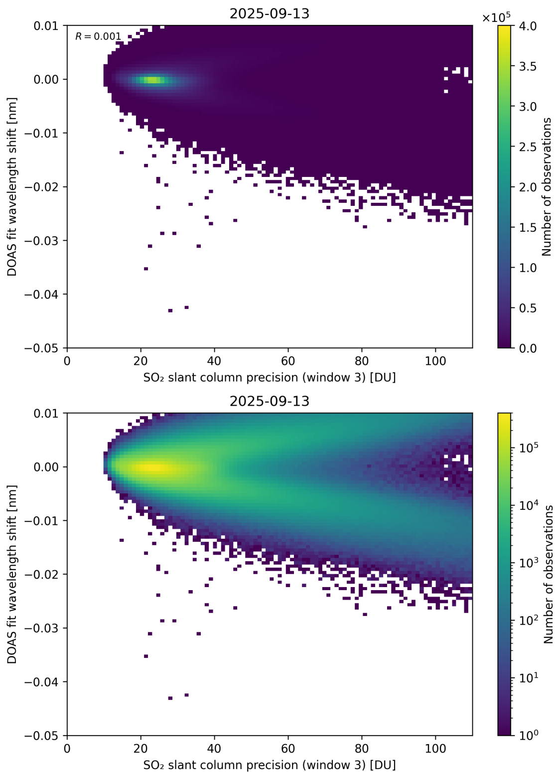
Figure 308: Scatter density plot of “SO 2 slant column precision (window 3)” against “DOAS fit wavelength shift” for 2025-09-12 to 2025-09-14.
