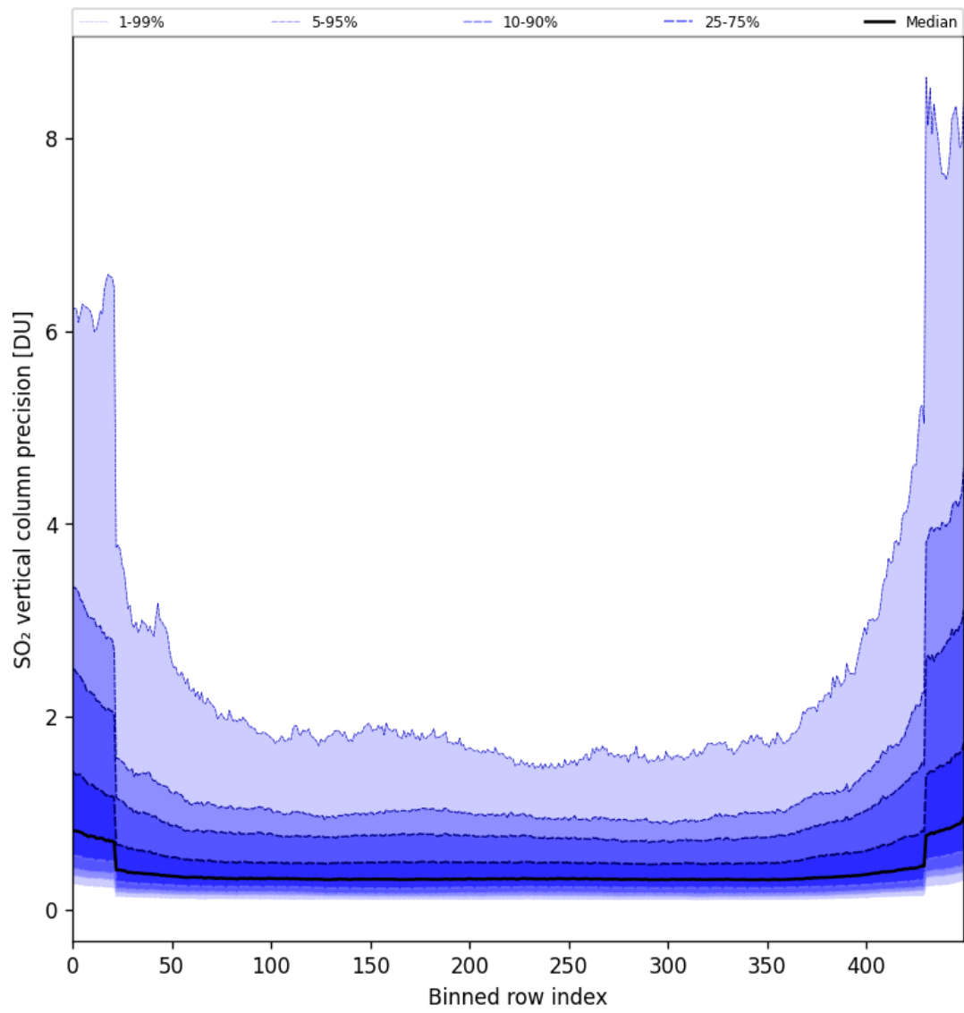
Figure 85: Along track statistics of “SO 2 vertical column precision” for 2025-09-12 to 2025-09-14
