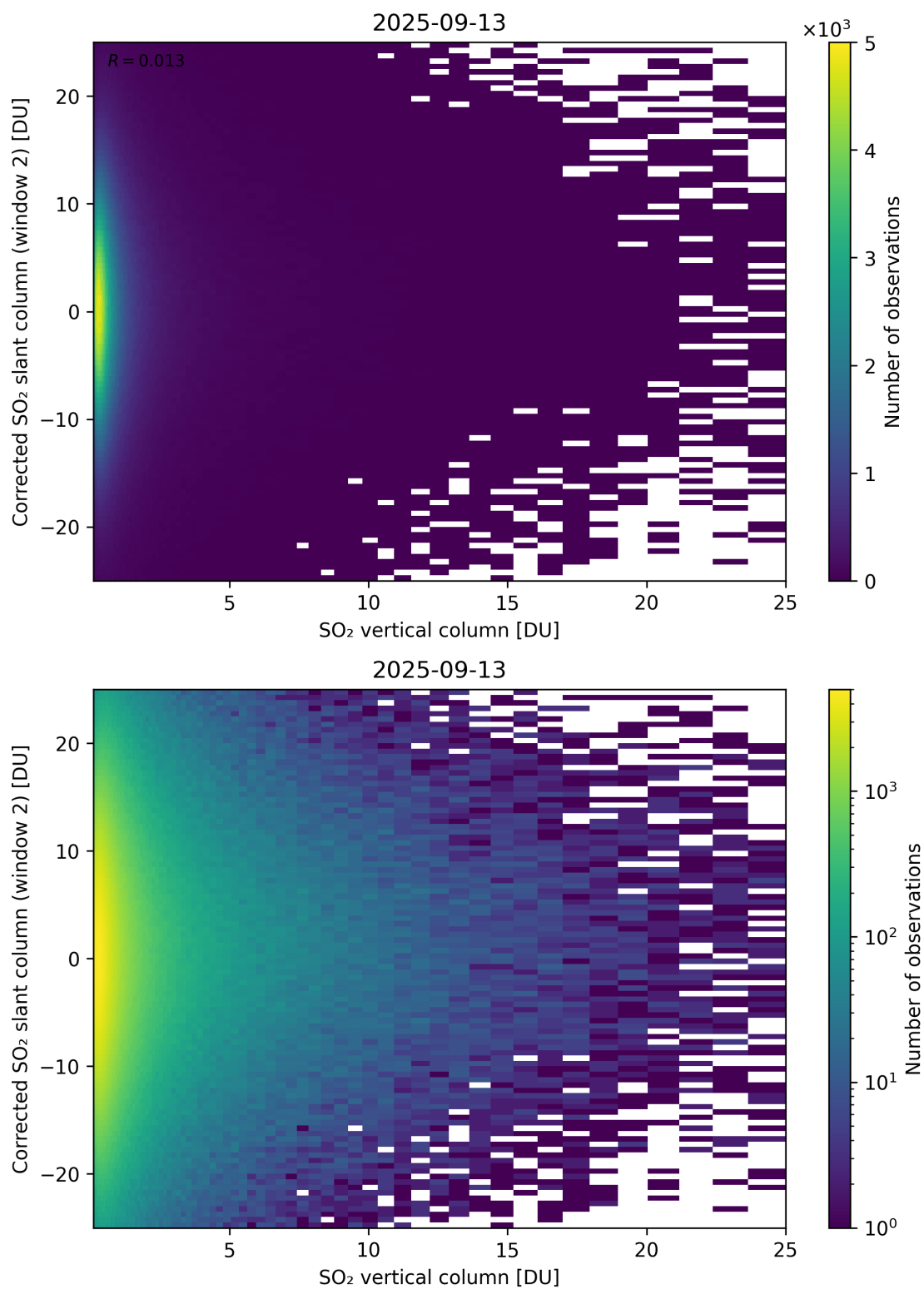
Figure 352: Scatter density plot of “SO 2 vertical column” against “Corrected SO 2 slant column (window 2)” for 2025-09-12 to 2025-09-14.
