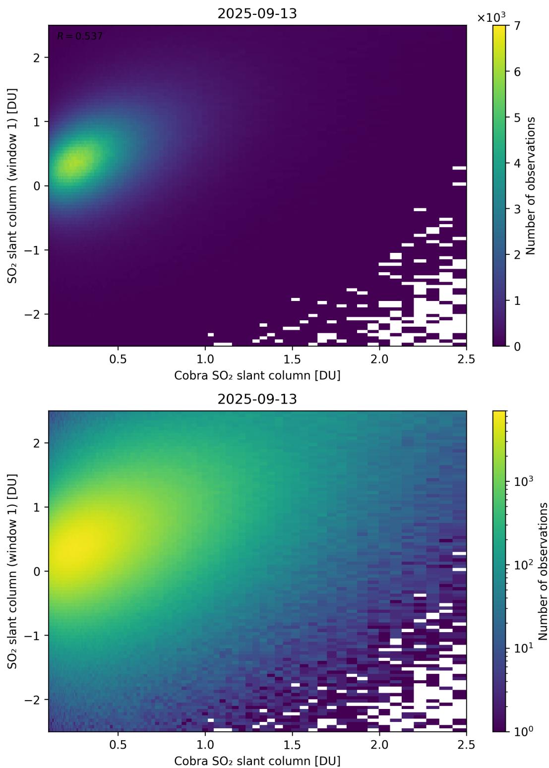
Figure 219: Scatter density plot of “Cobra SO 2 slant column” against “SO 2 slant column (window 1)” for 2025-09-12 to 2025-09-14.
