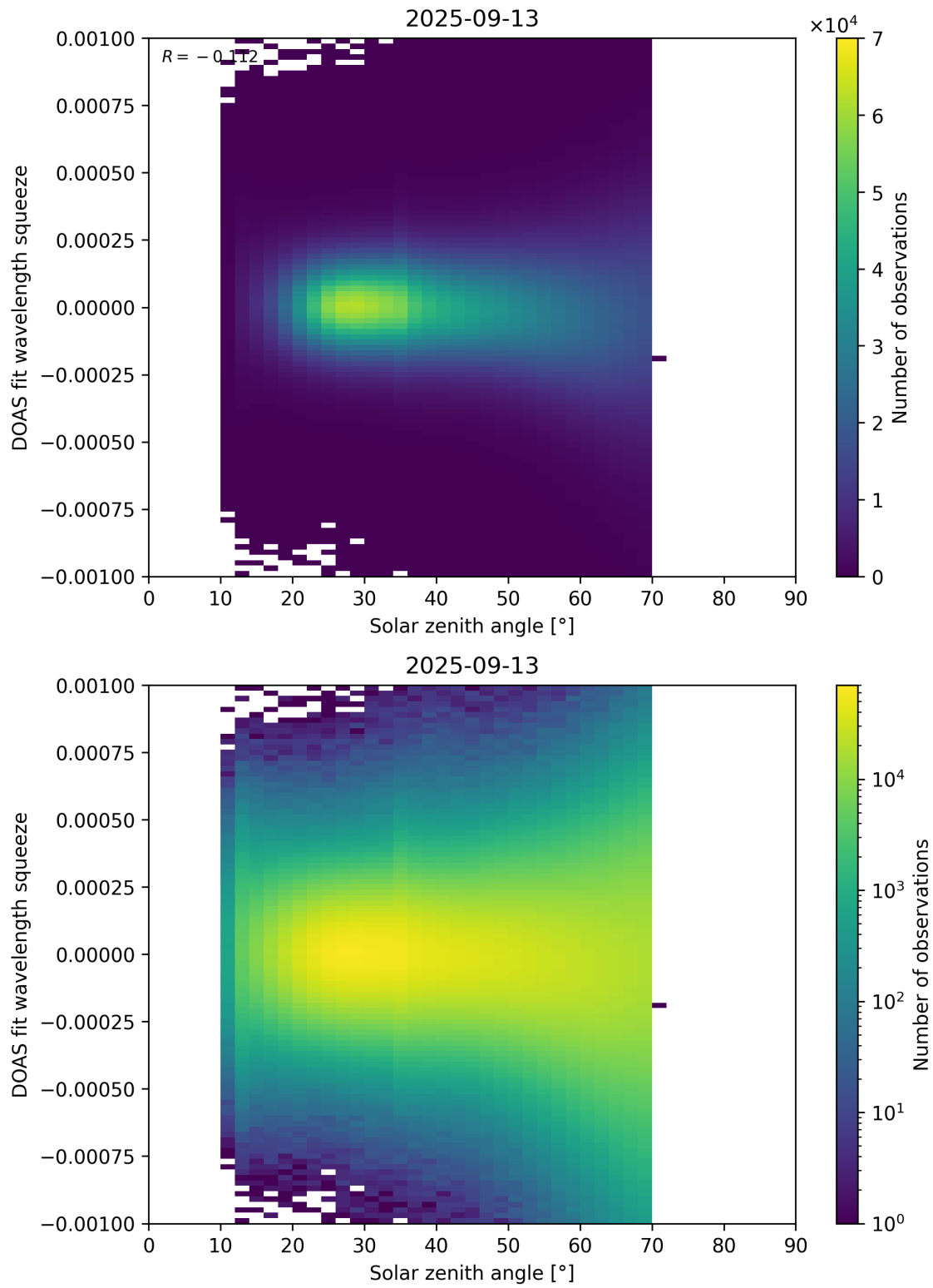
Figure 175: Scatter density plot of “Solar zenith angle” against “DOAS fit wavelength squeeze” for 2025-09-12 to 2025-09-14.
