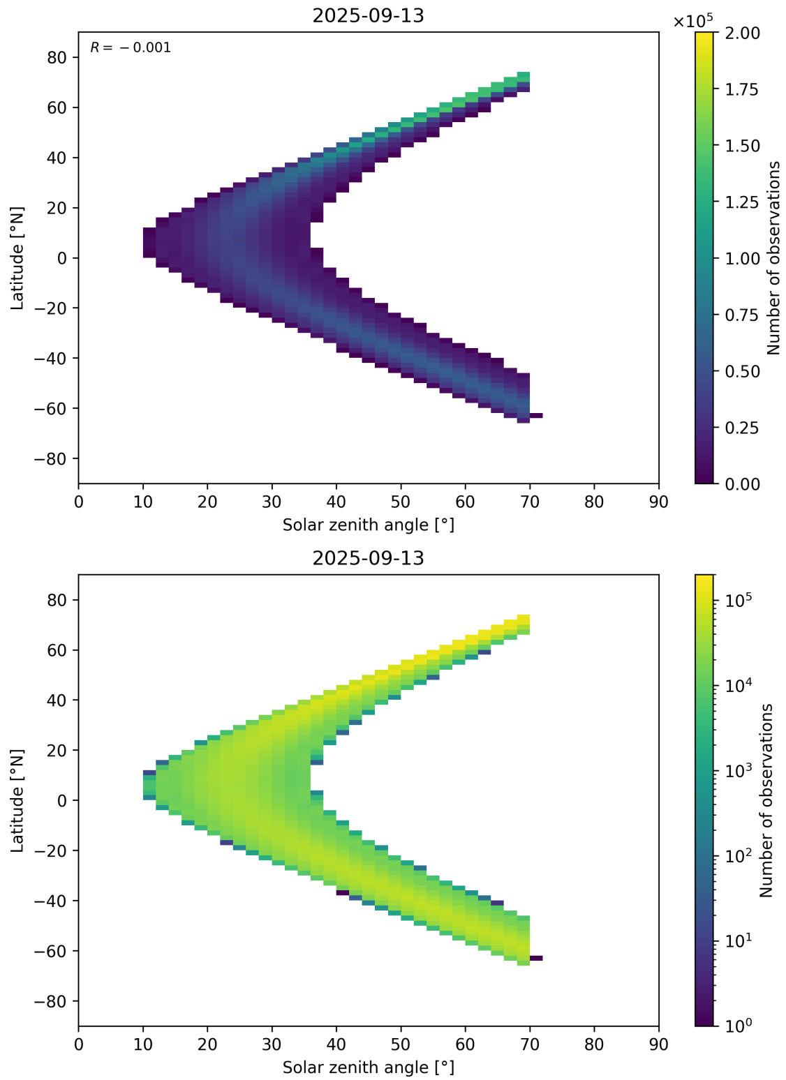
Figure 177: Scatter density plot of “Solar zenith angle” against “Latitude” for 2025-09-12 to 2025-09-14.
