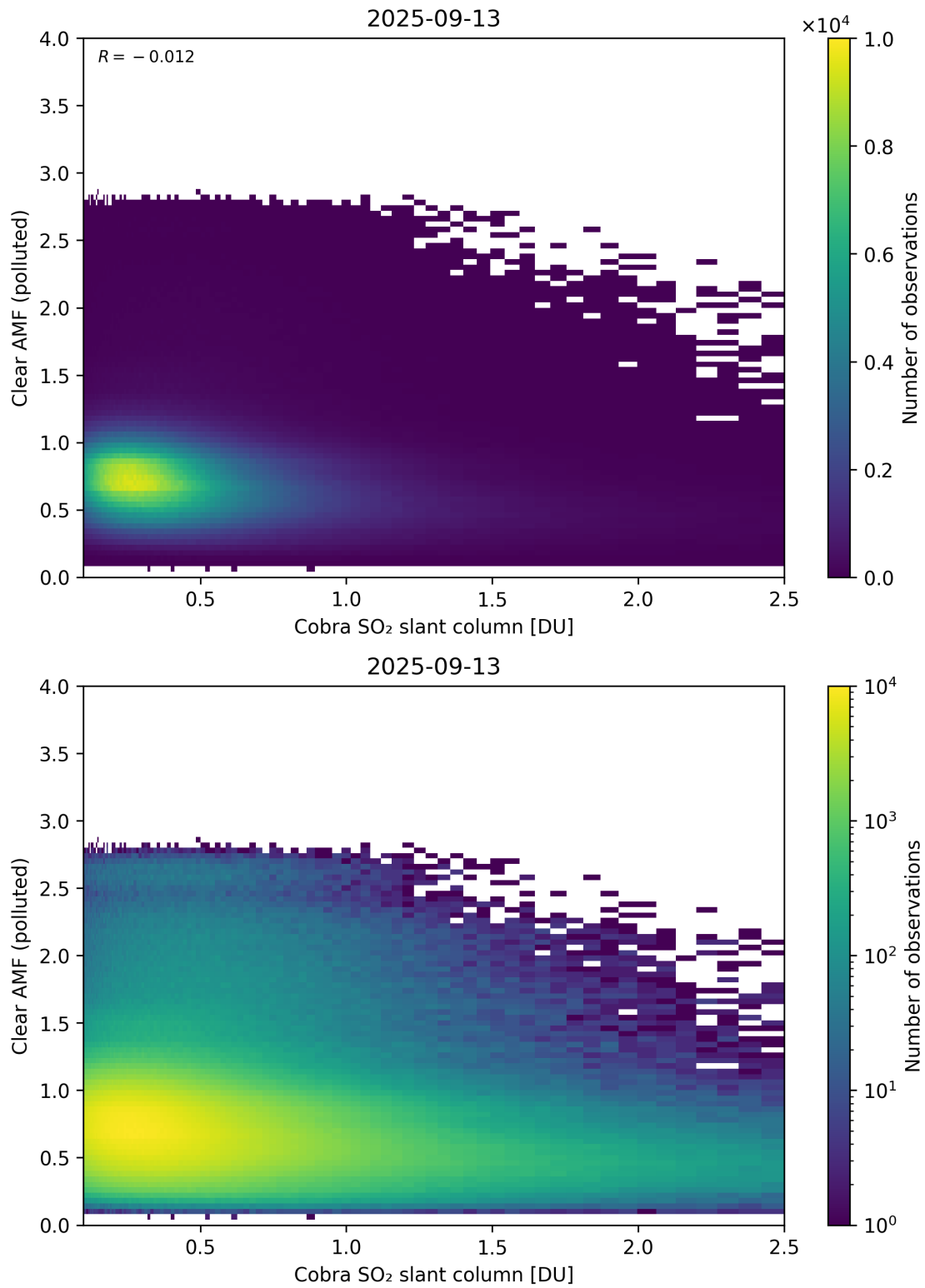
Figure 215: Scatter density plot of “Cobra SO 2 slant column” against “Clear AMF (polluted)” for 2025-09-12 to 2025-09-14.
