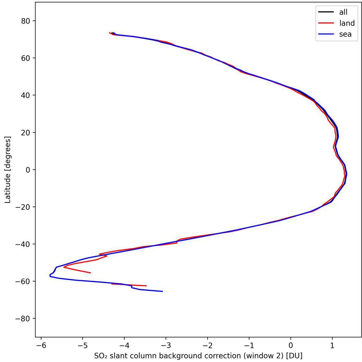
Figure 44: Zonal average of “SO 2 slant column background correction (window 2)” for 2025-09-12 to 2025-09-14.
