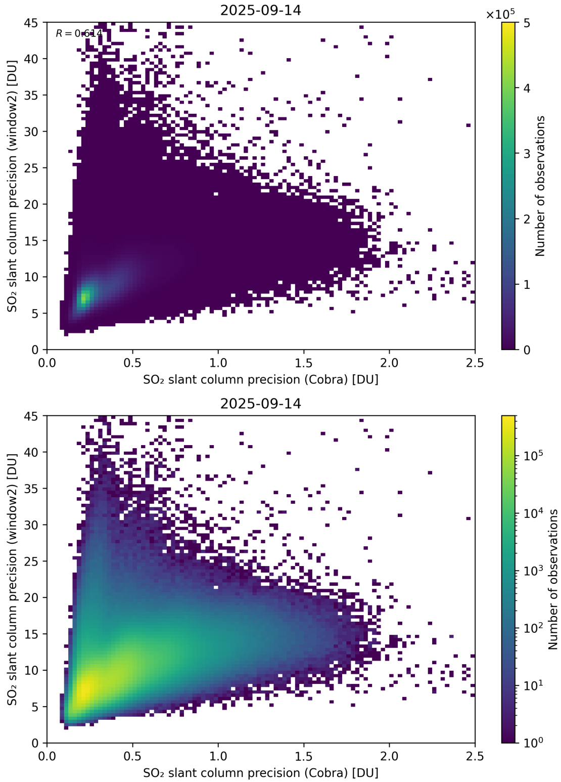
Figure 210: Scatter density plot of “SO 2 slant column precision (Cobra)” against “SO 2 slant column precision (window2)” for 2025-09-13 to 2025-09-15.
