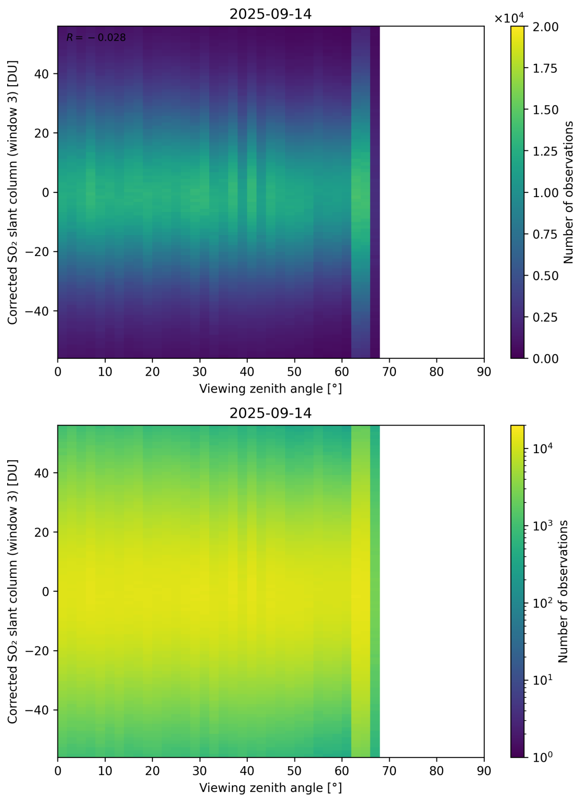
Figure 375: Scatter density plot of “Viewing zenith angle” against “Corrected SO 2 slant column (window 3)” for 2025-09-13 to 2025-09-15.
