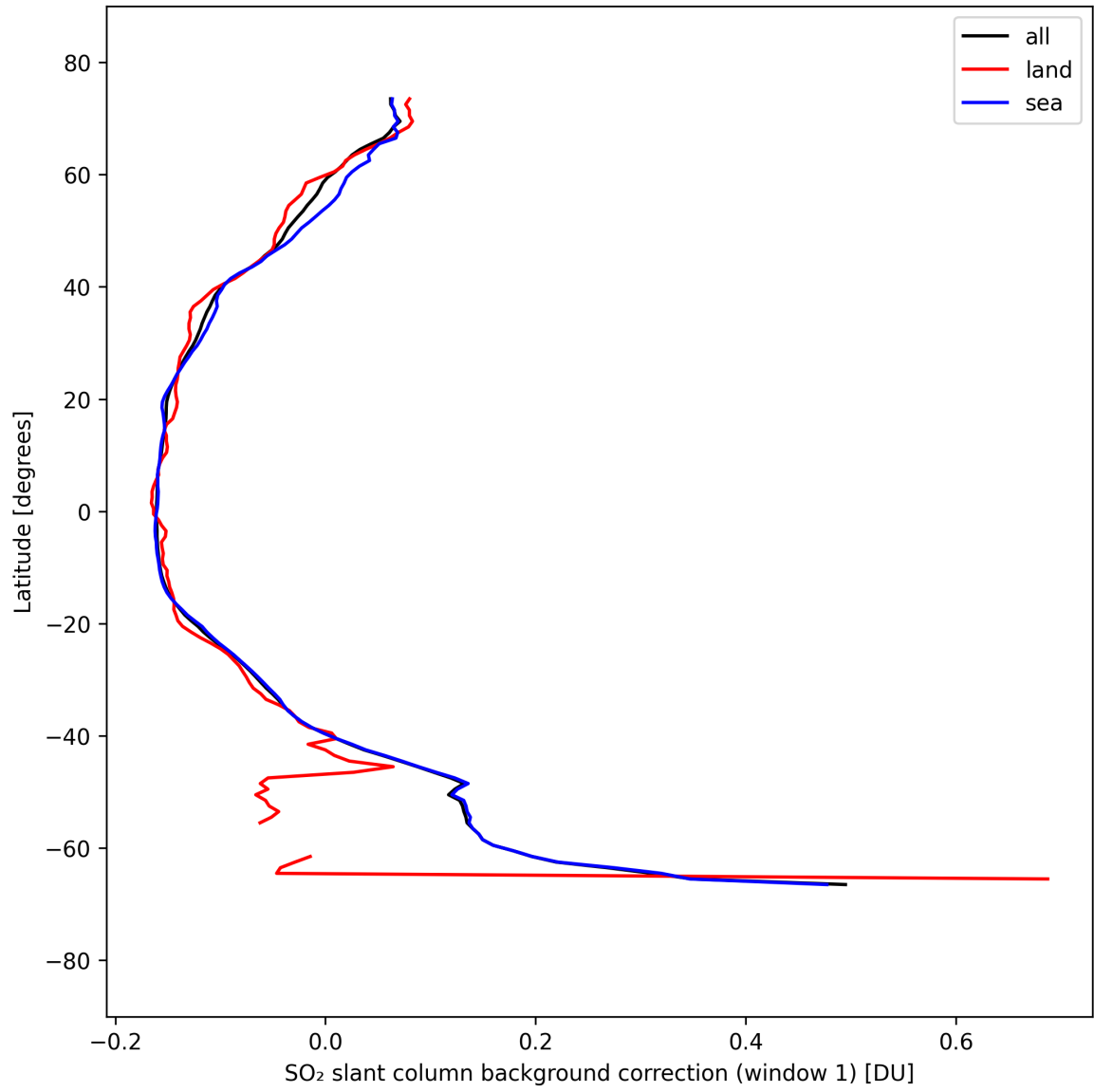
Figure 40: Zonal average of “SO 2 slant column background correction (window 1)” for 2025-09-13 to 2025-09-15.
