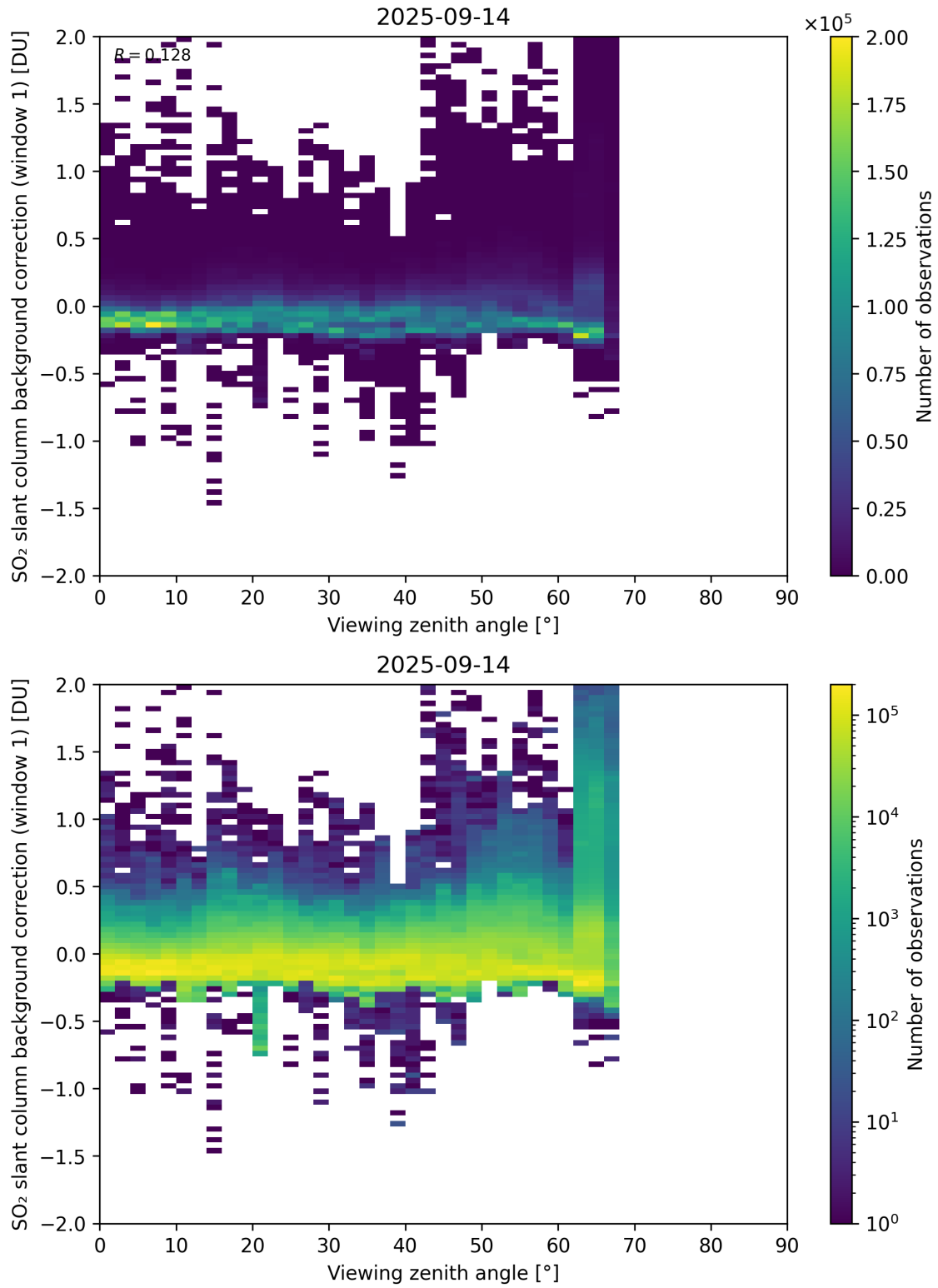
Figure 362: Scatter density plot of “Viewing zenith angle” against “SO 2 slant column background correction (window 1)” for 2025-09-13 to 2025-09-15.
