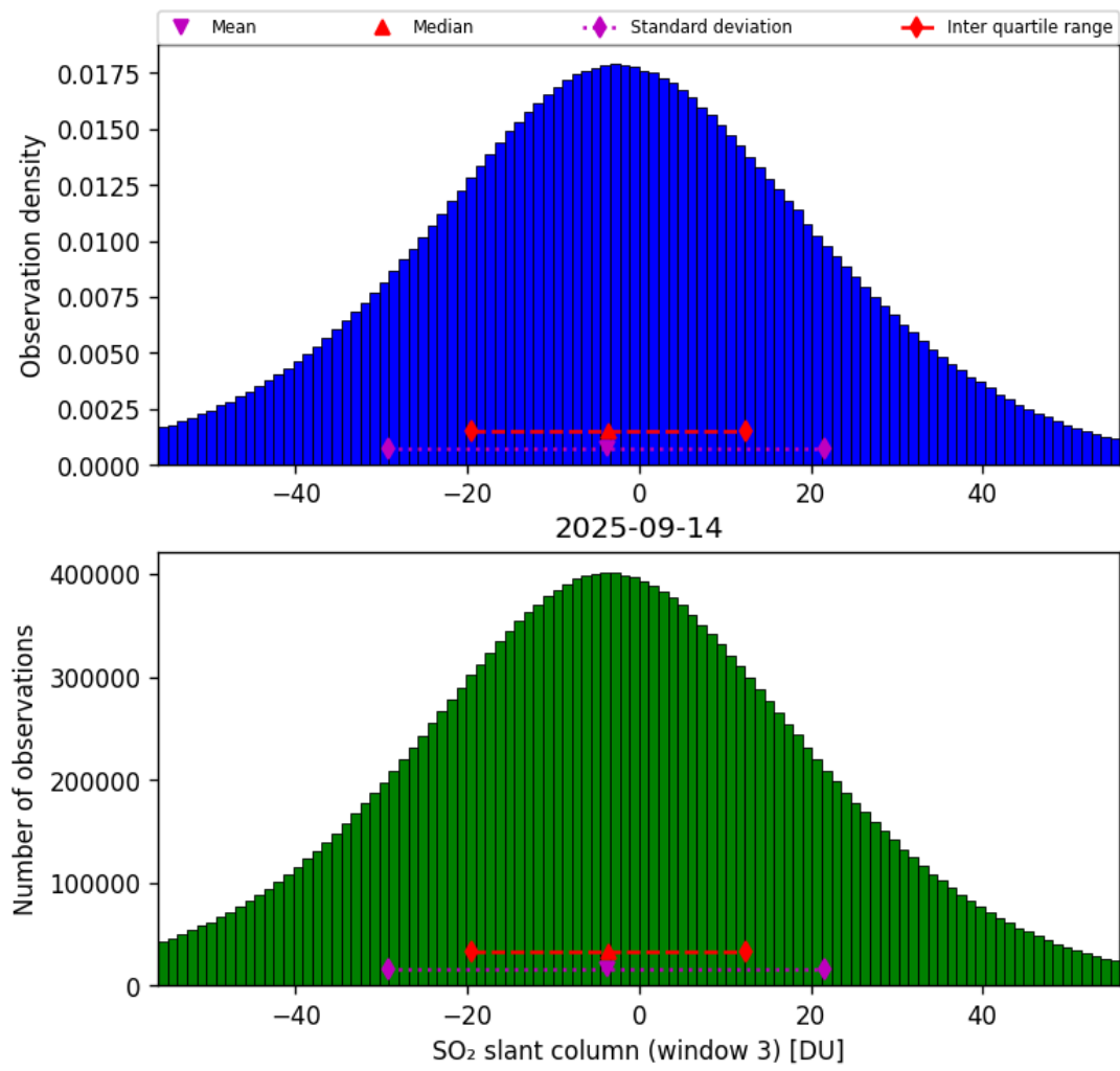
Figure 71: Histogram of “SO 2 slant column (window 3)” for 2025-09-13 to 2025-09-15
