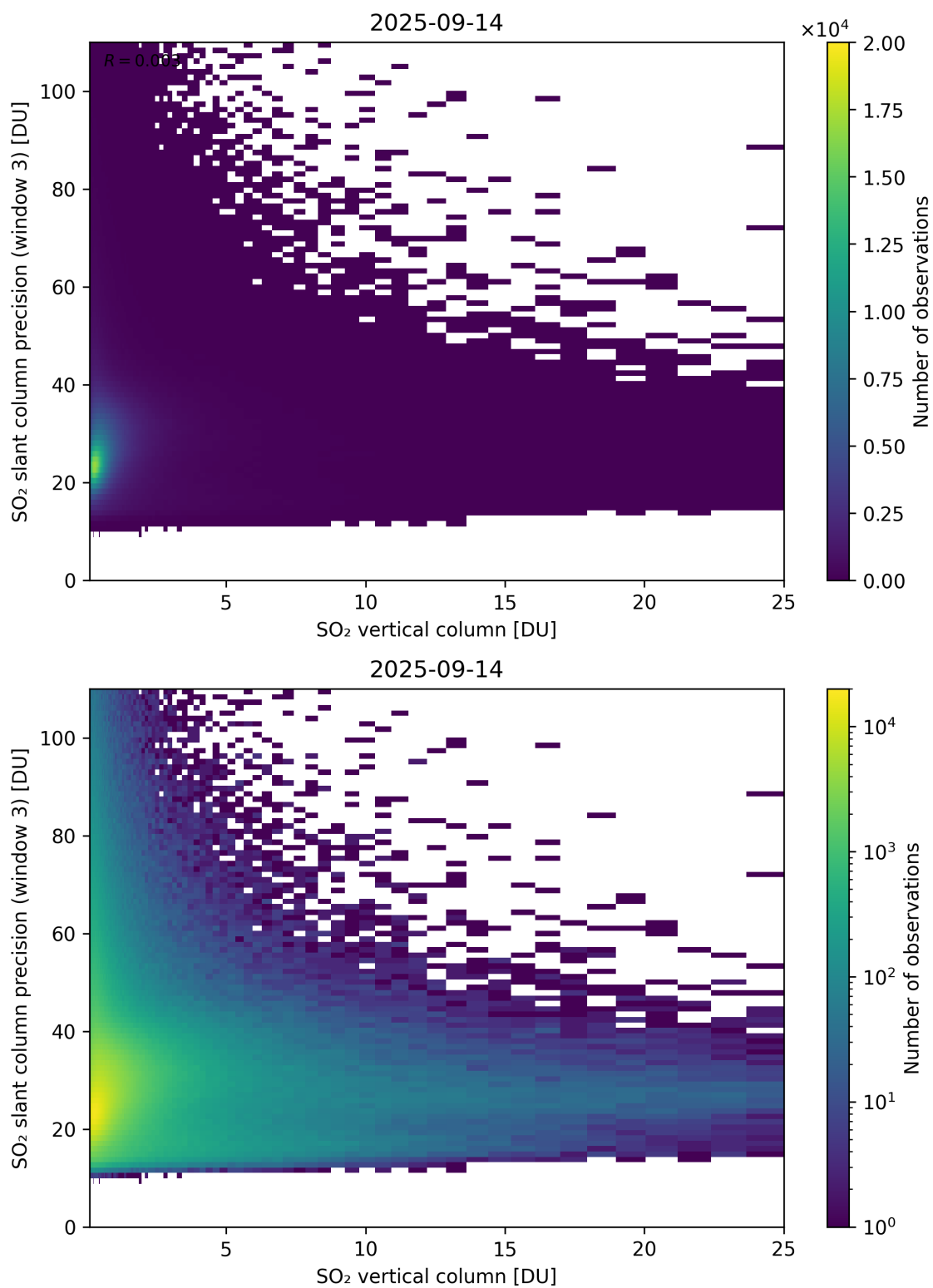
Figure 358: Scatter density plot of “SO 2 vertical column” against “SO 2 slant column precision (window 3)” for 2025-09-13 to 2025-09-15.
