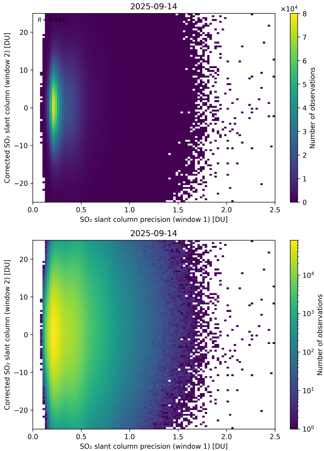
Figure 275: Scatter density plot of “SO 2 slant column precision (window 1)” against “Corrected SO 2 slant column (window 2)” for 2025-09-13 to 2025-09-15.
