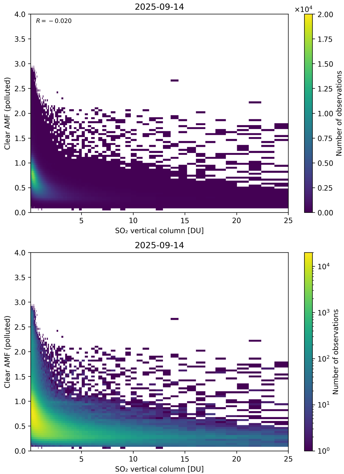
Figure 348: Scatter density plot of “SO 2 vertical column” against “Clear AMF (polluted)” for 2025-09-13 to 2025-09-15.
