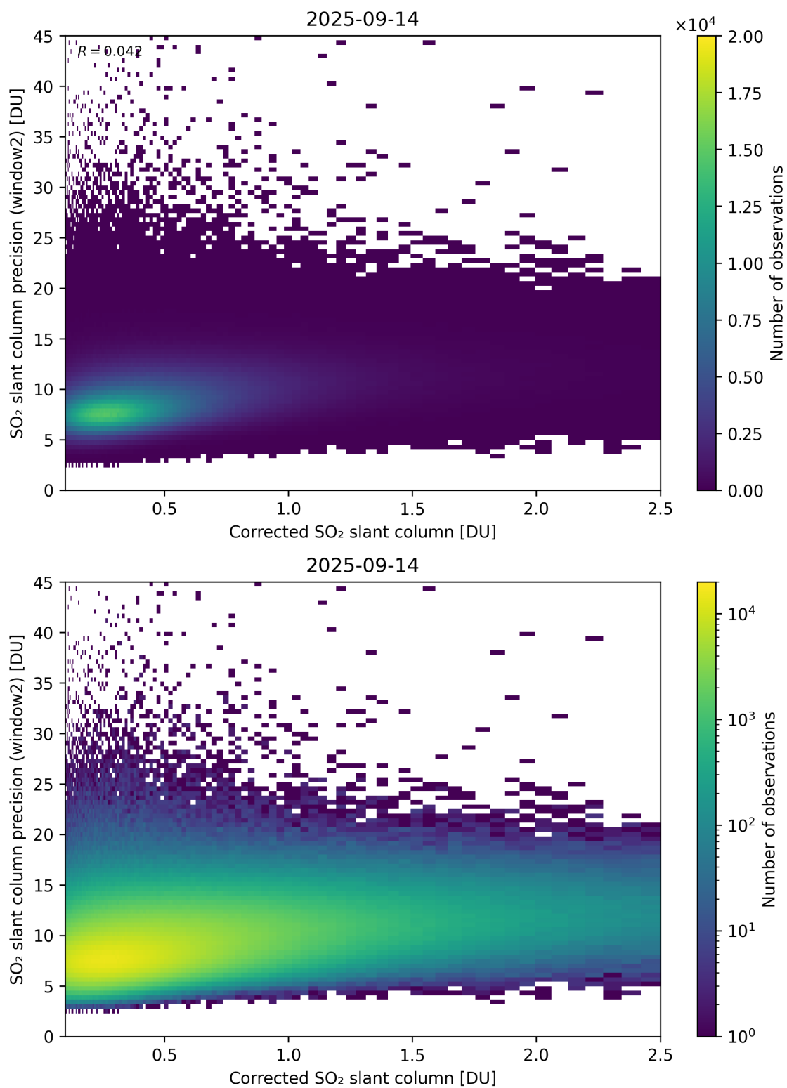
Figure 239: Scatter density plot of “Corrected SO 2 slant column” against “SO 2 slant column precision (window2)” for 2025-09-13 to 2025-09-15.
