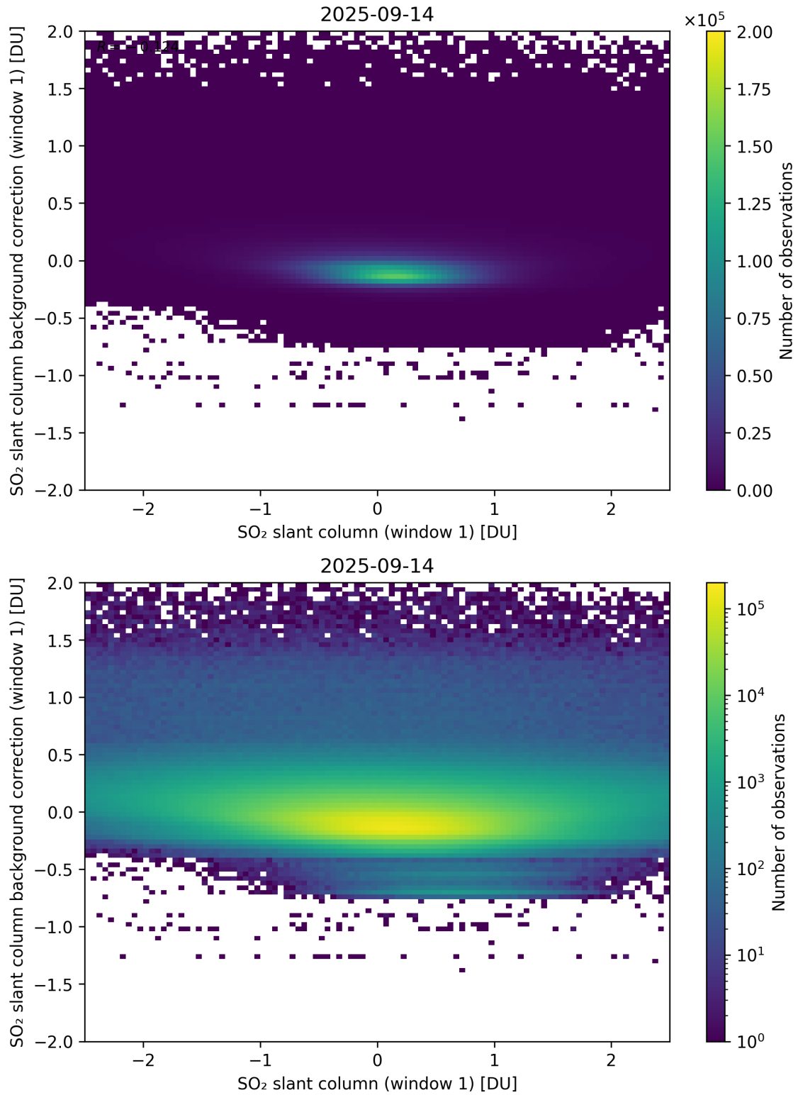
Figure 262: Scatter density plot of “SO 2 slant column (window 1)” against “SO 2 slant column background correction (window 1)” for 2025-09-13 to 2025-09-15.
