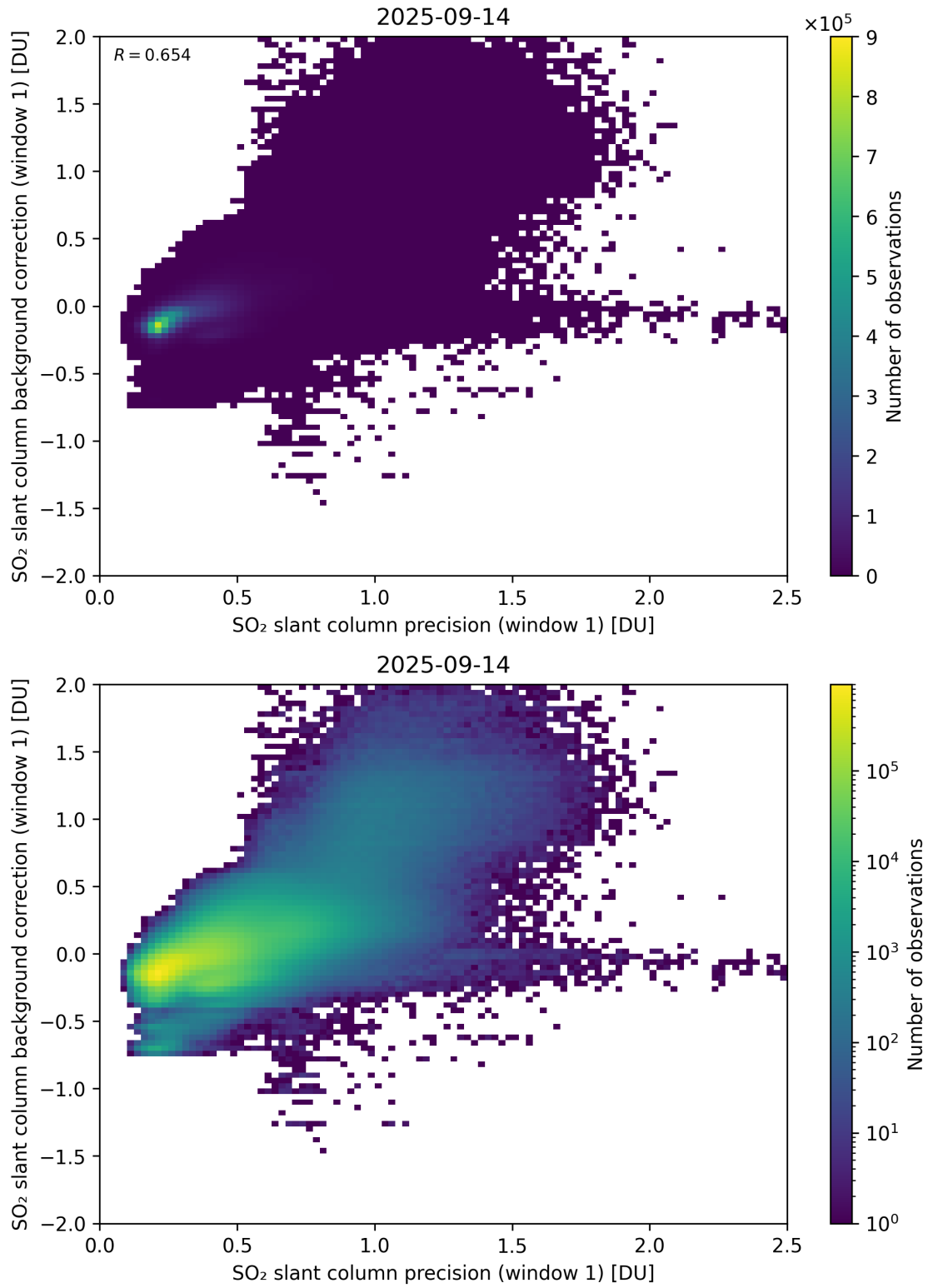
Figure 268: Scatter density plot of “SO 2 slant column precision (window 1)” against “SO 2 slant column background correction (window 1)” for 2025-09-13 to 2025-09-15.
