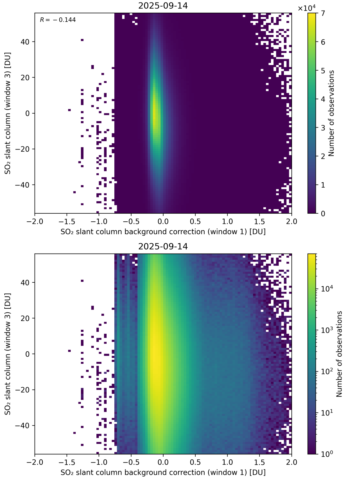
Figure 118: Scatter density plot of “SO 2 slant column background correction (window 1)” against “SO 2 slant column (window 3)” for 2025-09-13 to 2025-09-15.
