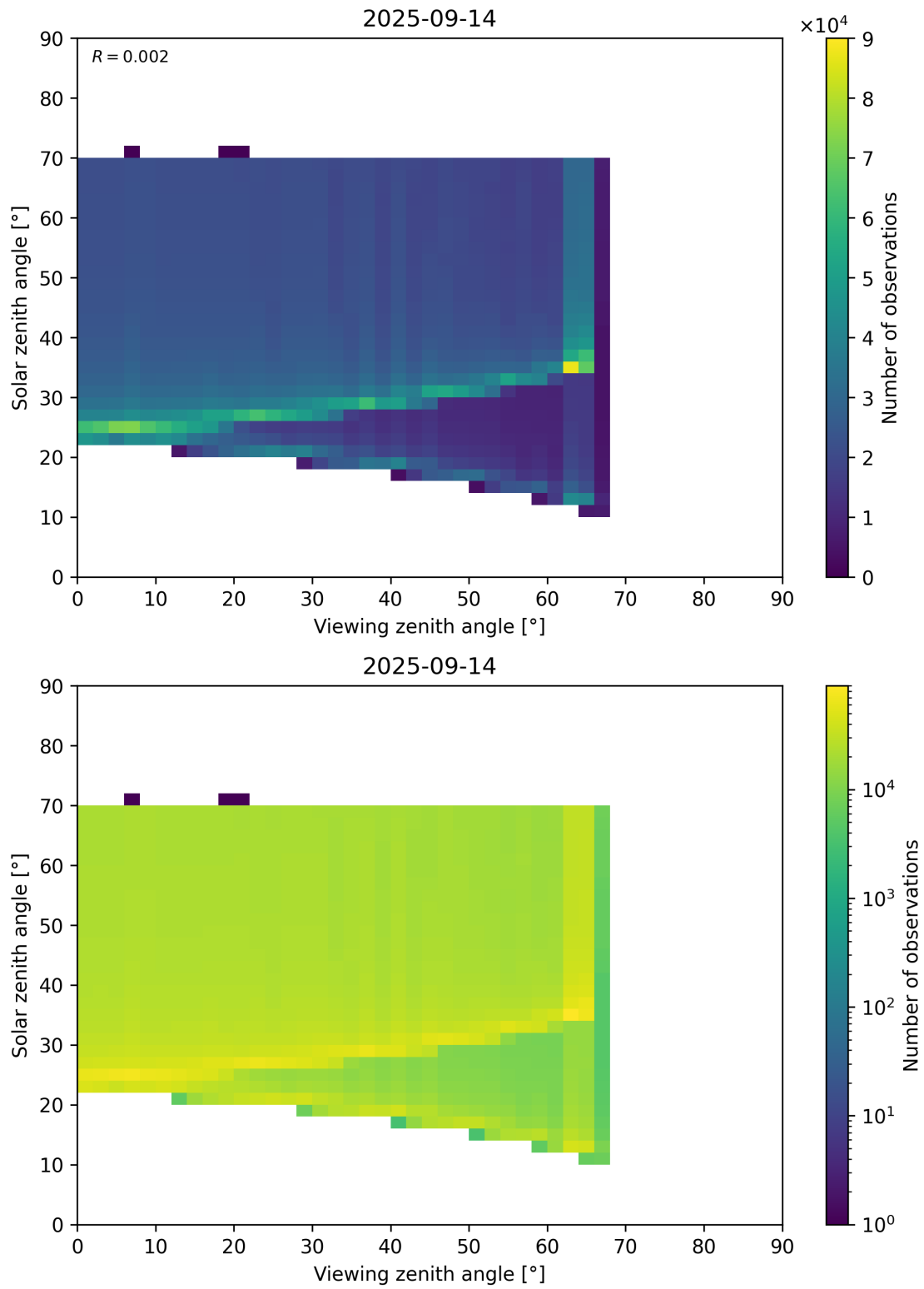
Figure 369: Scatter density plot of “Viewing zenith angle” against “Solar zenith angle” for 2025-09-13 to 2025-09-15.
