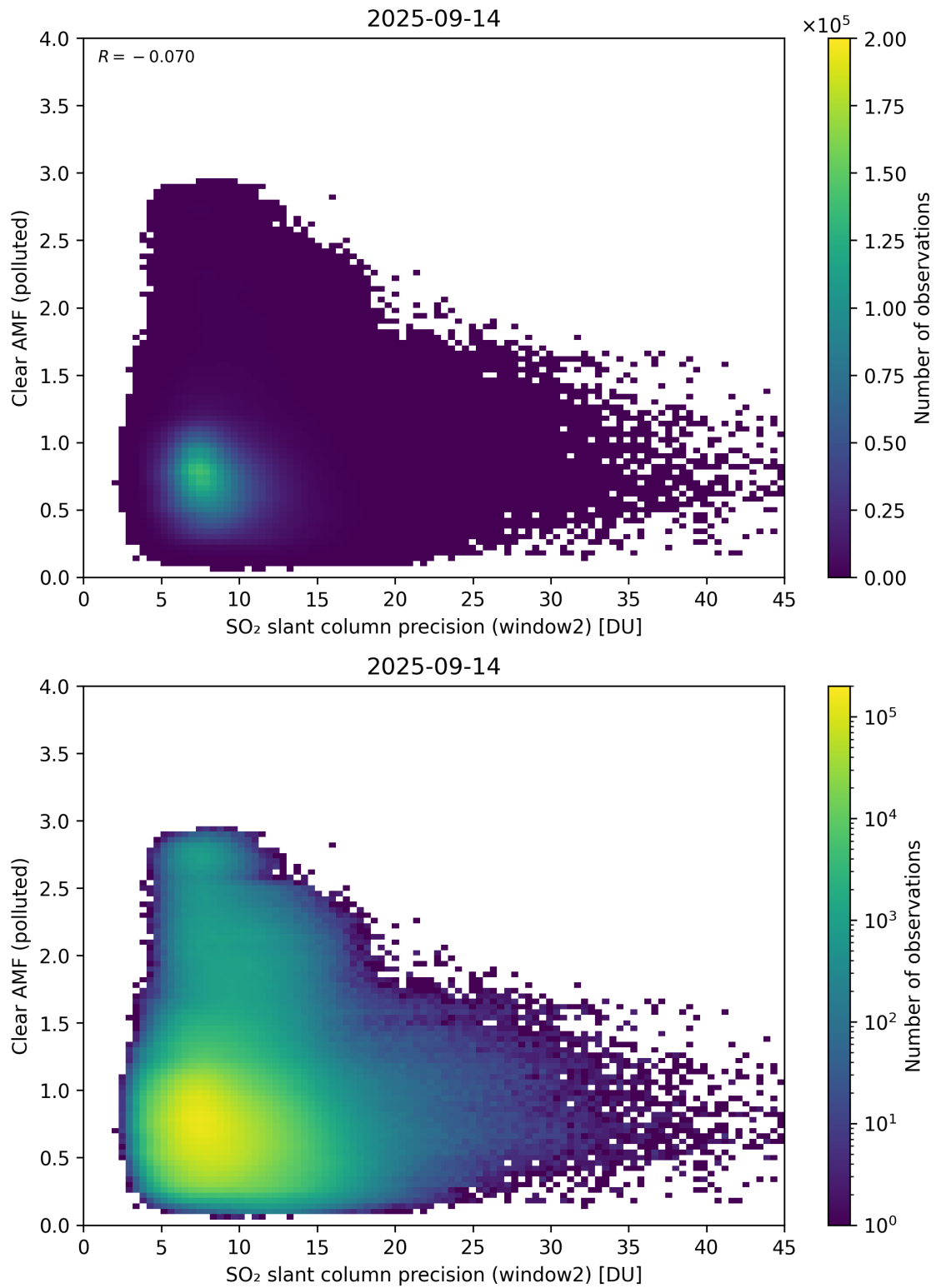
Figure 296: Scatter density plot of “SO 2 slant column precision (window2)” against “Clear AMF (polluted)” for 2025-09-13 to 2025-09-15.
