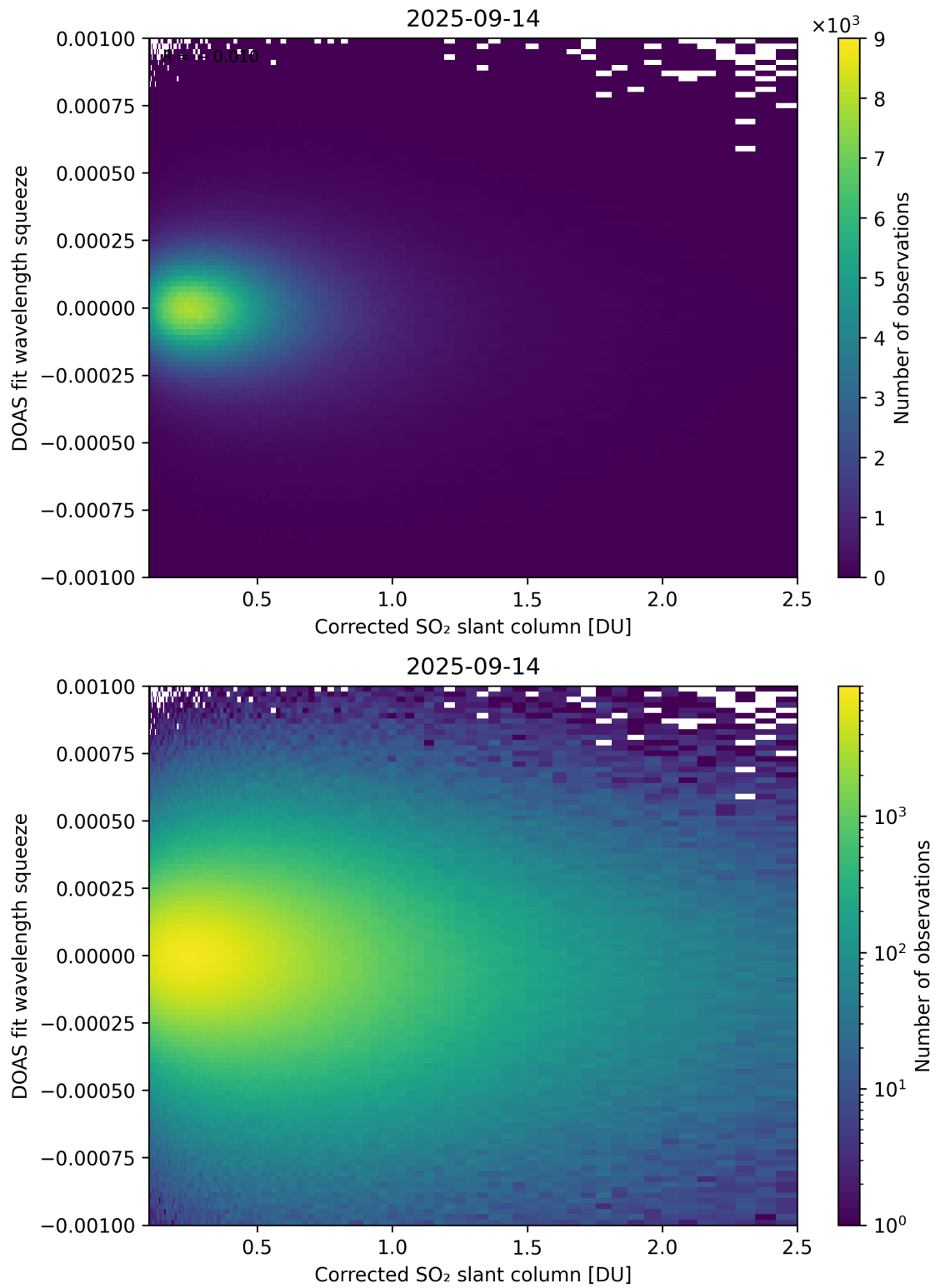
Figure 230: Scatter density plot of “Corrected SO 2 slant column” against “DOAS fit wavelength squeeze” for 2025-09-13 to 2025-09-15.
