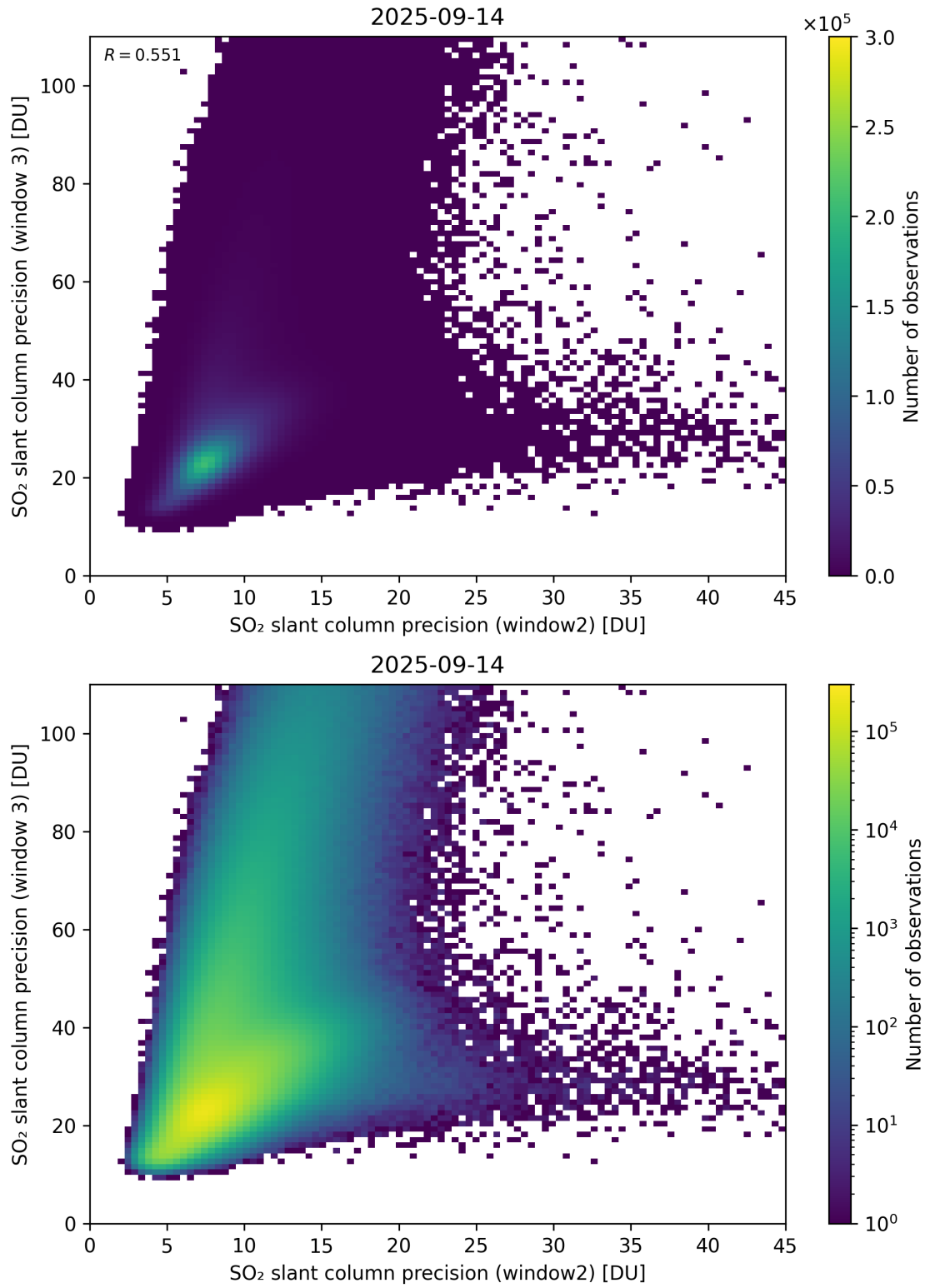
Figure 300: Scatter density plot of “SO 2 slant column precision (window2)” against “SO 2 slant column precision (window 3)” for 2025-09-13 to 2025-09-15.
