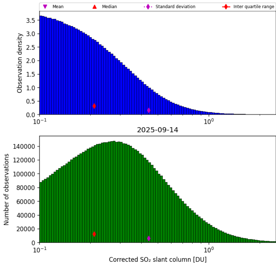
Figure 60: Histogram of "Corrected SO 2 slant column" for 2025-09-13 to 2025-09-15
