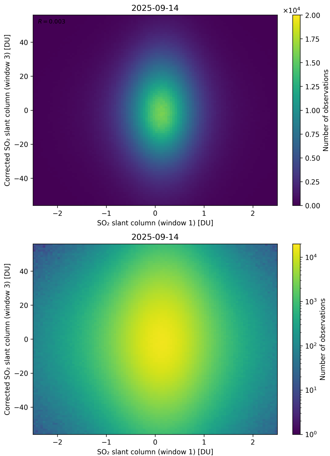
Figure 284: Scatter density plot of “SO 2 slant column (window 1)” against “Corrected SO 2 slant column (window 3)” for 2025-09-13 to 2025-09-15.
