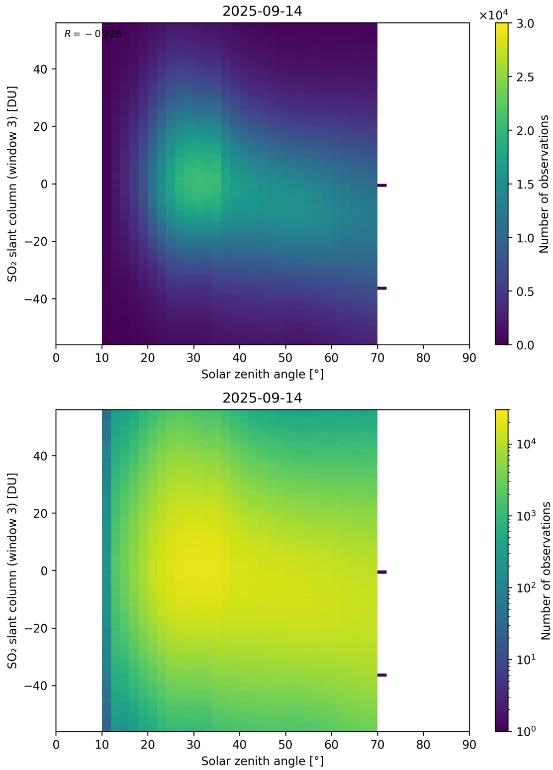
Figure 187: Scatter density plot of “Solar zenith angle” against “SO 2 slant column (window 3)” for 2025-09-13 to 2025-09-15.
