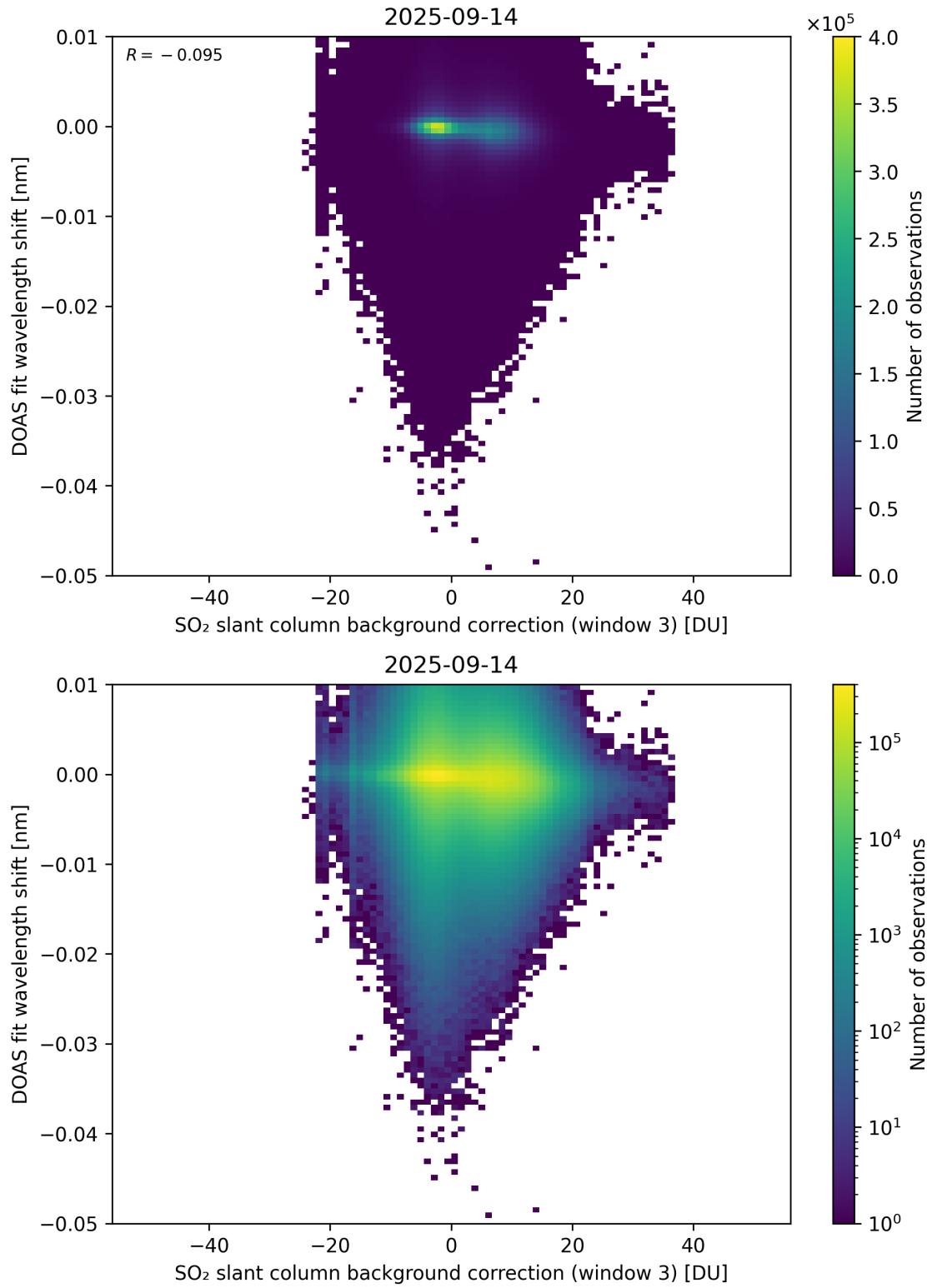
Figure 132: Scatter density plot of “SO 2 slant column background correction (window 3)” against “DOAS fit wavelength shift” for 2025-09-13 to 2025-09-15.
