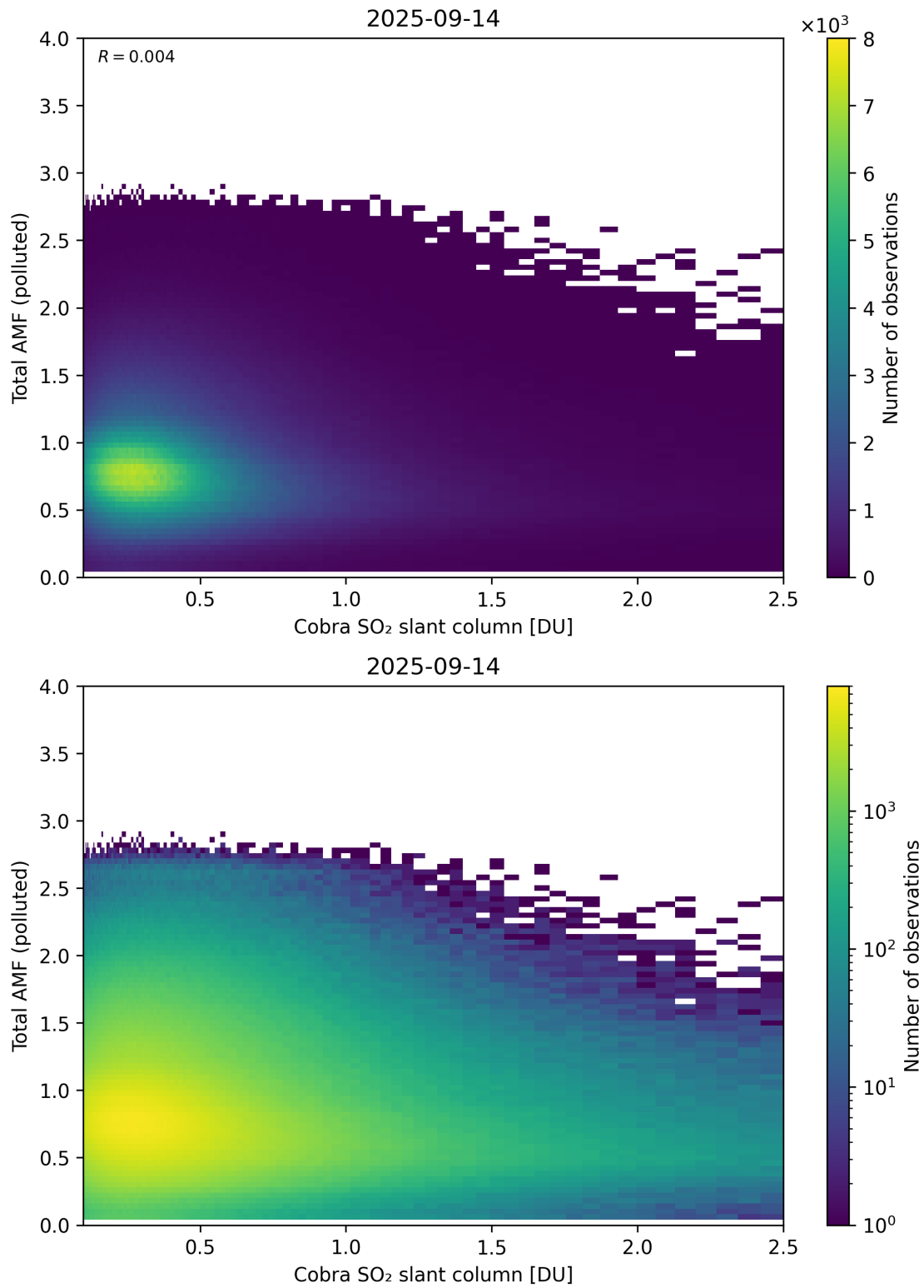
Figure 224: Scatter density plot of “Cobra SO 2 slant column” against “Total AMF (polluted)” for 2025-09-13 to 2025-09-15.
