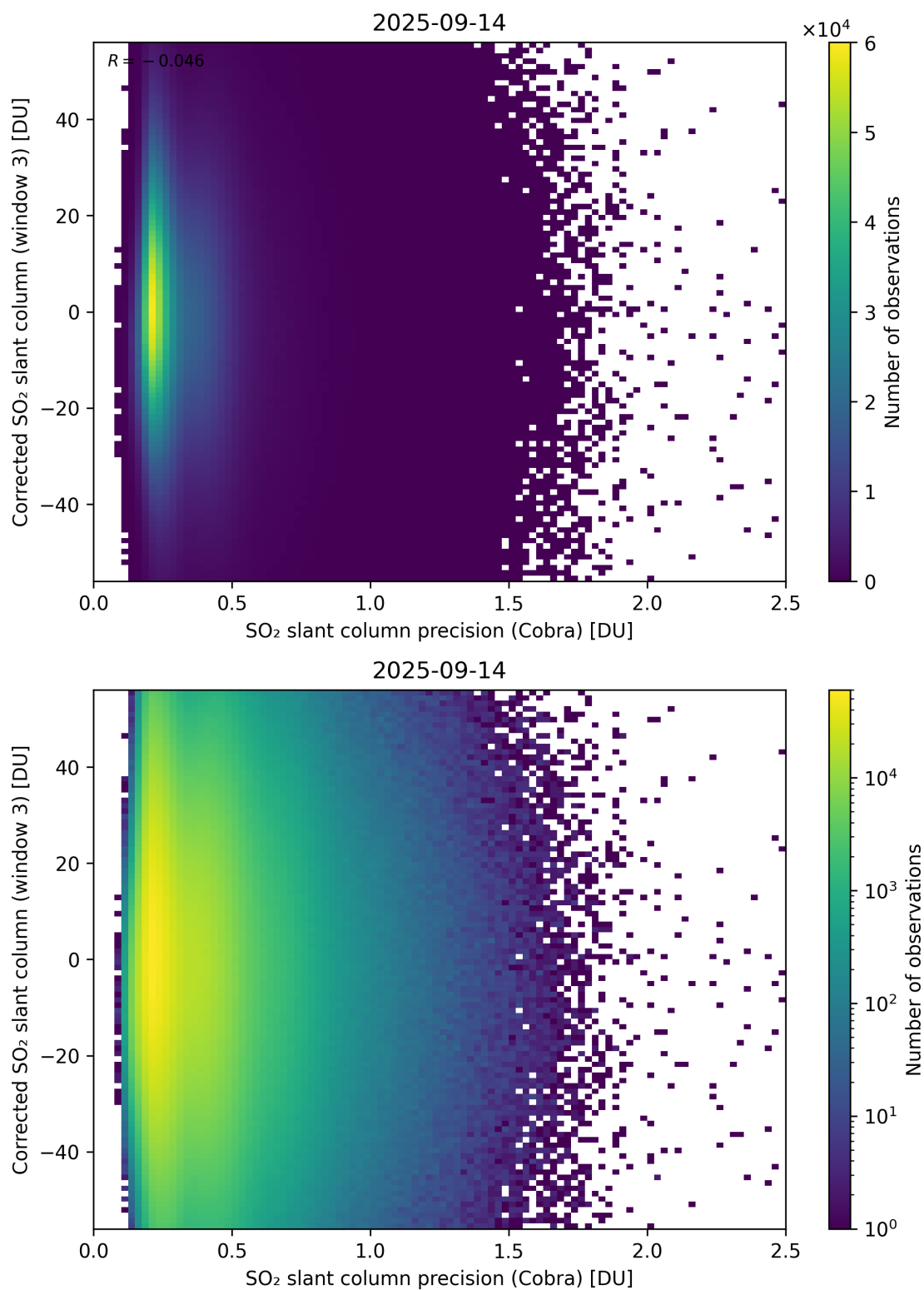
Figure 207: Scatter density plot of “SO 2 slant column precision (Cobra)” against “Corrected SO 2 slant column (window 3)” for 2025-09-13 to 2025-09-15.
