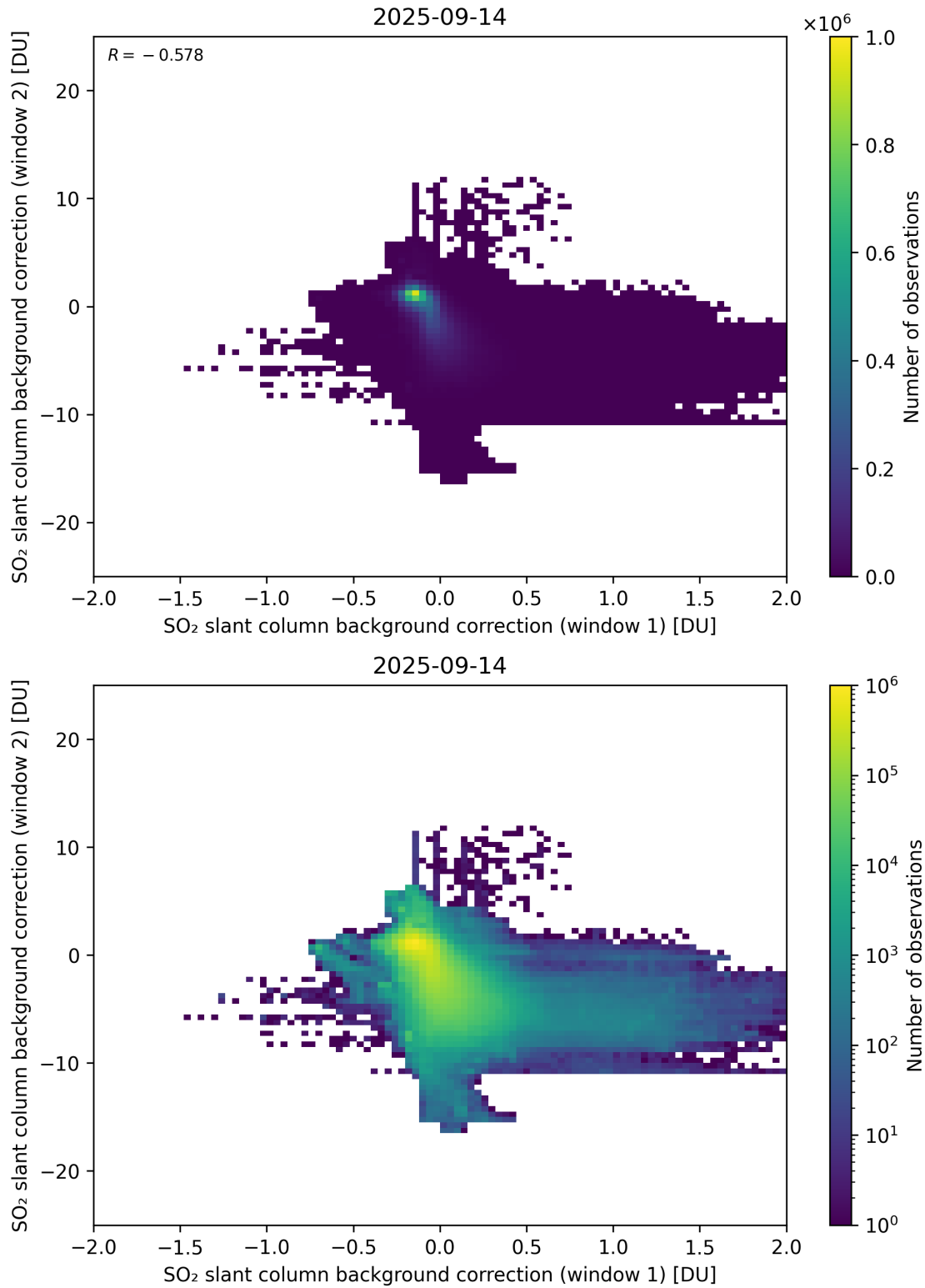
Figure 109: Scatter density plot of “SO 2 slant column background correction (window 1)” against “SO 2 slant column background correction (window 2)” for 2025-09-13 to 2025-09-15.
