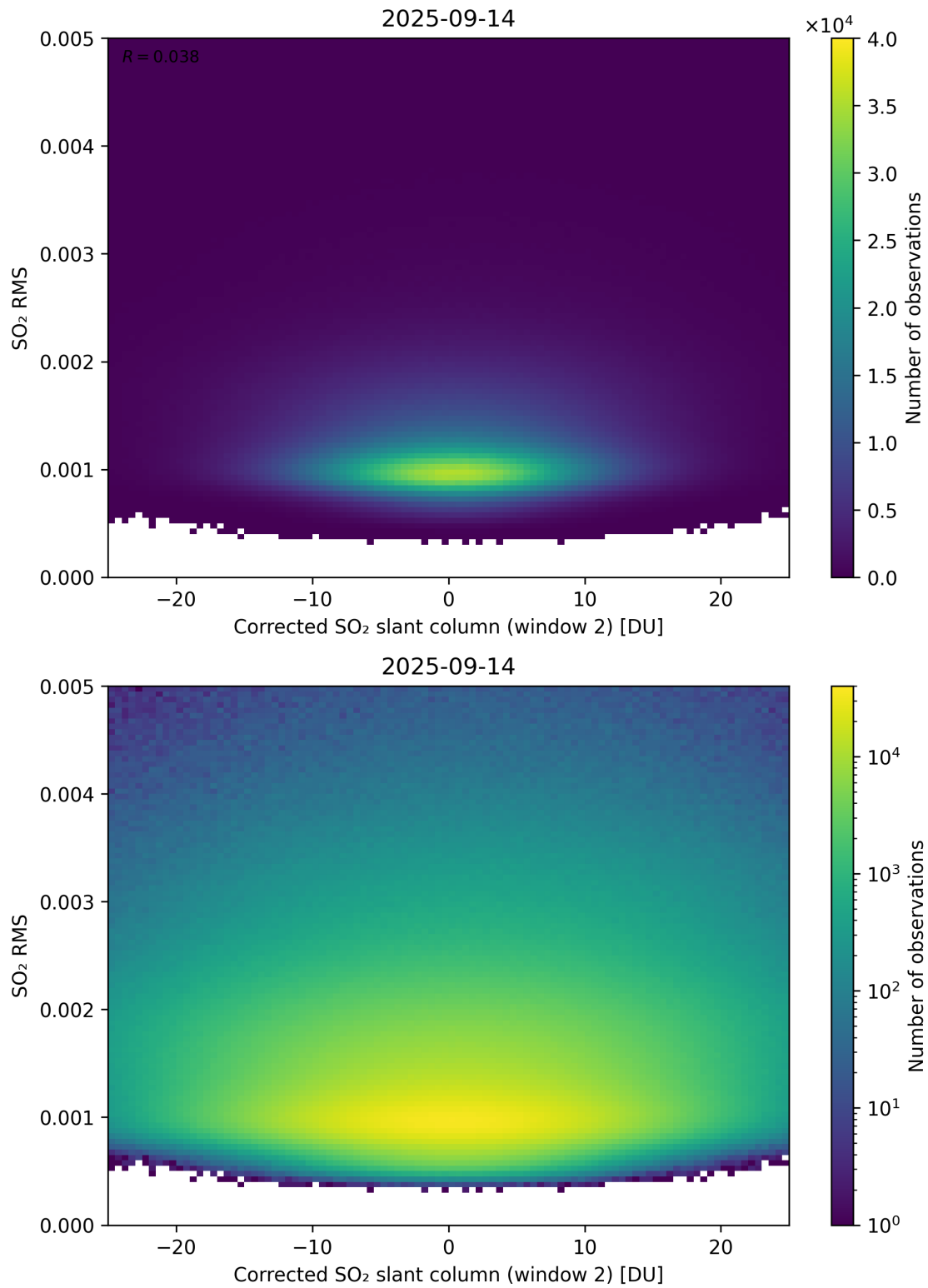
Figure 248: Scatter density plot of “Corrected SO 2 slant column (window 2)” against “SO 2 RMS” for 2025-09-13 to 2025-09-15.
