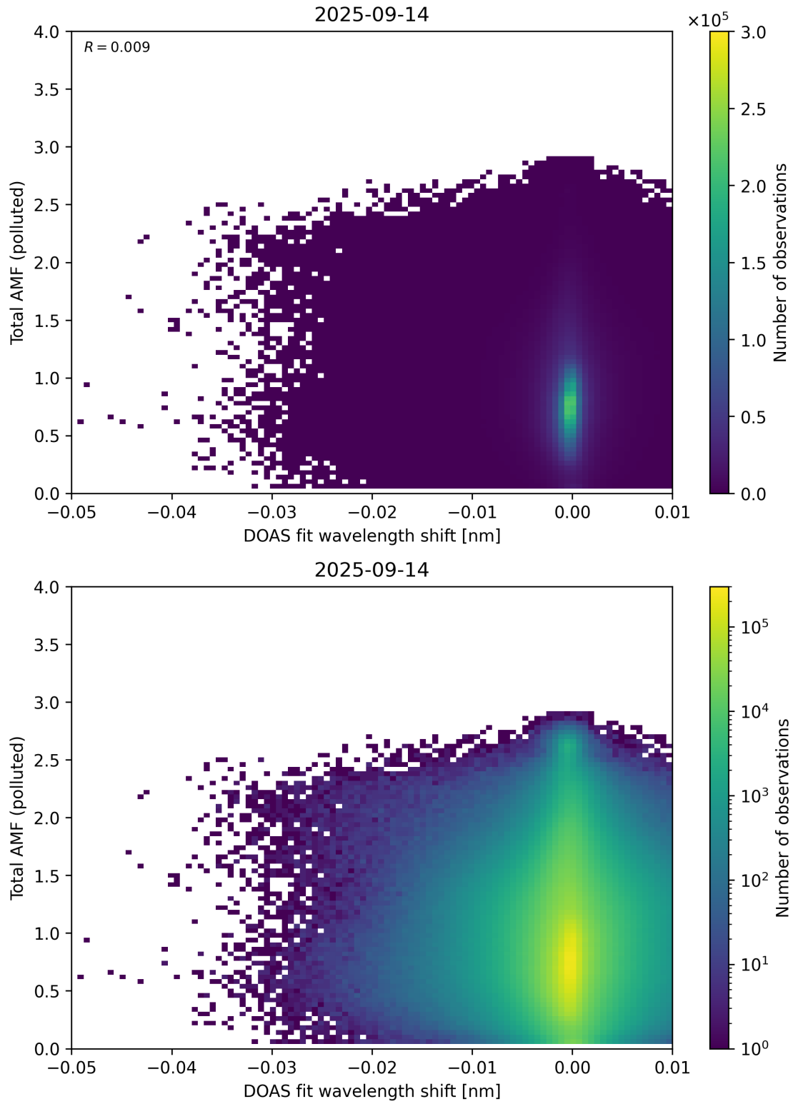
Figure 141: Scatter density plot of “DOAS fit wavelength shift” against “Total AMF (polluted)” for 2025-09-13 to 2025-09-15.
