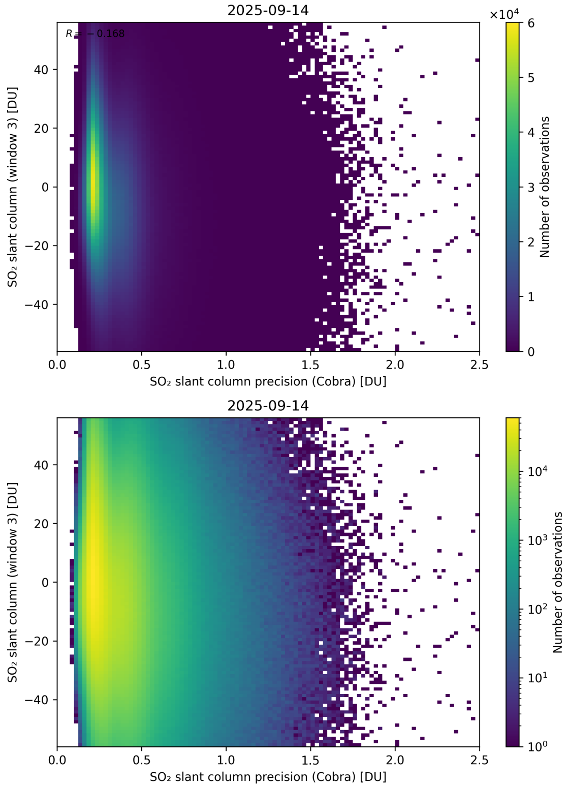
Figure 211: Scatter density plot of “SO 2 slant column precision (Cobra)” against “SO 2 slant column (window 3)” for 2025-09-13 to 2025-09-15.
