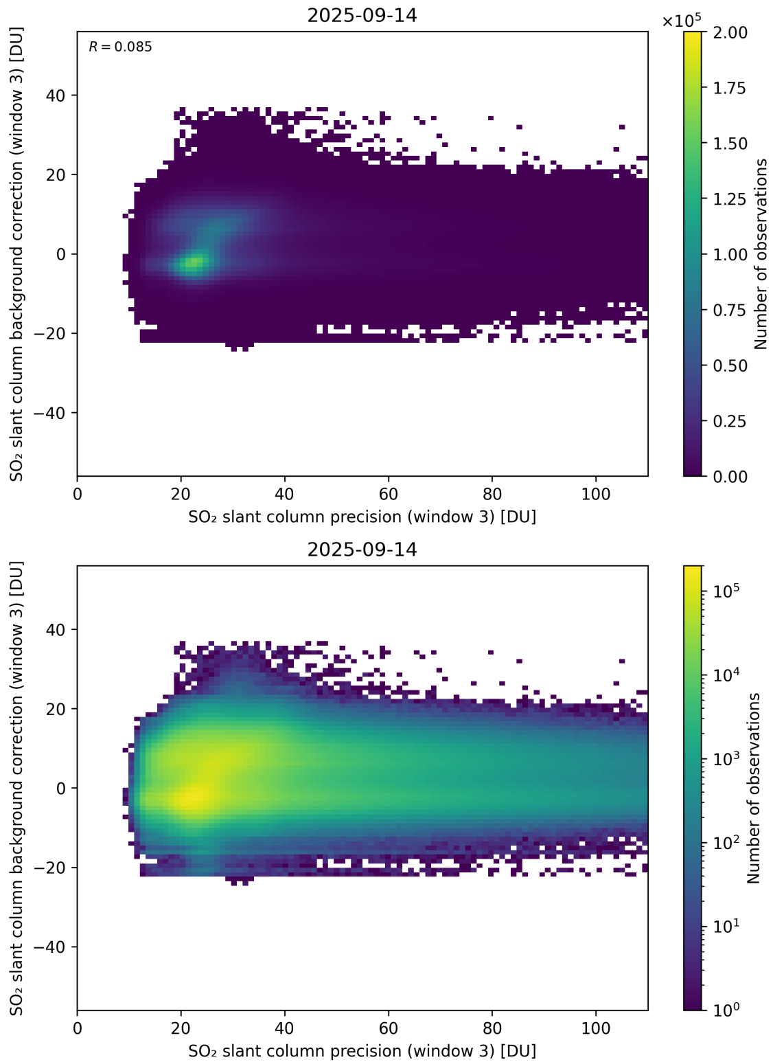
Figure 307: Scatter density plot of “SO 2 slant column precision (window 3)” against “SO 2 slant column background correction (window 3)” for 2025-09-13 to 2025-09-15.
