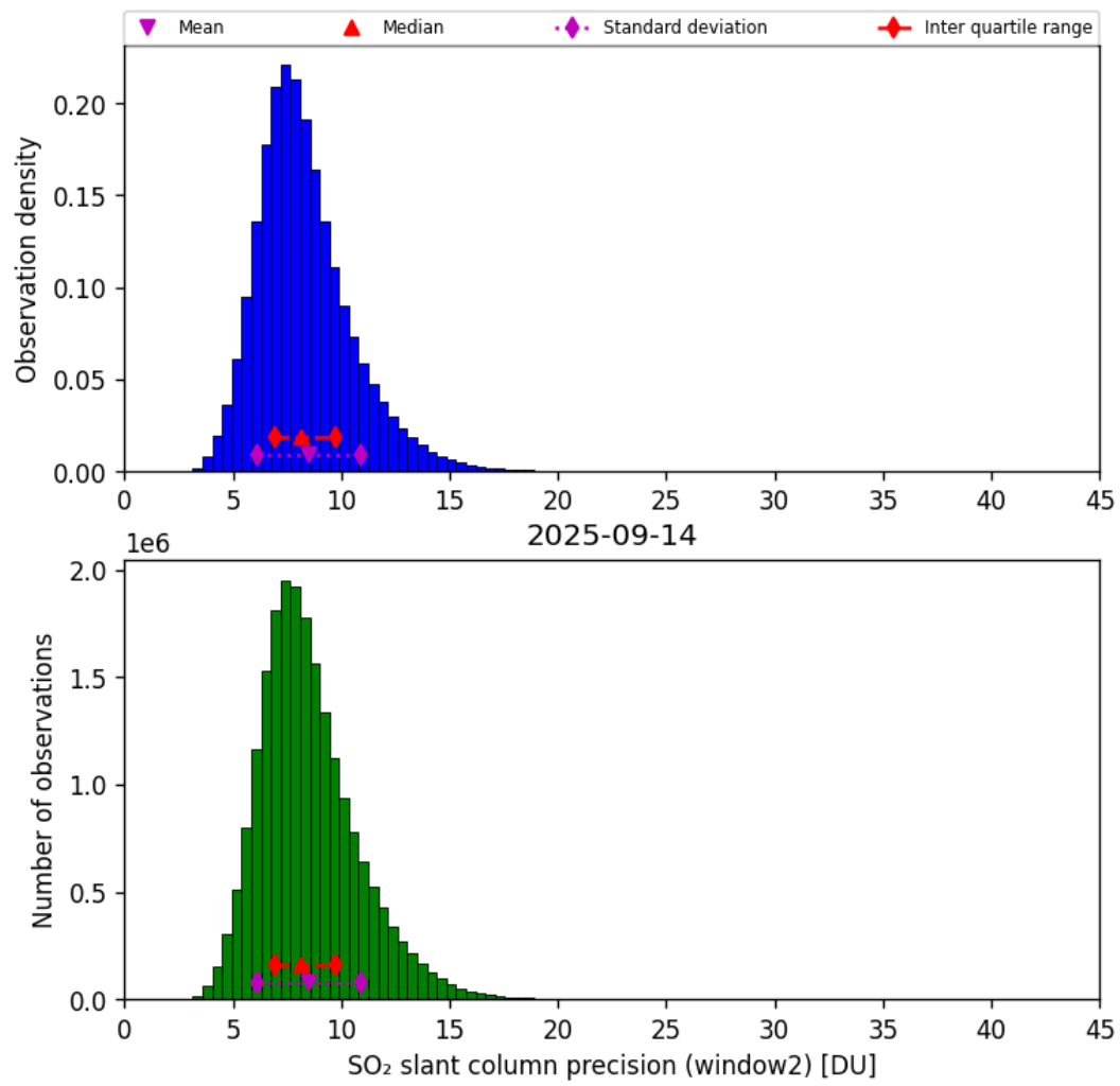
Figure 68: Histogram of “SO 2 slant column precision (window2)” for 2025-09-13 to 2025-09-15
