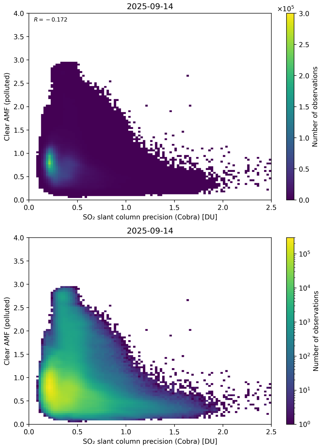
Figure 205: Scatter density plot of “SO 2 slant column precision (Cobra)” against “Clear AMF (polluted)” for 2025-09-13 to 2025-09-15.
