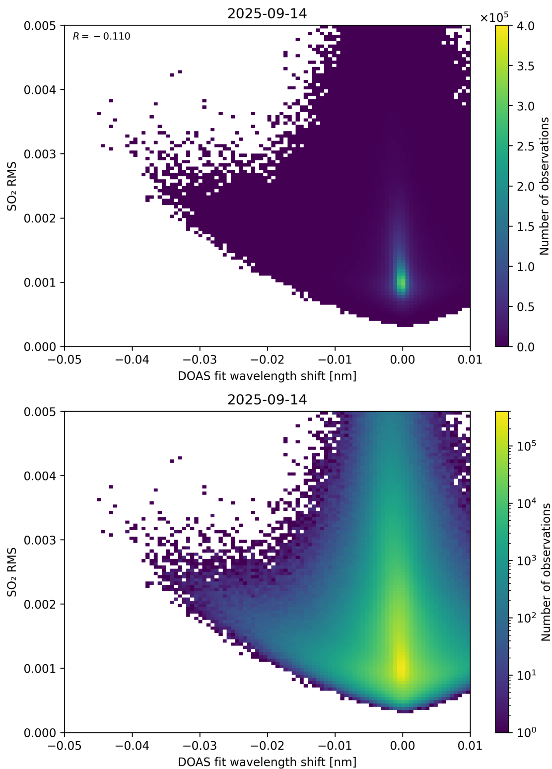
Figure 139: Scatter density plot of “DOAS fit wavelength shift” against “SO 2 RMS” for 2025-09-13 to 2025-09-15.
