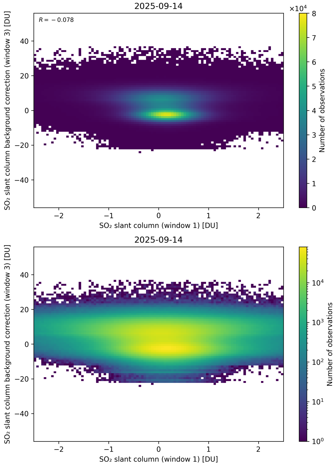
Figure 264: Scatter density plot of “SO 2 slant column (window 1)” against “SO 2 slant column background correction (window 3)” for 2025-09-13 to 2025-09-15.
