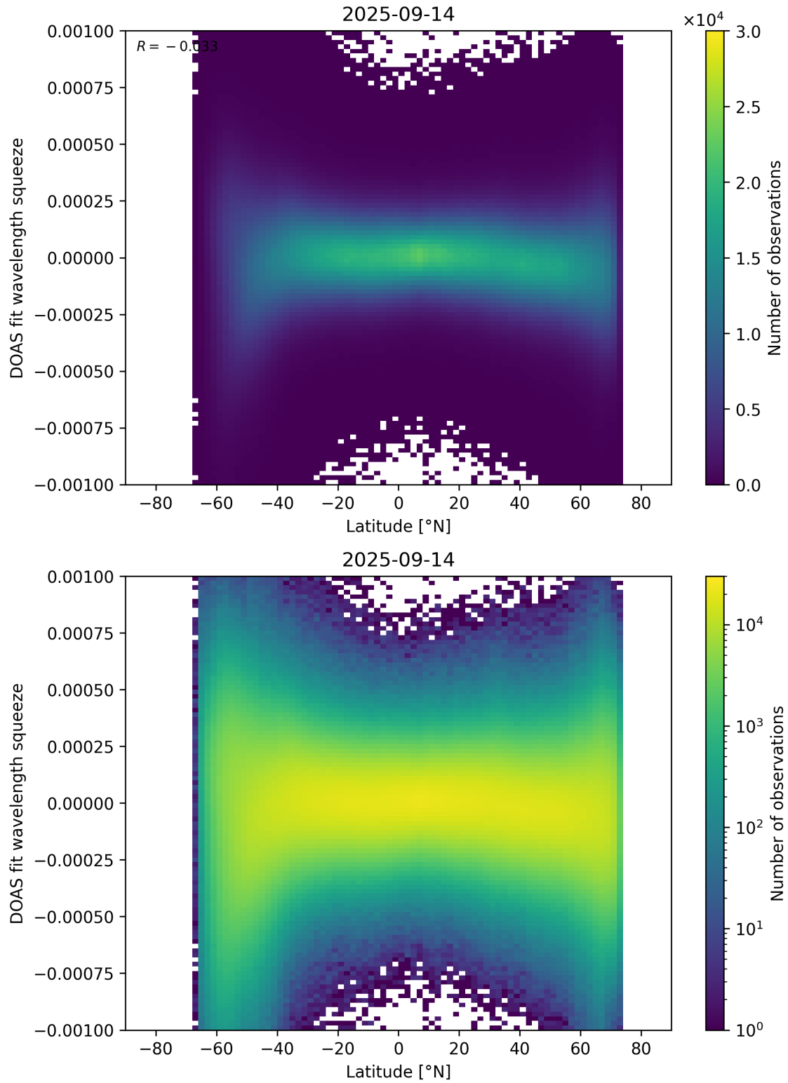
Figure 154: Scatter density plot of “Latitude” against “DOAS fit wavelength squeeze” for 2025-09-13 to 2025-09-15.
