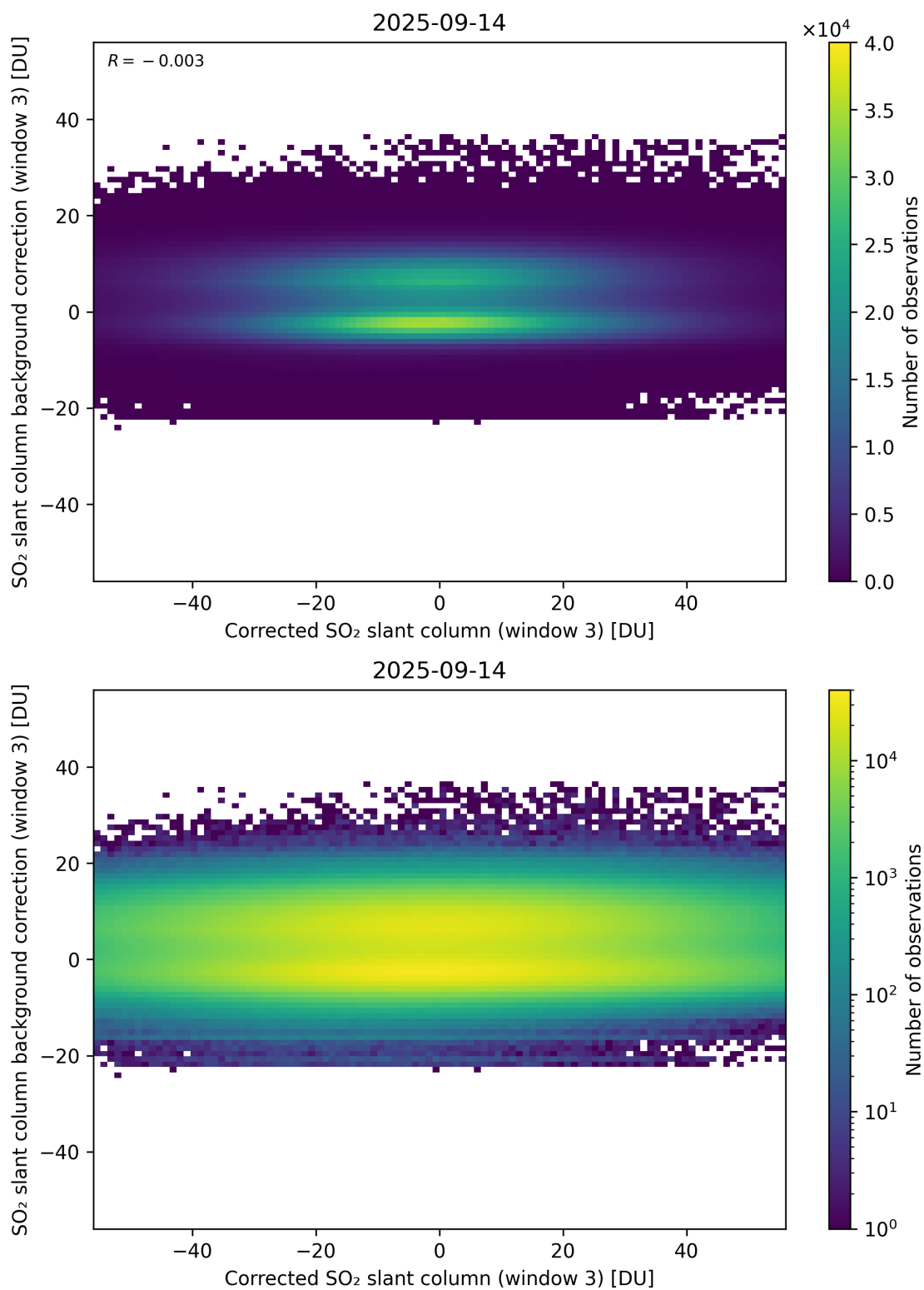
Figure 255: Scatter density plot of “Corrected SO 2 slant column (window 3)” against “SO 2 slant column background correction (window 3)” for 2025-09-13 to 2025-09-15.
