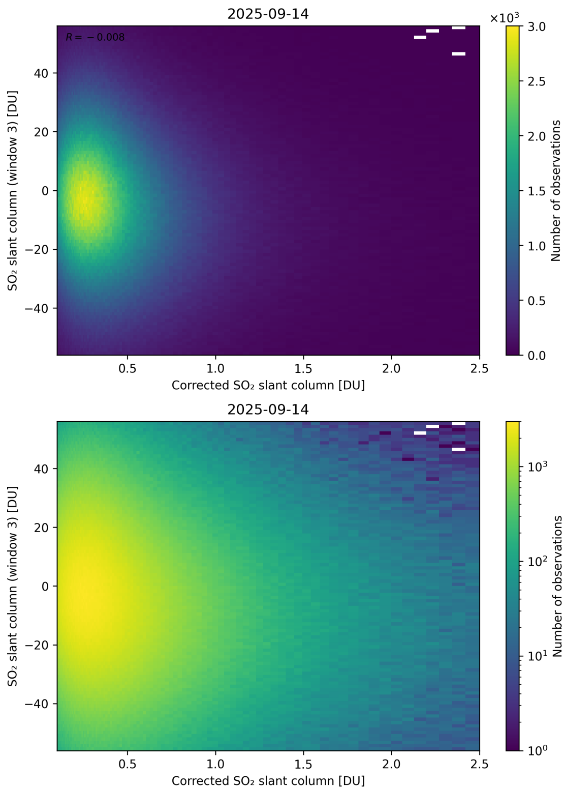
Figure 240: Scatter density plot of “Corrected SO 2 slant column” against “SO 2 slant column (window 3)” for 2025-09-13 to 2025-09-15.
