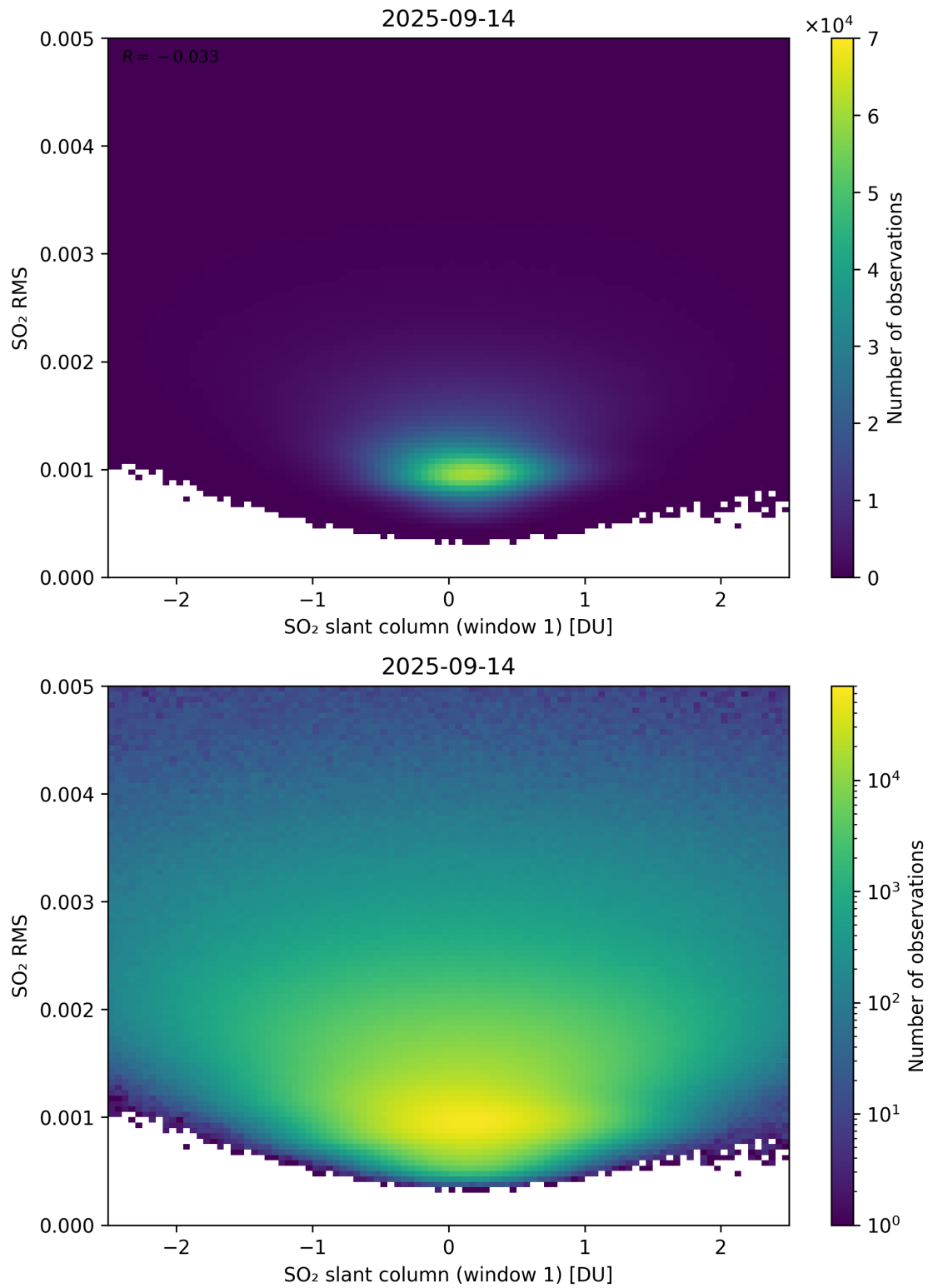
Figure 267: Scatter density plot of “SO 2 slant column (window 1)” against “SO 2 RMS” for 2025-09-13 to 2025-09-15.
