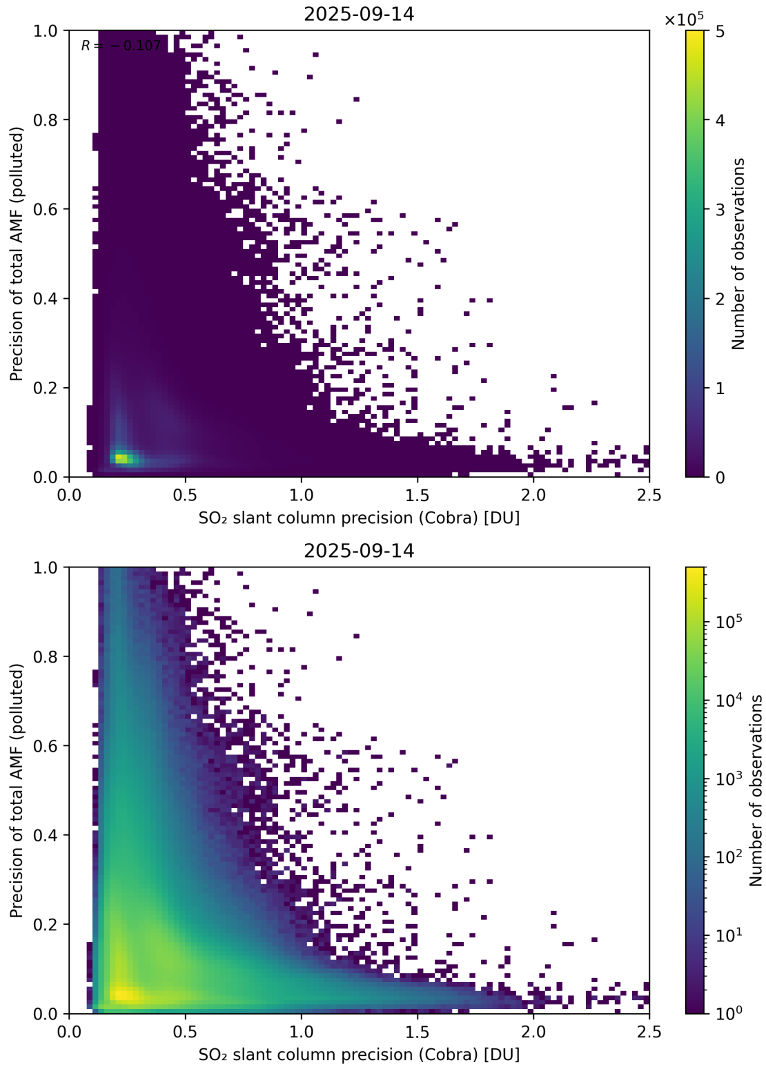
Figure 214: Scatter density plot of “SO 2 slant column precision (Cobra)” against “Precision of total AMF (polluted)” for 2025-09-13 to 2025-09-15.
