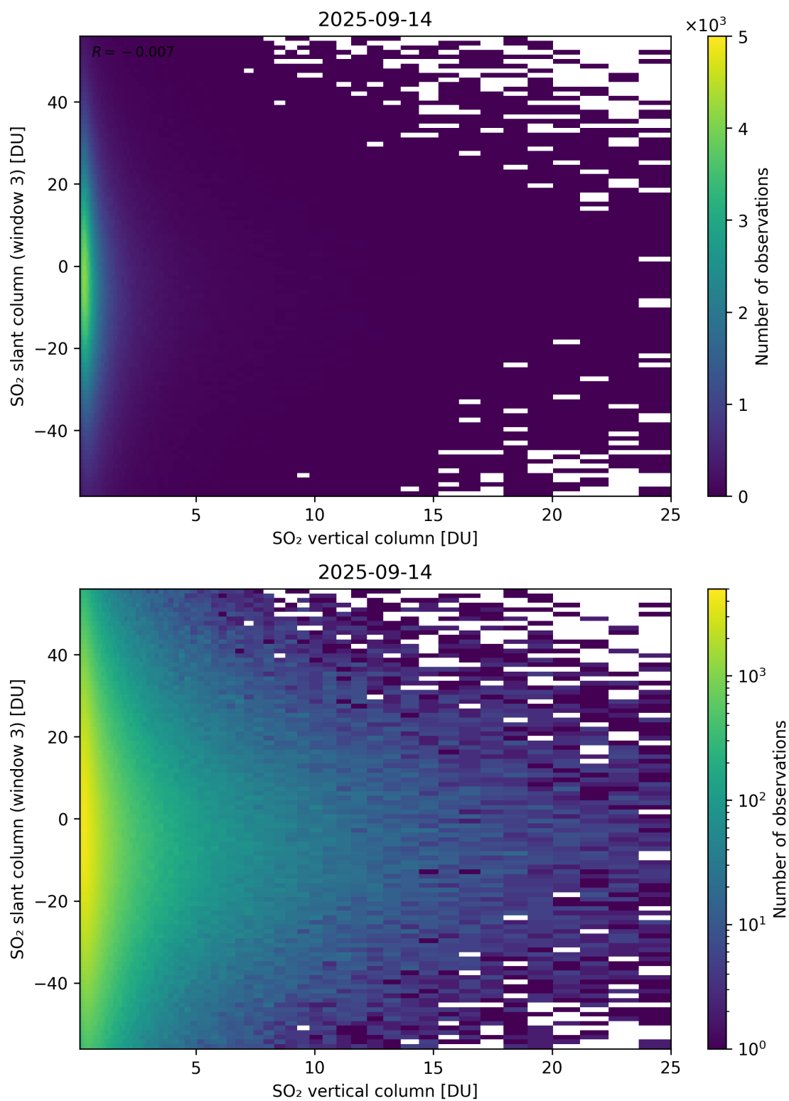
Figure 357: Scatter density plot of “SO 2 vertical column” against “SO 2 slant column (window 3)” for 2025-09-13 to 2025-09-15.
