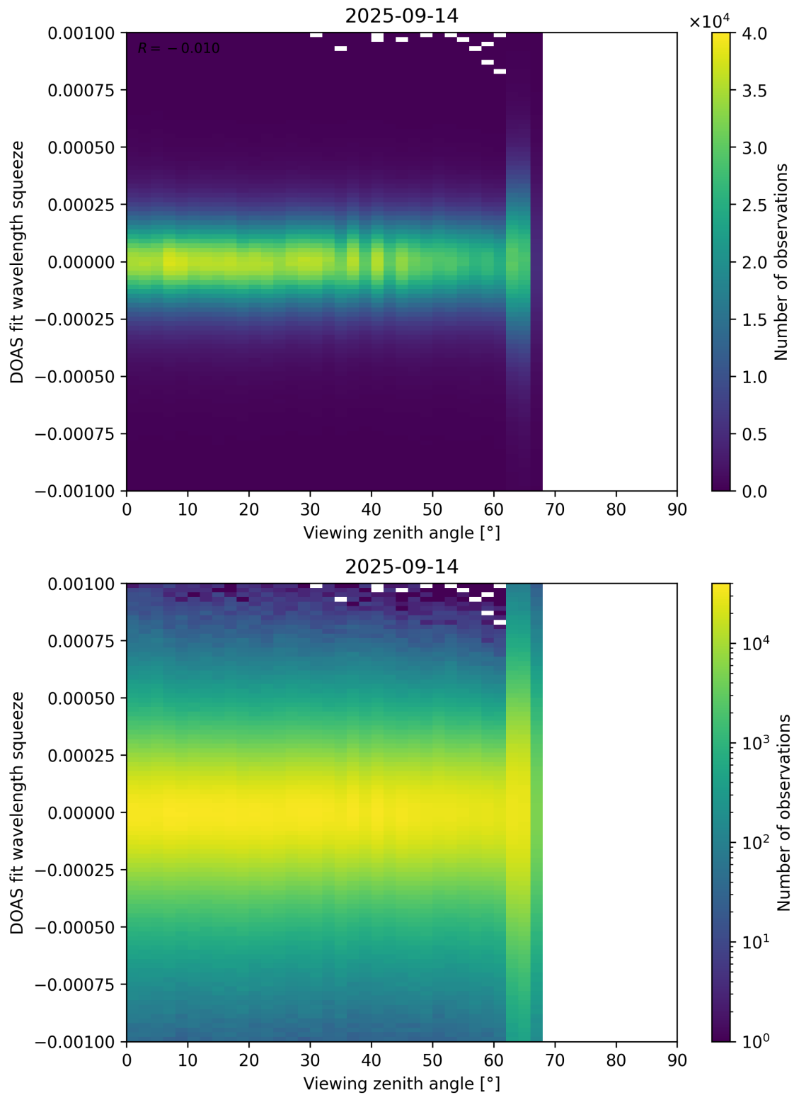
Figure 366: Scatter density plot of “Viewing zenith angle” against “DOAS fit wavelength squeeze” for 2025-09-13 to 2025-09-15.
