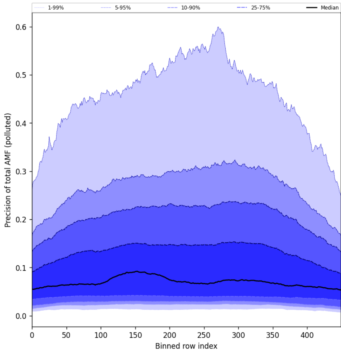
Figure 106: Along track statistics of “Precision of total AMF (polluted)” for 2025-09-13 to 2025-09-15
