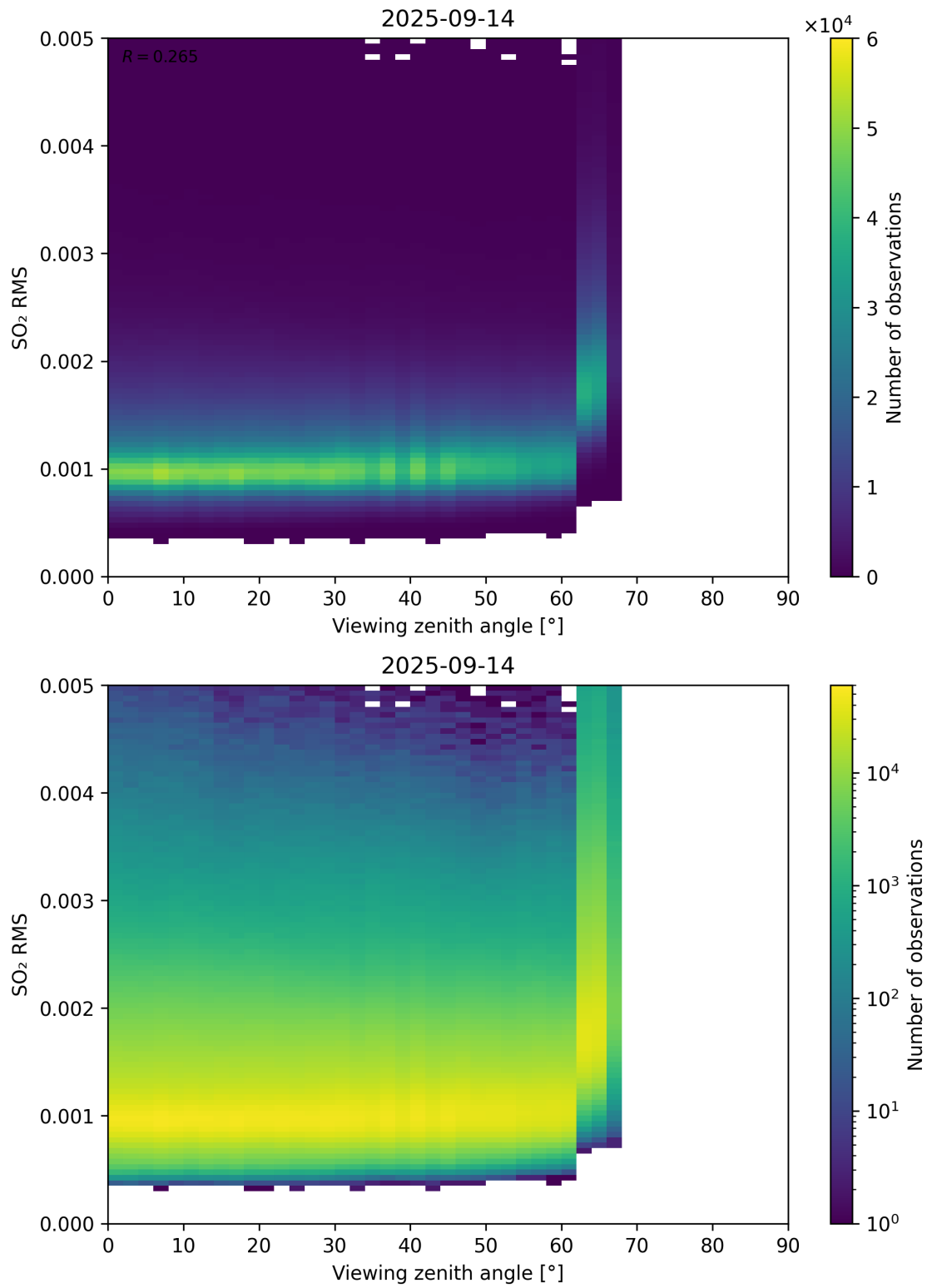
Figure 367: Scatter density plot of “Viewing zenith angle” against “SO 2 RMS” for 2025-09-13 to 2025-09-15.
