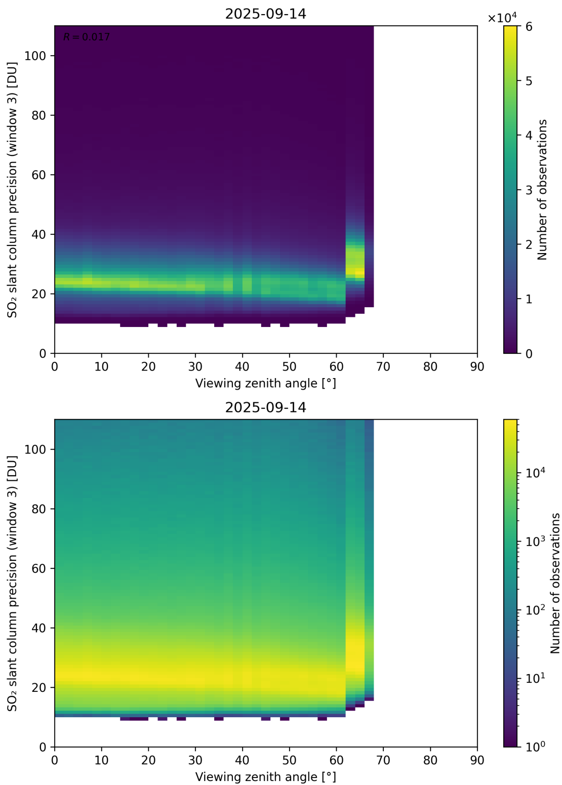
Figure 380: Scatter density plot of “Viewing zenith angle” against “SO 2 slant column precision (window 3)” for 2025-09-13 to 2025-09-15.
