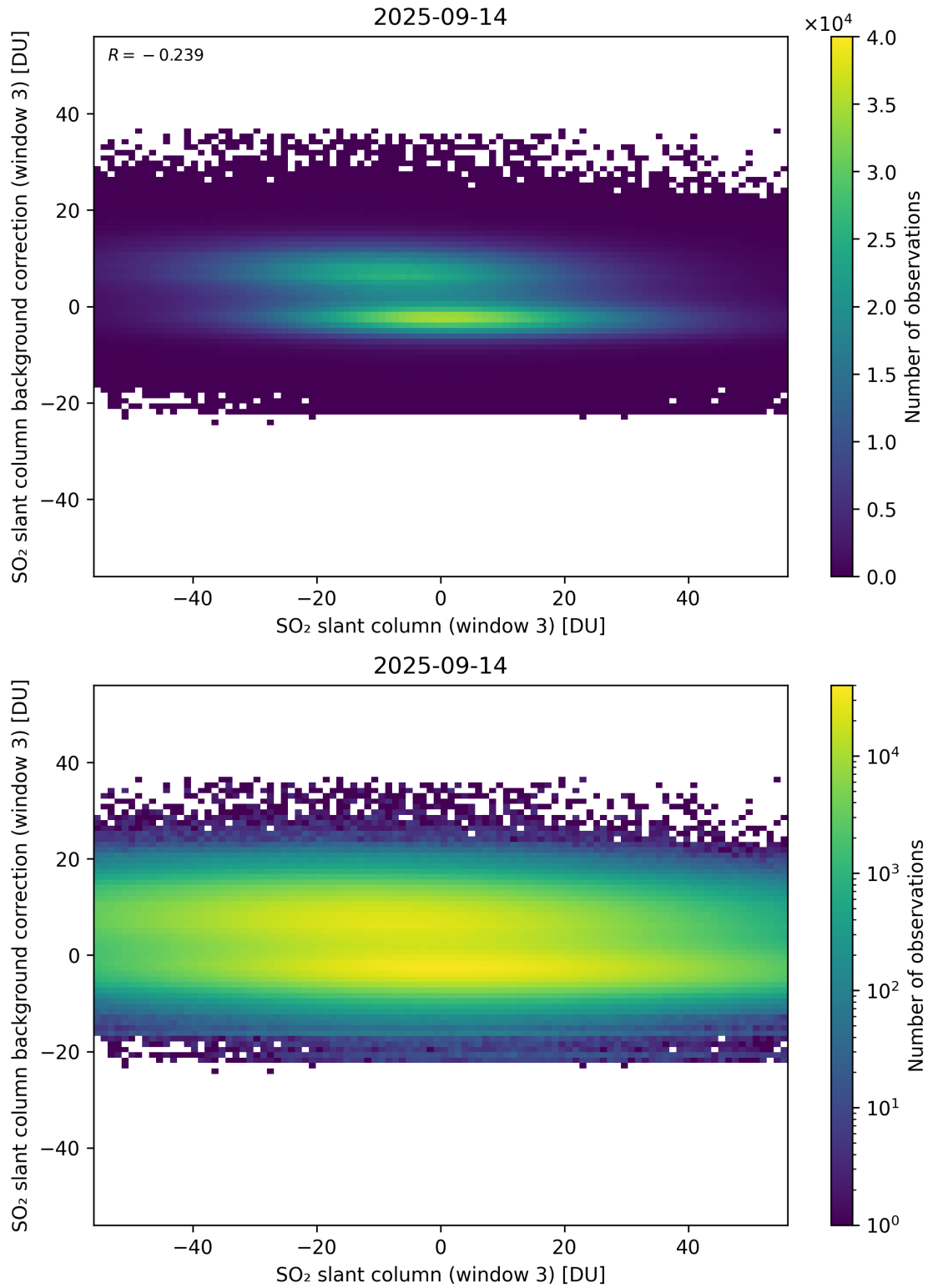
Figure 303: Scatter density plot of “SO 2 slant column (window 3)” against “SO 2 slant column background correction (window 3)” for 2025-09-13 to 2025-09-15.
