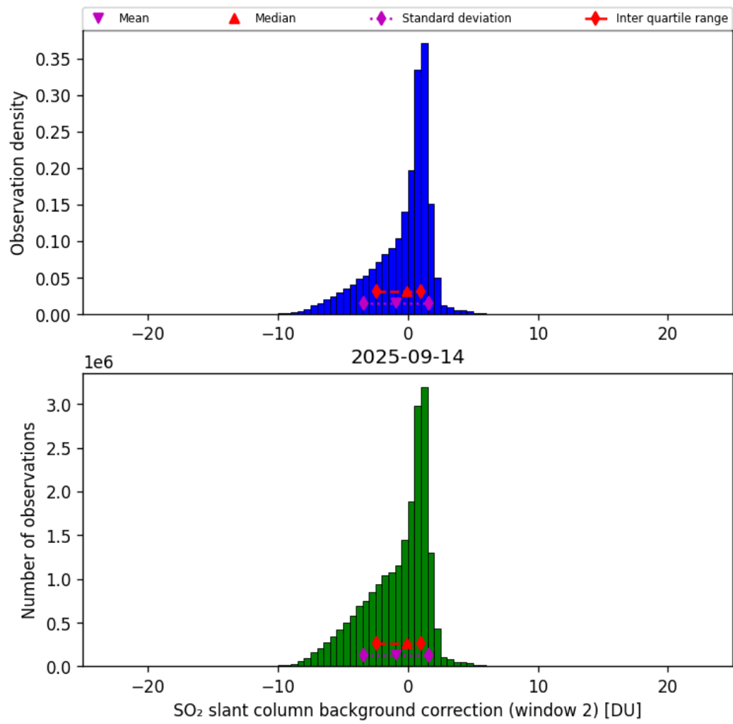
Figure 70: Histogram of “SO 2 slant column background correction (window 2)” for 2025-09-13 to 2025-09-15
