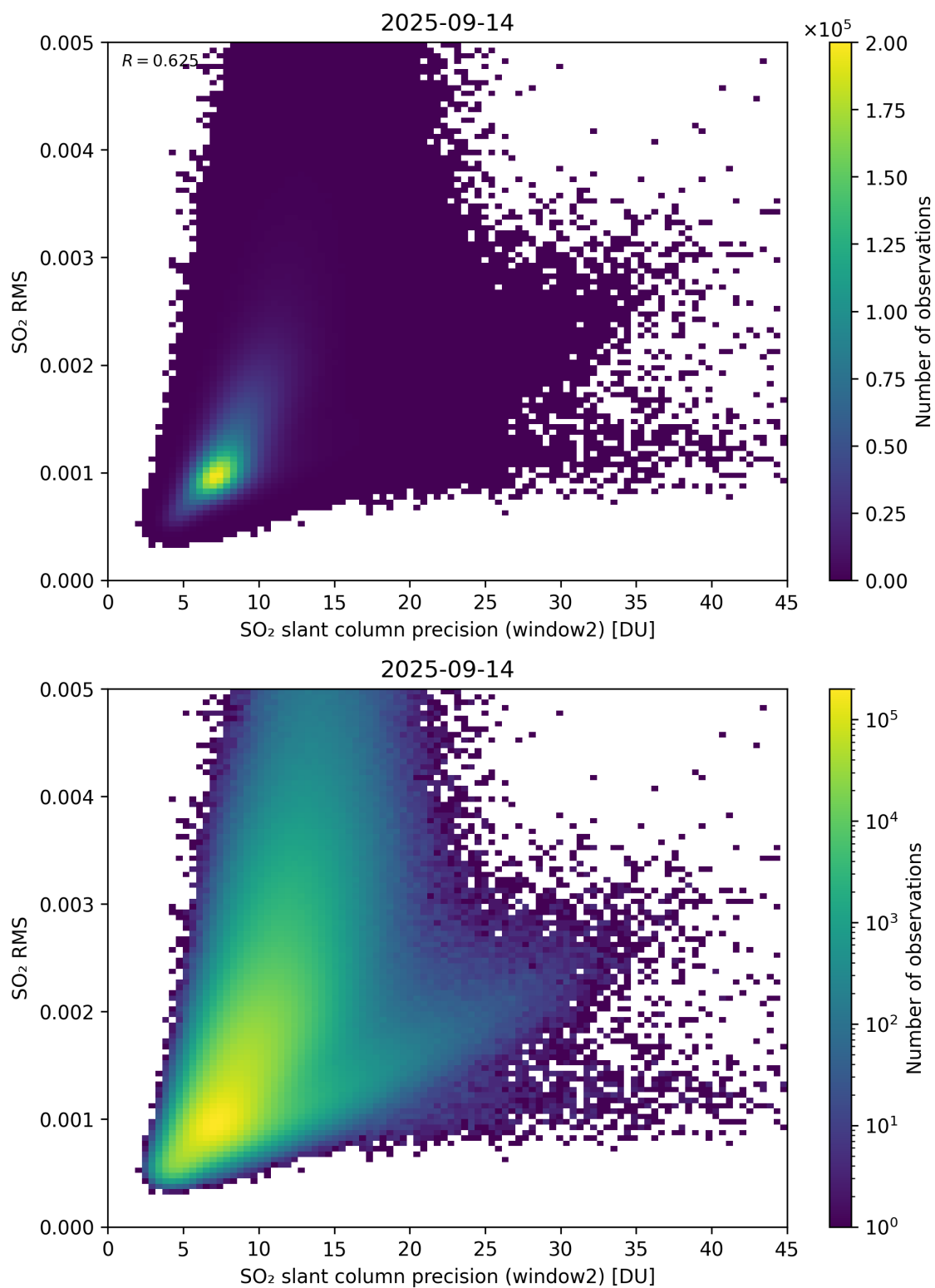
Figure 295: Scatter density plot of “SO 2 slant column precision (window2)” against “SO 2 RMS” for 2025-09-13 to 2025-09-15.
