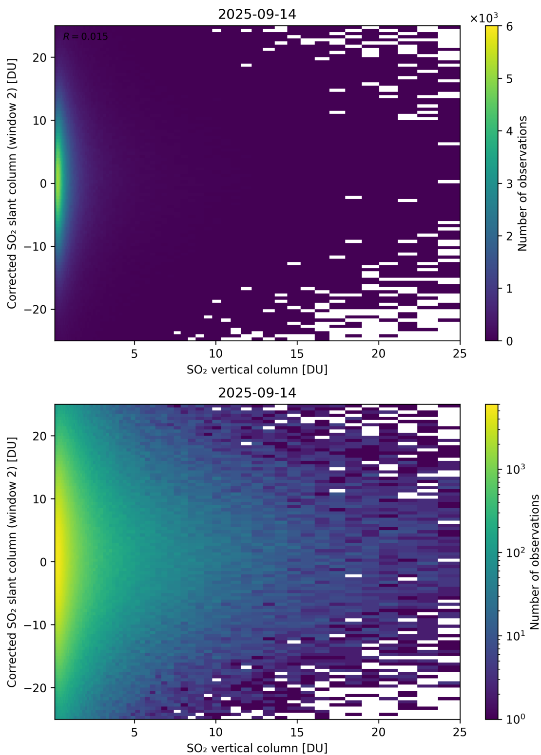
Figure 352: Scatter density plot of “SO 2 vertical column” against “Corrected SO 2 slant column (window 2)” for 2025-09-13 to 2025-09-15.
