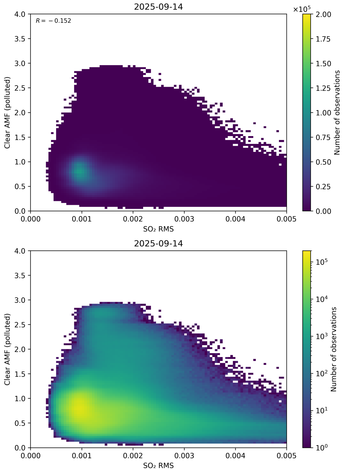
Figure 147: Scatter density plot of “SO 2 RMS” against “Clear AMF (polluted)” for 2025-09-13 to 2025-09-15.
