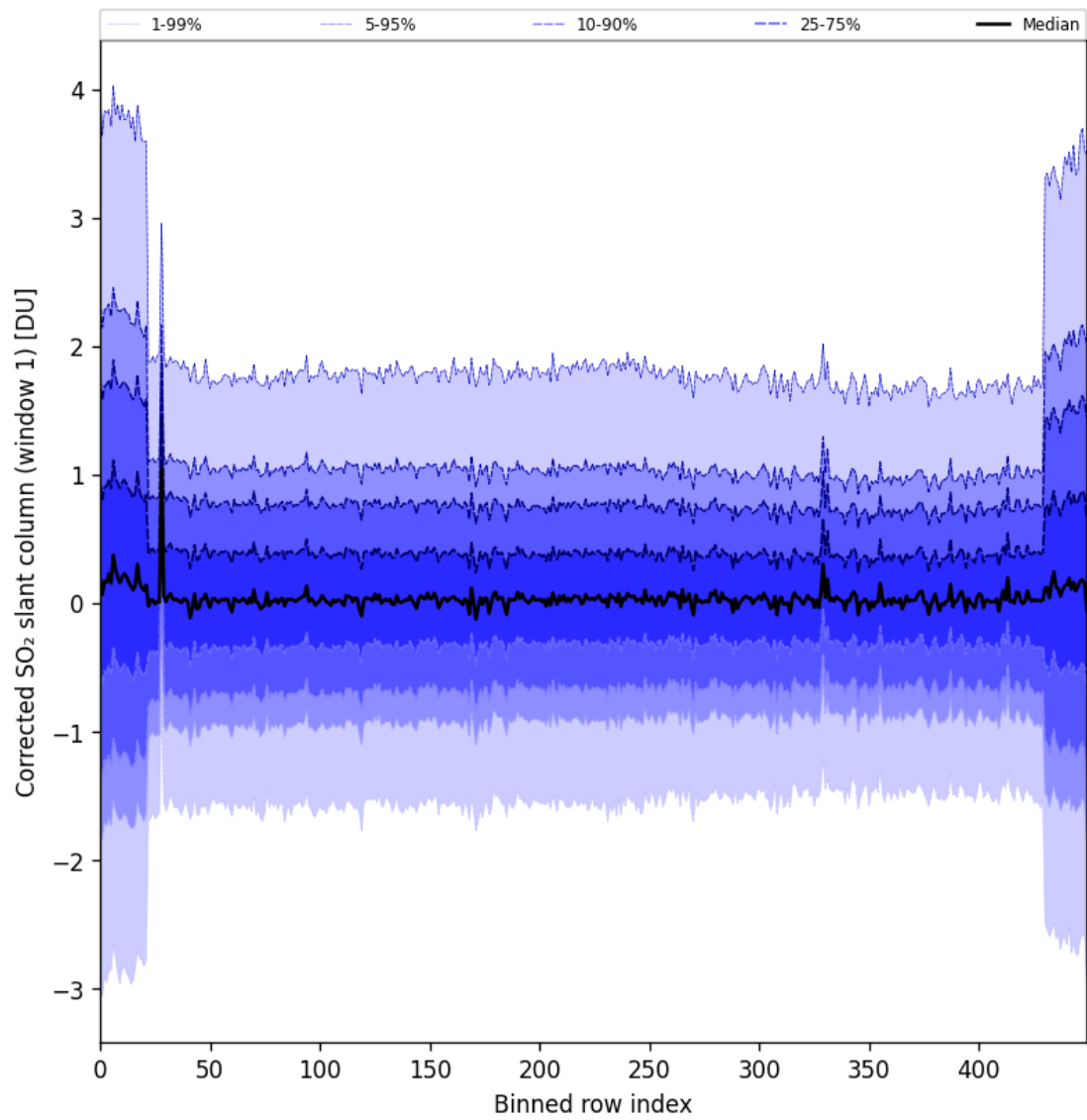
Figure 91: Along track statistics of “Corrected SO 2 slant column (window 1)” for 2025-09-13 to 2025-09-15
