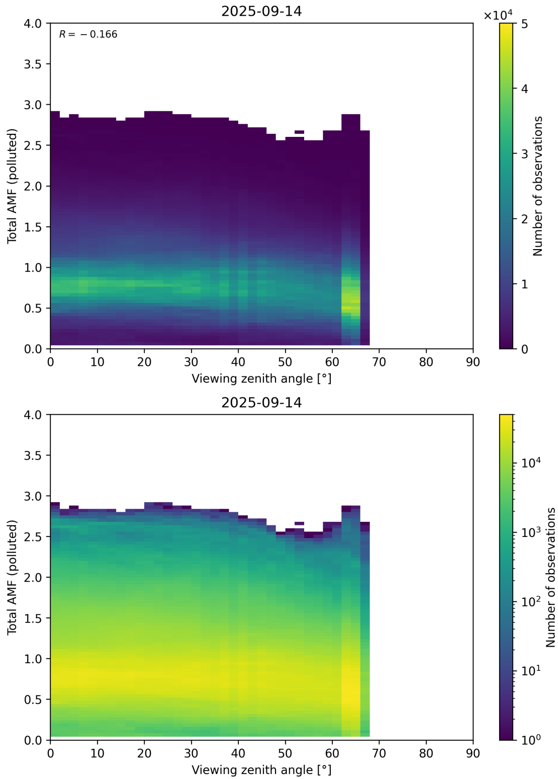
Figure 381: Scatter density plot of “Viewing zenith angle” against “Total AMF (polluted)” for 2025-09-13 to 2025-09-15.
