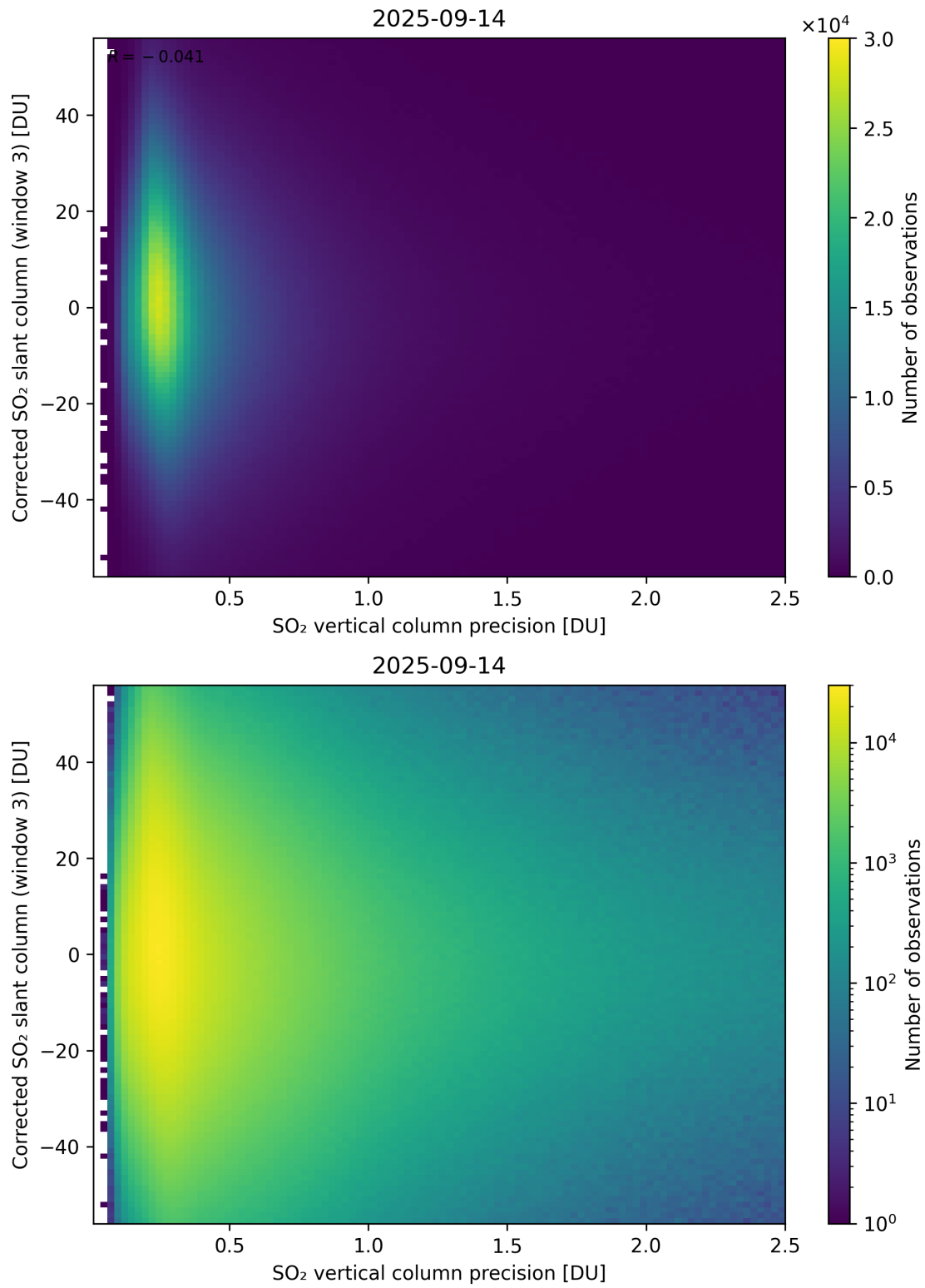
Figure 340: Scatter density plot of “SO 2 vertical column precision” against “Corrected SO 2 slant column (window 3)” for 2025-09-13 to 2025-09-15.
