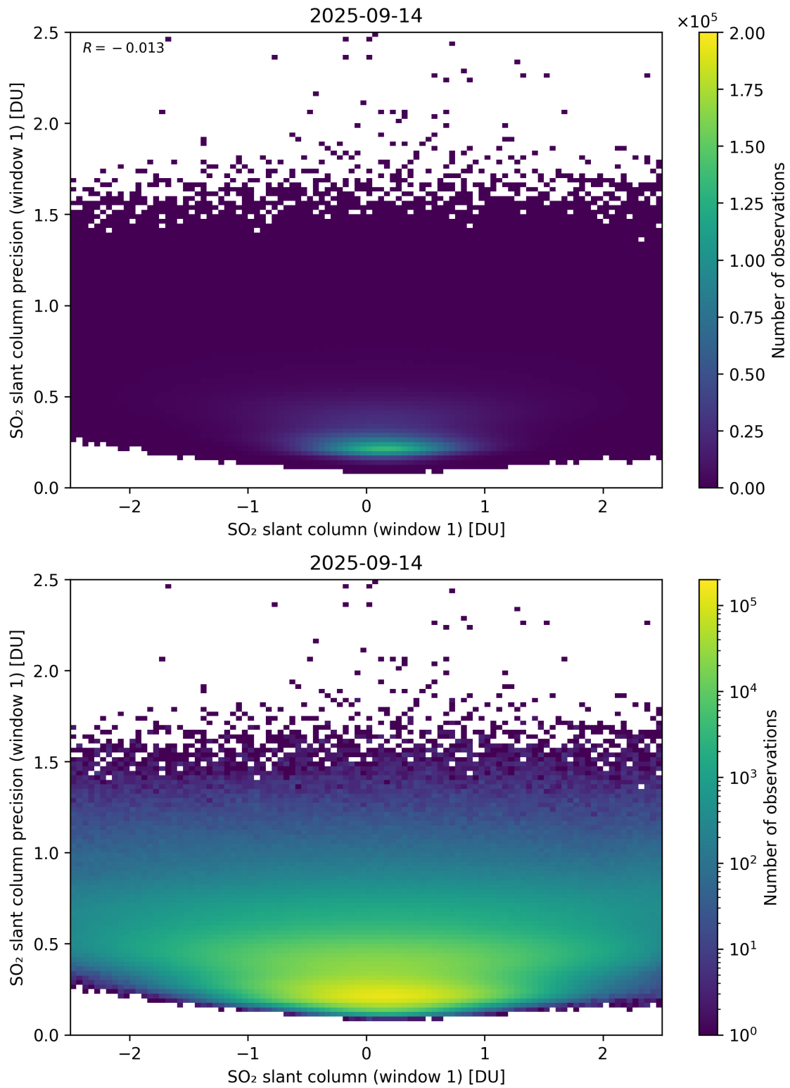
Figure 285: Scatter density plot of “SO 2 slant column (window 1)” against “SO 2 slant column precision (window 1)” for 2025-09-13 to 2025-09-15.
