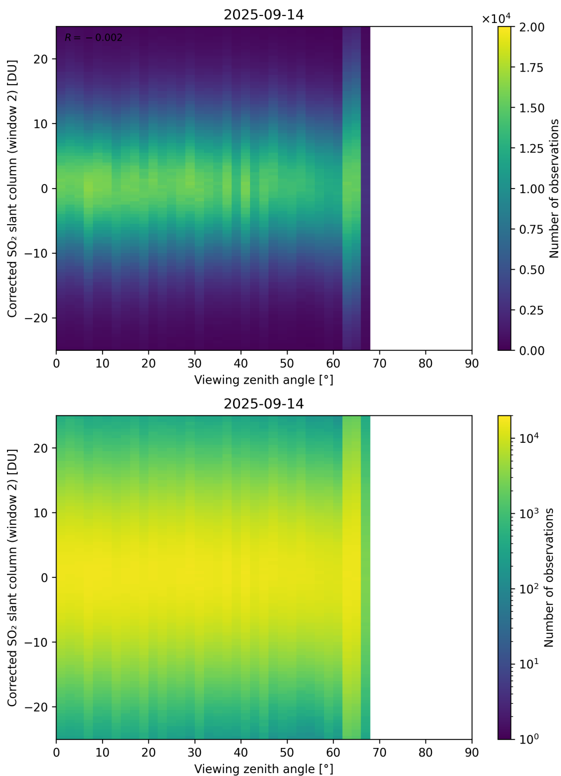
Figure 374: Scatter density plot of “Viewing zenith angle” against “Corrected SO 2 slant column (window 2)” for 2025-09-13 to 2025-09-15.
