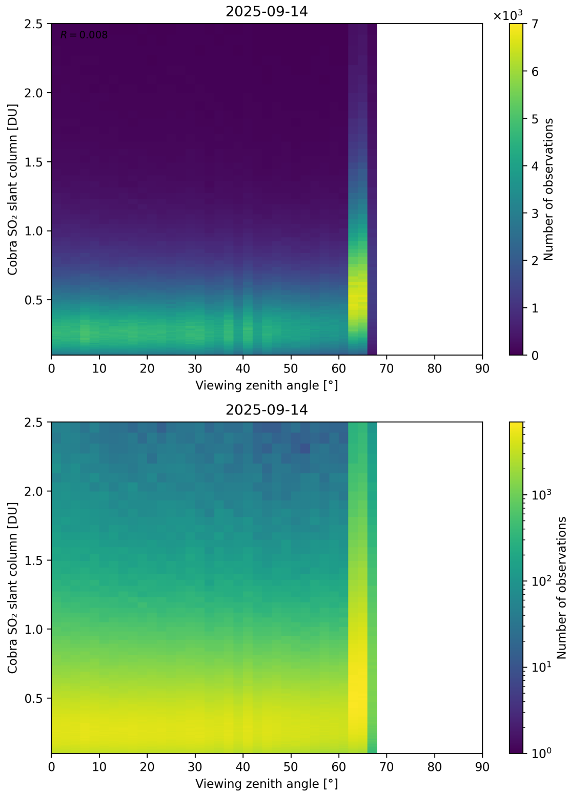
Figure 371: Scatter density plot of “Viewing zenith angle” against “Cobra SO 2 slant column” for 2025-09-13 to 2025-09-15.
