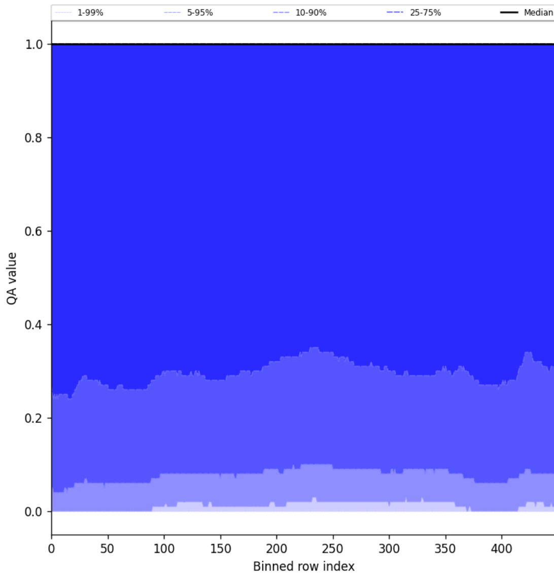
Figure 83: Along track statistics of “QA value” for 2025-09-13 to 2025-09-15
