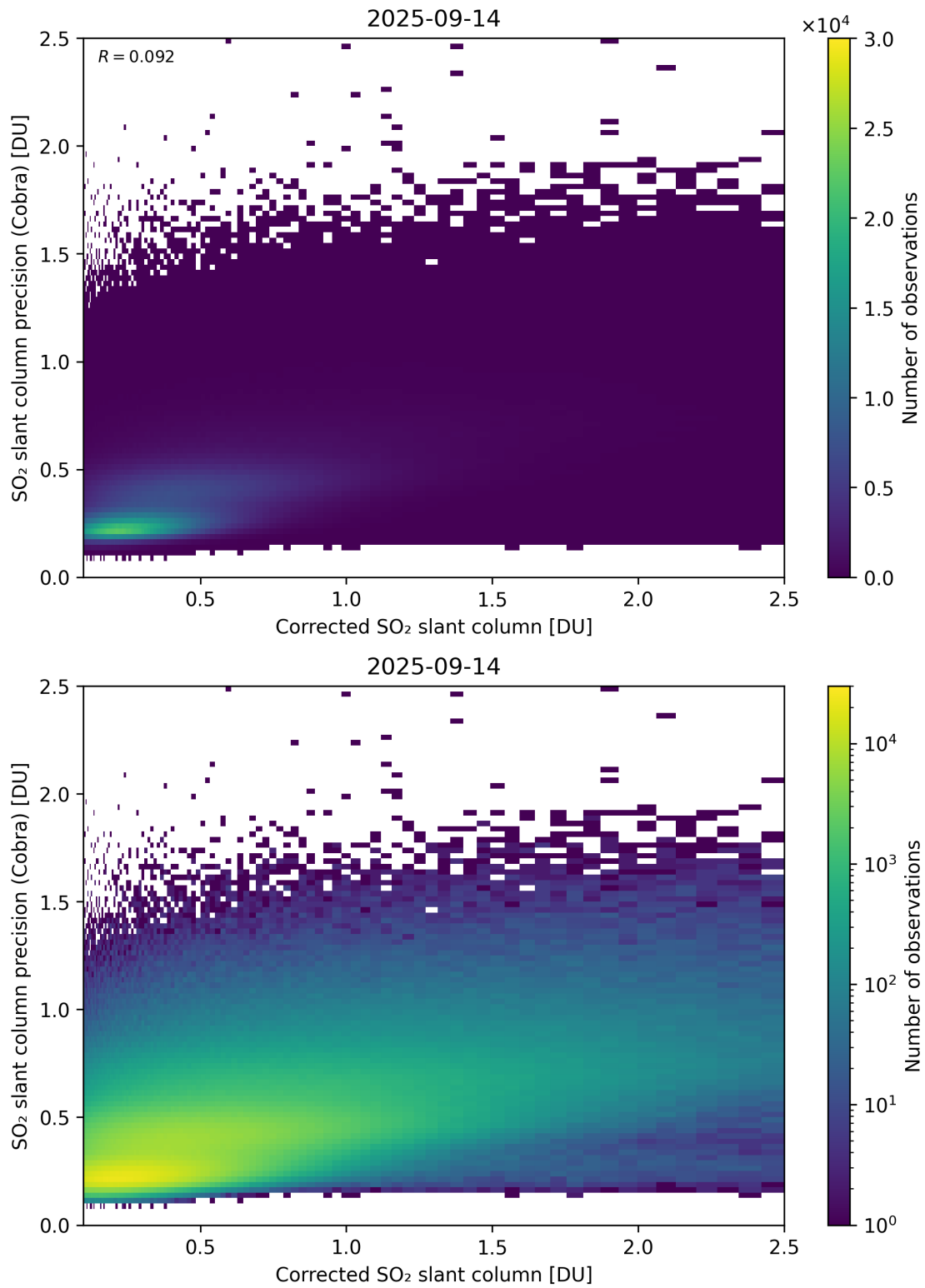
Figure 234: Scatter density plot of “Corrected SO 2 slant column” against “SO 2 slant column precision (Cobra)” for 2025-09-13 to 2025-09-15.
