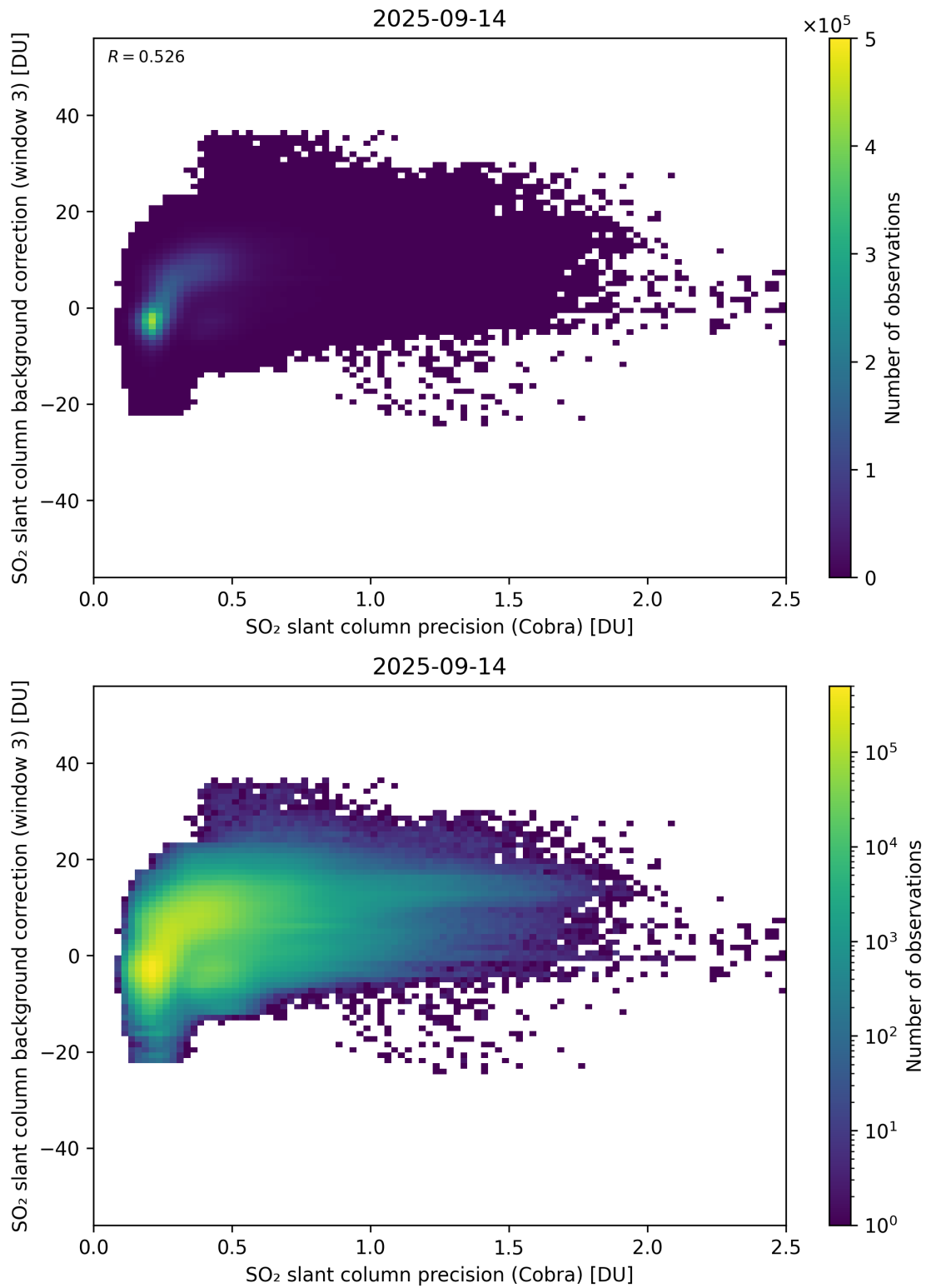
Figure 201: Scatter density plot of “SO 2 slant column precision (Cobra)” against “SO 2 slant column background correction (window 3)” for 2025-09-13 to 2025-09-15.
