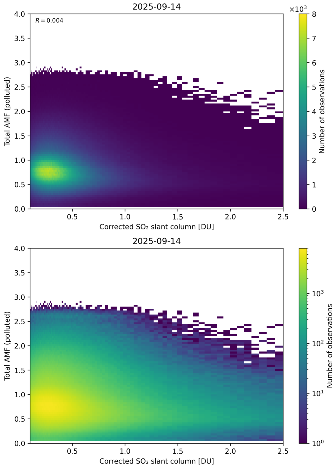
Figure 242: Scatter density plot of “Corrected SO 2 slant column” against “Total AMF (polluted)” for 2025-09-13 to 2025-09-15.
