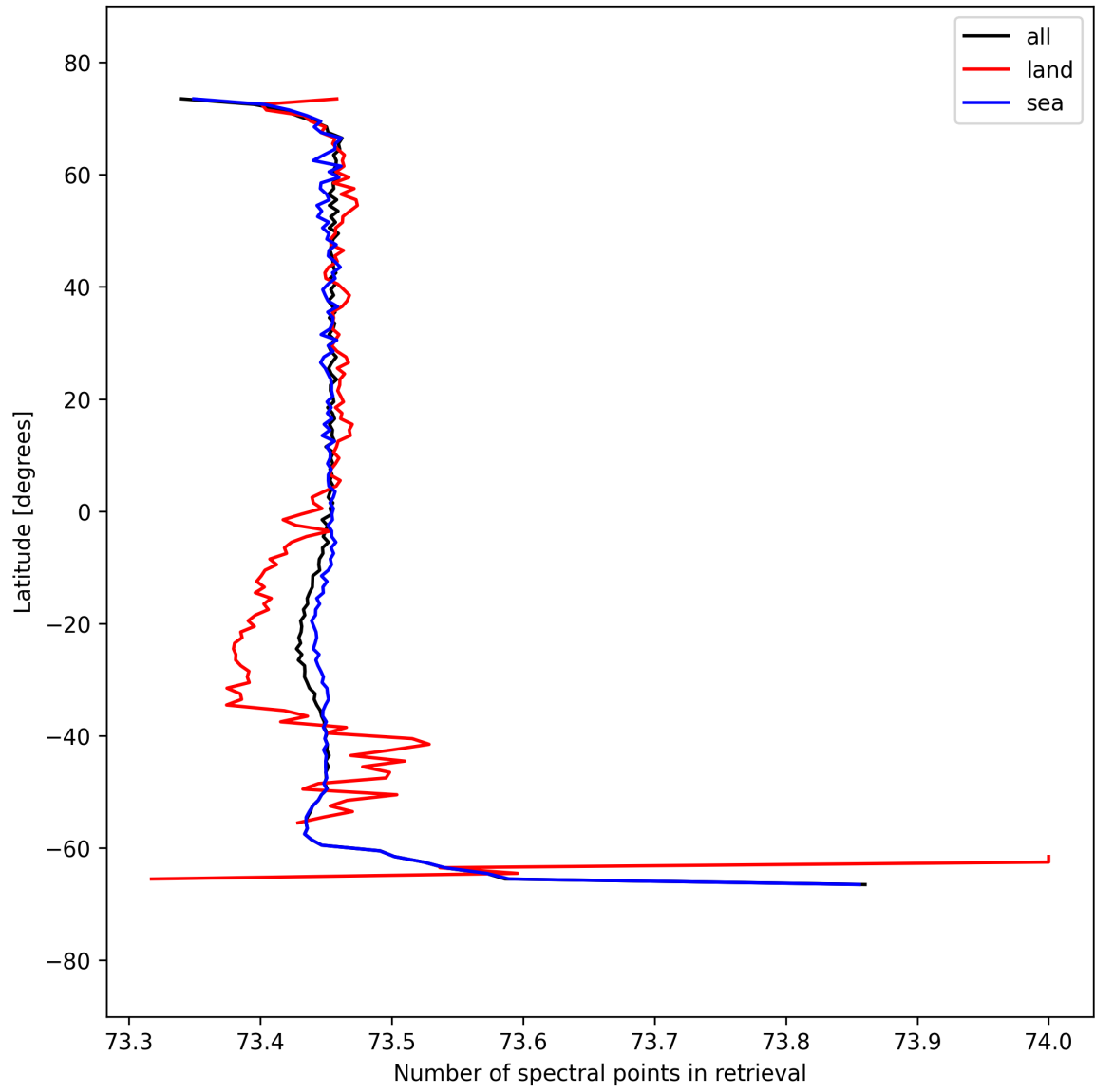
Figure 56: Zonal average of “Number of spectral points in retrieval” for 2025-09-13 to 2025-09-15.
