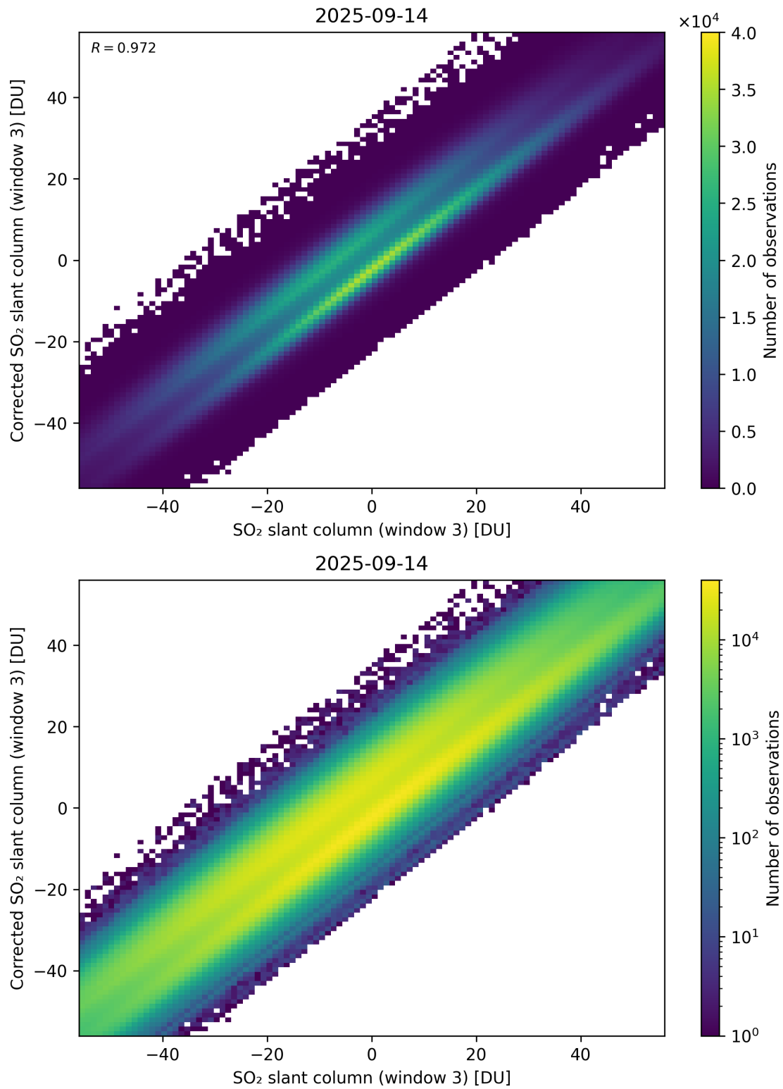
Figure 316: Scatter density plot of “SO 2 slant column (window 3)” against “Corrected SO 2 slant column (window 3)” for 2025-09-13 to 2025-09-15.
