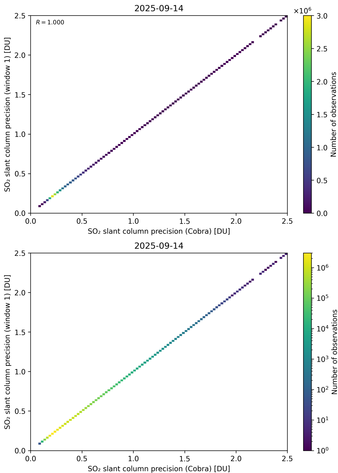
Figure 209: Scatter density plot of “SO 2 slant column precision (Cobra)” against “SO 2 slant column precision (window 1)” for 2025-09-13 to 2025-09-15.
