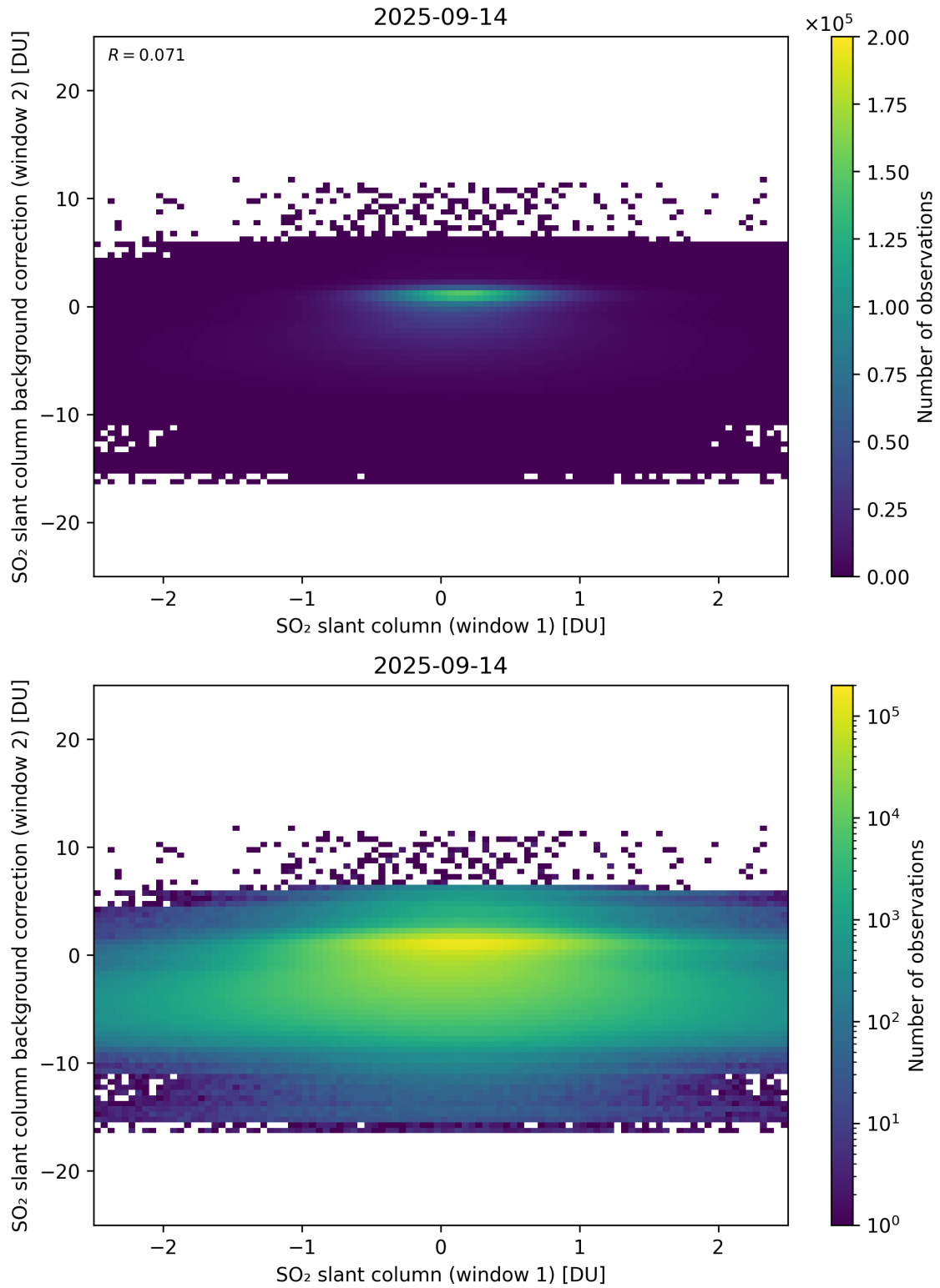
Figure 263: Scatter density plot of “SO 2 slant column (window 1)” against “SO 2 slant column background correction (window 2)” for 2025-09-13 to 2025-09-15.
