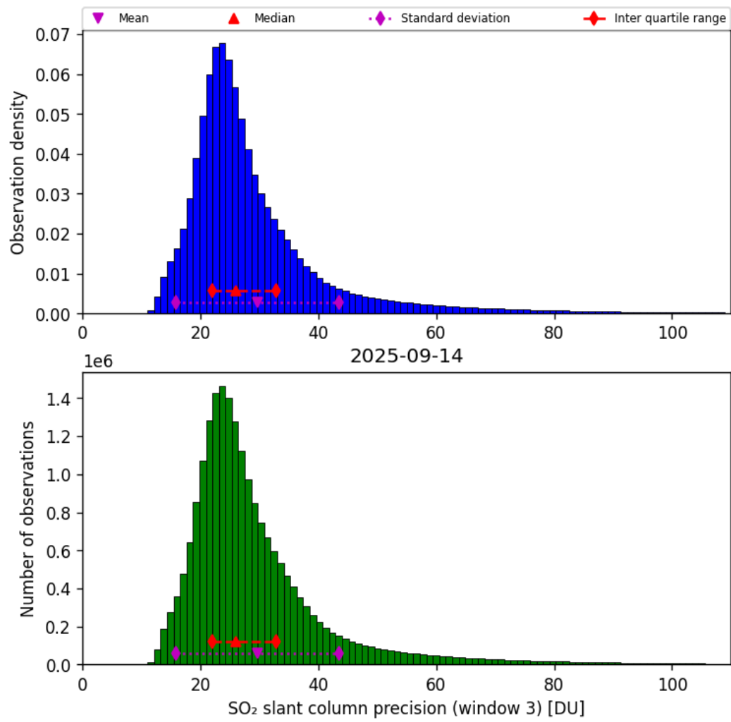
Figure 72: Histogram of “SO 2 slant column precision (window 3)” for 2025-09-13 to 2025-09-15
