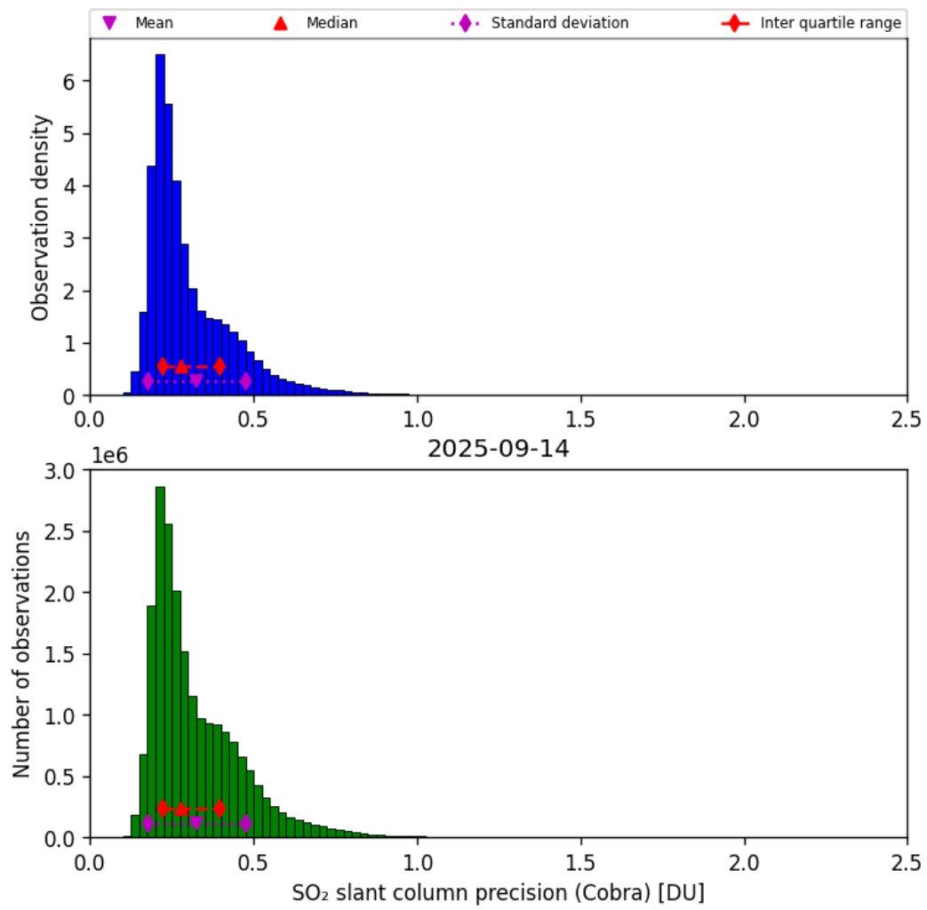
Figure 62: Histogram of “SO 2 slant column precision (Cobra)” for 2025-09-13 to 2025-09-15
