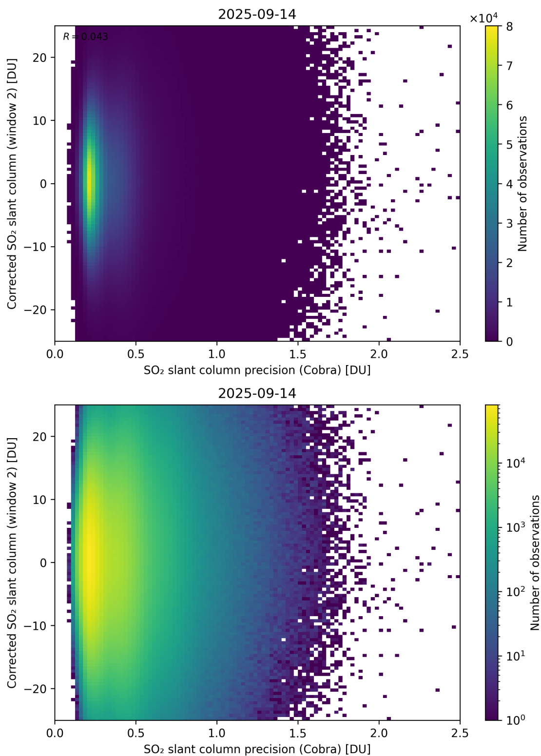
Figure 206: Scatter density plot of “SO 2 slant column precision (Cobra)” against “Corrected SO 2 slant column (window 2)” for 2025-09-13 to 2025-09-15.
