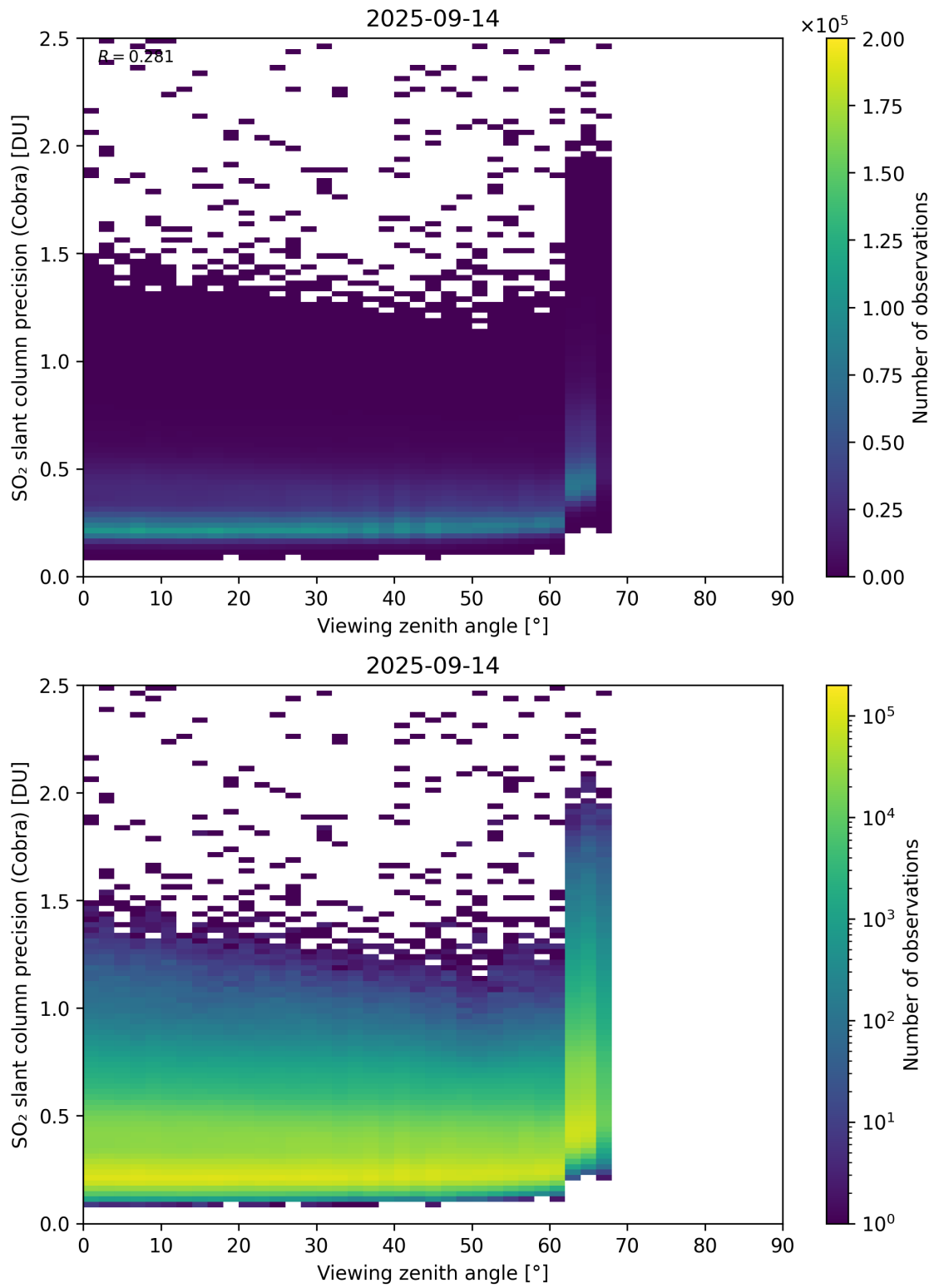
Figure 372: Scatter density plot of “Viewing zenith angle” against “SO 2 slant column precision (Cobra)” for 2025-09-13 to 2025-09-15.
