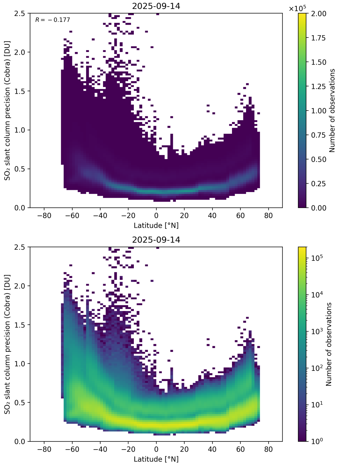
Figure 158: Scatter density plot of “Latitude” against “SO 2 slant column precision (Cobra)” for 2025-09-13 to 2025-09-15.
