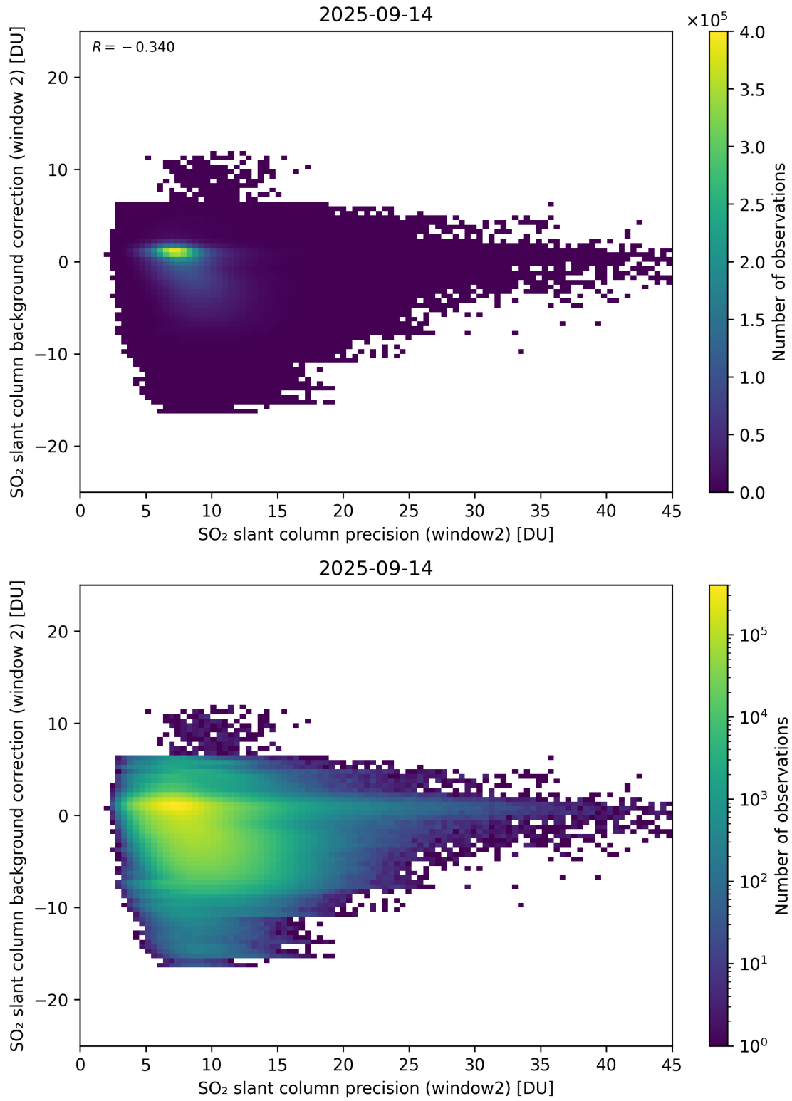
Figure 291: Scatter density plot of “SO 2 slant column precision (window2)” against “SO 2 slant column background correction (window 2)” for 2025-09-13 to 2025-09-15.
