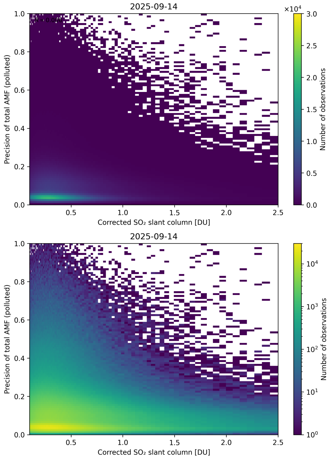
Figure 243: Scatter density plot of “Corrected SO 2 slant column” against “Precision of total AMF (polluted)” for 2025-09-13 to 2025-09-15.
