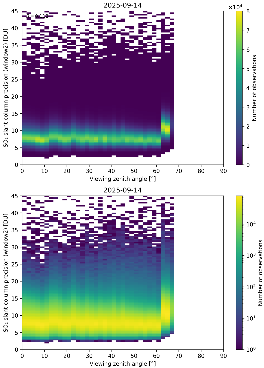
Figure 378: Scatter density plot of “Viewing zenith angle” against “SO 2 slant column precision (window2)” for 2025-09-13 to 2025-09-15.
