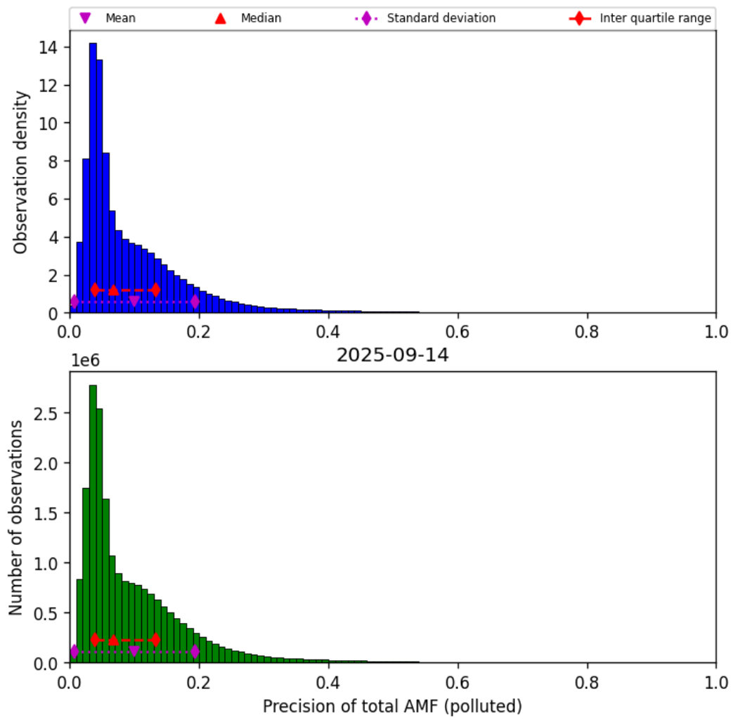
Figure 80: Histogram of “Precision of total AMF (polluted)” for 2025-09-13 to 2025-09-15
