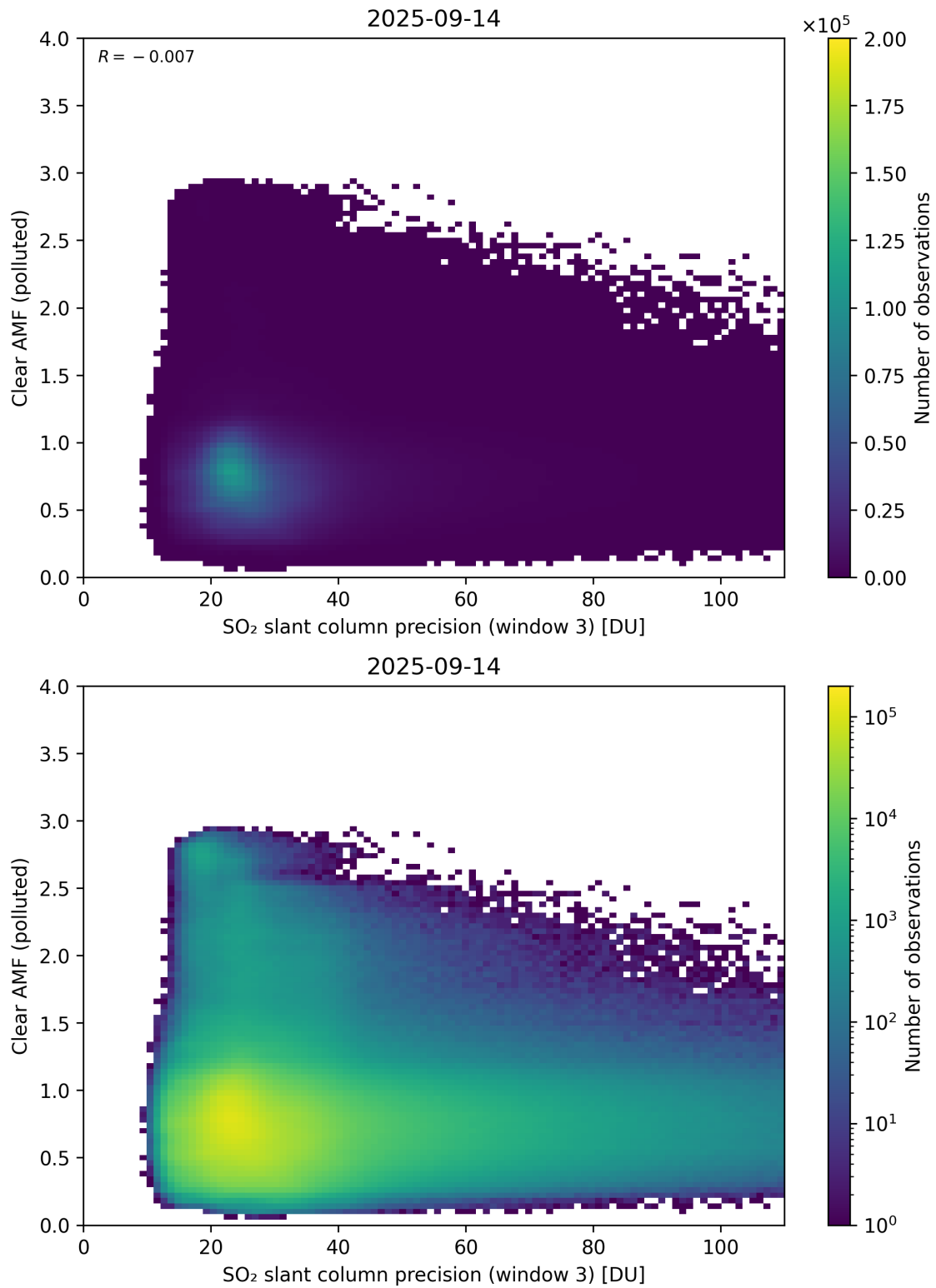
Figure 311: Scatter density plot of “SO 2 slant column precision (window 3)” against “Clear AMF (polluted)” for 2025-09-13 to 2025-09-15.
