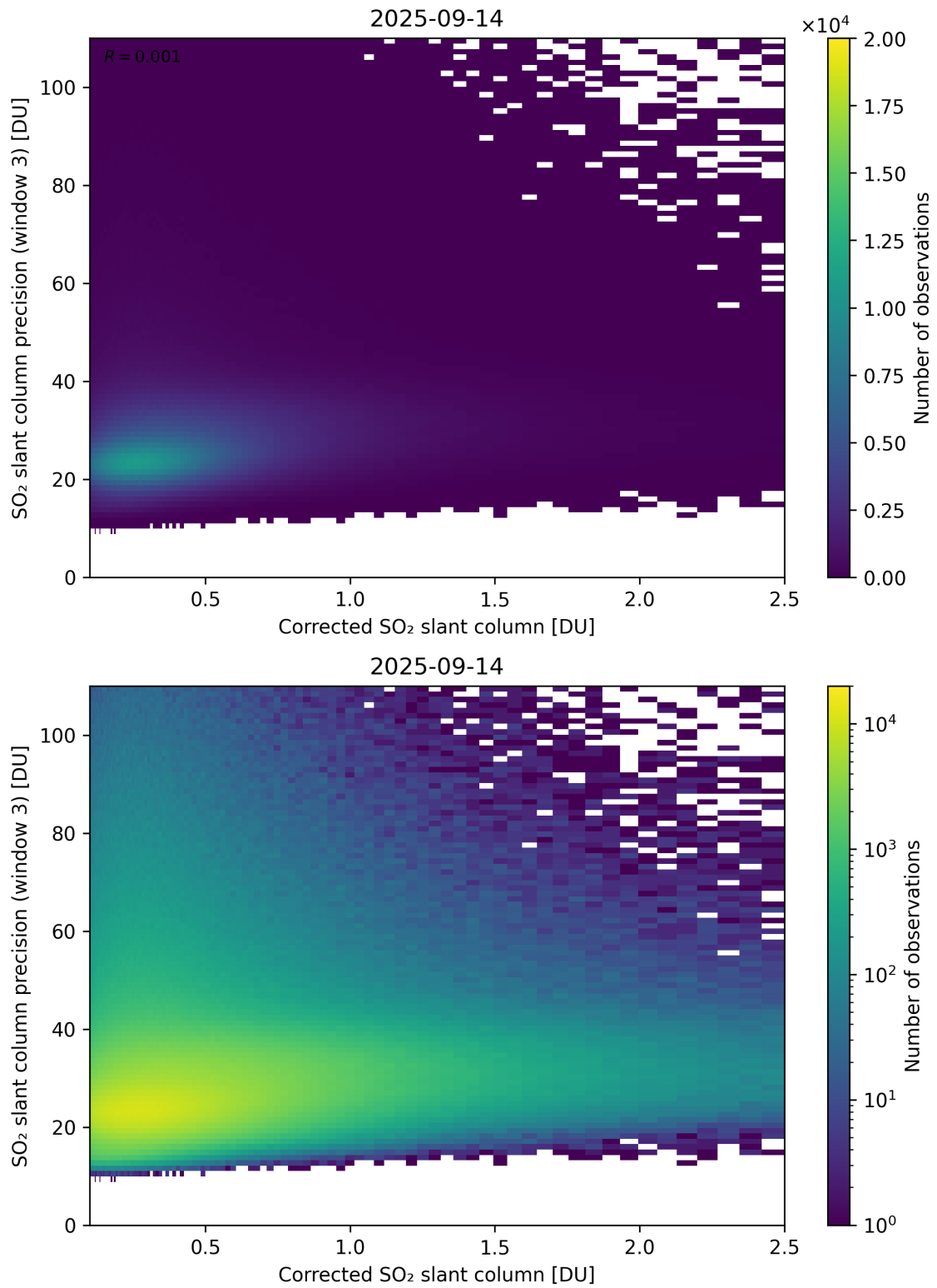
Figure 241: Scatter density plot of “Corrected SO 2 slant column” against “SO 2 slant column precision (window 3)” for 2025-09-13 to 2025-09-15.
