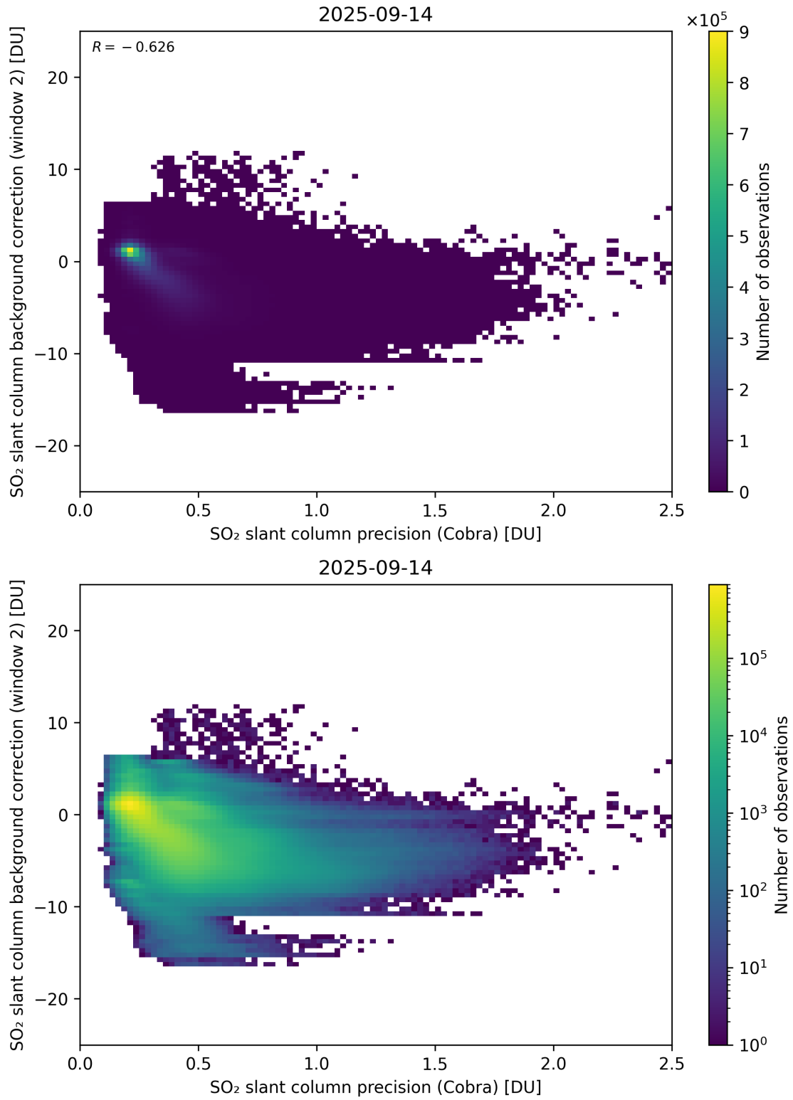
Figure 200: Scatter density plot of “SO 2 slant column precision (Cobra)” against “SO 2 slant column background correction (window 2)” for 2025-09-13 to 2025-09-15.
