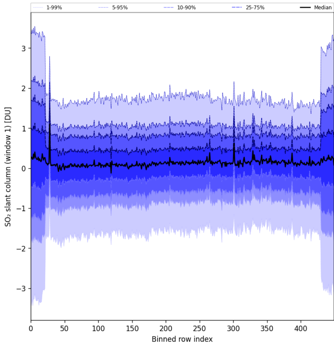
Figure 89: Along track statistics of “SO 2 slant column (window 1)” for 2025-09-13 to 2025-09-15
