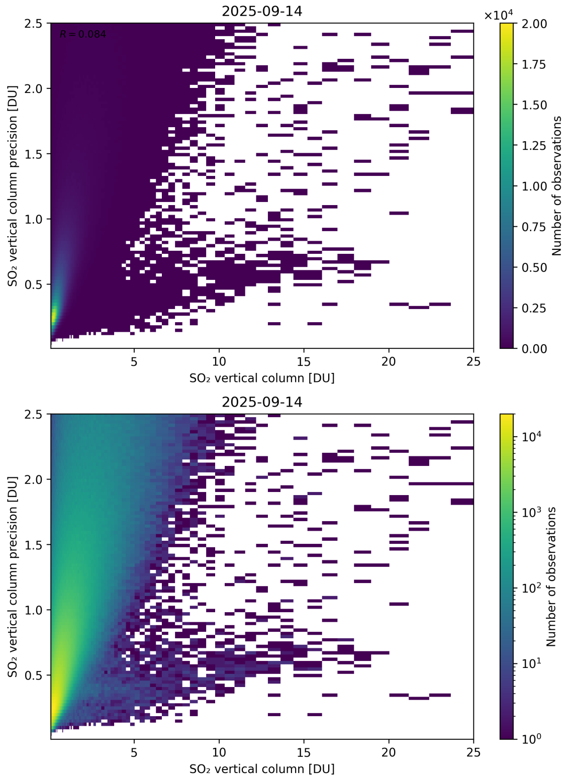
Figure 361: Scatter density plot of “SO 2 vertical column” against “SO 2 vertical column precision” for 2025-09-13 to 2025-09-15.
