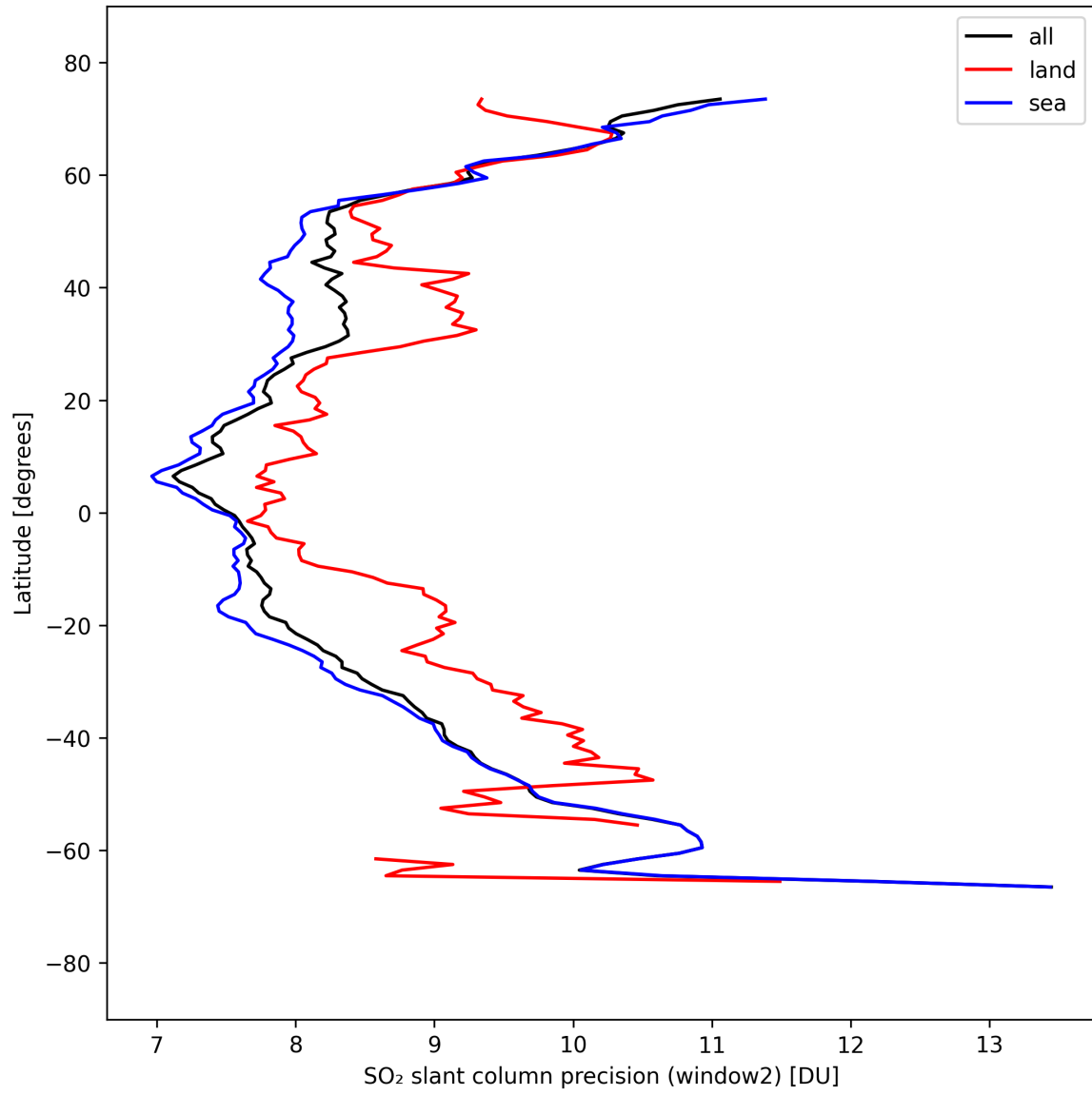
Figure 42: Zonal average of “SO 2 slant column precision (window2)” for 2025-09-13 to 2025-09-15.
