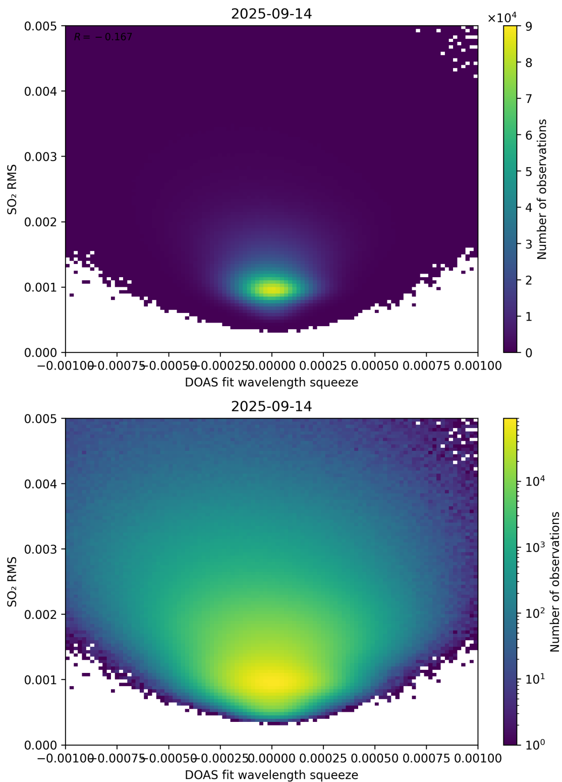
Figure 143: Scatter density plot of “DOAS fit wavelength squeeze” against “SO 2 RMS” for 2025-09-13 to 2025-09-15.
