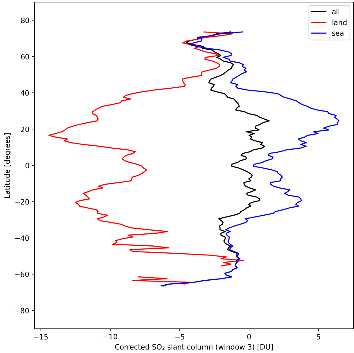
Figure 47: Zonal average of “Corrected SO 2 slant column (window 3)” for 2025-09-13 to 2025-09-15.
