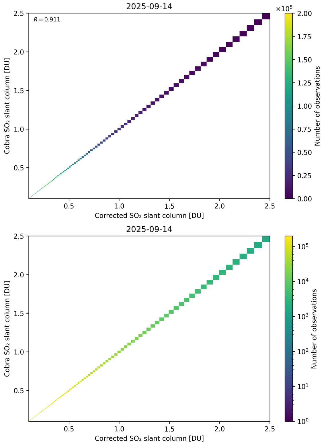
Figure 233: Scatter density plot of “Corrected SO 2 slant column” against “Cobra SO 2 slant column” for 2025-09-13 to 2025-09-15.
