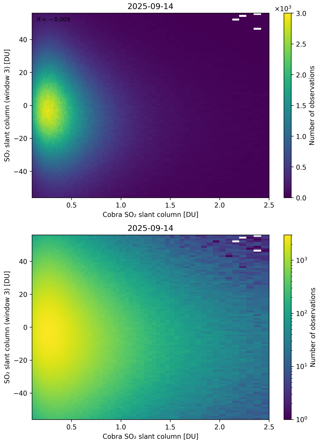
Figure 222: Scatter density plot of “Cobra SO 2 slant column” against “SO 2 slant column (window 3)” for 2025-09-13 to 2025-09-15.
