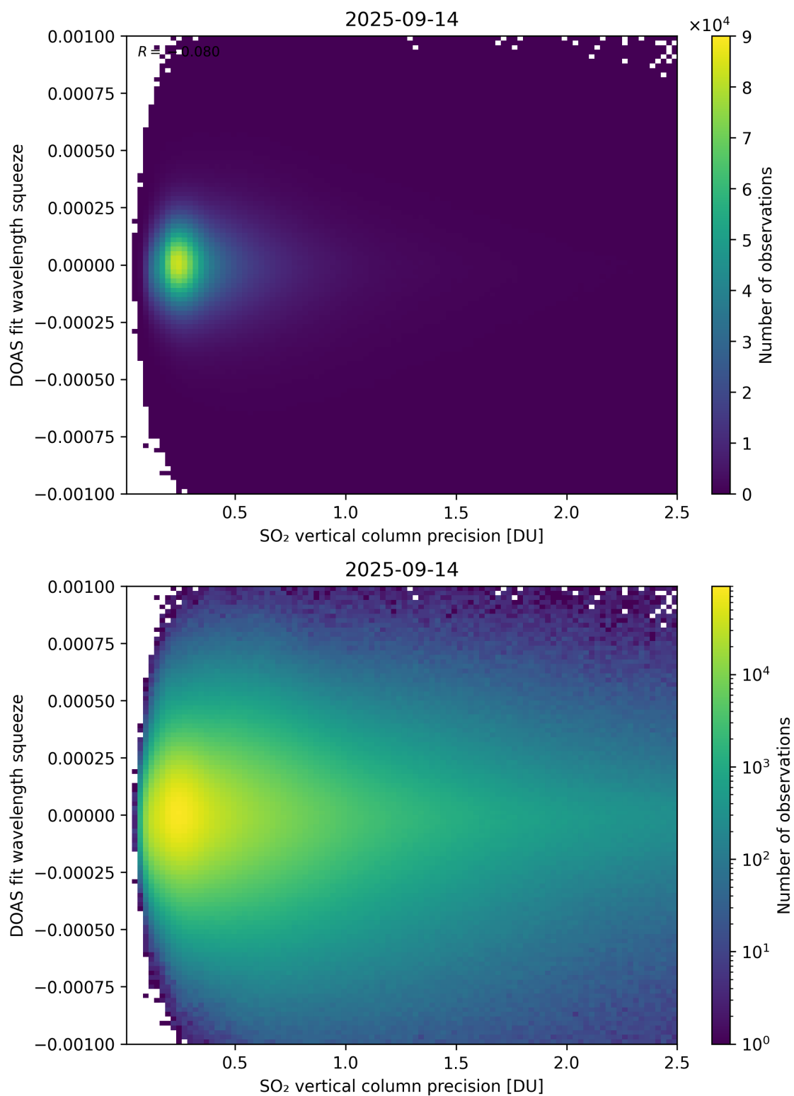
Figure 333: Scatter density plot of “SO 2 vertical column precision” against “DOAS fit wavelength squeeze” for 2025-09-13 to 2025-09-15.
