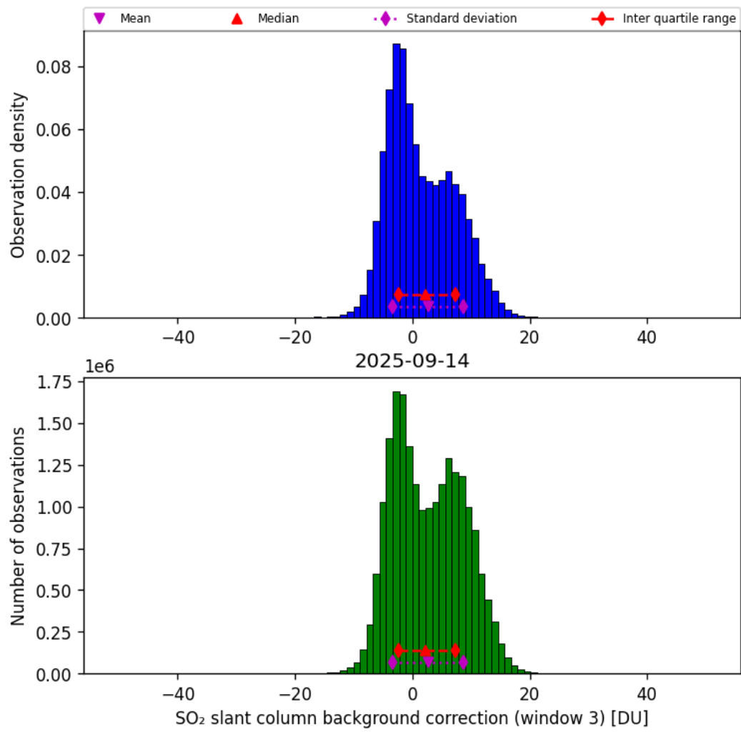
Figure 74: Histogram of “SO 2 slant column background correction (window 3)” for 2025-09-13 to 2025-09-15
