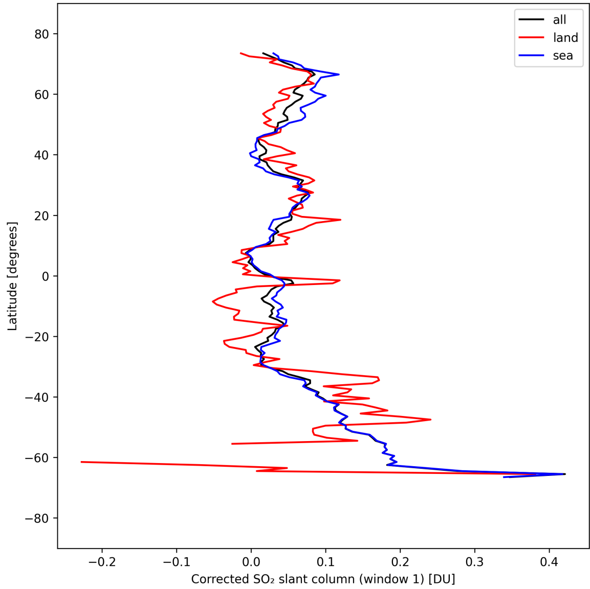
Figure 39: Zonal average of “Corrected SO 2 slant column (window 1)” for 2025-09-13 to 2025-09-15.
