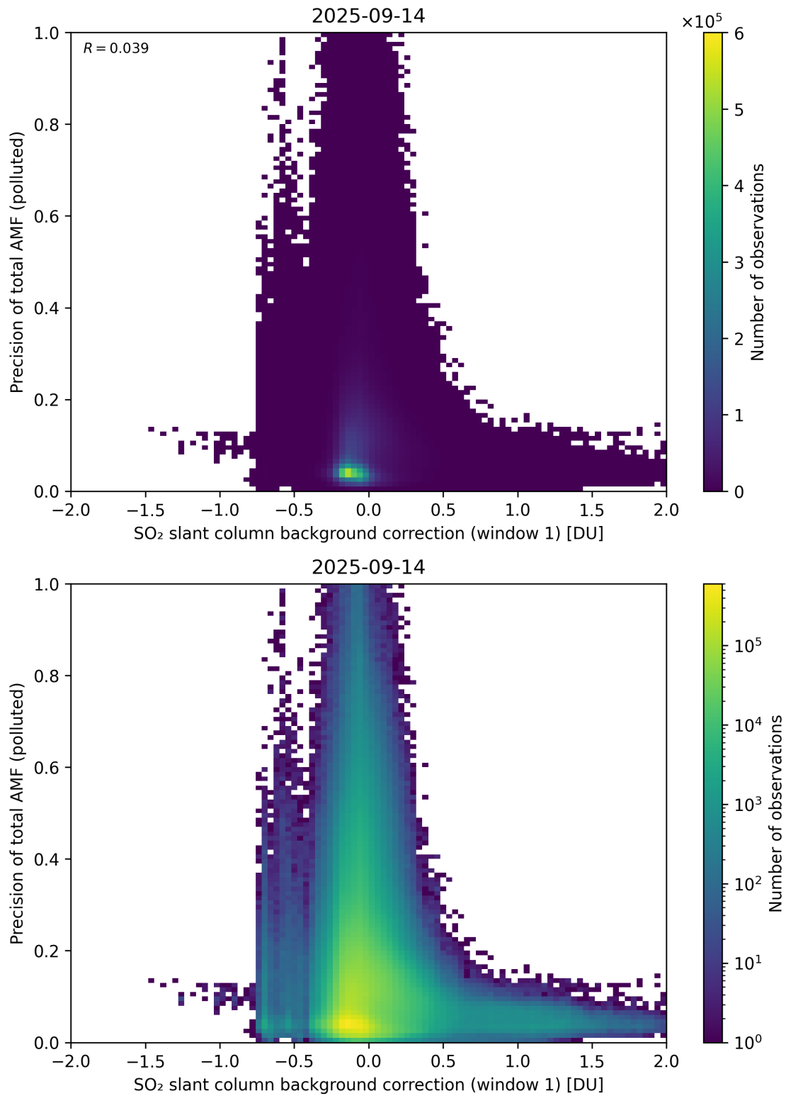
Figure 121: Scatter density plot of “SO 2 slant column background correction (window 1)” against “Precision of total AMF (polluted)” for 2025-09-13 to 2025-09-15.
