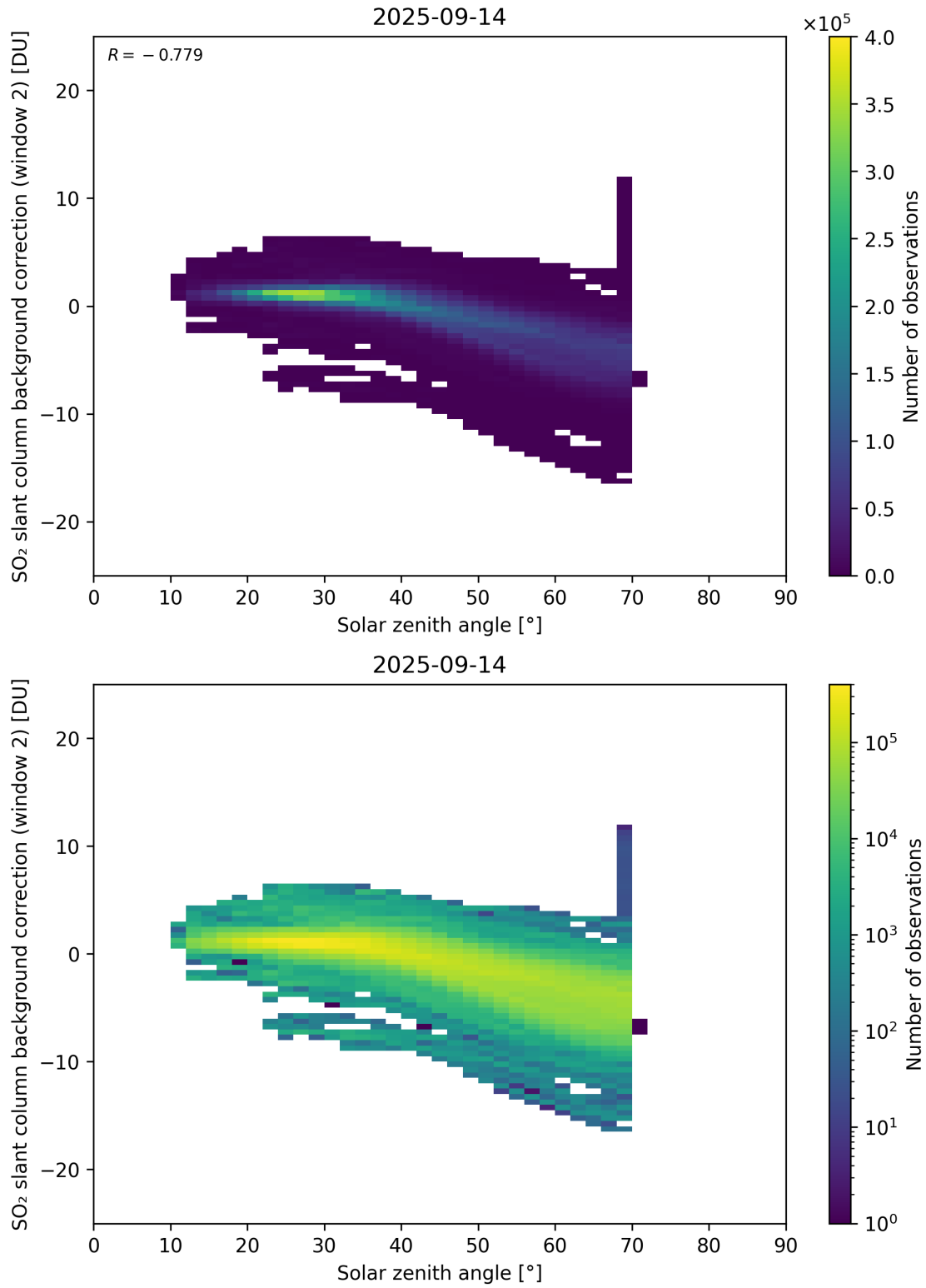
Figure 172: Scatter density plot of “Solar zenith angle” against “SO 2 slant column background correction (window 2)” for 2025-09-13 to 2025-09-15.
