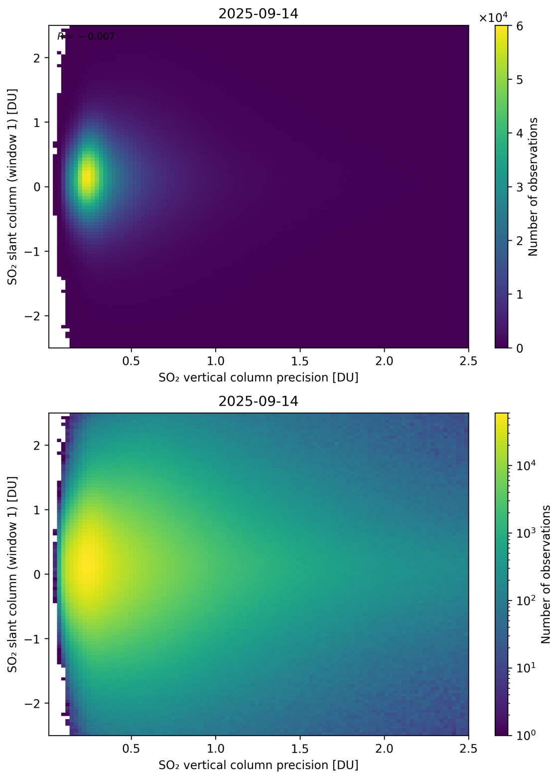
Figure 341: Scatter density plot of “SO 2 vertical column precision” against “SO 2 slant column (window 1)” for 2025-09-13 to 2025-09-15.
