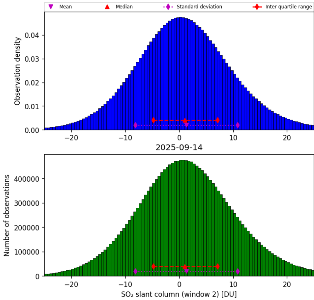
Figure 67: Histogram of “SO 2 slant column (window 2)” for 2025-09-13 to 2025-09-15
