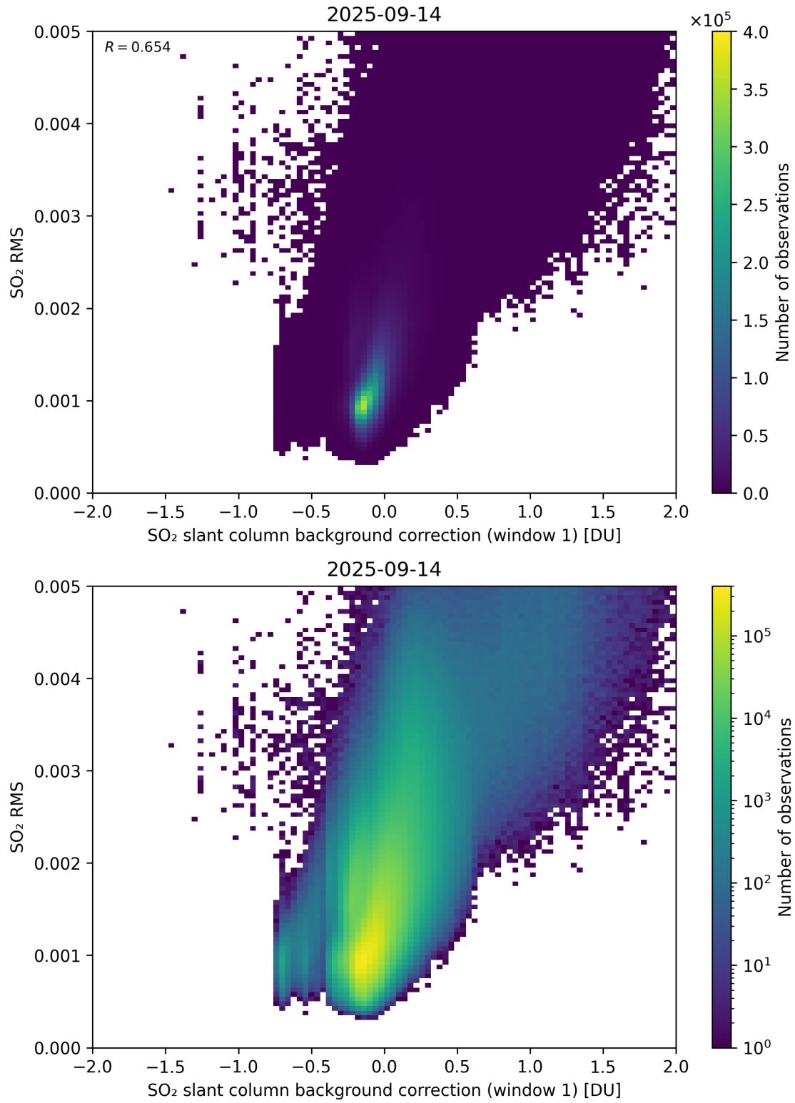
Figure 113: Scatter density plot of “SO 2 slant column background correction (window 1)” against “SO 2 RMS” for 2025-09-13 to 2025-09-15.
