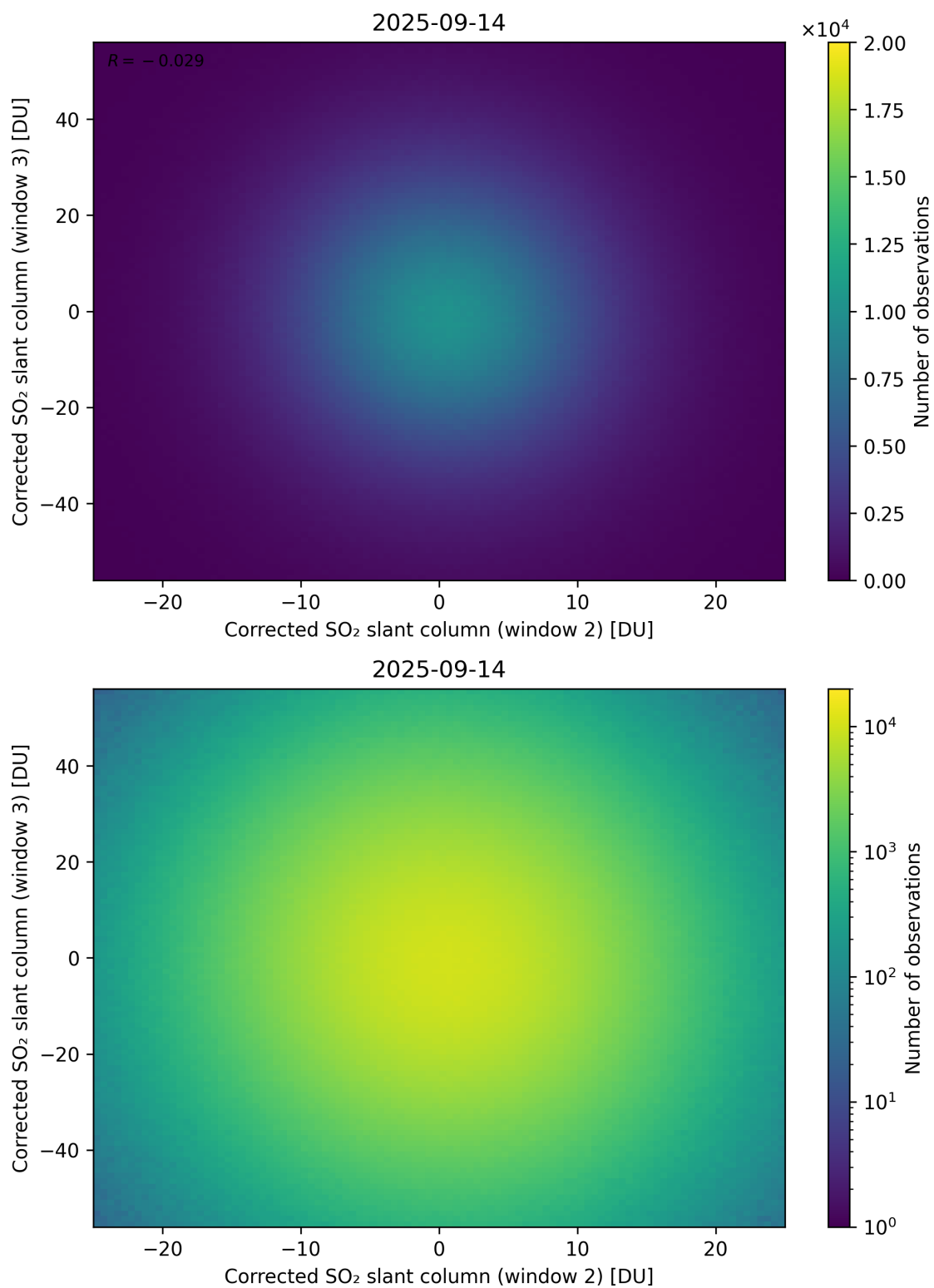
Figure 250: Scatter density plot of “Corrected SO 2 slant column (window 2)” against “Corrected SO 2 slant column (window 3)” for 2025-09-13 to 2025-09-15.
