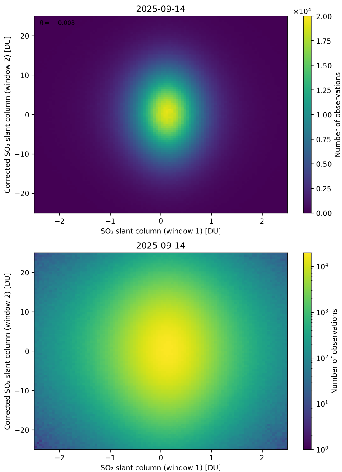
Figure 283: Scatter density plot of “SO 2 slant column (window 1)” against “Corrected SO 2 slant column (window 2)” for 2025-09-13 to 2025-09-15.
