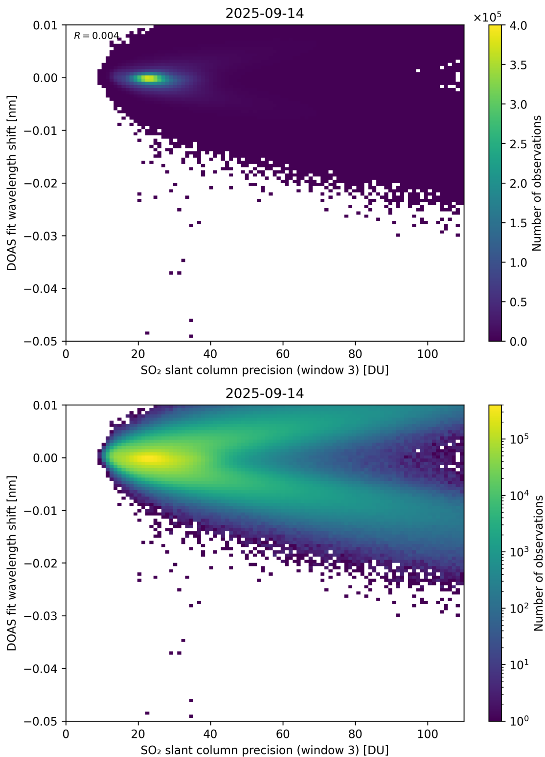
Figure 308: Scatter density plot of “SO 2 slant column precision (window 3)” against “DOAS fit wavelength shift” for 2025-09-13 to 2025-09-15.
