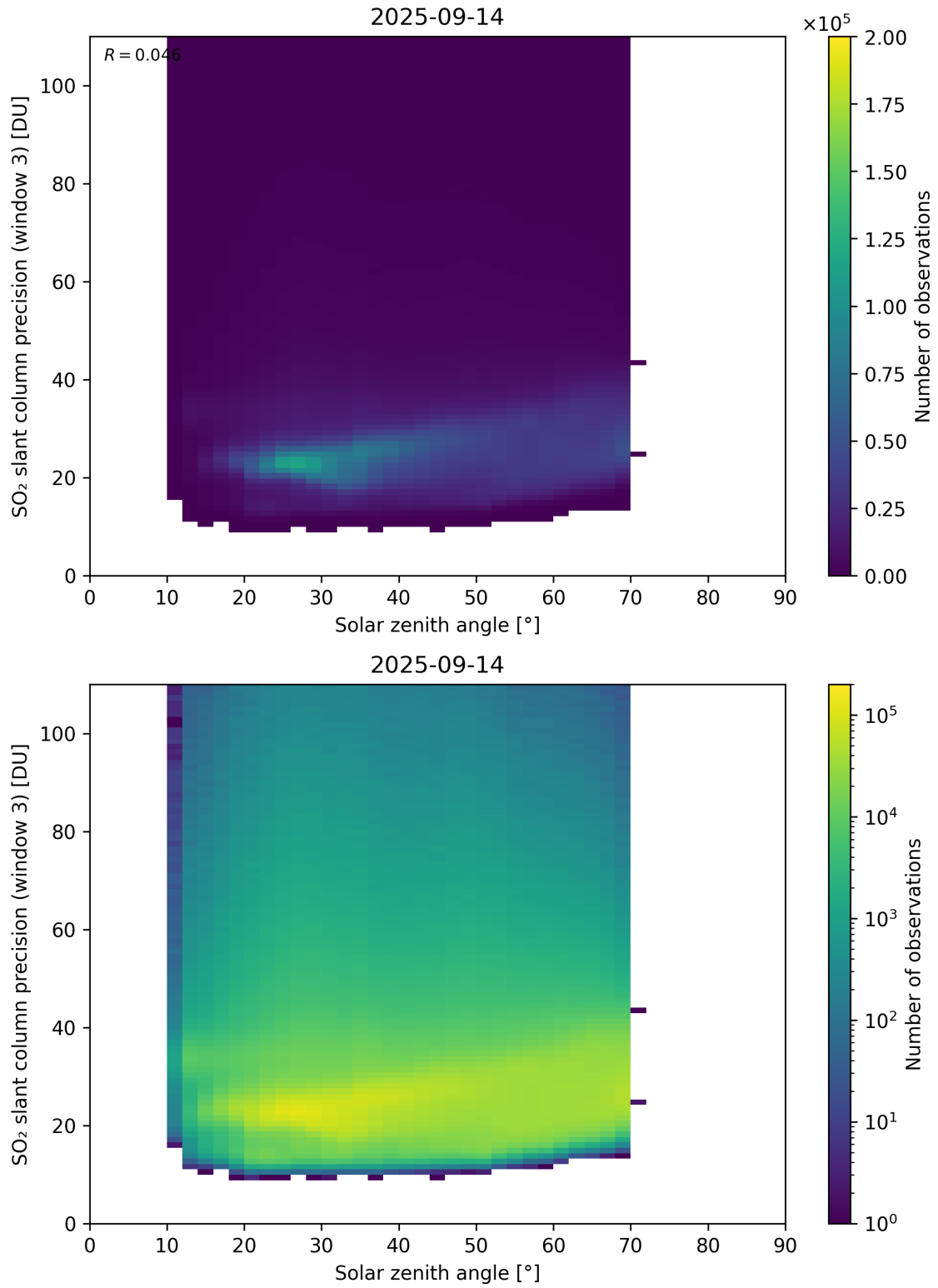
Figure 188: Scatter density plot of “Solar zenith angle” against “SO 2 slant column precision (window 3)” for 2025-09-13 to 2025-09-15.
