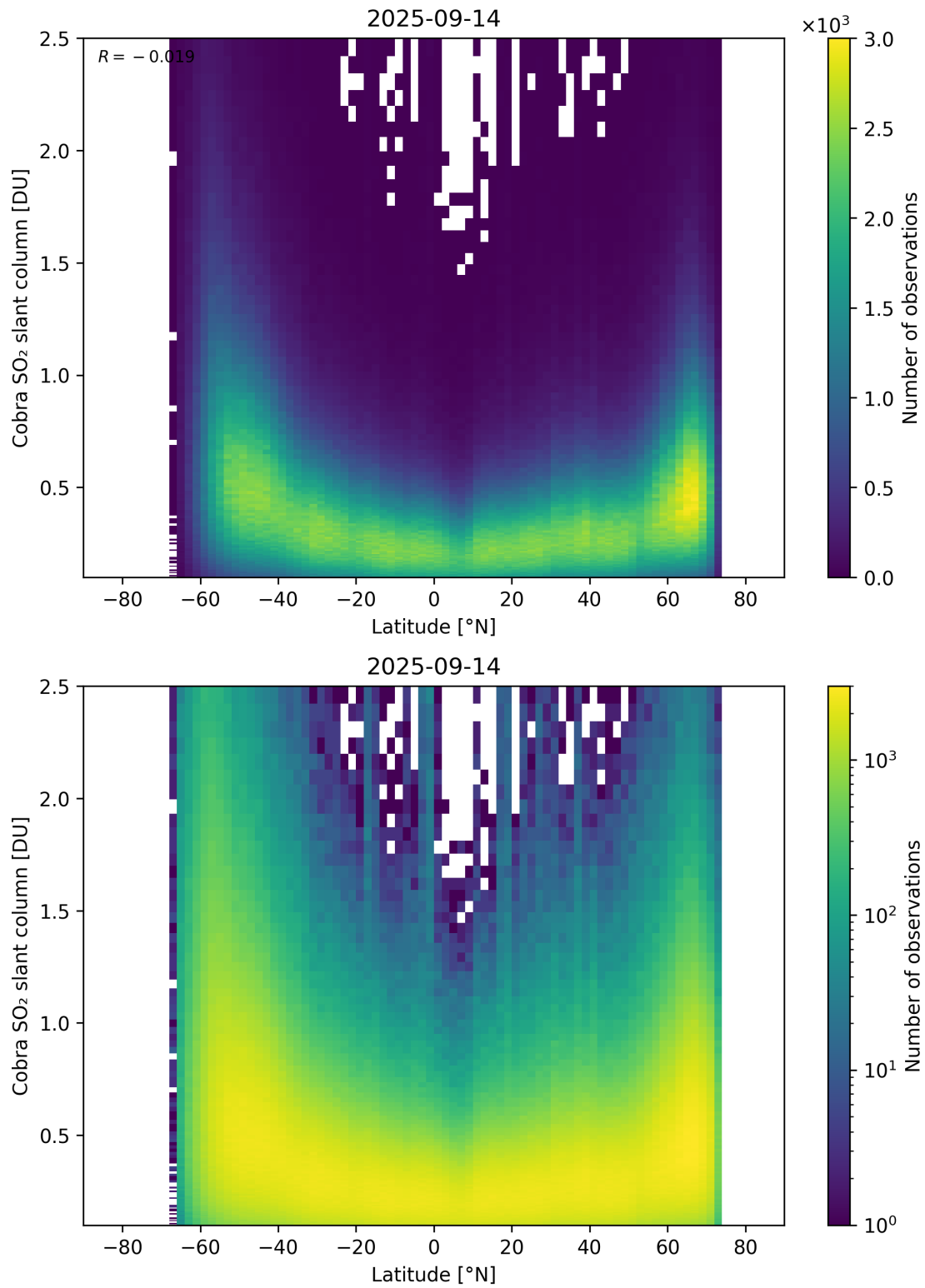
Figure 157: Scatter density plot of “Latitude” against “Cobra SO 2 slant column” for 2025-09-13 to 2025-09-15.
