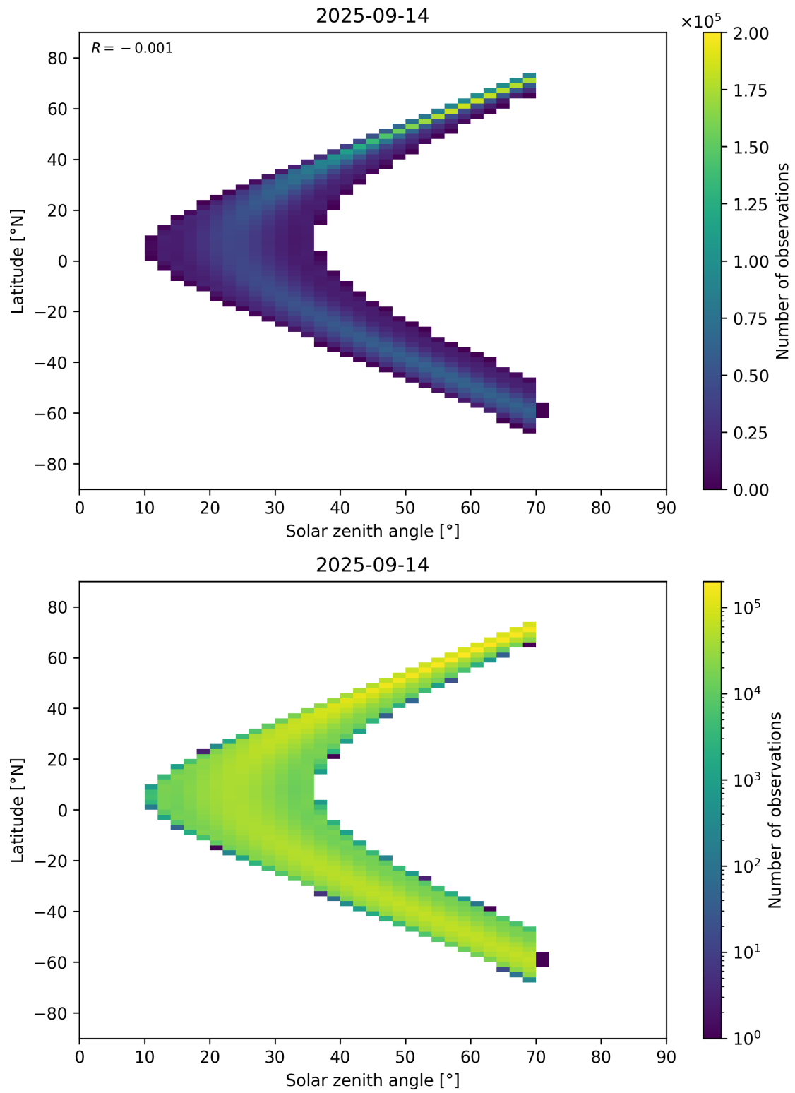
Figure 177: Scatter density plot of “Solar zenith angle” against “Latitude” for 2025-09-13 to 2025-09-15.
