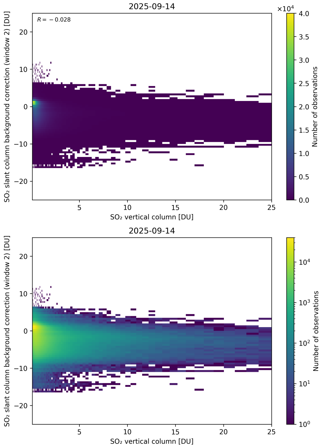
Figure 324: Scatter density plot of “SO 2 vertical column” against “SO 2 slant column background correction (window 2)” for 2025-09-13 to 2025-09-15.
