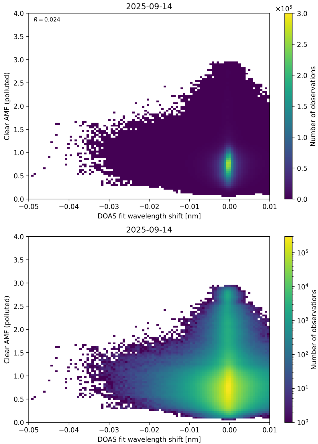
Figure 140: Scatter density plot of “DOAS fit wavelength shift” against “Clear AMF (polluted)” for 2025-09-13 to 2025-09-15.
