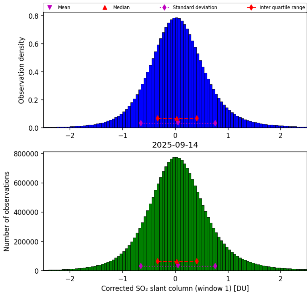
Figure 65: Histogram of “Corrected SO 2 slant column (window 1)” for 2025-09-13 to 2025-09-15
