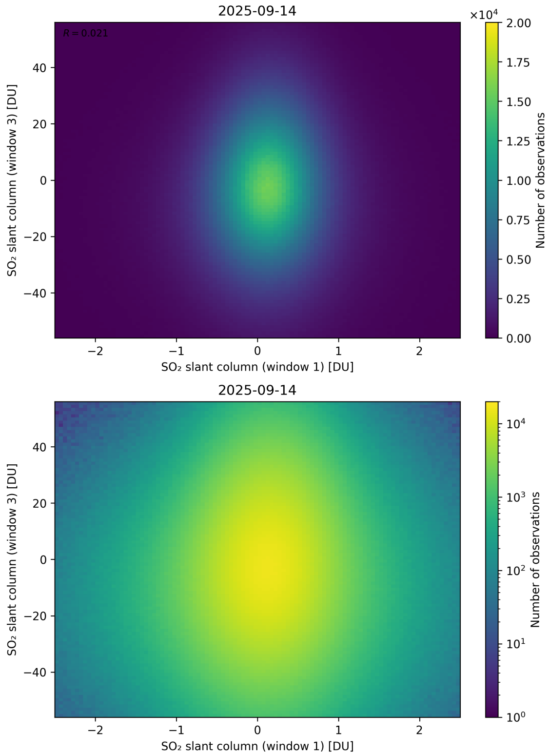
Figure 287: Scatter density plot of “SO 2 slant column (window 1)” against “SO 2 slant column (window 3)” for 2025-09-13 to 2025-09-15.
