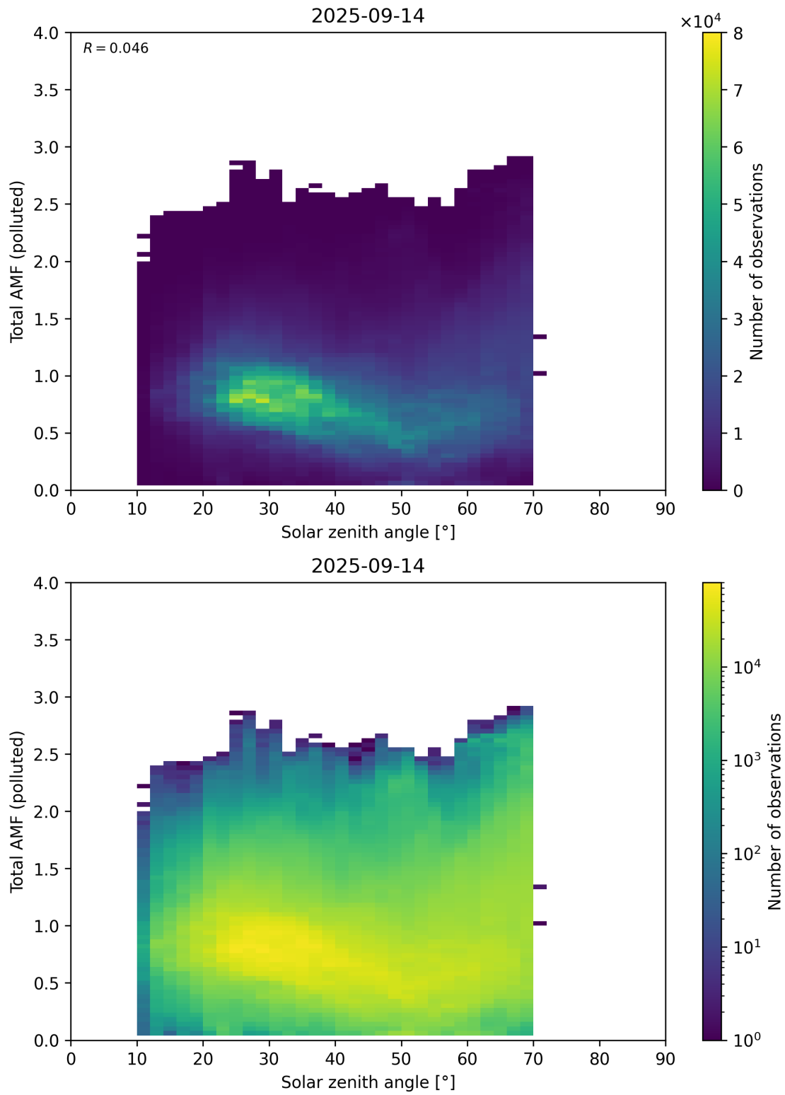
Figure 189: Scatter density plot of “Solar zenith angle” against “Total AMF (polluted)” for 2025-09-13 to 2025-09-15.
