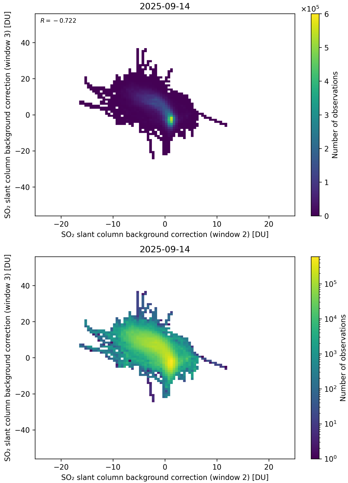
Figure 122: Scatter density plot of “SO 2 slant column background correction (window 2)” against “SO 2 slant column background correction (window 3)” for 2025-09-13 to 2025-09-15.
