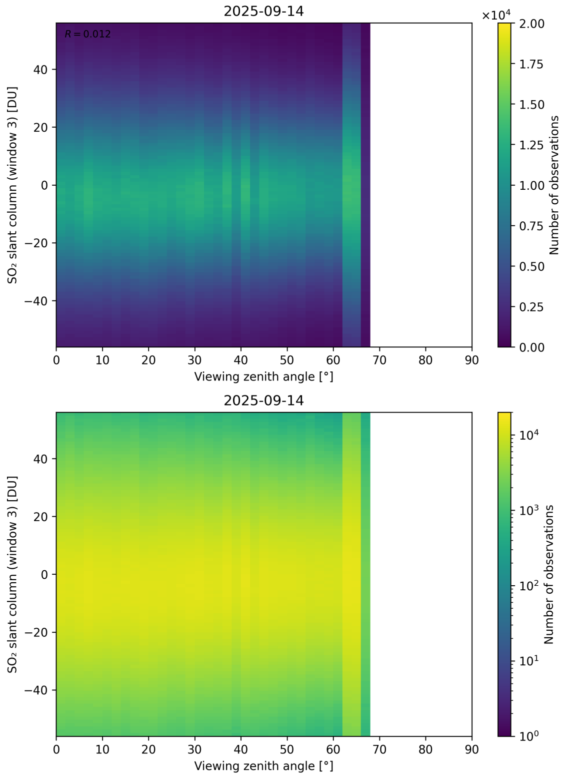
Figure 379: Scatter density plot of “Viewing zenith angle” against “SO 2 slant column (window 3)” for 2025-09-13 to 2025-09-15.
