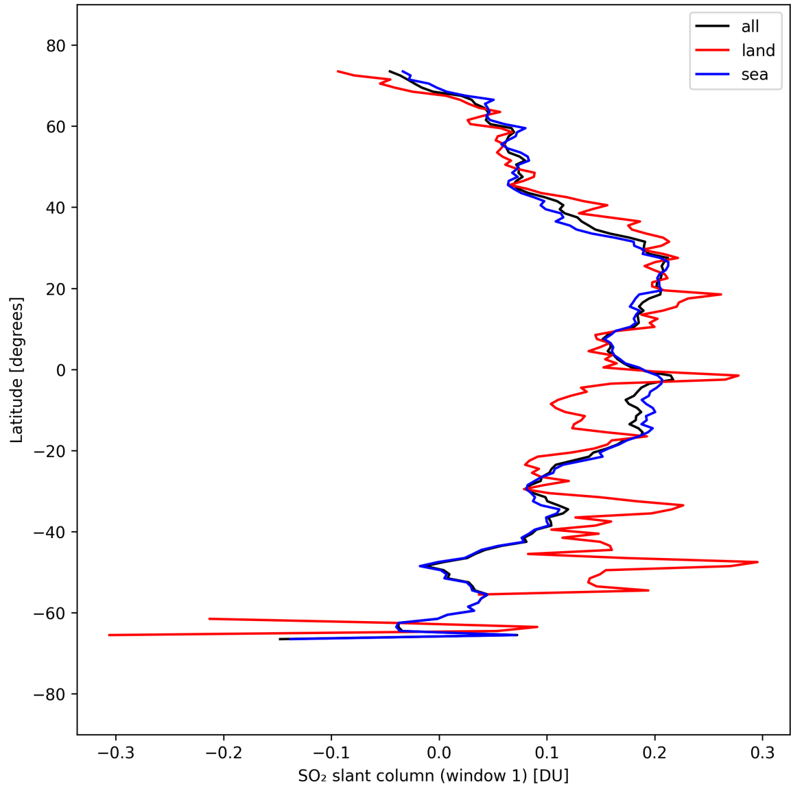
Figure 37: Zonal average of “SO 2 slant column (window 1)” for 2025-09-13 to 2025-09-15.
