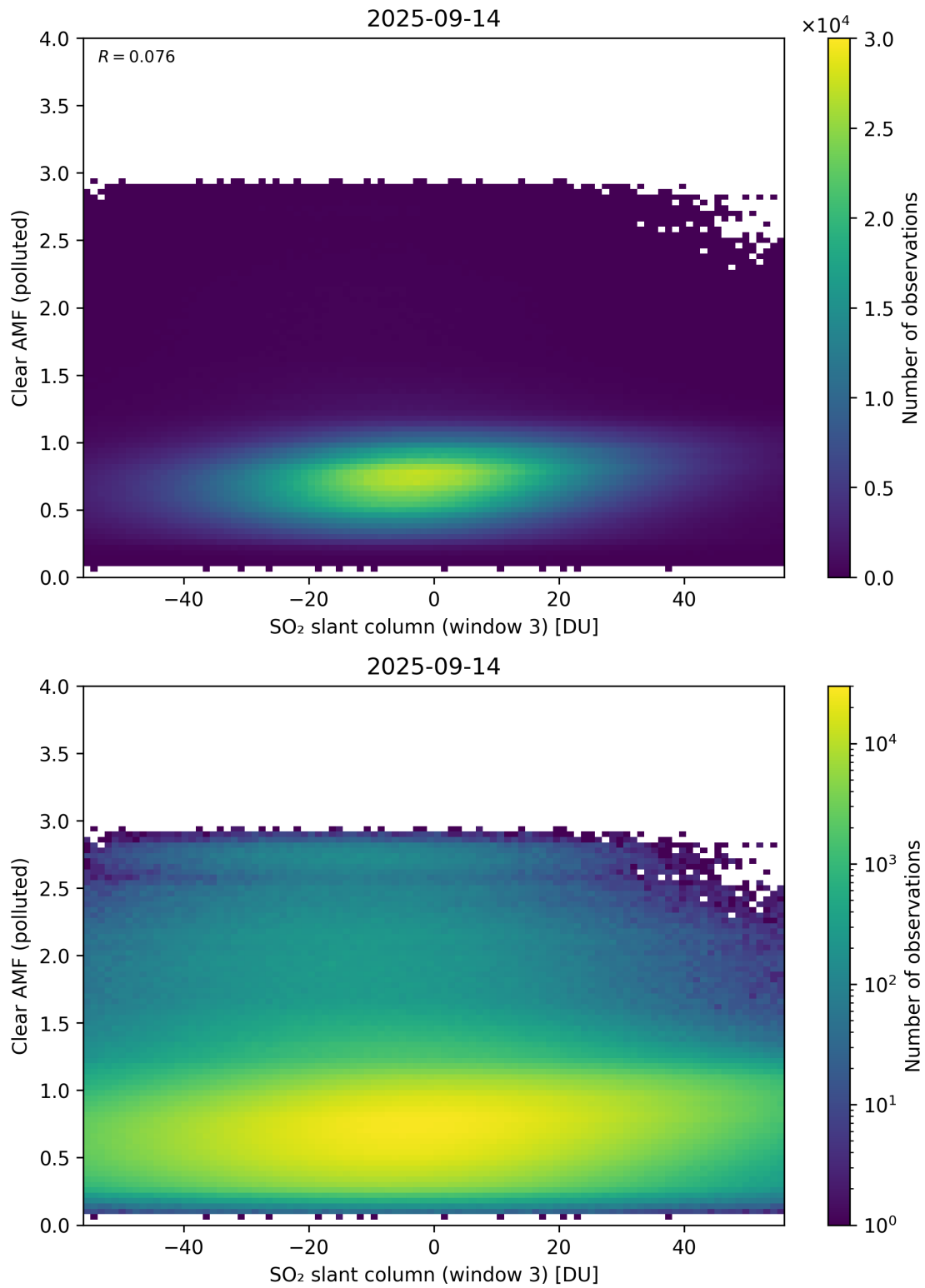
Figure 315: Scatter density plot of “SO 2 slant column (window 3)” against “Clear AMF (polluted)” for 2025-09-13 to 2025-09-15.
