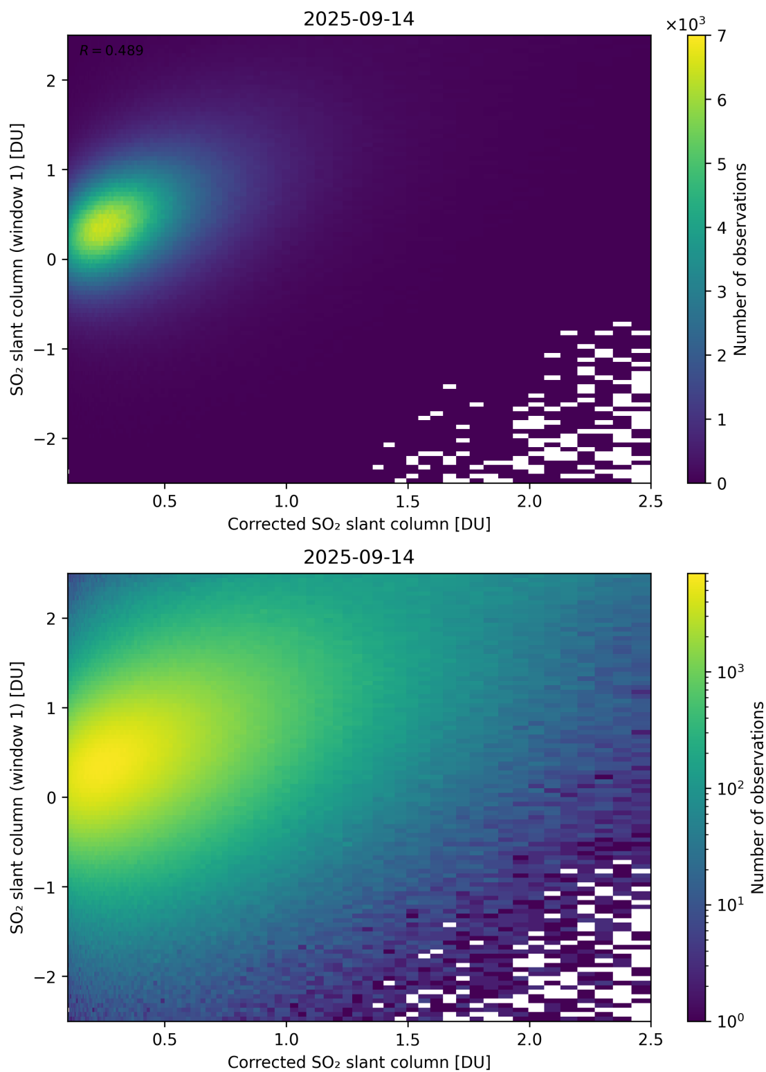
Figure 237: Scatter density plot of “Corrected SO 2 slant column” against “SO 2 slant column (window 1)” for 2025-09-13 to 2025-09-15.
