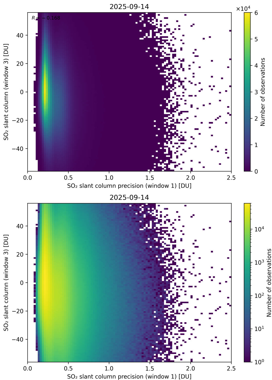
Figure 278: Scatter density plot of “SO 2 slant column precision (window 1)” against “SO 2 slant column (window 3)” for 2025-09-13 to 2025-09-15.
