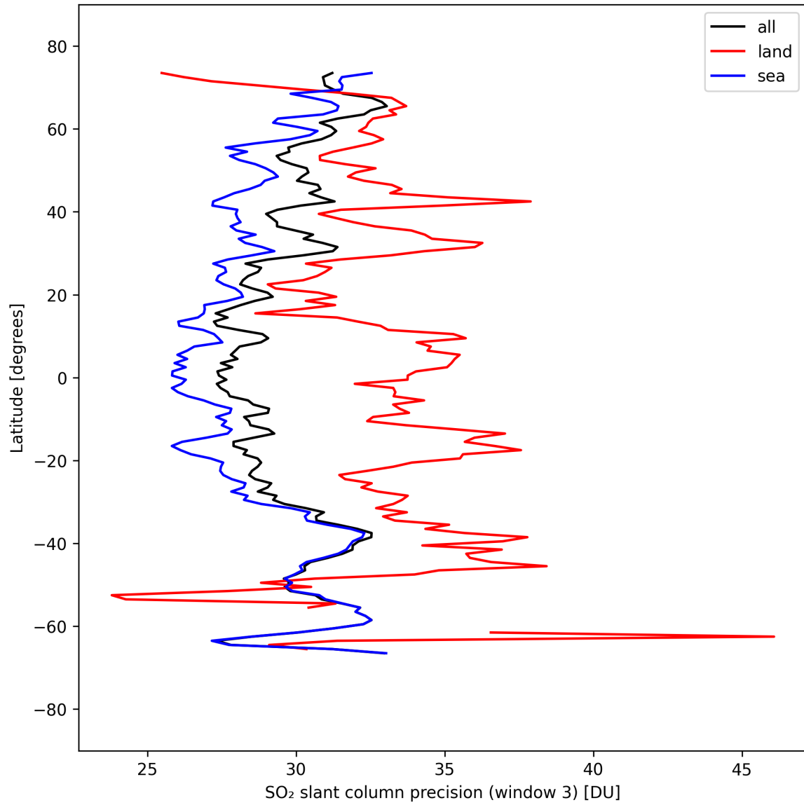
Figure 46: Zonal average of “SO 2 slant column precision (window 3)” for 2025-09-13 to 2025-09-15.
