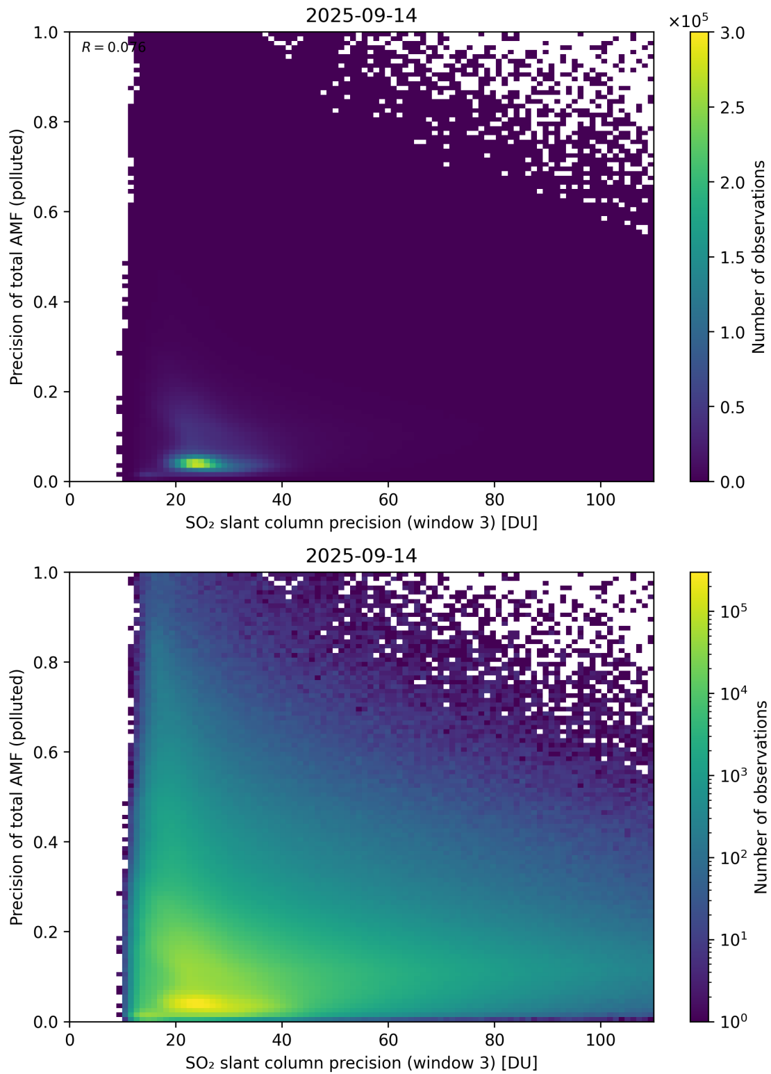
Figure 314: Scatter density plot of “SO 2 slant column precision (window 3)” against “Precision of total AMF (polluted)” for 2025-09-13 to 2025-09-15.
