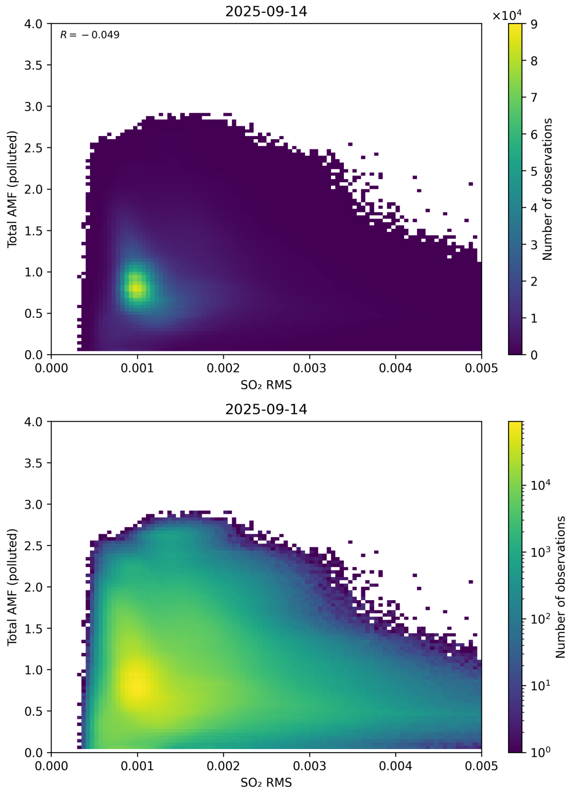
Figure 148: Scatter density plot of “SO 2 RMS” against “Total AMF (polluted)” for 2025-09-13 to 2025-09-15.
