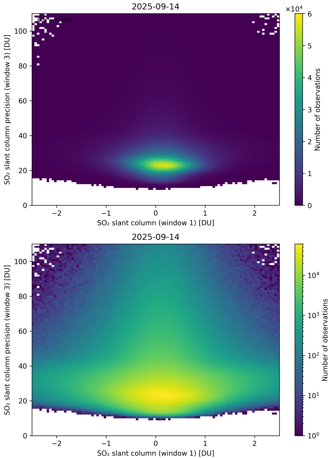
Figure 288: Scatter density plot of “SO 2 slant column (window 1)” against “SO 2 slant column precision (window 3)” for 2025-09-13 to 2025-09-15.
