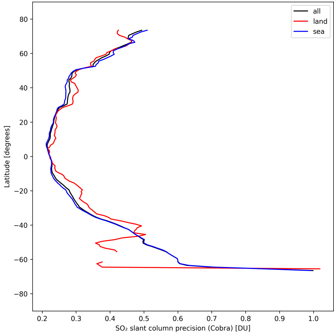
Figure 36: Zonal average of “SO 2 slant column precision (Cobra)” for 2025-09-13 to 2025-09-15.
