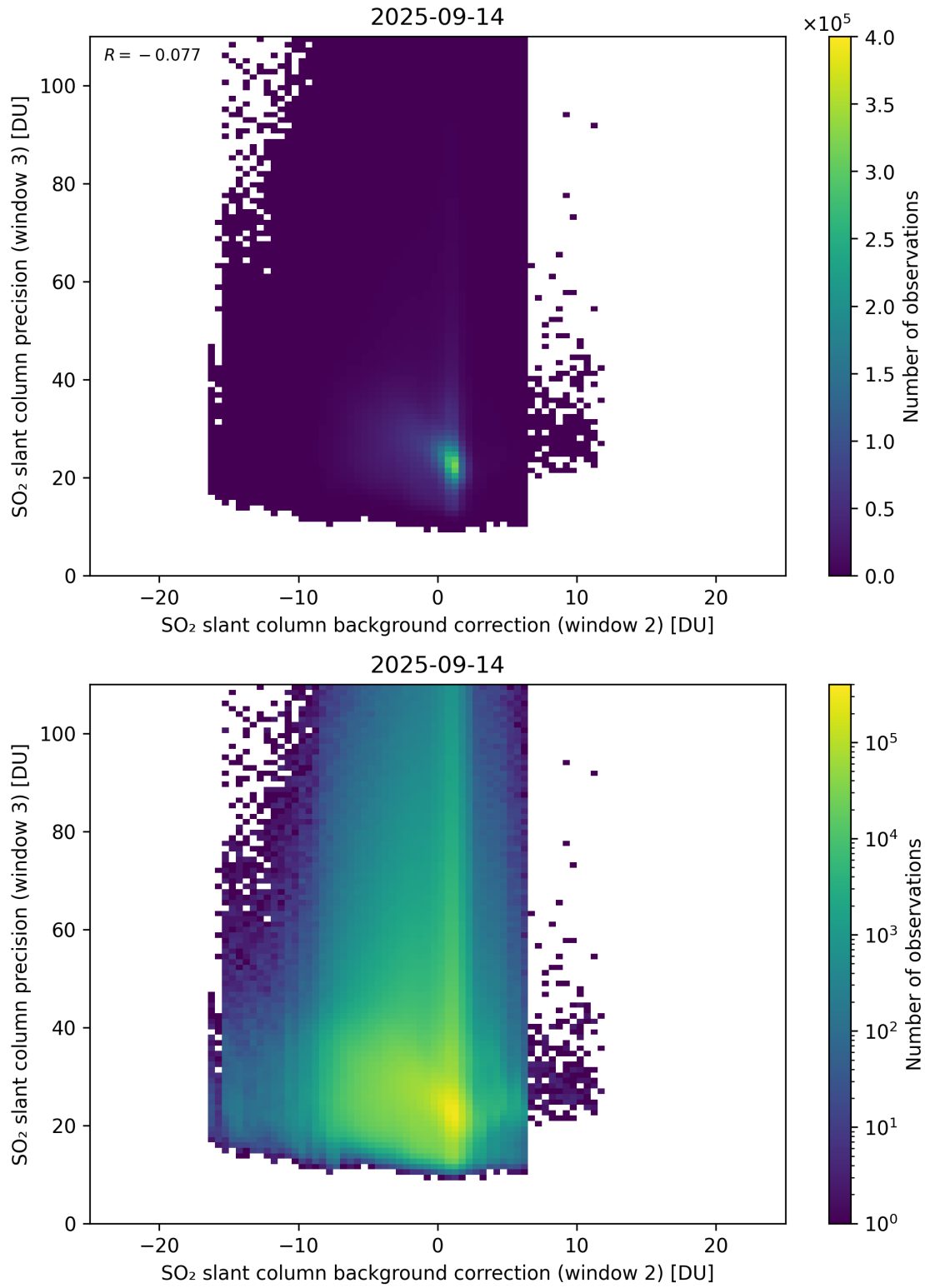
Figure 129: Scatter density plot of “SO 2 slant column background correction (window 2)” against “SO 2 slant column precision (window 3)” for 2025-09-13 to 2025-09-15.
