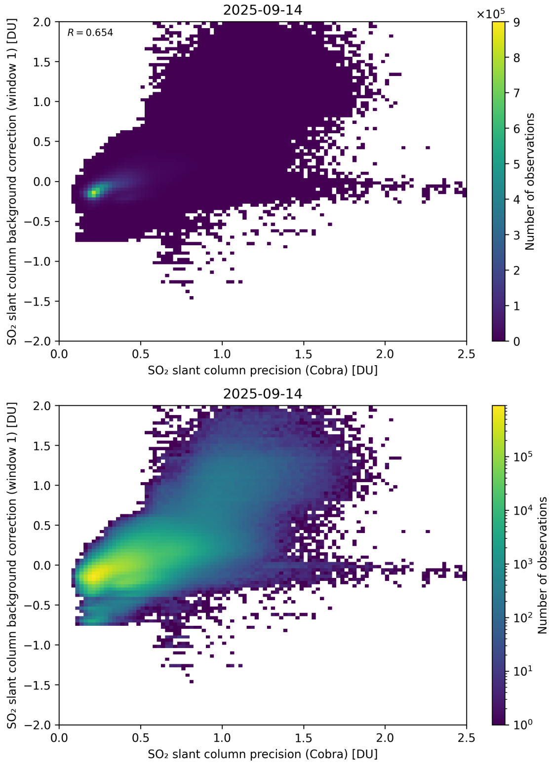
Figure 199: Scatter density plot of “SO 2 slant column precision (Cobra)” against “SO 2 slant column background correction (window 1)” for 2025-09-13 to 2025-09-15.
