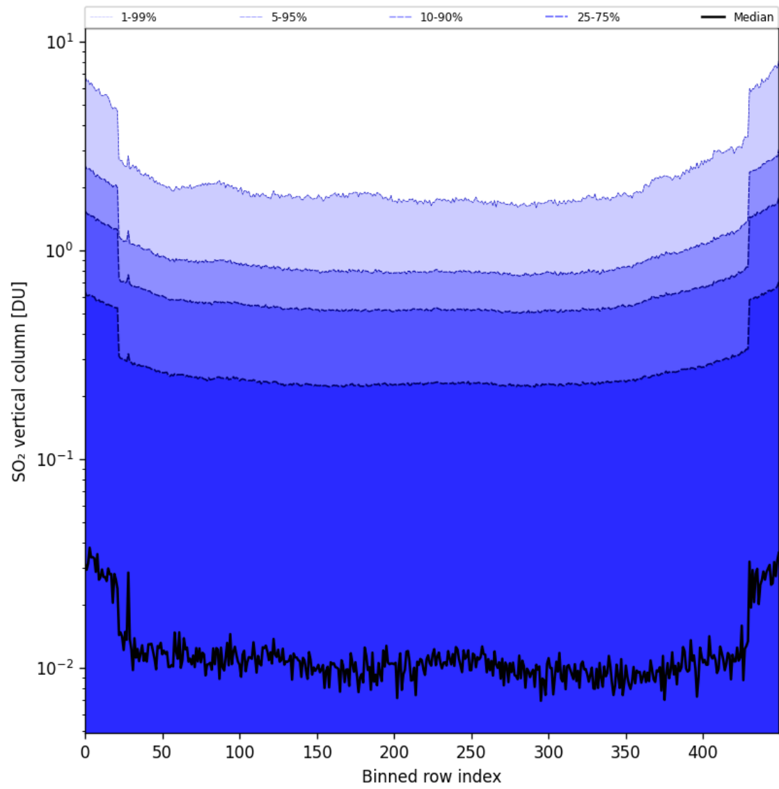
Figure 84: Along track statistics of “SO 2 vertical column” for 2025-09-13 to 2025-09-15
