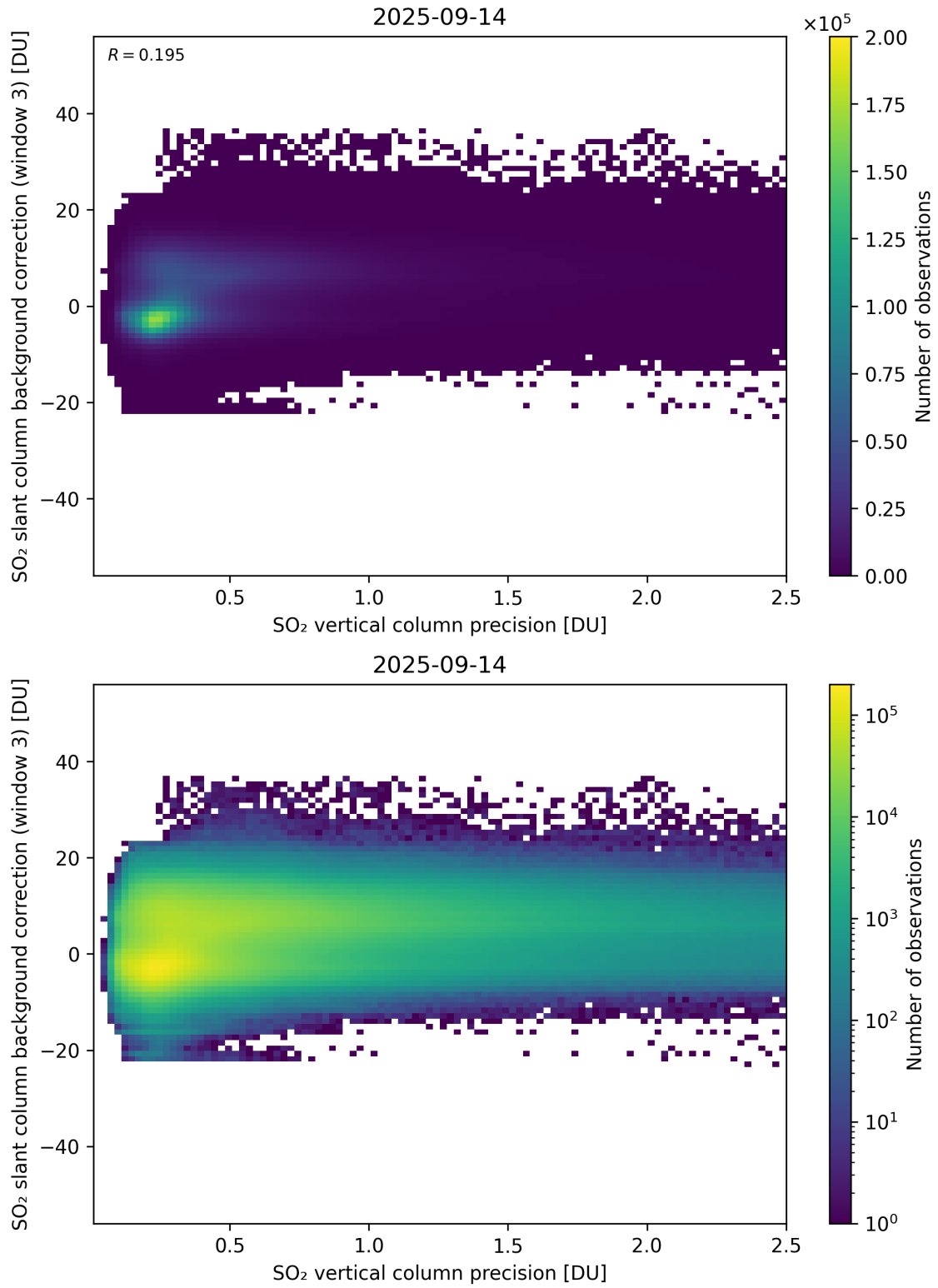
Figure 331: Scatter density plot of “SO 2 vertical column precision” against “SO 2 slant column background correction (window 3)” for 2025-09-13 to 2025-09-15.
