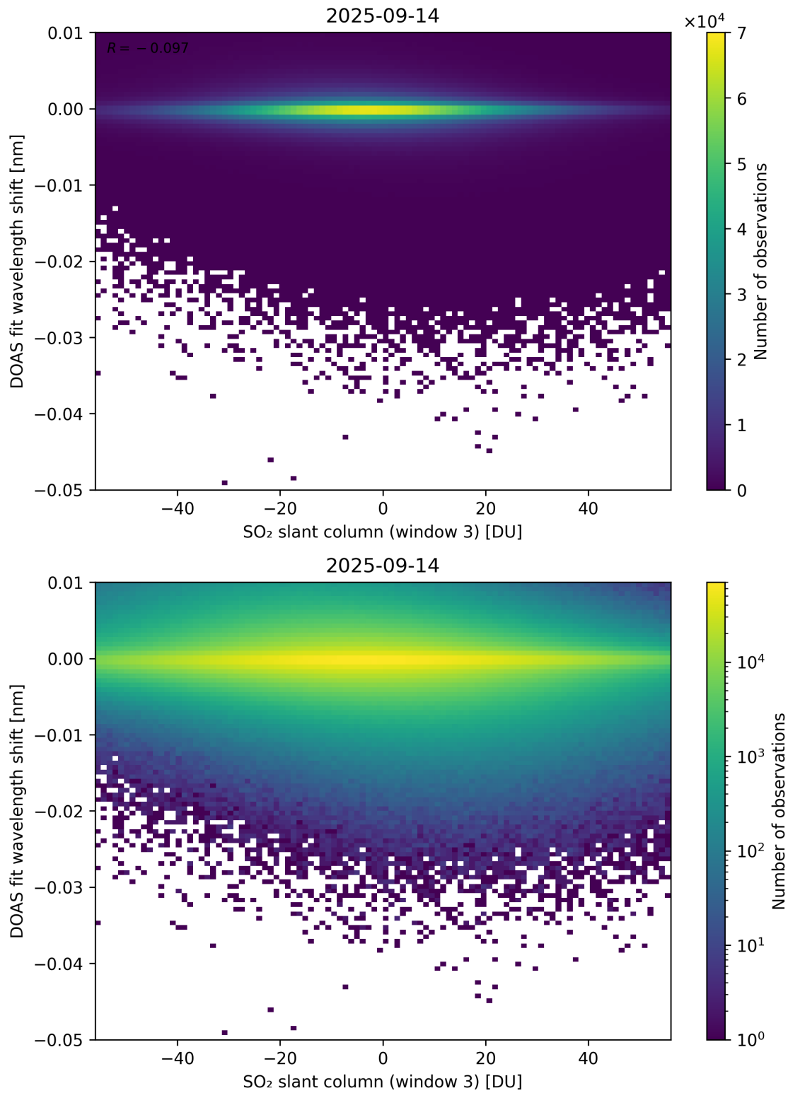
Figure 304: Scatter density plot of “SO 2 slant column (window 3)” against “DOAS fit wavelength shift” for 2025-09-13 to 2025-09-15.
