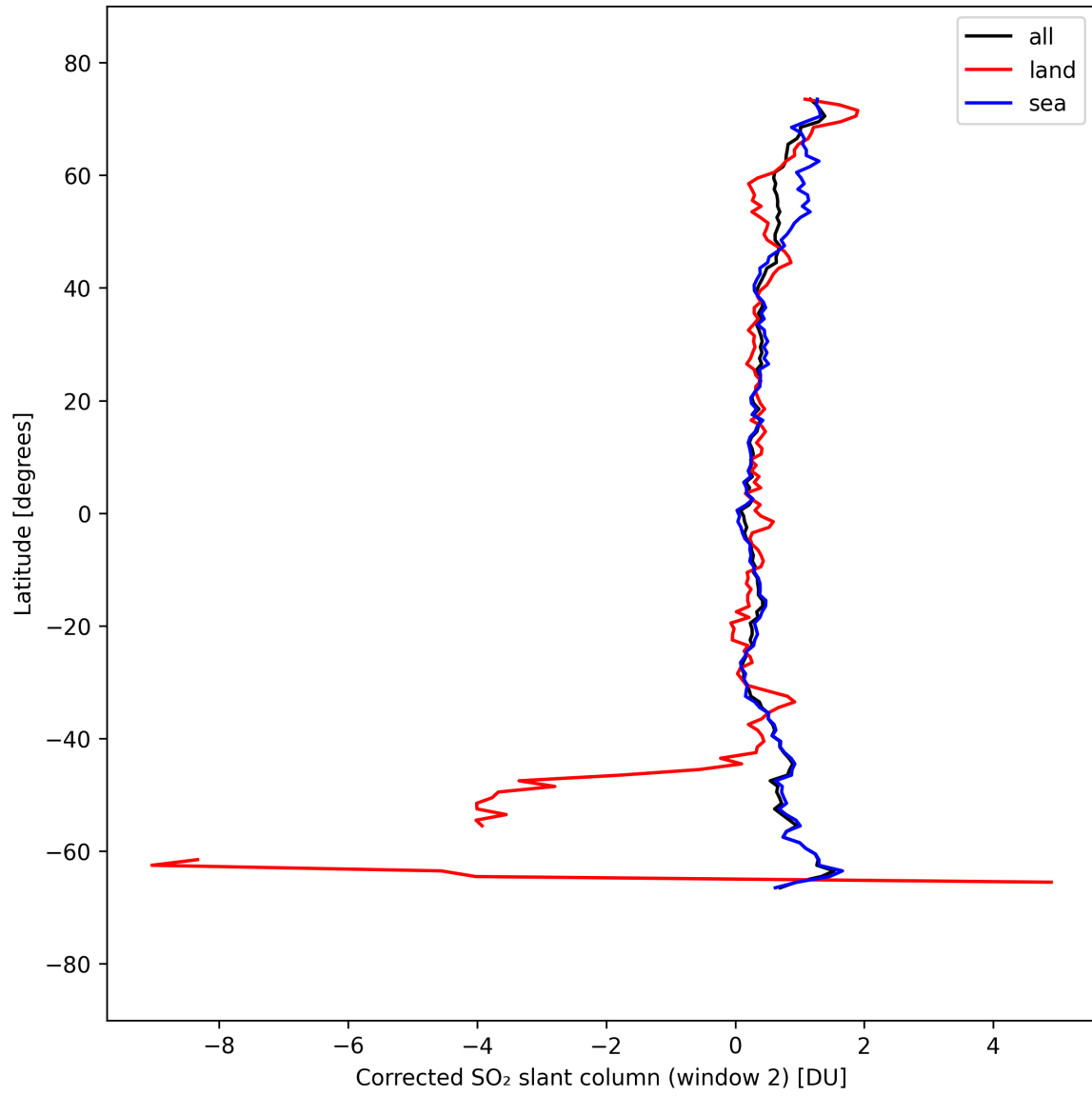
Figure 43: Zonal average of “Corrected SO 2 slant column (window 2)” for 2025-09-13 to 2025-09-15.
