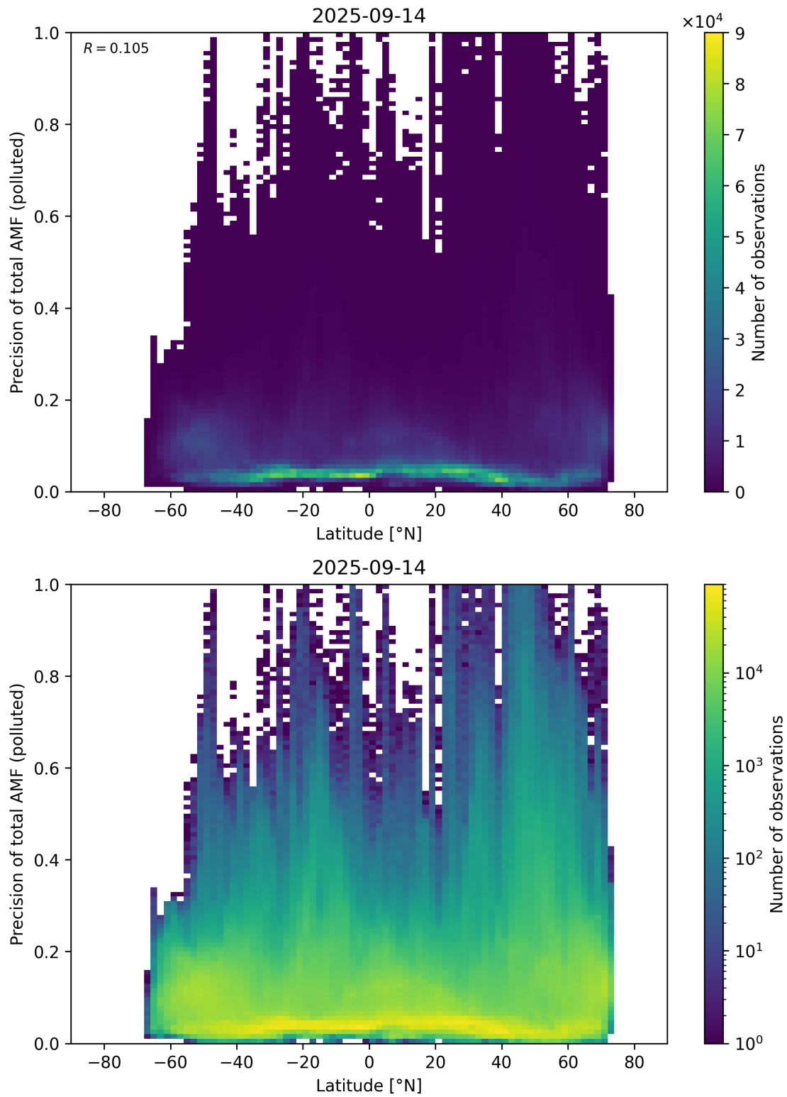
Figure 168: Scatter density plot of “Latitude” against “Precision of total AMF (polluted)” for 2025-09-13 to 2025-09-15.
