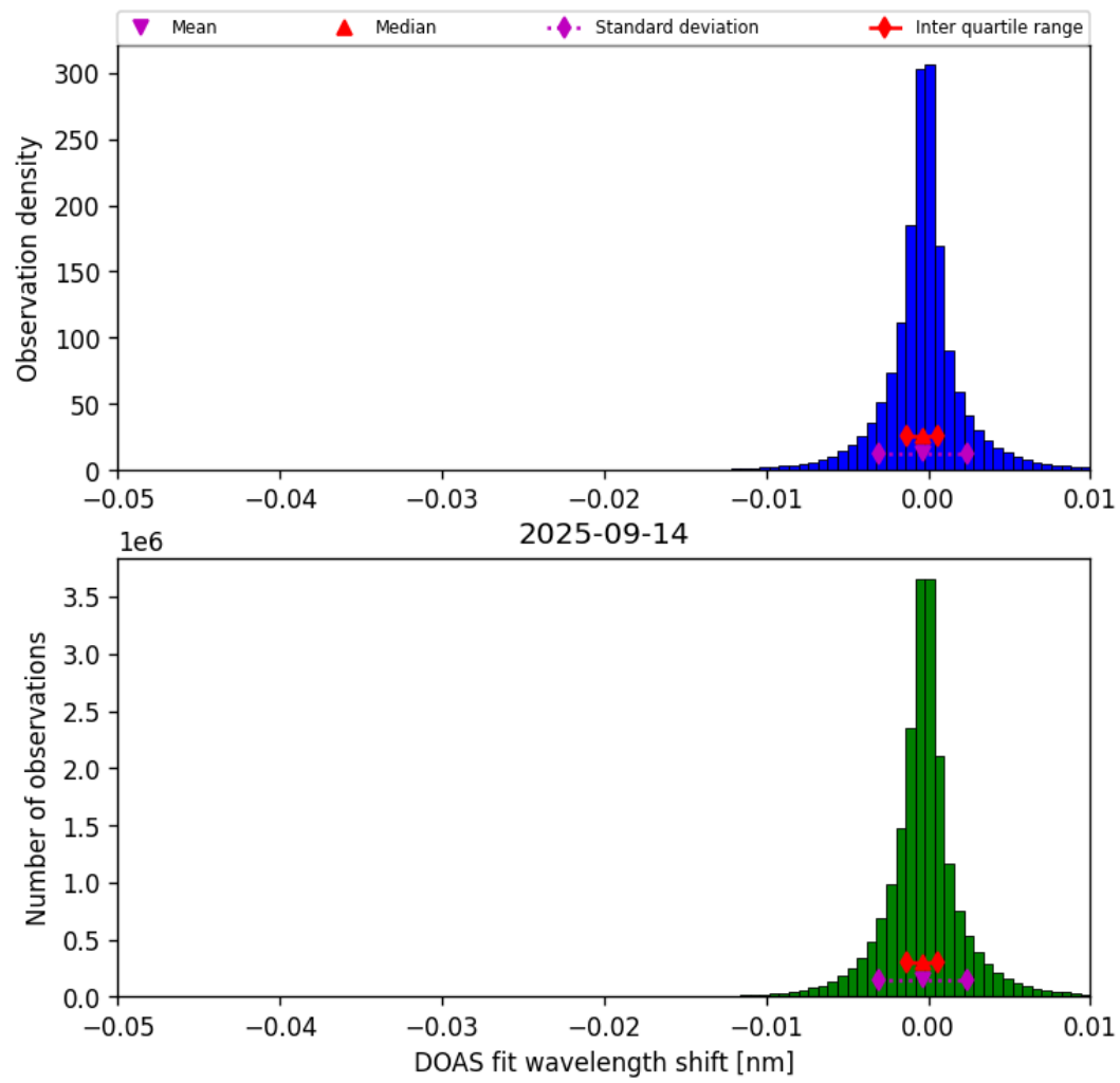
Figure 76: Histogram of “DOAS fit wavelength shift” for 2025-09-13 to 2025-09-15
