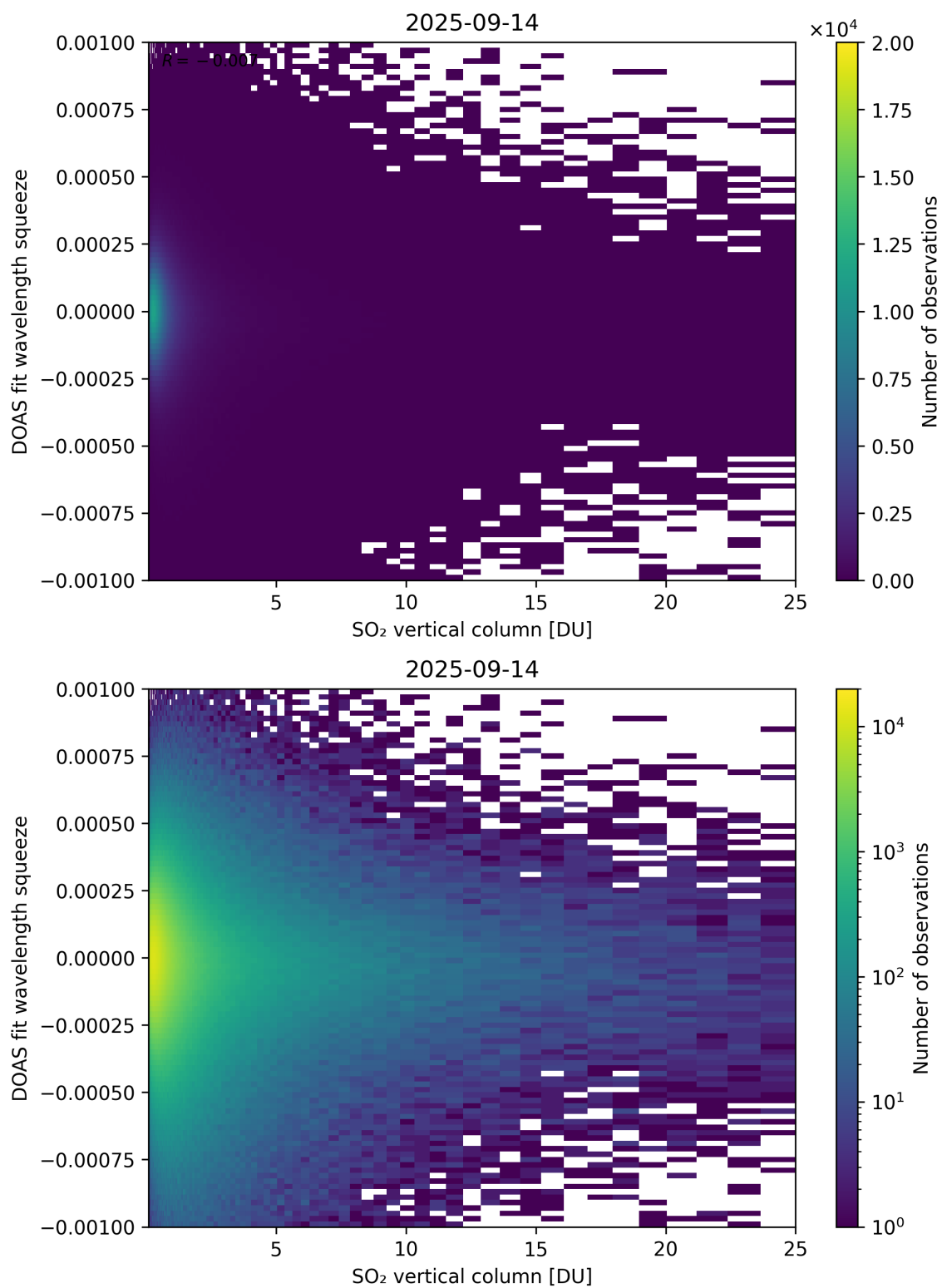
Figure 327: Scatter density plot of “SO 2 vertical column” against “DOAS fit wavelength squeeze” for 2025-09-13 to 2025-09-15.
