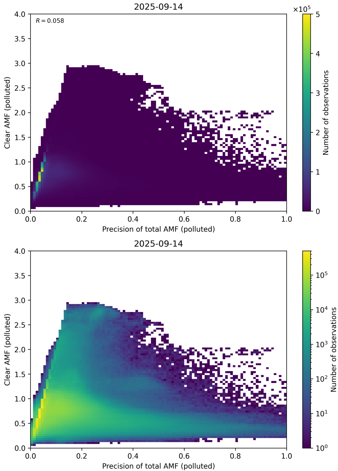
Figure 320: Scatter density plot of “Precision of total AMF (polluted)” against “Clear AMF (polluted)” for 2025-09-13 to 2025-09-15.
