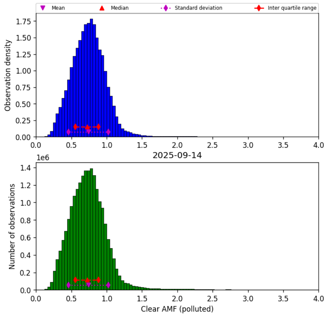
Figure 81: Histogram of “Clear AMF (polluted)” for 2025-09-13 to 2025-09-15
