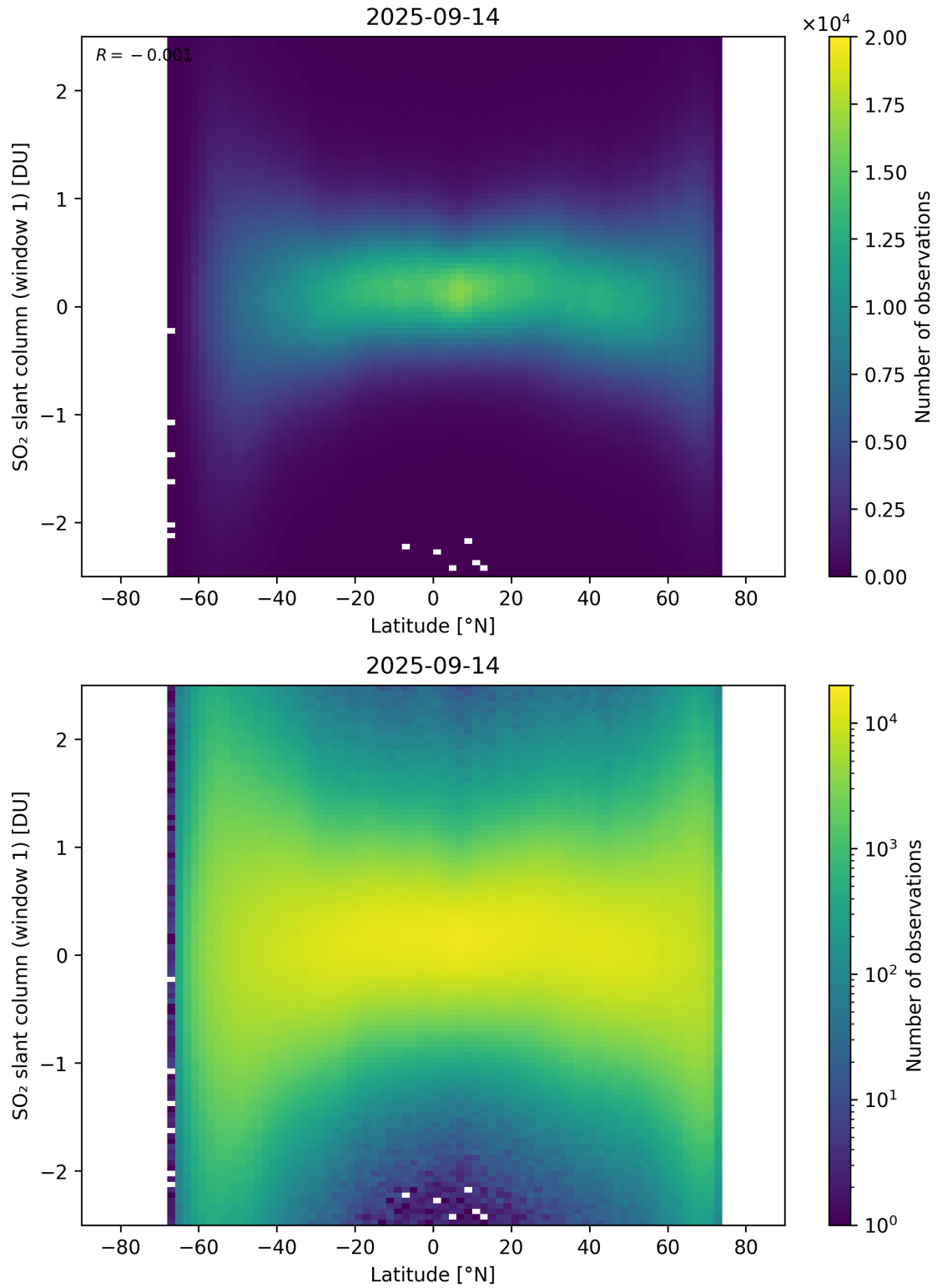
Figure 162: Scatter density plot of “Latitude” against “SO 2 slant column (window 1)” for 2025-09-13 to 2025-09-15.
