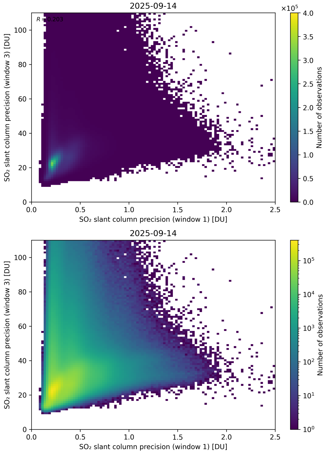
Figure 279: Scatter density plot of “SO 2 slant column precision (window 1)” against “SO 2 slant column precision (window 3)” for 2025-09-13 to 2025-09-15.
