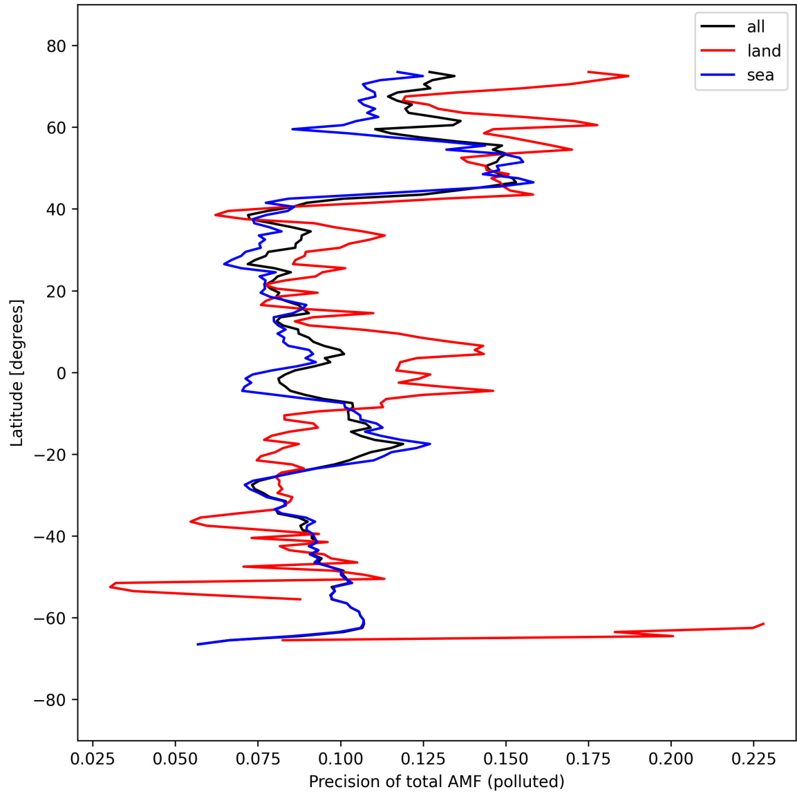
Figure 54: Zonal average of “Precision of total AMF (polluted)” for 2025-09-13 to 2025-09-15.
