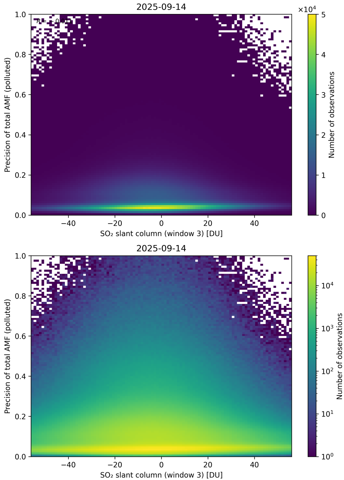
Figure 319: Scatter density plot of “SO 2 slant column (window 3)” against “Precision of total AMF (polluted)” for 2025-09-13 to 2025-09-15.
