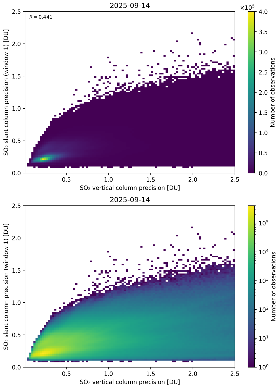
Figure 342: Scatter density plot of “SO 2 vertical column precision” against “SO 2 slant column precision (window 1)” for 2025-09-13 to 2025-09-15.
