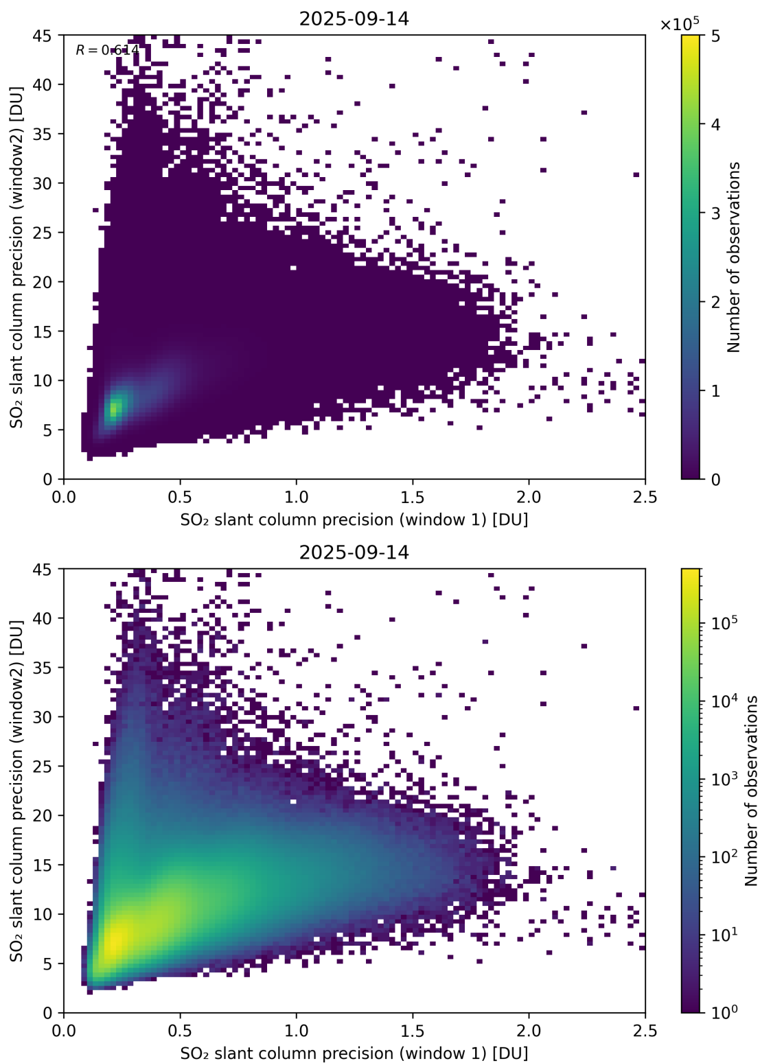
Figure 277: Scatter density plot of “SO 2 slant column precision (window 1)” against “SO 2 slant column precision (window2)” for 2025-09-13 to 2025-09-15.
