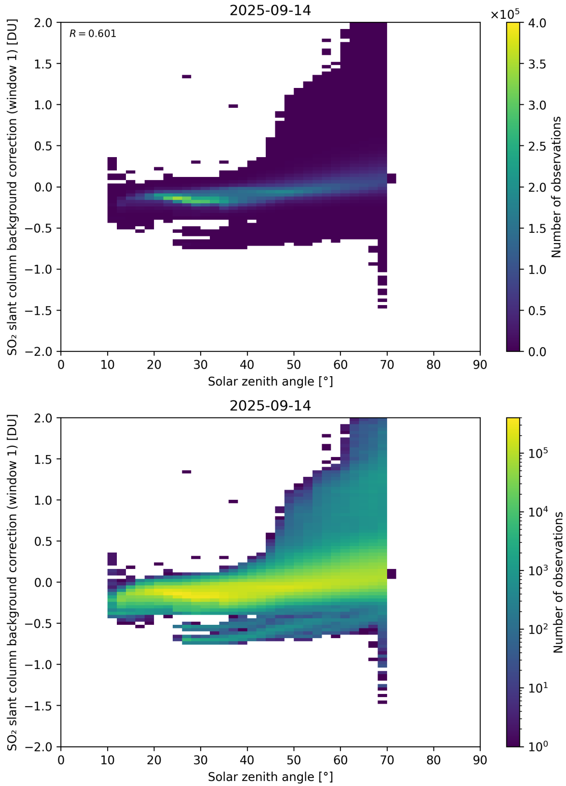
Figure 171: Scatter density plot of “Solar zenith angle” against “SO 2 slant column background correction (window 1)” for 2025-09-13 to 2025-09-15.
