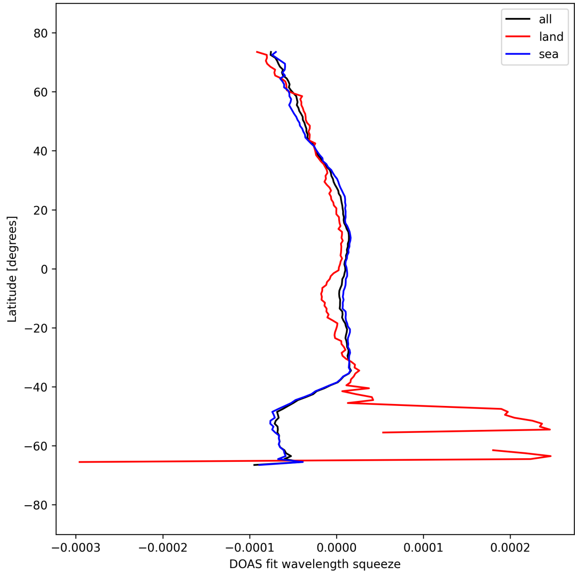
Figure 51: Zonal average of “DOAS fit wavelength squeeze” for 2025-09-13 to 2025-09-15.
