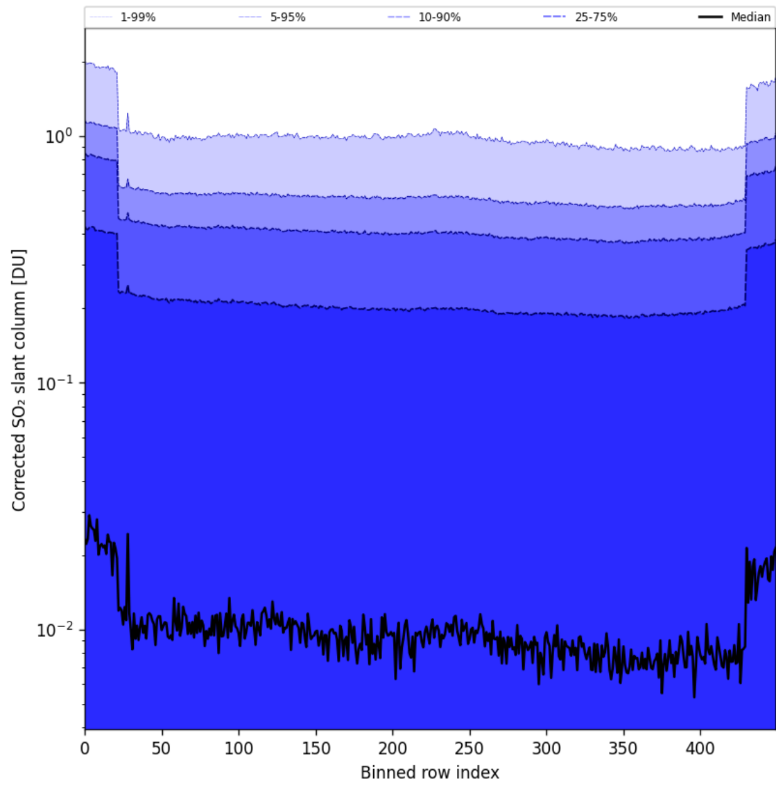
Figure 86: Along track statistics of “Corrected SO 2 slant column” for 2025-09-13 to 2025-09-15
