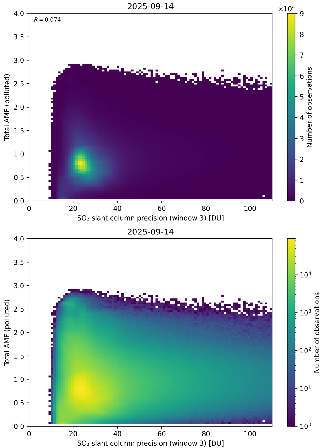
Figure 313: Scatter density plot of “SO 2 slant column precision (window 3)” against “Total AMF (polluted)” for 2025-09-13 to 2025-09-15.
