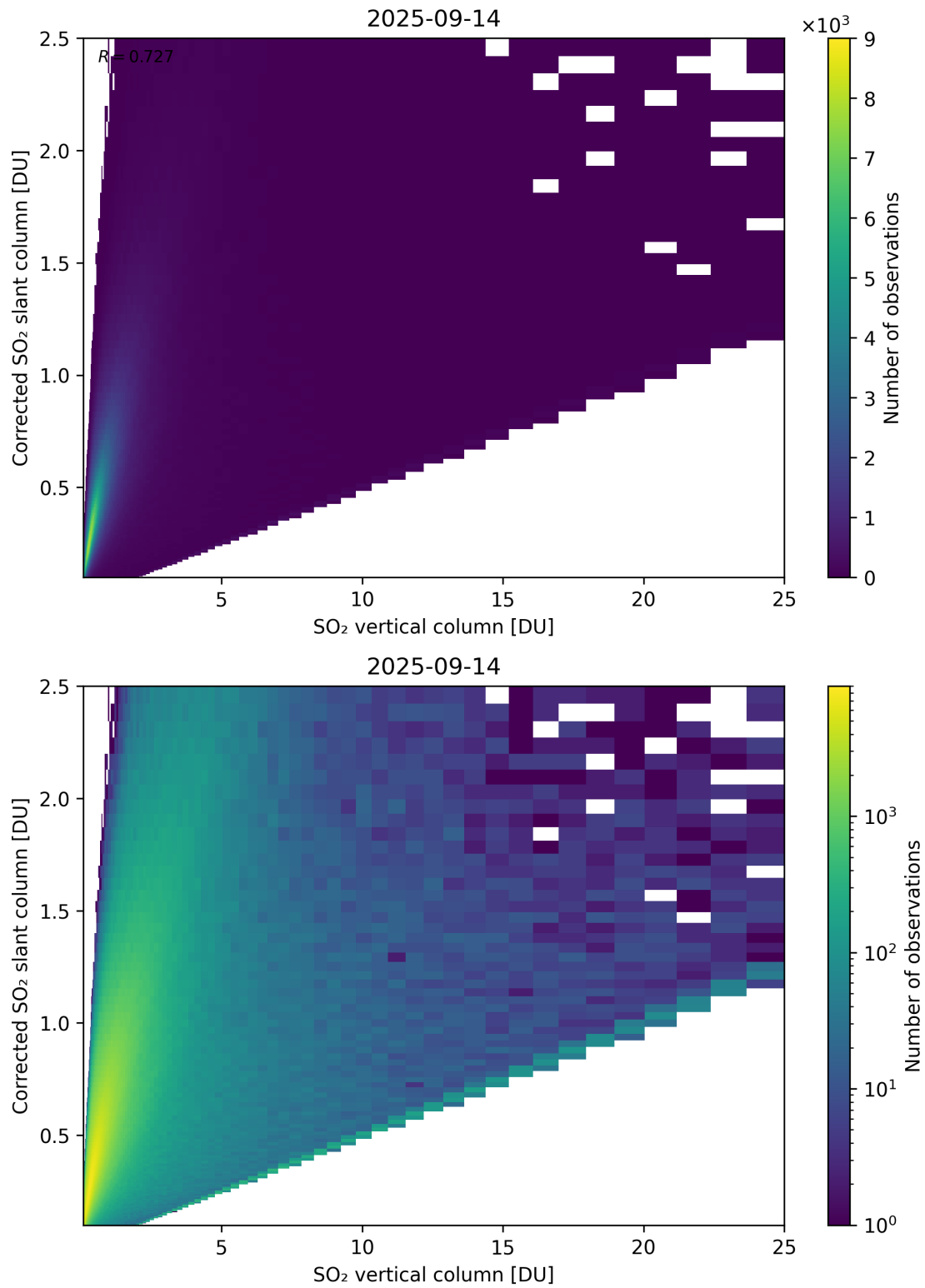
Figure 351: Scatter density plot of “SO 2 vertical column” against “Corrected SO 2 slant column” for 2025-09-13 to 2025-09-15.
