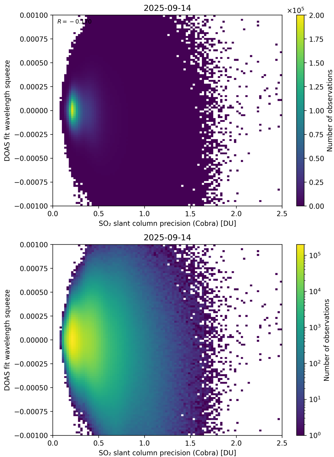
Figure 203: Scatter density plot of “SO 2 slant column precision (Cobra)” against “DOAS fit wavelength squeeze” for 2025-09-13 to 2025-09-15.
