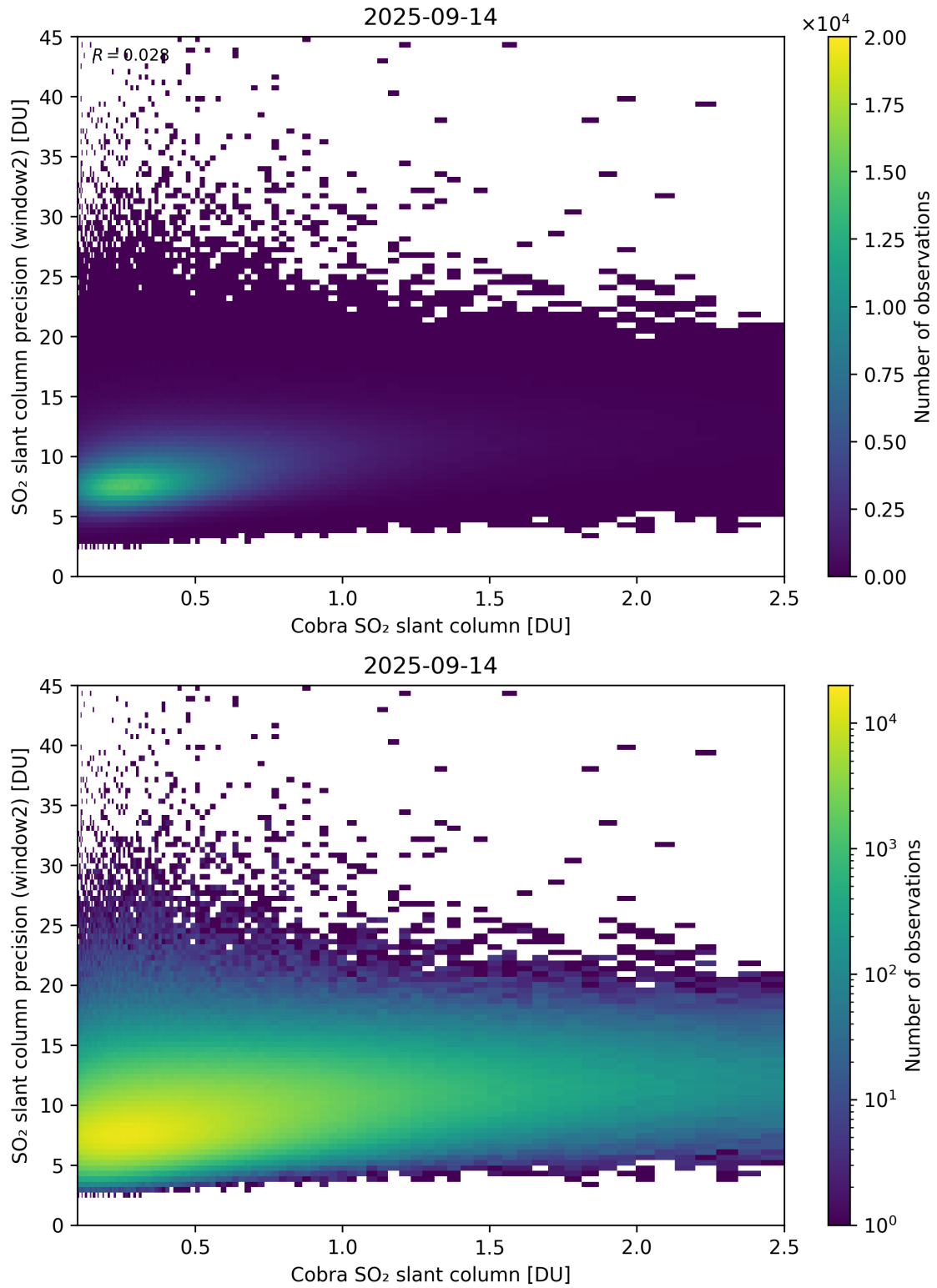
Figure 221: Scatter density plot of “Cobra SO 2 slant column” against “SO 2 slant column precision (window2)” for 2025-09-13 to 2025-09-15.
