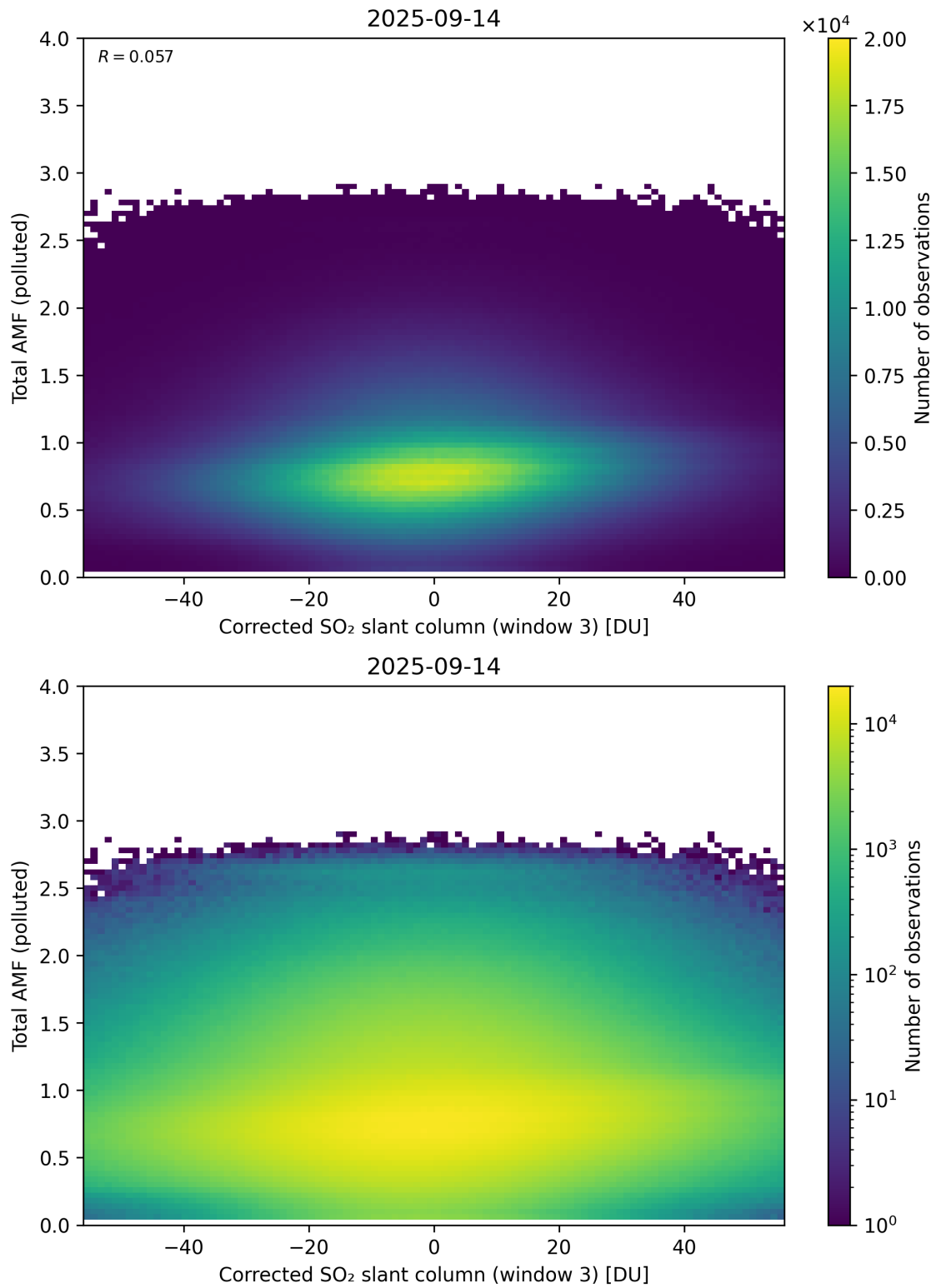
Figure 260: Scatter density plot of “Corrected SO 2 slant column (window 3)” against “Total AMF (polluted)” for 2025-09-13 to 2025-09-15.
