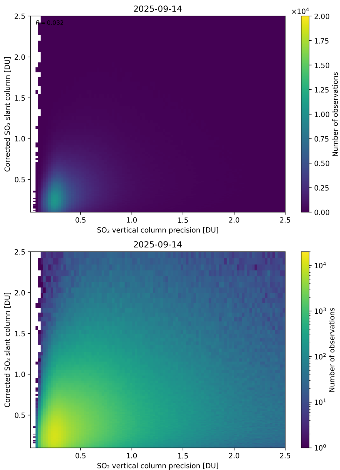
Figure 338: Scatter density plot of “SO 2 vertical column precision” against “Corrected SO 2 slant column” for 2025-09-13 to 2025-09-15.
