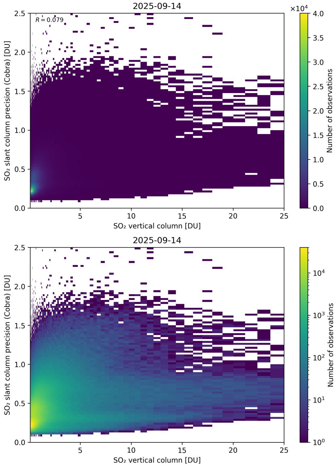
Figure 350: Scatter density plot of “SO 2 vertical column” against “SO 2 slant column precision (Cobra)” for 2025-09-13 to 2025-09-15.
