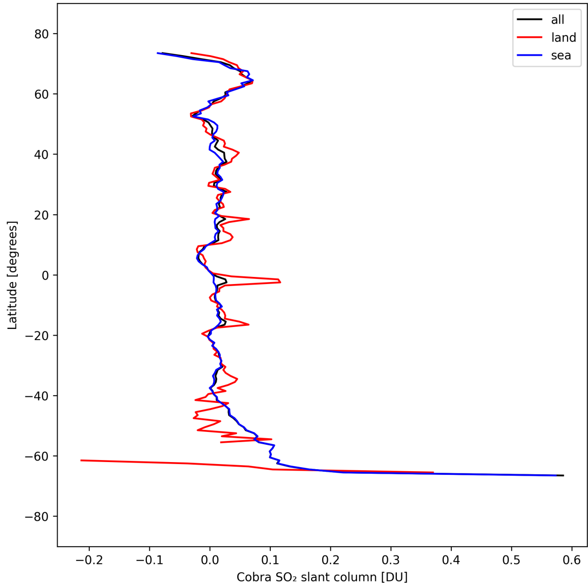
Figure 35: Zonal average of “Cobra SO 2 slant column” for 2025-09-13 to 2025-09-15.
