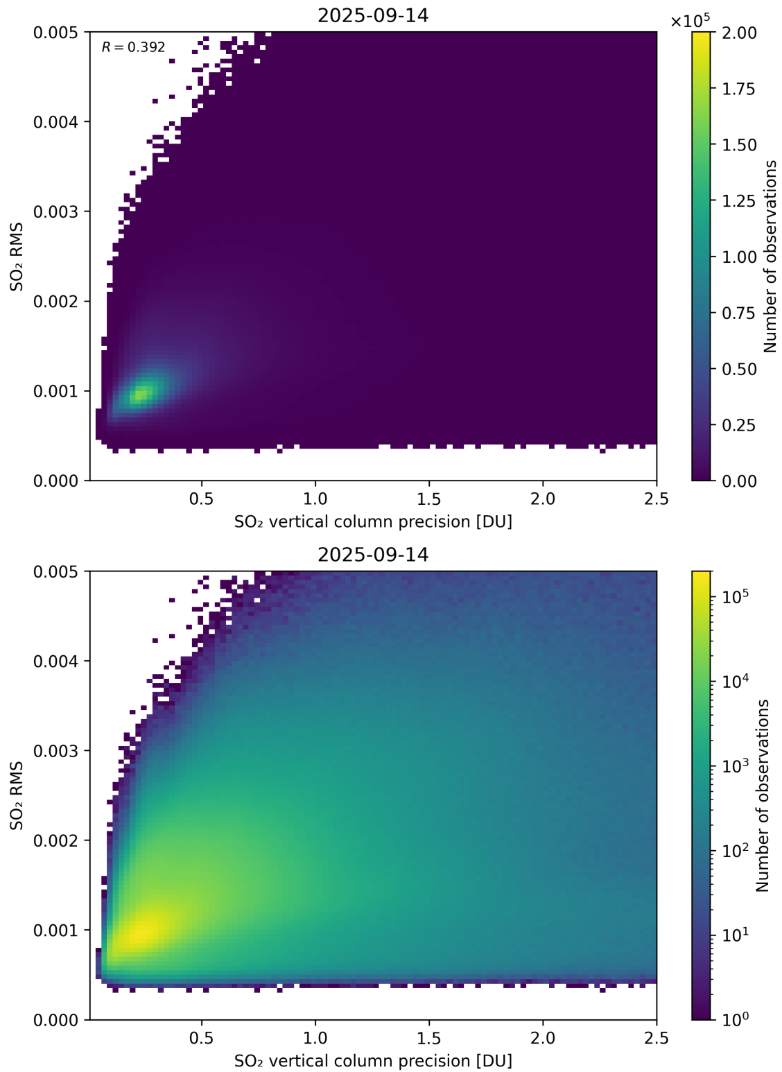
Figure 334: Scatter density plot of “SO 2 vertical column precision” against “SO 2 RMS” for 2025-09-13 to 2025-09-15.
