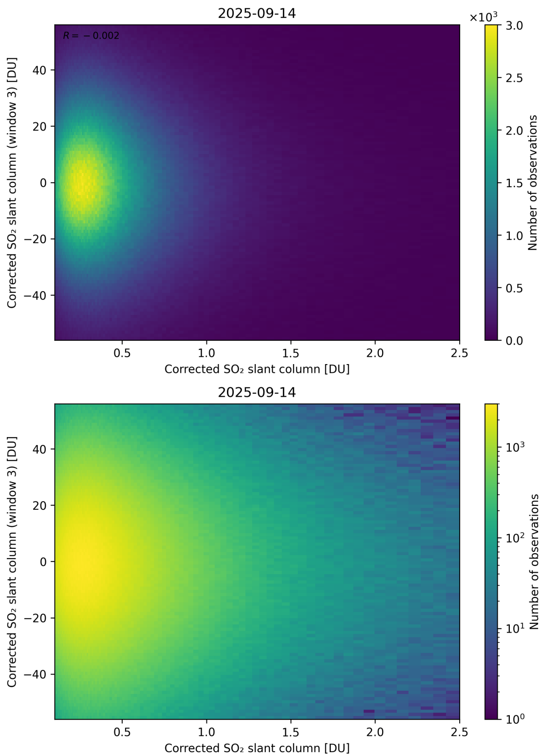
Figure 236: Scatter density plot of “Corrected SO 2 slant column” against “Corrected SO 2 slant column (window 3)” for 2025-09-13 to 2025-09-15.
