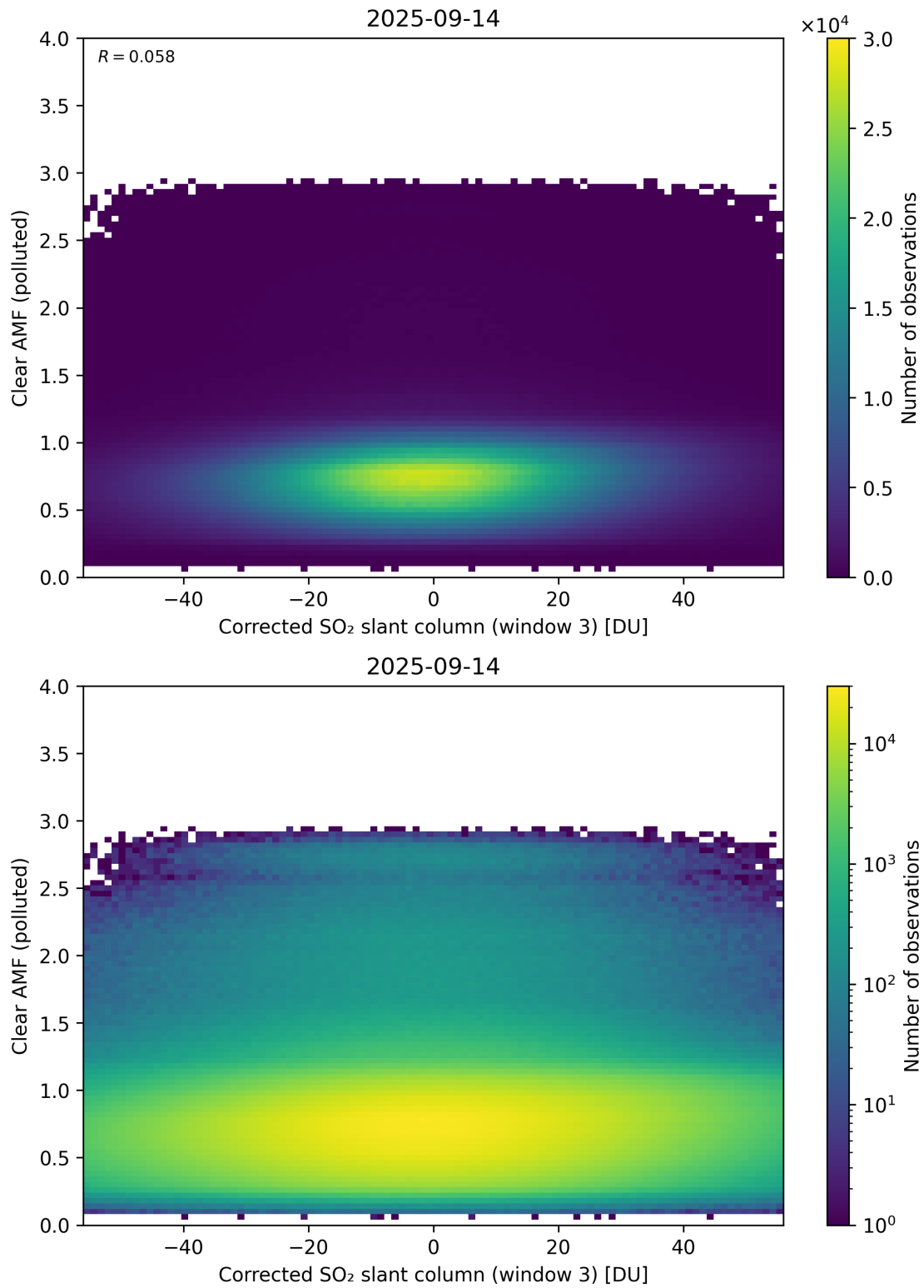
Figure 259: Scatter density plot of “Corrected SO 2 slant column (window 3)” against “Clear AMF (polluted)” for 2025-09-13 to 2025-09-15.
