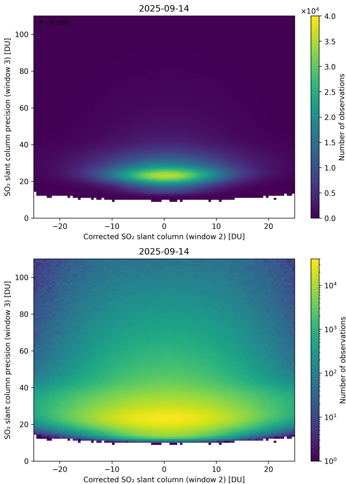
Figure 252: Scatter density plot of “Corrected SO 2 slant column (window 2)” against “SO 2 slant column precision (window 3)” for 2025-09-13 to 2025-09-15.
