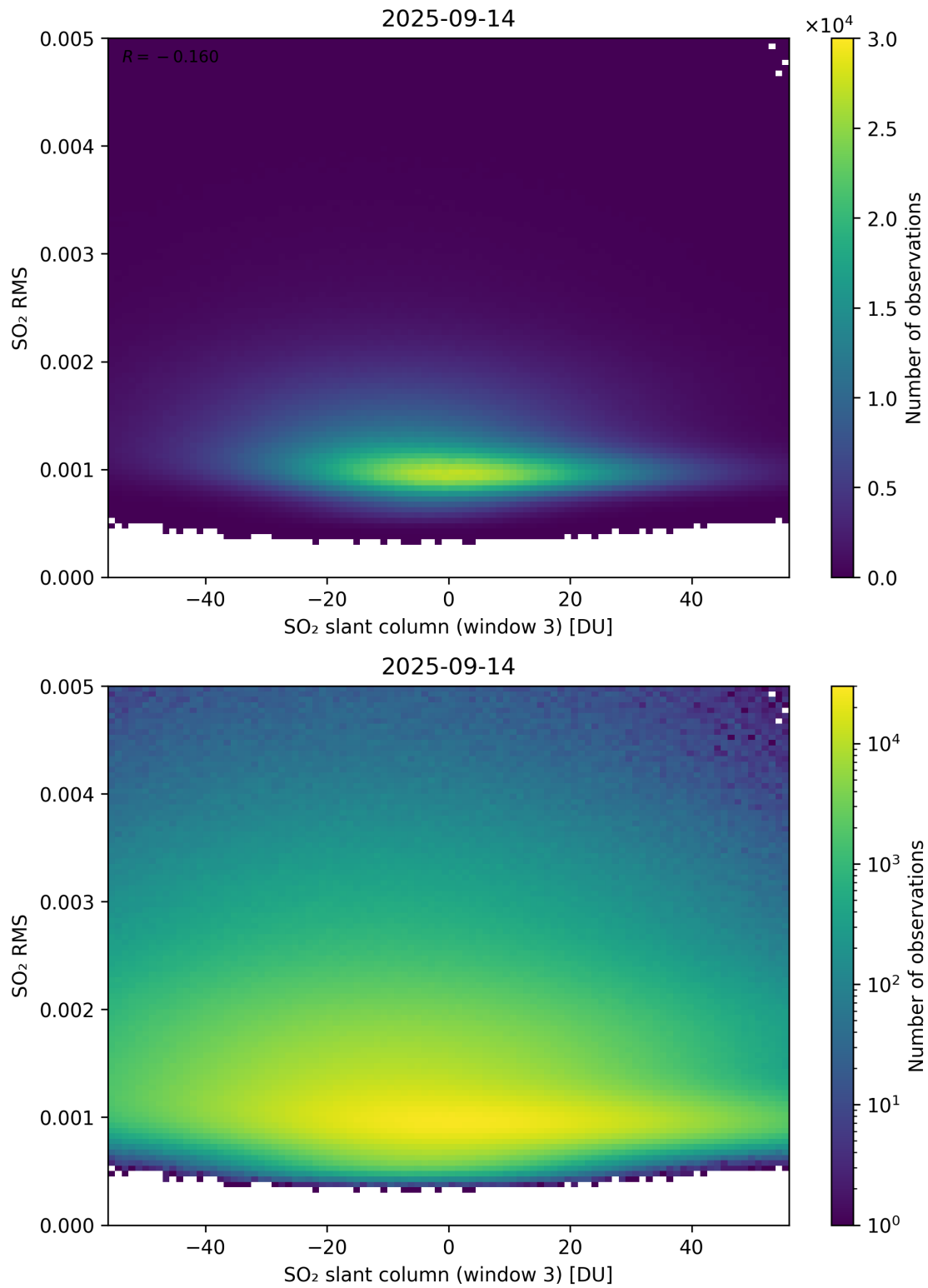
Figure 306: Scatter density plot of “SO 2 slant column (window 3)” against “SO 2 RMS” for 2025-09-13 to 2025-09-15.
