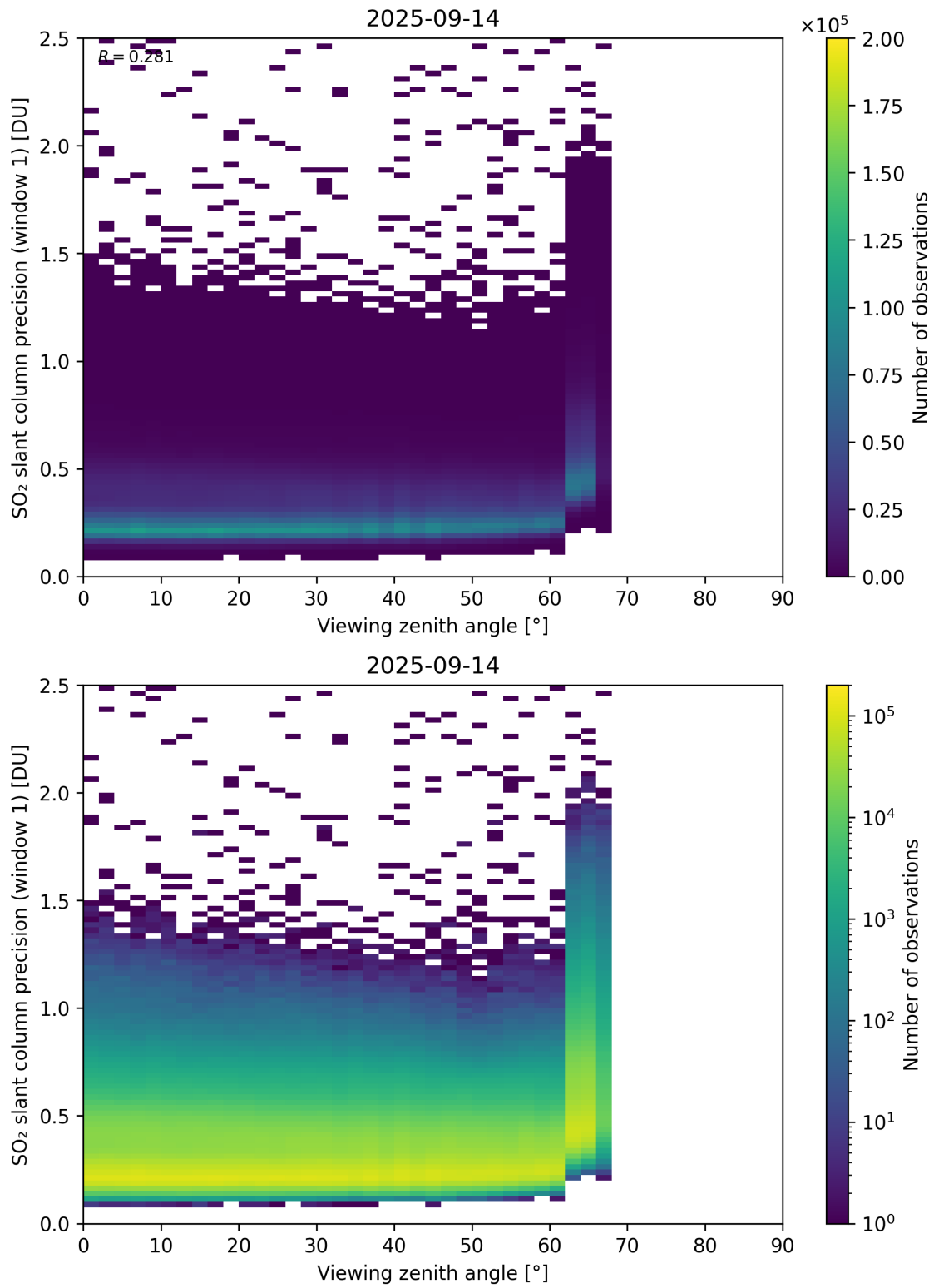
Figure 377: Scatter density plot of “Viewing zenith angle” against “SO 2 slant column precision (window 1)” for 2025-09-13 to 2025-09-15.
