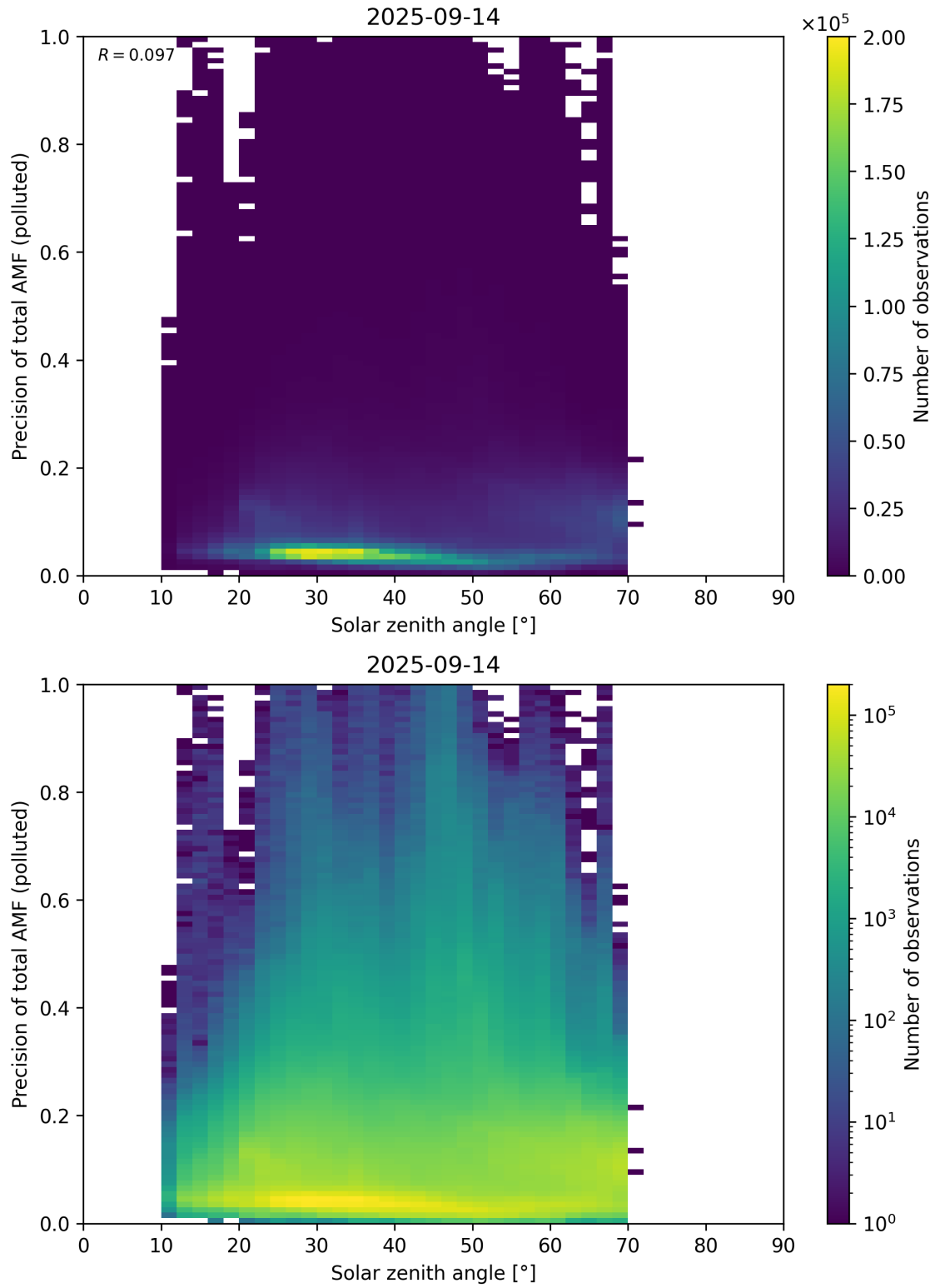
Figure 190: Scatter density plot of “Solar zenith angle” against “Precision of total AMF (polluted)” for 2025-09-13 to 2025-09-15.
