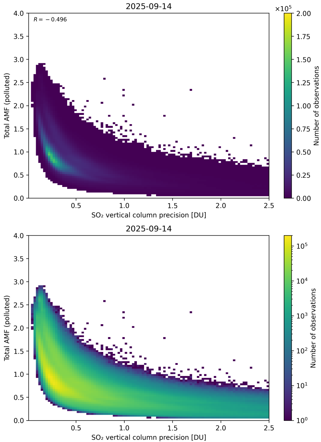
Figure 346: Scatter density plot of “SO 2 vertical column precision” against “Total AMF (polluted)” for 2025-09-13 to 2025-09-15.
