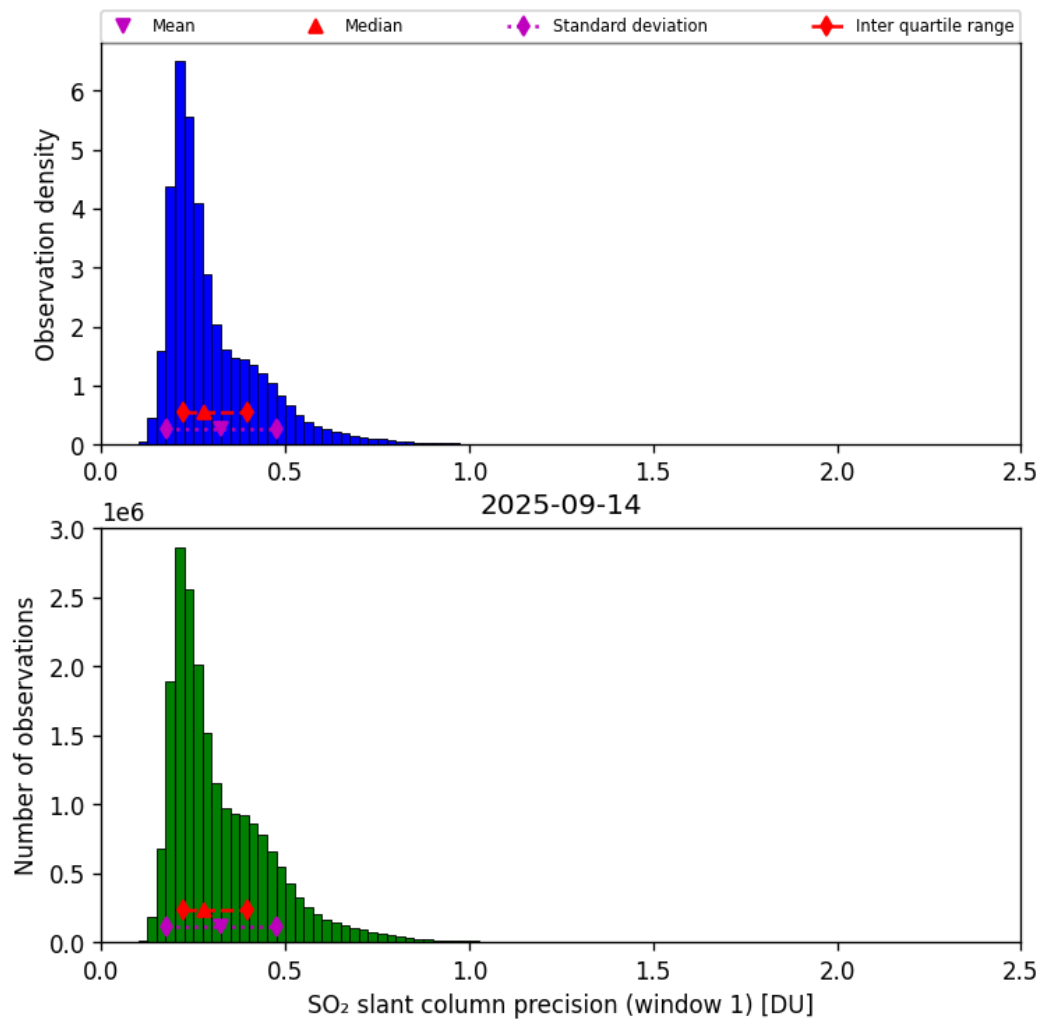
Figure 64: Histogram of “SO 2 slant column precision (window 1)” for 2025-09-13 to 2025-09-15
