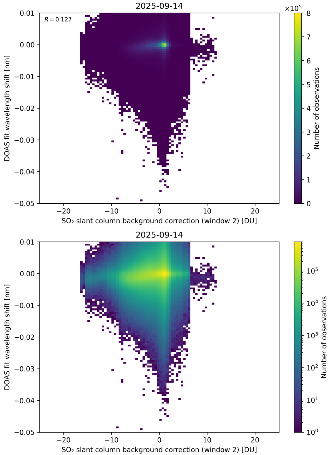
Figure 123: Scatter density plot of “SO 2 slant column background correction (window 2)” against “DOAS fit wavelength shift” for 2025-09-13 to 2025-09-15.
