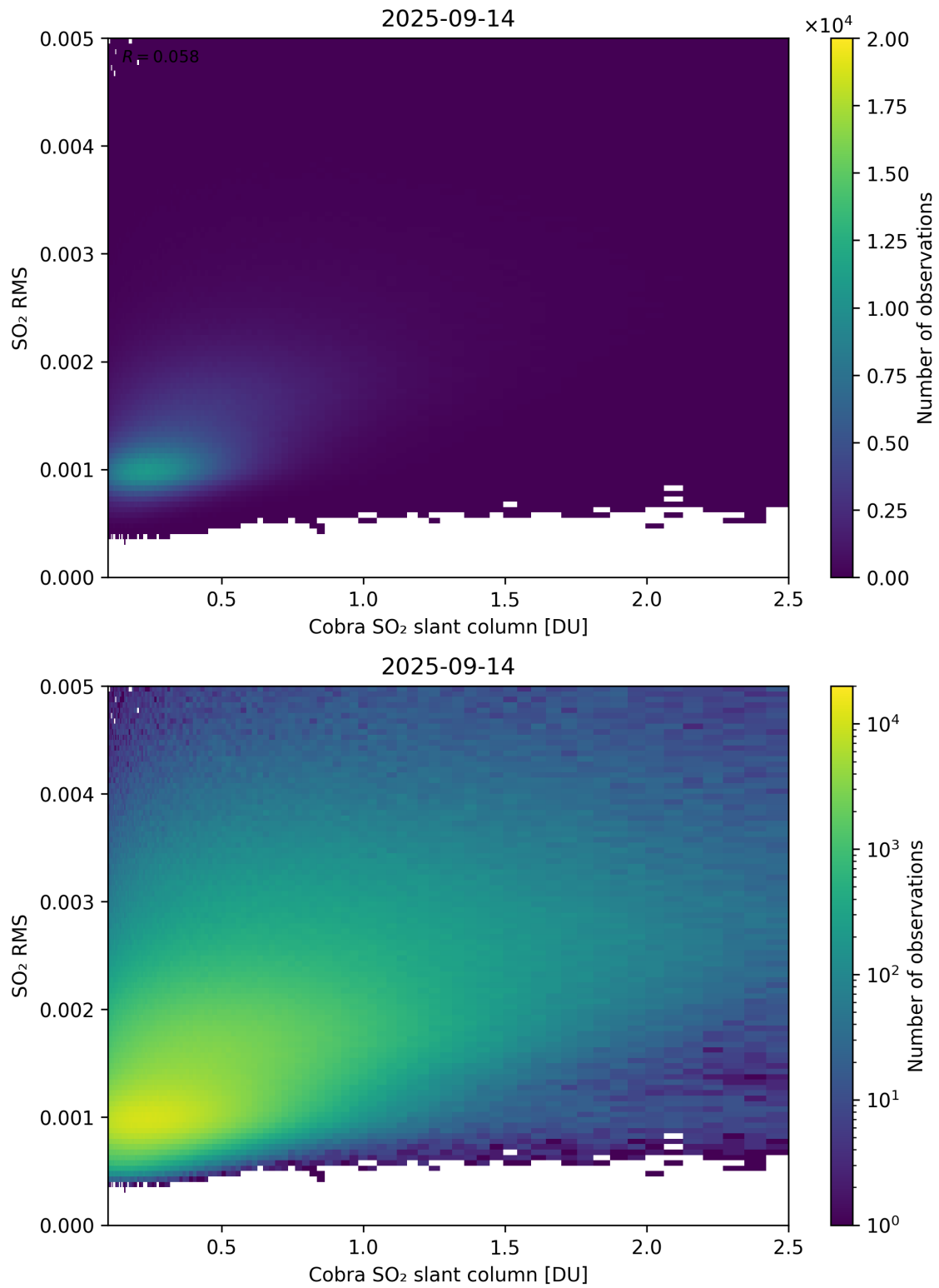
Figure 198: Scatter density plot of “Cobra SO 2 slant column” against “SO 2 RMS” for 2025-09-13 to 2025-09-15.
