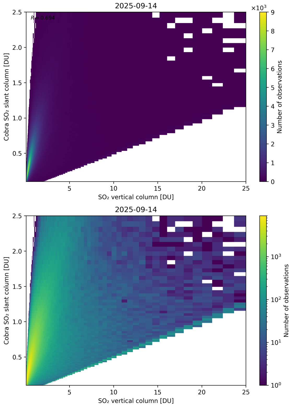
Figure 349: Scatter density plot of “SO 2 vertical column” against “Cobra SO 2 slant column” for 2025-09-13 to 2025-09-15.
