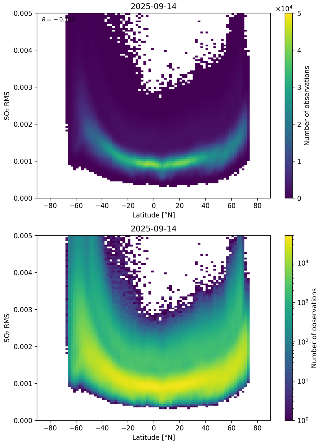
Figure 155: Scatter density plot of “Latitude” against “SO 2 RMS” for 2025-09-13 to 2025-09-15.
