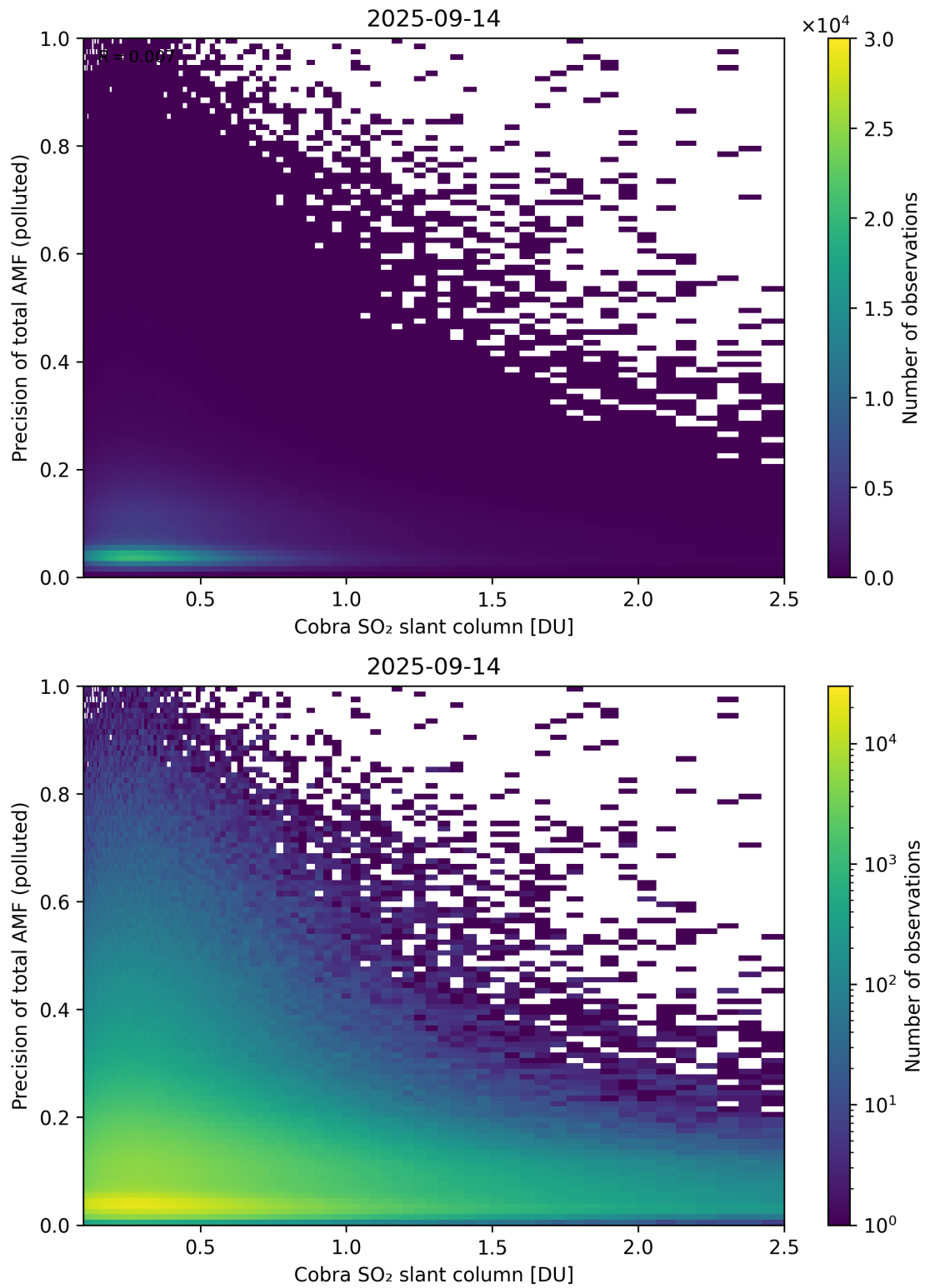
Figure 225: Scatter density plot of “Cobra SO 2 slant column” against “Precision of total AMF (polluted)” for 2025-09-13 to 2025-09-15.
