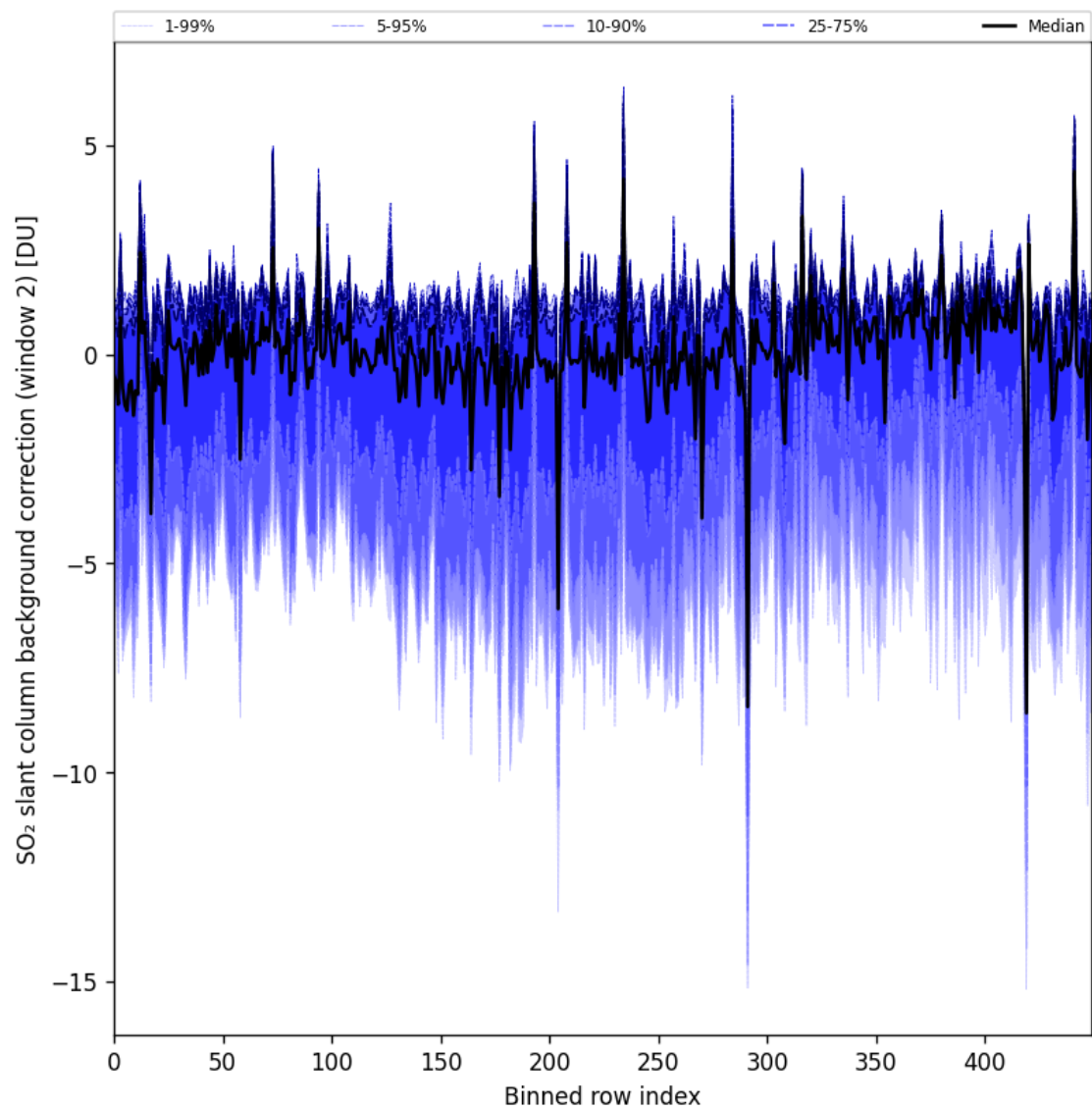
Figure 96: Along track statistics of “SO 2 slant column background correction (window 2)” for 2025-09-13 to 2025-09-15
