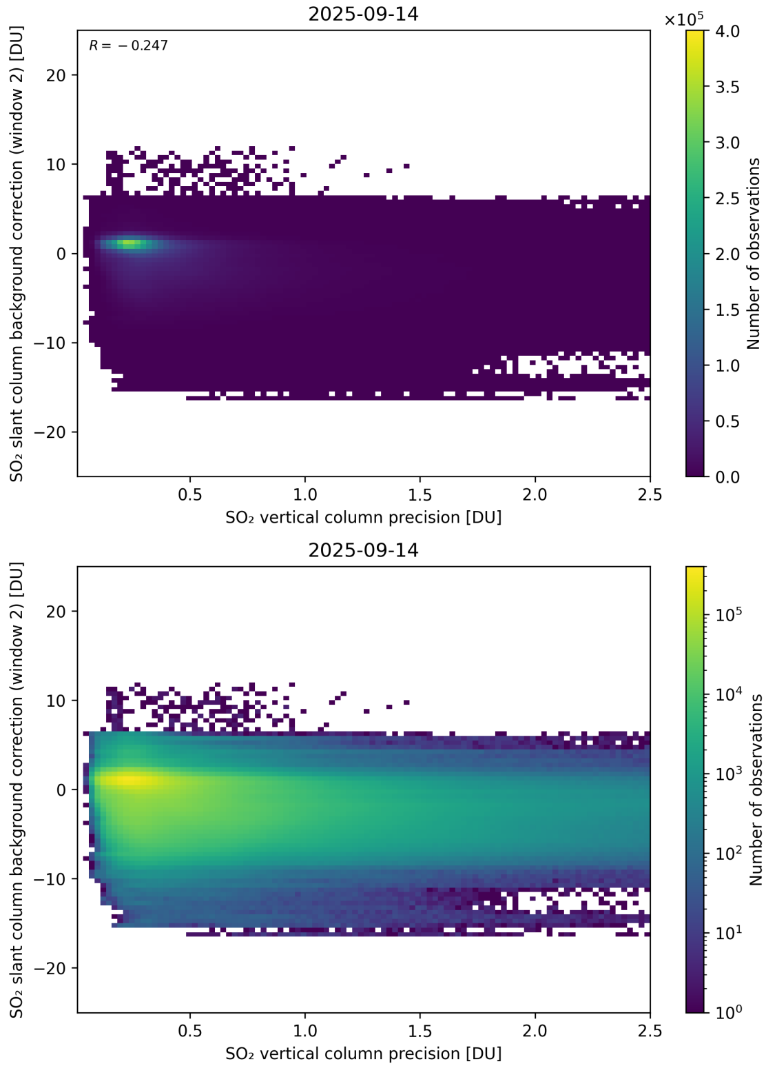
Figure 330: Scatter density plot of “SO 2 vertical column precision” against “SO 2 slant column background correction (window 2)” for 2025-09-13 to 2025-09-15.
