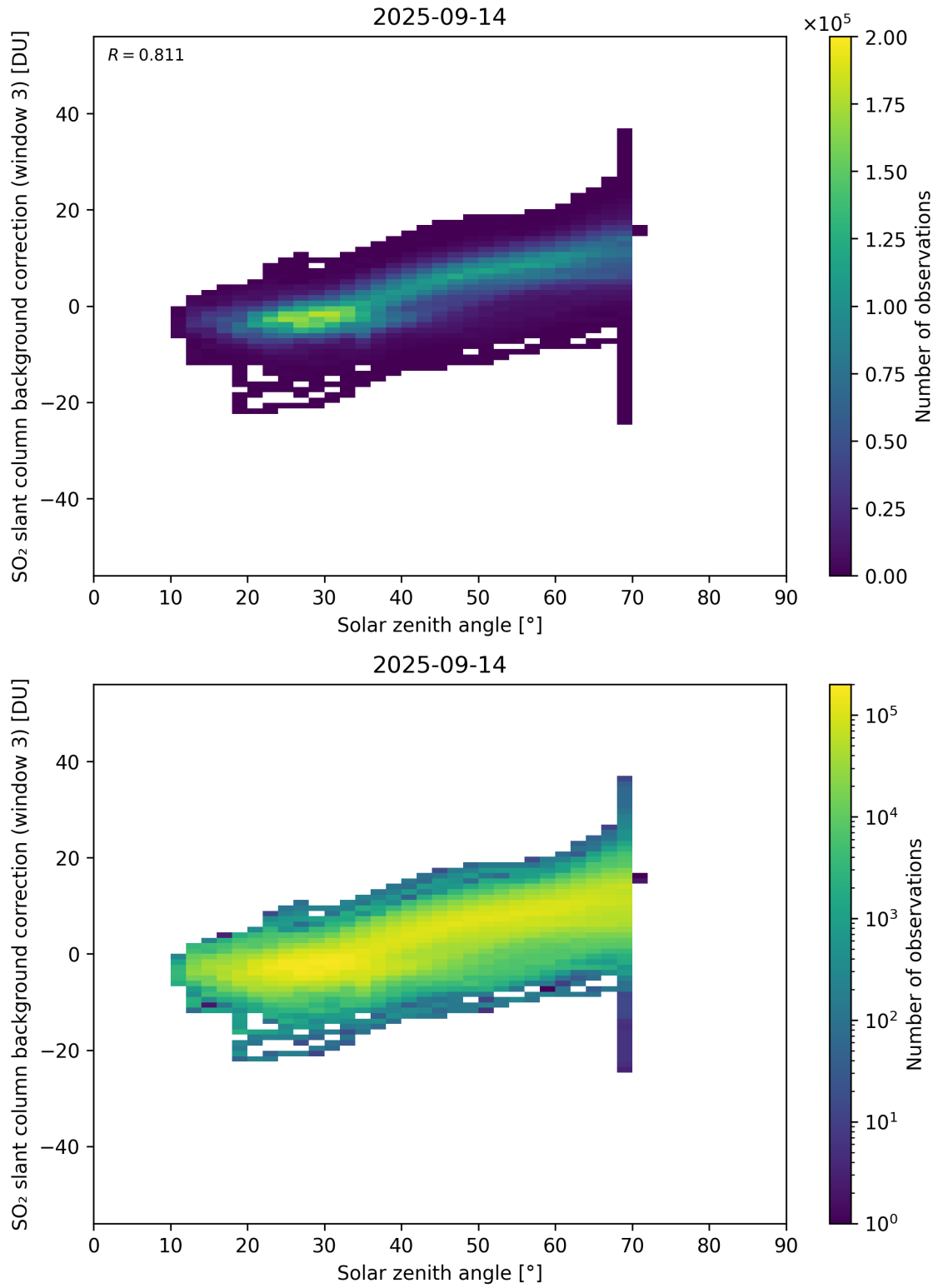
Figure 173: Scatter density plot of “Solar zenith angle” against “SO 2 slant column background correction (window 3)” for 2025-09-13 to 2025-09-15.
