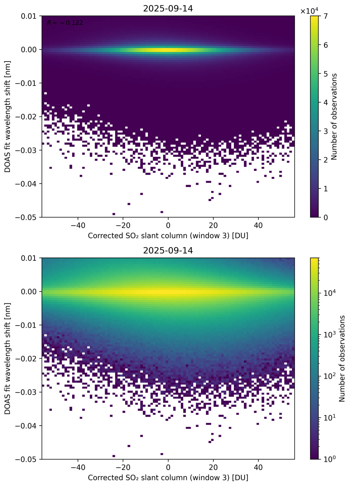
Figure 256: Scatter density plot of “Corrected SO 2 slant column (window 3)” against “DOAS fit wavelength shift” for 2025-09-13 to 2025-09-15.
