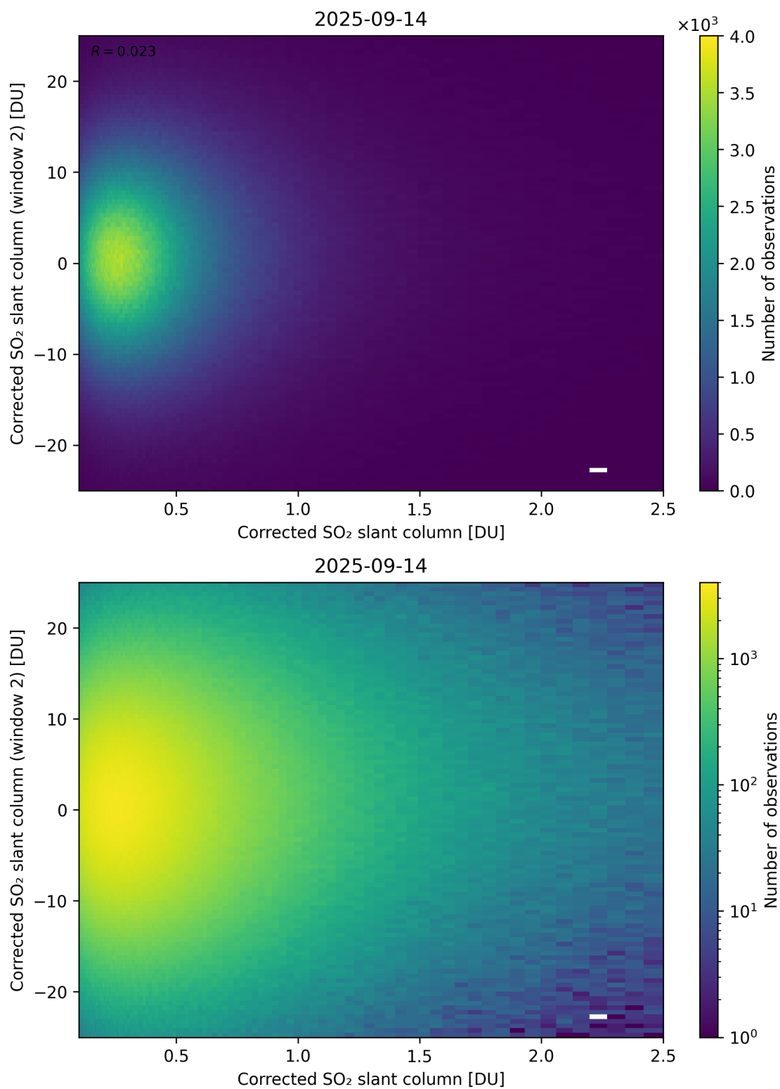
Figure 235: Scatter density plot of “Corrected SO 2 slant column” against “Corrected SO 2 slant column (window 2)” for 2025-09-13 to 2025-09-15.
