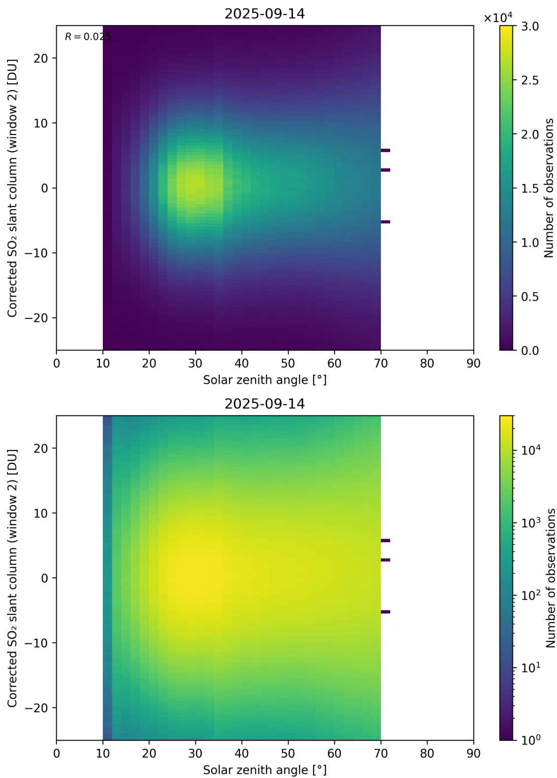
Figure 182: Scatter density plot of “Solar zenith angle” against “Corrected SO 2 slant column (window 2)” for 2025-09-13 to 2025-09-15.
