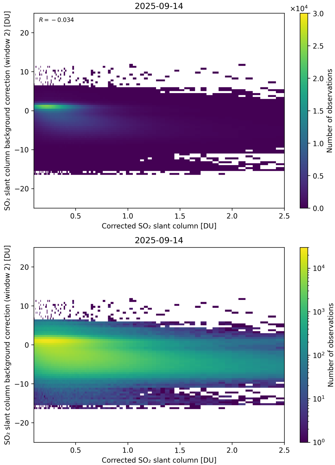
Figure 227: Scatter density plot of “Corrected SO 2 slant column” against “SO 2 slant column background correction (window 2)” for 2025-09-13 to 2025-09-15.
