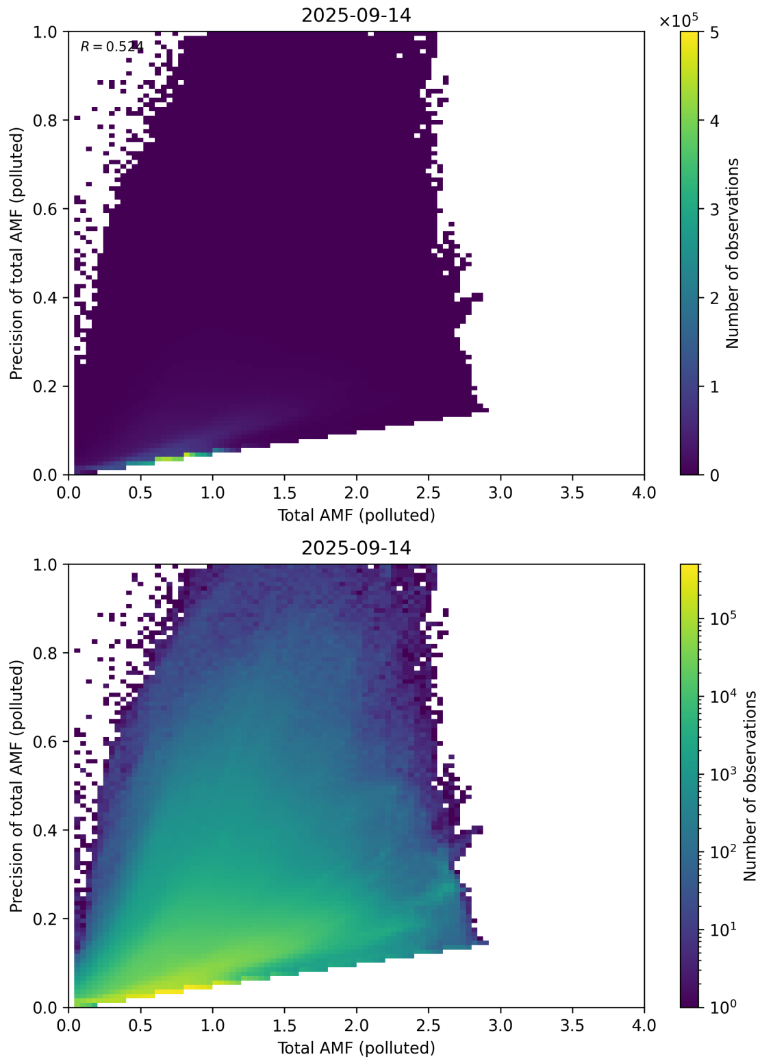
Figure 322: Scatter density plot of “Total AMF (polluted)” against “Precision of total AMF (polluted)” for 2025-09-13 to 2025-09-15.
