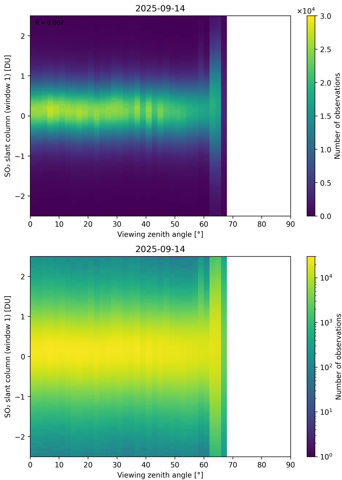
Figure 376: Scatter density plot of “Viewing zenith angle” against “SO 2 slant column (window 1)” for 2025-09-13 to 2025-09-15.
