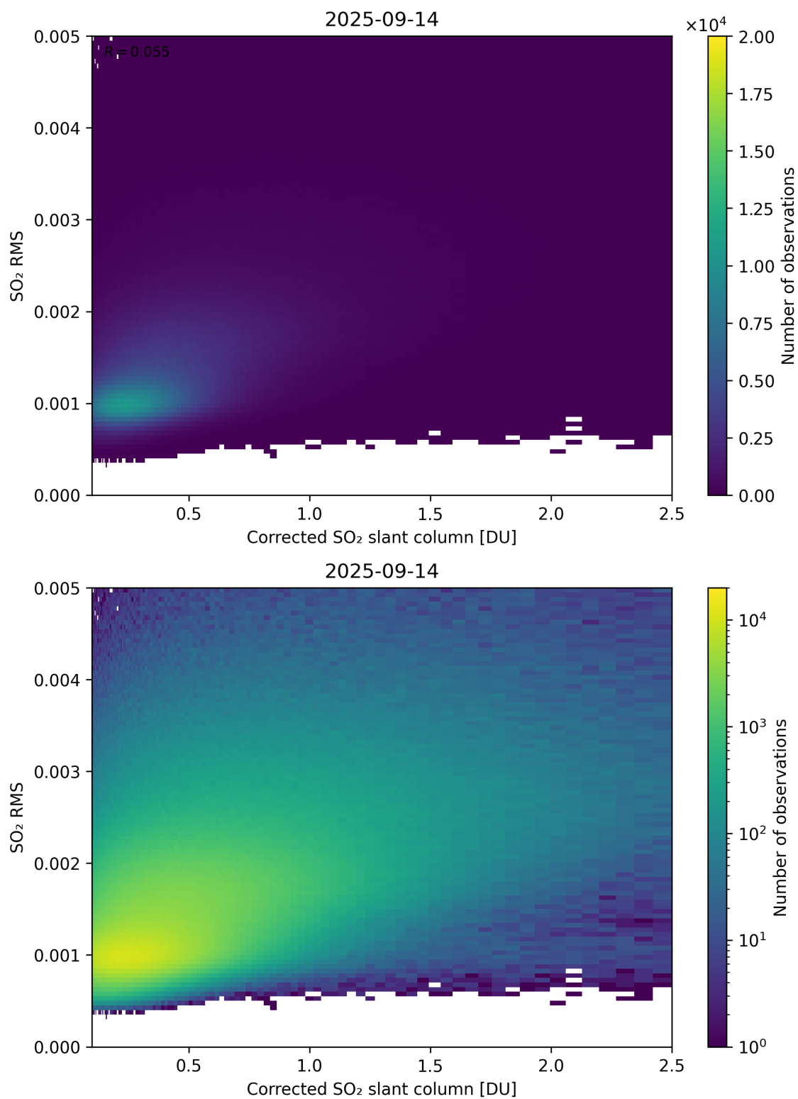
Figure 231: Scatter density plot of “Corrected SO 2 slant column” against “SO 2 RMS” for 2025-09-13 to 2025-09-15.
