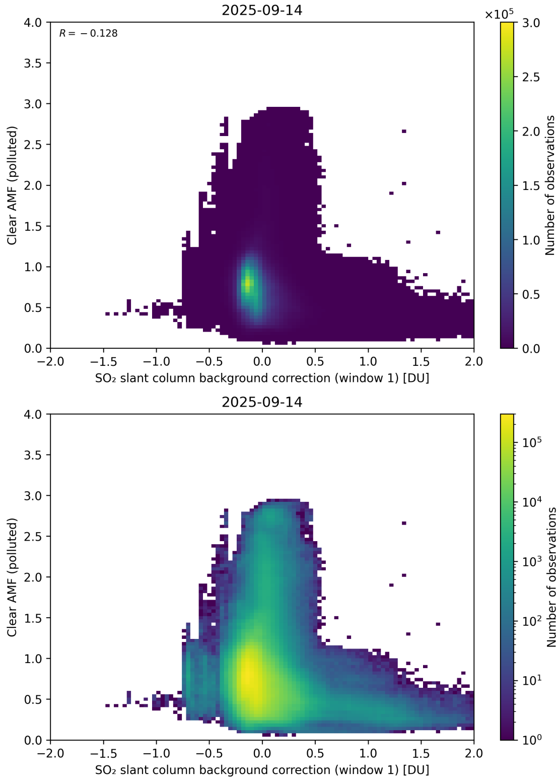
Figure 114: Scatter density plot of “SO 2 slant column background correction (window 1)” against “Clear AMF (polluted)” for 2025-09-13 to 2025-09-15.
