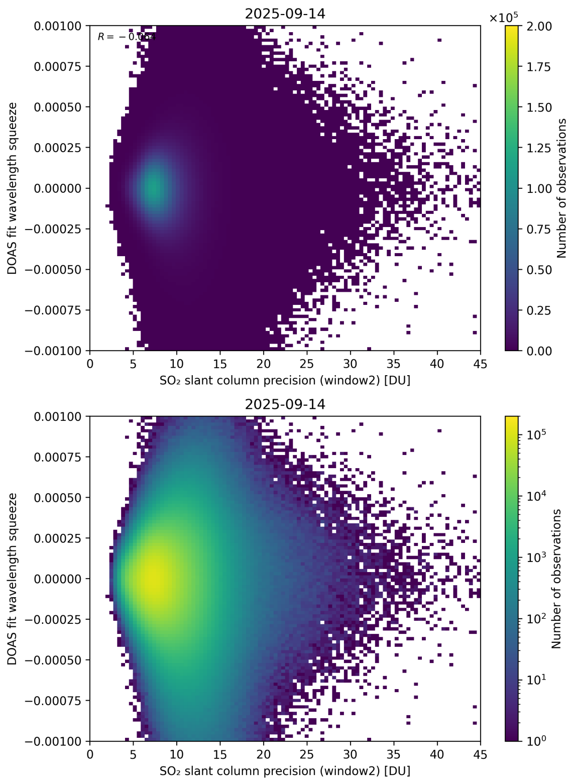
Figure 294: Scatter density plot of “SO 2 slant column precision (window2)” against “DOAS fit wavelength squeeze” for 2025-09-13 to 2025-09-15.
