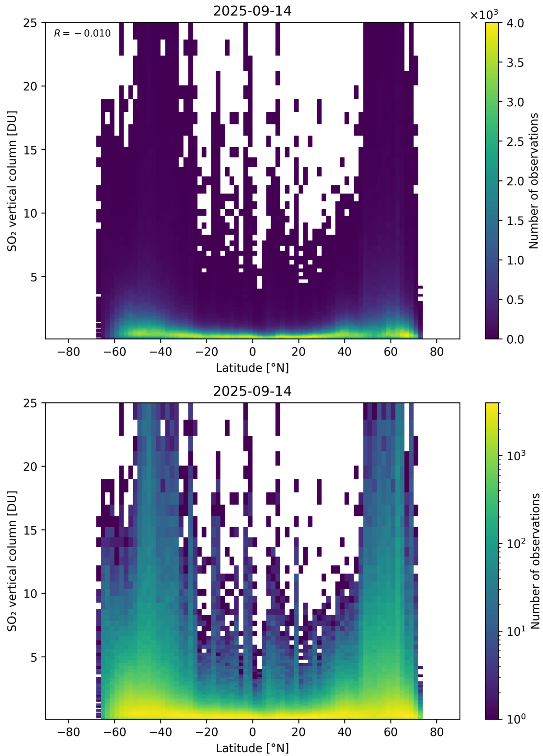
Figure 169: Scatter density plot of “Latitude” against “SO 2 vertical column” for 2025-09-13 to 2025-09-15.
