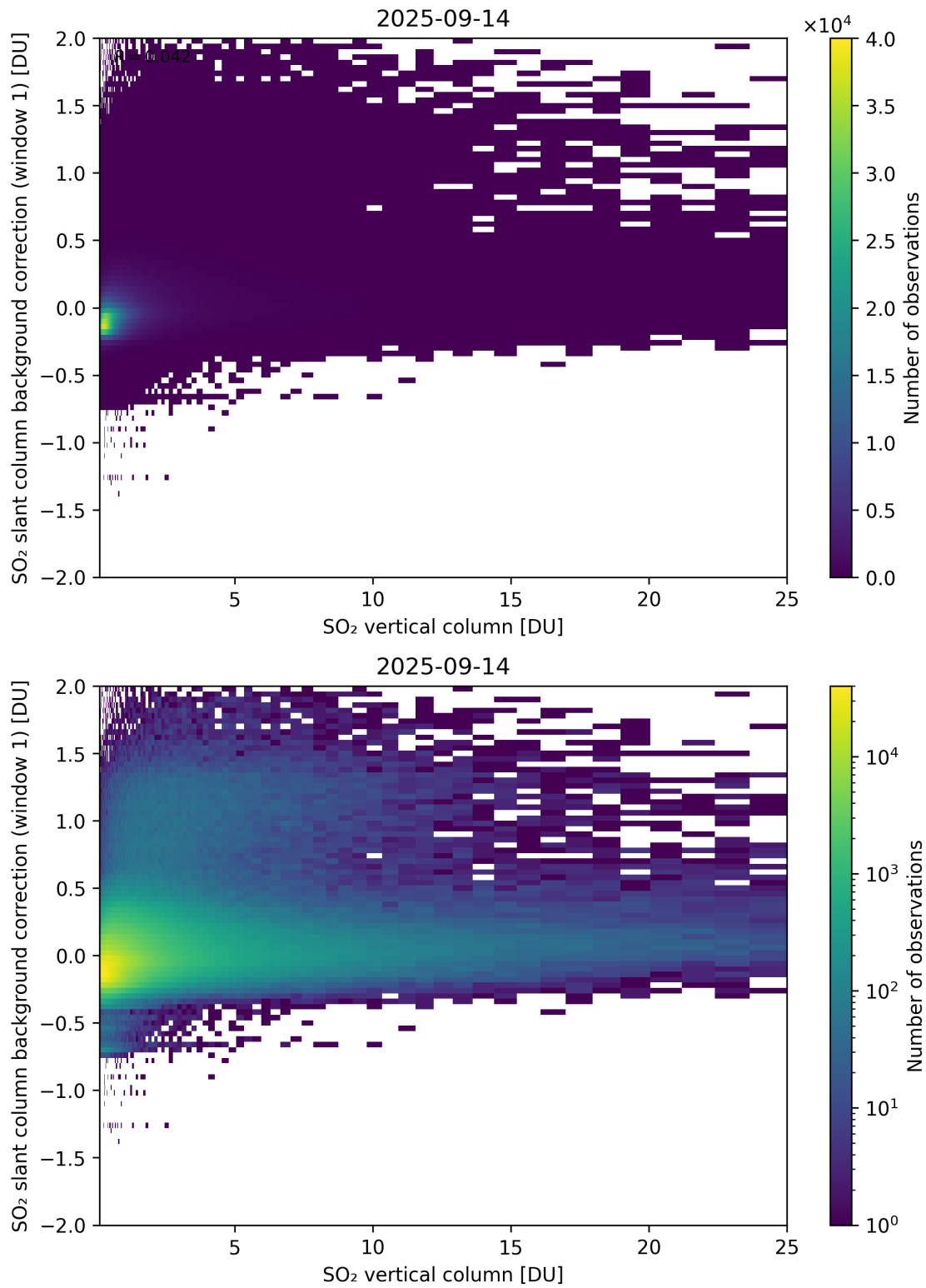
Figure 323: Scatter density plot of “SO 2 vertical column” against “SO 2 slant column background correction (window 1)” for 2025-09-13 to 2025-09-15.
