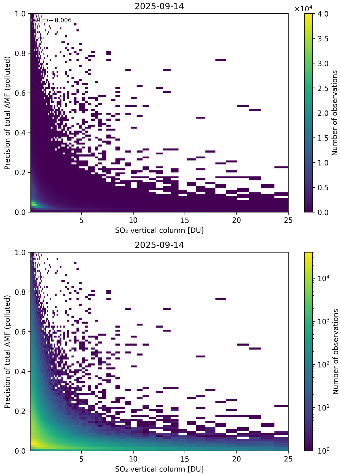
Figure 360: Scatter density plot of “SO 2 vertical column” against “Precision of total AMF (polluted)” for 2025-09-13 to 2025-09-15.
