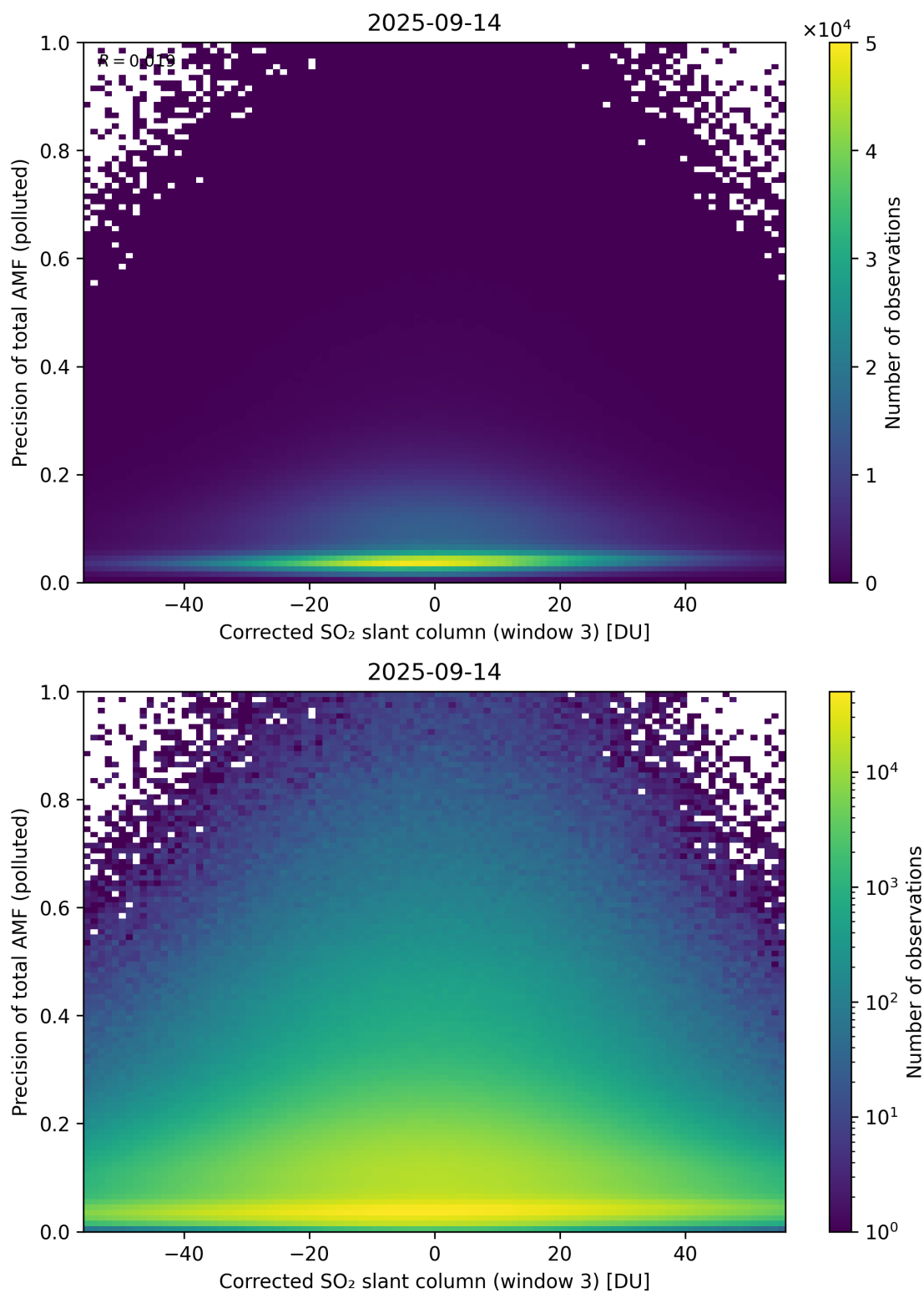
Figure 261: Scatter density plot of “Corrected SO 2 slant column (window 3)” against “Precision of total AMF (polluted)” for 2025-09-13 to 2025-09-15.
