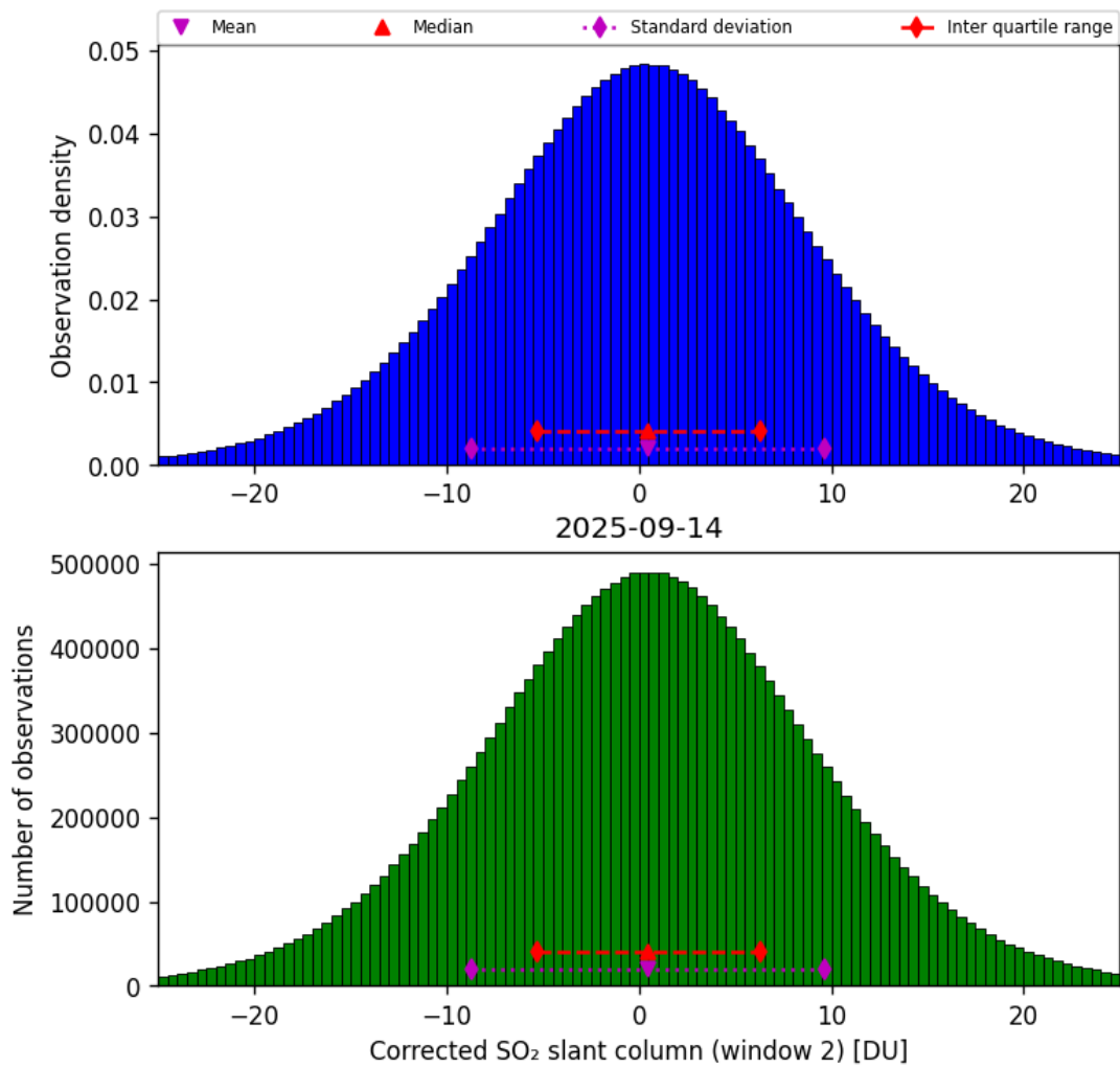
Figure 69: Histogram of “Corrected SO 2 slant column (window 2)” for 2025-09-13 to 2025-09-15
