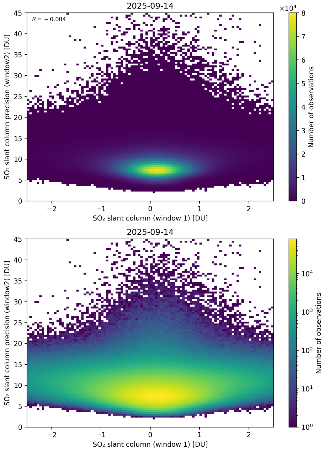
Figure 286: Scatter density plot of “SO 2 slant column (window 1)” against “SO 2 slant column precision (window2)” for 2025-09-13 to 2025-09-15.
