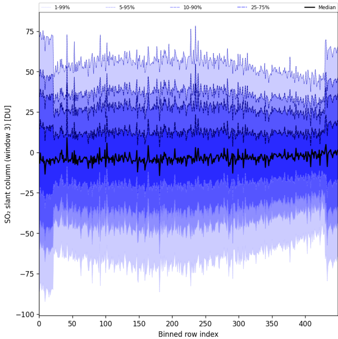
Figure 97: Along track statistics of “SO 2 slant column (window 3)” for 2025-09-13 to 2025-09-15
