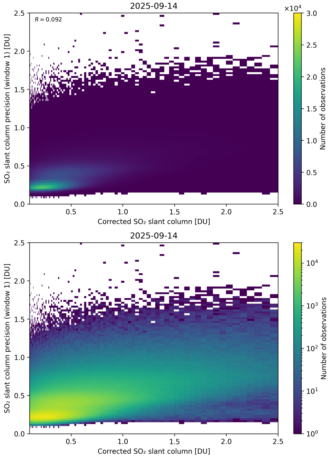
Figure 238: Scatter density plot of “Corrected SO 2 slant column” against “SO 2 slant column precision (window 1)” for 2025-09-13 to 2025-09-15.
