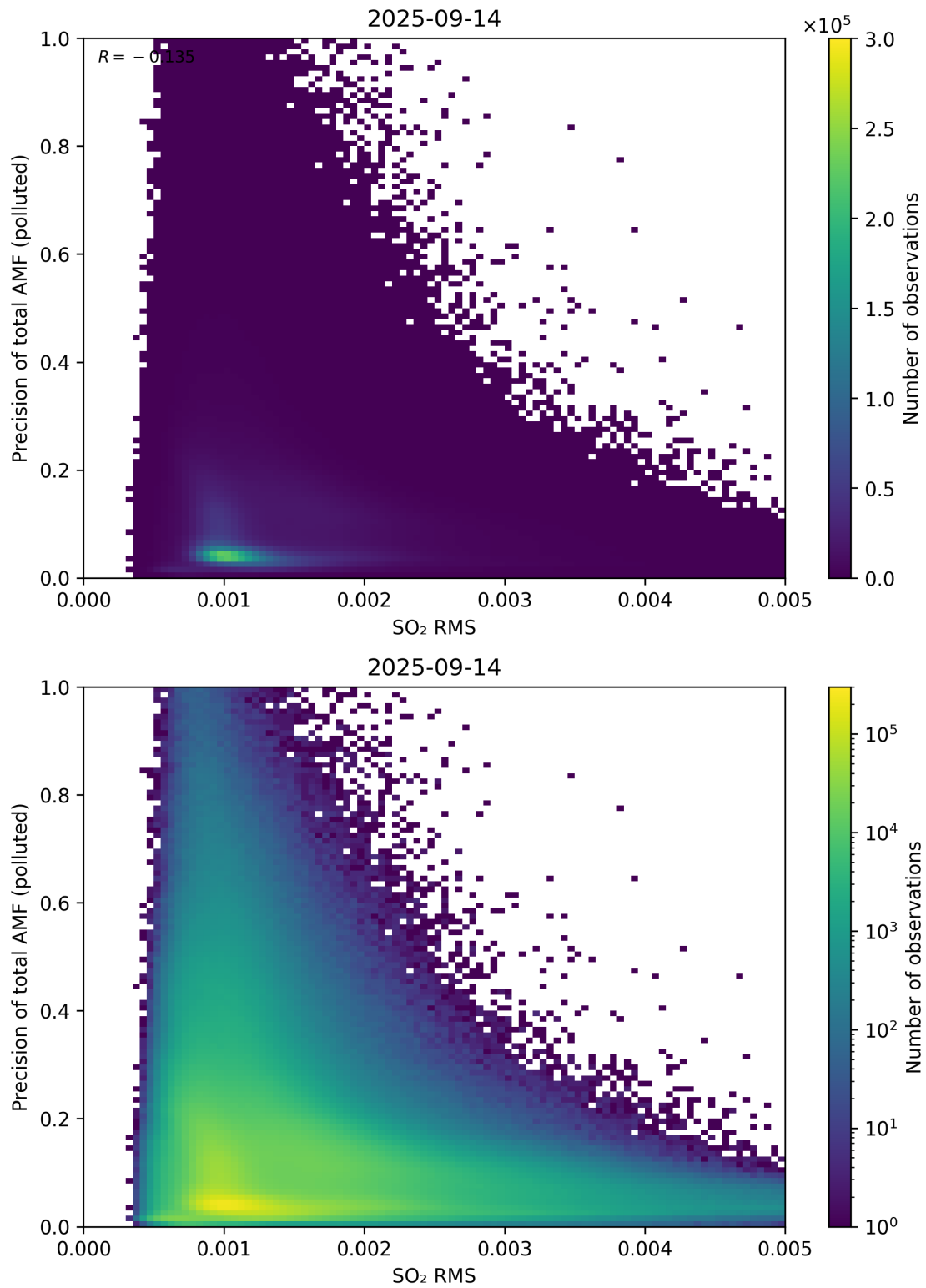
Figure 149: Scatter density plot of “SO 2 RMS” against “Precision of total AMF (polluted)” for 2025-09-13 to 2025-09-15.
