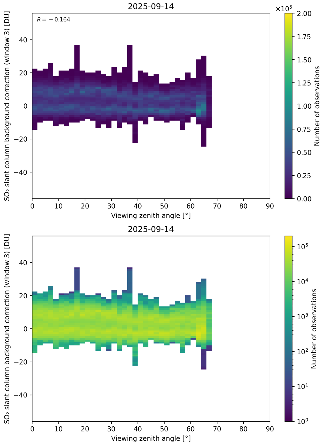
Figure 364: Scatter density plot of “Viewing zenith angle” against “SO 2 slant column background correction (window 3)” for 2025-09-13 to 2025-09-15.
