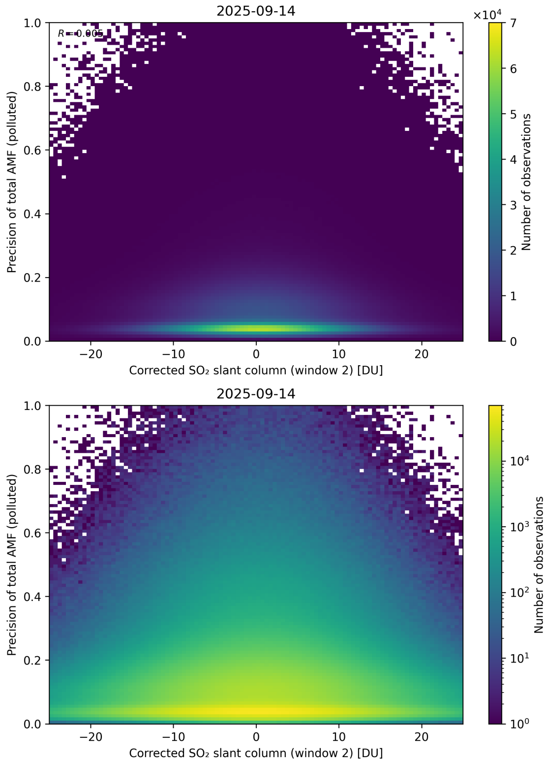
Figure 254: Scatter density plot of “Corrected SO 2 slant column (window 2)” against “Precision of total AMF (polluted)” for 2025-09-13 to 2025-09-15.
