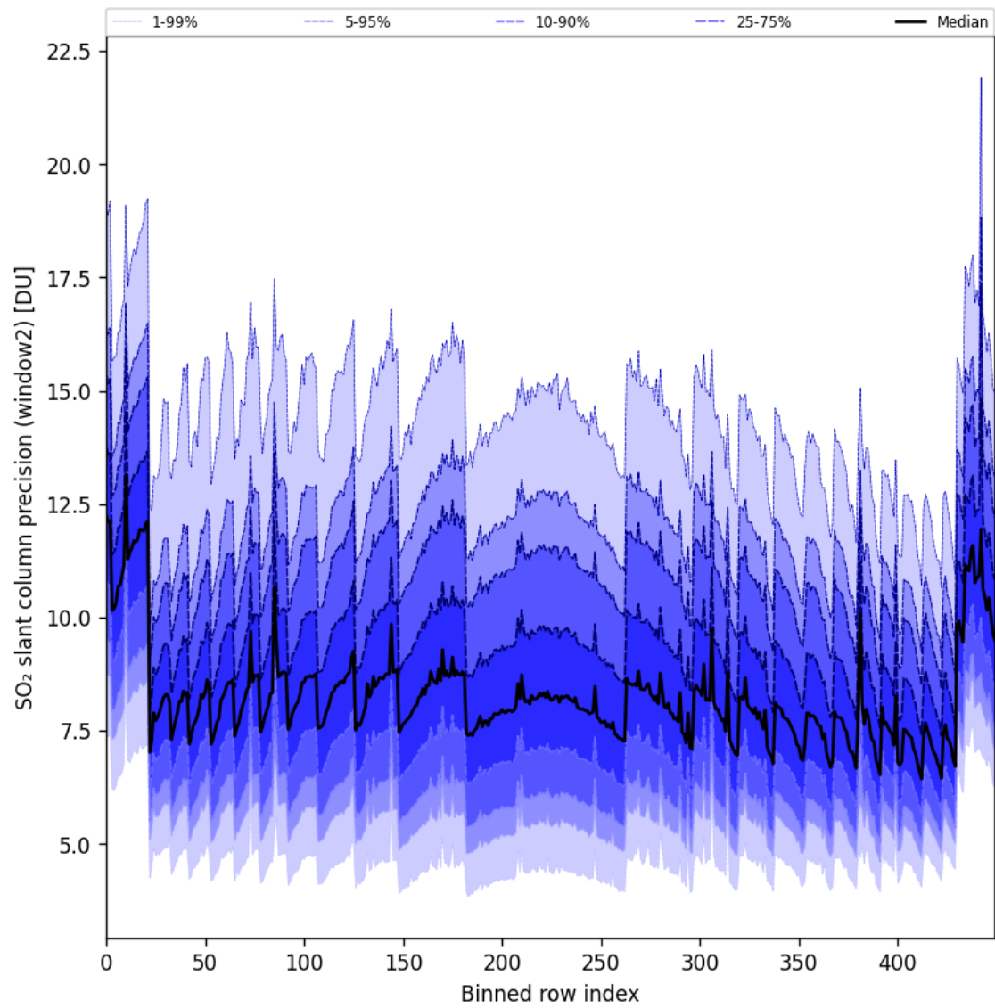
Figure 94: Along track statistics of “SO 2 slant column precision (window2)” for 2025-09-13 to 2025-09-15
