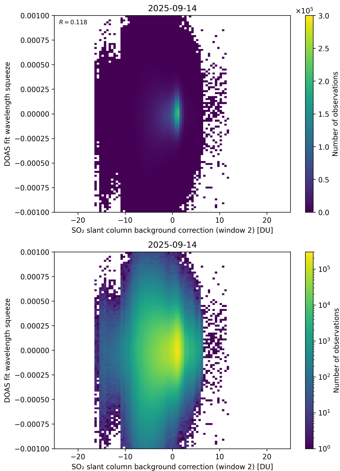
Figure 124: Scatter density plot of “SO 2 slant column background correction (window 2)” against “DOAS fit wavelength squeeze” for 2025-09-13 to 2025-09-15.
