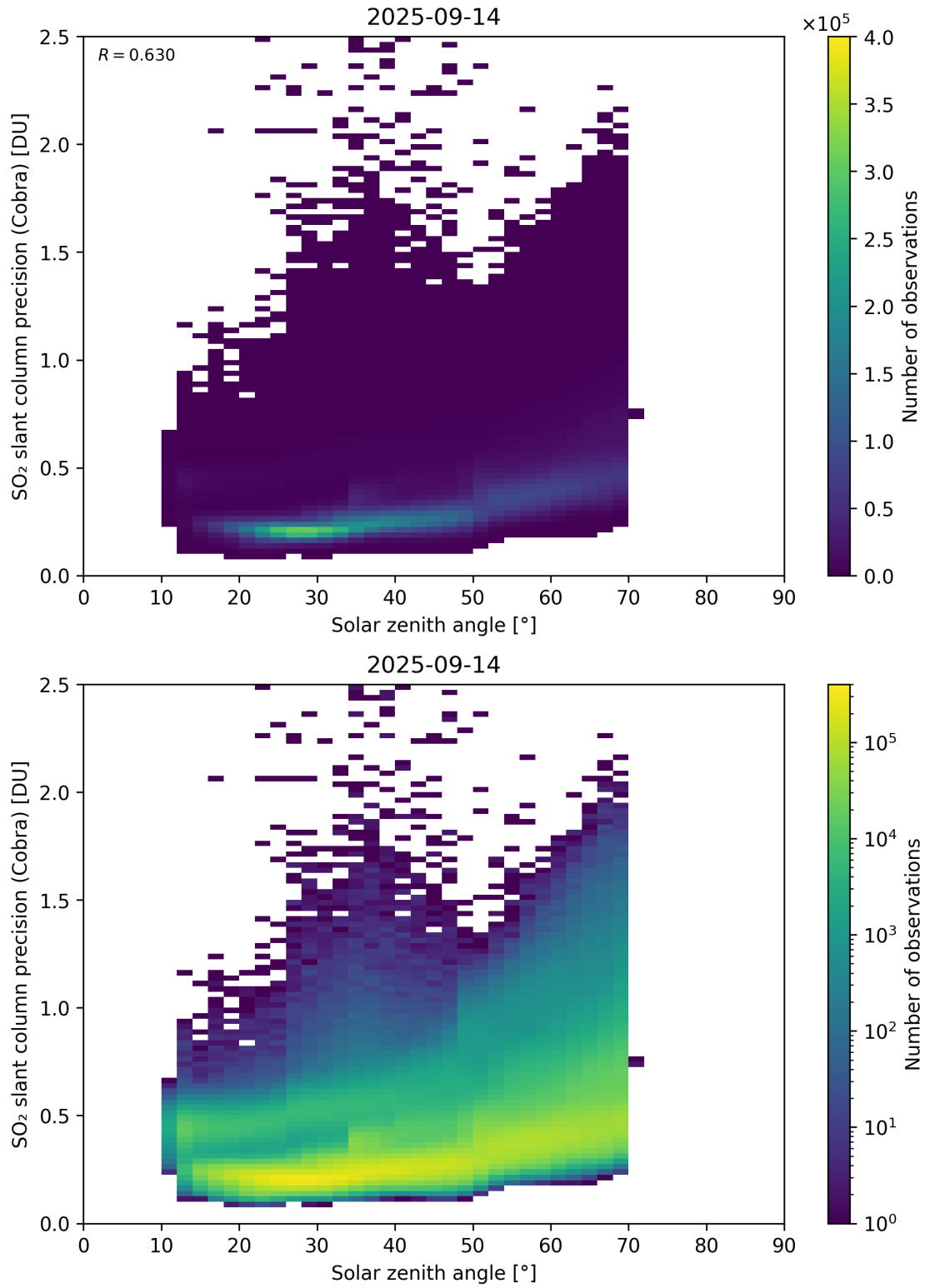
Figure 180: Scatter density plot of “Solar zenith angle” against “SO 2 slant column precision (Cobra)” for 2025-09-13 to 2025-09-15.
