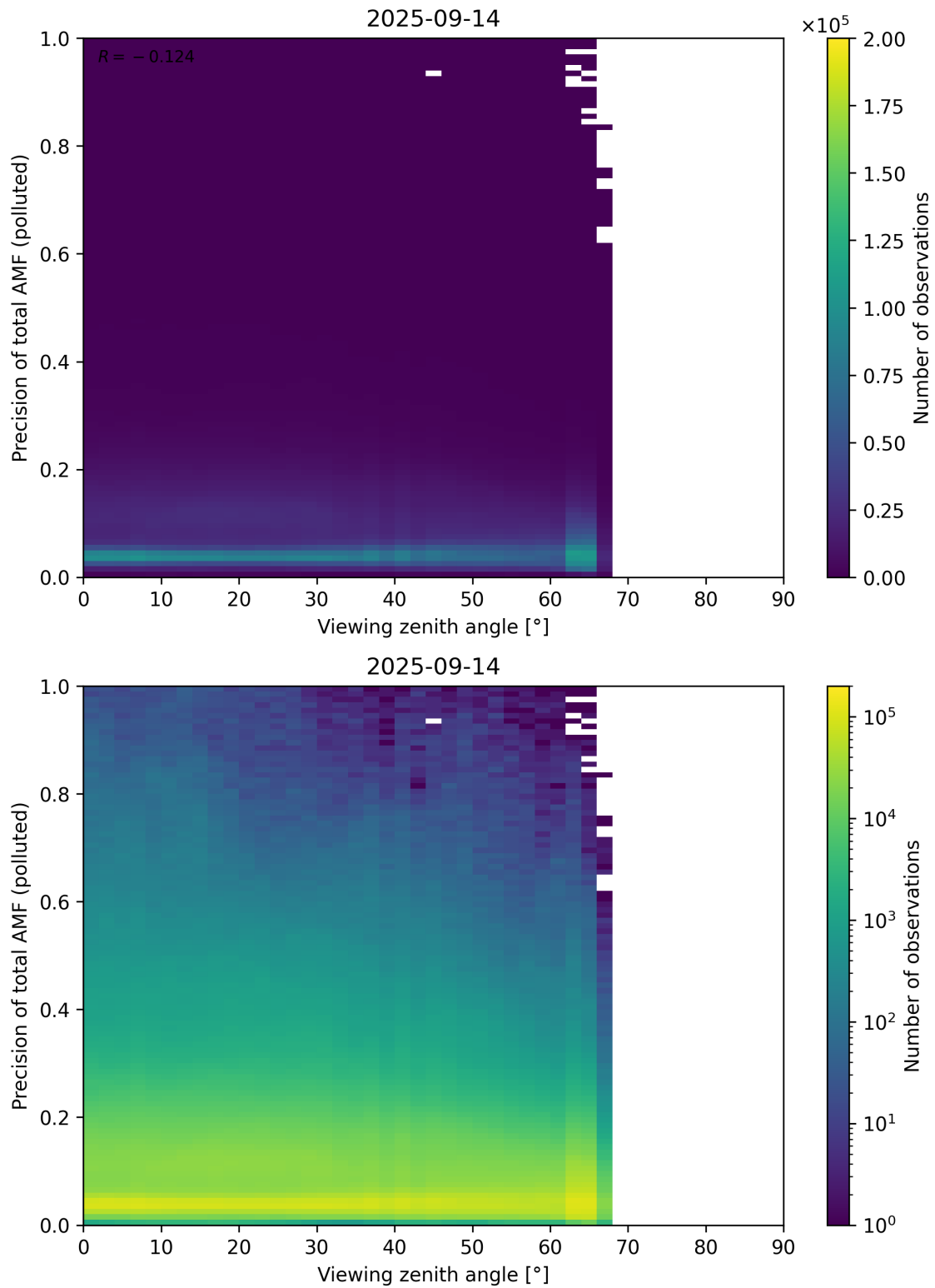
Figure 382: Scatter density plot of “Viewing zenith angle” against “Precision of total AMF (polluted)” for 2025-09-13 to 2025-09-15.
