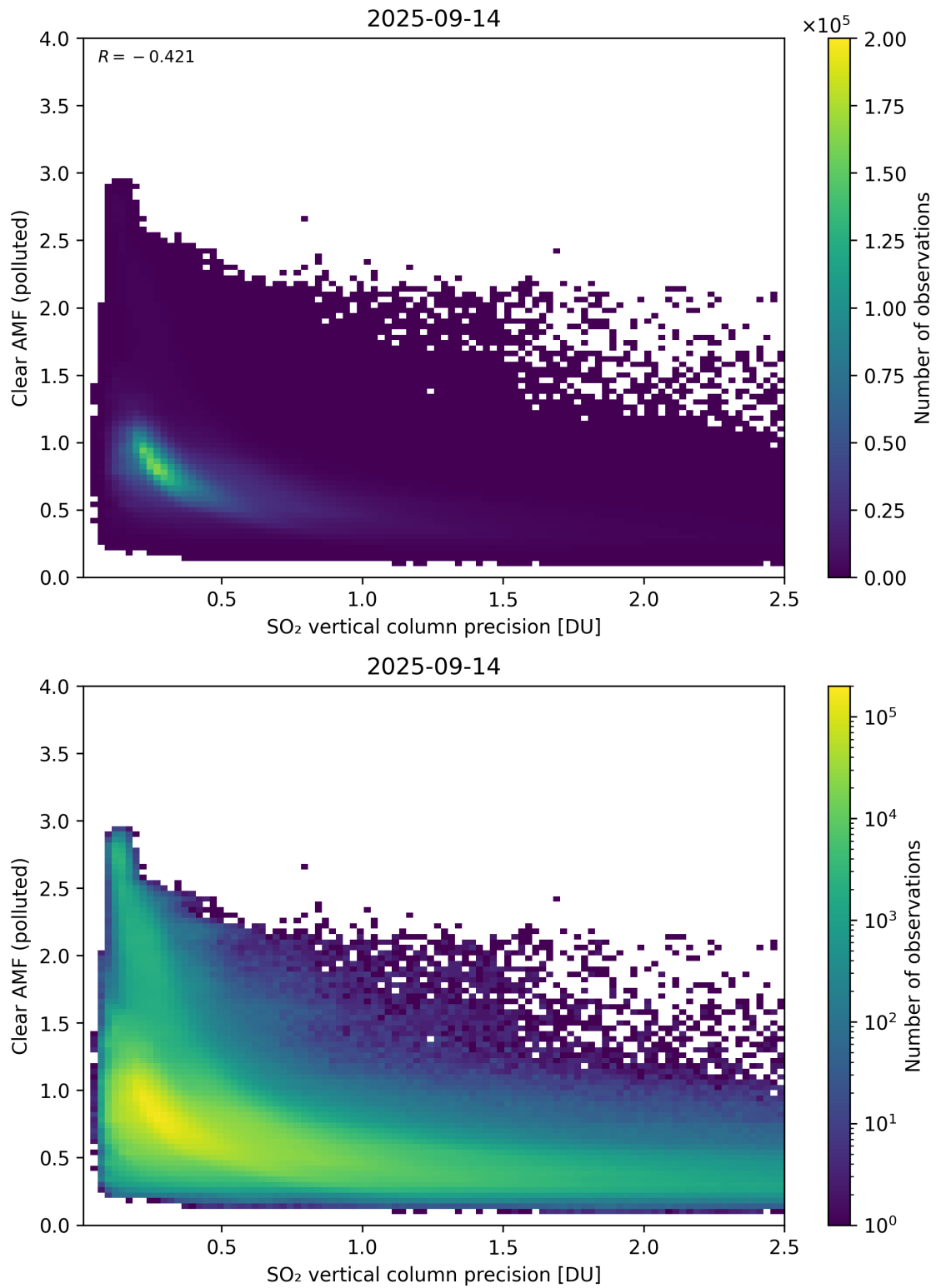
Figure 335: Scatter density plot of “SO 2 vertical column precision” against “Clear AMF (polluted)” for 2025-09-13 to 2025-09-15.
