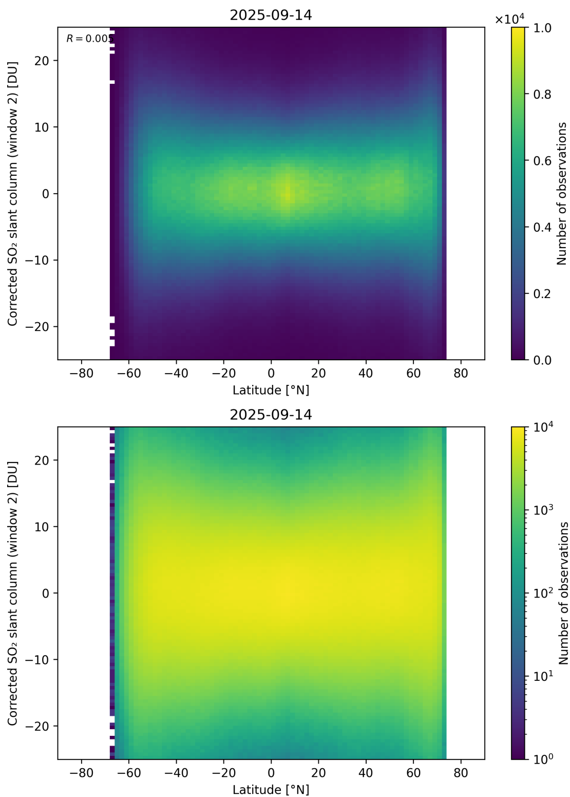
Figure 160: Scatter density plot of “Latitude” against “Corrected SO 2 slant column (window 2)” for 2025-09-13 to 2025-09-15.
