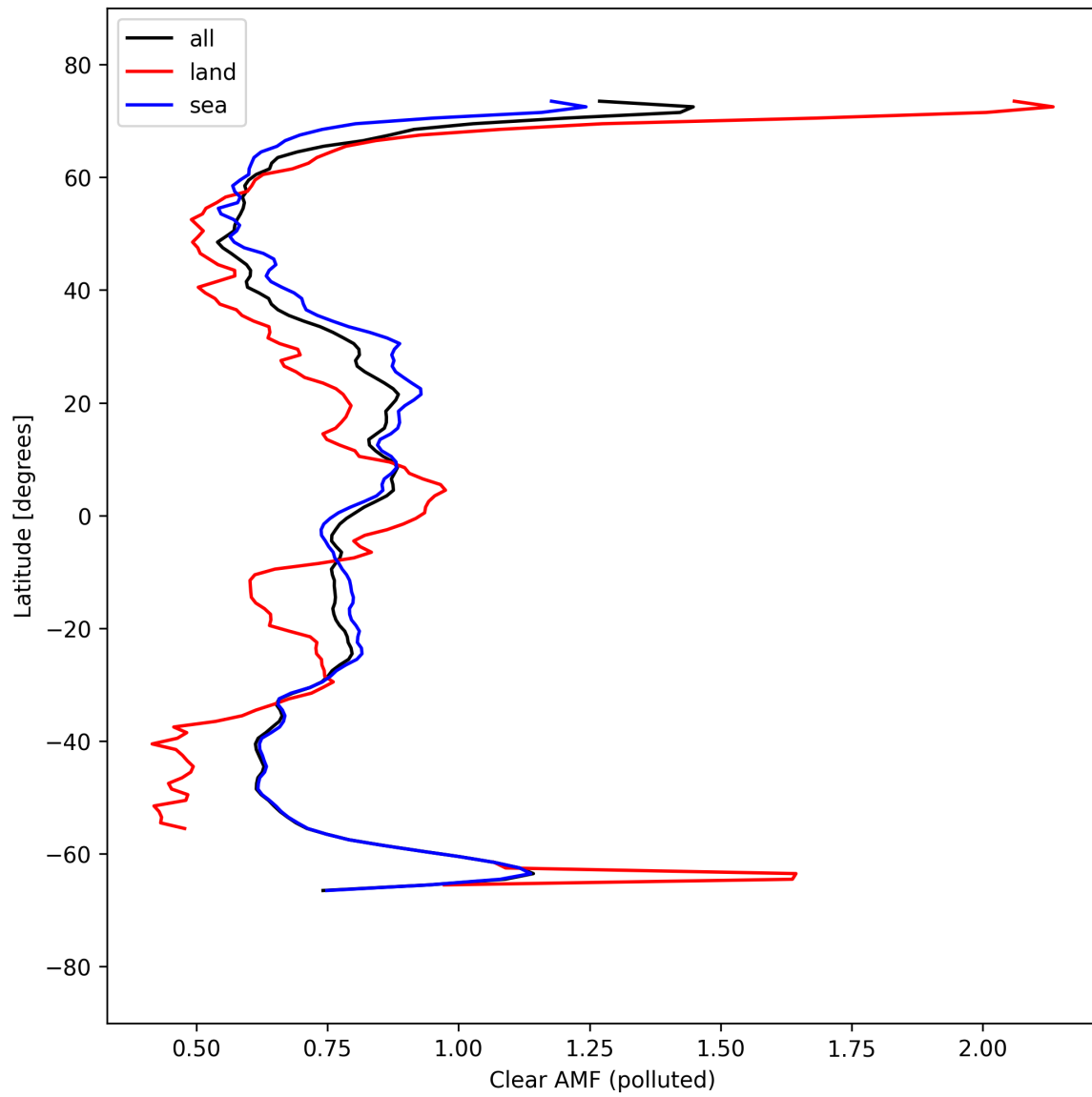
Figure 55: Zonal average of “Clear AMF (polluted)” for 2025-09-13 to 2025-09-15.
