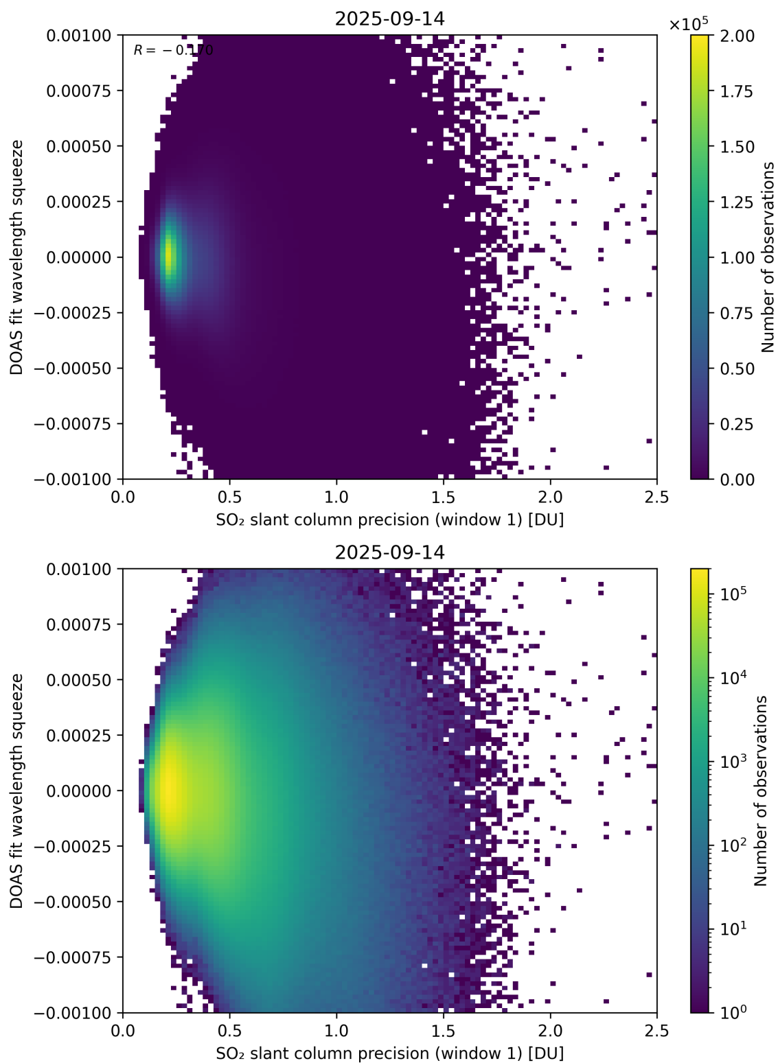
Figure 272: Scatter density plot of “SO 2 slant column precision (window 1)” against “DOAS fit wavelength squeeze” for 2025-09-13 to 2025-09-15.
