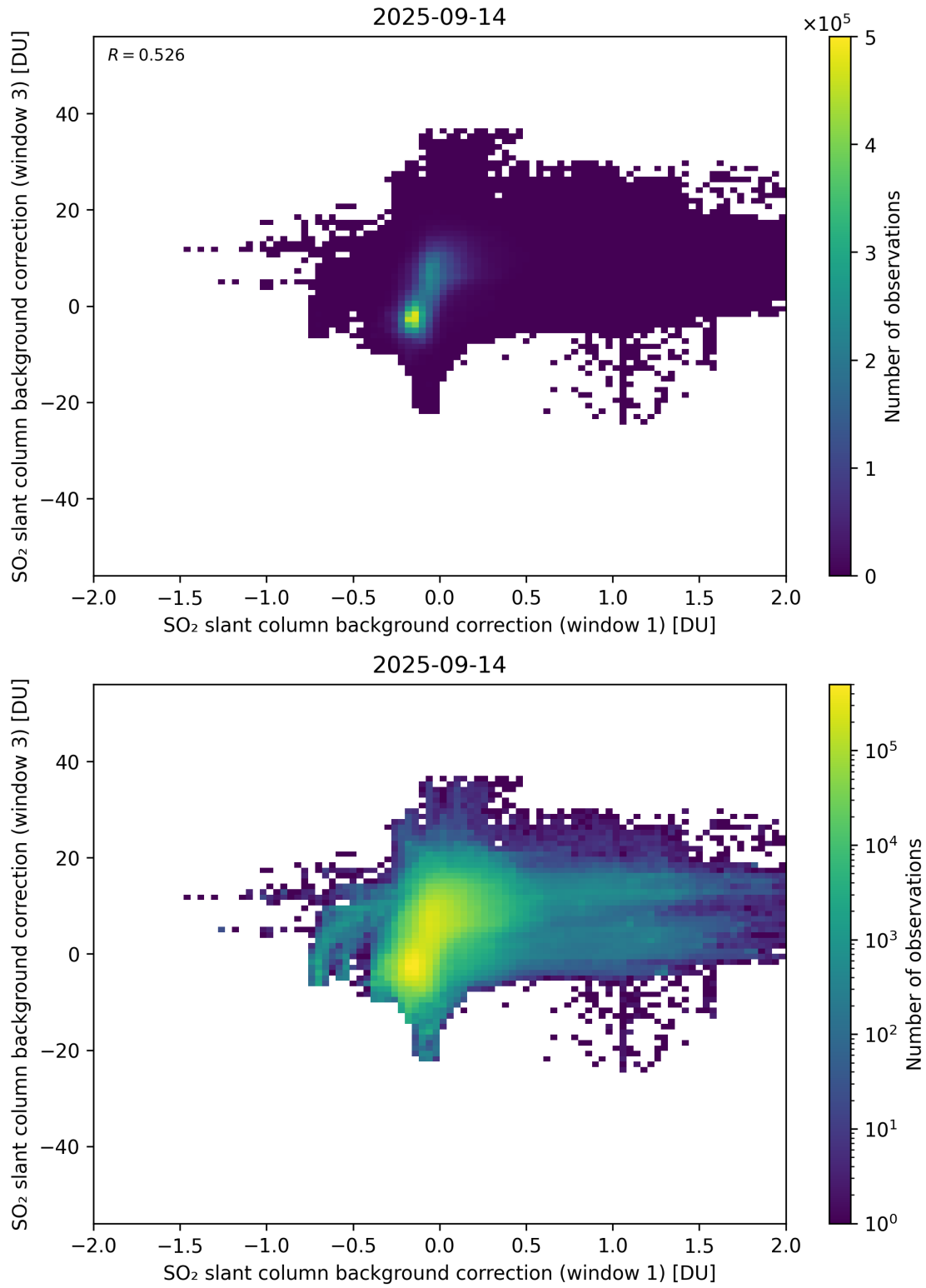
Figure 110: Scatter density plot of “SO 2 slant column background correction (window 1)” against “SO 2 slant column background correction (window 3)” for 2025-09-13 to 2025-09-15.
