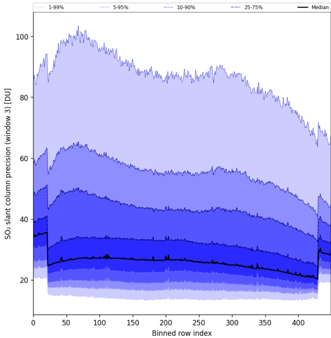
Figure 98: Along track statistics of “SO 2 slant column precision (window 3)” for 2025-09-13 to 2025-09-15
