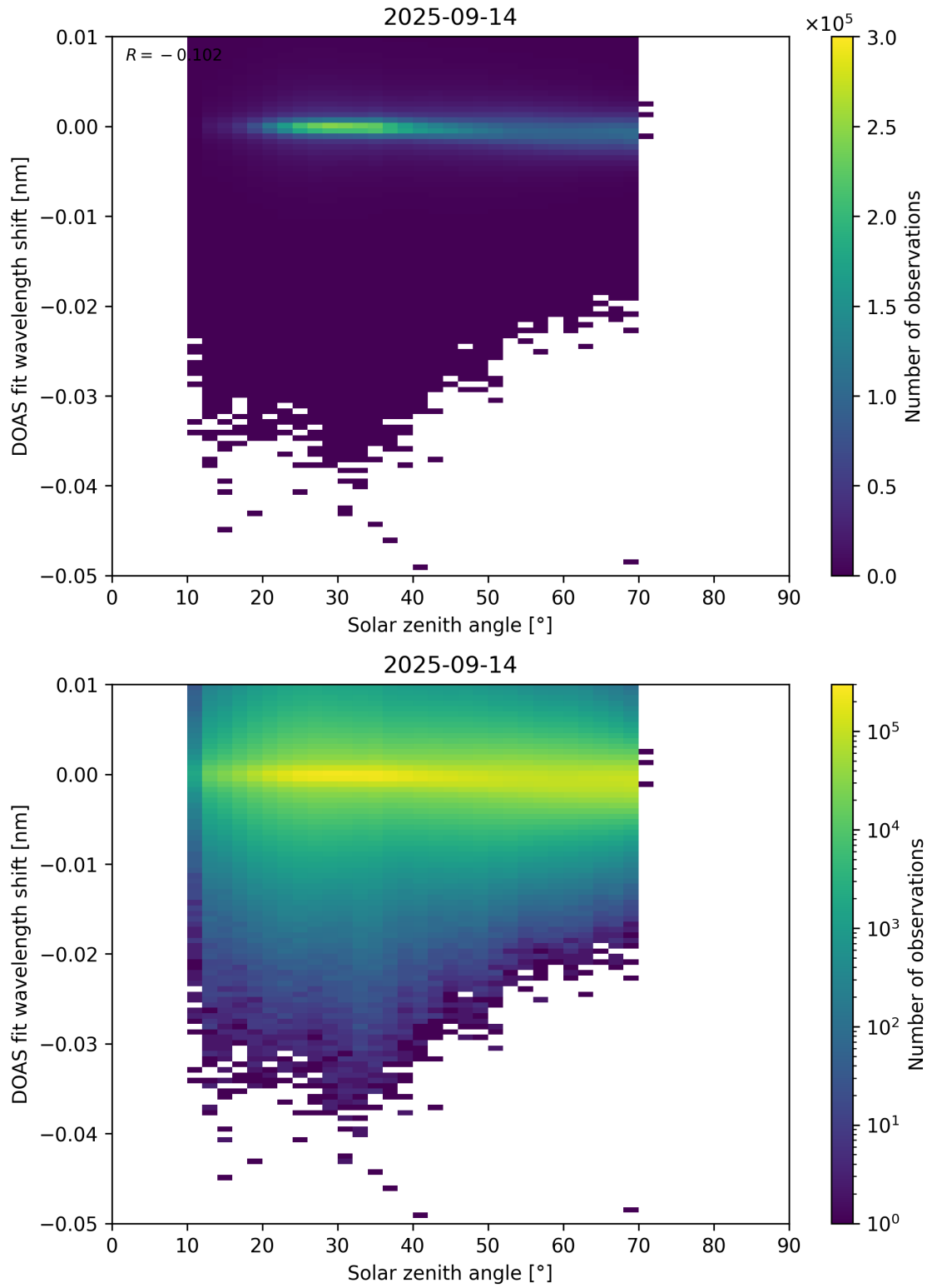
Figure 174: Scatter density plot of “Solar zenith angle” against “DOAS fit wavelength shift” for 2025-09-13 to 2025-09-15.
