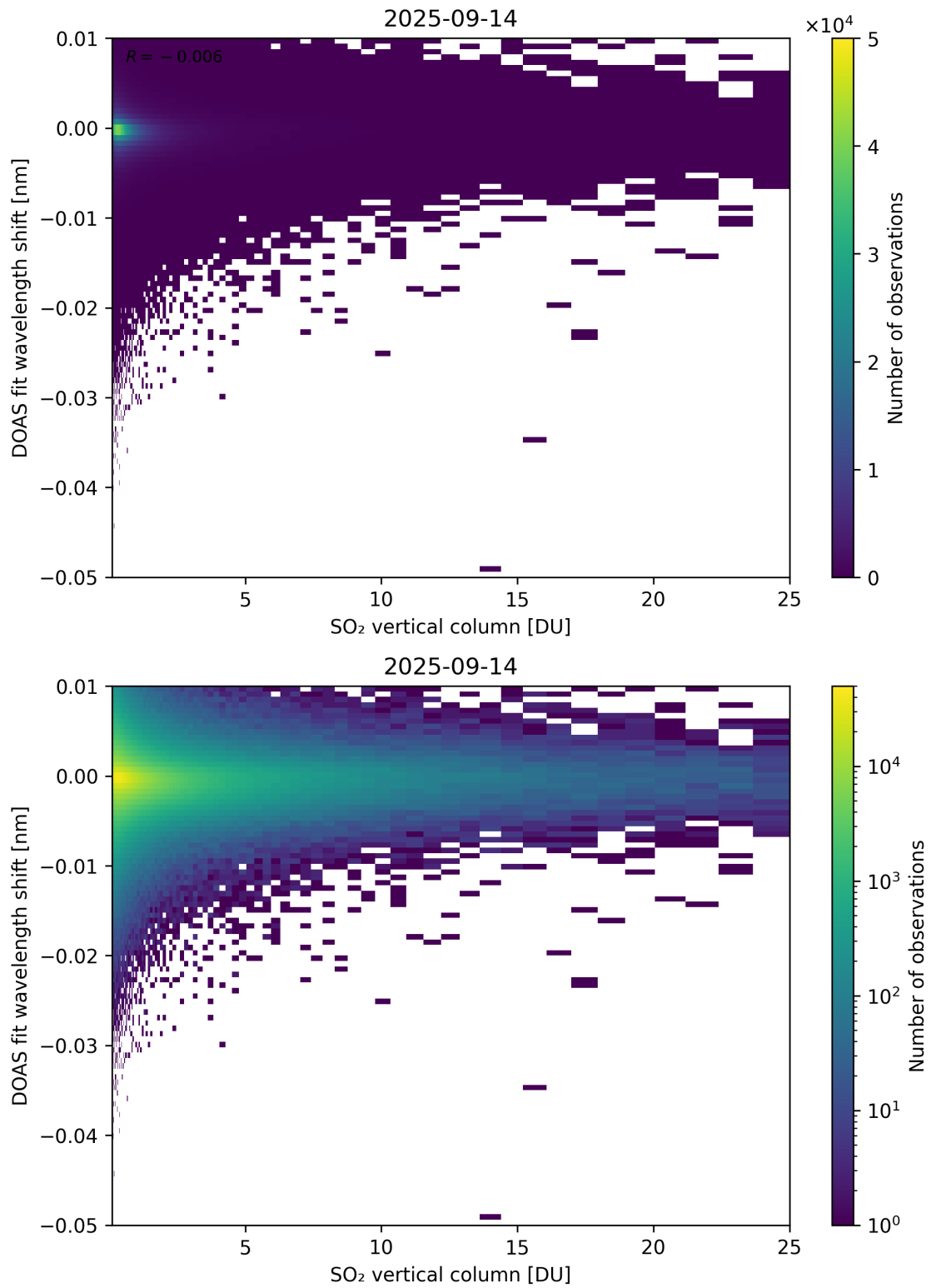
Figure 326: Scatter density plot of “SO 2 vertical column” against “DOAS fit wavelength shift” for 2025-09-13 to 2025-09-15.
