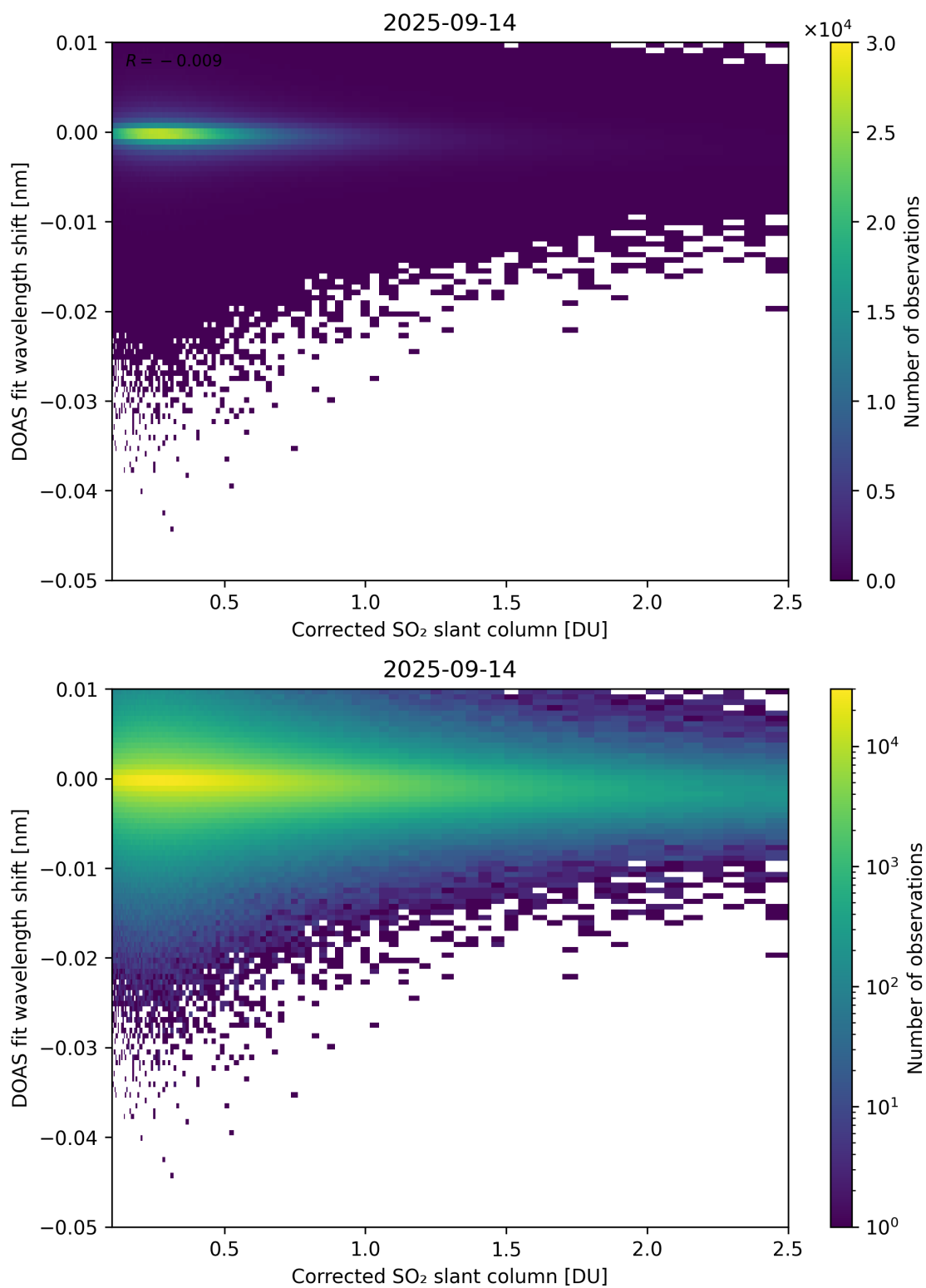
Figure 229: Scatter density plot of “Corrected SO 2 slant column” against “DOAS fit wavelength shift” for 2025-09-13 to 2025-09-15.
