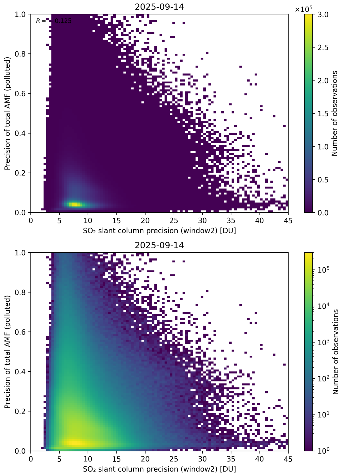
Figure 302: Scatter density plot of “SO 2 slant column precision (window2)” against “Precision of total AMF (polluted)” for 2025-09-13 to 2025-09-15.
