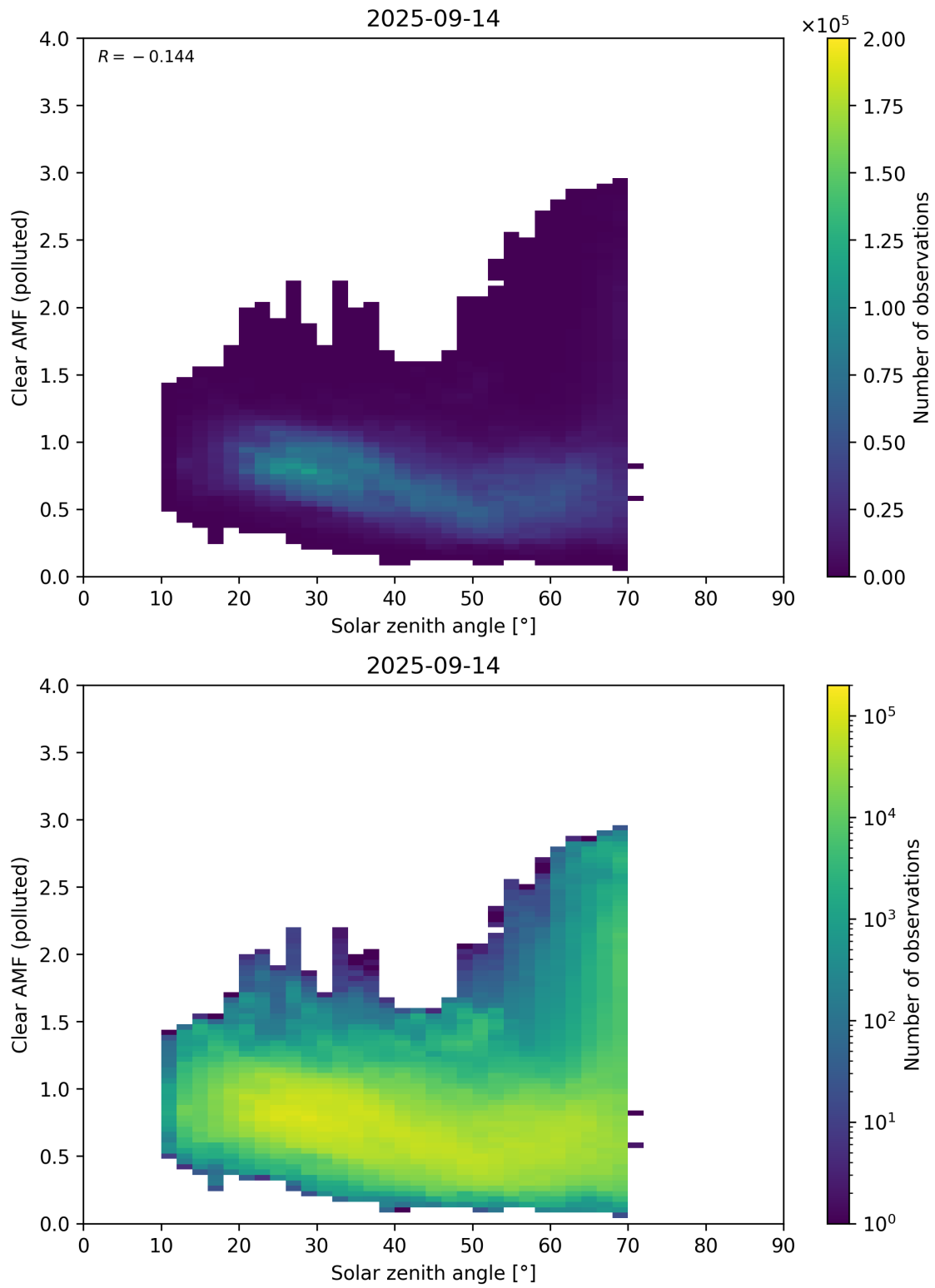
Figure 178: Scatter density plot of “Solar zenith angle” against “Clear AMF (polluted)” for 2025-09-13 to 2025-09-15.
