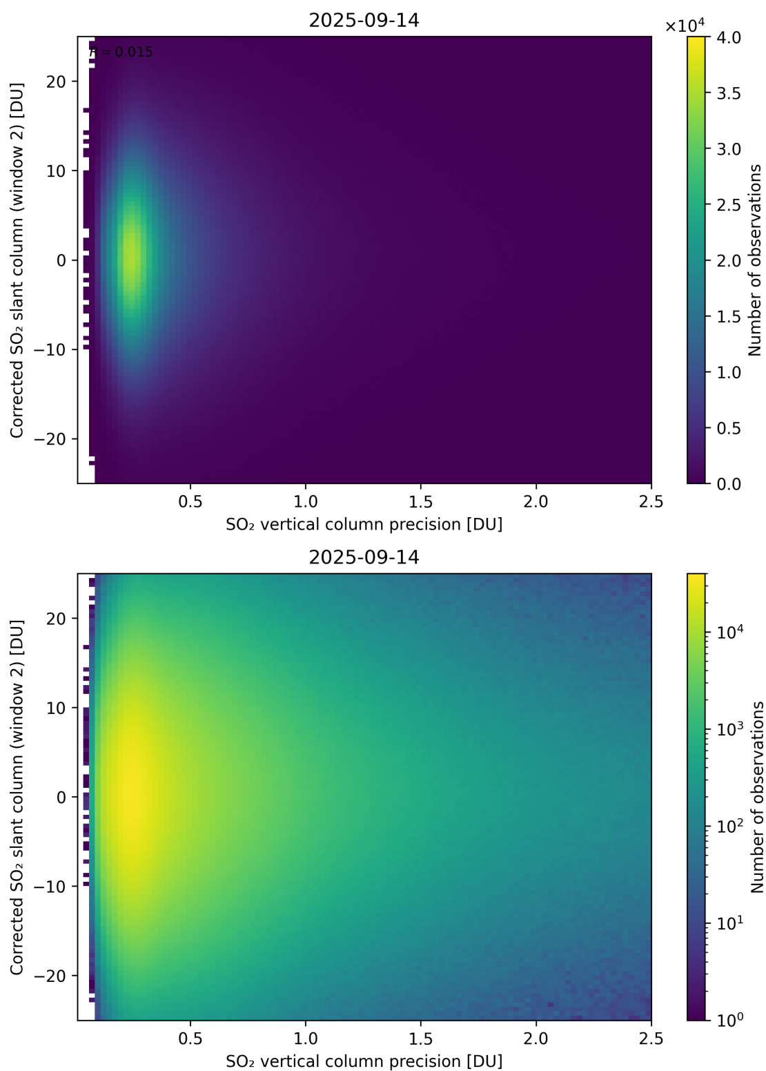
Figure 339: Scatter density plot of “SO 2 vertical column precision” against “Corrected SO 2 slant column (window 2)” for 2025-09-13 to 2025-09-15.
