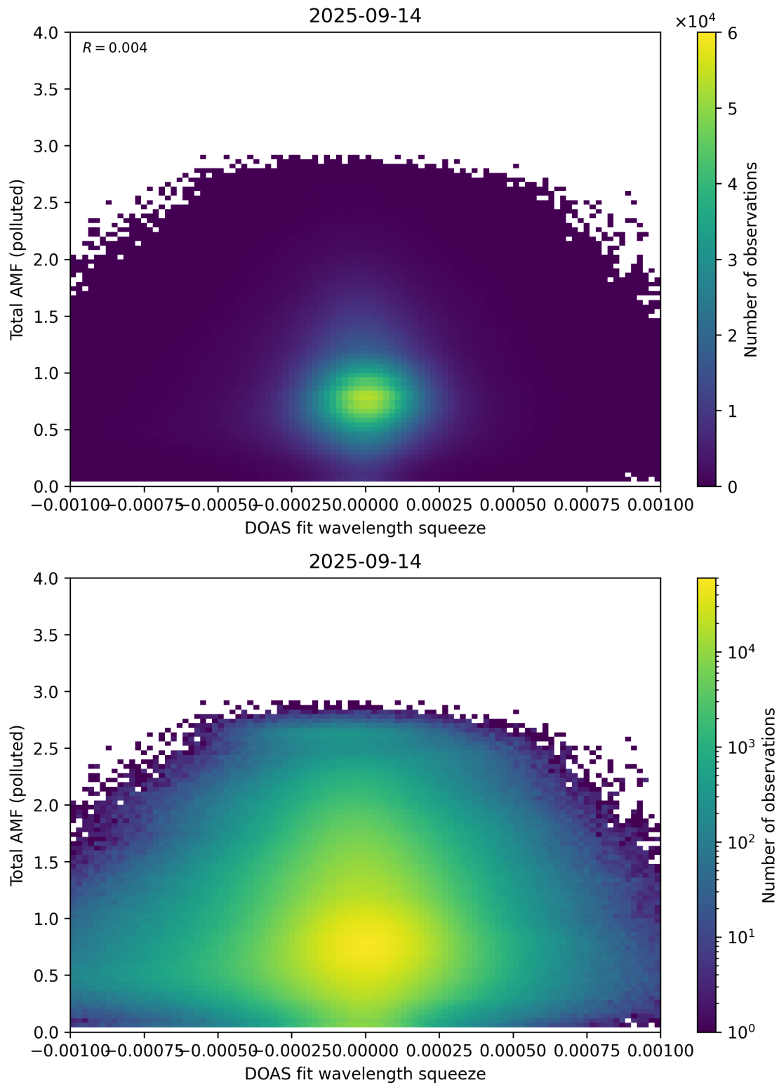
Figure 145: Scatter density plot of “DOAS fit wavelength squeeze” against “Total AMF (polluted)” for 2025-09-13 to 2025-09-15.
