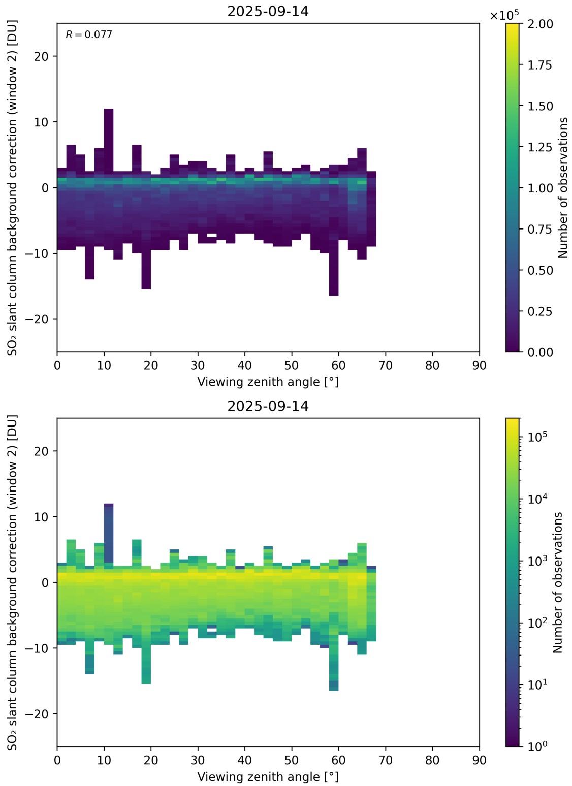
Figure 363: Scatter density plot of “Viewing zenith angle” against “SO 2 slant column background correction (window 2)” for 2025-09-13 to 2025-09-15.
