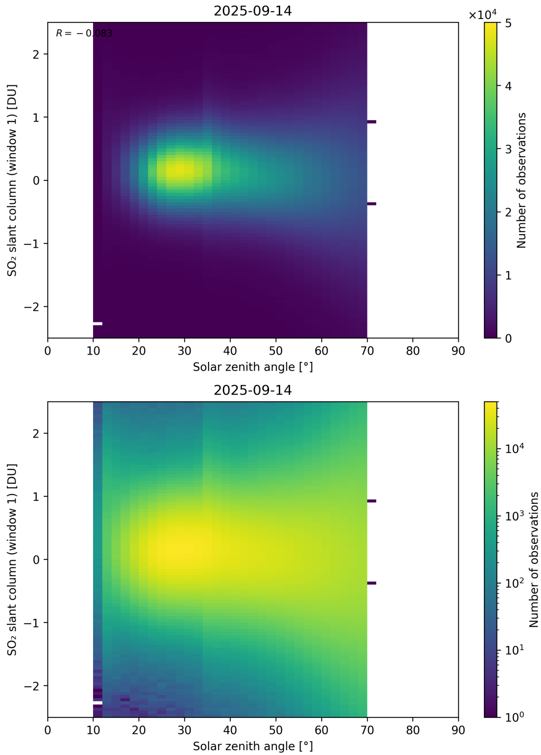
Figure 184: Scatter density plot of “Solar zenith angle” against “SO 2 slant column (window 1)” for 2025-09-13 to 2025-09-15.
