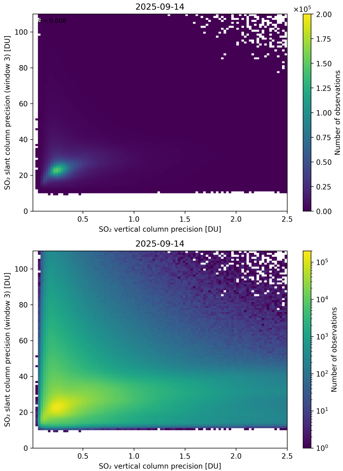
Figure 345: Scatter density plot of “SO 2 vertical column precision” against “SO 2 slant column precision (window 3)” for 2025-09-13 to 2025-09-15.
