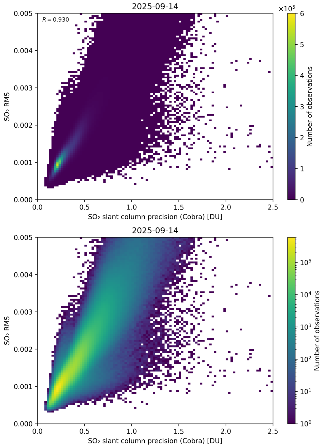
Figure 204: Scatter density plot of “SO 2 slant column precision (Cobra)” against “SO 2 RMS” for 2025-09-13 to 2025-09-15.
