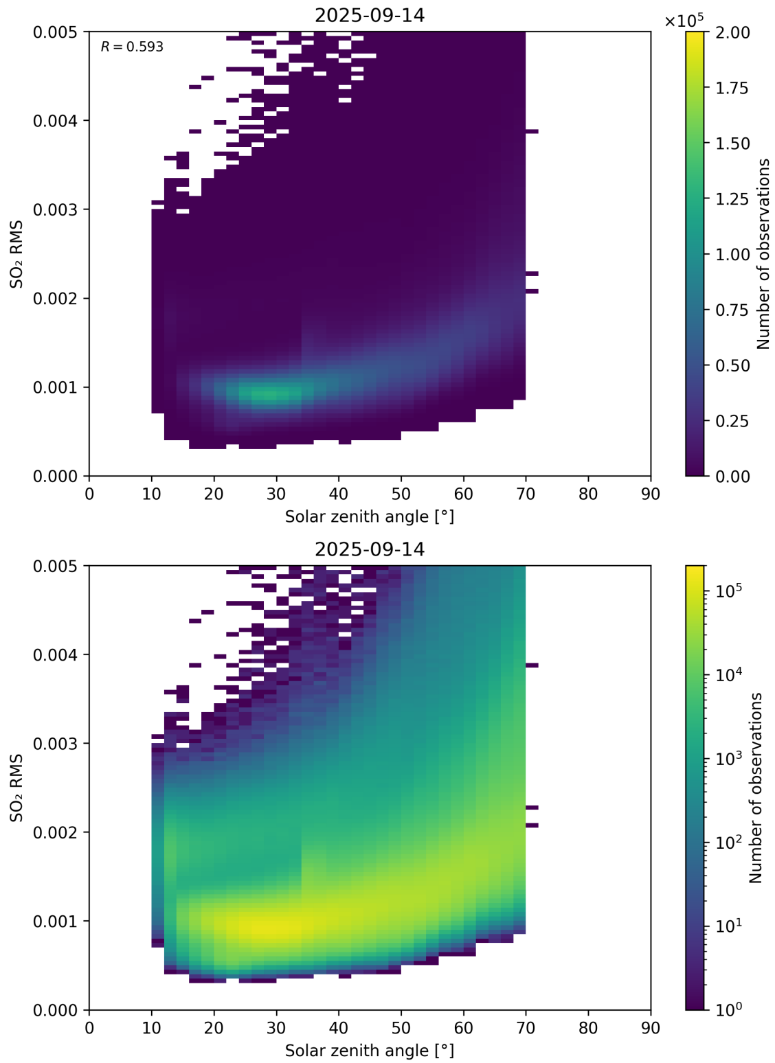
Figure 176: Scatter density plot of “Solar zenith angle” against “SO 2 RMS” for 2025-09-13 to 2025-09-15.
