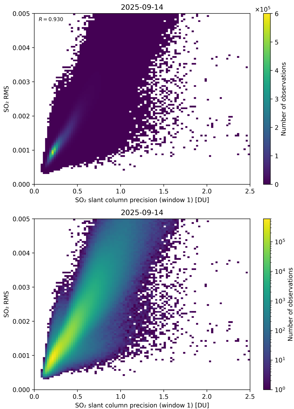
Figure 273: Scatter density plot of “SO 2 slant column precision (window 1)” against “SO 2 RMS” for 2025-09-13 to 2025-09-15.
