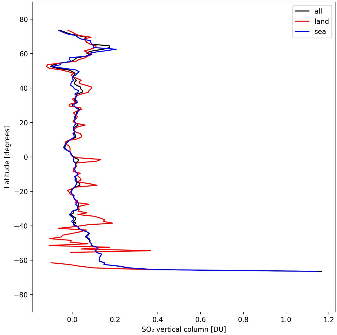
Figure 32: Zonal average of “SO 2 vertical column” for 2025-09-13 to 2025-09-15.
