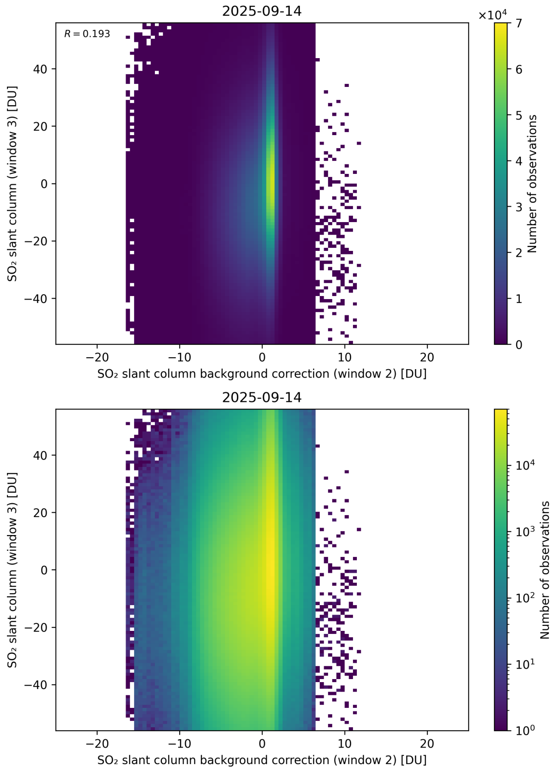
Figure 128: Scatter density plot of “SO 2 slant column background correction (window 2)” against “SO 2 slant column (window 3)” for 2025-09-13 to 2025-09-15.
