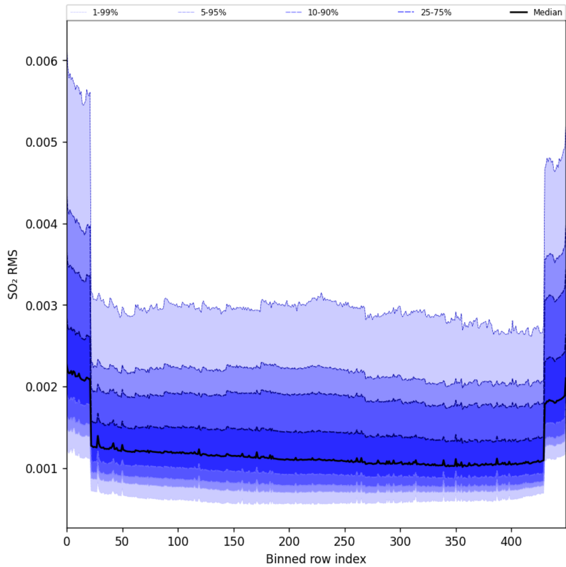
Figure 104: Along track statistics of “SO 2 RMS” for 2025-09-13 to 2025-09-15
