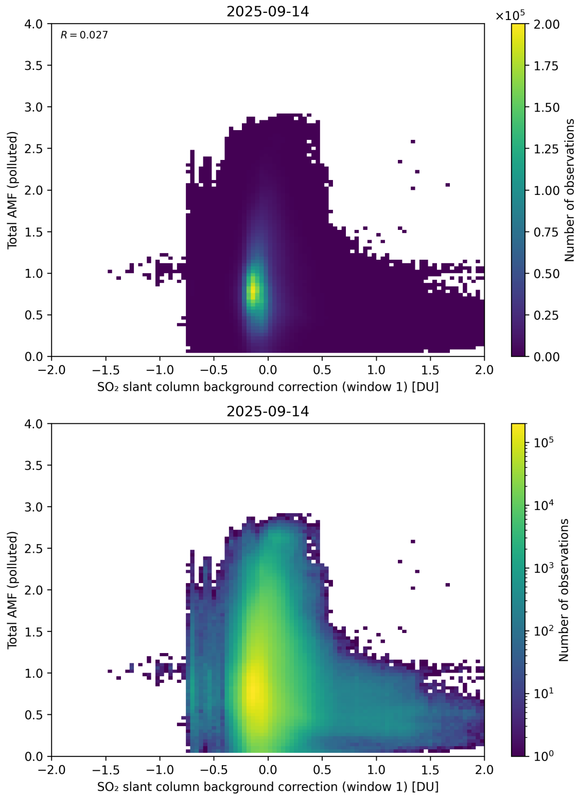
Figure 120: Scatter density plot of “SO 2 slant column background correction (window 1)” against “Total AMF (polluted)” for 2025-09-13 to 2025-09-15.
