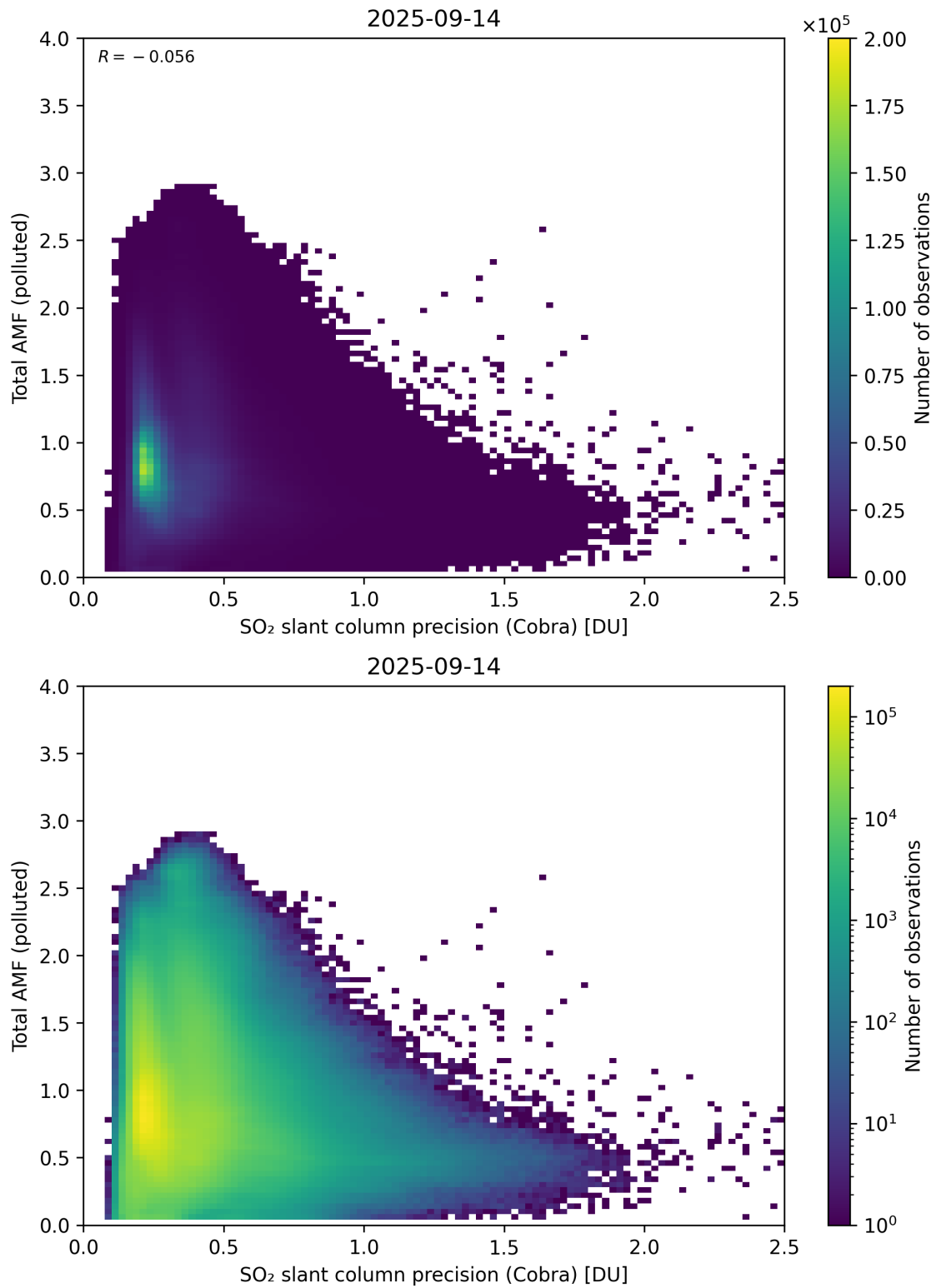
Figure 213: Scatter density plot of “SO 2 slant column precision (Cobra)” against “Total AMF (polluted)” for 2025-09-13 to 2025-09-15.
