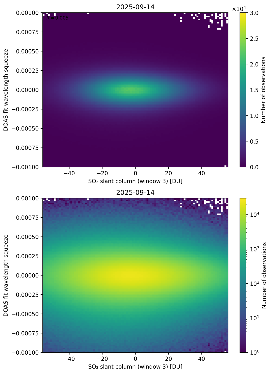
Figure 305: Scatter density plot of “SO 2 slant column (window 3)” against “DOAS fit wavelength squeeze” for 2025-09-13 to 2025-09-15.
