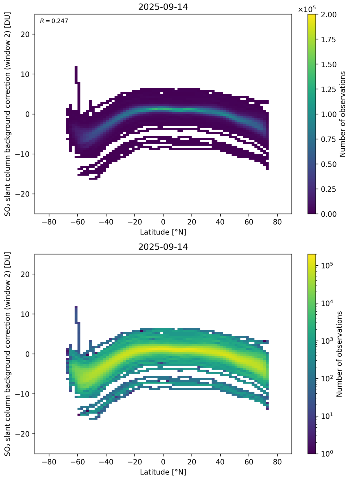
Figure 151: Scatter density plot of “Latitude” against “SO 2 slant column background correction (window 2)” for 2025-09-13 to 2025-09-15.
