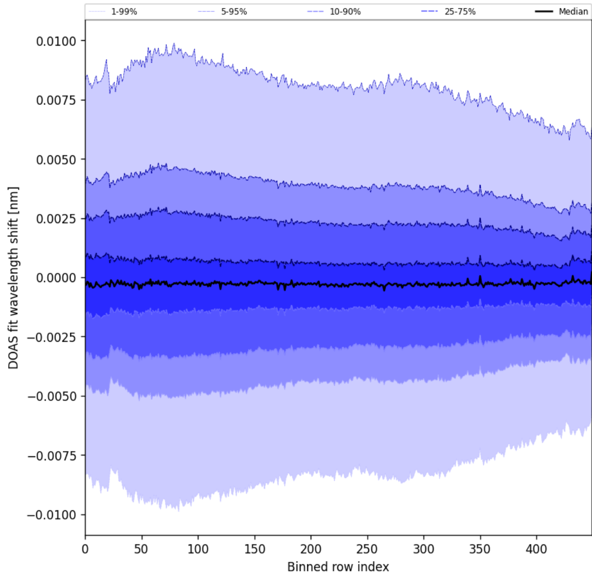
Figure 102: Along track statistics of “DOAS fit wavelength shift” for 2025-09-13 to 2025-09-15
