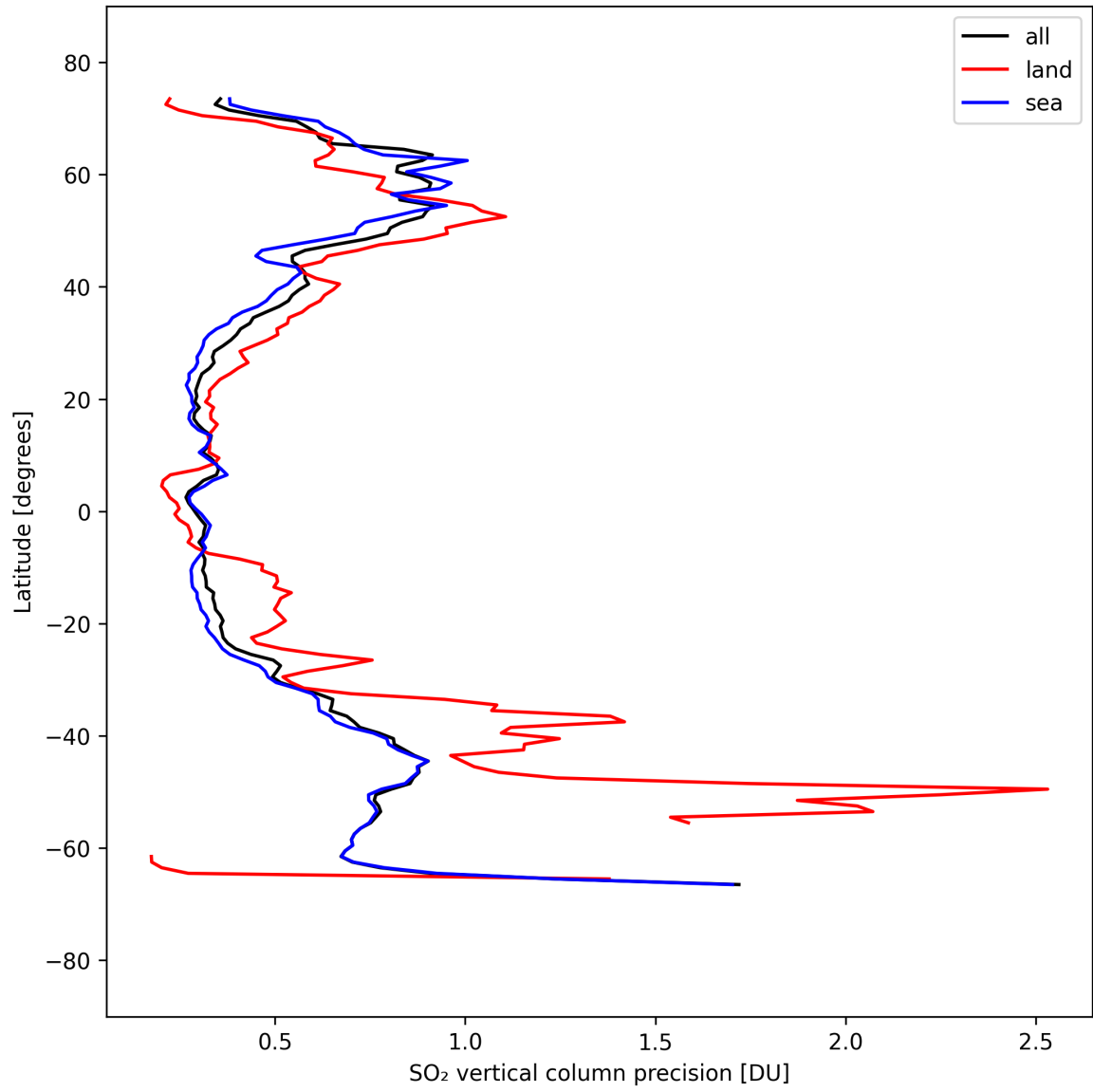
Figure 33: Zonal average of “SO 2 vertical column precision” for 2025-09-13 to 2025-09-15.
