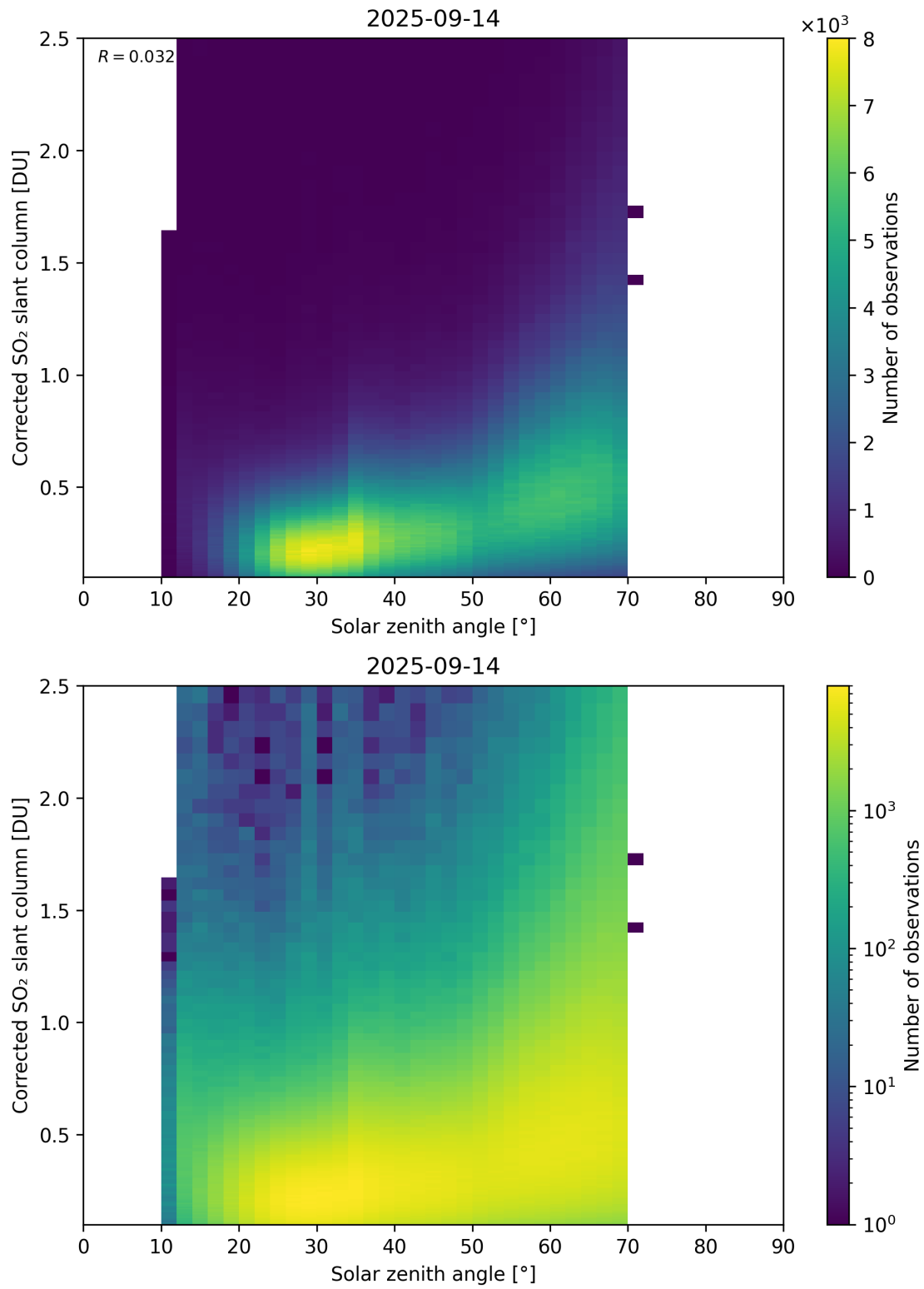
Figure 181: Scatter density plot of “Solar zenith angle” against “Corrected SO 2 slant column” for 2025-09-13 to 2025-09-15.
