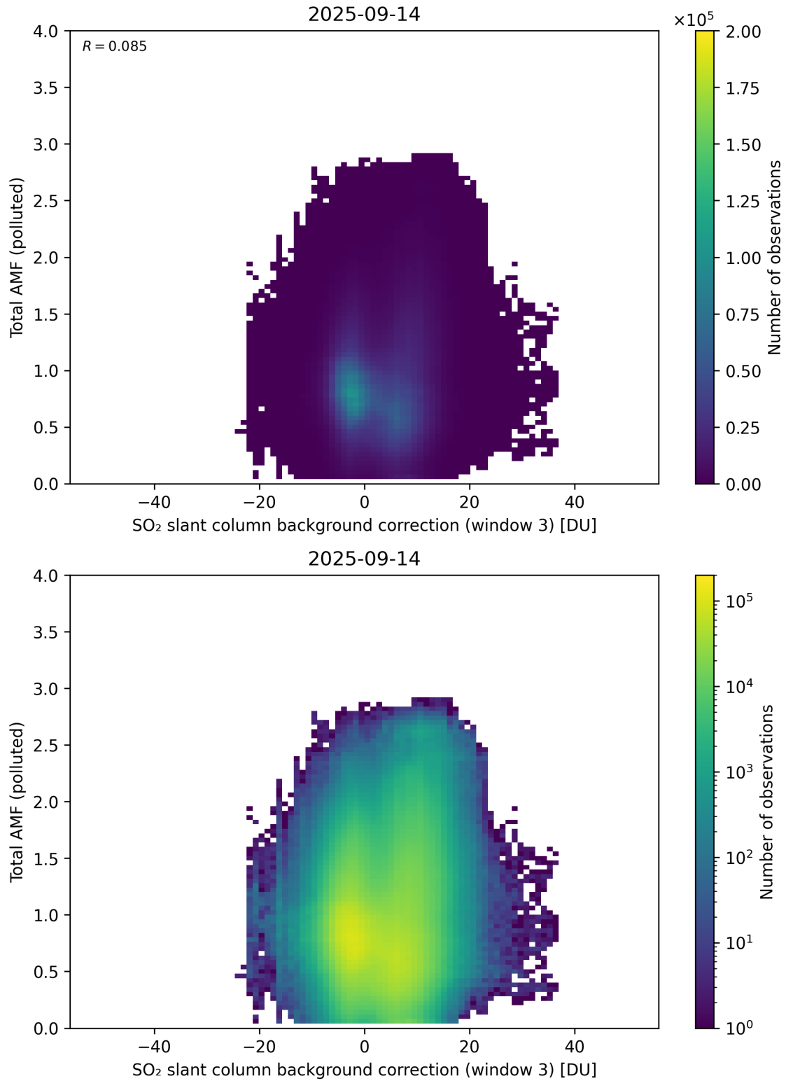
Figure 136: Scatter density plot of “SO 2 slant column background correction (window 3)” against “Total AMF (polluted)” for 2025-09-13 to 2025-09-15.
