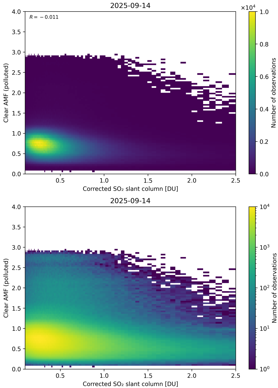
Figure 232: Scatter density plot of “Corrected SO 2 slant column” against “Clear AMF (polluted)” for 2025-09-13 to 2025-09-15.
