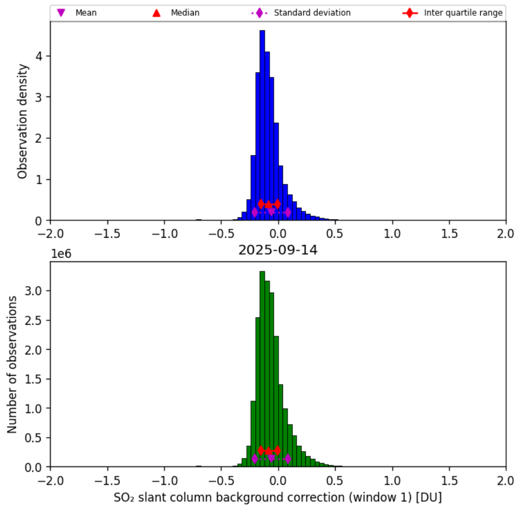
Figure 66: Histogram of “SO 2 slant column background correction (window 1)” for 2025-09-13 to 2025-09-15
