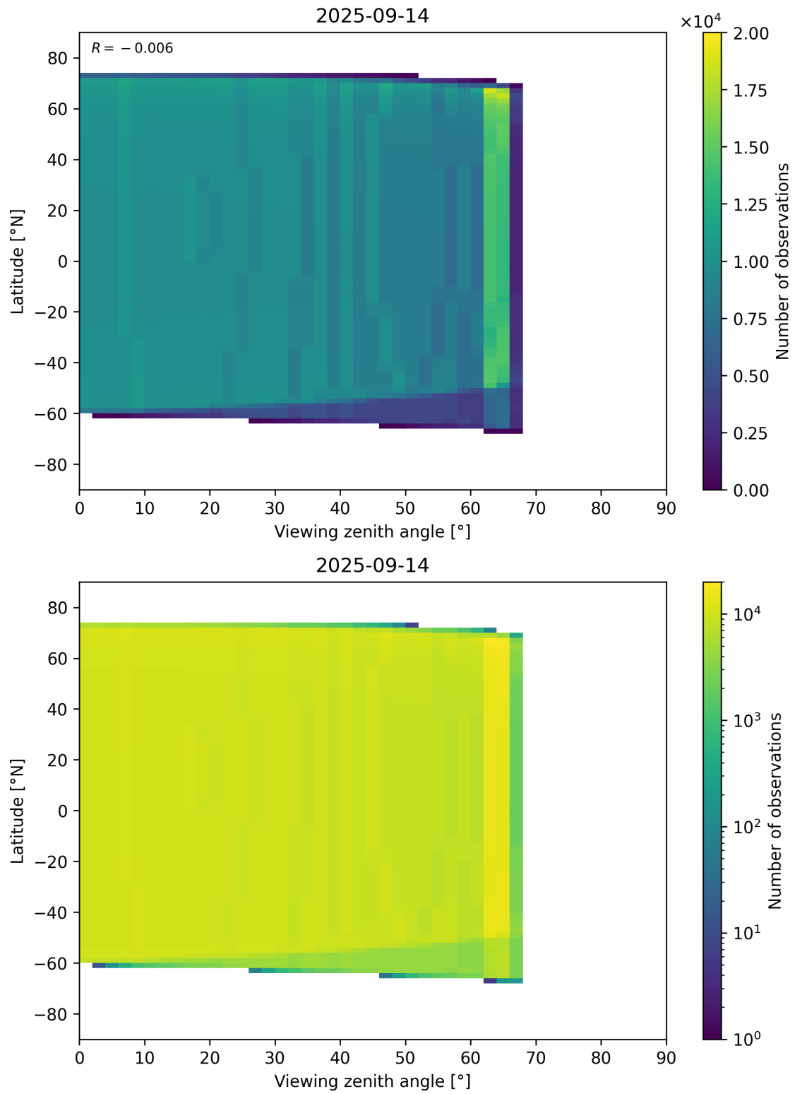
Figure 368: Scatter density plot of “Viewing zenith angle” against “Latitude” for 2025-09-13 to 2025-09-15.
