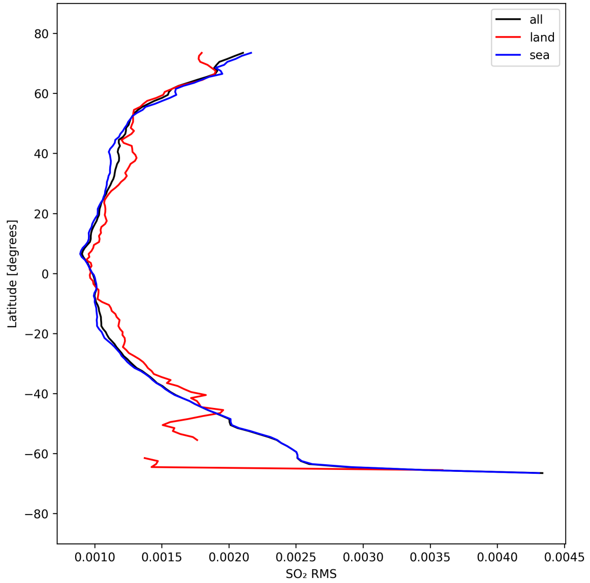
Figure 52: Zonal average of “SO 2 RMS” for 2025-09-13 to 2025-09-15.
