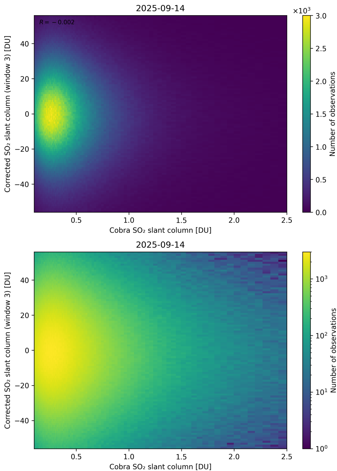
Figure 218: Scatter density plot of “Cobra SO 2 slant column” against “Corrected SO 2 slant column (window 3)” for 2025-09-13 to 2025-09-15.
