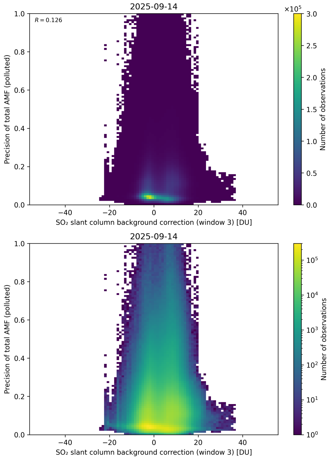
Figure 137: Scatter density plot of “SO 2 slant column background correction (window 3)” against “Precision of total AMF (polluted)” for 2025-09-13 to 2025-09-15.
