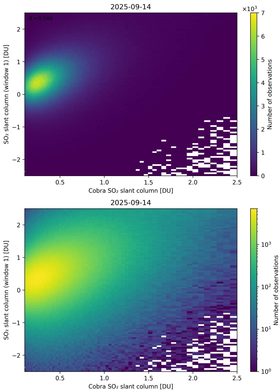
Figure 219: Scatter density plot of “Cobra SO 2 slant column” against “SO 2 slant column (window 1)” for 2025-09-13 to 2025-09-15.
