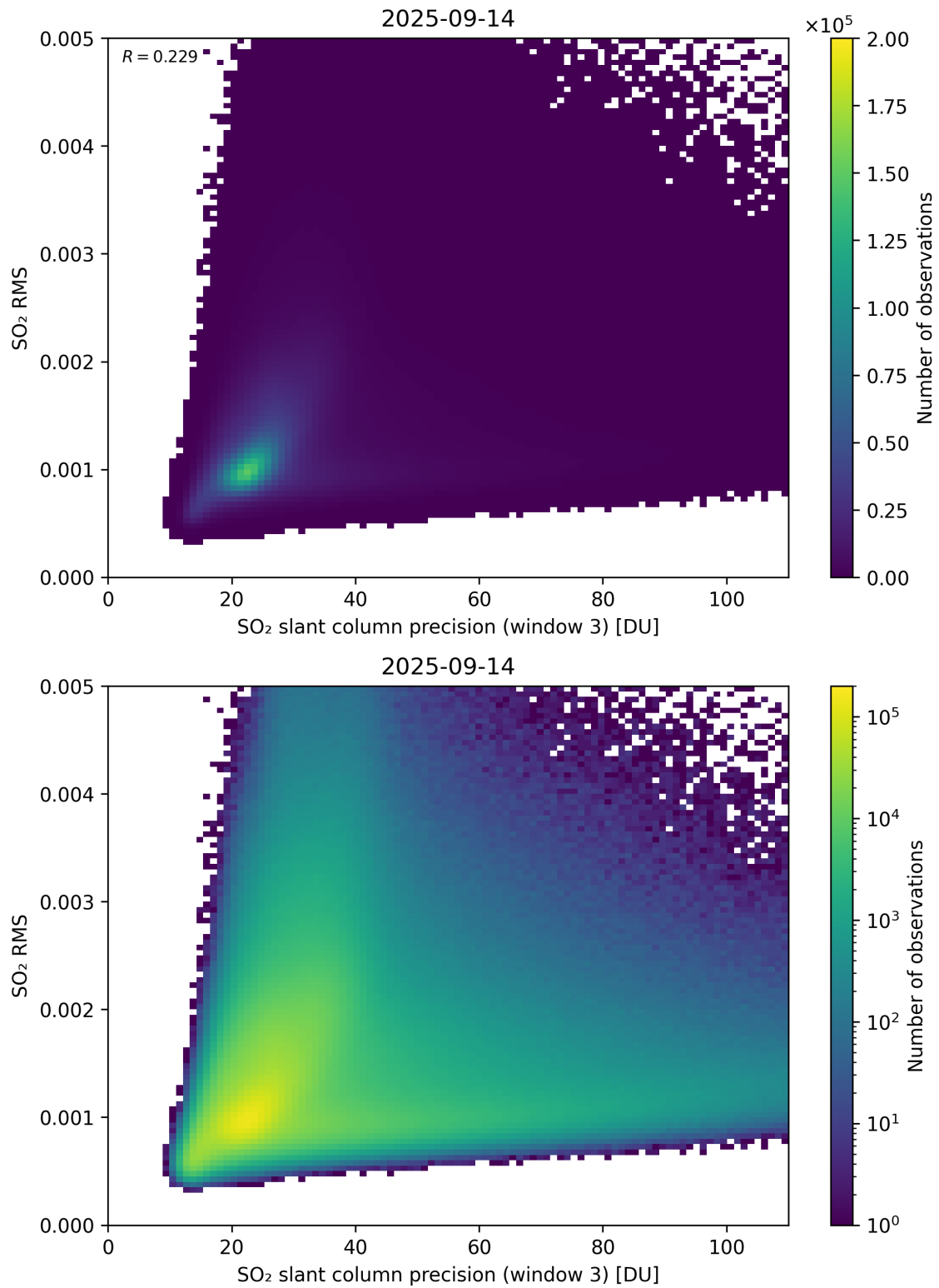
Figure 310: Scatter density plot of “SO 2 slant column precision (window 3)” against “SO 2 RMS” for 2025-09-13 to 2025-09-15.
