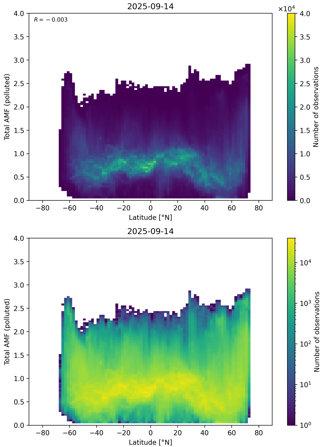
Figure 167: Scatter density plot of “Latitude” against “Total AMF (polluted)” for 2025-09-13 to 2025-09-15.
