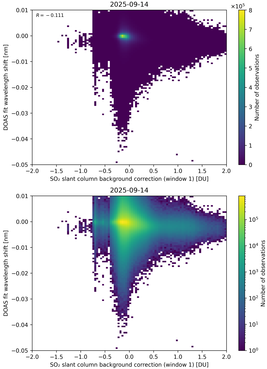
Figure 111: Scatter density plot of “SO 2 slant column background correction (window 1)” against “DOAS fit wavelength shift” for 2025-09-13 to 2025-09-15.
