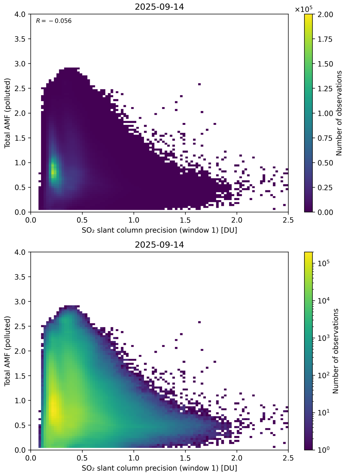
Figure 280: Scatter density plot of “SO 2 slant column precision (window 1)” against “Total AMF (polluted)” for 2025-09-13 to 2025-09-15.
