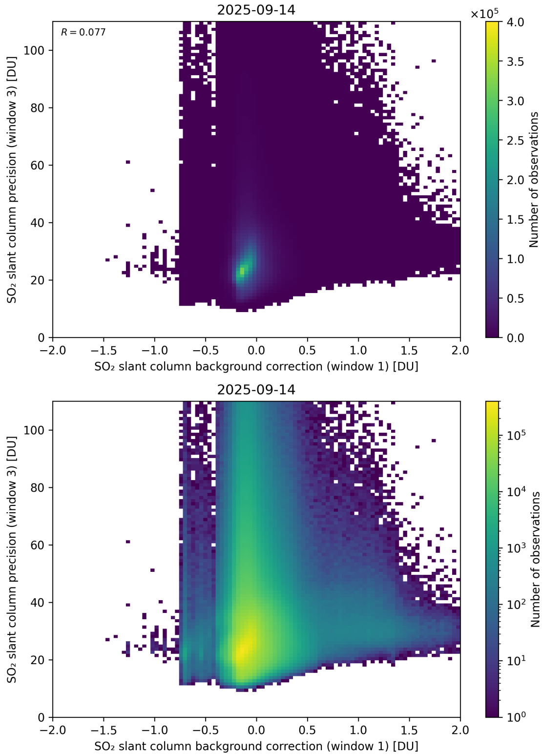
Figure 119: Scatter density plot of “SO 2 slant column background correction (window 1)” against “SO 2 slant column precision (window 3)” for 2025-09-13 to 2025-09-15.
