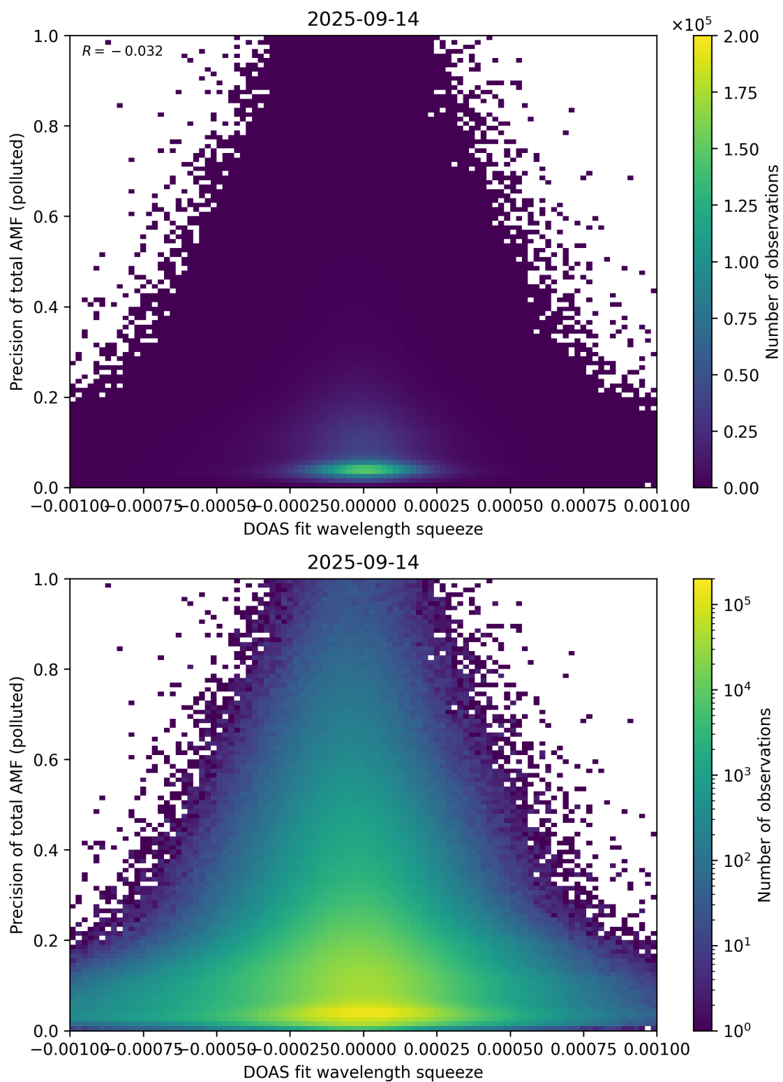
Figure 146: Scatter density plot of “DOAS fit wavelength squeeze” against “Precision of total AMF (polluted)” for 2025-09-13 to 2025-09-15.
