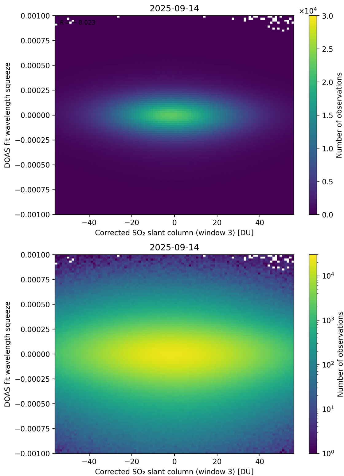
Figure 257: Scatter density plot of “Corrected SO 2 slant column (window 3)” against “DOAS fit wavelength squeeze” for 2025-09-13 to 2025-09-15.
