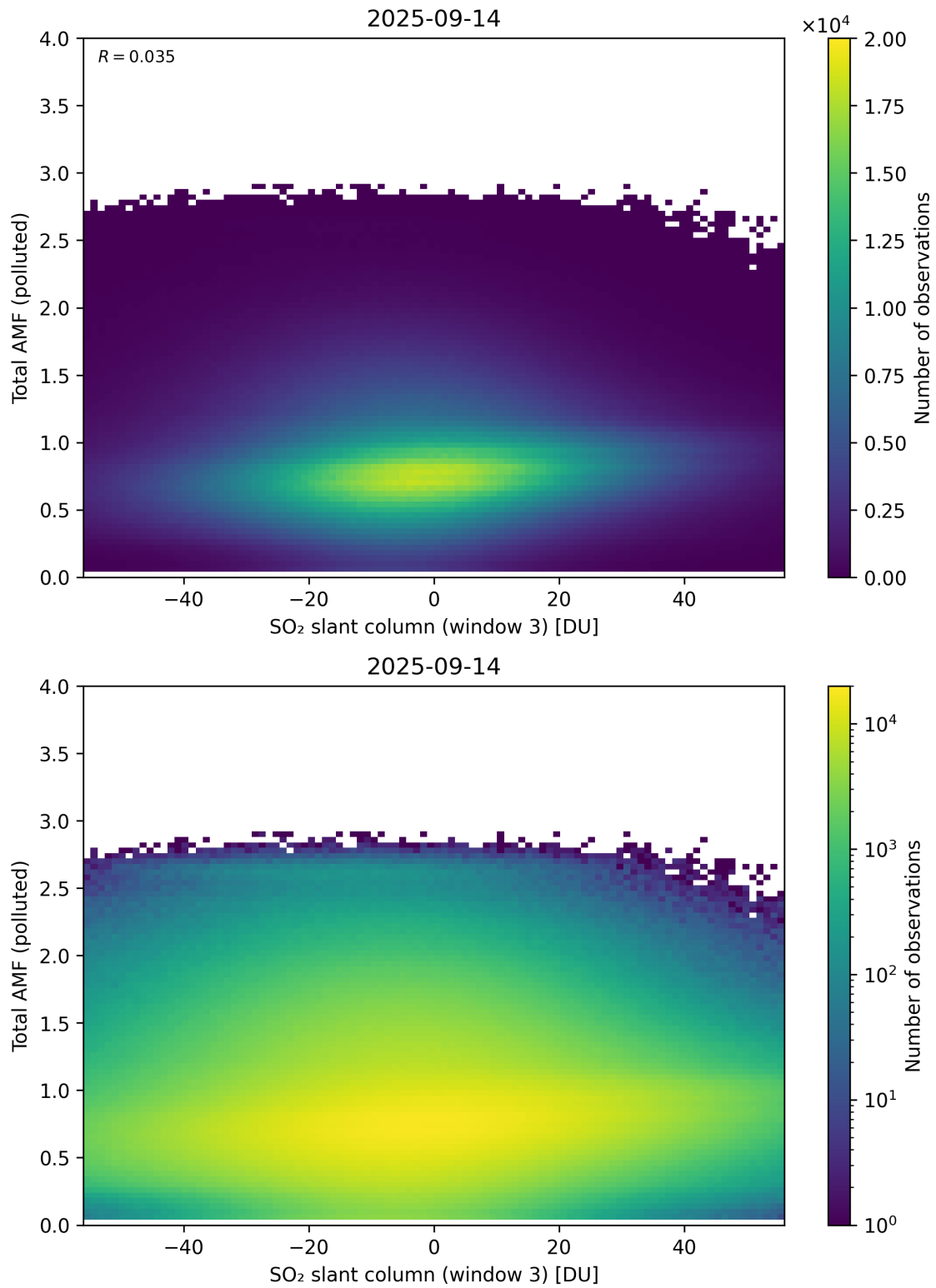
Figure 318: Scatter density plot of “SO 2 slant column (window 3)” against “Total AMF (polluted)” for 2025-09-13 to 2025-09-15.
