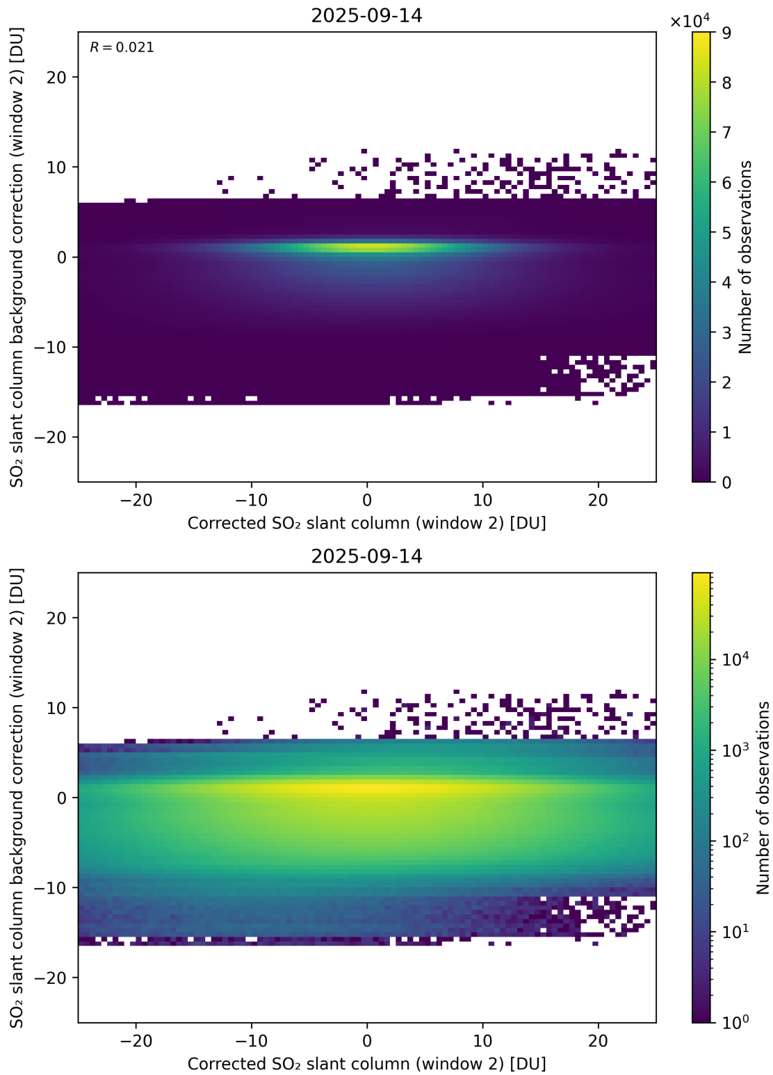
Figure 244: Scatter density plot of “Corrected SO 2 slant column (window 2)” against “SO 2 slant column background correction (window 2)” for 2025-09-13 to 2025-09-15.
