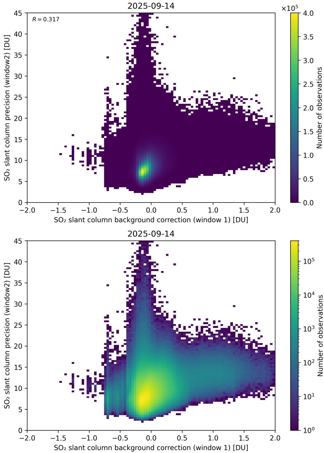
Figure 117: Scatter density plot of “SO 2 slant column background correction (window 1)” against “SO 2 slant column precision (window2)” for 2025-09-13 to 2025-09-15.
