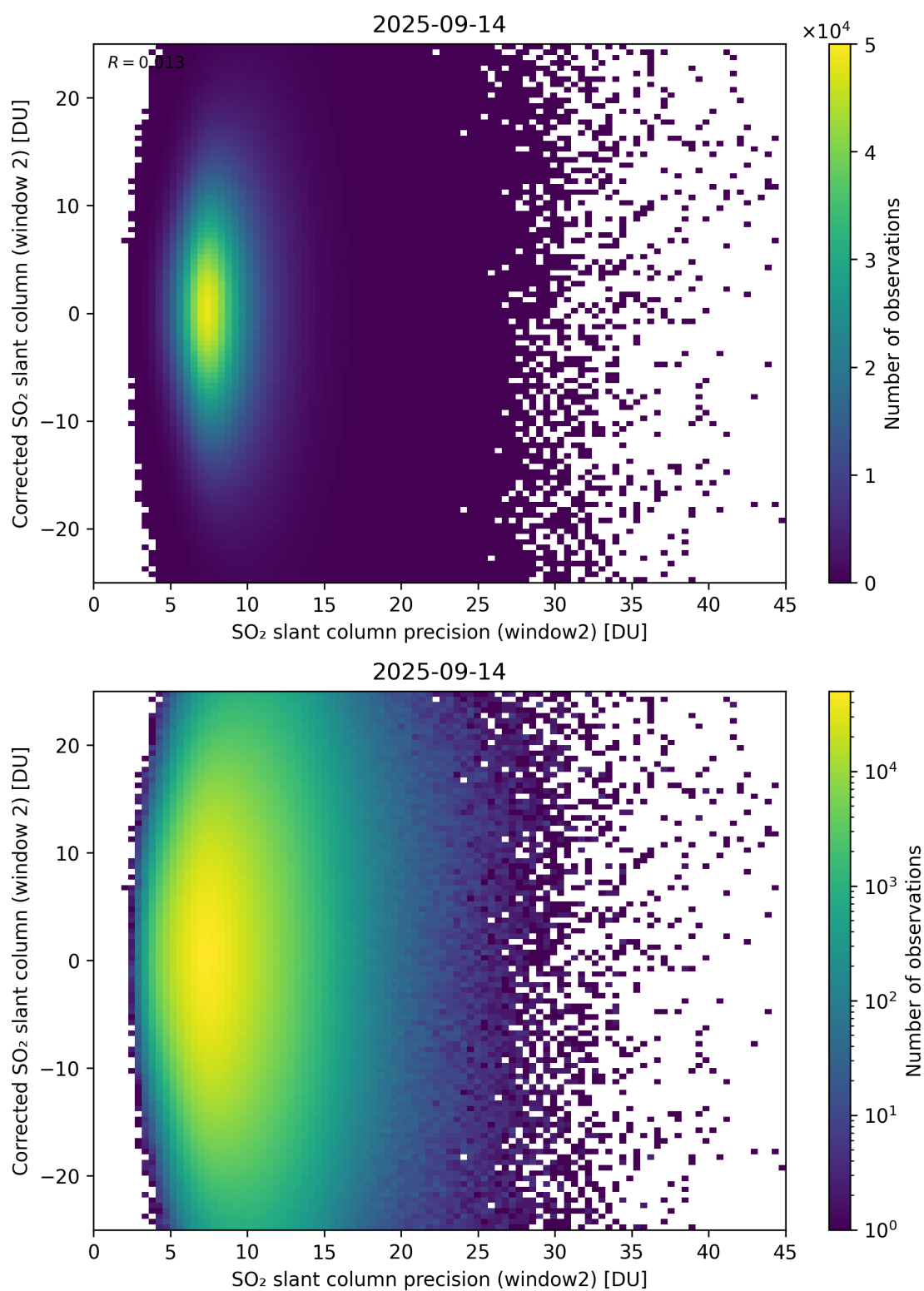
Figure 297: Scatter density plot of “SO 2 slant column precision (window2)” against “Corrected SO 2 slant column (window 2)” for 2025-09-13 to 2025-09-15.
