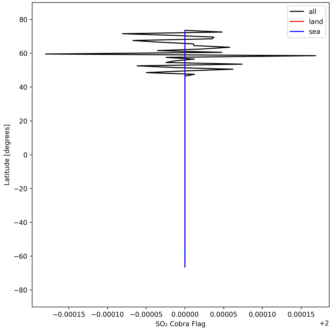
Figure 49: Zonal average of “SO 2 Cobra Flag” for 2025-09-13 to 2025-09-15.
