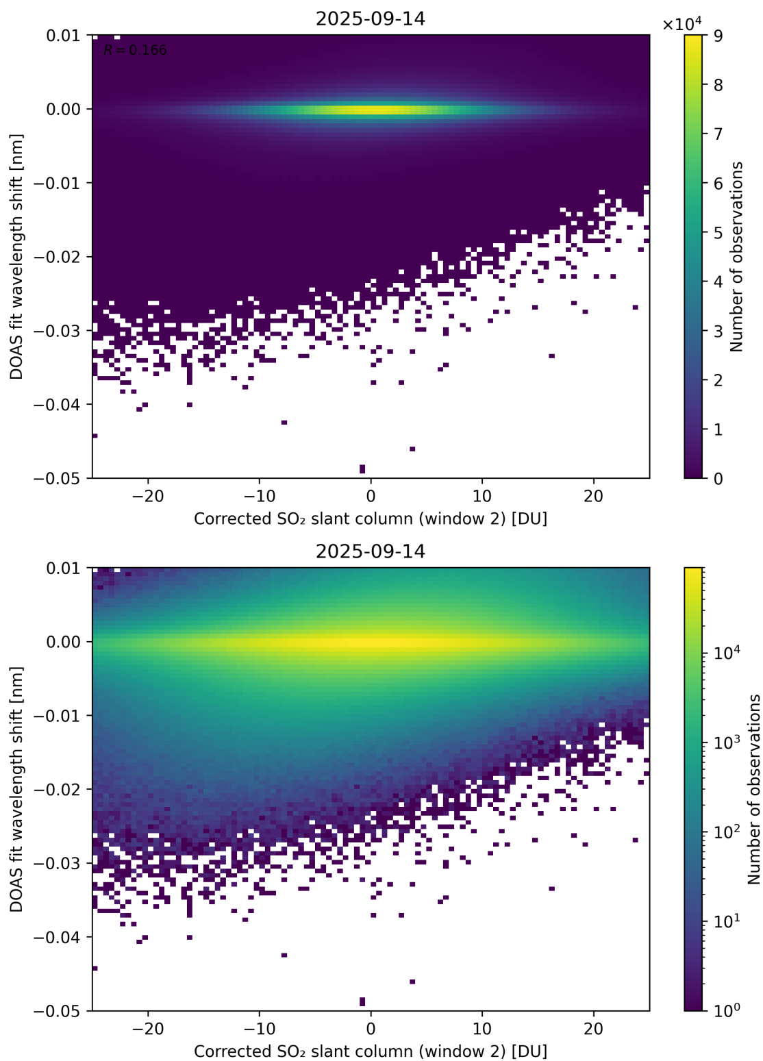
Figure 246: Scatter density plot of “Corrected SO 2 slant column (window 2)” against “DOAS fit wavelength shift” for 2025-09-13 to 2025-09-15.
