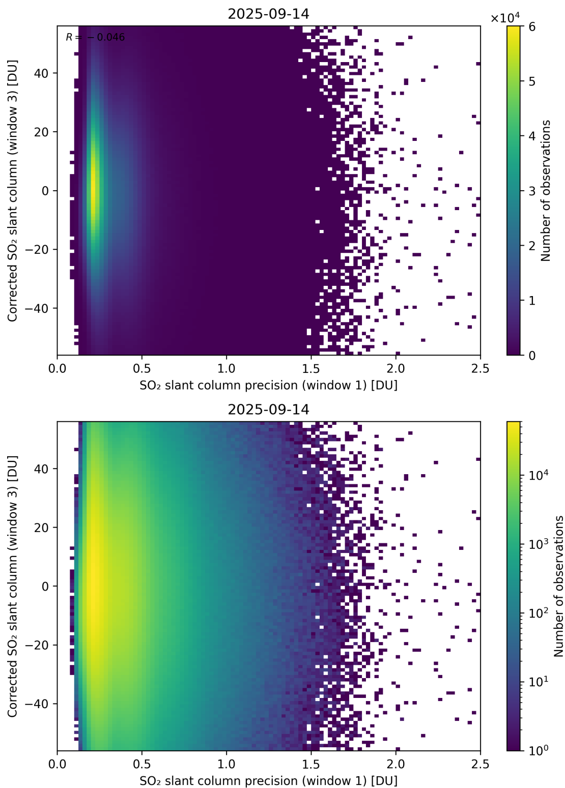
Figure 276: Scatter density plot of “SO 2 slant column precision (window 1)” against “Corrected SO 2 slant column (window 3)” for 2025-09-13 to 2025-09-15.
