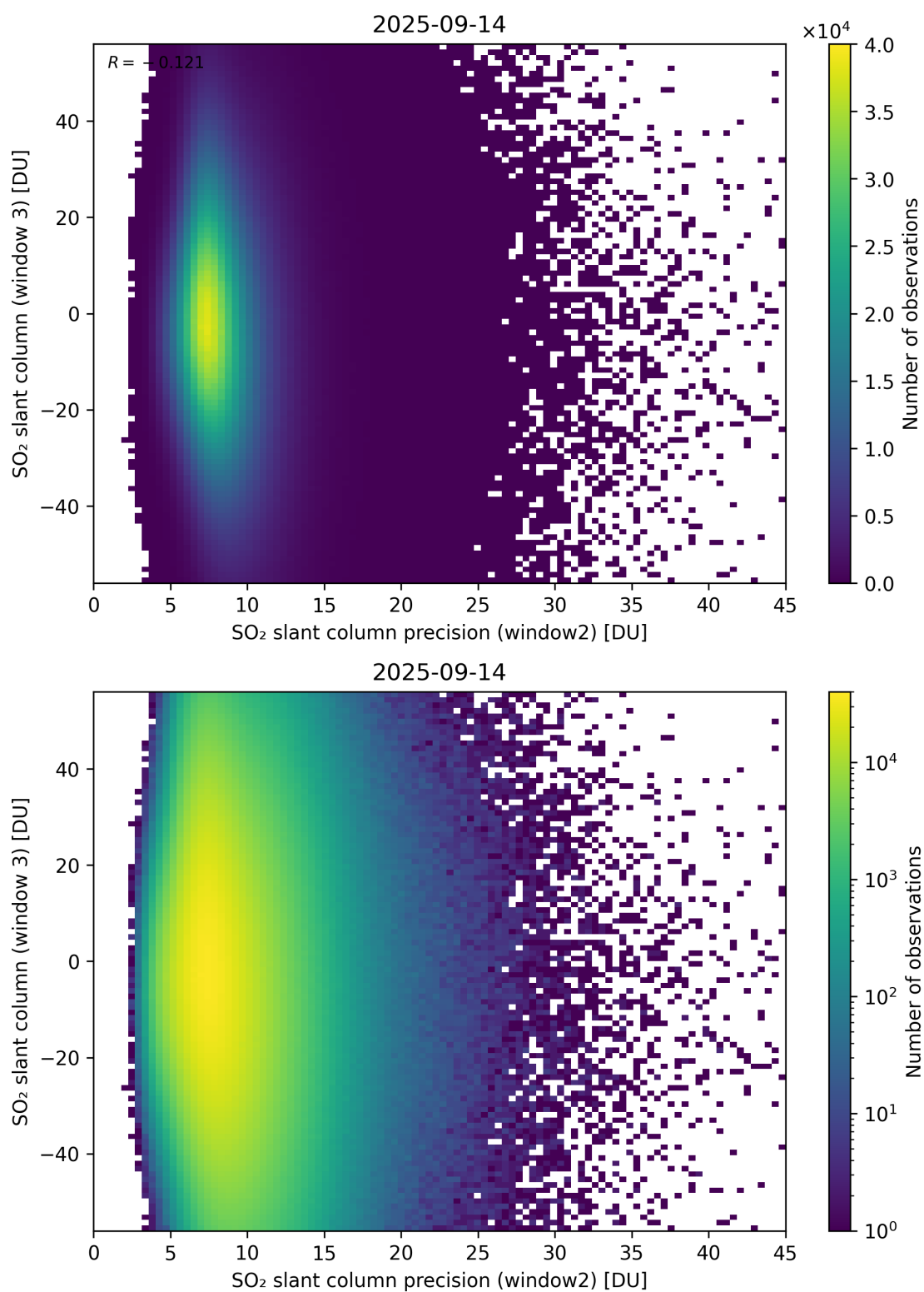
Figure 299: Scatter density plot of “SO 2 slant column precision (window2)” against “SO 2 slant column (window 3)” for 2025-09-13 to 2025-09-15.
