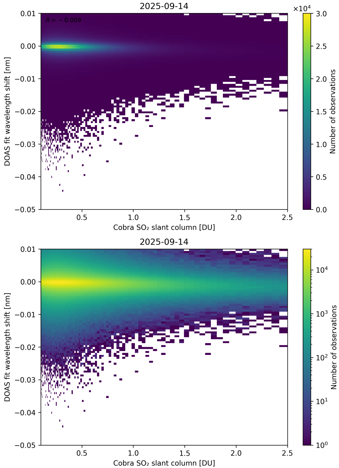
Figure 196: Scatter density plot of “Cobra SO 2 slant column” against “DOAS fit wavelength shift” for 2025-09-13 to 2025-09-15.
