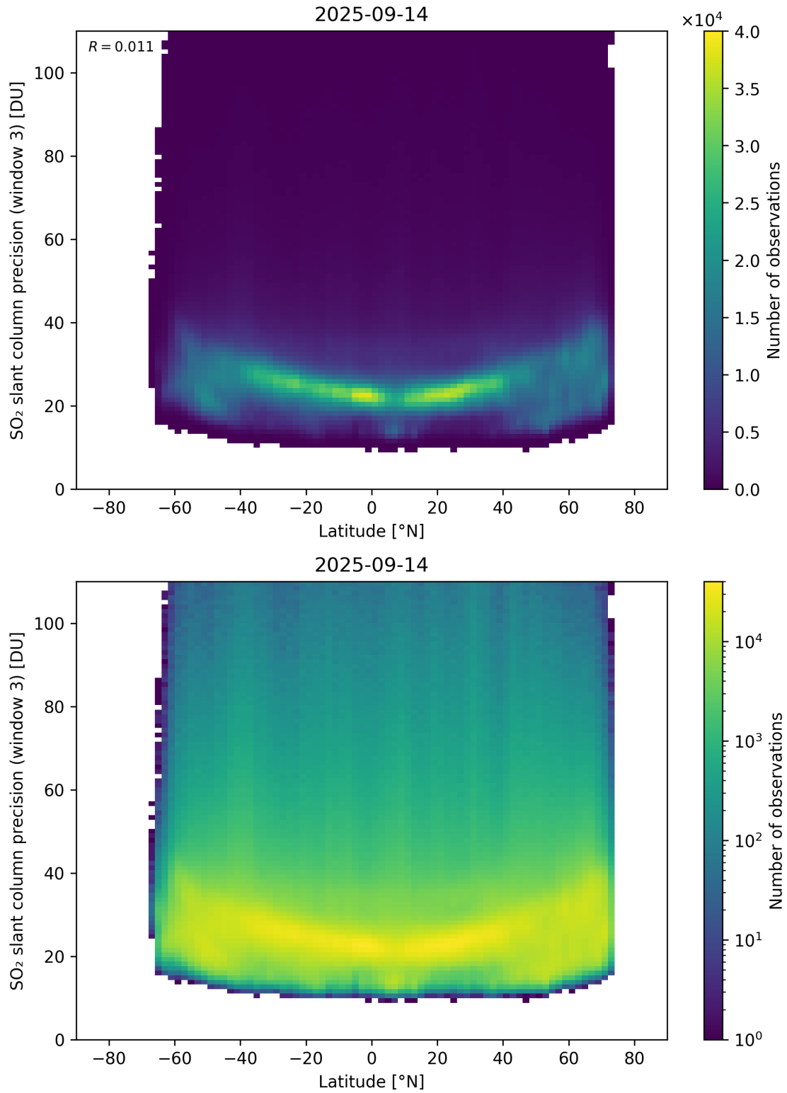
Figure 166: Scatter density plot of “Latitude” against “SO 2 slant column precision (window 3)” for 2025-09-13 to 2025-09-15.
