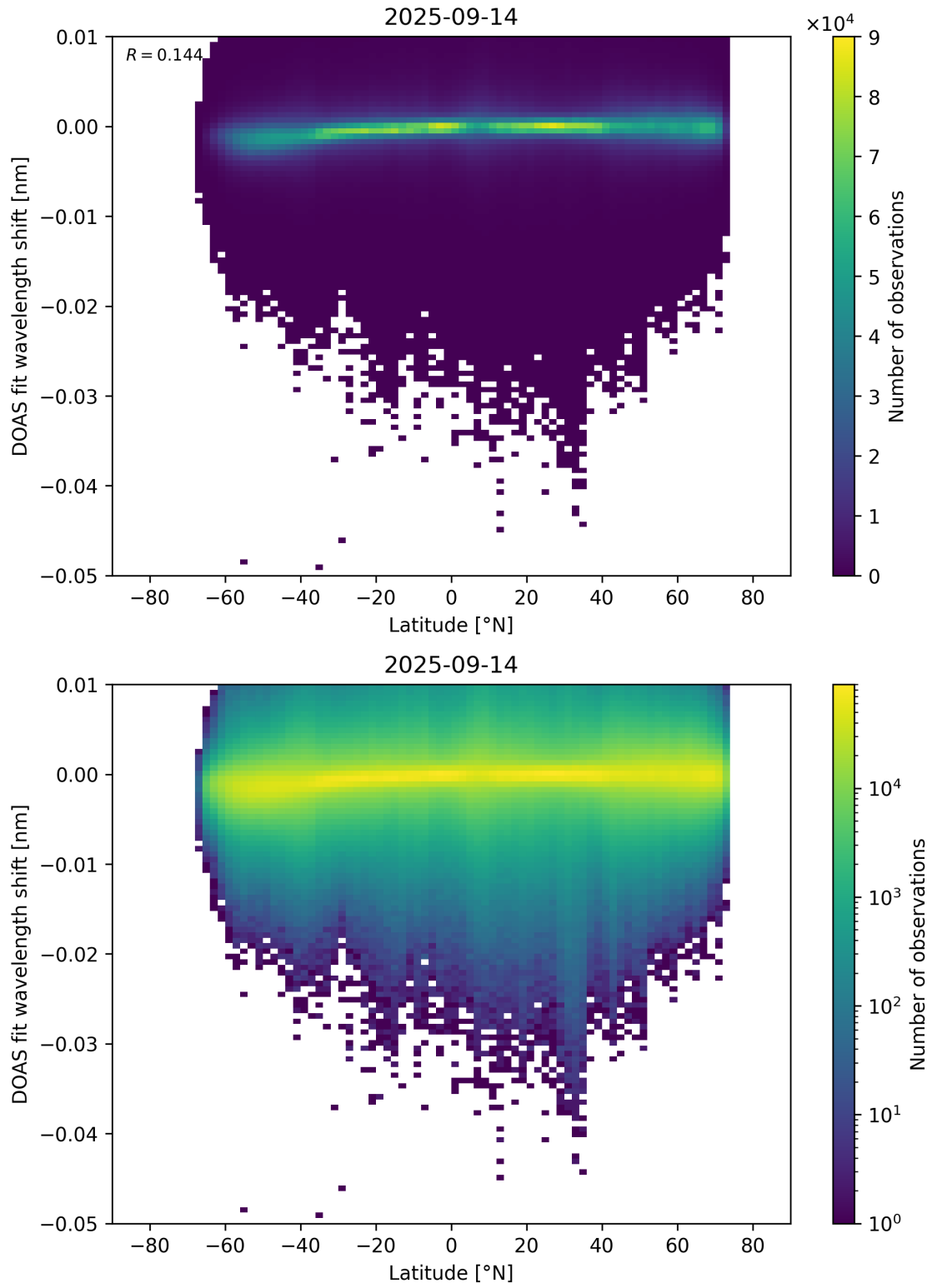
Figure 153: Scatter density plot of “Latitude” against “DOAS fit wavelength shift” for 2025-09-13 to 2025-09-15.
