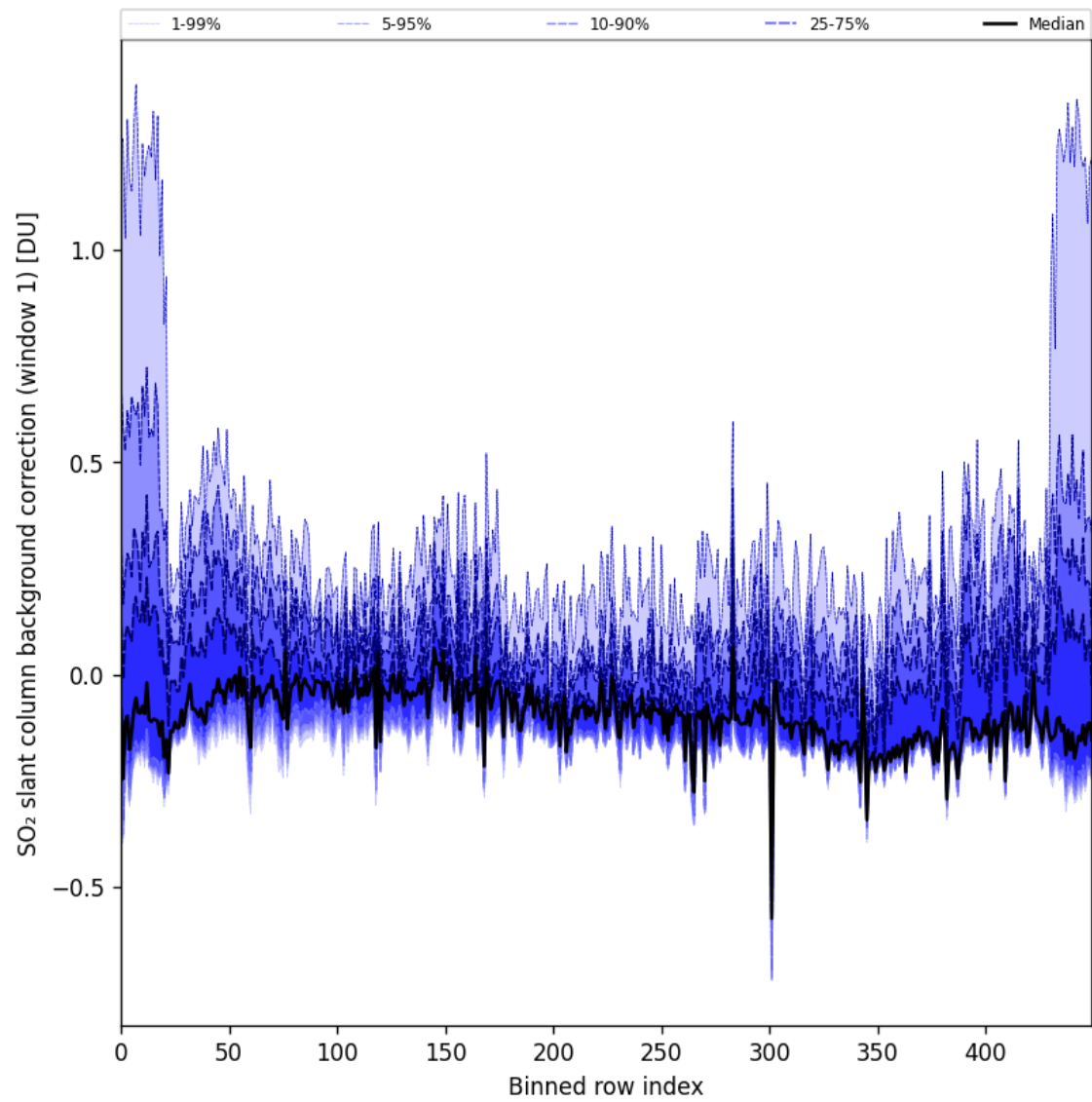
Figure 92: Along track statistics of “SO 2 slant column background correction (window 1)” for 2025-09-13 to 2025-09-15
