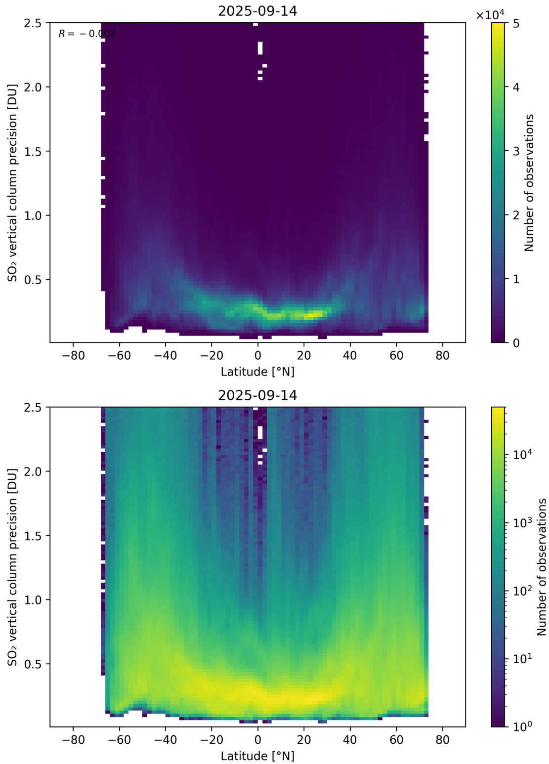
Figure 170: Scatter density plot of “Latitude” against “SO 2 vertical column precision” for 2025-09-13 to 2025-09-15.
