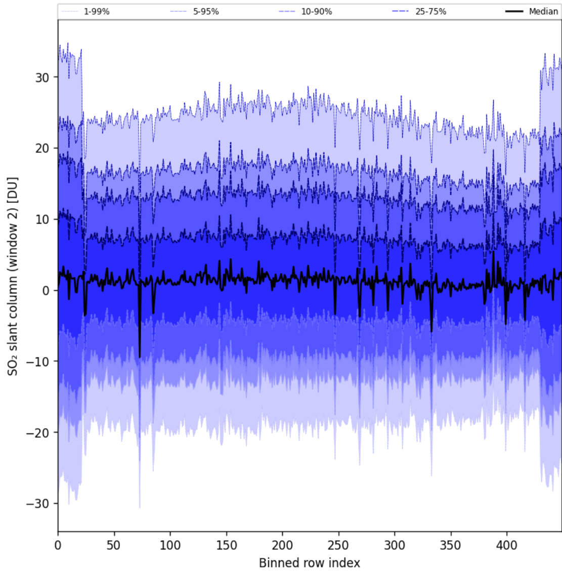
Figure 93: Along track statistics of “SO 2 slant column (window 2)” for 2025-09-13 to 2025-09-15
