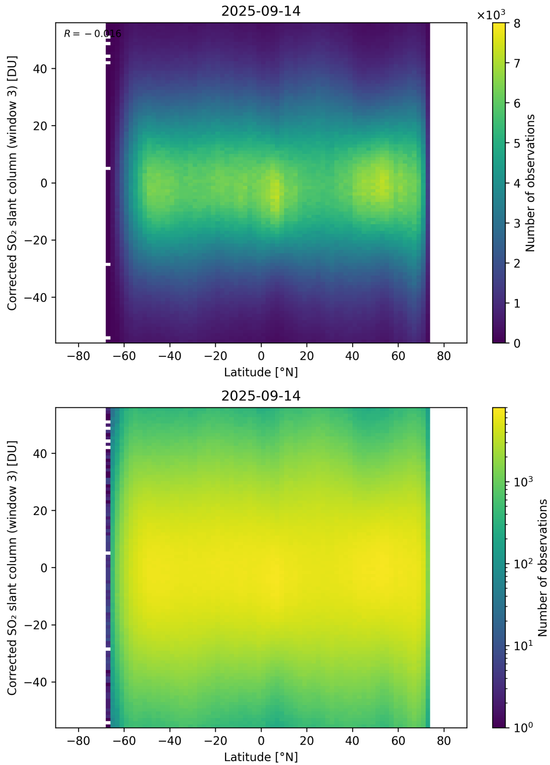
Figure 161: Scatter density plot of “Latitude” against “Corrected SO 2 slant column (window 3)” for 2025-09-13 to 2025-09-15.
