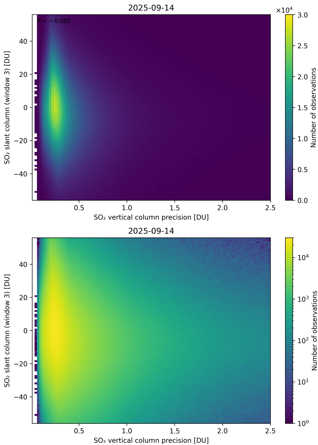
Figure 344: Scatter density plot of “SO 2 vertical column precision” against “SO 2 slant column (window 3)” for 2025-09-13 to 2025-09-15.
