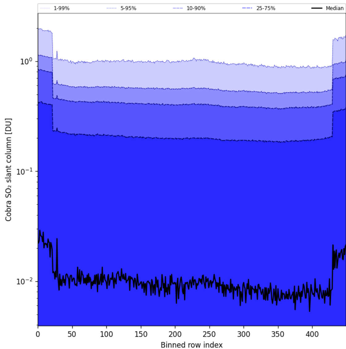
Figure 87: Along track statistics of “Cobra SO 2 slant column” for 2025-09-13 to 2025-09-15
