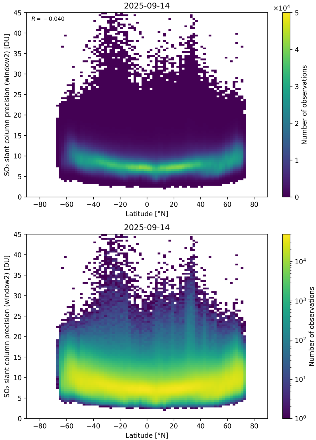
Figure 164: Scatter density plot of “Latitude” against “SO 2 slant column precision (window2)” for 2025-09-13 to 2025-09-15.
