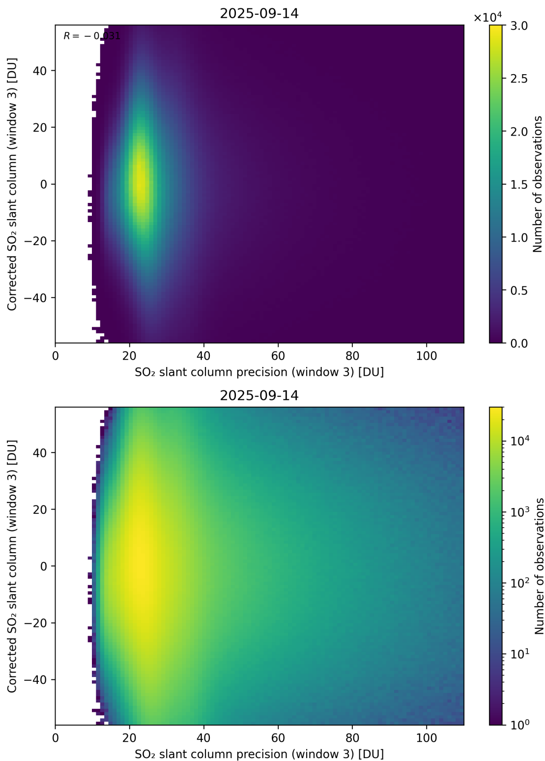
Figure 312: Scatter density plot of “SO 2 slant column precision (window 3)” against “Corrected SO 2 slant column (window 3)” for 2025-09-13 to 2025-09-15.
