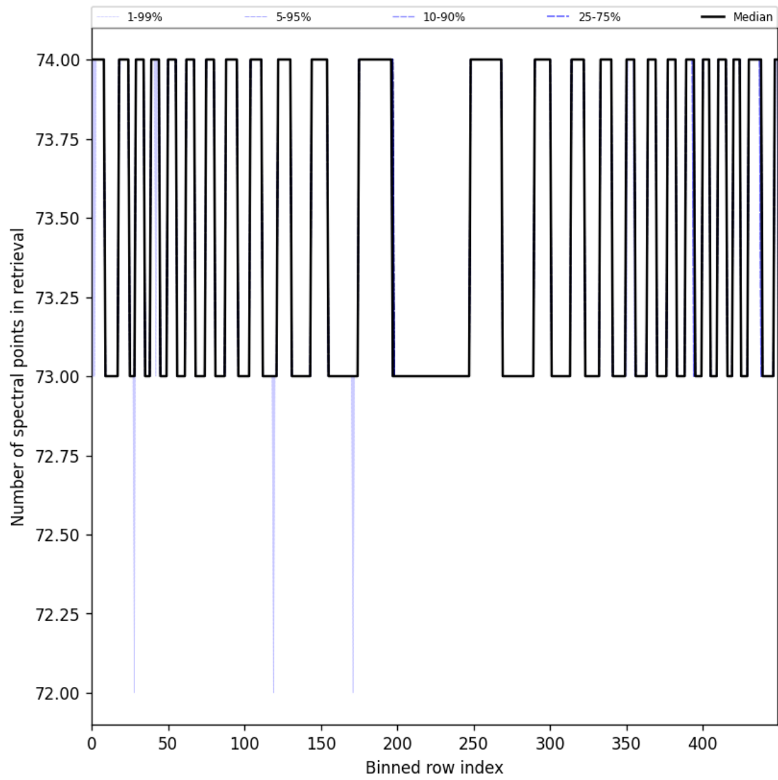
Figure 108: Along track statistics of “Number of spectral points in retrieval” for 2025-09-13 to 2025-09-15
