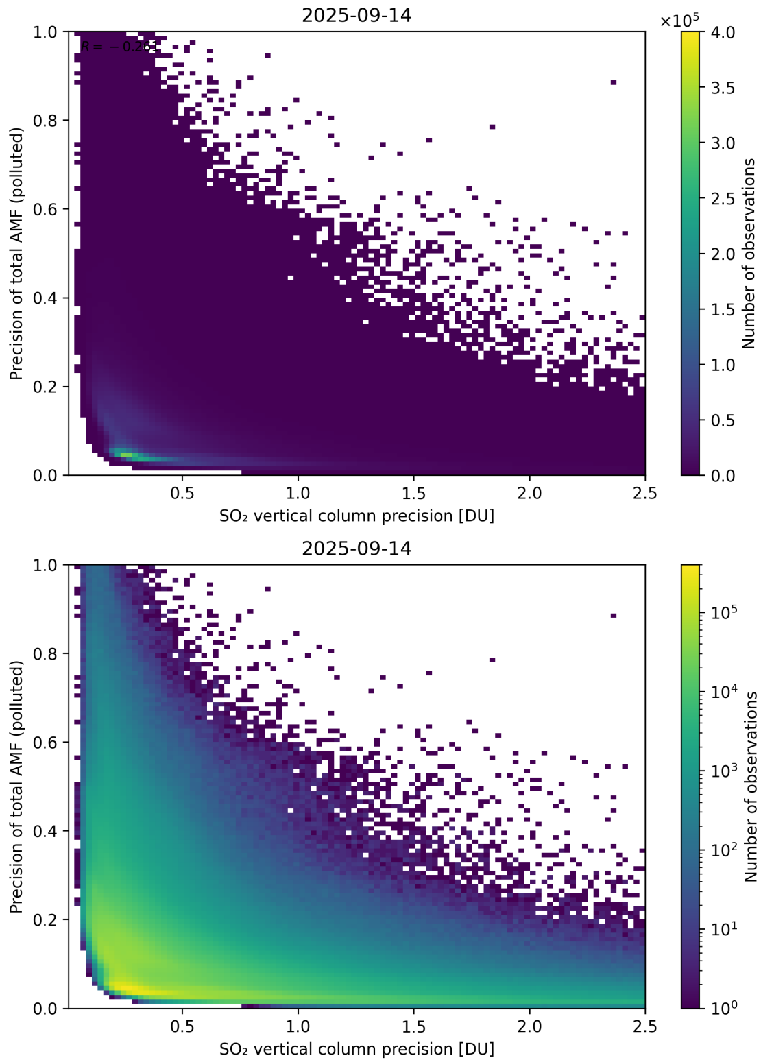
Figure 347: Scatter density plot of “SO 2 vertical column precision” against “Precision of total AMF (polluted)” for 2025-09-13 to 2025-09-15.
