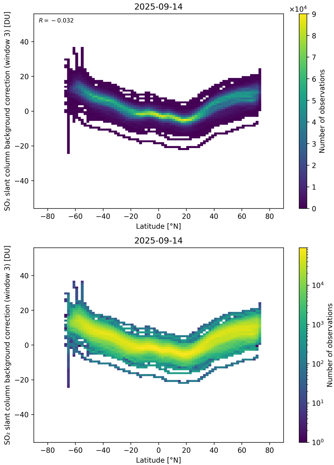
Figure 152: Scatter density plot of “Latitude” against “SO 2 slant column background correction (window 3)” for 2025-09-13 to 2025-09-15.
