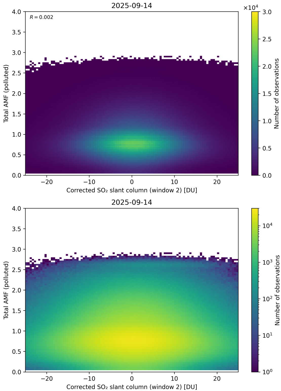
Figure 253: Scatter density plot of “Corrected SO 2 slant column (window 2)” against “Total AMF (polluted)” for 2025-09-13 to 2025-09-15.
