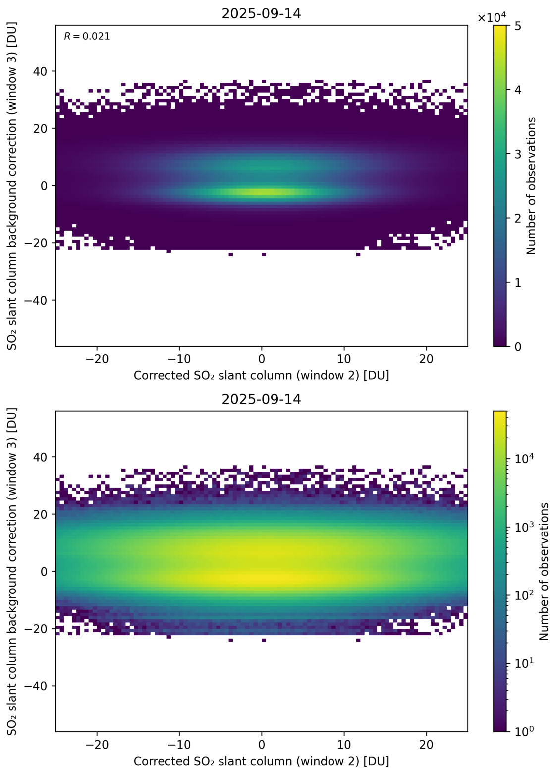
Figure 245: Scatter density plot of “Corrected SO 2 slant column (window 2)” against “SO 2 slant column background correction (window 3)” for 2025-09-13 to 2025-09-15.
