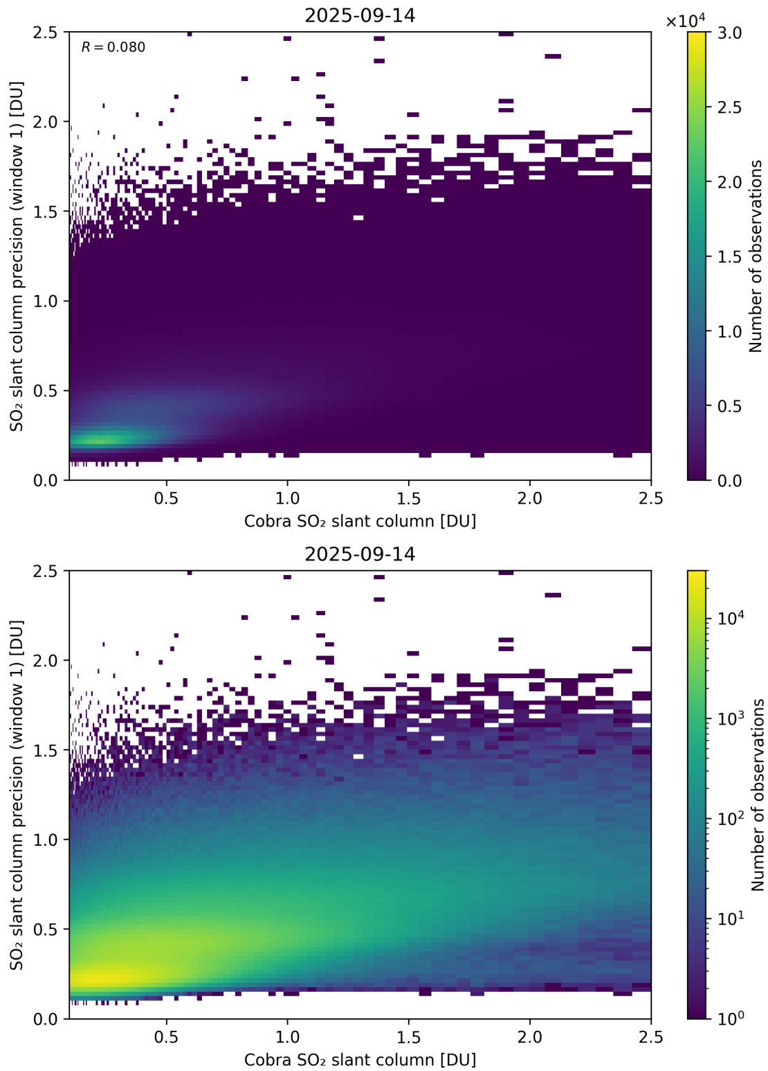
Figure 220: Scatter density plot of “Cobra SO 2 slant column” against “SO 2 slant column precision (window 1)” for 2025-09-13 to 2025-09-15.
