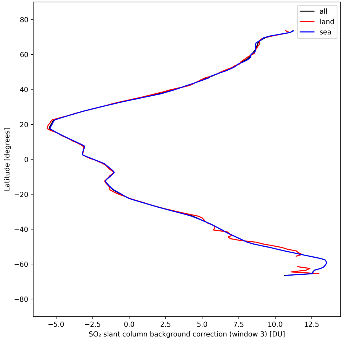
Figure 48: Zonal average of “SO 2 slant column background correction (window 3)” for 2025-09-13 to 2025-09-15.
