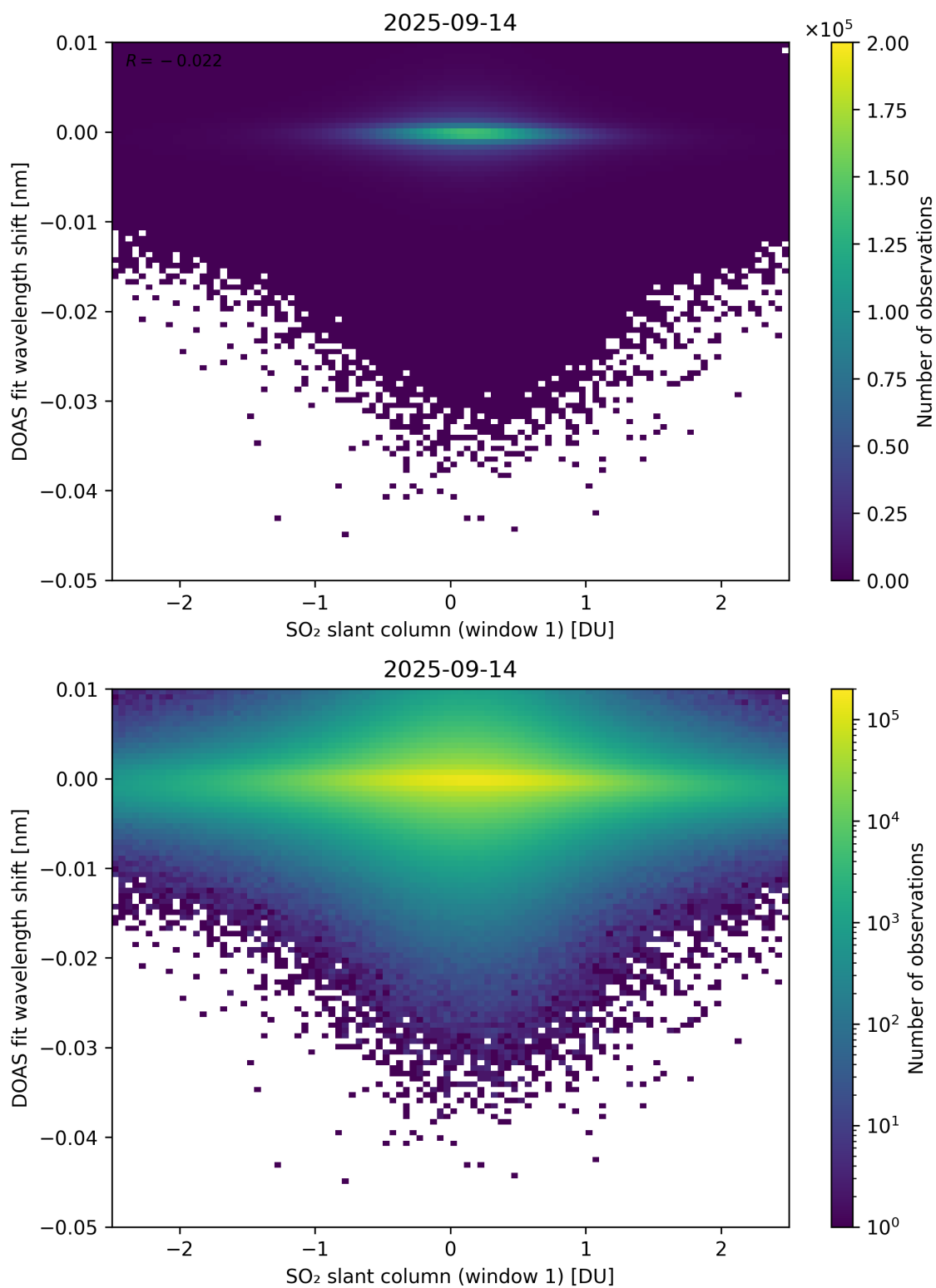
Figure 265: Scatter density plot of “SO 2 slant column (window 1)” against “DOAS fit wavelength shift” for 2025-09-13 to 2025-09-15.
