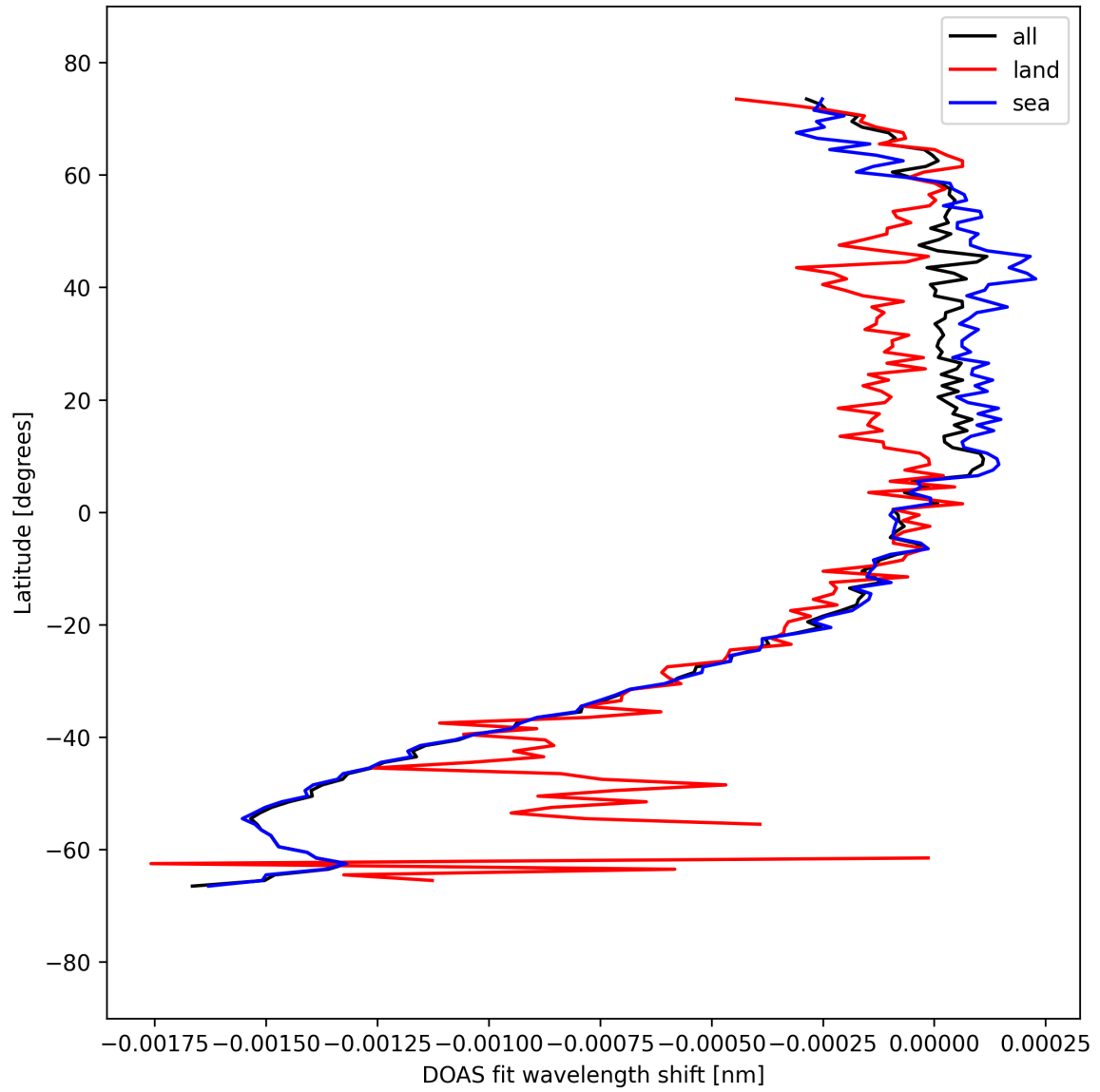
Figure 50: Zonal average of “DOAS fit wavelength shift” for 2025-09-13 to 2025-09-15.
