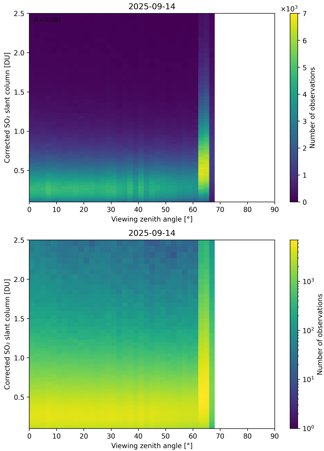
Figure 373: Scatter density plot of “Viewing zenith angle” against “Corrected SO 2 slant column” for 2025-09-13 to 2025-09-15.
