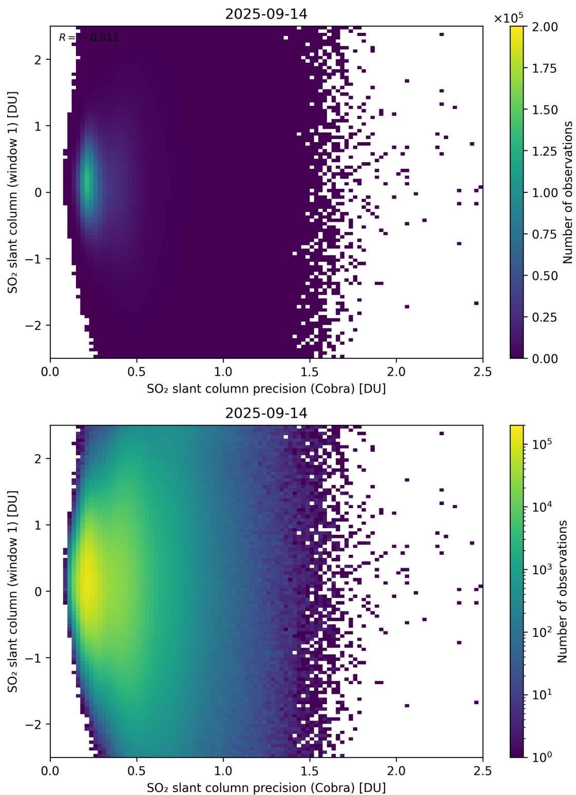
Figure 208: Scatter density plot of “SO 2 slant column precision (Cobra)” against “SO 2 slant column (window 1)” for 2025-09-13 to 2025-09-15.
