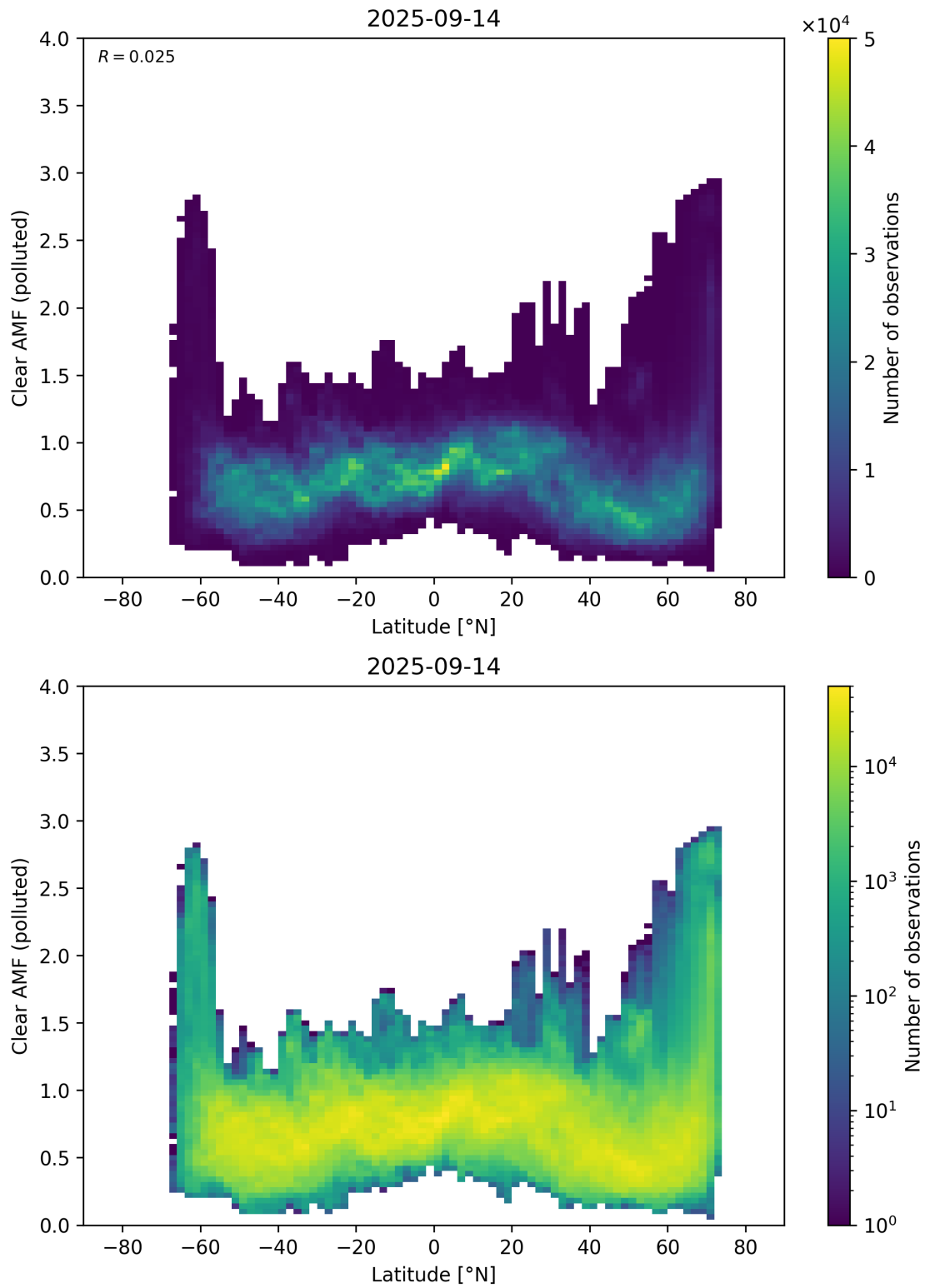
Figure 156: Scatter density plot of “Latitude” against “Clear AMF (polluted)” for 2025-09-13 to 2025-09-15.
