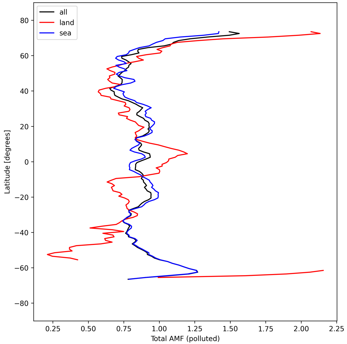
Figure 53: Zonal average of “Total AMF (polluted)” for 2025-09-13 to 2025-09-15.
