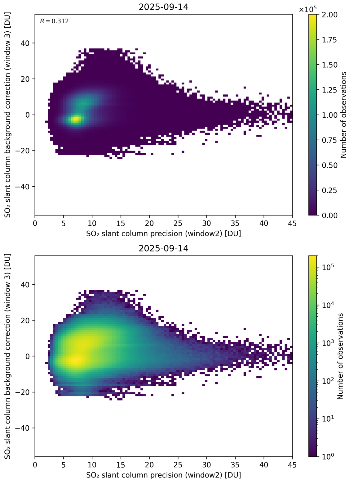
Figure 292: Scatter density plot of “SO 2 slant column precision (window2)” against “SO 2 slant column background correction (window 3)” for 2025-09-13 to 2025-09-15.
