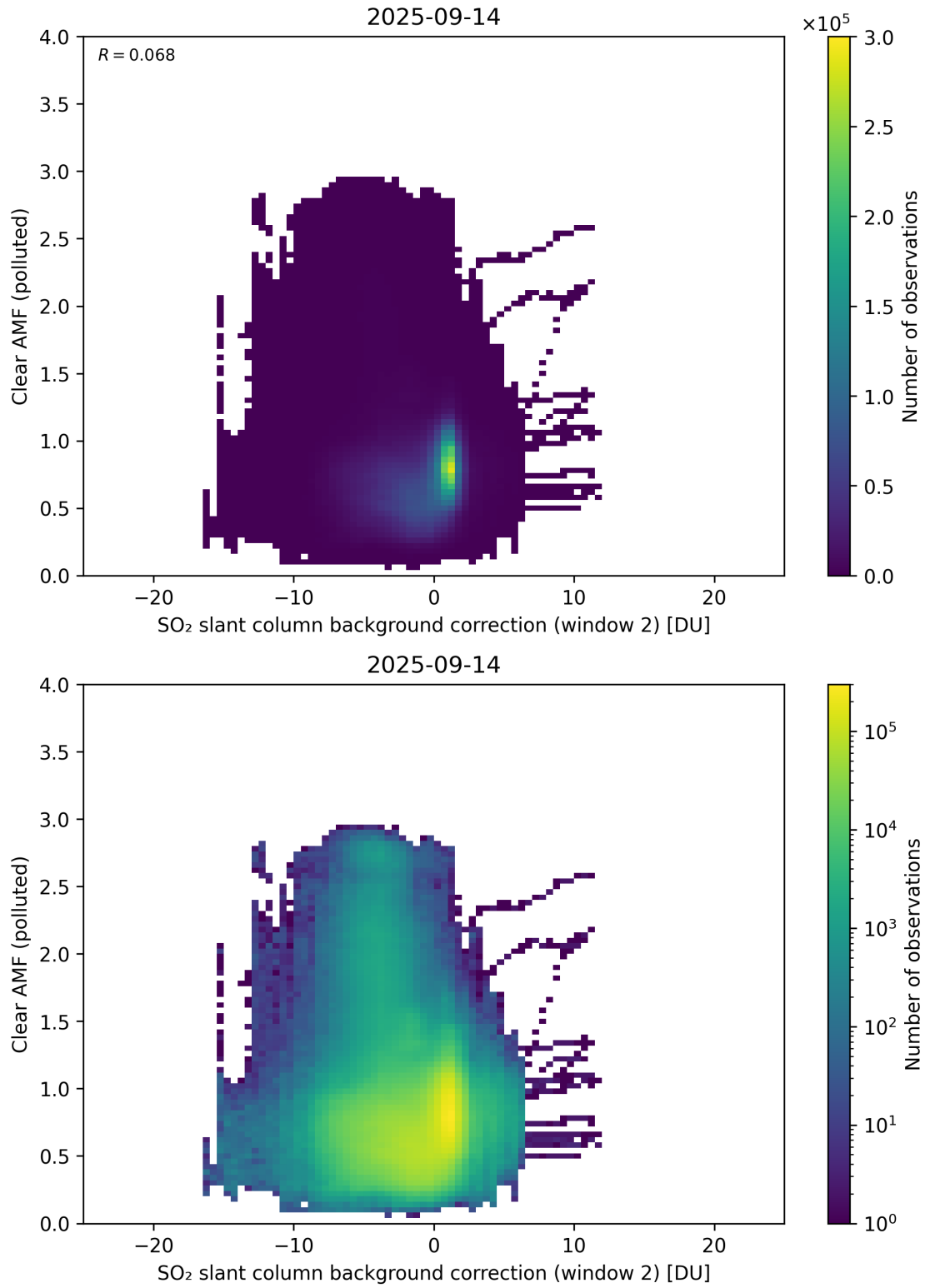
Figure 126: Scatter density plot of “SO 2 slant column background correction (window 2)” against “Clear AMF (polluted)” for 2025-09-13 to 2025-09-15.
