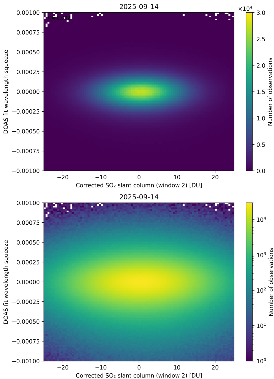
Figure 247: Scatter density plot of “Corrected SO 2 slant column (window 2)” against “DOAS fit wavelength squeeze” for 2025-09-13 to 2025-09-15.
