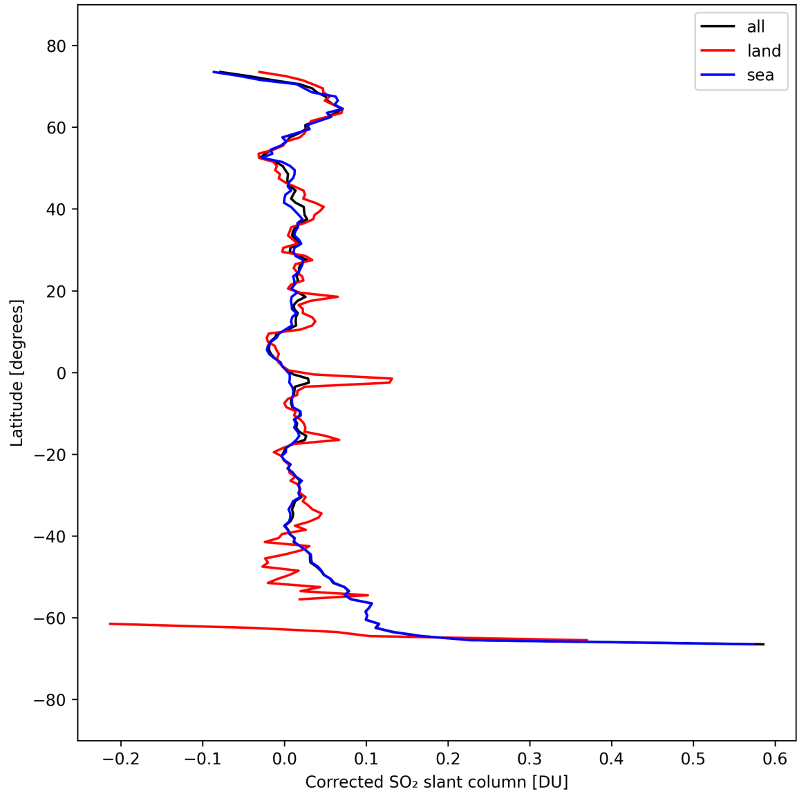
Figure 34: Zonal average of “Corrected SO 2 slant column” for 2025-09-13 to 2025-09-15.
