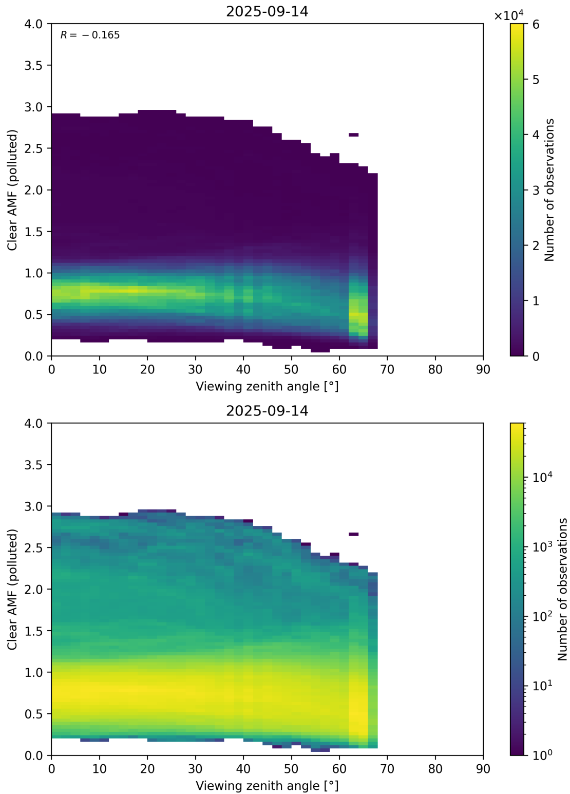
Figure 370: Scatter density plot of “Viewing zenith angle” against “Clear AMF (polluted)” for 2025-09-13 to 2025-09-15.
