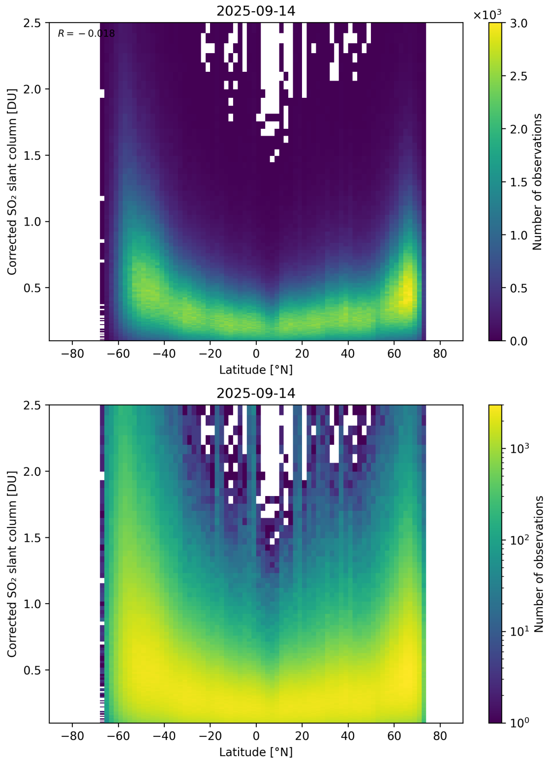
Figure 159: Scatter density plot of “Latitude” against “Corrected SO 2 slant column” for 2025-09-13 to 2025-09-15.
