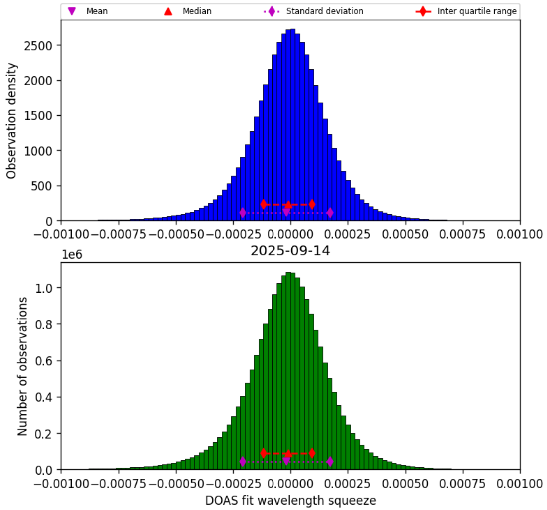
Figure 77: Histogram of “DOAS fit wavelength squeeze” for 2025-09-13 to 2025-09-15
