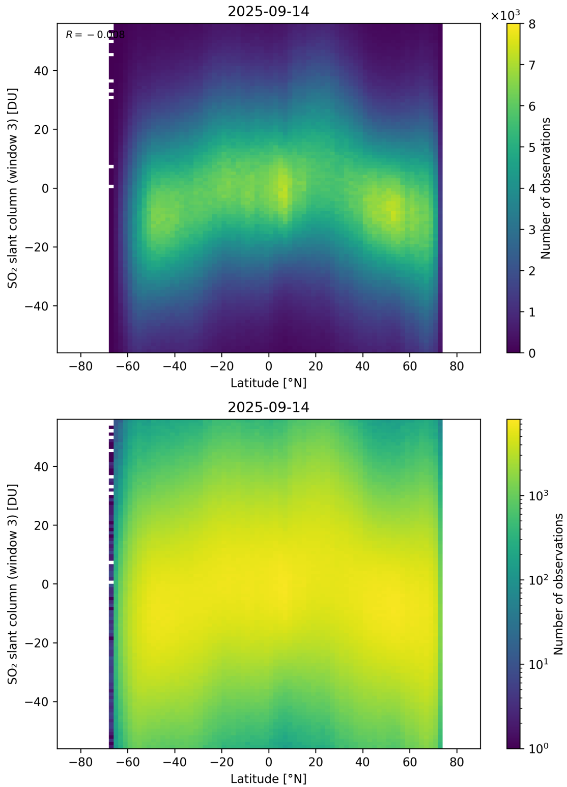
Figure 165: Scatter density plot of “Latitude” against “SO 2 slant column (window 3)” for 2025-09-13 to 2025-09-15.
