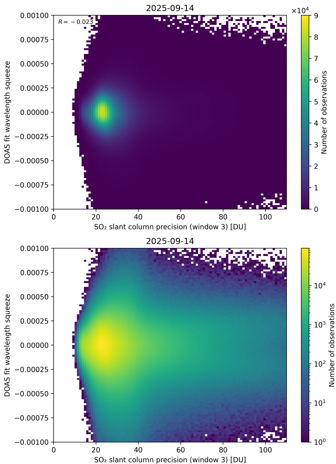
Figure 309: Scatter density plot of “SO 2 slant column precision (window 3)” against “DOAS fit wavelength squeeze” for 2025-09-13 to 2025-09-15.
