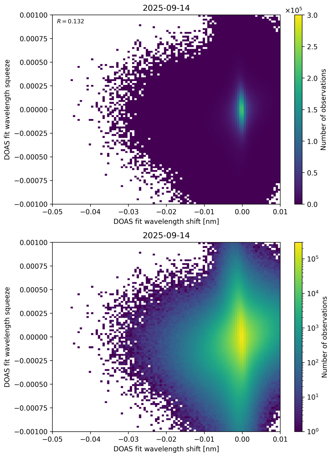
Figure 138: Scatter density plot of “DOAS fit wavelength shift” against “DOAS fit wavelength squeeze” for 2025-09-13 to 2025-09-15.
