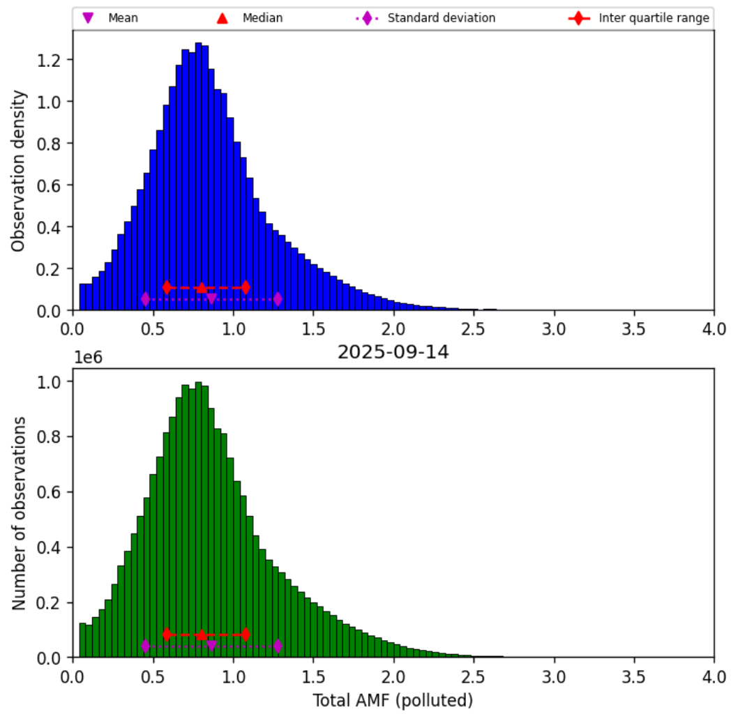
Figure 79: Histogram of “Total AMF (polluted)” for 2025-09-13 to 2025-09-15
