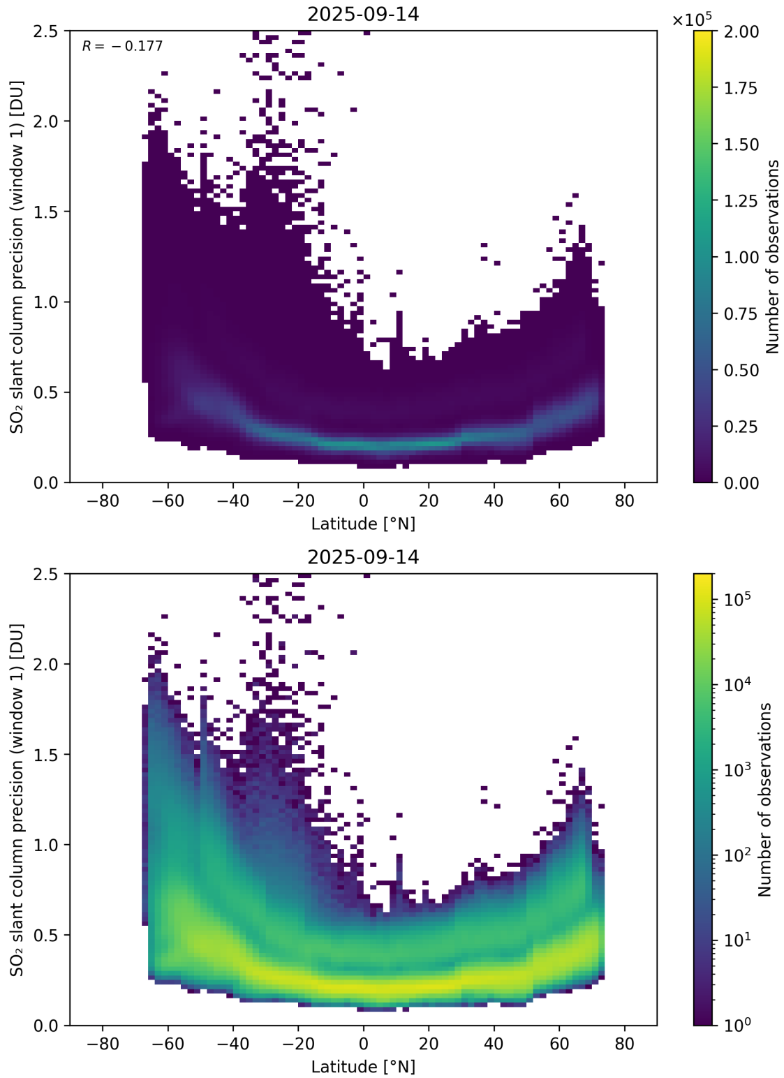
Figure 163: Scatter density plot of “Latitude” against “SO 2 slant column precision (window 1)” for 2025-09-13 to 2025-09-15.
