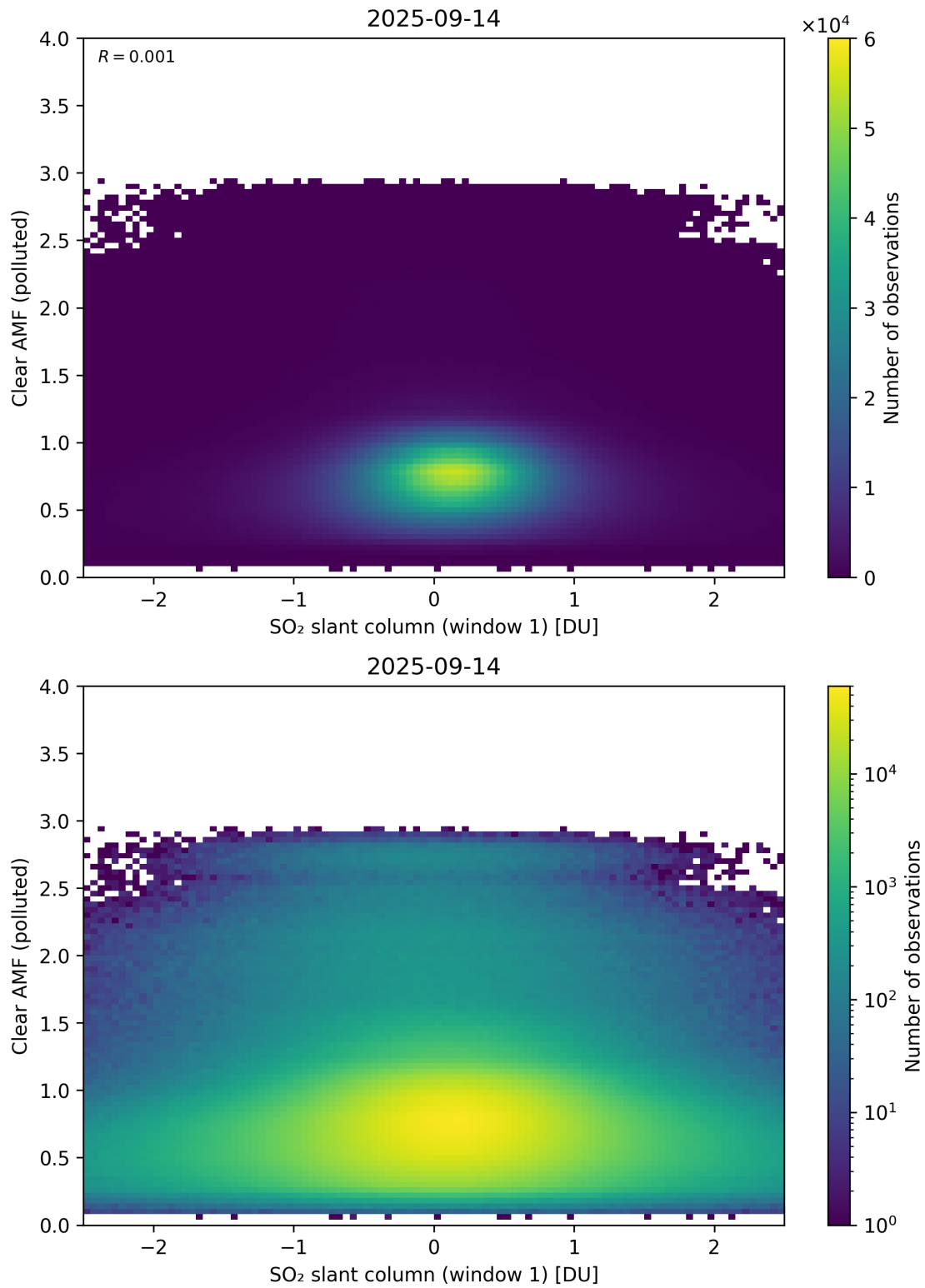
Figure 282: Scatter density plot of “SO 2 slant column (window 1)” against “Clear AMF (polluted)” for 2025-09-13 to 2025-09-15.
