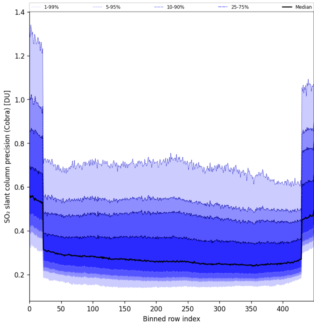
Figure 88: Along track statistics of “SO 2 slant column precision (Cobra)” for 2025-09-13 to 2025-09-15
