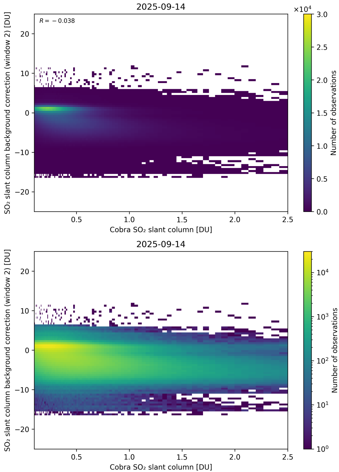
Figure 194: Scatter density plot of “Cobra SO 2 slant column” against “SO 2 slant column background correction (window 2)” for 2025-09-13 to 2025-09-15.
