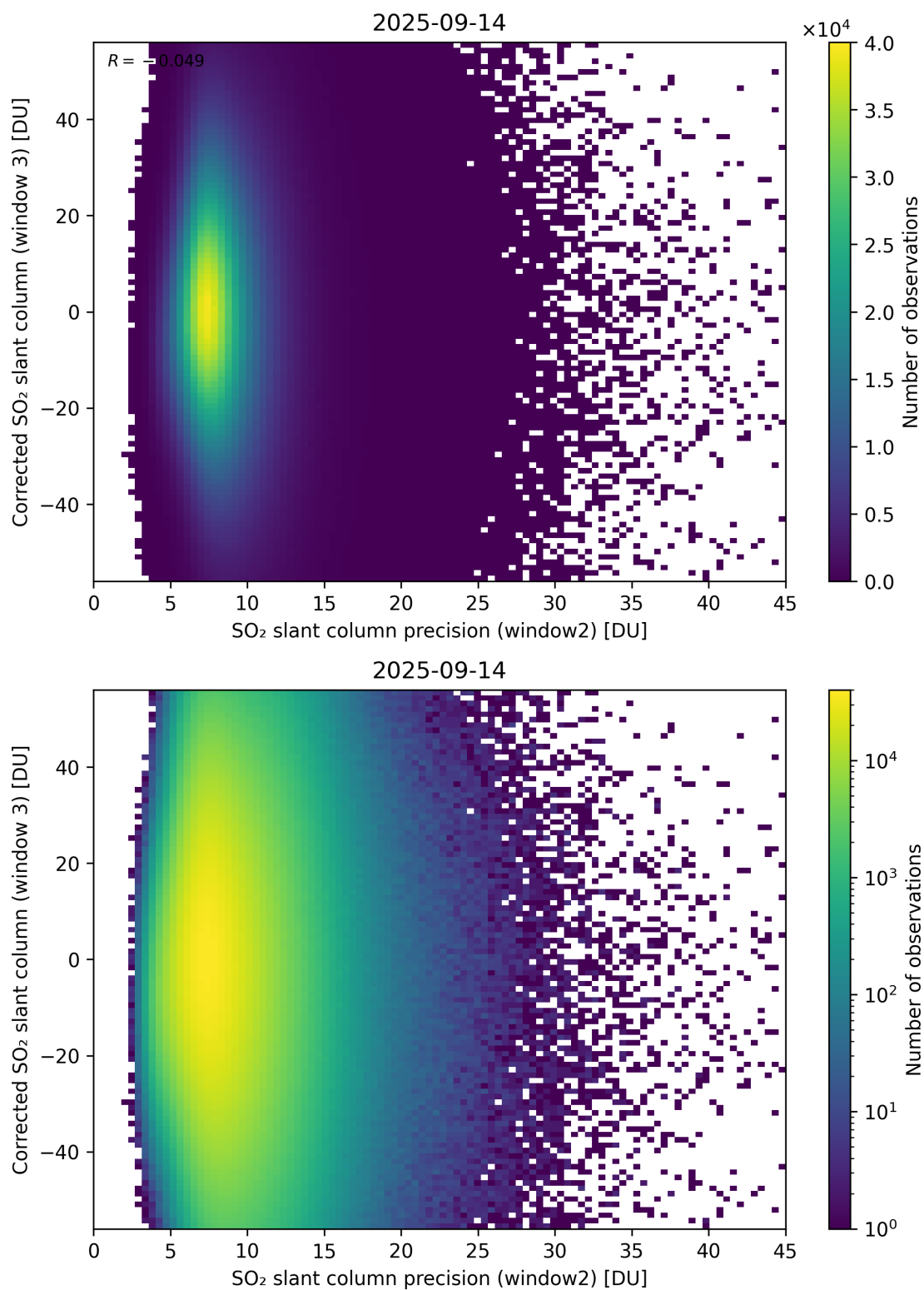
Figure 298: Scatter density plot of “SO 2 slant column precision (window2)” against “Corrected SO 2 slant column (window 3)” for 2025-09-13 to 2025-09-15.
