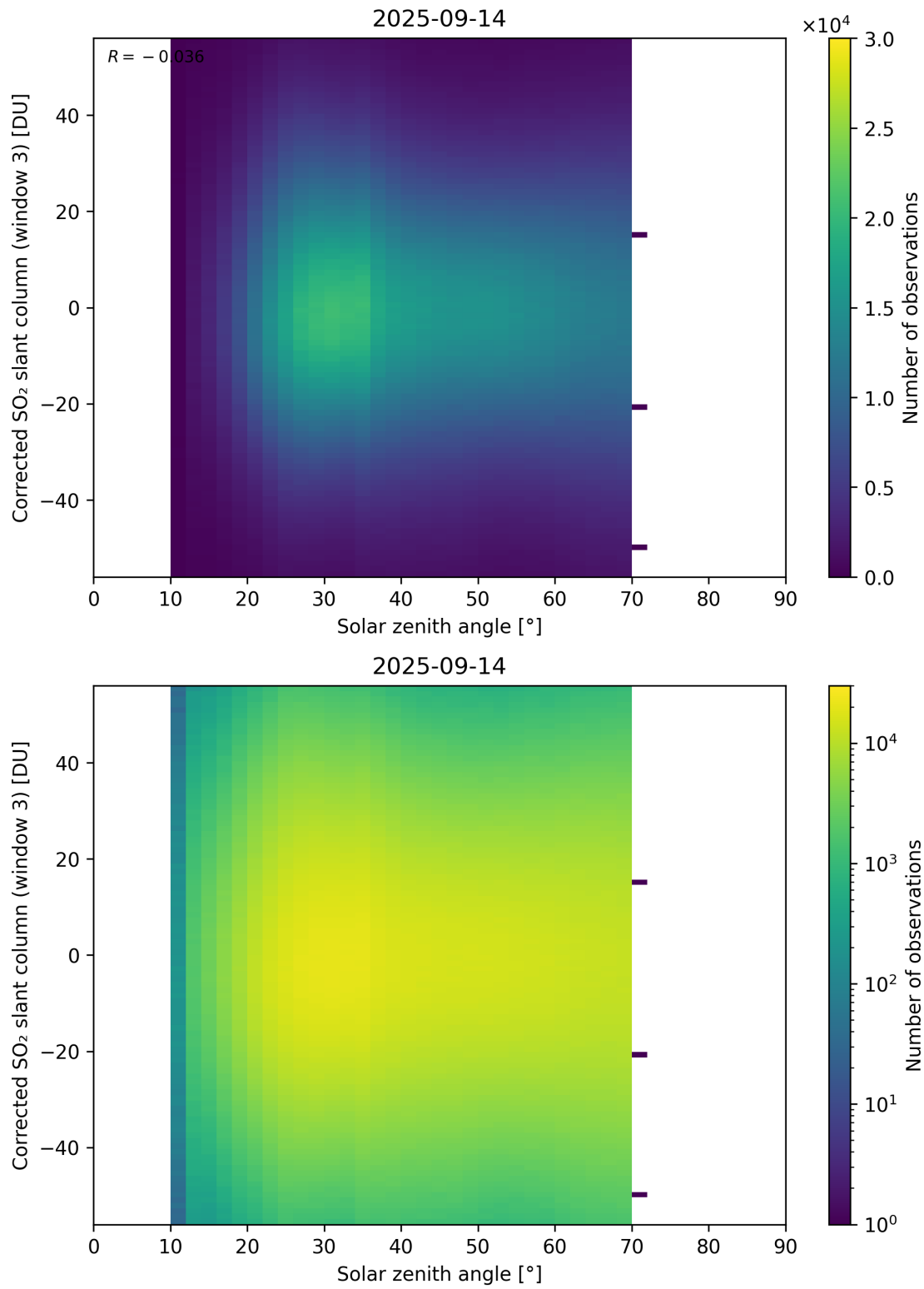
Figure 183: Scatter density plot of “Solar zenith angle” against “Corrected SO 2 slant column (window 3)” for 2025-09-13 to 2025-09-15.
