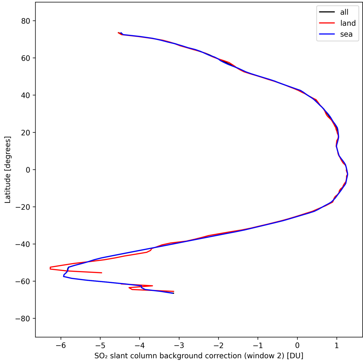
Figure 44: Zonal average of “SO 2 slant column background correction (window 2)” for 2025-09-13 to 2025-09-15.
