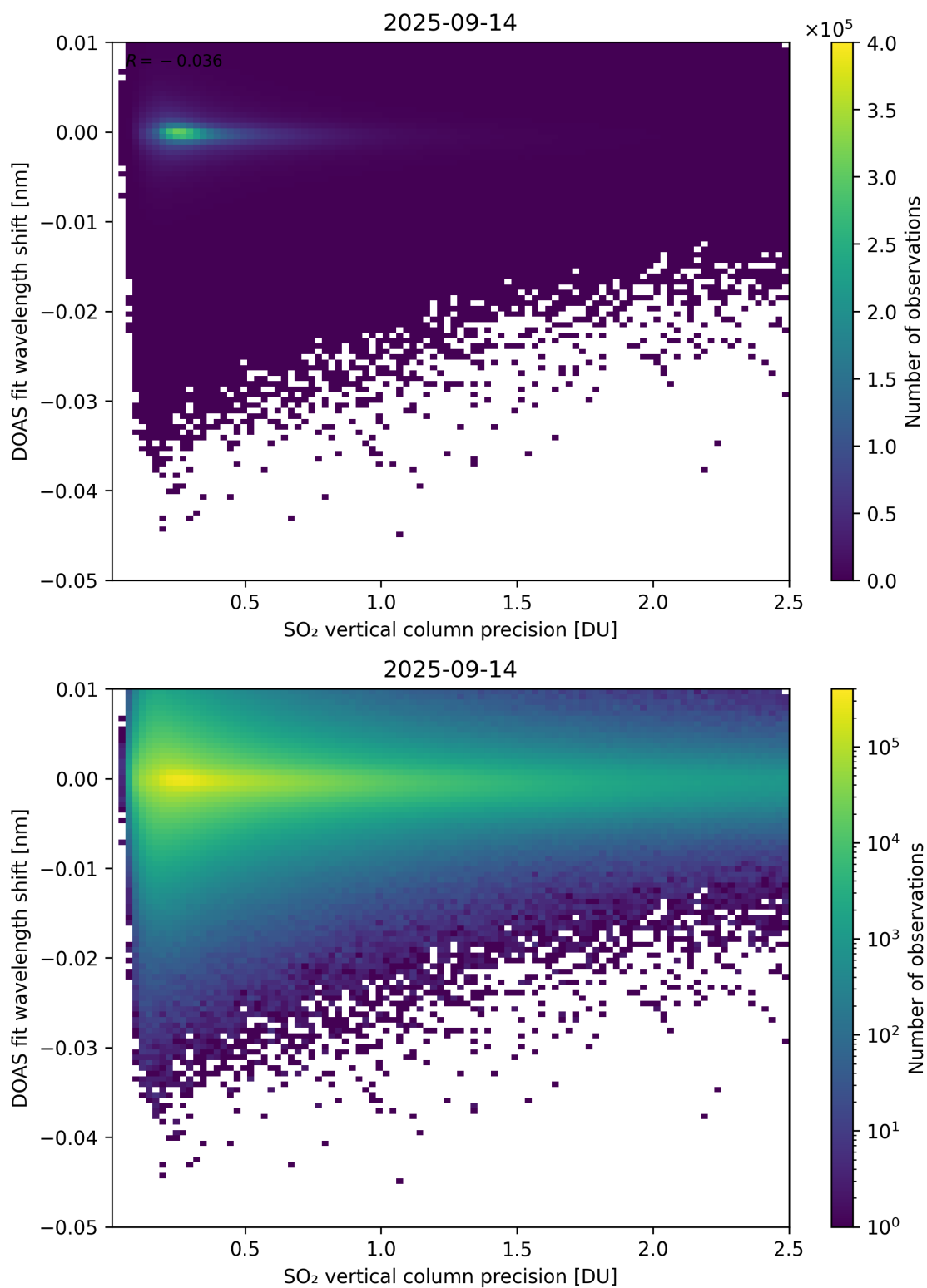
Figure 332: Scatter density plot of “SO 2 vertical column precision” against “DOAS fit wavelength shift” for 2025-09-13 to 2025-09-15.
