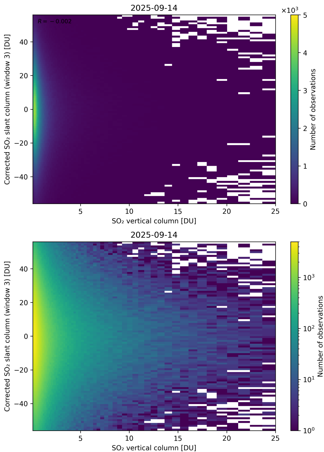
Figure 353: Scatter density plot of “SO 2 vertical column” against “Corrected SO 2 slant column (window 3)” for 2025-09-13 to 2025-09-15.
