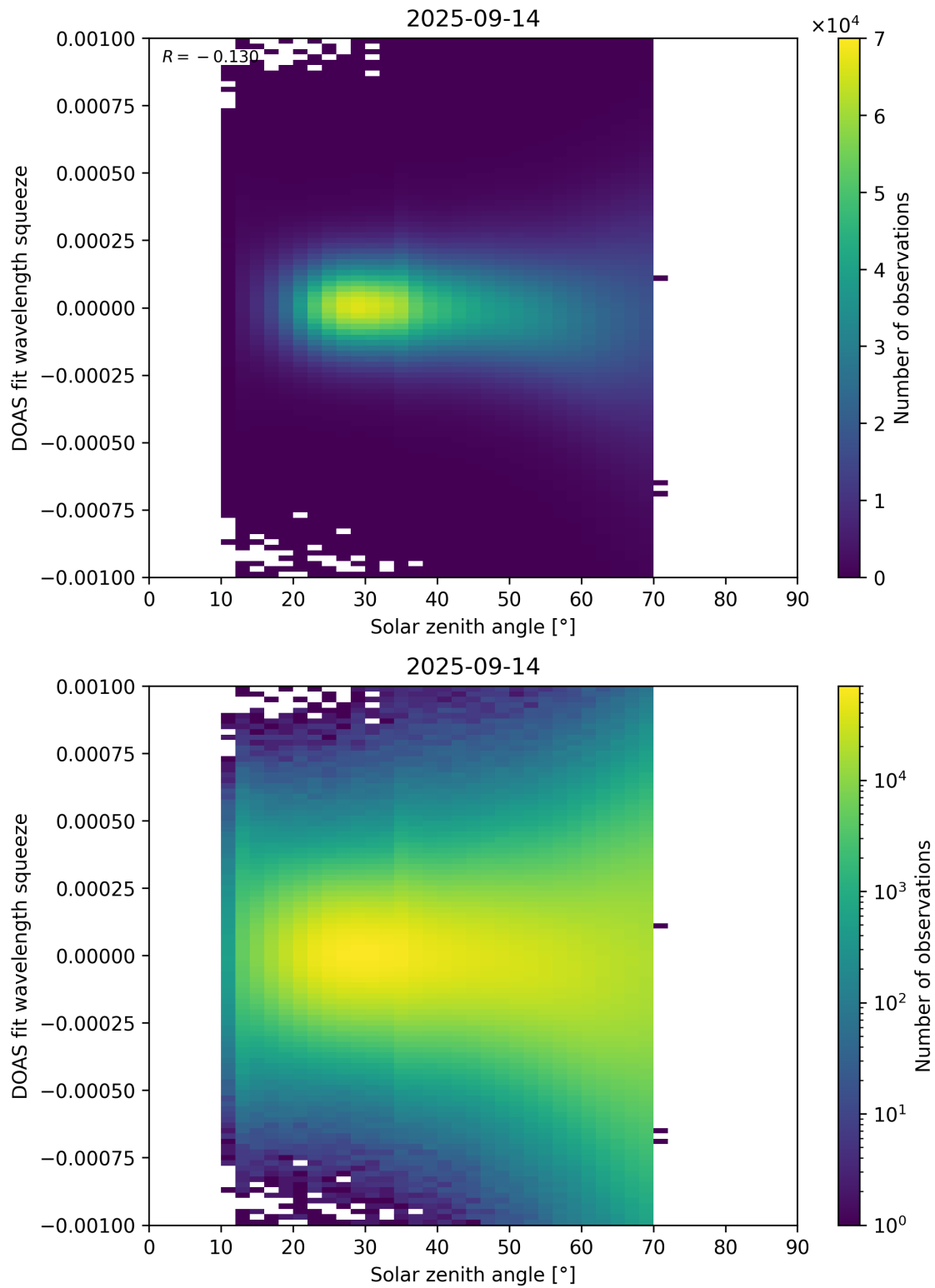
Figure 175: Scatter density plot of “Solar zenith angle” against “DOAS fit wavelength squeeze” for 2025-09-13 to 2025-09-15.
