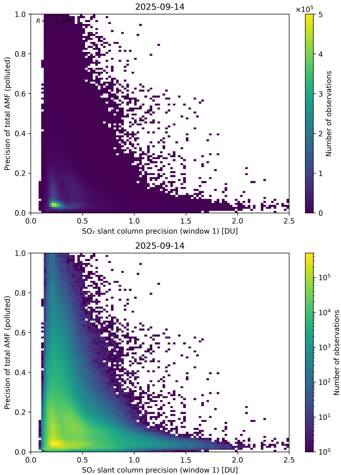
Figure 281: Scatter density plot of “SO 2 slant column precision (window 1)” against “Precision of total AMF (polluted)” for 2025-09-13 to 2025-09-15.
