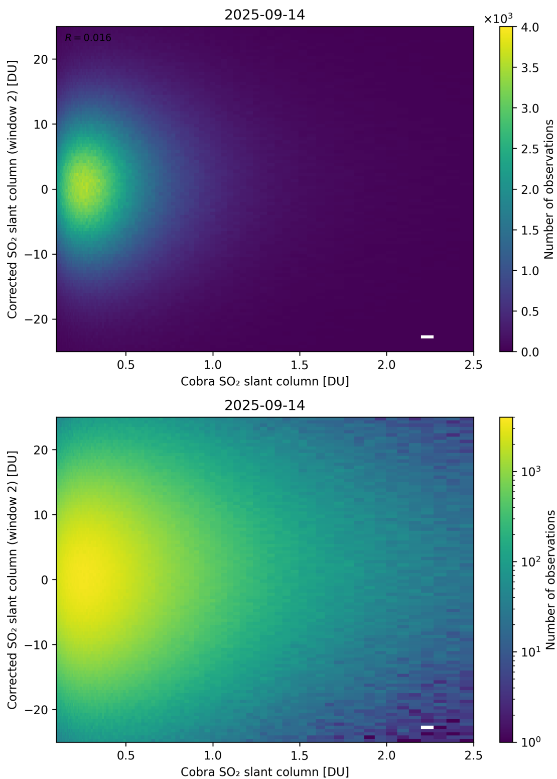
Figure 217: Scatter density plot of “Cobra SO 2 slant column” against “Corrected SO 2 slant column (window 2)” for 2025-09-13 to 2025-09-15.
