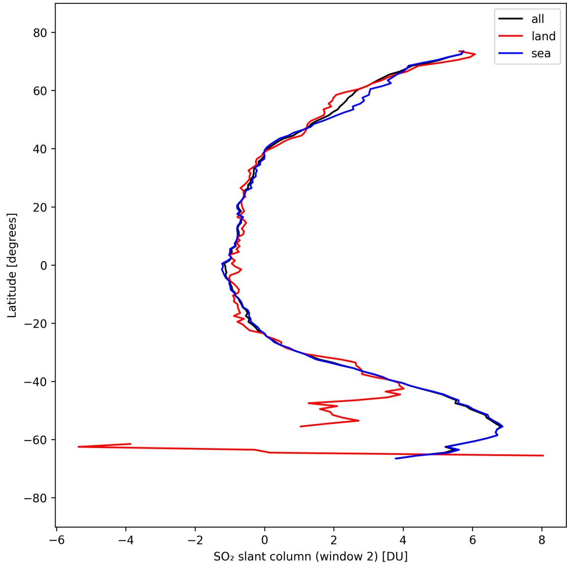
Figure 41: Zonal average of “SO 2 slant column (window 2)” for 2025-09-13 to 2025-09-15.
