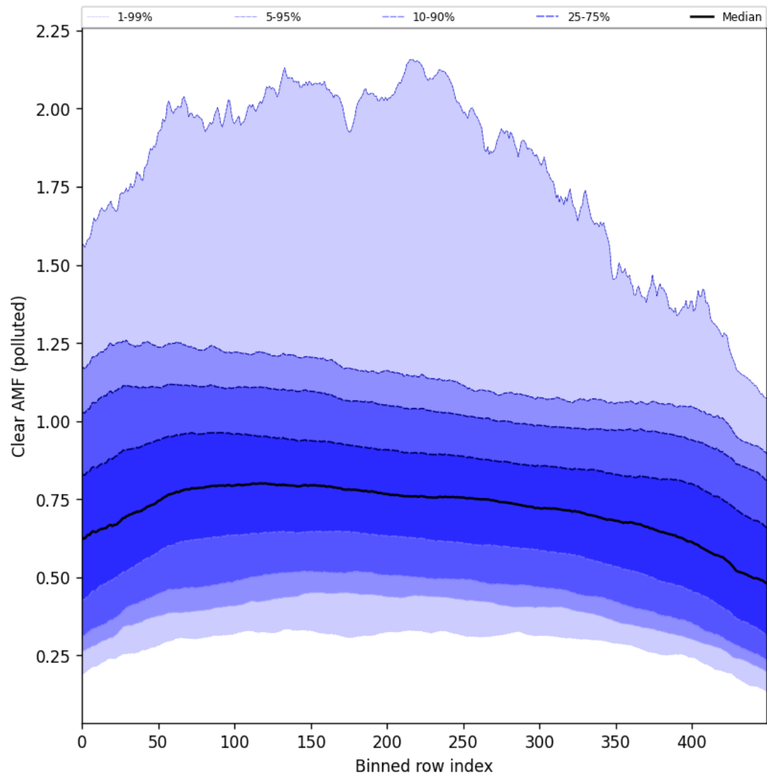
Figure 107: Along track statistics of “Clear AMF (polluted)” for 2025-09-13 to 2025-09-15
