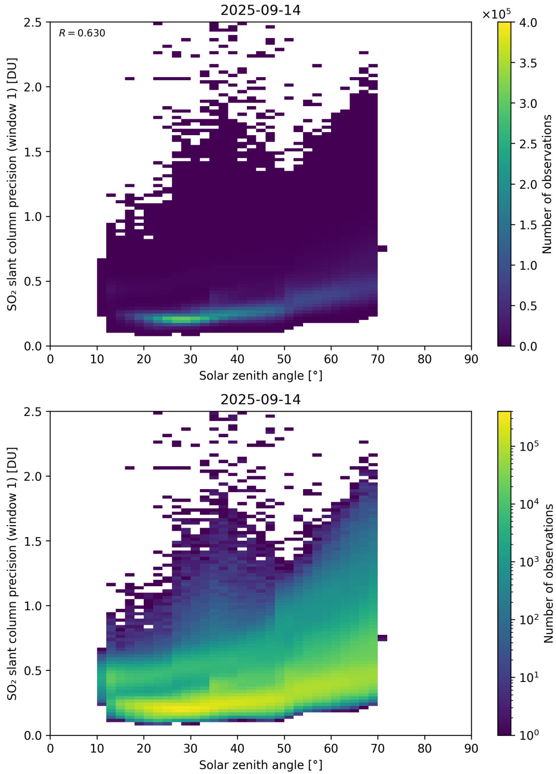
Figure 185: Scatter density plot of “Solar zenith angle” against “SO 2 slant column precision (window 1)” for 2025-09-13 to 2025-09-15.
