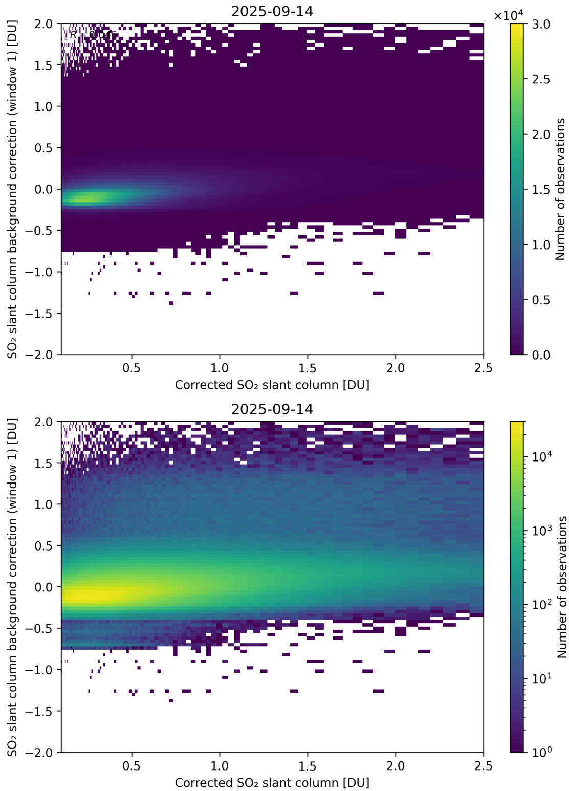
Figure 226: Scatter density plot of “Corrected SO 2 slant column” against “SO 2 slant column background correction (window 1)” for 2025-09-13 to 2025-09-15.
