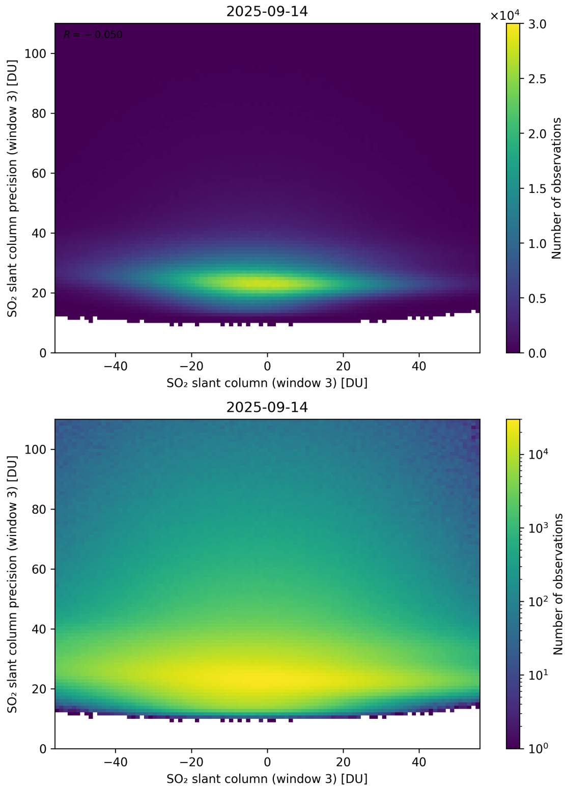
Figure 317: Scatter density plot of “SO 2 slant column (window 3)” against “SO 2 slant column precision (window 3)” for 2025-09-13 to 2025-09-15.
