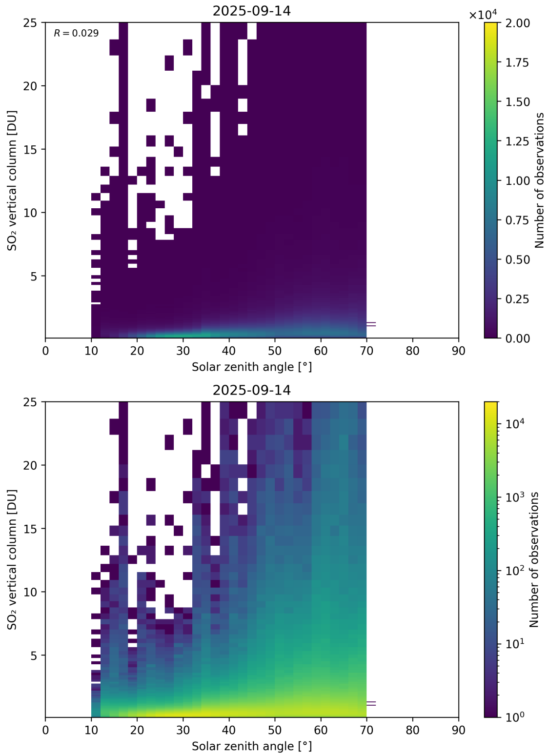
Figure 191: Scatter density plot of “Solar zenith angle” against “SO 2 vertical column” for 2025-09-13 to 2025-09-15.
