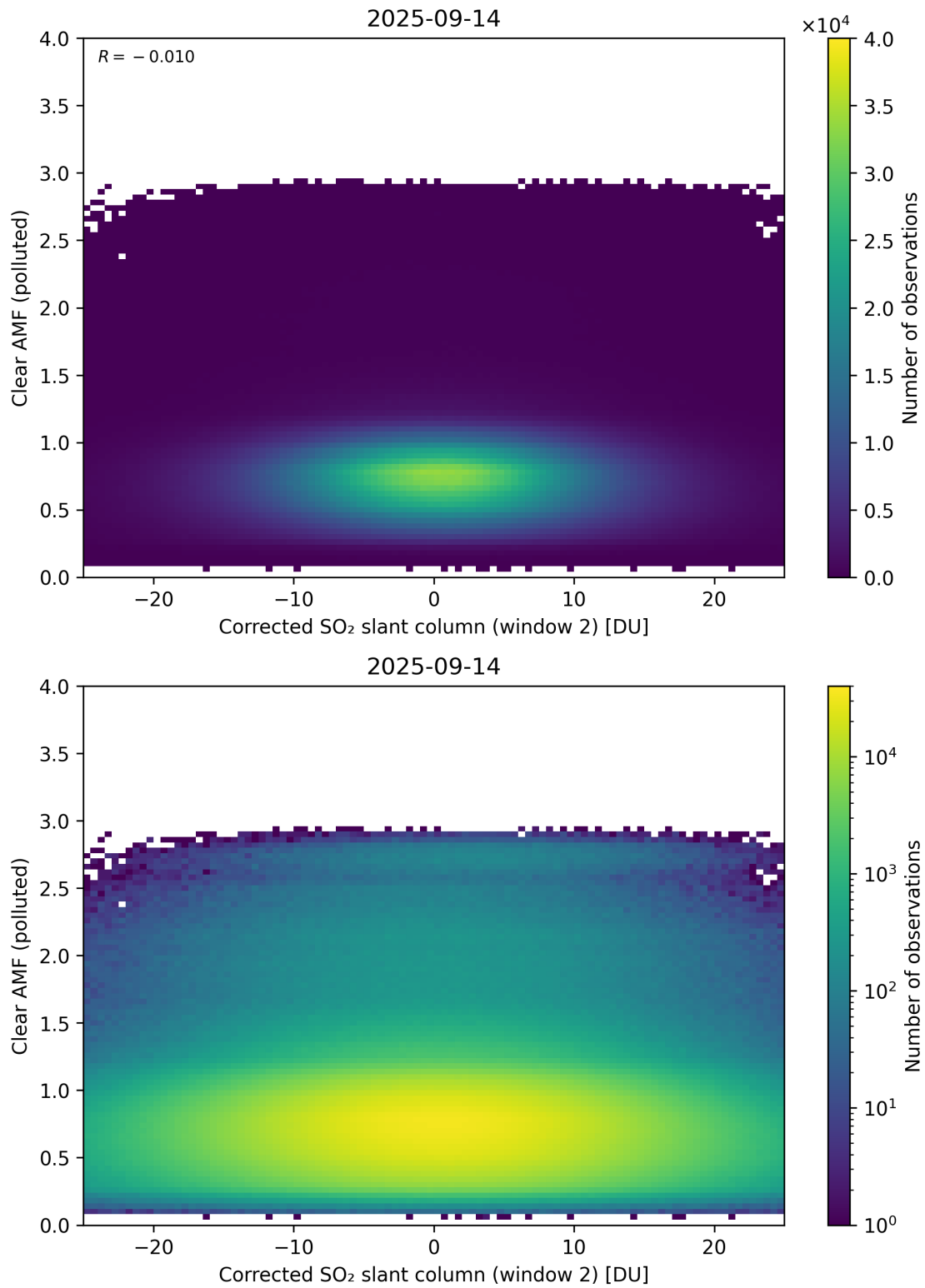
Figure 249: Scatter density plot of “Corrected SO 2 slant column (window 2)” against “Clear AMF (polluted)” for 2025-09-13 to 2025-09-15.
