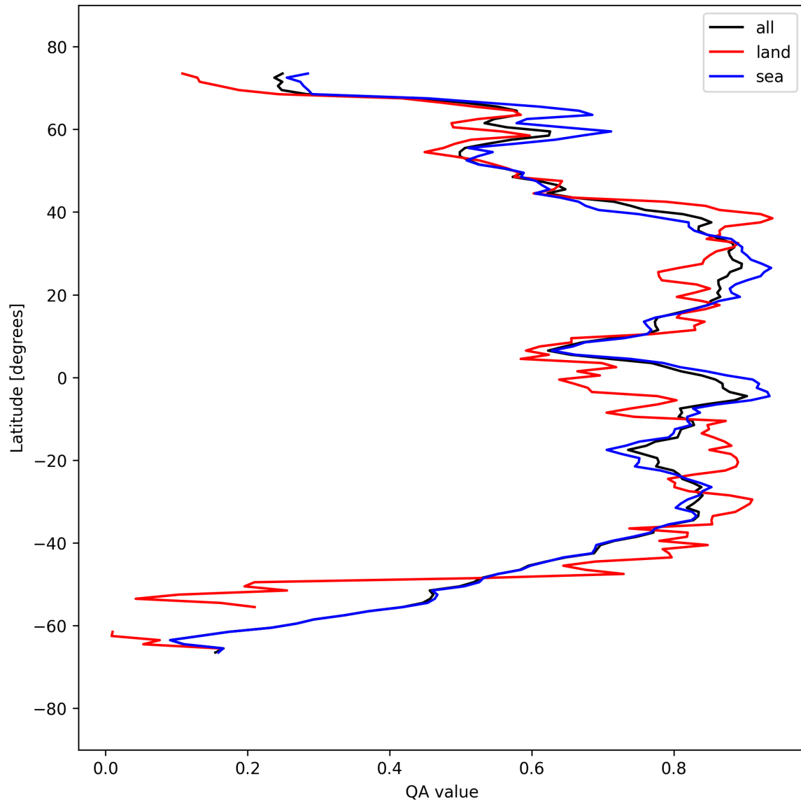
Figure 31: Zonal average of “QA value” for 2025-09-13 to 2025-09-15.
