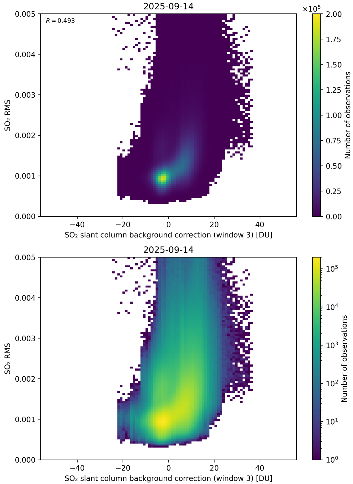
Figure 134: Scatter density plot of “SO 2 slant column background correction (window 3)” against “SO 2 RMS” for 2025-09-13 to 2025-09-15.
