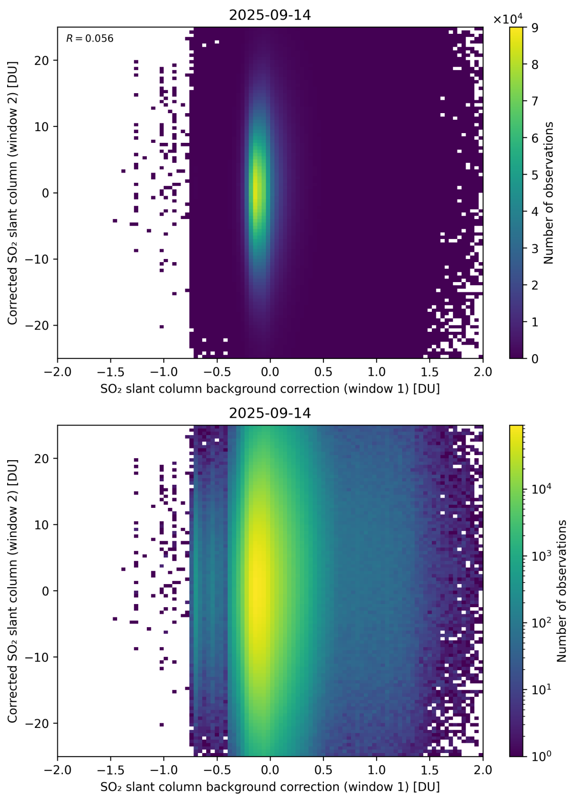
Figure 115: Scatter density plot of “SO 2 slant column background correction (window 1)” against “Corrected SO 2 slant column (window 2)” for 2025-09-13 to 2025-09-15.
