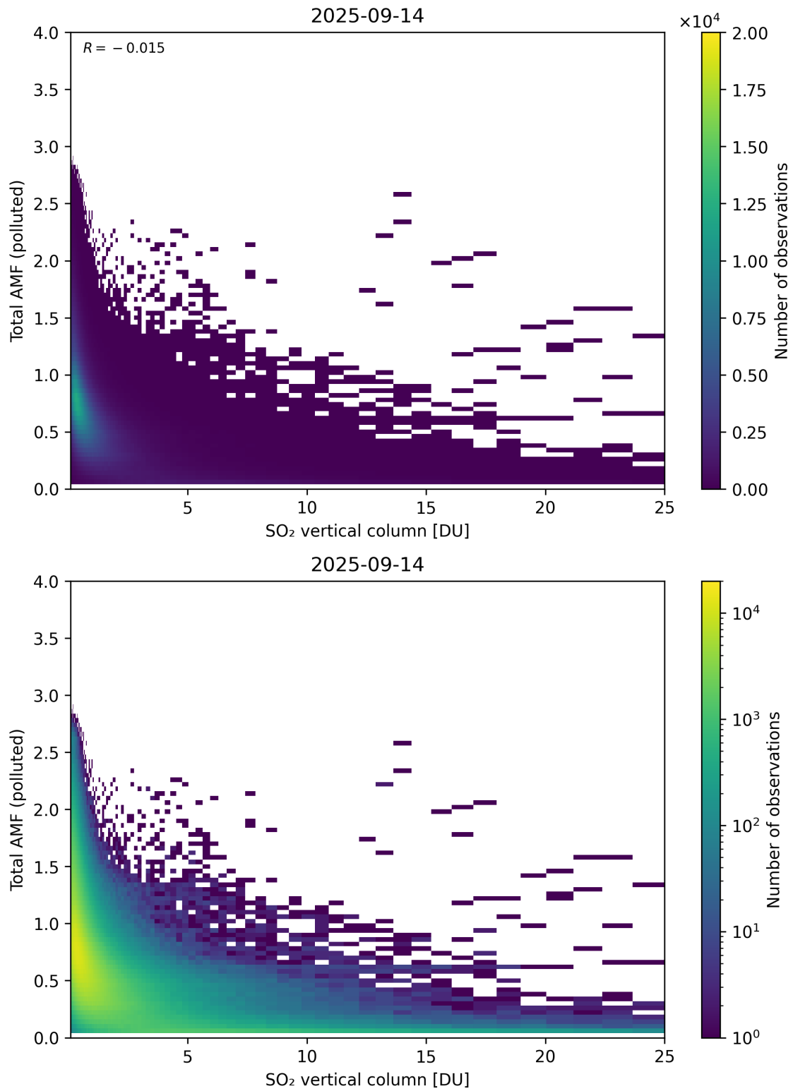
Figure 359: Scatter density plot of “SO 2 vertical column” against “Total AMF (polluted)” for 2025-09-13 to 2025-09-15.
