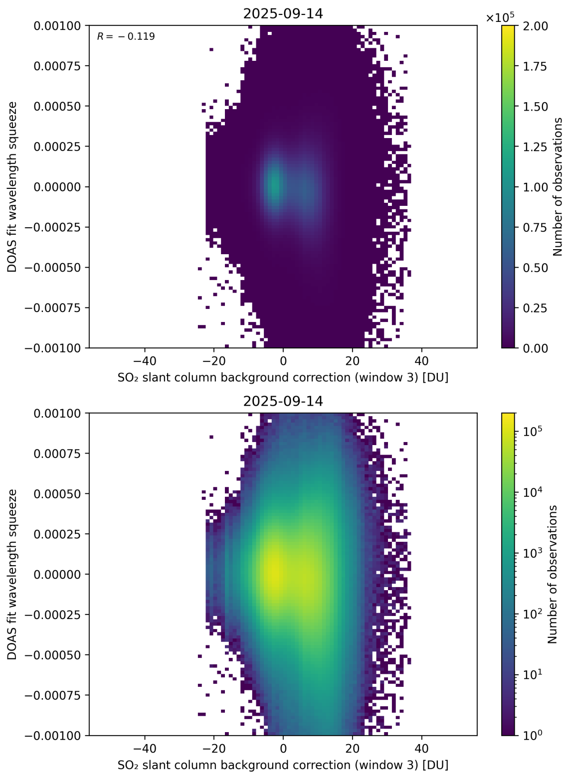
Figure 133: Scatter density plot of “SO 2 slant column background correction (window 3)” against “DOAS fit wavelength squeeze” for 2025-09-13 to 2025-09-15.
