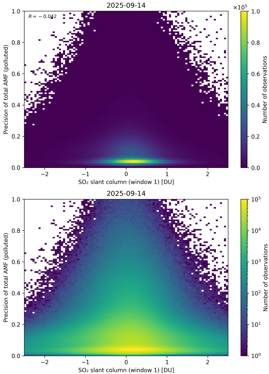
Figure 290: Scatter density plot of “SO 2 slant column (window 1)” against “Precision of total AMF (polluted)” for 2025-09-13 to 2025-09-15.
