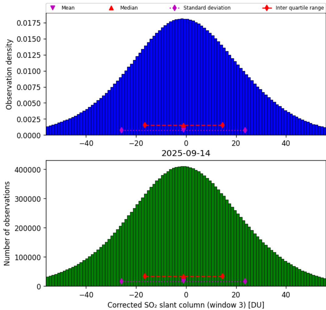
Figure 73: Histogram of “Corrected SO 2 slant column (window 3)” for 2025-09-13 to 2025-09-15
