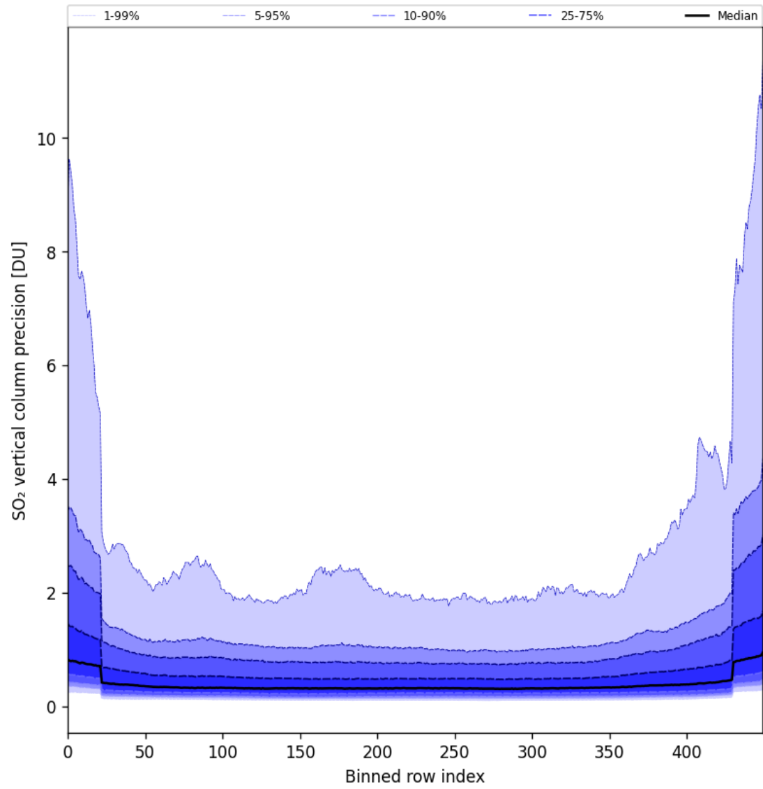
Figure 85: Along track statistics of “SO 2 vertical column precision” for 2025-09-13 to 2025-09-15
