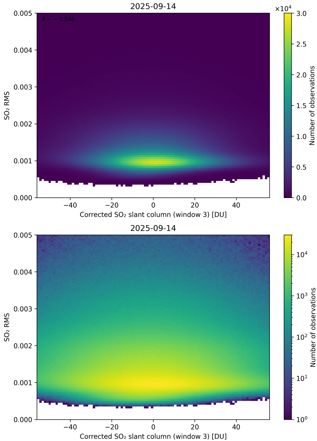
Figure 258: Scatter density plot of “Corrected SO 2 slant column (window 3)” against “SO 2 RMS” for 2025-09-13 to 2025-09-15.
