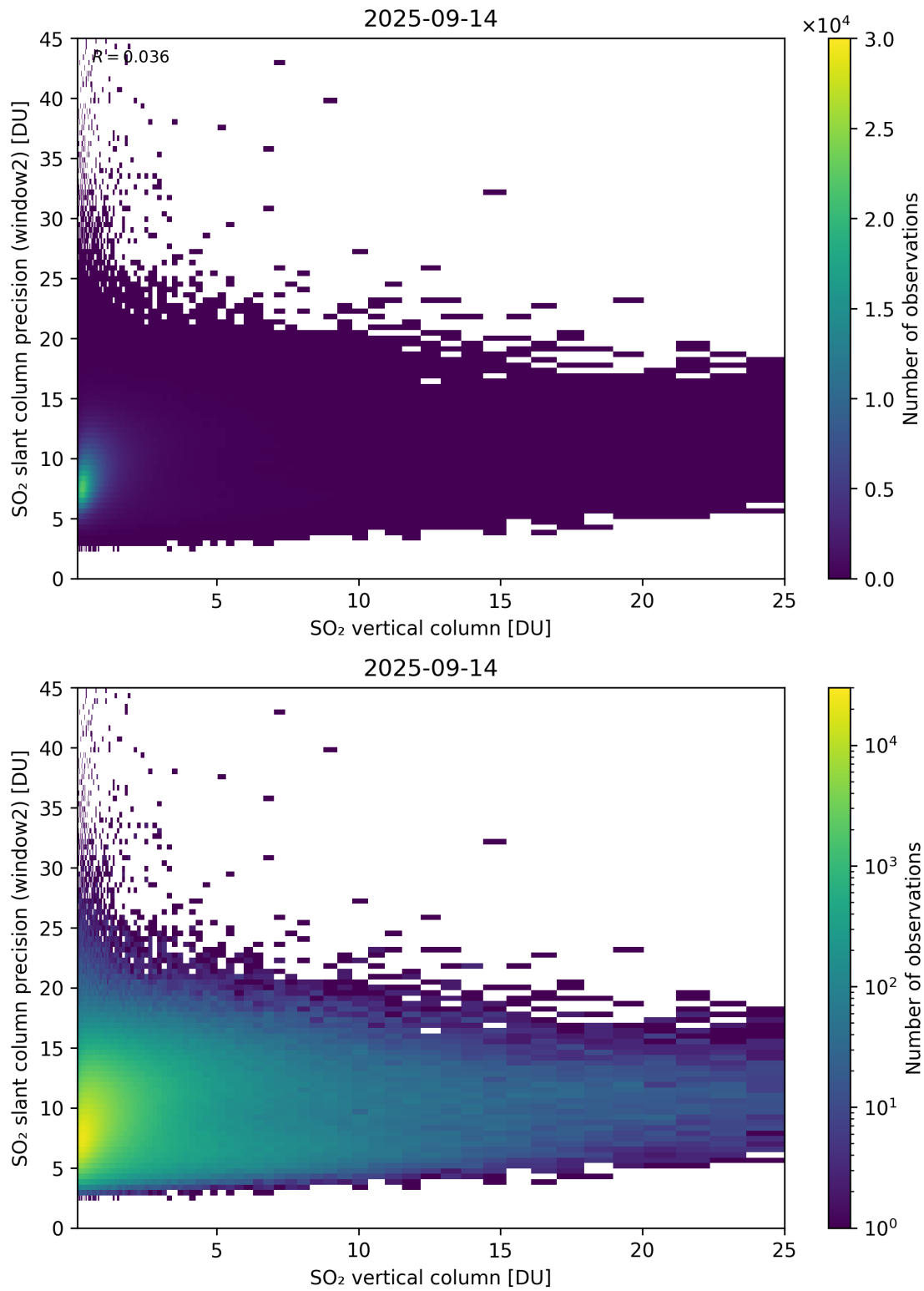
Figure 356: Scatter density plot of “SO 2 vertical column” against “SO 2 slant column precision (window2)” for 2025-09-13 to 2025-09-15.
