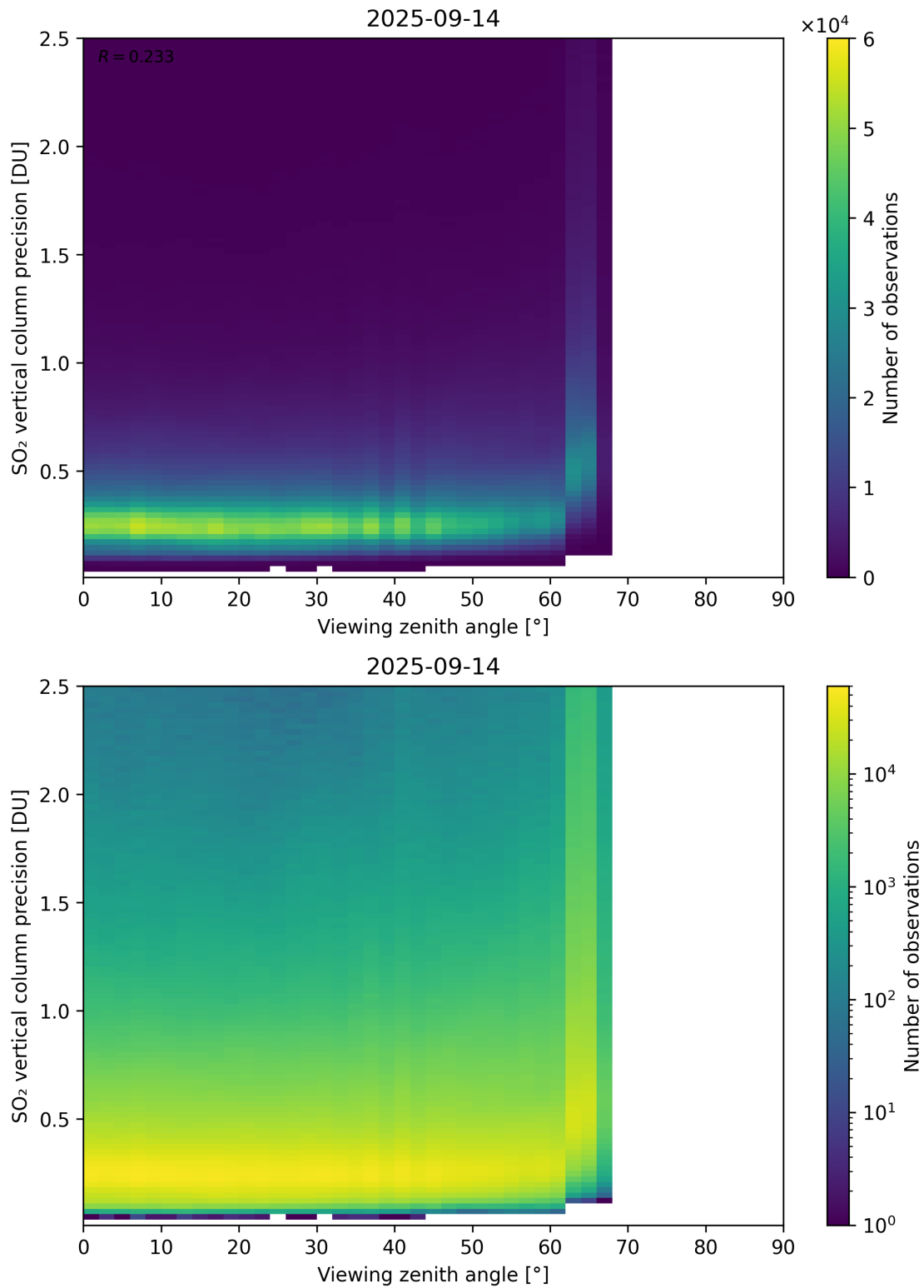
Figure 384: Scatter density plot of “Viewing zenith angle” against “SO 2 vertical column precision” for 2025-09-13 to 2025-09-15.
