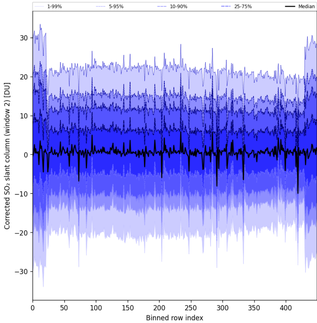
Figure 95: Along track statistics of “Corrected SO 2 slant column (window 2)” for 2025-09-13 to 2025-09-15
