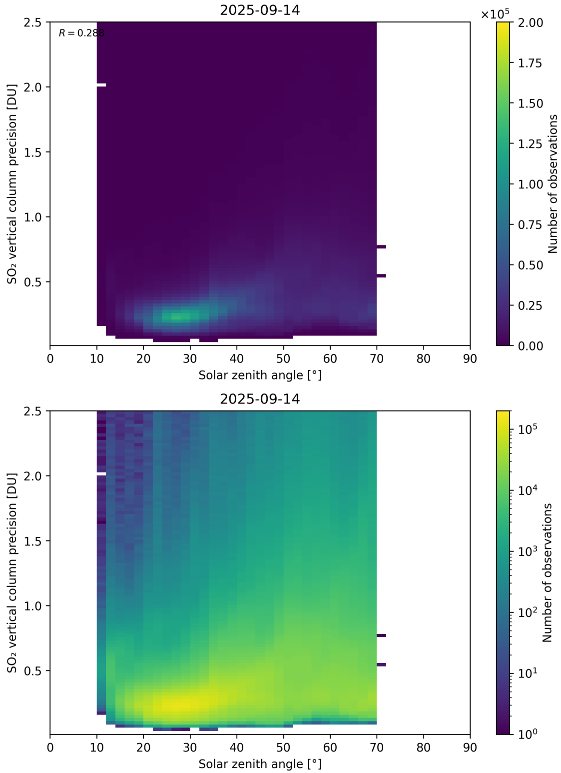
Figure 192: Scatter density plot of “Solar zenith angle” against “SO 2 vertical column precision” for 2025-09-13 to 2025-09-15.
