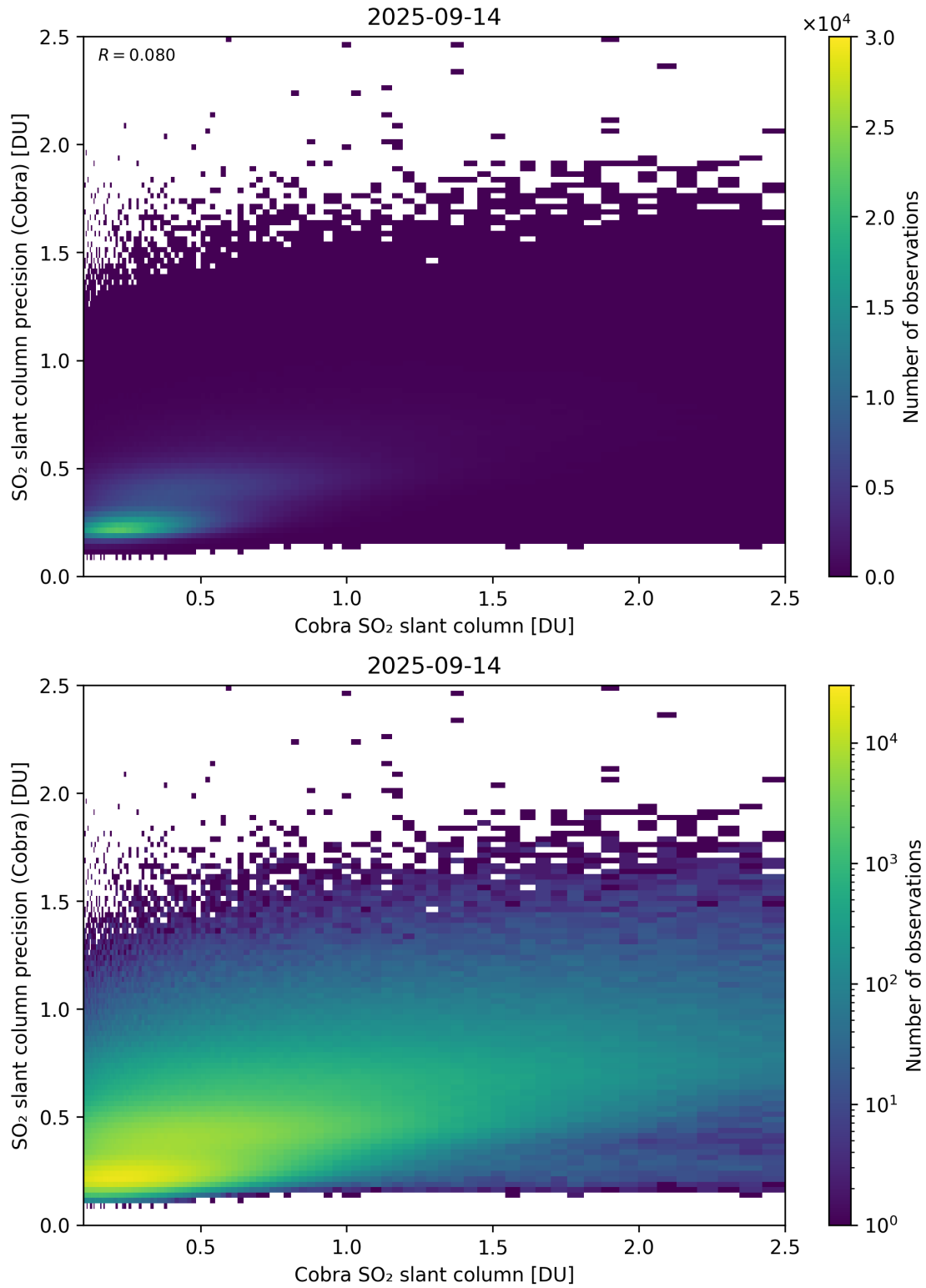
Figure 216: Scatter density plot of “Cobra SO 2 slant column” against “SO 2 slant column precision (Cobra)” for 2025-09-13 to 2025-09-15.
