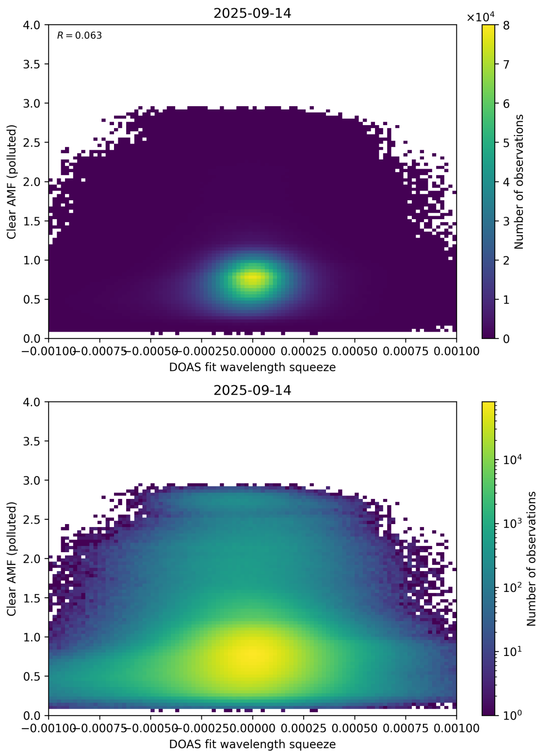
Figure 144: Scatter density plot of “DOAS fit wavelength squeeze” against “Clear AMF (polluted)” for 2025-09-13 to 2025-09-15.
