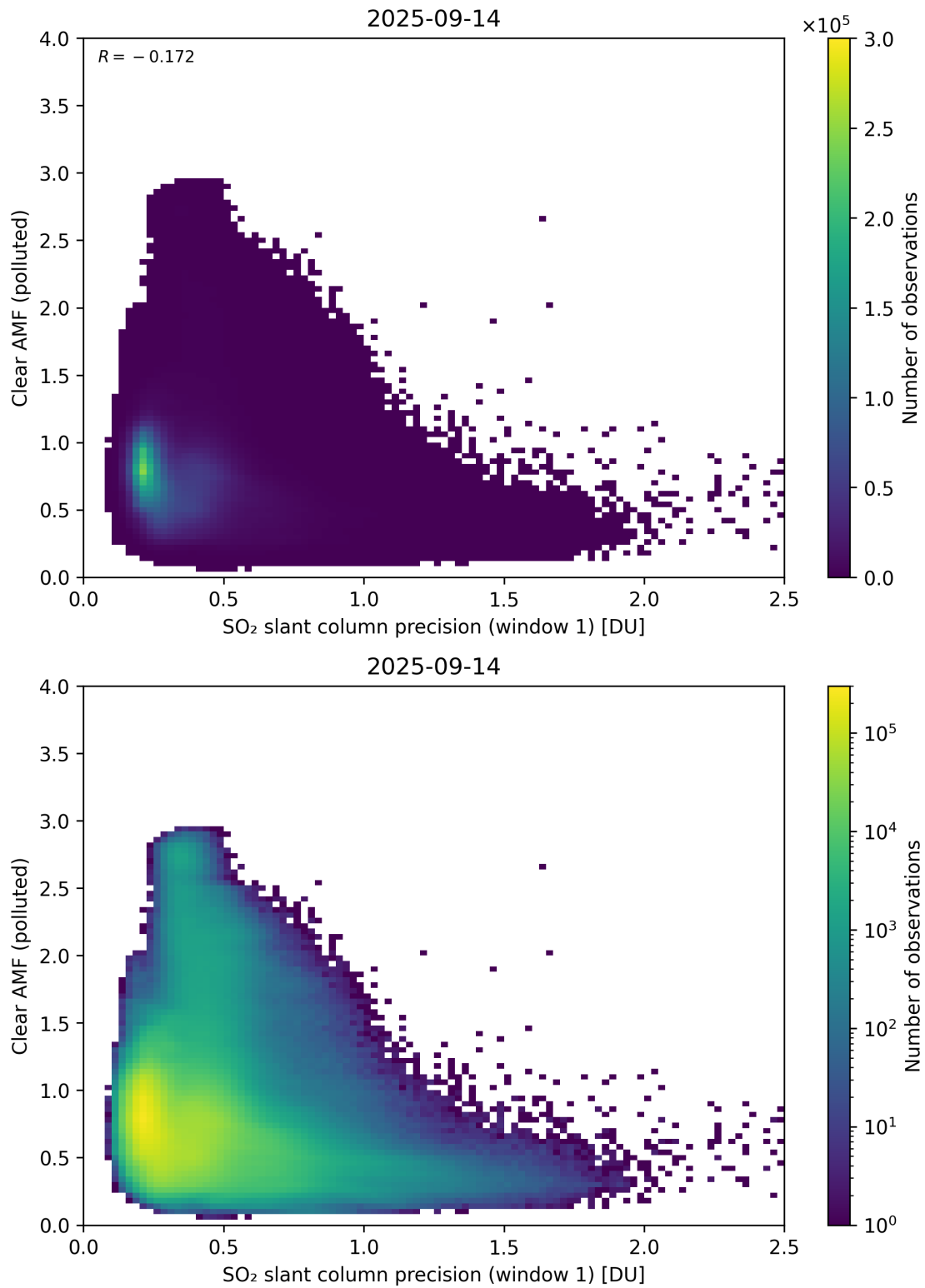
Figure 274: Scatter density plot of “SO 2 slant column precision (window 1)” against “Clear AMF (polluted)” for 2025-09-13 to 2025-09-15.
