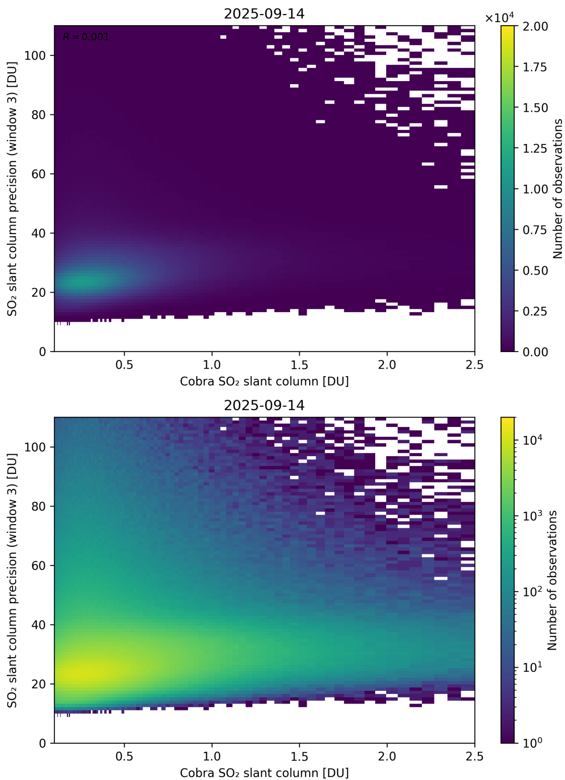
Figure 223: Scatter density plot of “Cobra SO 2 slant column” against “SO 2 slant column precision (window 3)” for 2025-09-13 to 2025-09-15.
