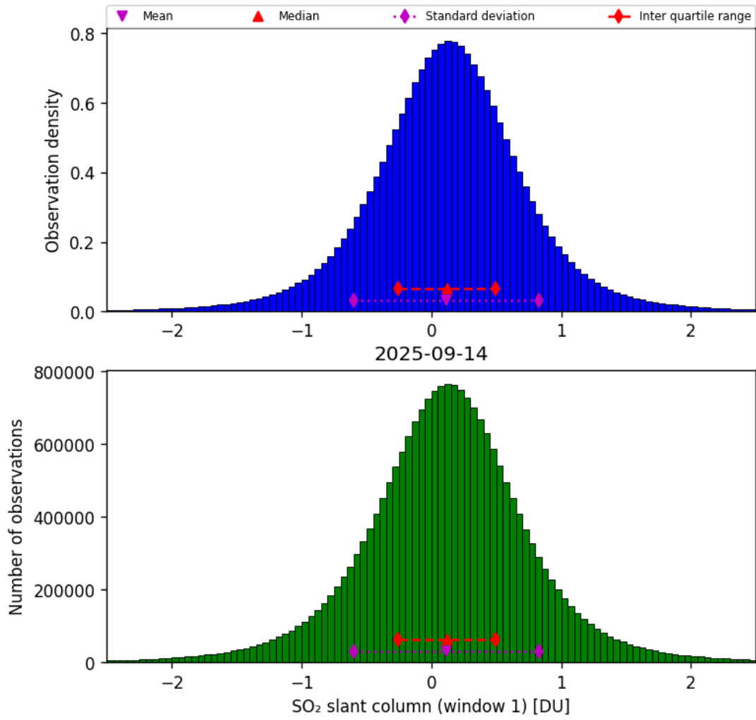
Figure 63: Histogram of “SO 2 slant column (window 1)” for 2025-09-13 to 2025-09-15
