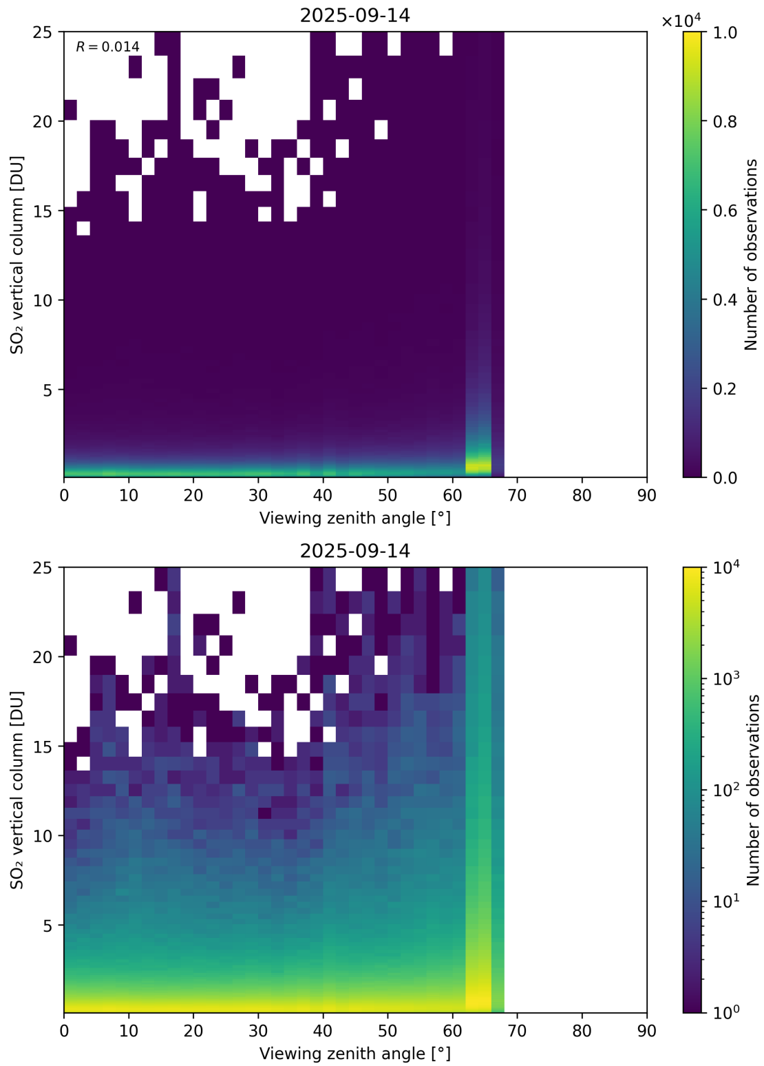
Figure 383: Scatter density plot of “Viewing zenith angle” against “SO 2 vertical column” for 2025-09-13 to 2025-09-15.
