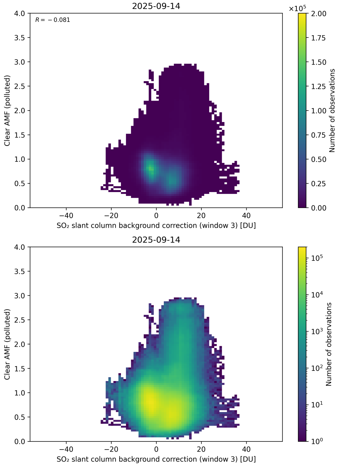
Figure 135: Scatter density plot of “SO 2 slant column background correction (window 3)” against “Clear AMF (polluted)” for 2025-09-13 to 2025-09-15.
