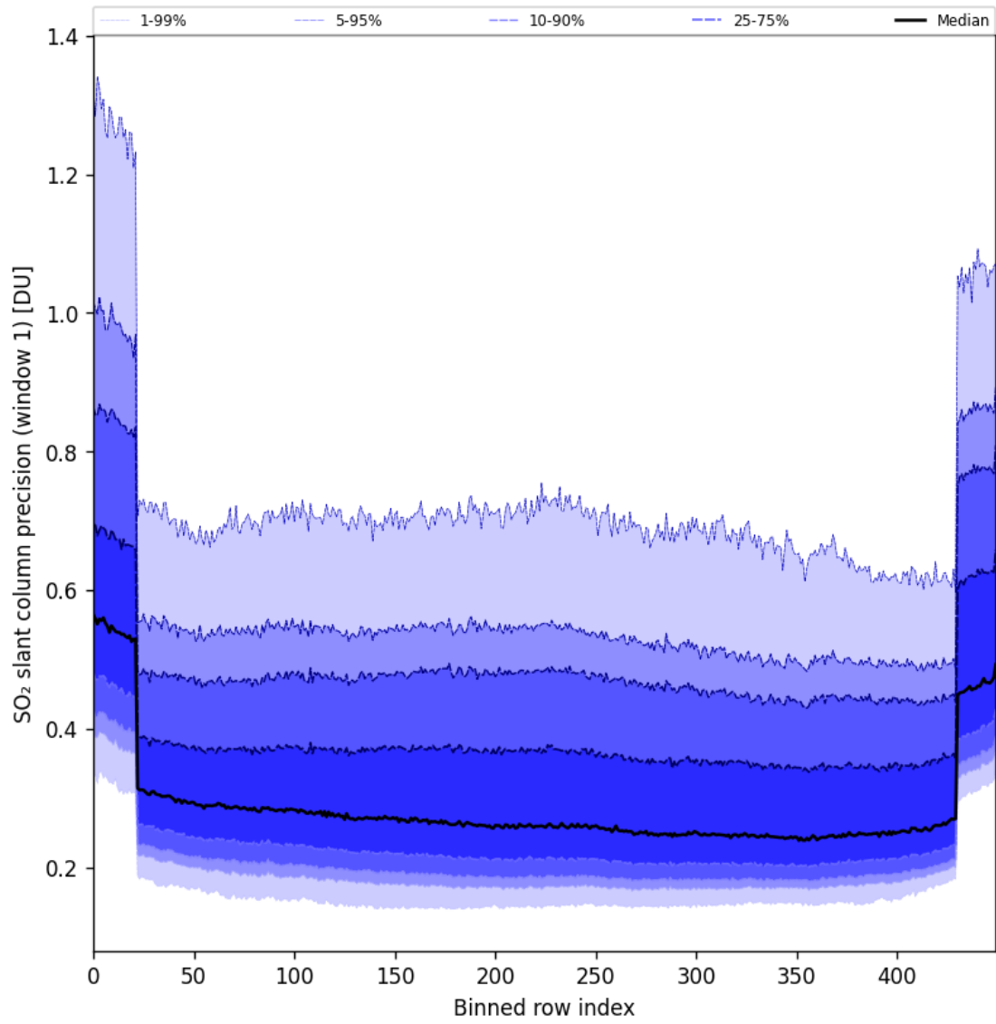
Figure 90: Along track statistics of “SO 2 slant column precision (window 1)” for 2025-09-13 to 2025-09-15
