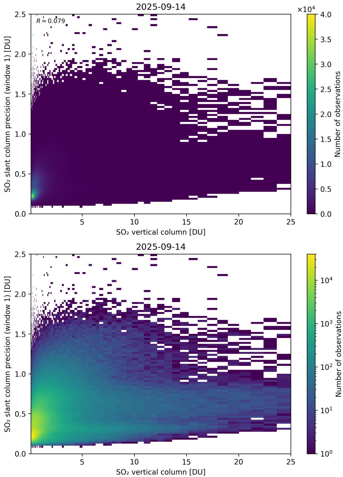
Figure 355: Scatter density plot of “SO 2 vertical column” against “SO 2 slant column precision (window 1)” for 2025-09-13 to 2025-09-15.
