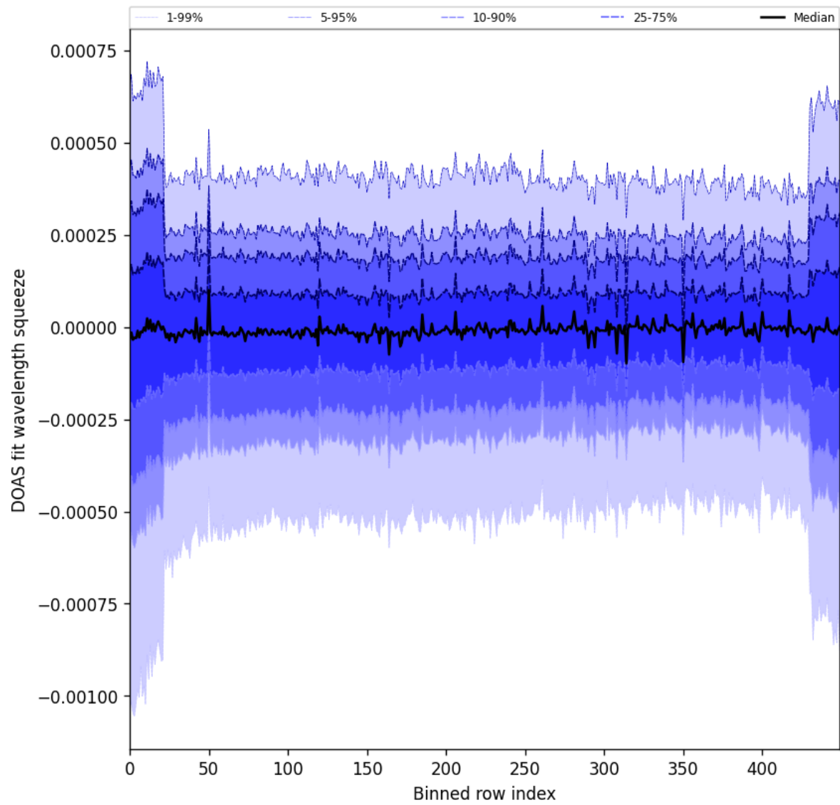
Figure 103: Along track statistics of “DOAS fit wavelength squeeze” for 2025-09-13 to 2025-09-15
