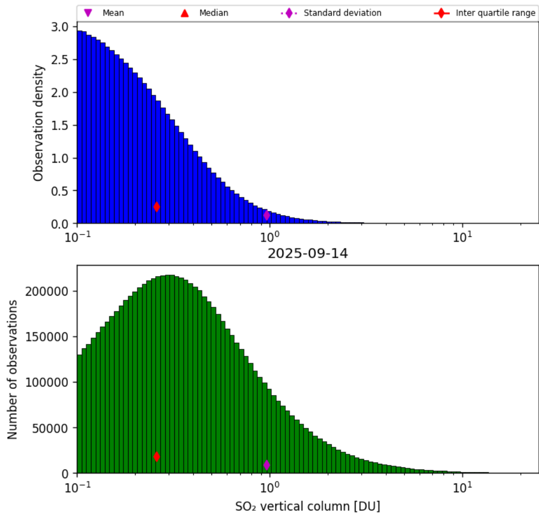
Figure 58: Histogram of “SO 2 vertical column” for 2025-09-13 to 2025-09-15
