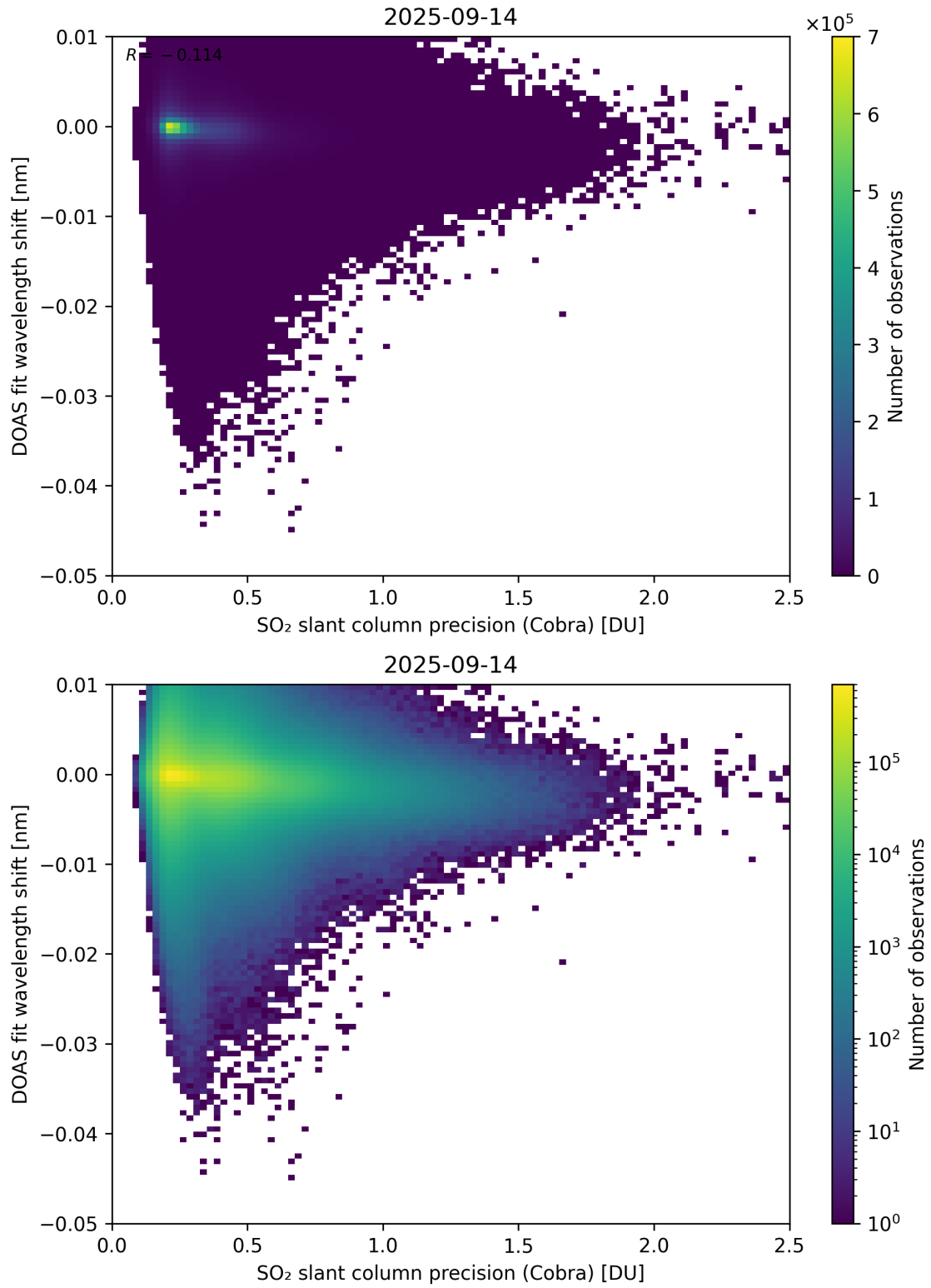
Figure 202: Scatter density plot of “SO 2 slant column precision (Cobra)” against “DOAS fit wavelength shift” for 2025-09-13 to 2025-09-15.
