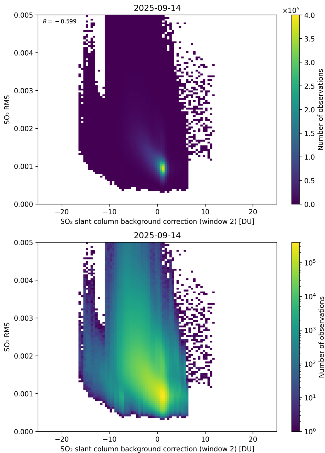
Figure 125: Scatter density plot of “SO 2 slant column background correction (window 2)” against “SO 2 RMS” for 2025-09-13 to 2025-09-15.
