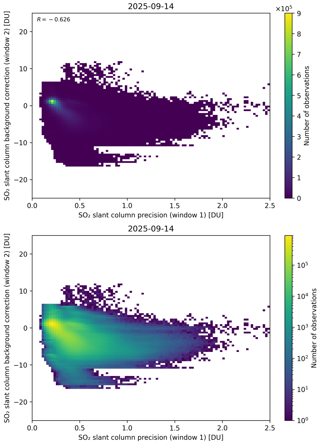
Figure 269: Scatter density plot of “SO 2 slant column precision (window 1)” against “SO 2 slant column background correction (window 2)” for 2025-09-13 to 2025-09-15.
