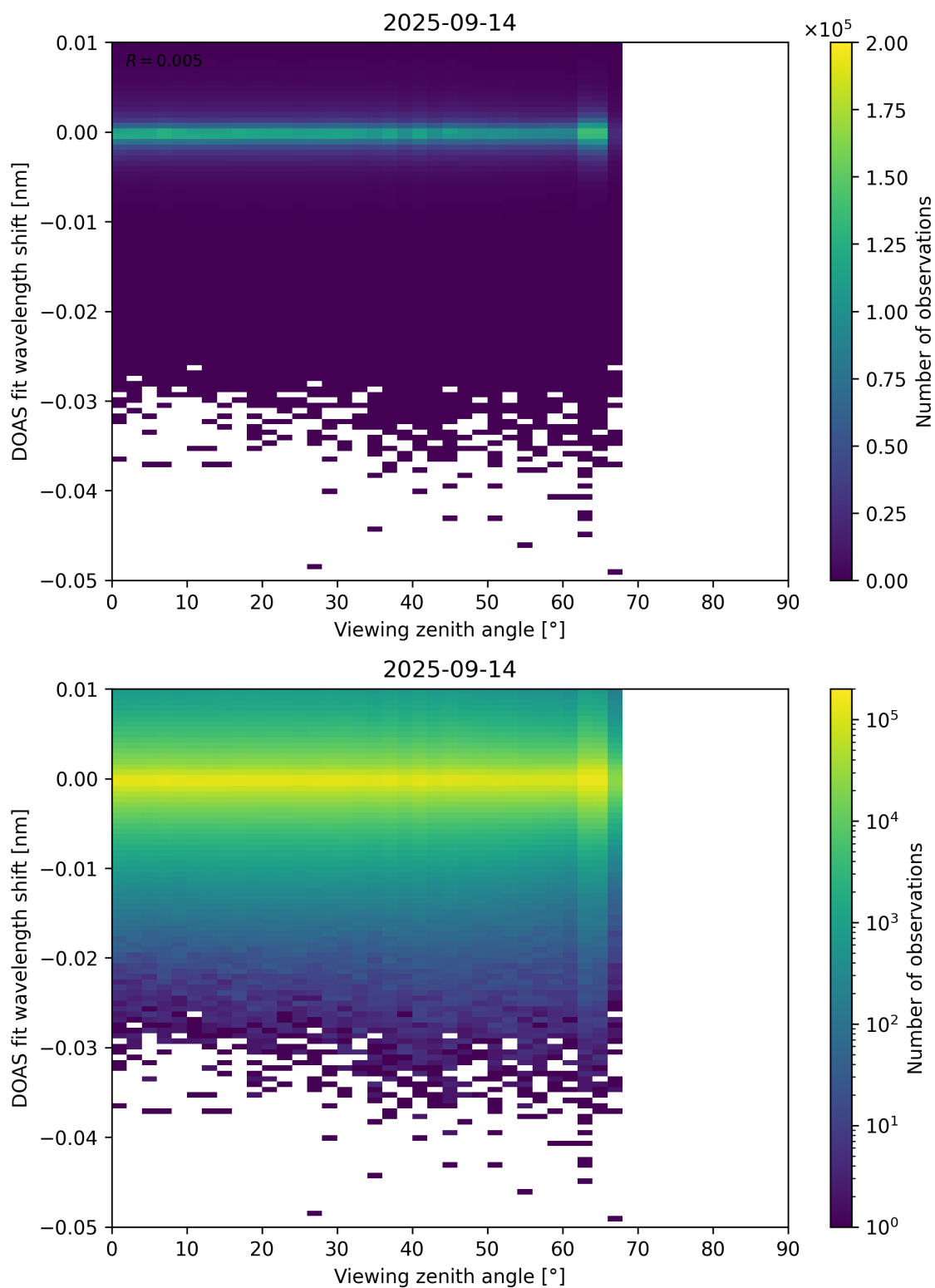
Figure 365: Scatter density plot of “Viewing zenith angle” against “DOAS fit wavelength shift” for 2025-09-13 to 2025-09-15.
