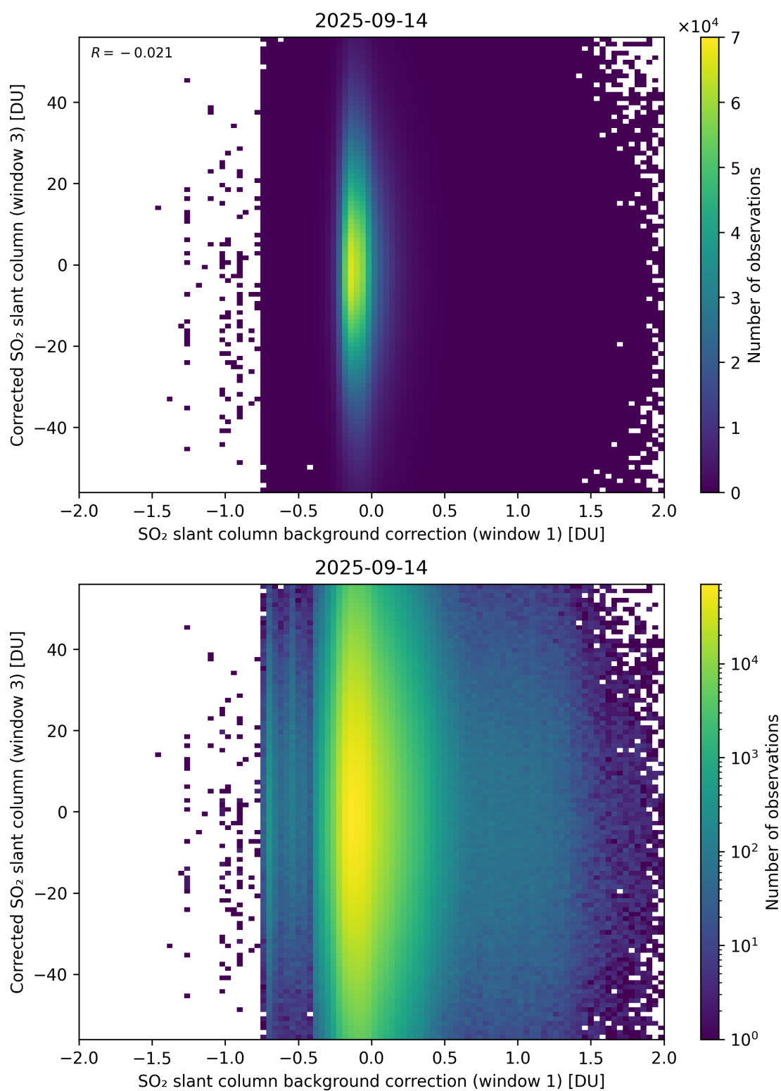
Figure 116: Scatter density plot of “SO 2 slant column background correction (window 1)” against “Corrected SO 2 slant column (window 3)” for 2025-09-13 to 2025-09-15.
