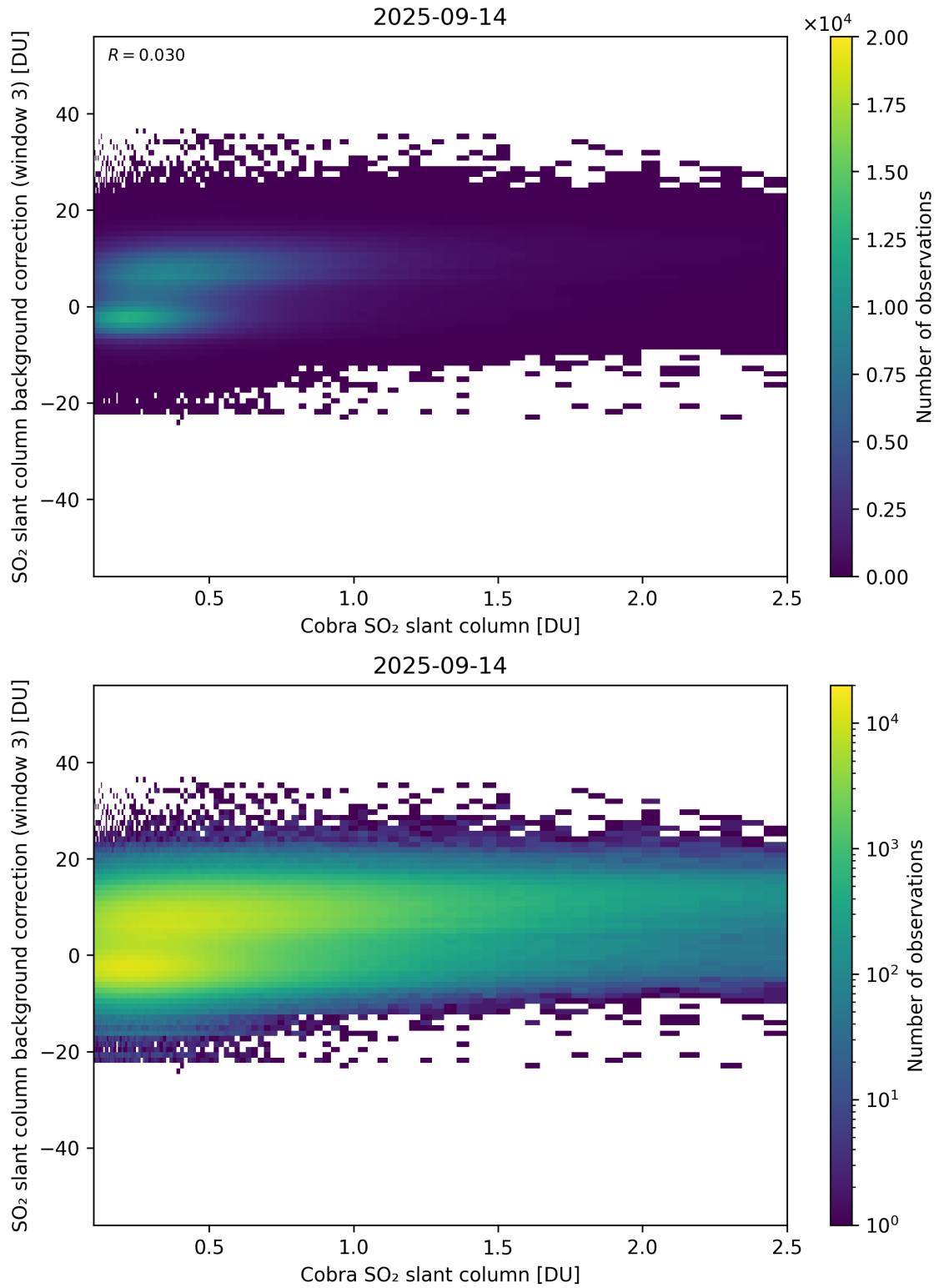
Figure 195: Scatter density plot of “Cobra SO 2 slant column” against “SO 2 slant column background correction (window 3)” for 2025-09-13 to 2025-09-15.
