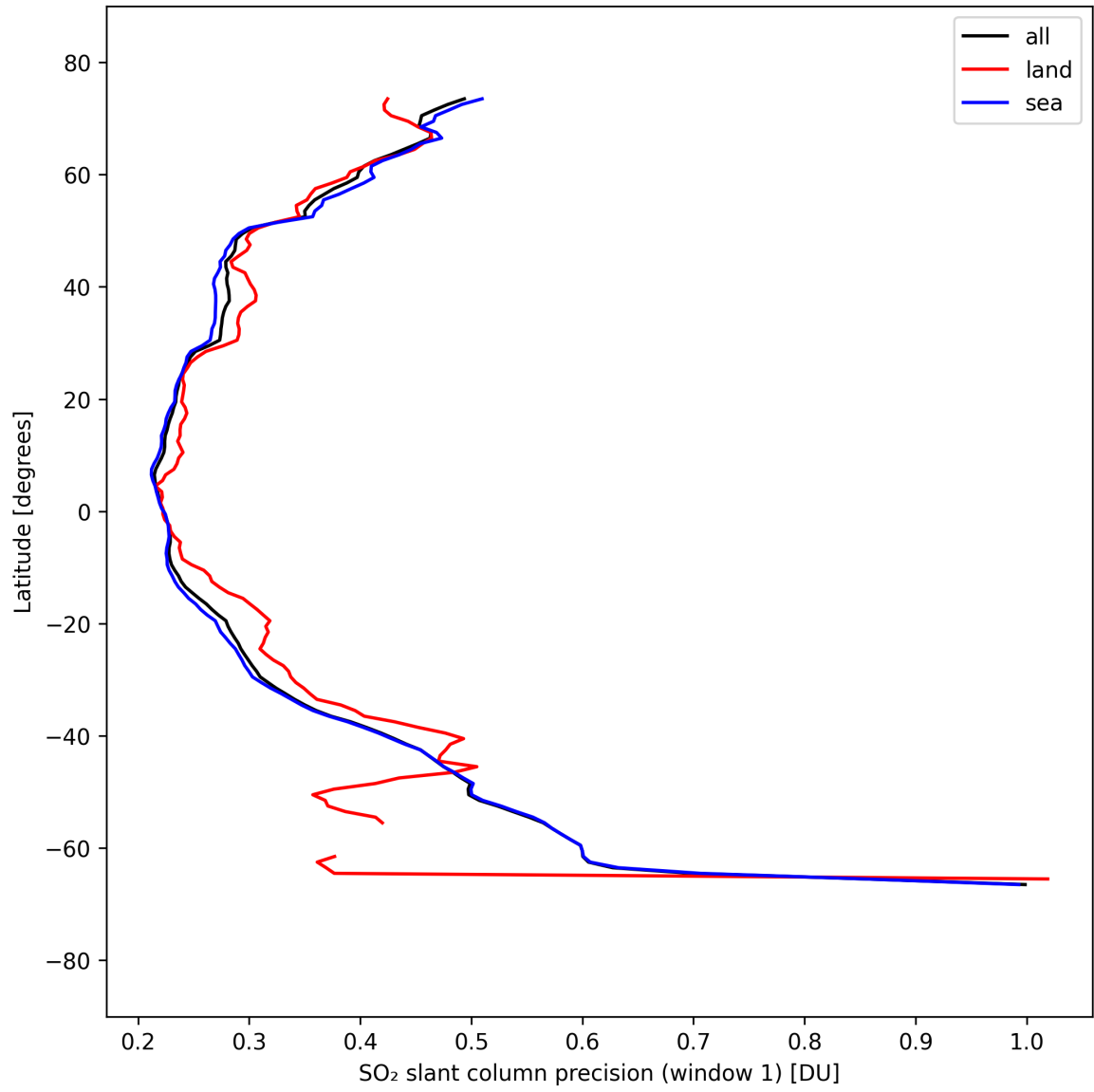
Figure 38: Zonal average of “SO 2 slant column precision (window 1)” for 2025-09-13 to 2025-09-15.
