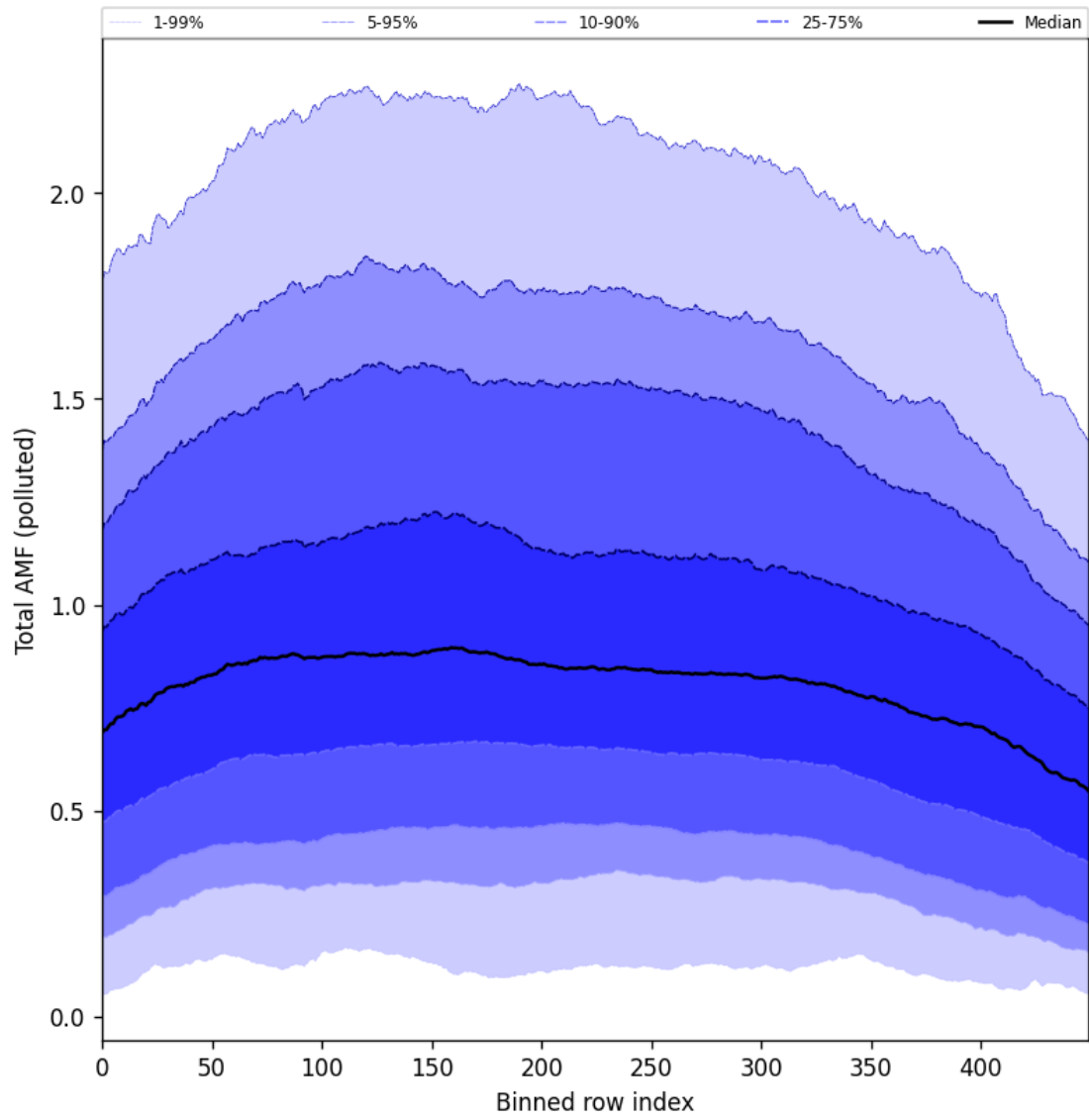
Figure 105: Along track statistics of “Total AMF (polluted)” for 2025-09-13 to 2025-09-15
