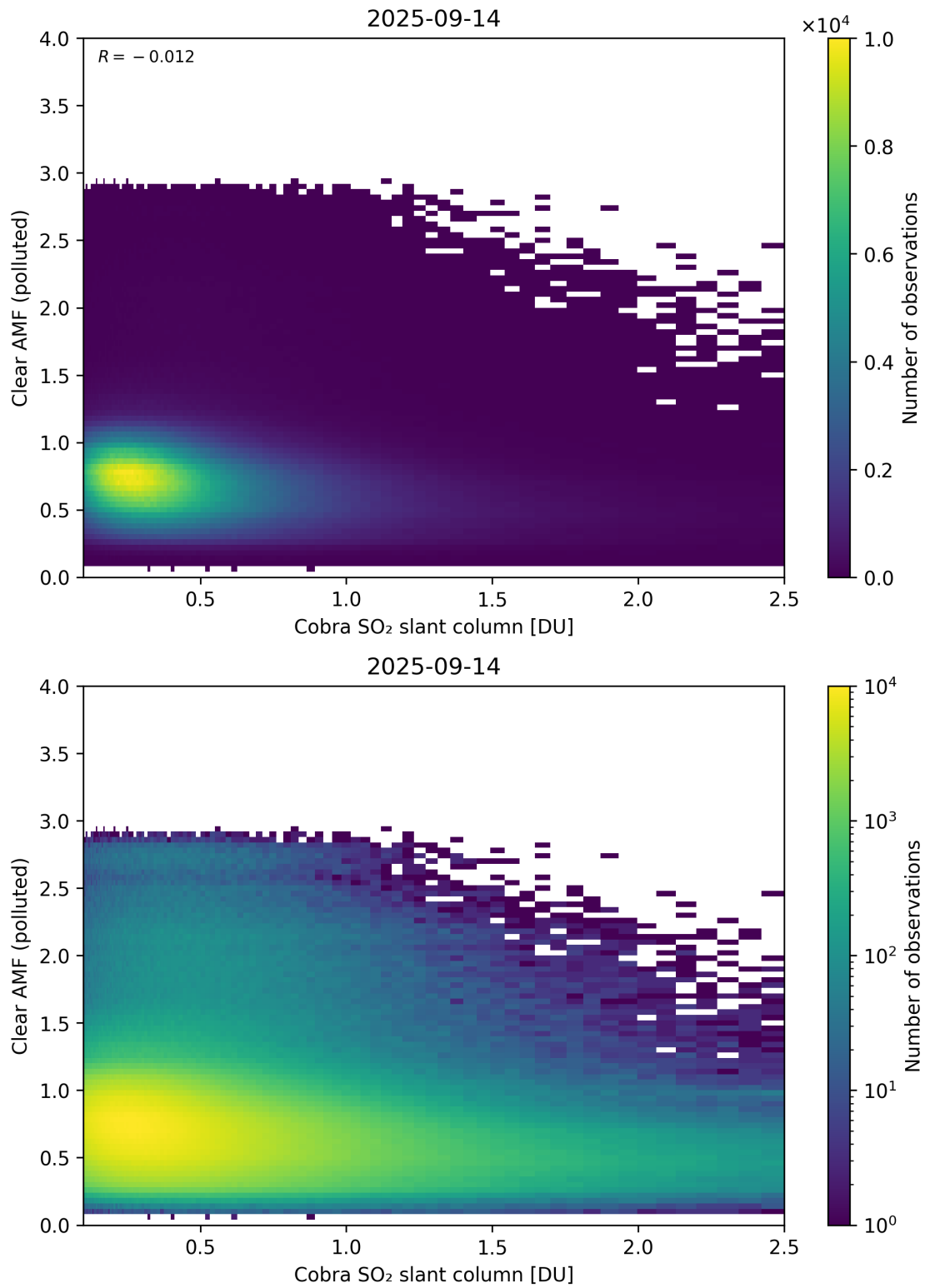
Figure 215: Scatter density plot of “Cobra SO 2 slant column” against “Clear AMF (polluted)” for 2025-09-13 to 2025-09-15.
