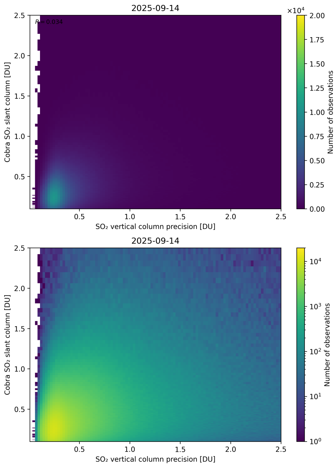
Figure 336: Scatter density plot of “SO 2 vertical column precision” against “Cobra SO 2 slant column” for 2025-09-13 to 2025-09-15.
