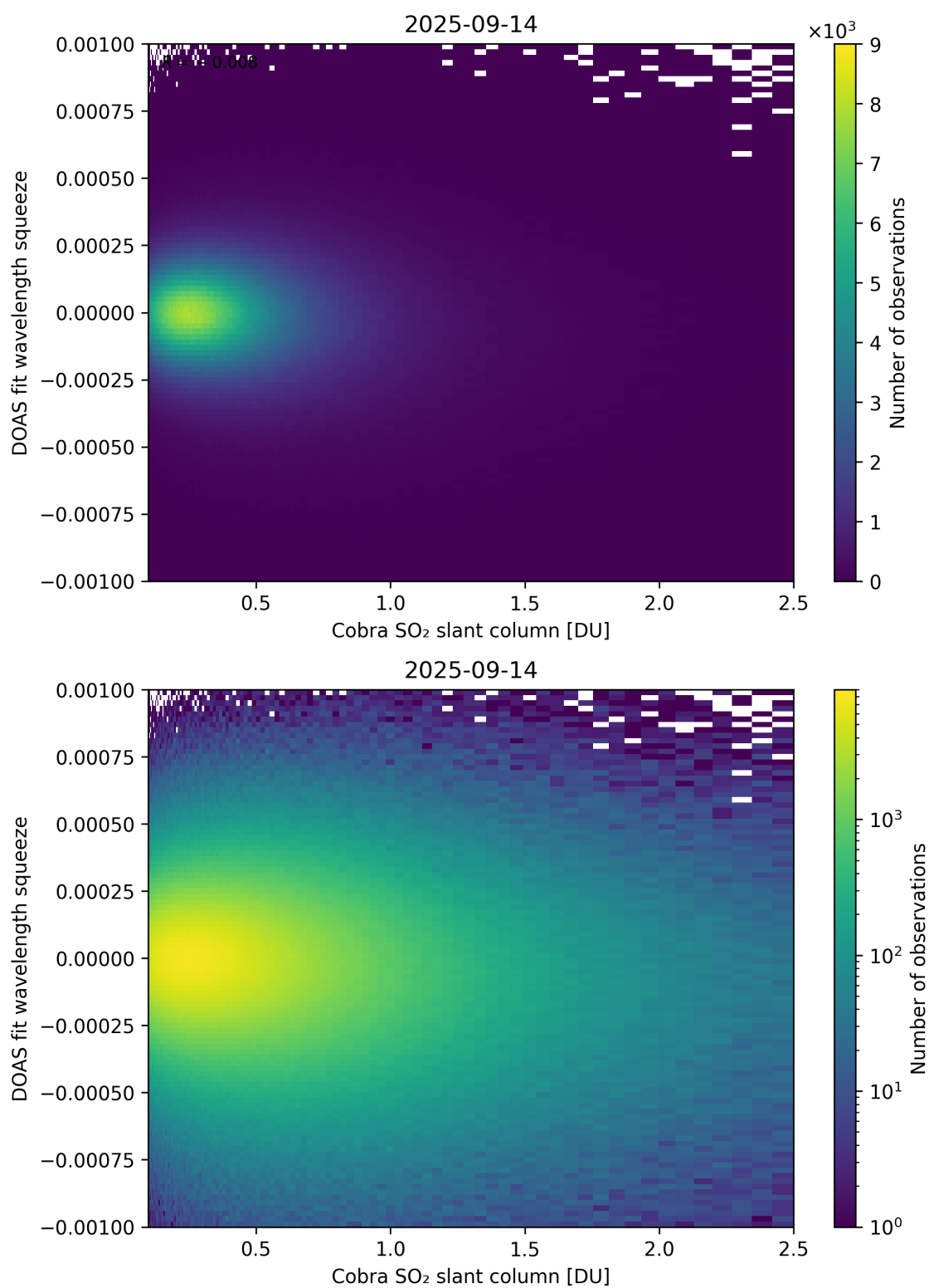
Figure 197: Scatter density plot of “Cobra SO 2 slant column” against “DOAS fit wavelength squeeze” for 2025-09-13 to 2025-09-15.
