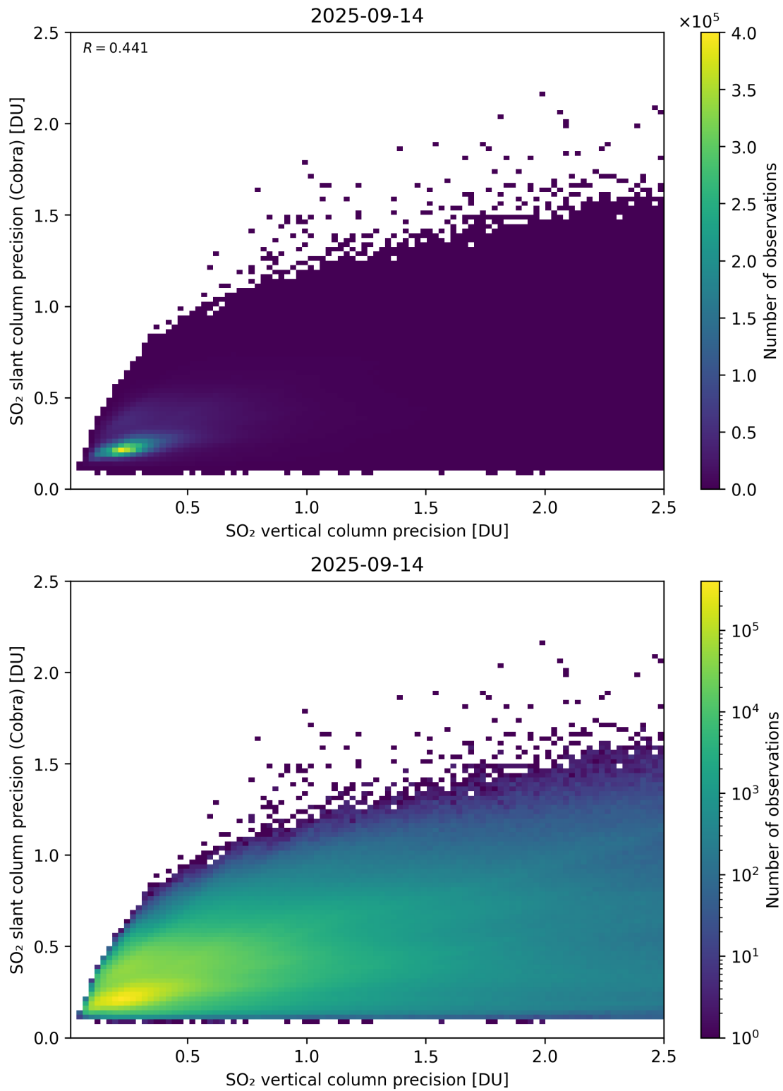
Figure 337: Scatter density plot of “SO 2 vertical column precision” against “SO 2 slant column precision (Cobra)” for 2025-09-13 to 2025-09-15.
