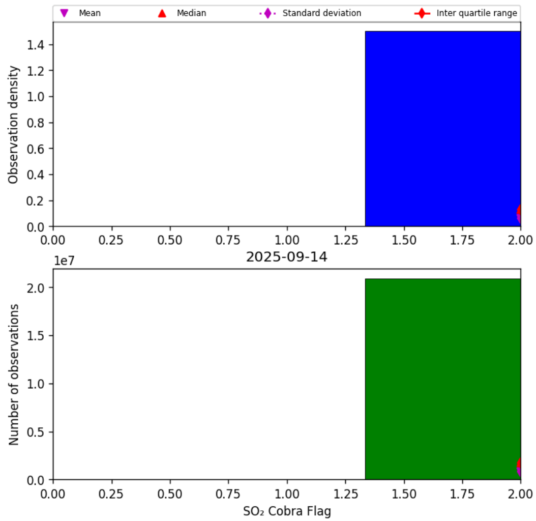
Figure 75: Histogram of "SO 2 Cobra Flag" for 2025-09-13 to 2025-09-15
