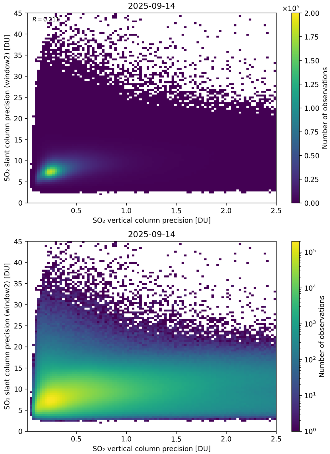
Figure 343: Scatter density plot of “SO 2 vertical column precision” against “SO 2 slant column precision (window2)” for 2025-09-13 to 2025-09-15.
