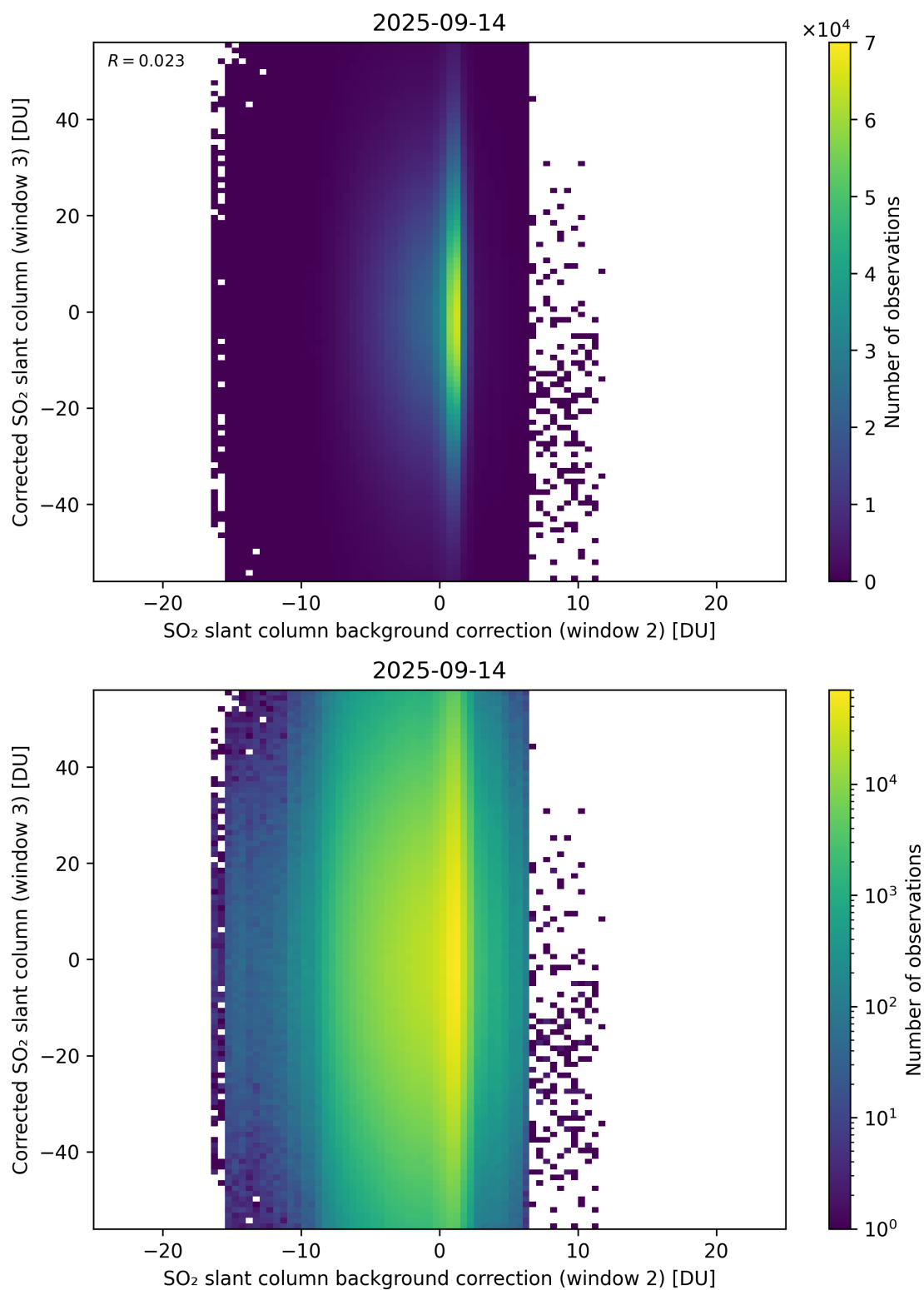
Figure 127: Scatter density plot of “SO 2 slant column background correction (window 2)” against “Corrected SO 2 slant column (window 3)” for 2025-09-13 to 2025-09-15.
