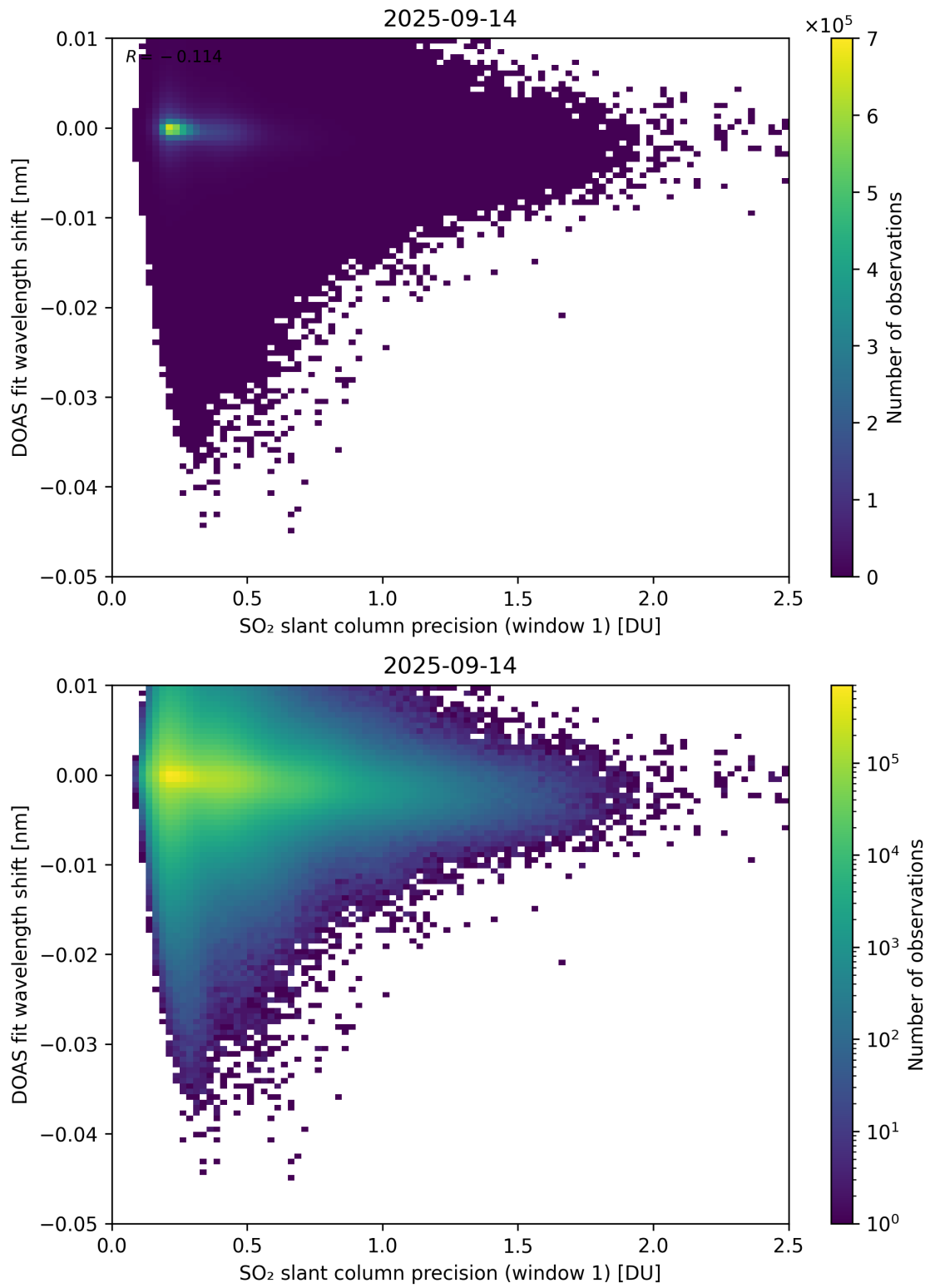
Figure 271: Scatter density plot of “SO 2 slant column precision (window 1)” against “DOAS fit wavelength shift” for 2025-09-13 to 2025-09-15.
