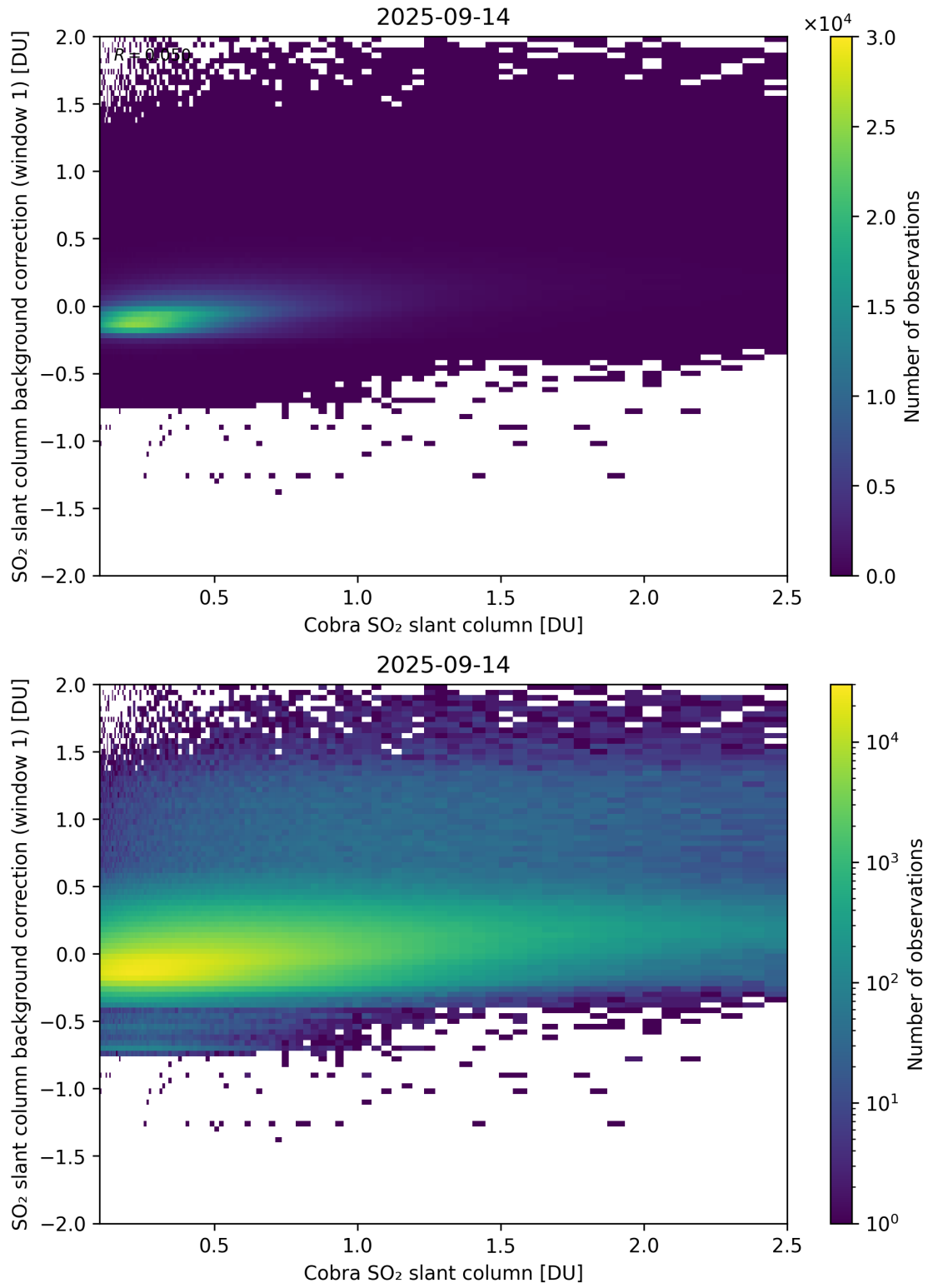
Figure 193: Scatter density plot of “Cobra SO 2 slant column” against “SO 2 slant column background correction (window 1)” for 2025-09-13 to 2025-09-15.
