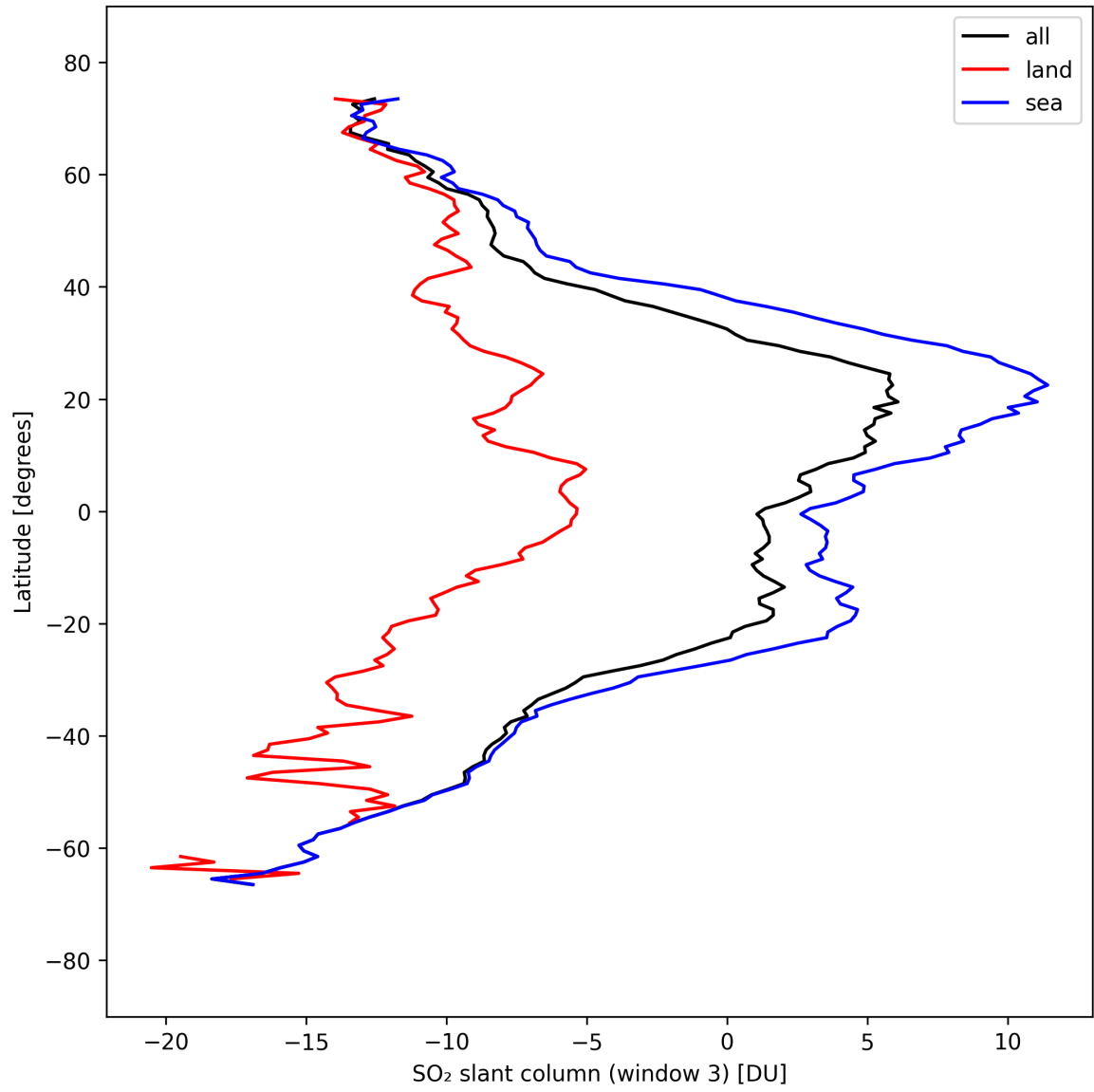
Figure 45: Zonal average of “SO 2 slant column (window 3)” for 2025-09-13 to 2025-09-15.
