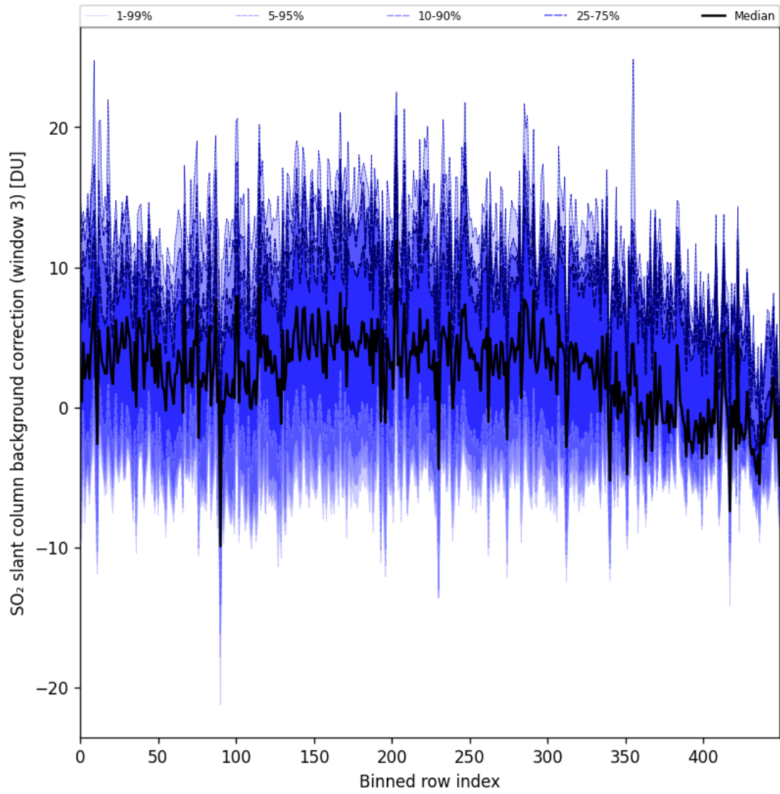
Figure 100: Along track statistics of “SO 2 slant column background correction (window 3)” for 2025-09-13 to 2025-09-15
