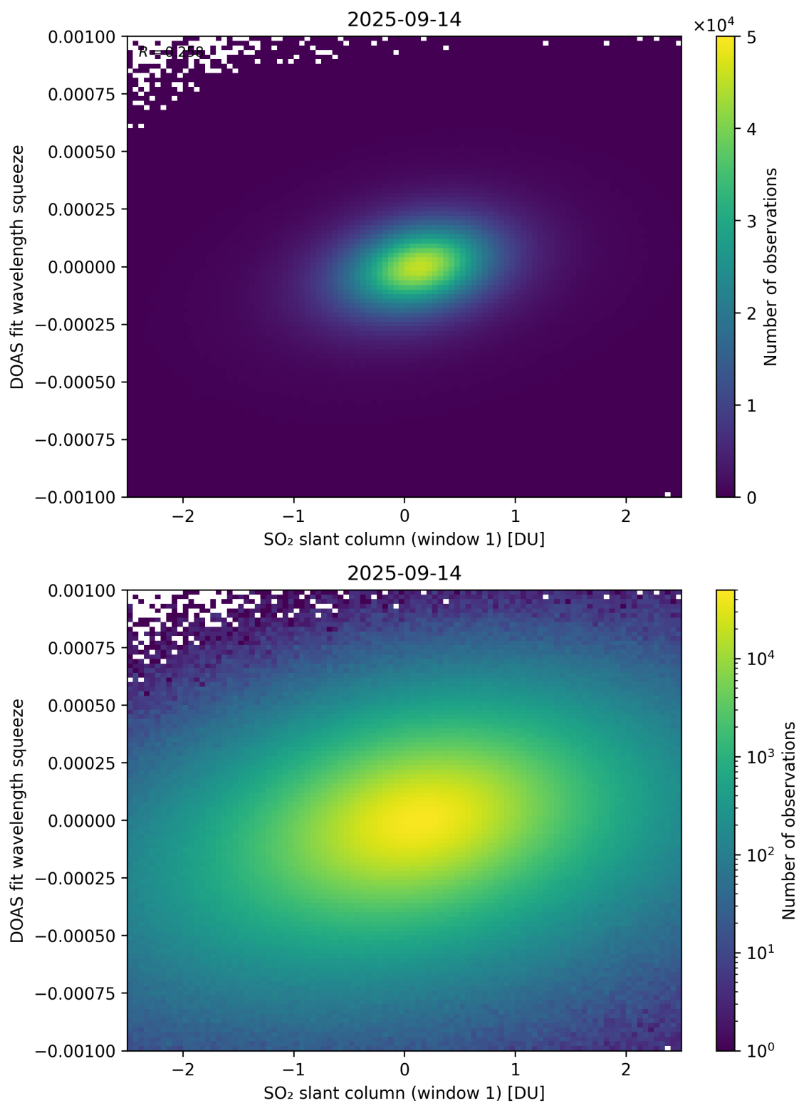
Figure 266: Scatter density plot of “SO 2 slant column (window 1)” against “DOAS fit wavelength squeeze” for 2025-09-13 to 2025-09-15.
