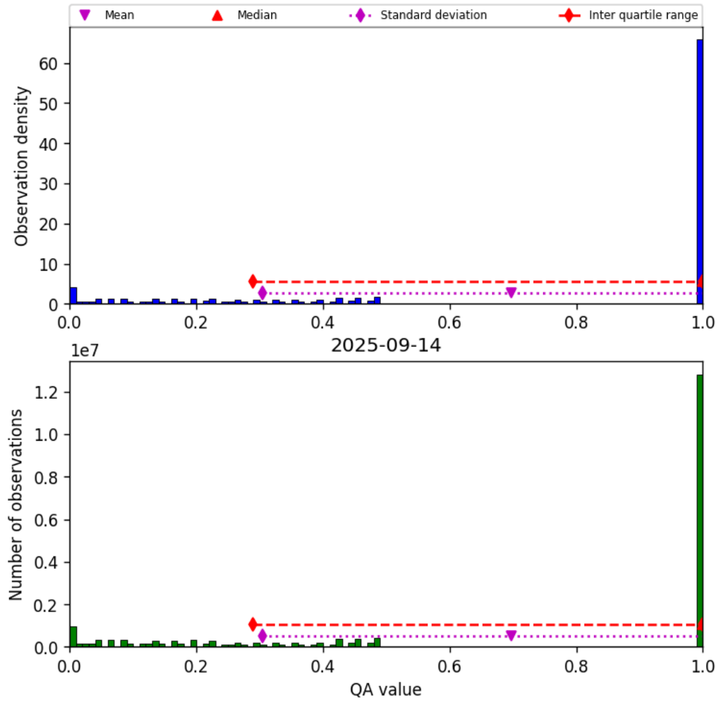
Figure 57: Histogram of “QA value” for 2025-09-13 to 2025-09-15
