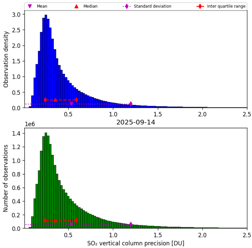
Figure 59: Histogram of “SO 2 vertical column precision” for 2025-09-13 to 2025-09-15
