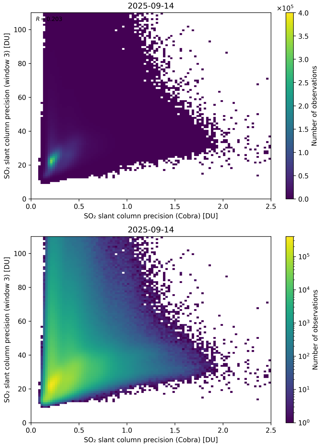
Figure 212: Scatter density plot of “SO 2 slant column precision (Cobra)” against “SO 2 slant column precision (window 3)” for 2025-09-13 to 2025-09-15.
