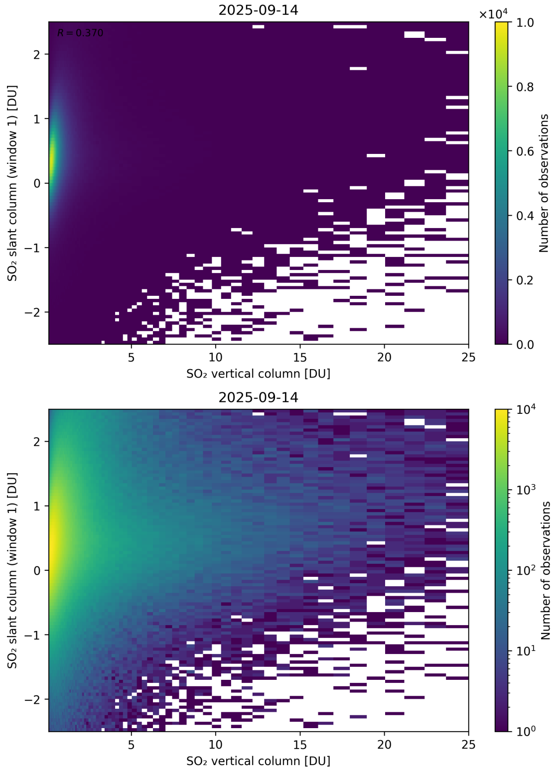
Figure 354: Scatter density plot of “SO 2 vertical column” against “SO 2 slant column (window 1)” for 2025-09-13 to 2025-09-15.
