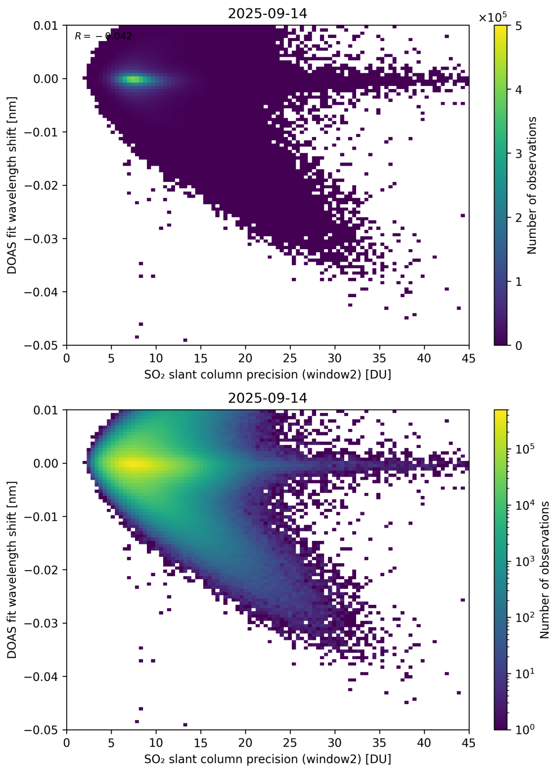
Figure 293: Scatter density plot of “SO 2 slant column precision (window2)” against “DOAS fit wavelength shift” for 2025-09-13 to 2025-09-15.
