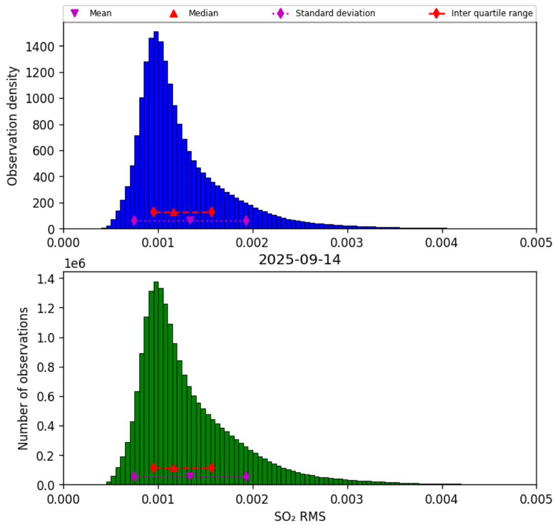
Figure 78: Histogram of “SO 2 RMS” for 2025-09-13 to 2025-09-15
