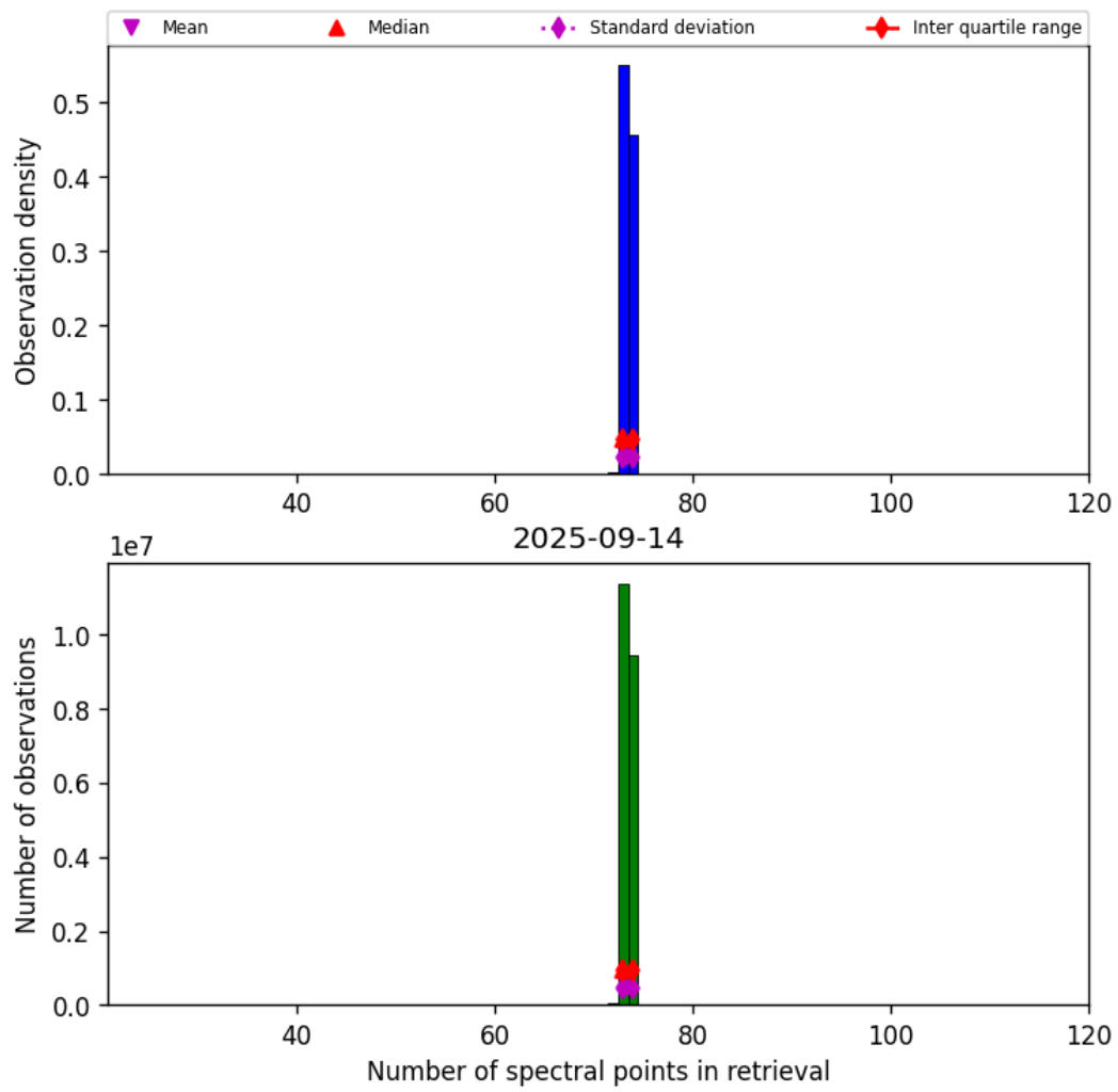
Figure 82: Histogram of “Number of spectral points in retrieval” for 2025-09-13 to 2025-09-15
