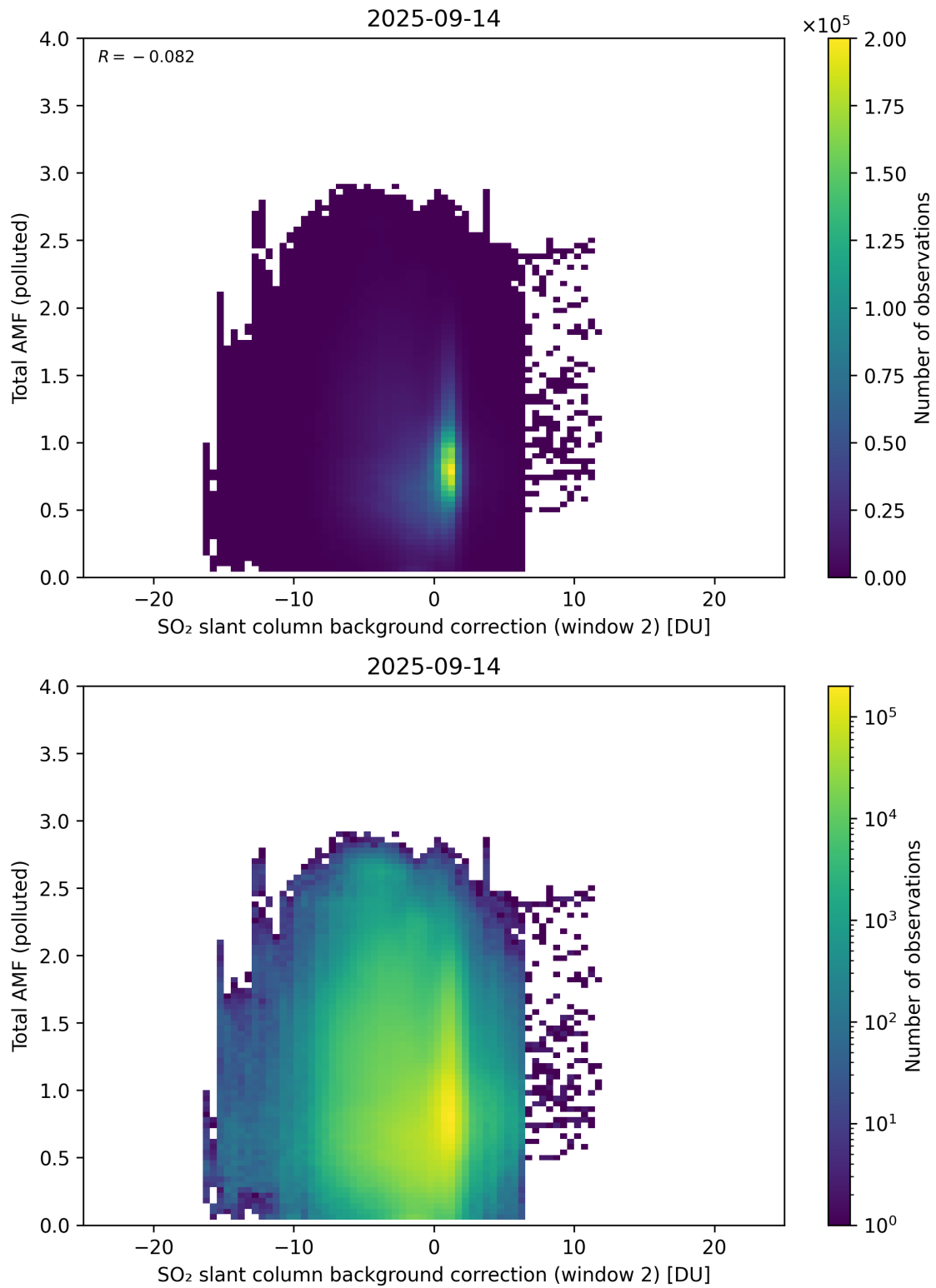
Figure 130: Scatter density plot of “SO 2 slant column background correction (window 2)” against “Total AMF (polluted)” for 2025-09-13 to 2025-09-15.
