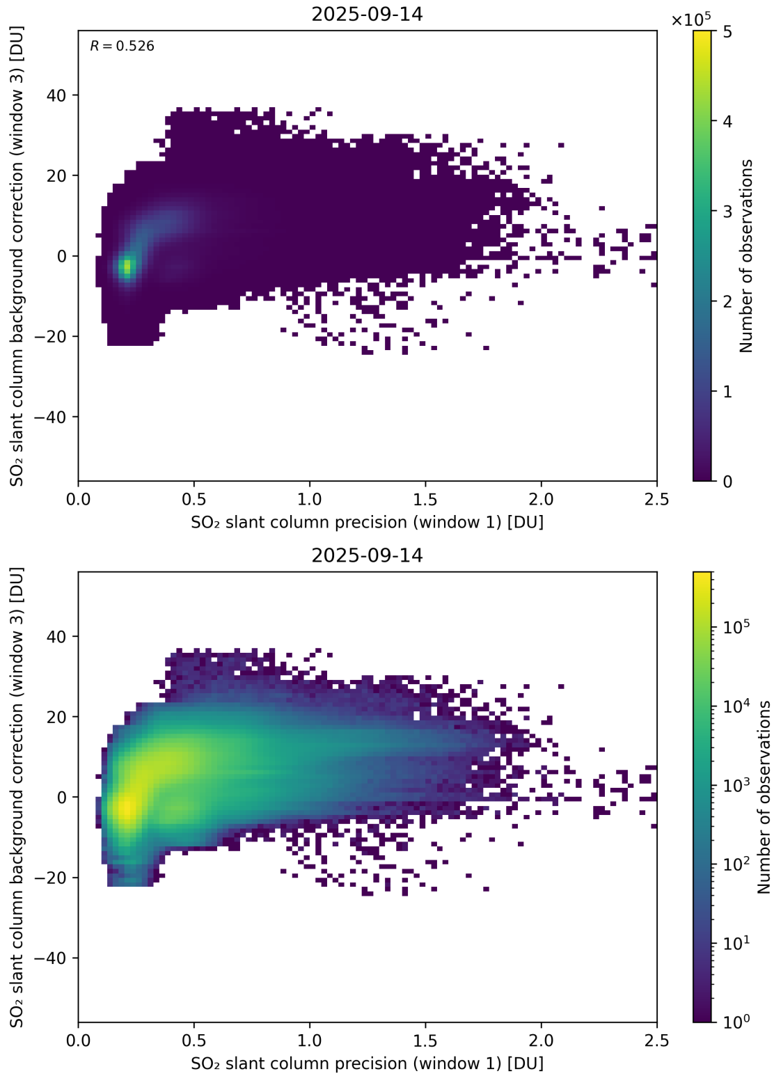
Figure 270: Scatter density plot of “SO 2 slant column precision (window 1)” against “SO 2 slant column background correction (window 3)” for 2025-09-13 to 2025-09-15.
