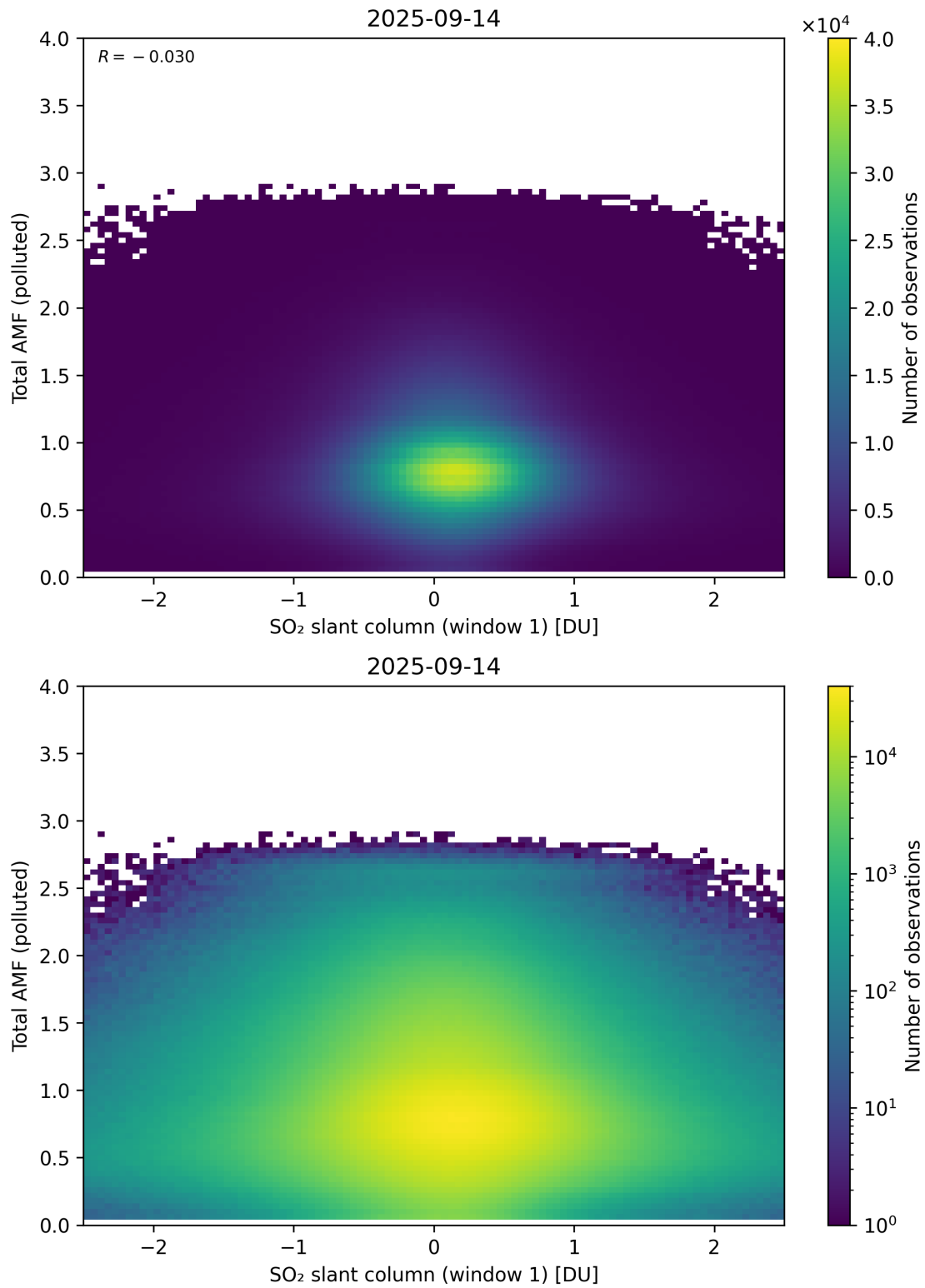
Figure 289: Scatter density plot of “SO 2 slant column (window 1)” against “Total AMF (polluted)” for 2025-09-13 to 2025-09-15.
