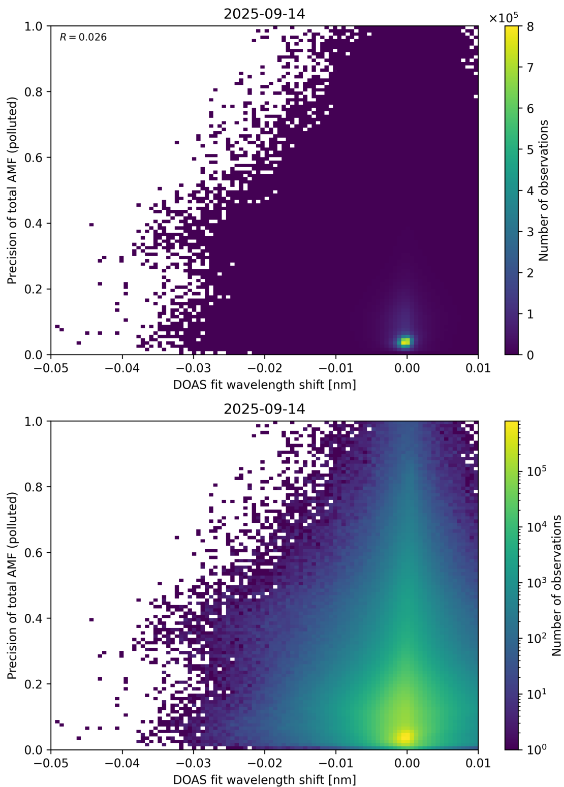
Figure 142: Scatter density plot of “DOAS fit wavelength shift” against “Precision of total AMF (polluted)” for 2025-09-13 to 2025-09-15.
