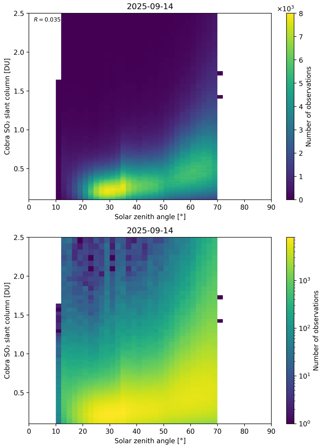
Figure 179: Scatter density plot of “Solar zenith angle” against “Cobra SO 2 slant column” for 2025-09-13 to 2025-09-15.
