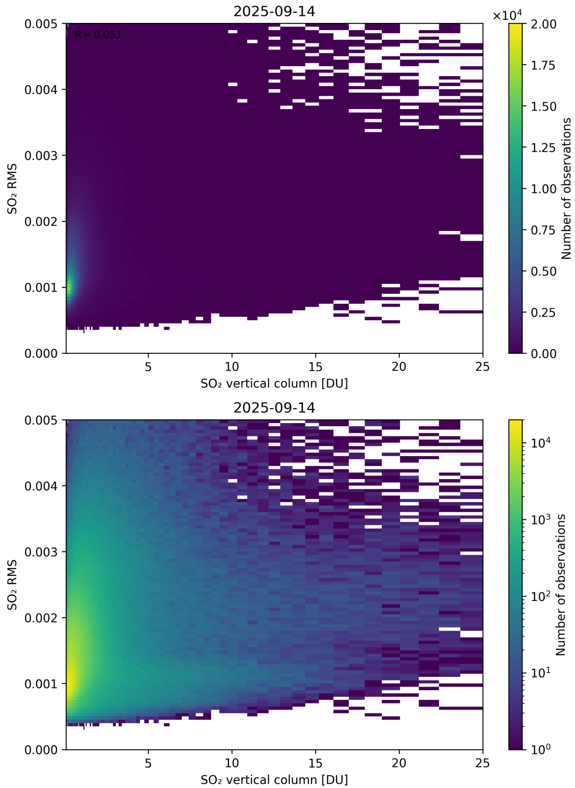
Figure 328: Scatter density plot of “SO 2 vertical column” against “SO 2 RMS” for 2025-09-13 to 2025-09-15.
