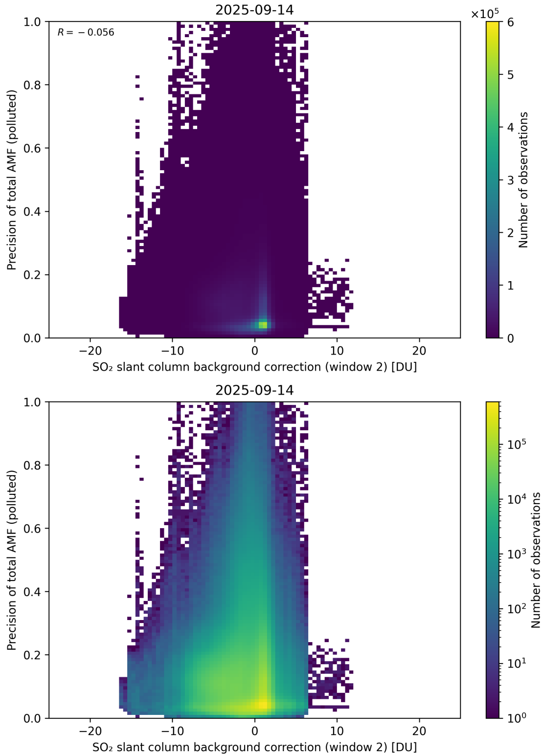
Figure 131: Scatter density plot of “SO 2 slant column background correction (window 2)” against “Precision of total AMF (polluted)” for 2025-09-13 to 2025-09-15.
