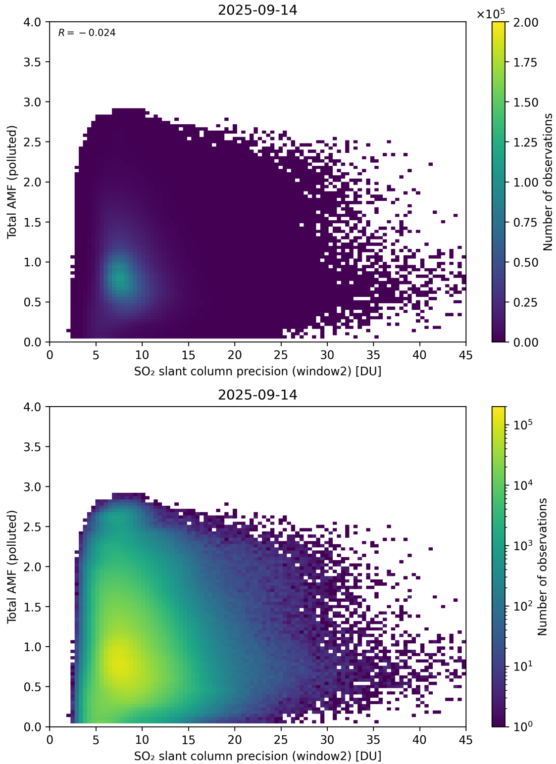
Figure 301: Scatter density plot of “SO 2 slant column precision (window2)” against “Total AMF (polluted)” for 2025-09-13 to 2025-09-15.
