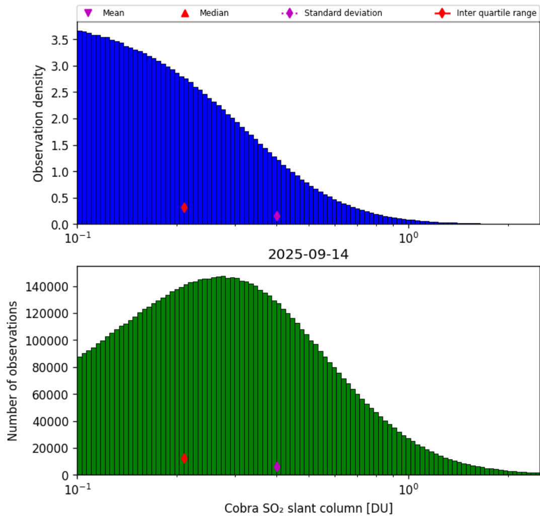
Figure 61: Histogram of “Cobra SO 2 slant column” for 2025-09-13 to 2025-09-15
