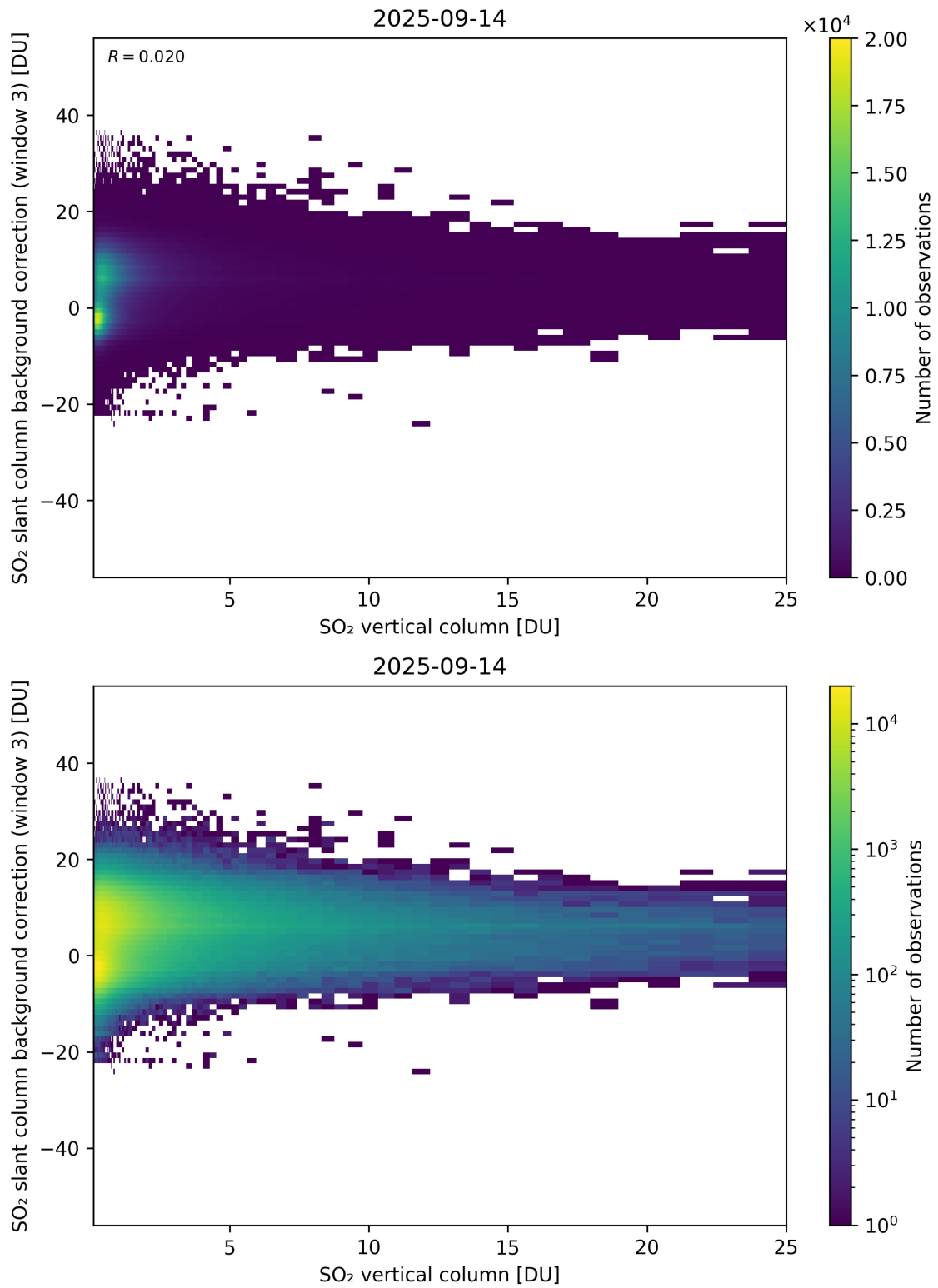
Figure 325: Scatter density plot of “SO 2 vertical column” against “SO 2 slant column background correction (window 3)” for 2025-09-13 to 2025-09-15.
