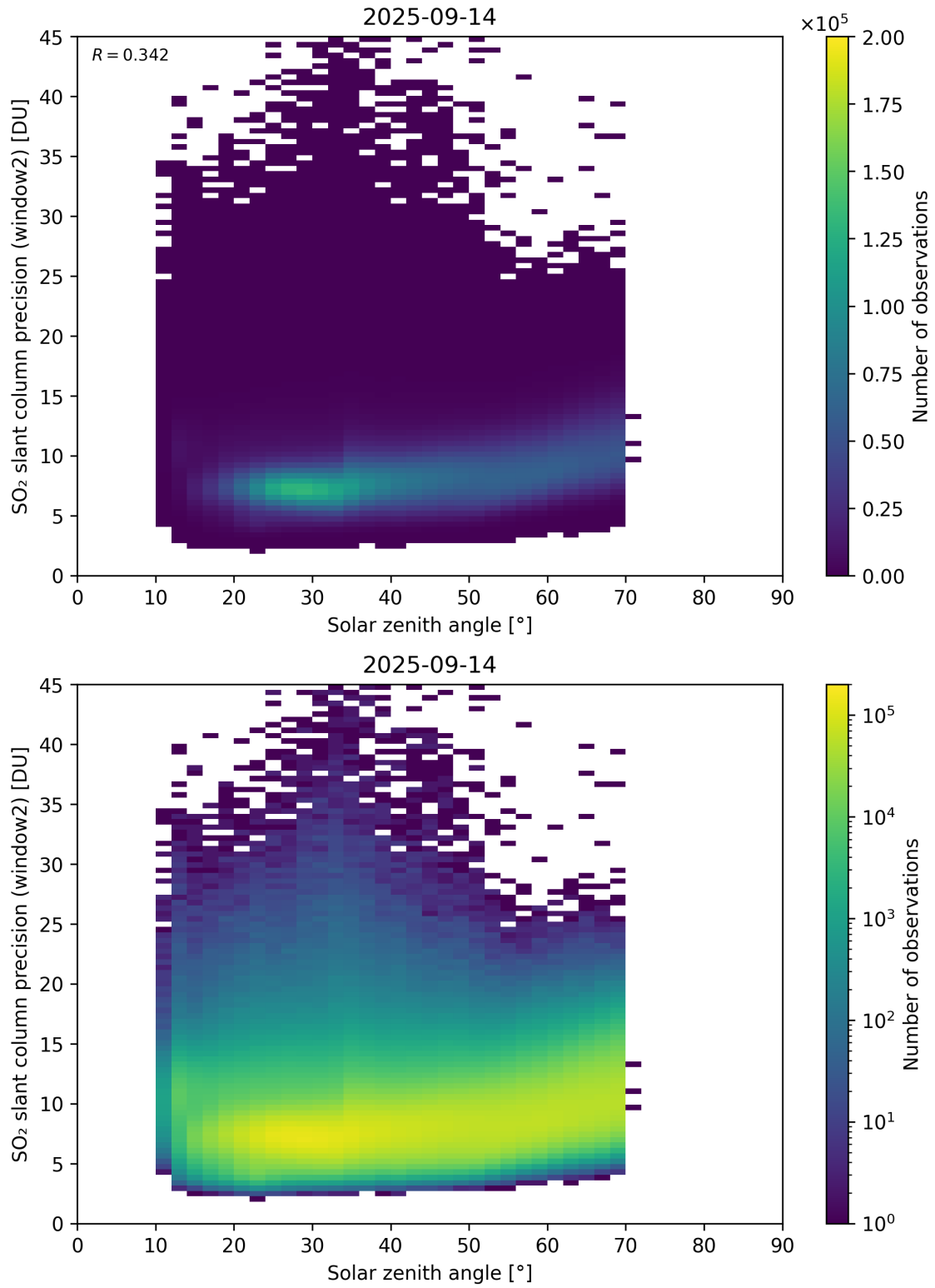
Figure 186: Scatter density plot of “Solar zenith angle” against “SO 2 slant column precision (window2)” for 2025-09-13 to 2025-09-15.
