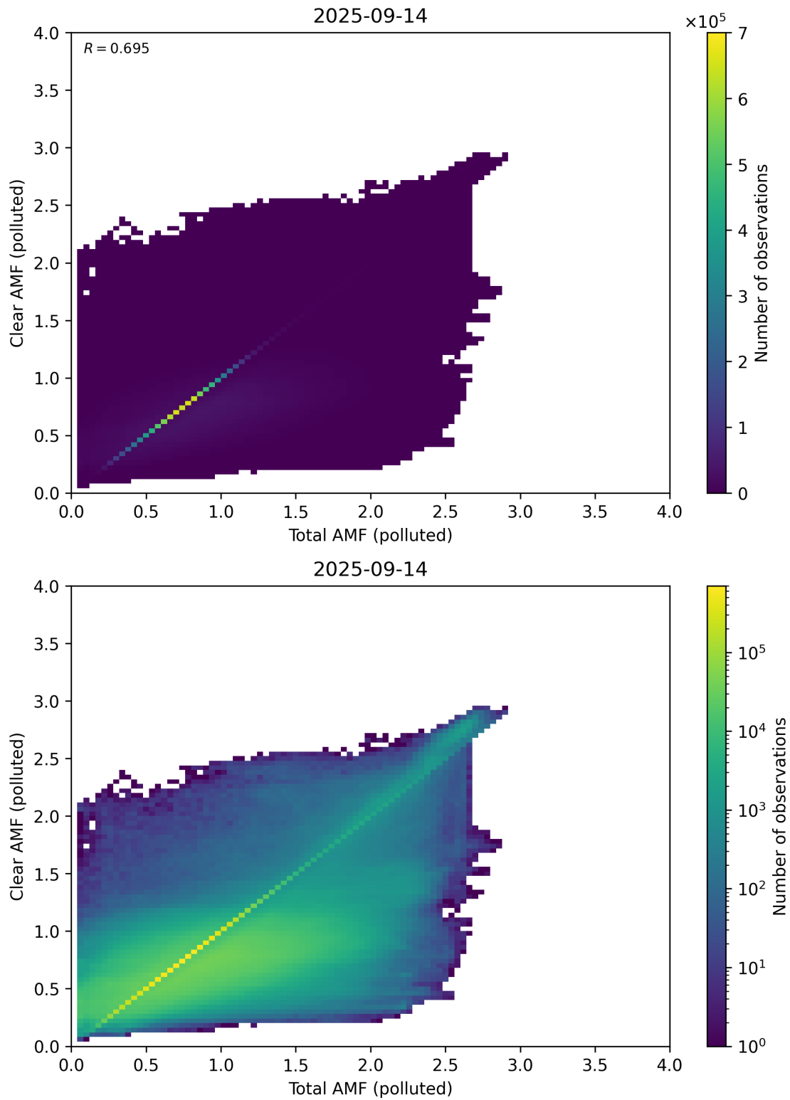
Figure 321: Scatter density plot of “Total AMF (polluted)” against “Clear AMF (polluted)” for 2025-09-13 to 2025-09-15.
