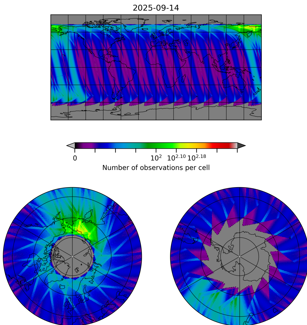
Figure 30: Map of the number of observations for 2025-09-13 to 2025-09-15
