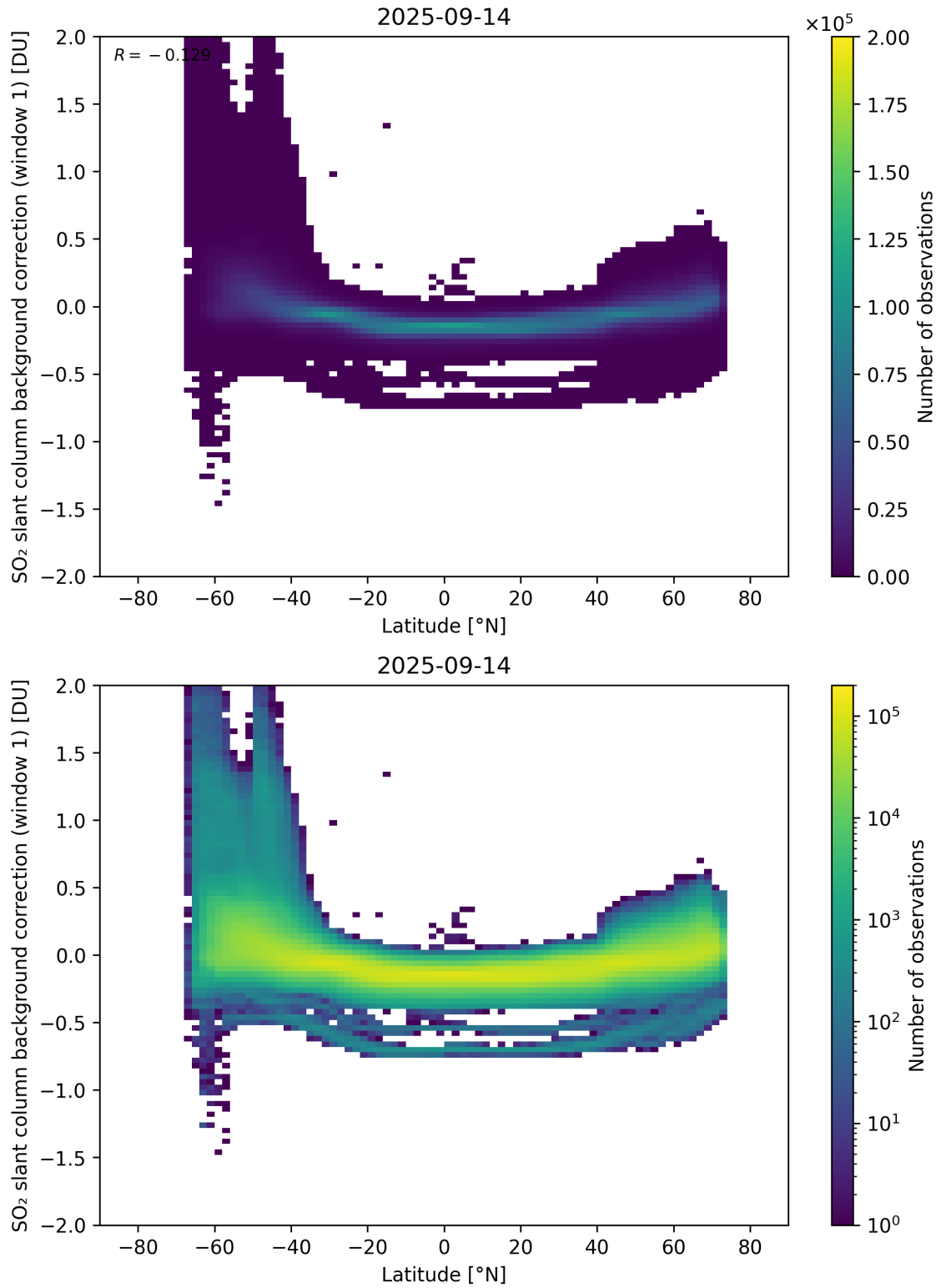
Figure 150: Scatter density plot of “Latitude” against “SO 2 slant column background correction (window 1)” for 2025-09-13 to 2025-09-15.
