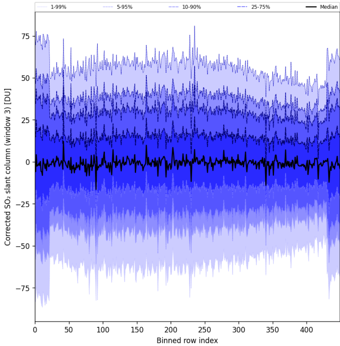
Figure 99: Along track statistics of “Corrected SO 2 slant column (window 3)” for 2025-09-13 to 2025-09-15
