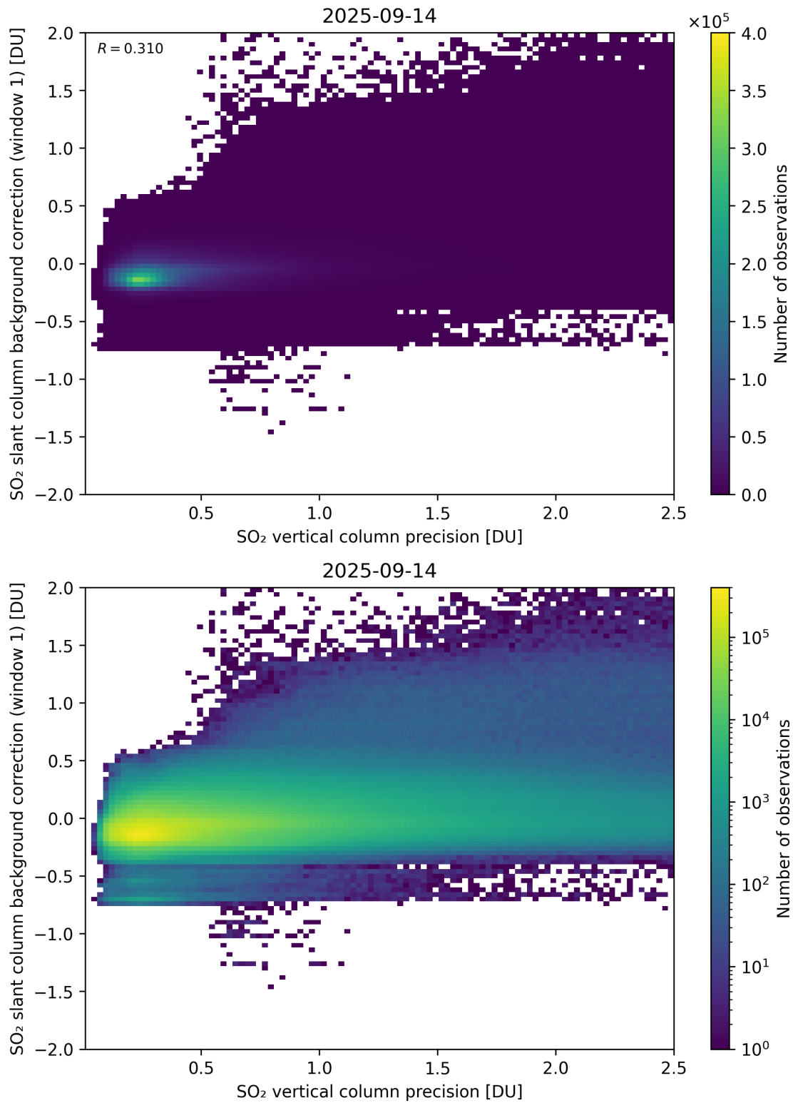
Figure 329: Scatter density plot of “SO 2 vertical column precision” against “SO 2 slant column background correction (window 1)” for 2025-09-13 to 2025-09-15.
