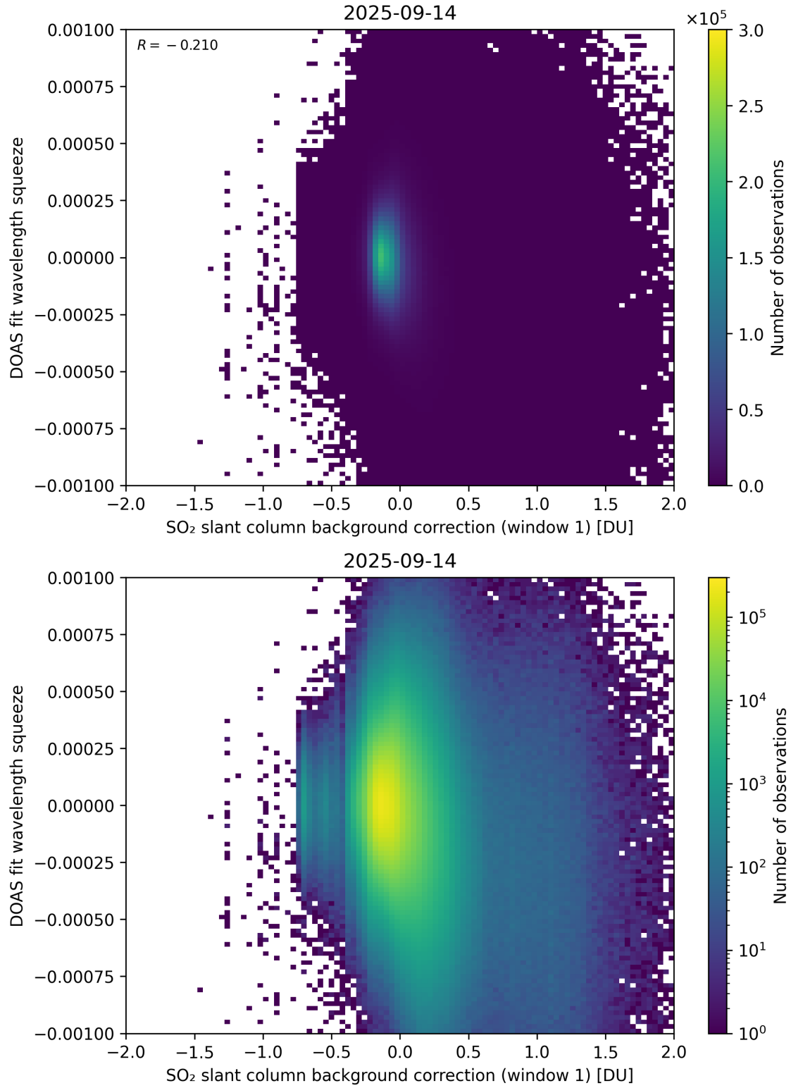
Figure 112: Scatter density plot of “SO 2 slant column background correction (window 1)” against “DOAS fit wavelength squeeze” for 2025-09-13 to 2025-09-15.
