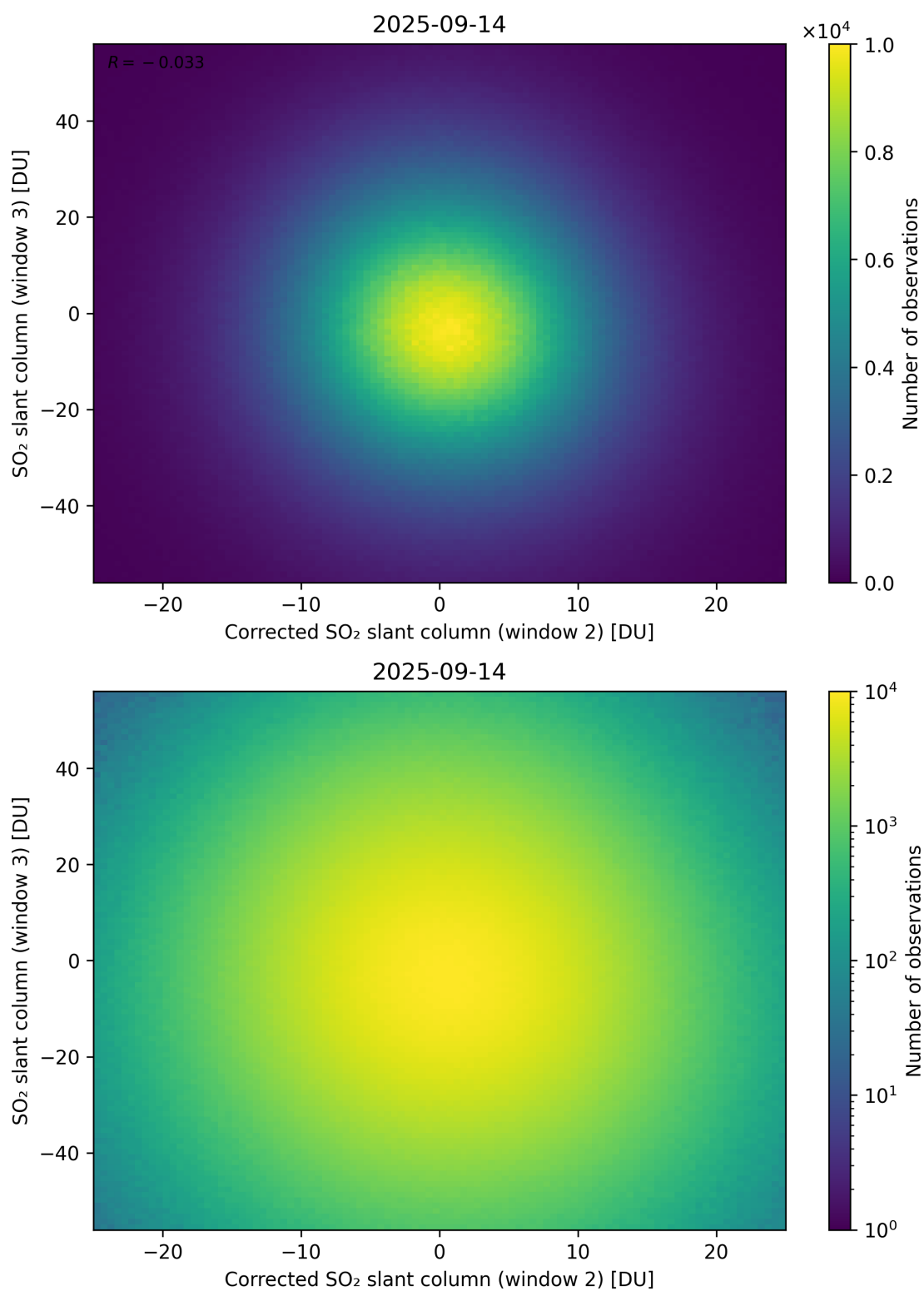
Figure 251: Scatter density plot of “Corrected SO 2 slant column (window 2)” against “SO 2 slant column (window 3)” for 2025-09-13 to 2025-09-15.
