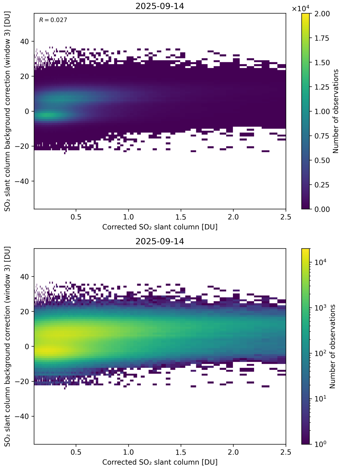
Figure 228: Scatter density plot of “Corrected SO 2 slant column” against “SO 2 slant column background correction (window 3)” for 2025-09-13 to 2025-09-15.
