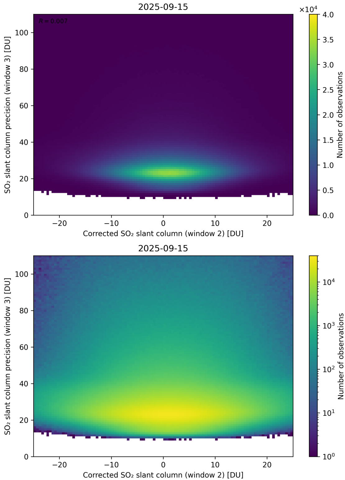
Figure 252: Scatter density plot of “Corrected SO 2 slant column (window 2)” against “SO 2 slant column precision (window 3)” for 2025-09-15 to 2025-09-16.
