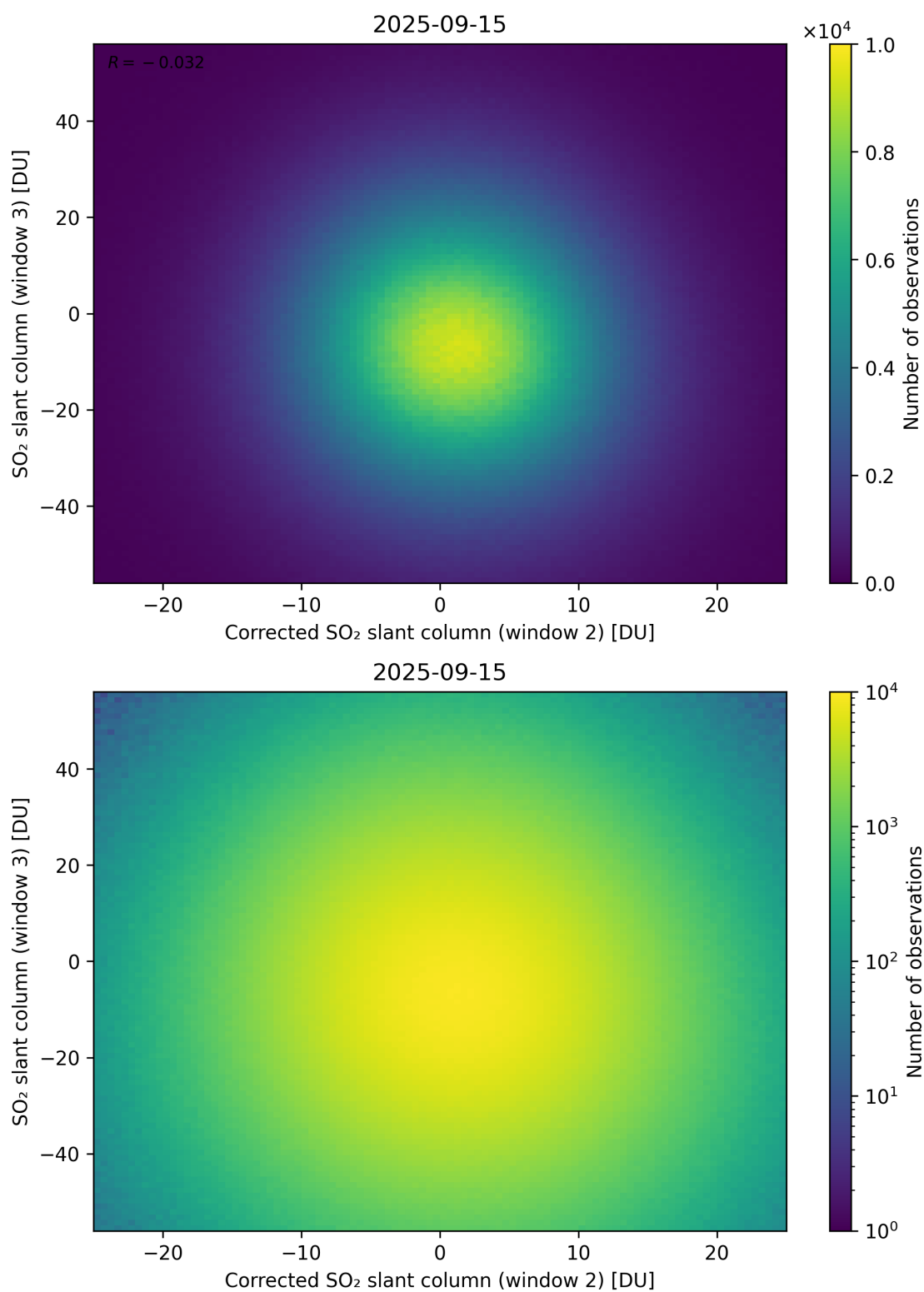
Figure 251: Scatter density plot of “Corrected SO 2 slant column (window 2)” against “SO 2 slant column (window 3)” for 2025-09-15 to 2025-09-16.
