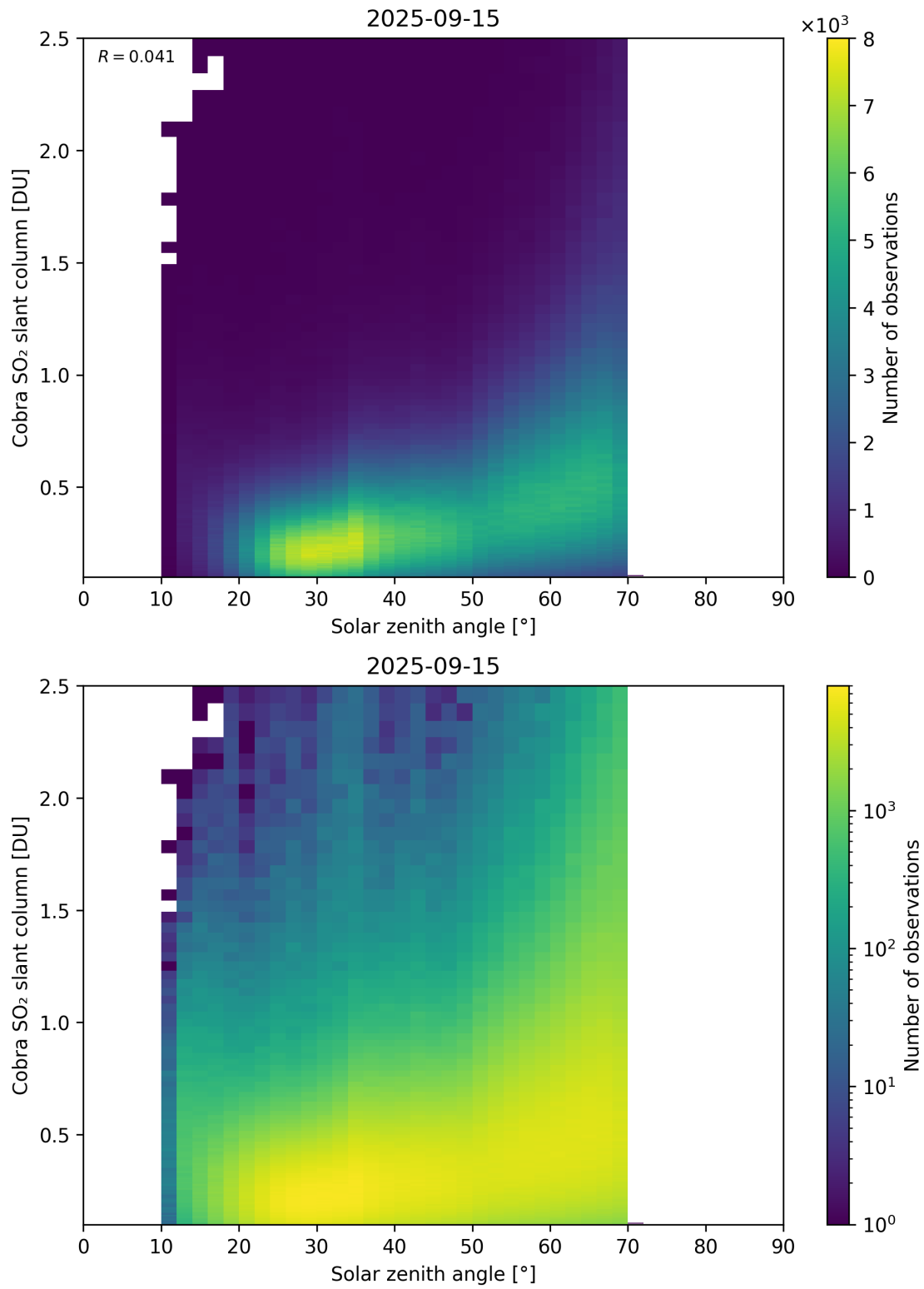
Figure 179: Scatter density plot of “Solar zenith angle” against “Cobra SO 2 slant column” for 2025-09-15 to 2025-09-16.
