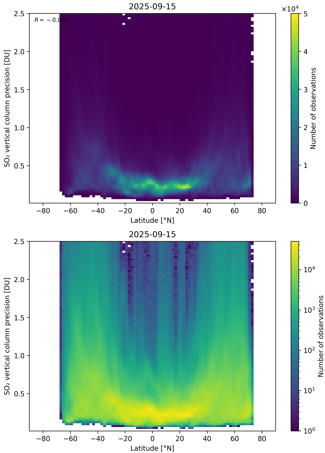
Figure 170: Scatter density plot of “Latitude” against “SO 2 vertical column precision” for 2025-09-15 to 2025-09-16.
