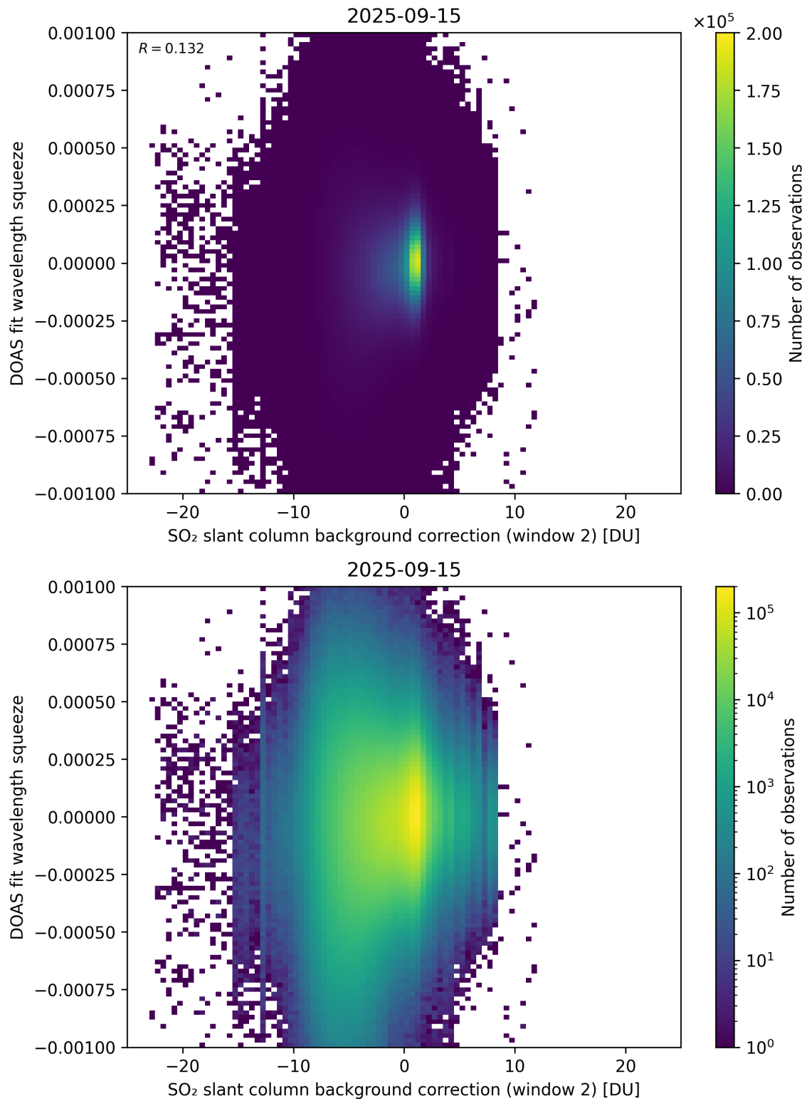
Figure 124: Scatter density plot of “SO 2 slant column background correction (window 2)” against “DOAS fit wavelength squeeze” for 2025-09-15 to 2025-09-16.
