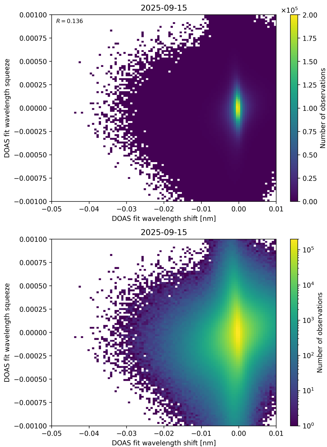
Figure 138: Scatter density plot of “DOAS fit wavelength shift” against “DOAS fit wavelength squeeze” for 2025-09-15 to 2025-09-16.
