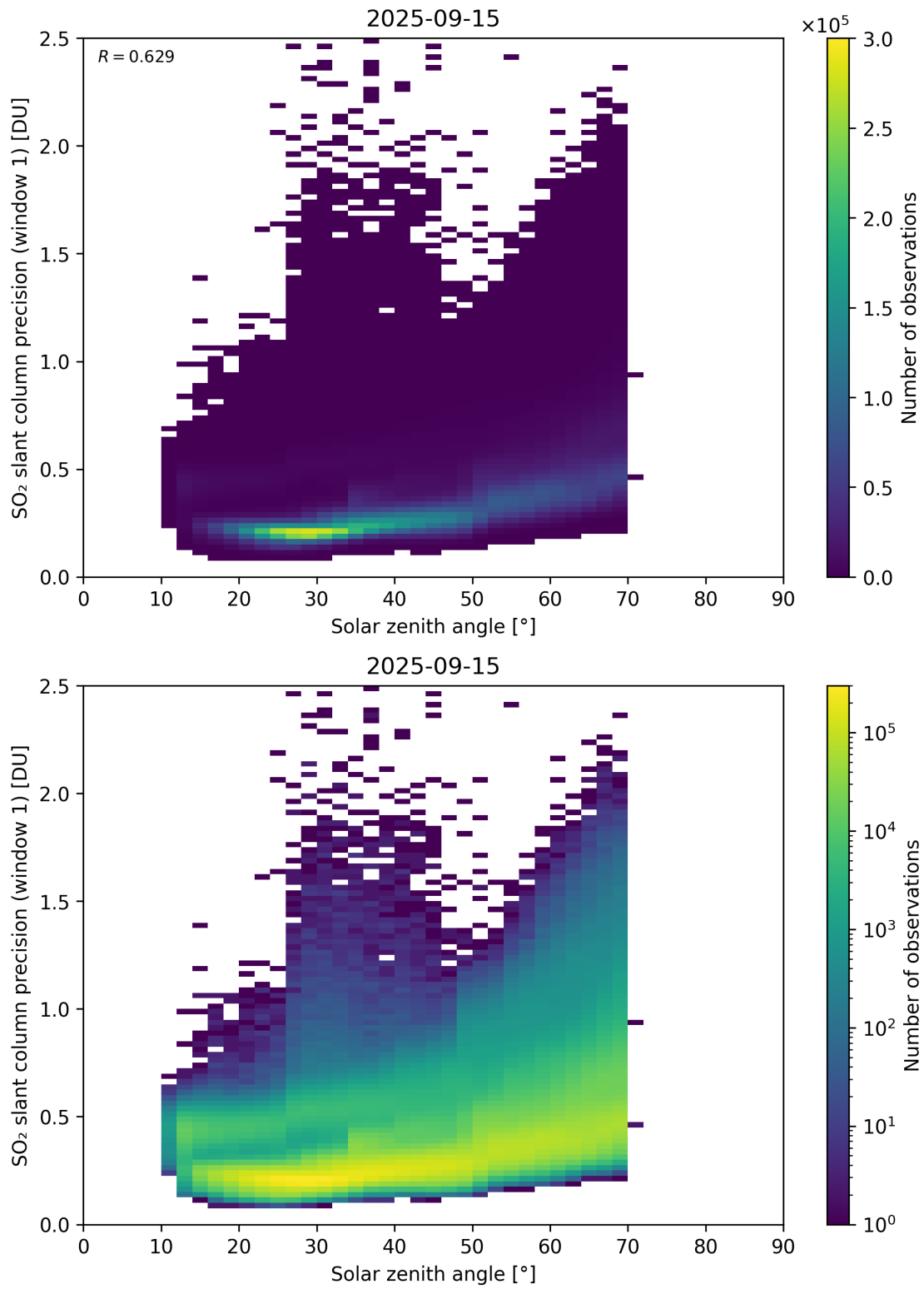
Figure 185: Scatter density plot of “Solar zenith angle” against “SO 2 slant column precision (window 1)” for 2025-09-15 to 2025-09-16.
