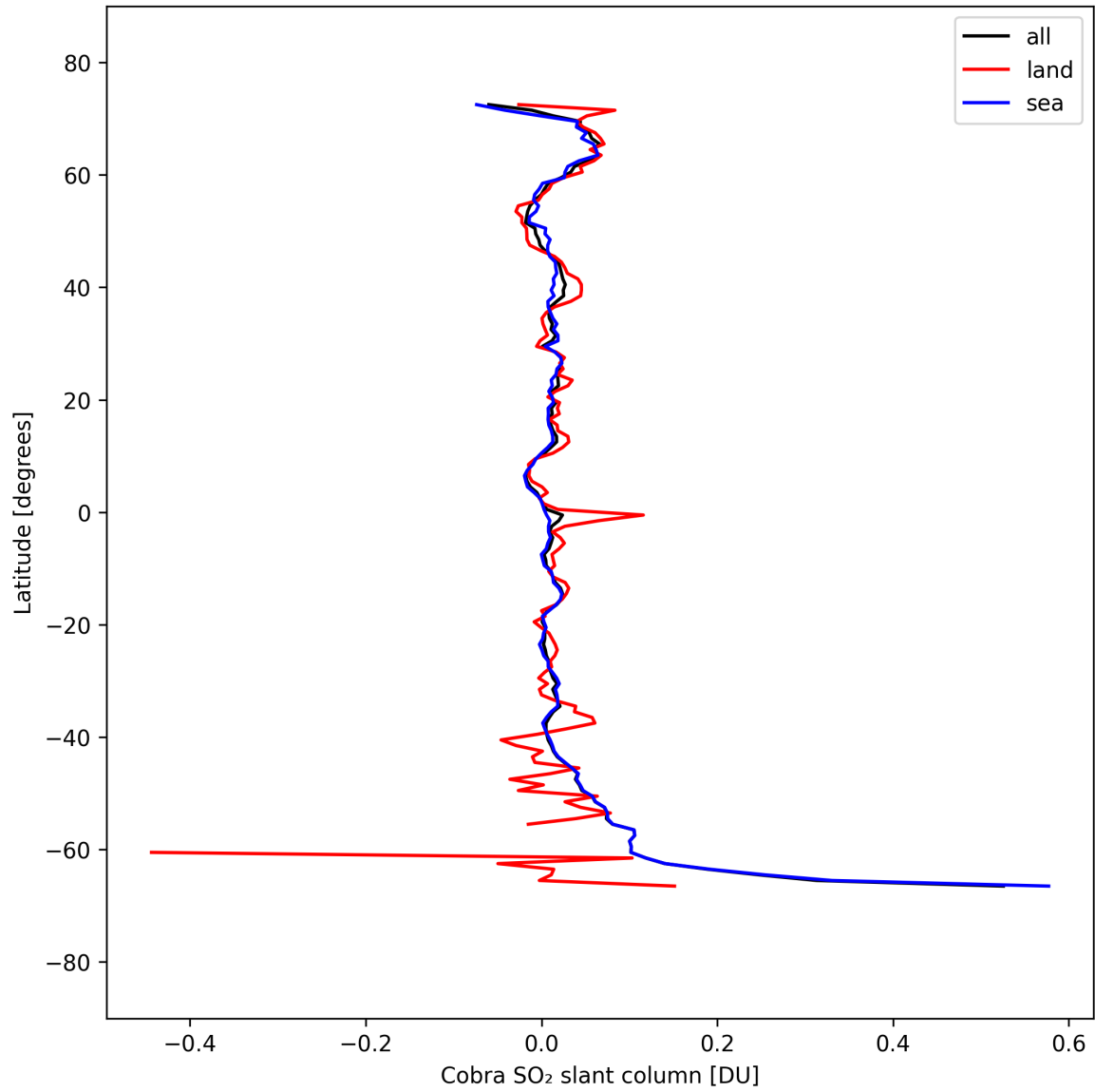
Figure 35: Zonal average of “Cobra SO 2 slant column” for 2025-09-15 to 2025-09-16.
