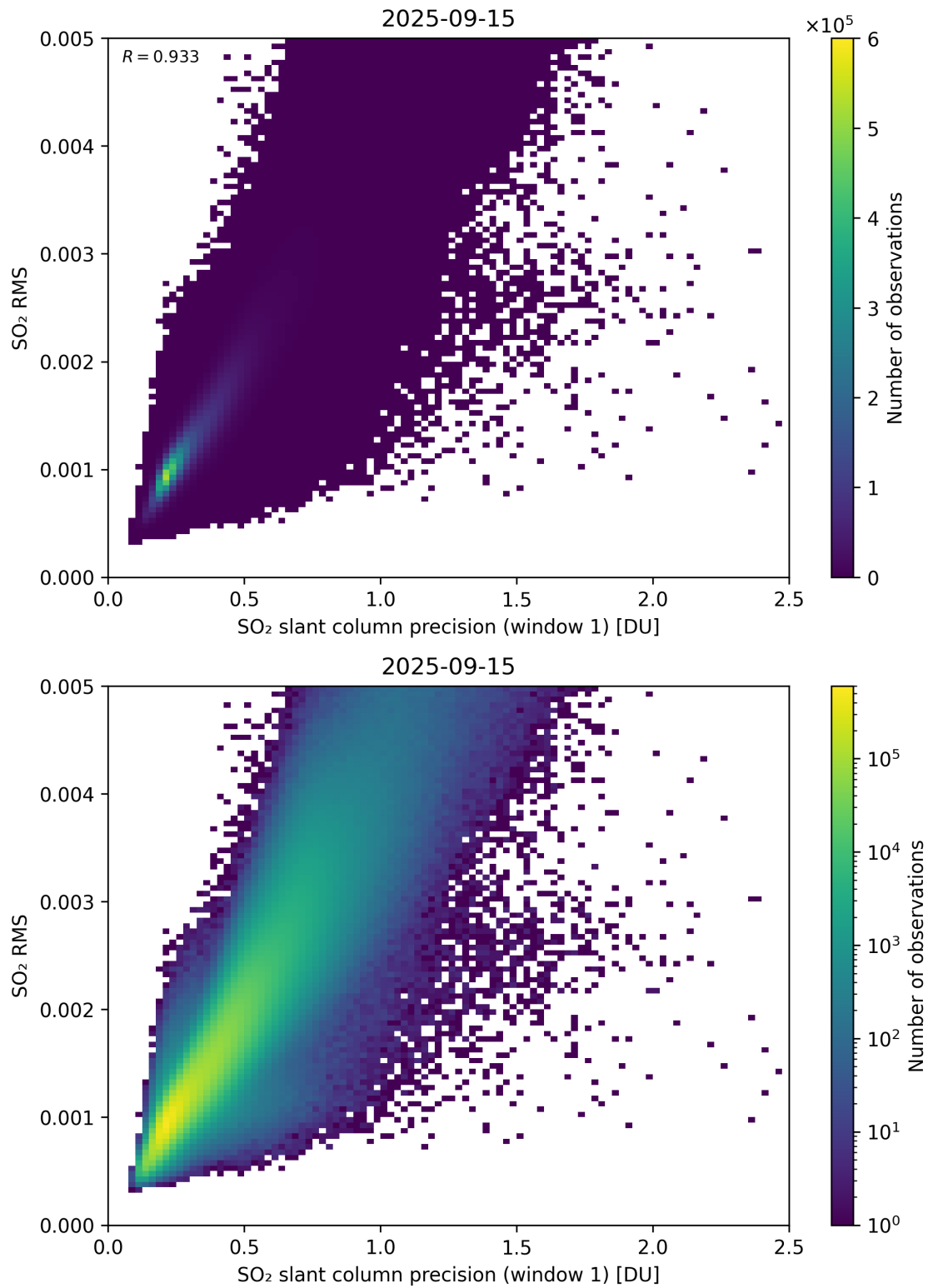
Figure 273: Scatter density plot of “SO 2 slant column precision (window 1)” against “SO 2 RMS” for 2025-09-15 to 2025-09-16.
