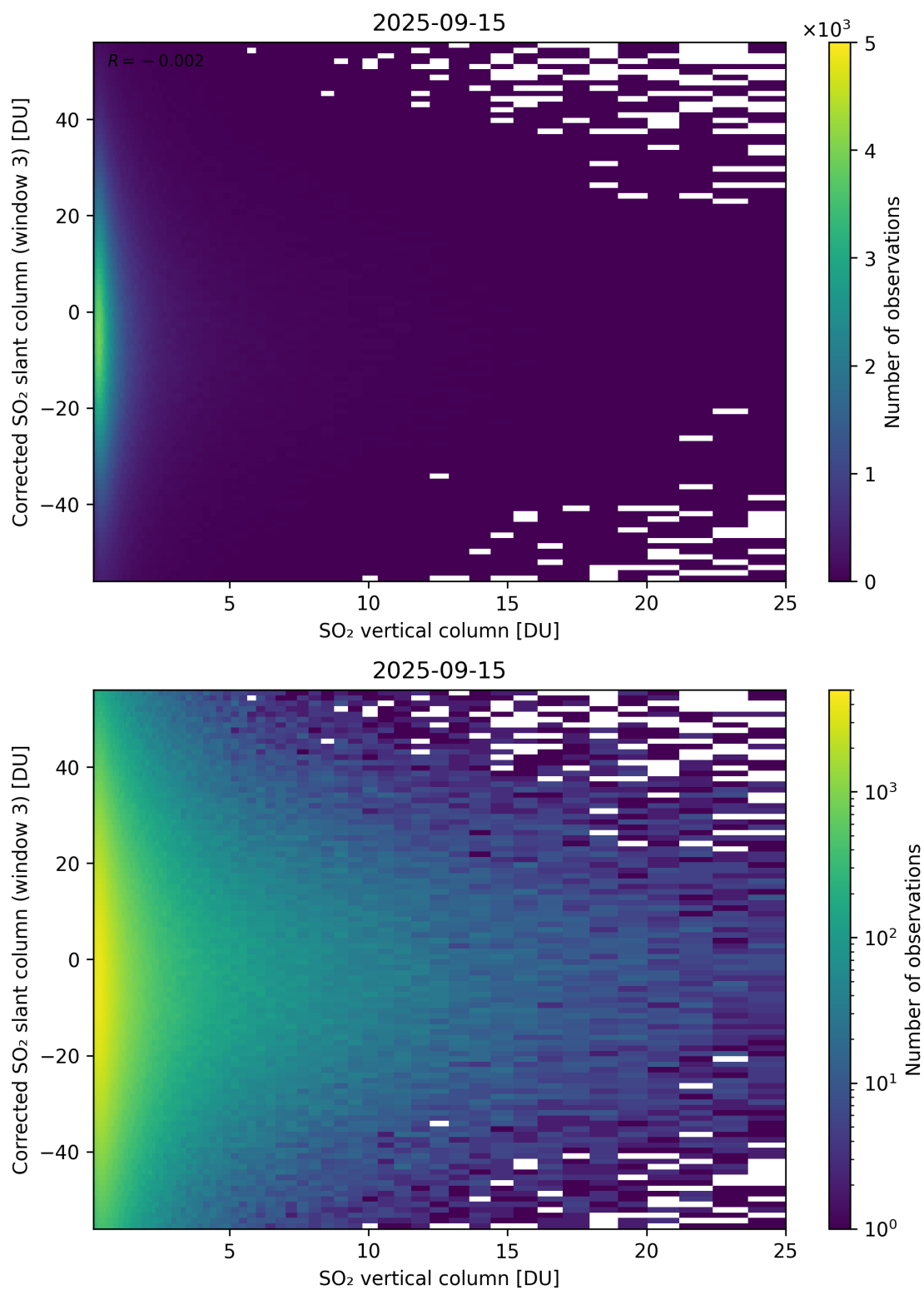
Figure 353: Scatter density plot of “SO 2 vertical column” against “Corrected SO 2 slant column (window 3)” for 2025-09-15 to 2025-09-16.
