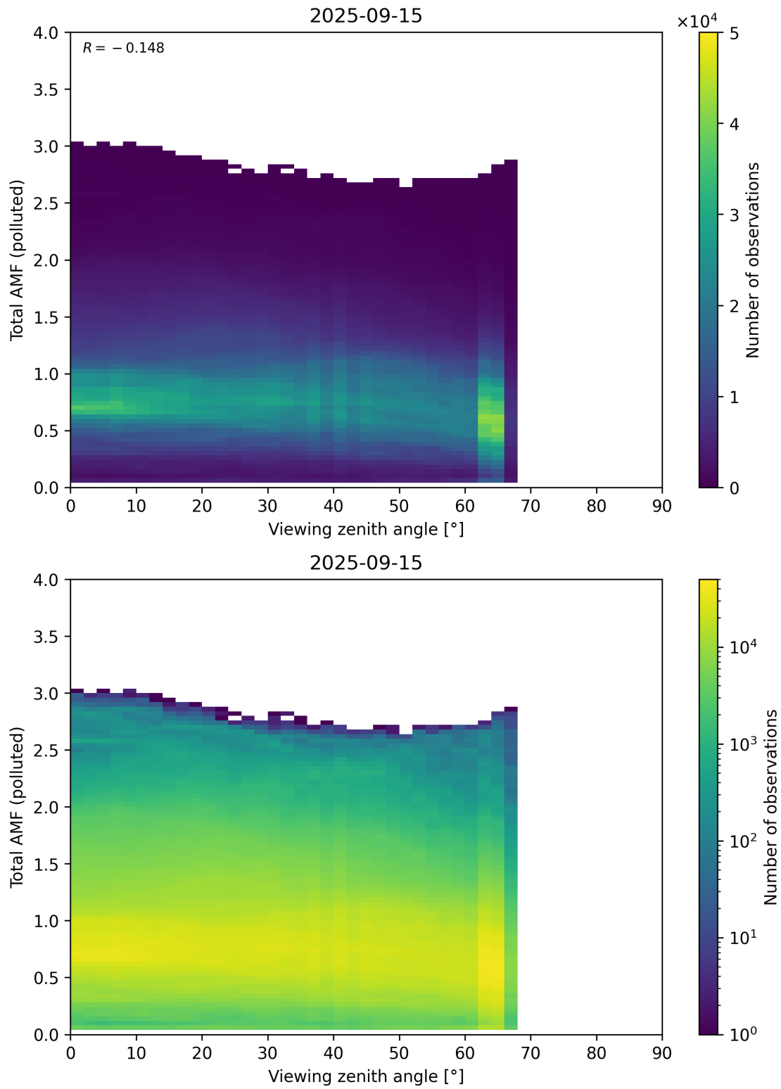
Figure 381: Scatter density plot of “Viewing zenith angle” against “Total AMF (polluted)” for 2025-09-15 to 2025-09-16.
