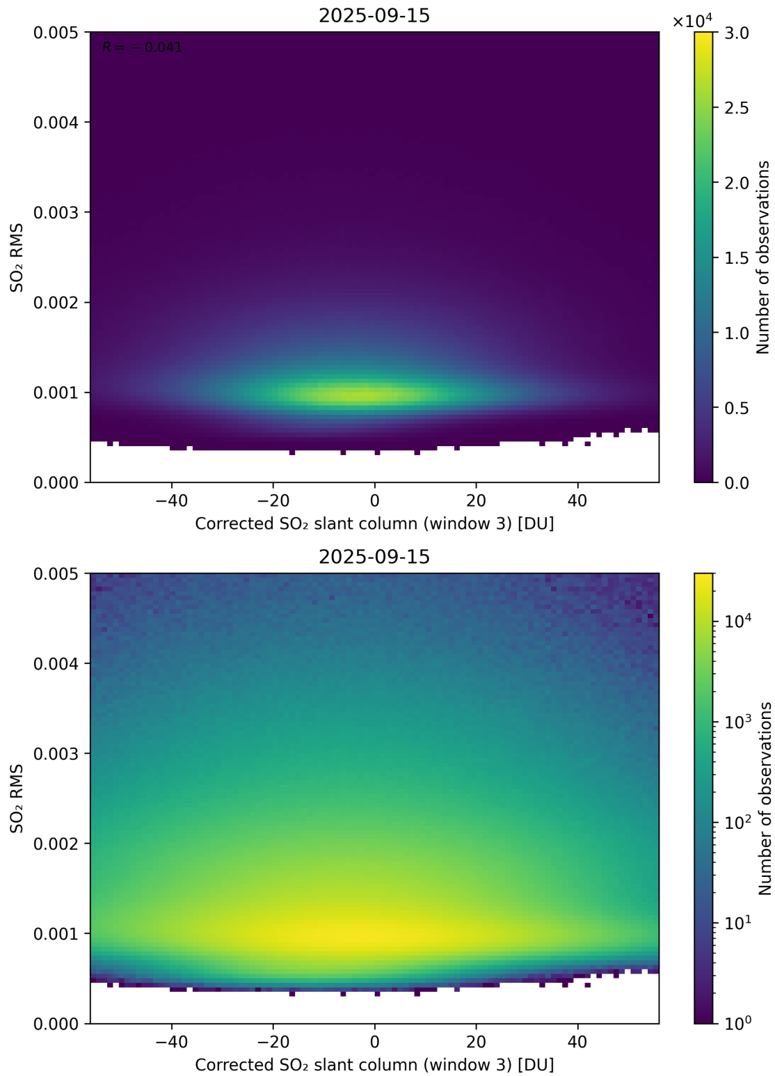
Figure 258: Scatter density plot of “Corrected SO 2 slant column (window 3)” against “SO 2 RMS” for 2025-09-15 to 2025-09-16.
