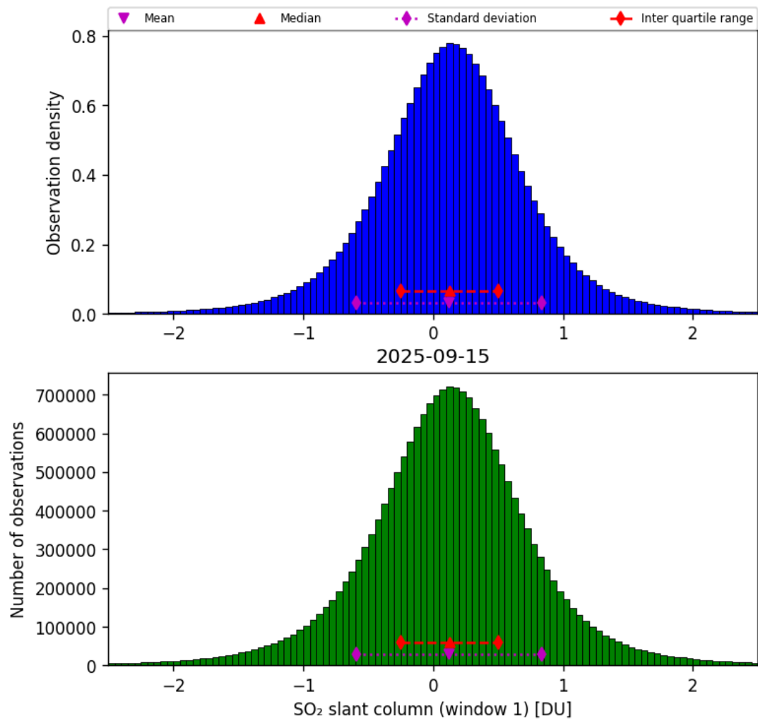
Figure 63: Histogram of “SO 2 slant column (window 1)” for 2025-09-15 to 2025-09-16
