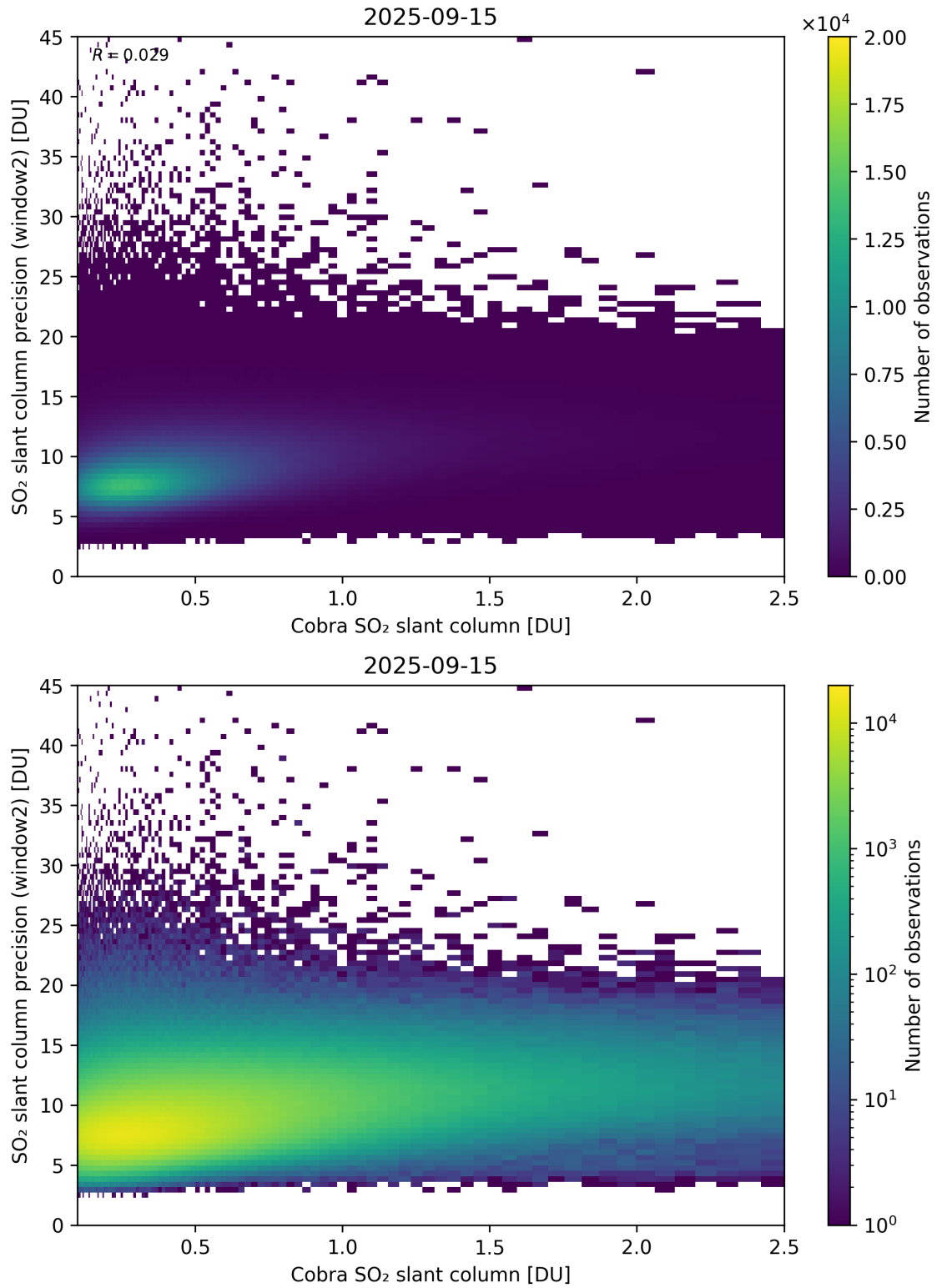
Figure 221: Scatter density plot of “Cobra SO 2 slant column” against “SO 2 slant column precision (window2)” for 2025-09-15 to 2025-09-16.
