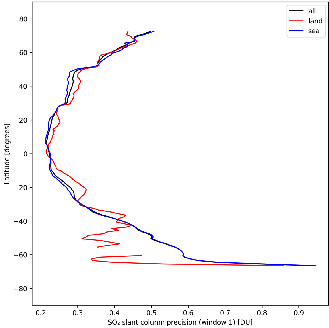
Figure 38: Zonal average of “SO 2 slant column precision (window 1)” for 2025-09-15 to 2025-09-16.
