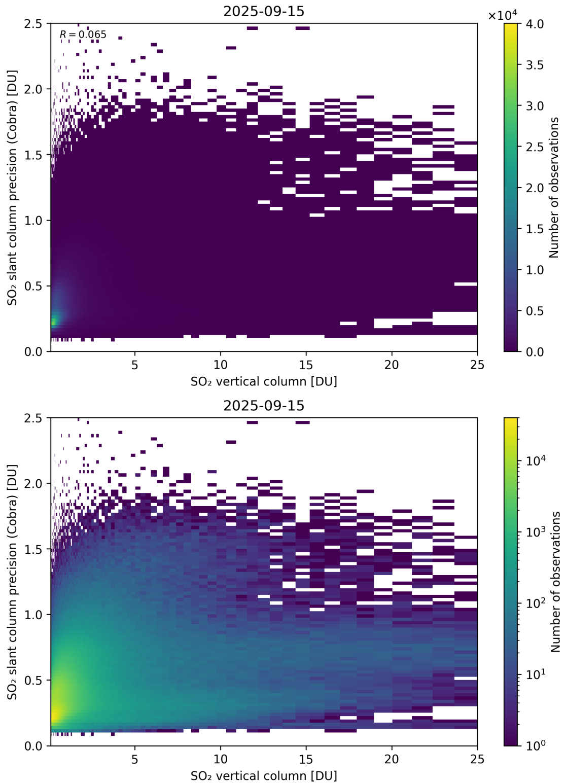
Figure 350: Scatter density plot of “SO 2 vertical column” against “SO 2 slant column precision (Cobra)” for 2025-09-15 to 2025-09-16.
