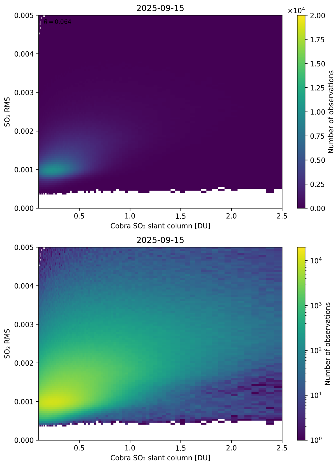
Figure 198: Scatter density plot of “Cobra SO 2 slant column” against “SO 2 RMS” for 2025-09-15 to 2025-09-16.
