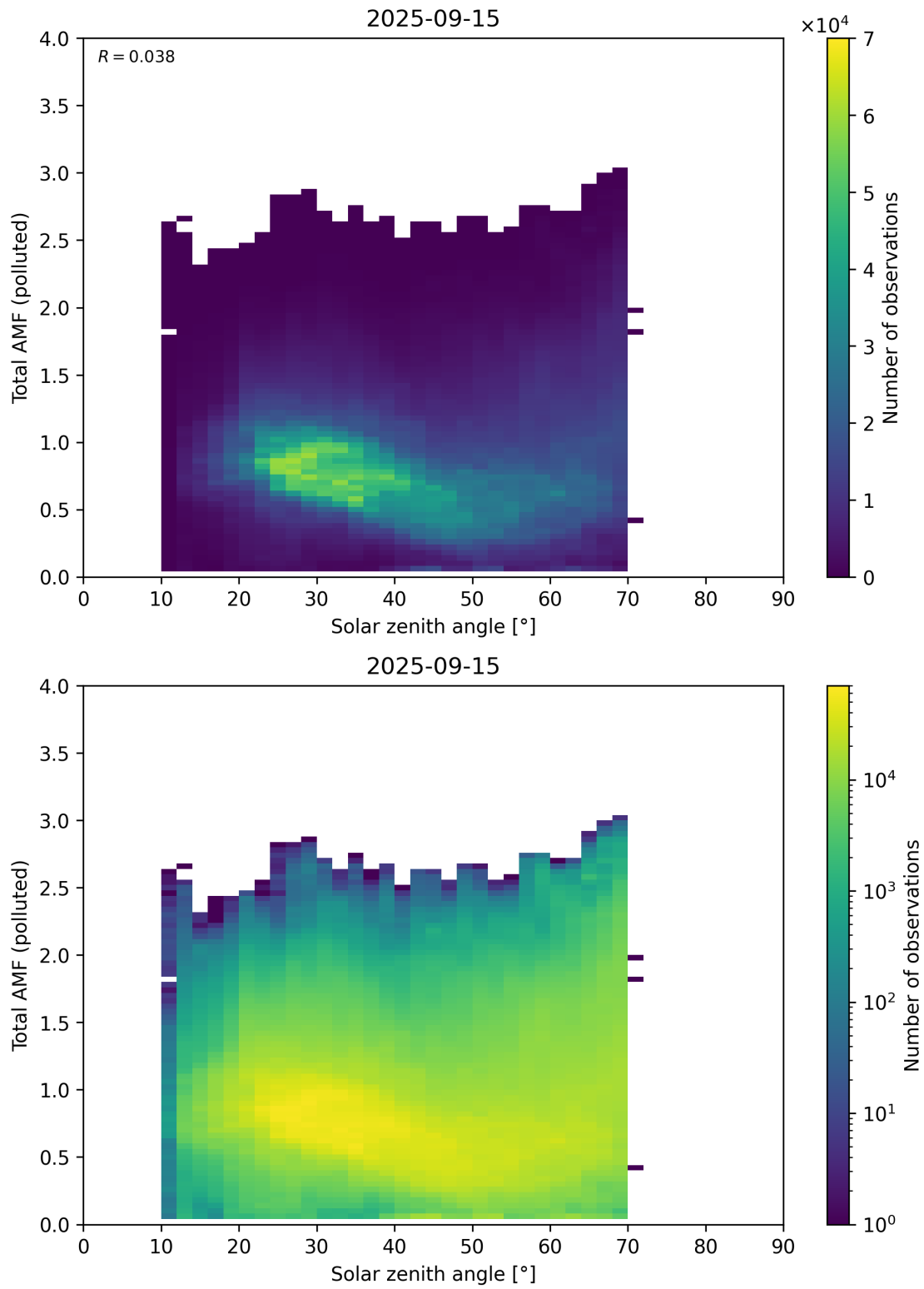
Figure 189: Scatter density plot of “Solar zenith angle” against “Total AMF (polluted)” for 2025-09-15 to 2025-09-16.
