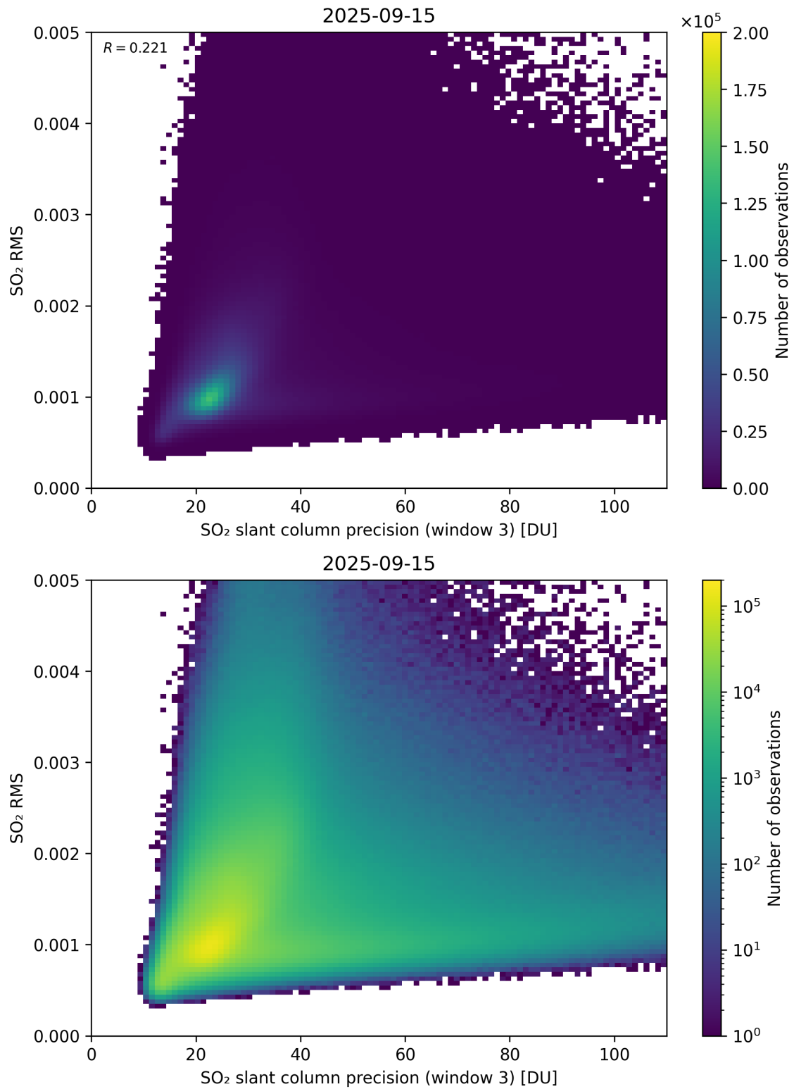
Figure 310: Scatter density plot of “SO 2 slant column precision (window 3)” against “SO 2 RMS” for 2025-09-15 to 2025-09-16.
