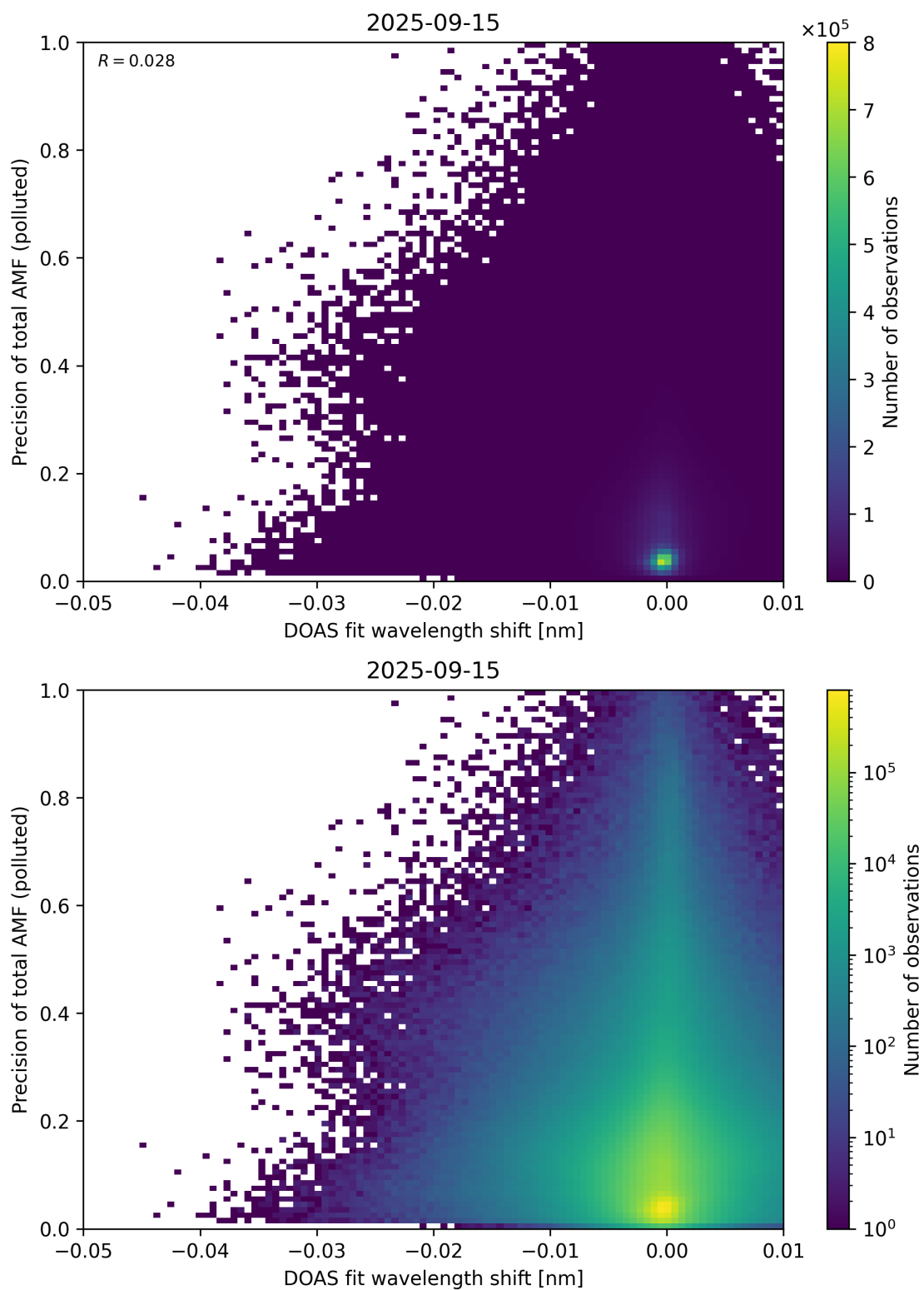
Figure 142: Scatter density plot of “DOAS fit wavelength shift” against “Precision of total AMF (polluted)” for 2025-09-15 to 2025-09-16.
