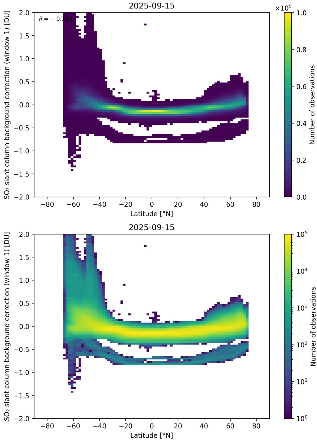
Figure 150: Scatter density plot of “Latitude” against “SO 2 slant column background correction (window 1)” for 2025-09-15 to 2025-09-16.
