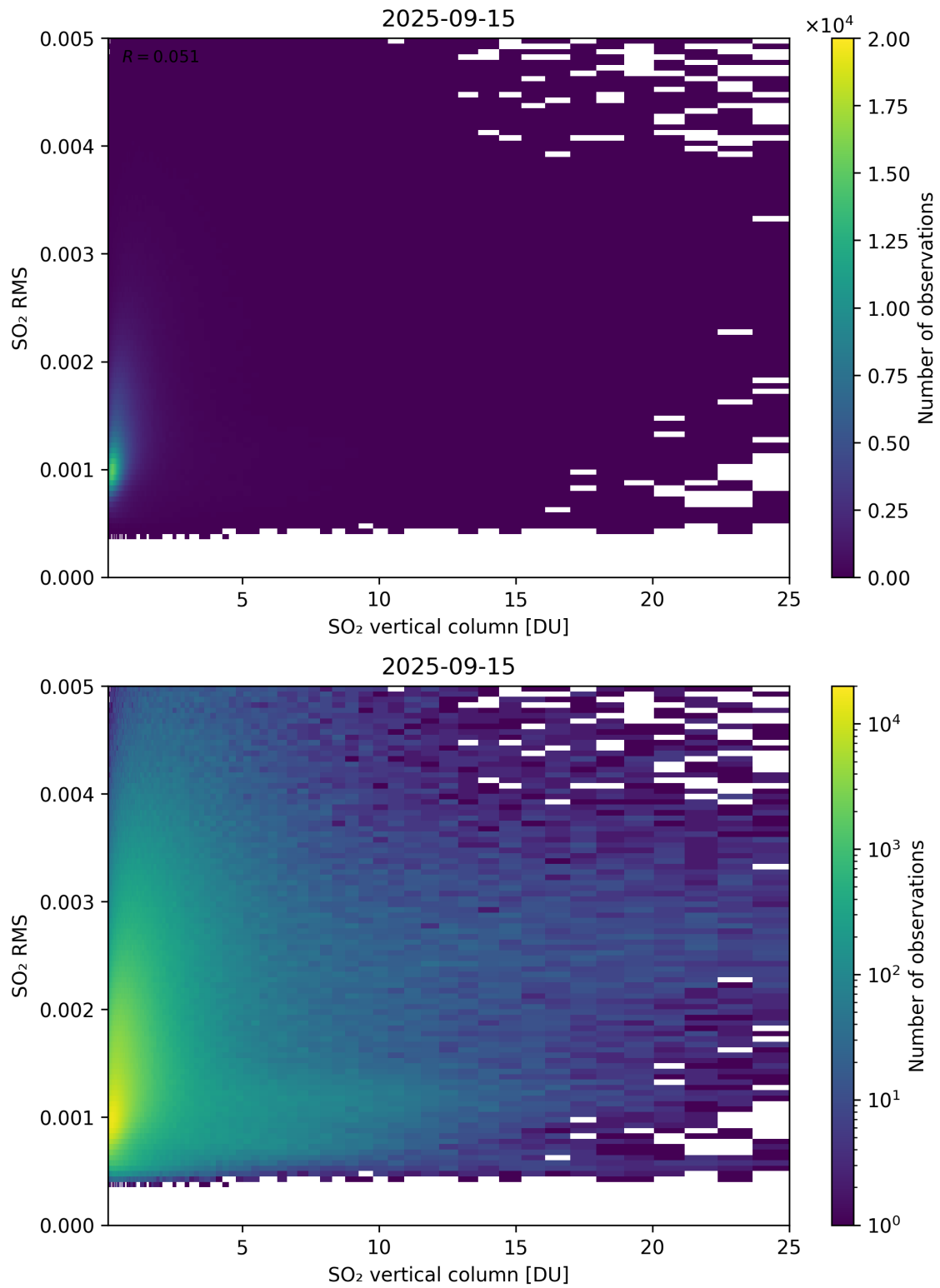
Figure 328: Scatter density plot of “SO 2 vertical column” against “SO 2 RMS” for 2025-09-15 to 2025-09-16.
