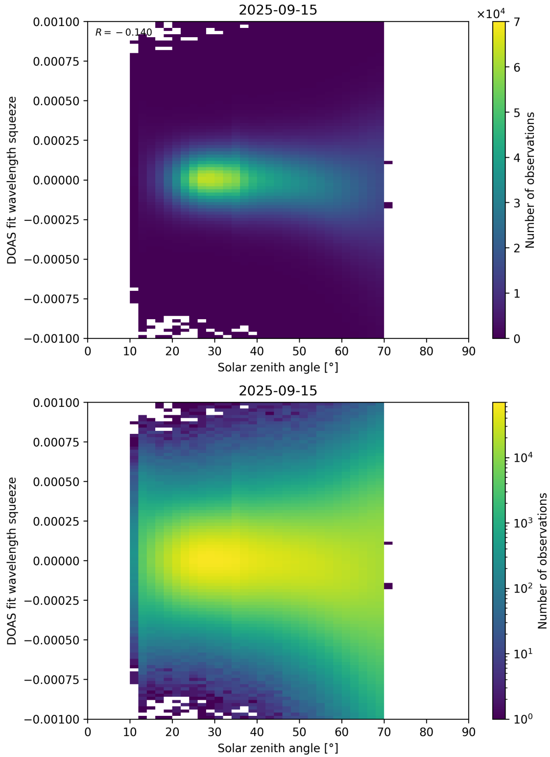
Figure 175: Scatter density plot of “Solar zenith angle” against “DOAS fit wavelength squeeze” for 2025-09-15 to 2025-09-16.
