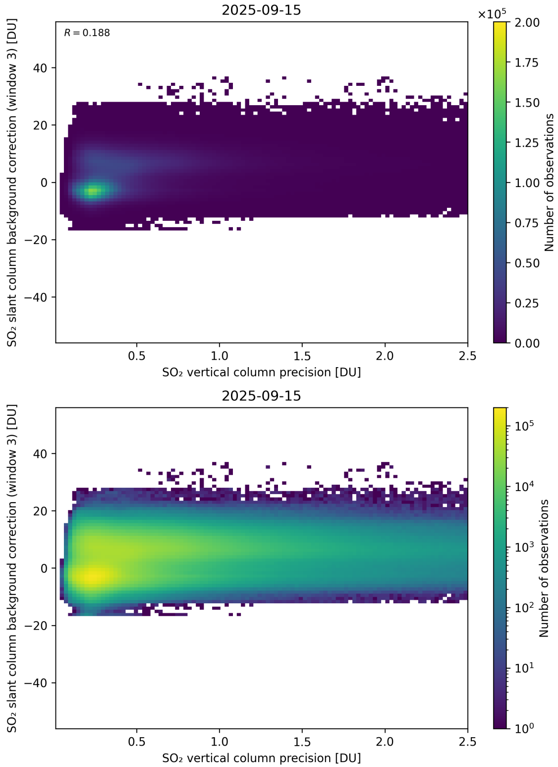
Figure 331: Scatter density plot of “SO 2 vertical column precision” against “SO 2 slant column background correction (window 3)” for 2025-09-15 to 2025-09-16.
