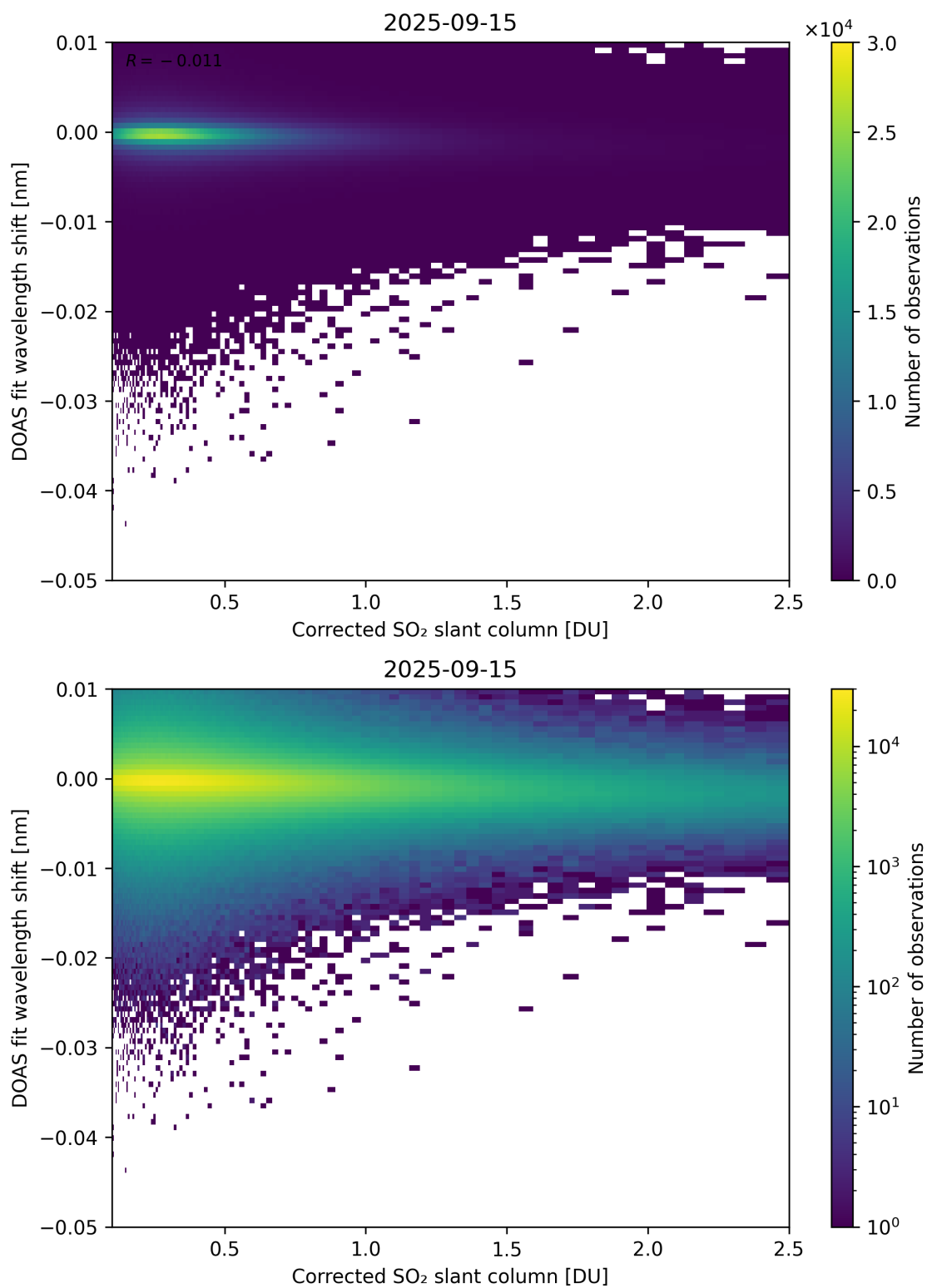
Figure 229: Scatter density plot of “Corrected SO 2 slant column” against “DOAS fit wavelength shift” for 2025-09-15 to 2025-09-16.
