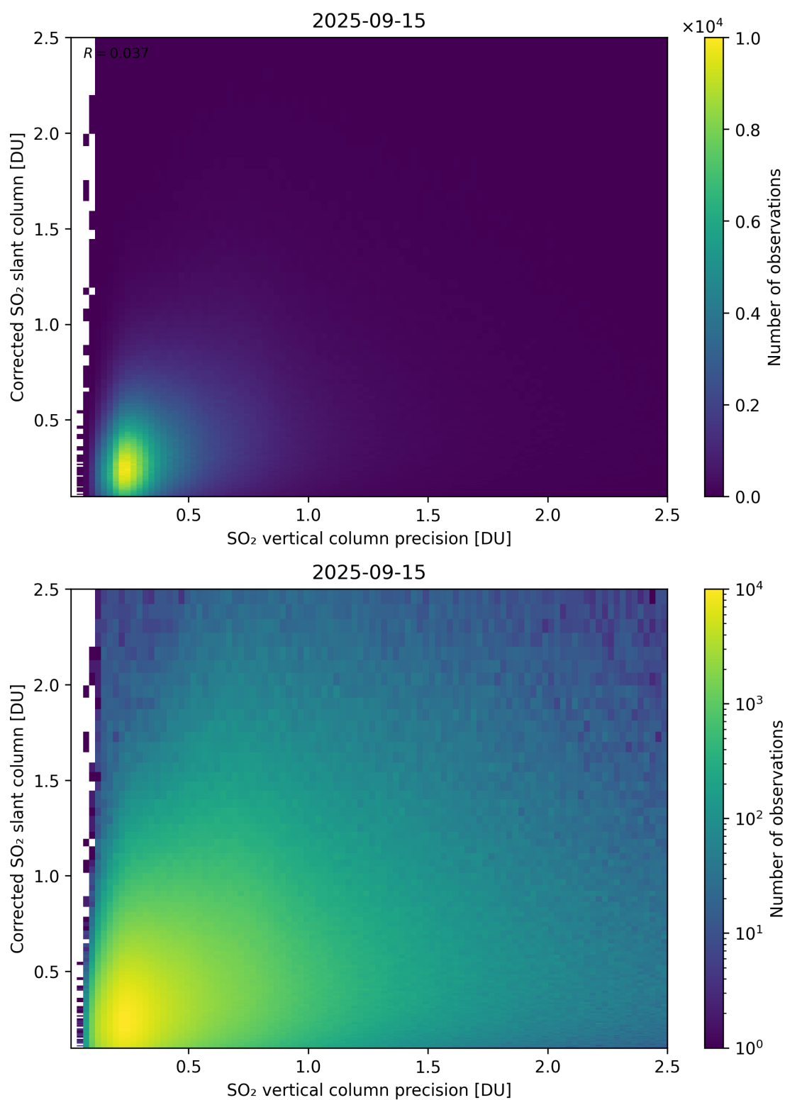
Figure 338: Scatter density plot of “SO 2 vertical column precision” against “Corrected SO 2 slant column” for 2025-09-15 to 2025-09-16.
