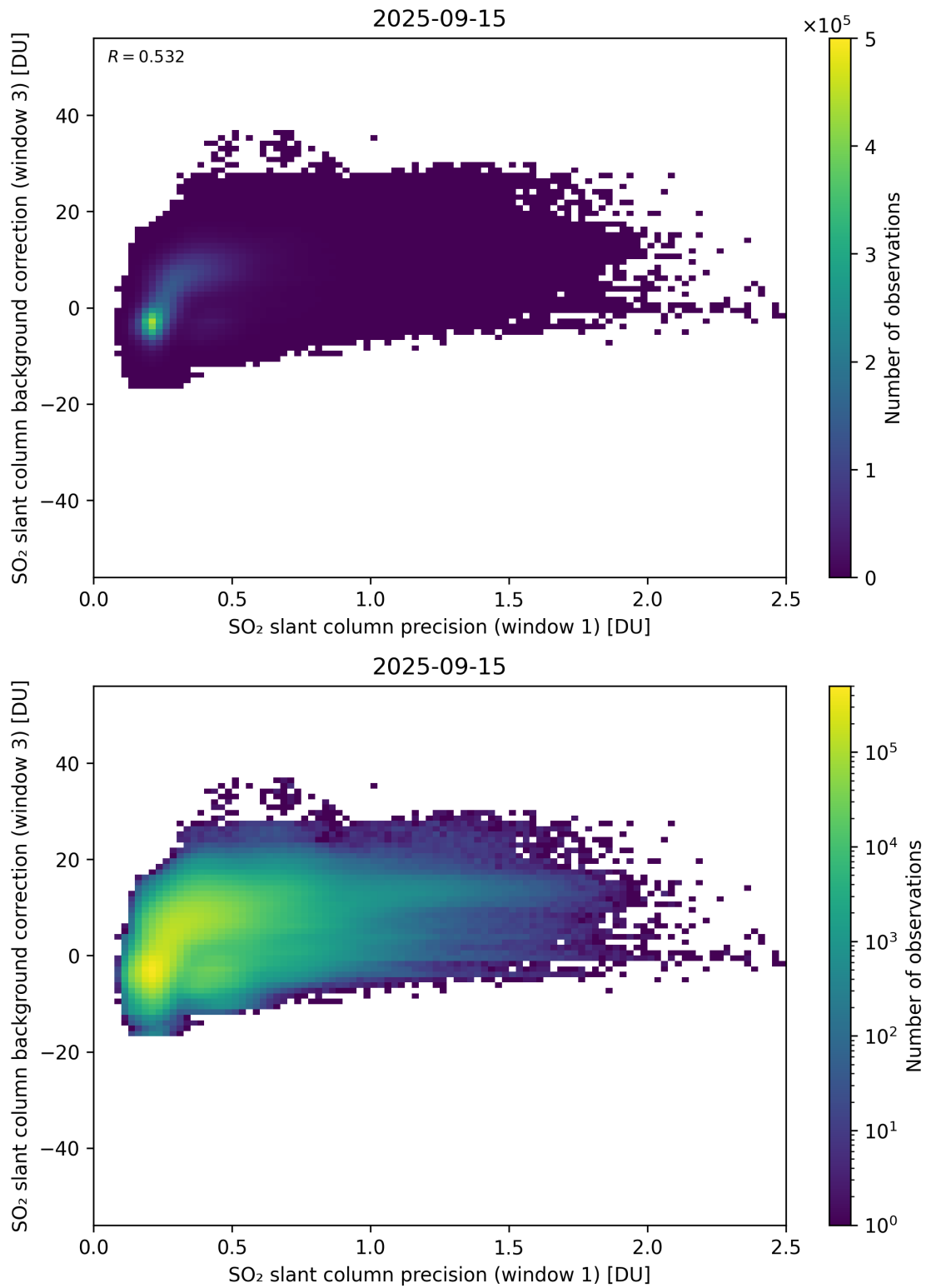
Figure 270: Scatter density plot of “SO 2 slant column precision (window 1)” against “SO 2 slant column background correction (window 3)” for 2025-09-15 to 2025-09-16.
