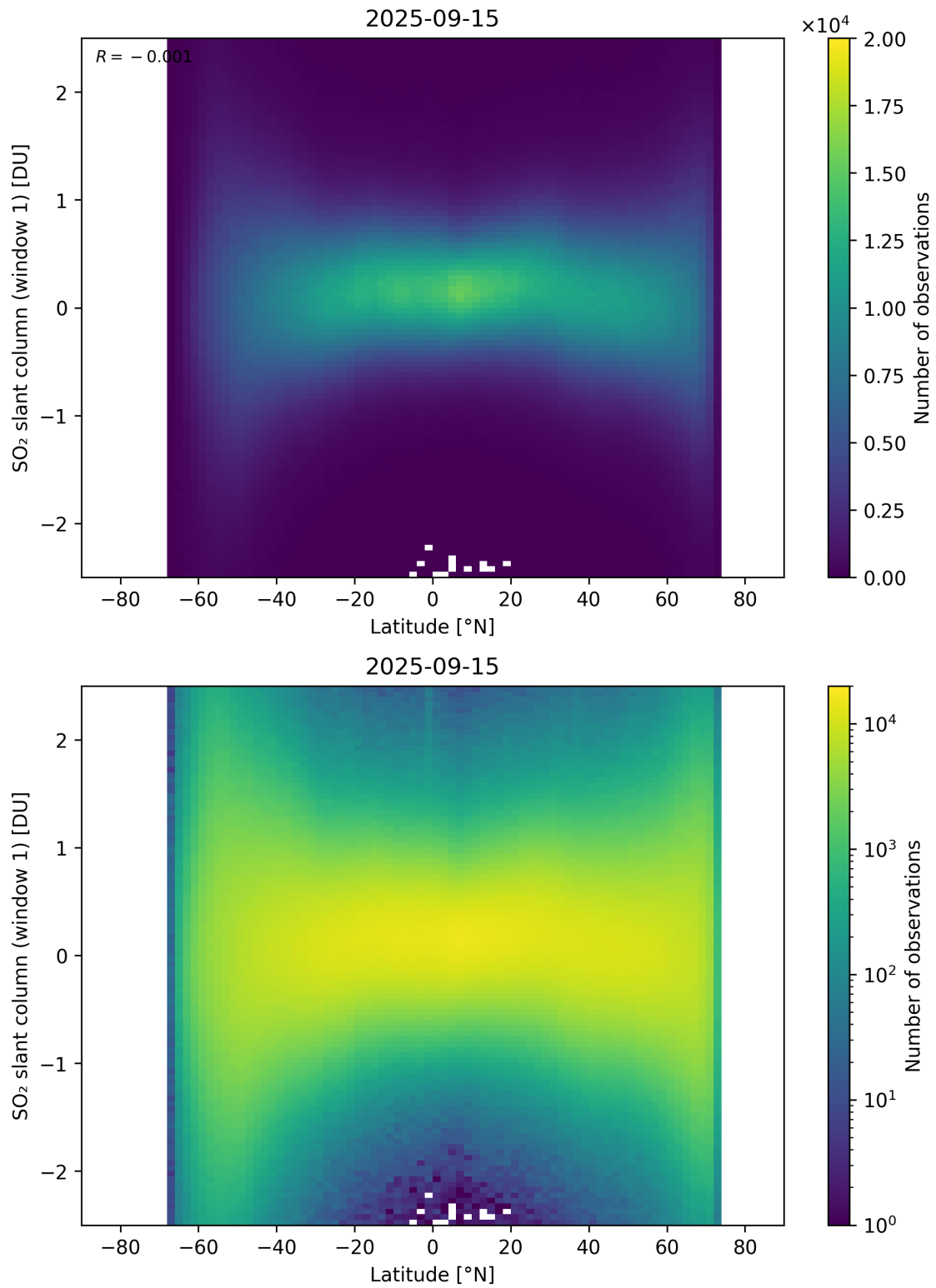
Figure 162: Scatter density plot of “Latitude” against “SO 2 slant column (window 1)” for 2025-09-15 to 2025-09-16.
