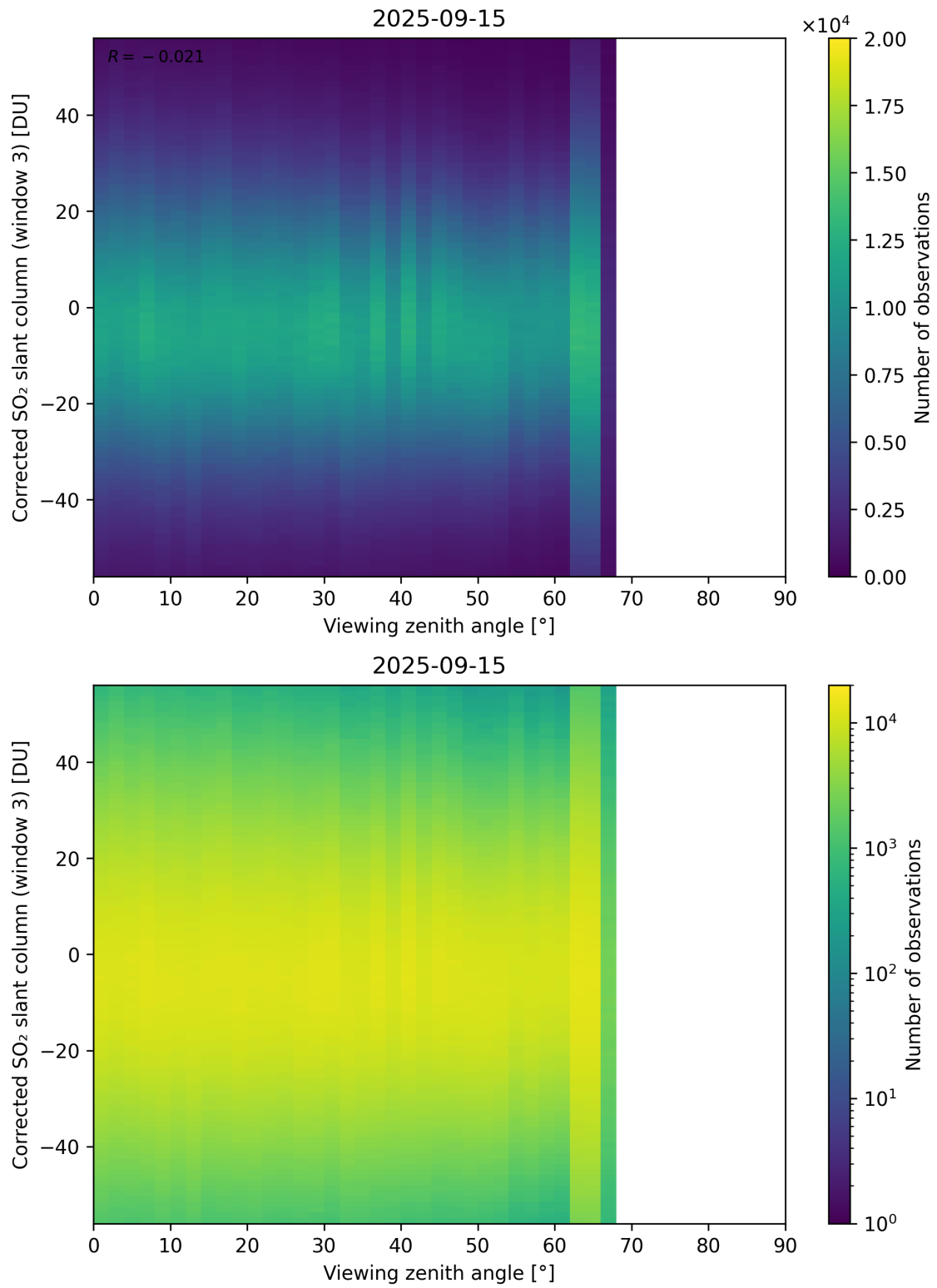
Figure 375: Scatter density plot of “Viewing zenith angle” against “Corrected SO 2 slant column (window 3)” for 2025-09-15 to 2025-09-16.
