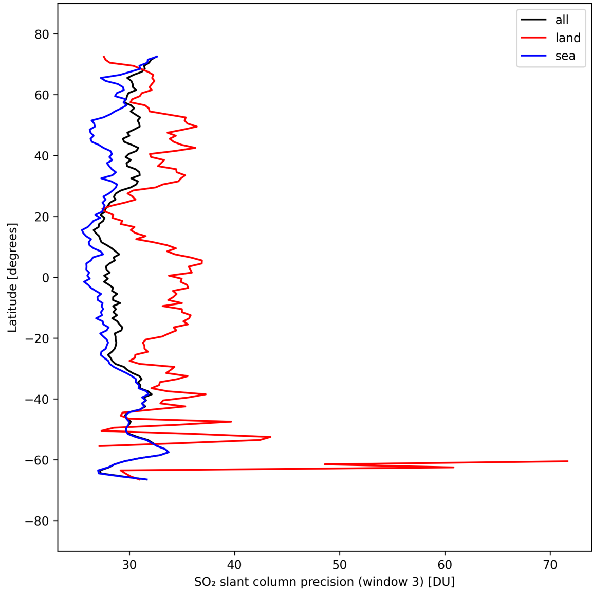
Figure 46: Zonal average of “SO 2 slant column precision (window 3)” for 2025-09-15 to 2025-09-16.
