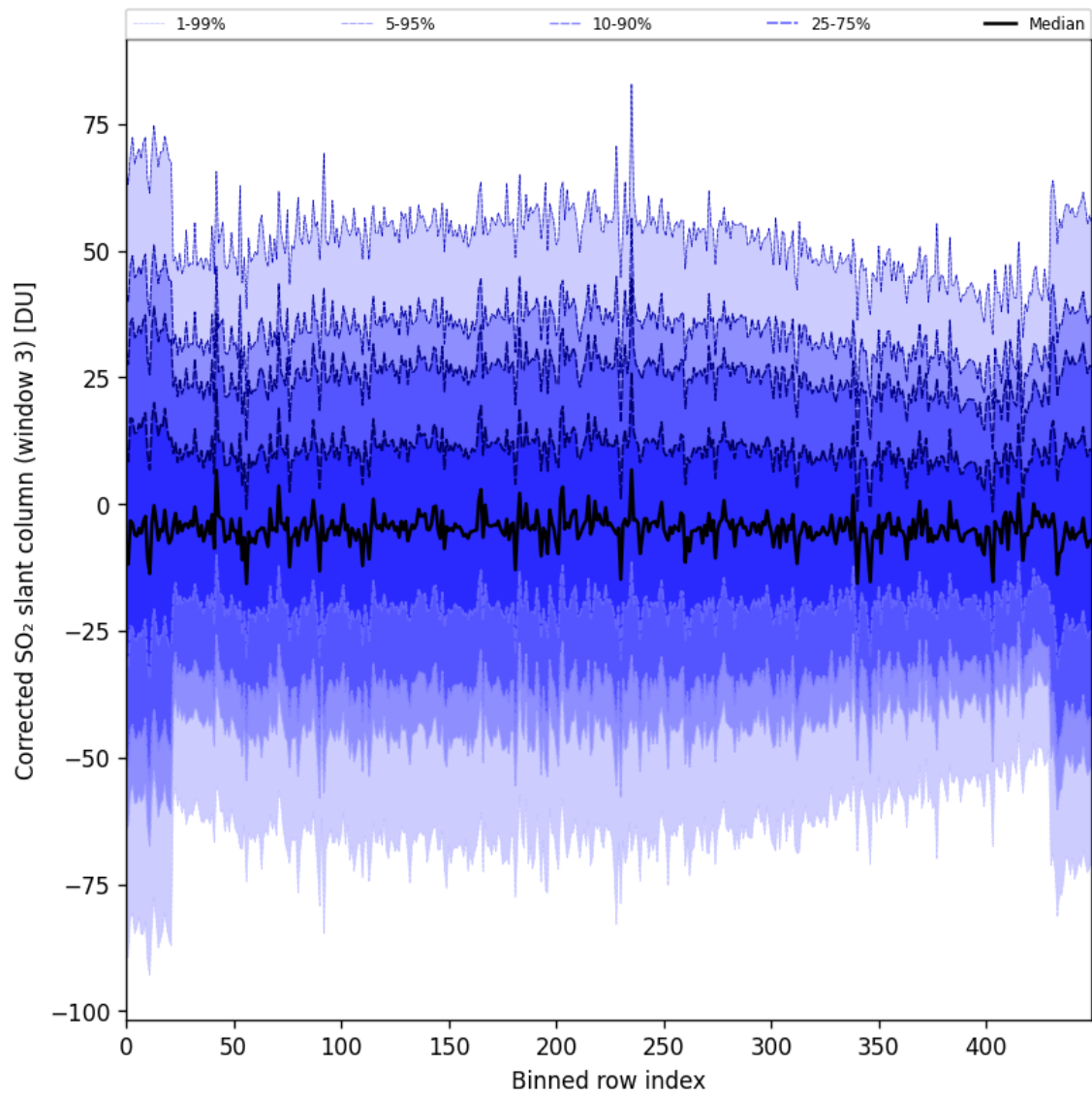
Figure 99: Along track statistics of “Corrected SO 2 slant column (window 3)” for 2025-09-15 to 2025-09-16
