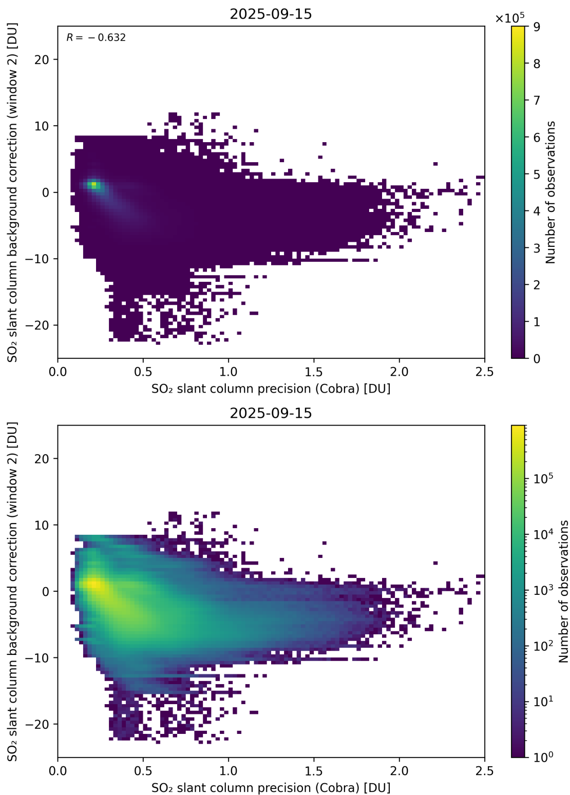
Figure 200: Scatter density plot of “SO 2 slant column precision (Cobra)” against “SO 2 slant column background correction (window 2)” for 2025-09-15 to 2025-09-16.
