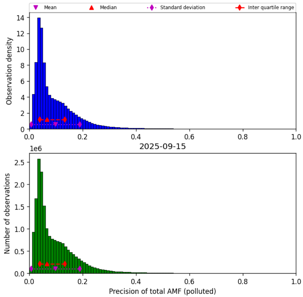
Figure 80: Histogram of “Precision of total AMF (polluted)” for 2025-09-15 to 2025-09-16
