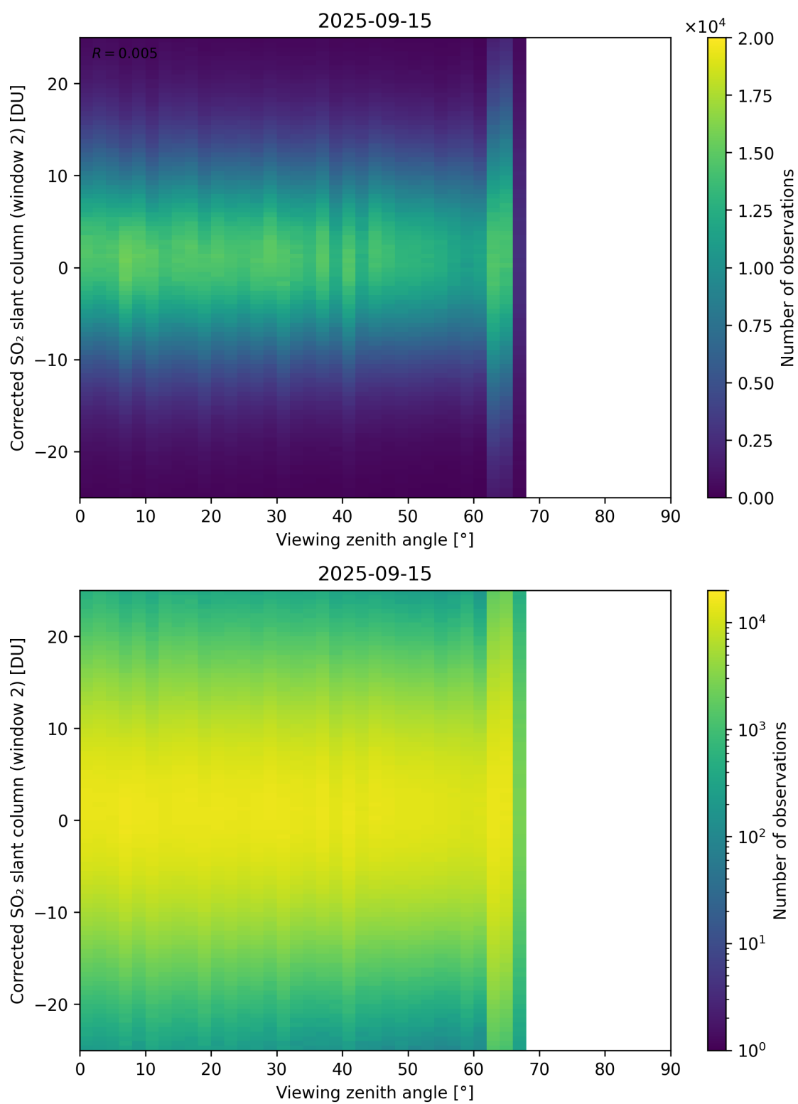
Figure 374: Scatter density plot of “Viewing zenith angle” against “Corrected SO 2 slant column (window 2)” for 2025-09-15 to 2025-09-16.
