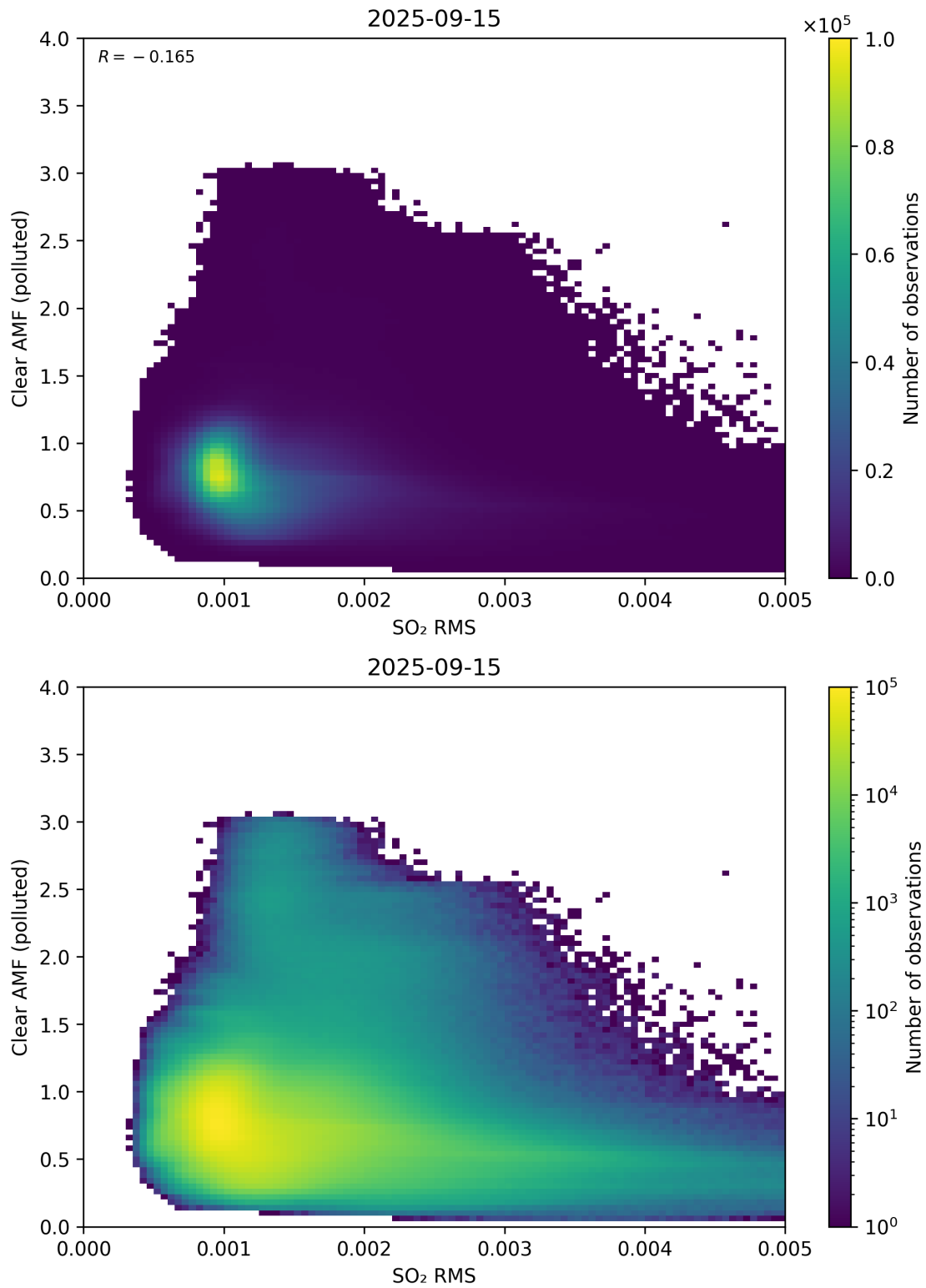
Figure 147: Scatter density plot of “SO 2 RMS” against “Clear AMF (polluted)” for 2025-09-15 to 2025-09-16.
