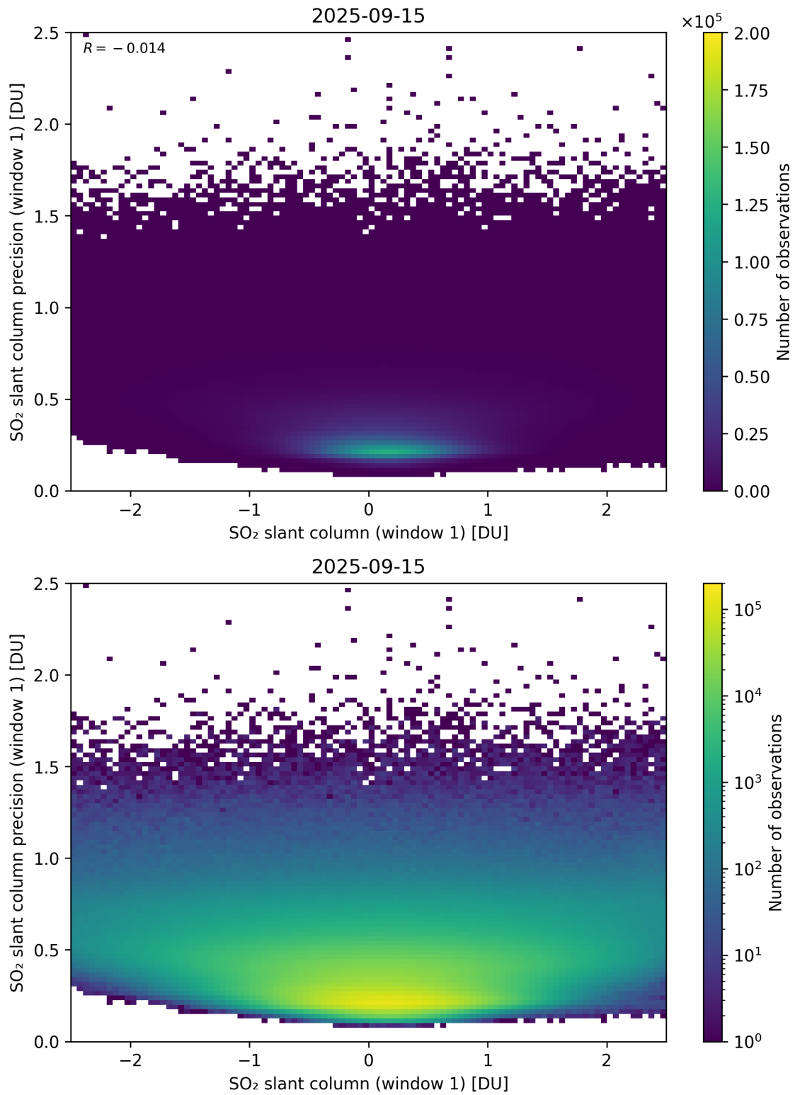
Figure 285: Scatter density plot of “SO 2 slant column (window 1)” against “SO 2 slant column precision (window 1)” for 2025-09-15 to 2025-09-16.
