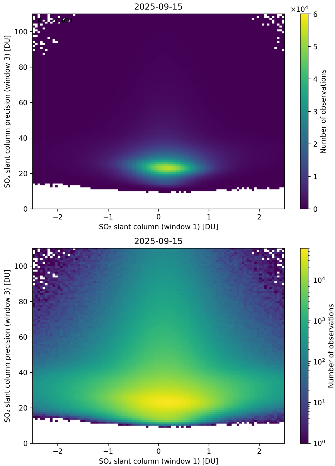
Figure 288: Scatter density plot of “SO 2 slant column (window 1)” against “SO 2 slant column precision (window 3)” for 2025-09-15 to 2025-09-16.
