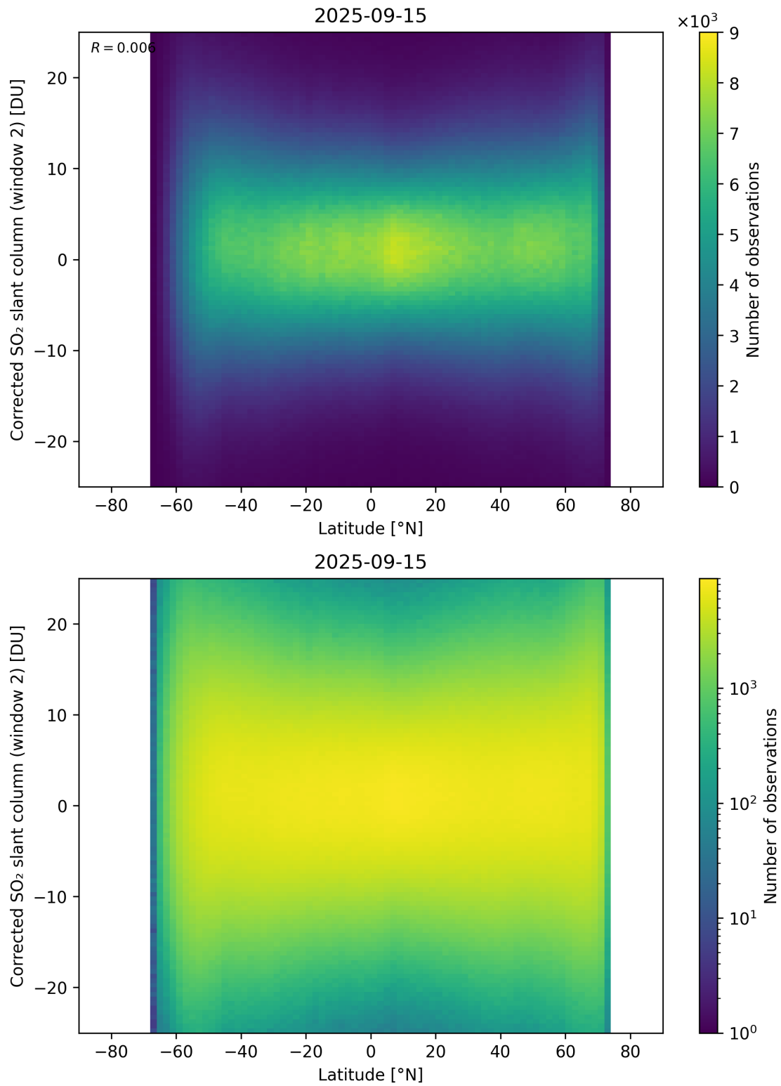
Figure 160: Scatter density plot of “Latitude” against “Corrected SO 2 slant column (window 2)” for 2025-09-15 to 2025-09-16.
