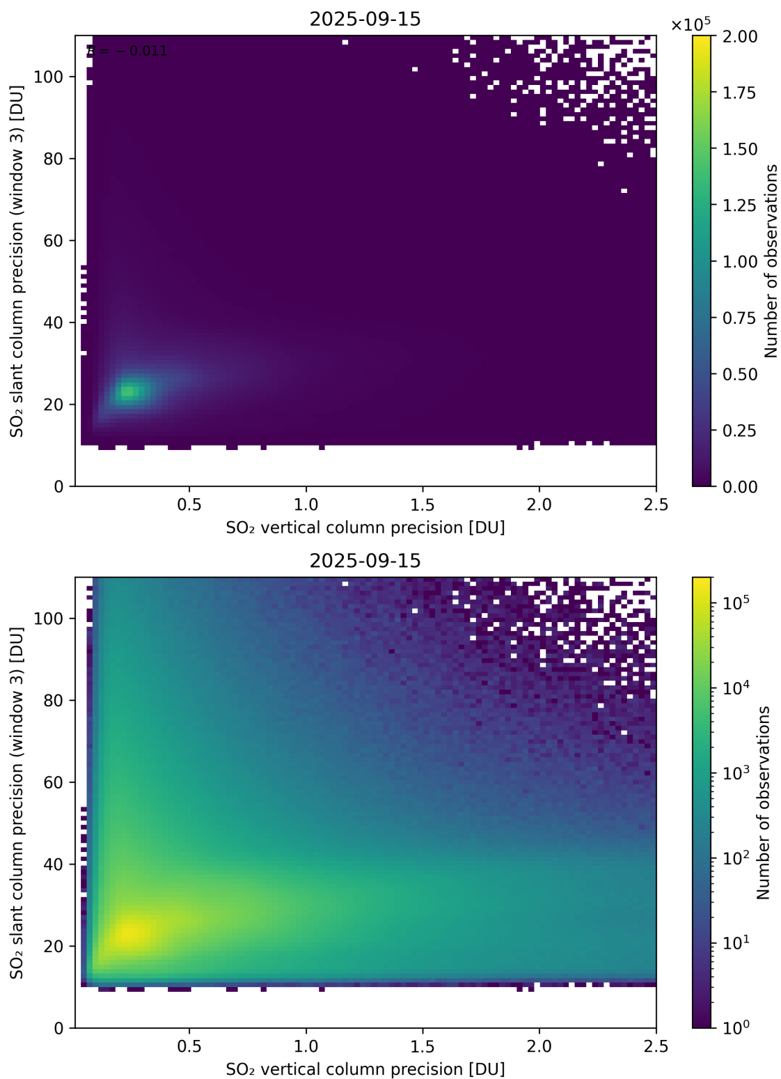
Figure 345: Scatter density plot of “SO 2 vertical column precision” against “SO 2 slant column precision (window 3)” for 2025-09-15 to 2025-09-16.
