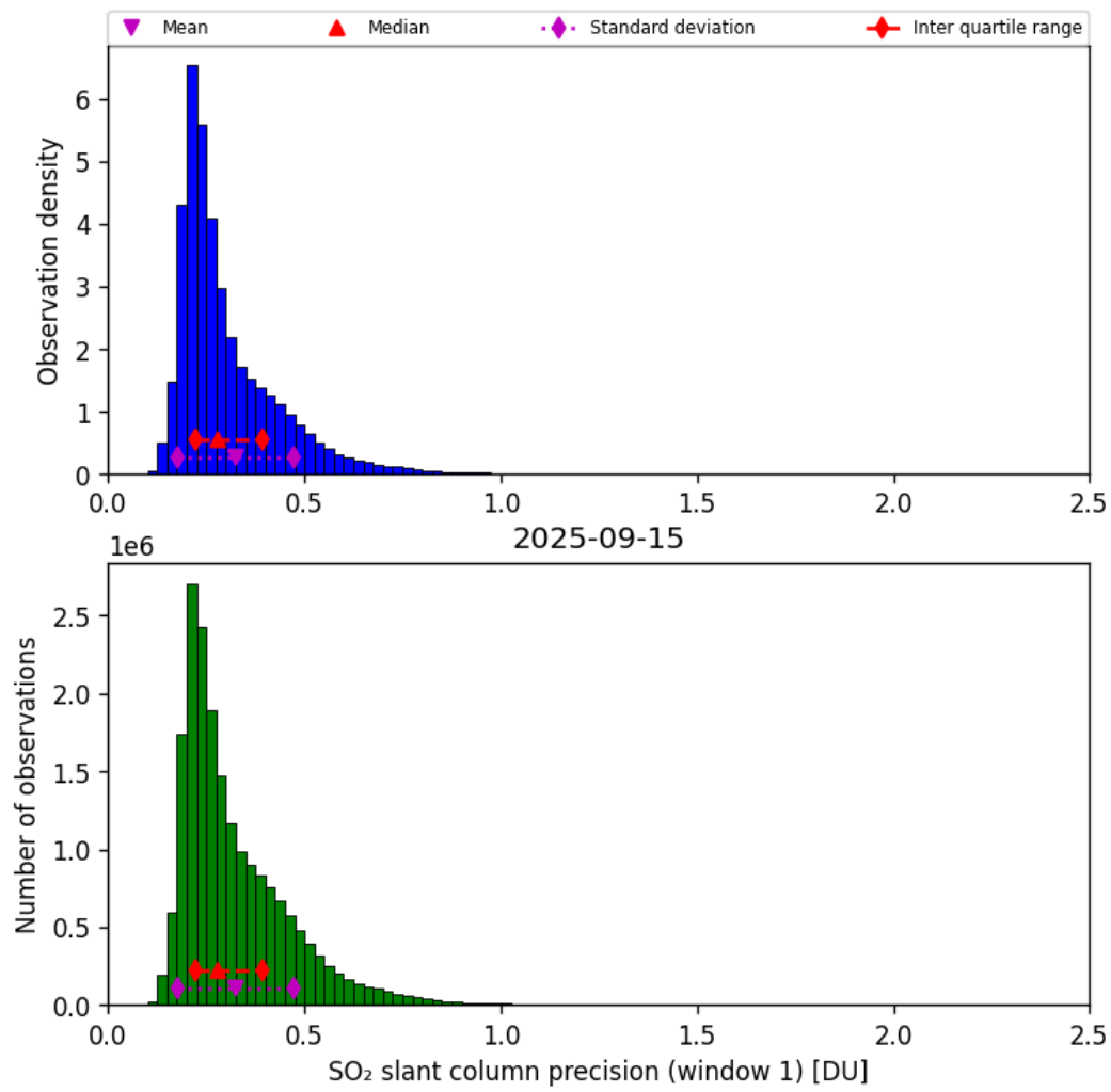
Figure 64: Histogram of “SO 2 slant column precision (window 1)” for 2025-09-15 to 2025-09-16
