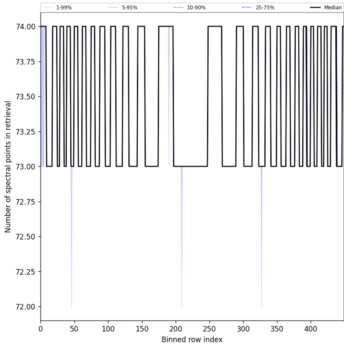
Figure 108: Along track statistics of “Number of spectral points in retrieval” for 2025-09-15 to 2025-09-16
