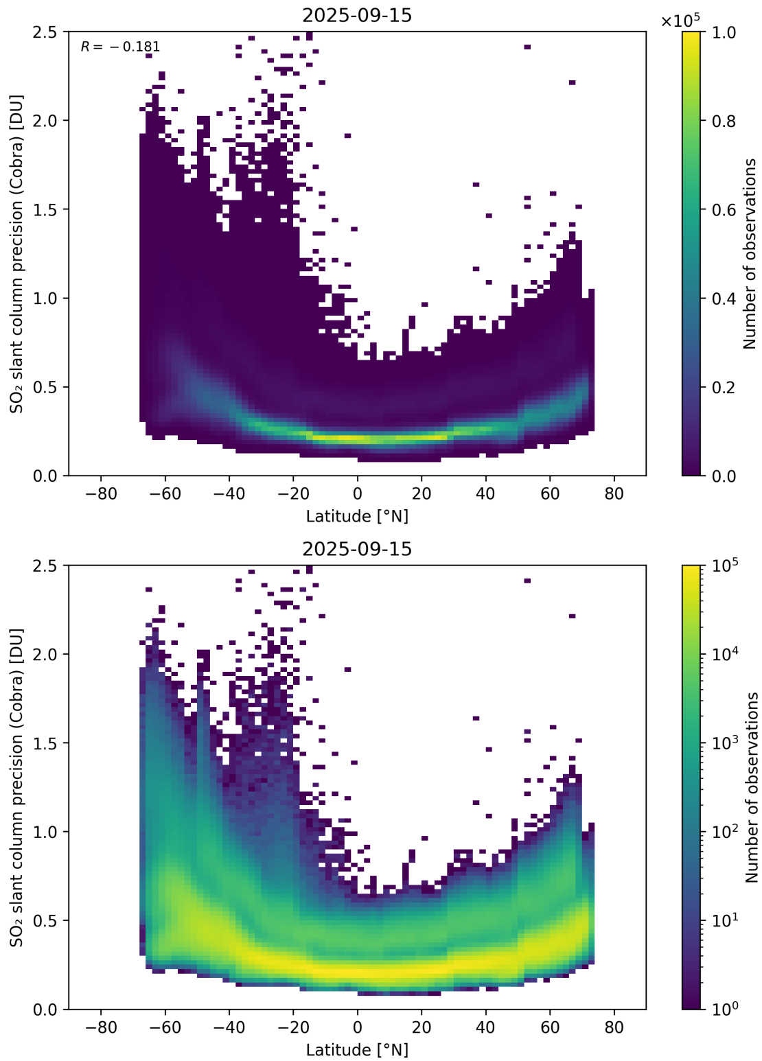
Figure 158: Scatter density plot of “Latitude” against “SO 2 slant column precision (Cobra)” for 2025-09-15 to 2025-09-16.
