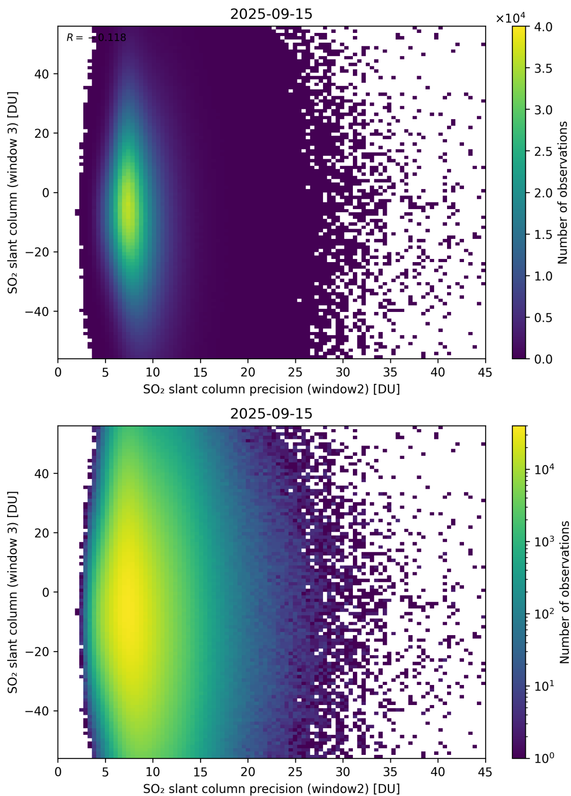
Figure 299: Scatter density plot of “SO 2 slant column precision (window2)” against “SO 2 slant column (window 3)” for 2025-09-15 to 2025-09-16.
