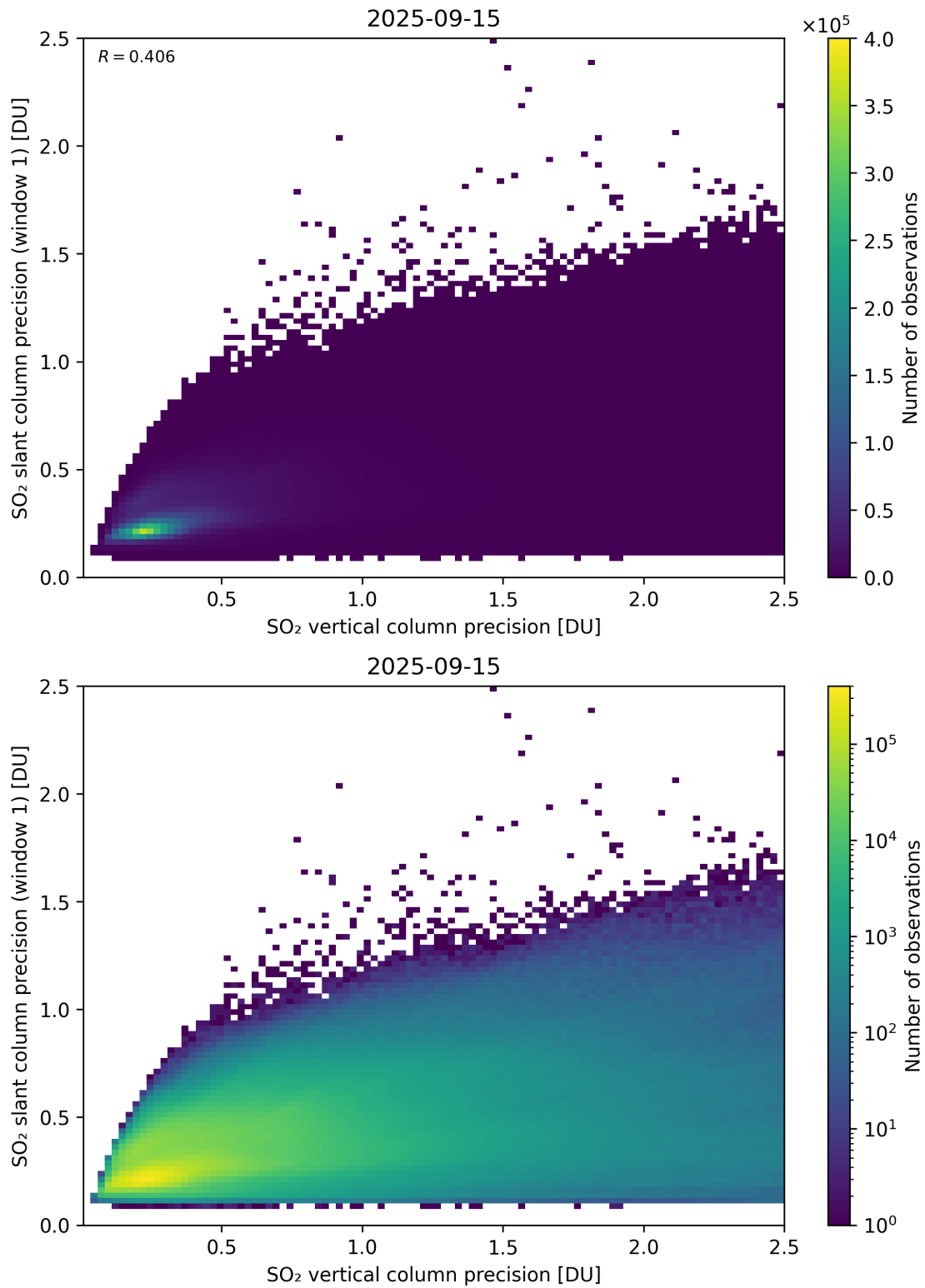
Figure 342: Scatter density plot of “SO 2 vertical column precision” against “SO 2 slant column precision (window 1)” for 2025-09-15 to 2025-09-16.
