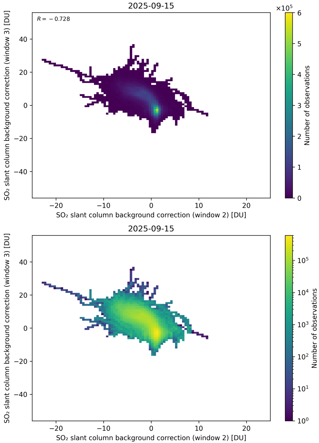
Figure 122: Scatter density plot of “SO 2 slant column background correction (window 2)” against “SO 2 slant column background correction (window 3)” for 2025-09-15 to 2025-09-16.
