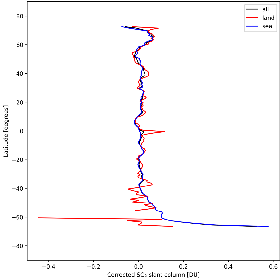
Figure 34: Zonal average of “Corrected SO 2 slant column” for 2025-09-15 to 2025-09-16.
