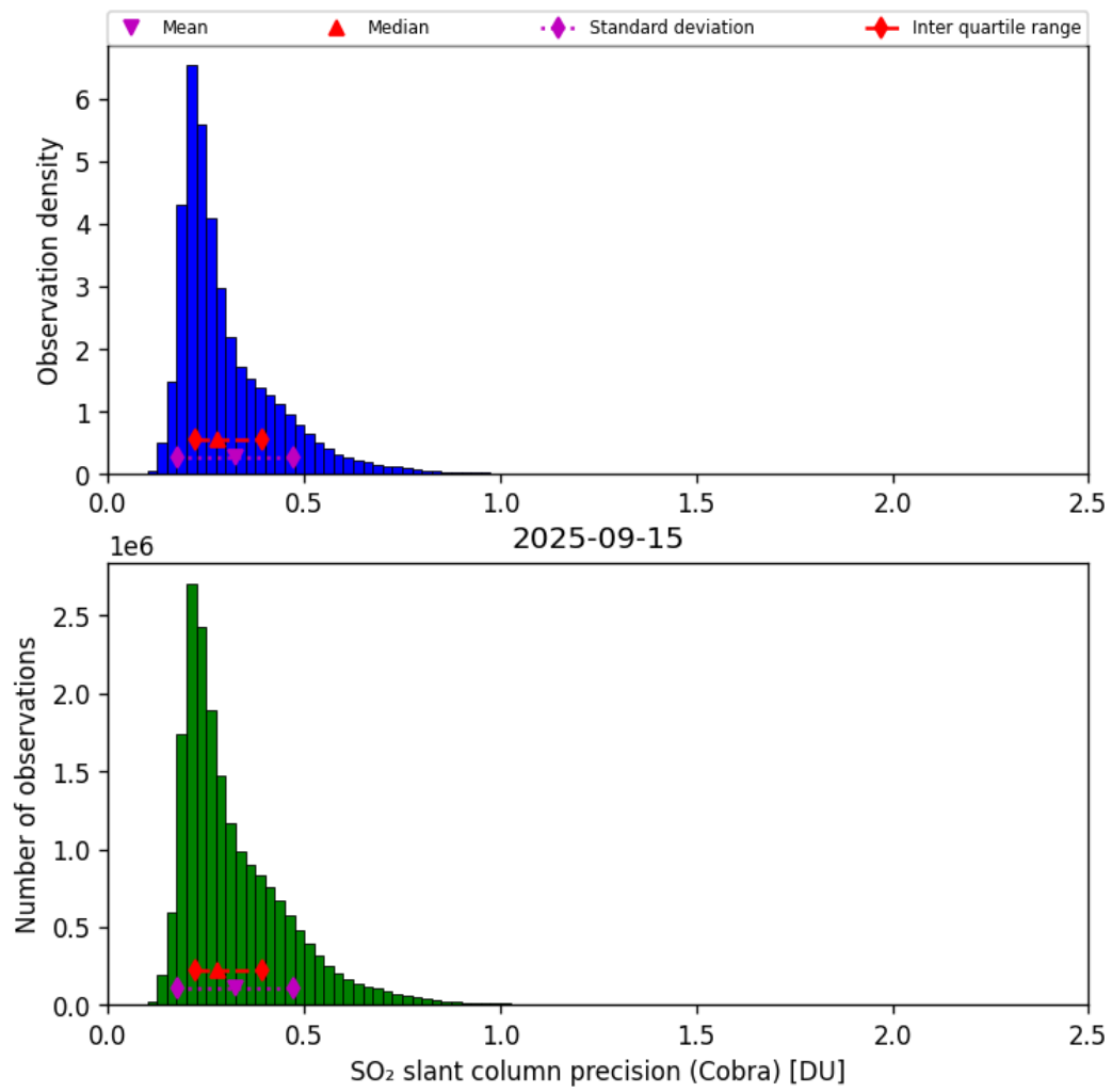
Figure 62: Histogram of “SO 2 slant column precision (Cobra)” for 2025-09-15 to 2025-09-16
