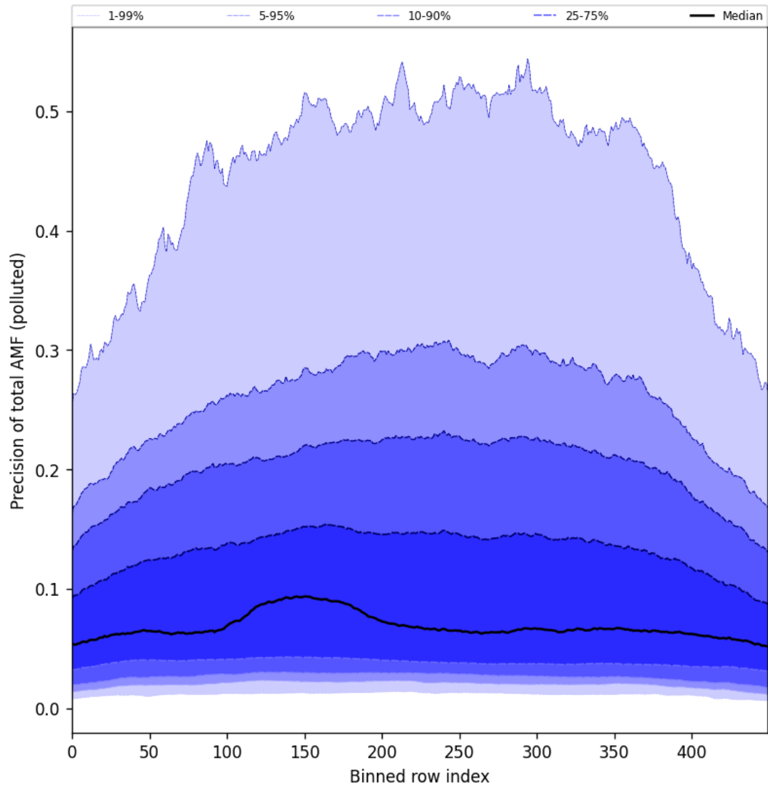
Figure 106: Along track statistics of “Precision of total AMF (polluted)” for 2025-09-15 to 2025-09-16
