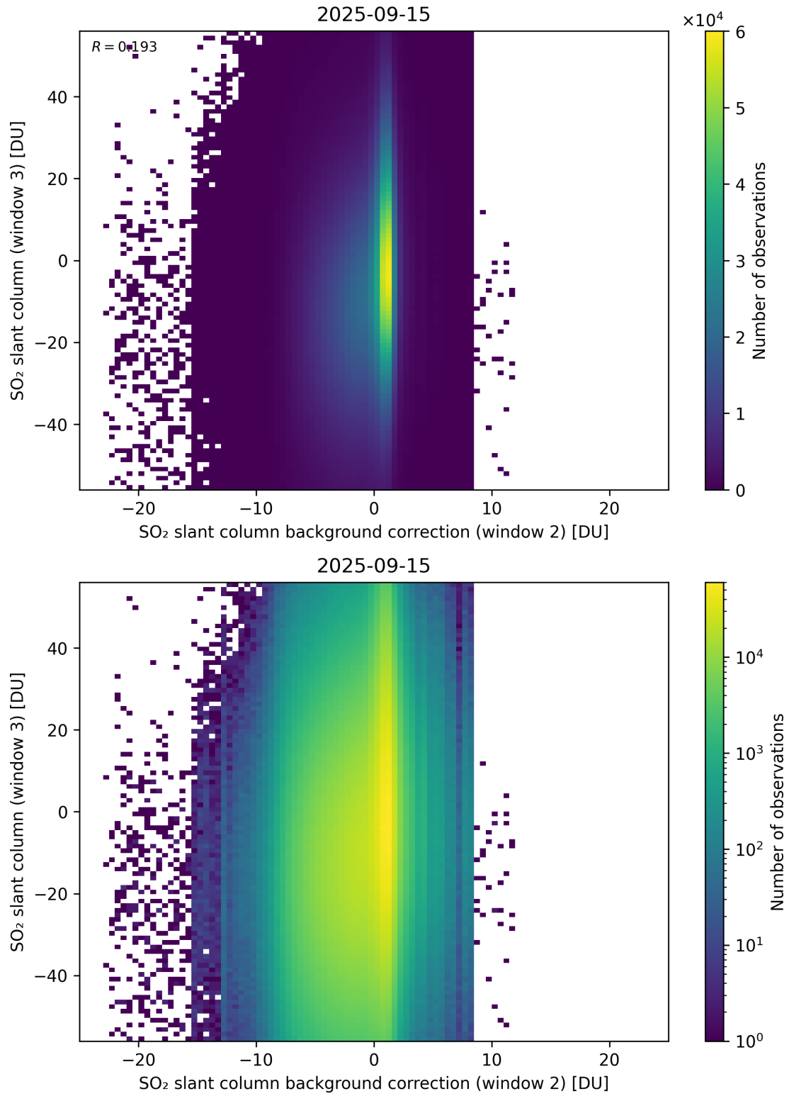
Figure 128: Scatter density plot of “SO 2 slant column background correction (window 2)” against “SO 2 slant column (window 3)” for 2025-09-15 to 2025-09-16.
