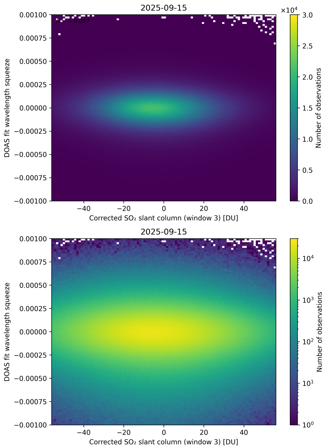
Figure 257: Scatter density plot of “Corrected SO 2 slant column (window 3)” against “DOAS fit wavelength squeeze” for 2025-09-15 to 2025-09-16.
