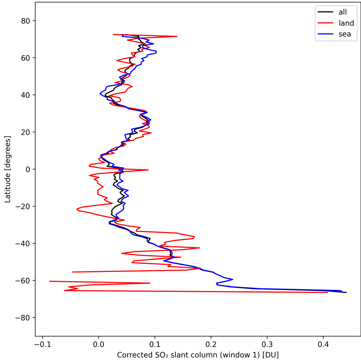
Figure 39: Zonal average of “Corrected SO 2 slant column (window 1)” for 2025-09-15 to 2025-09-16.
