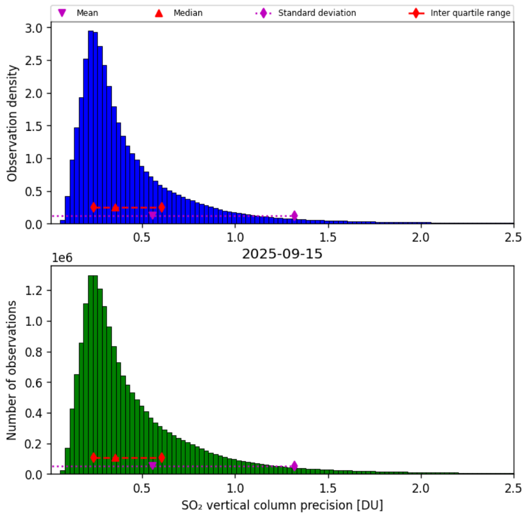
Figure 59: Histogram of “SO 2 vertical column precision” for 2025-09-15 to 2025-09-16
