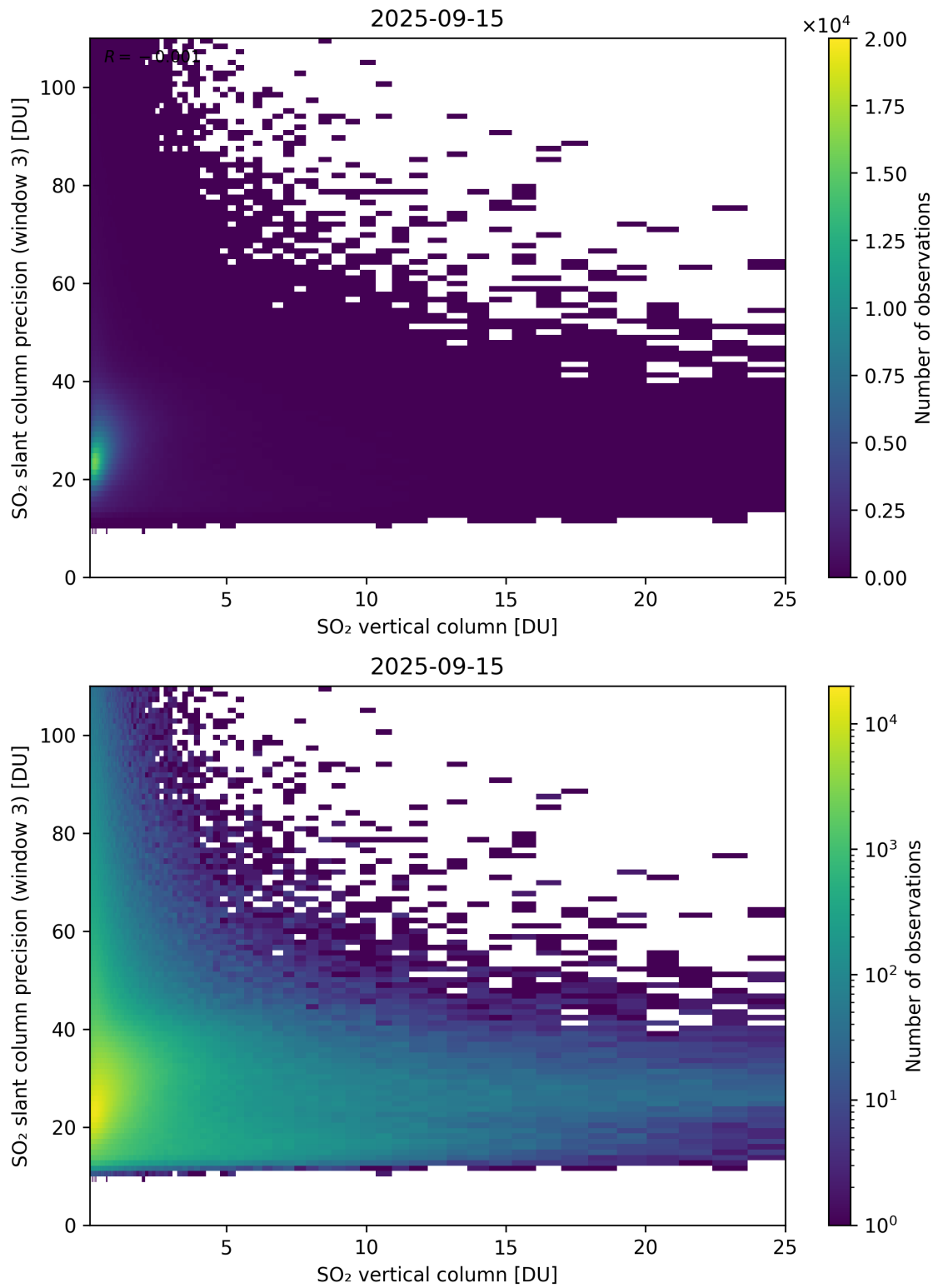
Figure 358: Scatter density plot of “SO 2 vertical column” against “SO 2 slant column precision (window 3)” for 2025-09-15 to 2025-09-16.
