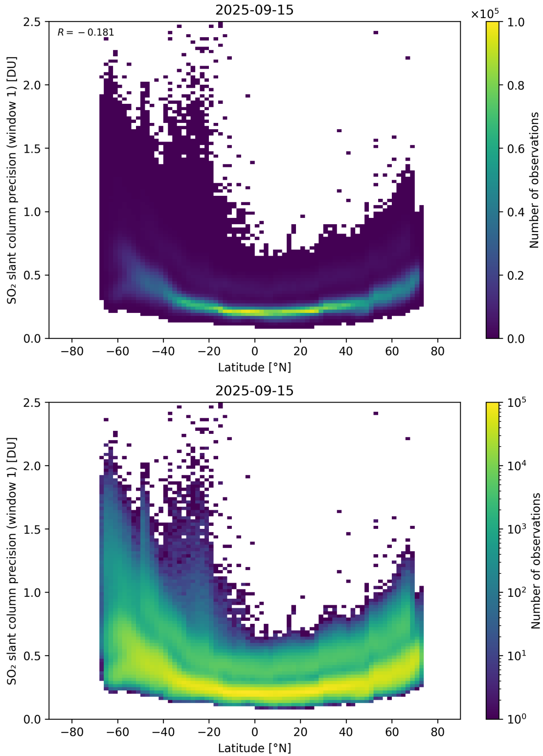
Figure 163: Scatter density plot of “Latitude” against “SO 2 slant column precision (window 1)” for 2025-09-15 to 2025-09-16.
