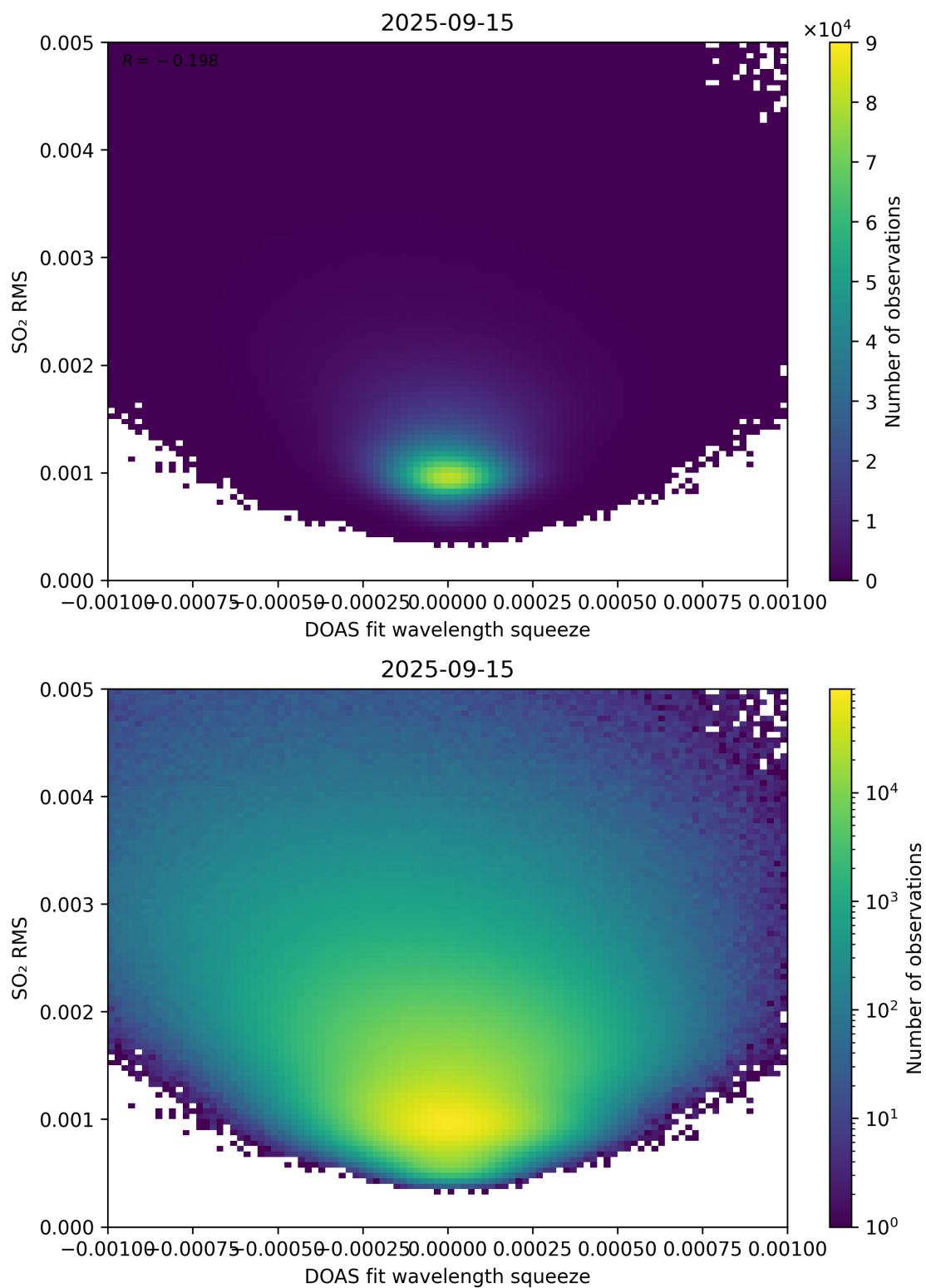
Figure 143: Scatter density plot of “DOAS fit wavelength squeeze” against “SO 2 RMS” for 2025-09-15 to 2025-09-16.
