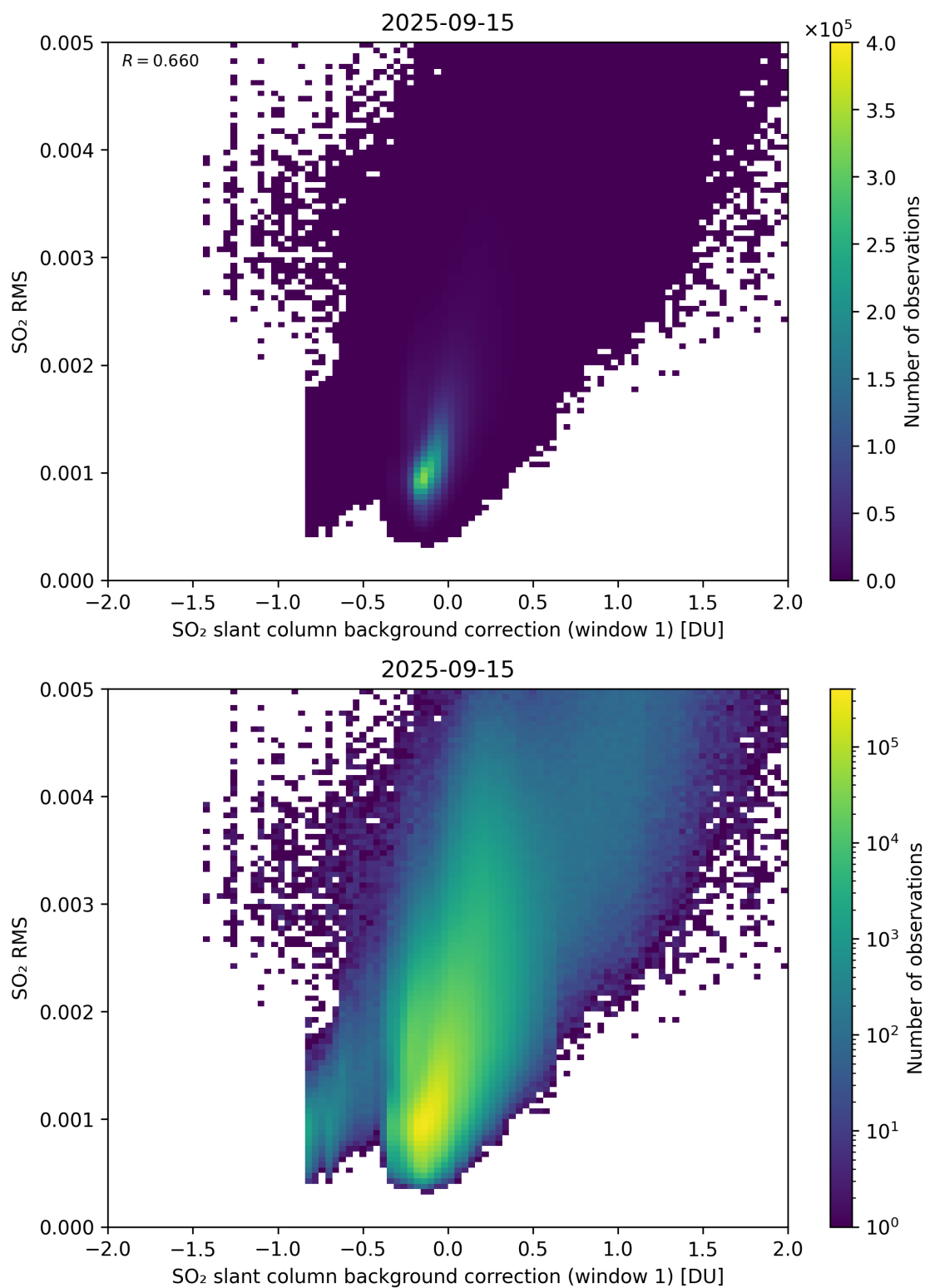
Figure 113: Scatter density plot of “SO 2 slant column background correction (window 1)” against “SO 2 RMS” for 2025-09-15 to 2025-09-16.
