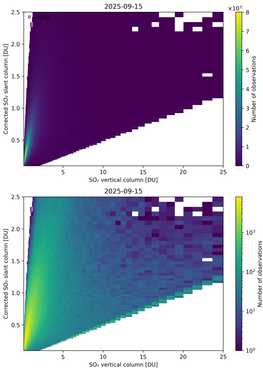
Figure 351: Scatter density plot of “SO 2 vertical column” against “Corrected SO 2 slant column” for 2025-09-15 to 2025-09-16.
