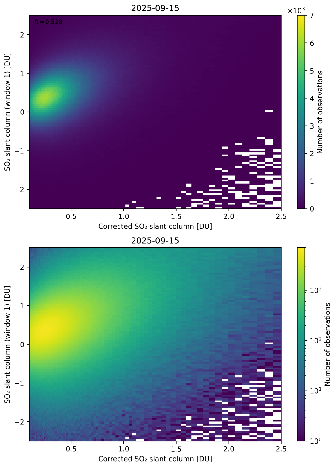
Figure 237: Scatter density plot of “Corrected SO 2 slant column” against “SO 2 slant column (window 1)” for 2025-09-15 to 2025-09-16.
