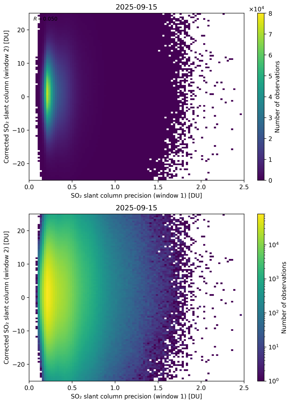
Figure 275: Scatter density plot of “SO 2 slant column precision (window 1)” against “Corrected SO 2 slant column (window 2)” for 2025-09-15 to 2025-09-16.
