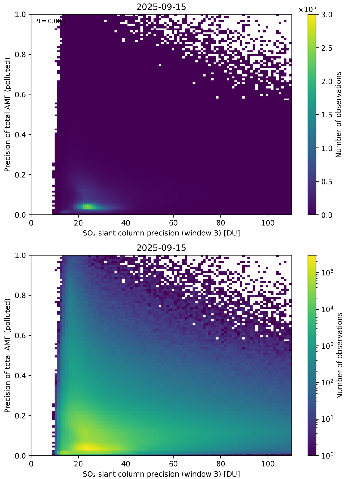
Figure 314: Scatter density plot of “SO 2 slant column precision (window 3)” against “Precision of total AMF (polluted)” for 2025-09-15 to 2025-09-16.
