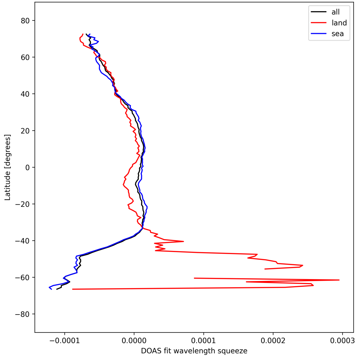
Figure 51: Zonal average of “DOAS fit wavelength squeeze” for 2025-09-15 to 2025-09-16.
