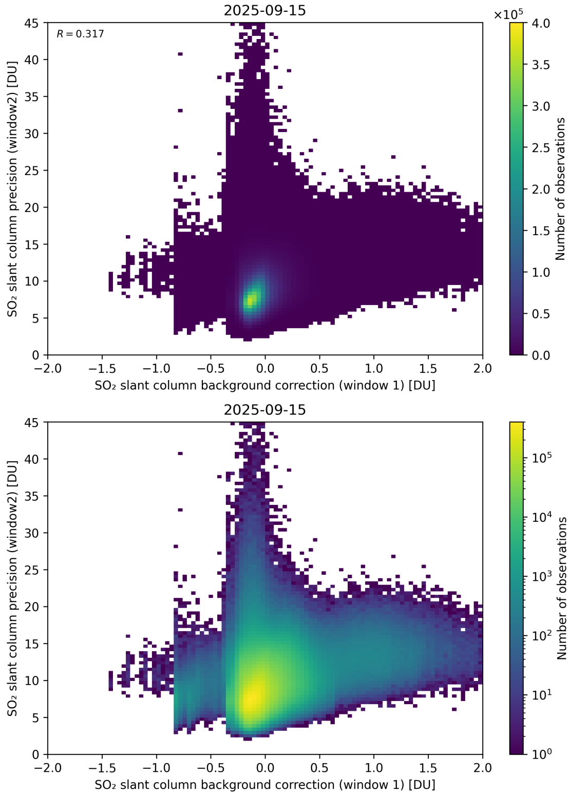
Figure 117: Scatter density plot of “SO 2 slant column background correction (window 1)” against “SO 2 slant column precision (window2)” for 2025-09-15 to 2025-09-16.
