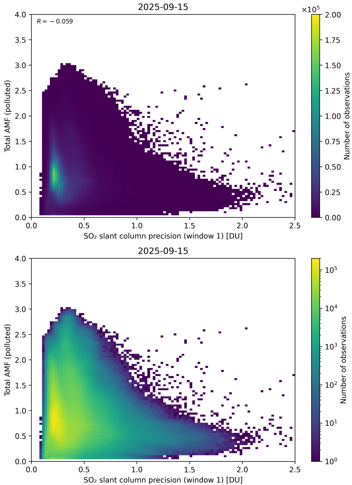
Figure 280: Scatter density plot of “SO 2 slant column precision (window 1)” against “Total AMF (polluted)” for 2025-09-15 to 2025-09-16.
