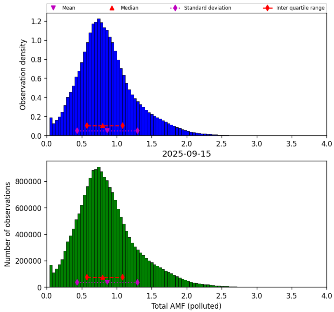
Figure 79: Histogram of “Total AMF (polluted)” for 2025-09-15 to 2025-09-16
