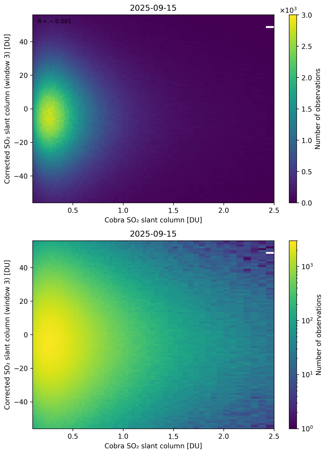
Figure 218: Scatter density plot of “Cobra SO 2 slant column” against “Corrected SO 2 slant column (window 3)” for 2025-09-15 to 2025-09-16.
