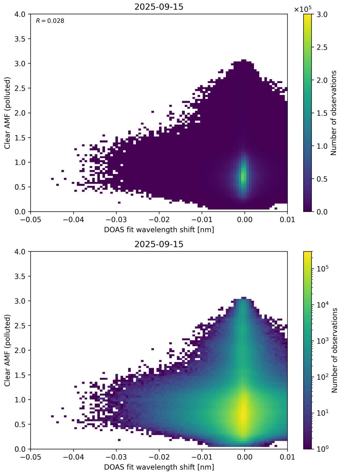
Figure 140: Scatter density plot of “DOAS fit wavelength shift” against “Clear AMF (polluted)” for 2025-09-15 to 2025-09-16.
