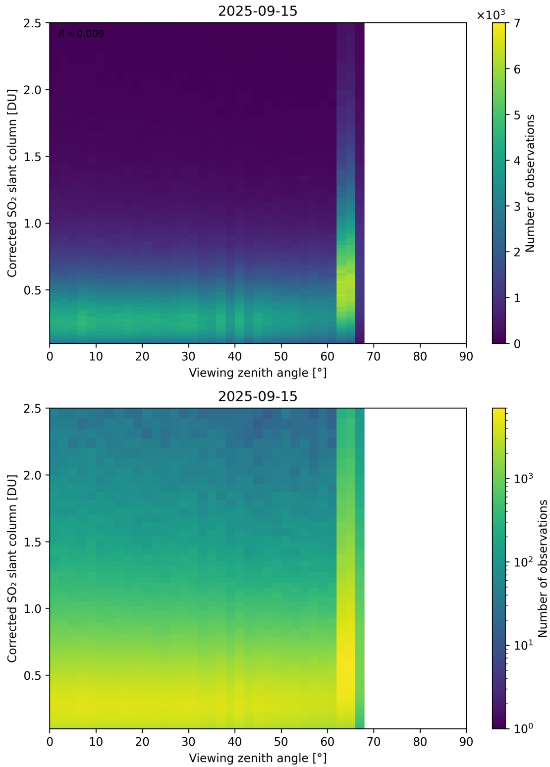
Figure 373: Scatter density plot of “Viewing zenith angle” against “Corrected SO 2 slant column” for 2025-09-15 to 2025-09-16.
