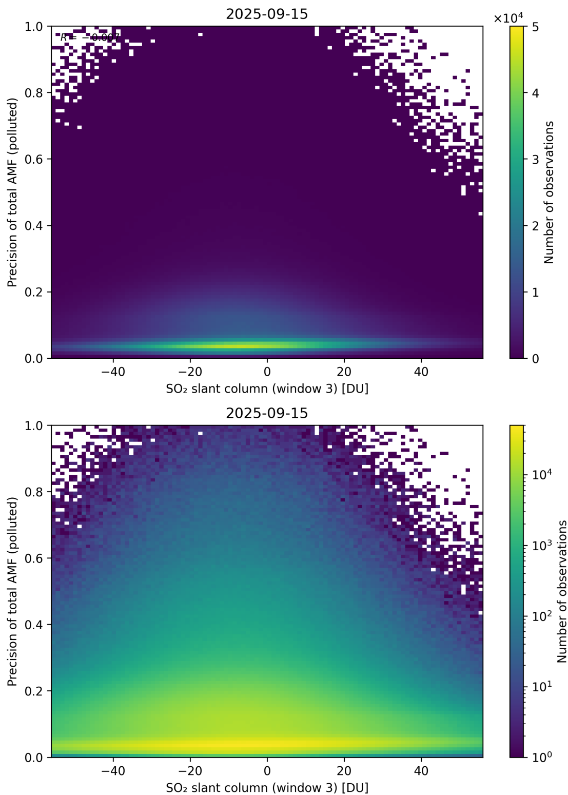
Figure 319: Scatter density plot of “SO 2 slant column (window 3)” against “Precision of total AMF (polluted)” for 2025-09-15 to 2025-09-16.
