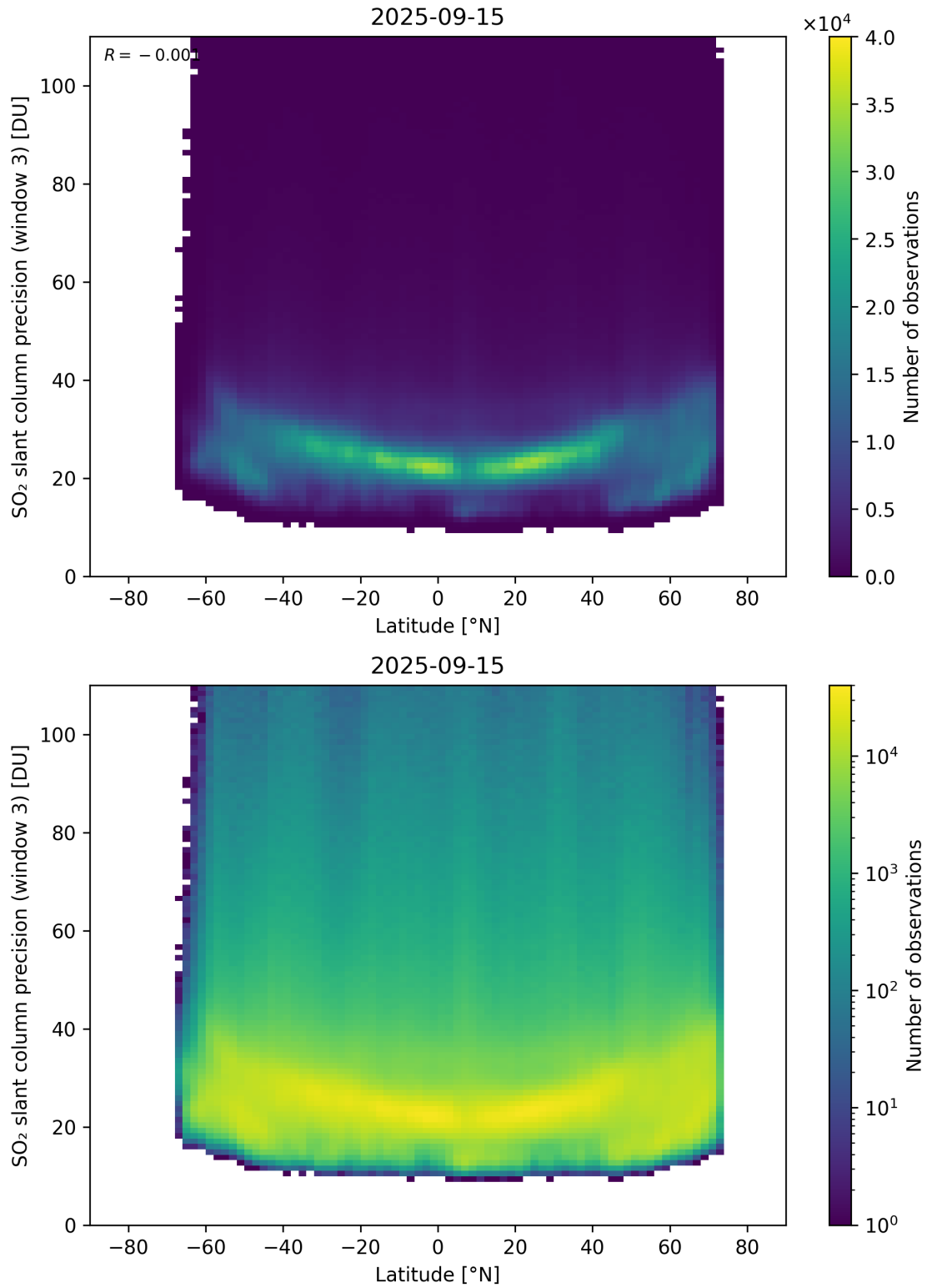
Figure 166: Scatter density plot of “Latitude” against “SO 2 slant column precision (window 3)” for 2025-09-15 to 2025-09-16.
