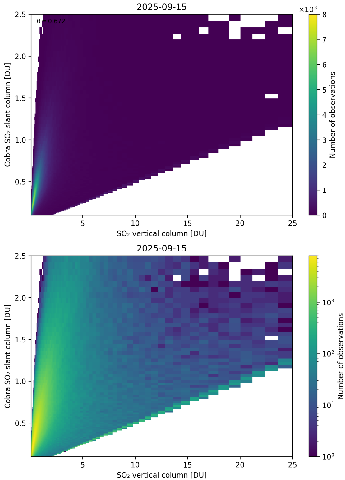
Figure 349: Scatter density plot of “SO 2 vertical column” against “Cobra SO 2 slant column” for 2025-09-15 to 2025-09-16.
