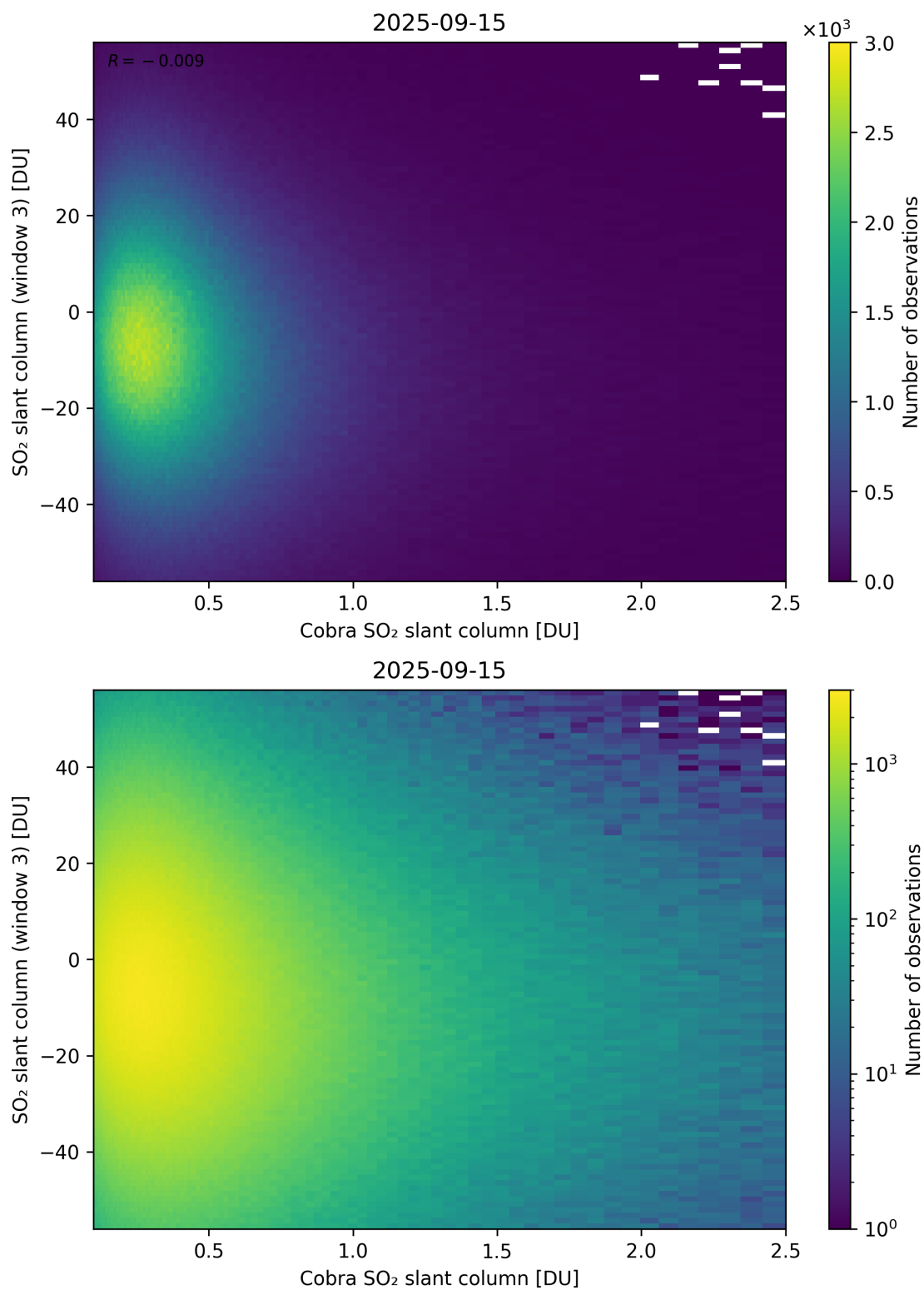
Figure 222: Scatter density plot of “Cobra SO 2 slant column” against “SO 2 slant column (window 3)” for 2025-09-15 to 2025-09-16.
