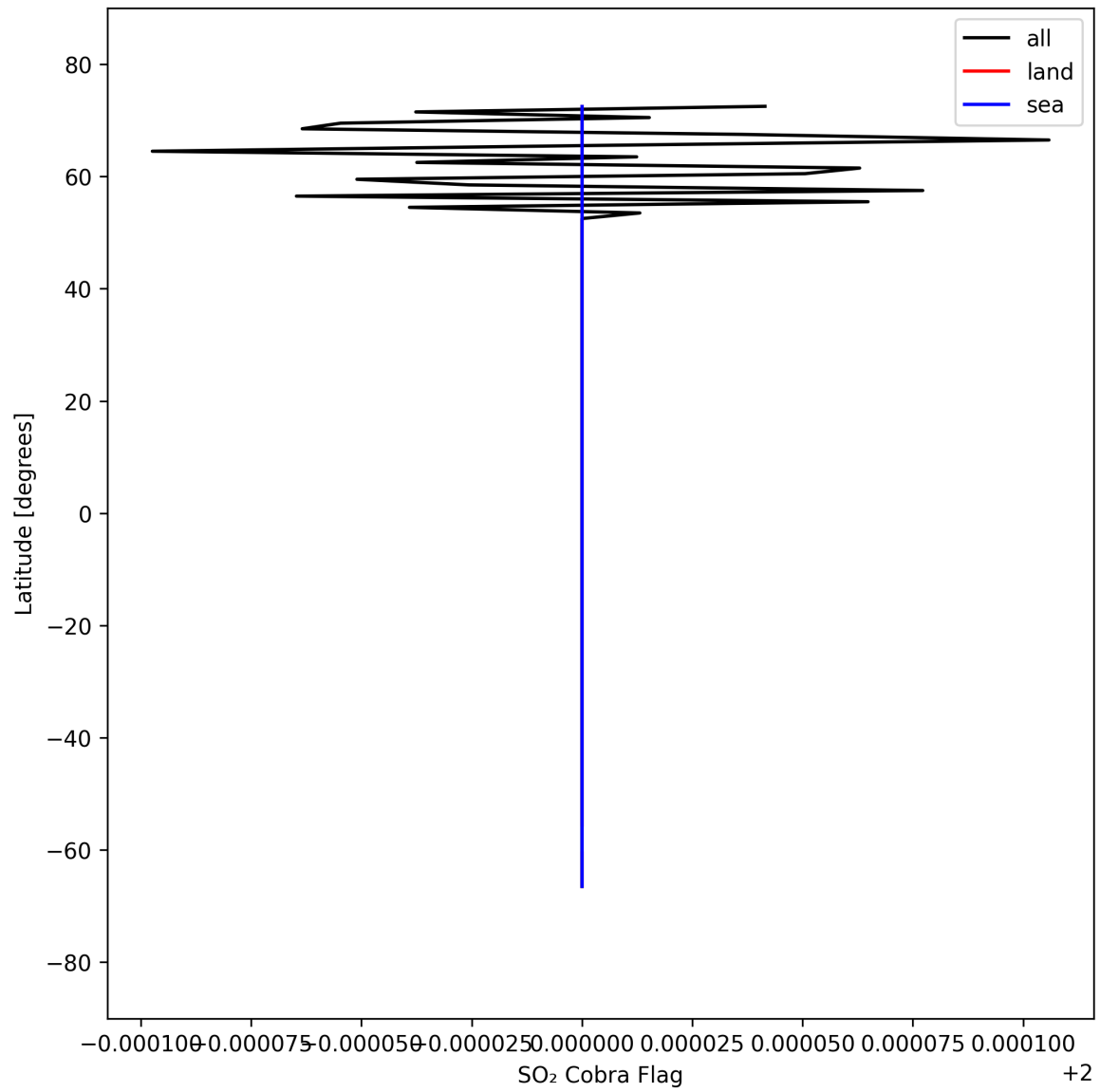
Figure 49: Zonal average of "SO 2 Cobra Flag" for 2025-09-15 to 2025-09-16.
