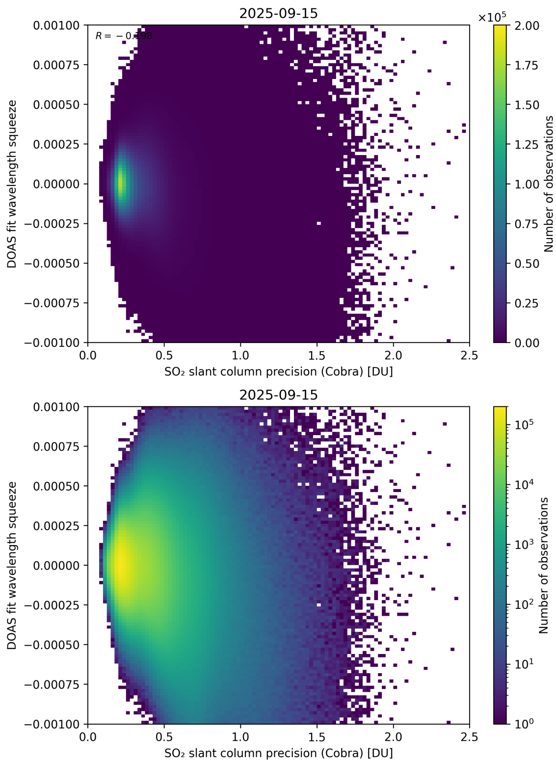
Figure 203: Scatter density plot of “SO 2 slant column precision (Cobra)” against “DOAS fit wavelength squeeze” for 2025-09-15 to 2025-09-16.
