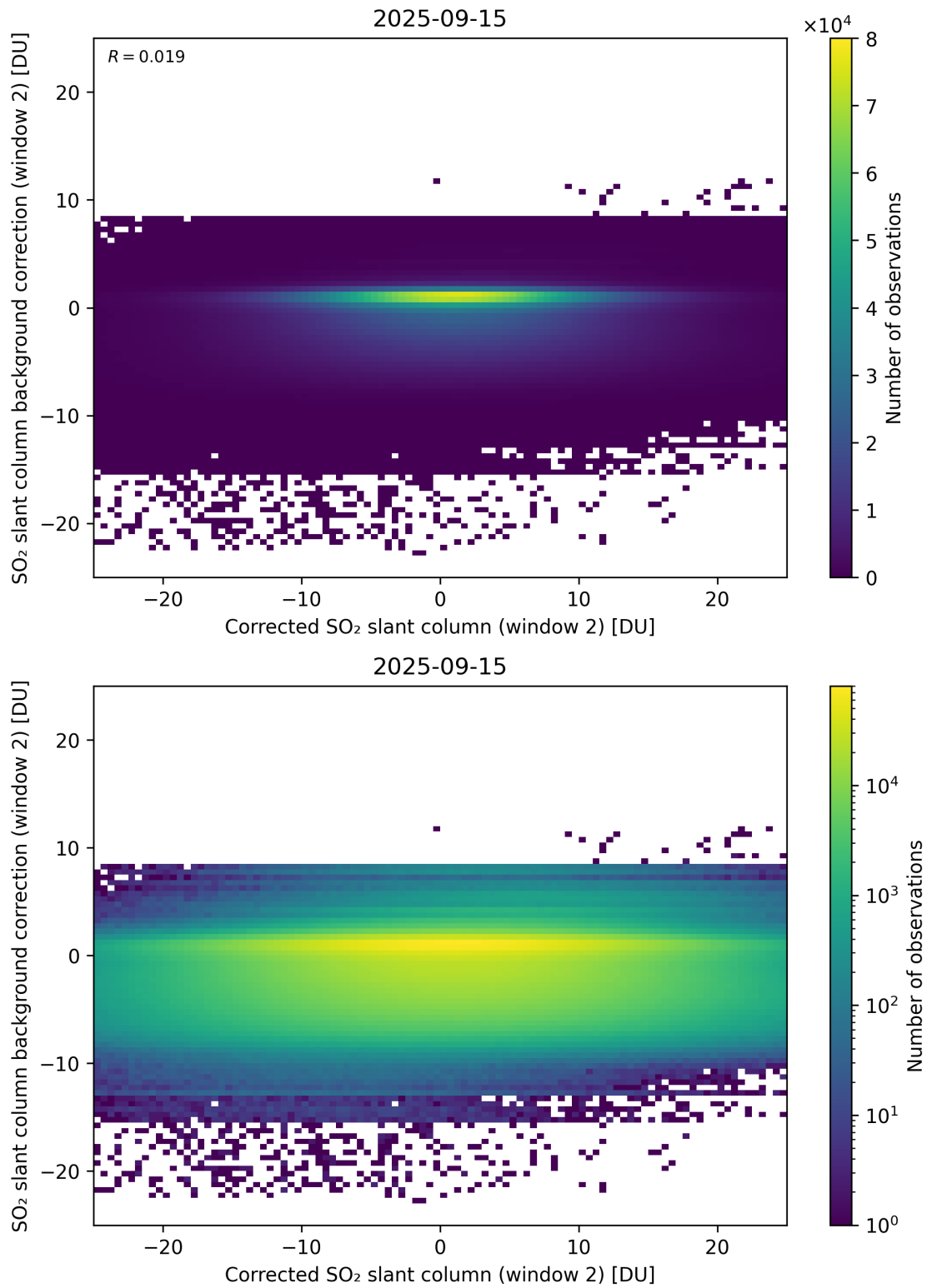
Figure 244: Scatter density plot of “Corrected SO 2 slant column (window 2)” against “SO 2 slant column background correction (window 2)” for 2025-09-15 to 2025-09-16.
