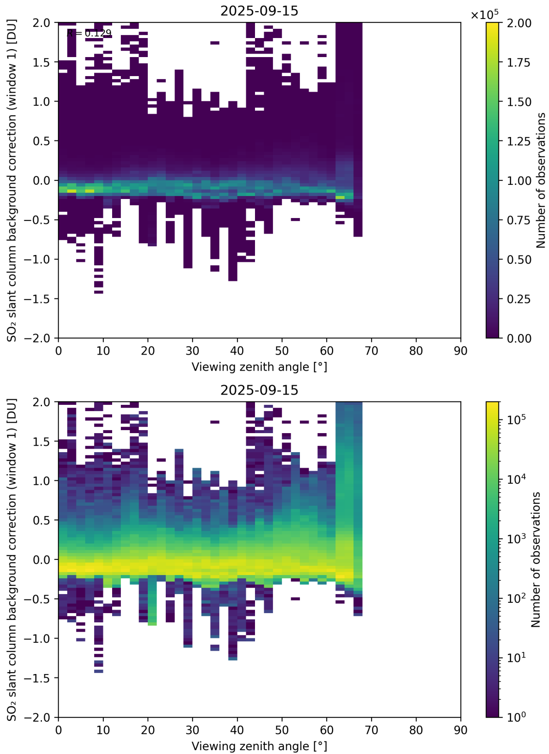
Figure 362: Scatter density plot of “Viewing zenith angle” against “SO 2 slant column background correction (window 1)” for 2025-09-15 to 2025-09-16.
