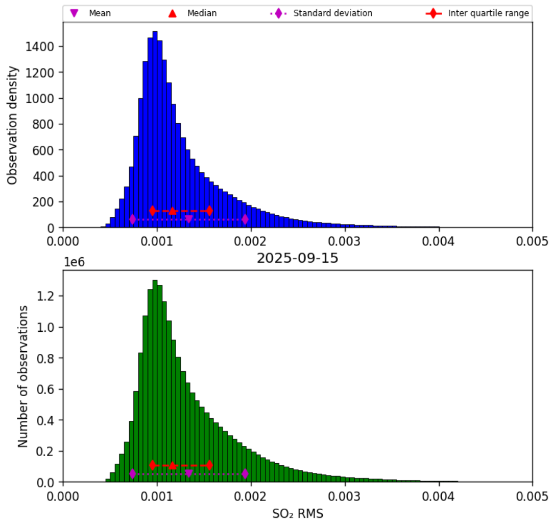
Figure 78: Histogram of “SO 2 RMS” for 2025-09-15 to 2025-09-16
