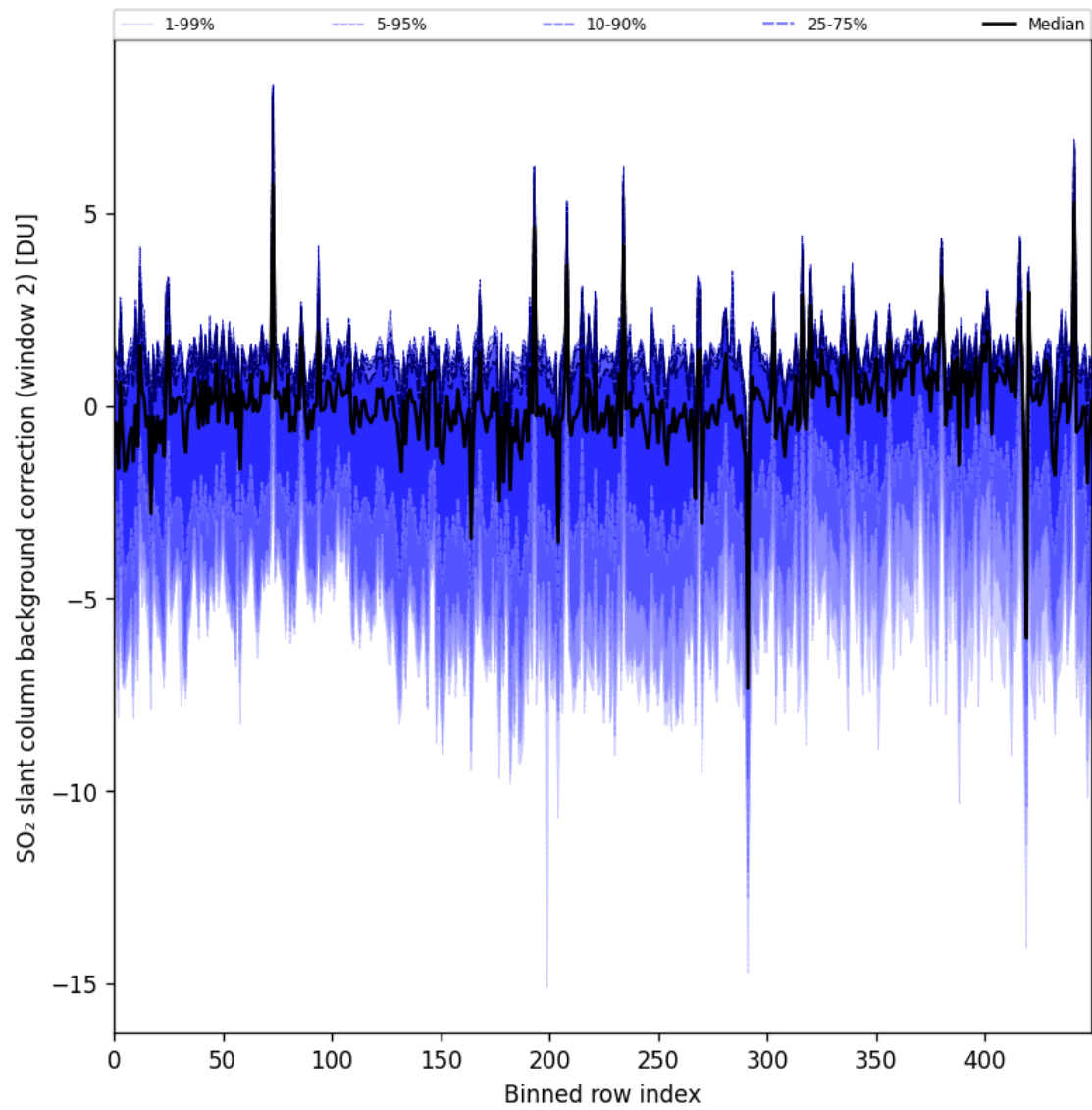
Figure 96: Along track statistics of “SO 2 slant column background correction (window 2)” for 2025-09-15 to 2025-09-16
