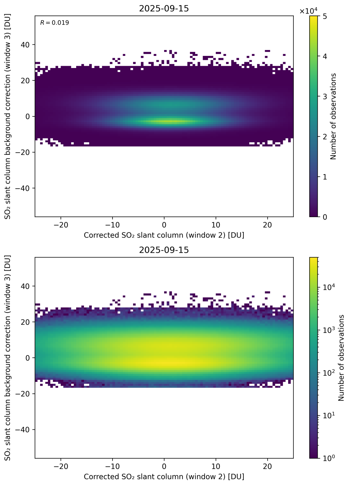
Figure 245: Scatter density plot of “Corrected SO 2 slant column (window 2)” against “SO 2 slant column background correction (window 3)” for 2025-09-15 to 2025-09-16.
