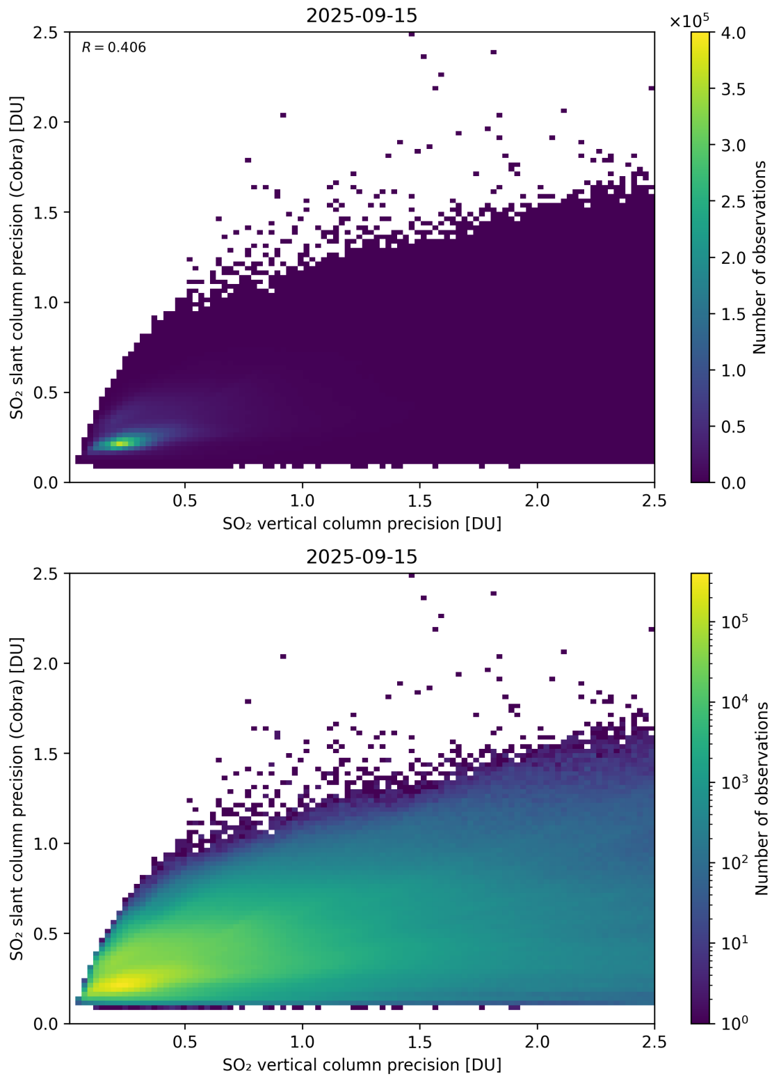
Figure 337: Scatter density plot of “SO 2 vertical column precision” against “SO 2 slant column precision (Cobra)” for 2025-09-15 to 2025-09-16.
