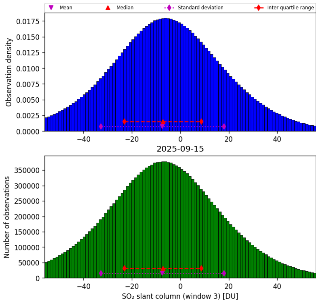
Figure 71: Histogram of “SO 2 slant column (window 3)” for 2025-09-15 to 2025-09-16
