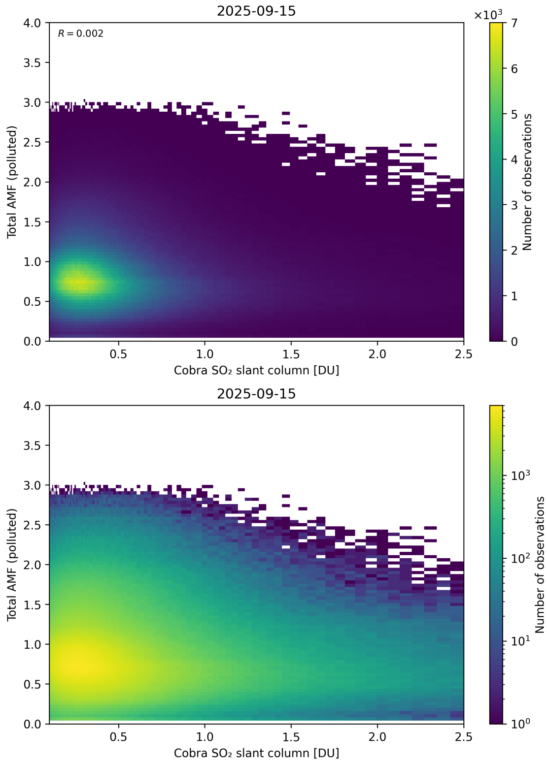
Figure 224: Scatter density plot of “Cobra SO 2 slant column” against “Total AMF (polluted)” for 2025-09-15 to 2025-09-16.
