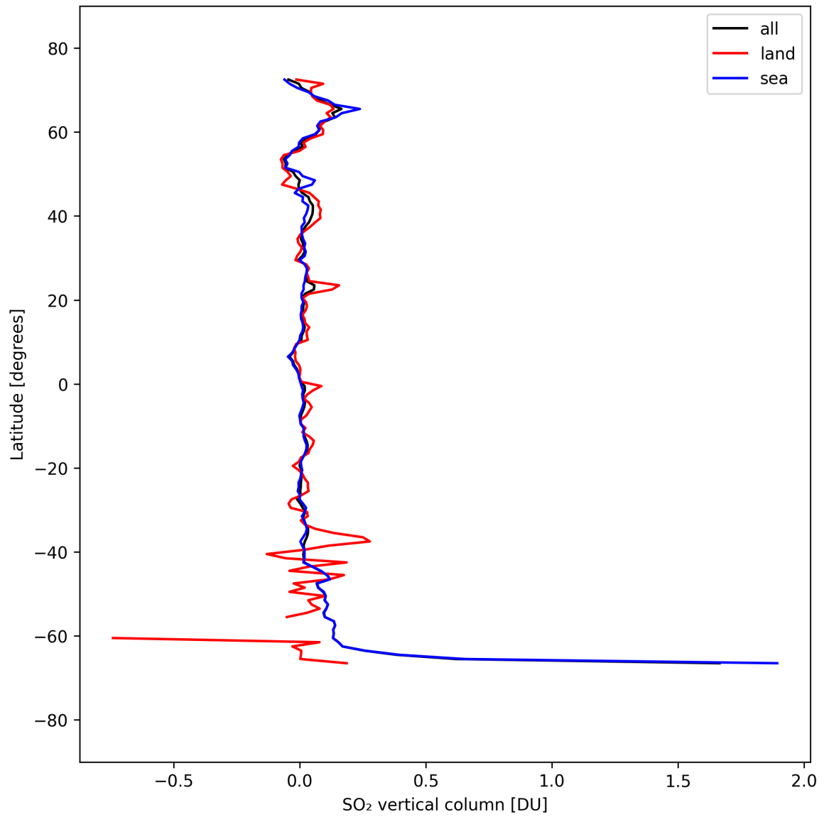
Figure 32: Zonal average of “SO 2 vertical column” for 2025-09-15 to 2025-09-16.
