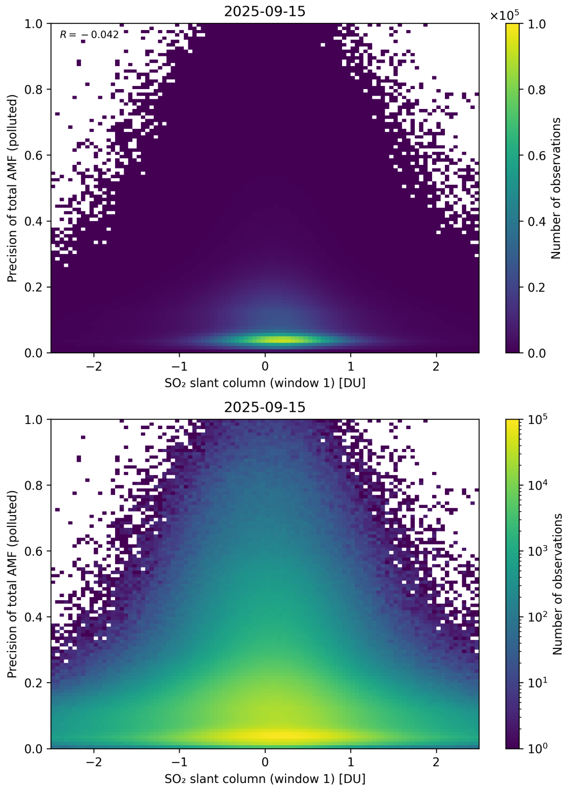
Figure 290: Scatter density plot of “SO 2 slant column (window 1)” against “Precision of total AMF (polluted)” for 2025-09-15 to 2025-09-16.
