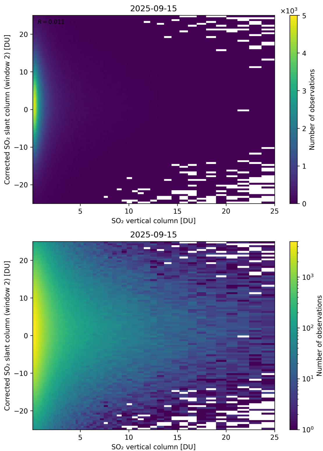
Figure 352: Scatter density plot of “SO 2 vertical column” against “Corrected SO 2 slant column (window 2)” for 2025-09-15 to 2025-09-16.
