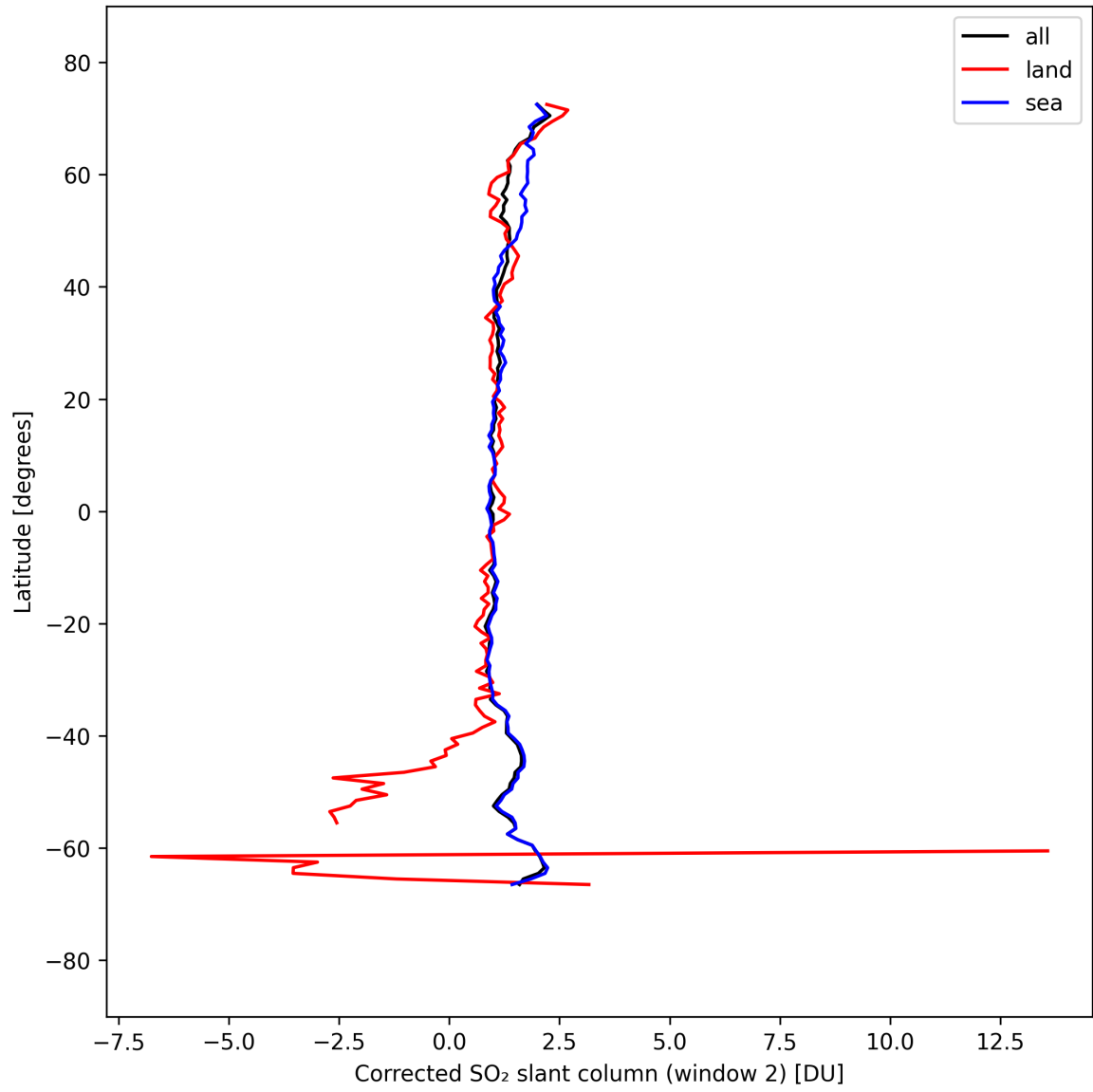
Figure 43: Zonal average of “Corrected SO 2 slant column (window 2)” for 2025-09-15 to 2025-09-16.
