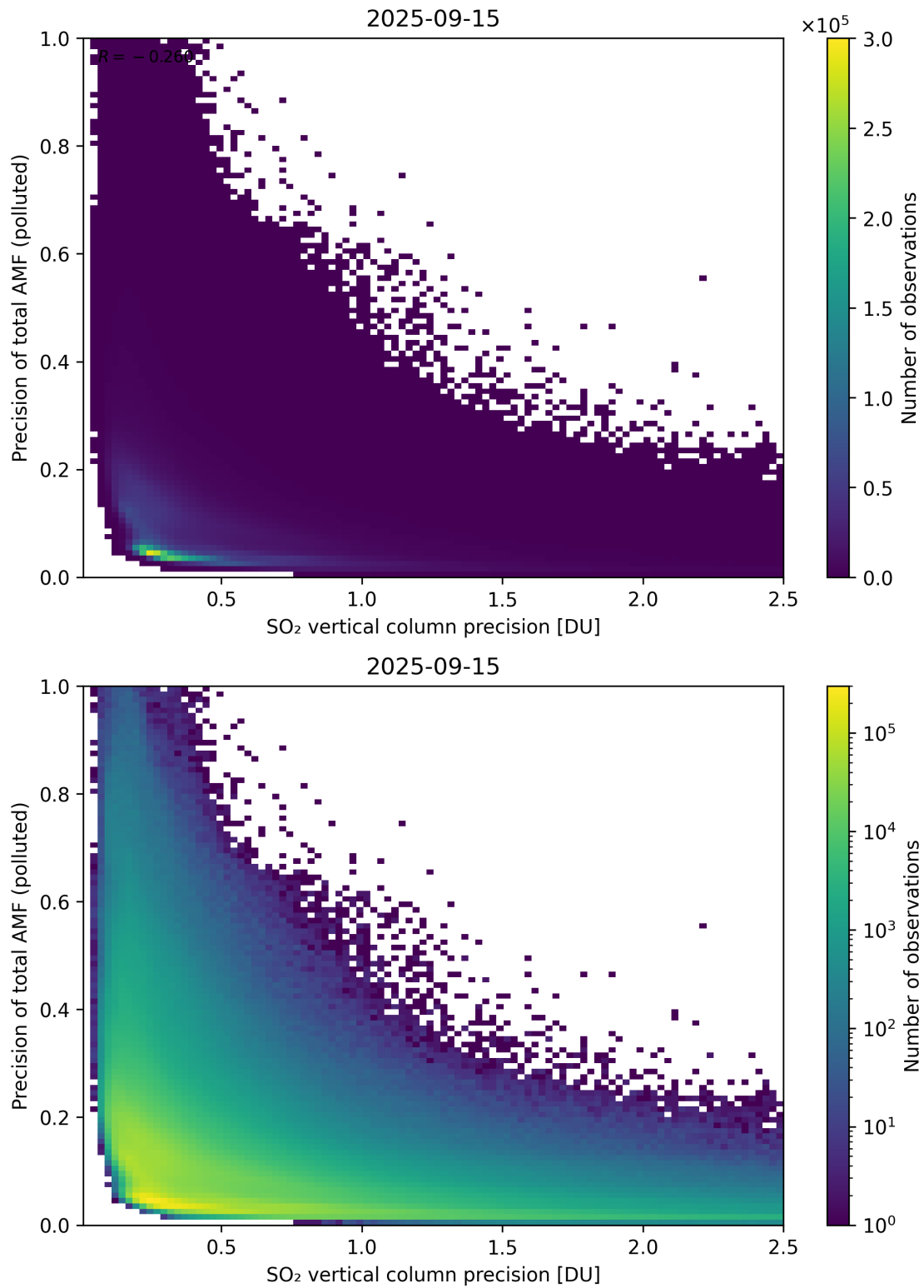
Figure 347: Scatter density plot of “SO 2 vertical column precision” against “Precision of total AMF (polluted)” for 2025-09-15 to 2025-09-16.
