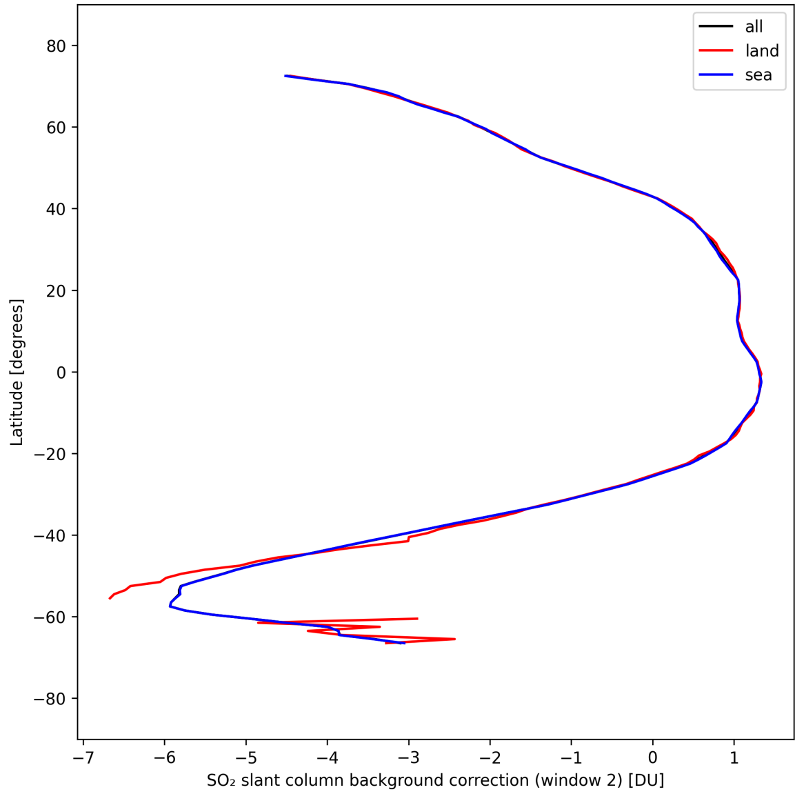
Figure 44: Zonal average of “SO 2 slant column background correction (window 2)” for 2025-09-15 to 2025-09-16.
