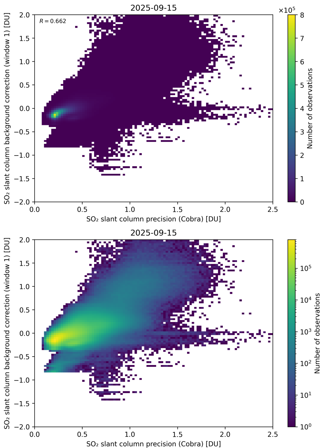
Figure 199: Scatter density plot of “SO 2 slant column precision (Cobra)” against “SO 2 slant column background correction (window 1)” for 2025-09-15 to 2025-09-16.
