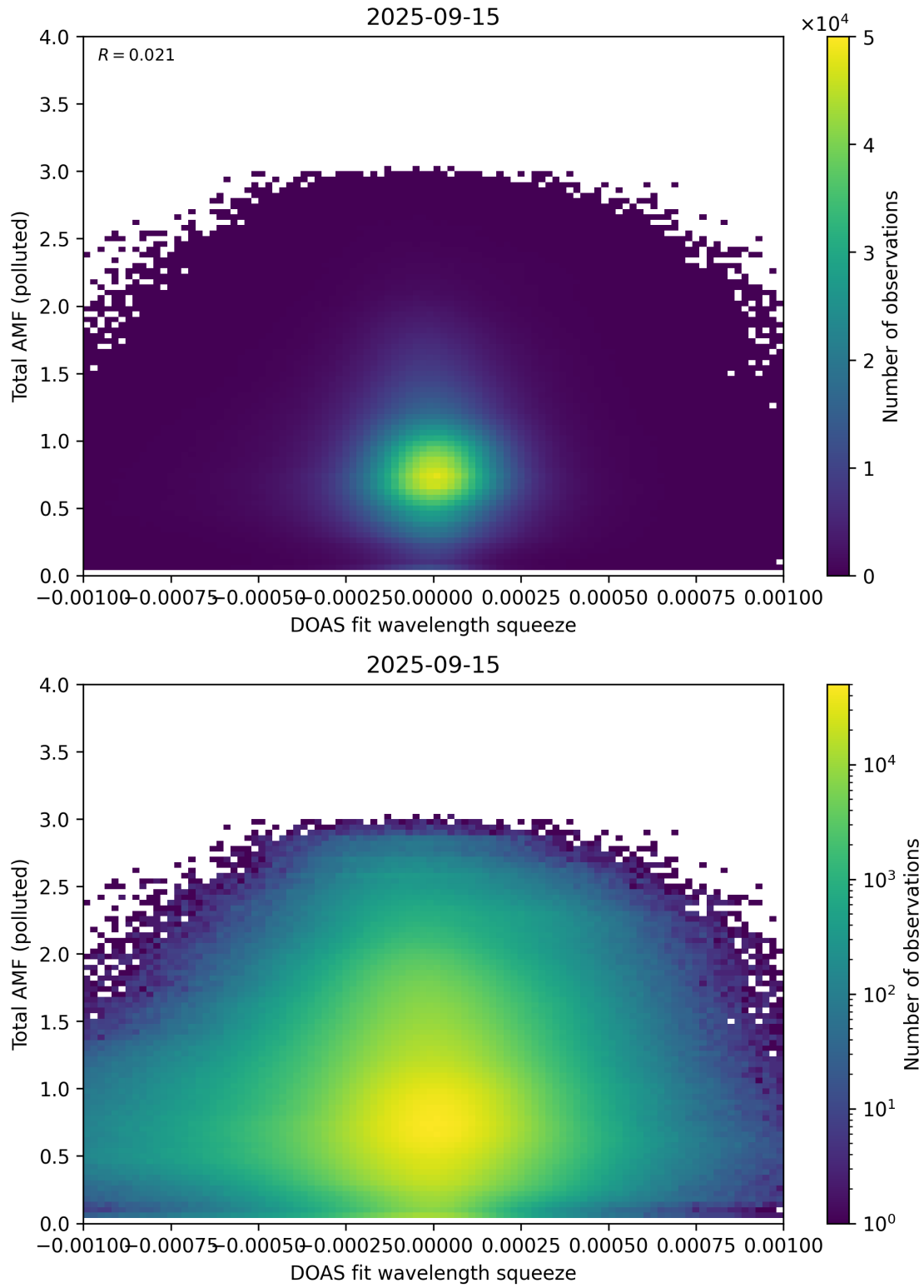
Figure 145: Scatter density plot of “DOAS fit wavelength squeeze” against “Total AMF (polluted)” for 2025-09-15 to 2025-09-16.
