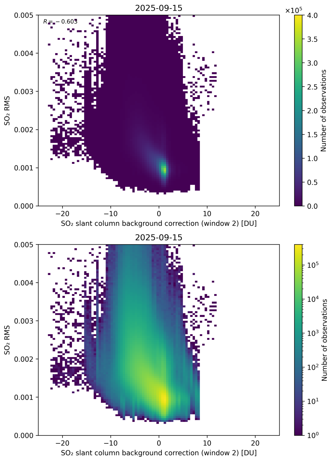
Figure 125: Scatter density plot of “SO 2 slant column background correction (window 2)” against “SO 2 RMS” for 2025-09-15 to 2025-09-16.
