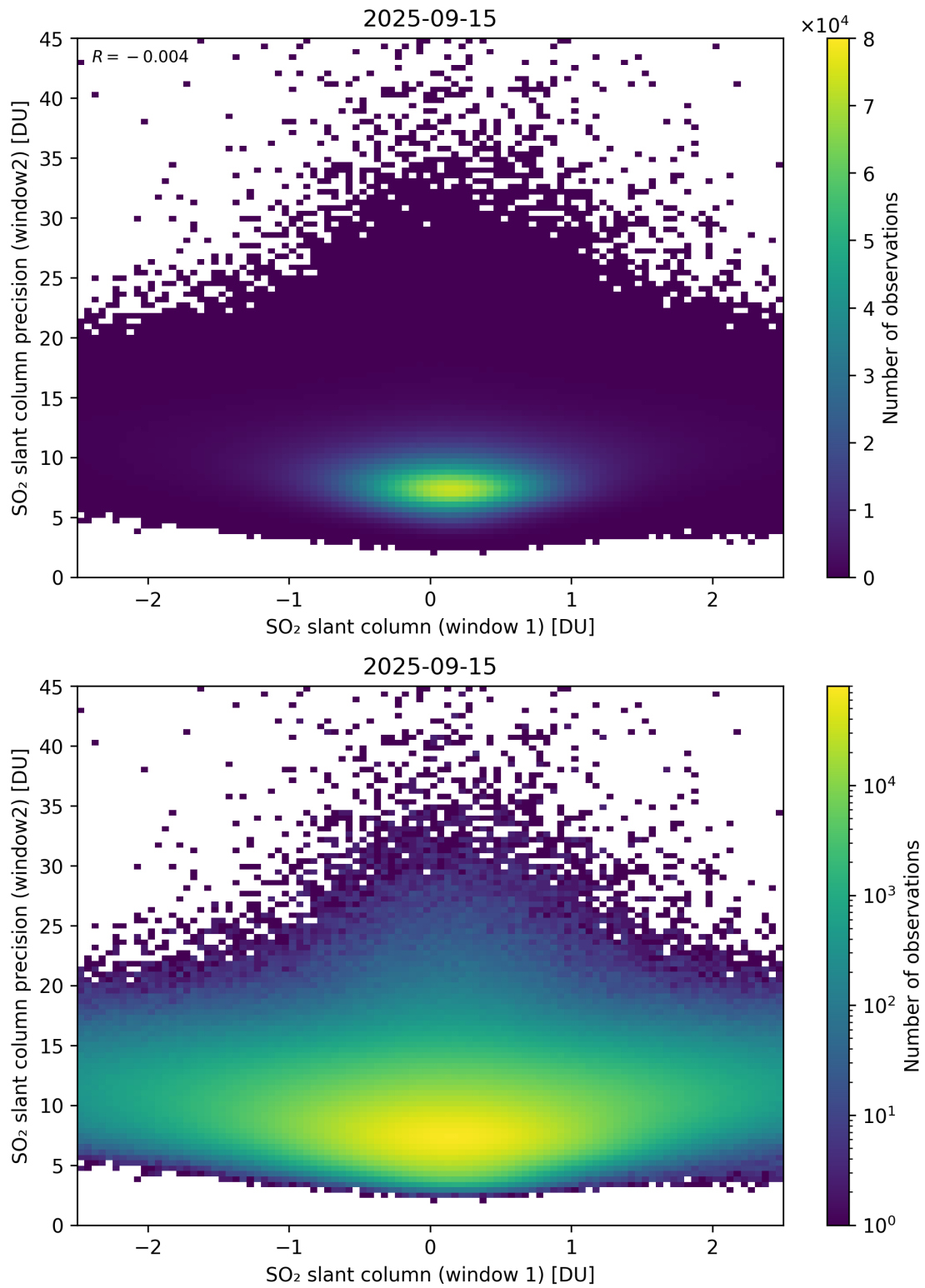
Figure 286: Scatter density plot of “SO 2 slant column (window 1)” against “SO 2 slant column precision (window2)” for 2025-09-15 to 2025-09-16.
