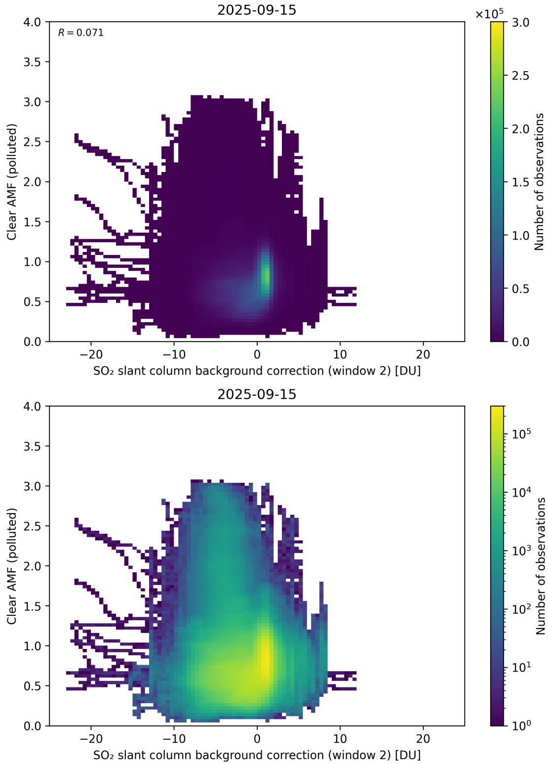
Figure 126: Scatter density plot of “SO 2 slant column background correction (window 2)” against “Clear AMF (polluted)” for 2025-09-15 to 2025-09-16.
