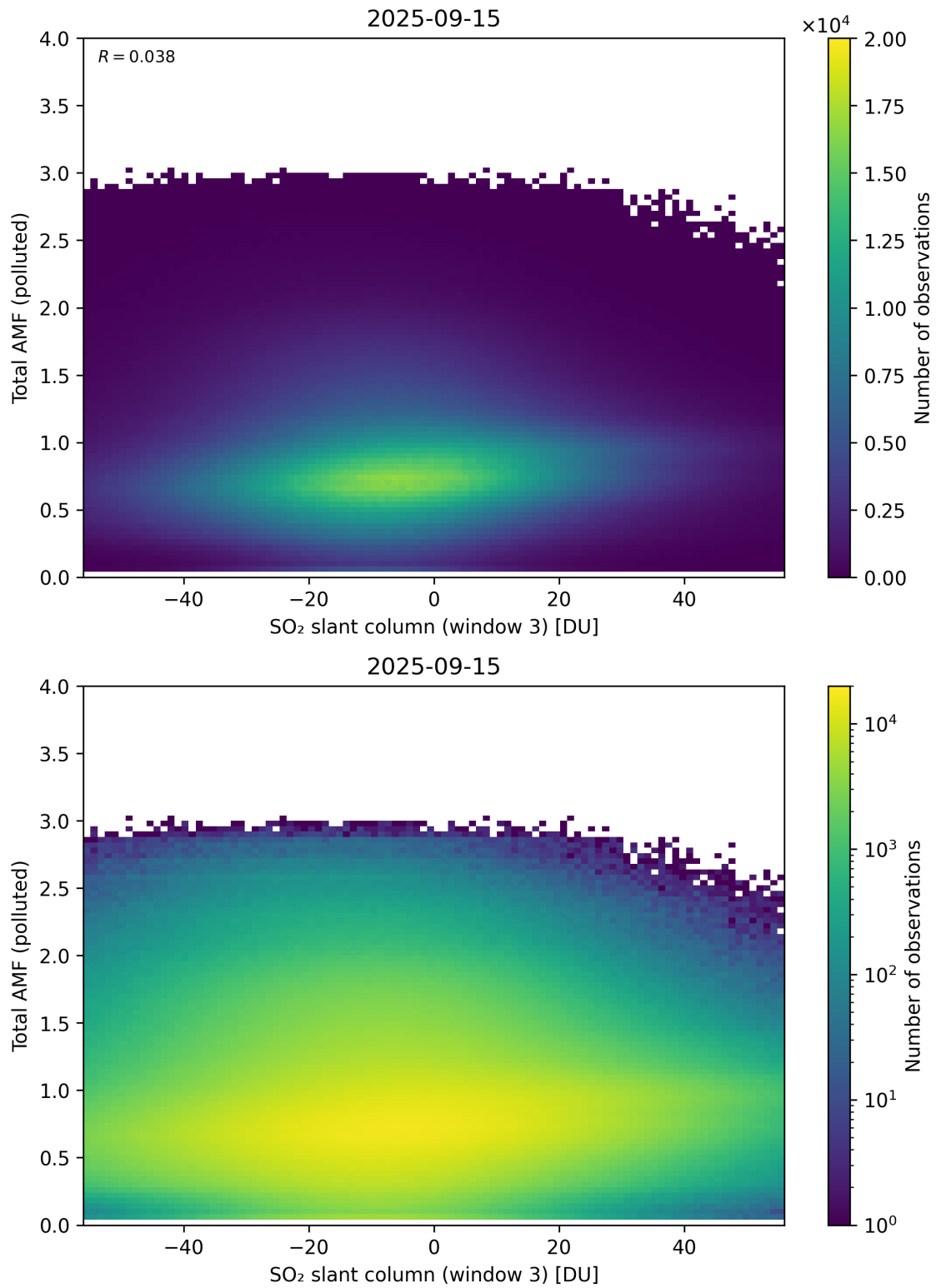
Figure 318: Scatter density plot of “SO 2 slant column (window 3)” against “Total AMF (polluted)” for 2025-09-15 to 2025-09-16.
