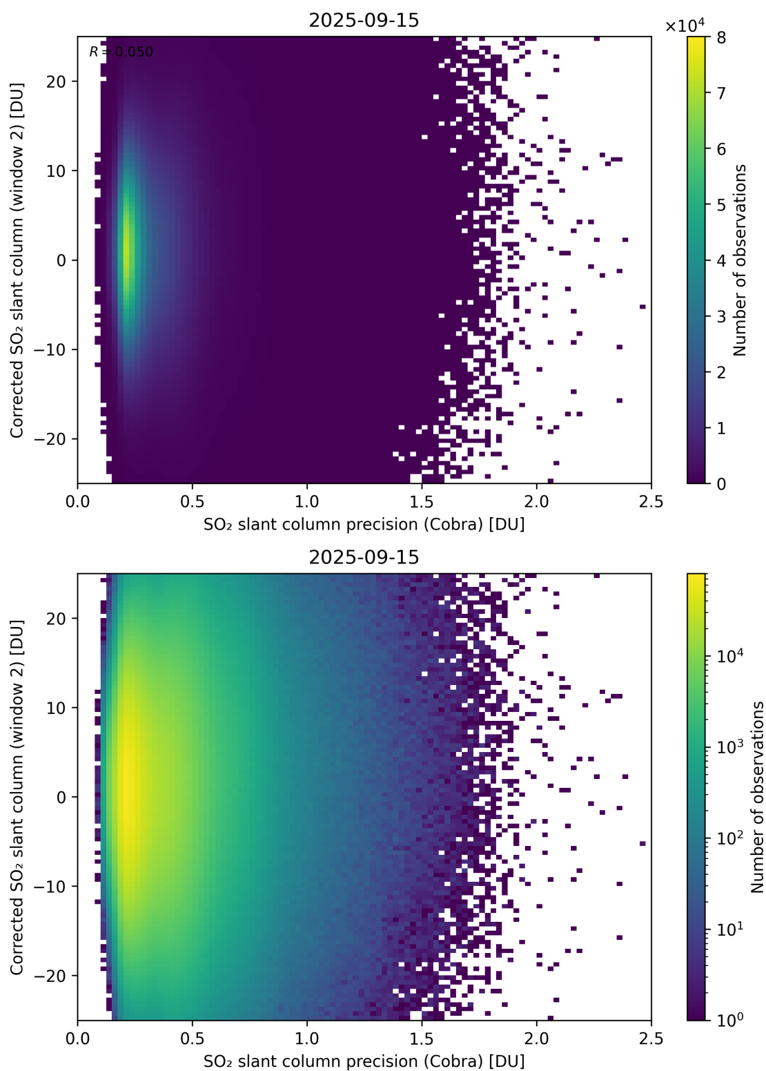
Figure 206: Scatter density plot of “SO 2 slant column precision (Cobra)” against “Corrected SO 2 slant column (window 2)” for 2025-09-15 to 2025-09-16.
