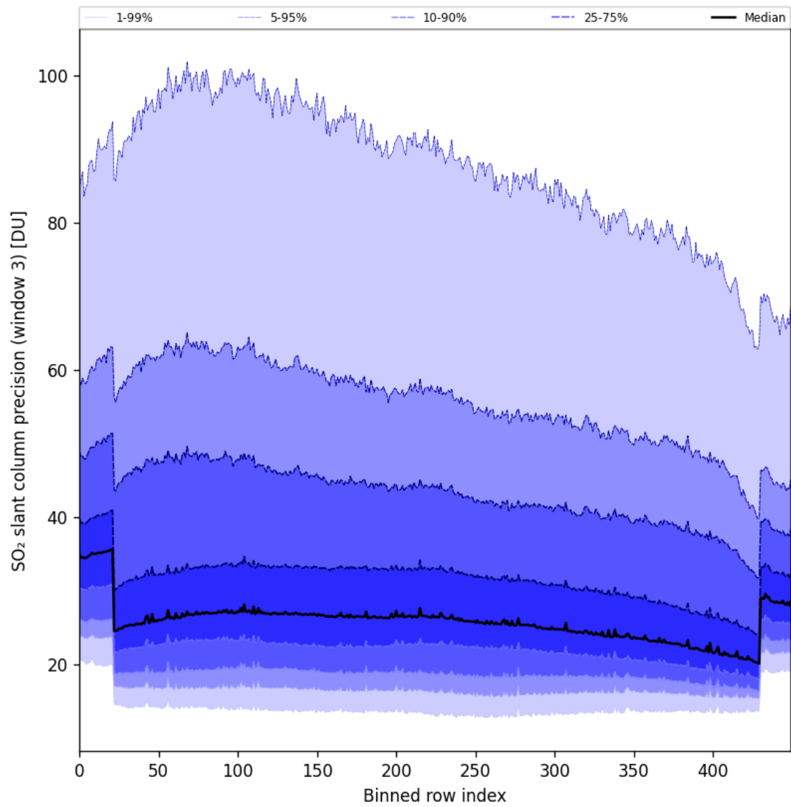
Figure 98: Along track statistics of “SO 2 slant column precision (window 3)” for 2025-09-15 to 2025-09-16
