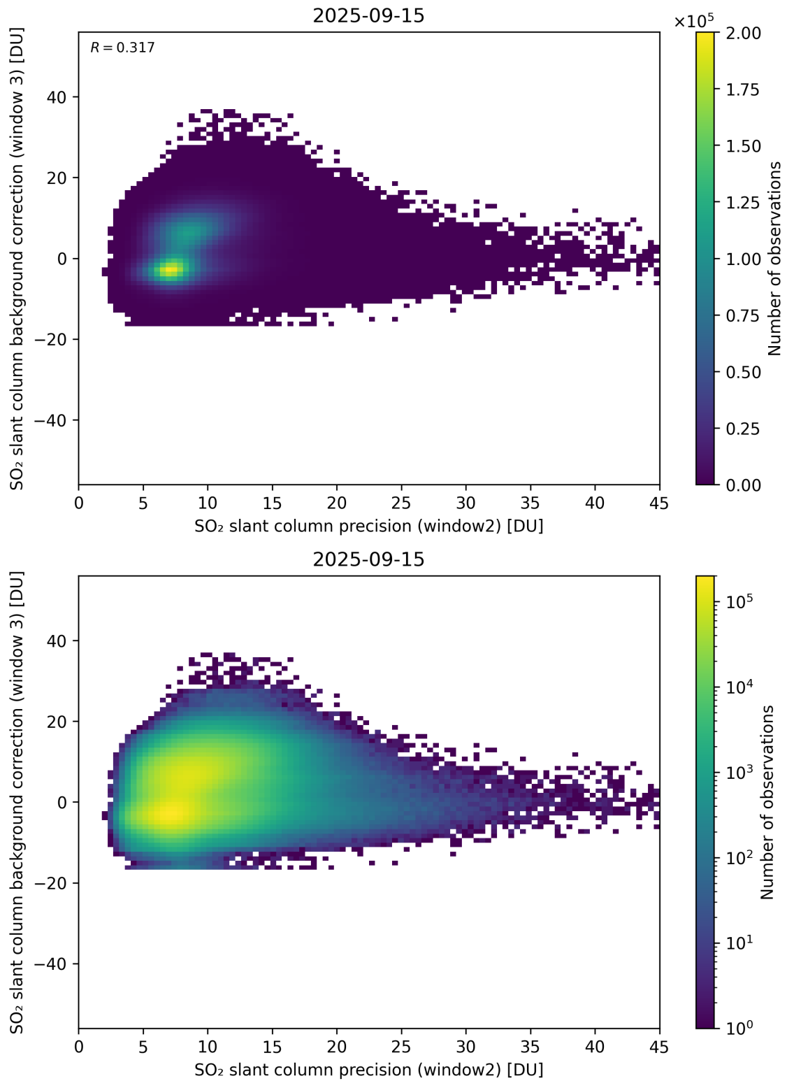
Figure 292: Scatter density plot of “SO 2 slant column precision (window2)” against “SO 2 slant column background correction (window 3)” for 2025-09-15 to 2025-09-16.
