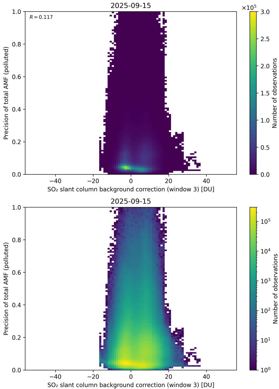
Figure 137: Scatter density plot of “SO 2 slant column background correction (window 3)” against “Precision of total AMF (polluted)” for 2025-09-15 to 2025-09-16.
