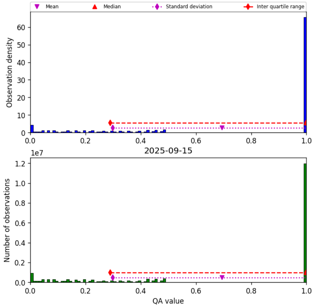
Figure 57: Histogram of “QA value” for 2025-09-15 to 2025-09-16
