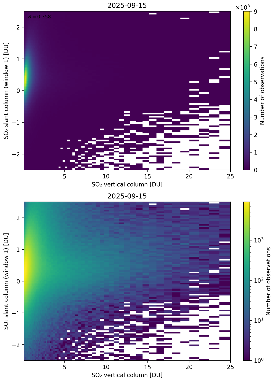
Figure 354: Scatter density plot of “SO 2 vertical column” against “SO 2 slant column (window 1)” for 2025-09-15 to 2025-09-16.
