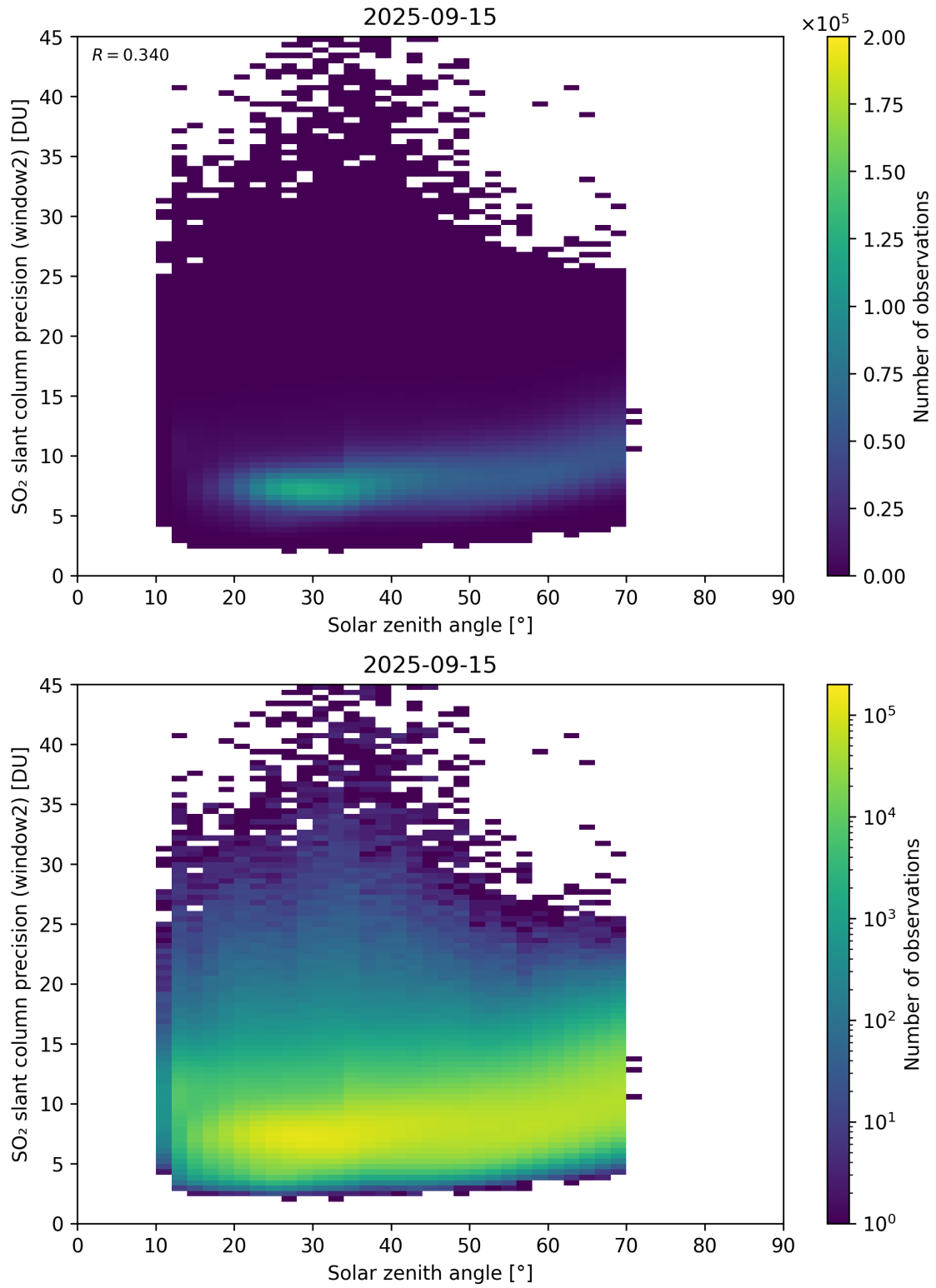
Figure 186: Scatter density plot of “Solar zenith angle” against “SO 2 slant column precision (window2)” for 2025-09-15 to 2025-09-16.
