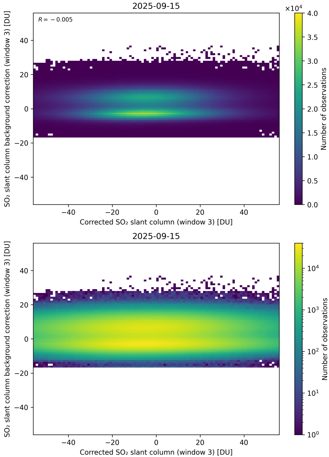
Figure 255: Scatter density plot of “Corrected SO 2 slant column (window 3)” against “SO 2 slant column background correction (window 3)” for 2025-09-15 to 2025-09-16.
