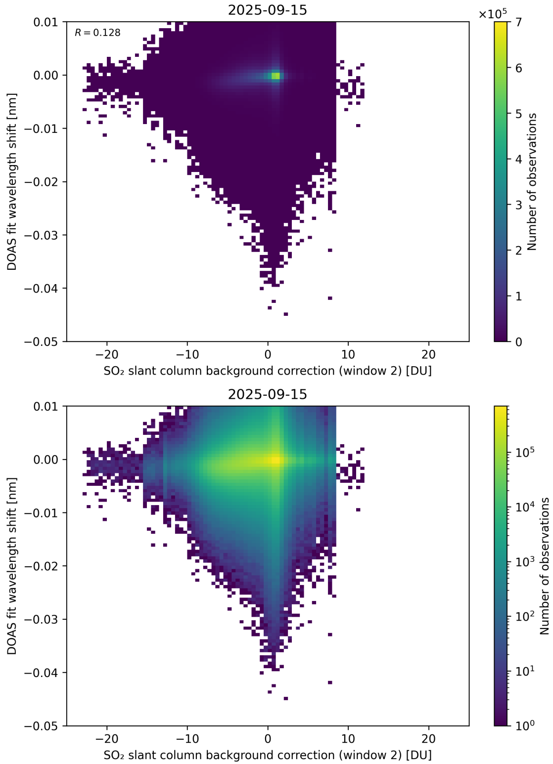
Figure 123: Scatter density plot of “SO 2 slant column background correction (window 2)” against “DOAS fit wavelength shift” for 2025-09-15 to 2025-09-16.
