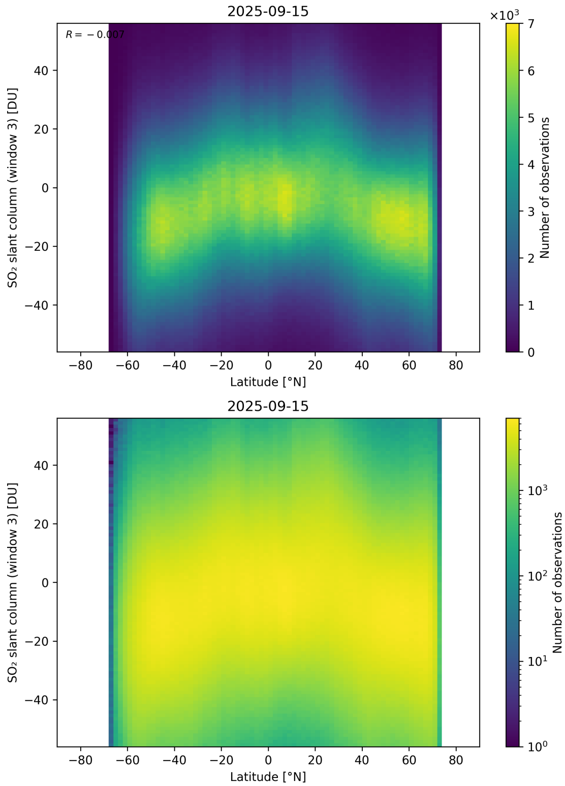
Figure 165: Scatter density plot of “Latitude” against “SO 2 slant column (window 3)” for 2025-09-15 to 2025-09-16.
