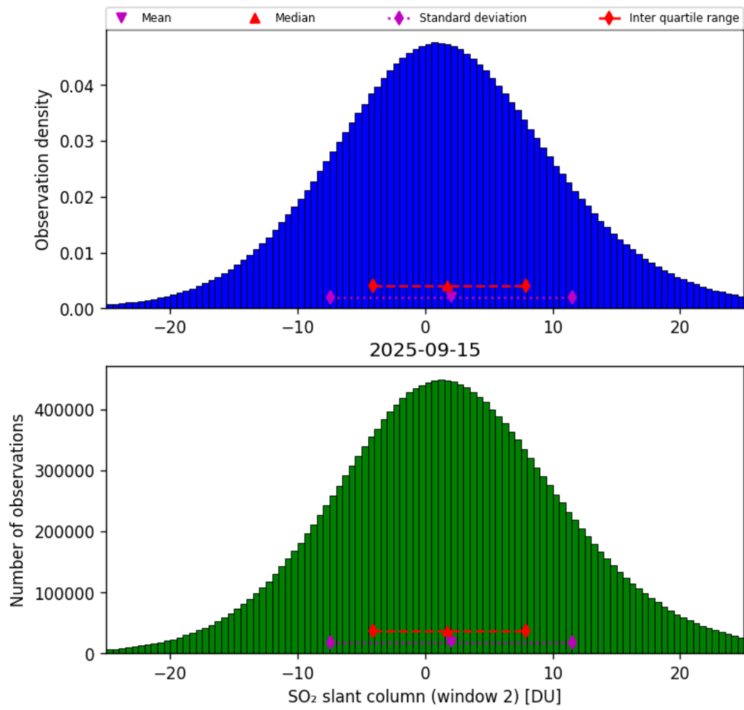
Figure 67: Histogram of “SO 2 slant column (window 2)” for 2025-09-15 to 2025-09-16
