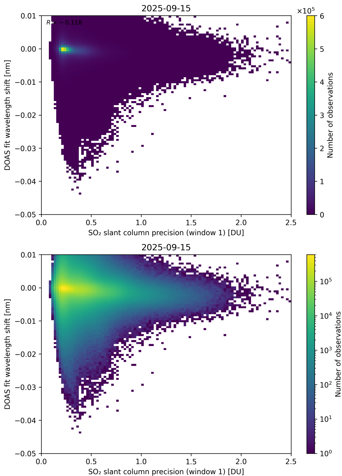
Figure 271: Scatter density plot of “SO 2 slant column precision (window 1)” against “DOAS fit wavelength shift” for 2025-09-15 to 2025-09-16.
