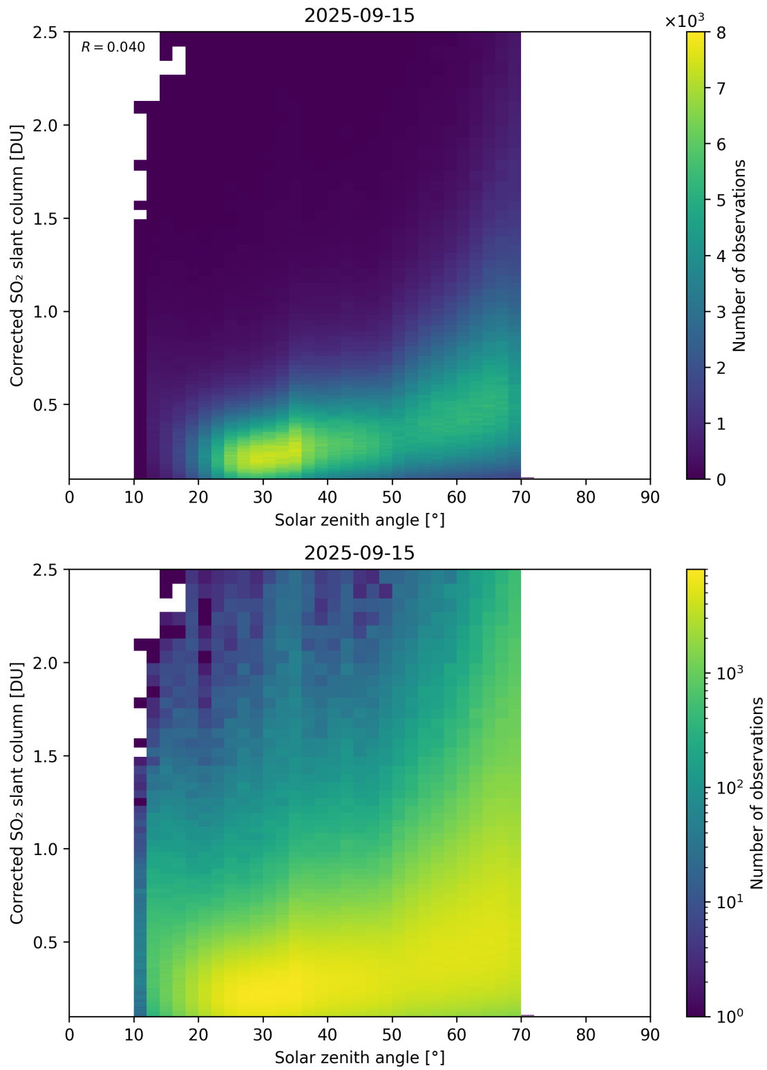
Figure 181: Scatter density plot of “Solar zenith angle” against “Corrected SO 2 slant column” for 2025-09-15 to 2025-09-16.
