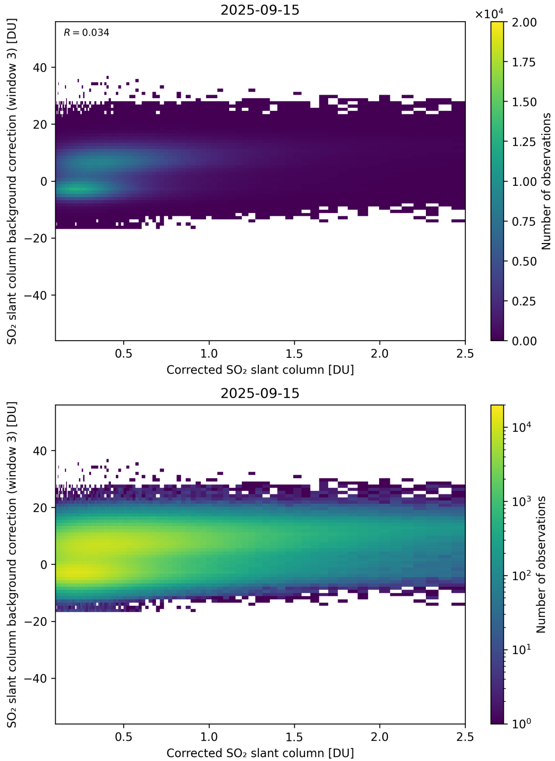
Figure 228: Scatter density plot of “Corrected SO 2 slant column” against “SO 2 slant column background correction (window 3)” for 2025-09-15 to 2025-09-16.
