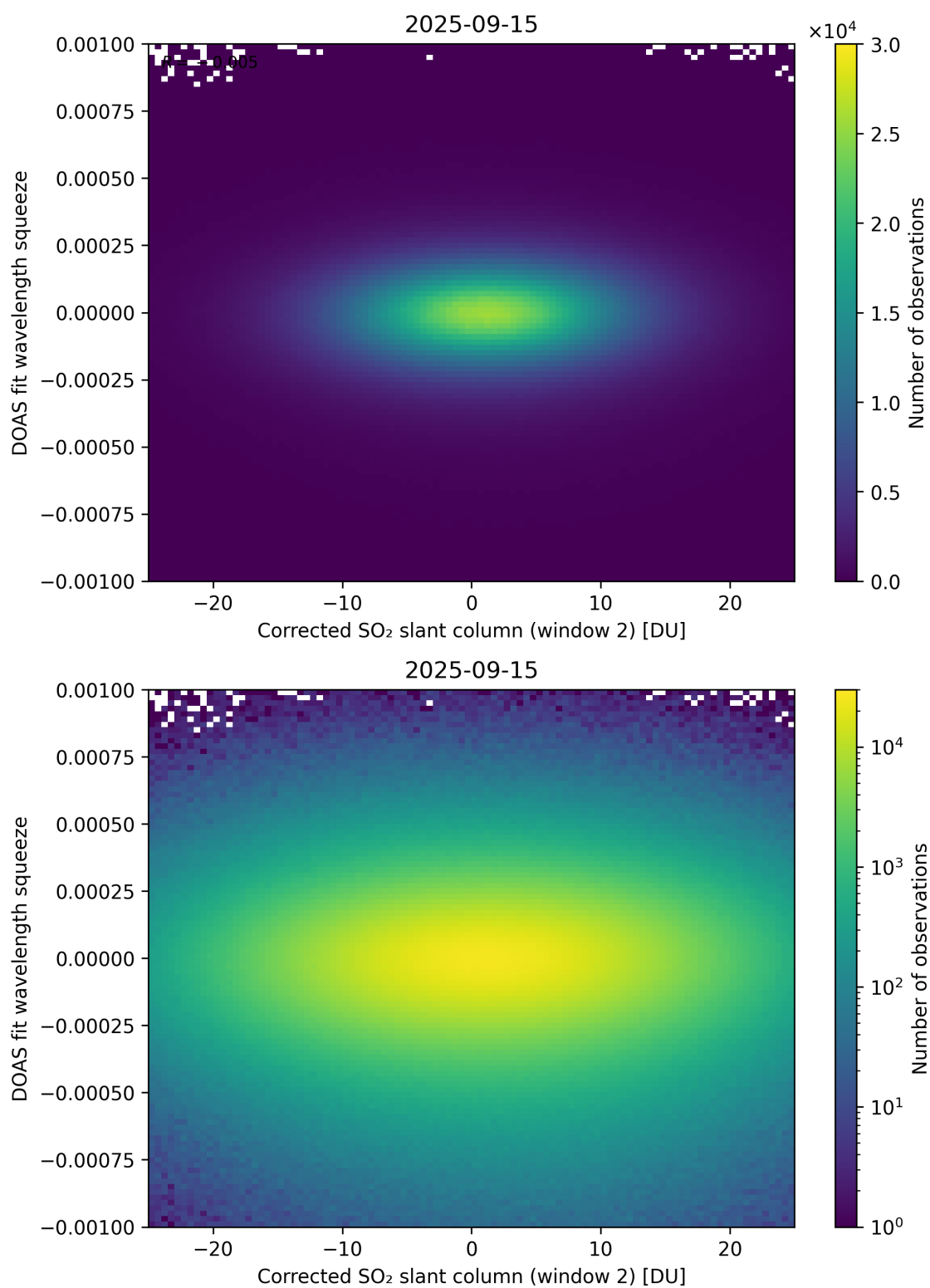
Figure 247: Scatter density plot of “Corrected SO 2 slant column (window 2)” against “DOAS fit wavelength squeeze” for 2025-09-15 to 2025-09-16.
