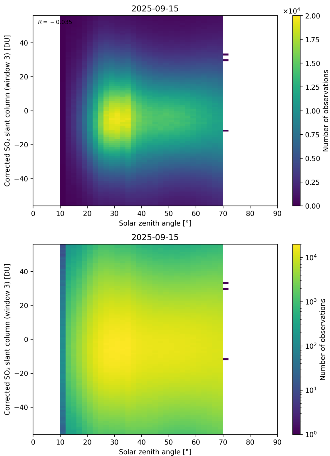
Figure 183: Scatter density plot of “Solar zenith angle” against “Corrected SO 2 slant column (window 3)” for 2025-09-15 to 2025-09-16.
