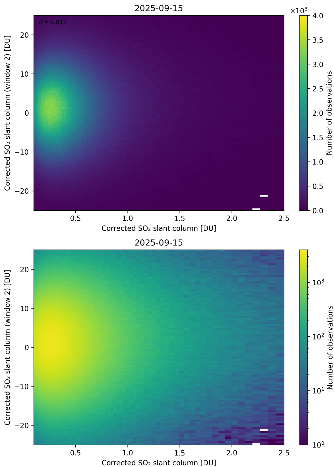
Figure 235: Scatter density plot of “Corrected SO 2 slant column” against “Corrected SO 2 slant column (window 2)” for 2025-09-15 to 2025-09-16.
