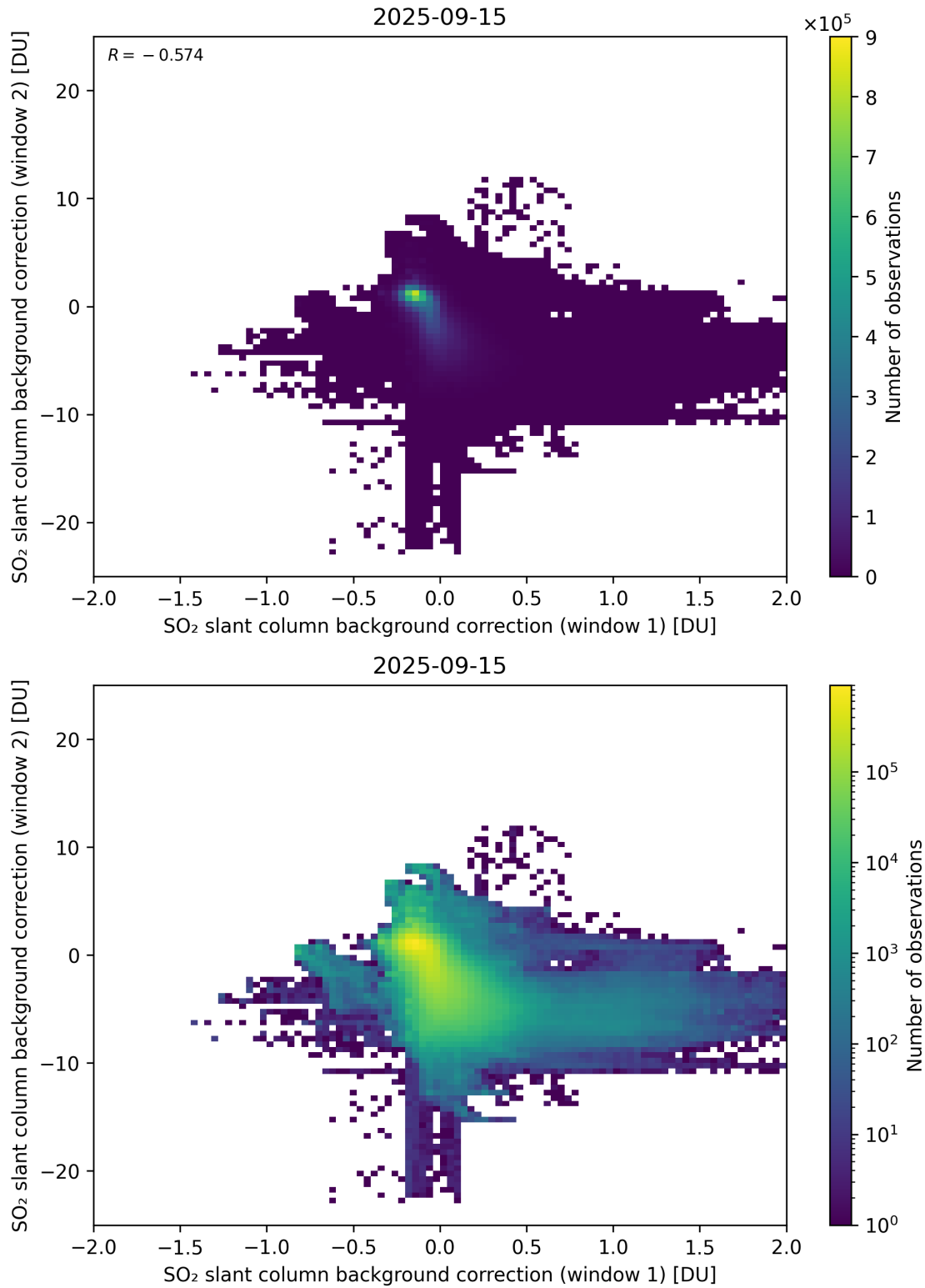
Figure 109: Scatter density plot of “SO 2 slant column background correction (window 1)” against “SO 2 slant column background correction (window 2)” for 2025-09-15 to 2025-09-16.
