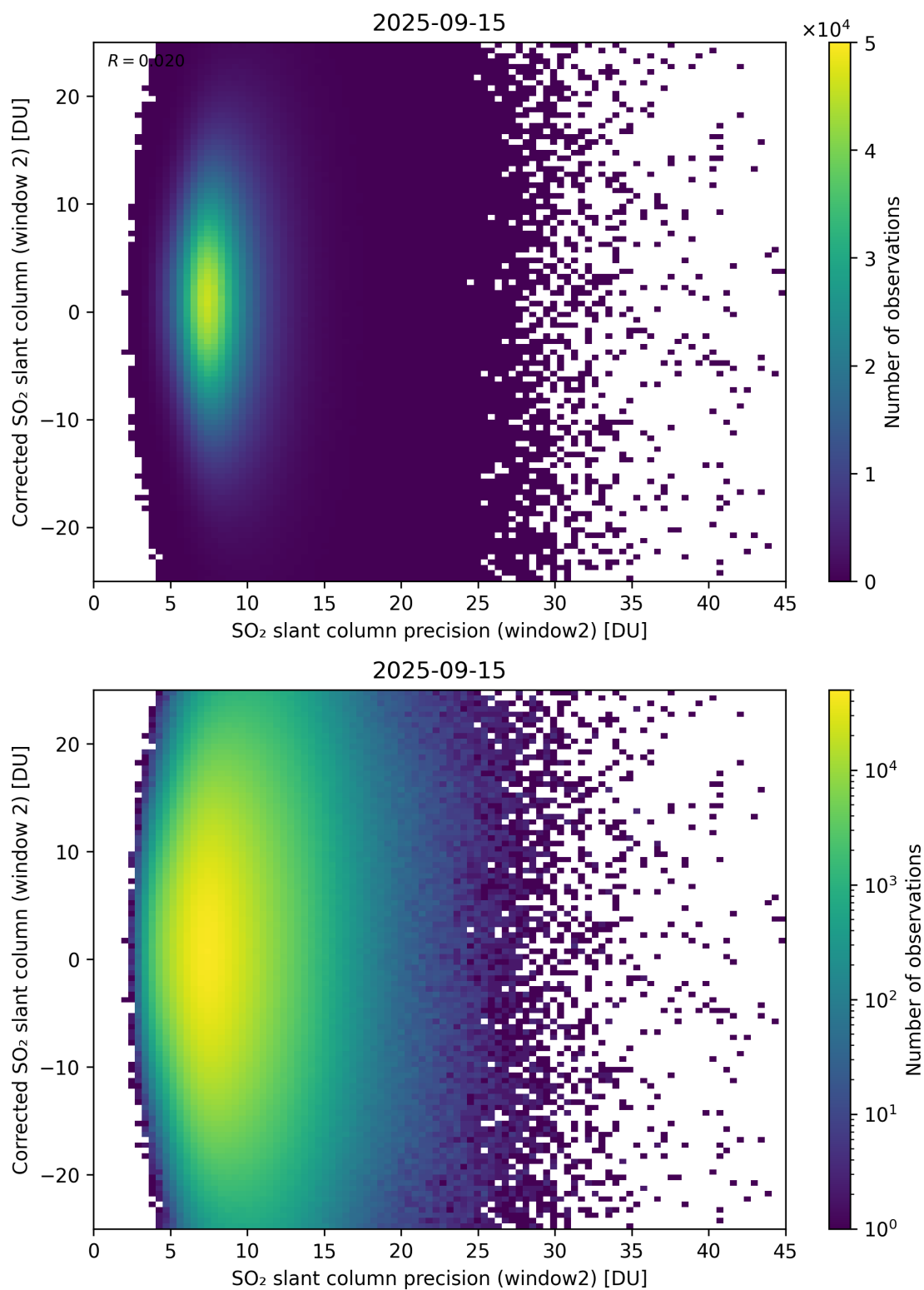
Figure 297: Scatter density plot of “SO 2 slant column precision (window2)” against “Corrected SO 2 slant column (window 2)” for 2025-09-15 to 2025-09-16.
