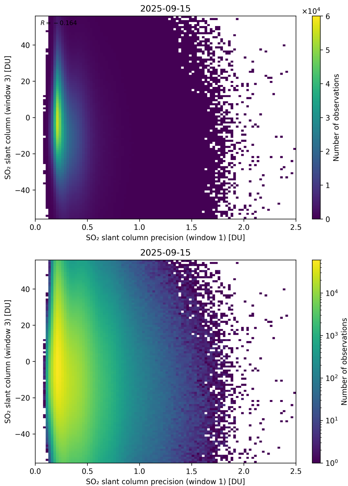
Figure 278: Scatter density plot of “SO 2 slant column precision (window 1)” against “SO 2 slant column (window 3)” for 2025-09-15 to 2025-09-16.
