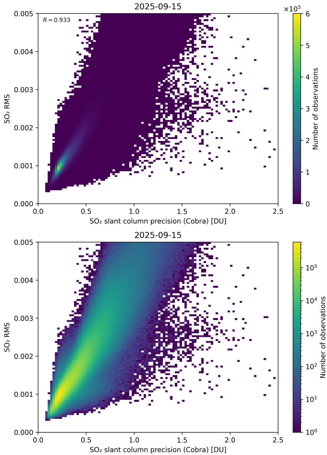
Figure 204: Scatter density plot of “SO 2 slant column precision (Cobra)” against “SO 2 RMS” for 2025-09-15 to 2025-09-16.
