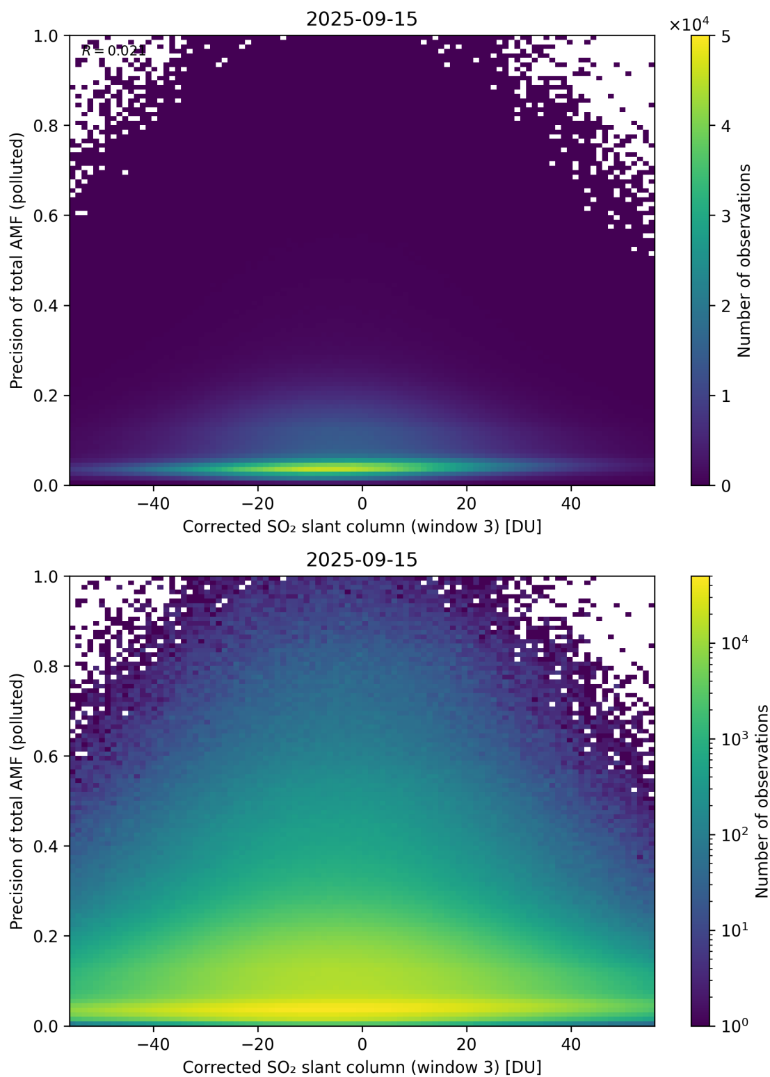
Figure 261: Scatter density plot of “Corrected SO 2 slant column (window 3)” against “Precision of total AMF (polluted)” for 2025-09-15 to 2025-09-16.
