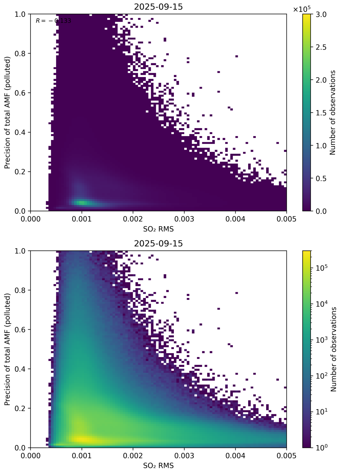
Figure 149: Scatter density plot of “SO 2 RMS” against “Precision of total AMF (polluted)” for 2025-09-15 to 2025-09-16.
