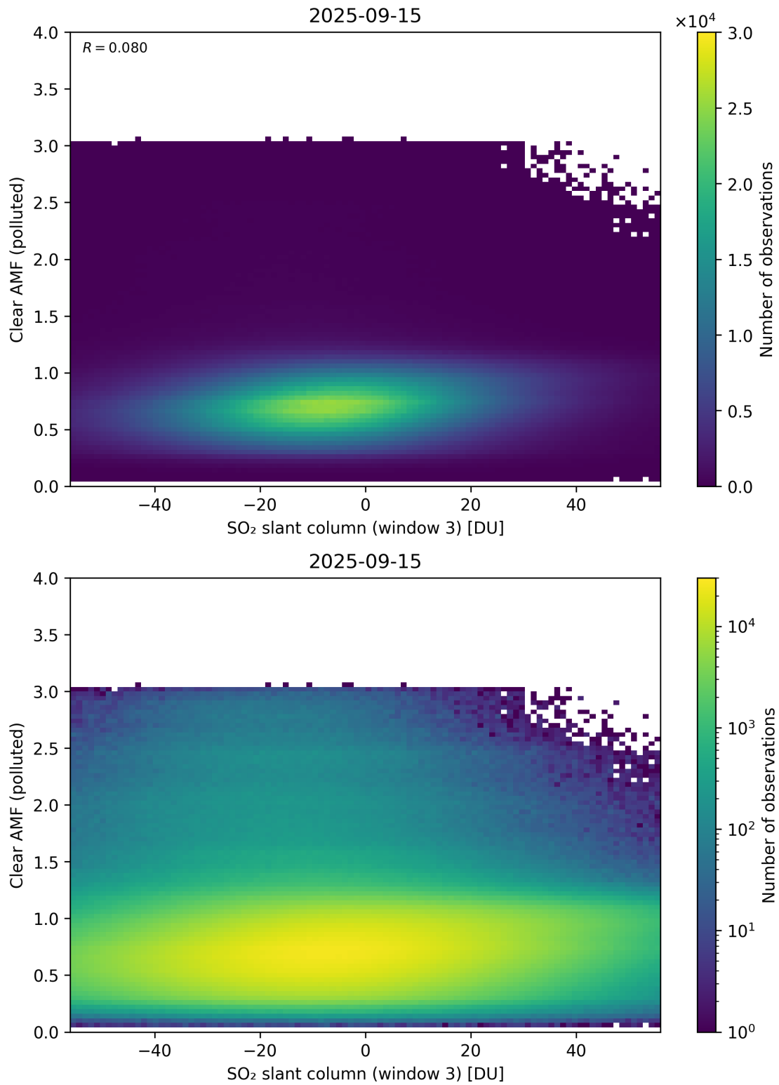
Figure 315: Scatter density plot of “SO 2 slant column (window 3)” against “Clear AMF (polluted)” for 2025-09-15 to 2025-09-16.
