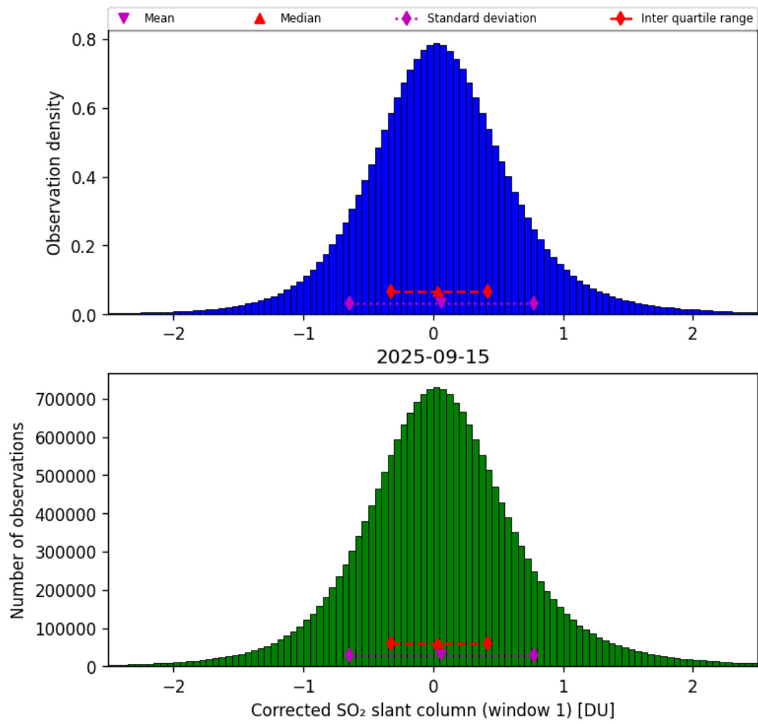
Figure 65: Histogram of “Corrected SO 2 slant column (window 1)” for 2025-09-15 to 2025-09-16
