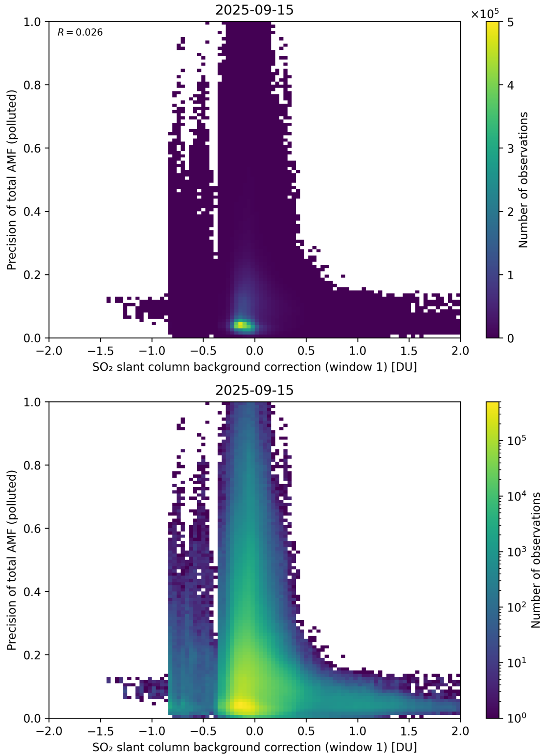
Figure 121: Scatter density plot of “SO 2 slant column background correction (window 1)” against “Precision of total AMF (polluted)” for 2025-09-15 to 2025-09-16.
