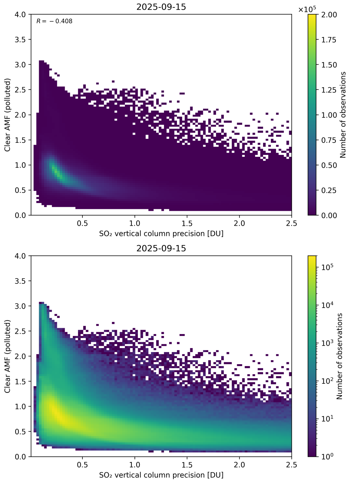
Figure 335: Scatter density plot of “SO 2 vertical column precision” against “Clear AMF (polluted)” for 2025-09-15 to 2025-09-16.
