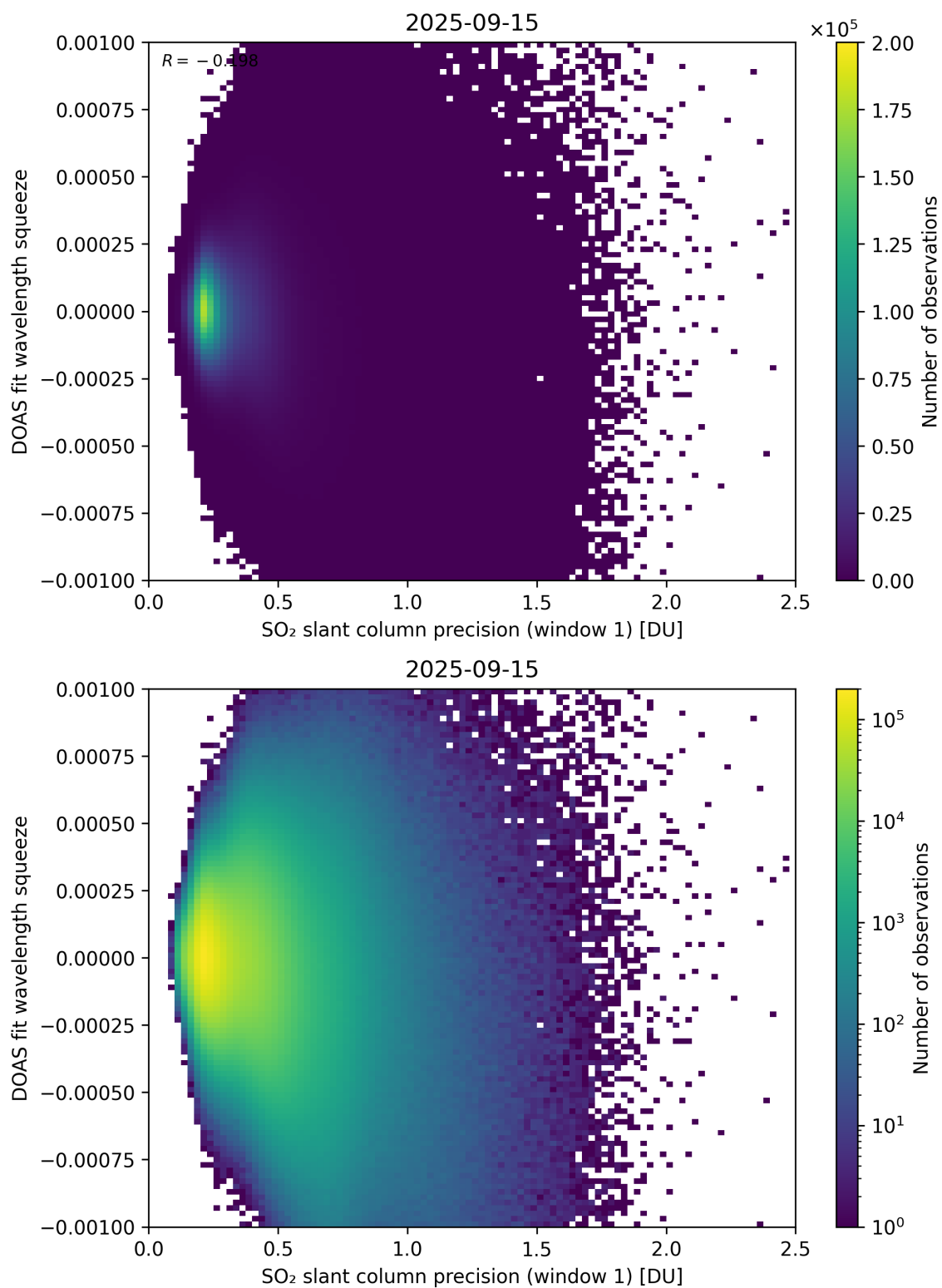
Figure 272: Scatter density plot of “SO 2 slant column precision (window 1)” against “DOAS fit wavelength squeeze” for 2025-09-15 to 2025-09-16.
