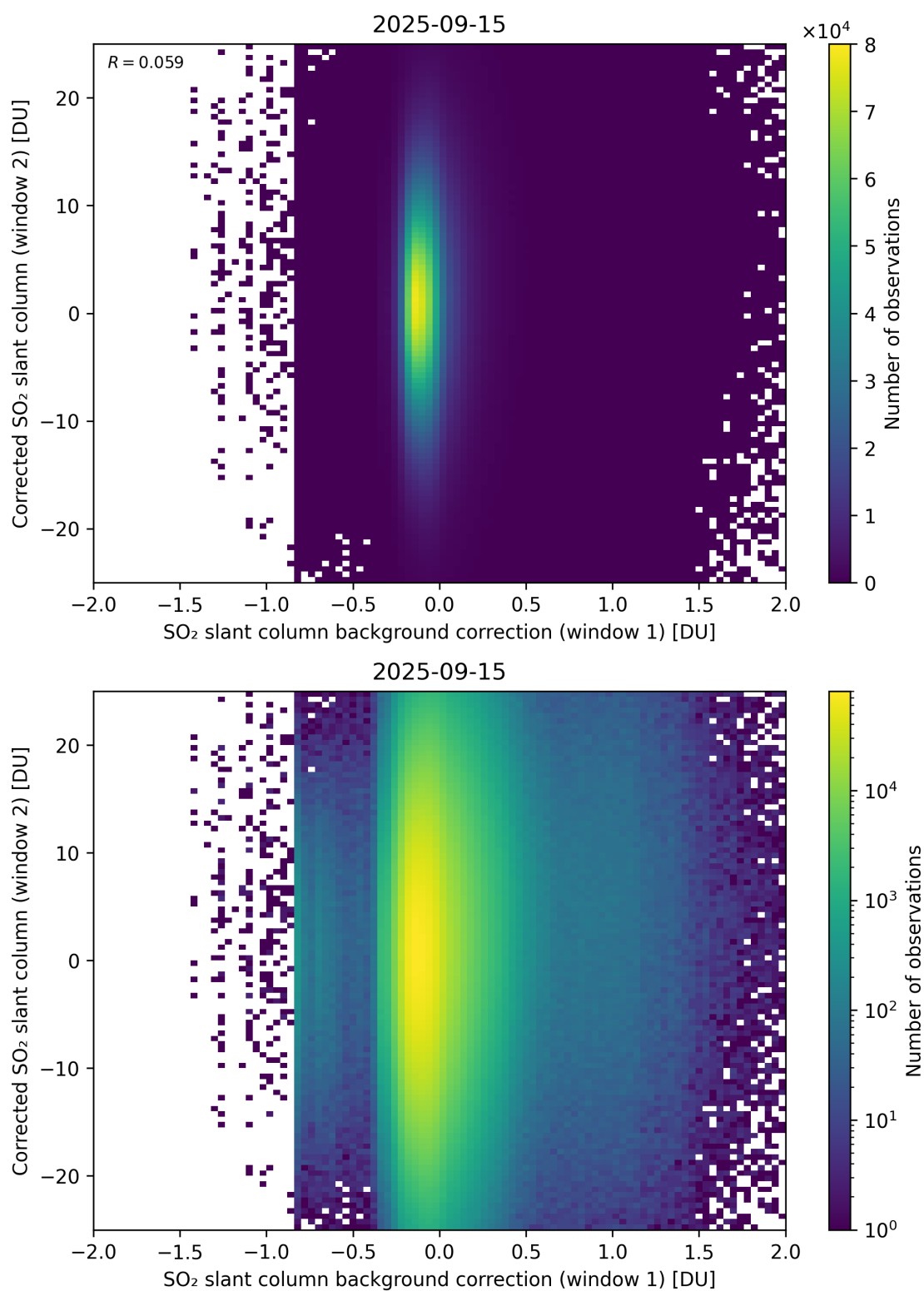
Figure 115: Scatter density plot of “SO 2 slant column background correction (window 1)” against “Corrected SO 2 slant column (window 2)” for 2025-09-15 to 2025-09-16.
