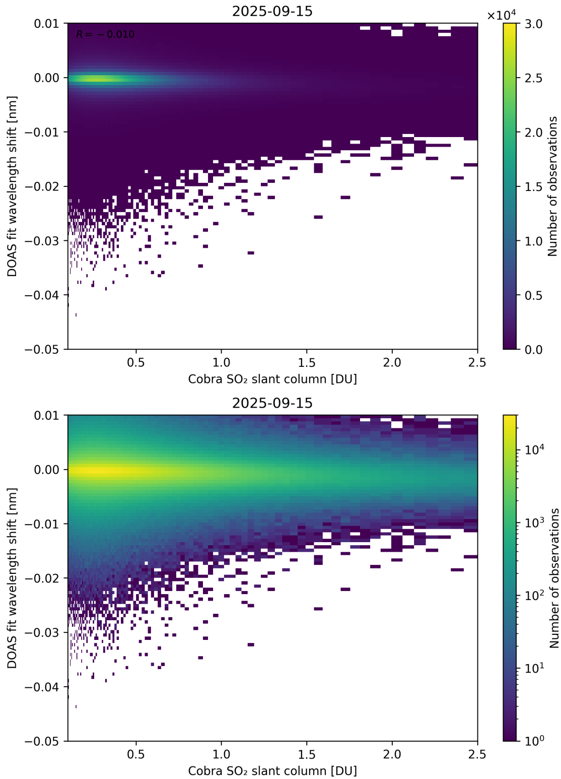
Figure 196: Scatter density plot of “Cobra SO 2 slant column” against “DOAS fit wavelength shift” for 2025-09-15 to 2025-09-16.
