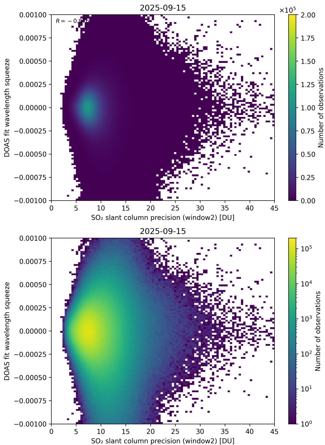
Figure 294: Scatter density plot of “SO 2 slant column precision (window2)” against “DOAS fit wavelength squeeze” for 2025-09-15 to 2025-09-16.
