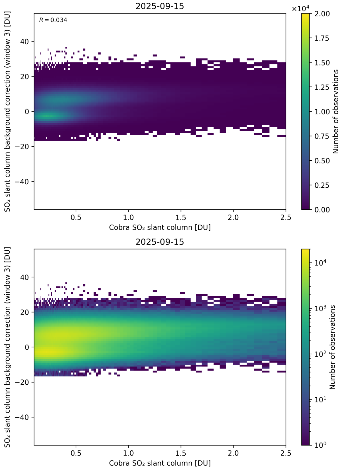
Figure 195: Scatter density plot of “Cobra SO 2 slant column” against “SO 2 slant column background correction (window 3)” for 2025-09-15 to 2025-09-16.
