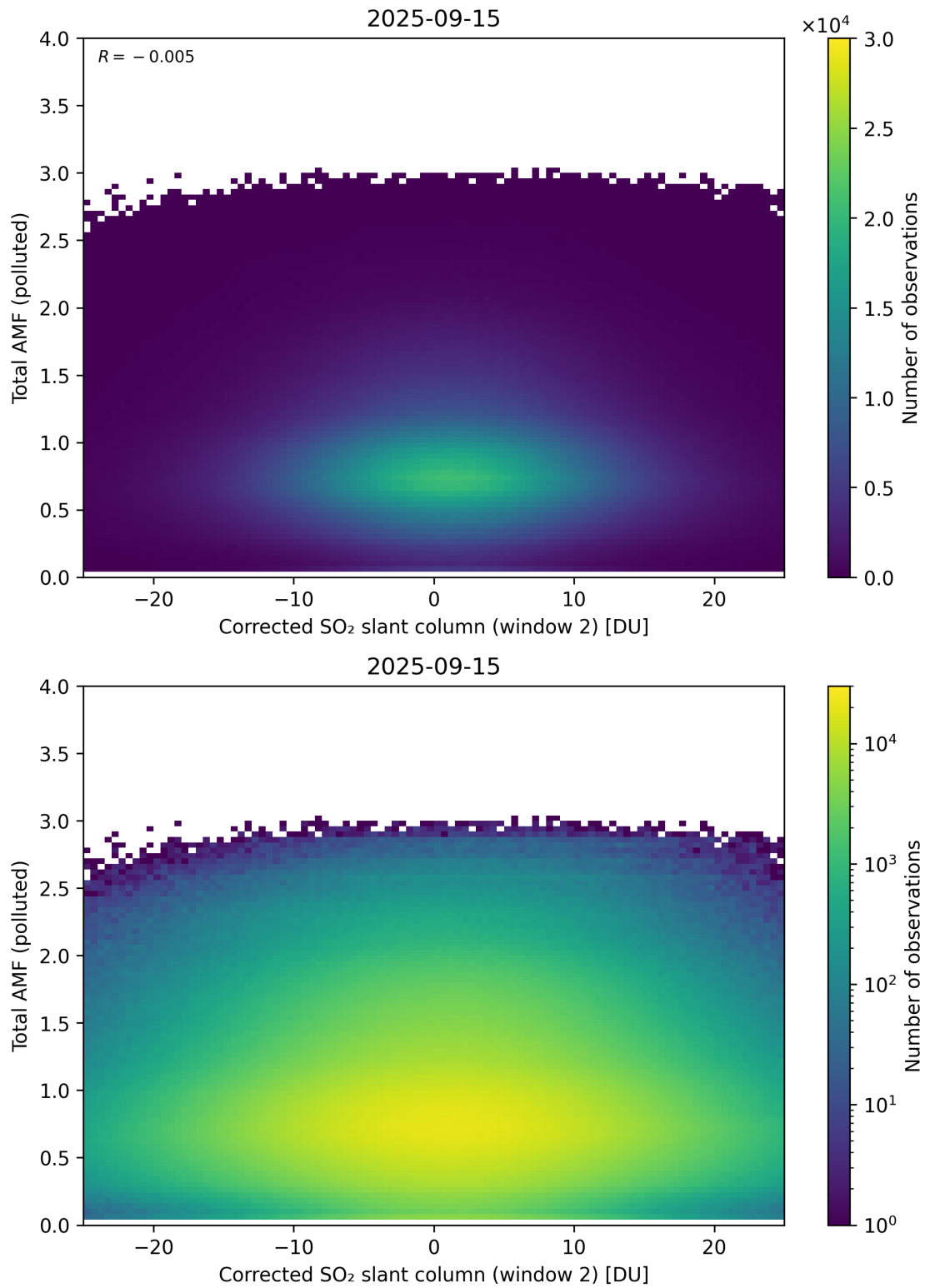
Figure 253: Scatter density plot of “Corrected SO 2 slant column (window 2)” against “Total AMF (polluted)” for 2025-09-15 to 2025-09-16.
