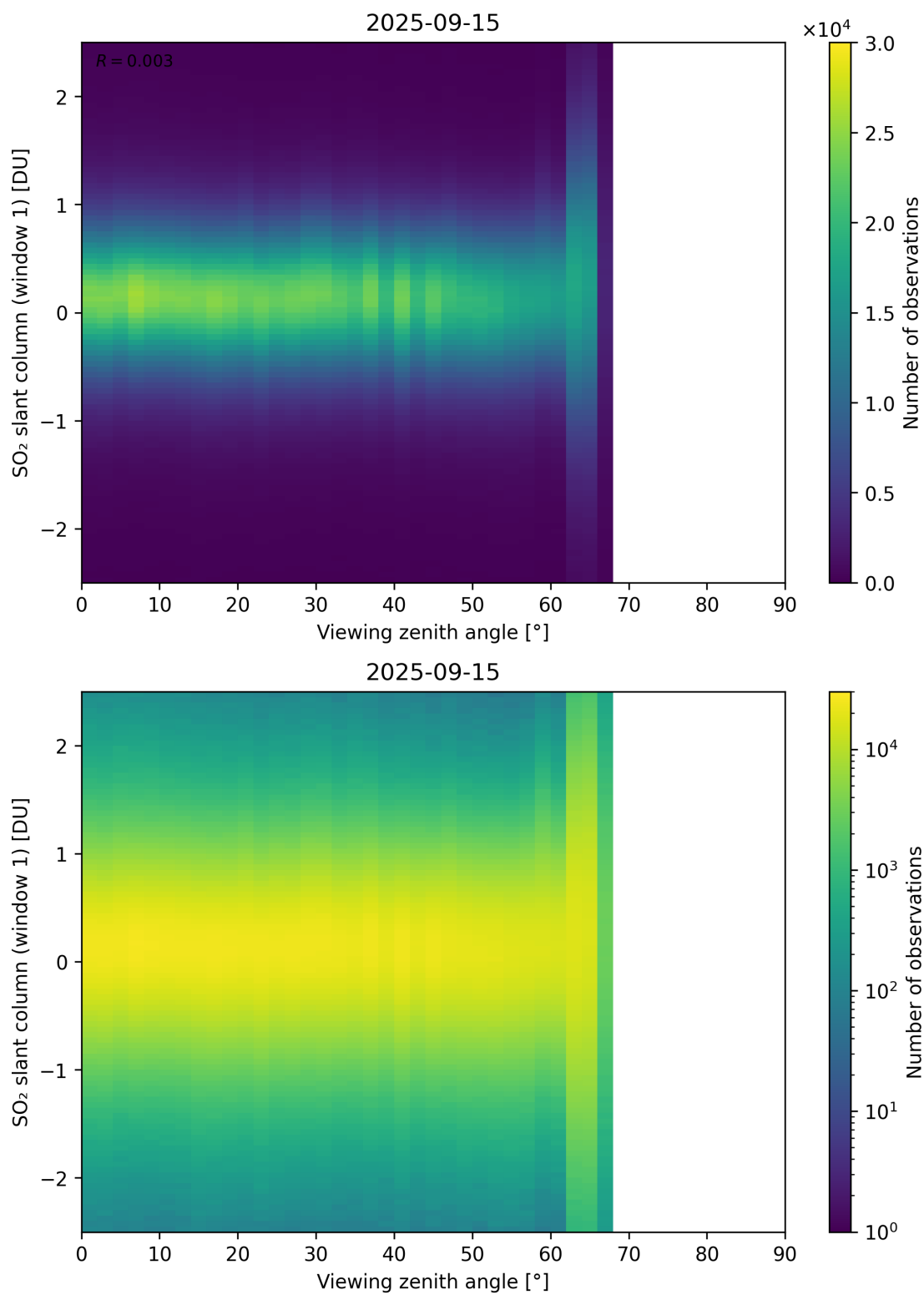
Figure 376: Scatter density plot of “Viewing zenith angle” against “SO 2 slant column (window 1)” for 2025-09-15 to 2025-09-16.
