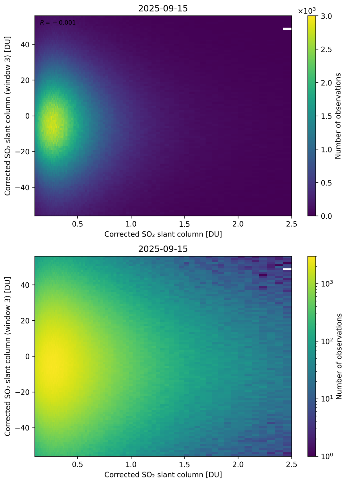
Figure 236: Scatter density plot of “Corrected SO 2 slant column” against “Corrected SO 2 slant column (window 3)” for 2025-09-15 to 2025-09-16.
