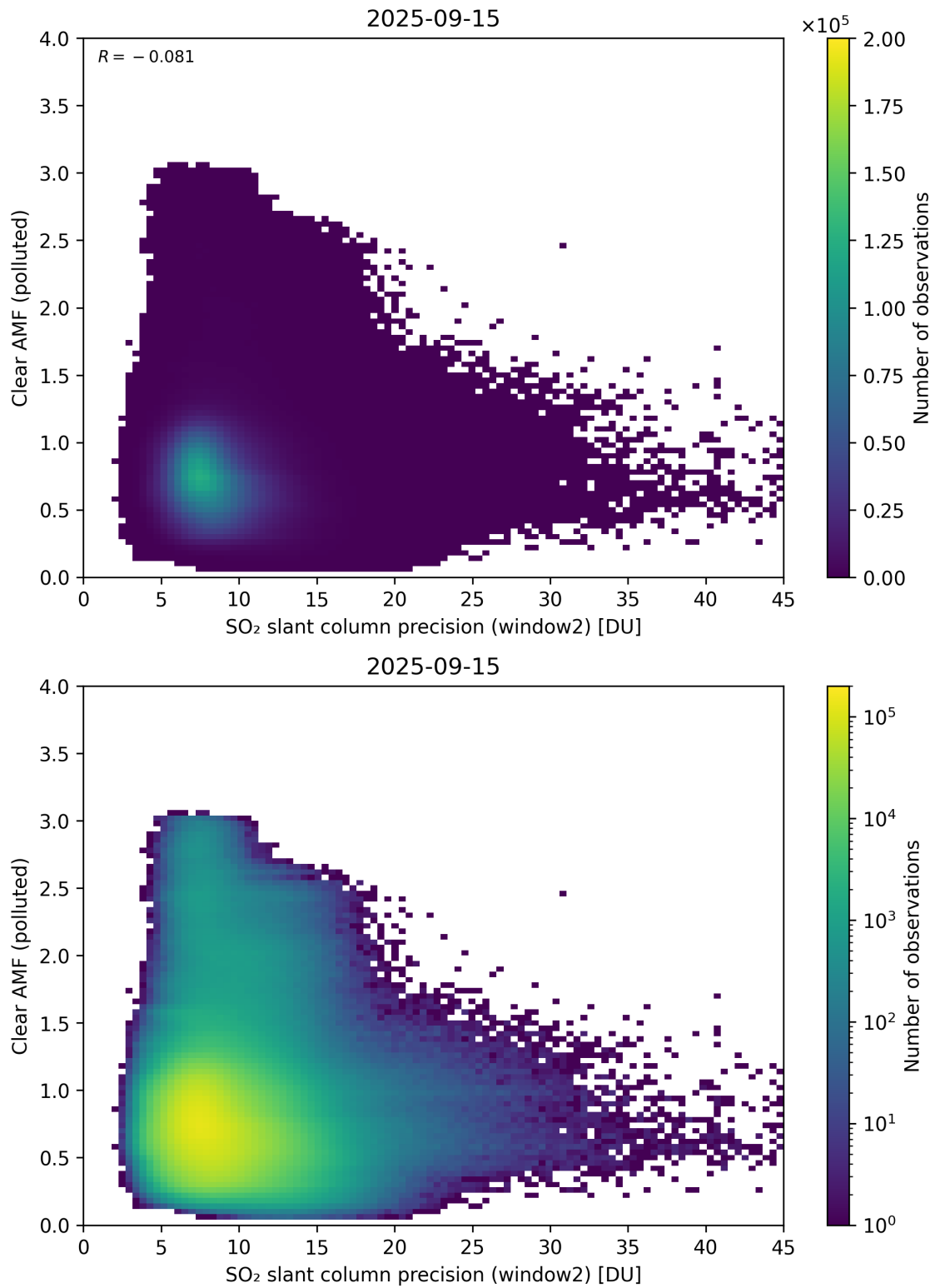
Figure 296: Scatter density plot of “SO 2 slant column precision (window2)” against “Clear AMF (polluted)” for 2025-09-15 to 2025-09-16.
