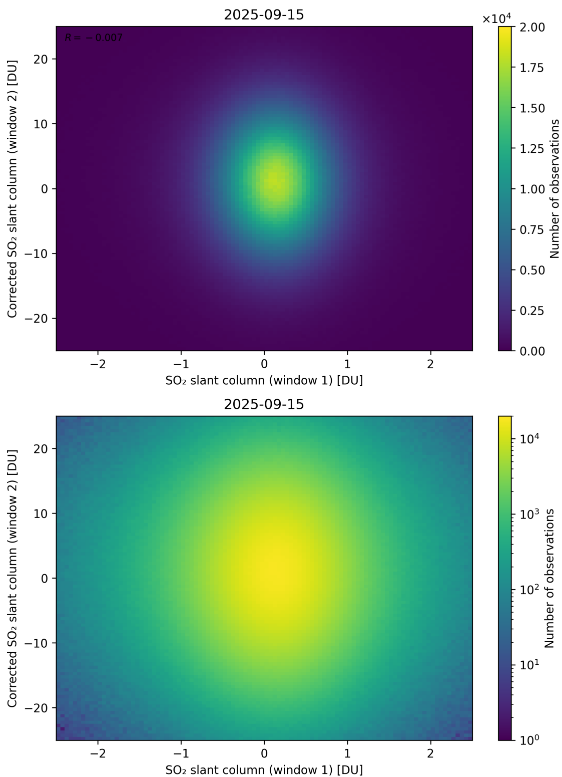
Figure 283: Scatter density plot of “SO 2 slant column (window 1)” against “Corrected SO 2 slant column (window 2)” for 2025-09-15 to 2025-09-16.
