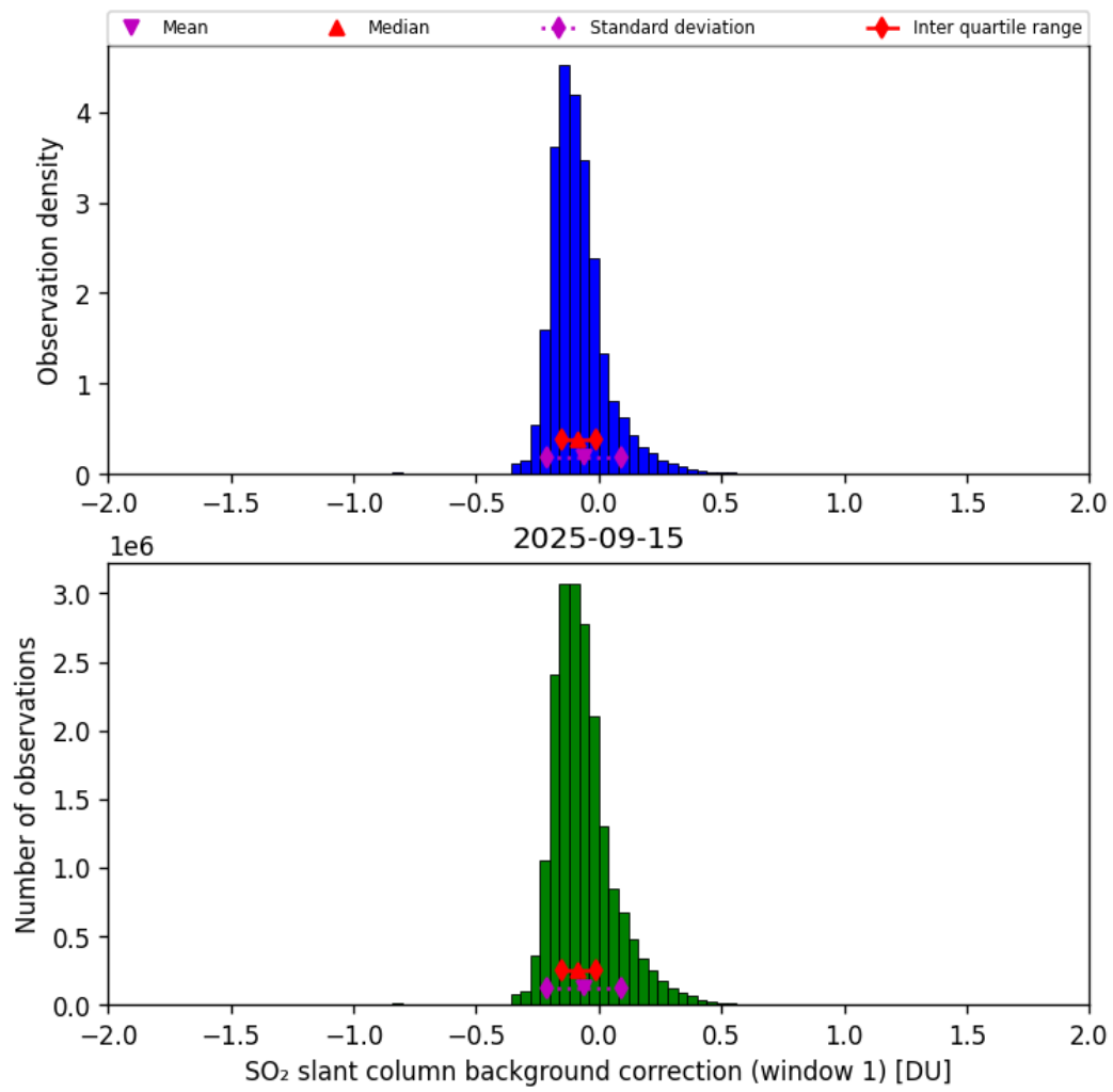
Figure 66: Histogram of “SO 2 slant column background correction (window 1)” for 2025-09-15 to 2025-09-16
