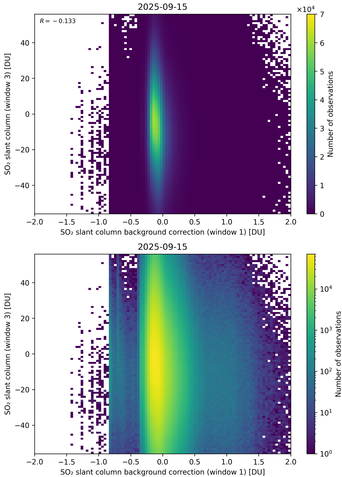
Figure 118: Scatter density plot of “SO 2 slant column background correction (window 1)” against “SO 2 slant column (window 3)” for 2025-09-15 to 2025-09-16.
