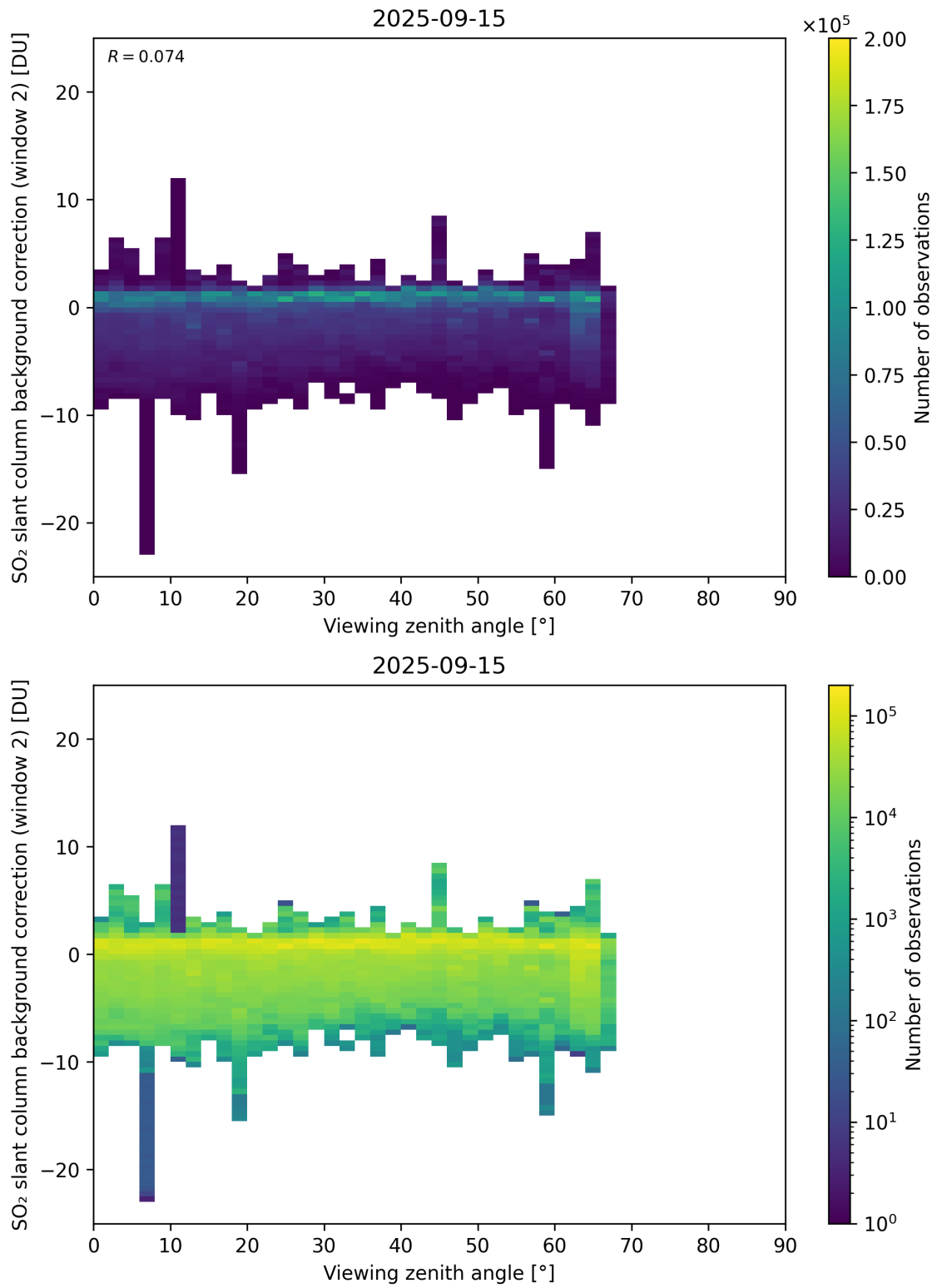
Figure 363: Scatter density plot of “Viewing zenith angle” against “SO 2 slant column background correction (window 2)” for 2025-09-15 to 2025-09-16.
