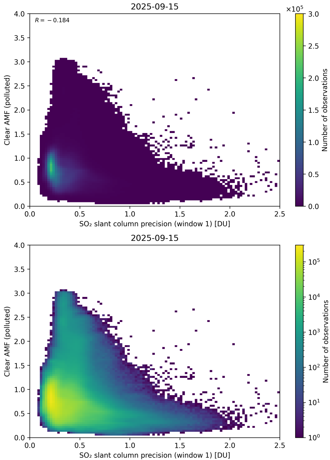
Figure 274: Scatter density plot of “SO 2 slant column precision (window 1)” against “Clear AMF (polluted)” for 2025-09-15 to 2025-09-16.
