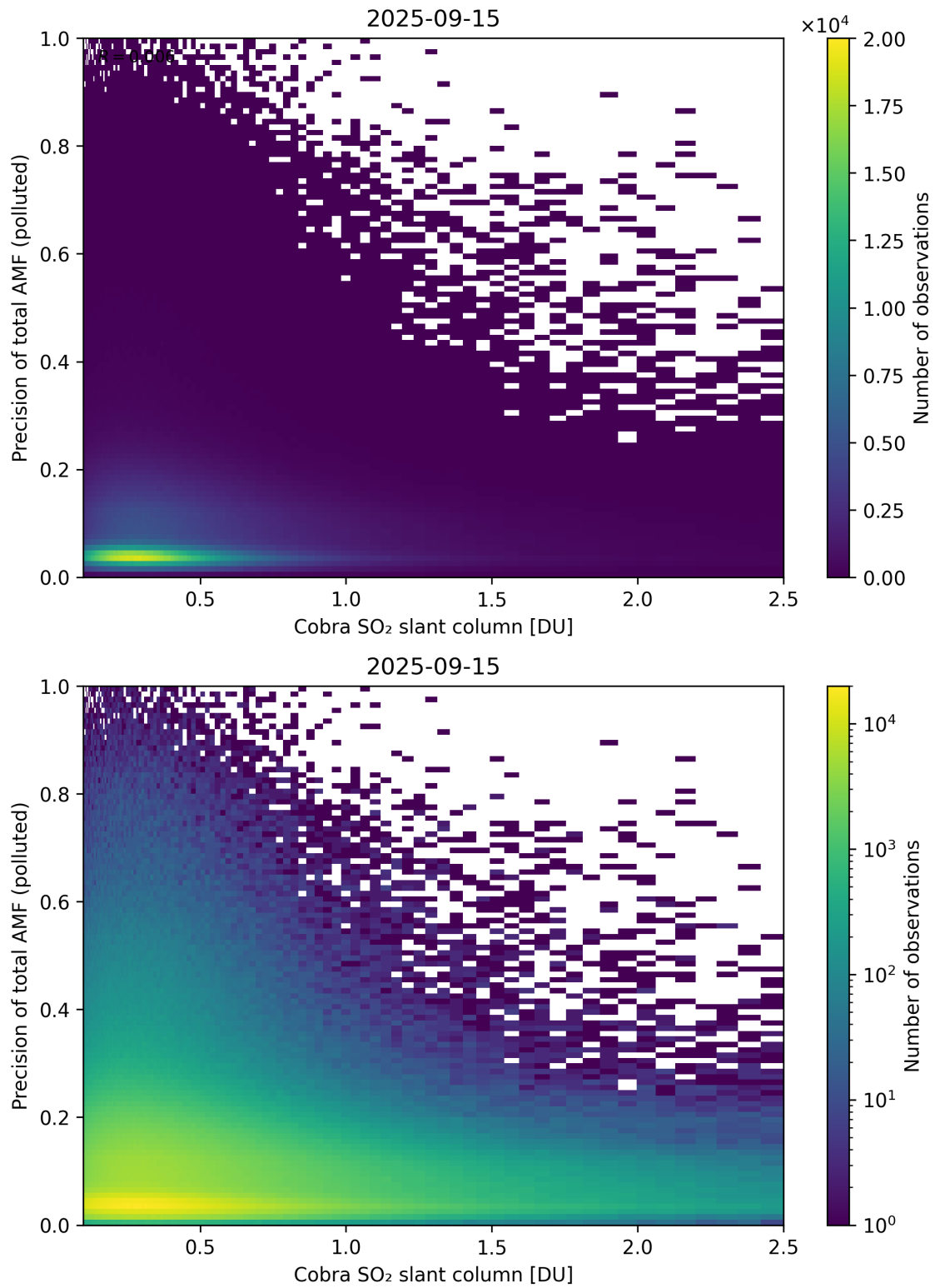
Figure 225: Scatter density plot of “Cobra SO 2 slant column” against “Precision of total AMF (polluted)” for 2025-09-15 to 2025-09-16.
