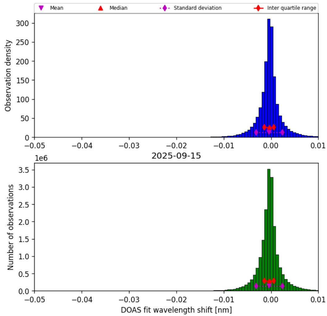
Figure 76: Histogram of “DOAS fit wavelength shift” for 2025-09-15 to 2025-09-16
