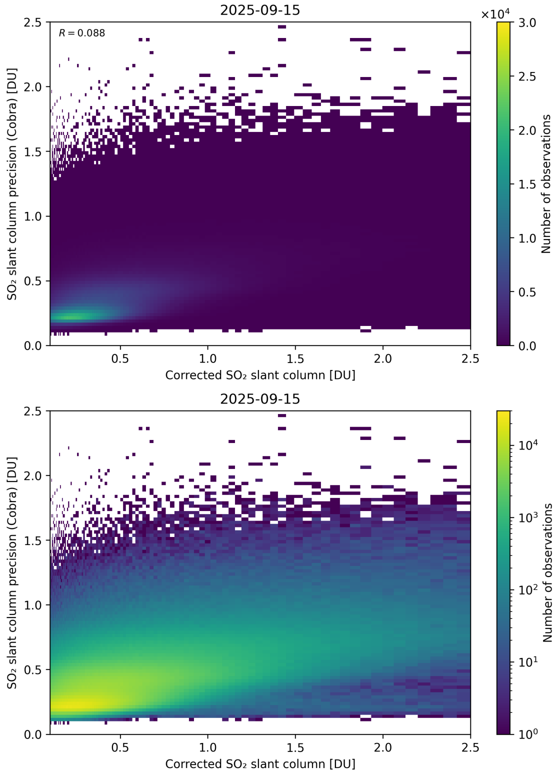
Figure 234: Scatter density plot of “Corrected SO 2 slant column” against “SO 2 slant column precision (Cobra)” for 2025-09-15 to 2025-09-16.
