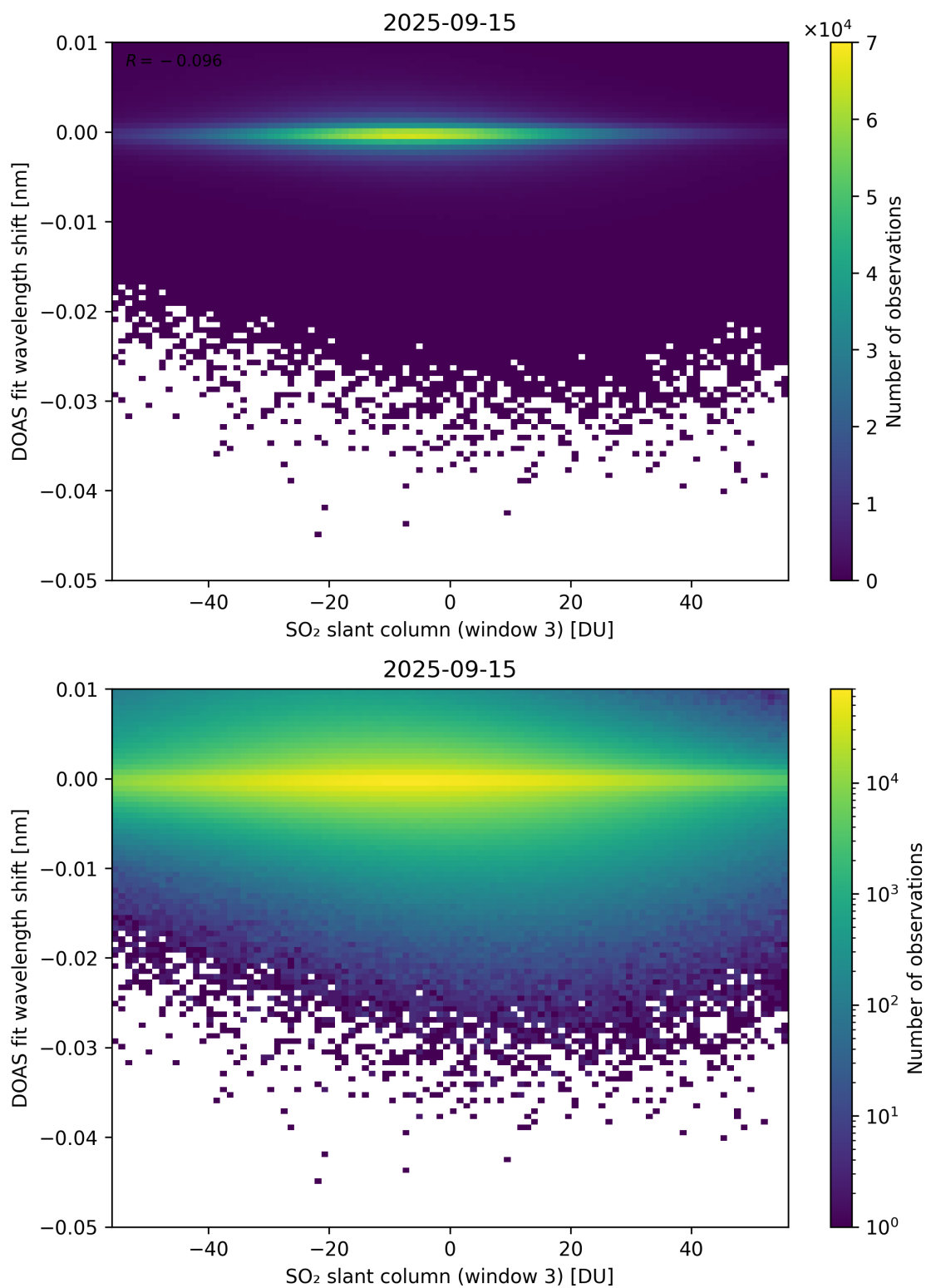
Figure 304: Scatter density plot of “SO 2 slant column (window 3)” against “DOAS fit wavelength shift” for 2025-09-15 to 2025-09-16.
