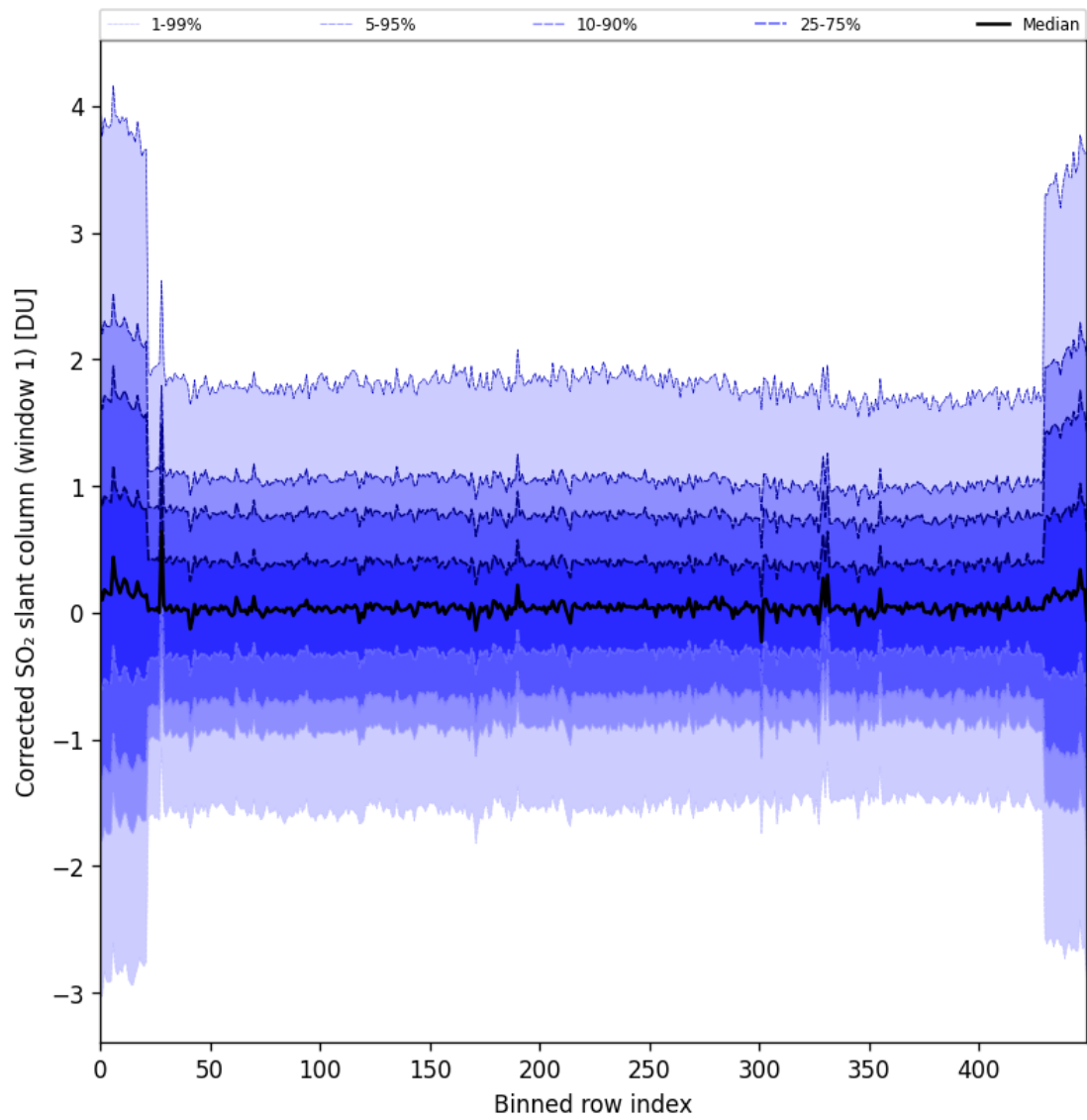
Figure 91: Along track statistics of “Corrected SO 2 slant column (window 1)” for 2025-09-15 to 2025-09-16
