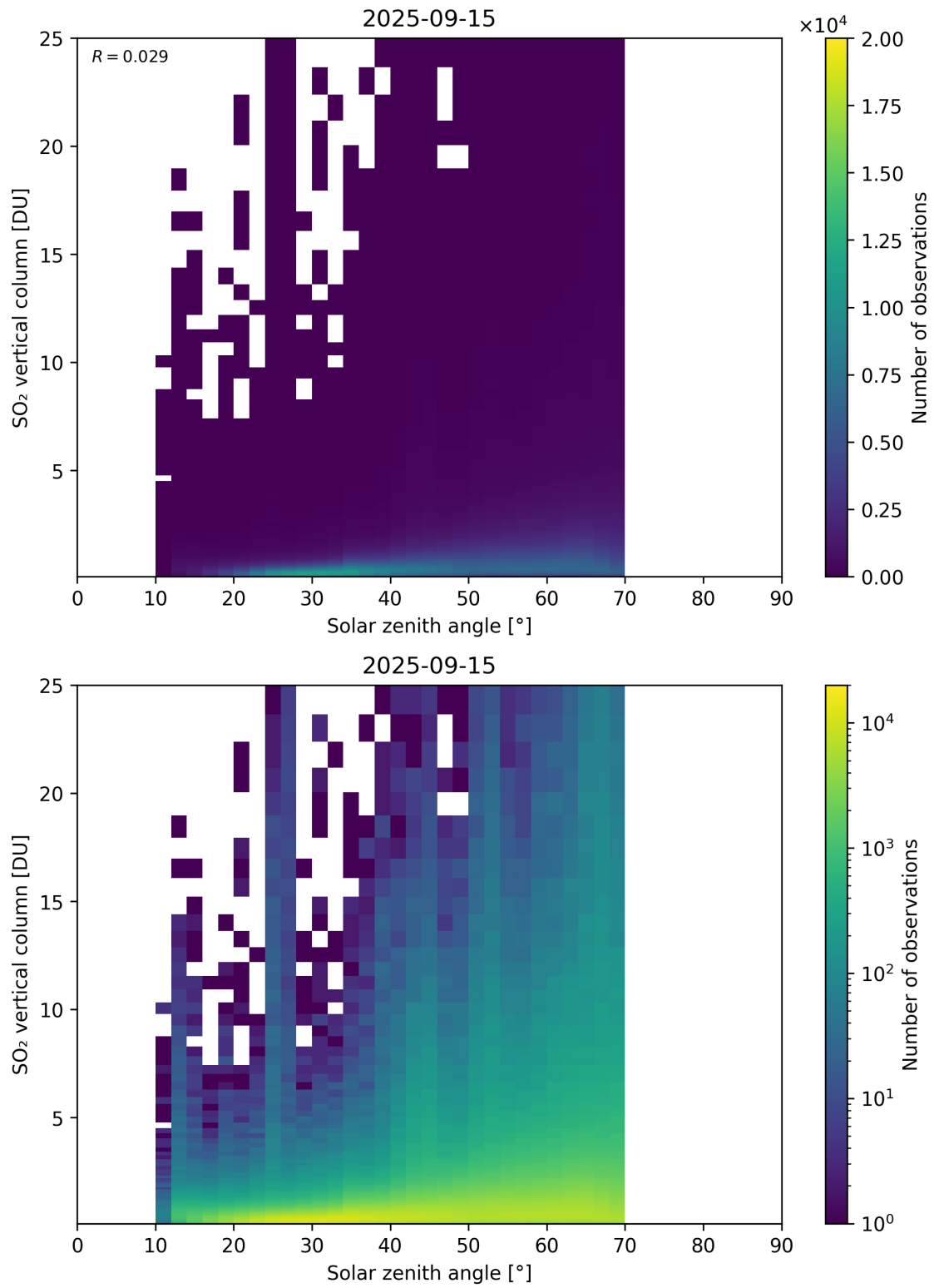
Figure 191: Scatter density plot of “Solar zenith angle” against “SO 2 vertical column” for 2025-09-15 to 2025-09-16.
