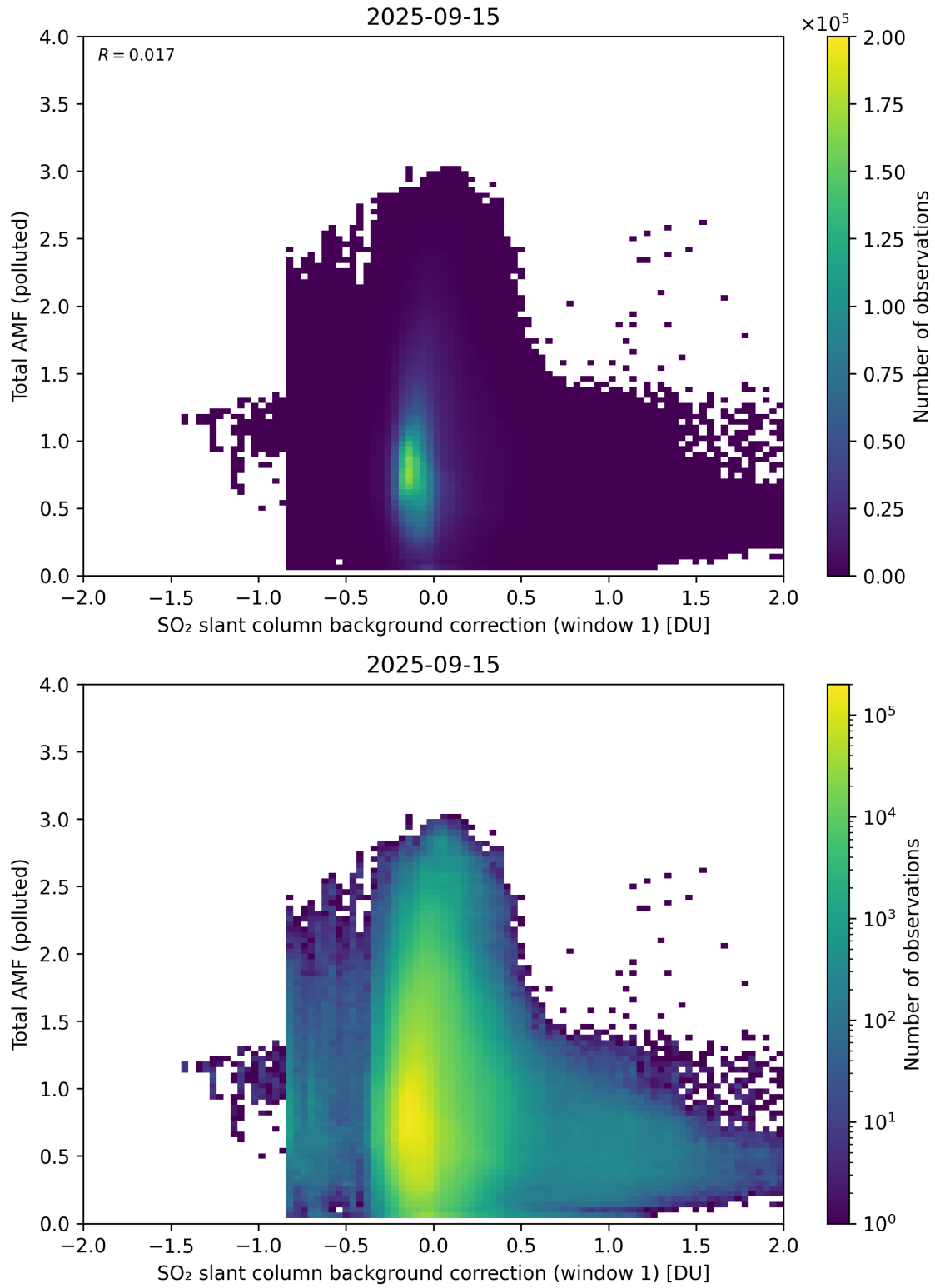
Figure 120: Scatter density plot of “SO 2 slant column background correction (window 1)” against “Total AMF (polluted)” for 2025-09-15 to 2025-09-16.
