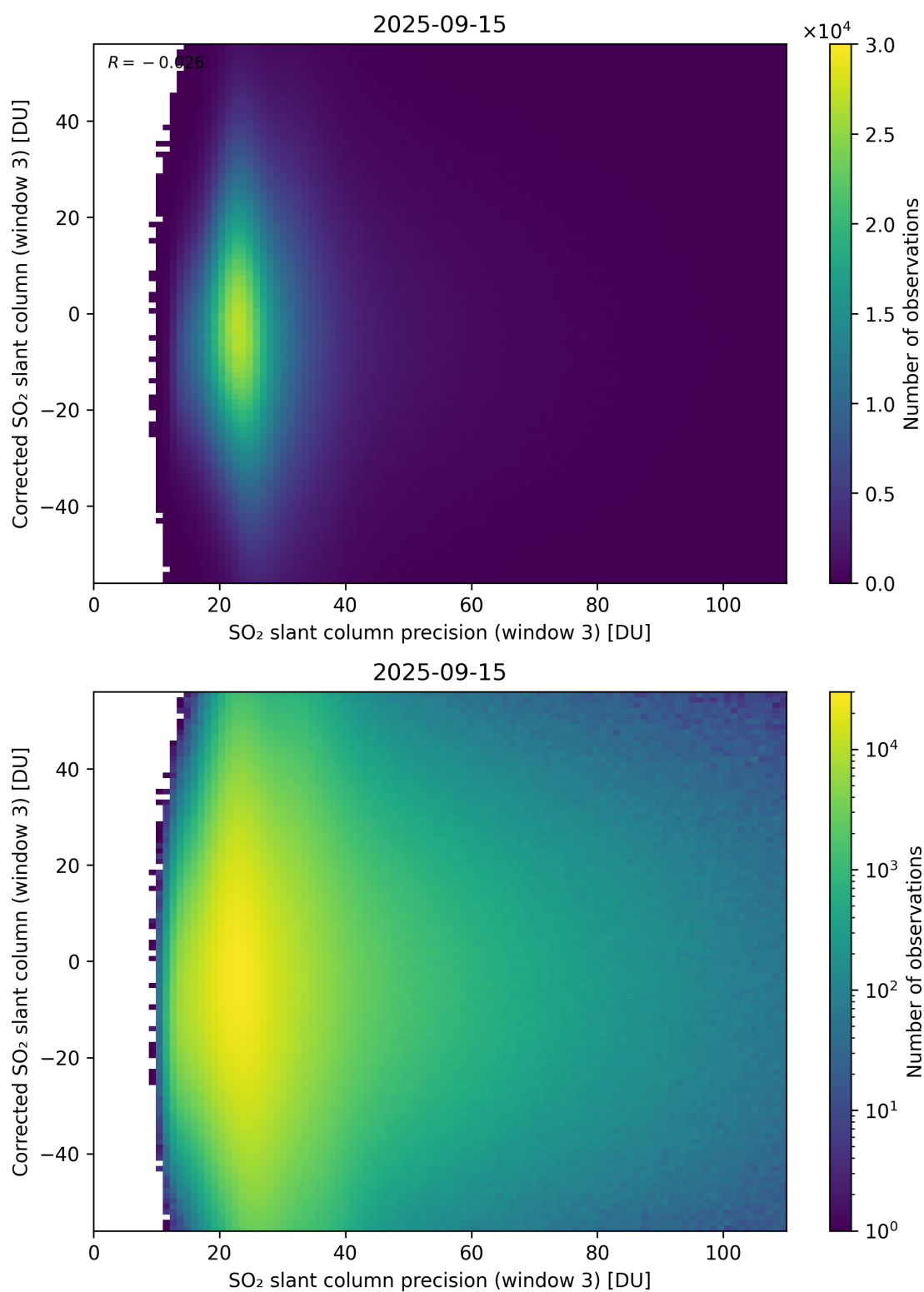
Figure 312: Scatter density plot of “SO 2 slant column precision (window 3)” against “Corrected SO 2 slant column (window 3)” for 2025-09-15 to 2025-09-16.
