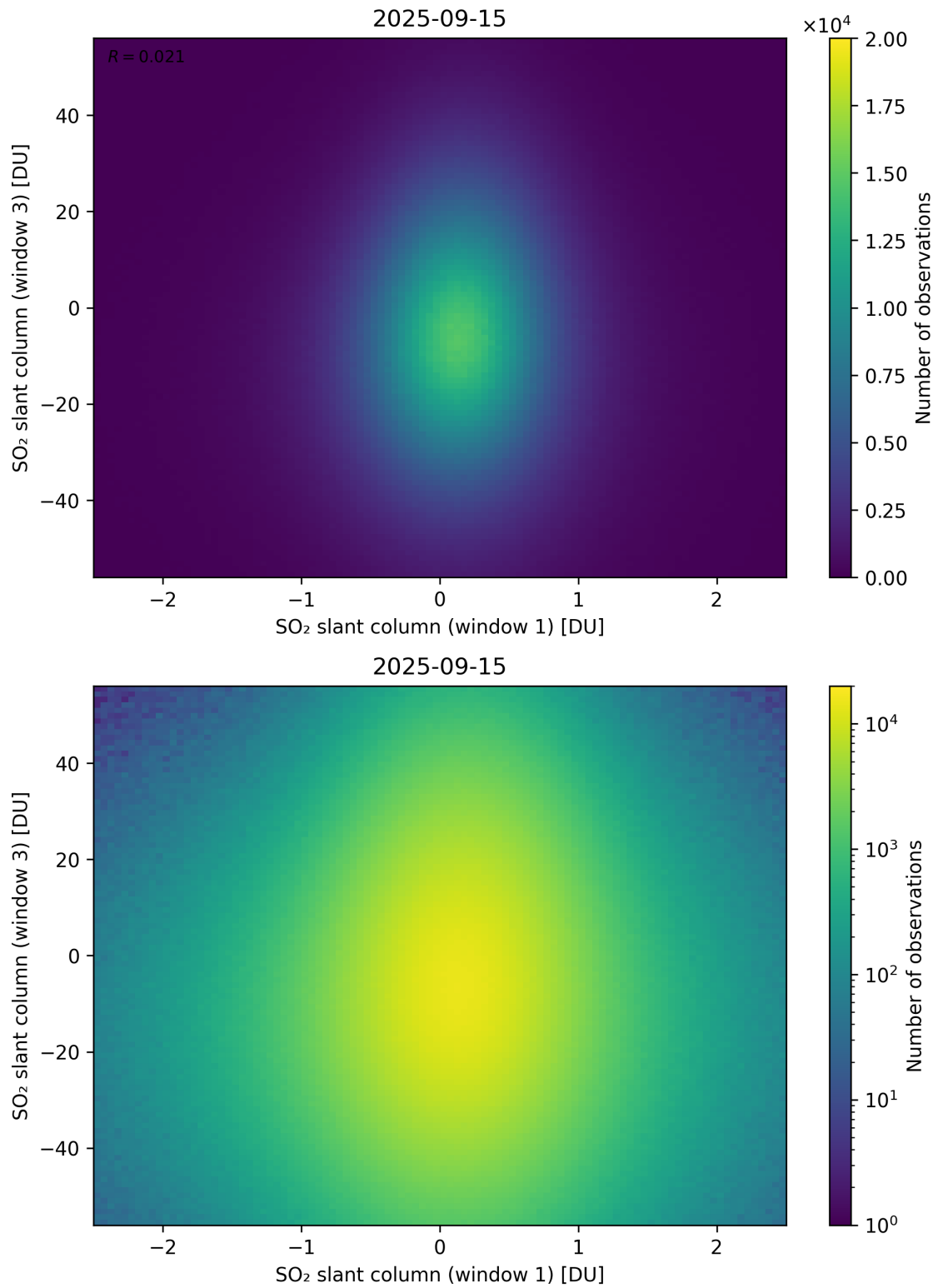
Figure 287: Scatter density plot of “SO 2 slant column (window 1)” against “SO 2 slant column (window 3)” for 2025-09-15 to 2025-09-16.
