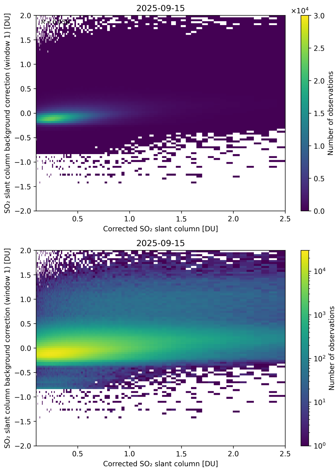
Figure 226: Scatter density plot of “Corrected SO 2 slant column” against “SO 2 slant column background correction (window 1)” for 2025-09-15 to 2025-09-16.
