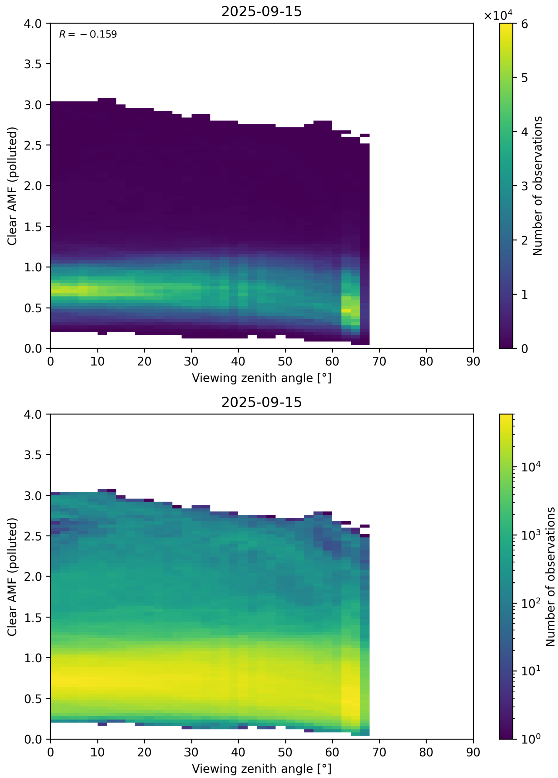
Figure 370: Scatter density plot of “Viewing zenith angle” against “Clear AMF (polluted)” for 2025-09-15 to 2025-09-16.
