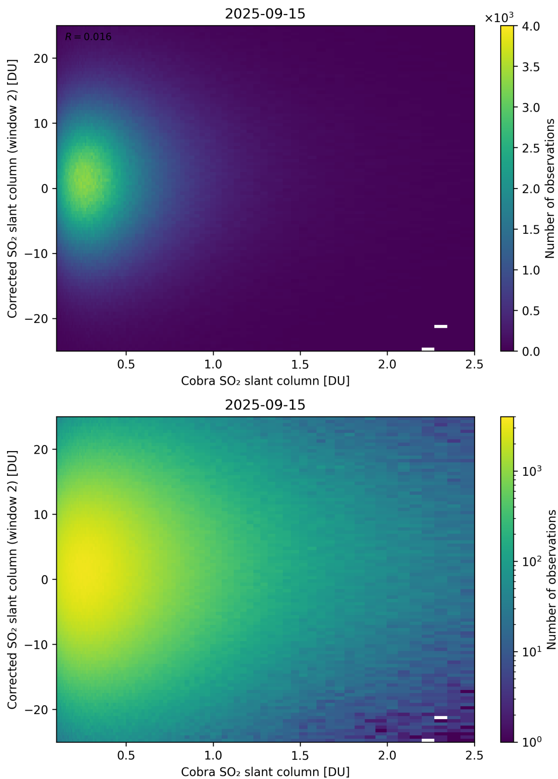
Figure 217: Scatter density plot of “Cobra SO 2 slant column” against “Corrected SO 2 slant column (window 2)” for 2025-09-15 to 2025-09-16.
