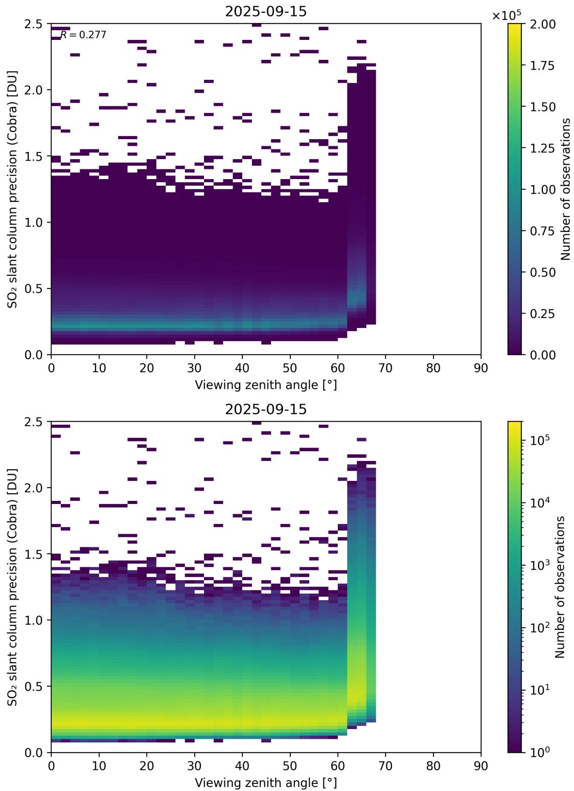
Figure 372: Scatter density plot of “Viewing zenith angle” against “SO 2 slant column precision (Cobra)” for 2025-09-15 to 2025-09-16.
