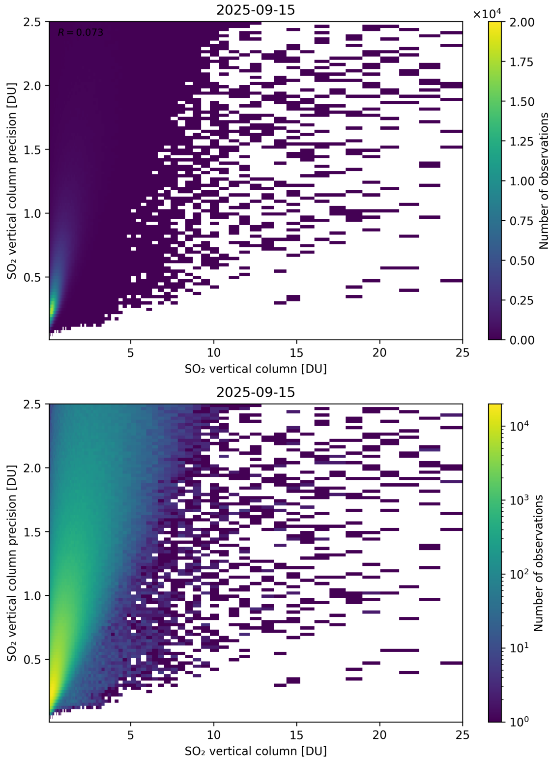
Figure 361: Scatter density plot of “SO 2 vertical column” against “SO 2 vertical column precision” for 2025-09-15 to 2025-09-16.
