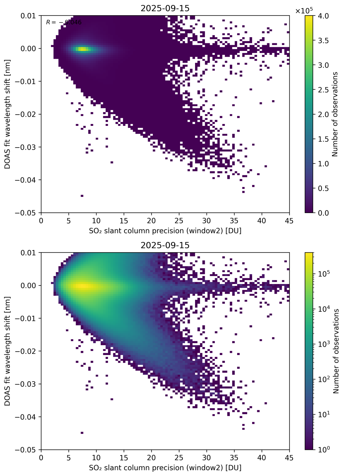
Figure 293: Scatter density plot of “SO 2 slant column precision (window2)” against “DOAS fit wavelength shift” for 2025-09-15 to 2025-09-16.
