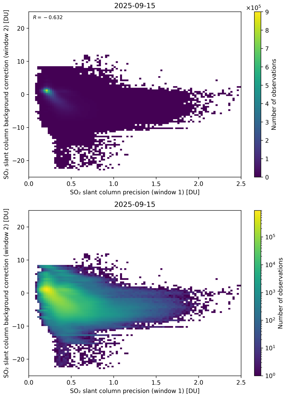
Figure 269: Scatter density plot of “SO 2 slant column precision (window 1)” against “SO 2 slant column background correction (window 2)” for 2025-09-15 to 2025-09-16.
