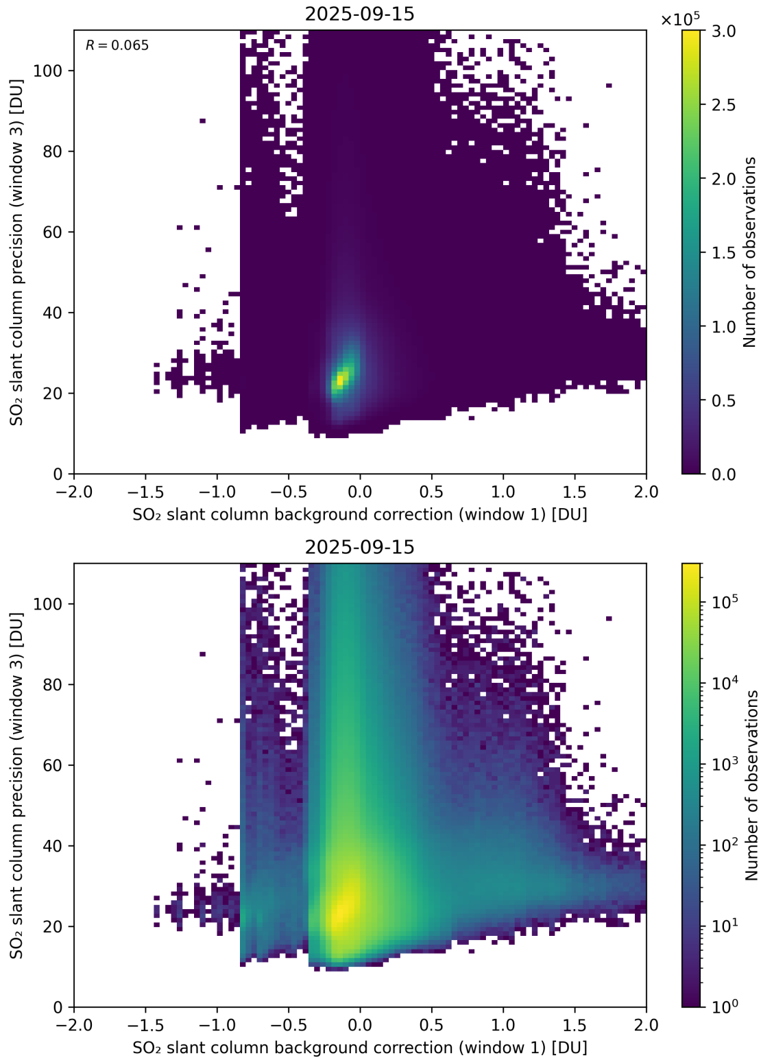
Figure 119: Scatter density plot of “SO 2 slant column background correction (window 1)” against “SO 2 slant column precision (window 3)” for 2025-09-15 to 2025-09-16.
