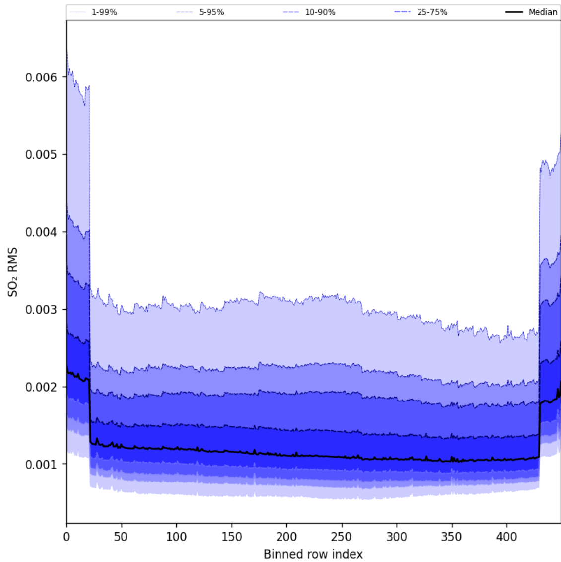
Figure 104: Along track statistics of “SO 2 RMS” for 2025-09-15 to 2025-09-16
