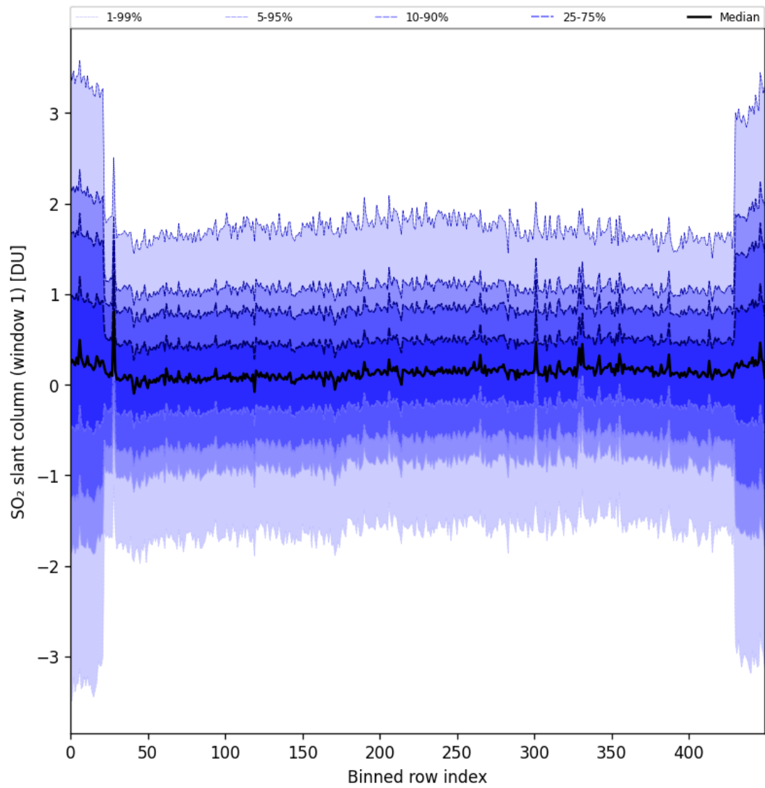
Figure 89: Along track statistics of “SO 2 slant column (window 1)” for 2025-09-15 to 2025-09-16
