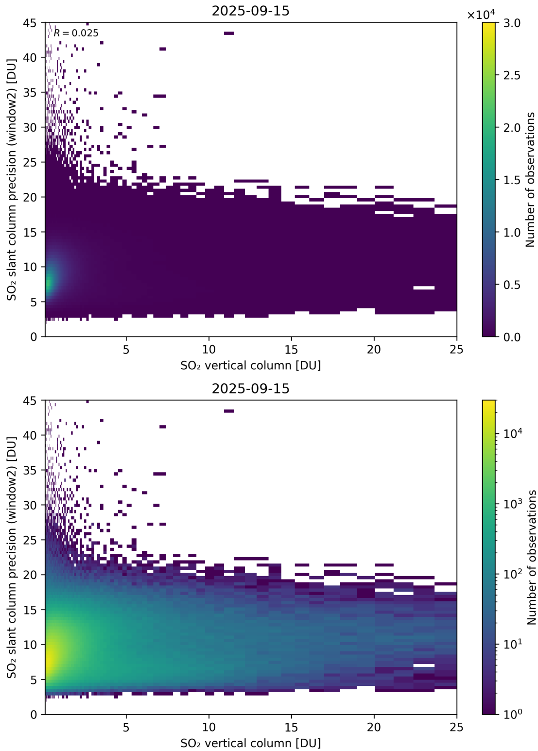
Figure 356: Scatter density plot of “SO 2 vertical column” against “SO 2 slant column precision (window2)” for 2025-09-15 to 2025-09-16.
