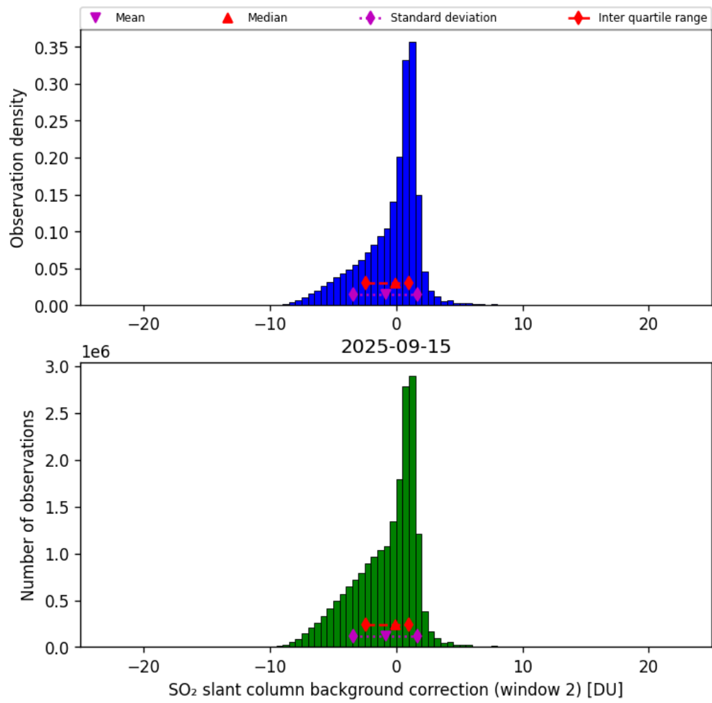
Figure 70: Histogram of “SO 2 slant column background correction (window 2)” for 2025-09-15 to 2025-09-16
