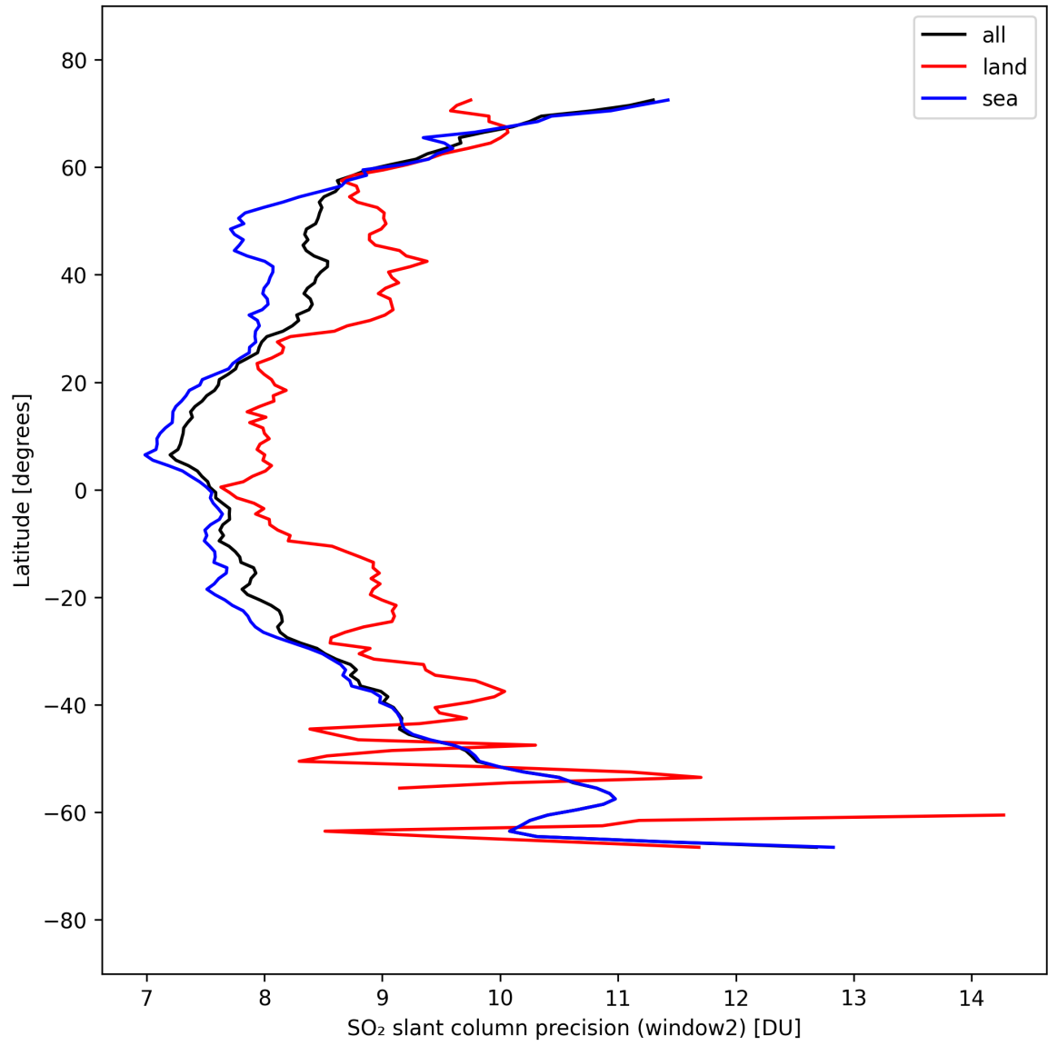
Figure 42: Zonal average of “SO 2 slant column precision (window2)” for 2025-09-15 to 2025-09-16.
