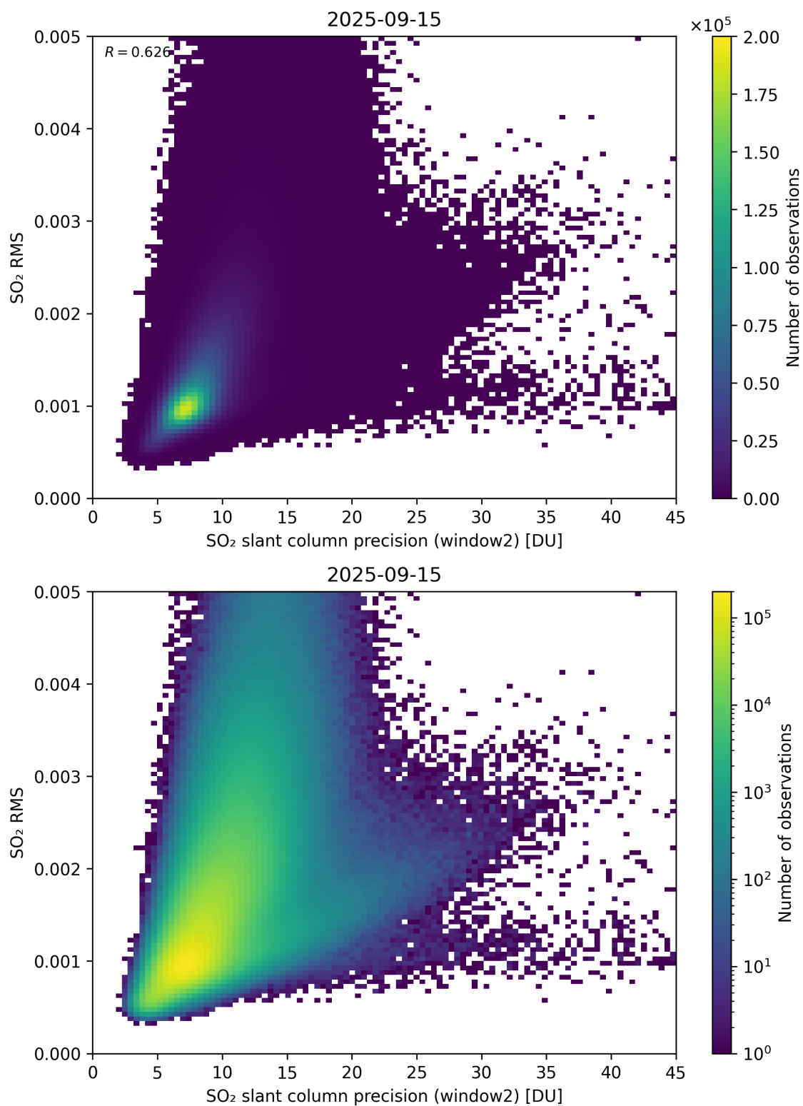
Figure 295: Scatter density plot of “SO 2 slant column precision (window2)” against “SO 2 RMS” for 2025-09-15 to 2025-09-16.
