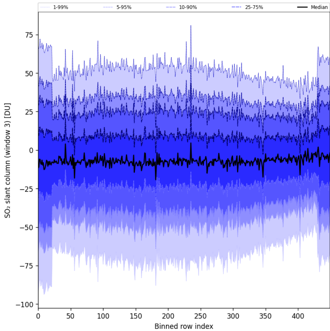
Figure 97: Along track statistics of “SO 2 slant column (window 3)” for 2025-09-15 to 2025-09-16
