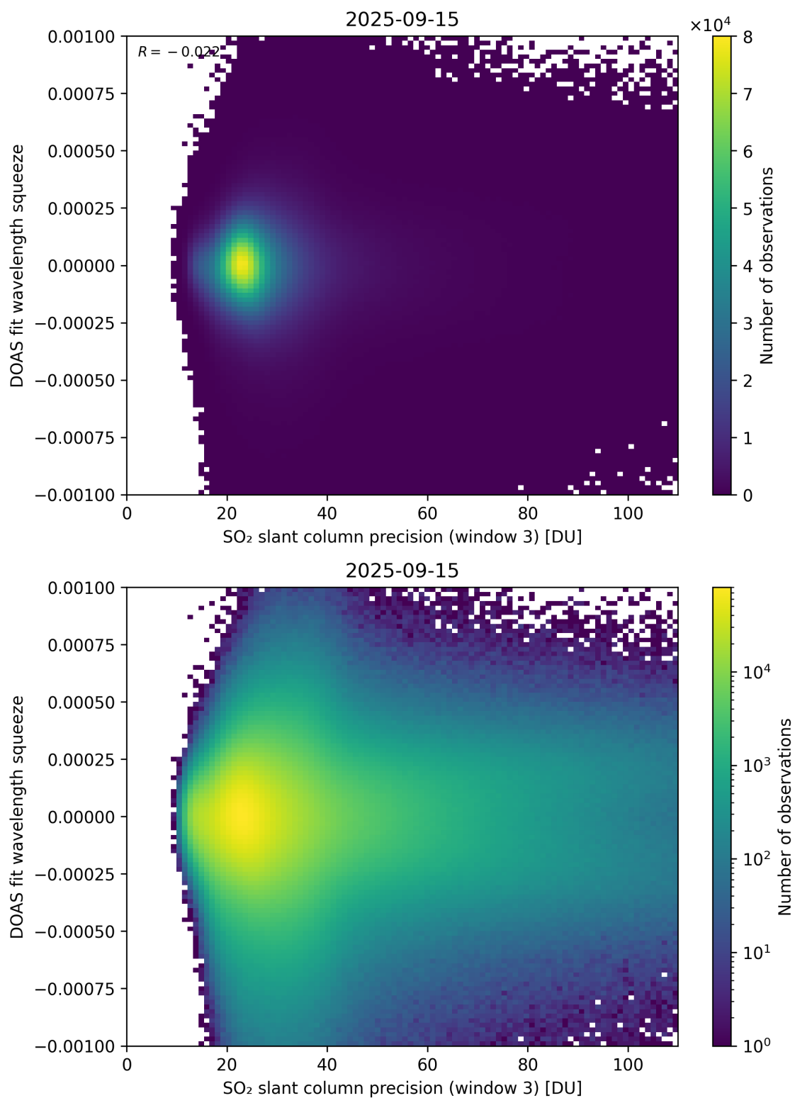
Figure 309: Scatter density plot of “SO 2 slant column precision (window 3)” against “DOAS fit wavelength squeeze” for 2025-09-15 to 2025-09-16.
