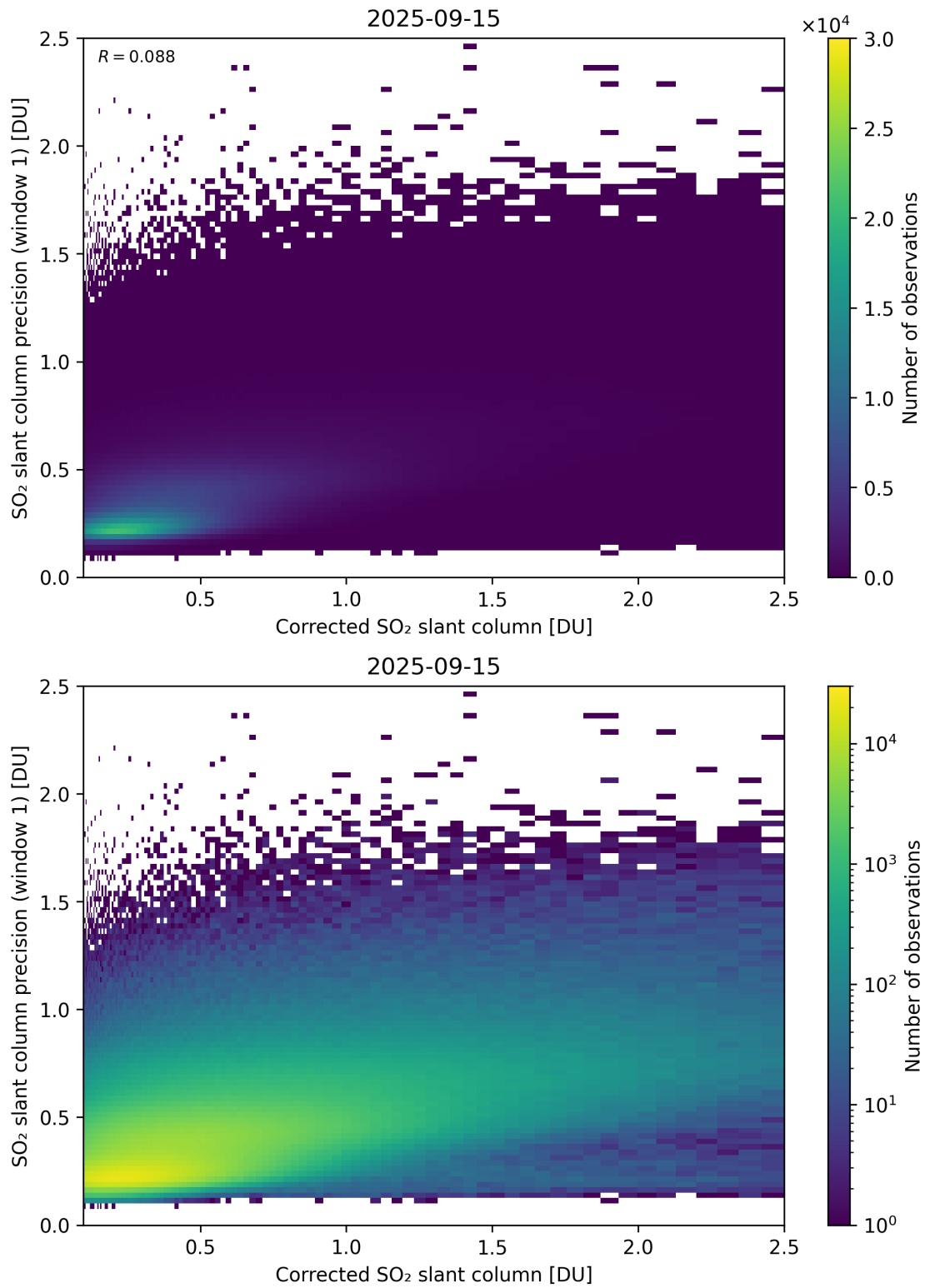
Figure 238: Scatter density plot of “Corrected SO 2 slant column” against “SO 2 slant column precision (window 1)” for 2025-09-15 to 2025-09-16.
