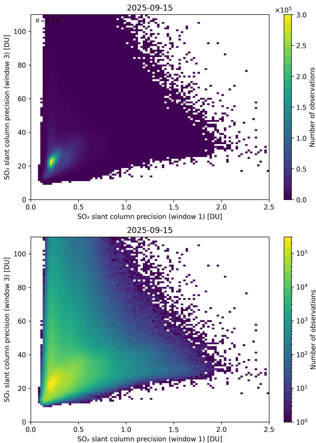
Figure 279: Scatter density plot of “SO 2 slant column precision (window 1)” against “SO 2 slant column precision (window 3)” for 2025-09-15 to 2025-09-16.
