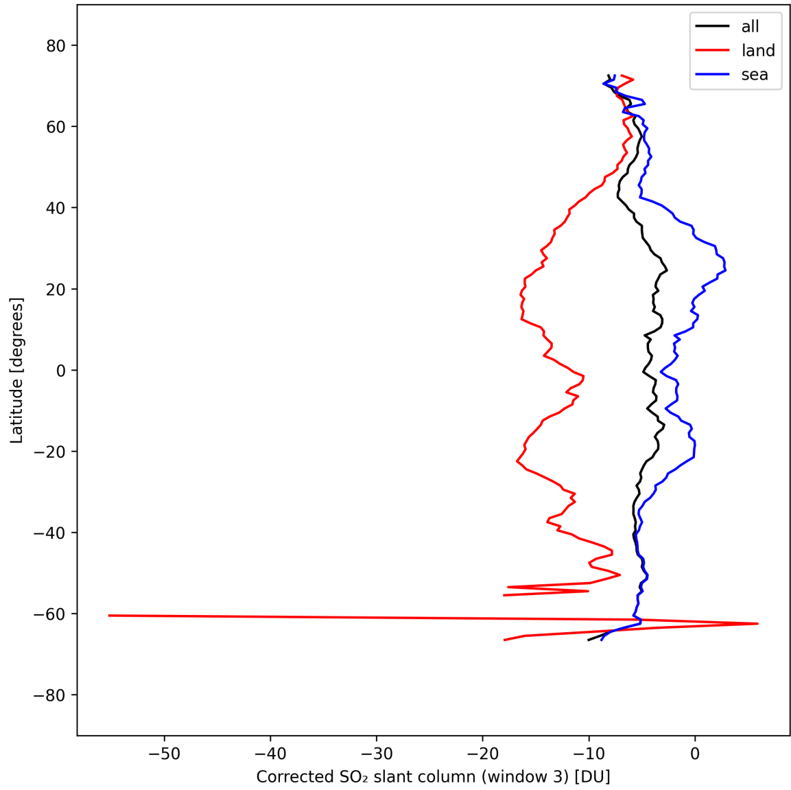
Figure 47: Zonal average of “Corrected SO 2 slant column (window 3)” for 2025-09-15 to 2025-09-16.
