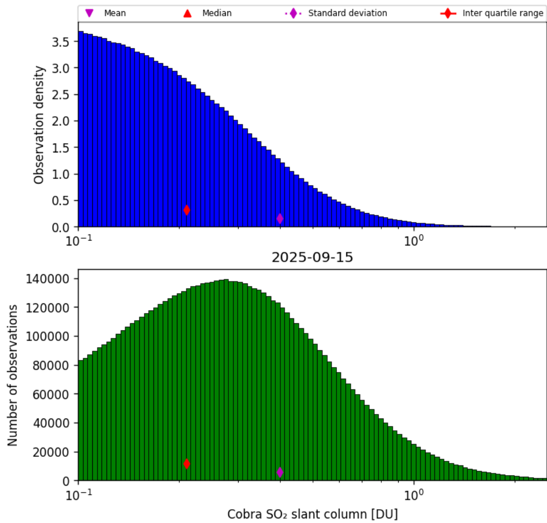
Figure 61: Histogram of “Cobra SO 2 slant column” for 2025-09-15 to 2025-09-16
