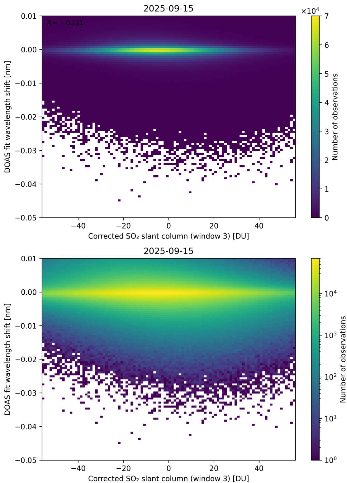
Figure 256: Scatter density plot of “Corrected SO 2 slant column (window 3)” against “DOAS fit wavelength shift” for 2025-09-15 to 2025-09-16.
