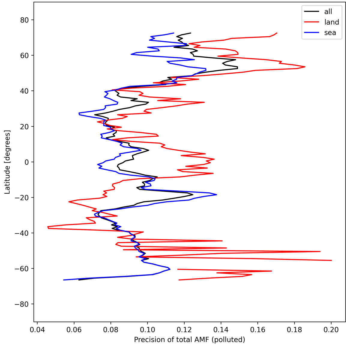
Figure 54: Zonal average of “Precision of total AMF (polluted)” for 2025-09-15 to 2025-09-16.
