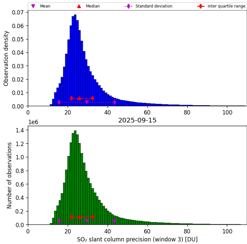
Figure 72: Histogram of “SO 2 slant column precision (window 3)” for 2025-09-15 to 2025-09-16
