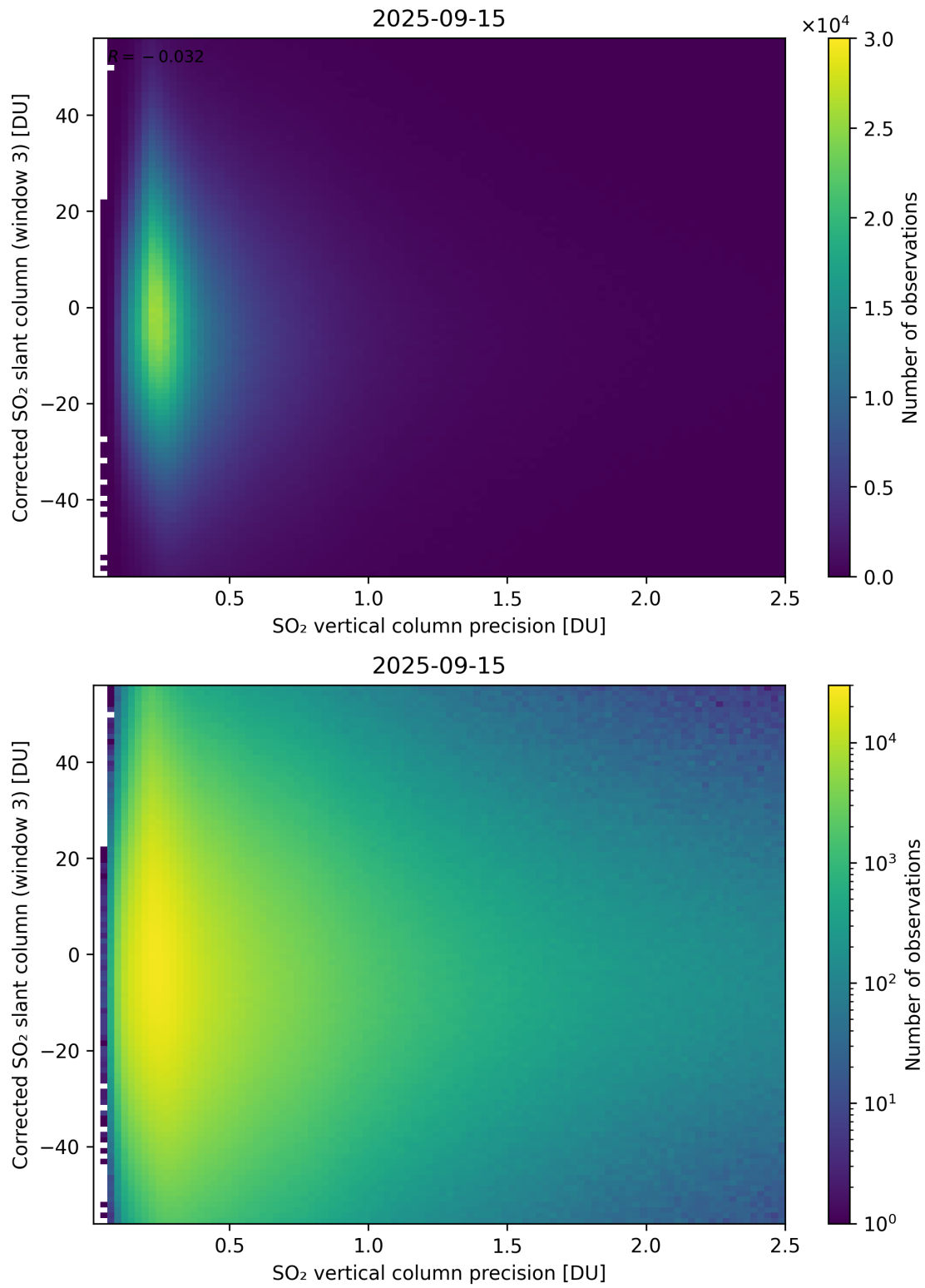
Figure 340: Scatter density plot of “SO 2 vertical column precision” against “Corrected SO 2 slant column (window 3)” for 2025-09-15 to 2025-09-16.
