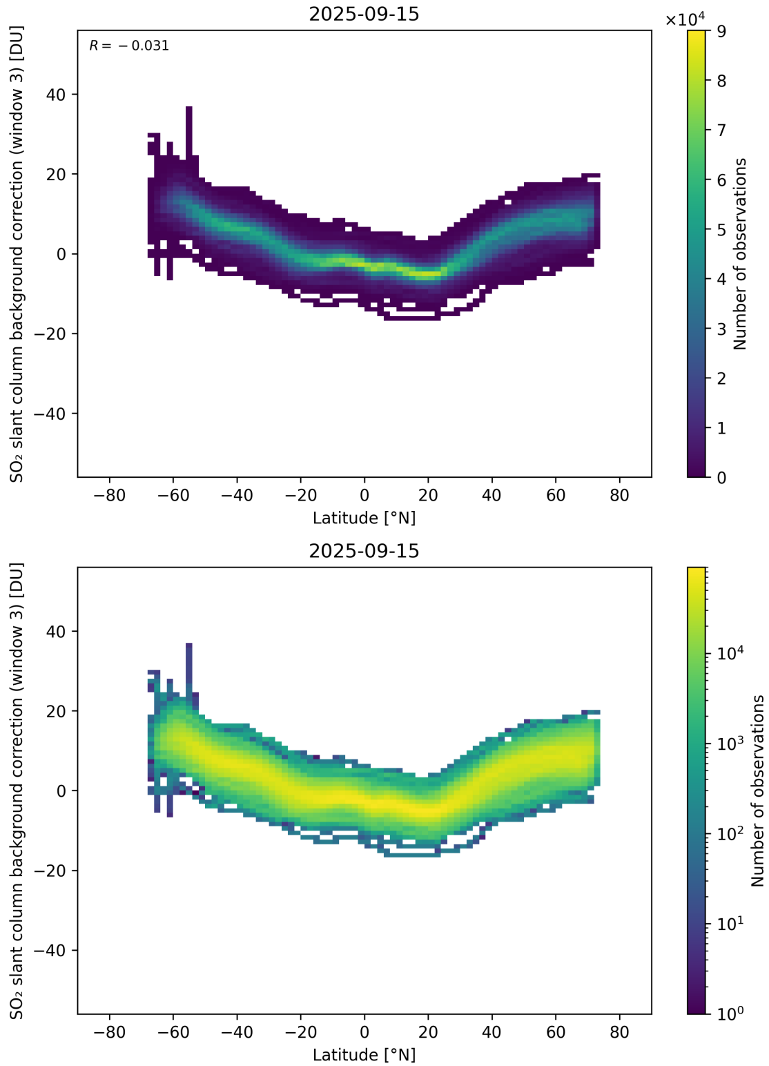
Figure 152: Scatter density plot of “Latitude” against “SO 2 slant column background correction (window 3)” for 2025-09-15 to 2025-09-16.
