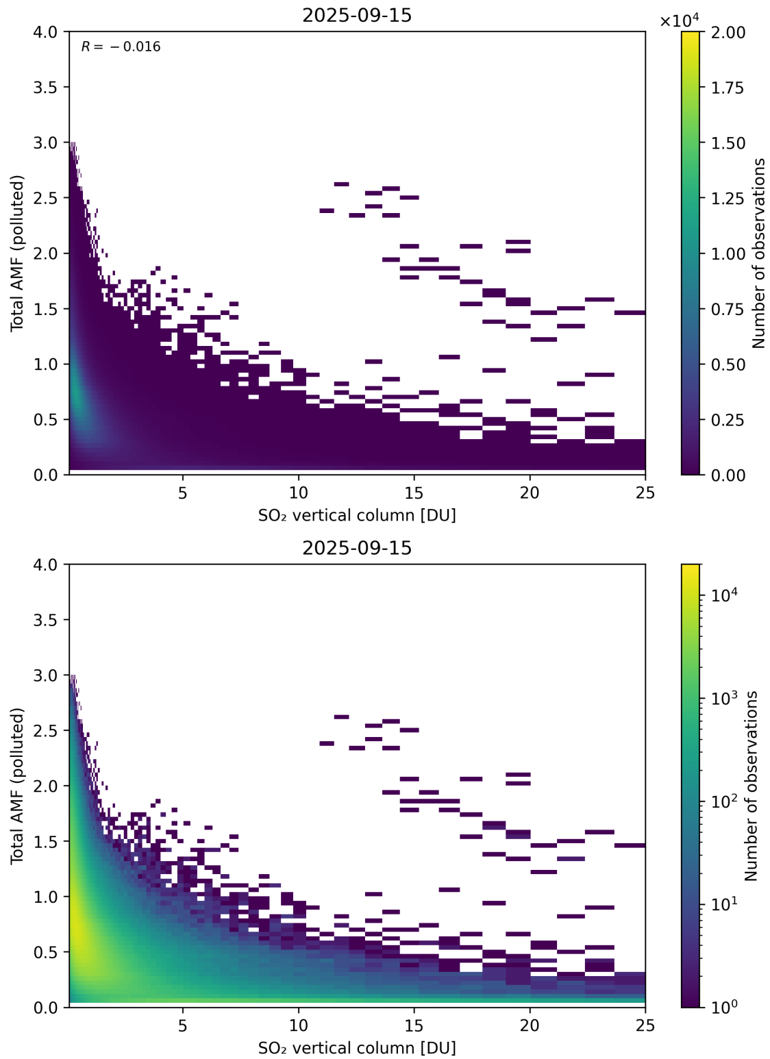
Figure 359: Scatter density plot of “SO 2 vertical column” against “Total AMF (polluted)” for 2025-09-15 to 2025-09-16.
