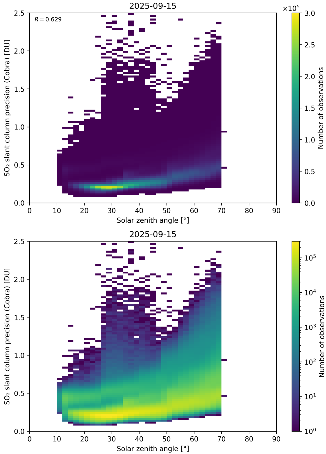
Figure 180: Scatter density plot of “Solar zenith angle” against “SO 2 slant column precision (Cobra)” for 2025-09-15 to 2025-09-16.
