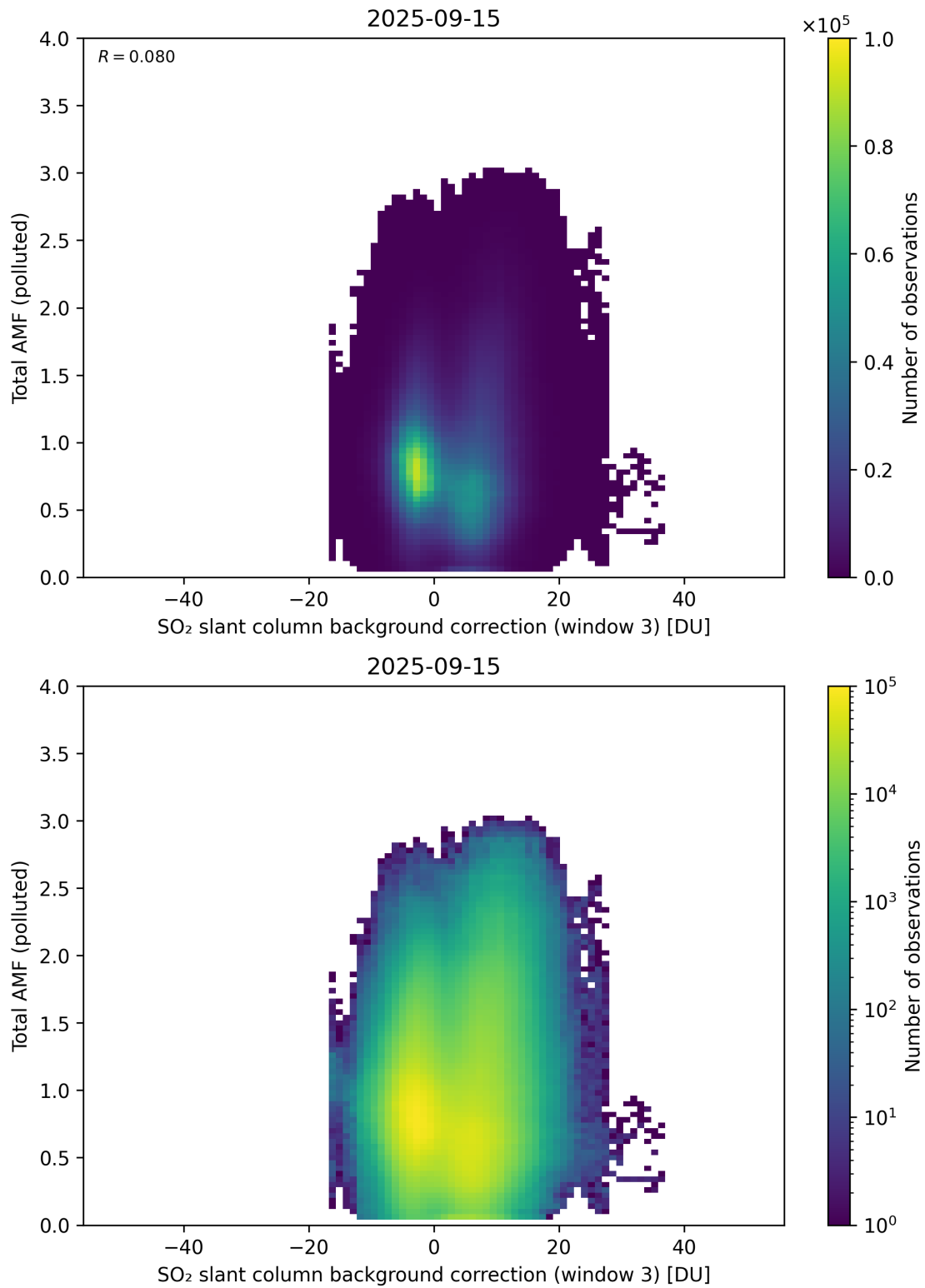
Figure 136: Scatter density plot of “SO 2 slant column background correction (window 3)” against “Total AMF (polluted)” for 2025-09-15 to 2025-09-16.
