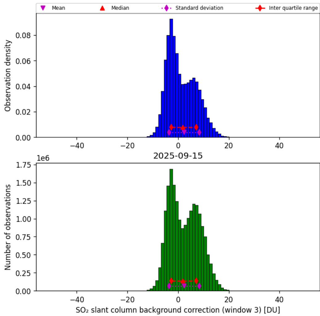
Figure 74: Histogram of “SO 2 slant column background correction (window 3)” for 2025-09-15 to 2025-09-16
