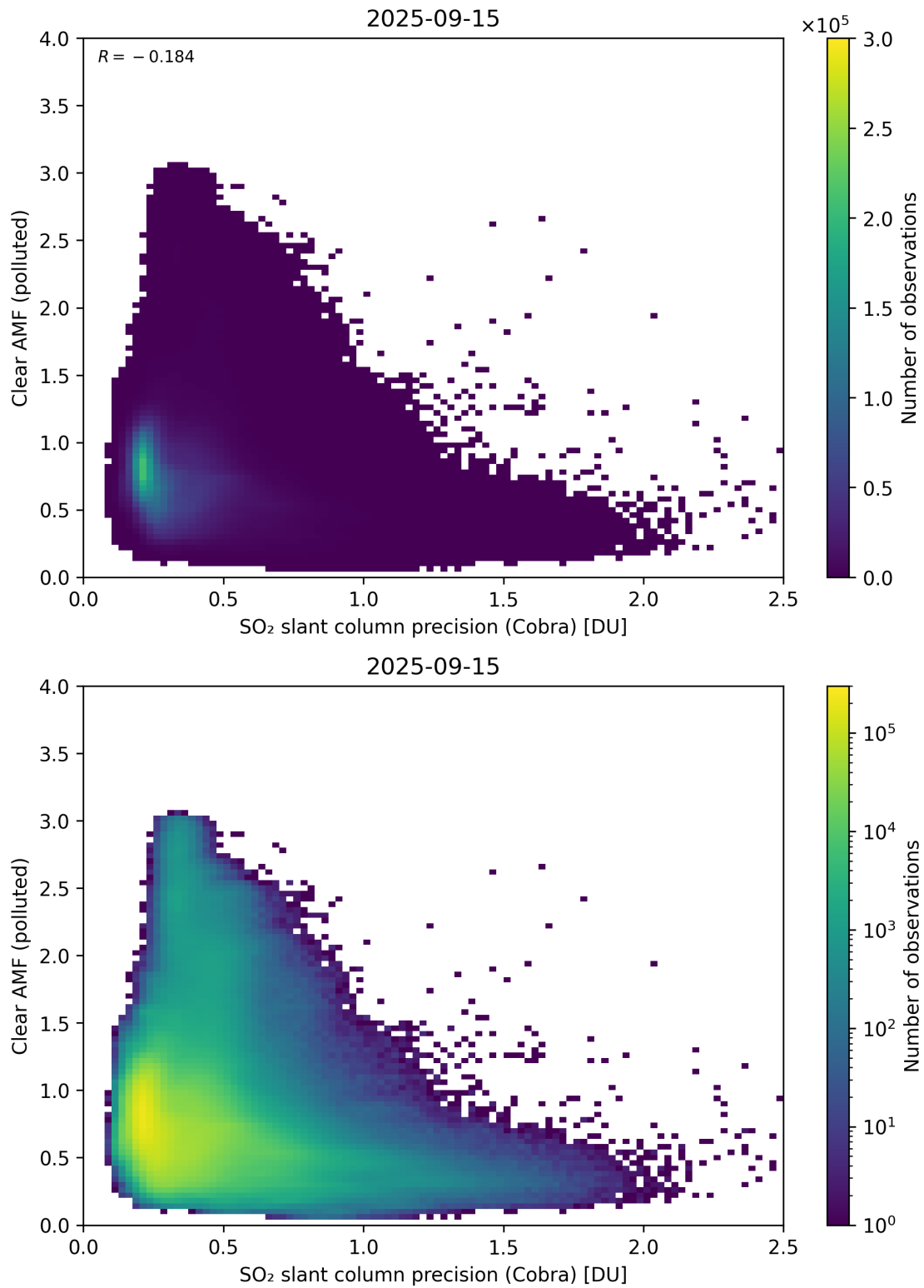
Figure 205: Scatter density plot of “SO 2 slant column precision (Cobra)” against “Clear AMF (polluted)” for 2025-09-15 to 2025-09-16.
