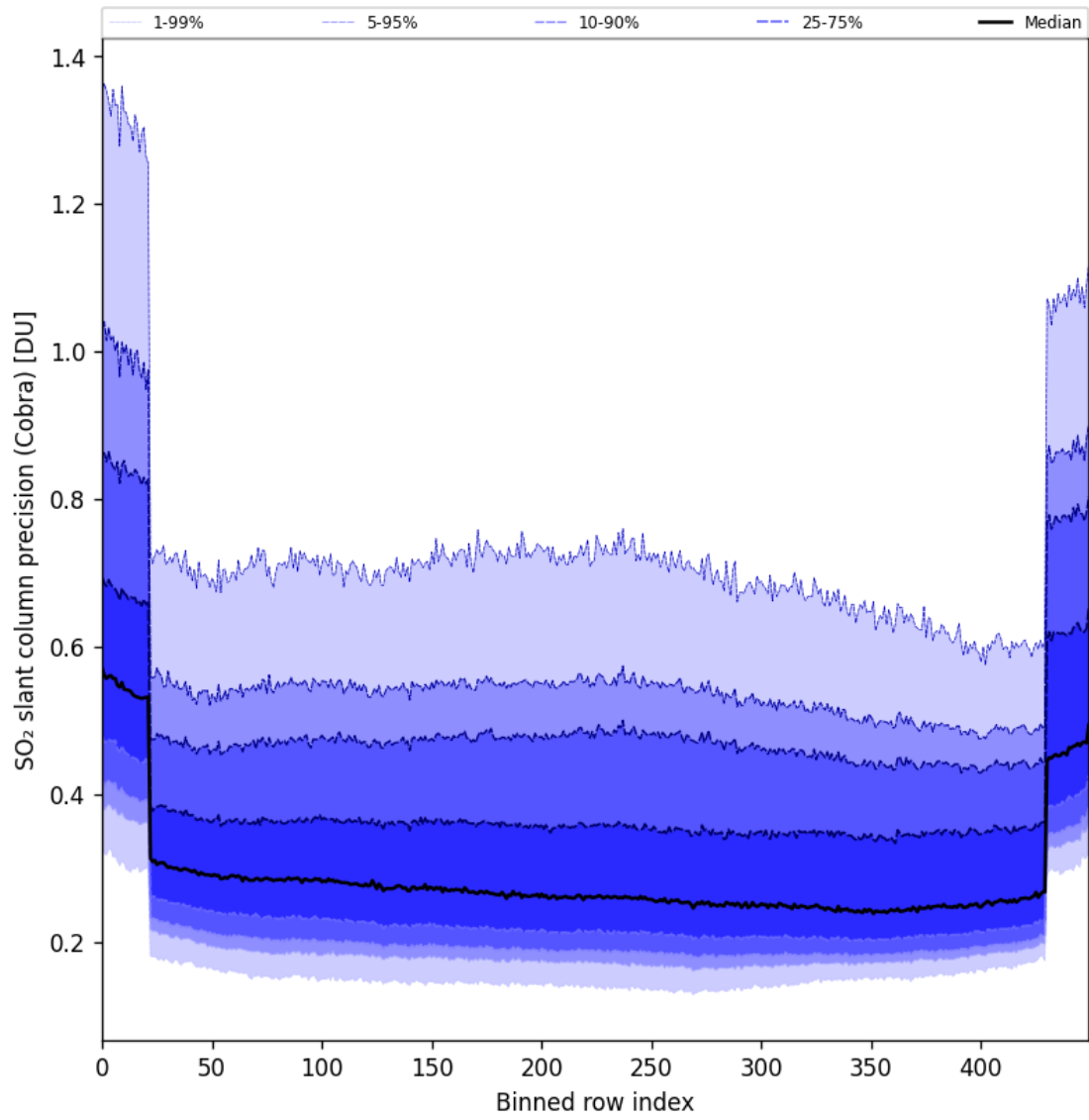
Figure 88: Along track statistics of “SO 2 slant column precision (Cobra)” for 2025-09-15 to 2025-09-16
