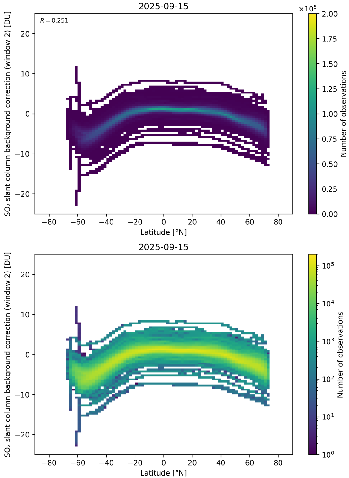
Figure 151: Scatter density plot of “Latitude” against “SO 2 slant column background correction (window 2)” for 2025-09-15 to 2025-09-16.
