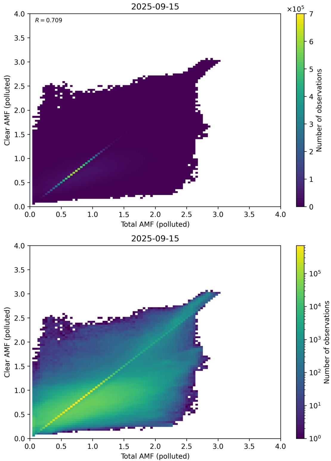
Figure 321: Scatter density plot of “Total AMF (polluted)” against “Clear AMF (polluted)” for 2025-09-15 to 2025-09-16.
