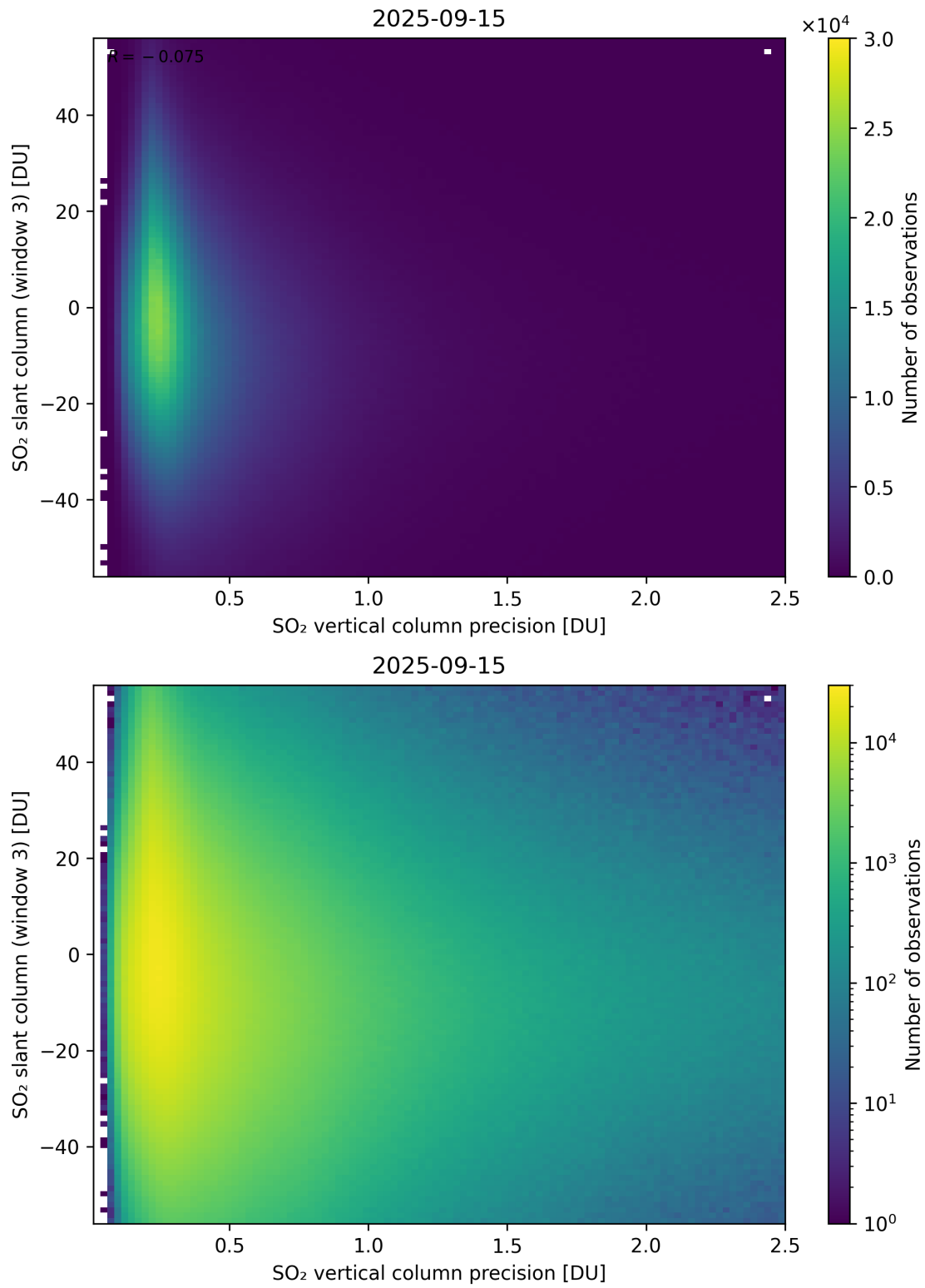
Figure 344: Scatter density plot of “SO 2 vertical column precision” against “SO 2 slant column (window 3)” for 2025-09-15 to 2025-09-16.
