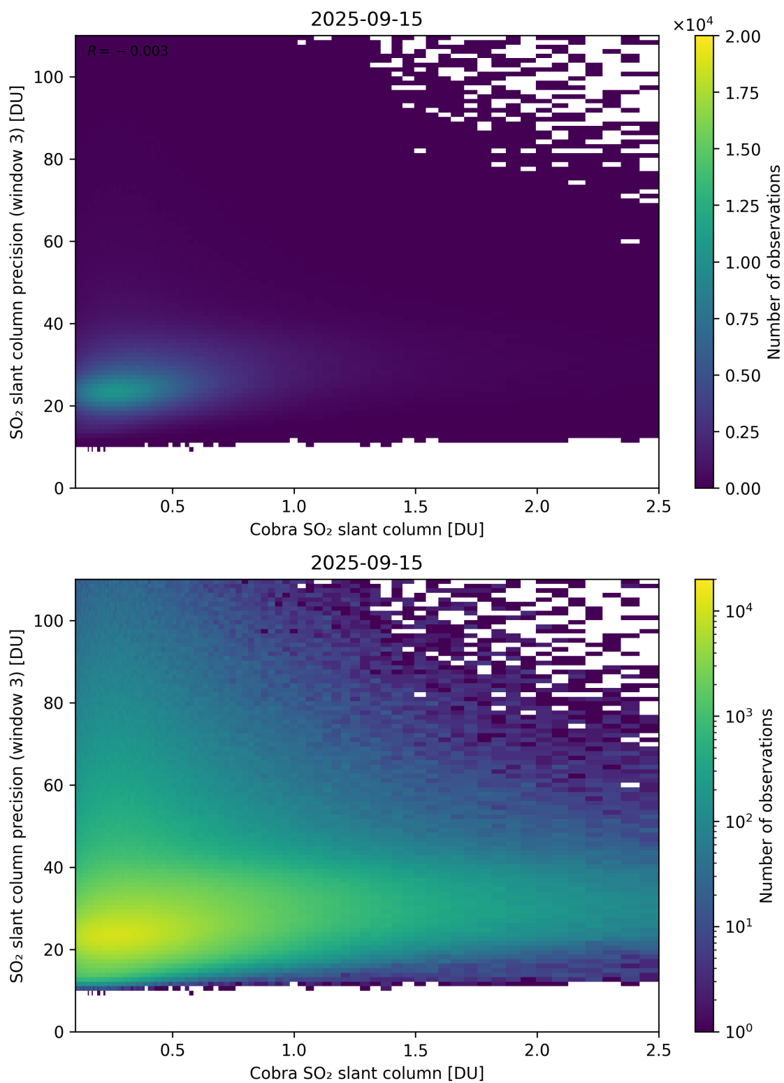
Figure 223: Scatter density plot of “Cobra SO 2 slant column” against “SO 2 slant column precision (window 3)” for 2025-09-15 to 2025-09-16.
