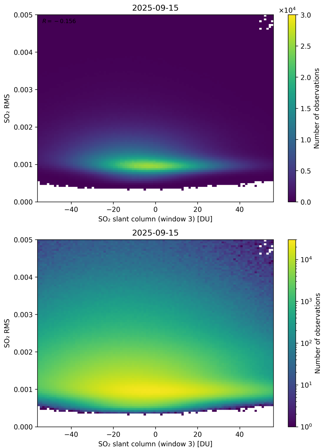
Figure 306: Scatter density plot of “SO 2 slant column (window 3)” against “SO 2 RMS” for 2025-09-15 to 2025-09-16.
