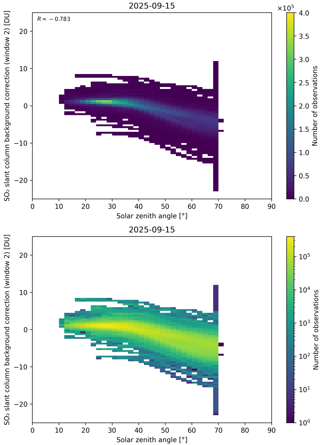
Figure 172: Scatter density plot of “Solar zenith angle” against “SO 2 slant column background correction (window 2)” for 2025-09-15 to 2025-09-16.
