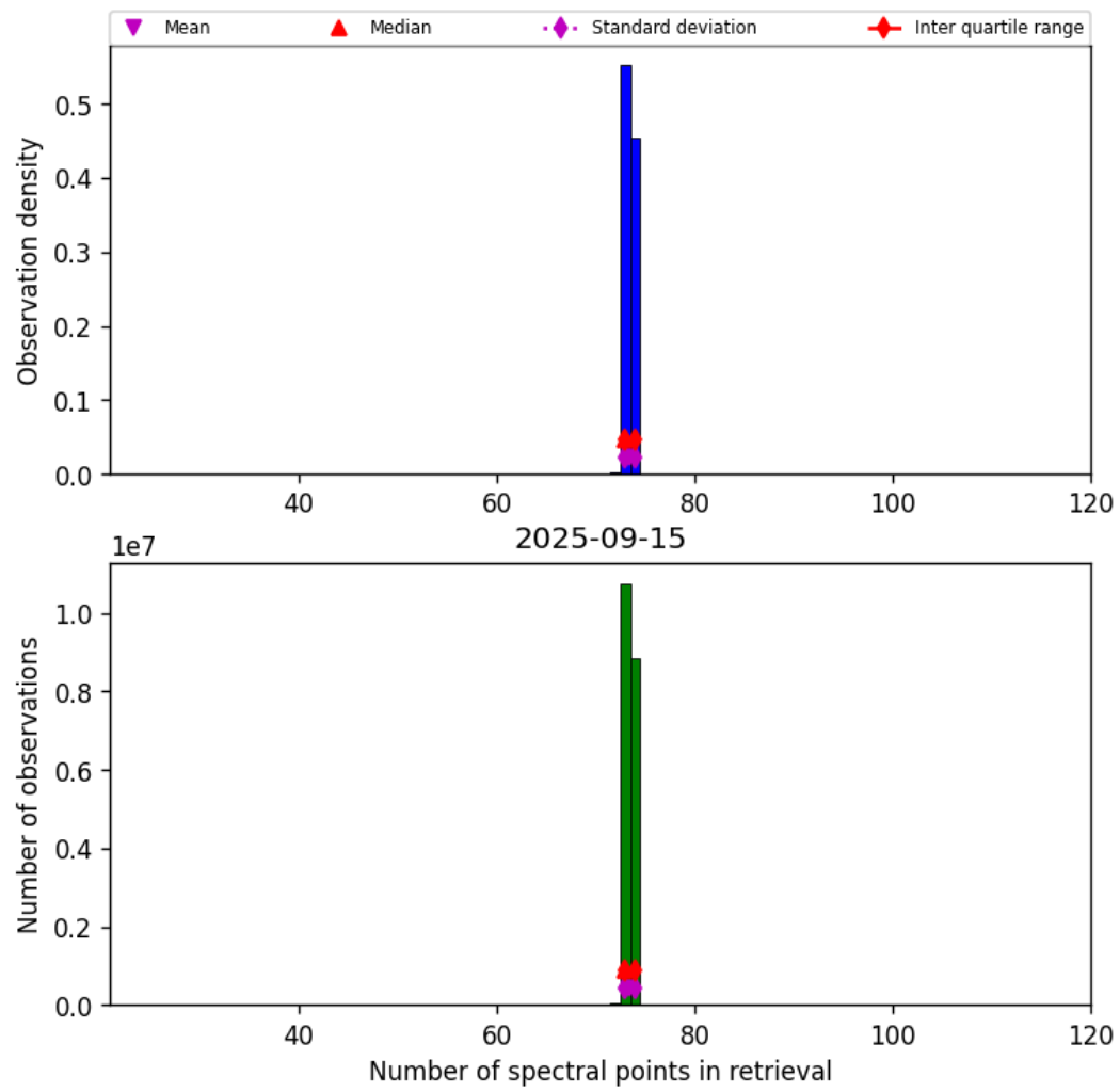
Figure 82: Histogram of “Number of spectral points in retrieval” for 2025-09-15 to 2025-09-16
