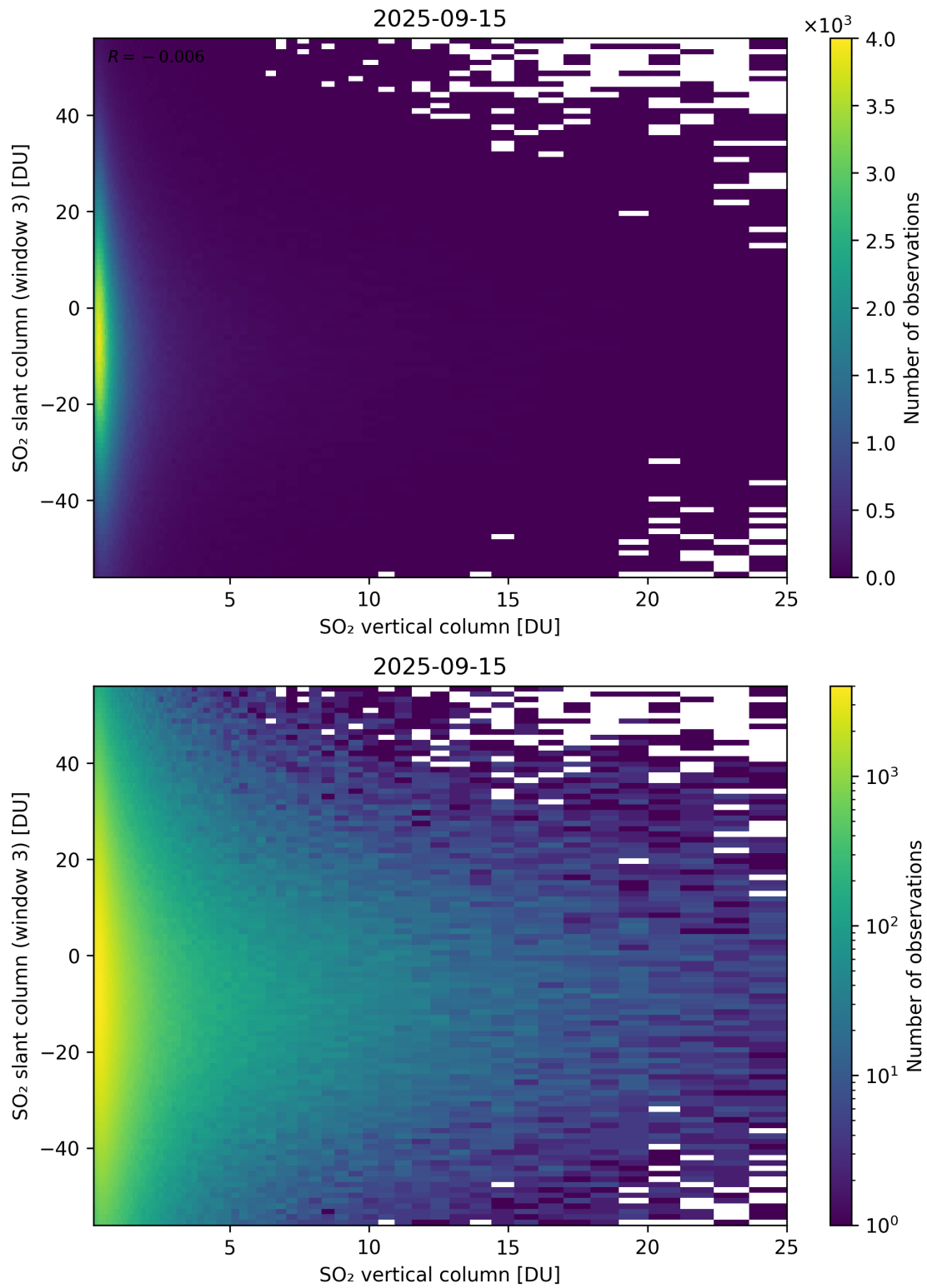
Figure 357: Scatter density plot of “SO 2 vertical column” against “SO 2 slant column (window 3)” for 2025-09-15 to 2025-09-16.
