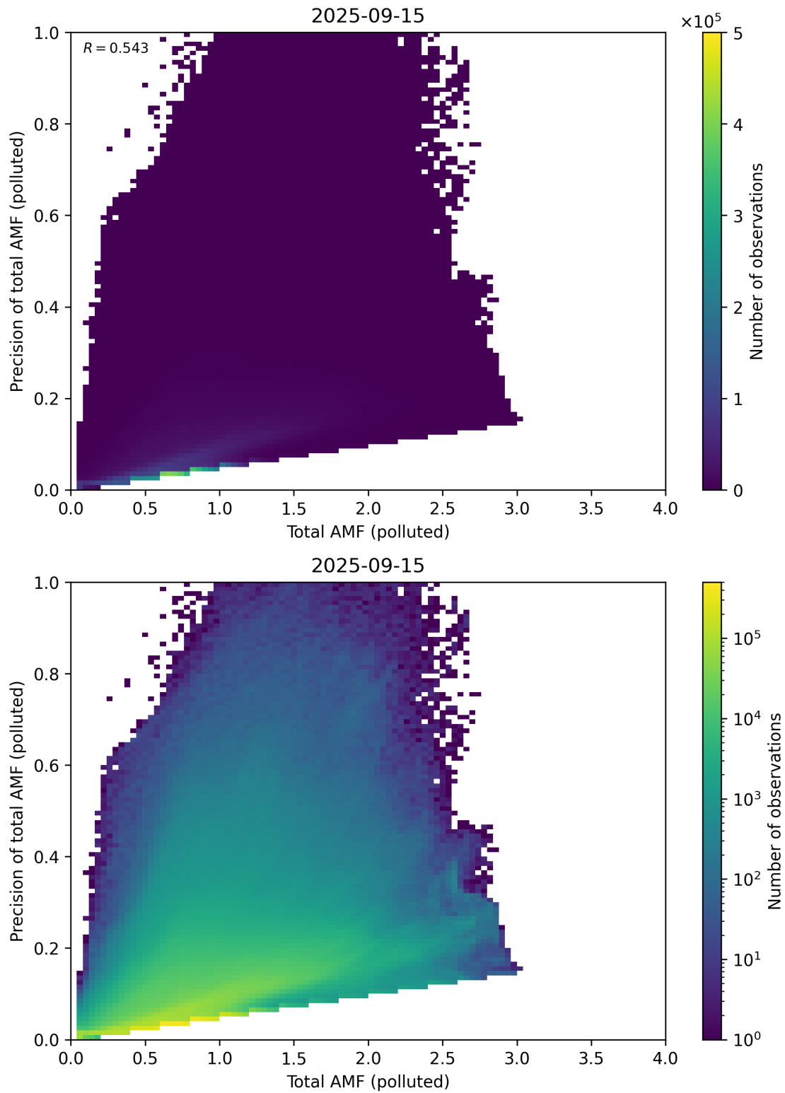
Figure 322: Scatter density plot of “Total AMF (polluted)” against “Precision of total AMF (polluted)” for 2025-09-15 to 2025-09-16.
