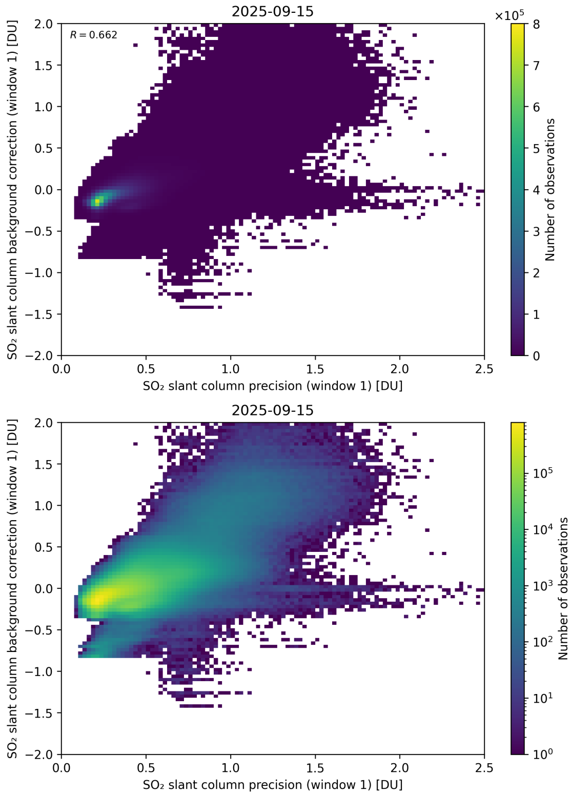
Figure 268: Scatter density plot of “SO 2 slant column precision (window 1)” against “SO 2 slant column background correction (window 1)” for 2025-09-15 to 2025-09-16.
