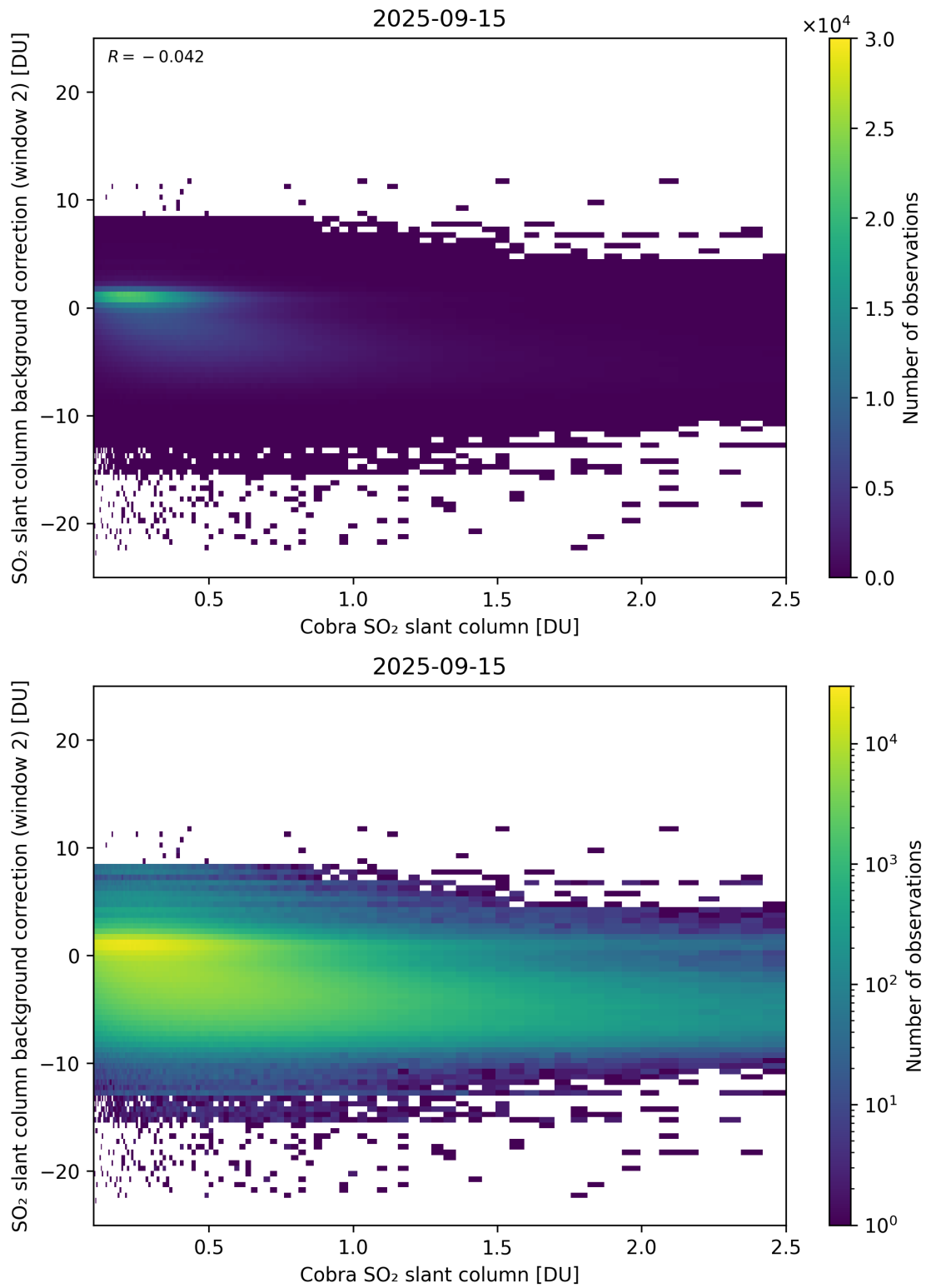
Figure 194: Scatter density plot of “Cobra SO 2 slant column” against “SO 2 slant column background correction (window 2)” for 2025-09-15 to 2025-09-16.
