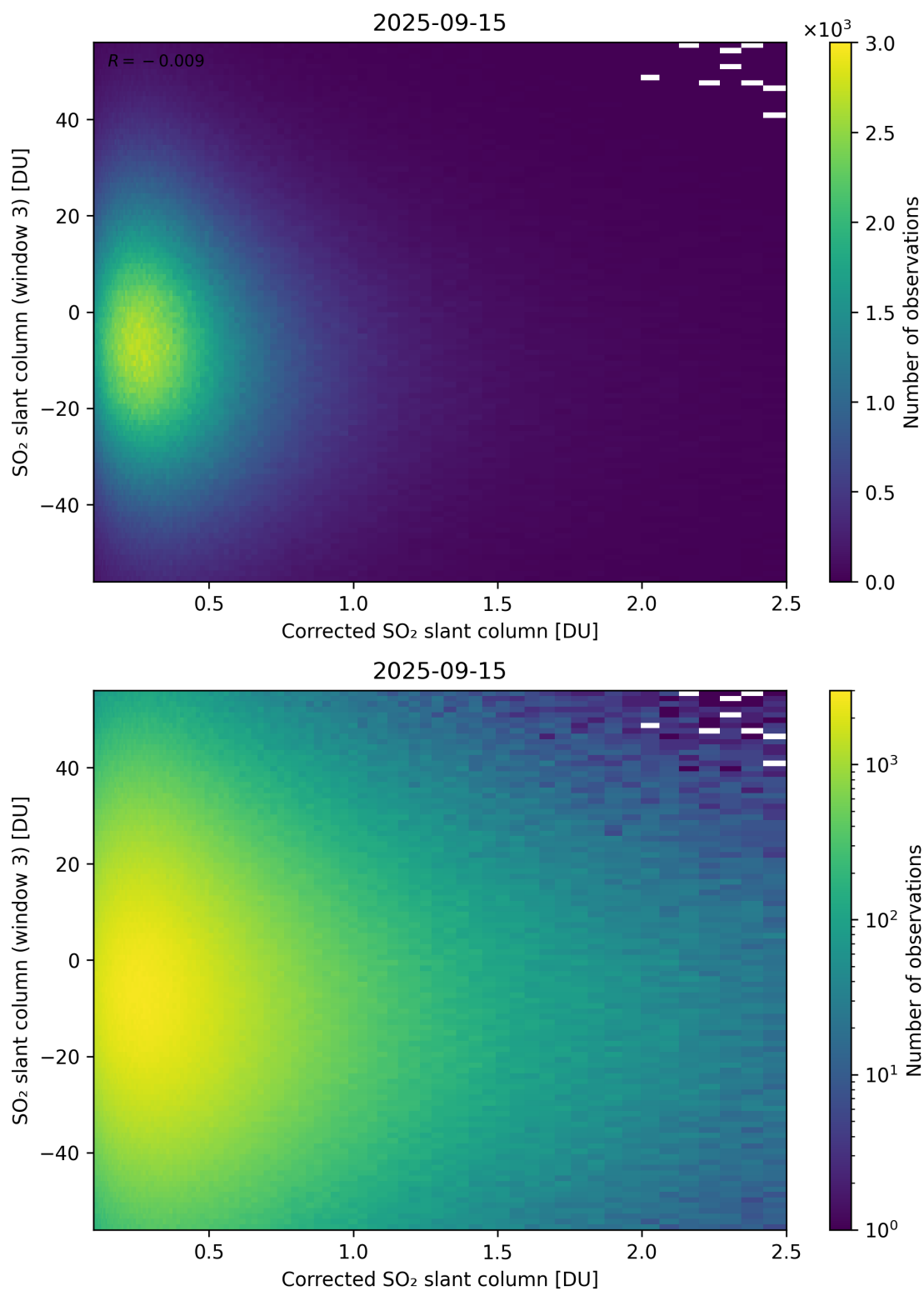
Figure 240: Scatter density plot of “Corrected SO 2 slant column” against “SO 2 slant column (window 3)” for 2025-09-15 to 2025-09-16.
