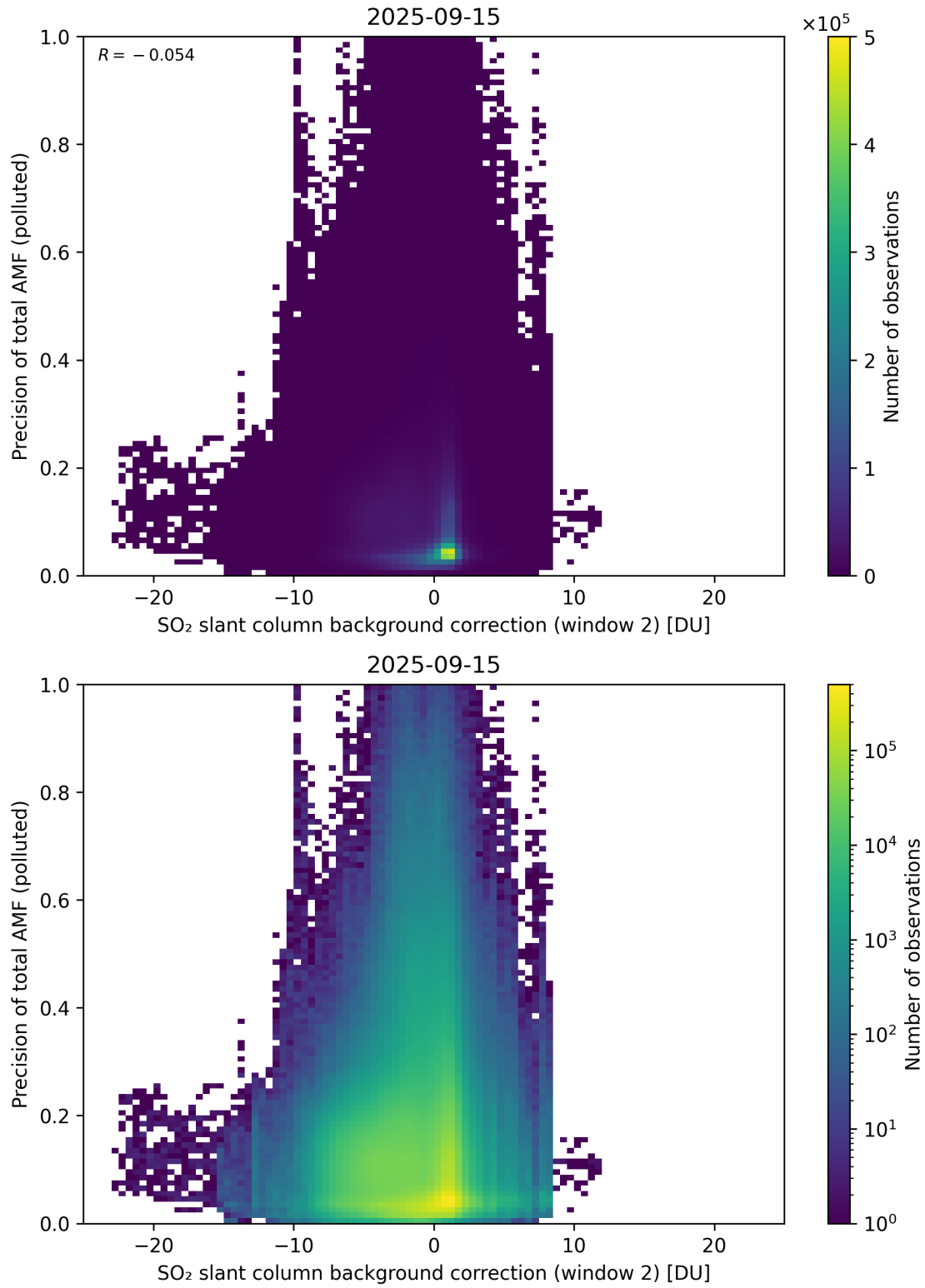
Figure 131: Scatter density plot of “SO 2 slant column background correction (window 2)” against “Precision of total AMF (polluted)” for 2025-09-15 to 2025-09-16.
