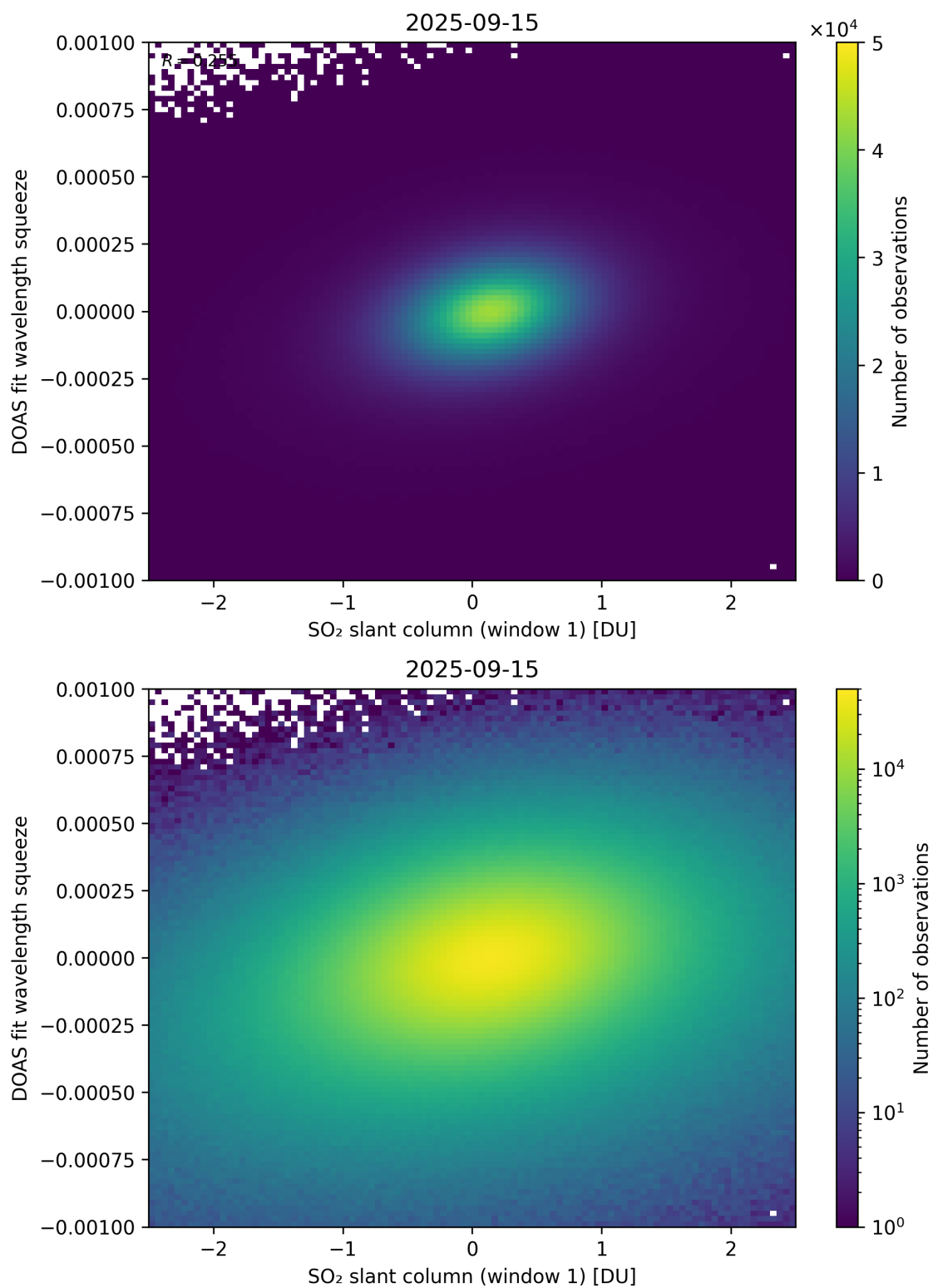
Figure 266: Scatter density plot of “SO 2 slant column (window 1)” against “DOAS fit wavelength squeeze” for 2025-09-15 to 2025-09-16.
