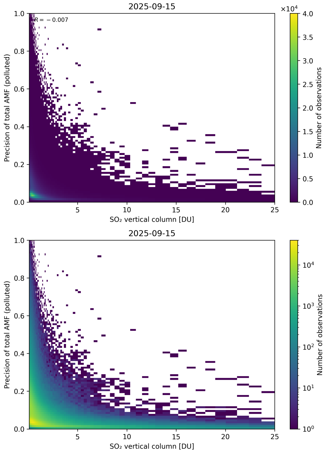
Figure 360: Scatter density plot of “SO 2 vertical column” against “Precision of total AMF (polluted)” for 2025-09-15 to 2025-09-16.
