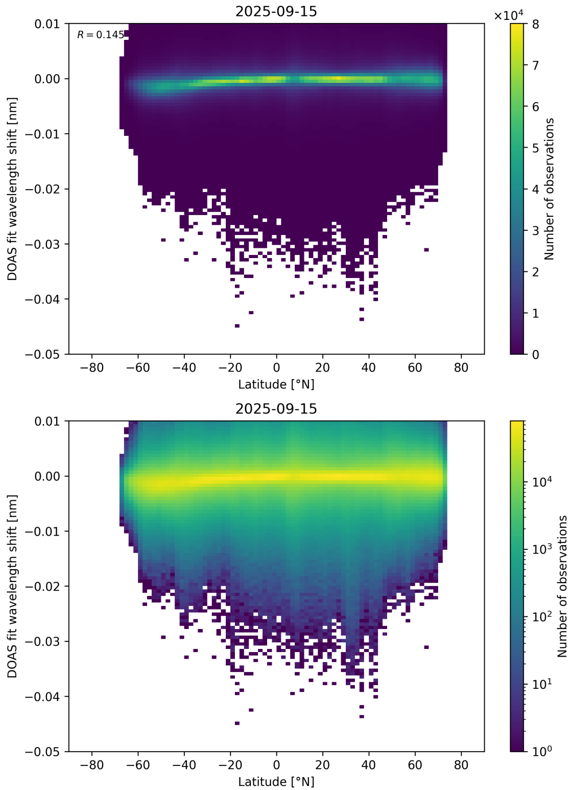
Figure 153: Scatter density plot of “Latitude” against “DOAS fit wavelength shift” for 2025-09-15 to 2025-09-16.
