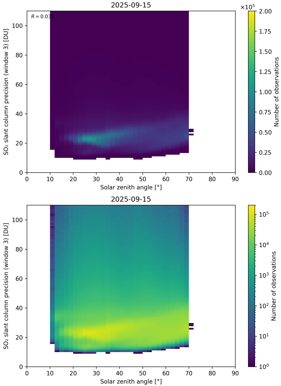
Figure 188: Scatter density plot of “Solar zenith angle” against “SO 2 slant column precision (window 3)” for 2025-09-15 to 2025-09-16.
