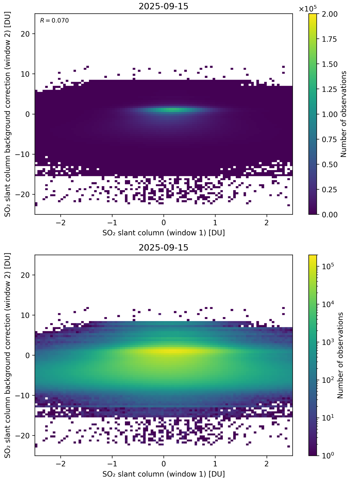
Figure 263: Scatter density plot of “SO 2 slant column (window 1)” against “SO 2 slant column background correction (window 2)” for 2025-09-15 to 2025-09-16.
