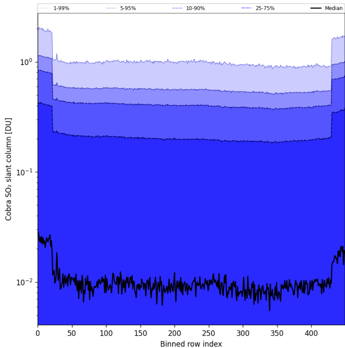
Figure 87: Along track statistics of “Cobra SO 2 slant column” for 2025-09-15 to 2025-09-16
