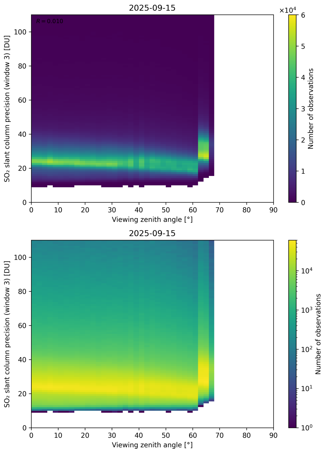
Figure 380: Scatter density plot of “Viewing zenith angle” against “SO 2 slant column precision (window 3)” for 2025-09-15 to 2025-09-16.
