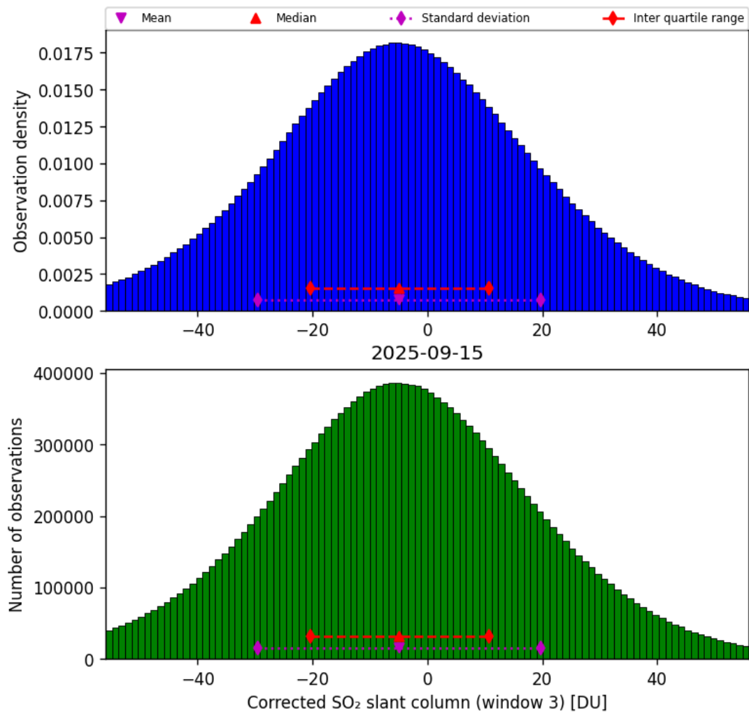
Figure 73: Histogram of “Corrected SO 2 slant column (window 3)” for 2025-09-15 to 2025-09-16
