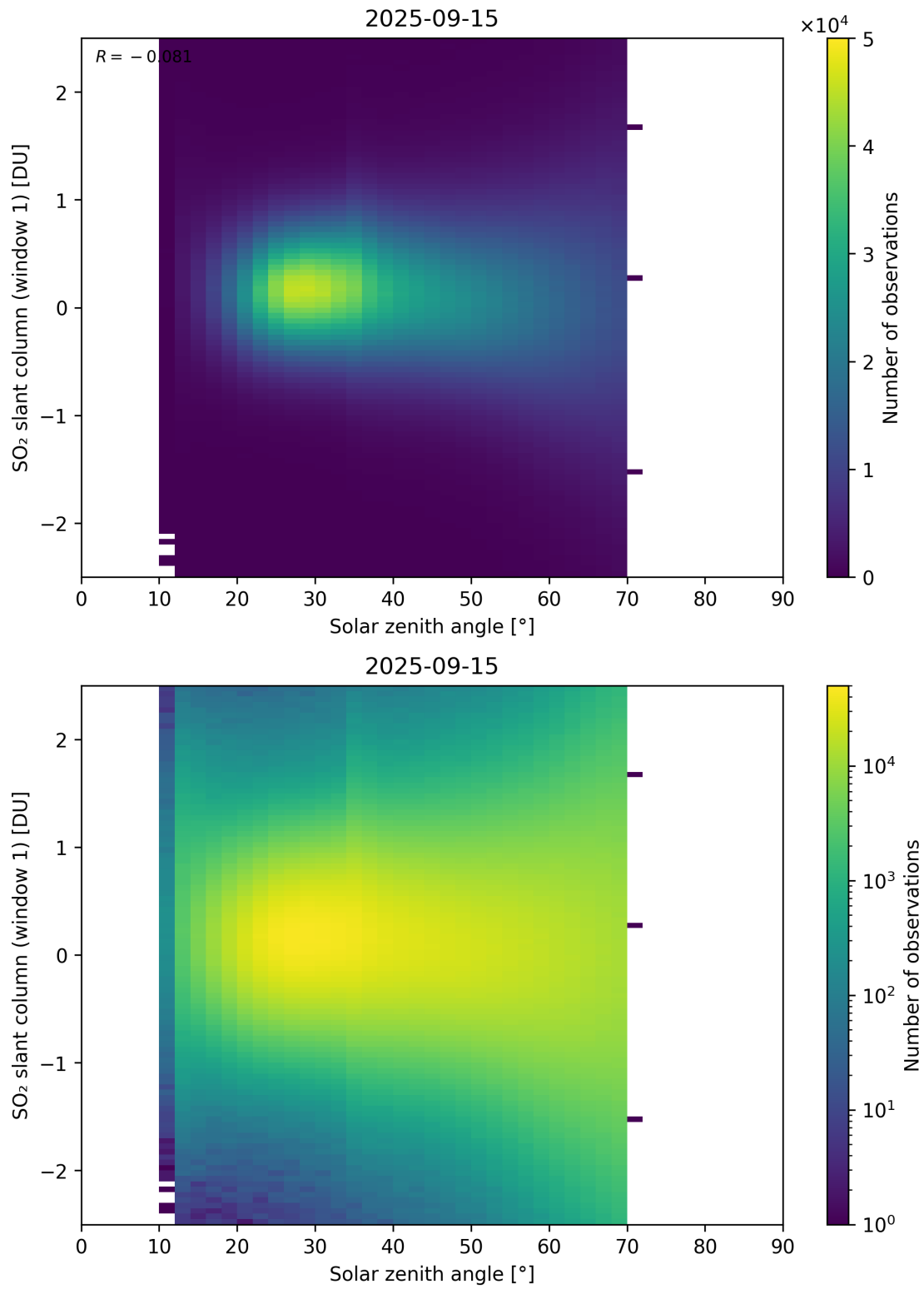
Figure 184: Scatter density plot of “Solar zenith angle” against “SO 2 slant column (window 1)” for 2025-09-15 to 2025-09-16.
