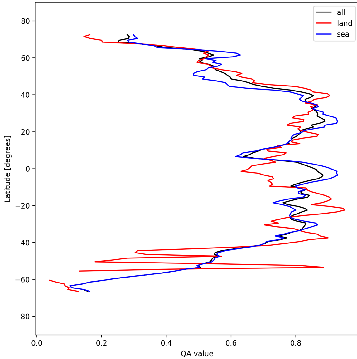
Figure 31: Zonal average of “QA value” for 2025-09-15 to 2025-09-16.
