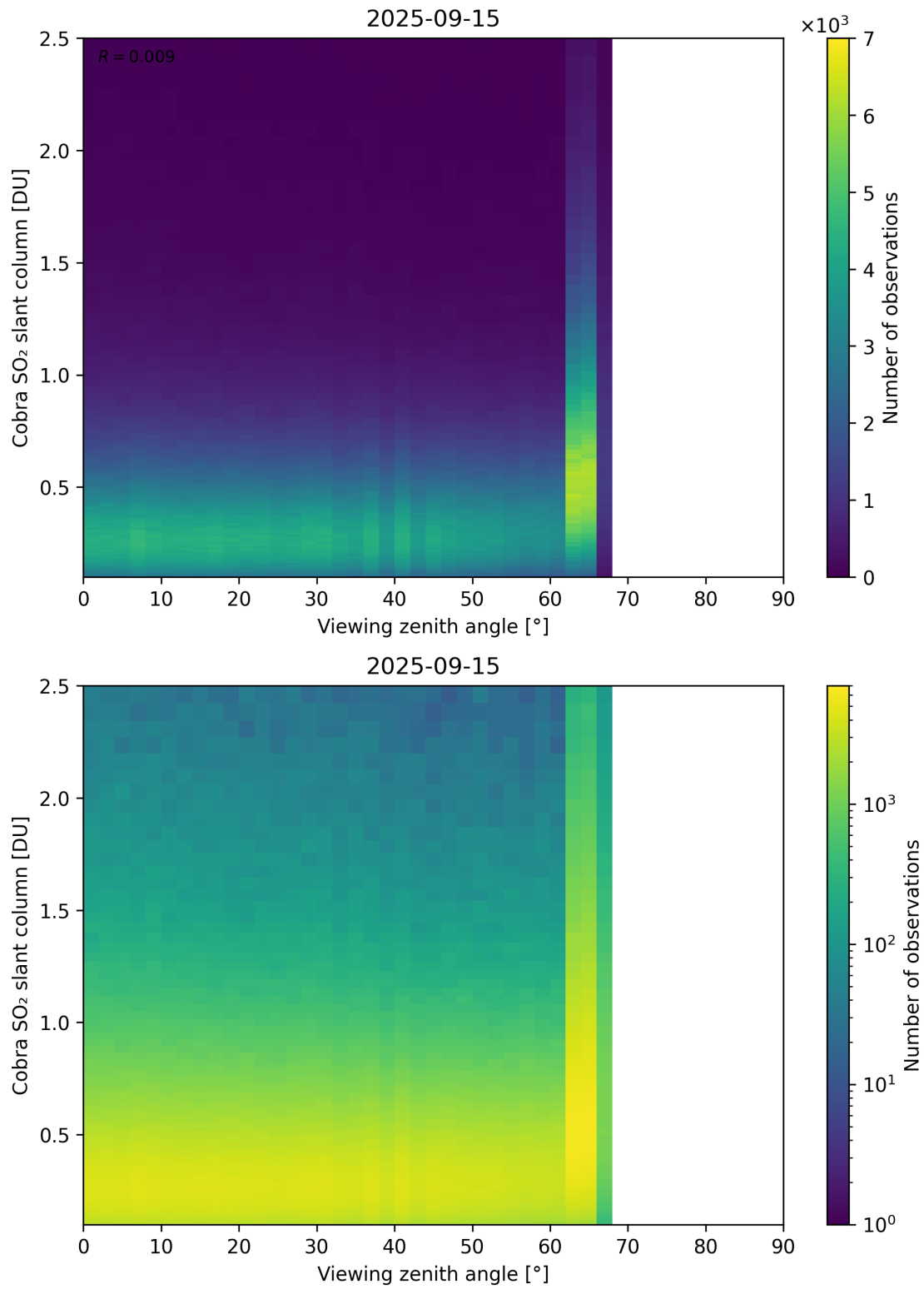
Figure 371: Scatter density plot of “Viewing zenith angle” against “Cobra SO 2 slant column” for 2025-09-15 to 2025-09-16.
