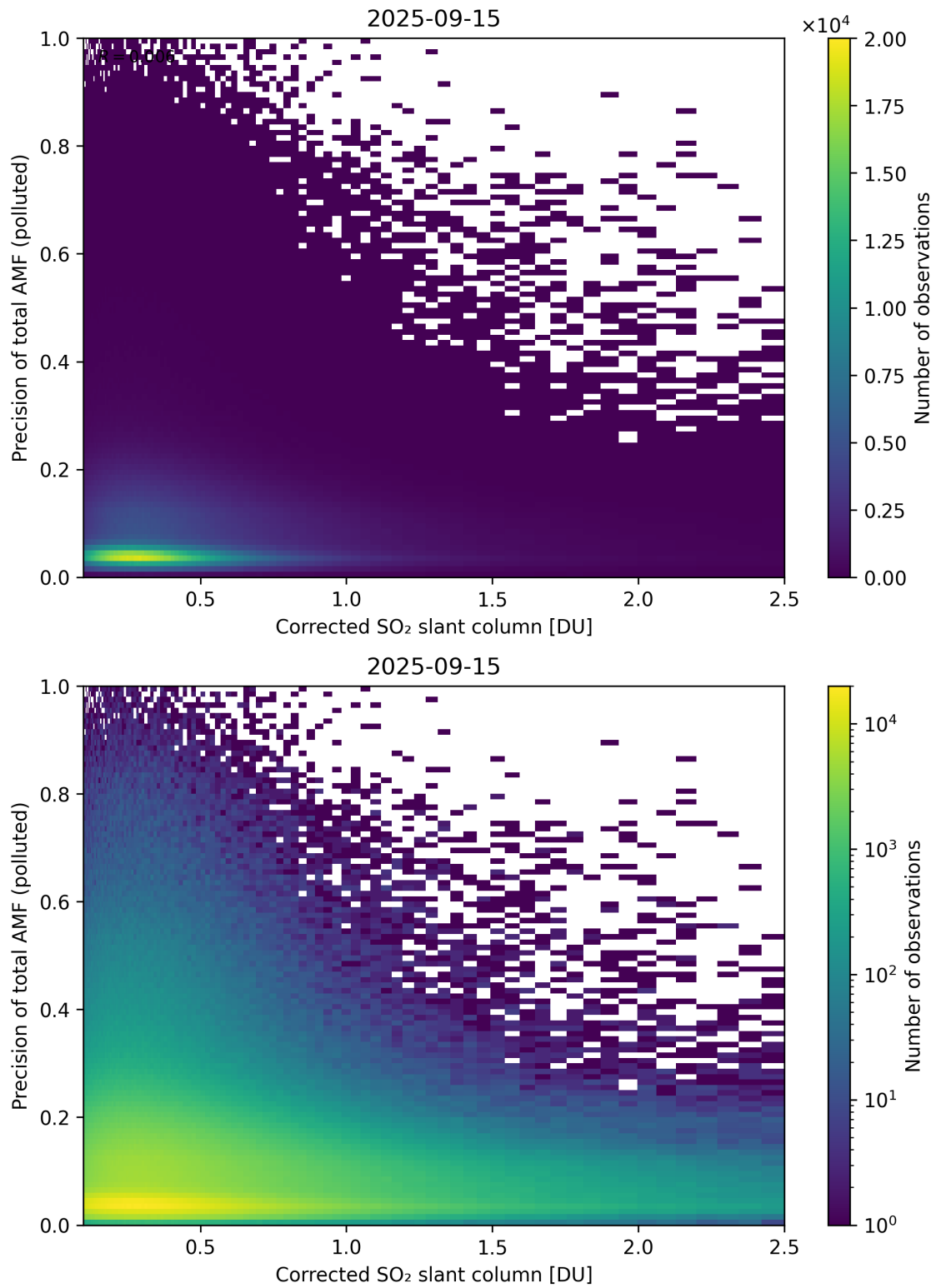
Figure 243: Scatter density plot of “Corrected SO 2 slant column” against “Precision of total AMF (polluted)” for 2025-09-15 to 2025-09-16.
