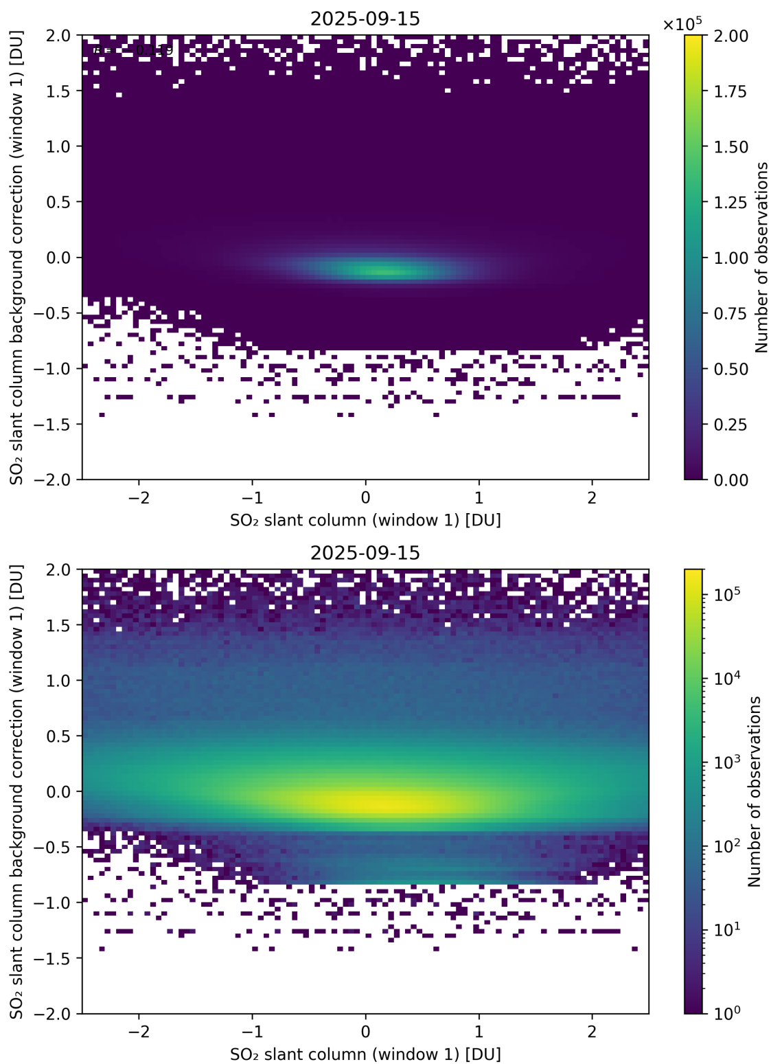
Figure 262: Scatter density plot of “SO 2 slant column (window 1)” against “SO 2 slant column background correction (window 1)” for 2025-09-15 to 2025-09-16.
