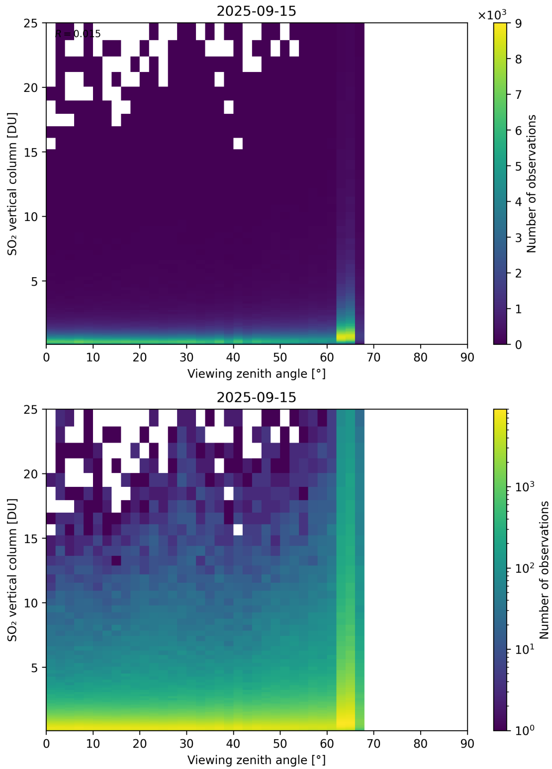
Figure 383: Scatter density plot of “Viewing zenith angle” against “SO 2 vertical column” for 2025-09-15 to 2025-09-16.
