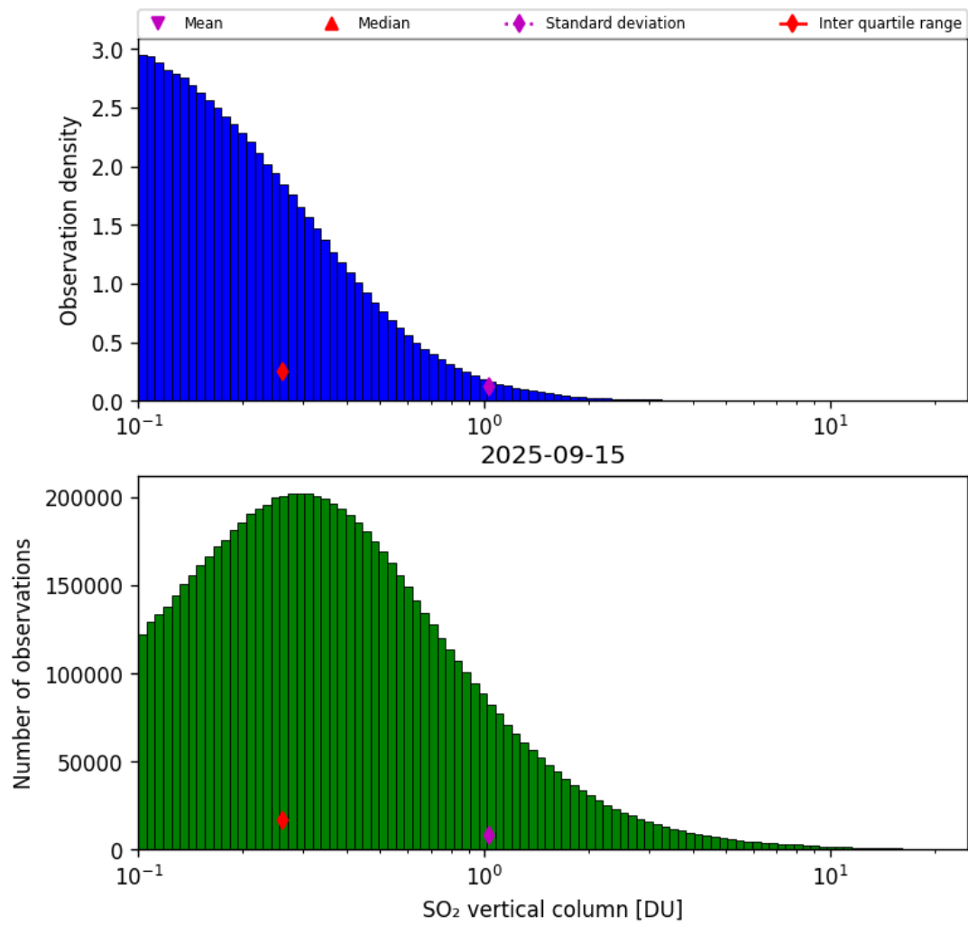
Figure 58: Histogram of “SO 2 vertical column” for 2025-09-15 to 2025-09-16
