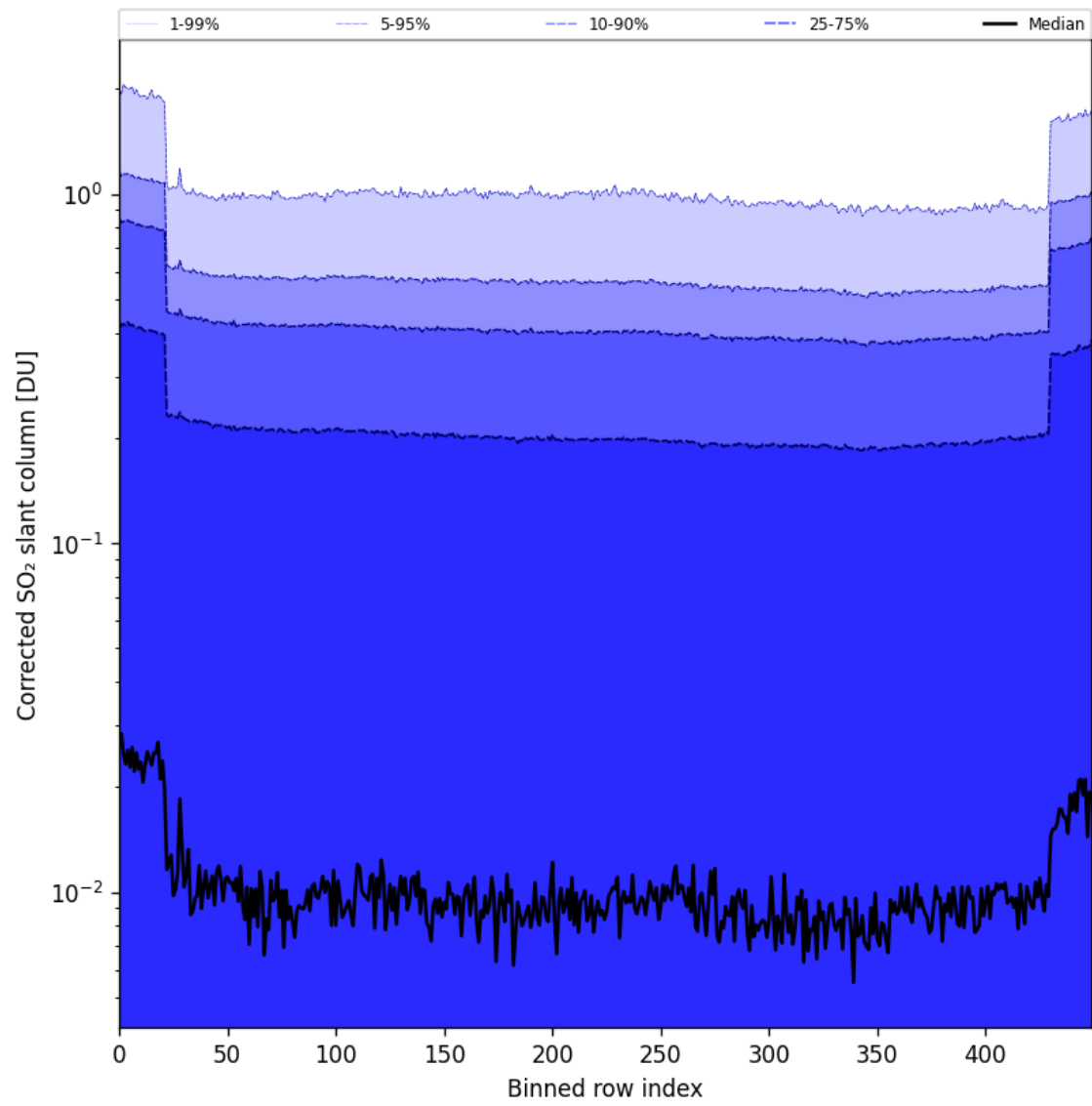
Figure 86: Along track statistics of “Corrected SO 2 slant column” for 2025-09-15 to 2025-09-16
