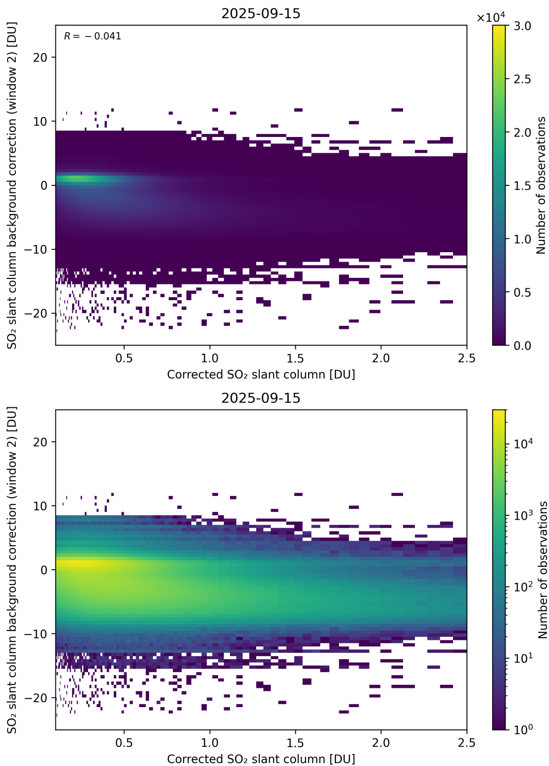
Figure 227: Scatter density plot of “Corrected SO 2 slant column” against “SO 2 slant column background correction (window 2)” for 2025-09-15 to 2025-09-16.
