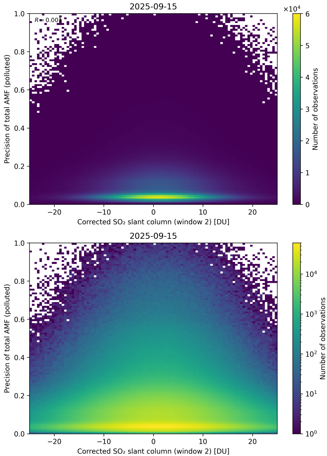
Figure 254: Scatter density plot of “Corrected SO 2 slant column (window 2)” against “Precision of total AMF (polluted)” for 2025-09-15 to 2025-09-16.
