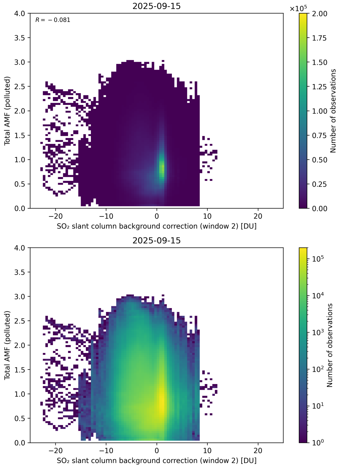
Figure 130: Scatter density plot of “SO 2 slant column background correction (window 2)” against “Total AMF (polluted)” for 2025-09-15 to 2025-09-16.
