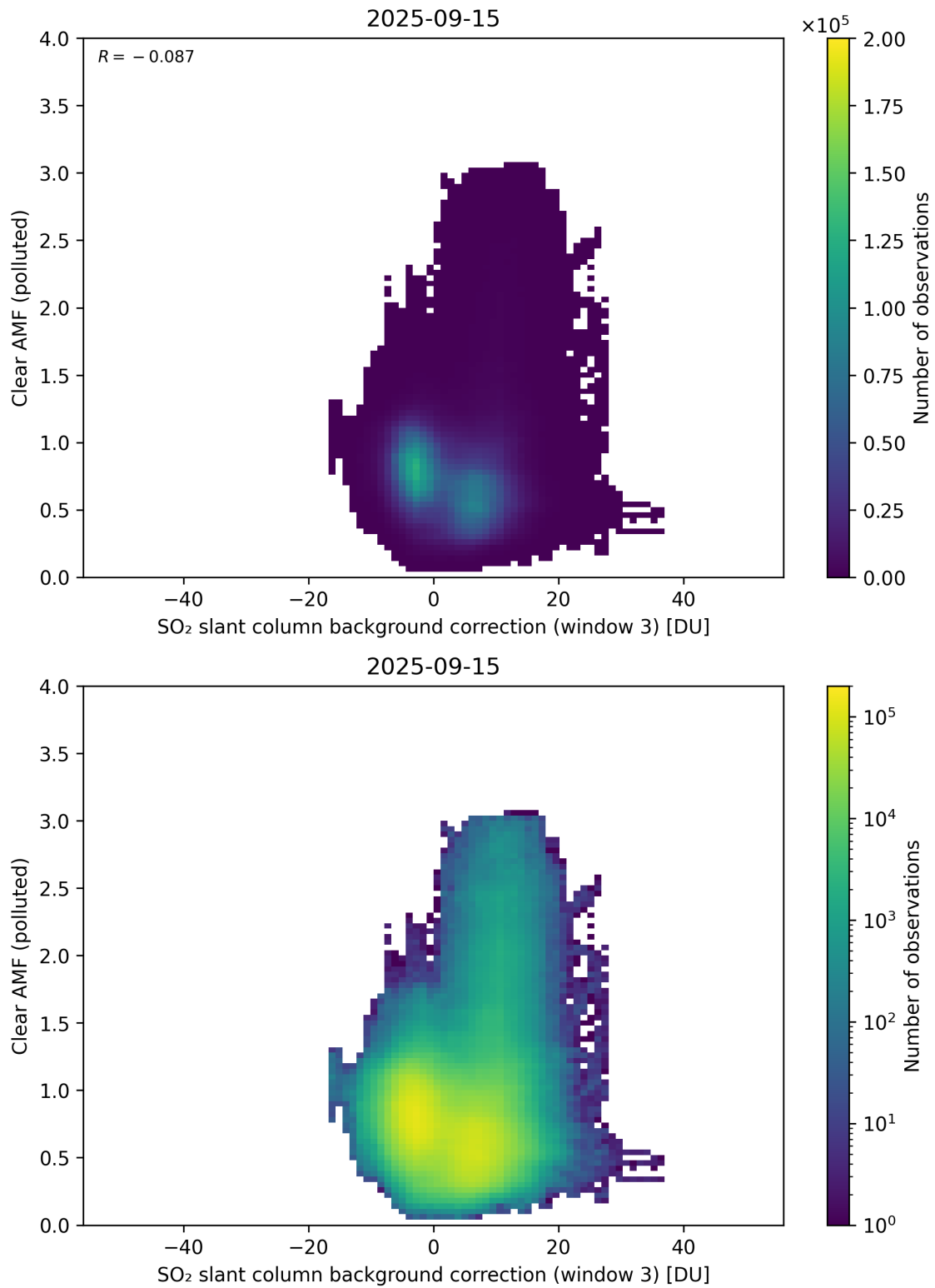
Figure 135: Scatter density plot of “SO 2 slant column background correction (window 3)” against “Clear AMF (polluted)” for 2025-09-15 to 2025-09-16.
