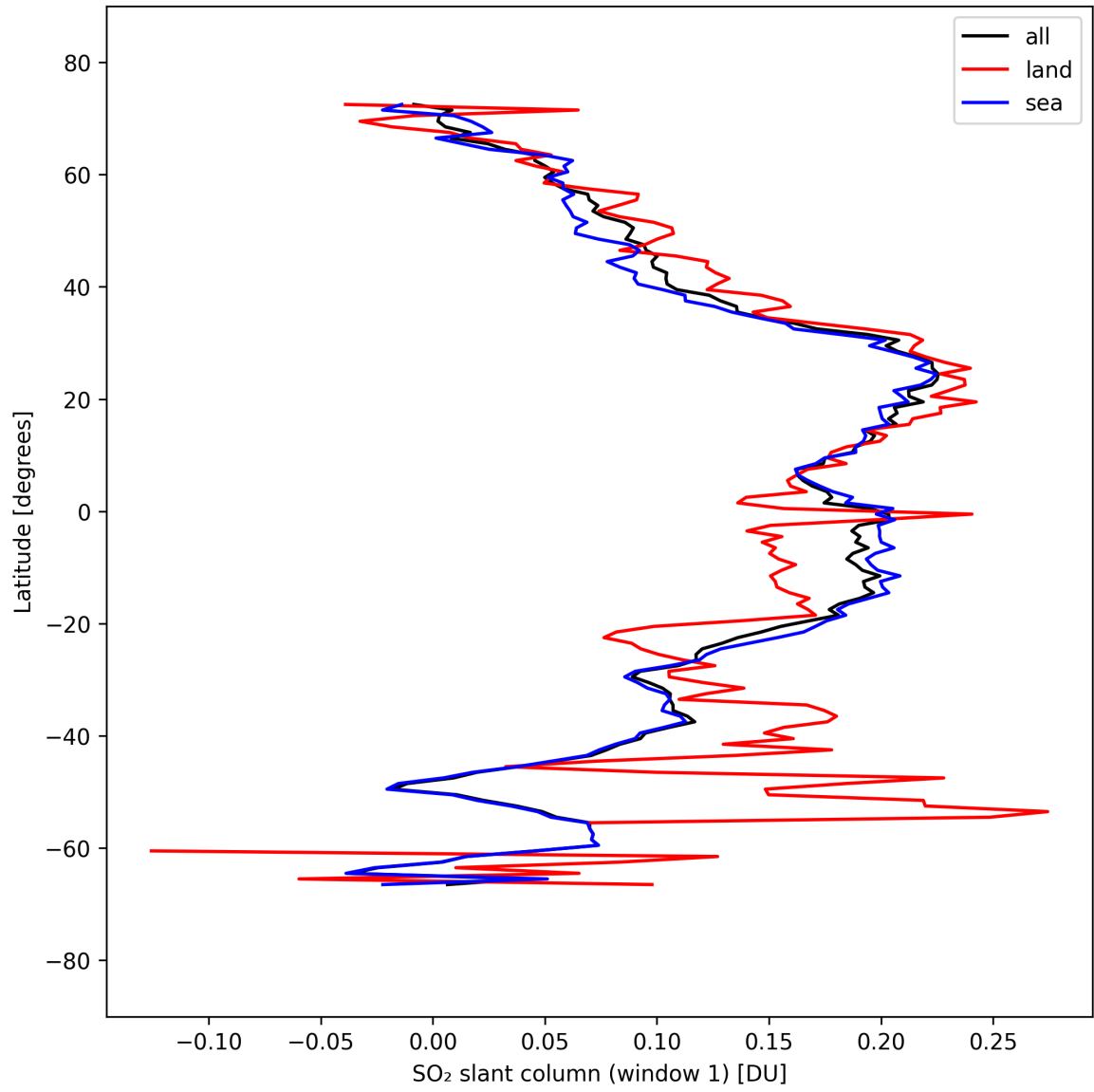
Figure 37: Zonal average of “SO 2 slant column (window 1)” for 2025-09-15 to 2025-09-16.
