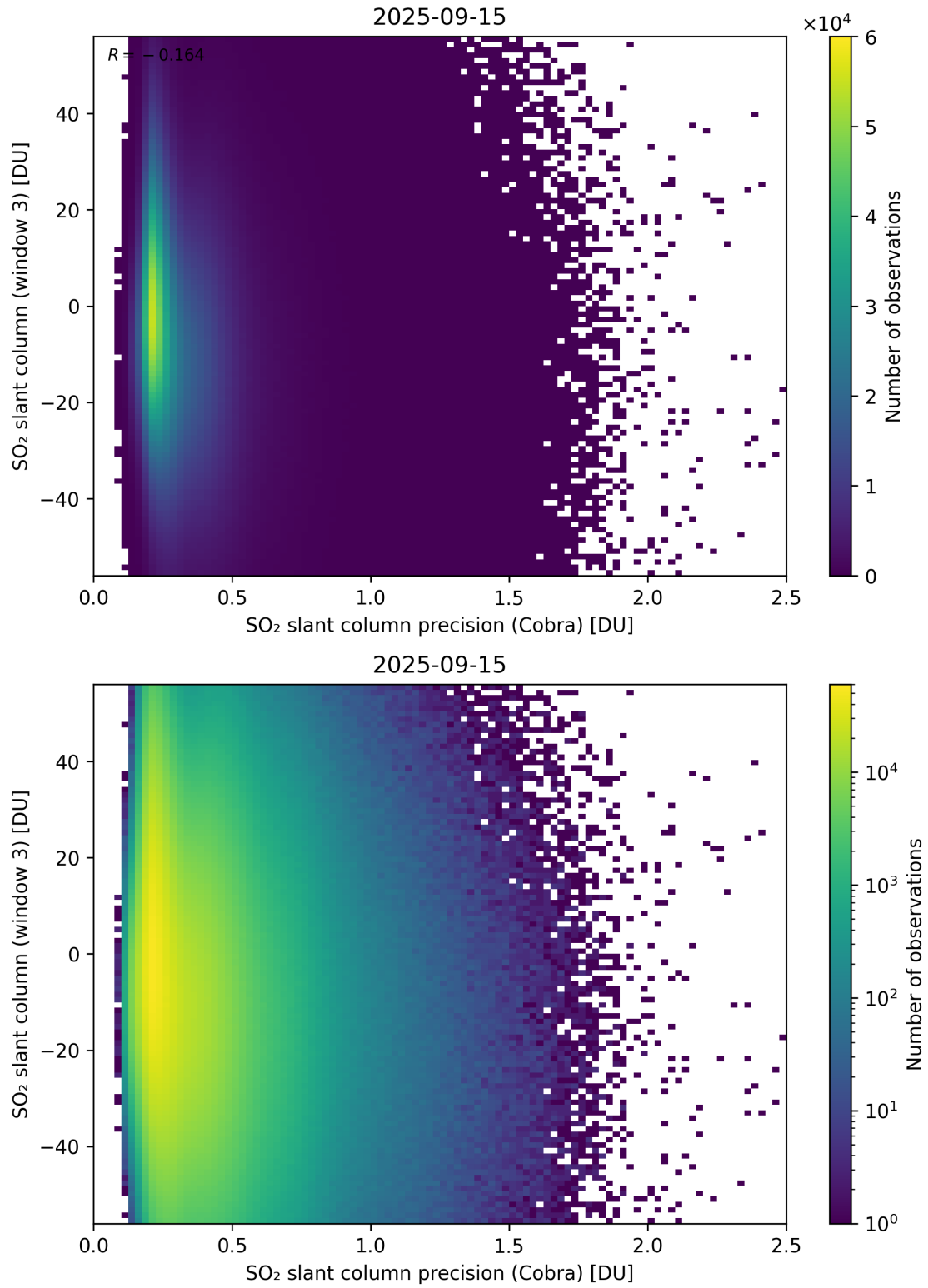
Figure 211: Scatter density plot of “SO 2 slant column precision (Cobra)” against “SO 2 slant column (window 3)” for 2025-09-15 to 2025-09-16.
