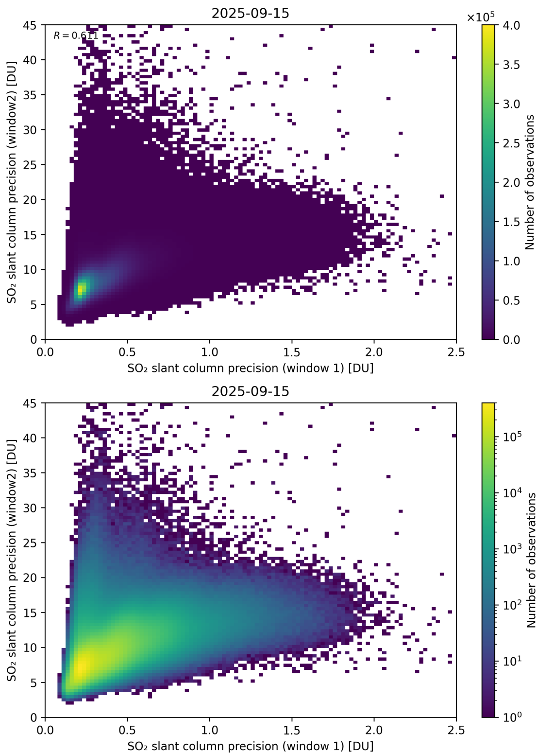
Figure 277: Scatter density plot of “SO 2 slant column precision (window 1)” against “SO 2 slant column precision (window2)” for 2025-09-15 to 2025-09-16.
