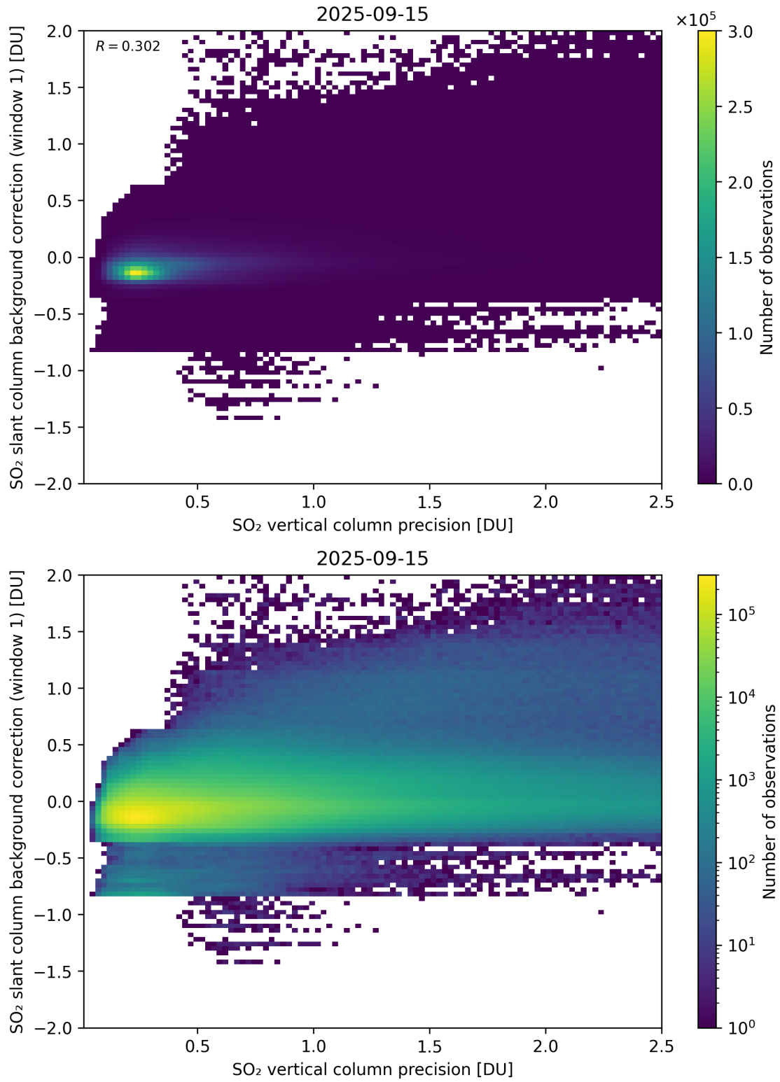
Figure 329: Scatter density plot of “SO 2 vertical column precision” against “SO 2 slant column background correction (window 1)” for 2025-09-15 to 2025-09-16.
