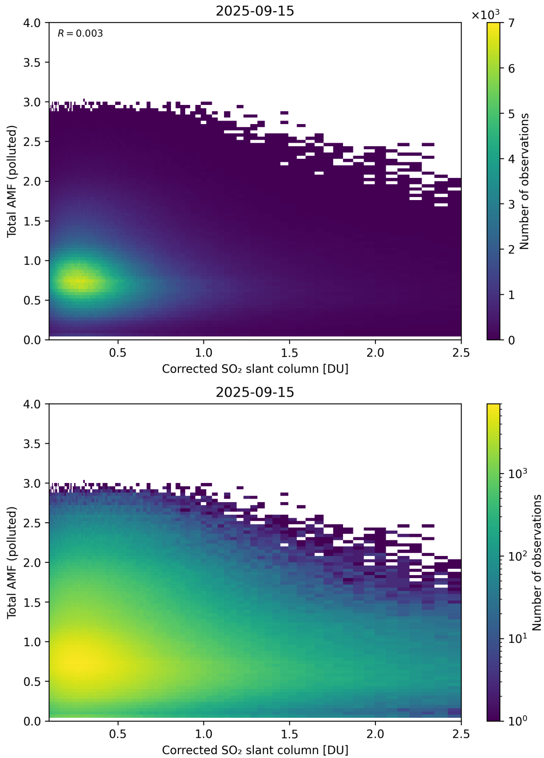
Figure 242: Scatter density plot of “Corrected SO 2 slant column” against “Total AMF (polluted)” for 2025-09-15 to 2025-09-16.
