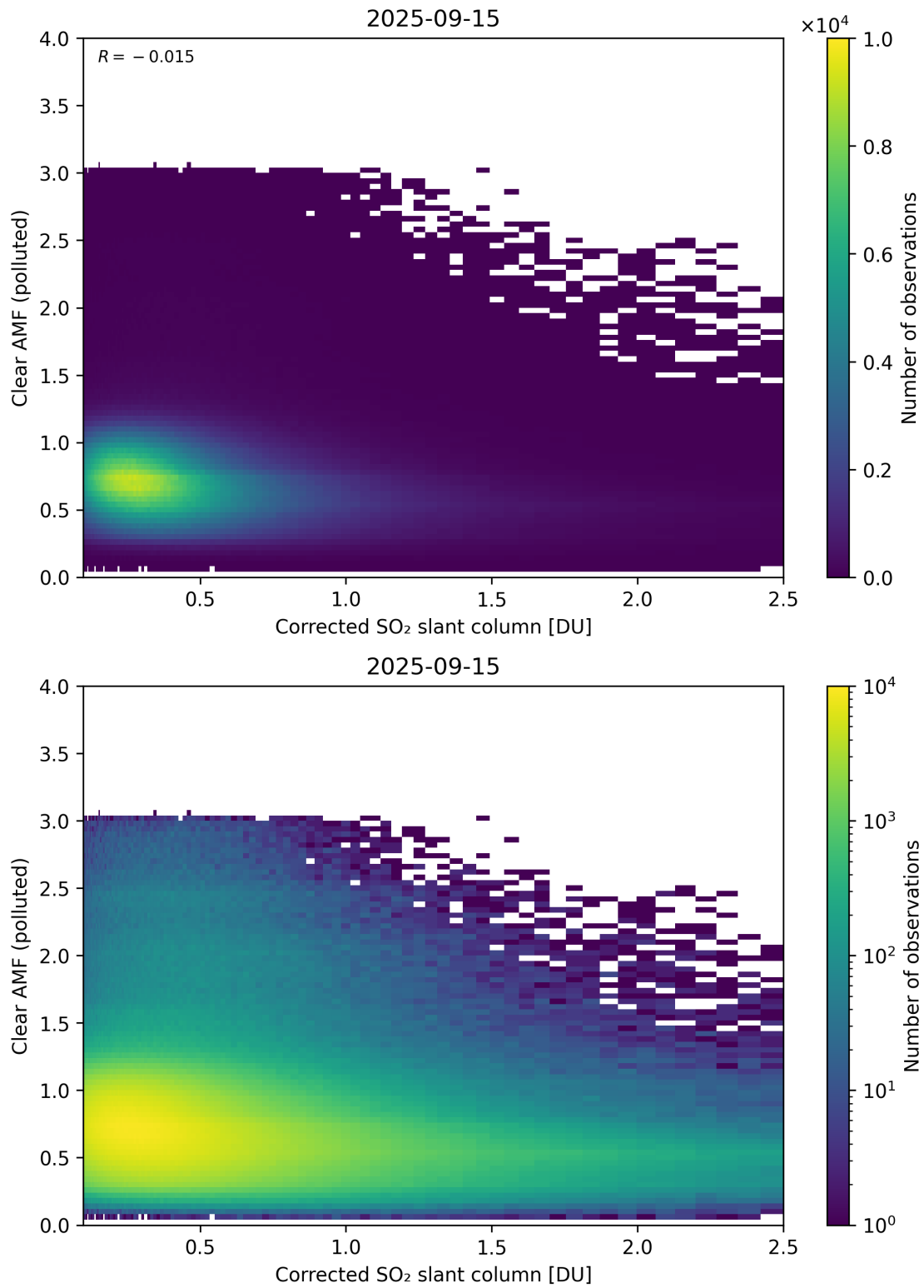
Figure 232: Scatter density plot of “Corrected SO 2 slant column” against “Clear AMF (polluted)” for 2025-09-15 to 2025-09-16.
