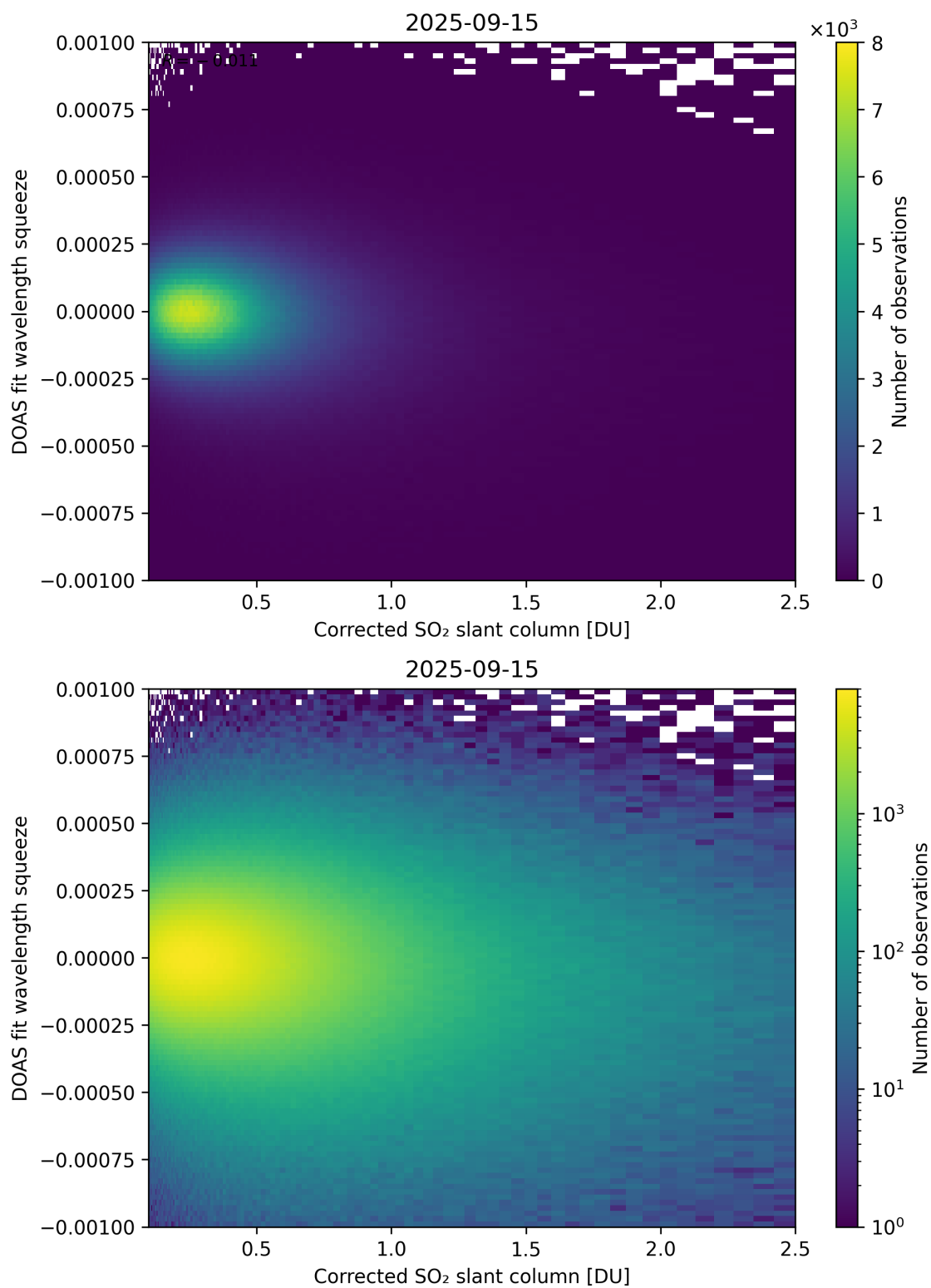
Figure 230: Scatter density plot of “Corrected SO 2 slant column” against “DOAS fit wavelength squeeze” for 2025-09-15 to 2025-09-16.
