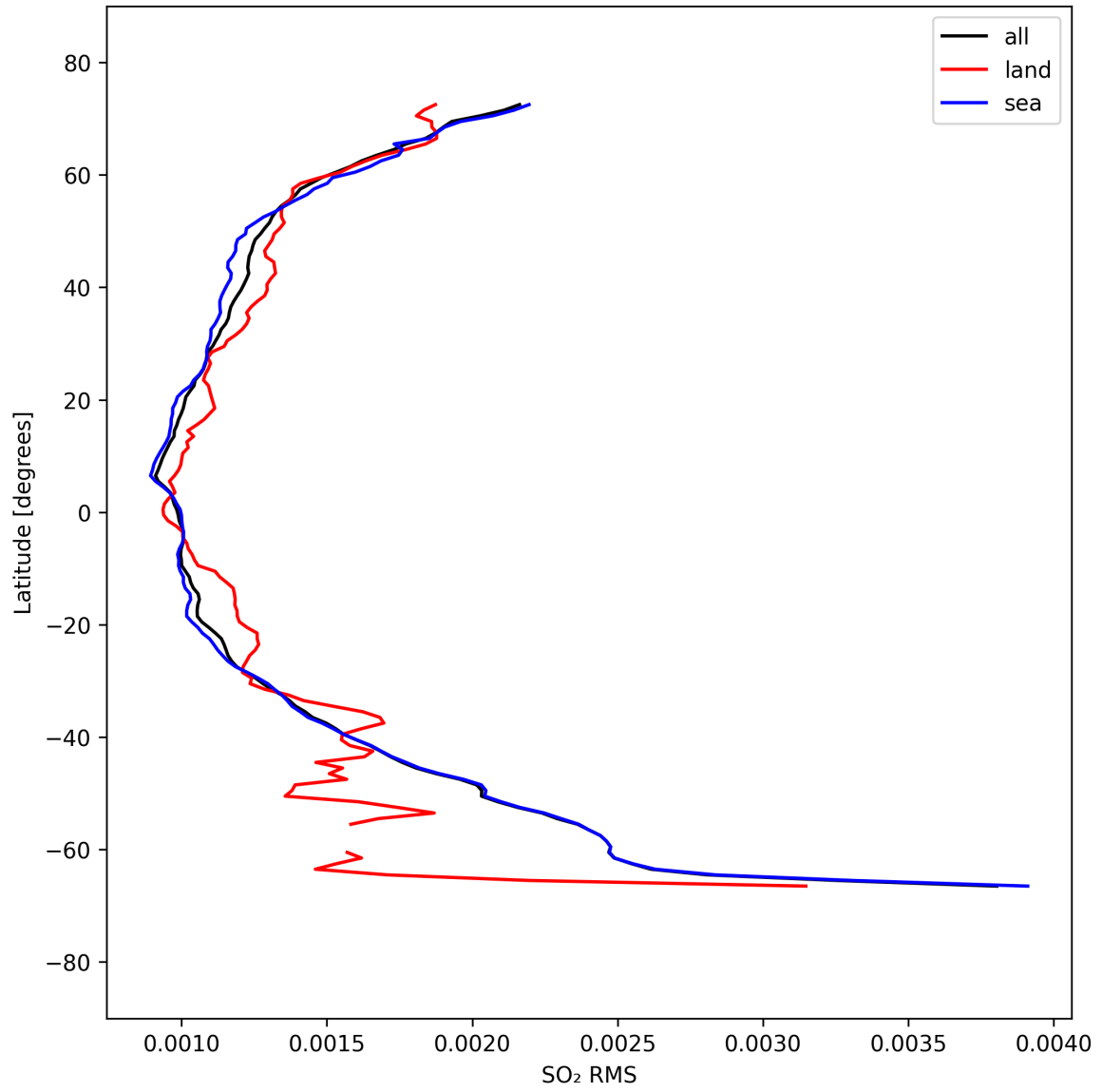
Figure 52: Zonal average of “SO 2 RMS” for 2025-09-15 to 2025-09-16.
