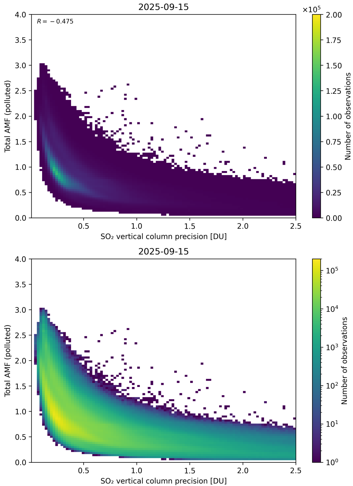
Figure 346: Scatter density plot of “SO 2 vertical column precision” against “Total AMF (polluted)” for 2025-09-15 to 2025-09-16.
