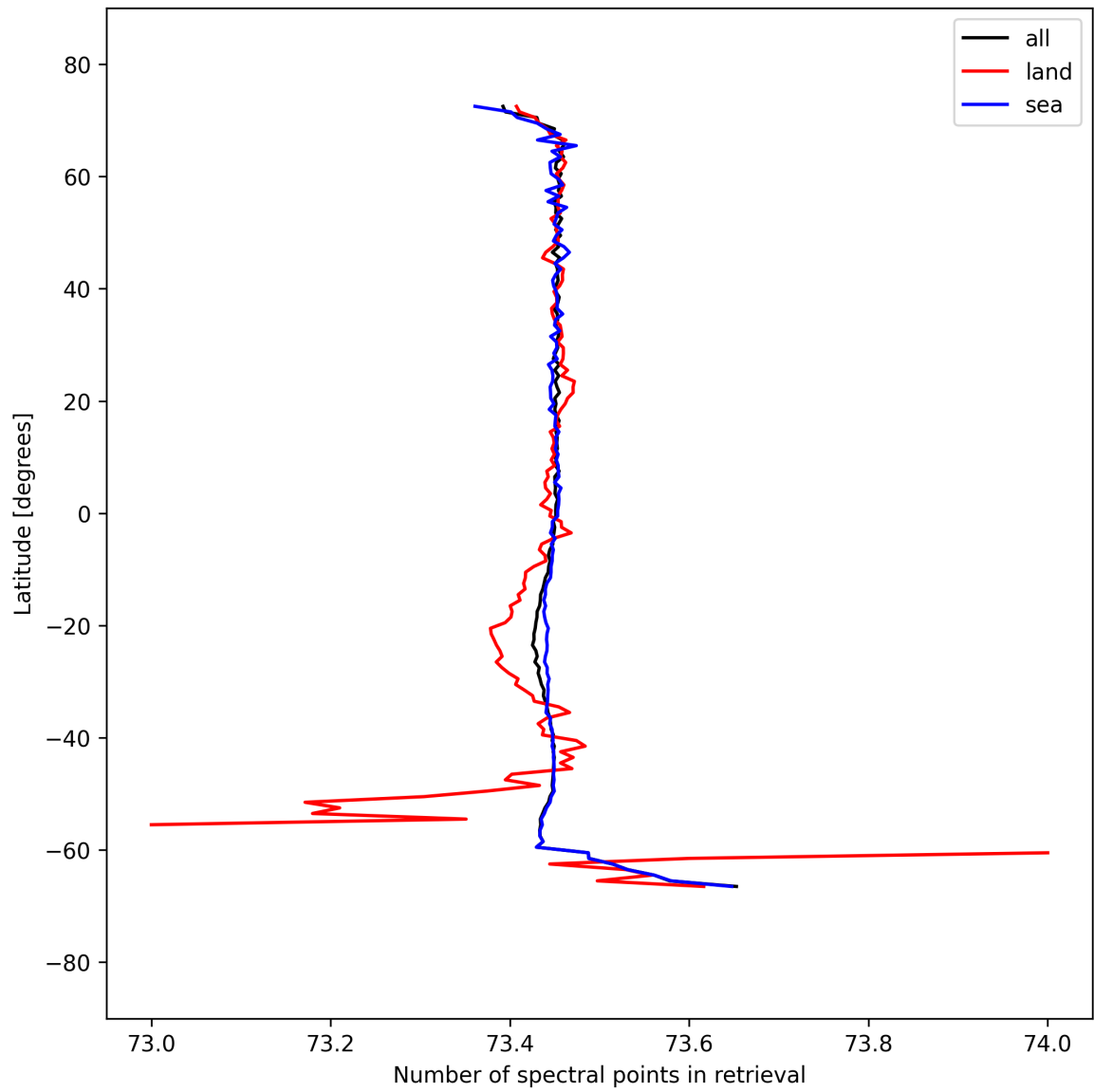
Figure 56: Zonal average of “Number of spectral points in retrieval” for 2025-09-15 to 2025-09-16.
