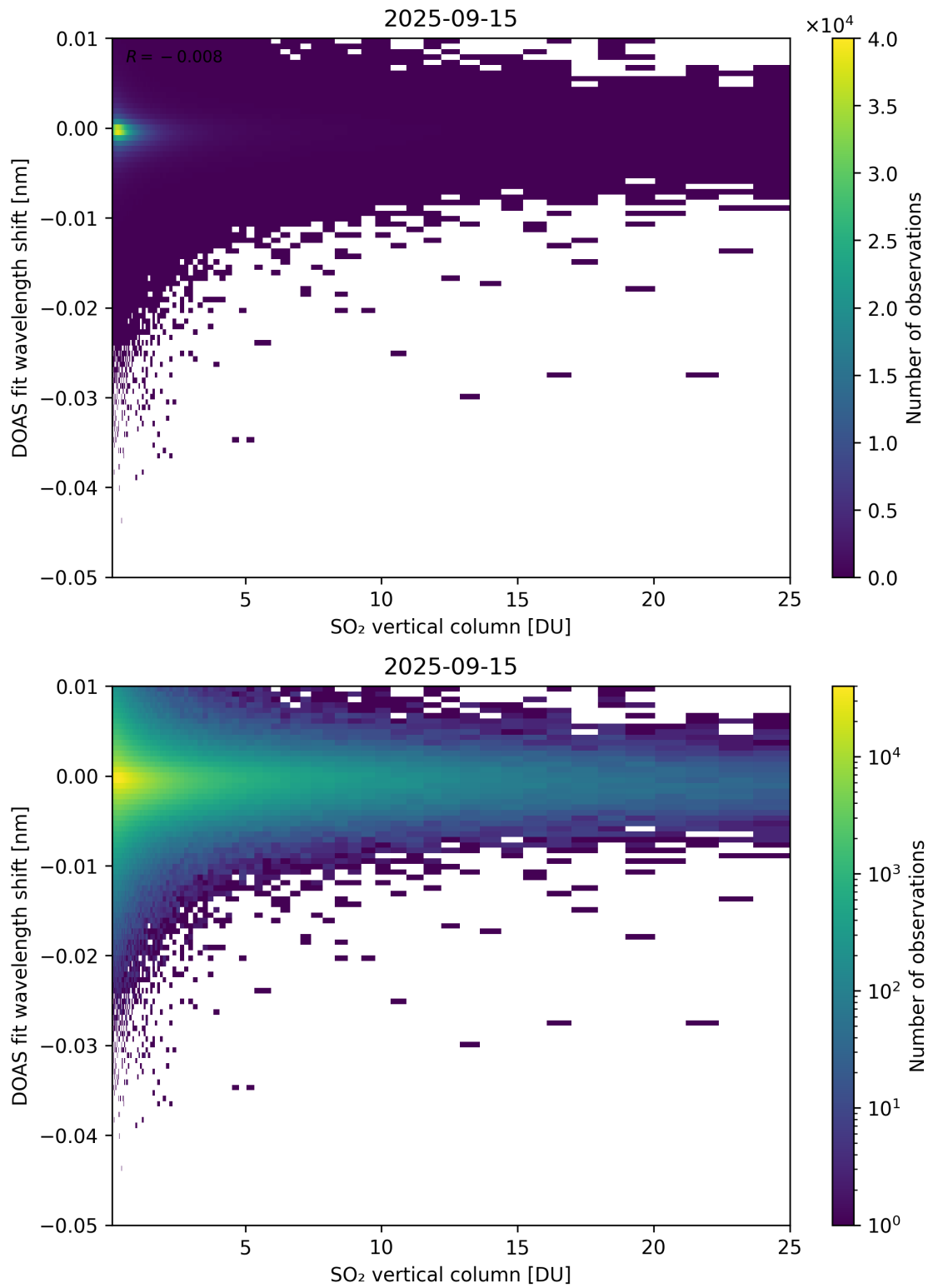
Figure 326: Scatter density plot of “SO 2 vertical column” against “DOAS fit wavelength shift” for 2025-09-15 to 2025-09-16.
