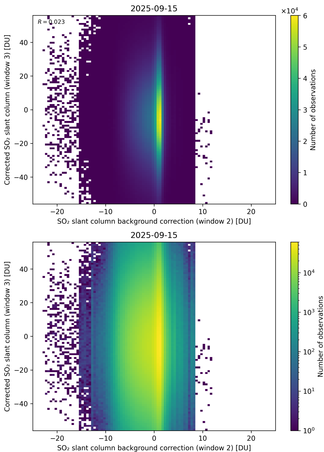
Figure 127: Scatter density plot of “SO 2 slant column background correction (window 2)” against “Corrected SO 2 slant column (window 3)” for 2025-09-15 to 2025-09-16.
