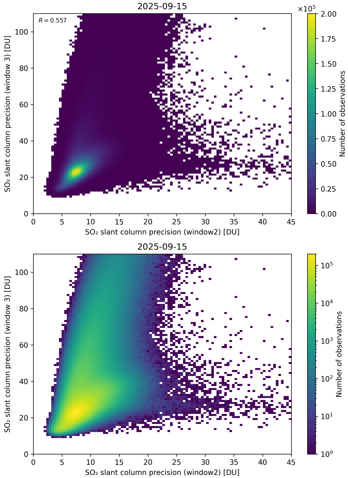
Figure 300: Scatter density plot of “SO 2 slant column precision (window2)” against “SO 2 slant column precision (window 3)” for 2025-09-15 to 2025-09-16.
