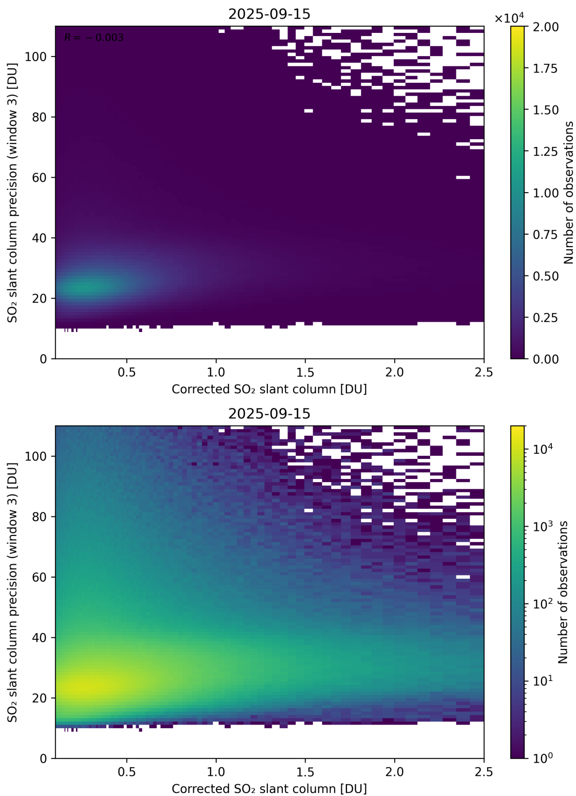
Figure 241: Scatter density plot of “Corrected SO 2 slant column” against “SO 2 slant column precision (window 3)” for 2025-09-15 to 2025-09-16.
