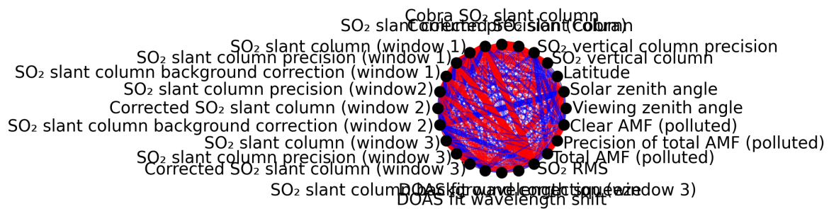
Figure 1: Map of correlation graph for 2025-09-15 to 2025-09-16.
