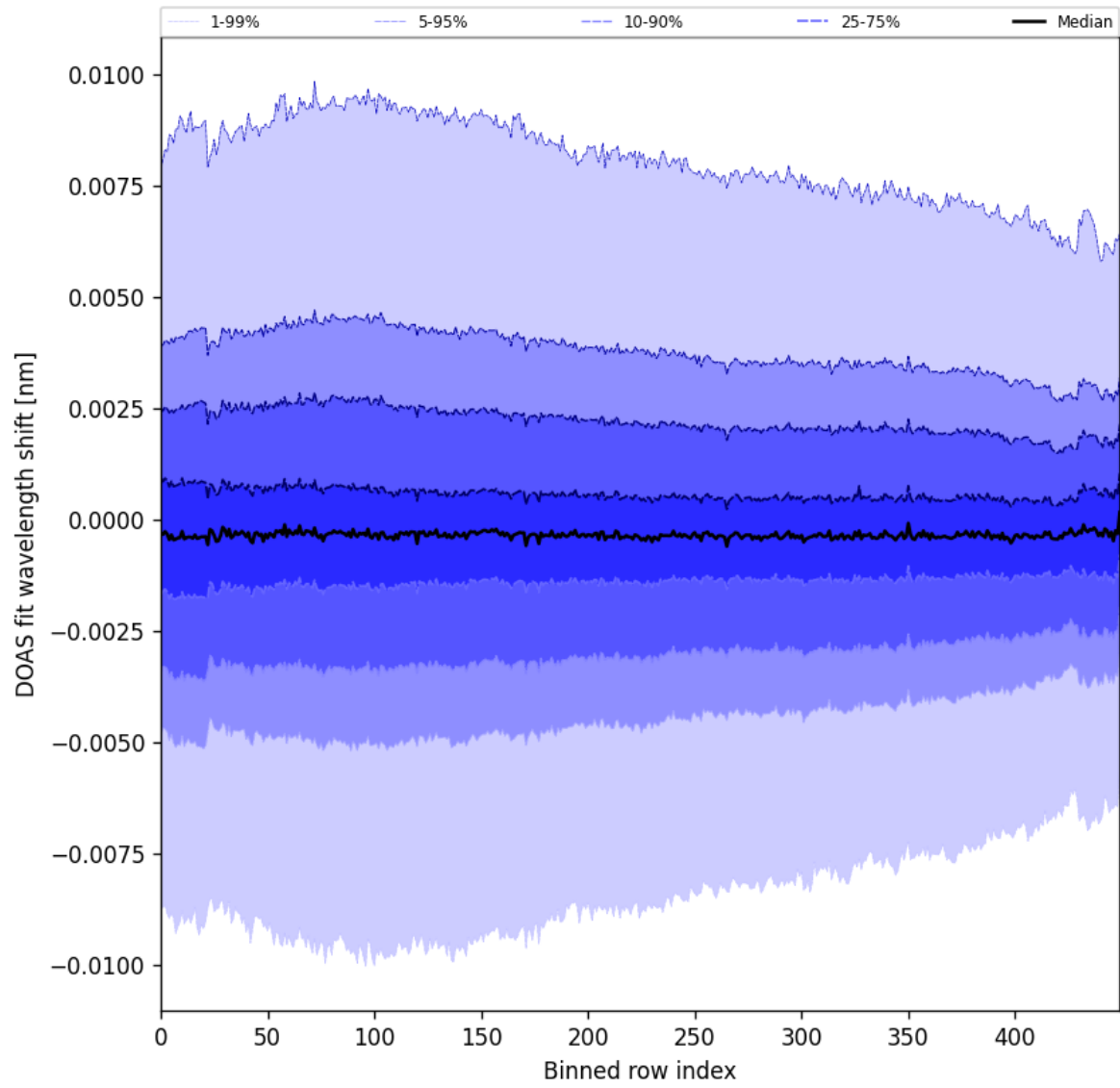
Figure 102: Along track statistics of “DOAS fit wavelength shift” for 2025-09-15 to 2025-09-16
