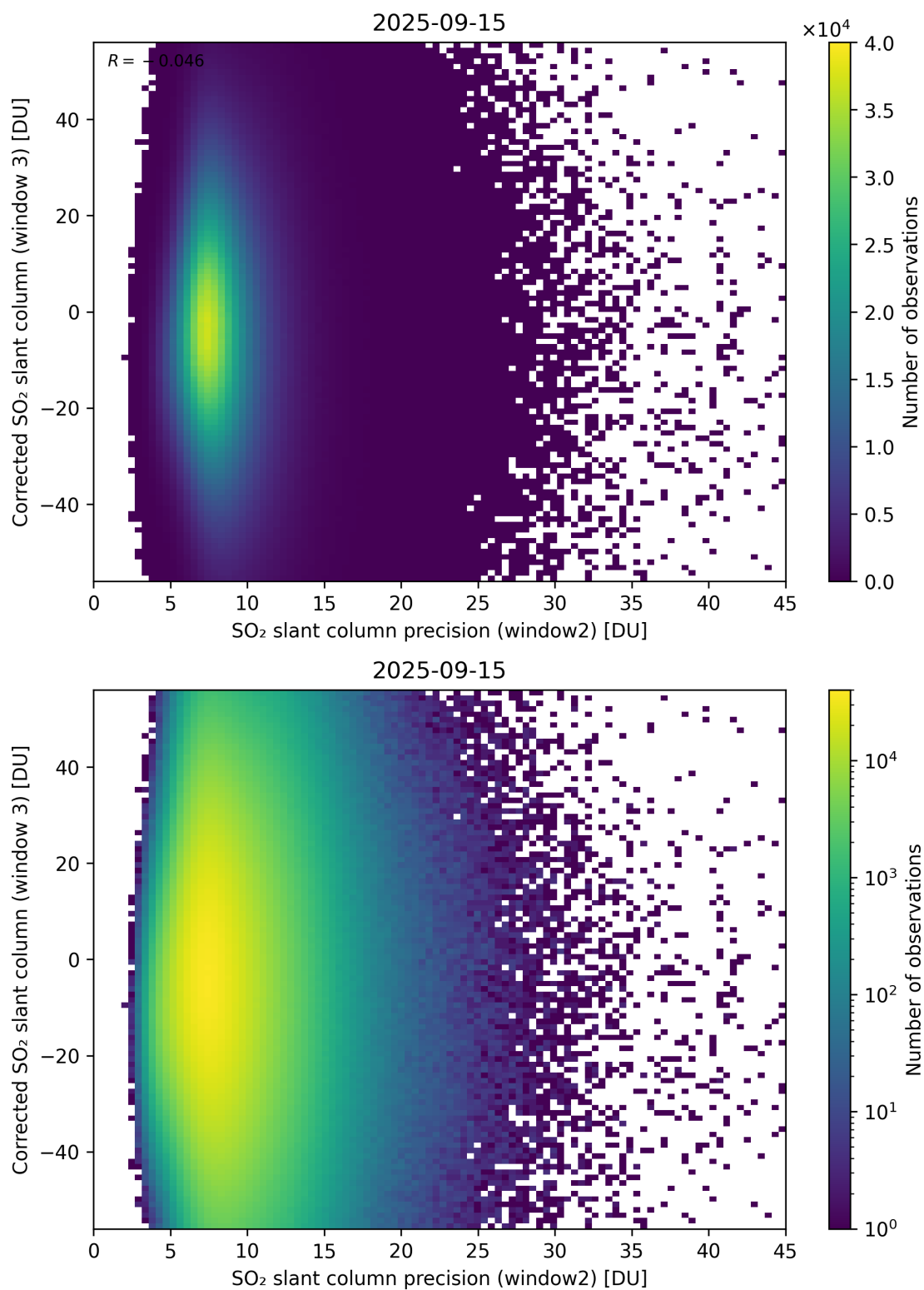
Figure 298: Scatter density plot of “SO 2 slant column precision (window2)” against “Corrected SO 2 slant column (window 3)” for 2025-09-15 to 2025-09-16.
