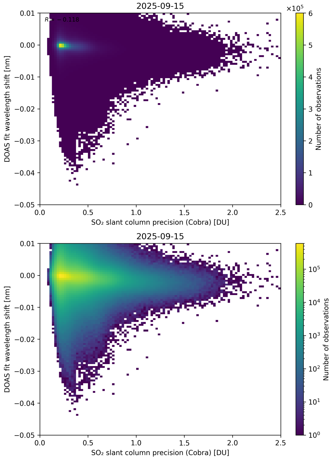
Figure 202: Scatter density plot of “SO 2 slant column precision (Cobra)” against “DOAS fit wavelength shift” for 2025-09-15 to 2025-09-16.
