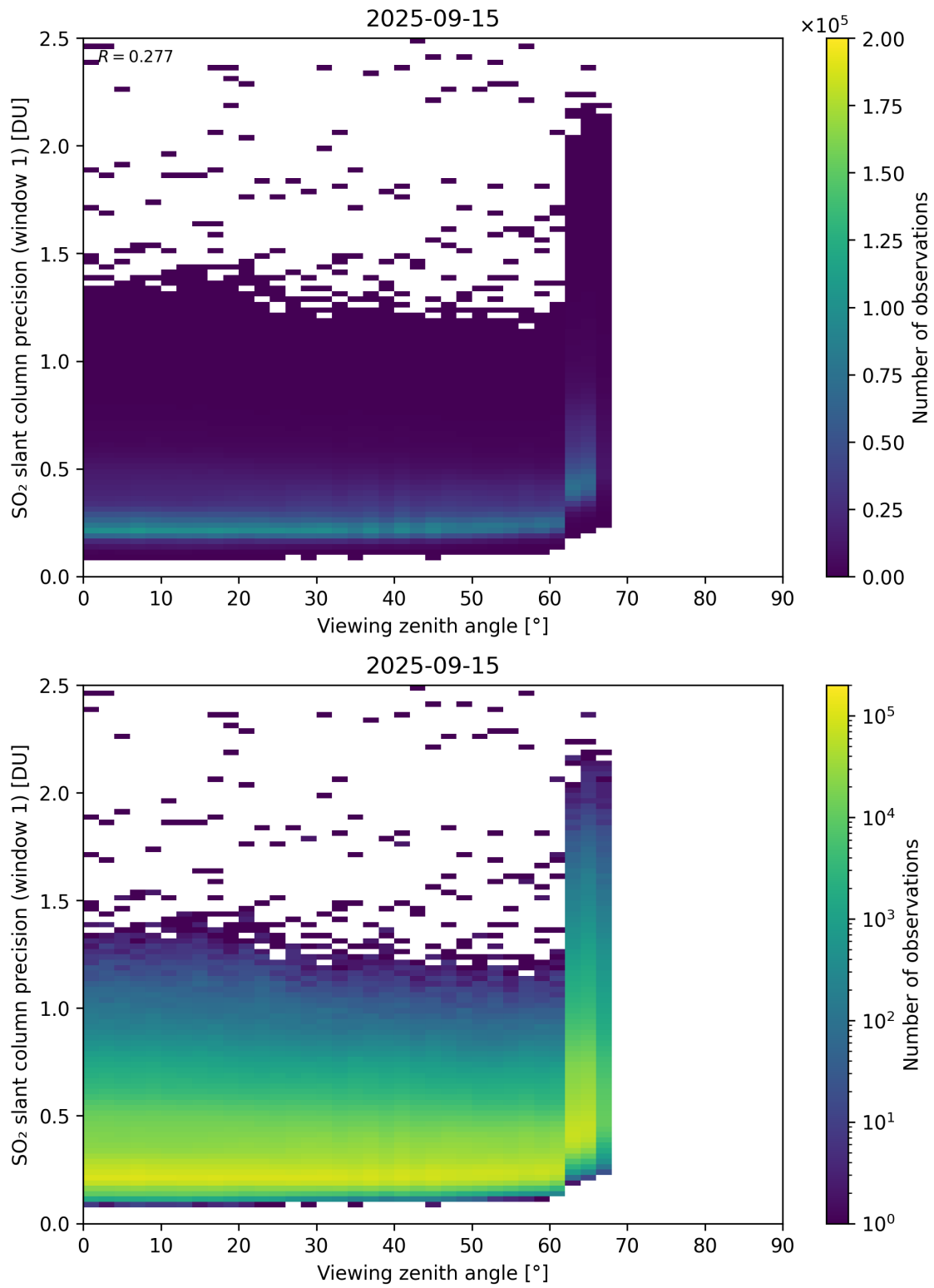
Figure 377: Scatter density plot of “Viewing zenith angle” against “SO 2 slant column precision (window 1)” for 2025-09-15 to 2025-09-16.
