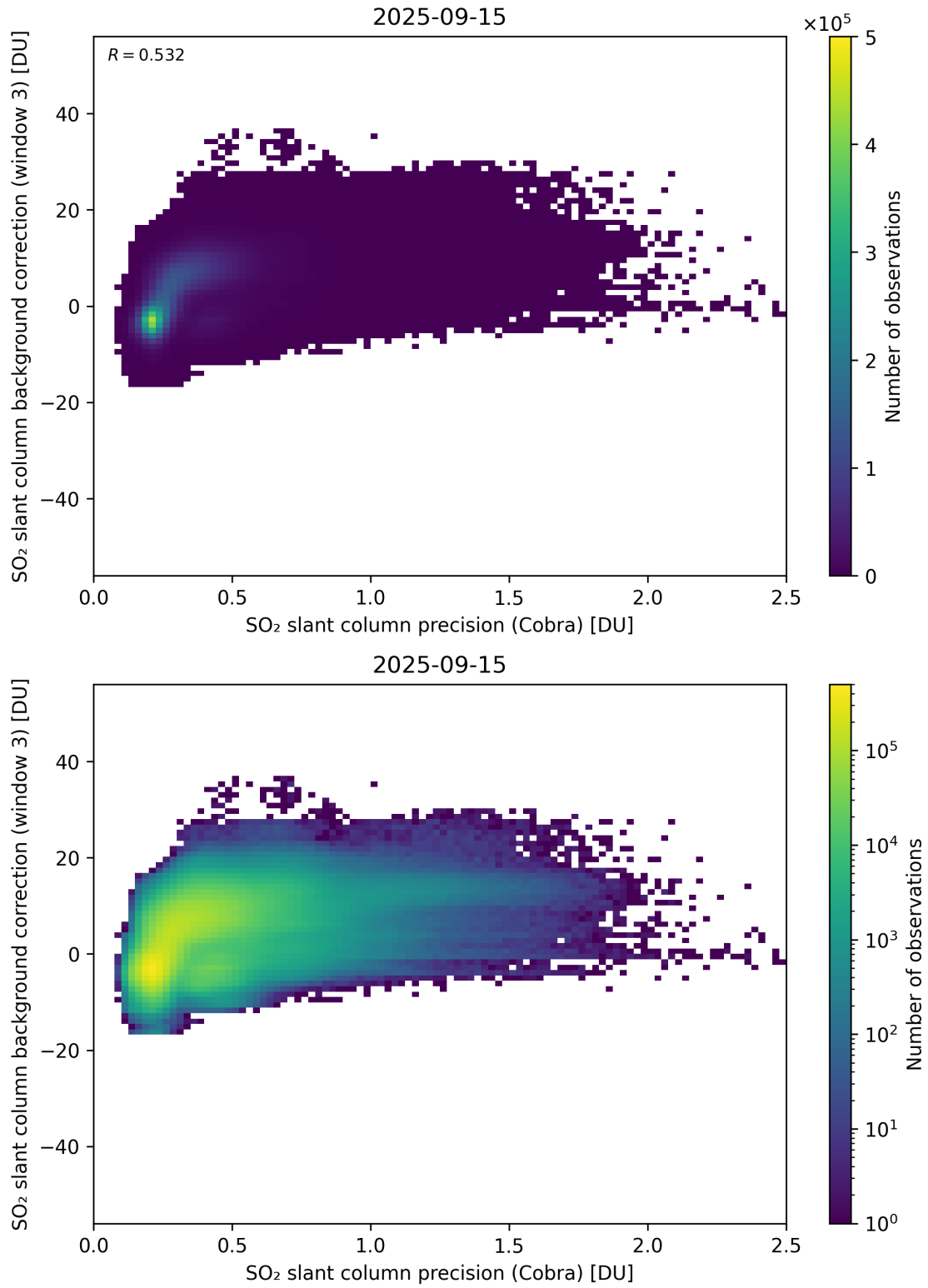
Figure 201: Scatter density plot of “SO 2 slant column precision (Cobra)” against “SO 2 slant column background correction (window 3)” for 2025-09-15 to 2025-09-16.
