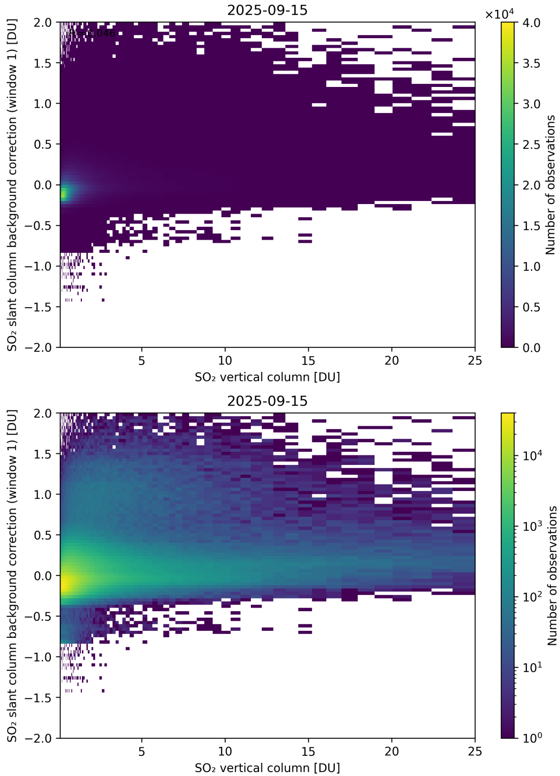
Figure 323: Scatter density plot of “SO 2 vertical column” against “SO 2 slant column background correction (window 1)” for 2025-09-15 to 2025-09-16.
