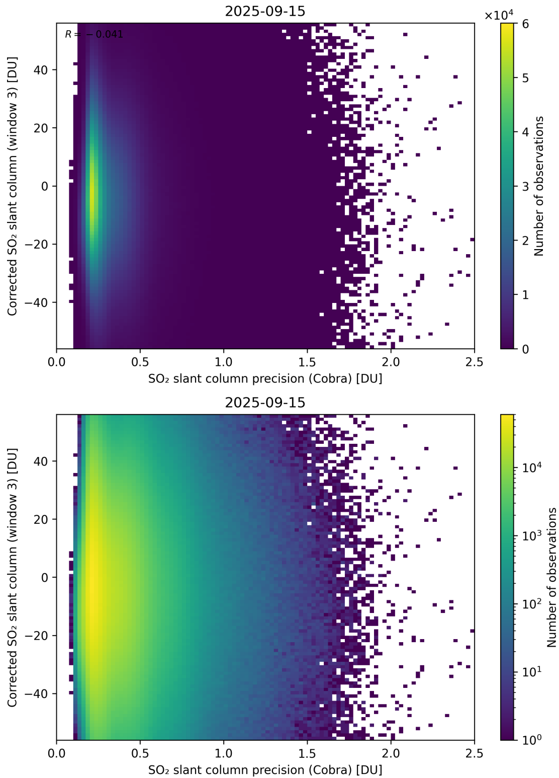
Figure 207: Scatter density plot of “SO 2 slant column precision (Cobra)” against “Corrected SO 2 slant column (window 3)” for 2025-09-15 to 2025-09-16.
