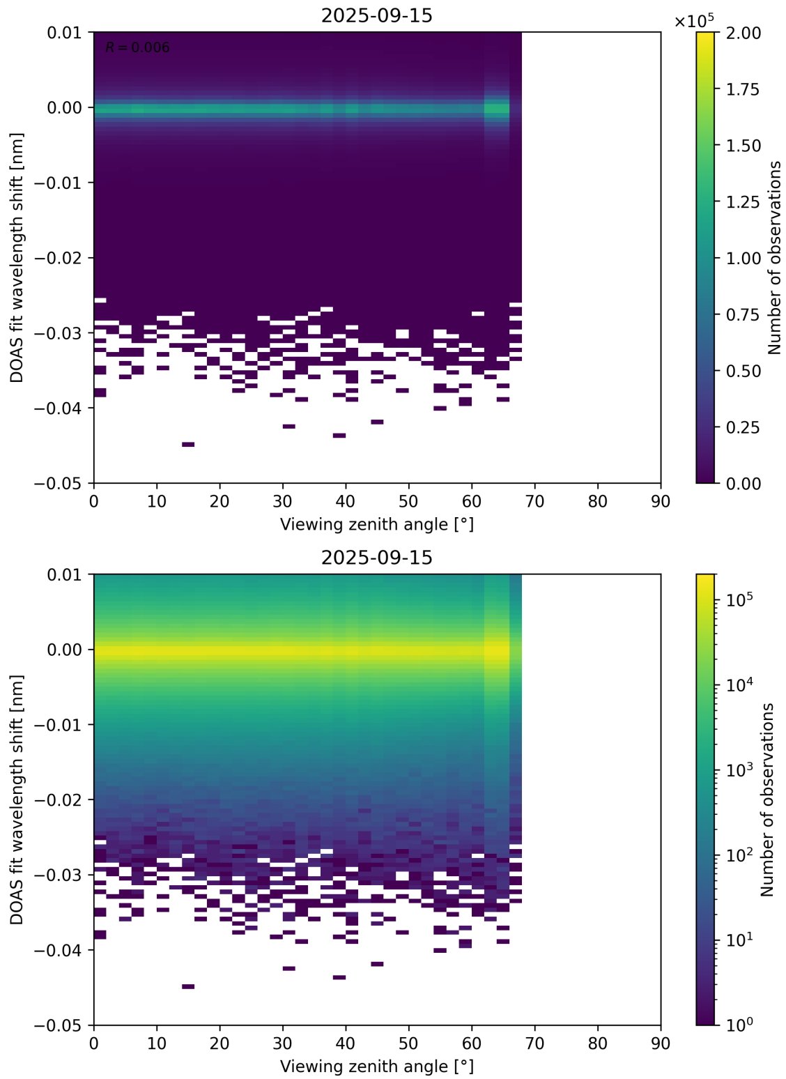
Figure 365: Scatter density plot of “Viewing zenith angle” against “DOAS fit wavelength shift” for 2025-09-15 to 2025-09-16.
