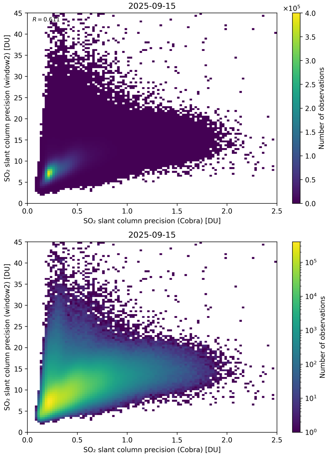
Figure 210: Scatter density plot of “SO 2 slant column precision (Cobra)” against “SO 2 slant column precision (window2)” for 2025-09-15 to 2025-09-16.
