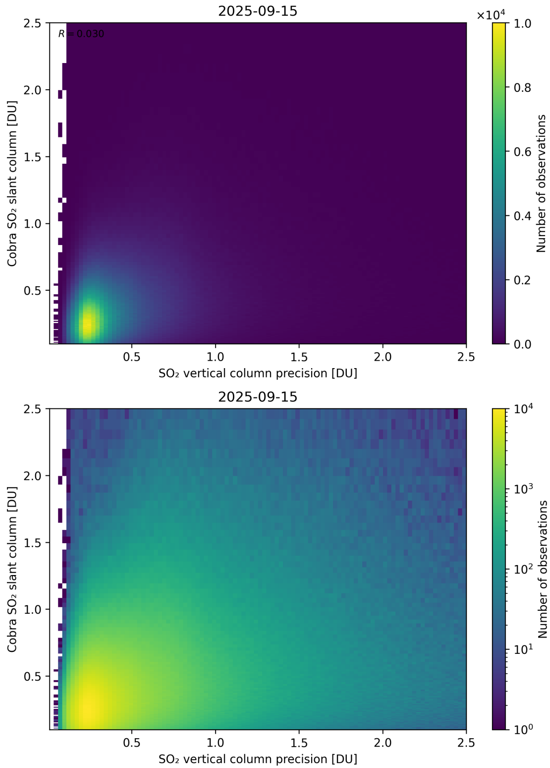
Figure 336: Scatter density plot of “SO 2 vertical column precision” against “Cobra SO 2 slant column” for 2025-09-15 to 2025-09-16.
