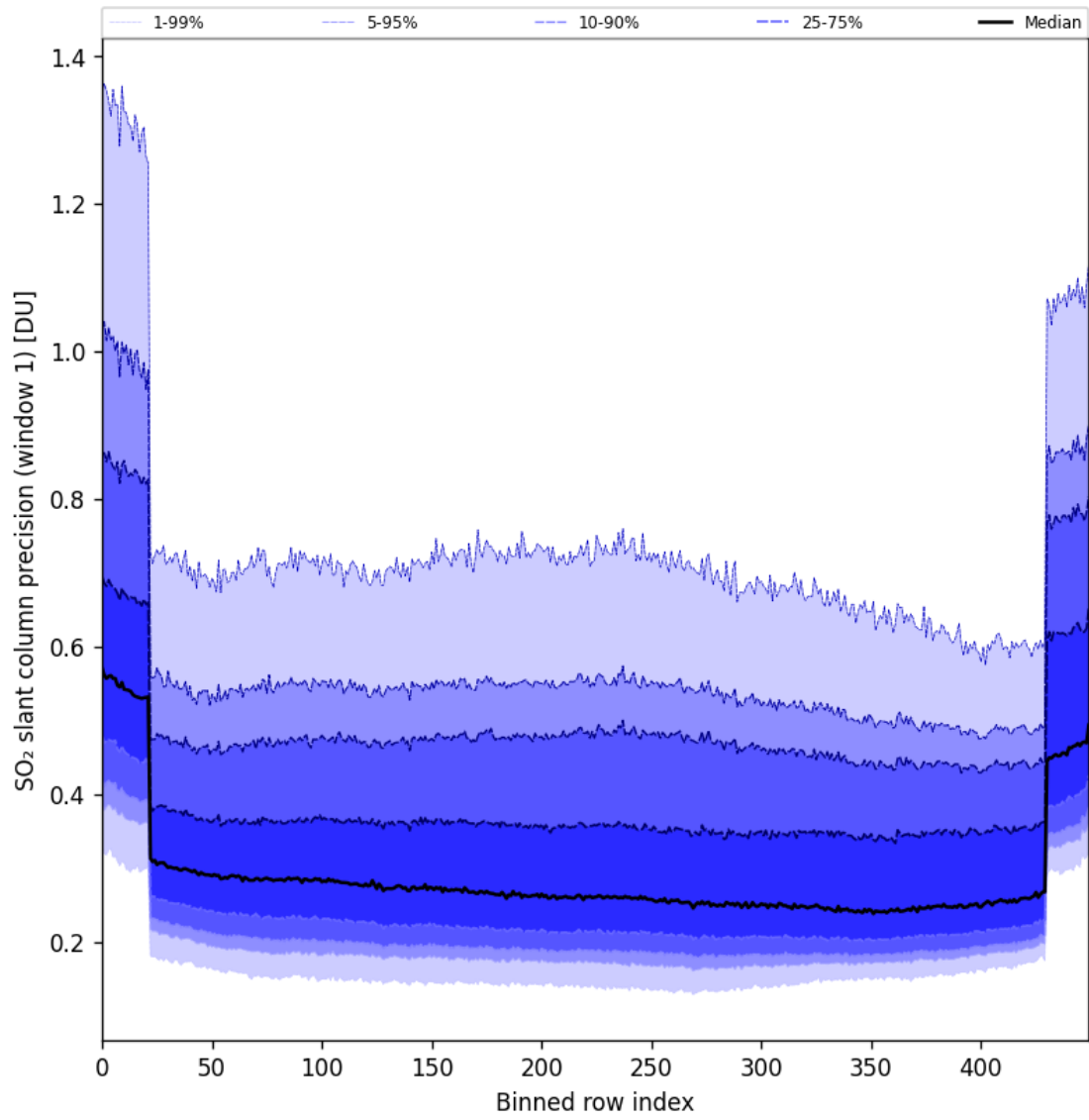
Figure 90: Along track statistics of “SO 2 slant column precision (window 1)” for 2025-09-15 to 2025-09-16
