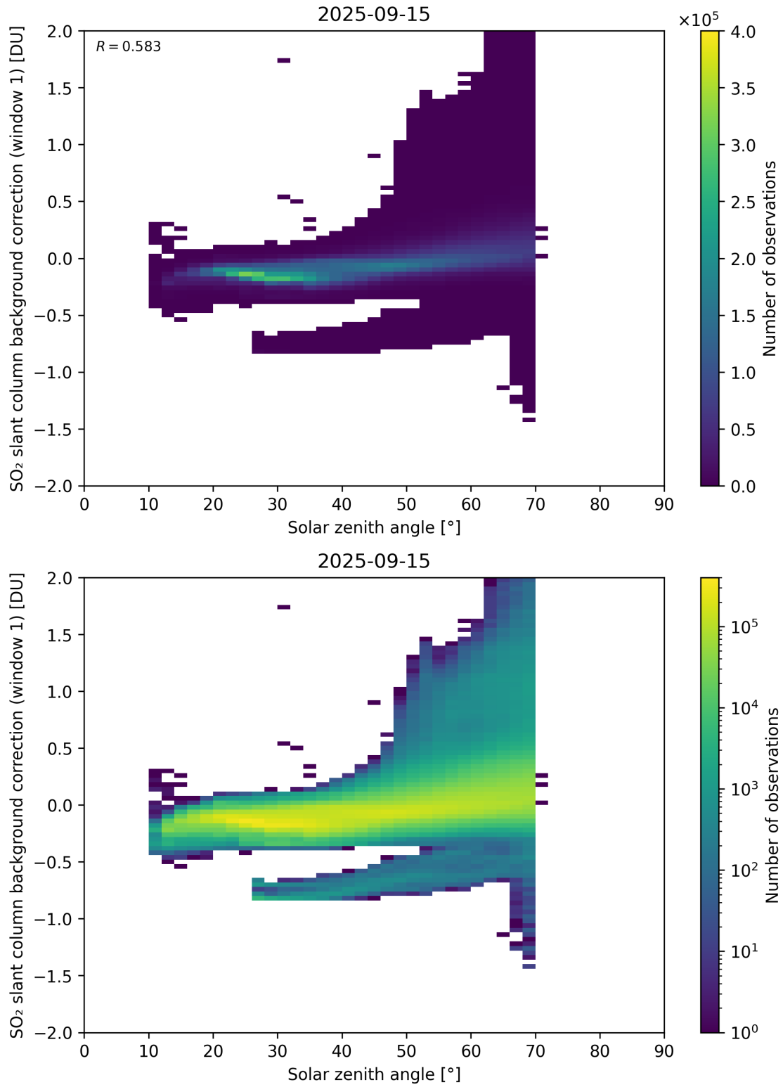
Figure 171: Scatter density plot of “Solar zenith angle” against “SO 2 slant column background correction (window 1)” for 2025-09-15 to 2025-09-16.
