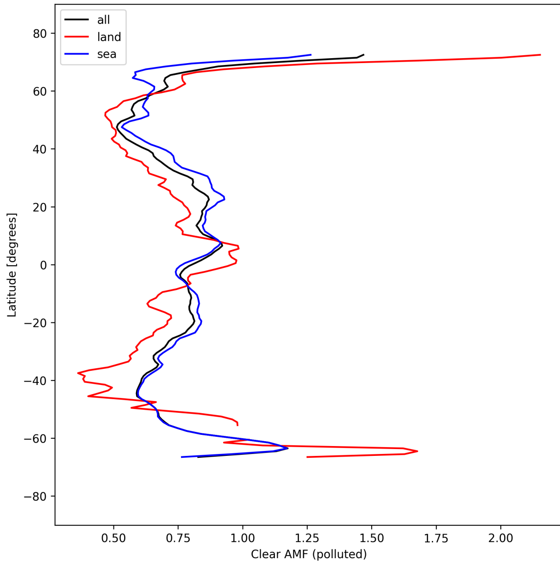
Figure 55: Zonal average of “Clear AMF (polluted)” for 2025-09-15 to 2025-09-16.
