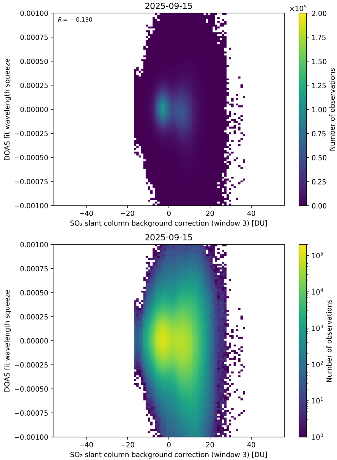
Figure 133: Scatter density plot of “SO 2 slant column background correction (window 3)” against “DOAS fit wavelength squeeze” for 2025-09-15 to 2025-09-16.
