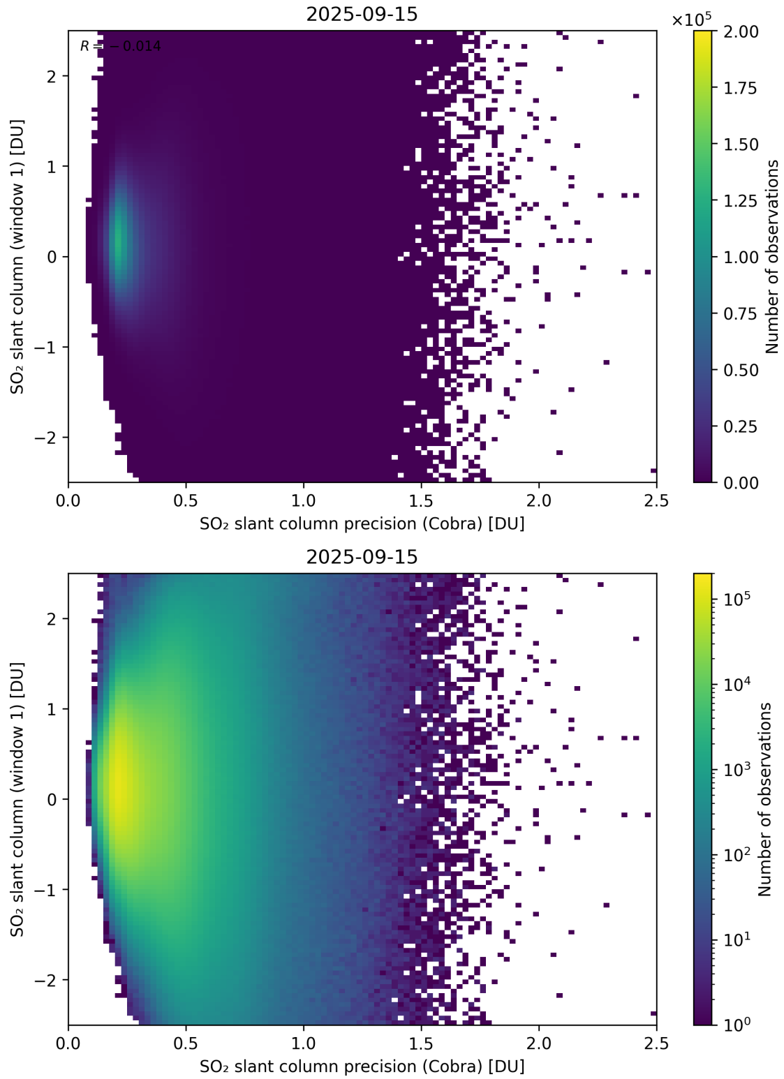
Figure 208: Scatter density plot of “SO 2 slant column precision (Cobra)” against “SO 2 slant column (window 1)” for 2025-09-15 to 2025-09-16.
