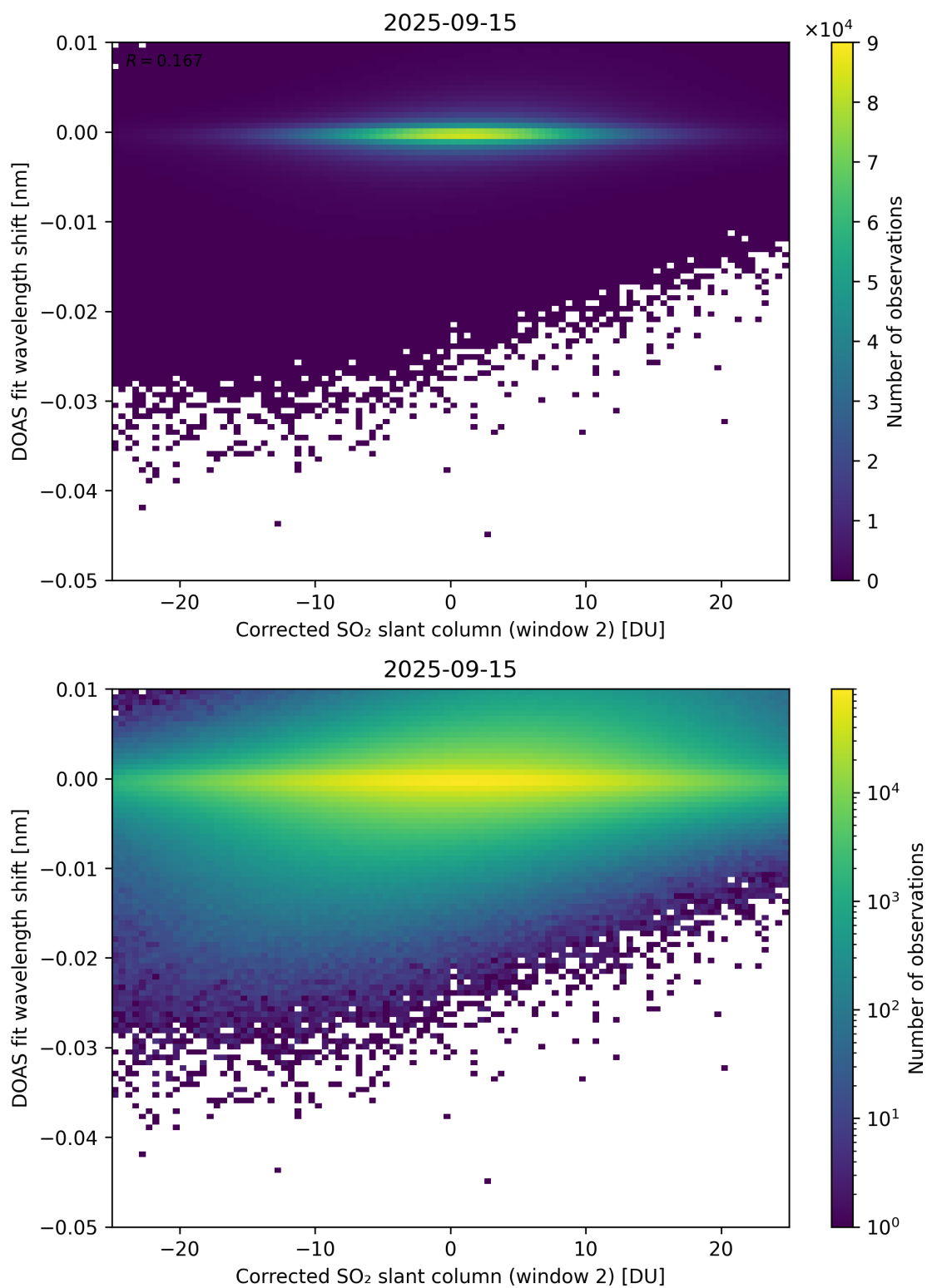
Figure 246: Scatter density plot of “Corrected SO 2 slant column (window 2)” against “DOAS fit wavelength shift” for 2025-09-15 to 2025-09-16.
