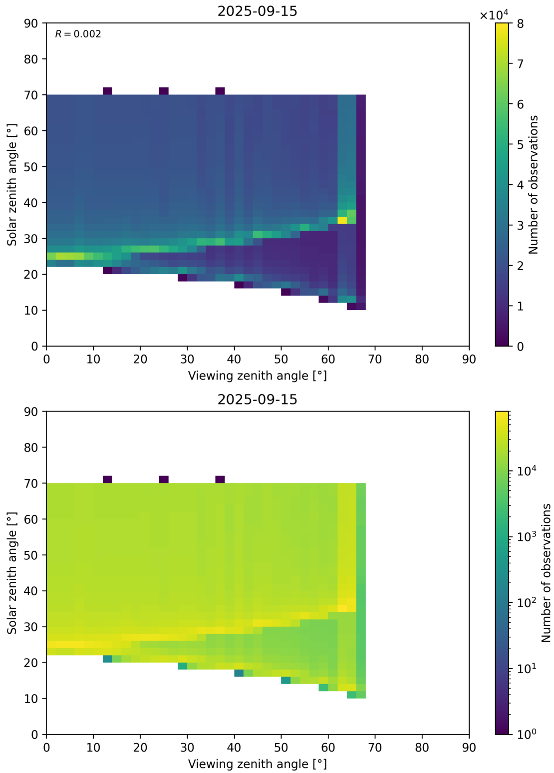
Figure 369: Scatter density plot of “Viewing zenith angle” against “Solar zenith angle” for 2025-09-15 to 2025-09-16.
