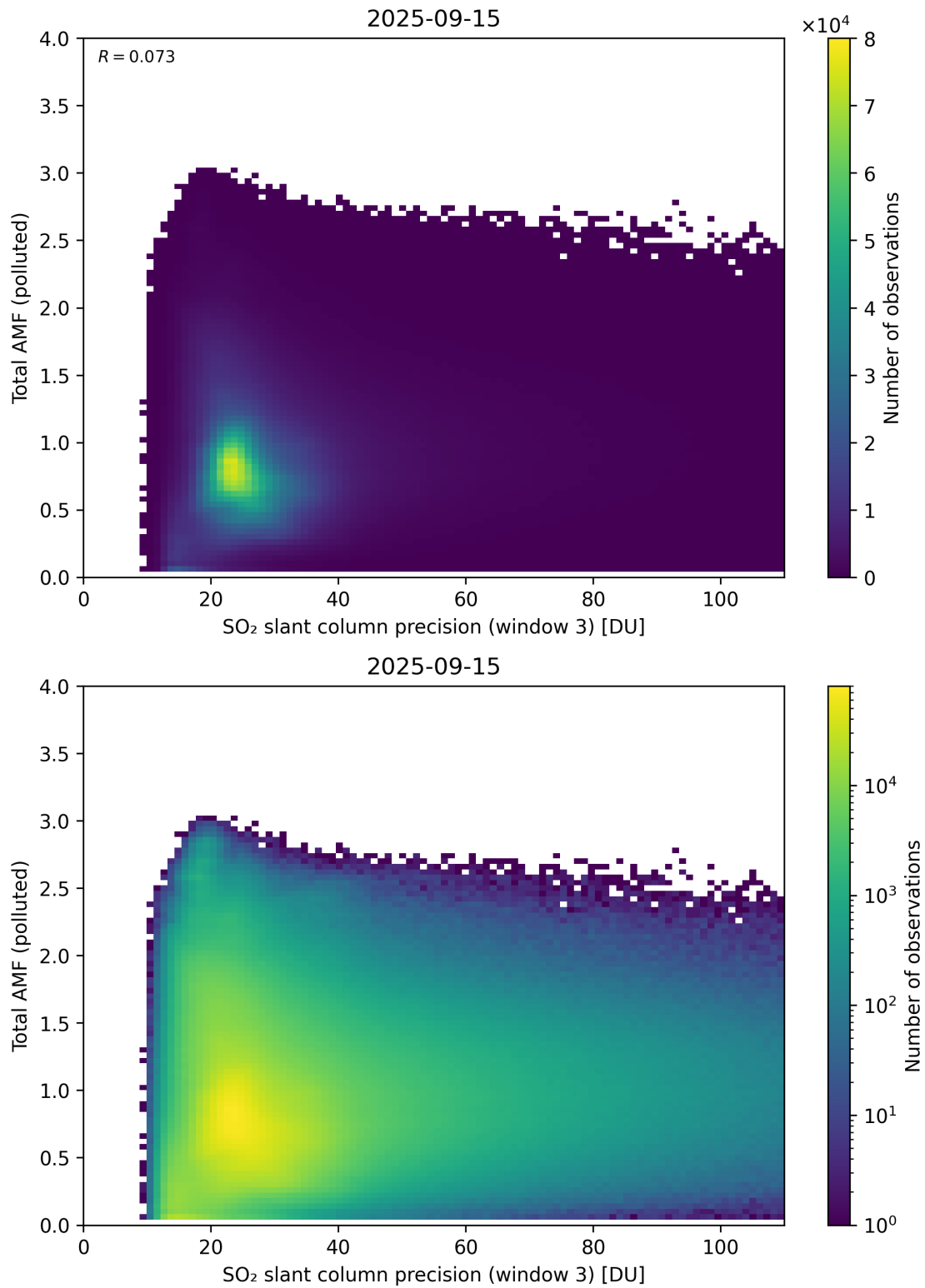
Figure 313: Scatter density plot of “SO 2 slant column precision (window 3)” against “Total AMF (polluted)” for 2025-09-15 to 2025-09-16.
