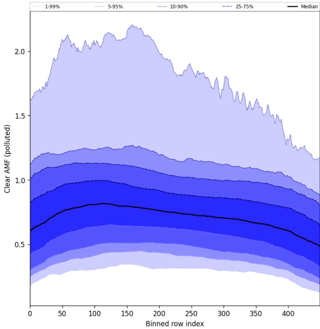
Figure 107: Along track statistics of “Clear AMF (polluted)” for 2025-09-15 to 2025-09-16
