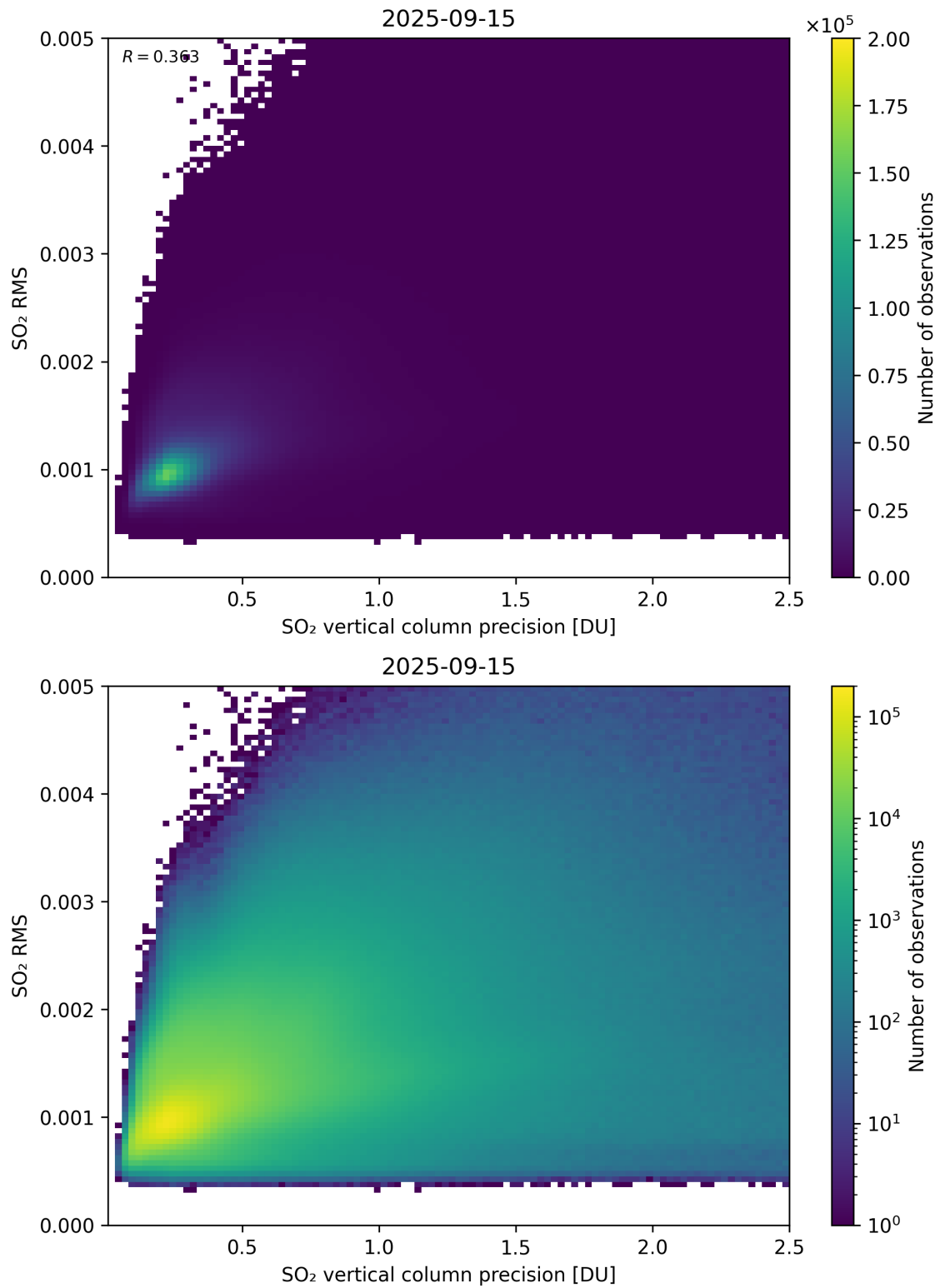
Figure 334: Scatter density plot of “SO 2 vertical column precision” against “SO 2 RMS” for 2025-09-15 to 2025-09-16.
