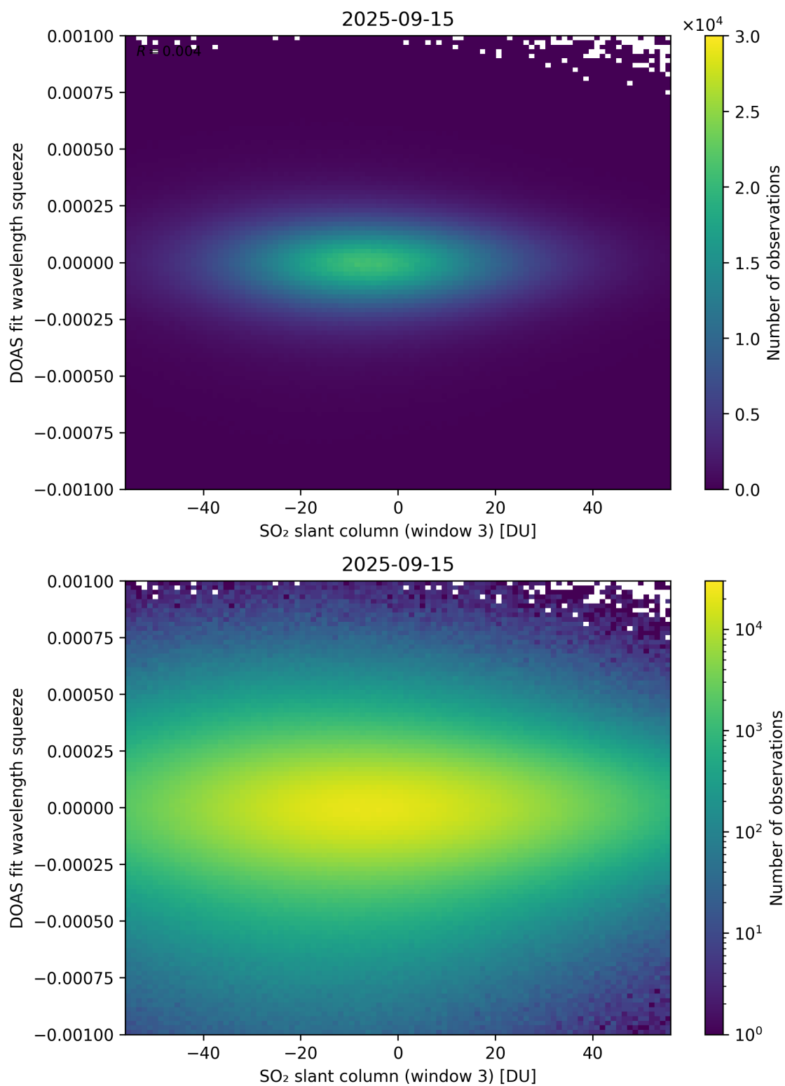
Figure 305: Scatter density plot of “SO 2 slant column (window 3)” against “DOAS fit wavelength squeeze” for 2025-09-15 to 2025-09-16.
