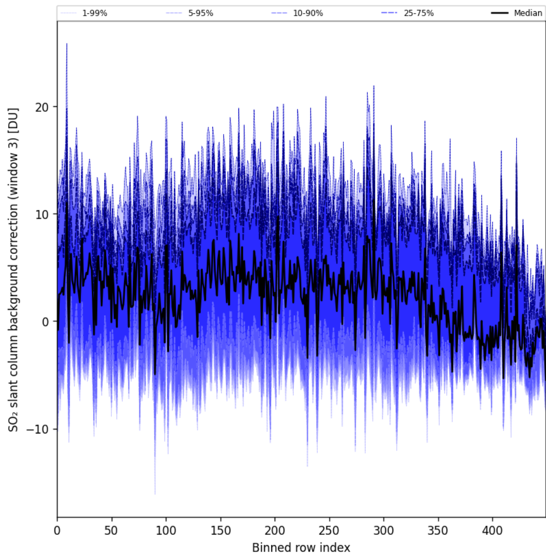
Figure 100: Along track statistics of “SO 2 slant column background correction (window 3)” for 2025-09-15 to 2025-09-16
