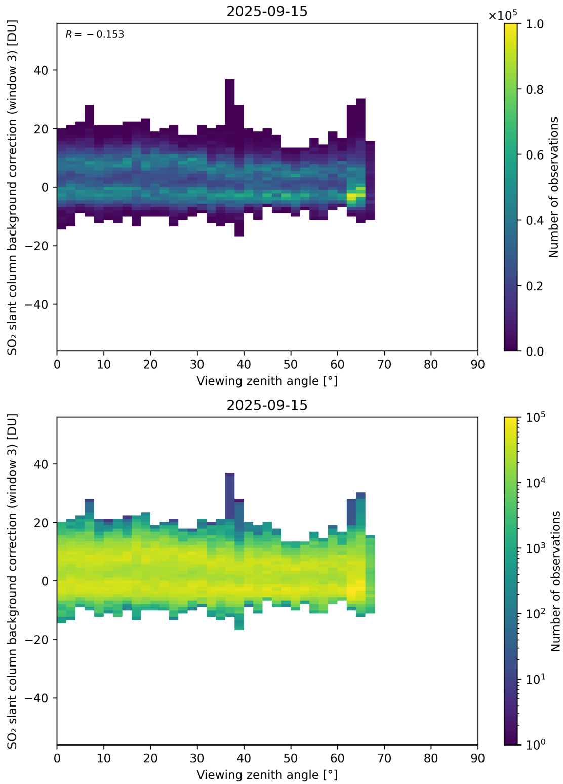
Figure 364: Scatter density plot of “Viewing zenith angle” against “SO 2 slant column background correction (window 3)” for 2025-09-15 to 2025-09-16.
