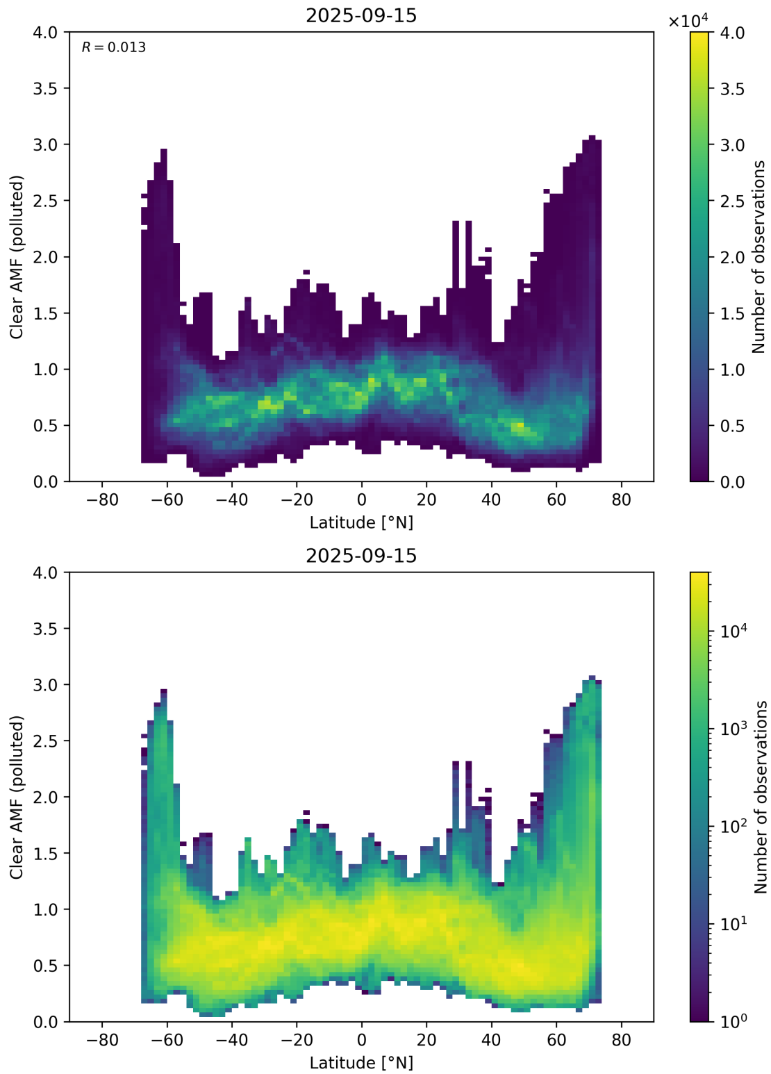
Figure 156: Scatter density plot of “Latitude” against “Clear AMF (polluted)” for 2025-09-15 to 2025-09-16.
