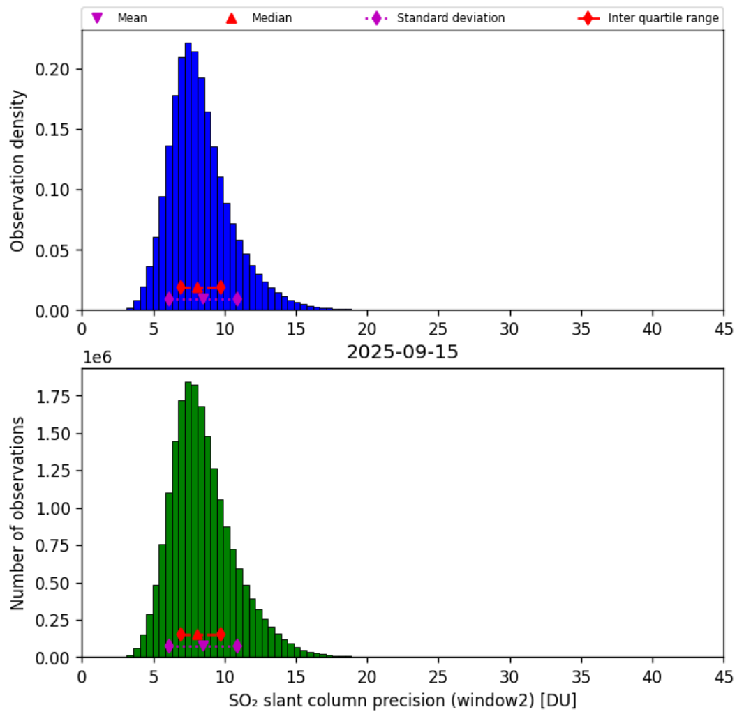
Figure 68: Histogram of “SO 2 slant column precision (window2)” for 2025-09-15 to 2025-09-16
