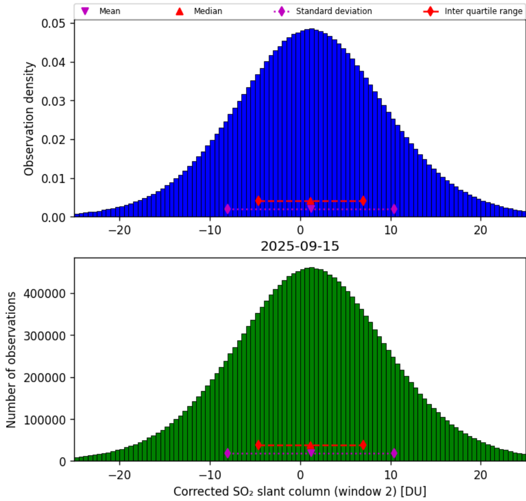
Figure 69: Histogram of “Corrected SO 2 slant column (window 2)” for 2025-09-15 to 2025-09-16
