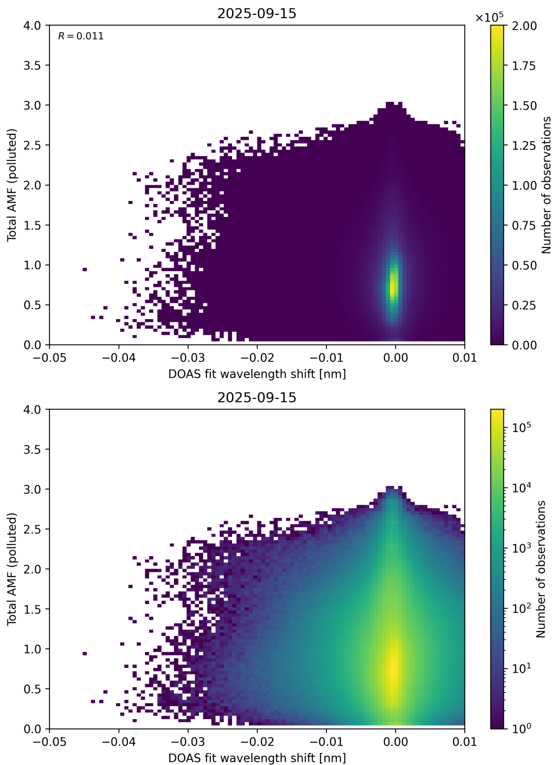
Figure 141: Scatter density plot of “DOAS fit wavelength shift” against “Total AMF (polluted)” for 2025-09-15 to 2025-09-16.
