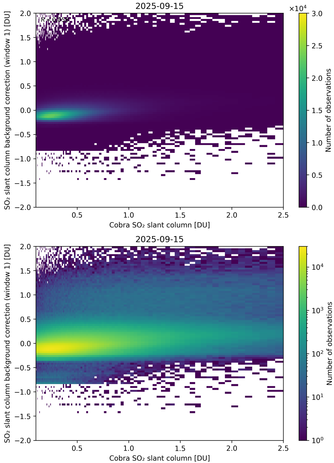
Figure 193: Scatter density plot of “Cobra SO 2 slant column” against “SO 2 slant column background correction (window 1)” for 2025-09-15 to 2025-09-16.
