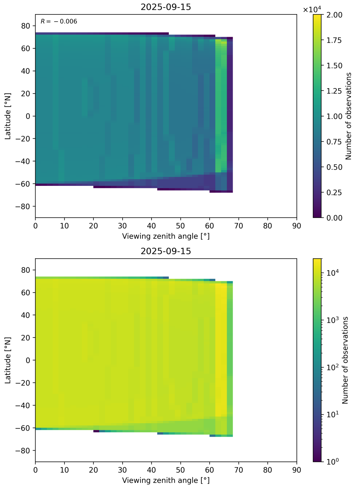
Figure 368: Scatter density plot of “Viewing zenith angle” against “Latitude” for 2025-09-15 to 2025-09-16.
