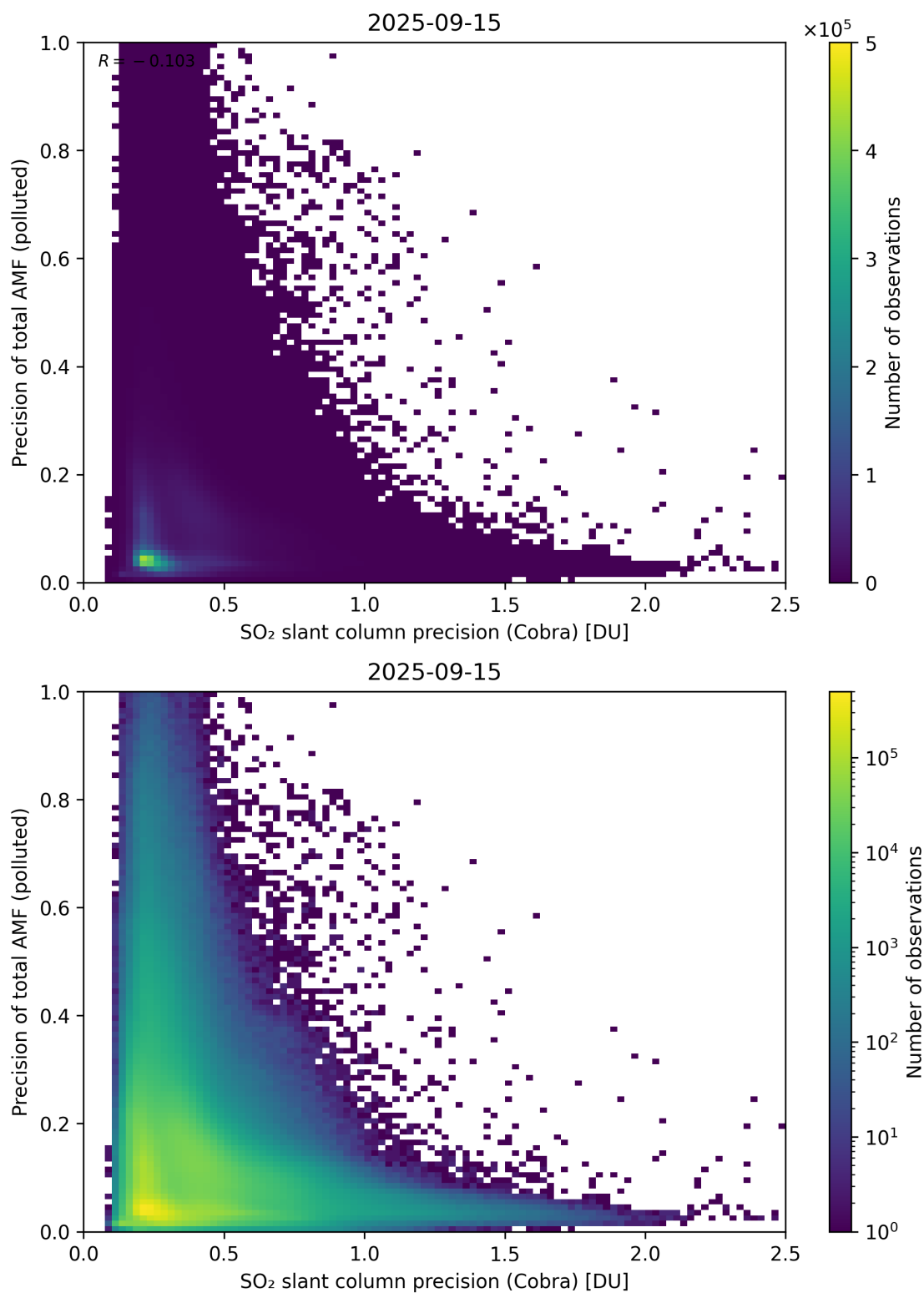
Figure 214: Scatter density plot of “SO 2 slant column precision (Cobra)” against “Precision of total AMF (polluted)” for 2025-09-15 to 2025-09-16.
