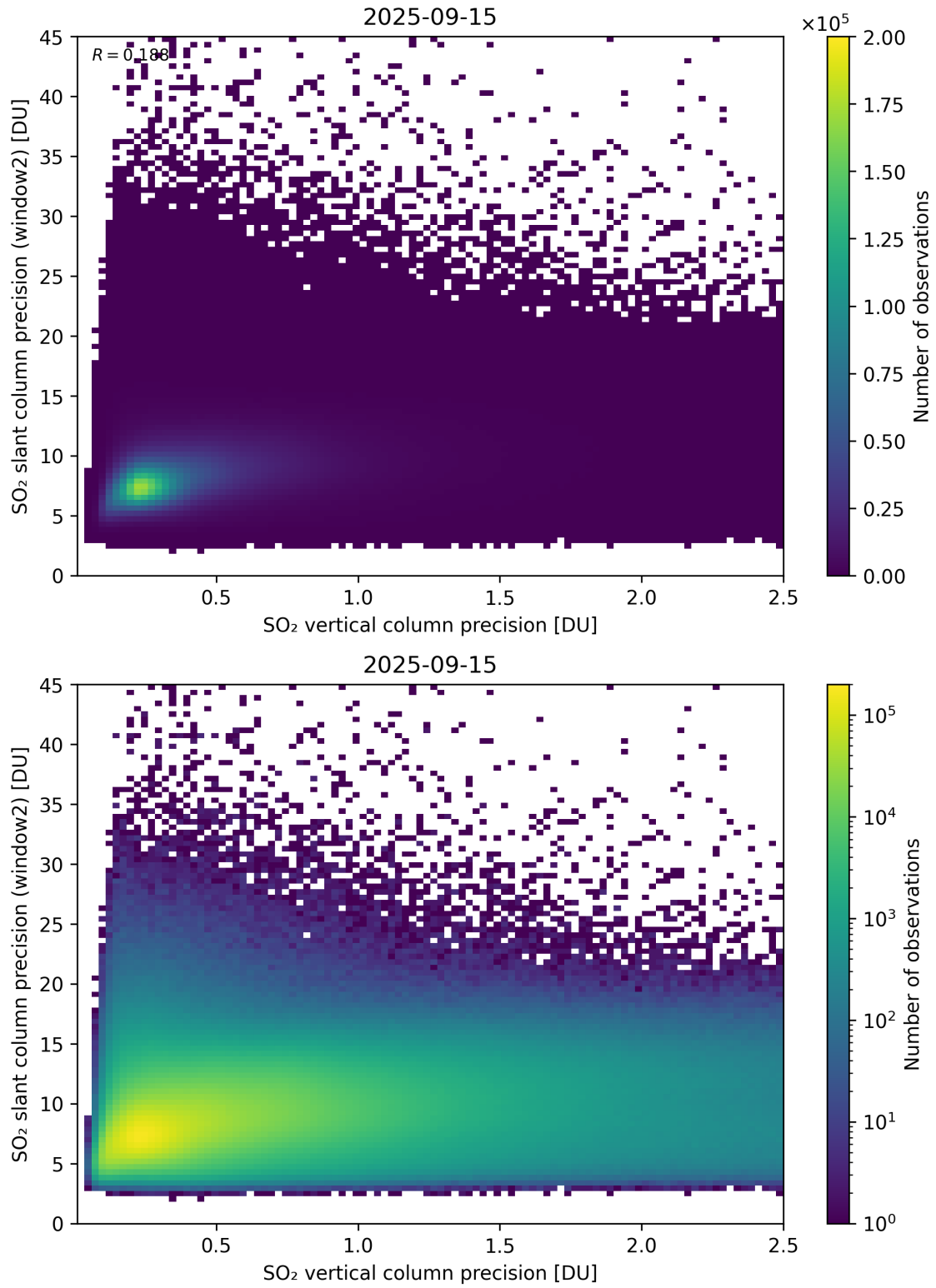
Figure 343: Scatter density plot of “SO 2 vertical column precision” against “SO 2 slant column precision (window2)” for 2025-09-15 to 2025-09-16.
