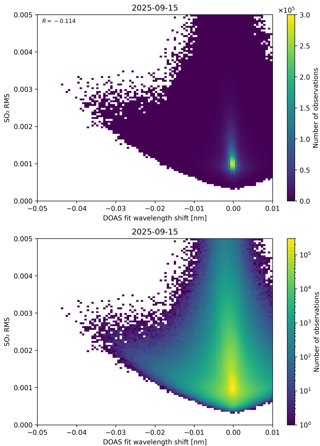
Figure 139: Scatter density plot of “DOAS fit wavelength shift” against “SO 2 RMS” for 2025-09-15 to 2025-09-16.
