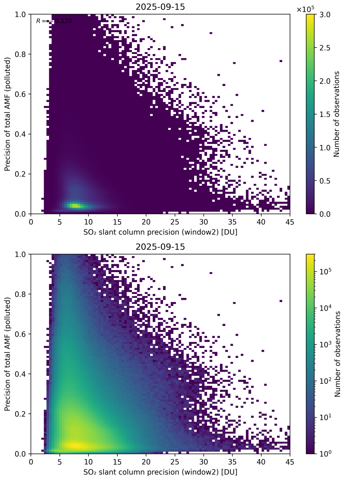
Figure 302: Scatter density plot of “SO 2 slant column precision (window2)” against “Precision of total AMF (polluted)” for 2025-09-15 to 2025-09-16.
