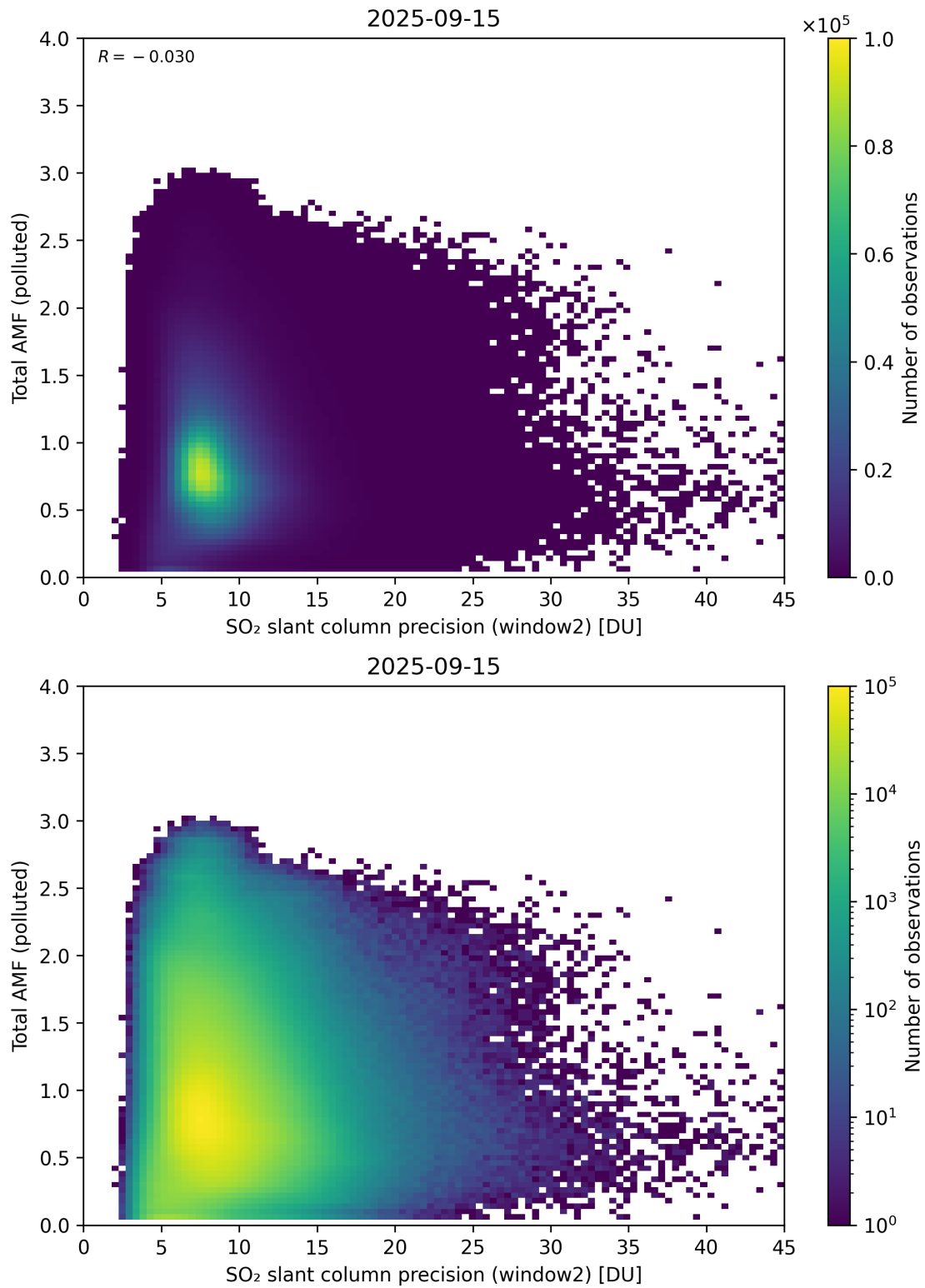
Figure 301: Scatter density plot of “SO 2 slant column precision (window2)” against “Total AMF (polluted)” for 2025-09-15 to 2025-09-16.
