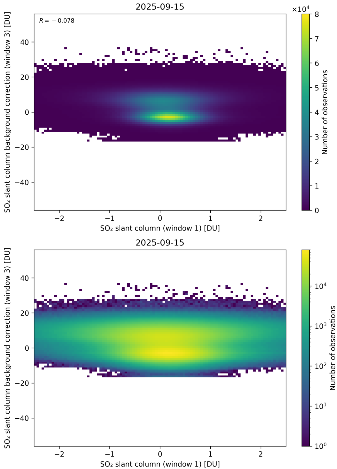
Figure 264: Scatter density plot of “SO 2 slant column (window 1)” against “SO 2 slant column background correction (window 3)” for 2025-09-15 to 2025-09-16.
