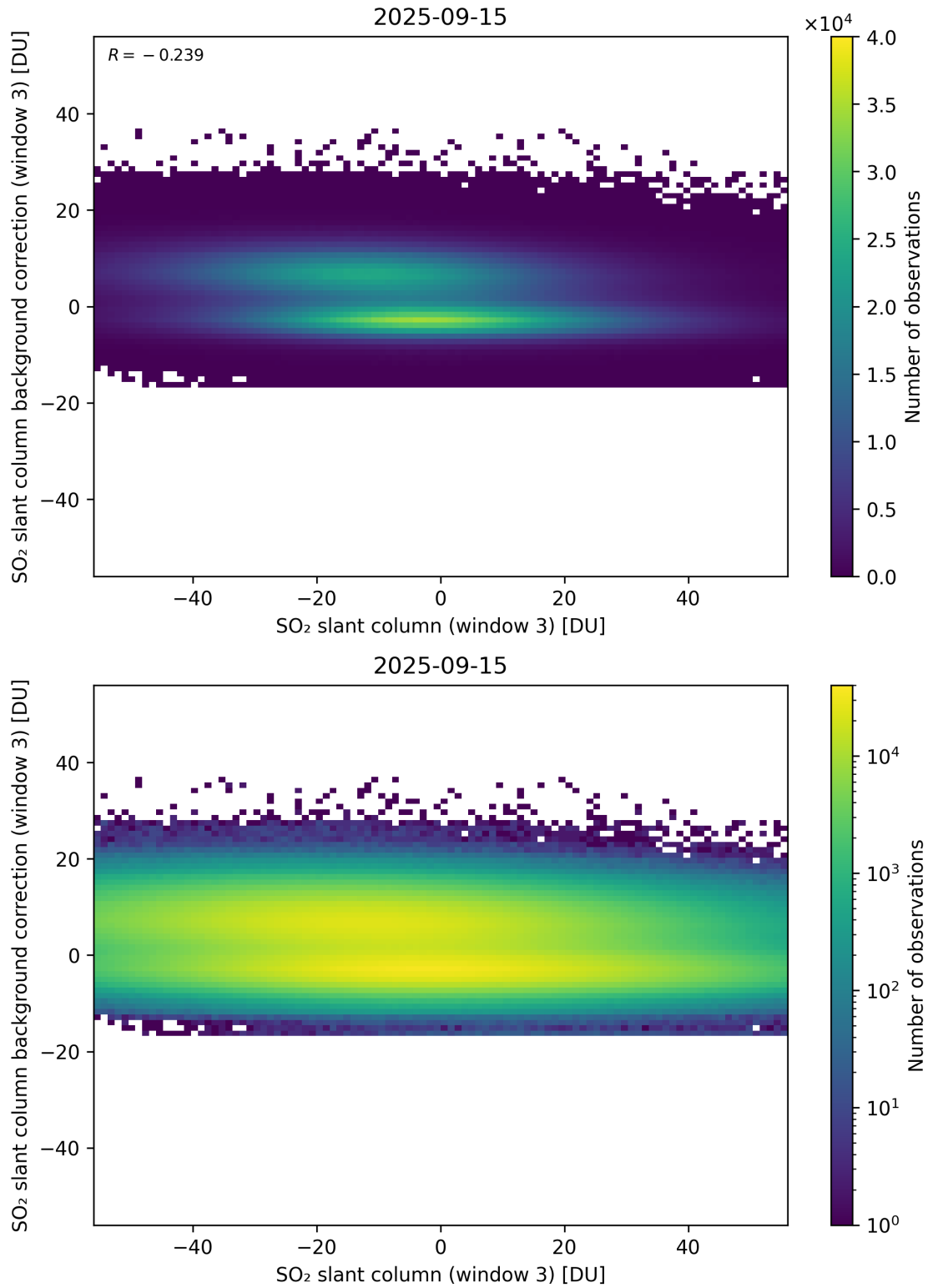
Figure 303: Scatter density plot of “SO 2 slant column (window 3)” against “SO 2 slant column background correction (window 3)” for 2025-09-15 to 2025-09-16.
