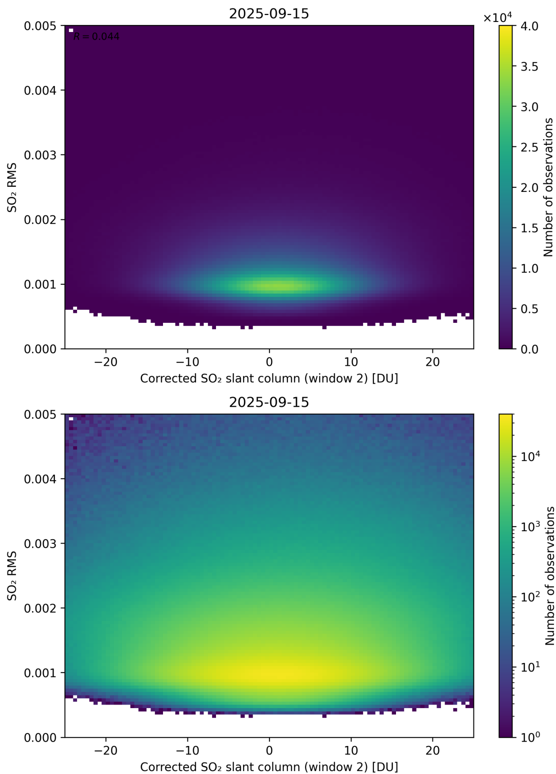
Figure 248: Scatter density plot of “Corrected SO 2 slant column (window 2)” against “SO 2 RMS” for 2025-09-15 to 2025-09-16.
