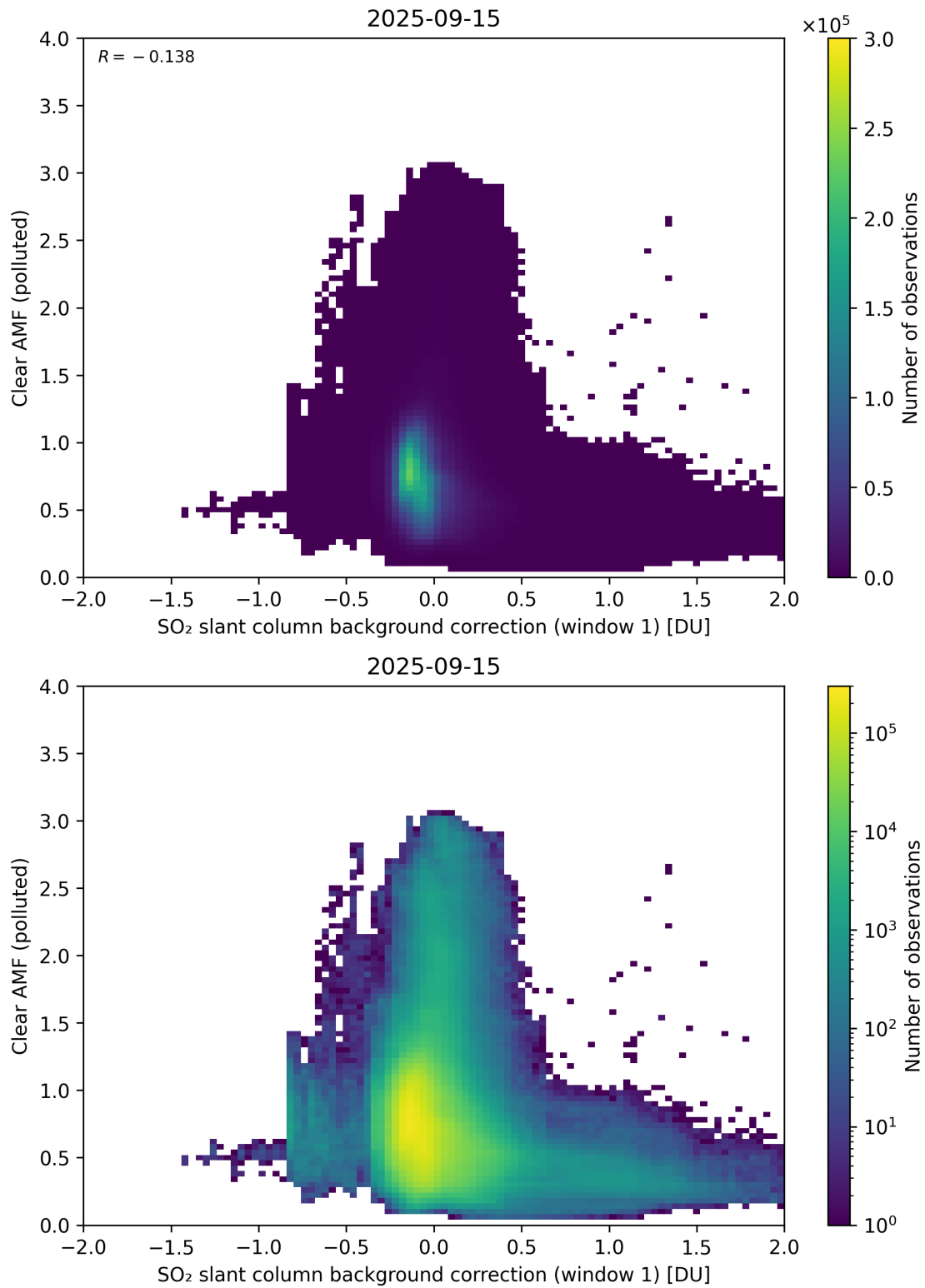
Figure 114: Scatter density plot of “SO 2 slant column background correction (window 1)” against “Clear AMF (polluted)” for 2025-09-15 to 2025-09-16.
