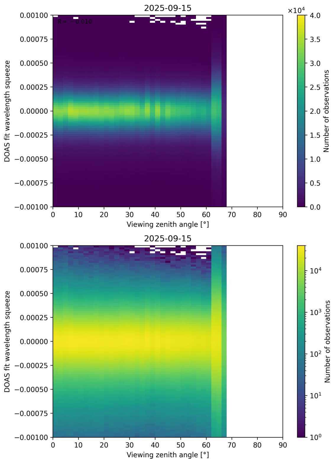
Figure 366: Scatter density plot of “Viewing zenith angle” against “DOAS fit wavelength squeeze” for 2025-09-15 to 2025-09-16.
