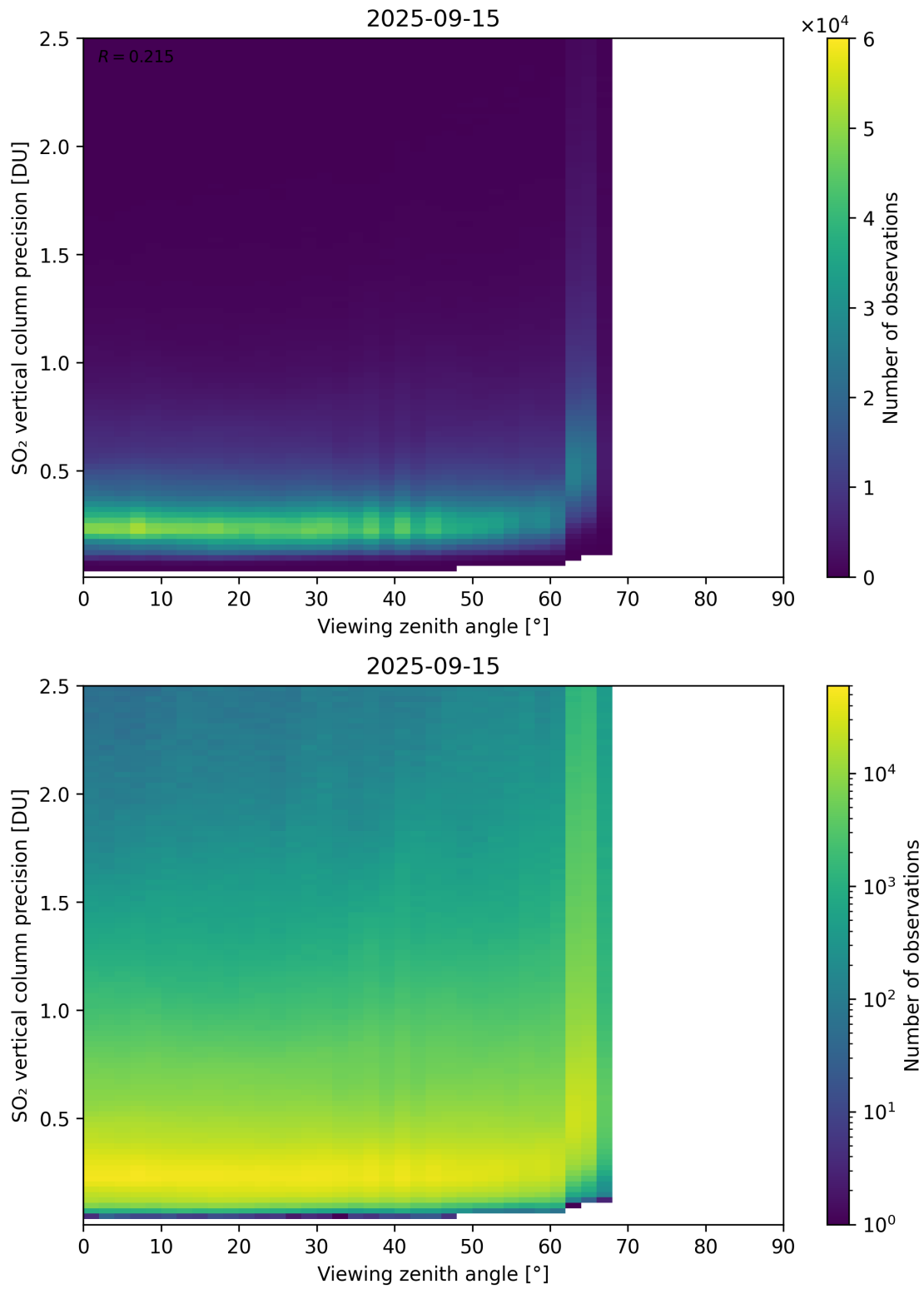
Figure 384: Scatter density plot of “Viewing zenith angle” against “SO 2 vertical column precision” for 2025-09-15 to 2025-09-16.
