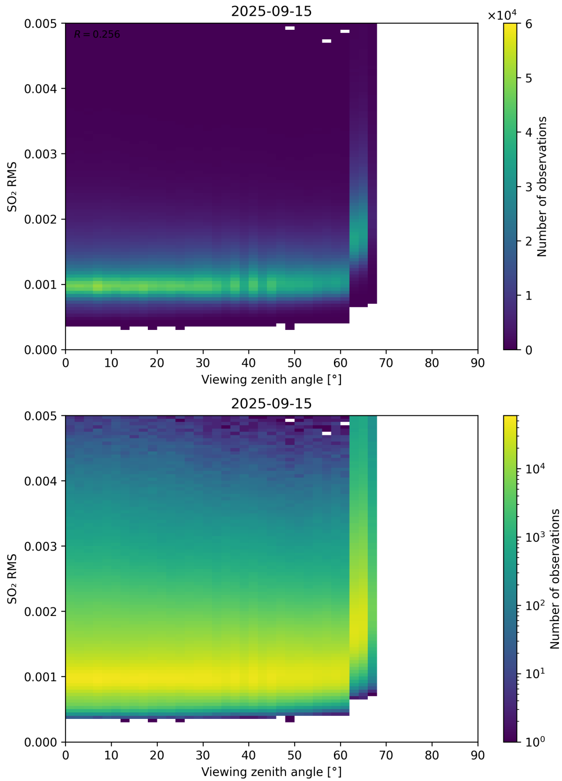
Figure 367: Scatter density plot of “Viewing zenith angle” against “SO 2 RMS” for 2025-09-15 to 2025-09-16.
