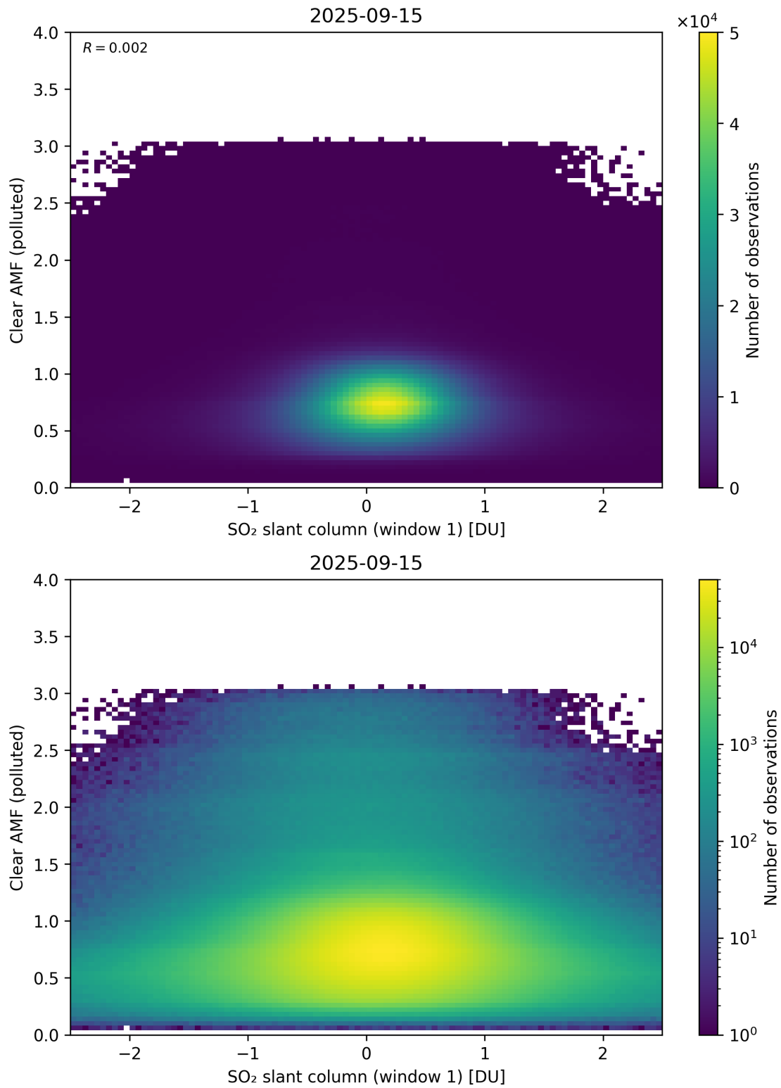
Figure 282: Scatter density plot of “SO 2 slant column (window 1)” against “Clear AMF (polluted)” for 2025-09-15 to 2025-09-16.
