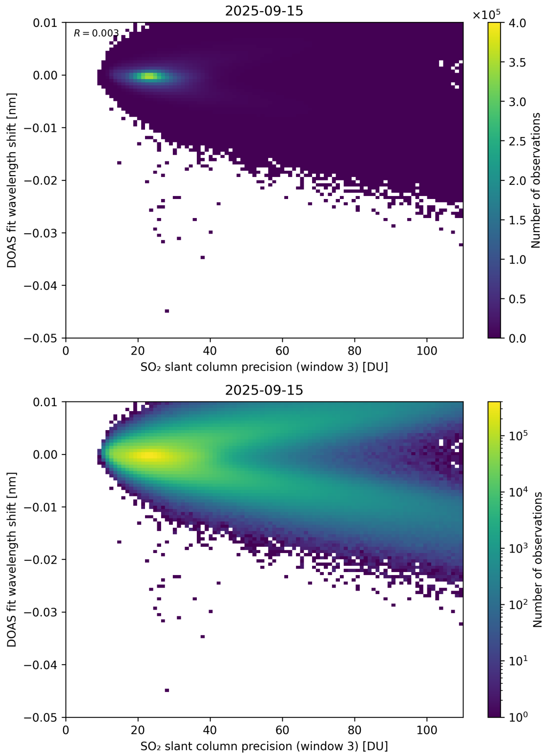
Figure 308: Scatter density plot of “SO 2 slant column precision (window 3)” against “DOAS fit wavelength shift” for 2025-09-15 to 2025-09-16.
