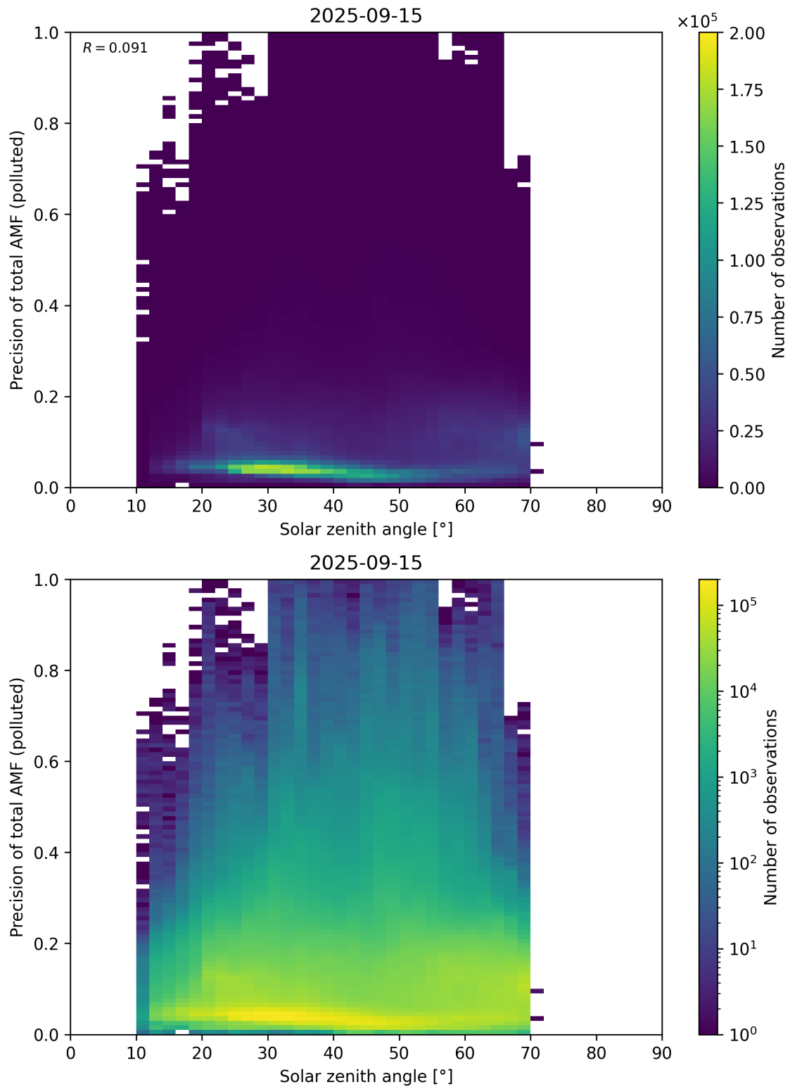
Figure 190: Scatter density plot of “Solar zenith angle” against “Precision of total AMF (polluted)” for 2025-09-15 to 2025-09-16.
