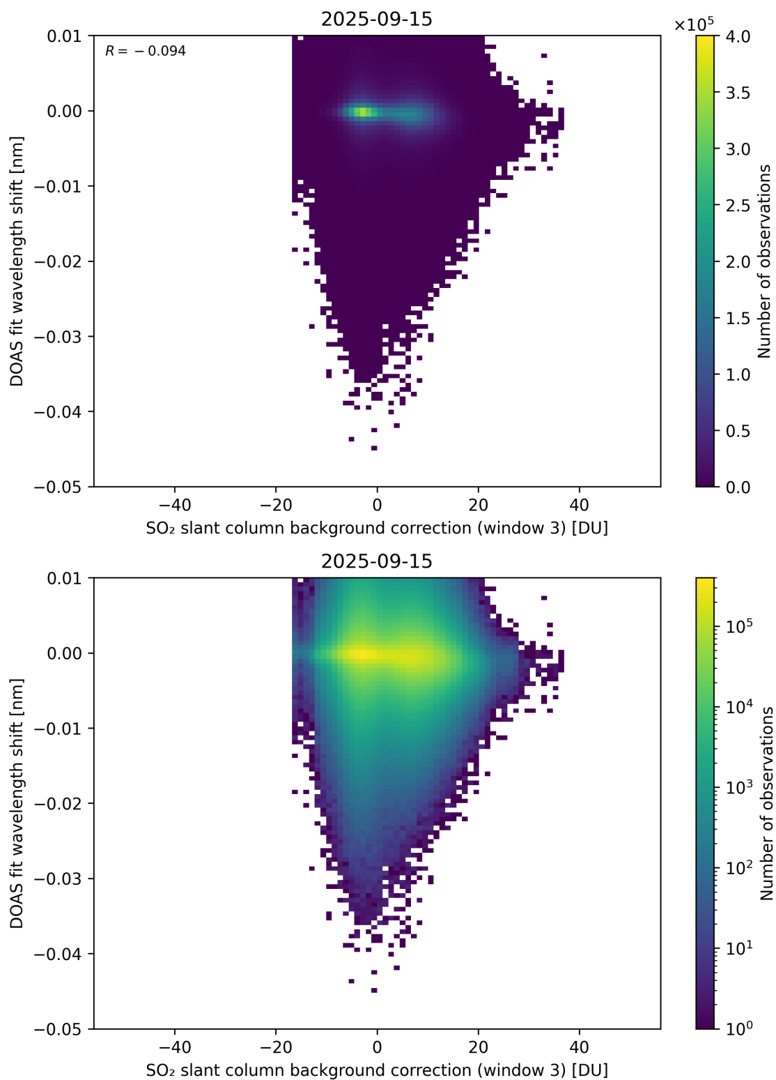
Figure 132: Scatter density plot of “SO 2 slant column background correction (window 3)” against “DOAS fit wavelength shift” for 2025-09-15 to 2025-09-16.
