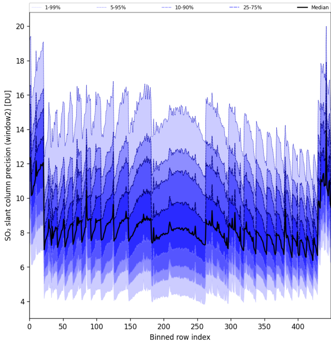
Figure 94: Along track statistics of “SO 2 slant column precision (window2)” for 2025-09-15 to 2025-09-16
