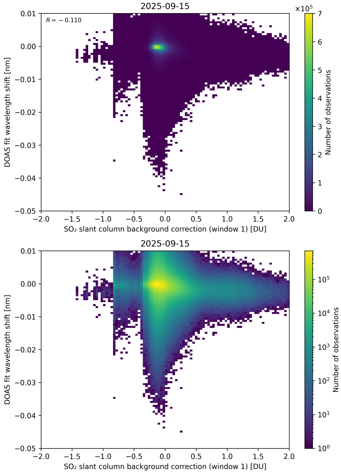
Figure 111: Scatter density plot of “SO 2 slant column background correction (window 1)” against “DOAS fit wavelength shift” for 2025-09-15 to 2025-09-16.
