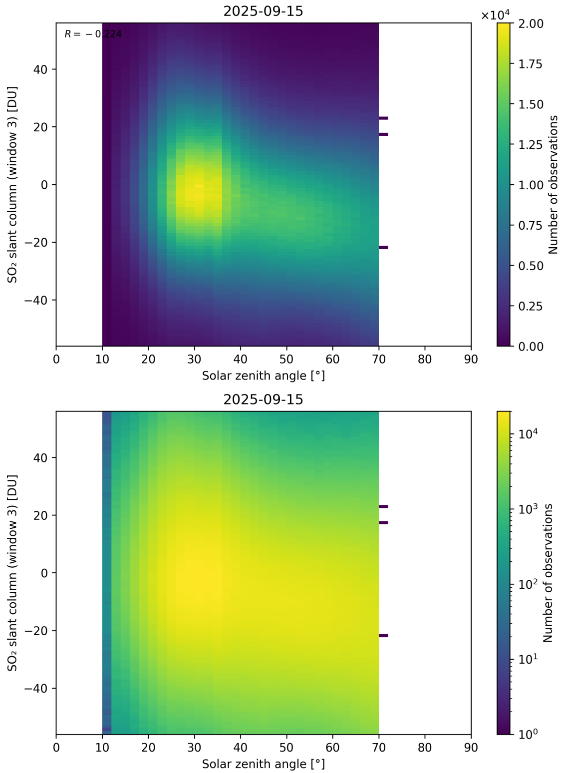
Figure 187: Scatter density plot of “Solar zenith angle” against “SO 2 slant column (window 3)” for 2025-09-15 to 2025-09-16.
