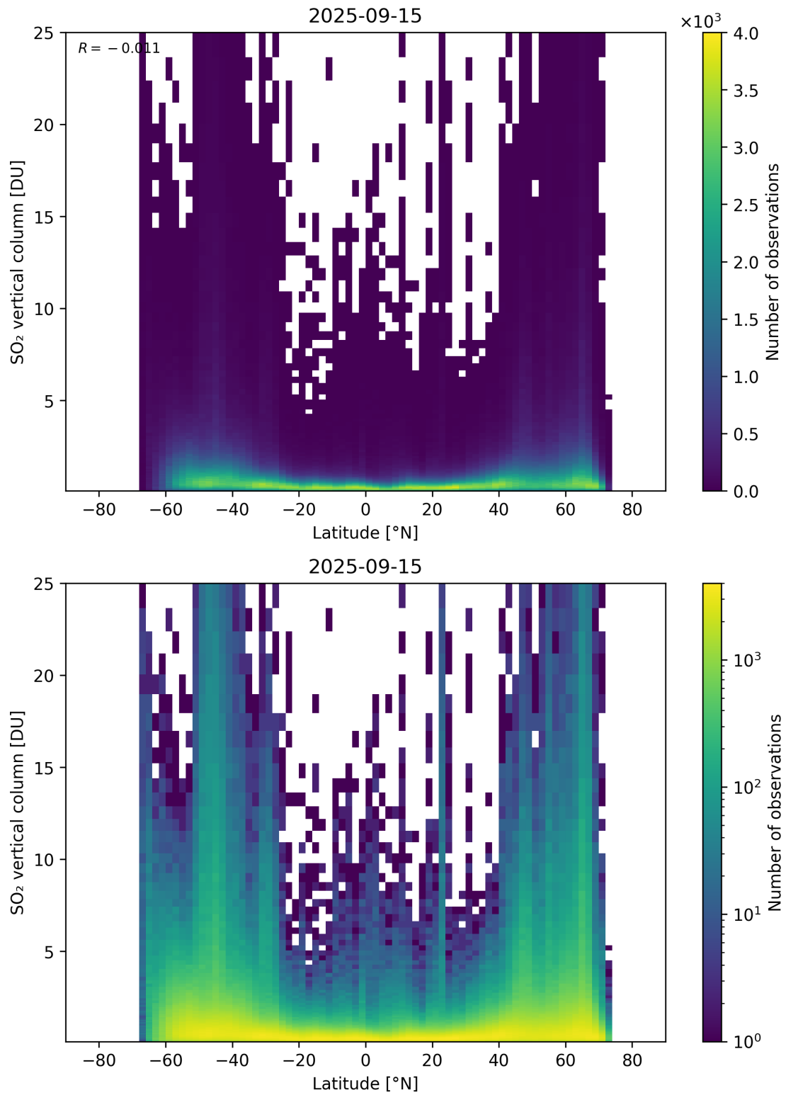
Figure 169: Scatter density plot of “Latitude” against “SO 2 vertical column” for 2025-09-15 to 2025-09-16.
