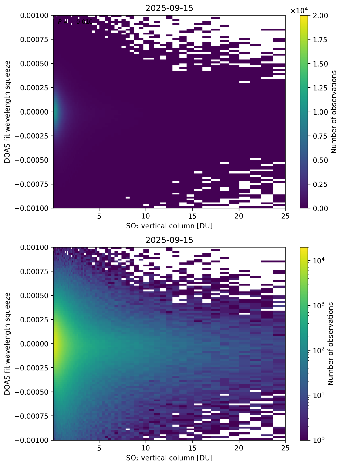
Figure 327: Scatter density plot of “SO 2 vertical column” against “DOAS fit wavelength squeeze” for 2025-09-15 to 2025-09-16.
