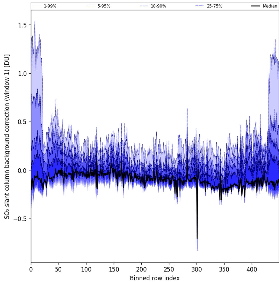
Figure 92: Along track statistics of “SO 2 slant column background correction (window 1)” for 2025-09-15 to 2025-09-16
