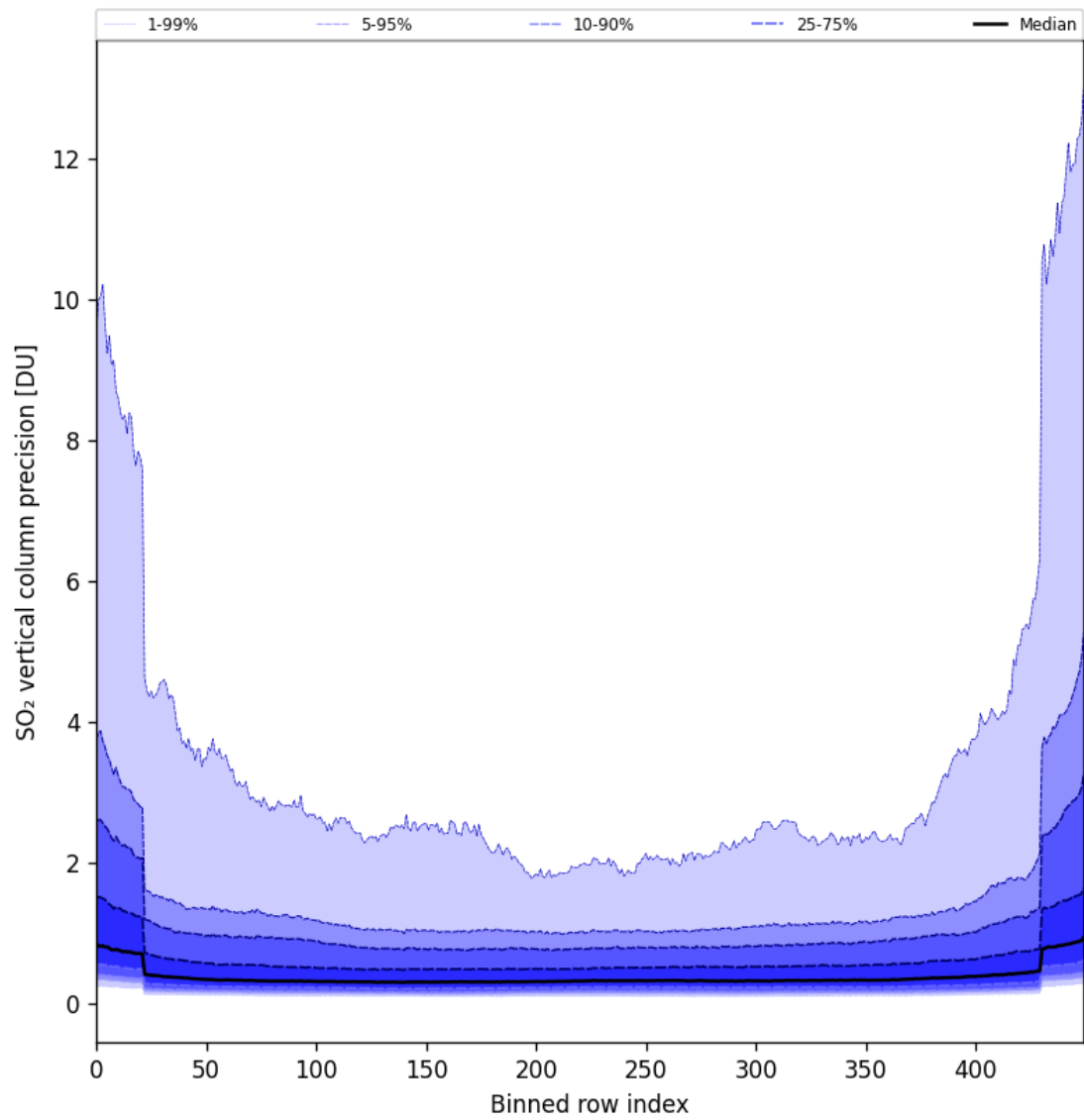
Figure 85: Along track statistics of “SO 2 vertical column precision” for 2025-09-15 to 2025-09-16
