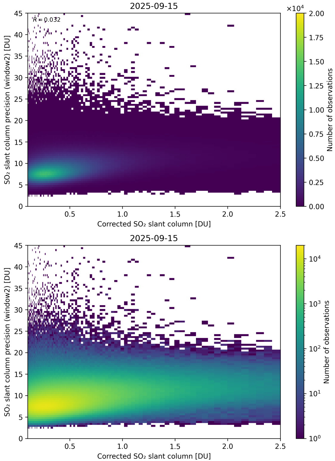
Figure 239: Scatter density plot of “Corrected SO 2 slant column” against “SO 2 slant column precision (window2)” for 2025-09-15 to 2025-09-16.
