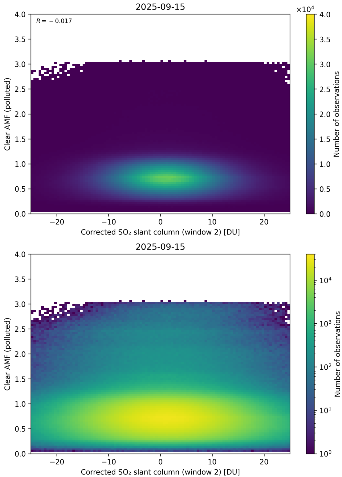
Figure 249: Scatter density plot of “Corrected SO 2 slant column (window 2)” against “Clear AMF (polluted)” for 2025-09-15 to 2025-09-16.
