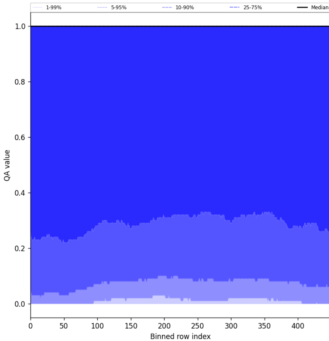
Figure 83: Along track statistics of “QA value” for 2025-09-15 to 2025-09-16
