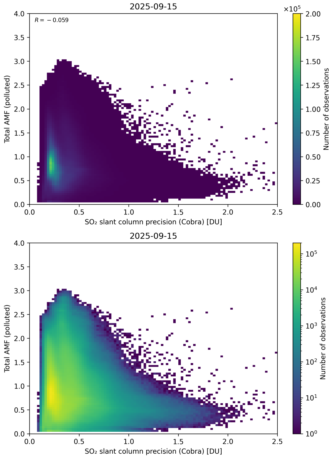
Figure 213: Scatter density plot of “SO 2 slant column precision (Cobra)” against “Total AMF (polluted)” for 2025-09-15 to 2025-09-16.
