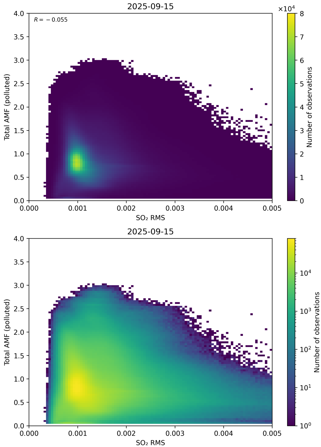
Figure 148: Scatter density plot of “SO 2 RMS” against “Total AMF (polluted)” for 2025-09-15 to 2025-09-16.
