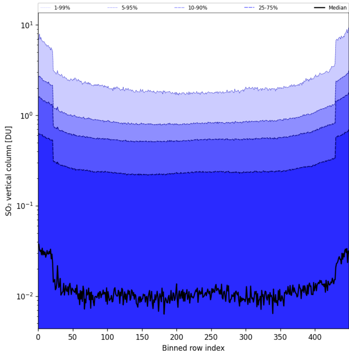
Figure 84: Along track statistics of “SO 2 vertical column” for 2025-09-15 to 2025-09-16
