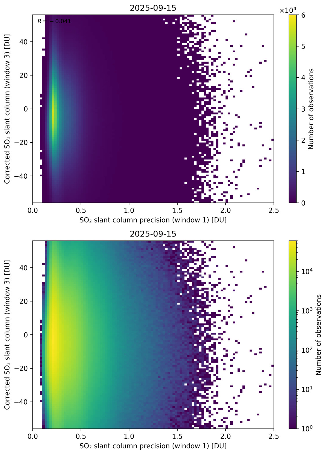
Figure 276: Scatter density plot of “SO 2 slant column precision (window 1)” against “Corrected SO 2 slant column (window 3)” for 2025-09-15 to 2025-09-16.
