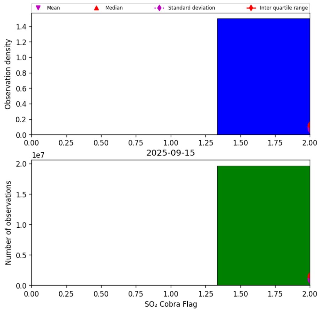
Figure 75: Histogram of “SO 2 Cobra Flag” for 2025-09-15 to 2025-09-16
