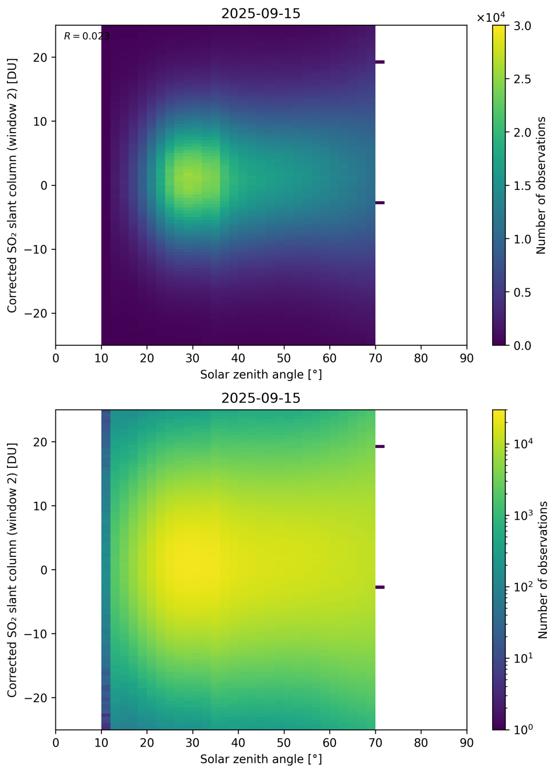
Figure 182: Scatter density plot of “Solar zenith angle” against “Corrected SO 2 slant column (window 2)” for 2025-09-15 to 2025-09-16.
