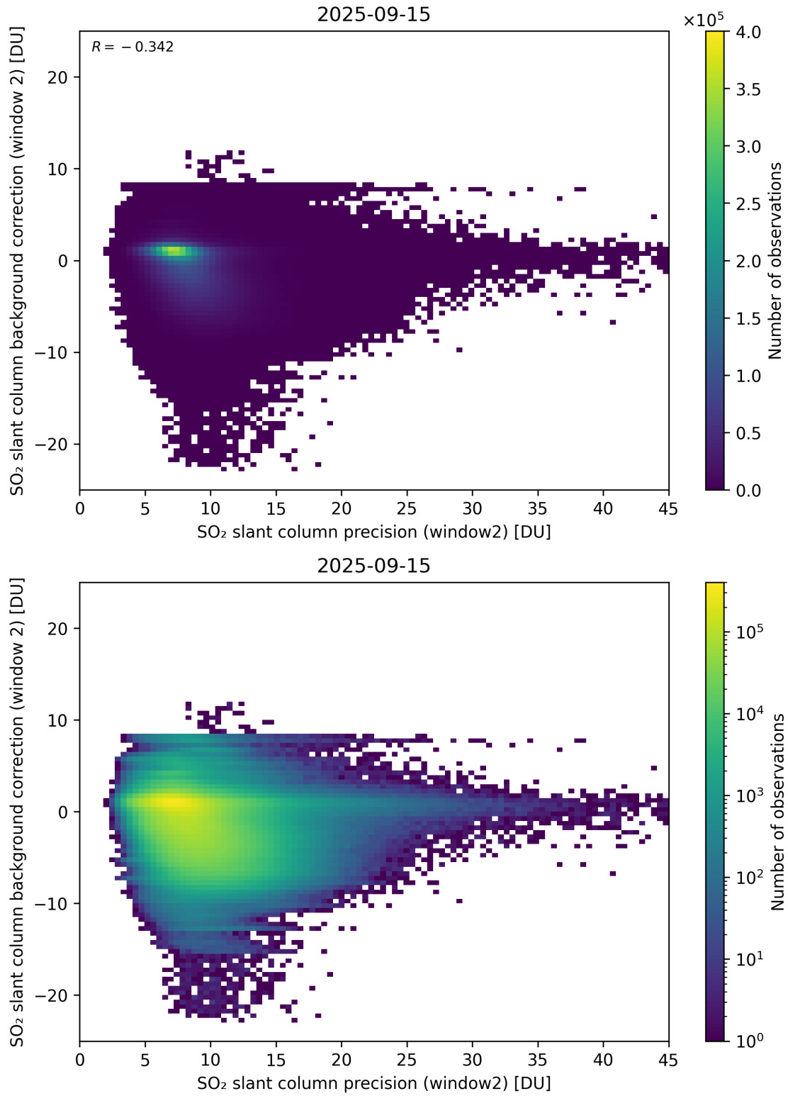
Figure 291: Scatter density plot of “SO 2 slant column precision (window2)” against “SO 2 slant column background correction (window 2)” for 2025-09-15 to 2025-09-16.
