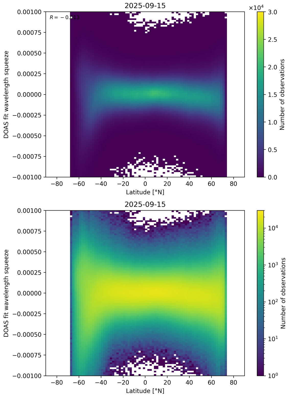
Figure 154: Scatter density plot of “Latitude” against “DOAS fit wavelength squeeze” for 2025-09-15 to 2025-09-16.
