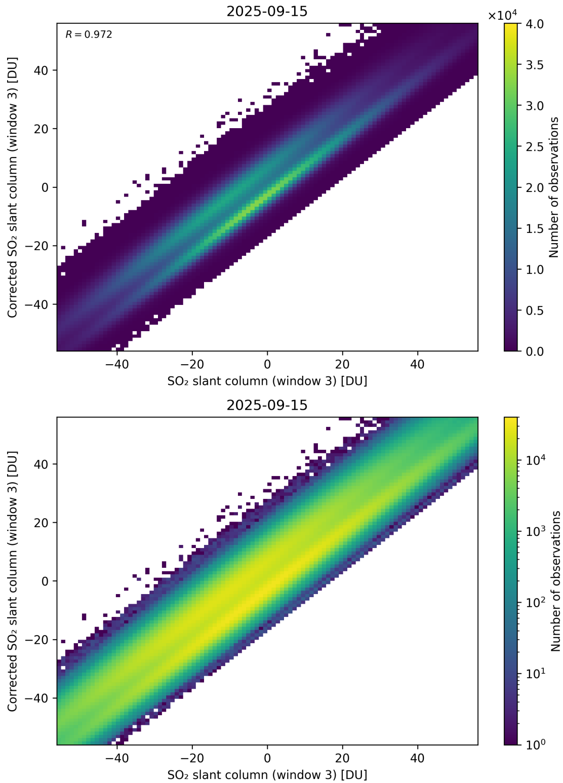
Figure 316: Scatter density plot of “SO 2 slant column (window 3)” against “Corrected SO 2 slant column (window 3)” for 2025-09-15 to 2025-09-16.
