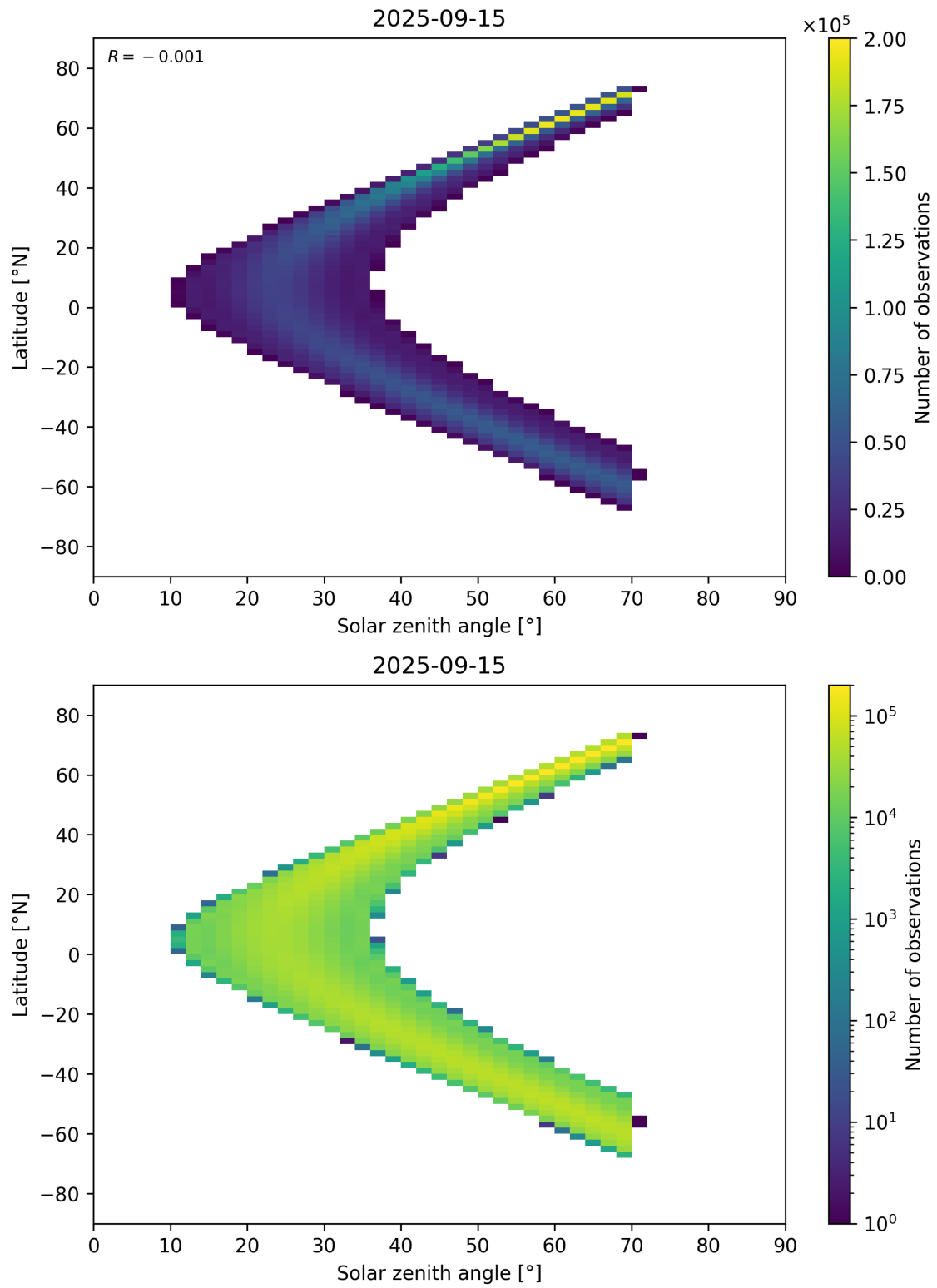
Figure 177: Scatter density plot of “Solar zenith angle” against “Latitude” for 2025-09-15 to 2025-09-16.
