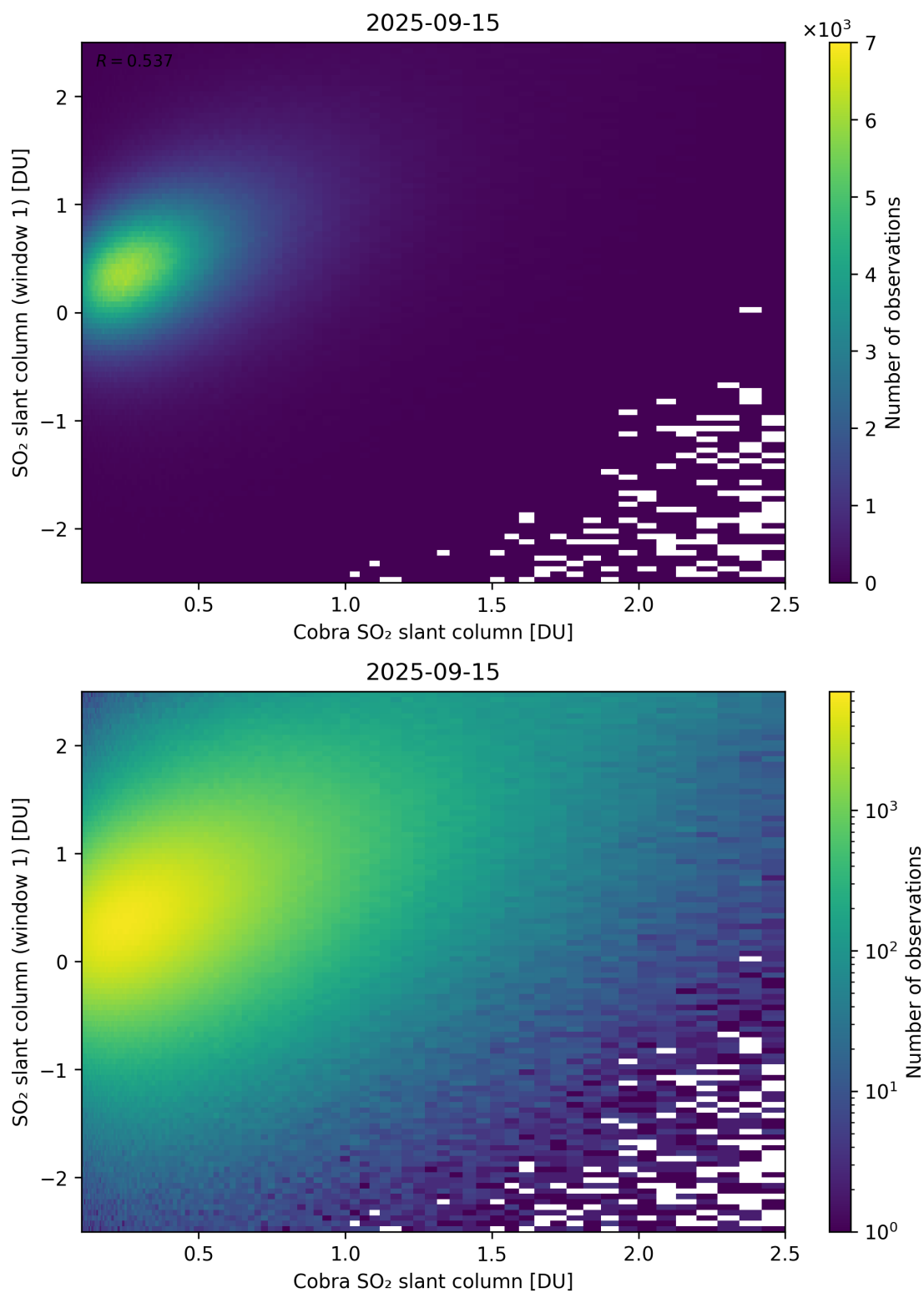
Figure 219: Scatter density plot of “Cobra SO 2 slant column” against “SO 2 slant column (window 1)” for 2025-09-15 to 2025-09-16.
