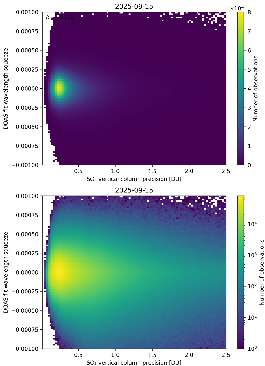
Figure 333: Scatter density plot of “SO 2 vertical column precision” against “DOAS fit wavelength squeeze” for 2025-09-15 to 2025-09-16.
