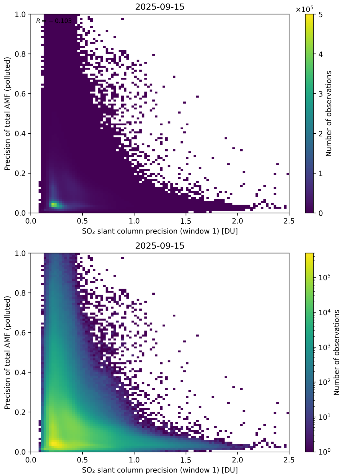
Figure 281: Scatter density plot of “SO 2 slant column precision (window 1)” against “Precision of total AMF (polluted)” for 2025-09-15 to 2025-09-16.
