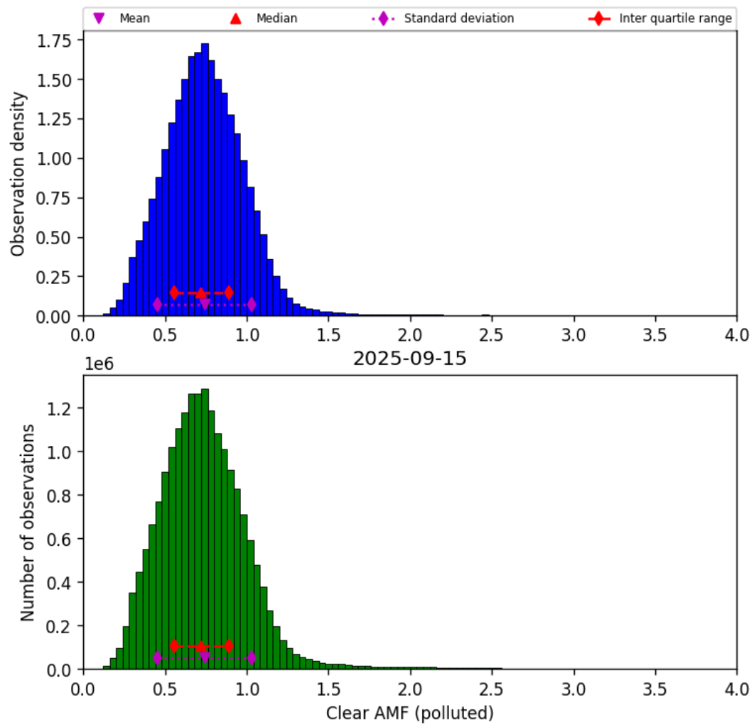
Figure 81: Histogram of "Clear AMF (polluted)" for 2025-09-15 to 2025-09-16
