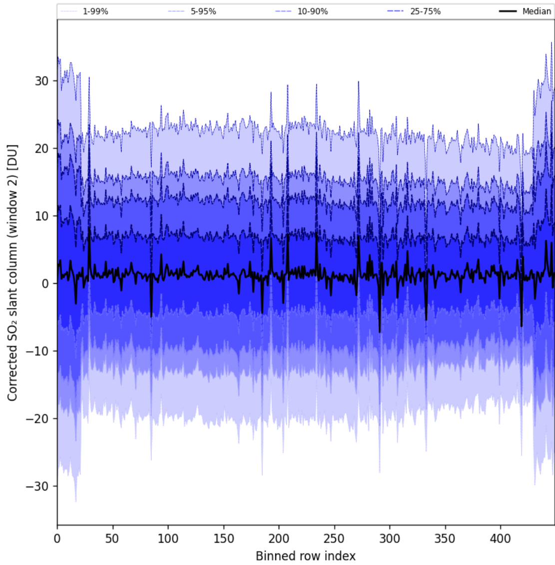
Figure 95: Along track statistics of “Corrected SO 2 slant column (window 2)” for 2025-09-15 to 2025-09-16
