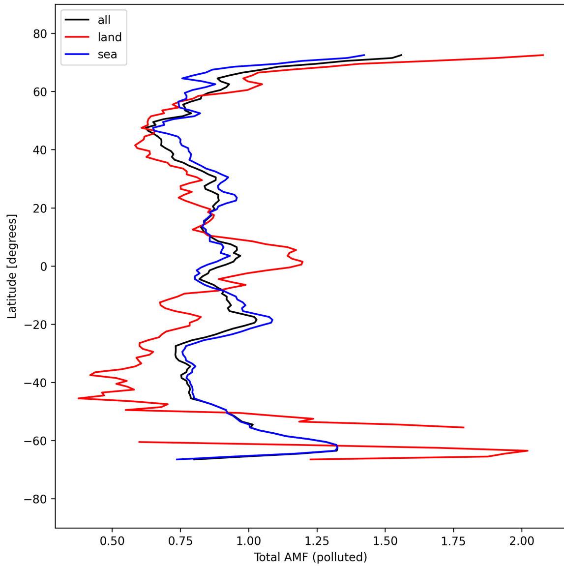
Figure 53: Zonal average of “Total AMF (polluted)” for 2025-09-15 to 2025-09-16.
