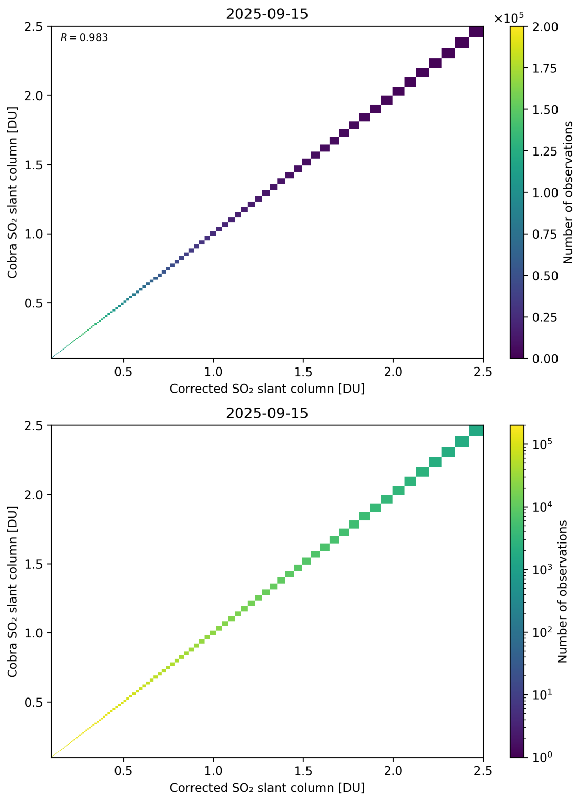
Figure 233: Scatter density plot of “Corrected SO 2 slant column” against “Cobra SO 2 slant column” for 2025-09-15 to 2025-09-16.
