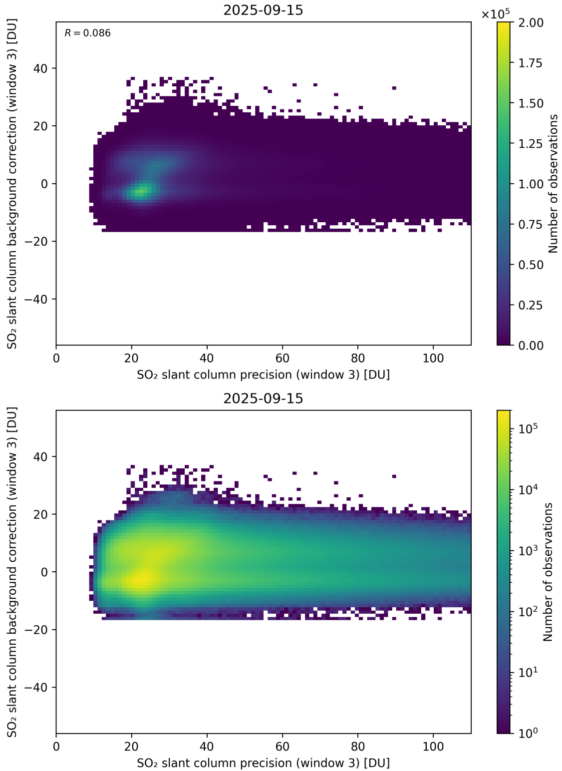
Figure 307: Scatter density plot of “SO 2 slant column precision (window 3)” against “SO 2 slant column background correction (window 3)” for 2025-09-15 to 2025-09-16.
