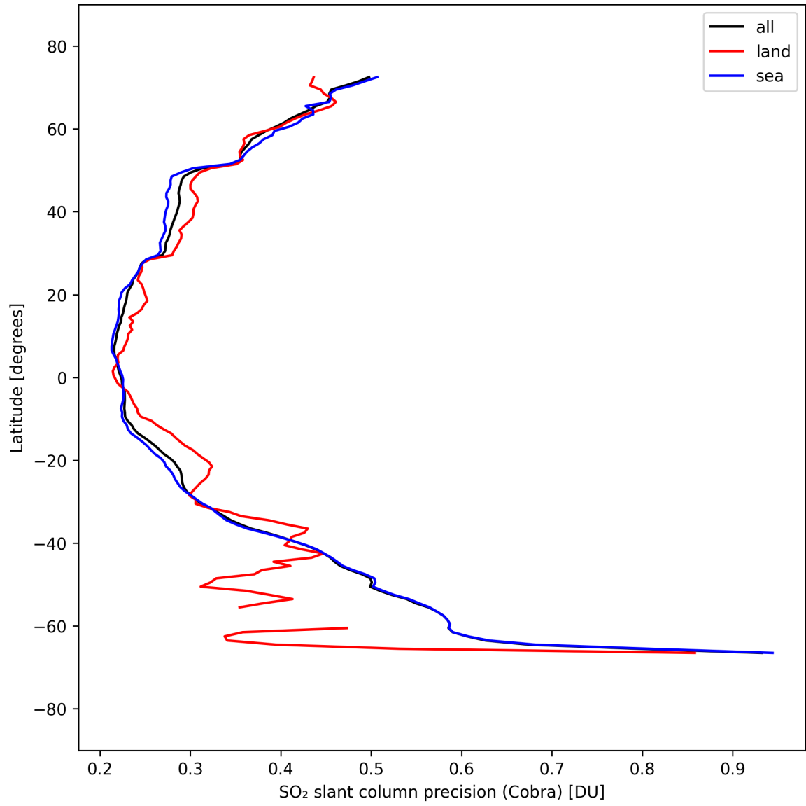
Figure 36: Zonal average of “SO 2 slant column precision (Cobra)” for 2025-09-15 to 2025-09-16.
