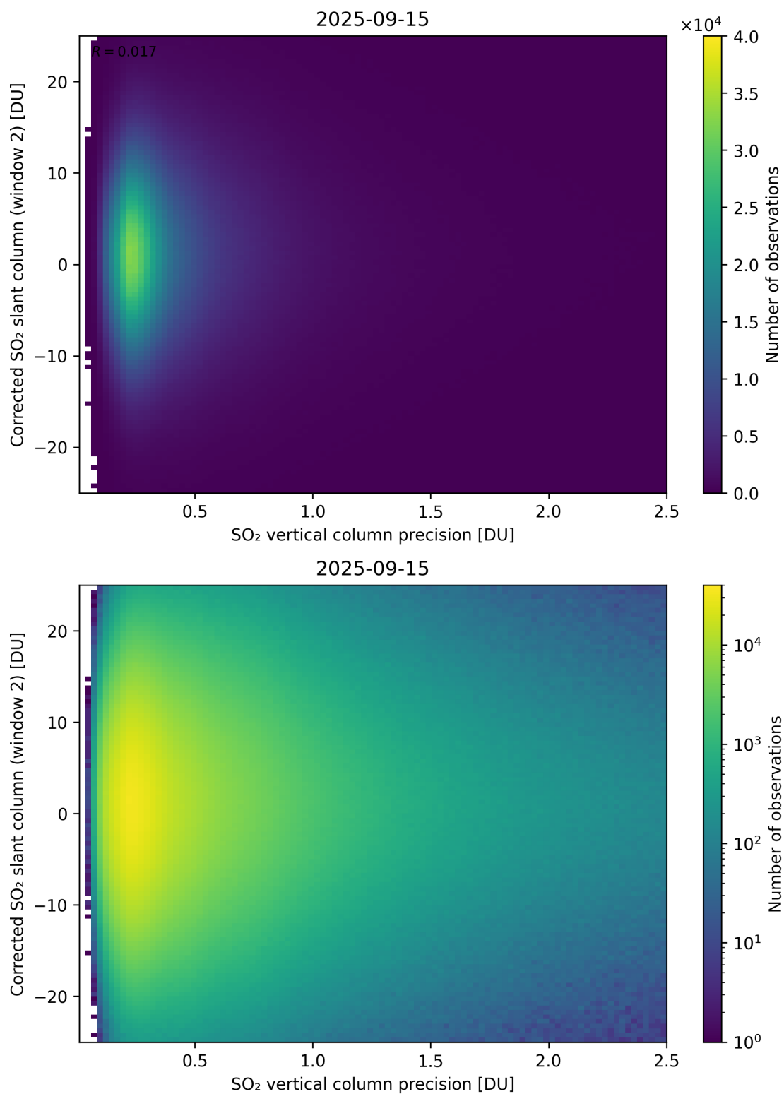
Figure 339: Scatter density plot of “SO 2 vertical column precision” against “Corrected SO 2 slant column (window 2)” for 2025-09-15 to 2025-09-16.
