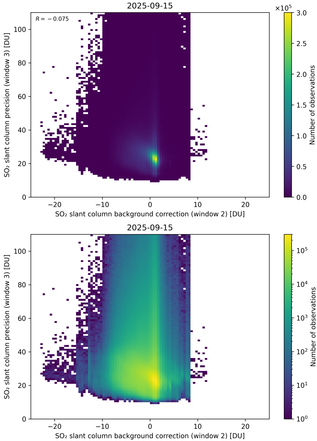
Figure 129: Scatter density plot of “SO 2 slant column background correction (window 2)” against “SO 2 slant column precision (window 3)” for 2025-09-15 to 2025-09-16.
