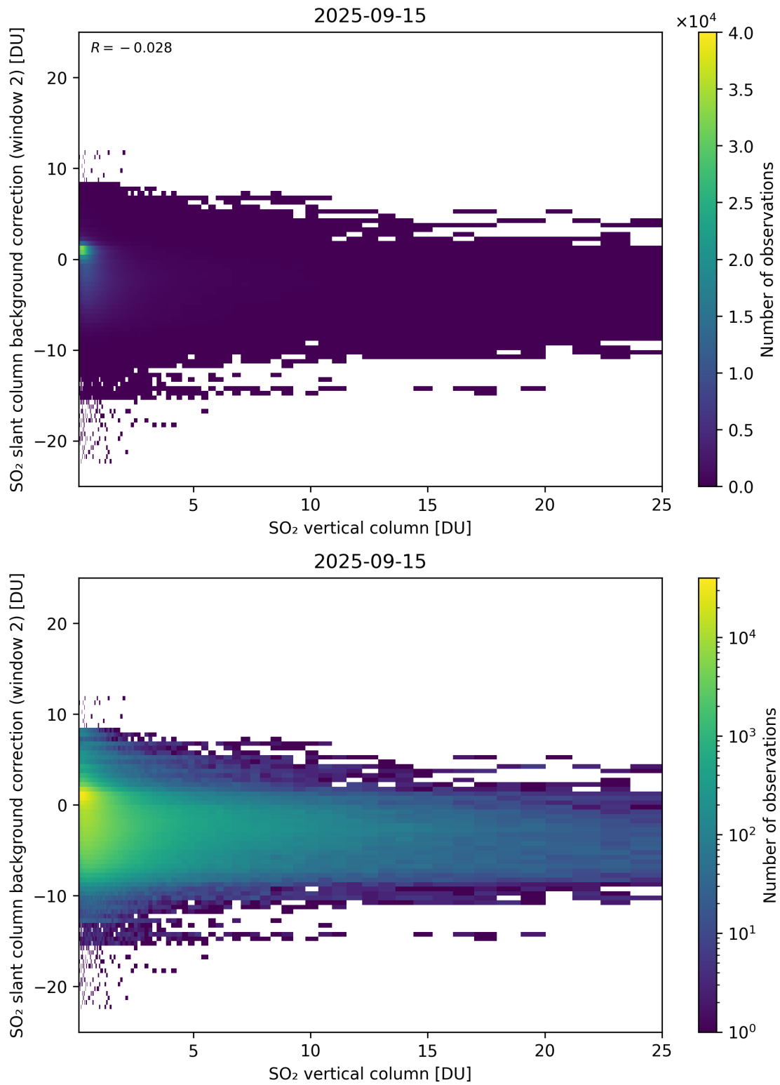
Figure 324: Scatter density plot of “SO 2 vertical column” against “SO 2 slant column background correction (window 2)” for 2025-09-15 to 2025-09-16.
