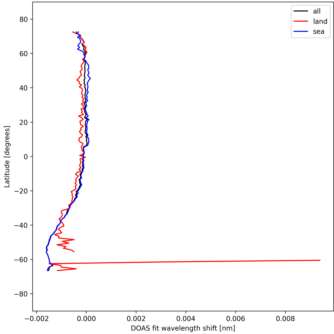
Figure 50: Zonal average of "DOAS fit wavelength shift" for 2025-09-15 to 2025-09-16.
