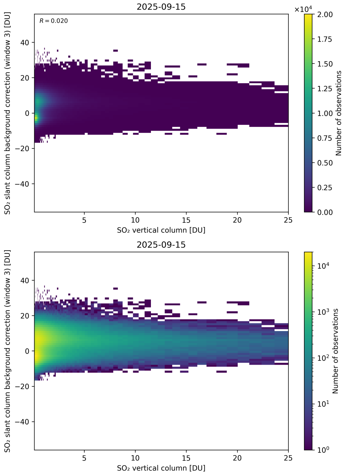
Figure 325: Scatter density plot of “SO 2 vertical column” against “SO 2 slant column background correction (window 3)” for 2025-09-15 to 2025-09-16.
