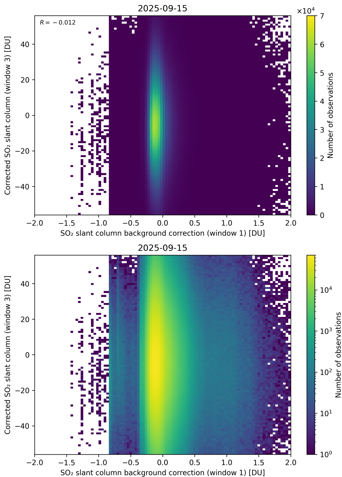
Figure 116: Scatter density plot of “SO 2 slant column background correction (window 1)” against “Corrected SO 2 slant column (window 3)” for 2025-09-15 to 2025-09-16.
