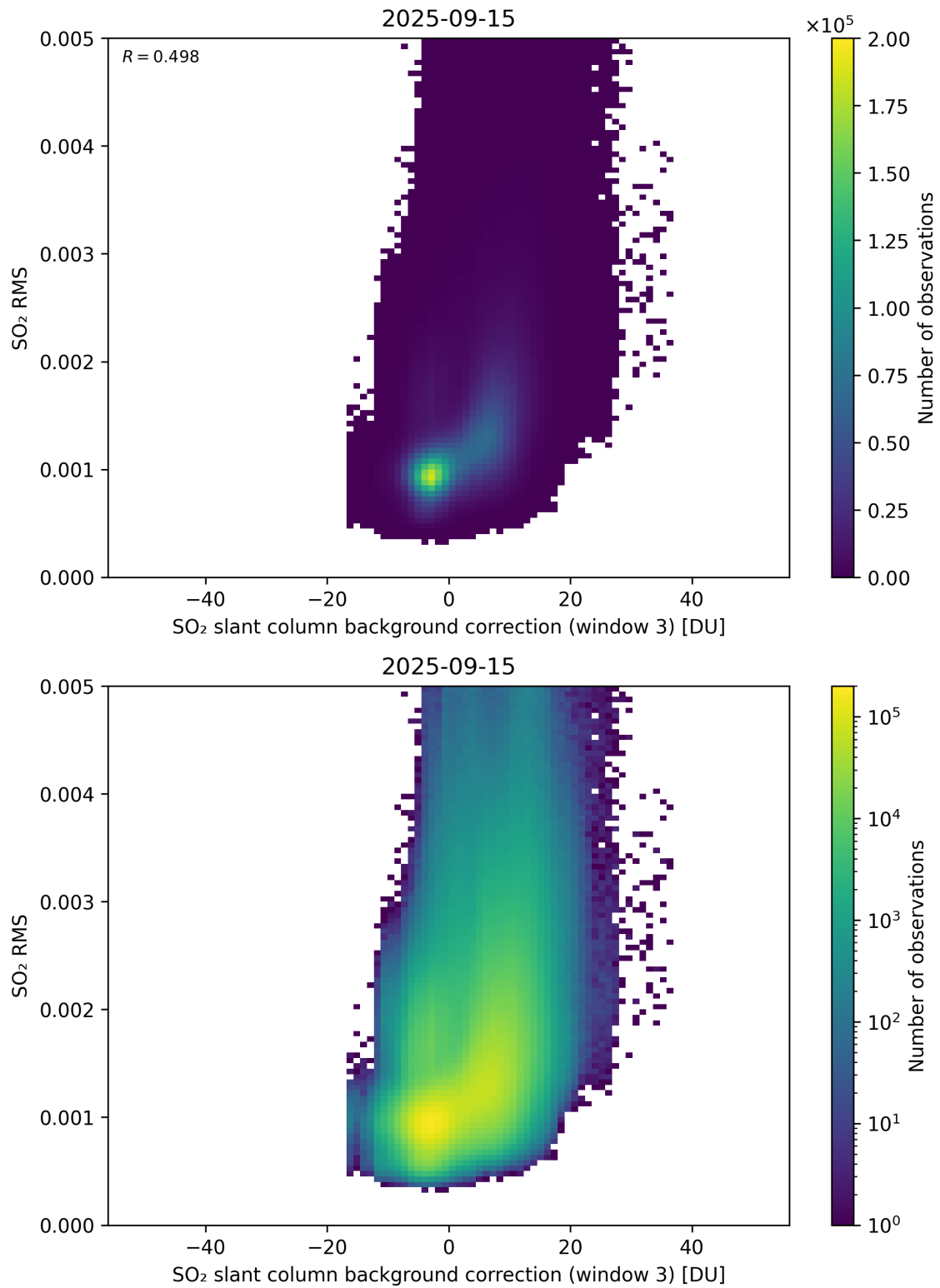
Figure 134: Scatter density plot of “SO 2 slant column background correction (window 3)” against “SO 2 RMS” for 2025-09-15 to 2025-09-16.
