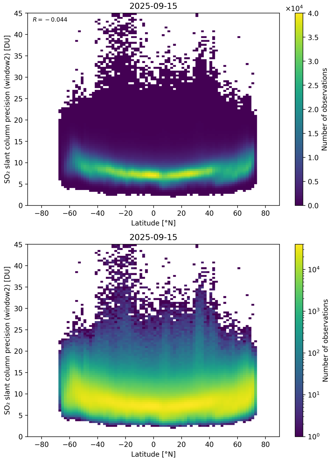
Figure 164: Scatter density plot of “Latitude” against “SO 2 slant column precision (window2)” for 2025-09-15 to 2025-09-16.
