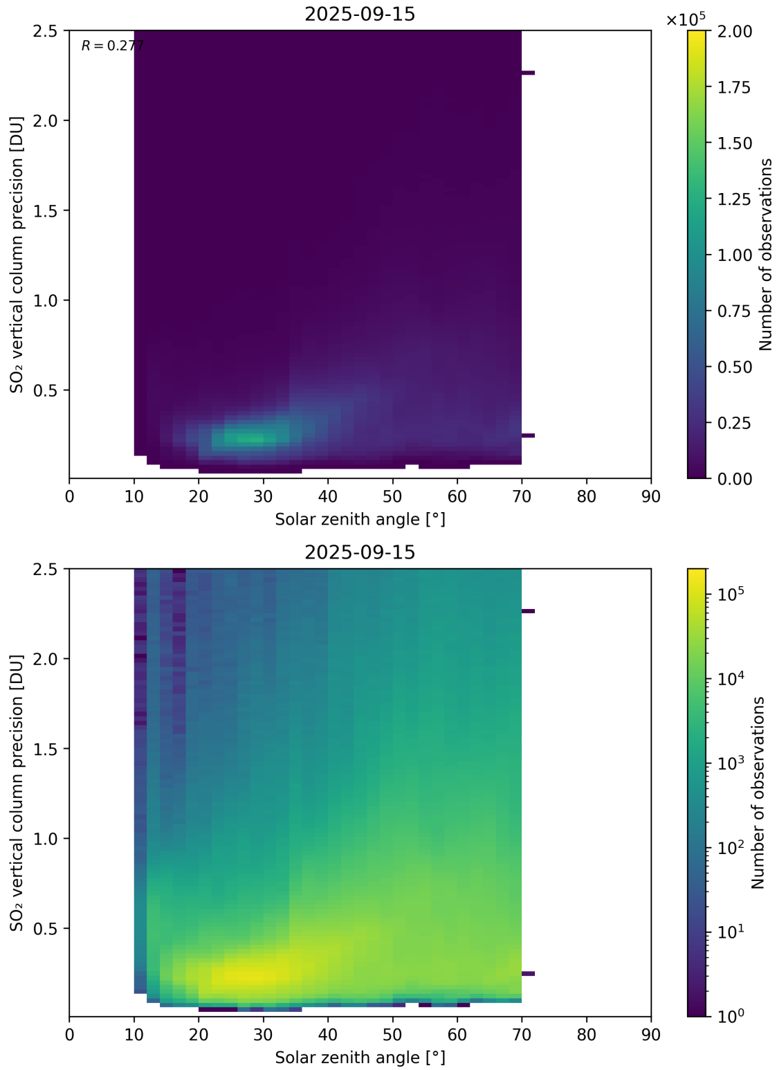
Figure 192: Scatter density plot of “Solar zenith angle” against “SO 2 vertical column precision” for 2025-09-15 to 2025-09-16.
