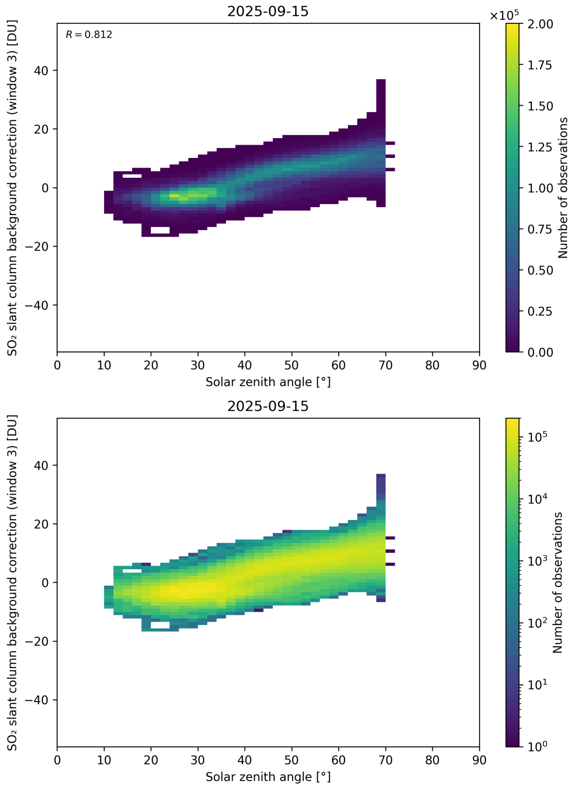
Figure 173: Scatter density plot of “Solar zenith angle” against “SO 2 slant column background correction (window 3)” for 2025-09-15 to 2025-09-16.
