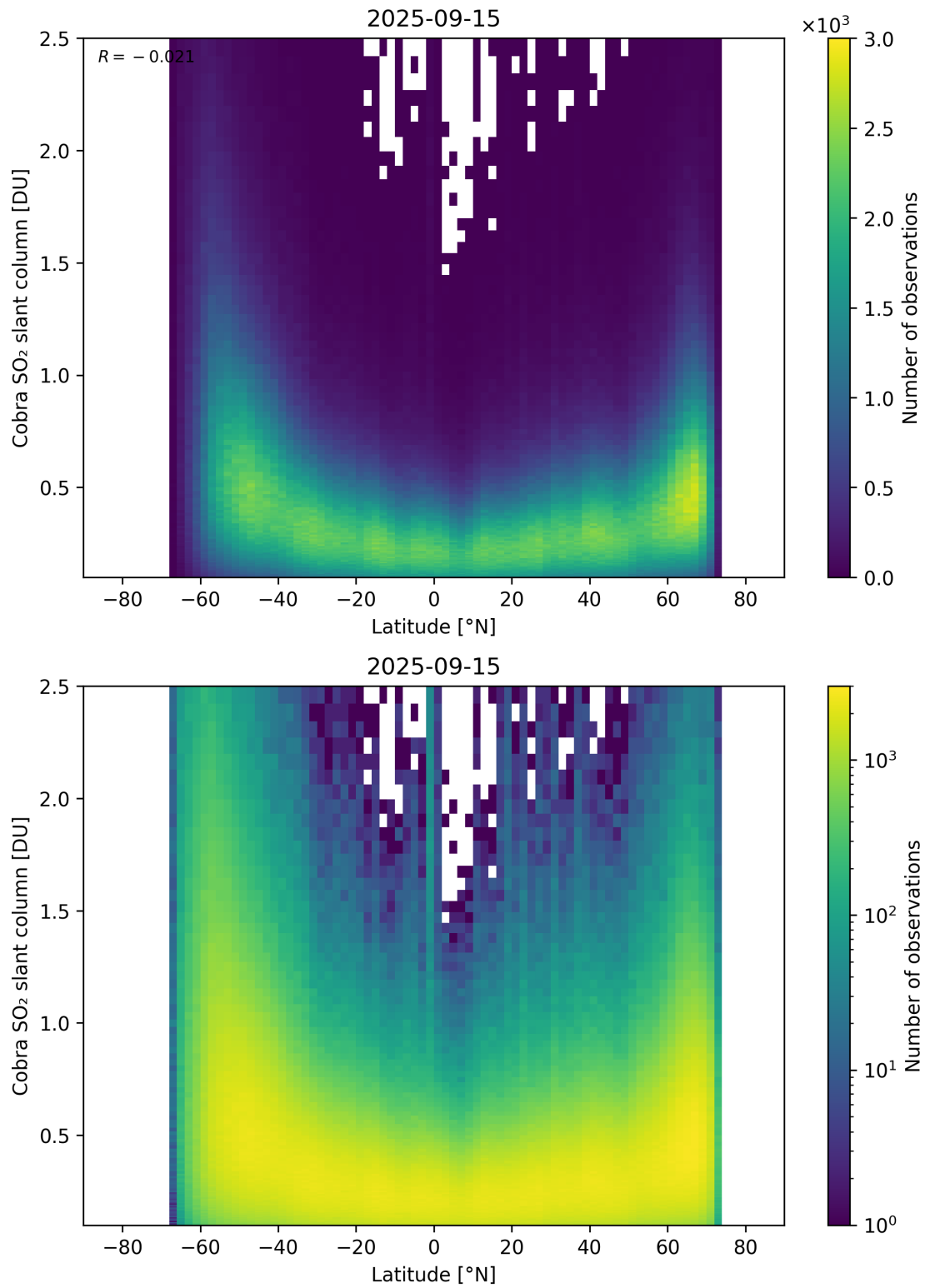
Figure 157: Scatter density plot of “Latitude” against “Cobra SO 2 slant column” for 2025-09-15 to 2025-09-16.
