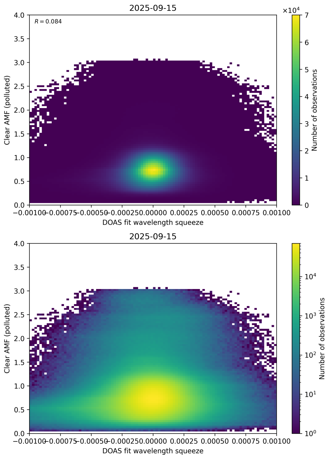
Figure 144: Scatter density plot of “DOAS fit wavelength squeeze” against “Clear AMF (polluted)” for 2025-09-15 to 2025-09-16.
