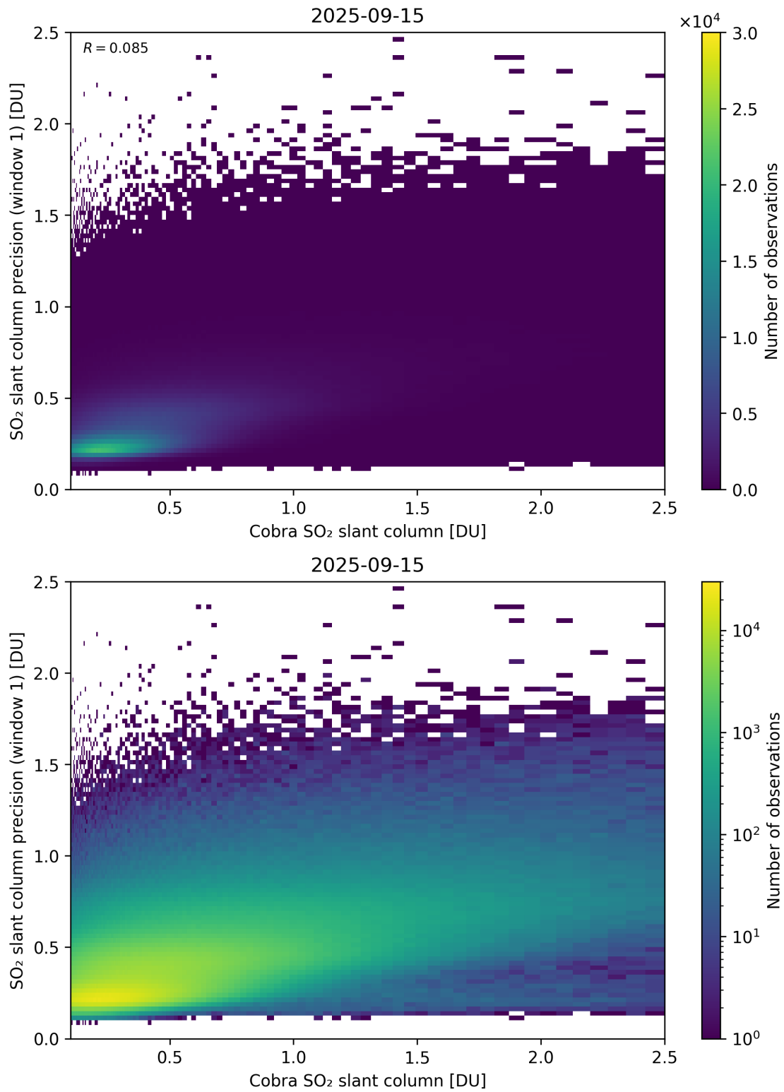
Figure 220: Scatter density plot of “Cobra SO 2 slant column” against “SO 2 slant column precision (window 1)” for 2025-09-15 to 2025-09-16.
