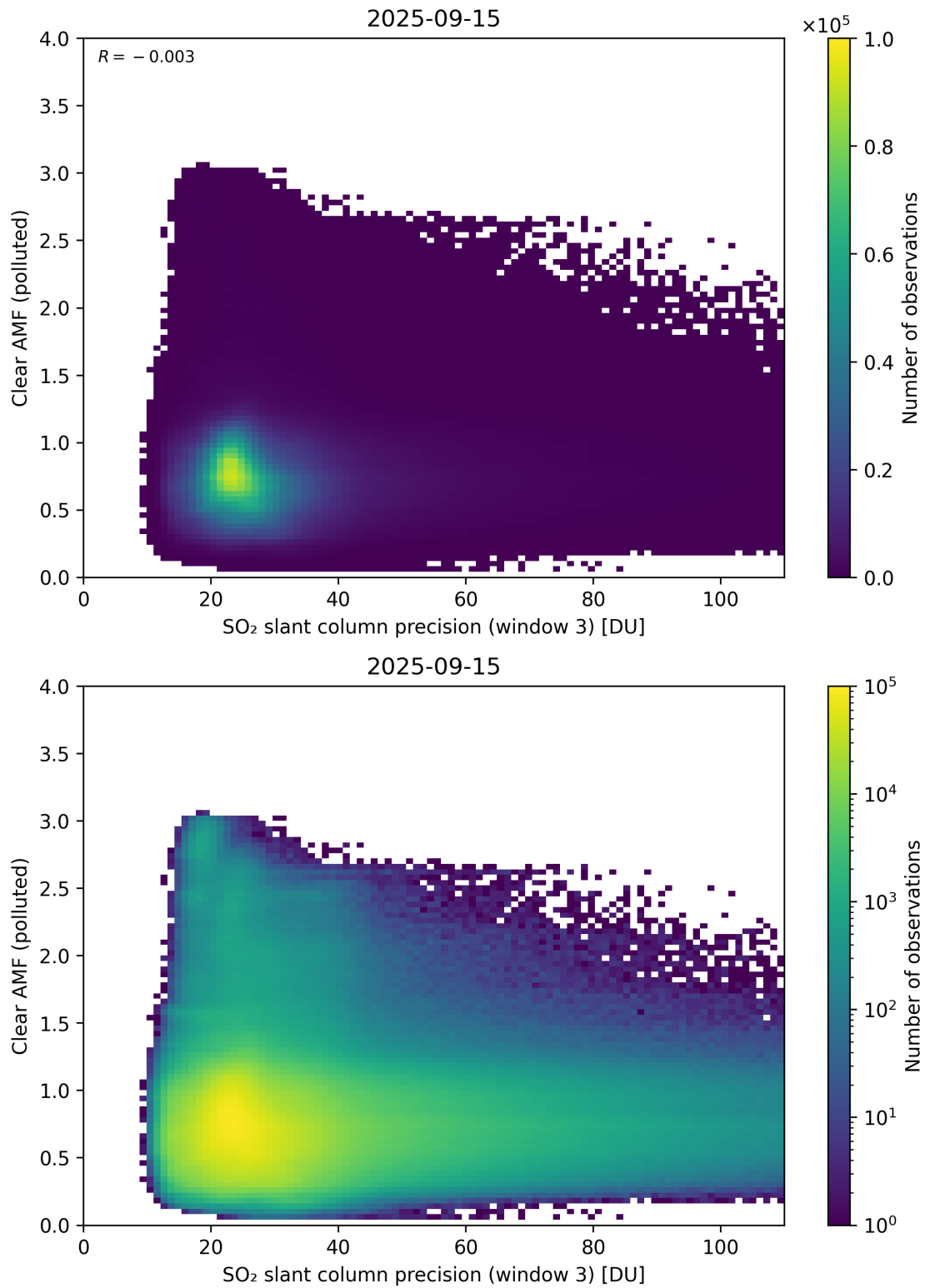
Figure 311: Scatter density plot of “SO 2 slant column precision (window 3)” against “Clear AMF (polluted)” for 2025-09-15 to 2025-09-16.
