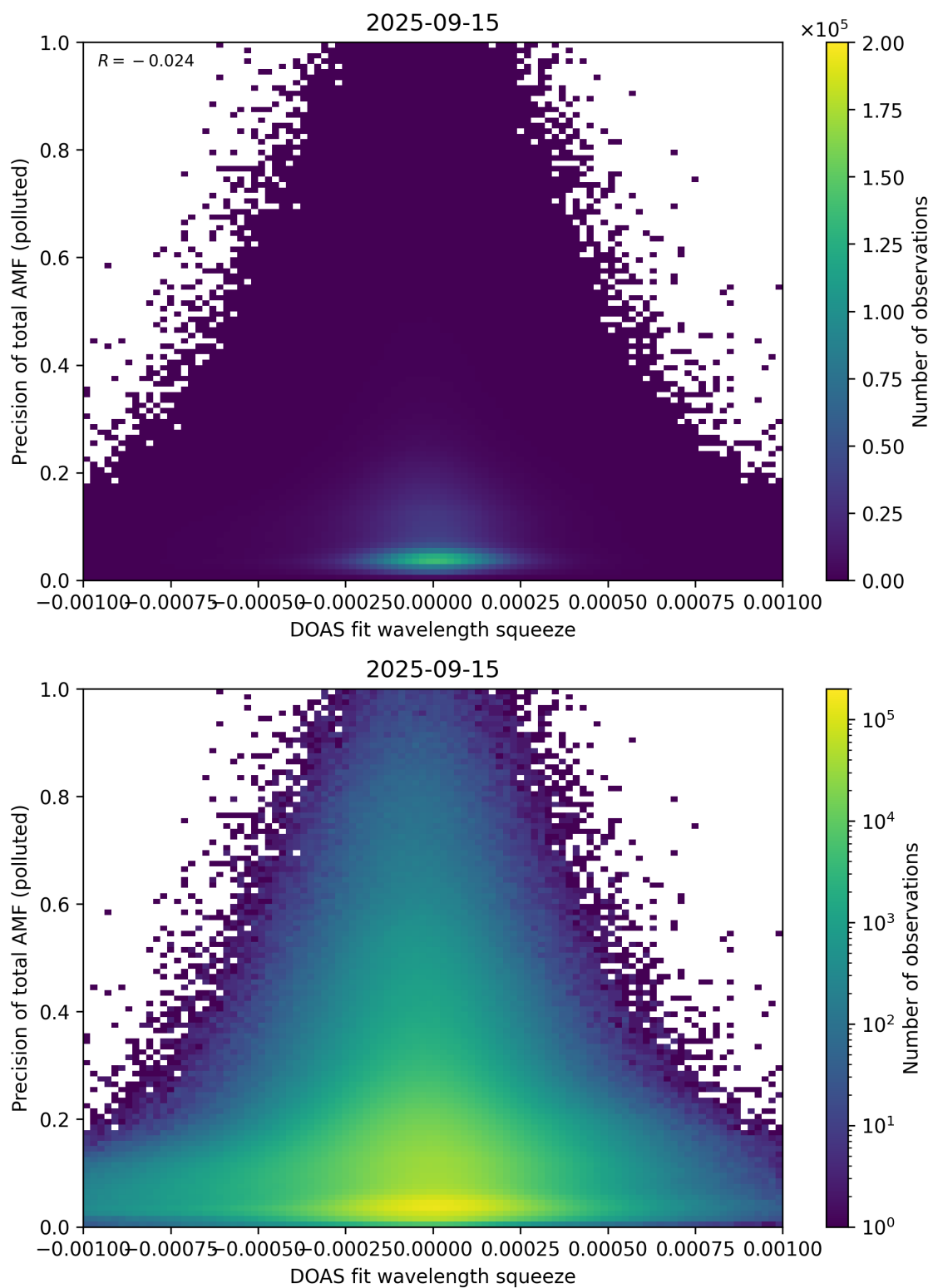
Figure 146: Scatter density plot of “DOAS fit wavelength squeeze” against “Precision of total AMF (polluted)” for 2025-09-15 to 2025-09-16.
