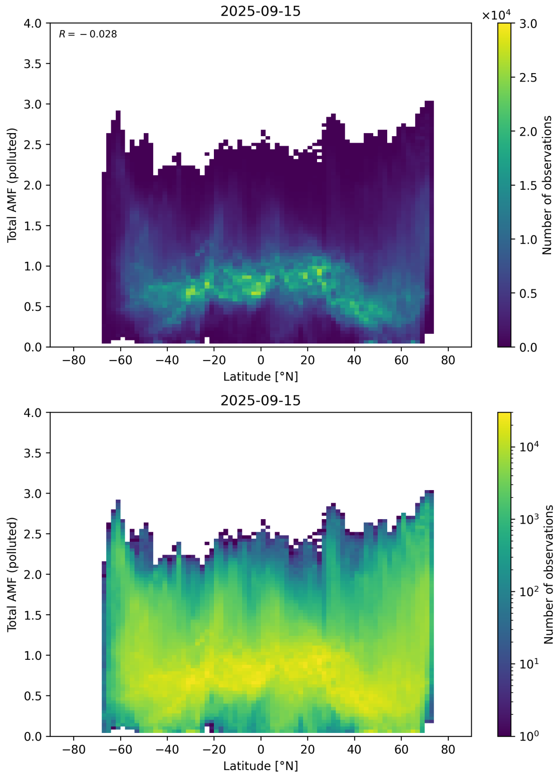
Figure 167: Scatter density plot of “Latitude” against “Total AMF (polluted)” for 2025-09-15 to 2025-09-16.
