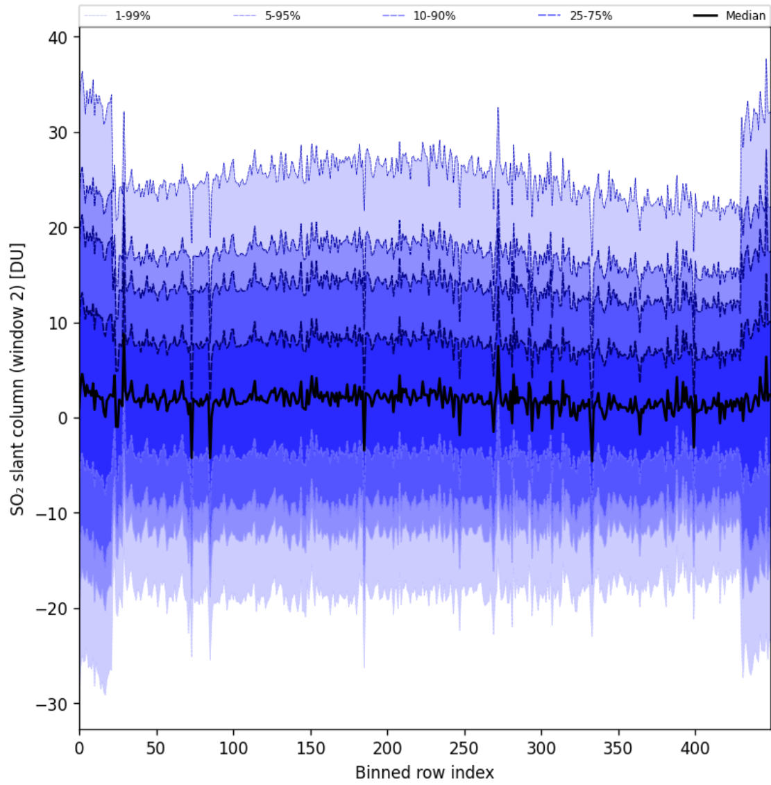
Figure 93: Along track statistics of “SO 2 slant column (window 2)” for 2025-09-15 to 2025-09-16
