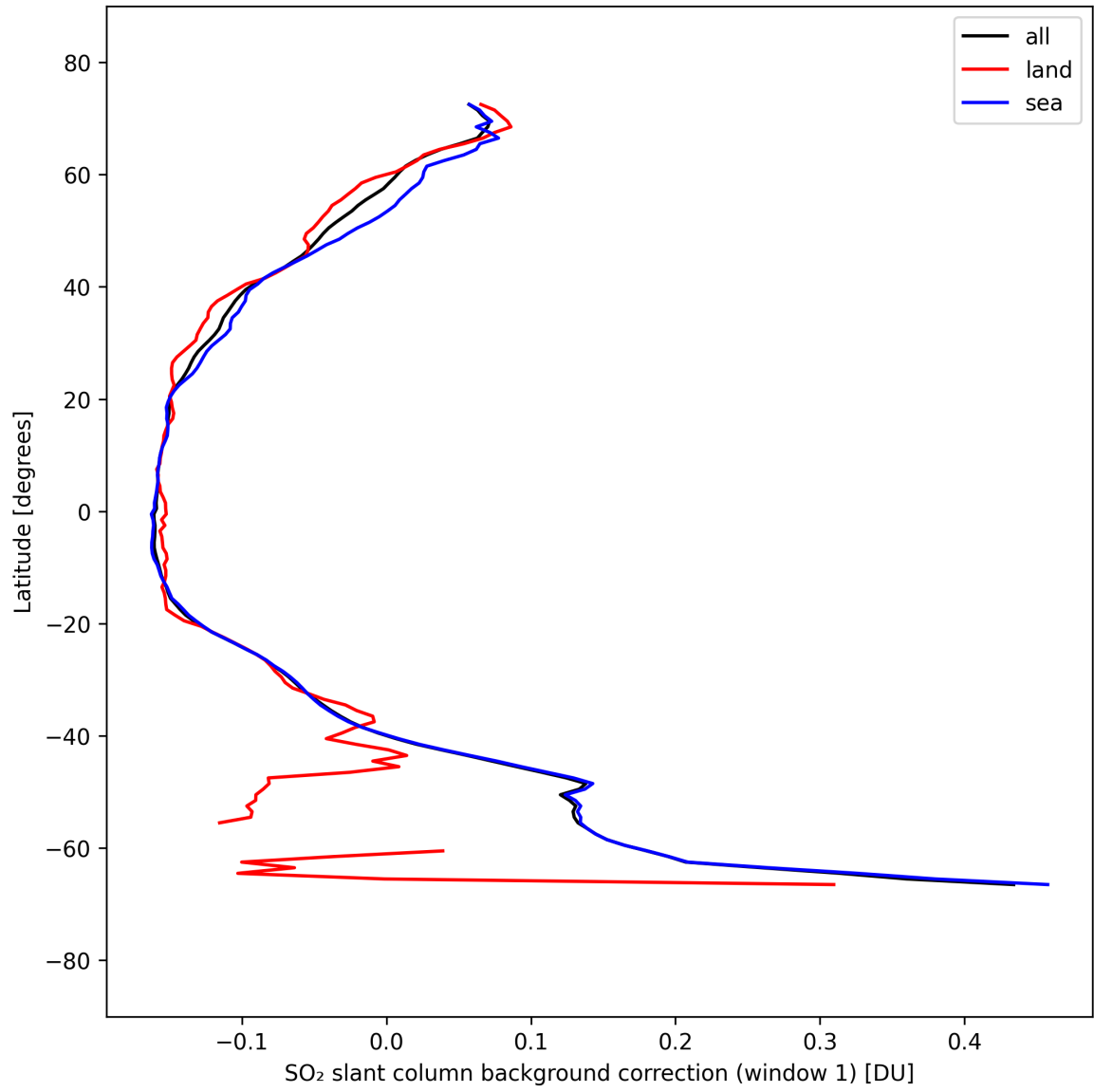
Figure 40: Zonal average of “SO 2 slant column background correction (window 1)” for 2025-09-15 to 2025-09-16.
