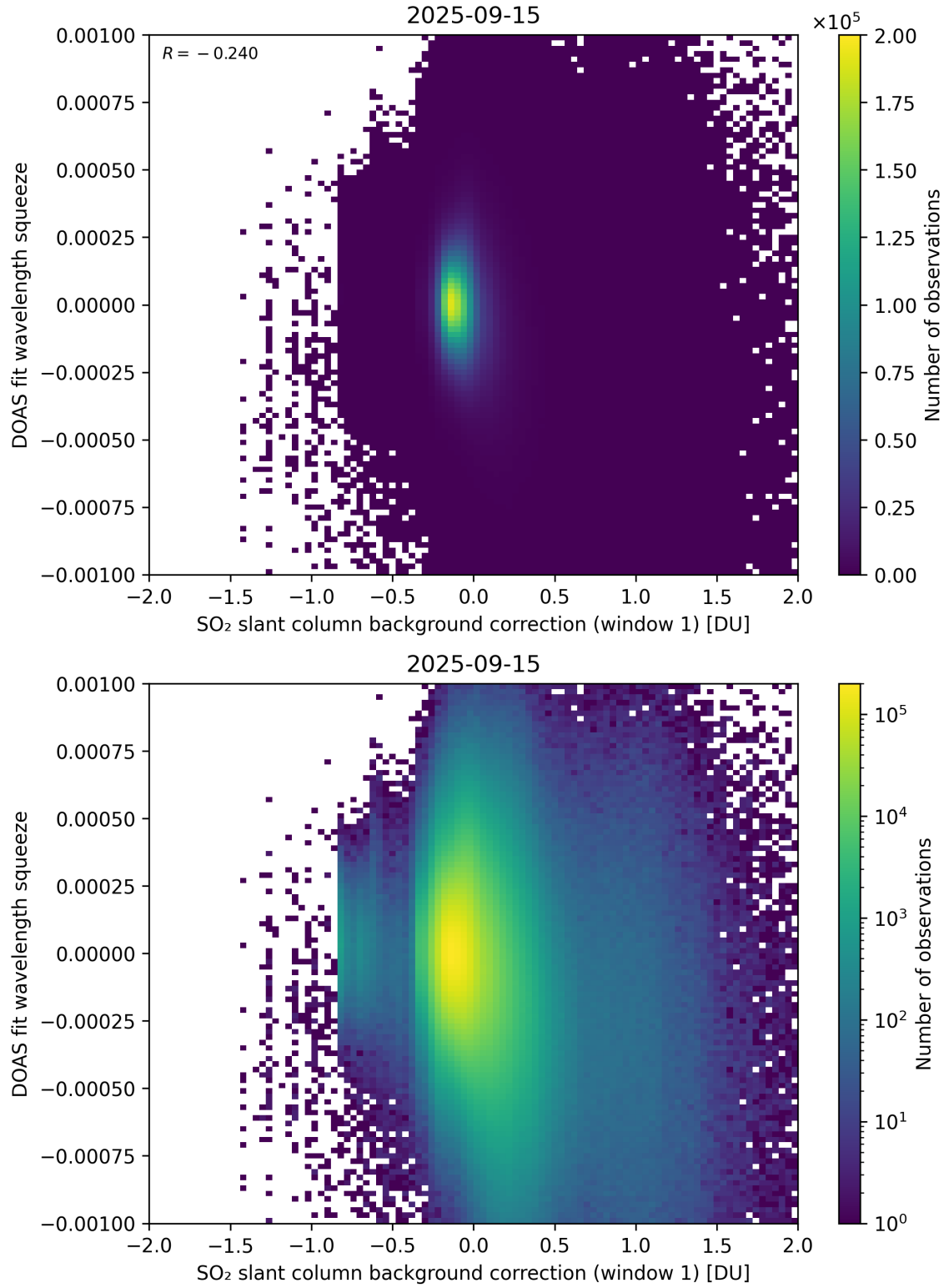
Figure 112: Scatter density plot of “SO 2 slant column background correction (window 1)” against “DOAS fit wavelength squeeze” for 2025-09-15 to 2025-09-16.
