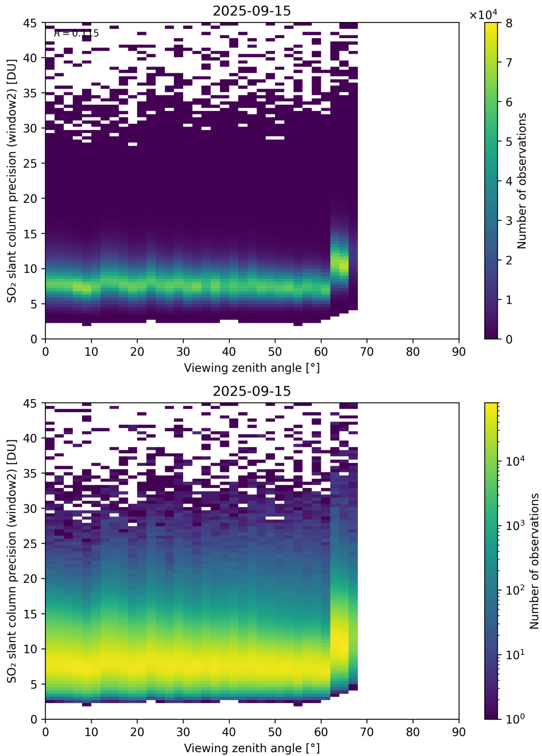
Figure 378: Scatter density plot of “Viewing zenith angle” against “SO 2 slant column precision (window2)” for 2025-09-15 to 2025-09-16.
