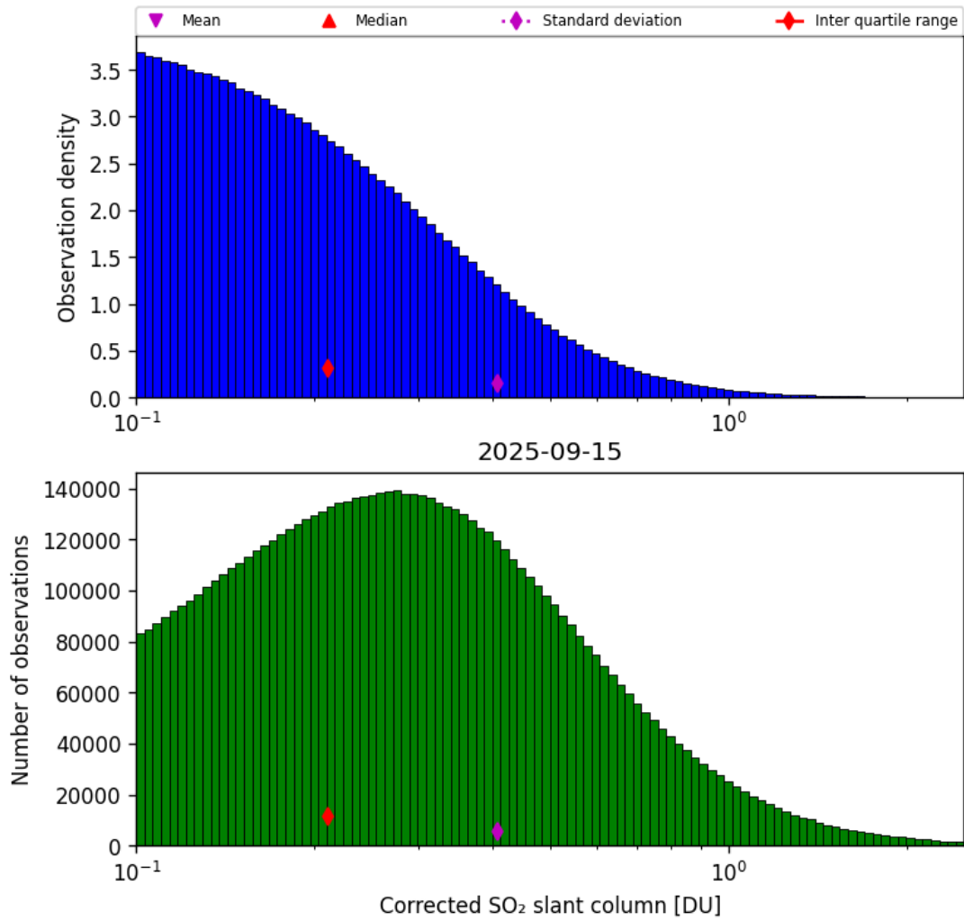
Figure 60: Histogram of “Corrected SO 2 slant column” for 2025-09-15 to 2025-09-16
