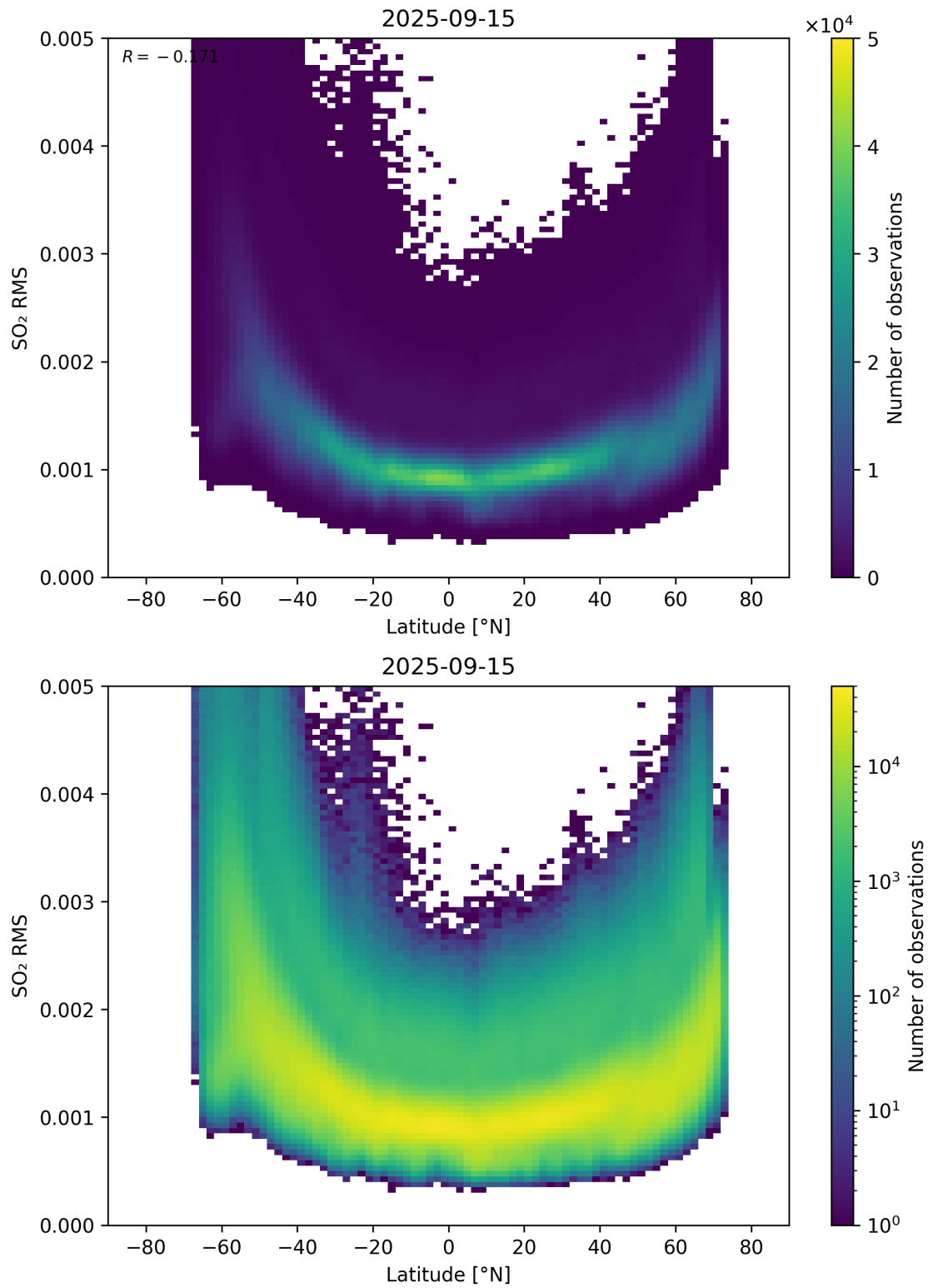
Figure 155: Scatter density plot of “Latitude” against “SO 2 RMS” for 2025-09-15 to 2025-09-16.
