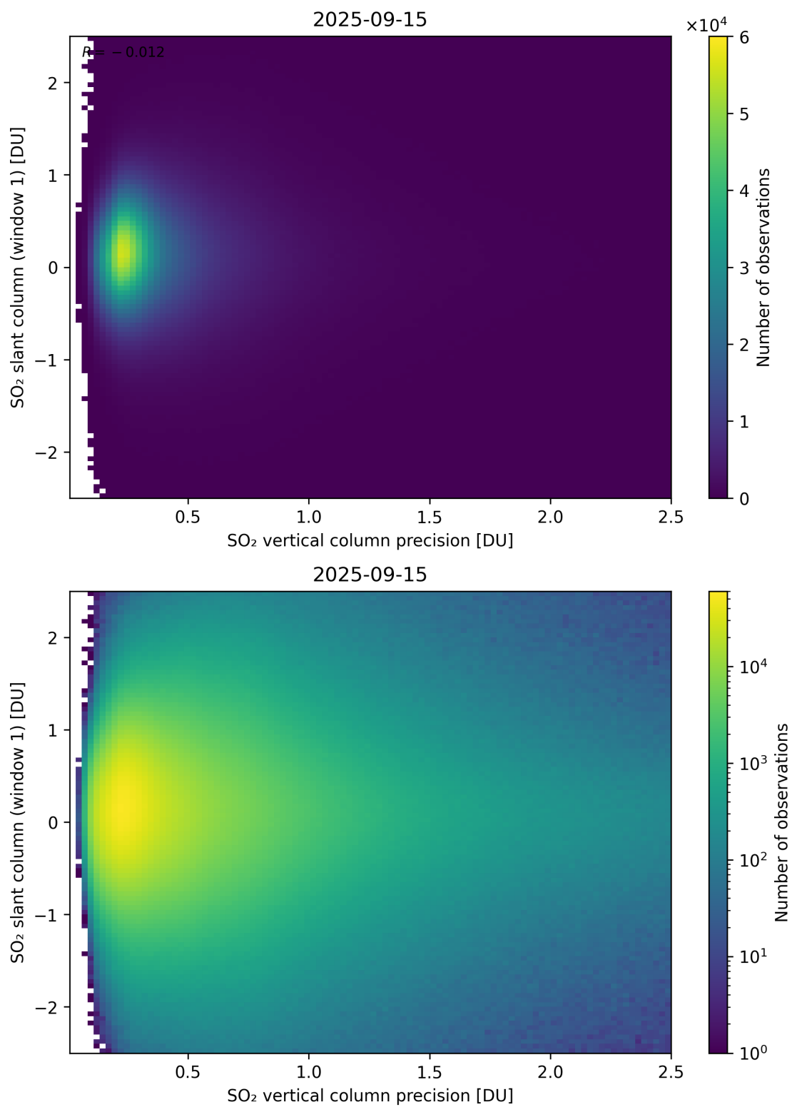
Figure 341: Scatter density plot of “SO 2 vertical column precision” against “SO 2 slant column (window 1)” for 2025-09-15 to 2025-09-16.
