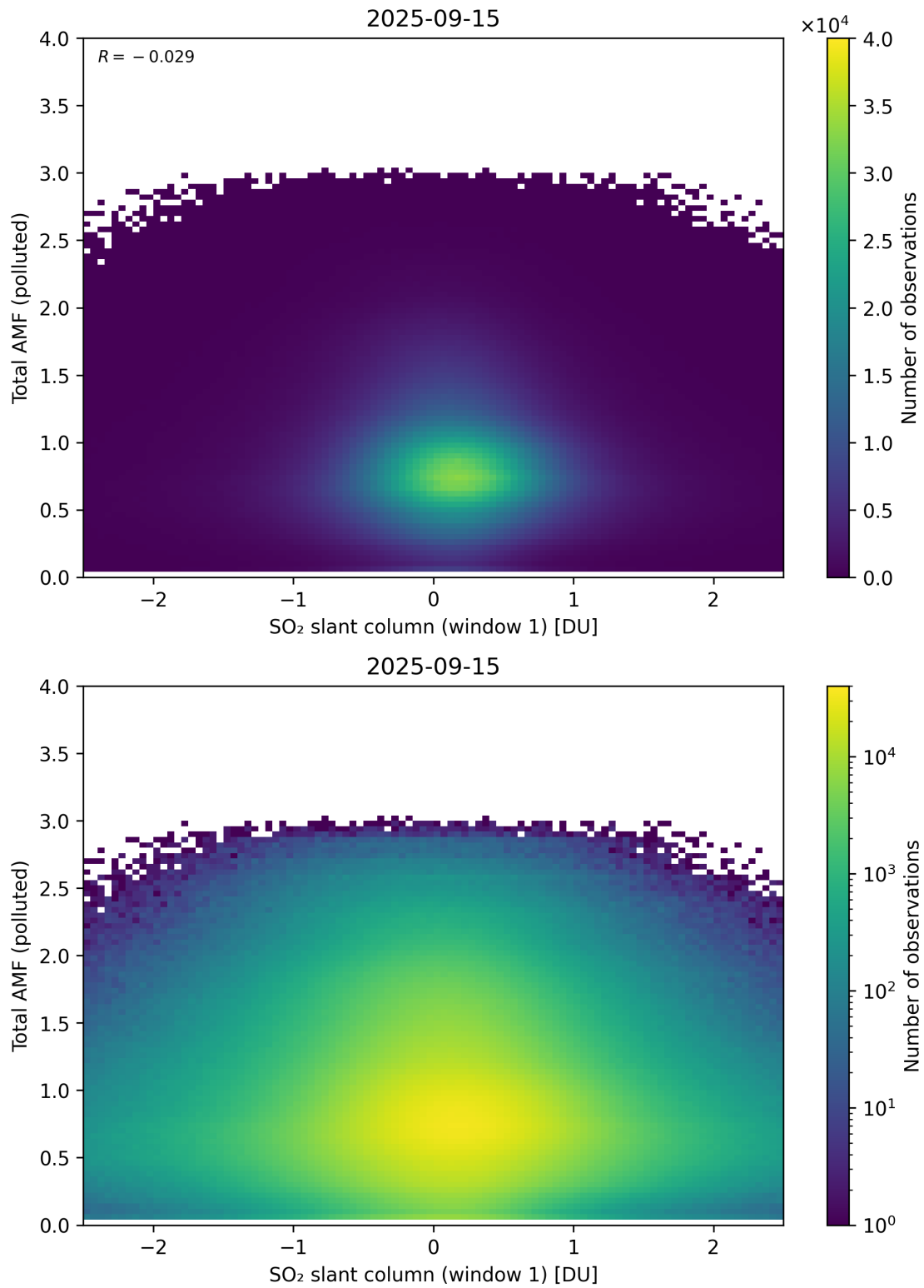
Figure 289: Scatter density plot of “SO 2 slant column (window 1)” against “Total AMF (polluted)” for 2025-09-15 to 2025-09-16.
