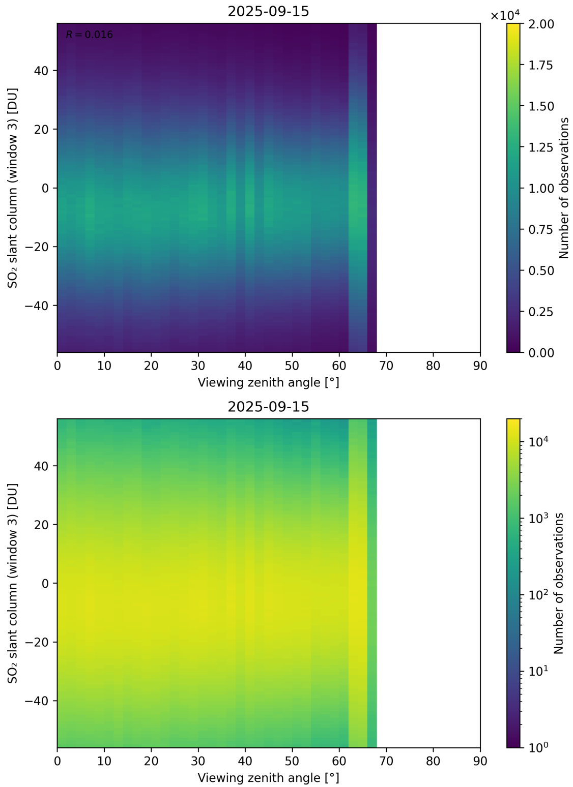
Figure 379: Scatter density plot of “Viewing zenith angle” against “SO 2 slant column (window 3)” for 2025-09-15 to 2025-09-16.
