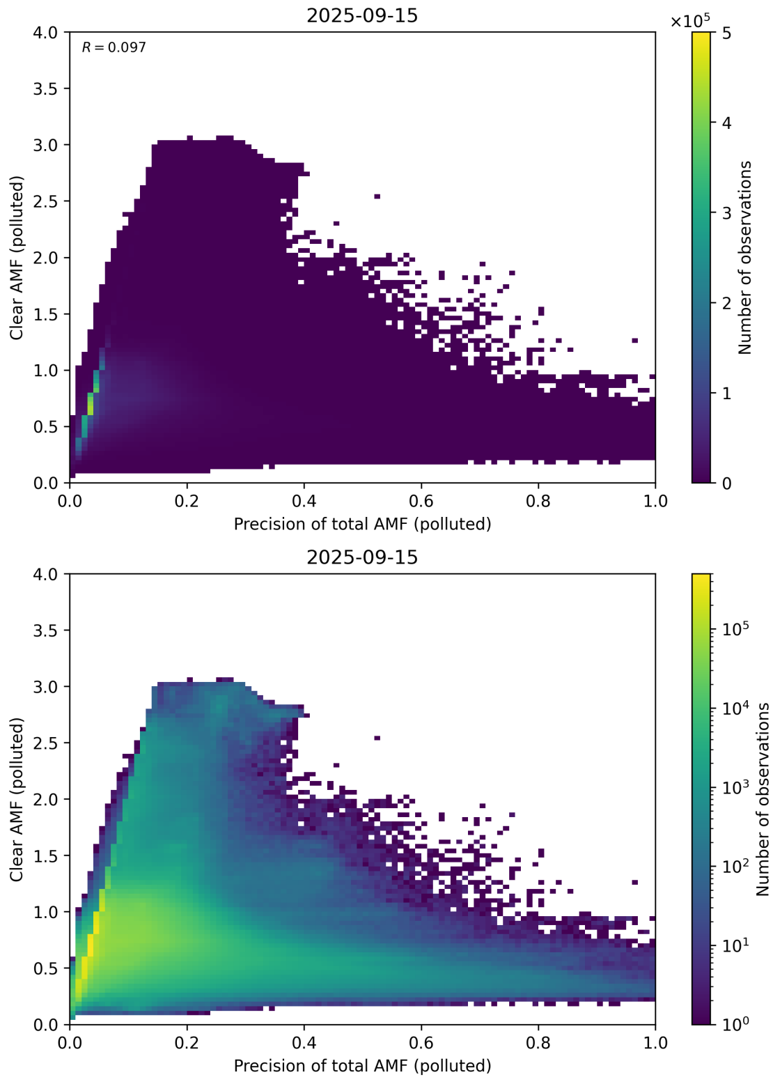
Figure 320: Scatter density plot of “Precision of total AMF (polluted)” against “Clear AMF (polluted)” for 2025-09-15 to 2025-09-16.
