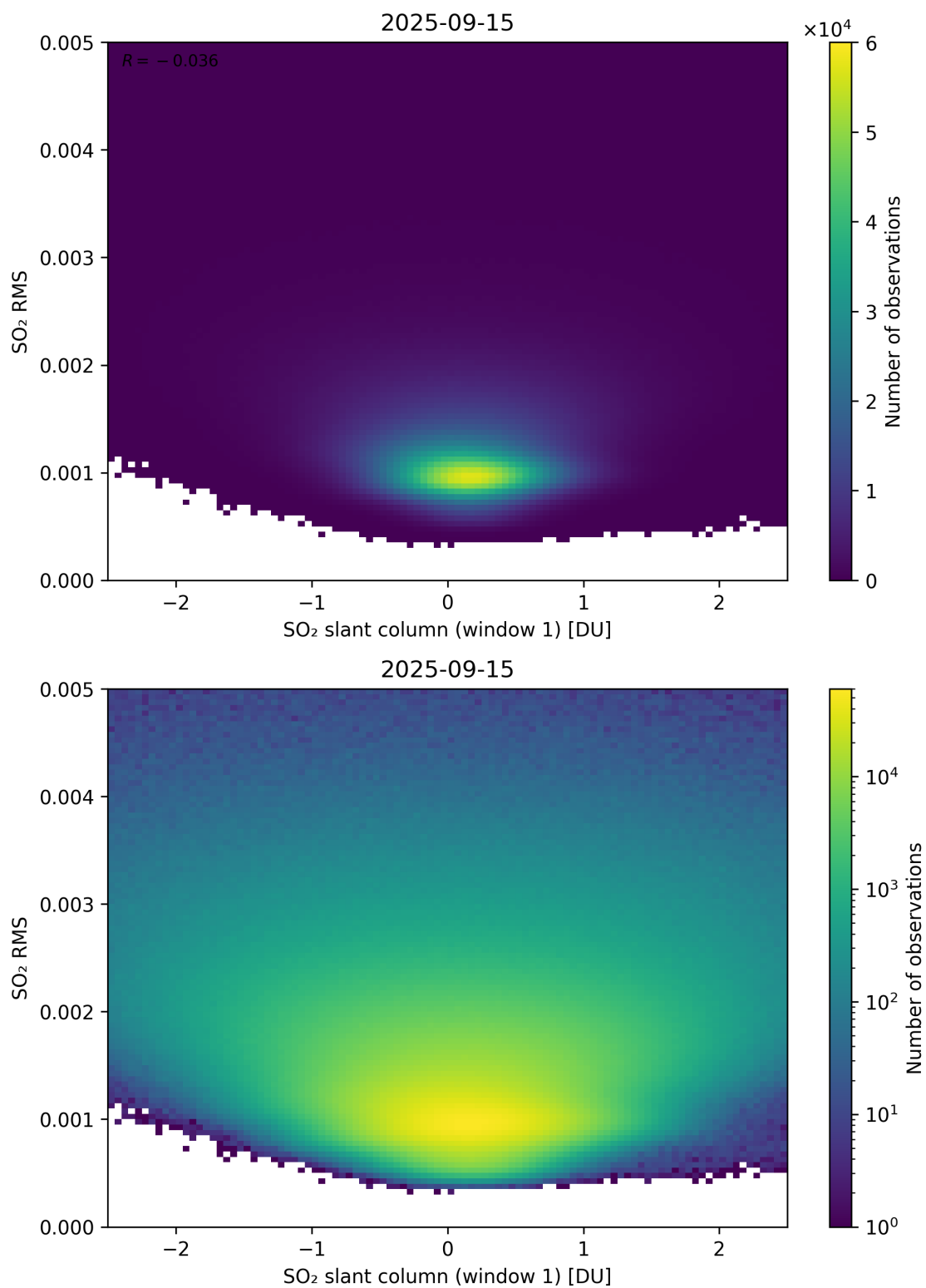
Figure 267: Scatter density plot of “SO 2 slant column (window 1)” against “SO 2 RMS” for 2025-09-15 to 2025-09-16.
