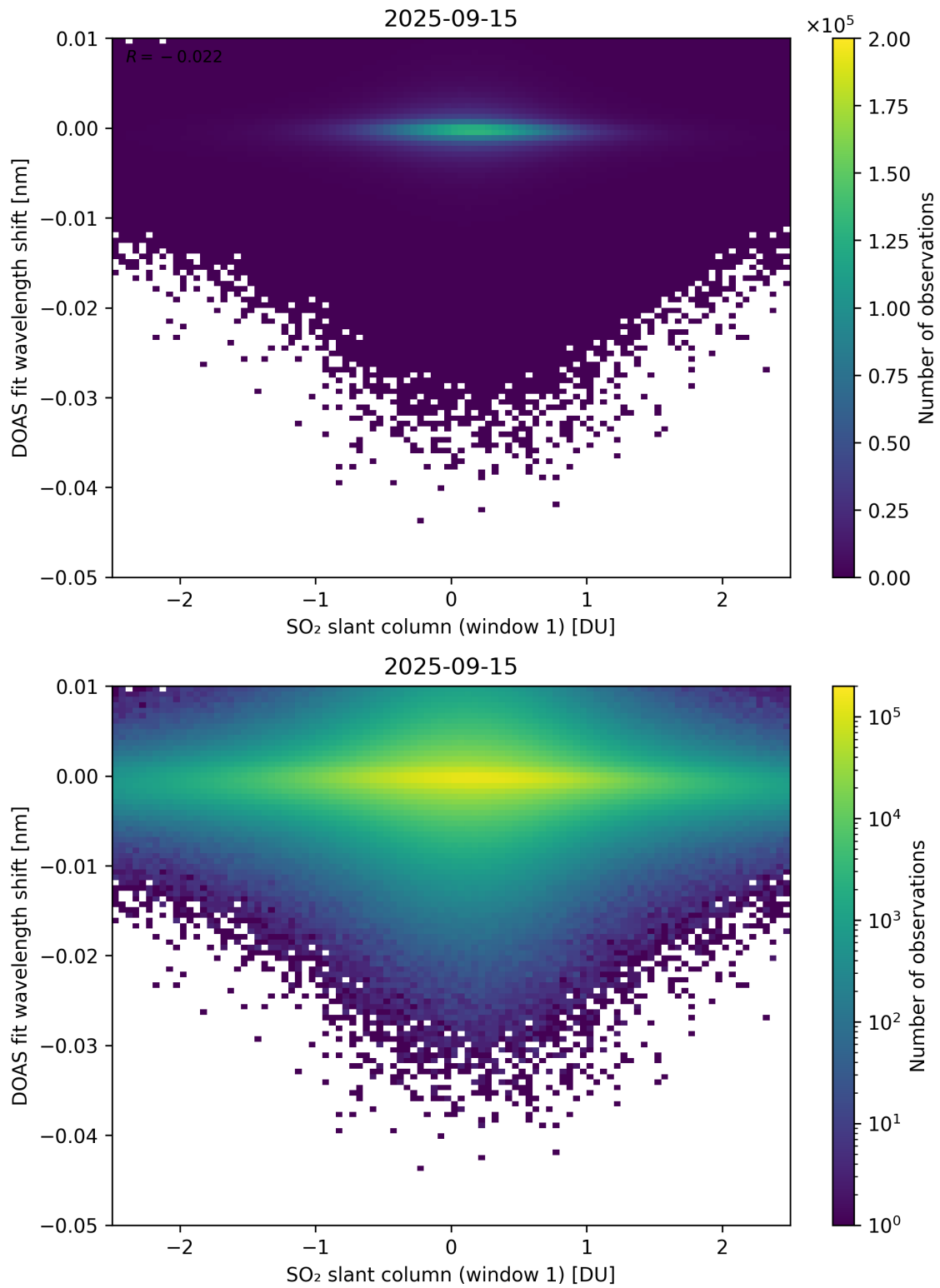
Figure 265: Scatter density plot of “SO 2 slant column (window 1)” against “DOAS fit wavelength shift” for 2025-09-15 to 2025-09-16.
