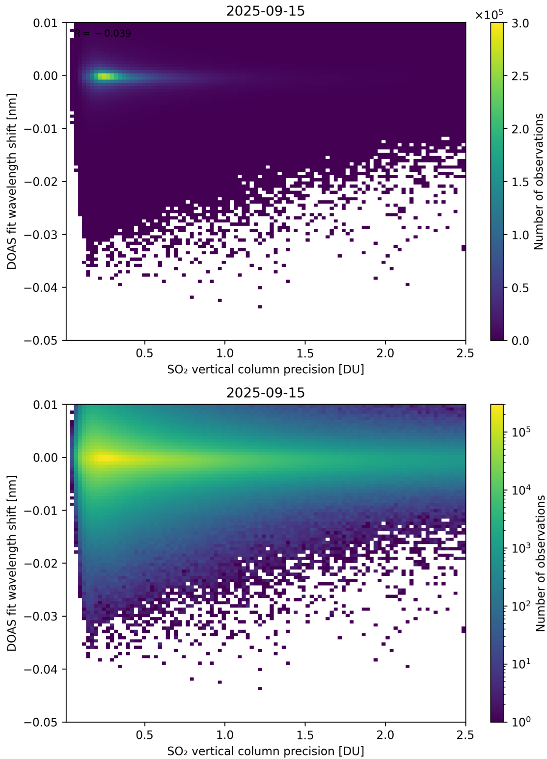
Figure 332: Scatter density plot of “SO 2 vertical column precision” against “DOAS fit wavelength shift” for 2025-09-15 to 2025-09-16.
