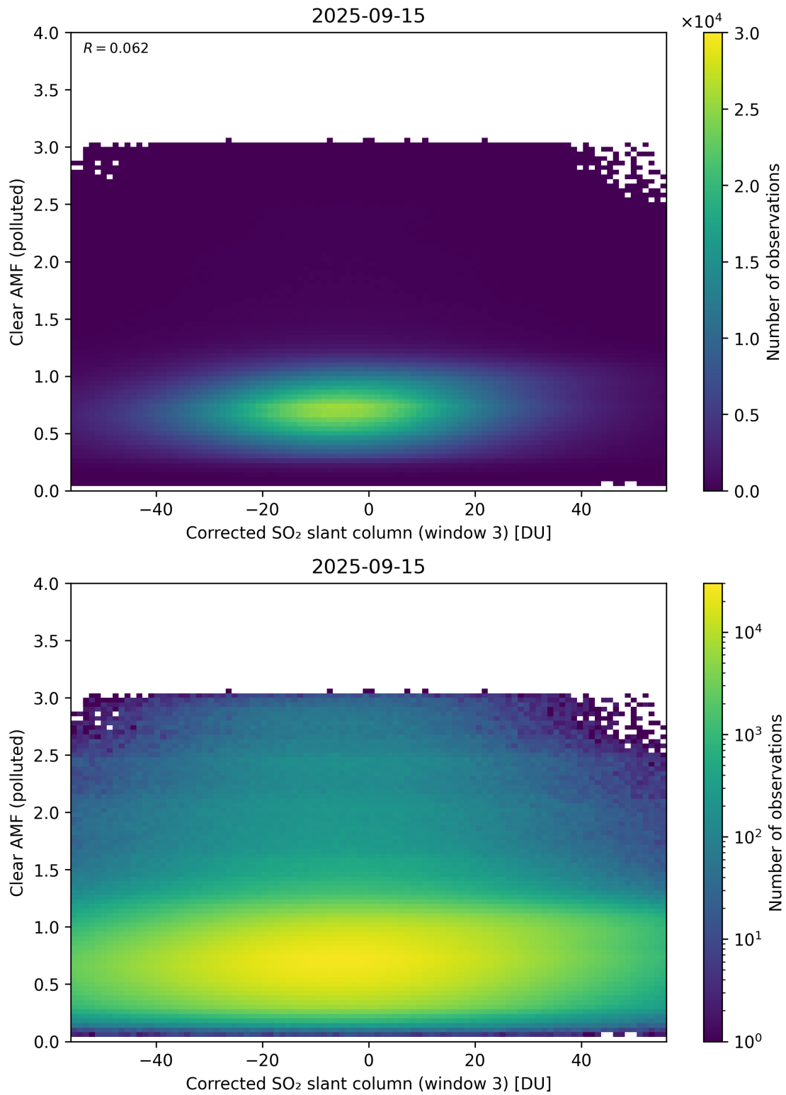
Figure 259: Scatter density plot of “Corrected SO 2 slant column (window 3)” against “Clear AMF (polluted)” for 2025-09-15 to 2025-09-16.
