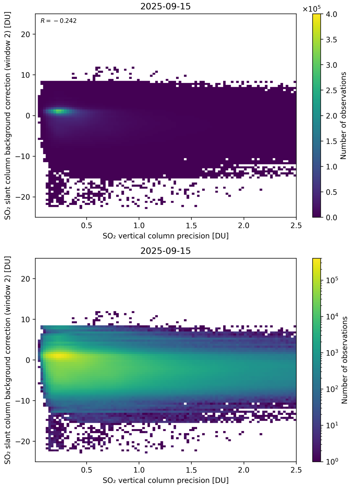
Figure 330: Scatter density plot of “SO 2 vertical column precision” against “SO 2 slant column background correction (window 2)” for 2025-09-15 to 2025-09-16.
