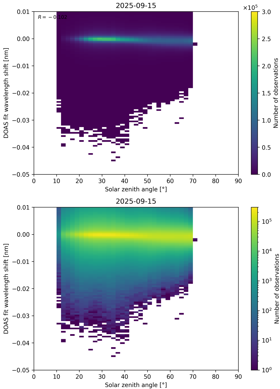
Figure 174: Scatter density plot of “Solar zenith angle” against “DOAS fit wavelength shift” for 2025-09-15 to 2025-09-16.
