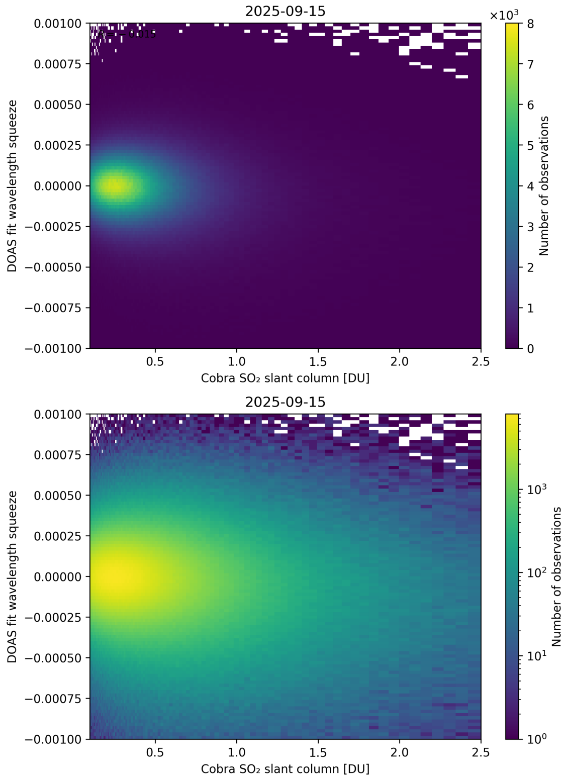
Figure 197: Scatter density plot of “Cobra SO 2 slant column” against “DOAS fit wavelength squeeze” for 2025-09-15 to 2025-09-16.
