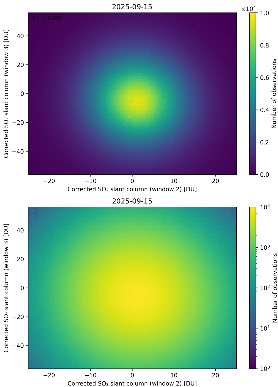
Figure 250: Scatter density plot of “Corrected SO 2 slant column (window 2)” against “Corrected SO 2 slant column (window 3)” for 2025-09-15 to 2025-09-16.
