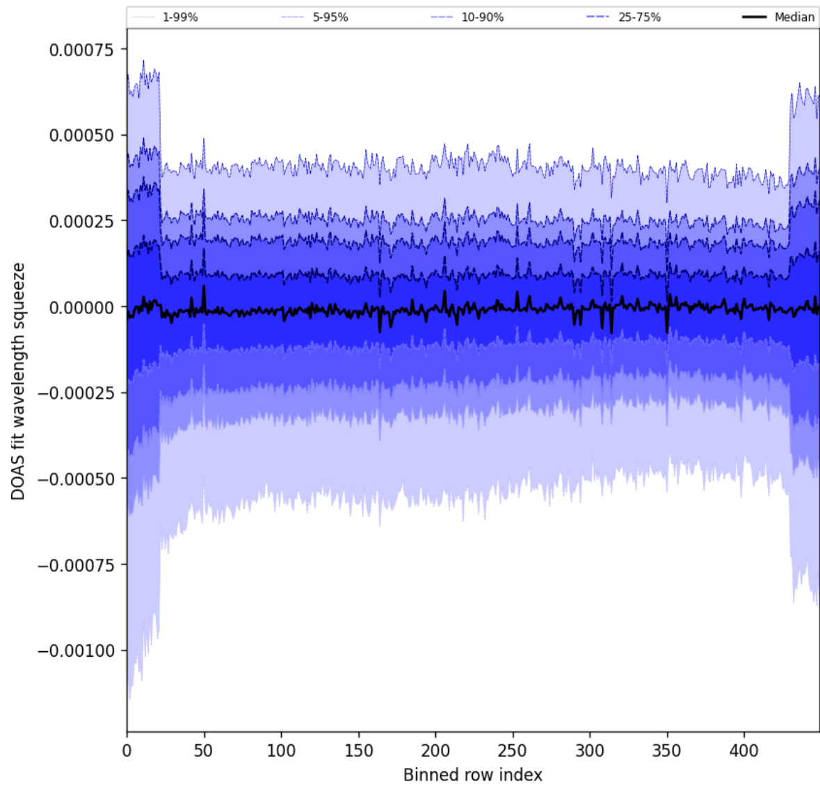
Figure 103: Along track statistics of “DOAS fit wavelength squeeze” for 2025-09-15 to 2025-09-16
