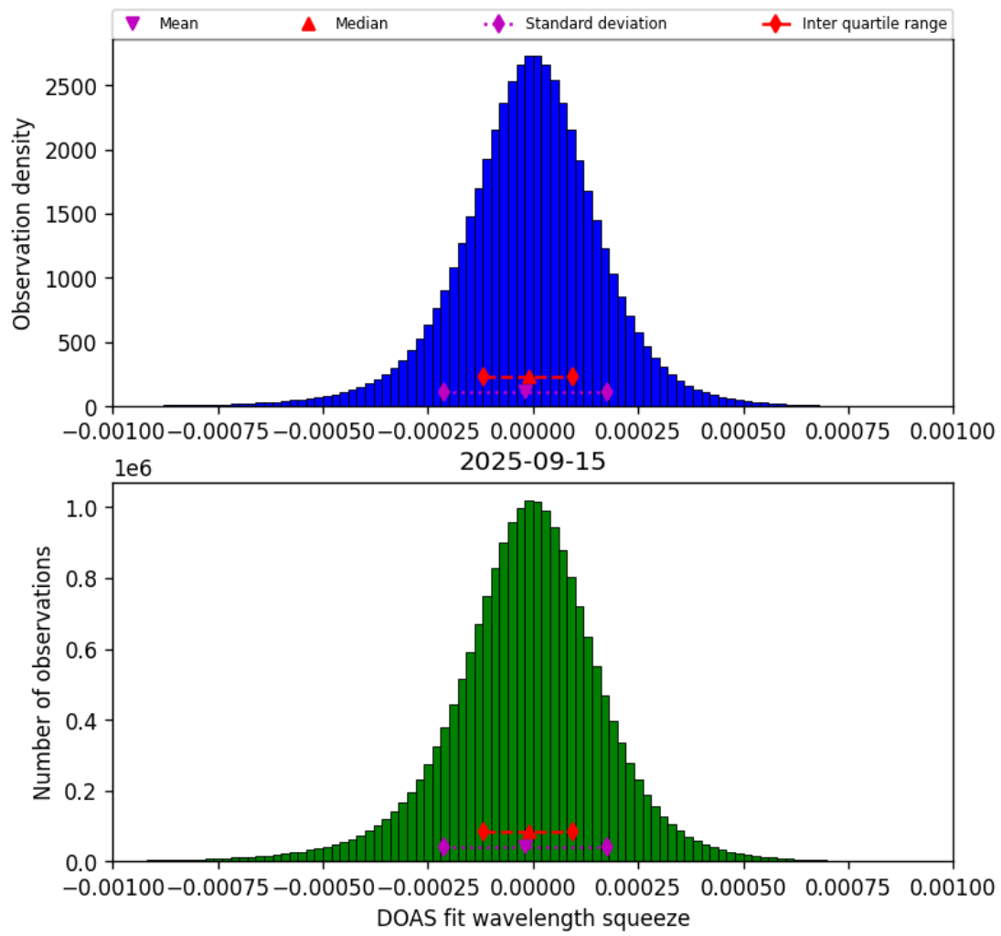
Figure 77: Histogram of “DOAS fit wavelength squeeze” for 2025-09-15 to 2025-09-16
