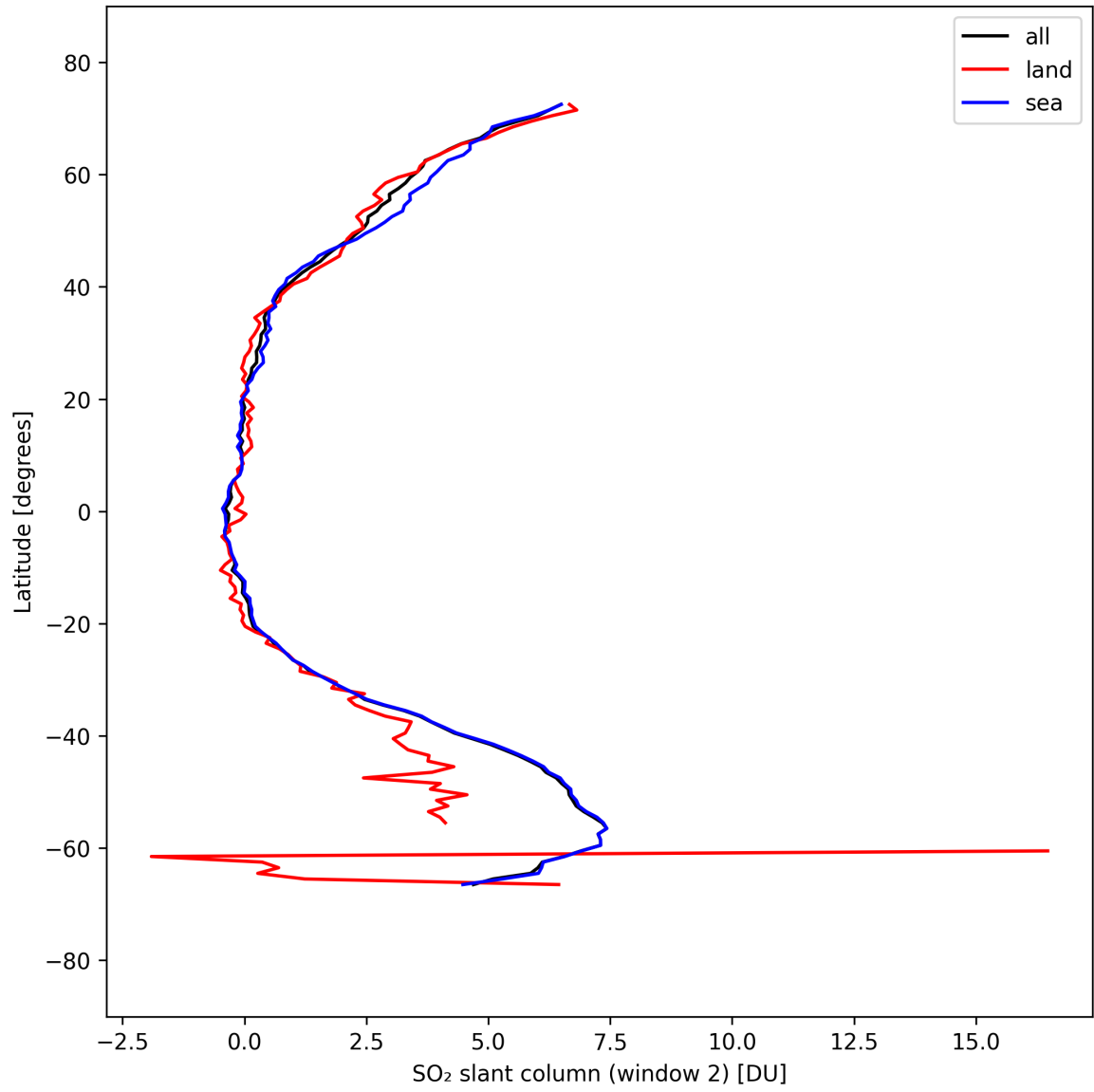
Figure 41: Zonal average of “SO 2 slant column (window 2)” for 2025-09-15 to 2025-09-16.
