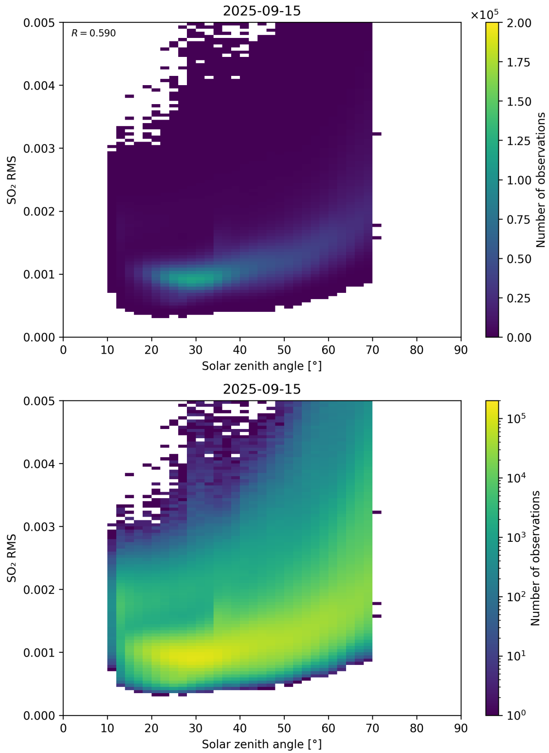
Figure 176: Scatter density plot of “Solar zenith angle” against “SO 2 RMS” for 2025-09-15 to 2025-09-16.
