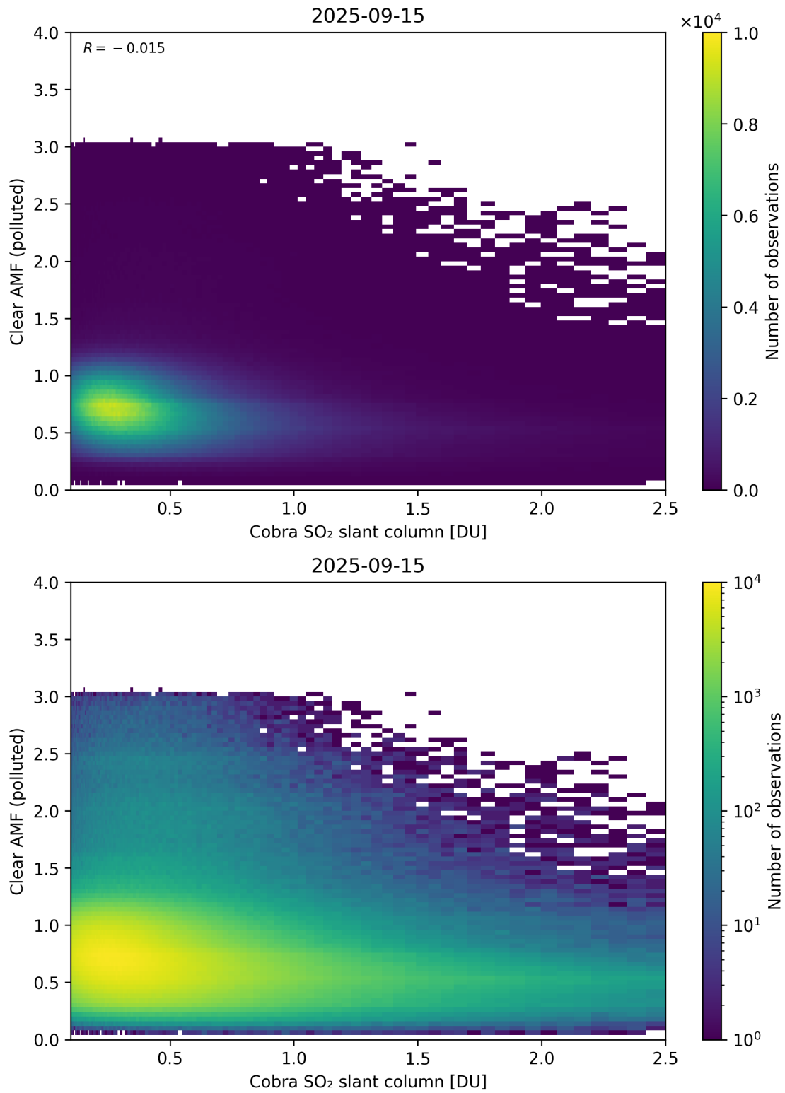
Figure 215: Scatter density plot of “Cobra SO 2 slant column” against “Clear AMF (polluted)” for 2025-09-15 to 2025-09-16.
