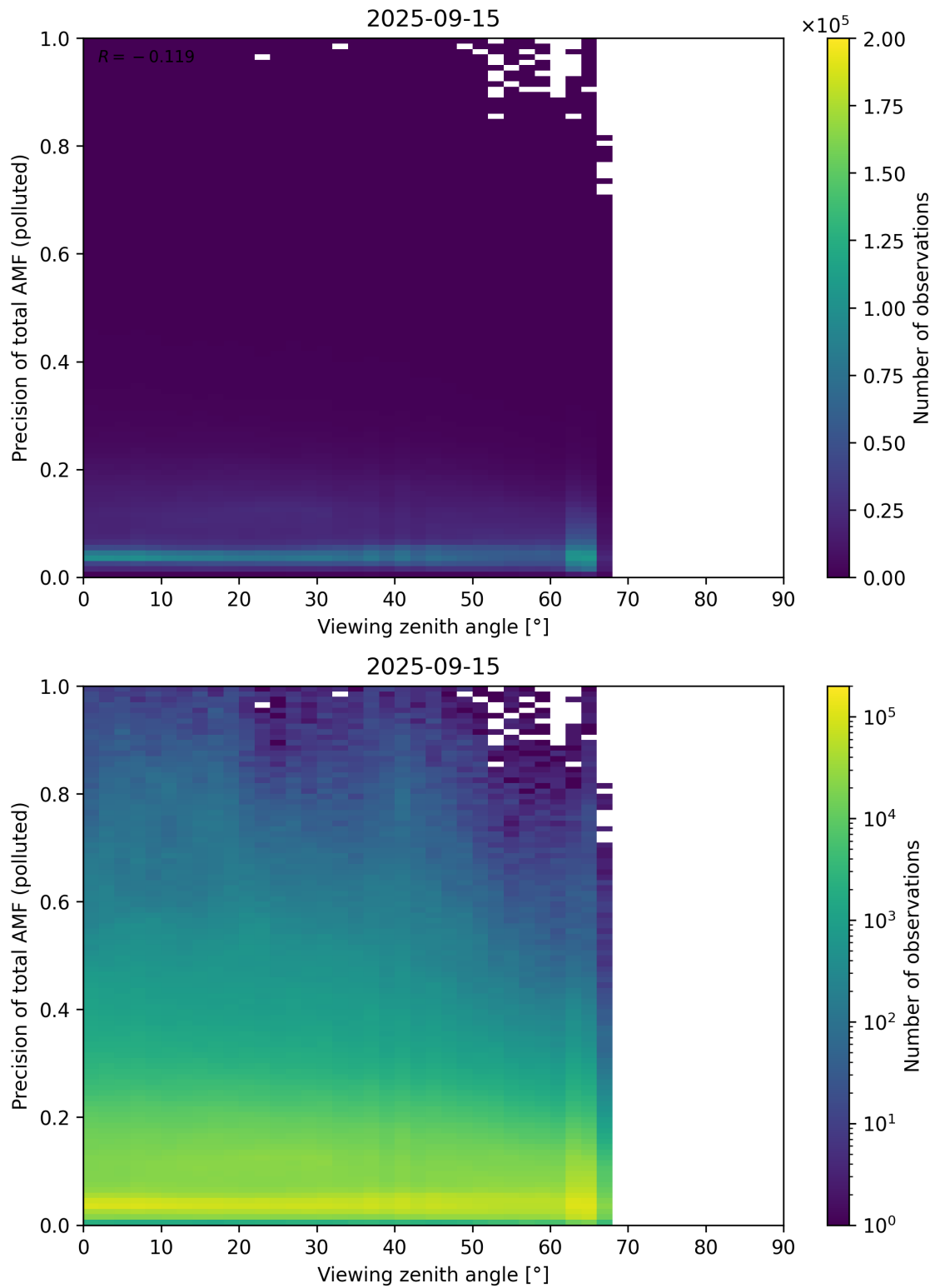
Figure 382: Scatter density plot of “Viewing zenith angle” against “Precision of total AMF (polluted)” for 2025-09-15 to 2025-09-16.
