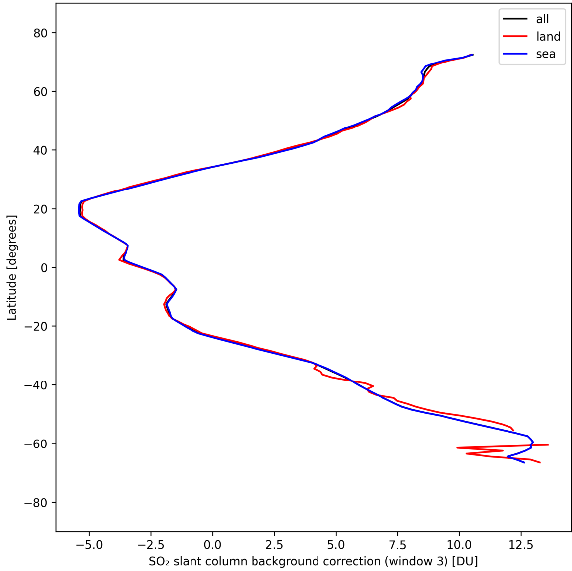
Figure 48: Zonal average of “SO 2 slant column background correction (window 3)” for 2025-09-15 to 2025-09-16.
