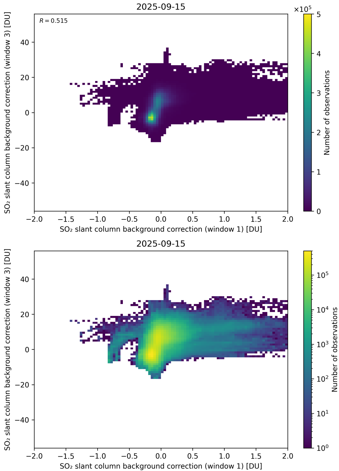
Figure 110: Scatter density plot of “SO 2 slant column background correction (window 1)” against “SO 2 slant column background correction (window 3)” for 2025-09-15 to 2025-09-16.
