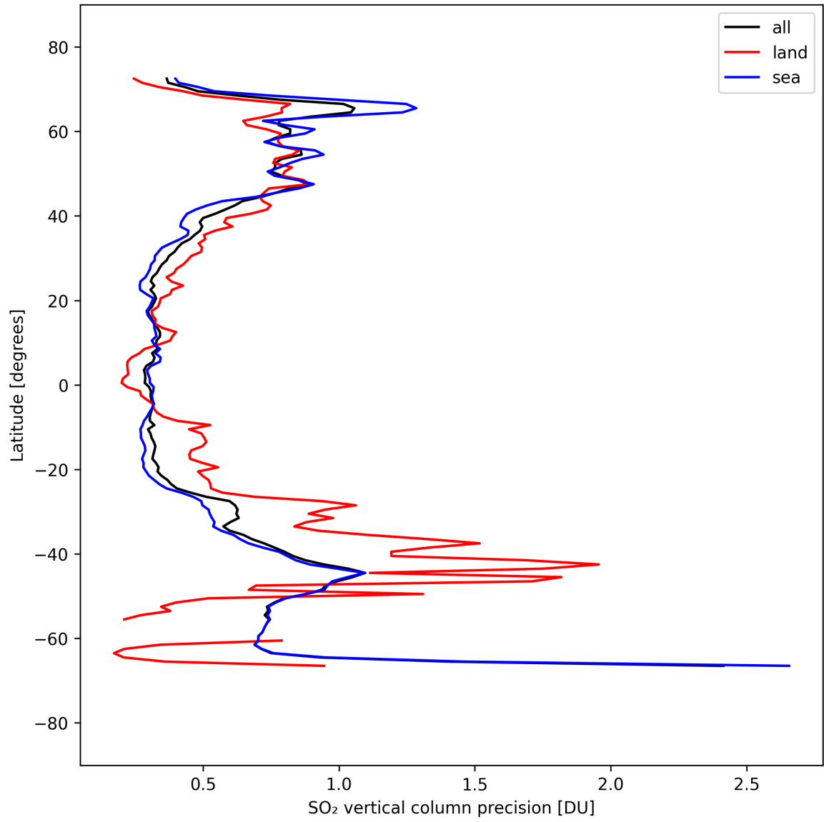
Figure 33: Zonal average of “SO 2 vertical column precision” for 2025-09-15 to 2025-09-16.
