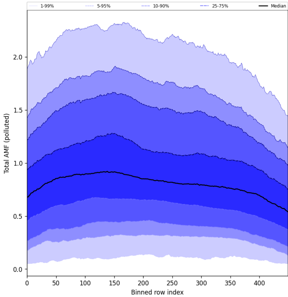
Figure 105: Along track statistics of “Total AMF (polluted)” for 2025-09-15 to 2025-09-16
