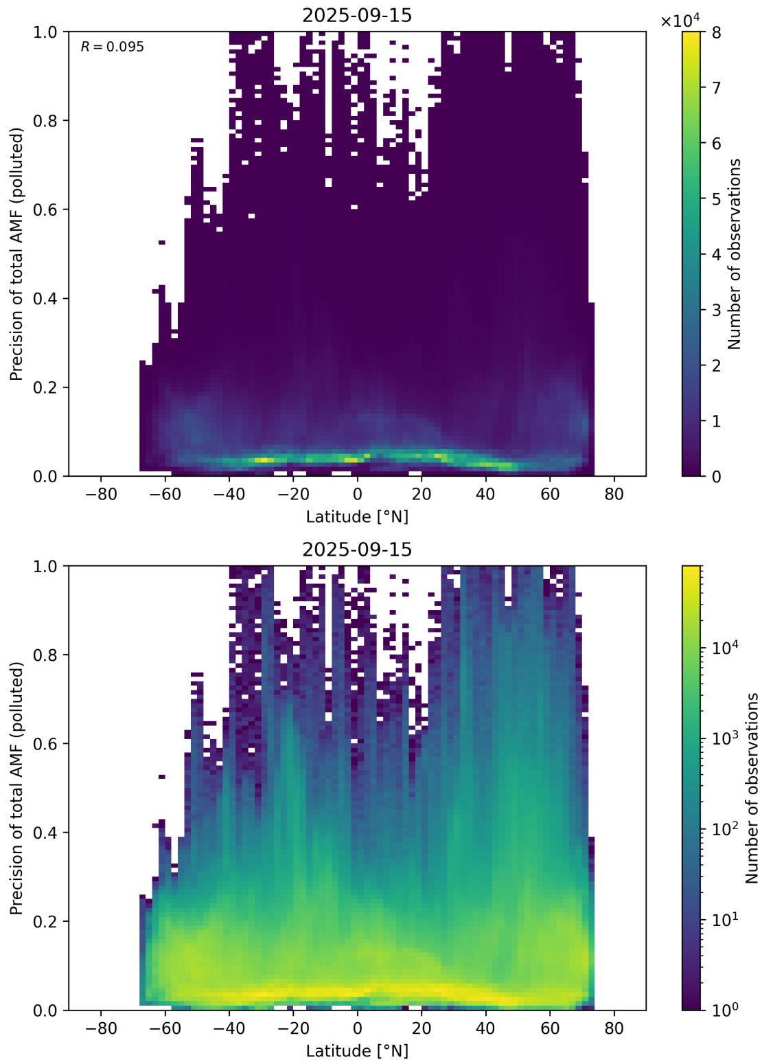
Figure 168: Scatter density plot of “Latitude” against “Precision of total AMF (polluted)” for 2025-09-15 to 2025-09-16.
