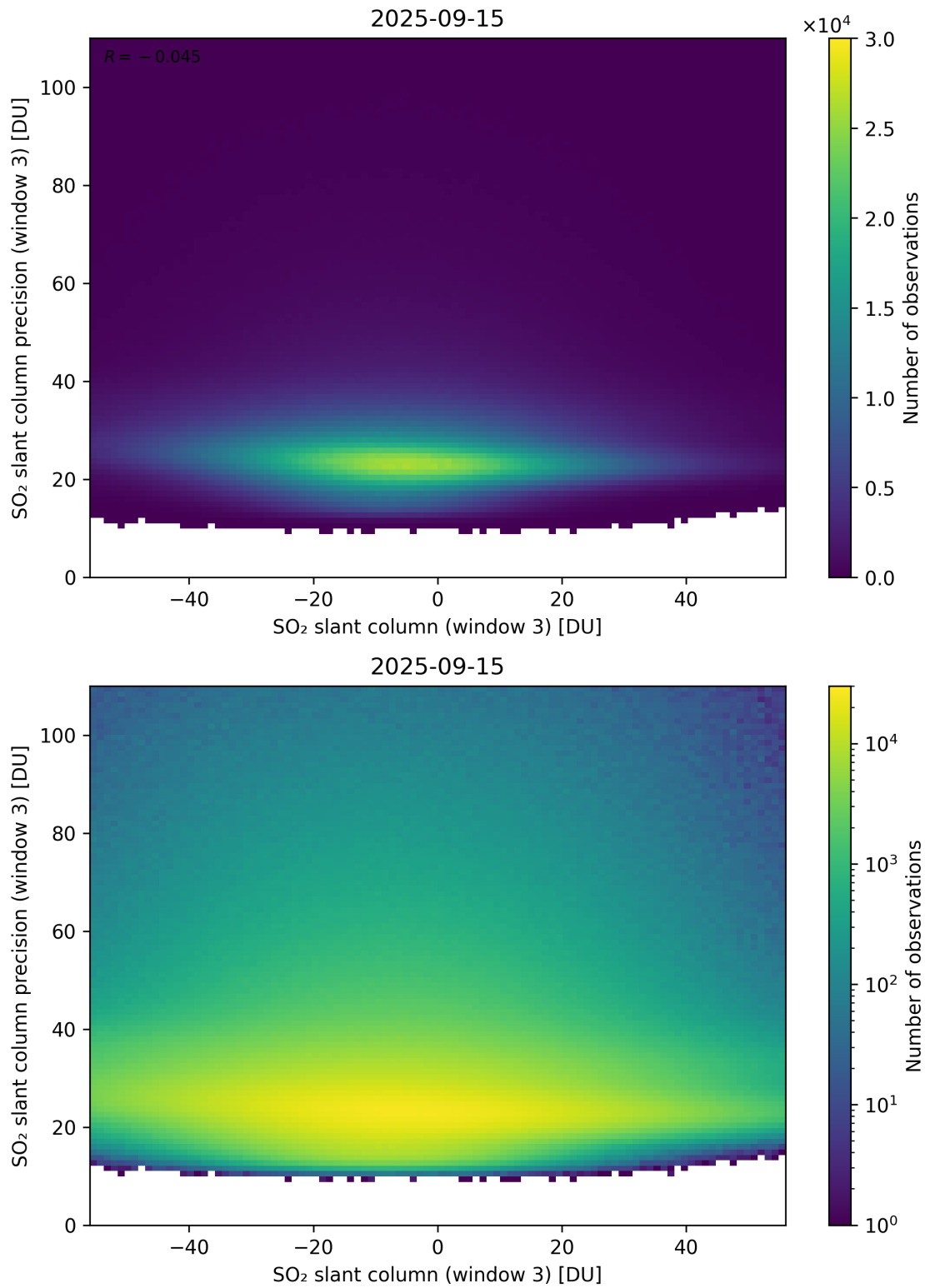
Figure 317: Scatter density plot of “SO 2 slant column (window 3)” against “SO 2 slant column precision (window 3)” for 2025-09-15 to 2025-09-16.
