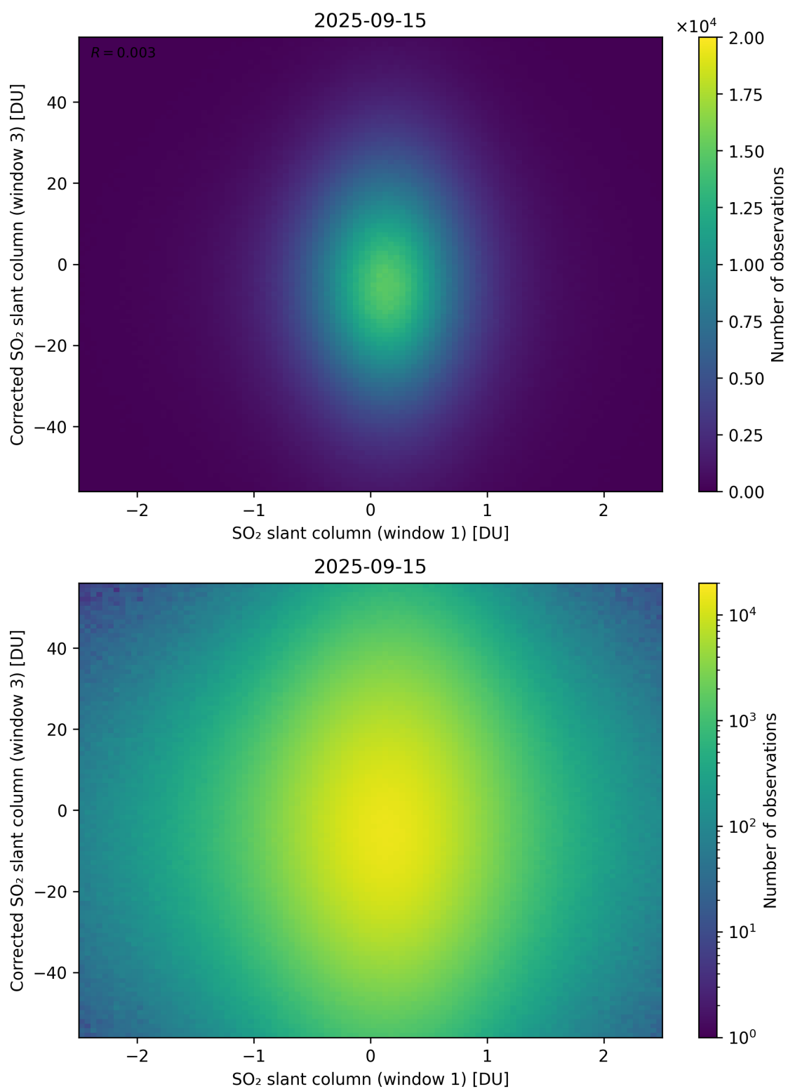
Figure 284: Scatter density plot of “SO 2 slant column (window 1)” against “Corrected SO 2 slant column (window 3)” for 2025-09-15 to 2025-09-16.
