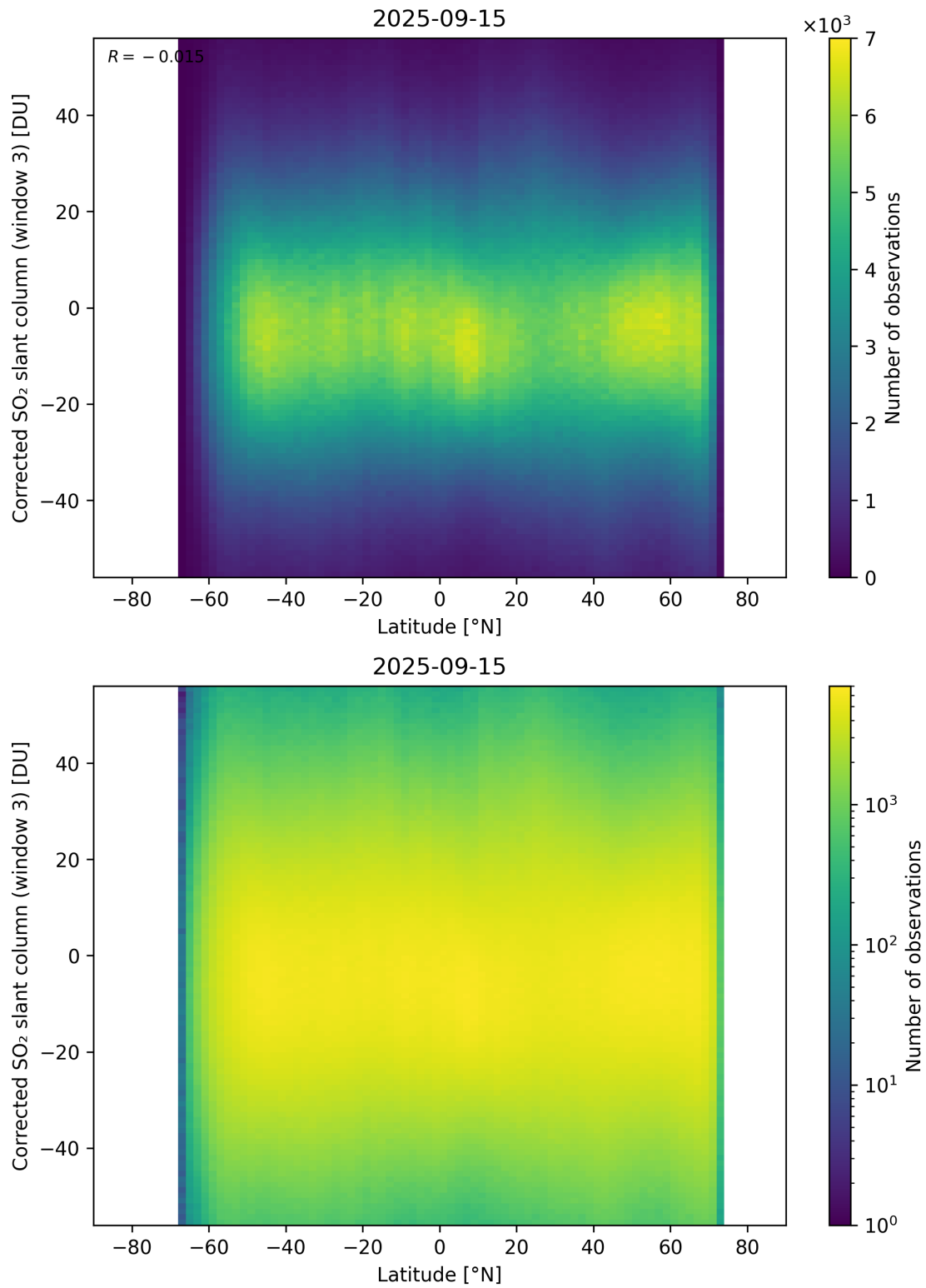
Figure 161: Scatter density plot of “Latitude” against “Corrected SO 2 slant column (window 3)” for 2025-09-15 to 2025-09-16.
