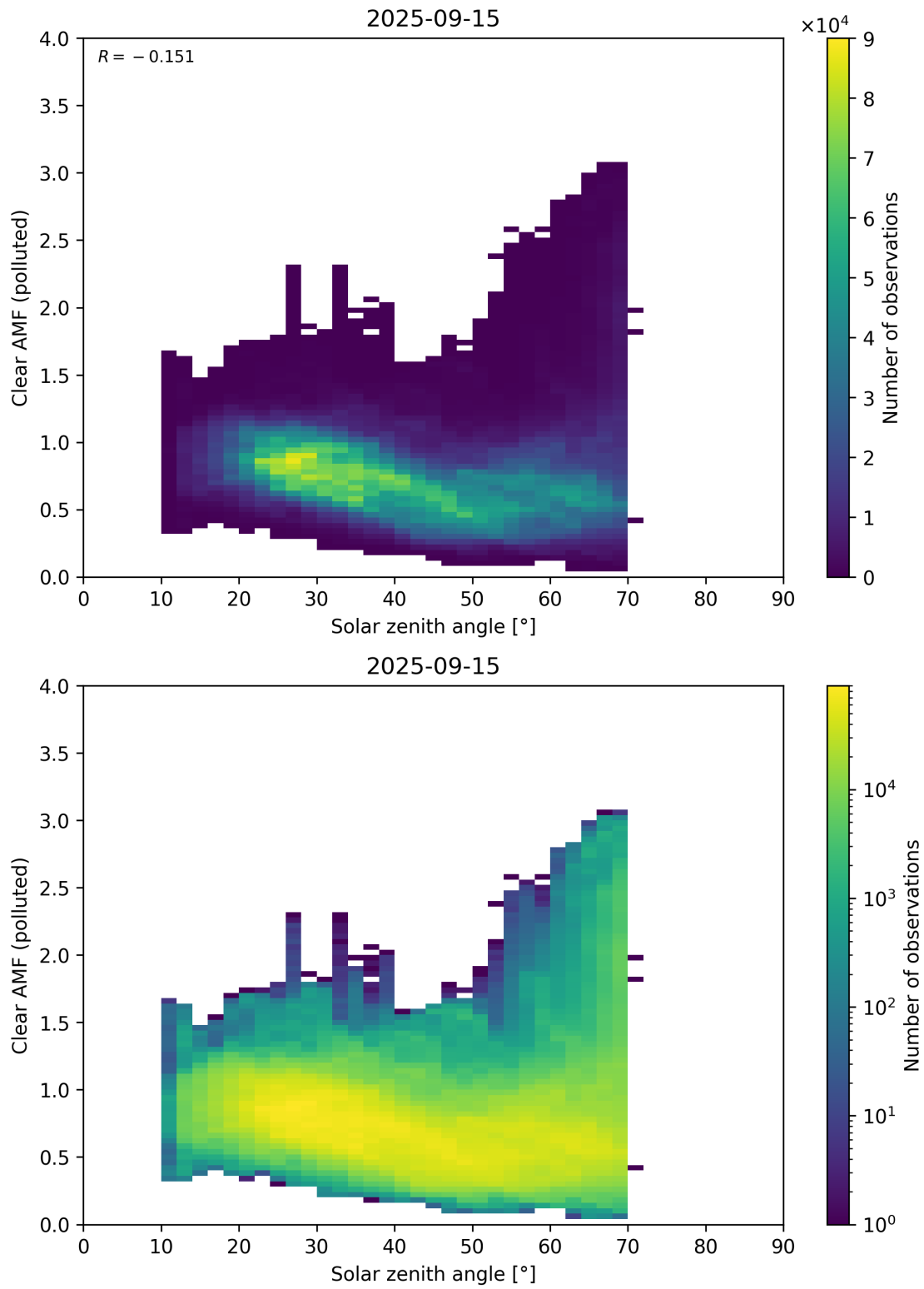
Figure 178: Scatter density plot of “Solar zenith angle” against “Clear AMF (polluted)” for 2025-09-15 to 2025-09-16.
