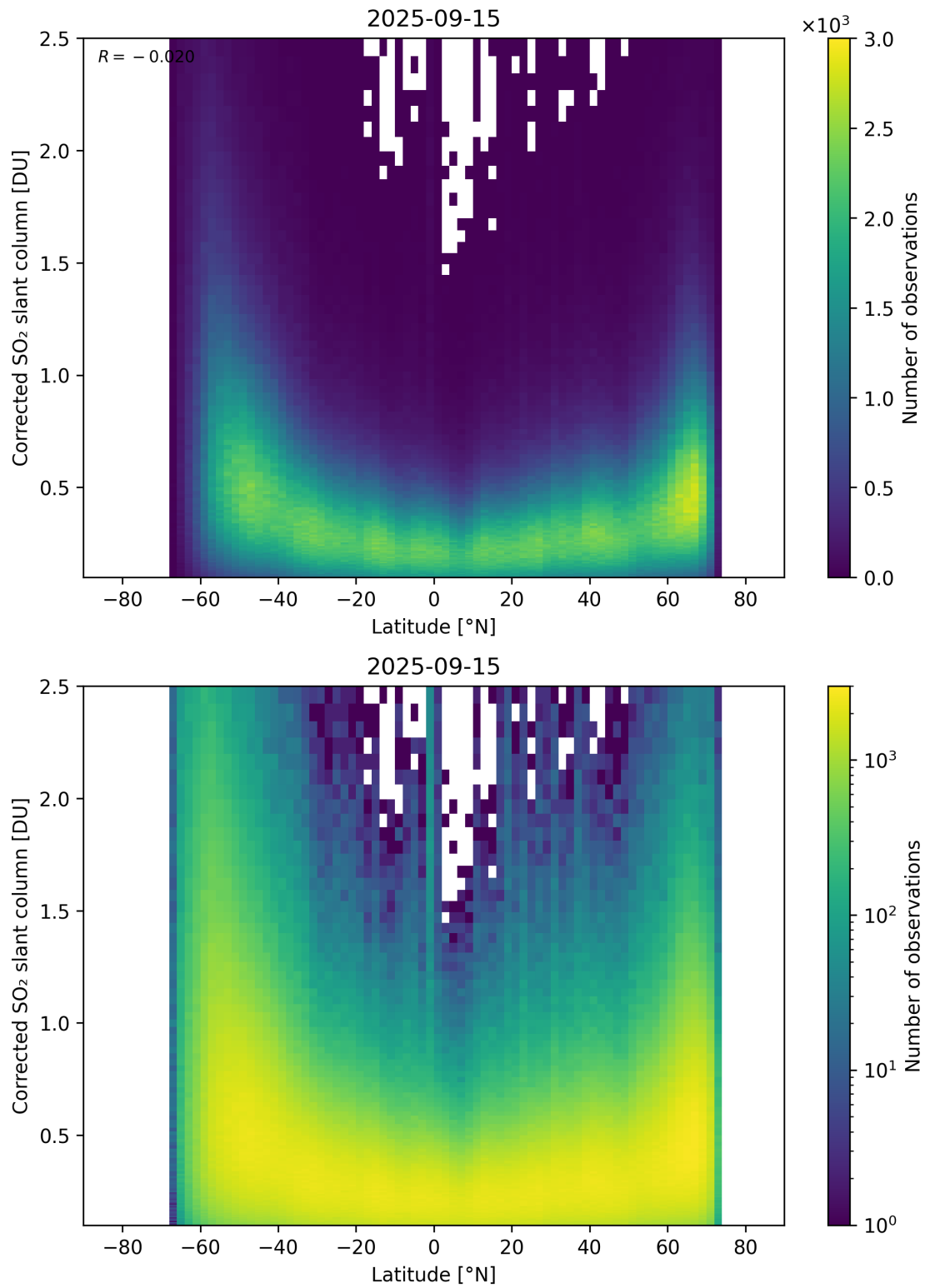
Figure 159: Scatter density plot of “Latitude” against “Corrected SO 2 slant column” for 2025-09-15 to 2025-09-16.
