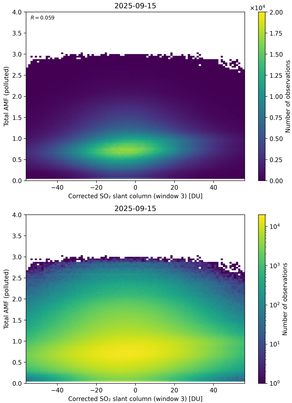
Figure 260: Scatter density plot of “Corrected SO 2 slant column (window 3)” against “Total AMF (polluted)” for 2025-09-15 to 2025-09-16.
