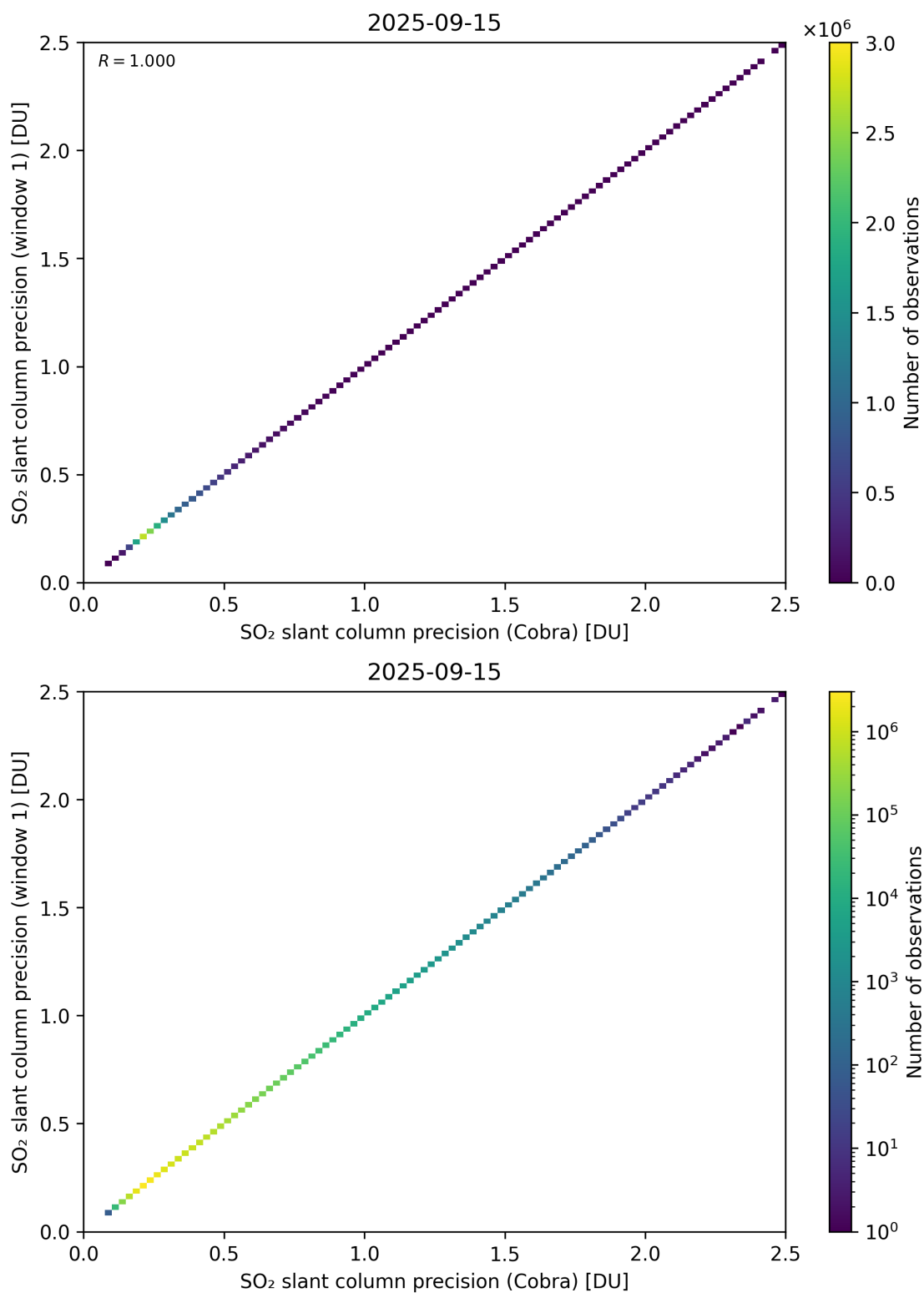
Figure 209: Scatter density plot of “SO 2 slant column precision (Cobra)” against “SO 2 slant column precision (window 1)” for 2025-09-15 to 2025-09-16.
