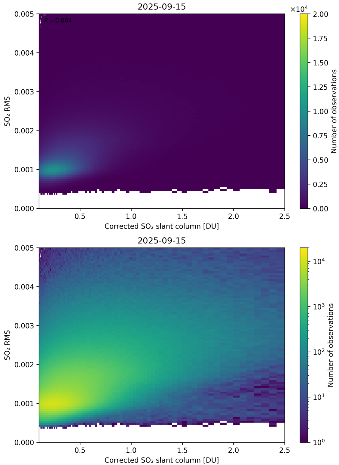
Figure 231: Scatter density plot of “Corrected SO 2 slant column” against “SO 2 RMS” for 2025-09-15 to 2025-09-16.
