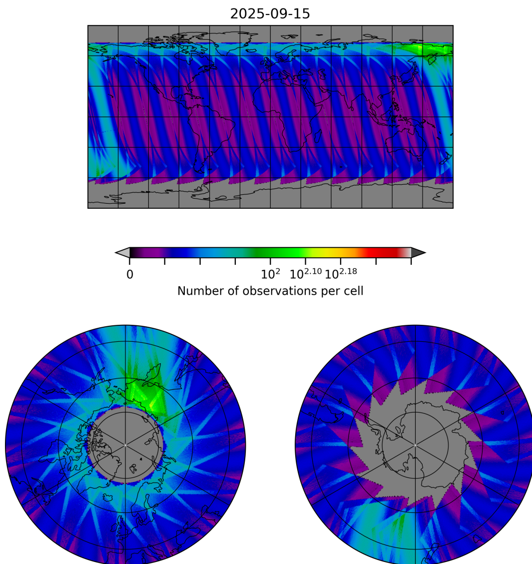
Figure 30: Map of the number of observations for 2025-09-15 to 2025-09-16
