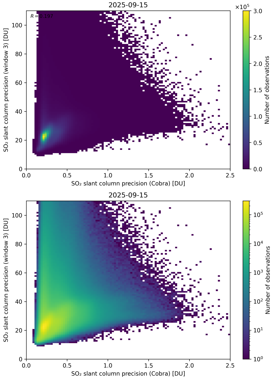
Figure 212: Scatter density plot of “SO 2 slant column precision (Cobra)” against “SO 2 slant column precision (window 3)” for 2025-09-15 to 2025-09-16.
