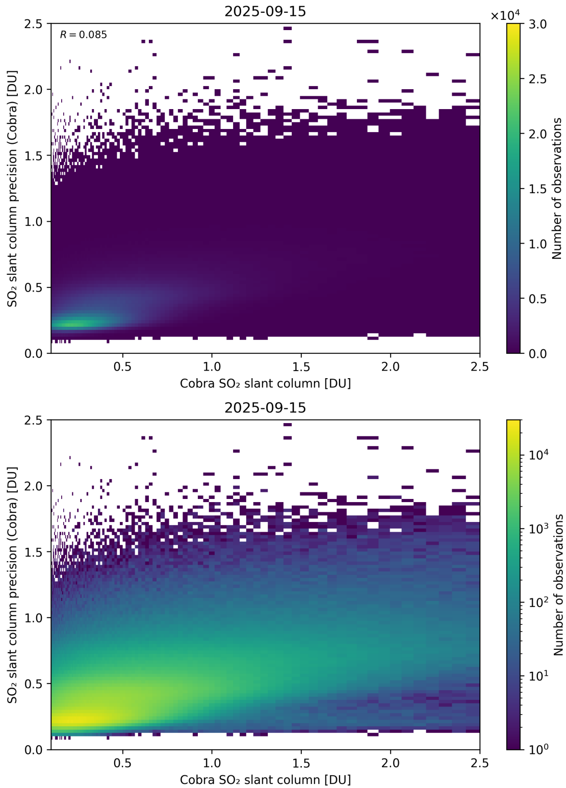
Figure 216: Scatter density plot of “Cobra SO 2 slant column” against “SO 2 slant column precision (Cobra)” for 2025-09-15 to 2025-09-16.
