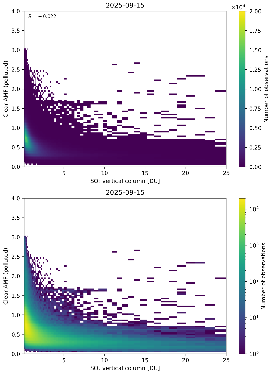
Figure 348: Scatter density plot of “SO 2 vertical column” against “Clear AMF (polluted)” for 2025-09-15 to 2025-09-16.
