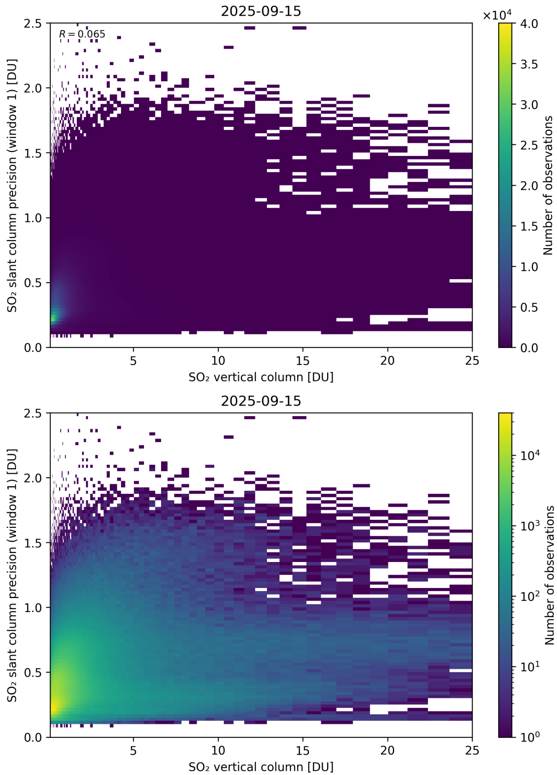
Figure 355: Scatter density plot of “SO 2 vertical column” against “SO 2 slant column precision (window 1)” for 2025-09-15 to 2025-09-16.
