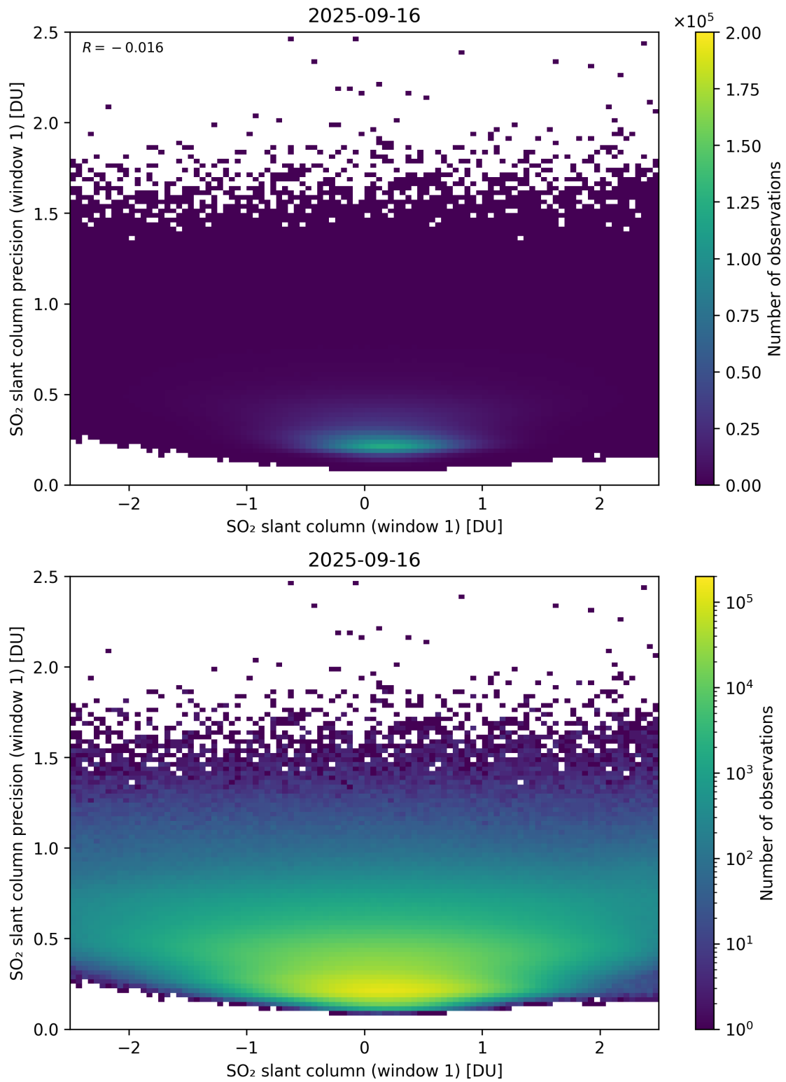
Figure 285: Scatter density plot of “SO 2 slant column (window 1)” against “SO 2 slant column precision (window 1)” for 2025-09-15 to 2025-09-17.
