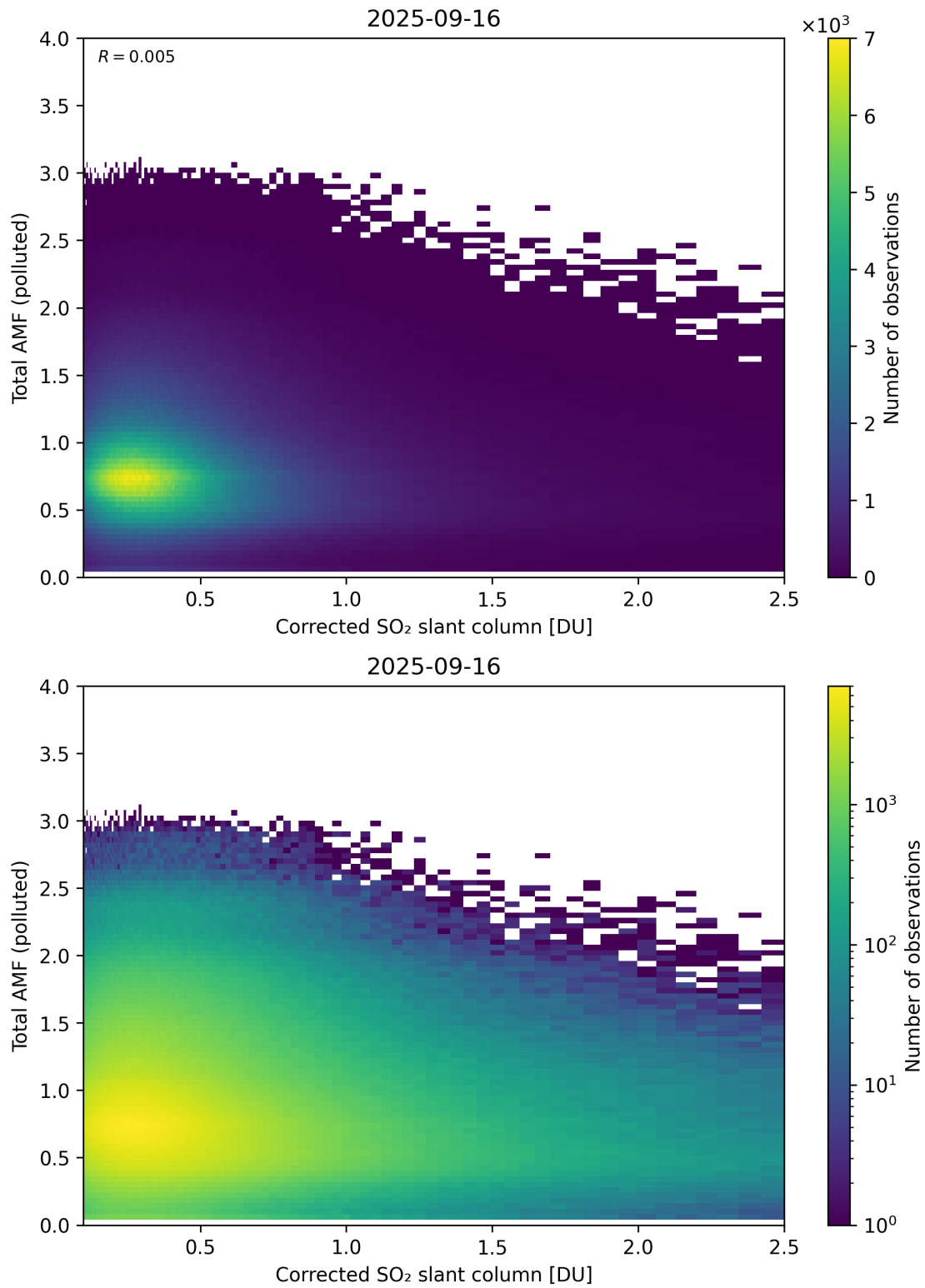
Figure 242: Scatter density plot of “Corrected SO 2 slant column” against “Total AMF (polluted)” for 2025-09-15 to 2025-09-17.
