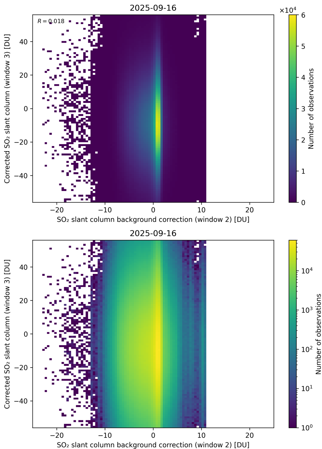
Figure 127: Scatter density plot of “SO 2 slant column background correction (window 2)” against “Corrected SO 2 slant column (window 3)” for 2025-09-15 to 2025-09-17.
