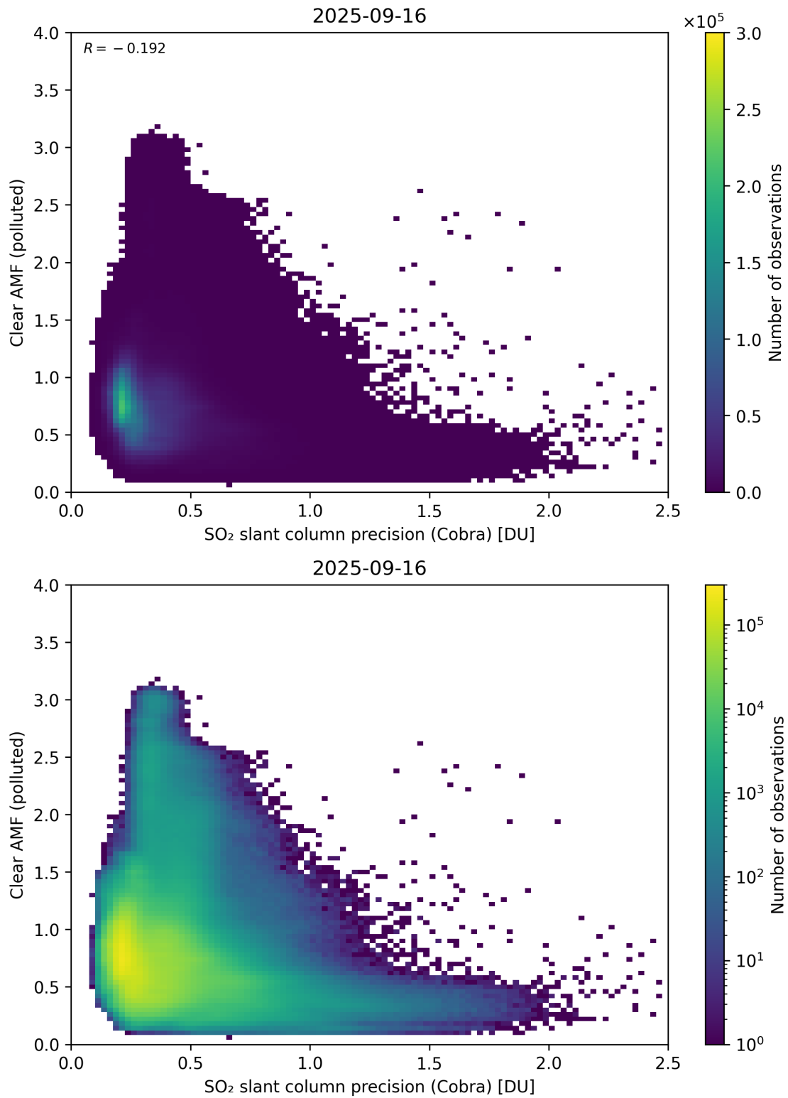
Figure 205: Scatter density plot of “SO 2 slant column precision (Cobra)” against “Clear AMF (polluted)” for 2025-09-15 to 2025-09-17.
