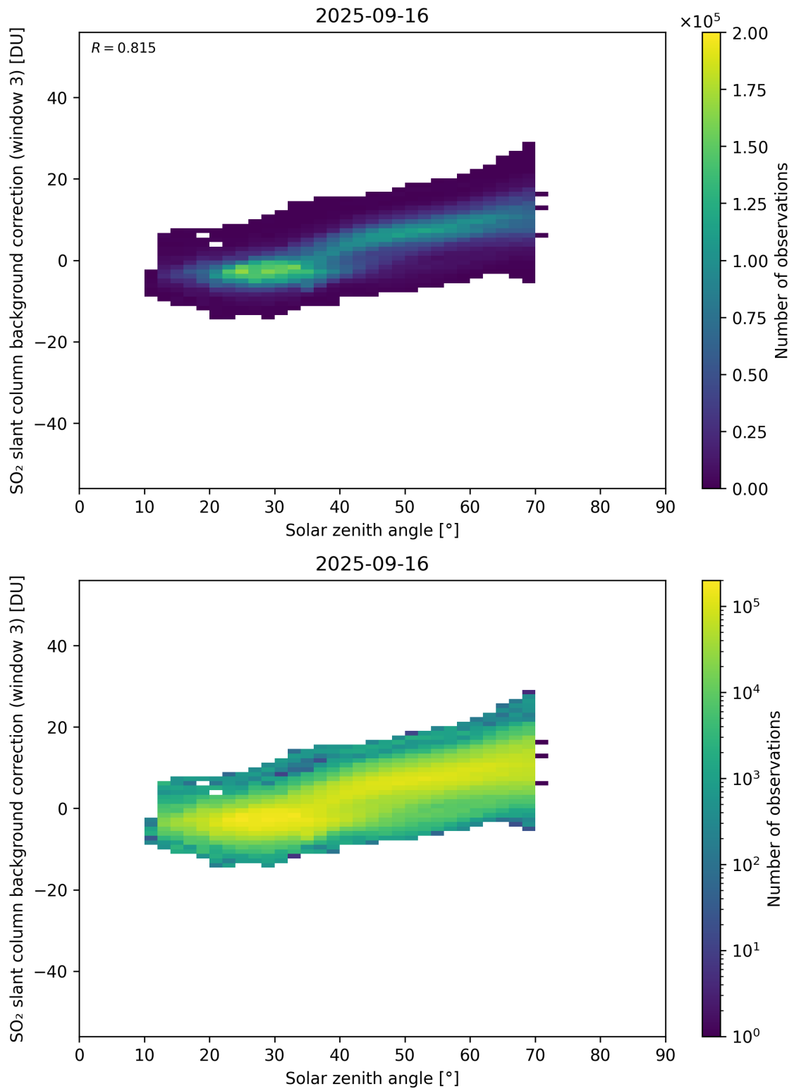
Figure 173: Scatter density plot of “Solar zenith angle” against “SO 2 slant column background correction (window 3)” for 2025-09-15 to 2025-09-17.
