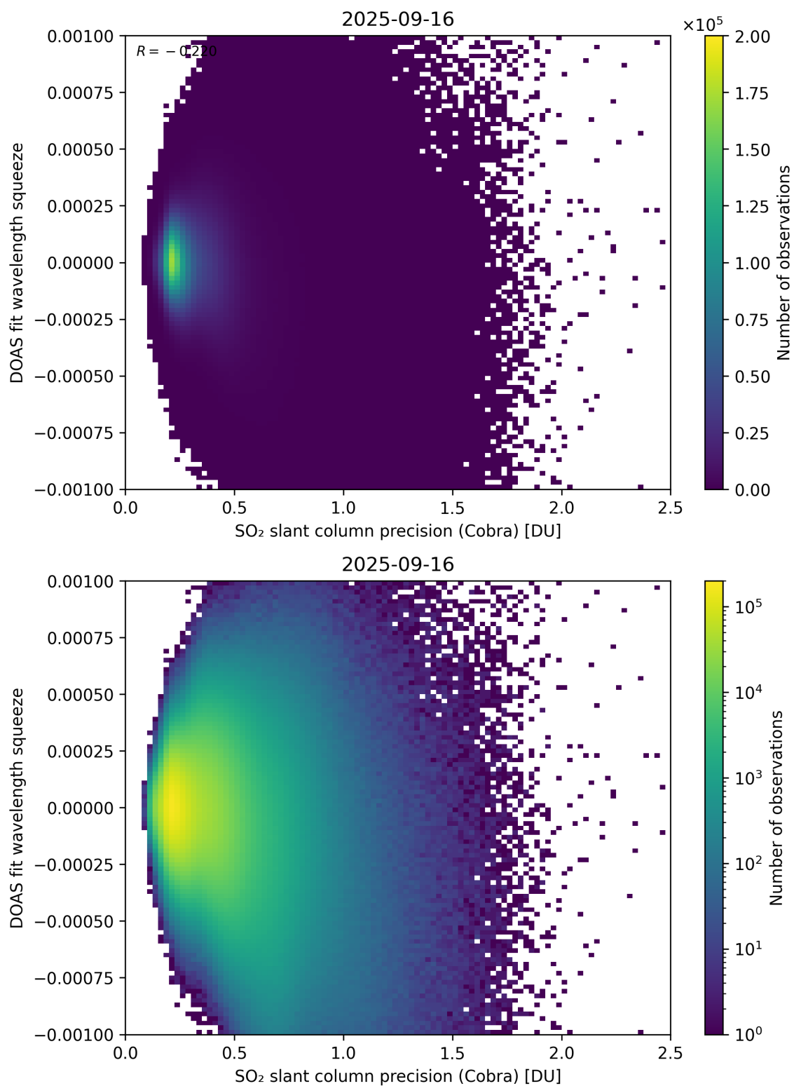
Figure 203: Scatter density plot of “SO 2 slant column precision (Cobra)” against “DOAS fit wavelength squeeze” for 2025-09-15 to 2025-09-17.
