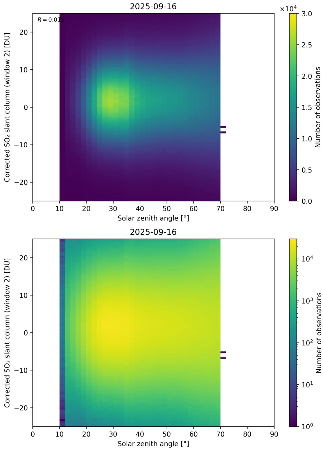
Figure 182: Scatter density plot of “Solar zenith angle” against “Corrected SO 2 slant column (window 2)” for 2025-09-15 to 2025-09-17.
