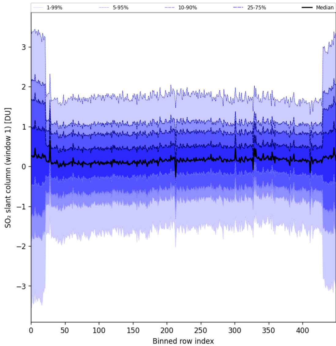
Figure 89: Along track statistics of “SO 2 slant column (window 1)” for 2025-09-15 to 2025-09-17
