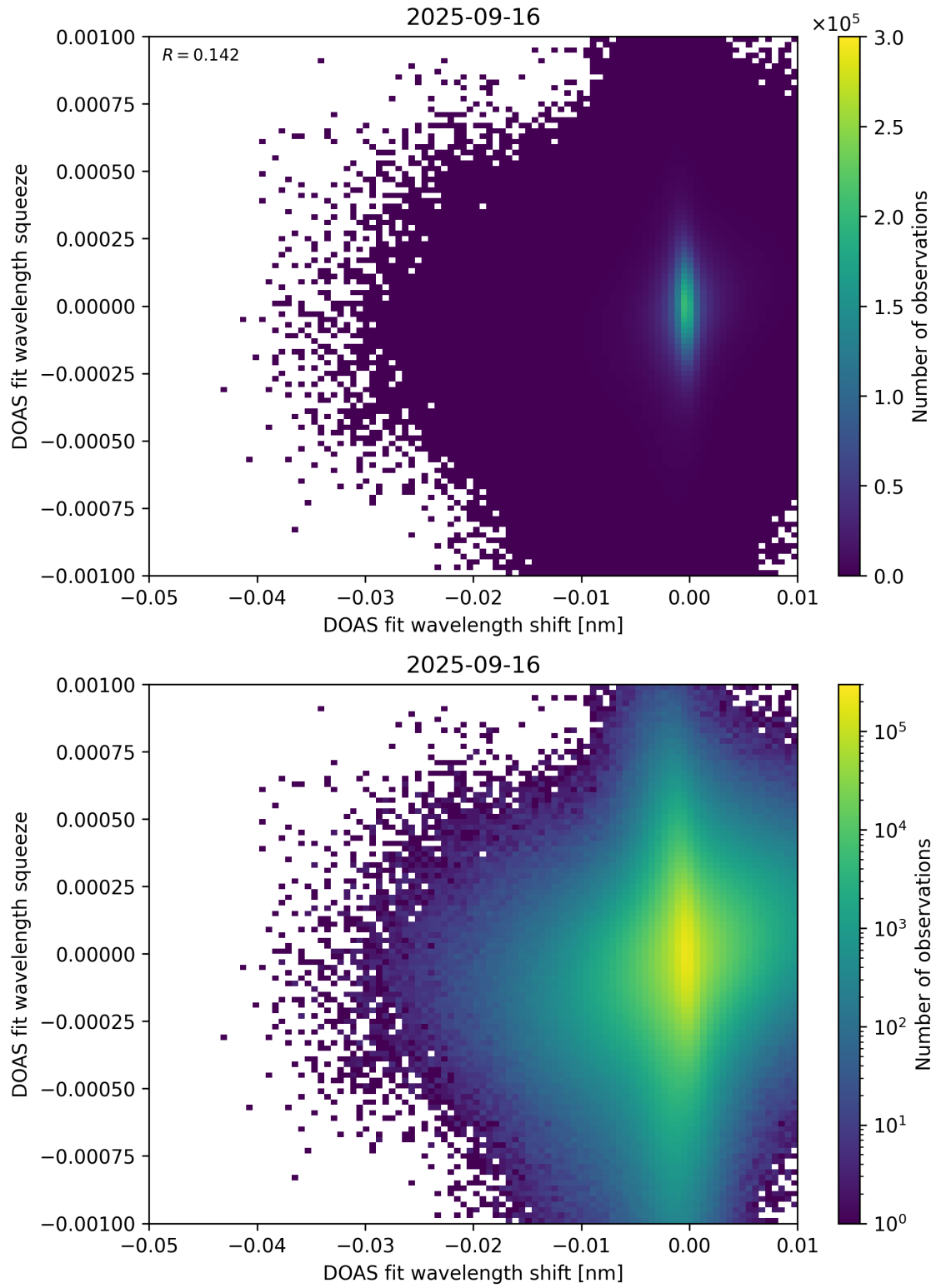
Figure 138: Scatter density plot of “DOAS fit wavelength shift” against “DOAS fit wavelength squeeze” for 2025-09-15 to 2025-09-17.
