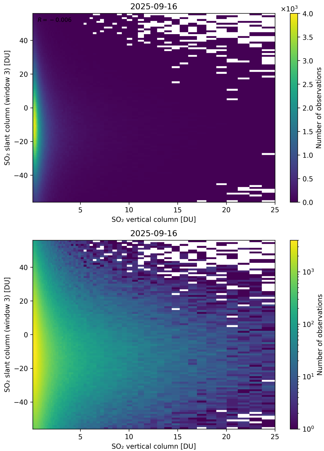
Figure 357: Scatter density plot of “SO 2 vertical column” against “SO 2 slant column (window 3)” for 2025-09-15 to 2025-09-17.
