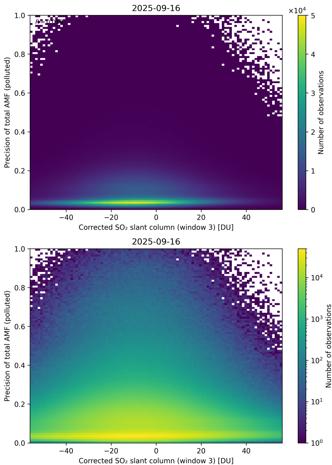
Figure 261: Scatter density plot of “Corrected SO 2 slant column (window 3)” against “Precision of total AMF (polluted)” for 2025-09-15 to 2025-09-17.
