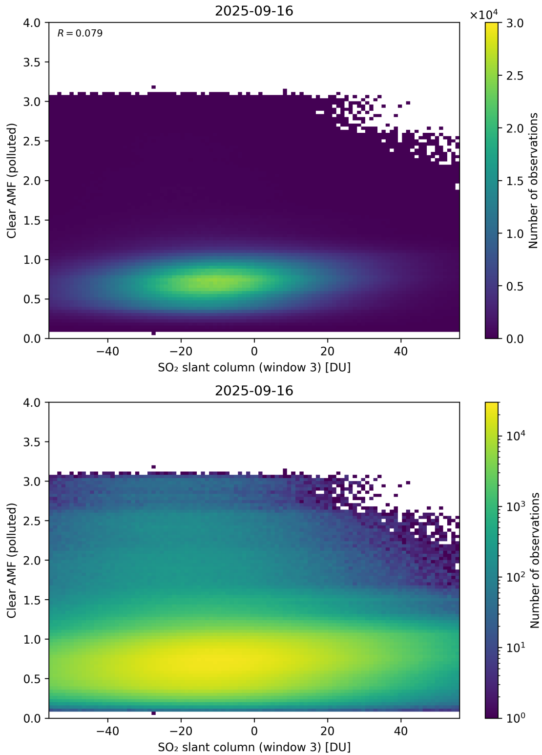
Figure 315: Scatter density plot of “SO 2 slant column (window 3)” against “Clear AMF (polluted)” for 2025-09-15 to 2025-09-17.
