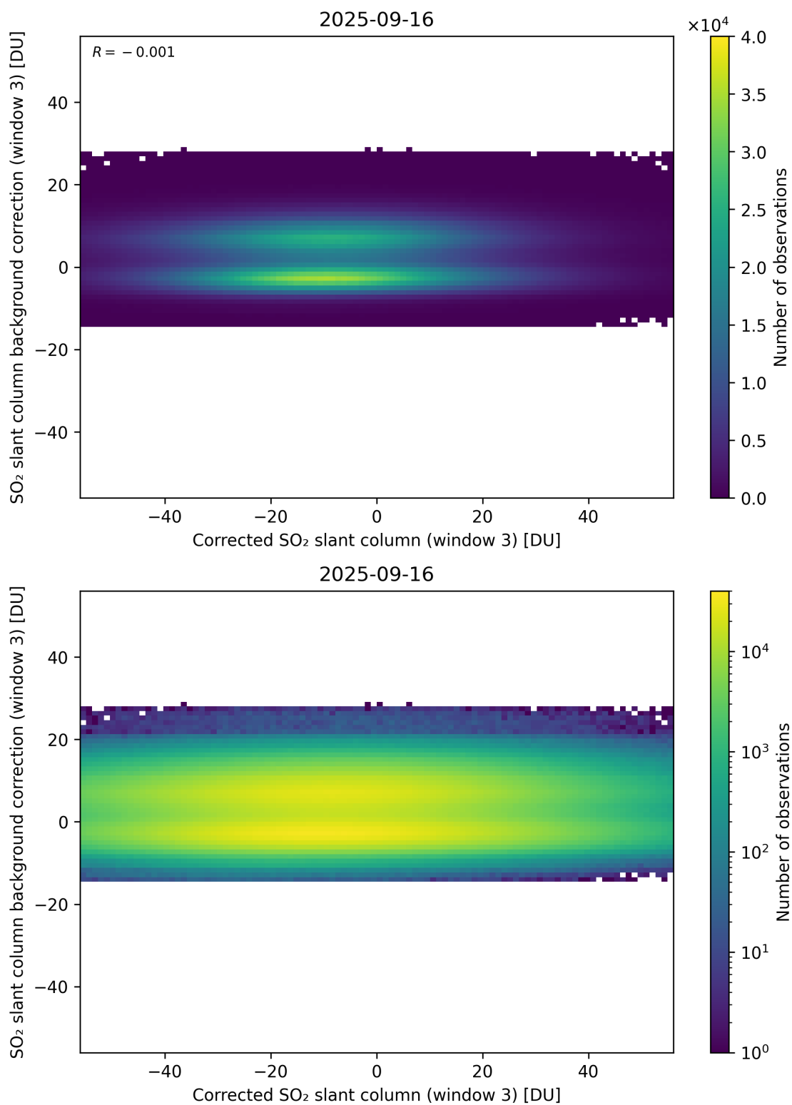
Figure 255: Scatter density plot of “Corrected SO 2 slant column (window 3)” against “SO 2 slant column background correction (window 3)” for 2025-09-15 to 2025-09-17.
