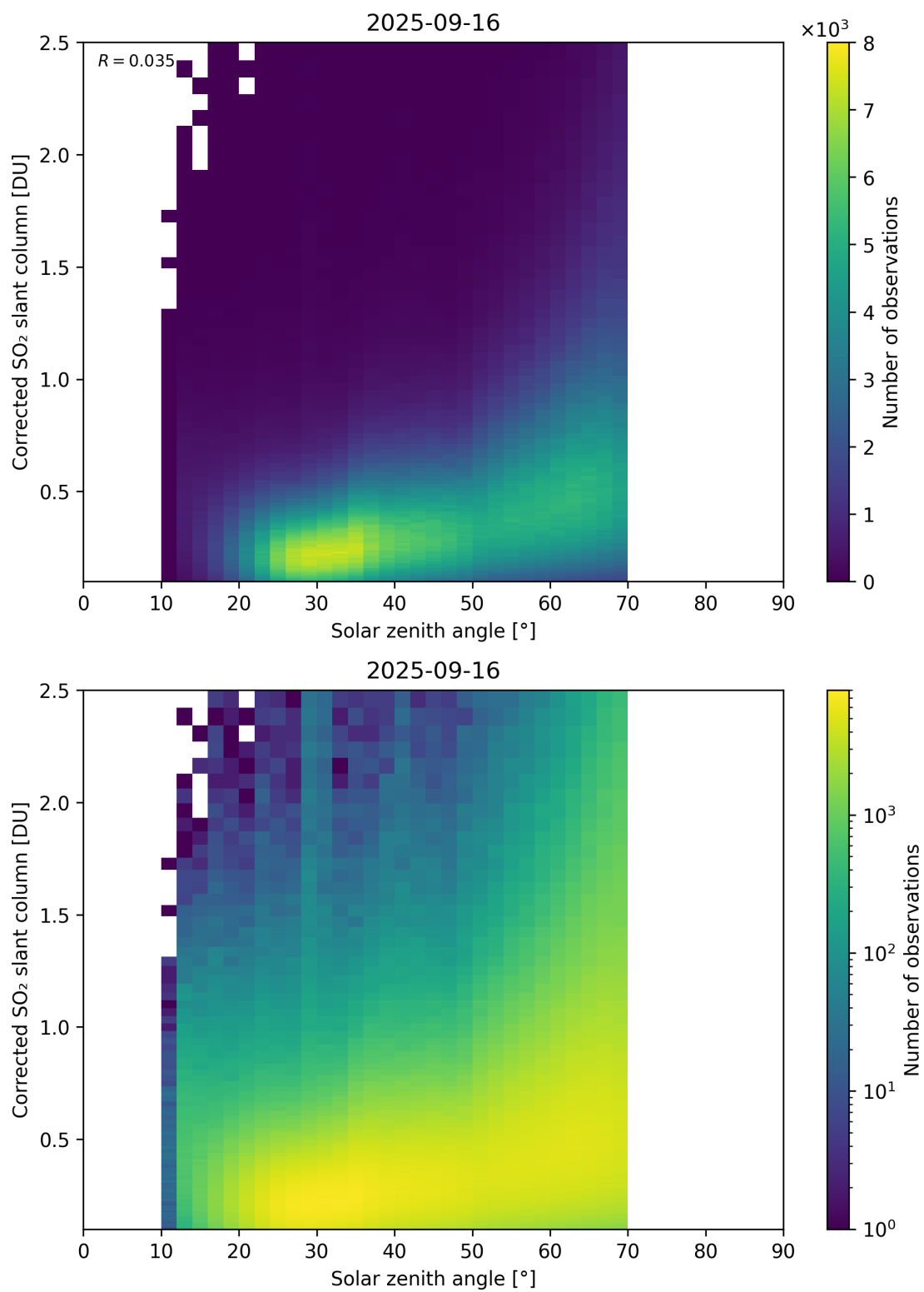
Figure 181: Scatter density plot of “Solar zenith angle” against “Corrected SO 2 slant column” for 2025-09-15 to 2025-09-17.
