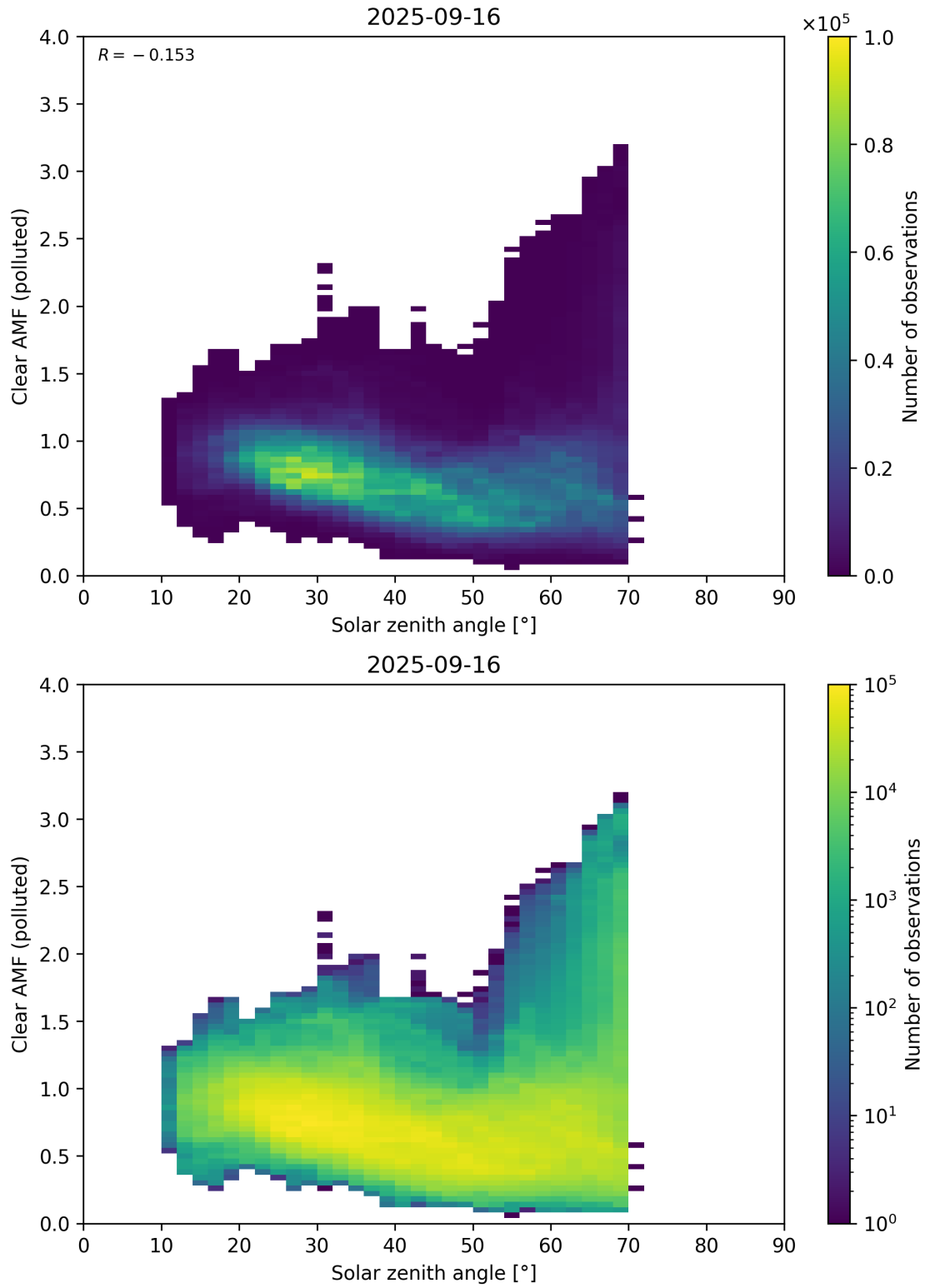
Figure 178: Scatter density plot of “Solar zenith angle” against “Clear AMF (polluted)” for 2025-09-15 to 2025-09-17.
