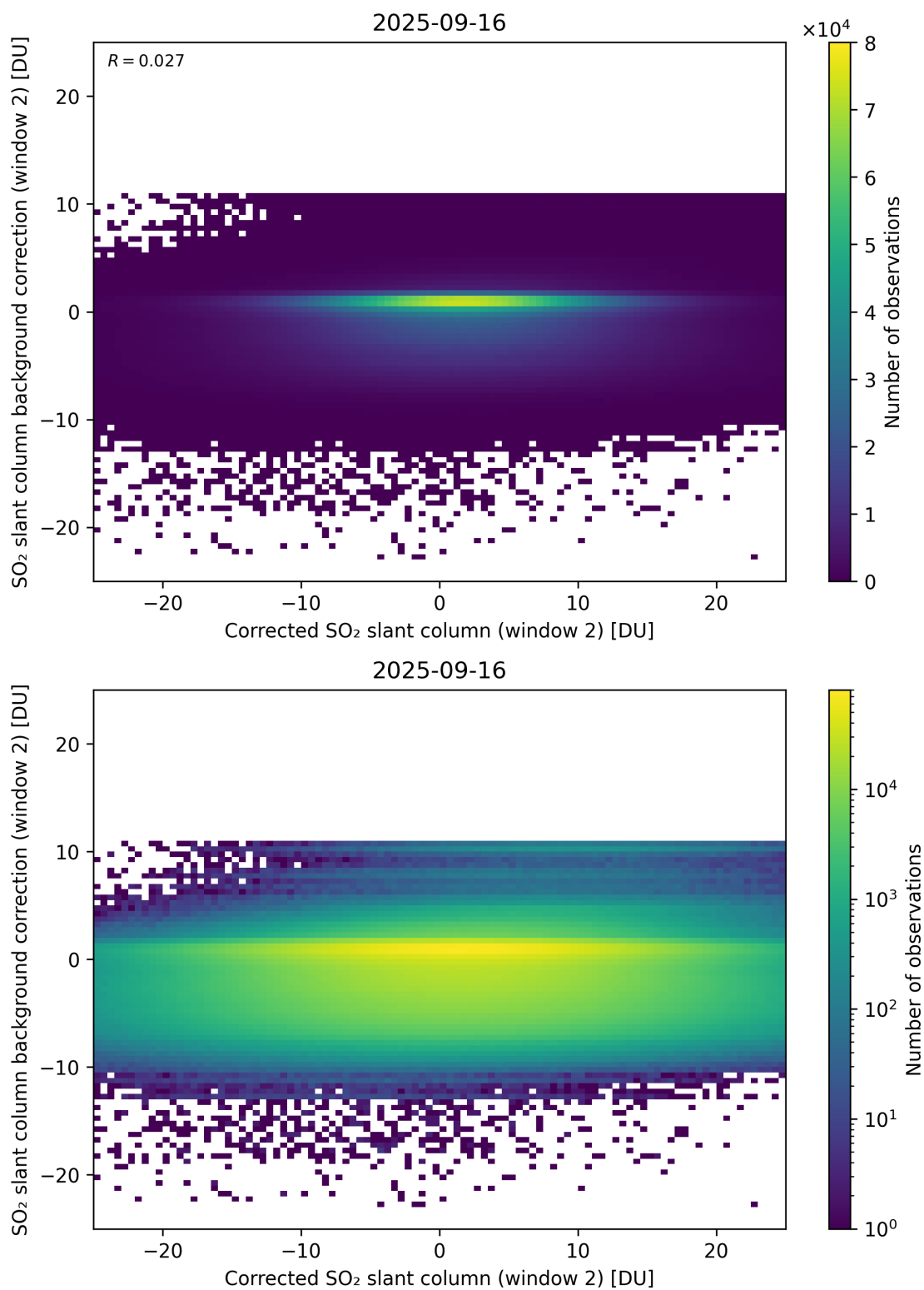
Figure 244: Scatter density plot of “Corrected SO 2 slant column (window 2)” against “SO 2 slant column background correction (window 2)” for 2025-09-15 to 2025-09-17.
