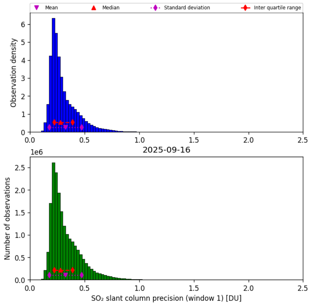
Figure 64: Histogram of “SO 2 slant column precision (window 1)” for 2025-09-15 to 2025-09-17
