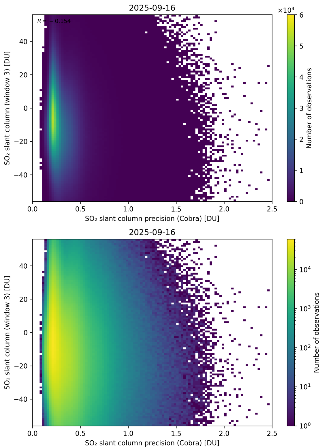
Figure 211: Scatter density plot of “SO 2 slant column precision (Cobra)” against “SO 2 slant column (window 3)” for 2025-09-15 to 2025-09-17.
