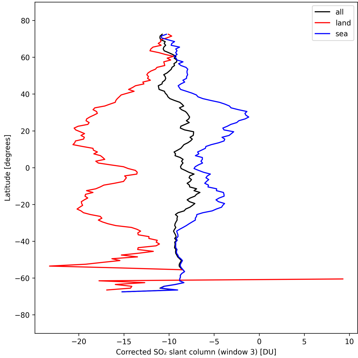
Figure 47: Zonal average of “Corrected SO 2 slant column (window 3)” for 2025-09-15 to 2025-09-17.
