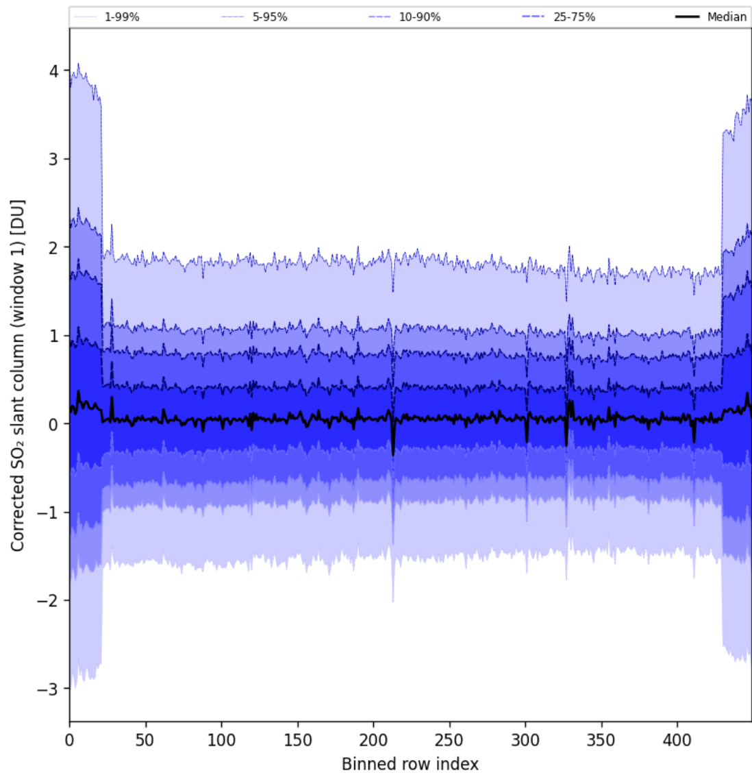
Figure 91: Along track statistics of “Corrected SO 2 slant column (window 1)” for 2025-09-15 to 2025-09-17
