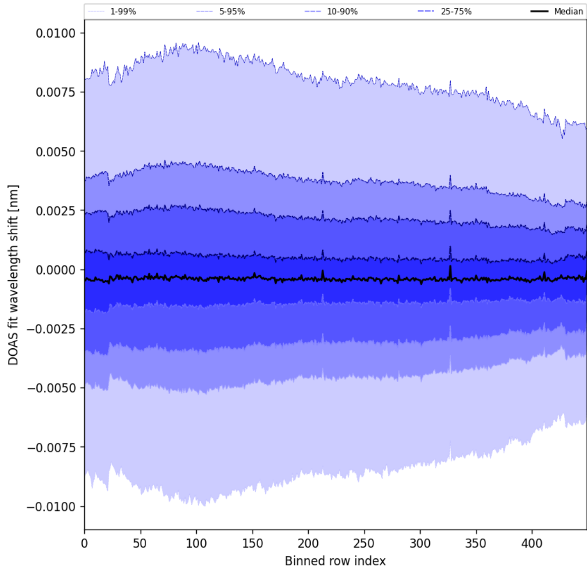
Figure 102: Along track statistics of “DOAS fit wavelength shift” for 2025-09-15 to 2025-09-17
