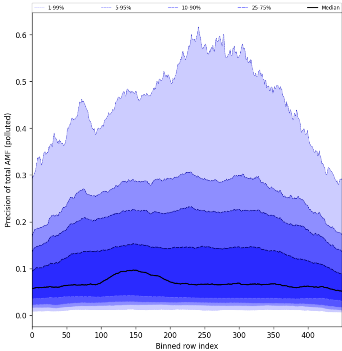
Figure 106: Along track statistics of “Precision of total AMF (polluted)” for 2025-09-15 to 2025-09-17
