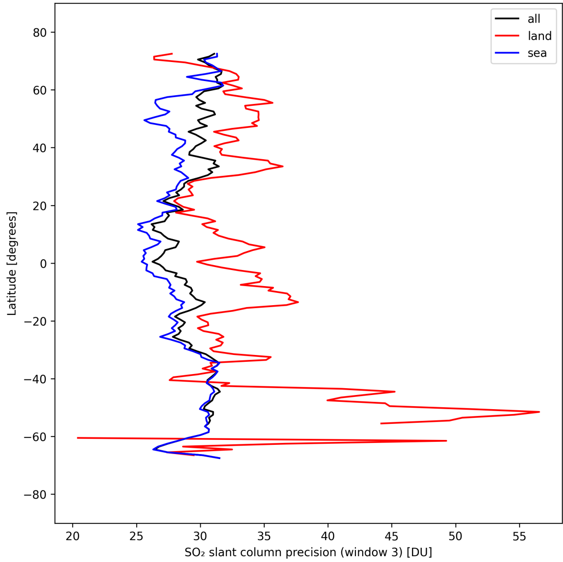
Figure 46: Zonal average of “SO 2 slant column precision (window 3)” for 2025-09-15 to 2025-09-17.
