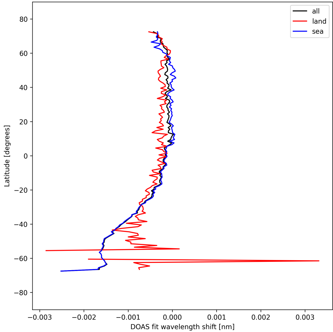
Figure 50: Zonal average of “DOAS fit wavelength shift” for 2025-09-15 to 2025-09-17.
