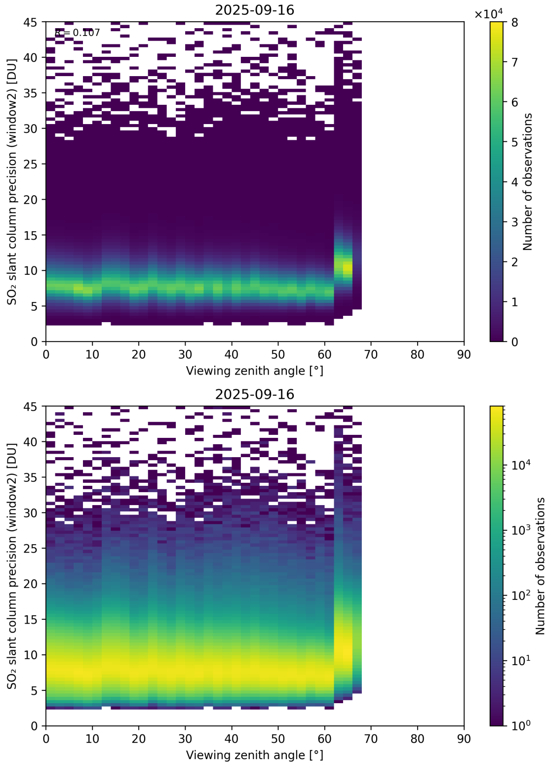
Figure 378: Scatter density plot of “Viewing zenith angle” against “SO 2 slant column precision (window2)” for 2025-09-15 to 2025-09-17.
