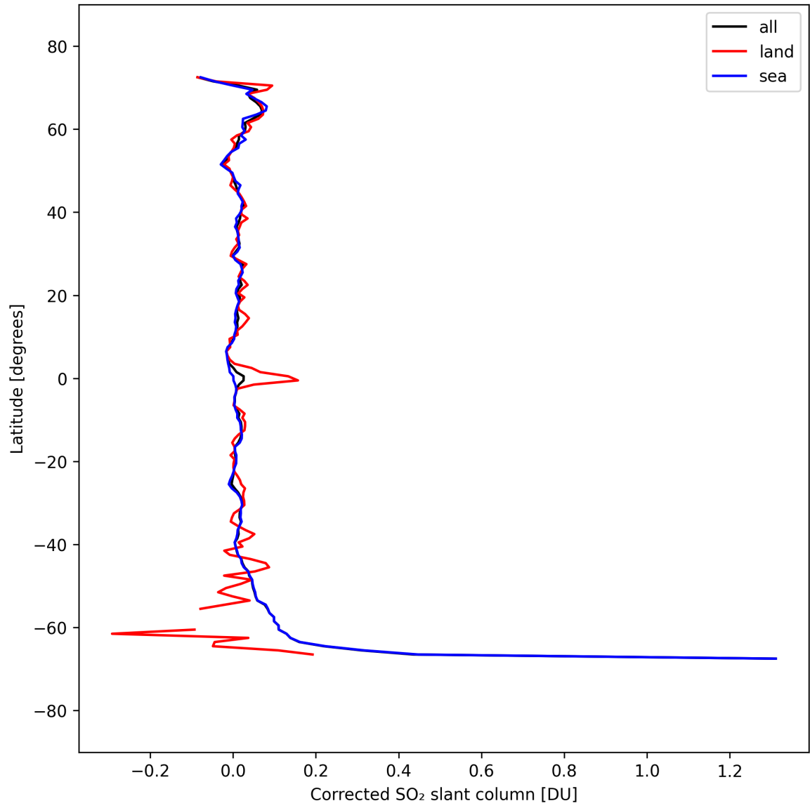
Figure 34: Zonal average of “Corrected SO 2 slant column” for 2025-09-15 to 2025-09-17.
