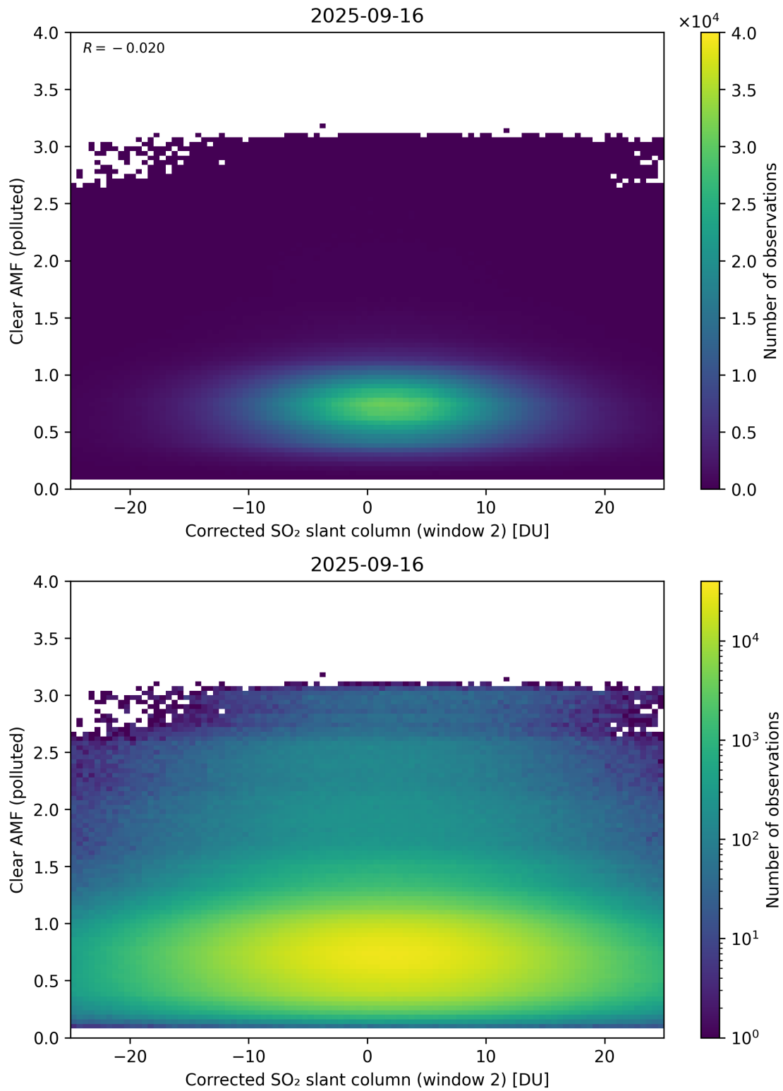
Figure 249: Scatter density plot of “Corrected SO 2 slant column (window 2)” against “Clear AMF (polluted)” for 2025-09-15 to 2025-09-17.
