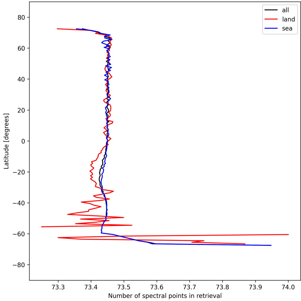
Figure 56: Zonal average of “Number of spectral points in retrieval” for 2025-09-15 to 2025-09-17.
