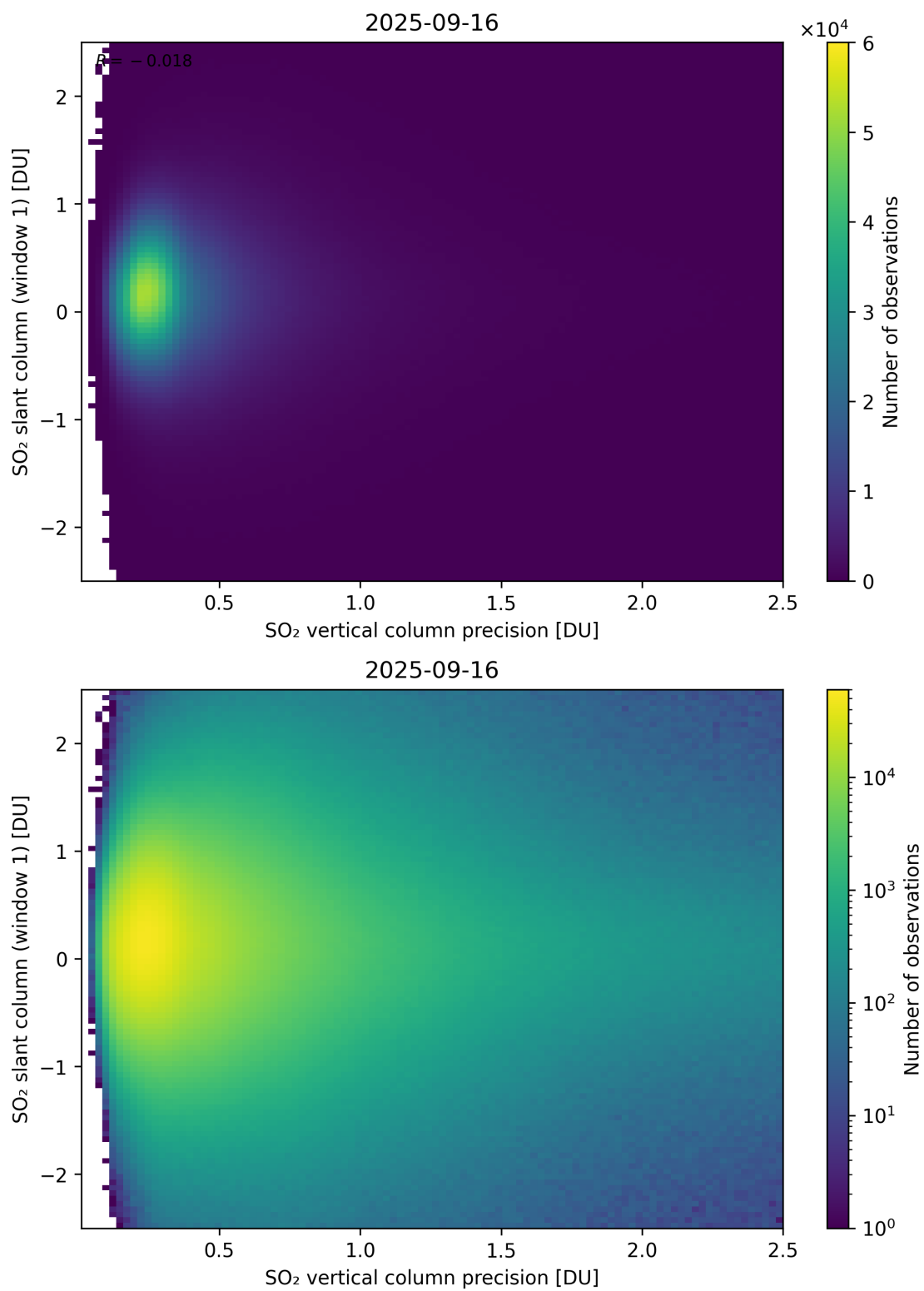
Figure 341: Scatter density plot of “SO 2 vertical column precision” against “SO 2 slant column (window 1)” for 2025-09-15 to 2025-09-17.
