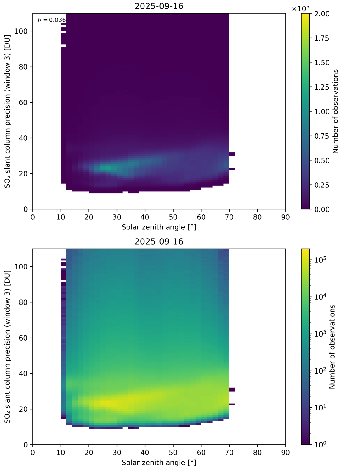
Figure 188: Scatter density plot of “Solar zenith angle” against “SO 2 slant column precision (window 3)” for 2025-09-15 to 2025-09-17.
