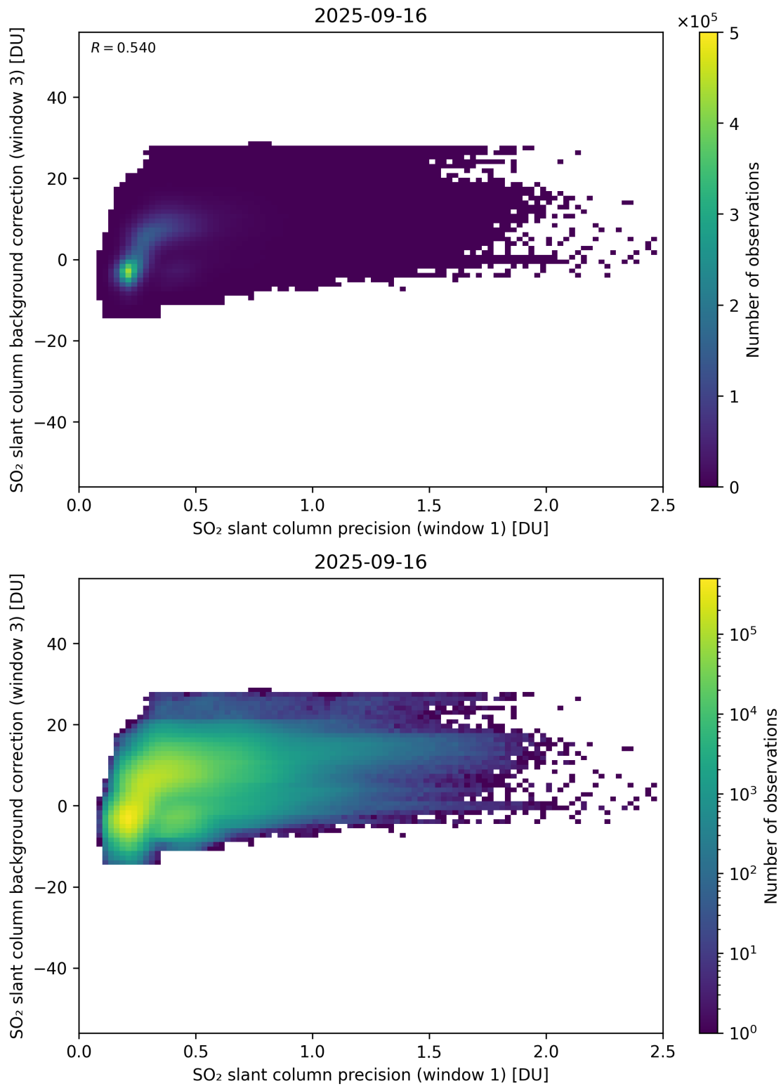
Figure 270: Scatter density plot of “SO 2 slant column precision (window 1)” against “SO 2 slant column background correction (window 3)” for 2025-09-15 to 2025-09-17.
