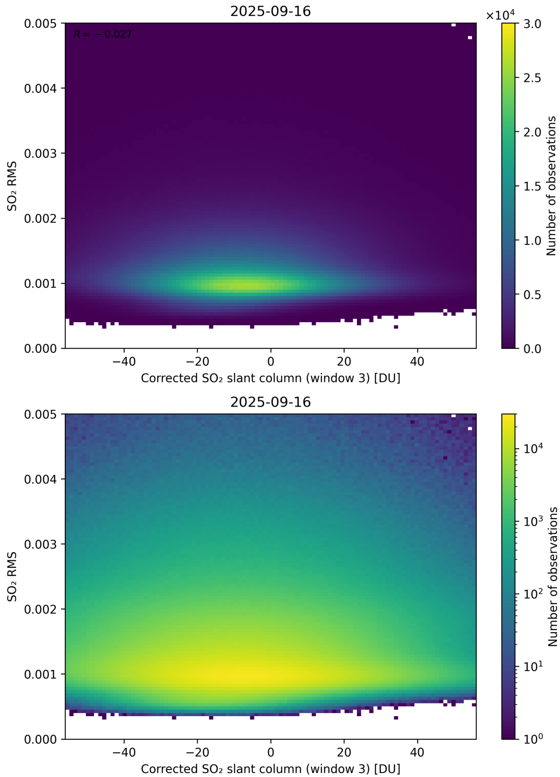
Figure 258: Scatter density plot of “Corrected SO 2 slant column (window 3)” against “SO 2 RMS” for 2025-09-15 to 2025-09-17.
