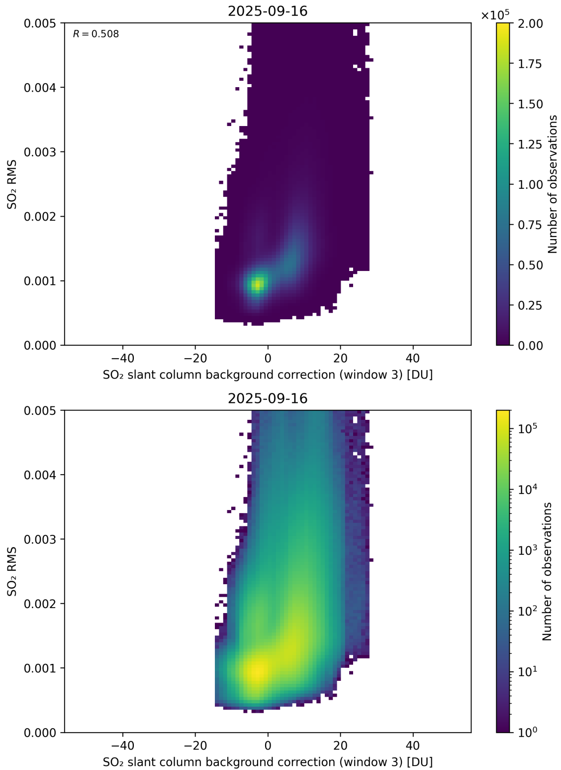
Figure 134: Scatter density plot of “SO 2 slant column background correction (window 3)” against “SO 2 RMS” for 2025-09-15 to 2025-09-17.
