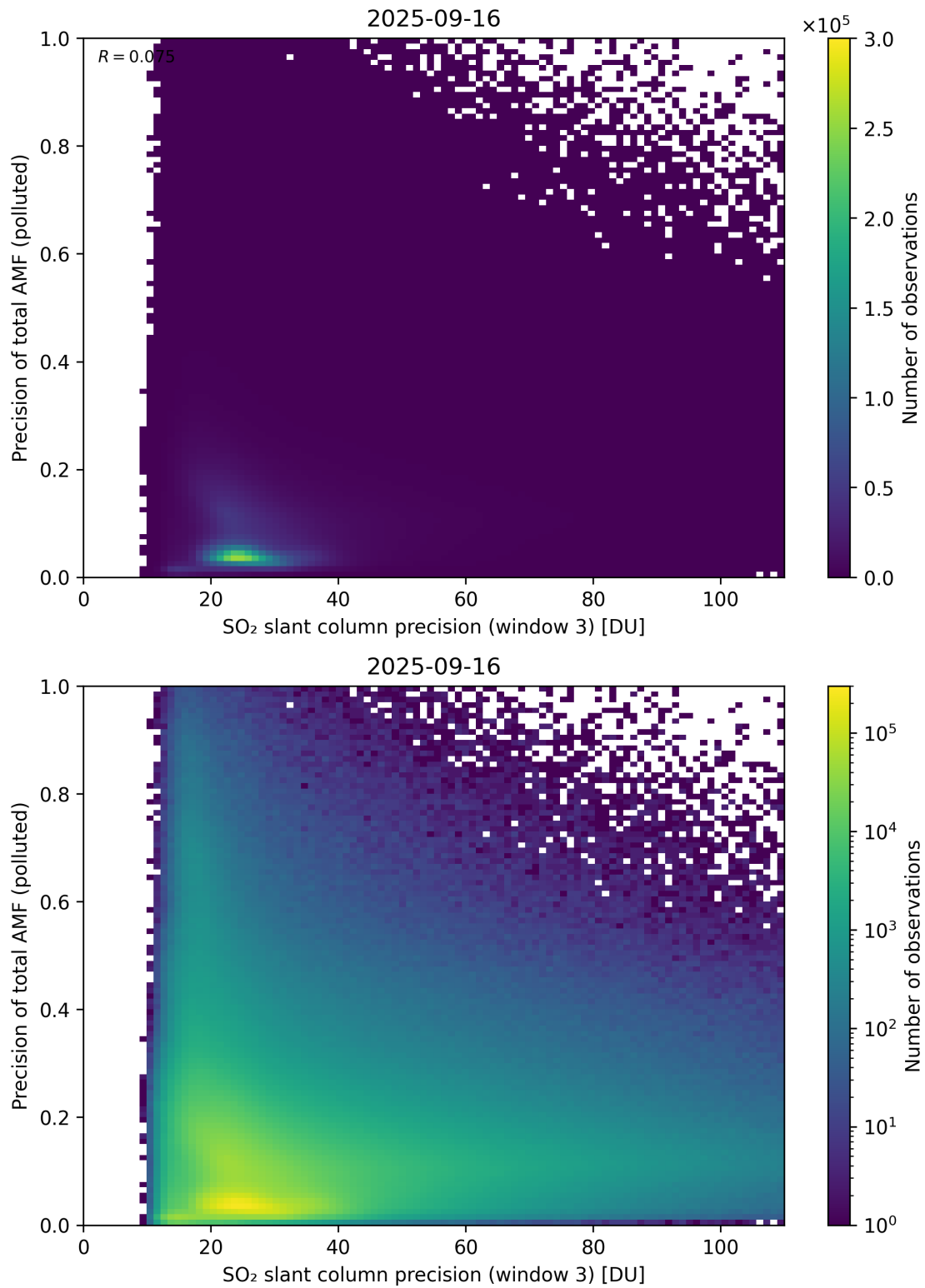
Figure 314: Scatter density plot of “SO 2 slant column precision (window 3)” against “Precision of total AMF (polluted)” for 2025-09-15 to 2025-09-17.
