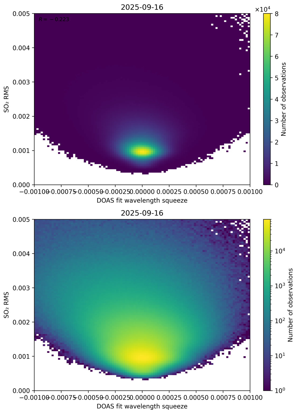
Figure 143: Scatter density plot of “DOAS fit wavelength squeeze” against “SO 2 RMS” for 2025-09-15 to 2025-09-17.
