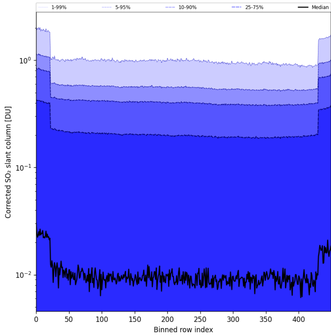
Figure 86: Along track statistics of “Corrected SO 2 slant column” for 2025-09-15 to 2025-09-17
