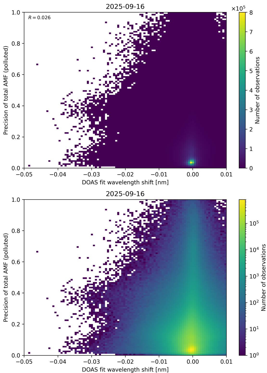
Figure 142: Scatter density plot of “DOAS fit wavelength shift” against “Precision of total AMF (polluted)” for 2025-09-15 to 2025-09-17.
