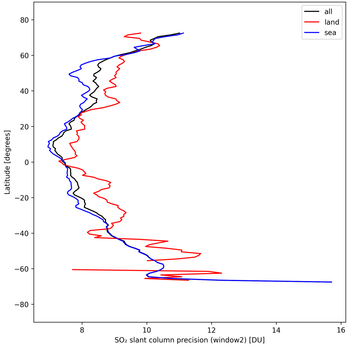
Figure 42: Zonal average of "SO 2 slant column precision (window2)" for 2025-09-15 to 2025-09-17.
