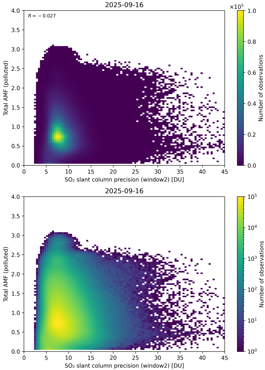
Figure 301: Scatter density plot of “SO 2 slant column precision (window2)” against “Total AMF (polluted)” for 2025-09-15 to 2025-09-17.
