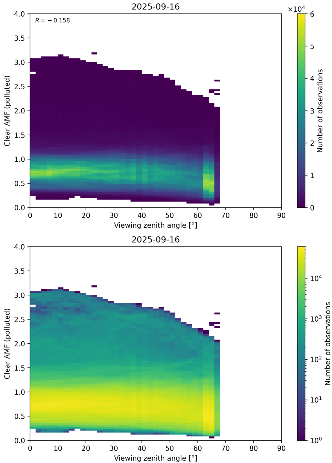
Figure 370: Scatter density plot of “Viewing zenith angle” against “Clear AMF (polluted)” for 2025-09-15 to 2025-09-17.
