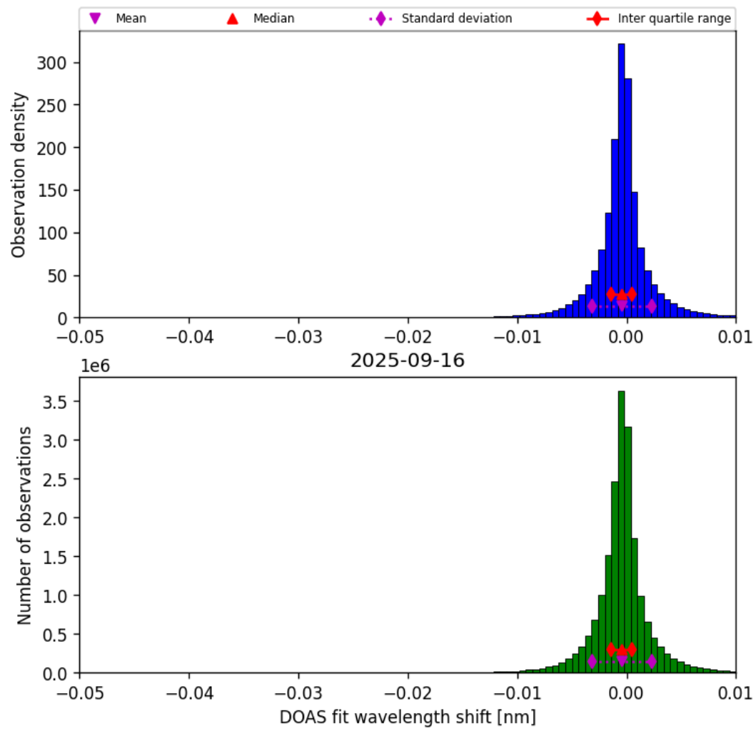
Figure 76: Histogram of “DOAS fit wavelength shift” for 2025-09-15 to 2025-09-17
