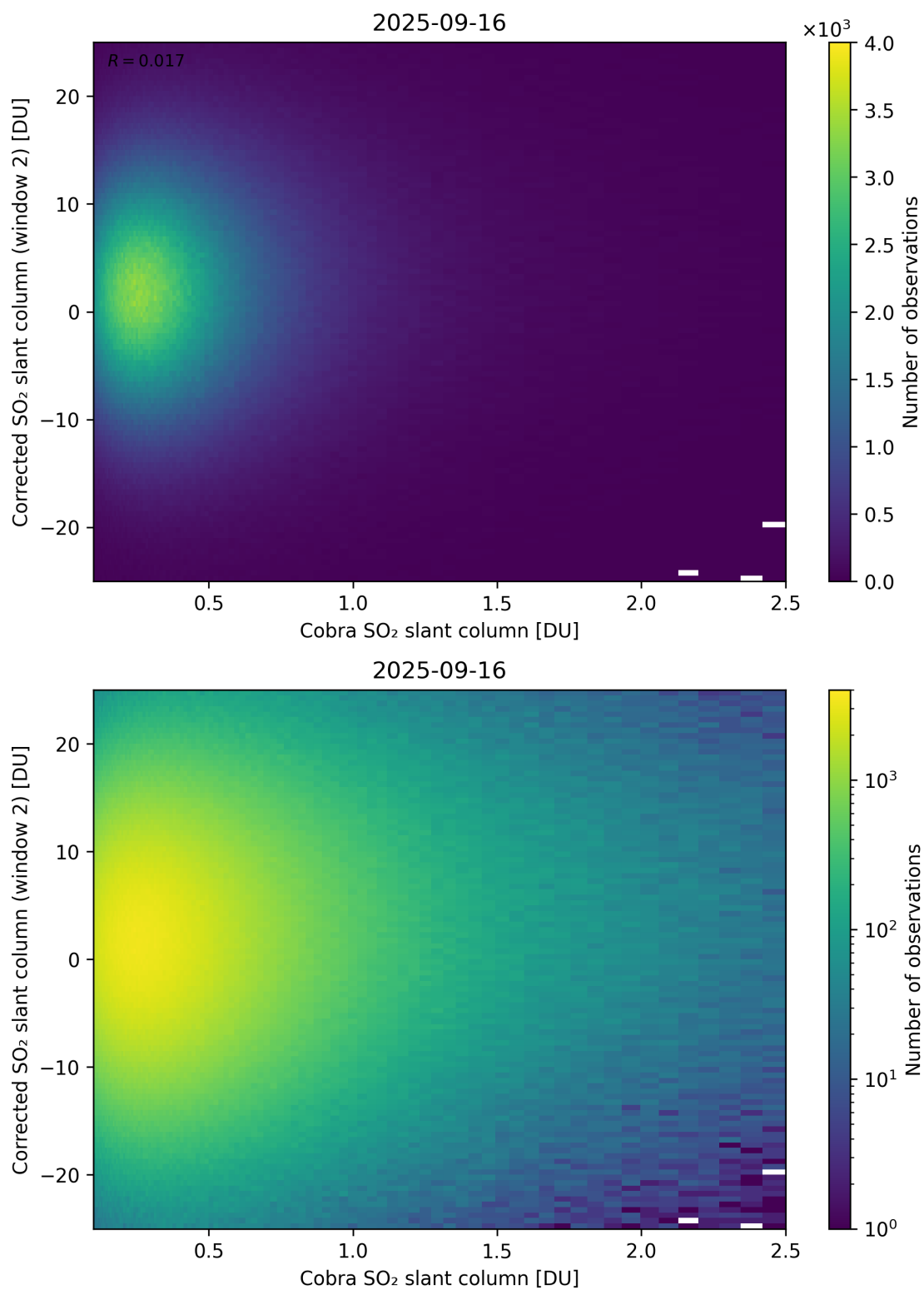
Figure 217: Scatter density plot of “Cobra SO 2 slant column” against “Corrected SO 2 slant column (window 2)” for 2025-09-15 to 2025-09-17.
