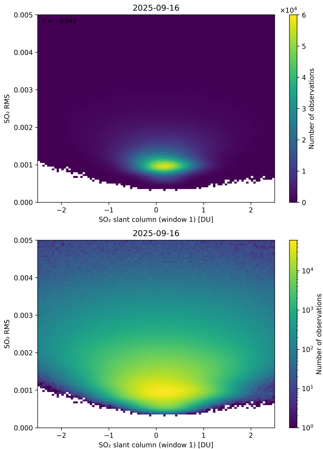
Figure 267: Scatter density plot of “SO 2 slant column (window 1)” against “SO 2 RMS” for 2025-09-15 to 2025-09-17.
