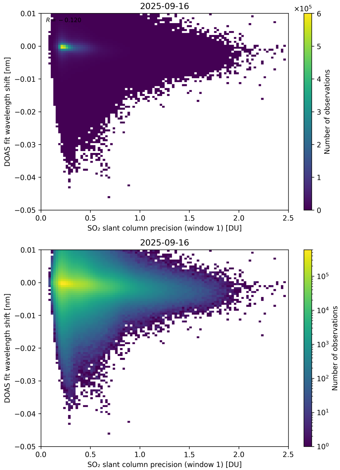
Figure 271: Scatter density plot of “SO 2 slant column precision (window 1)” against “DOAS fit wavelength shift” for 2025-09-15 to 2025-09-17.
