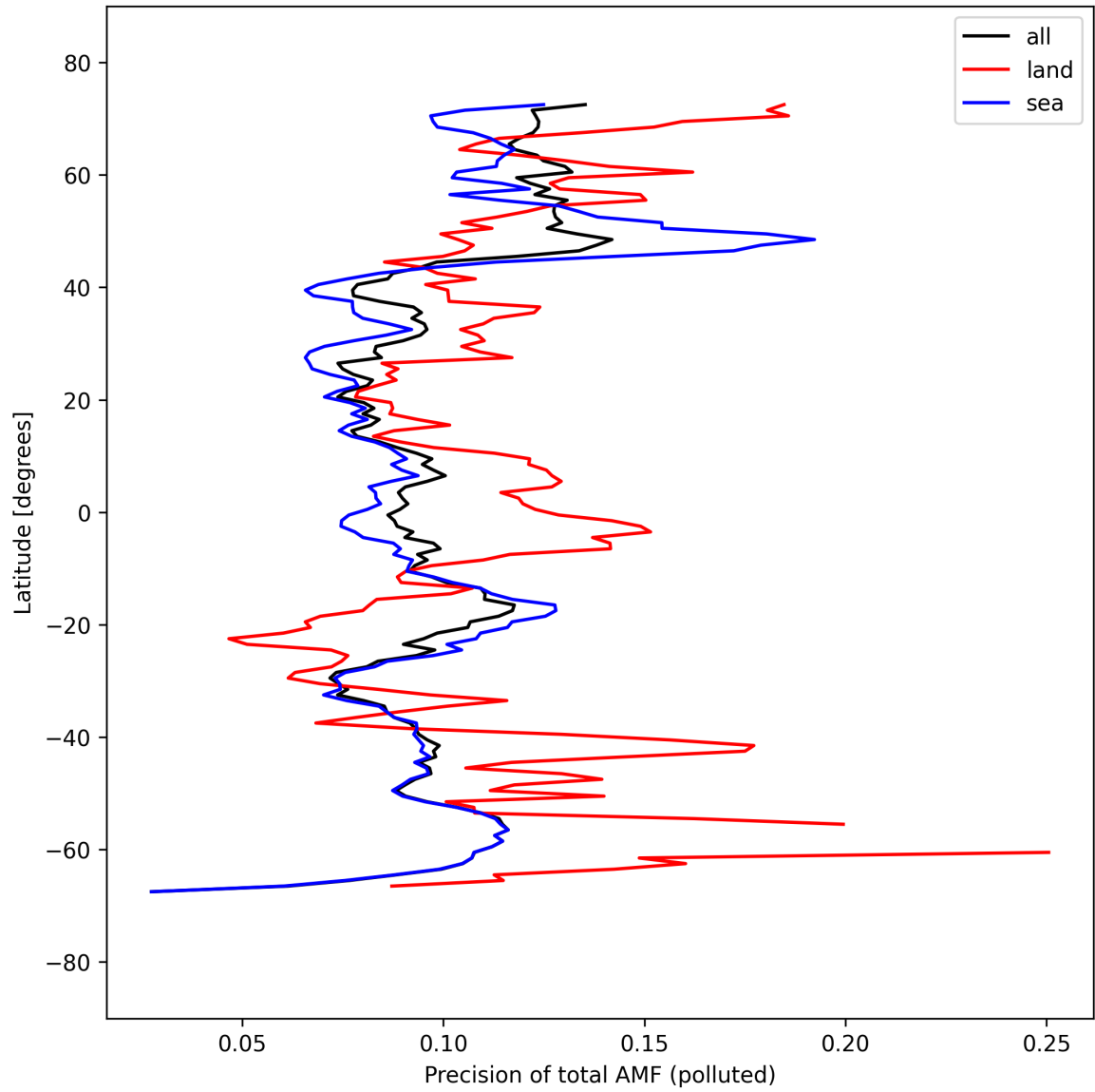
Figure 54: Zonal average of “Precision of total AMF (polluted)” for 2025-09-15 to 2025-09-17.
