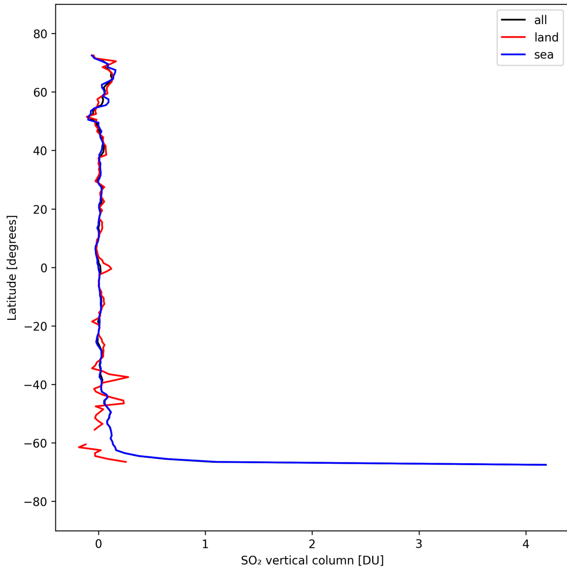
Figure 32: Zonal average of “SO 2 vertical column” for 2025-09-15 to 2025-09-17.
