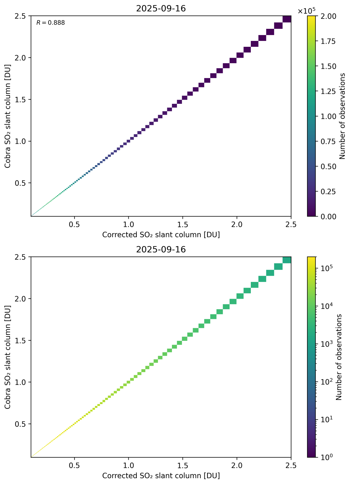
Figure 233: Scatter density plot of “Corrected SO 2 slant column” against “Cobra SO 2 slant column” for 2025-09-15 to 2025-09-17.
