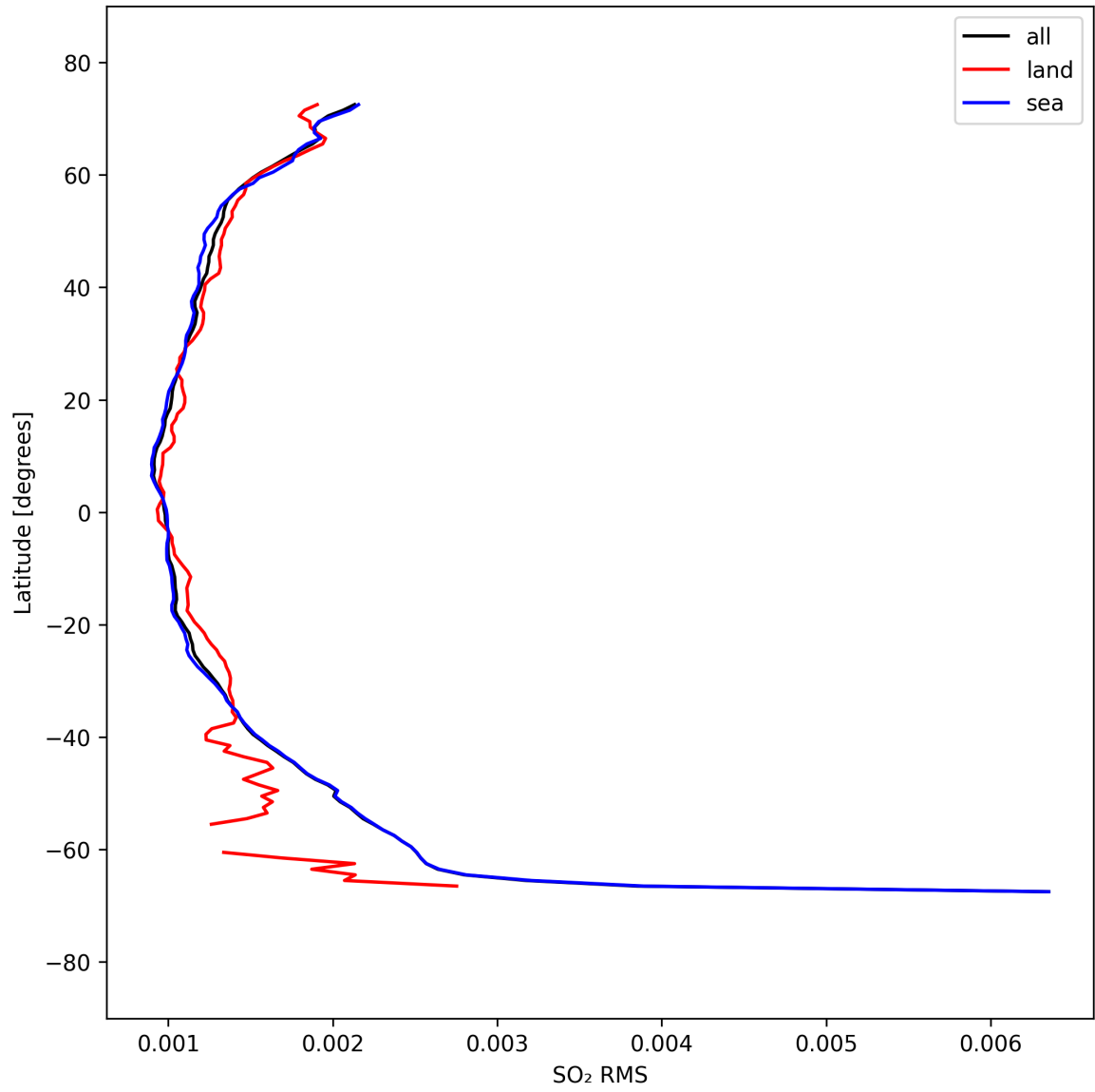
Figure 52: Zonal average of “SO 2 RMS” for 2025-09-15 to 2025-09-17.
