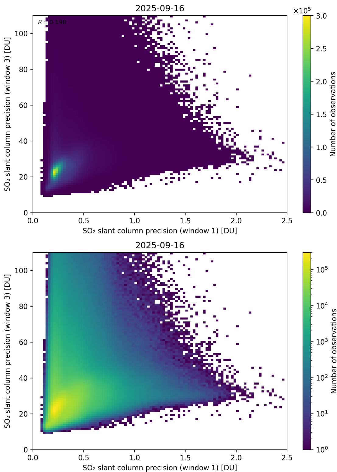
Figure 279: Scatter density plot of “SO 2 slant column precision (window 1)” against “SO 2 slant column precision (window 3)” for 2025-09-15 to 2025-09-17.
