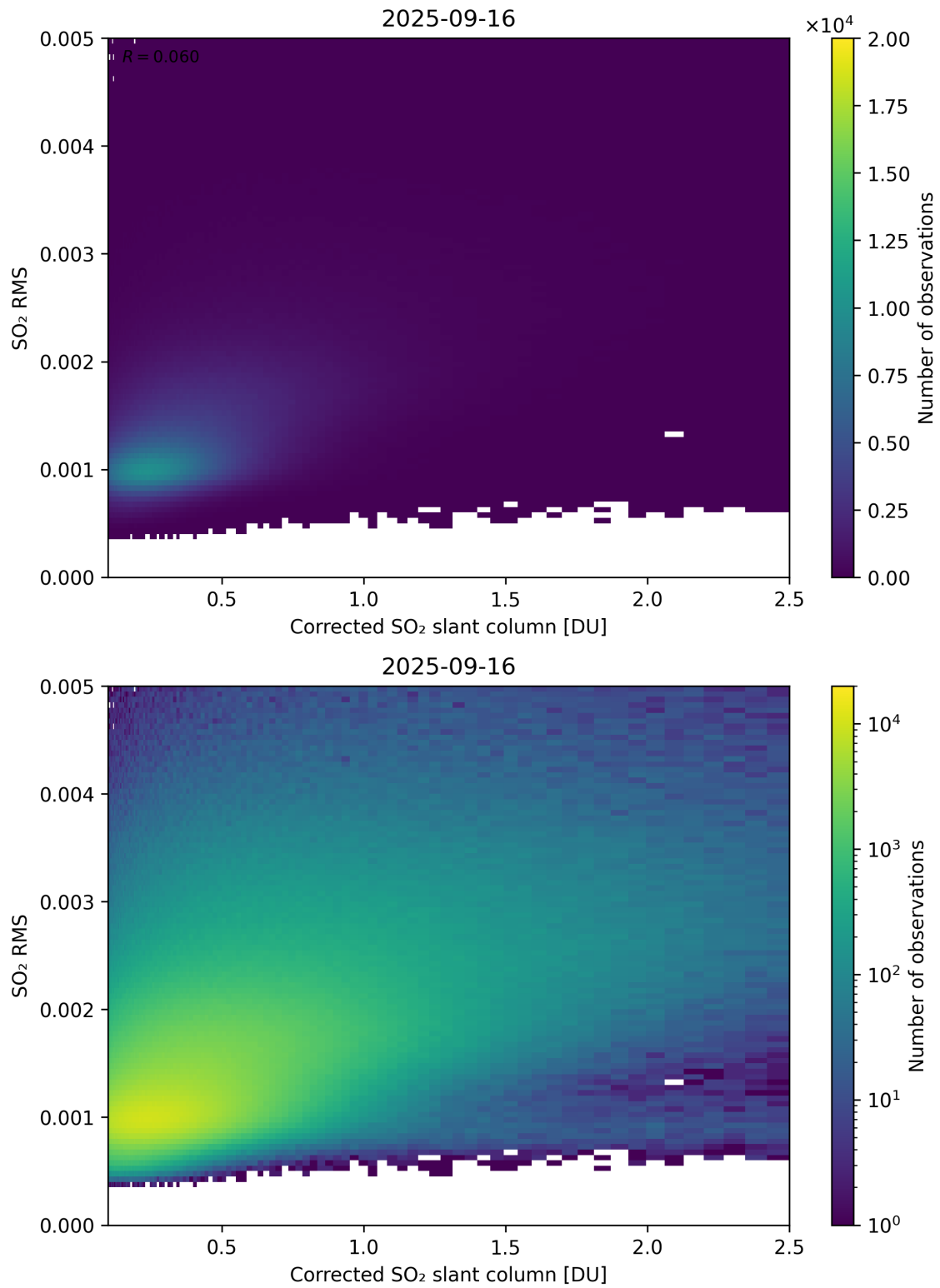
Figure 231: Scatter density plot of “Corrected SO 2 slant column” against “SO 2 RMS” for 2025-09-15 to 2025-09-17.
