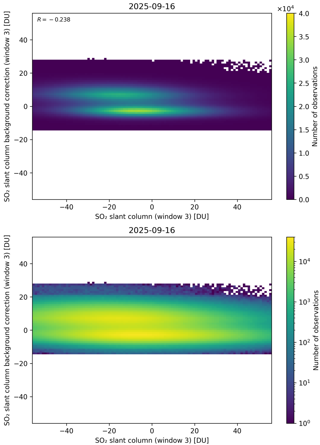
Figure 303: Scatter density plot of “SO 2 slant column (window 3)” against “SO 2 slant column background correction (window 3)” for 2025-09-15 to 2025-09-17.
