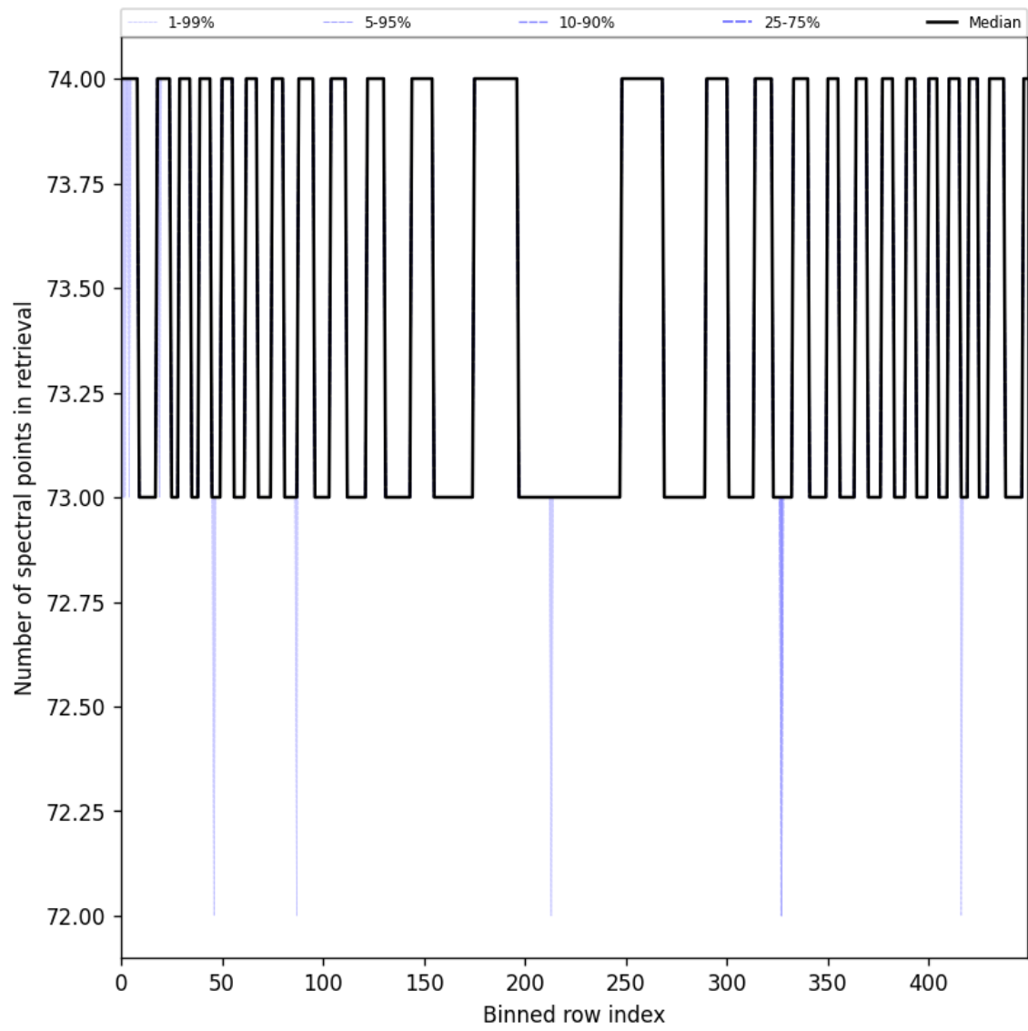
Figure 108: Along track statistics of “Number of spectral points in retrieval” for 2025-09-15 to 2025-09-17
