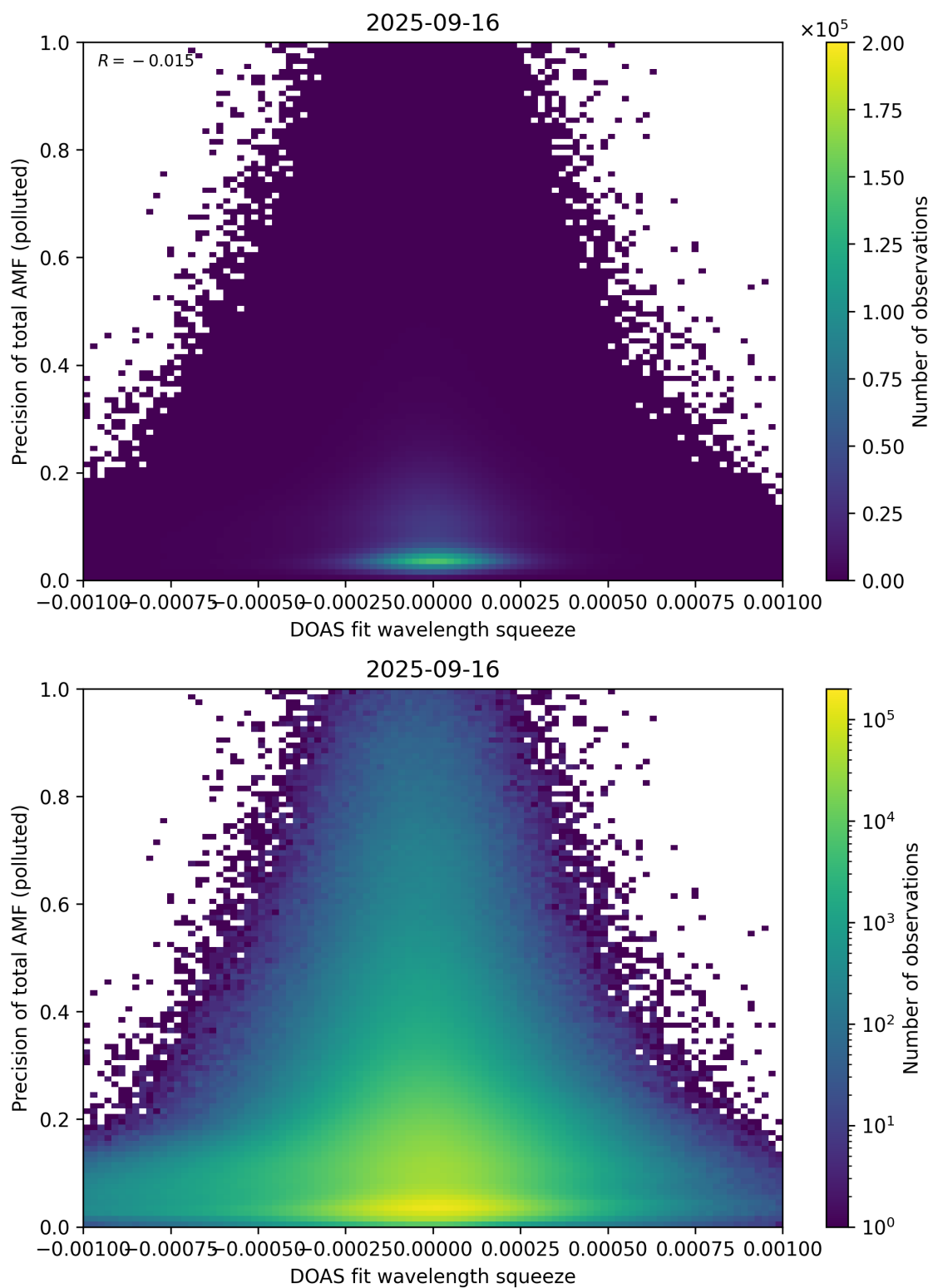
Figure 146: Scatter density plot of “DOAS fit wavelength squeeze” against “Precision of total AMF (polluted)” for 2025-09-15 to 2025-09-17.
