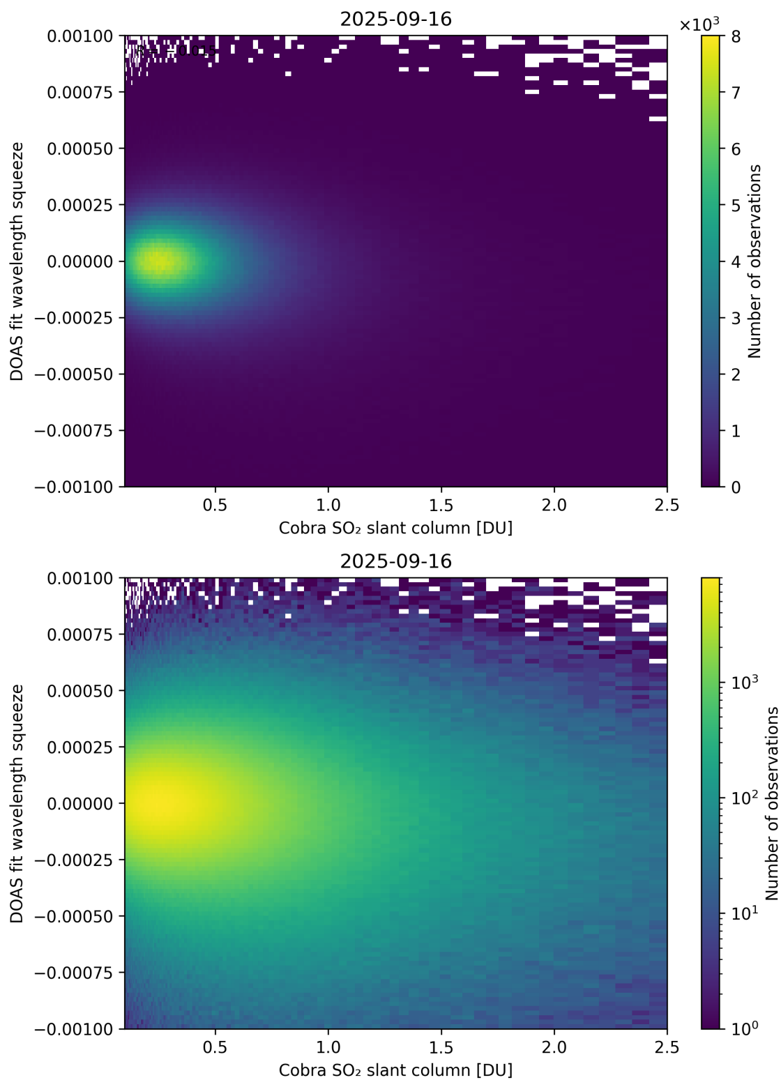
Figure 197: Scatter density plot of “Cobra SO 2 slant column” against “DOAS fit wavelength squeeze” for 2025-09-15 to 2025-09-17.
