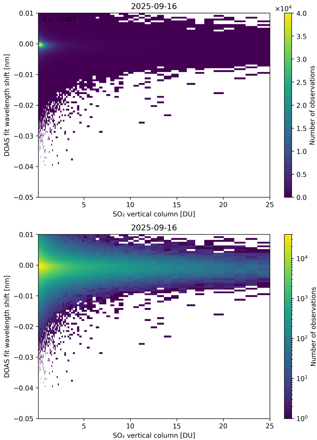
Figure 326: Scatter density plot of “SO 2 vertical column” against “DOAS fit wavelength shift” for 2025-09-15 to 2025-09-17.
