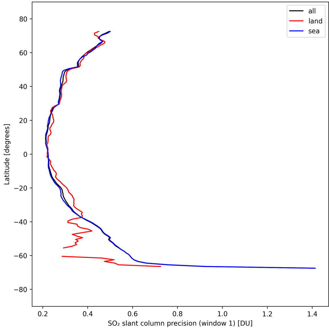
Figure 38: Zonal average of “SO 2 slant column precision (window 1)” for 2025-09-15 to 2025-09-17.
