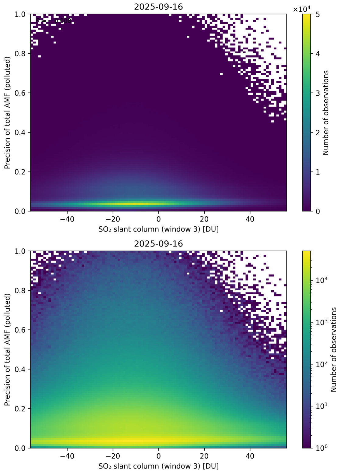
Figure 319: Scatter density plot of “SO 2 slant column (window 3)” against “Precision of total AMF (polluted)” for 2025-09-15 to 2025-09-17.
