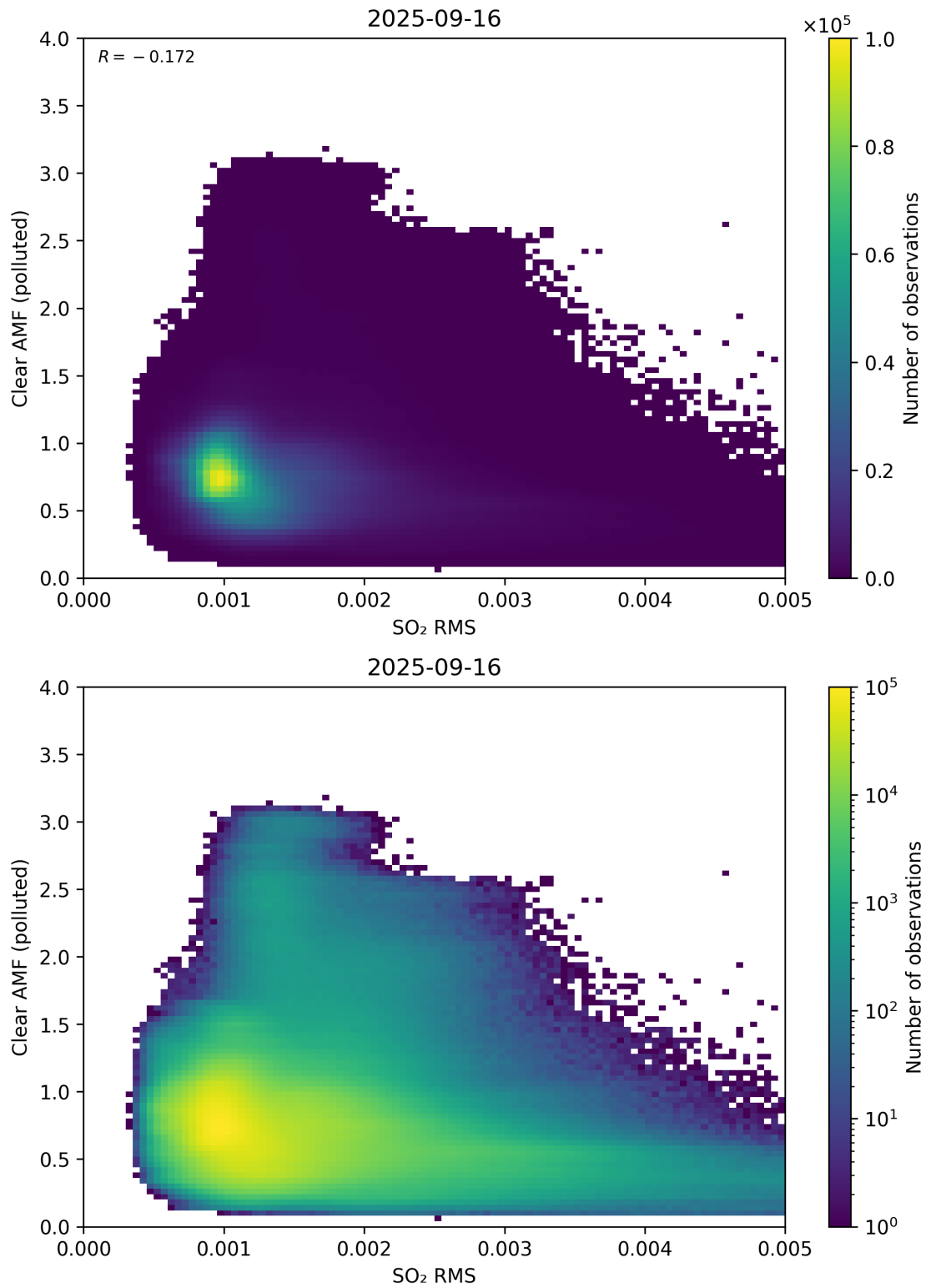
Figure 147: Scatter density plot of “SO 2 RMS” against “Clear AMF (polluted)” for 2025-09-15 to 2025-09-17.
