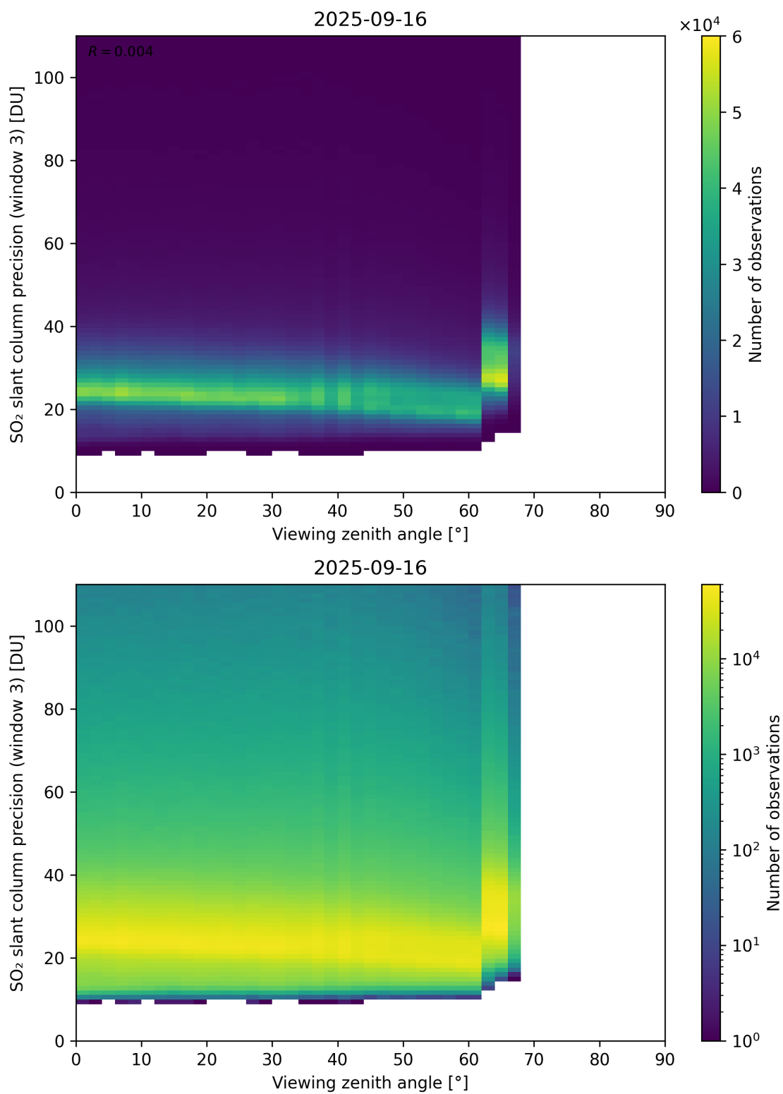
Figure 380: Scatter density plot of “Viewing zenith angle” against “SO 2 slant column precision (window 3)” for 2025-09-15 to 2025-09-17.
