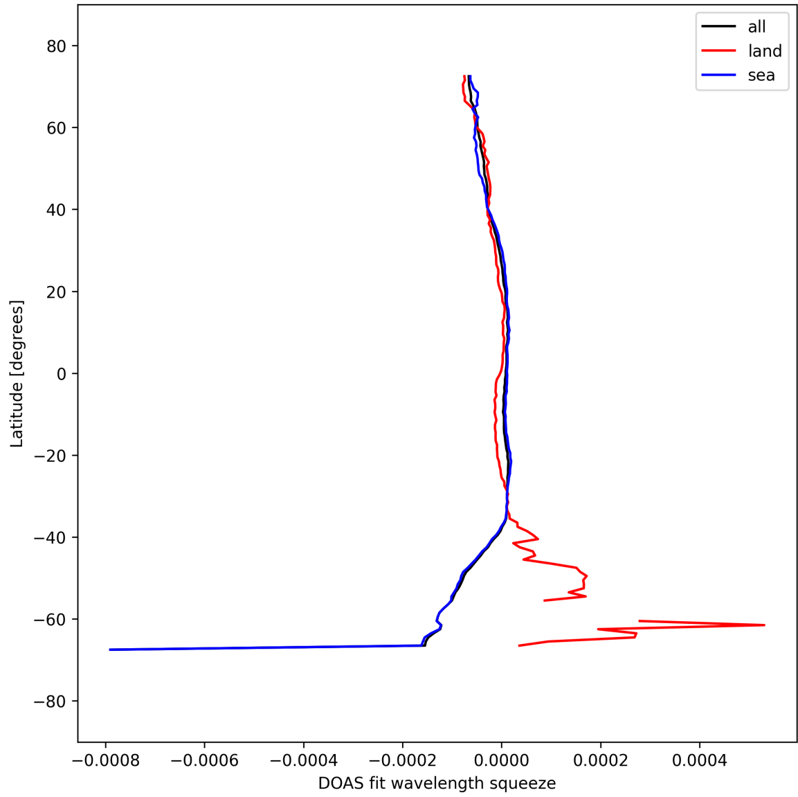
Figure 51: Zonal average of “DOAS fit wavelength squeeze” for 2025-09-15 to 2025-09-17.
