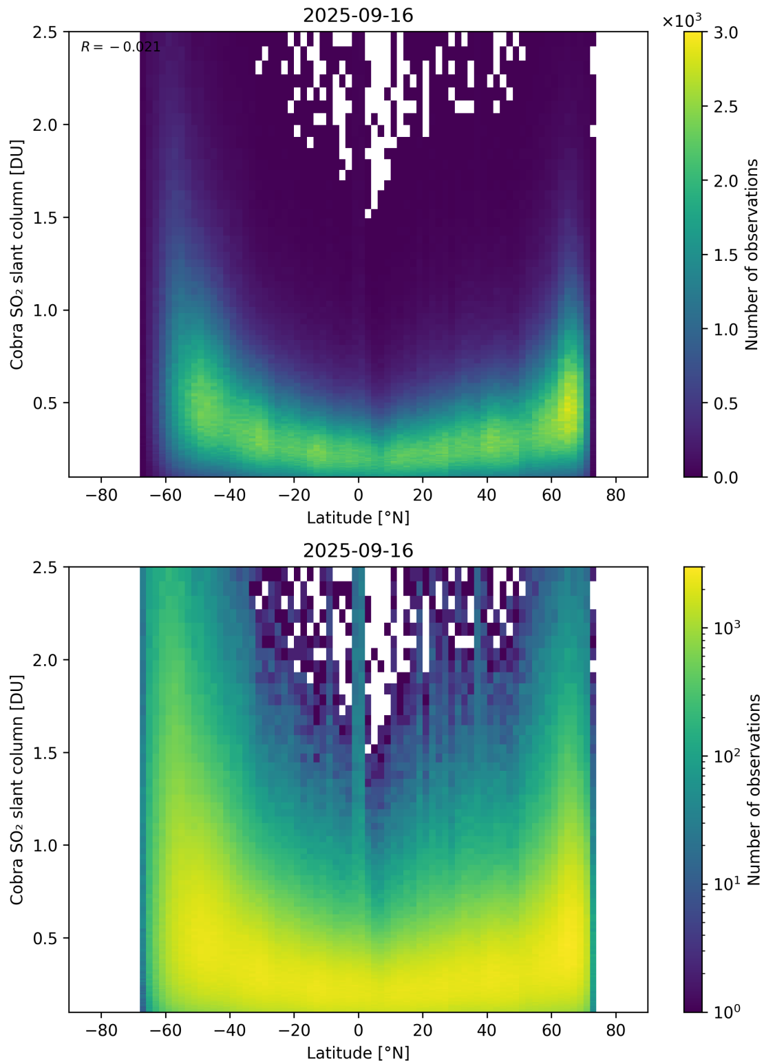
Figure 157: Scatter density plot of “Latitude” against “Cobra SO 2 slant column” for 2025-09-15 to 2025-09-17.
