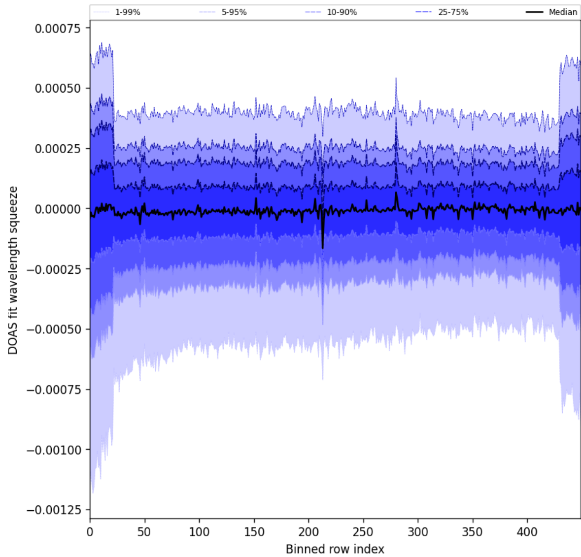
Figure 103: Along track statistics of “DOAS fit wavelength squeeze” for 2025-09-15 to 2025-09-17
