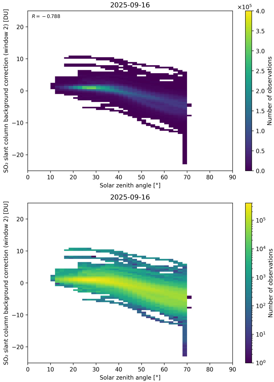
Figure 172: Scatter density plot of “Solar zenith angle” against “SO 2 slant column background correction (window 2)” for 2025-09-15 to 2025-09-17.
