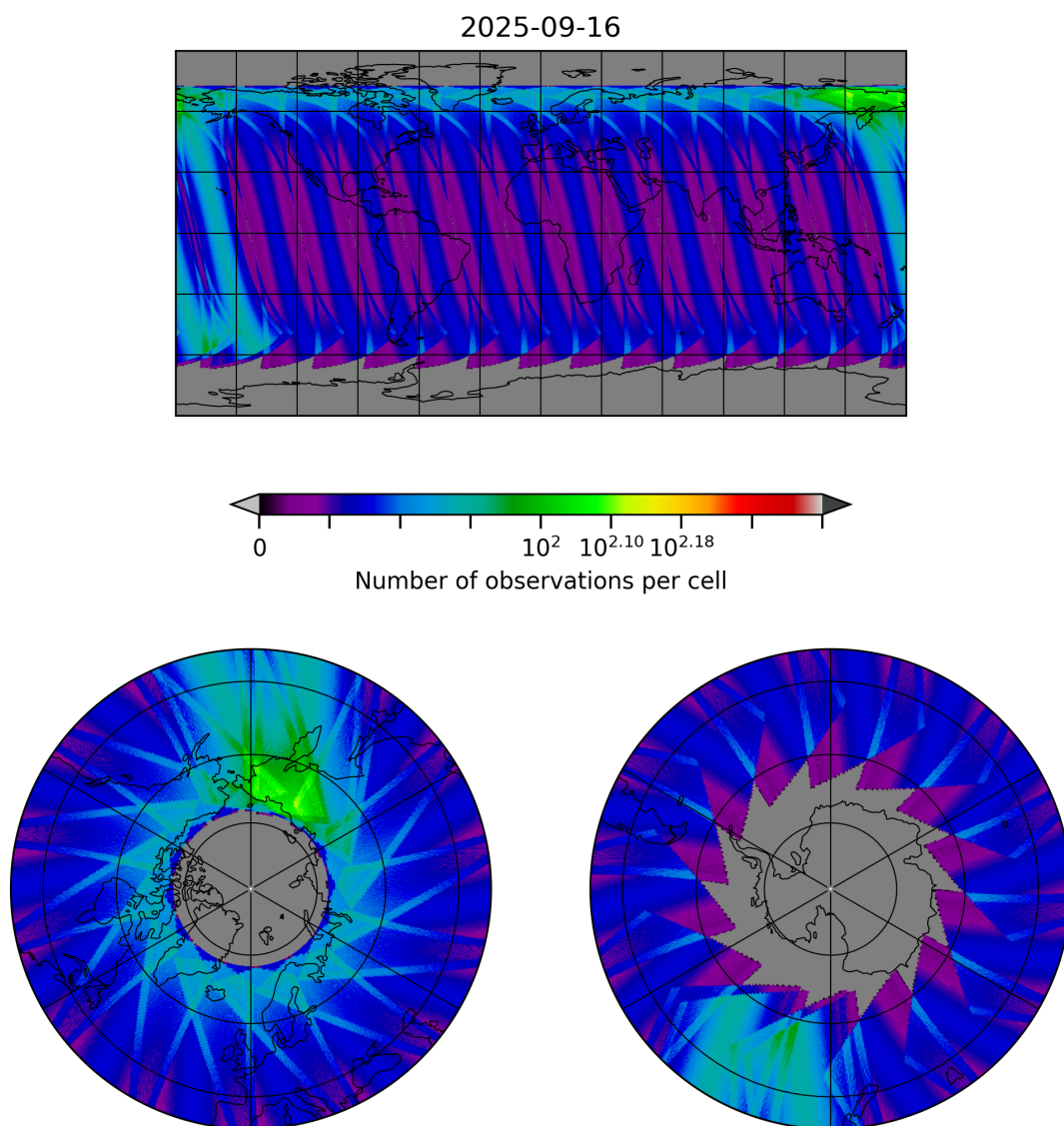
Figure 30: Map of the number of observations for 2025-09-15 to 2025-09-17
