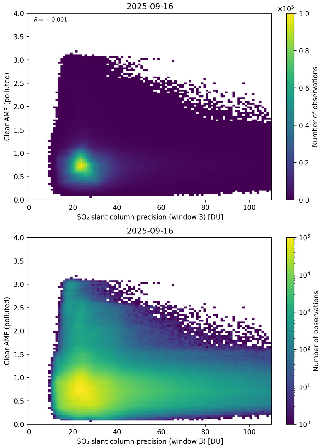
Figure 311: Scatter density plot of “SO 2 slant column precision (window 3)” against “Clear AMF (polluted)” for 2025-09-15 to 2025-09-17.
