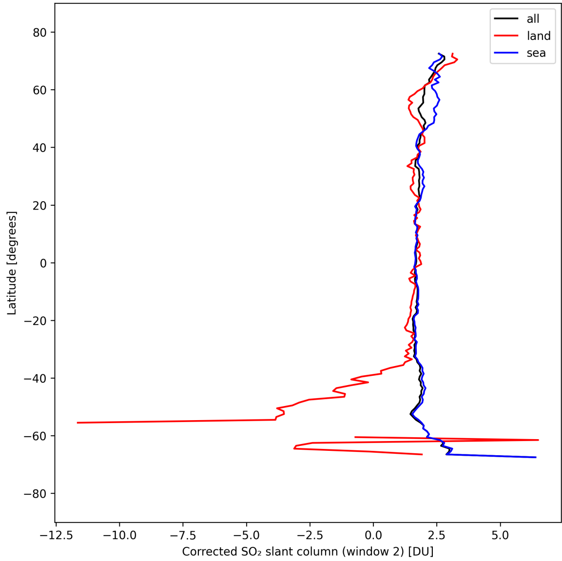
Figure 43: Zonal average of “Corrected SO 2 slant column (window 2)” for 2025-09-15 to 2025-09-17.
