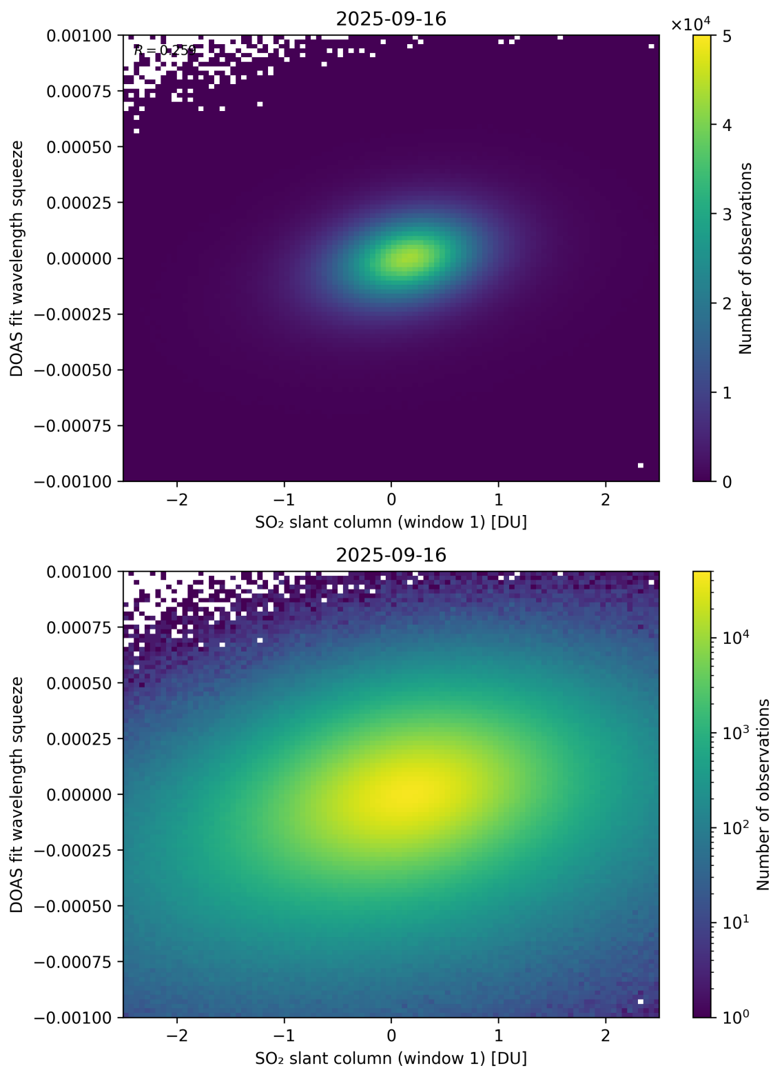
Figure 266: Scatter density plot of “SO 2 slant column (window 1)” against “DOAS fit wavelength squeeze” for 2025-09-15 to 2025-09-17.
