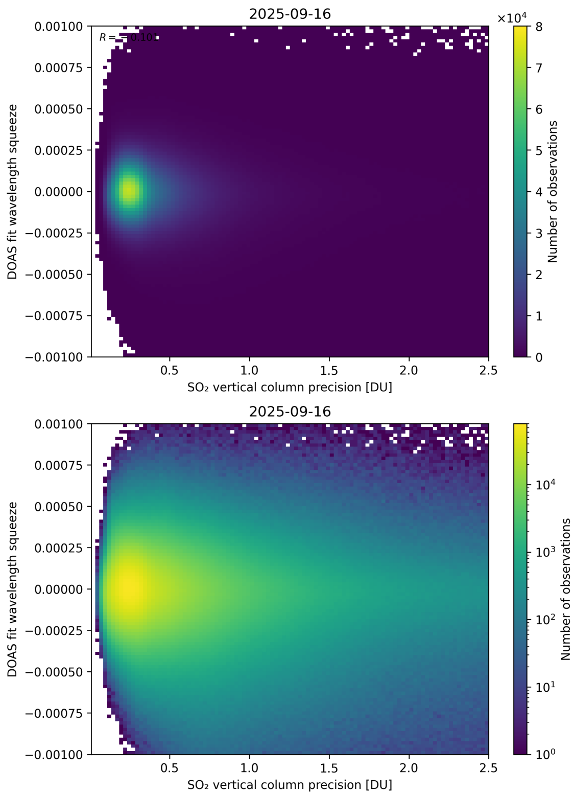
Figure 333: Scatter density plot of “SO 2 vertical column precision” against “DOAS fit wavelength squeeze” for 2025-09-15 to 2025-09-17.
