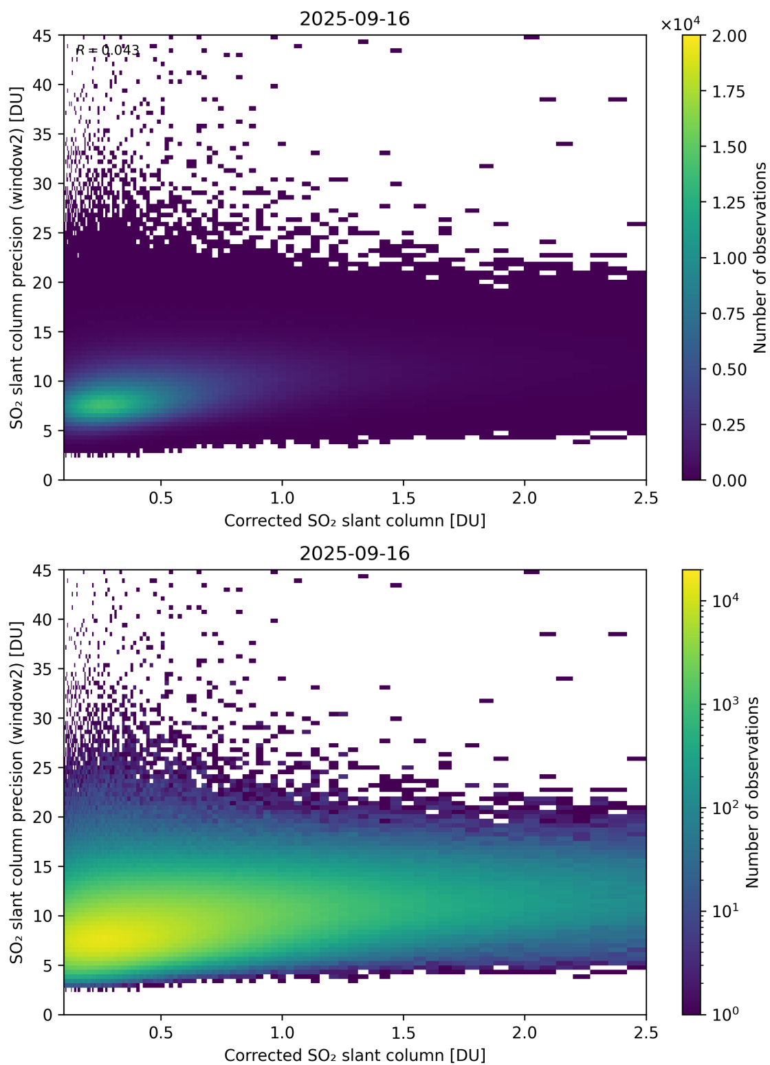
Figure 239: Scatter density plot of “Corrected SO 2 slant column” against “SO 2 slant column precision (window2)” for 2025-09-15 to 2025-09-17.
