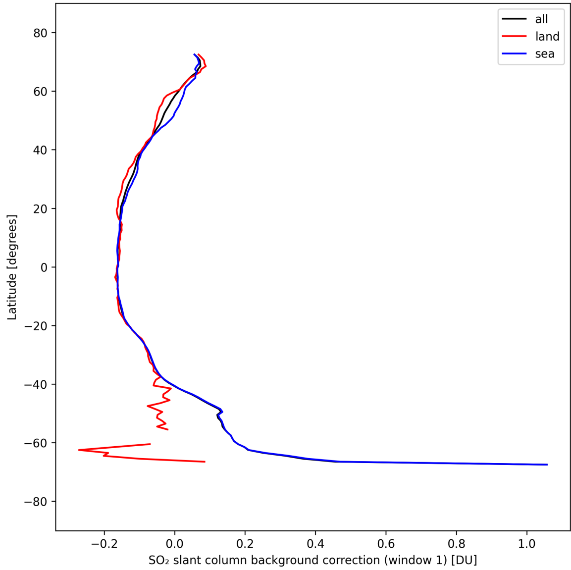
Figure 40: Zonal average of “SO 2 slant column background correction (window 1)” for 2025-09-15 to 2025-09-17.
