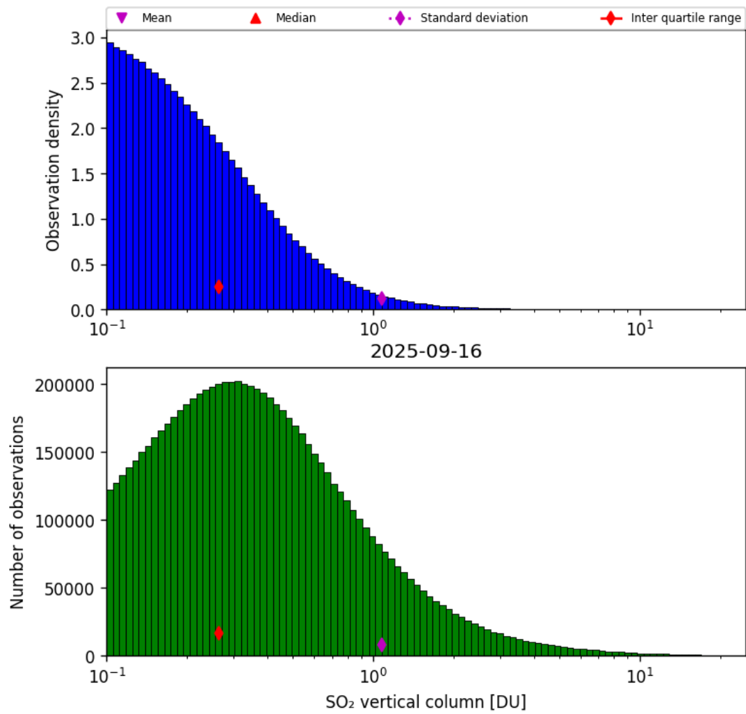
Figure 58: Histogram of “SO 2 vertical column” for 2025-09-15 to 2025-09-17
