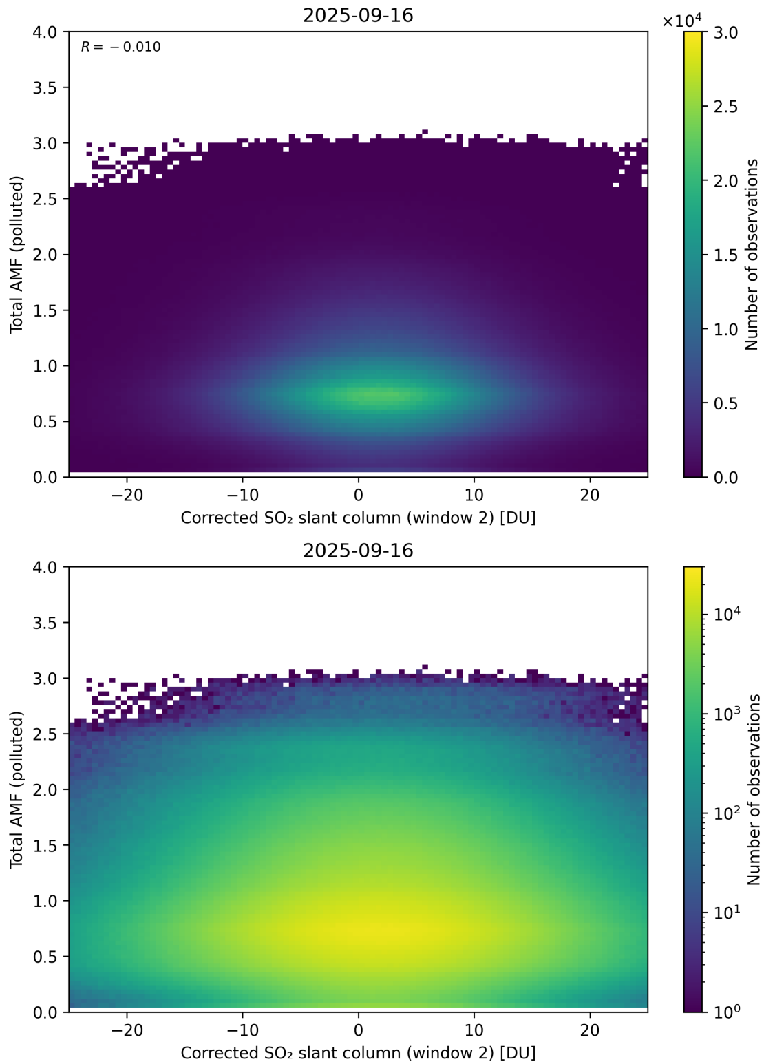
Figure 253: Scatter density plot of “Corrected SO 2 slant column (window 2)” against “Total AMF (polluted)” for 2025-09-15 to 2025-09-17.
