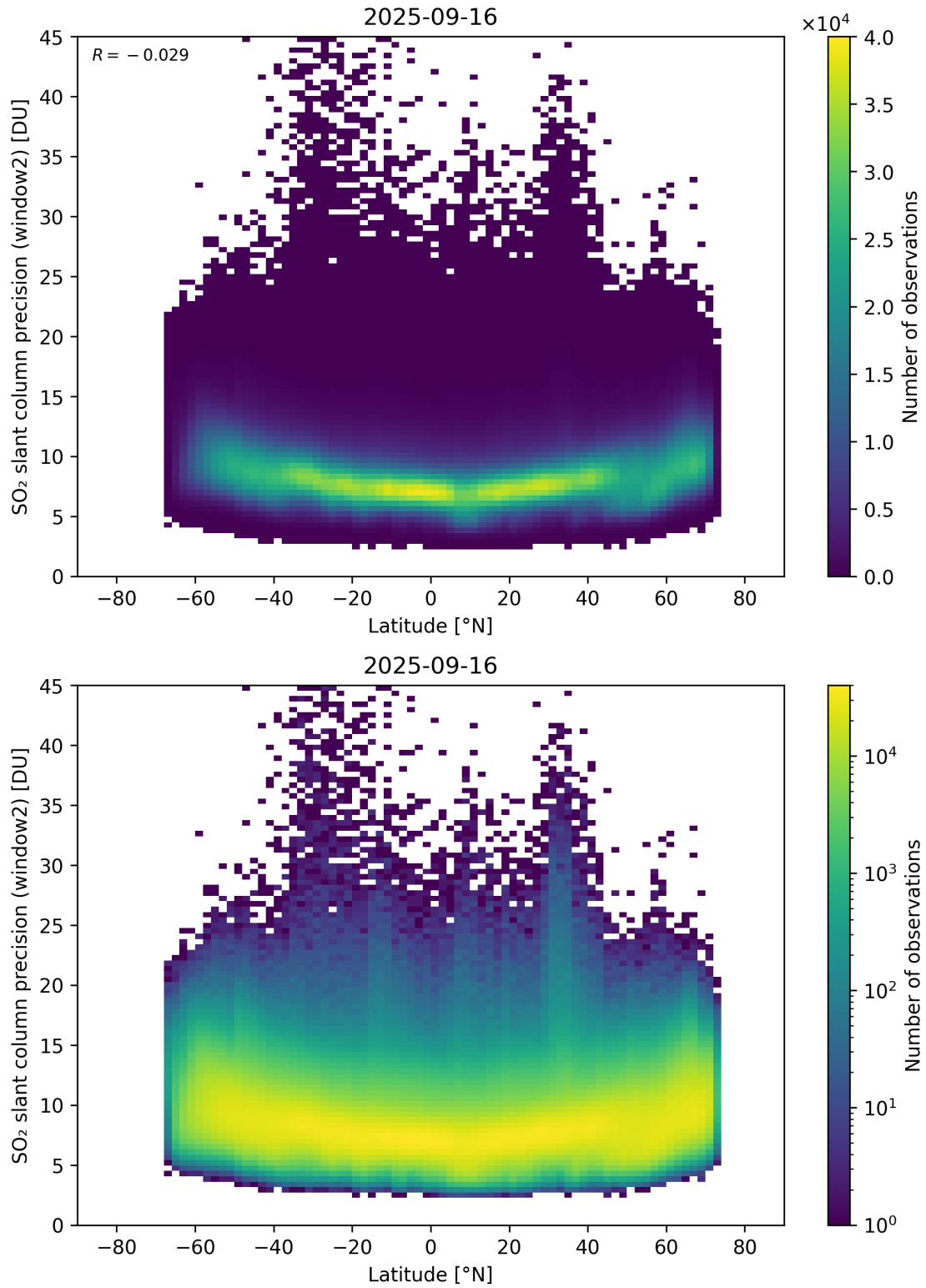
Figure 164: Scatter density plot of “Latitude” against “SO 2 slant column precision (window2)” for 2025-09-15 to 2025-09-17.
