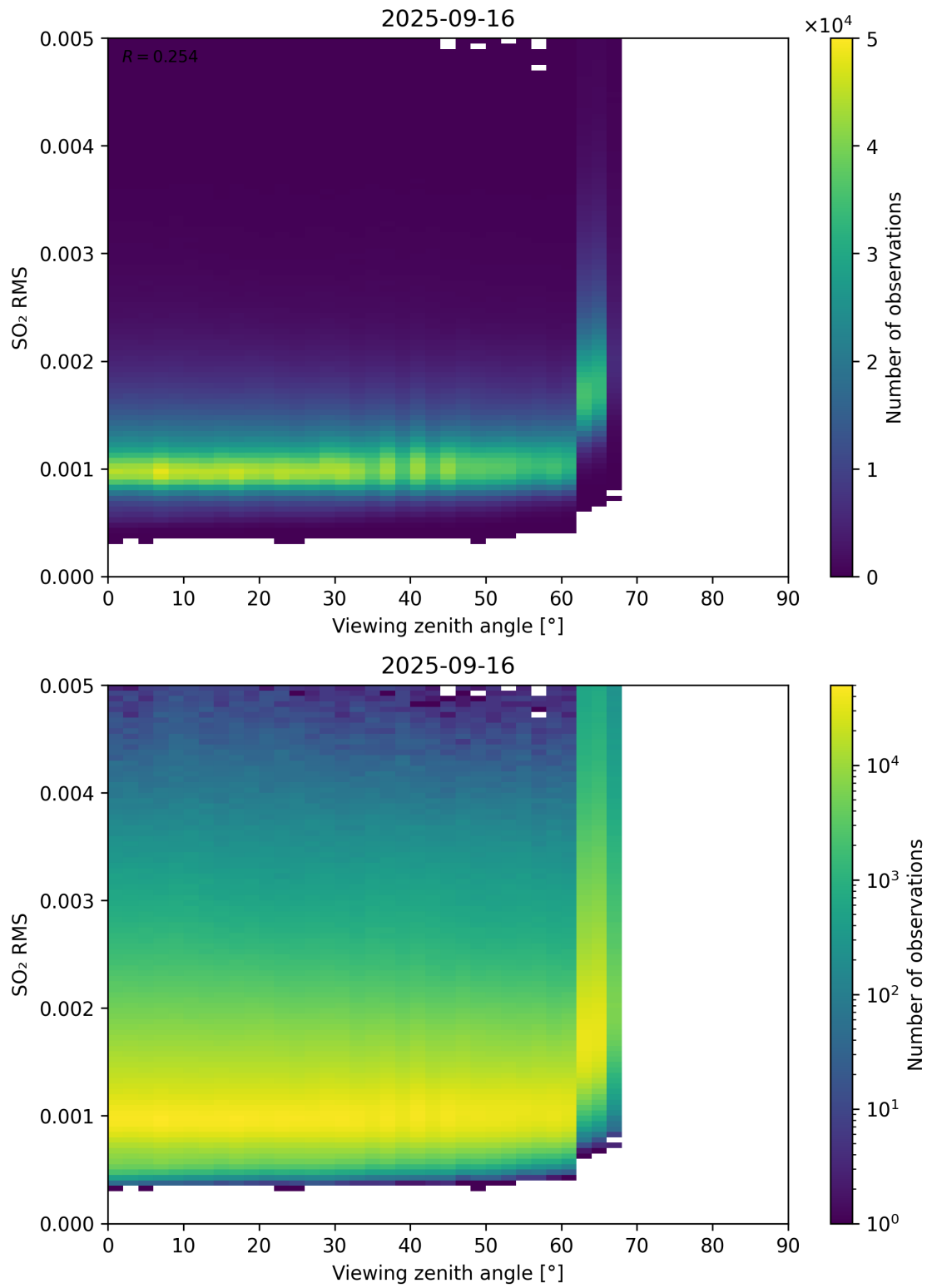
Figure 367: Scatter density plot of “Viewing zenith angle” against “SO 2 RMS” for 2025-09-15 to 2025-09-17.
