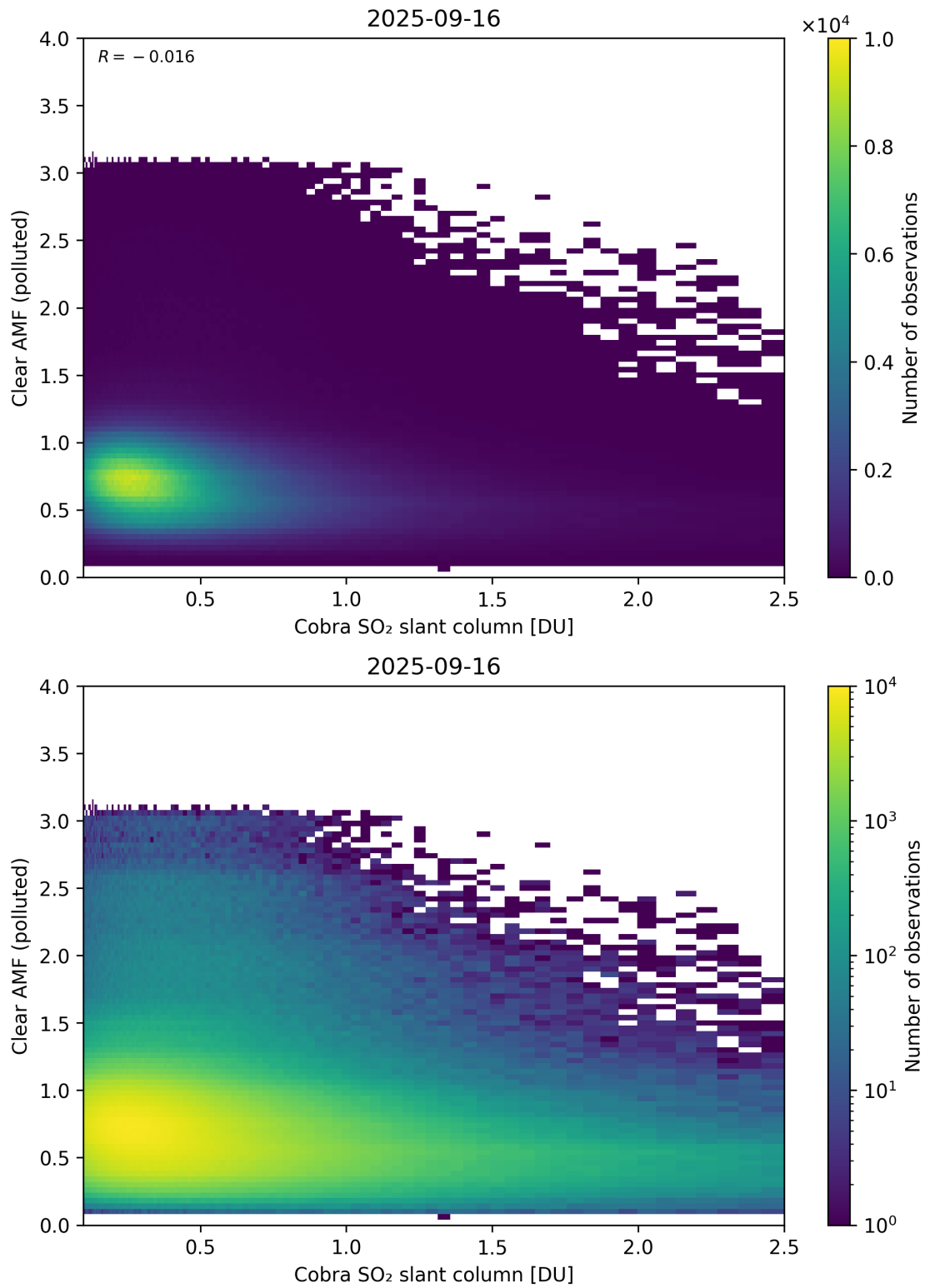
Figure 215: Scatter density plot of “Cobra SO 2 slant column” against “Clear AMF (polluted)” for 2025-09-15 to 2025-09-17.
