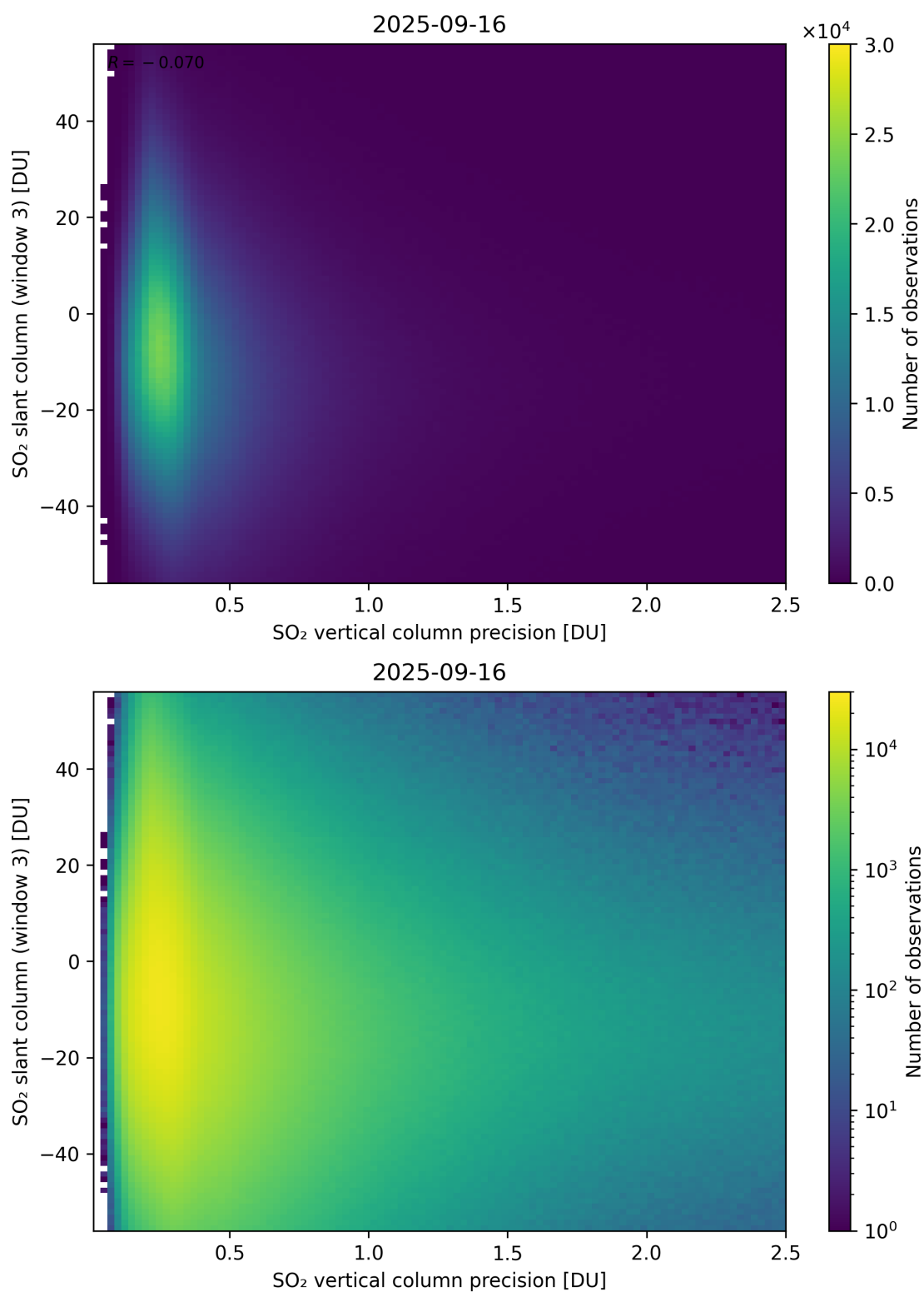
Figure 344: Scatter density plot of “SO 2 vertical column precision” against “SO 2 slant column (window 3)” for 2025-09-15 to 2025-09-17.
