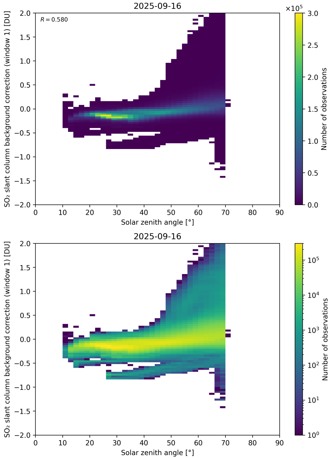
Figure 171: Scatter density plot of “Solar zenith angle” against “SO 2 slant column background correction (window 1)” for 2025-09-15 to 2025-09-17.
