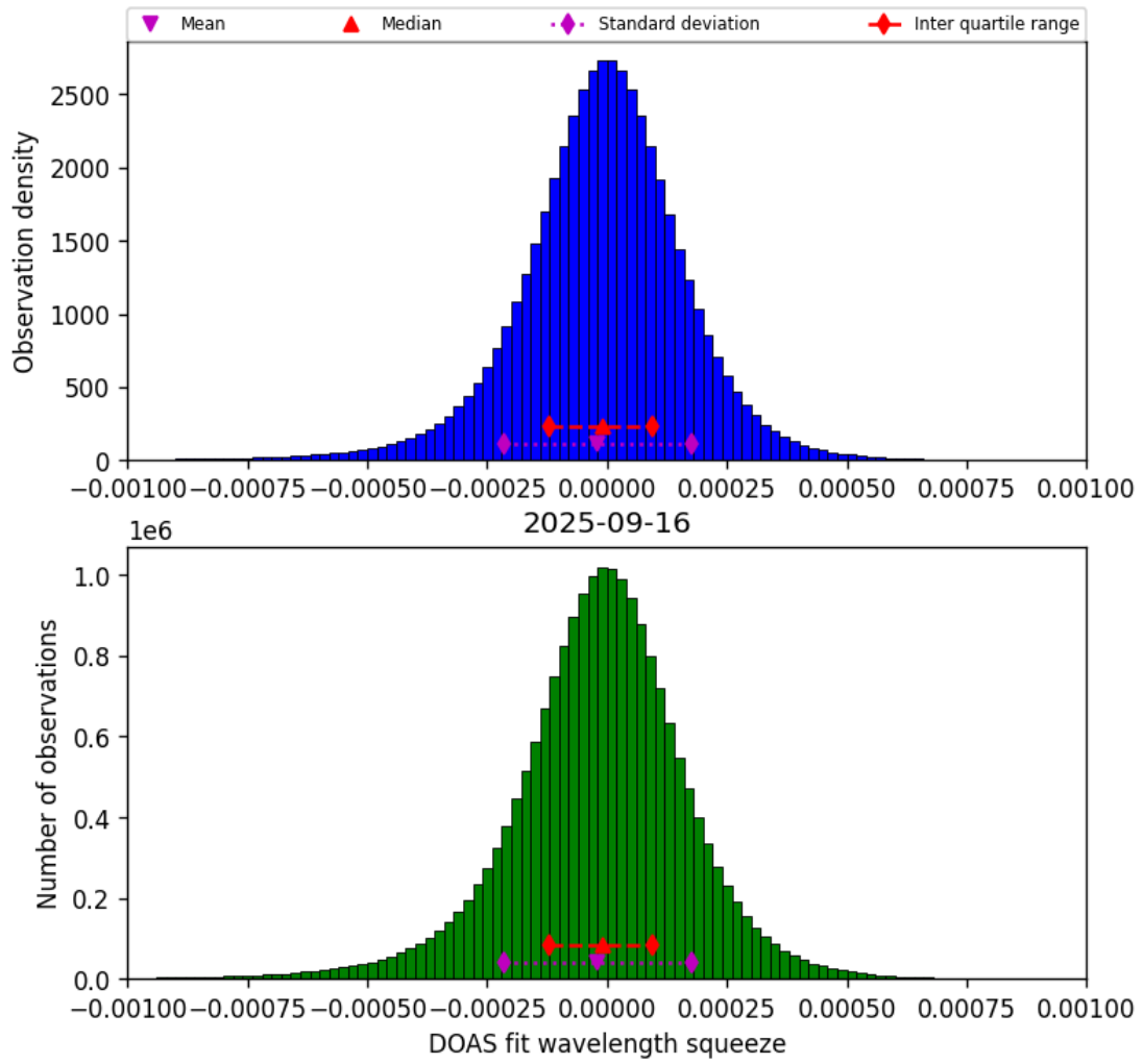
Figure 77: Histogram of “DOAS fit wavelength squeeze” for 2025-09-15 to 2025-09-17
