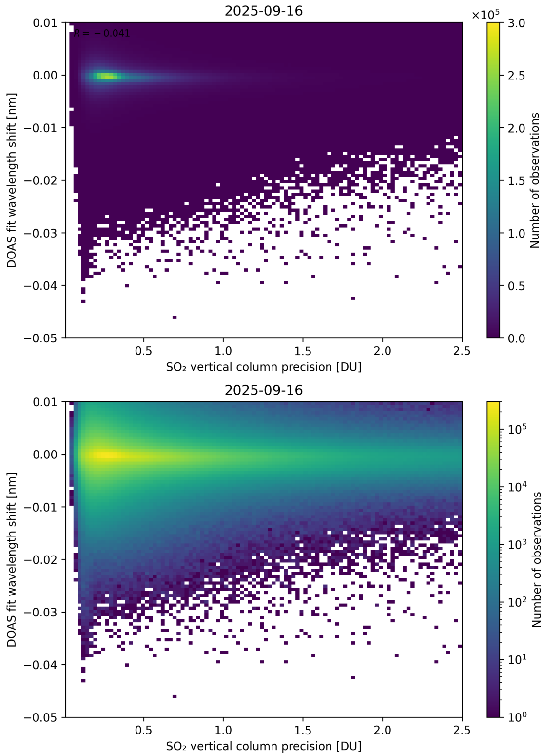
Figure 332: Scatter density plot of “SO 2 vertical column precision” against “DOAS fit wavelength shift” for 2025-09-15 to 2025-09-17.
