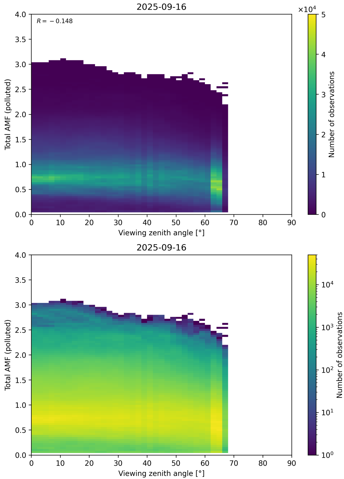
Figure 381: Scatter density plot of “Viewing zenith angle” against “Total AMF (polluted)” for 2025-09-15 to 2025-09-17.
