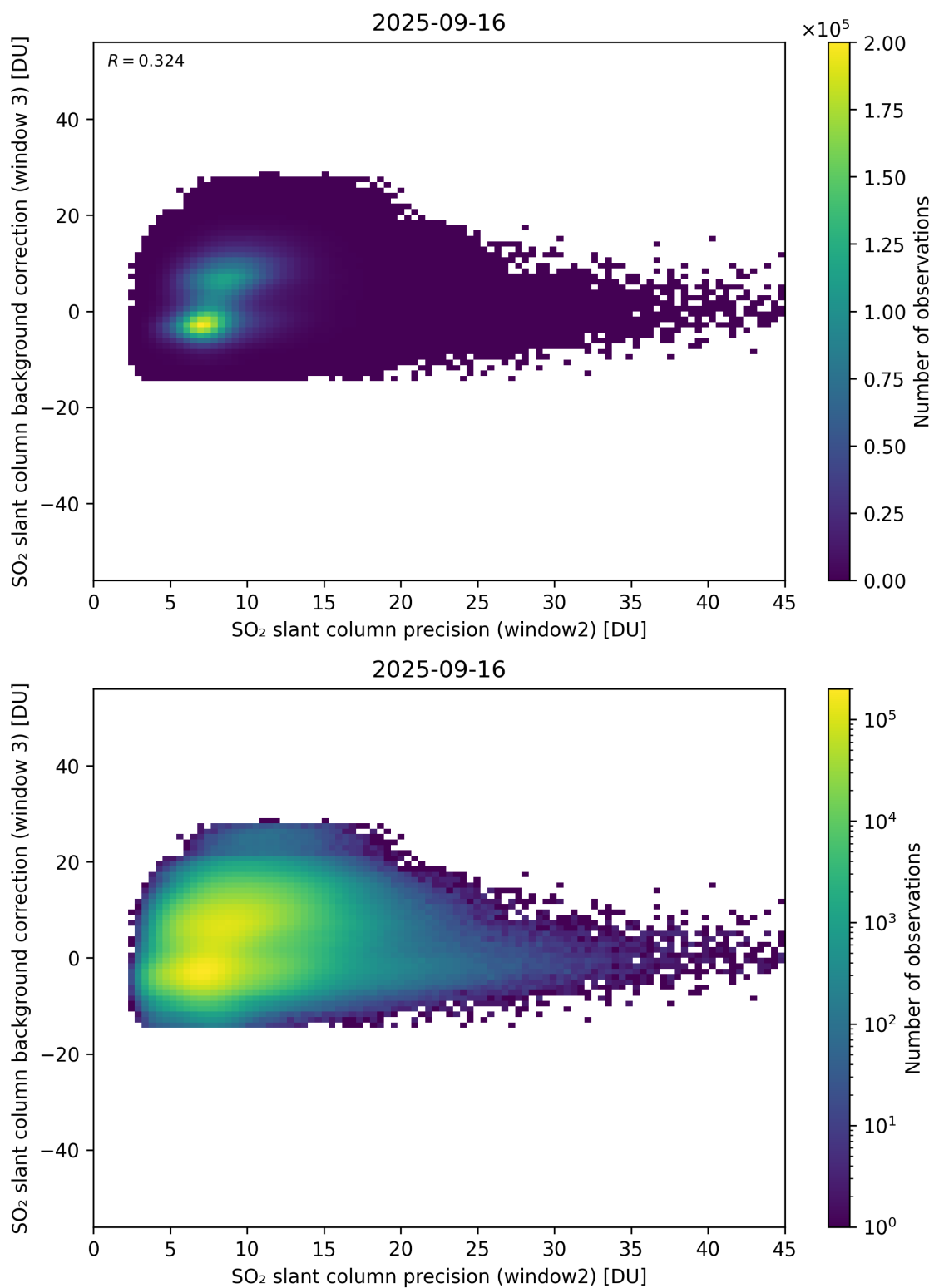
Figure 292: Scatter density plot of “SO 2 slant column precision (window2)” against “SO 2 slant column background correction (window 3)” for 2025-09-15 to 2025-09-17.
