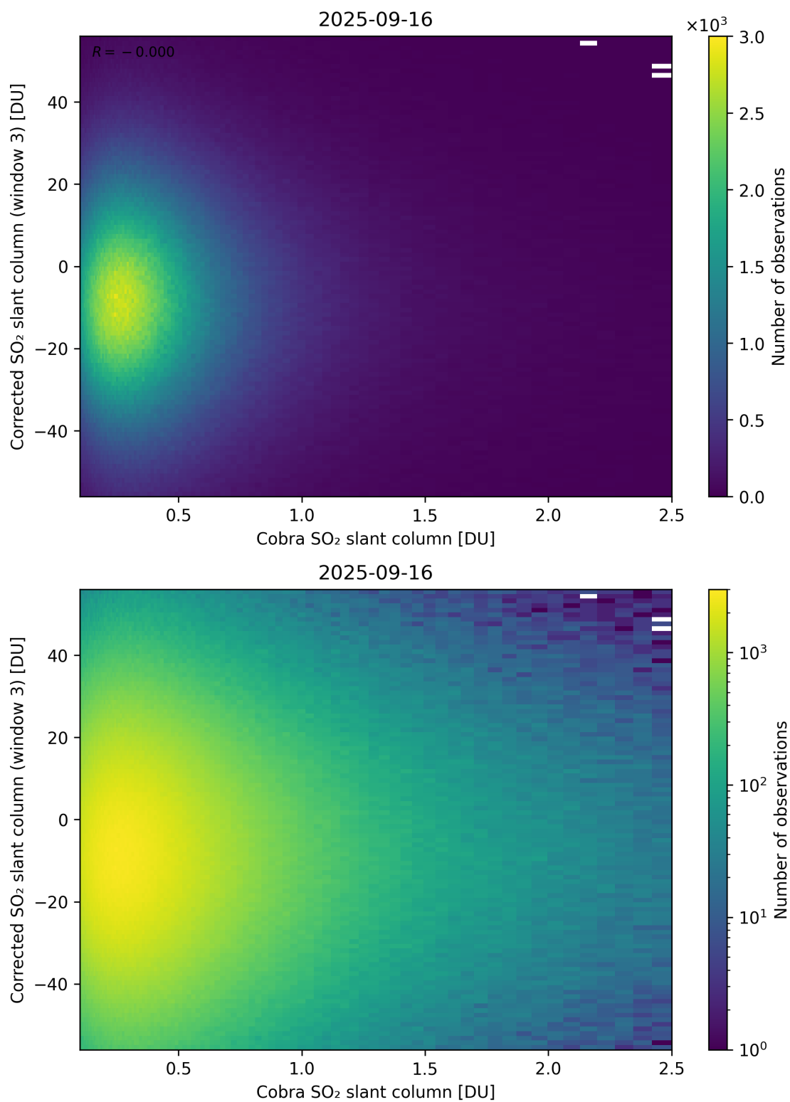
Figure 218: Scatter density plot of “Cobra SO 2 slant column” against “Corrected SO 2 slant column (window 3)” for 2025-09-15 to 2025-09-17.
