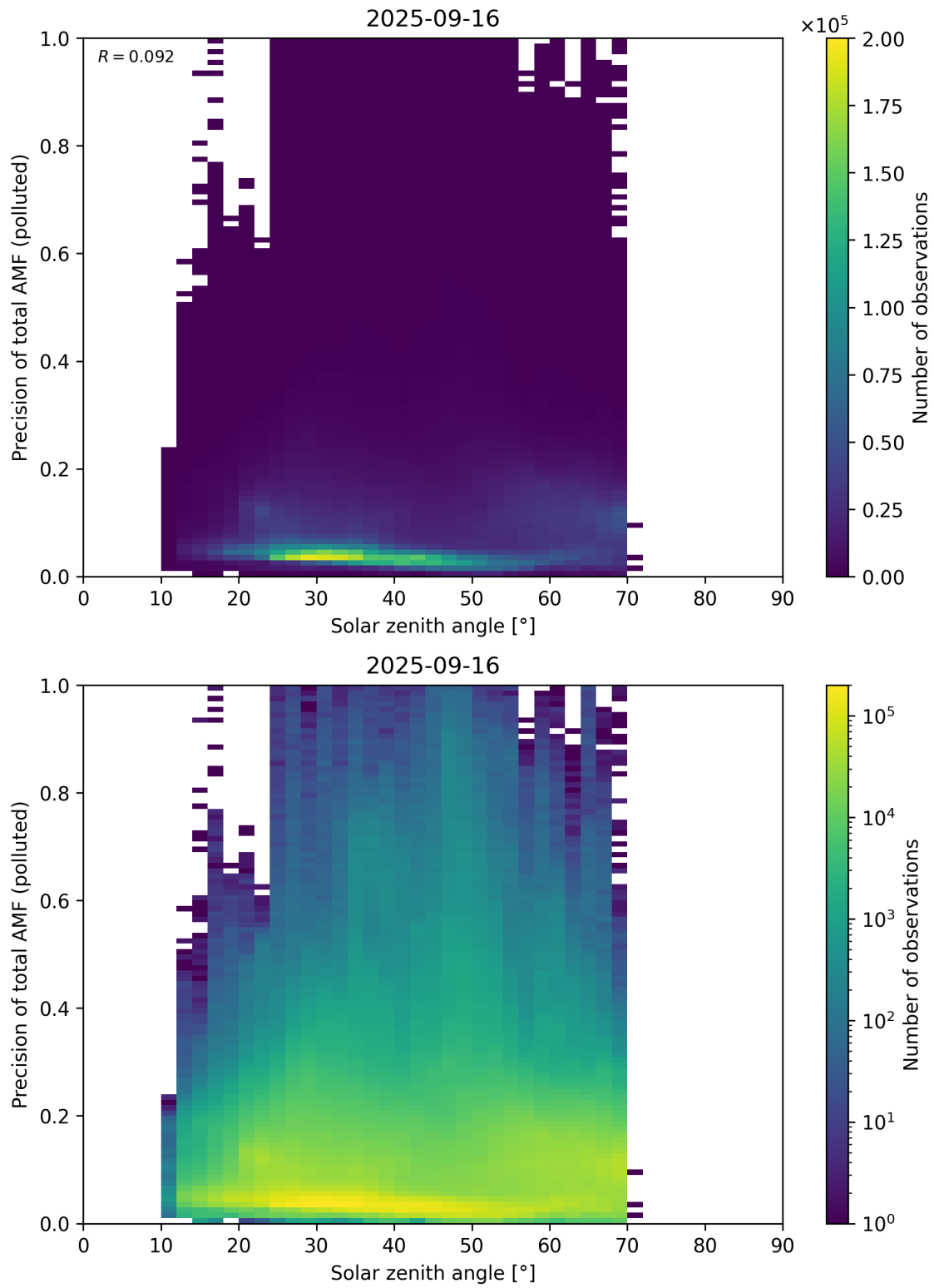
Figure 190: Scatter density plot of “Solar zenith angle” against “Precision of total AMF (polluted)” for 2025-09-15 to 2025-09-17.
