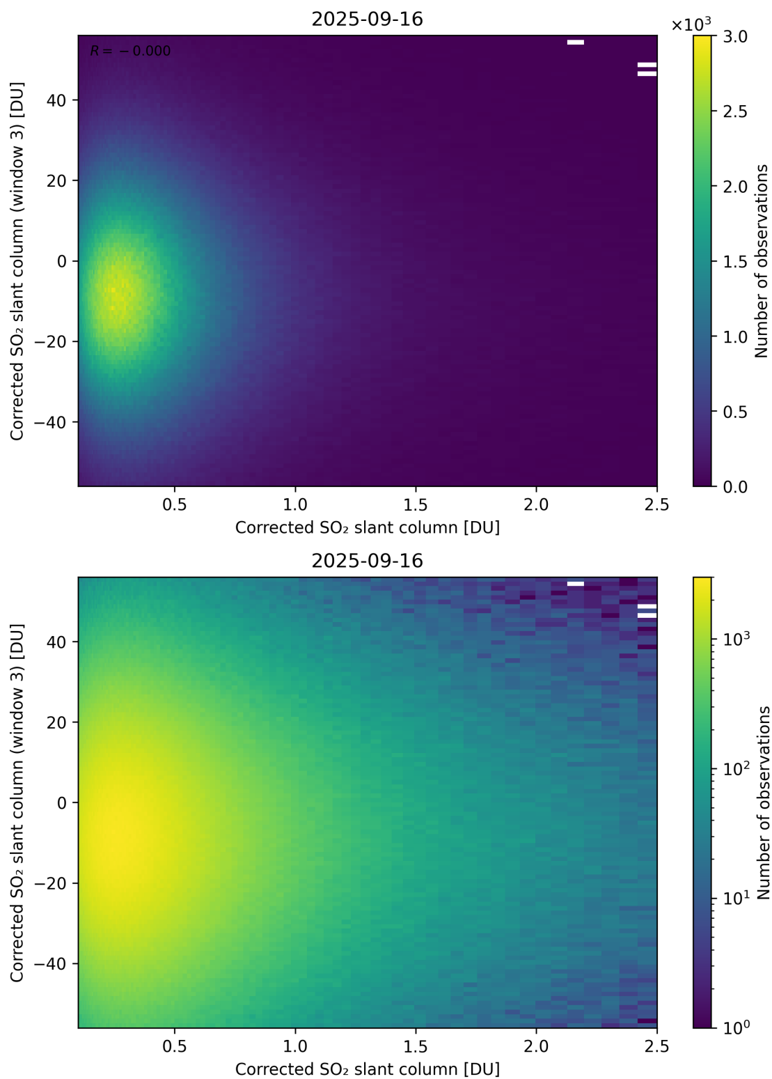
Figure 236: Scatter density plot of “Corrected SO 2 slant column” against “Corrected SO 2 slant column (window 3)” for 2025-09-15 to 2025-09-17.
