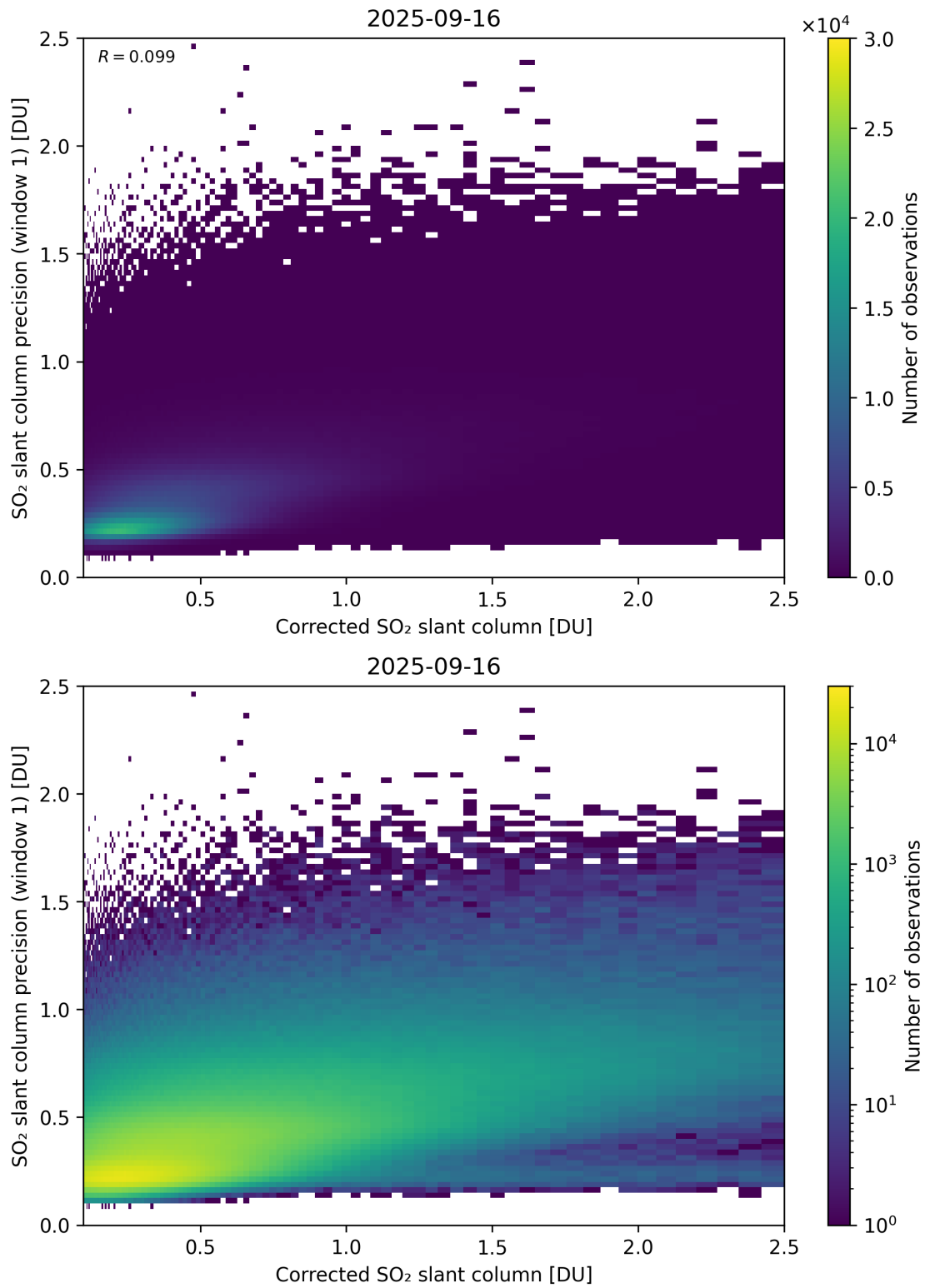
Figure 238: Scatter density plot of “Corrected SO 2 slant column” against “SO 2 slant column precision (window 1)” for 2025-09-15 to 2025-09-17.
