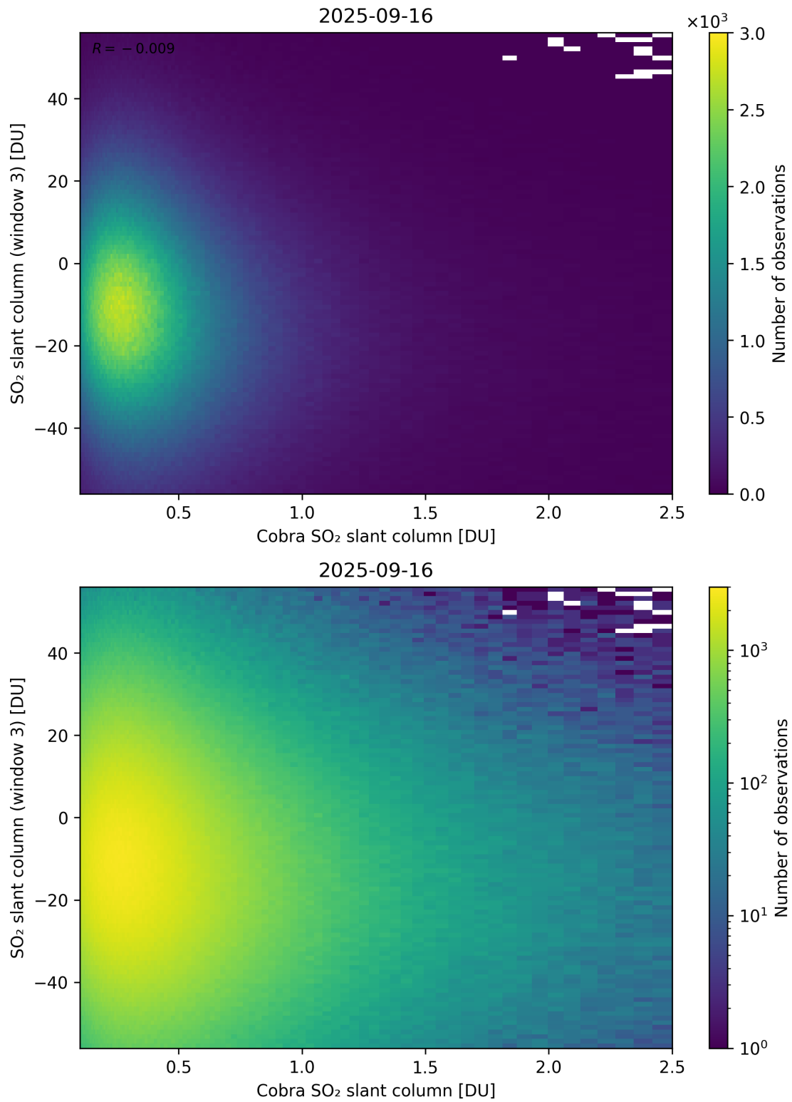
Figure 222: Scatter density plot of “Cobra SO 2 slant column” against “SO 2 slant column (window 3)” for 2025-09-15 to 2025-09-17.
