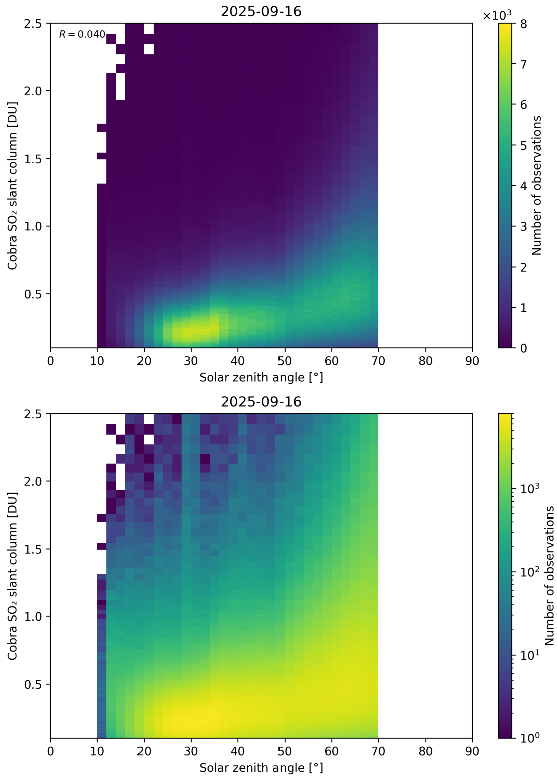
Figure 179: Scatter density plot of “Solar zenith angle” against “Cobra SO 2 slant column” for 2025-09-15 to 2025-09-17.
