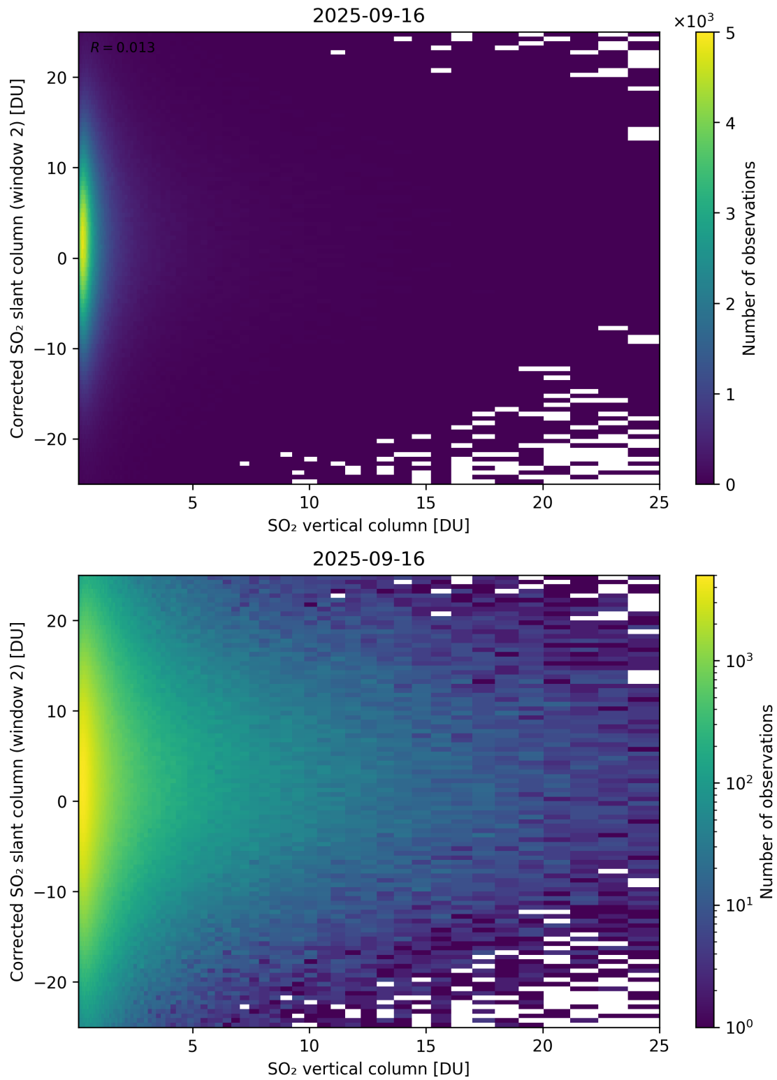
Figure 352: Scatter density plot of “SO 2 vertical column” against “Corrected SO 2 slant column (window 2)” for 2025-09-15 to 2025-09-17.
