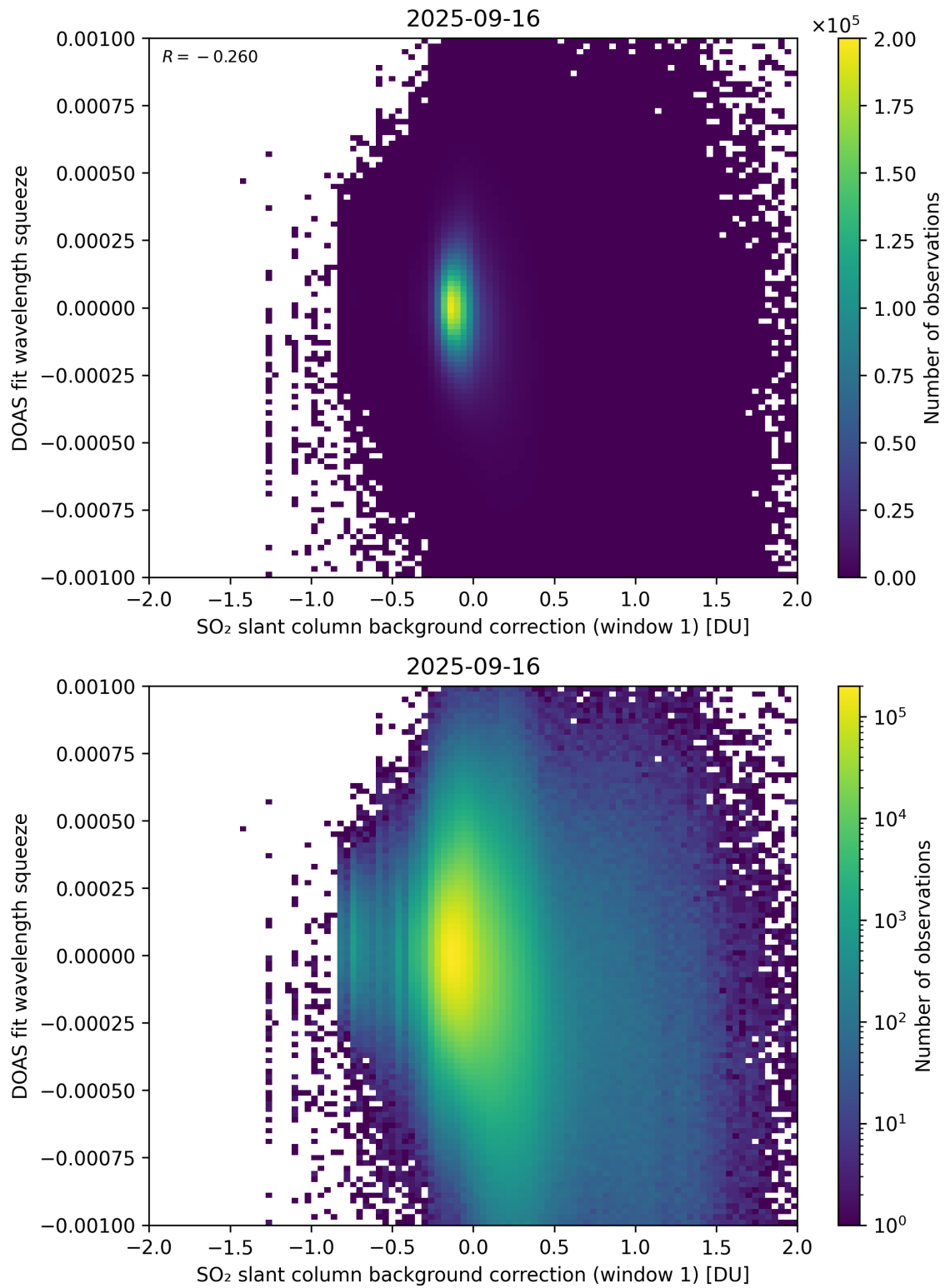
Figure 112: Scatter density plot of “SO 2 slant column background correction (window 1)” against “DOAS fit wavelength squeeze” for 2025-09-15 to 2025-09-17.
