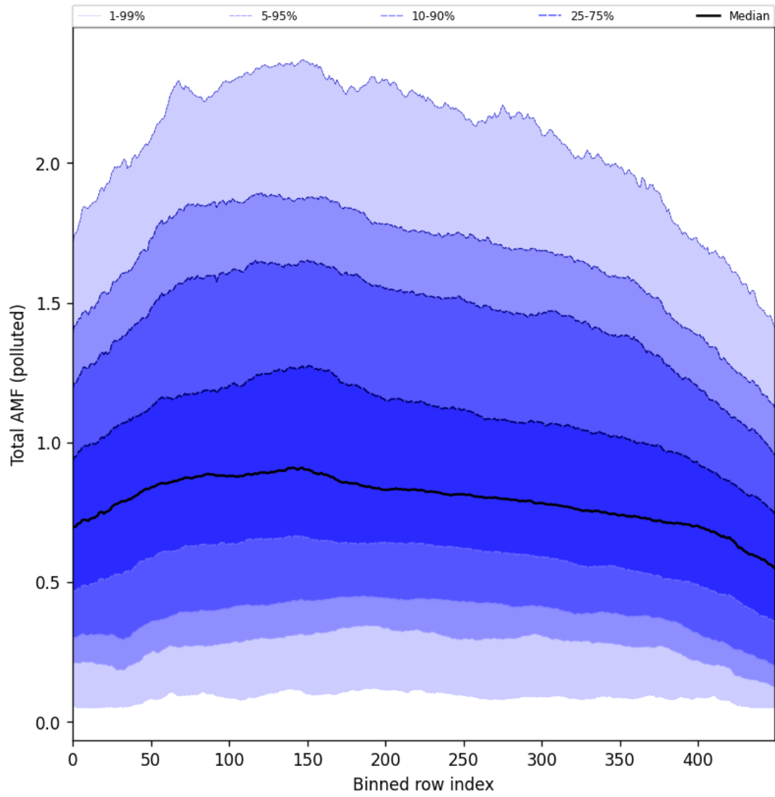
Figure 105: Along track statistics of “Total AMF (polluted)” for 2025-09-15 to 2025-09-17
