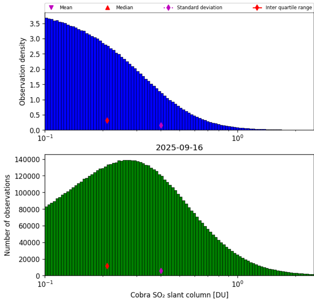
Figure 61: Histogram of “Cobra SO 2 slant column” for 2025-09-15 to 2025-09-17
