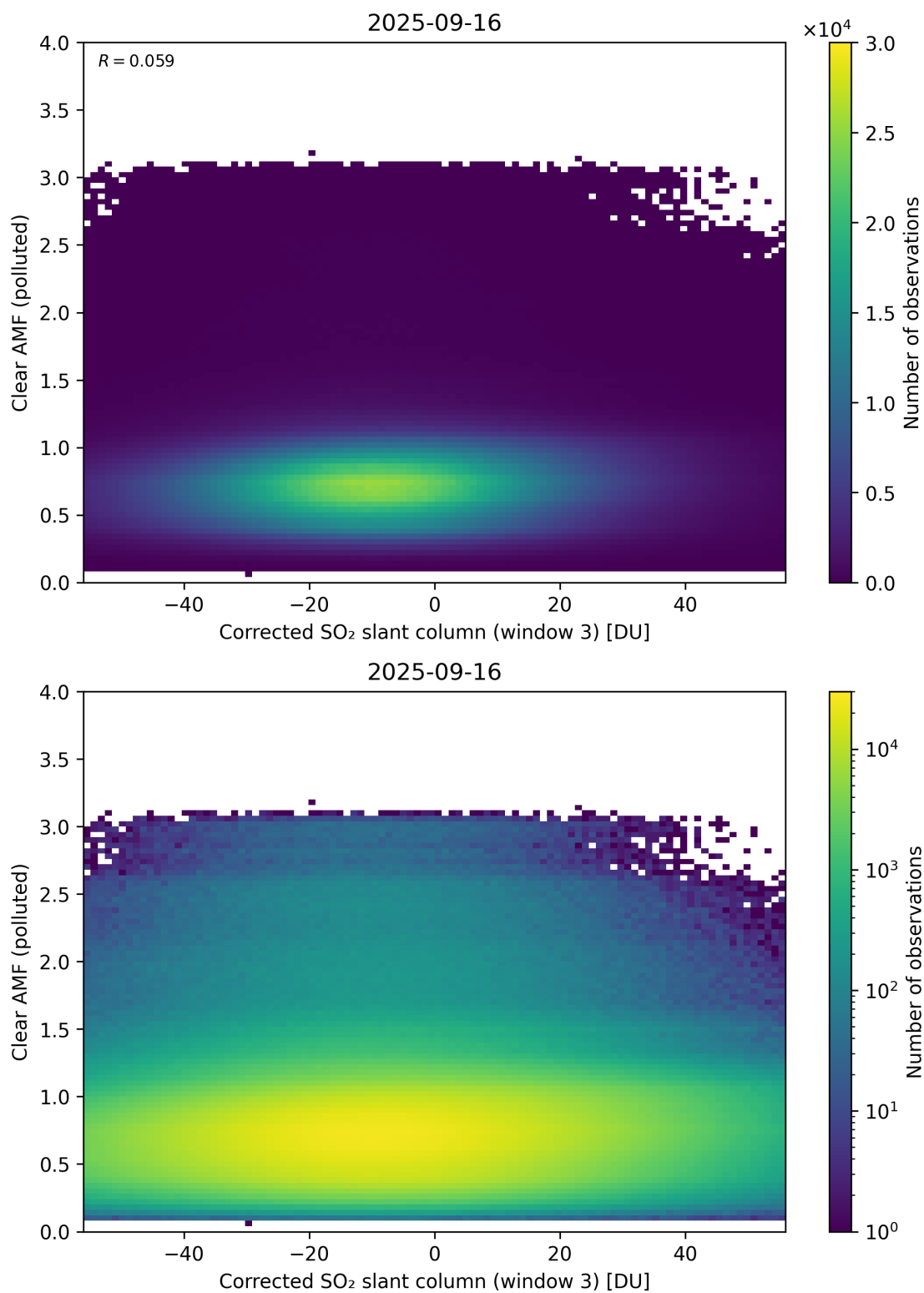
Figure 259: Scatter density plot of “Corrected SO 2 slant column (window 3)” against “Clear AMF (polluted)” for 2025-09-15 to 2025-09-17.
