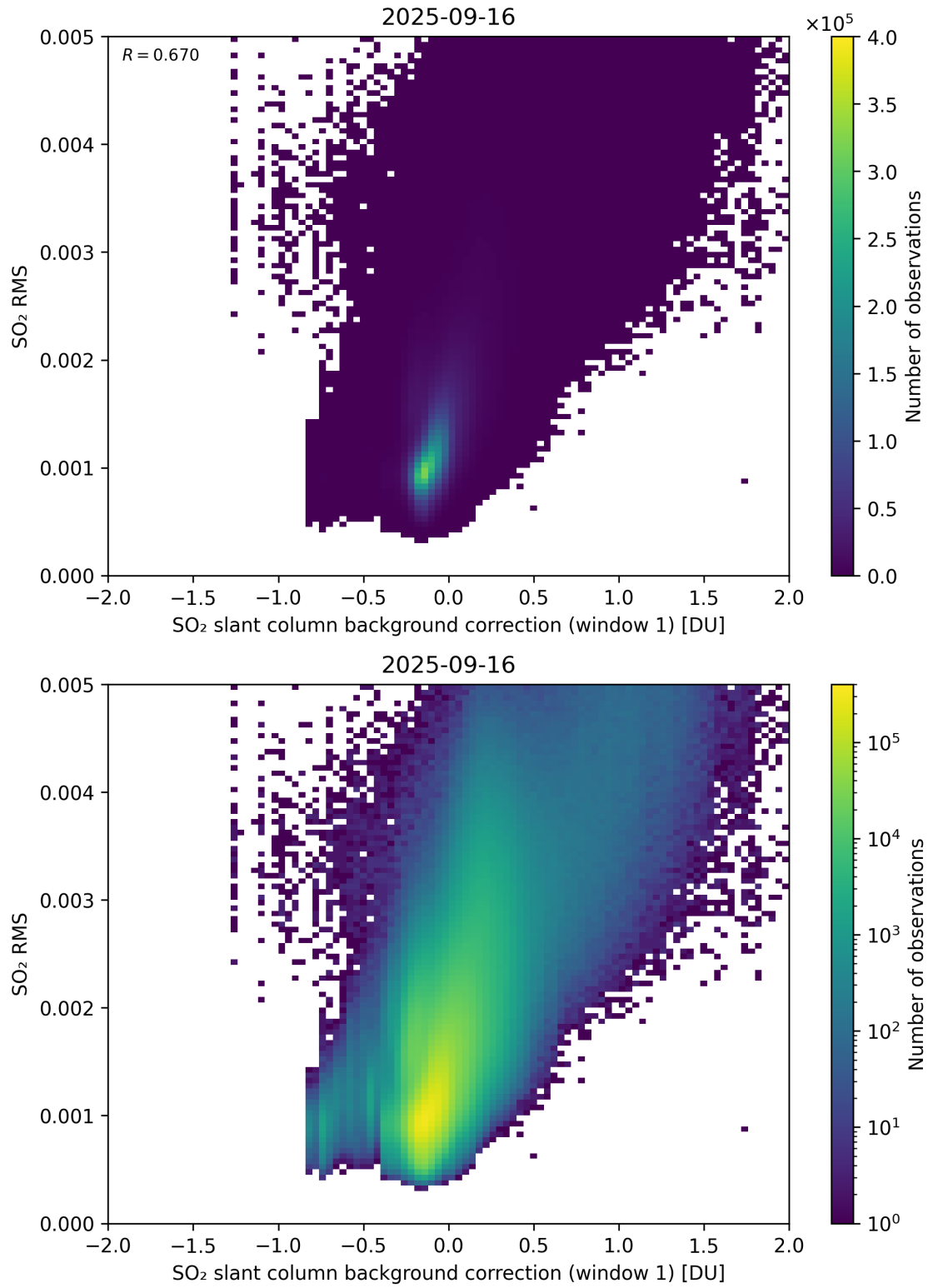
Figure 113: Scatter density plot of “SO 2 slant column background correction (window 1)” against “SO 2 RMS” for 2025-09-15 to 2025-09-17.
