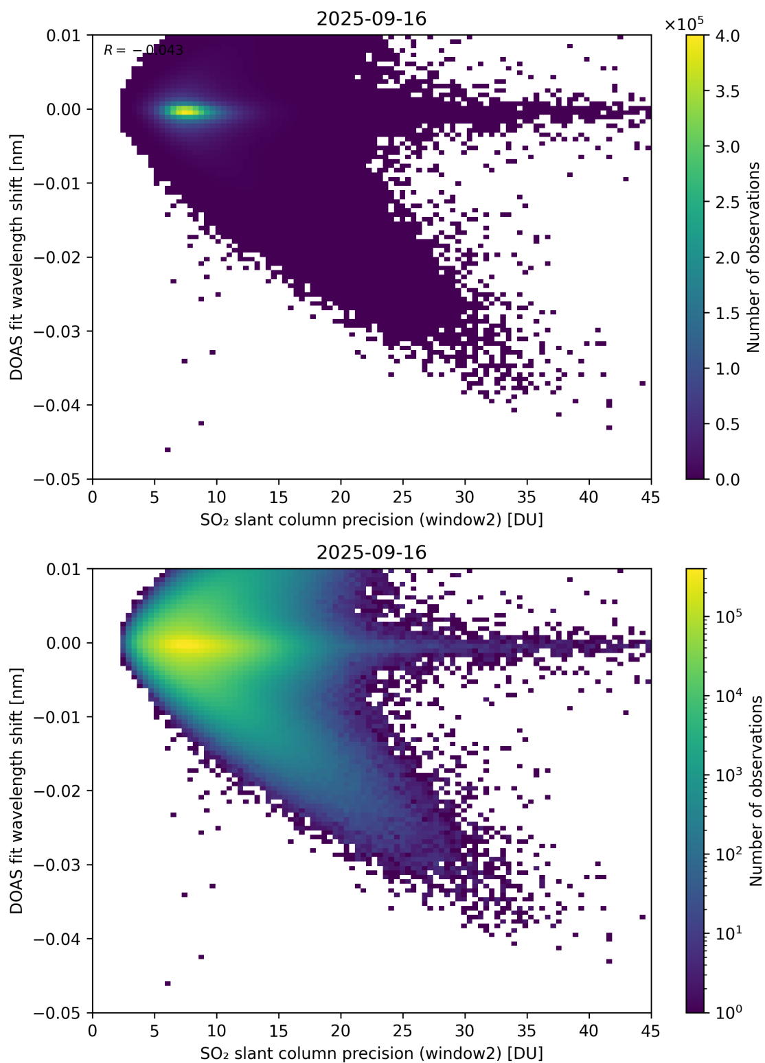
Figure 293: Scatter density plot of “SO 2 slant column precision (window2)” against “DOAS fit wavelength shift” for 2025-09-15 to 2025-09-17.
