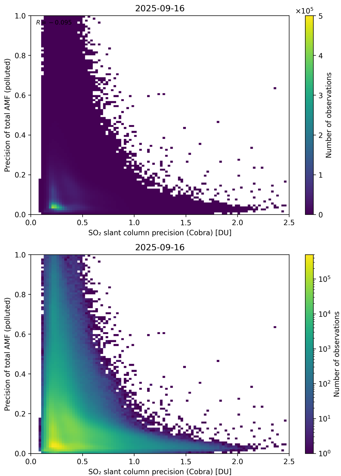
Figure 214: Scatter density plot of “SO 2 slant column precision (Cobra)” against “Precision of total AMF (polluted)” for 2025-09-15 to 2025-09-17.
