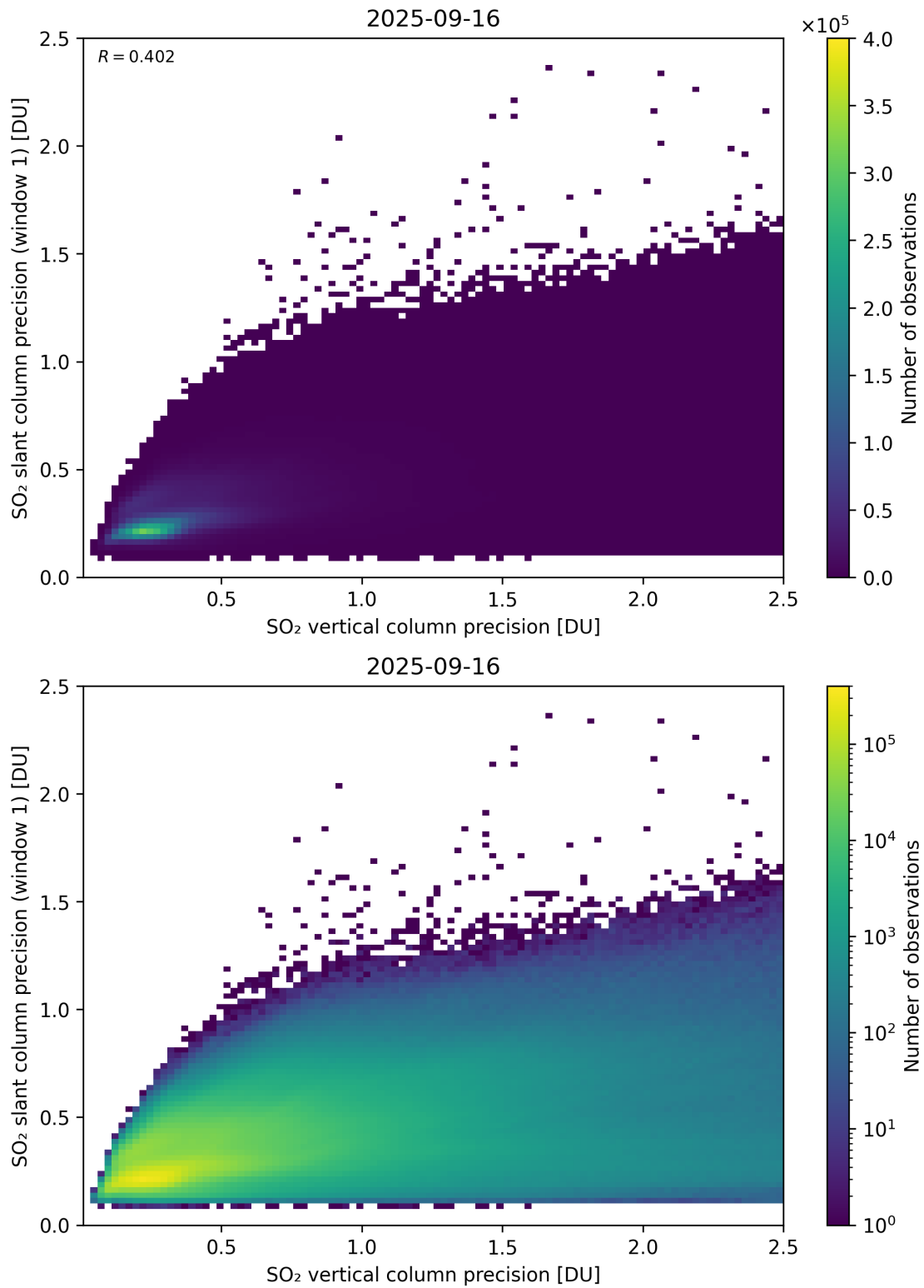
Figure 342: Scatter density plot of “SO 2 vertical column precision” against “SO 2 slant column precision (window 1)” for 2025-09-15 to 2025-09-17.
