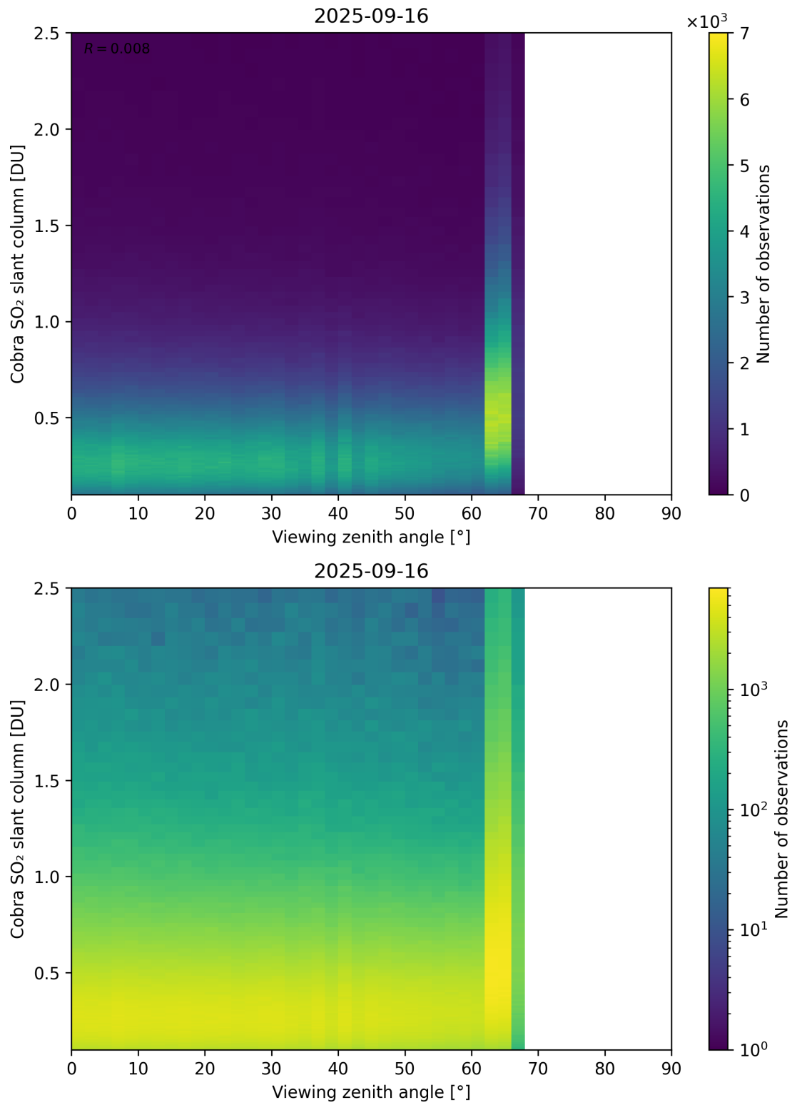
Figure 371: Scatter density plot of “Viewing zenith angle” against “Cobra SO 2 slant column” for 2025-09-15 to 2025-09-17.
