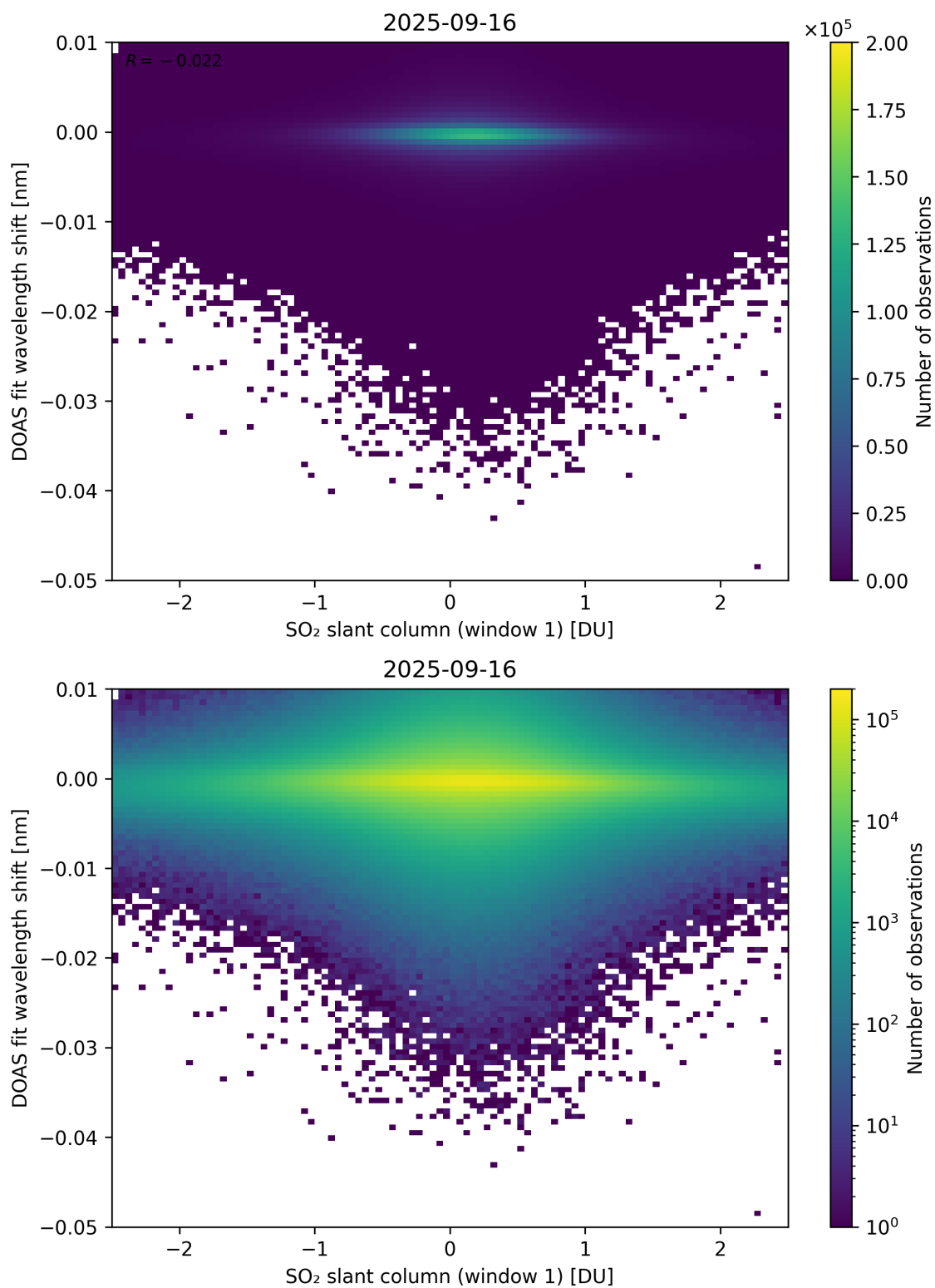
Figure 265: Scatter density plot of “SO 2 slant column (window 1)” against “DOAS fit wavelength shift” for 2025-09-15 to 2025-09-17.
