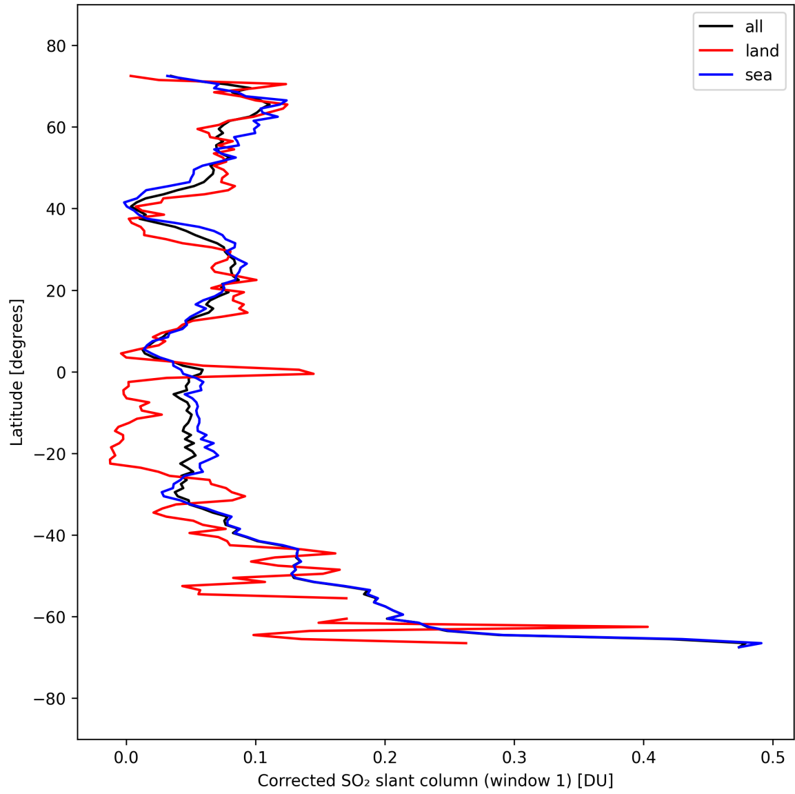
Figure 39: Zonal average of “Corrected SO 2 slant column (window 1)” for 2025-09-15 to 2025-09-17.
