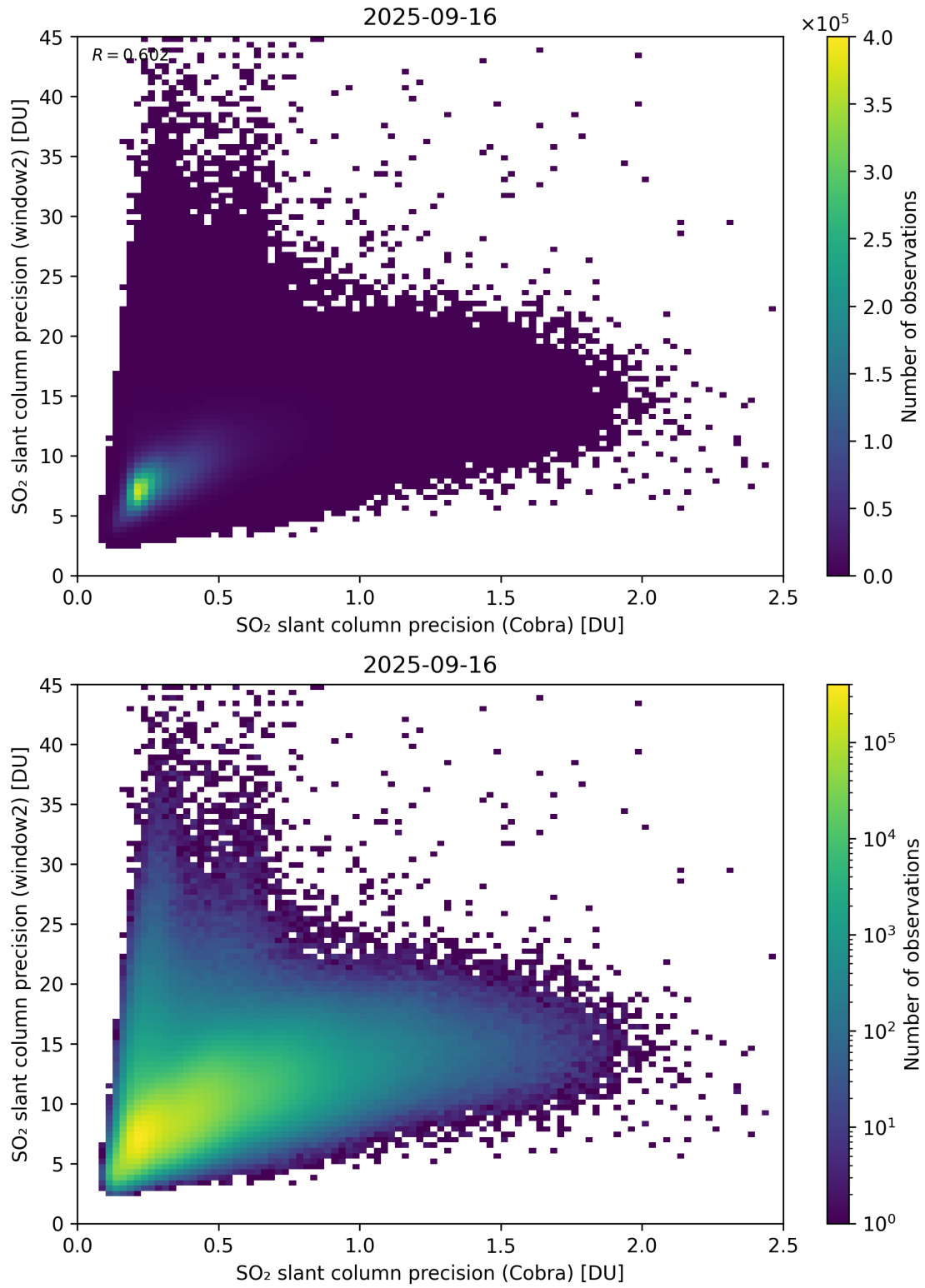
Figure 210: Scatter density plot of “SO 2 slant column precision (Cobra)” against “SO 2 slant column precision (window2)” for 2025-09-15 to 2025-09-17.
