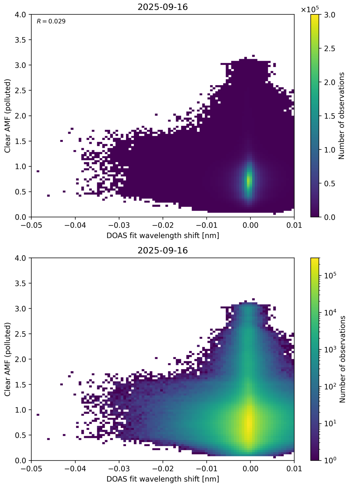
Figure 140: Scatter density plot of “DOAS fit wavelength shift” against “Clear AMF (polluted)” for 2025-09-15 to 2025-09-17.
