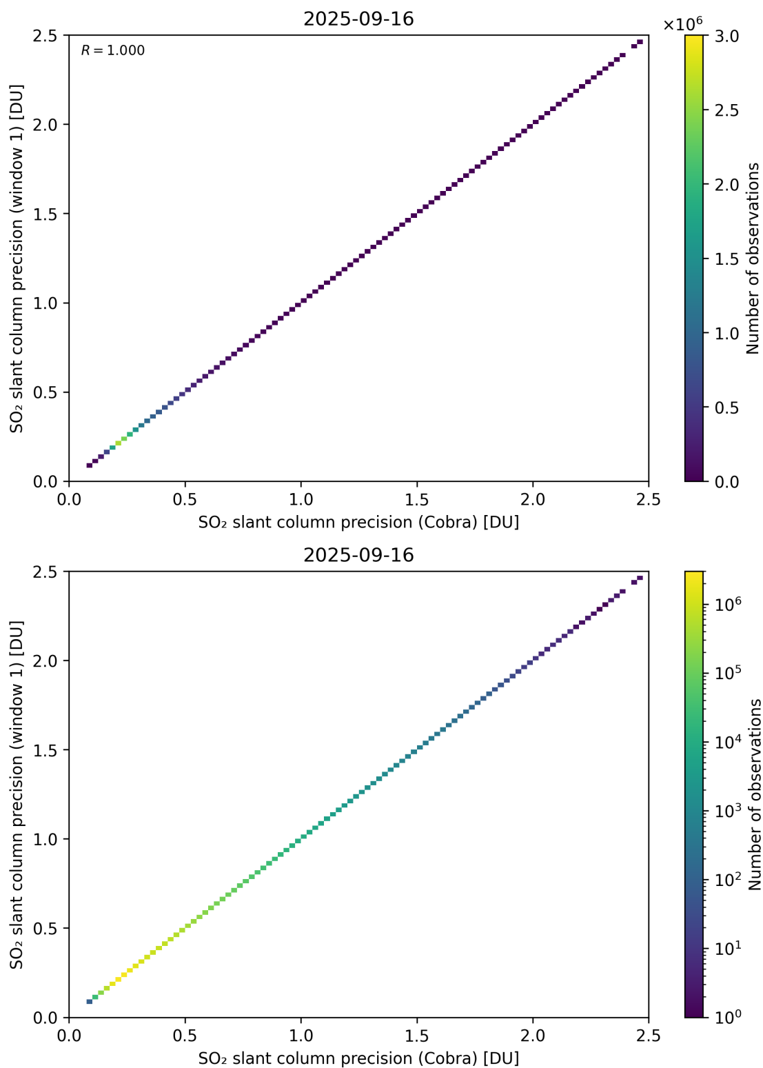
Figure 209: Scatter density plot of “SO 2 slant column precision (Cobra)” against “SO 2 slant column precision (window 1)” for 2025-09-15 to 2025-09-17.
