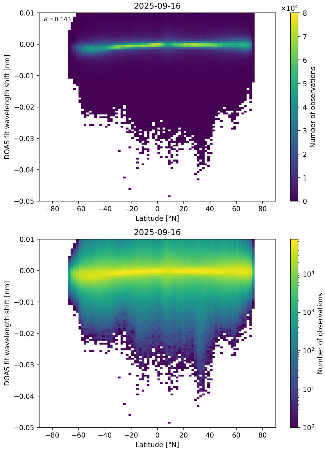
Figure 153: Scatter density plot of “Latitude” against “DOAS fit wavelength shift” for 2025-09-15 to 2025-09-17.
