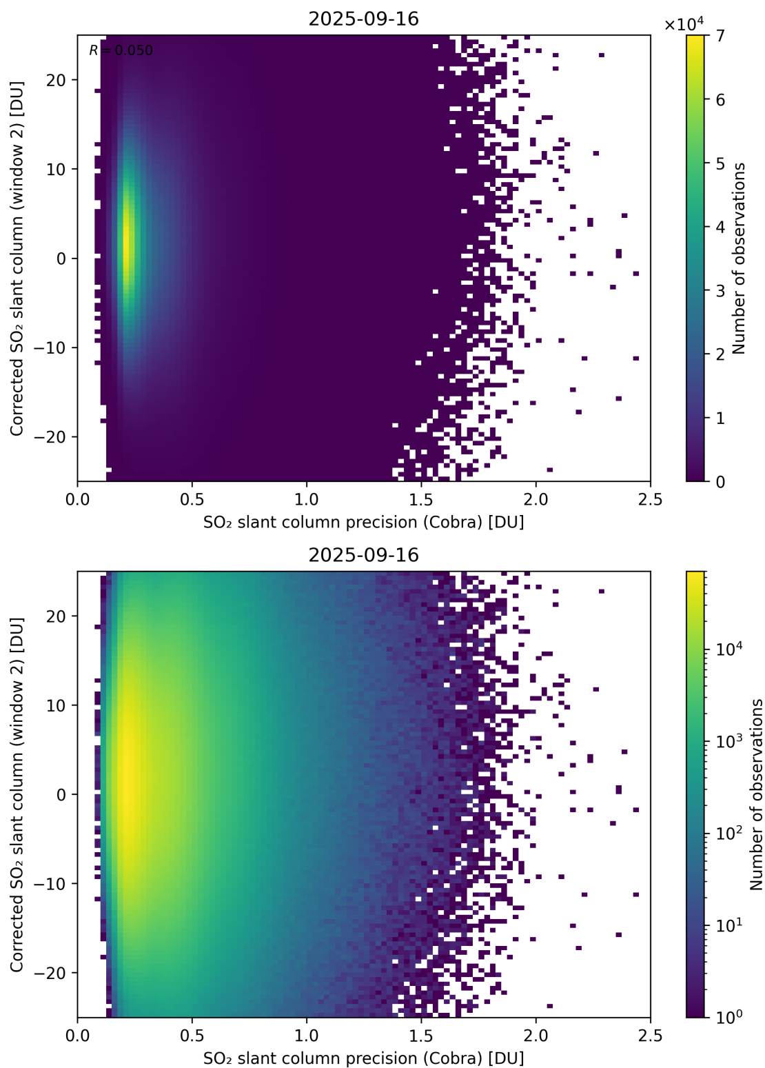
Figure 206: Scatter density plot of “SO 2 slant column precision (Cobra)” against “Corrected SO 2 slant column (window 2)” for 2025-09-15 to 2025-09-17.
