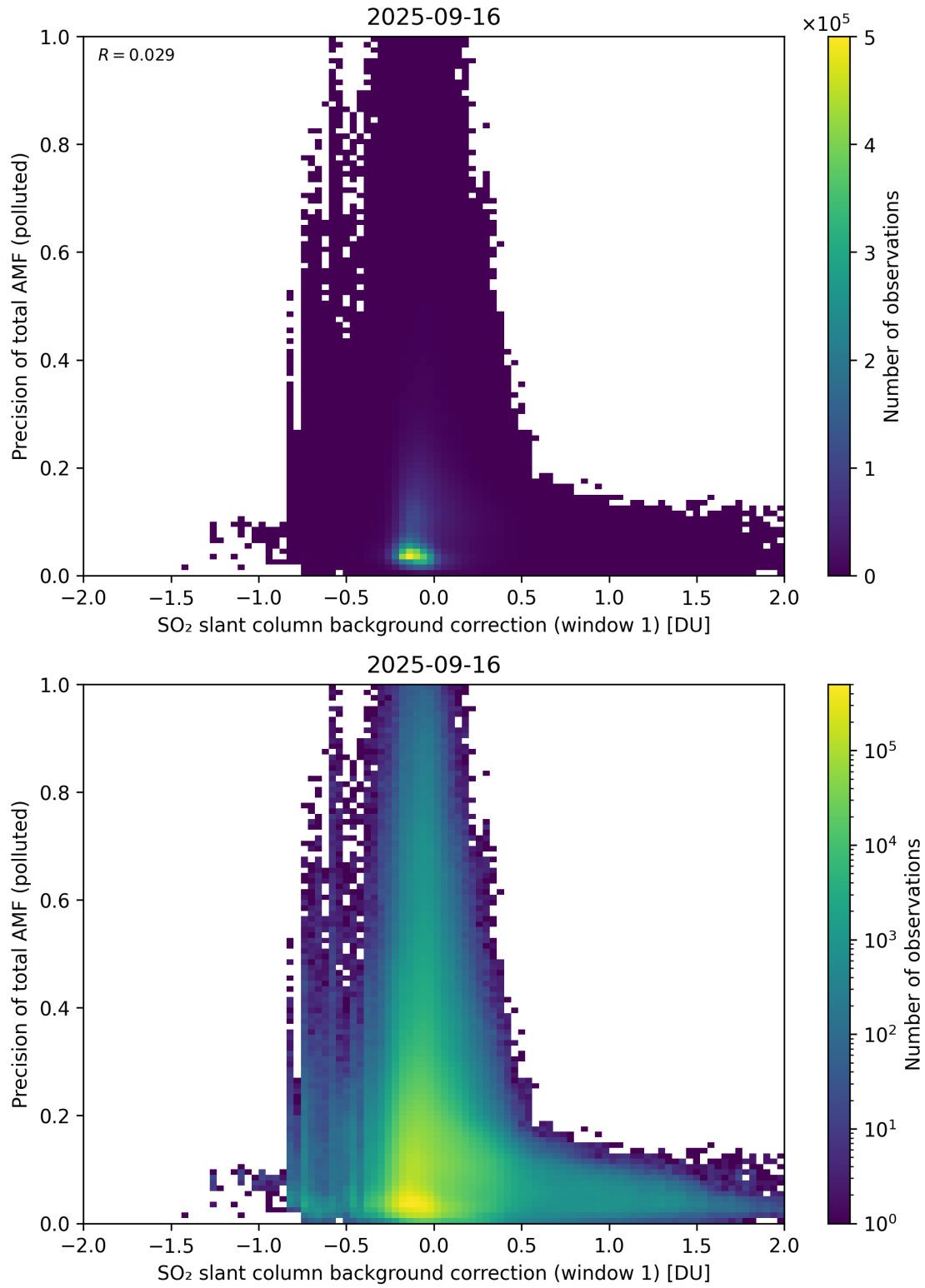
Figure 121: Scatter density plot of “SO 2 slant column background correction (window 1)” against “Precision of total AMF (polluted)” for 2025-09-15 to 2025-09-17.
