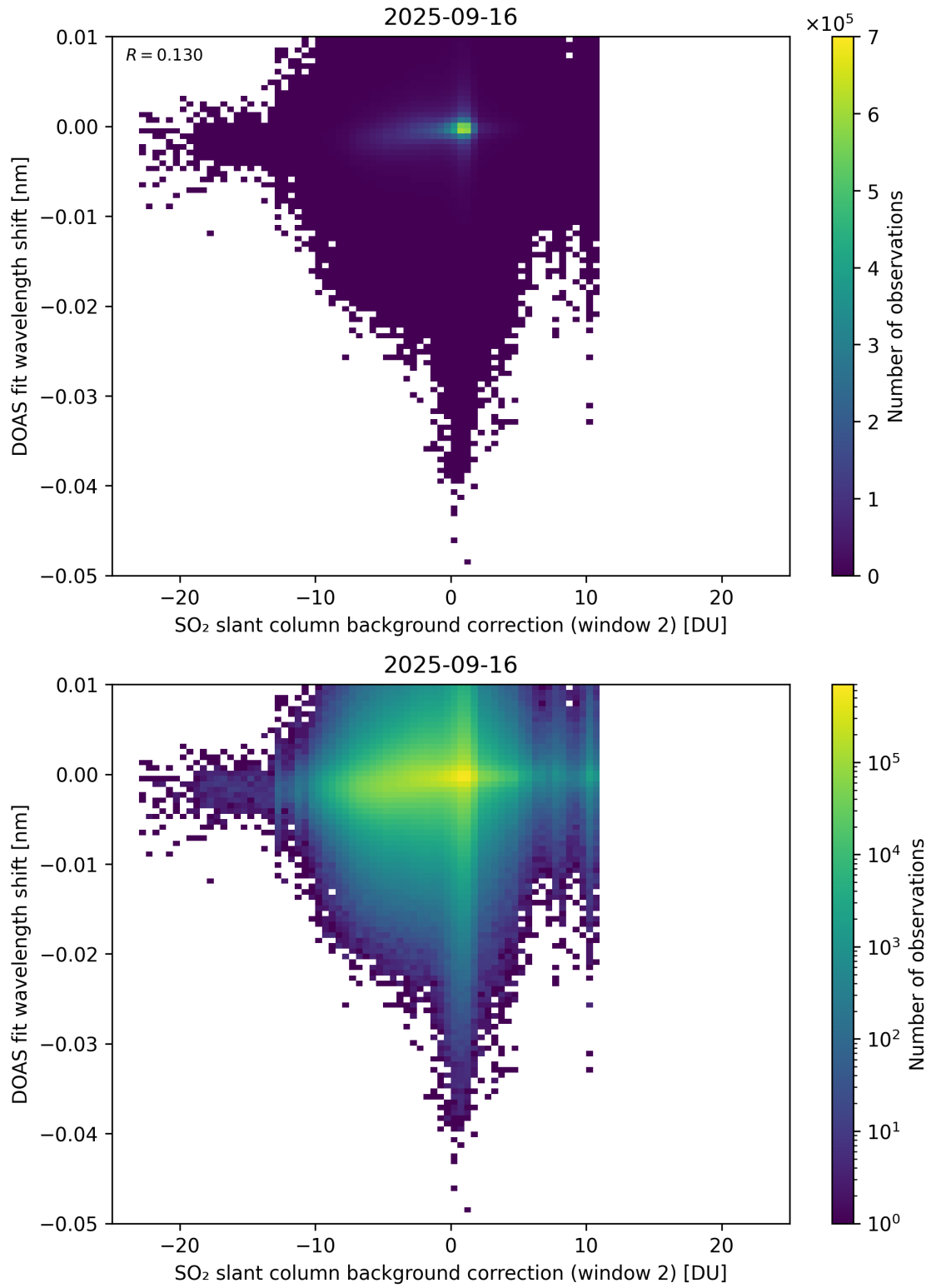
Figure 123: Scatter density plot of “SO 2 slant column background correction (window 2)” against “DOAS fit wavelength shift” for 2025-09-15 to 2025-09-17.
