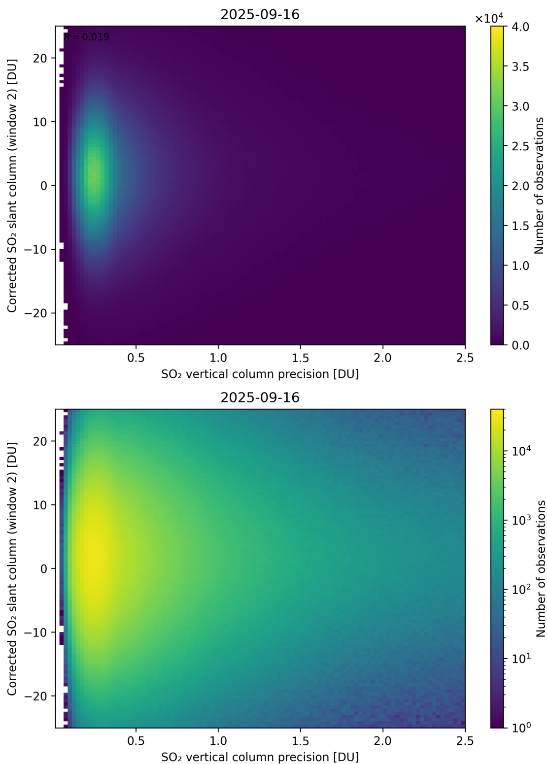
Figure 339: Scatter density plot of “SO 2 vertical column precision” against “Corrected SO 2 slant column (window 2)” for 2025-09-15 to 2025-09-17.
