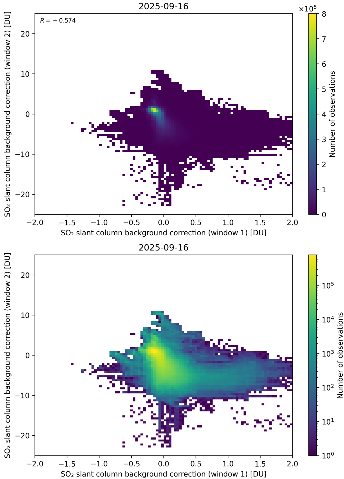
Figure 109: Scatter density plot of “SO 2 slant column background correction (window 1)” against “SO 2 slant column background correction (window 2)” for 2025-09-15 to 2025-09-17.
