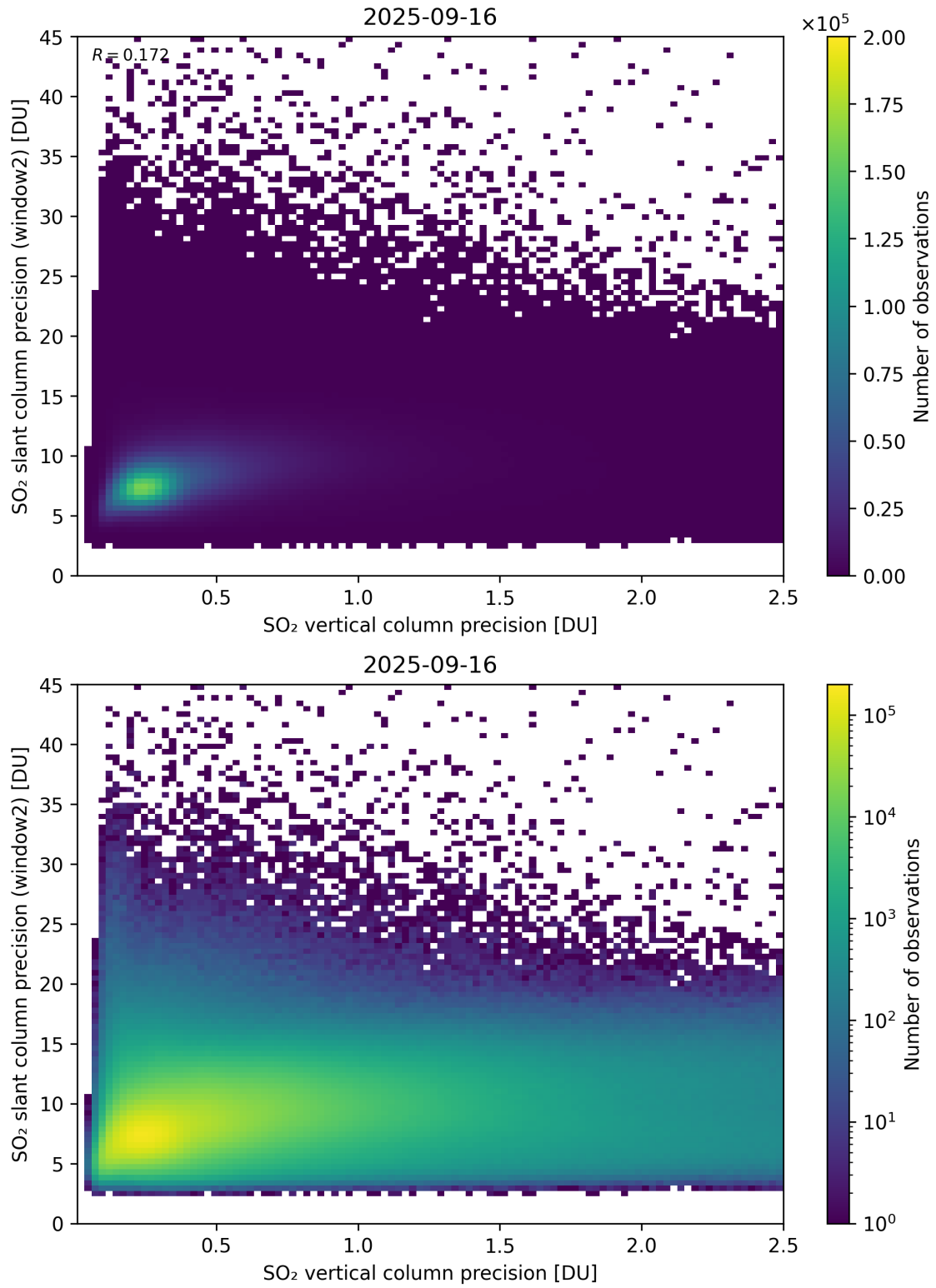
Figure 343: Scatter density plot of “SO 2 vertical column precision” against “SO 2 slant column precision (window2)” for 2025-09-15 to 2025-09-17.
