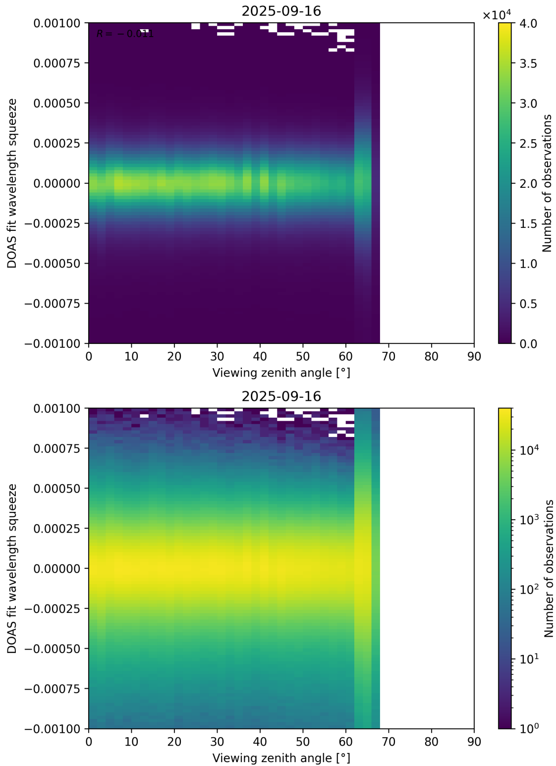
Figure 366: Scatter density plot of “Viewing zenith angle” against “DOAS fit wavelength squeeze” for 2025-09-15 to 2025-09-17.
