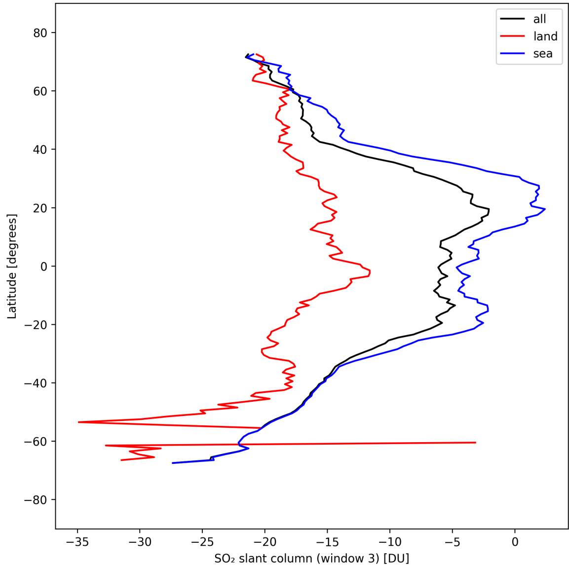
Figure 45: Zonal average of “SO 2 slant column (window 3)” for 2025-09-15 to 2025-09-17.
