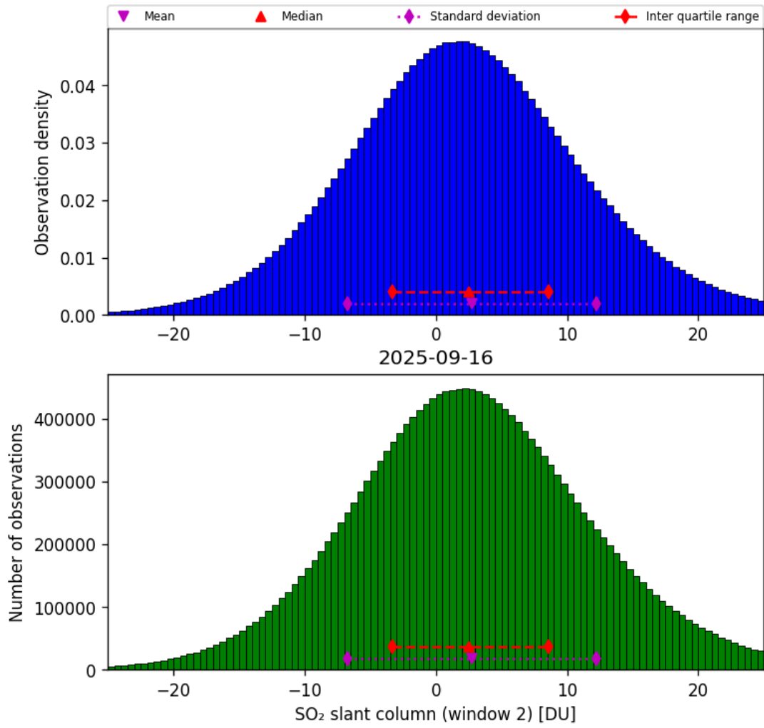
Figure 67: Histogram of “SO 2 slant column (window 2)” for 2025-09-15 to 2025-09-17
