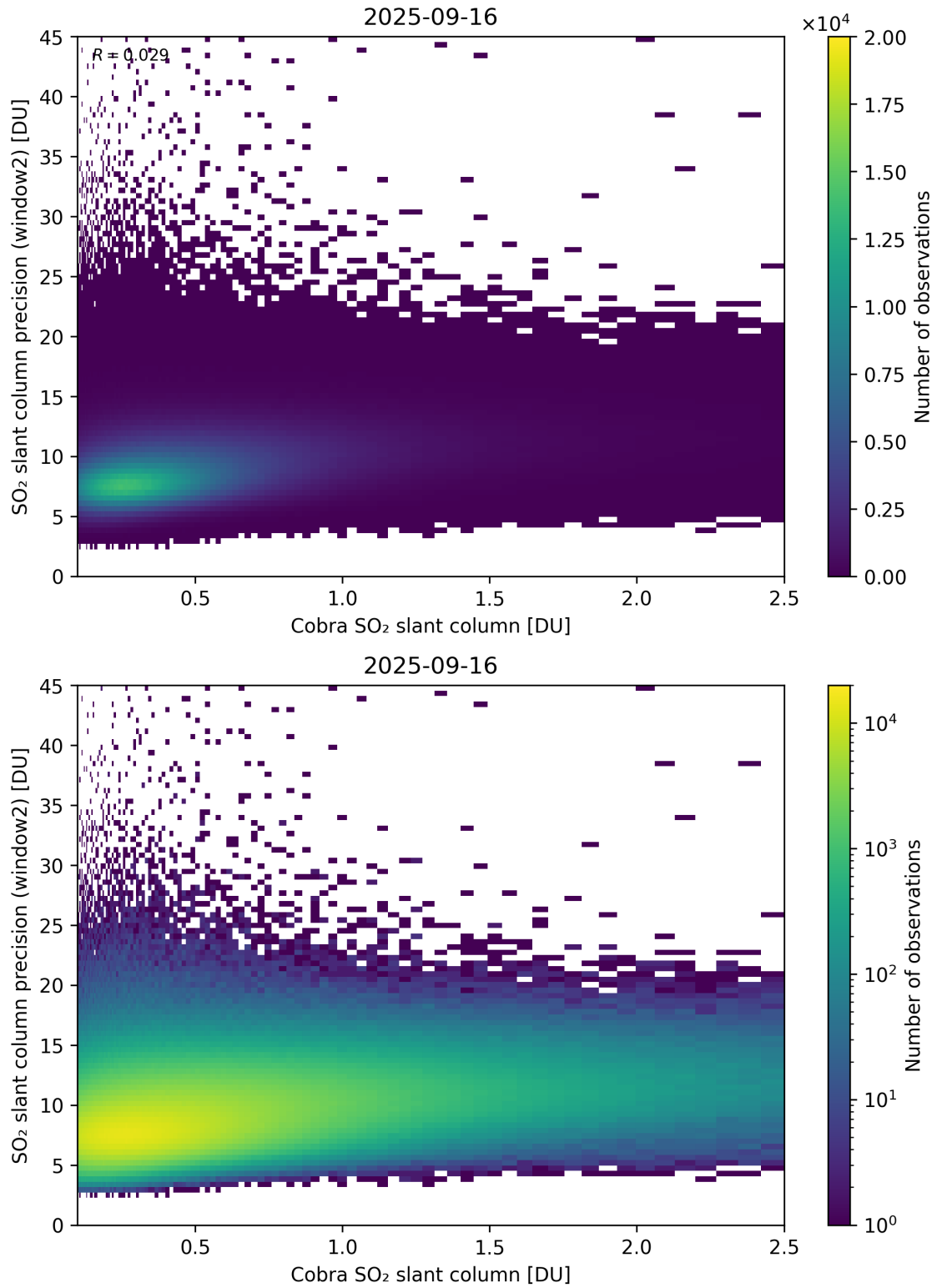
Figure 221: Scatter density plot of “Cobra SO 2 slant column” against “SO 2 slant column precision (window2)” for 2025-09-15 to 2025-09-17.
