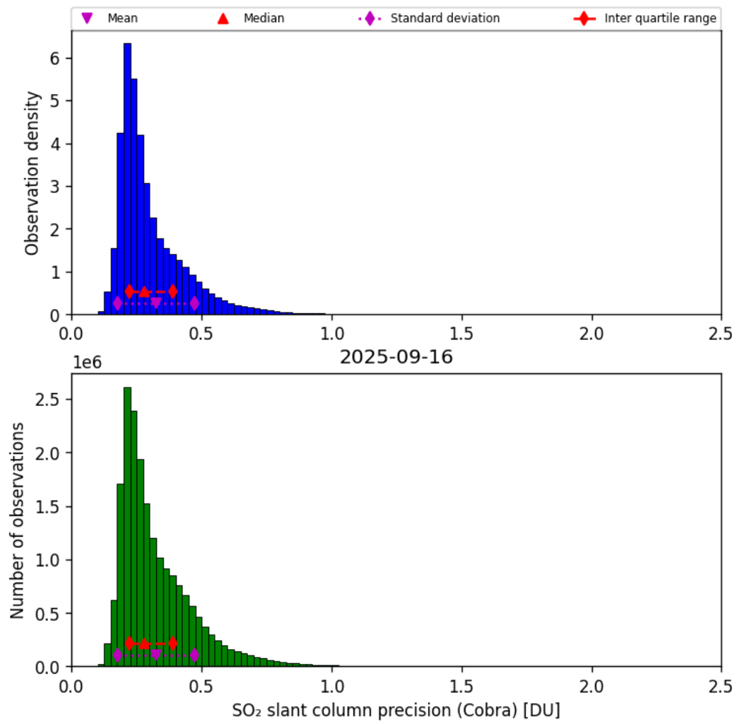
Figure 62: Histogram of “SO 2 slant column precision (Cobra)” for 2025-09-15 to 2025-09-17
