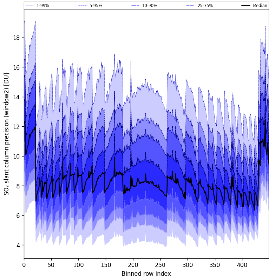
Figure 94: Along track statistics of “SO 2 slant column precision (window2)” for 2025-09-15 to 2025-09-17
