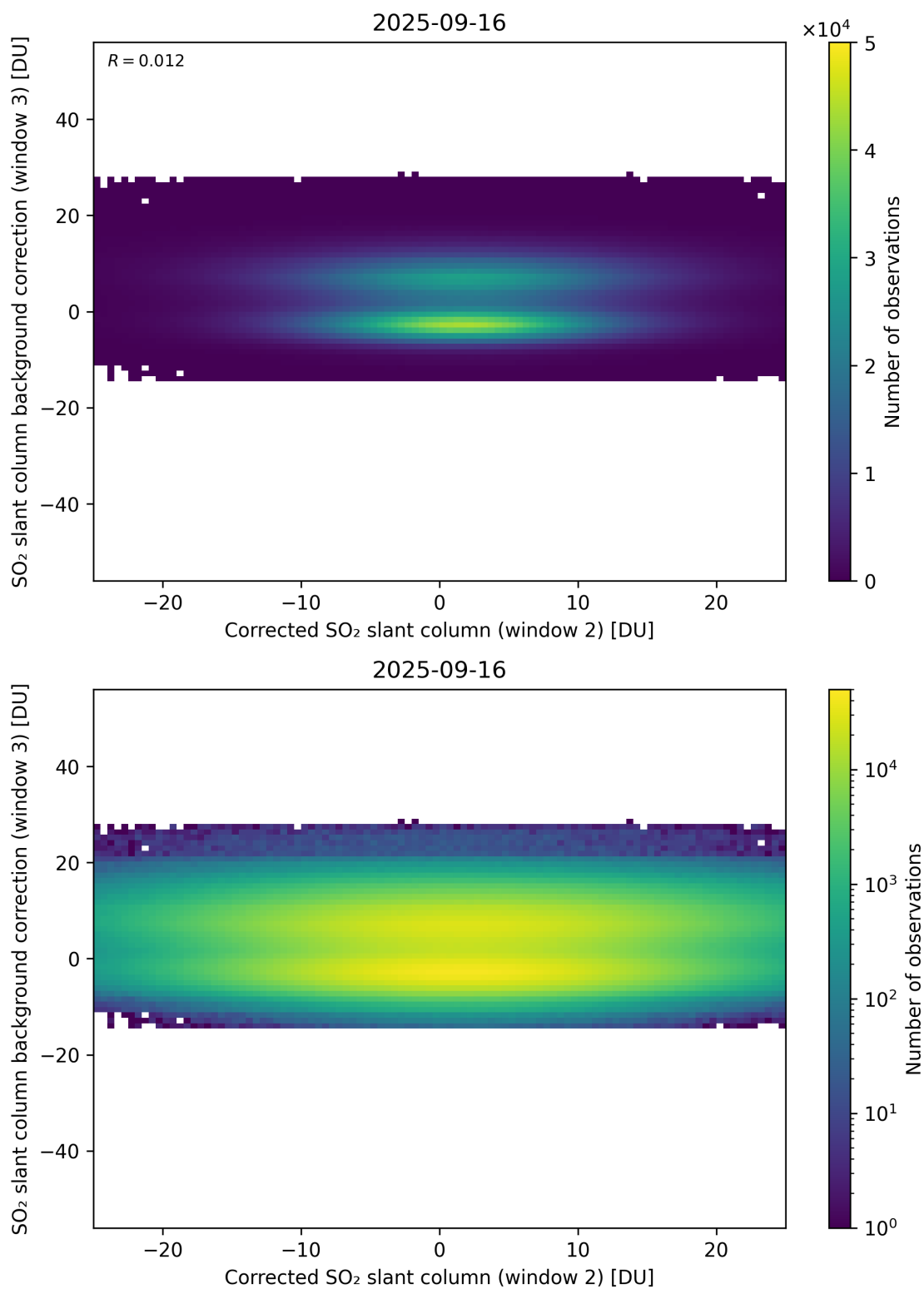
Figure 245: Scatter density plot of “Corrected SO 2 slant column (window 2)” against “SO 2 slant column background correction (window 3)” for 2025-09-15 to 2025-09-17.
