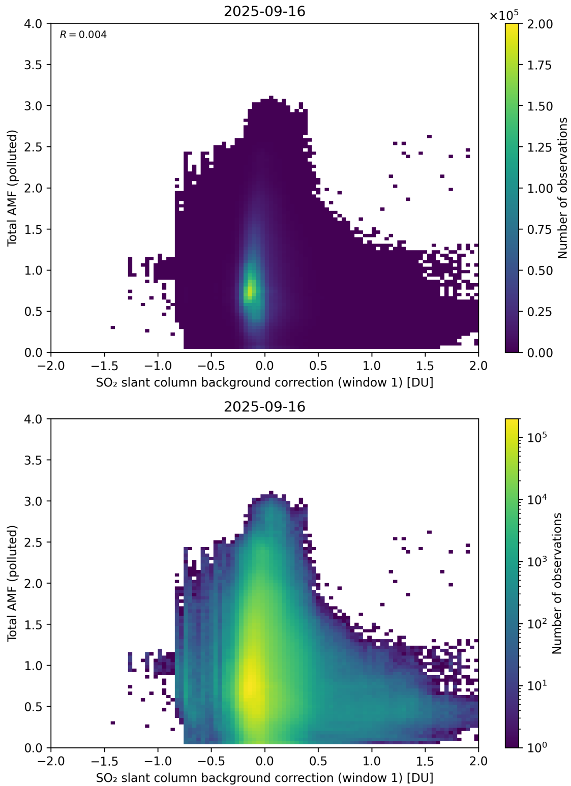
Figure 120: Scatter density plot of “SO 2 slant column background correction (window 1)” against “Total AMF (polluted)” for 2025-09-15 to 2025-09-17.
