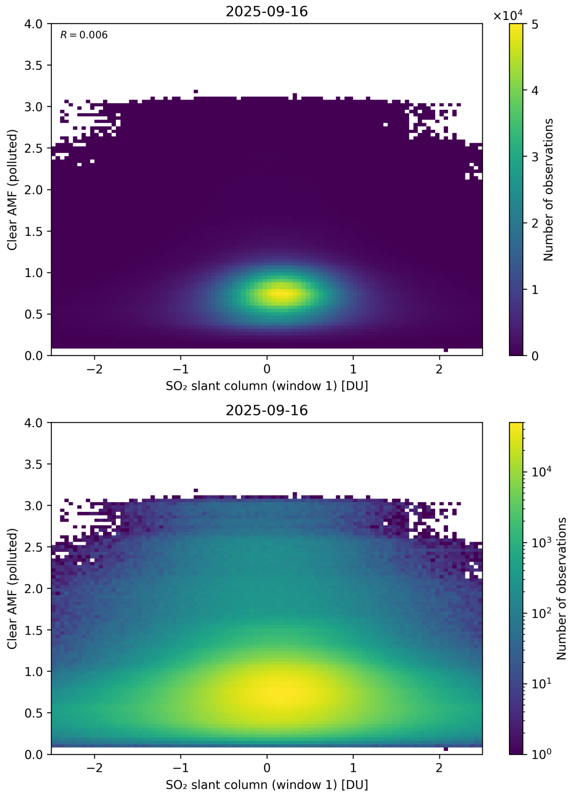
Figure 282: Scatter density plot of “SO 2 slant column (window 1)” against “Clear AMF (polluted)” for 2025-09-15 to 2025-09-17.
