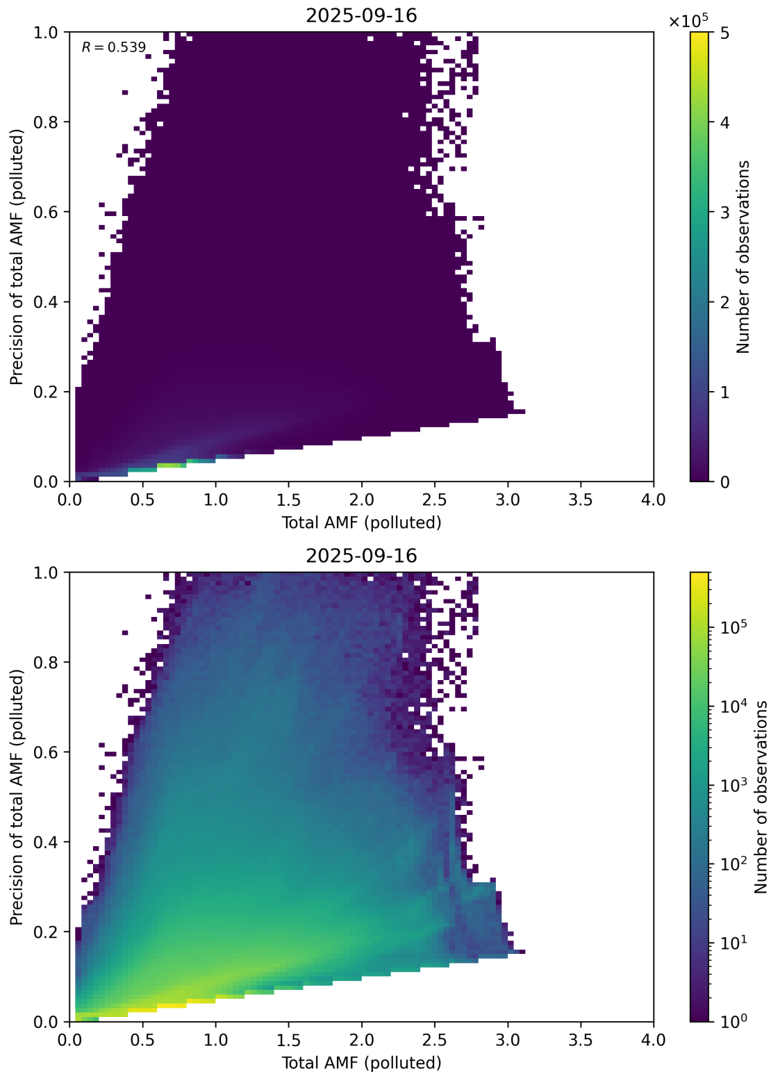
Figure 322: Scatter density plot of “Total AMF (polluted)” against “Precision of total AMF (polluted)” for 2025-09-15 to 2025-09-17.
