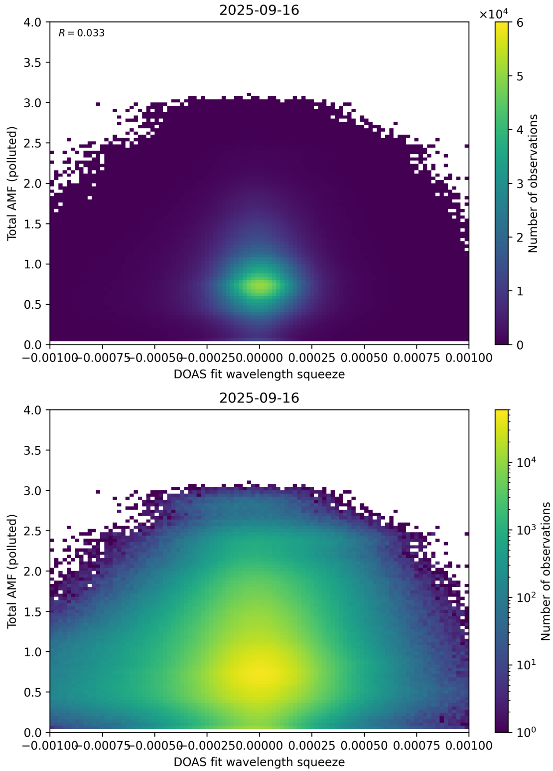
Figure 145: Scatter density plot of “DOAS fit wavelength squeeze” against “Total AMF (polluted)” for 2025-09-15 to 2025-09-17.
