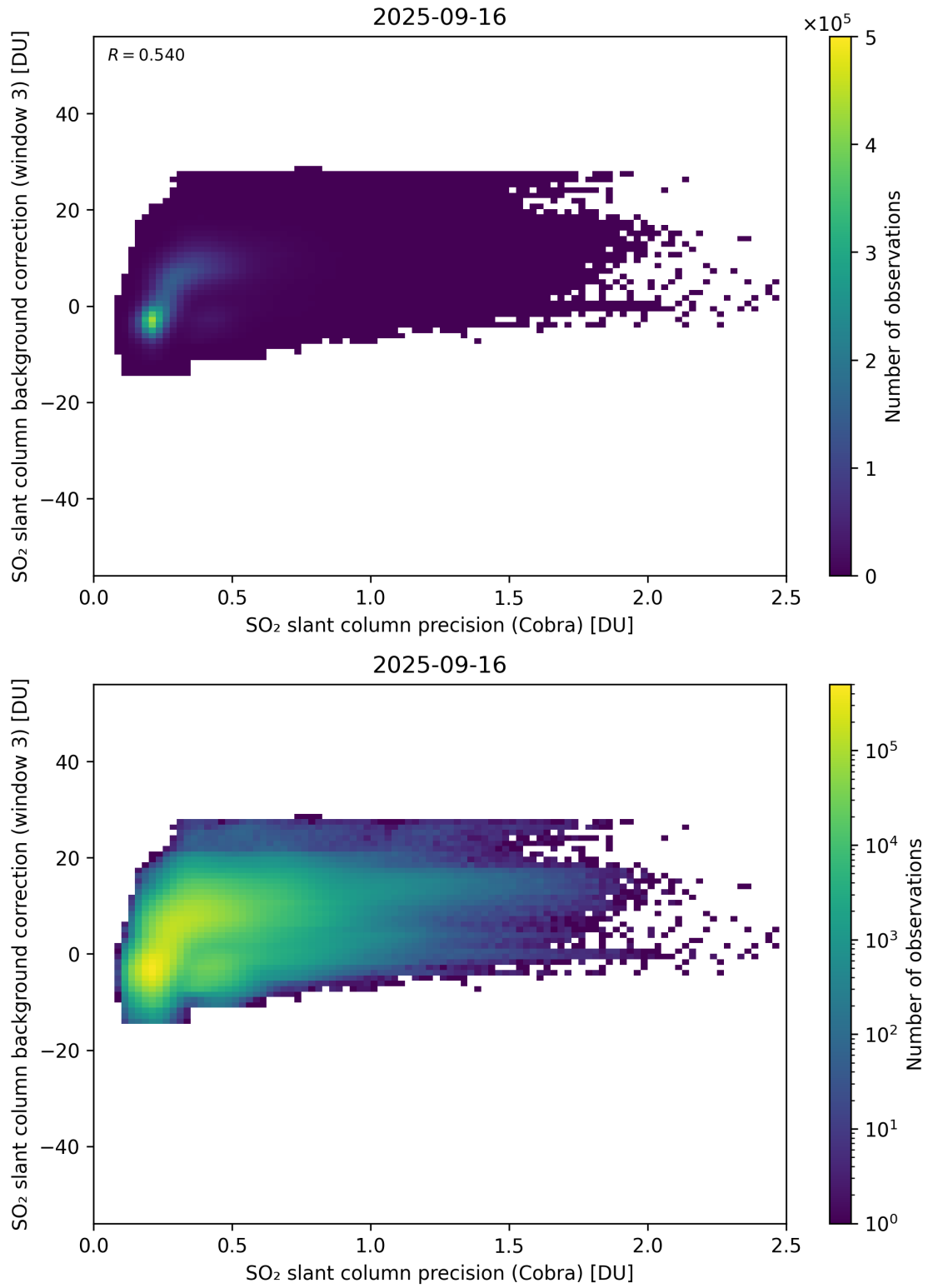
Figure 201: Scatter density plot of “SO 2 slant column precision (Cobra)” against “SO 2 slant column background correction (window 3)” for 2025-09-15 to 2025-09-17.
