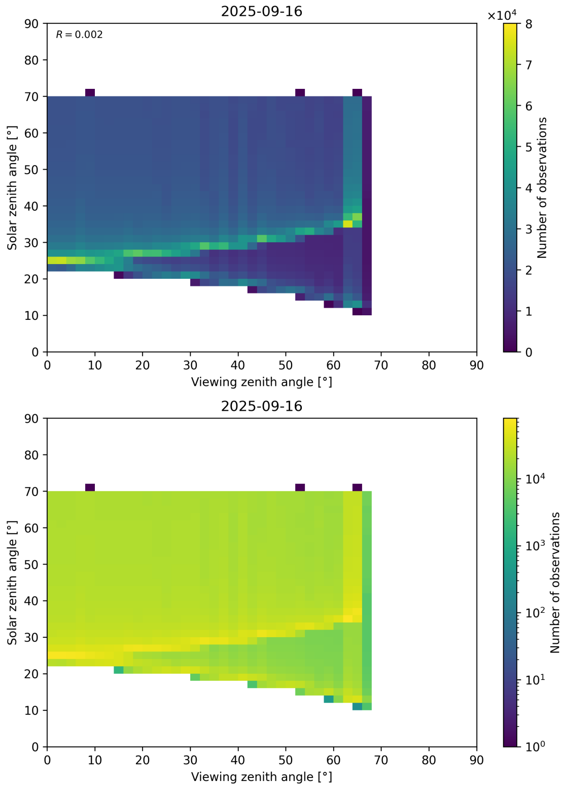
Figure 369: Scatter density plot of “Viewing zenith angle” against “Solar zenith angle” for 2025-09-15 to 2025-09-17.
