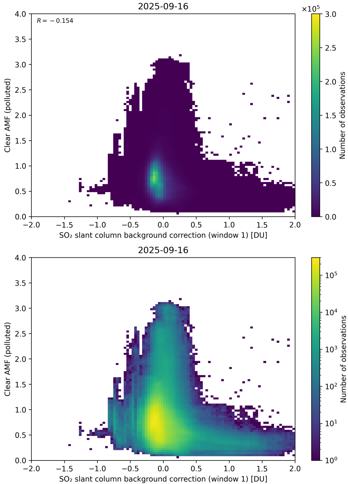
Figure 114: Scatter density plot of “SO 2 slant column background correction (window 1)” against “Clear AMF (polluted)” for 2025-09-15 to 2025-09-17.
