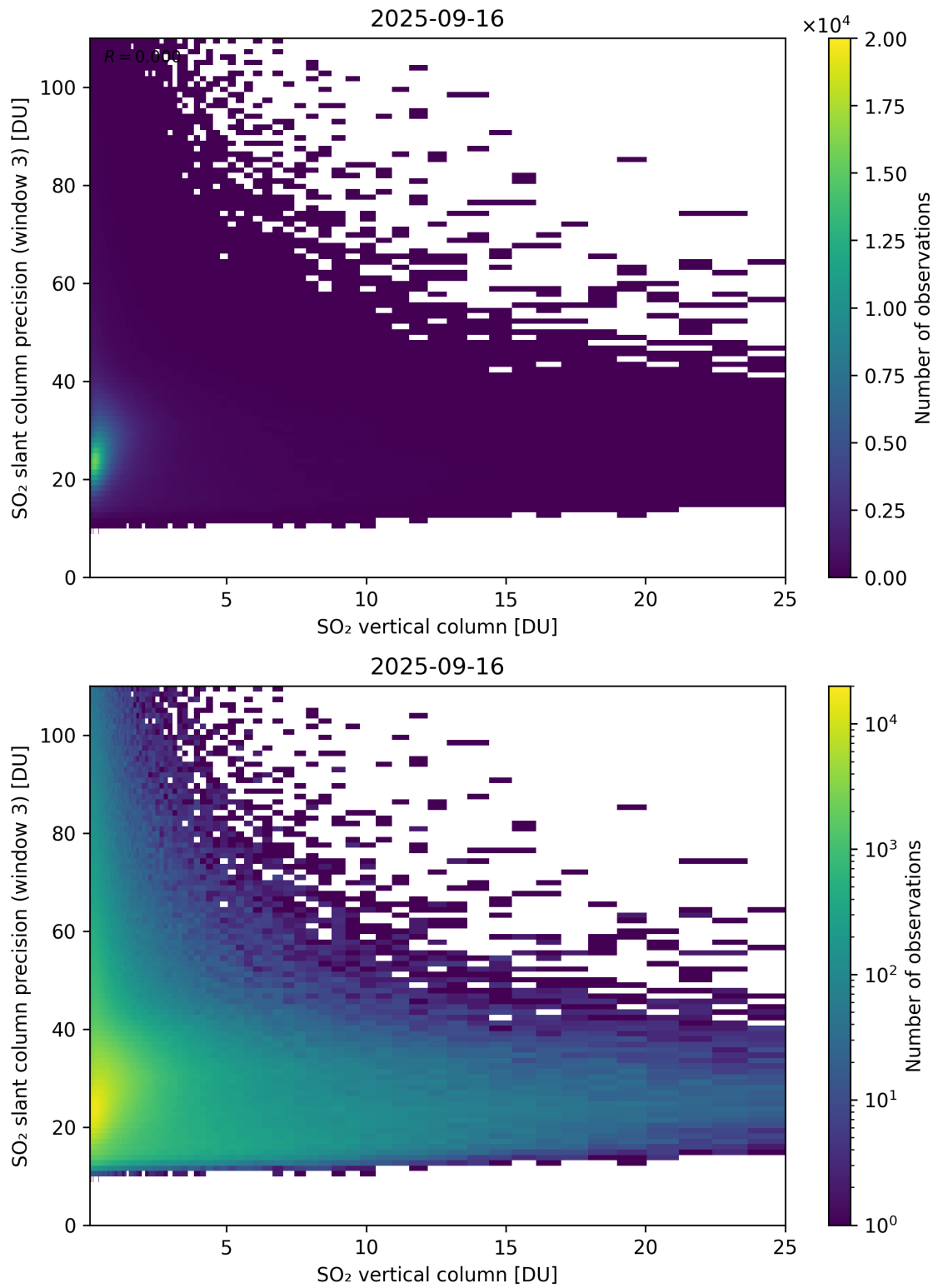
Figure 358: Scatter density plot of “SO 2 vertical column” against “SO 2 slant column precision (window 3)” for 2025-09-15 to 2025-09-17.
