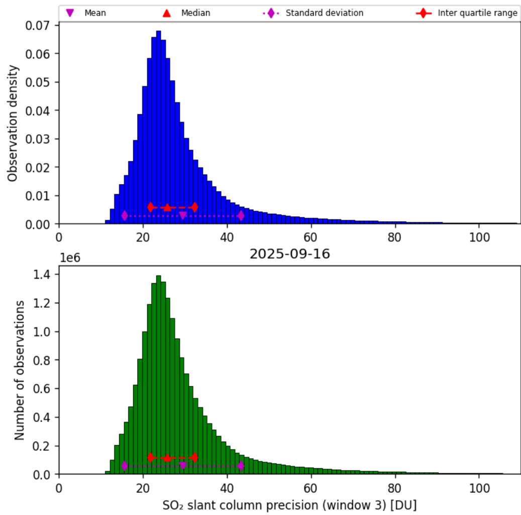
Figure 72: Histogram of “SO 2 slant column precision (window 3)” for 2025-09-15 to 2025-09-17
