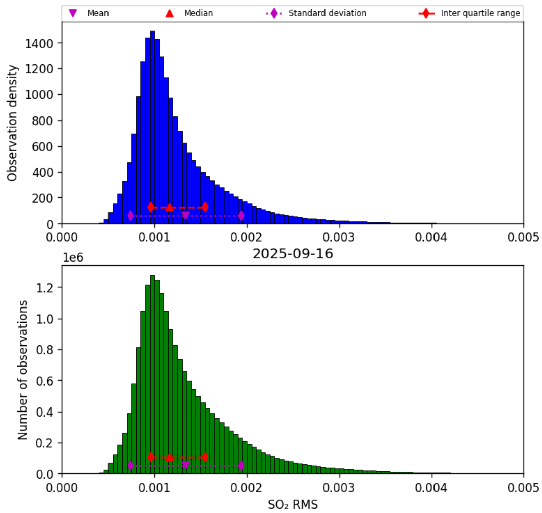
Figure 78: Histogram of “SO 2 RMS” for 2025-09-15 to 2025-09-17
