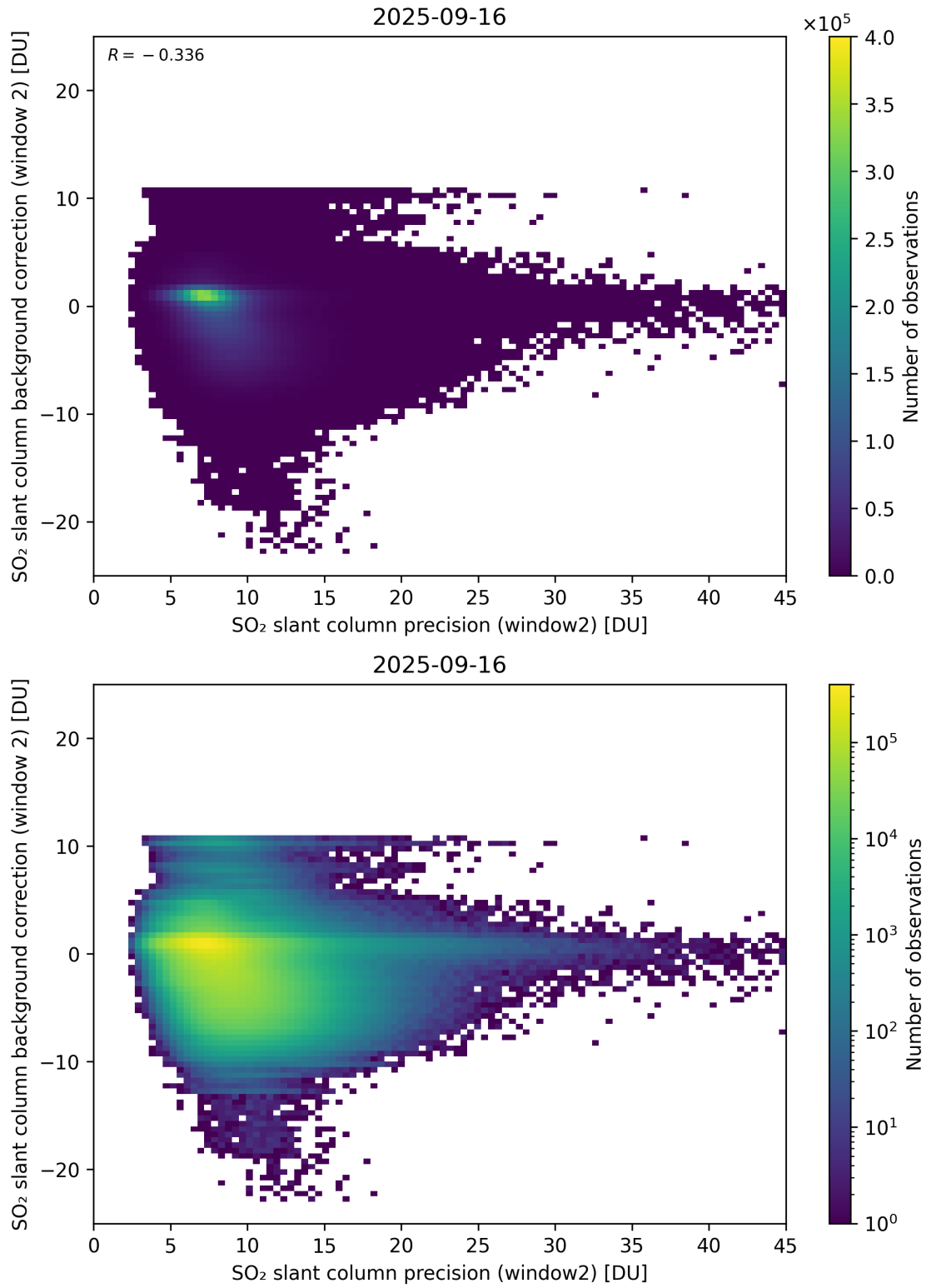
Figure 291: Scatter density plot of “SO 2 slant column precision (window2)” against “SO 2 slant column background correction (window 2)” for 2025-09-15 to 2025-09-17.
