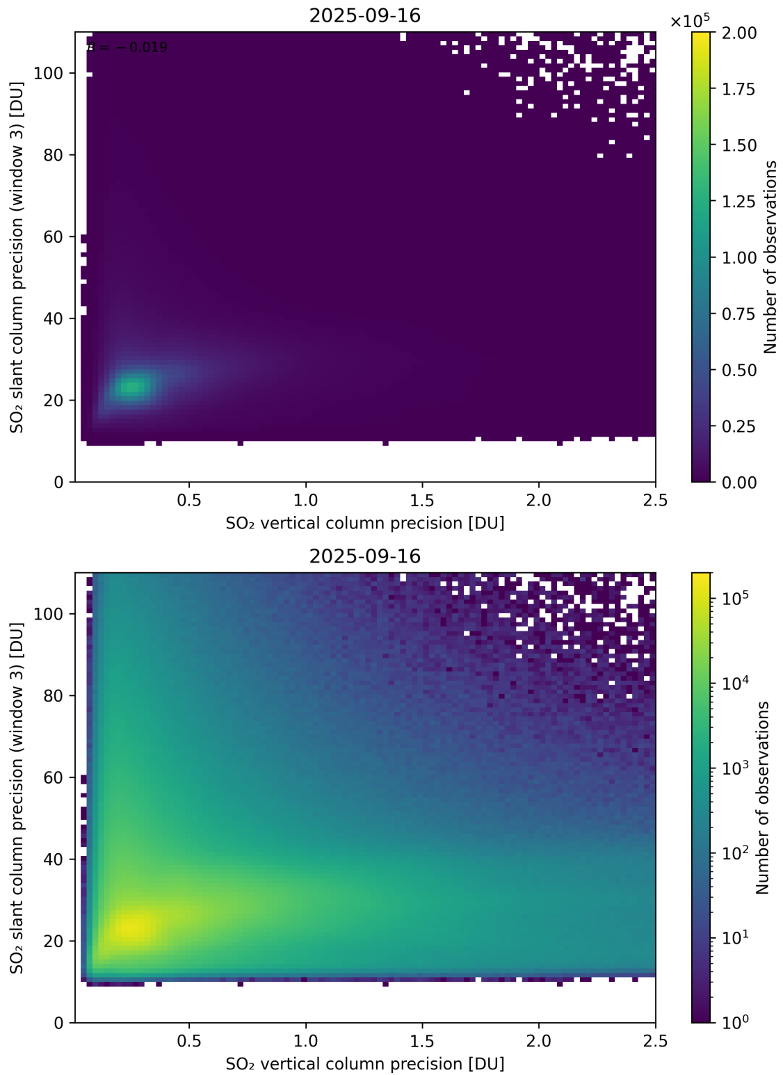
Figure 345: Scatter density plot of “SO 2 vertical column precision” against “SO 2 slant column precision (window 3)” for 2025-09-15 to 2025-09-17.
