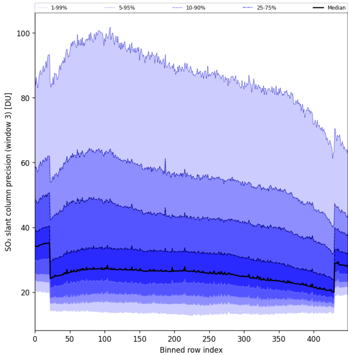
Figure 98: Along track statistics of “SO 2 slant column precision (window 3)” for 2025-09-15 to 2025-09-17
