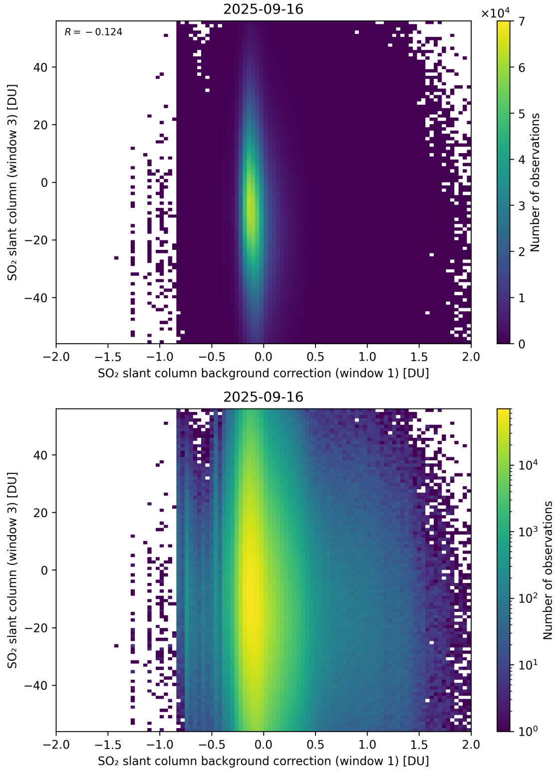
Figure 118: Scatter density plot of “SO 2 slant column background correction (window 1)” against “SO 2 slant column (window 3)” for 2025-09-15 to 2025-09-17.
