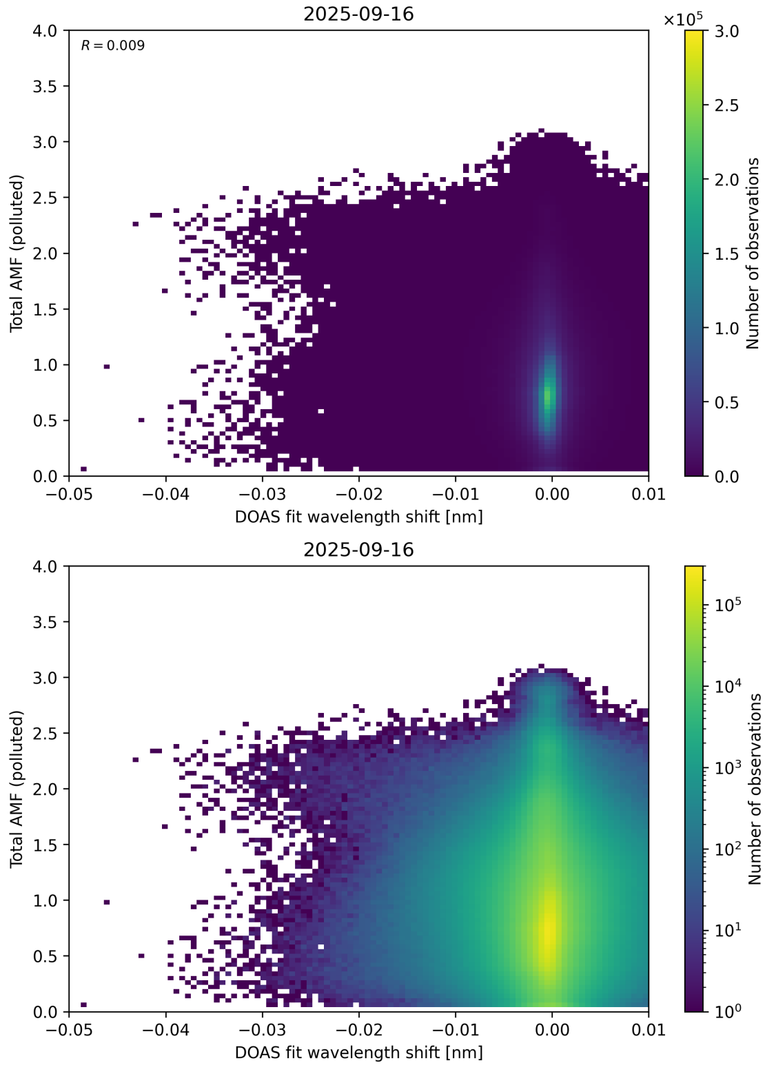
Figure 141: Scatter density plot of “DOAS fit wavelength shift” against “Total AMF (polluted)” for 2025-09-15 to 2025-09-17.
