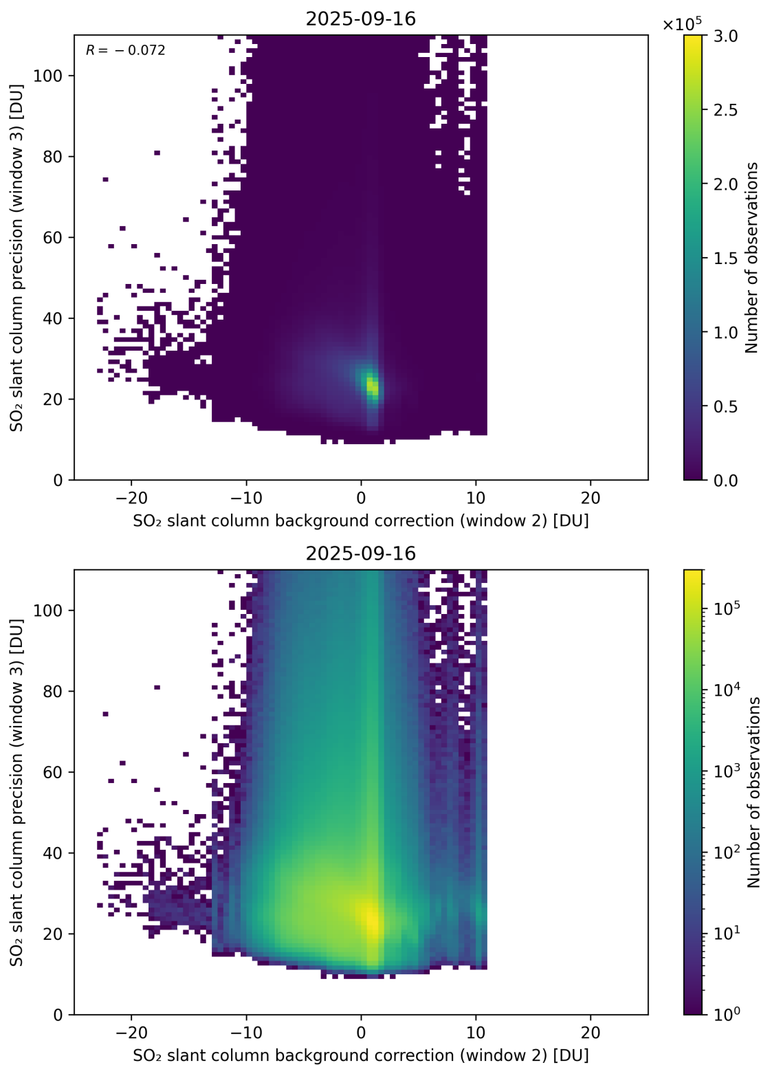
Figure 129: Scatter density plot of “SO 2 slant column background correction (window 2)” against “SO 2 slant column precision (window 3)” for 2025-09-15 to 2025-09-17.
