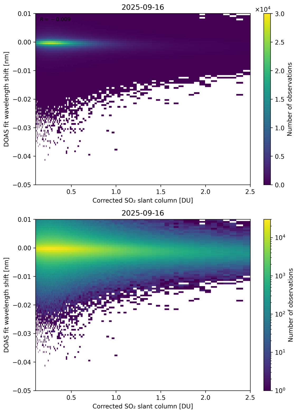
Figure 229: Scatter density plot of “Corrected SO 2 slant column” against “DOAS fit wavelength shift” for 2025-09-15 to 2025-09-17.
