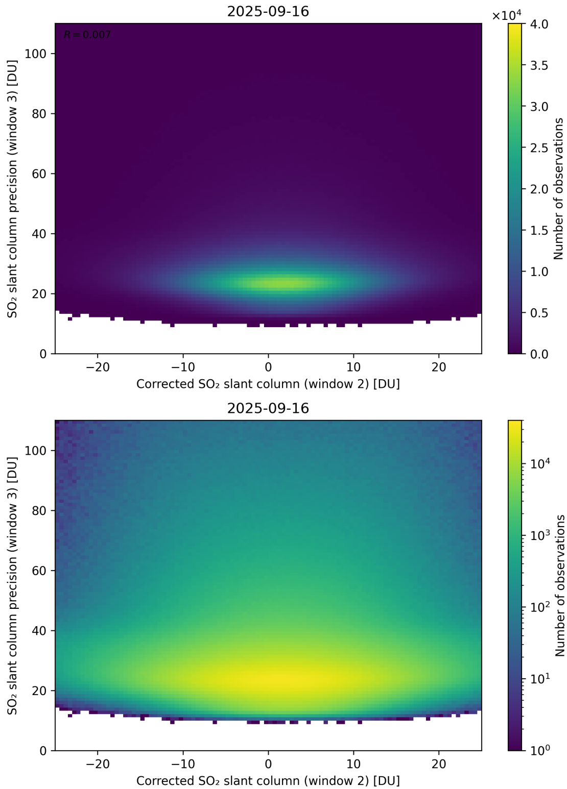
Figure 252: Scatter density plot of “Corrected SO 2 slant column (window 2)” against “SO 2 slant column precision (window 3)” for 2025-09-15 to 2025-09-17.
