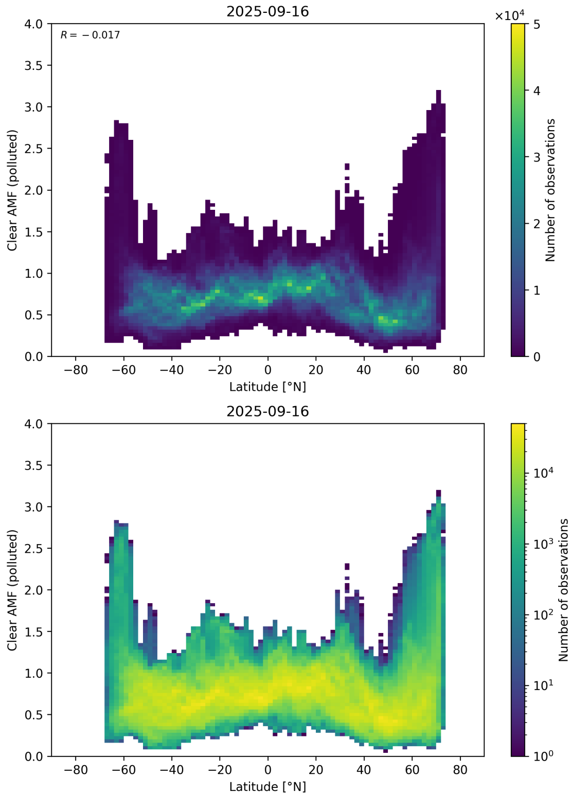
Figure 156: Scatter density plot of “Latitude” against “Clear AMF (polluted)” for 2025-09-15 to 2025-09-17.
