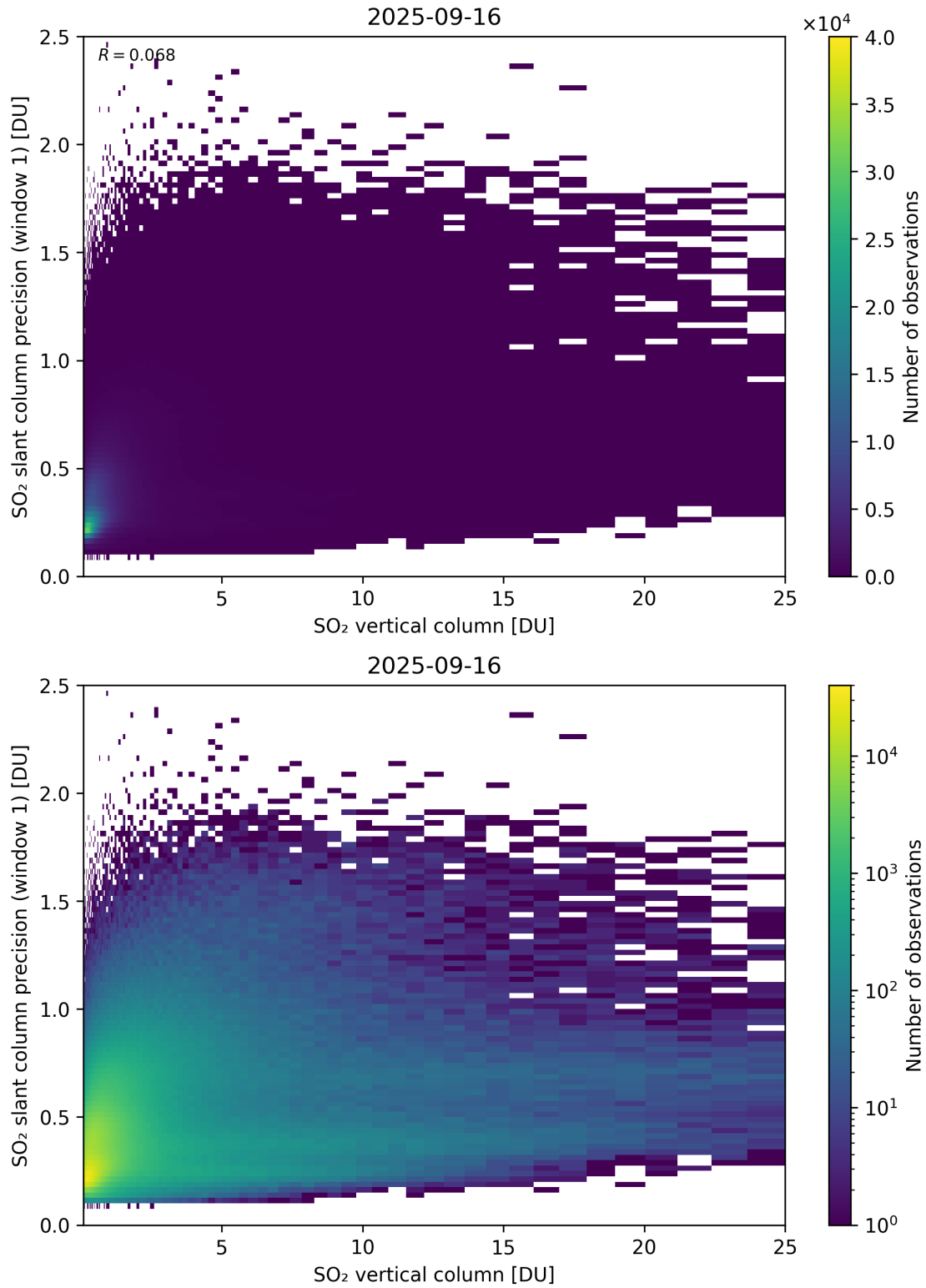
Figure 355: Scatter density plot of “SO 2 vertical column” against “SO 2 slant column precision (window 1)” for 2025-09-15 to 2025-09-17.
