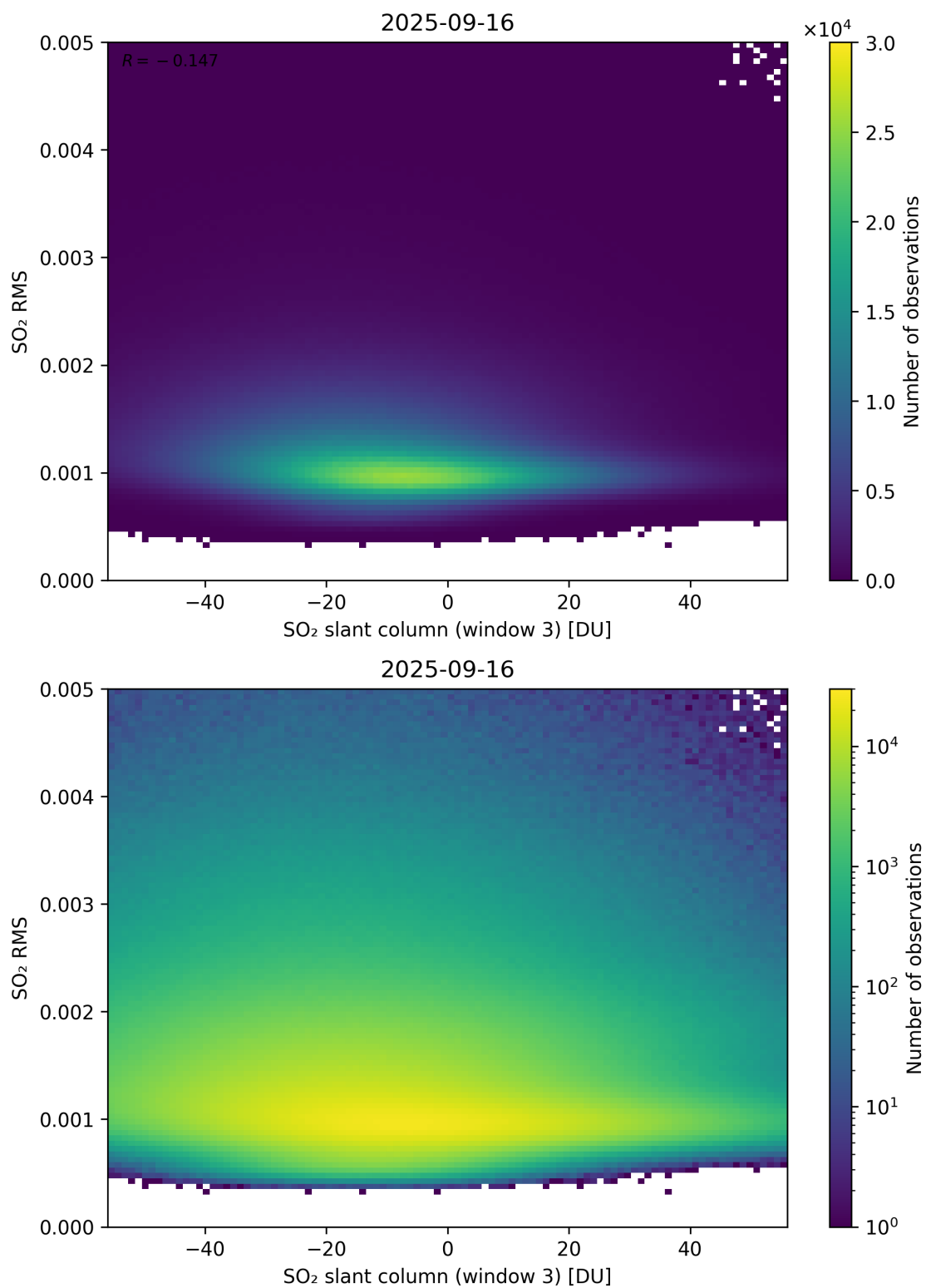
Figure 306: Scatter density plot of “SO 2 slant column (window 3)” against “SO 2 RMS” for 2025-09-15 to 2025-09-17.
