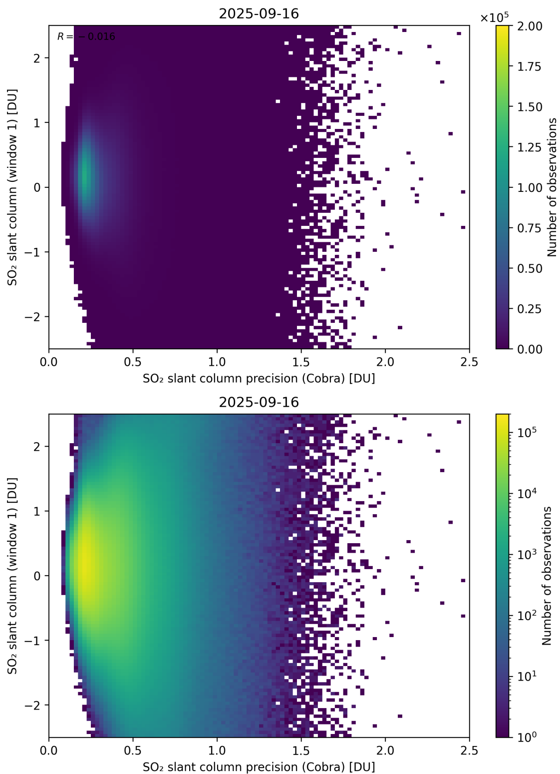
Figure 208: Scatter density plot of “SO 2 slant column precision (Cobra)” against “SO 2 slant column (window 1)” for 2025-09-15 to 2025-09-17.
