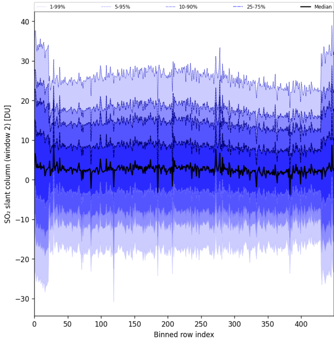
Figure 93: Along track statistics of “SO 2 slant column (window 2)” for 2025-09-15 to 2025-09-17
