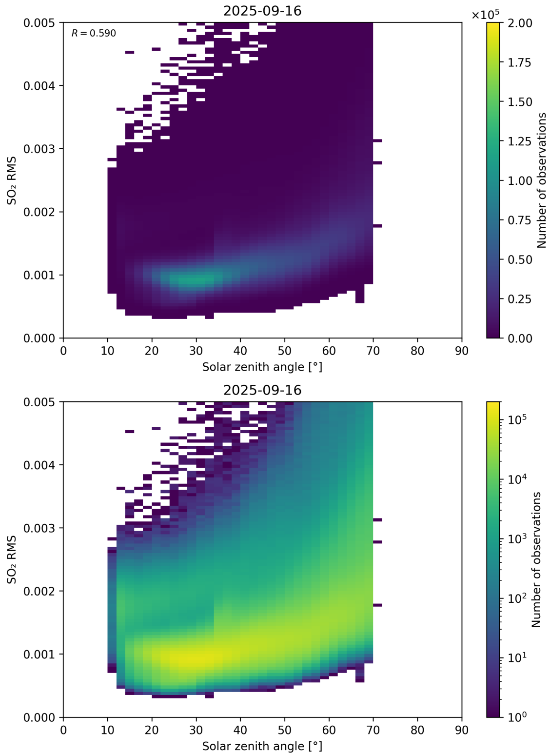
Figure 176: Scatter density plot of “Solar zenith angle” against “SO 2 RMS” for 2025-09-15 to 2025-09-17.
