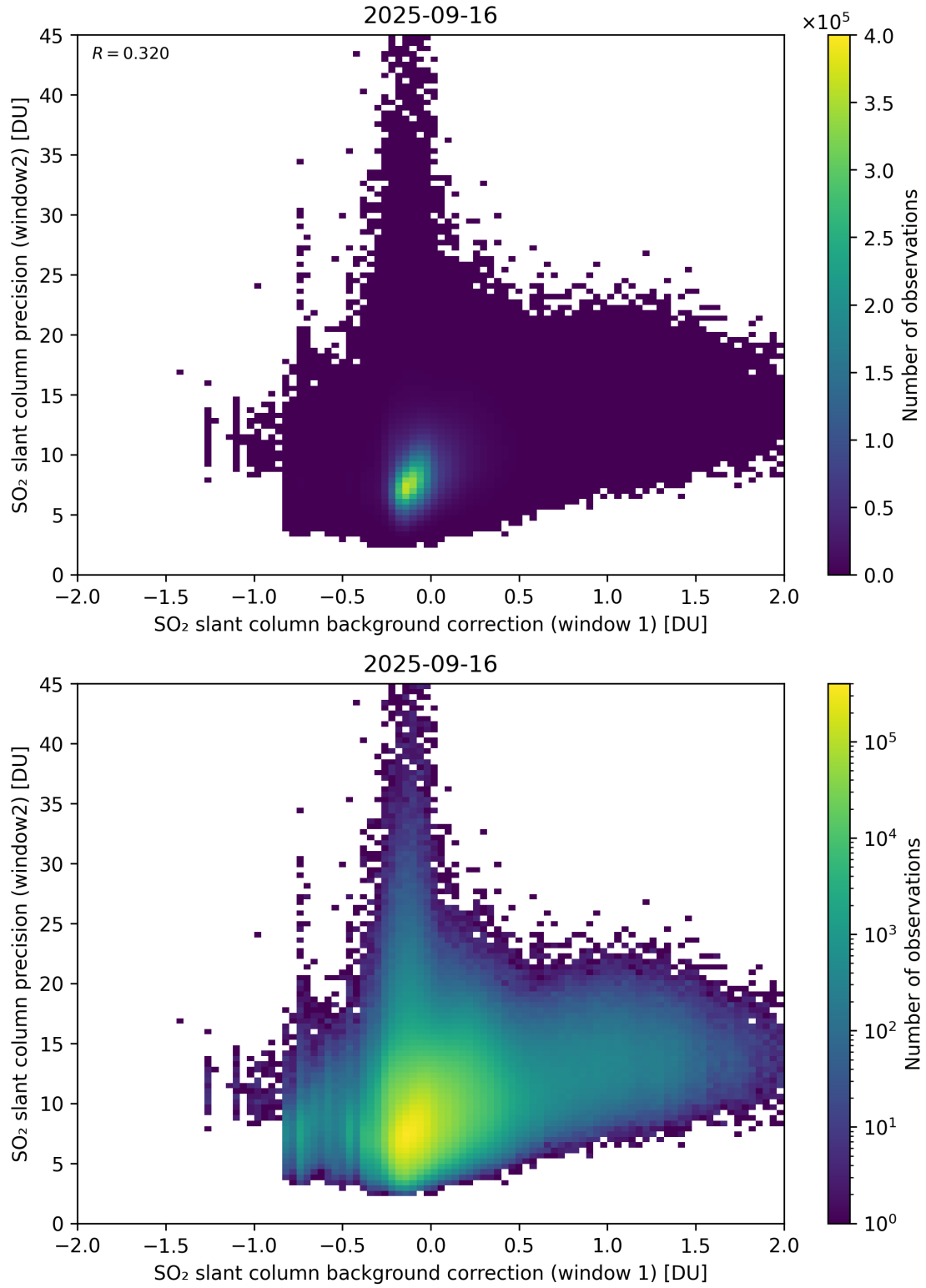
Figure 117: Scatter density plot of “SO 2 slant column background correction (window 1)” against “SO 2 slant column precision (window2)” for 2025-09-15 to 2025-09-17.
