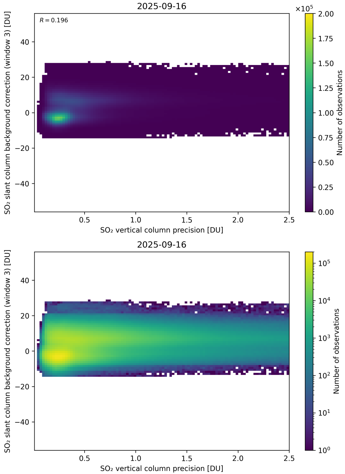
Figure 331: Scatter density plot of “SO 2 vertical column precision” against “SO 2 slant column background correction (window 3)” for 2025-09-15 to 2025-09-17.
