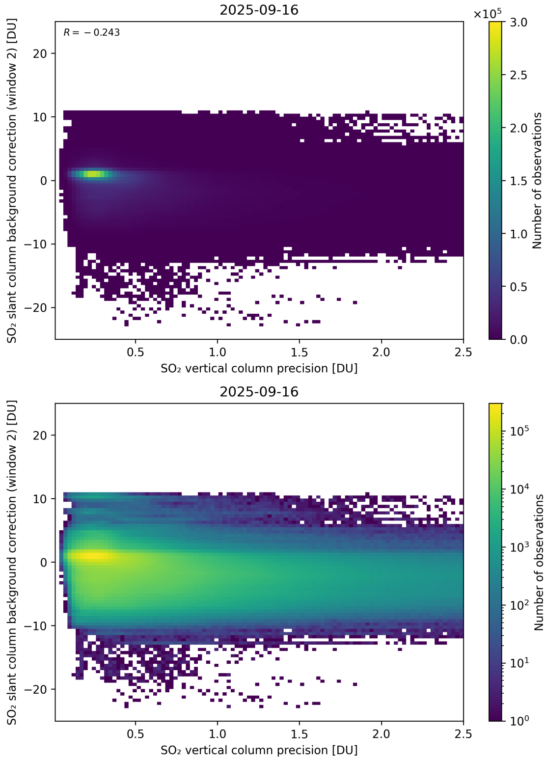
Figure 330: Scatter density plot of “SO 2 vertical column precision” against “SO 2 slant column background correction (window 2)” for 2025-09-15 to 2025-09-17.
