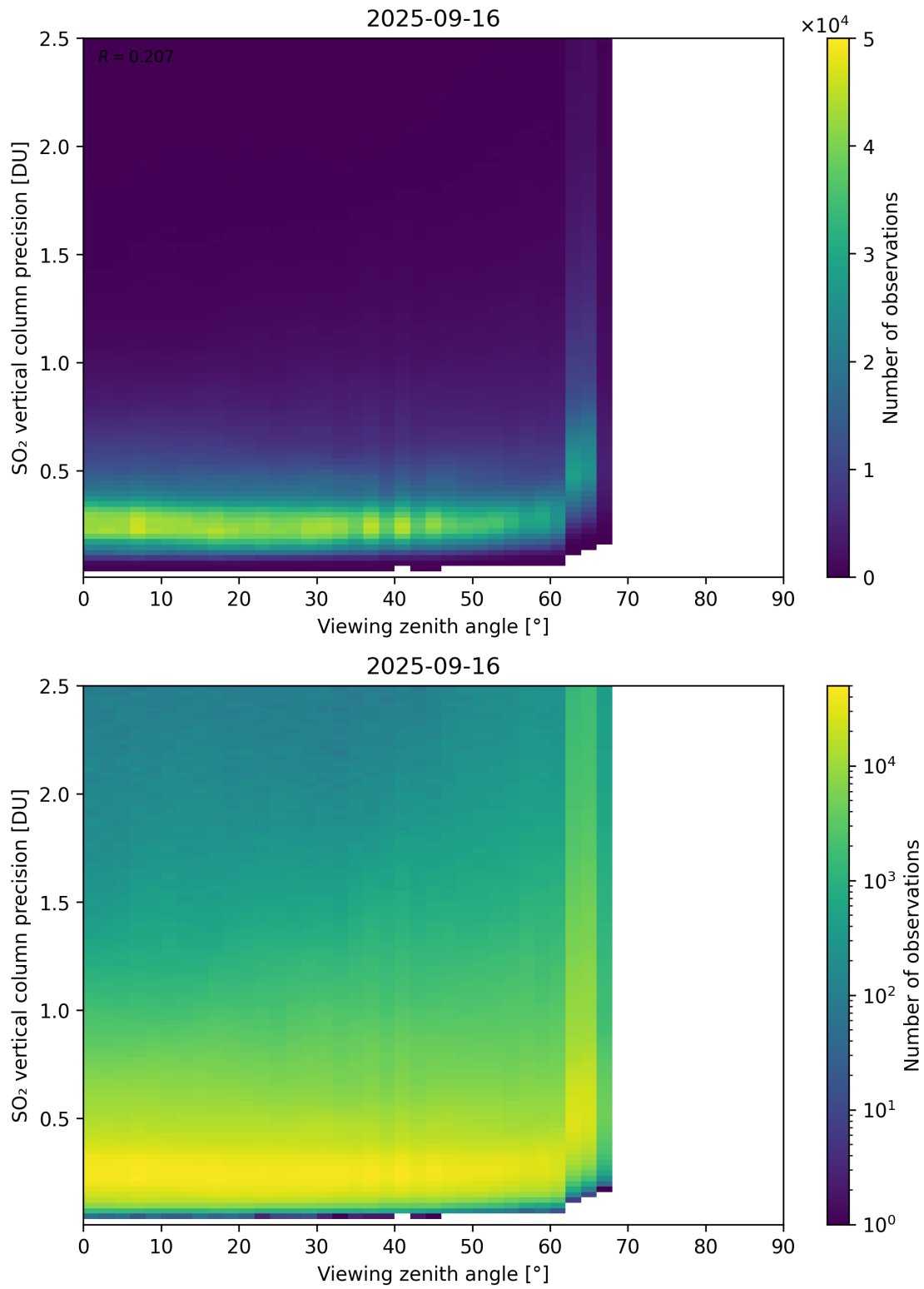
Figure 384: Scatter density plot of “Viewing zenith angle” against “SO 2 vertical column precision” for 2025-09-15 to 2025-09-17.
