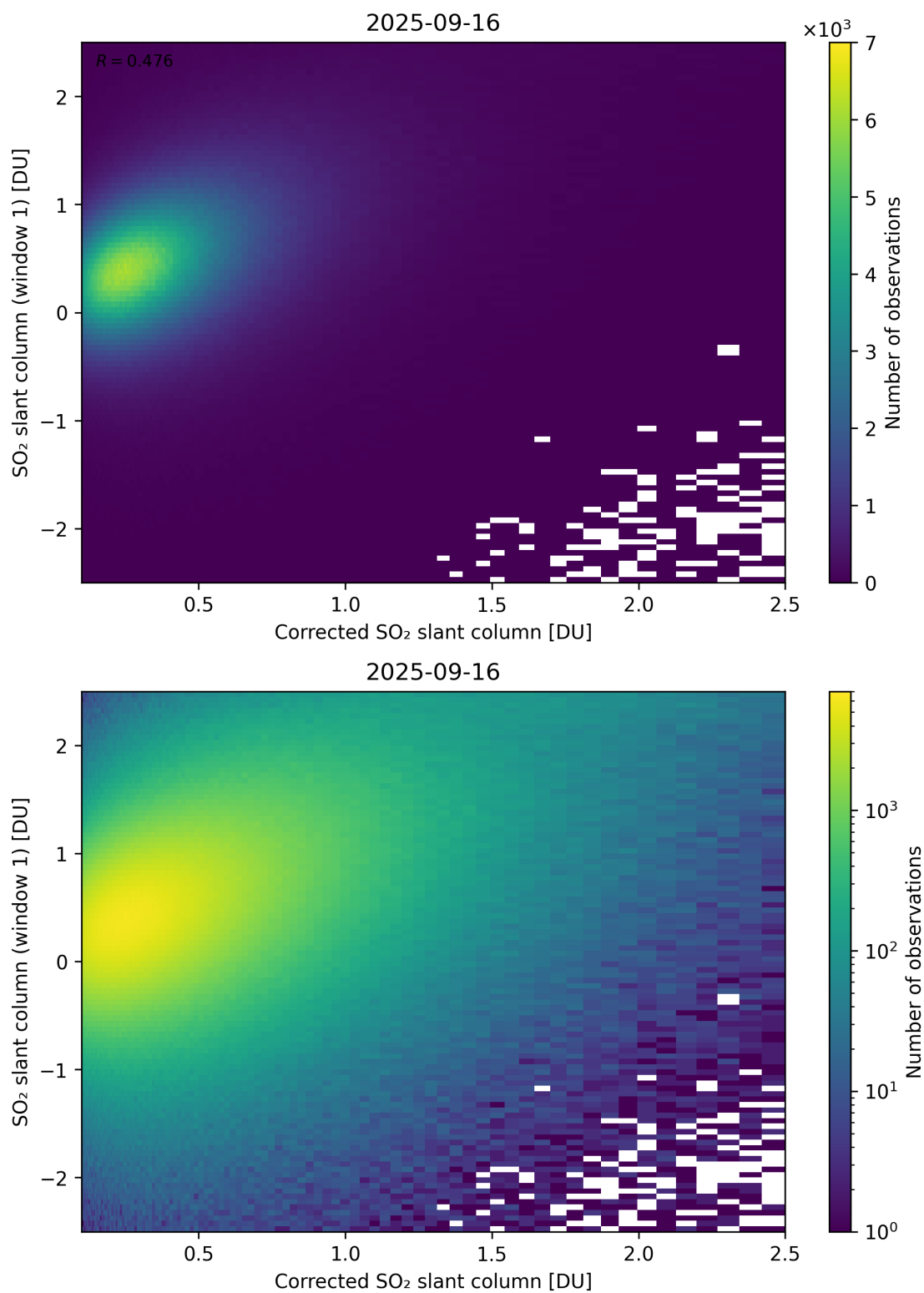
Figure 237: Scatter density plot of “Corrected SO 2 slant column” against “SO 2 slant column (window 1)” for 2025-09-15 to 2025-09-17.
