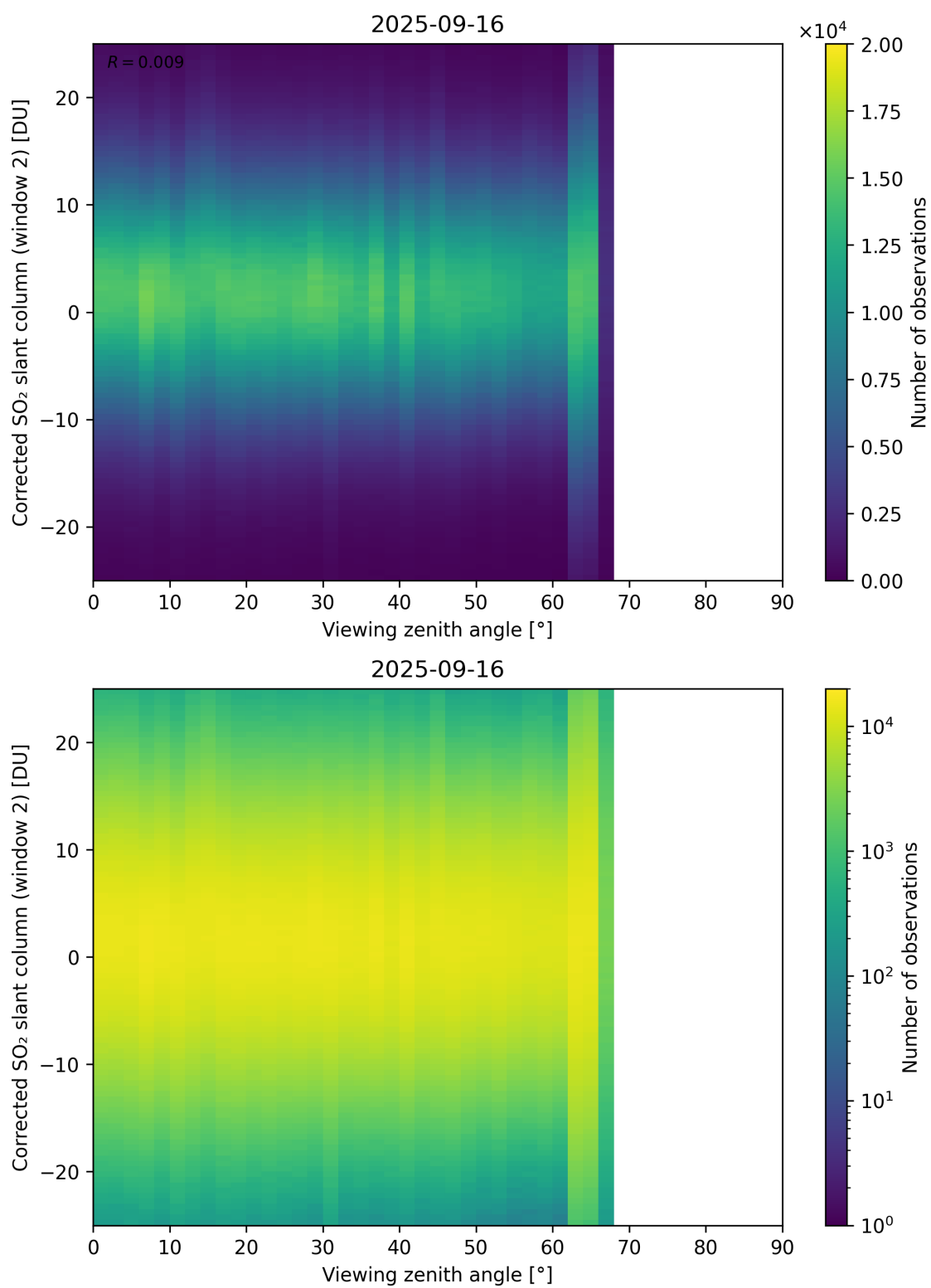
Figure 374: Scatter density plot of “Viewing zenith angle” against “Corrected SO 2 slant column (window 2)” for 2025-09-15 to 2025-09-17.
