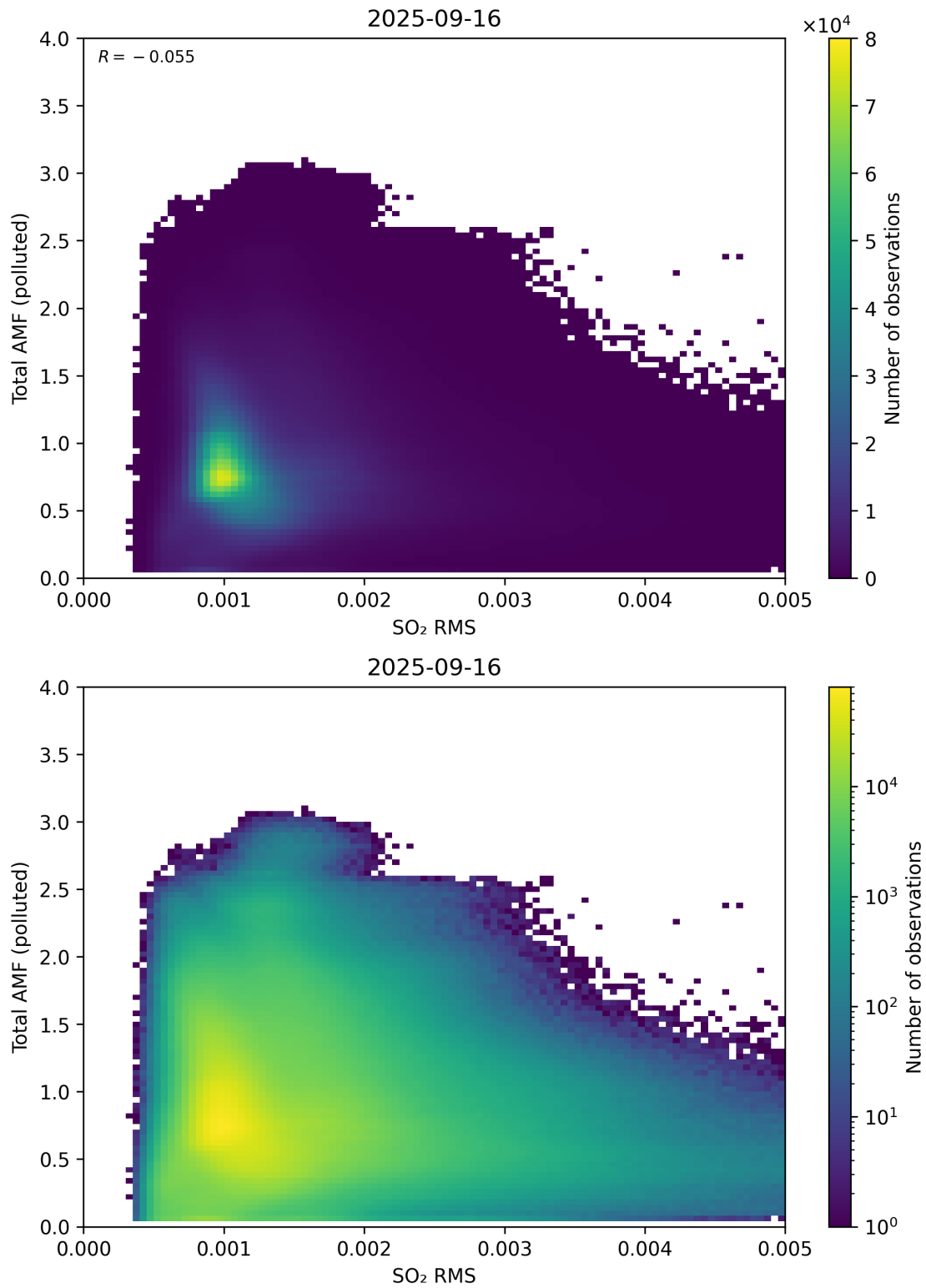
Figure 148: Scatter density plot of “SO 2 RMS” against “Total AMF (polluted)” for 2025-09-15 to 2025-09-17.
