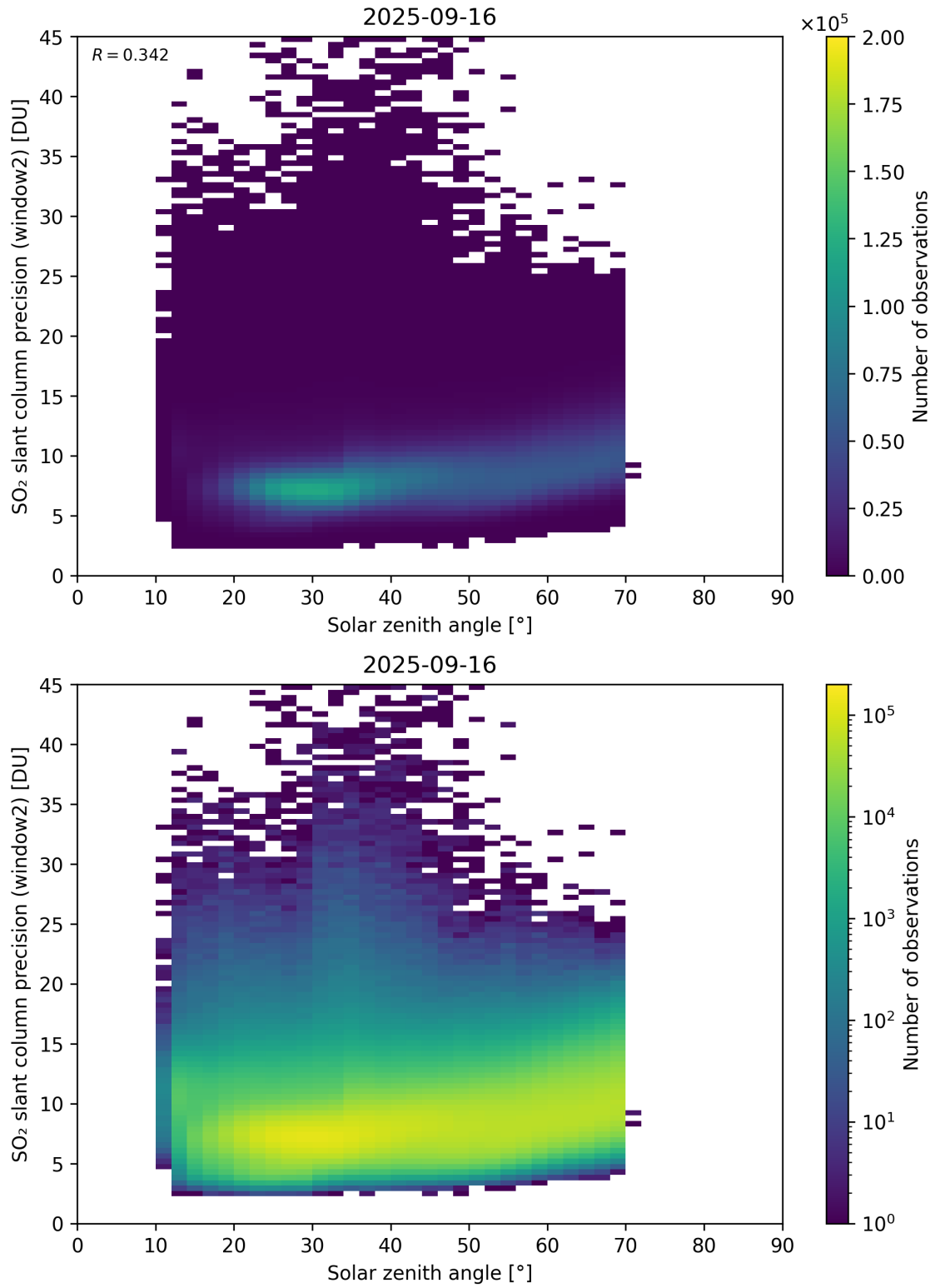
Figure 186: Scatter density plot of “Solar zenith angle” against “SO 2 slant column precision (window2)” for 2025-09-15 to 2025-09-17.
