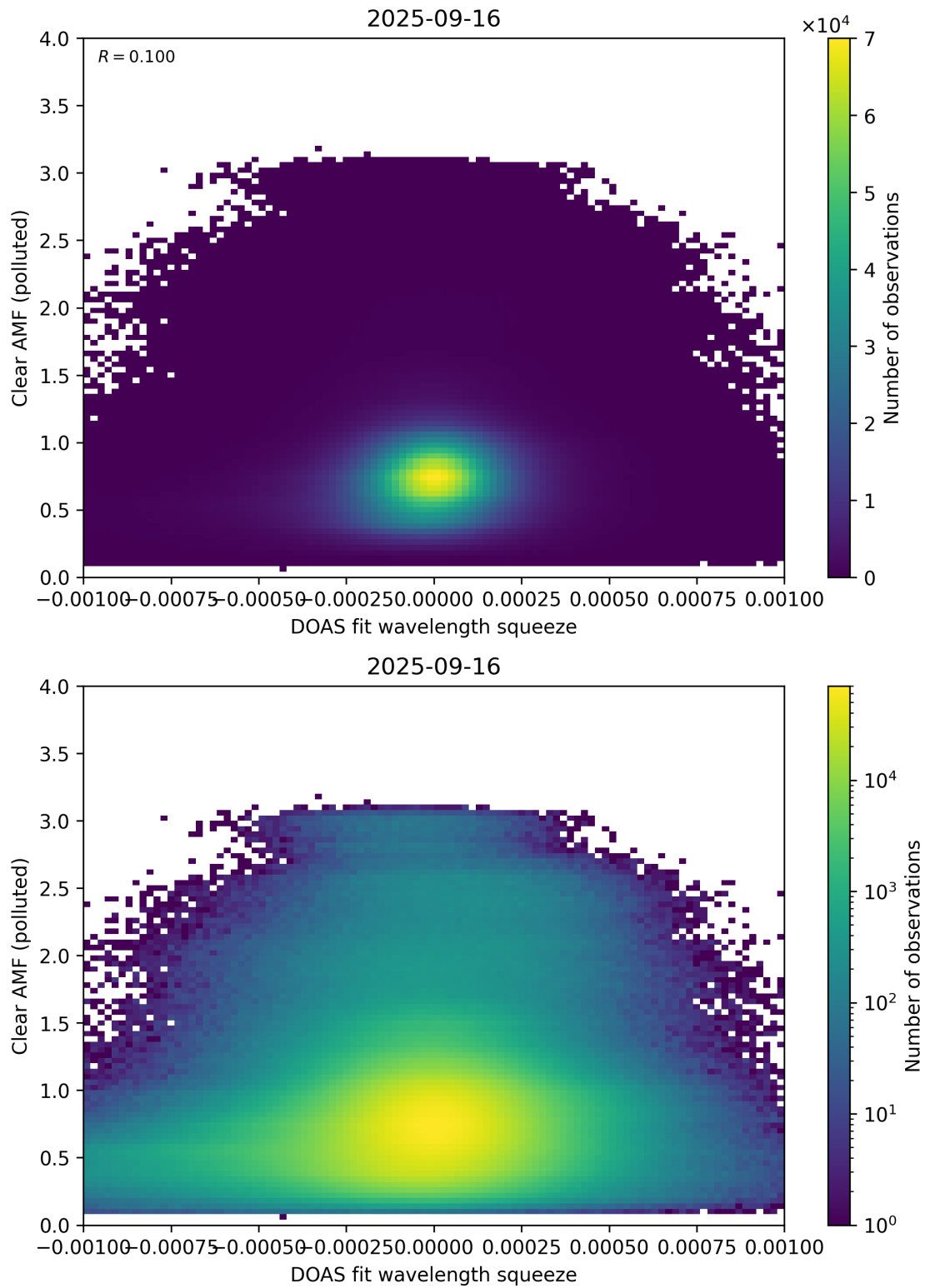
Figure 144: Scatter density plot of “DOAS fit wavelength squeeze” against “Clear AMF (polluted)” for 2025-09-15 to 2025-09-17.
