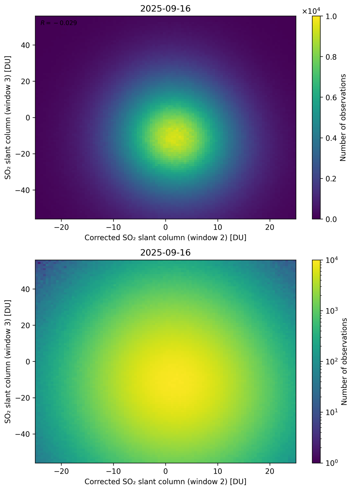
Figure 251: Scatter density plot of “Corrected SO 2 slant column (window 2)” against “SO 2 slant column (window 3)” for 2025-09-15 to 2025-09-17.
