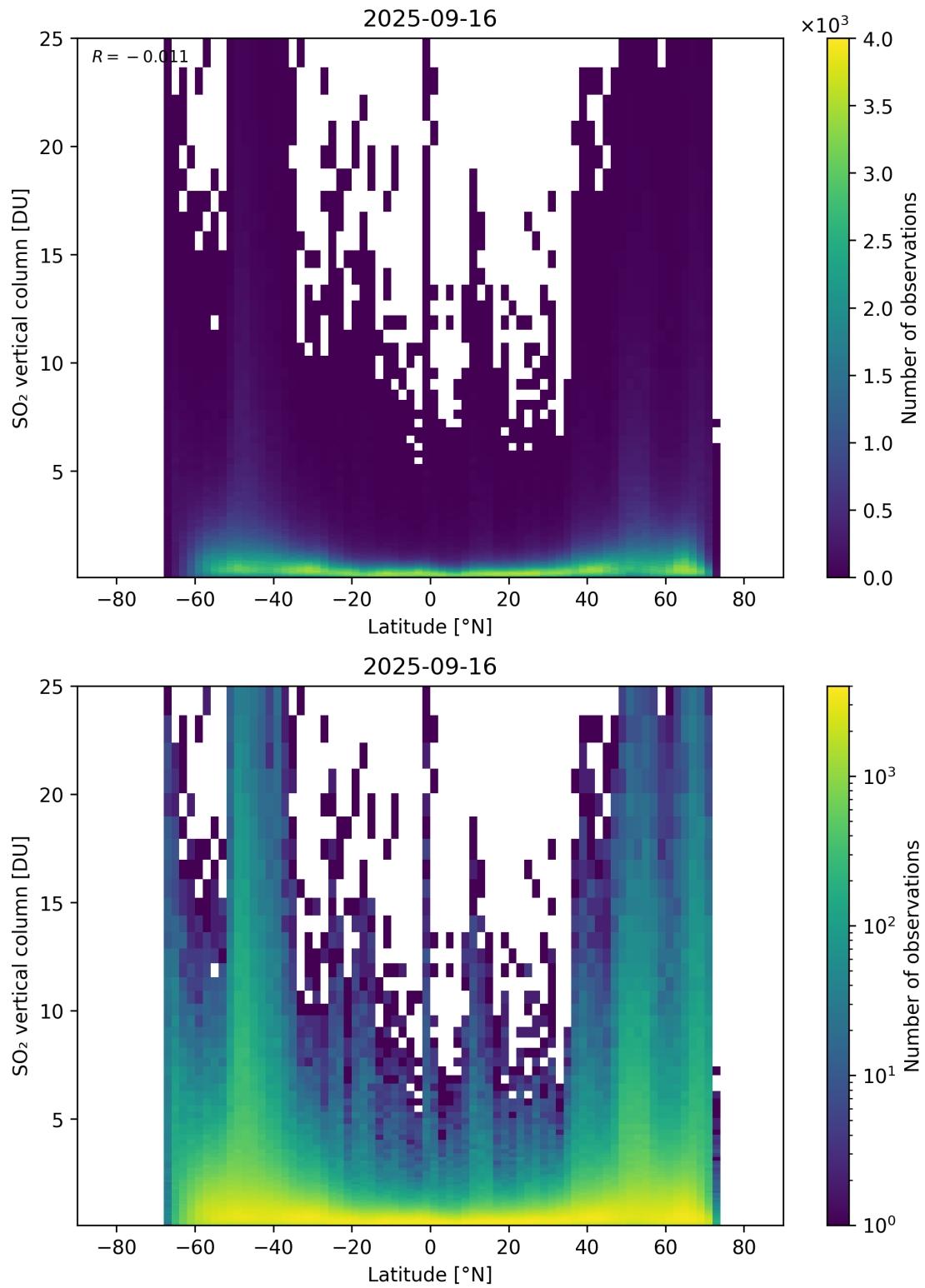
Figure 169: Scatter density plot of “Latitude” against “SO 2 vertical column” for 2025-09-15 to 2025-09-17.
