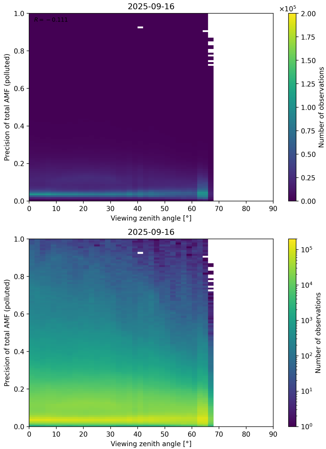
Figure 382: Scatter density plot of “Viewing zenith angle” against “Precision of total AMF (polluted)” for 2025-09-15 to 2025-09-17.
