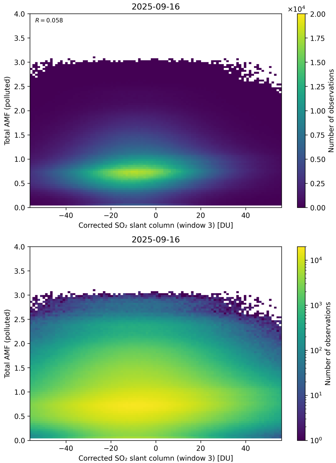
Figure 260: Scatter density plot of “Corrected SO 2 slant column (window 3)” against “Total AMF (polluted)” for 2025-09-15 to 2025-09-17.
