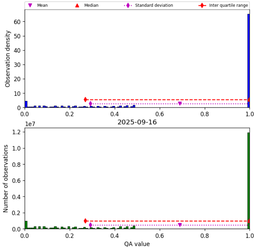
Figure 57: Histogram of “QA value” for 2025-09-15 to 2025-09-17
