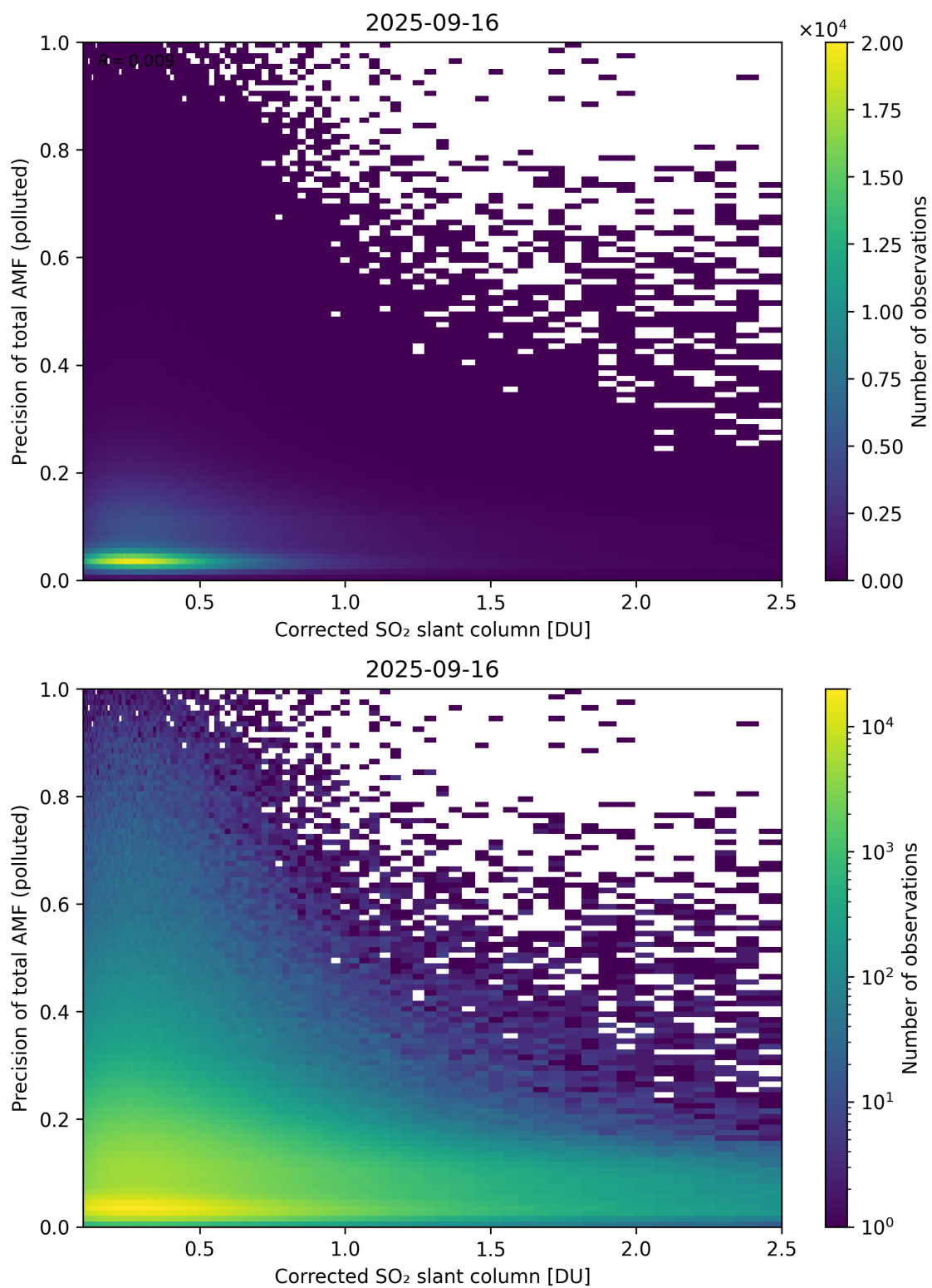
Figure 243: Scatter density plot of “Corrected SO 2 slant column” against “Precision of total AMF (polluted)” for 2025-09-15 to 2025-09-17.
