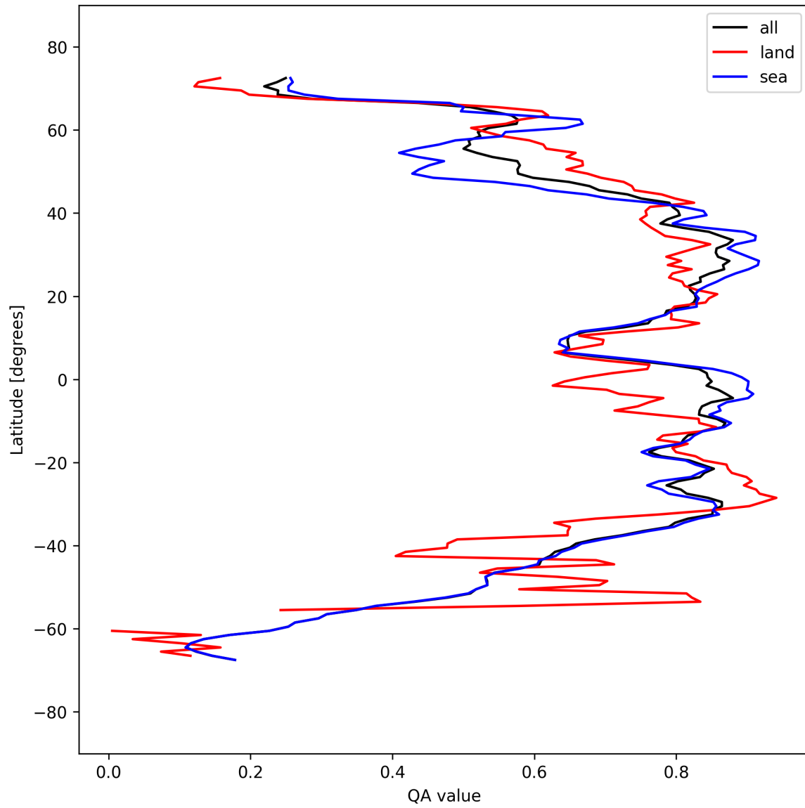
Figure 31: Zonal average of “QA value” for 2025-09-15 to 2025-09-17.
