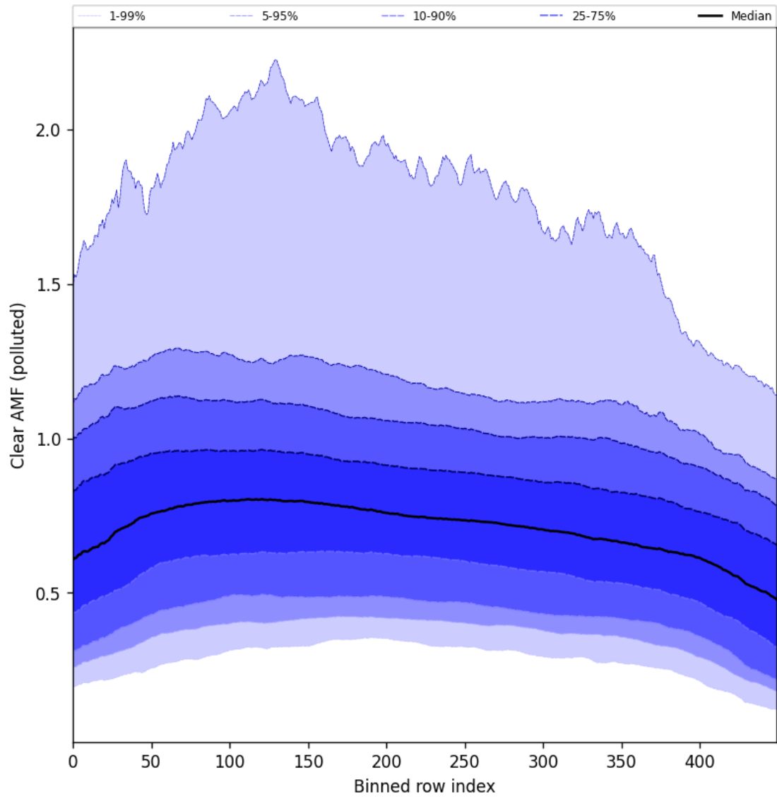
Figure 107: Along track statistics of “Clear AMF (polluted)” for 2025-09-15 to 2025-09-17
