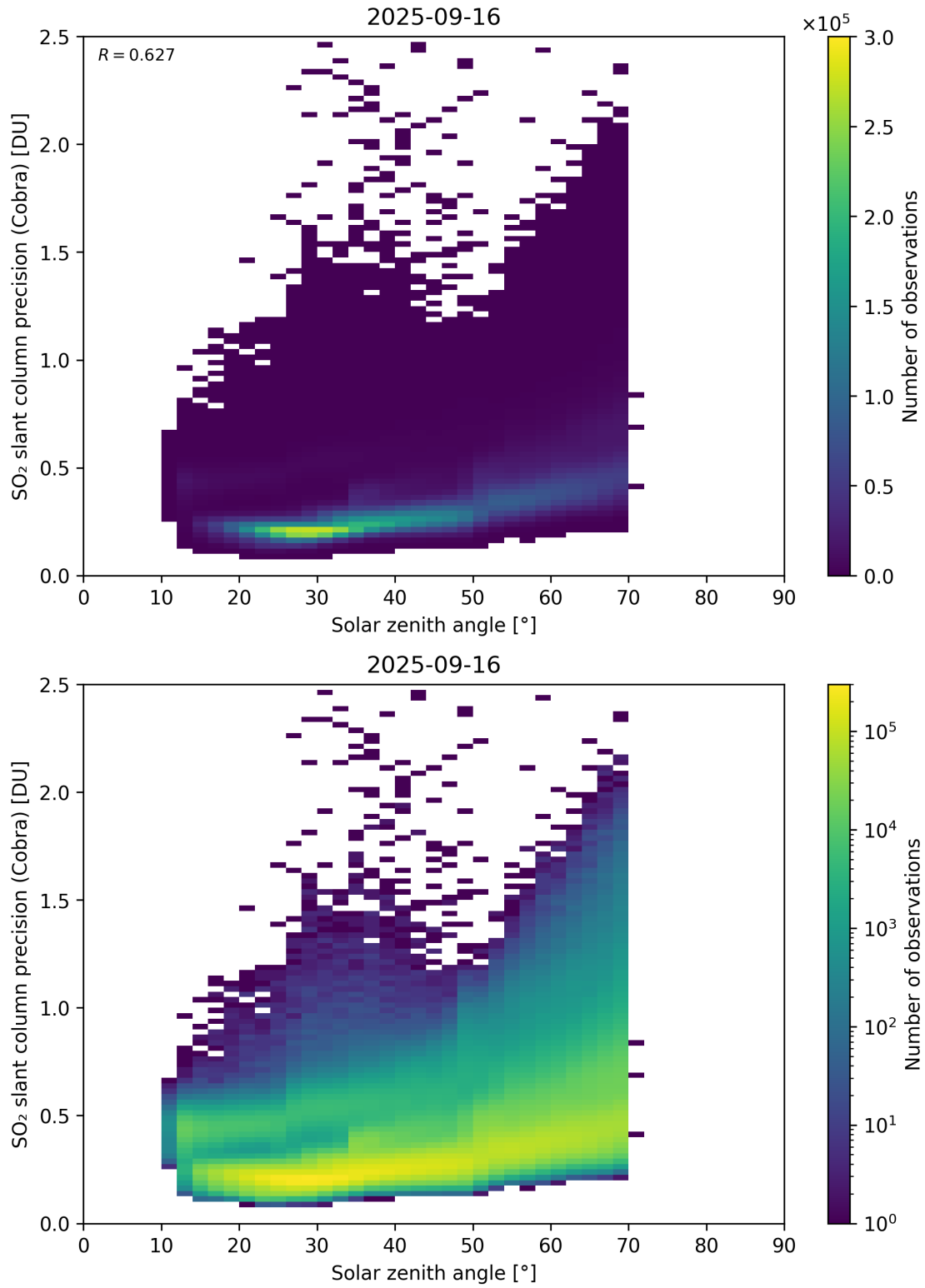
Figure 180: Scatter density plot of “Solar zenith angle” against “SO 2 slant column precision (Cobra)” for 2025-09-15 to 2025-09-17.
