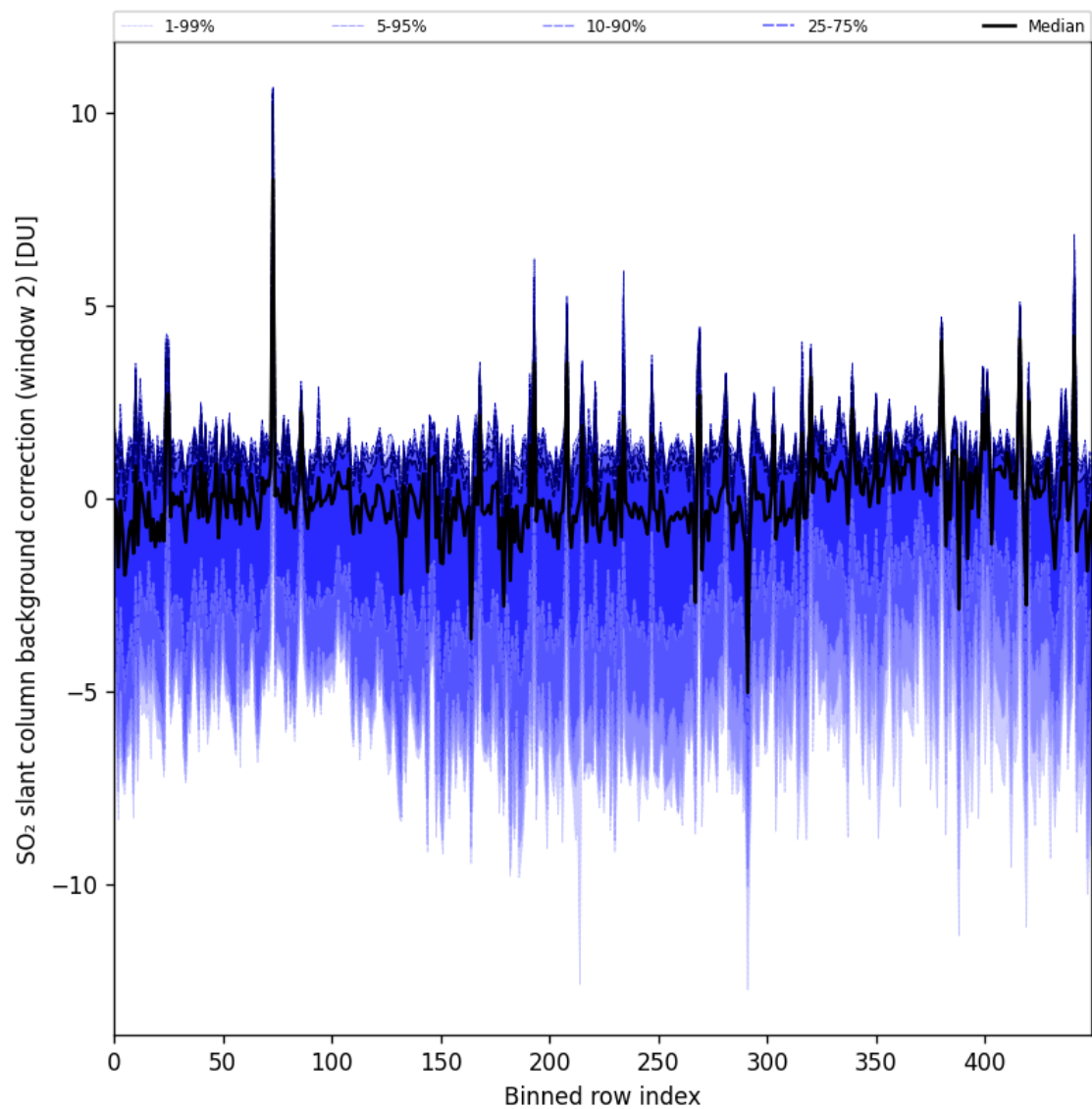
Figure 96: Along track statistics of “SO 2 slant column background correction (window 2)” for 2025-09-15 to 2025-09-17
