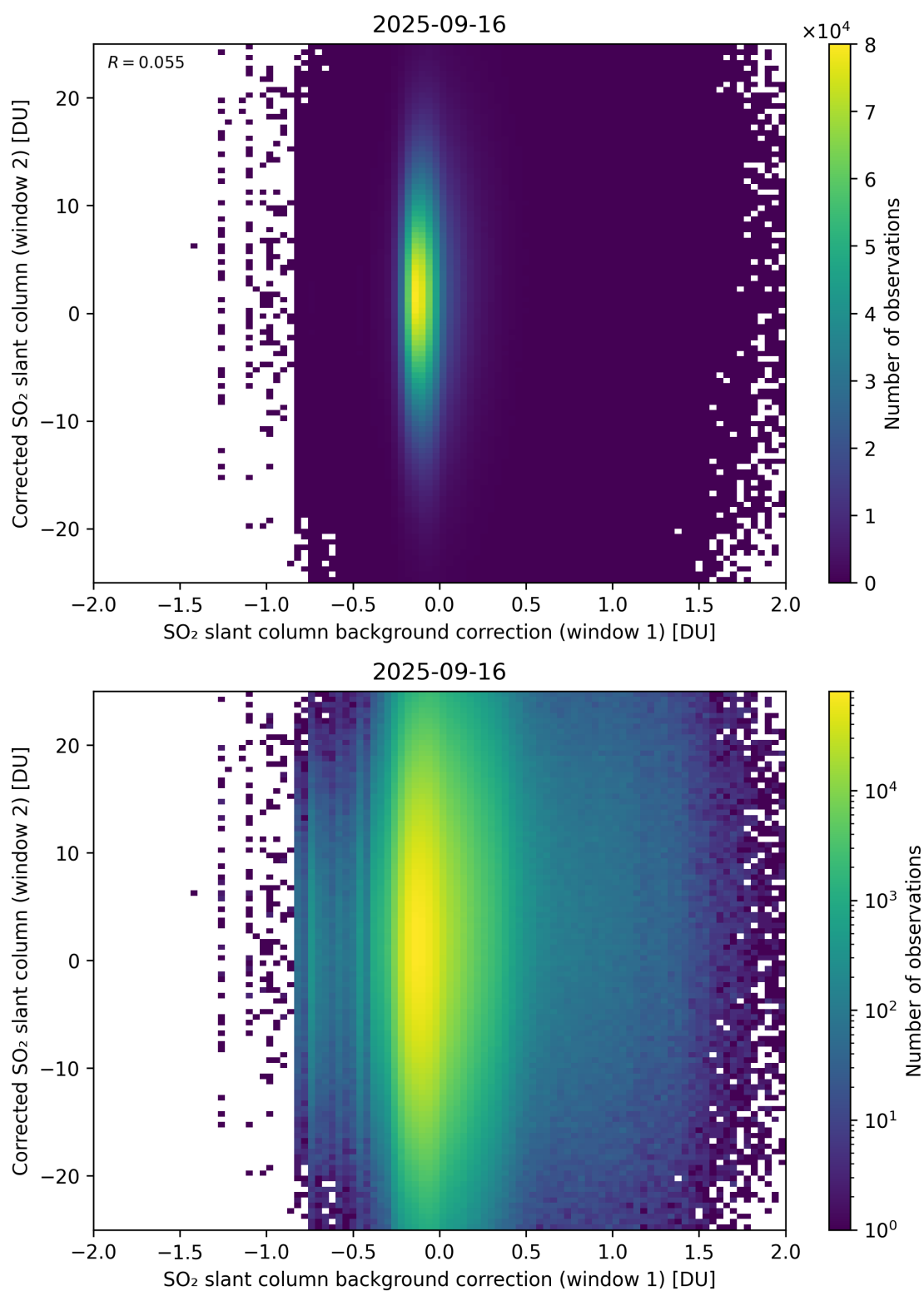
Figure 115: Scatter density plot of “SO 2 slant column background correction (window 1)” against “Corrected SO 2 slant column (window 2)” for 2025-09-15 to 2025-09-17.
