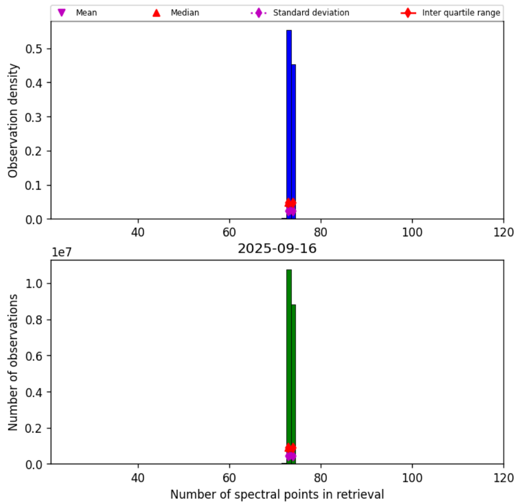
Figure 82: Histogram of “Number of spectral points in retrieval” for 2025-09-15 to 2025-09-17
