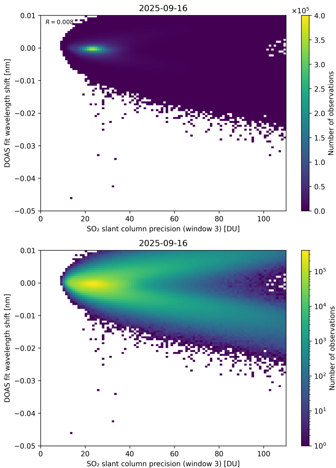
Figure 308: Scatter density plot of “SO 2 slant column precision (window 3)” against “DOAS fit wavelength shift” for 2025-09-15 to 2025-09-17.
