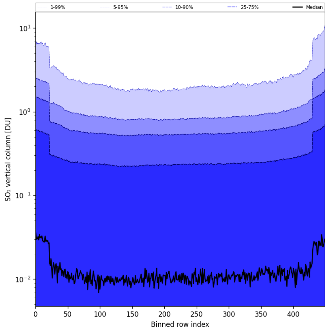
Figure 84: Along track statistics of “SO 2 vertical column” for 2025-09-15 to 2025-09-17
