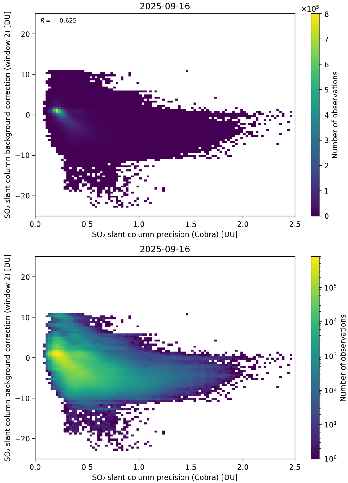
Figure 200: Scatter density plot of “SO 2 slant column precision (Cobra)” against “SO 2 slant column background correction (window 2)” for 2025-09-15 to 2025-09-17.
