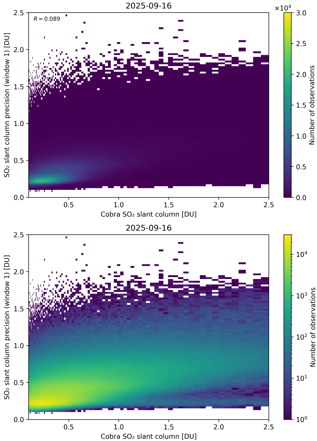
Figure 220: Scatter density plot of “Cobra SO 2 slant column” against “SO 2 slant column precision (window 1)” for 2025-09-15 to 2025-09-17.
