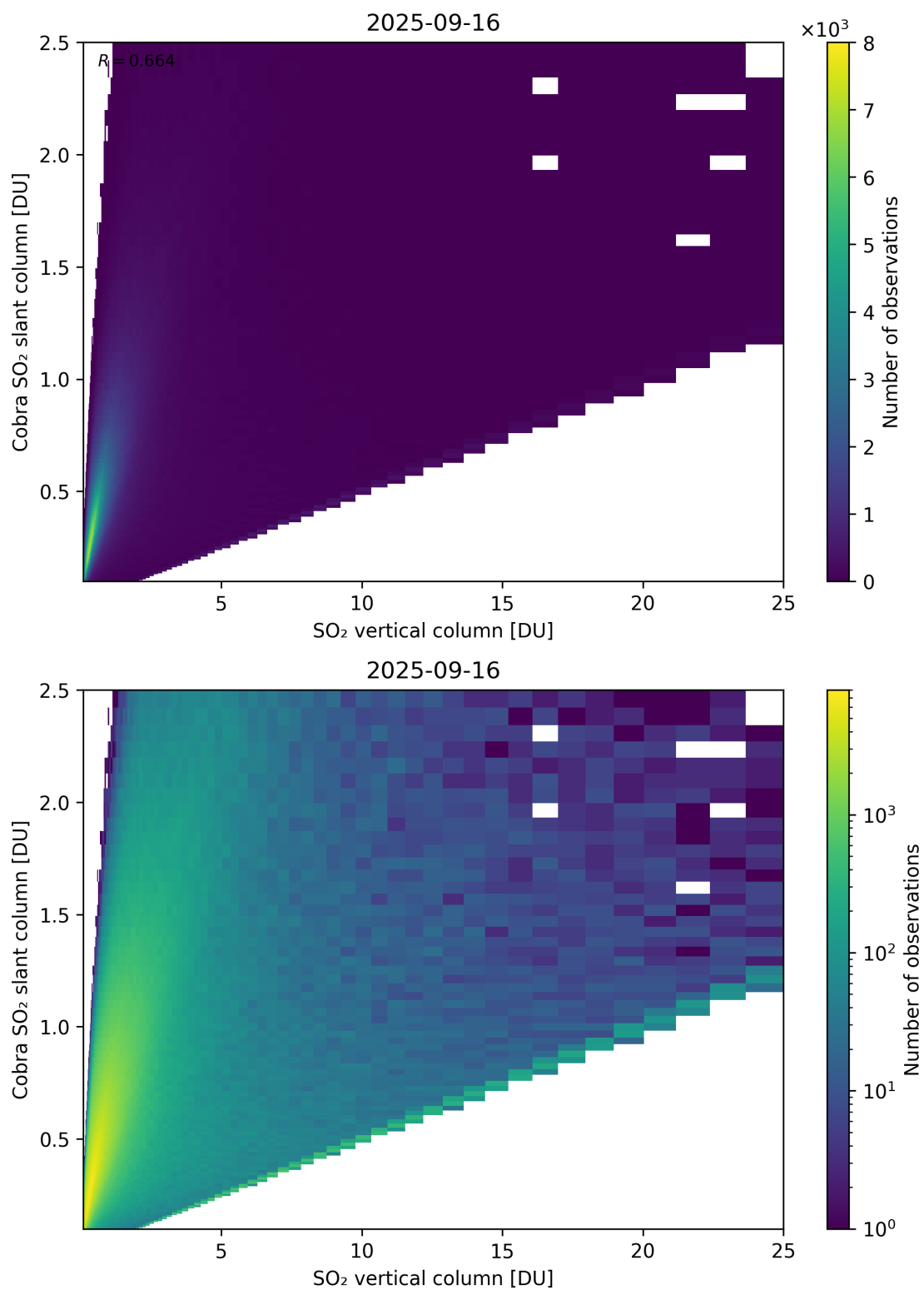
Figure 349: Scatter density plot of “SO 2 vertical column” against “Cobra SO 2 slant column” for 2025-09-15 to 2025-09-17.
