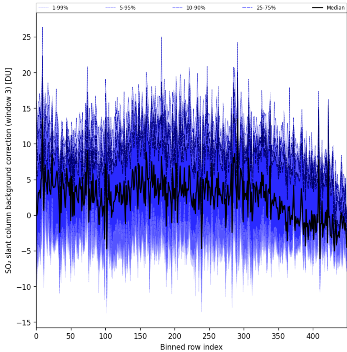
Figure 100: Along track statistics of “SO 2 slant column background correction (window 3)” for 2025-09-15 to 2025-09-17
