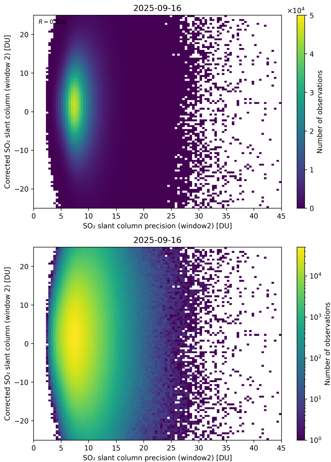
Figure 297: Scatter density plot of “SO 2 slant column precision (window2)” against “Corrected SO 2 slant column (window 2)” for 2025-09-15 to 2025-09-17.
