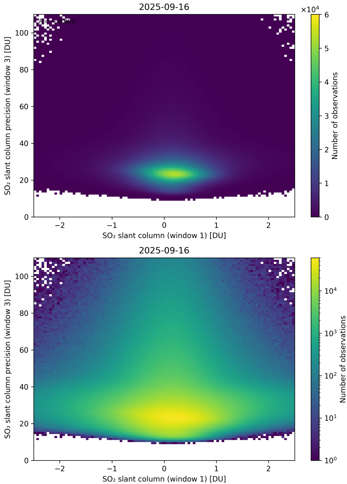
Figure 288: Scatter density plot of “SO 2 slant column (window 1)” against “SO 2 slant column precision (window 3)” for 2025-09-15 to 2025-09-17.
