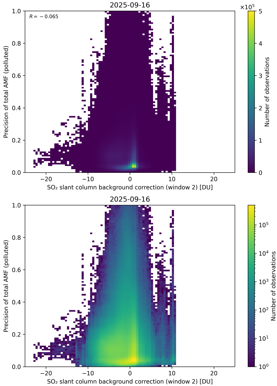
Figure 131: Scatter density plot of “SO 2 slant column background correction (window 2)” against “Precision of total AMF (polluted)” for 2025-09-15 to 2025-09-17.
