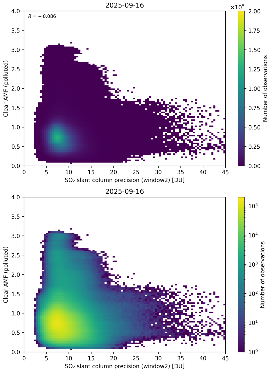
Figure 296: Scatter density plot of “SO 2 slant column precision (window2)” against “Clear AMF (polluted)” for 2025-09-15 to 2025-09-17.
