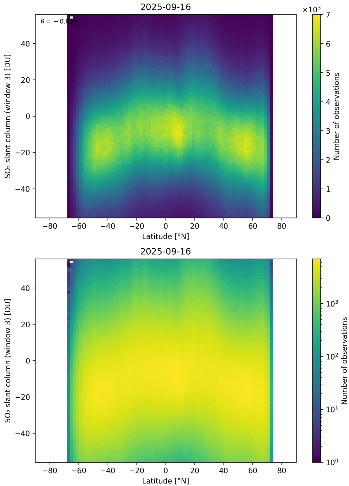
Figure 165: Scatter density plot of “Latitude” against “SO 2 slant column (window 3)” for 2025-09-15 to 2025-09-17.
