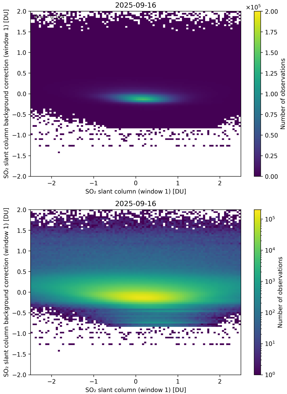
Figure 262: Scatter density plot of “SO 2 slant column (window 1)” against “SO 2 slant column background correction (window 1)” for 2025-09-15 to 2025-09-17.
