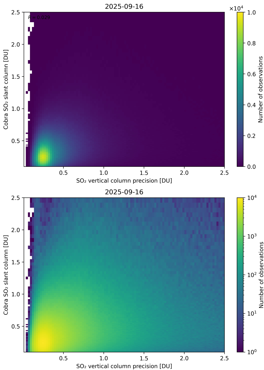
Figure 336: Scatter density plot of “SO 2 vertical column precision” against “Cobra SO 2 slant column” for 2025-09-15 to 2025-09-17.
