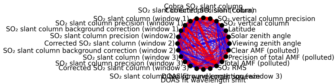
Figure 1: Map of correlation graph for 2025-09-15 to 2025-09-17.
