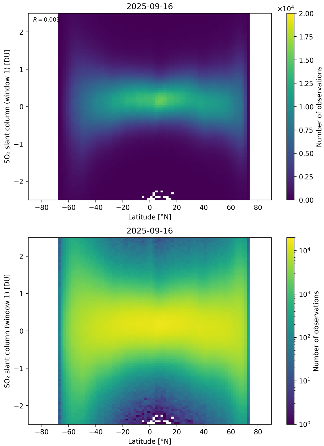
Figure 162: Scatter density plot of “Latitude” against “SO 2 slant column (window 1)” for 2025-09-15 to 2025-09-17.
