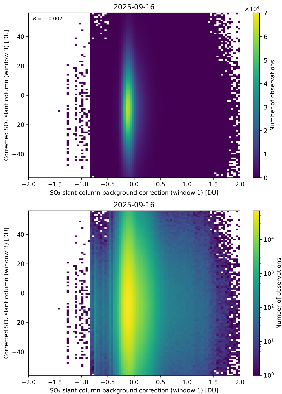
Figure 116: Scatter density plot of “SO 2 slant column background correction (window 1)” against “Corrected SO 2 slant column (window 3)” for 2025-09-15 to 2025-09-17.
