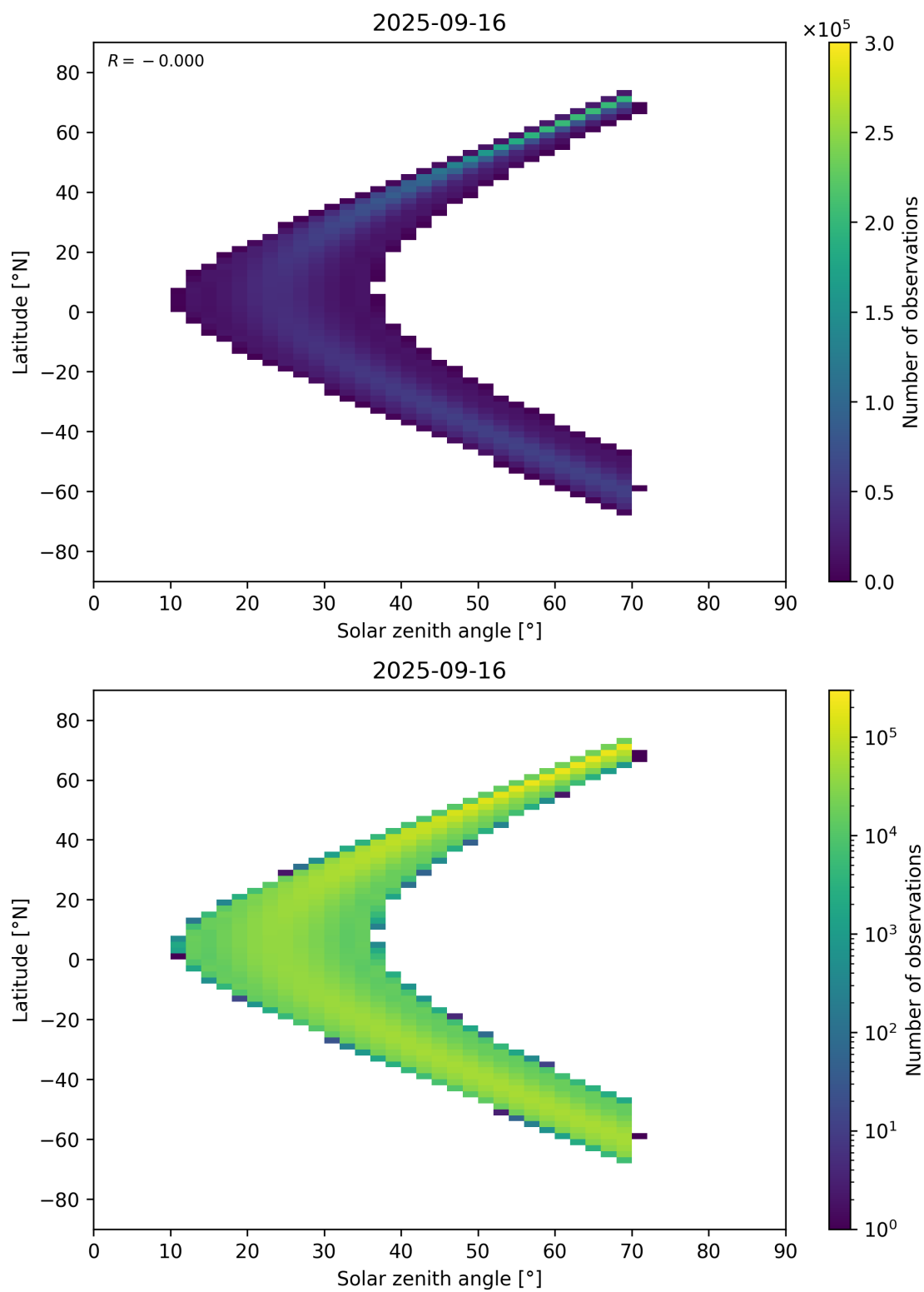
Figure 177: Scatter density plot of “Solar zenith angle” against “Latitude” for 2025-09-15 to 2025-09-17.
