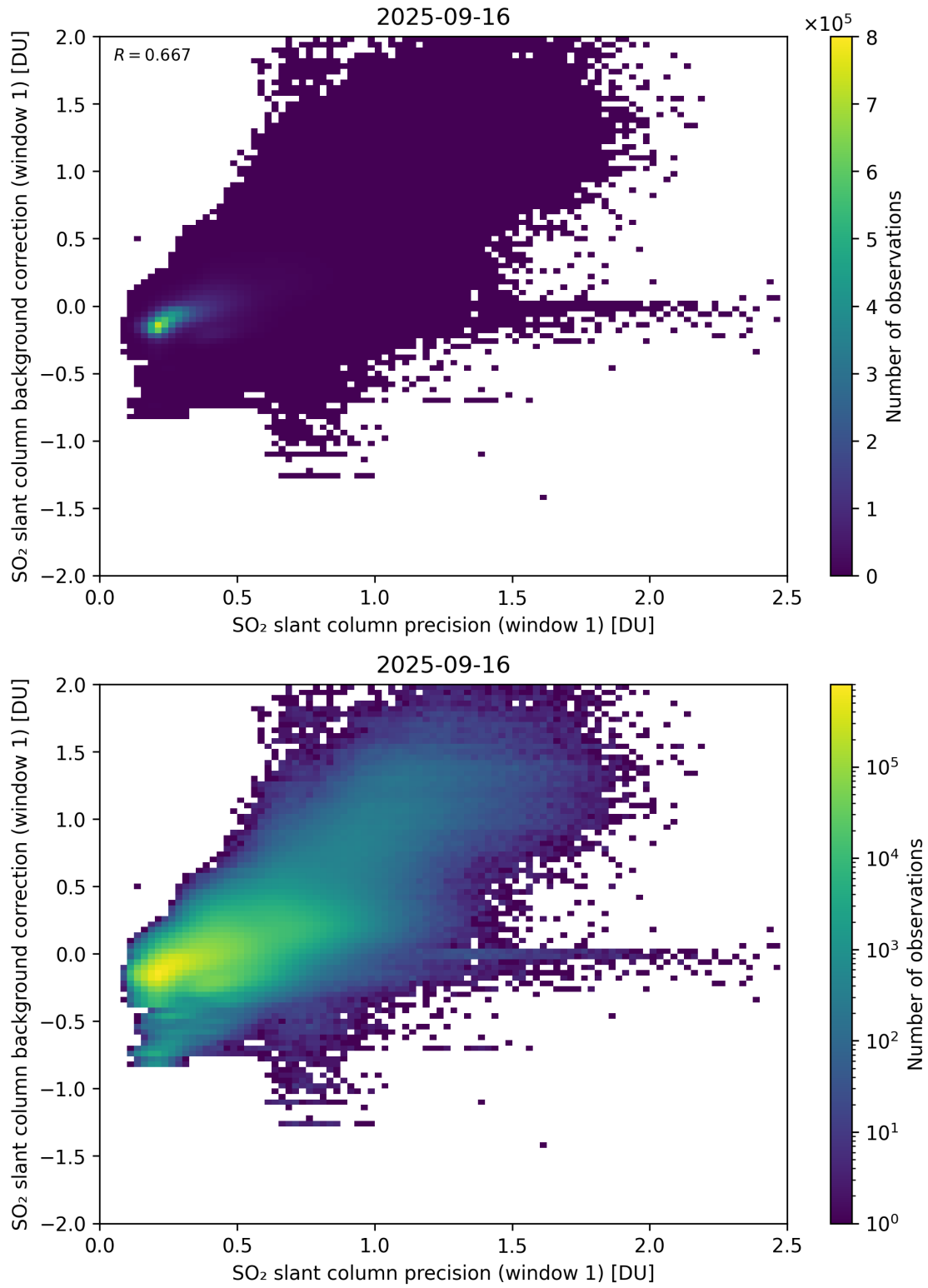
Figure 268: Scatter density plot of “SO 2 slant column precision (window 1)” against “SO 2 slant column background correction (window 1)” for 2025-09-15 to 2025-09-17.
