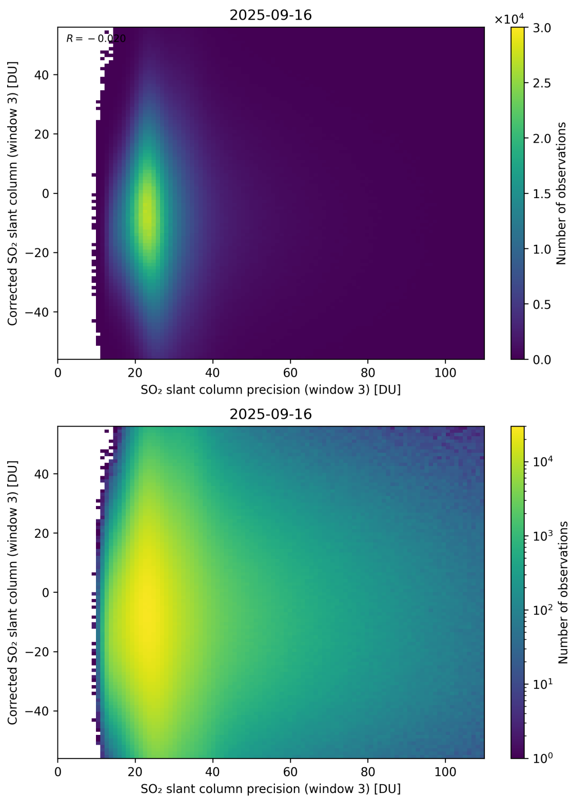
Figure 312: Scatter density plot of “SO 2 slant column precision (window 3)” against “Corrected SO 2 slant column (window 3)” for 2025-09-15 to 2025-09-17.
