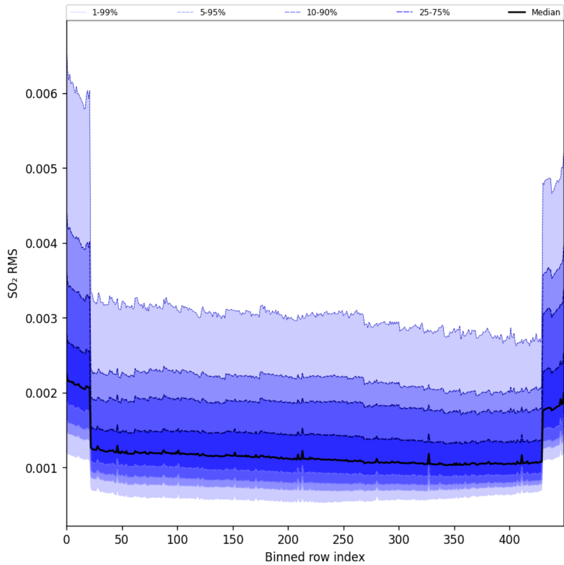
Figure 104: Along track statistics of “SO 2 RMS” for 2025-09-15 to 2025-09-17
