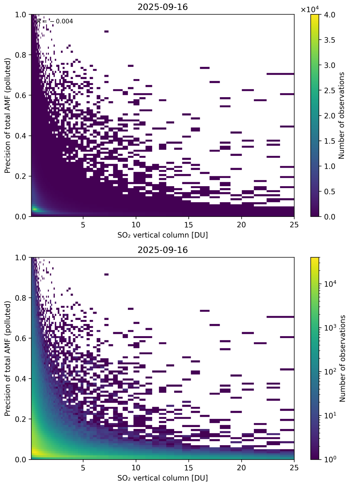
Figure 360: Scatter density plot of “SO 2 vertical column” against “Precision of total AMF (polluted)” for 2025-09-15 to 2025-09-17.
