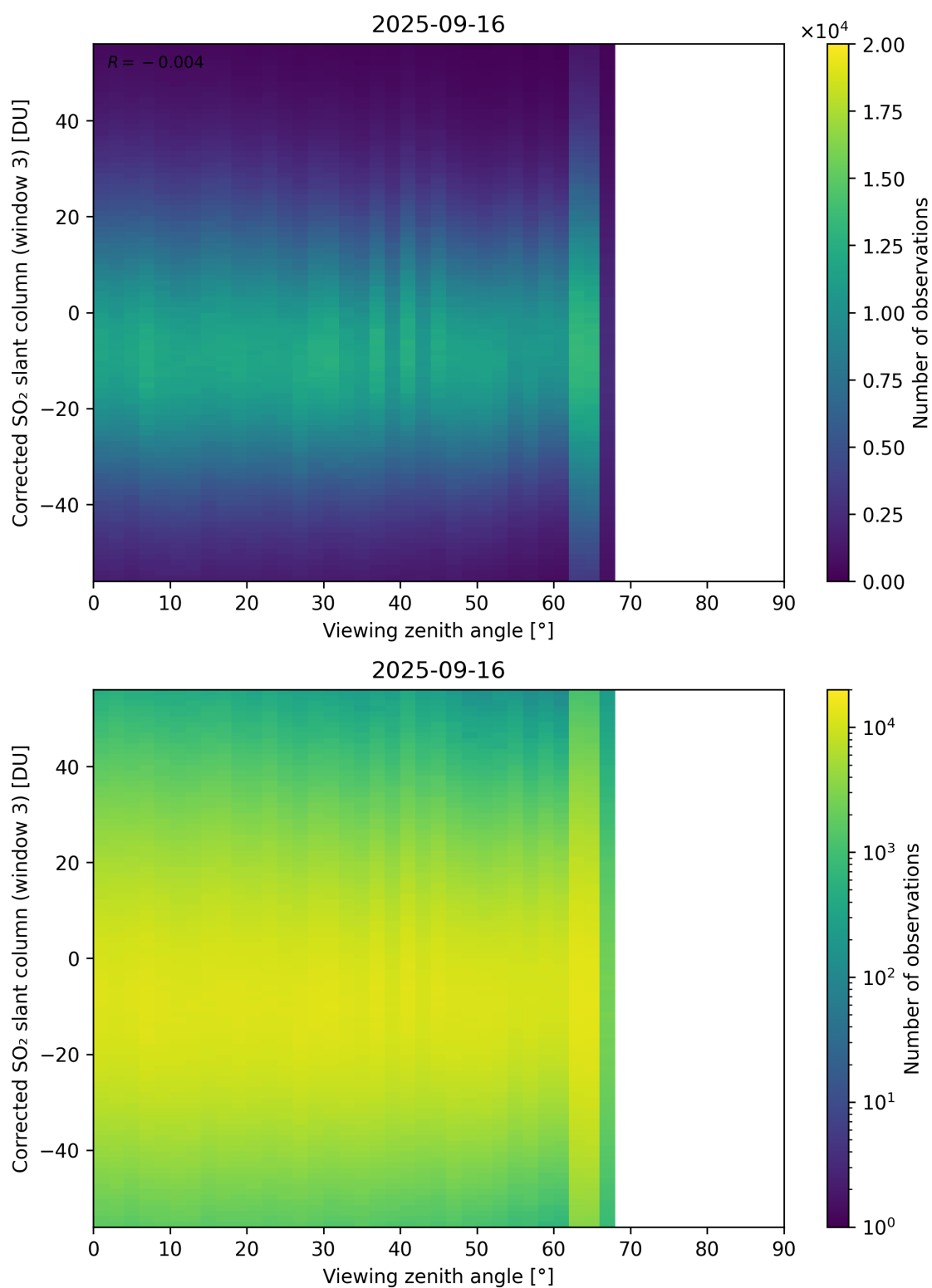
Figure 375: Scatter density plot of “Viewing zenith angle” against “Corrected SO 2 slant column (window 3)” for 2025-09-15 to 2025-09-17.
