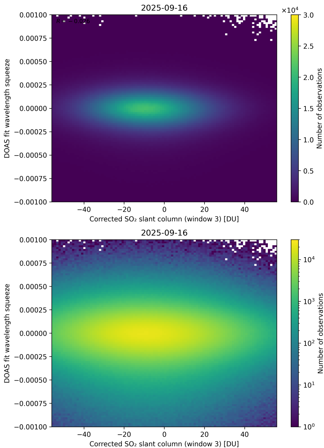
Figure 257: Scatter density plot of “Corrected SO 2 slant column (window 3)” against “DOAS fit wavelength squeeze” for 2025-09-15 to 2025-09-17.
