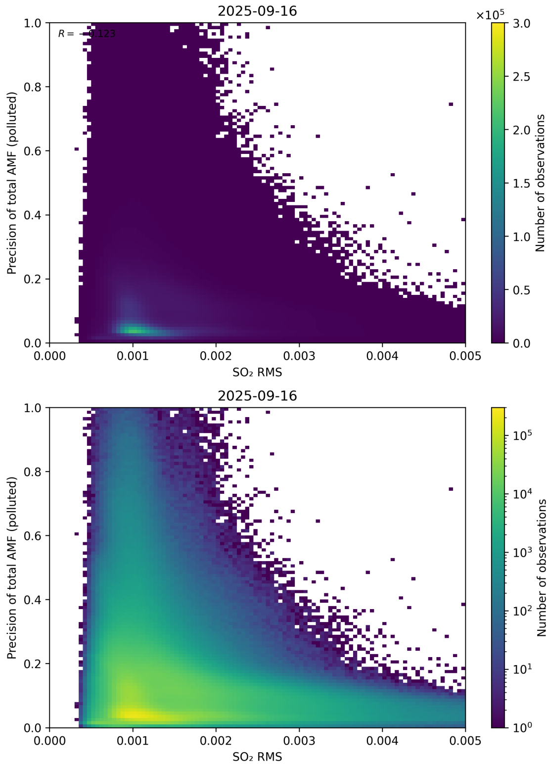
Figure 149: Scatter density plot of “SO 2 RMS” against “Precision of total AMF (polluted)” for 2025-09-15 to 2025-09-17.
