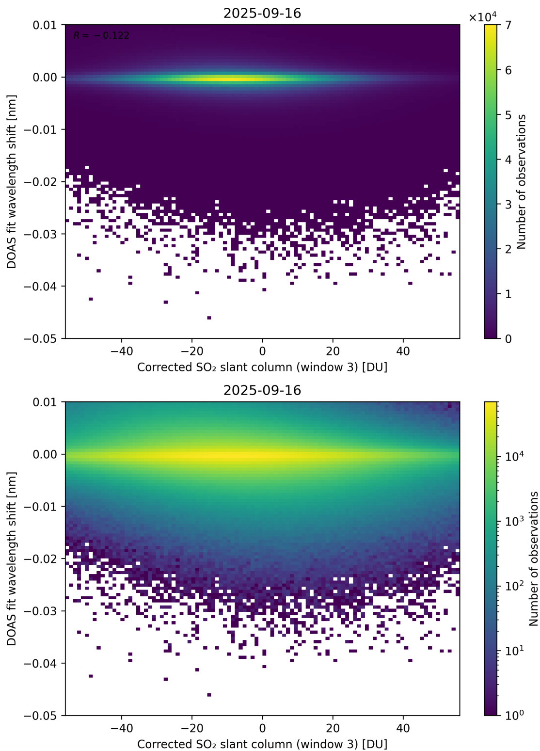
Figure 256: Scatter density plot of “Corrected SO 2 slant column (window 3)” against “DOAS fit wavelength shift” for 2025-09-15 to 2025-09-17.
