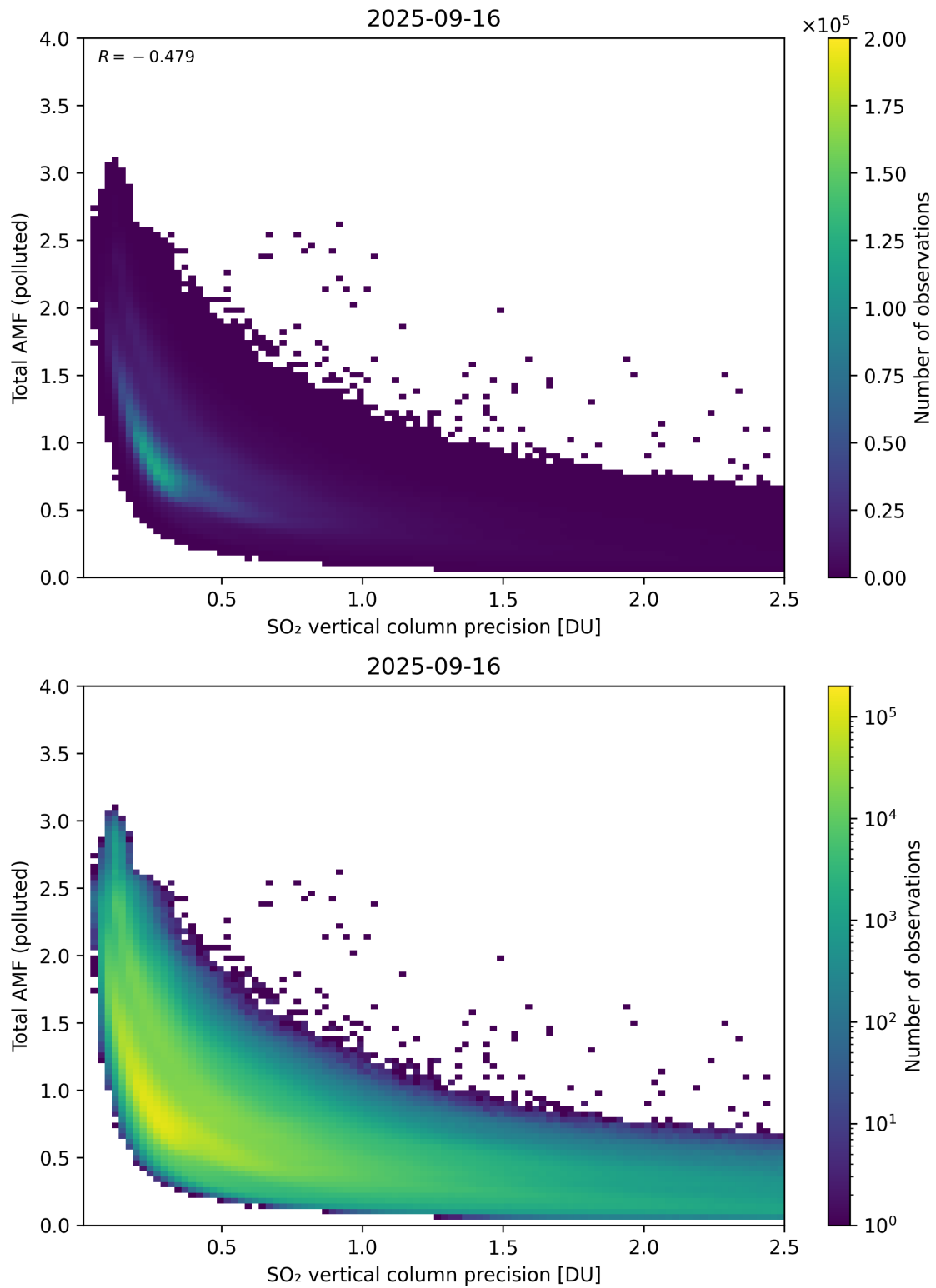
Figure 346: Scatter density plot of “SO 2 vertical column precision” against “Total AMF (polluted)” for 2025-09-15 to 2025-09-17.
