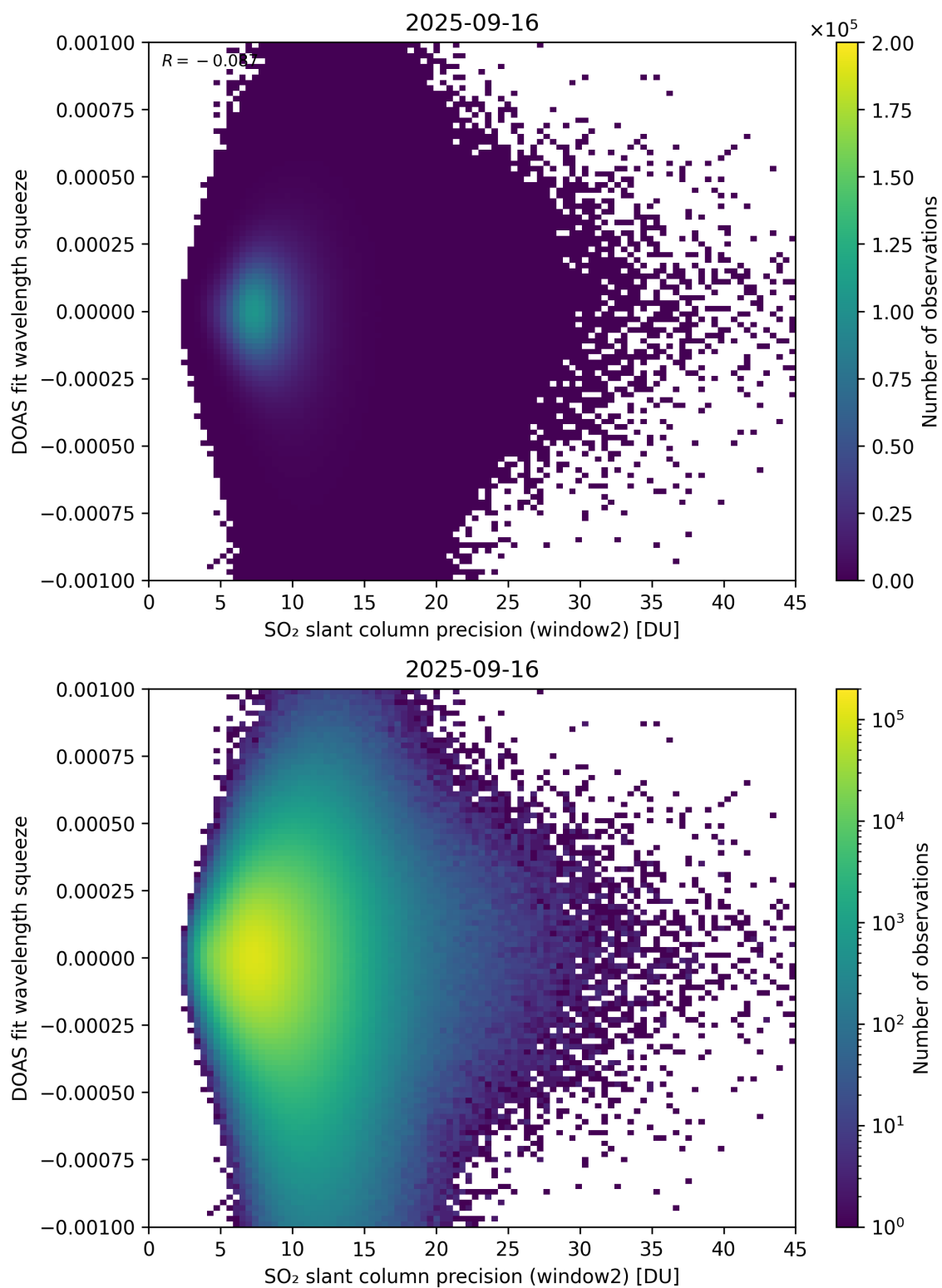
Figure 294: Scatter density plot of “SO 2 slant column precision (window2)” against “DOAS fit wavelength squeeze” for 2025-09-15 to 2025-09-17.
