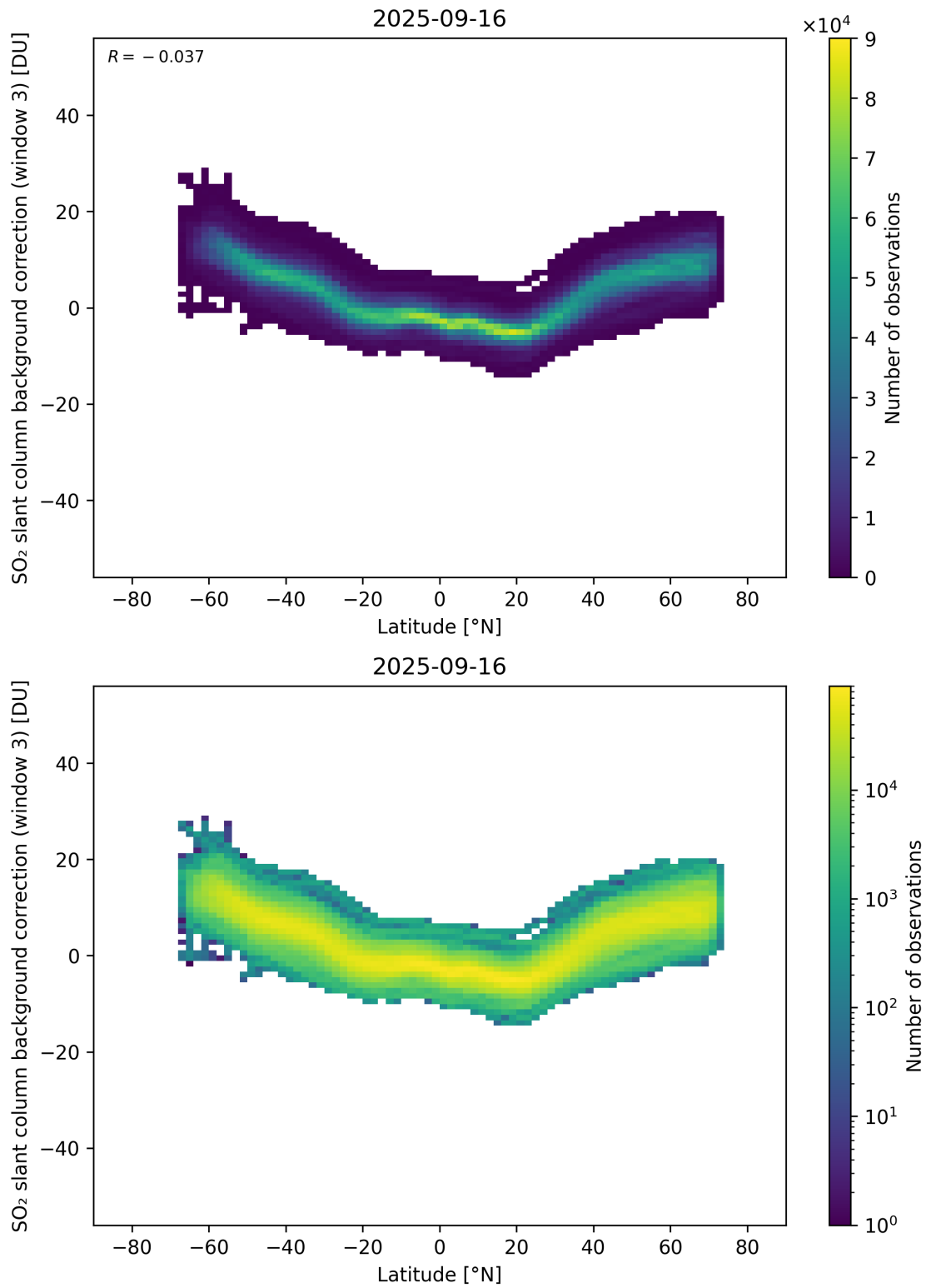
Figure 152: Scatter density plot of “Latitude” against “SO 2 slant column background correction (window 3)” for 2025-09-15 to 2025-09-17.
