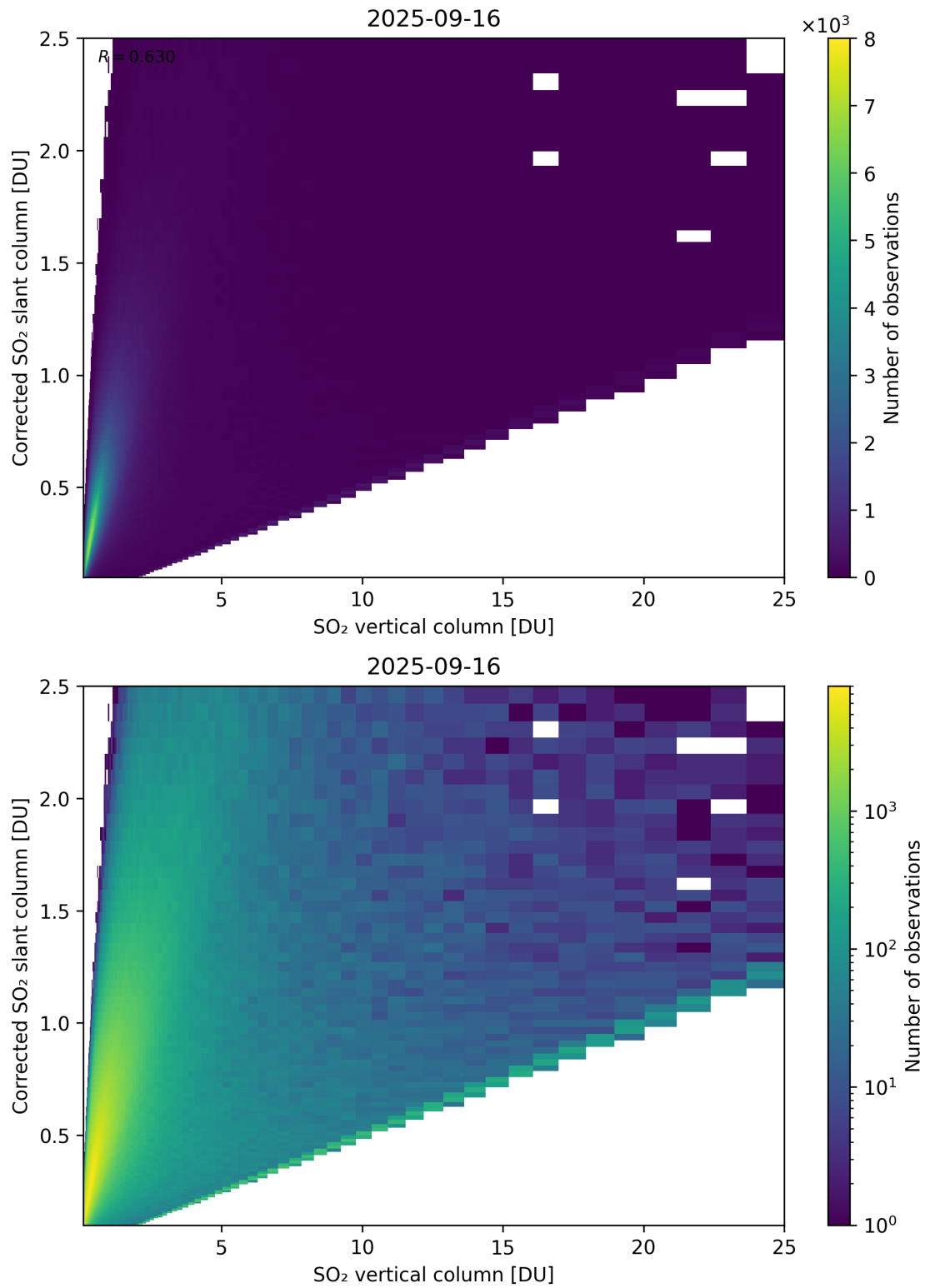
Figure 351: Scatter density plot of “SO 2 vertical column” against “Corrected SO 2 slant column” for 2025-09-15 to 2025-09-17.
