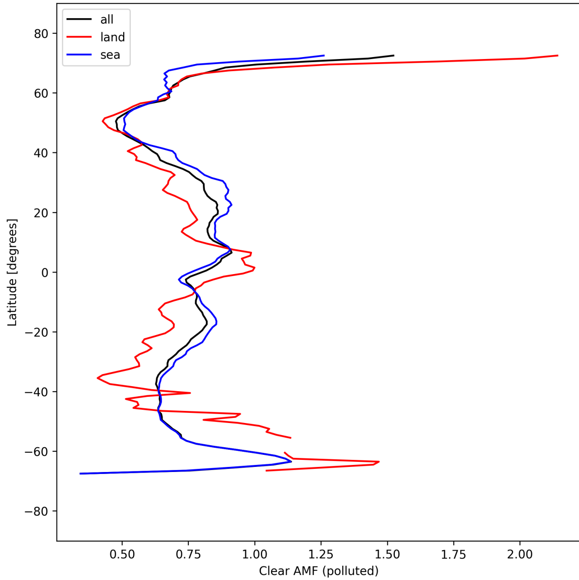
Figure 55: Zonal average of “Clear AMF (polluted)” for 2025-09-15 to 2025-09-17.
