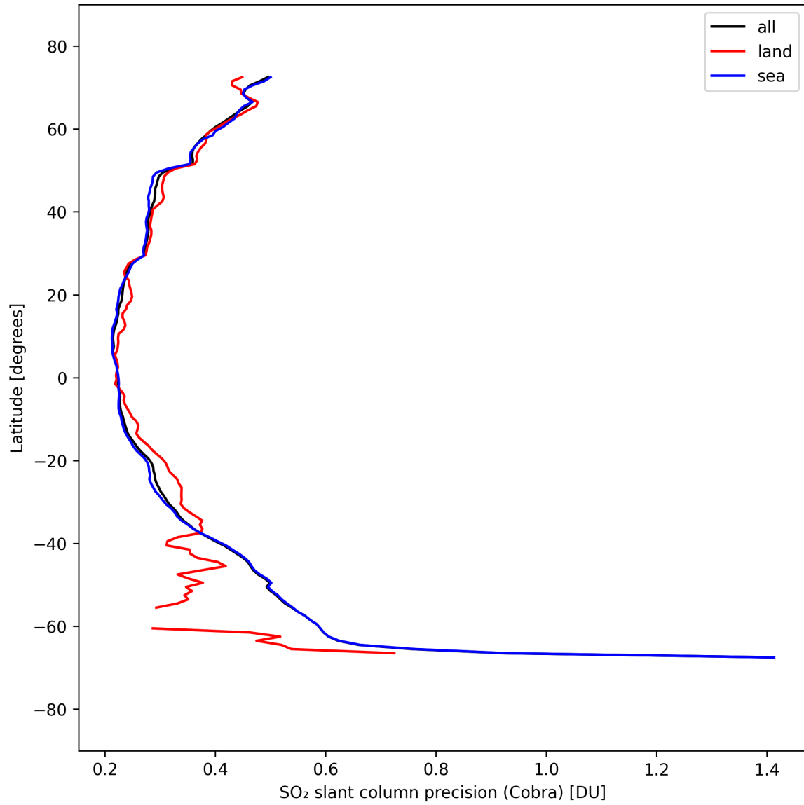
Figure 36: Zonal average of “SO 2 slant column precision (Cobra)” for 2025-09-15 to 2025-09-17.
