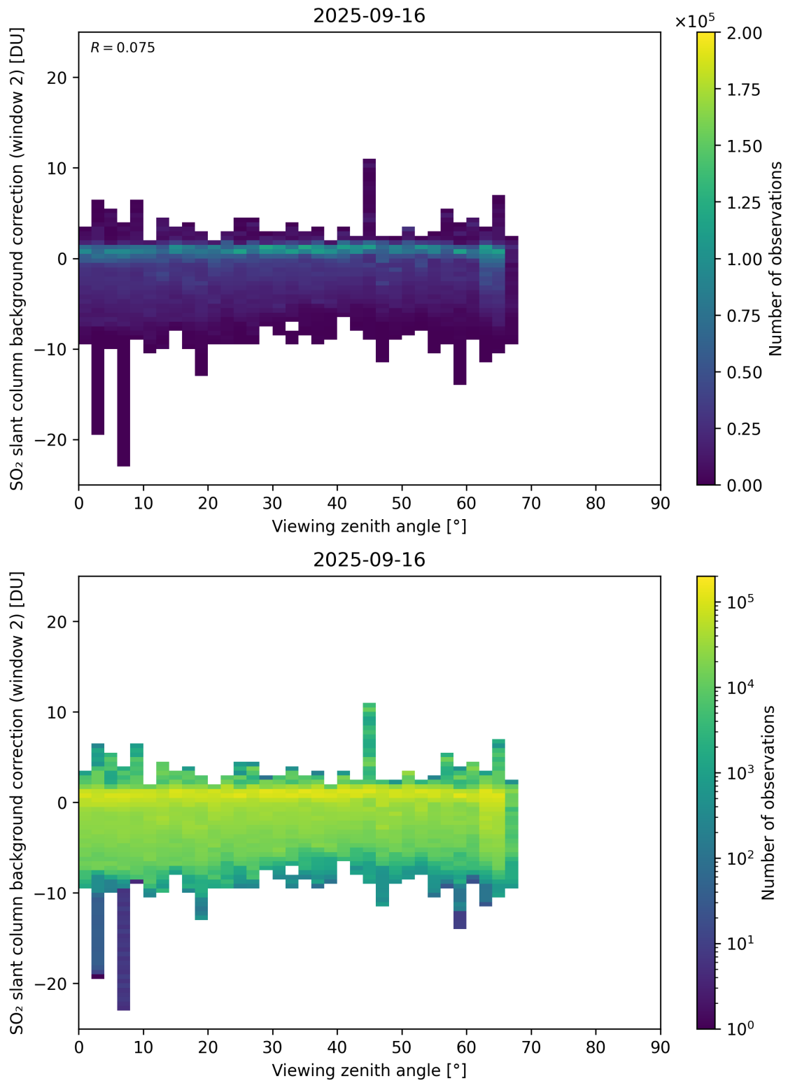
Figure 363: Scatter density plot of “Viewing zenith angle” against “SO 2 slant column background correction (window 2)” for 2025-09-15 to 2025-09-17.
