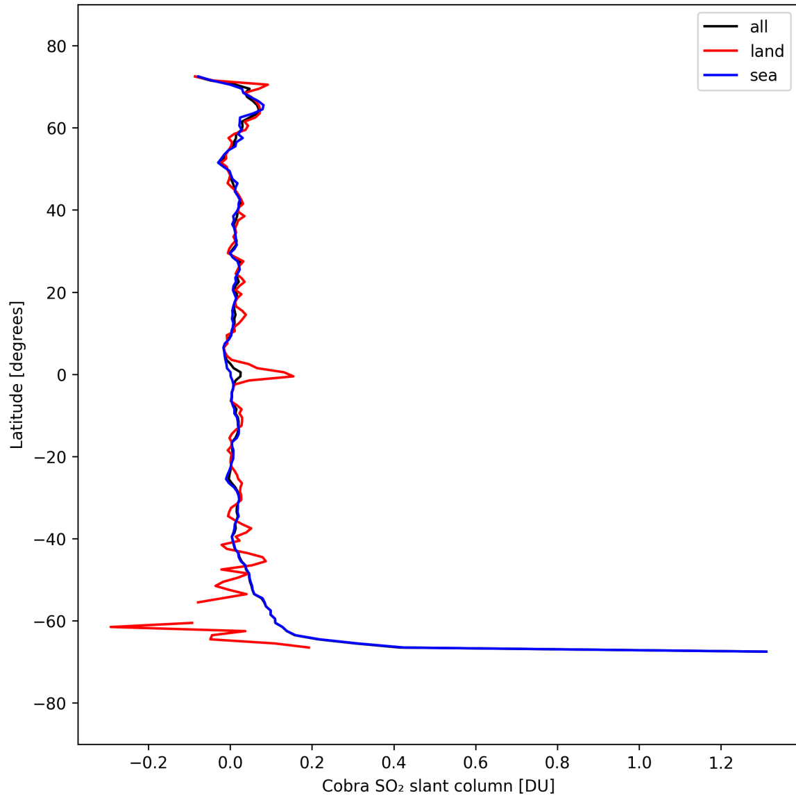
Figure 35: Zonal average of “Cobra SO 2 slant column” for 2025-09-15 to 2025-09-17.
