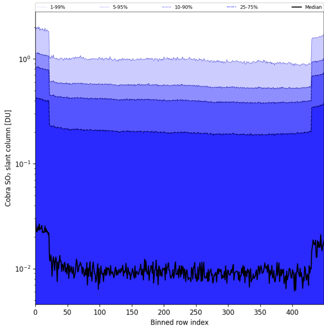
Figure 87: Along track statistics of “Cobra SO 2 slant column” for 2025-09-15 to 2025-09-17
