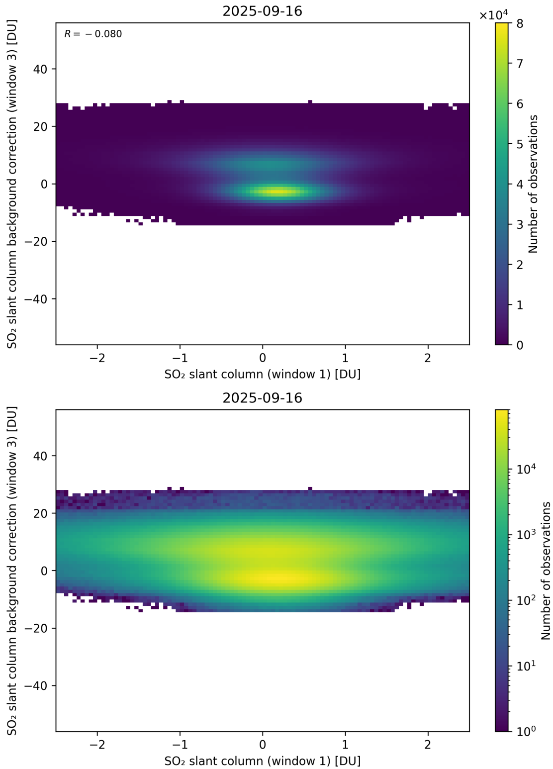
Figure 264: Scatter density plot of “SO 2 slant column (window 1)” against “SO 2 slant column background correction (window 3)” for 2025-09-15 to 2025-09-17.
