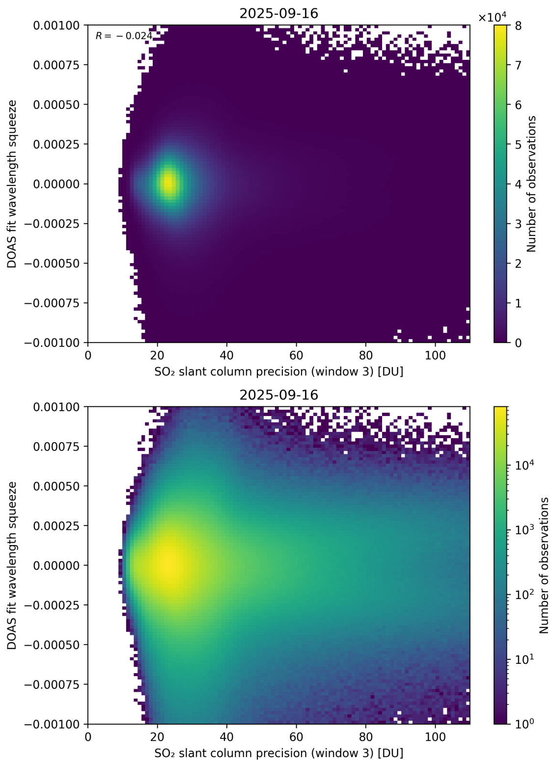
Figure 309: Scatter density plot of “SO 2 slant column precision (window 3)” against “DOAS fit wavelength squeeze” for 2025-09-15 to 2025-09-17.
