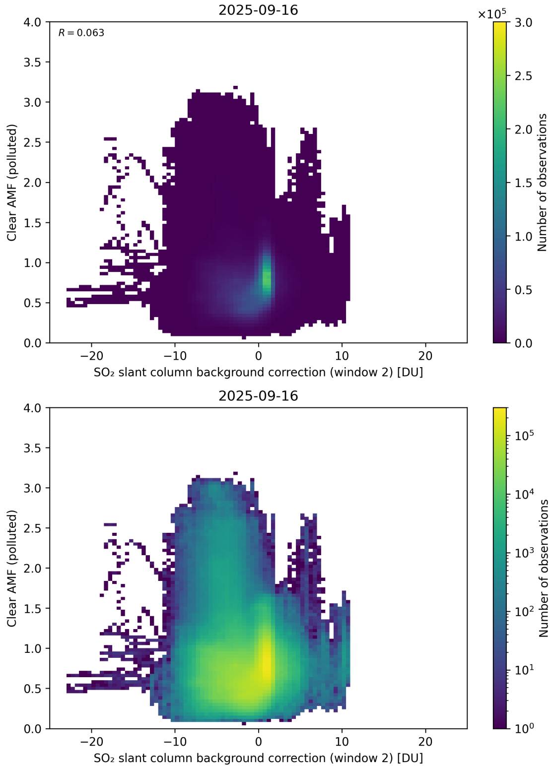
Figure 126: Scatter density plot of “SO 2 slant column background correction (window 2)” against “Clear AMF (polluted)” for 2025-09-15 to 2025-09-17.
