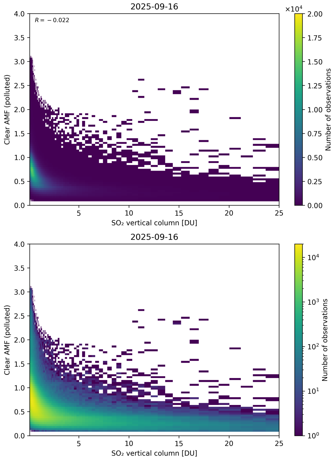
Figure 348: Scatter density plot of “SO 2 vertical column” against “Clear AMF (polluted)” for 2025-09-15 to 2025-09-17.
