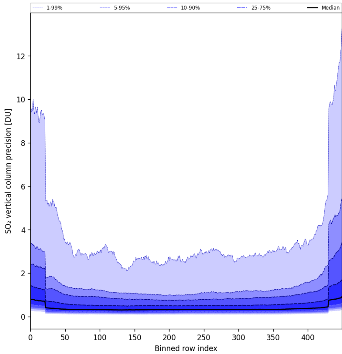
Figure 85: Along track statistics of “SO 2 vertical column precision” for 2025-09-15 to 2025-09-17
