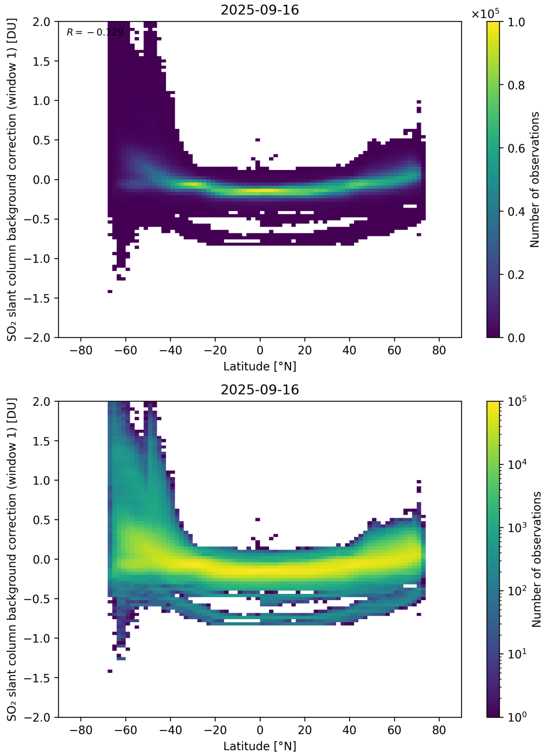
Figure 150: Scatter density plot of “Latitude” against “SO 2 slant column background correction (window 1)” for 2025-09-15 to 2025-09-17.
