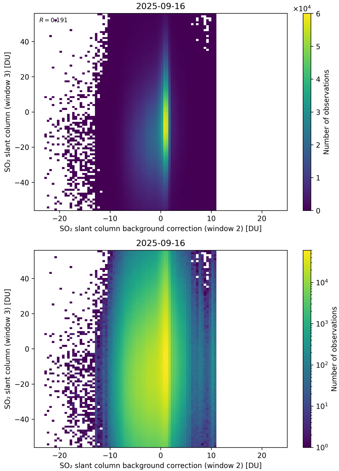
Figure 128: Scatter density plot of “SO 2 slant column background correction (window 2)” against “SO 2 slant column (window 3)” for 2025-09-15 to 2025-09-17.
