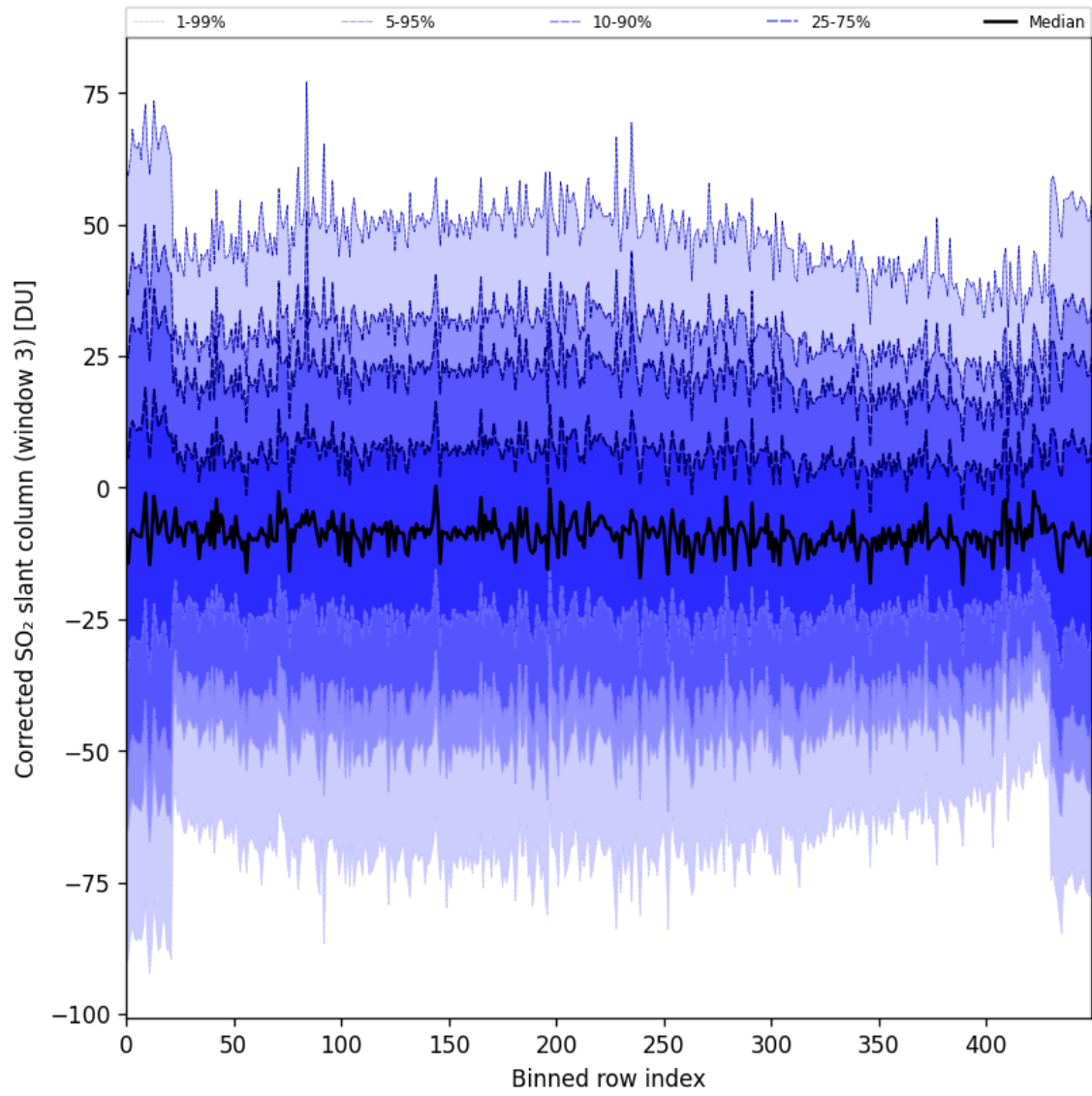
Figure 99: Along track statistics of “Corrected SO 2 slant column (window 3)” for 2025-09-15 to 2025-09-17
