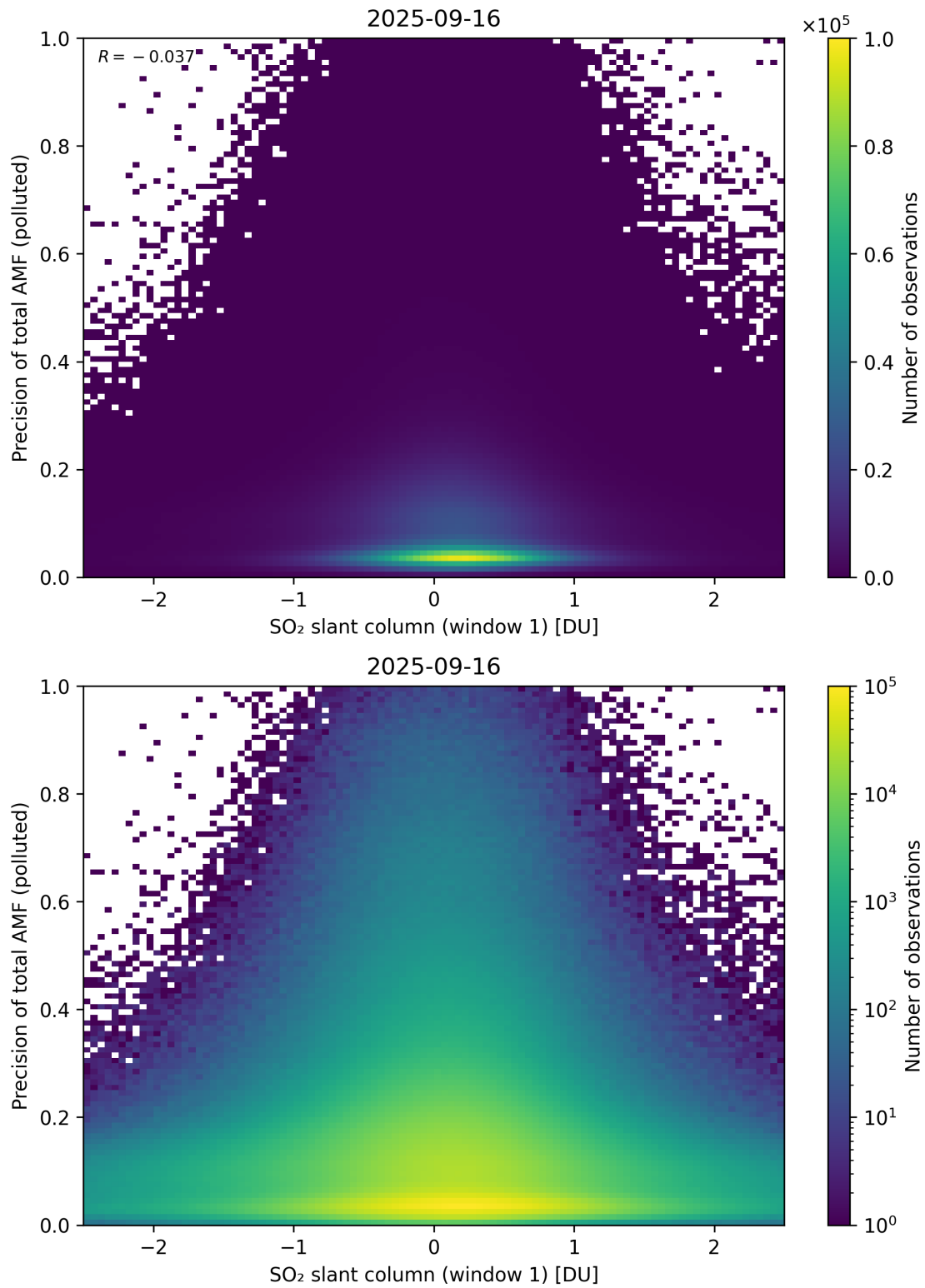
Figure 290: Scatter density plot of “SO 2 slant column (window 1)” against “Precision of total AMF (polluted)” for 2025-09-15 to 2025-09-17.
