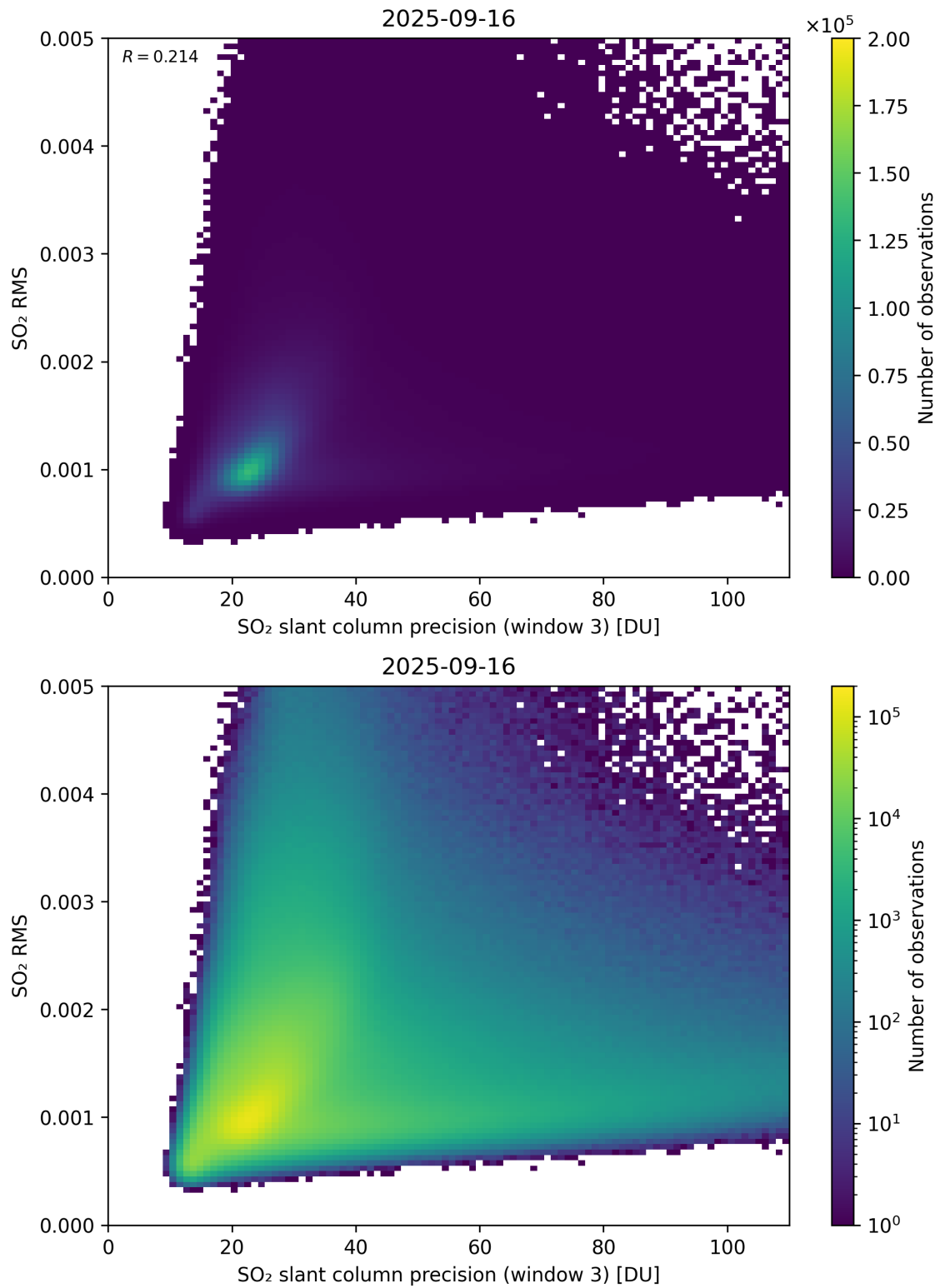
Figure 310: Scatter density plot of “SO 2 slant column precision (window 3)” against “SO 2 RMS” for 2025-09-15 to 2025-09-17.
