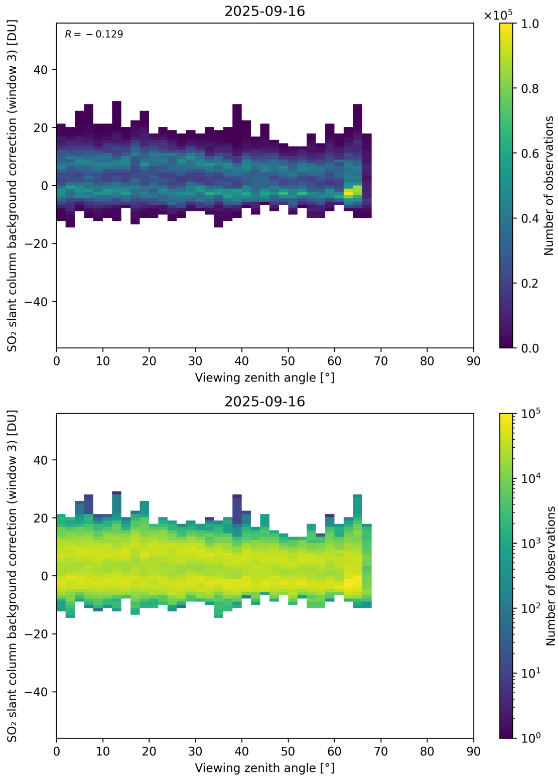
Figure 364: Scatter density plot of “Viewing zenith angle” against “SO 2 slant column background correction (window 3)” for 2025-09-15 to 2025-09-17.
