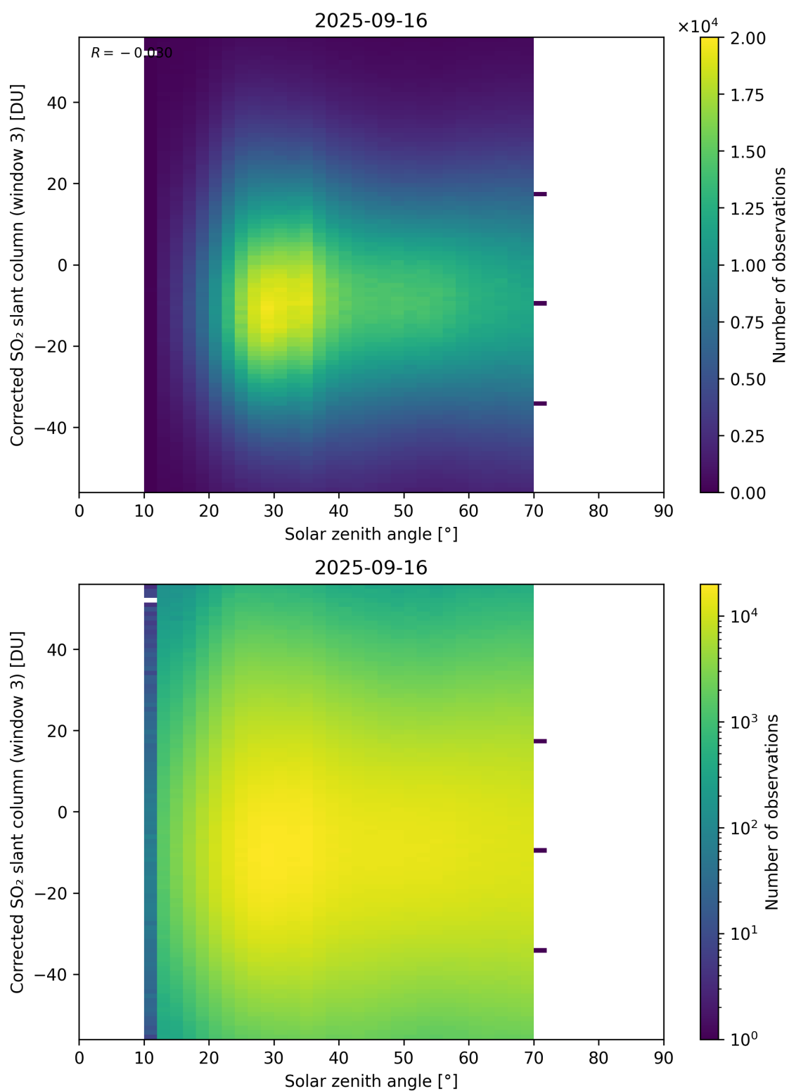
Figure 183: Scatter density plot of “Solar zenith angle” against “Corrected SO 2 slant column (window 3)” for 2025-09-15 to 2025-09-17.
