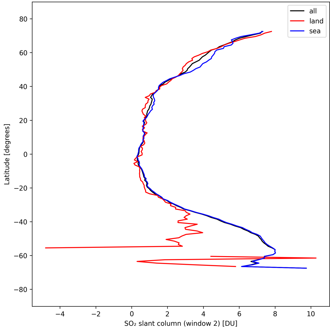
Figure 41: Zonal average of “SO 2 slant column (window 2)” for 2025-09-15 to 2025-09-17.
