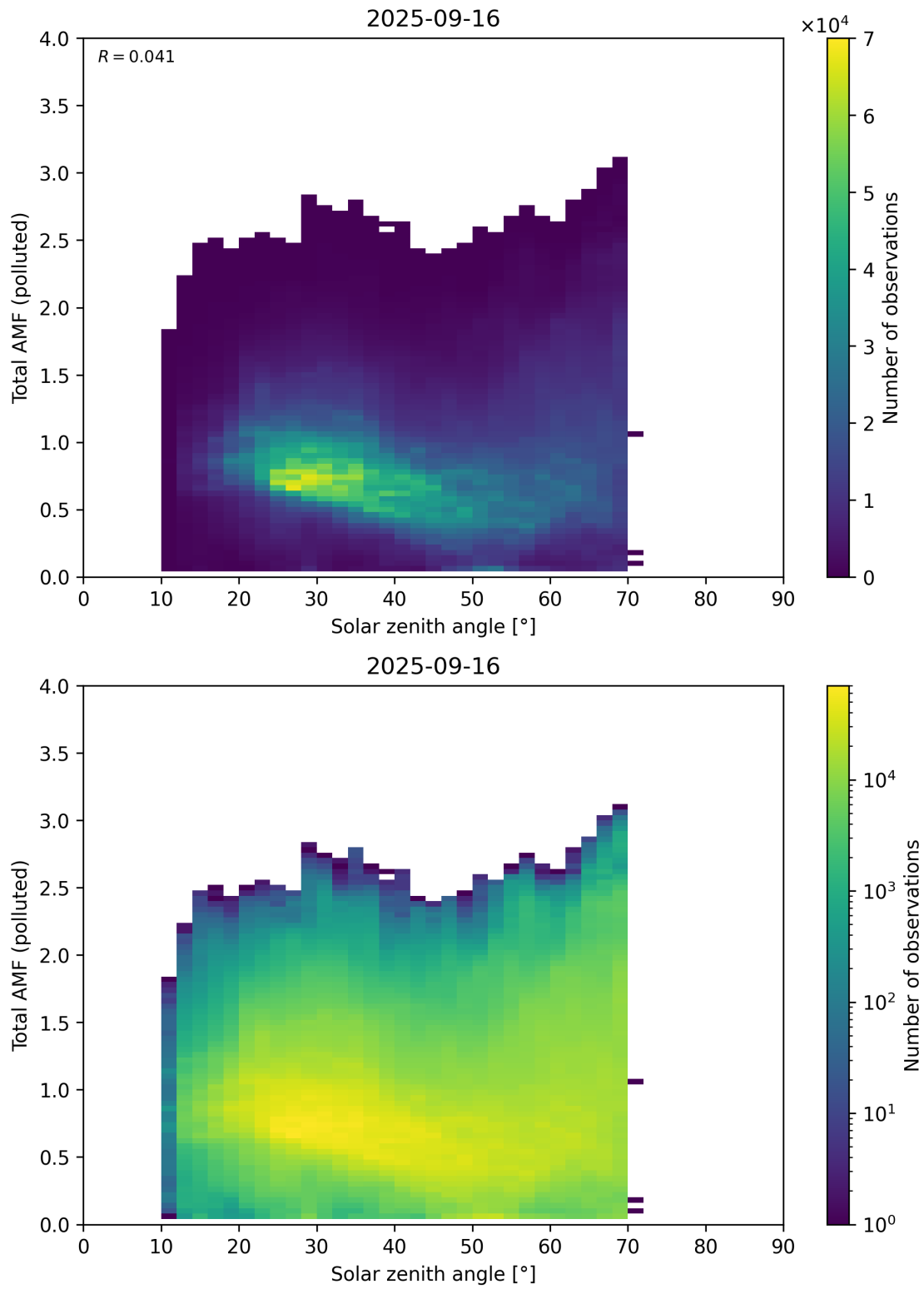
Figure 189: Scatter density plot of “Solar zenith angle” against “Total AMF (polluted)” for 2025-09-15 to 2025-09-17.
