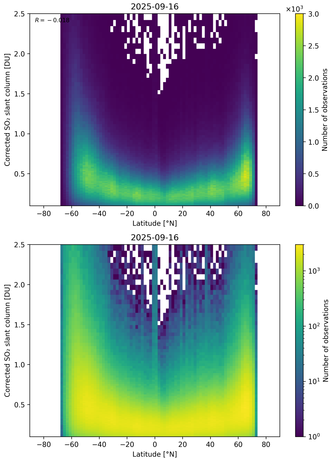
Figure 159: Scatter density plot of “Latitude” against “Corrected SO 2 slant column” for 2025-09-15 to 2025-09-17.
