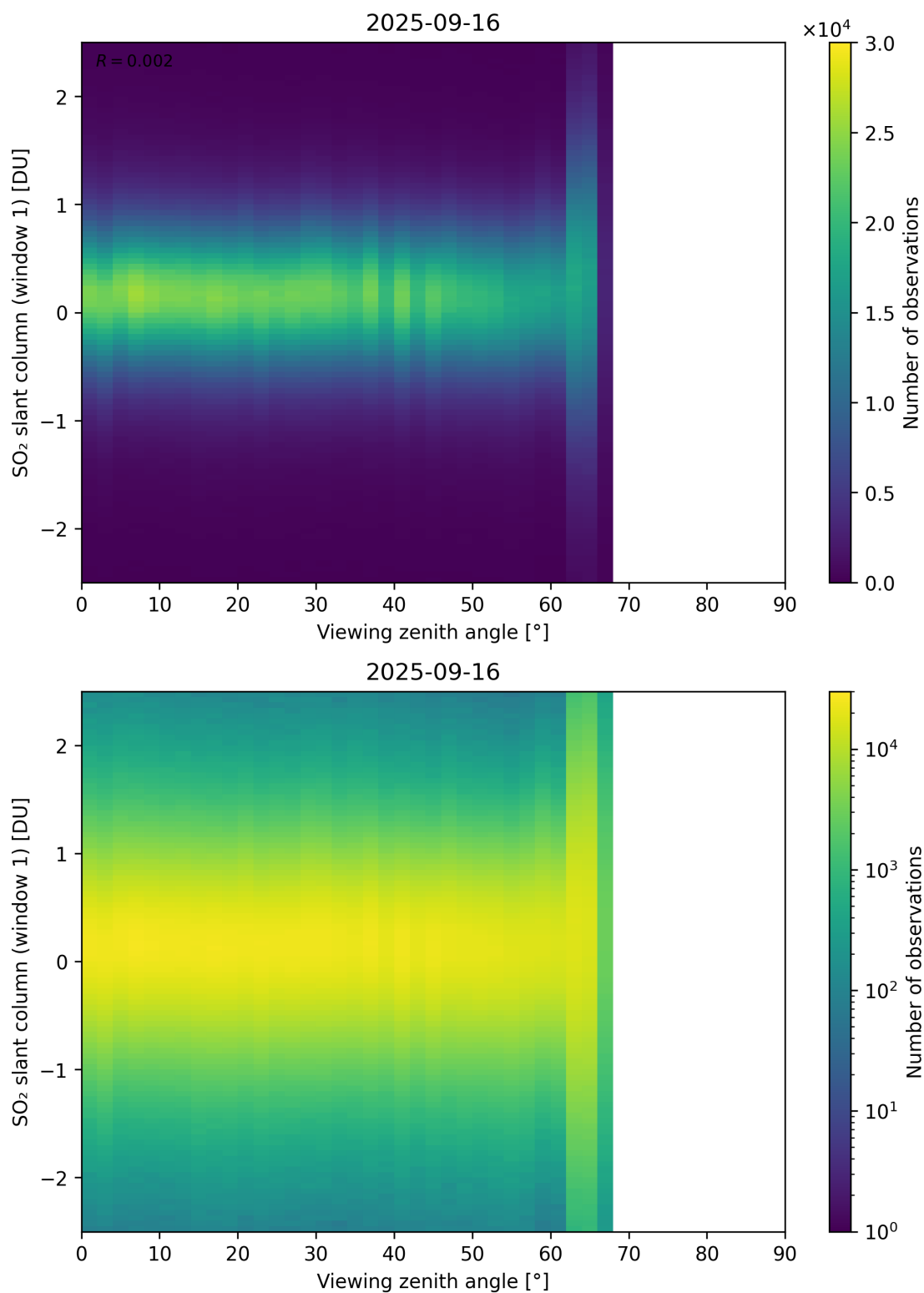
Figure 376: Scatter density plot of “Viewing zenith angle” against “SO 2 slant column (window 1)” for 2025-09-15 to 2025-09-17.
