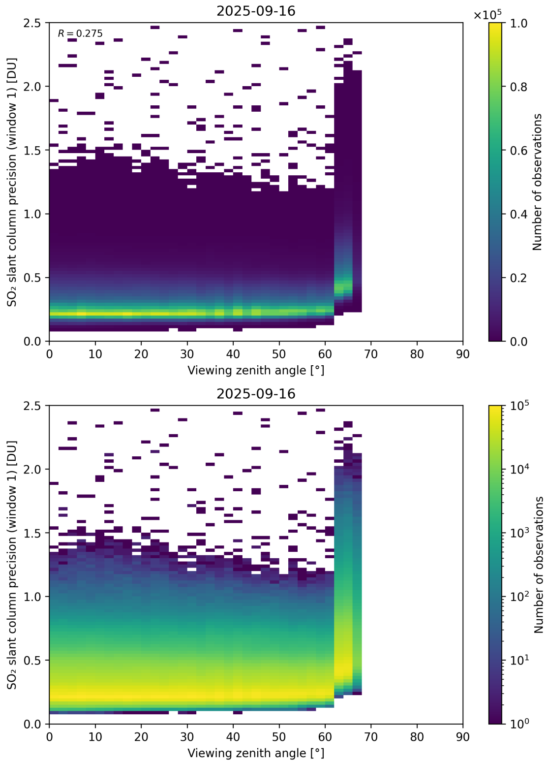
Figure 377: Scatter density plot of “Viewing zenith angle” against “SO 2 slant column precision (window 1)” for 2025-09-15 to 2025-09-17.
