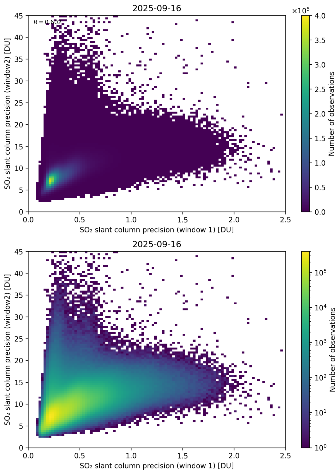
Figure 277: Scatter density plot of “SO 2 slant column precision (window 1)” against “SO 2 slant column precision (window 2)” for 2025-09-15 to 2025-09-17.
