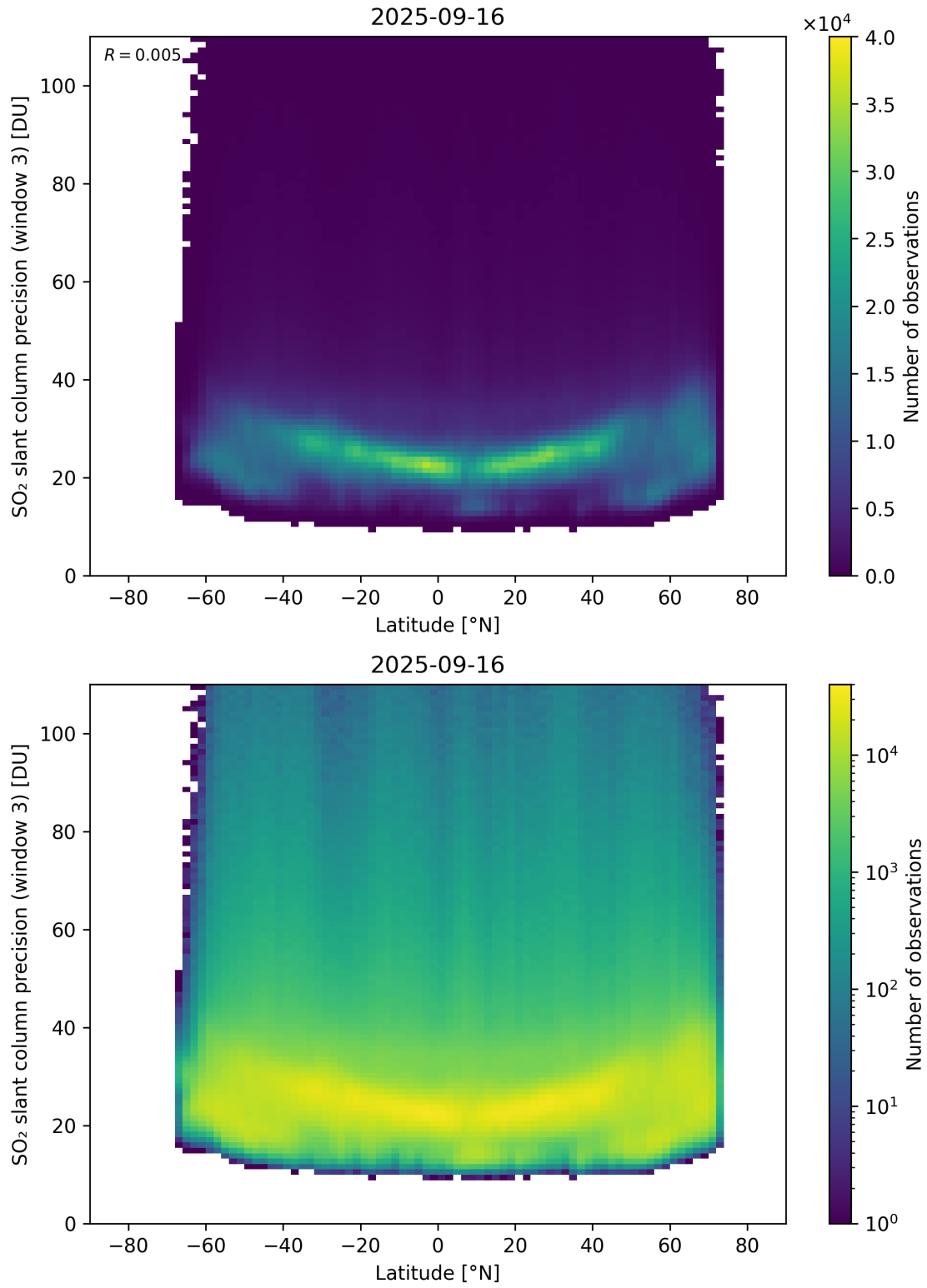
Figure 166: Scatter density plot of “Latitude” against “SO 2 slant column precision (window 3)” for 2025-09-15 to 2025-09-17.
