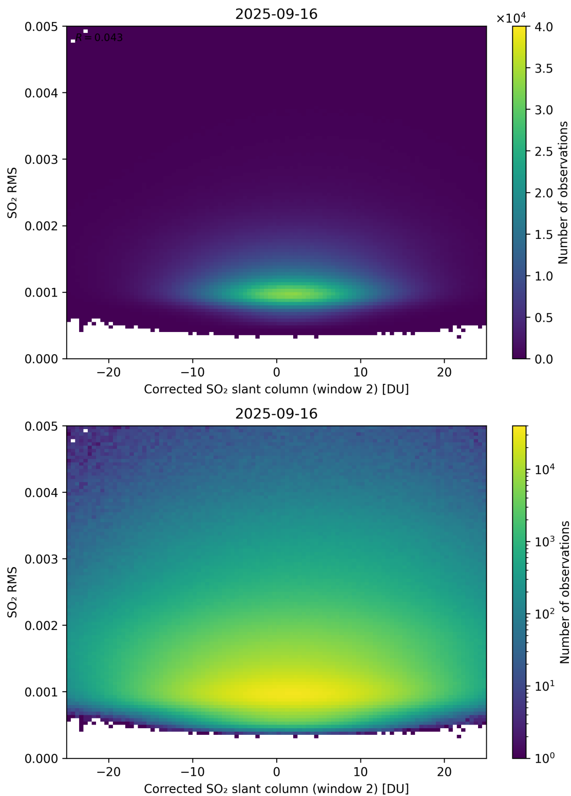
Figure 248: Scatter density plot of “Corrected SO 2 slant column (window 2)” against “SO 2 RMS” for 2025-09-15 to 2025-09-17.
