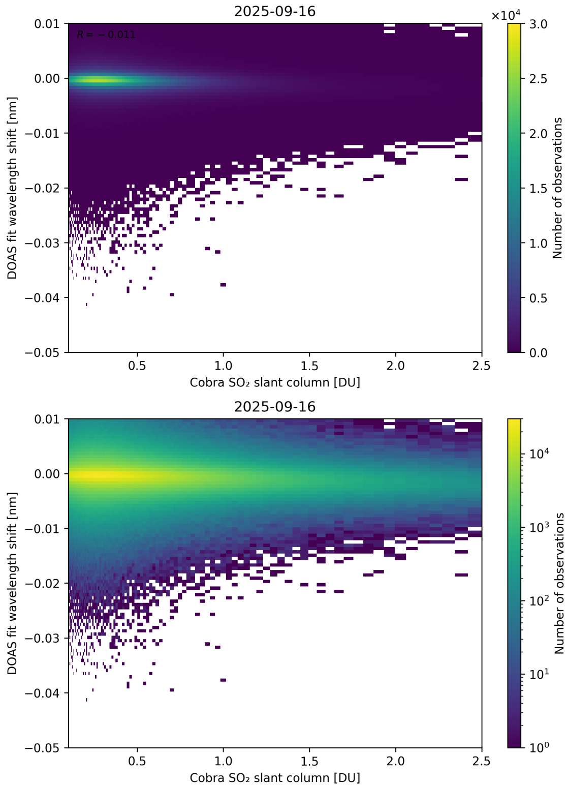
Figure 196: Scatter density plot of “Cobra SO 2 slant column” against “DOAS fit wavelength shift” for 2025-09-15 to 2025-09-17.
