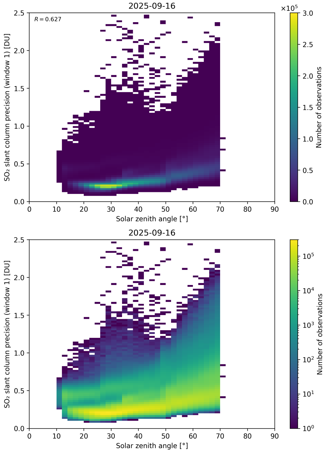
Figure 185: Scatter density plot of “Solar zenith angle” against “SO 2 slant column precision (window 1)” for 2025-09-15 to 2025-09-17.
