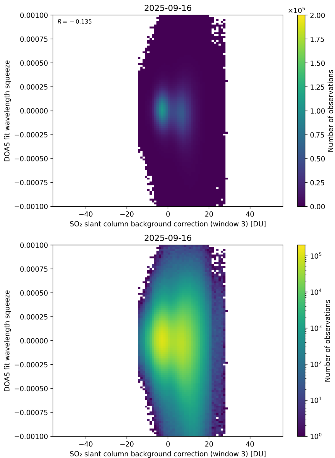
Figure 133: Scatter density plot of “SO 2 slant column background correction (window 3)” against “DOAS fit wavelength squeeze” for 2025-09-15 to 2025-09-17.
