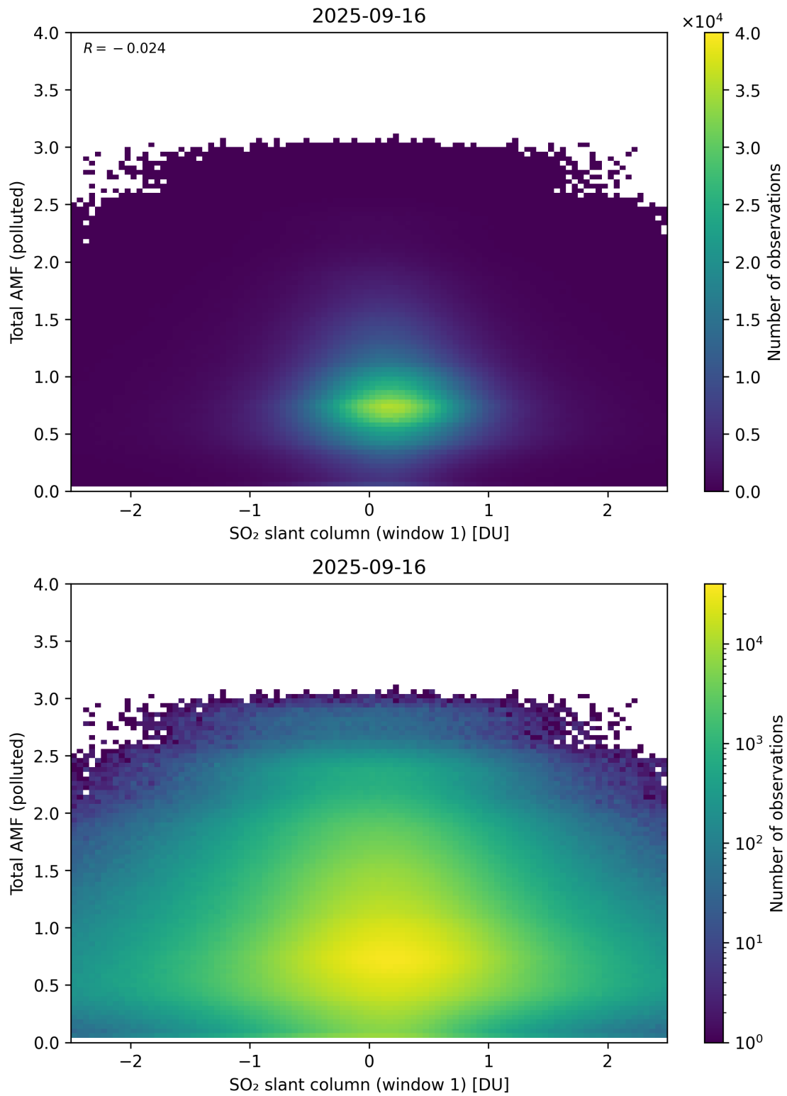
Figure 289: Scatter density plot of “SO 2 slant column (window 1)” against “Total AMF (polluted)” for 2025-09-15 to 2025-09-17.
