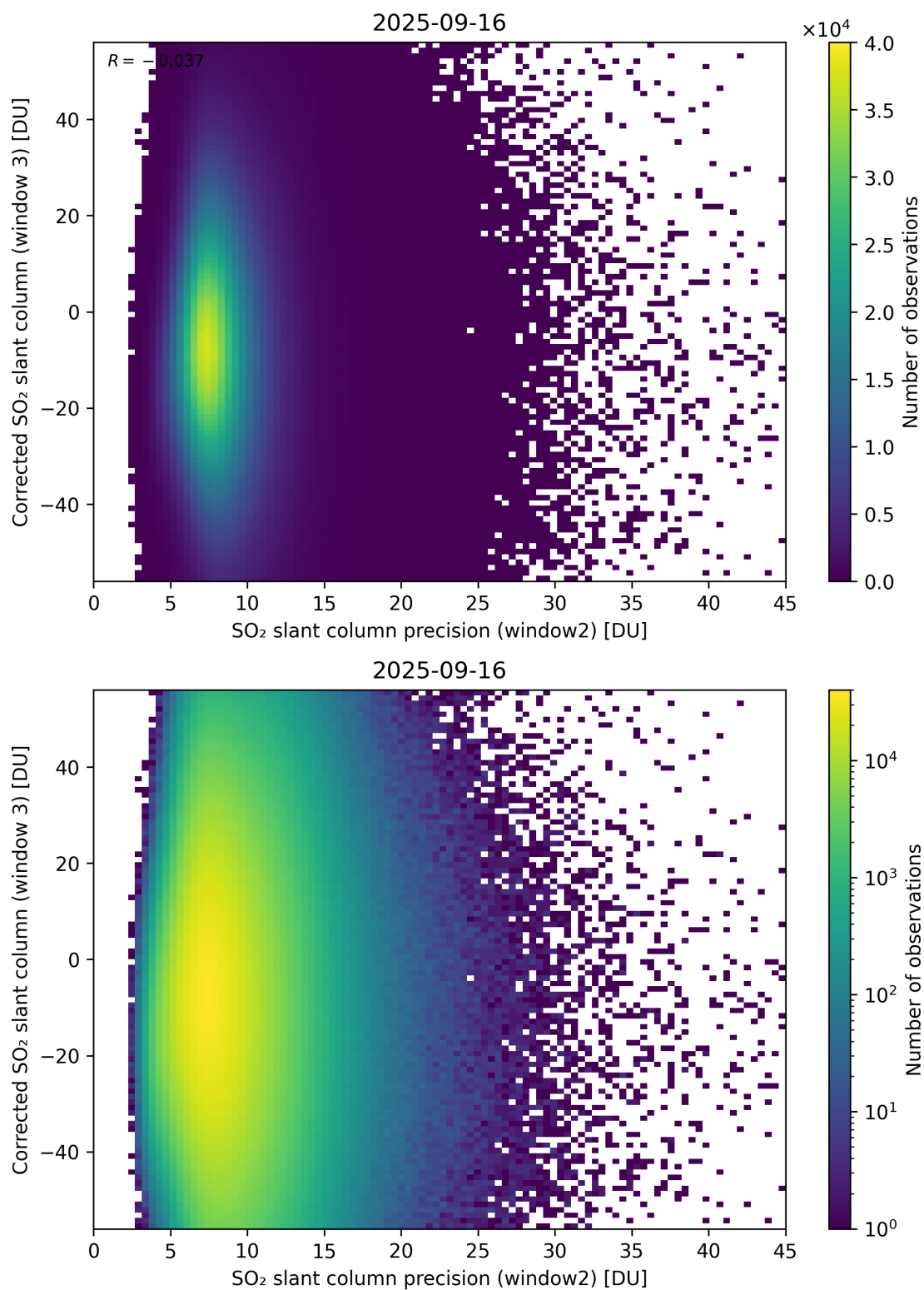
Figure 298: Scatter density plot of “SO 2 slant column precision (window2)” against “Corrected SO 2 slant column (window 3)” for 2025-09-15 to 2025-09-17.
