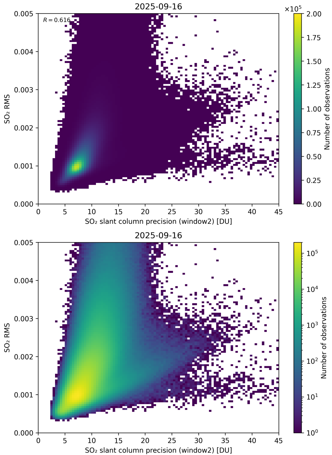
Figure 295: Scatter density plot of “SO 2 slant column precision (window2)” against “SO 2 RMS” for 2025-09-15 to 2025-09-17.
