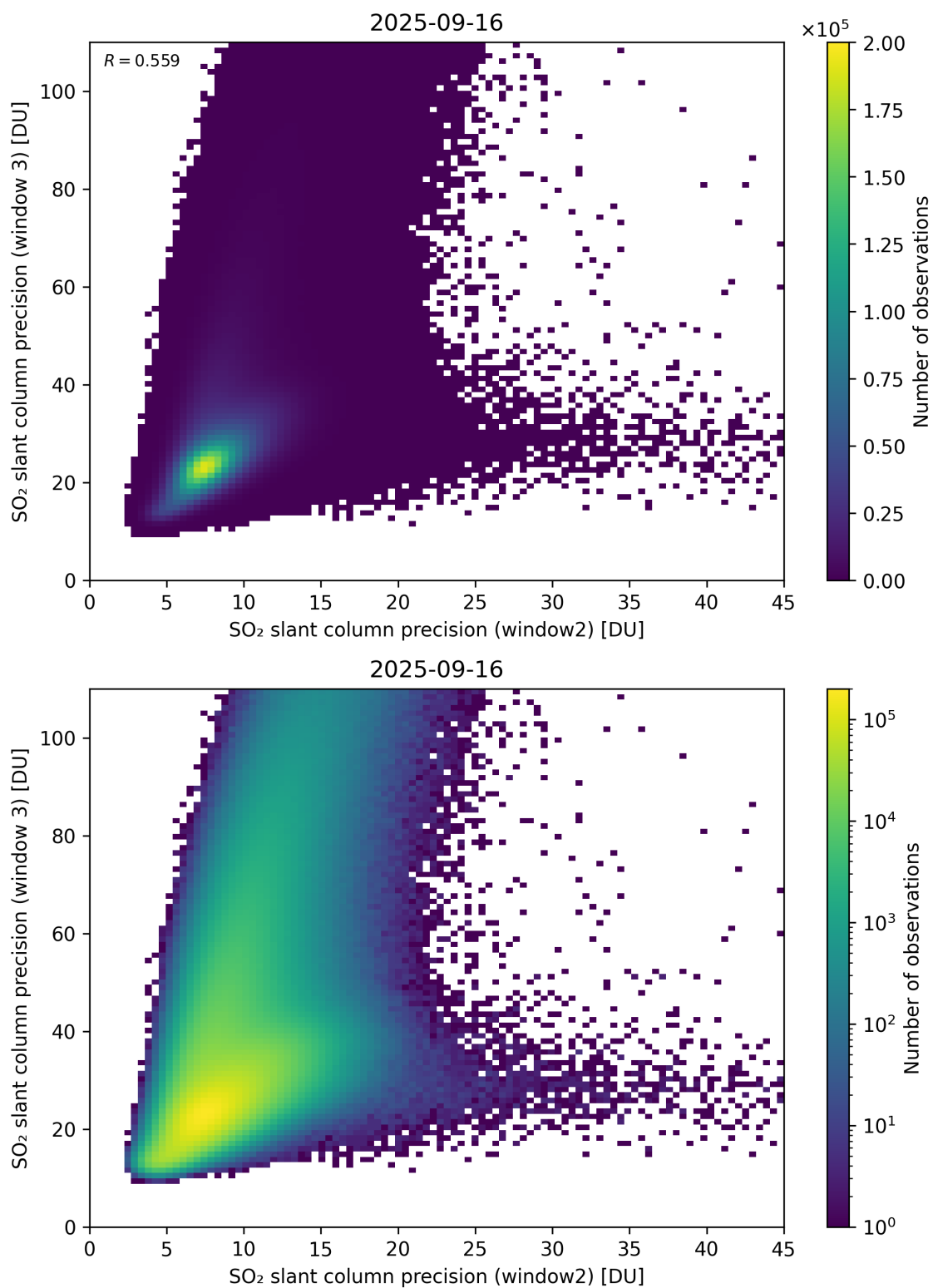
Figure 300: Scatter density plot of “SO 2 slant column precision (window2)” against “SO 2 slant column precision (window 3)” for 2025-09-15 to 2025-09-17.
