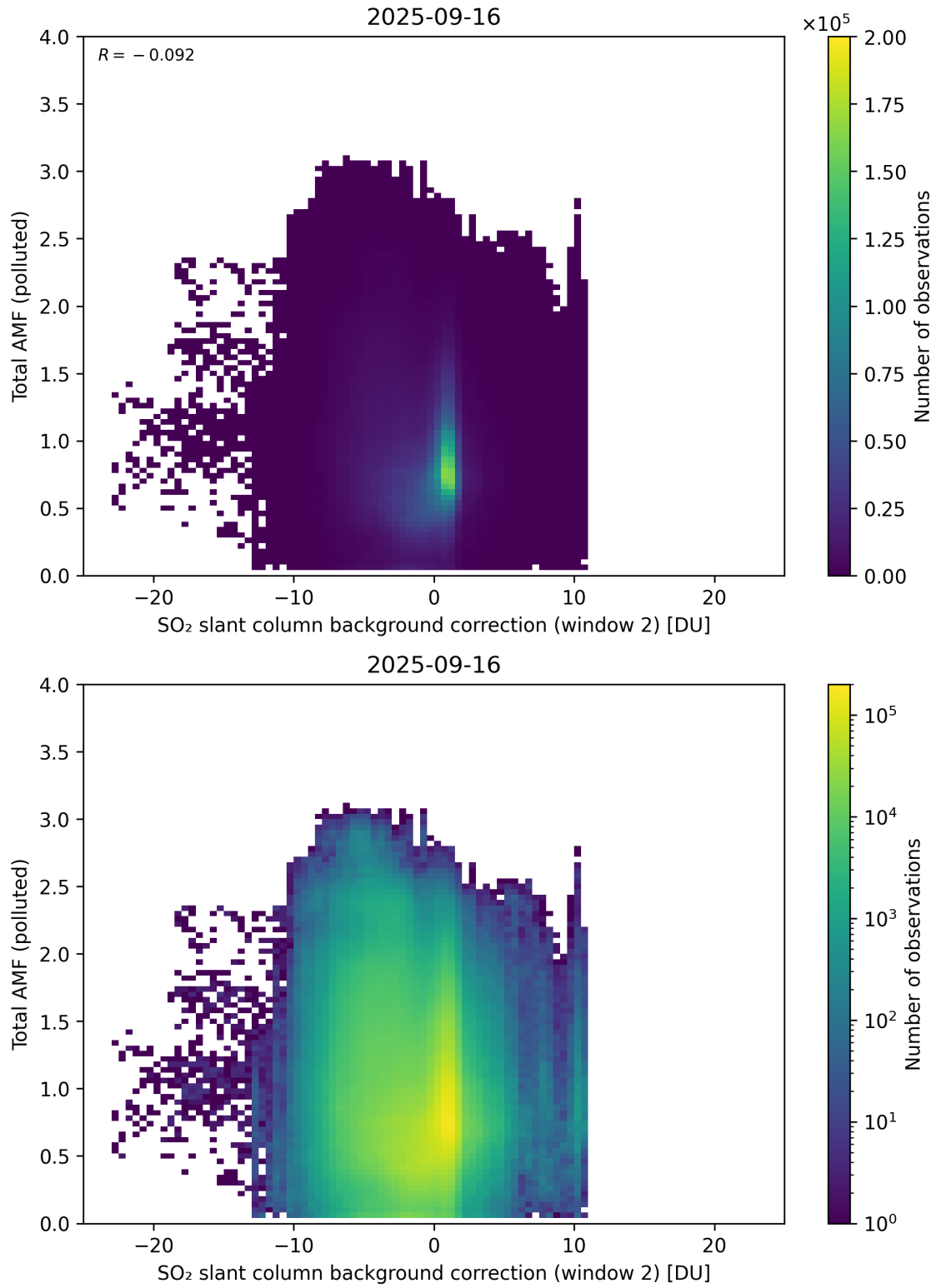
Figure 130: Scatter density plot of “SO 2 slant column background correction (window 2)” against “Total AMF (polluted)” for 2025-09-15 to 2025-09-17.
