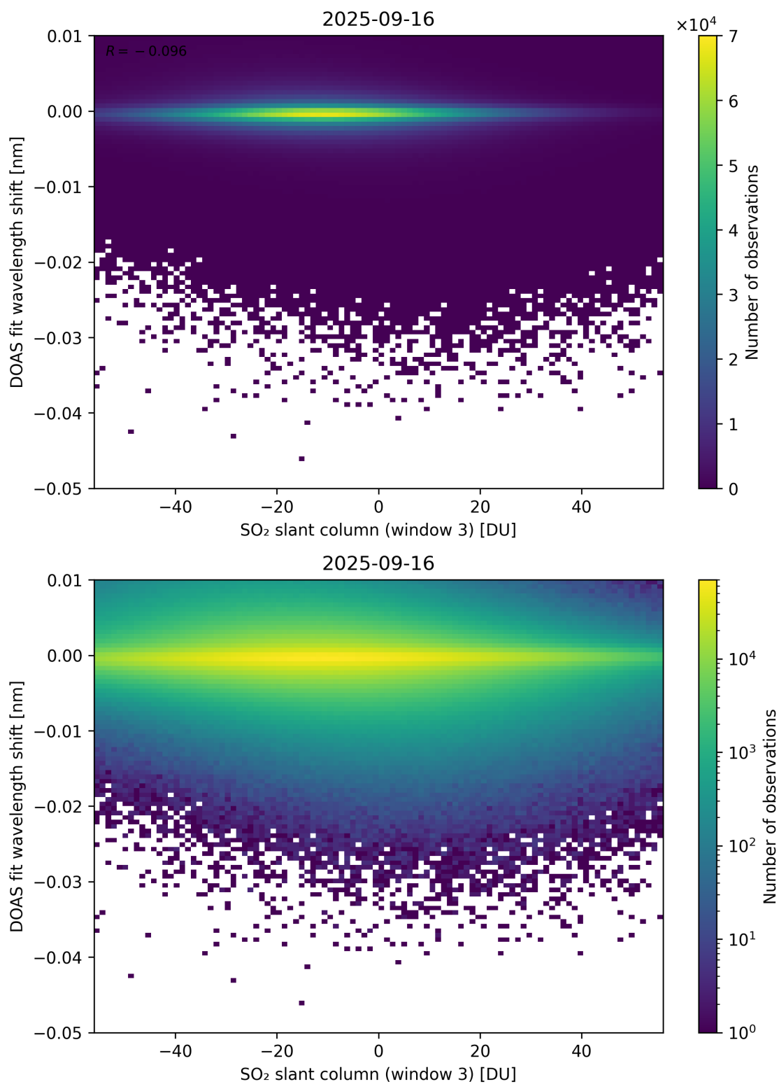
Figure 304: Scatter density plot of “SO 2 slant column (window 3)” against “DOAS fit wavelength shift” for 2025-09-15 to 2025-09-17.
