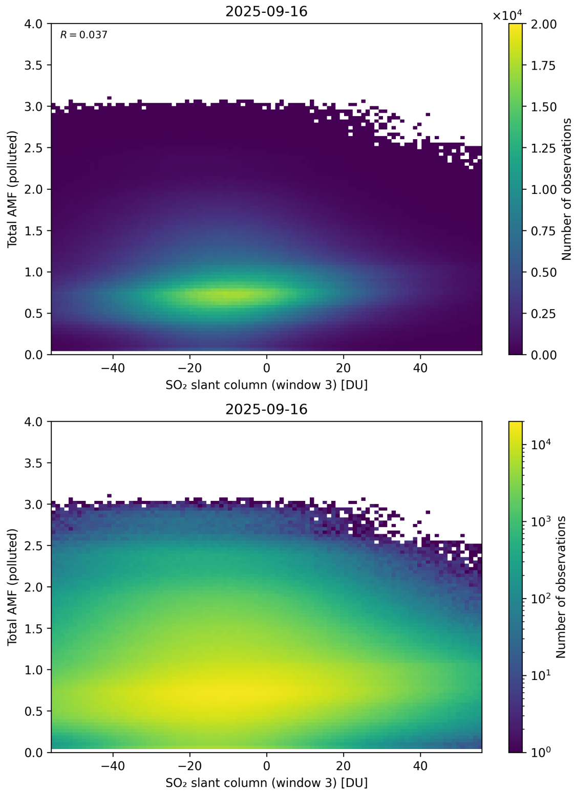
Figure 318: Scatter density plot of “SO 2 slant column (window 3)” against “Total AMF (polluted)” for 2025-09-15 to 2025-09-17.
