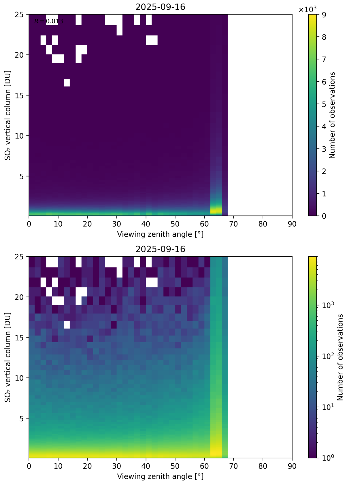
Figure 383: Scatter density plot of “Viewing zenith angle” against “SO 2 vertical column” for 2025-09-15 to 2025-09-17.
