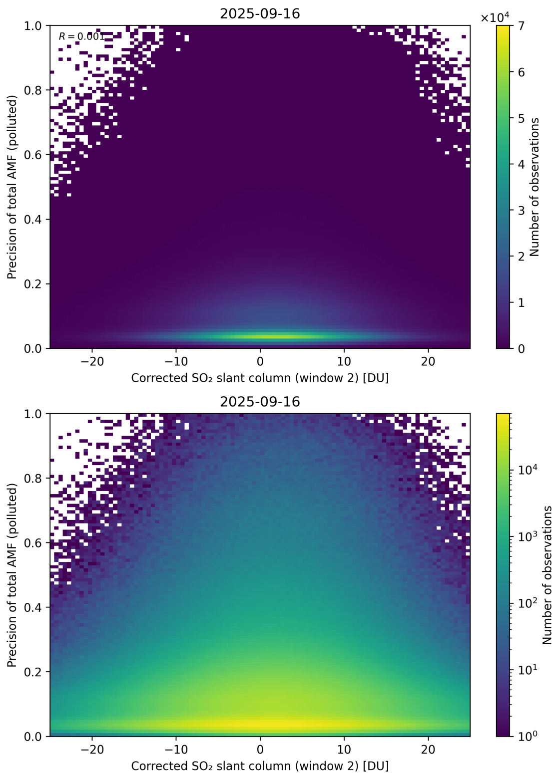
Figure 254: Scatter density plot of “Corrected SO 2 slant column (window 2)” against “Precision of total AMF (polluted)” for 2025-09-15 to 2025-09-17.
