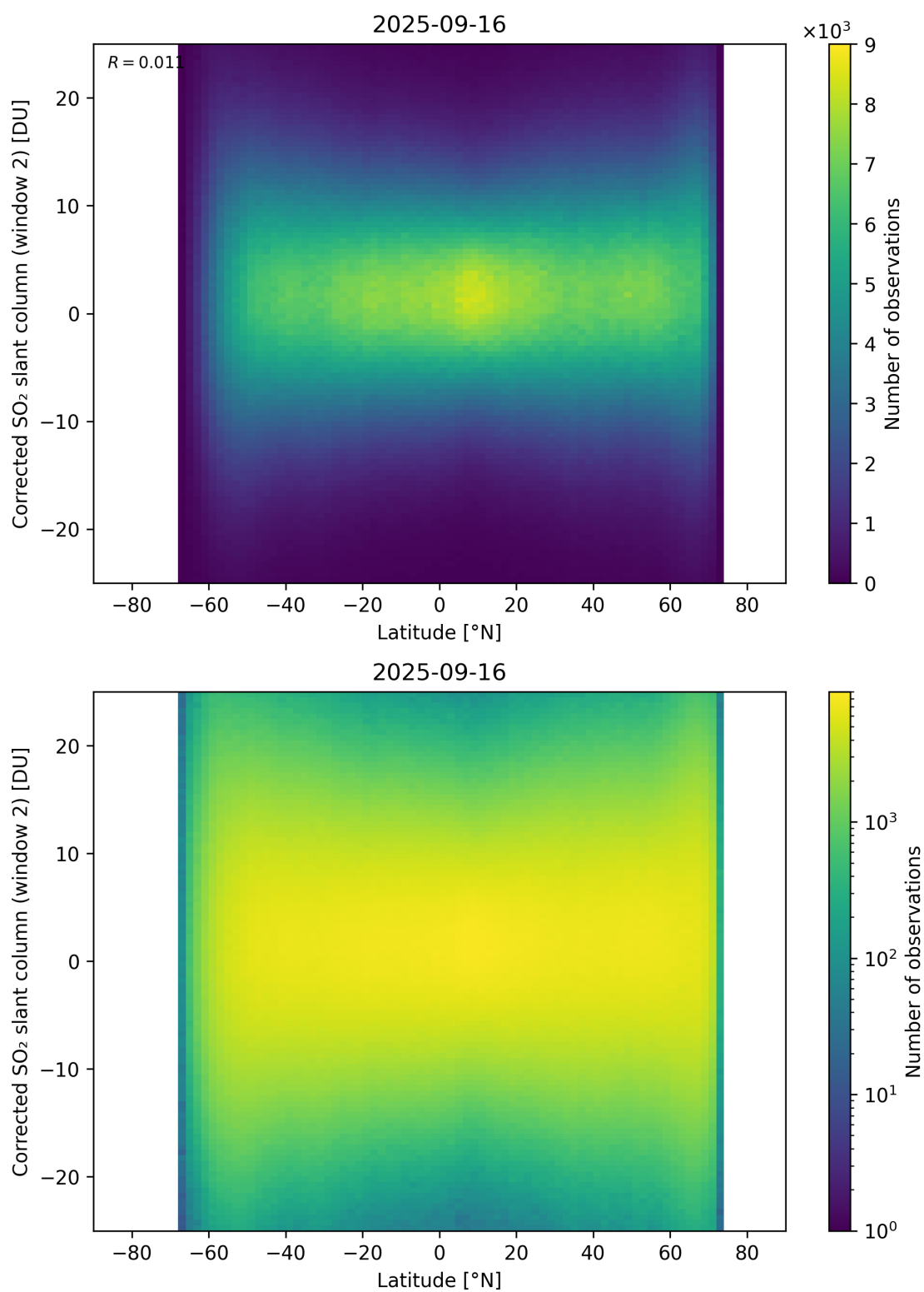
Figure 160: Scatter density plot of “Latitude” against “Corrected SO 2 slant column (window 2)” for 2025-09-15 to 2025-09-17.
