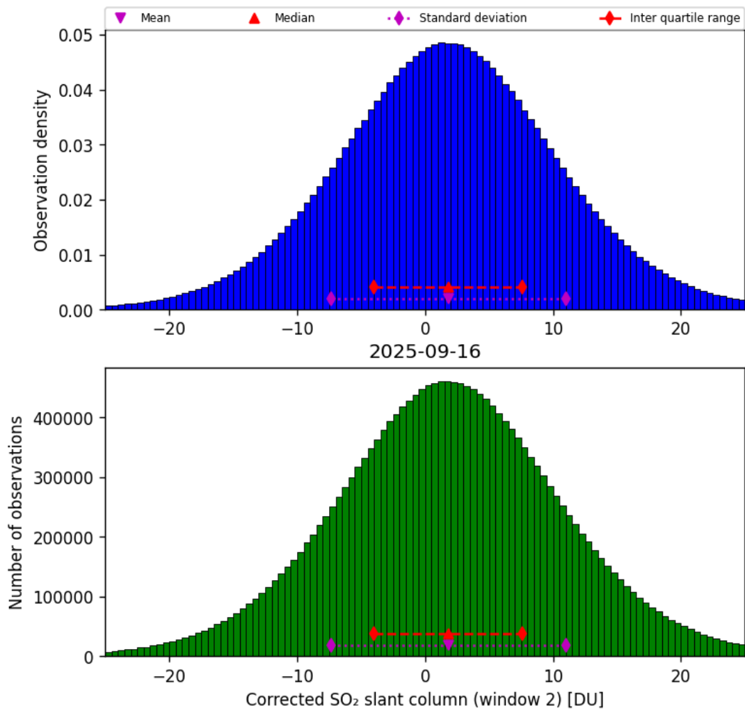
Figure 69: Histogram of “Corrected SO 2 slant column (window 2)” for 2025-09-15 to 2025-09-17
