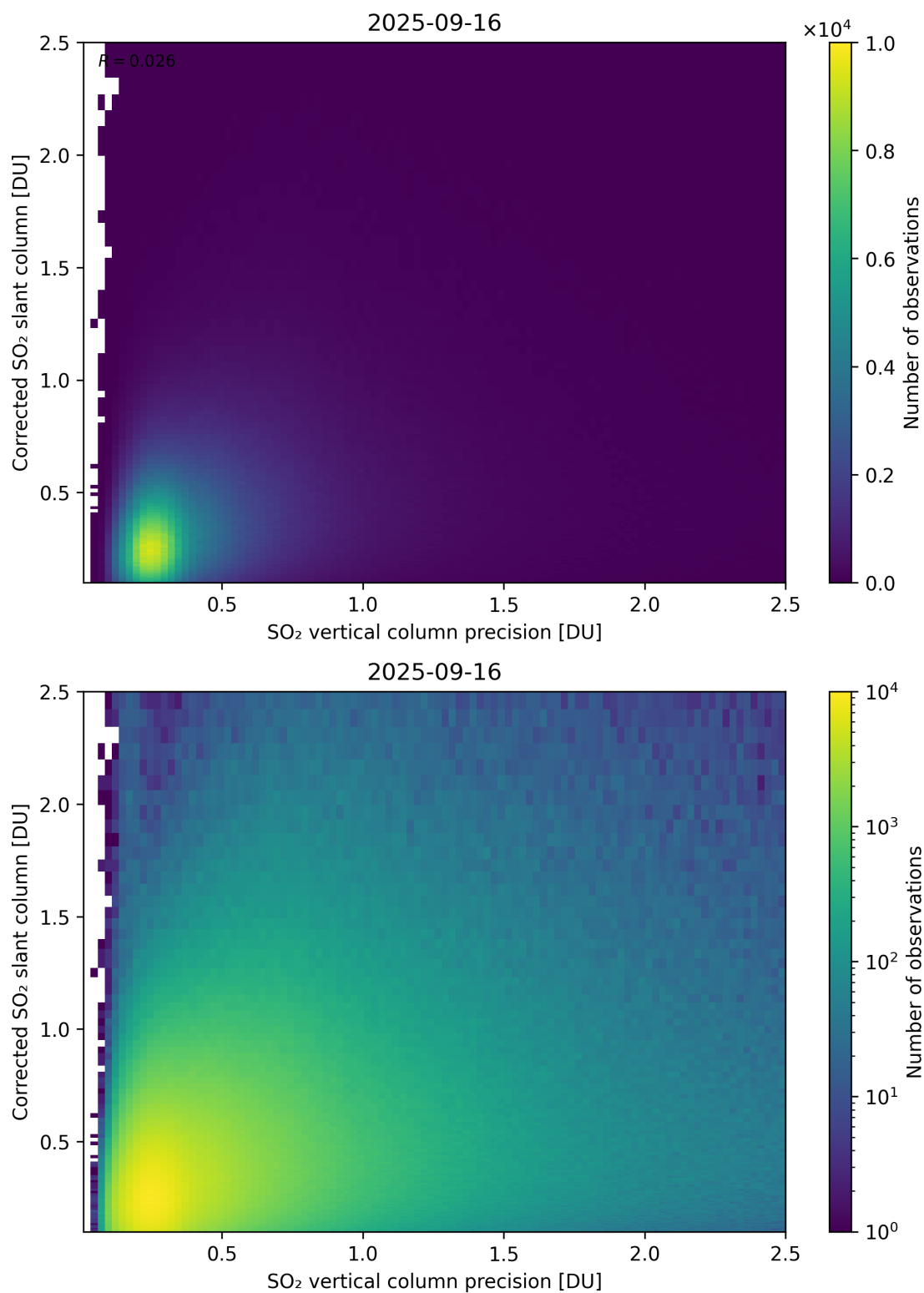
Figure 338: Scatter density plot of “SO 2 vertical column precision” against “Corrected SO 2 slant column” for 2025-09-15 to 2025-09-17.
