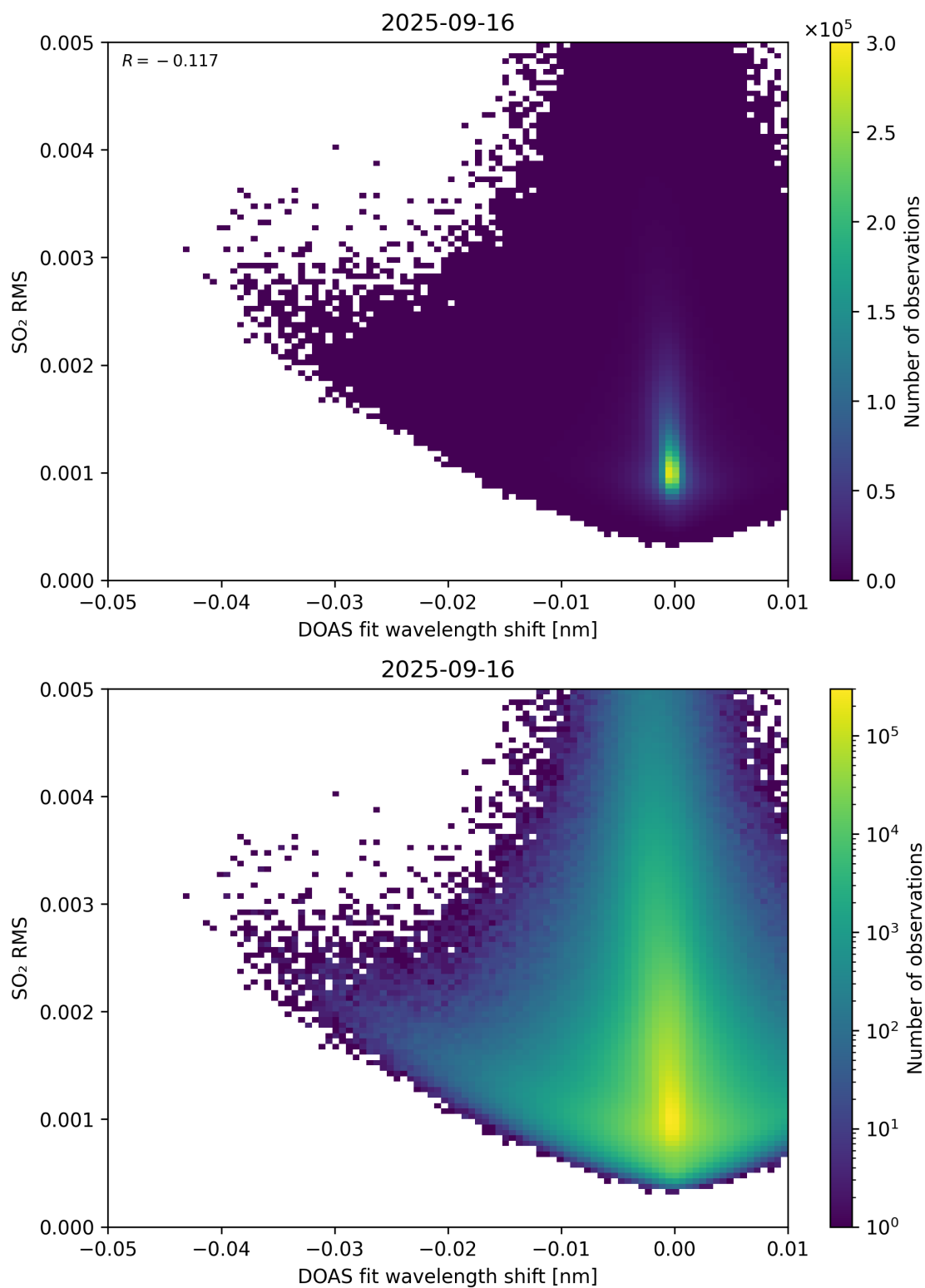
Figure 139: Scatter density plot of “DOAS fit wavelength shift” against “SO 2 RMS” for 2025-09-15 to 2025-09-17.
