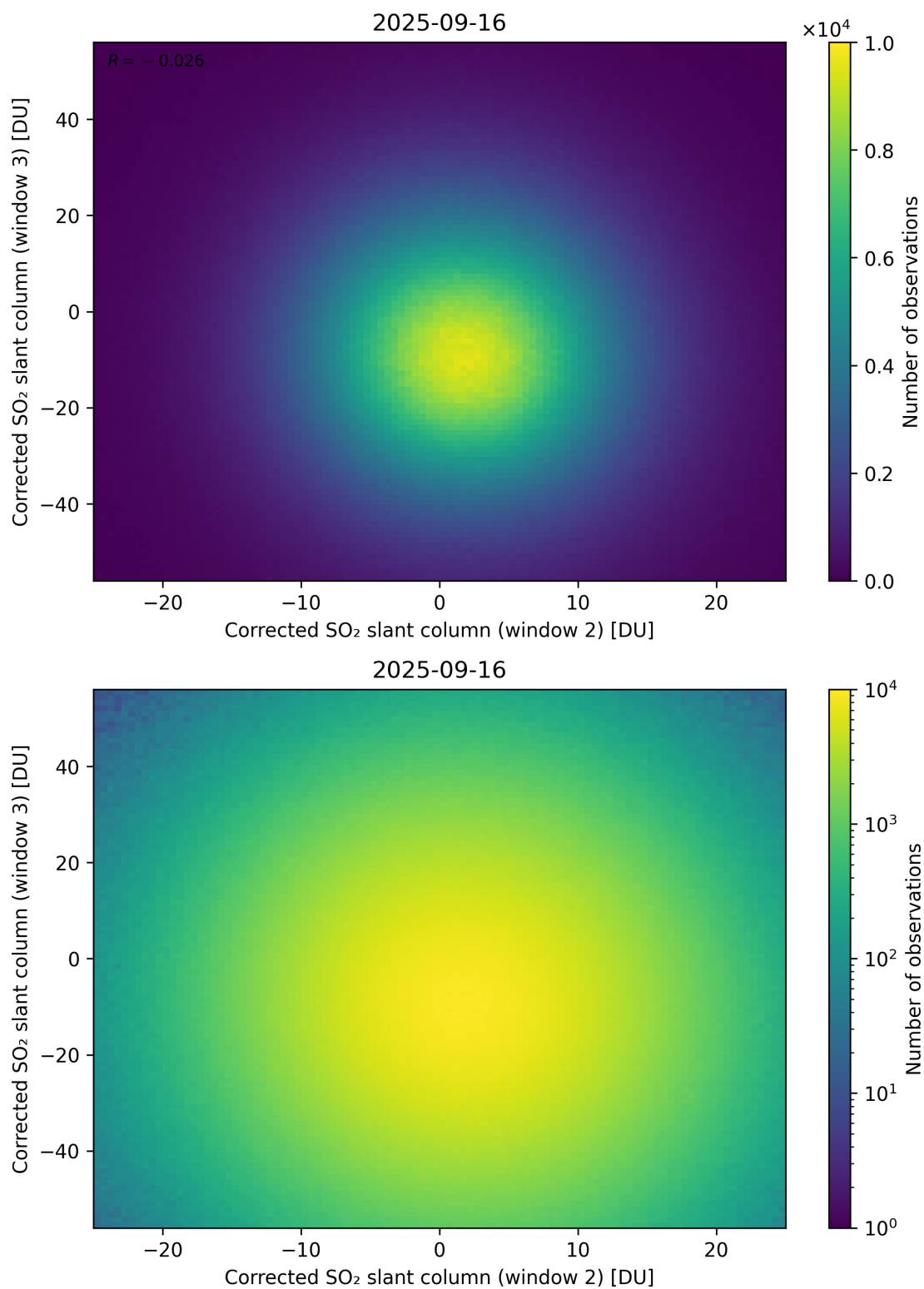
Figure 250: Scatter density plot of “Corrected SO 2 slant column (window 2)” against “Corrected SO 2 slant column (window 3)” for 2025-09-15 to 2025-09-17.
