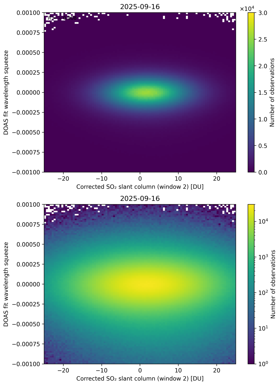
Figure 247: Scatter density plot of “Corrected SO 2 slant column (window 2)” against “DOAS fit wavelength squeeze” for 2025-09-15 to 2025-09-17.
