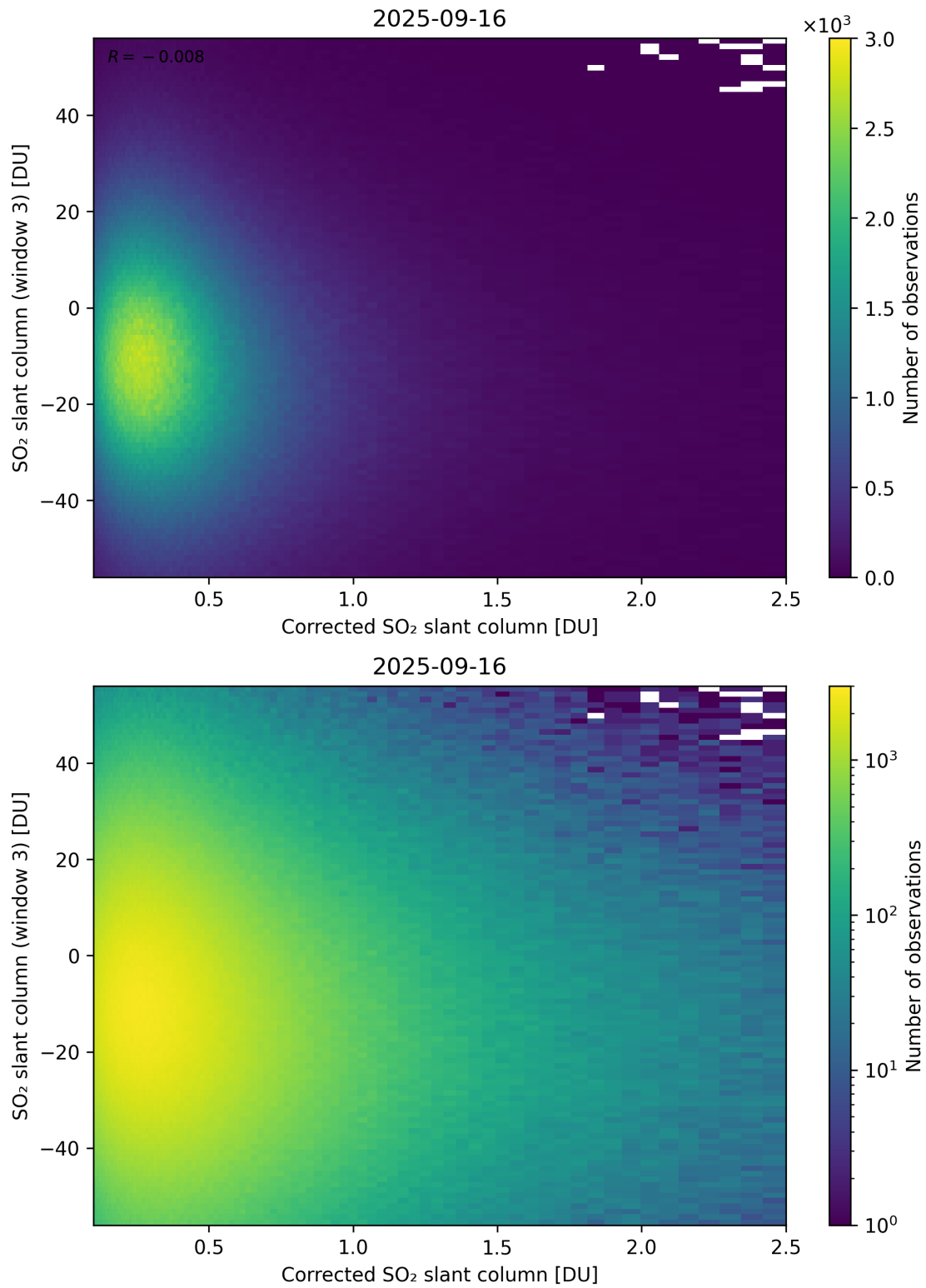
Figure 240: Scatter density plot of “Corrected SO 2 slant column” against “SO 2 slant column (window 3)” for 2025-09-15 to 2025-09-17.
