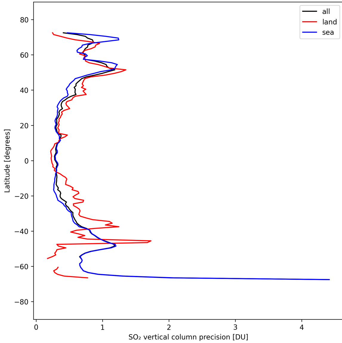
Figure 33: Zonal average of “SO 2 vertical column precision” for 2025-09-15 to 2025-09-17.
