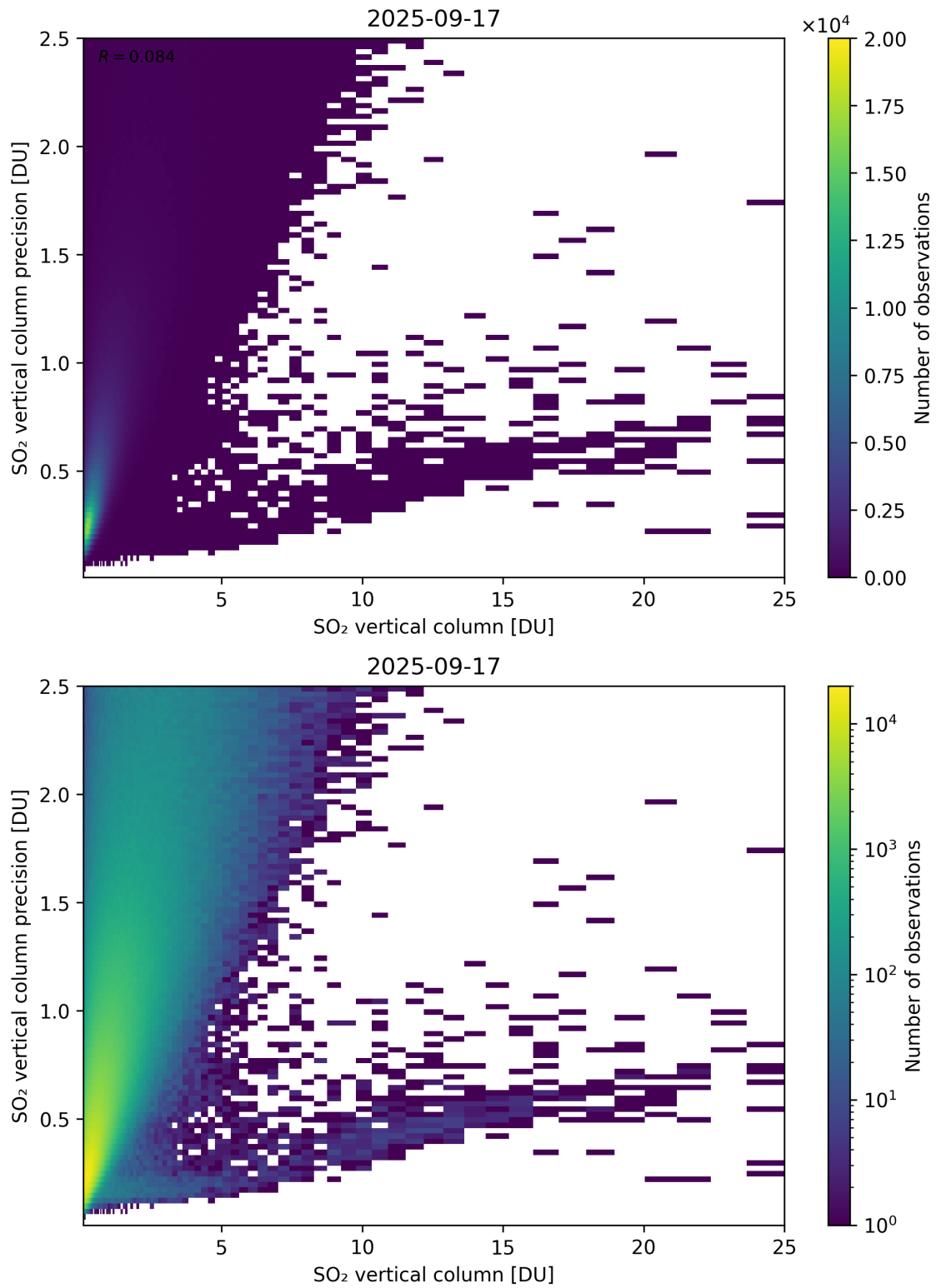
Figure 361: Scatter density plot of “SO 2 vertical column” against “SO 2 vertical column precision” for 2025-09-16 to 2025-09-18.
