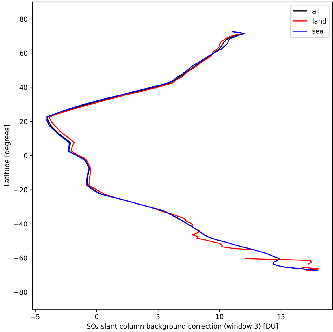
Figure 48: Zonal average of “SO 2 slant column background correction (window 3)” for 2025-09-16 to 2025-09-18.
