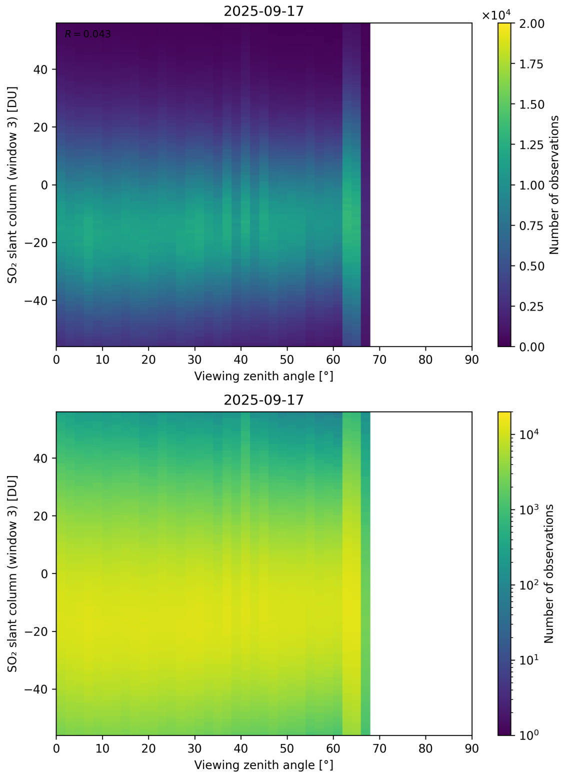
Figure 379: Scatter density plot of “Viewing zenith angle” against “SO 2 slant column (window 3)” for 2025-09-16 to 2025-09-18.
