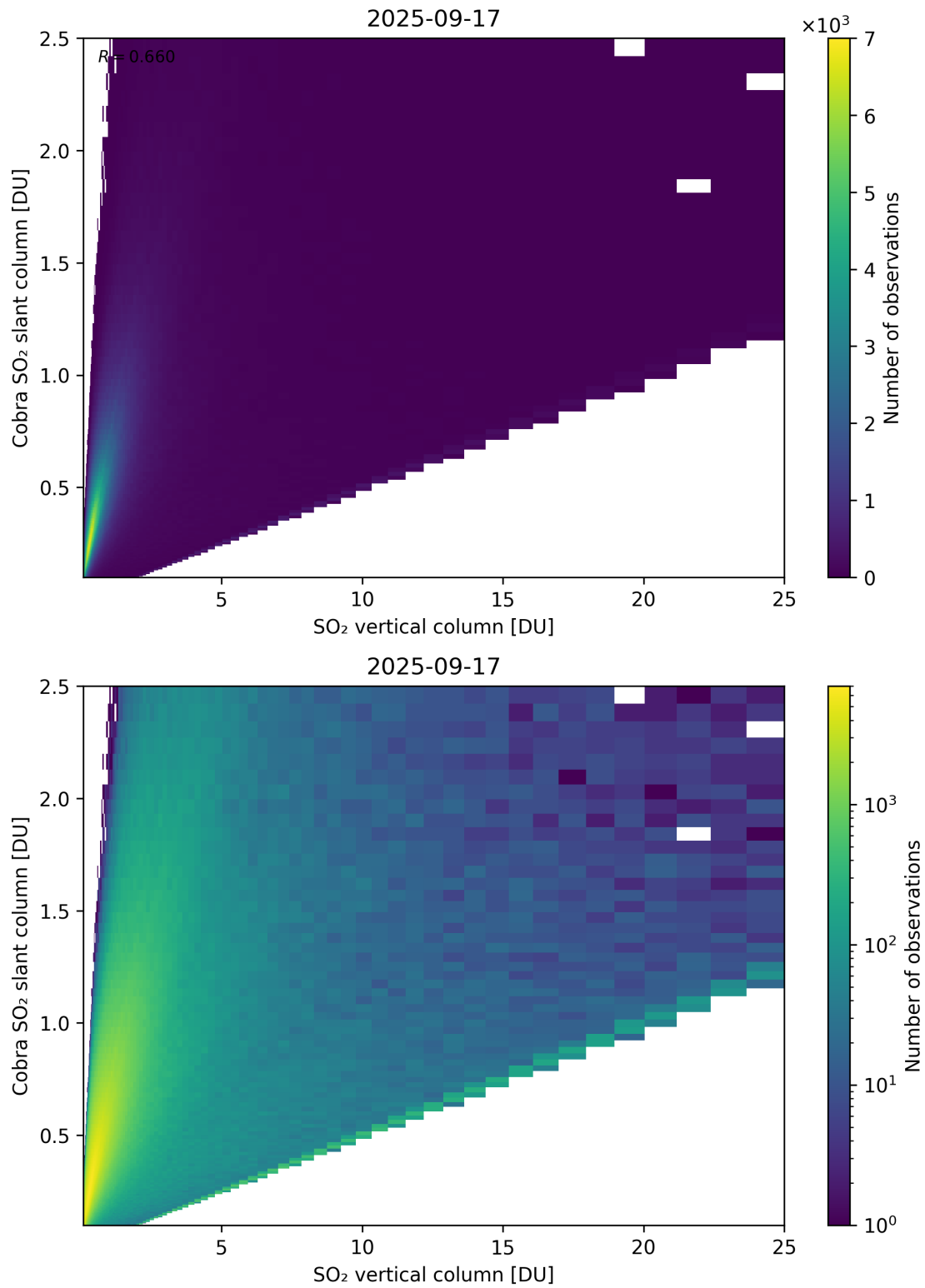
Figure 349: Scatter density plot of “SO 2 vertical column” against “Cobra SO 2 slant column” for 2025-09-16 to 2025-09-18.
