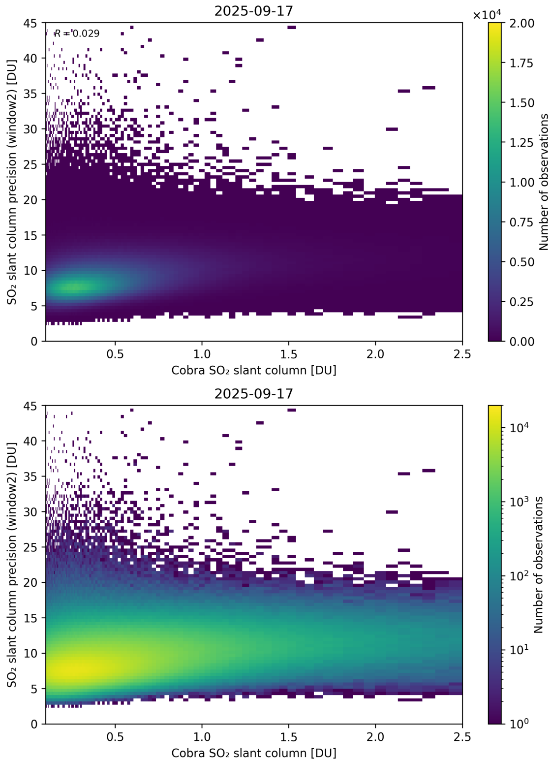
Figure 221: Scatter density plot of “Cobra SO 2 slant column” against “SO 2 slant column precision (window2)” for 2025-09-16 to 2025-09-18.
