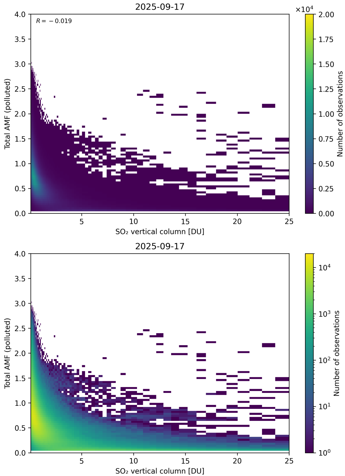
Figure 359: Scatter density plot of “SO 2 vertical column” against “Total AMF (polluted)” for 2025-09-16 to 2025-09-18.
