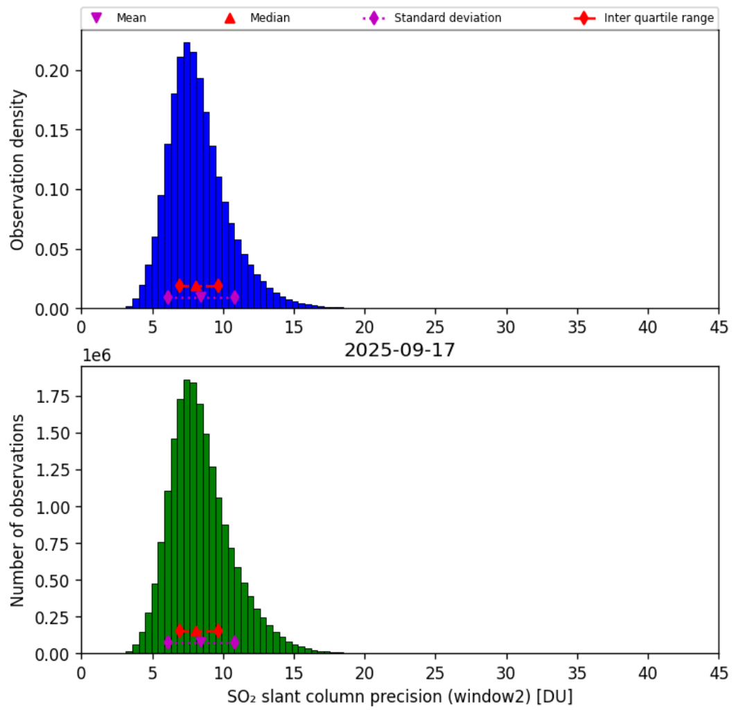
Figure 68: Histogram of “SO 2 slant column precision (window2)” for 2025-09-16 to 2025-09-18
