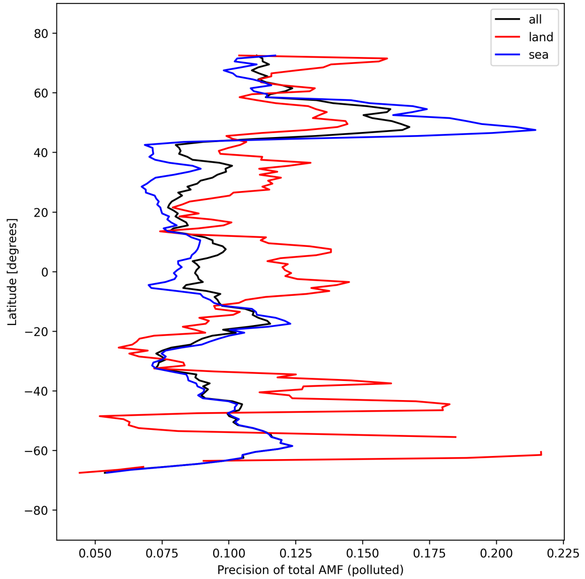
Figure 54: Zonal average of “Precision of total AMF (polluted)” for 2025-09-16 to 2025-09-18.
