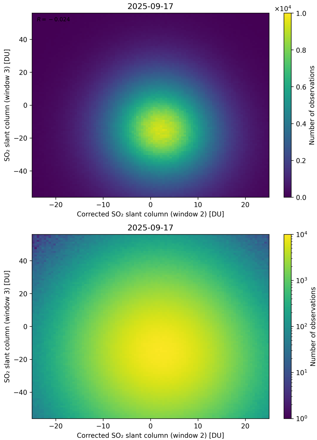
Figure 251: Scatter density plot of “Corrected SO 2 slant column (window 2)” against “SO 2 slant column (window 3)” for 2025-09-16 to 2025-09-18.
