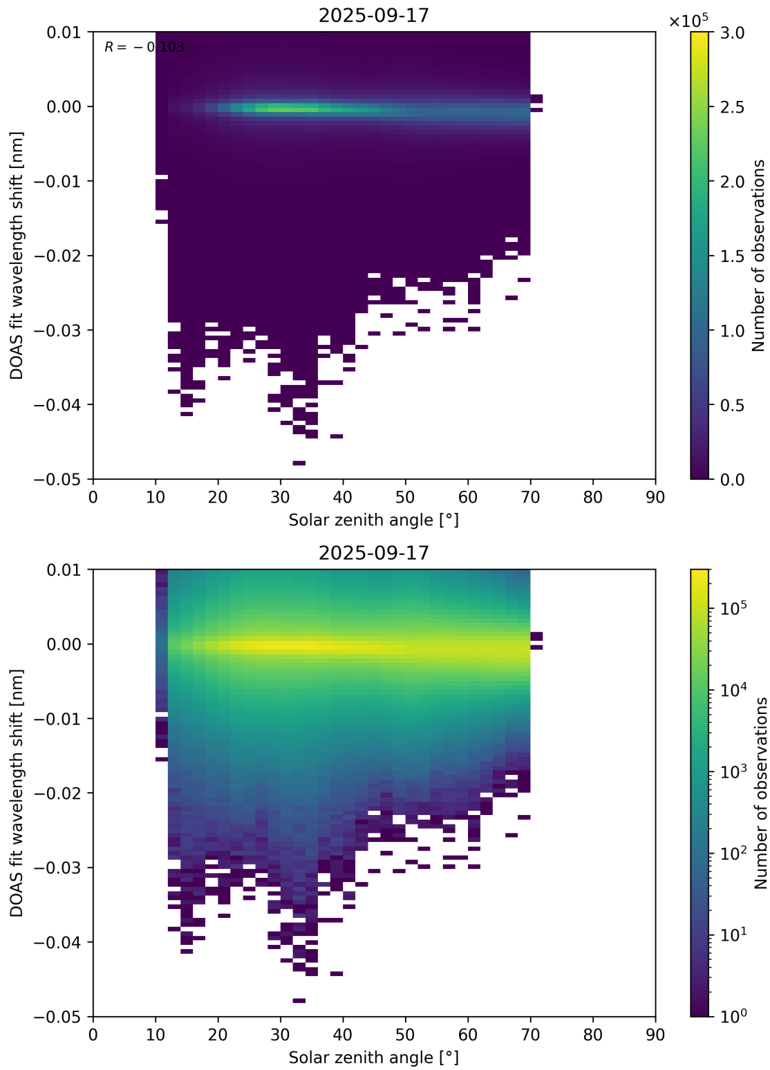
Figure 174: Scatter density plot of “Solar zenith angle” against “DOAS fit wavelength shift” for 2025-09-16 to 2025-09-18.
