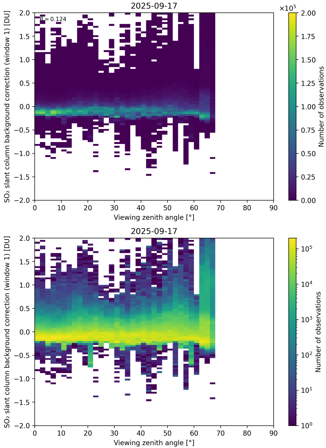
Figure 362: Scatter density plot of “Viewing zenith angle” against “SO 2 slant column background correction (window 1)” for 2025-09-16 to 2025-09-18.
