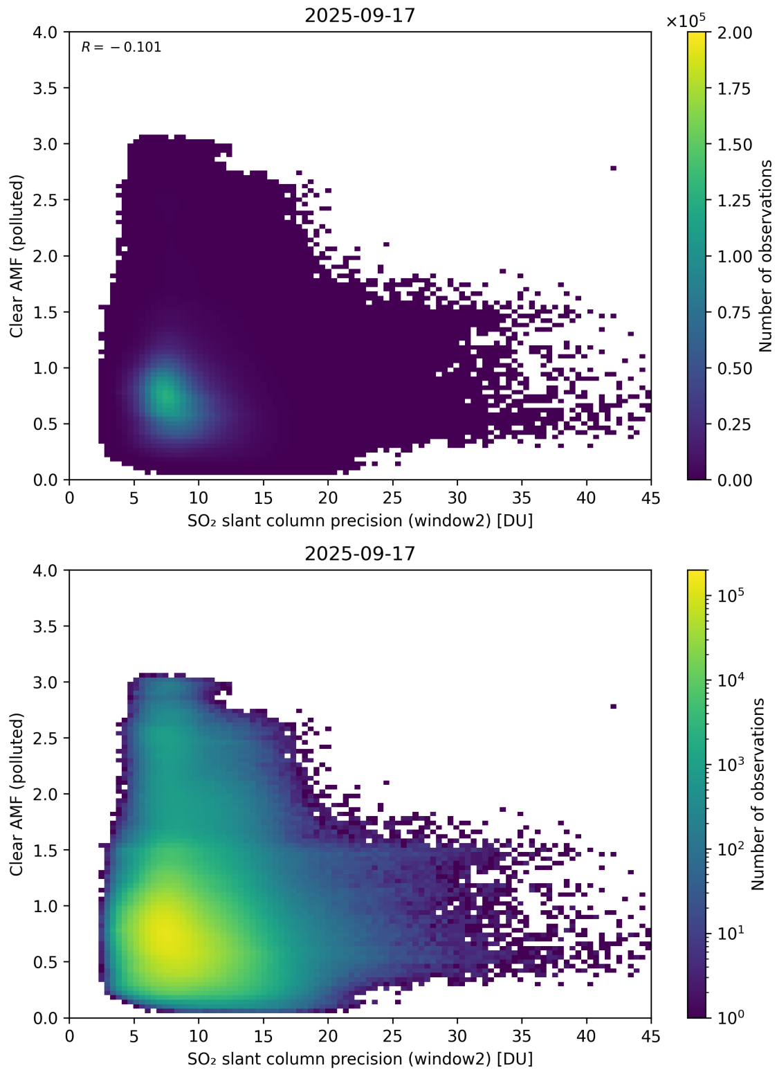
Figure 296: Scatter density plot of “SO 2 slant column precision (window2)” against “Clear AMF (polluted)” for 2025-09-16 to 2025-09-18.
