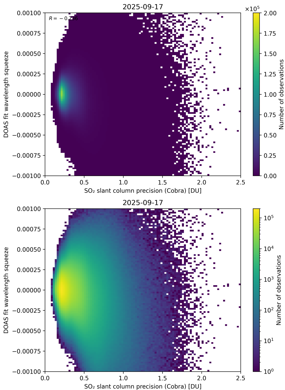
Figure 203: Scatter density plot of “SO 2 slant column precision (Cobra)” against “DOAS fit wavelength squeeze” for 2025-09-16 to 2025-09-18.
