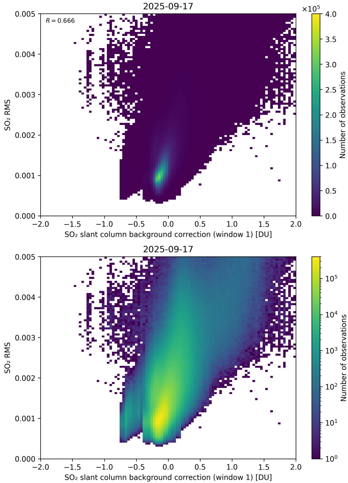
Figure 113: Scatter density plot of “SO 2 slant column background correction (window 1)” against “SO 2 RMS” for 2025-09-16 to 2025-09-18.
