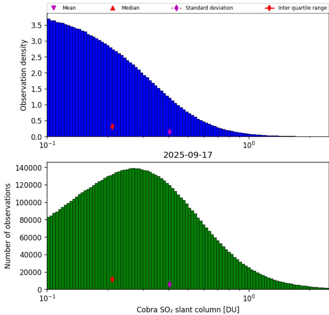
Figure 61: Histogram of “Cobra SO 2 slant column” for 2025-09-16 to 2025-09-18
