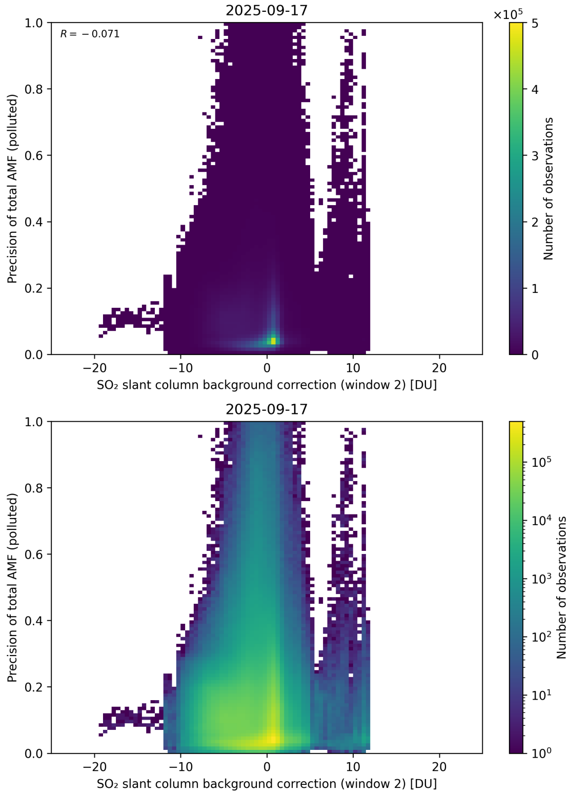
Figure 131: Scatter density plot of “SO 2 slant column background correction (window 2)” against “Precision of total AMF (polluted)” for 2025-09-16 to 2025-09-18.
