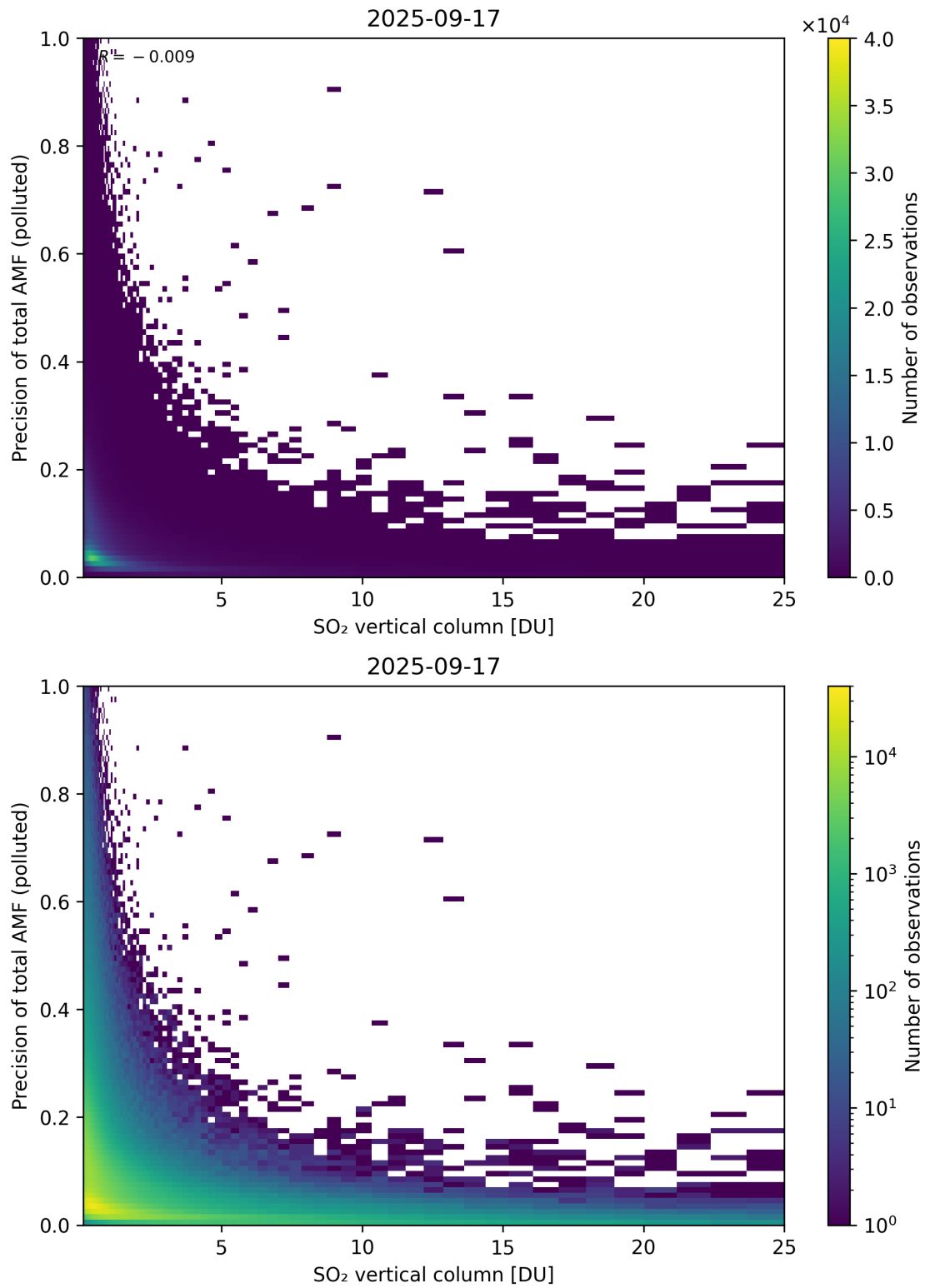
Figure 360: Scatter density plot of “SO 2 vertical column” against “Precision of total AMF (polluted)” for 2025-09-16 to 2025-09-18.
