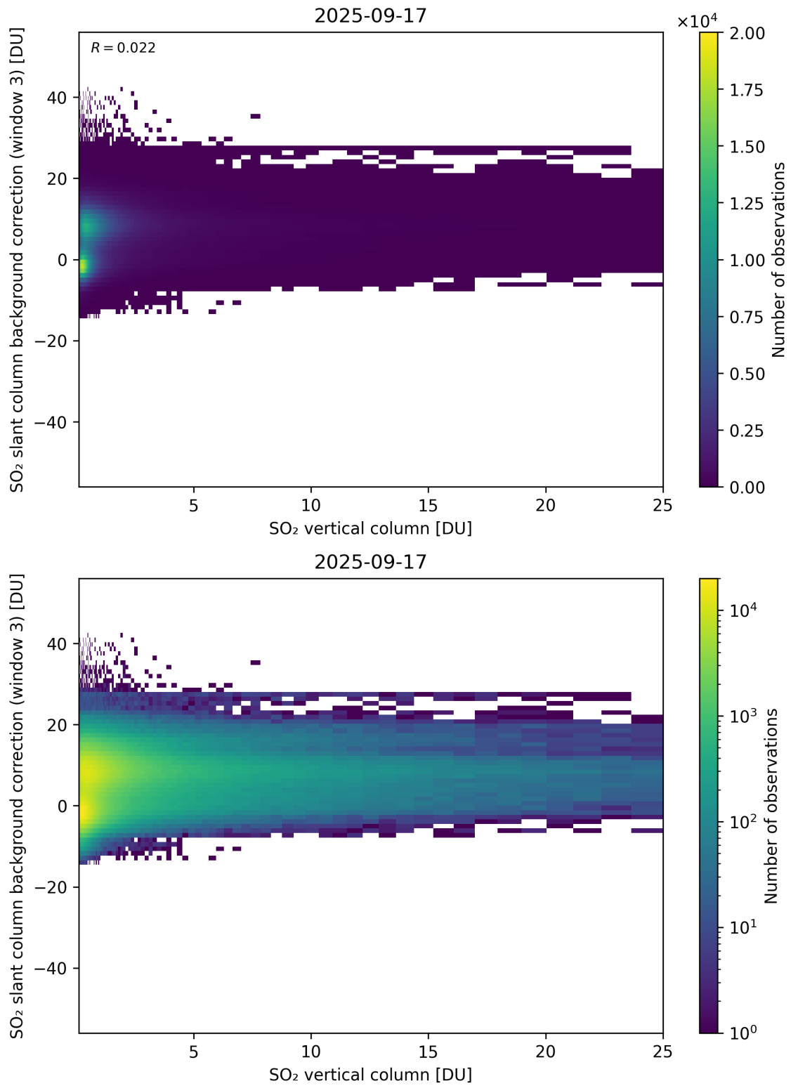
Figure 325: Scatter density plot of “SO 2 vertical column” against “SO 2 slant column background correction (window 3)” for 2025-09-16 to 2025-09-18.
