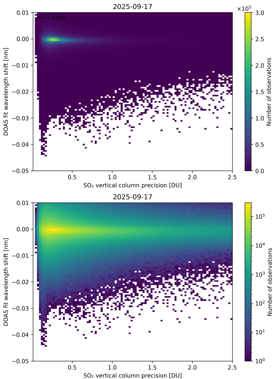
Figure 332: Scatter density plot of “SO 2 vertical column precision” against “DOAS fit wavelength shift” for 2025-09-16 to 2025-09-18.
