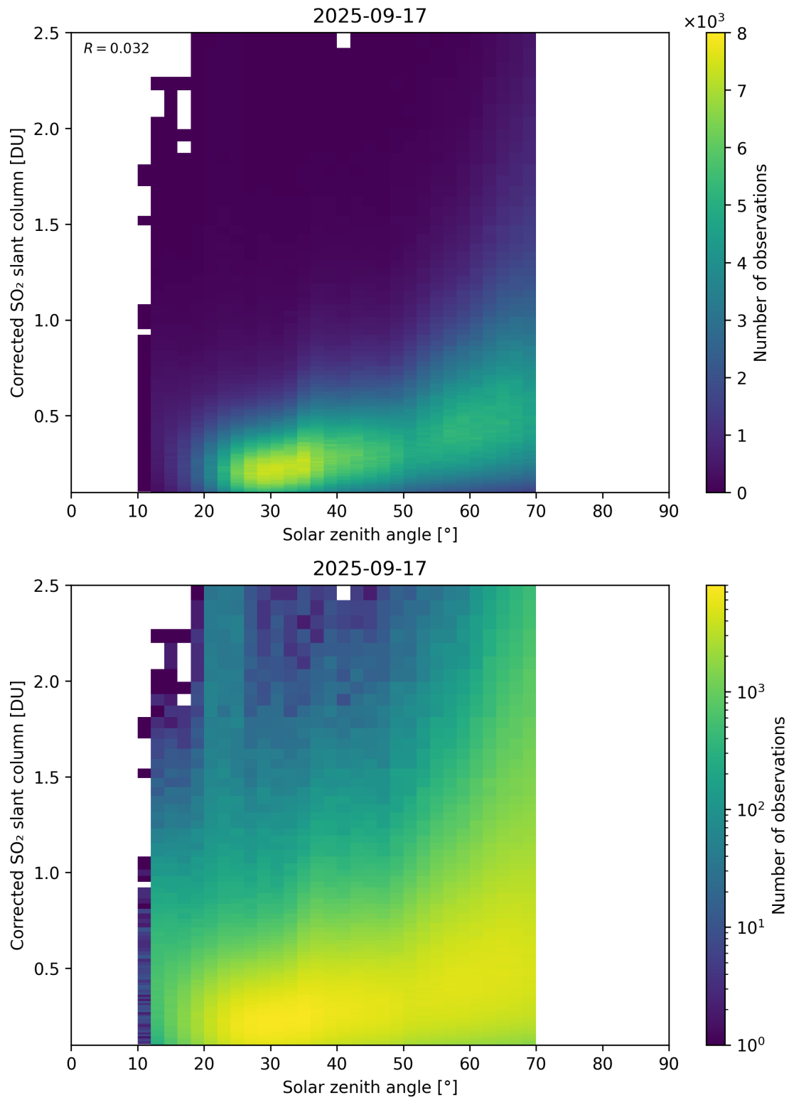
Figure 181: Scatter density plot of “Solar zenith angle” against “Corrected SO 2 slant column” for 2025-09-16 to 2025-09-18.
