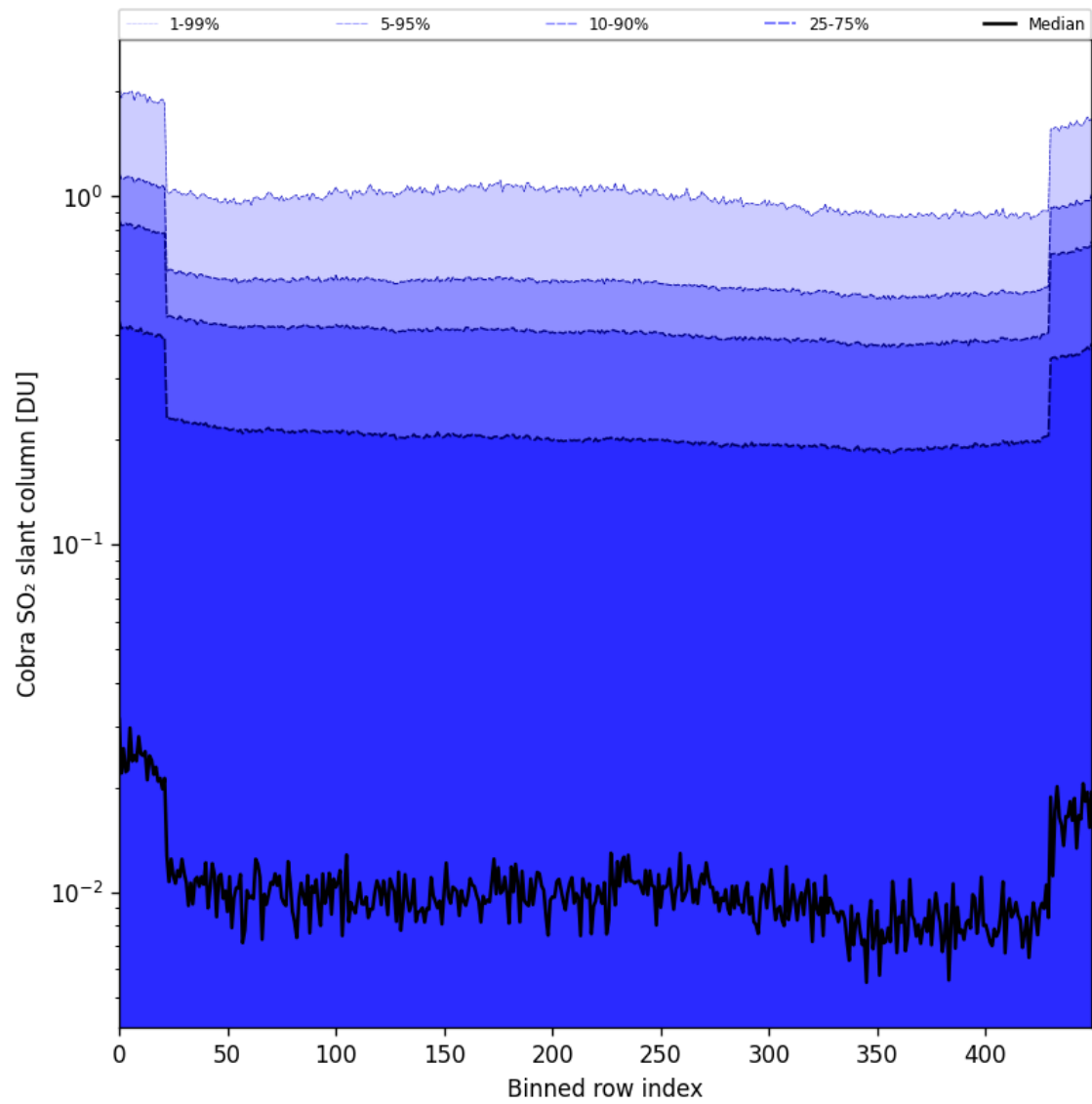
Figure 87: Along track statistics of “Cobra SO 2 slant column” for 2025-09-16 to 2025-09-18
