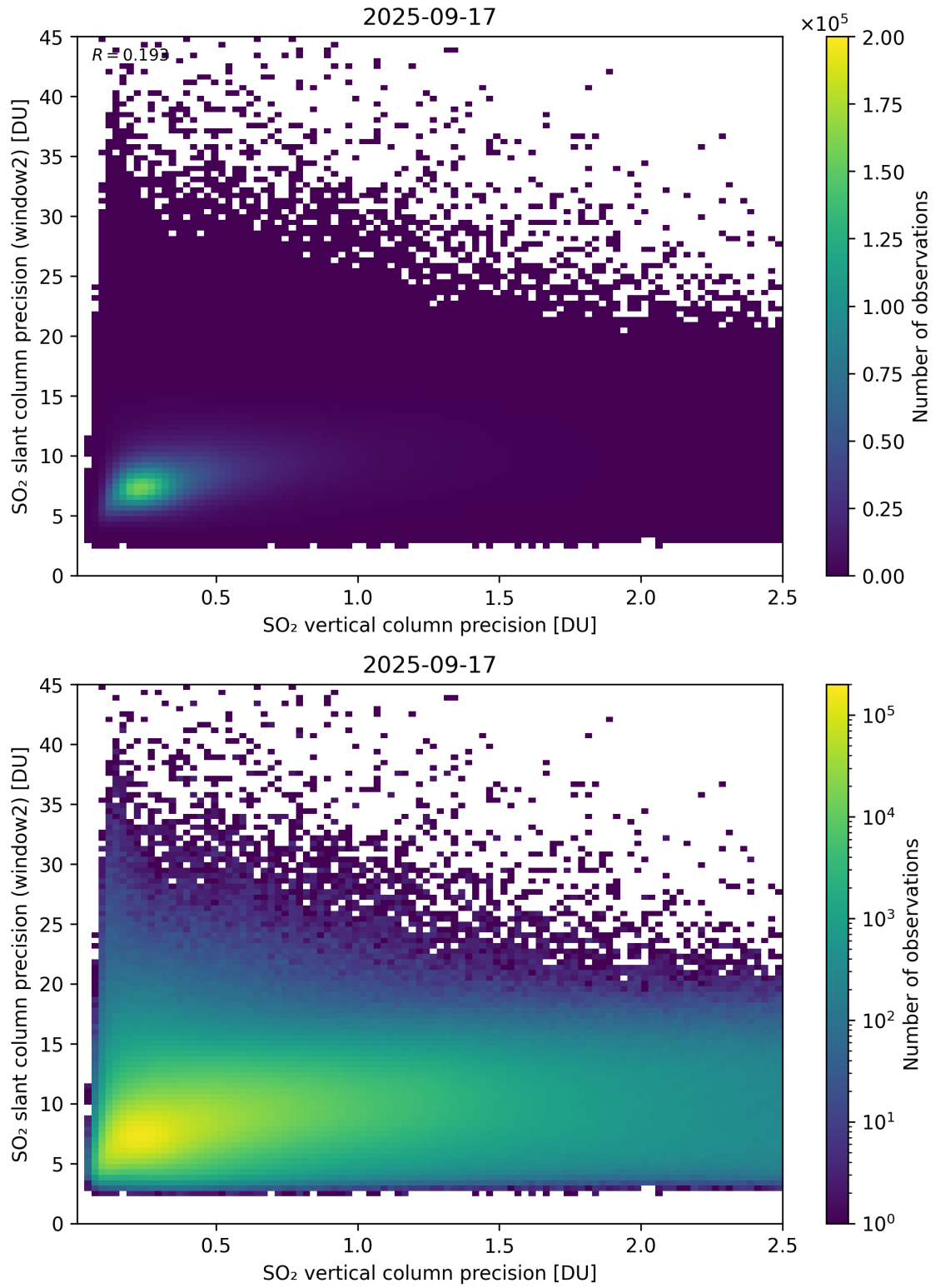
Figure 343: Scatter density plot of “SO 2 vertical column precision” against “SO 2 slant column precision (window2)” for 2025-09-16 to 2025-09-18.
