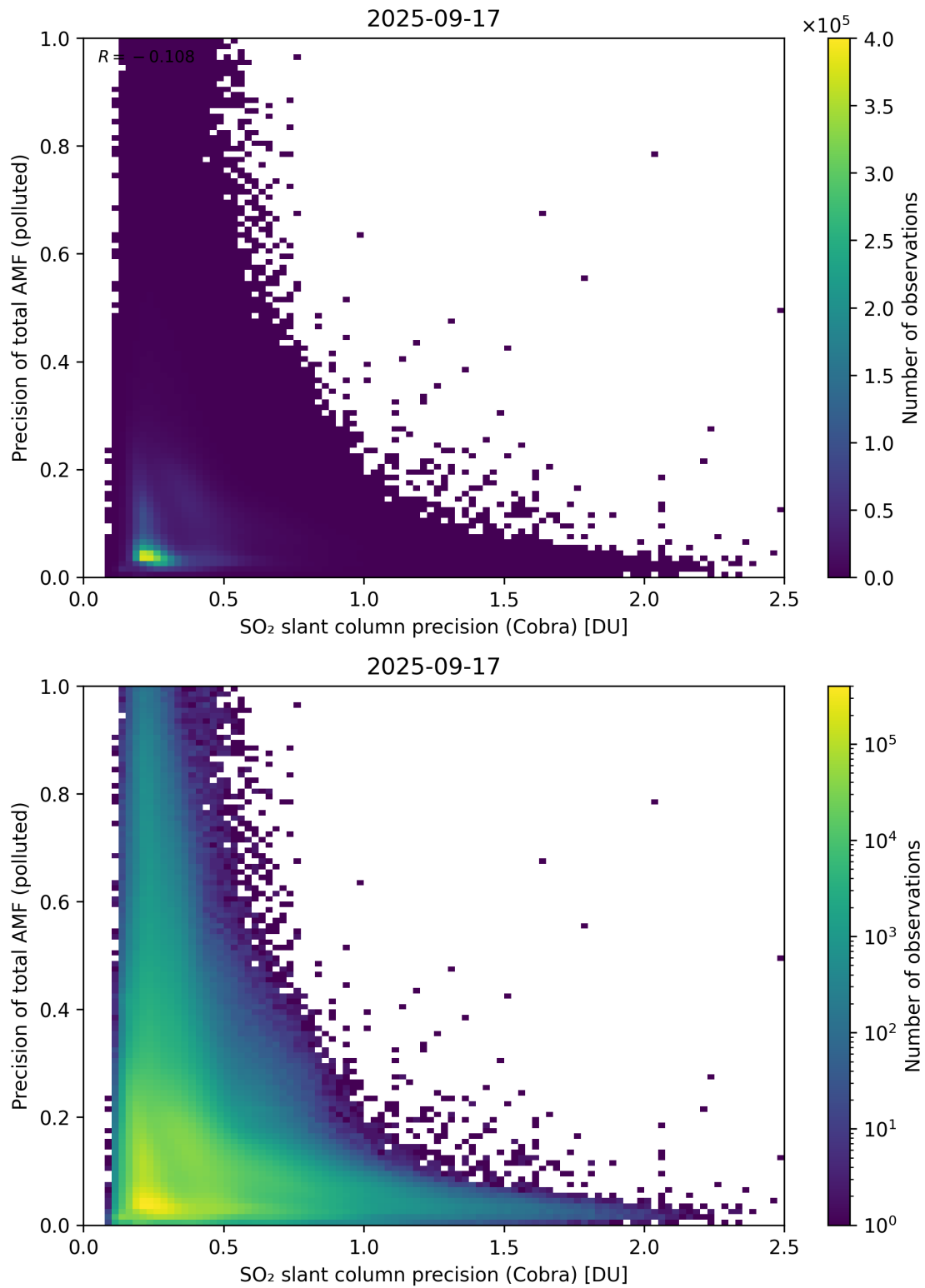
Figure 214: Scatter density plot of “SO 2 slant column precision (Cobra)” against “Precision of total AMF (polluted)” for 2025-09-16 to 2025-09-18.
