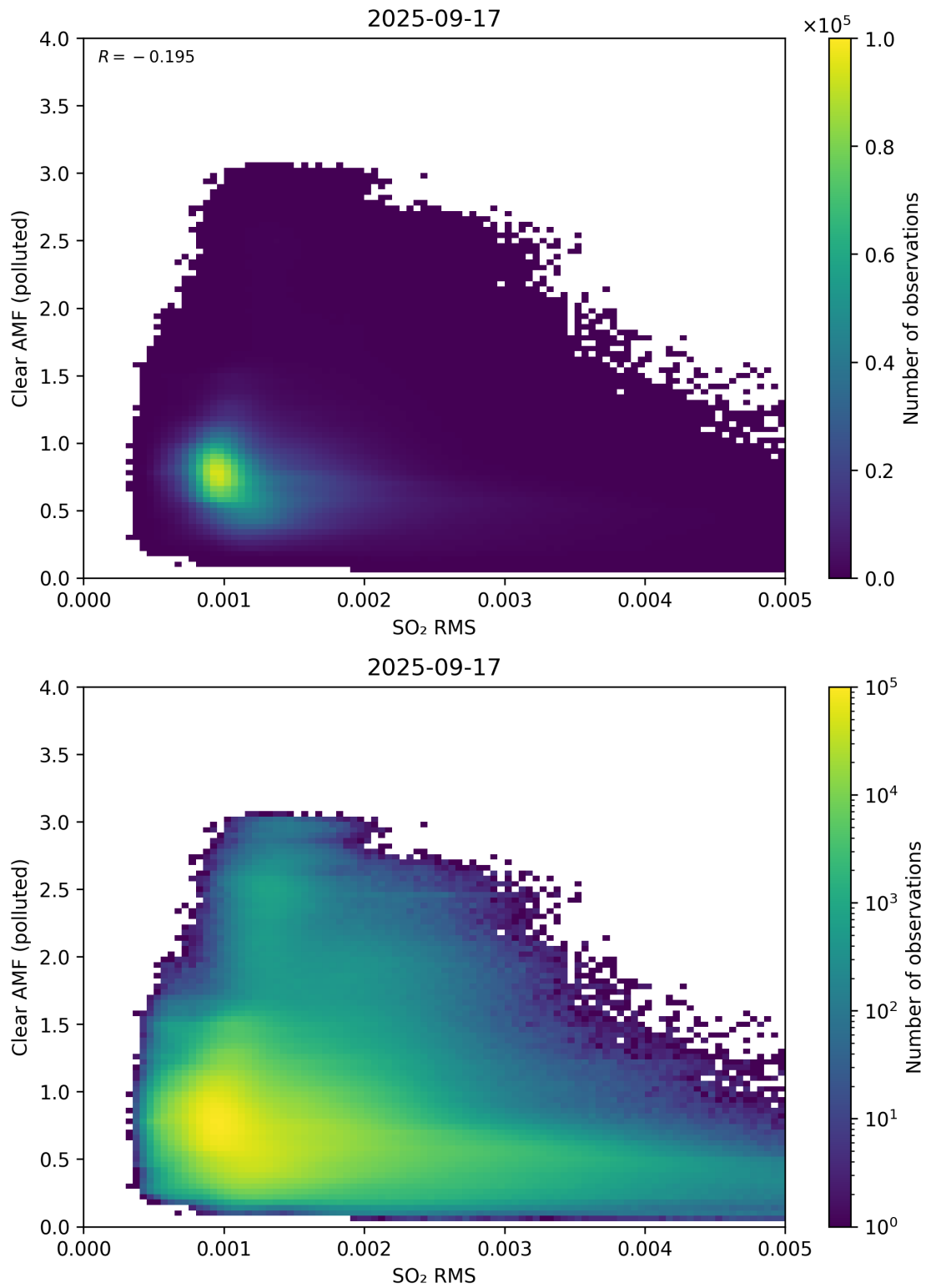
Figure 147: Scatter density plot of “SO 2 RMS” against “Clear AMF (polluted)” for 2025-09-16 to 2025-09-18.
