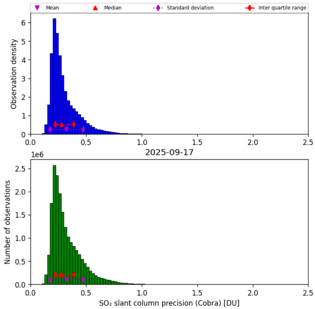
Figure 62: Histogram of “SO 2 slant column precision (Cobra)” for 2025-09-16 to 2025-09-18
