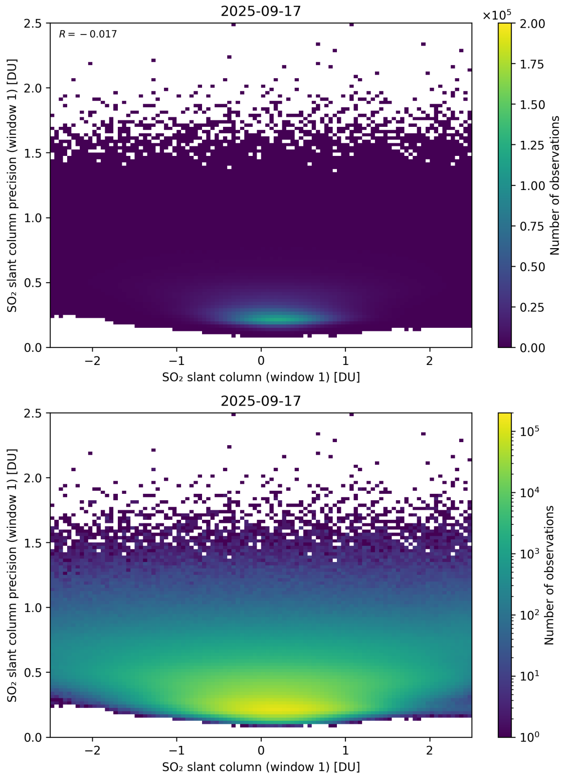
Figure 285: Scatter density plot of “SO 2 slant column (window 1)” against “SO 2 slant column precision (window 1)” for 2025-09-16 to 2025-09-18.
