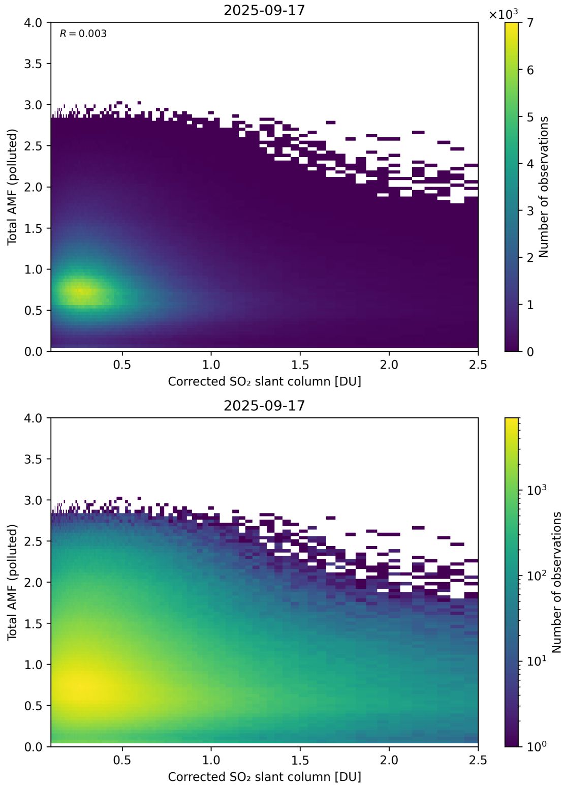
Figure 242: Scatter density plot of “Corrected SO 2 slant column” against “Total AMF (polluted)” for 2025-09-16 to 2025-09-18.
