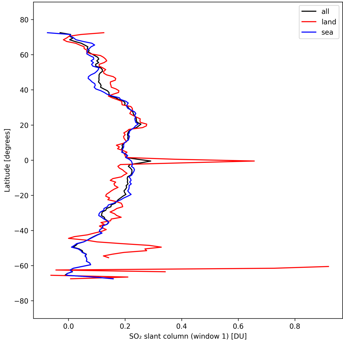
Figure 37: Zonal average of “SO 2 slant column (window 1)” for 2025-09-16 to 2025-09-18.
