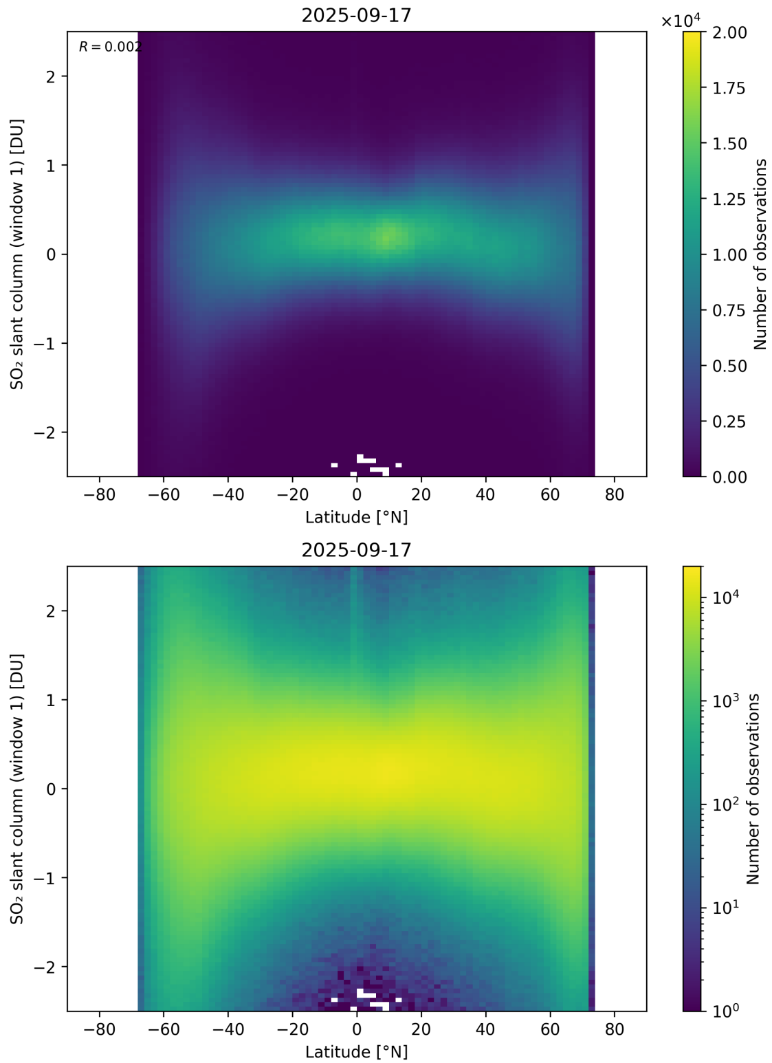
Figure 162: Scatter density plot of “Latitude” against “SO 2 slant column (window 1)” for 2025-09-16 to 2025-09-18.
