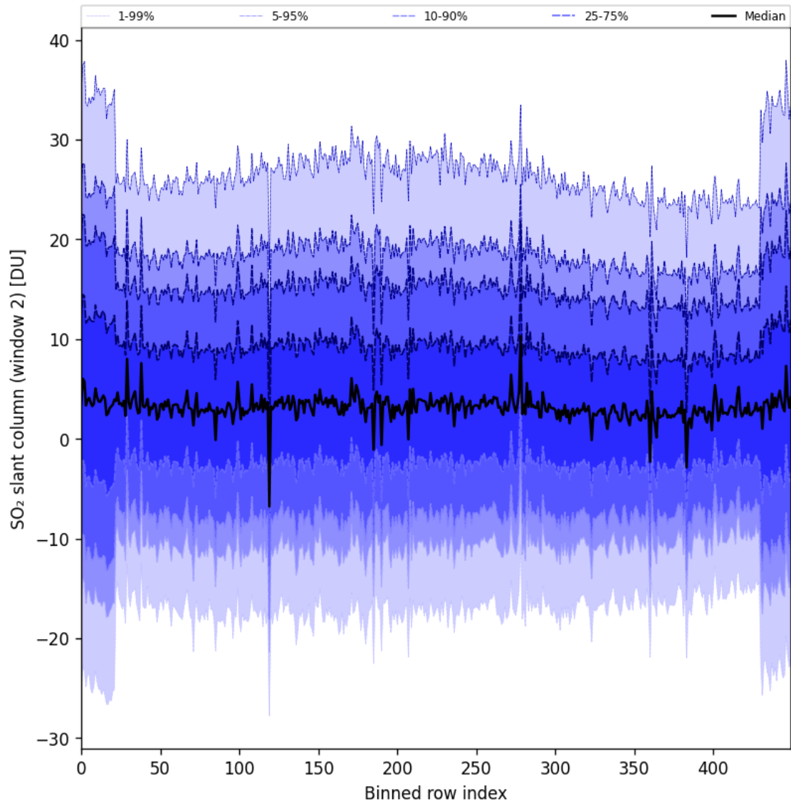
Figure 93: Along track statistics of “SO 2 slant column (window 2)” for 2025-09-16 to 2025-09-18
