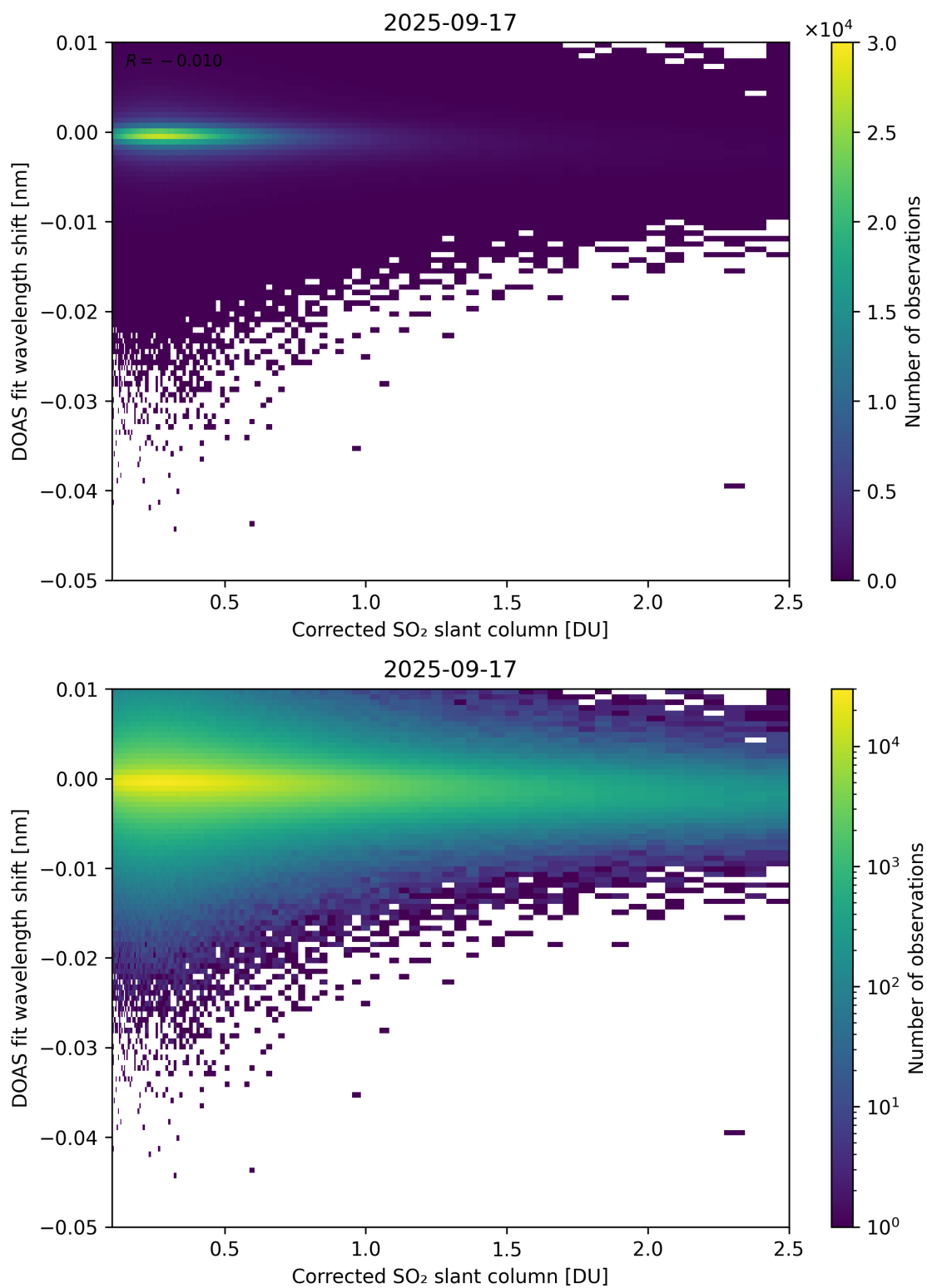
Figure 229: Scatter density plot of “Corrected SO 2 slant column” against “DOAS fit wavelength shift” for 2025-09-16 to 2025-09-18.
