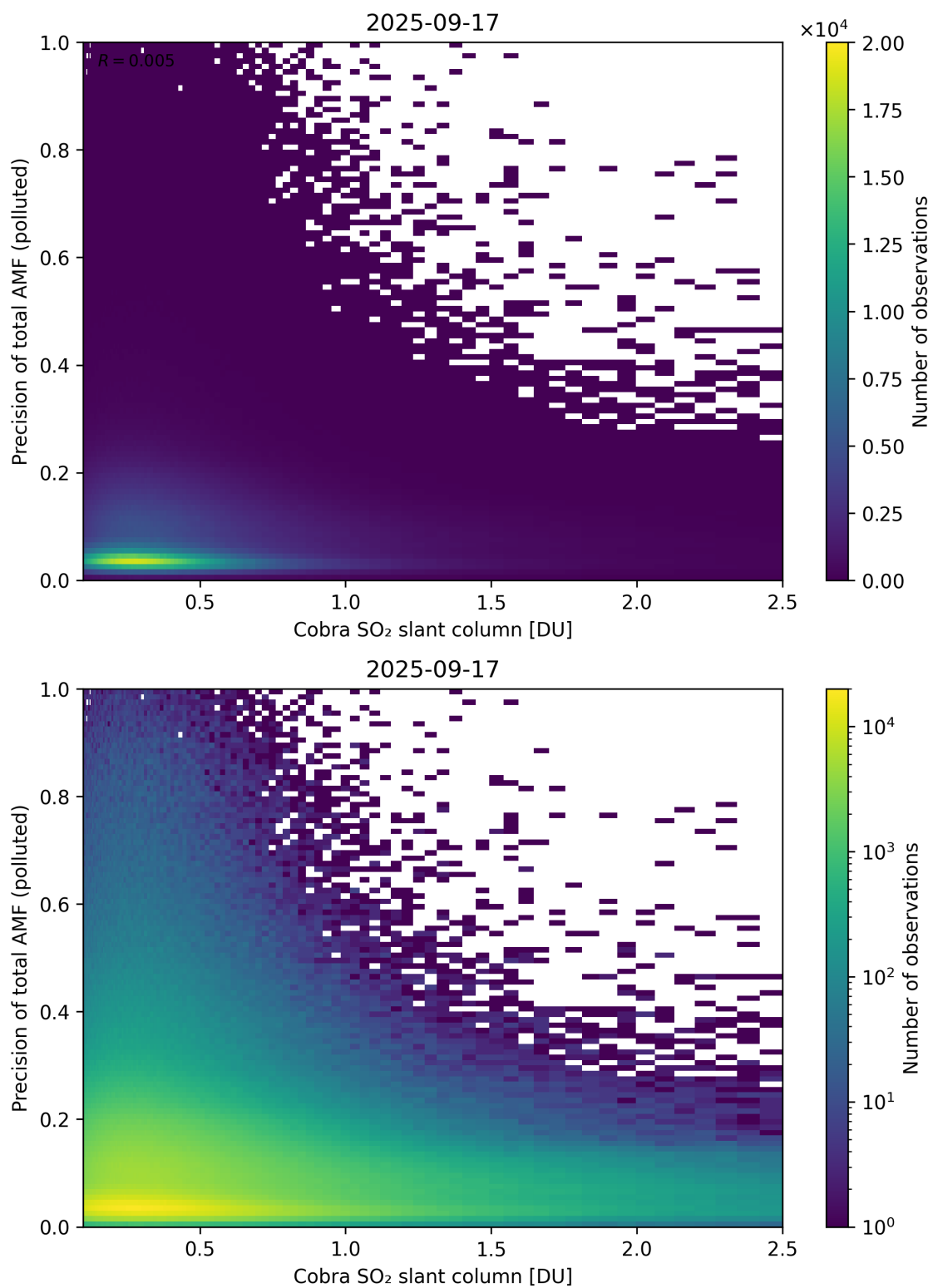
Figure 225: Scatter density plot of “Cobra SO 2 slant column” against “Precision of total AMF (polluted)” for 2025-09-16 to 2025-09-18.
