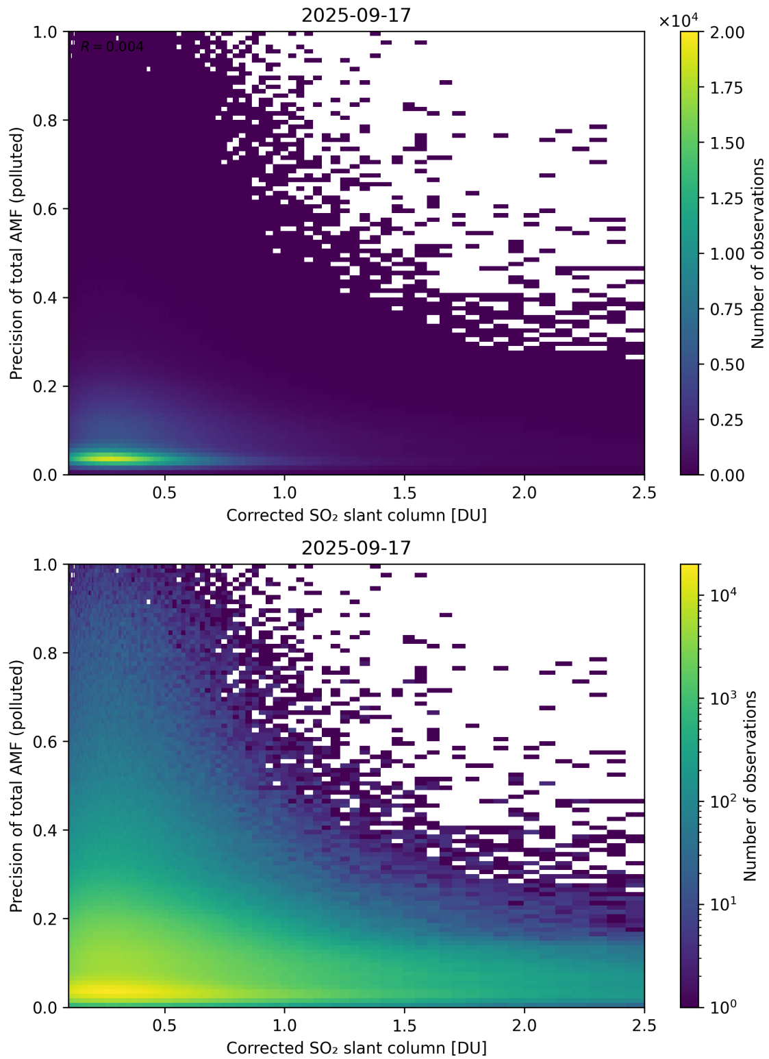
Figure 243: Scatter density plot of “Corrected SO 2 slant column” against “Precision of total AMF (polluted)” for 2025-09-16 to 2025-09-18.
