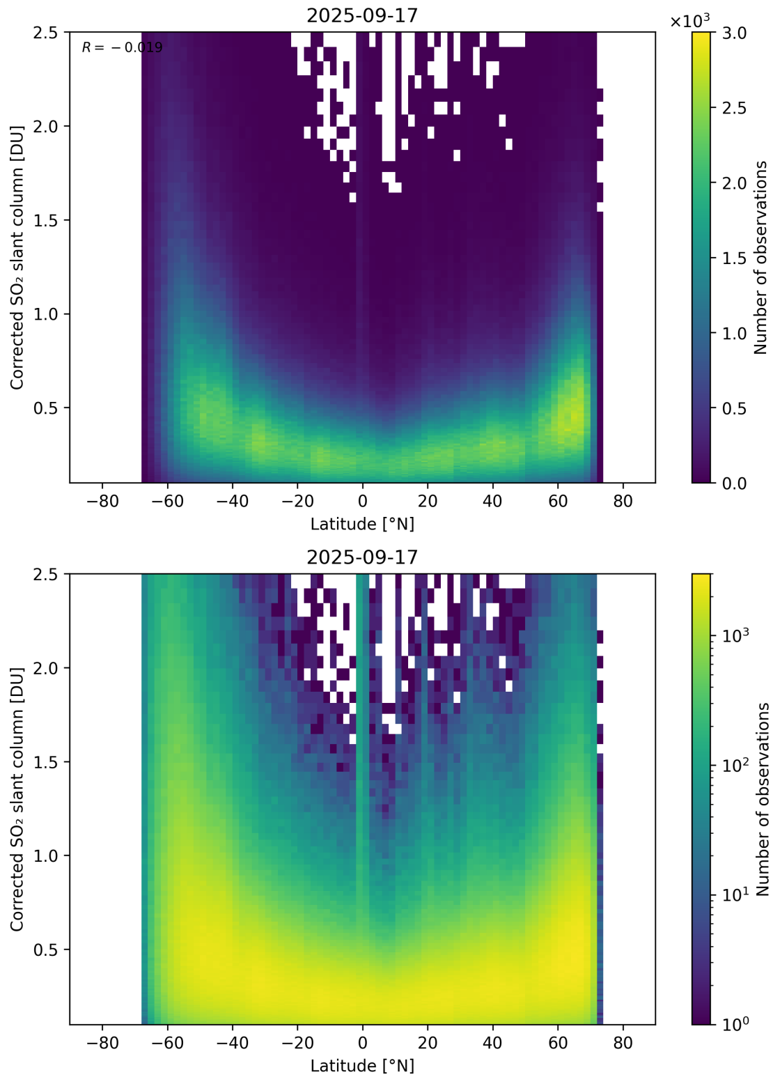
Figure 159: Scatter density plot of “Latitude” against “Corrected SO 2 slant column” for 2025-09-16 to 2025-09-18.
