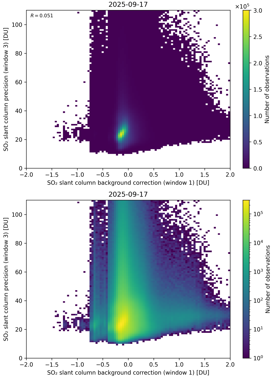
Figure 119: Scatter density plot of “SO 2 slant column background correction (window 1)” against “SO 2 slant column precision (window 3)” for 2025-09-16 to 2025-09-18.
