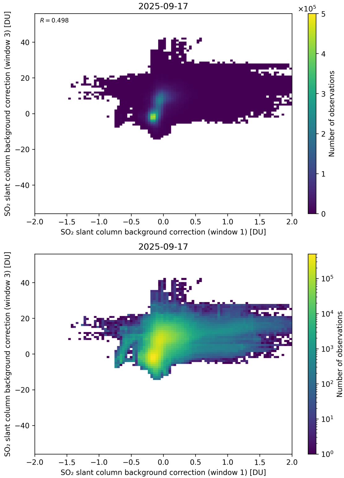
Figure 110: Scatter density plot of “SO 2 slant column background correction (window 1)” against “SO 2 slant column background correction (window 3)” for 2025-09-16 to 2025-09-18.
