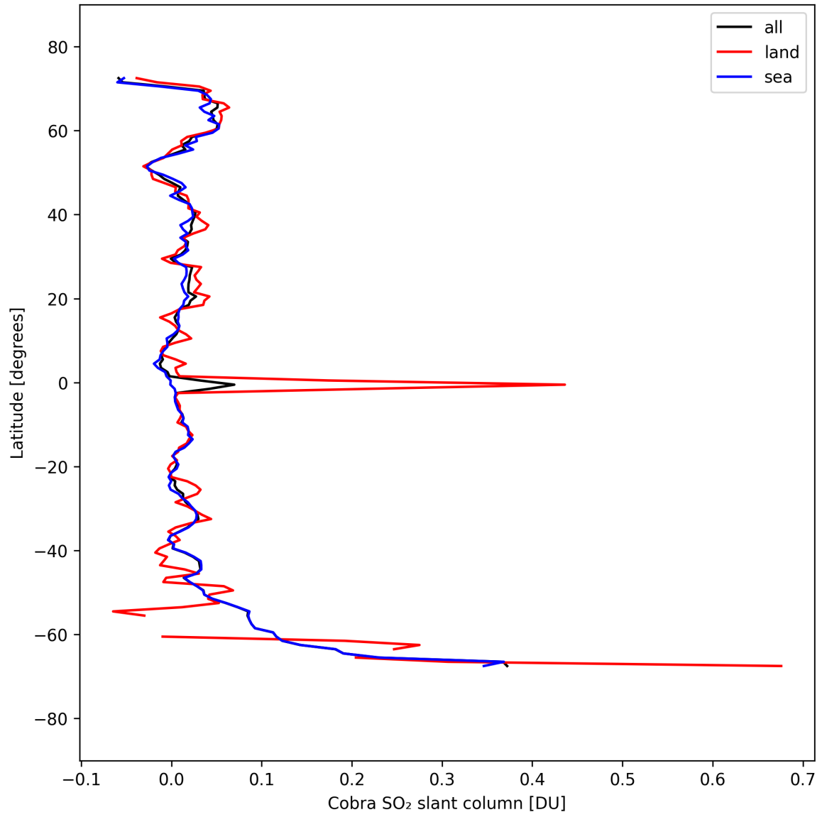
Figure 35: Zonal average of “Cobra SO 2 slant column” for 2025-09-16 to 2025-09-18.
