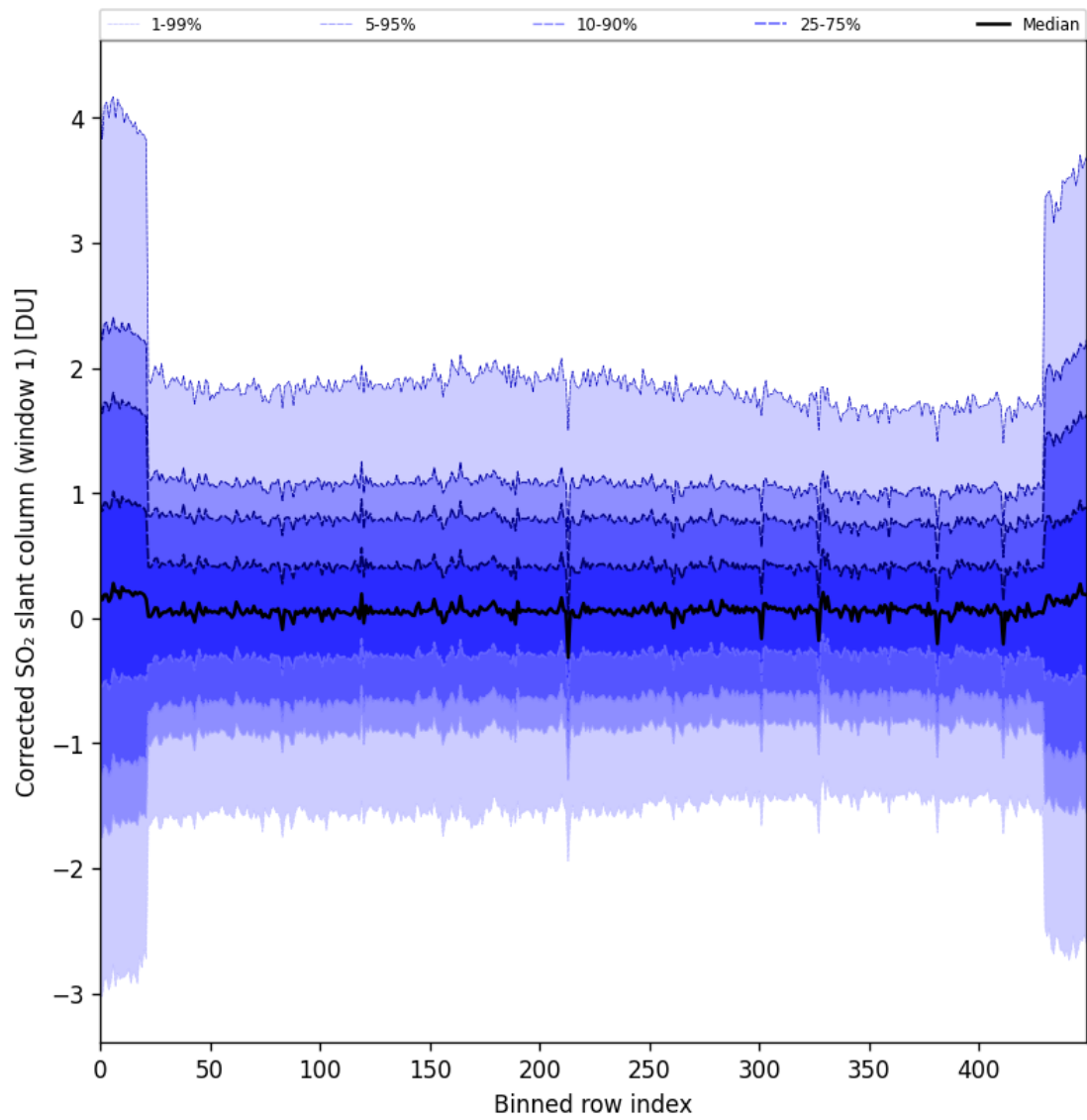
Figure 91: Along track statistics of “Corrected SO 2 slant column (window 1)” for 2025-09-16 to 2025-09-18
