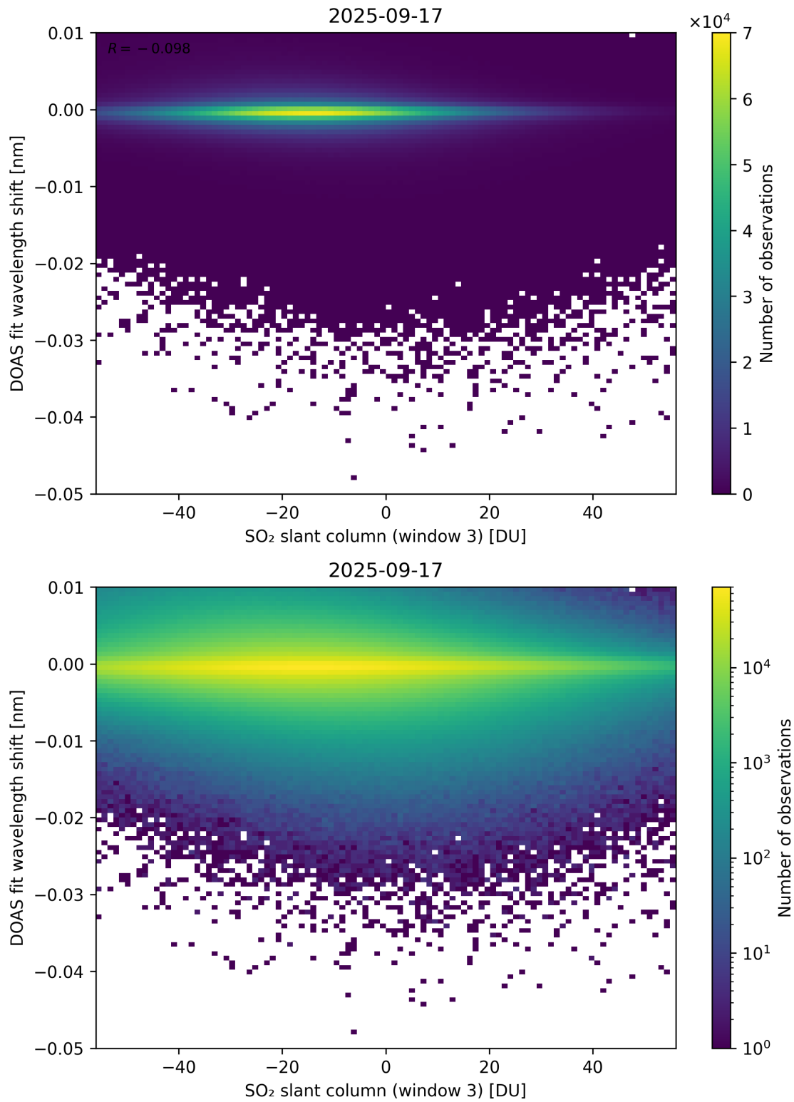
Figure 304: Scatter density plot of “SO 2 slant column (window 3)” against “DOAS fit wavelength shift” for 2025-09-16 to 2025-09-18.
