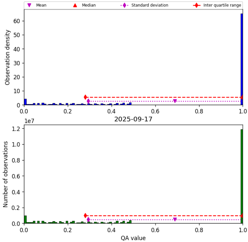
Figure 57: Histogram of “QA value” for 2025-09-16 to 2025-09-18
