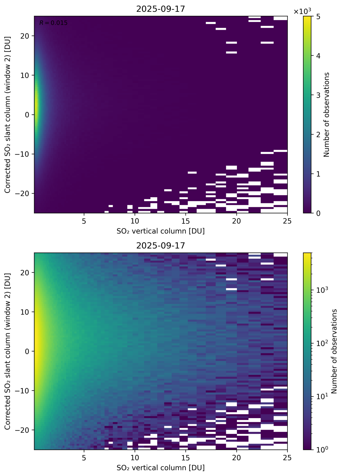
Figure 352: Scatter density plot of “SO 2 vertical column” against “Corrected SO 2 slant column (window 2)” for 2025-09-16 to 2025-09-18.
