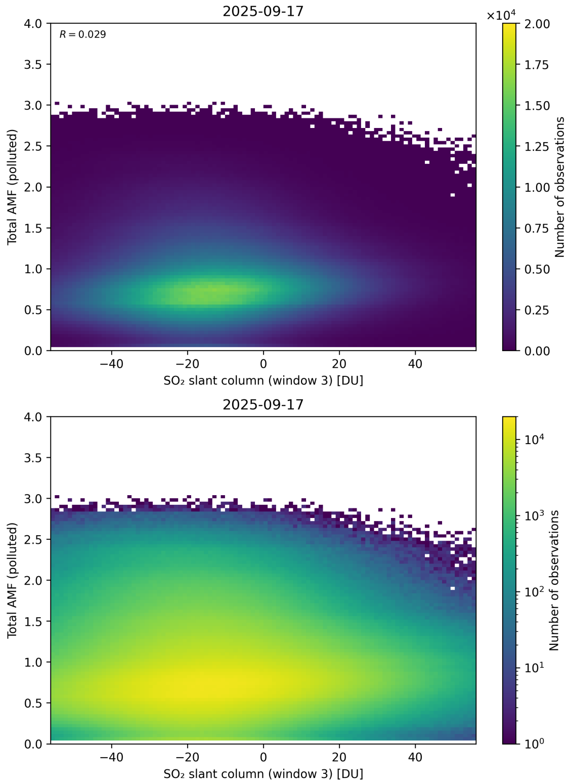
Figure 318: Scatter density plot of “SO 2 slant column (window 3)” against “Total AMF (polluted)” for 2025-09-16 to 2025-09-18.
