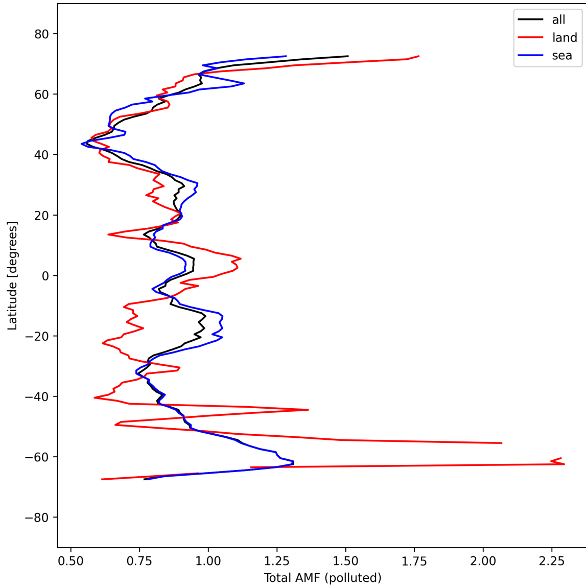
Figure 53: Zonal average of “Total AMF (polluted)” for 2025-09-16 to 2025-09-18.
