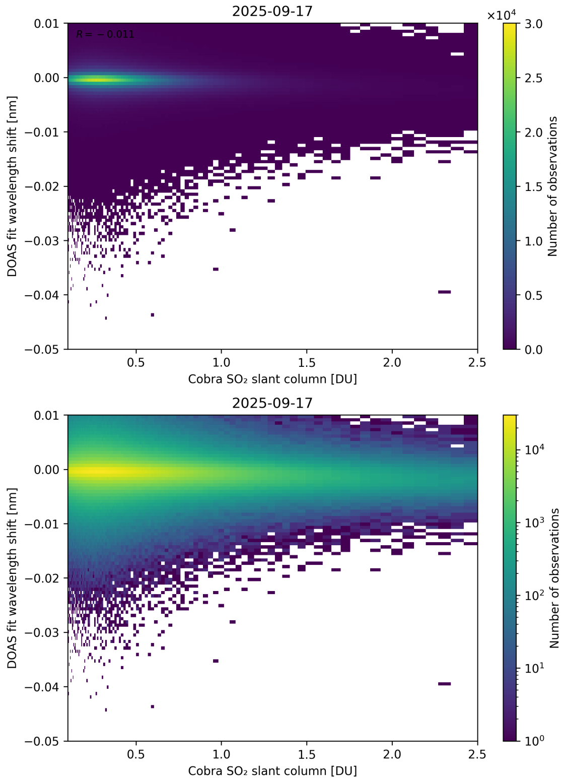
Figure 196: Scatter density plot of “Cobra SO 2 slant column” against “DOAS fit wavelength shift” for 2025-09-16 to 2025-09-18.
