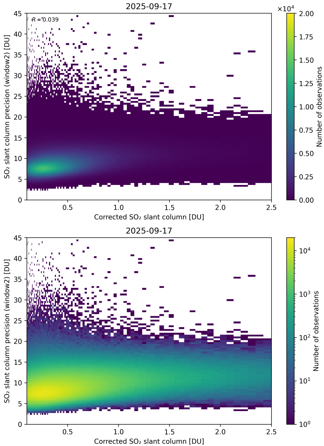
Figure 239: Scatter density plot of “Corrected SO 2 slant column” against “SO 2 slant column precision (window2)” for 2025-09-16 to 2025-09-18.
