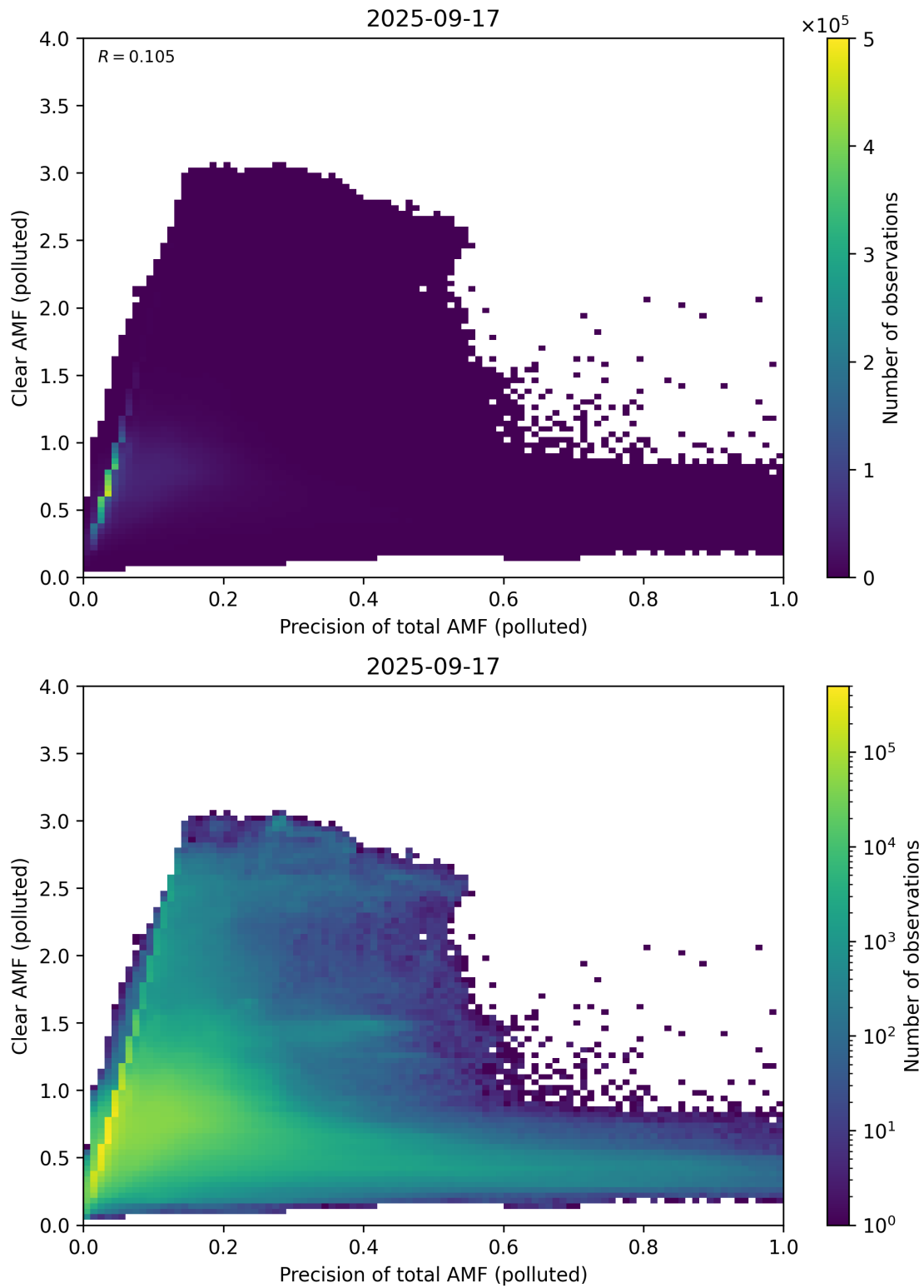
Figure 320: Scatter density plot of “Precision of total AMF (polluted)” against “Clear AMF (polluted)” for 2025-09-16 to 2025-09-18.
