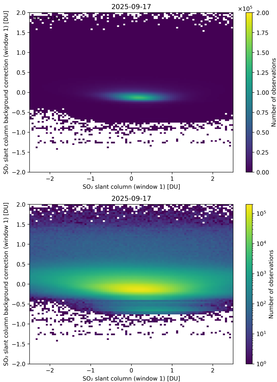
Figure 262: Scatter density plot of “SO 2 slant column (window 1)” against “SO 2 slant column background correction (window 1)” for 2025-09-16 to 2025-09-18.
