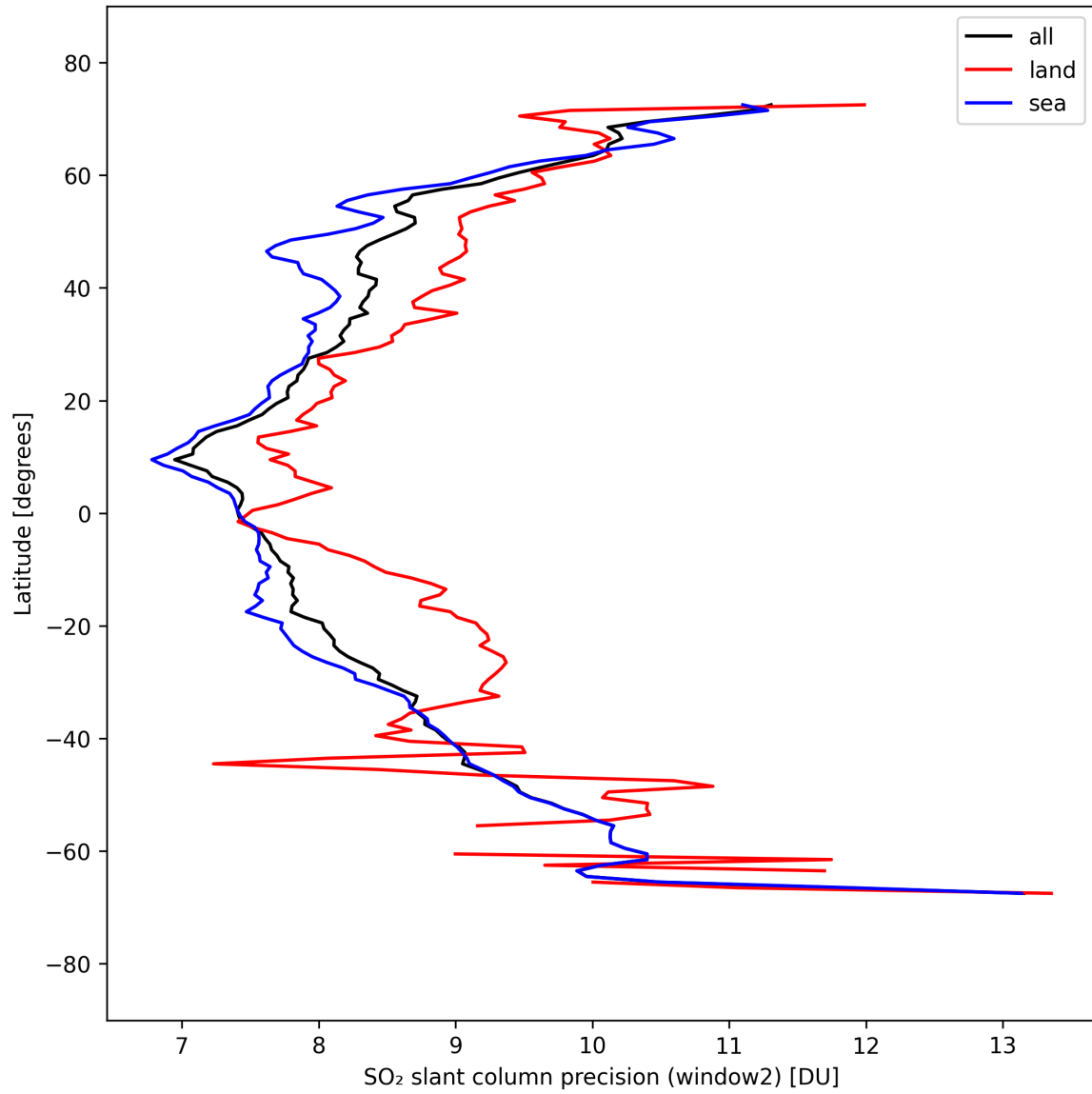
Figure 42: Zonal average of "SO 2 slant column precision (window2)" for 2025-09-16 to 2025-09-18.
