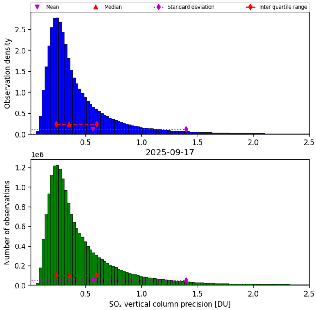
Figure 59: Histogram of “SO 2 vertical column precision” for 2025-09-16 to 2025-09-18
