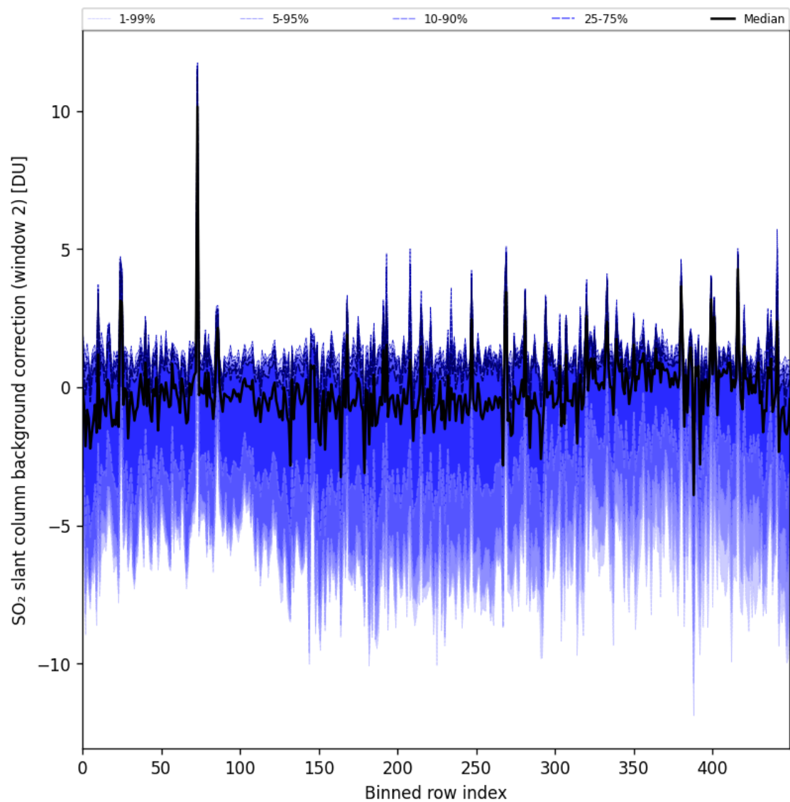
Figure 96: Along track statistics of “SO 2 slant column background correction (window 2)” for 2025-09-16 to 2025-09-18
