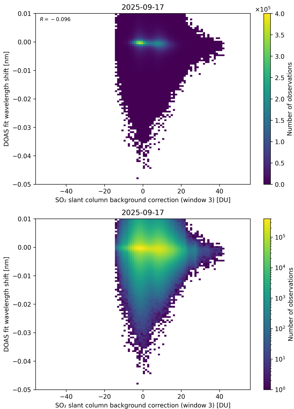
Figure 132: Scatter density plot of “SO 2 slant column background correction (window 3)” against “DOAS fit wavelength shift” for 2025-09-16 to 2025-09-18.
