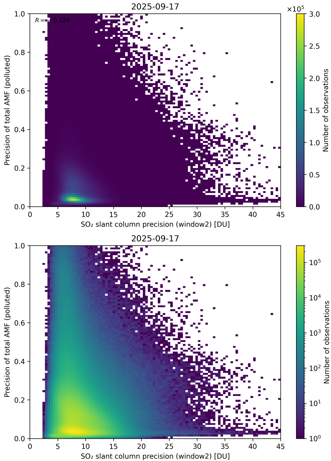
Figure 302: Scatter density plot of “SO 2 slant column precision (window2)” against “Precision of total AMF (polluted)” for 2025-09-16 to 2025-09-18.
