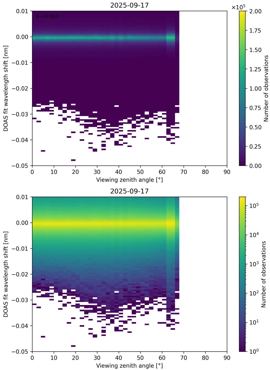
Figure 365: Scatter density plot of “Viewing zenith angle” against “DOAS fit wavelength shift” for 2025-09-16 to 2025-09-18.
