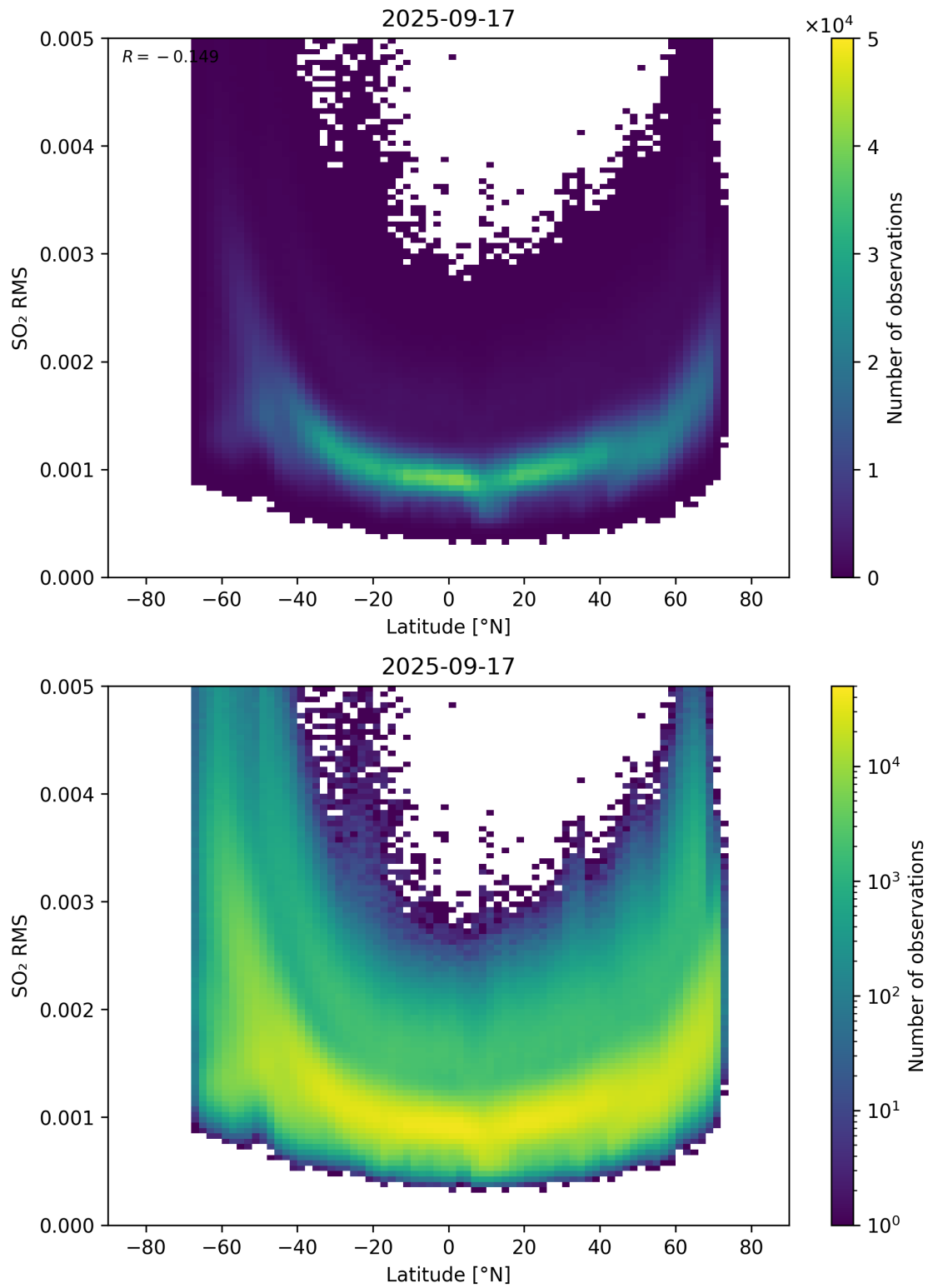
Figure 155: Scatter density plot of “Latitude” against “SO 2 RMS” for 2025-09-16 to 2025-09-18.
