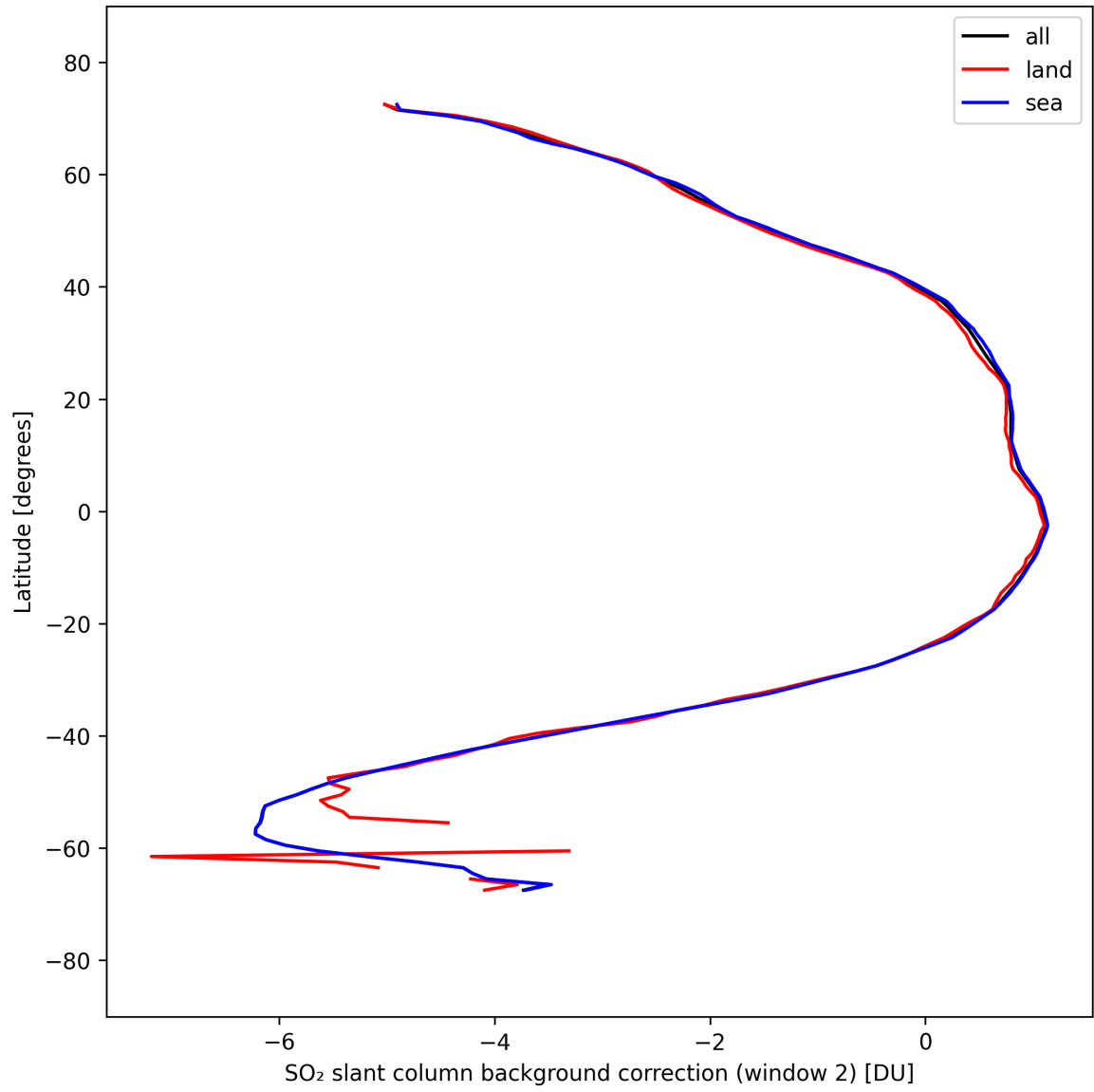
Figure 44: Zonal average of “SO 2 slant column background correction (window 2)” for 2025-09-16 to 2025-09-18.
