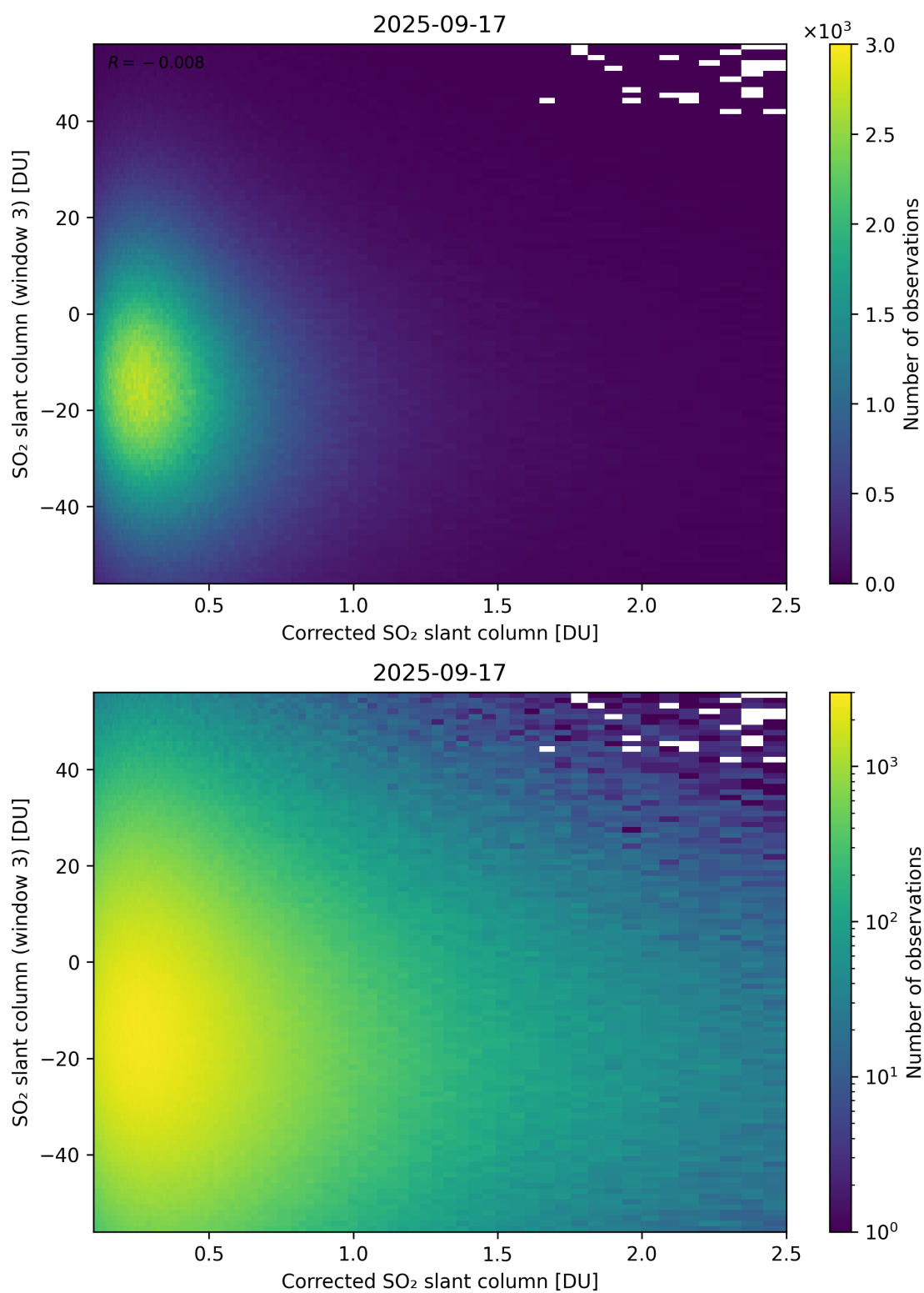
Figure 240: Scatter density plot of “Corrected SO 2 slant column” against “SO 2 slant column (window 3)” for 2025-09-16 to 2025-09-18.
