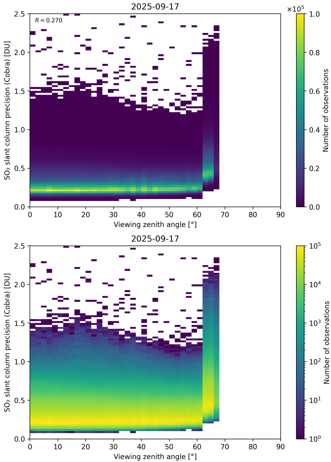
Figure 372: Scatter density plot of “Viewing zenith angle” against “SO 2 slant column precision (Cobra)” for 2025-09-16 to 2025-09-18.
