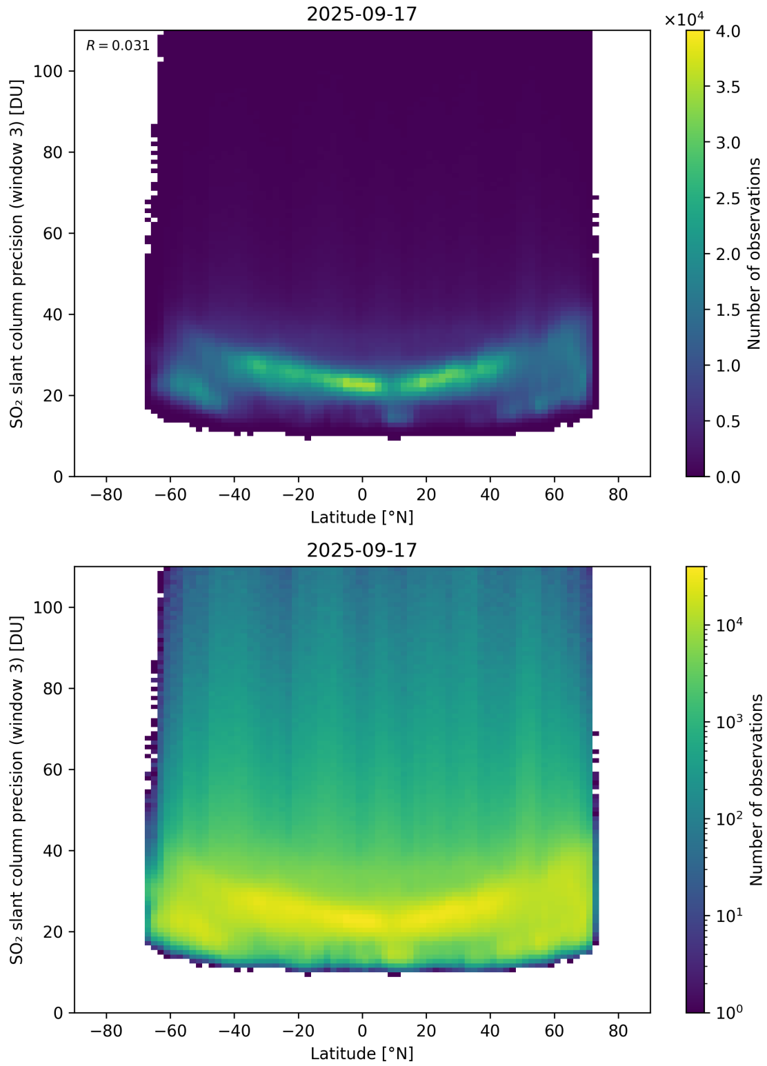
Figure 166: Scatter density plot of “Latitude” against “SO 2 slant column precision (window 3)” for 2025-09-16 to 2025-09-18.
