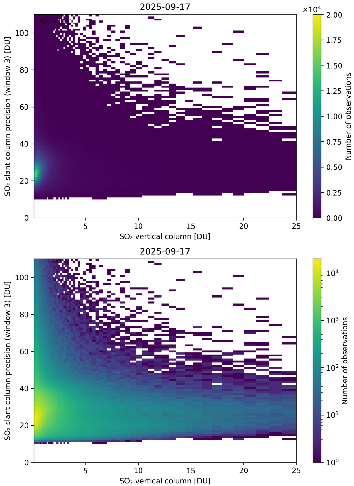
Figure 358: Scatter density plot of “SO 2 vertical column” against “SO 2 slant column precision (window 3)” for 2025-09-16 to 2025-09-18.
