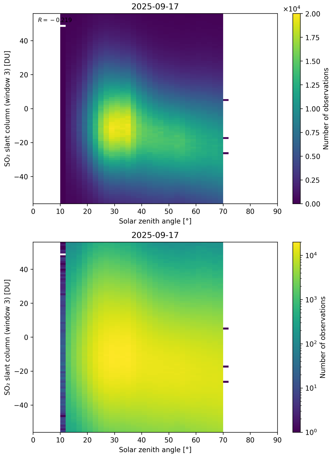
Figure 187: Scatter density plot of “Solar zenith angle” against “SO 2 slant column (window 3)” for 2025-09-16 to 2025-09-18.
