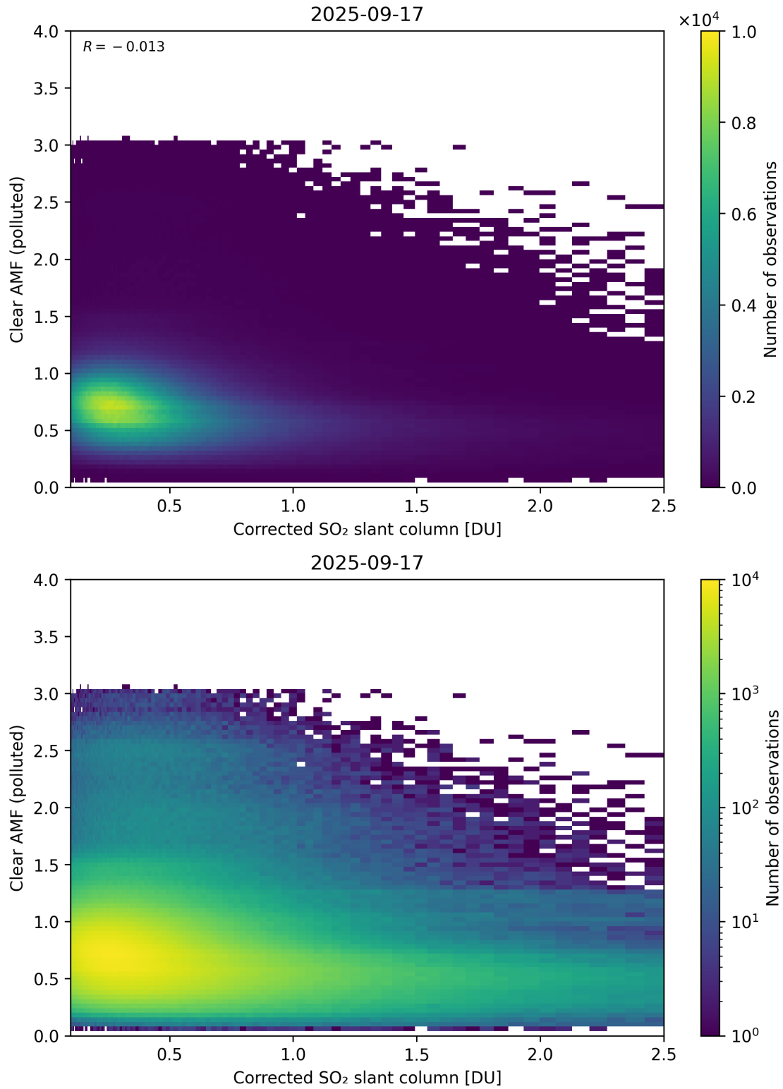
Figure 232: Scatter density plot of “Corrected SO 2 slant column” against “Clear AMF (polluted)” for 2025-09-16 to 2025-09-18.
