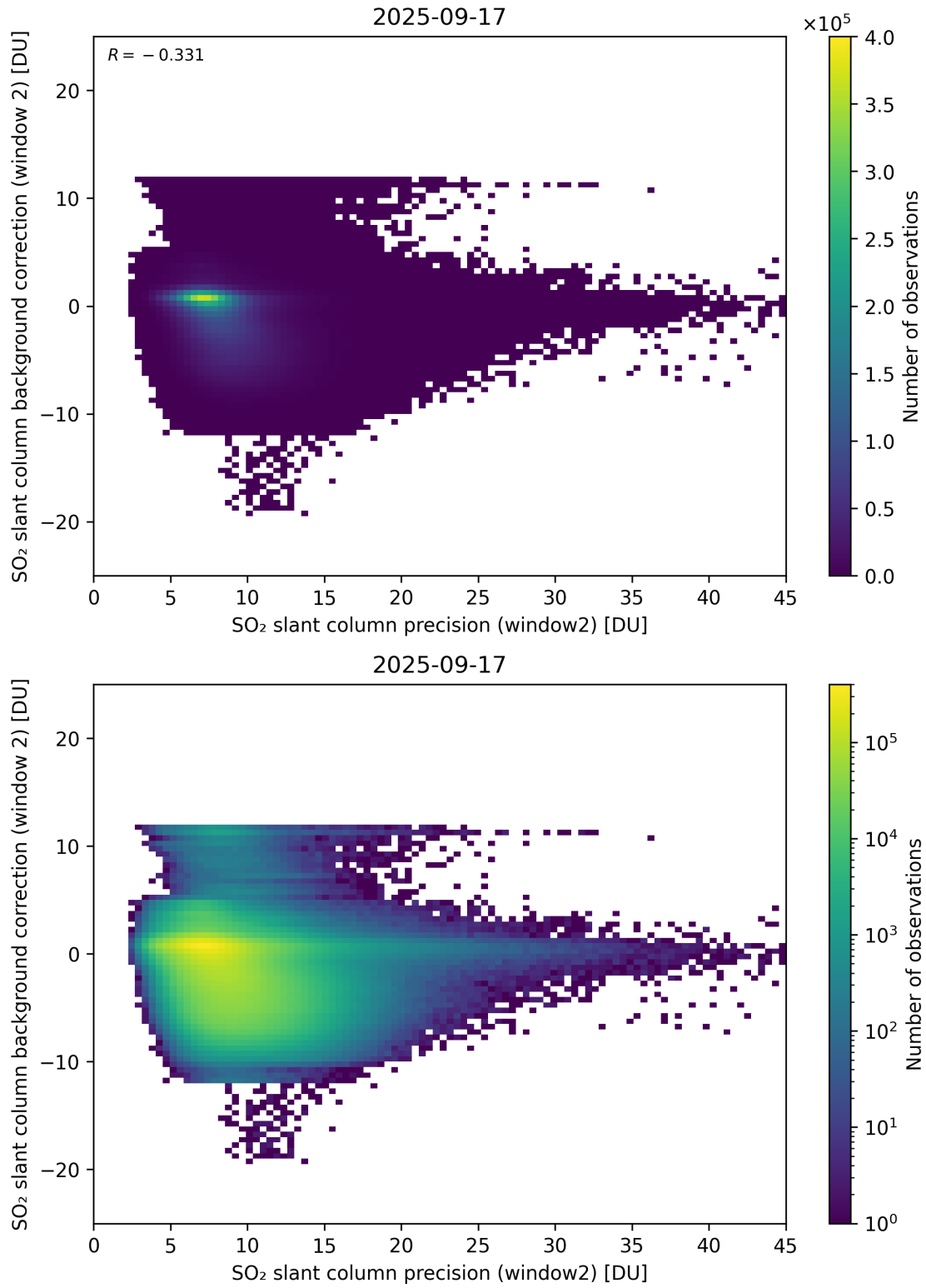
Figure 291: Scatter density plot of “SO 2 slant column precision (window2)” against “SO 2 slant column background correction (window 2)” for 2025-09-16 to 2025-09-18.
