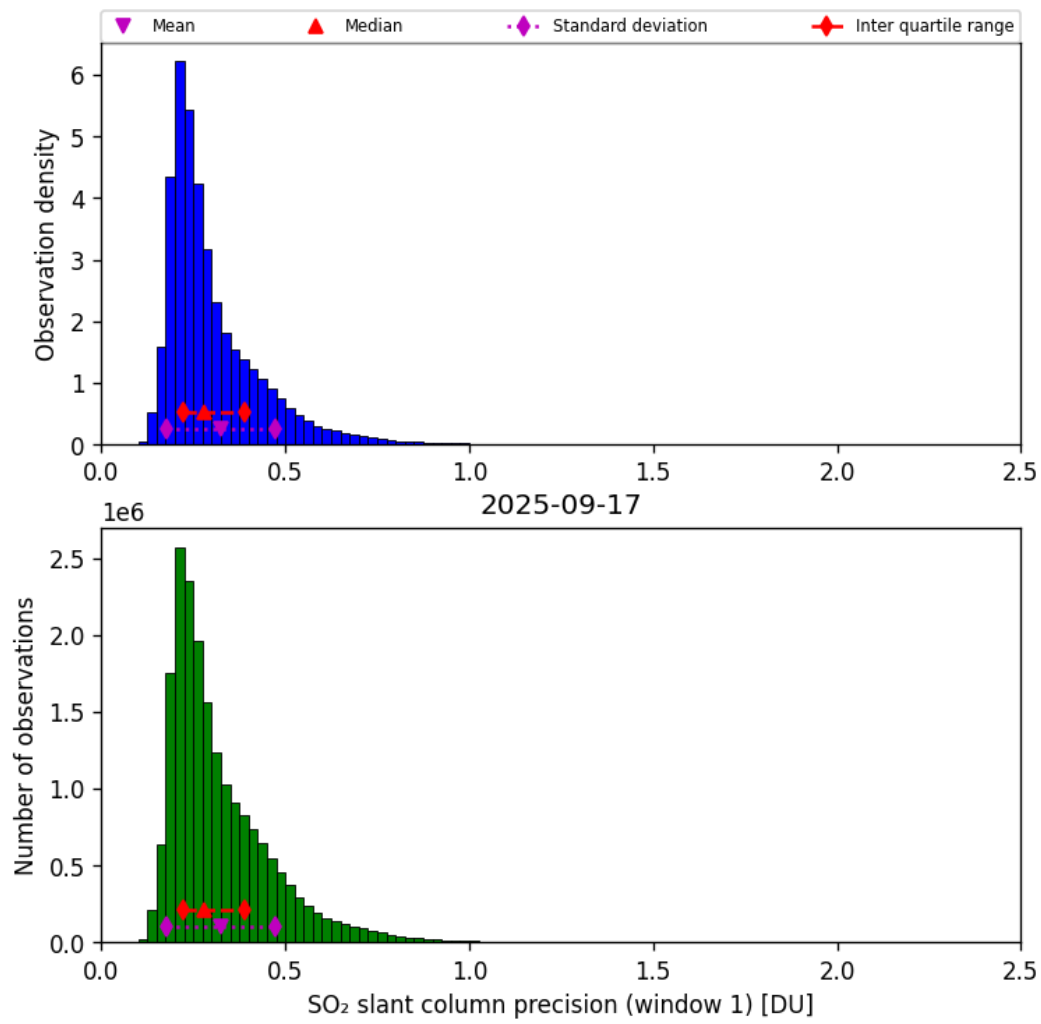
Figure 64: Histogram of “SO 2 slant column precision (window 1)” for 2025-09-16 to 2025-09-18
