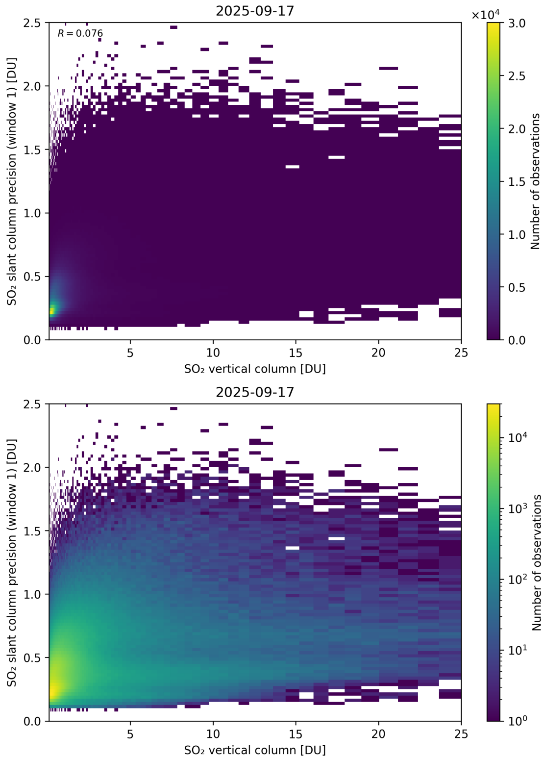
Figure 355: Scatter density plot of “SO 2 vertical column” against “SO 2 slant column precision (window 1)” for 2025-09-16 to 2025-09-18.
