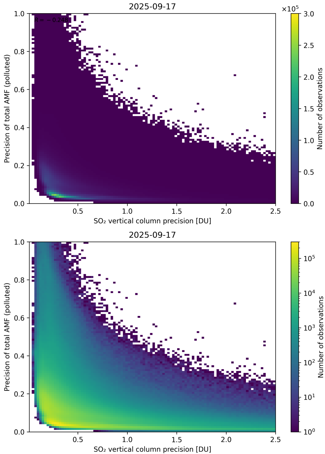
Figure 347: Scatter density plot of “SO 2 vertical column precision” against “Precision of total AMF (polluted)” for 2025-09-16 to 2025-09-18.
