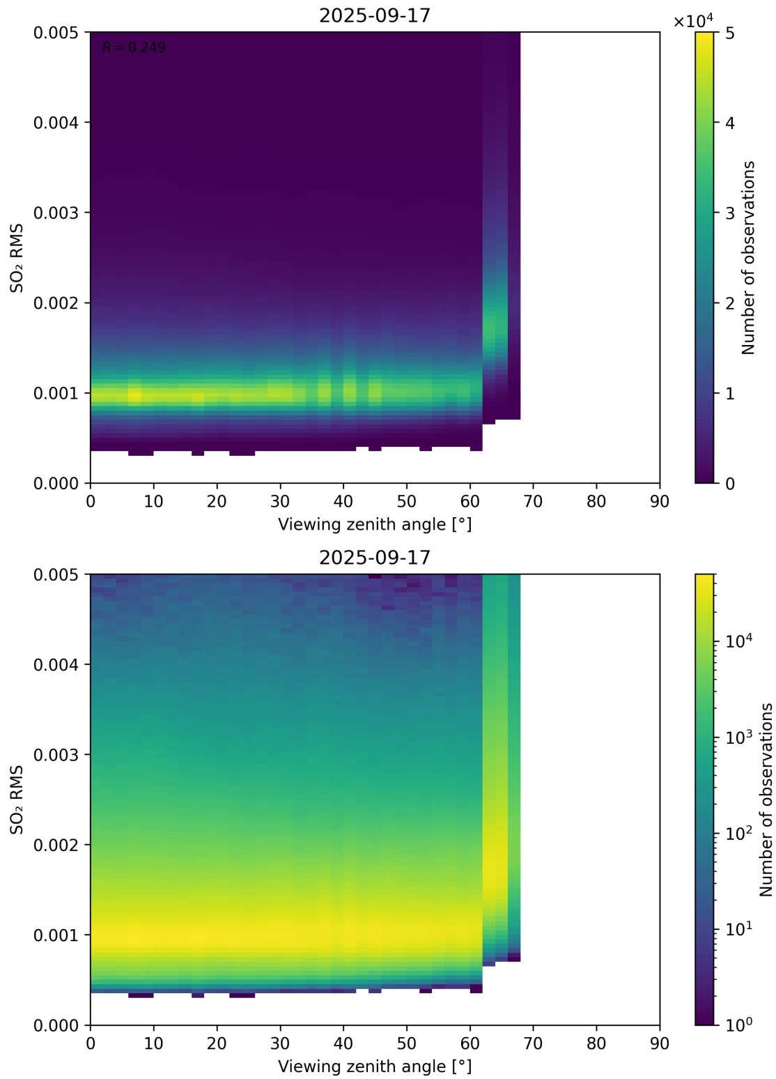
Figure 367: Scatter density plot of “Viewing zenith angle” against “SO 2 RMS” for 2025-09-16 to 2025-09-18.
