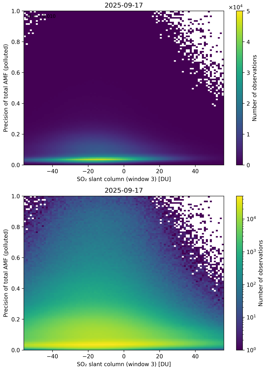
Figure 319: Scatter density plot of “SO 2 slant column (window 3)” against “Precision of total AMF (polluted)” for 2025-09-16 to 2025-09-18.
