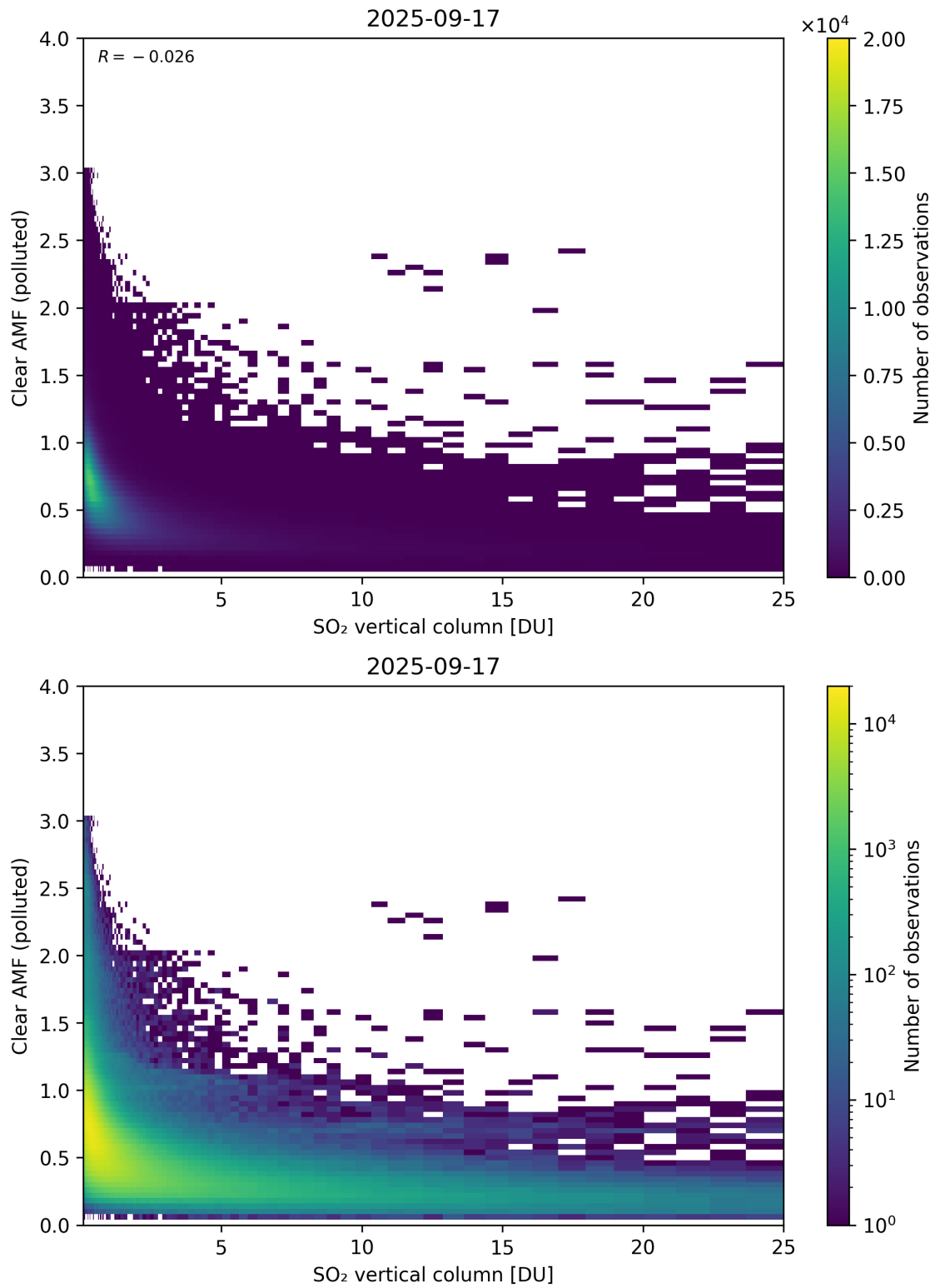
Figure 348: Scatter density plot of “SO 2 vertical column” against “Clear AMF (polluted)” for 2025-09-16 to 2025-09-18.
