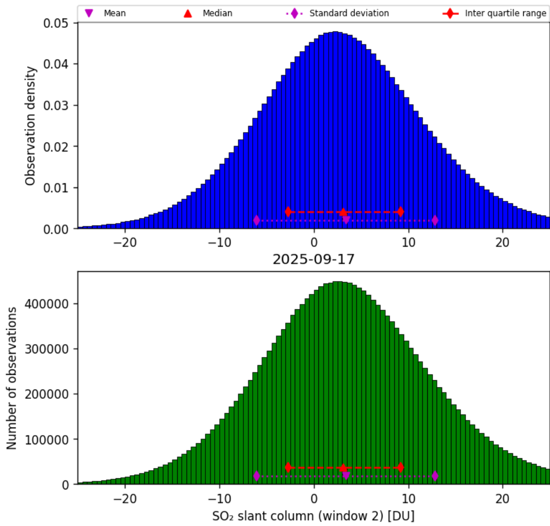
Figure 67: Histogram of “SO 2 slant column (window 2)” for 2025-09-16 to 2025-09-18
