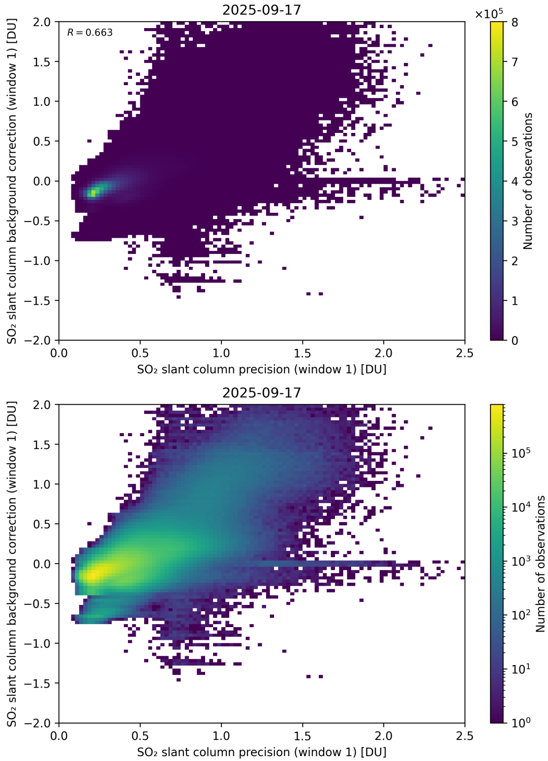
Figure 268: Scatter density plot of “SO 2 slant column precision (window 1)” against “SO 2 slant column background correction (window 1)” for 2025-09-16 to 2025-09-18.
