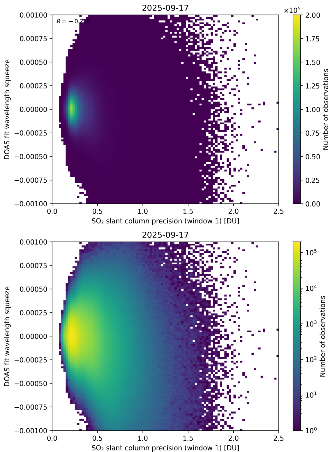
Figure 272: Scatter density plot of “SO 2 slant column precision (window 1)” against “DOAS fit wavelength squeeze” for 2025-09-16 to 2025-09-18.
