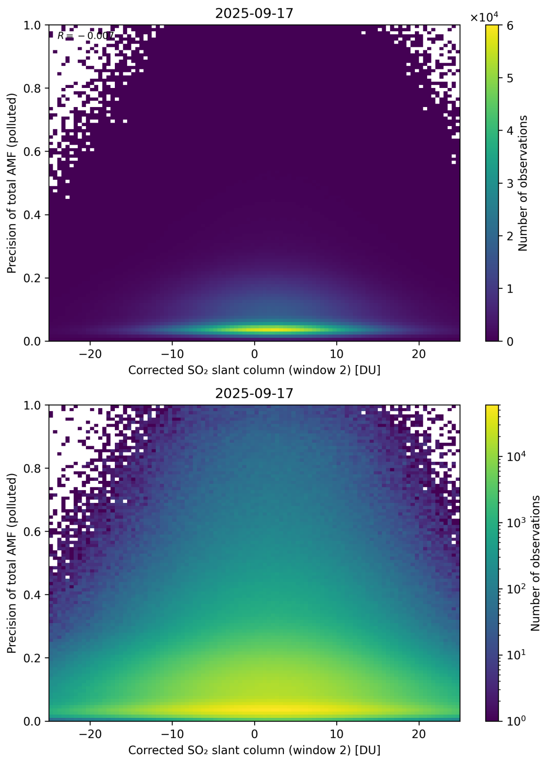
Figure 254: Scatter density plot of “Corrected SO 2 slant column (window 2)” against “Precision of total AMF (polluted)” for 2025-09-16 to 2025-09-18.
