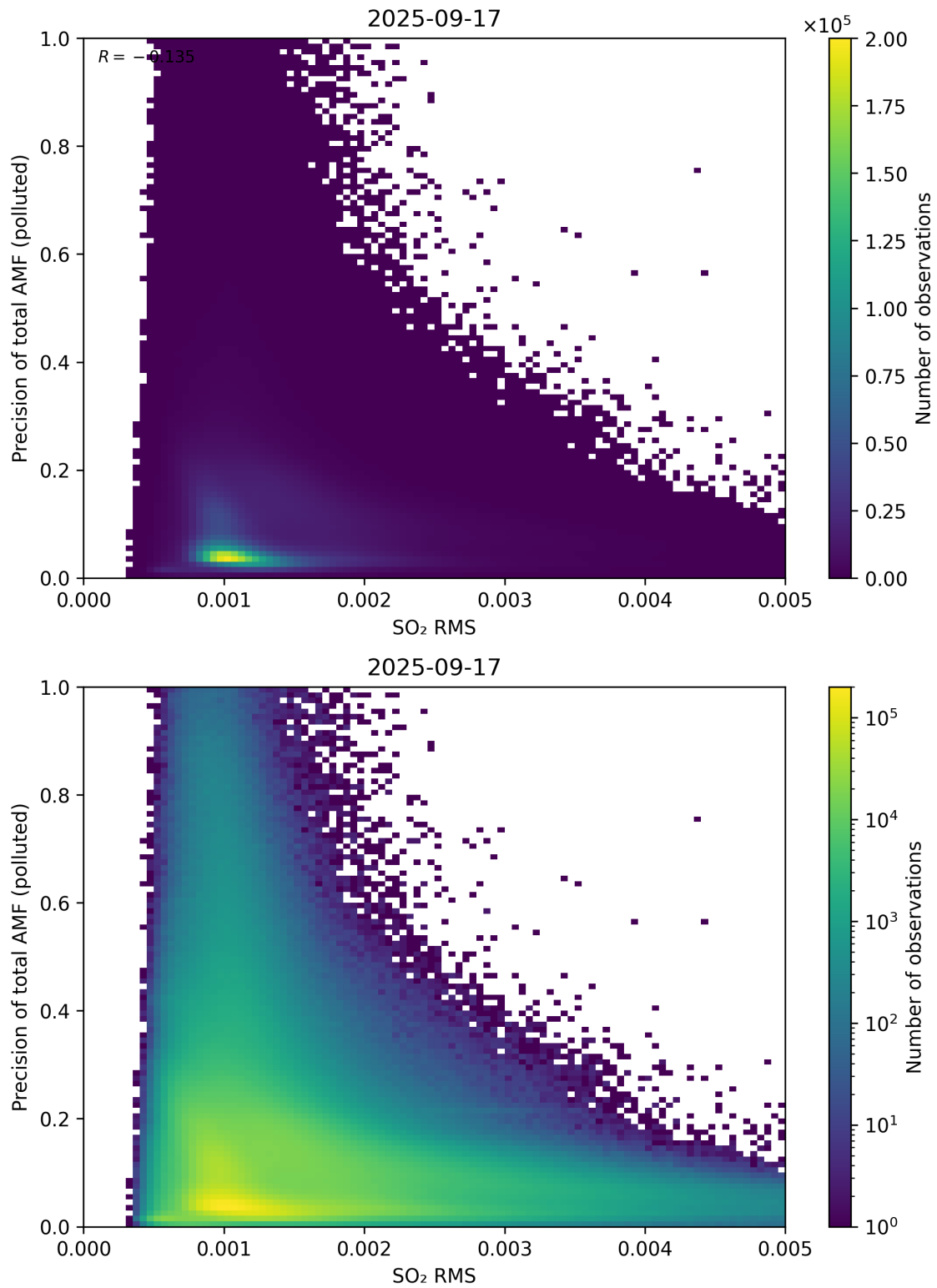
Figure 149: Scatter density plot of “SO 2 RMS” against “Precision of total AMF (polluted)” for 2025-09-16 to 2025-09-18.
