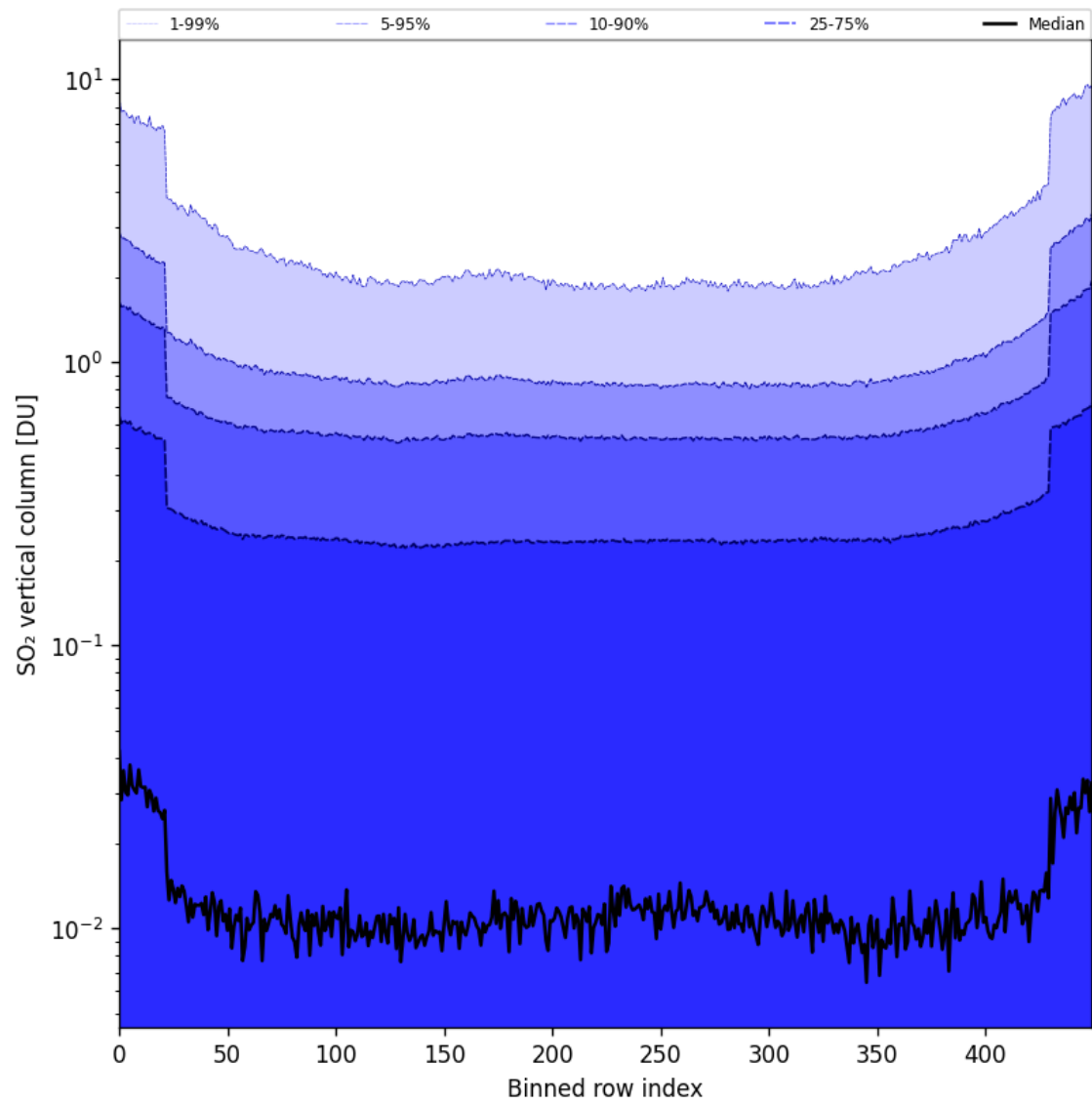
Figure 84: Along track statistics of “SO 2 vertical column” for 2025-09-16 to 2025-09-18
