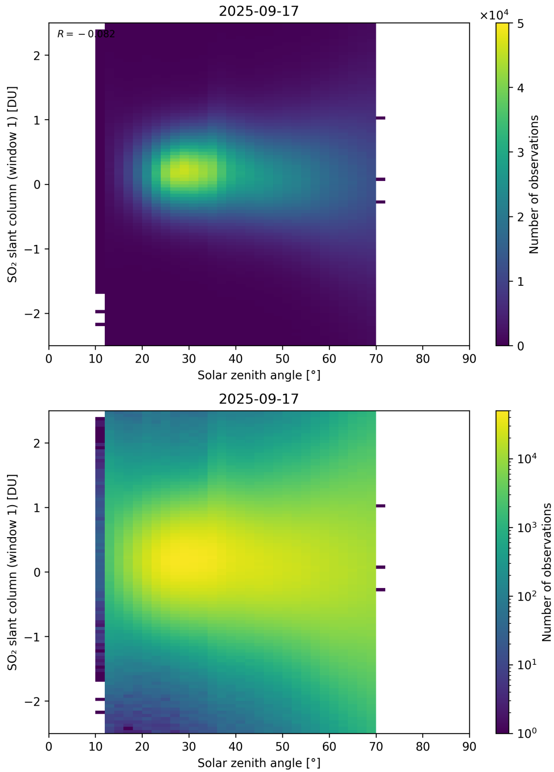
Figure 184: Scatter density plot of “Solar zenith angle” against “SO 2 slant column (window 1)” for 2025-09-16 to 2025-09-18.
