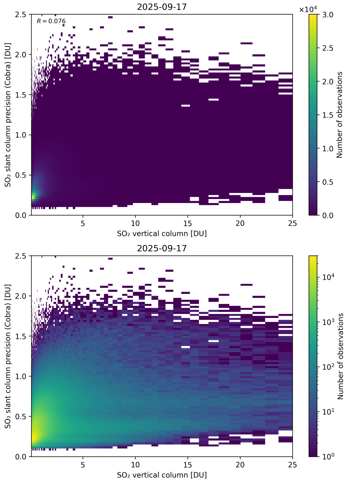
Figure 350: Scatter density plot of “SO 2 vertical column” against “SO 2 slant column precision (Cobra)” for 2025-09-16 to 2025-09-18.
