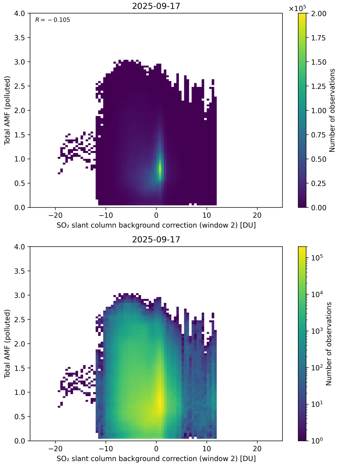
Figure 130: Scatter density plot of “SO 2 slant column background correction (window 2)” against “Total AMF (polluted)” for 2025-09-16 to 2025-09-18.
