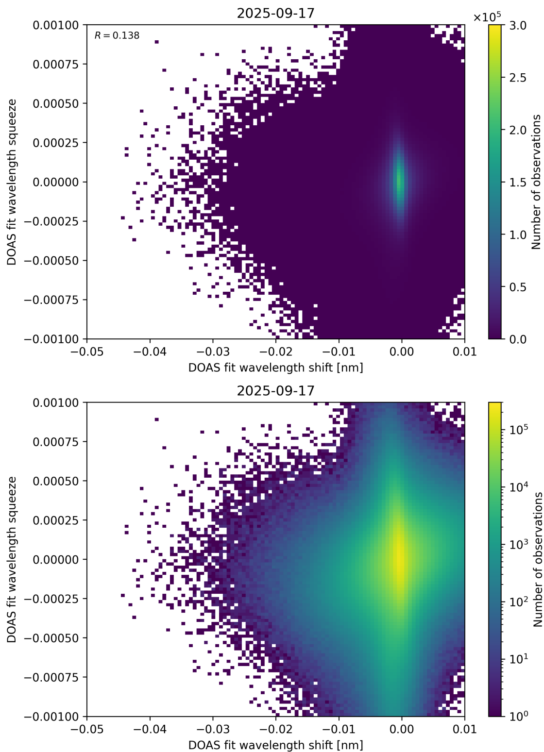
Figure 138: Scatter density plot of “DOAS fit wavelength shift” against “DOAS fit wavelength squeeze” for 2025-09-16 to 2025-09-18.
