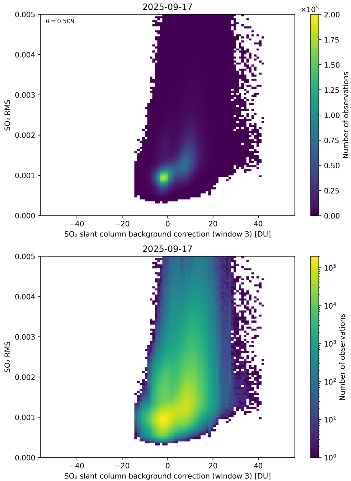
Figure 134: Scatter density plot of “SO 2 slant column background correction (window 3)” against “SO 2 RMS” for 2025-09-16 to 2025-09-18.
