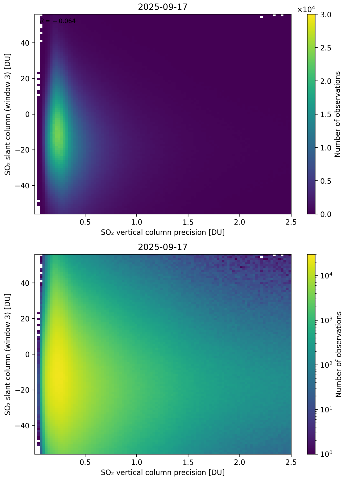
Figure 344: Scatter density plot of “SO 2 vertical column precision” against “SO 2 slant column (window 3)” for 2025-09-16 to 2025-09-18.
