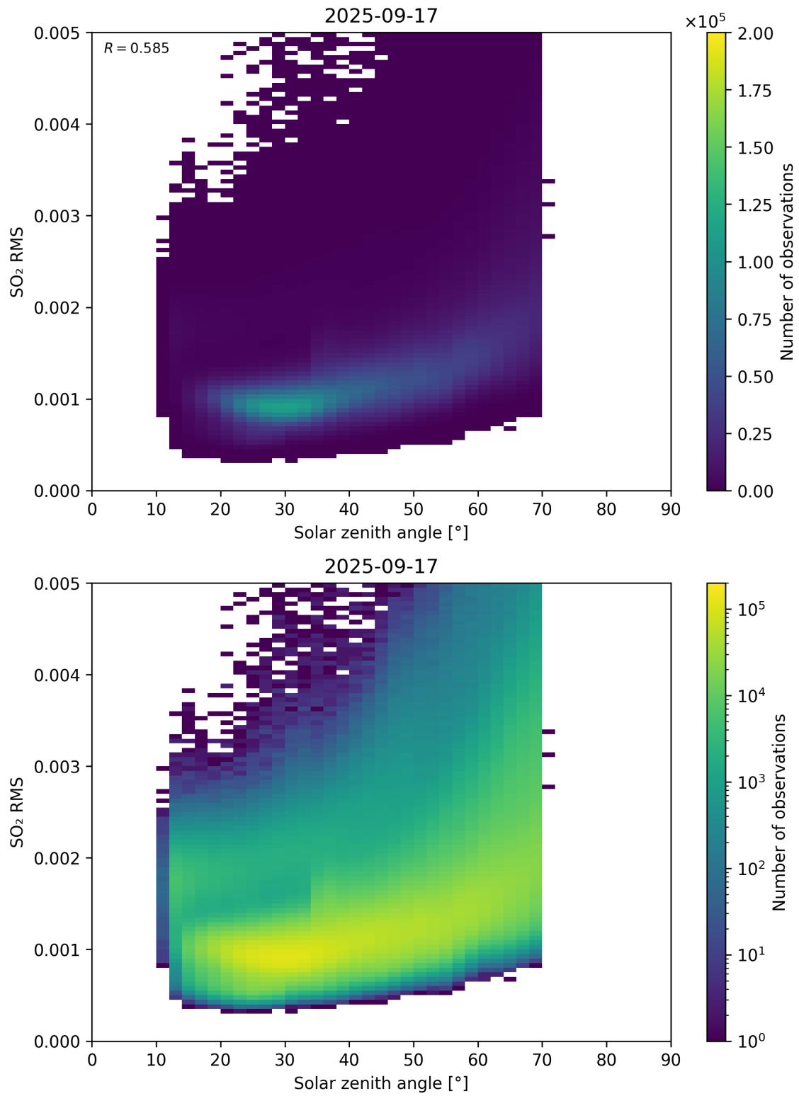
Figure 176: Scatter density plot of “Solar zenith angle” against “SO 2 RMS” for 2025-09-16 to 2025-09-18.
