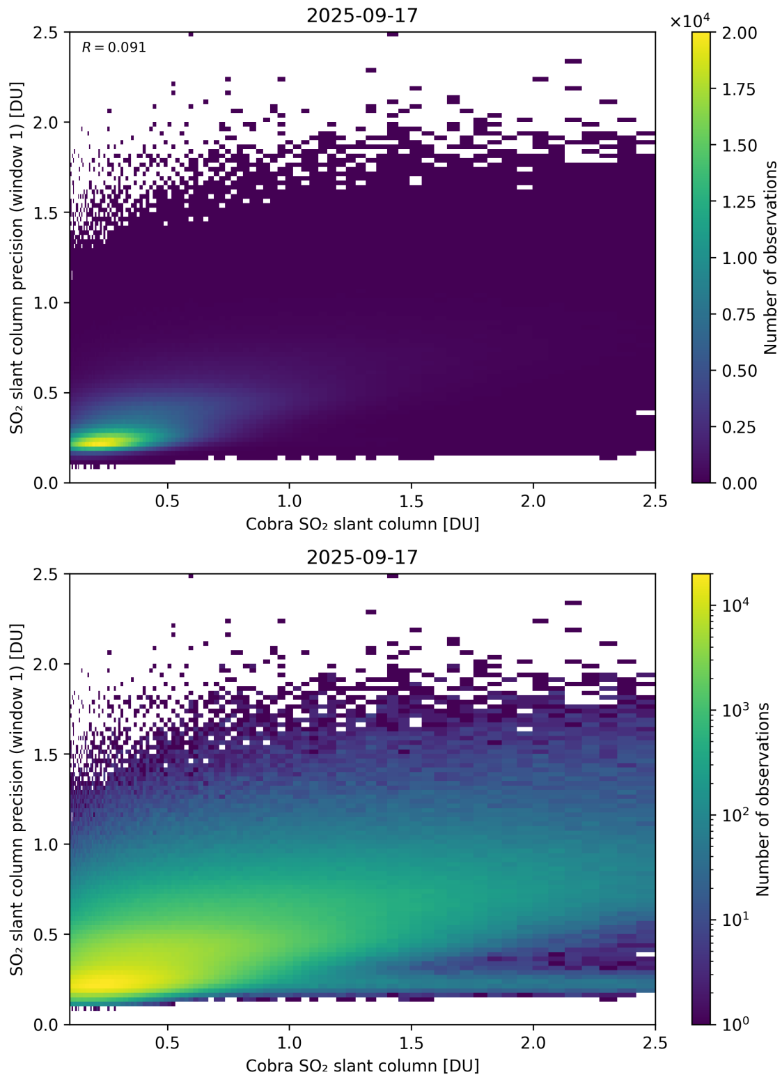
Figure 220: Scatter density plot of “Cobra SO 2 slant column” against “SO 2 slant column precision (window 1)” for 2025-09-16 to 2025-09-18.
