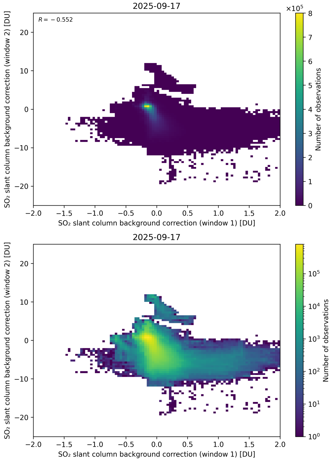
Figure 109: Scatter density plot of “SO 2 slant column background correction (window 1)” against “SO 2 slant column background correction (window 2)” for 2025-09-16 to 2025-09-18.
