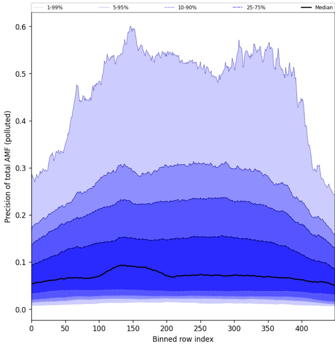
Figure 106: Along track statistics of “Precision of total AMF (polluted)” for 2025-09-16 to 2025-09-18
