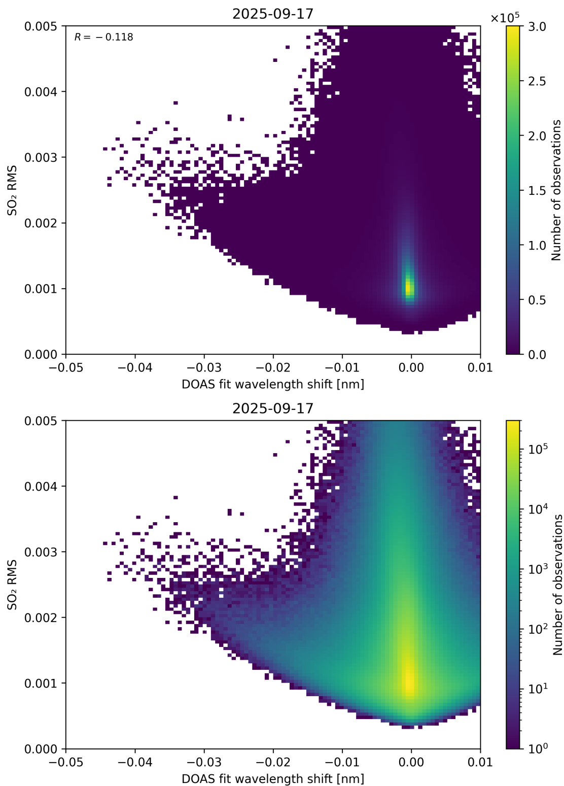
Figure 139: Scatter density plot of “DOAS fit wavelength shift” against “SO 2 RMS” for 2025-09-16 to 2025-09-18.
