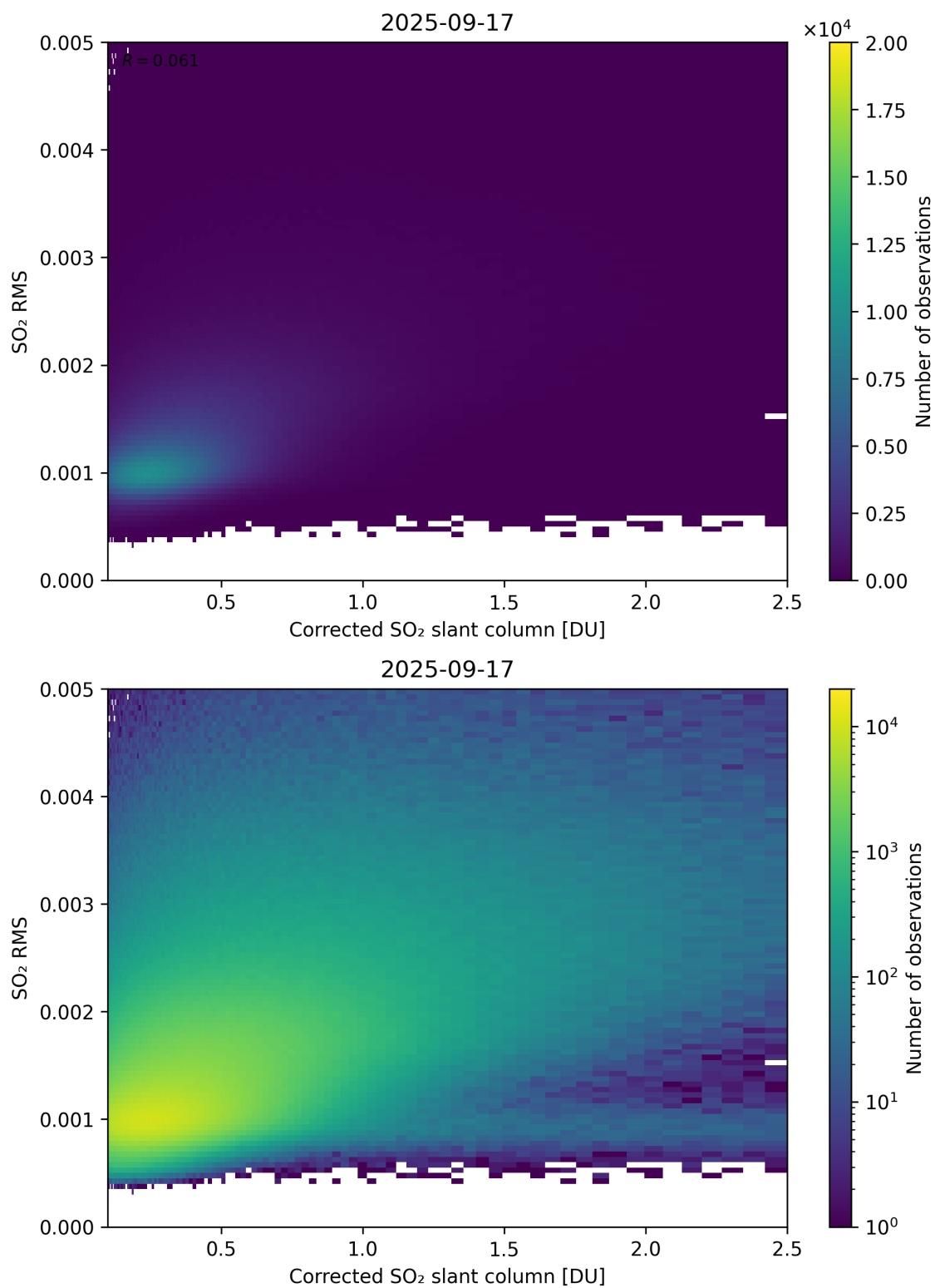
Figure 231: Scatter density plot of “Corrected SO 2 slant column” against “SO 2 RMS” for 2025-09-16 to 2025-09-18.
