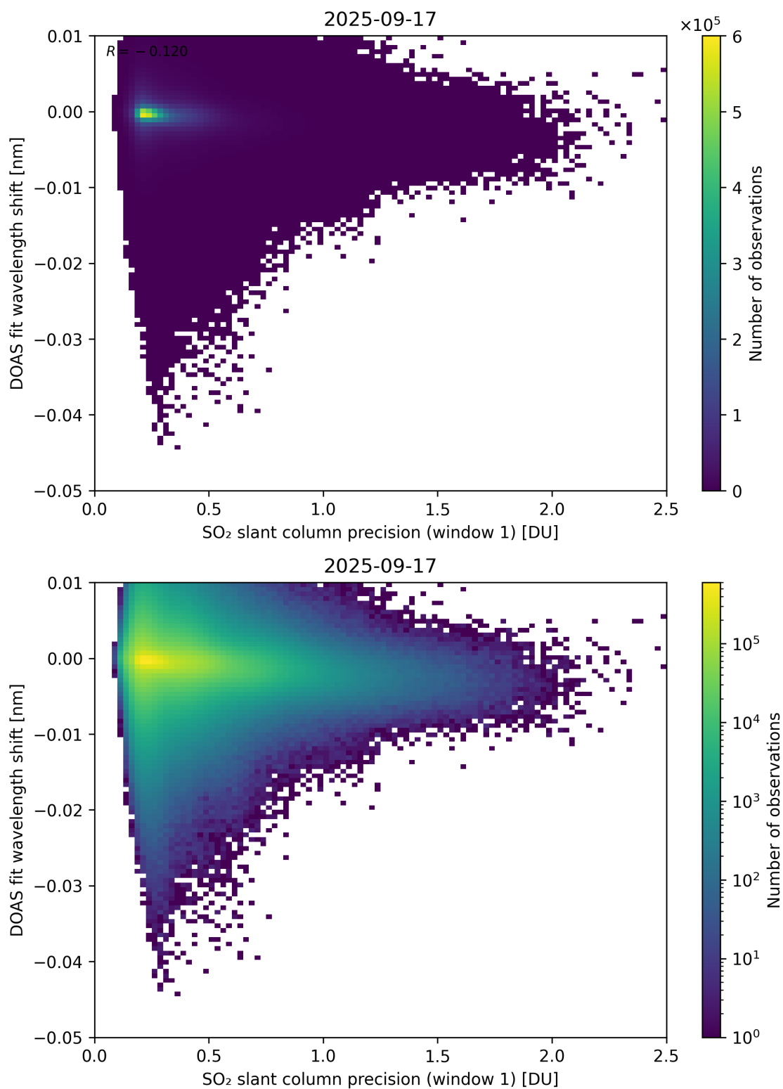
Figure 271: Scatter density plot of “SO 2 slant column precision (window 1)” against “DOAS fit wavelength shift” for 2025-09-16 to 2025-09-18.
