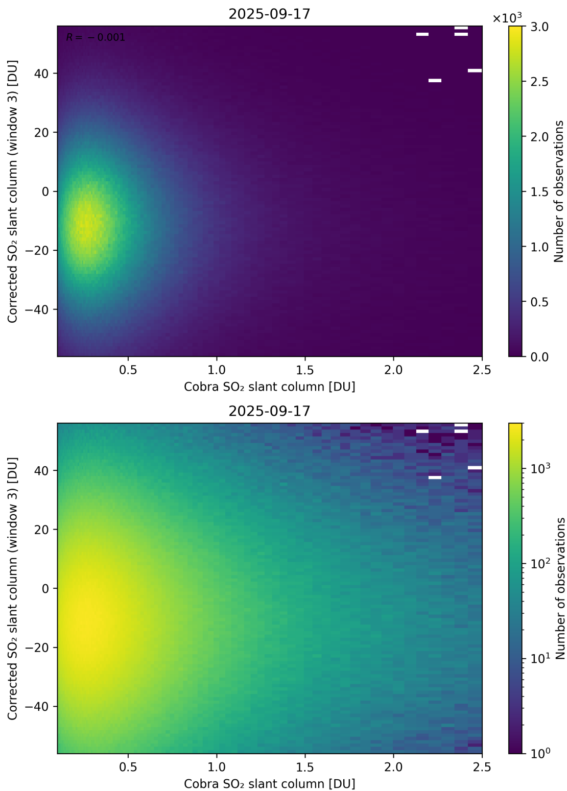
Figure 218: Scatter density plot of “Cobra SO 2 slant column” against “Corrected SO 2 slant column (window 3)” for 2025-09-16 to 2025-09-18.
