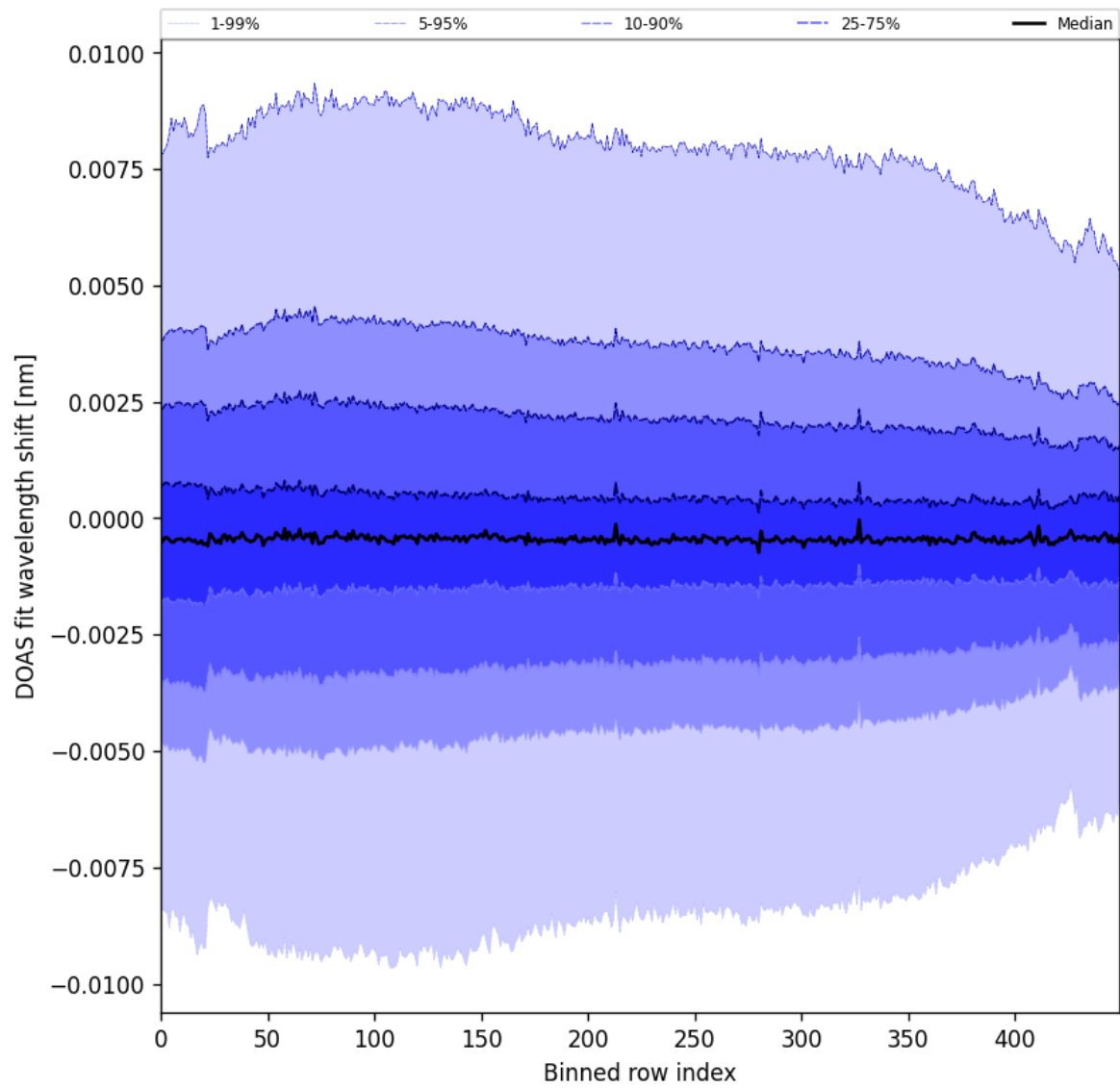
Figure 102: Along track statistics of “DOAS fit wavelength shift” for 2025-09-16 to 2025-09-18
