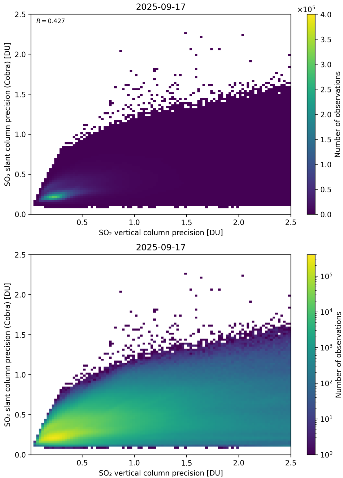
Figure 337: Scatter density plot of “SO 2 vertical column precision” against “SO 2 slant column precision (Cobra)” for 2025-09-16 to 2025-09-18.
