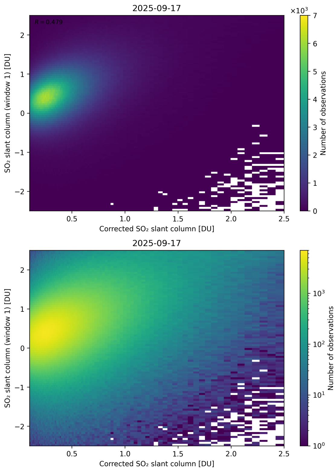
Figure 237: Scatter density plot of “Corrected SO 2 slant column” against “SO 2 slant column (window 1)” for 2025-09-16 to 2025-09-18.
