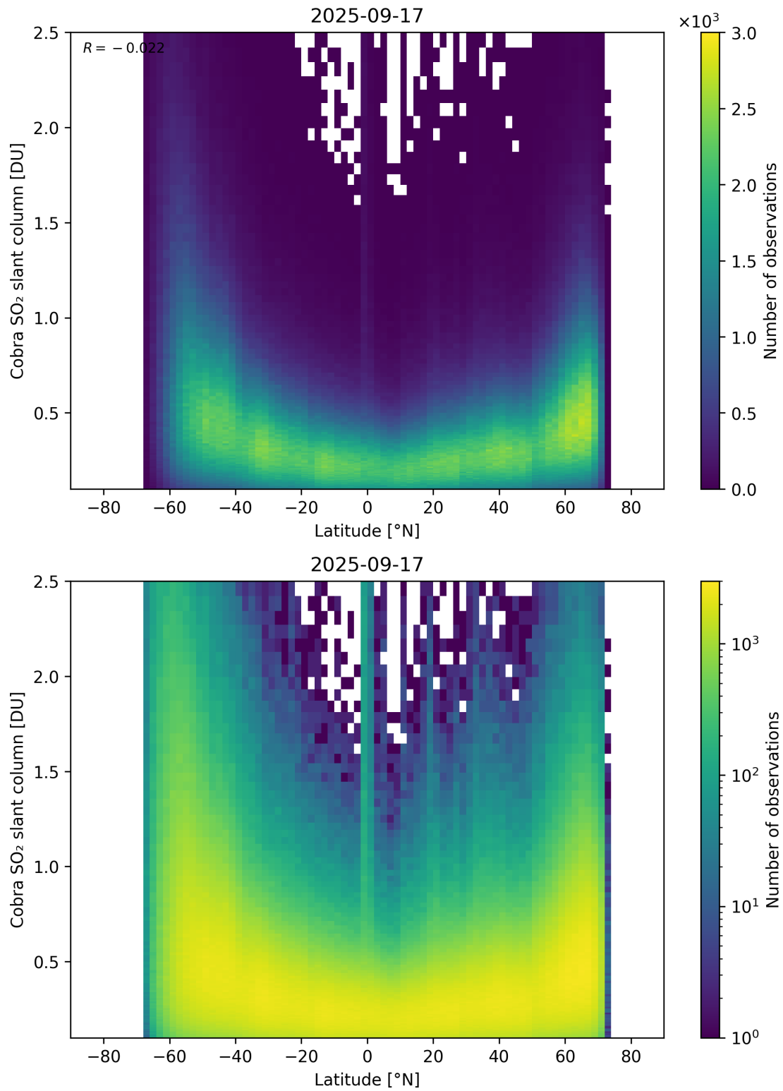
Figure 157: Scatter density plot of “Latitude” against “Cobra SO 2 slant column” for 2025-09-16 to 2025-09-18.
