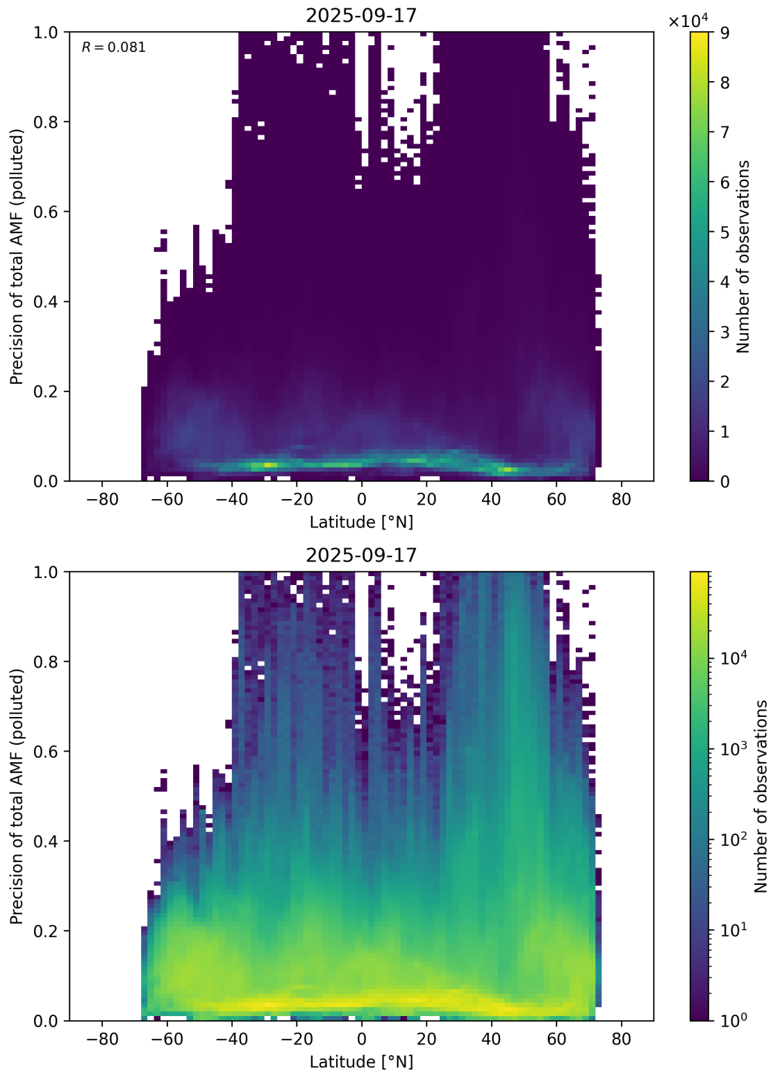
Figure 168: Scatter density plot of “Latitude” against “Precision of total AMF (polluted)” for 2025-09-16 to 2025-09-18.
