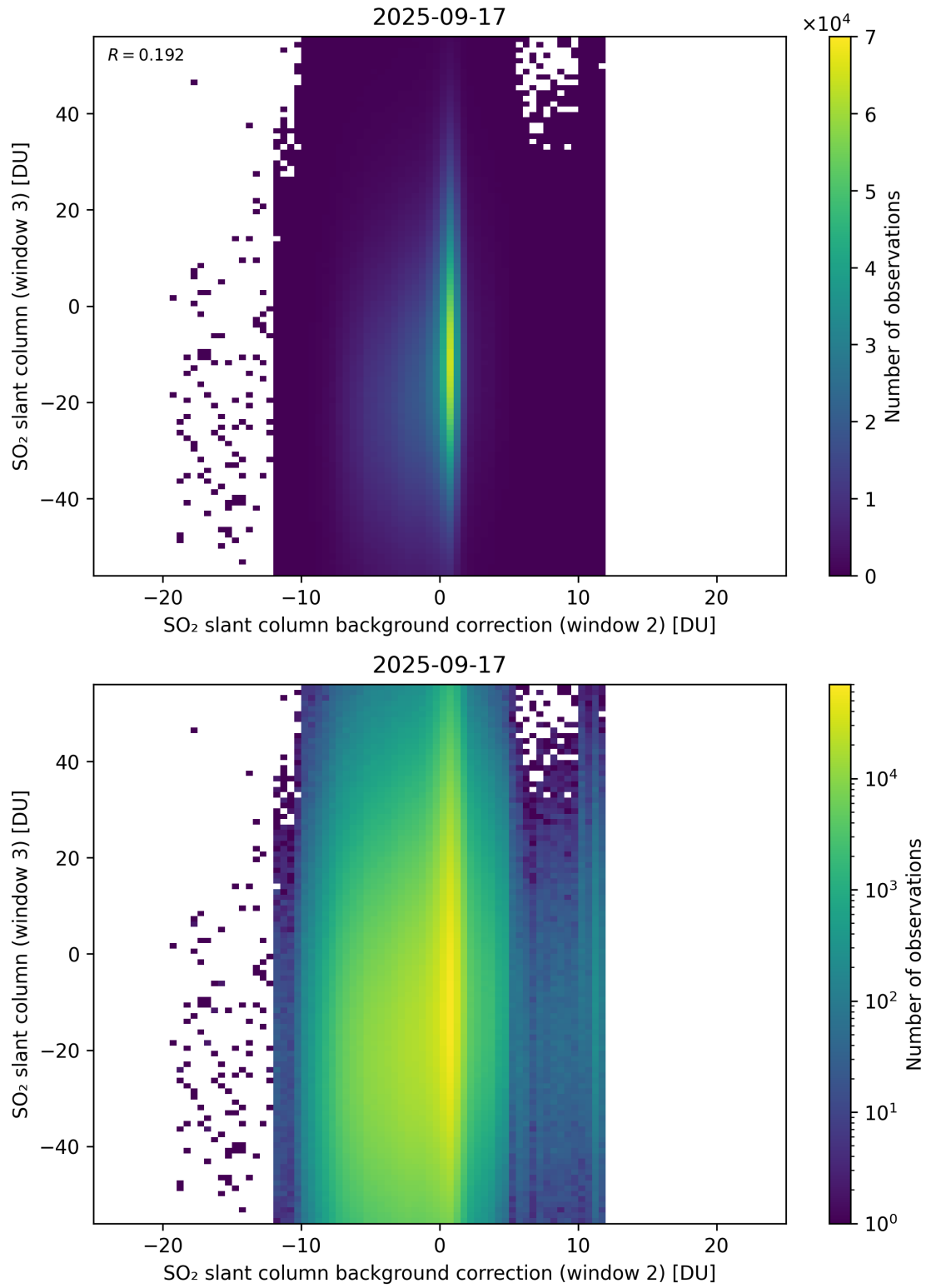
Figure 128: Scatter density plot of “SO 2 slant column background correction (window 2)” against “SO 2 slant column (window 3)” for 2025-09-16 to 2025-09-18.
