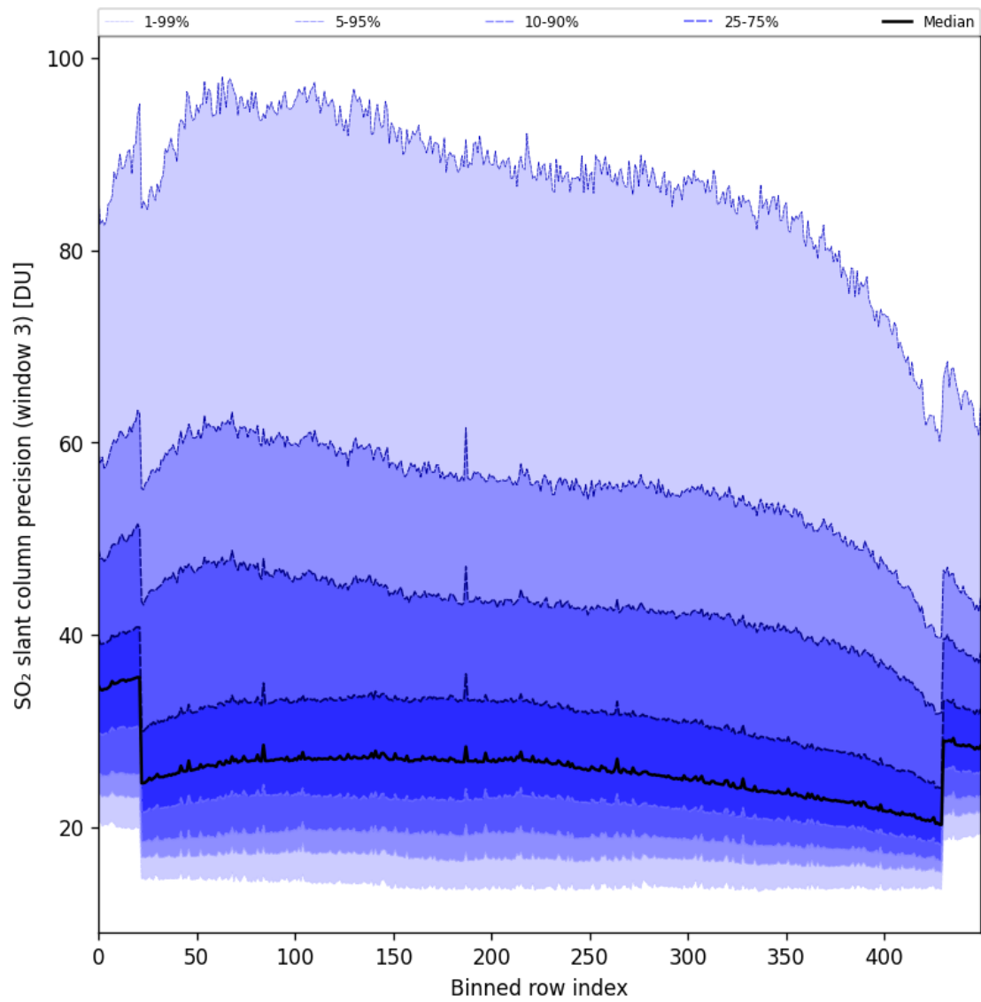
Figure 98: Along track statistics of “SO 2 slant column precision (window 3)” for 2025-09-16 to 2025-09-18
