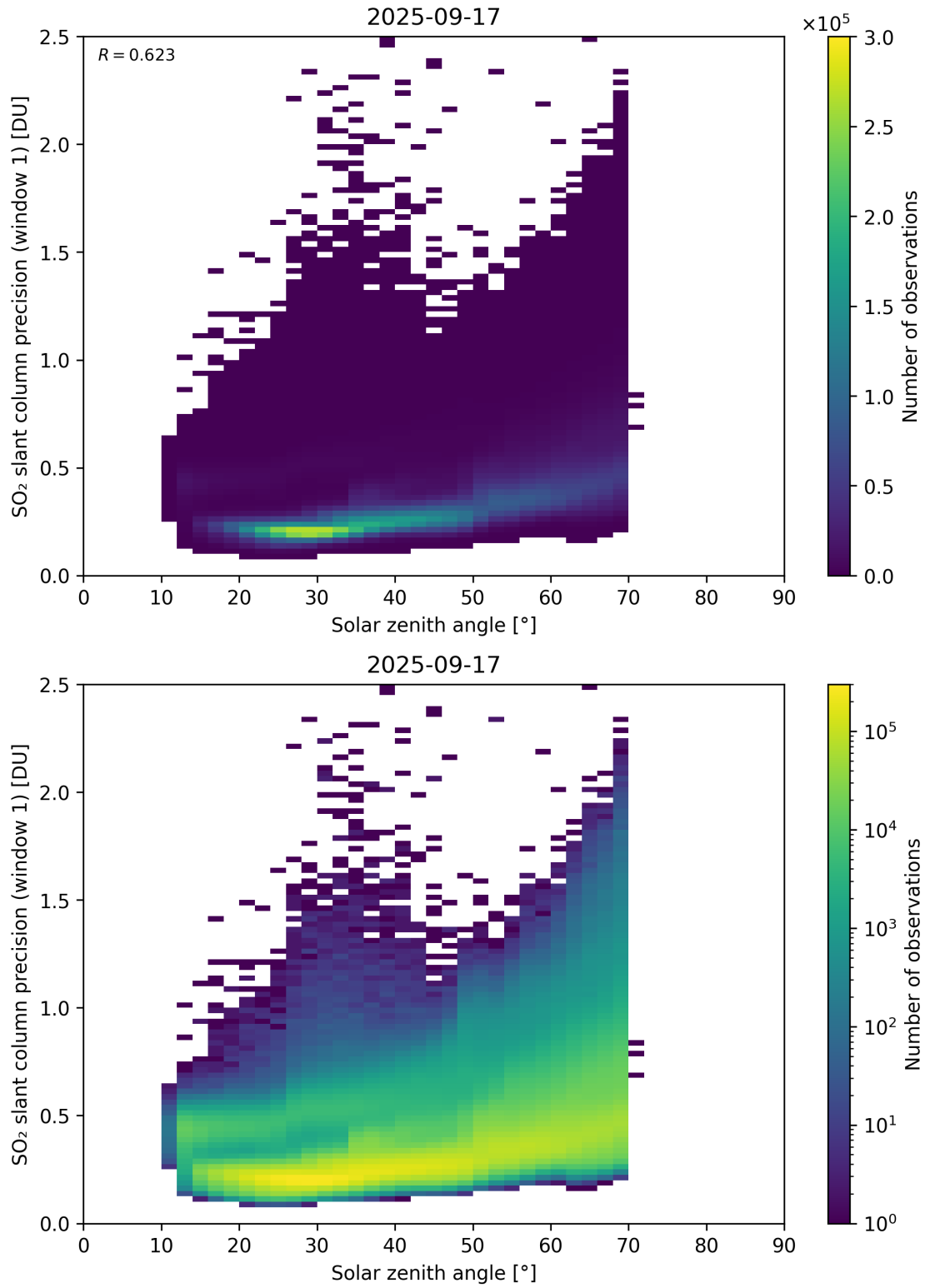
Figure 185: Scatter density plot of “Solar zenith angle” against “SO 2 slant column precision (window 1)” for 2025-09-16 to 2025-09-18.
