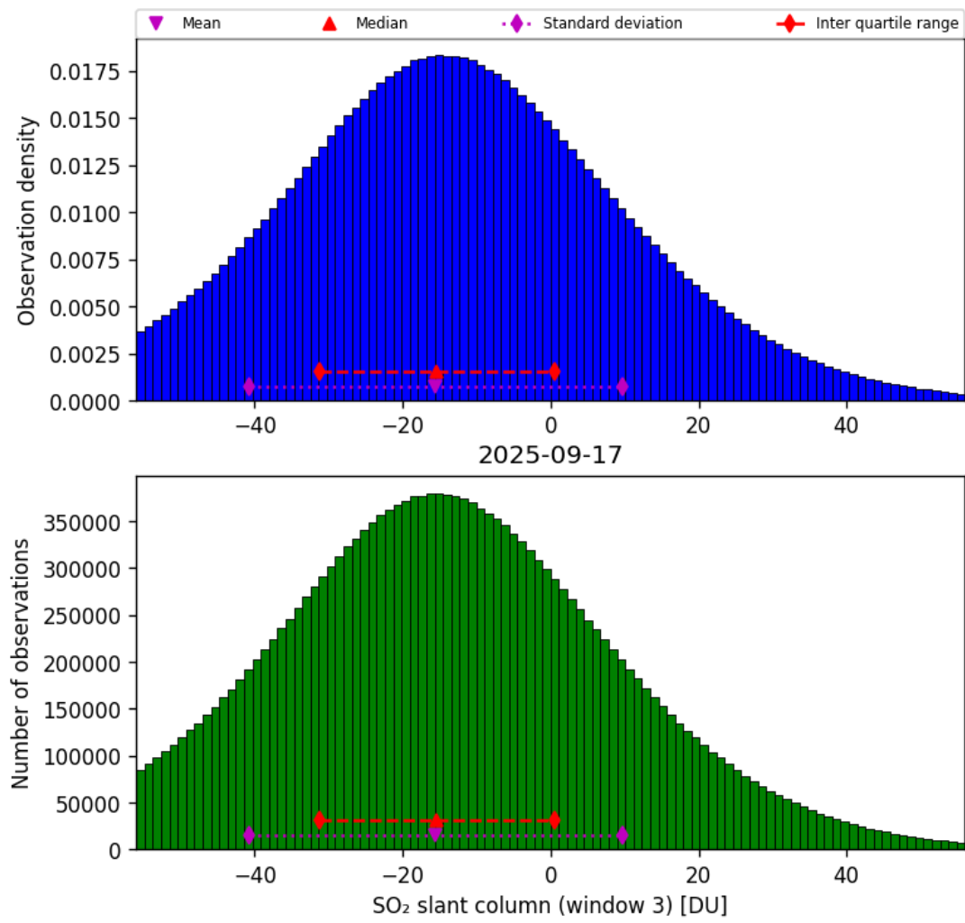
Figure 71: Histogram of “SO 2 slant column (window 3)” for 2025-09-16 to 2025-09-18
