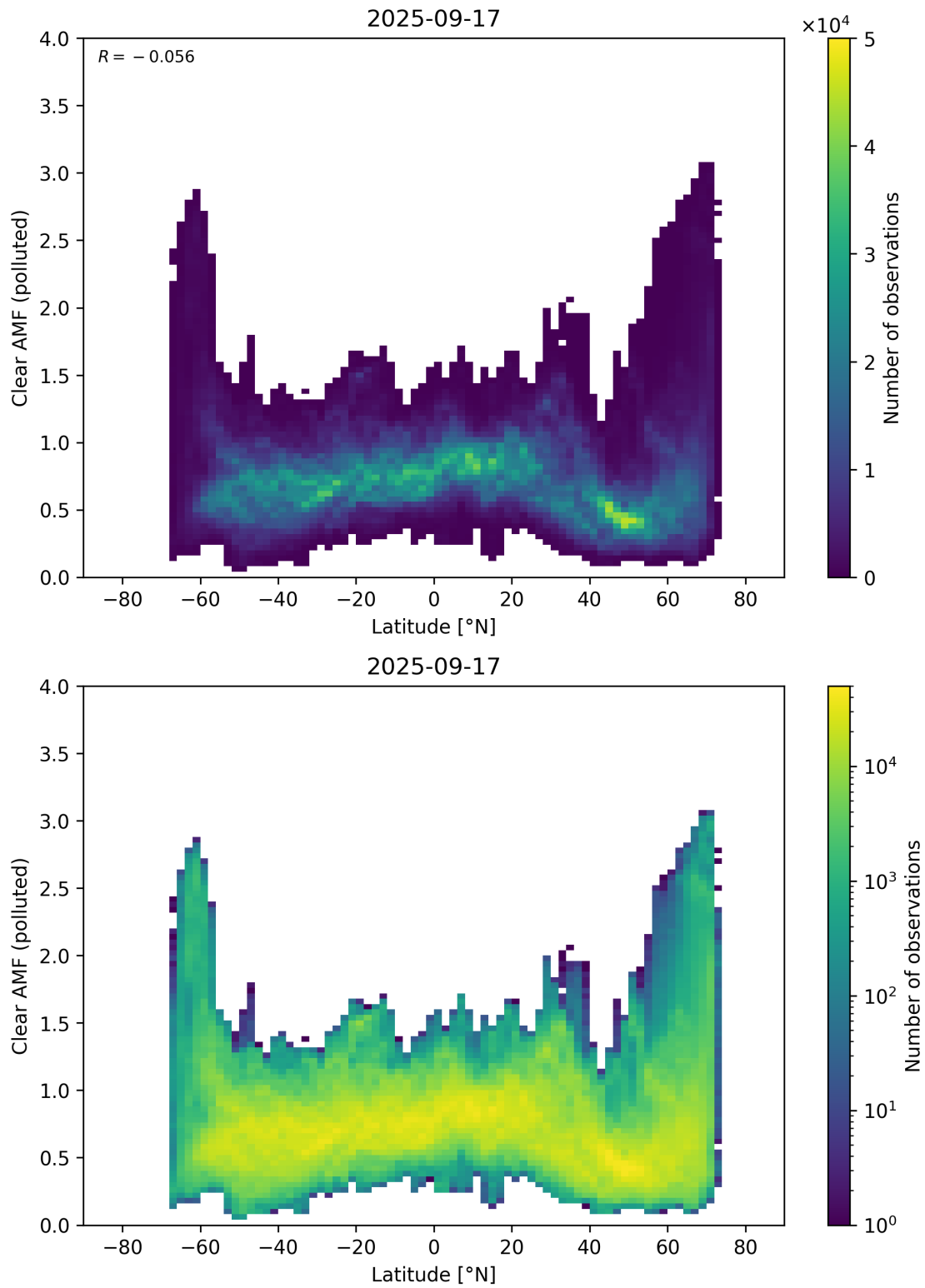
Figure 156: Scatter density plot of “Latitude” against “Clear AMF (polluted)” for 2025-09-16 to 2025-09-18.
