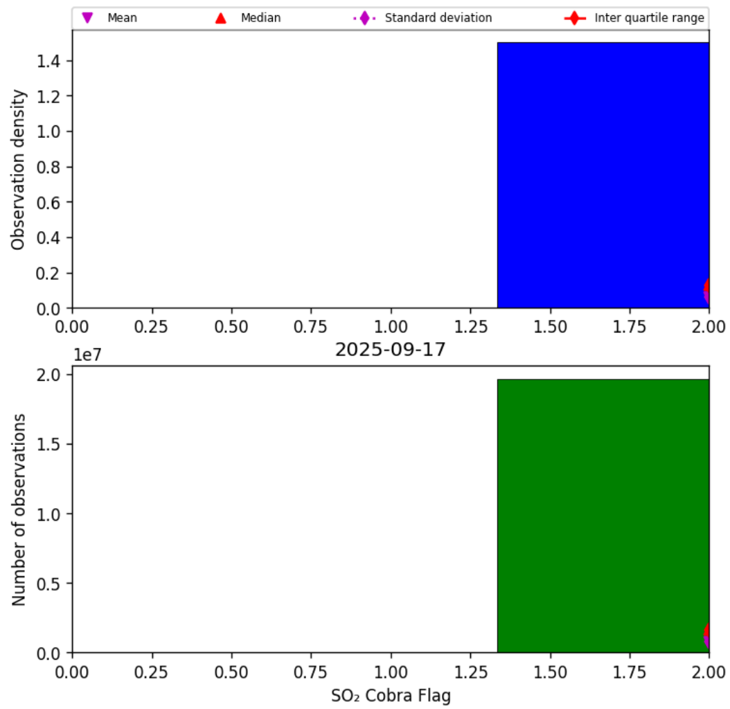
Figure 75: Histogram of "SO 2 Cobra Flag" for 2025-09-16 to 2025-09-18
