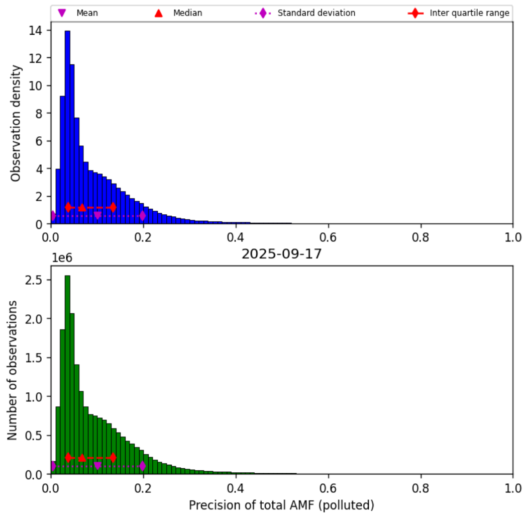
Figure 80: Histogram of “Precision of total AMF (polluted)” for 2025-09-16 to 2025-09-18
