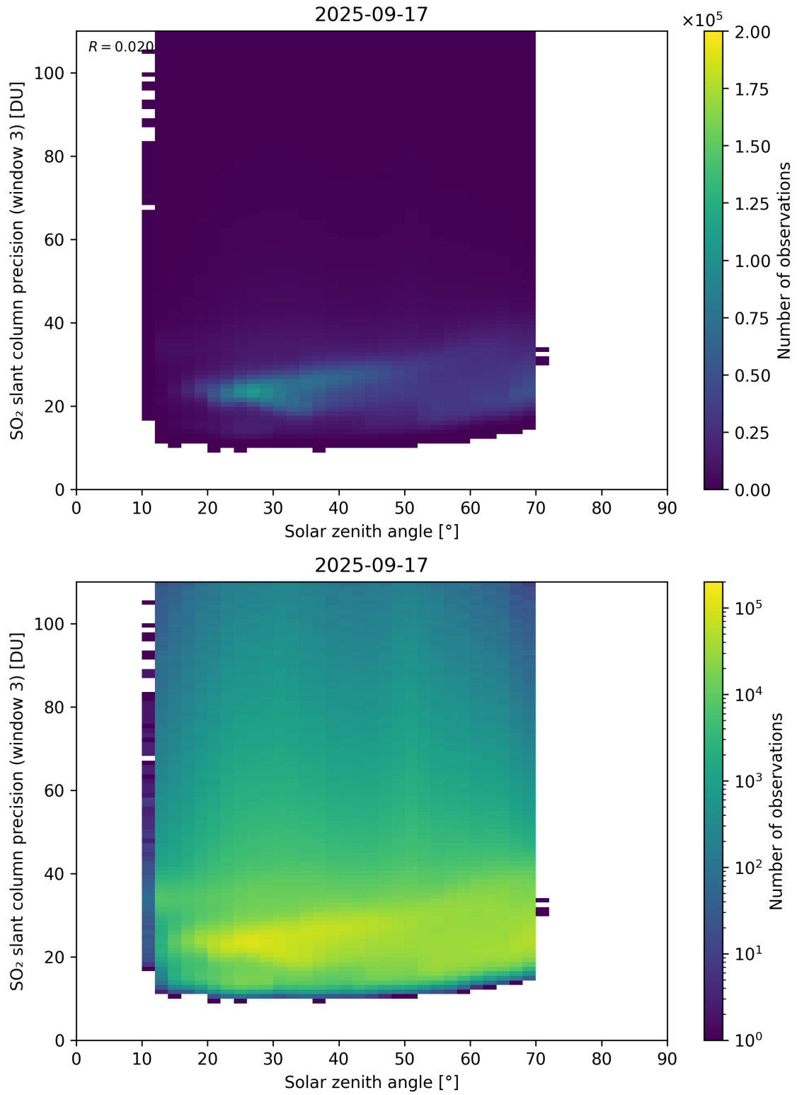
Figure 188: Scatter density plot of “Solar zenith angle” against “SO 2 slant column precision (window 3)” for 2025-09-16 to 2025-09-18.
