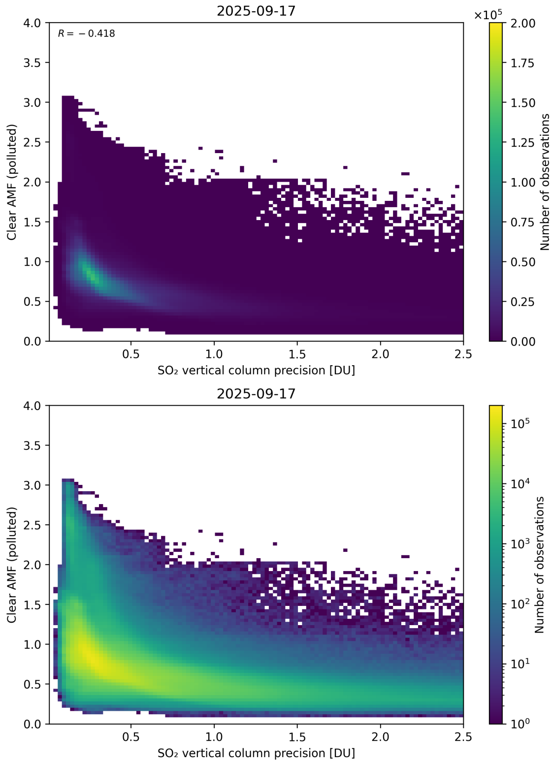
Figure 335: Scatter density plot of “SO 2 vertical column precision” against “Clear AMF (polluted)” for 2025-09-16 to 2025-09-18.
