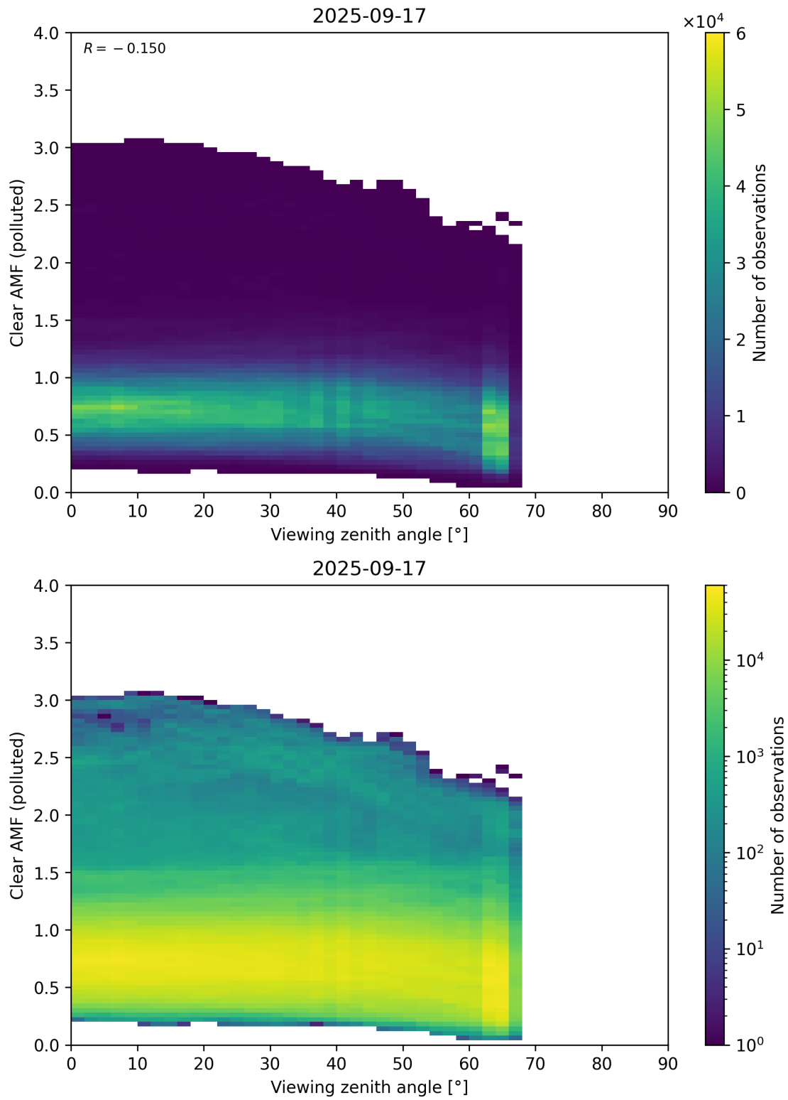
Figure 370: Scatter density plot of “Viewing zenith angle” against “Clear AMF (polluted)” for 2025-09-16 to 2025-09-18.
