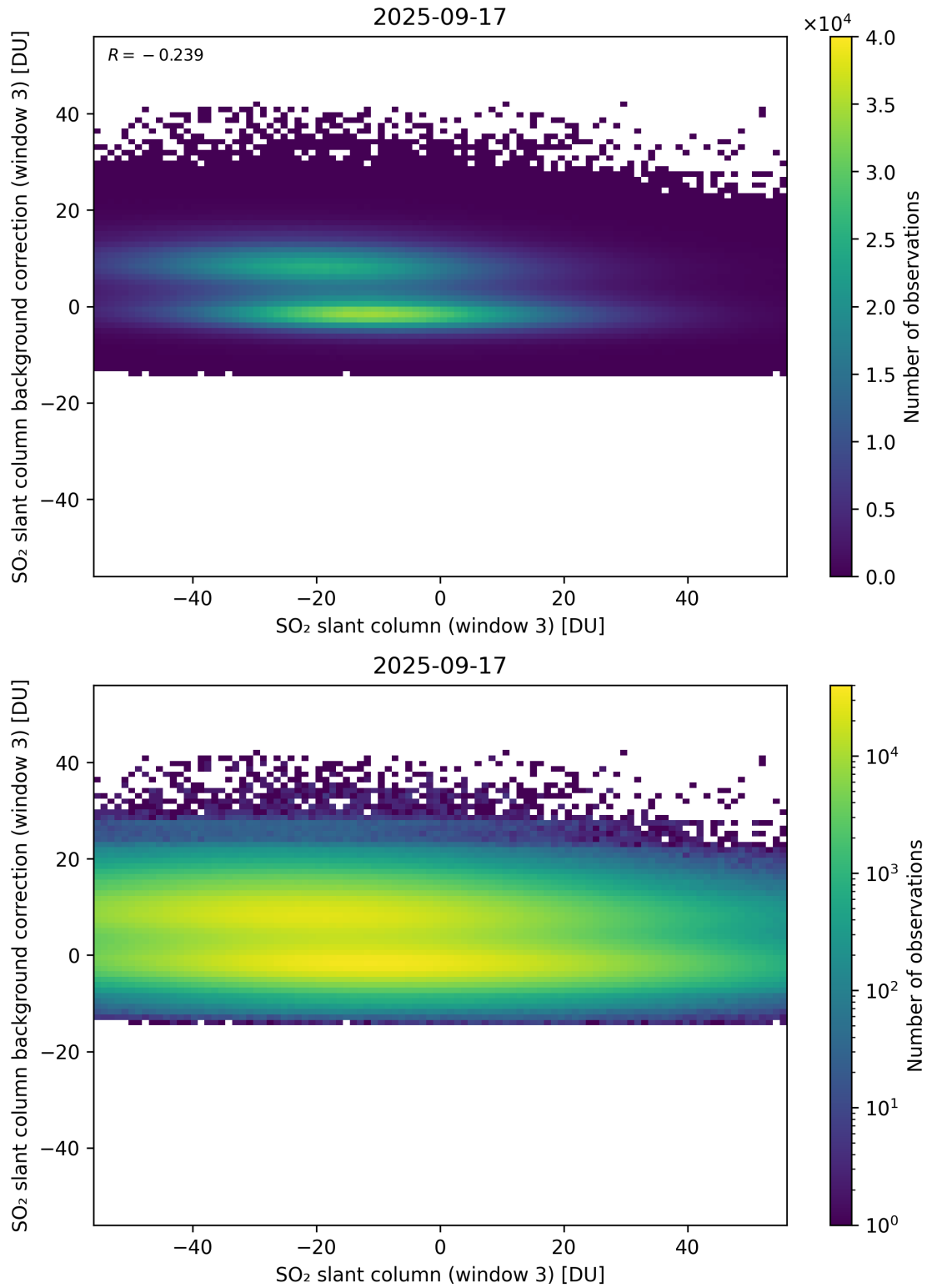
Figure 303: Scatter density plot of “SO 2 slant column (window 3)” against “SO 2 slant column background correction (window 3)” for 2025-09-16 to 2025-09-18.
