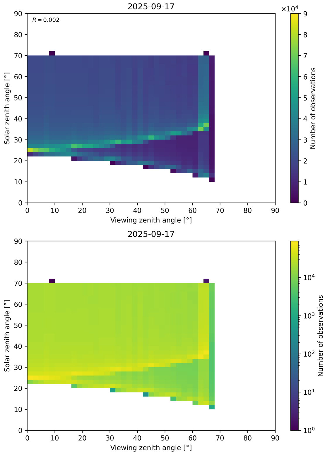
Figure 369: Scatter density plot of “Viewing zenith angle” against “Solar zenith angle” for 2025-09-16 to 2025-09-18.
