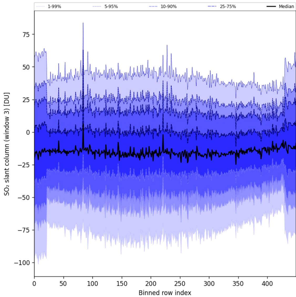
Figure 97: Along track statistics of “SO 2 slant column (window 3)” for 2025-09-16 to 2025-09-18
