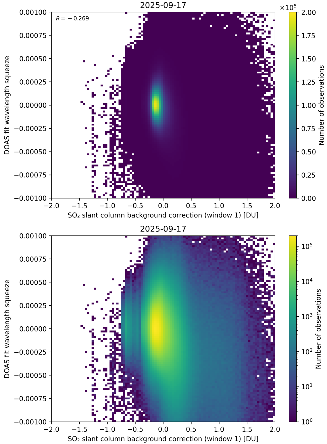
Figure 112: Scatter density plot of “SO 2 slant column background correction (window 1)” against “DOAS fit wavelength squeeze” for 2025-09-16 to 2025-09-18.
