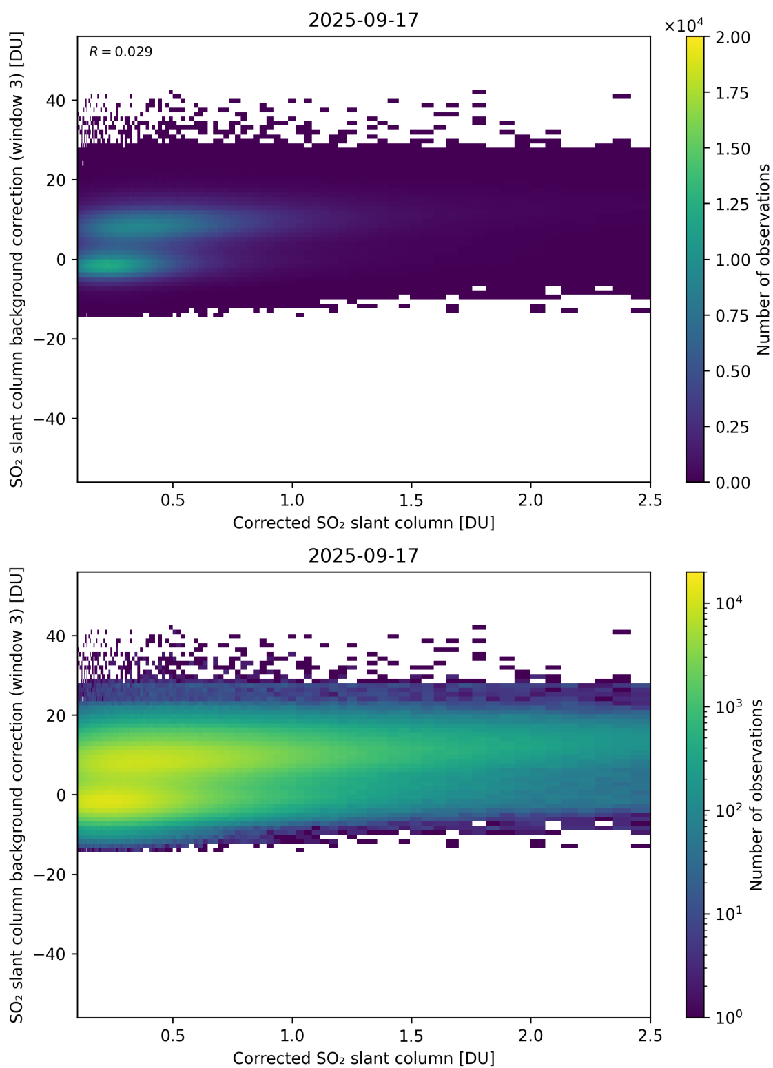
Figure 228: Scatter density plot of “Corrected SO 2 slant column” against “SO 2 slant column background correction (window 3)” for 2025-09-16 to 2025-09-18.
