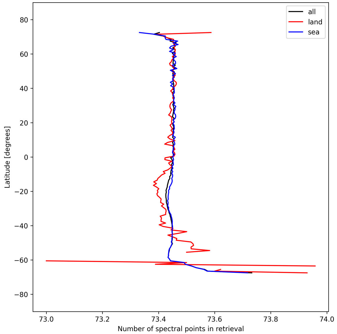
Figure 56: Zonal average of “Number of spectral points in retrieval” for 2025-09-16 to 2025-09-18.
