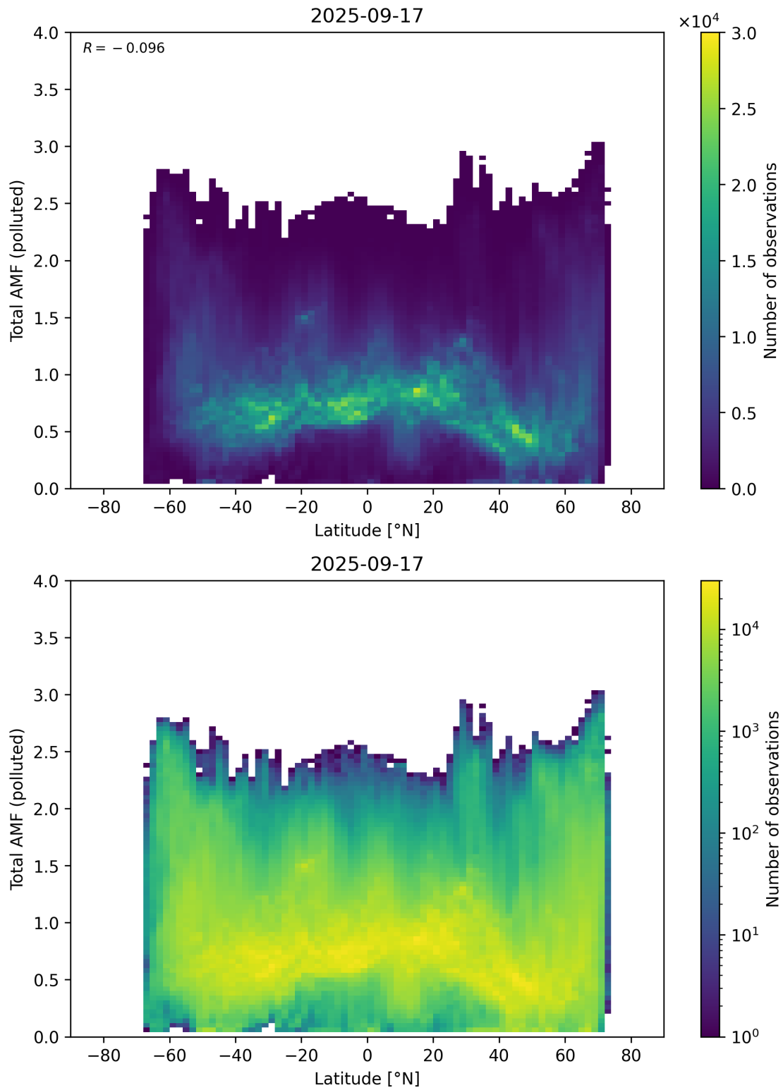
Figure 167: Scatter density plot of “Latitude” against “Total AMF (polluted)” for 2025-09-16 to 2025-09-18.
