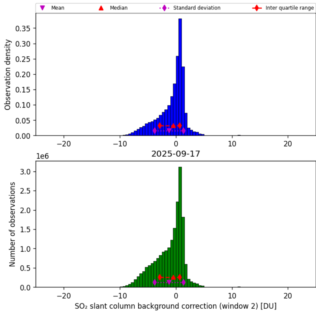
Figure 70: Histogram of “SO 2 slant column background correction (window 2)” for 2025-09-16 to 2025-09-18
