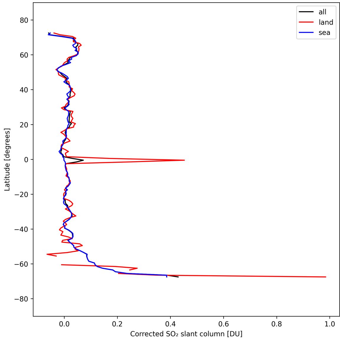
Figure 34: Zonal average of “Corrected SO 2 slant column” for 2025-09-16 to 2025-09-18.
