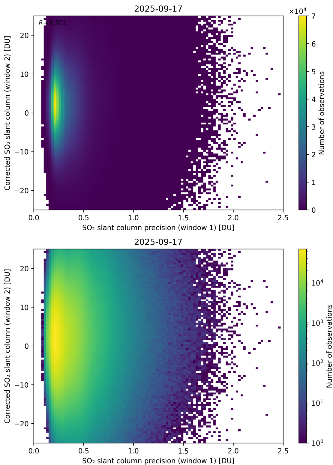
Figure 275: Scatter density plot of “SO 2 slant column precision (window 1)” against “Corrected SO 2 slant column (window 2)” for 2025-09-16 to 2025-09-18.
