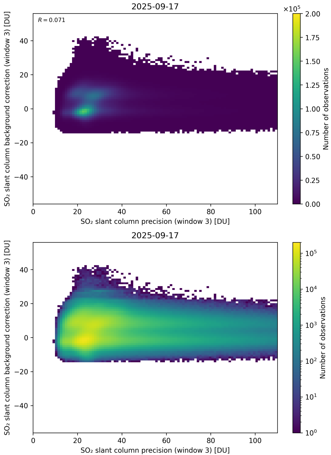
Figure 307: Scatter density plot of “SO 2 slant column precision (window 3)” against “SO 2 slant column background correction (window 3)” for 2025-09-16 to 2025-09-18.
