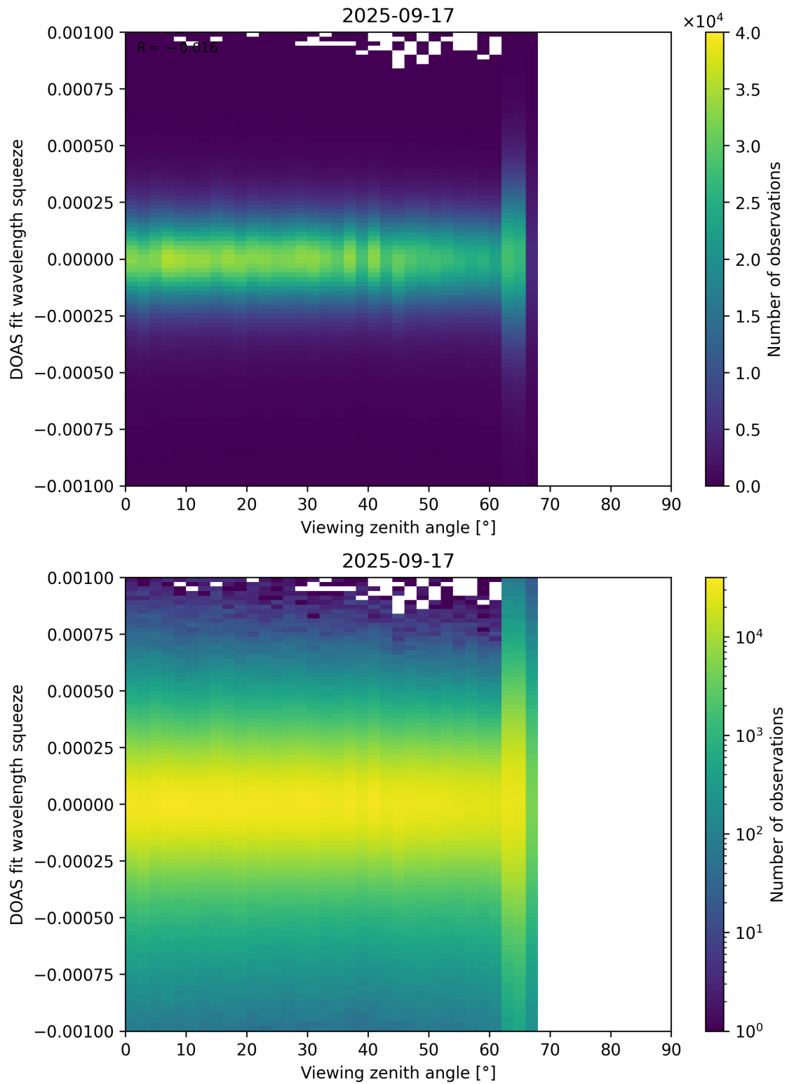
Figure 366: Scatter density plot of “Viewing zenith angle” against “DOAS fit wavelength squeeze” for 2025-09-16 to 2025-09-18.
