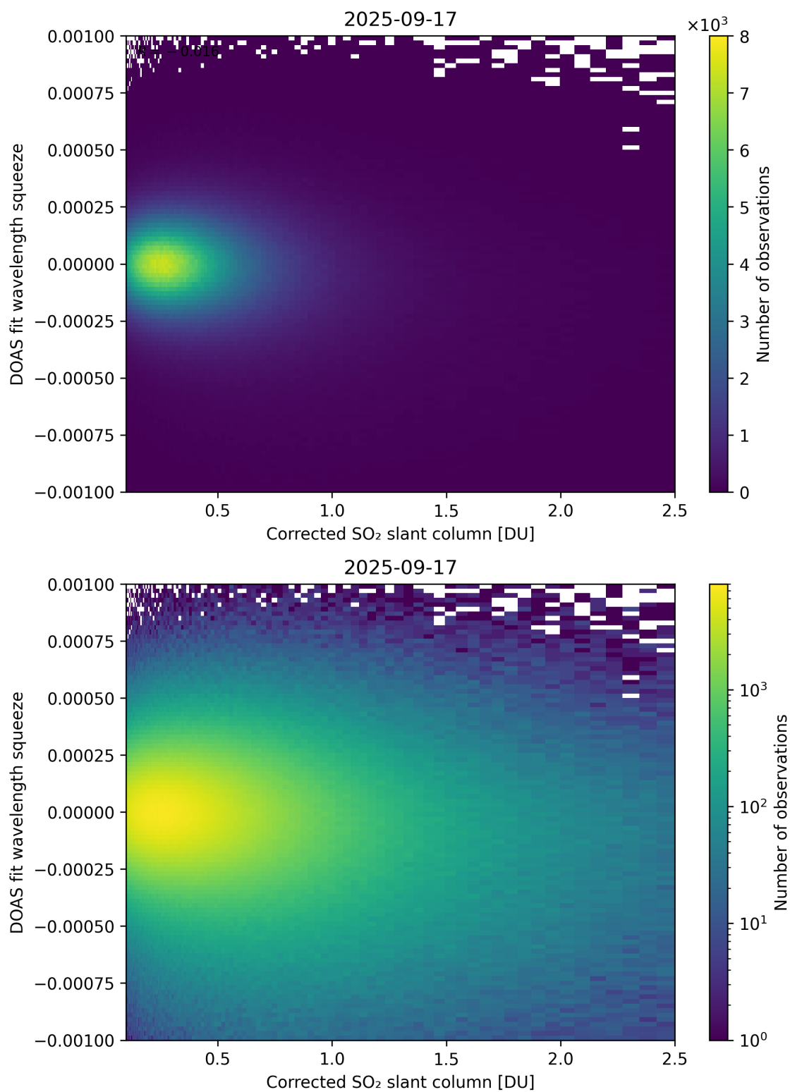
Figure 230: Scatter density plot of "Corrected SO 2 slant column" against "DOAS fit wavelength squeeze" for 2025-09-16 to 2025-09-18.
