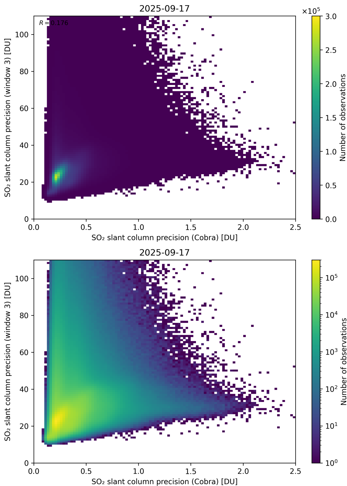
Figure 212: Scatter density plot of “SO 2 slant column precision (Cobra)” against “SO 2 slant column precision (window 3)” for 2025-09-16 to 2025-09-18.
