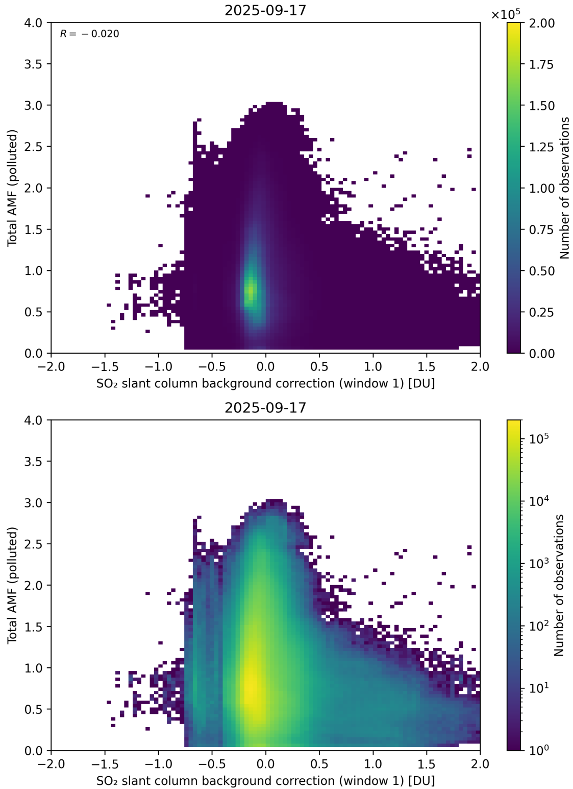
Figure 120: Scatter density plot of “SO 2 slant column background correction (window 1)” against “Total AMF (polluted)” for 2025-09-16 to 2025-09-18.
