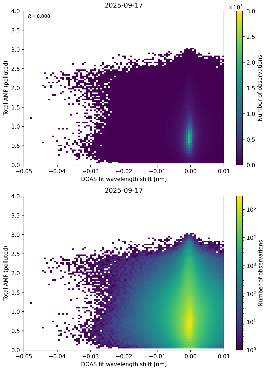
Figure 141: Scatter density plot of “DOAS fit wavelength shift” against “Total AMF (polluted)” for 2025-09-16 to 2025-09-18.
