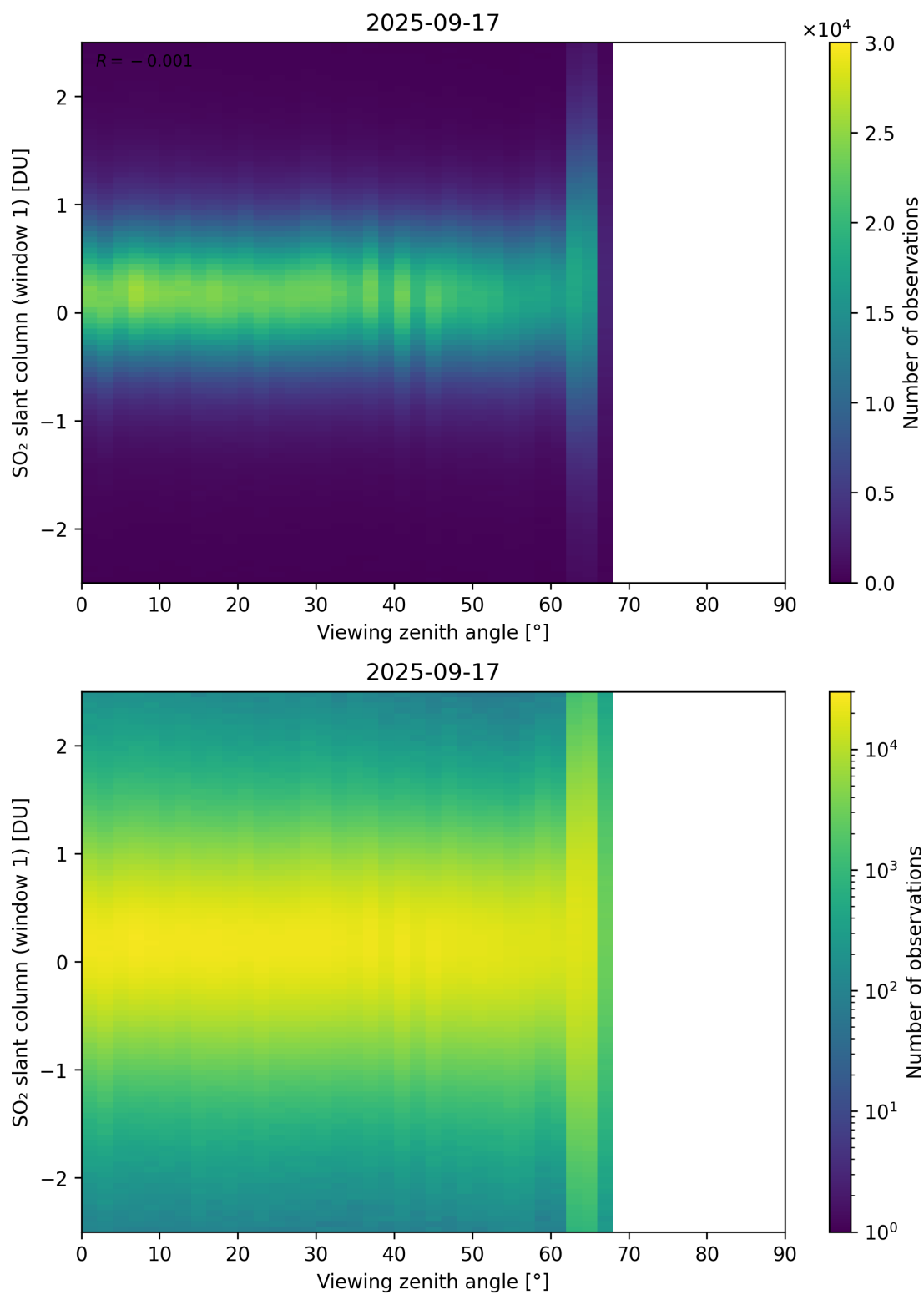
Figure 376: Scatter density plot of “Viewing zenith angle” against “SO 2 slant column (window 1)” for 2025-09-16 to 2025-09-18.
