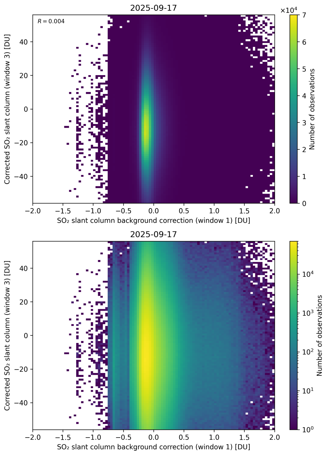
Figure 116: Scatter density plot of “SO 2 slant column background correction (window 1)” against “Corrected SO 2 slant column (window 3)” for 2025-09-16 to 2025-09-18.
