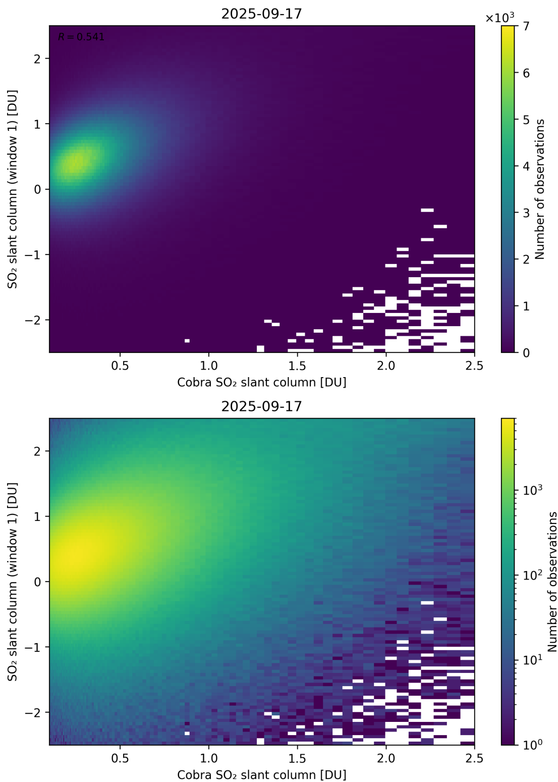
Figure 219: Scatter density plot of “Cobra SO 2 slant column” against “SO 2 slant column (window 1)” for 2025-09-16 to 2025-09-18.
