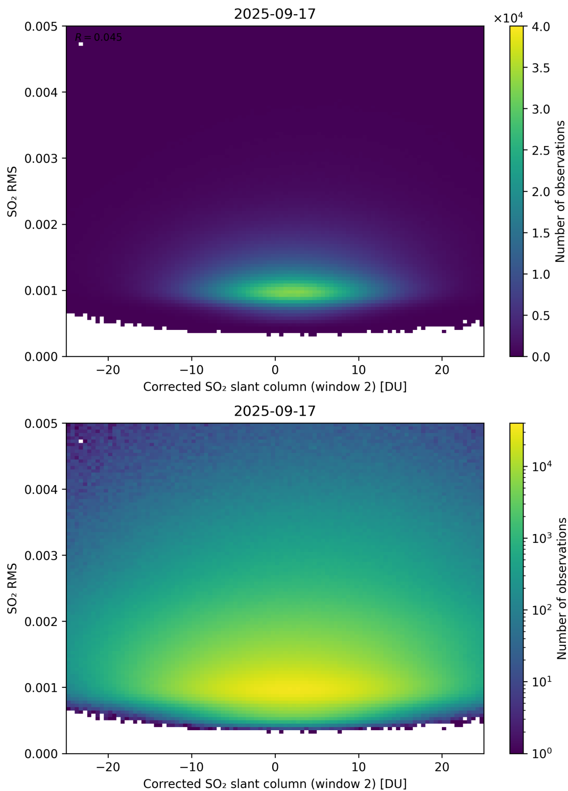
Figure 248: Scatter density plot of “Corrected SO 2 slant column (window 2)” against “SO 2 RMS” for 2025-09-16 to 2025-09-18.
