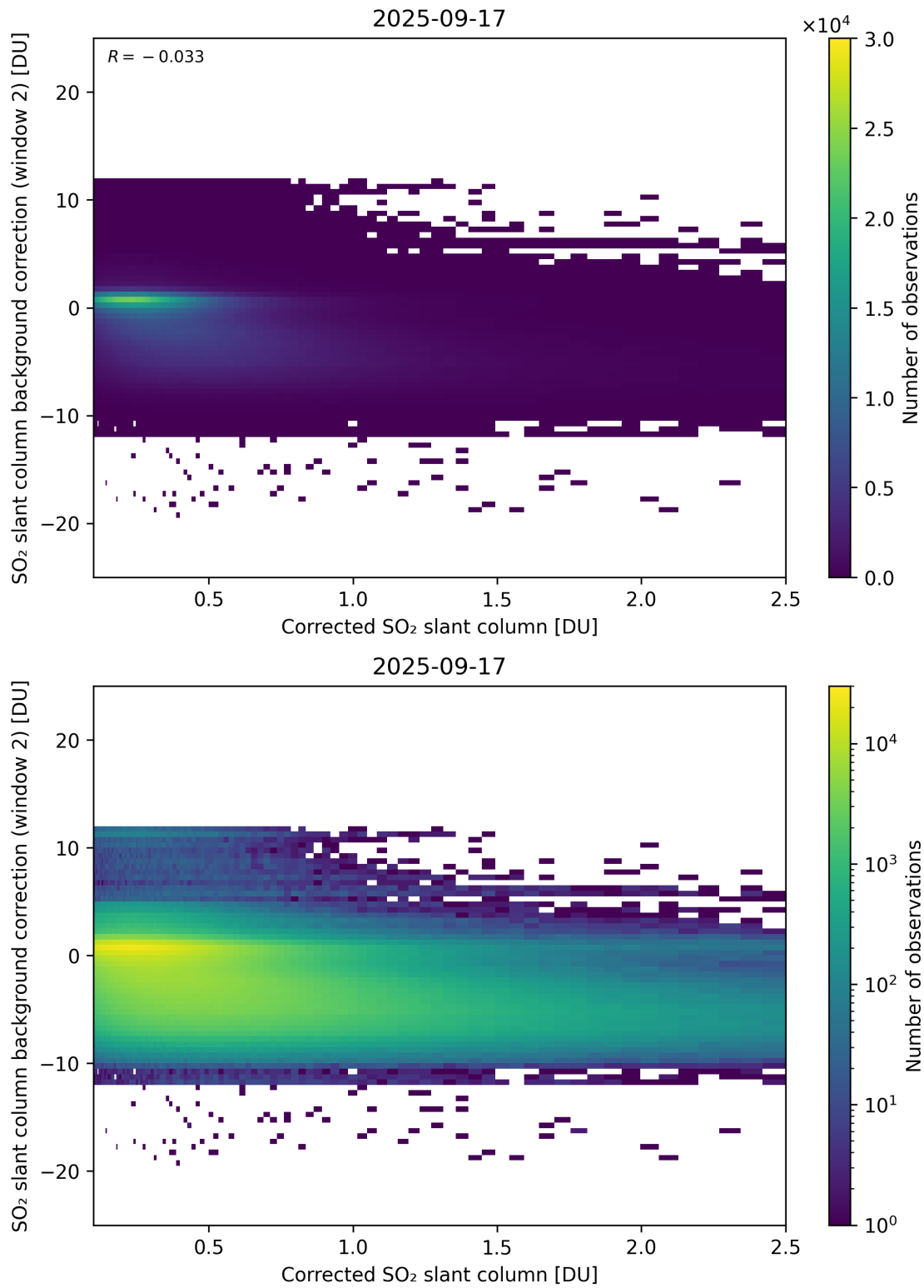
Figure 227: Scatter density plot of “Corrected SO 2 slant column” against “SO 2 slant column background correction (window 2)” for 2025-09-16 to 2025-09-18.
