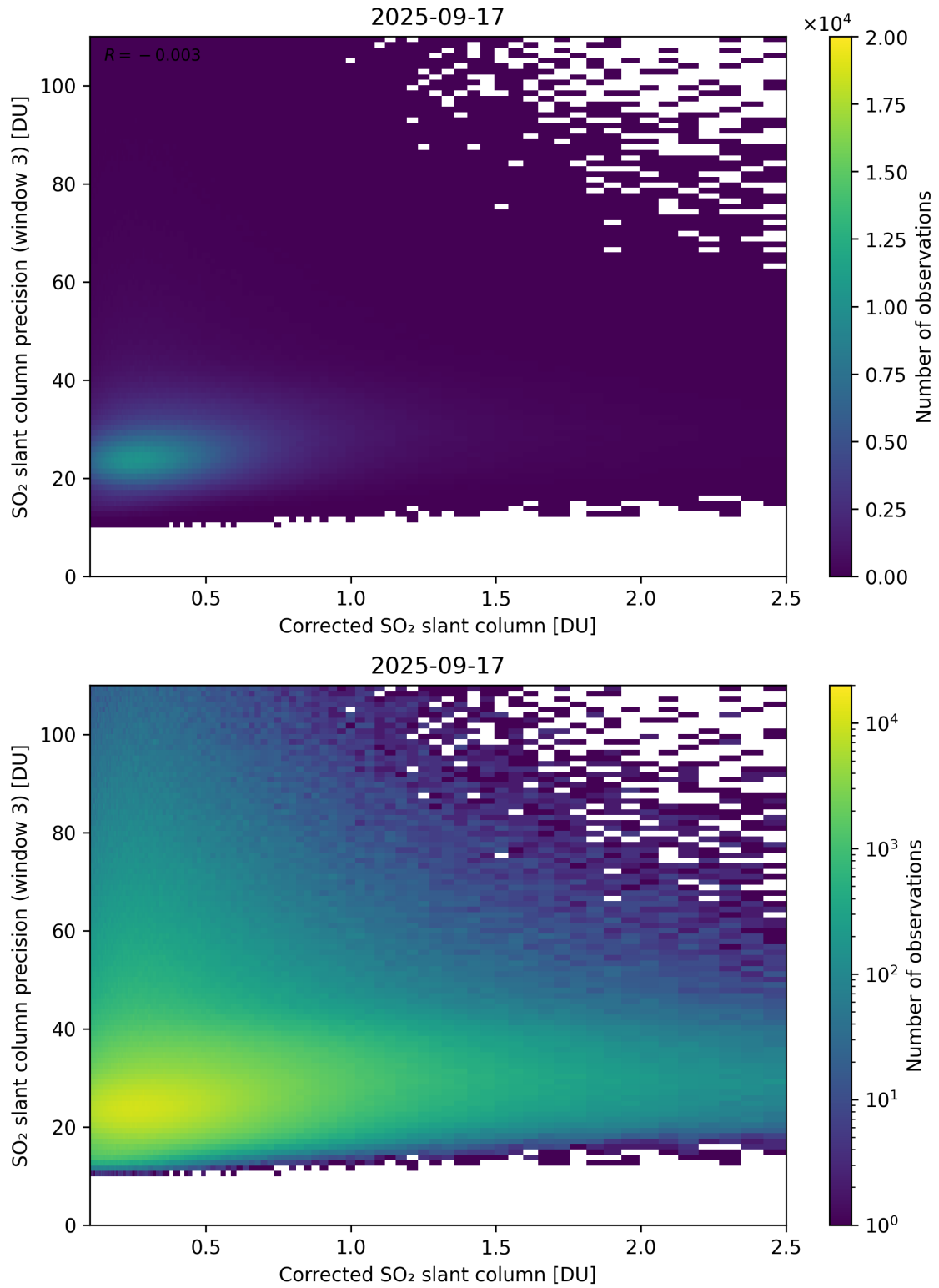
Figure 241: Scatter density plot of “Corrected SO 2 slant column” against “SO 2 slant column precision (window 3)” for 2025-09-16 to 2025-09-18.
