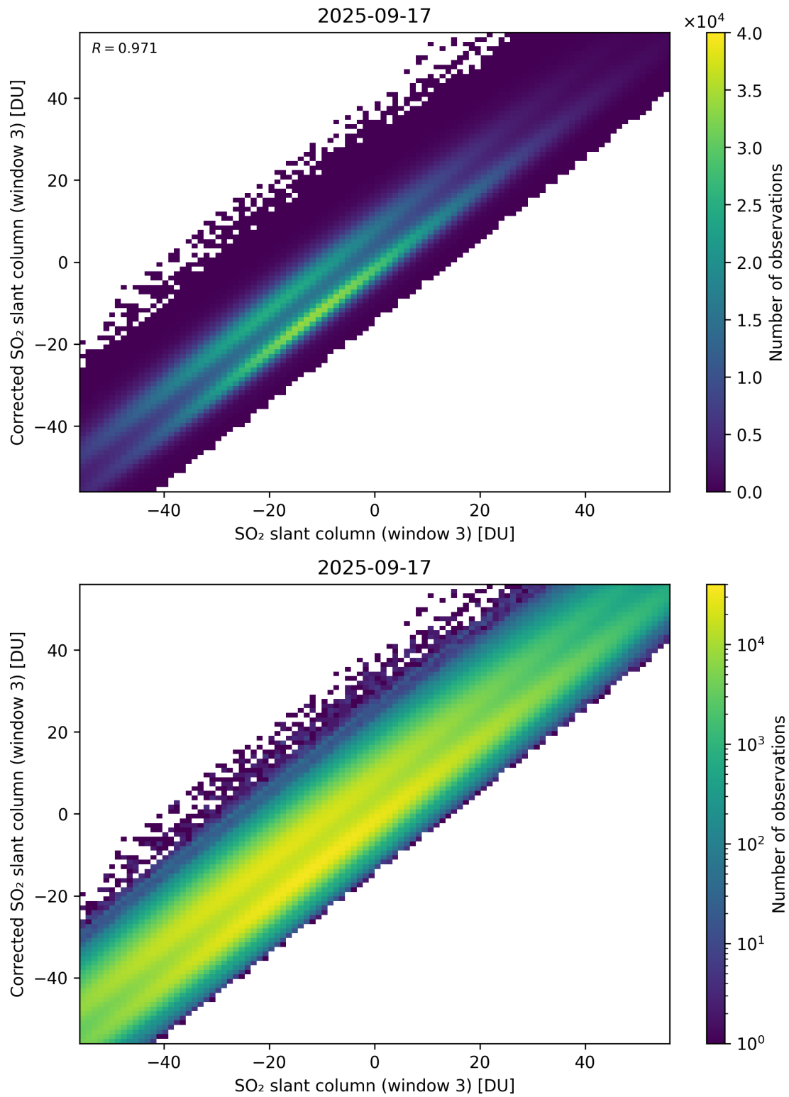
Figure 316: Scatter density plot of “SO 2 slant column (window 3)” against “Corrected SO 2 slant column (window 3)” for 2025-09-16 to 2025-09-18.
