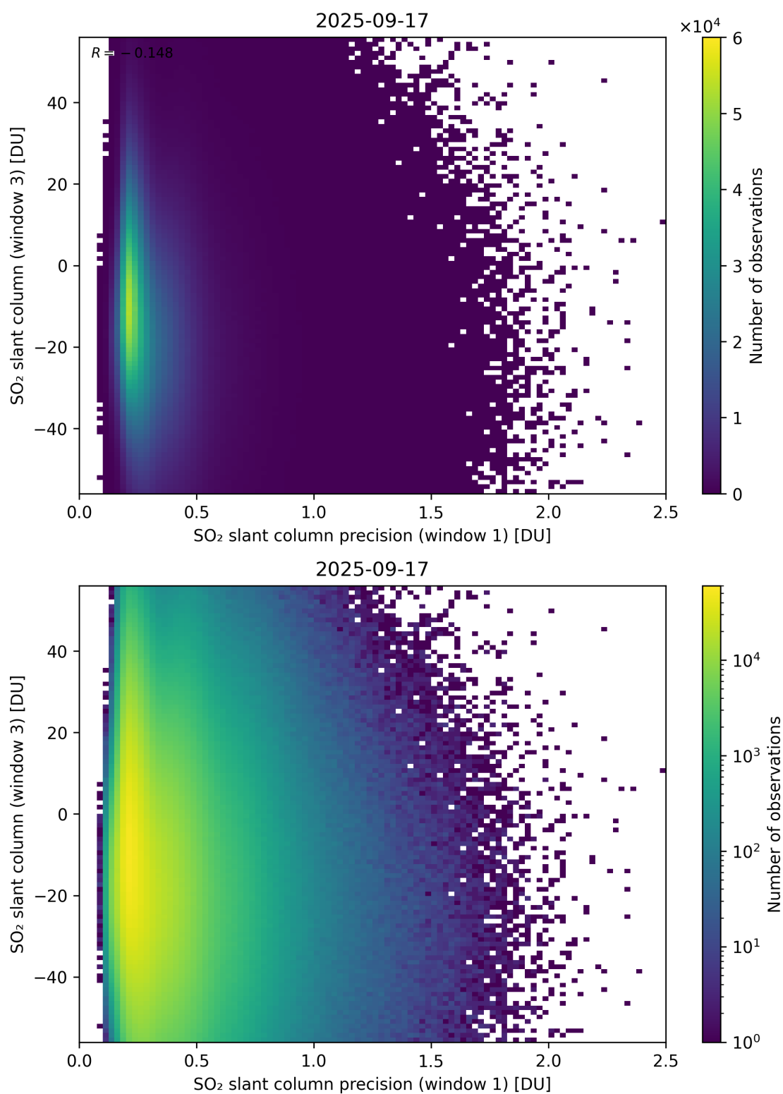
Figure 278: Scatter density plot of “SO 2 slant column precision (window 1)” against “SO 2 slant column (window 3)” for 2025-09-16 to 2025-09-18.
