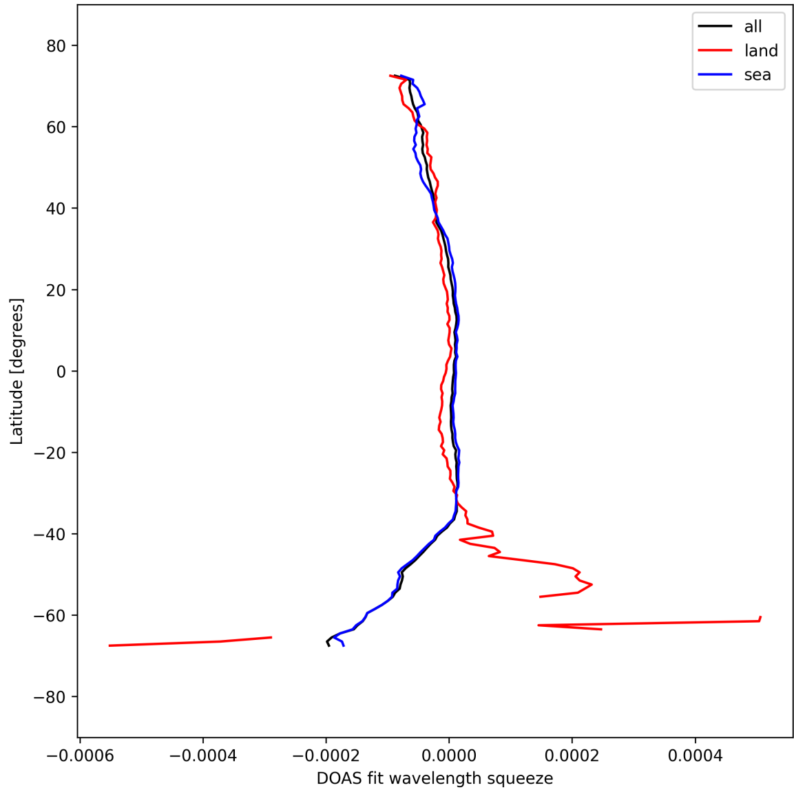
Figure 51: Zonal average of “DOAS fit wavelength squeeze” for 2025-09-16 to 2025-09-18.
