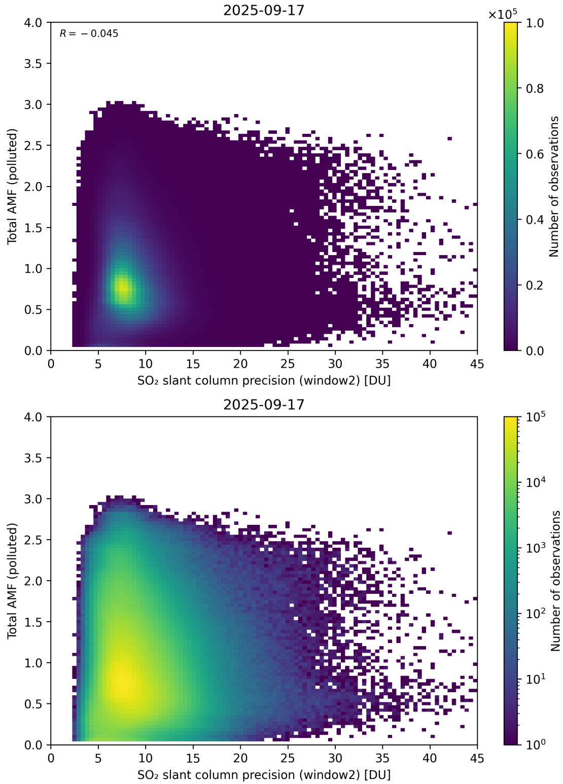
Figure 301: Scatter density plot of “SO 2 slant column precision (window2)” against “Total AMF (polluted)” for 2025-09-16 to 2025-09-18.
