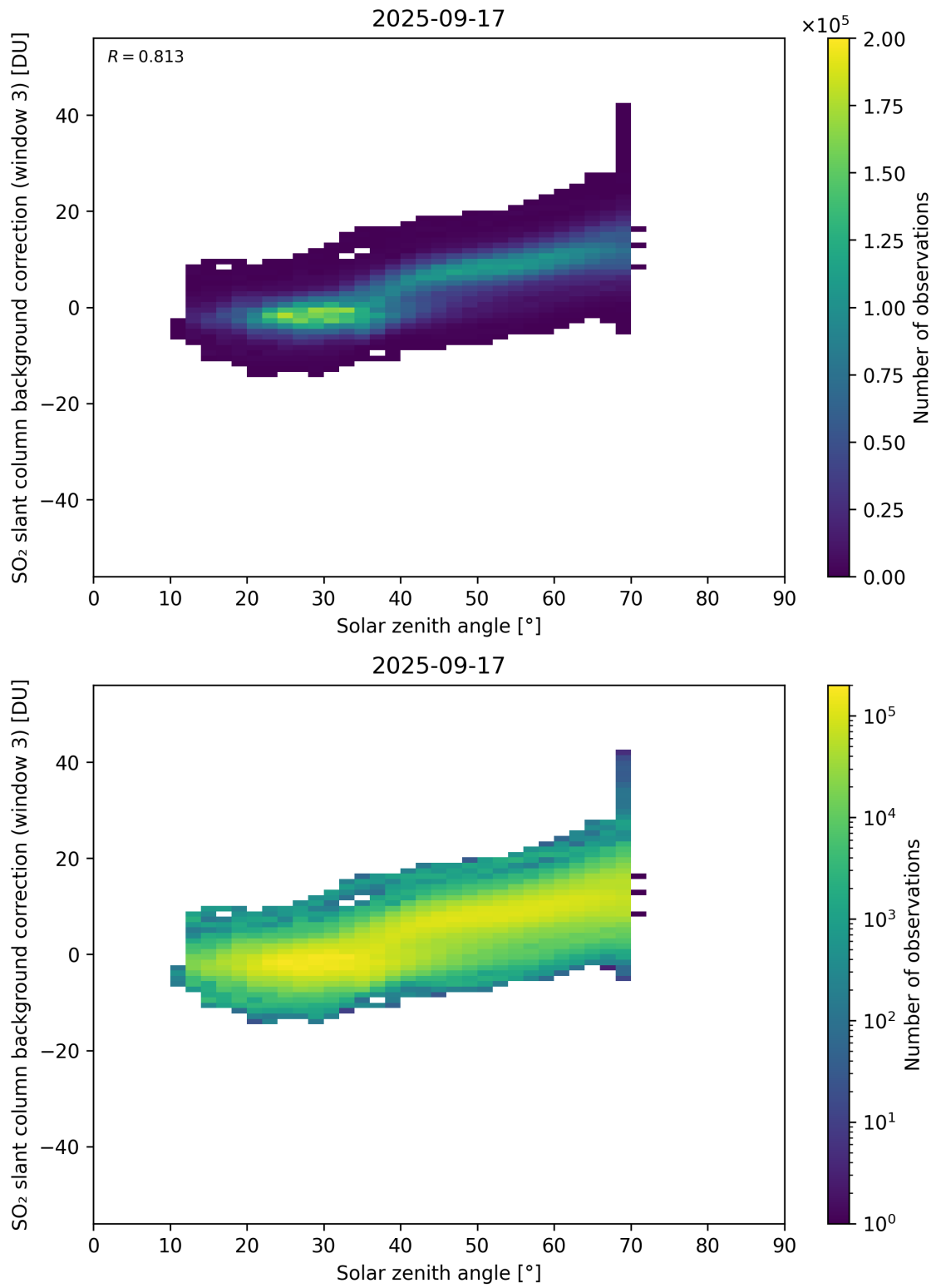
Figure 173: Scatter density plot of “Solar zenith angle” against “SO 2 slant column background correction (window 3)” for 2025-09-16 to 2025-09-18.
