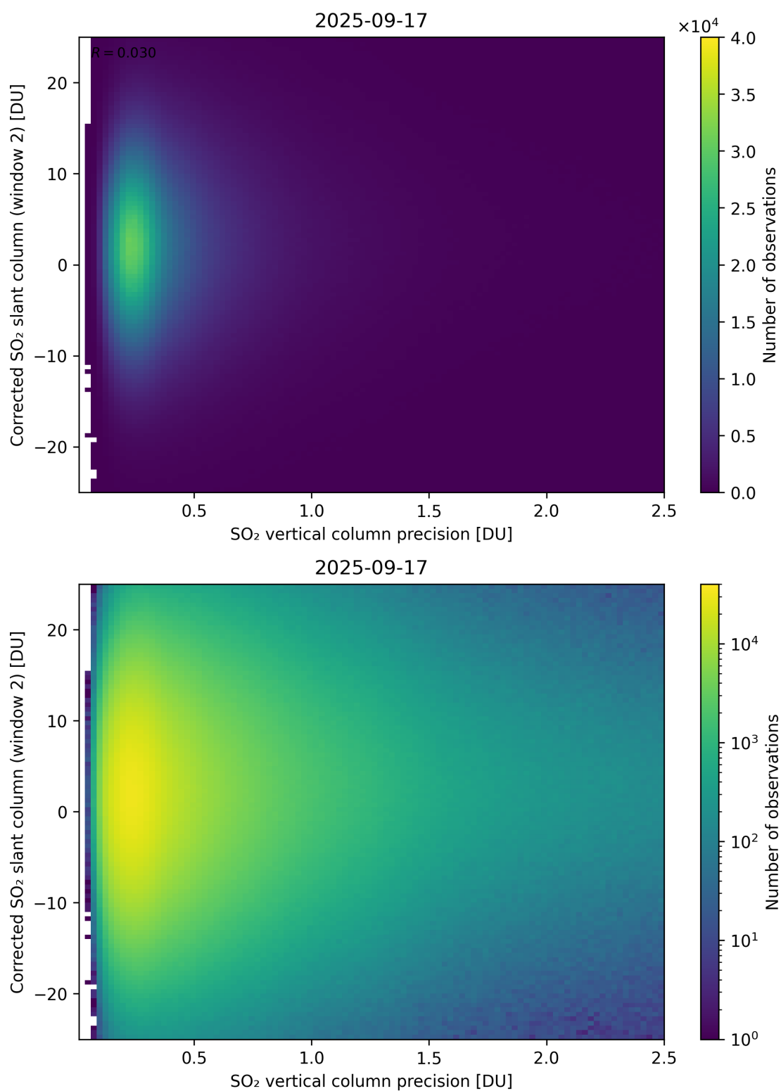
Figure 339: Scatter density plot of “SO 2 vertical column precision” against “Corrected SO 2 slant column (window 2)” for 2025-09-16 to 2025-09-18.
