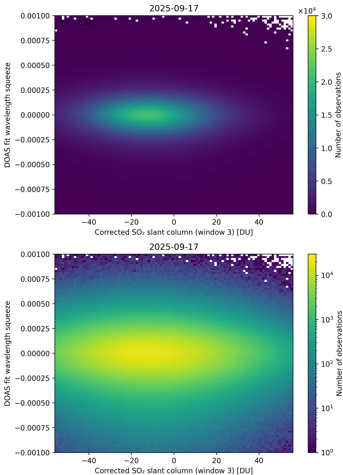
Figure 257: Scatter density plot of “Corrected SO 2 slant column (window 3)” against “DOAS fit wavelength squeeze” for 2025-09-16 to 2025-09-18.
