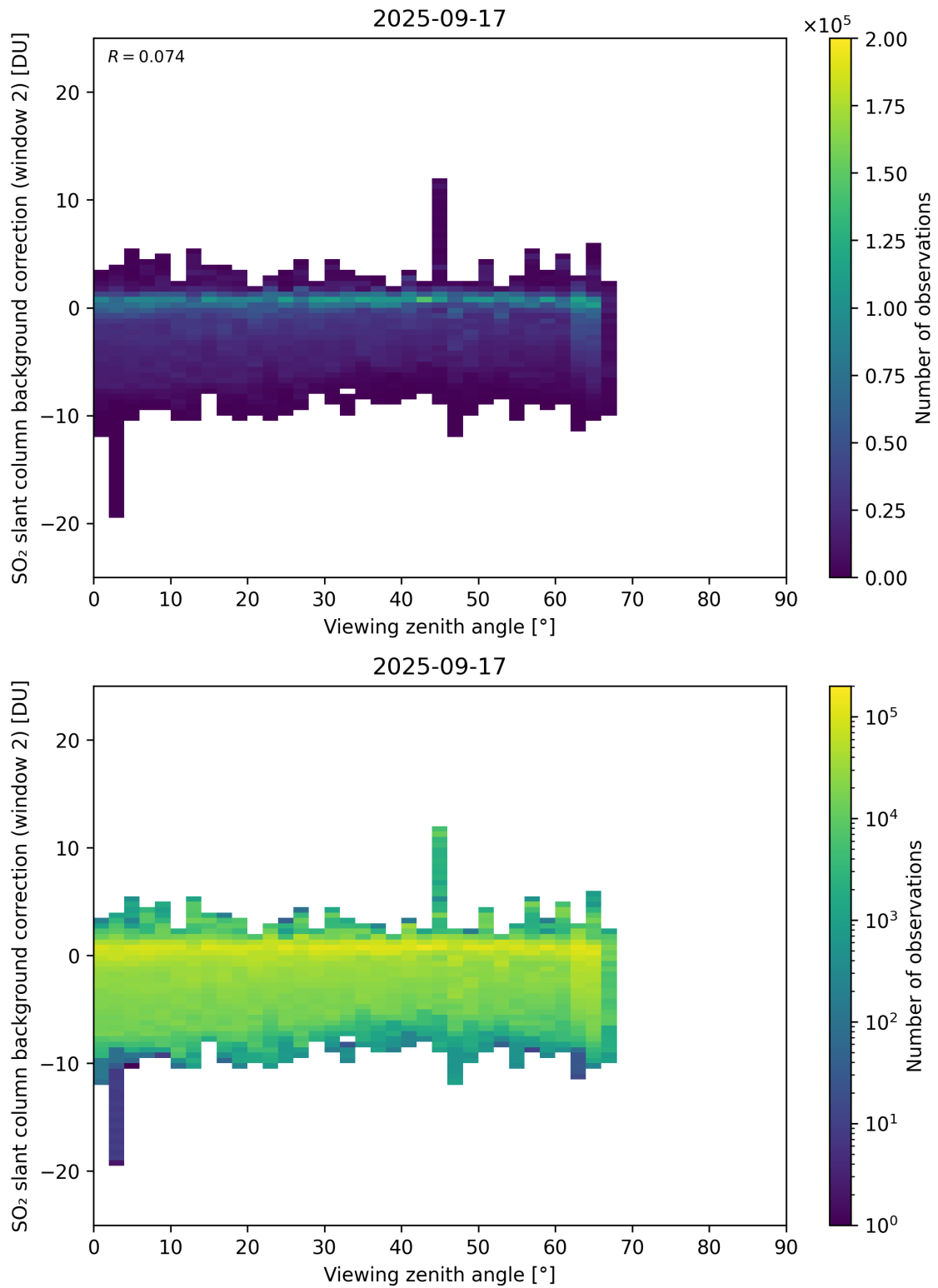
Figure 363: Scatter density plot of “Viewing zenith angle” against “SO 2 slant column background correction (window 2)” for 2025-09-16 to 2025-09-18.
