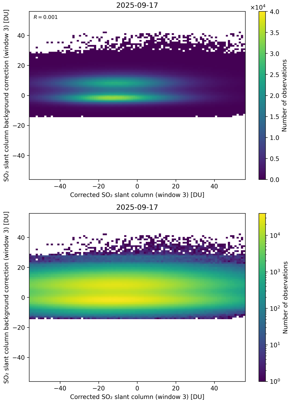
Figure 255: Scatter density plot of “Corrected SO 2 slant column (window 3)” against “SO 2 slant column background correction (window 3)” for 2025-09-16 to 2025-09-18.
