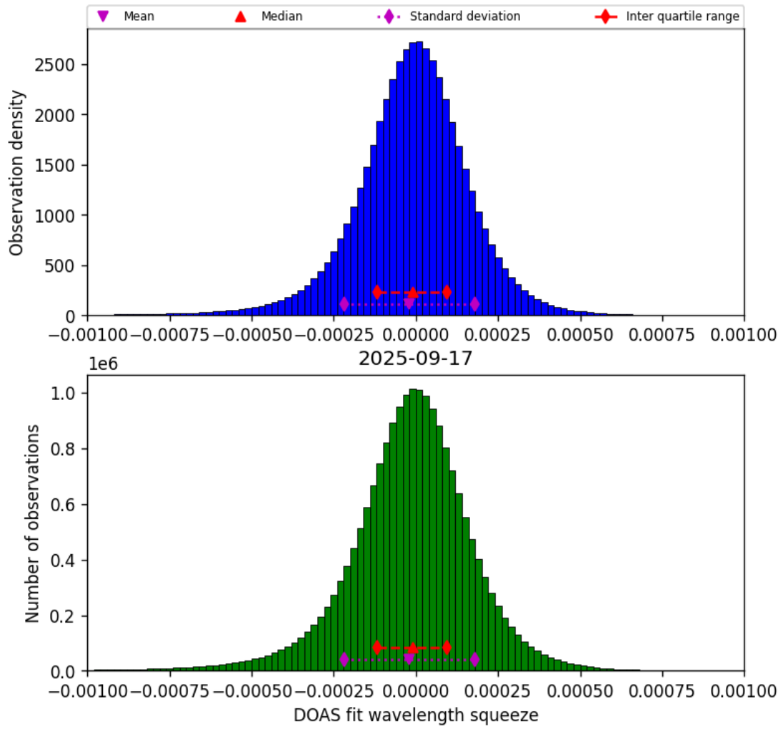
Figure 77: Histogram of “DOAS fit wavelength squeeze” for 2025-09-16 to 2025-09-18
