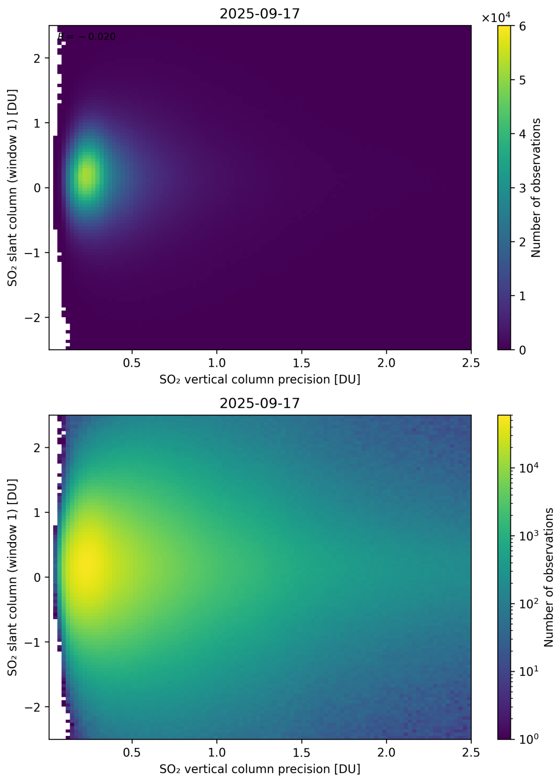
Figure 341: Scatter density plot of “SO 2 vertical column precision” against “SO 2 slant column (window 1)” for 2025-09-16 to 2025-09-18.
