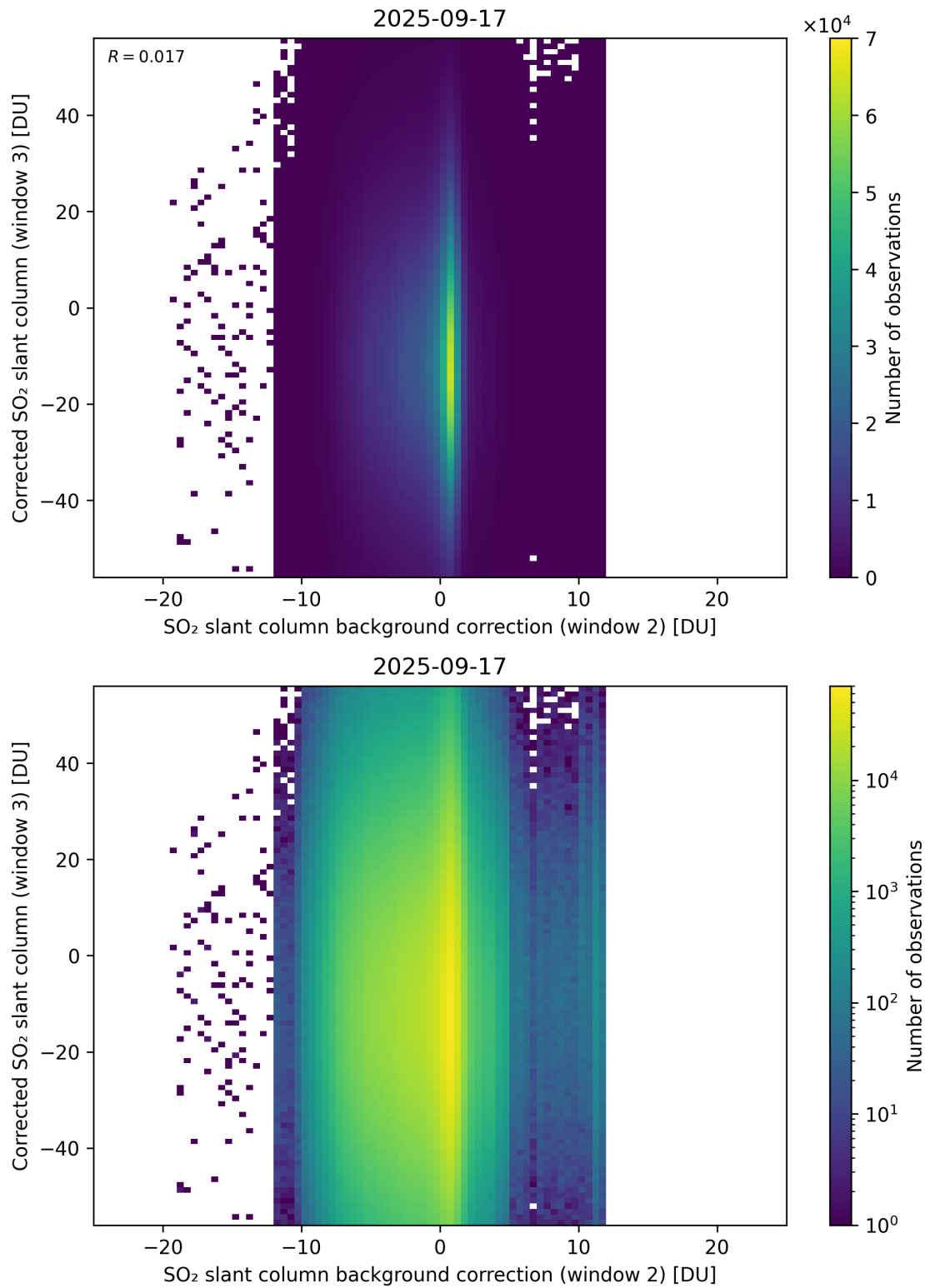
Figure 127: Scatter density plot of “SO 2 slant column background correction (window 2)” against “Corrected SO 2 slant column (window 3)” for 2025-09-16 to 2025-09-18.
