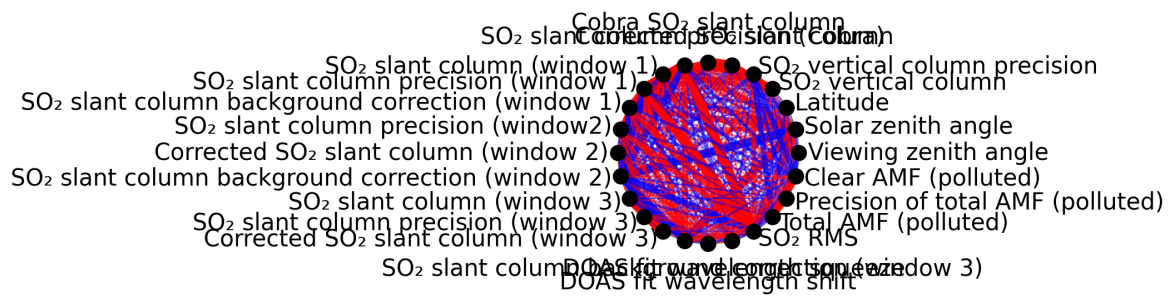
Figure 1: Map of correlation graph for 2025-09-16 to 2025-09-18.
