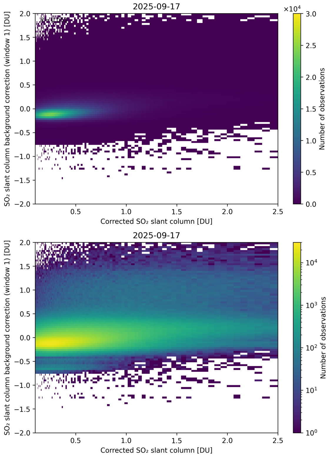
Figure 226: Scatter density plot of “Corrected SO 2 slant column” against “SO 2 slant column background correction (window 1)” for 2025-09-16 to 2025-09-18.
