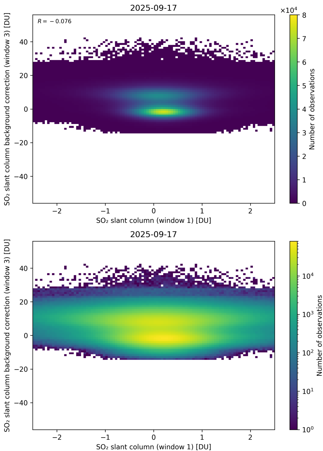
Figure 264: Scatter density plot of “SO 2 slant column (window 1)” against “SO 2 slant column background correction (window 3)” for 2025-09-16 to 2025-09-18.
