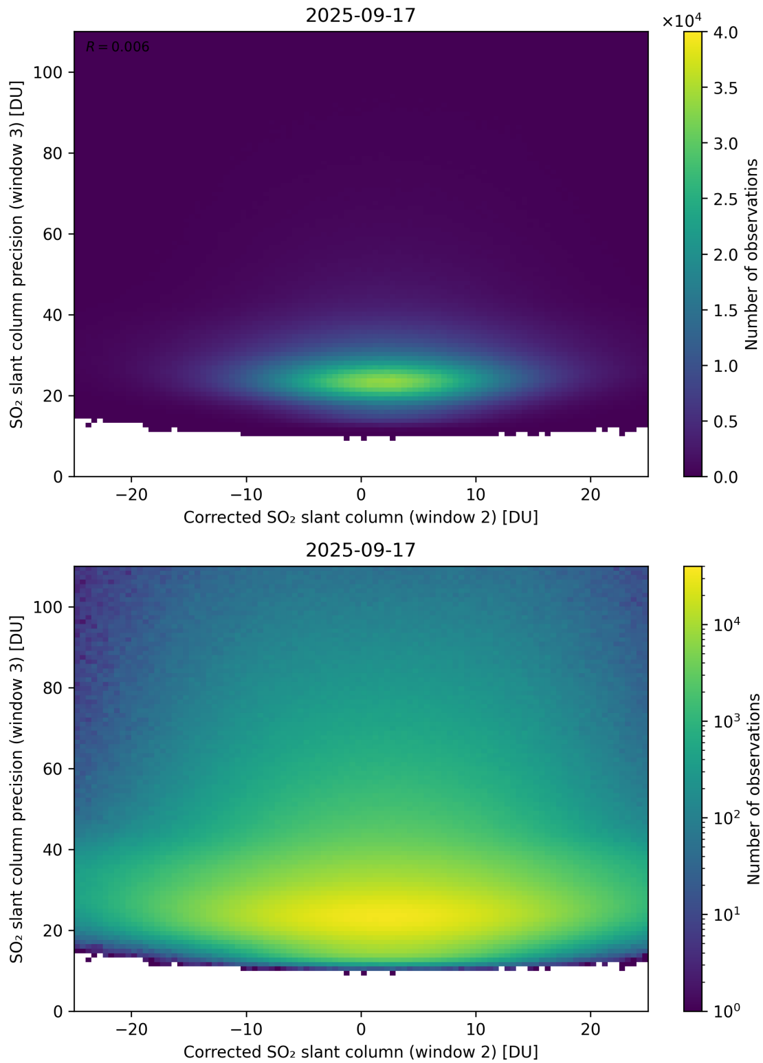
Figure 252: Scatter density plot of “Corrected SO 2 slant column (window 2)” against “SO 2 slant column precision (window 3)” for 2025-09-16 to 2025-09-18.
