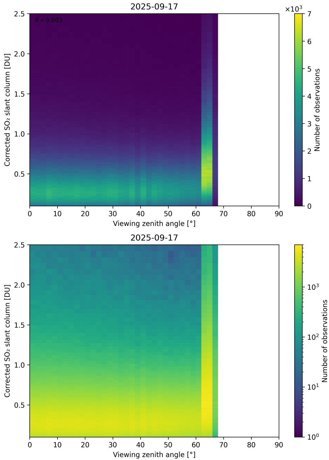
Figure 373: Scatter density plot of “Viewing zenith angle” against “Corrected SO 2 slant column” for 2025-09-16 to 2025-09-18.
