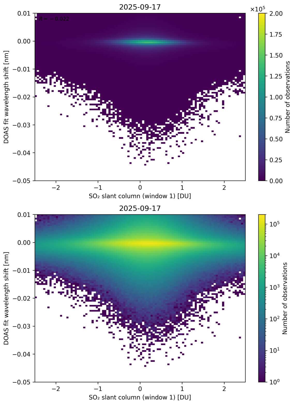
Figure 265: Scatter density plot of “SO 2 slant column (window 1)” against “DOAS fit wavelength shift” for 2025-09-16 to 2025-09-18.
