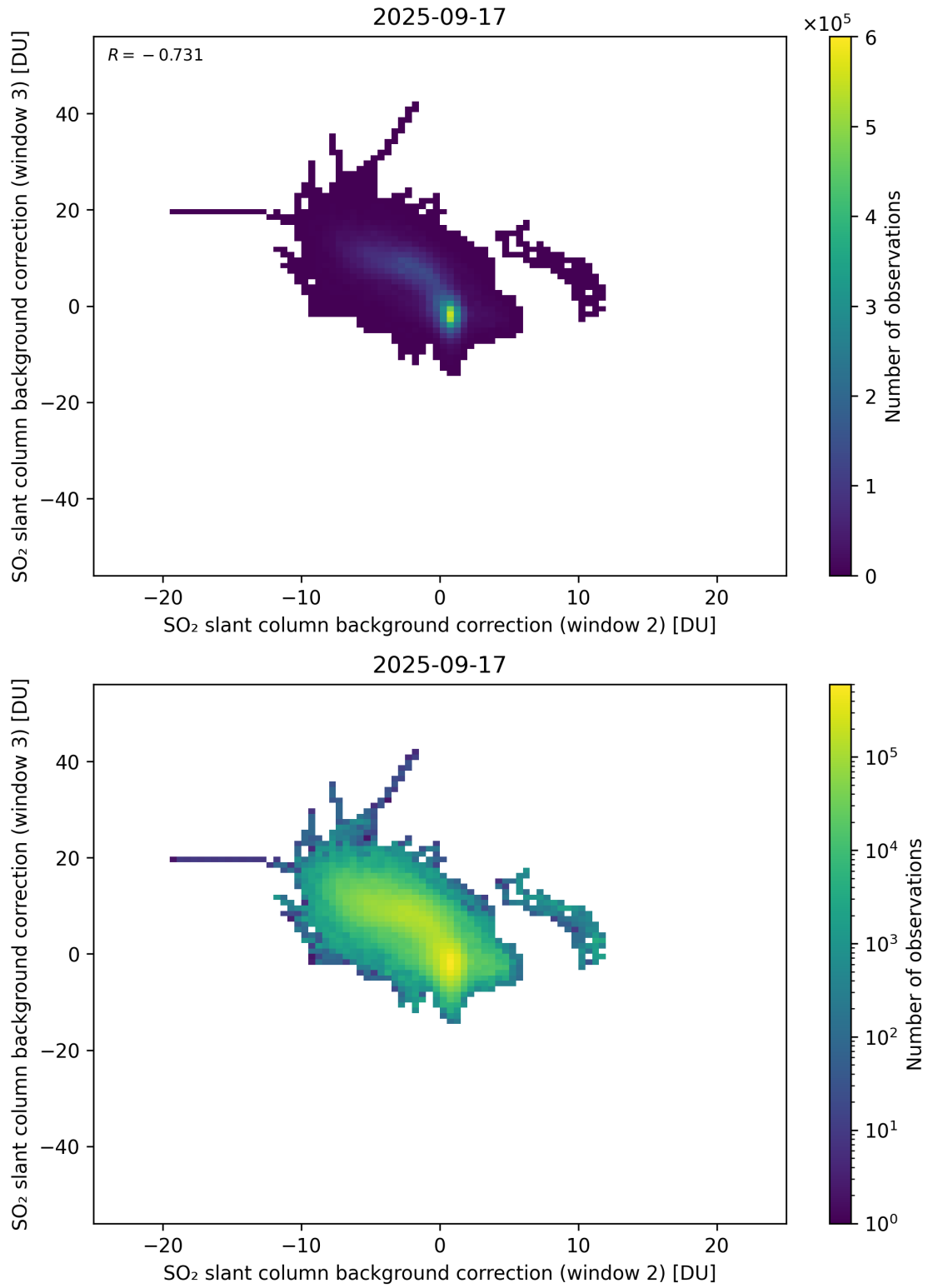
Figure 122: Scatter density plot of “SO 2 slant column background correction (window 2)” against “SO 2 slant column background correction (window 3)” for 2025-09-16 to 2025-09-18.
