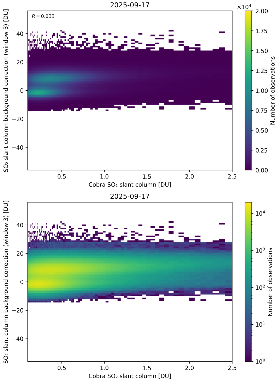
Figure 195: Scatter density plot of “Cobra SO 2 slant column” against “SO 2 slant column background correction (window 3)” for 2025-09-16 to 2025-09-18.
