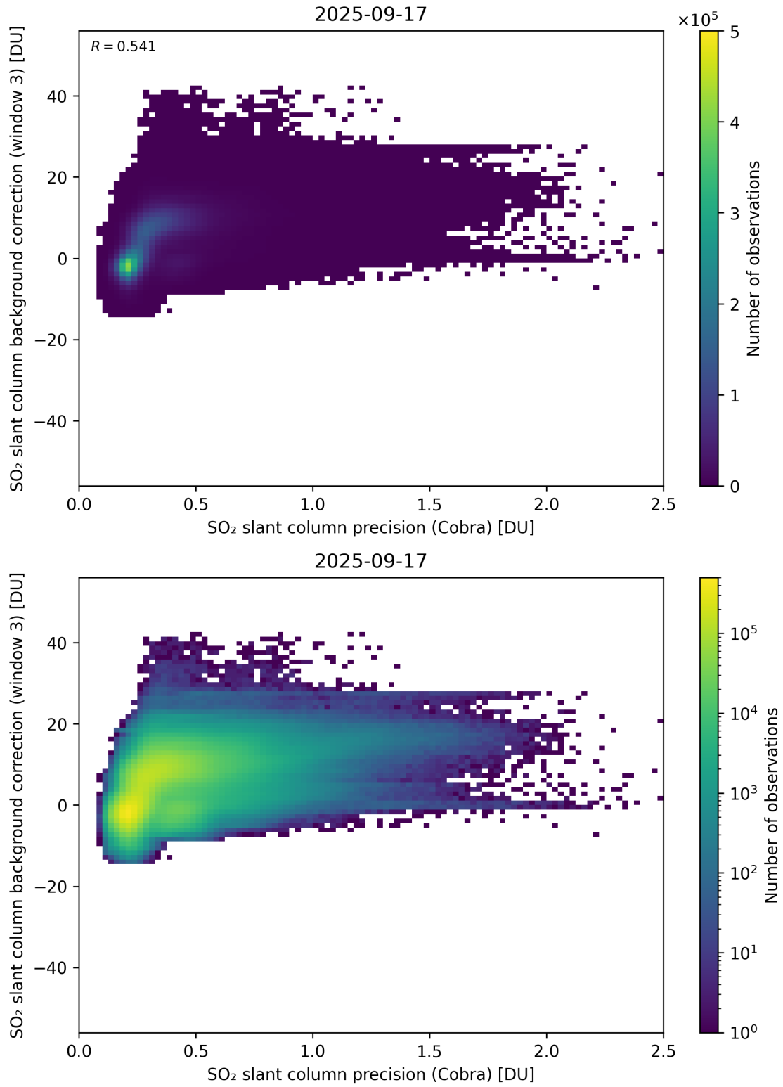
Figure 201: Scatter density plot of “SO 2 slant column precision (Cobra)” against “SO 2 slant column background correction (window 3)” for 2025-09-16 to 2025-09-18.
