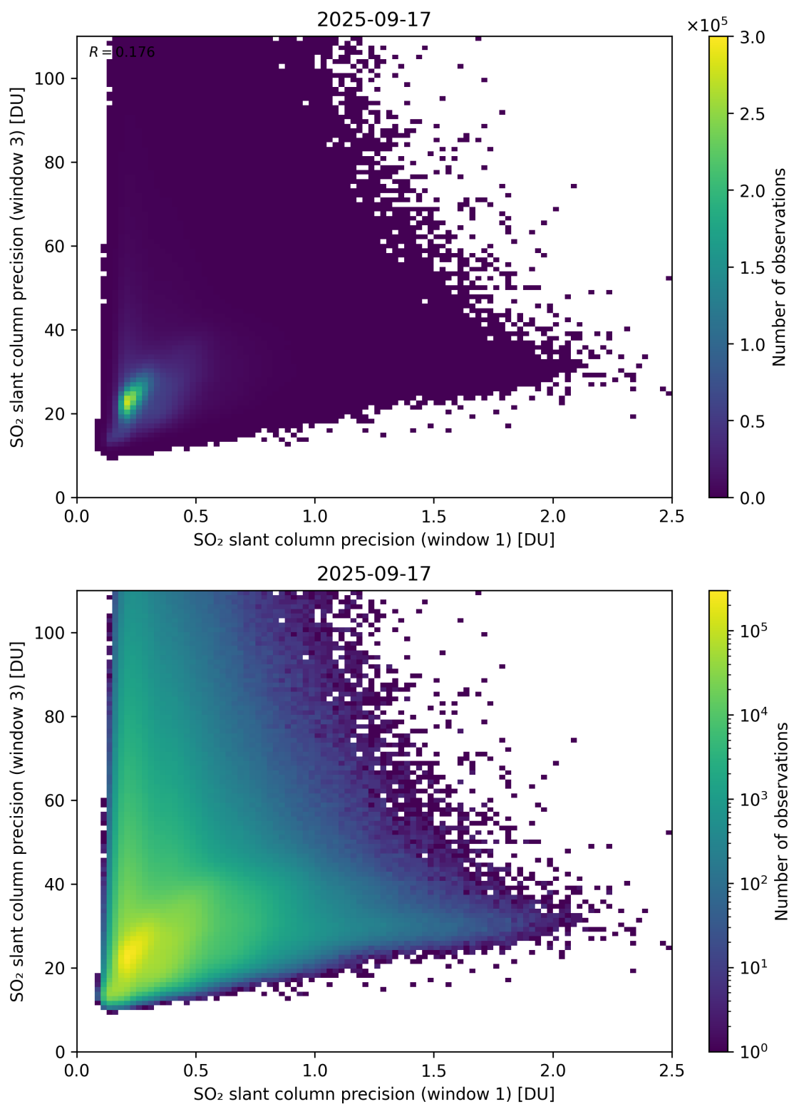
Figure 279: Scatter density plot of “SO 2 slant column precision (window 1)” against “SO 2 slant column precision (window 3)” for 2025-09-16 to 2025-09-18.
