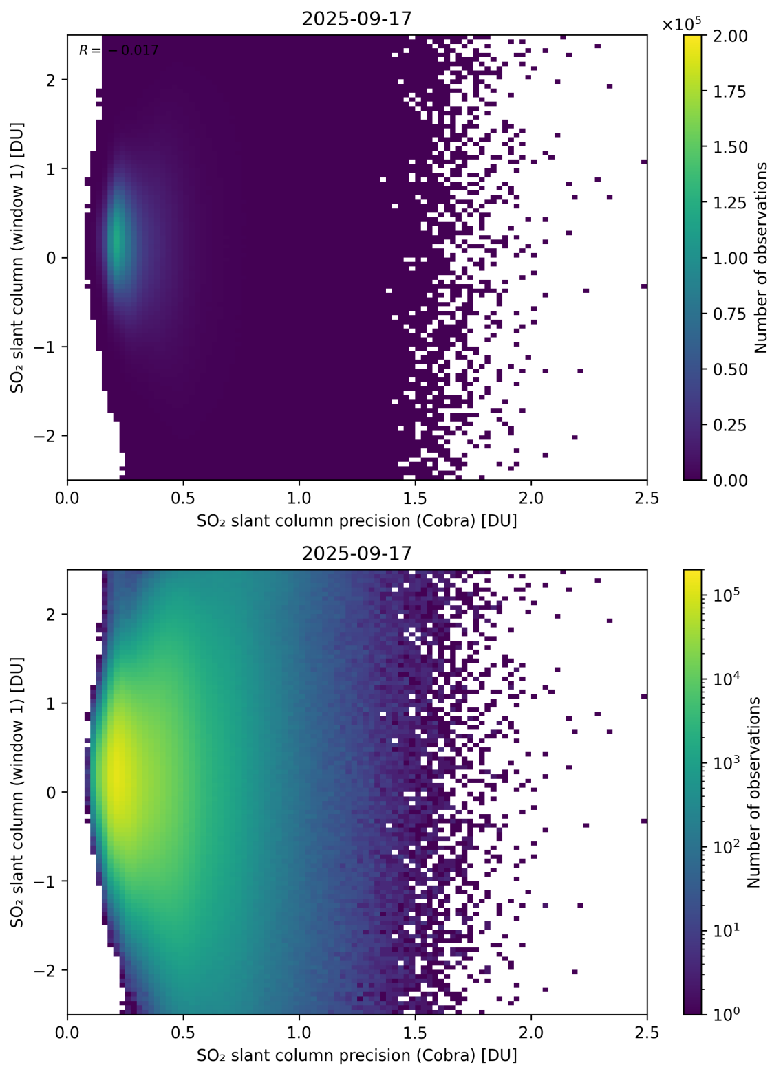
Figure 208: Scatter density plot of “SO 2 slant column precision (Cobra)” against “SO 2 slant column (window 1)” for 2025-09-16 to 2025-09-18.
