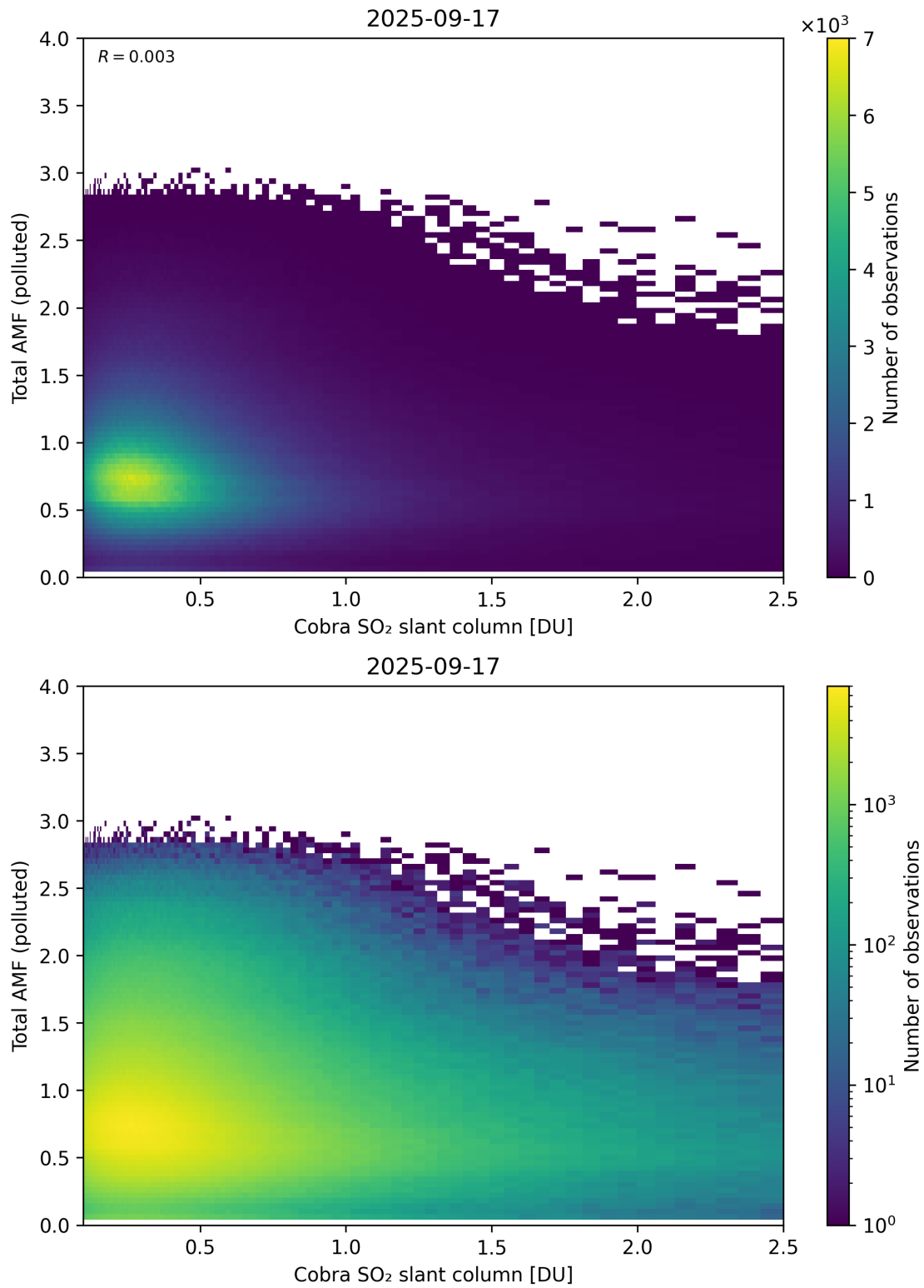
Figure 224: Scatter density plot of “Cobra SO 2 slant column” against “Total AMF (polluted)” for 2025-09-16 to 2025-09-18.
