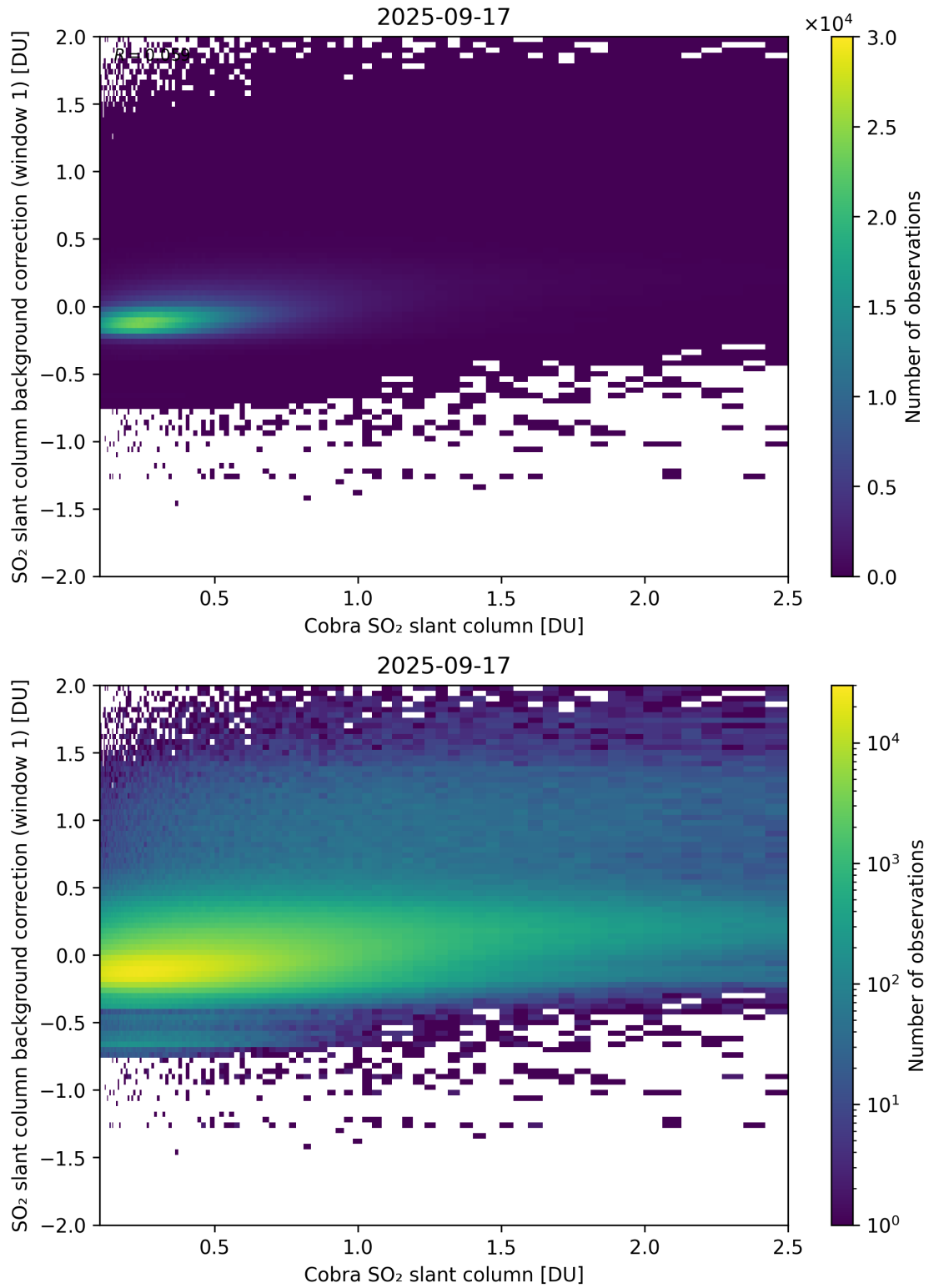
Figure 193: Scatter density plot of “Cobra SO 2 slant column” against “SO 2 slant column background correction (window 1)” for 2025-09-16 to 2025-09-18.
