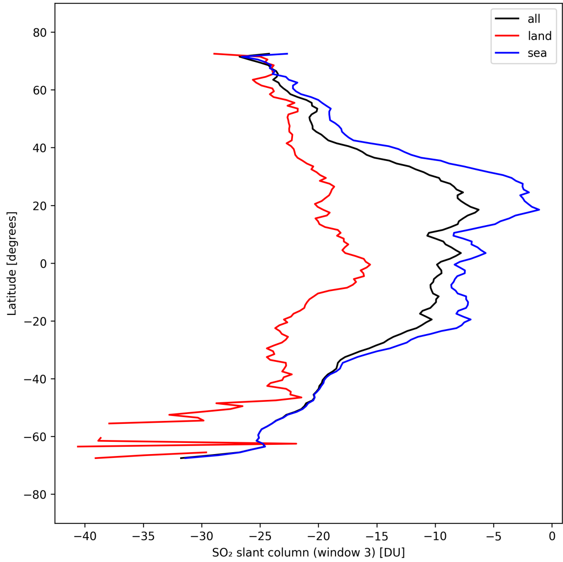
Figure 45: Zonal average of “SO 2 slant column (window 3)” for 2025-09-16 to 2025-09-18.
