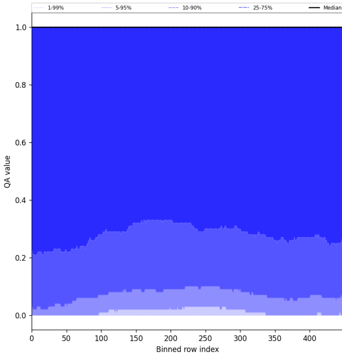
Figure 83: Along track statistics of “QA value” for 2025-09-16 to 2025-09-18
