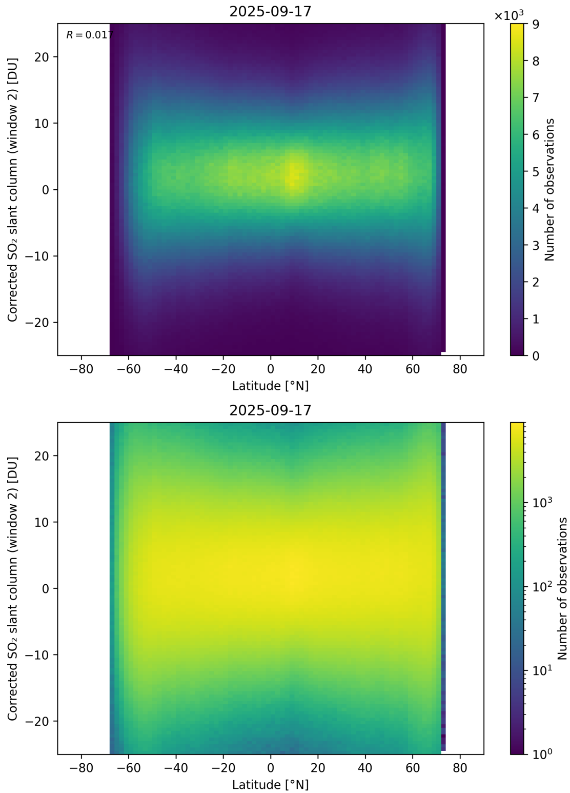
Figure 160: Scatter density plot of “Latitude” against “Corrected SO 2 slant column (window 2)” for 2025-09-16 to 2025-09-18.
