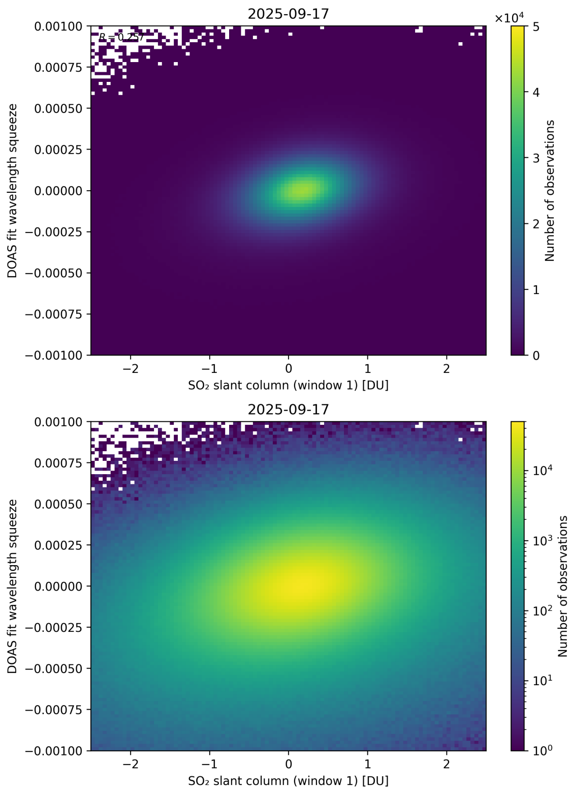
Figure 266: Scatter density plot of “SO 2 slant column (window 1)” against “DOAS fit wavelength squeeze” for 2025-09-16 to 2025-09-18.
