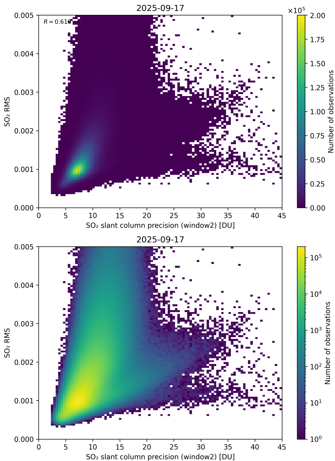
Figure 295: Scatter density plot of “SO 2 slant column precision (window2)” against “SO 2 RMS” for 2025-09-16 to 2025-09-18.
