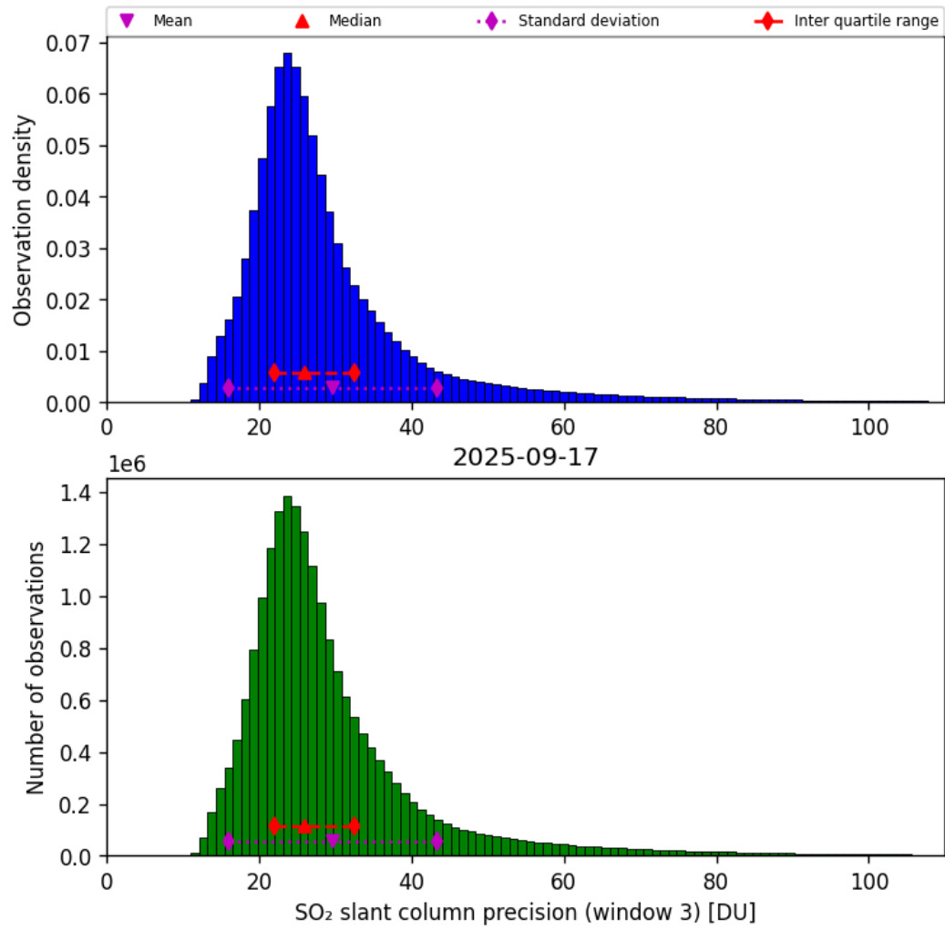
Figure 72: Histogram of “SO 2 slant column precision (window 3)” for 2025-09-16 to 2025-09-18
