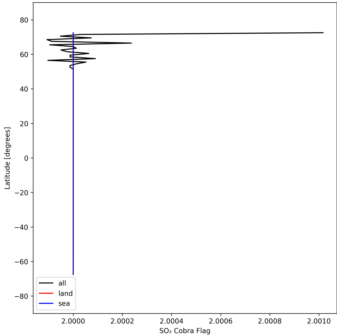
Figure 49: Zonal average of "SO 2 Cobra Flag" for 2025-09-16 to 2025-09-18.
