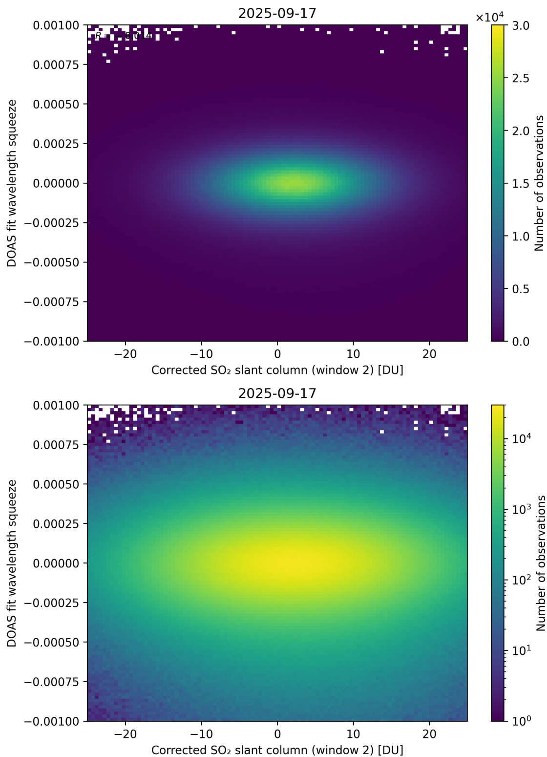
Figure 247: Scatter density plot of “Corrected SO 2 slant column (window 2)” against “DOAS fit wavelength squeeze” for 2025-09-16 to 2025-09-18.
