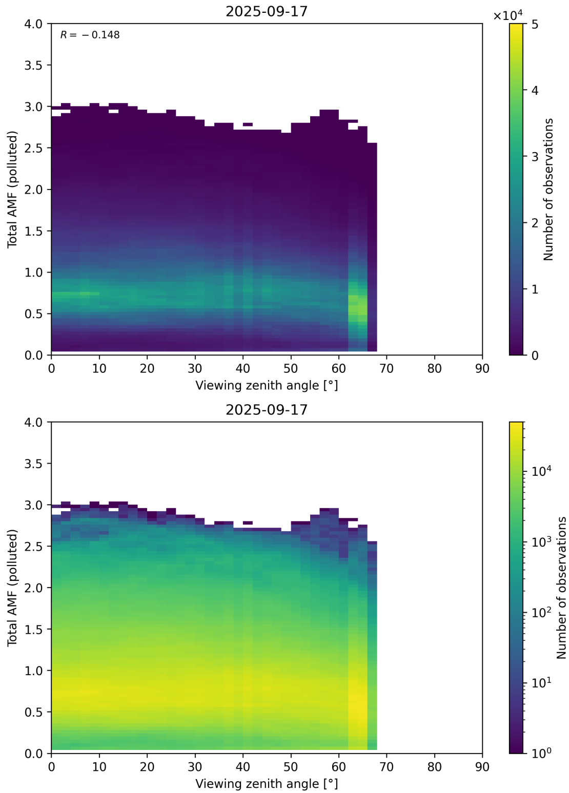
Figure 381: Scatter density plot of “Viewing zenith angle” against “Total AMF (polluted)” for 2025-09-16 to 2025-09-18.
