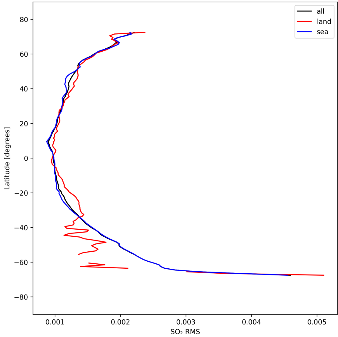
Figure 52: Zonal average of “SO 2 RMS” for 2025-09-16 to 2025-09-18.
