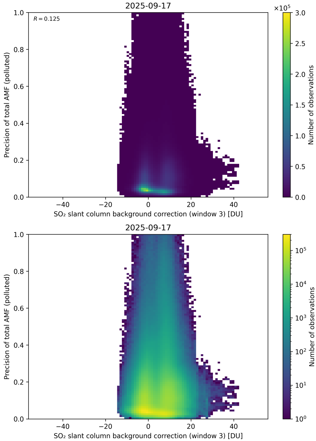
Figure 137: Scatter density plot of “SO 2 slant column background correction (window 3)” against “Precision of total AMF (polluted)” for 2025-09-16 to 2025-09-18.
