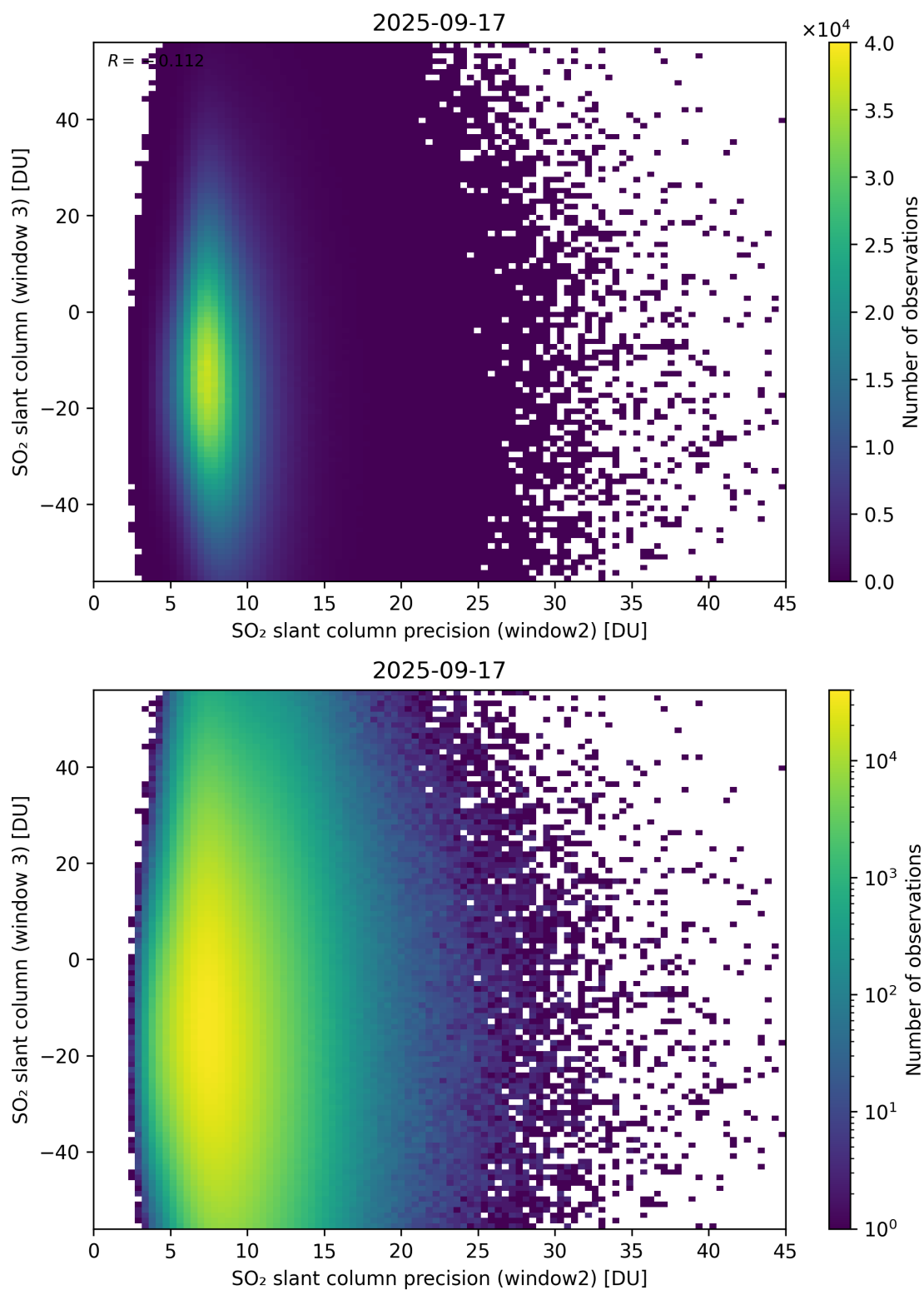
Figure 299: Scatter density plot of “SO 2 slant column precision (window2)” against “SO 2 slant column (window 3)” for 2025-09-16 to 2025-09-18.
