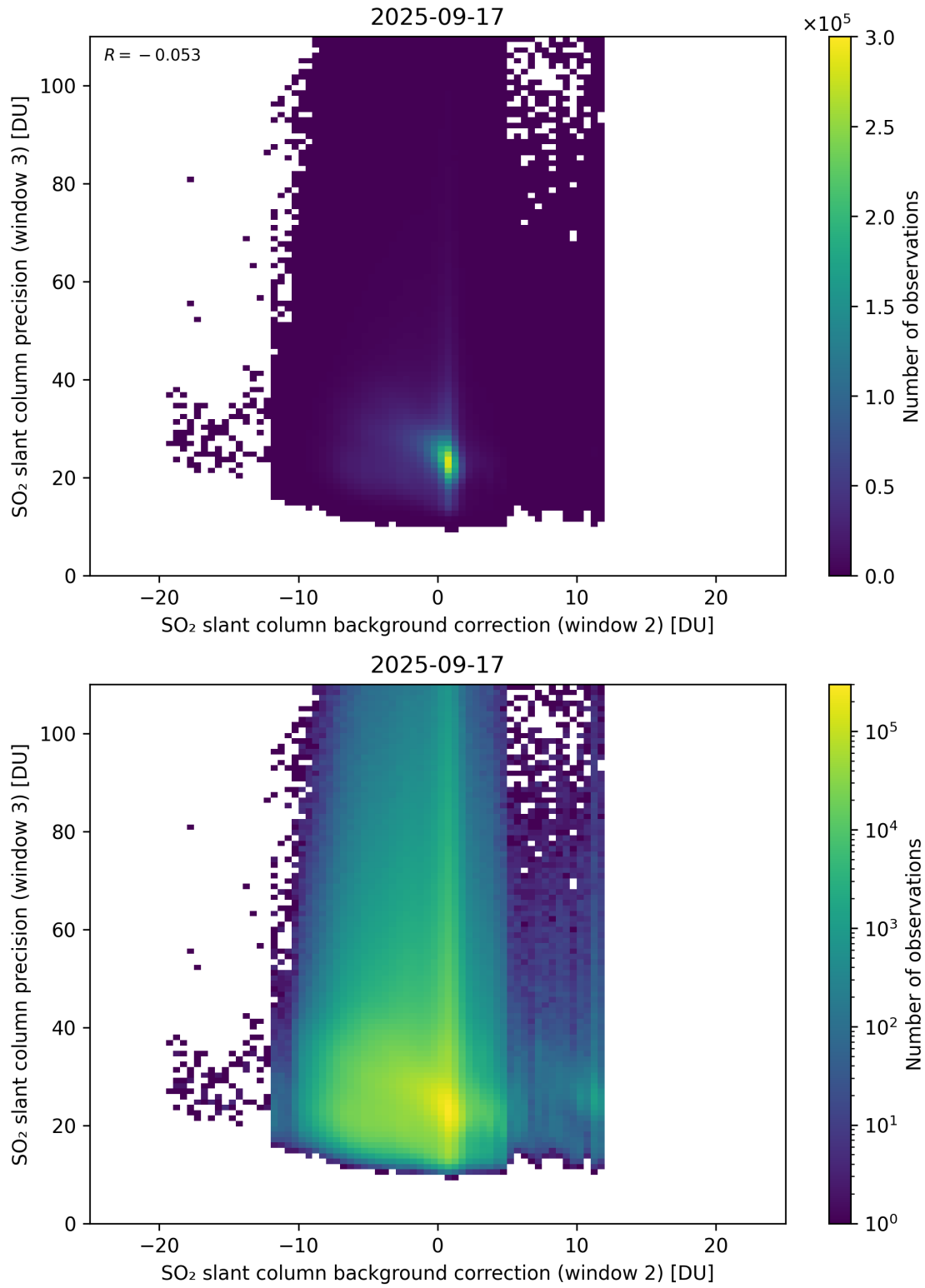
Figure 129: Scatter density plot of “SO 2 slant column background correction (window 2)” against “SO 2 slant column precision (window 3)” for 2025-09-16 to 2025-09-18.
