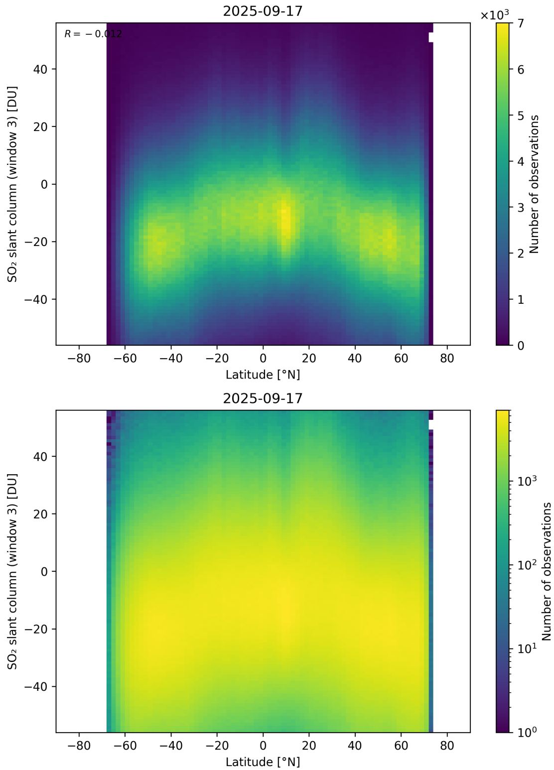
Figure 165: Scatter density plot of “Latitude” against “SO 2 slant column (window 3)” for 2025-09-16 to 2025-09-18.
