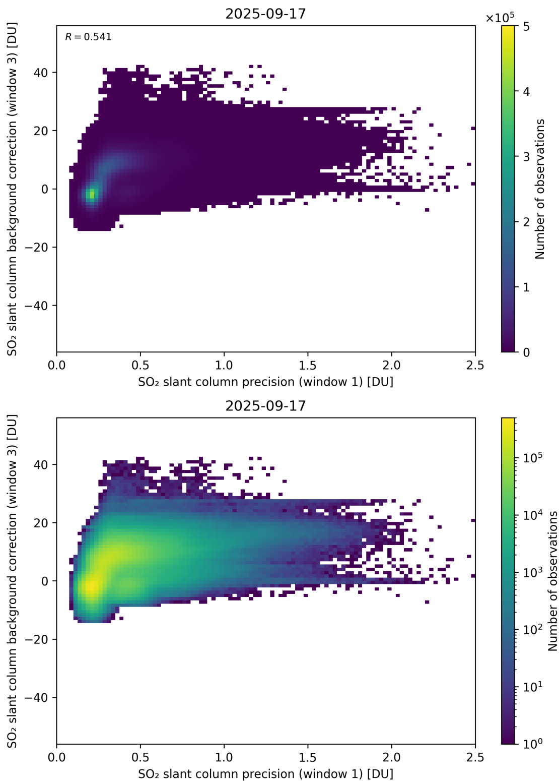
Figure 270: Scatter density plot of “SO 2 slant column precision (window 1)” against “SO 2 slant column background correction (window 3)” for 2025-09-16 to 2025-09-18.
