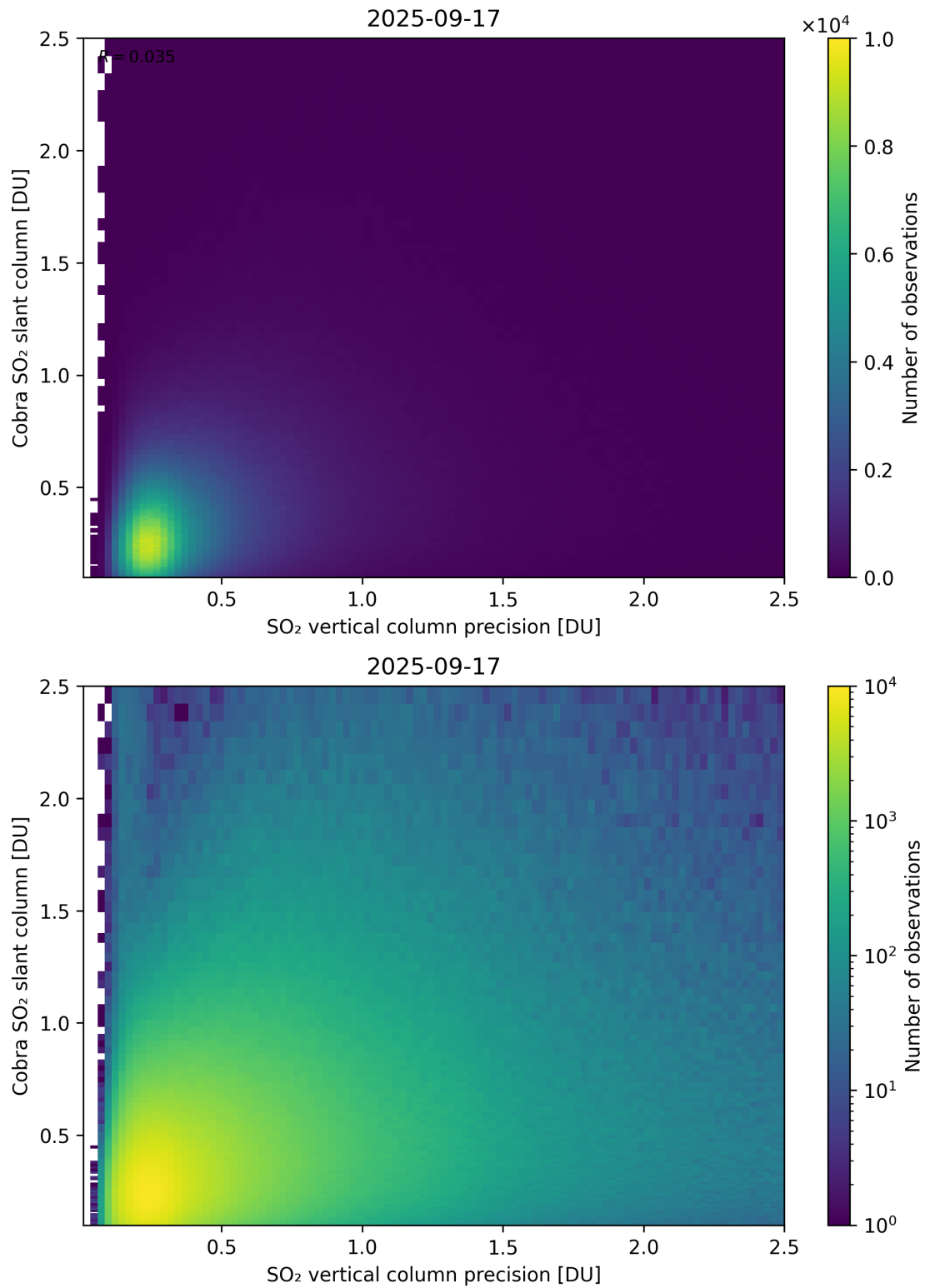
Figure 336: Scatter density plot of “SO 2 vertical column precision” against “Cobra SO 2 slant column” for 2025-09-16 to 2025-09-18.
