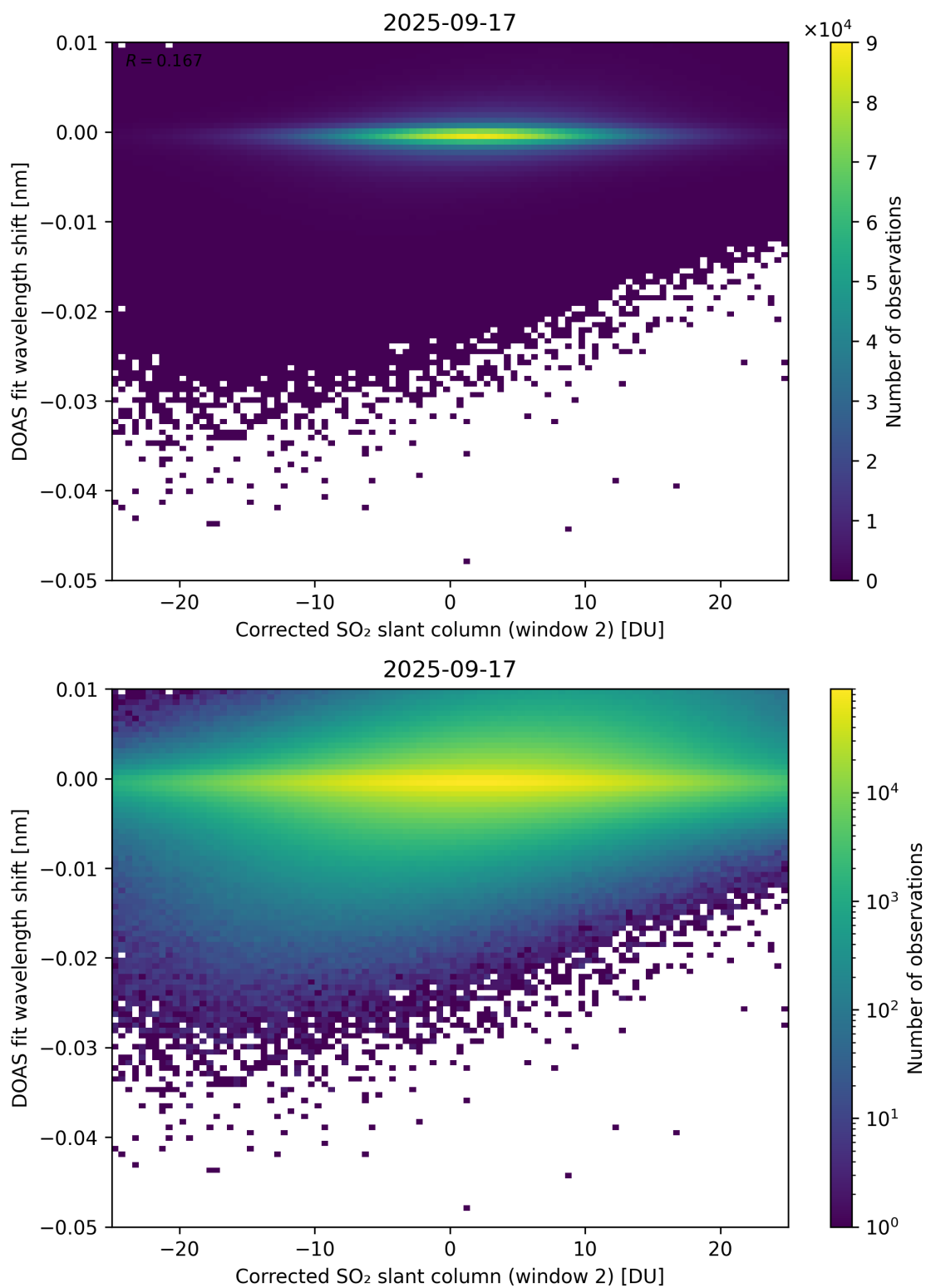
Figure 246: Scatter density plot of “Corrected SO 2 slant column (window 2)” against “DOAS fit wavelength shift” for 2025-09-16 to 2025-09-18.
