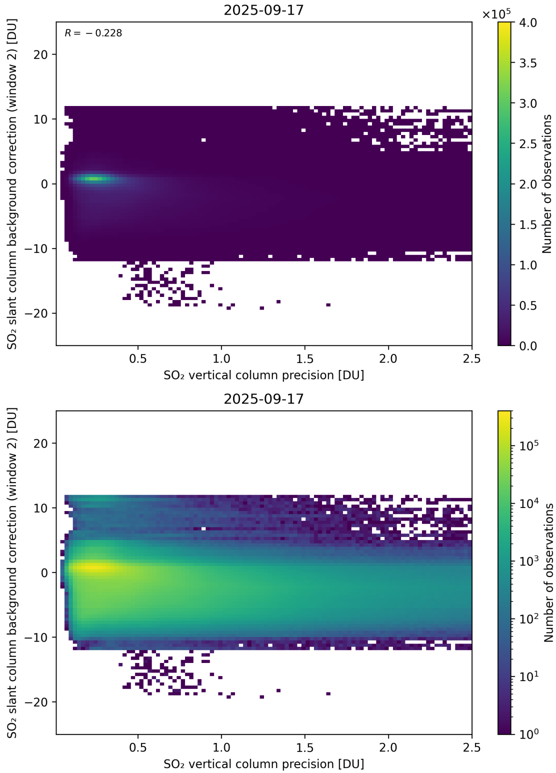
Figure 330: Scatter density plot of “SO 2 vertical column precision” against “SO 2 slant column background correction (window 2)” for 2025-09-16 to 2025-09-18.
