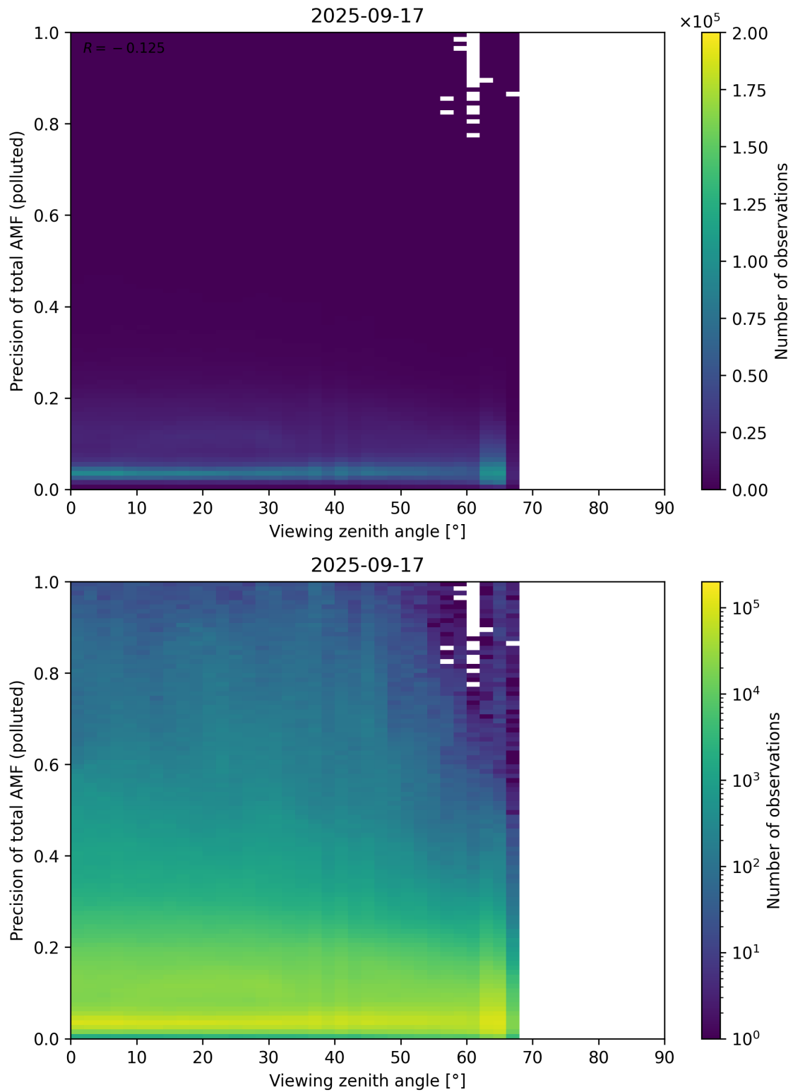
Figure 382: Scatter density plot of “Viewing zenith angle” against “Precision of total AMF (polluted)” for 2025-09-16 to 2025-09-18.
