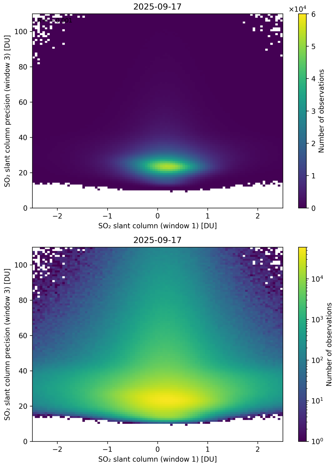
Figure 288: Scatter density plot of “SO 2 slant column (window 1)” against “SO 2 slant column precision (window 3)” for 2025-09-16 to 2025-09-18.
