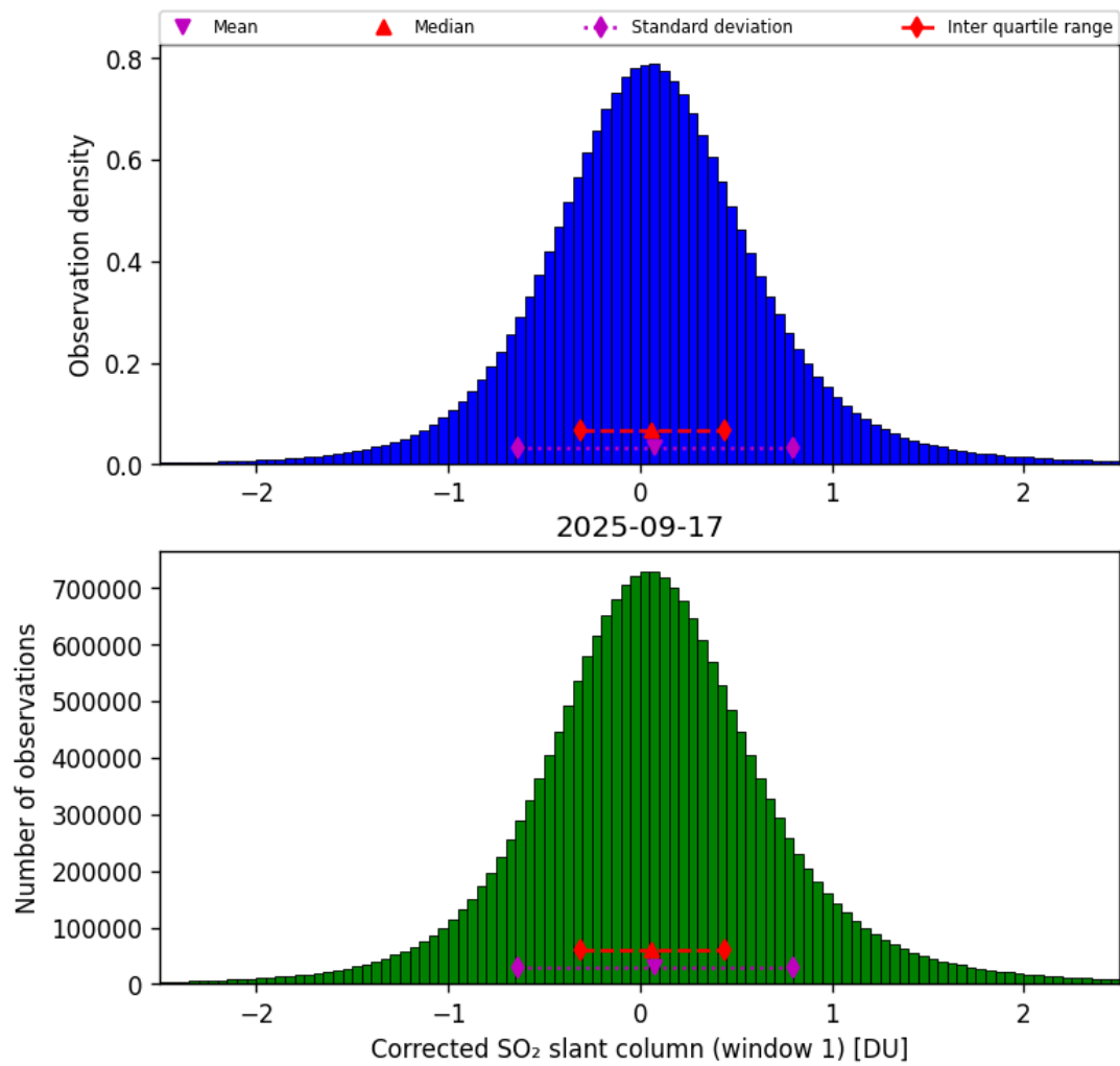
Figure 65: Histogram of “Corrected SO 2 slant column (window 1)” for 2025-09-16 to 2025-09-18
