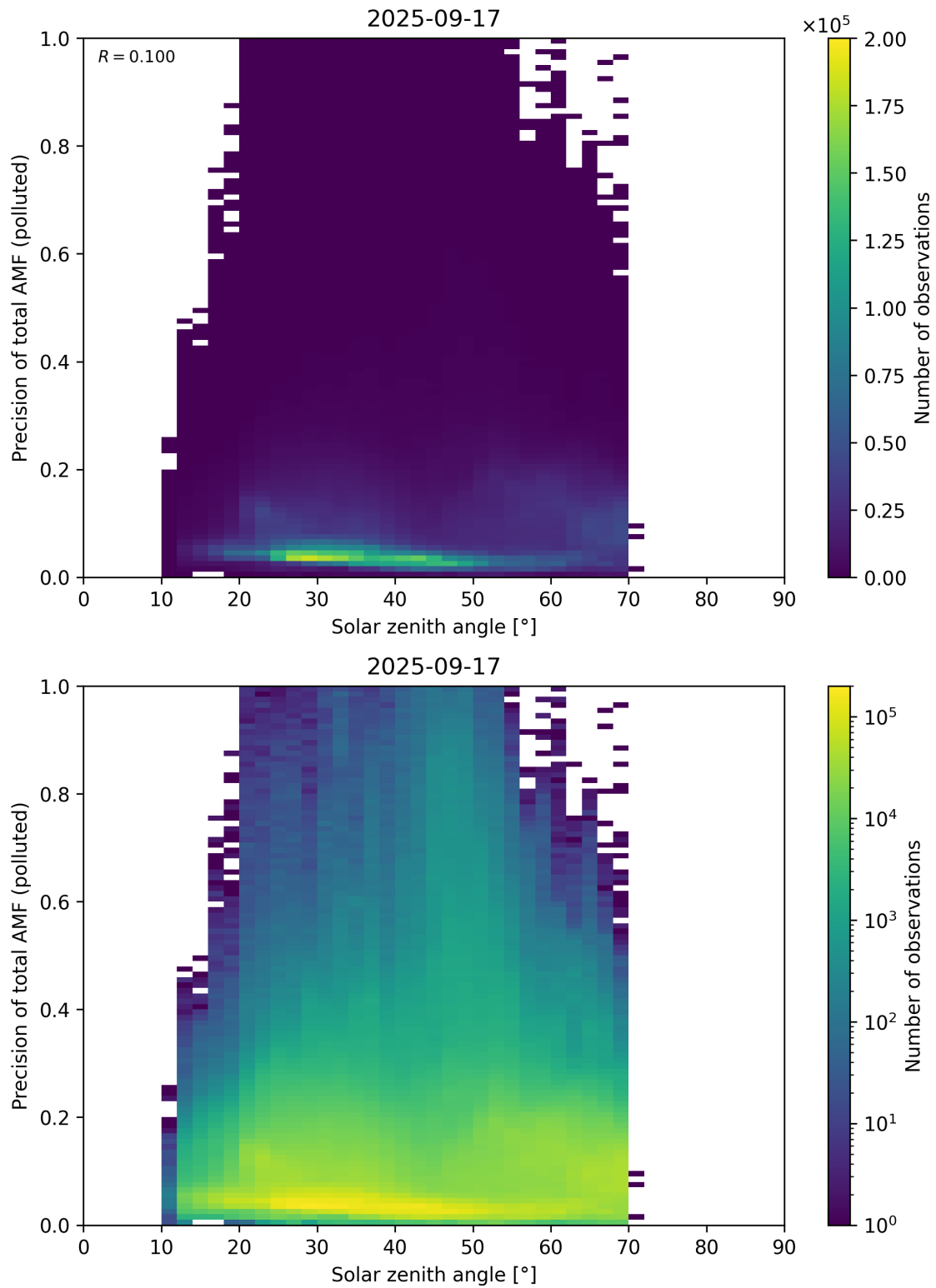
Figure 190: Scatter density plot of “Solar zenith angle” against “Precision of total AMF (polluted)” for 2025-09-16 to 2025-09-18.
