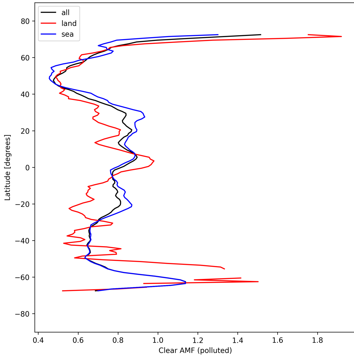
Figure 55: Zonal average of “Clear AMF (polluted)” for 2025-09-16 to 2025-09-18.
