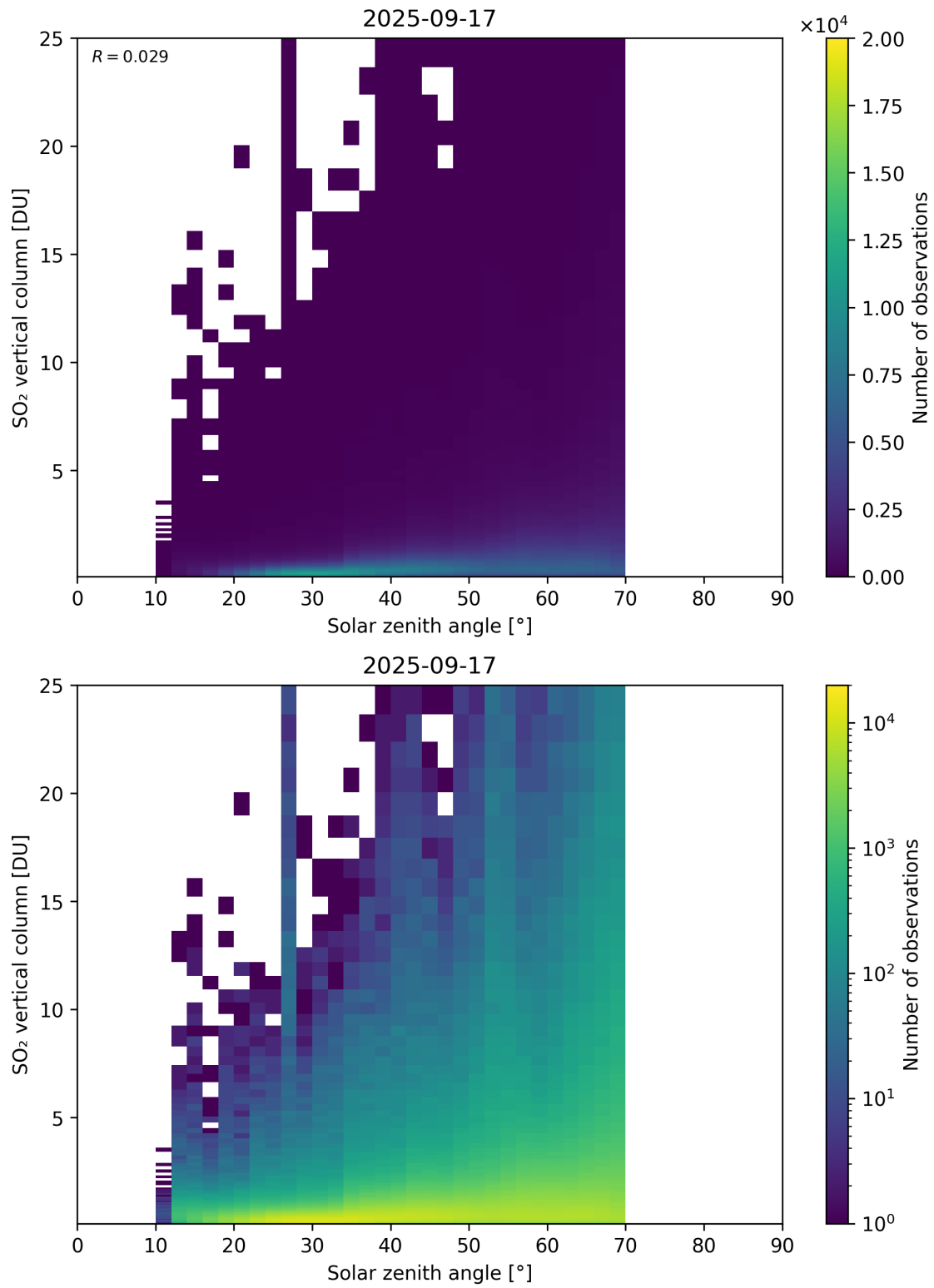
Figure 191: Scatter density plot of “Solar zenith angle” against “SO 2 vertical column” for 2025-09-16 to 2025-09-18.
