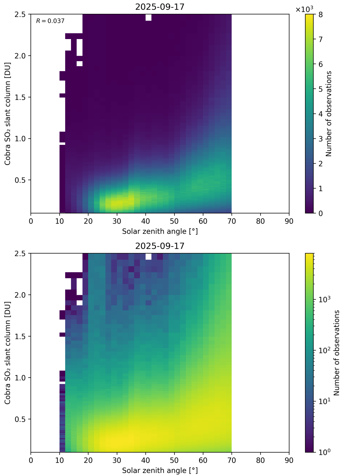
Figure 179: Scatter density plot of “Solar zenith angle” against “Cobra SO 2 slant column” for 2025-09-16 to 2025-09-18.
