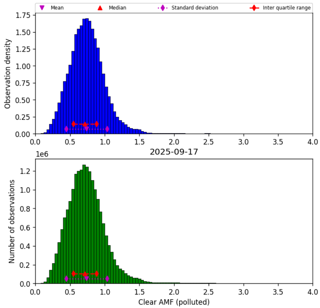
Figure 81: Histogram of “Clear AMF (polluted)” for 2025-09-16 to 2025-09-18
