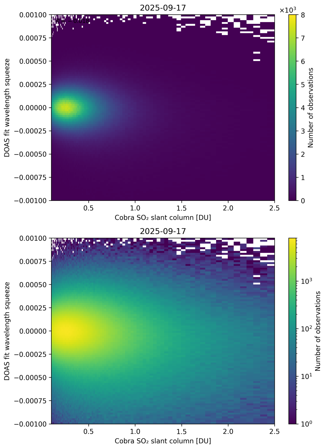
Figure 197: Scatter density plot of “Cobra SO 2 slant column” against “DOAS fit wavelength squeeze” for 2025-09-16 to 2025-09-18.
