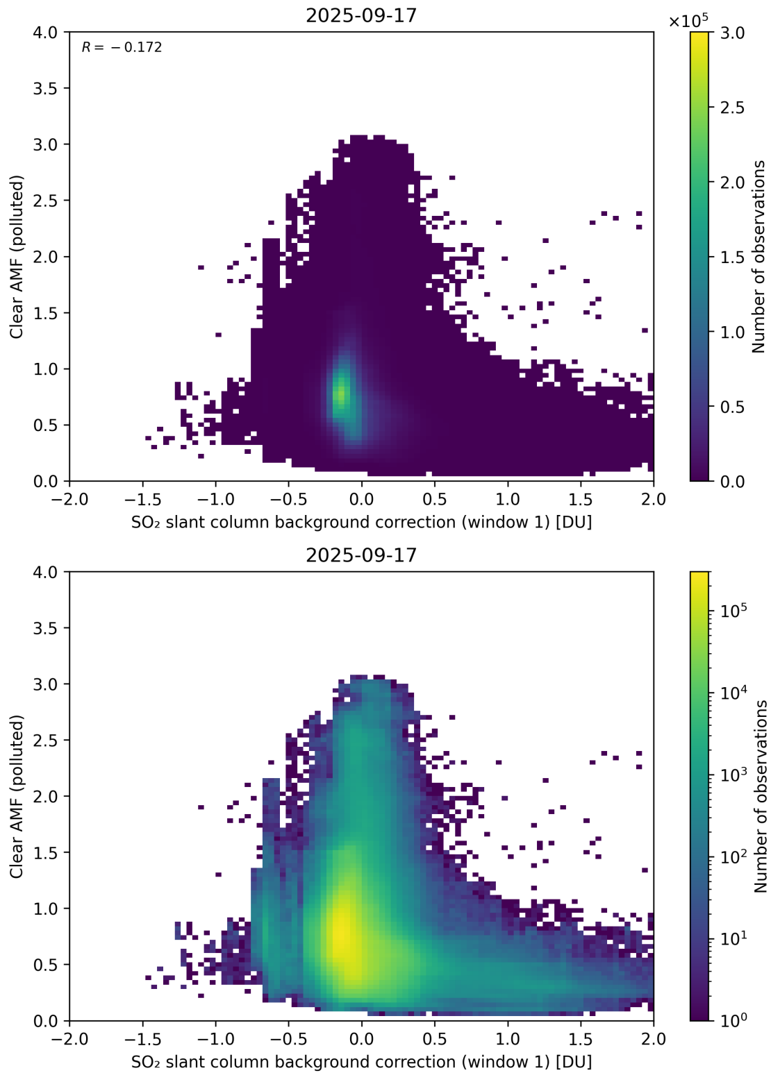
Figure 114: Scatter density plot of “SO 2 slant column background correction (window 1)” against “Clear AMF (polluted)” for 2025-09-16 to 2025-09-18.
