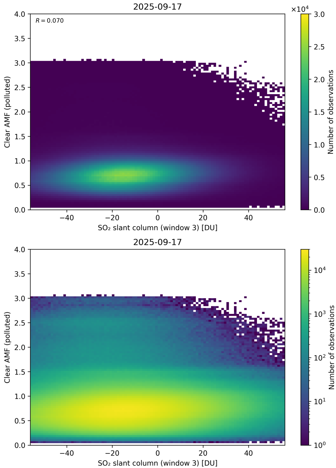
Figure 315: Scatter density plot of “SO 2 slant column (window 3)” against “Clear AMF (polluted)” for 2025-09-16 to 2025-09-18.
