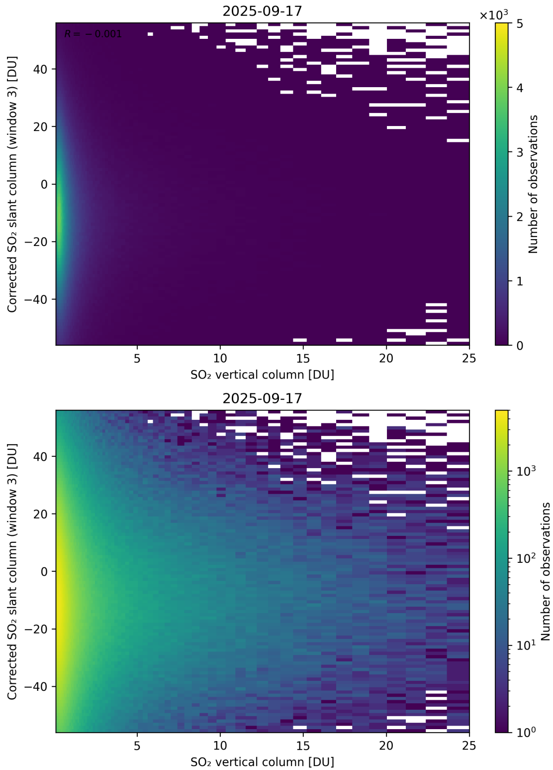
Figure 353: Scatter density plot of “SO 2 vertical column” against “Corrected SO 2 slant column (window 3)” for 2025-09-16 to 2025-09-18.
