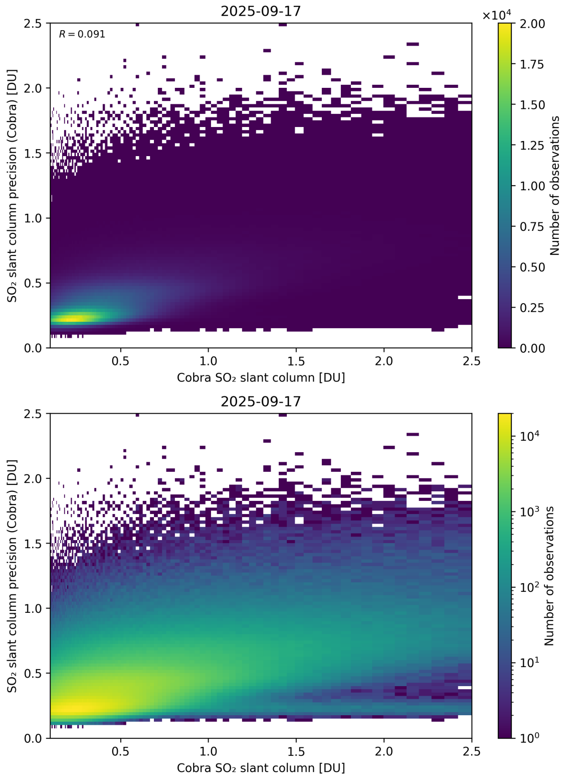
Figure 216: Scatter density plot of “Cobra SO 2 slant column” against “SO 2 slant column precision (Cobra)” for 2025-09-16 to 2025-09-18.
