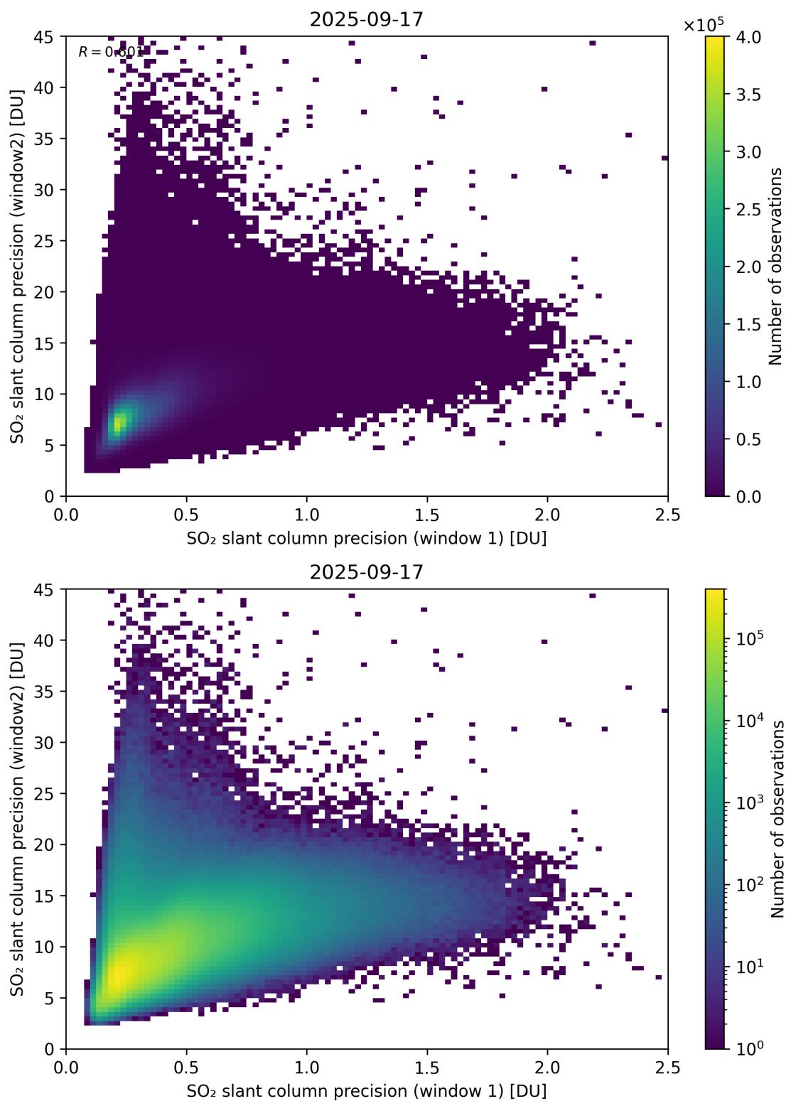
Figure 277: Scatter density plot of “SO 2 slant column precision (window 1)” against “SO 2 slant column precision (window 2)” for 2025-09-16 to 2025-09-18.
