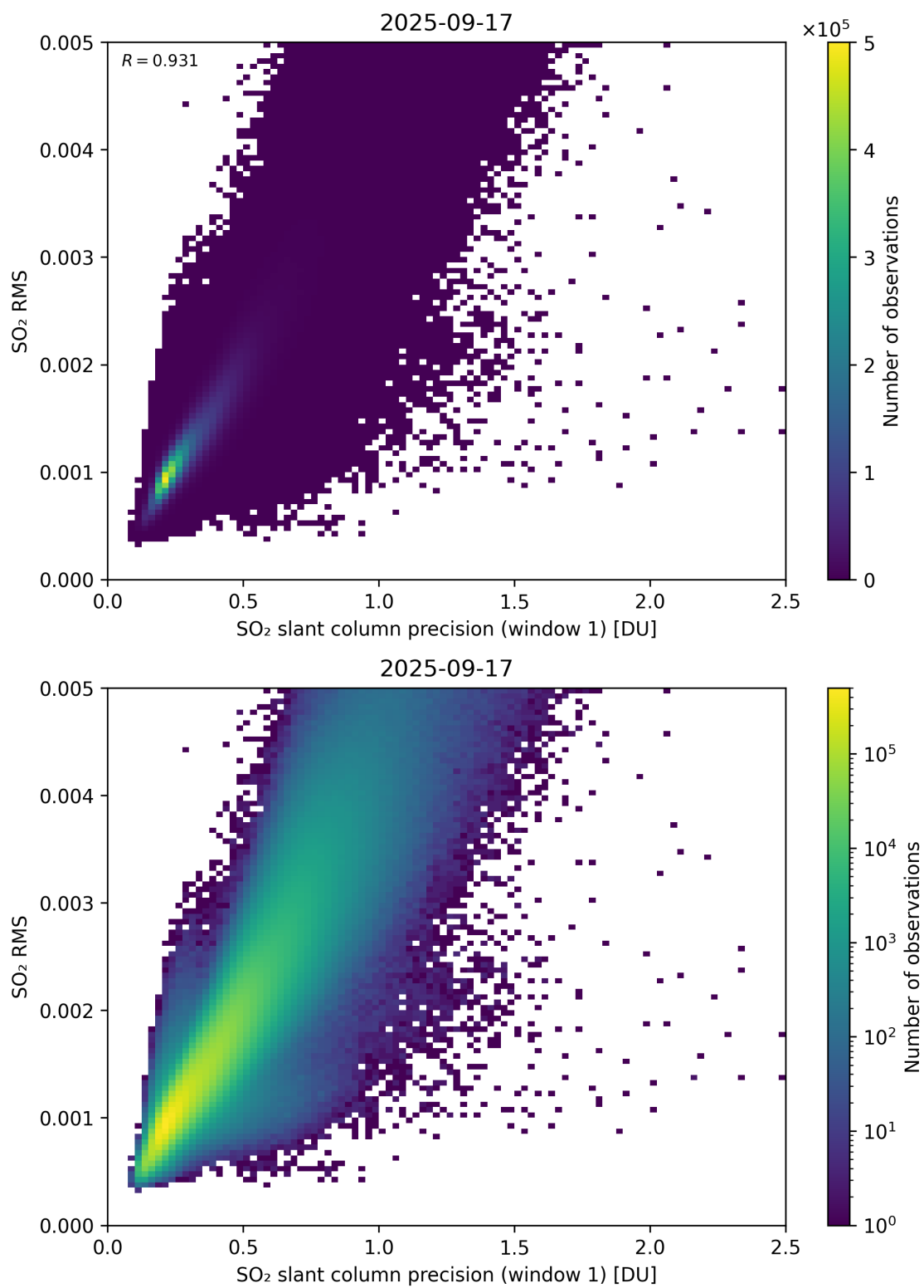
Figure 273: Scatter density plot of “SO 2 slant column precision (window 1)” against “SO 2 RMS” for 2025-09-16 to 2025-09-18.
