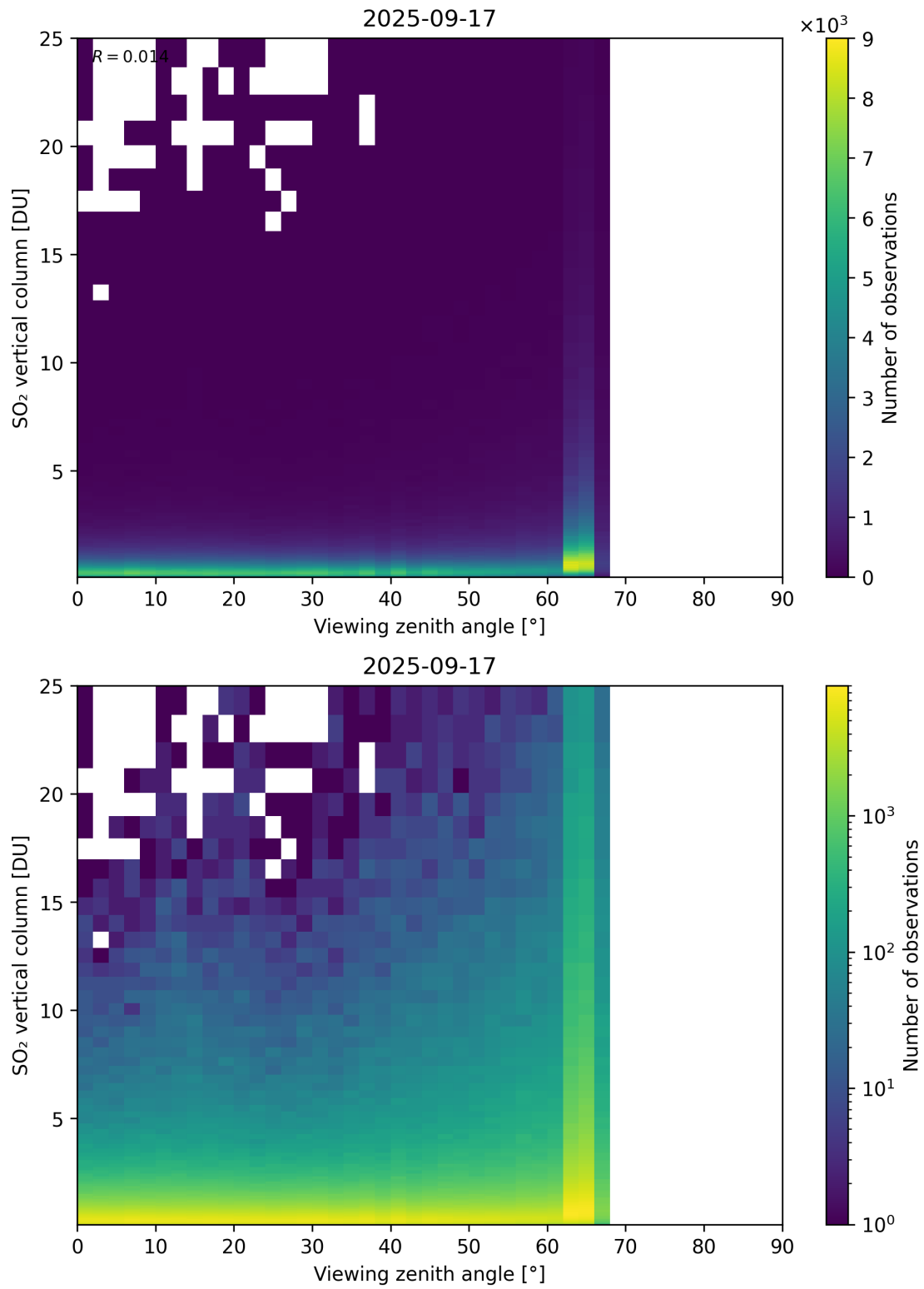
Figure 383: Scatter density plot of “Viewing zenith angle” against “SO 2 vertical column” for 2025-09-16 to 2025-09-18.
