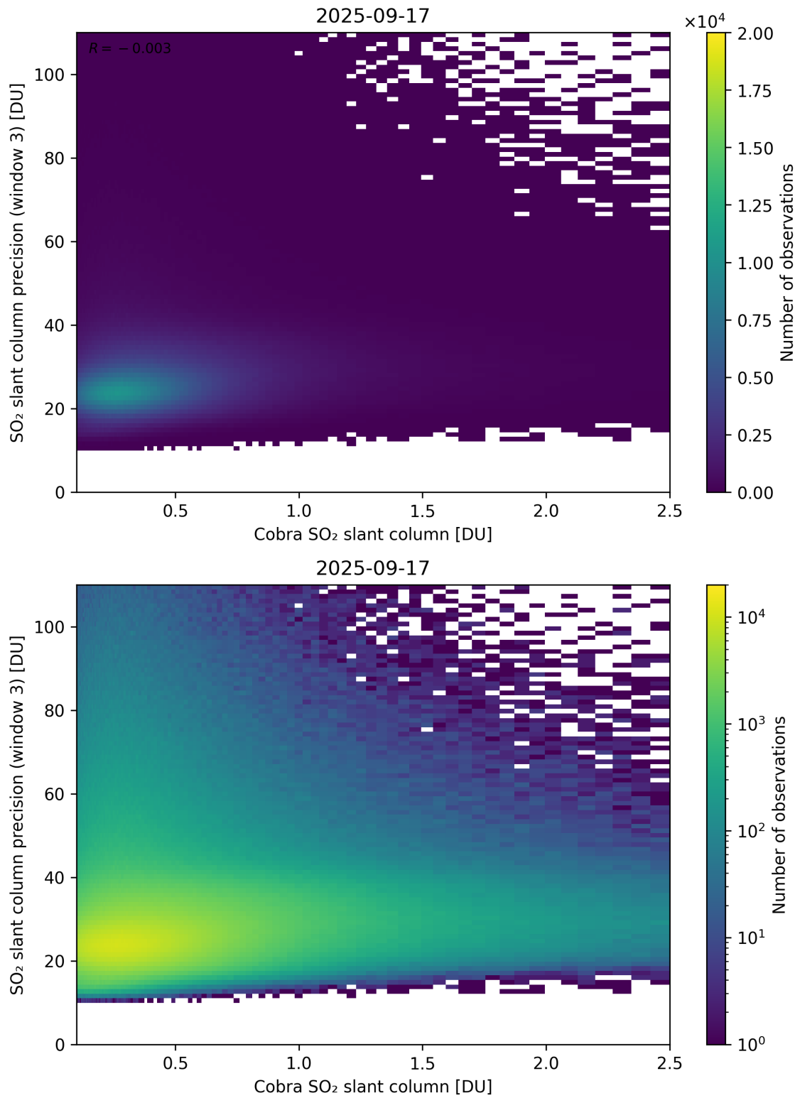
Figure 223: Scatter density plot of “Cobra SO 2 slant column” against “SO 2 slant column precision (window 3)” for 2025-09-16 to 2025-09-18.
