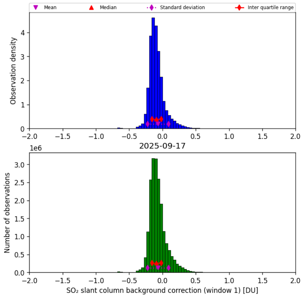
Figure 66: Histogram of “SO 2 slant column background correction (window 1)” for 2025-09-16 to 2025-09-18
