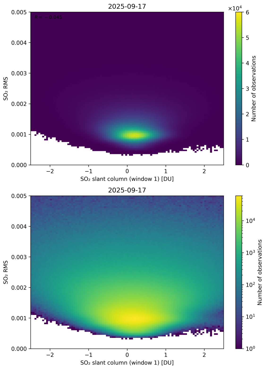
Figure 267: Scatter density plot of “SO 2 slant column (window 1)” against “SO 2 RMS” for 2025-09-16 to 2025-09-18.
