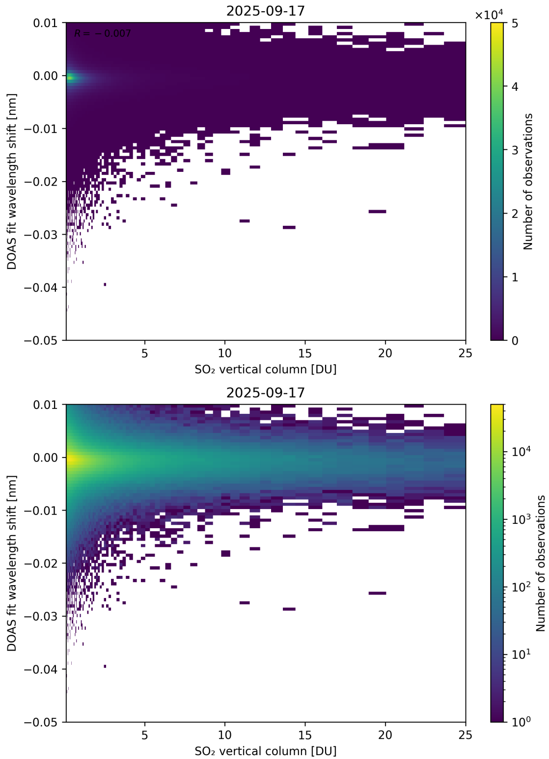
Figure 326: Scatter density plot of “SO 2 vertical column” against “DOAS fit wavelength shift” for 2025-09-16 to 2025-09-18.
