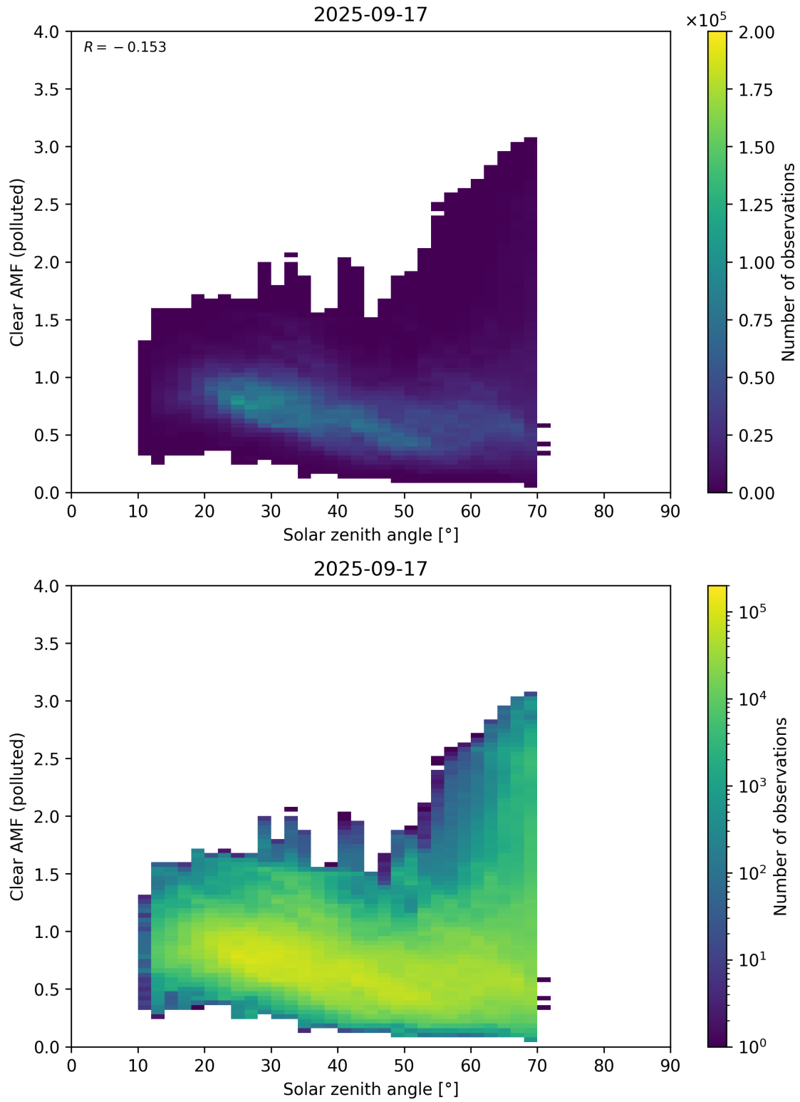
Figure 178: Scatter density plot of “Solar zenith angle” against “Clear AMF (polluted)” for 2025-09-16 to 2025-09-18.
