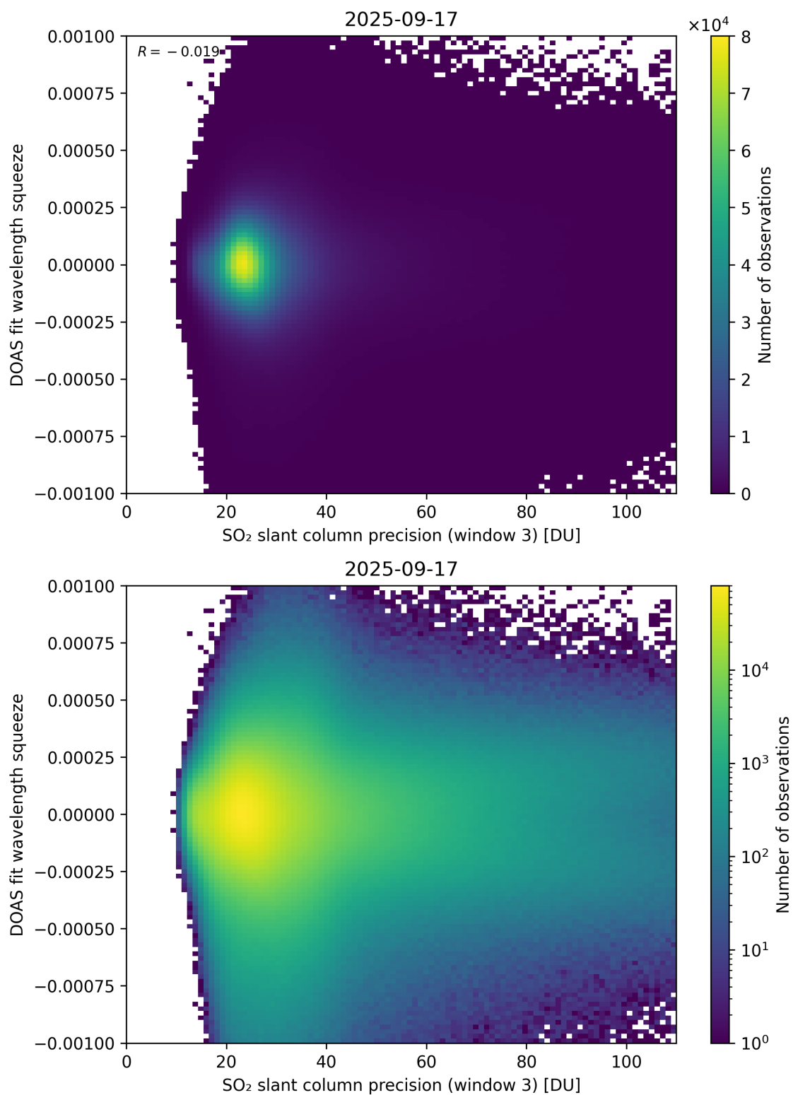
Figure 309: Scatter density plot of “SO 2 slant column precision (window 3)” against “DOAS fit wavelength squeeze” for 2025-09-16 to 2025-09-18.
