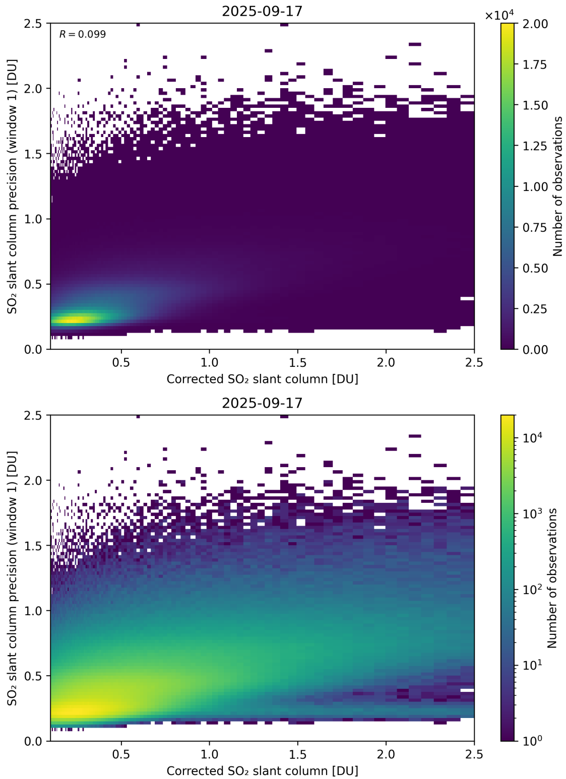
Figure 238: Scatter density plot of “Corrected SO 2 slant column” against “SO 2 slant column precision (window 1)” for 2025-09-16 to 2025-09-18.
