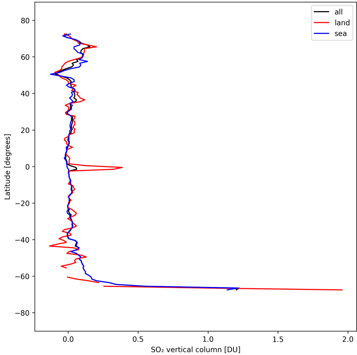
Figure 32: Zonal average of “SO 2 vertical column” for 2025-09-16 to 2025-09-18.
