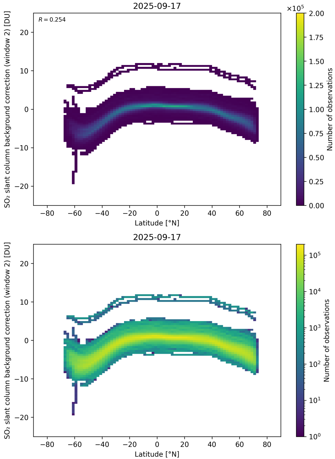
Figure 151: Scatter density plot of “Latitude” against “SO 2 slant column background correction (window 2)” for 2025-09-16 to 2025-09-18.
