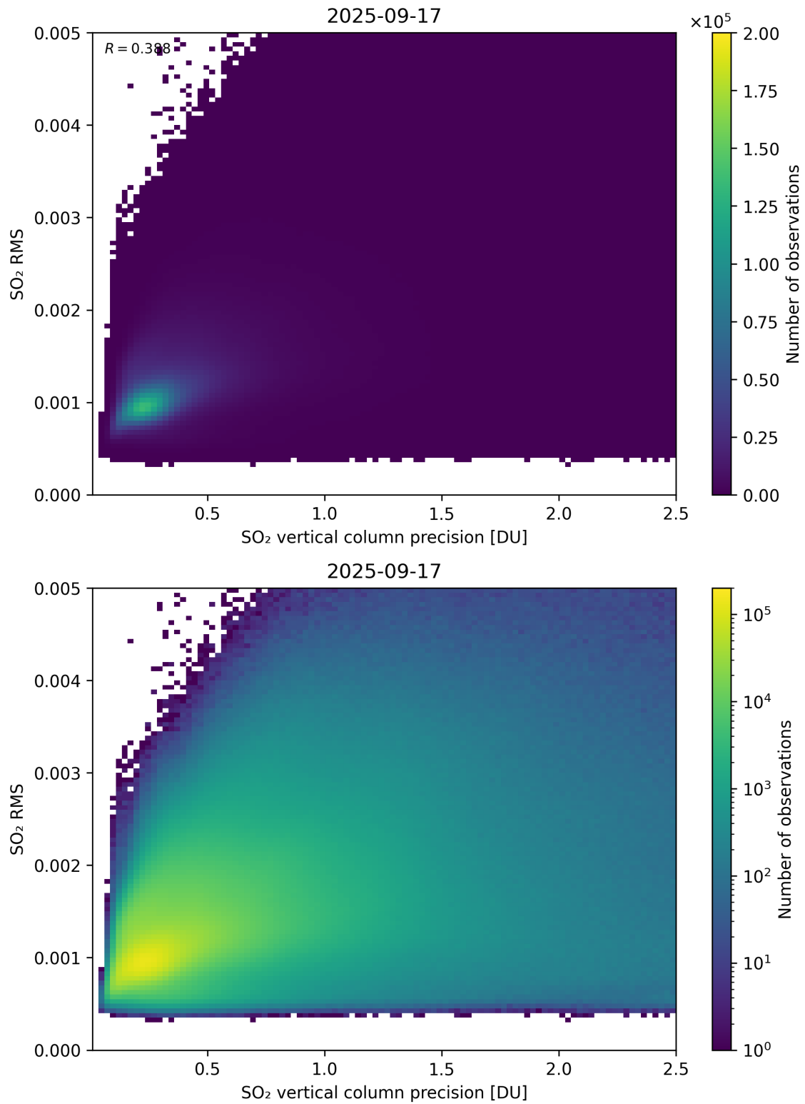
Figure 334: Scatter density plot of “SO 2 vertical column precision” against “SO 2 RMS” for 2025-09-16 to 2025-09-18.
