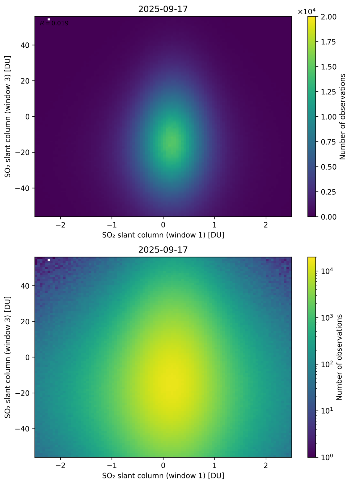
Figure 287: Scatter density plot of “SO 2 slant column (window 1)” against “SO 2 slant column (window 3)” for 2025-09-16 to 2025-09-18.
