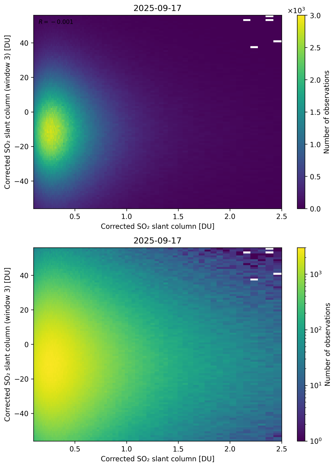
Figure 236: Scatter density plot of “Corrected SO 2 slant column” against “Corrected SO 2 slant column (window 3)” for 2025-09-16 to 2025-09-18.
