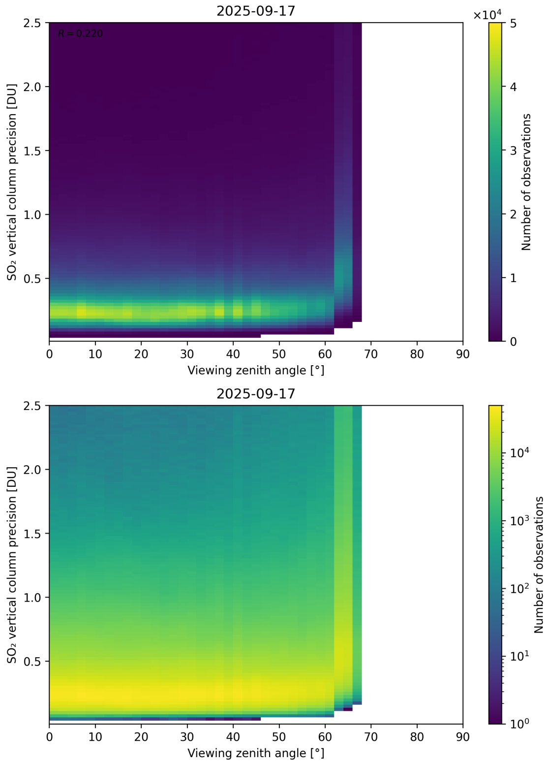
Figure 384: Scatter density plot of “Viewing zenith angle” against “SO 2 vertical column precision” for 2025-09-16 to 2025-09-18.
