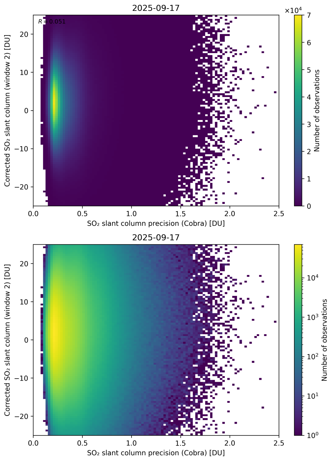
Figure 206: Scatter density plot of “SO 2 slant column precision (Cobra)” against “Corrected SO 2 slant column (window 2)” for 2025-09-16 to 2025-09-18.
