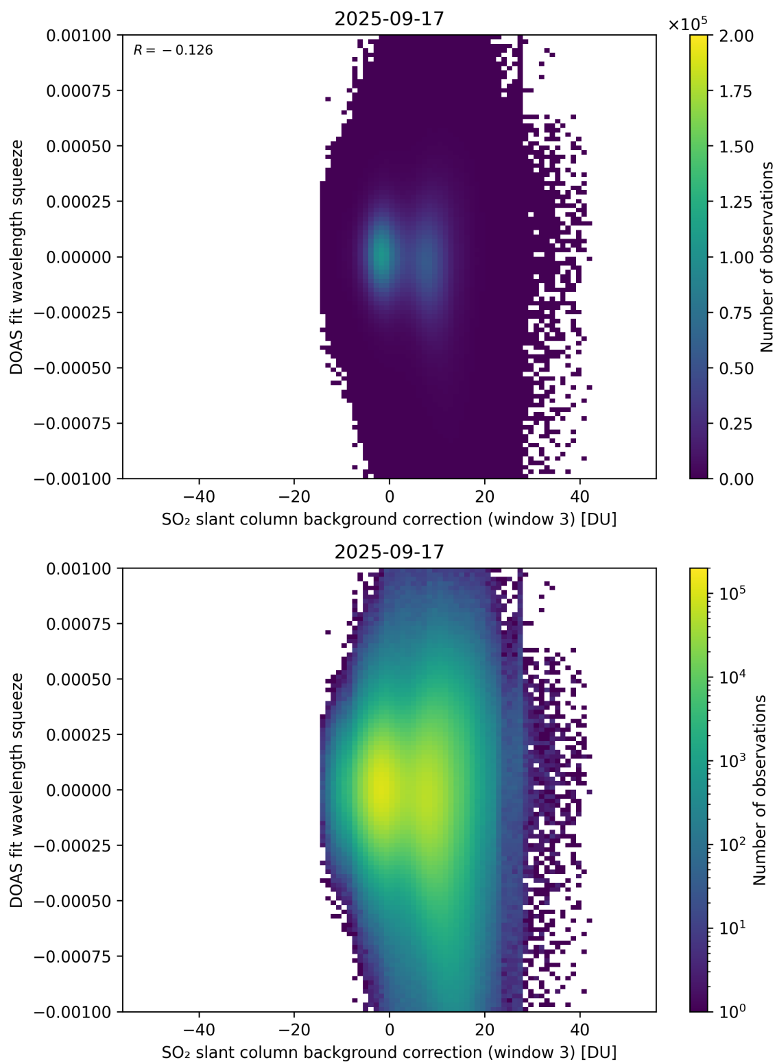
Figure 133: Scatter density plot of “SO 2 slant column background correction (window 3)” against “DOAS fit wavelength squeeze” for 2025-09-16 to 2025-09-18.
