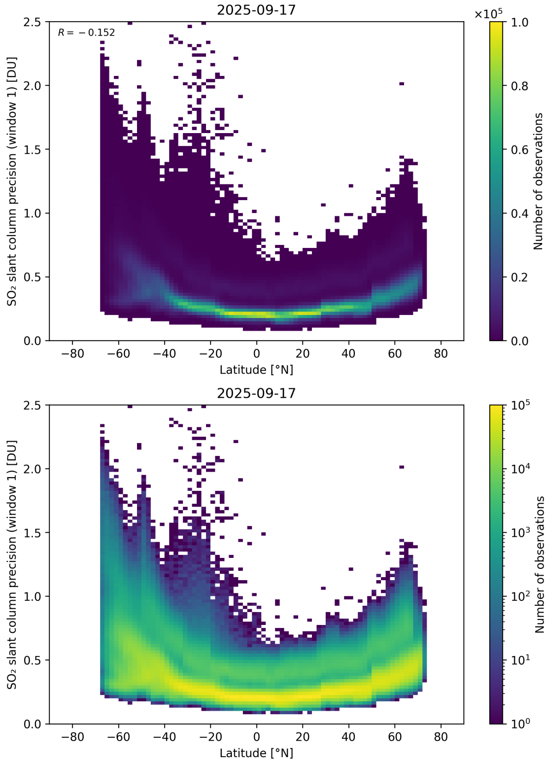
Figure 163: Scatter density plot of “Latitude” against “SO 2 slant column precision (window 1)” for 2025-09-16 to 2025-09-18.
