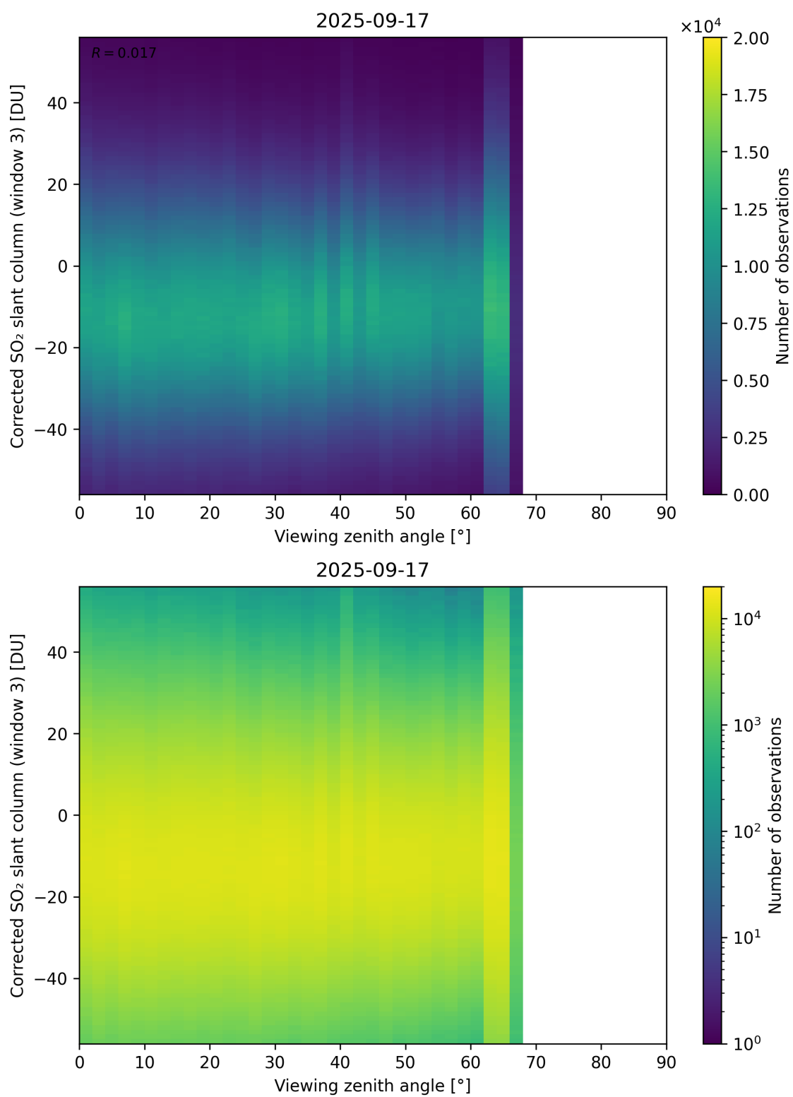
Figure 375: Scatter density plot of “Viewing zenith angle” against “Corrected SO 2 slant column (window 3)” for 2025-09-16 to 2025-09-18.
