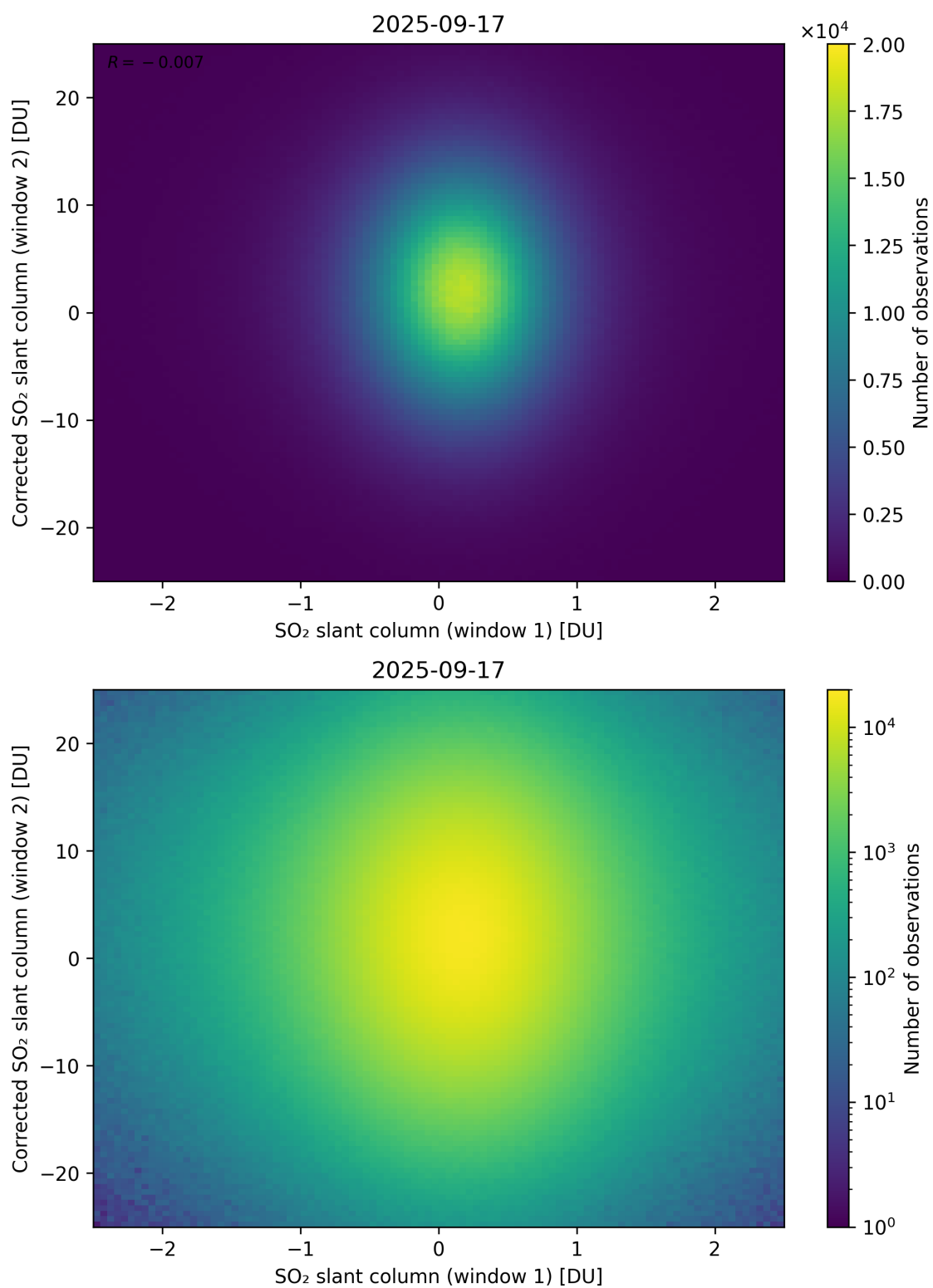
Figure 283: Scatter density plot of “SO 2 slant column (window 1)” against “Corrected SO 2 slant column (window 2)” for 2025-09-16 to 2025-09-18.
