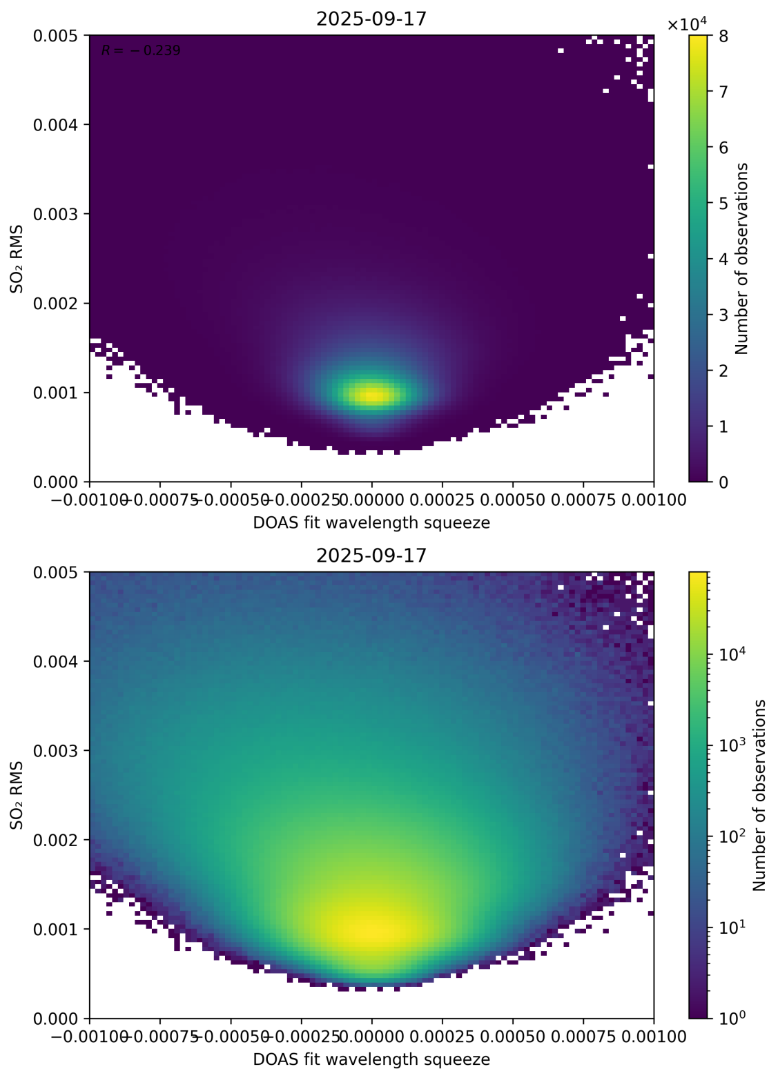
Figure 143: Scatter density plot of “DOAS fit wavelength squeeze” against “SO 2 RMS” for 2025-09-16 to 2025-09-18.
