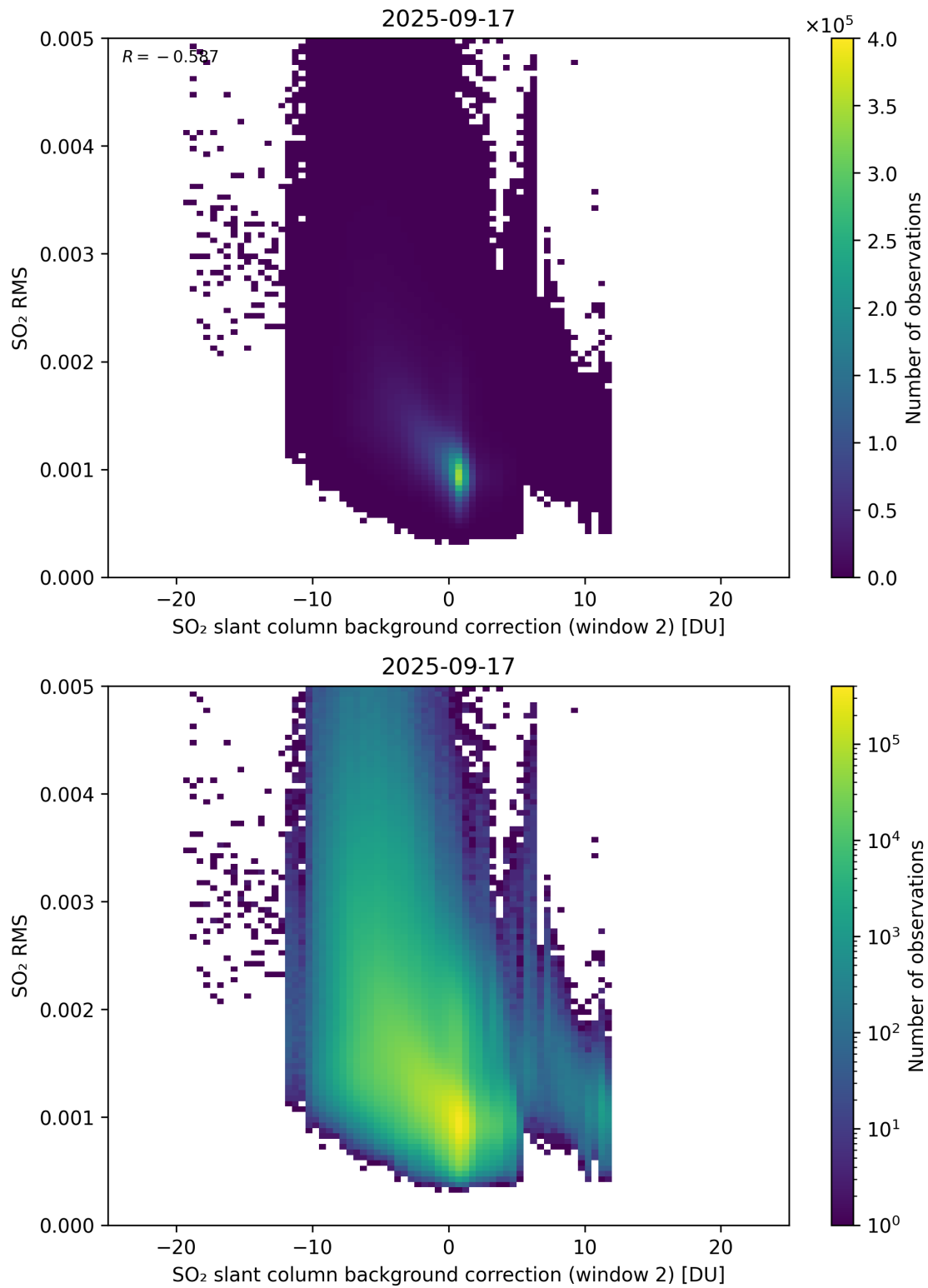
Figure 125: Scatter density plot of “SO 2 slant column background correction (window 2)” against “SO 2 RMS” for 2025-09-16 to 2025-09-18.
