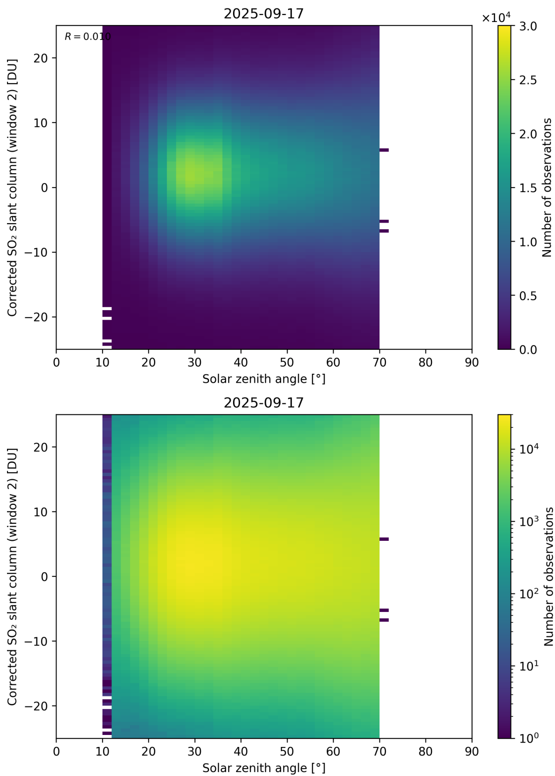
Figure 182: Scatter density plot of “Solar zenith angle” against “Corrected SO 2 slant column (window 2)” for 2025-09-16 to 2025-09-18.
