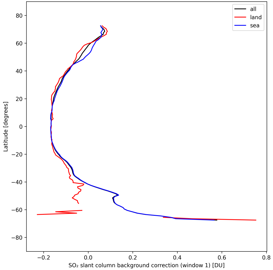
Figure 40: Zonal average of “SO 2 slant column background correction (window 1)” for 2025-09-16 to 2025-09-18.
