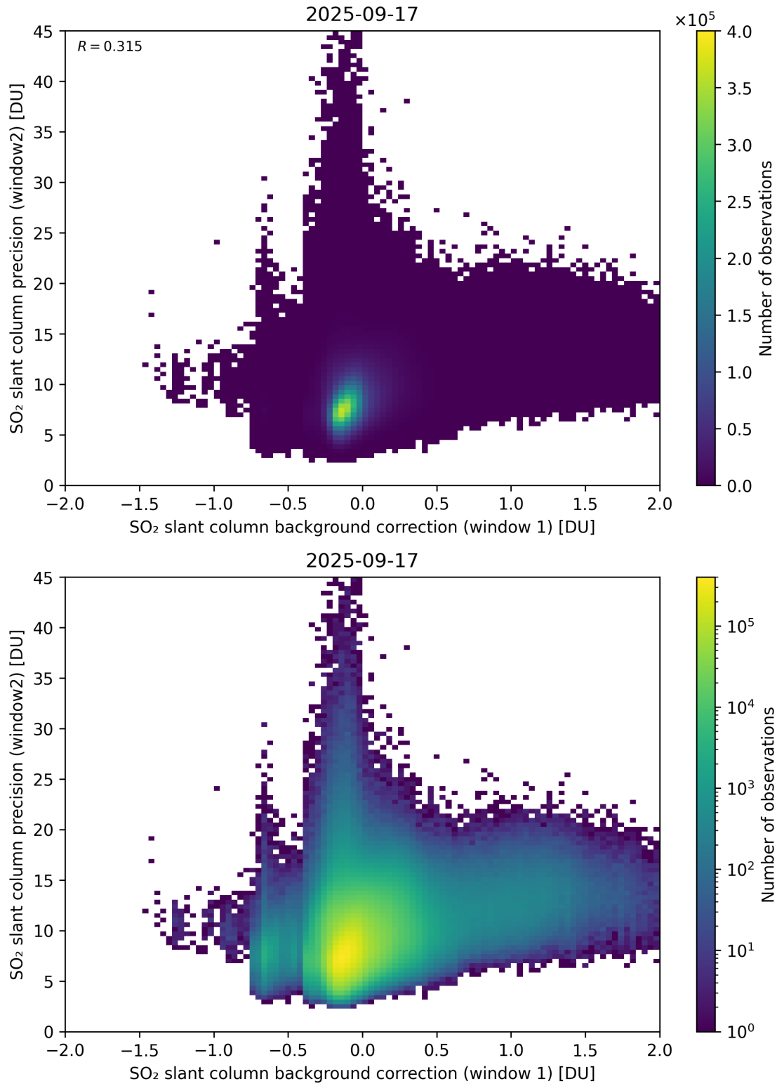
Figure 117: Scatter density plot of “SO 2 slant column background correction (window 1)” against “SO 2 slant column precision (window2)” for 2025-09-16 to 2025-09-18.
