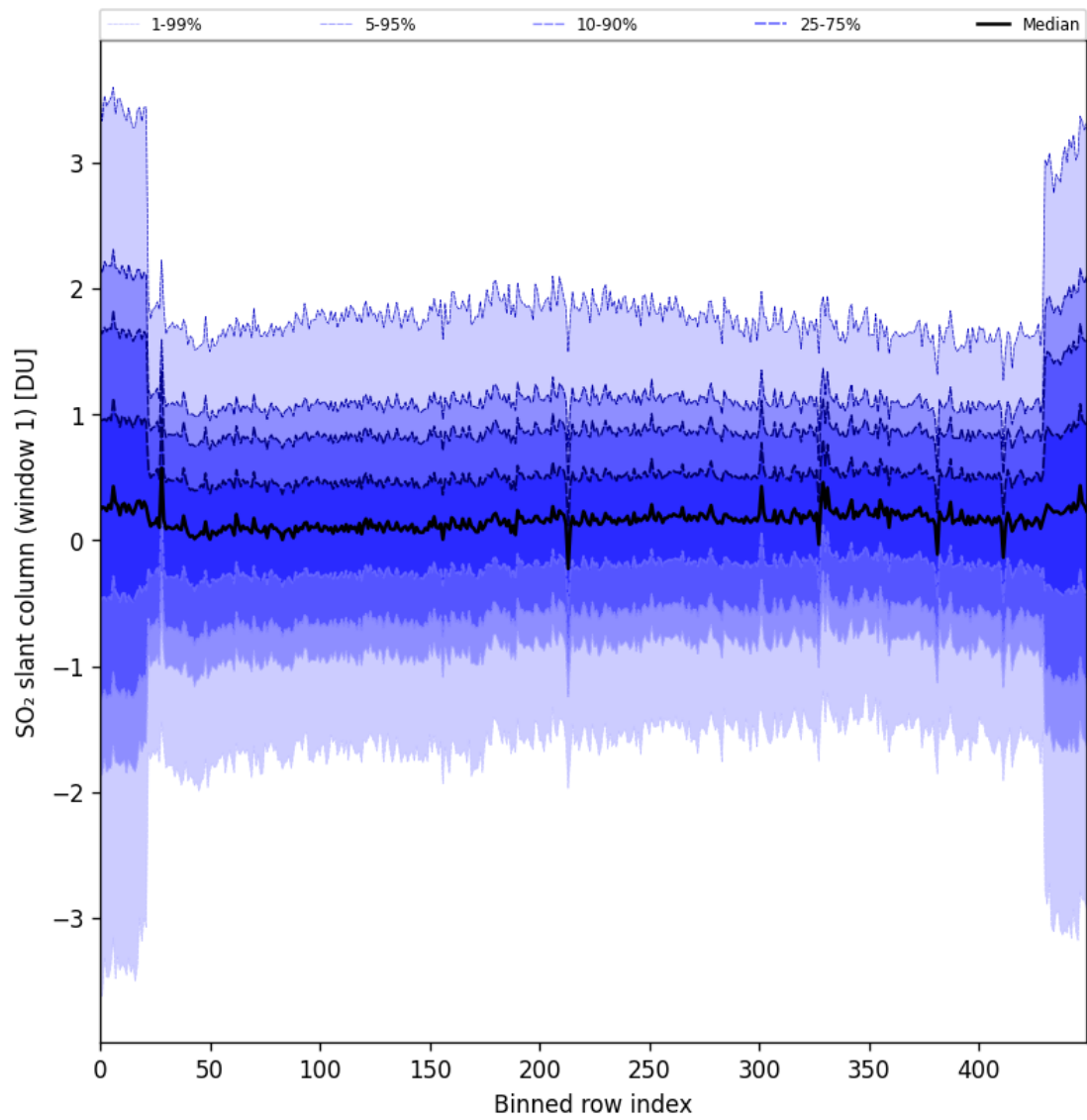
Figure 89: Along track statistics of “SO 2 slant column (window 1)” for 2025-09-16 to 2025-09-18
