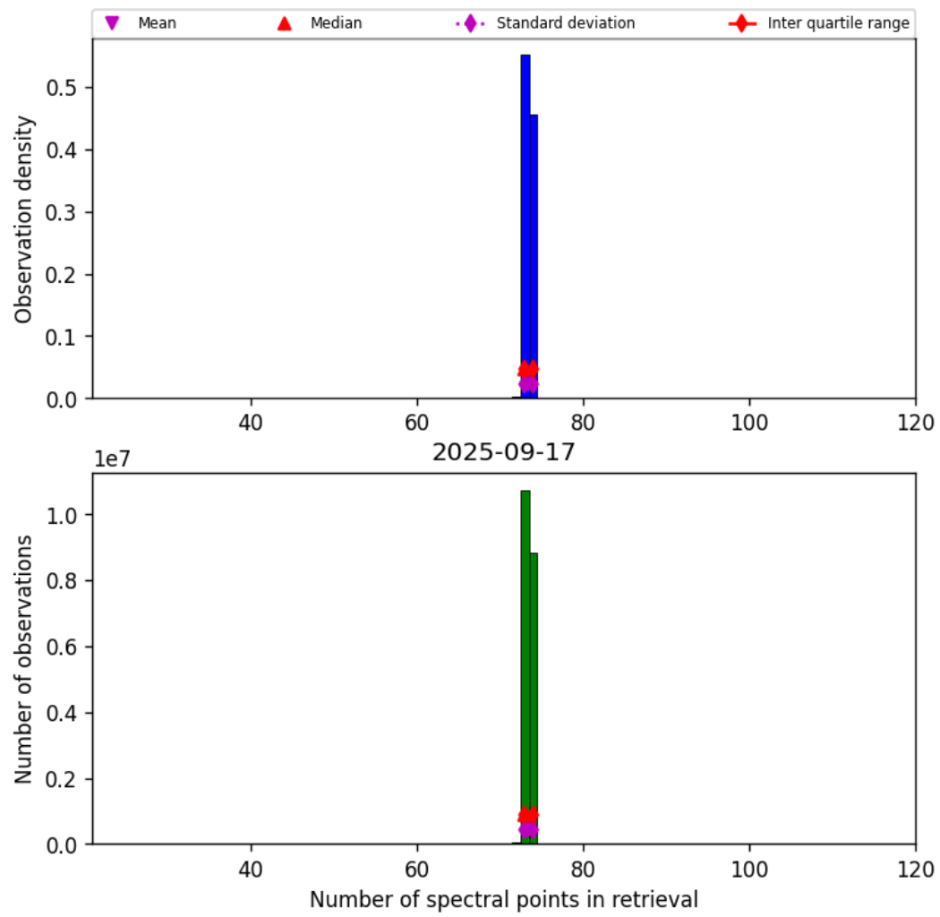
Figure 82: Histogram of “Number of spectral points in retrieval” for 2025-09-16 to 2025-09-18
