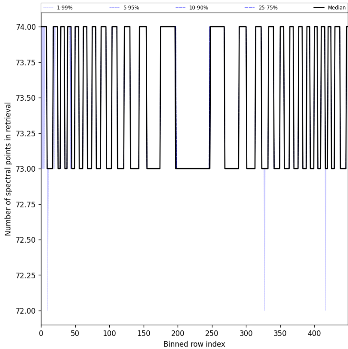
Figure 108: Along track statistics of “Number of spectral points in retrieval” for 2025-09-16 to 2025-09-18
