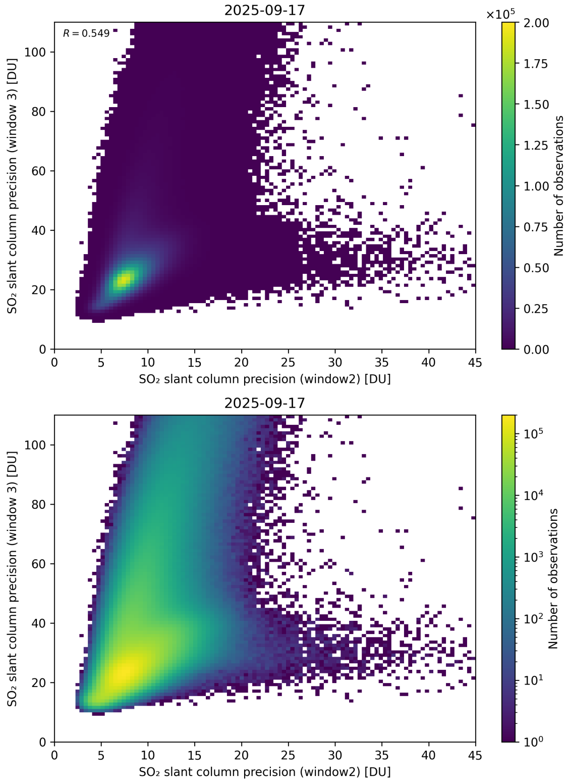
Figure 300: Scatter density plot of “SO 2 slant column precision (window2)” against “SO 2 slant column precision (window 3)” for 2025-09-16 to 2025-09-18.
