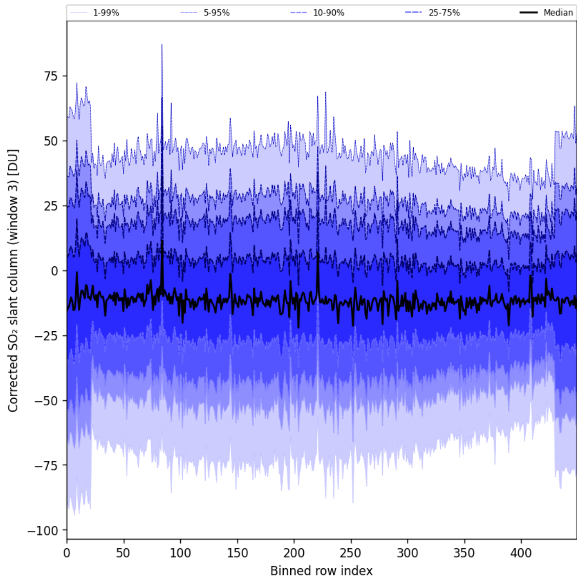
Figure 99: Along track statistics of “Corrected SO 2 slant column (window 3)” for 2025-09-16 to 2025-09-18
