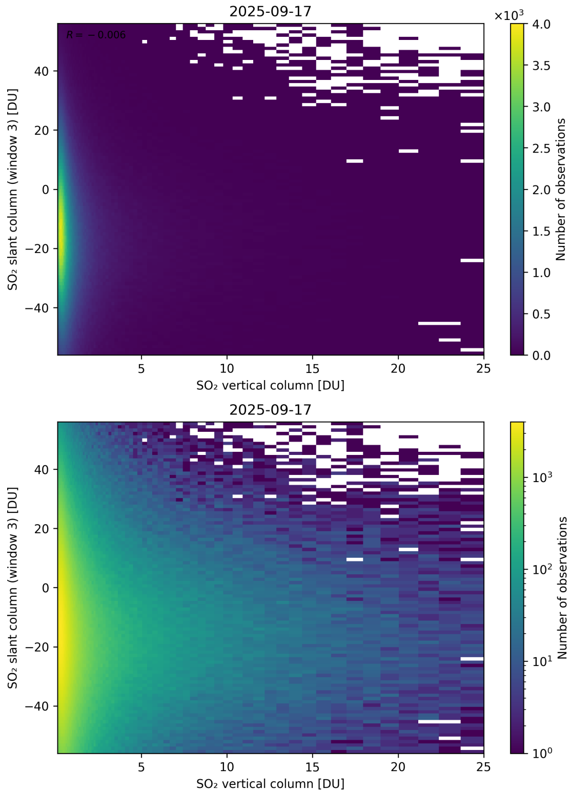
Figure 357: Scatter density plot of “SO 2 vertical column” against “SO 2 slant column (window 3)” for 2025-09-16 to 2025-09-18.
