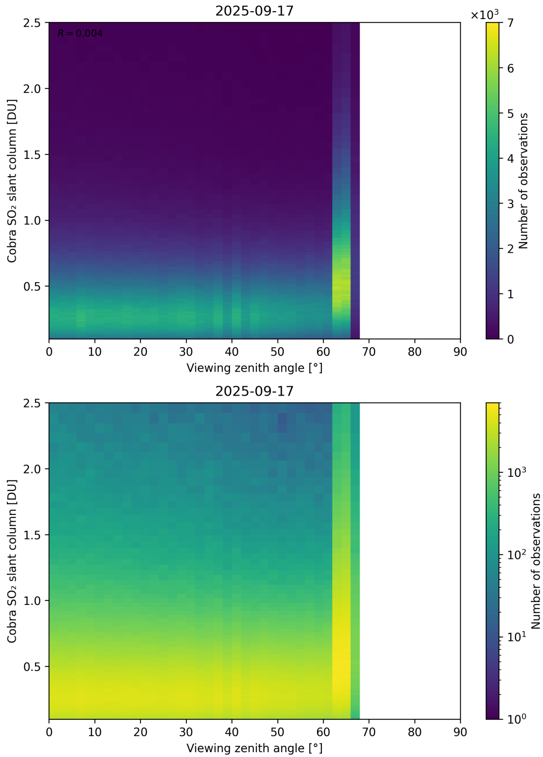
Figure 371: Scatter density plot of “Viewing zenith angle” against “Cobra SO 2 slant column” for 2025-09-16 to 2025-09-18.
