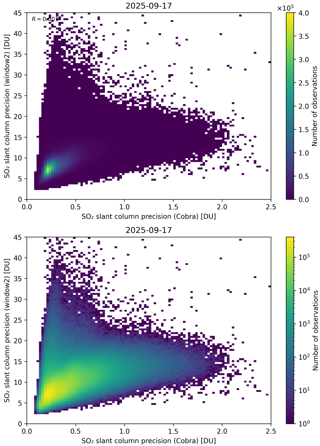
Figure 210: Scatter density plot of “SO 2 slant column precision (Cobra)” against “SO 2 slant column precision (window2)” for 2025-09-16 to 2025-09-18.
