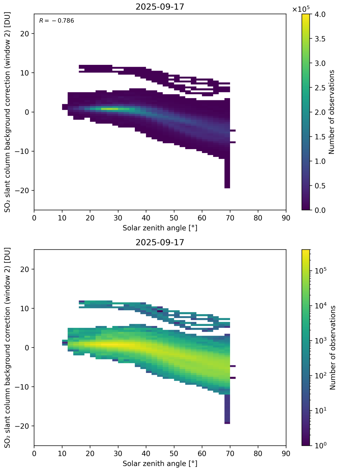
Figure 172: Scatter density plot of “Solar zenith angle” against “SO 2 slant column background correction (window 2)” for 2025-09-16 to 2025-09-18.
