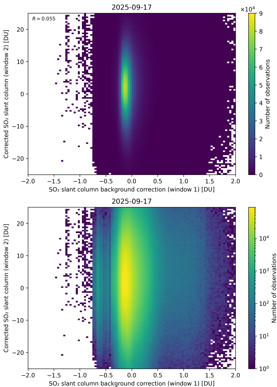
Figure 115: Scatter density plot of “SO 2 slant column background correction (window 1)” against “Corrected SO 2 slant column (window 2)” for 2025-09-16 to 2025-09-18.
