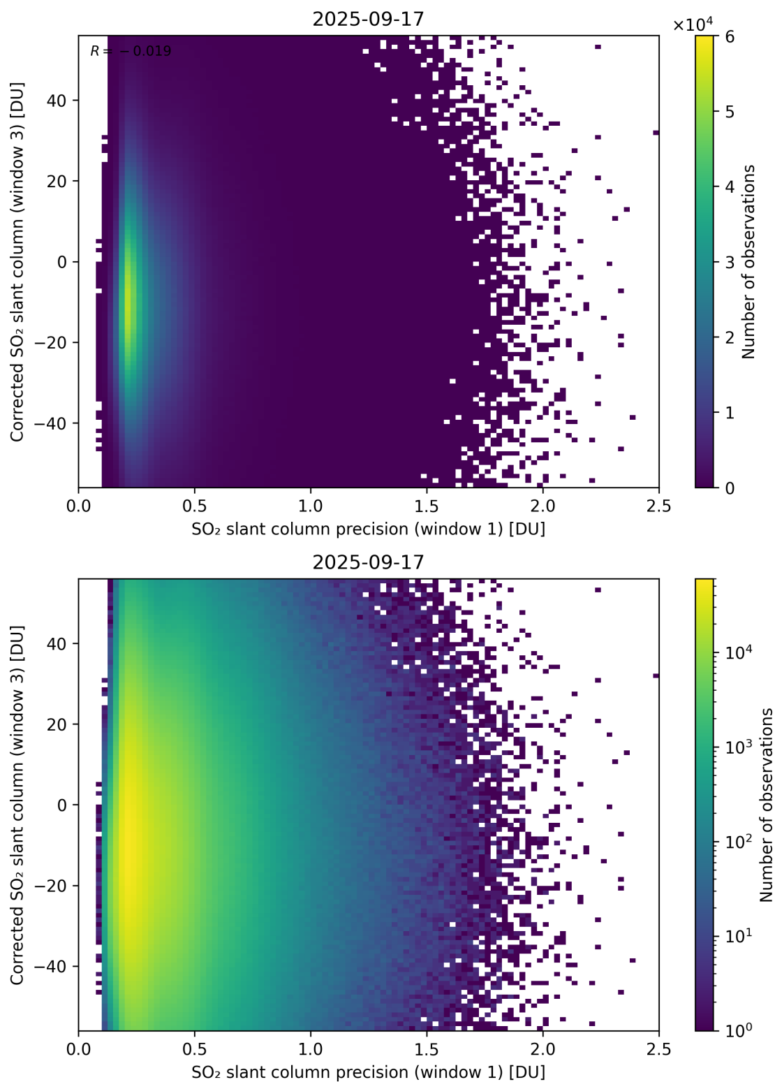
Figure 276: Scatter density plot of “SO 2 slant column precision (window 1)” against “Corrected SO 2 slant column (window 3)” for 2025-09-16 to 2025-09-18.
