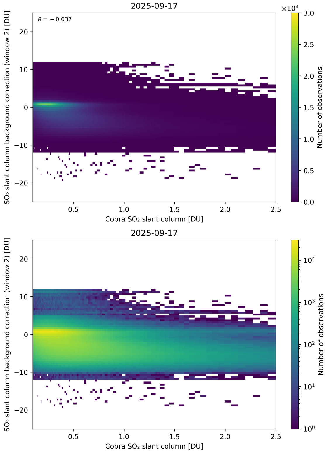
Figure 194: Scatter density plot of “Cobra SO 2 slant column” against “SO 2 slant column background correction (window 2)” for 2025-09-16 to 2025-09-18.
