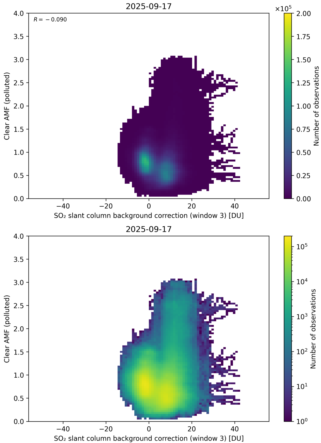
Figure 135: Scatter density plot of “SO 2 slant column background correction (window 3)” against “Clear AMF (polluted)” for 2025-09-16 to 2025-09-18.
