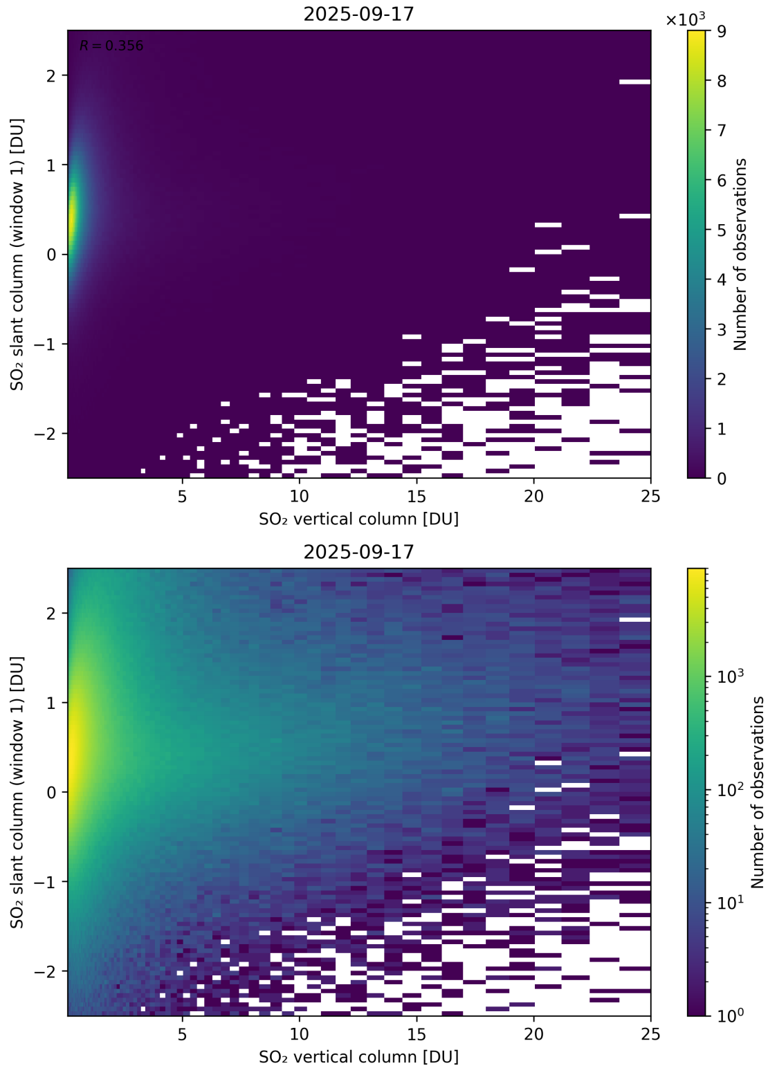
Figure 354: Scatter density plot of “SO 2 vertical column” against “SO 2 slant column (window 1)” for 2025-09-16 to 2025-09-18.
