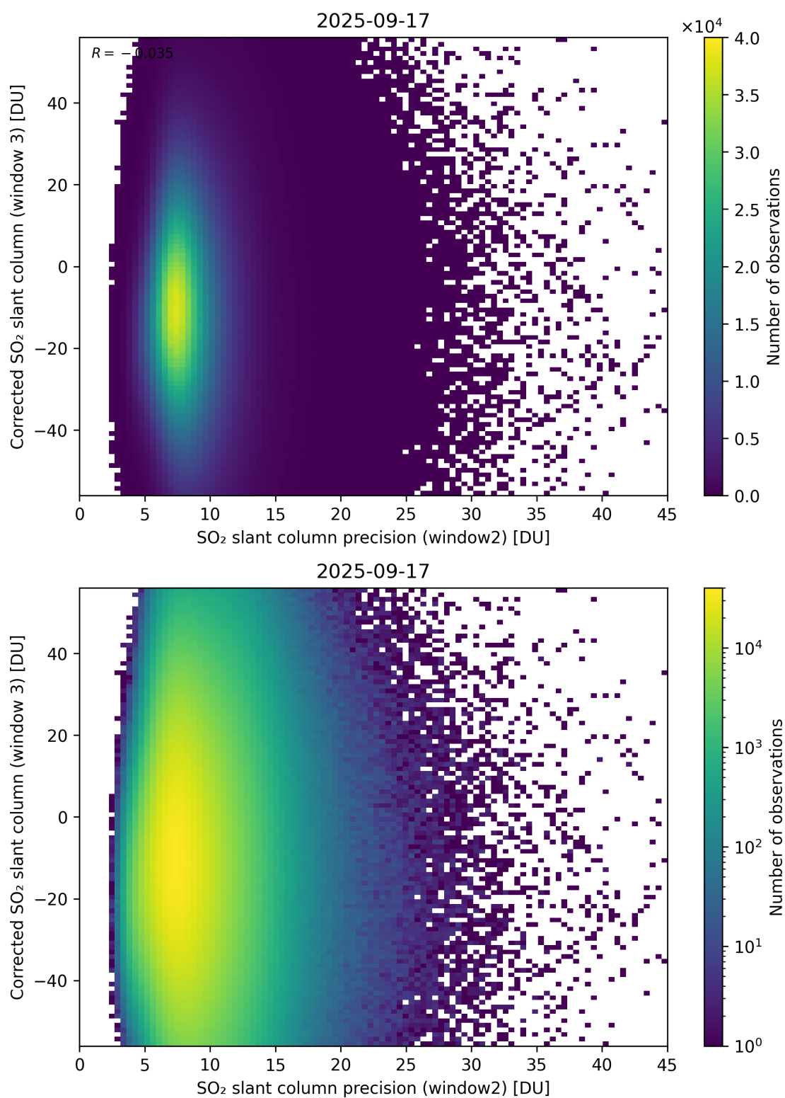
Figure 298: Scatter density plot of “SO 2 slant column precision (window2)” against “Corrected SO 2 slant column (window 3)” for 2025-09-16 to 2025-09-18.
