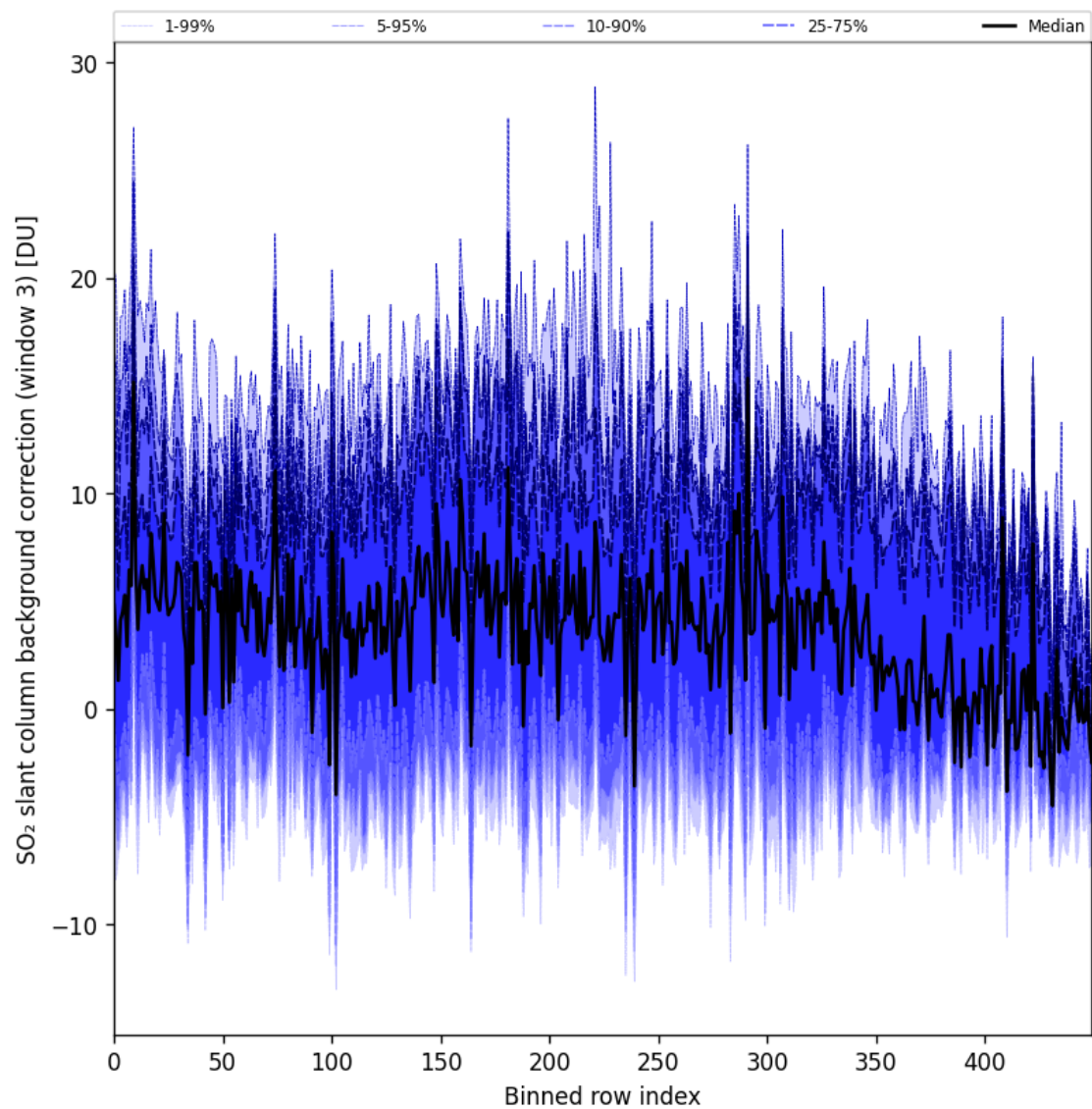
Figure 100: Along track statistics of “SO 2 slant column background correction (window 3)” for 2025-09-16 to 2025-09-18
