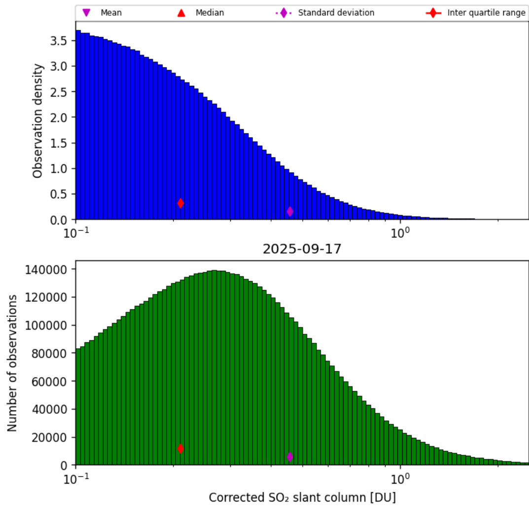
Figure 60: Histogram of "Corrected SO 2 slant column" for 2025-09-16 to 2025-09-18
