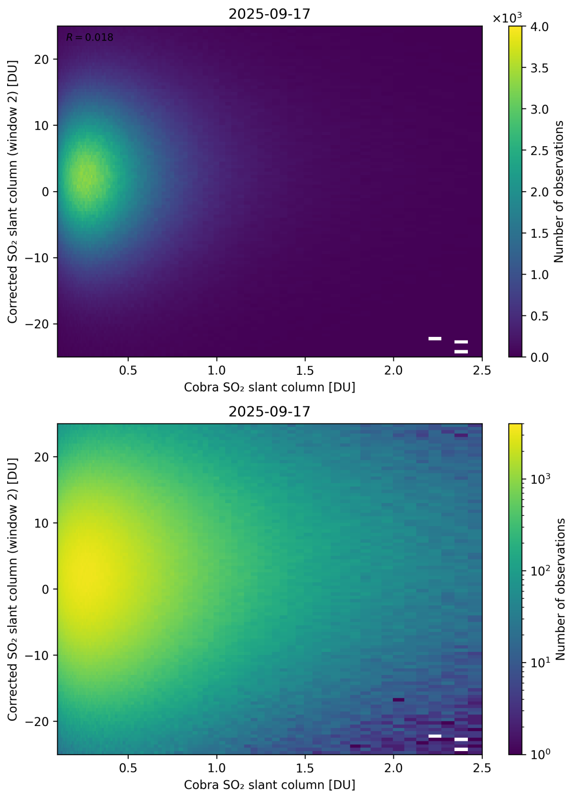
Figure 217: Scatter density plot of “Cobra SO 2 slant column” against “Corrected SO 2 slant column (window 2)” for 2025-09-16 to 2025-09-18.
