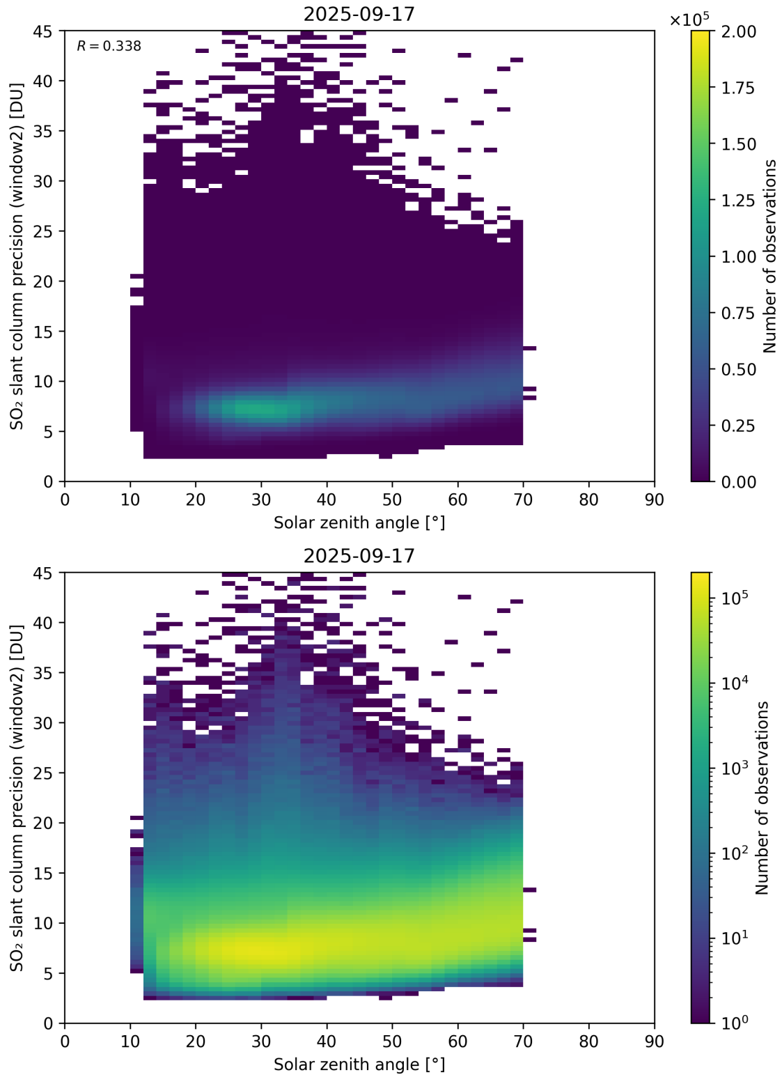
Figure 186: Scatter density plot of “Solar zenith angle” against “SO 2 slant column precision (window2)” for 2025-09-16 to 2025-09-18.
