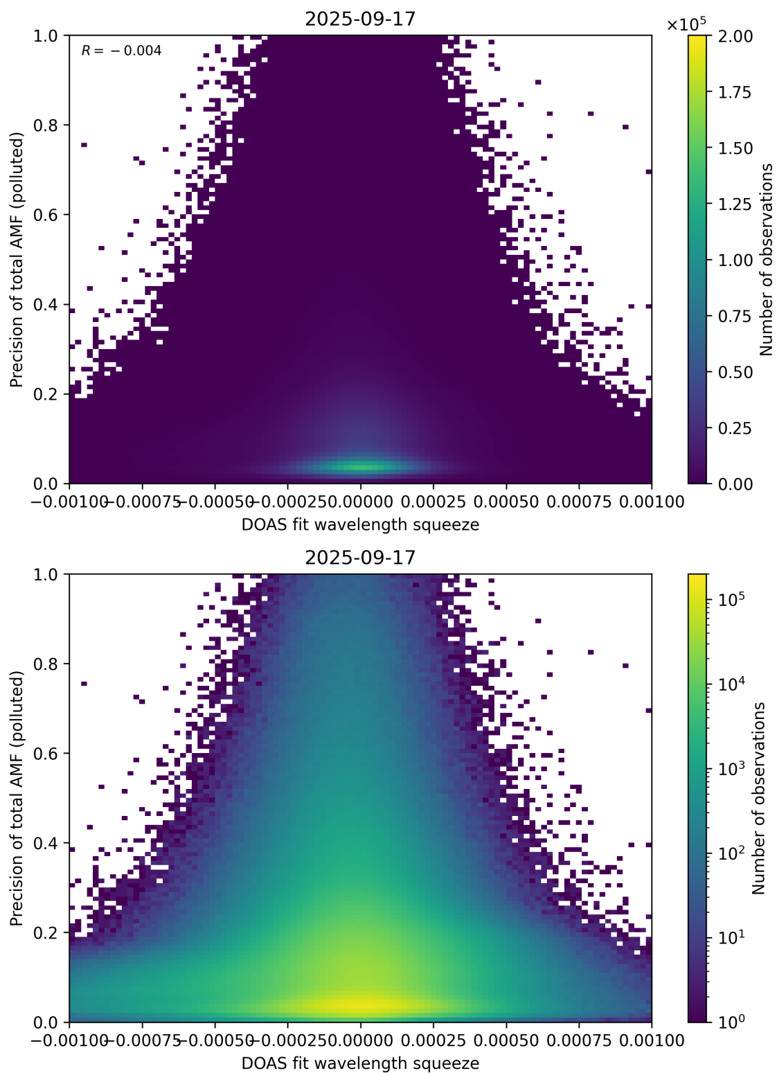
Figure 146: Scatter density plot of “DOAS fit wavelength squeeze” against “Precision of total AMF (polluted)” for 2025-09-16 to 2025-09-18.
