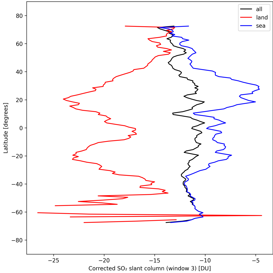
Figure 47: Zonal average of “Corrected SO 2 slant column (window 3)” for 2025-09-16 to 2025-09-18.
