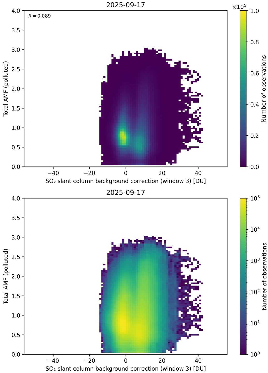
Figure 136: Scatter density plot of “SO 2 slant column background correction (window 3)” against “Total AMF (polluted)” for 2025-09-16 to 2025-09-18.
