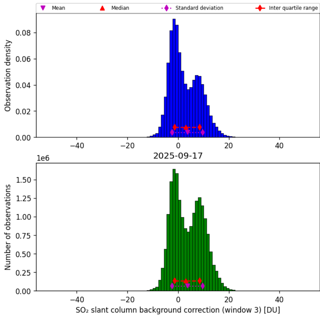
Figure 74: Histogram of “SO 2 slant column background correction (window 3)” for 2025-09-16 to 2025-09-18
