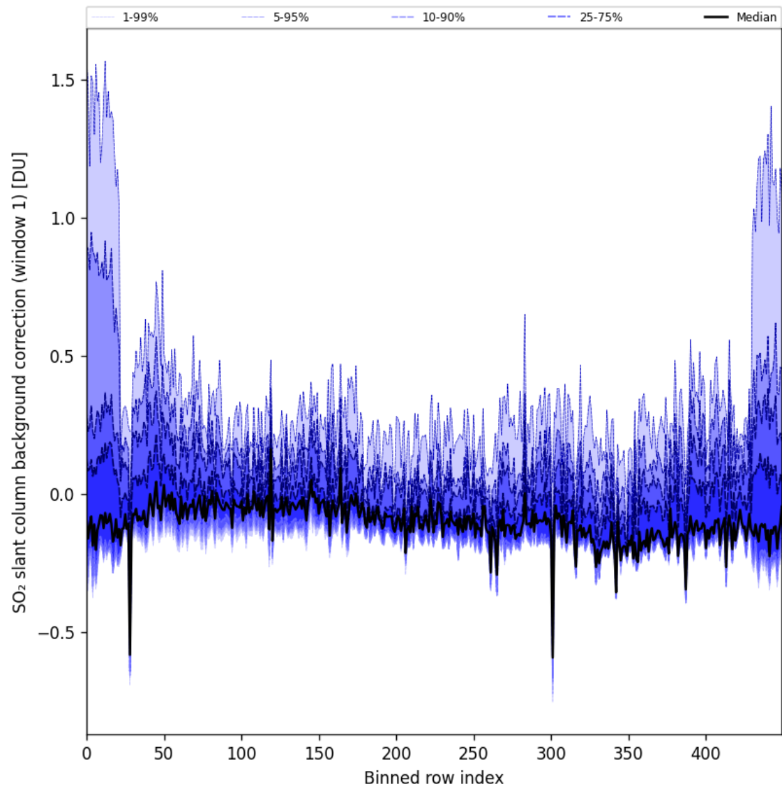
Figure 92: Along track statistics of “SO 2 slant column background correction (window 1)” for 2025-09-16 to 2025-09-18
