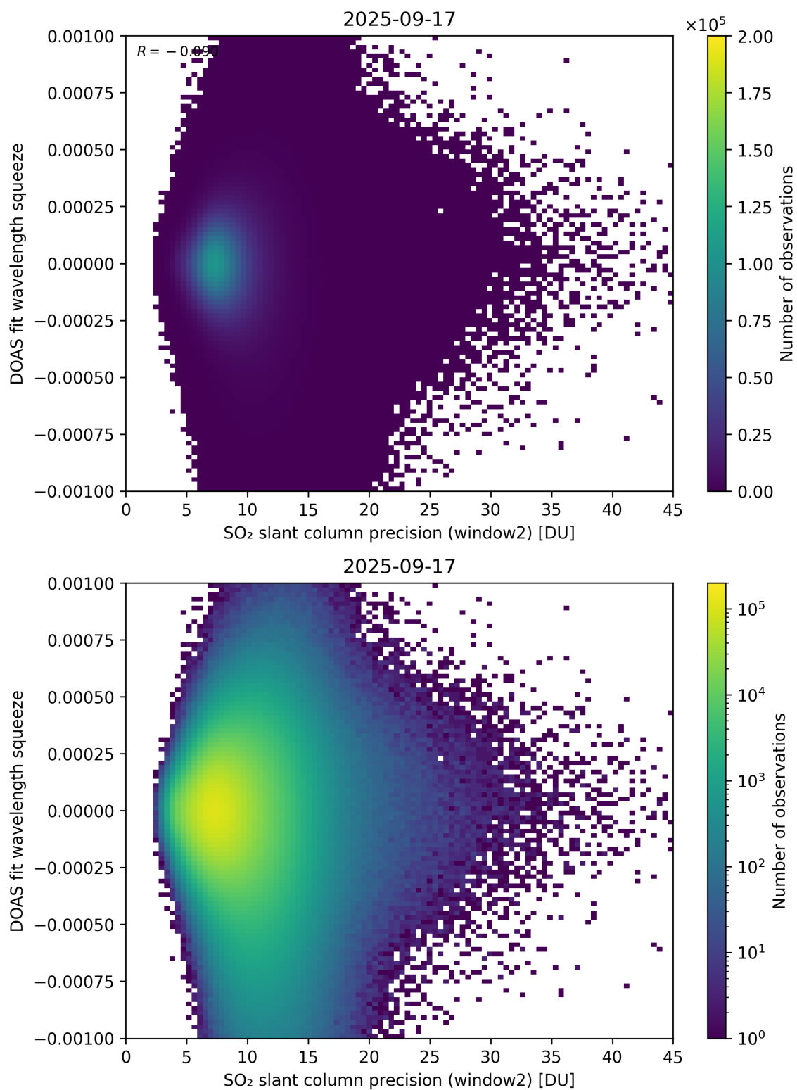
Figure 294: Scatter density plot of “SO 2 slant column precision (window2)” against “DOAS fit wavelength squeeze” for 2025-09-16 to 2025-09-18.
