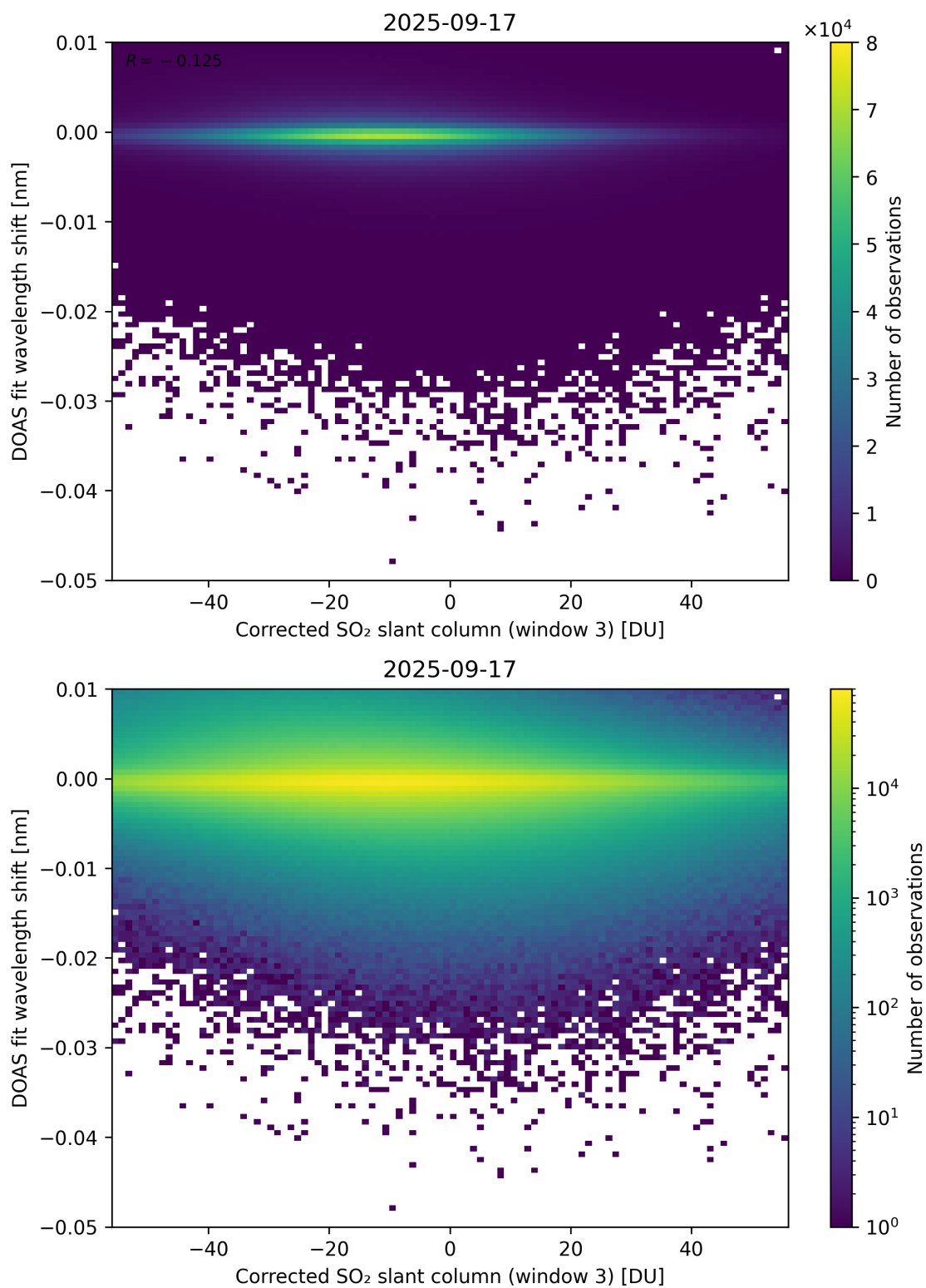
Figure 256: Scatter density plot of “Corrected SO 2 slant column (window 3)” against “DOAS fit wavelength shift” for 2025-09-16 to 2025-09-18.
