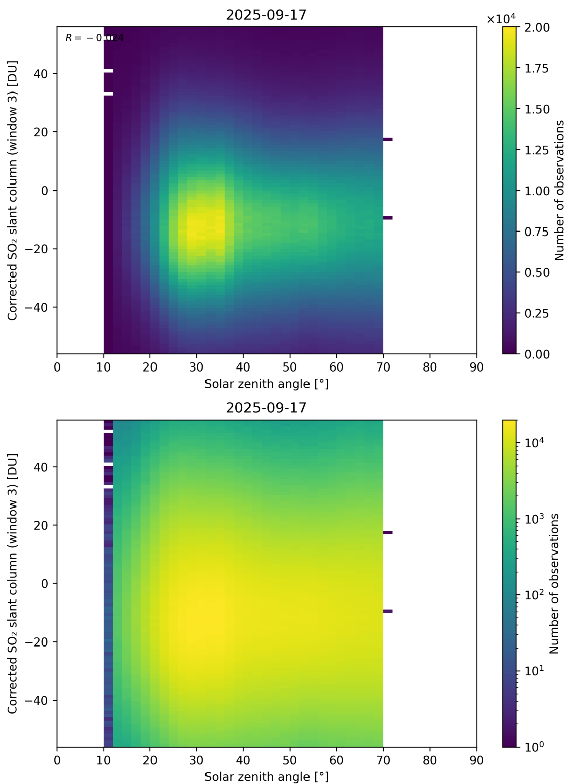
Figure 183: Scatter density plot of “Solar zenith angle” against “Corrected SO 2 slant column (window 3)” for 2025-09-16 to 2025-09-18.
