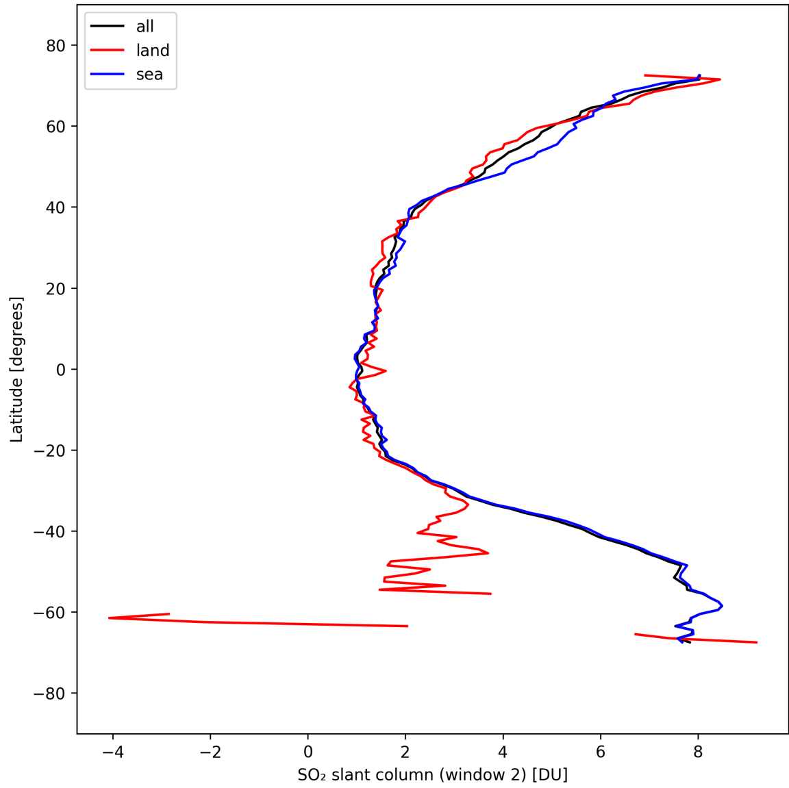
Figure 41: Zonal average of “SO 2 slant column (window 2)” for 2025-09-16 to 2025-09-18.
