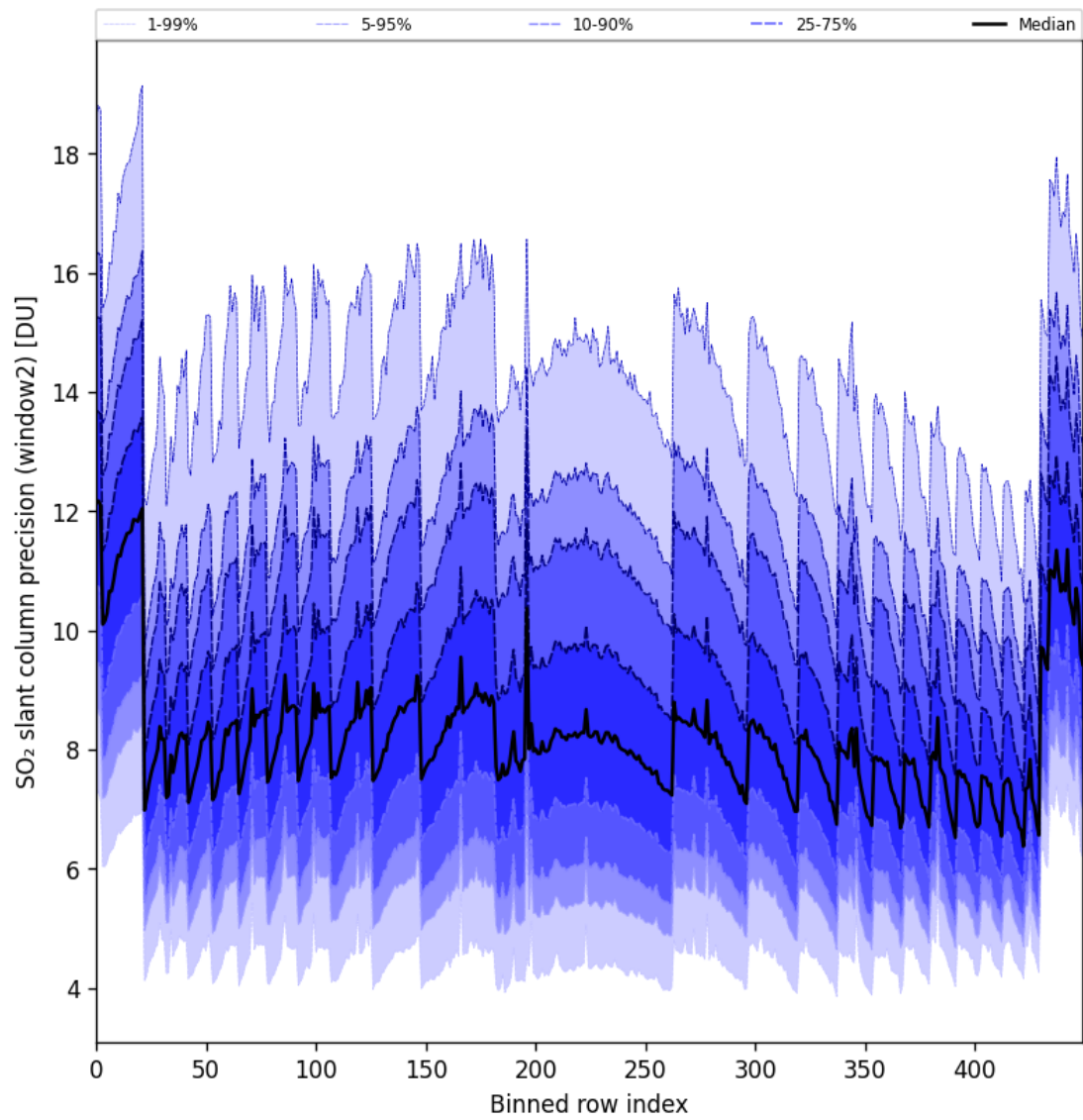
Figure 94: Along track statistics of “SO 2 slant column precision (window2)” for 2025-09-16 to 2025-09-18
