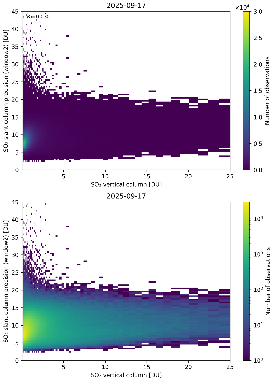
Figure 356: Scatter density plot of “SO 2 vertical column” against “SO 2 slant column precision (window2)” for 2025-09-16 to 2025-09-18.
