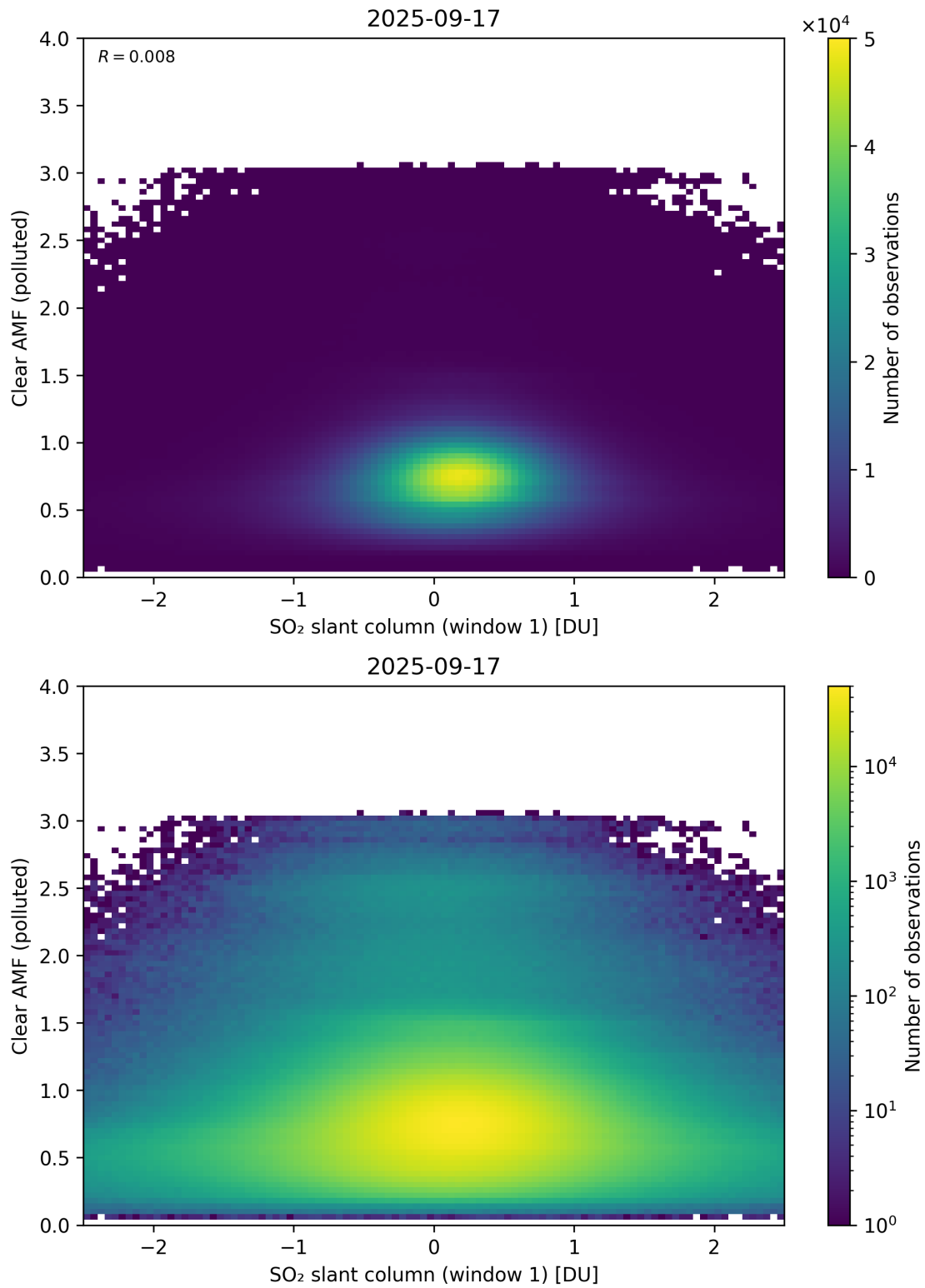
Figure 282: Scatter density plot of “SO 2 slant column (window 1)” against “Clear AMF (polluted)” for 2025-09-16 to 2025-09-18.
