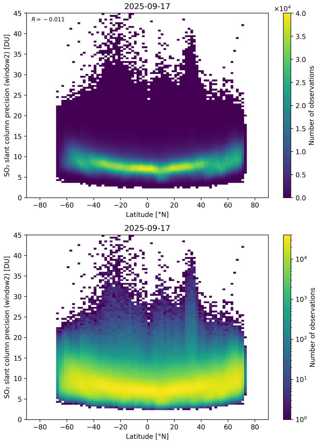
Figure 164: Scatter density plot of “Latitude” against “SO 2 slant column precision (window2)” for 2025-09-16 to 2025-09-18.
