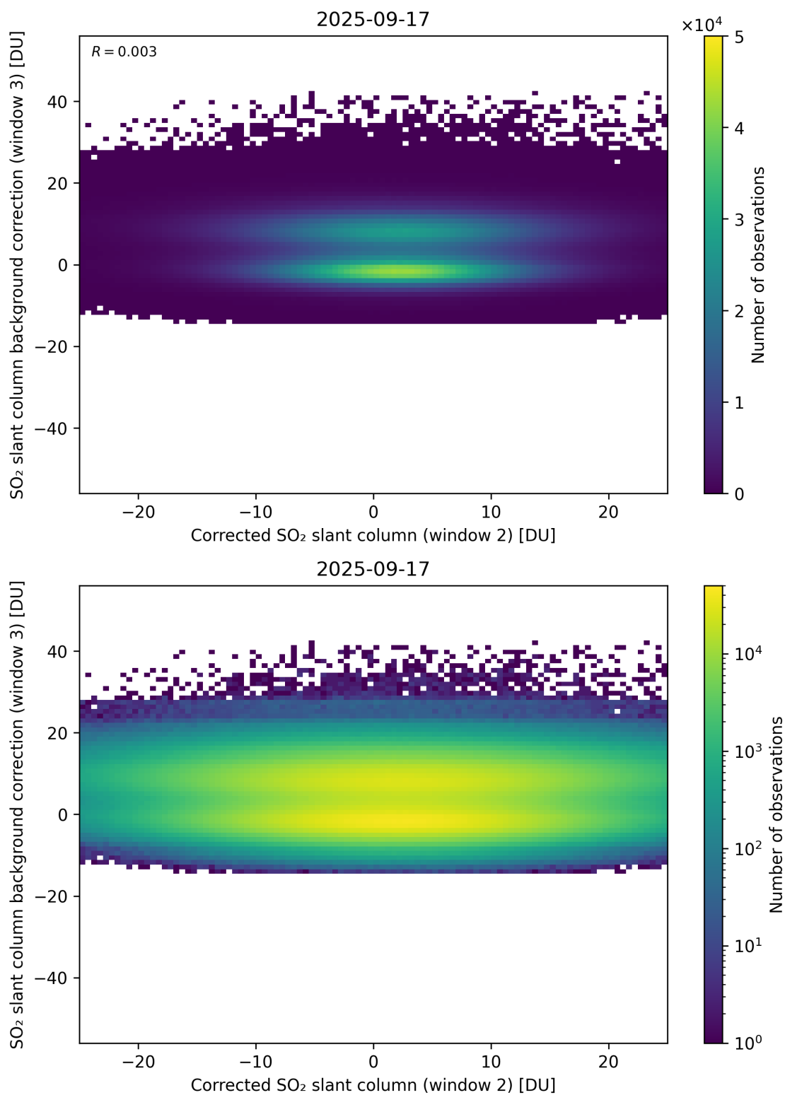
Figure 245: Scatter density plot of “Corrected SO 2 slant column (window 2)” against “SO 2 slant column background correction (window 3)” for 2025-09-16 to 2025-09-18.
