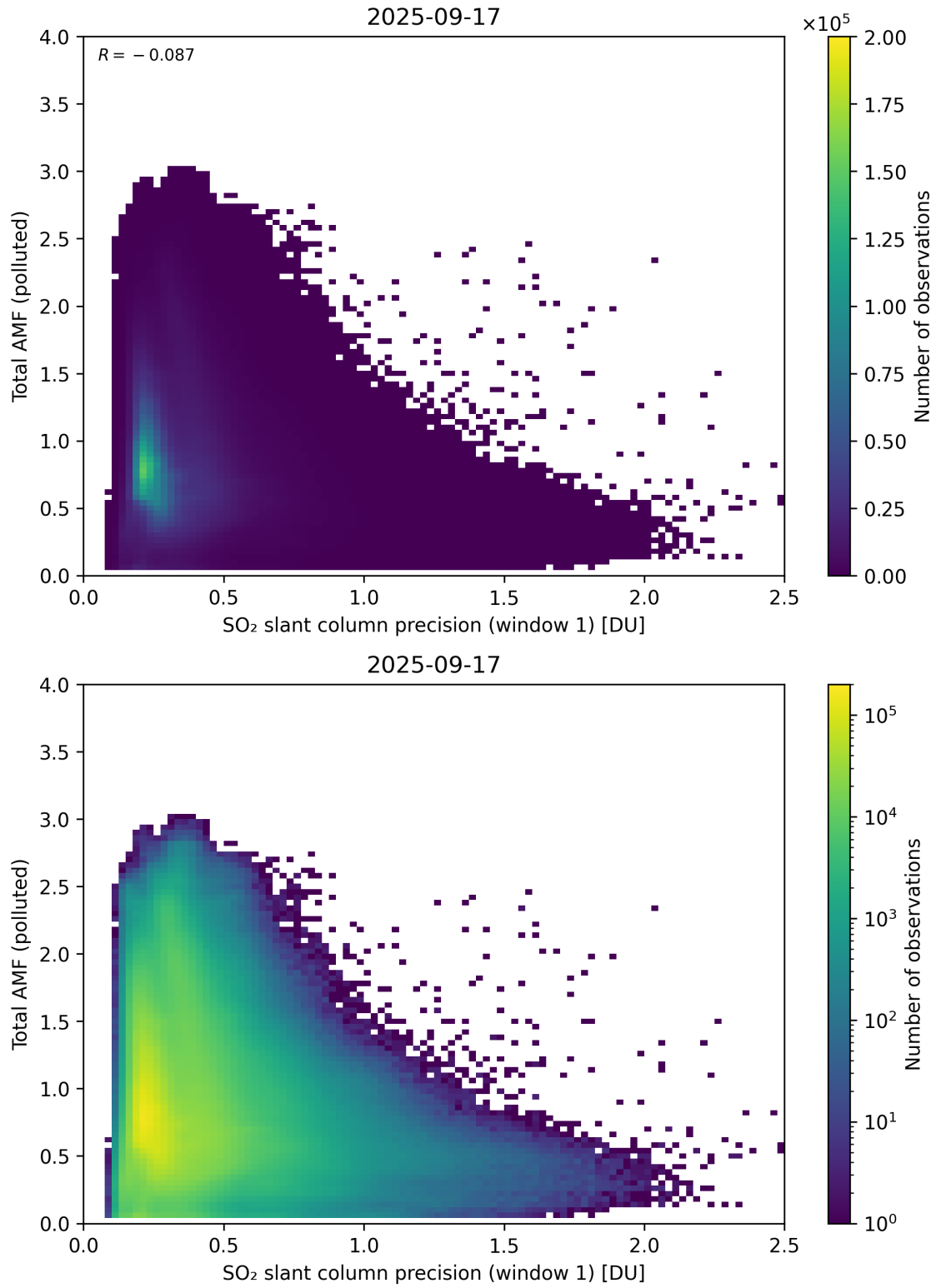
Figure 280: Scatter density plot of “SO 2 slant column precision (window 1)” against “Total AMF (polluted)” for 2025-09-16 to 2025-09-18.
