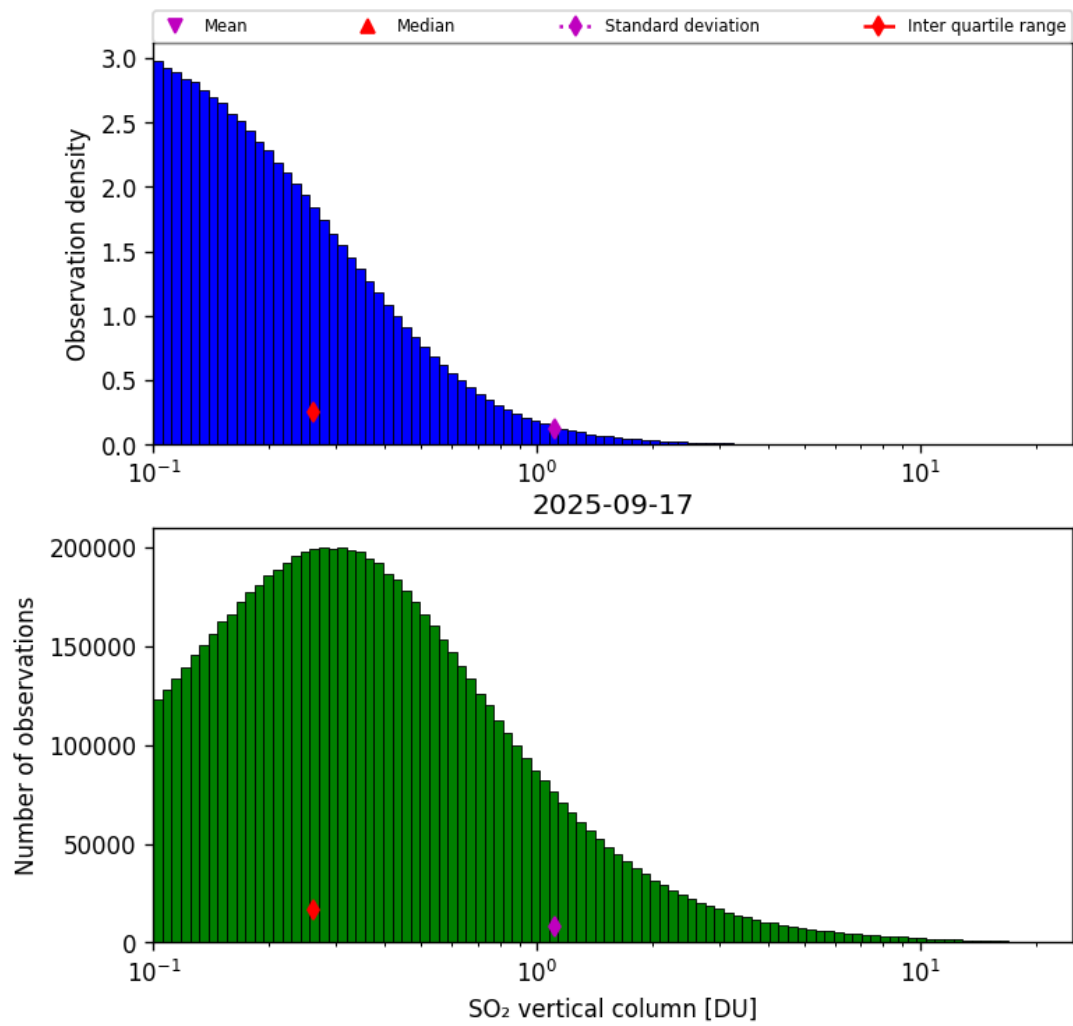
Figure 58: Histogram of “SO 2 vertical column” for 2025-09-16 to 2025-09-18
