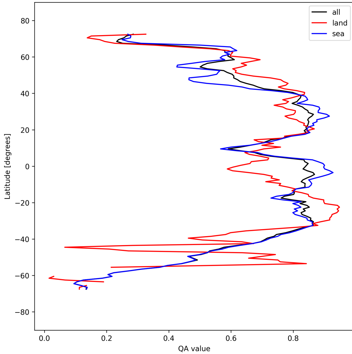
Figure 31: Zonal average of “QA value” for 2025-09-16 to 2025-09-18.
