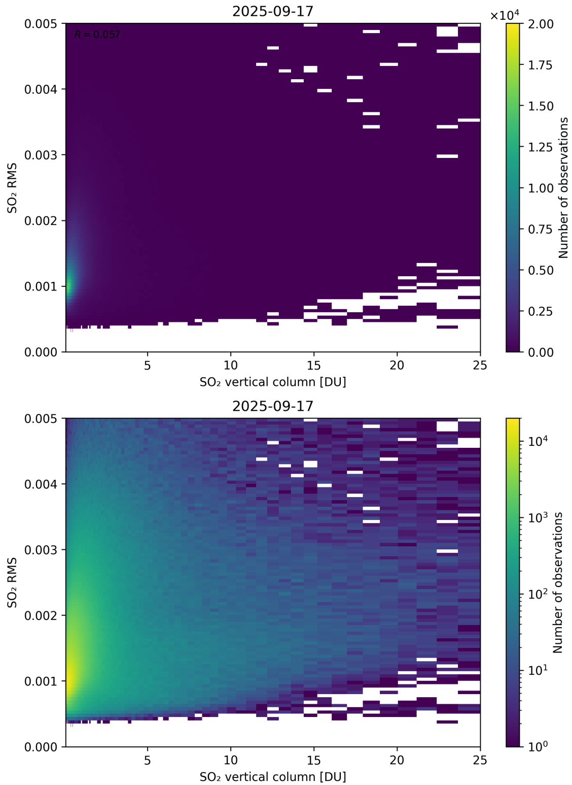
Figure 328: Scatter density plot of “SO 2 vertical column” against “SO 2 RMS” for 2025-09-16 to 2025-09-18.
