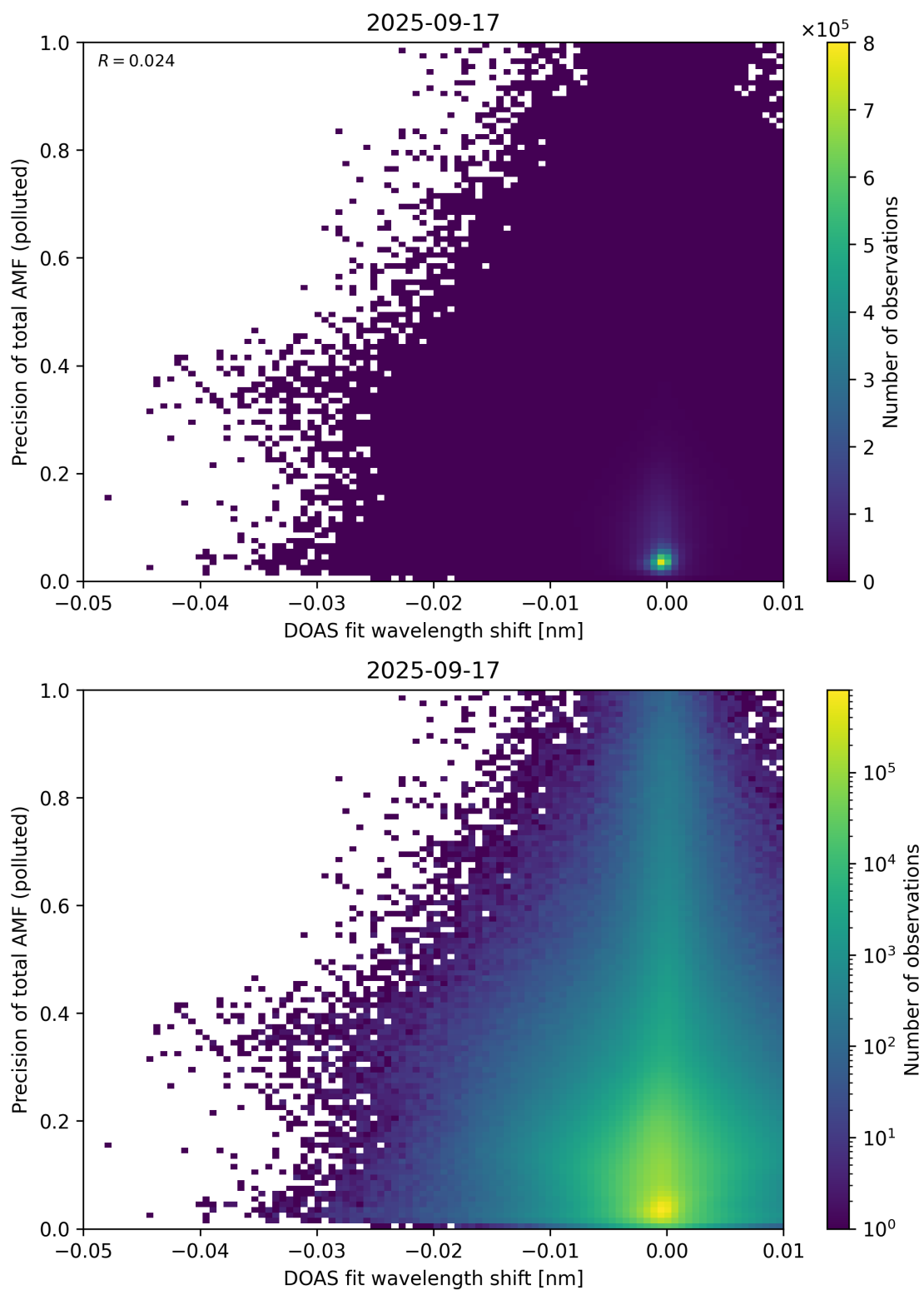
Figure 142: Scatter density plot of “DOAS fit wavelength shift” against “Precision of total AMF (polluted)” for 2025-09-16 to 2025-09-18.
