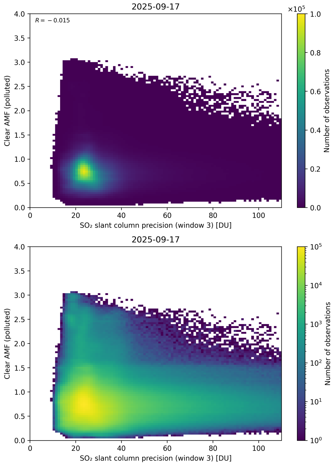
Figure 311: Scatter density plot of “SO 2 slant column precision (window 3)” against “Clear AMF (polluted)” for 2025-09-16 to 2025-09-18.
