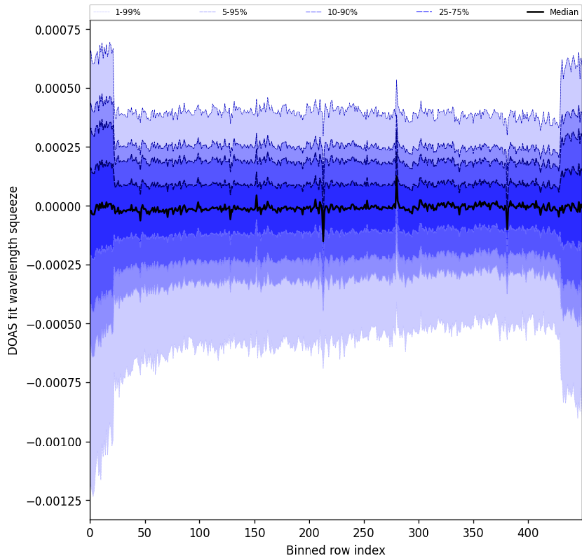
Figure 103: Along track statistics of “DOAS fit wavelength squeeze” for 2025-09-16 to 2025-09-18
