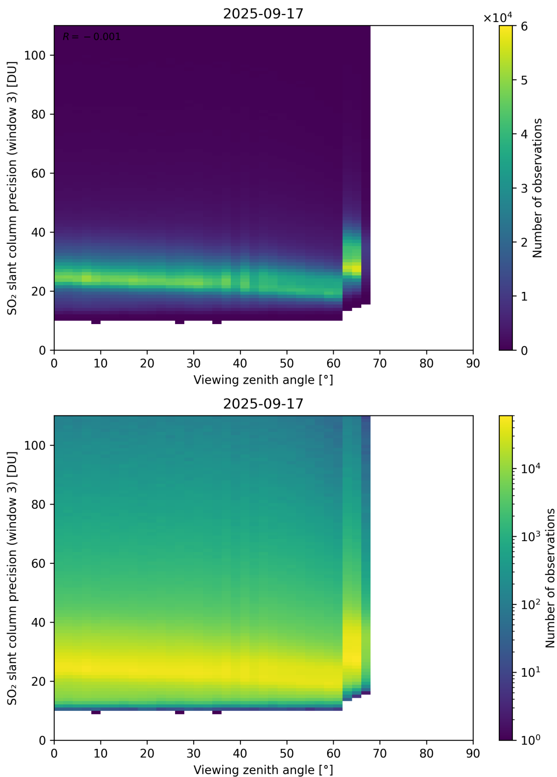
Figure 380: Scatter density plot of “Viewing zenith angle” against “SO 2 slant column precision (window 3)” for 2025-09-16 to 2025-09-18.
