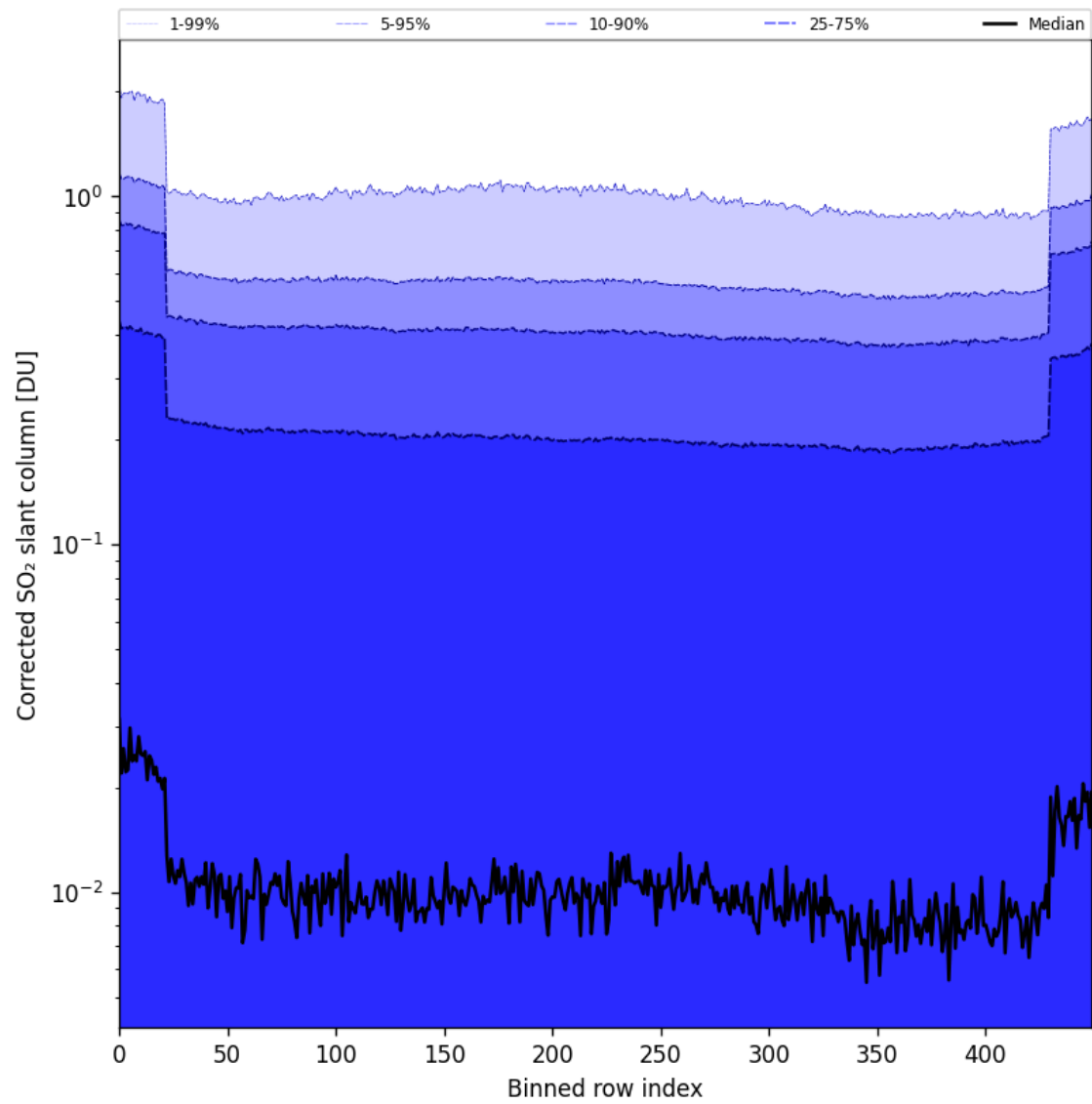
Figure 86: Along track statistics of “Corrected SO 2 slant column” for 2025-09-16 to 2025-09-18
