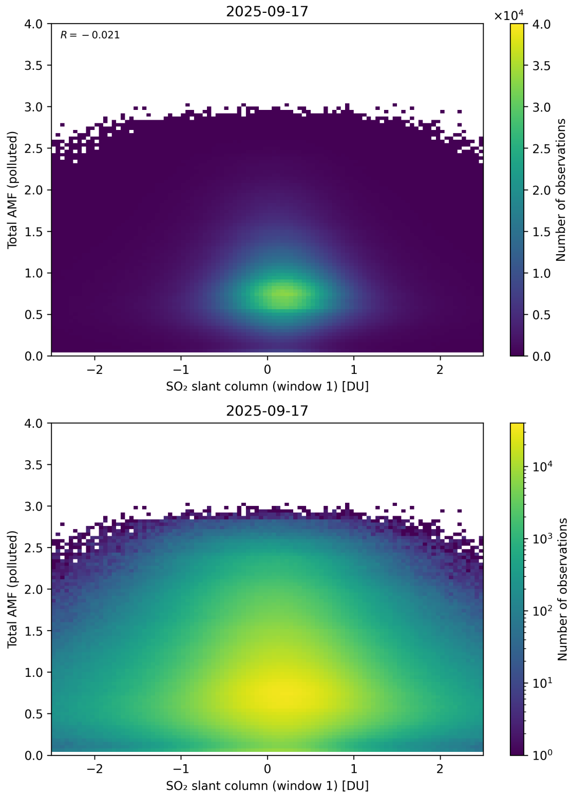
Figure 289: Scatter density plot of “SO 2 slant column (window 1)” against “Total AMF (polluted)” for 2025-09-16 to 2025-09-18.
