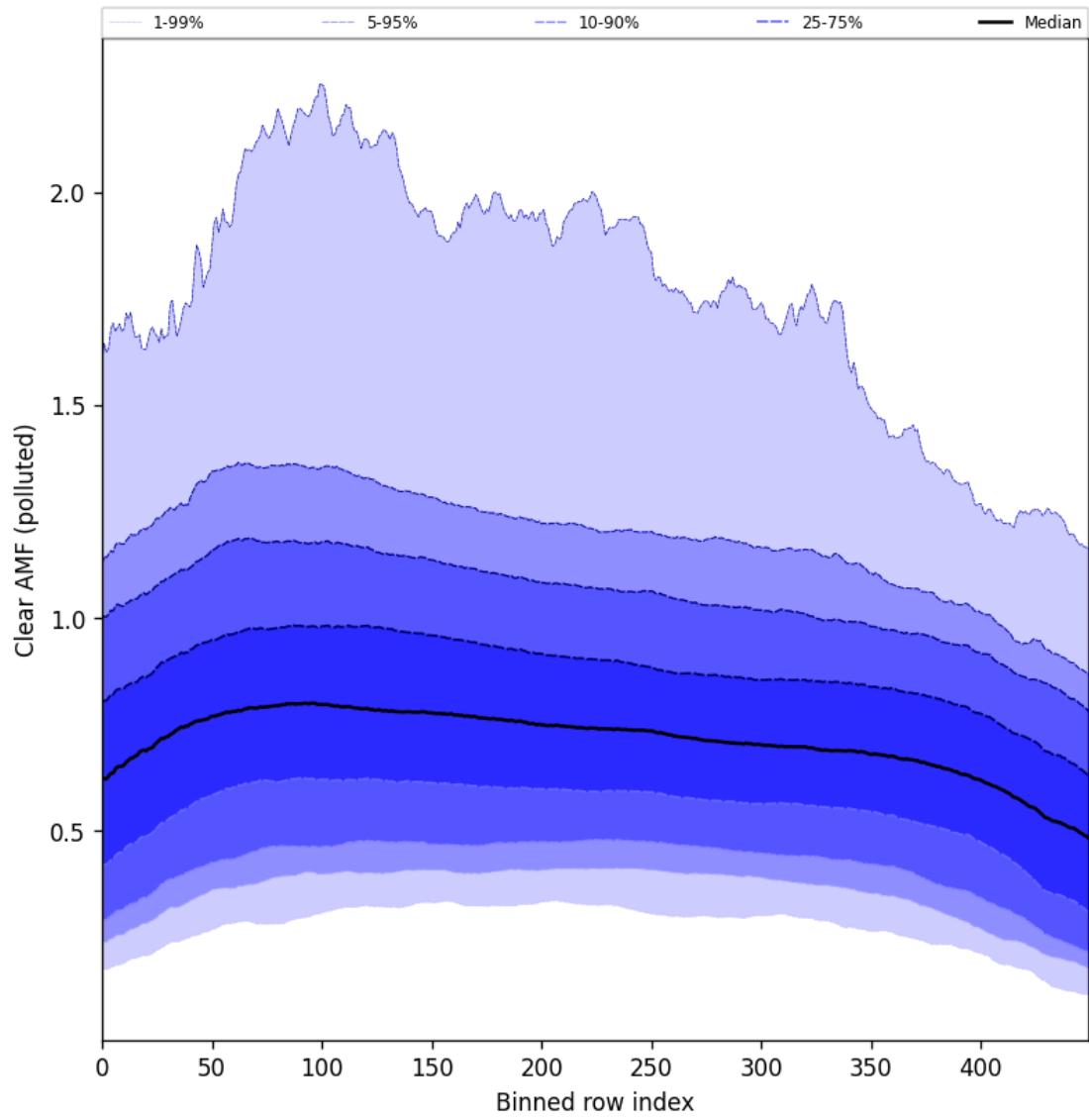
Figure 107: Along track statistics of “Clear AMF (polluted)” for 2025-09-16 to 2025-09-18
