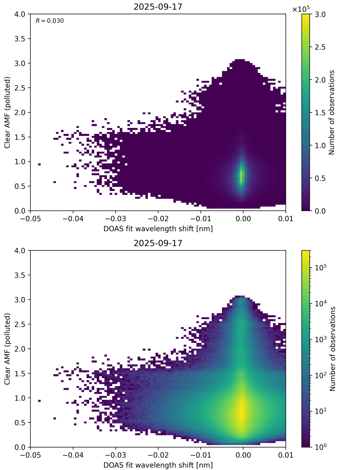
Figure 140: Scatter density plot of “DOAS fit wavelength shift” against “Clear AMF (polluted)” for 2025-09-16 to 2025-09-18.
