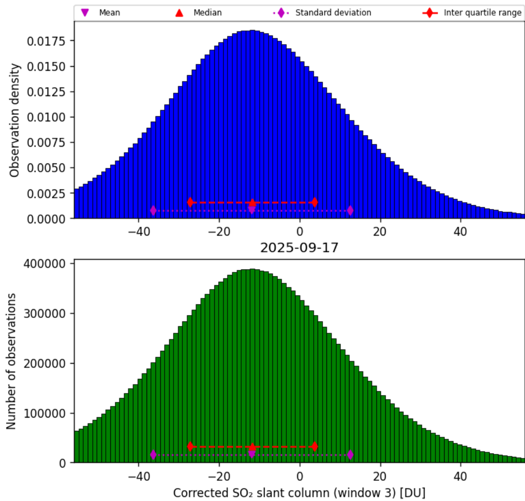
Figure 73: Histogram of “Corrected SO 2 slant column (window 3)” for 2025-09-16 to 2025-09-18
