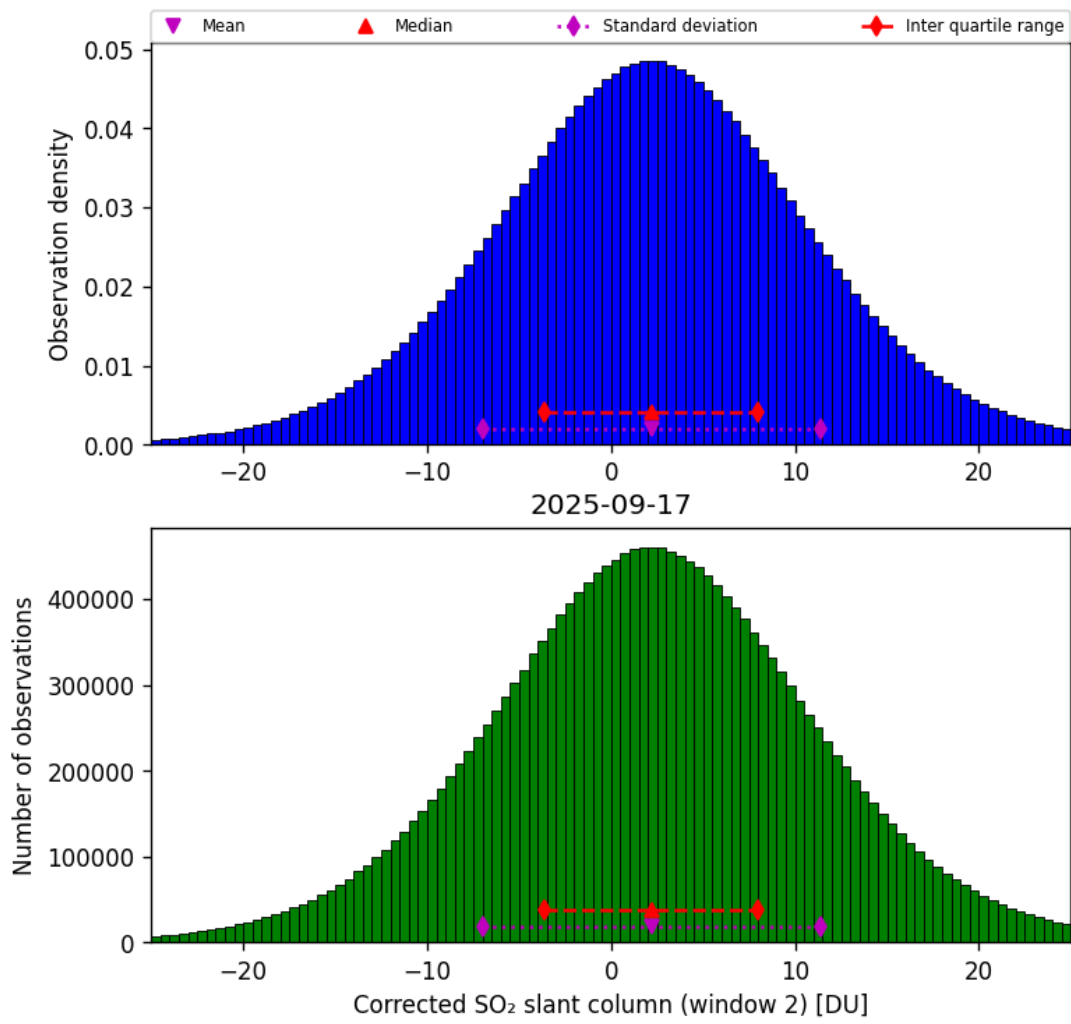
Figure 69: Histogram of “Corrected SO 2 slant column (window 2)” for 2025-09-16 to 2025-09-18
