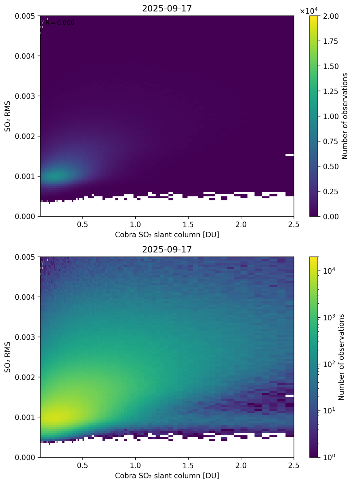
Figure 198: Scatter density plot of “Cobra SO 2 slant column” against “SO 2 RMS” for 2025-09-16 to 2025-09-18.
