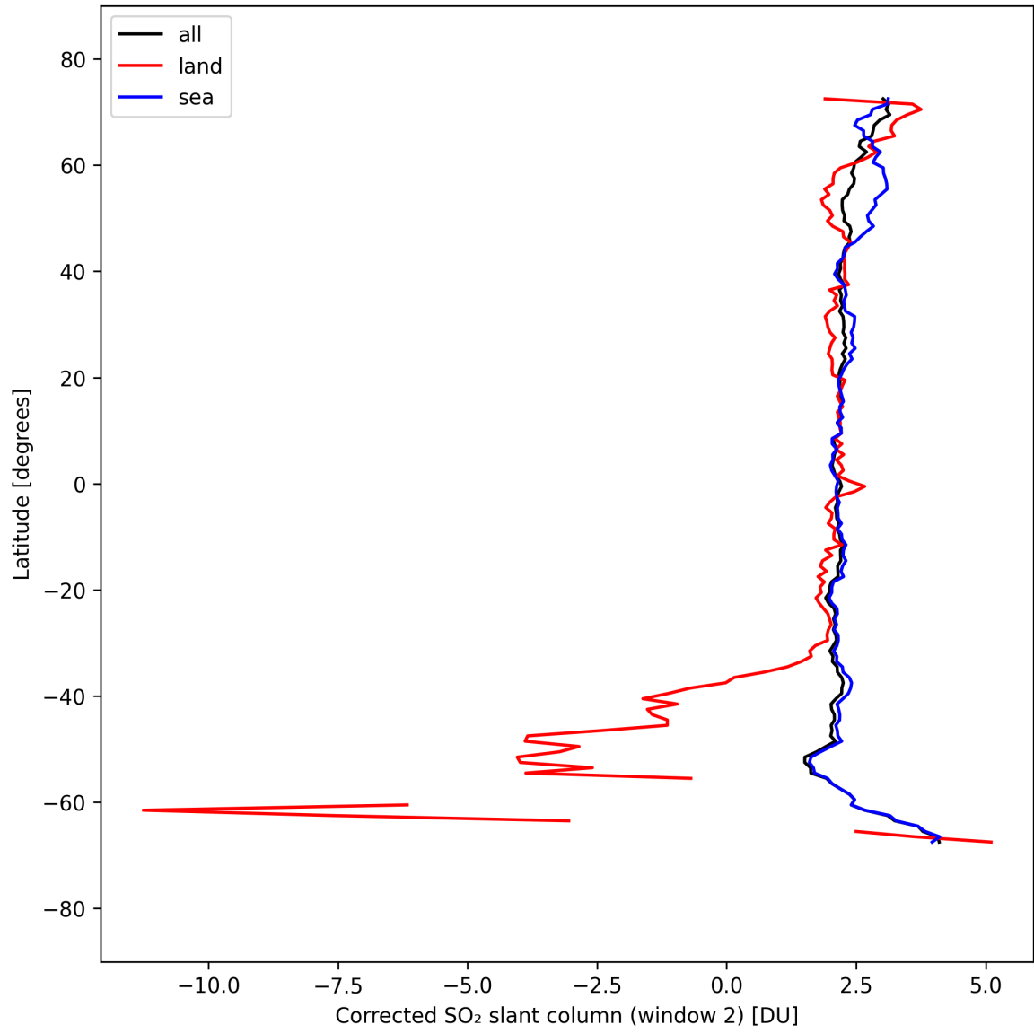
Figure 43: Zonal average of “Corrected SO 2 slant column (window 2)” for 2025-09-16 to 2025-09-18.
