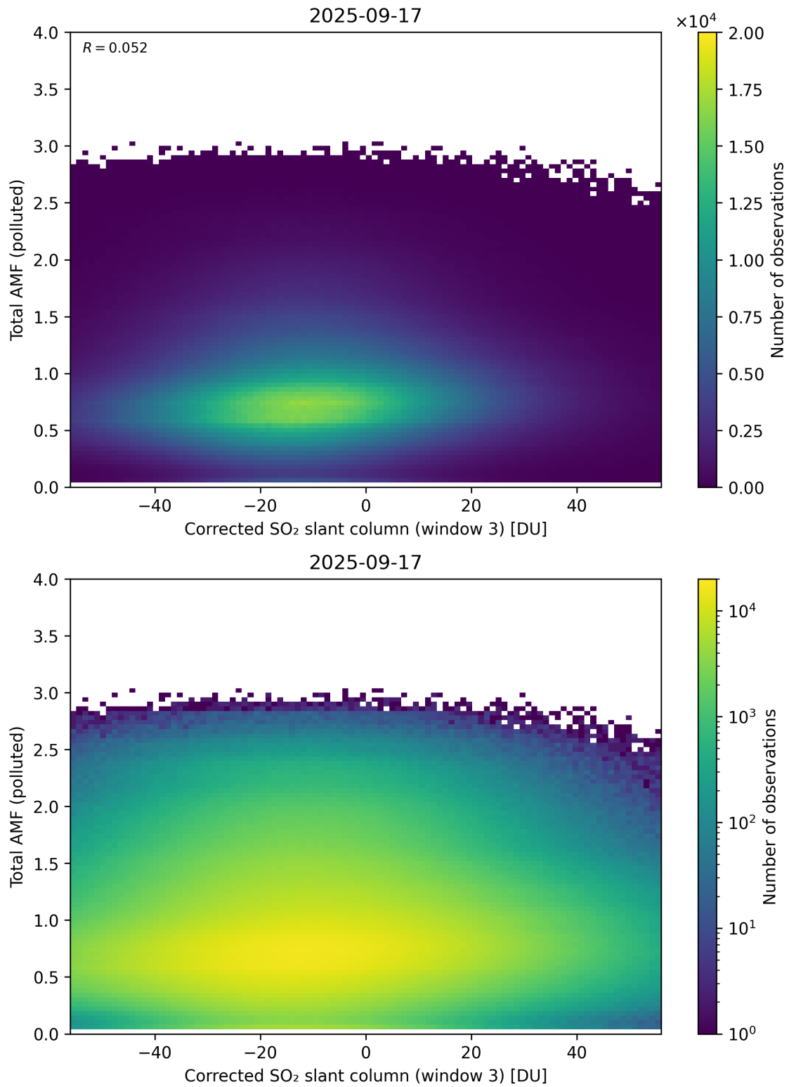
Figure 260: Scatter density plot of “Corrected SO 2 slant column (window 3)” against “Total AMF (polluted)” for 2025-09-16 to 2025-09-18.
