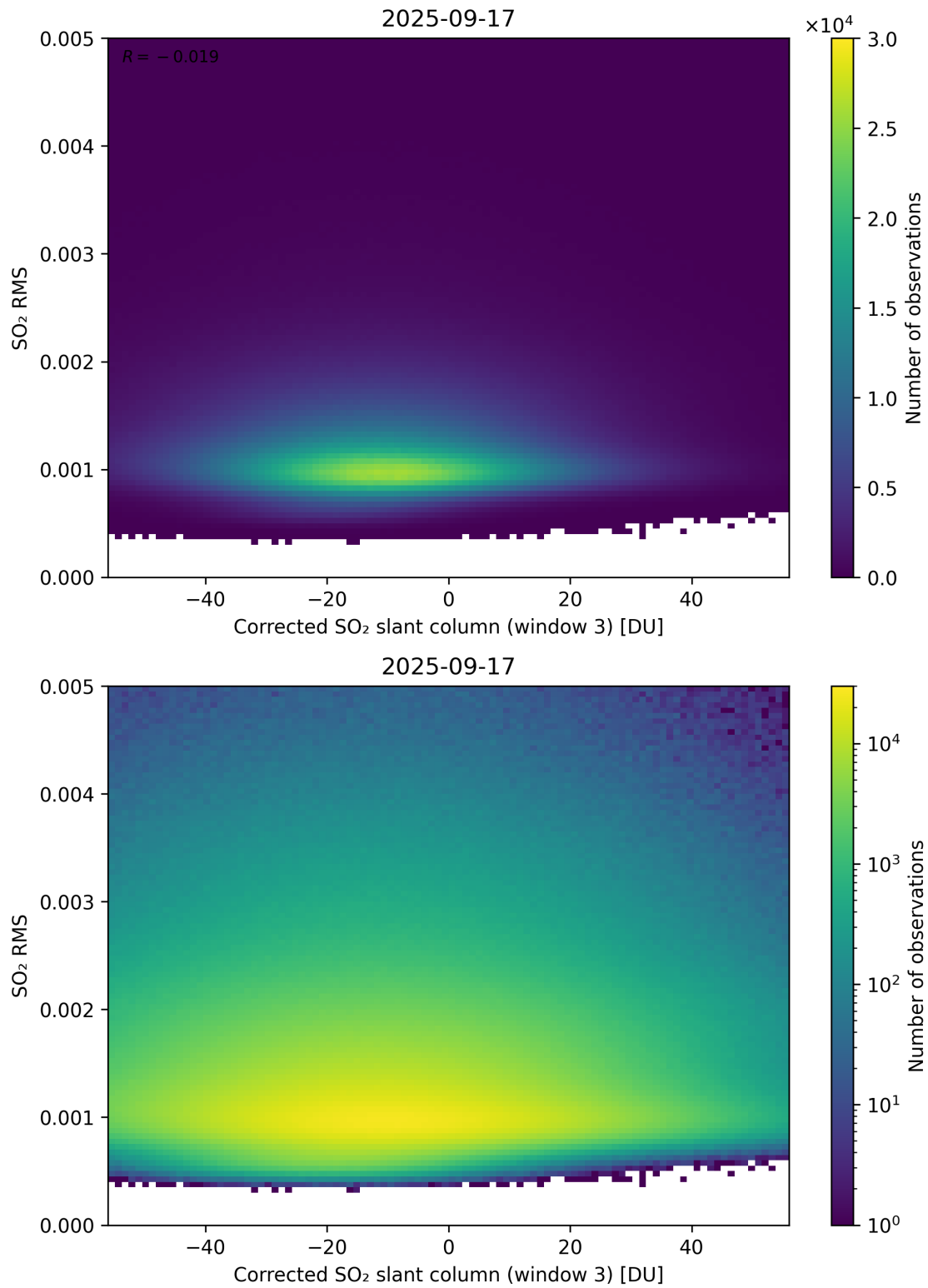
Figure 258: Scatter density plot of “Corrected SO 2 slant column (window 3)” against “SO 2 RMS” for 2025-09-16 to 2025-09-18.
