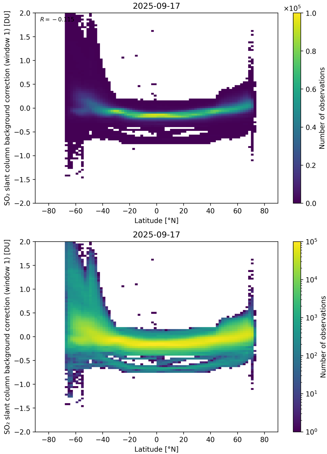
Figure 150: Scatter density plot of “Latitude” against “SO 2 slant column background correction (window 1)” for 2025-09-16 to 2025-09-18.
