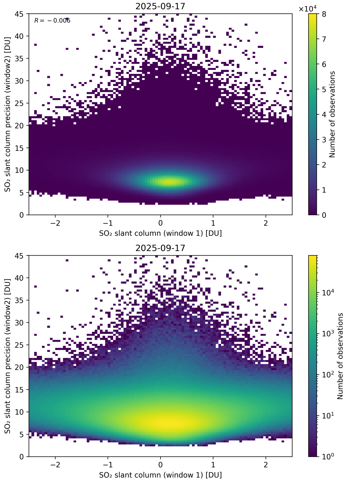
Figure 286: Scatter density plot of “SO 2 slant column (window 1)” against “SO 2 slant column precision (window2)” for 2025-09-16 to 2025-09-18.
