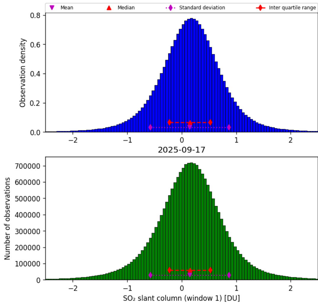
Figure 63: Histogram of “SO 2 slant column (window 1)” for 2025-09-16 to 2025-09-18
