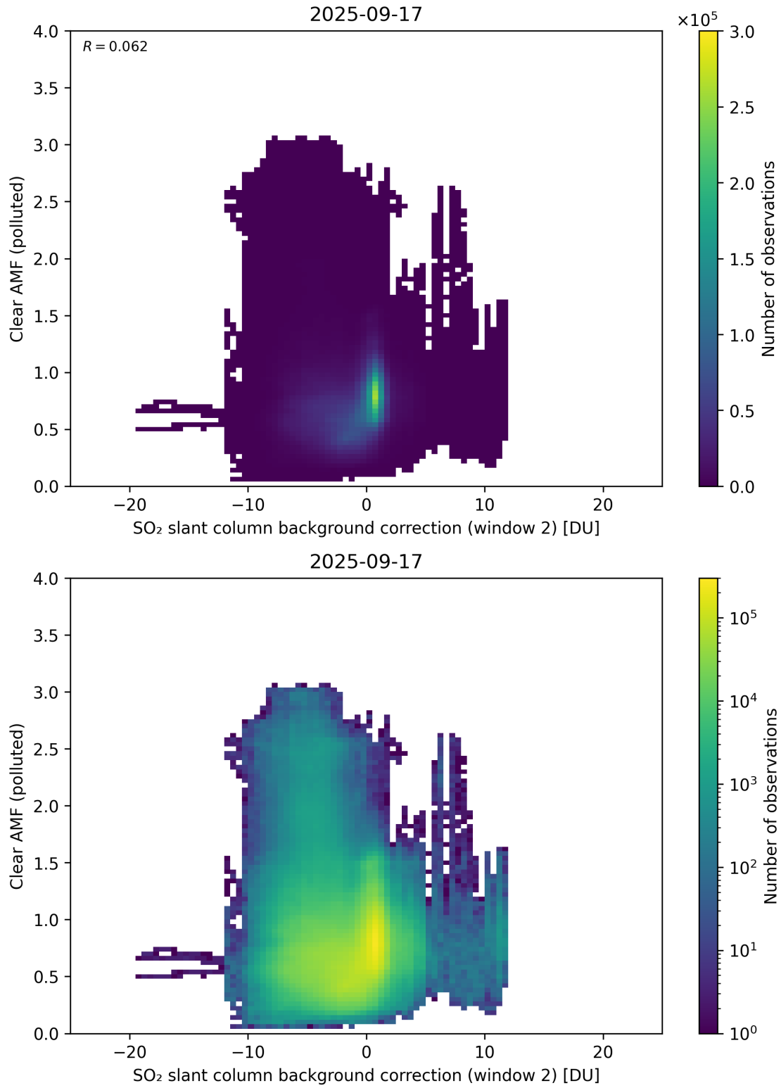
Figure 126: Scatter density plot of “SO 2 slant column background correction (window 2)” against “Clear AMF (polluted)” for 2025-09-16 to 2025-09-18.
