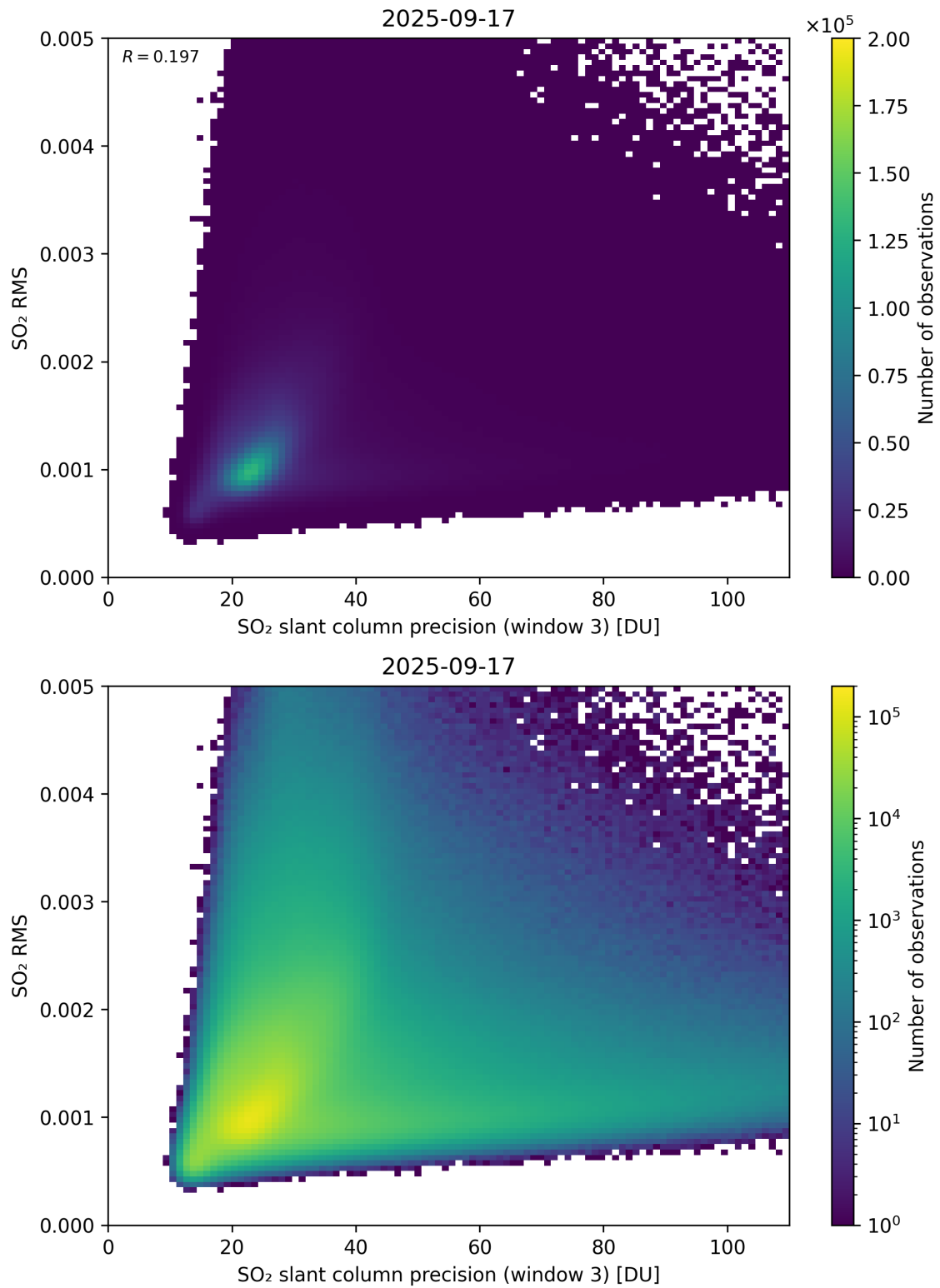
Figure 310: Scatter density plot of “SO 2 slant column precision (window 3)” against “SO 2 RMS” for 2025-09-16 to 2025-09-18.
