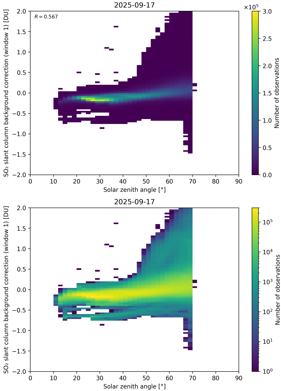
Figure 171: Scatter density plot of “Solar zenith angle” against “SO 2 slant column background correction (window 1)” for 2025-09-16 to 2025-09-18.
