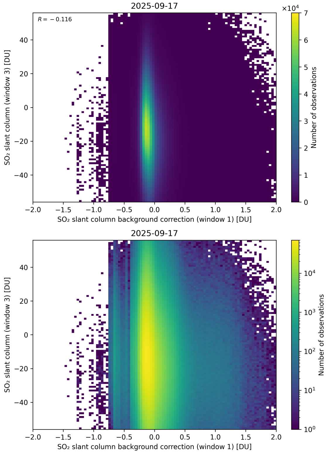
Figure 118: Scatter density plot of “SO 2 slant column background correction (window 1)” against “SO 2 slant column (window 3)” for 2025-09-16 to 2025-09-18.
