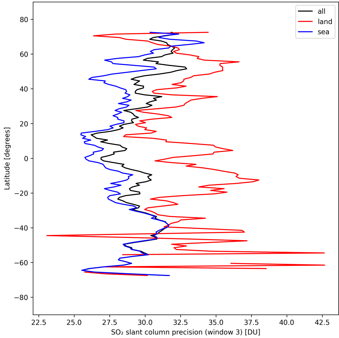
Figure 46: Zonal average of “SO 2 slant column precision (window 3)” for 2025-09-16 to 2025-09-18.
