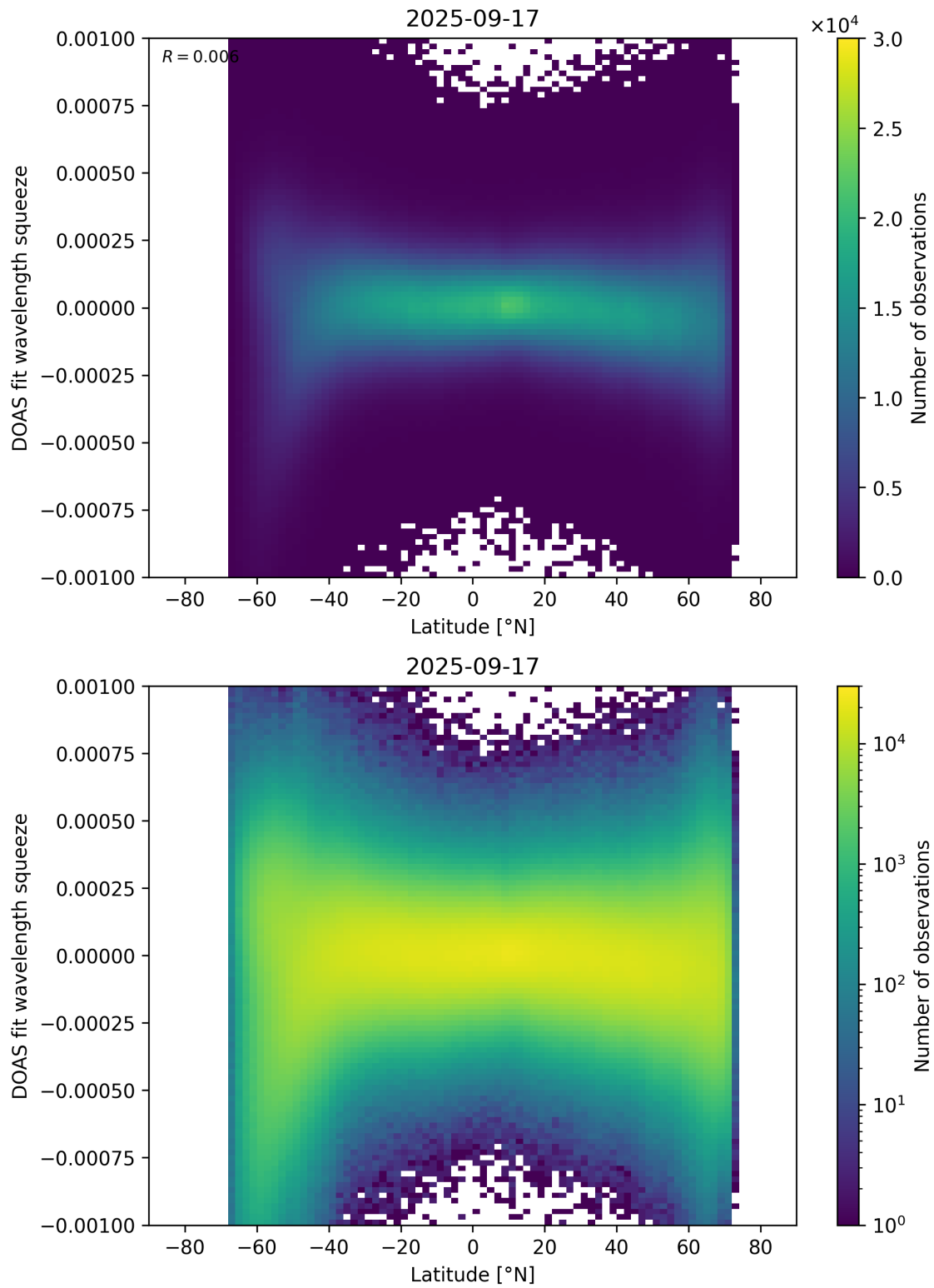
Figure 154: Scatter density plot of “Latitude” against “DOAS fit wavelength squeeze” for 2025-09-16 to 2025-09-18.
