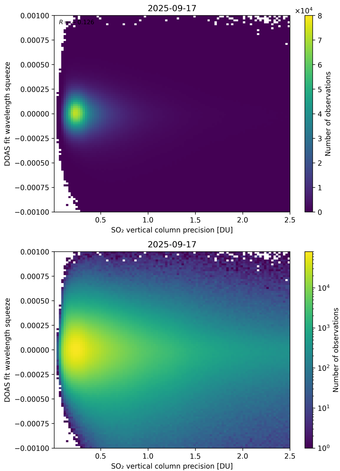
Figure 333: Scatter density plot of “SO 2 vertical column precision” against “DOAS fit wavelength squeeze” for 2025-09-16 to 2025-09-18.
