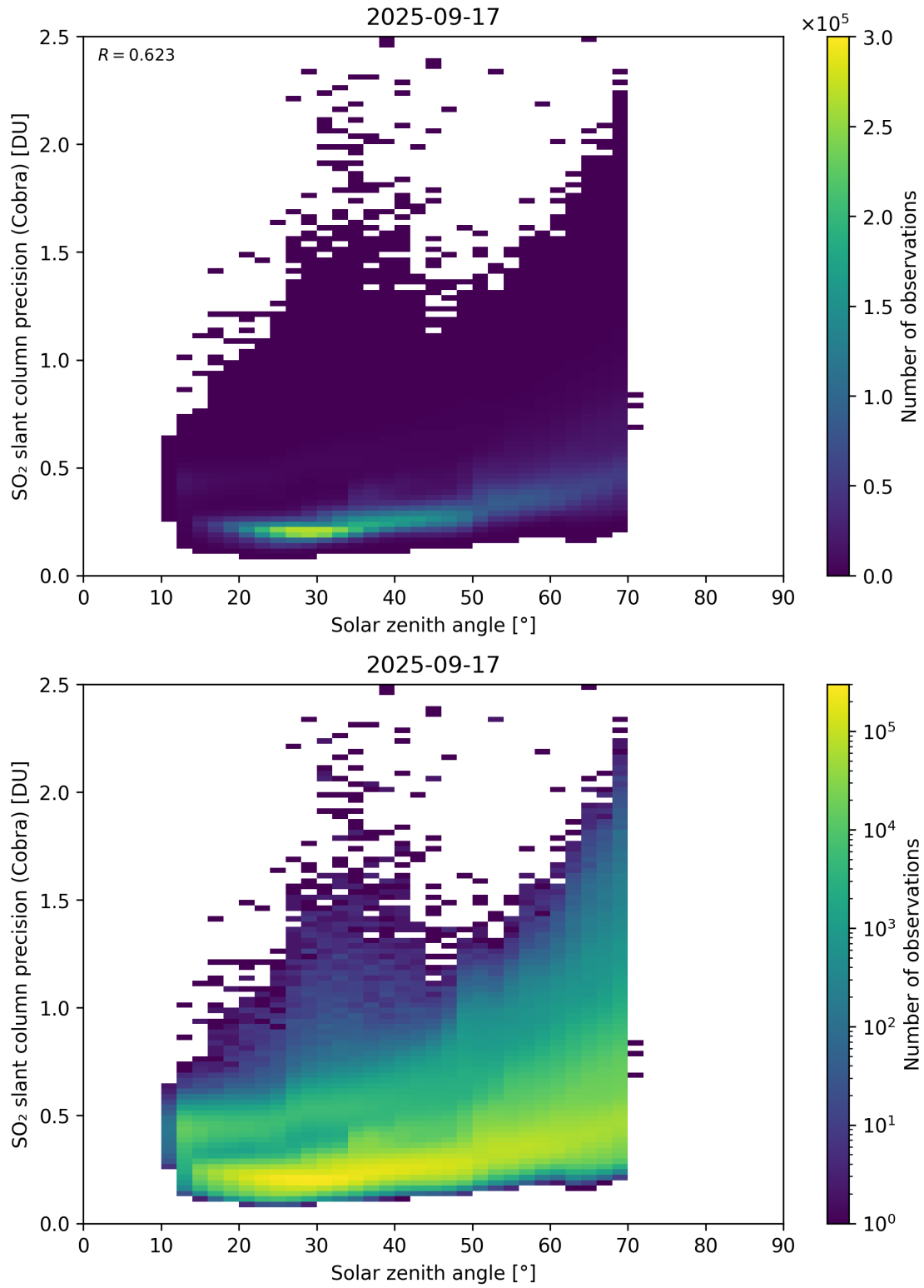
Figure 180: Scatter density plot of “Solar zenith angle” against “SO 2 slant column precision (Cobra)” for 2025-09-16 to 2025-09-18.
