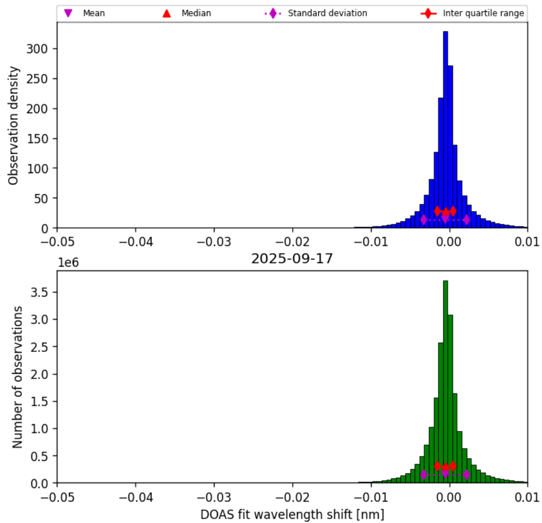
Figure 76: Histogram of “DOAS fit wavelength shift” for 2025-09-16 to 2025-09-18
