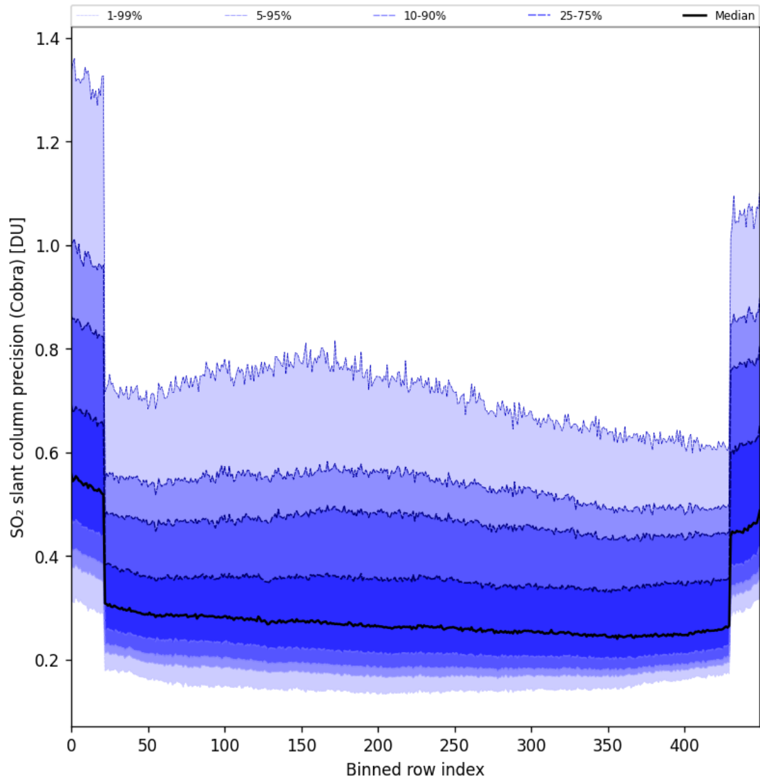
Figure 88: Along track statistics of “SO 2 slant column precision (Cobra)” for 2025-09-16 to 2025-09-18
