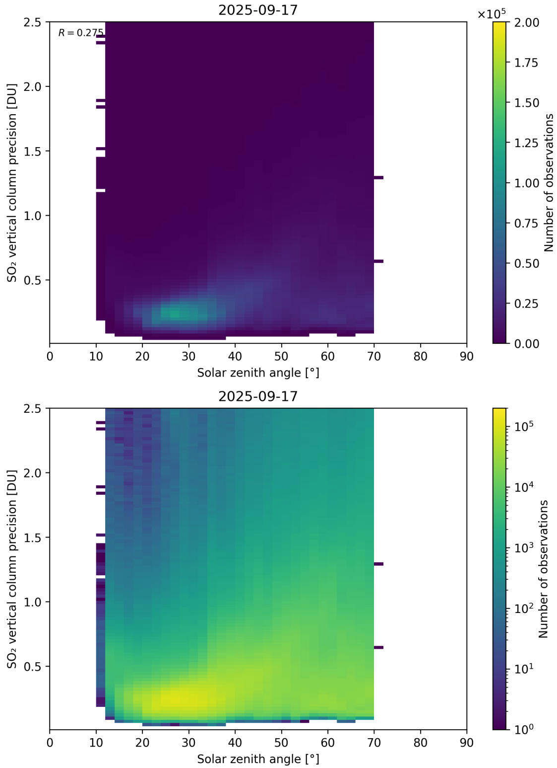
Figure 192: Scatter density plot of “Solar zenith angle” against “SO 2 vertical column precision” for 2025-09-16 to 2025-09-18.
