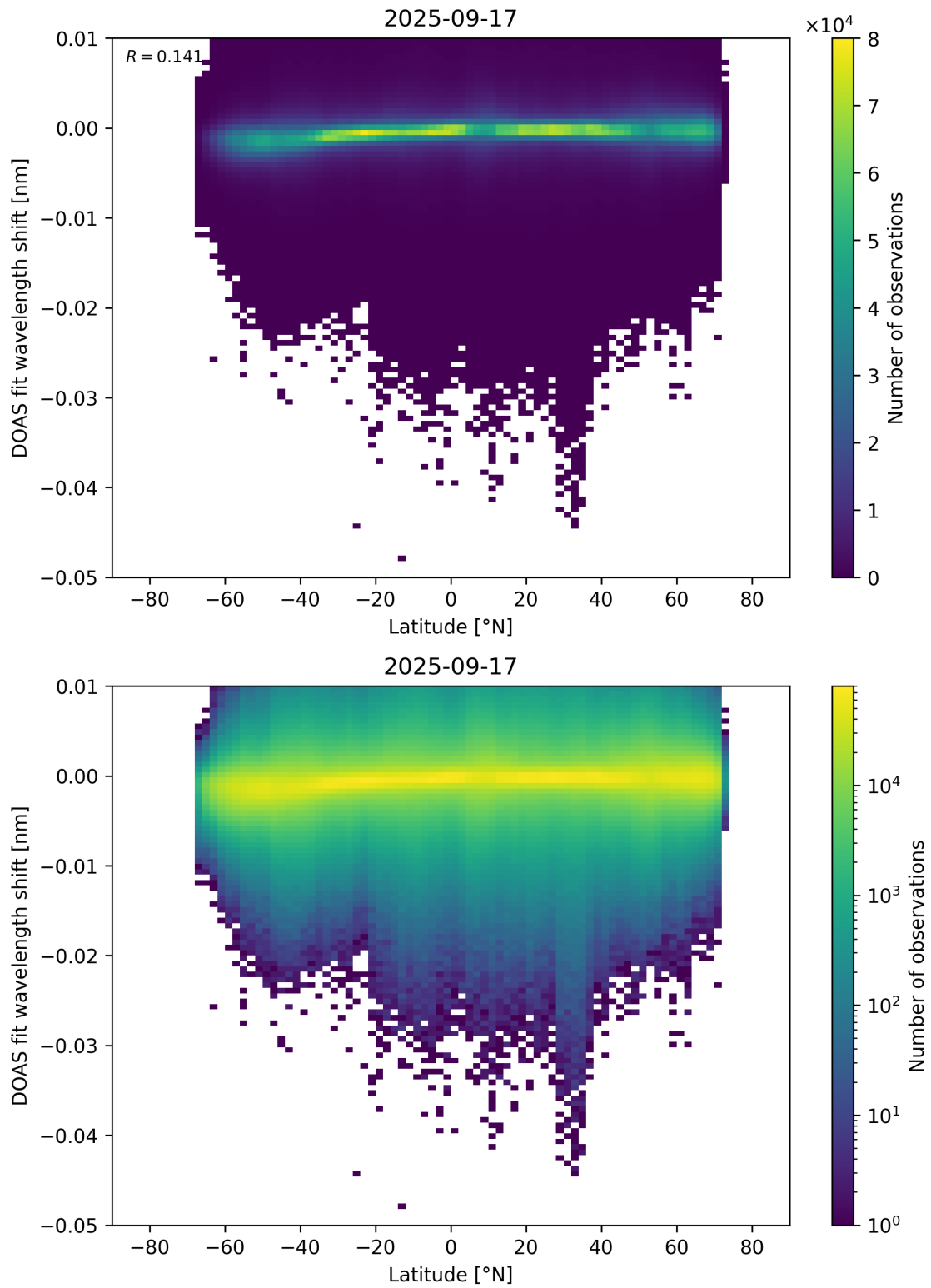
Figure 153: Scatter density plot of “Latitude” against “DOAS fit wavelength shift” for 2025-09-16 to 2025-09-18.
