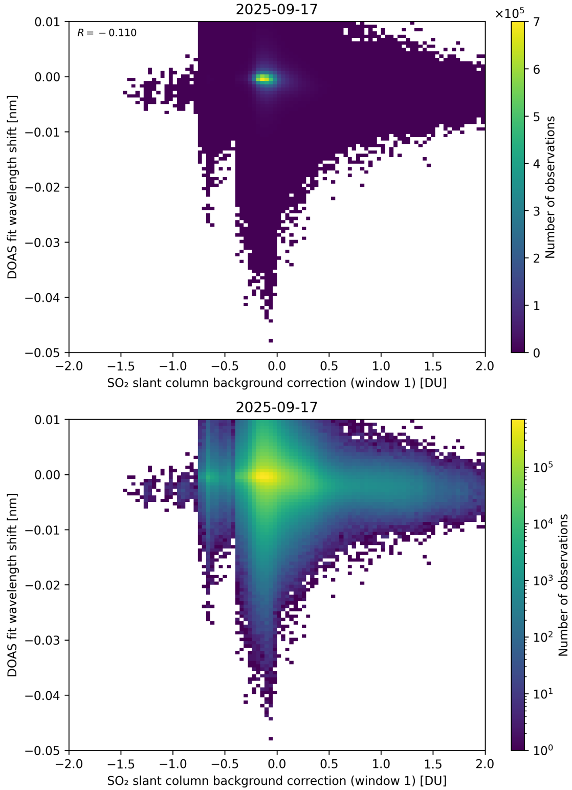
Figure 111: Scatter density plot of “SO 2 slant column background correction (window 1)” against “DOAS fit wavelength shift” for 2025-09-16 to 2025-09-18.
