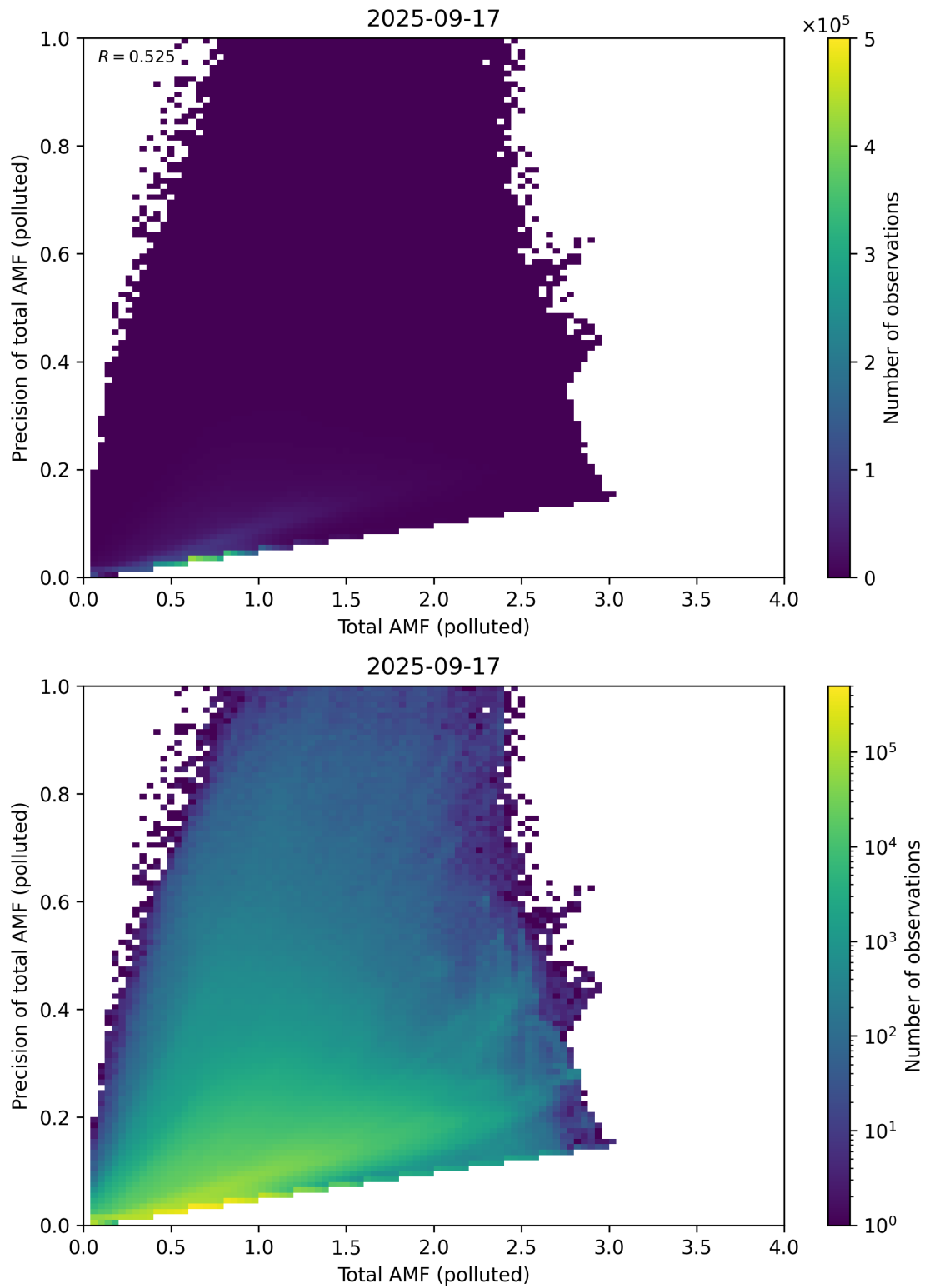
Figure 322: Scatter density plot of “Total AMF (polluted)” against “Precision of total AMF (polluted)” for 2025-09-16 to 2025-09-18.
