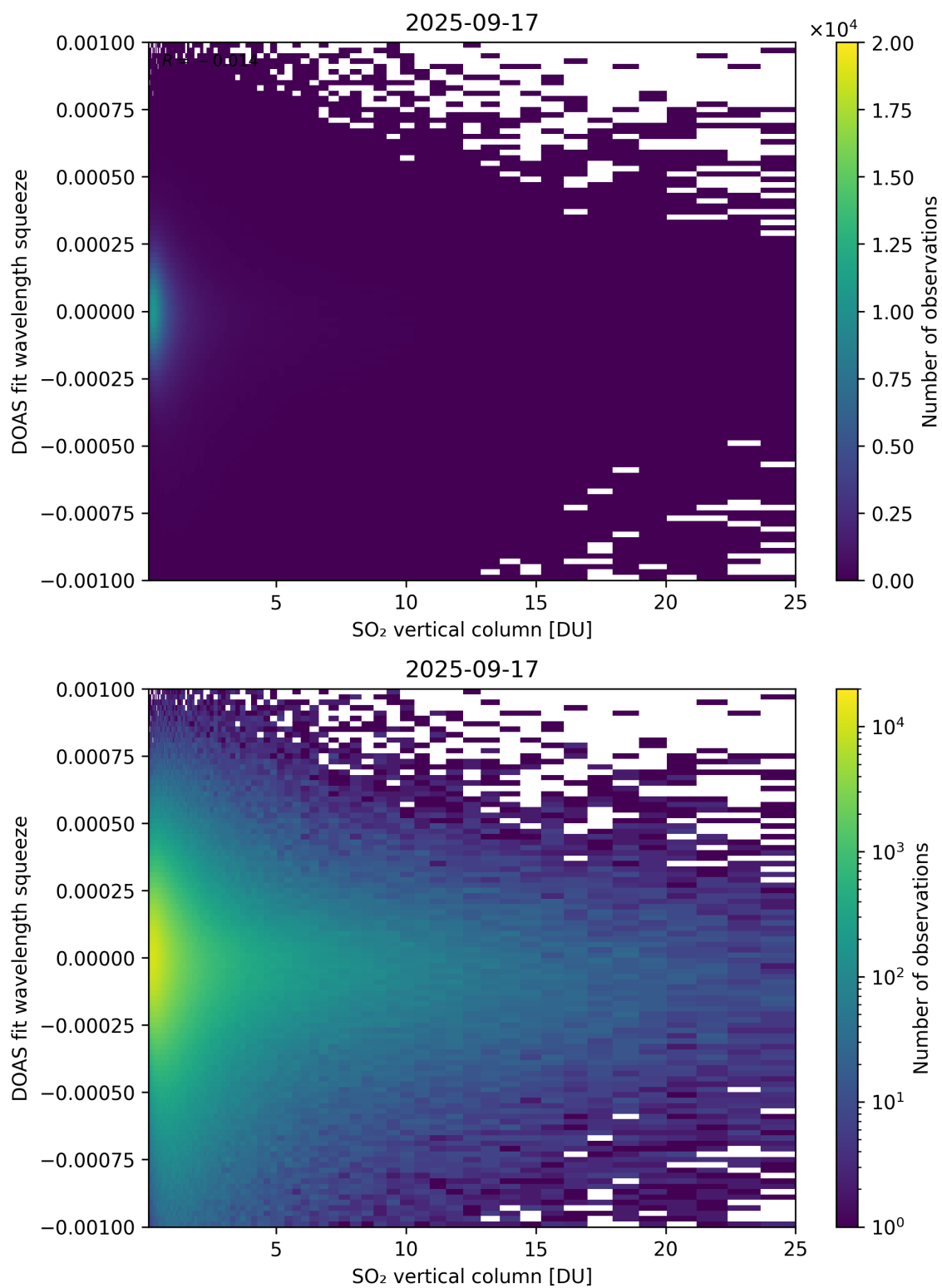
Figure 327: Scatter density plot of “SO 2 vertical column” against “DOAS fit wavelength squeeze” for 2025-09-16 to 2025-09-18.
