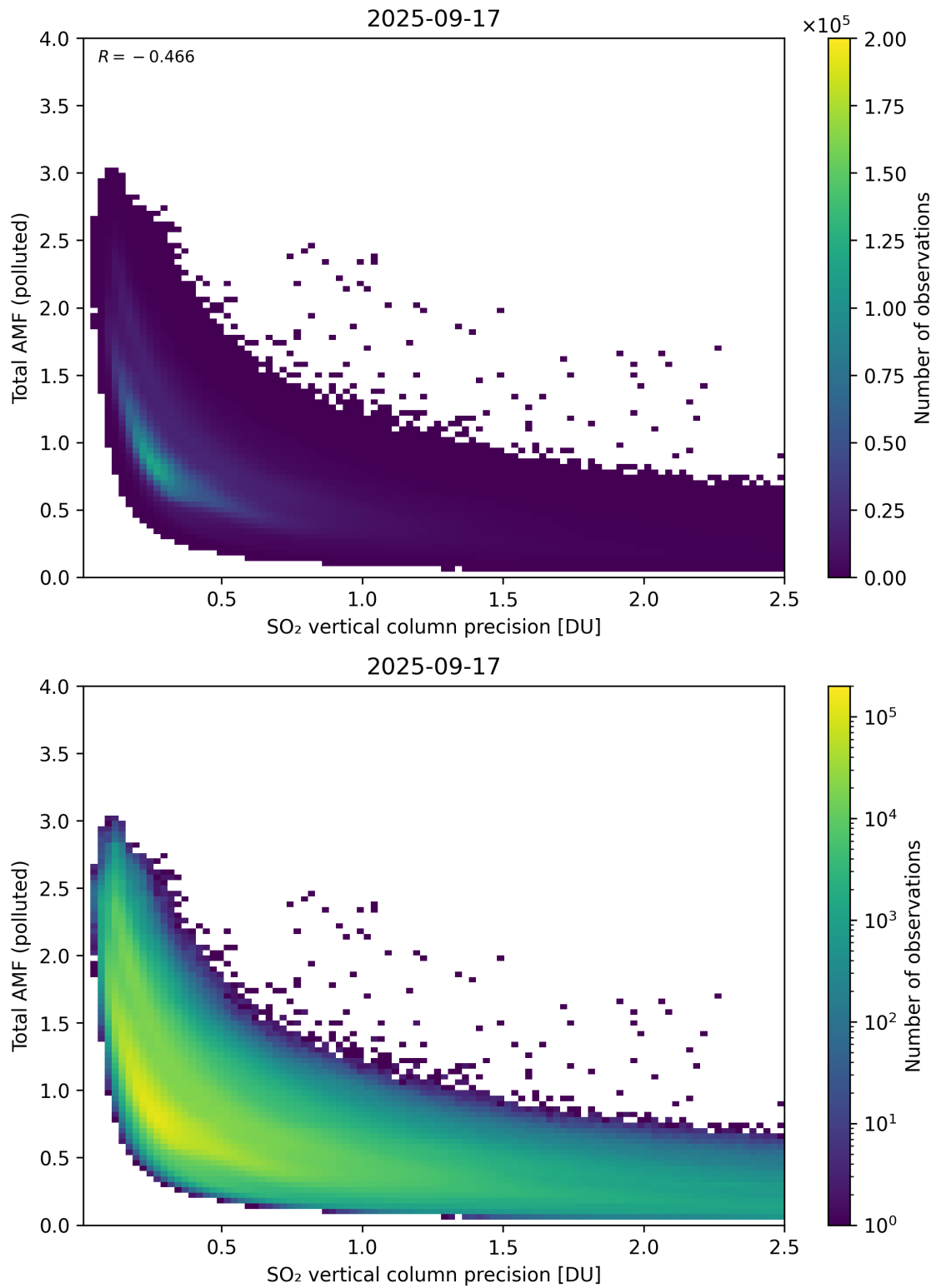
Figure 346: Scatter density plot of “SO 2 vertical column precision” against “Total AMF (polluted)” for 2025-09-16 to 2025-09-18.
