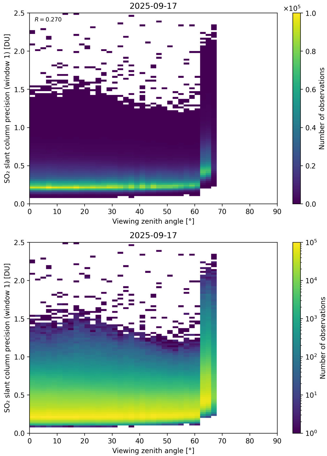
Figure 377: Scatter density plot of “Viewing zenith angle” against “SO 2 slant column precision (window 1)” for 2025-09-16 to 2025-09-18.
