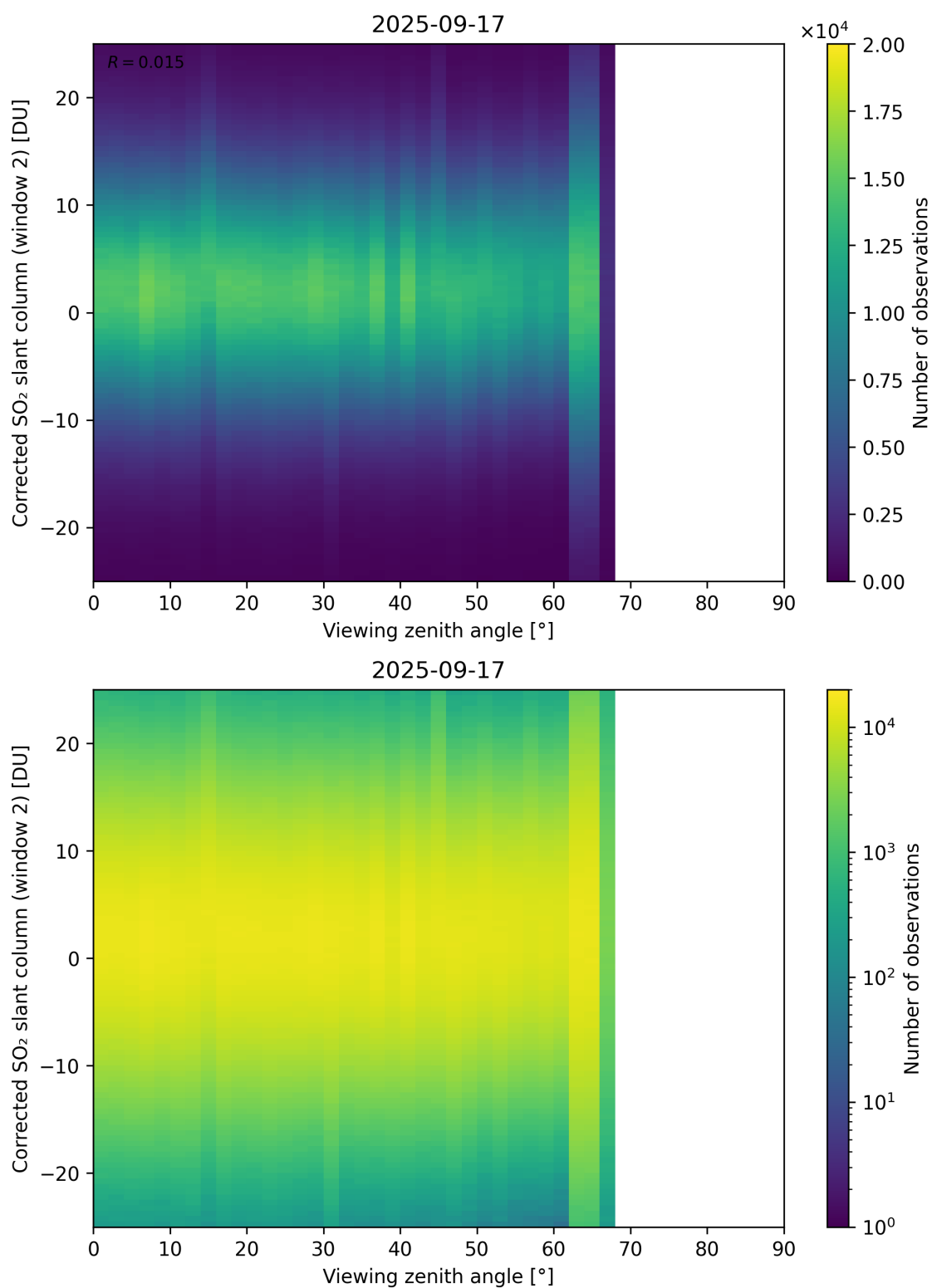
Figure 374: Scatter density plot of “Viewing zenith angle” against “Corrected SO 2 slant column (window 2)” for 2025-09-16 to 2025-09-18.
