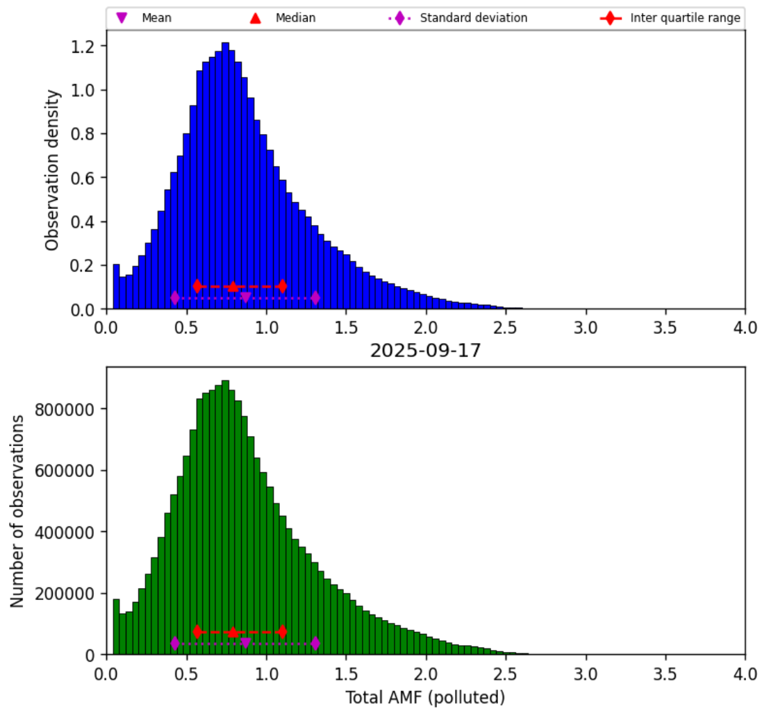
Figure 79: Histogram of “Total AMF (polluted)” for 2025-09-16 to 2025-09-18
