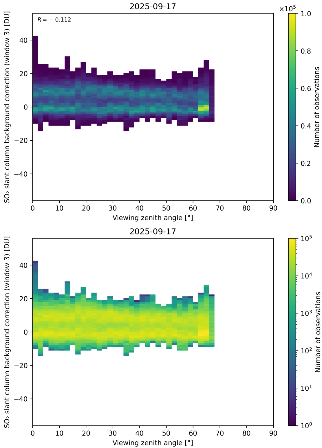
Figure 364: Scatter density plot of “Viewing zenith angle” against “SO 2 slant column background correction (window 3)” for 2025-09-16 to 2025-09-18.
