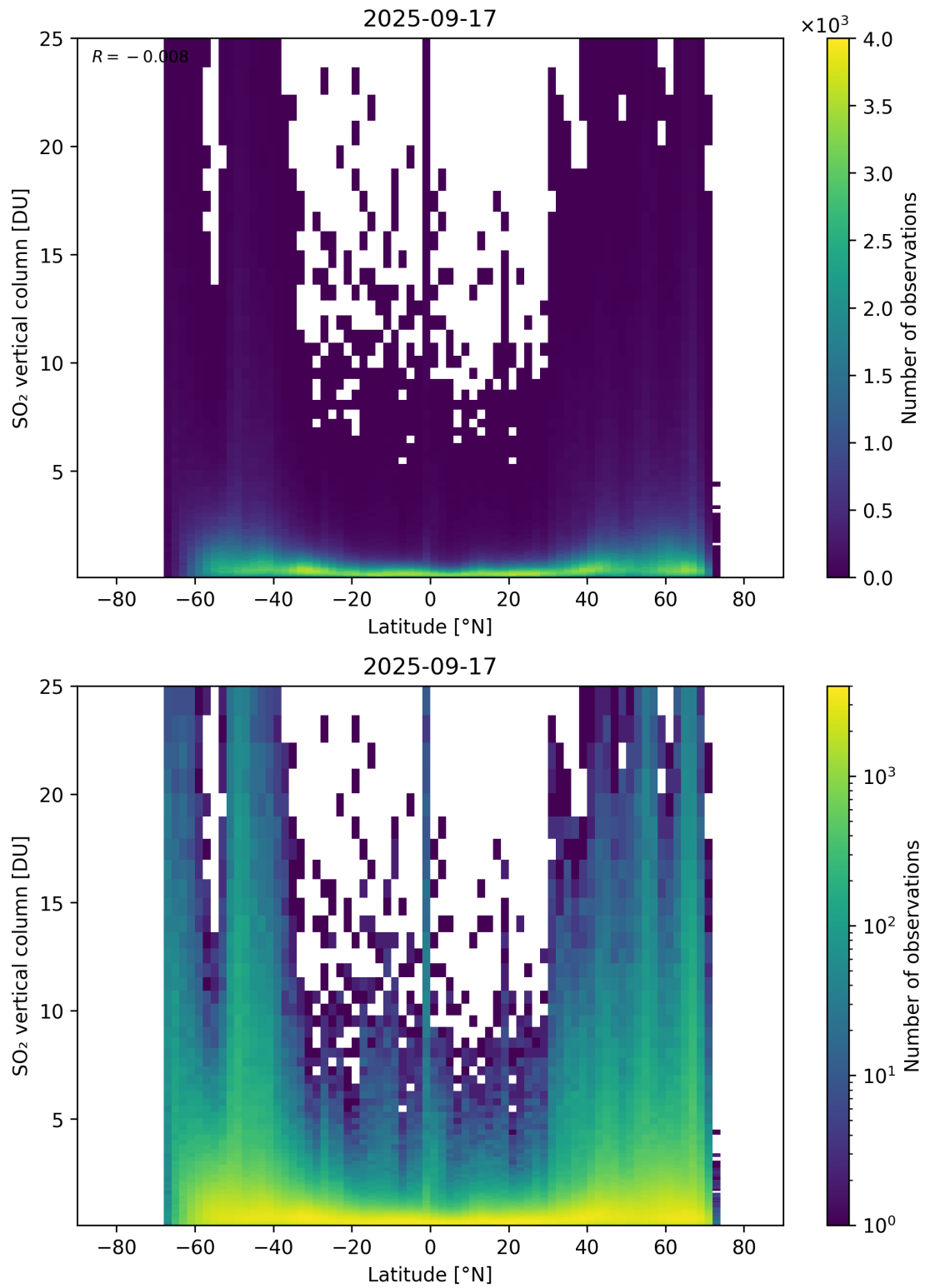
Figure 169: Scatter density plot of “Latitude” against “SO 2 vertical column” for 2025-09-16 to 2025-09-18.
