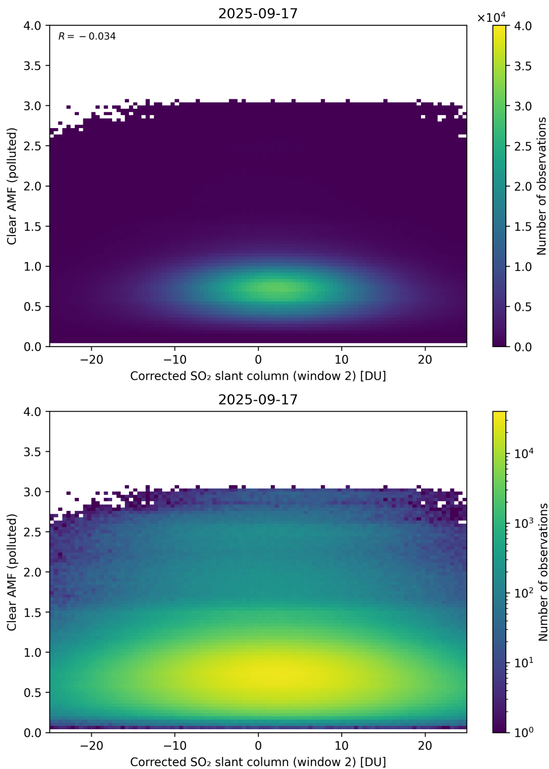
Figure 249: Scatter density plot of “Corrected SO 2 slant column (window 2)” against “Clear AMF (polluted)” for 2025-09-16 to 2025-09-18.
