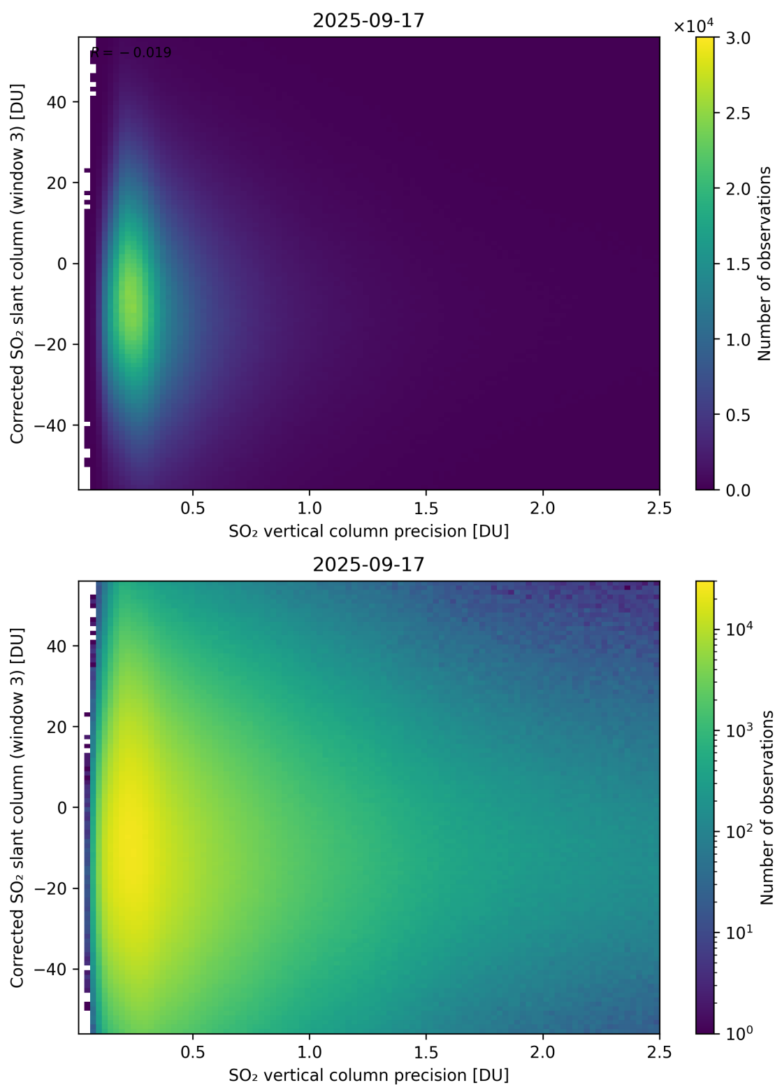
Figure 340: Scatter density plot of “SO 2 vertical column precision” against “Corrected SO 2 slant column (window 3)” for 2025-09-16 to 2025-09-18.
