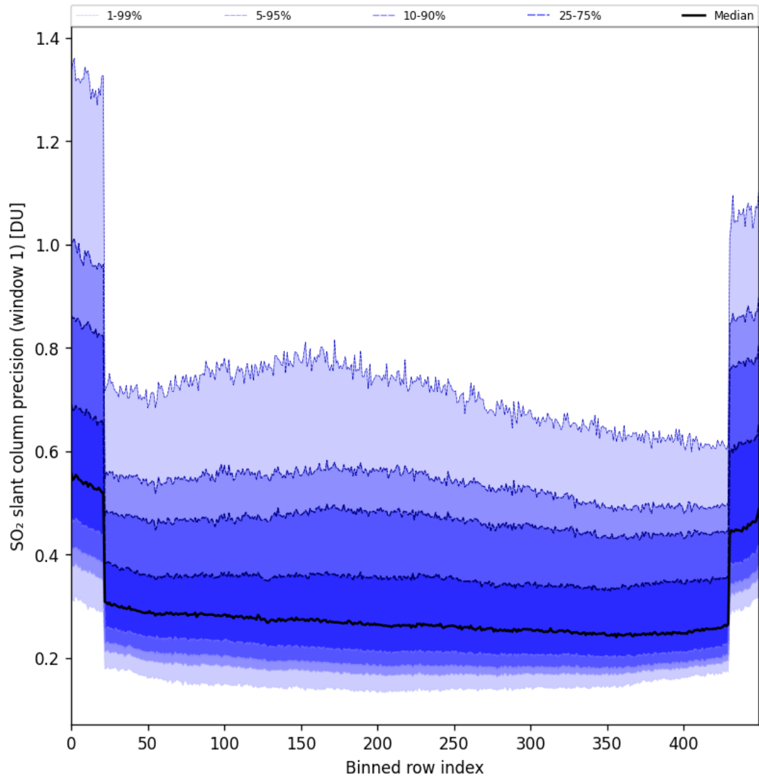
Figure 90: Along track statistics of “SO 2 slant column precision (window 1)” for 2025-09-16 to 2025-09-18
