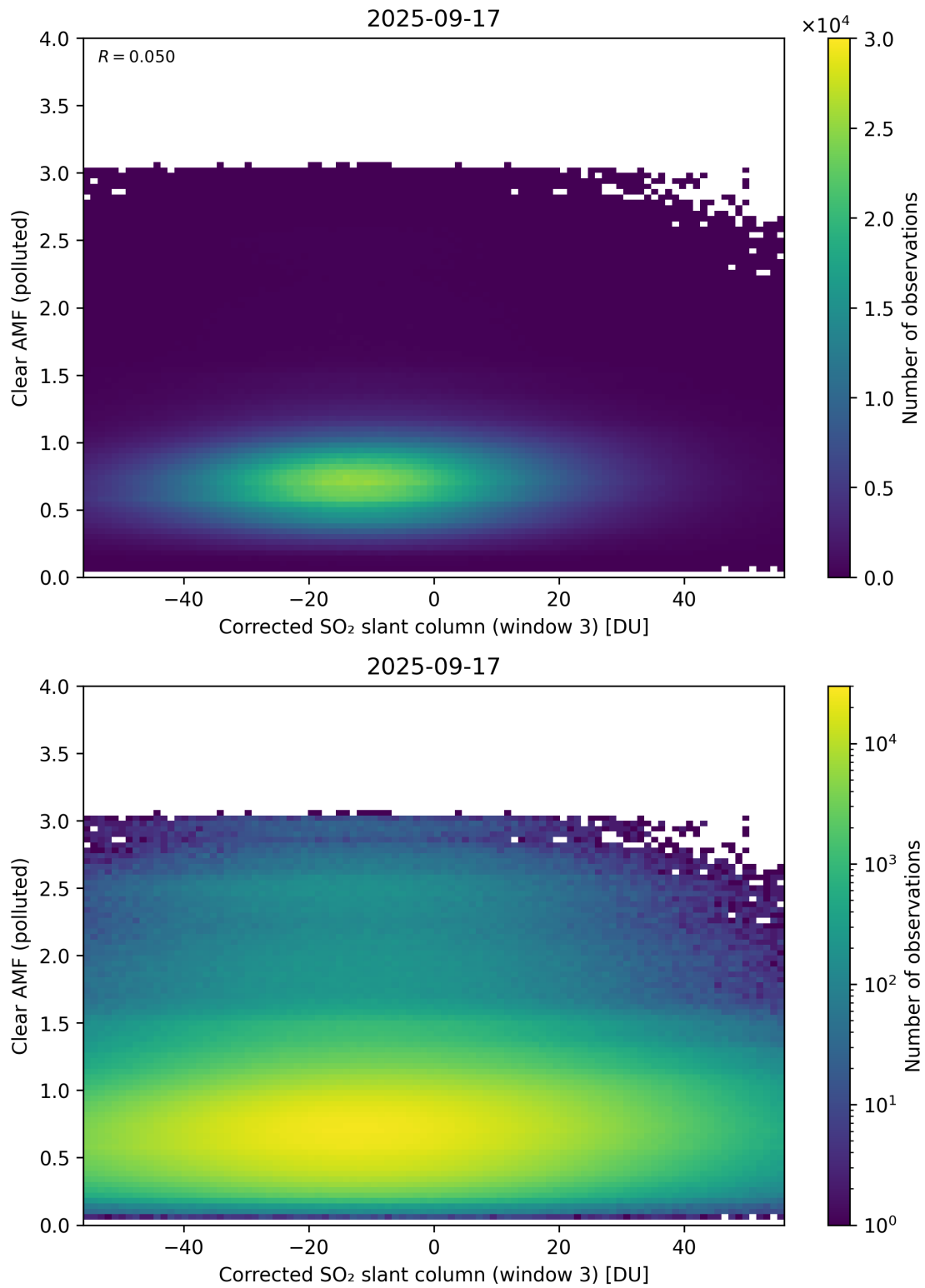
Figure 259: Scatter density plot of “Corrected SO 2 slant column (window 3)” against “Clear AMF (polluted)” for 2025-09-16 to 2025-09-18.
