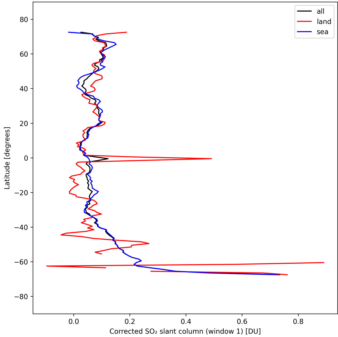
Figure 39: Zonal average of “Corrected SO 2 slant column (window 1)” for 2025-09-16 to 2025-09-18.
