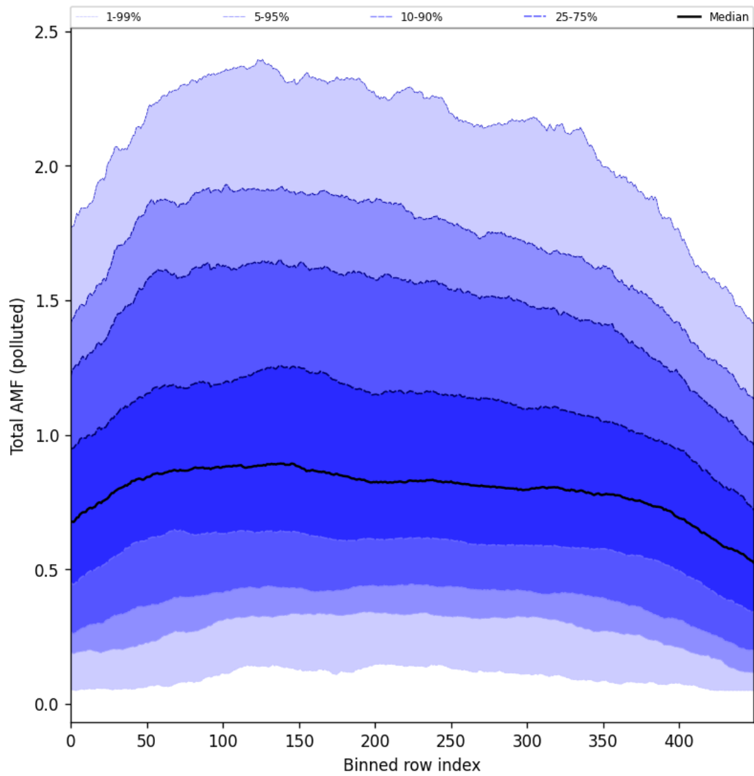
Figure 105: Along track statistics of “Total AMF (polluted)” for 2025-09-16 to 2025-09-18
