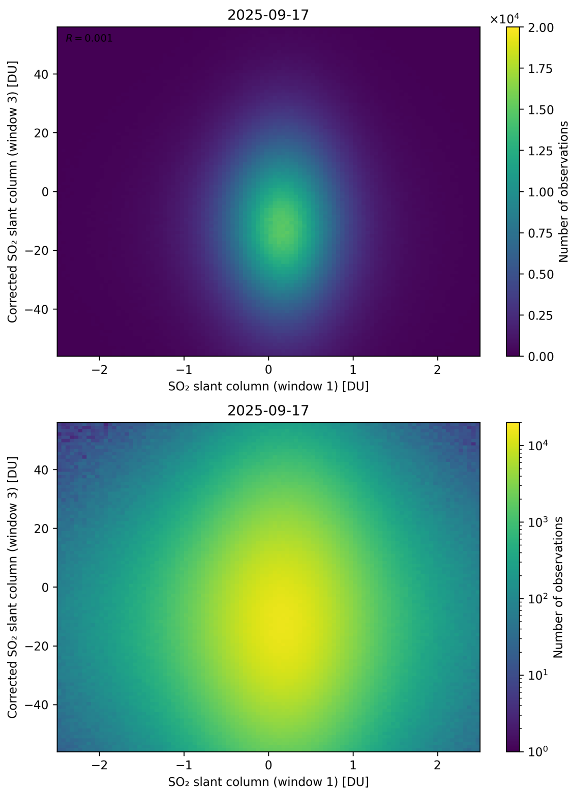
Figure 284: Scatter density plot of “SO 2 slant column (window 1)” against “Corrected SO 2 slant column (window 3)” for 2025-09-16 to 2025-09-18.
