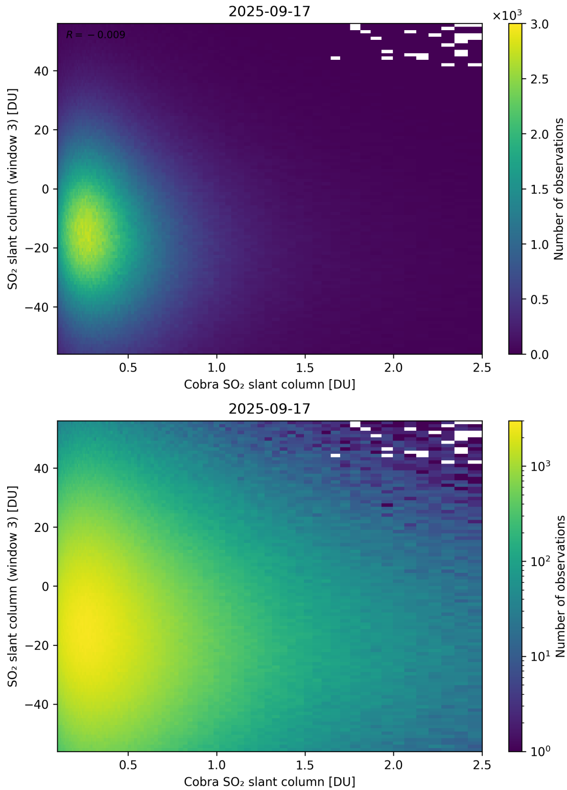
Figure 222: Scatter density plot of “Cobra SO 2 slant column” against “SO 2 slant column (window 3)” for 2025-09-16 to 2025-09-18.
