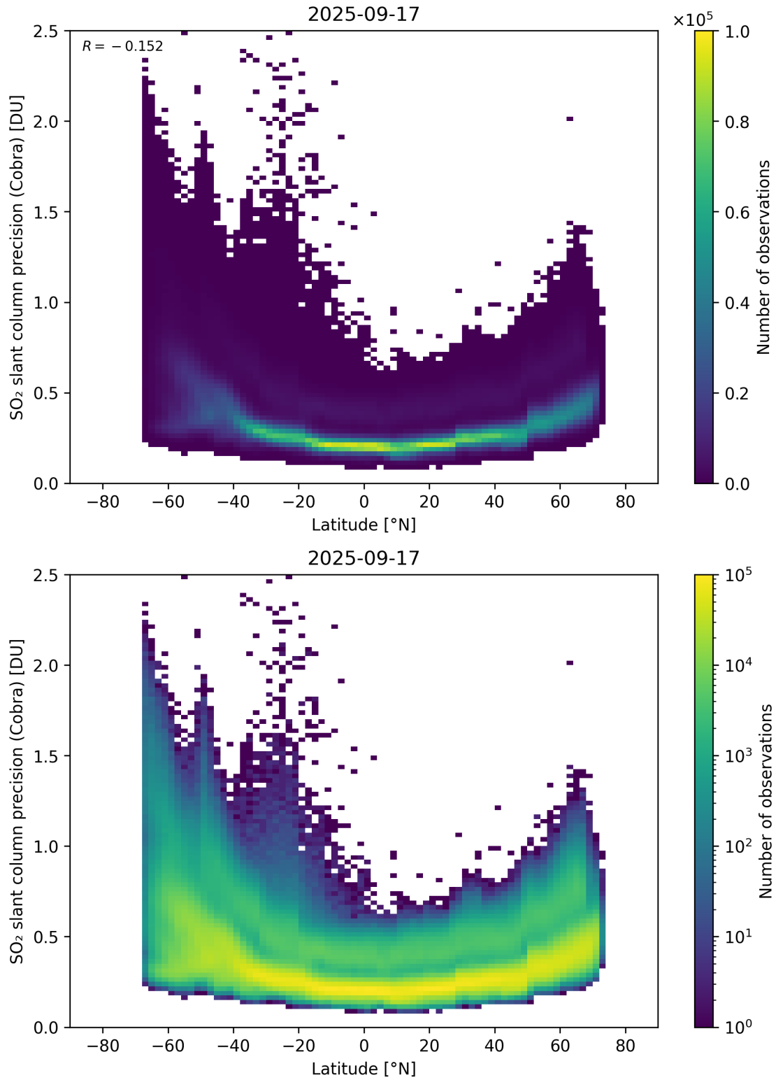
Figure 158: Scatter density plot of “Latitude” against “SO 2 slant column precision (Cobra)” for 2025-09-16 to 2025-09-18.
