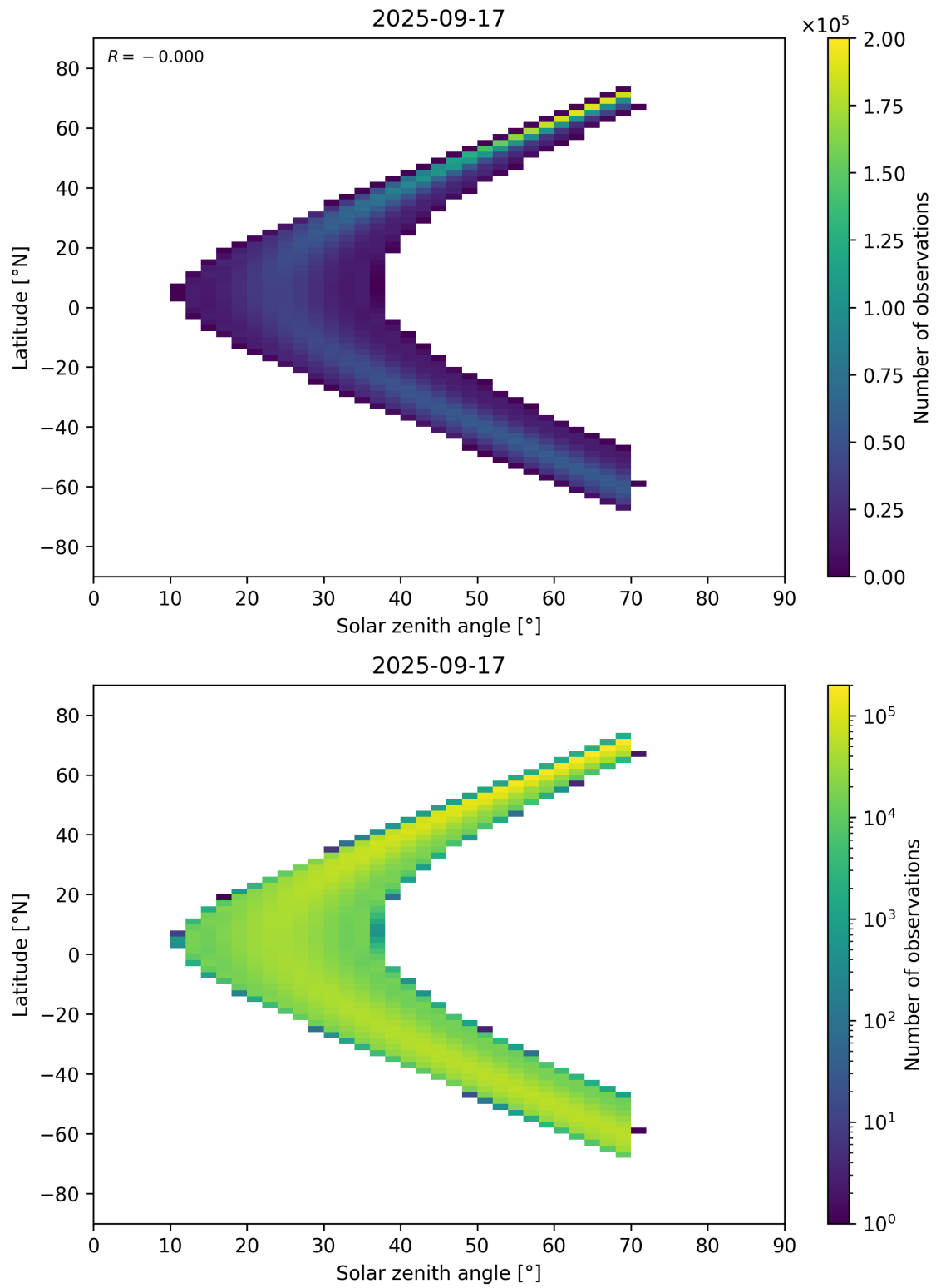
Figure 177: Scatter density plot of “Solar zenith angle” against “Latitude” for 2025-09-16 to 2025-09-18.
