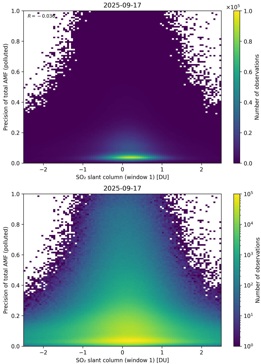
Figure 290: Scatter density plot of “SO 2 slant column (window 1)” against “Precision of total AMF (polluted)” for 2025-09-16 to 2025-09-18.
