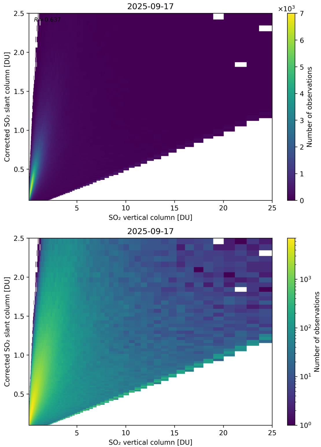
Figure 351: Scatter density plot of “SO 2 vertical column” against “Corrected SO 2 slant column” for 2025-09-16 to 2025-09-18.
