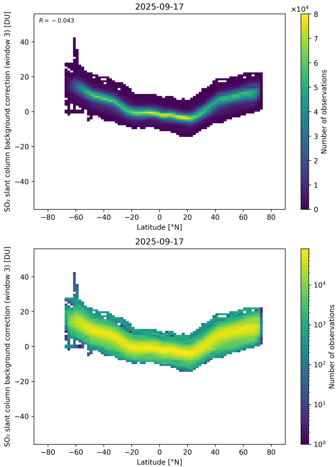
Figure 152: Scatter density plot of “Latitude” against “SO 2 slant column background correction (window 3)” for 2025-09-16 to 2025-09-18.
