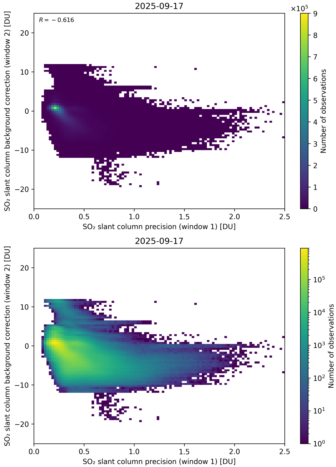
Figure 269: Scatter density plot of “SO 2 slant column precision (window 1)” against “SO 2 slant column background correction (window 2)” for 2025-09-16 to 2025-09-18.
