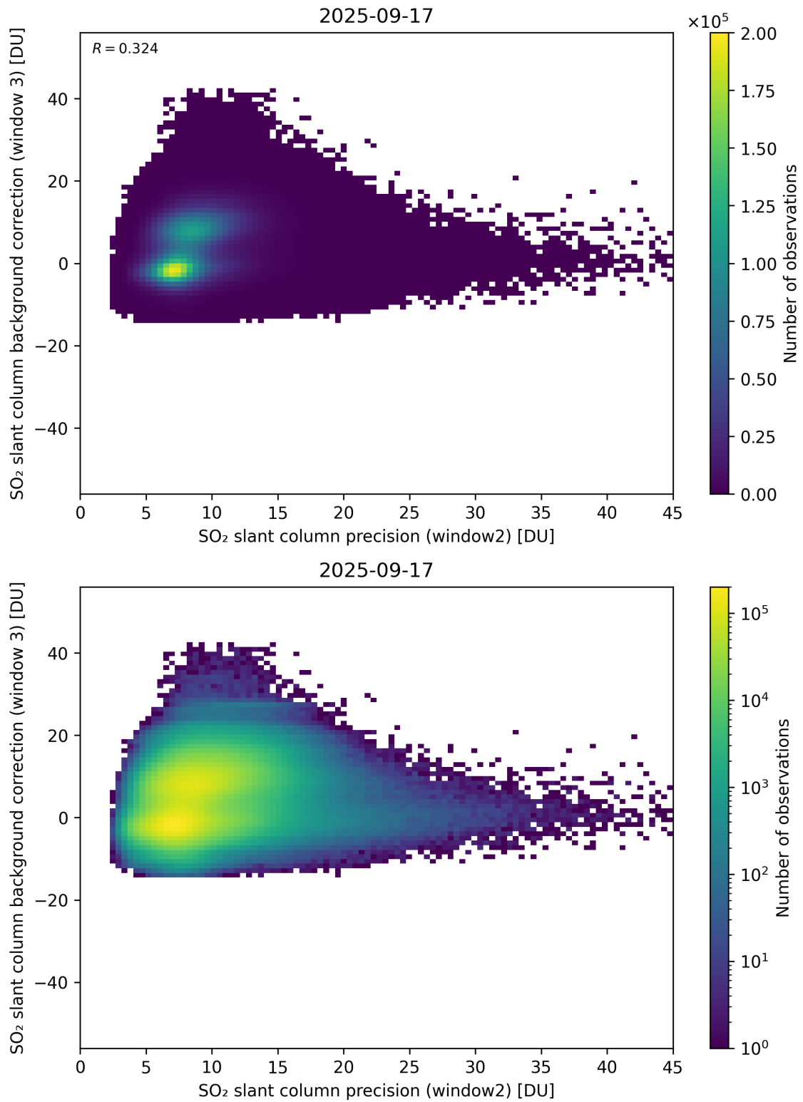
Figure 292: Scatter density plot of “SO 2 slant column precision (window2)” against “SO 2 slant column background correction (window 3)” for 2025-09-16 to 2025-09-18.
