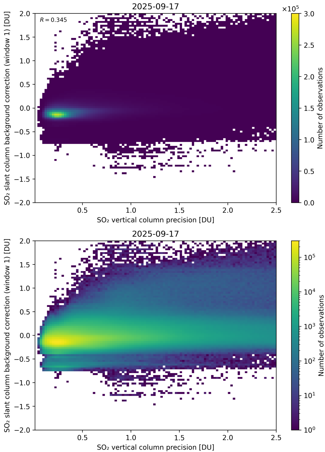
Figure 329: Scatter density plot of “SO 2 vertical column precision” against “SO 2 slant column background correction (window 1)” for 2025-09-16 to 2025-09-18.
