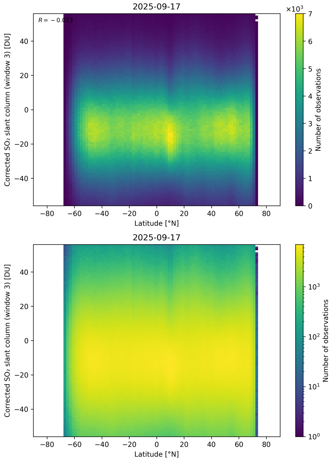
Figure 161: Scatter density plot of “Latitude” against “Corrected SO 2 slant column (window 3)” for 2025-09-16 to 2025-09-18.
