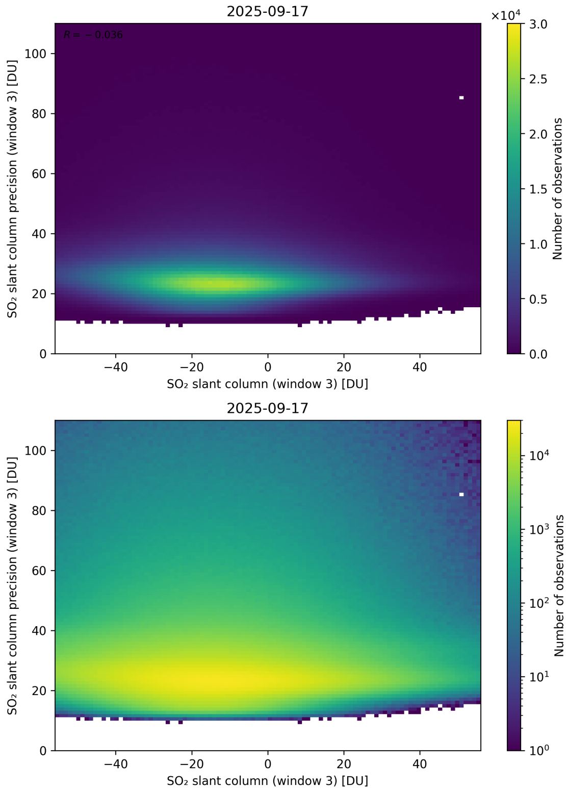
Figure 317: Scatter density plot of “SO 2 slant column (window 3)” against “SO 2 slant column precision (window 3)” for 2025-09-16 to 2025-09-18.
