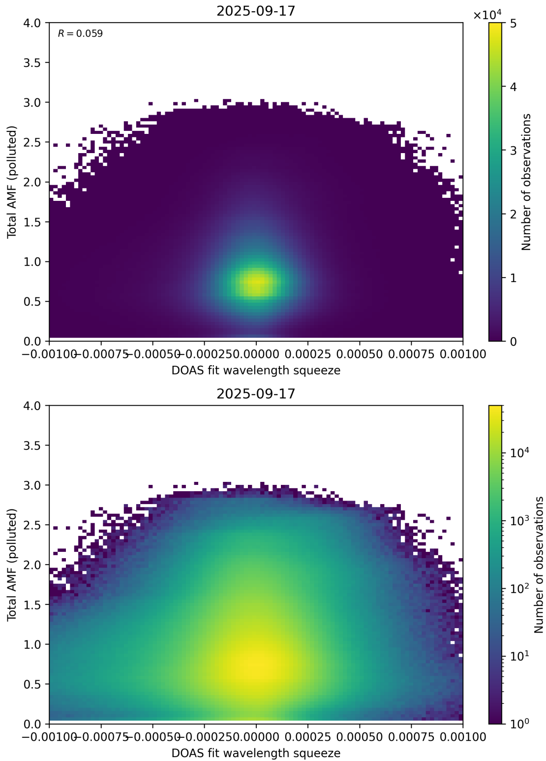
Figure 145: Scatter density plot of “DOAS fit wavelength squeeze” against “Total AMF (polluted)” for 2025-09-16 to 2025-09-18.
