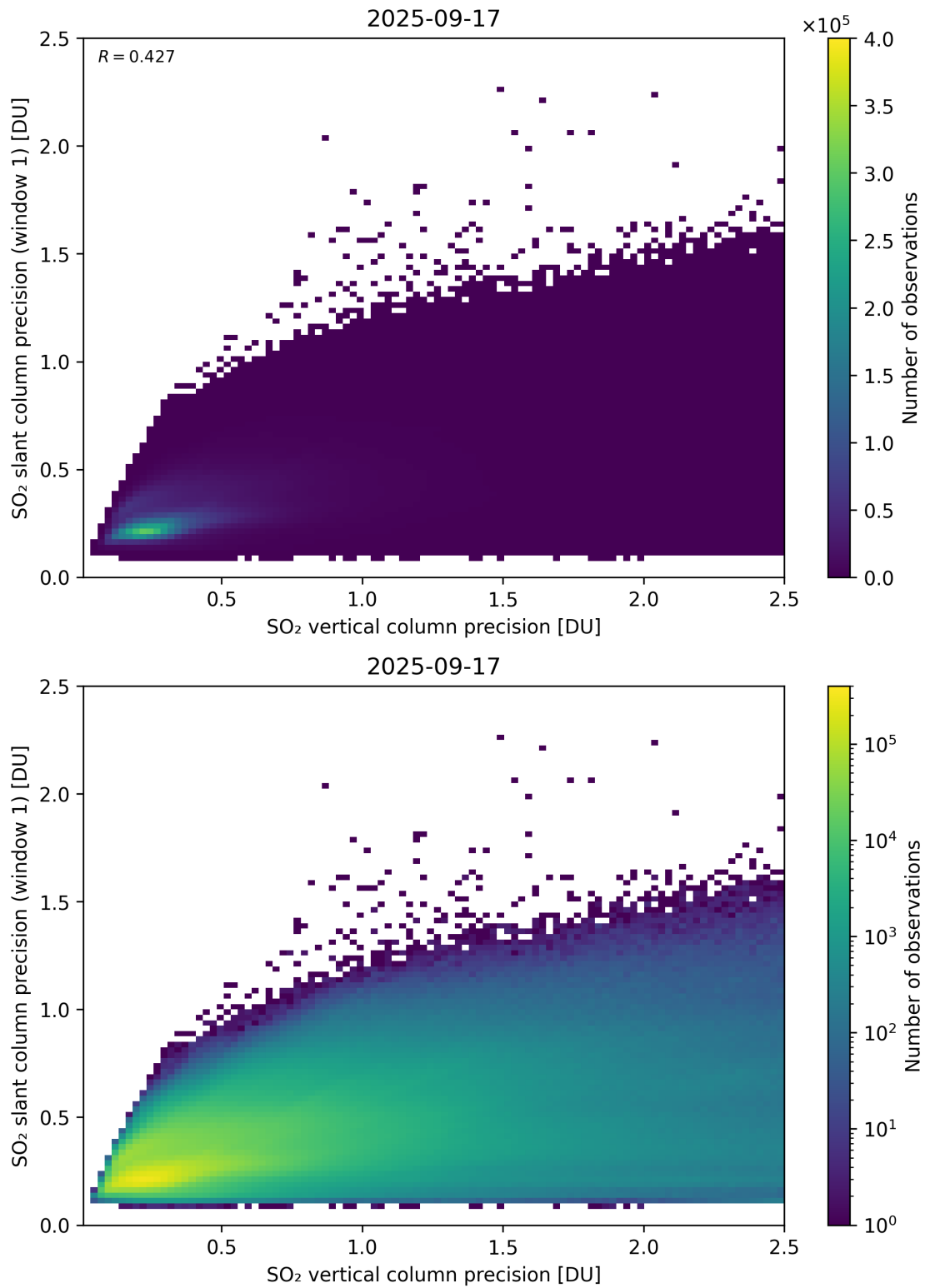
Figure 342: Scatter density plot of “SO 2 vertical column precision” against “SO 2 slant column precision (window 1)” for 2025-09-16 to 2025-09-18.
