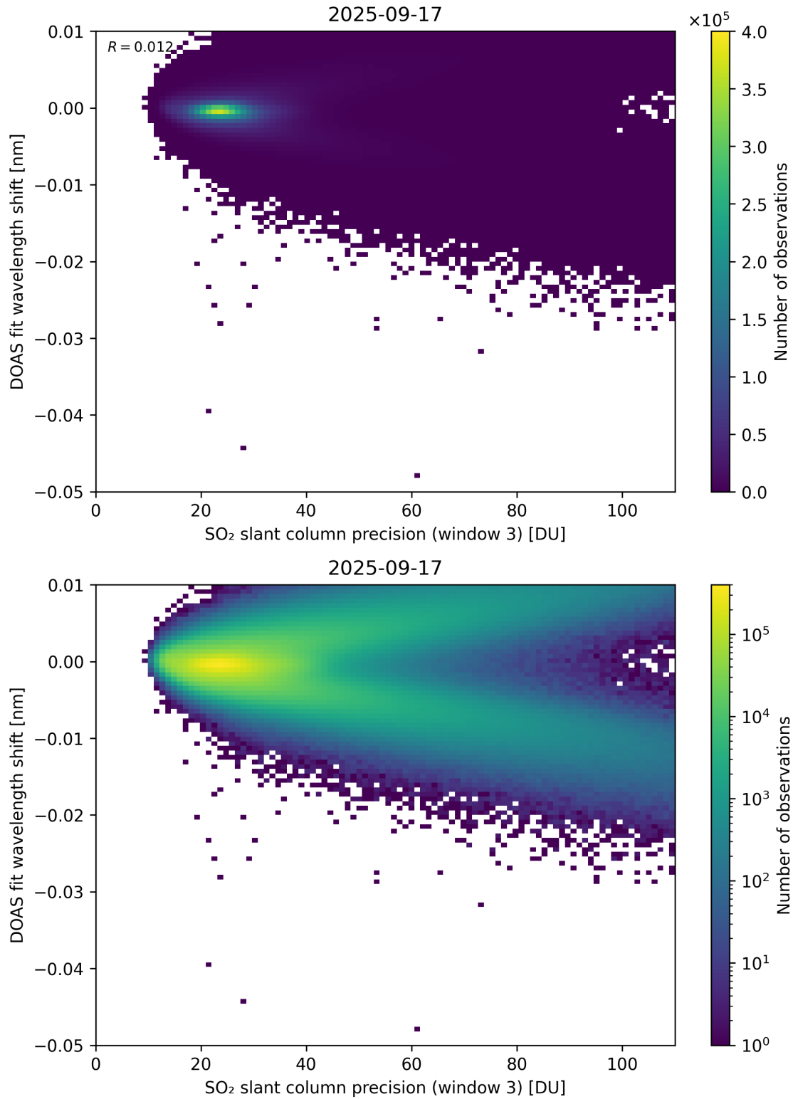
Figure 308: Scatter density plot of “SO 2 slant column precision (window 3)” against “DOAS fit wavelength shift” for 2025-09-16 to 2025-09-18.
