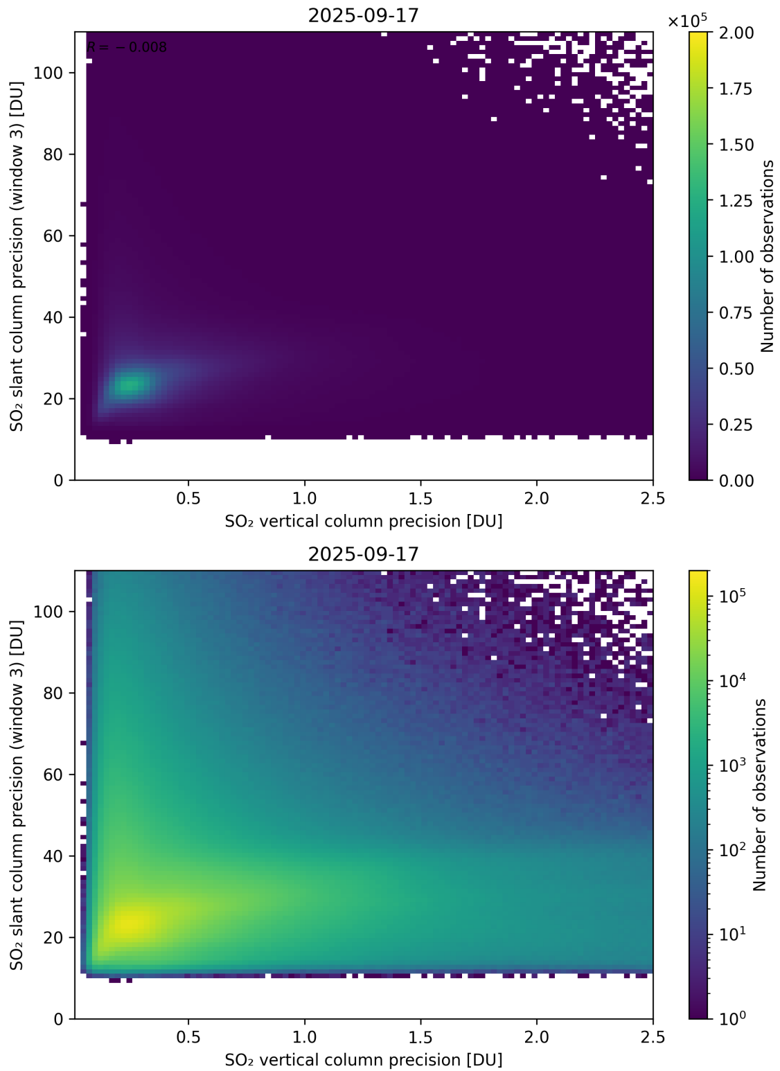
Figure 345: Scatter density plot of “SO 2 vertical column precision” against “SO 2 slant column precision (window 3)” for 2025-09-16 to 2025-09-18.
