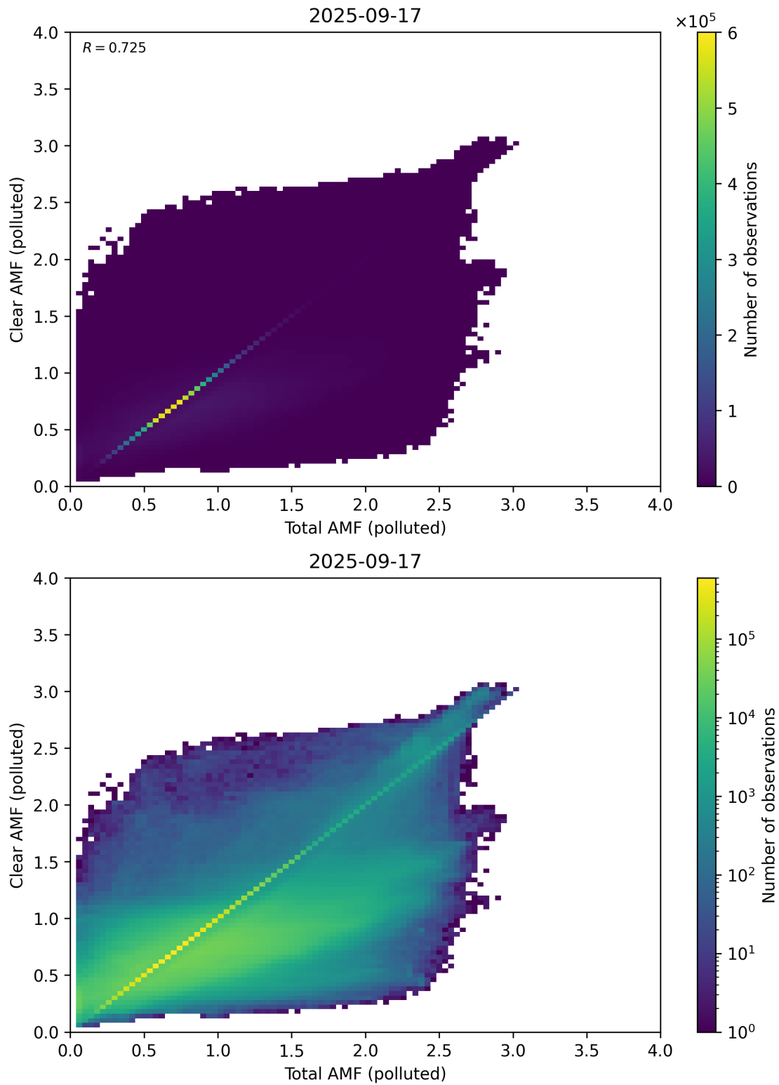
Figure 321: Scatter density plot of “Total AMF (polluted)” against “Clear AMF (polluted)” for 2025-09-16 to 2025-09-18.
