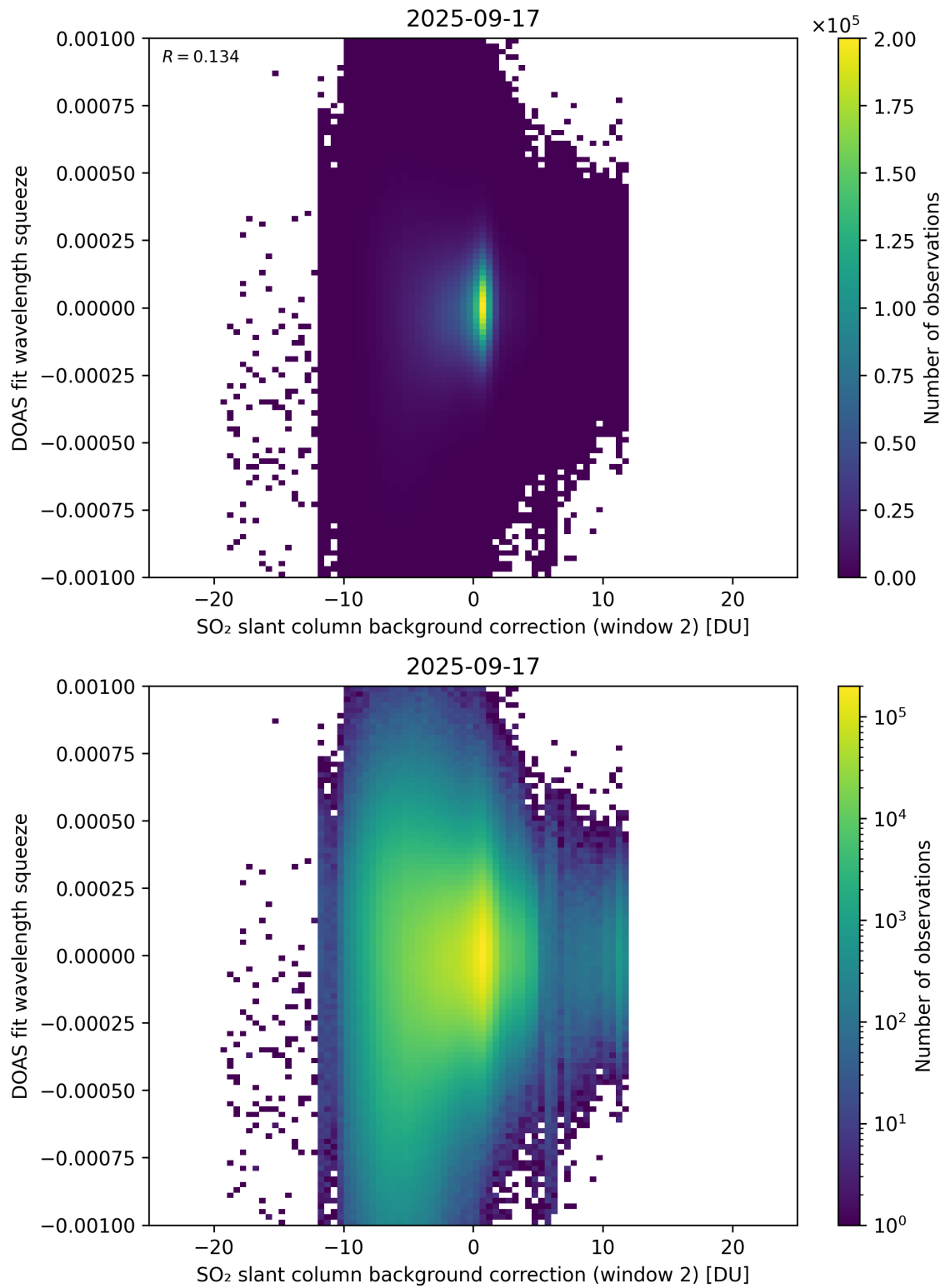
Figure 124: Scatter density plot of “SO 2 slant column background correction (window 2)” against “DOAS fit wavelength squeeze” for 2025-09-16 to 2025-09-18.
