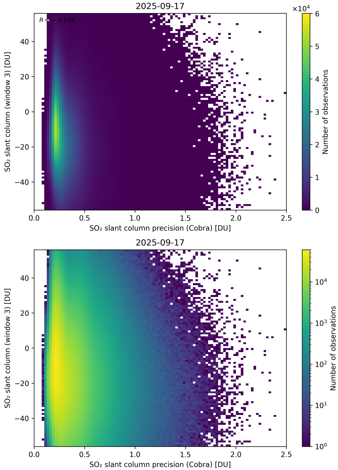
Figure 211: Scatter density plot of “SO 2 slant column precision (Cobra)” against “SO 2 slant column (window 3)” for 2025-09-16 to 2025-09-18.
