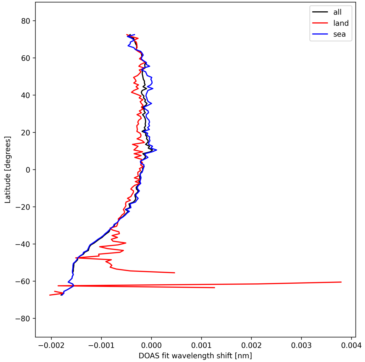
Figure 50: Zonal average of “DOAS fit wavelength shift” for 2025-09-16 to 2025-09-18.
