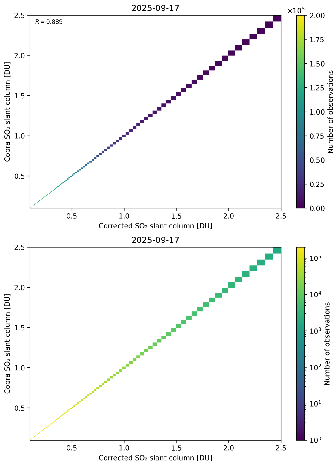
Figure 233: Scatter density plot of “Corrected SO 2 slant column” against “Cobra SO 2 slant column” for 2025-09-16 to 2025-09-18.
