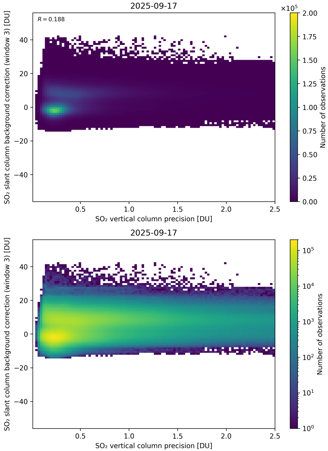
Figure 331: Scatter density plot of “SO 2 vertical column precision” against “SO 2 slant column background correction (window 3)” for 2025-09-16 to 2025-09-18.
