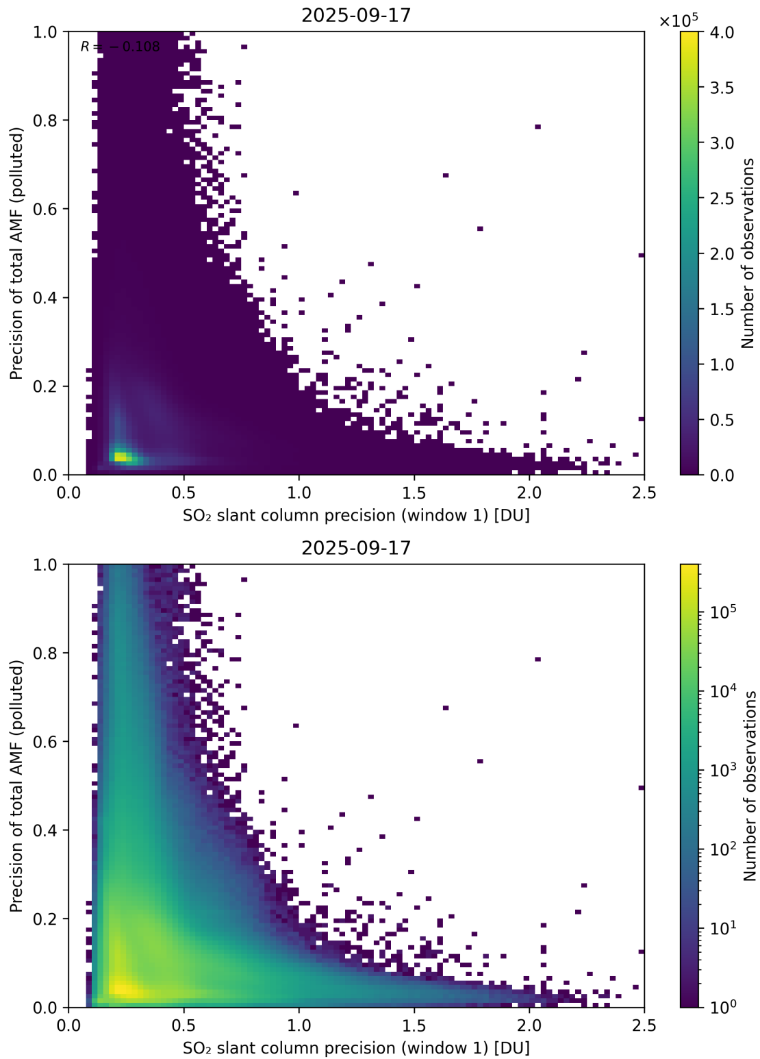
Figure 281: Scatter density plot of “SO 2 slant column precision (window 1)” against “Precision of total AMF (polluted)” for 2025-09-16 to 2025-09-18.
