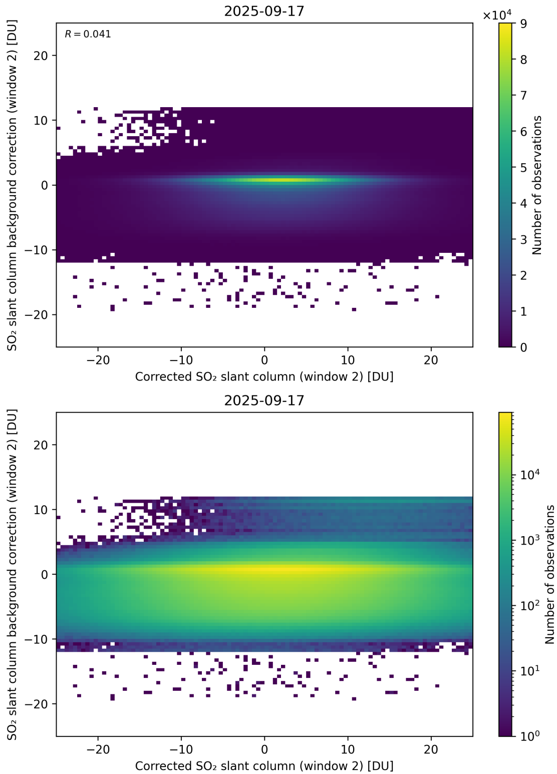
Figure 244: Scatter density plot of “Corrected SO 2 slant column (window 2)” against “SO 2 slant column background correction (window 2)” for 2025-09-16 to 2025-09-18.
