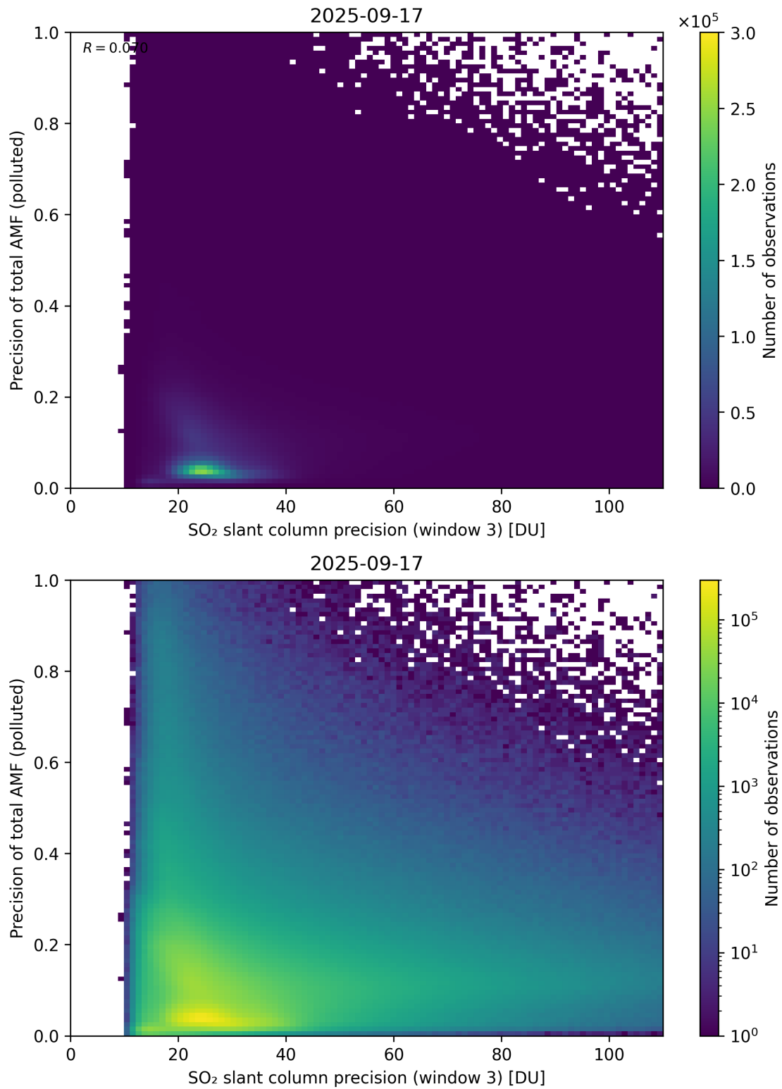
Figure 314: Scatter density plot of “SO 2 slant column precision (window 3)” against “Precision of total AMF (polluted)” for 2025-09-16 to 2025-09-18.
