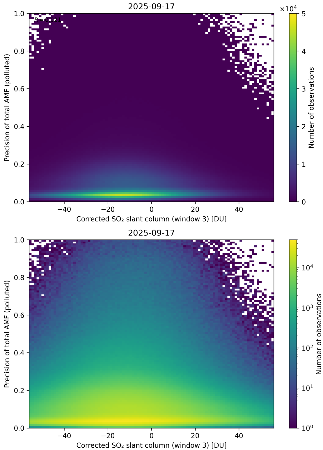
Figure 261: Scatter density plot of “Corrected SO 2 slant column (window 3)” against “Precision of total AMF (polluted)” for 2025-09-16 to 2025-09-18.
