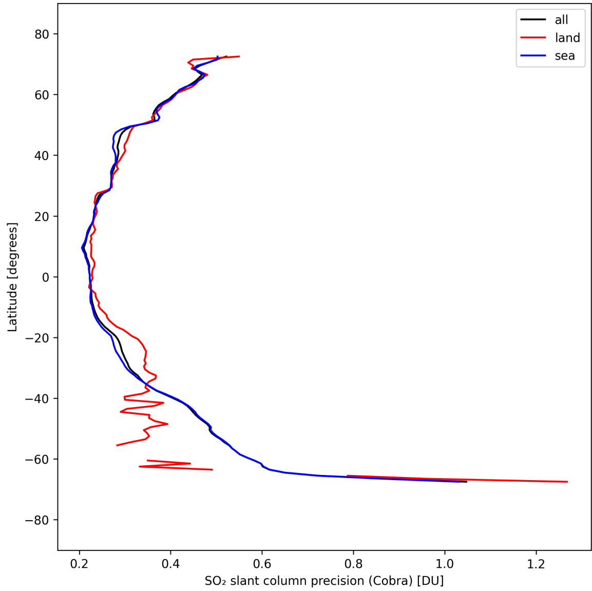
Figure 36: Zonal average of “SO 2 slant column precision (Cobra)” for 2025-09-16 to 2025-09-18.
