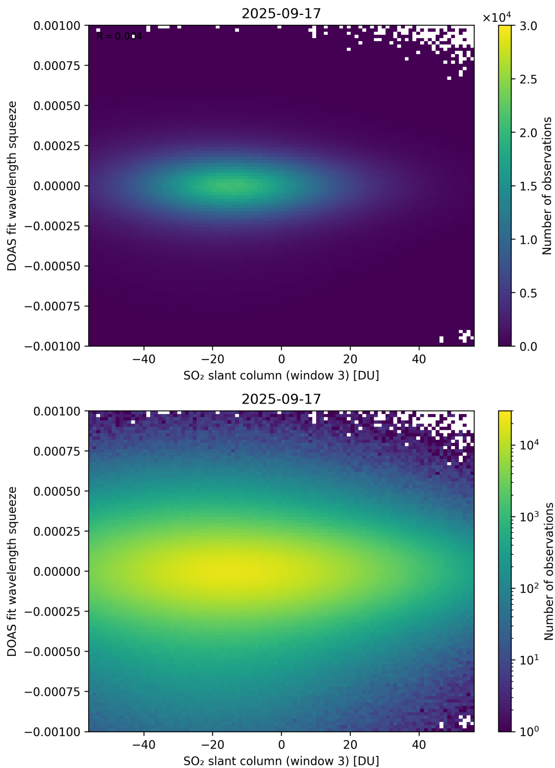
Figure 305: Scatter density plot of “SO 2 slant column (window 3)” against “DOAS fit wavelength squeeze” for 2025-09-16 to 2025-09-18.
