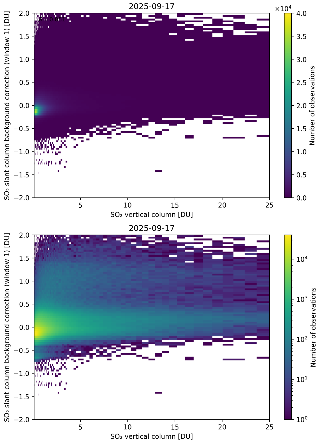
Figure 323: Scatter density plot of “SO 2 vertical column” against “SO 2 slant column background correction (window 1)” for 2025-09-16 to 2025-09-18.
