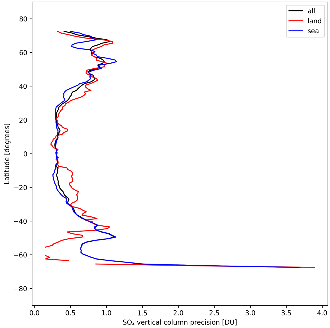
Figure 33: Zonal average of “SO 2 vertical column precision” for 2025-09-16 to 2025-09-18.
