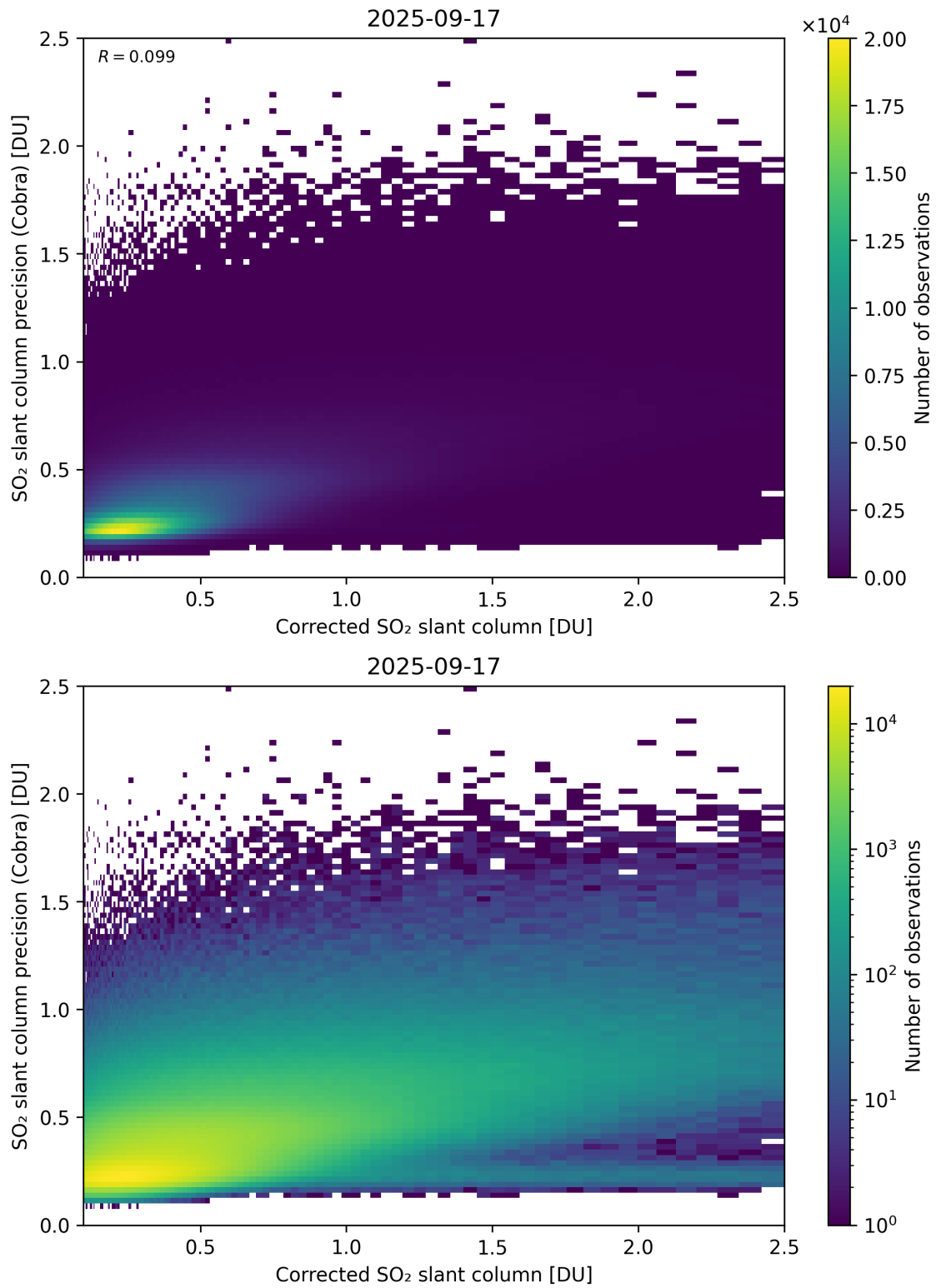
Figure 234: Scatter density plot of “Corrected SO 2 slant column” against “SO 2 slant column precision (Cobra)” for 2025-09-16 to 2025-09-18.
