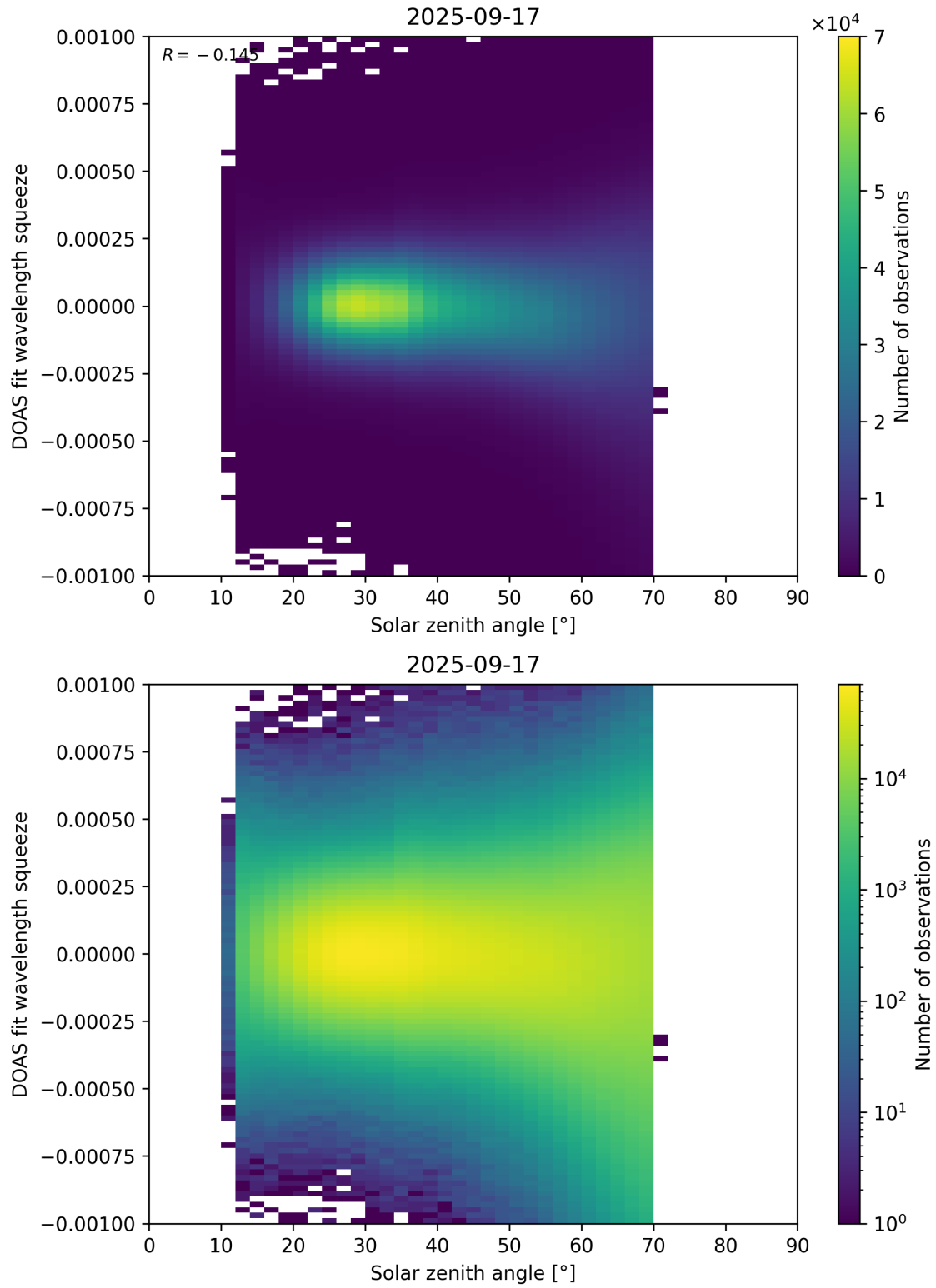
Figure 175: Scatter density plot of “Solar zenith angle” against “DOAS fit wavelength squeeze” for 2025-09-16 to 2025-09-18.
