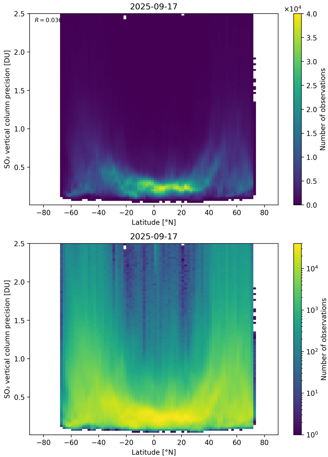
Figure 170: Scatter density plot of “Latitude” against “SO 2 vertical column precision” for 2025-09-16 to 2025-09-18.
