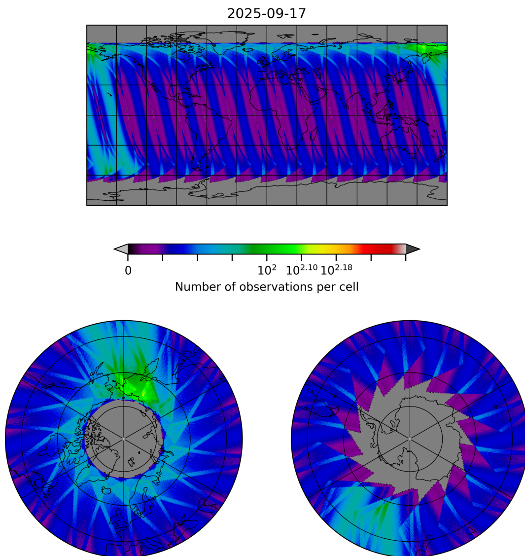
Figure 30: Map of the number of observations for 2025-09-16 to 2025-09-18
