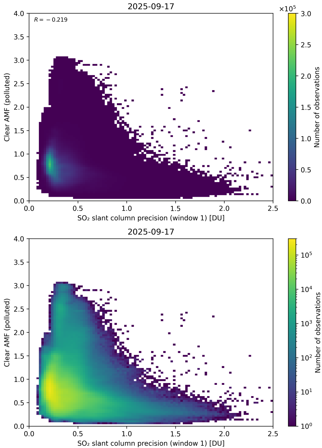
Figure 274: Scatter density plot of “SO 2 slant column precision (window 1)” against “Clear AMF (polluted)” for 2025-09-16 to 2025-09-18.
