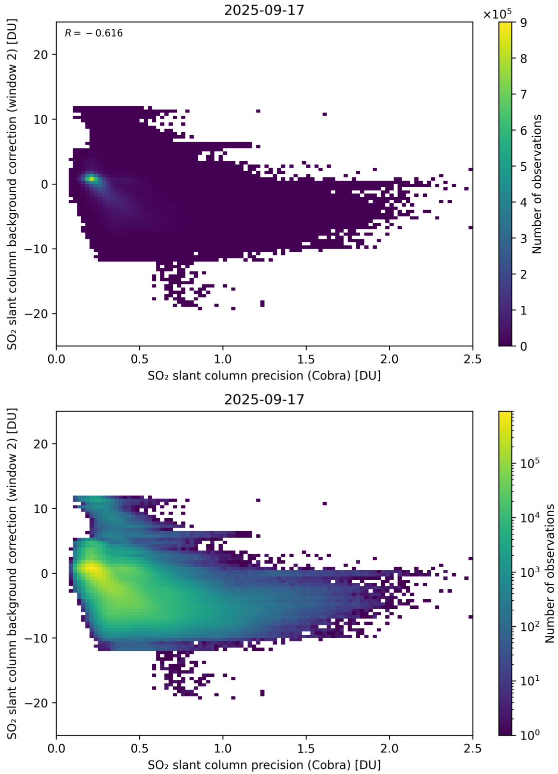
Figure 200: Scatter density plot of “SO 2 slant column precision (Cobra)” against “SO 2 slant column background correction (window 2)” for 2025-09-16 to 2025-09-18.
