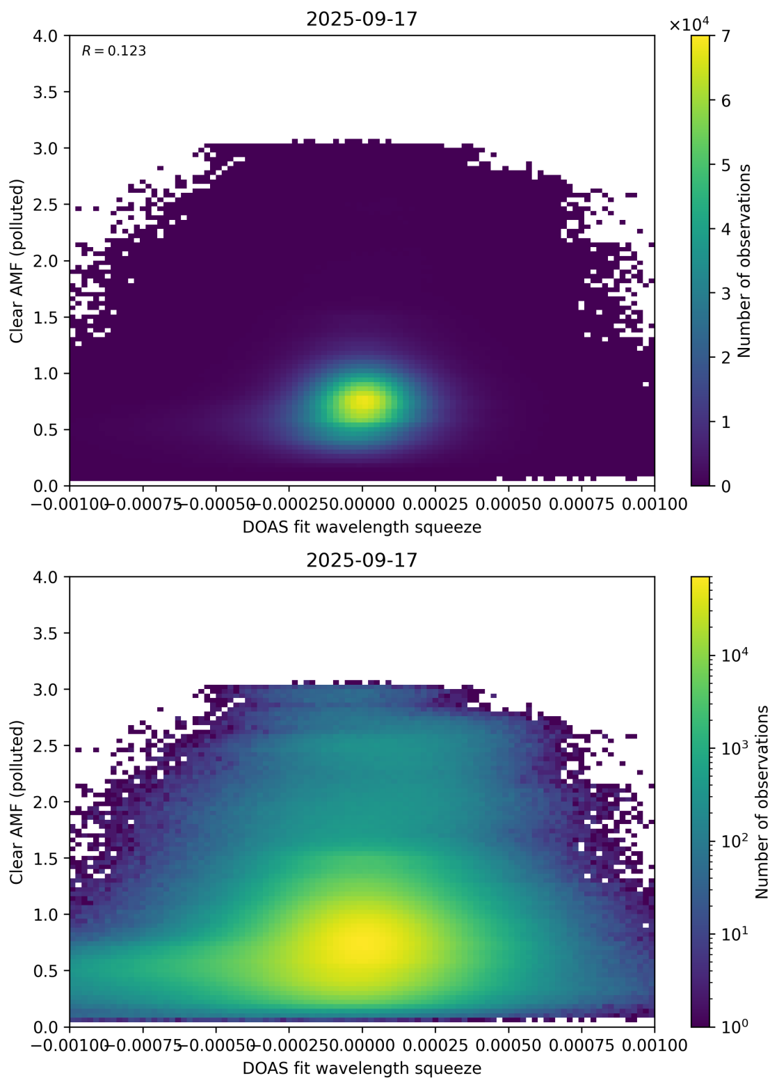
Figure 144: Scatter density plot of “DOAS fit wavelength squeeze” against “Clear AMF (polluted)” for 2025-09-16 to 2025-09-18.
