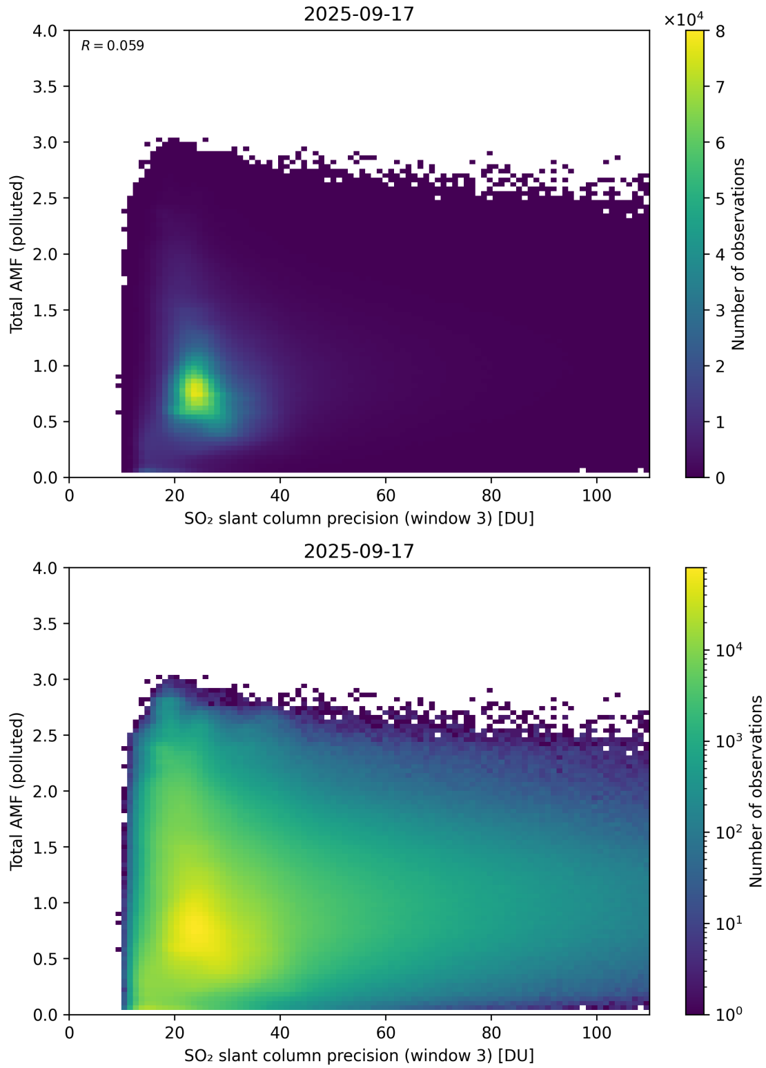
Figure 313: Scatter density plot of “SO 2 slant column precision (window 3)” against “Total AMF (polluted)” for 2025-09-16 to 2025-09-18.
