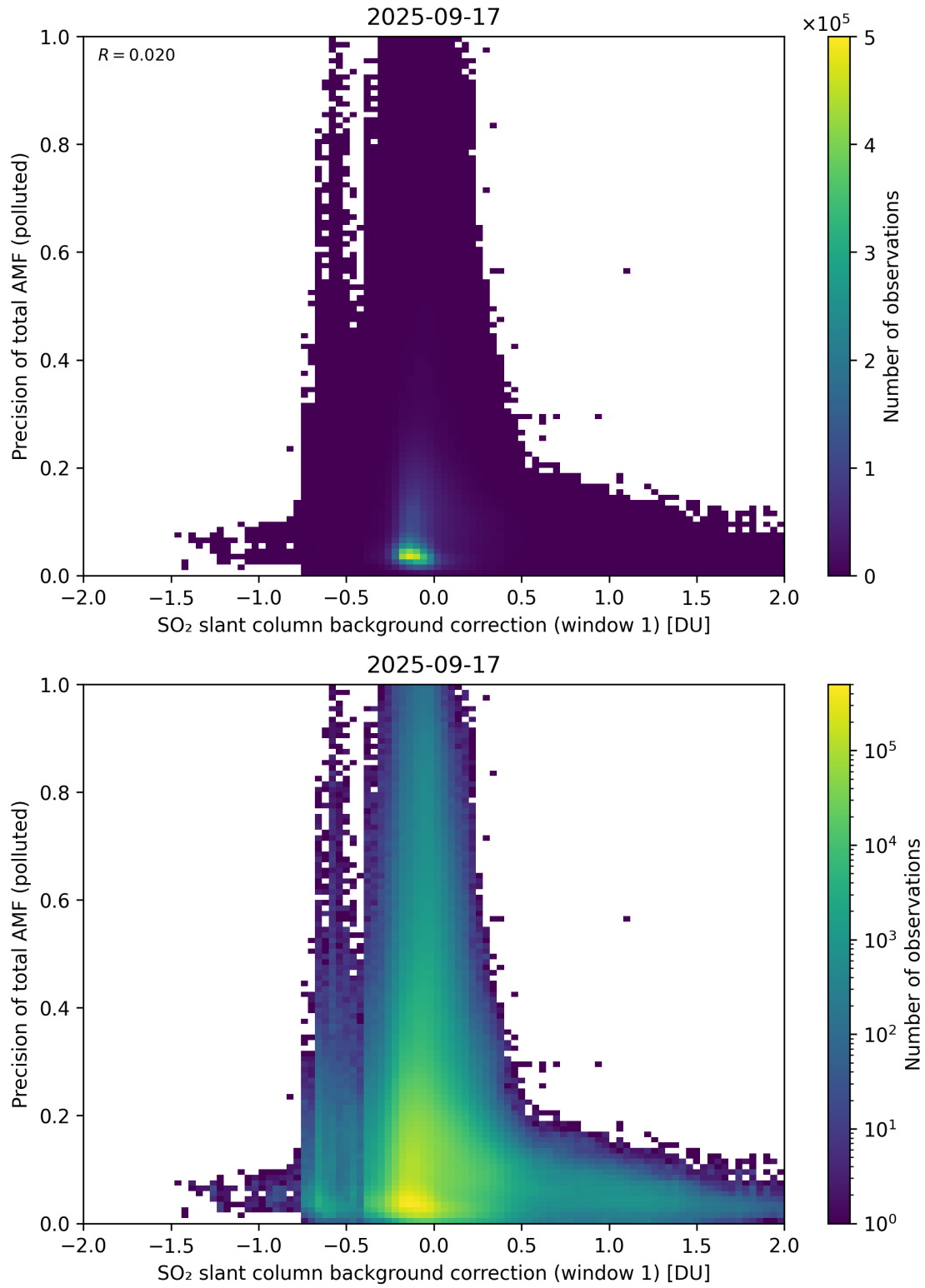
Figure 121: Scatter density plot of “SO 2 slant column background correction (window 1)” against “Precision of total AMF (polluted)” for 2025-09-16 to 2025-09-18.
