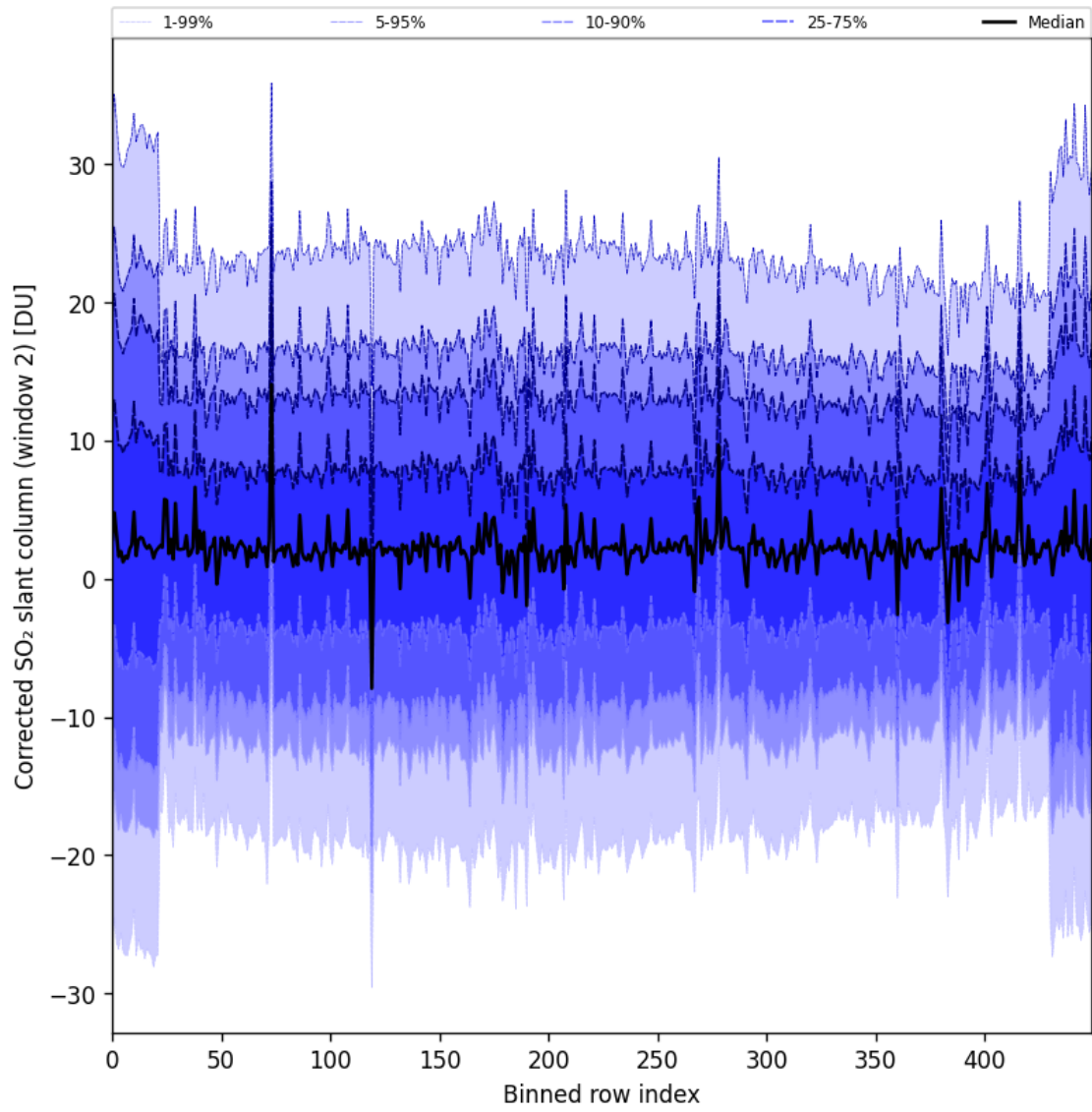
Figure 95: Along track statistics of “Corrected SO 2 slant column (window 2)” for 2025-09-16 to 2025-09-18
