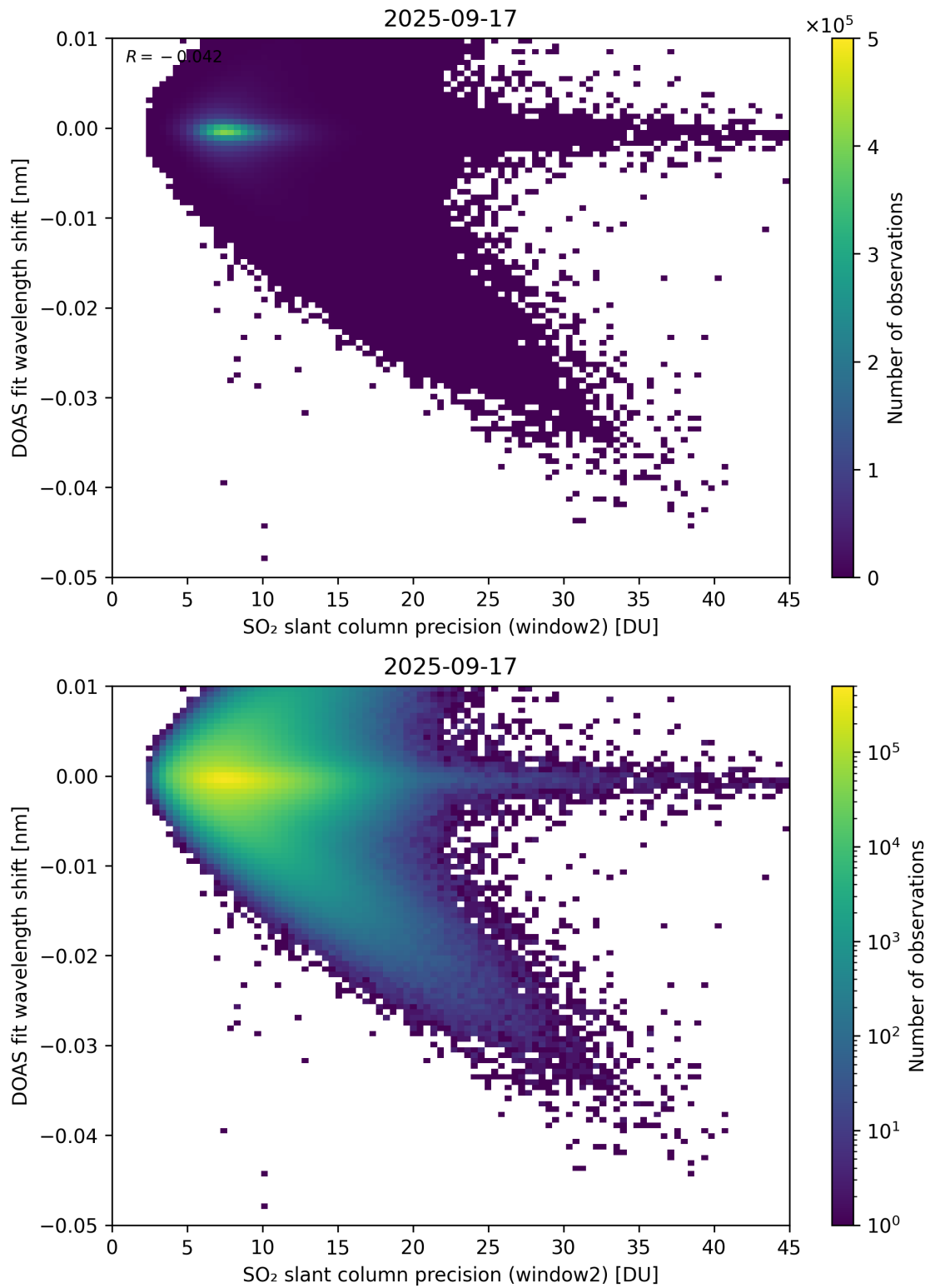
Figure 293: Scatter density plot of “SO 2 slant column precision (window2)” against “DOAS fit wavelength shift” for 2025-09-16 to 2025-09-18.
