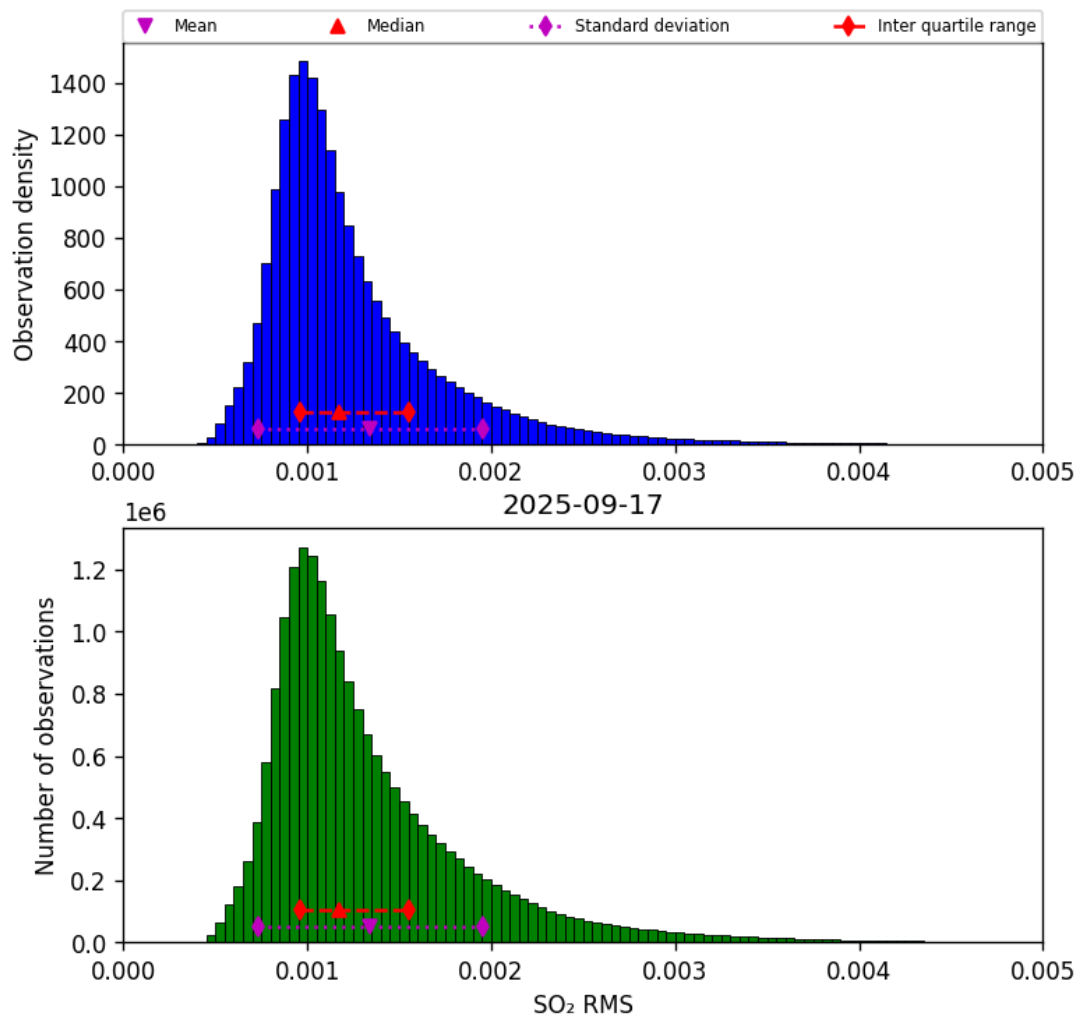
Figure 78: Histogram of “SO 2 RMS” for 2025-09-16 to 2025-09-18
