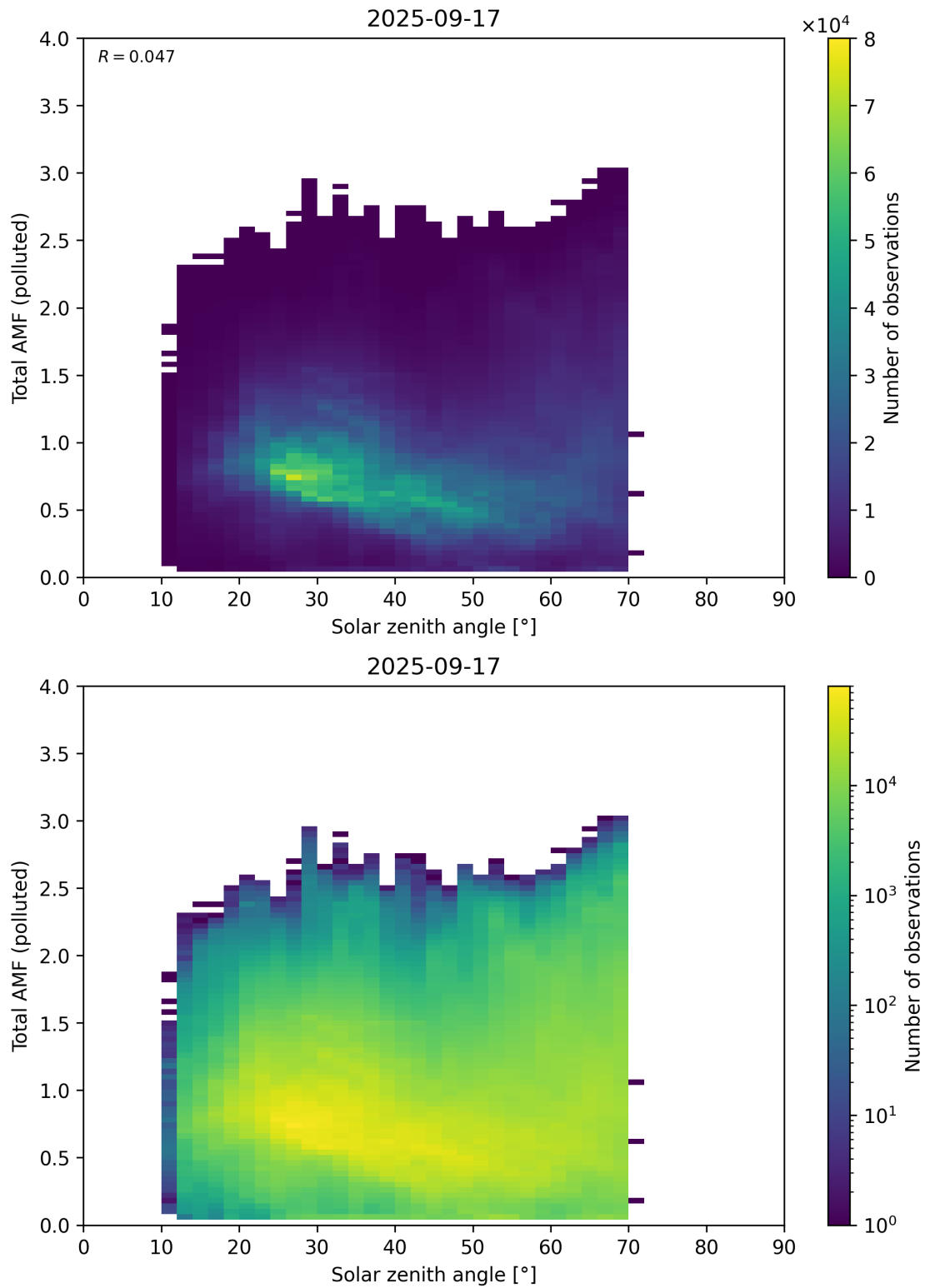
Figure 189: Scatter density plot of “Solar zenith angle” against “Total AMF (polluted)” for 2025-09-16 to 2025-09-18.
