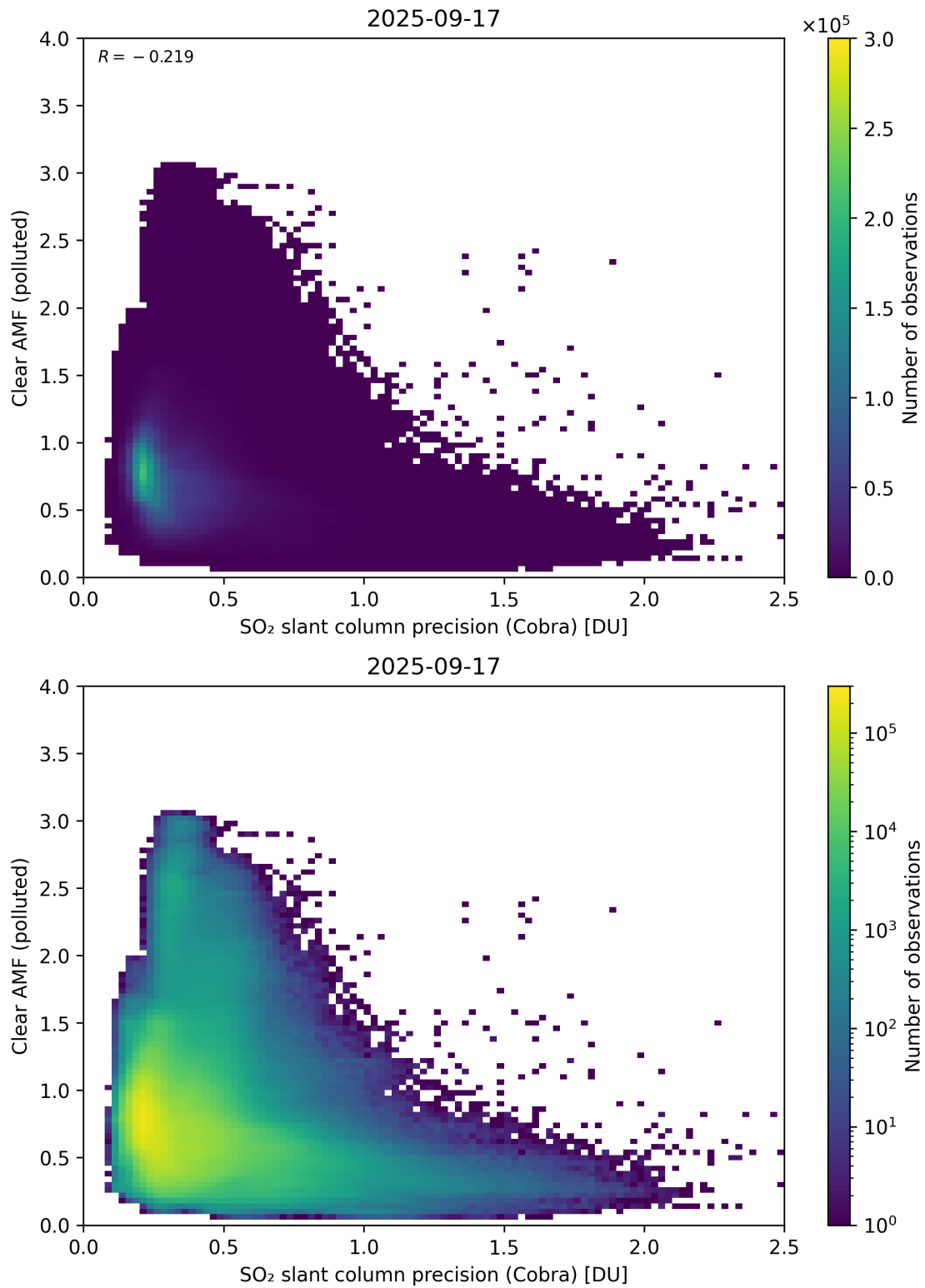
Figure 205: Scatter density plot of “SO 2 slant column precision (Cobra)” against “Clear AMF (polluted)” for 2025-09-16 to 2025-09-18.
