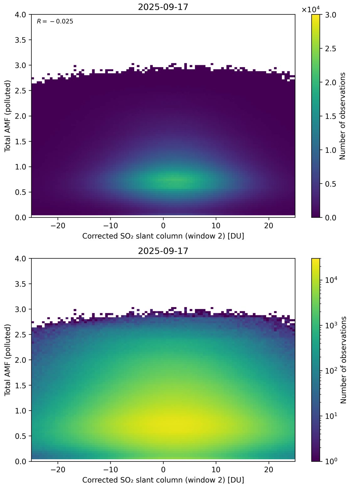
Figure 253: Scatter density plot of “Corrected SO 2 slant column (window 2)” against “Total AMF (polluted)” for 2025-09-16 to 2025-09-18.
