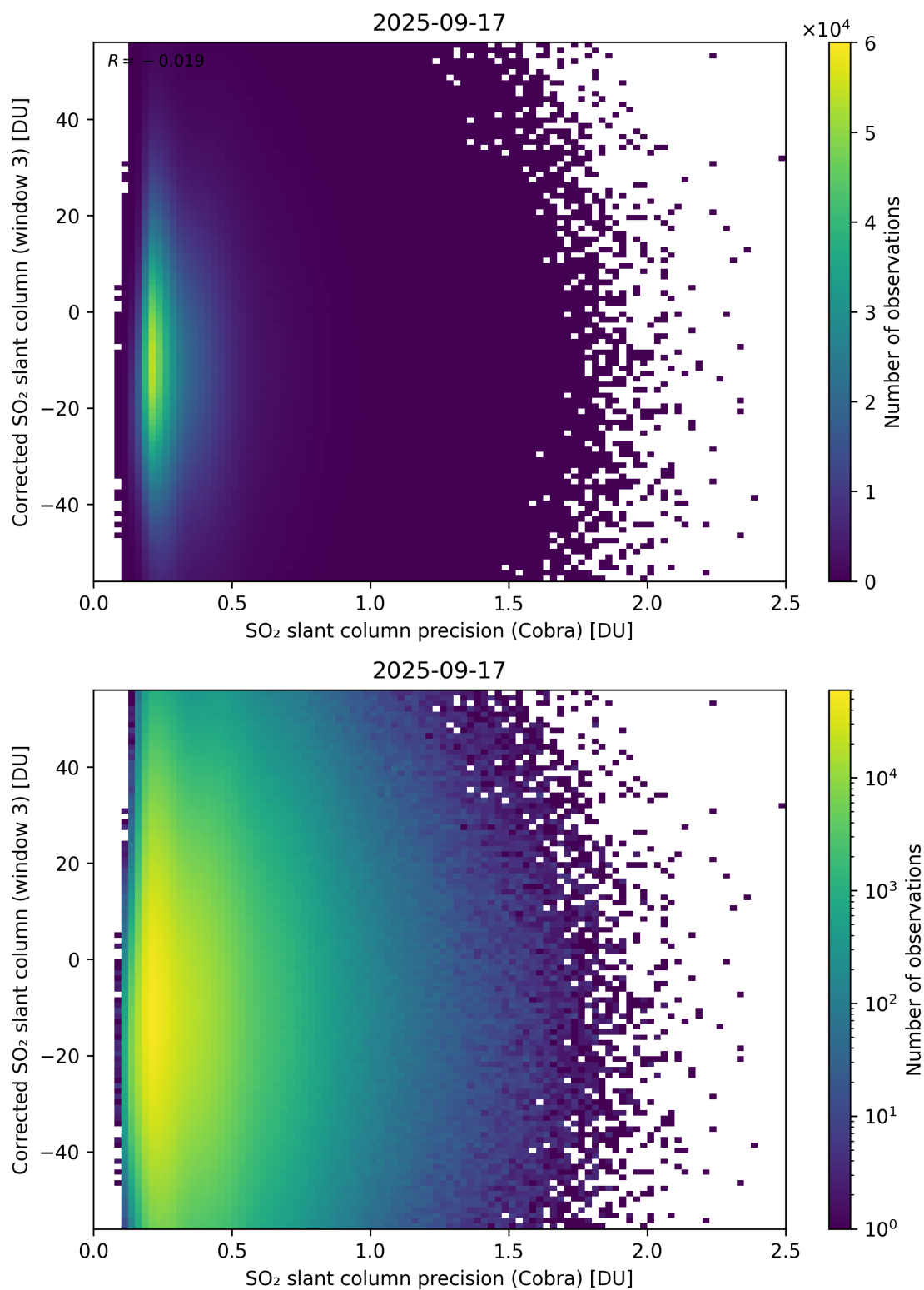
Figure 207: Scatter density plot of “SO 2 slant column precision (Cobra)” against “Corrected SO 2 slant column (window 3)” for 2025-09-16 to 2025-09-18.
