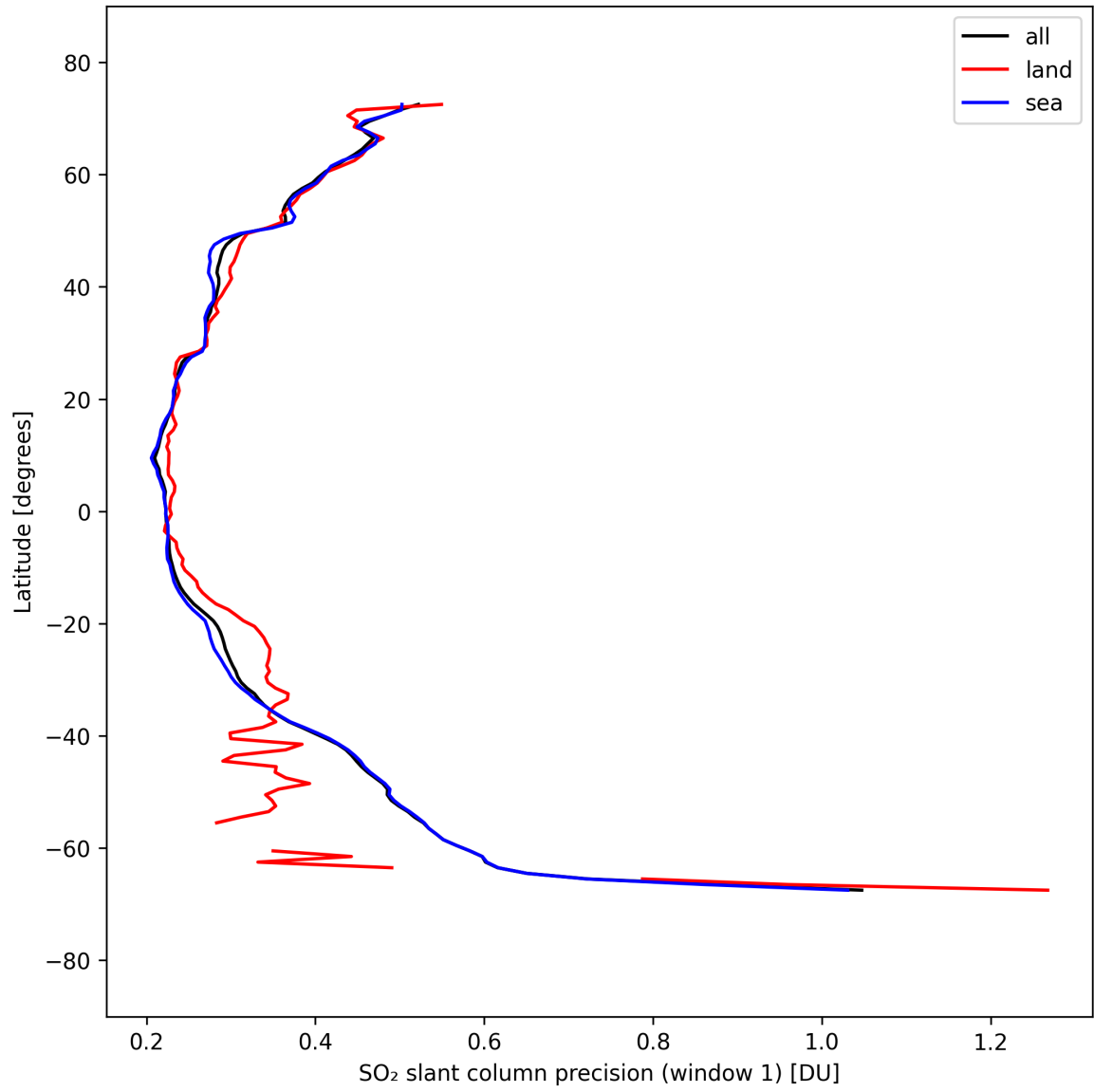
Figure 38: Zonal average of “SO 2 slant column precision (window 1)” for 2025-09-16 to 2025-09-18.
