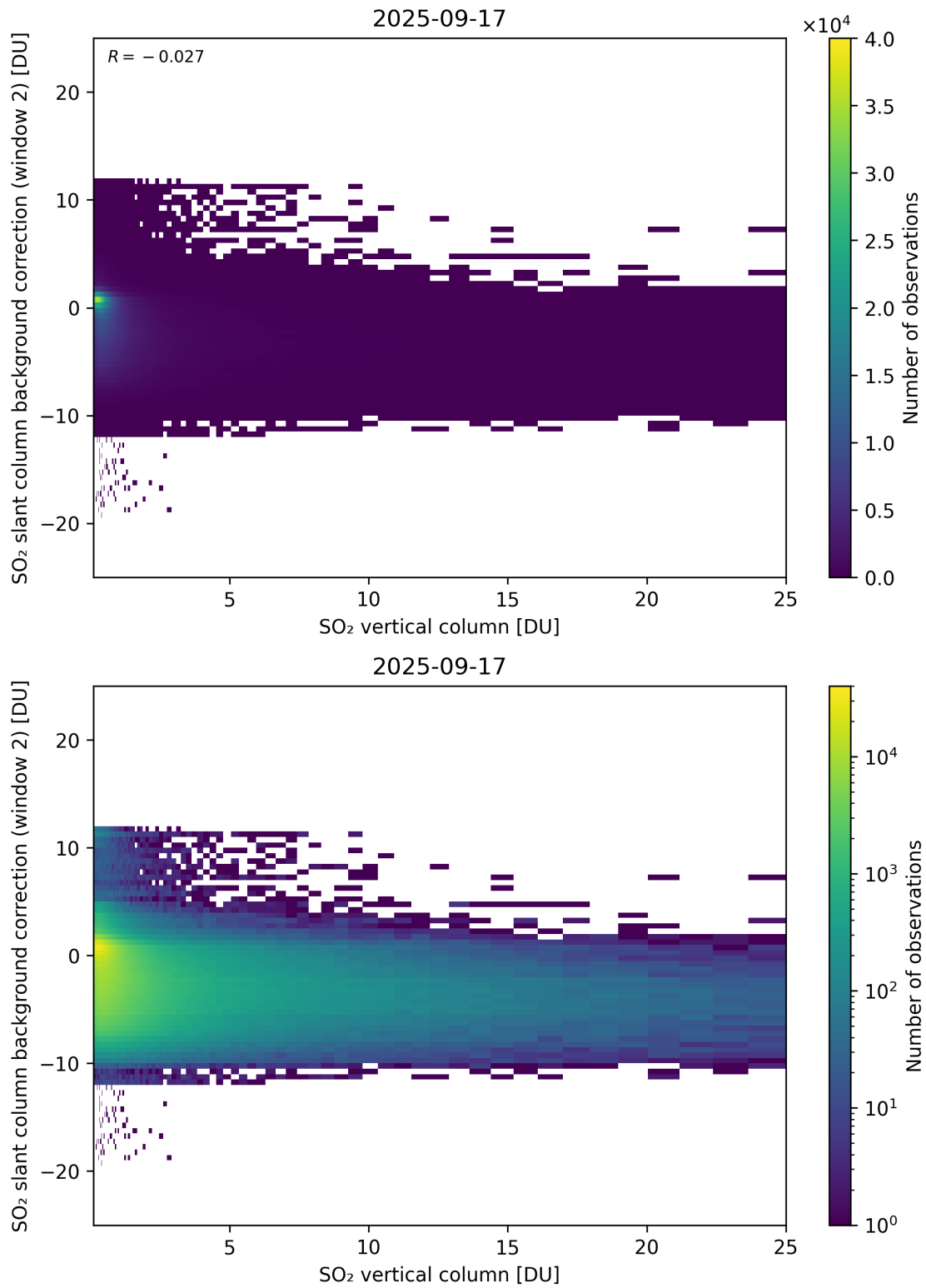
Figure 324: Scatter density plot of “SO 2 vertical column” against “SO 2 slant column background correction (window 2)” for 2025-09-16 to 2025-09-18.
