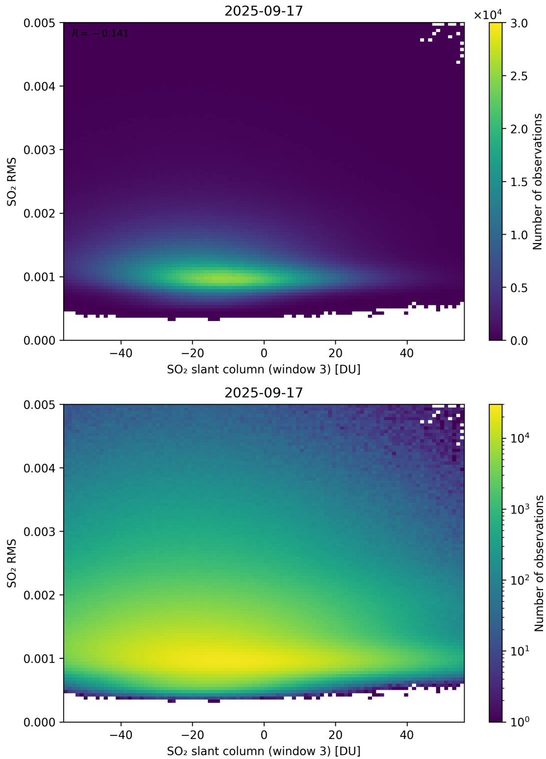
Figure 306: Scatter density plot of “SO 2 slant column (window 3)” against “SO 2 RMS” for 2025-09-16 to 2025-09-18.
