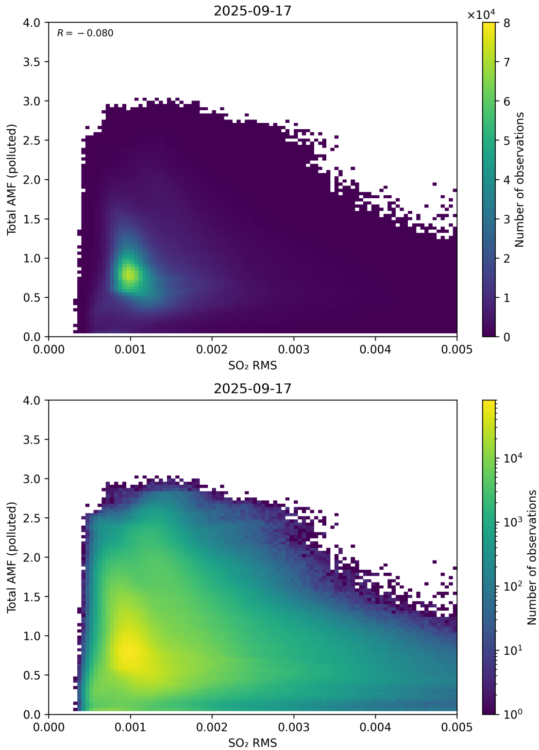
Figure 148: Scatter density plot of “SO 2 RMS” against “Total AMF (polluted)” for 2025-09-16 to 2025-09-18.
