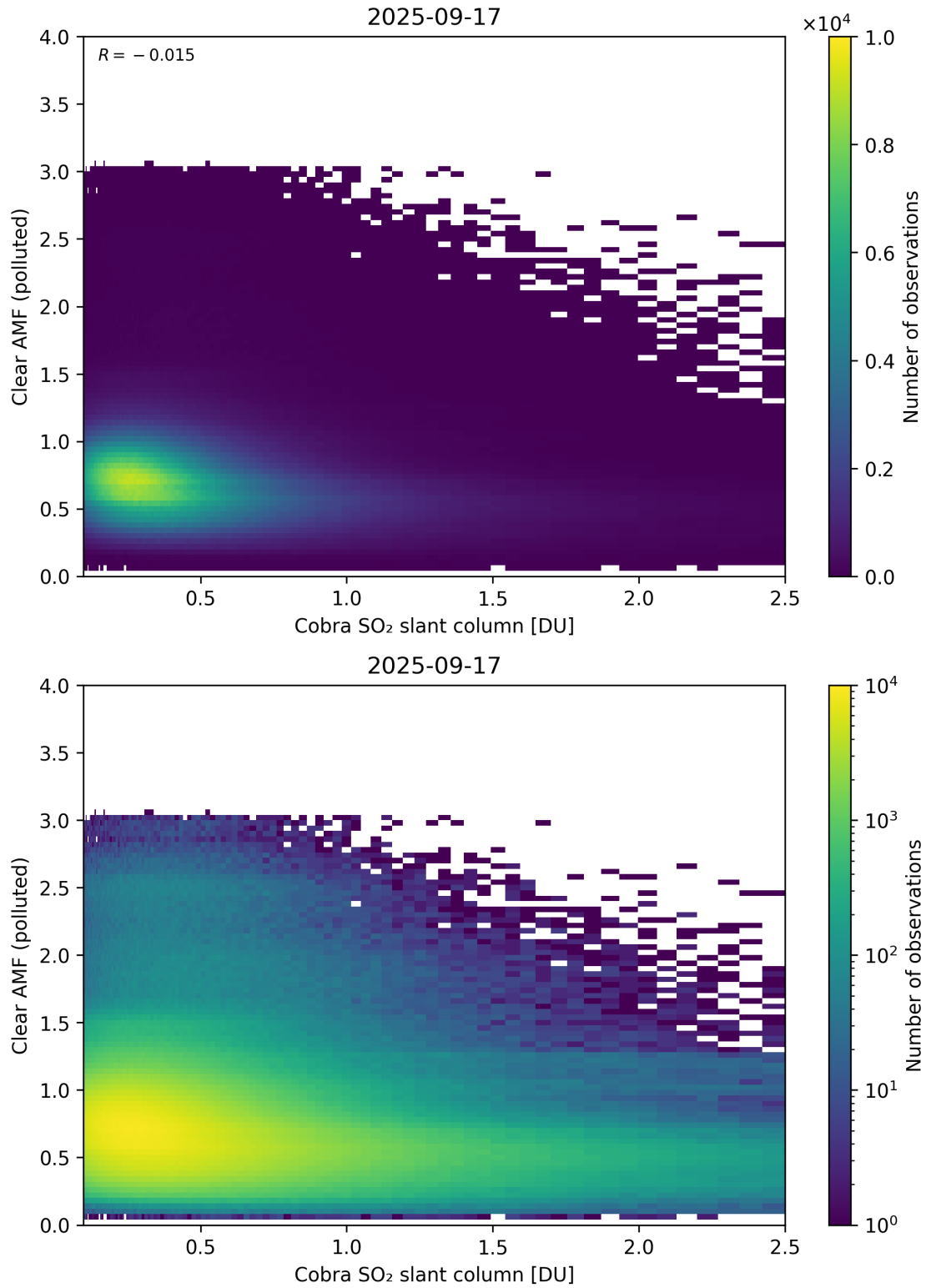
Figure 215: Scatter density plot of “Cobra SO 2 slant column” against “Clear AMF (polluted)” for 2025-09-16 to 2025-09-18.
