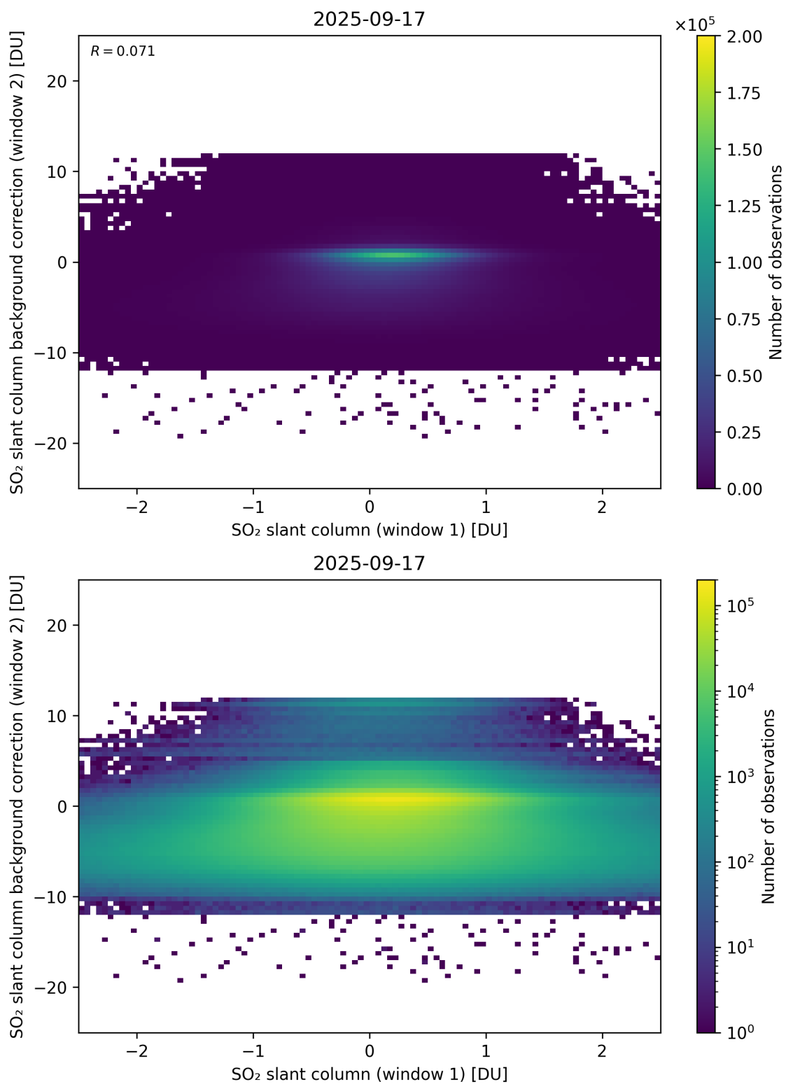
Figure 263: Scatter density plot of “SO 2 slant column (window 1)” against “SO 2 slant column background correction (window 2)” for 2025-09-16 to 2025-09-18.
