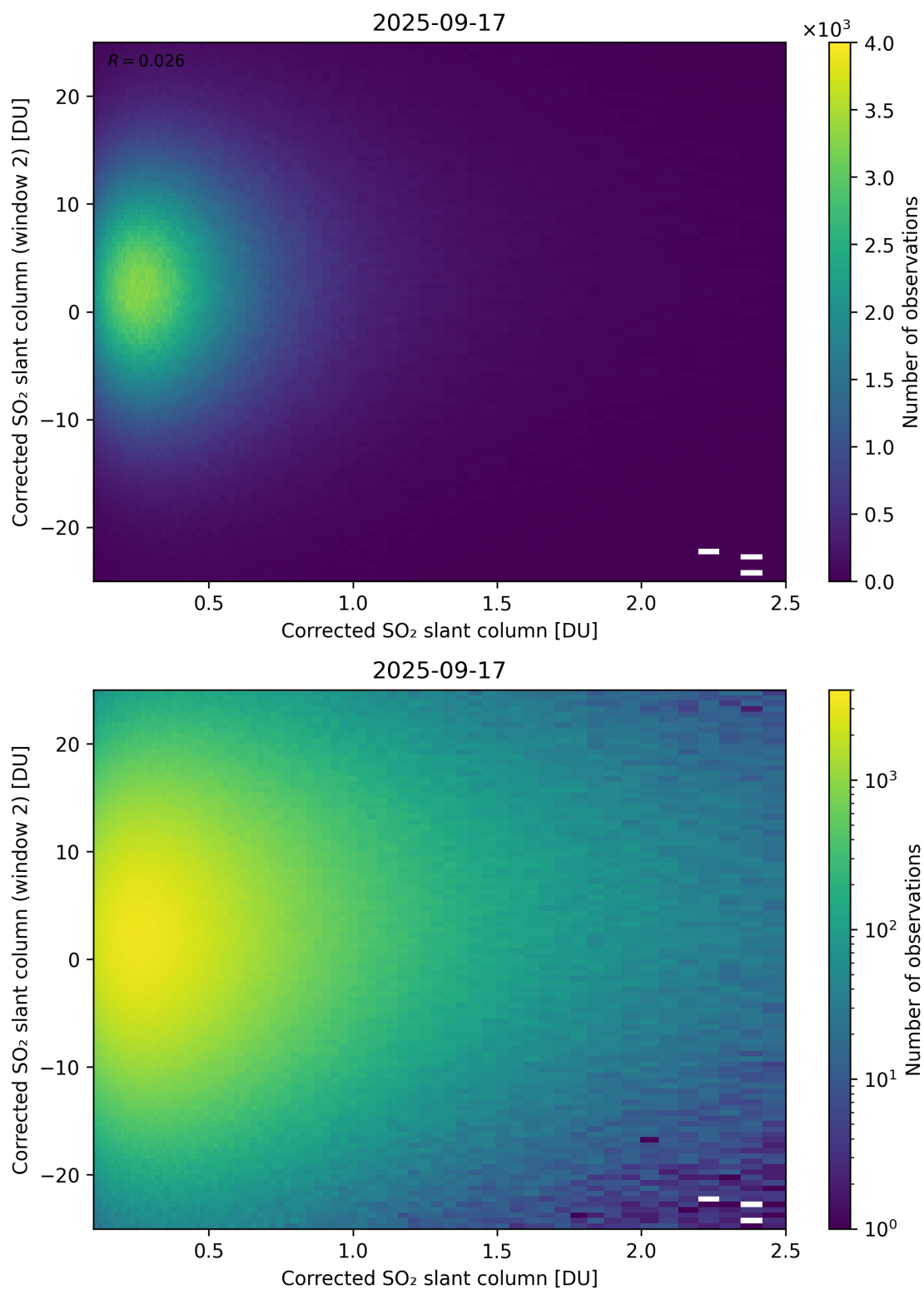
Figure 235: Scatter density plot of “Corrected SO 2 slant column” against “Corrected SO 2 slant column (window 2)” for 2025-09-16 to 2025-09-18.
