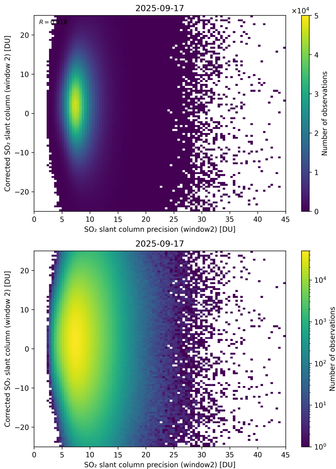
Figure 297: Scatter density plot of “SO 2 slant column precision (window2)” against “Corrected SO 2 slant column (window 2)” for 2025-09-16 to 2025-09-18.
