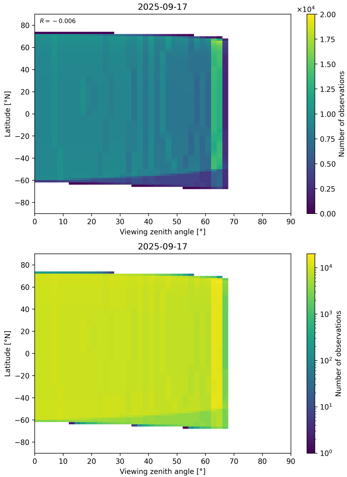
Figure 368: Scatter density plot of “Viewing zenith angle” against “Latitude” for 2025-09-16 to 2025-09-18.
