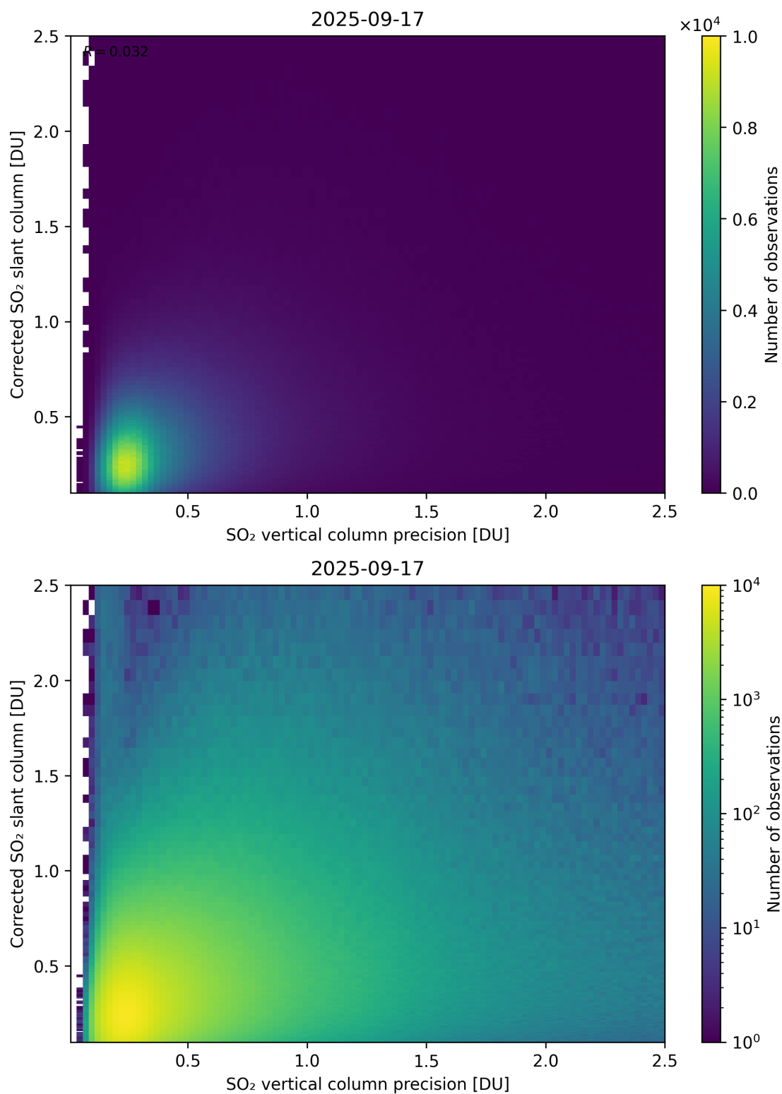
Figure 338: Scatter density plot of “SO 2 vertical column precision” against “Corrected SO 2 slant column” for 2025-09-16 to 2025-09-18.
