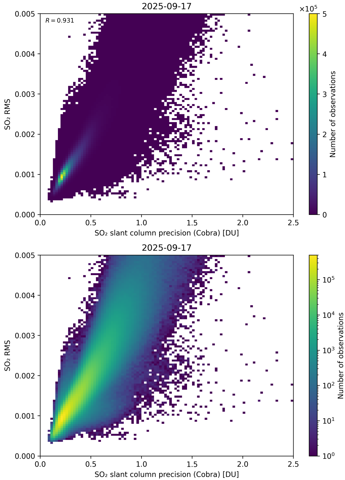
Figure 204: Scatter density plot of “SO 2 slant column precision (Cobra)” against “SO 2 RMS” for 2025-09-16 to 2025-09-18.
