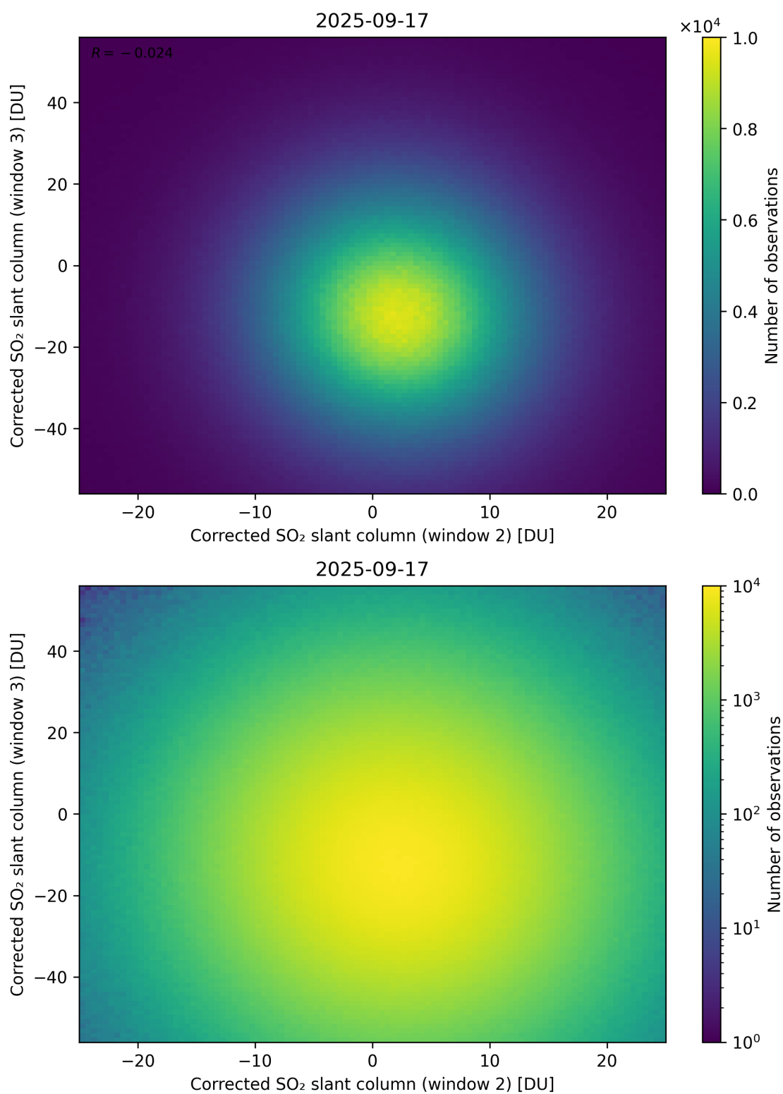
Figure 250: Scatter density plot of “Corrected SO 2 slant column (window 2)” against “Corrected SO 2 slant column (window 3)” for 2025-09-16 to 2025-09-18.
