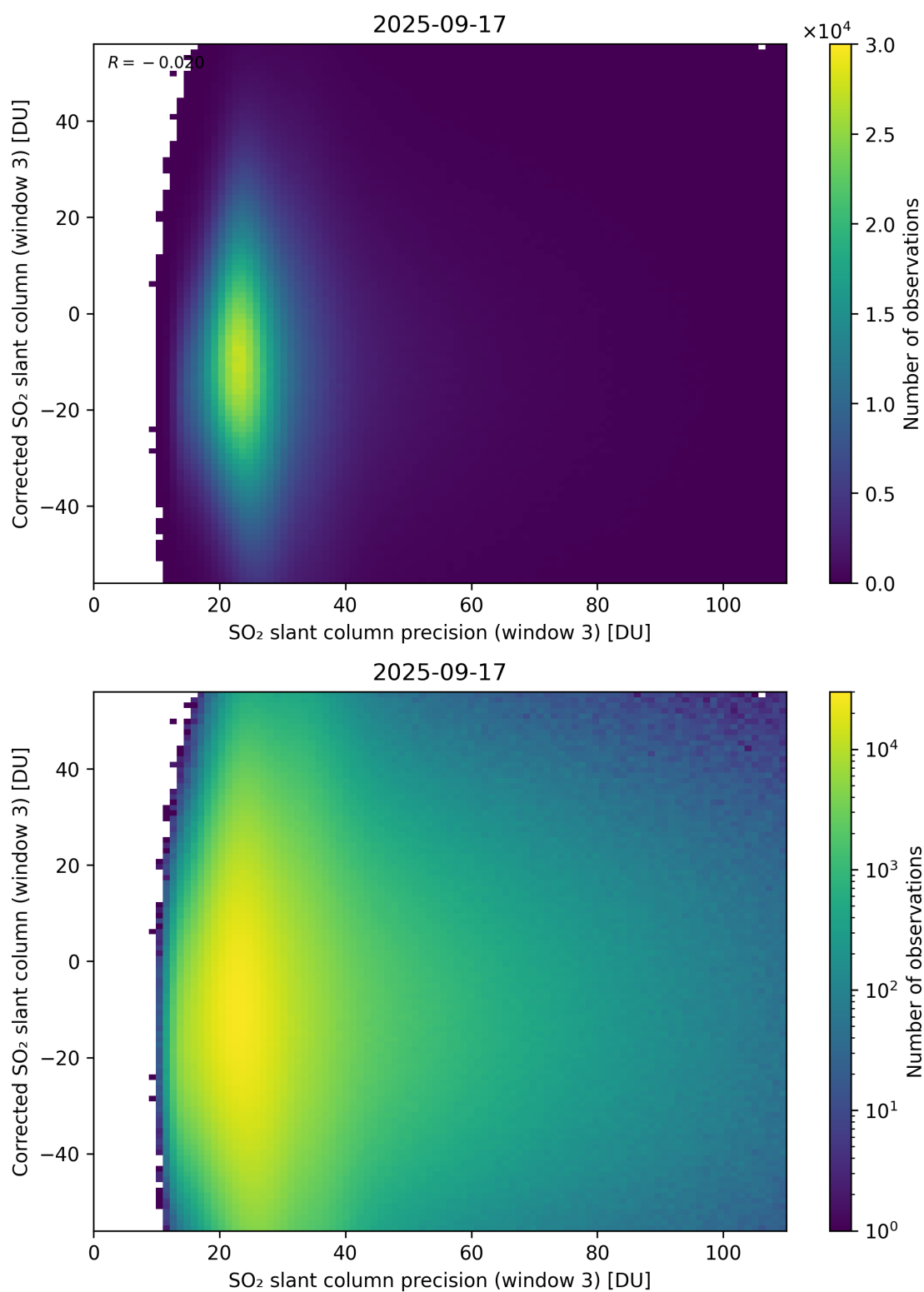
Figure 312: Scatter density plot of “SO 2 slant column precision (window 3)” against “Corrected SO 2 slant column (window 3)” for 2025-09-16 to 2025-09-18.
