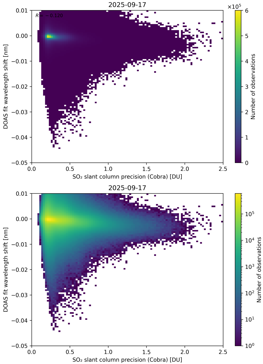
Figure 202: Scatter density plot of “SO 2 slant column precision (Cobra)” against “DOAS fit wavelength shift” for 2025-09-16 to 2025-09-18.
