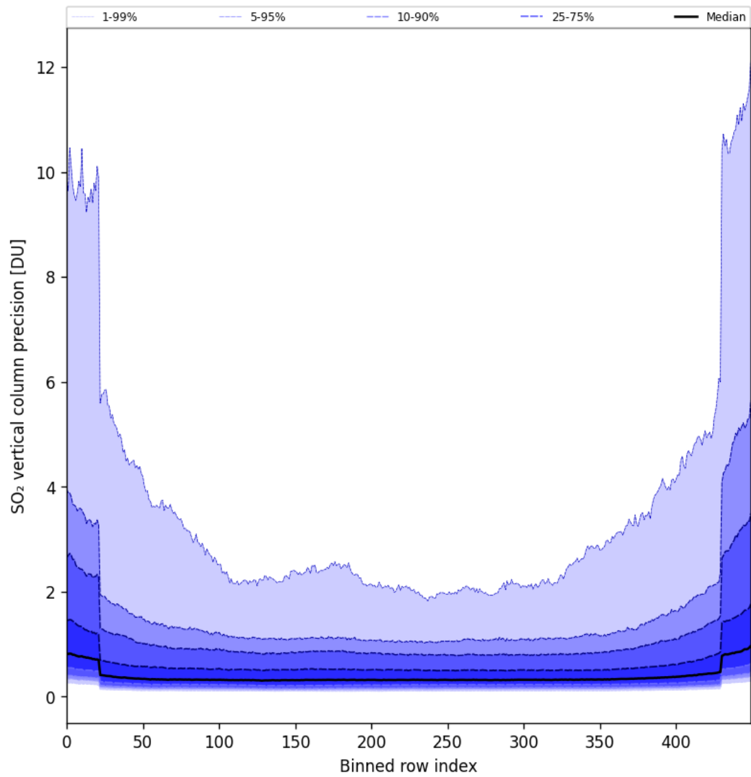
Figure 85: Along track statistics of “SO 2 vertical column precision” for 2025-09-16 to 2025-09-18
