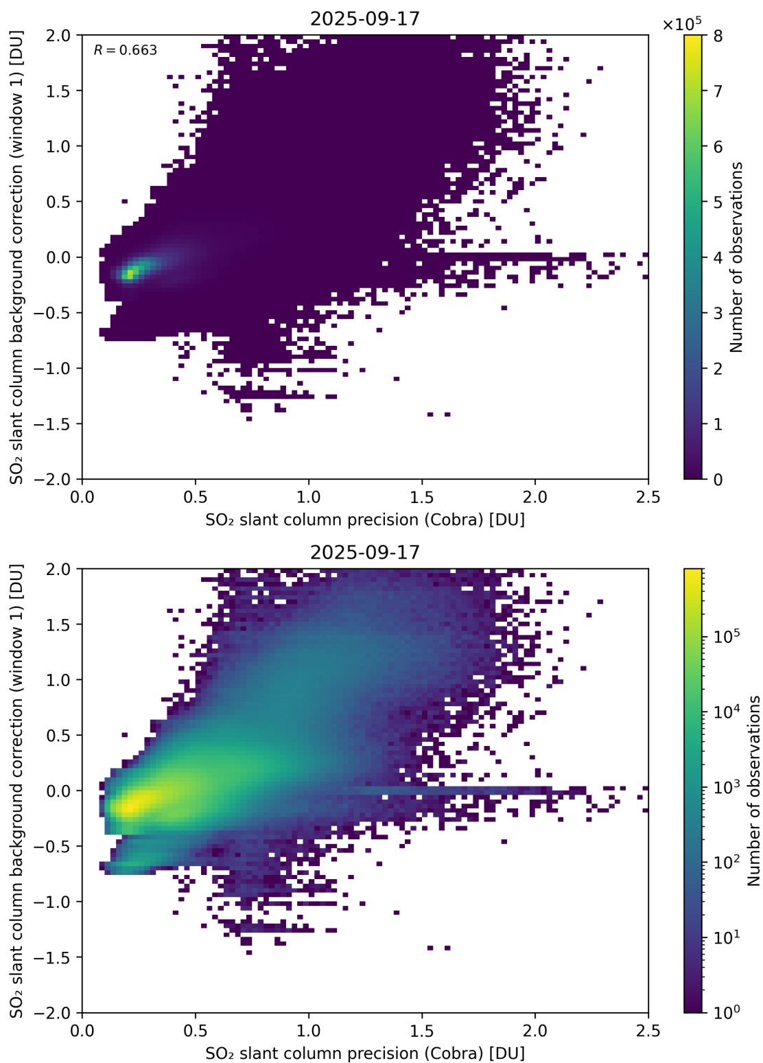
Figure 199: Scatter density plot of “SO 2 slant column precision (Cobra)” against “SO 2 slant column background correction (window 1)” for 2025-09-16 to 2025-09-18.
