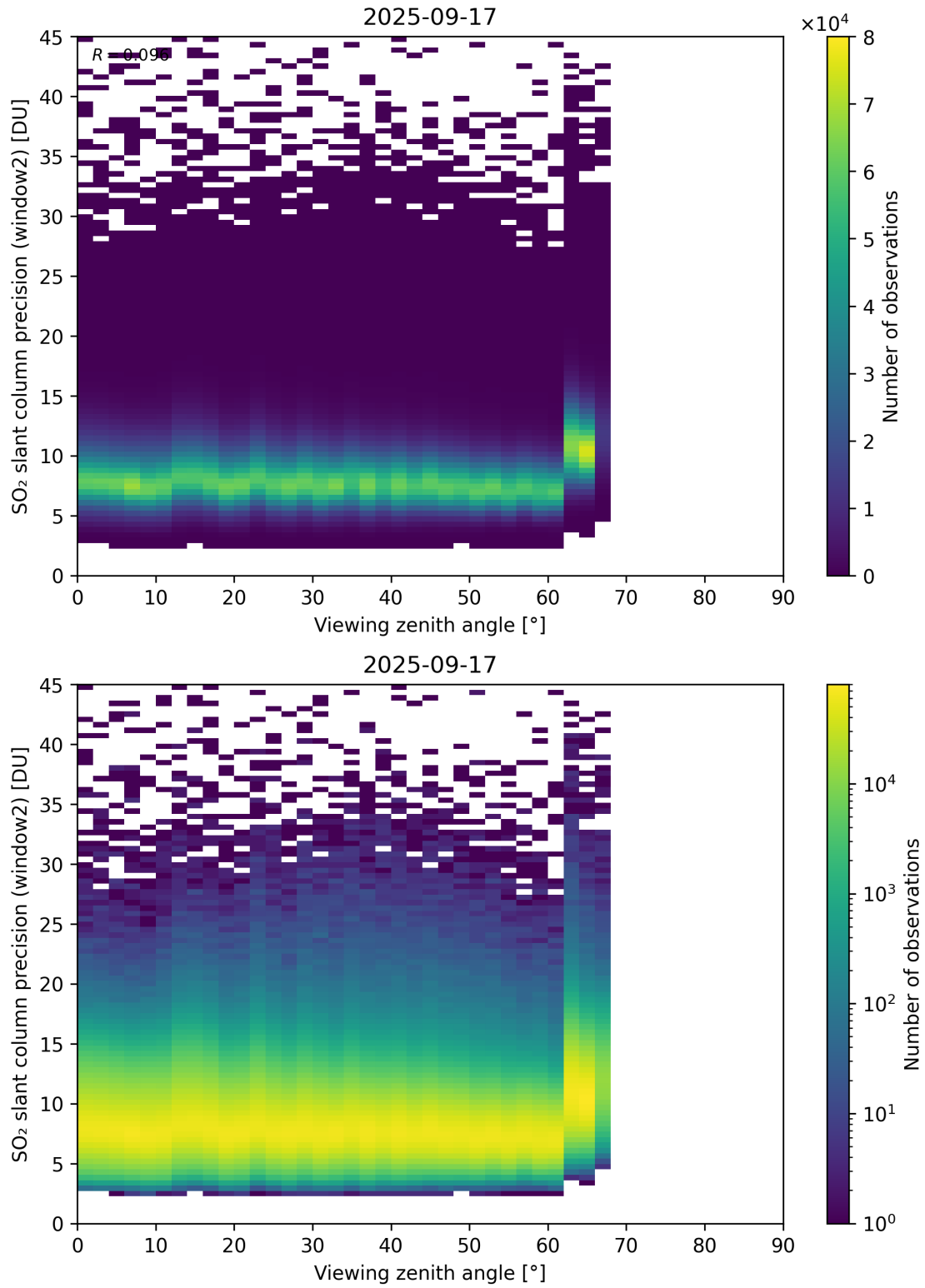
Figure 378: Scatter density plot of “Viewing zenith angle” against “SO 2 slant column precision (window2)” for 2025-09-16 to 2025-09-18.
