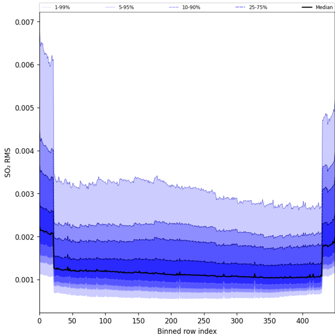
Figure 104: Along track statistics of “SO 2 RMS” for 2025-09-16 to 2025-09-18
