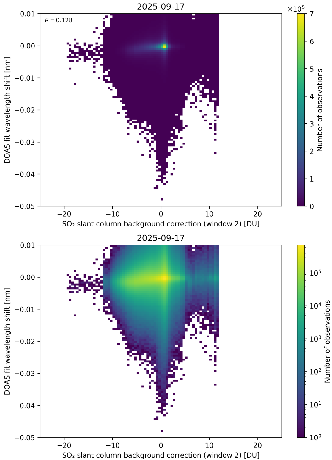
Figure 123: Scatter density plot of “SO 2 slant column background correction (window 2)” against “DOAS fit wavelength shift” for 2025-09-16 to 2025-09-18.
