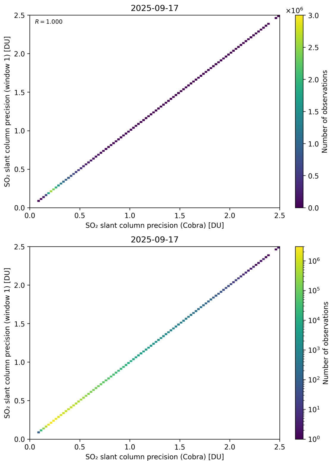
Figure 209: Scatter density plot of “SO 2 slant column precision (Cobra)” against “SO 2 slant column precision (window 1)” for 2025-09-16 to 2025-09-18.
