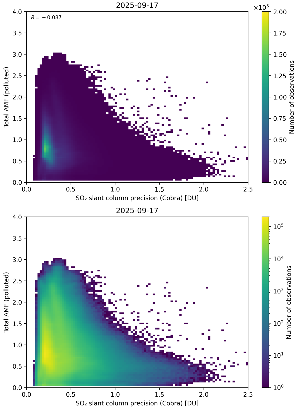
Figure 213: Scatter density plot of “SO 2 slant column precision (Cobra)” against “Total AMF (polluted)” for 2025-09-16 to 2025-09-18.
