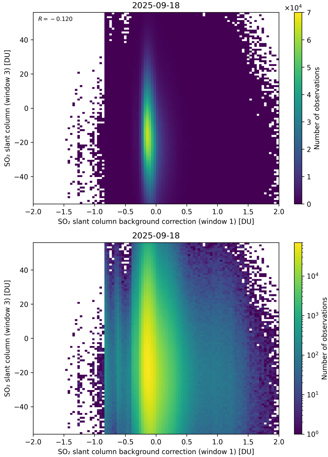
Figure 118: Scatter density plot of “SO 2 slant column background correction (window 1)” against “SO 2 slant column (window 3)” for 2025-09-17 to 2025-09-19.
