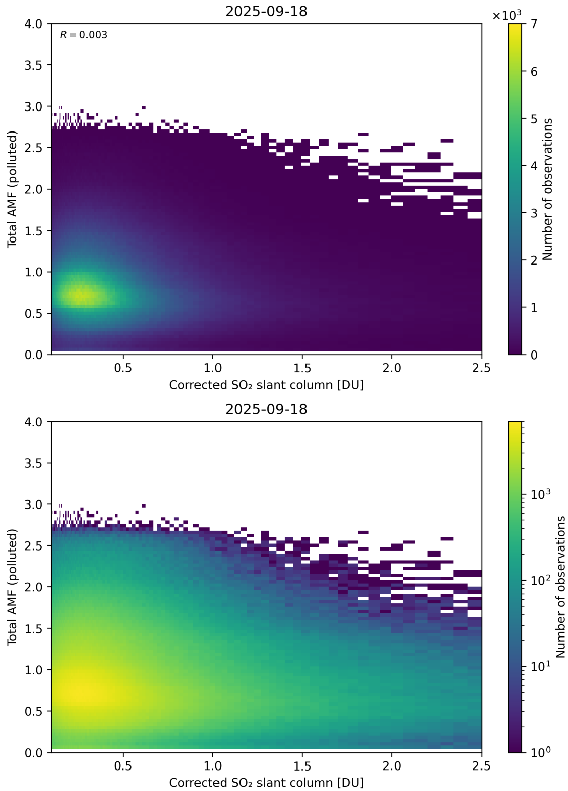
Figure 242: Scatter density plot of “Corrected SO 2 slant column” against “Total AMF (polluted)” for 2025-09-17 to 2025-09-19.
