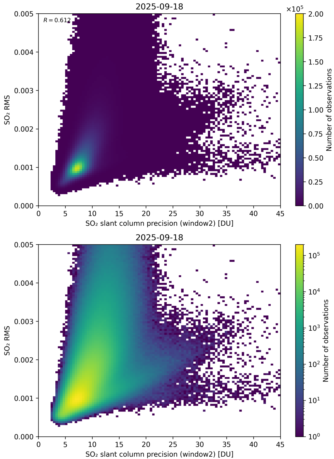
Figure 295: Scatter density plot of “SO 2 slant column precision (window2)” against “SO 2 RMS” for 2025-09-17 to 2025-09-19.
