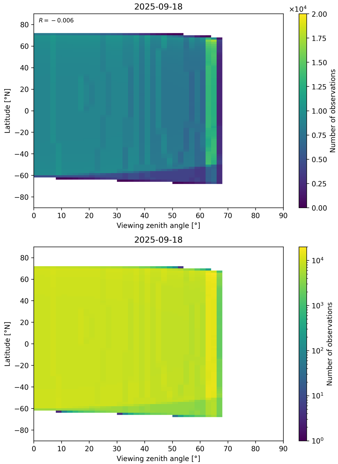
Figure 368: Scatter density plot of “Viewing zenith angle” against “Latitude” for 2025-09-17 to 2025-09-19.
