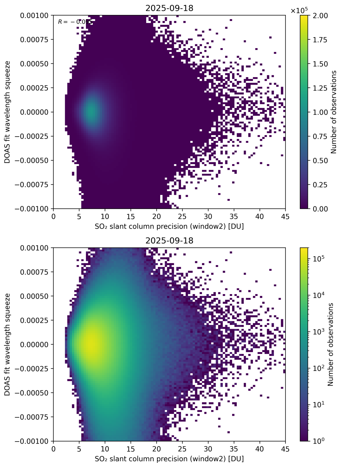
Figure 294: Scatter density plot of “SO 2 slant column precision (window2)” against “DOAS fit wavelength squeeze” for 2025-09-17 to 2025-09-19.
