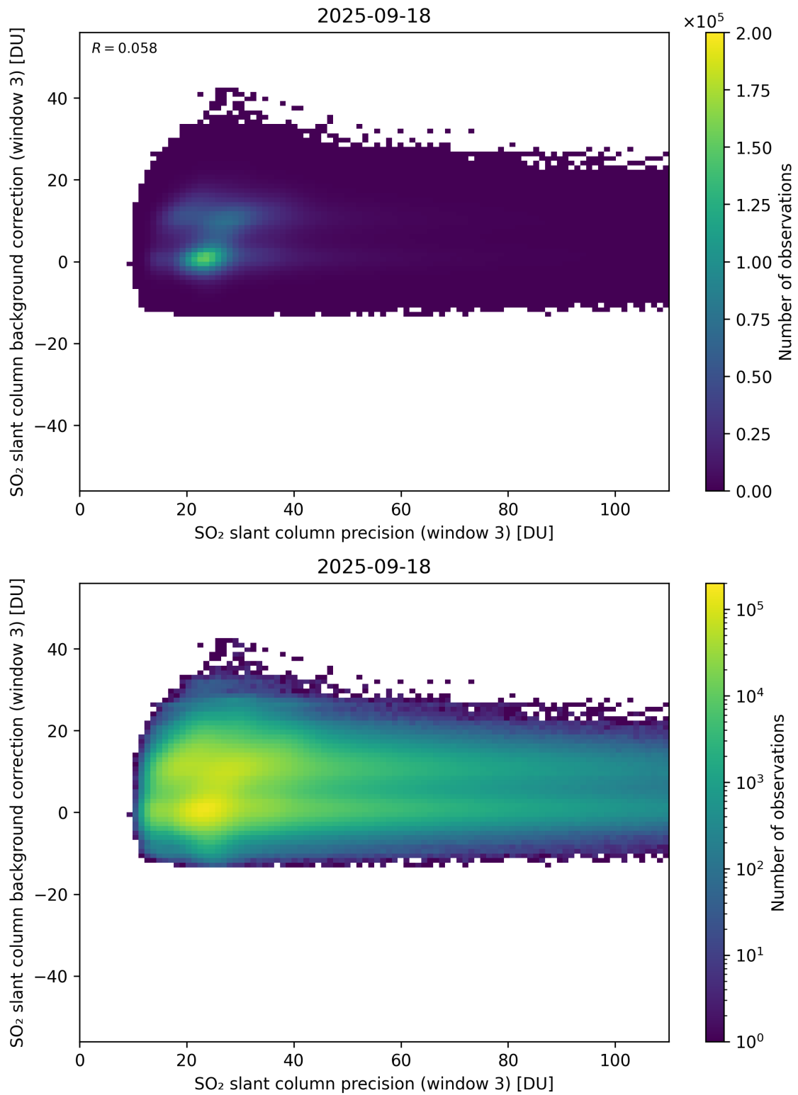
Figure 307: Scatter density plot of “SO 2 slant column precision (window 3)” against “SO 2 slant column background correction (window 3)” for 2025-09-17 to 2025-09-19.
