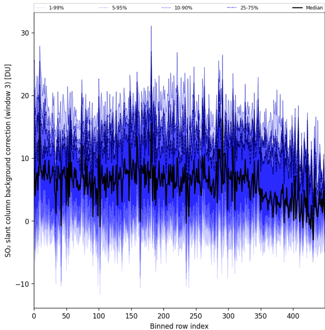
Figure 100: Along track statistics of “SO 2 slant column background correction (window 3)” for 2025-09-17 to 2025-09-19
