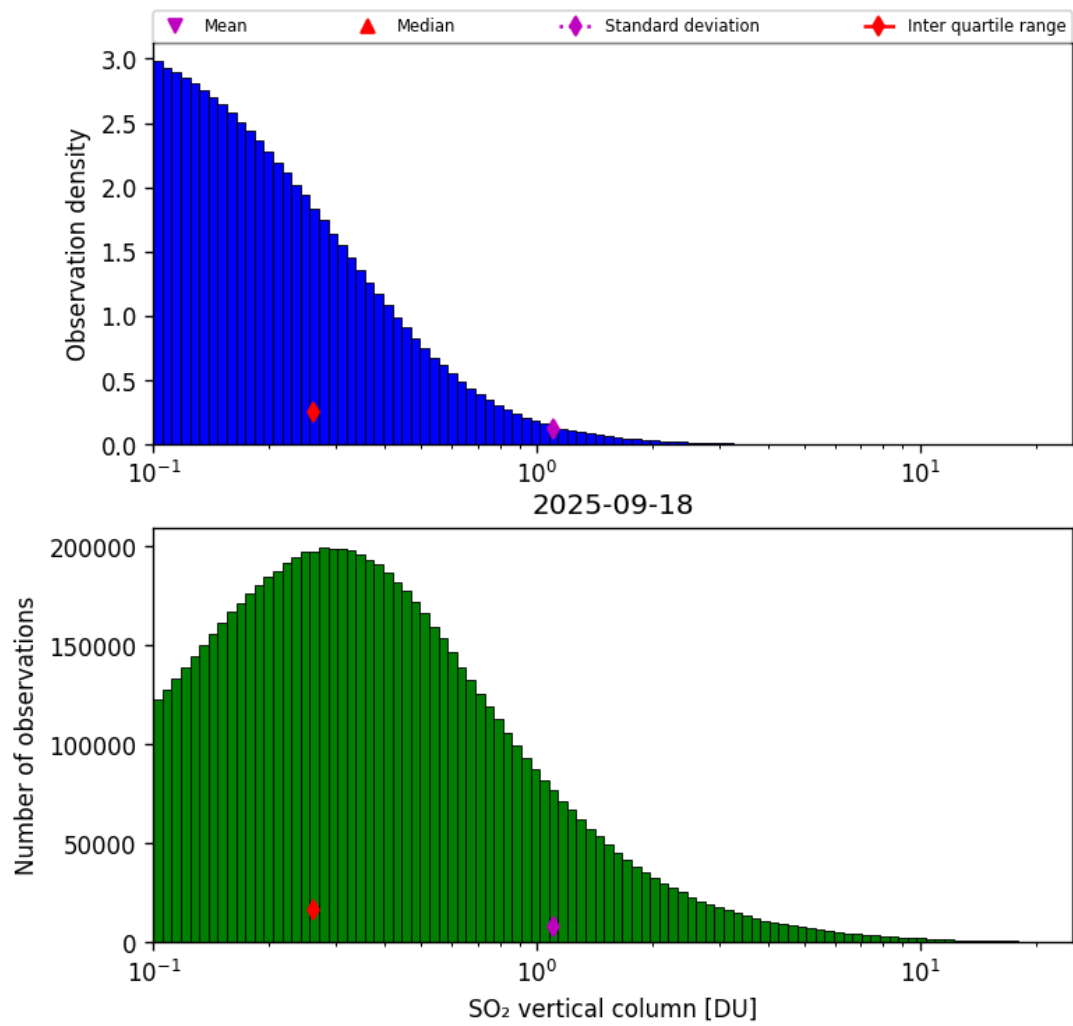
Figure 58: Histogram of “SO 2 vertical column” for 2025-09-17 to 2025-09-19
