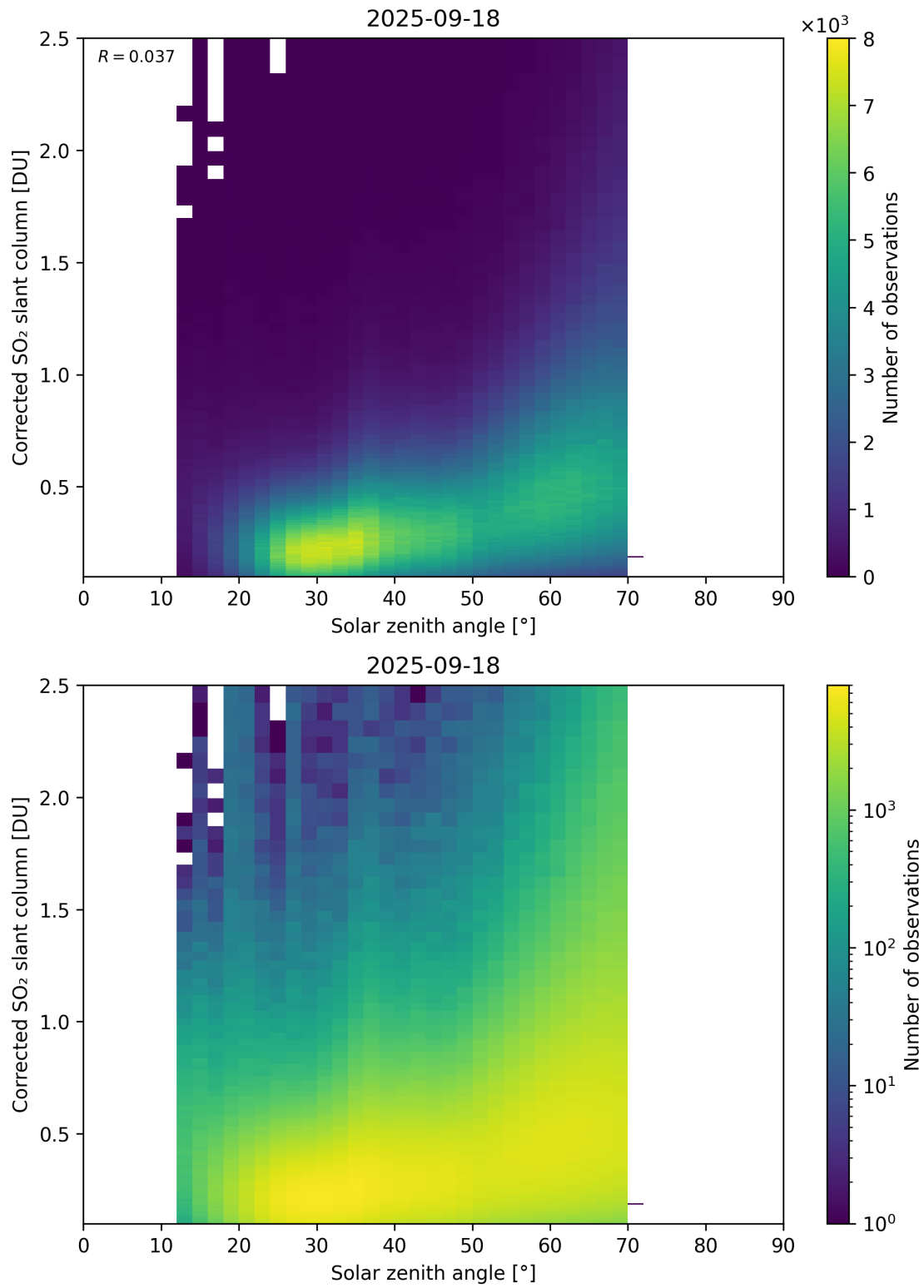
Figure 181: Scatter density plot of “Solar zenith angle” against “Corrected SO 2 slant column” for 2025-09-17 to 2025-09-19.
