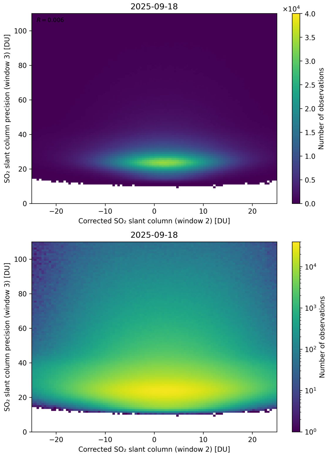
Figure 252: Scatter density plot of “Corrected SO 2 slant column (window 2)” against “SO 2 slant column precision (window 3)” for 2025-09-17 to 2025-09-19.
