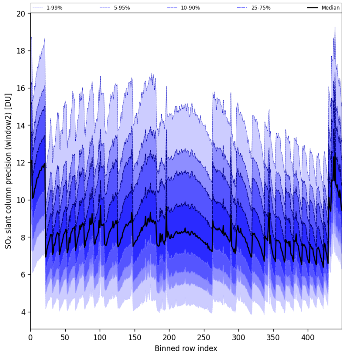
Figure 94: Along track statistics of “SO 2 slant column precision (window2)” for 2025-09-17 to 2025-09-19
