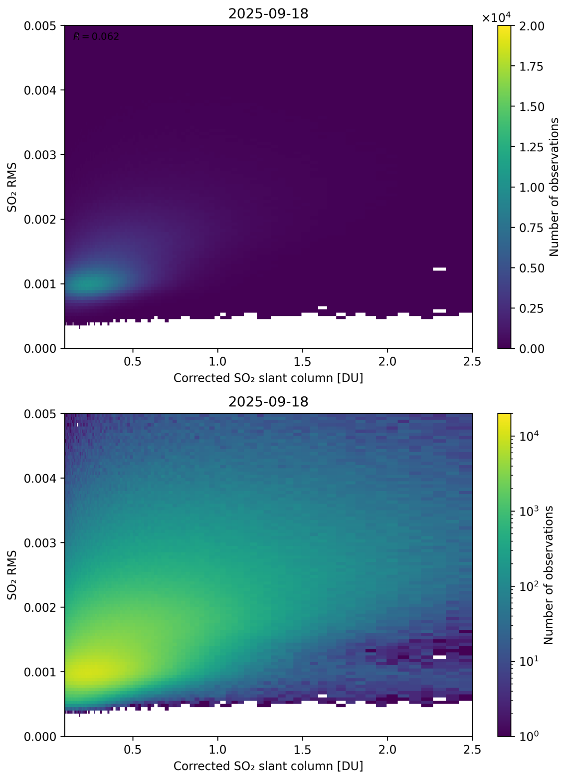
Figure 231: Scatter density plot of “Corrected SO 2 slant column” against “SO 2 RMS” for 2025-09-17 to 2025-09-19.
