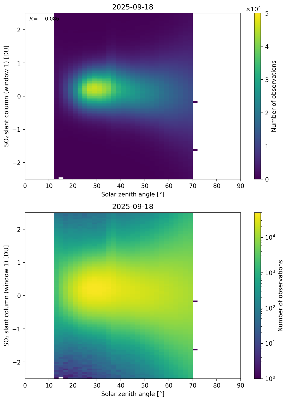
Figure 184: Scatter density plot of “Solar zenith angle” against “SO 2 slant column (window 1)” for 2025-09-17 to 2025-09-19.
