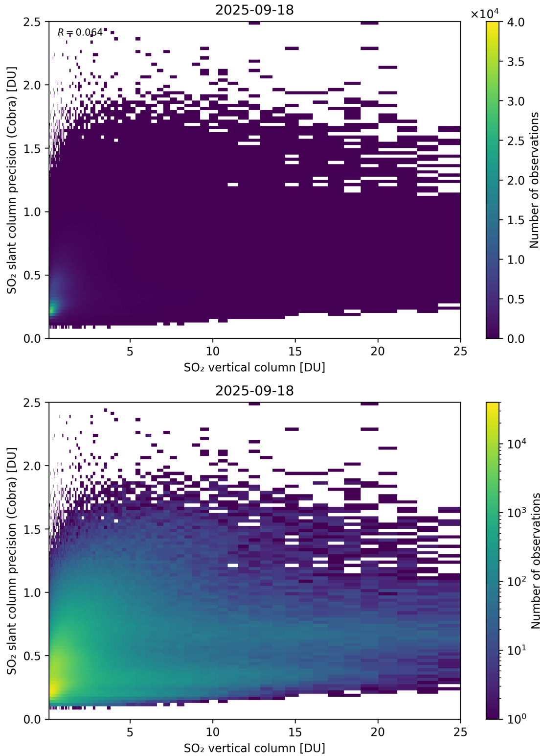
Figure 350: Scatter density plot of “SO 2 vertical column” against “SO 2 slant column precision (Cobra)” for 2025-09-17 to 2025-09-19.
