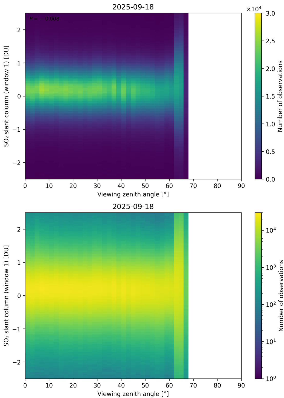
Figure 376: Scatter density plot of “Viewing zenith angle” against “SO 2 slant column (window 1)” for 2025-09-17 to 2025-09-19.
