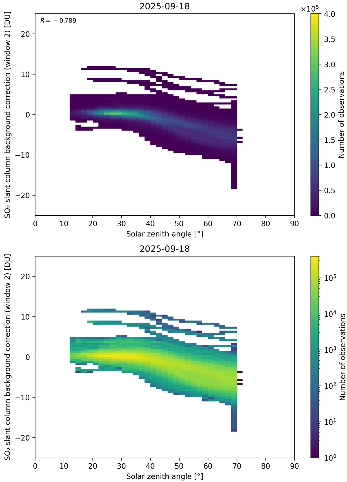
Figure 172: Scatter density plot of “Solar zenith angle” against “SO 2 slant column background correction (window 2)” for 2025-09-17 to 2025-09-19.
