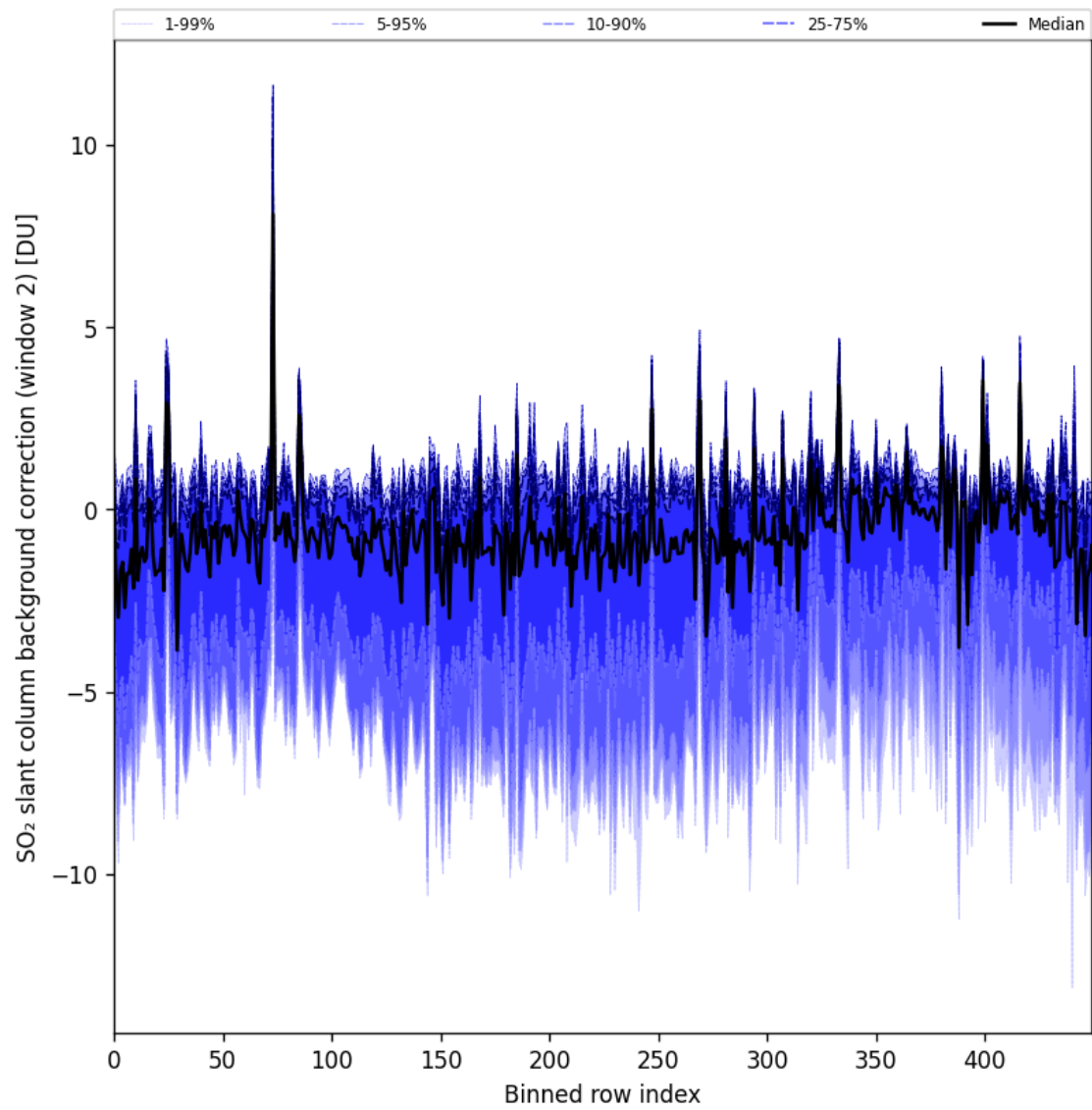
Figure 96: Along track statistics of “SO 2 slant column background correction (window 2)” for 2025-09-17 to 2025-09-19
