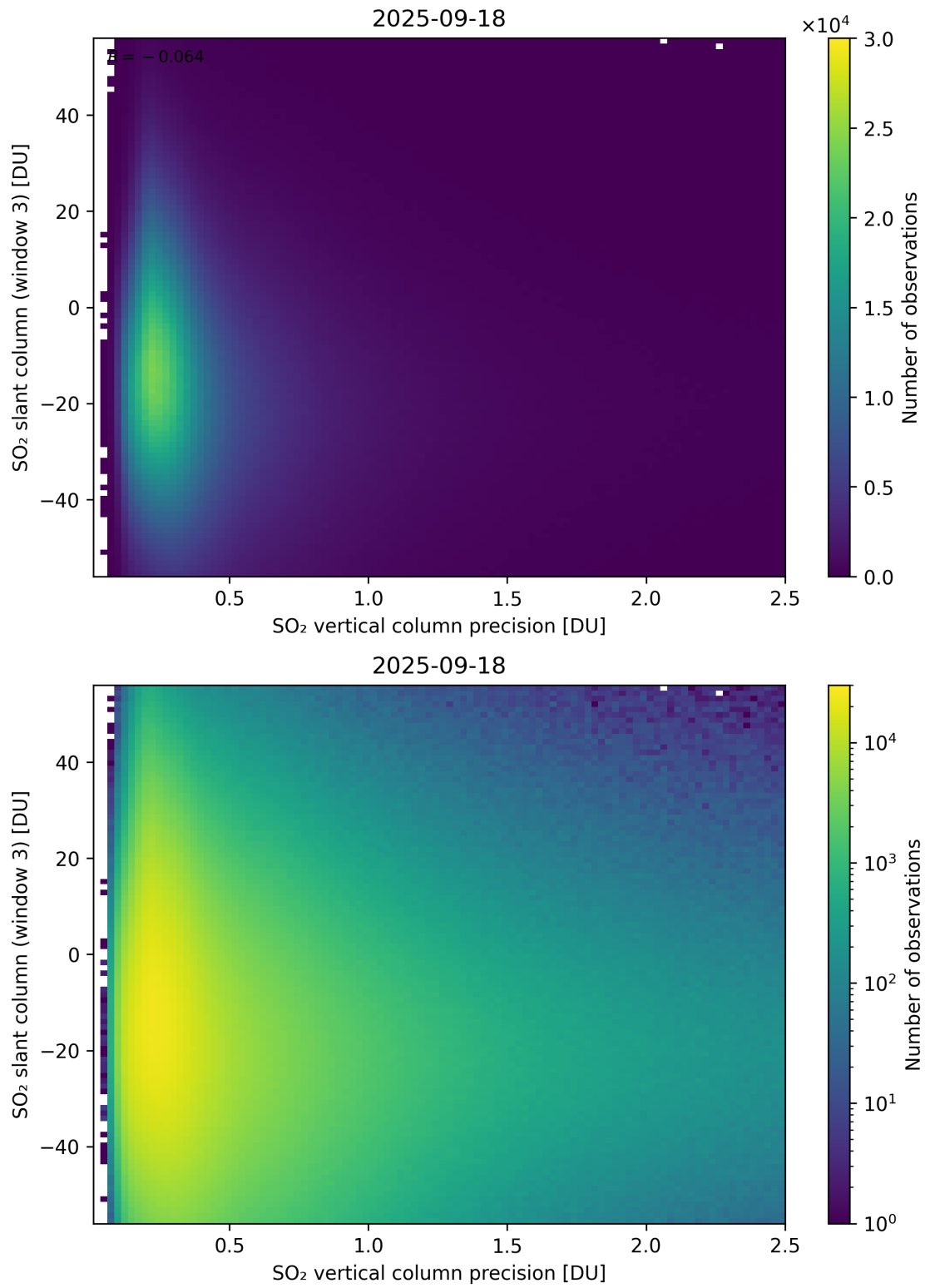
Figure 344: Scatter density plot of “SO 2 vertical column precision” against “SO 2 slant column (window 3)” for 2025-09-17 to 2025-09-19.
