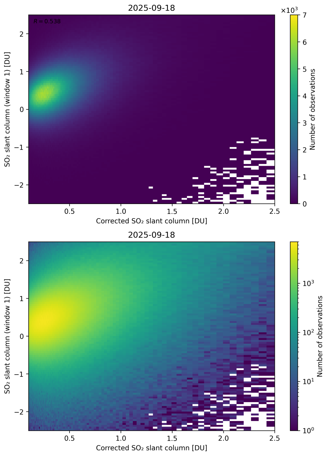
Figure 237: Scatter density plot of “Corrected SO 2 slant column” against “SO 2 slant column (window 1)” for 2025-09-17 to 2025-09-19.
