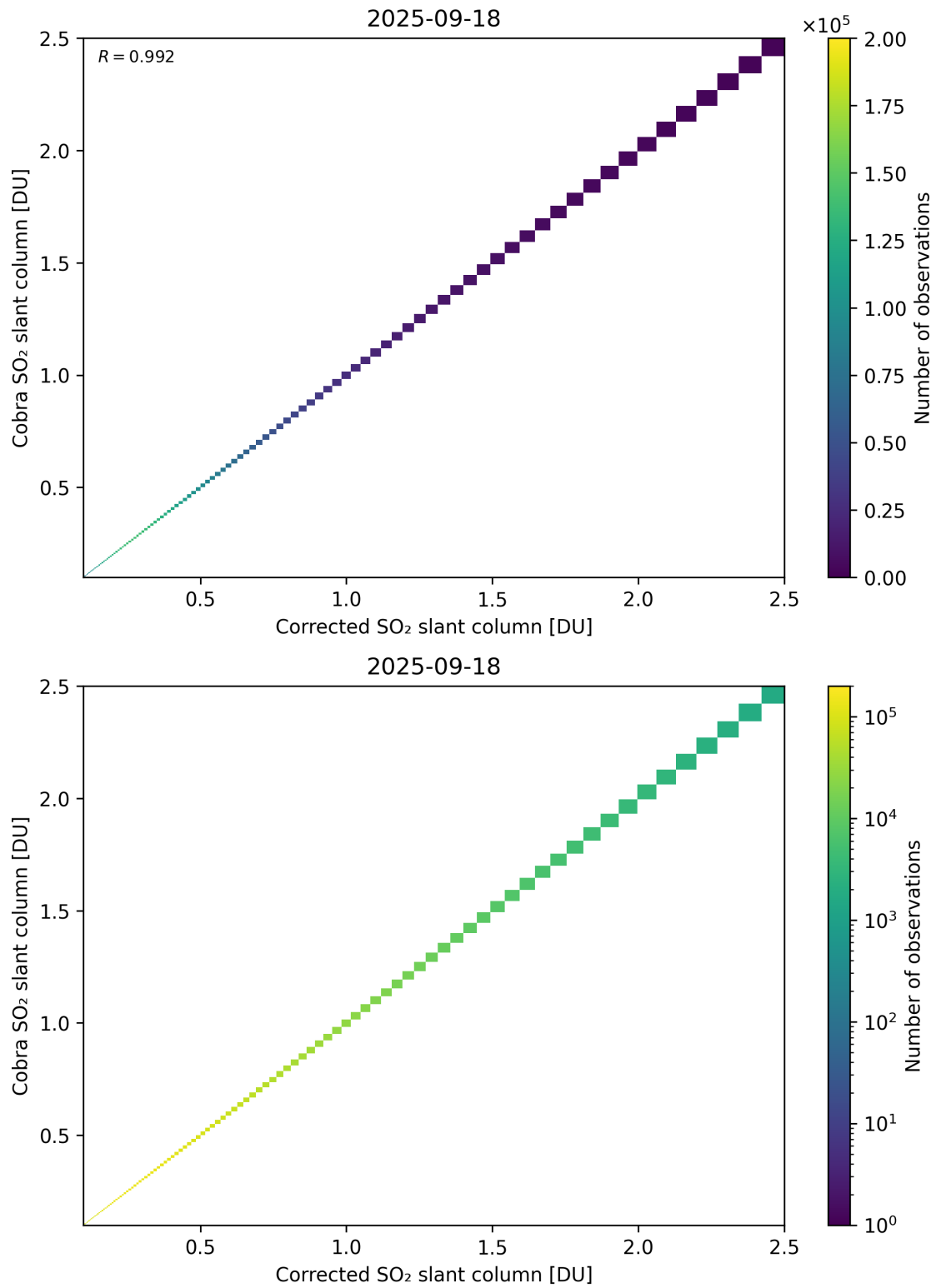
Figure 233: Scatter density plot of “Corrected SO 2 slant column” against “Cobra SO 2 slant column” for 2025-09-17 to 2025-09-19.
