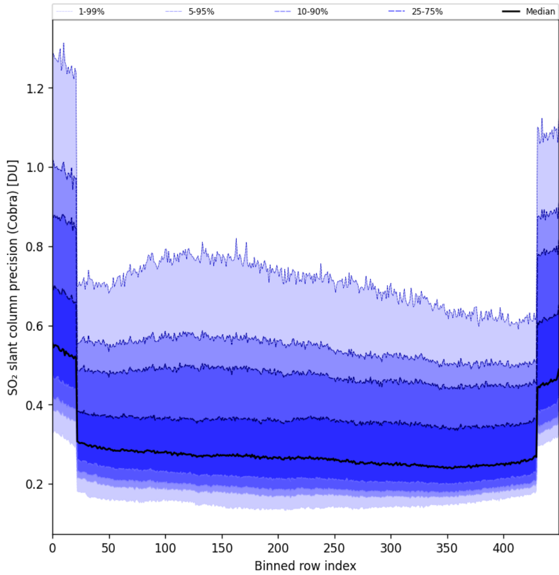
Figure 88: Along track statistics of “SO 2 slant column precision (Cobra)” for 2025-09-17 to 2025-09-19
