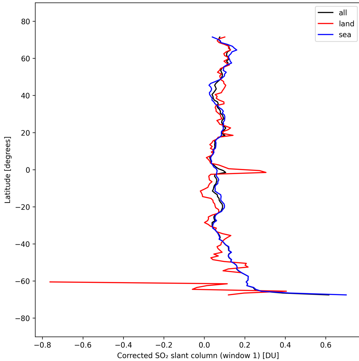
Figure 39: Zonal average of “Corrected SO 2 slant column (window 1)” for 2025-09-17 to 2025-09-19.
