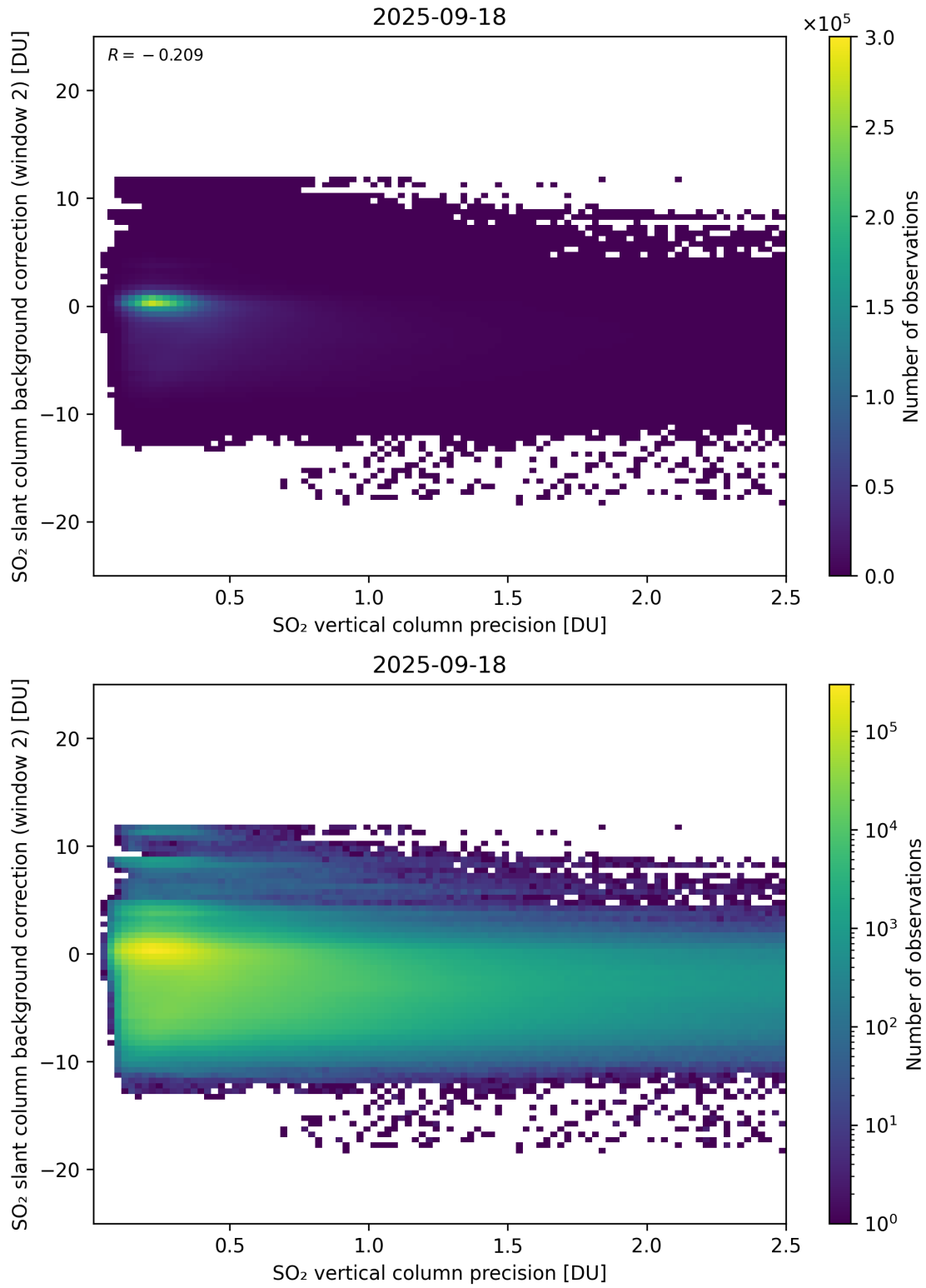
Figure 330: Scatter density plot of “SO 2 vertical column precision” against “SO 2 slant column background correction (window 2)” for 2025-09-17 to 2025-09-19.
