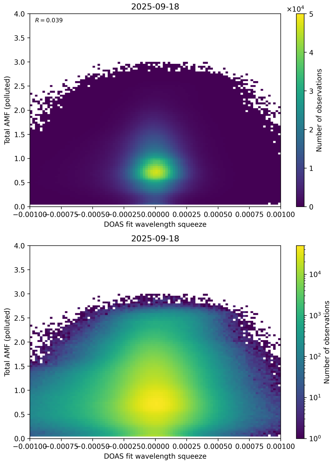
Figure 145: Scatter density plot of “DOAS fit wavelength squeeze” against “Total AMF (polluted)” for 2025-09-17 to 2025-09-19.
