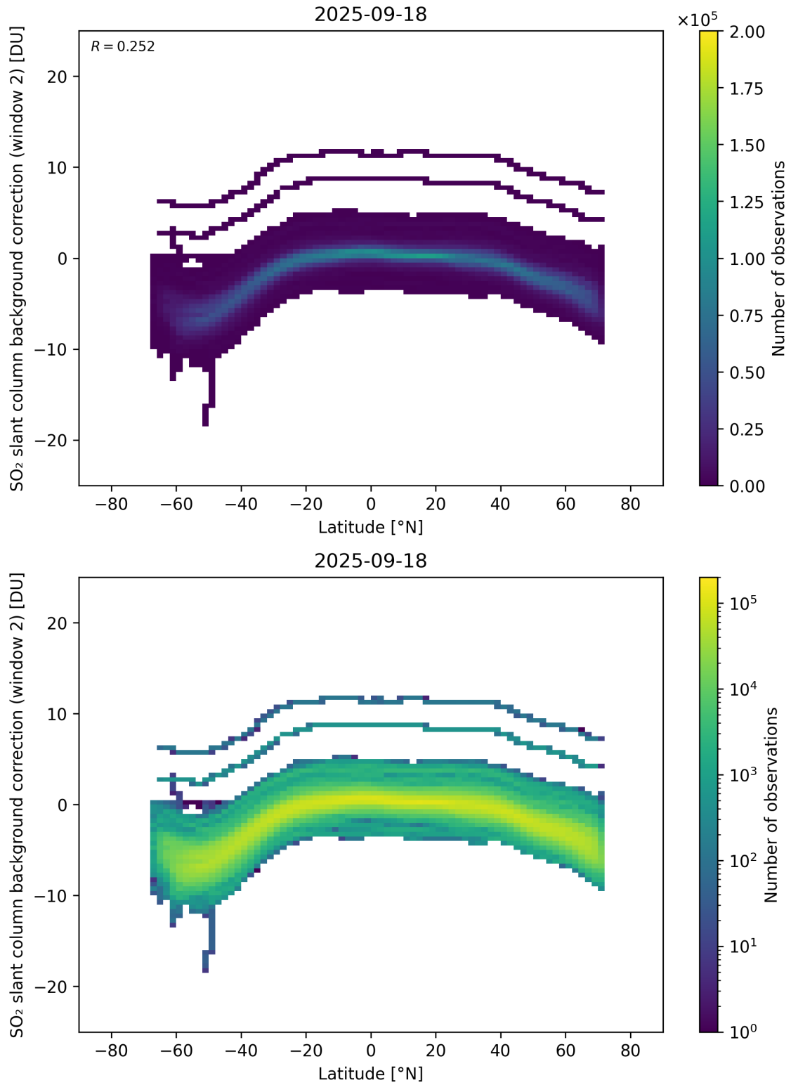
Figure 151: Scatter density plot of “Latitude” against “SO 2 slant column background correction (window 2)” for 2025-09-17 to 2025-09-19.
