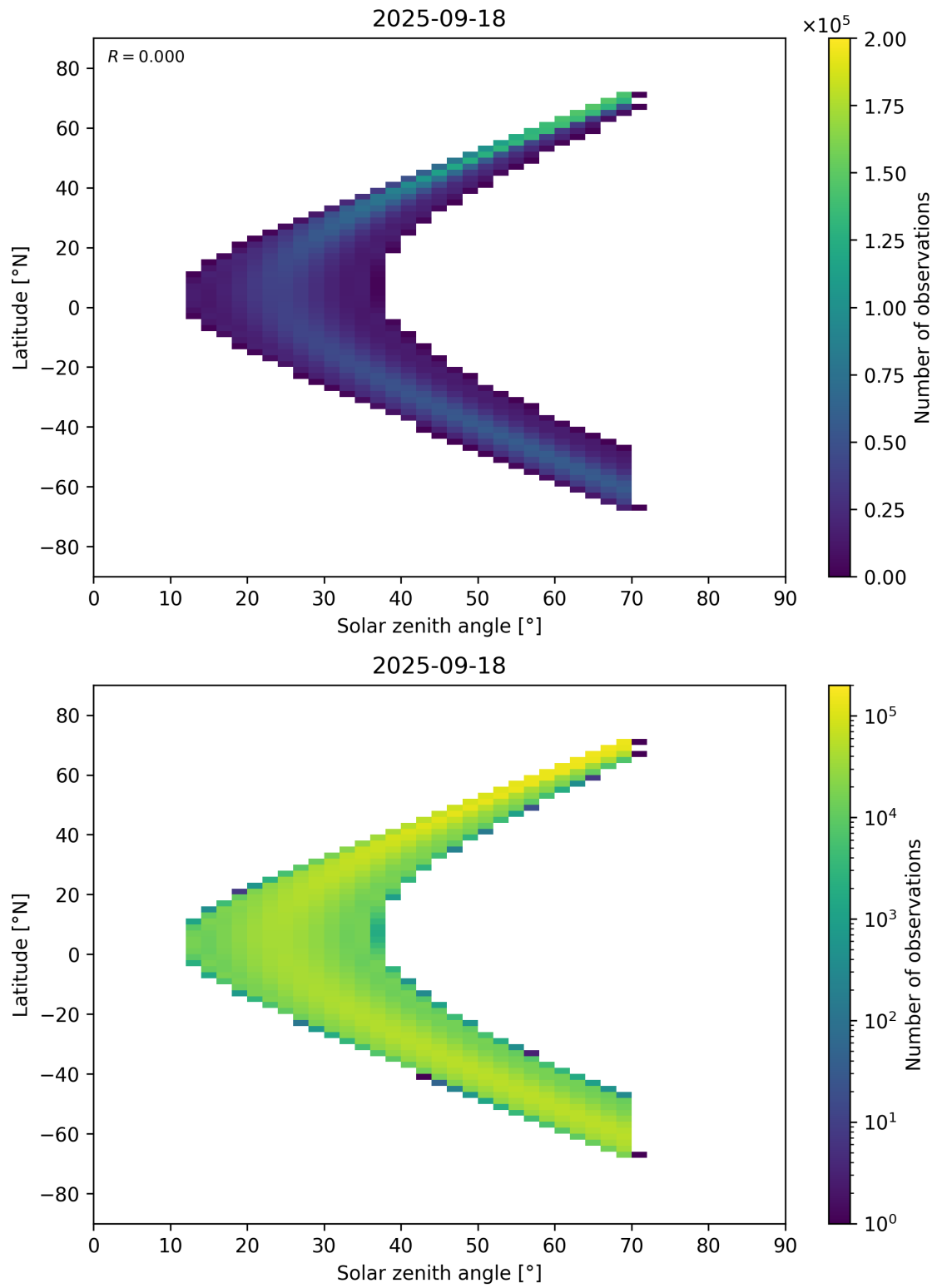
Figure 177: Scatter density plot of “Solar zenith angle” against “Latitude” for 2025-09-17 to 2025-09-19.
