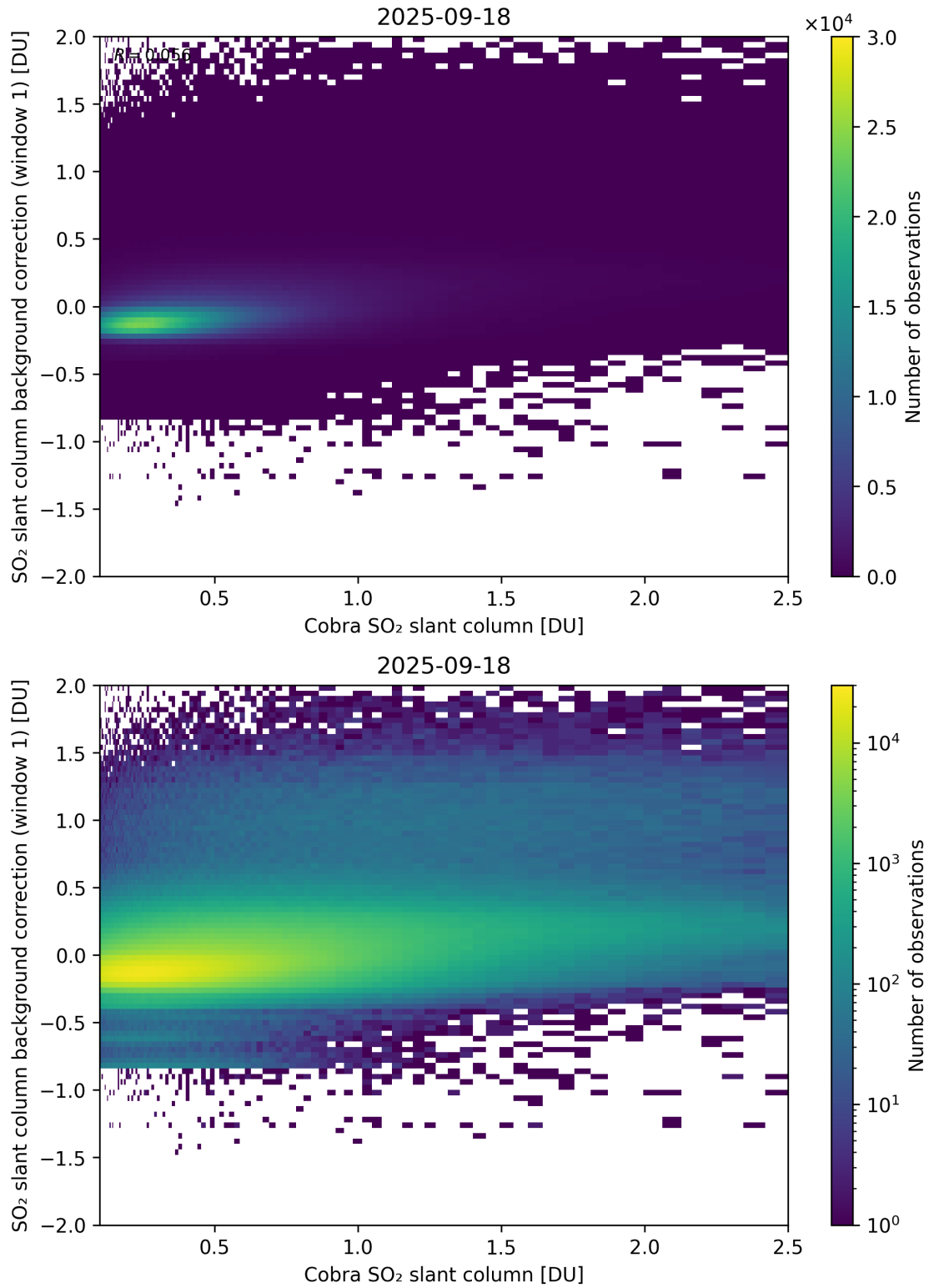
Figure 193: Scatter density plot of “Cobra SO 2 slant column” against “SO 2 slant column background correction (window 1)” for 2025-09-17 to 2025-09-19.
