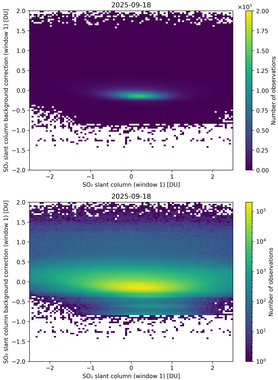
Figure 262: Scatter density plot of “SO 2 slant column (window 1)” against “SO 2 slant column background correction (window 1)” for 2025-09-17 to 2025-09-19.
