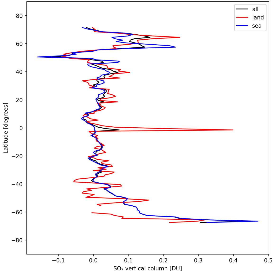
Figure 32: Zonal average of “SO 2 vertical column” for 2025-09-17 to 2025-09-19.
