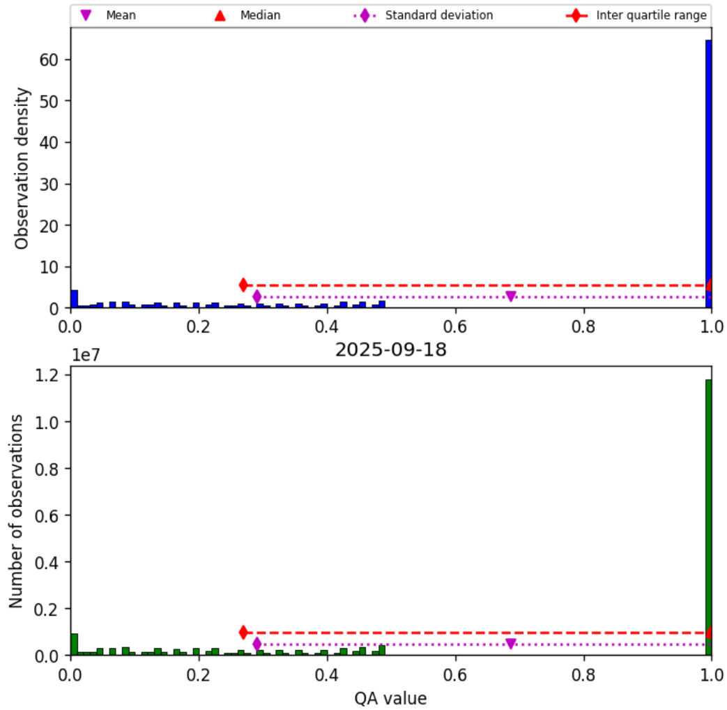
Figure 57: Histogram of “QA value” for 2025-09-17 to 2025-09-19
