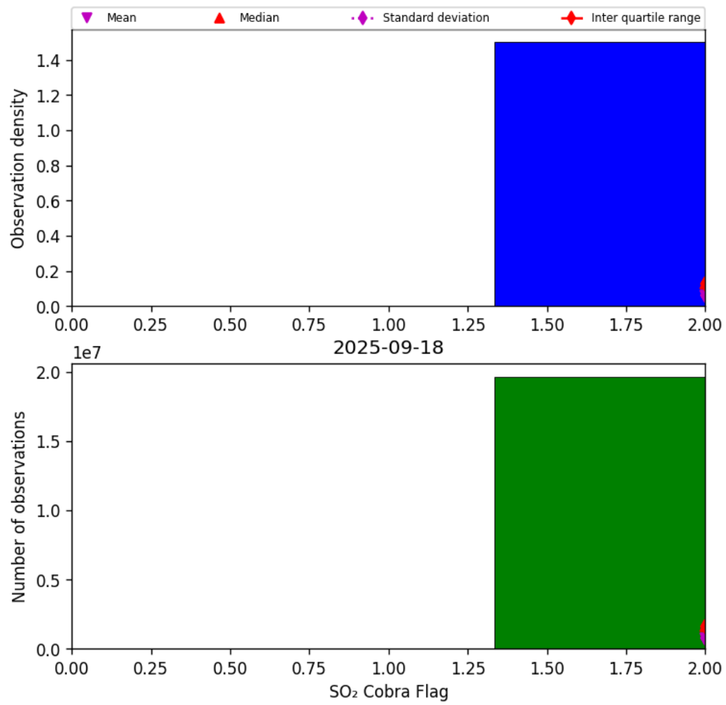
Figure 75: Histogram of "SO 2 Cobra Flag" for 2025-09-17 to 2025-09-19
