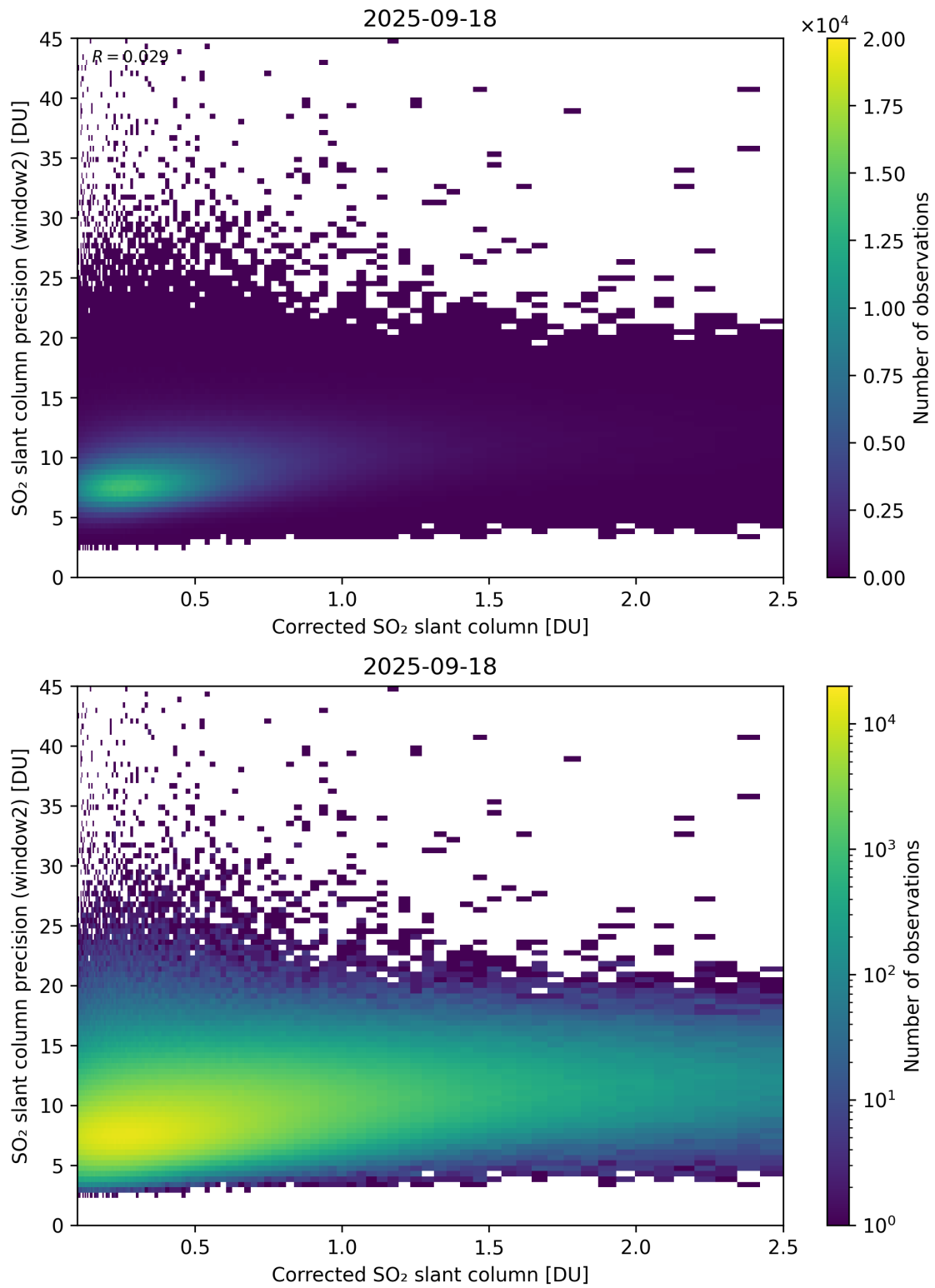
Figure 239: Scatter density plot of “Corrected SO 2 slant column” against “SO 2 slant column precision (window2)” for 2025-09-17 to 2025-09-19.
