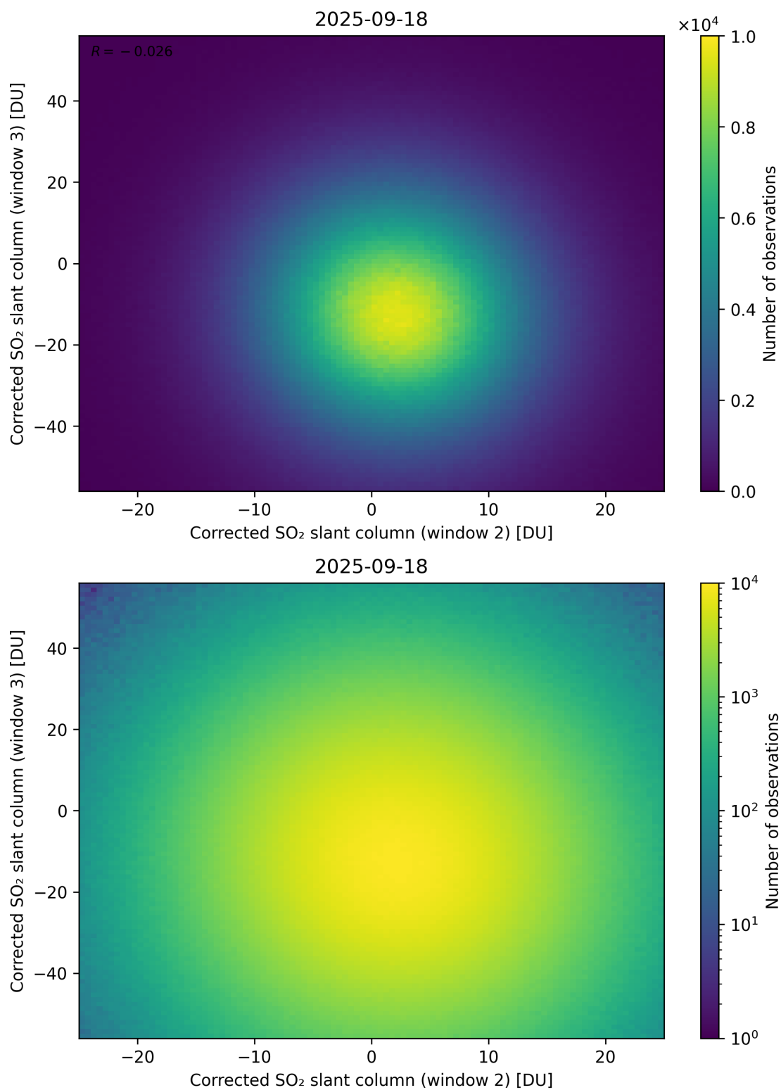
Figure 250: Scatter density plot of “Corrected SO 2 slant column (window 2)” against “Corrected SO 2 slant column (window 3)” for 2025-09-17 to 2025-09-19.
