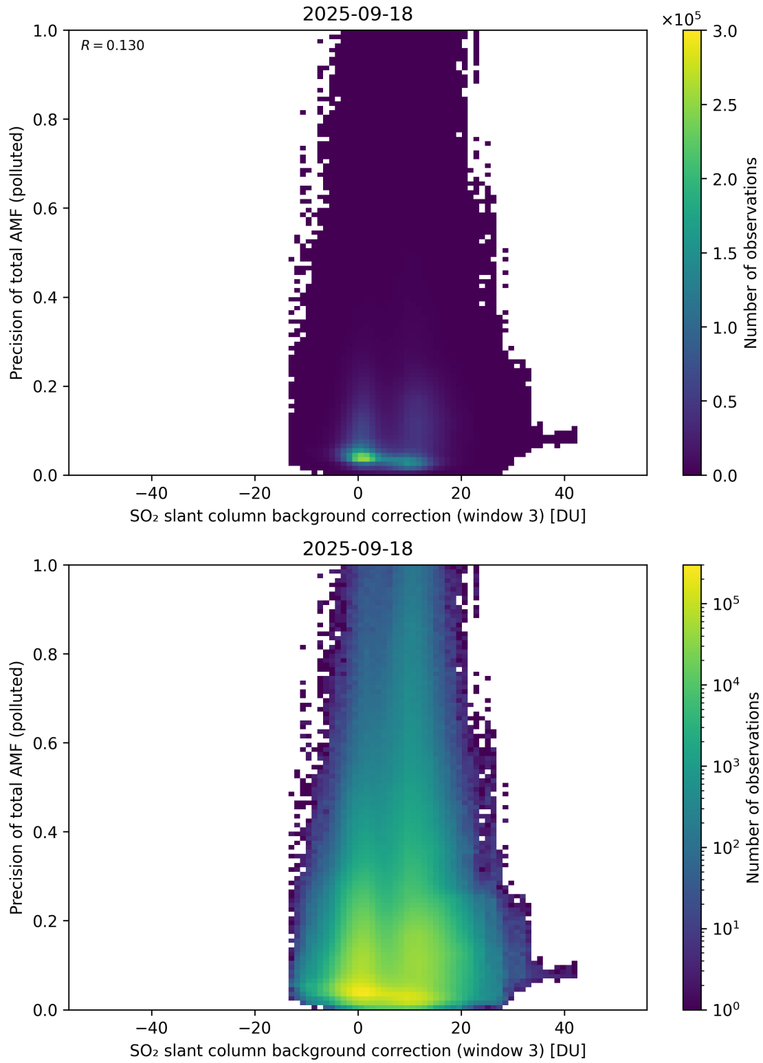
Figure 137: Scatter density plot of “SO 2 slant column background correction (window 3)” against “Precision of total AMF (polluted)” for 2025-09-17 to 2025-09-19.
