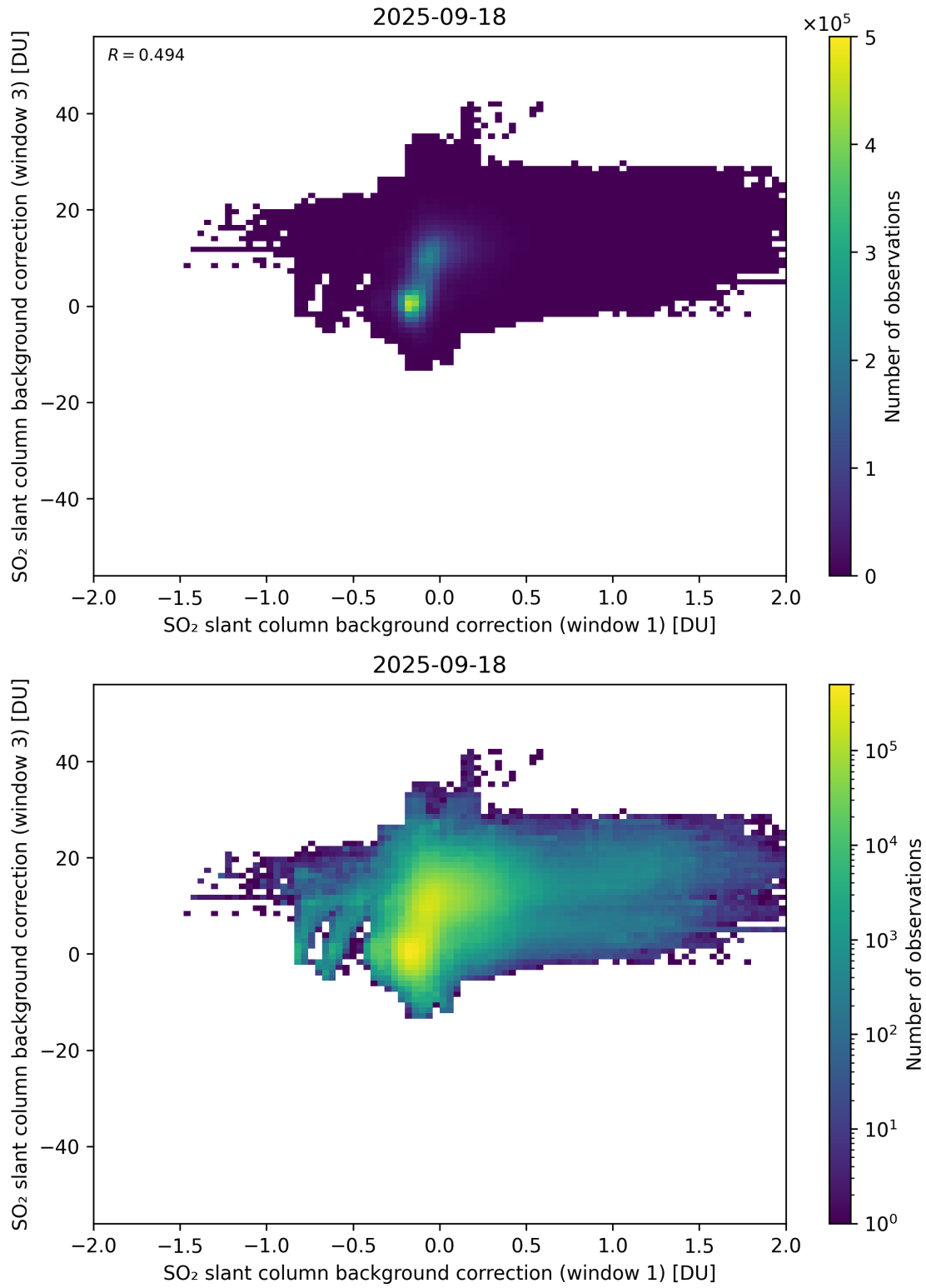
Figure 110: Scatter density plot of “SO 2 slant column background correction (window 1)” against “SO 2 slant column background correction (window 3)” for 2025-09-17 to 2025-09-19.
