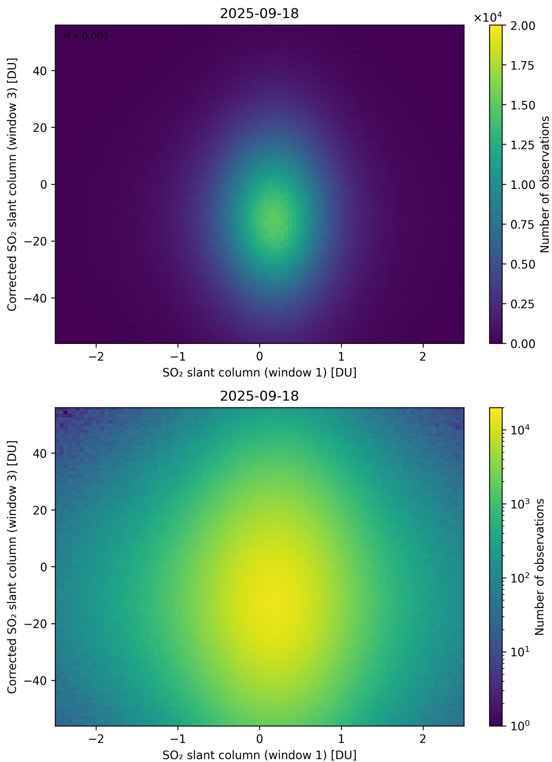
Figure 284: Scatter density plot of “SO 2 slant column (window 1)” against “Corrected SO 2 slant column (window 3)” for 2025-09-17 to 2025-09-19.
