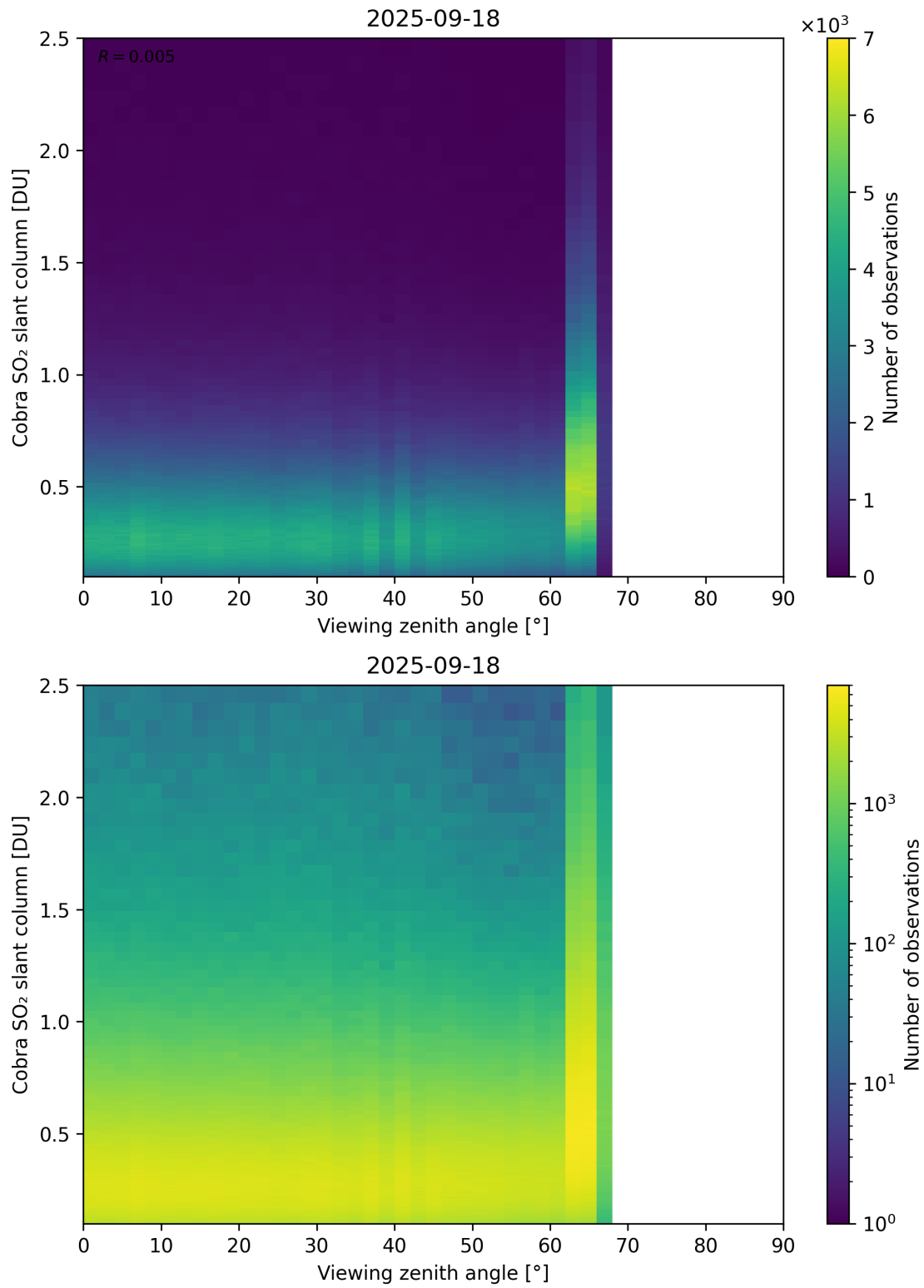
Figure 371: Scatter density plot of “Viewing zenith angle” against “Cobra SO 2 slant column” for 2025-09-17 to 2025-09-19.
