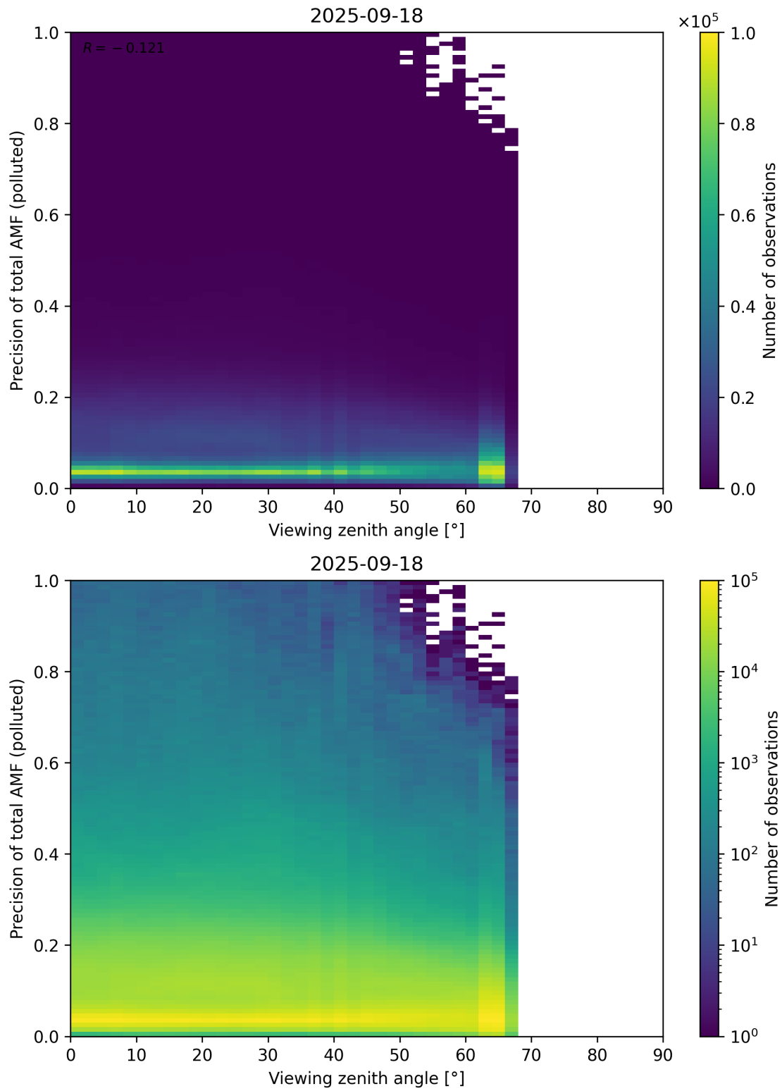
Figure 382: Scatter density plot of “Viewing zenith angle” against “Precision of total AMF (polluted)” for 2025-09-17 to 2025-09-19.
