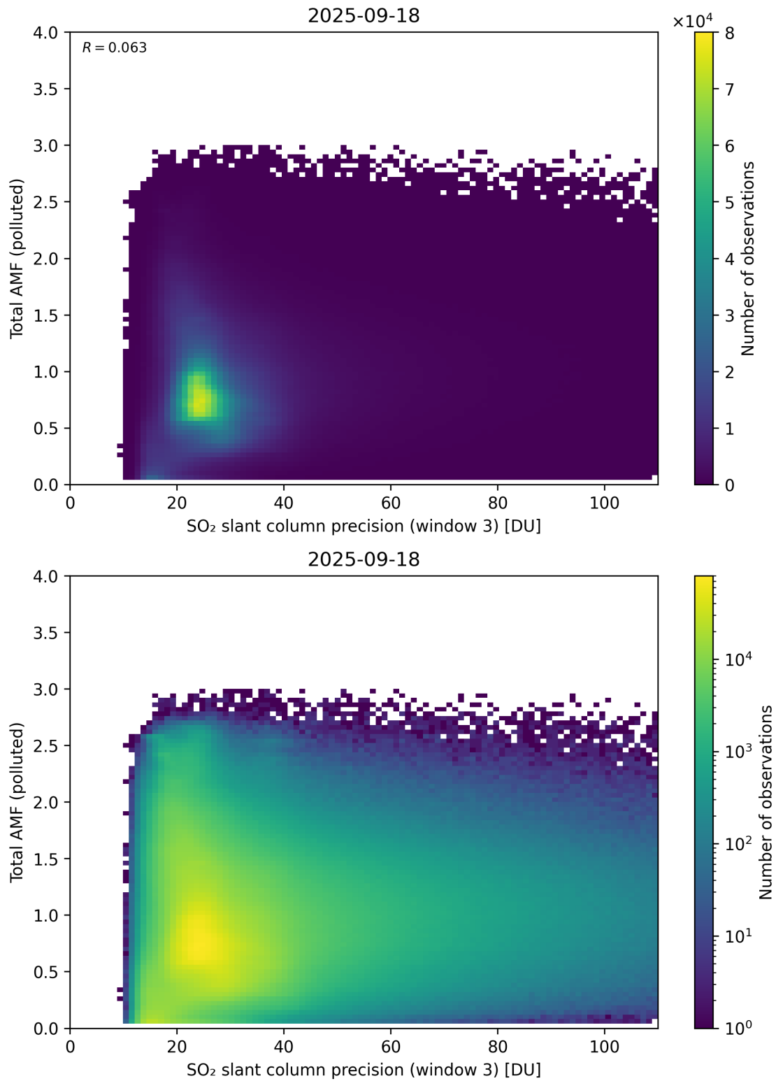
Figure 313: Scatter density plot of “SO 2 slant column precision (window 3)” against “Total AMF (polluted)” for 2025-09-17 to 2025-09-19.
