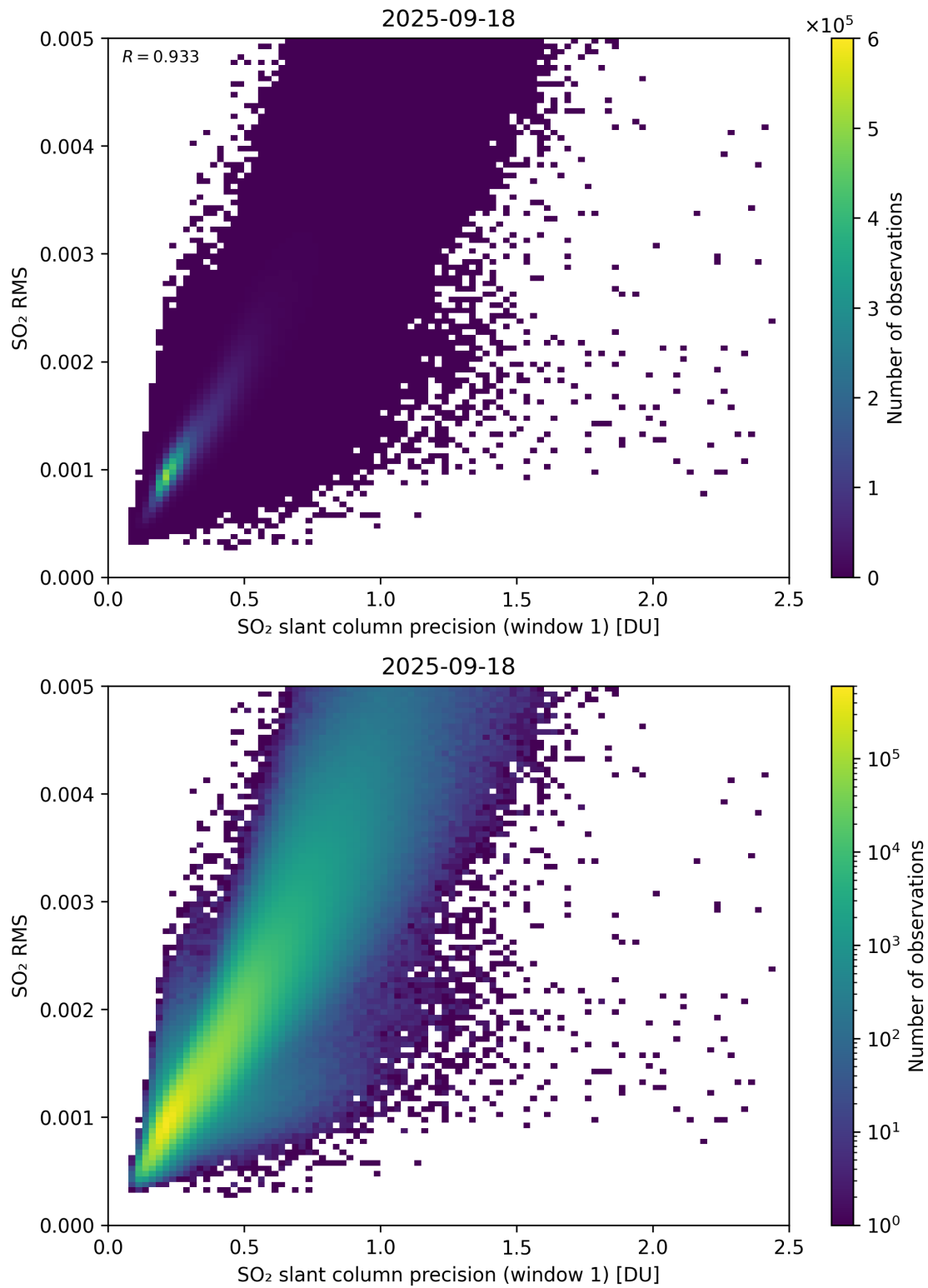
Figure 273: Scatter density plot of “SO 2 slant column precision (window 1)” against “SO 2 RMS” for 2025-09-17 to 2025-09-19.
