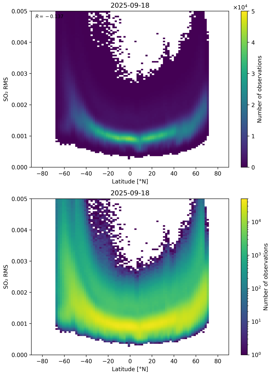
Figure 155: Scatter density plot of “Latitude” against “SO 2 RMS” for 2025-09-17 to 2025-09-19.
