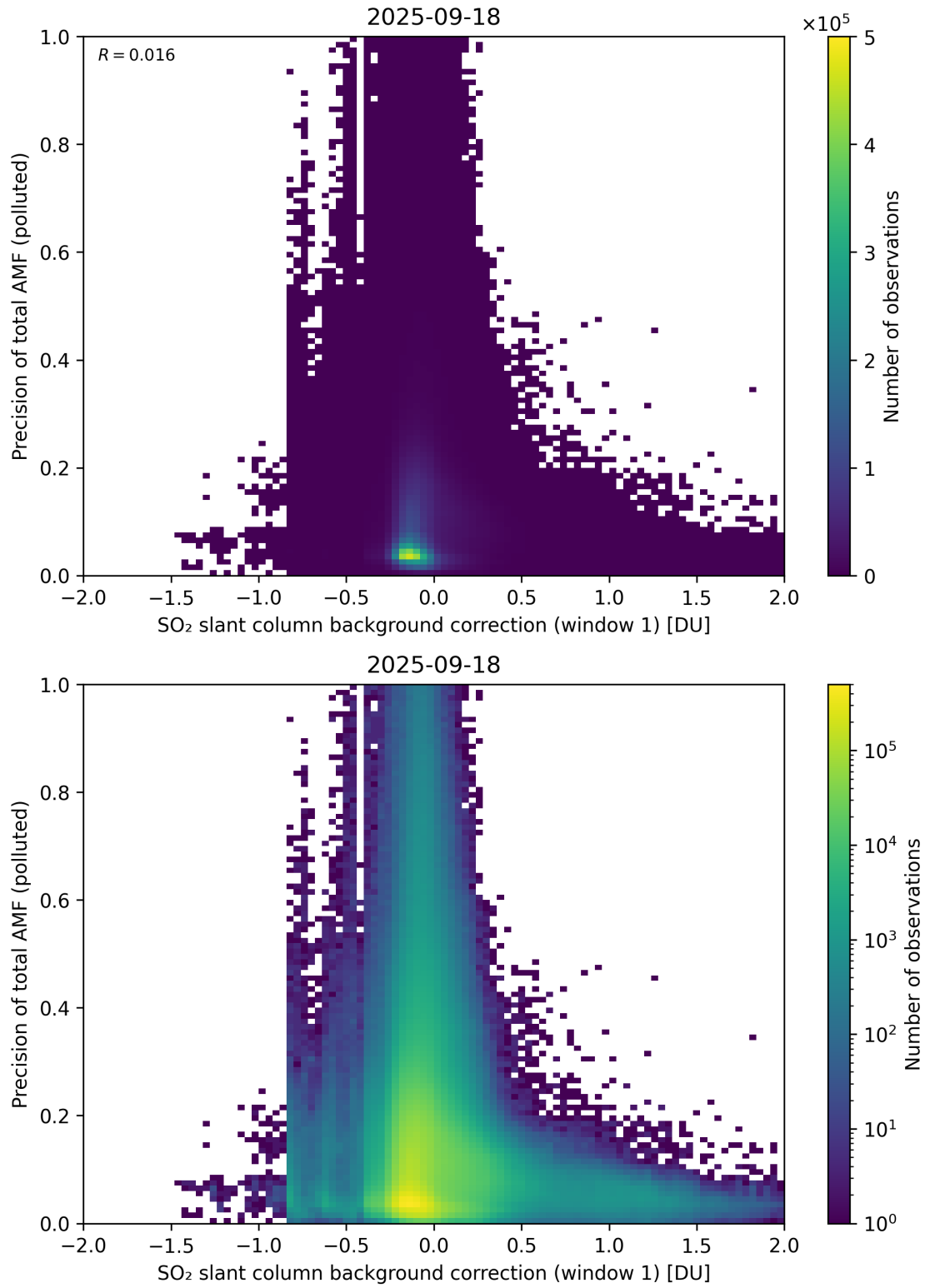
Figure 121: Scatter density plot of “SO 2 slant column background correction (window 1)” against “Precision of total AMF (polluted)” for 2025-09-17 to 2025-09-19.
