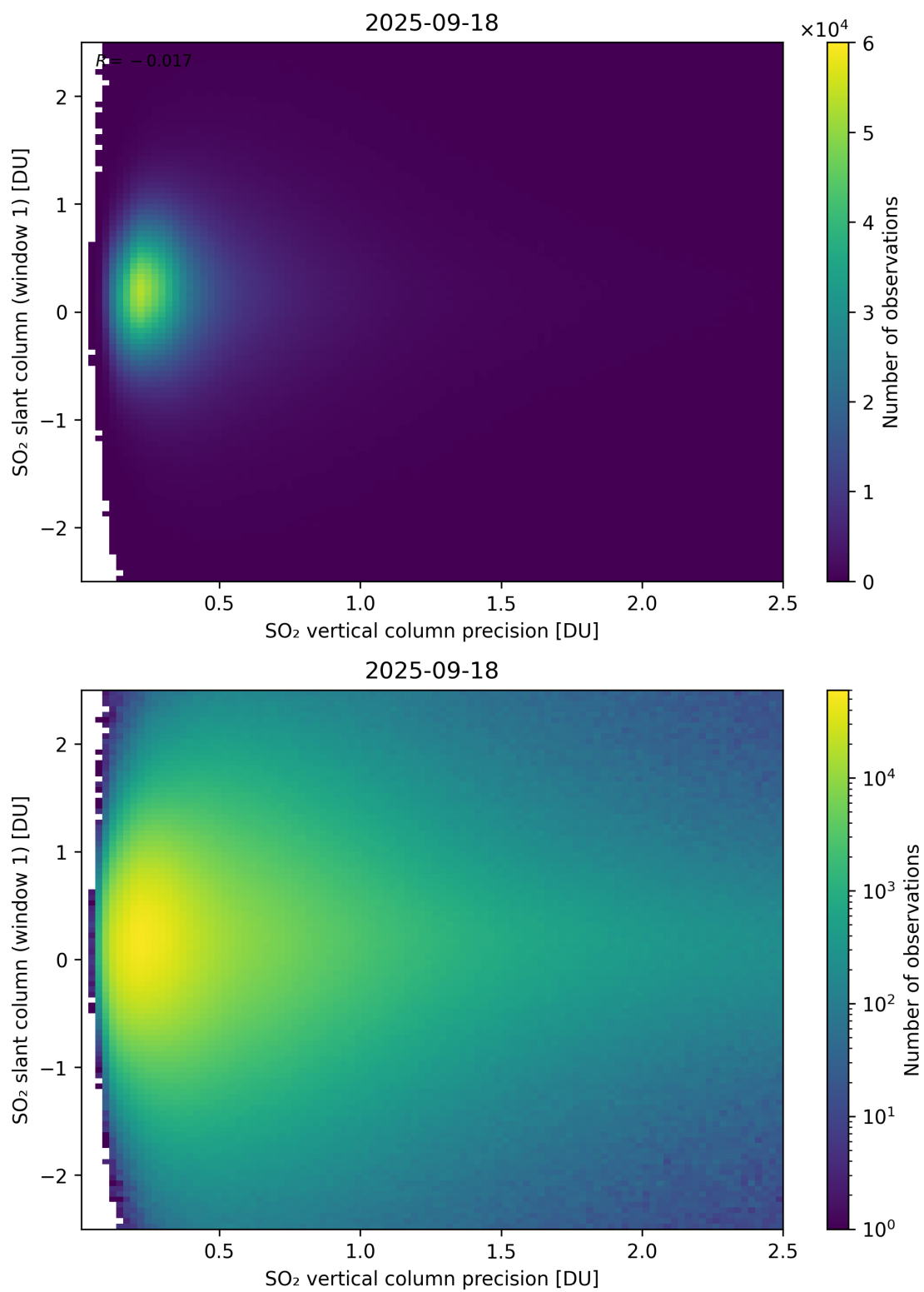
Figure 341: Scatter density plot of “SO 2 vertical column precision” against “SO 2 slant column (window 1)” for 2025-09-17 to 2025-09-19.
