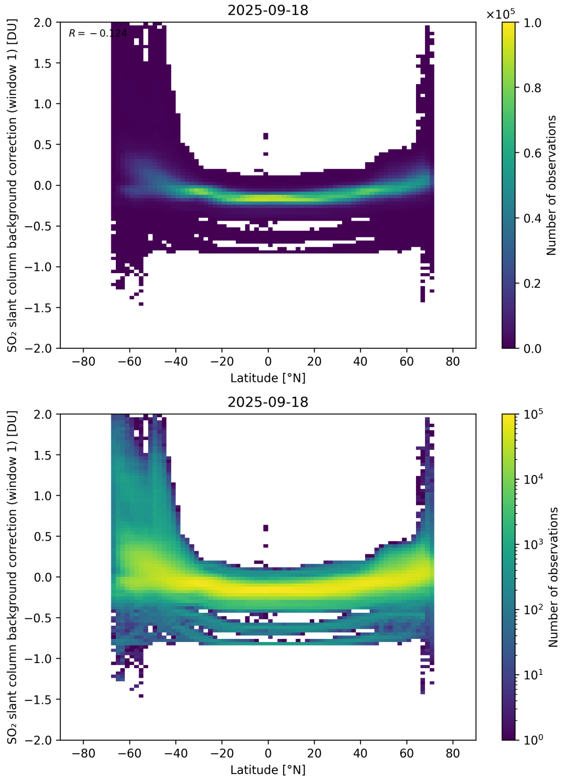
Figure 150: Scatter density plot of “Latitude” against “SO 2 slant column background correction (window 1)” for 2025-09-17 to 2025-09-19.
