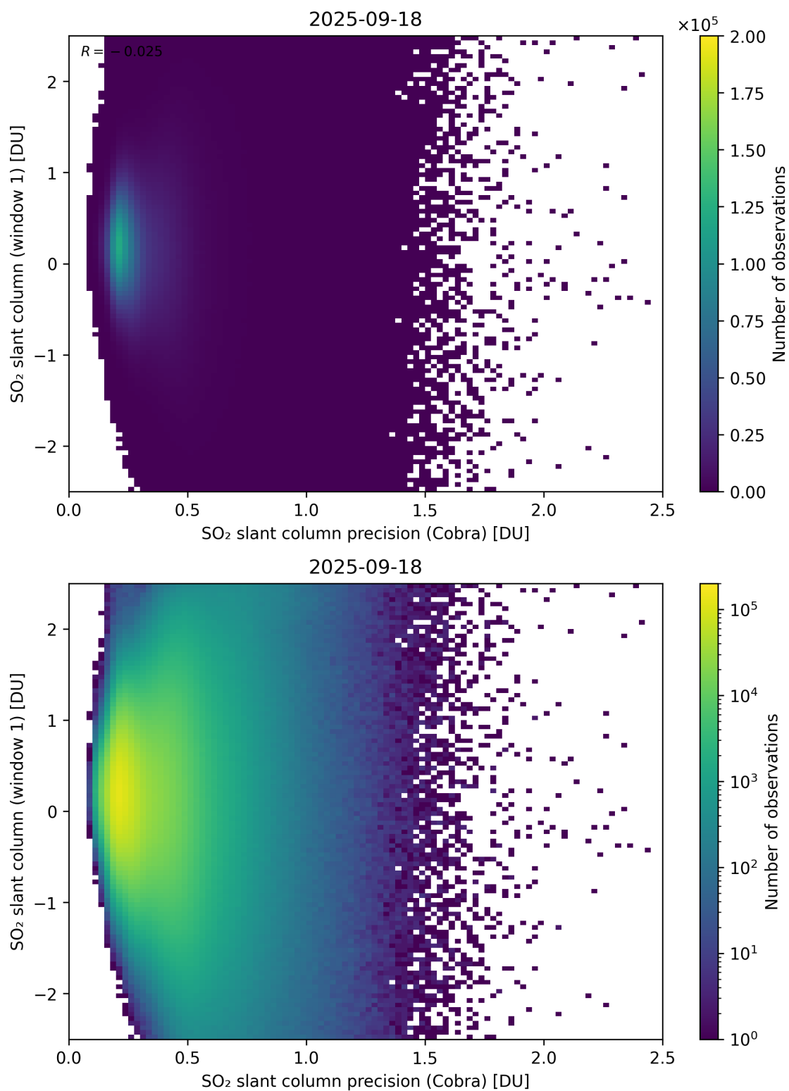
Figure 208: Scatter density plot of “SO 2 slant column precision (Cobra)” against “SO 2 slant column (window 1)” for 2025-09-17 to 2025-09-19.
