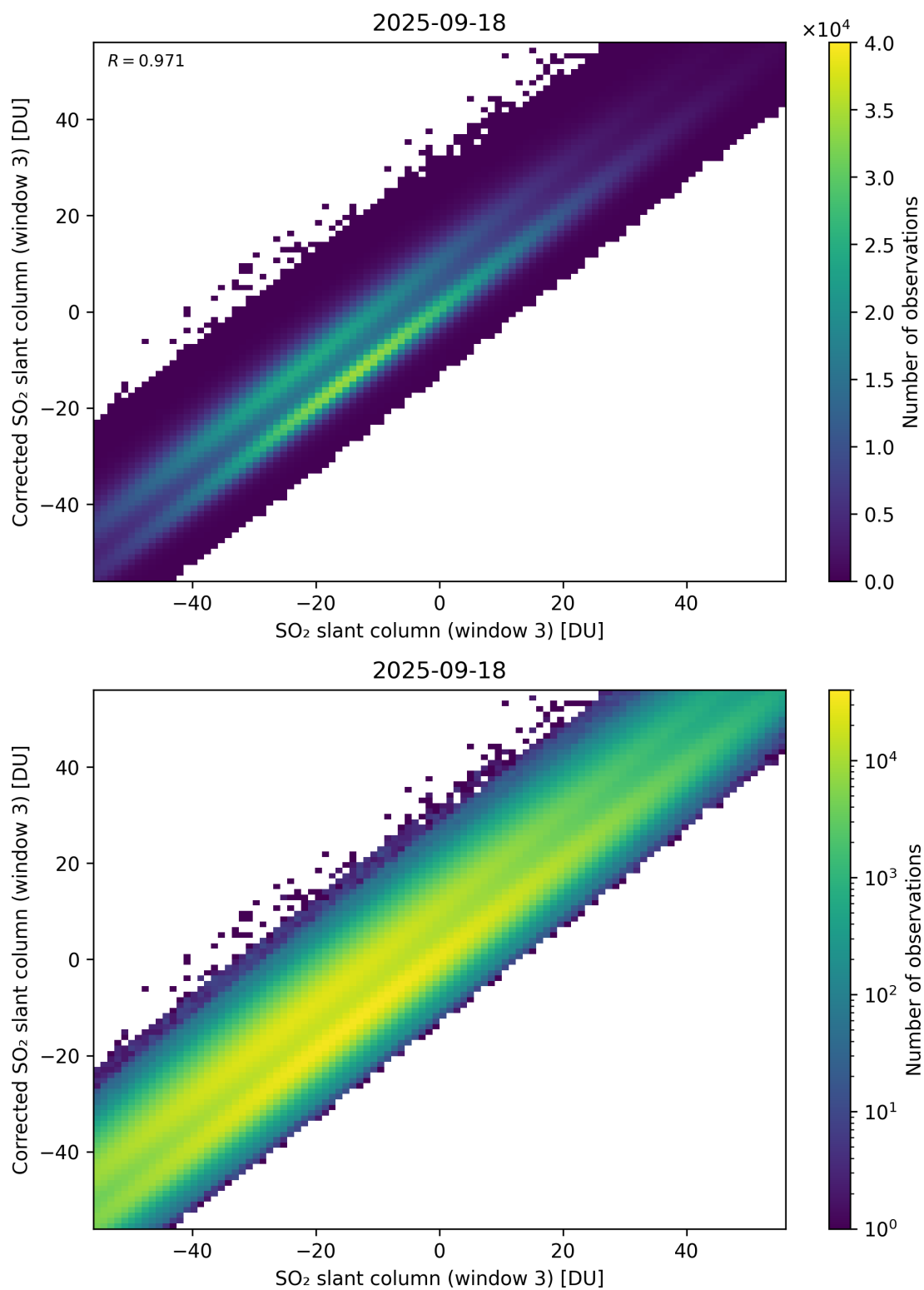
Figure 316: Scatter density plot of “SO 2 slant column (window 3)” against “Corrected SO 2 slant column (window 3)” for 2025-09-17 to 2025-09-19.
