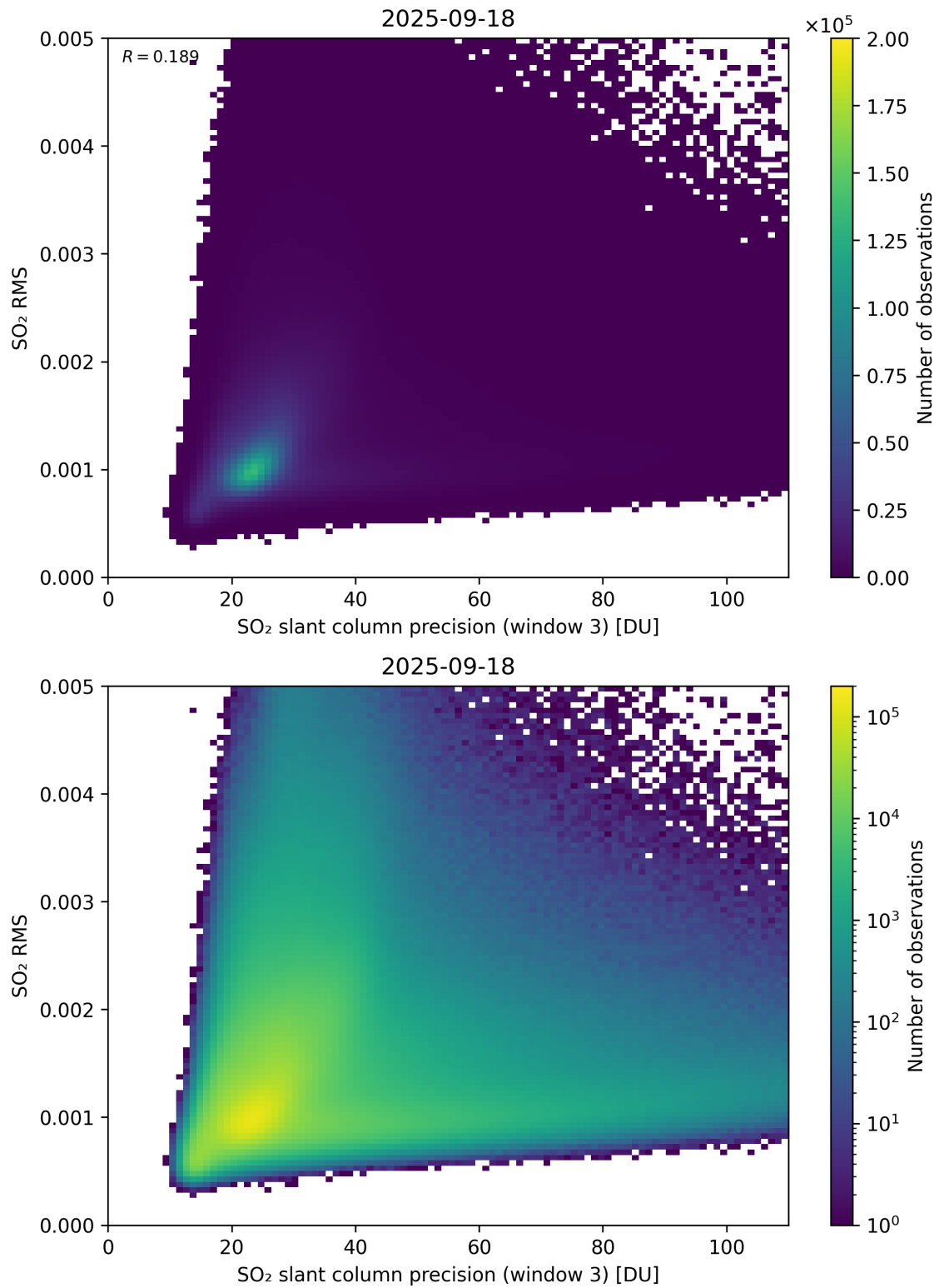
Figure 310: Scatter density plot of “SO 2 slant column precision (window 3)” against “SO 2 RMS” for 2025-09-17 to 2025-09-19.
