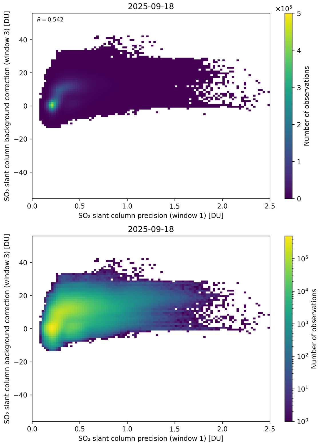
Figure 270: Scatter density plot of “SO 2 slant column precision (window 1)” against “SO 2 slant column background correction (window 3)” for 2025-09-17 to 2025-09-19.
