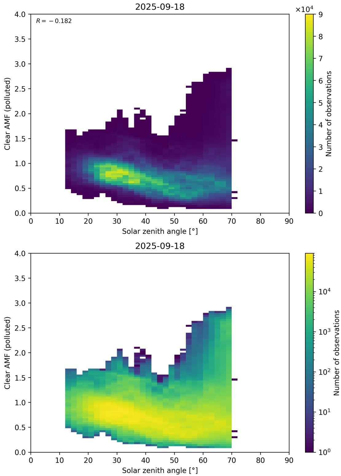
Figure 178: Scatter density plot of “Solar zenith angle” against “Clear AMF (polluted)” for 2025-09-17 to 2025-09-19.
