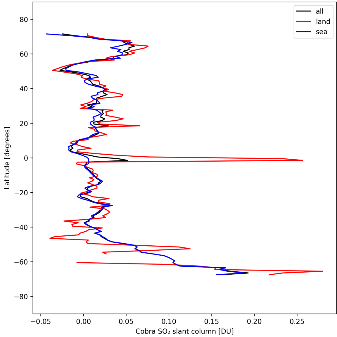
Figure 35: Zonal average of “Cobra SO 2 slant column” for 2025-09-17 to 2025-09-19.
