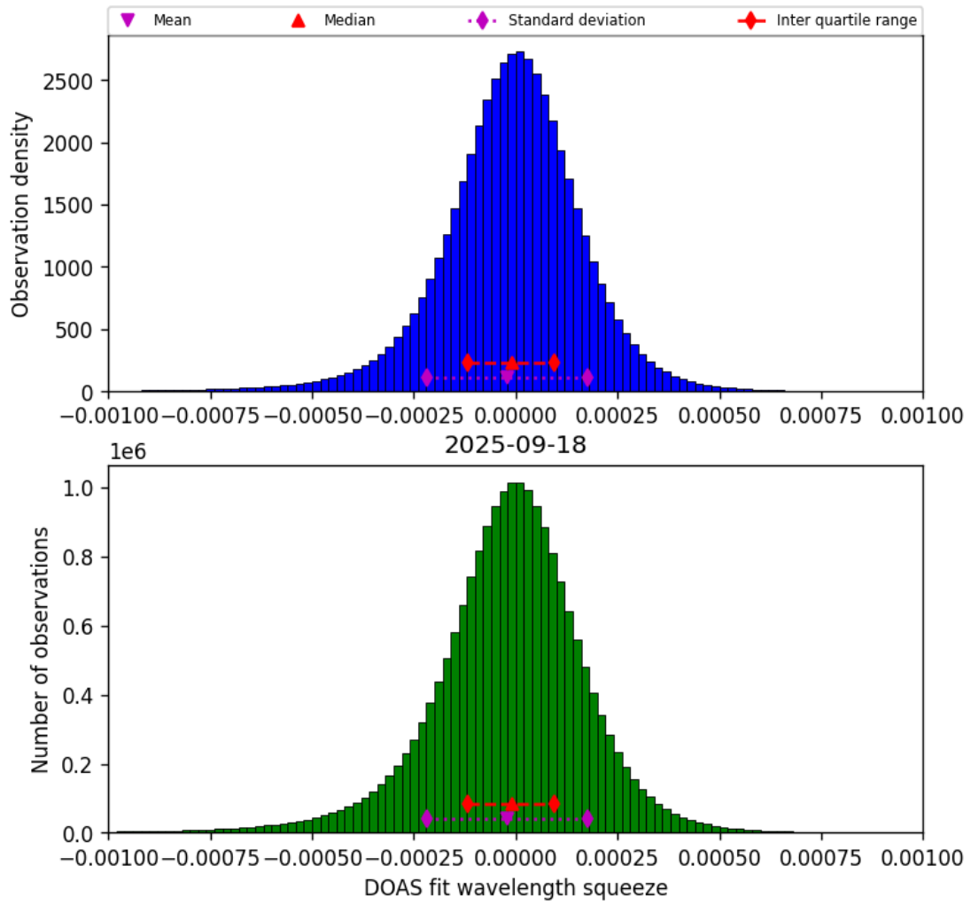
Figure 77: Histogram of “DOAS fit wavelength squeeze” for 2025-09-17 to 2025-09-19
