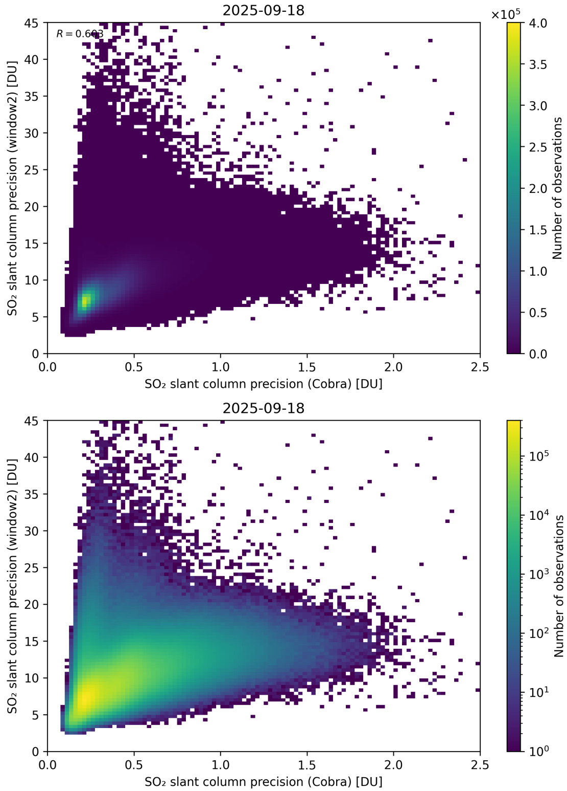
Figure 210: Scatter density plot of “SO 2 slant column precision (Cobra)” against “SO 2 slant column precision (window2)” for 2025-09-17 to 2025-09-19.
