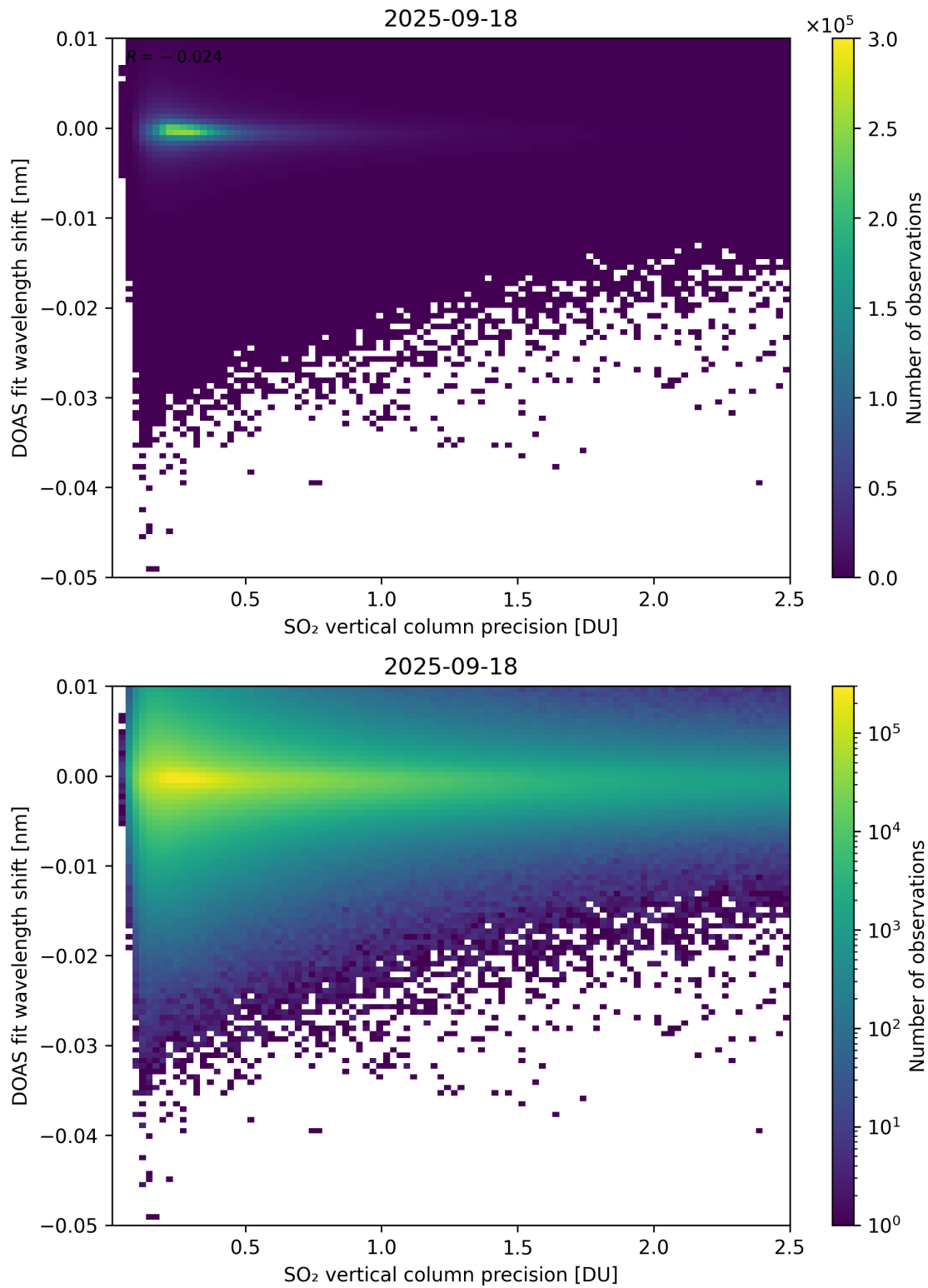
Figure 332: Scatter density plot of “SO 2 vertical column precision” against “DOAS fit wavelength shift” for 2025-09-17 to 2025-09-19.
