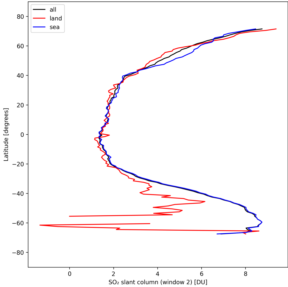
Figure 41: Zonal average of “SO 2 slant column (window 2)” for 2025-09-17 to 2025-09-19.
