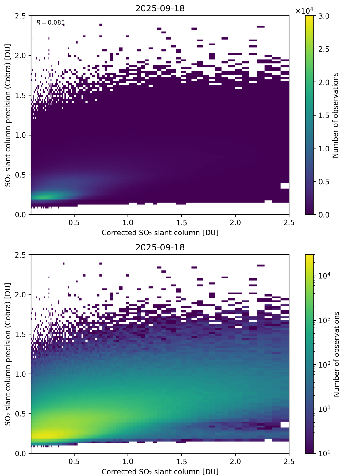
Figure 234: Scatter density plot of “Corrected SO 2 slant column” against “SO 2 slant column precision (Cobra)” for 2025-09-17 to 2025-09-19.
