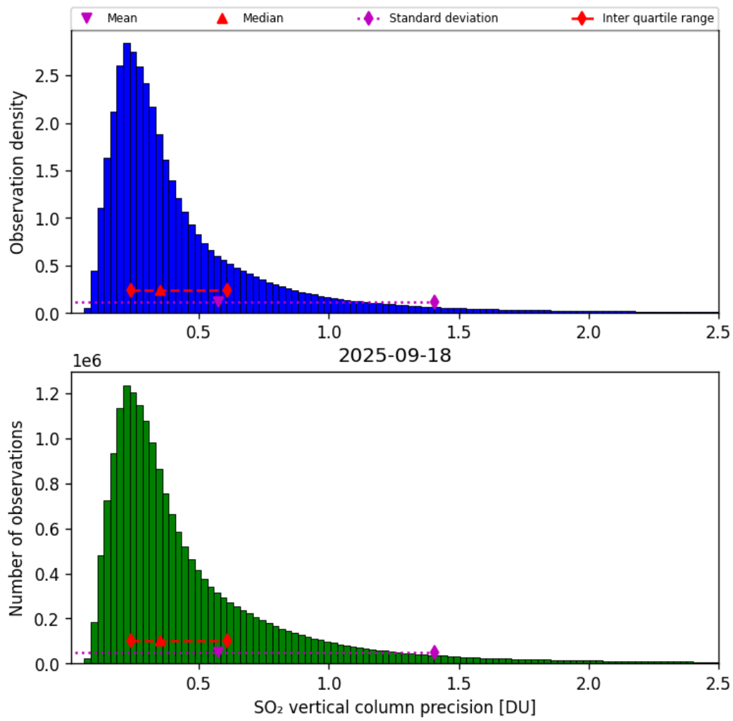
Figure 59: Histogram of “SO 2 vertical column precision” for 2025-09-17 to 2025-09-19
