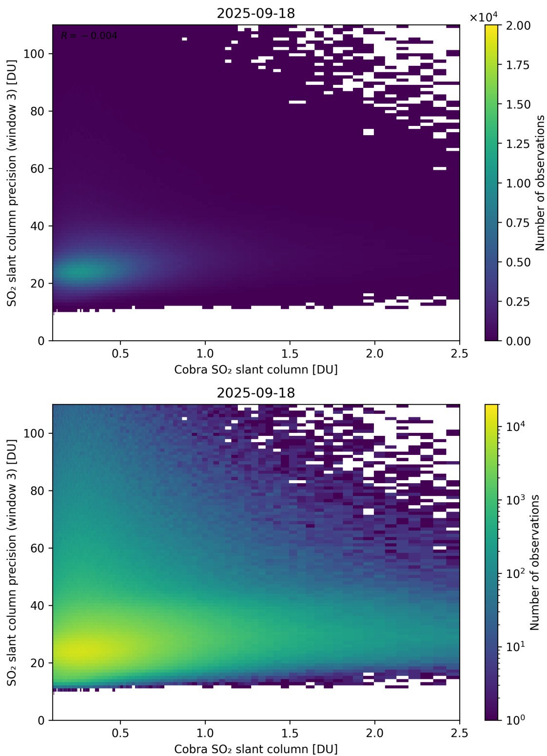
Figure 223: Scatter density plot of “Cobra SO 2 slant column” against “SO 2 slant column precision (window 3)” for 2025-09-17 to 2025-09-19.
