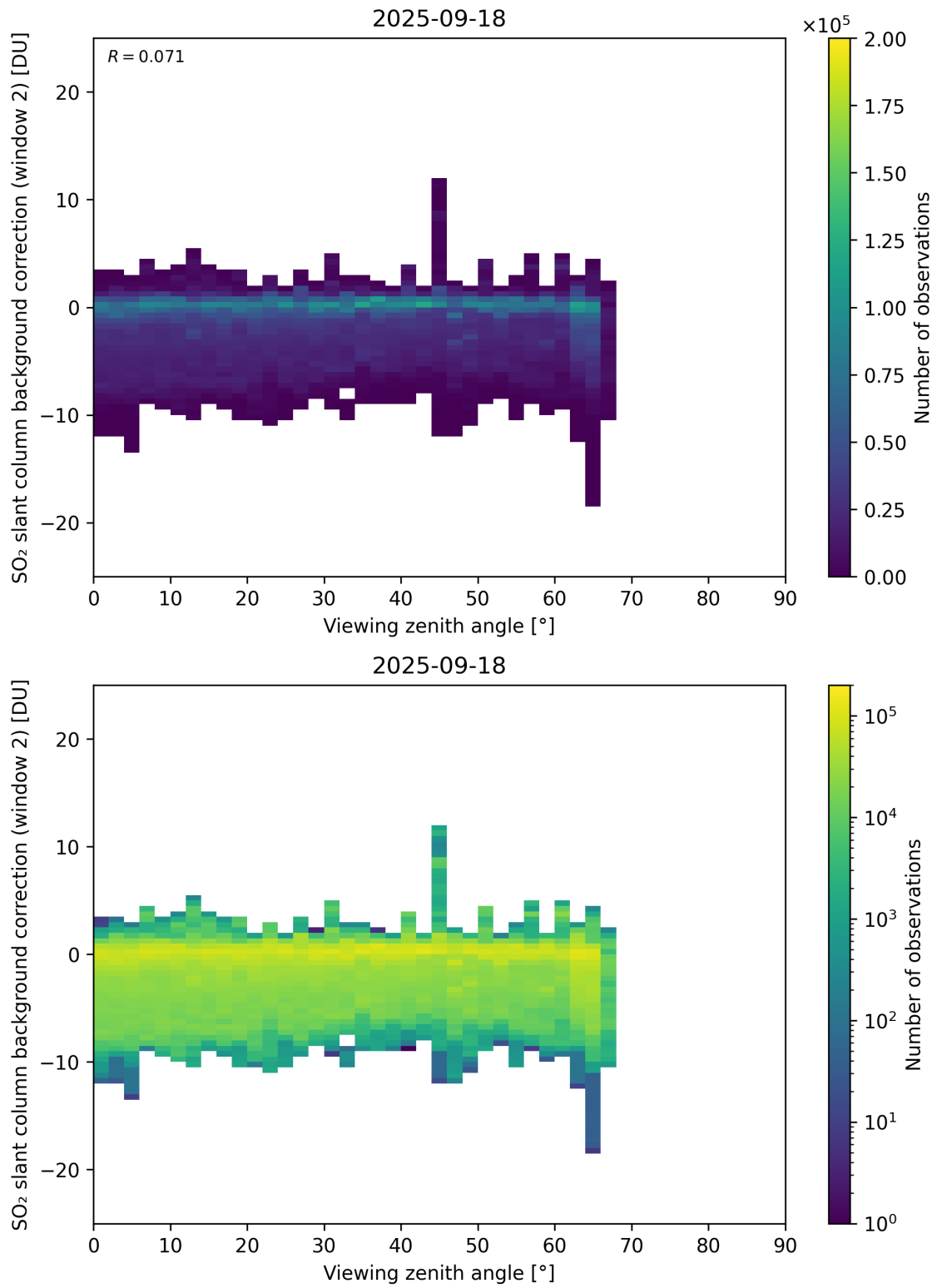
Figure 363: Scatter density plot of “Viewing zenith angle” against “SO 2 slant column background correction (window 2)” for 2025-09-17 to 2025-09-19.
