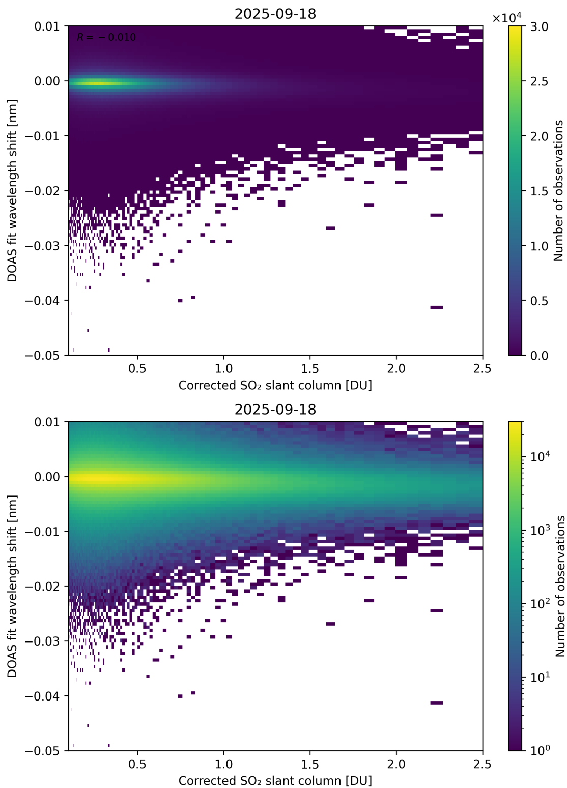
Figure 229: Scatter density plot of “Corrected SO 2 slant column” against “DOAS fit wavelength shift” for 2025-09-17 to 2025-09-19.
