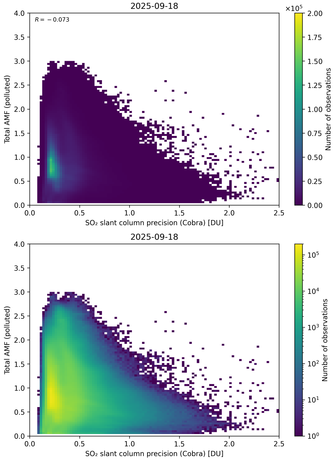
Figure 213: Scatter density plot of “SO 2 slant column precision (Cobra)” against “Total AMF (polluted)” for 2025-09-17 to 2025-09-19.
