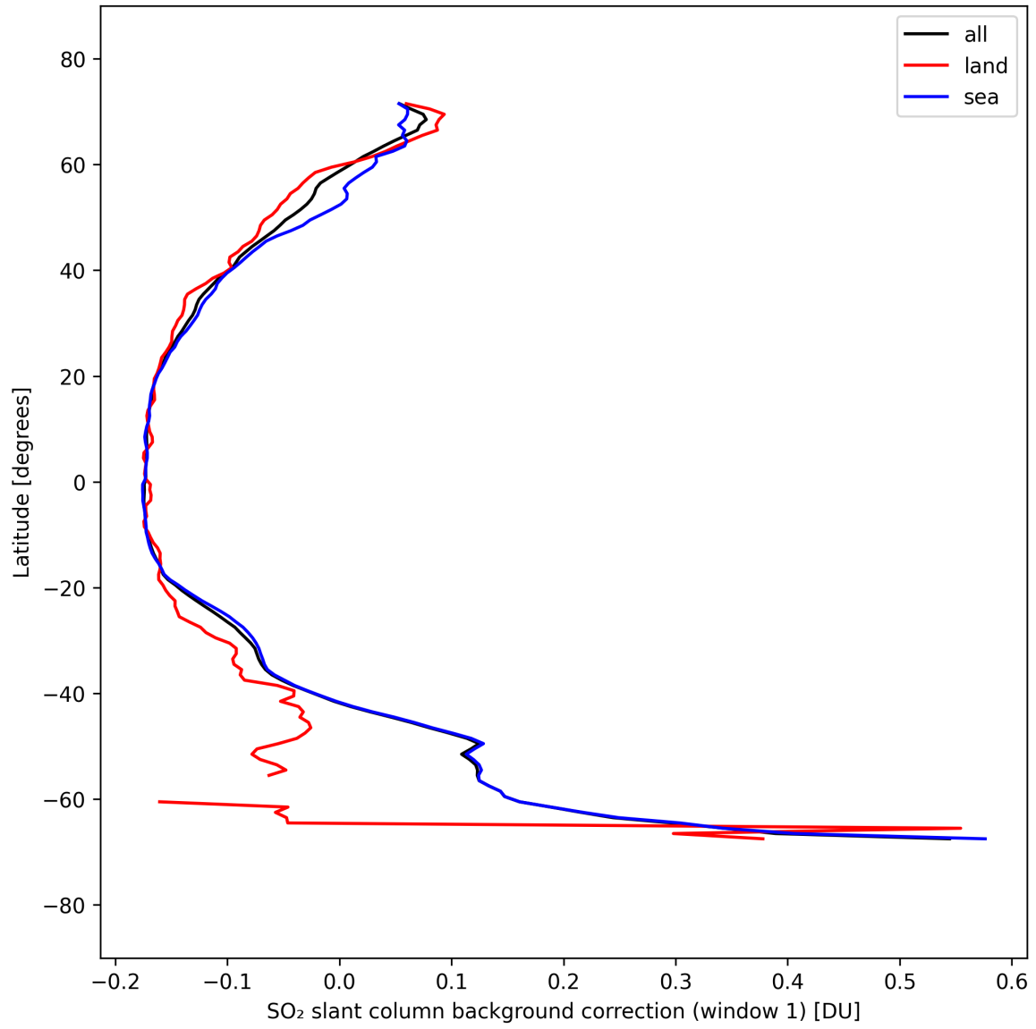
Figure 40: Zonal average of “SO 2 slant column background correction (window 1)” for 2025-09-17 to 2025-09-19.
