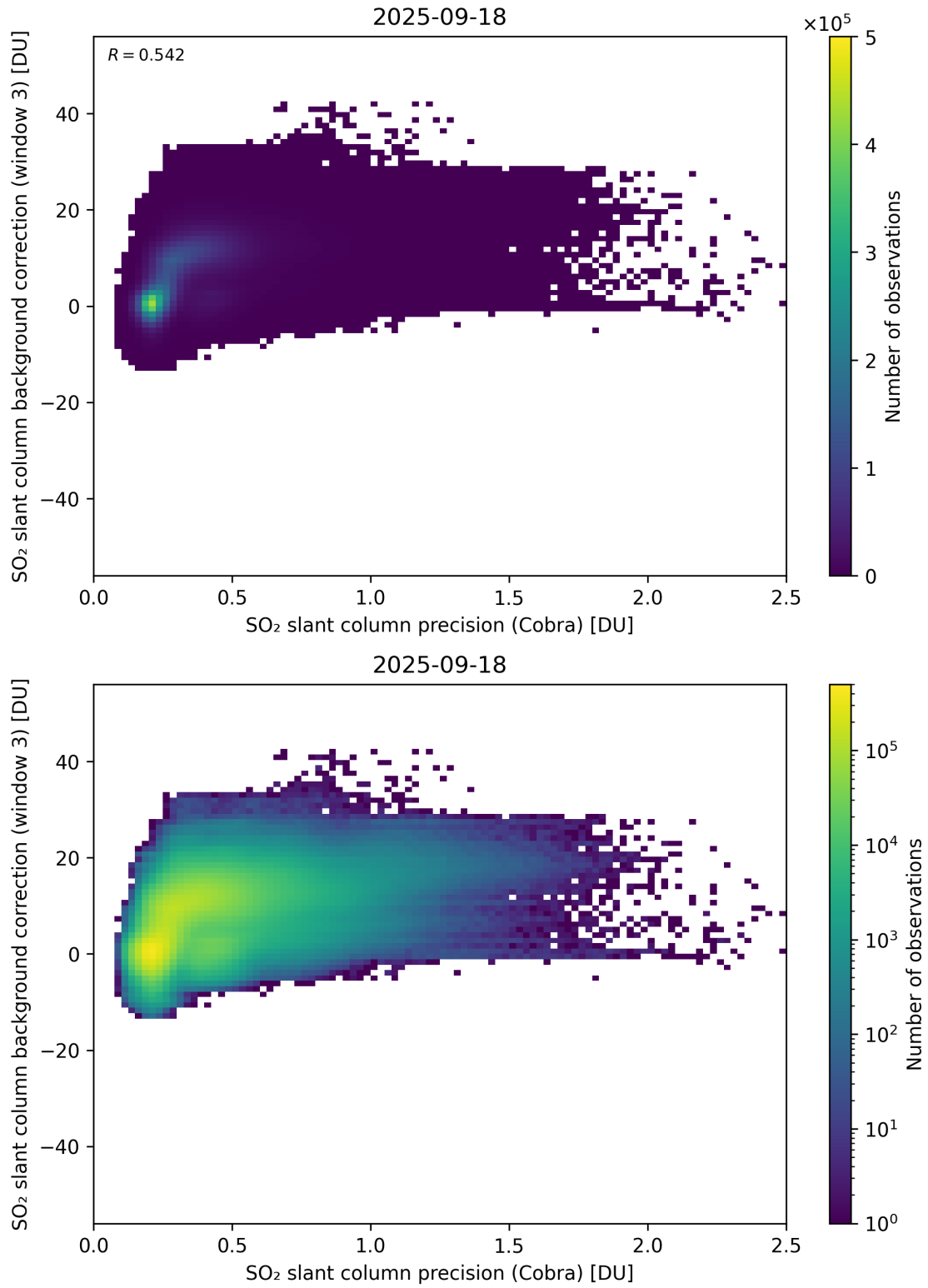
Figure 201: Scatter density plot of “SO 2 slant column precision (Cobra)” against “SO 2 slant column background correction (window 3)” for 2025-09-17 to 2025-09-19.
