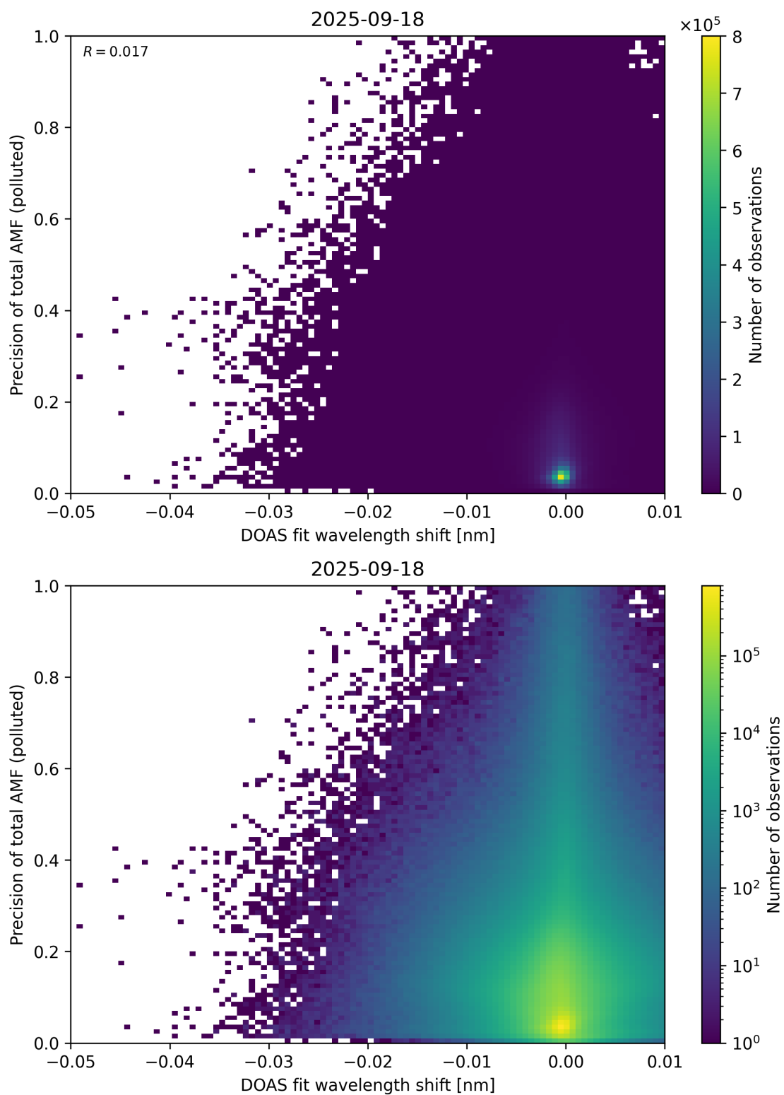
Figure 142: Scatter density plot of “DOAS fit wavelength shift” against “Precision of total AMF (polluted)” for 2025-09-17 to 2025-09-19.
