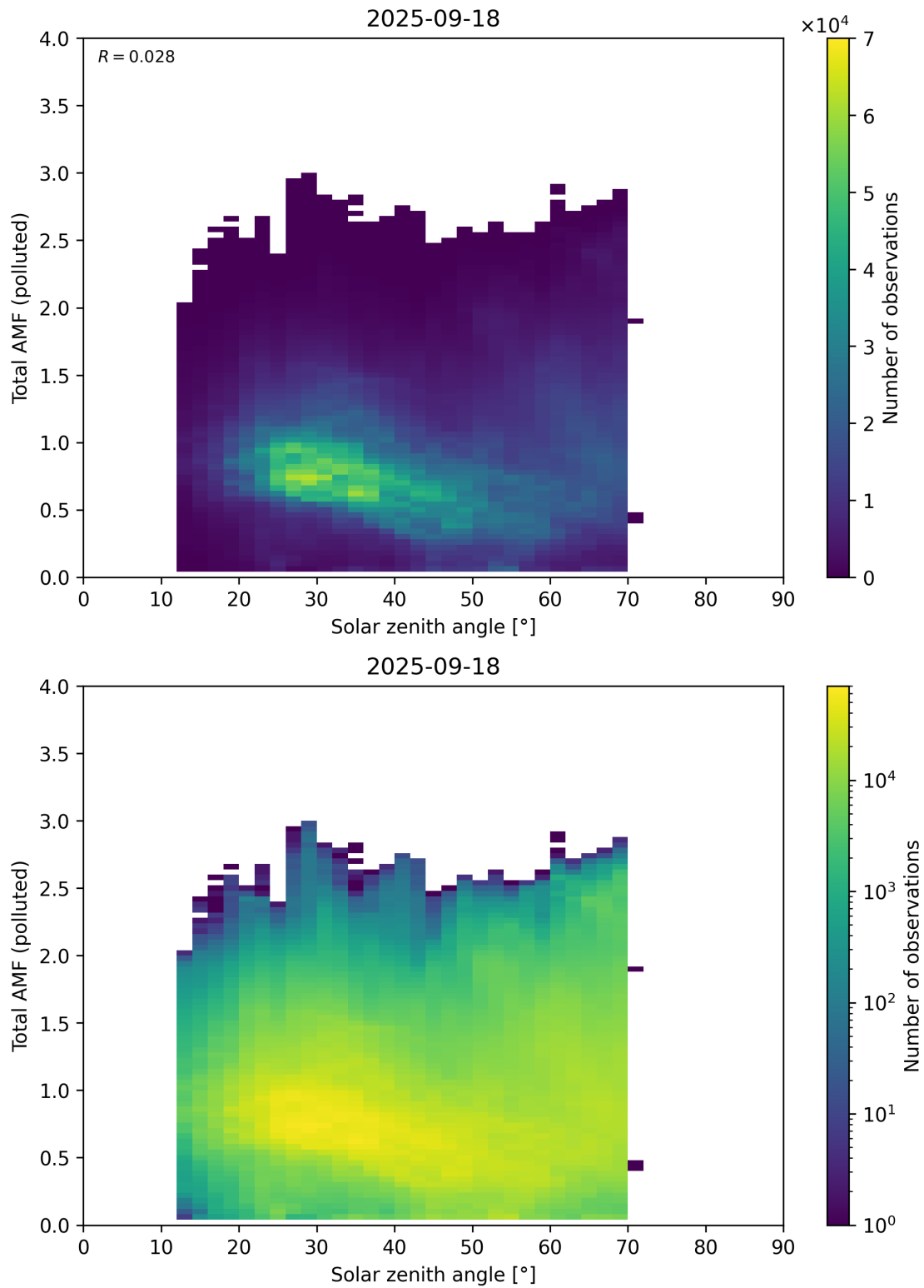
Figure 189: Scatter density plot of “Solar zenith angle” against “Total AMF (polluted)” for 2025-09-17 to 2025-09-19.
