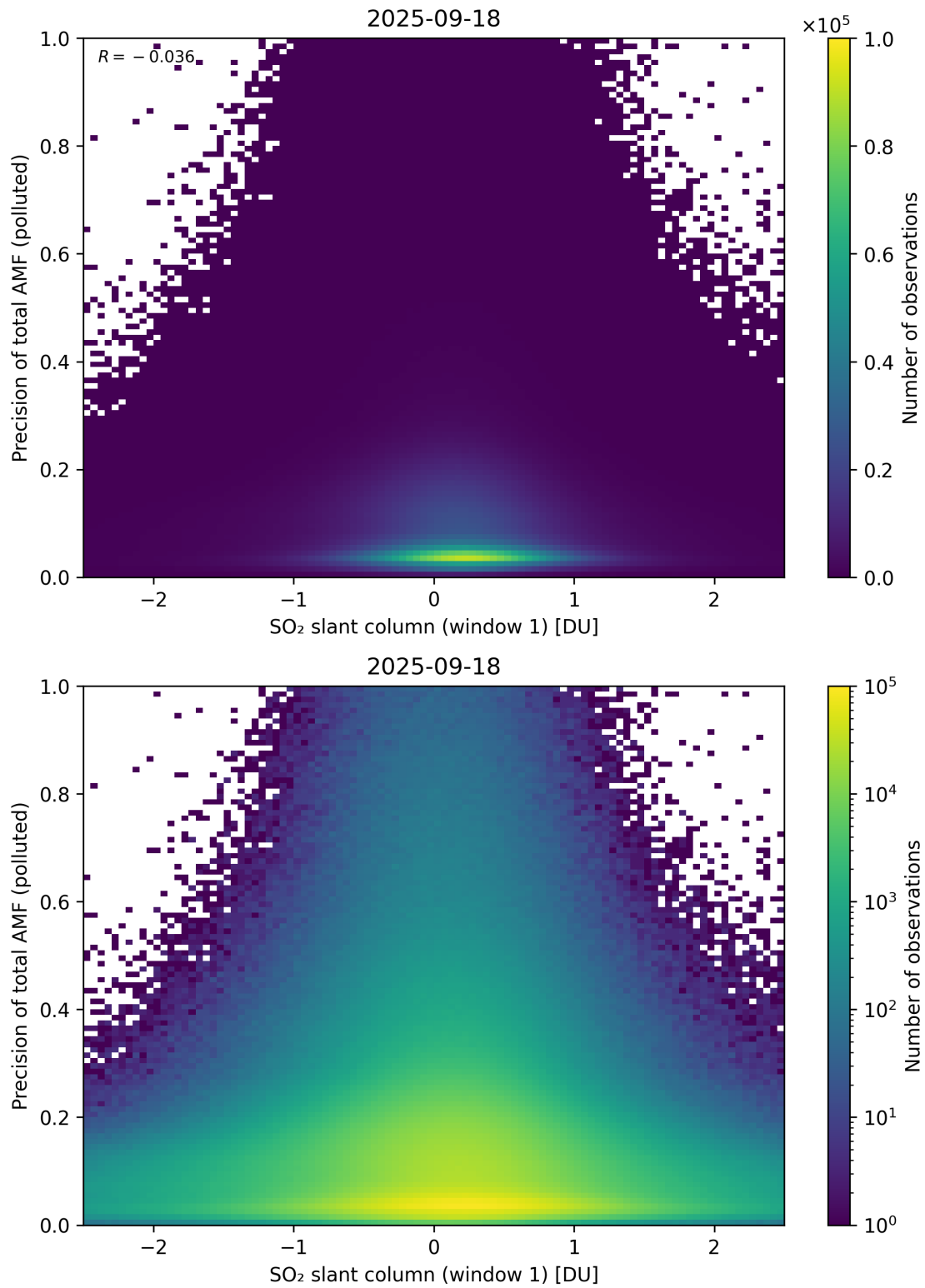
Figure 290: Scatter density plot of “SO 2 slant column (window 1)” against “Precision of total AMF (polluted)” for 2025-09-17 to 2025-09-19.
