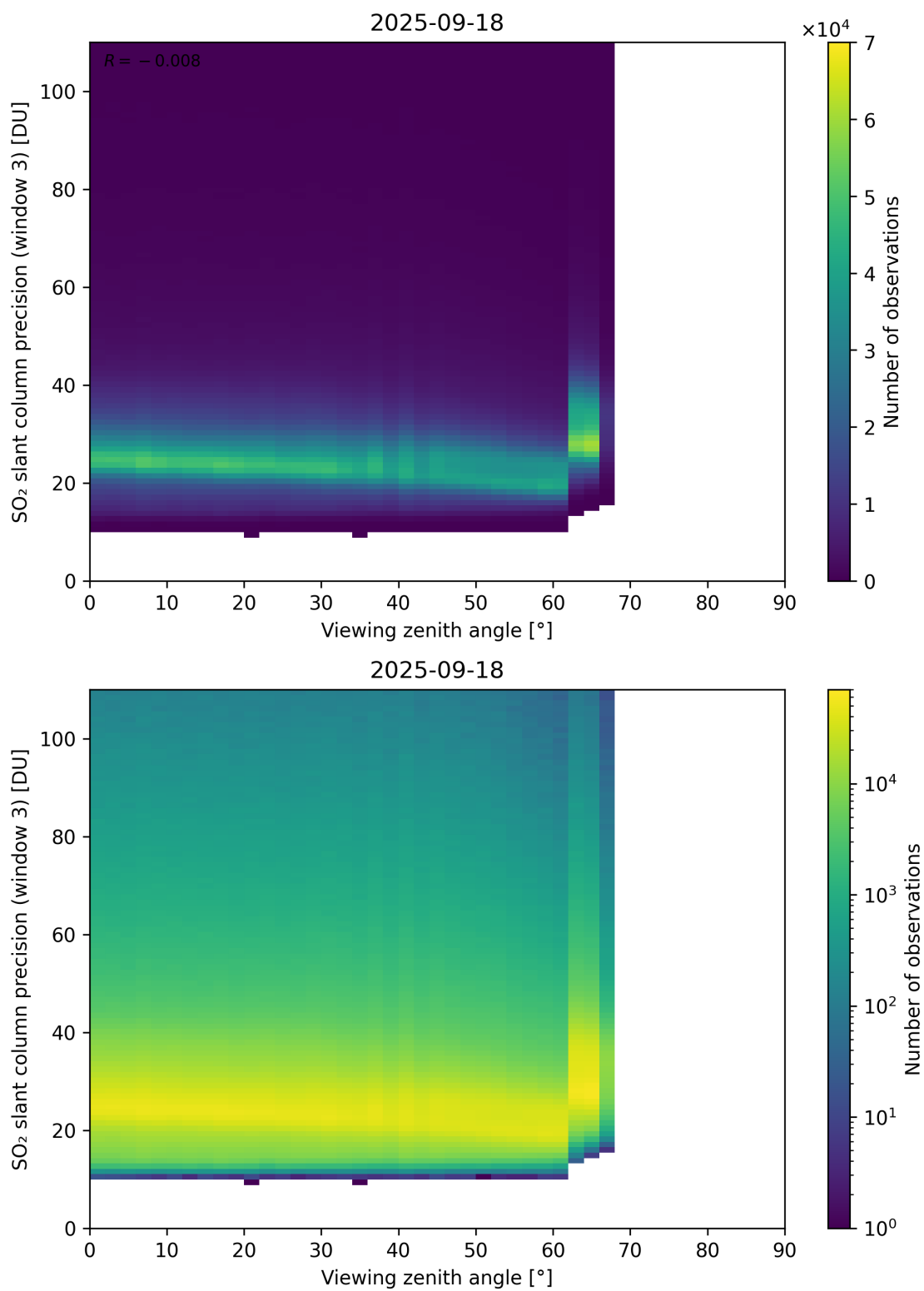
Figure 380: Scatter density plot of “Viewing zenith angle” against “SO 2 slant column precision (window 3)” for 2025-09-17 to 2025-09-19.
