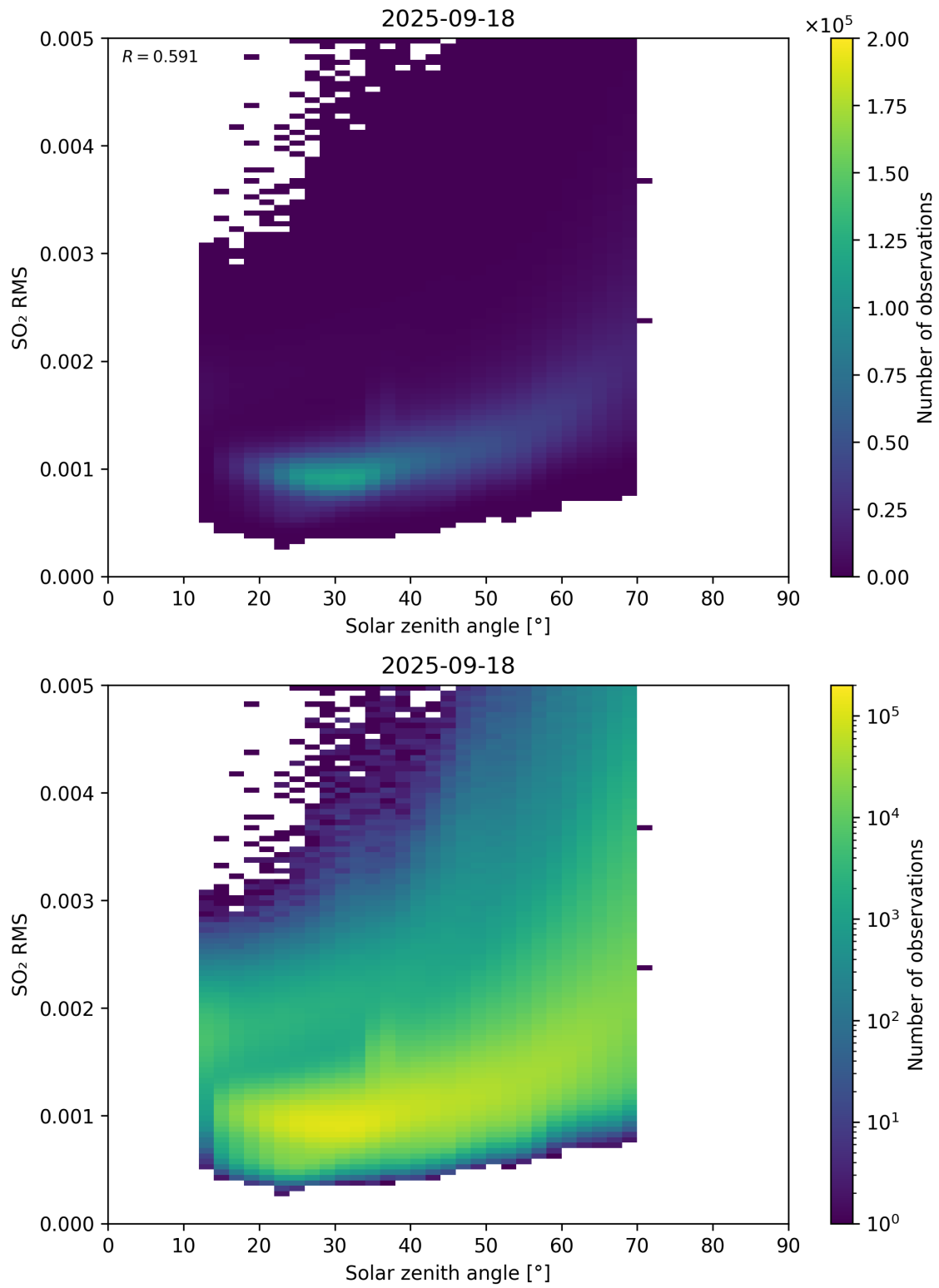
Figure 176: Scatter density plot of “Solar zenith angle” against “SO 2 RMS” for 2025-09-17 to 2025-09-19.
