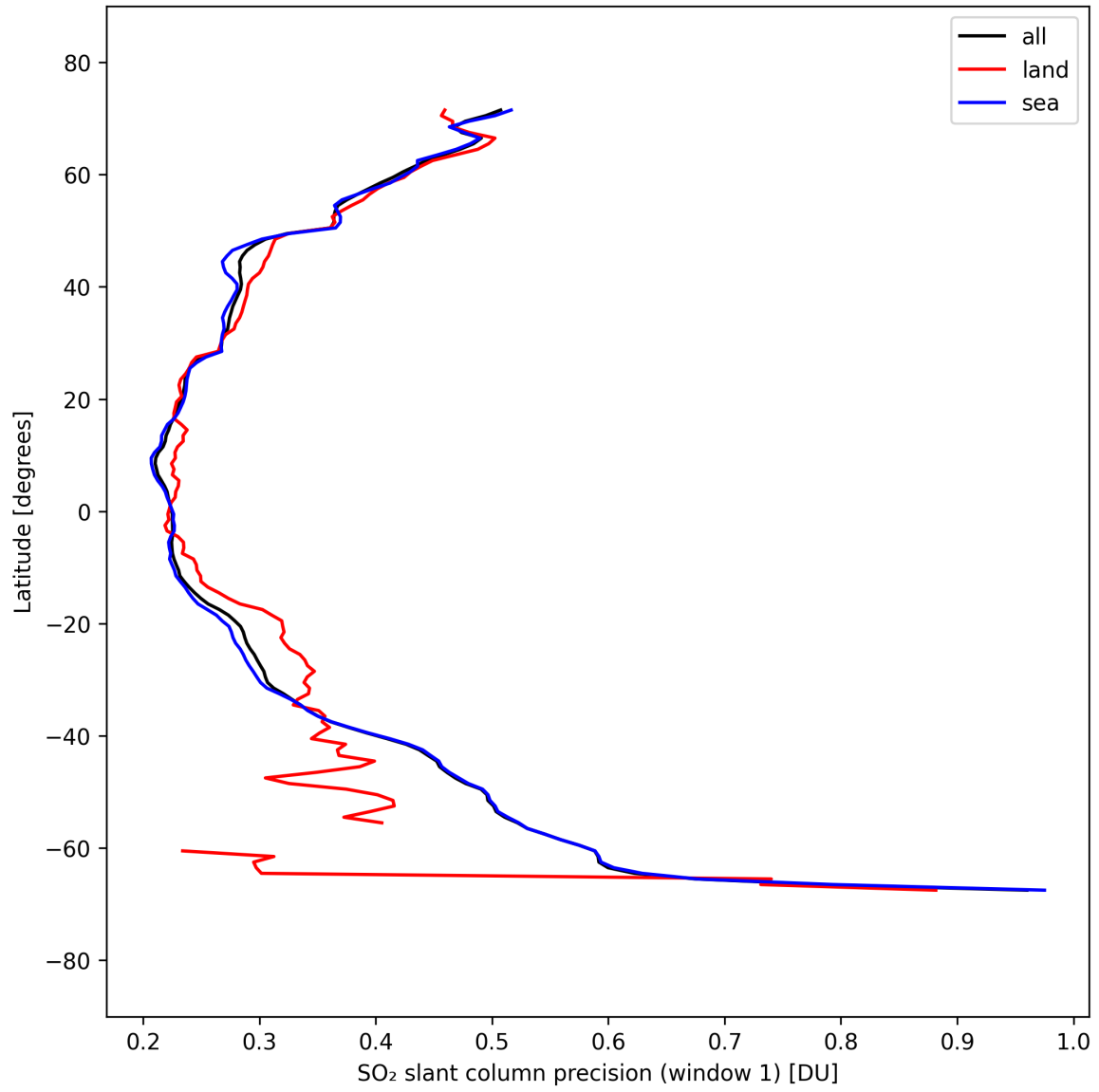
Figure 38: Zonal average of “SO 2 slant column precision (window 1)” for 2025-09-17 to 2025-09-19.
