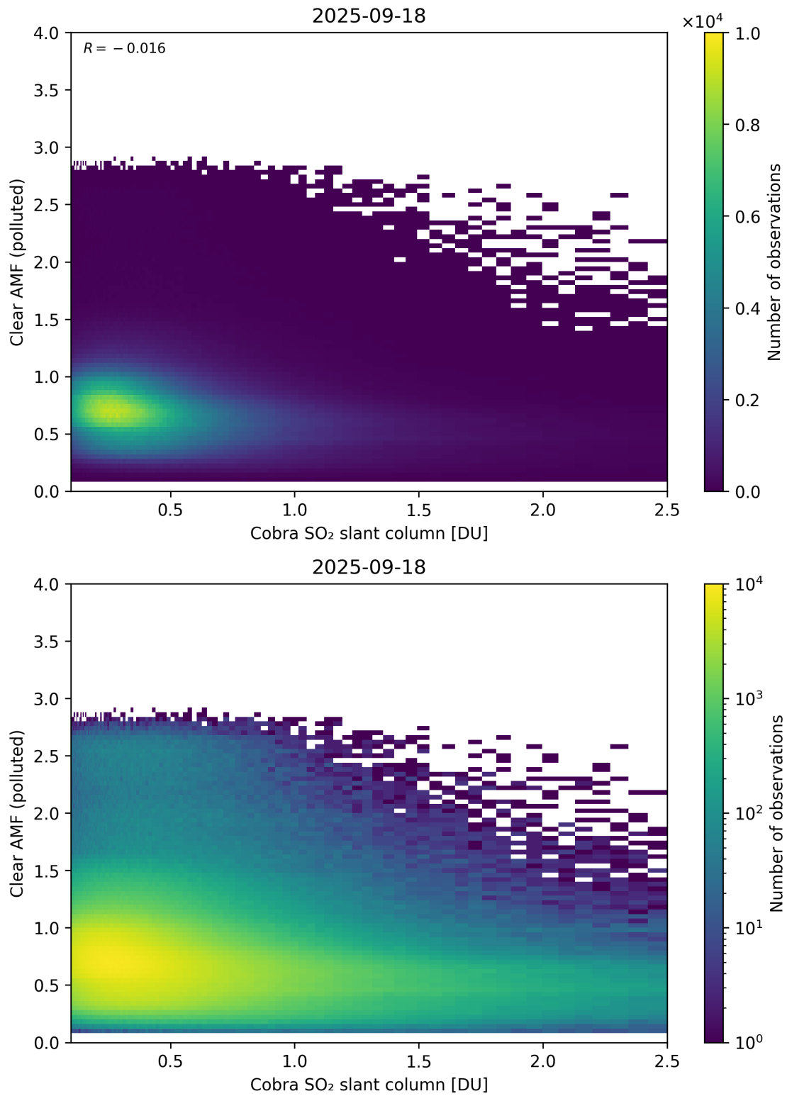
Figure 215: Scatter density plot of “Cobra SO 2 slant column” against “Clear AMF (polluted)” for 2025-09-17 to 2025-09-19.
