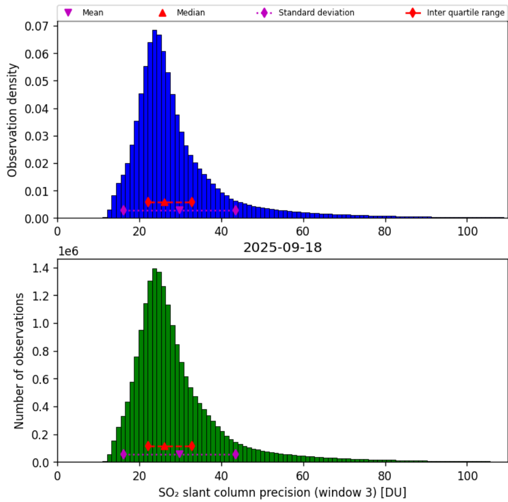
Figure 72: Histogram of “SO 2 slant column precision (window 3)” for 2025-09-17 to 2025-09-19
