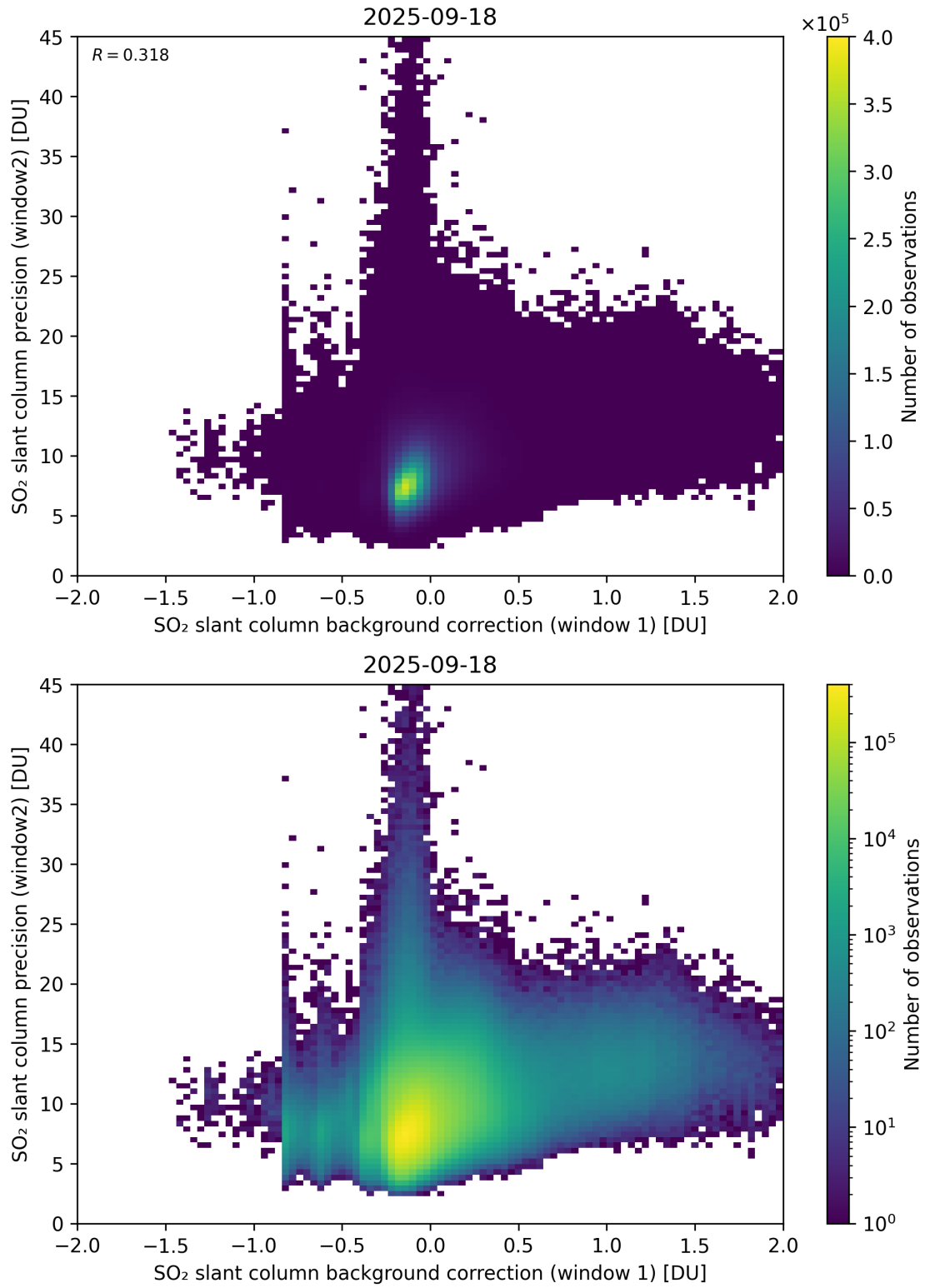
Figure 117: Scatter density plot of “SO 2 slant column background correction (window 1)” against “SO 2 slant column precision (window2)” for 2025-09-17 to 2025-09-19.
