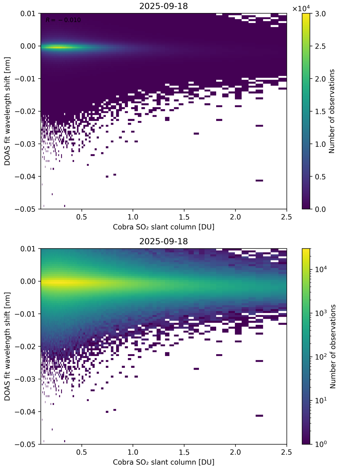
Figure 196: Scatter density plot of “Cobra SO 2 slant column” against “DOAS fit wavelength shift” for 2025-09-17 to 2025-09-19.
