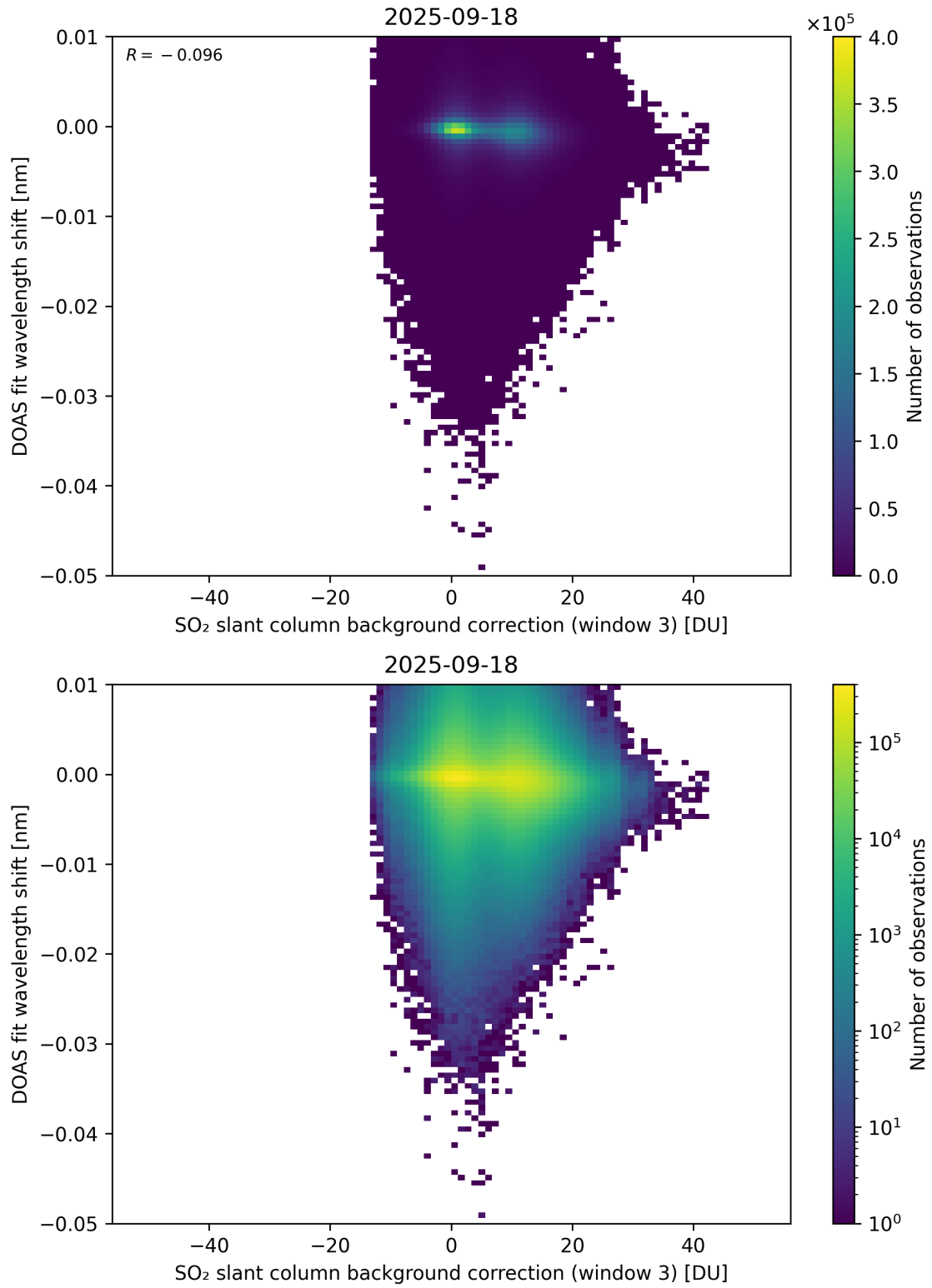
Figure 132: Scatter density plot of “SO 2 slant column background correction (window 3)” against “DOAS fit wavelength shift” for 2025-09-17 to 2025-09-19.
