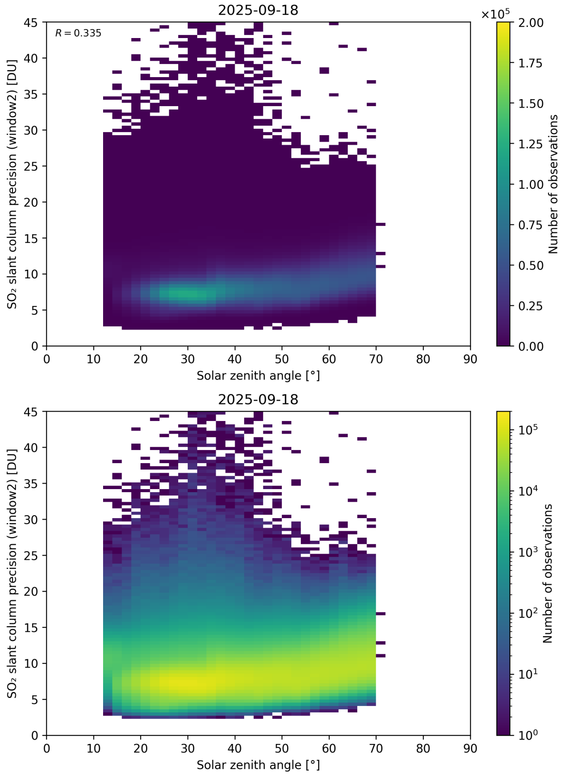
Figure 186: Scatter density plot of “Solar zenith angle” against “SO 2 slant column precision (window2)” for 2025-09-17 to 2025-09-19.
