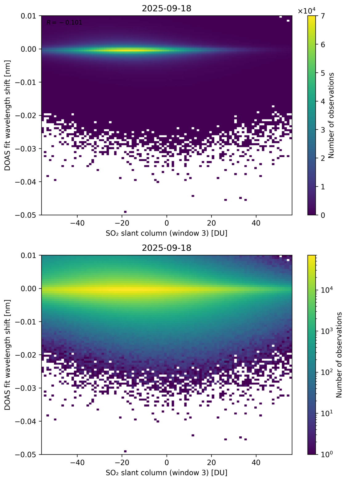
Figure 304: Scatter density plot of “SO 2 slant column (window 3)” against “DOAS fit wavelength shift” for 2025-09-17 to 2025-09-19.
