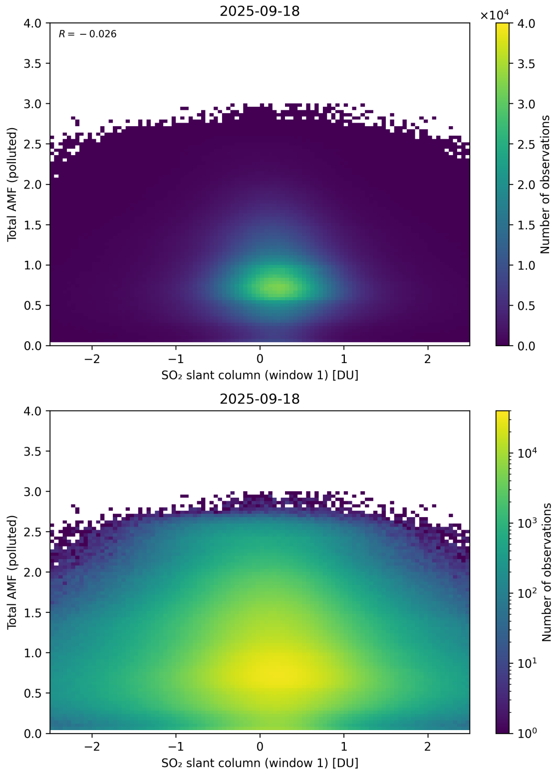
Figure 289: Scatter density plot of “SO 2 slant column (window 1)” against “Total AMF (polluted)” for 2025-09-17 to 2025-09-19.
