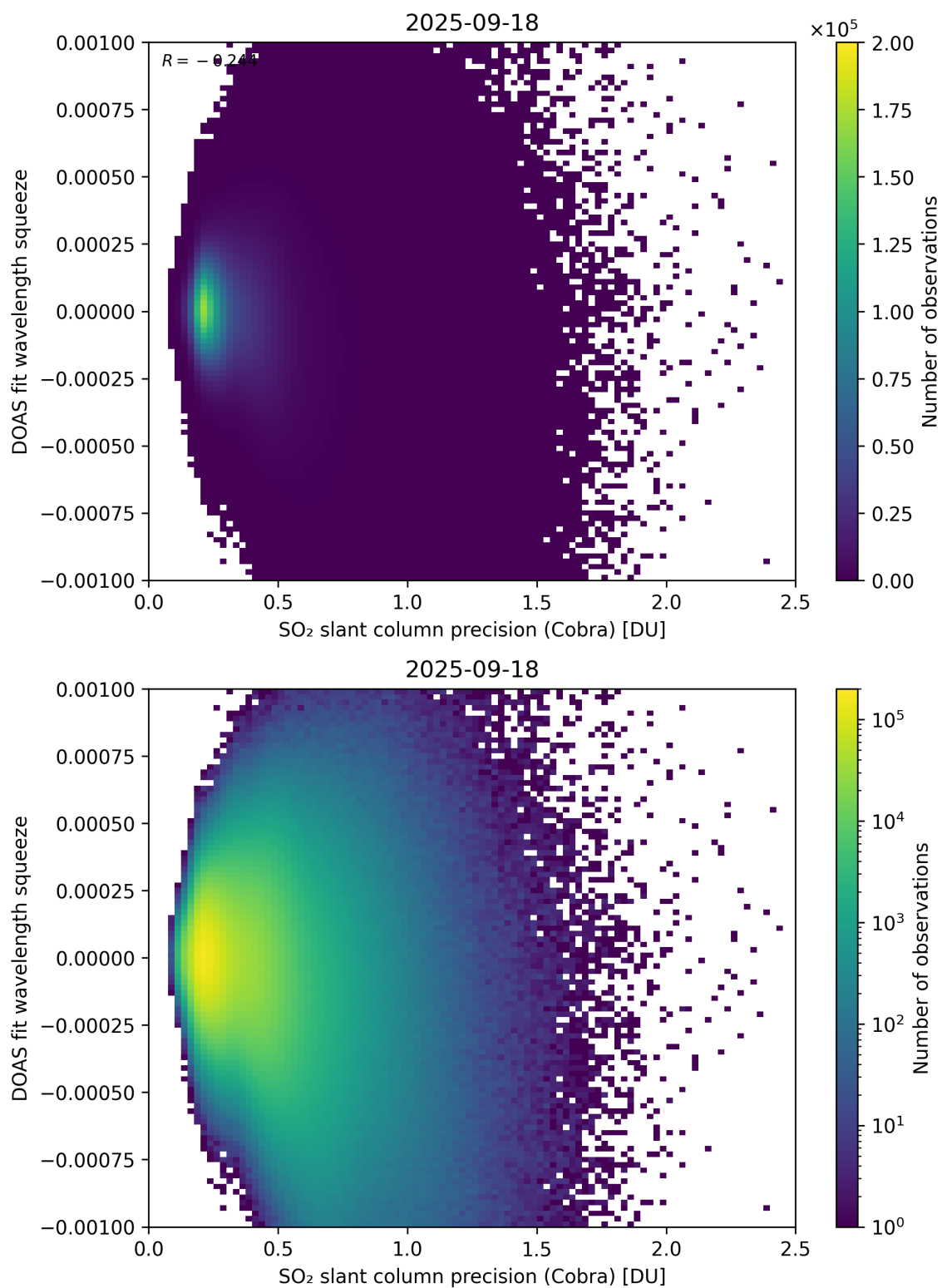
Figure 203: Scatter density plot of “SO 2 slant column precision (Cobra)” against “DOAS fit wavelength squeeze” for 2025-09-17 to 2025-09-19.
