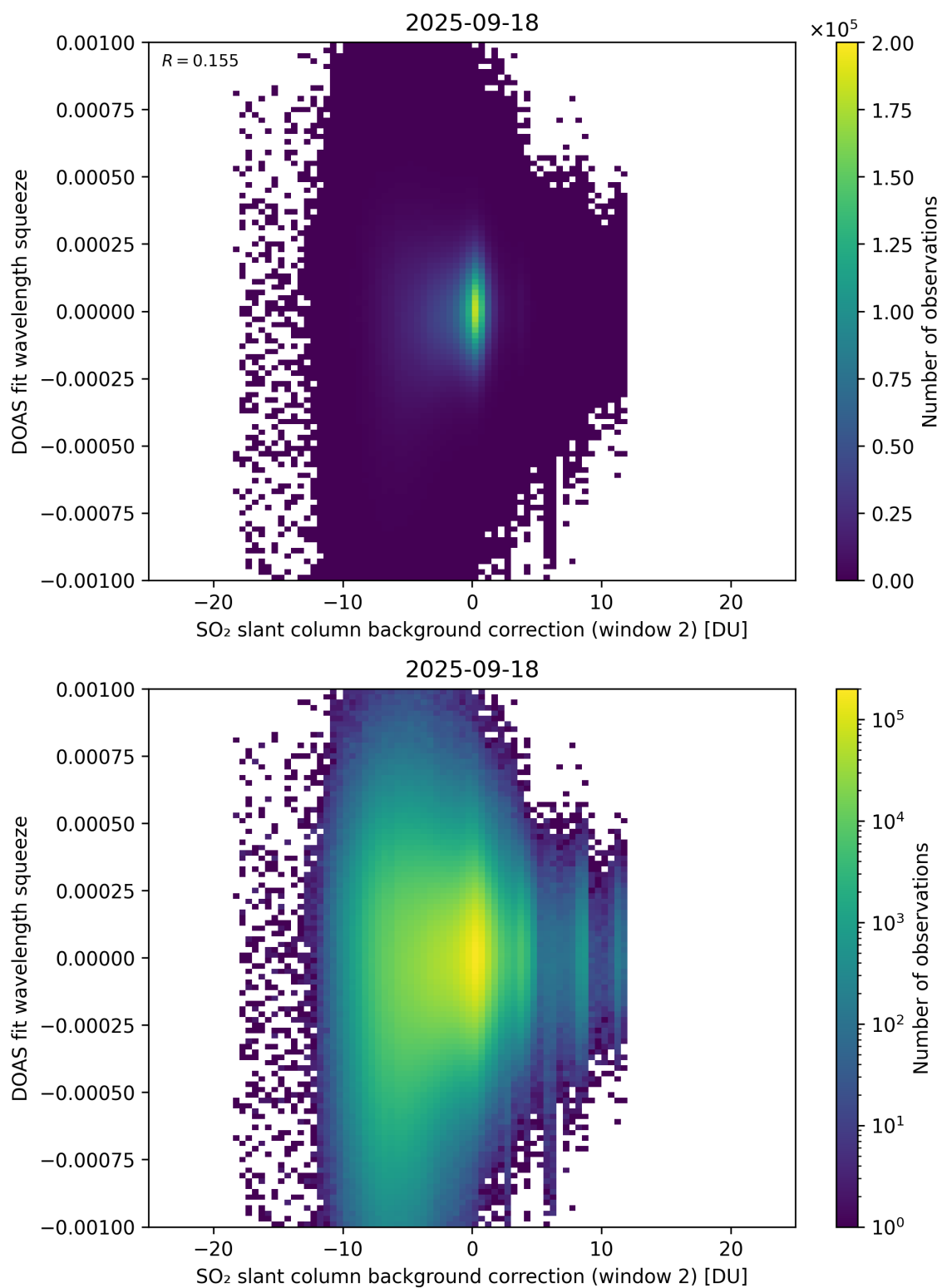
Figure 124: Scatter density plot of “SO 2 slant column background correction (window 2)” against “DOAS fit wavelength squeeze” for 2025-09-17 to 2025-09-19.
