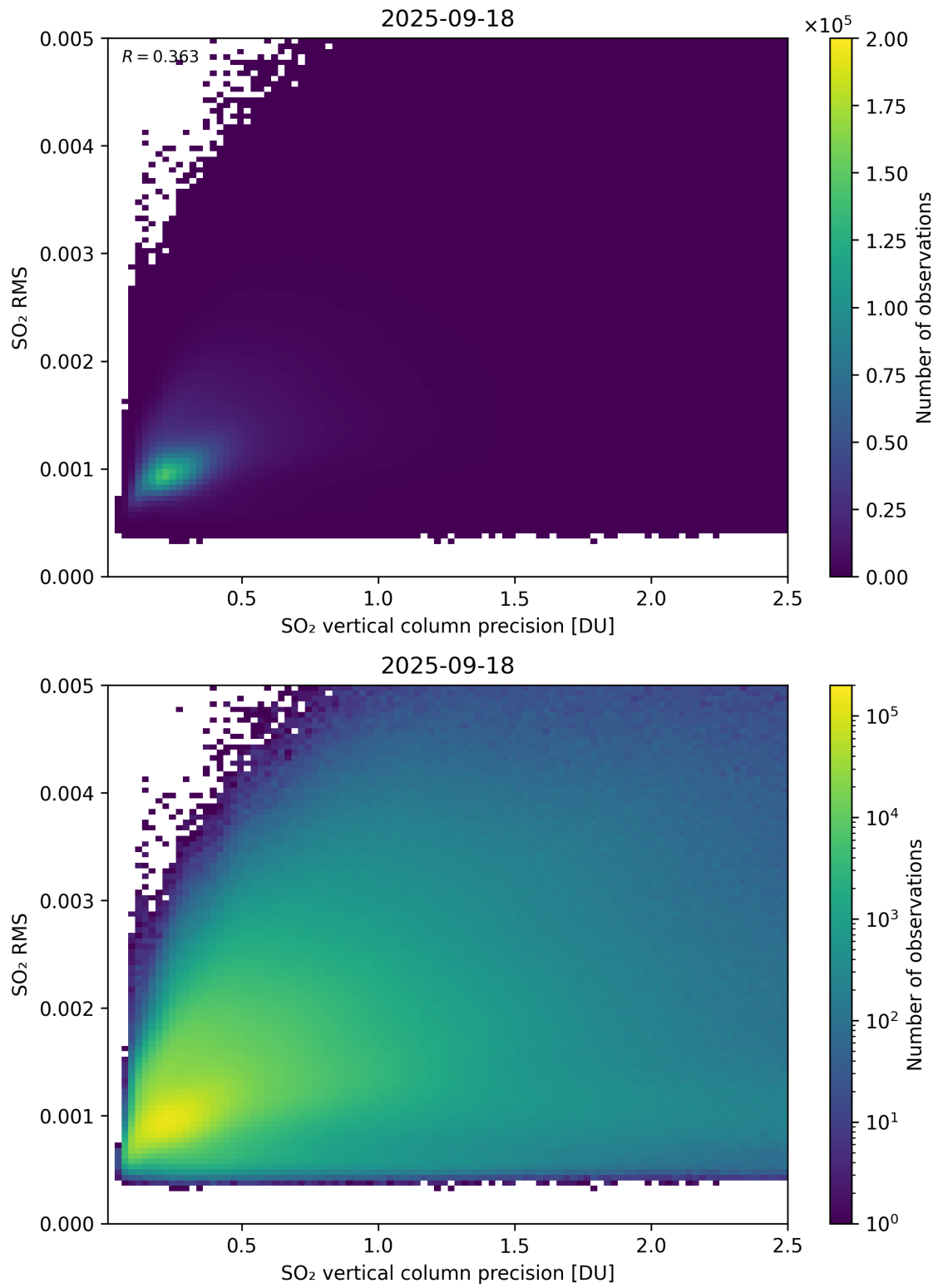
Figure 334: Scatter density plot of “SO 2 vertical column precision” against “SO 2 RMS” for 2025-09-17 to 2025-09-19.
