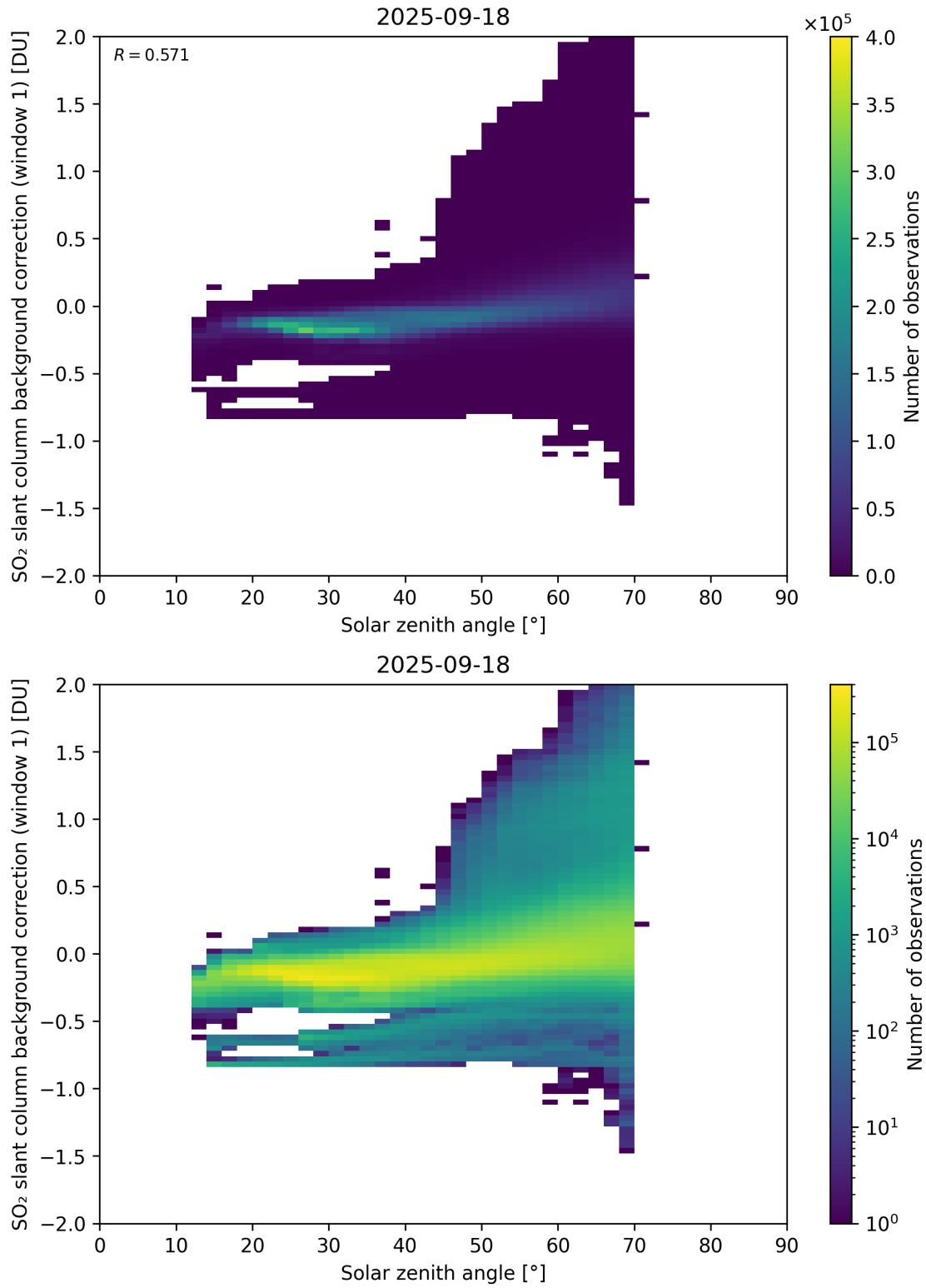
Figure 171: Scatter density plot of “Solar zenith angle” against “SO 2 slant column background correction (window 1)” for 2025-09-17 to 2025-09-19.
