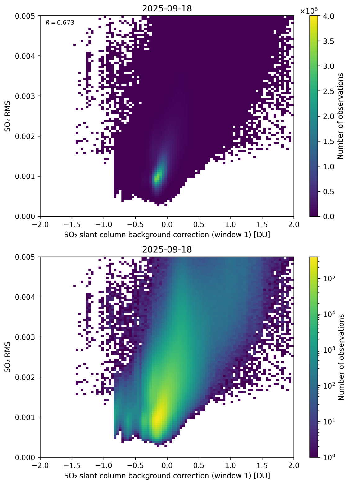
Figure 113: Scatter density plot of “SO 2 slant column background correction (window 1)” against “SO 2 RMS” for 2025-09-17 to 2025-09-19.
