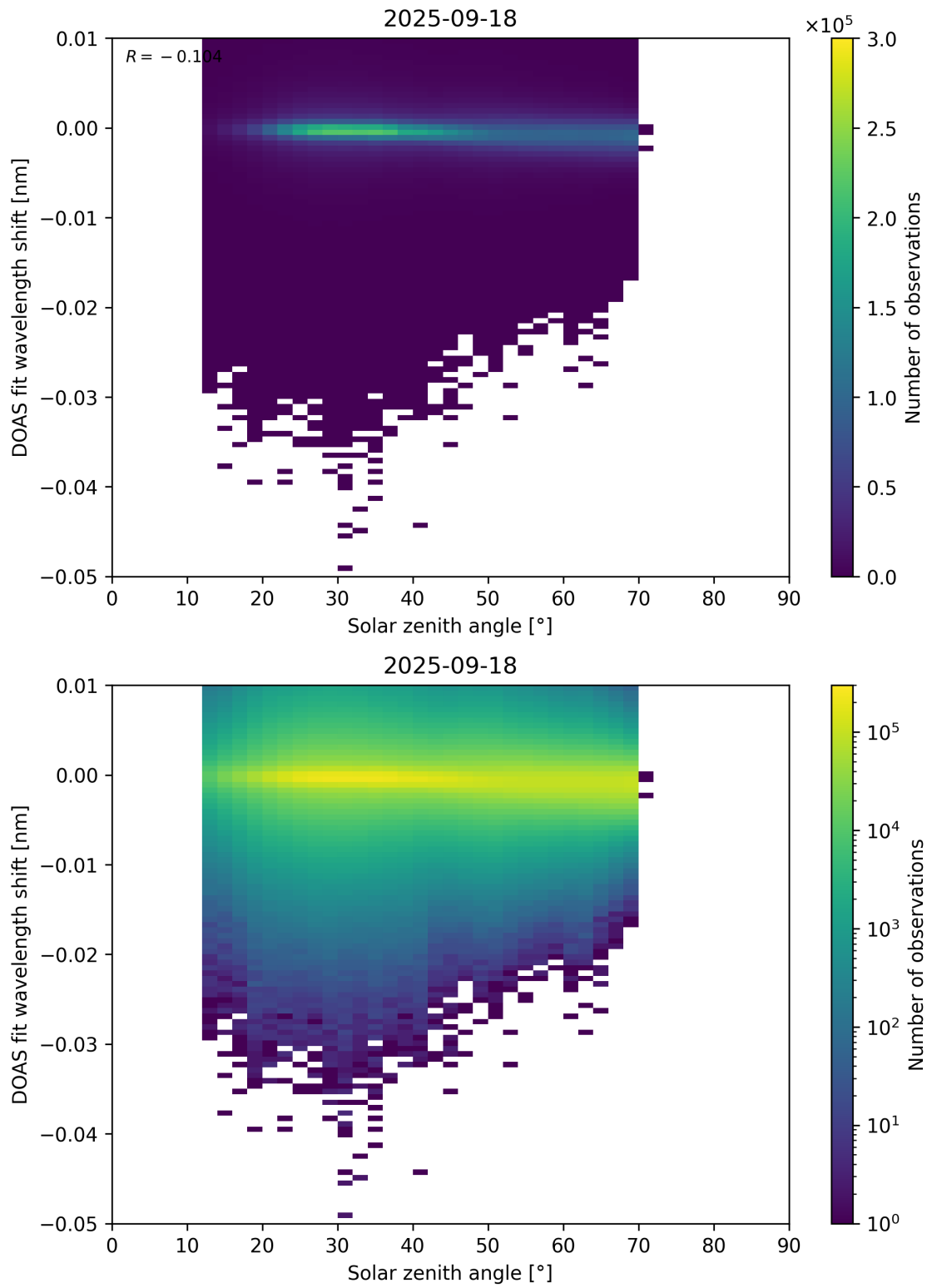
Figure 174: Scatter density plot of “Solar zenith angle” against “DOAS fit wavelength shift” for 2025-09-17 to 2025-09-19.
