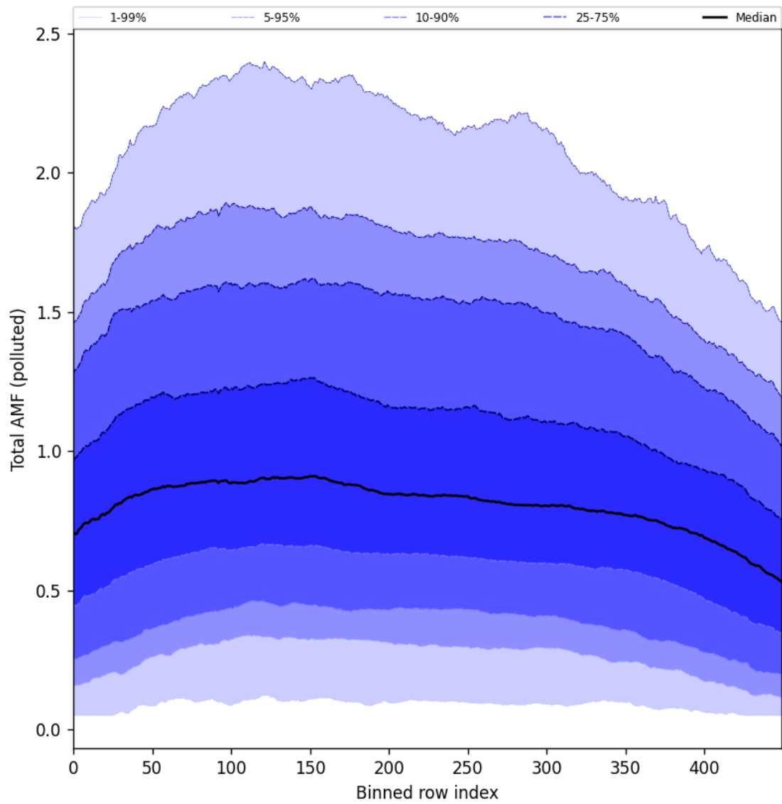
Figure 105: Along track statistics of “Total AMF (polluted)” for 2025-09-17 to 2025-09-19
