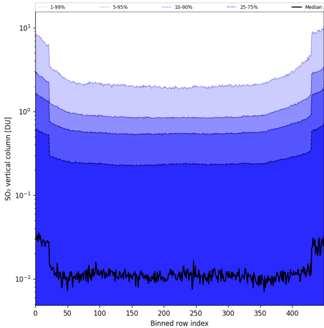
Figure 84: Along track statistics of “SO 2 vertical column” for 2025-09-17 to 2025-09-19
