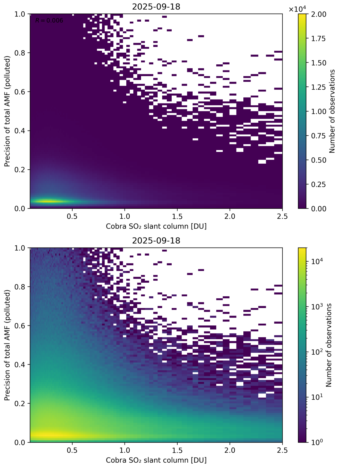
Figure 225: Scatter density plot of “Cobra SO 2 slant column” against “Precision of total AMF (polluted)” for 2025-09-17 to 2025-09-19.
