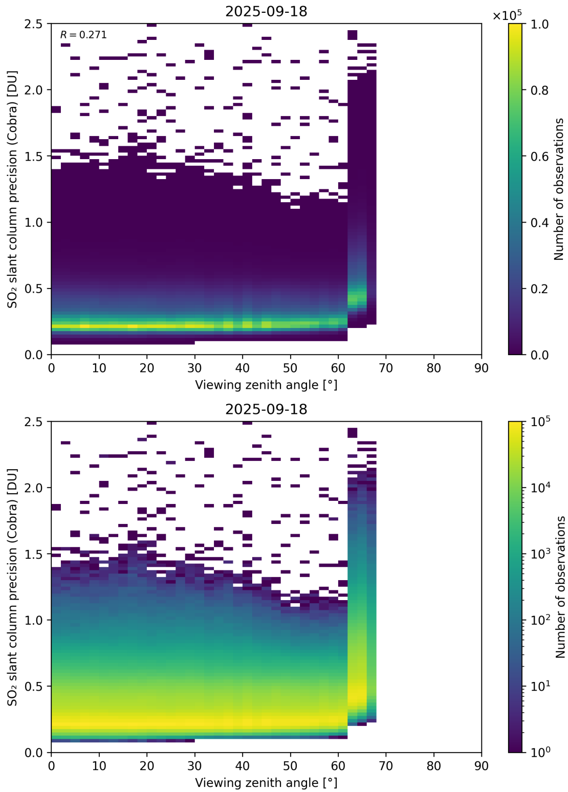
Figure 372: Scatter density plot of “Viewing zenith angle” against “SO 2 slant column precision (Cobra)” for 2025-09-17 to 2025-09-19.
