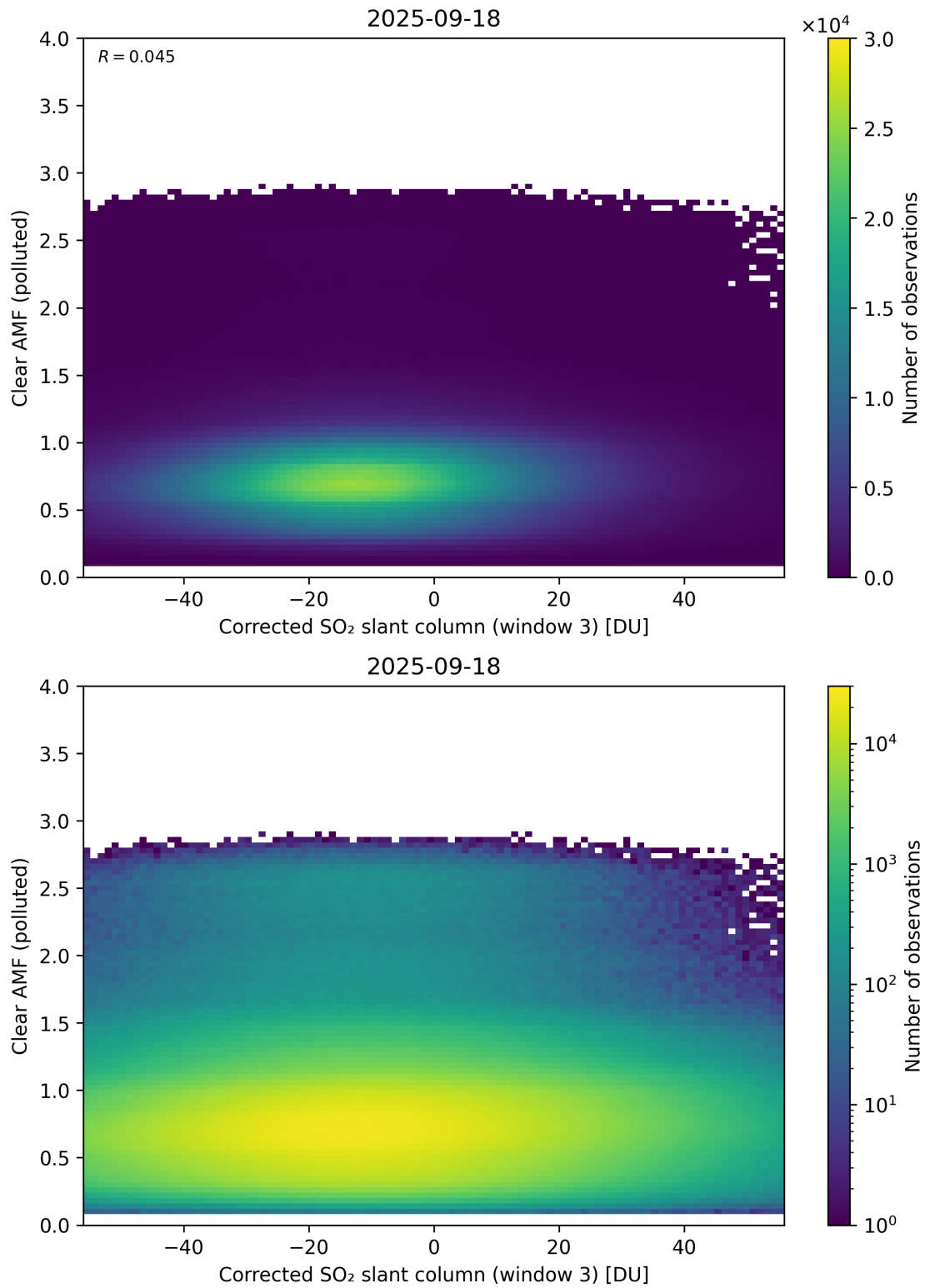
Figure 259: Scatter density plot of “Corrected SO 2 slant column (window 3)” against “Clear AMF (polluted)” for 2025-09-17 to 2025-09-19.
