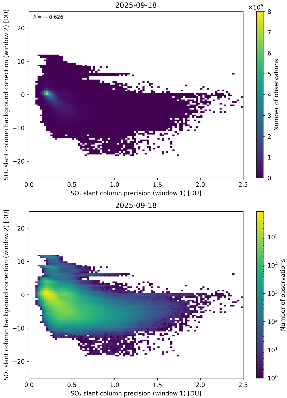
Figure 269: Scatter density plot of “SO 2 slant column precision (window 1)” against “SO 2 slant column background correction (window 2)” for 2025-09-17 to 2025-09-19.
