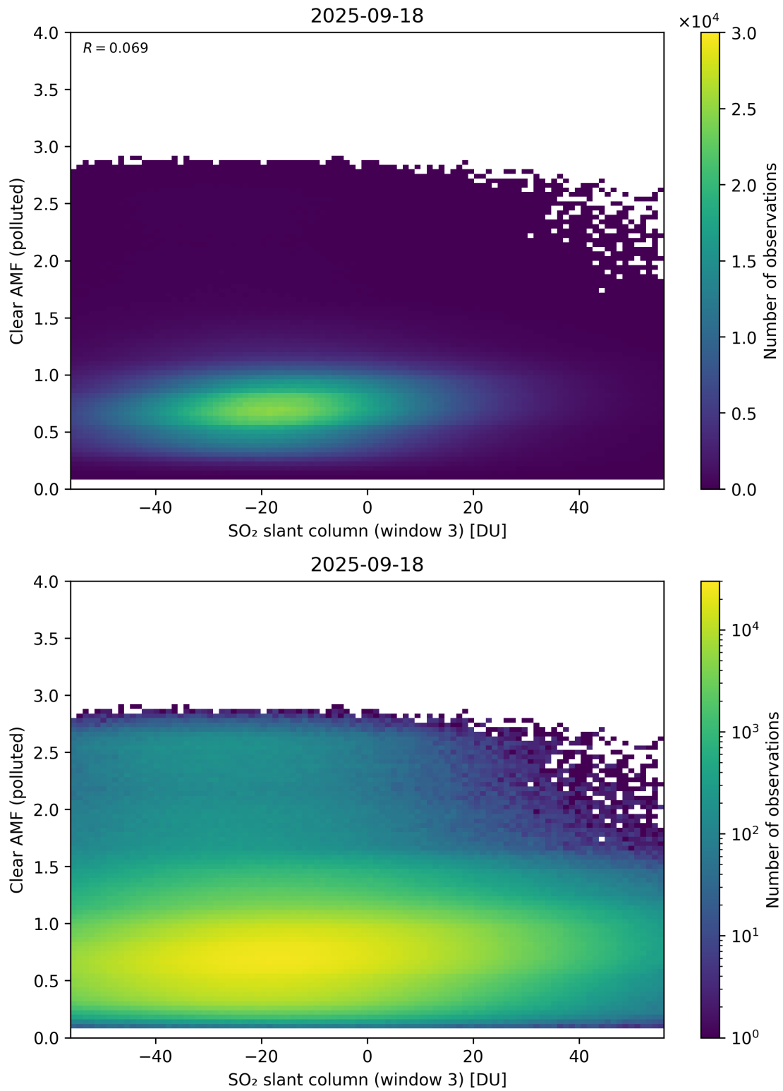
Figure 315: Scatter density plot of “SO 2 slant column (window 3)” against “Clear AMF (polluted)” for 2025-09-17 to 2025-09-19.
