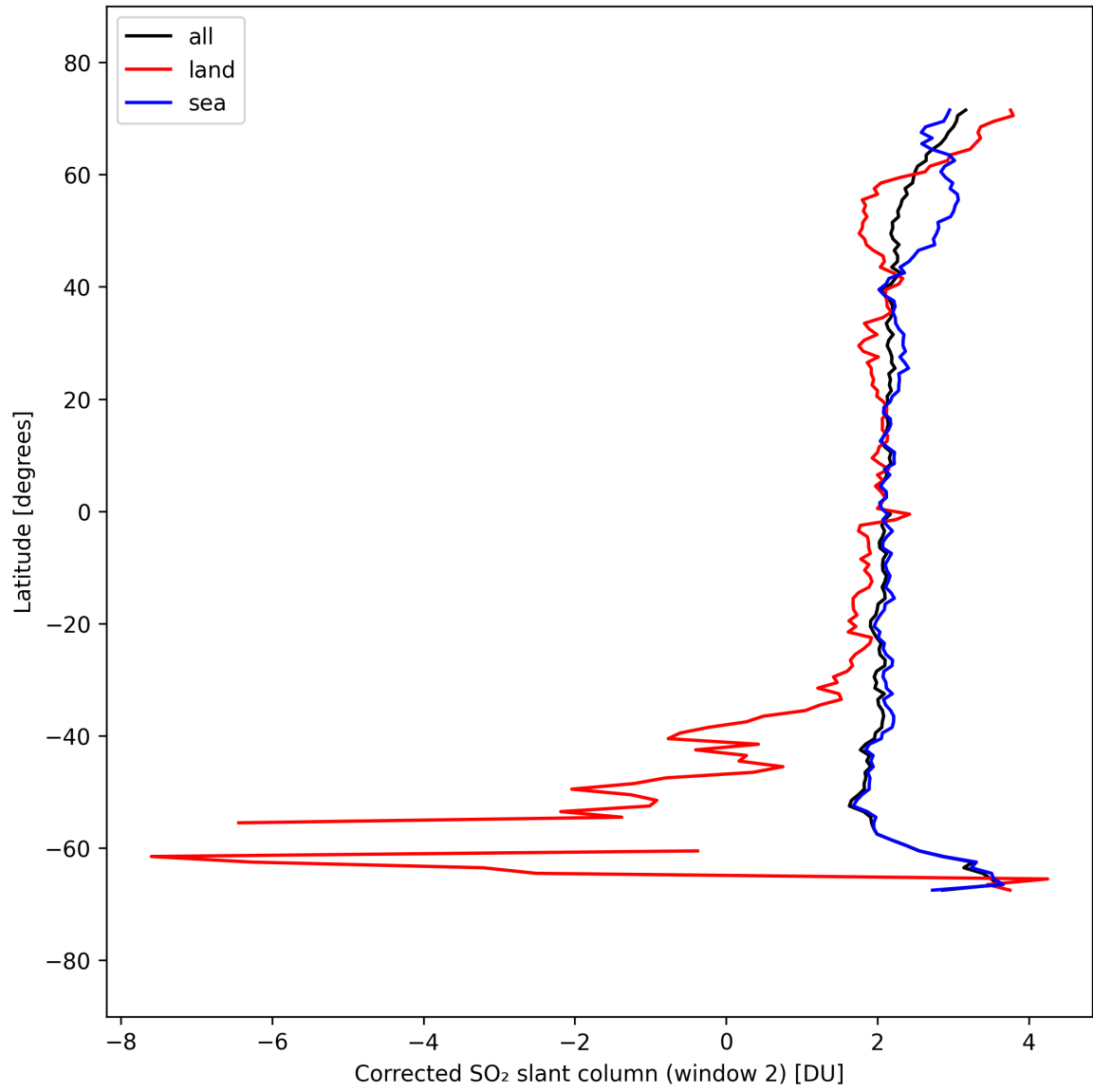
Figure 43: Zonal average of “Corrected SO 2 slant column (window 2)” for 2025-09-17 to 2025-09-19.
