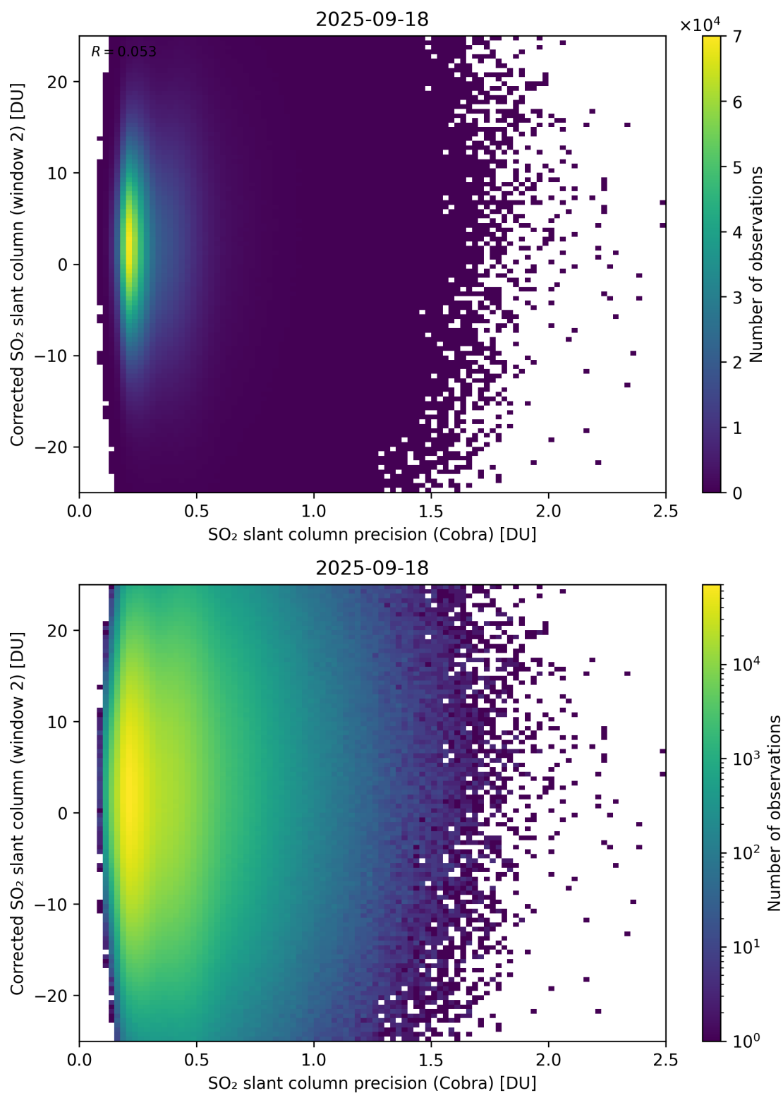
Figure 206: Scatter density plot of “SO 2 slant column precision (Cobra)” against “Corrected SO 2 slant column (window 2)” for 2025-09-17 to 2025-09-19.
