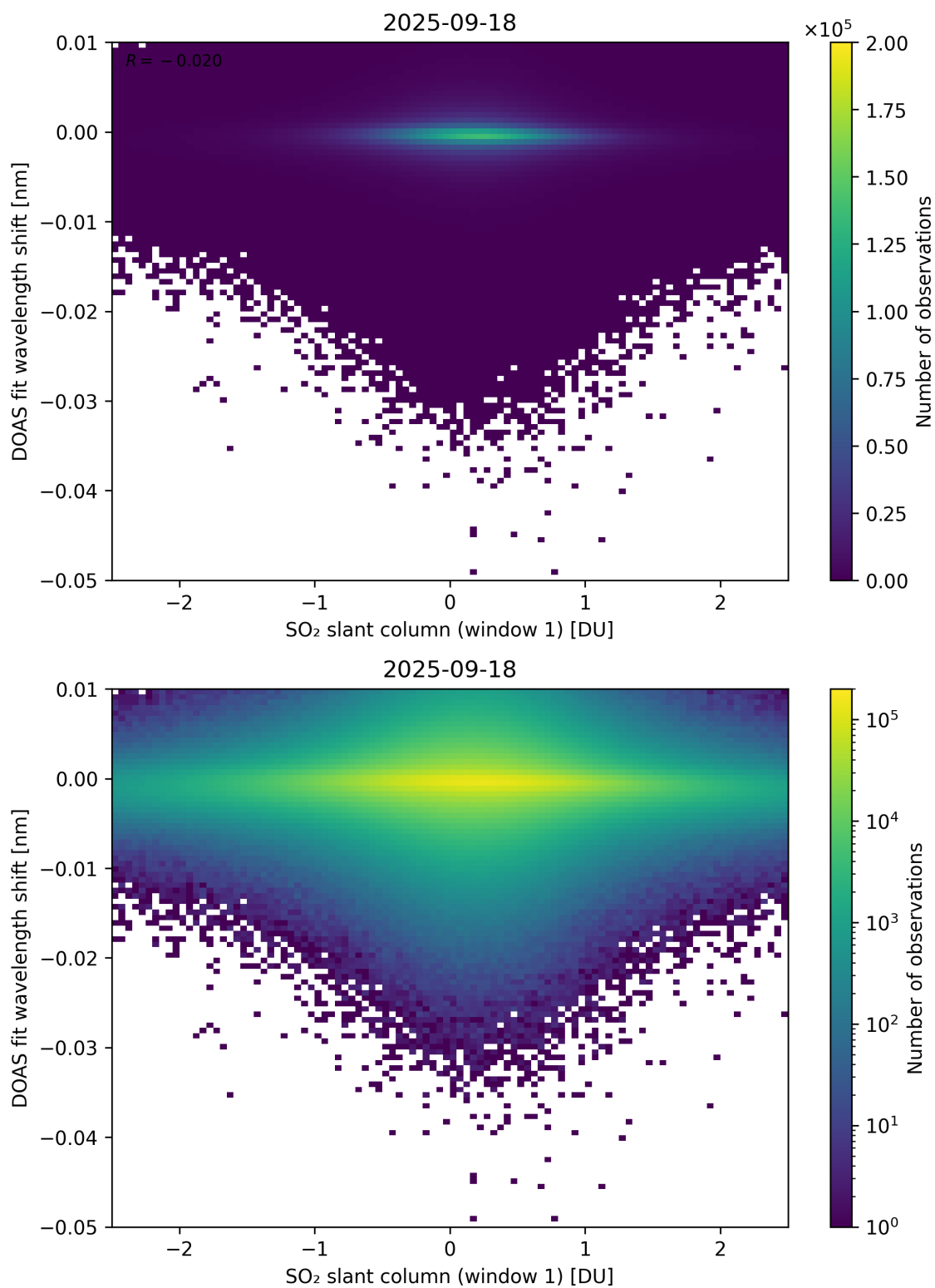
Figure 265: Scatter density plot of “SO 2 slant column (window 1)” against “DOAS fit wavelength shift” for 2025-09-17 to 2025-09-19.
