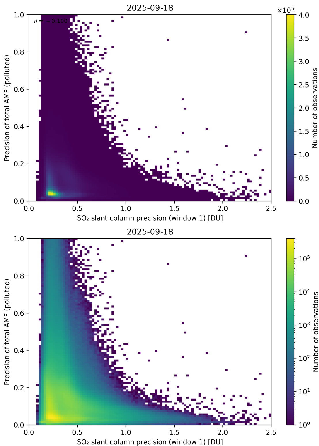
Figure 281: Scatter density plot of “SO 2 slant column precision (window 1)” against “Precision of total AMF (polluted)” for 2025-09-17 to 2025-09-19.
