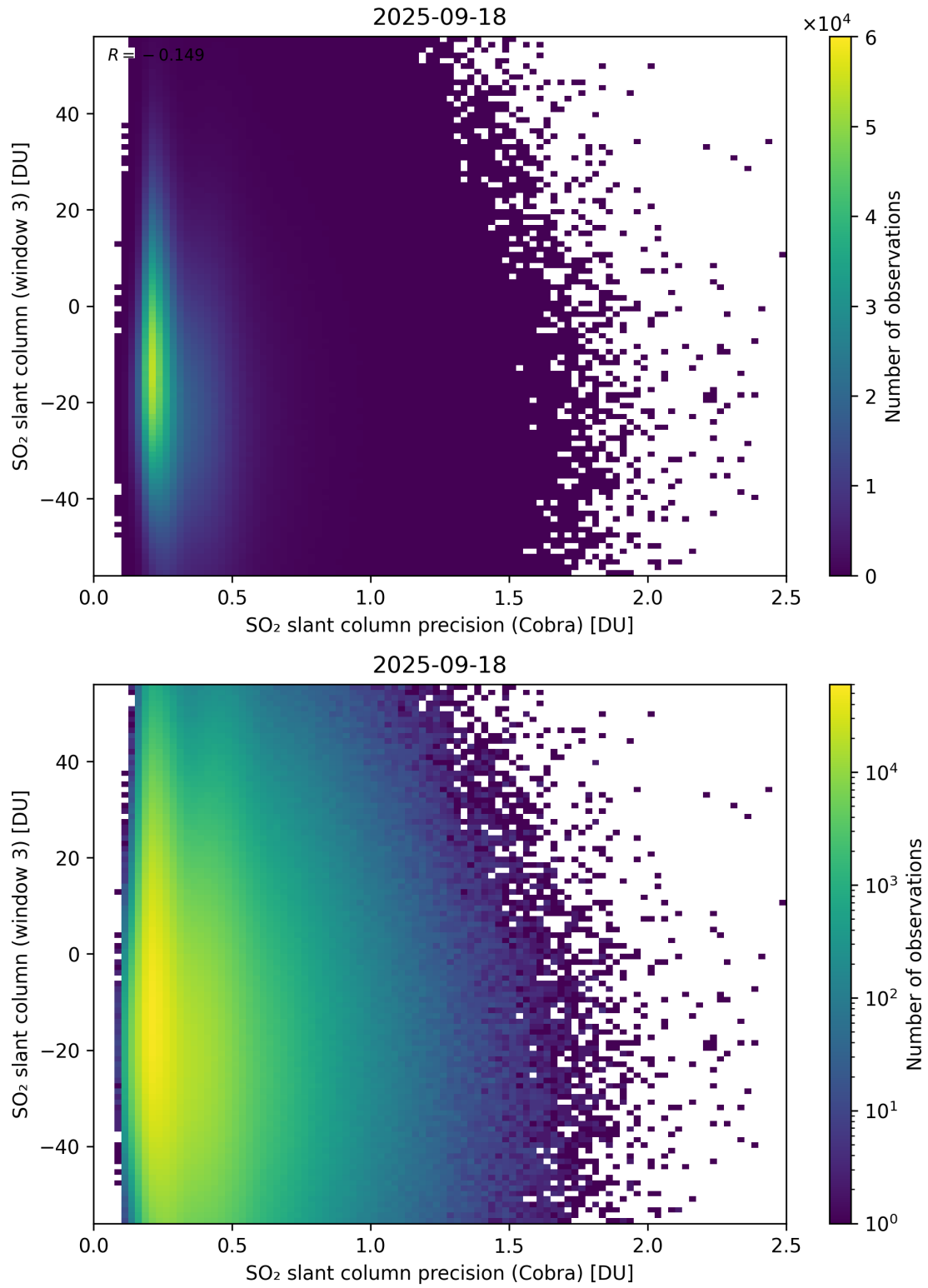
Figure 211: Scatter density plot of “SO 2 slant column precision (Cobra)” against “SO 2 slant column (window 3)” for 2025-09-17 to 2025-09-19.
