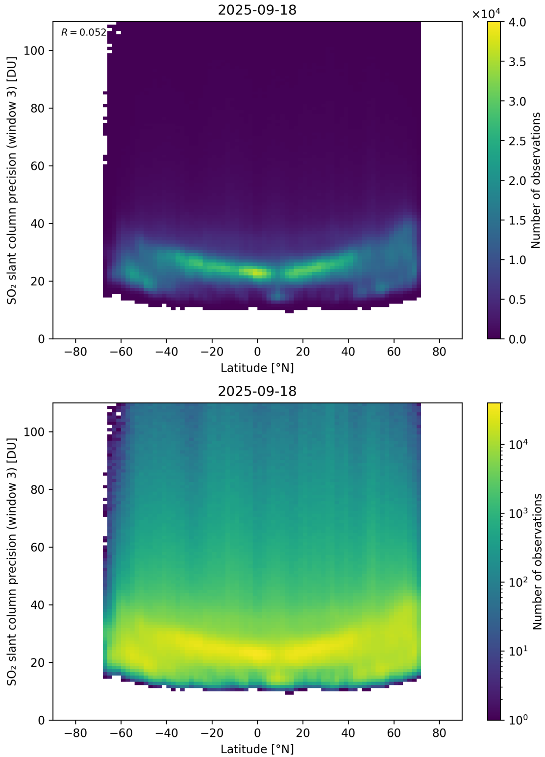
Figure 166: Scatter density plot of “Latitude” against “SO 2 slant column precision (window 3)” for 2025-09-17 to 2025-09-19.
