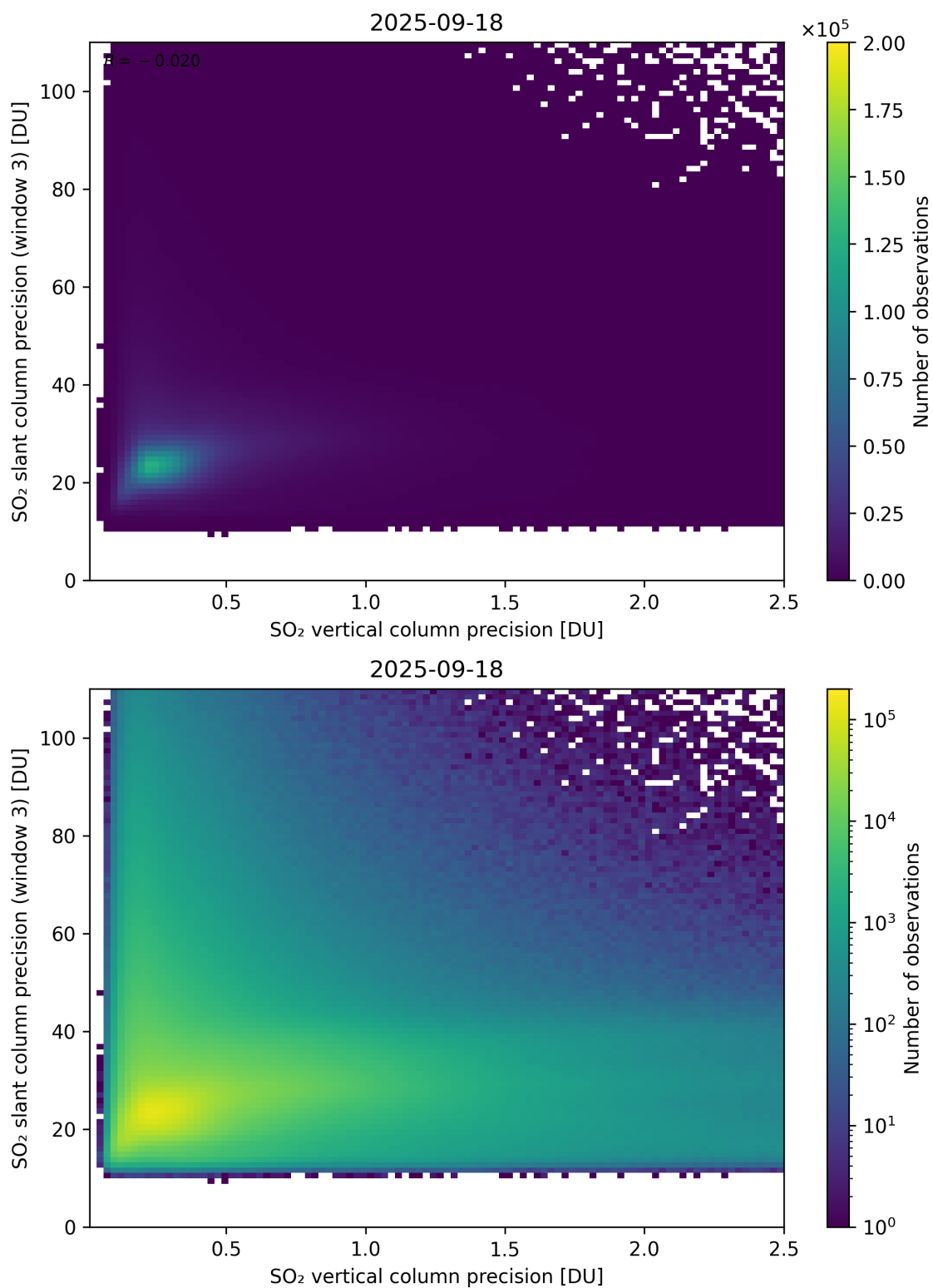
Figure 345: Scatter density plot of “SO 2 vertical column precision” against “SO 2 slant column precision (window 3)” for 2025-09-17 to 2025-09-19.
