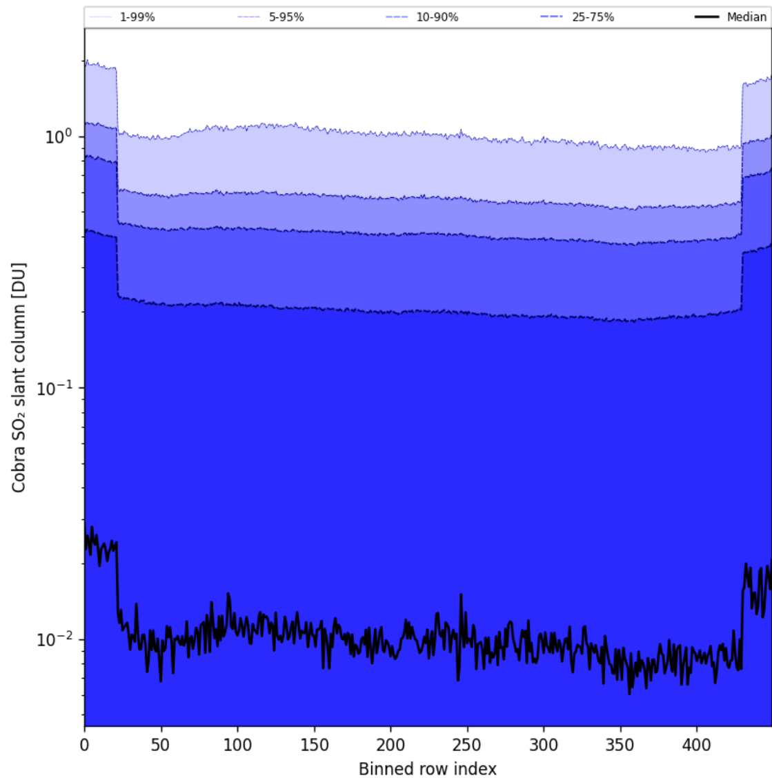
Figure 87: Along track statistics of “Cobra SO 2 slant column” for 2025-09-17 to 2025-09-19
