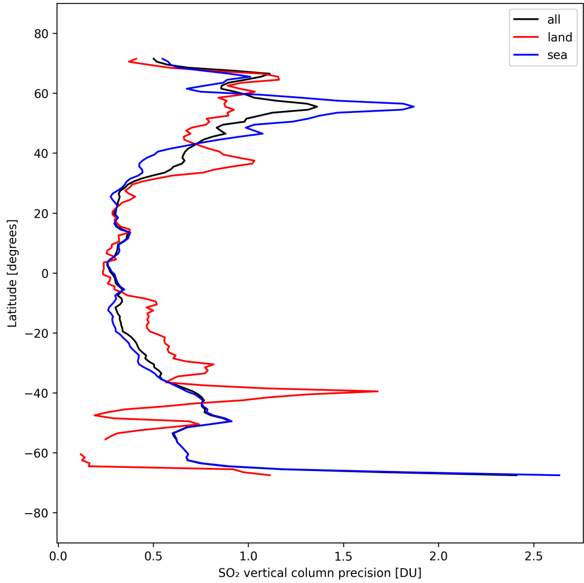
Figure 33: Zonal average of “SO 2 vertical column precision” for 2025-09-17 to 2025-09-19.
