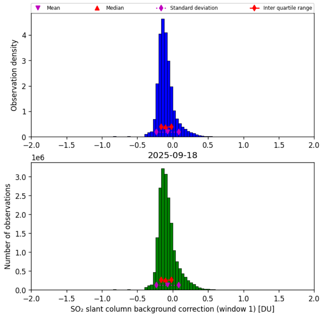
Figure 66: Histogram of “SO 2 slant column background correction (window 1)” for 2025-09-17 to 2025-09-19
