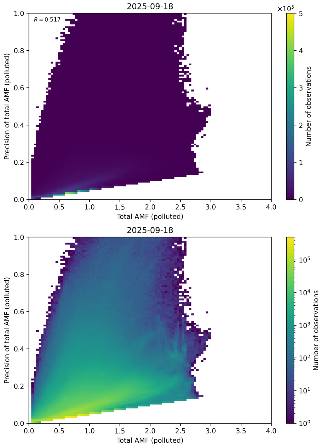
Figure 322: Scatter density plot of “Total AMF (polluted)” against “Precision of total AMF (polluted)” for 2025-09-17 to 2025-09-19.
