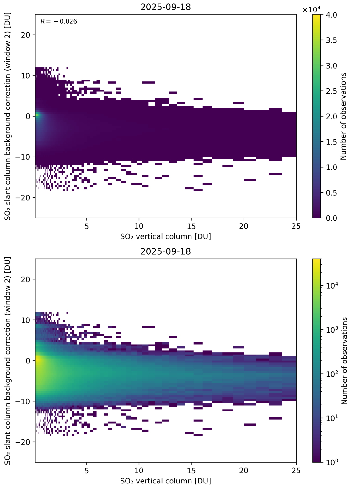
Figure 324: Scatter density plot of “SO 2 vertical column” against “SO 2 slant column background correction (window 2)” for 2025-09-17 to 2025-09-19.
