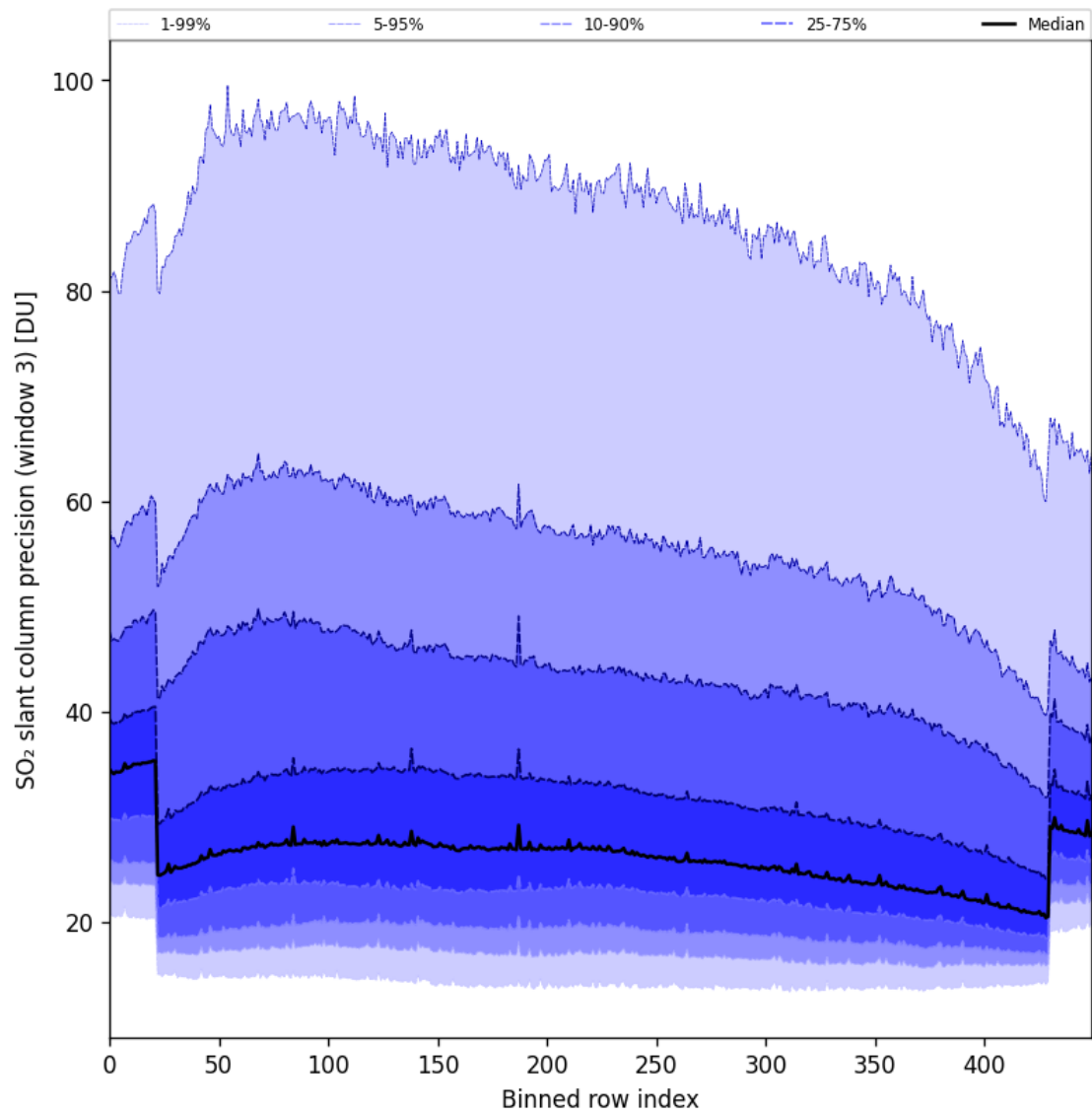
Figure 98: Along track statistics of “SO 2 slant column precision (window 3)” for 2025-09-17 to 2025-09-19
