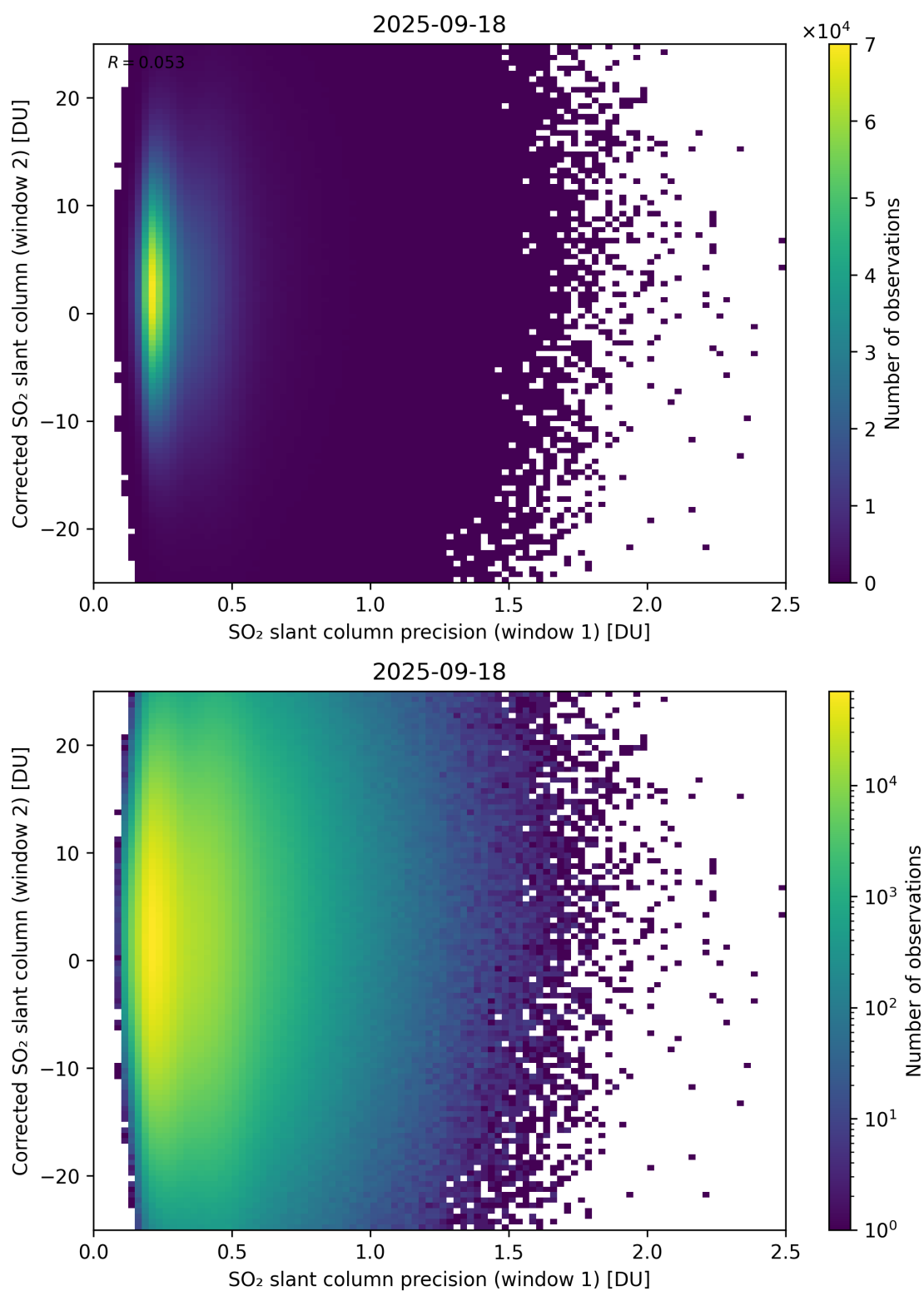
Figure 275: Scatter density plot of “SO 2 slant column precision (window 1)” against “Corrected SO 2 slant column (window 2)” for 2025-09-17 to 2025-09-19.
