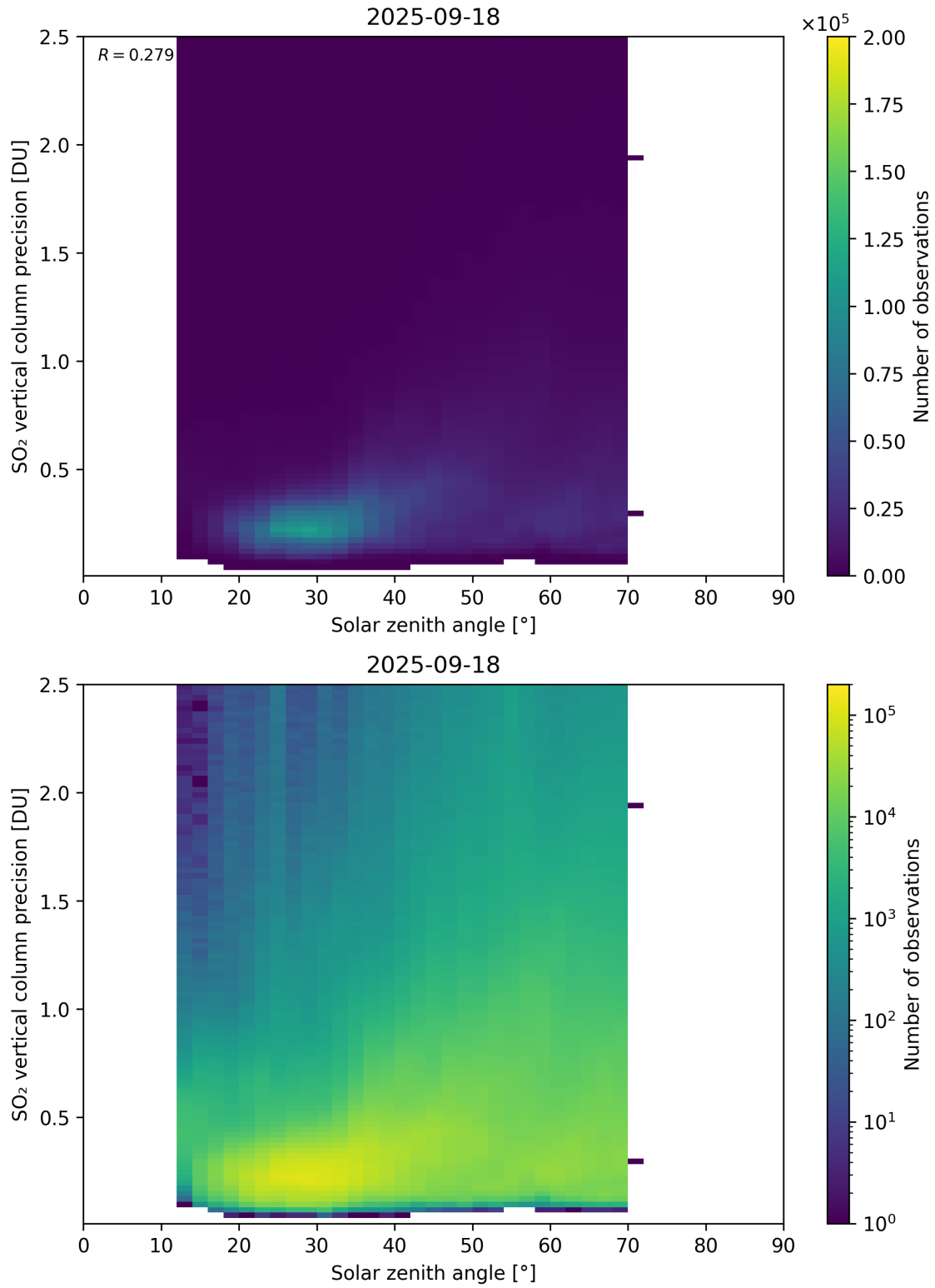
Figure 192: Scatter density plot of “Solar zenith angle” against “SO 2 vertical column precision” for 2025-09-17 to 2025-09-19.
