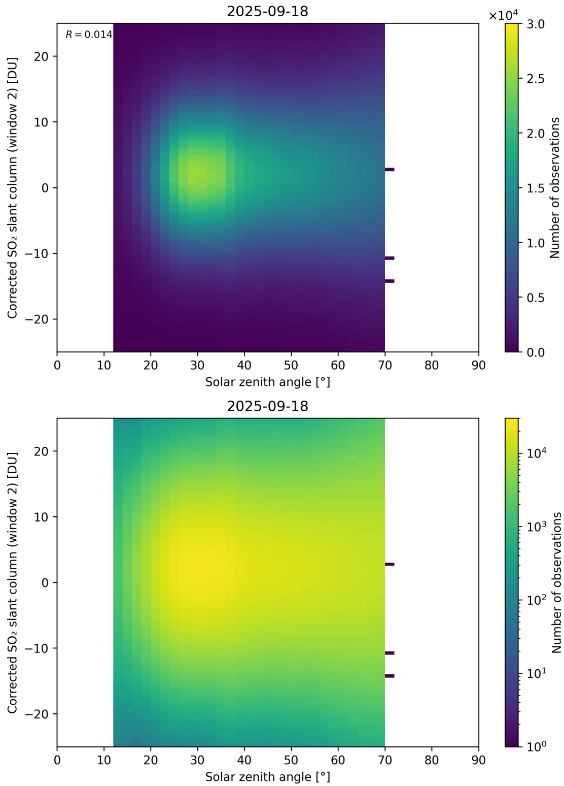
Figure 182: Scatter density plot of “Solar zenith angle” against “Corrected SO 2 slant column (window 2)” for 2025-09-17 to 2025-09-19.
