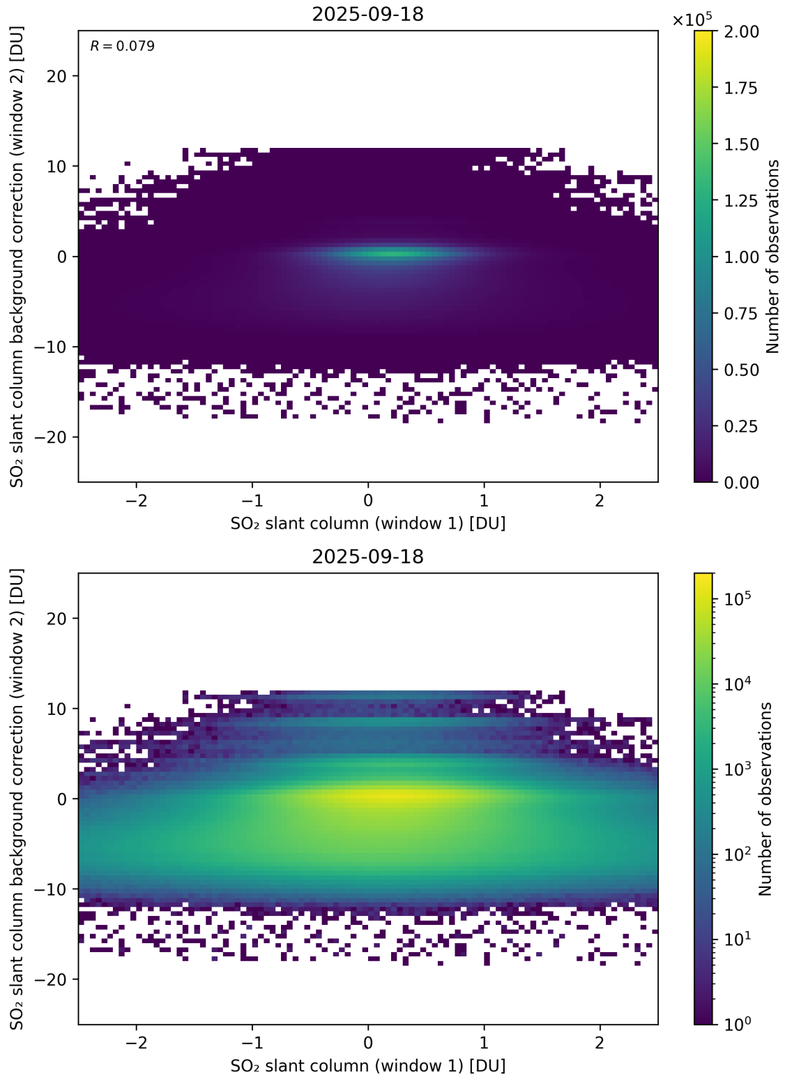
Figure 263: Scatter density plot of “SO 2 slant column (window 1)” against “SO 2 slant column background correction (window 2)” for 2025-09-17 to 2025-09-19.
