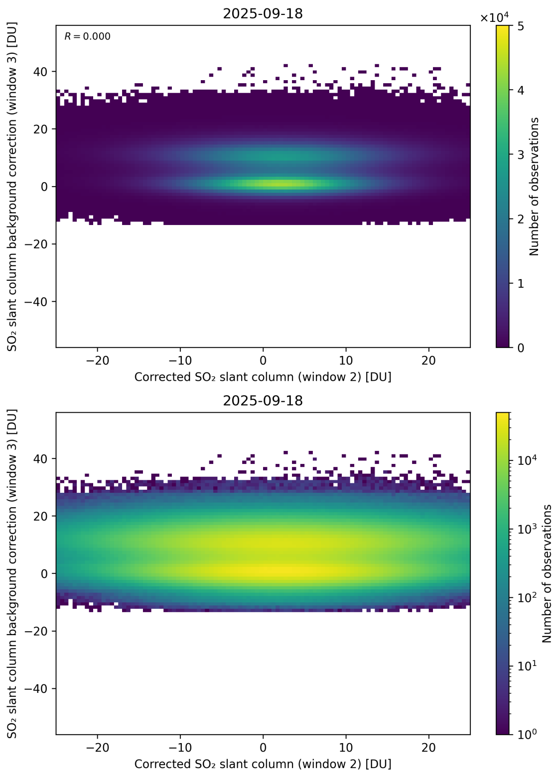
Figure 245: Scatter density plot of “Corrected SO 2 slant column (window 2)” against “SO 2 slant column background correction (window 3)” for 2025-09-17 to 2025-09-19.
