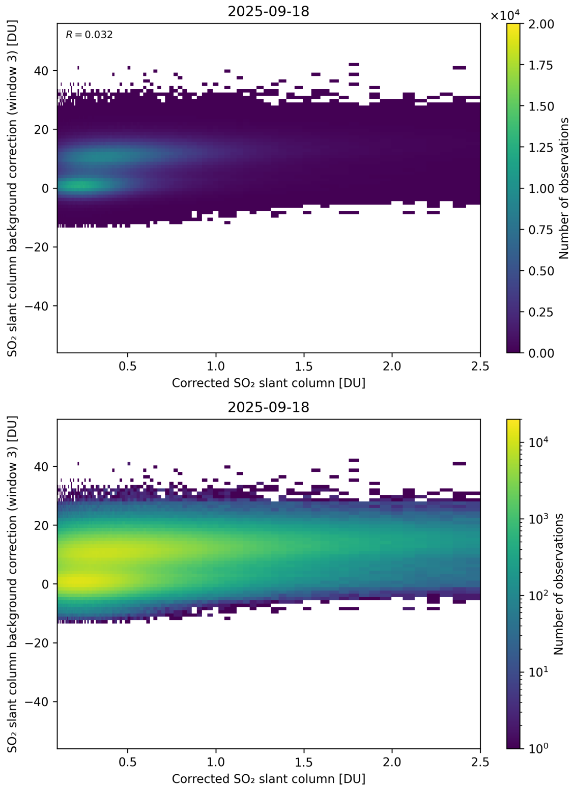
Figure 228: Scatter density plot of “Corrected SO 2 slant column” against “SO 2 slant column background correction (window 3)” for 2025-09-17 to 2025-09-19.
