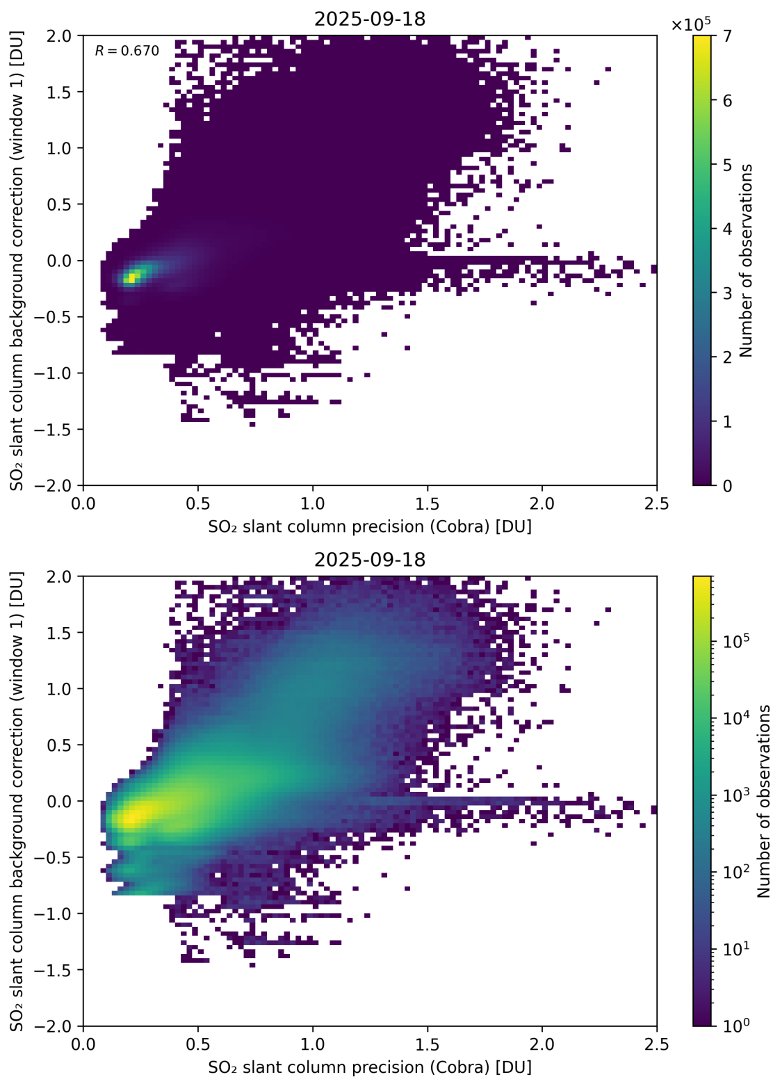
Figure 199: Scatter density plot of “SO 2 slant column precision (Cobra)” against “SO 2 slant column background correction (window 1)” for 2025-09-17 to 2025-09-19.
