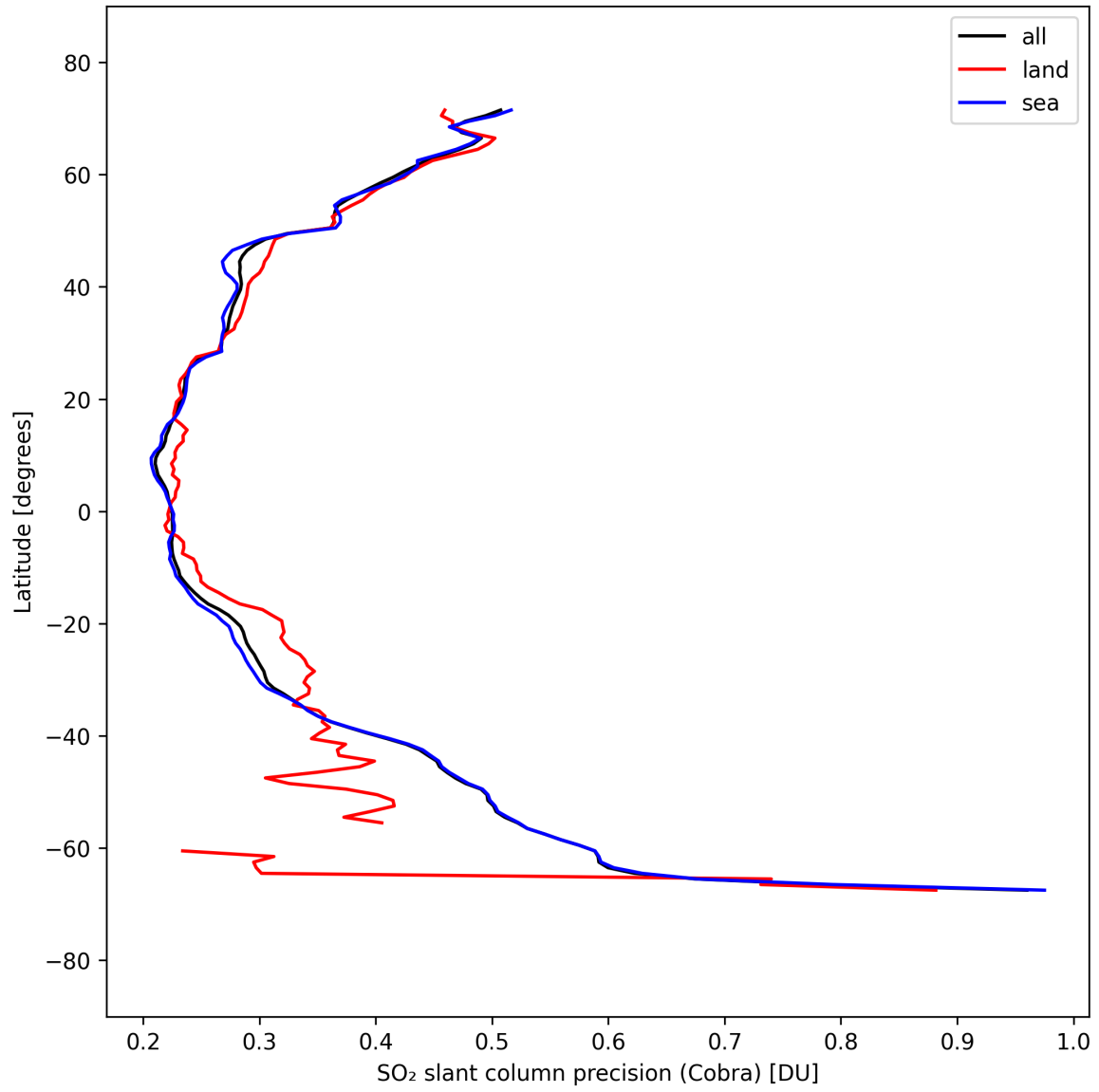
Figure 36: Zonal average of “SO 2 slant column precision (Cobra)” for 2025-09-17 to 2025-09-19.
