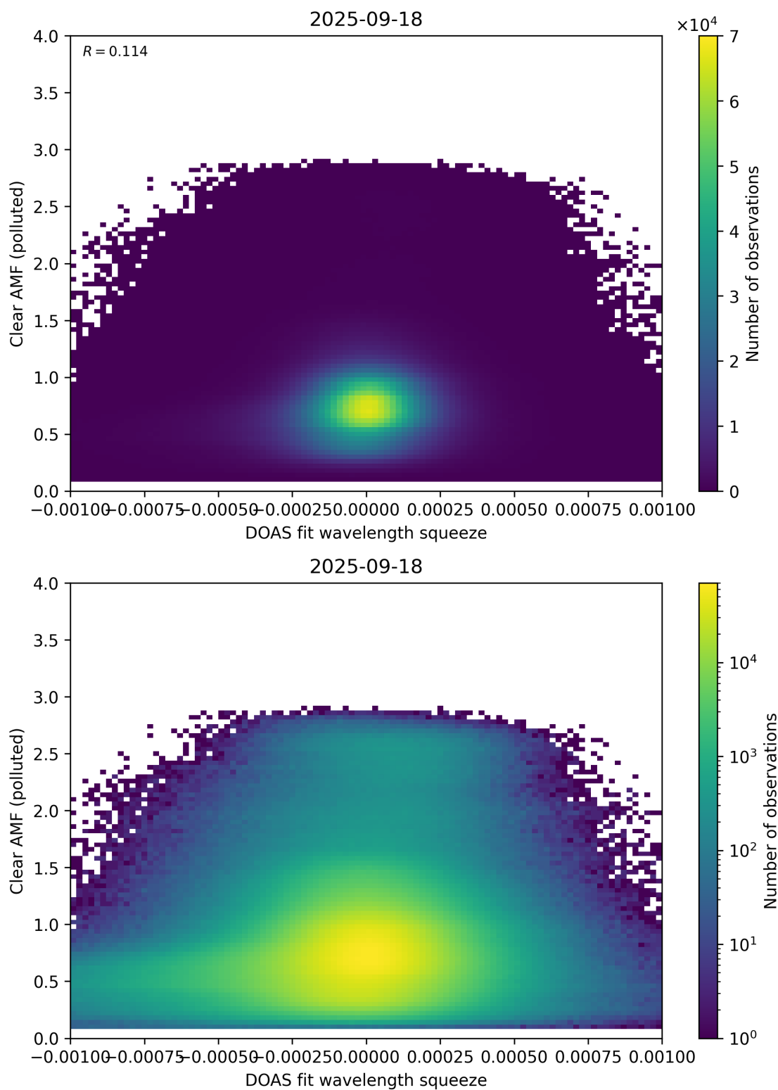
Figure 144: Scatter density plot of “DOAS fit wavelength squeeze” against “Clear AMF (polluted)” for 2025-09-17 to 2025-09-19.
