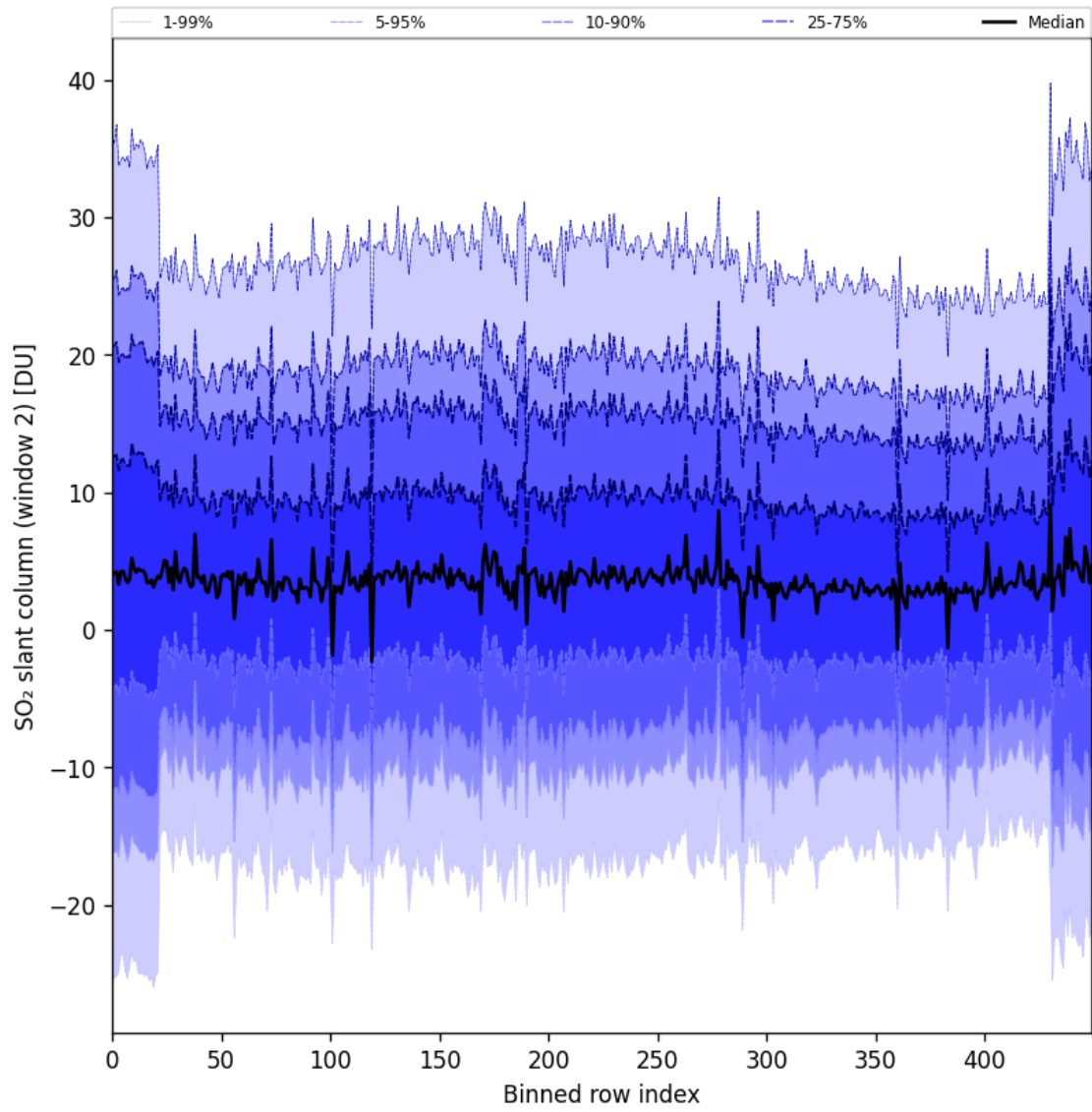
Figure 93: Along track statistics of “SO 2 slant column (window 2)” for 2025-09-17 to 2025-09-19
