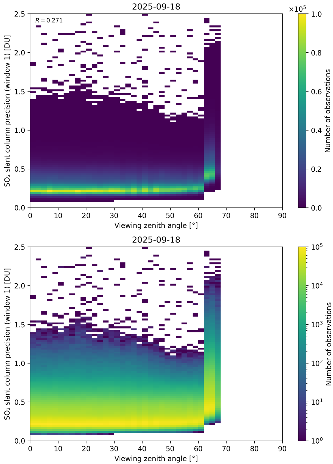
Figure 377: Scatter density plot of “Viewing zenith angle” against “SO 2 slant column precision (window 1)” for 2025-09-17 to 2025-09-19.
