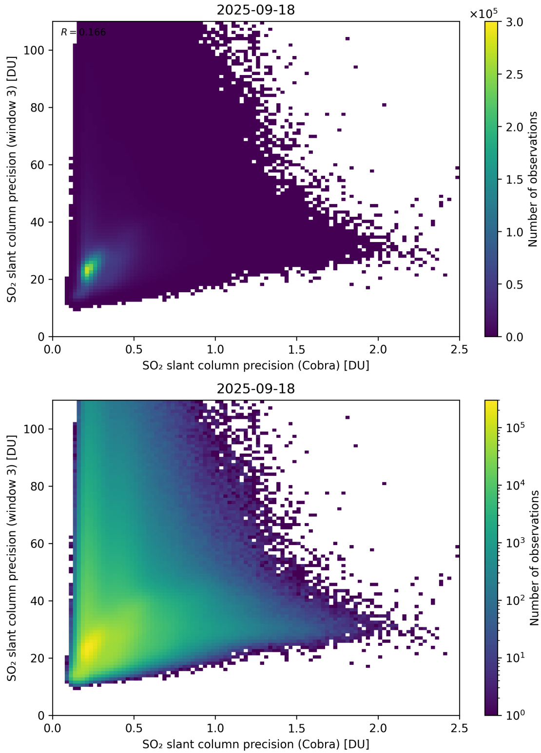
Figure 212: Scatter density plot of “SO 2 slant column precision (Cobra)” against “SO 2 slant column precision (window 3)” for 2025-09-17 to 2025-09-19.
