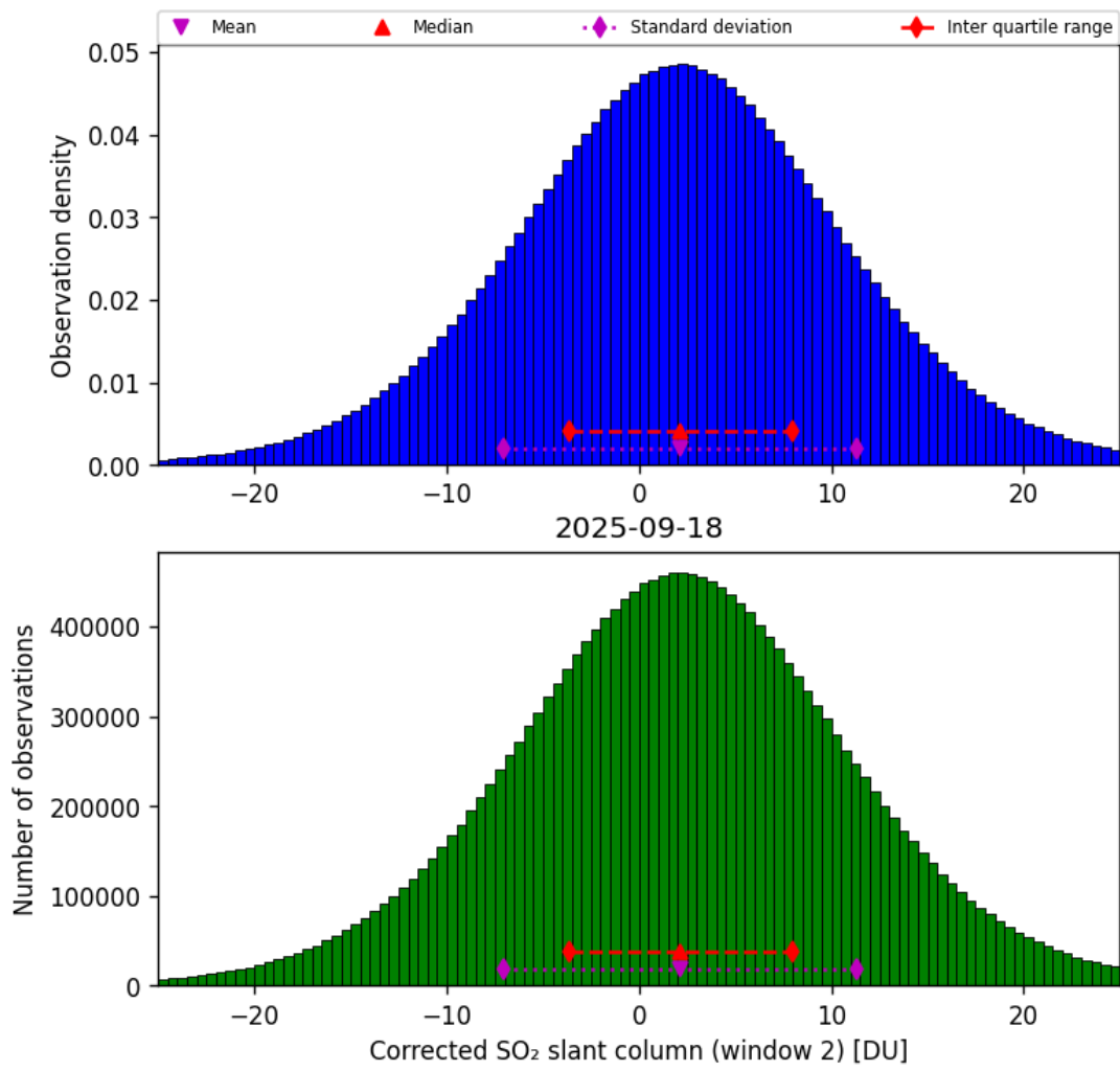
Figure 69: Histogram of “Corrected SO 2 slant column (window 2)” for 2025-09-17 to 2025-09-19
