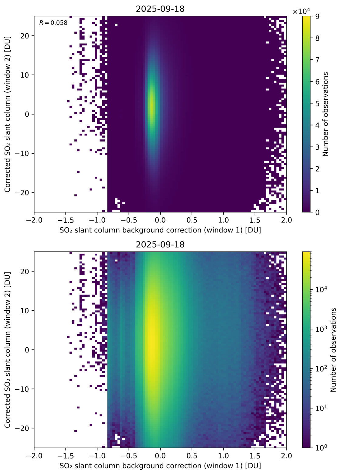
Figure 115: Scatter density plot of “SO 2 slant column background correction (window 1)” against “Corrected SO 2 slant column (window 2)” for 2025-09-17 to 2025-09-19.
