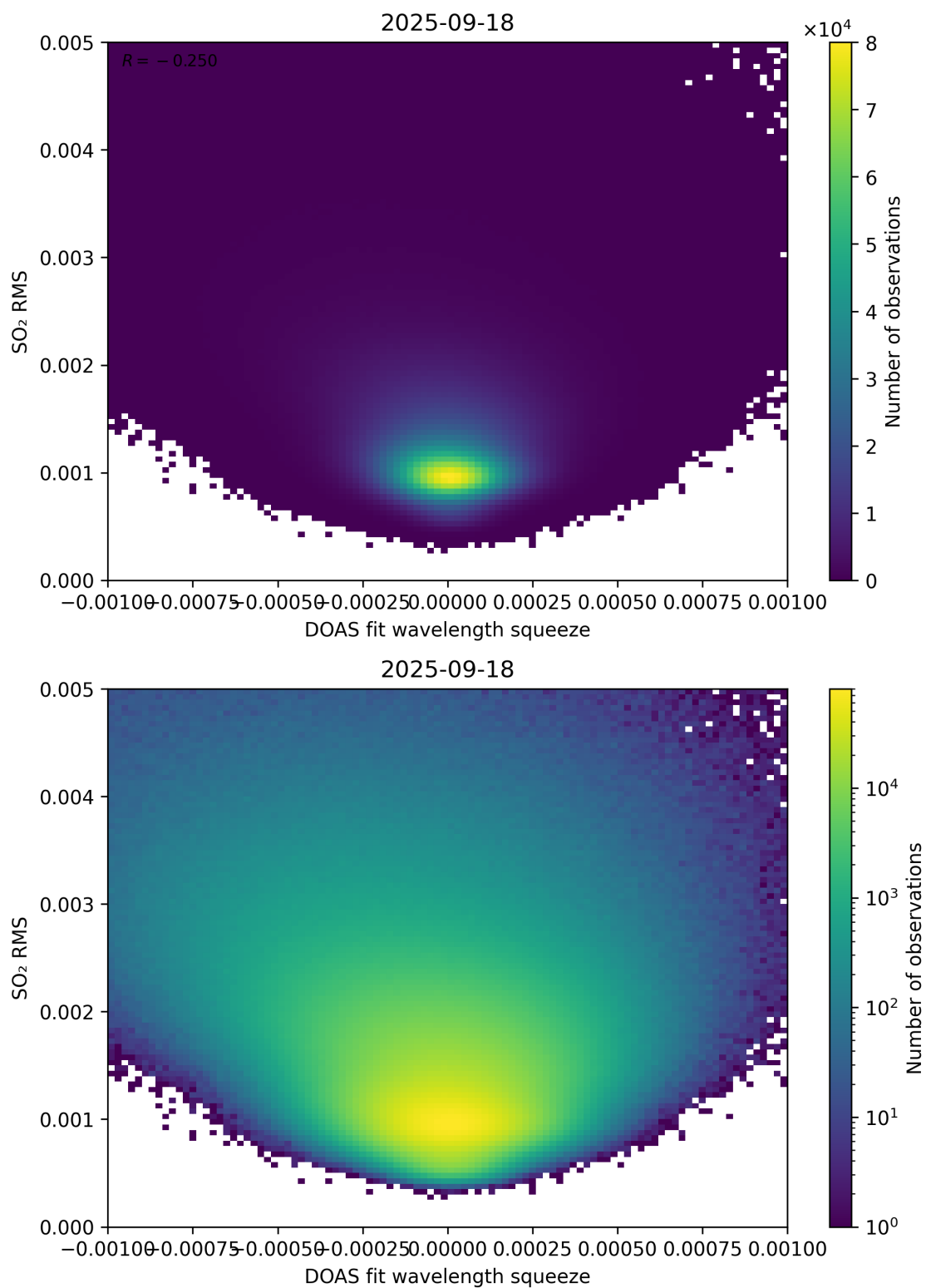
Figure 143: Scatter density plot of “DOAS fit wavelength squeeze” against “SO 2 RMS” for 2025-09-17 to 2025-09-19.
