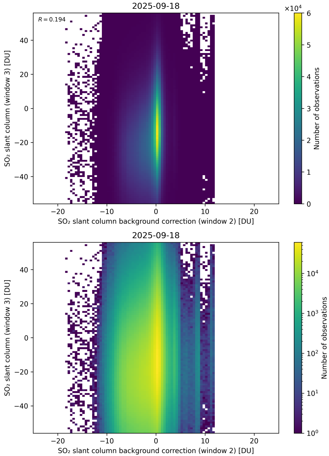
Figure 128: Scatter density plot of “SO 2 slant column background correction (window 2)” against “SO 2 slant column (window 3)” for 2025-09-17 to 2025-09-19.
