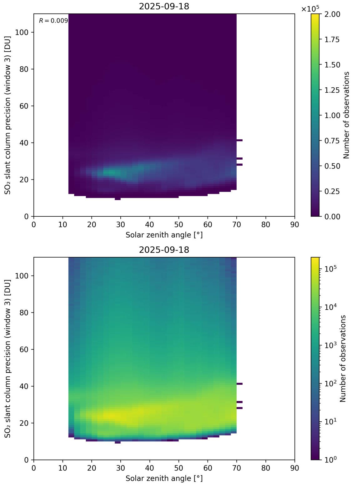
Figure 188: Scatter density plot of “Solar zenith angle” against “SO 2 slant column precision (window 3)” for 2025-09-17 to 2025-09-19.
