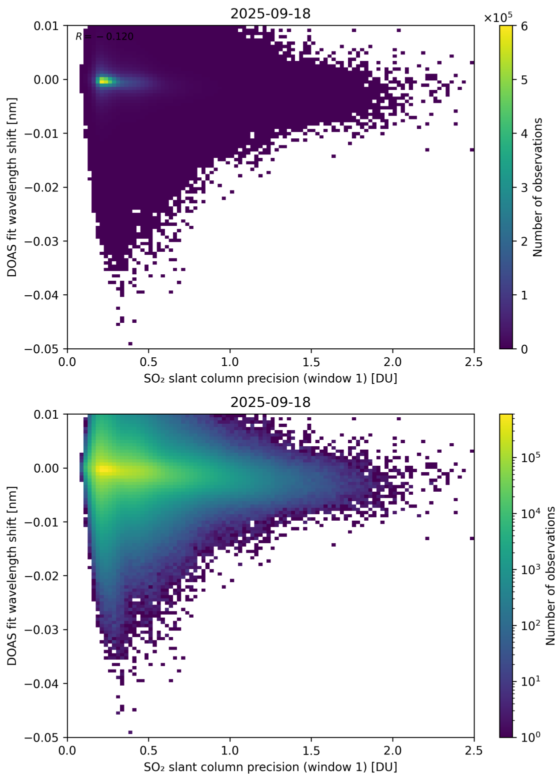
Figure 271: Scatter density plot of “SO 2 slant column precision (window 1)” against “DOAS fit wavelength shift” for 2025-09-17 to 2025-09-19.
