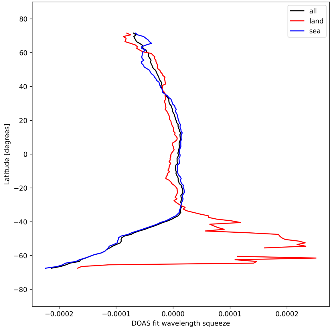
Figure 51: Zonal average of “DOAS fit wavelength squeeze” for 2025-09-17 to 2025-09-19.
