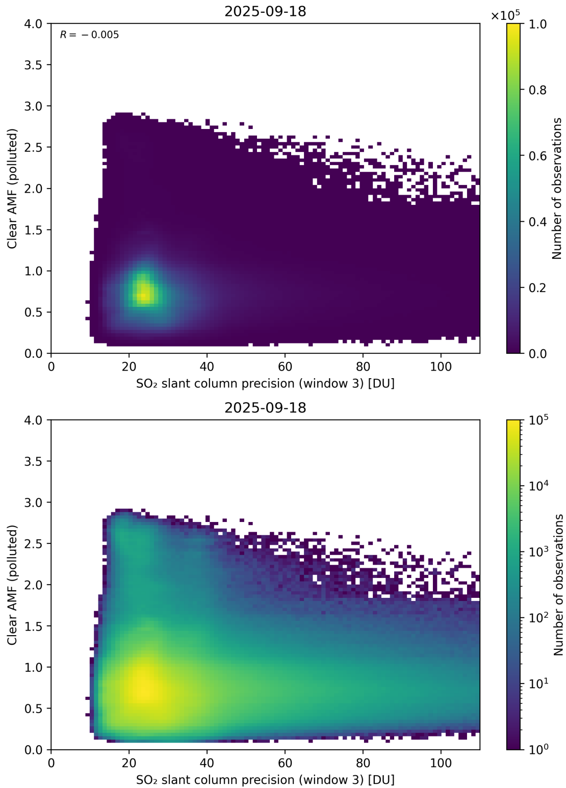
Figure 311: Scatter density plot of “SO 2 slant column precision (window 3)” against “Clear AMF (polluted)” for 2025-09-17 to 2025-09-19.
