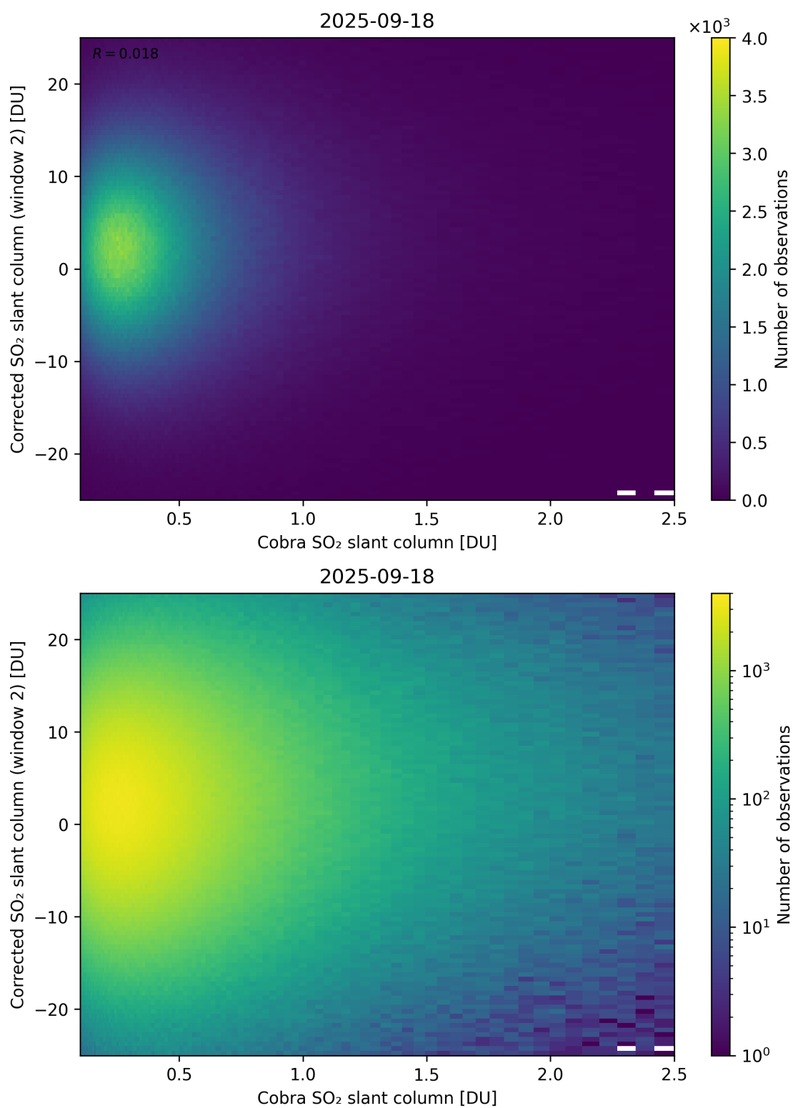
Figure 217: Scatter density plot of “Cobra SO 2 slant column” against “Corrected SO 2 slant column (window 2)” for 2025-09-17 to 2025-09-19.
