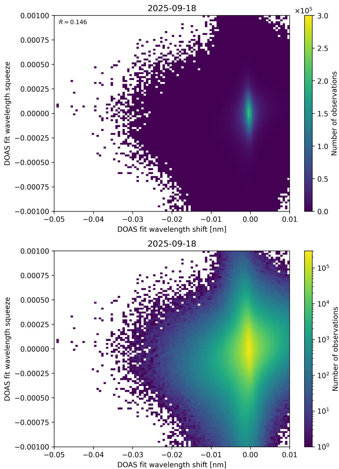
Figure 138: Scatter density plot of “DOAS fit wavelength shift” against “DOAS fit wavelength squeeze” for 2025-09-17 to 2025-09-19.
