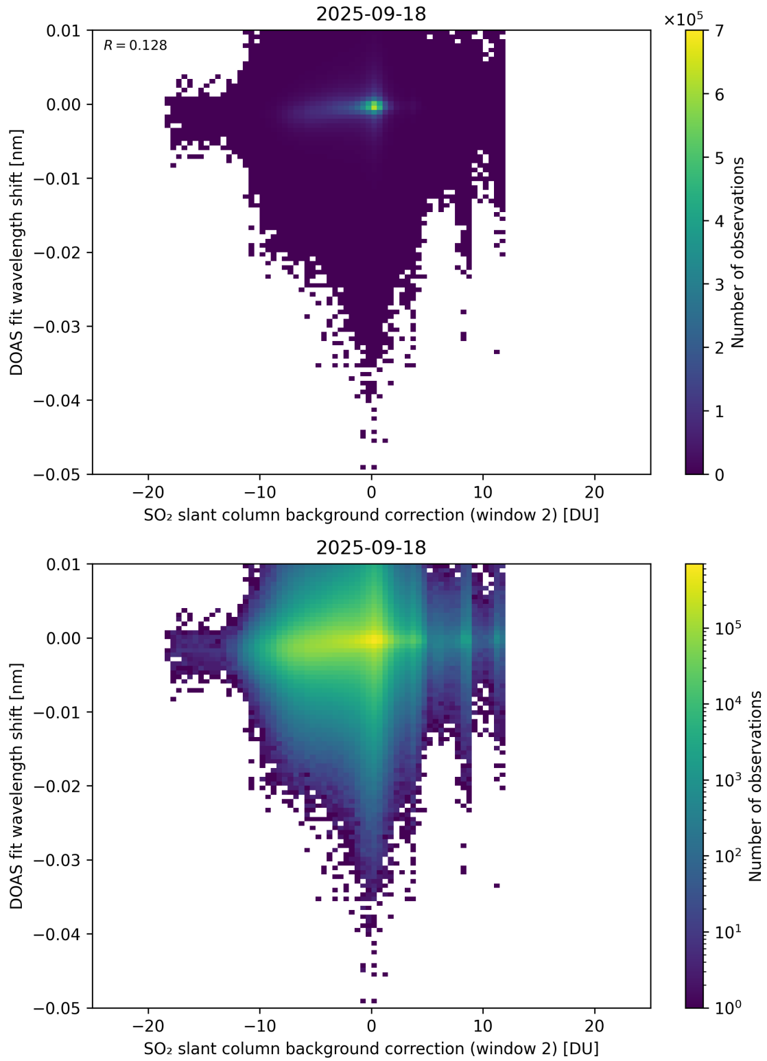
Figure 123: Scatter density plot of “SO 2 slant column background correction (window 2)” against “DOAS fit wavelength shift” for 2025-09-17 to 2025-09-19.
