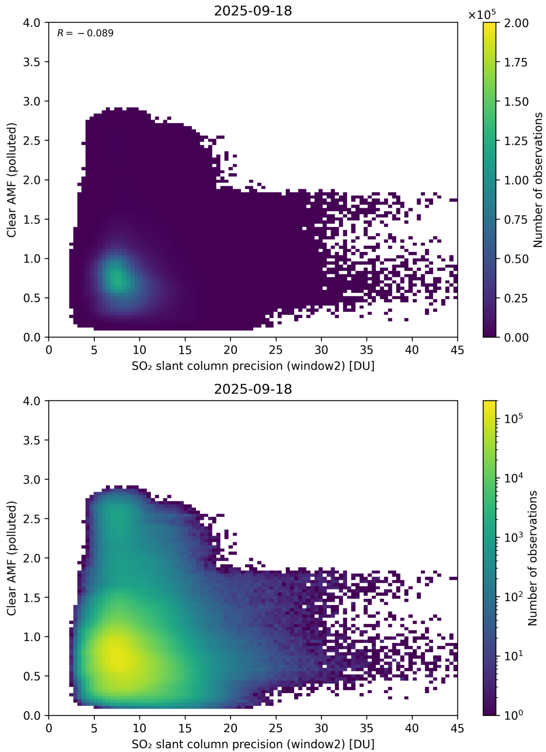
Figure 296: Scatter density plot of “SO 2 slant column precision (window2)” against “Clear AMF (polluted)” for 2025-09-17 to 2025-09-19.
