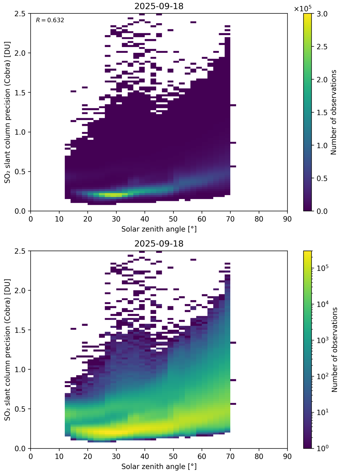
Figure 180: Scatter density plot of “Solar zenith angle” against “SO 2 slant column precision (Cobra)” for 2025-09-17 to 2025-09-19.
