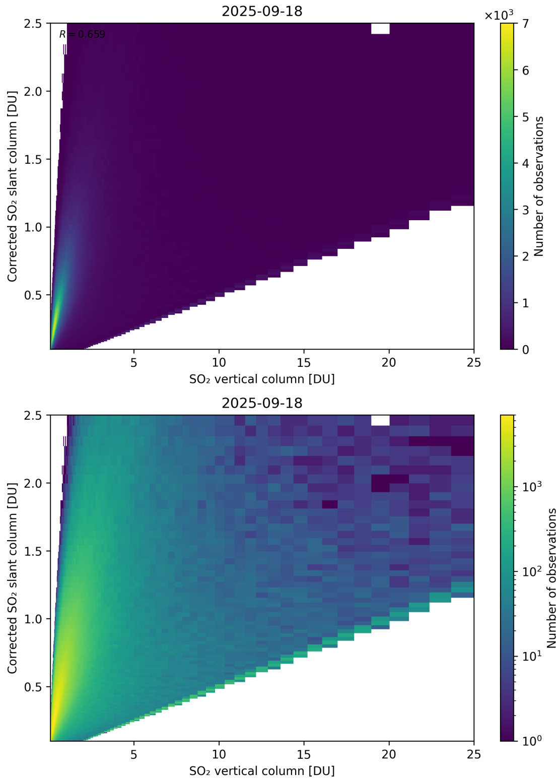
Figure 351: Scatter density plot of “SO 2 vertical column” against “Corrected SO 2 slant column” for 2025-09-17 to 2025-09-19.
