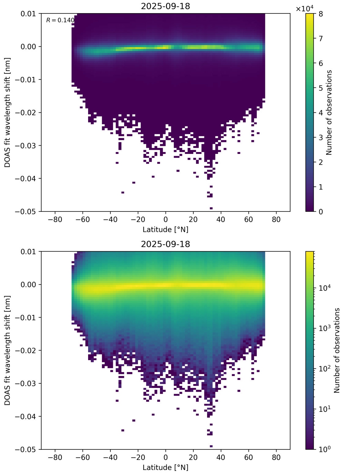
Figure 153: Scatter density plot of “Latitude” against “DOAS fit wavelength shift” for 2025-09-17 to 2025-09-19.
