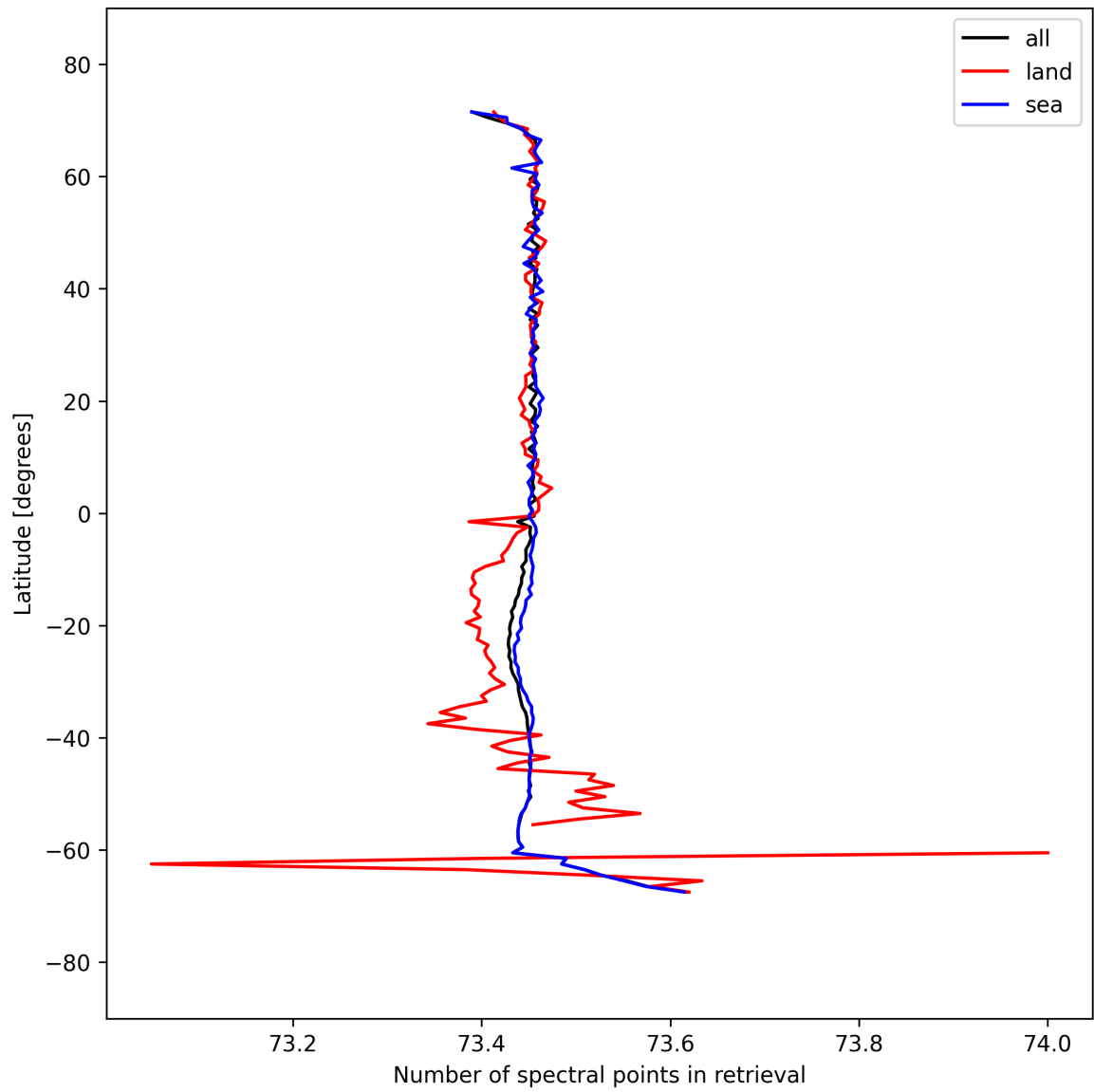
Figure 56: Zonal average of “Number of spectral points in retrieval” for 2025-09-17 to 2025-09-19.
