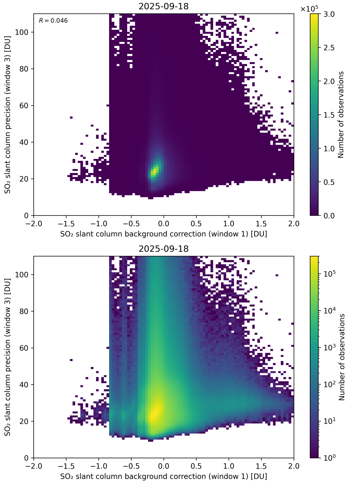
Figure 119: Scatter density plot of “SO 2 slant column background correction (window 1)” against “SO 2 slant column precision (window 3)” for 2025-09-17 to 2025-09-19.
