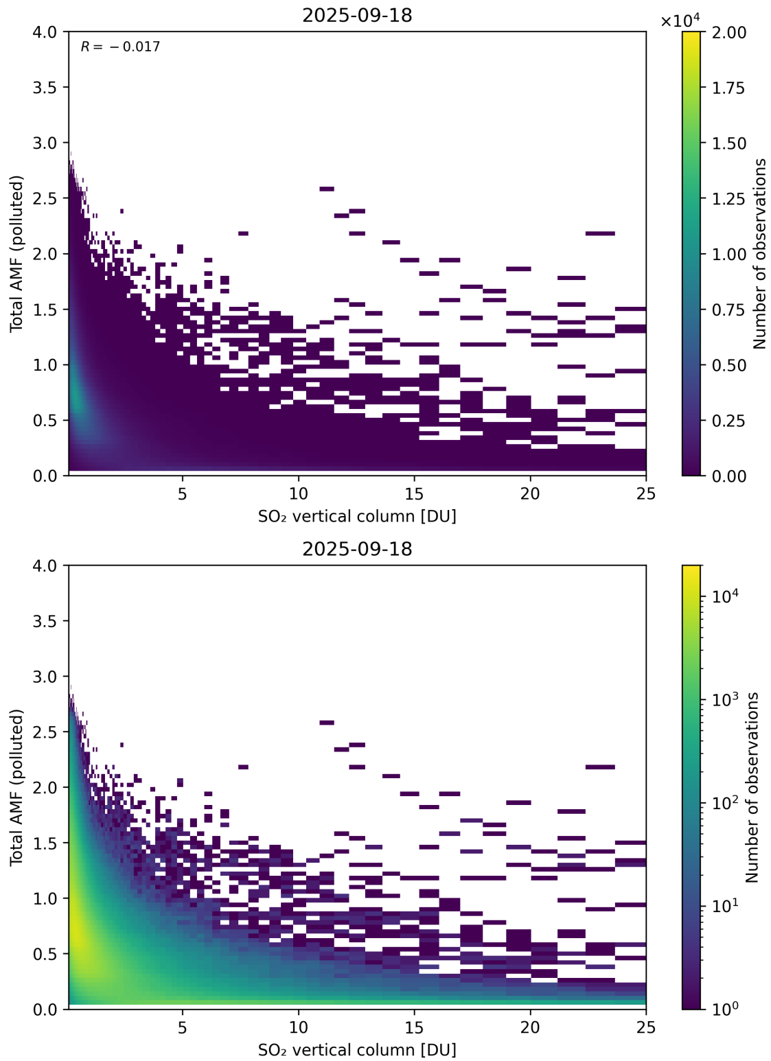
Figure 359: Scatter density plot of “SO 2 vertical column” against “Total AMF (polluted)” for 2025-09-17 to 2025-09-19.
