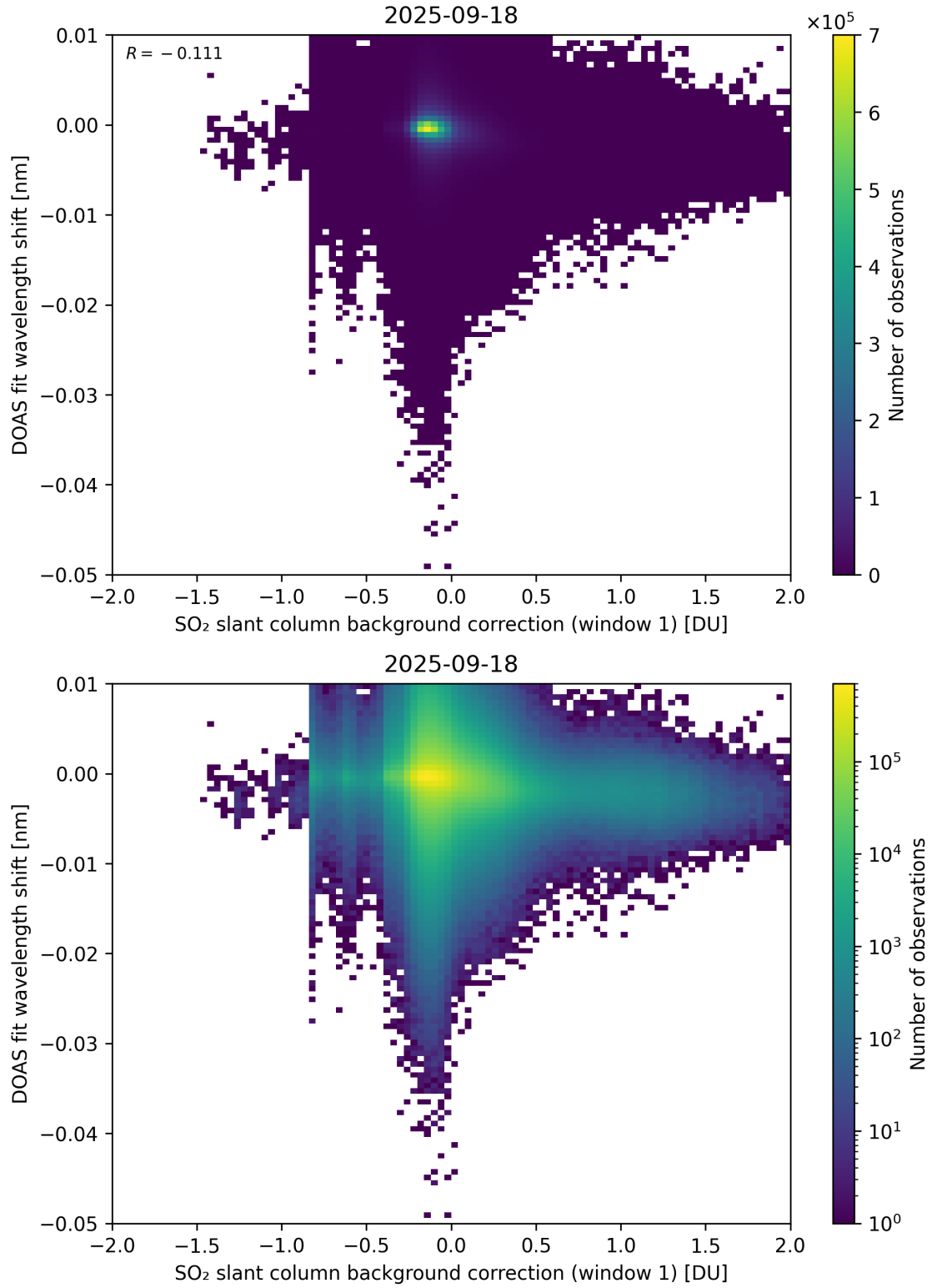
Figure 111: Scatter density plot of “SO 2 slant column background correction (window 1)” against “DOAS fit wavelength shift” for 2025-09-17 to 2025-09-19.
