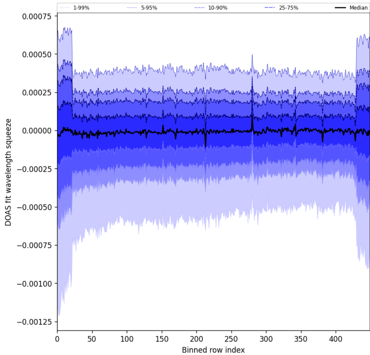
Figure 103: Along track statistics of “DOAS fit wavelength squeeze” for 2025-09-17 to 2025-09-19
