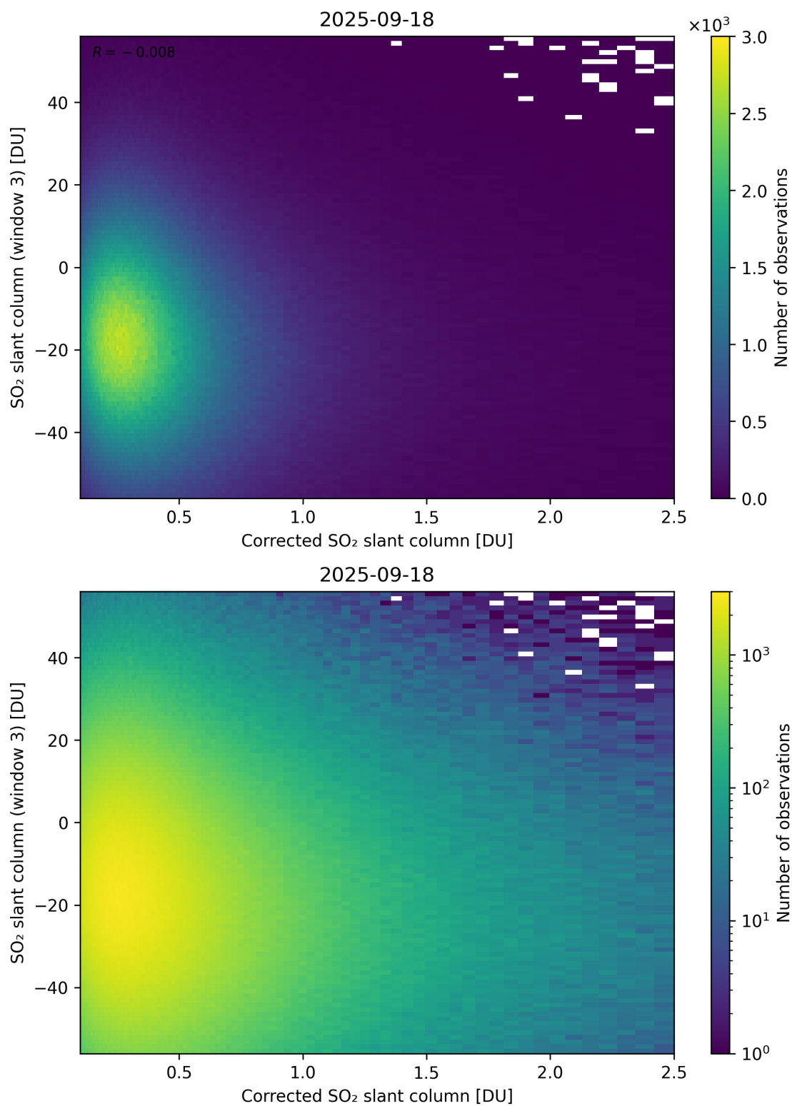
Figure 240: Scatter density plot of “Corrected SO 2 slant column” against “SO 2 slant column (window 3)” for 2025-09-17 to 2025-09-19.
