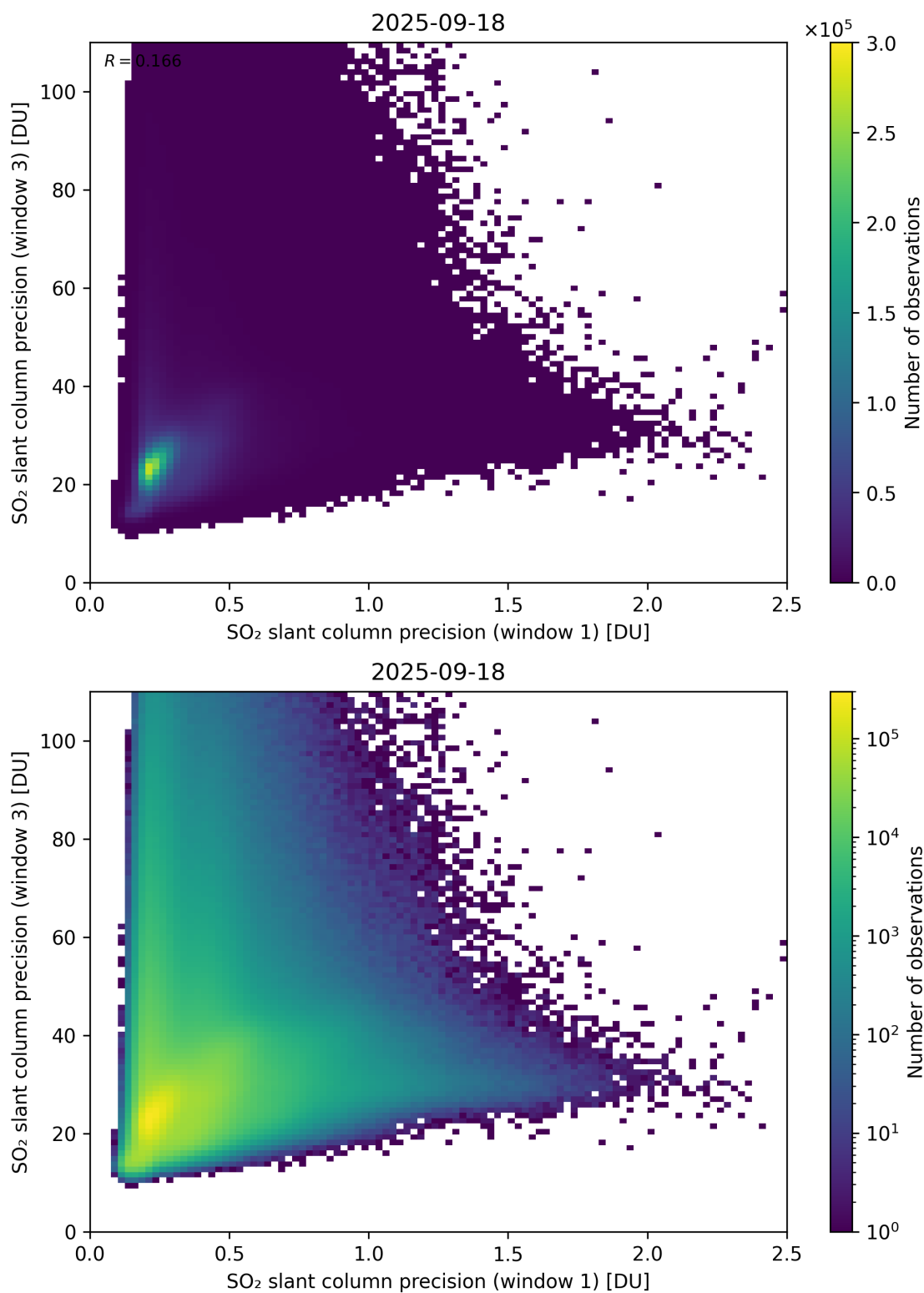
Figure 279: Scatter density plot of “SO 2 slant column precision (window 1)” against “SO 2 slant column precision (window 3)” for 2025-09-17 to 2025-09-19.
