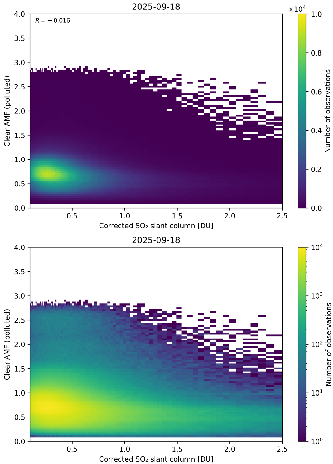
Figure 232: Scatter density plot of “Corrected SO 2 slant column” against “Clear AMF (polluted)” for 2025-09-17 to 2025-09-19.
