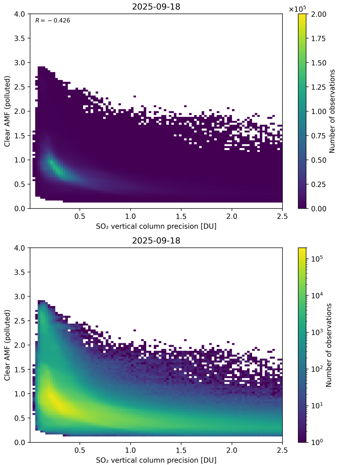
Figure 335: Scatter density plot of “SO 2 vertical column precision” against “Clear AMF (polluted)” for 2025-09-17 to 2025-09-19.
