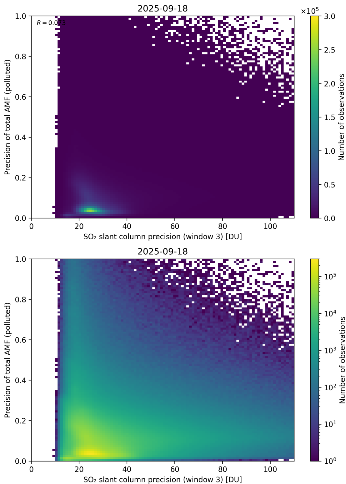
Figure 314: Scatter density plot of “SO 2 slant column precision (window 3)” against “Precision of total AMF (polluted)” for 2025-09-17 to 2025-09-19.
