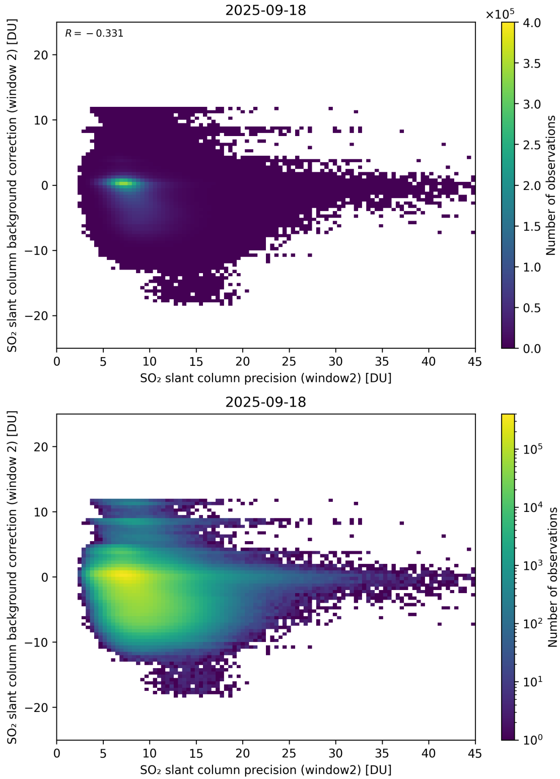
Figure 291: Scatter density plot of “SO 2 slant column precision (window2)” against “SO 2 slant column background correction (window 2)” for 2025-09-17 to 2025-09-19.
