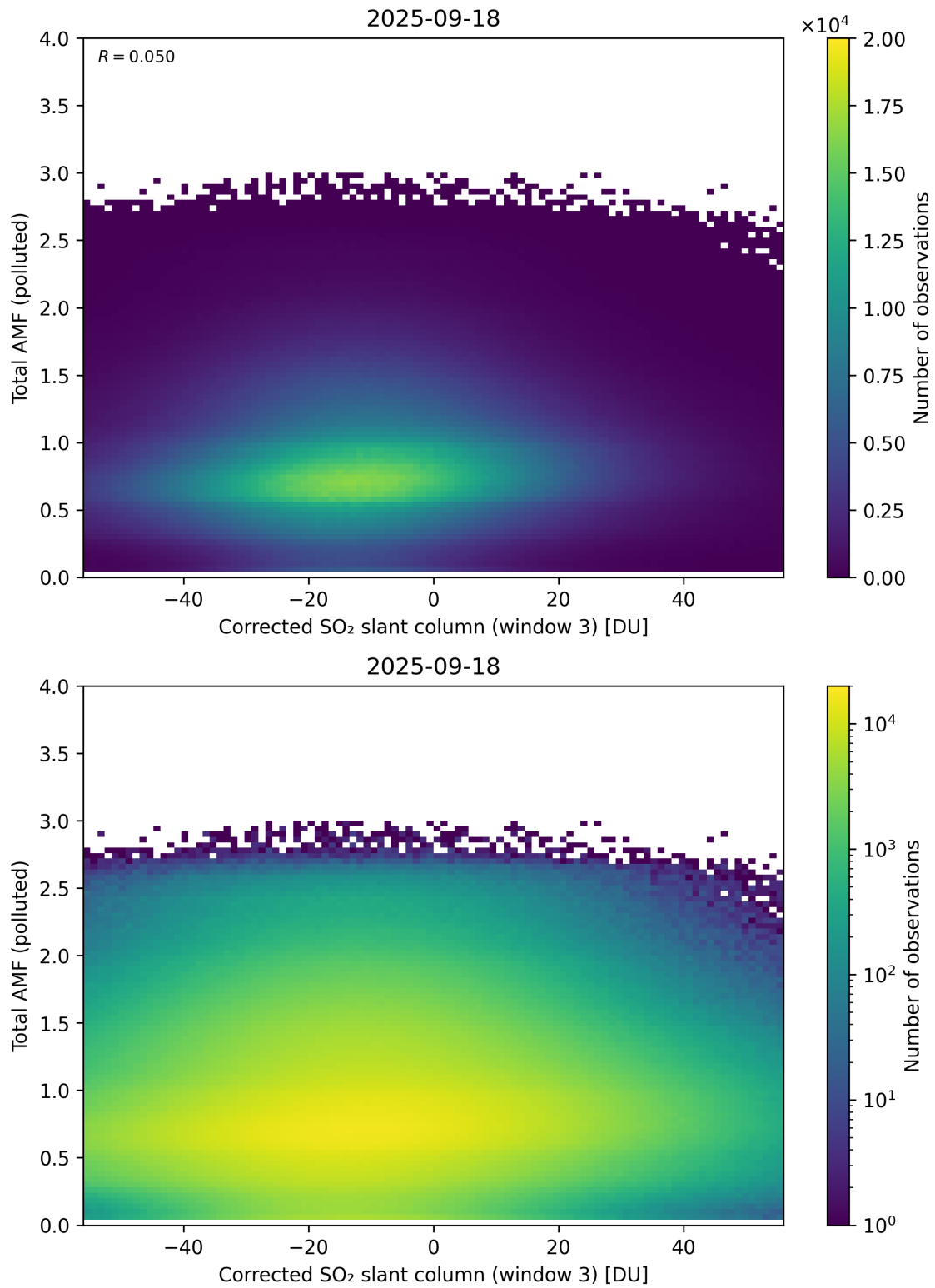
Figure 260: Scatter density plot of “Corrected SO 2 slant column (window 3)” against “Total AMF (polluted)” for 2025-09-17 to 2025-09-19.
