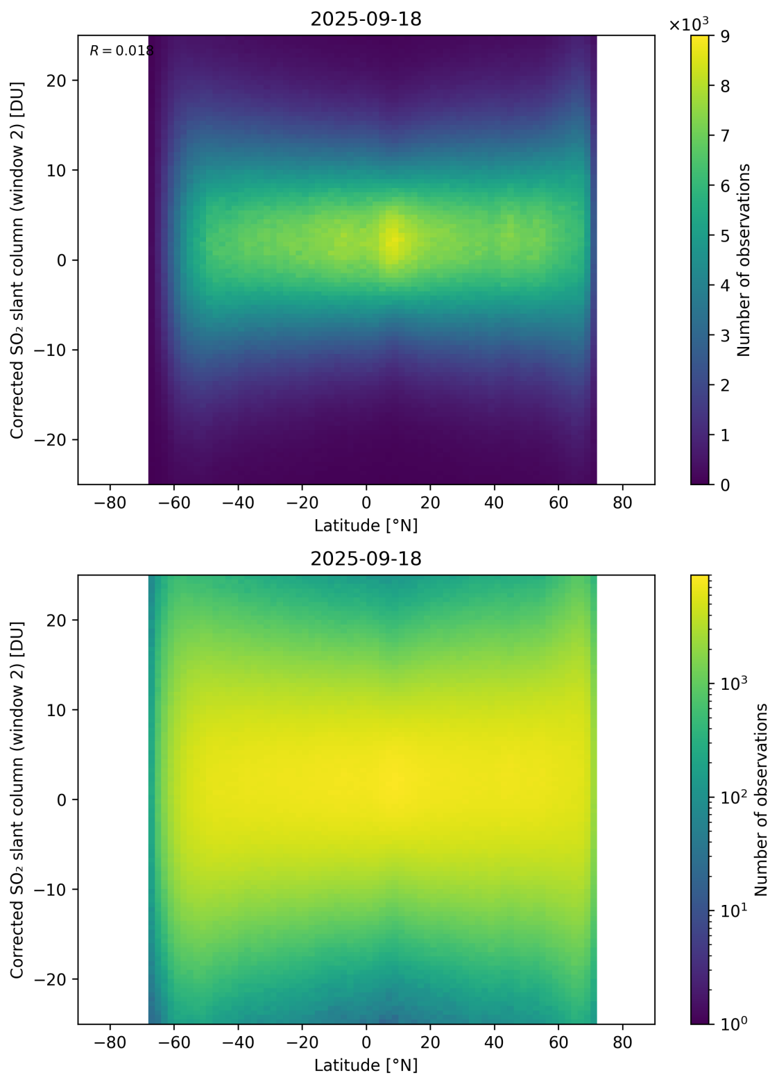
Figure 160: Scatter density plot of “Latitude” against “Corrected SO 2 slant column (window 2)” for 2025-09-17 to 2025-09-19.
