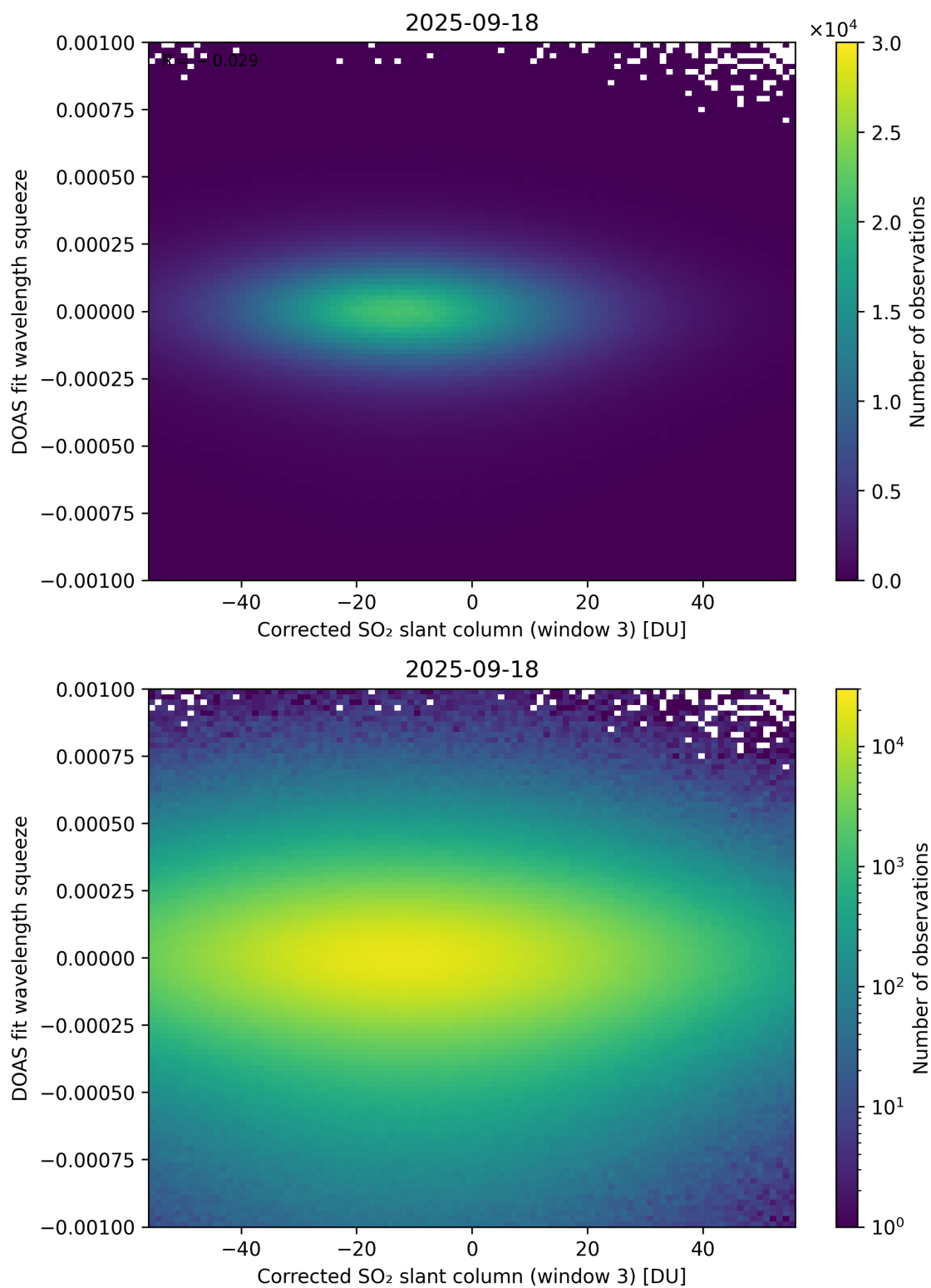
Figure 257: Scatter density plot of “Corrected SO 2 slant column (window 3)” against “DOAS fit wavelength squeeze” for 2025-09-17 to 2025-09-19.
