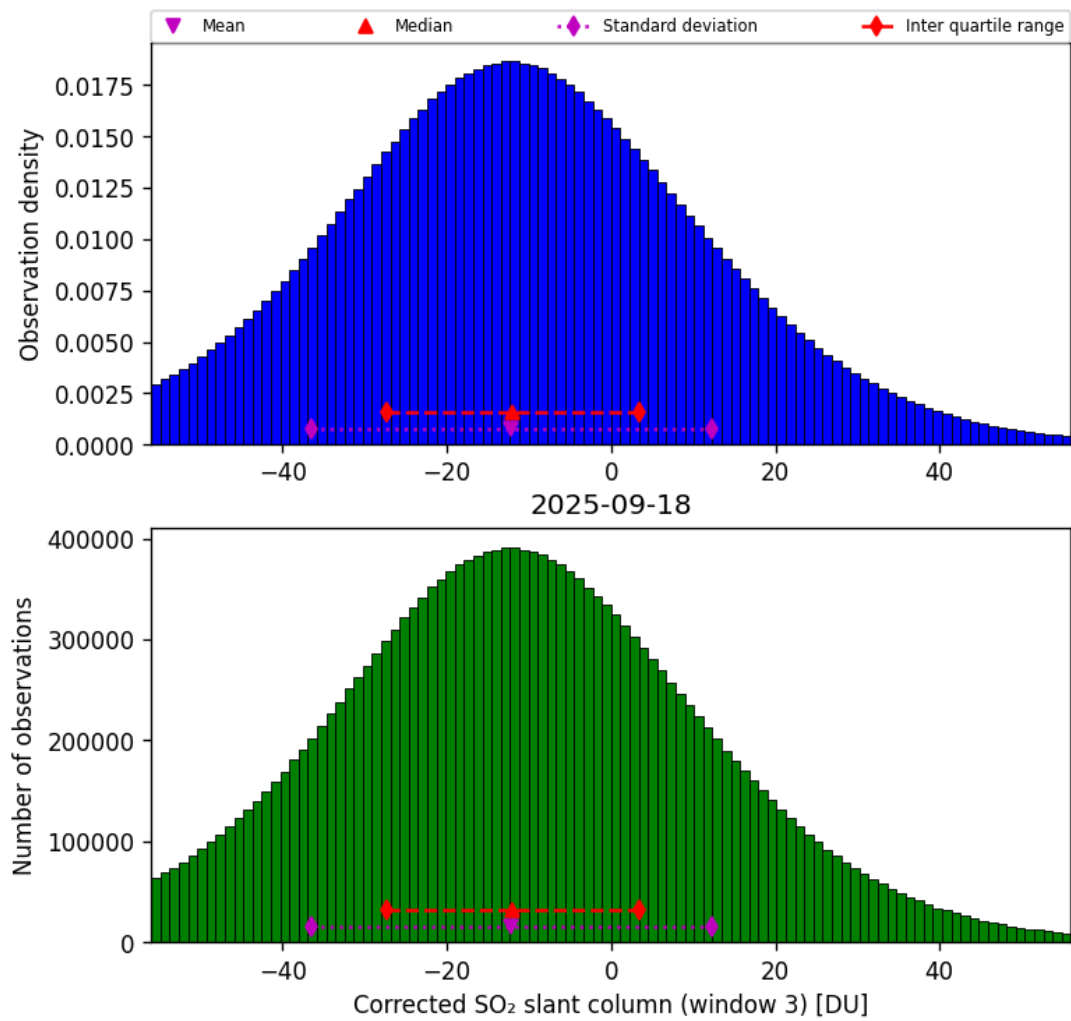
Figure 73: Histogram of "Corrected SO 2 slant column (window 3)" for 2025-09-17 to 2025-09-19
