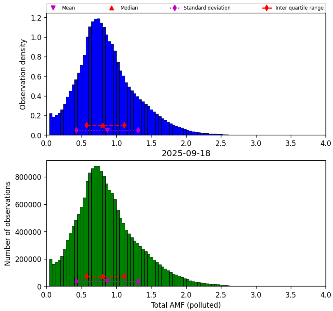
Figure 79: Histogram of “Total AMF (polluted)” for 2025-09-17 to 2025-09-19
