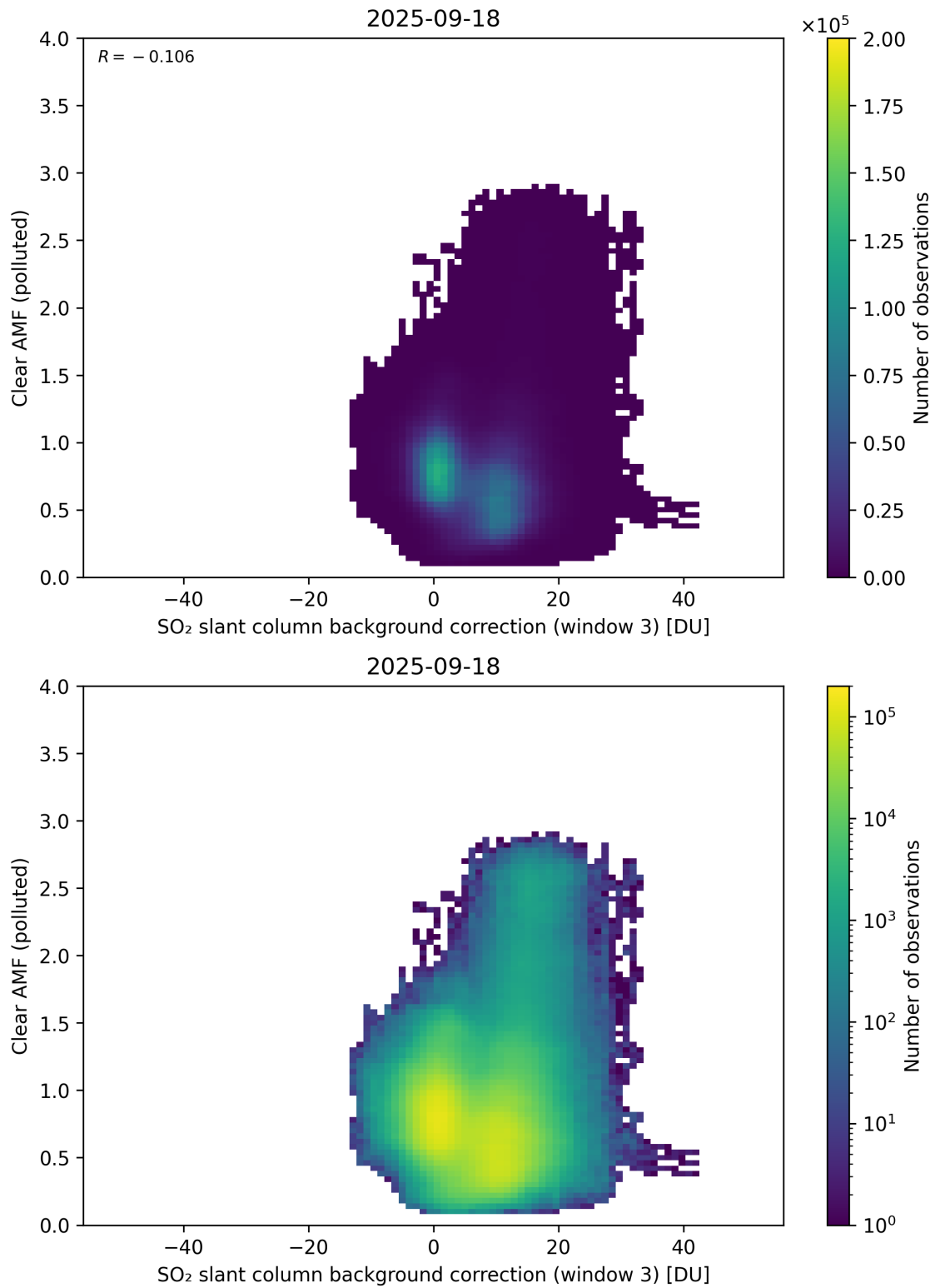
Figure 135: Scatter density plot of “SO 2 slant column background correction (window 3)” against “Clear AMF (polluted)” for 2025-09-17 to 2025-09-19.
