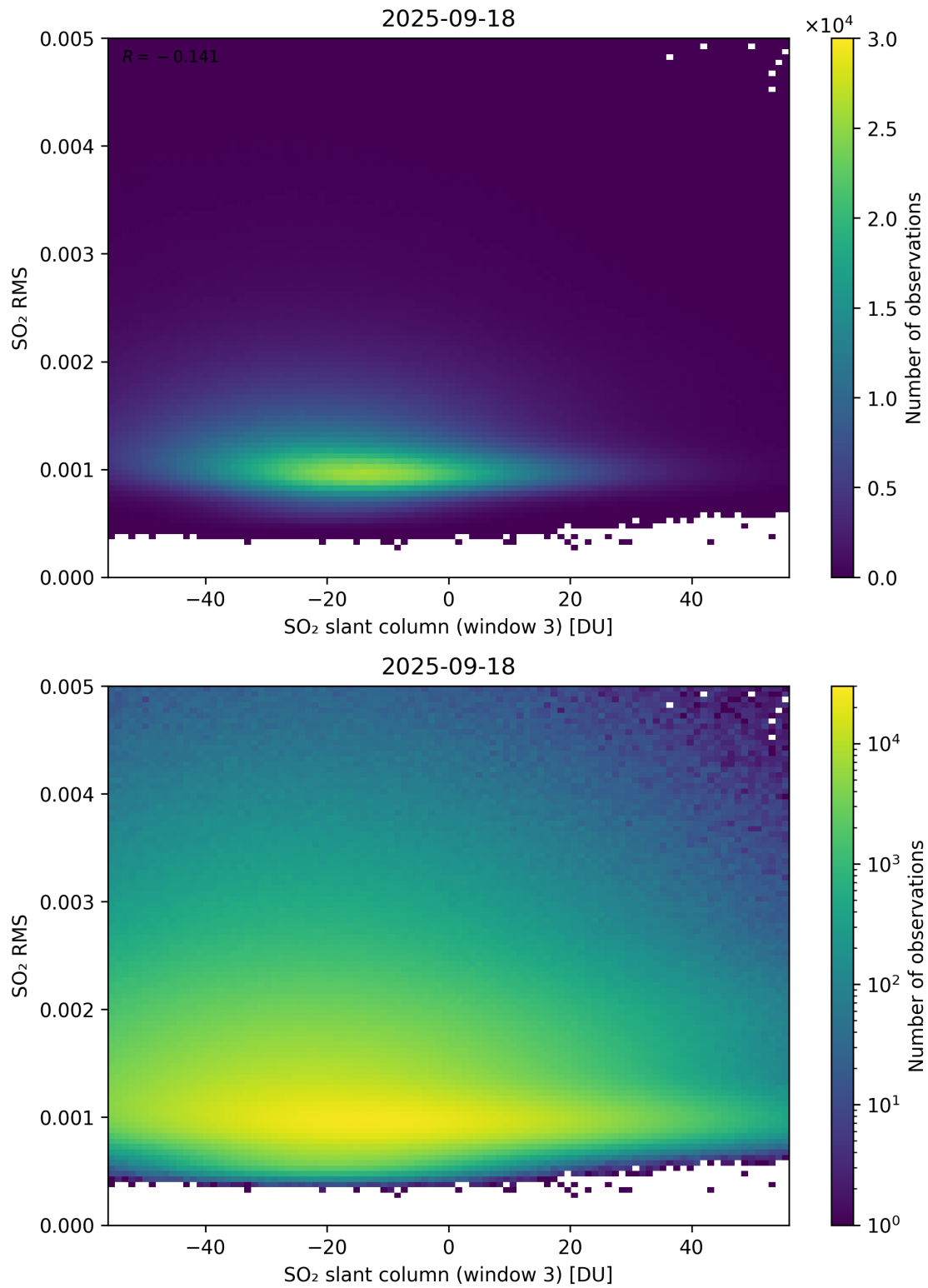
Figure 306: Scatter density plot of “SO 2 slant column (window 3)” against “SO 2 RMS” for 2025-09-17 to 2025-09-19.
