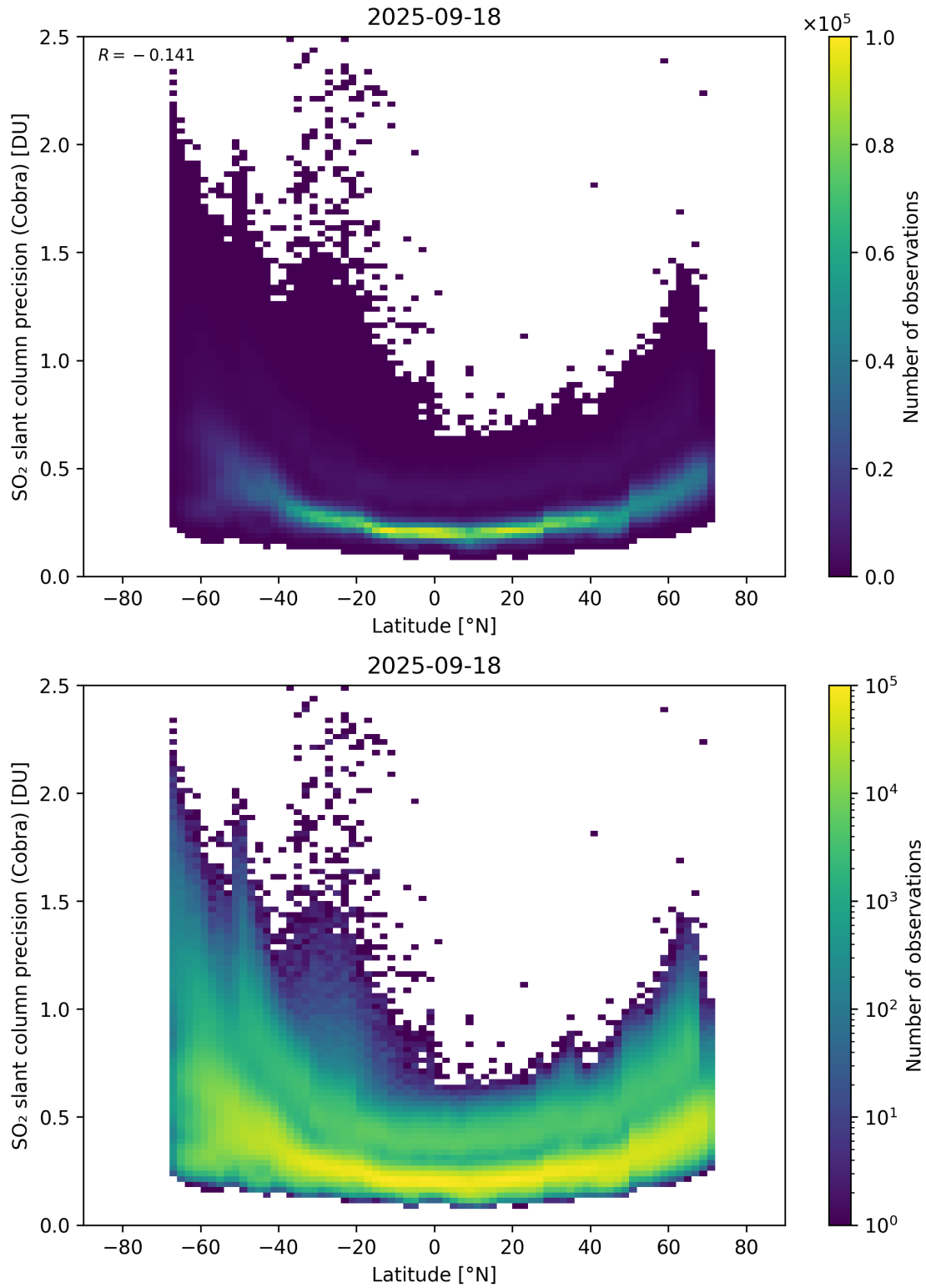
Figure 158: Scatter density plot of “Latitude” against “SO 2 slant column precision (Cobra)” for 2025-09-17 to 2025-09-19.
