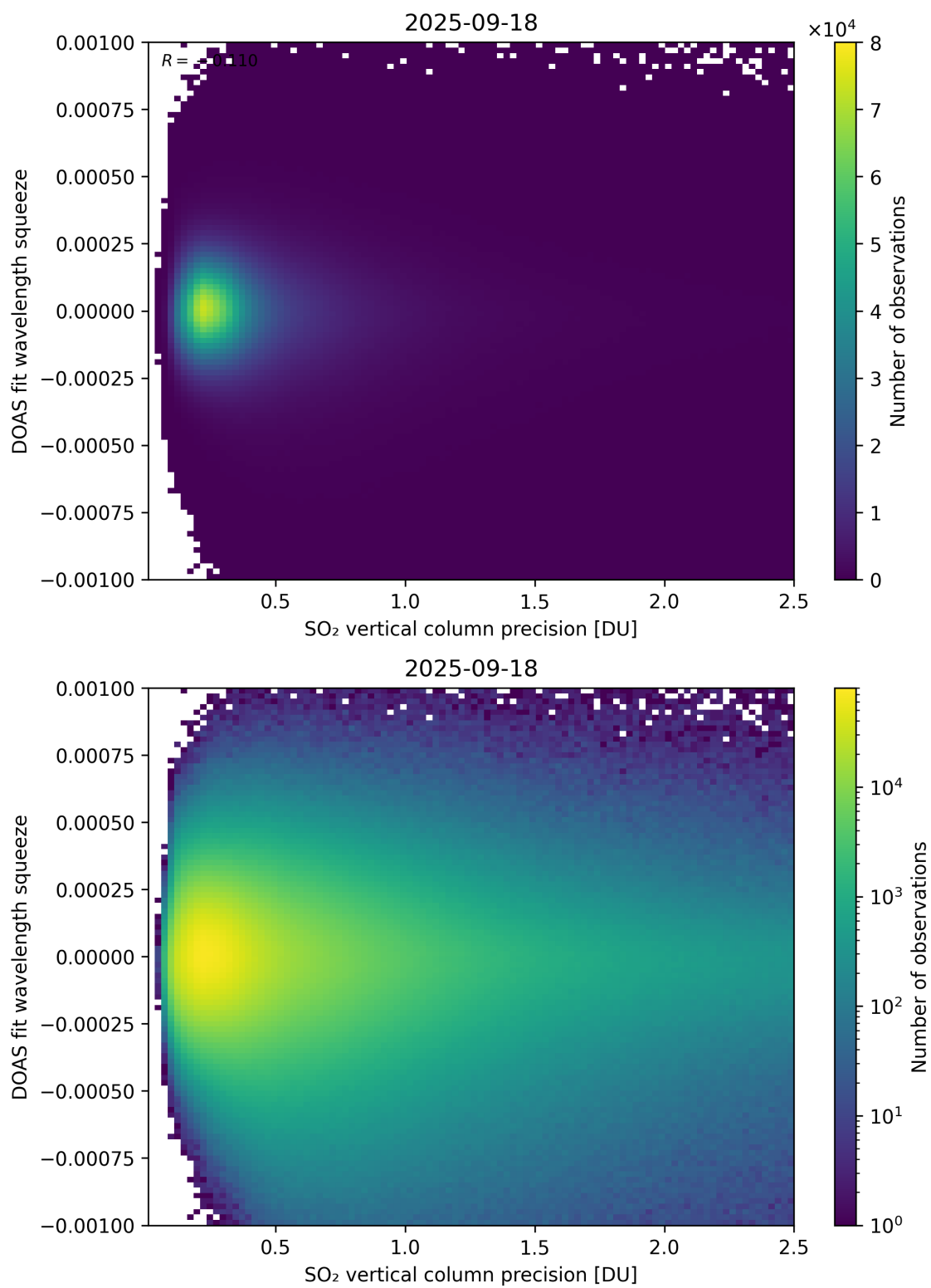
Figure 333: Scatter density plot of “SO 2 vertical column precision” against “DOAS fit wavelength squeeze” for 2025-09-17 to 2025-09-19.
