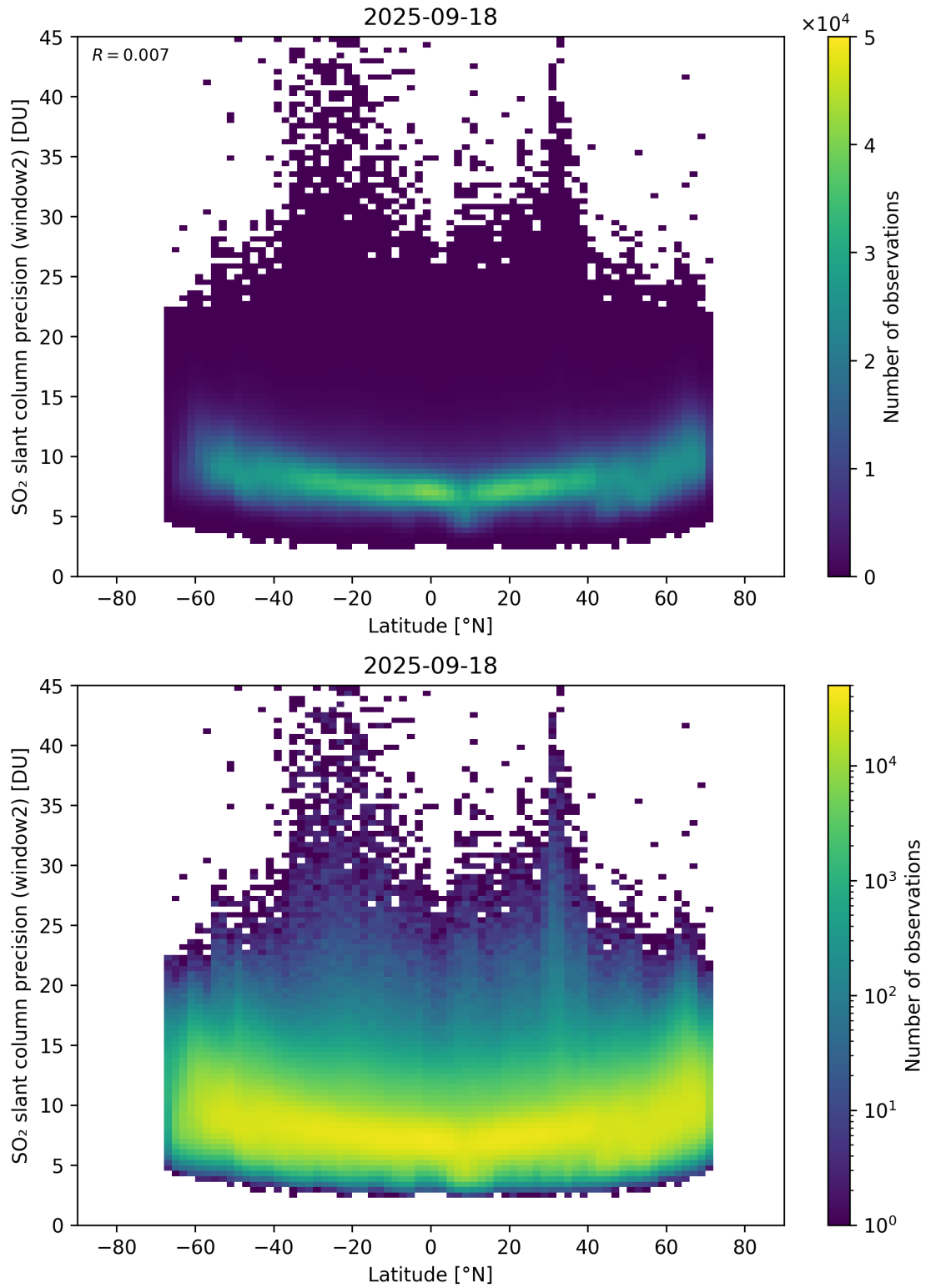
Figure 164: Scatter density plot of “Latitude” against “SO 2 slant column precision (window2)” for 2025-09-17 to 2025-09-19.
