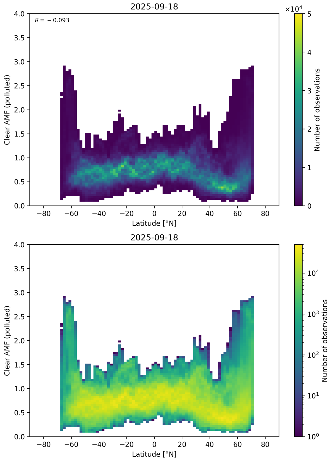
Figure 156: Scatter density plot of “Latitude” against “Clear AMF (polluted)” for 2025-09-17 to 2025-09-19.
