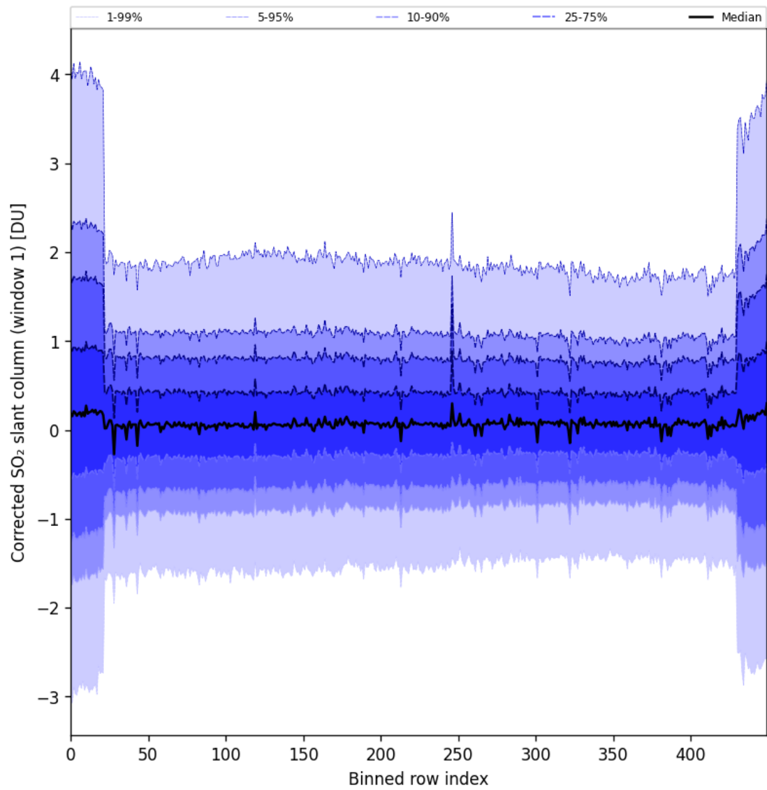
Figure 91: Along track statistics of “Corrected SO 2 slant column (window 1)” for 2025-09-17 to 2025-09-19
