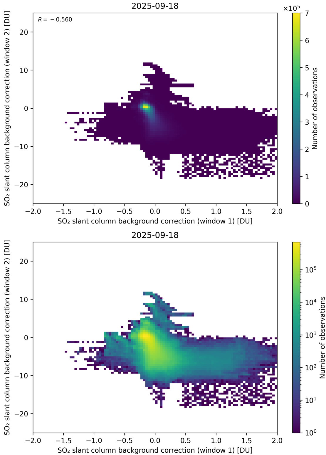
Figure 109: Scatter density plot of “SO 2 slant column background correction (window 1)” against “SO 2 slant column background correction (window 2)” for 2025-09-17 to 2025-09-19.
