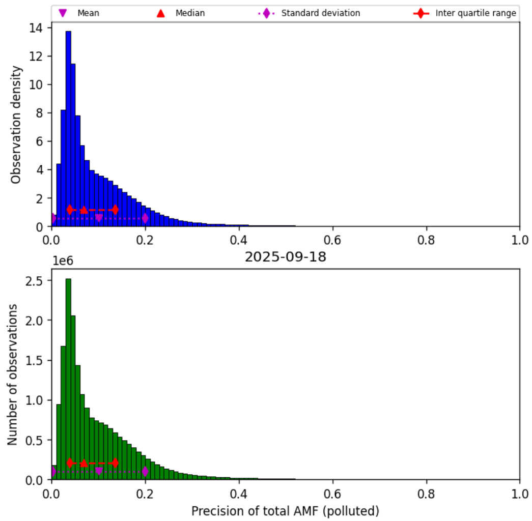
Figure 80: Histogram of “Precision of total AMF (polluted)” for 2025-09-17 to 2025-09-19
