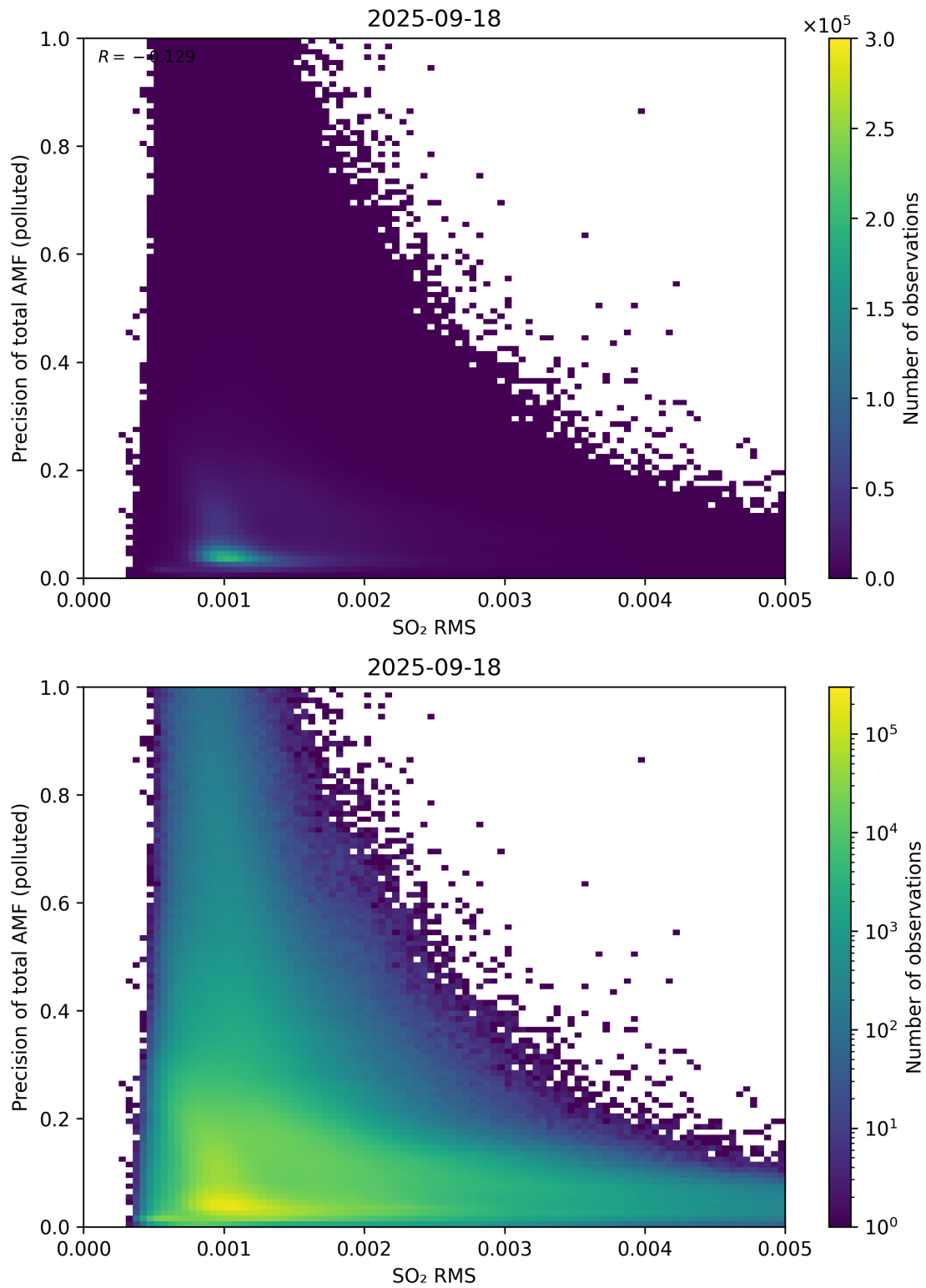
Figure 149: Scatter density plot of “SO 2 RMS” against “Precision of total AMF (polluted)” for 2025-09-17 to 2025-09-19.
