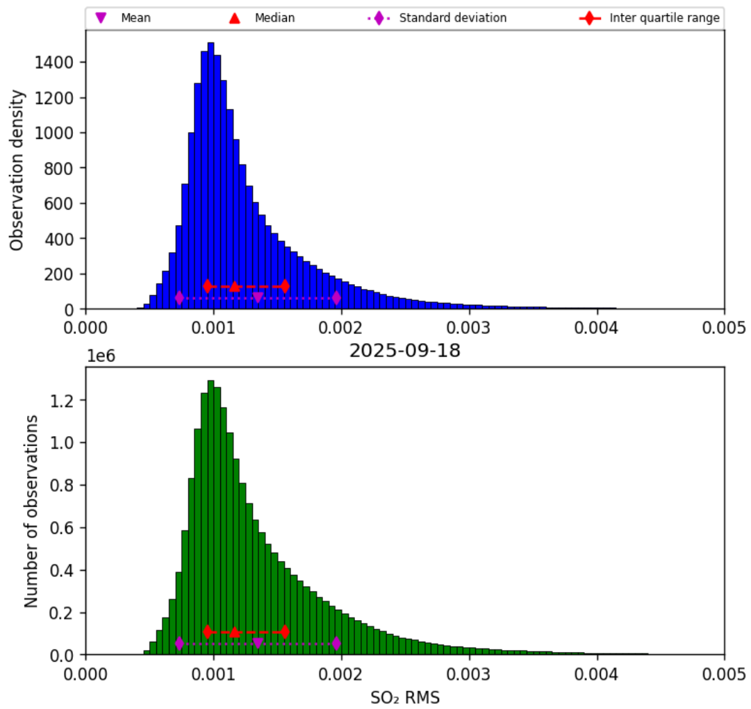
Figure 78: Histogram of “SO 2 RMS” for 2025-09-17 to 2025-09-19
