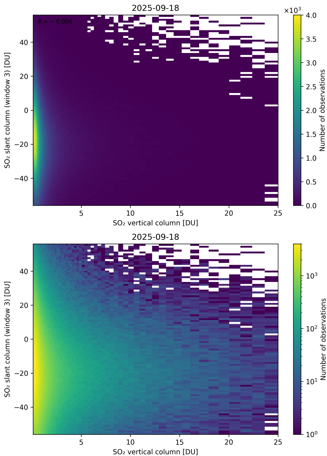
Figure 357: Scatter density plot of “SO 2 vertical column” against “SO 2 slant column (window 3)” for 2025-09-17 to 2025-09-19.
