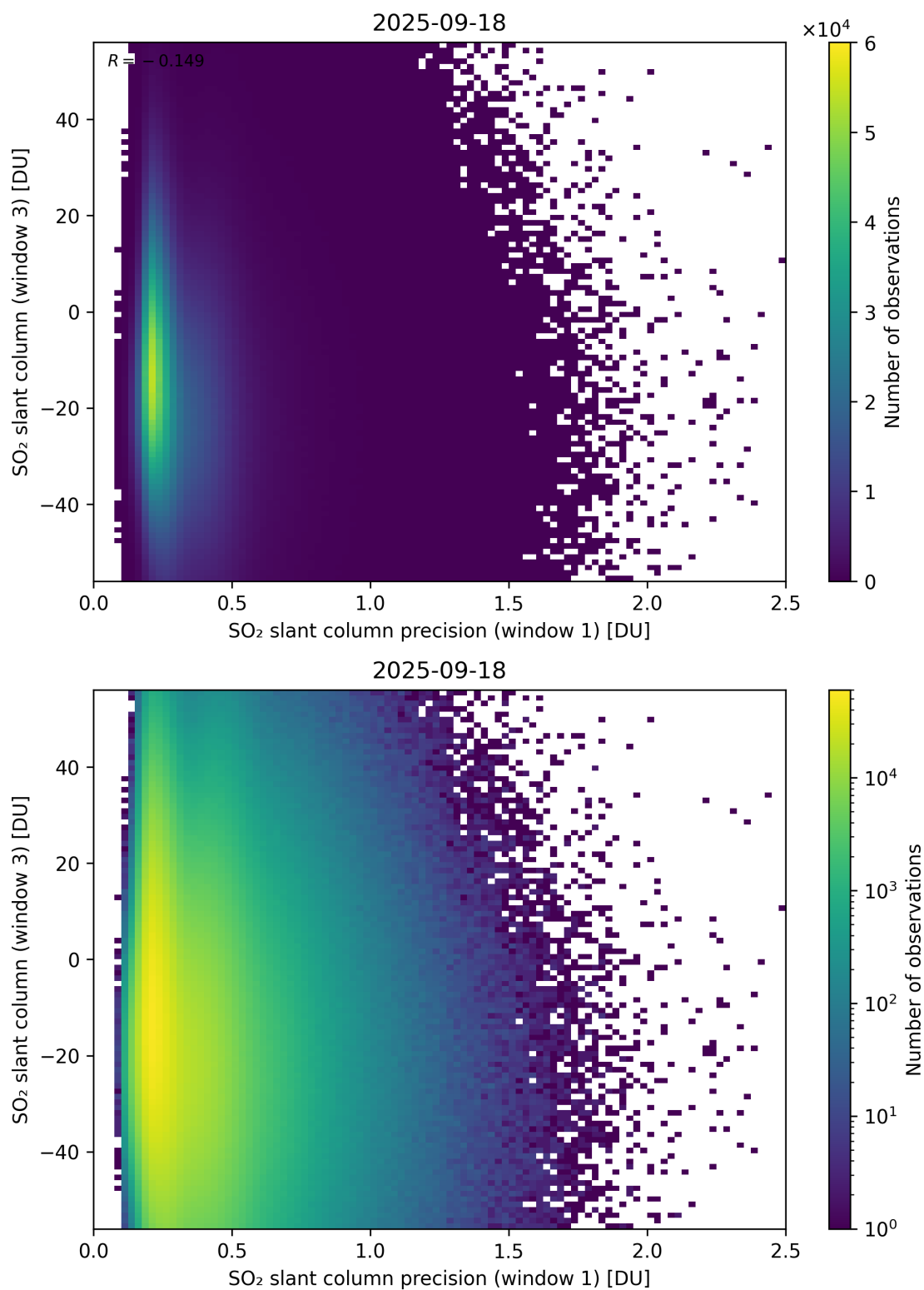
Figure 278: Scatter density plot of “SO 2 slant column precision (window 1)” against “SO 2 slant column (window 3)” for 2025-09-17 to 2025-09-19.
