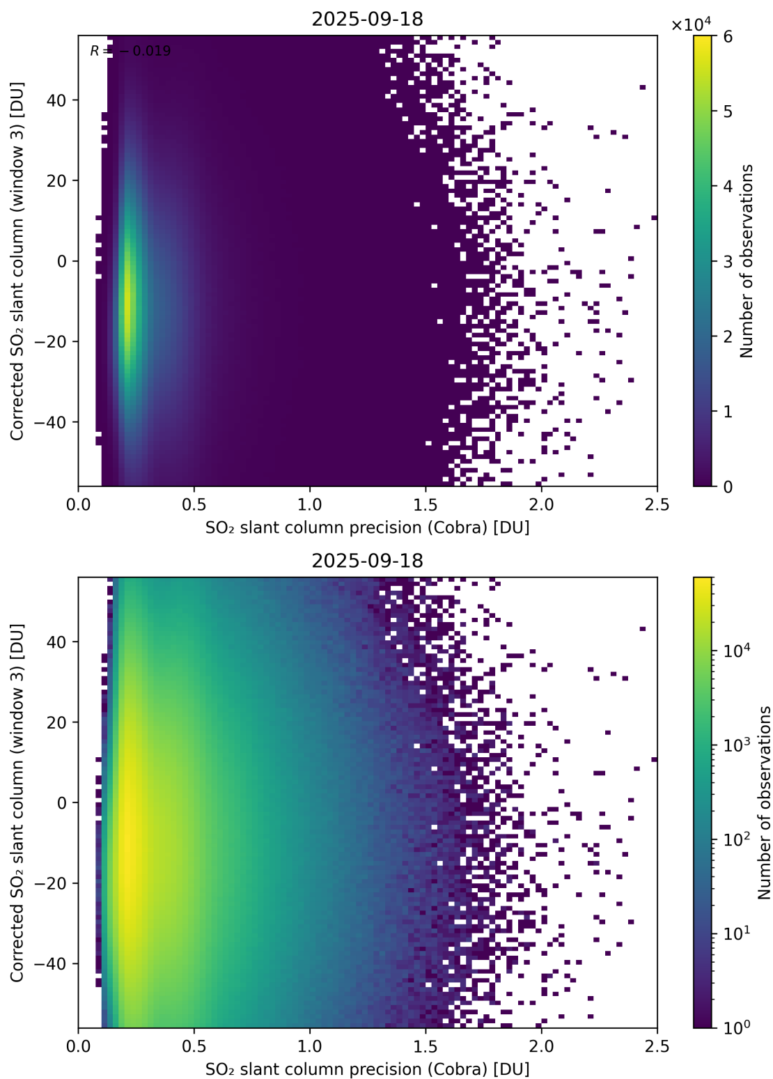
Figure 207: Scatter density plot of “SO 2 slant column precision (Cobra)” against “Corrected SO 2 slant column (window 3)” for 2025-09-17 to 2025-09-19.
