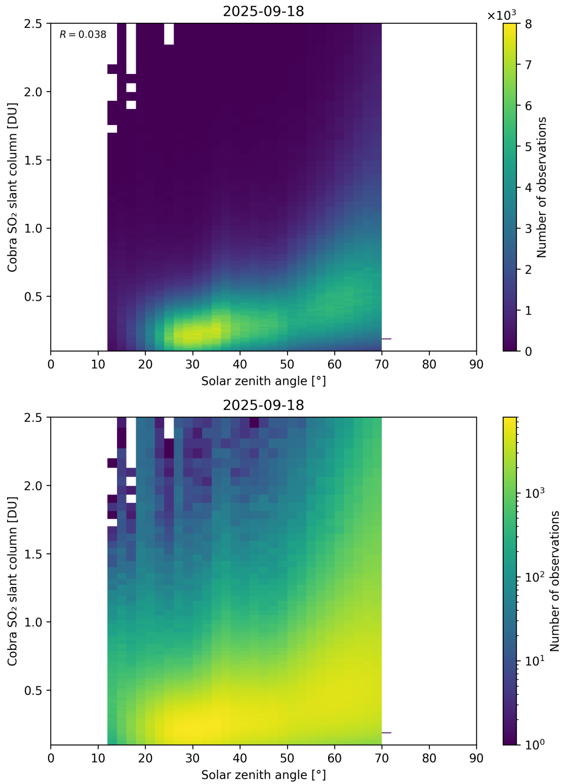
Figure 179: Scatter density plot of “Solar zenith angle” against “Cobra SO 2 slant column” for 2025-09-17 to 2025-09-19.
