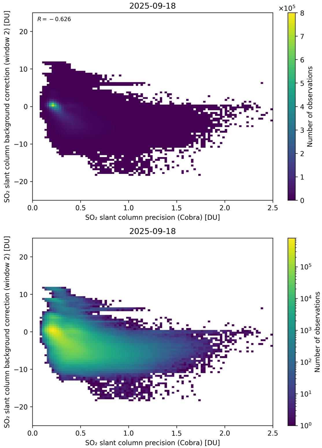
Figure 200: Scatter density plot of “SO 2 slant column precision (Cobra)” against “SO 2 slant column background correction (window 2)” for 2025-09-17 to 2025-09-19.
