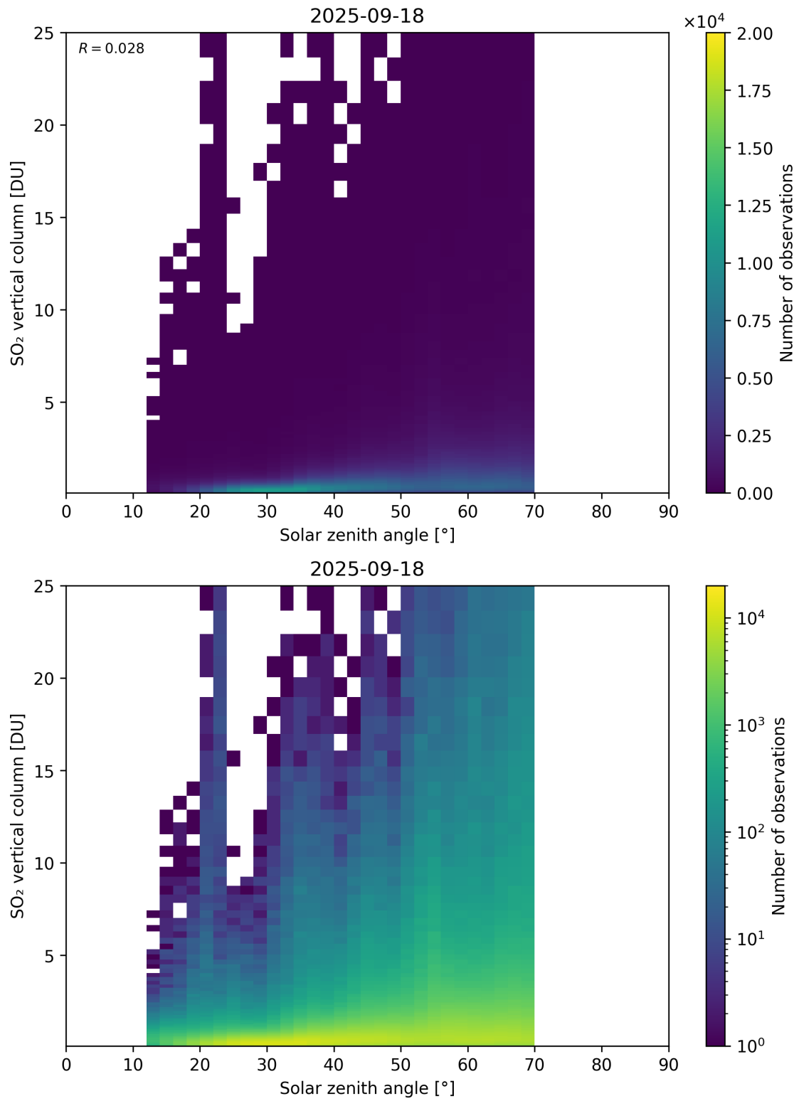
Figure 191: Scatter density plot of “Solar zenith angle” against “SO 2 vertical column” for 2025-09-17 to 2025-09-19.
