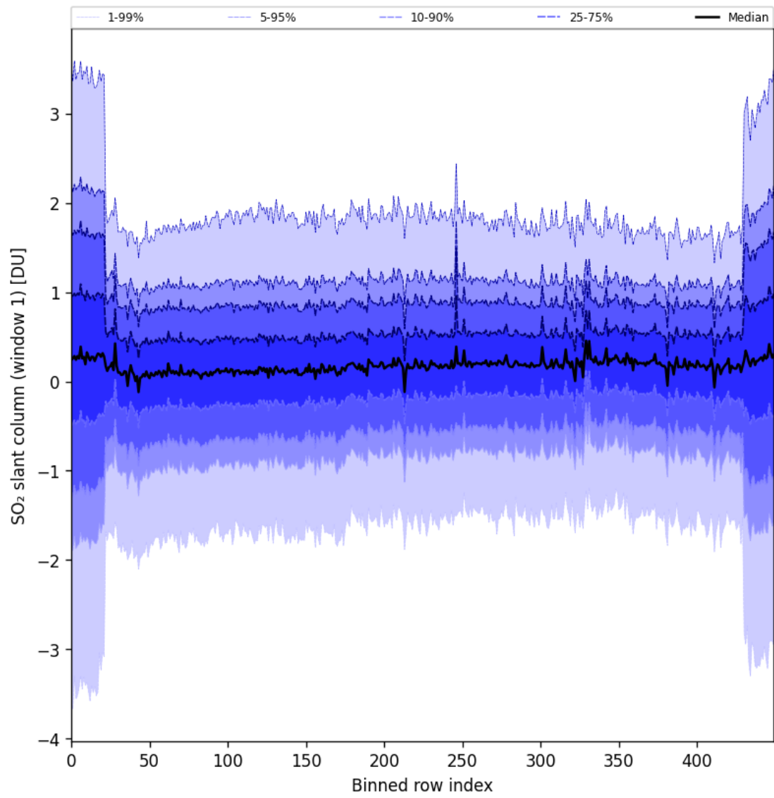
Figure 89: Along track statistics of “SO 2 slant column (window 1)” for 2025-09-17 to 2025-09-19
