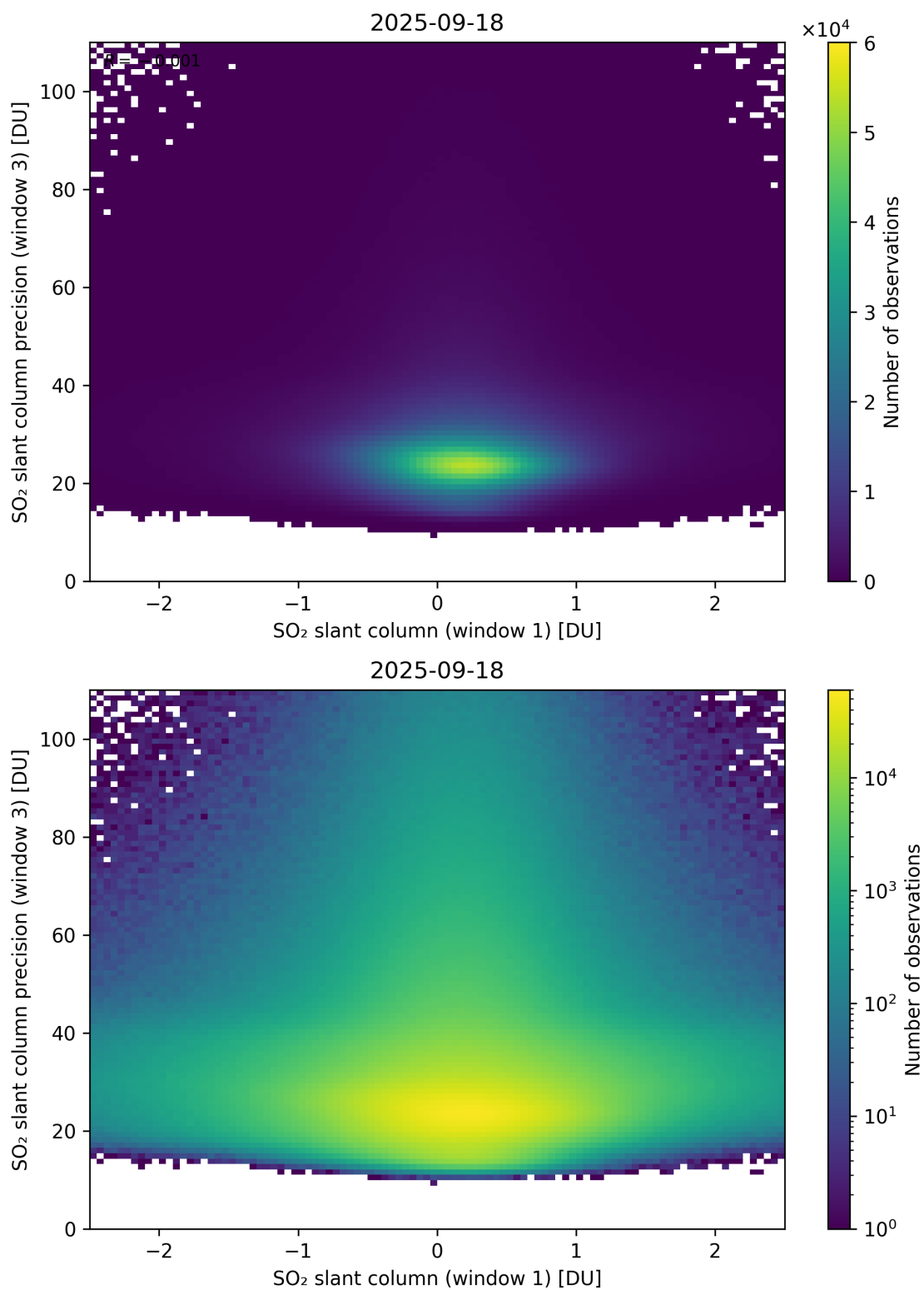
Figure 288: Scatter density plot of “SO 2 slant column (window 1)” against “SO 2 slant column precision (window 3)” for 2025-09-17 to 2025-09-19.
