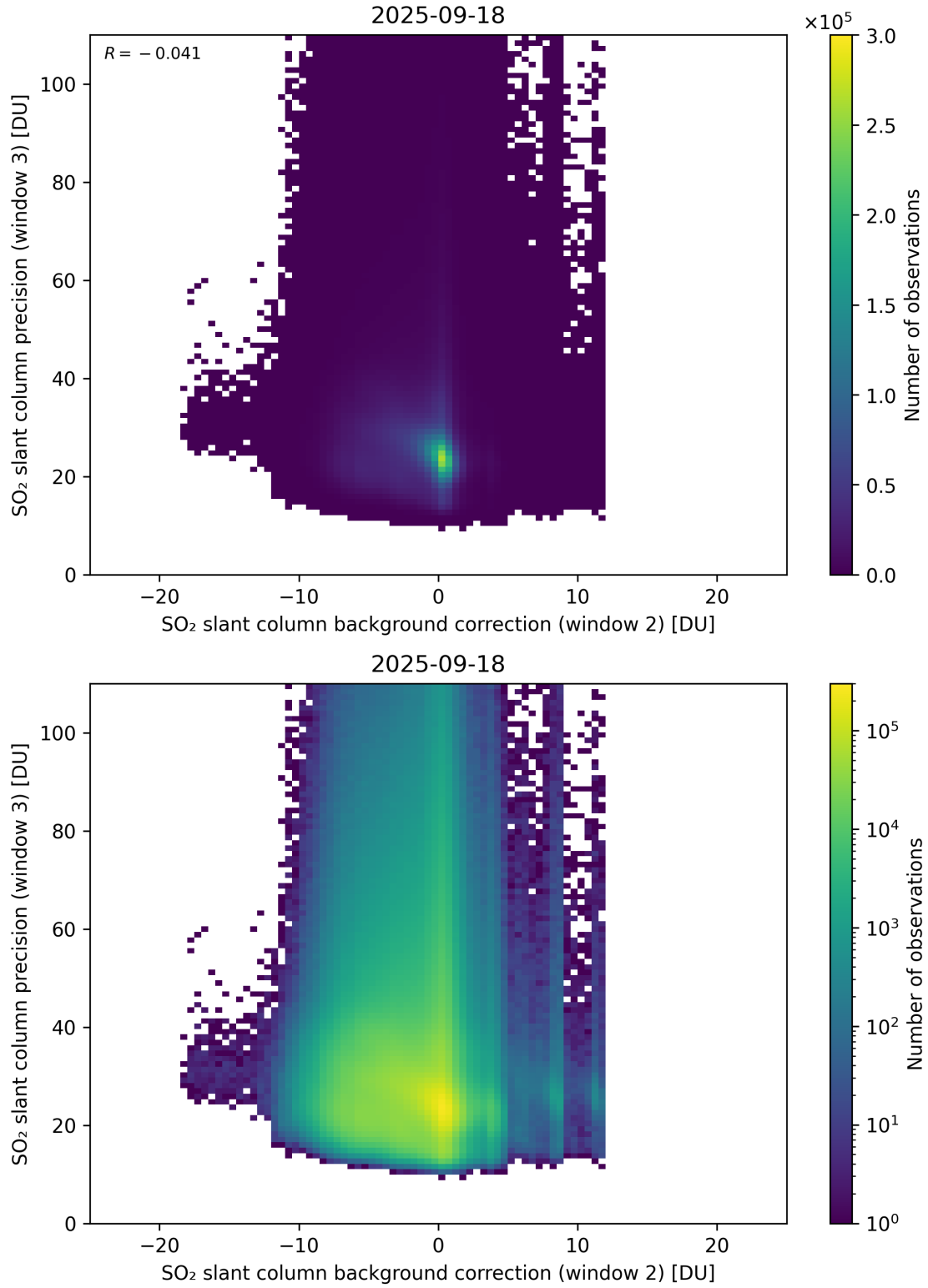
Figure 129: Scatter density plot of “SO 2 slant column background correction (window 2)” against “SO 2 slant column precision (window 3)” for 2025-09-17 to 2025-09-19.
