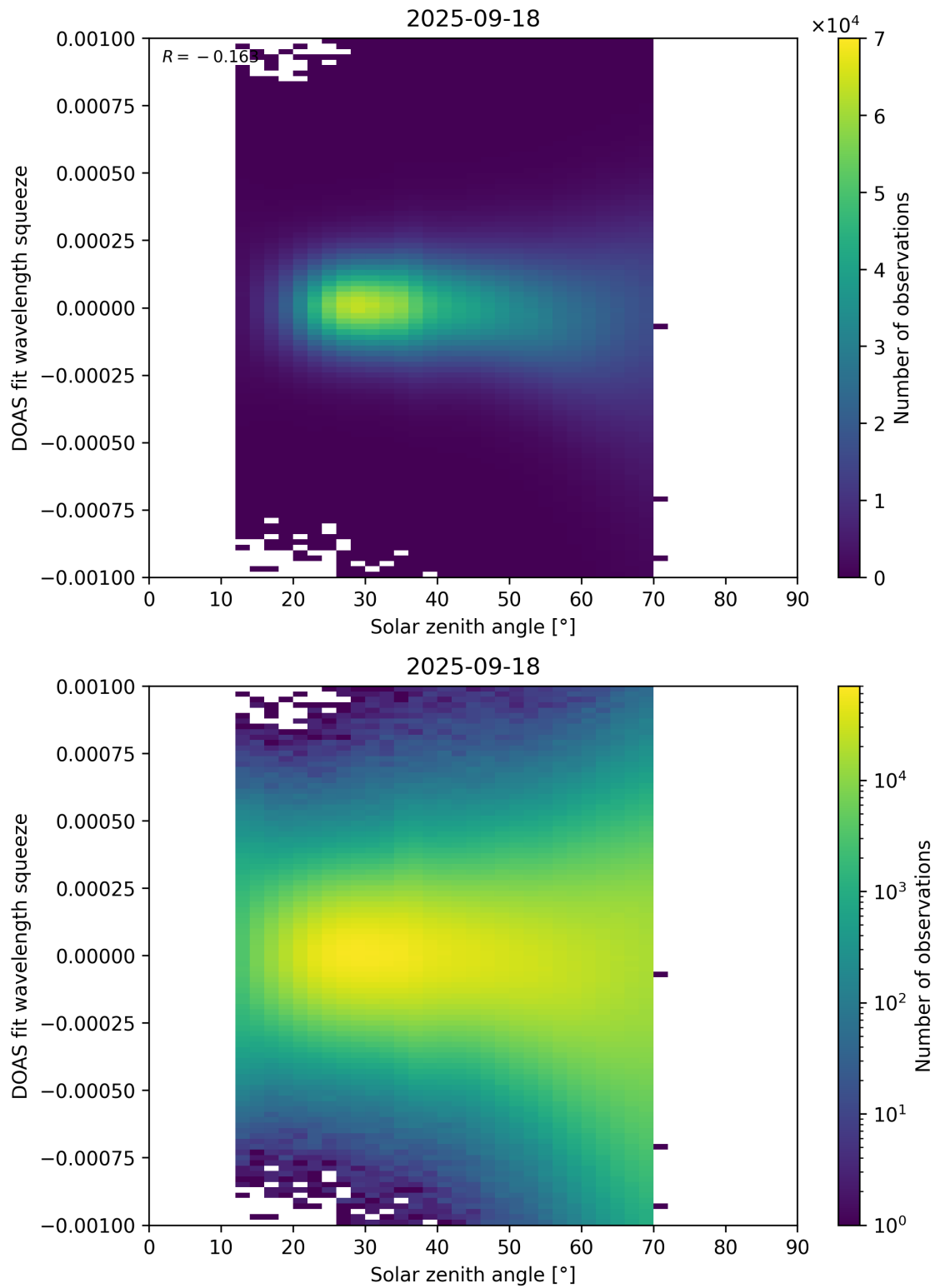
Figure 175: Scatter density plot of “Solar zenith angle” against “DOAS fit wavelength squeeze” for 2025-09-17 to 2025-09-19.
