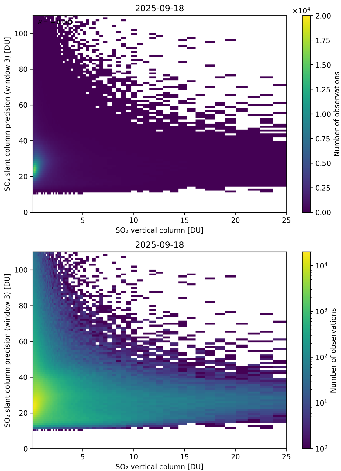
Figure 358: Scatter density plot of “SO 2 vertical column” against “SO 2 slant column precision (window 3)” for 2025-09-17 to 2025-09-19.
