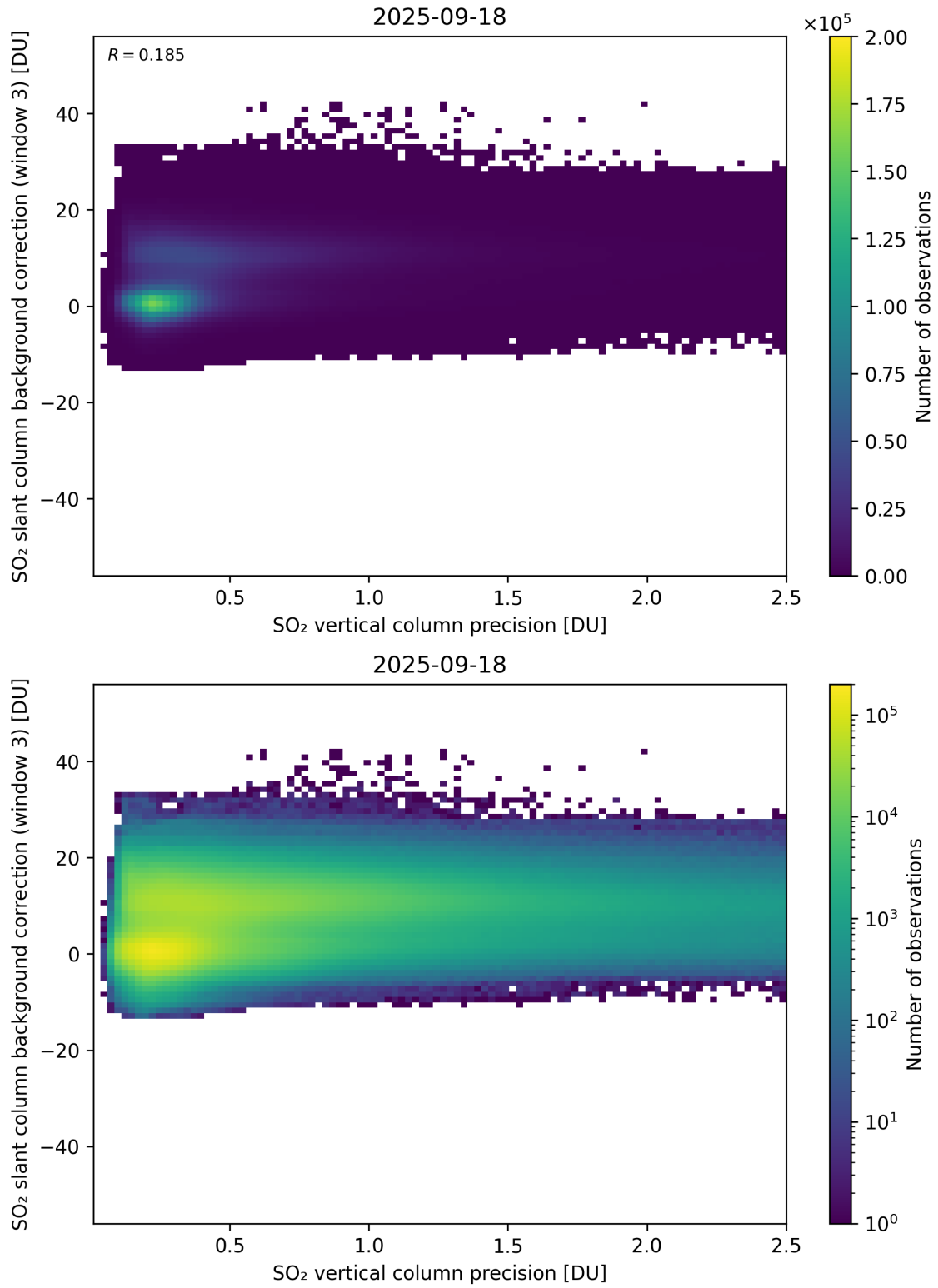
Figure 331: Scatter density plot of “SO 2 vertical column precision” against “SO 2 slant column background correction (window 3)” for 2025-09-17 to 2025-09-19.
