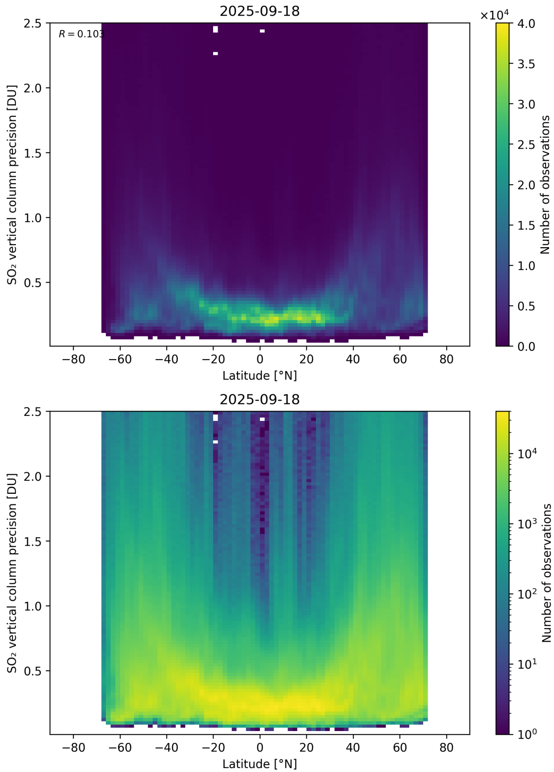
Figure 170: Scatter density plot of “Latitude” against “SO 2 vertical column precision” for 2025-09-17 to 2025-09-19.
