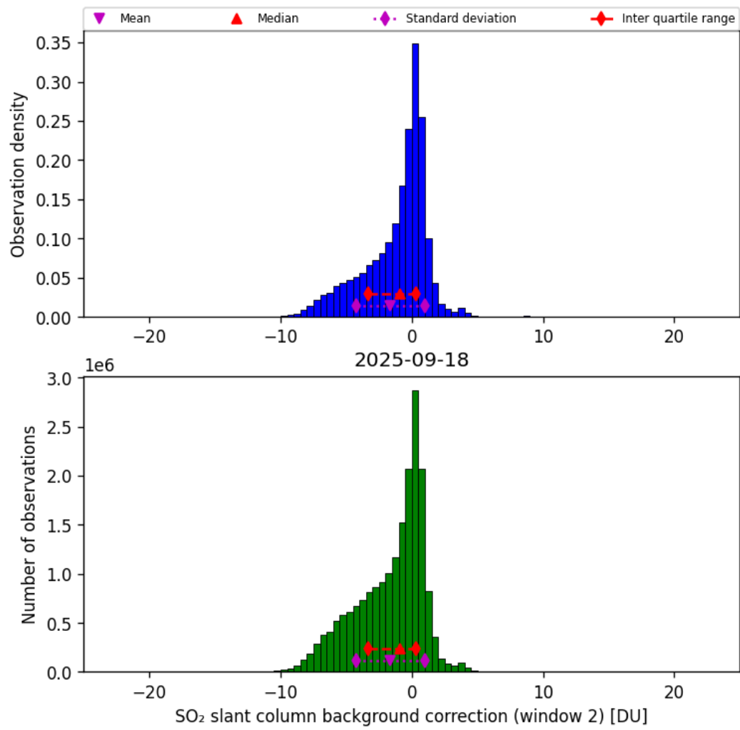
Figure 70: Histogram of “SO 2 slant column background correction (window 2)” for 2025-09-17 to 2025-09-19
