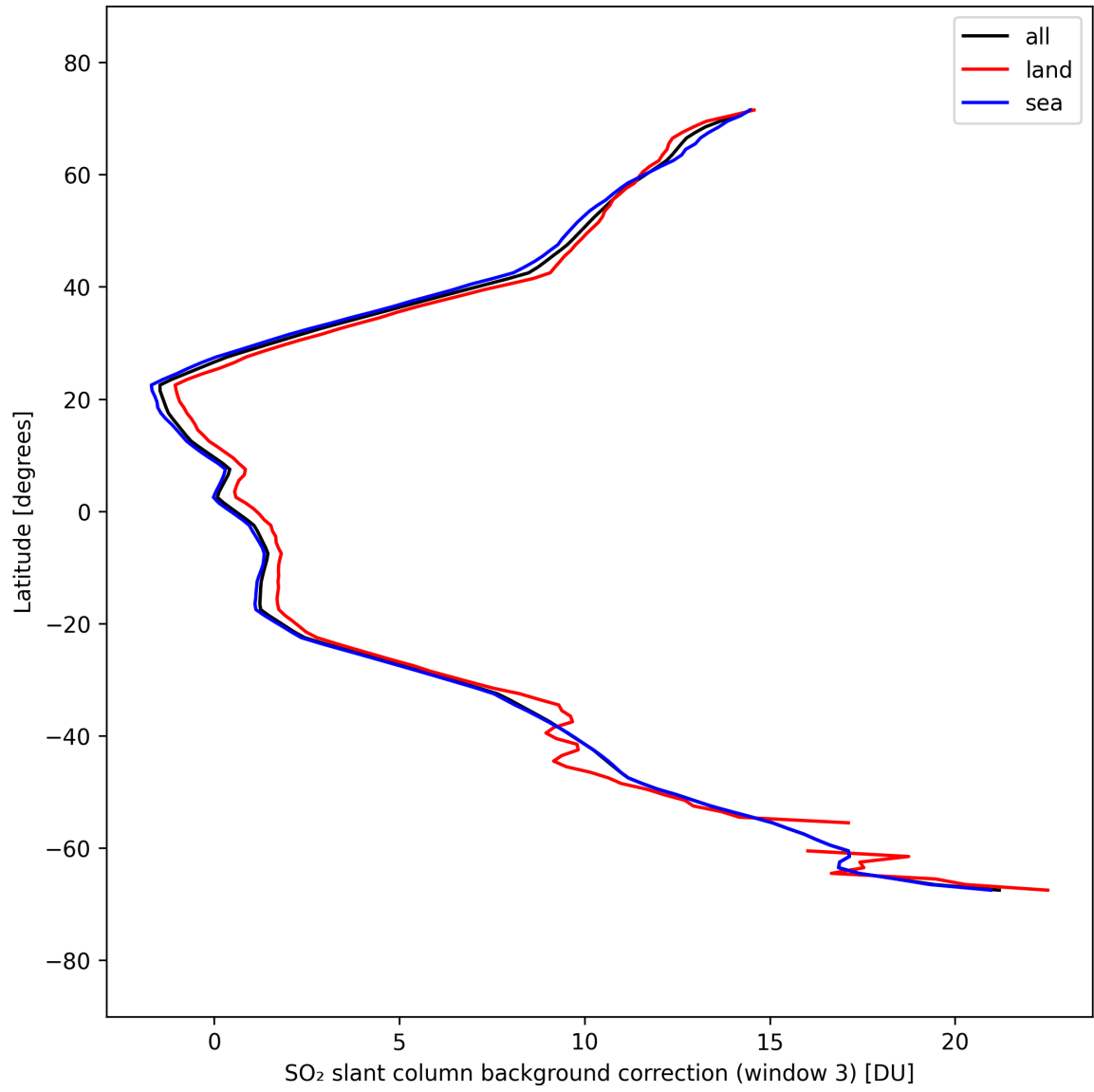
Figure 48: Zonal average of “SO 2 slant column background correction (window 3)” for 2025-09-17 to 2025-09-19.
