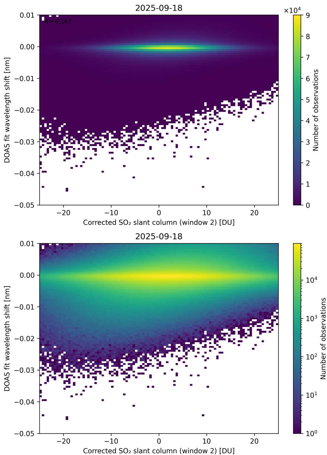
Figure 246: Scatter density plot of “Corrected SO 2 slant column (window 2)” against “DOAS fit wavelength shift” for 2025-09-17 to 2025-09-19.
