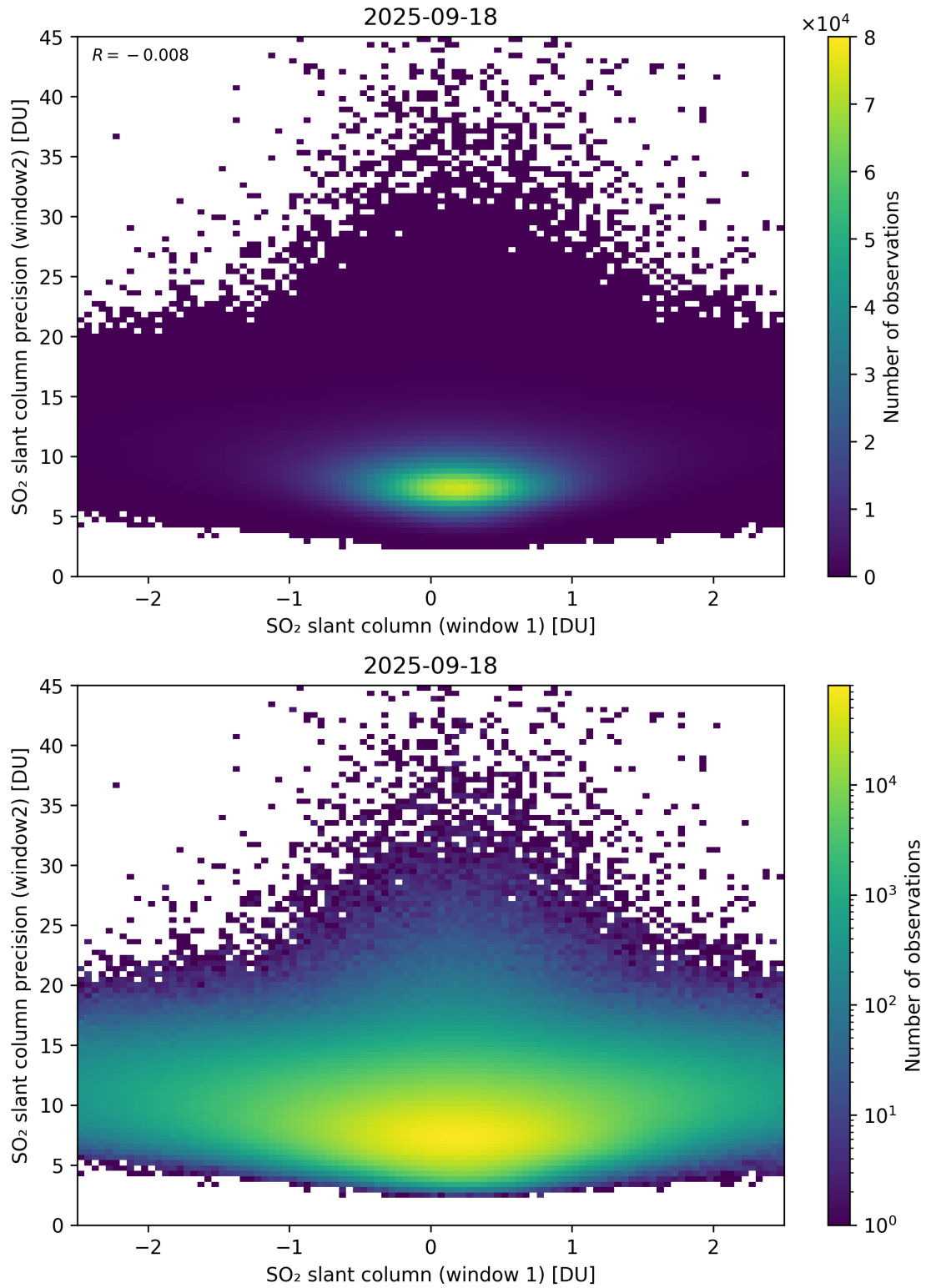
Figure 286: Scatter density plot of “SO 2 slant column (window 1)” against “SO 2 slant column precision (window2)” for 2025-09-17 to 2025-09-19.
