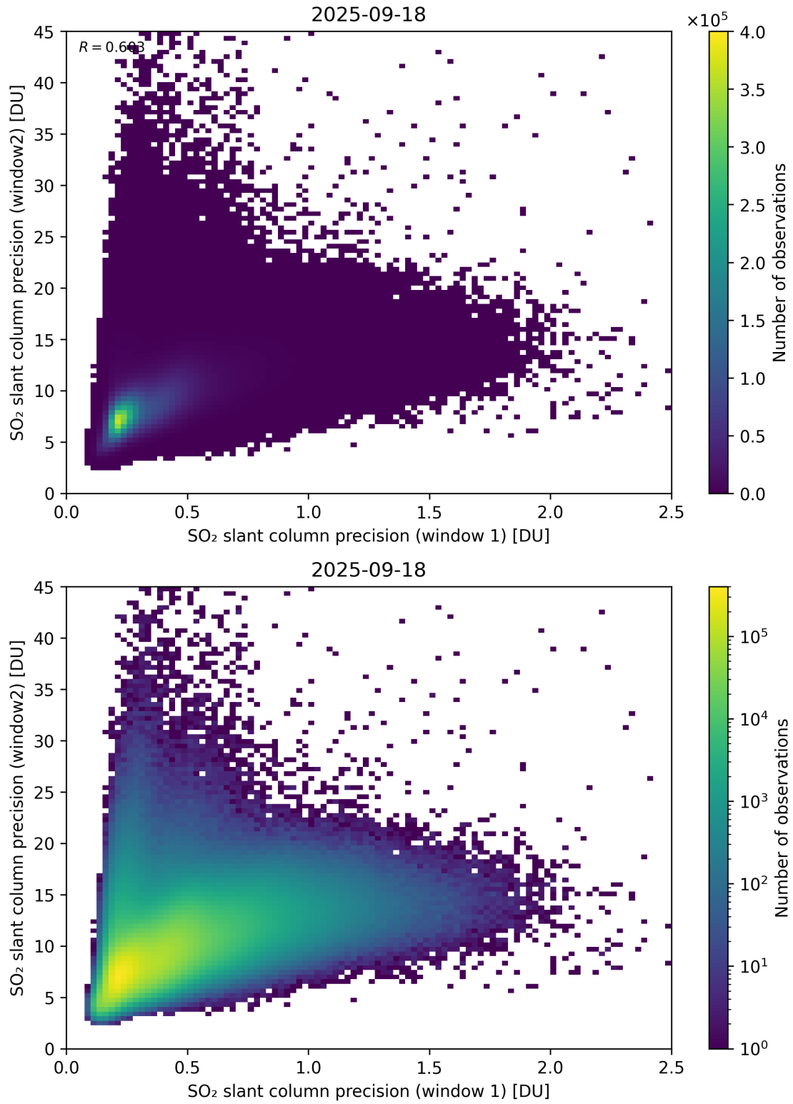
Figure 277: Scatter density plot of “SO 2 slant column precision (window 1)” against “SO 2 slant column precision (window2)” for 2025-09-17 to 2025-09-19.
