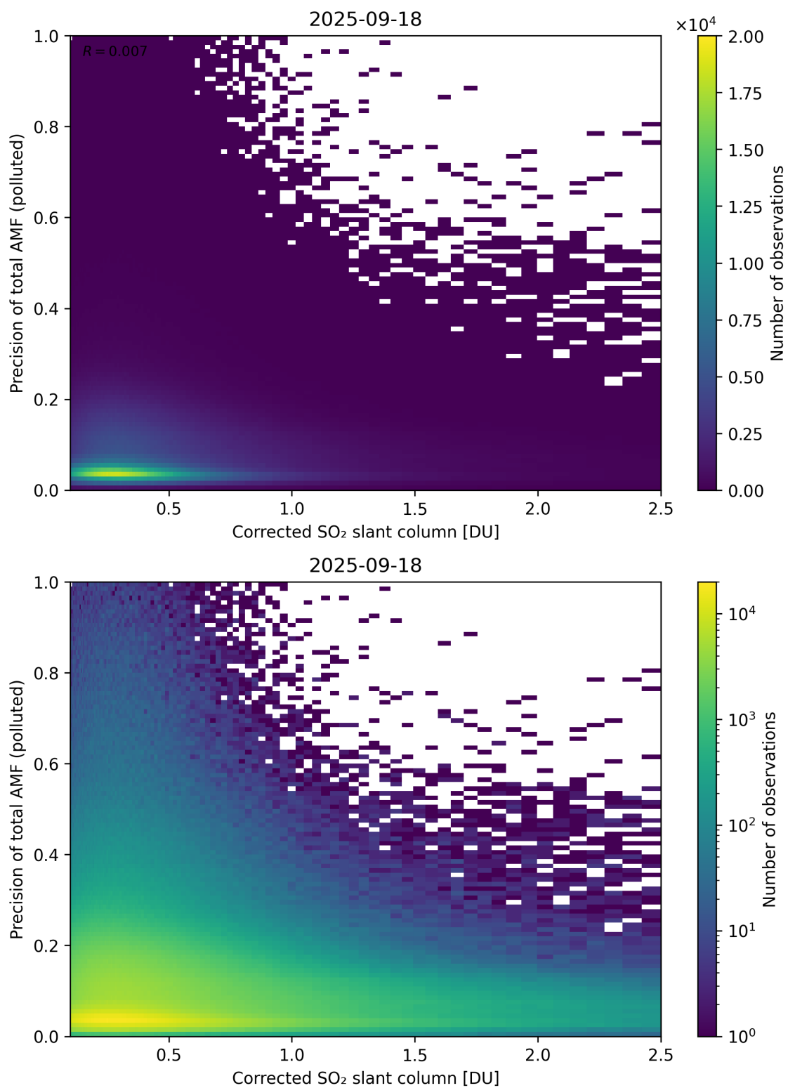
Figure 243: Scatter density plot of “Corrected SO 2 slant column” against “Precision of total AMF (polluted)” for 2025-09-17 to 2025-09-19.
