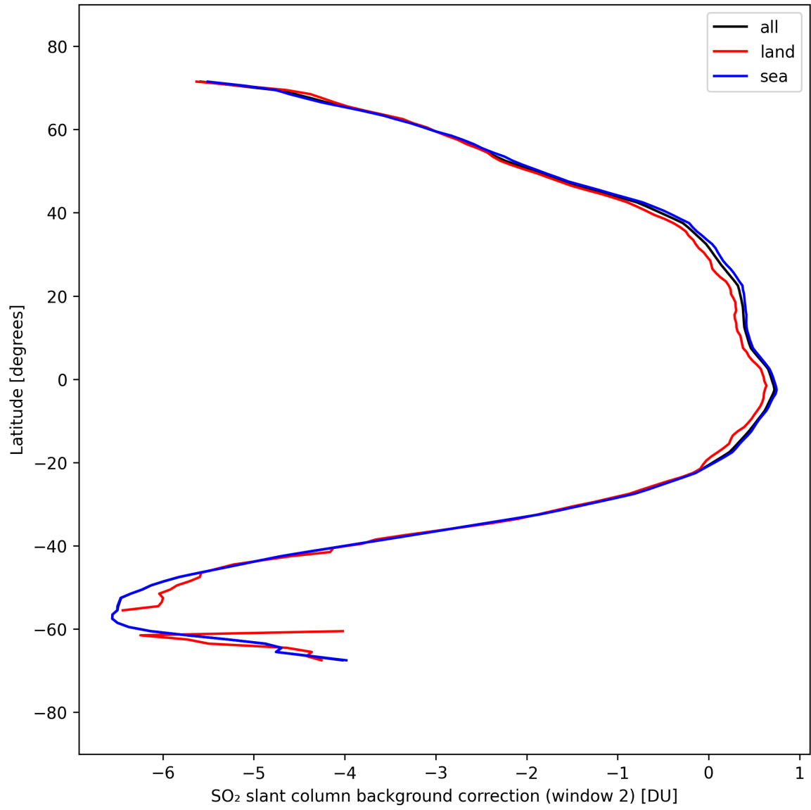
Figure 44: Zonal average of “SO 2 slant column background correction (window 2)” for 2025-09-17 to 2025-09-19.
