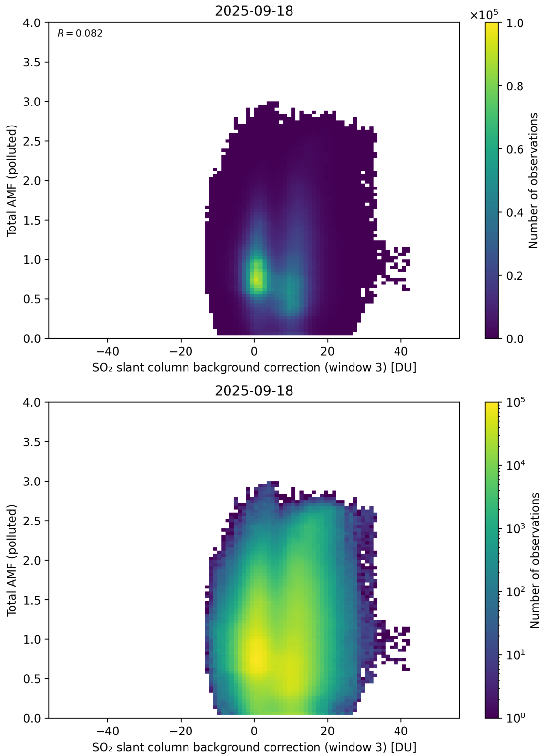
Figure 136: Scatter density plot of “SO 2 slant column background correction (window 3)” against “Total AMF (polluted)” for 2025-09-17 to 2025-09-19.
