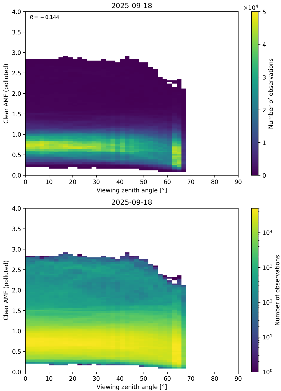
Figure 370: Scatter density plot of “Viewing zenith angle” against “Clear AMF (polluted)” for 2025-09-17 to 2025-09-19.
