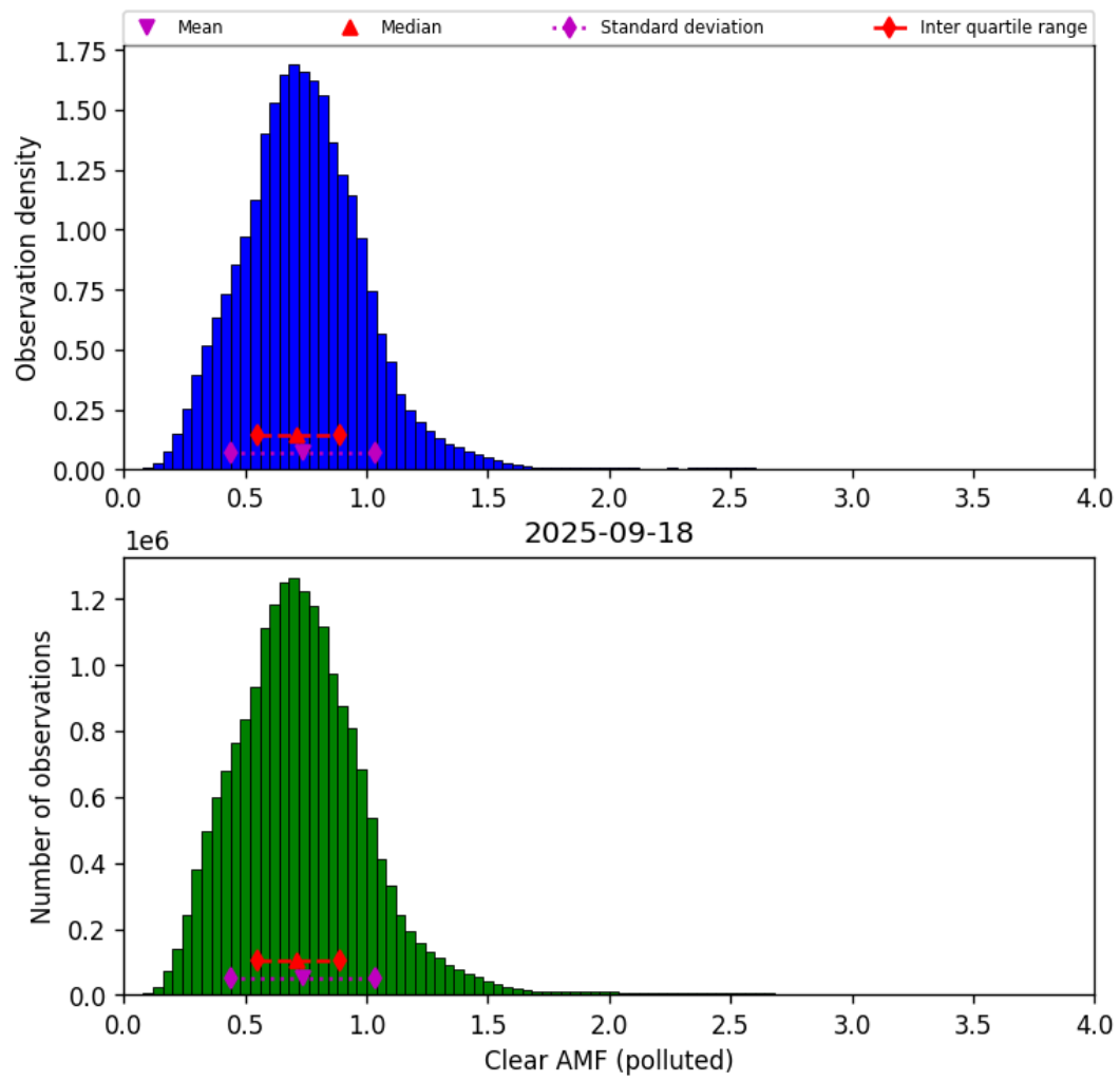
Figure 81: Histogram of “Clear AMF (polluted)” for 2025-09-17 to 2025-09-19
