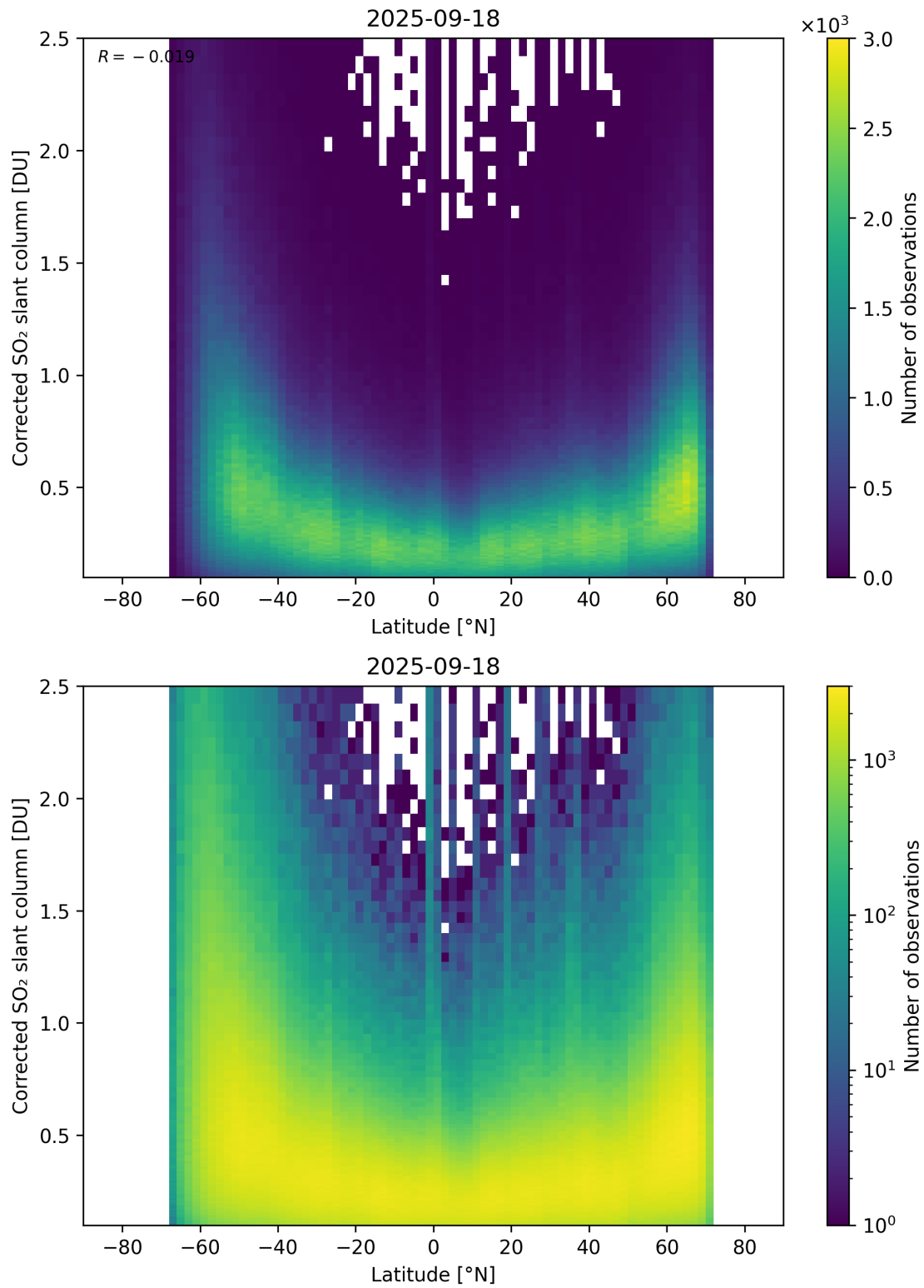
Figure 159: Scatter density plot of “Latitude” against “Corrected SO 2 slant column” for 2025-09-17 to 2025-09-19.
