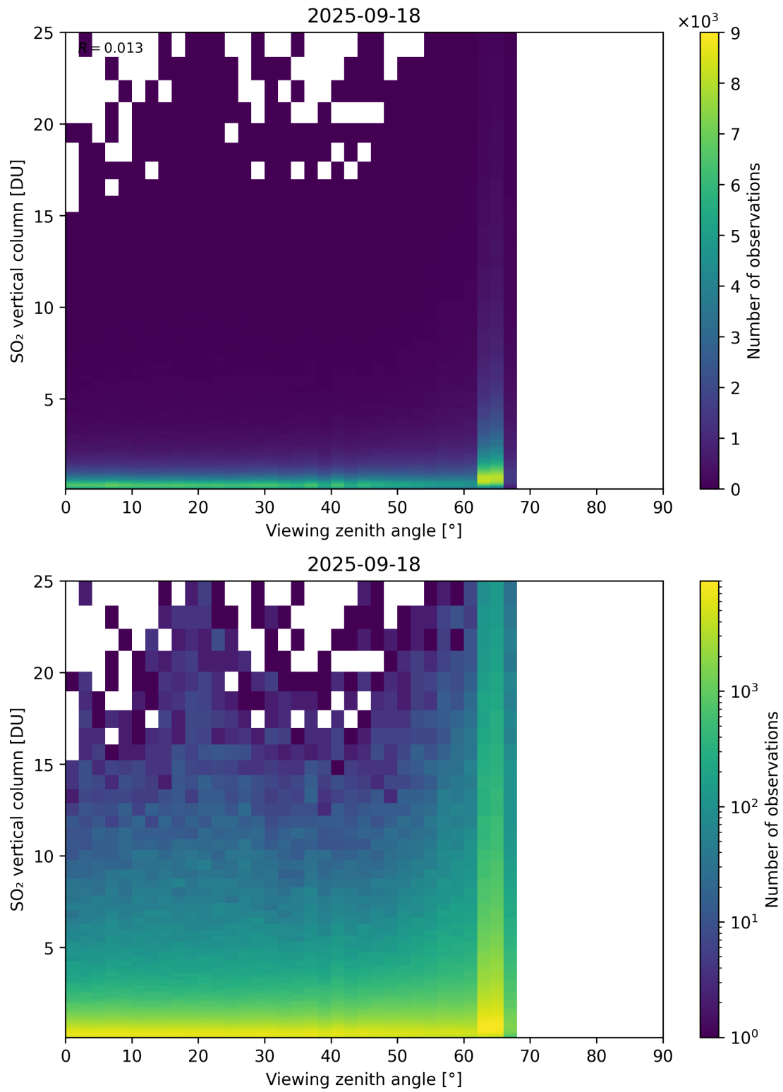
Figure 383: Scatter density plot of “Viewing zenith angle” against “SO 2 vertical column” for 2025-09-17 to 2025-09-19.
