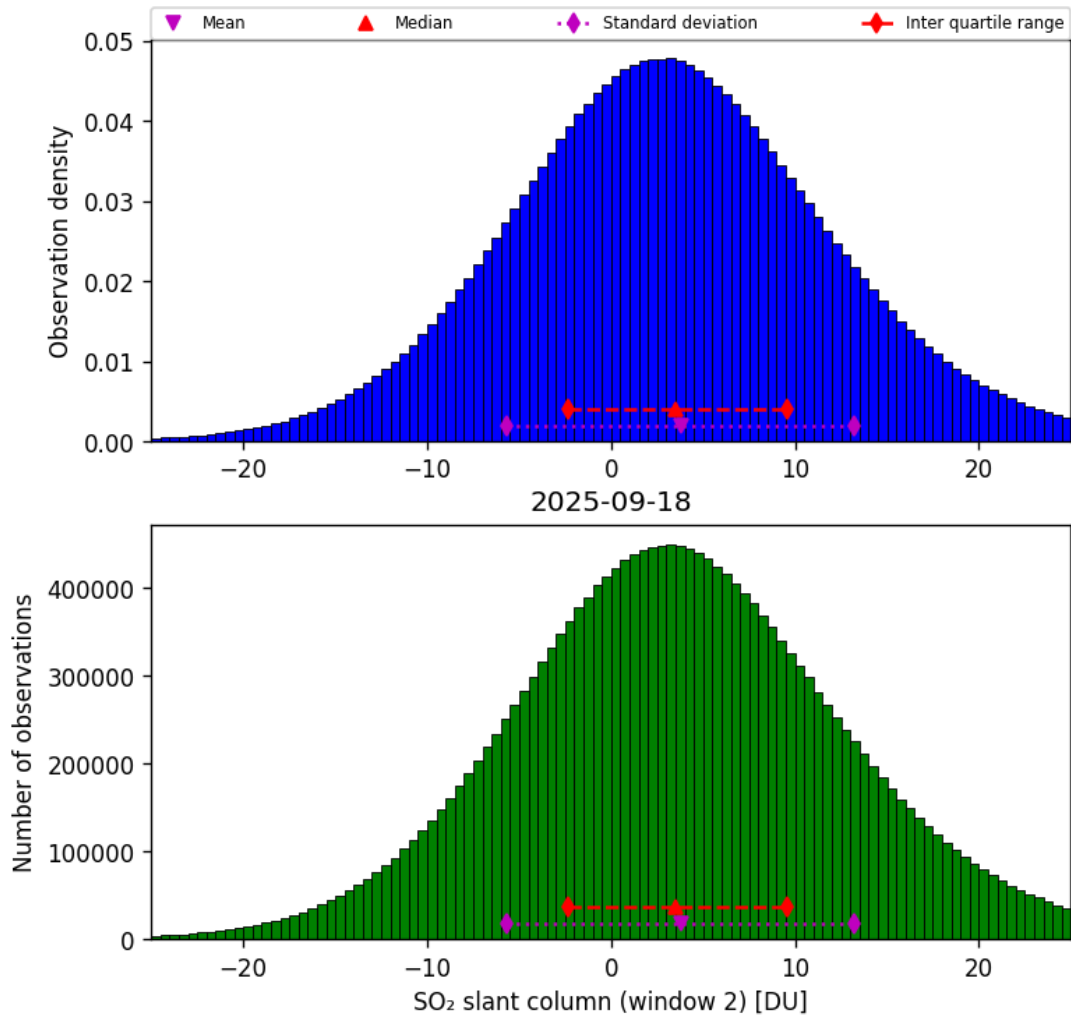
Figure 67: Histogram of “SO 2 slant column (window 2)” for 2025-09-17 to 2025-09-19
