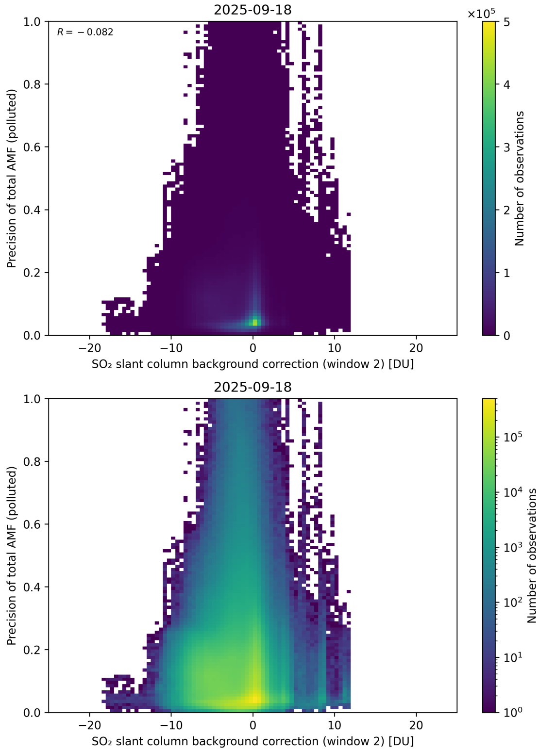
Figure 131: Scatter density plot of “SO 2 slant column background correction (window 2)” against “Precision of total AMF (polluted)” for 2025-09-17 to 2025-09-19.
