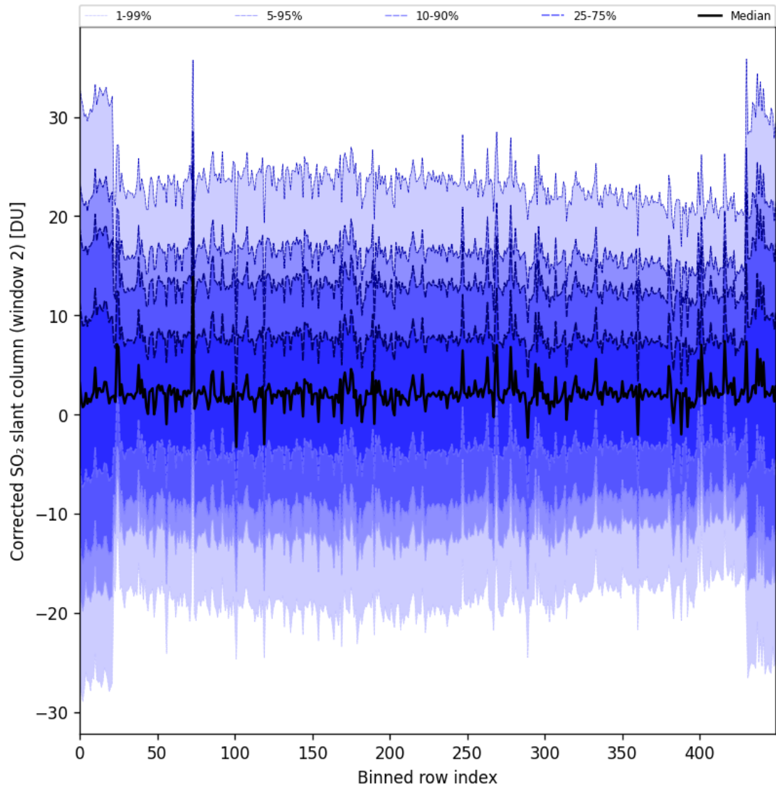
Figure 95: Along track statistics of “Corrected SO 2 slant column (window 2)” for 2025-09-17 to 2025-09-19
