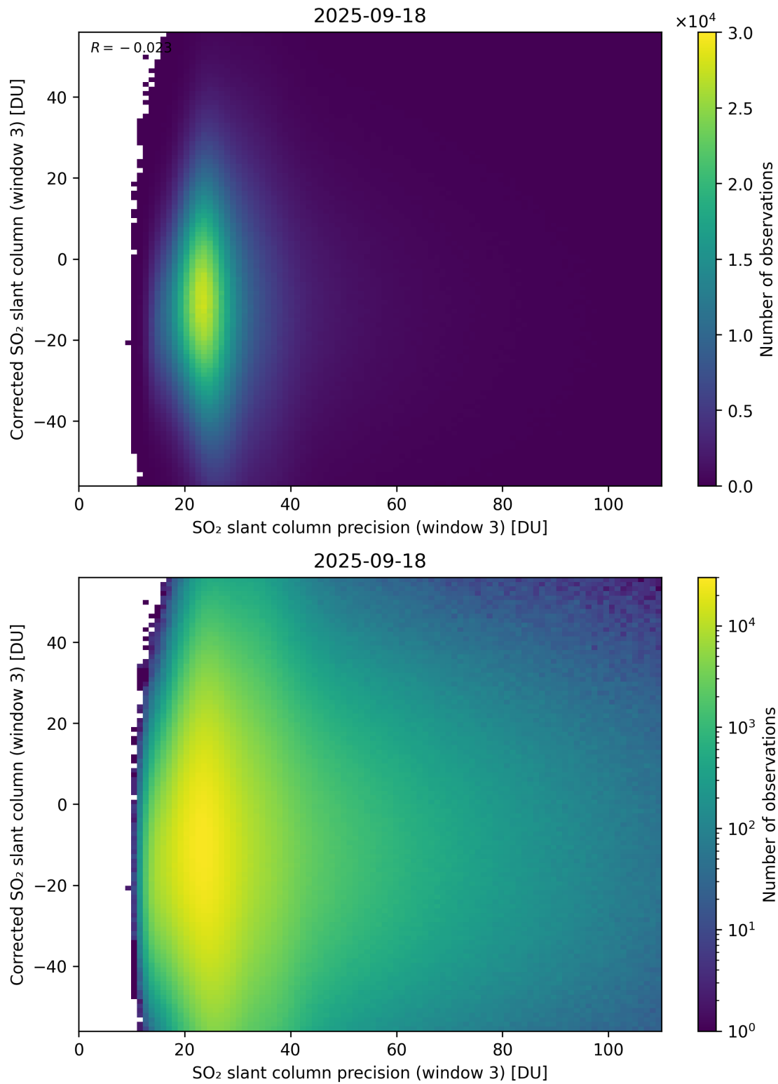
Figure 312: Scatter density plot of “SO 2 slant column precision (window 3)” against “Corrected SO 2 slant column (window 3)” for 2025-09-17 to 2025-09-19.
