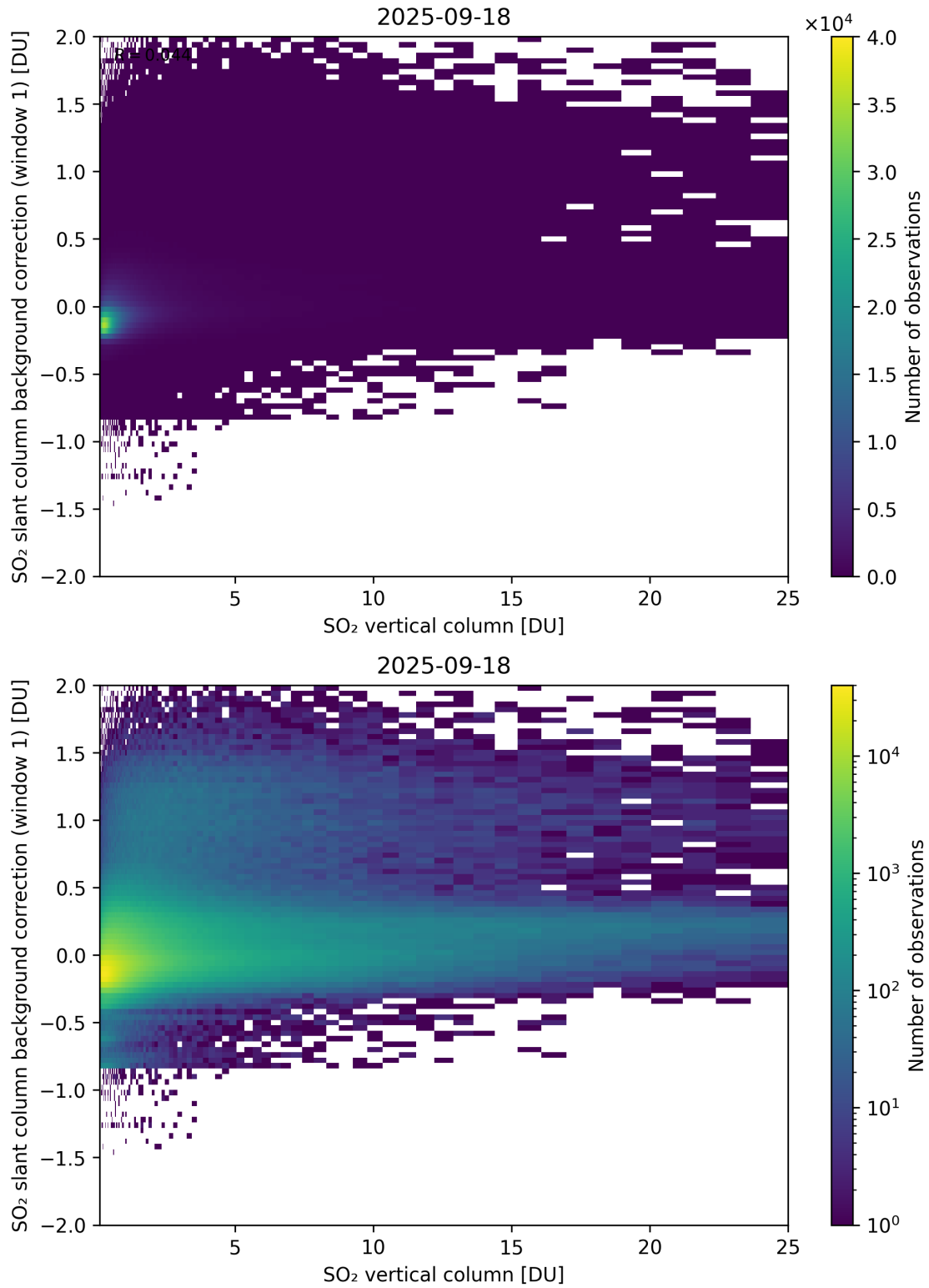
Figure 323: Scatter density plot of “SO 2 vertical column” against “SO 2 slant column background correction (window 1)” for 2025-09-17 to 2025-09-19.
