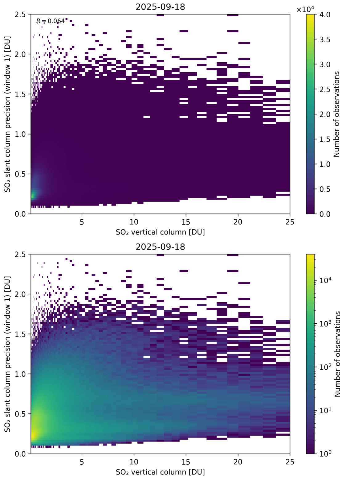
Figure 355: Scatter density plot of “SO 2 vertical column” against “SO 2 slant column precision (window 1)” for 2025-09-17 to 2025-09-19.
