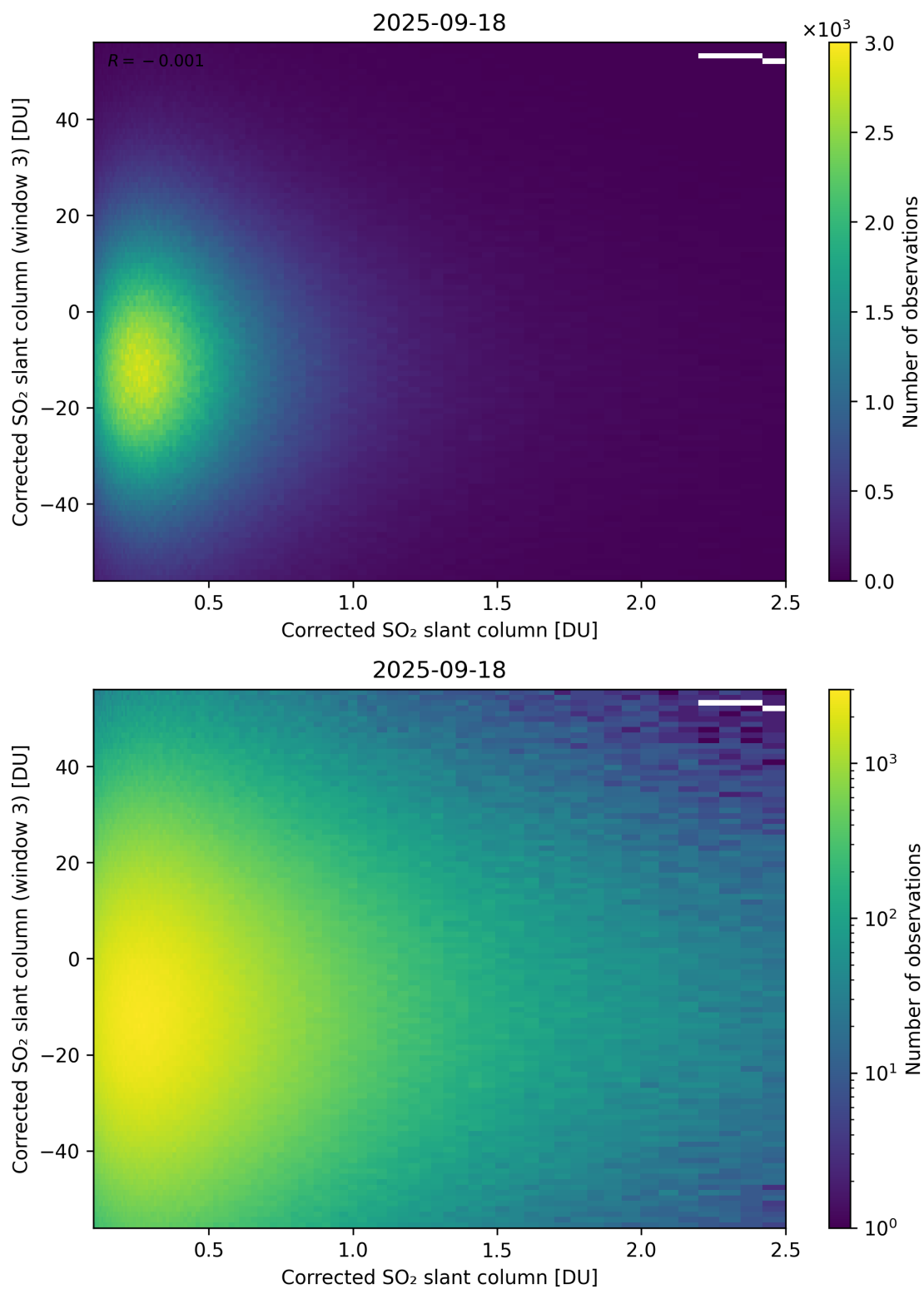
Figure 236: Scatter density plot of “Corrected SO 2 slant column” against “Corrected SO 2 slant column (window 3)” for 2025-09-17 to 2025-09-19.
