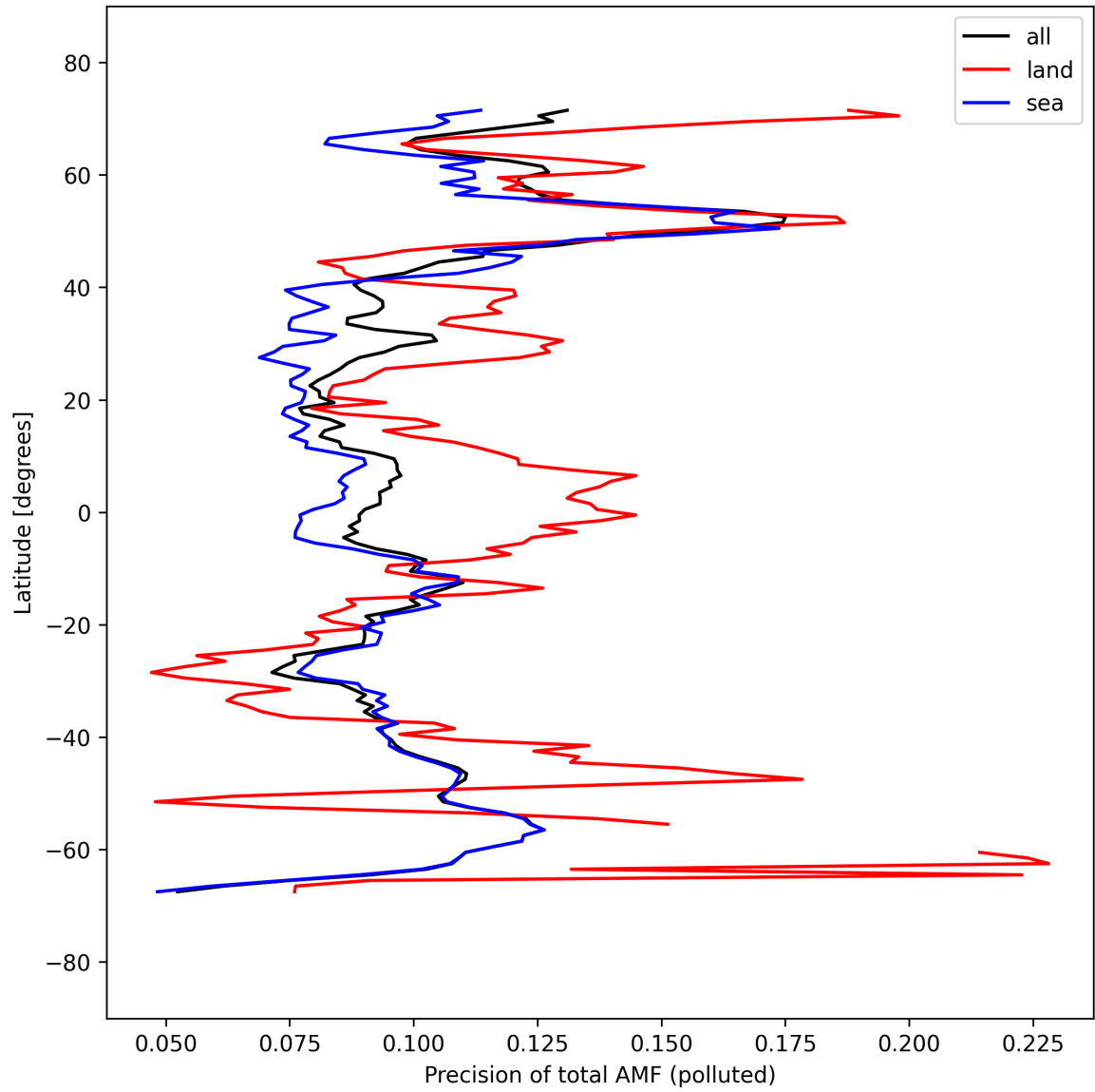
Figure 54: Zonal average of “Precision of total AMF (polluted)” for 2025-09-17 to 2025-09-19.
