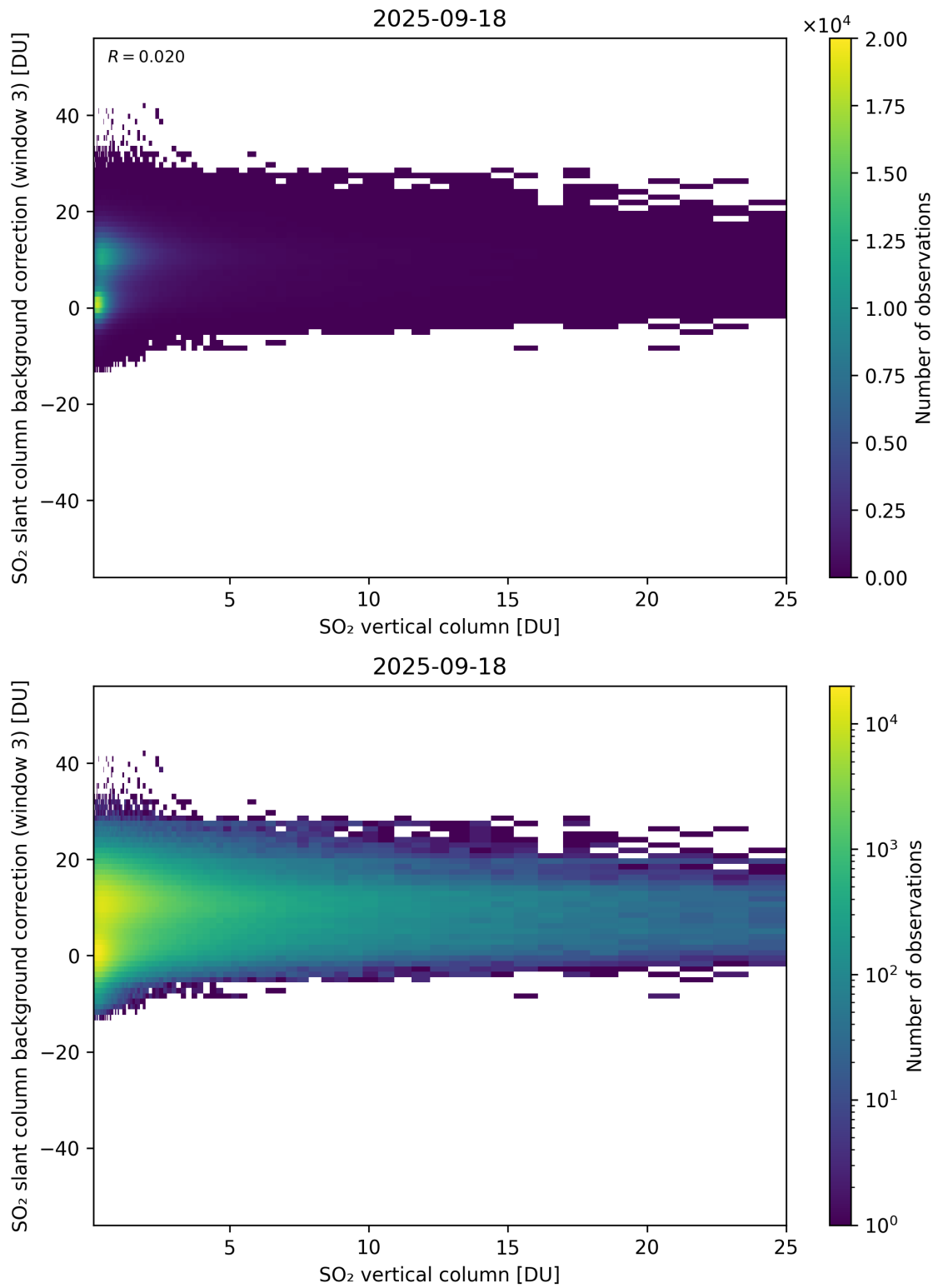
Figure 325: Scatter density plot of “SO 2 vertical column” against “SO 2 slant column background correction (window 3)” for 2025-09-17 to 2025-09-19.
