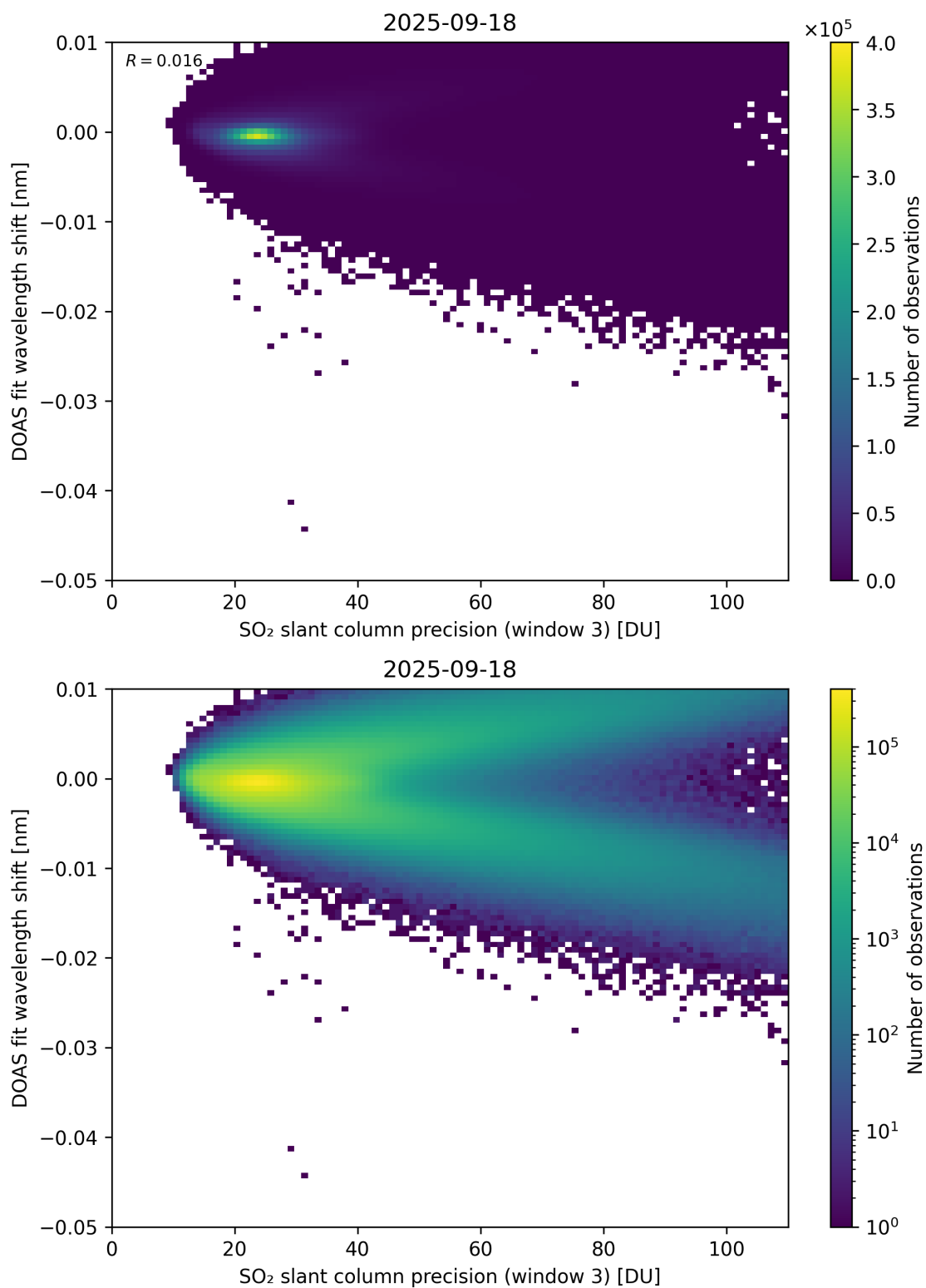
Figure 308: Scatter density plot of “SO 2 slant column precision (window 3)” against “DOAS fit wavelength shift” for 2025-09-17 to 2025-09-19.
