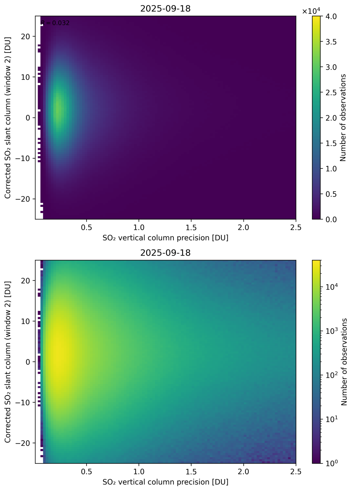
Figure 339: Scatter density plot of “SO 2 vertical column precision” against “Corrected SO 2 slant column (window 2)” for 2025-09-17 to 2025-09-19.
