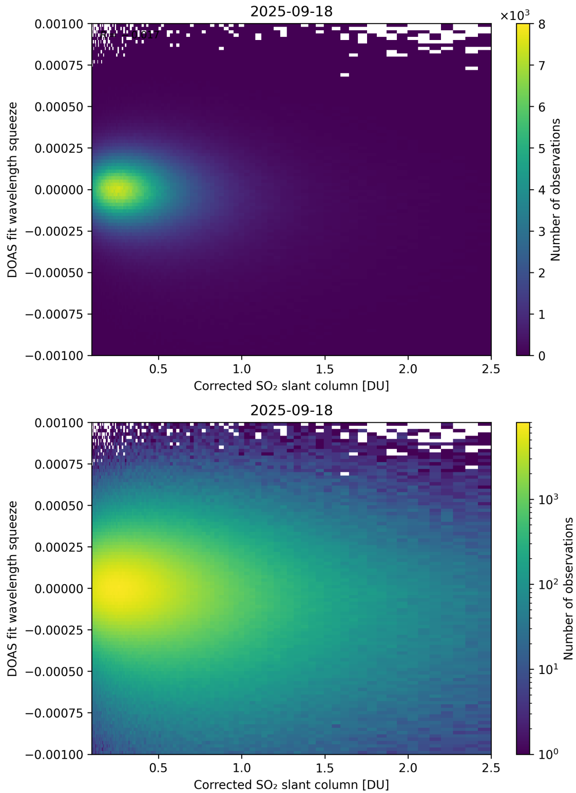
Figure 230: Scatter density plot of “Corrected SO 2 slant column” against “DOAS fit wavelength squeeze” for 2025-09-17 to 2025-09-19.
