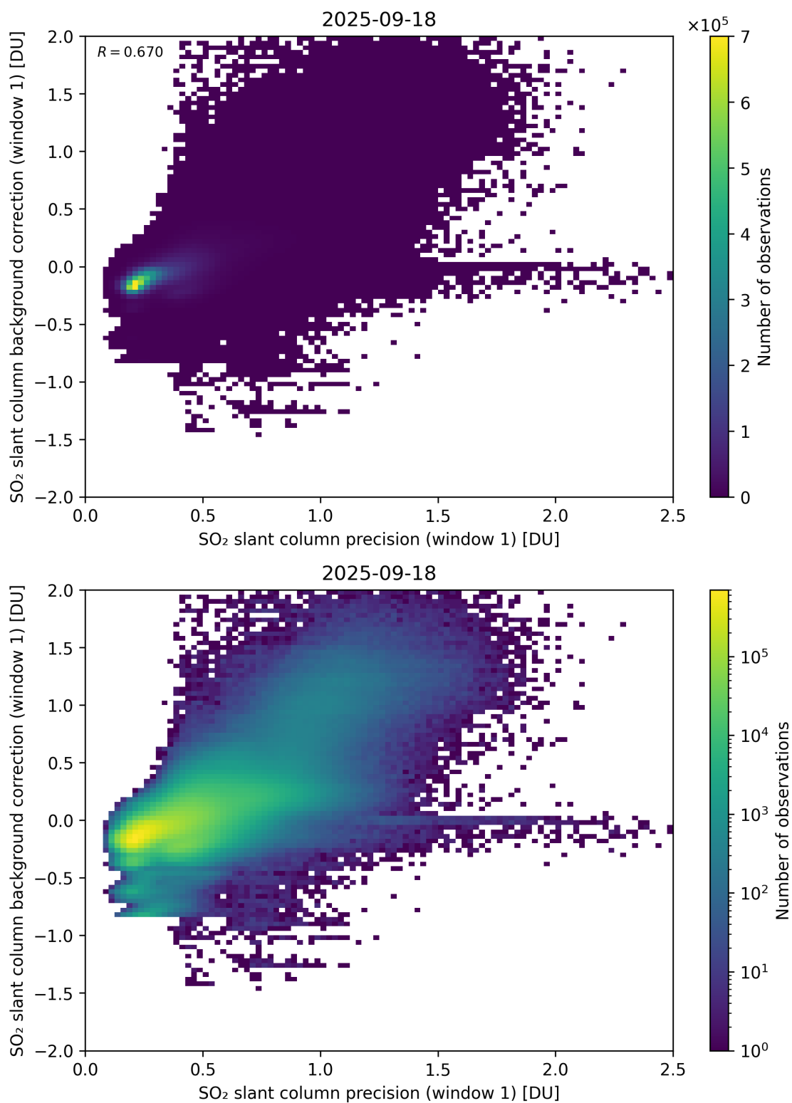
Figure 268: Scatter density plot of “SO 2 slant column precision (window 1)” against “SO 2 slant column background correction (window 1)” for 2025-09-17 to 2025-09-19.
