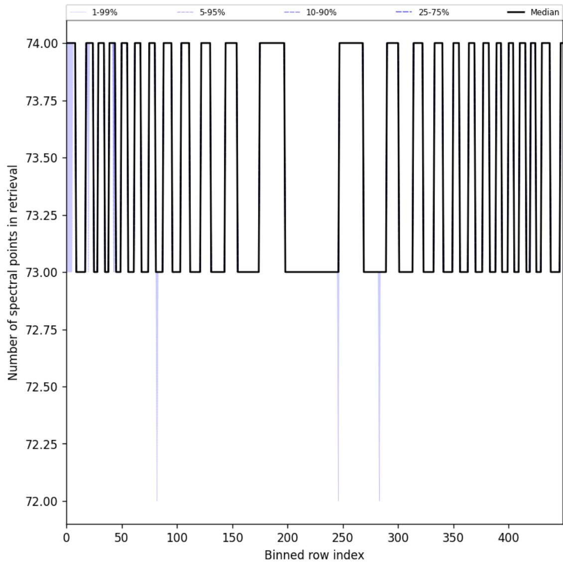
Figure 108: Along track statistics of “Number of spectral points in retrieval” for 2025-09-17 to 2025-09-19
