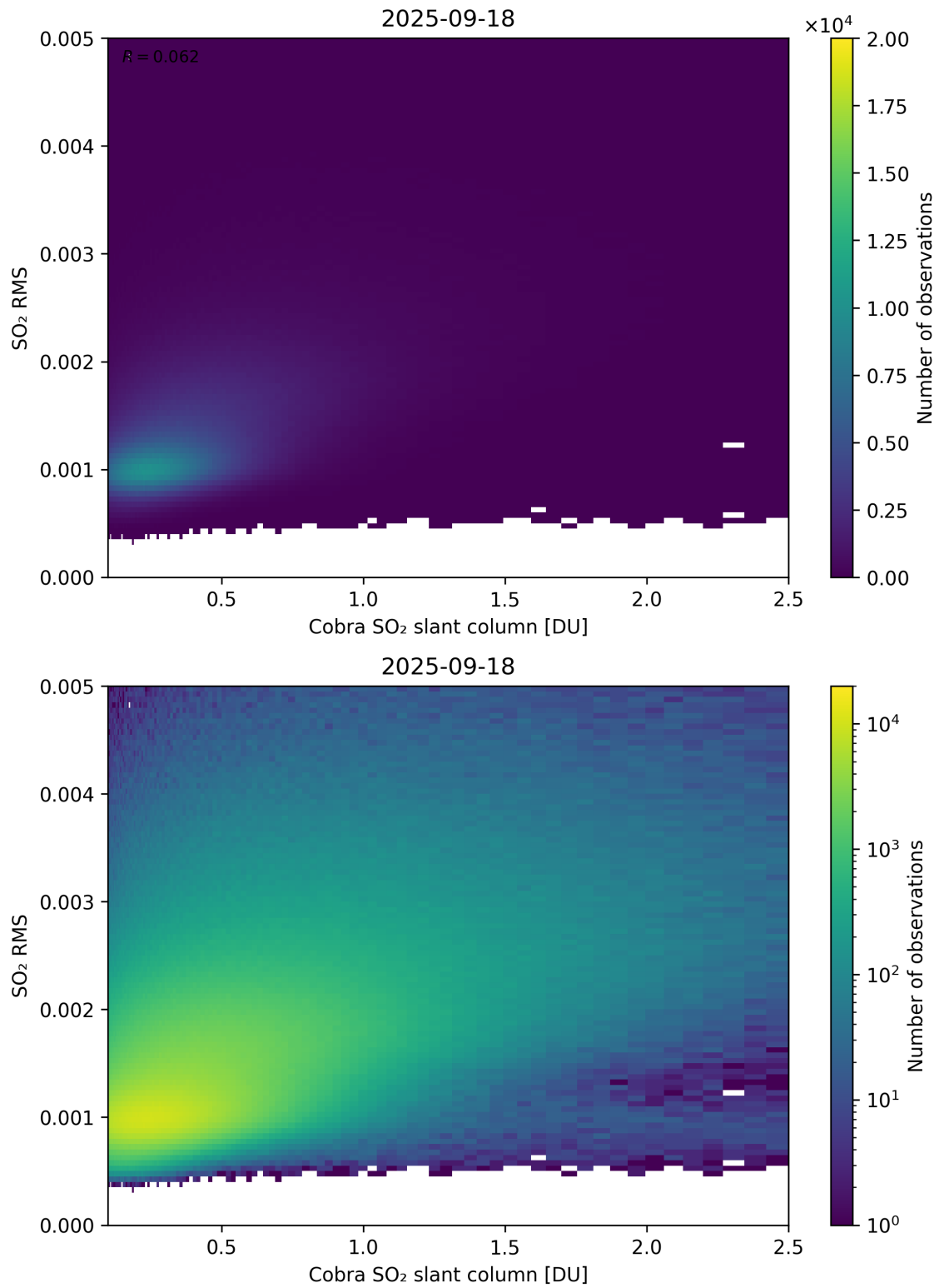
Figure 198: Scatter density plot of “Cobra SO 2 slant column” against “SO 2 RMS” for 2025-09-17 to 2025-09-19.
