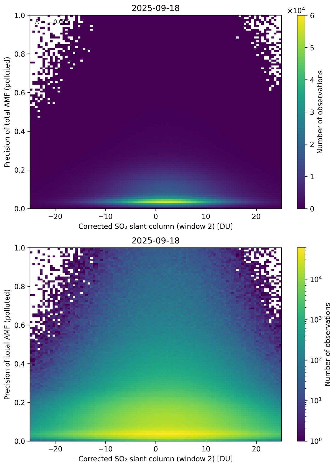
Figure 254: Scatter density plot of “Corrected SO 2 slant column (window 2)” against “Precision of total AMF (polluted)” for 2025-09-17 to 2025-09-19.
