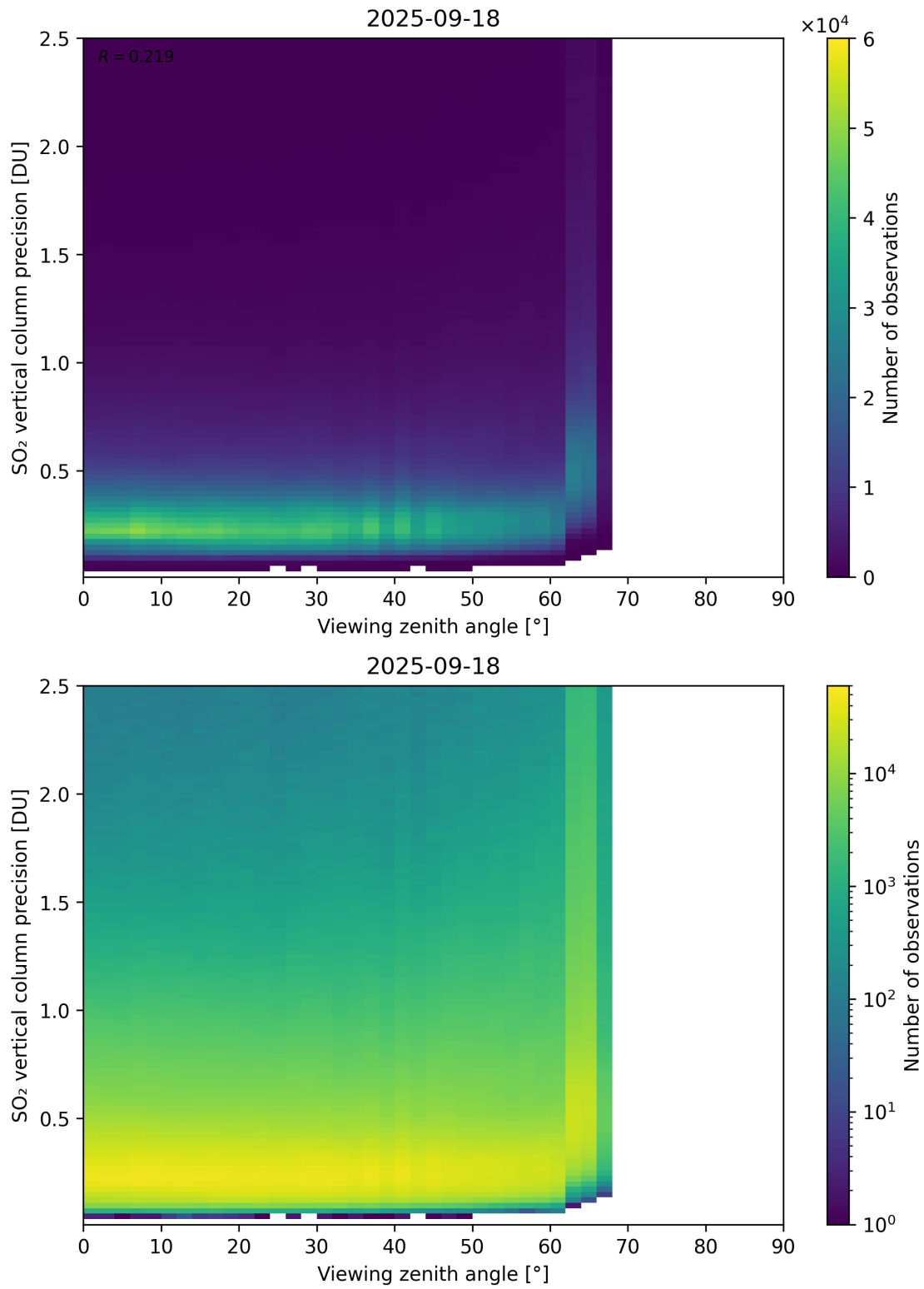
Figure 384: Scatter density plot of “Viewing zenith angle” against “SO 2 vertical column precision” for 2025-09-17 to 2025-09-19.
