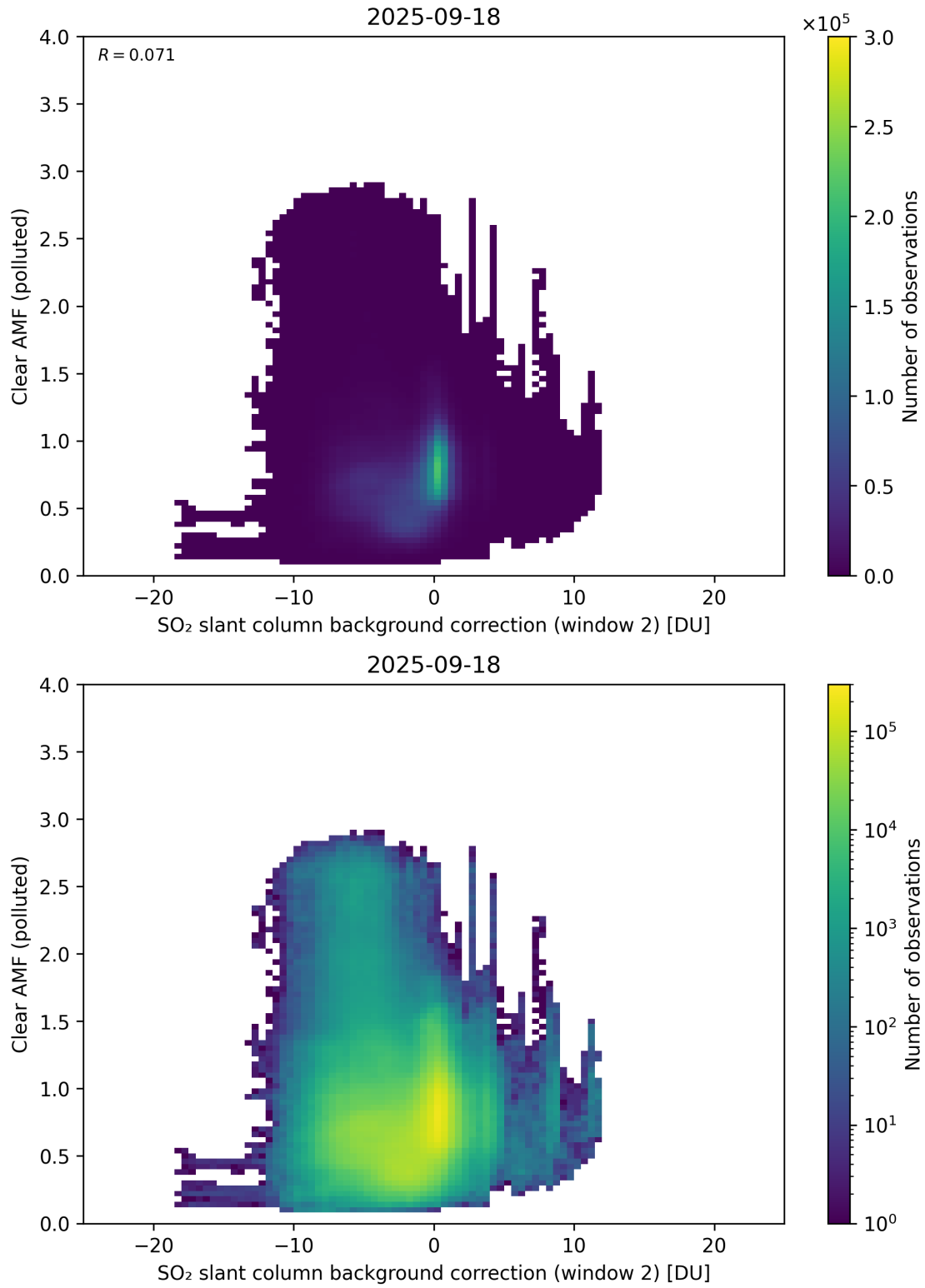
Figure 126: Scatter density plot of “SO 2 slant column background correction (window 2)” against “Clear AMF (polluted)” for 2025-09-17 to 2025-09-19.
