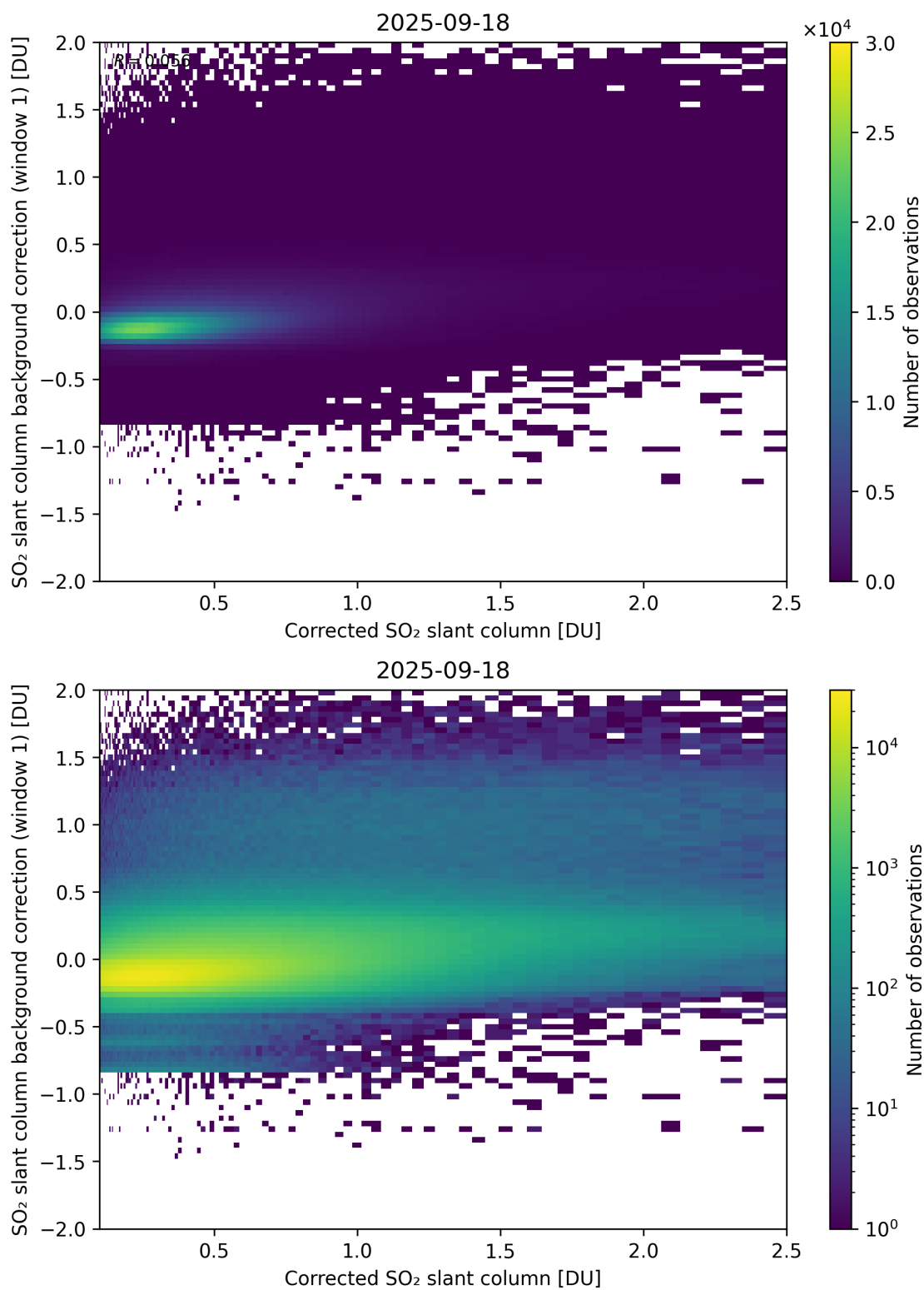
Figure 226: Scatter density plot of “Corrected SO 2 slant column” against “SO 2 slant column background correction (window 1)” for 2025-09-17 to 2025-09-19.
