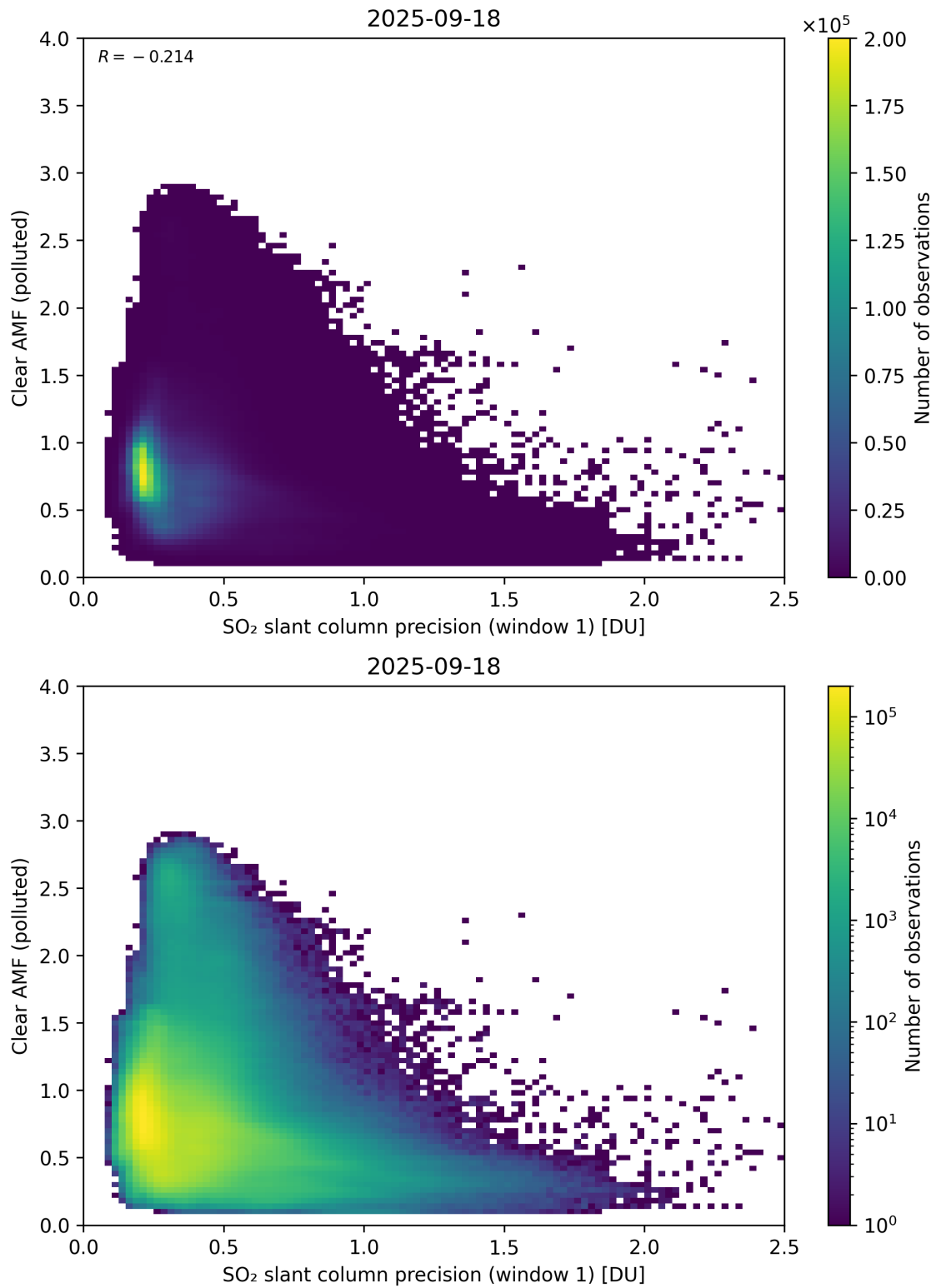
Figure 274: Scatter density plot of “SO 2 slant column precision (window 1)” against “Clear AMF (polluted)” for 2025-09-17 to 2025-09-19.
