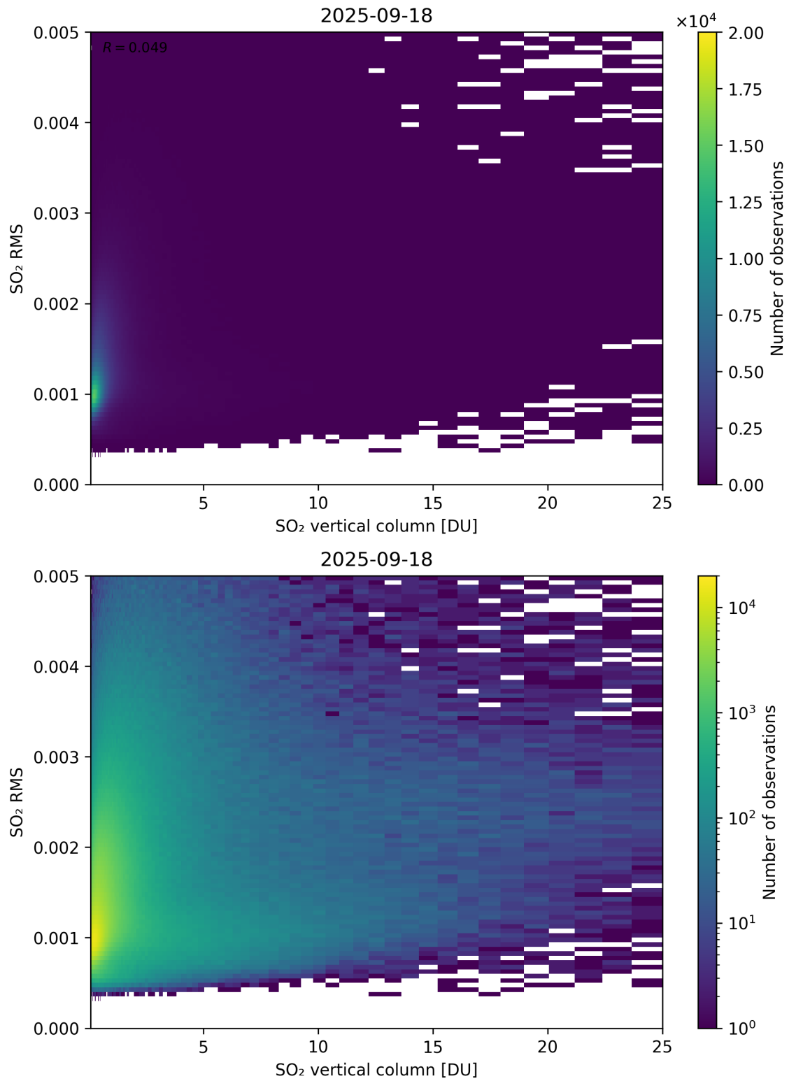
Figure 328: Scatter density plot of “SO 2 vertical column” against “SO 2 RMS” for 2025-09-17 to 2025-09-19.
