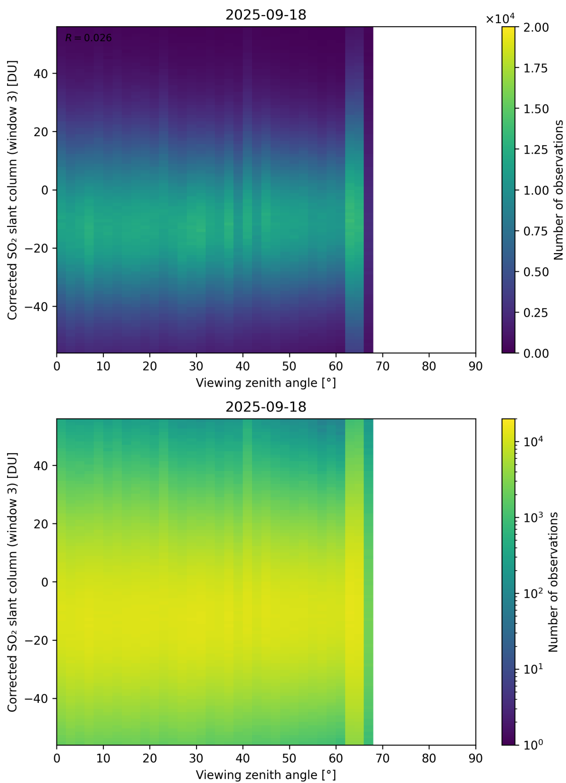
Figure 375: Scatter density plot of “Viewing zenith angle” against “Corrected SO 2 slant column (window 3)” for 2025-09-17 to 2025-09-19.
