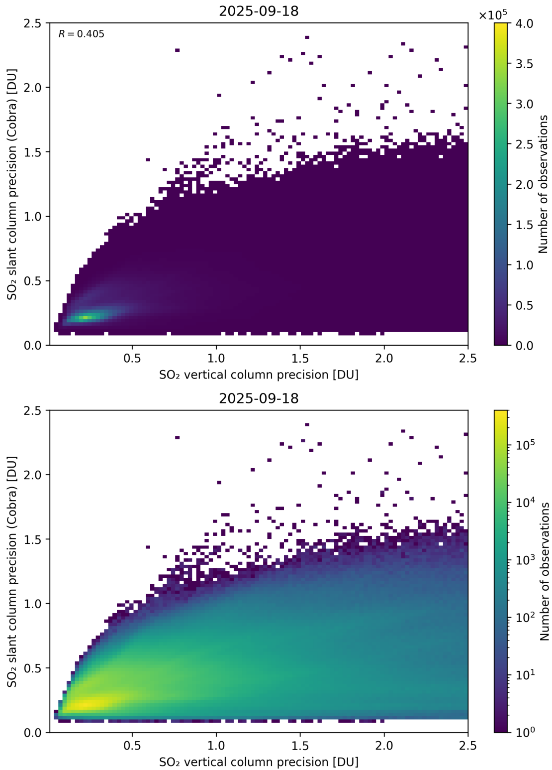
Figure 337: Scatter density plot of “SO 2 vertical column precision” against “SO 2 slant column precision (Cobra)” for 2025-09-17 to 2025-09-19.
