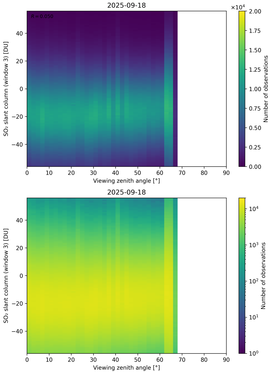
Figure 379: Scatter density plot of “Viewing zenith angle” against “SO 2 slant column (window 3)” for 2025-09-17 to 2025-09-19.
