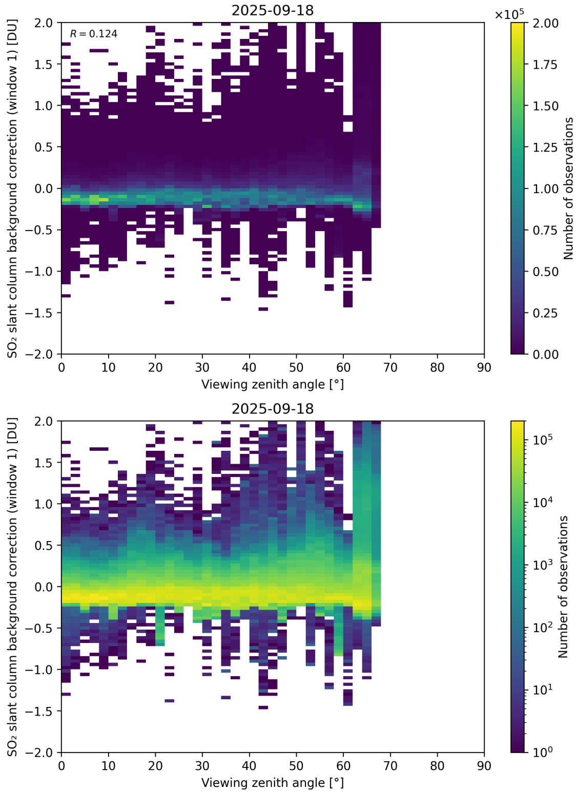
Figure 362: Scatter density plot of “Viewing zenith angle” against “SO 2 slant column background correction (window 1)” for 2025-09-17 to 2025-09-19.
