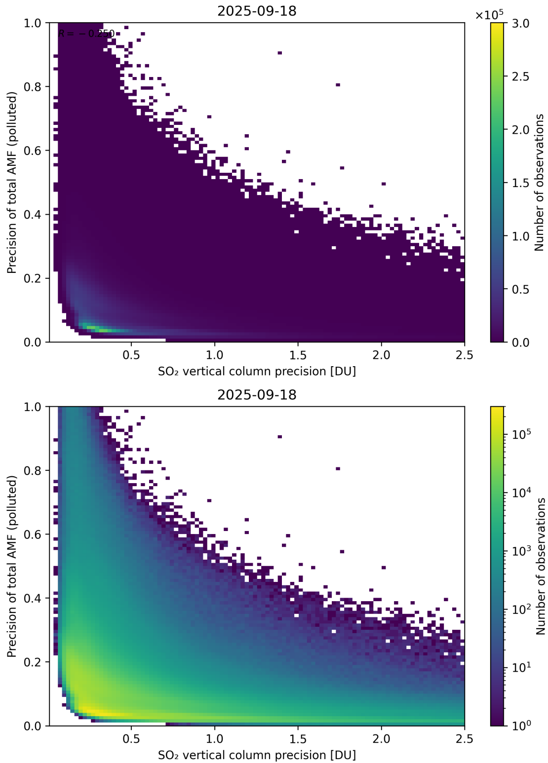
Figure 347: Scatter density plot of “SO 2 vertical column precision” against “Precision of total AMF (polluted)” for 2025-09-17 to 2025-09-19.
