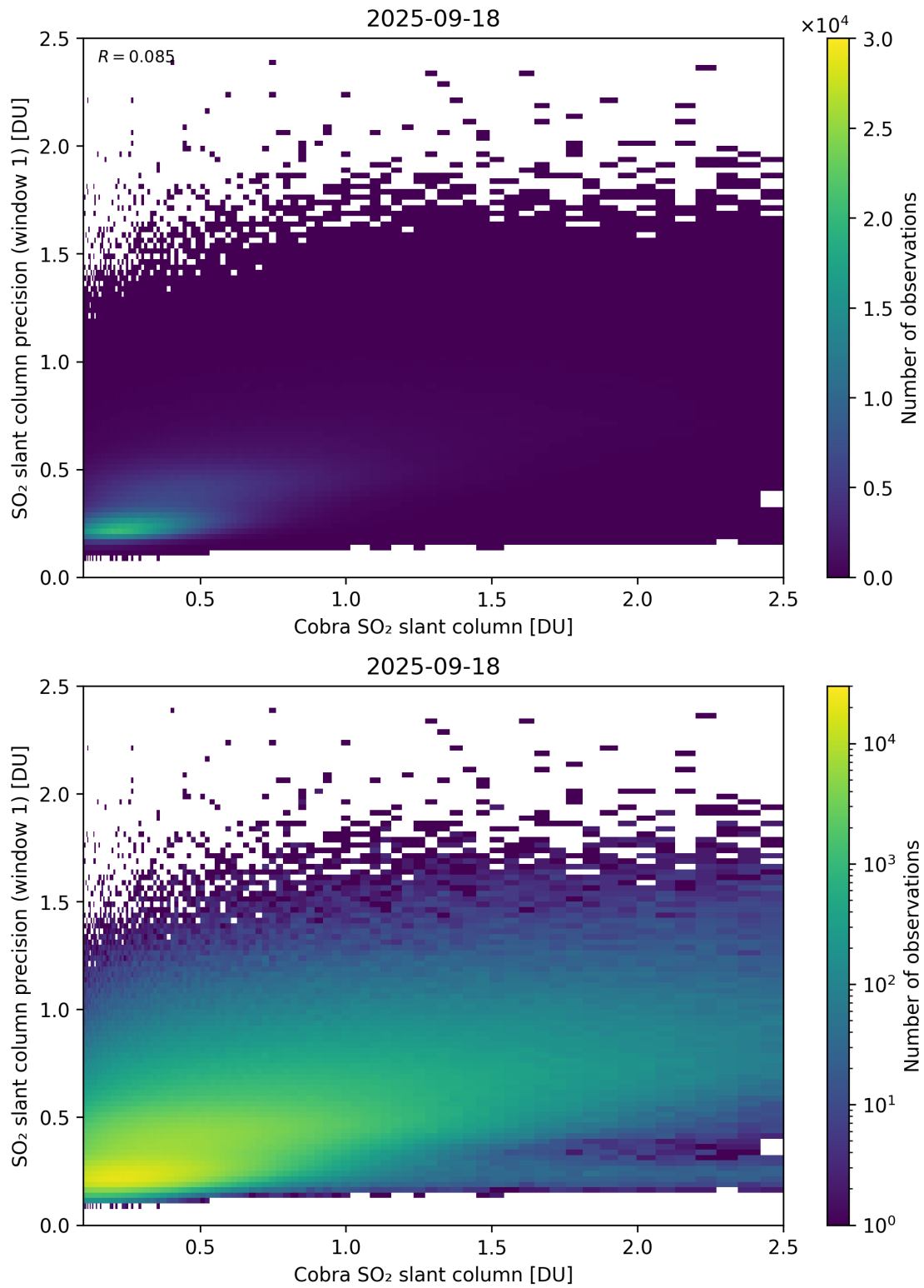
Figure 220: Scatter density plot of “Cobra SO 2 slant column” against “SO 2 slant column precision (window 1)” for 2025-09-17 to 2025-09-19.
