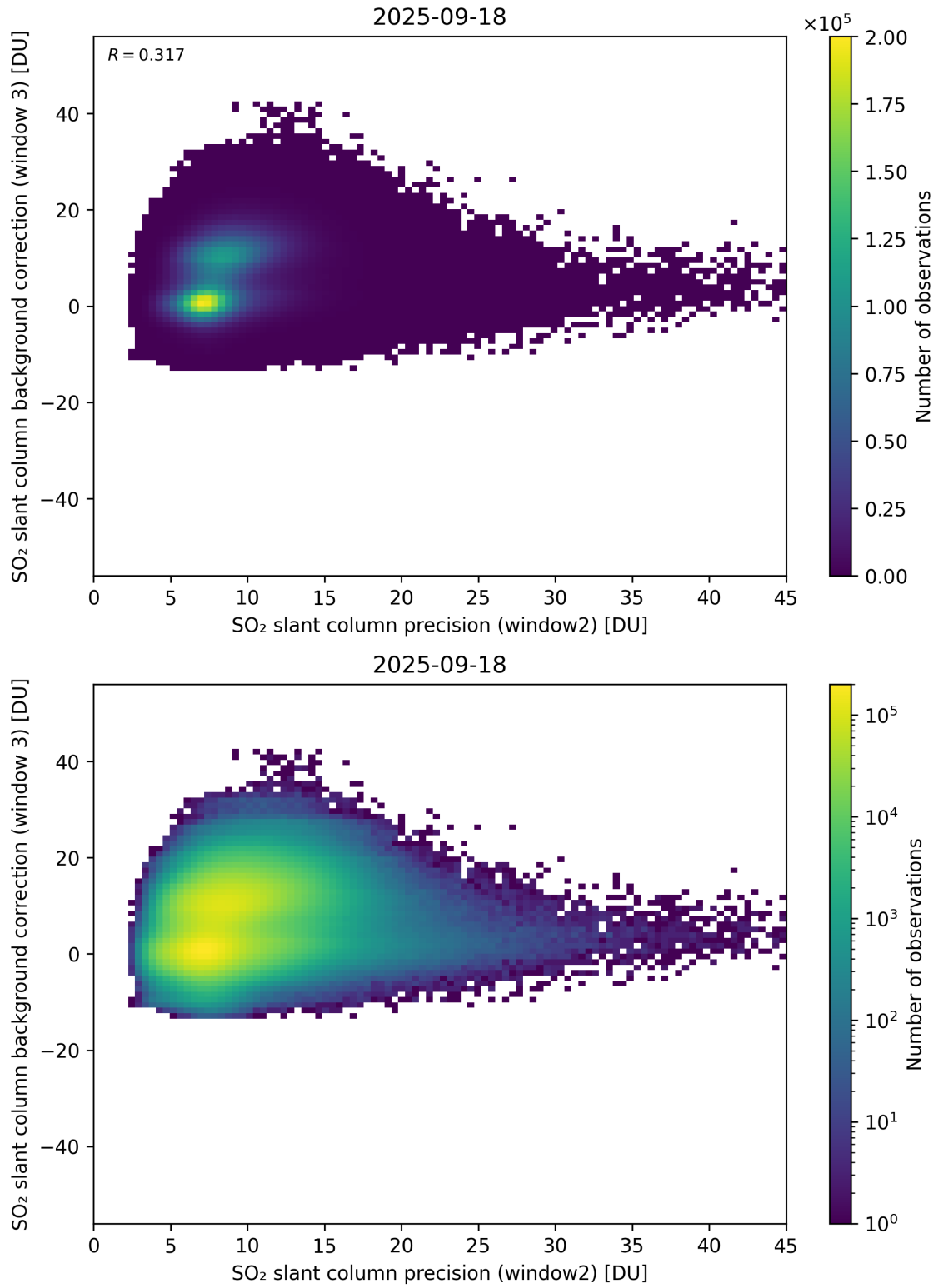
Figure 292: Scatter density plot of “SO 2 slant column precision (window2)” against “SO 2 slant column background correction (window 3)” for 2025-09-17 to 2025-09-19.
