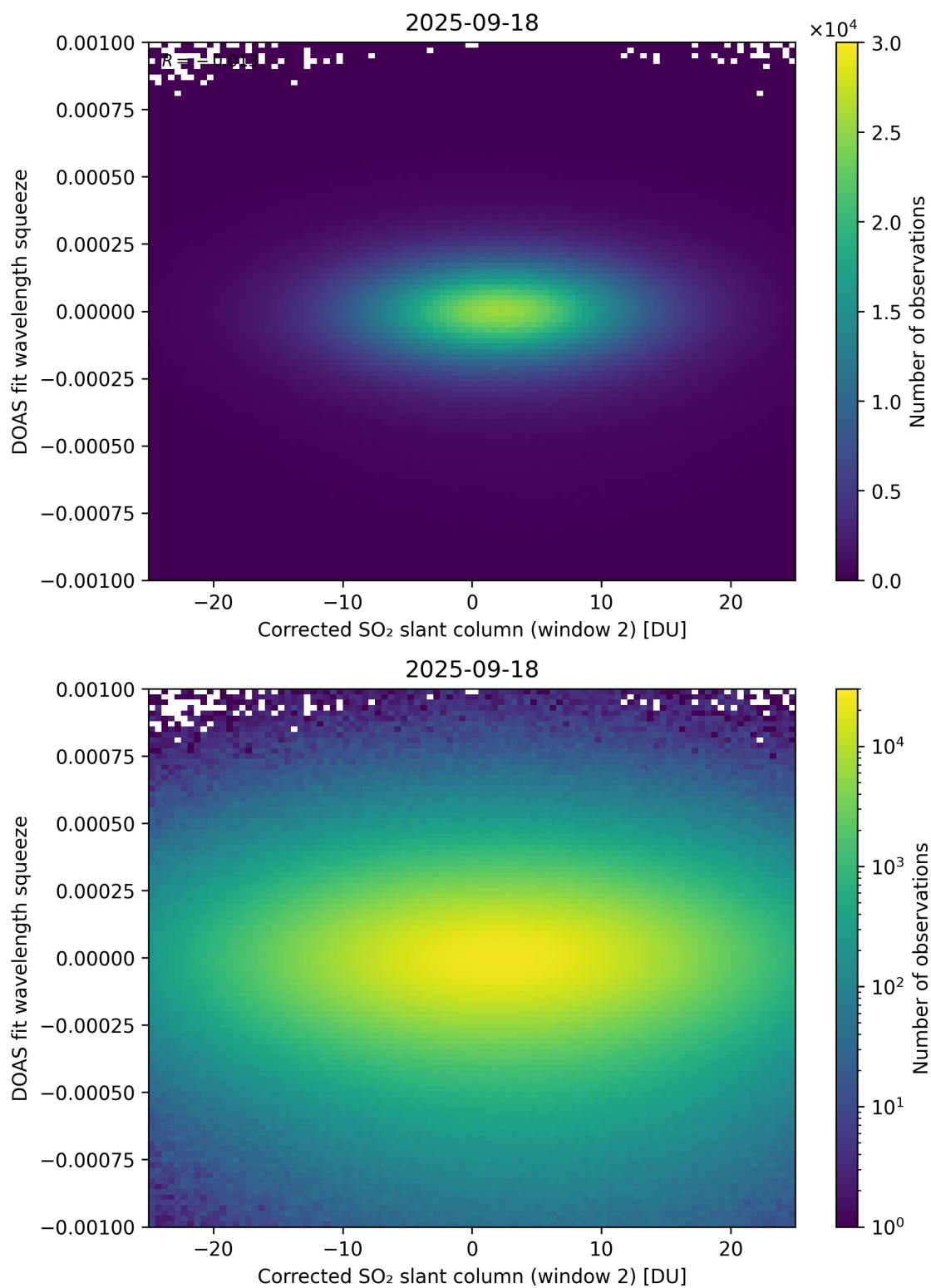
Figure 247: Scatter density plot of “Corrected SO 2 slant column (window 2)” against “DOAS fit wavelength squeeze” for 2025-09-17 to 2025-09-19.
