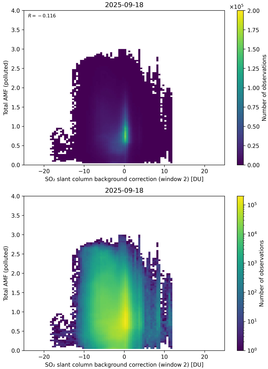
Figure 130: Scatter density plot of “SO 2 slant column background correction (window 2)” against “Total AMF (polluted)” for 2025-09-17 to 2025-09-19.
