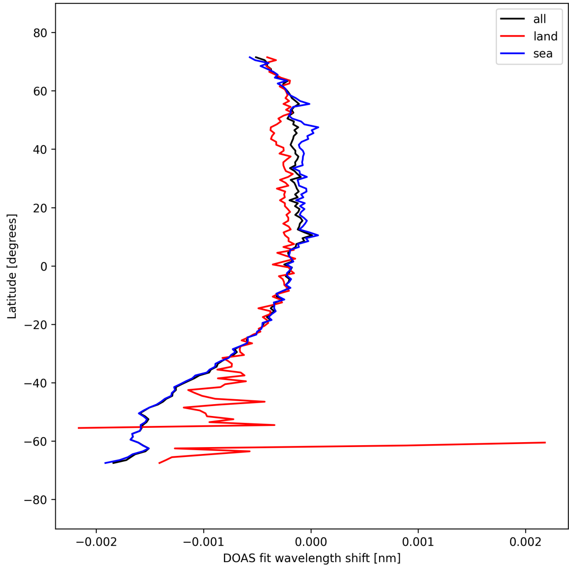
Figure 50: Zonal average of "DOAS fit wavelength shift" for 2025-09-17 to 2025-09-19.
