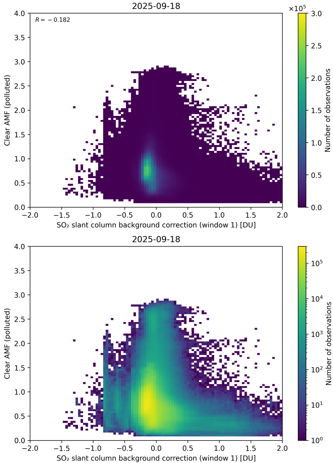
Figure 114: Scatter density plot of “SO 2 slant column background correction (window 1)” against “Clear AMF (polluted)” for 2025-09-17 to 2025-09-19.
