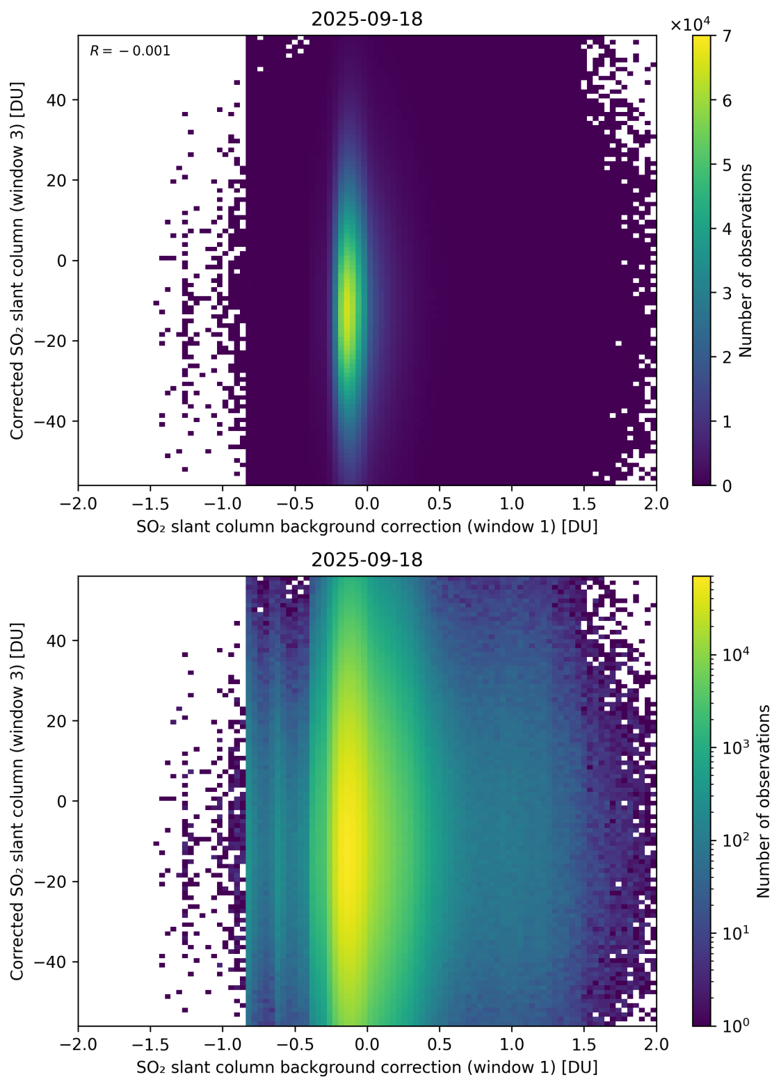
Figure 116: Scatter density plot of “SO 2 slant column background correction (window 1)” against “Corrected SO 2 slant column (window 3)” for 2025-09-17 to 2025-09-19.
