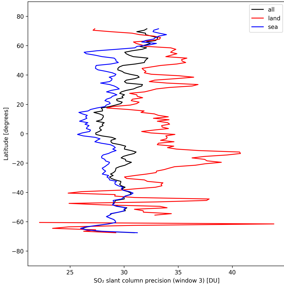
Figure 46: Zonal average of “SO 2 slant column precision (window 3)” for 2025-09-17 to 2025-09-19.
