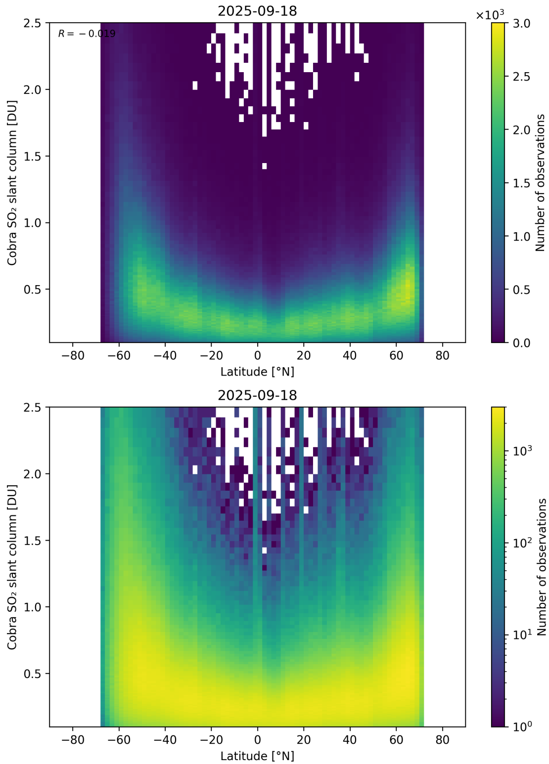
Figure 157: Scatter density plot of “Latitude” against “Cobra SO 2 slant column” for 2025-09-17 to 2025-09-19.
