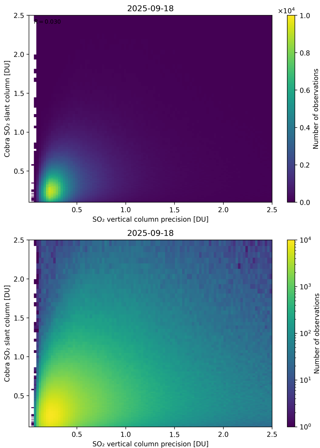
Figure 336: Scatter density plot of “SO 2 vertical column precision” against “Cobra SO 2 slant column” for 2025-09-17 to 2025-09-19.
