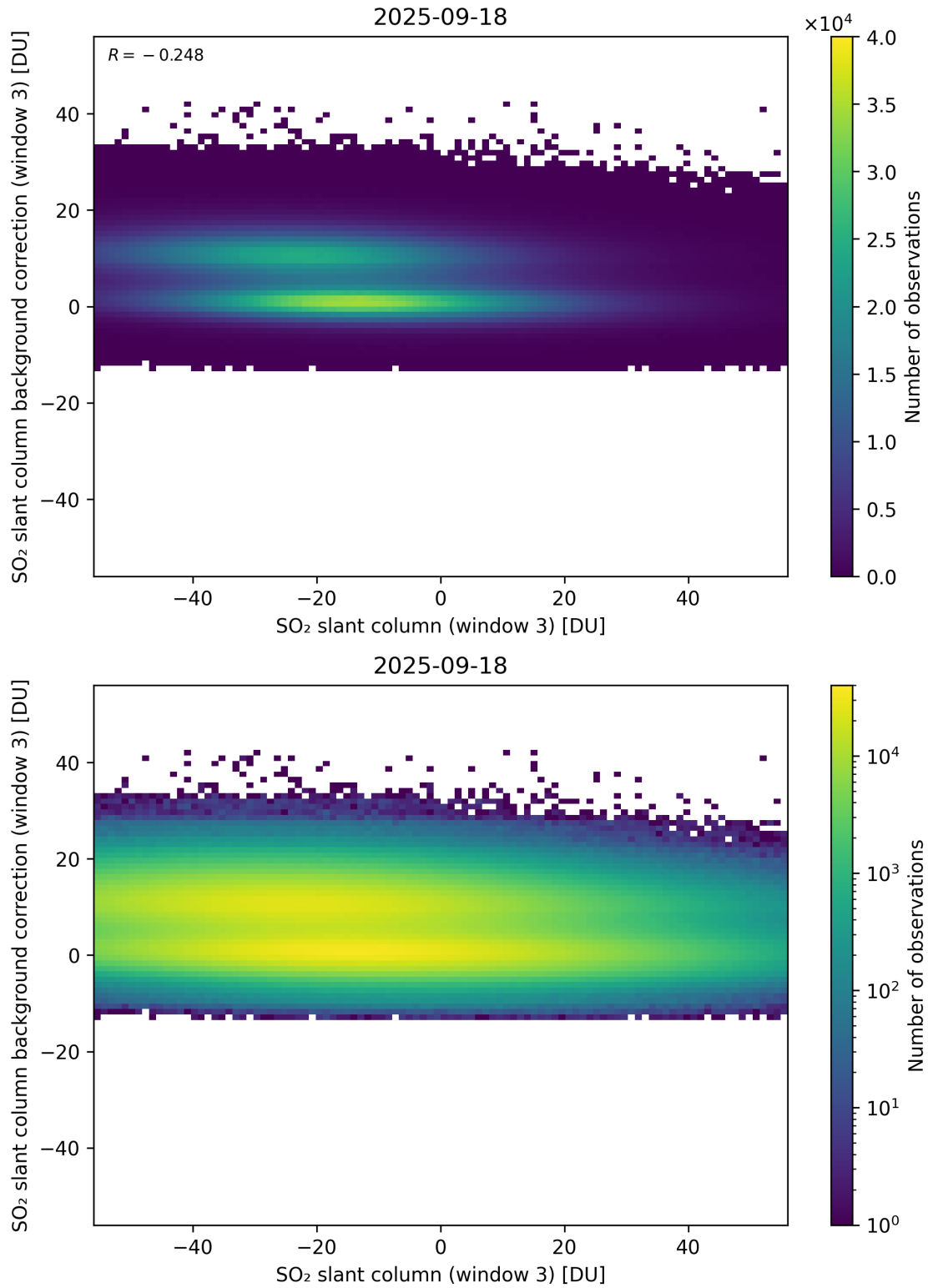
Figure 303: Scatter density plot of “SO 2 slant column (window 3)” against “SO 2 slant column background correction (window 3)” for 2025-09-17 to 2025-09-19.
