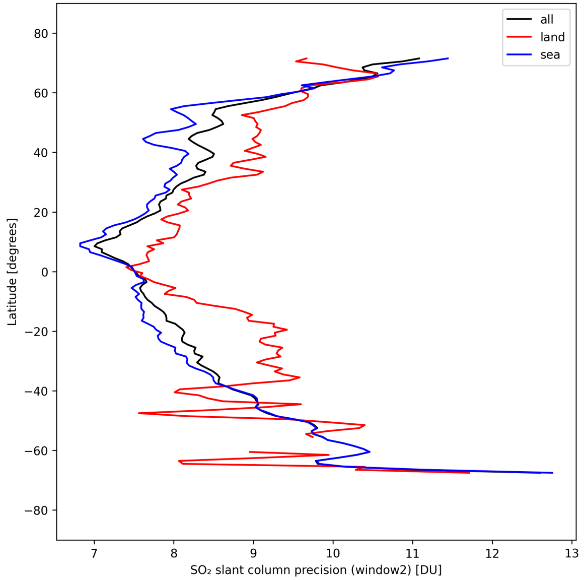
Figure 42: Zonal average of “SO 2 slant column precision (window2)” for 2025-09-17 to 2025-09-19.
