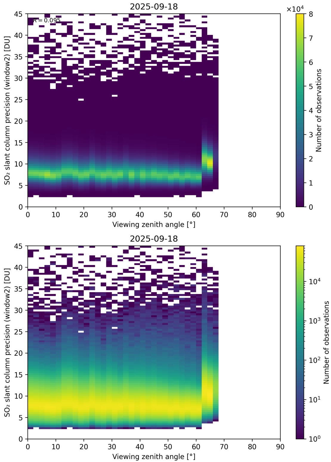
Figure 378: Scatter density plot of “Viewing zenith angle” against “SO 2 slant column precision (window2)” for 2025-09-17 to 2025-09-19.
