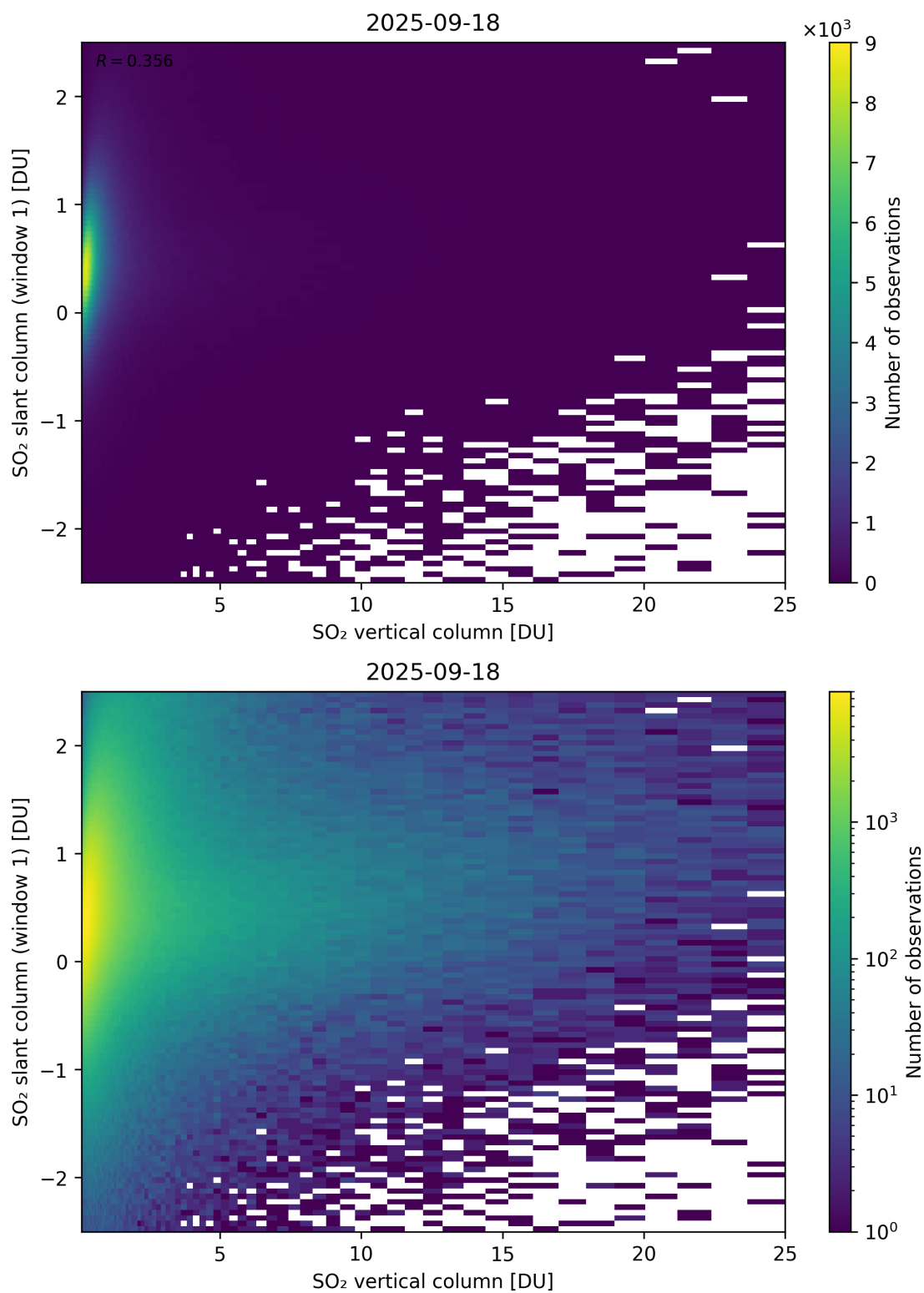
Figure 354: Scatter density plot of “SO 2 vertical column” against “SO 2 slant column (window 1)” for 2025-09-17 to 2025-09-19.
