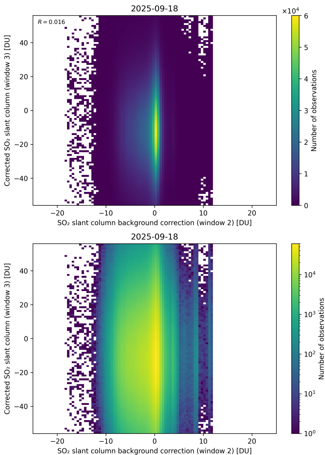
Figure 127: Scatter density plot of “SO 2 slant column background correction (window 2)” against “Corrected SO 2 slant column (window 3)” for 2025-09-17 to 2025-09-19.
