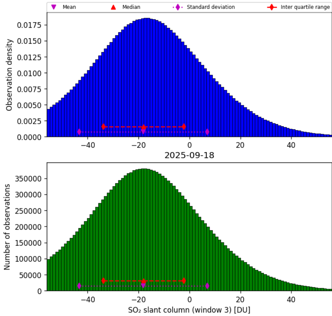
Figure 71: Histogram of “SO 2 slant column (window 3)” for 2025-09-17 to 2025-09-19
