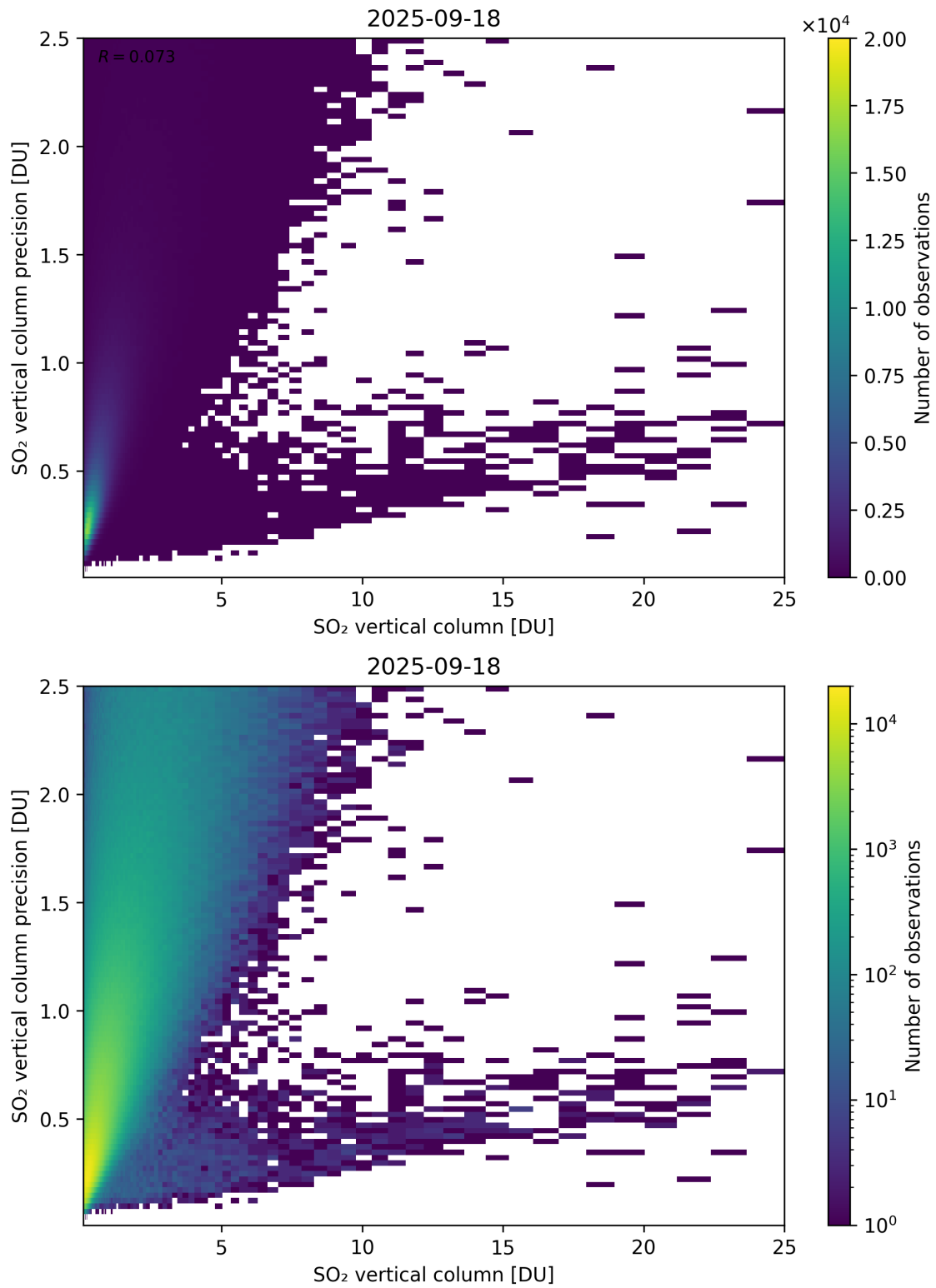
Figure 361: Scatter density plot of “SO 2 vertical column” against “SO 2 vertical column precision” for 2025-09-17 to 2025-09-19.
