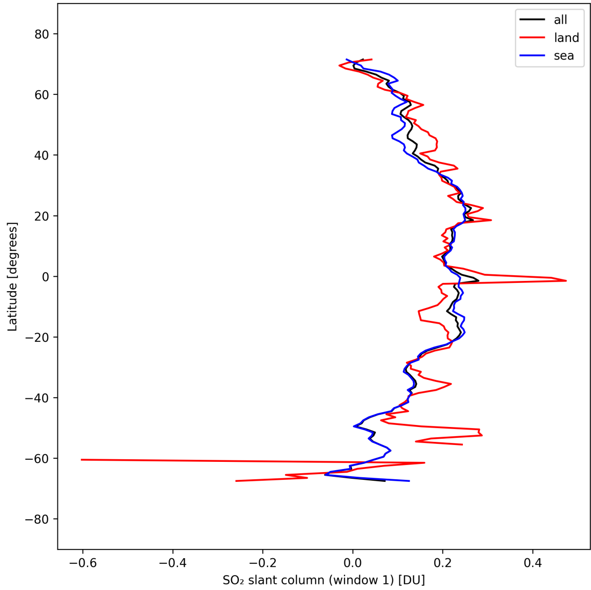
Figure 37: Zonal average of “SO 2 slant column (window 1)” for 2025-09-17 to 2025-09-19.
