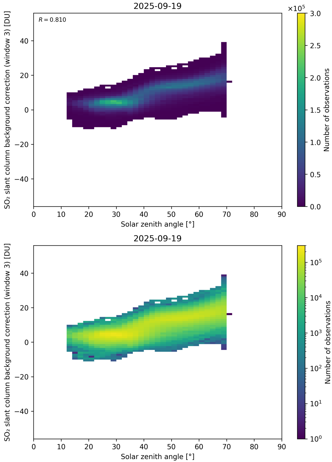
Figure 173: Scatter density plot of “Solar zenith angle” against “SO 2 slant column background correction (window 3)” for 2025-09-18 to 2025-09-20.
