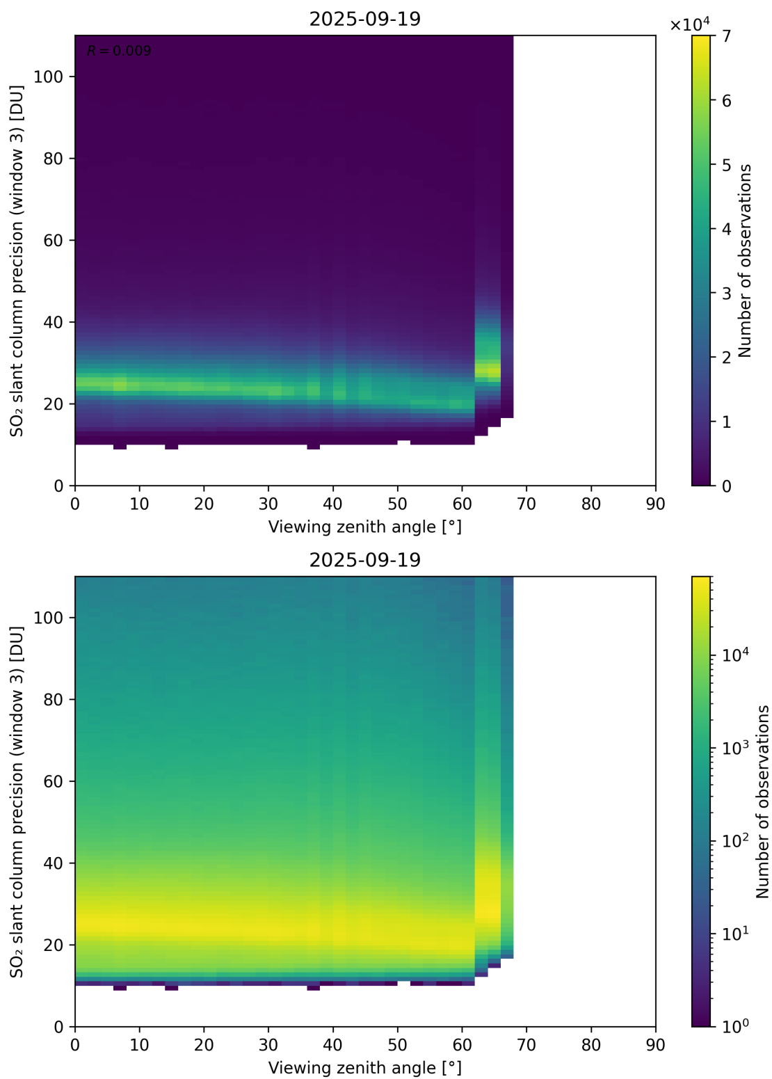
Figure 380: Scatter density plot of “Viewing zenith angle” against “SO 2 slant column precision (window 3)” for 2025-09-18 to 2025-09-20.
