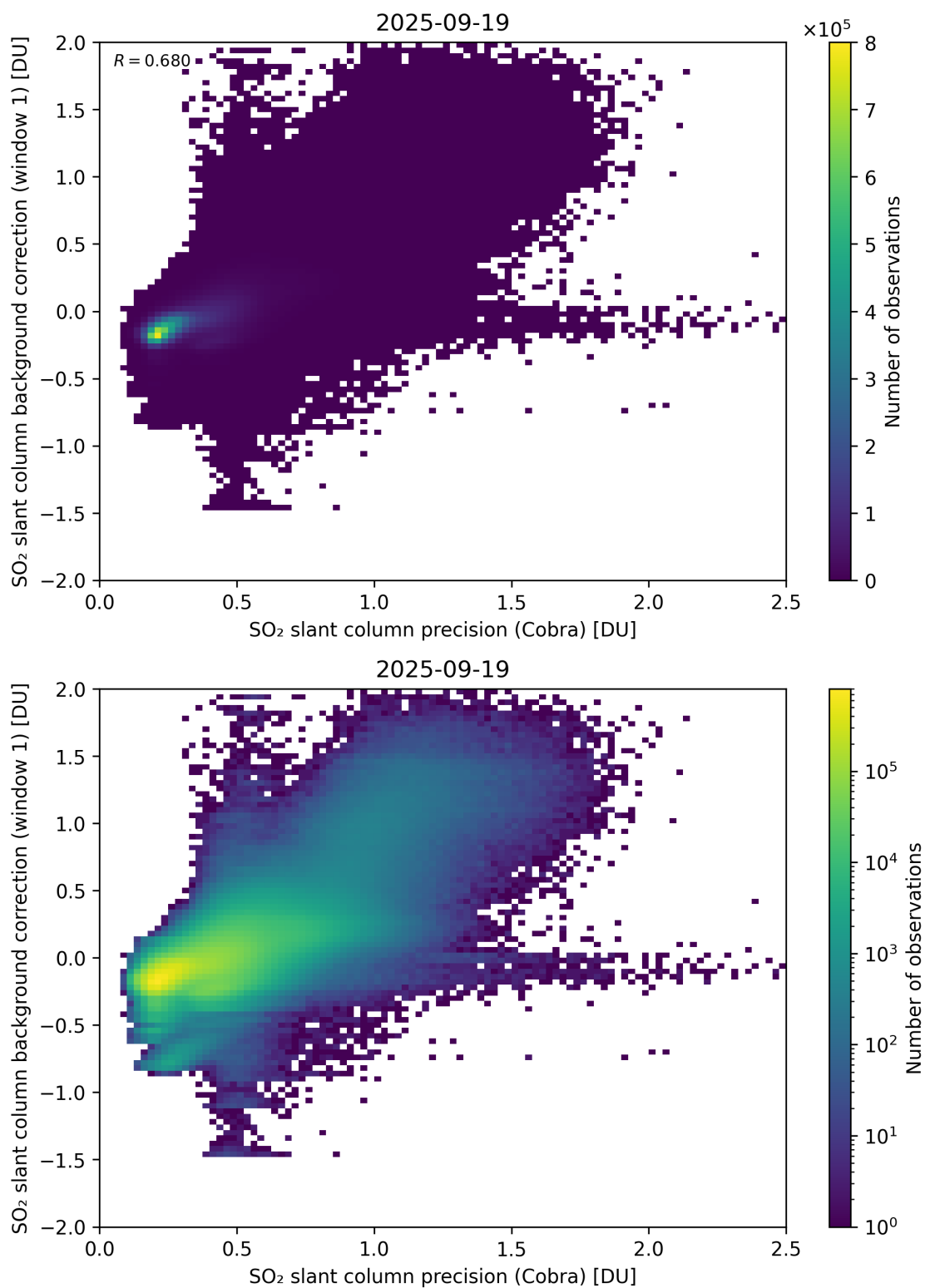
Figure 199: Scatter density plot of “SO 2 slant column precision (Cobra)” against “SO 2 slant column background correction (window 1)” for 2025-09-18 to 2025-09-20.
