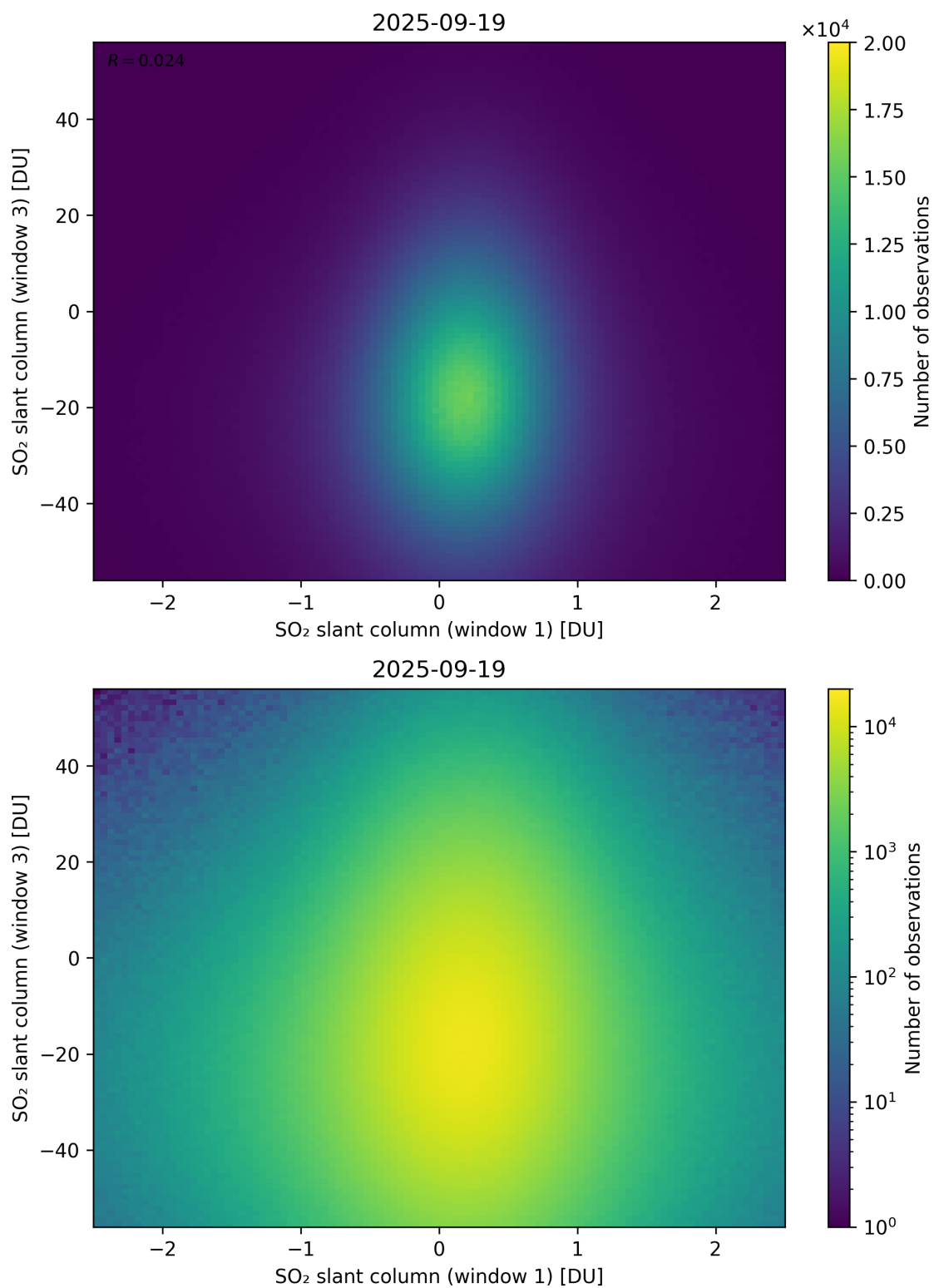
Figure 287: Scatter density plot of “SO 2 slant column (window 1)” against “SO 2 slant column (window 3)” for 2025-09-18 to 2025-09-20.
