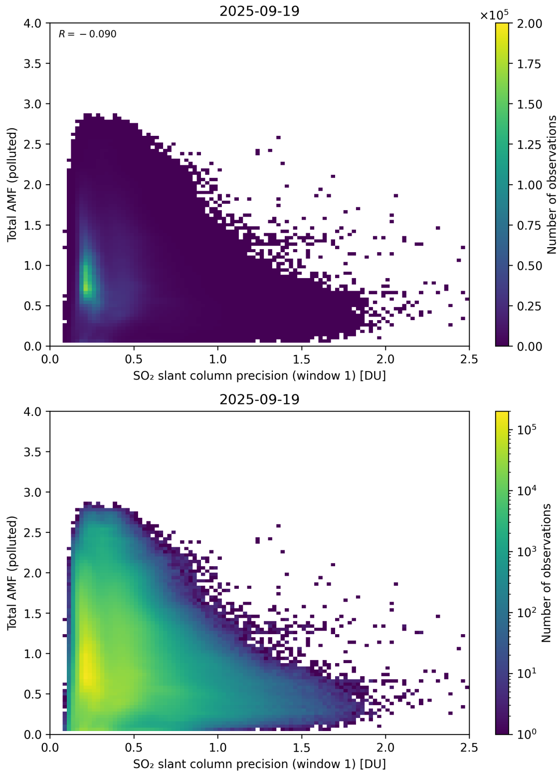
Figure 280: Scatter density plot of “SO 2 slant column precision (window 1)” against “Total AMF (polluted)” for 2025-09-18 to 2025-09-20.
