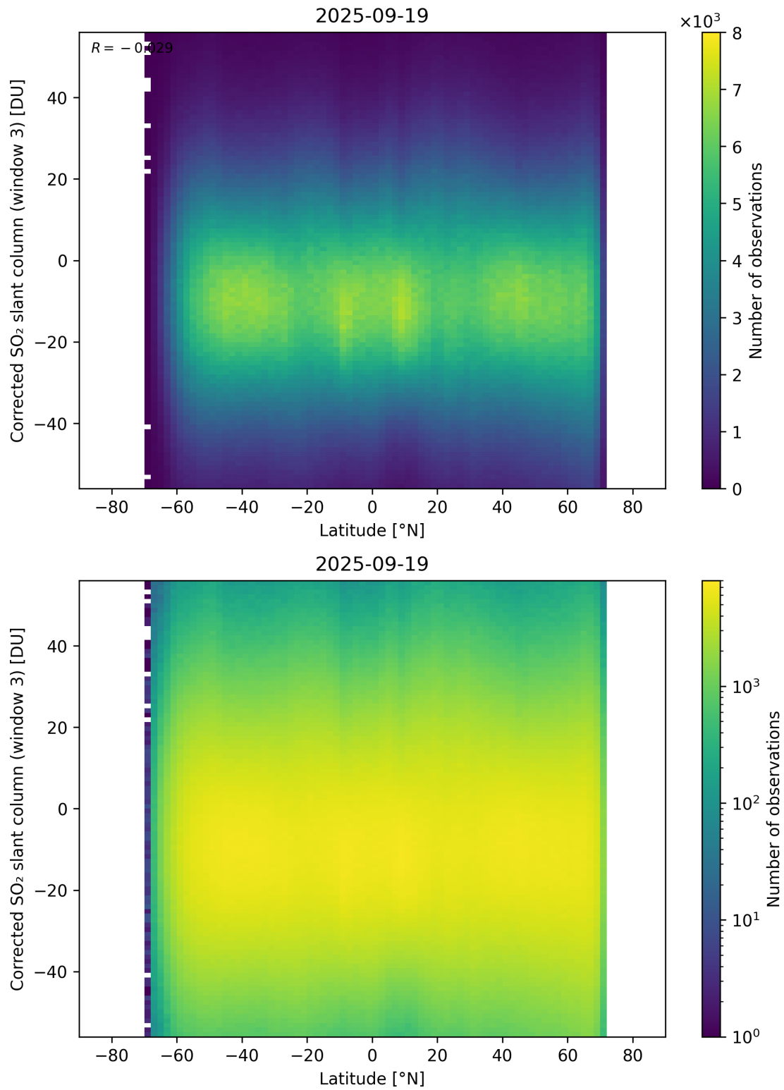
Figure 161: Scatter density plot of “Latitude” against “Corrected SO 2 slant column (window 3)” for 2025-09-18 to 2025-09-20.
