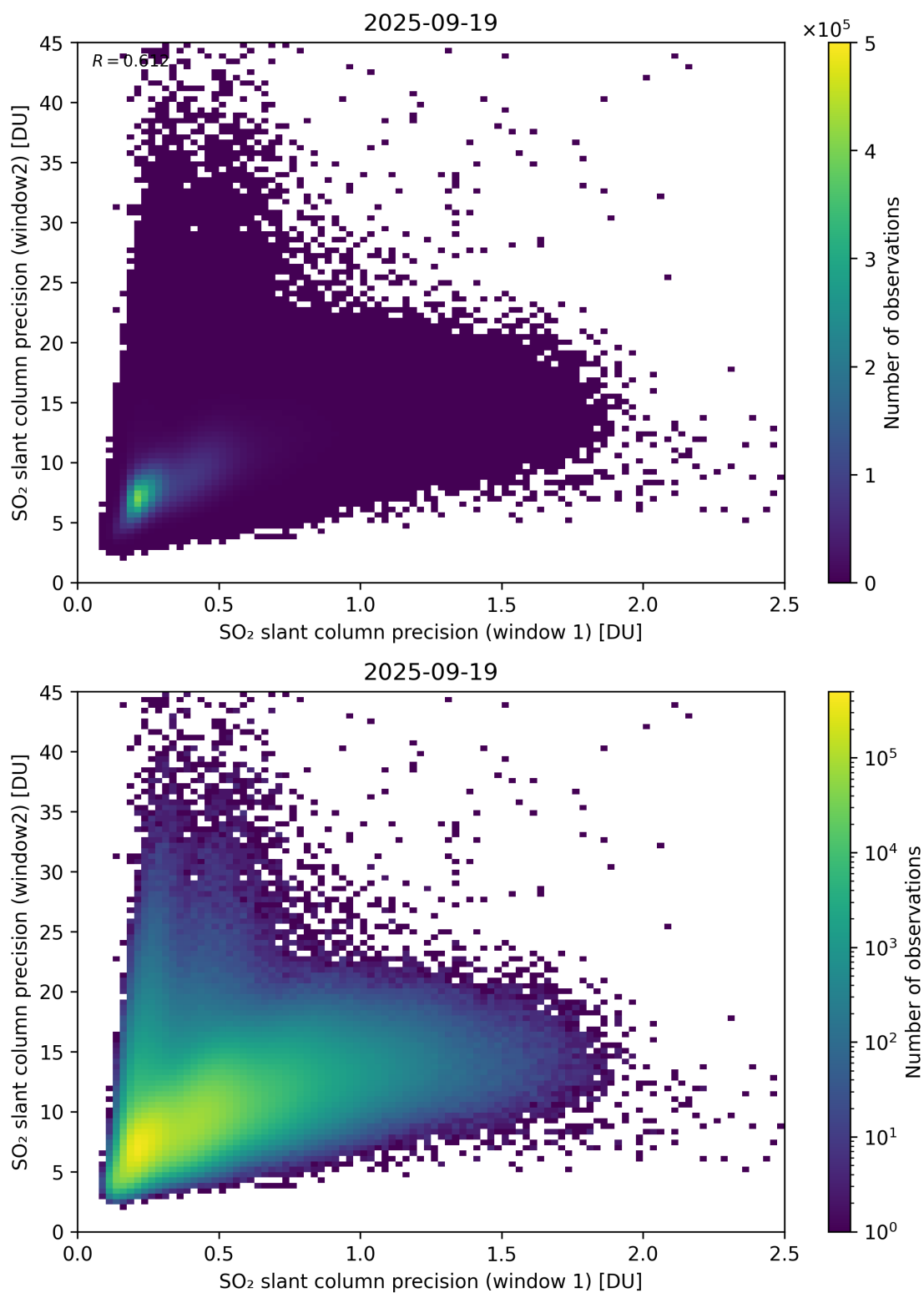
Figure 277: Scatter density plot of “SO 2 slant column precision (window 1)” against “SO 2 slant column precision (window 2)” for 2025-09-18 to 2025-09-20.
