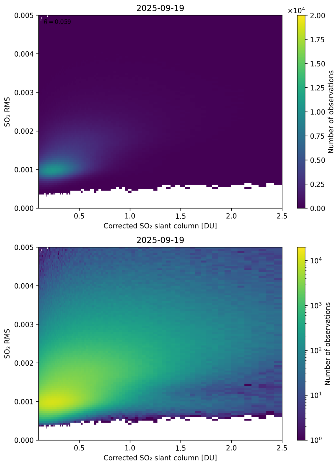
Figure 231: Scatter density plot of “Corrected SO 2 slant column” against “SO 2 RMS” for 2025-09-18 to 2025-09-20.
