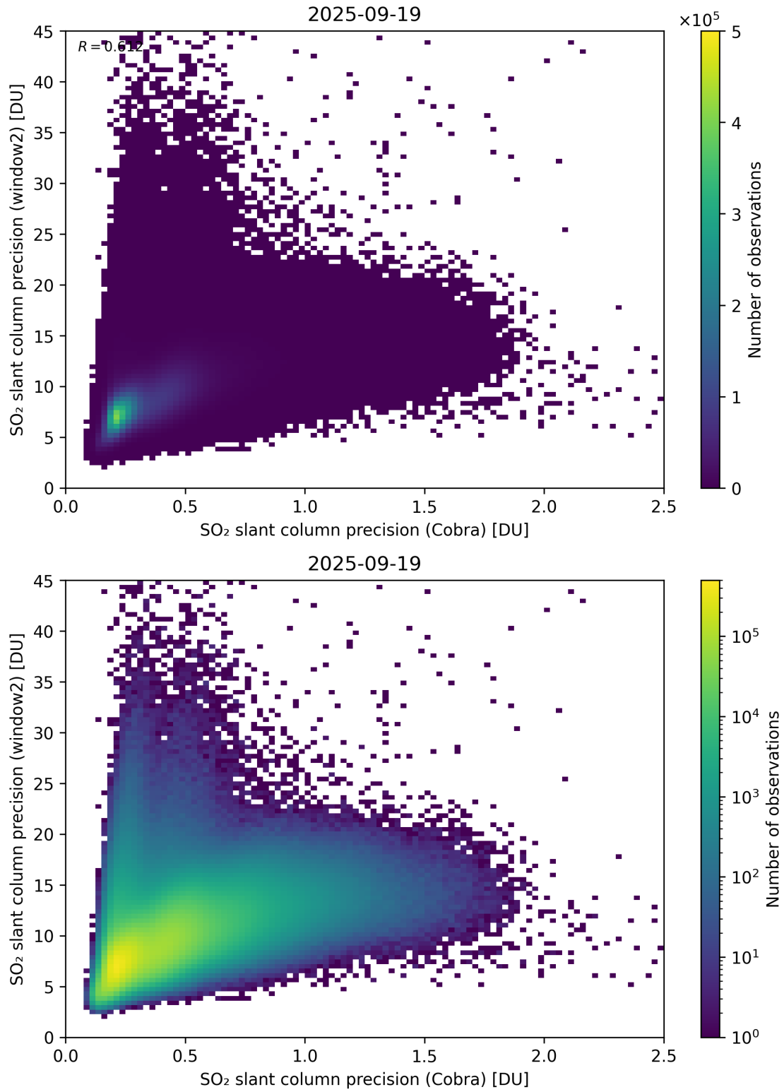
Figure 210: Scatter density plot of “SO 2 slant column precision (Cobra)” against “SO 2 slant column precision (window2)” for 2025-09-18 to 2025-09-20.
