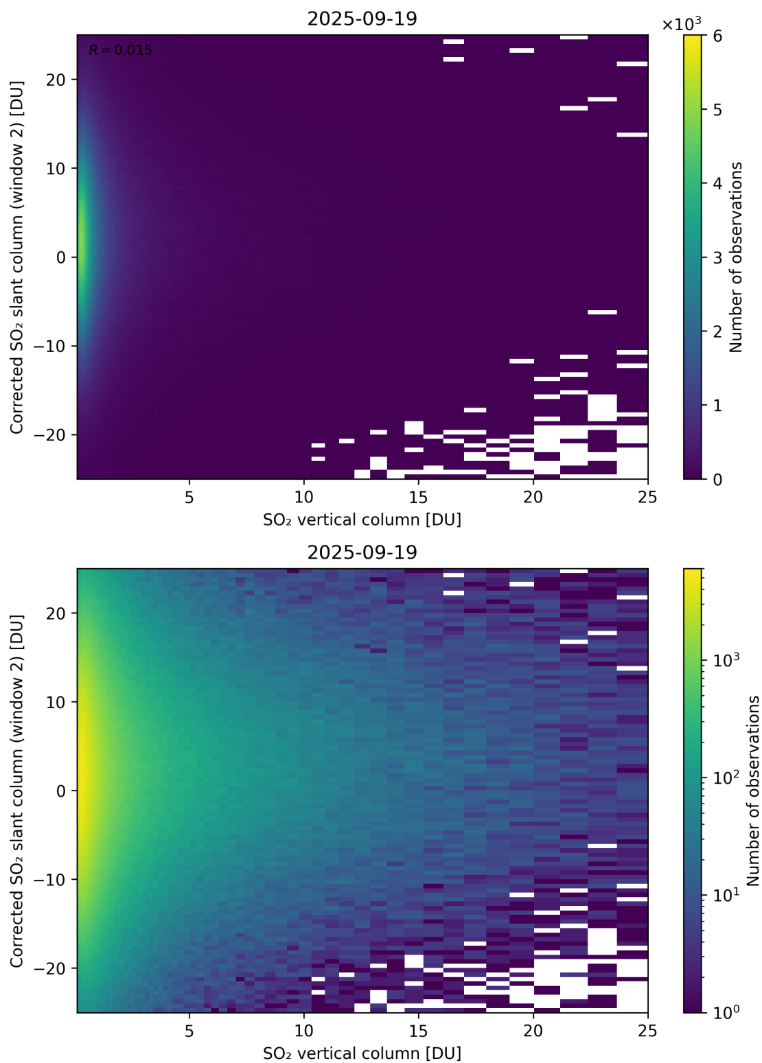
Figure 352: Scatter density plot of “SO 2 vertical column” against “Corrected SO 2 slant column (window 2)” for 2025-09-18 to 2025-09-20.
