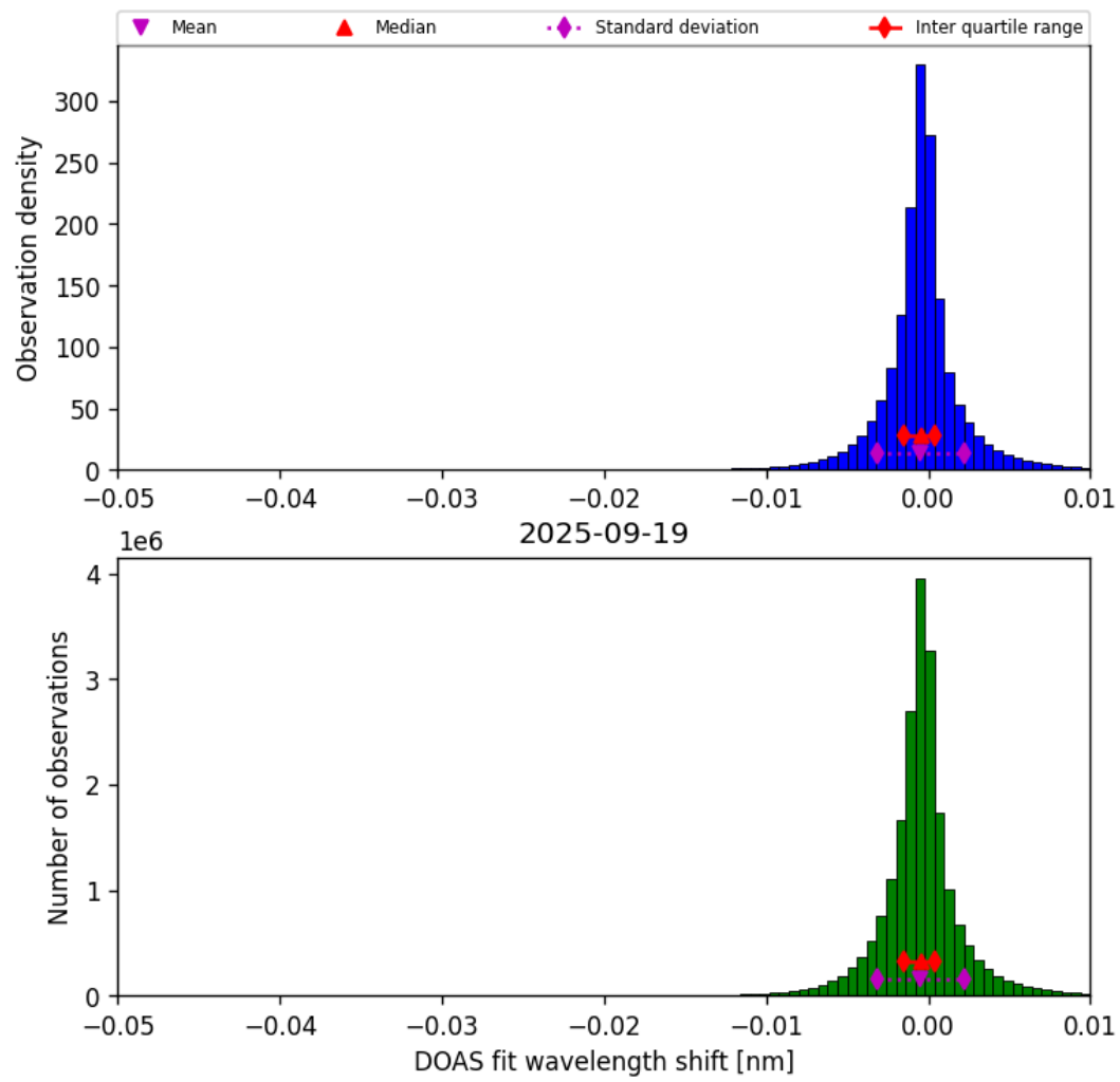
Figure 76: Histogram of “DOAS fit wavelength shift” for 2025-09-18 to 2025-09-20
