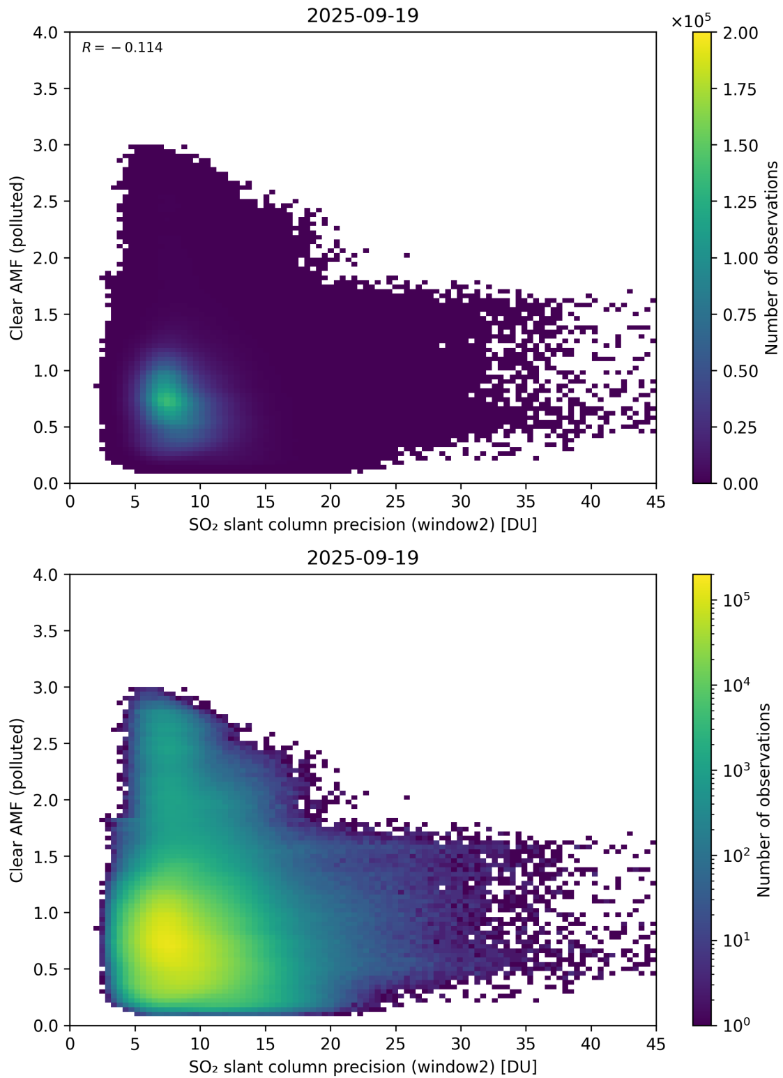
Figure 296: Scatter density plot of “SO 2 slant column precision (window2)” against “Clear AMF (polluted)” for 2025-09-18 to 2025-09-20.
