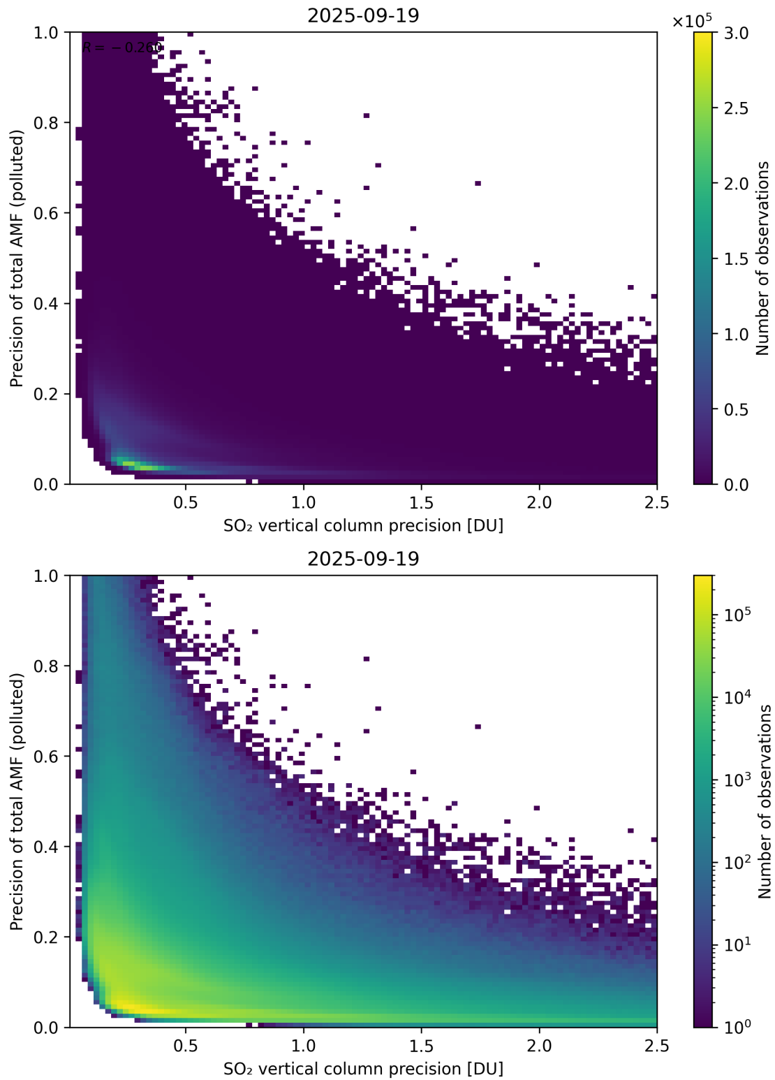
Figure 347: Scatter density plot of “SO 2 vertical column precision” against “Precision of total AMF (polluted)” for 2025-09-18 to 2025-09-20.
