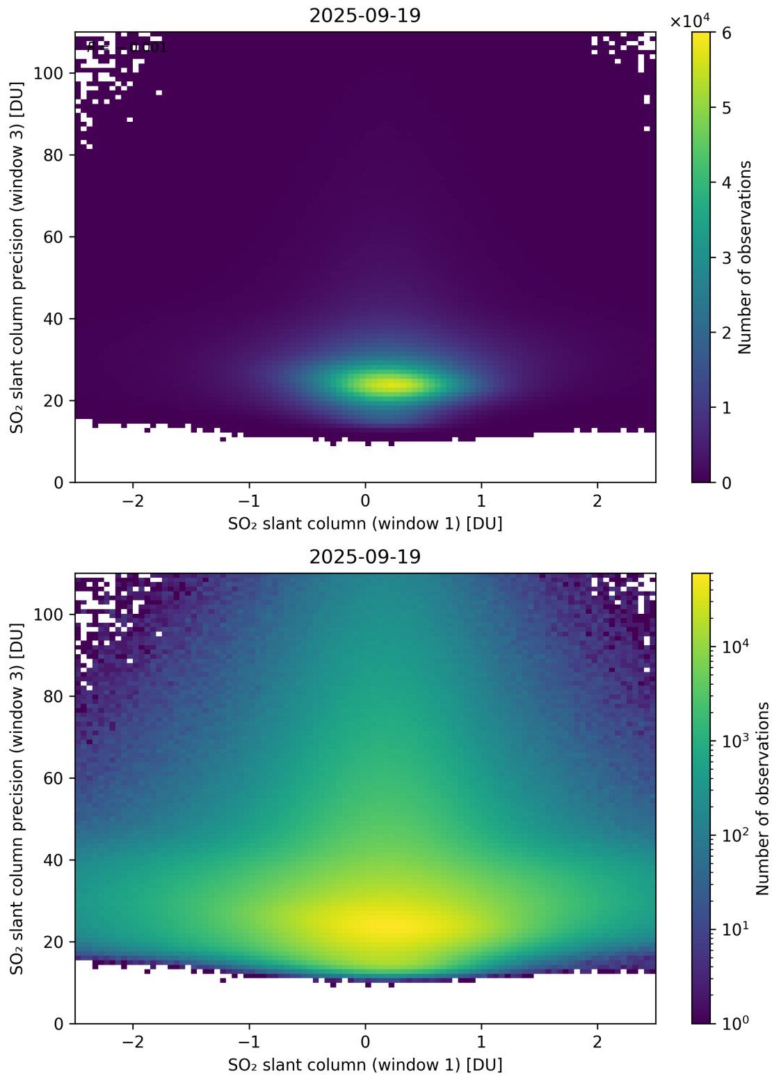
Figure 288: Scatter density plot of “SO 2 slant column (window 1)” against “SO 2 slant column precision (window 3)” for 2025-09-18 to 2025-09-20.
