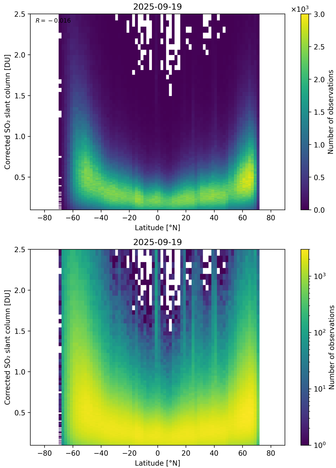
Figure 159: Scatter density plot of “Latitude” against “Corrected SO 2 slant column” for 2025-09-18 to 2025-09-20.
