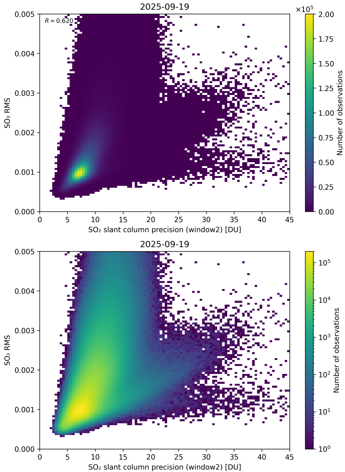
Figure 295: Scatter density plot of “SO 2 slant column precision (window2)” against “SO 2 RMS” for 2025-09-18 to 2025-09-20.
