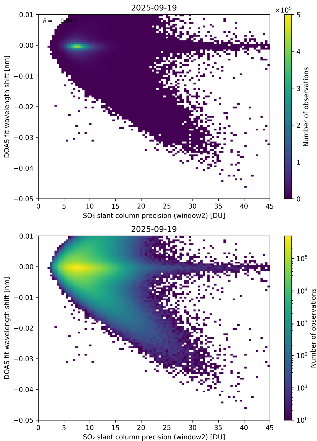
Figure 293: Scatter density plot of “SO 2 slant column precision (window2)” against “DOAS fit wavelength shift” for 2025-09-18 to 2025-09-20.
