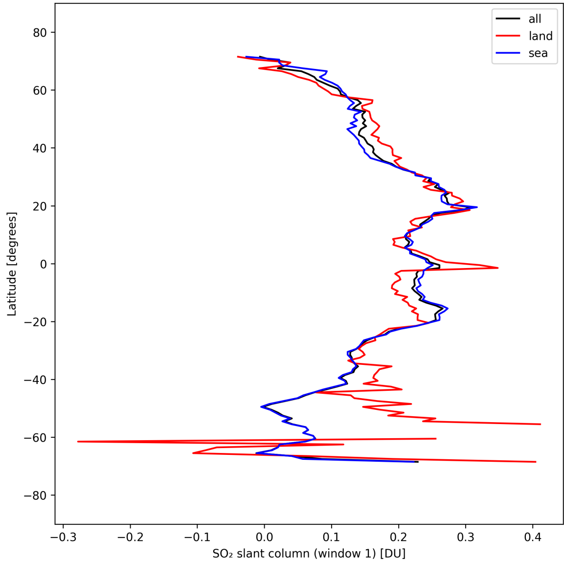
Figure 37: Zonal average of “SO 2 slant column (window 1)” for 2025-09-18 to 2025-09-20.
