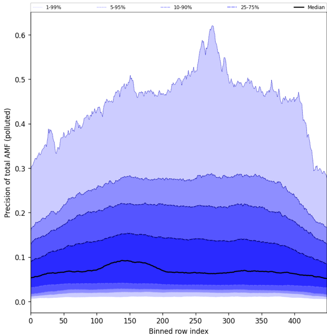
Figure 106: Along track statistics of “Precision of total AMF (polluted)” for 2025-09-18 to 2025-09-20
