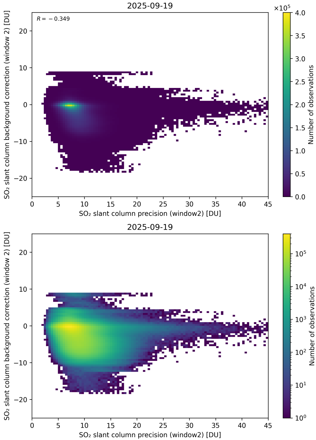
Figure 291: Scatter density plot of “SO 2 slant column precision (window2)” against “SO 2 slant column background correction (window 2)” for 2025-09-18 to 2025-09-20.
