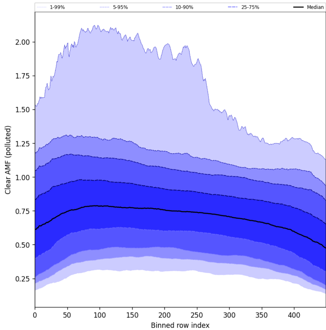
Figure 107: Along track statistics of “Clear AMF (polluted)” for 2025-09-18 to 2025-09-20
