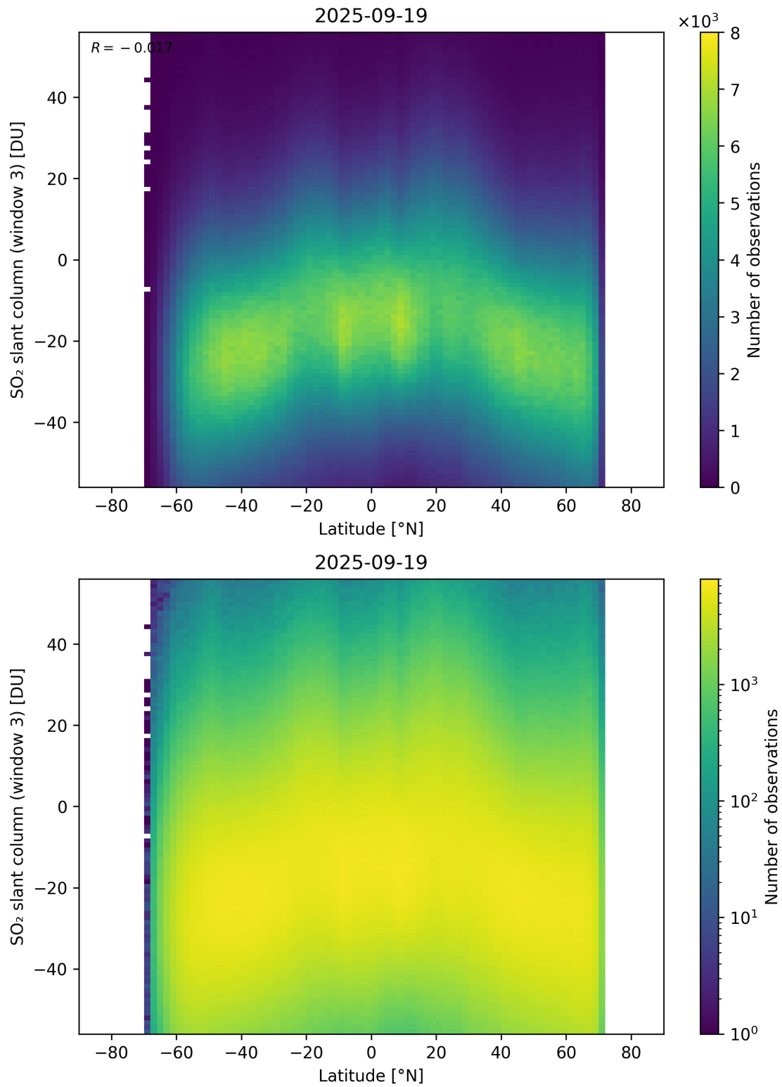
Figure 165: Scatter density plot of “Latitude” against “SO 2 slant column (window 3)” for 2025-09-18 to 2025-09-20.
