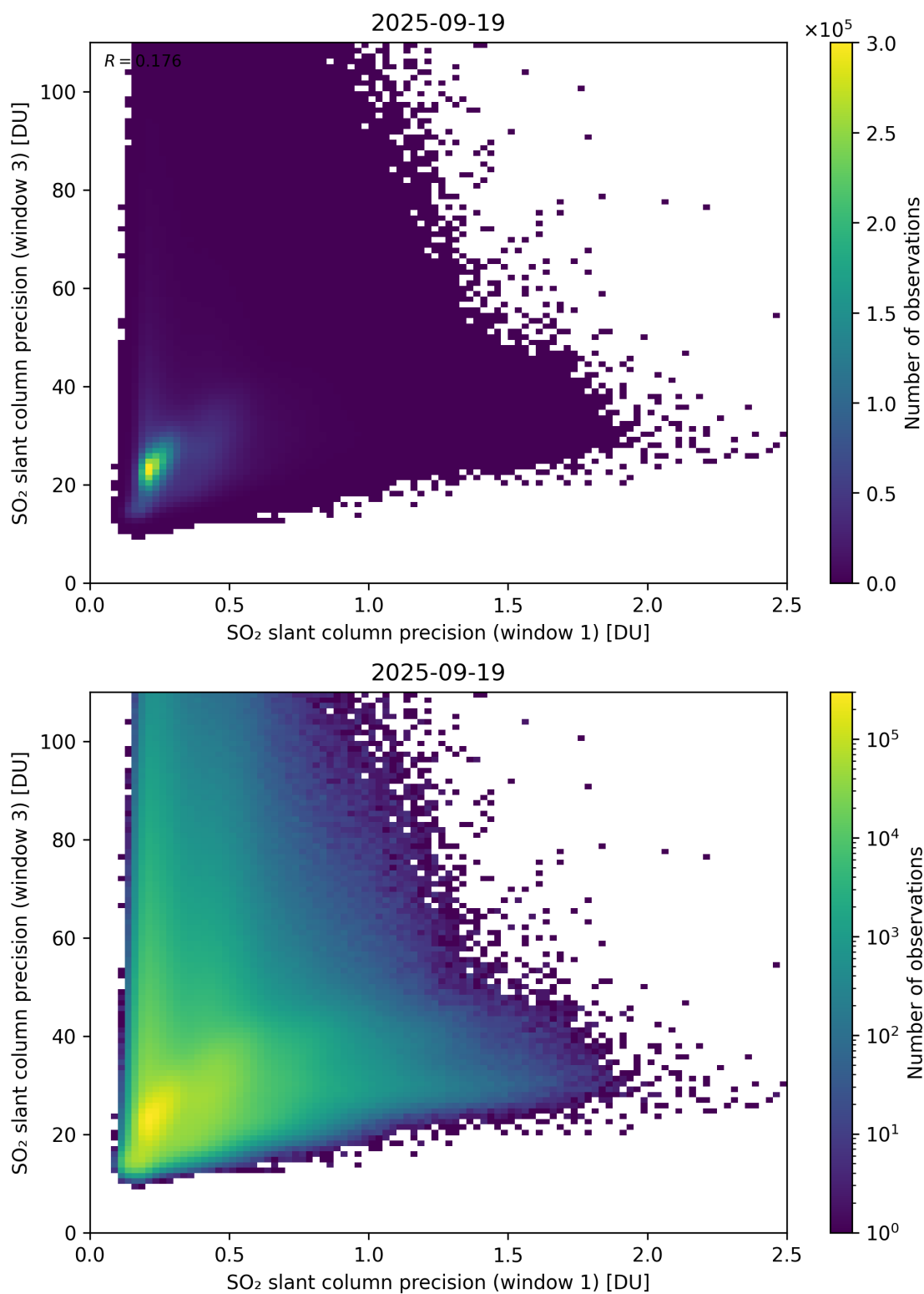
Figure 279: Scatter density plot of “SO 2 slant column precision (window 1)” against “SO 2 slant column precision (window 3)” for 2025-09-18 to 2025-09-20.
