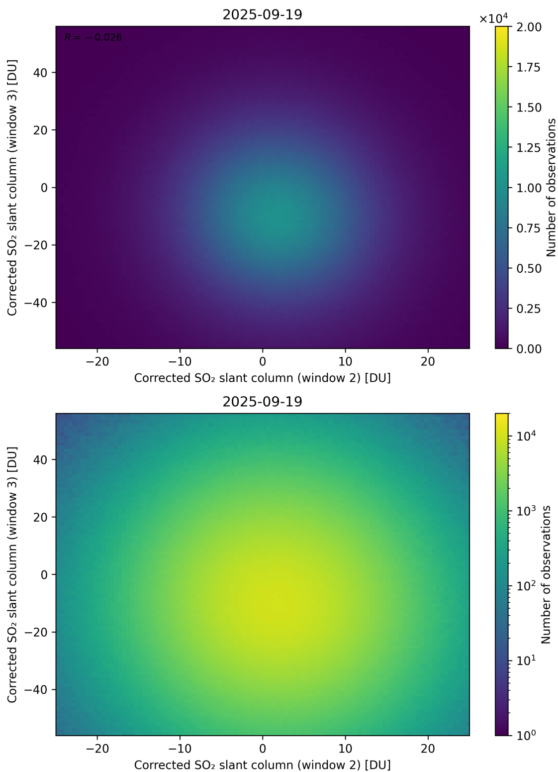
Figure 250: Scatter density plot of “Corrected SO 2 slant column (window 2)” against “Corrected SO 2 slant column (window 3)” for 2025-09-18 to 2025-09-20.
