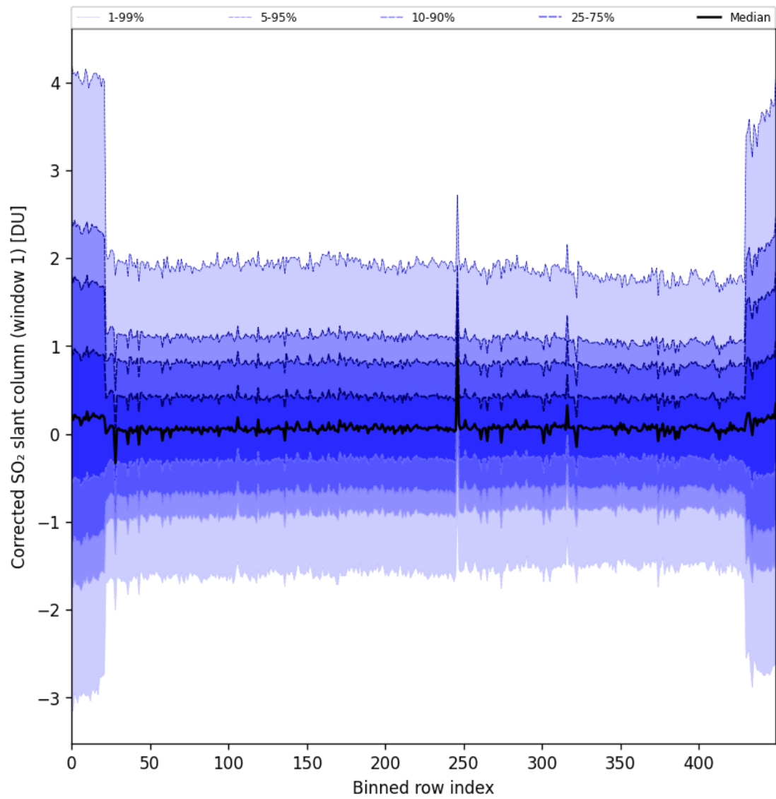
Figure 91: Along track statistics of “Corrected SO 2 slant column (window 1)” for 2025-09-18 to 2025-09-20
