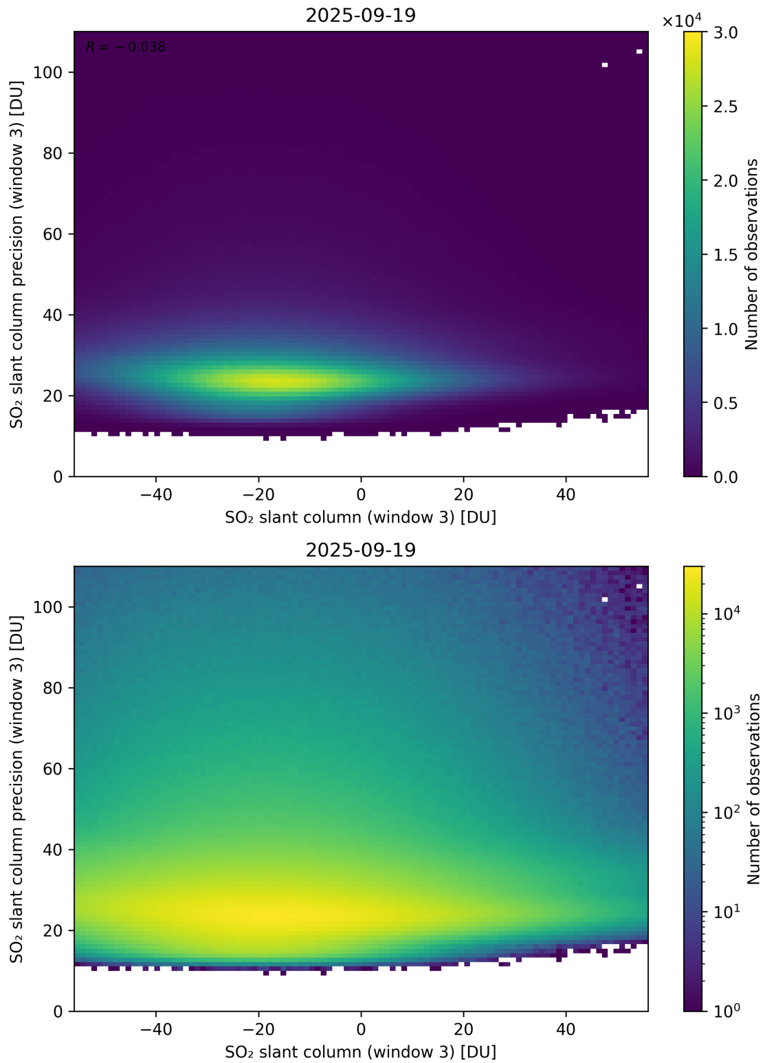
Figure 317: Scatter density plot of “SO 2 slant column (window 3)” against “SO 2 slant column precision (window 3)” for 2025-09-18 to 2025-09-20.
