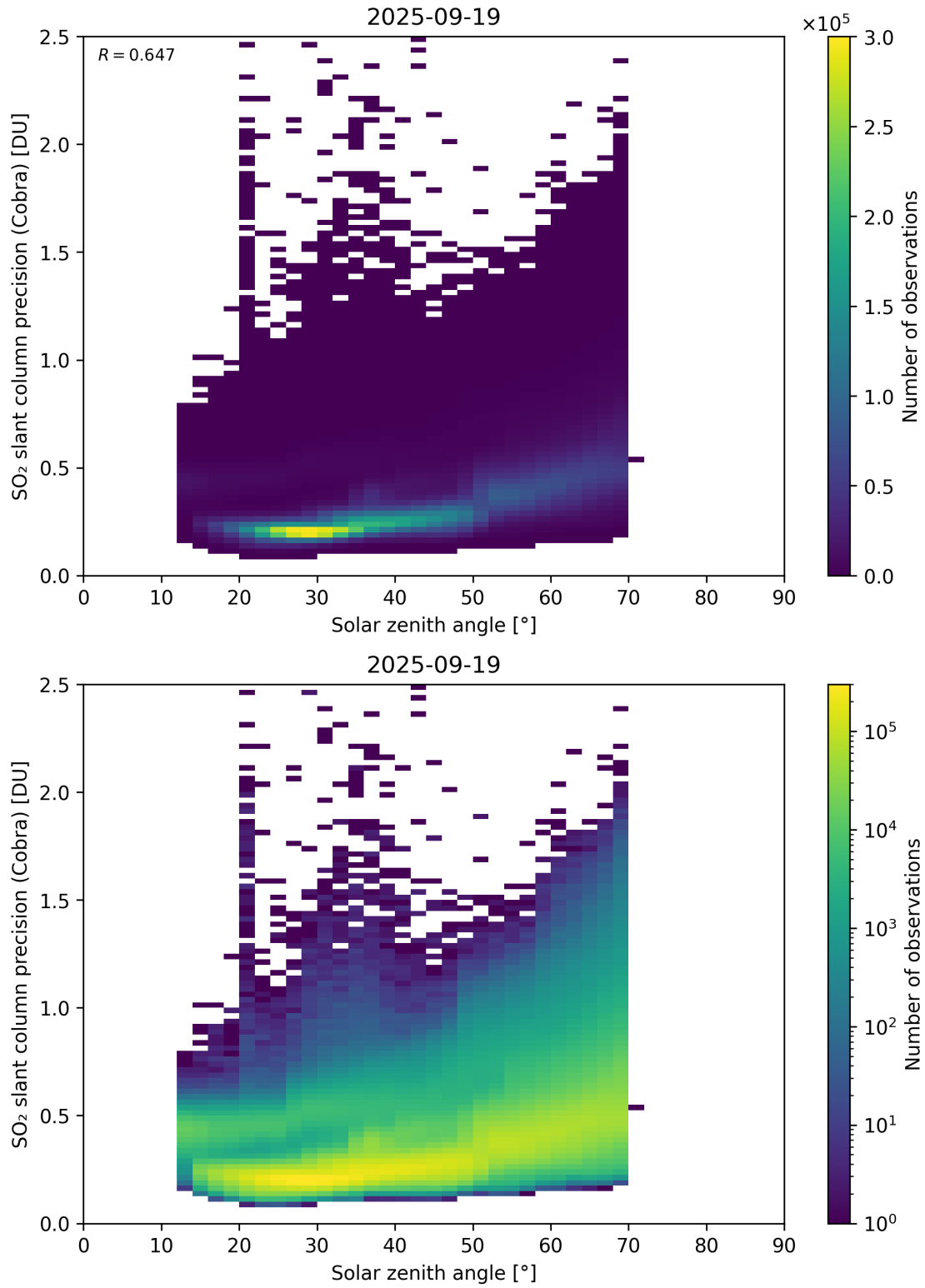
Figure 180: Scatter density plot of “Solar zenith angle” against “SO 2 slant column precision (Cobra)” for 2025-09-18 to 2025-09-20.
