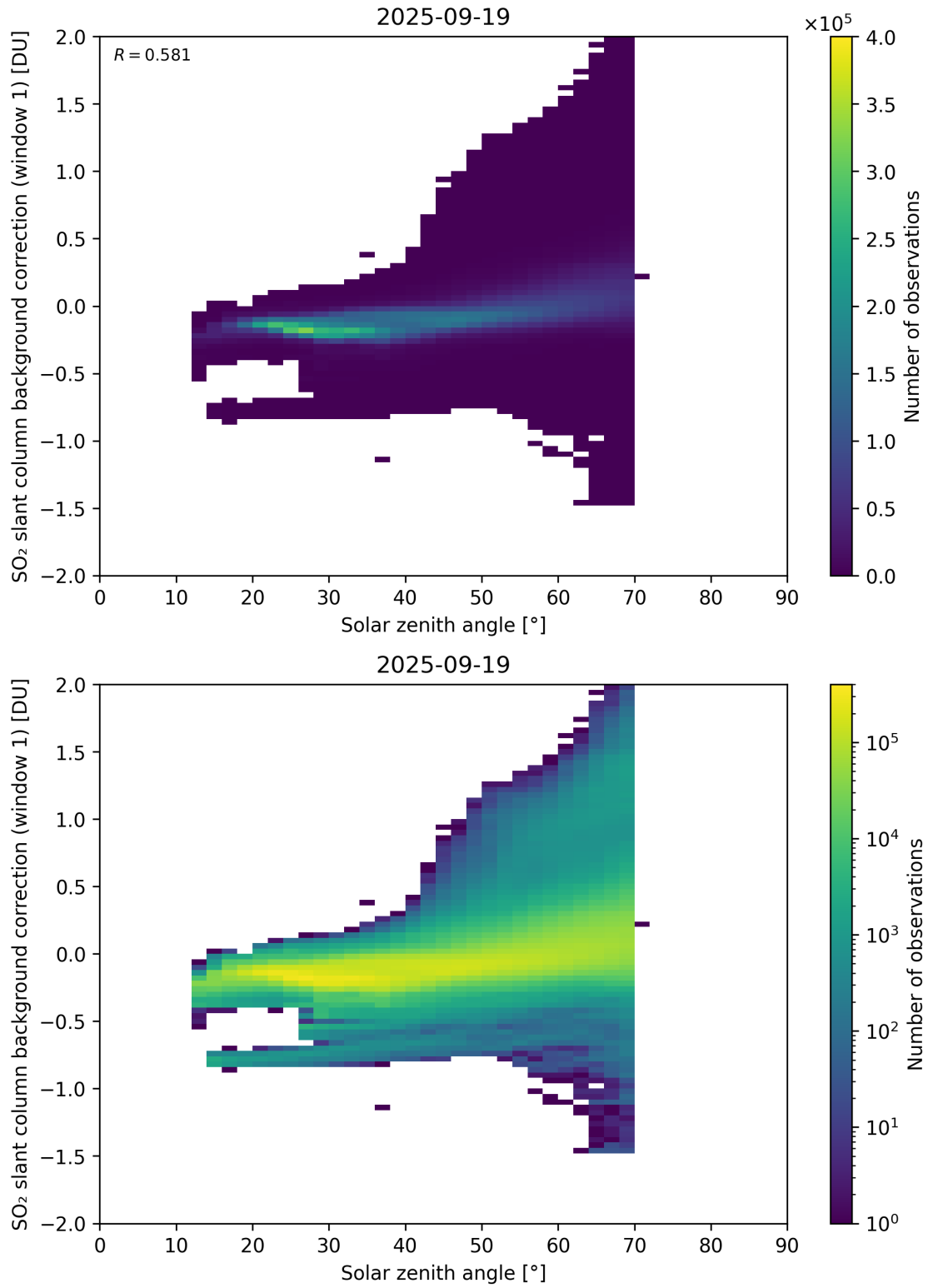
Figure 171: Scatter density plot of “Solar zenith angle” against “SO 2 slant column background correction (window 1)” for 2025-09-18 to 2025-09-20.
