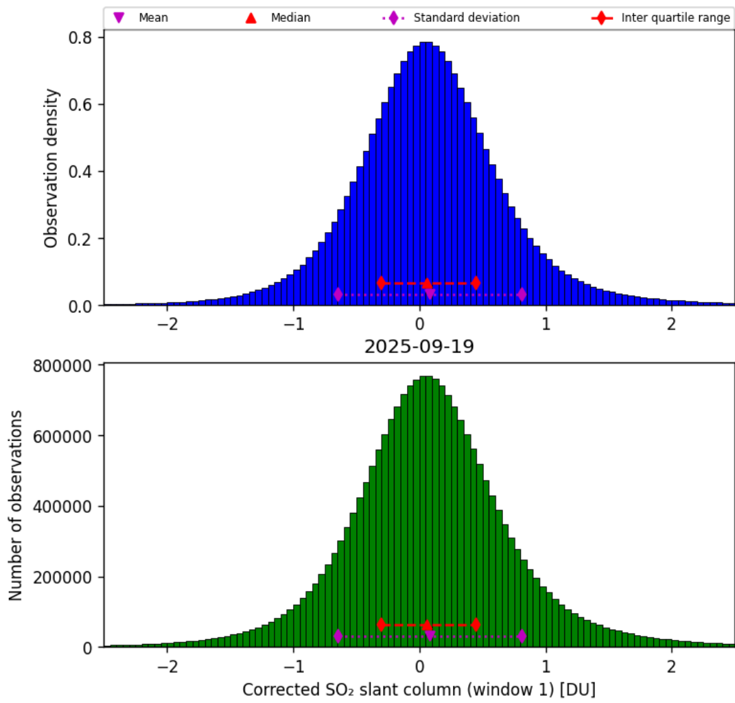
Figure 65: Histogram of “Corrected SO 2 slant column (window 1)” for 2025-09-18 to 2025-09-20
