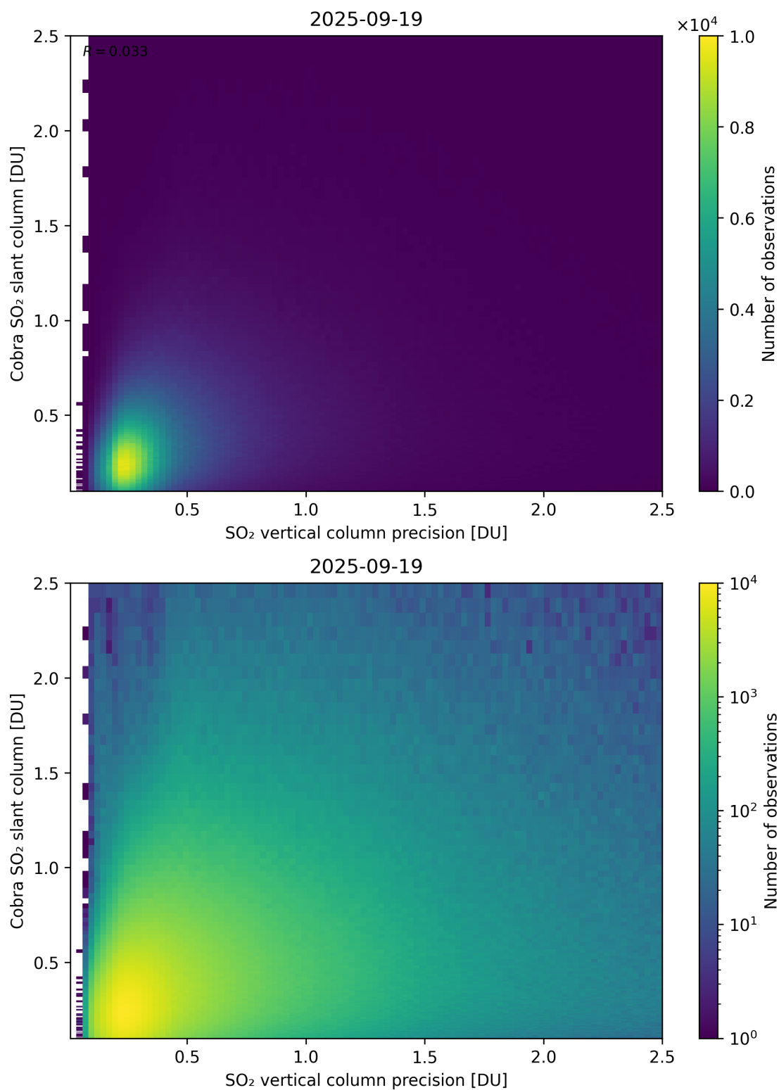
Figure 336: Scatter density plot of “SO 2 vertical column precision” against “Cobra SO 2 slant column” for 2025-09-18 to 2025-09-20.
