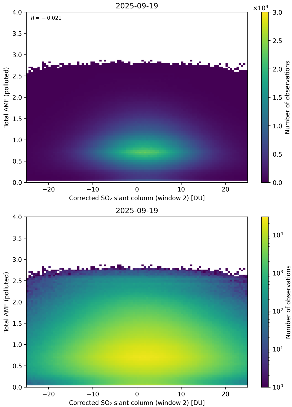
Figure 253: Scatter density plot of “Corrected SO 2 slant column (window 2)” against “Total AMF (polluted)” for 2025-09-18 to 2025-09-20.
