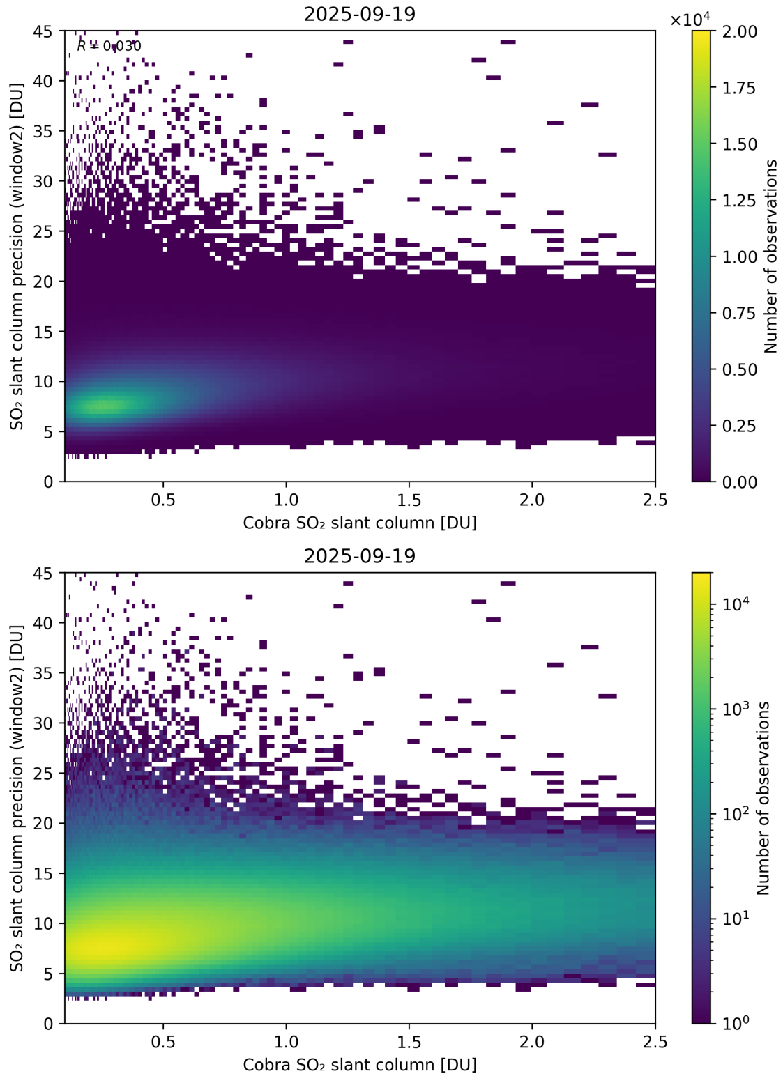
Figure 221: Scatter density plot of “Cobra SO 2 slant column” against “SO 2 slant column precision (window2)” for 2025-09-18 to 2025-09-20.
