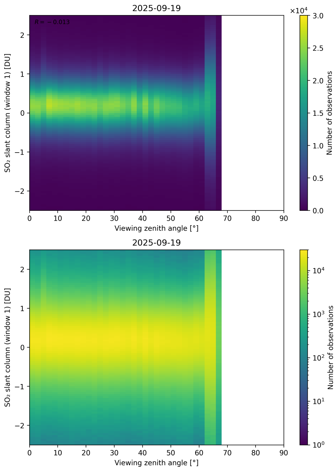
Figure 376: Scatter density plot of “Viewing zenith angle” against “SO 2 slant column (window 1)” for 2025-09-18 to 2025-09-20.
