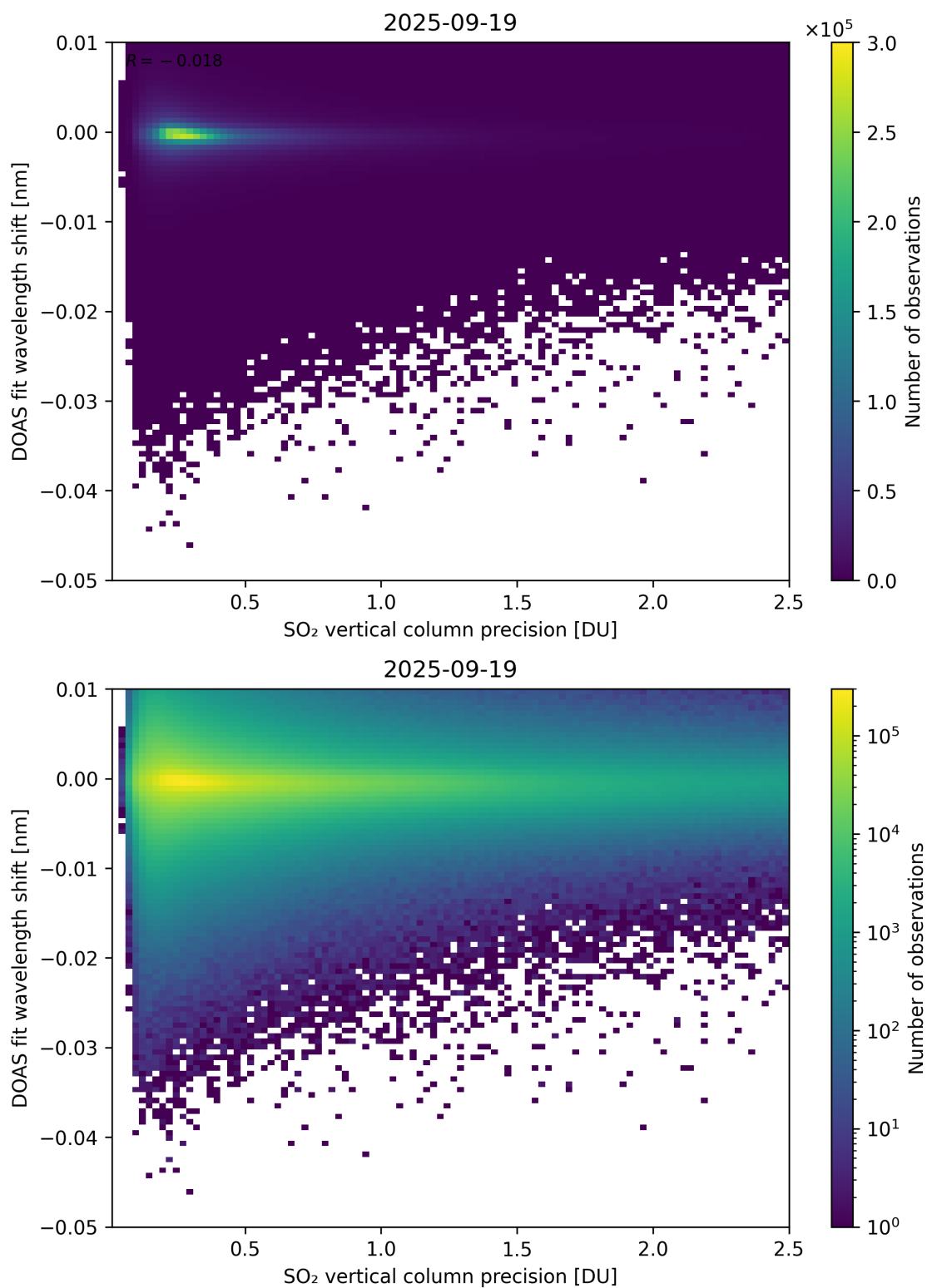
Figure 332: Scatter density plot of “SO 2 vertical column precision” against “DOAS fit wavelength shift” for 2025-09-18 to 2025-09-20.
