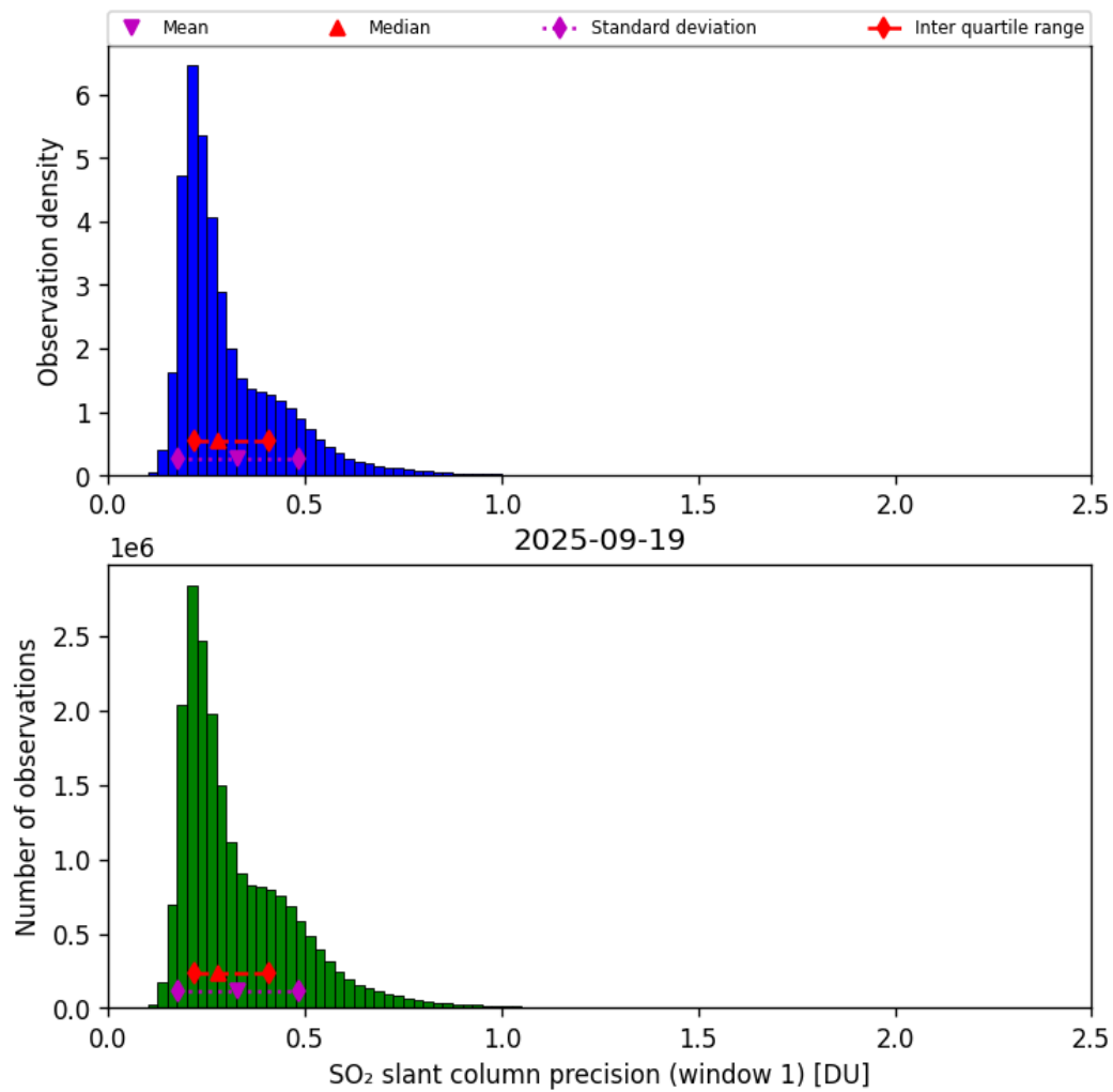
Figure 64: Histogram of “SO 2 slant column precision (window 1)” for 2025-09-18 to 2025-09-20
