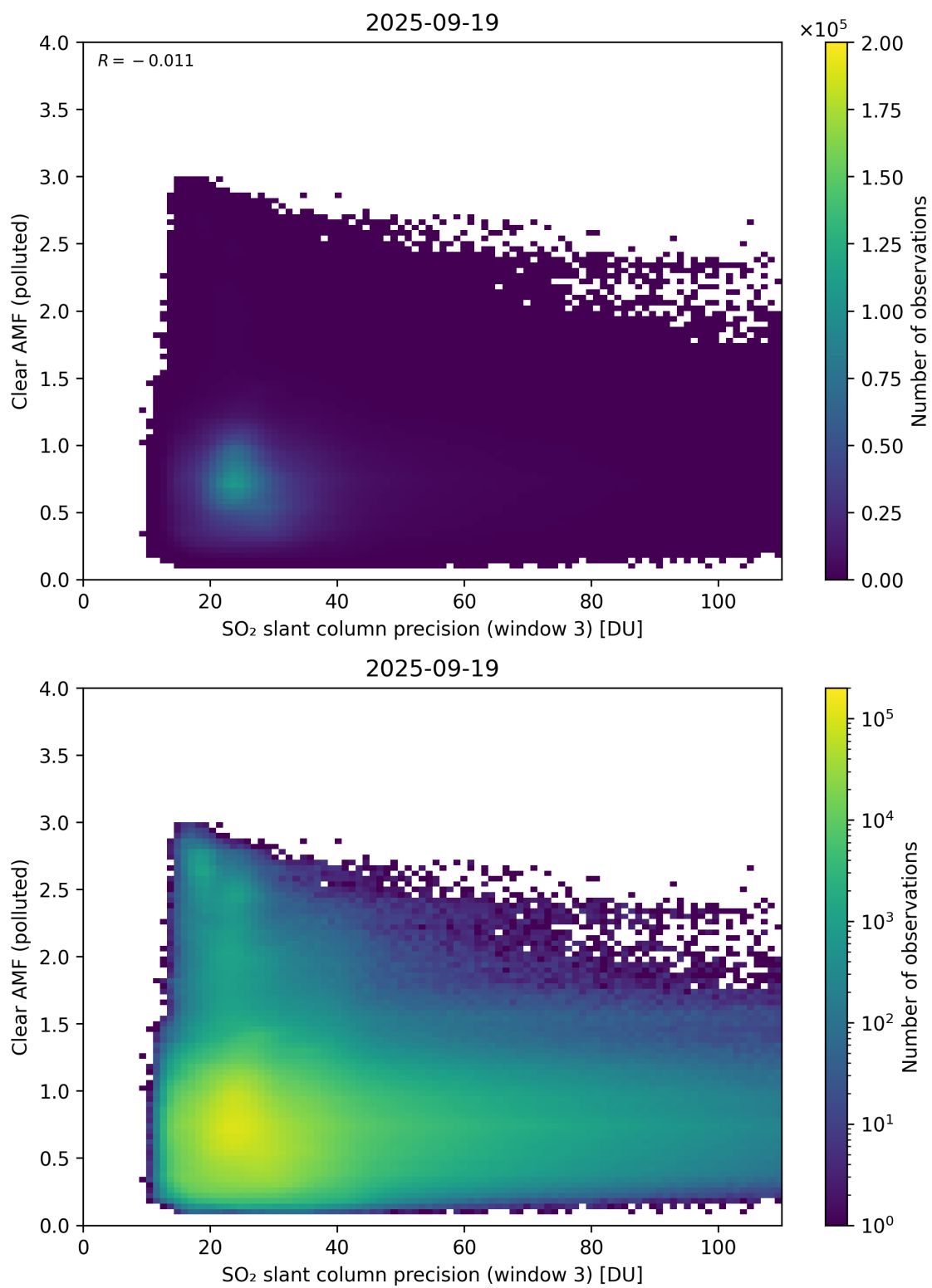
Figure 311: Scatter density plot of “SO 2 slant column precision (window 3)” against “Clear AMF (polluted)” for 2025-09-18 to 2025-09-20.
