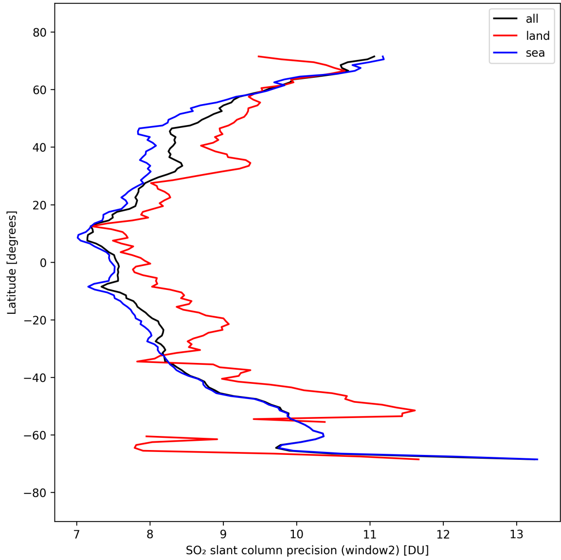
Figure 42: Zonal average of “SO 2 slant column precision (window2)” for 2025-09-18 to 2025-09-20.
