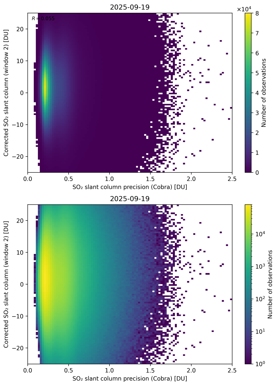
Figure 206: Scatter density plot of “SO 2 slant column precision (Cobra)” against “Corrected SO 2 slant column (window 2)” for 2025-09-18 to 2025-09-20.
