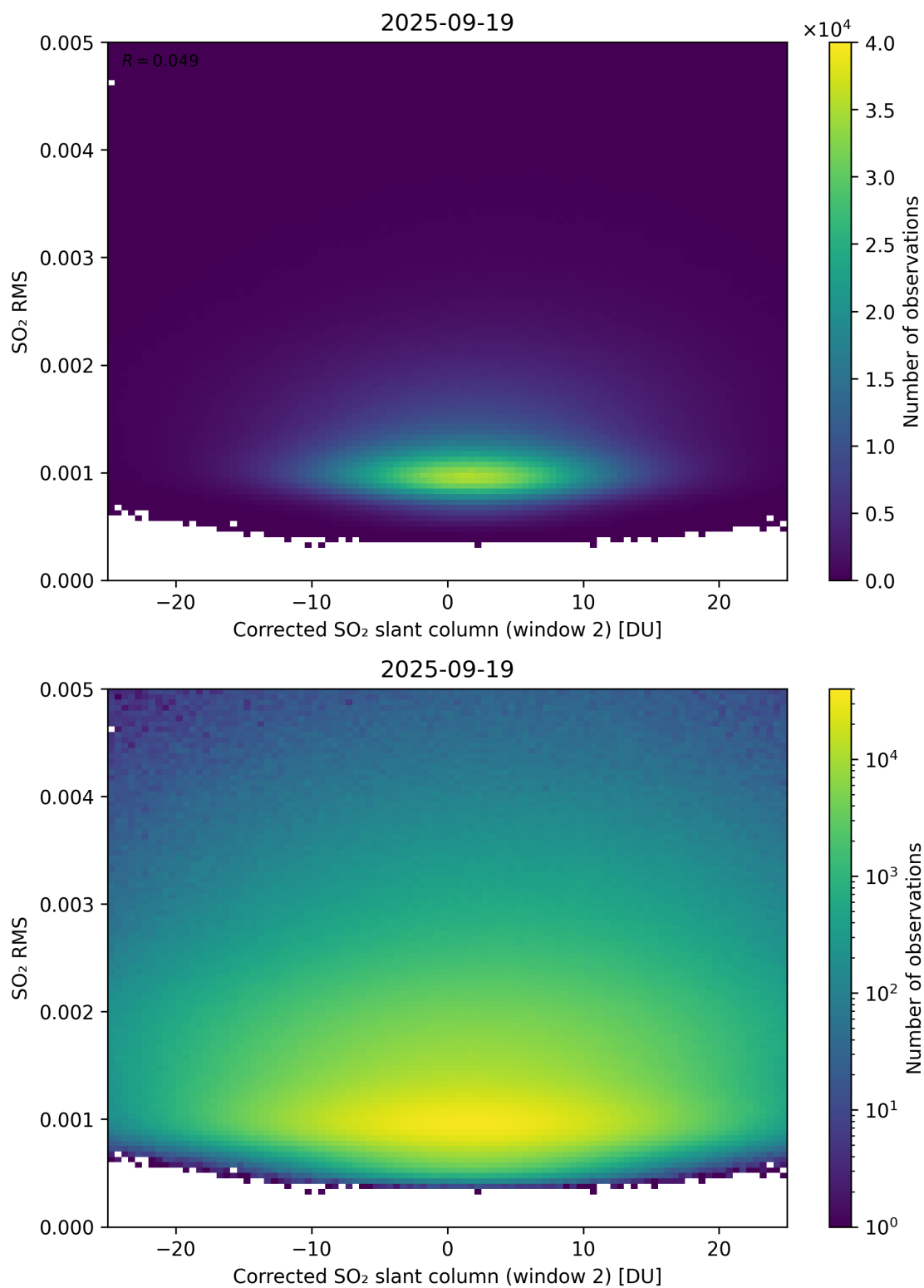
Figure 248: Scatter density plot of “Corrected SO 2 slant column (window 2)” against “SO 2 RMS” for 2025-09-18 to 2025-09-20.
