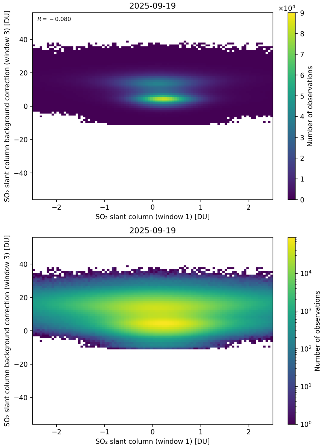
Figure 264: Scatter density plot of “SO 2 slant column (window 1)” against “SO 2 slant column background correction (window 3)” for 2025-09-18 to 2025-09-20.
