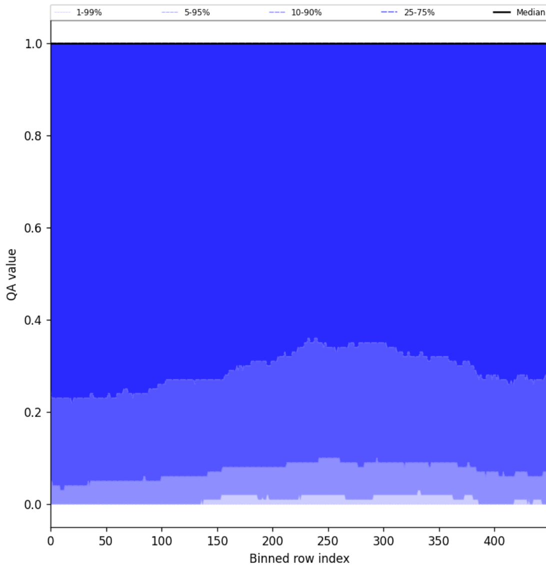
Figure 83: Along track statistics of “QA value” for 2025-09-18 to 2025-09-20
