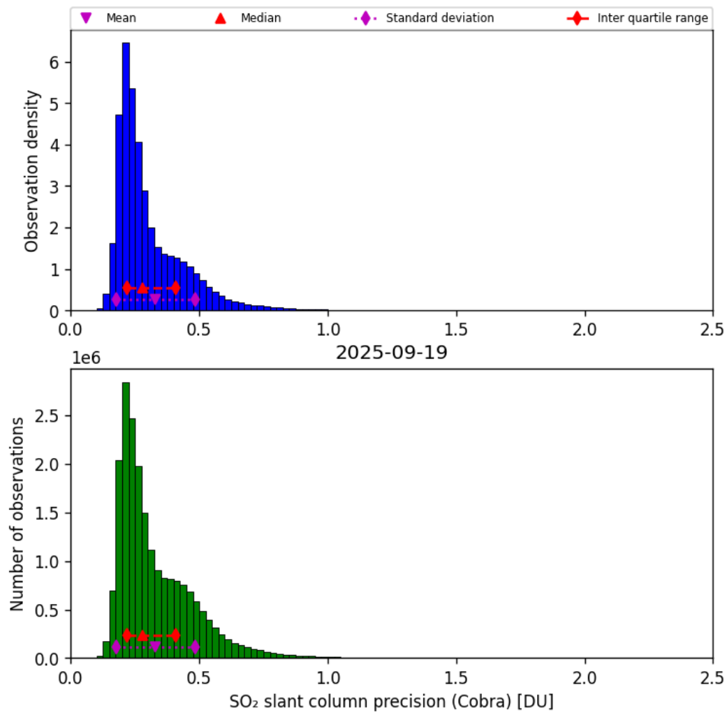
Figure 62: Histogram of “SO 2 slant column precision (Cobra)” for 2025-09-18 to 2025-09-20
