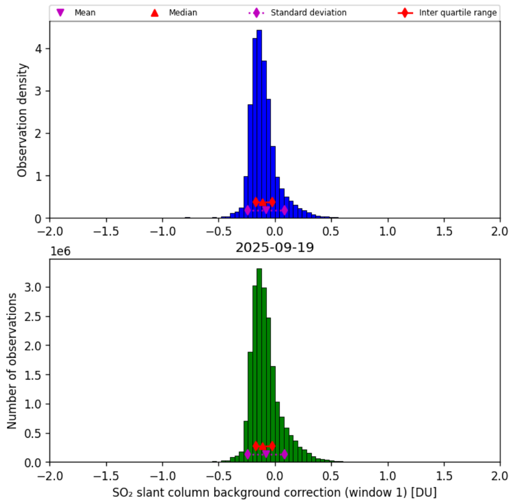
Figure 66: Histogram of “SO 2 slant column background correction (window 1)” for 2025-09-18 to 2025-09-20
