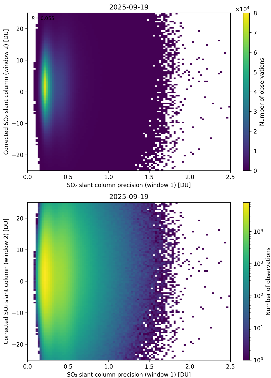
Figure 275: Scatter density plot of “SO 2 slant column precision (window 1)” against “Corrected SO 2 slant column (window 2)” for 2025-09-18 to 2025-09-20.
