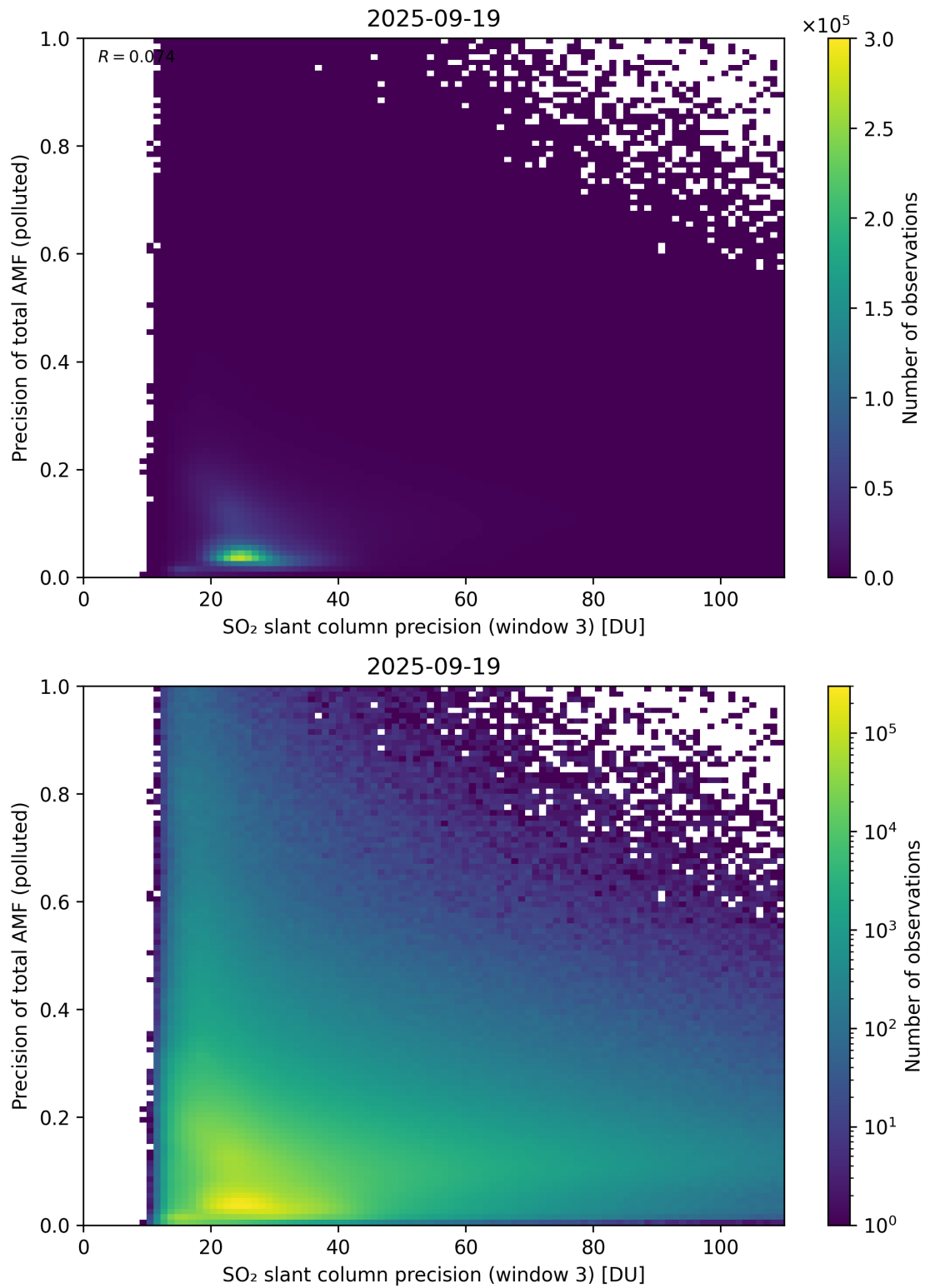
Figure 314: Scatter density plot of “SO 2 slant column precision (window 3)” against “Precision of total AMF (polluted)” for 2025-09-18 to 2025-09-20.
