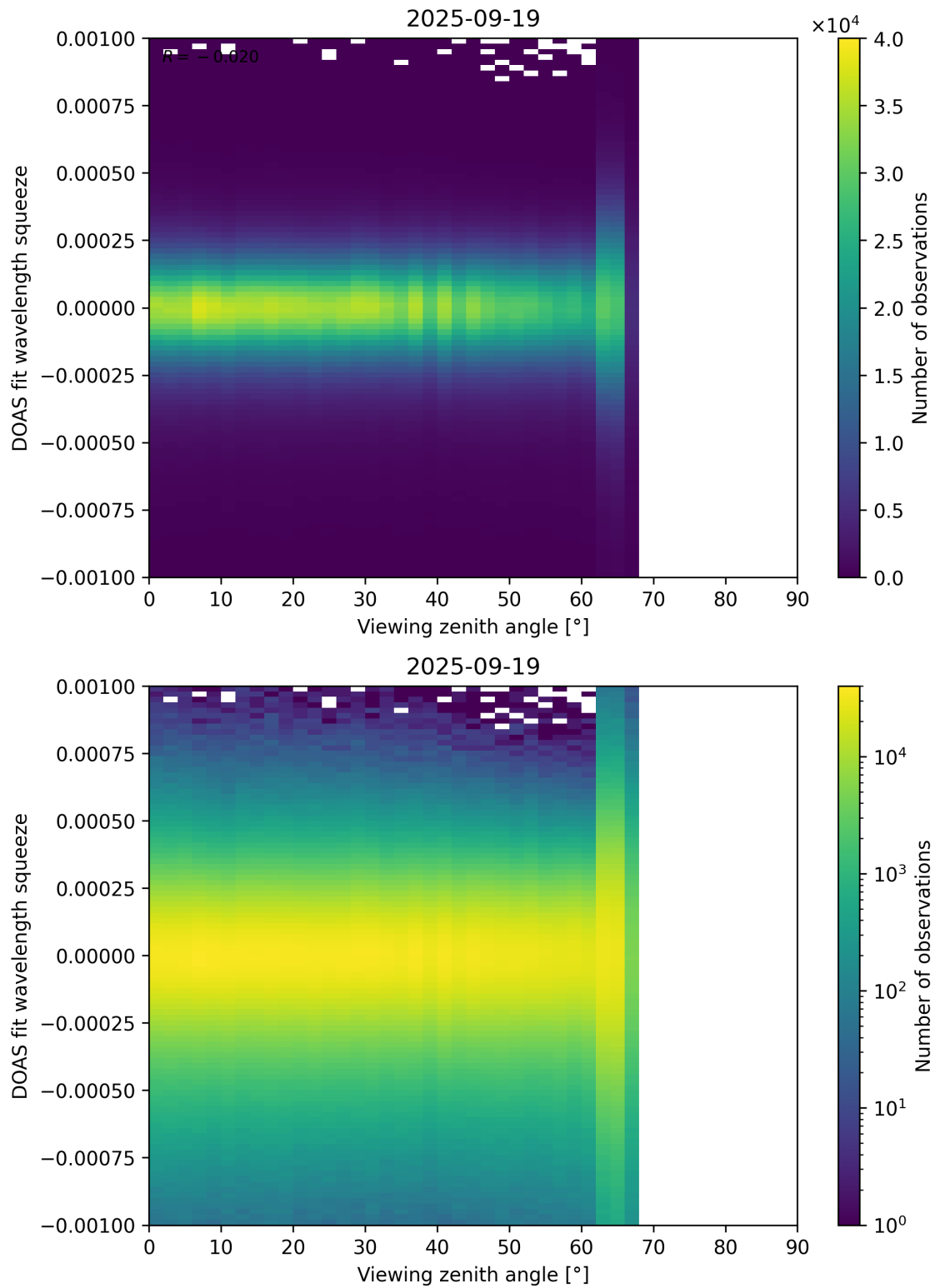
Figure 366: Scatter density plot of “Viewing zenith angle” against “DOAS fit wavelength squeeze” for 2025-09-18 to 2025-09-20.
