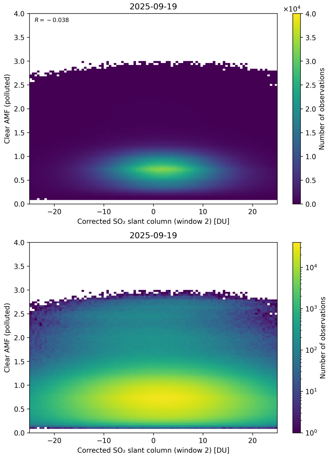
Figure 249: Scatter density plot of “Corrected SO 2 slant column (window 2)” against “Clear AMF (polluted)” for 2025-09-18 to 2025-09-20.
