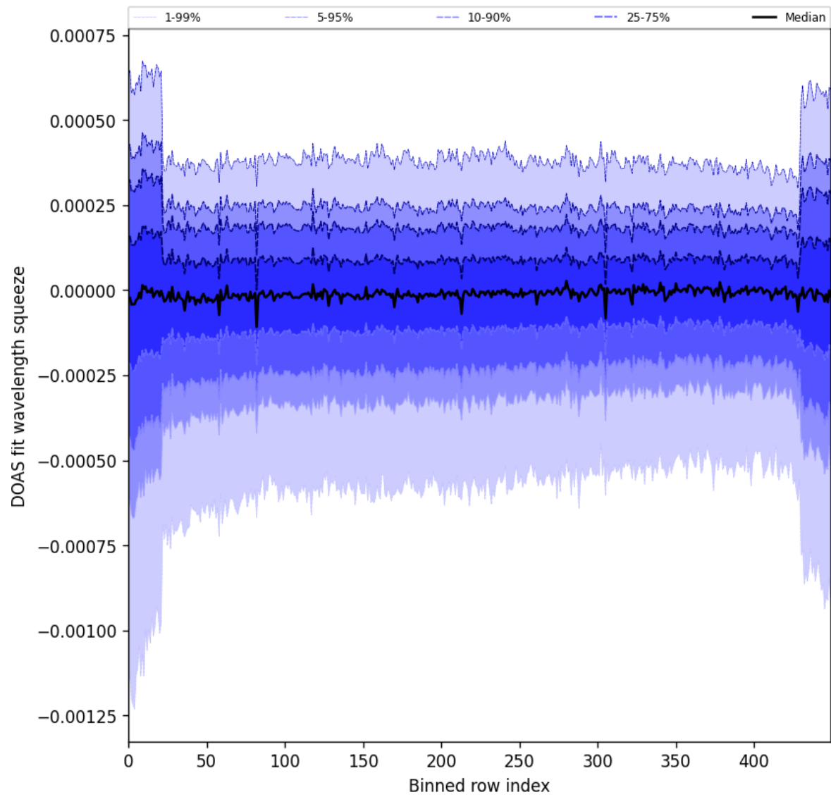
Figure 103: Along track statistics of “DOAS fit wavelength squeeze” for 2025-09-18 to 2025-09-20
