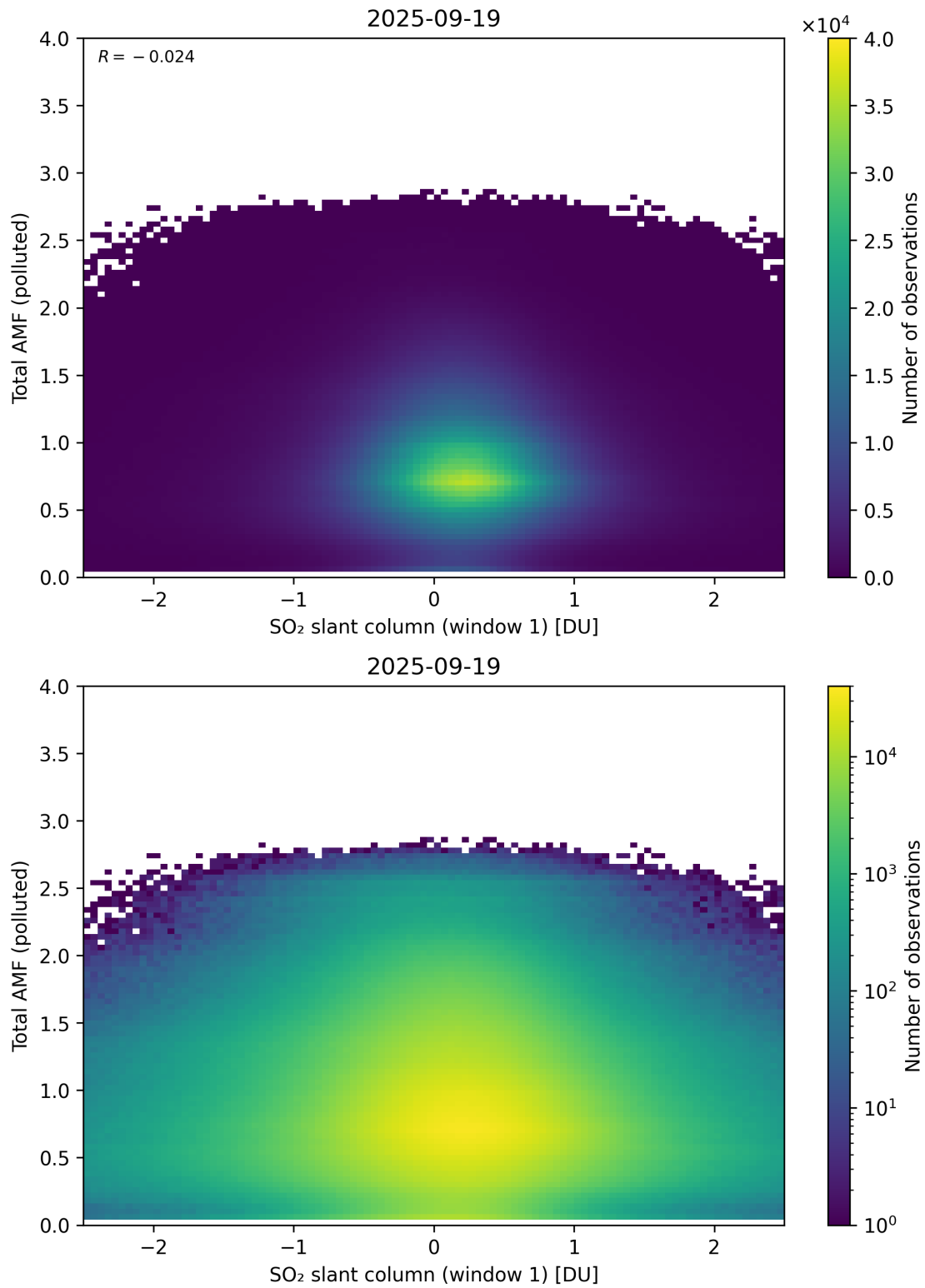
Figure 289: Scatter density plot of “SO 2 slant column (window 1)” against “Total AMF (polluted)” for 2025-09-18 to 2025-09-20.
