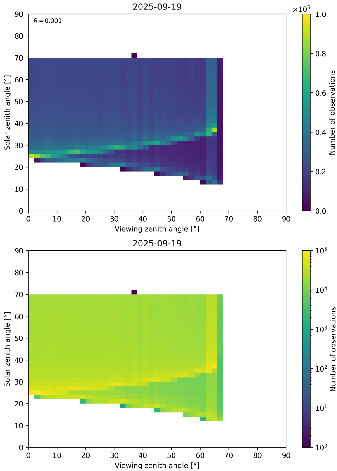
Figure 369: Scatter density plot of “Viewing zenith angle” against “Solar zenith angle” for 2025-09-18 to 2025-09-20.
