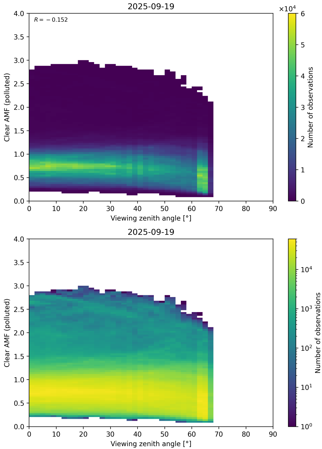
Figure 370: Scatter density plot of “Viewing zenith angle” against “Clear AMF (polluted)” for 2025-09-18 to 2025-09-20.
