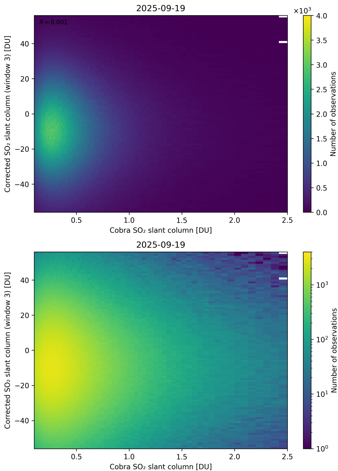
Figure 218: Scatter density plot of “Cobra SO 2 slant column” against “Corrected SO 2 slant column (window 3)” for 2025-09-18 to 2025-09-20.
