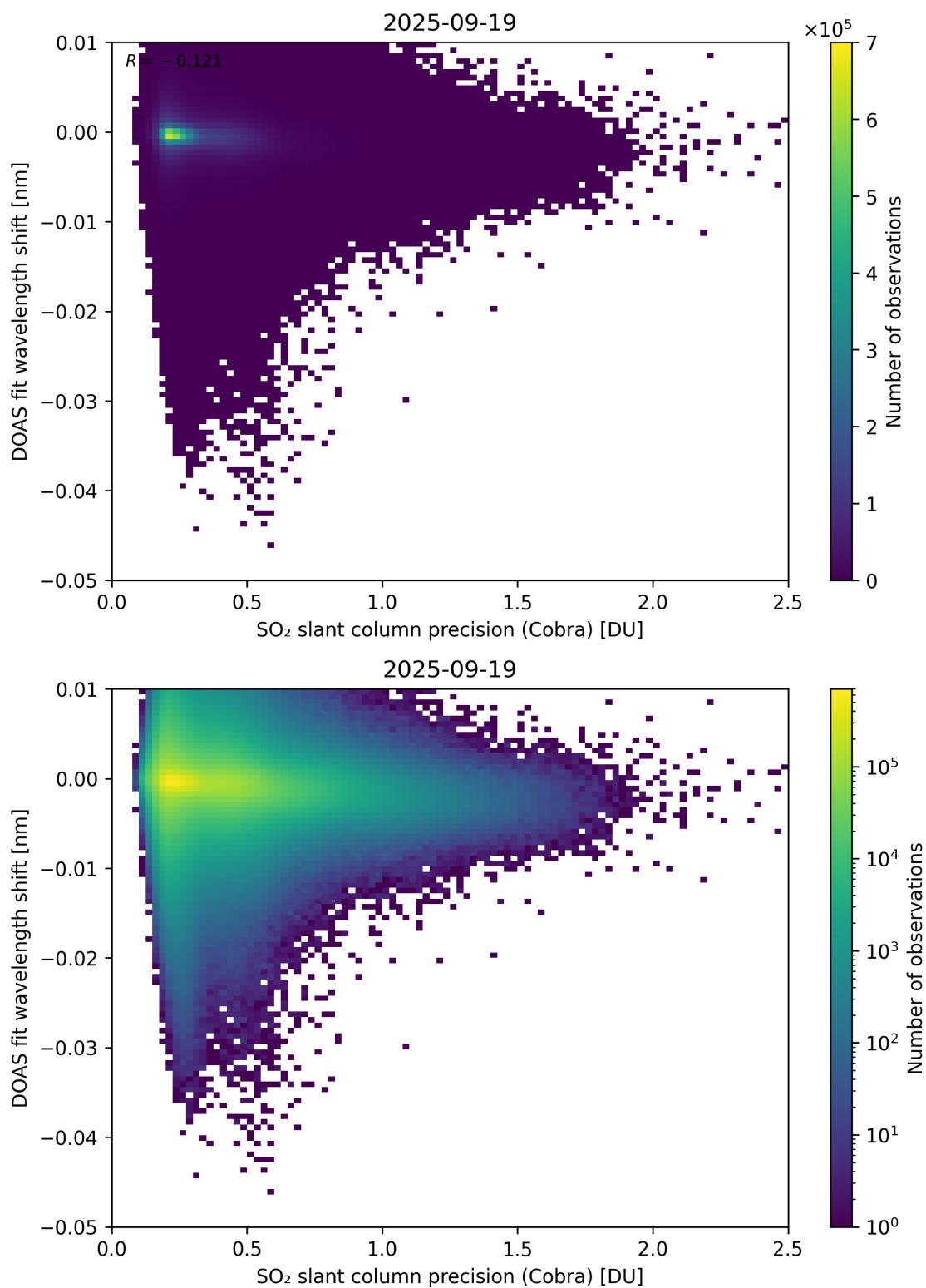
Figure 202: Scatter density plot of “SO 2 slant column precision (Cobra)” against “DOAS fit wavelength shift” for 2025-09-18 to 2025-09-20.
