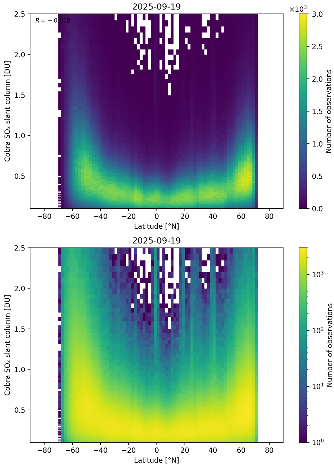
Figure 157: Scatter density plot of “Latitude” against “Cobra SO 2 slant column” for 2025-09-18 to 2025-09-20.
