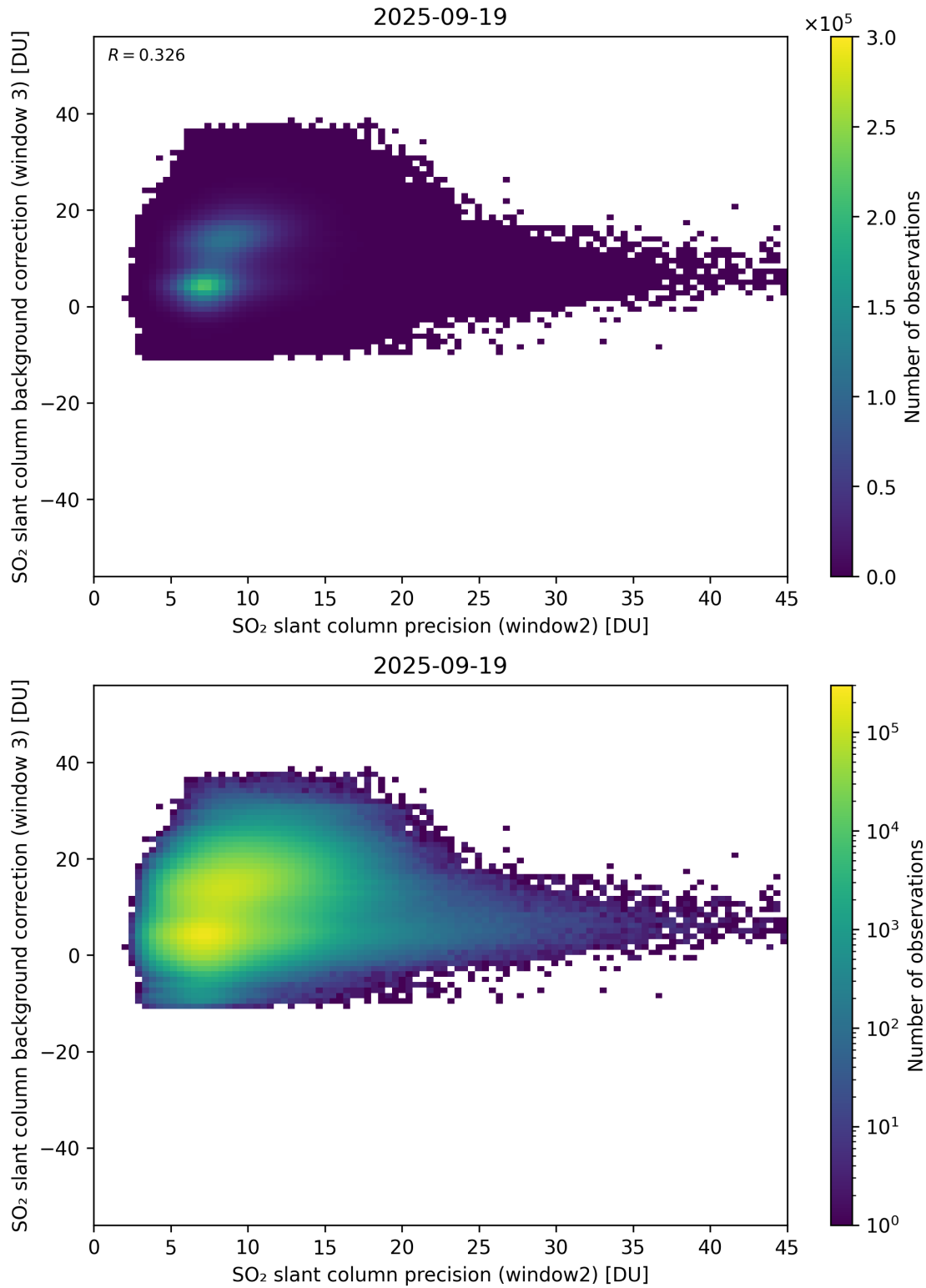
Figure 292: Scatter density plot of “SO 2 slant column precision (window2)” against “SO 2 slant column background correction (window 3)” for 2025-09-18 to 2025-09-20.
