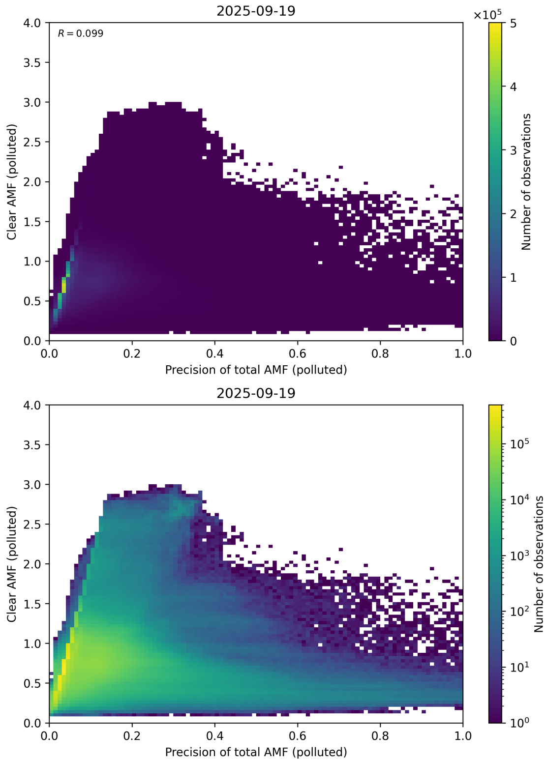
Figure 320: Scatter density plot of “Precision of total AMF (polluted)” against “Clear AMF (polluted)” for 2025-09-18 to 2025-09-20.
