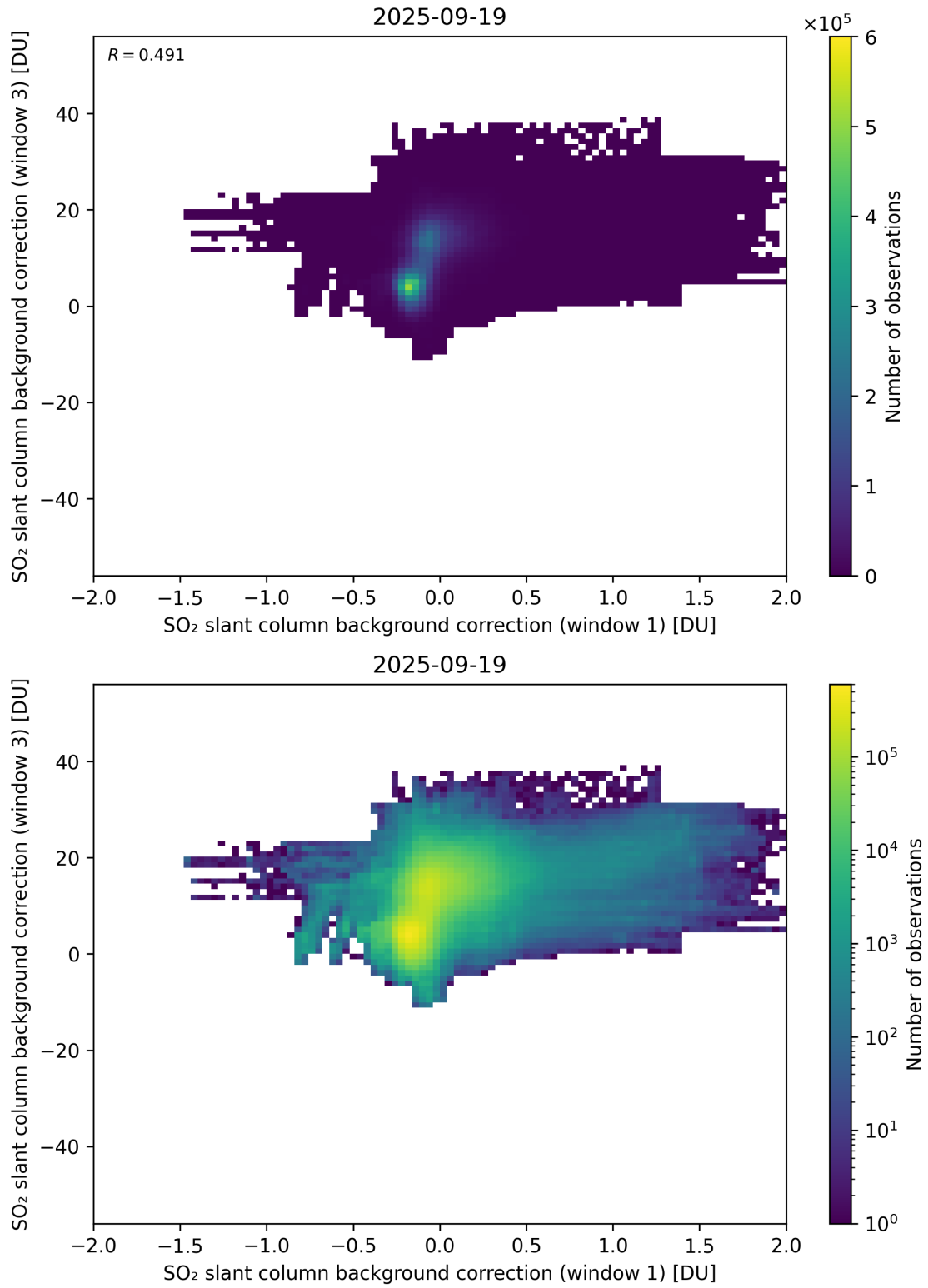
Figure 110: Scatter density plot of “SO 2 slant column background correction (window 1)” against “SO 2 slant column background correction (window 3)” for 2025-09-18 to 2025-09-20.
