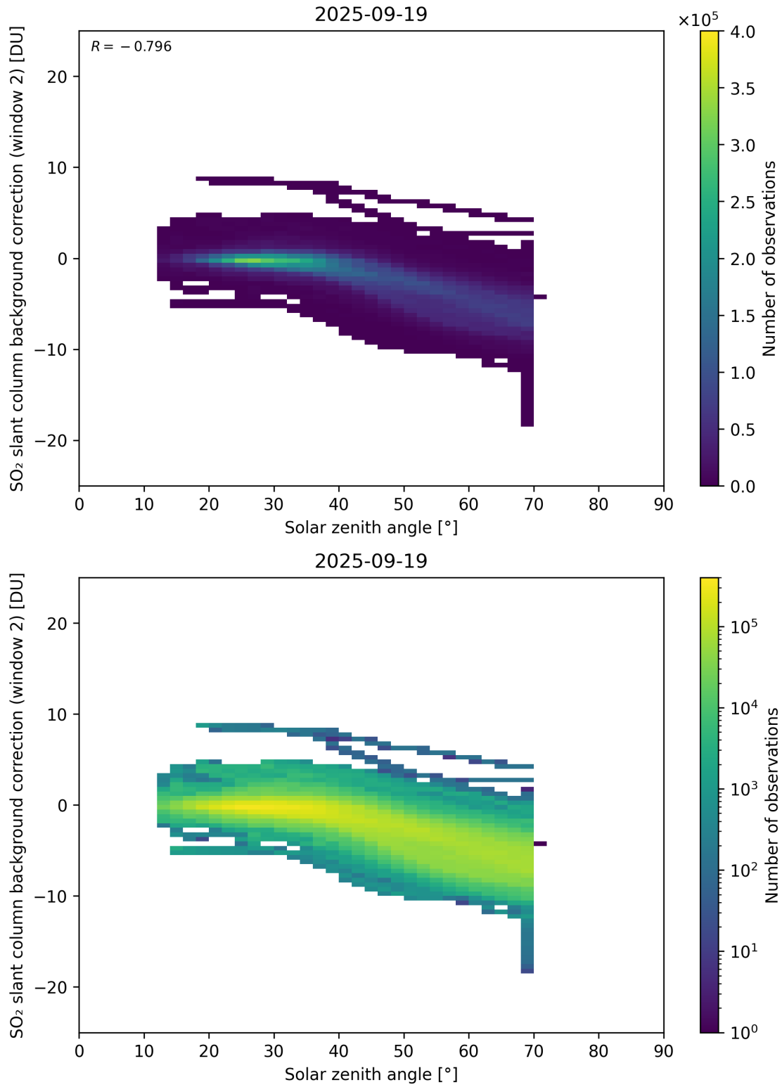
Figure 172: Scatter density plot of “Solar zenith angle” against “SO 2 slant column background correction (window 2)” for 2025-09-18 to 2025-09-20.
