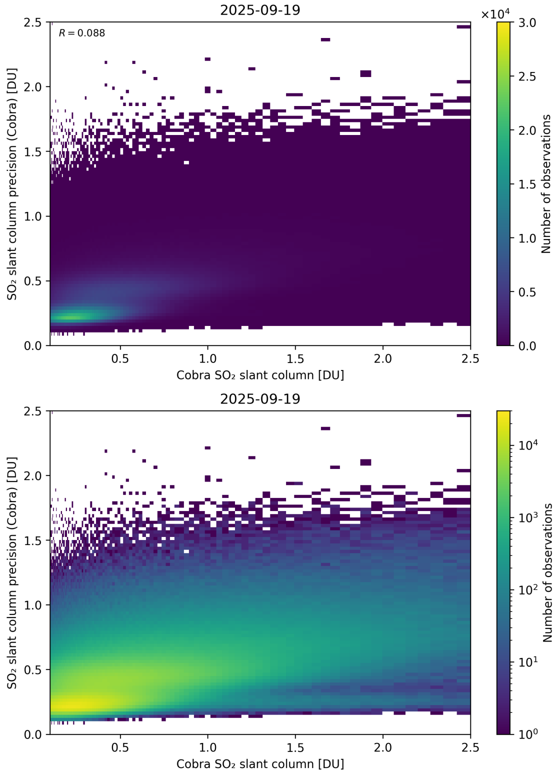
Figure 216: Scatter density plot of “Cobra SO 2 slant column” against “SO 2 slant column precision (Cobra)” for 2025-09-18 to 2025-09-20.
