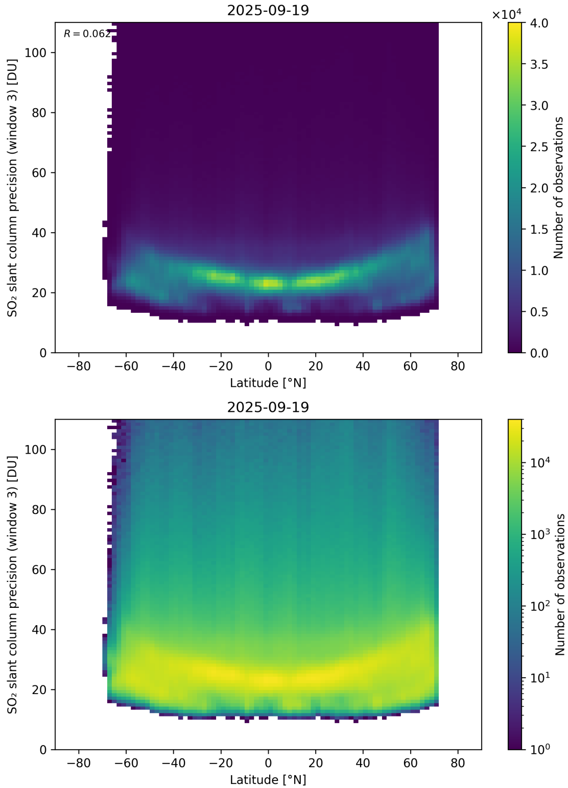
Figure 166: Scatter density plot of “Latitude” against “SO 2 slant column precision (window 3)” for 2025-09-18 to 2025-09-20.
