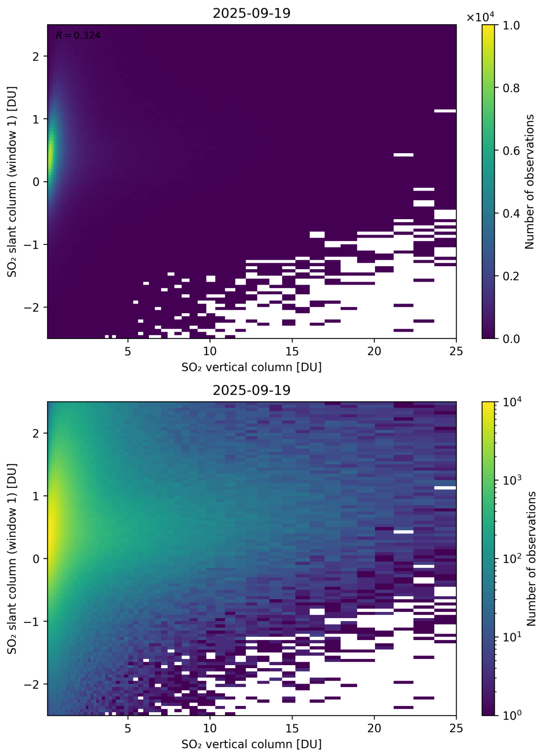
Figure 354: Scatter density plot of “SO 2 vertical column” against “SO 2 slant column (window 1)” for 2025-09-18 to 2025-09-20.
