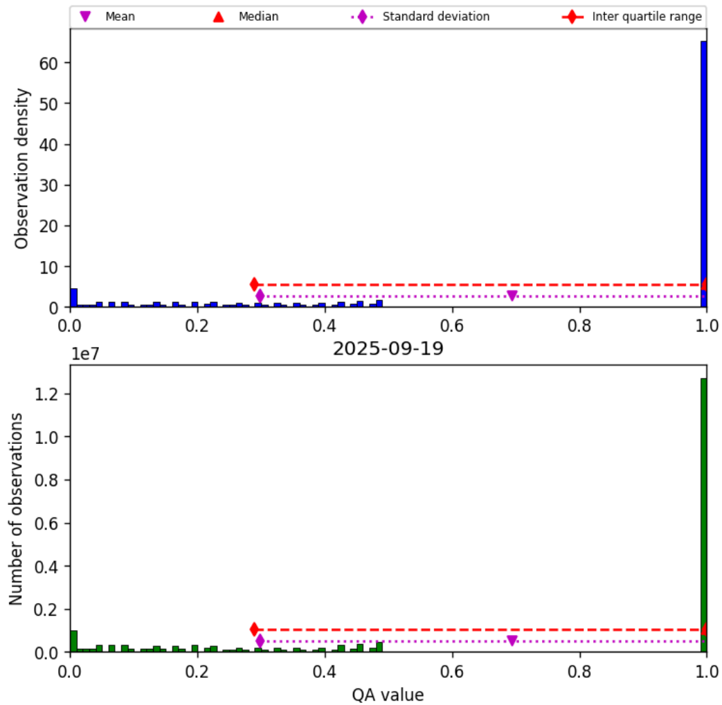
Figure 57: Histogram of “QA value” for 2025-09-18 to 2025-09-20
