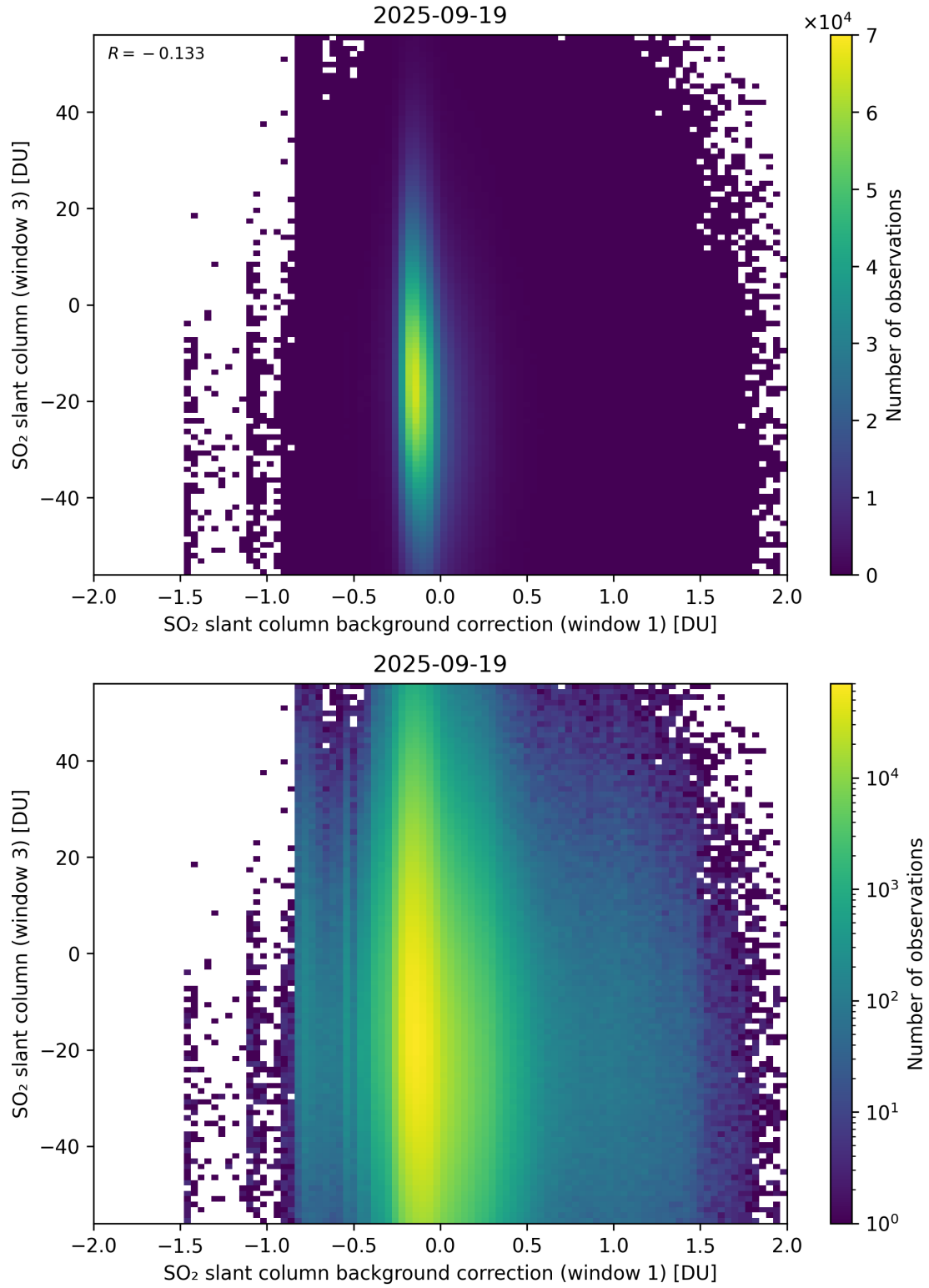
Figure 118: Scatter density plot of “SO 2 slant column background correction (window 1)” against “SO 2 slant column (window 3)” for 2025-09-18 to 2025-09-20.
