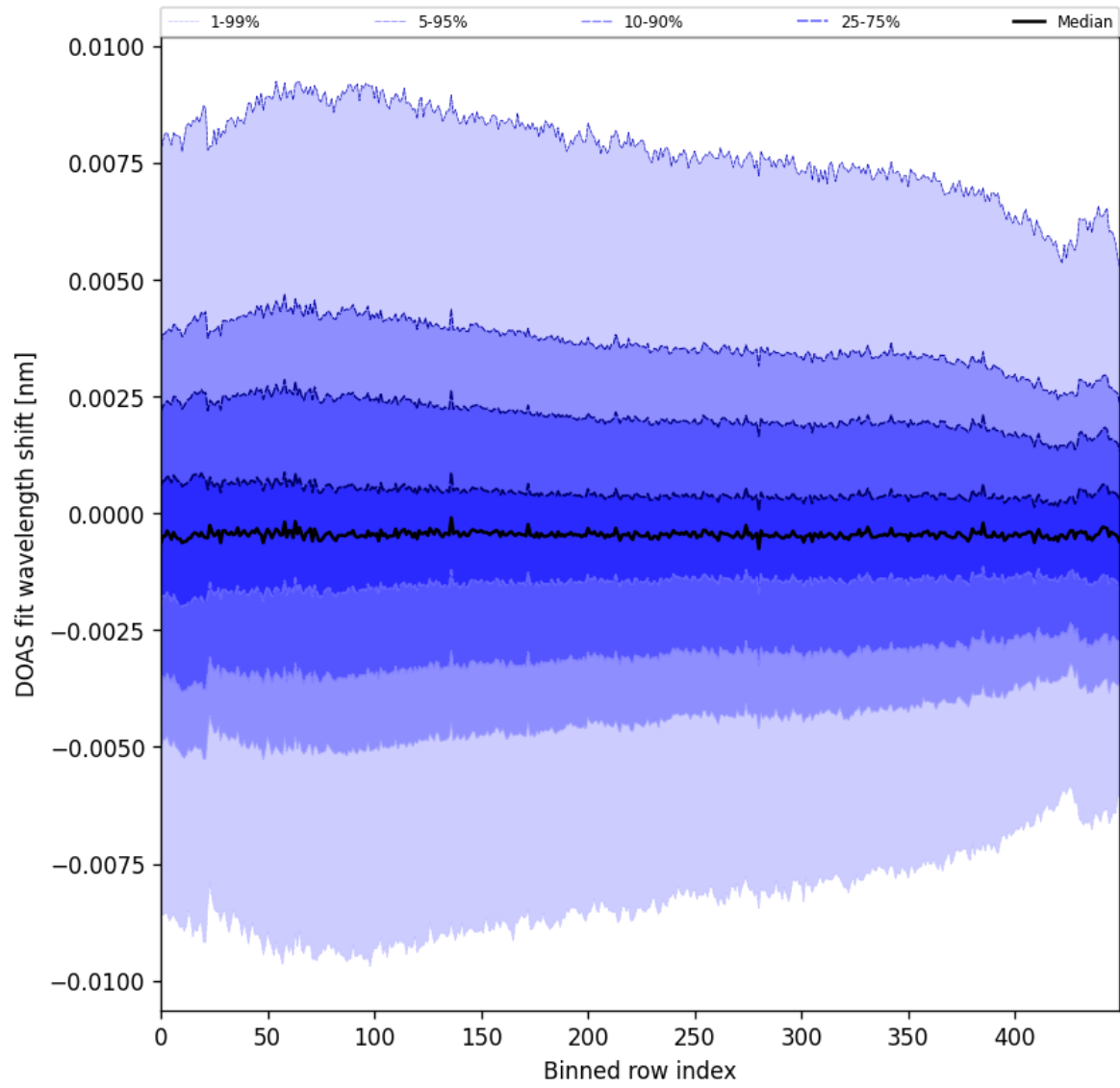
Figure 102: Along track statistics of “DOAS fit wavelength shift” for 2025-09-18 to 2025-09-20
