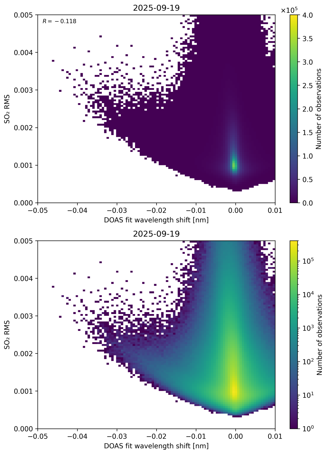
Figure 139: Scatter density plot of “DOAS fit wavelength shift” against “SO 2 RMS” for 2025-09-18 to 2025-09-20.
