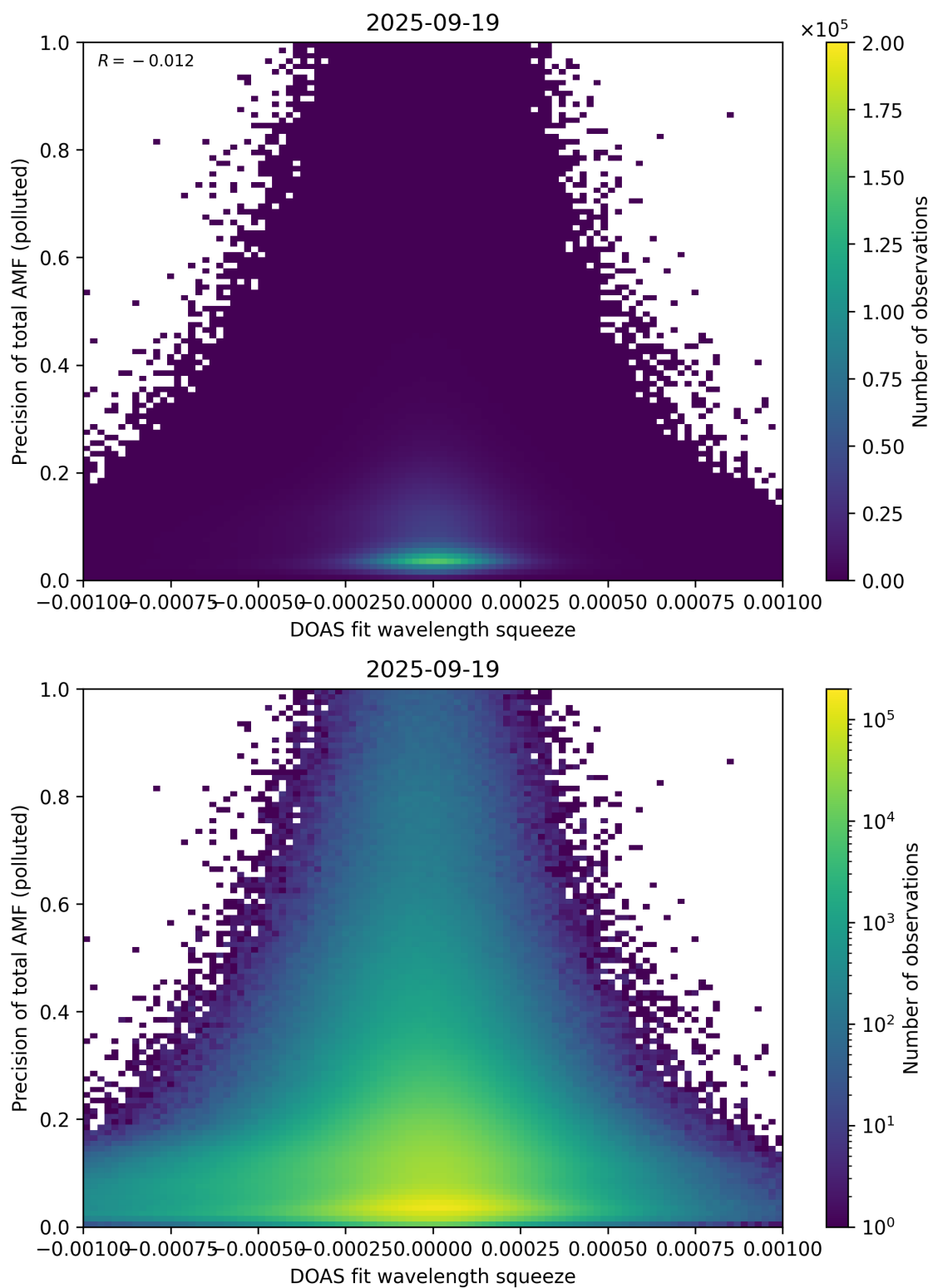
Figure 146: Scatter density plot of “DOAS fit wavelength squeeze” against “Precision of total AMF (polluted)” for 2025-09-18 to 2025-09-20.
