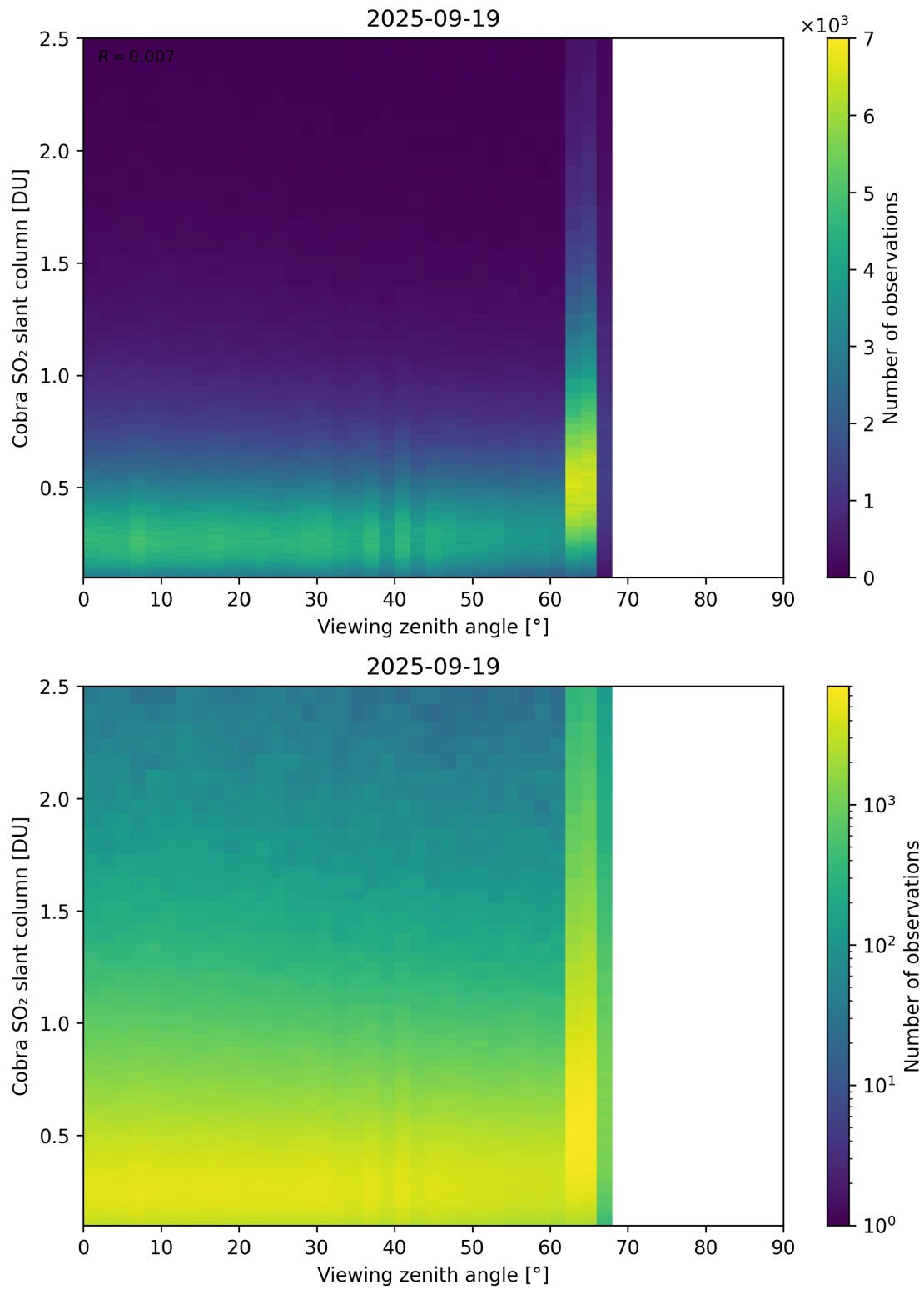
Figure 371: Scatter density plot of “Viewing zenith angle” against “Cobra SO 2 slant column” for 2025-09-18 to 2025-09-20.
