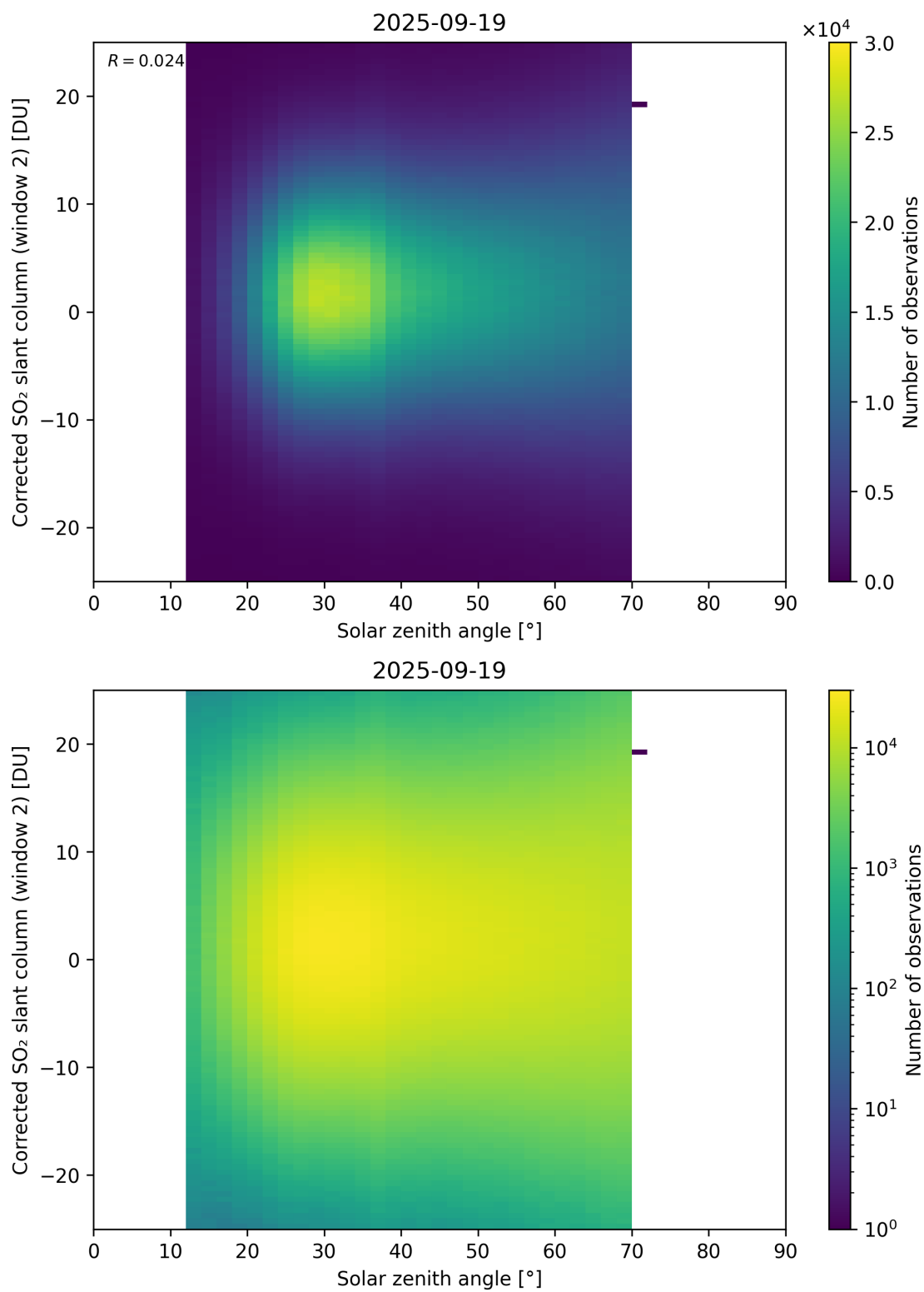
Figure 182: Scatter density plot of “Solar zenith angle” against “Corrected SO 2 slant column (window 2)” for 2025-09-18 to 2025-09-20.
