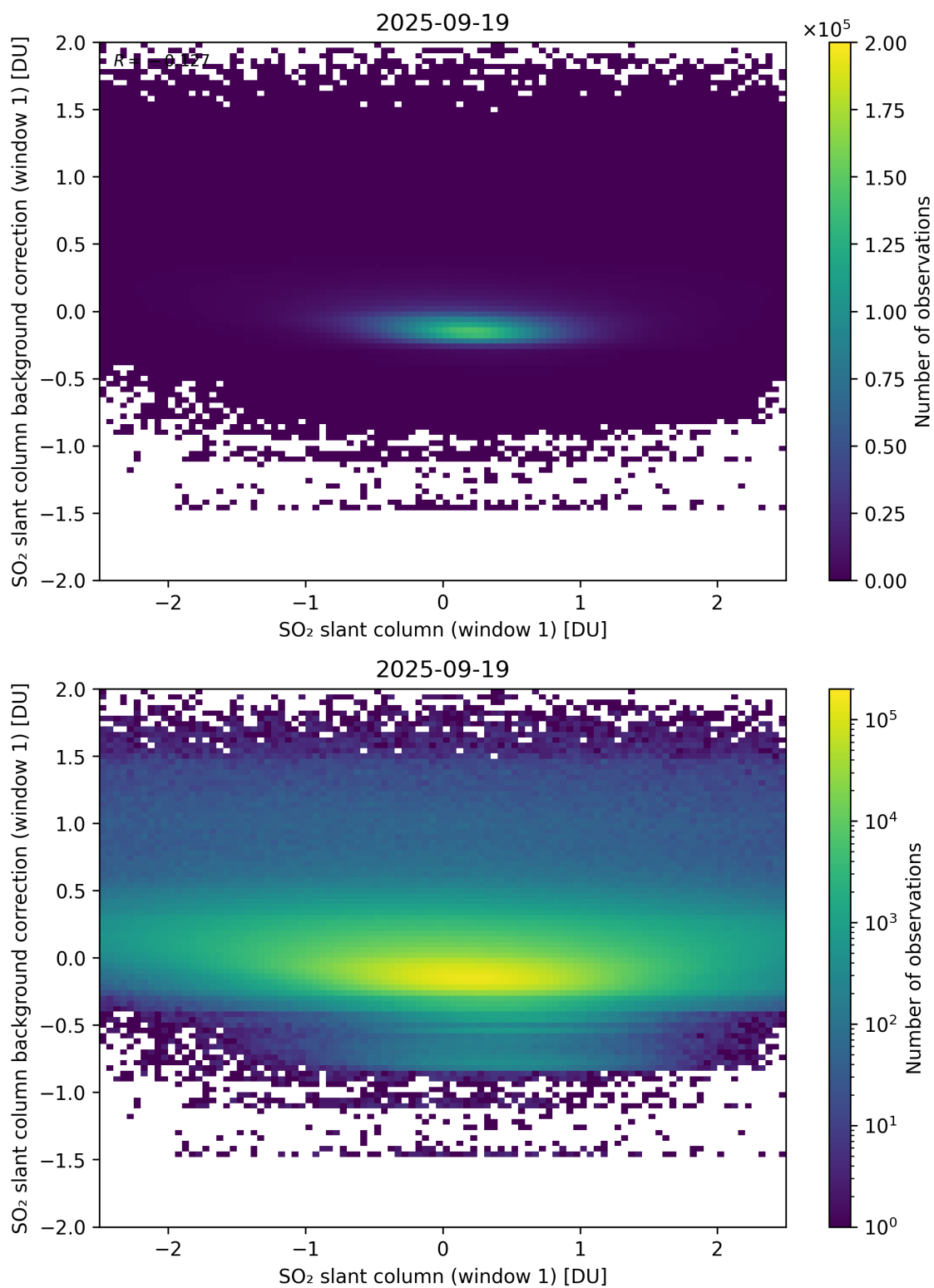
Figure 262: Scatter density plot of “SO 2 slant column (window 1)” against “SO 2 slant column background correction (window 1)” for 2025-09-18 to 2025-09-20.
