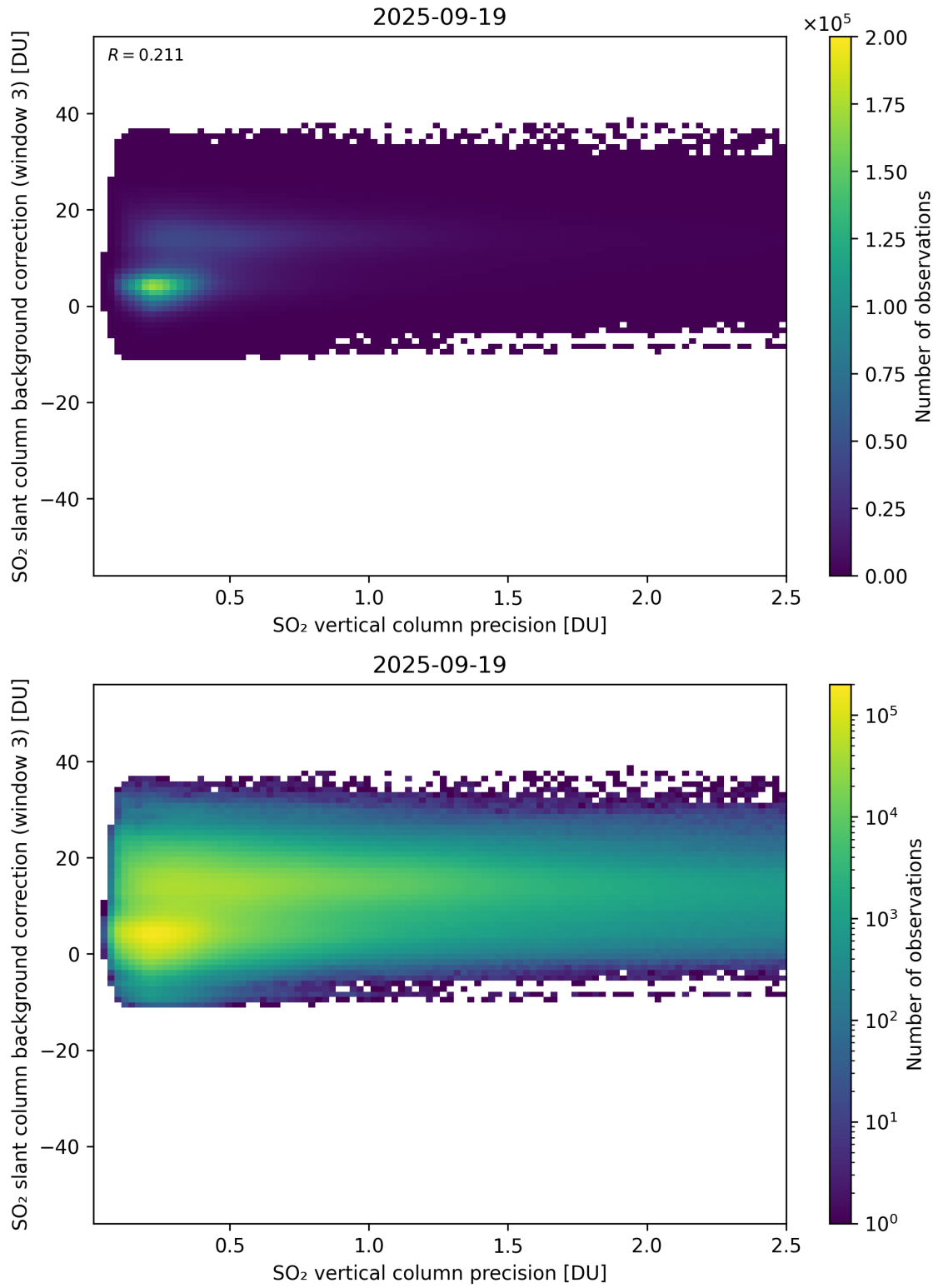
Figure 331: Scatter density plot of “SO 2 vertical column precision” against “SO 2 slant column background correction (window 3)” for 2025-09-18 to 2025-09-20.
