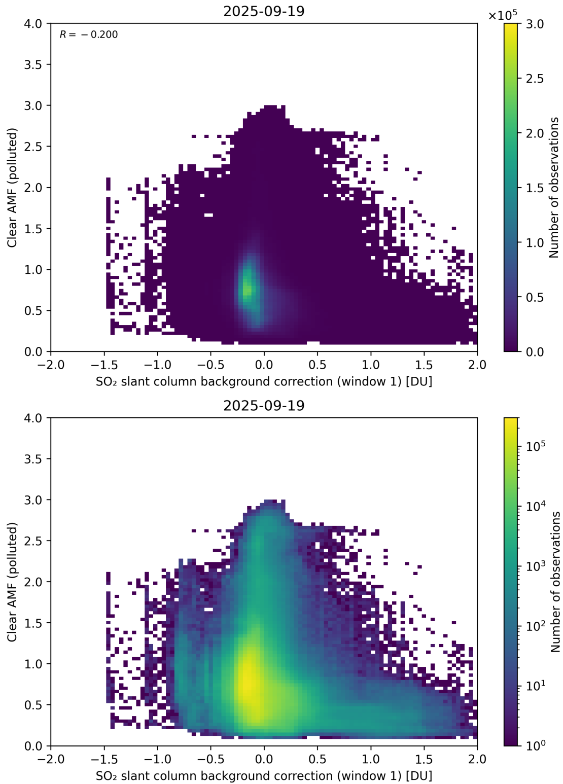
Figure 114: Scatter density plot of “SO 2 slant column background correction (window 1)” against “Clear AMF (polluted)” for 2025-09-18 to 2025-09-20.
