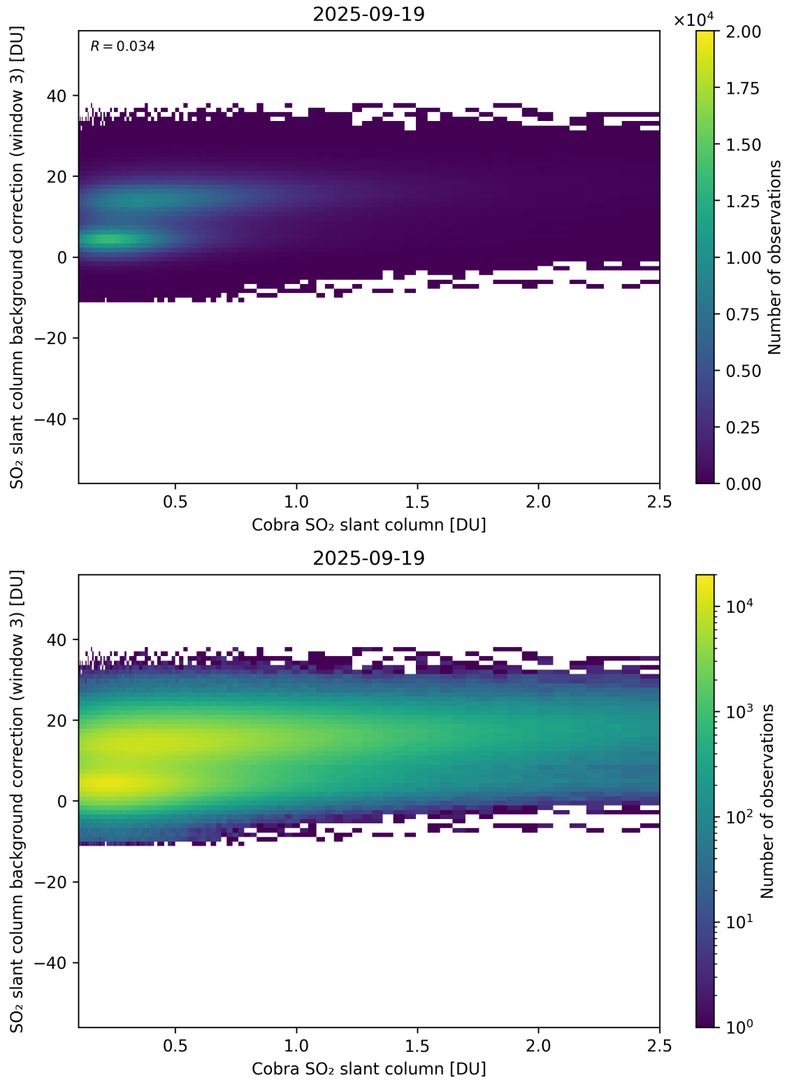
Figure 195: Scatter density plot of “Cobra SO 2 slant column” against “SO 2 slant column background correction (window 3)” for 2025-09-18 to 2025-09-20.
