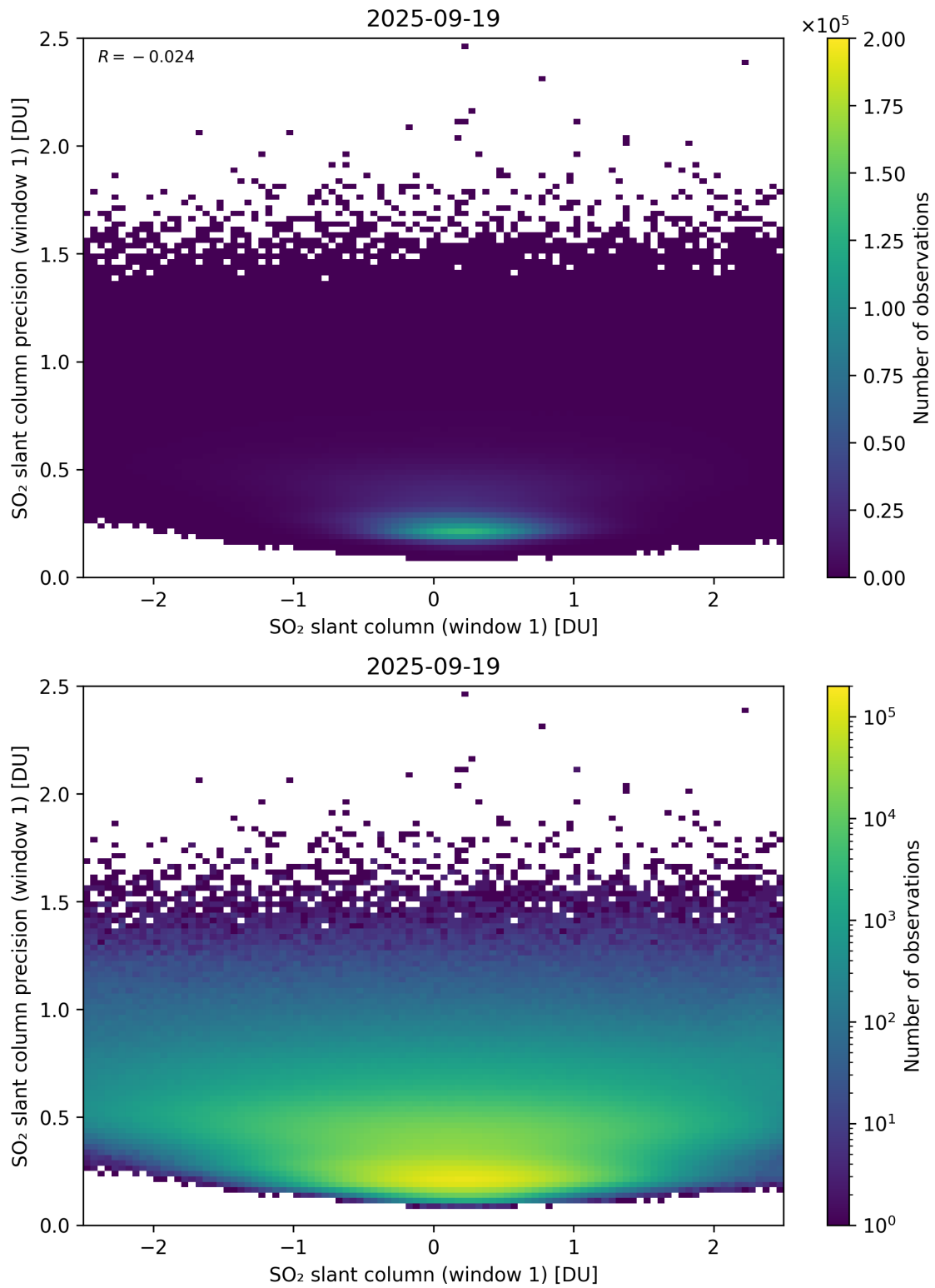
Figure 285: Scatter density plot of “SO 2 slant column (window 1)” against “SO 2 slant column precision (window 1)” for 2025-09-18 to 2025-09-20.
