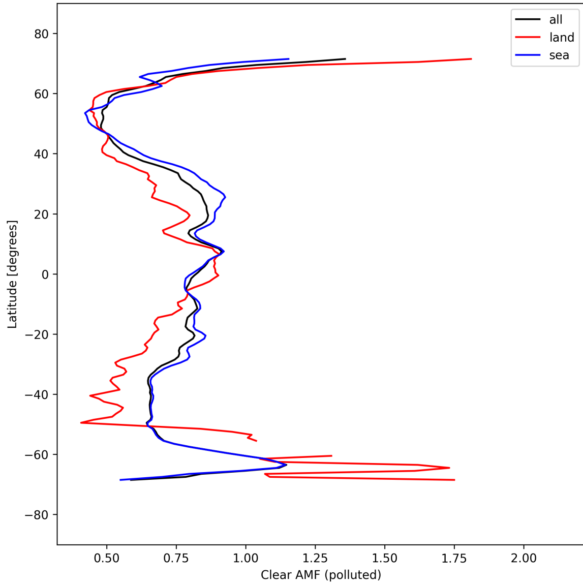
Figure 55: Zonal average of “Clear AMF (polluted)” for 2025-09-18 to 2025-09-20.
