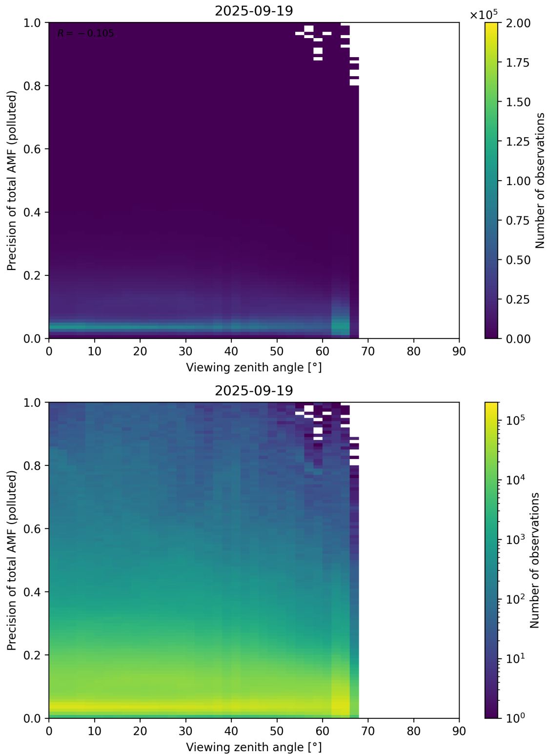
Figure 382: Scatter density plot of “Viewing zenith angle” against “Precision of total AMF (polluted)” for 2025-09-18 to 2025-09-20.
