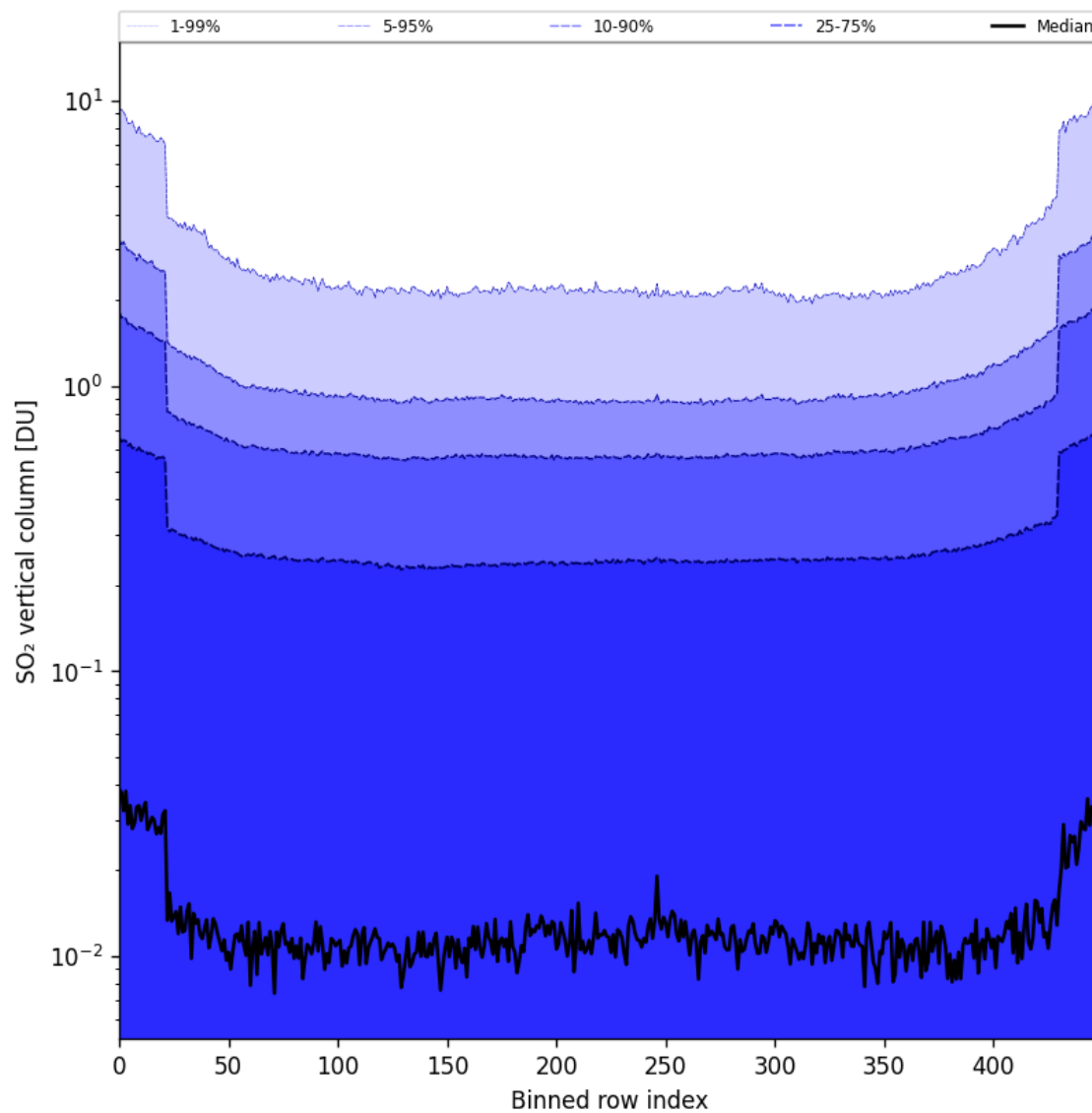
Figure 84: Along track statistics of “SO 2 vertical column” for 2025-09-18 to 2025-09-20
