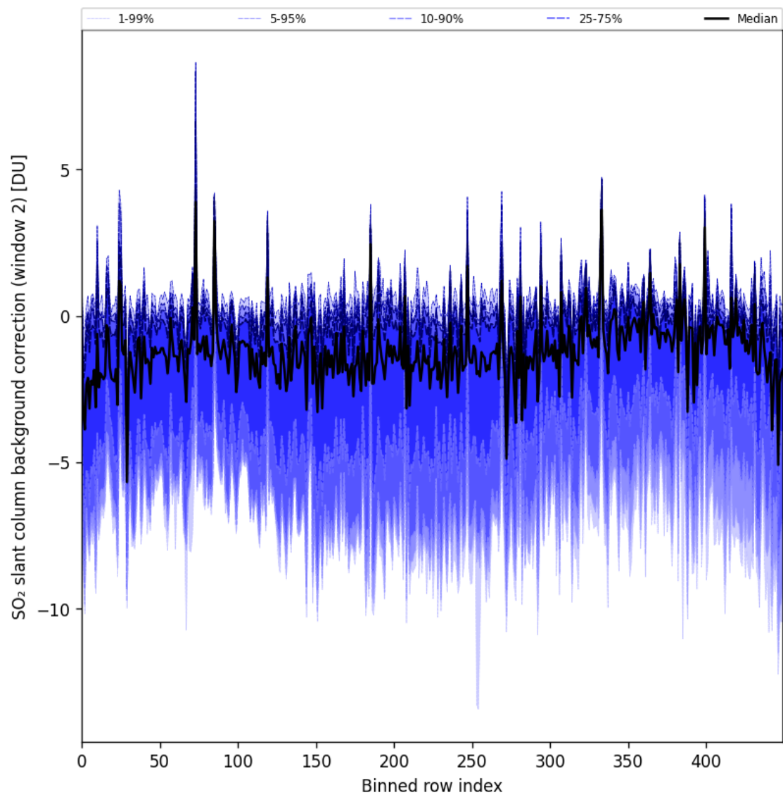
Figure 96: Along track statistics of “SO 2 slant column background correction (window 2)” for 2025-09-18 to 2025-09-20
