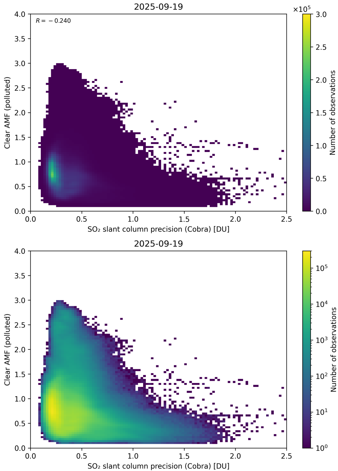
Figure 205: Scatter density plot of “SO 2 slant column precision (Cobra)” against “Clear AMF (polluted)” for 2025-09-18 to 2025-09-20.
