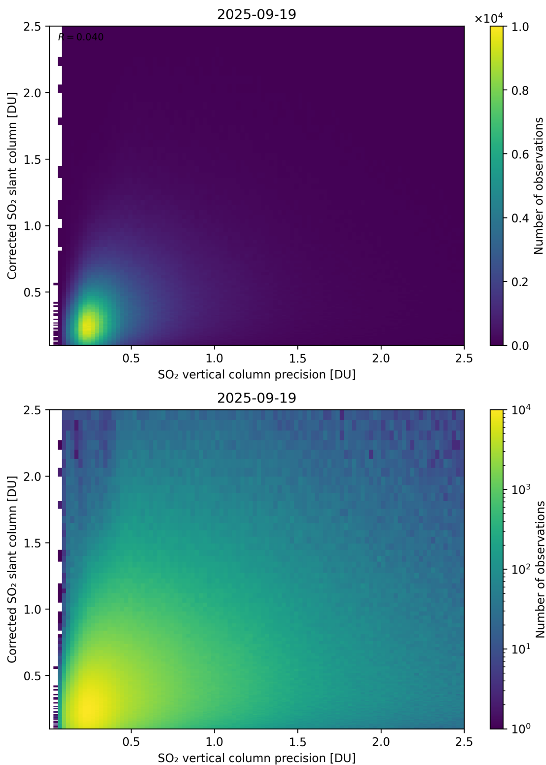
Figure 338: Scatter density plot of “SO 2 vertical column precision” against “Corrected SO 2 slant column” for 2025-09-18 to 2025-09-20.
