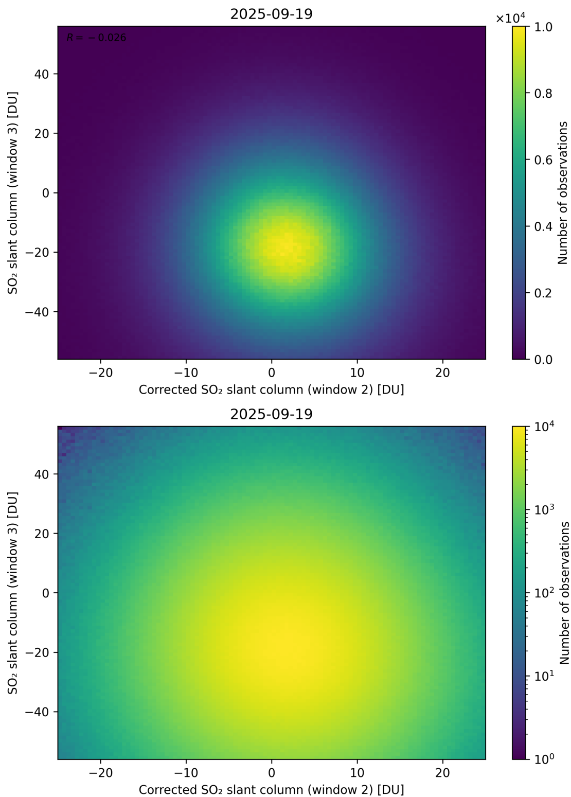
Figure 251: Scatter density plot of “Corrected SO 2 slant column (window 2)” against “SO 2 slant column (window 3)” for 2025-09-18 to 2025-09-20.
