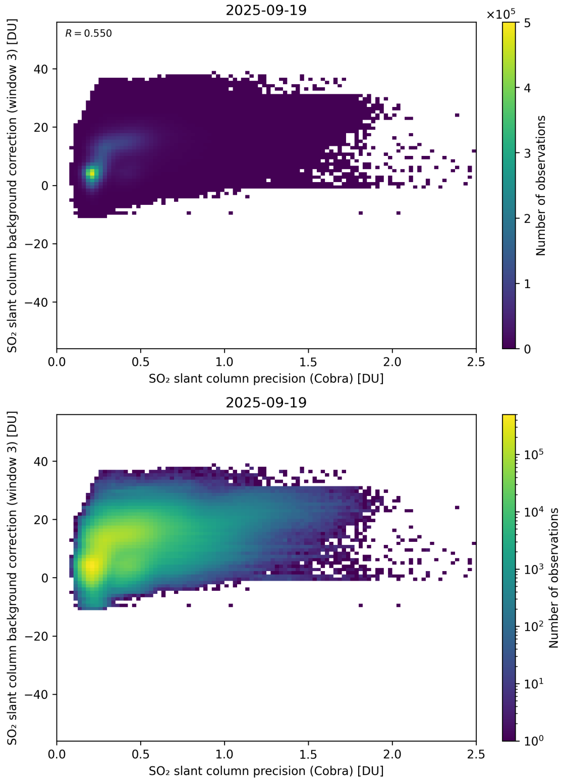
Figure 201: Scatter density plot of “SO 2 slant column precision (Cobra)” against “SO 2 slant column background correction (window 3)” for 2025-09-18 to 2025-09-20.
