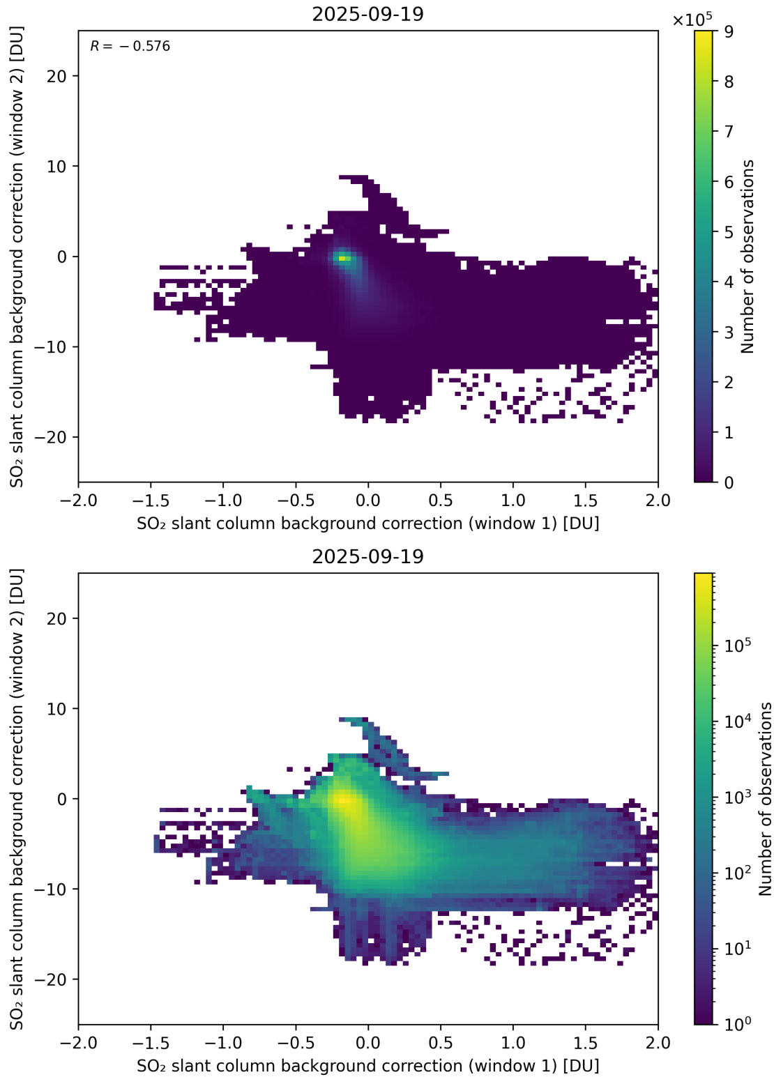
Figure 109: Scatter density plot of “SO 2 slant column background correction (window 1)” against “SO 2 slant column background correction (window 2)” for 2025-09-18 to 2025-09-20.
