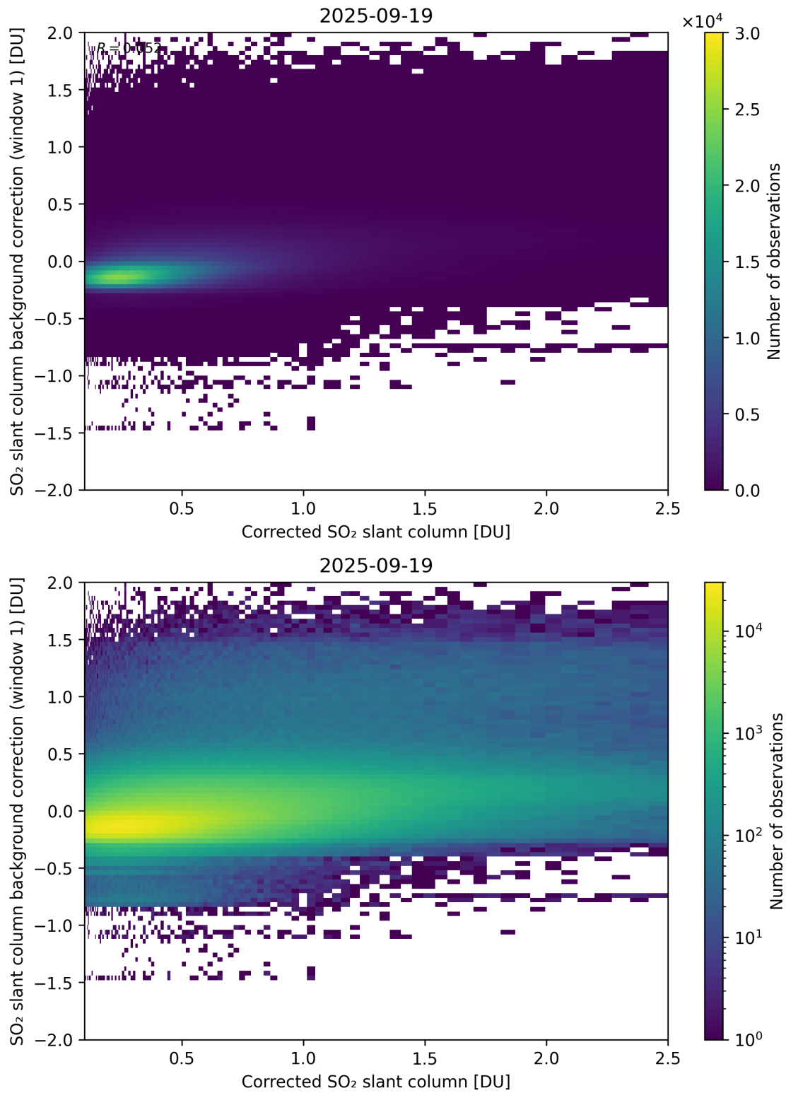
Figure 226: Scatter density plot of “Corrected SO 2 slant column” against “SO 2 slant column background correction (window 1)” for 2025-09-18 to 2025-09-20.
