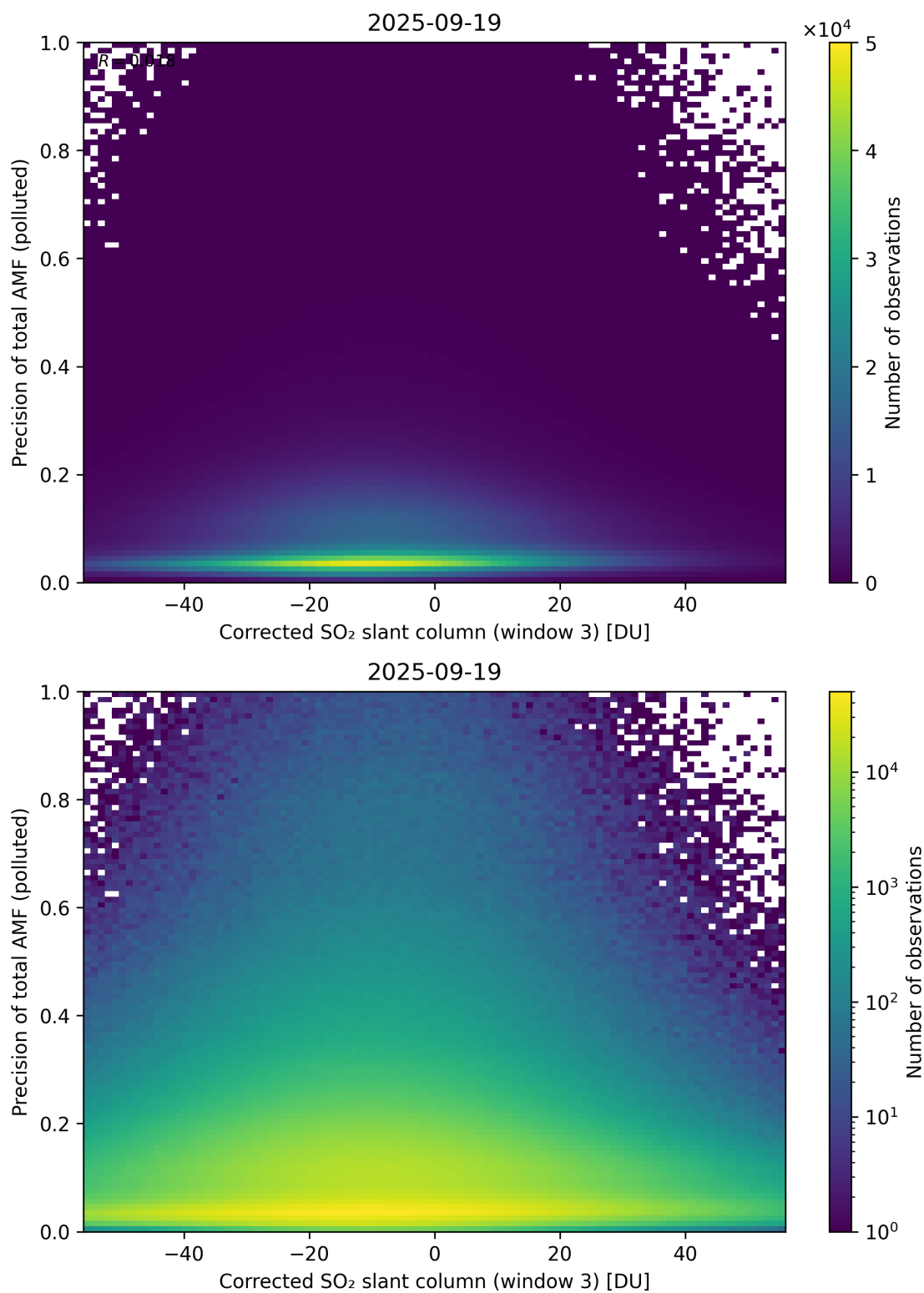
Figure 261: Scatter density plot of “Corrected SO 2 slant column (window 3)” against “Precision of total AMF (polluted)” for 2025-09-18 to 2025-09-20.
