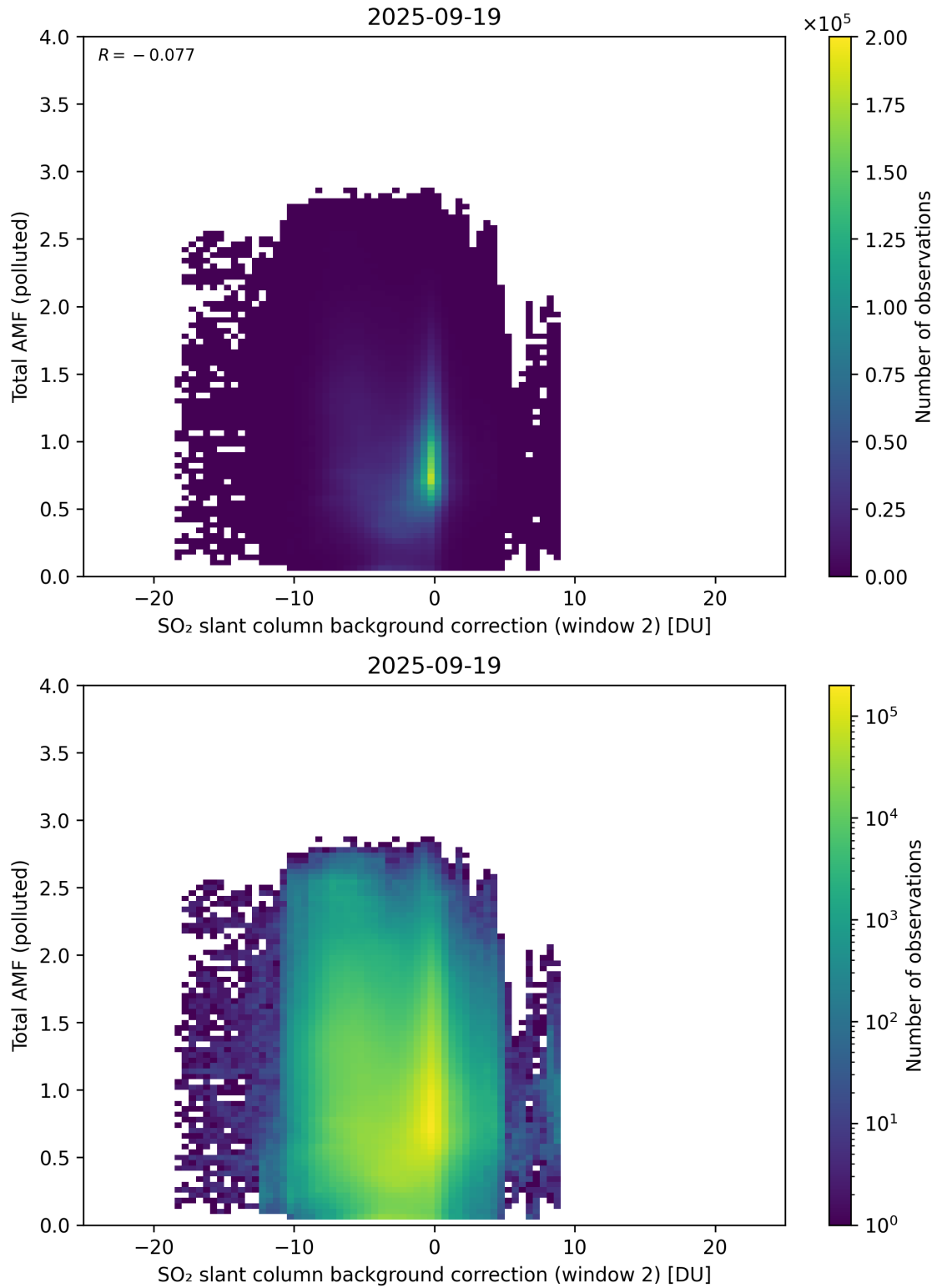
Figure 130: Scatter density plot of “SO 2 slant column background correction (window 2)” against “Total AMF (polluted)” for 2025-09-18 to 2025-09-20.
