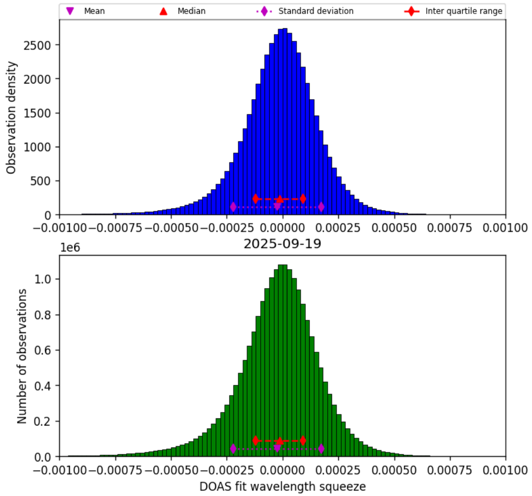
Figure 77: Histogram of “DOAS fit wavelength squeeze” for 2025-09-18 to 2025-09-20
