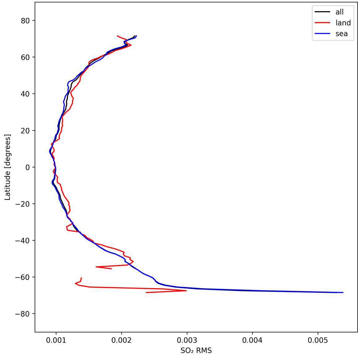
Figure 52: Zonal average of “SO 2 RMS” for 2025-09-18 to 2025-09-20.
