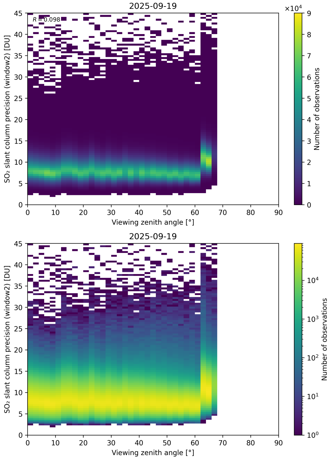
Figure 378: Scatter density plot of “Viewing zenith angle” against “SO 2 slant column precision (window2)” for 2025-09-18 to 2025-09-20.
