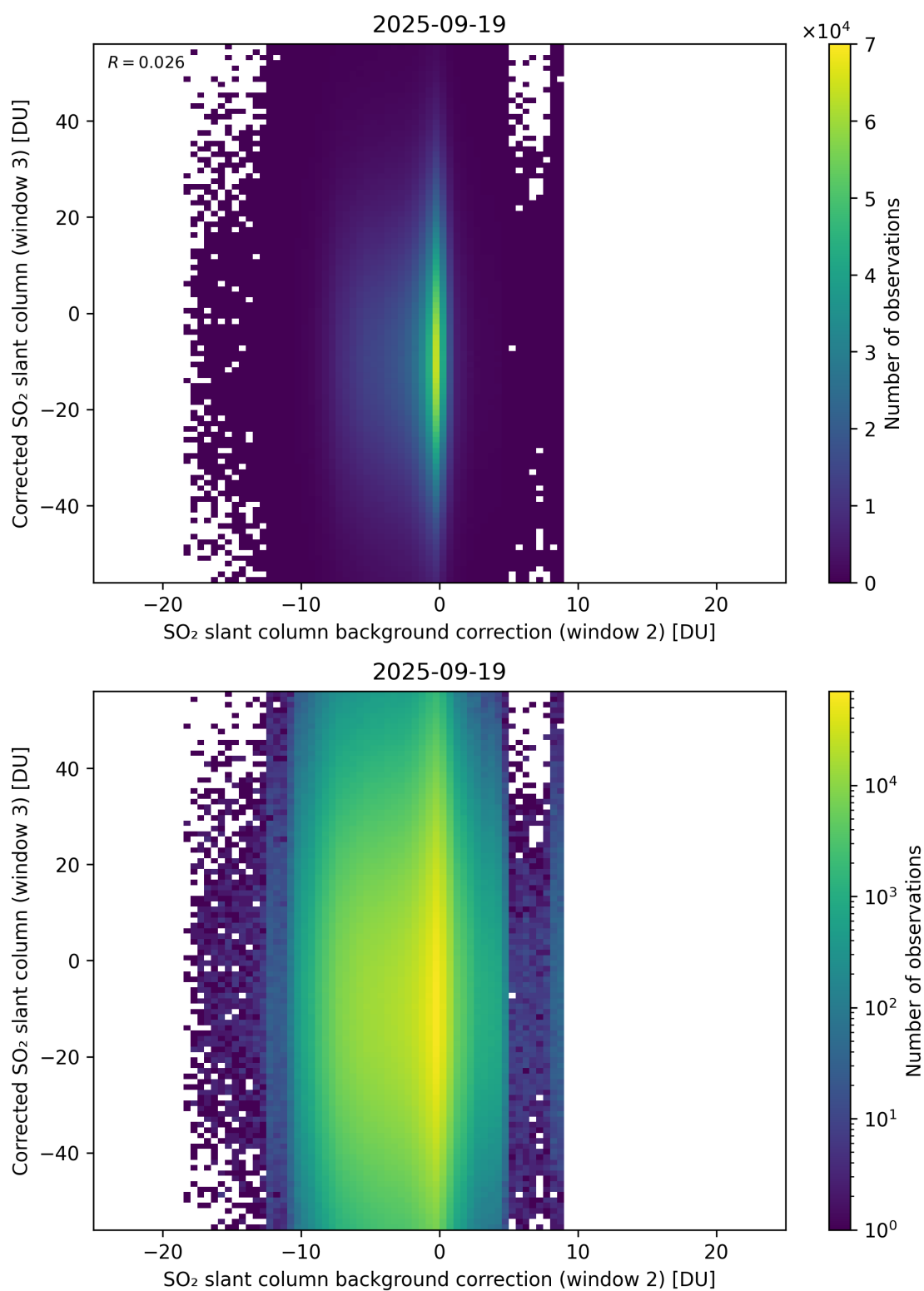
Figure 127: Scatter density plot of “SO 2 slant column background correction (window 2)” against “Corrected SO 2 slant column (window 3)” for 2025-09-18 to 2025-09-20.
