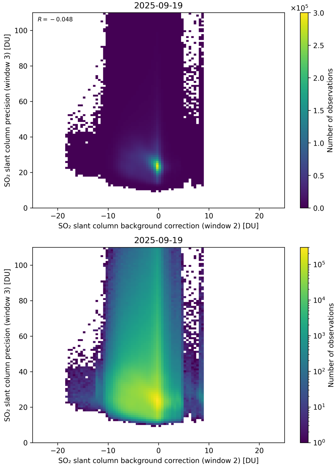
Figure 129: Scatter density plot of “SO 2 slant column background correction (window 2)” against “SO 2 slant column precision (window 3)” for 2025-09-18 to 2025-09-20.
