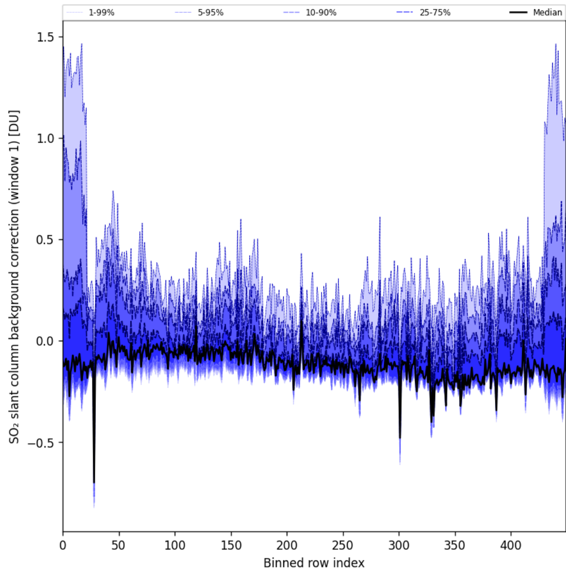
Figure 92: Along track statistics of “SO 2 slant column background correction (window 1)” for 2025-09-18 to 2025-09-20
