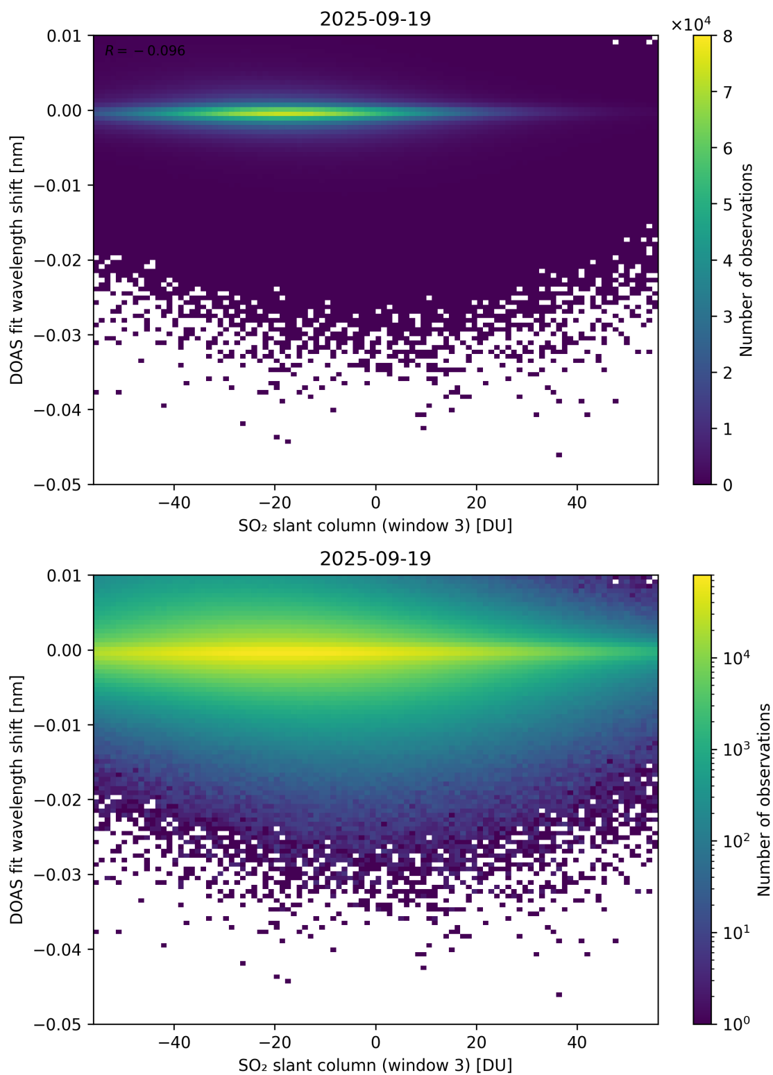
Figure 304: Scatter density plot of “SO 2 slant column (window 3)” against “DOAS fit wavelength shift” for 2025-09-18 to 2025-09-20.
