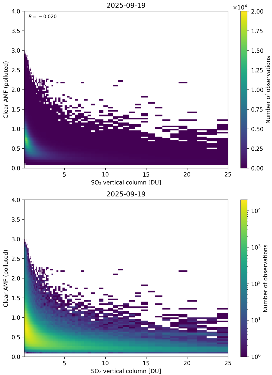
Figure 348: Scatter density plot of “SO 2 vertical column” against “Clear AMF (polluted)” for 2025-09-18 to 2025-09-20.
