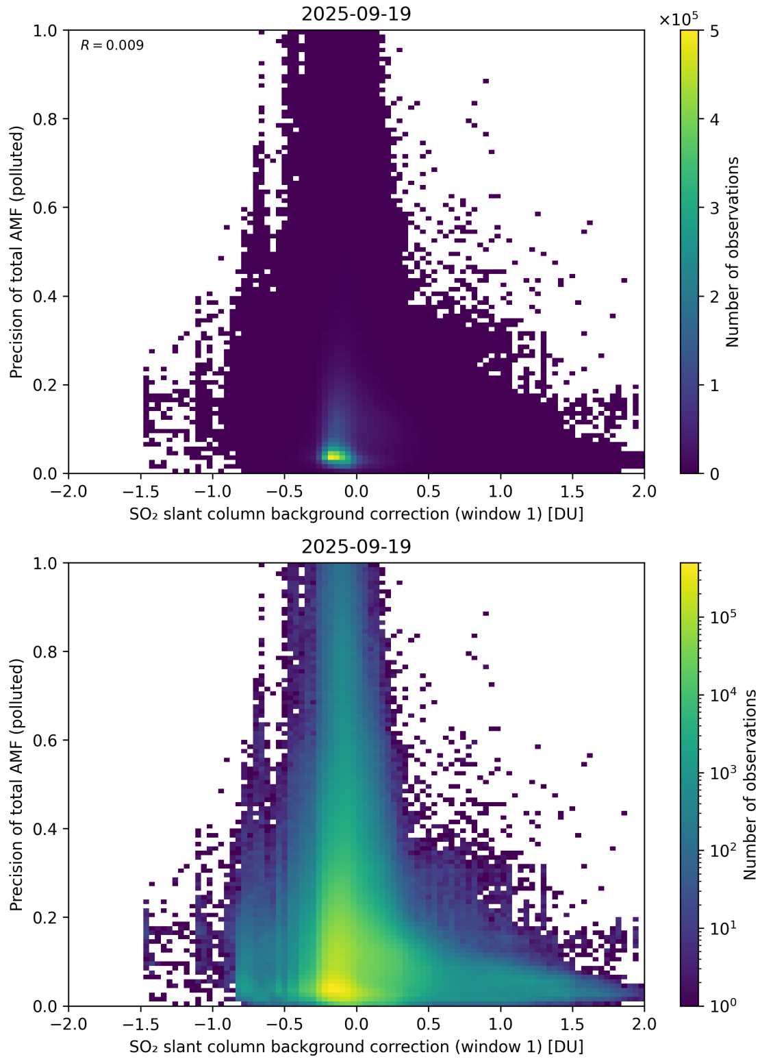
Figure 121: Scatter density plot of “SO 2 slant column background correction (window 1)” against “Precision of total AMF (polluted)” for 2025-09-18 to 2025-09-20.
