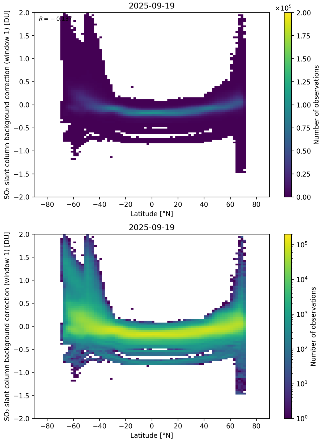
Figure 150: Scatter density plot of “Latitude” against “SO 2 slant column background correction (window 1)” for 2025-09-18 to 2025-09-20.
