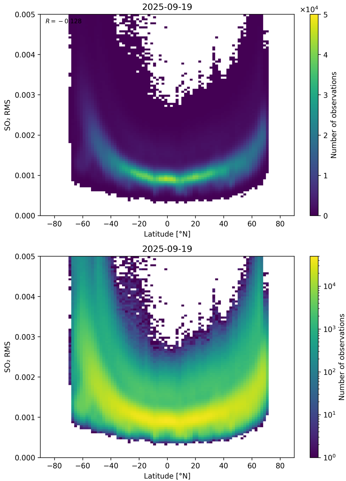
Figure 155: Scatter density plot of “Latitude” against “SO 2 RMS” for 2025-09-18 to 2025-09-20.
