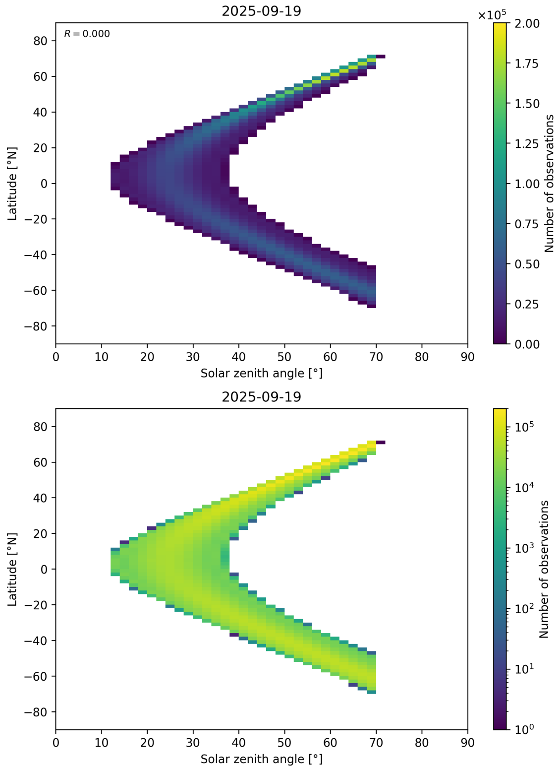
Figure 177: Scatter density plot of “Solar zenith angle” against “Latitude” for 2025-09-18 to 2025-09-20.
