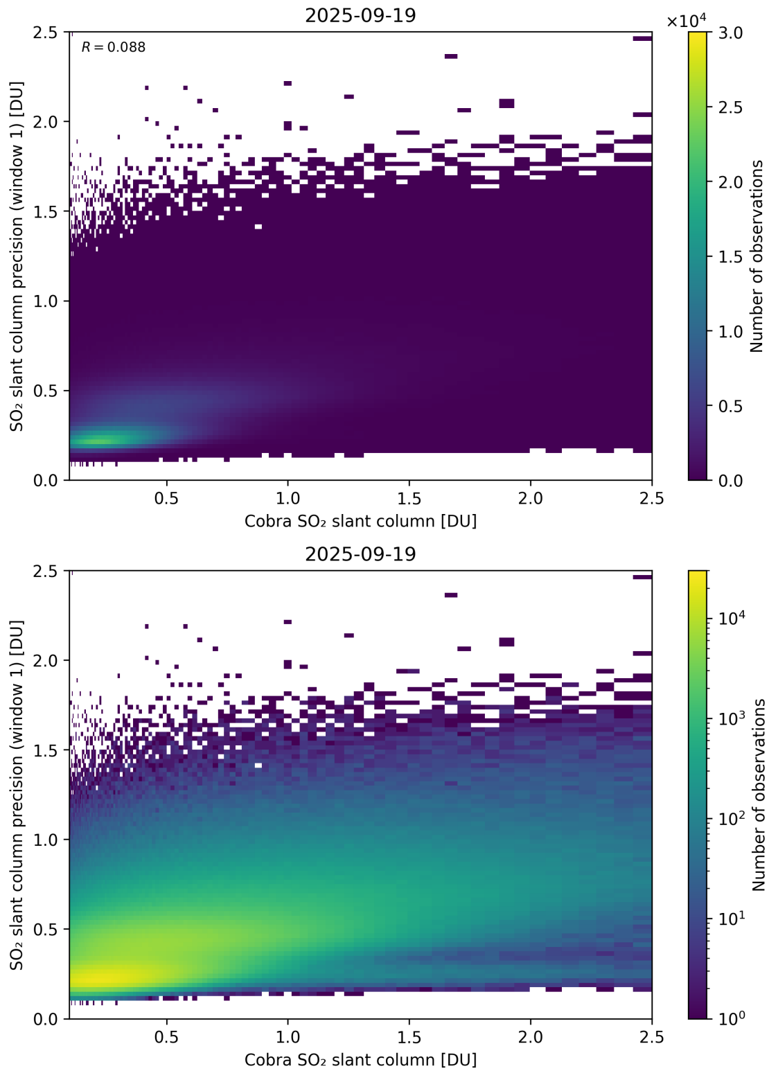
Figure 220: Scatter density plot of “Cobra SO 2 slant column” against “SO 2 slant column precision (window 1)” for 2025-09-18 to 2025-09-20.
