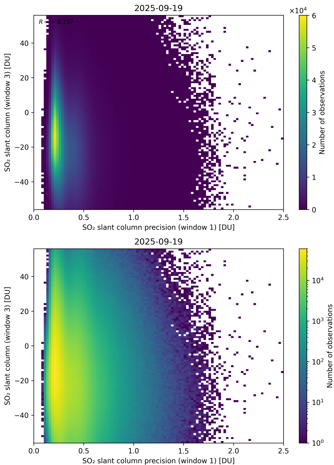
Figure 278: Scatter density plot of “SO 2 slant column precision (window 1)” against “SO 2 slant column (window 3)” for 2025-09-18 to 2025-09-20.
