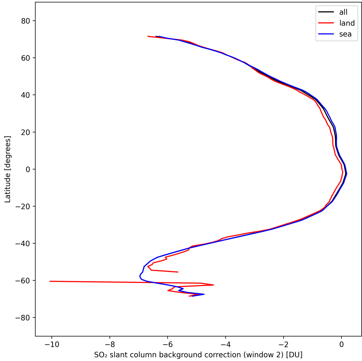
Figure 44: Zonal average of “SO 2 slant column background correction (window 2)” for 2025-09-18 to 2025-09-20.
