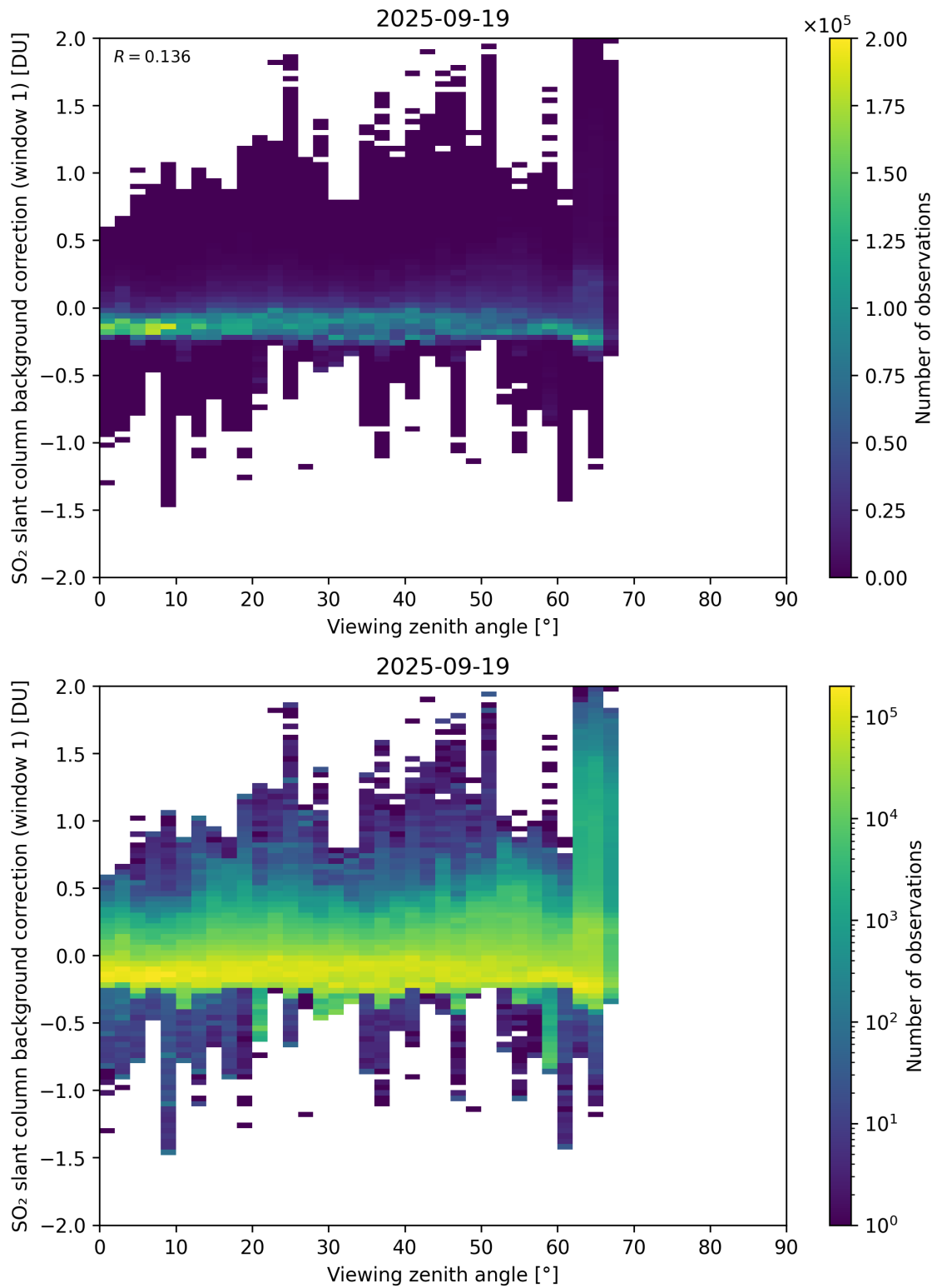
Figure 362: Scatter density plot of “Viewing zenith angle” against “SO 2 slant column background correction (window 1)” for 2025-09-18 to 2025-09-20.
