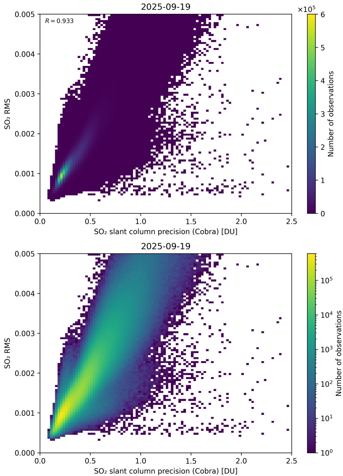
Figure 204: Scatter density plot of “SO 2 slant column precision (Cobra)” against “SO 2 RMS” for 2025-09-18 to 2025-09-20.
