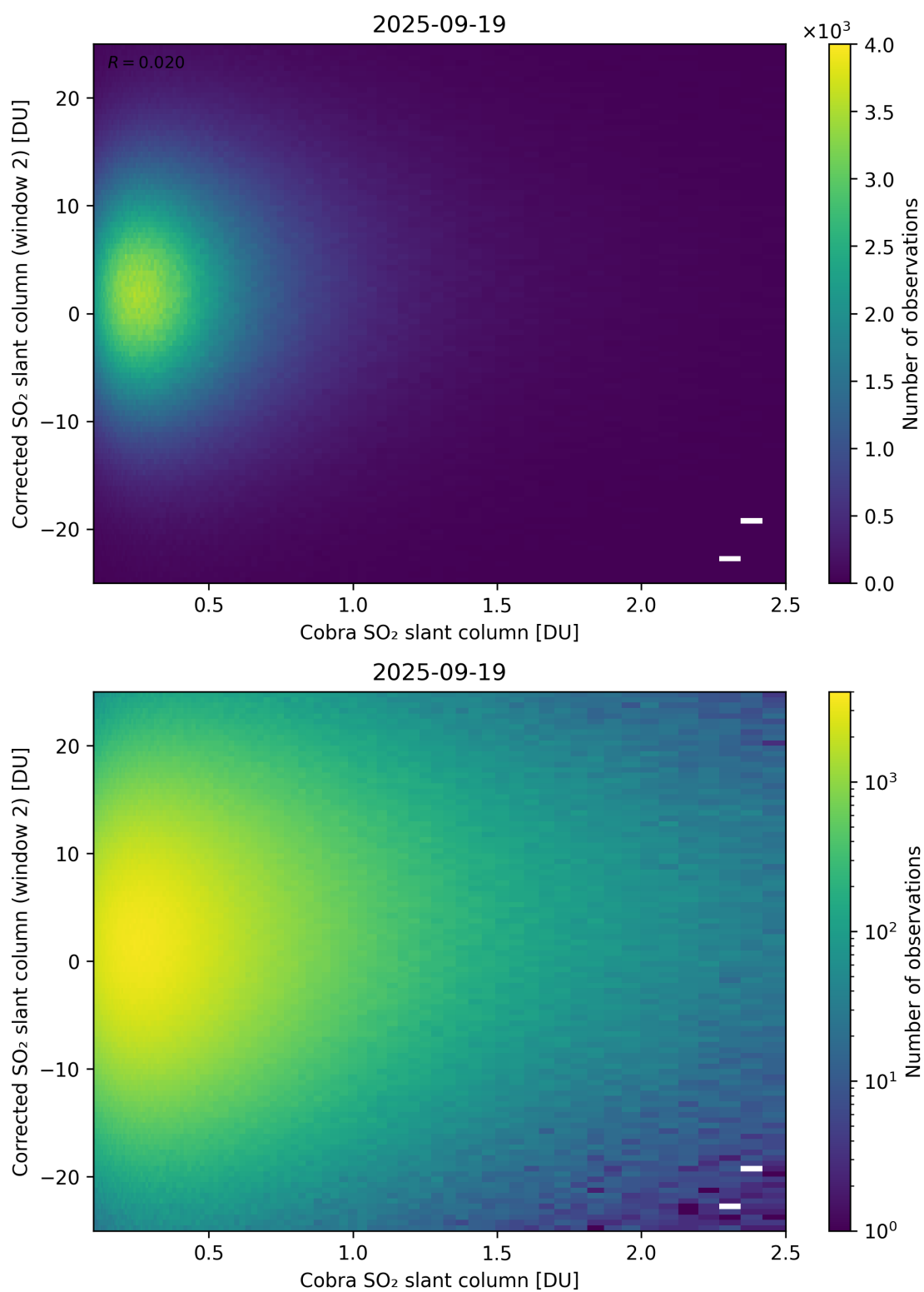
Figure 217: Scatter density plot of “Cobra SO 2 slant column” against “Corrected SO 2 slant column (window 2)” for 2025-09-18 to 2025-09-20.
