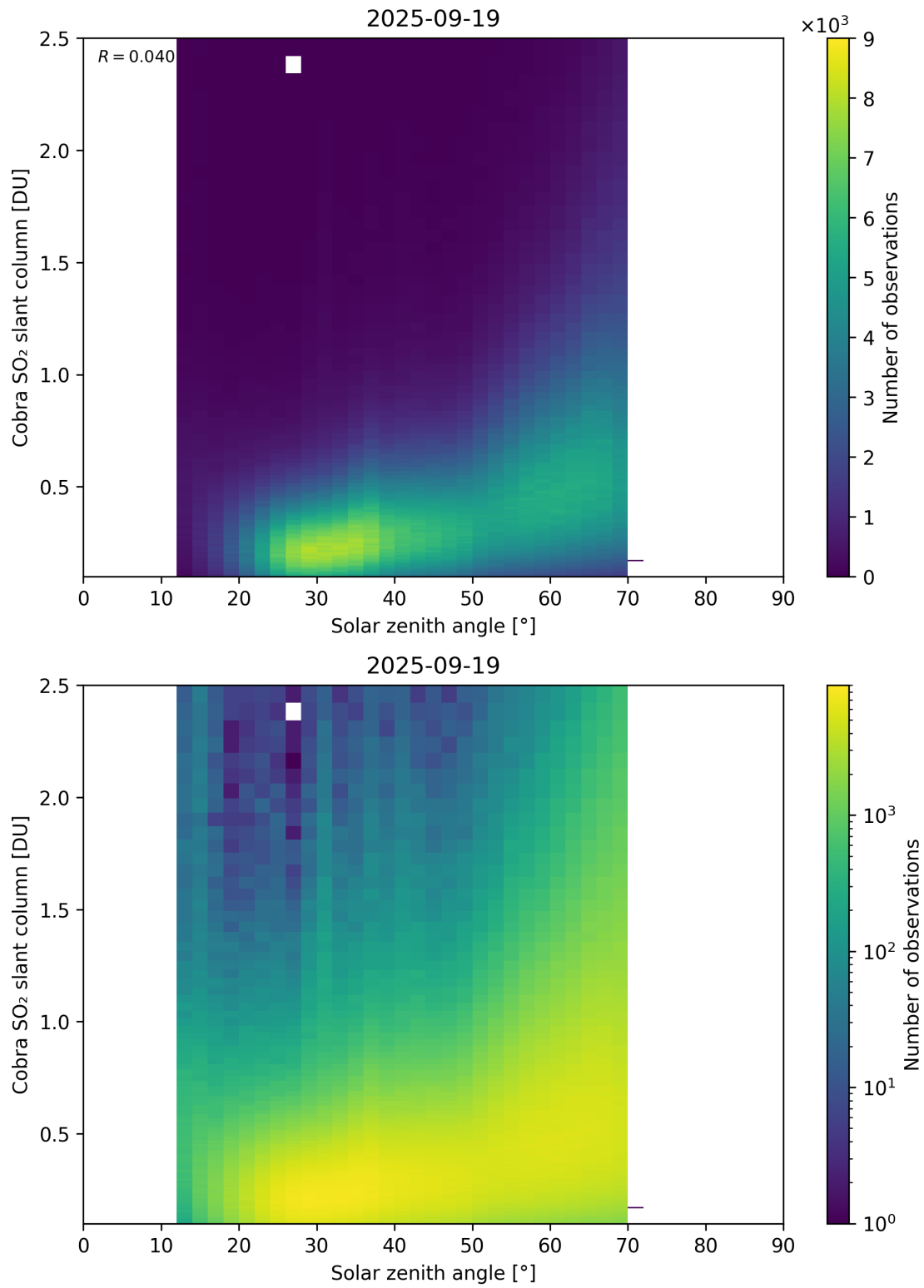
Figure 179: Scatter density plot of “Solar zenith angle” against “Cobra SO 2 slant column” for 2025-09-18 to 2025-09-20.
