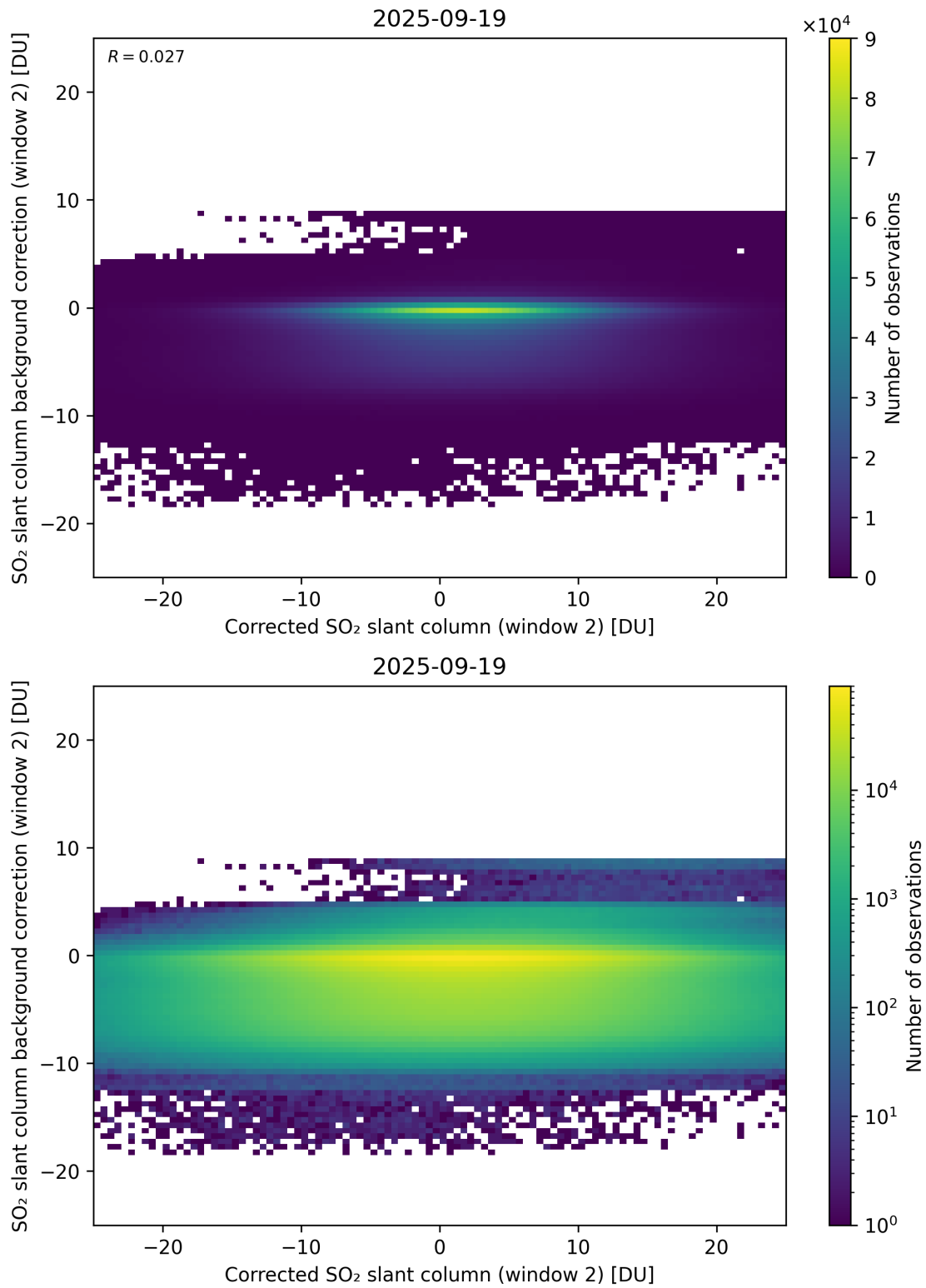
Figure 244: Scatter density plot of “Corrected SO 2 slant column (window 2)” against “SO 2 slant column background correction (window 2)” for 2025-09-18 to 2025-09-20.
