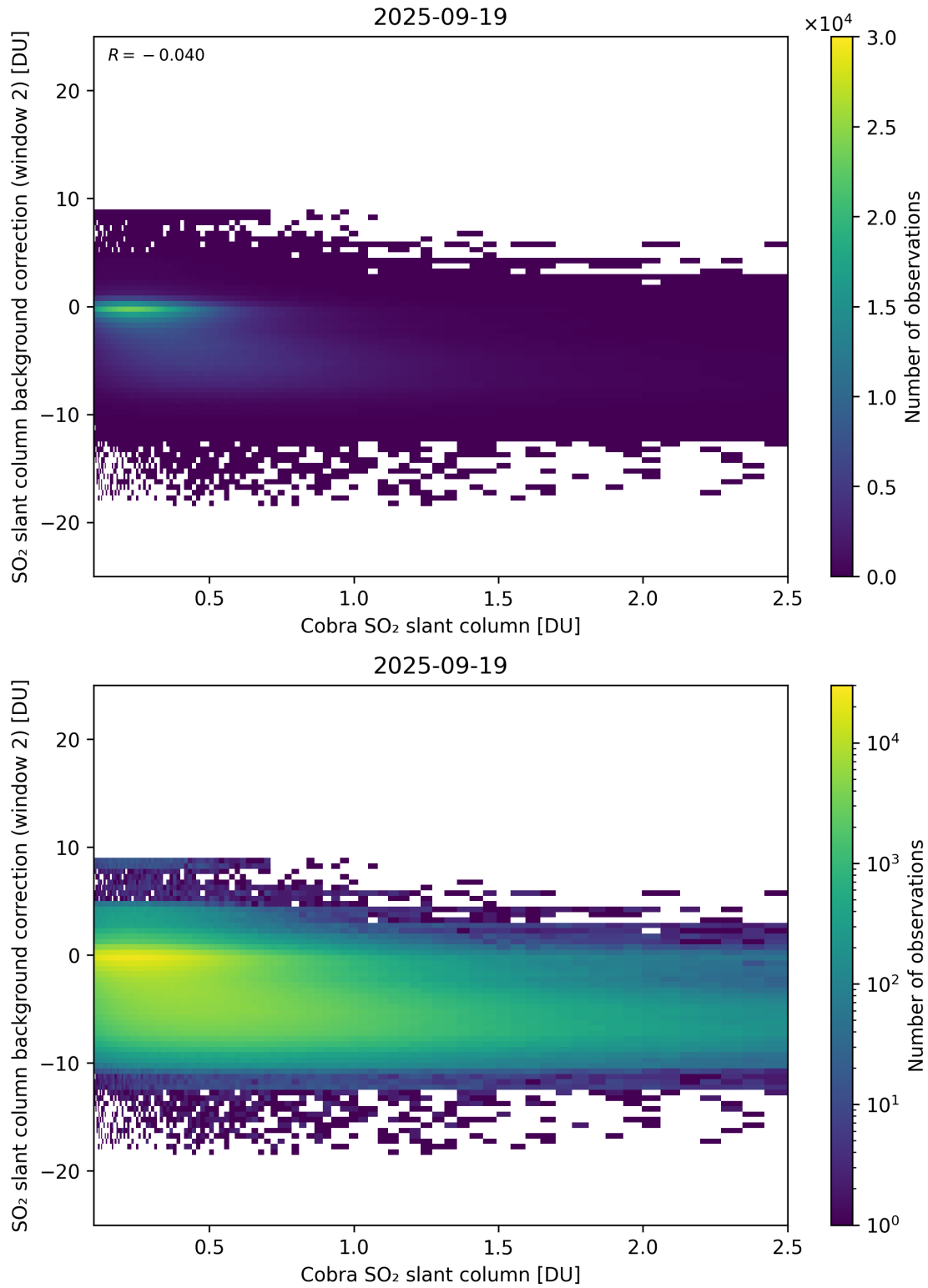
Figure 194: Scatter density plot of “Cobra SO 2 slant column” against “SO 2 slant column background correction (window 2)” for 2025-09-18 to 2025-09-20.
