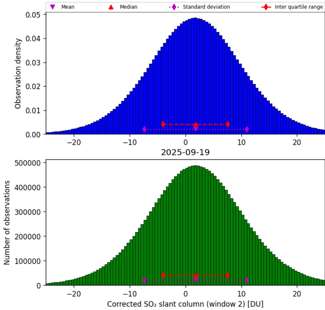
Figure 69: Histogram of “Corrected SO 2 slant column (window 2)” for 2025-09-18 to 2025-09-20
