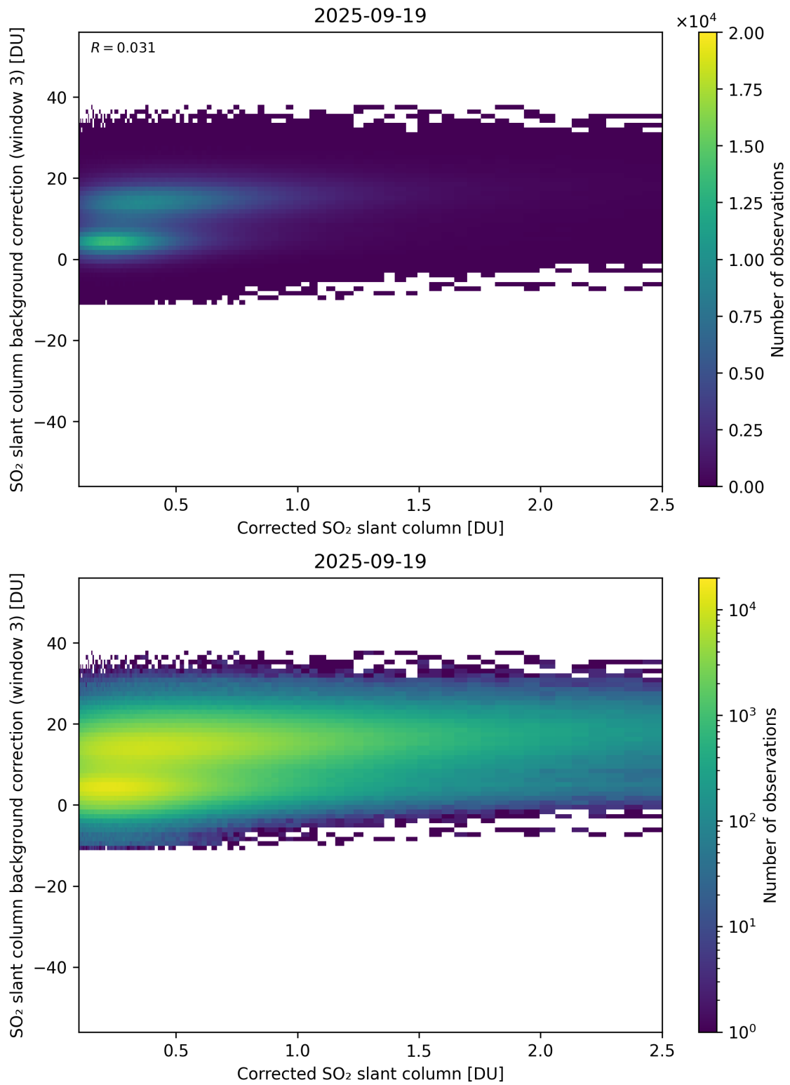
Figure 228: Scatter density plot of “Corrected SO 2 slant column” against “SO 2 slant column background correction (window 3)” for 2025-09-18 to 2025-09-20.
