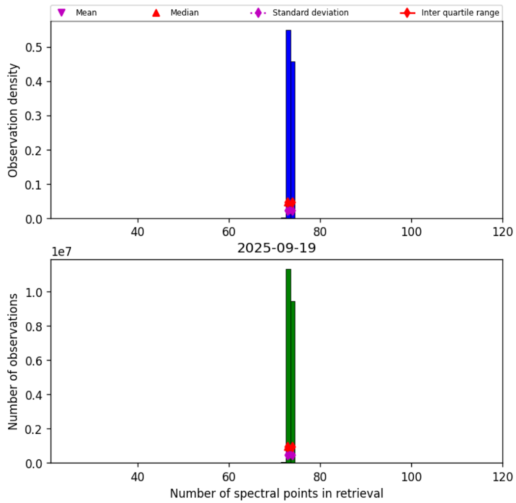
Figure 82: Histogram of “Number of spectral points in retrieval” for 2025-09-18 to 2025-09-20
