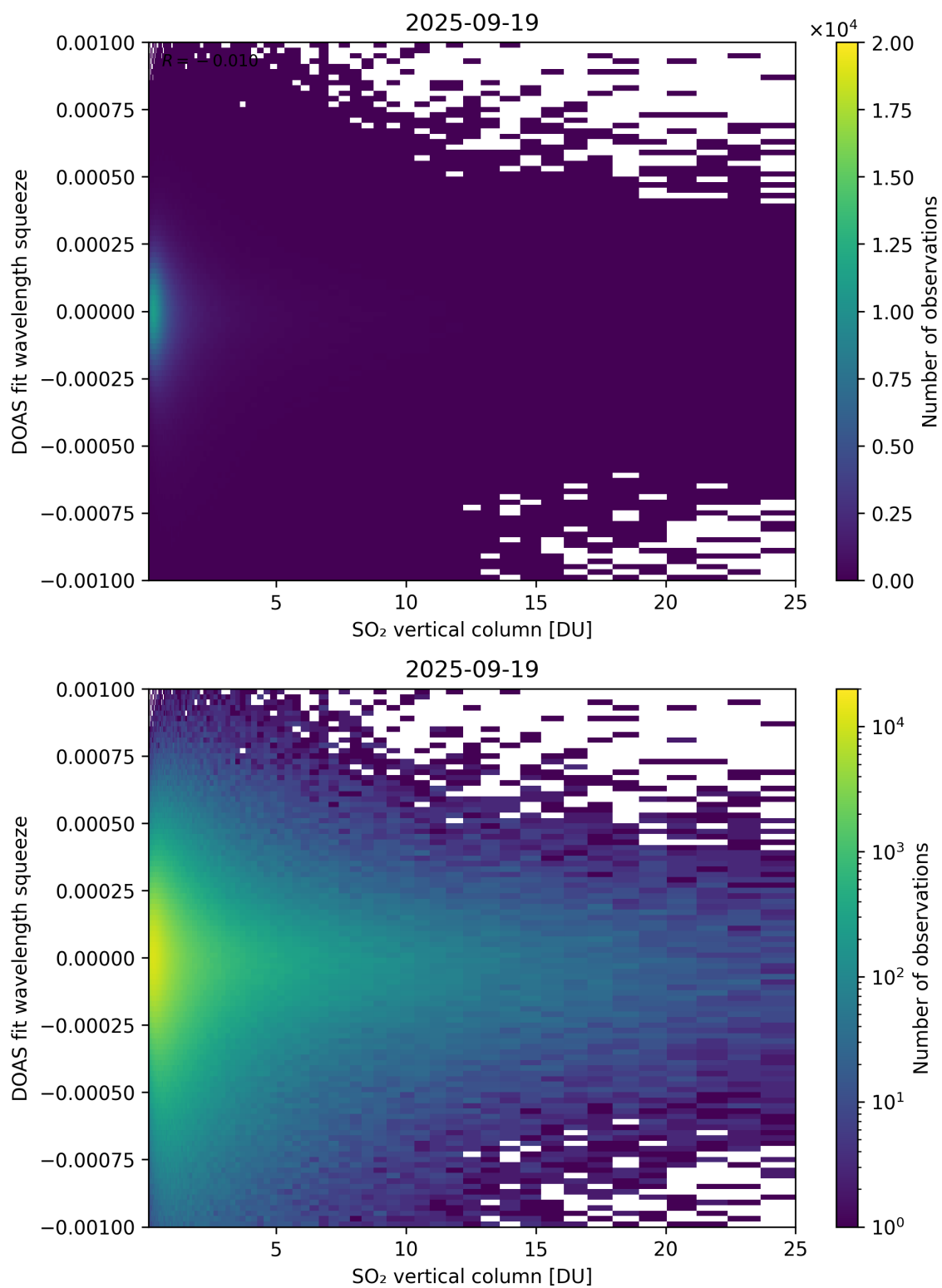
Figure 327: Scatter density plot of “SO 2 vertical column” against “DOAS fit wavelength squeeze” for 2025-09-18 to 2025-09-20.
