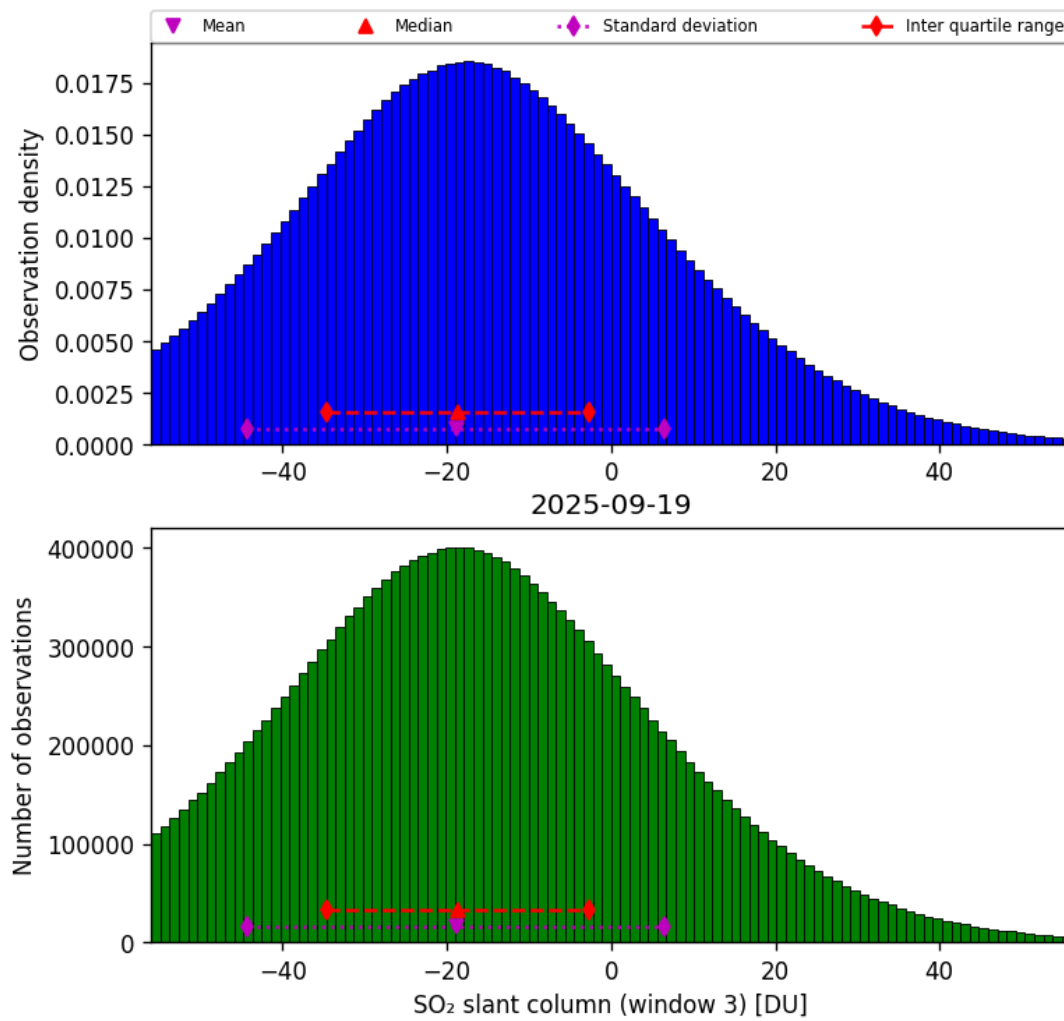
Figure 71: Histogram of “SO 2 slant column (window 3)” for 2025-09-18 to 2025-09-20
