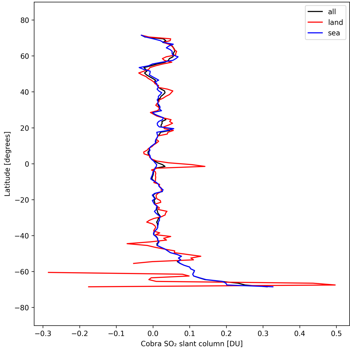
Figure 35: Zonal average of "Cobra SO 2 slant column" for 2025-09-18 to 2025-09-20.
