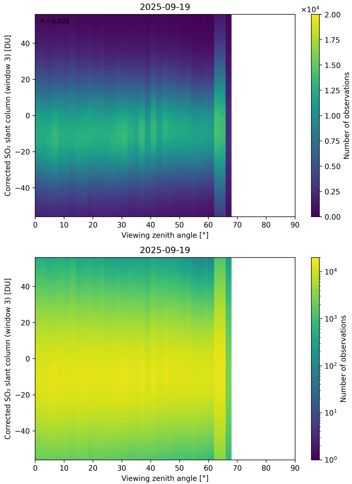
Figure 375: Scatter density plot of “Viewing zenith angle” against “Corrected SO 2 slant column (window 3)” for 2025-09-18 to 2025-09-20.
