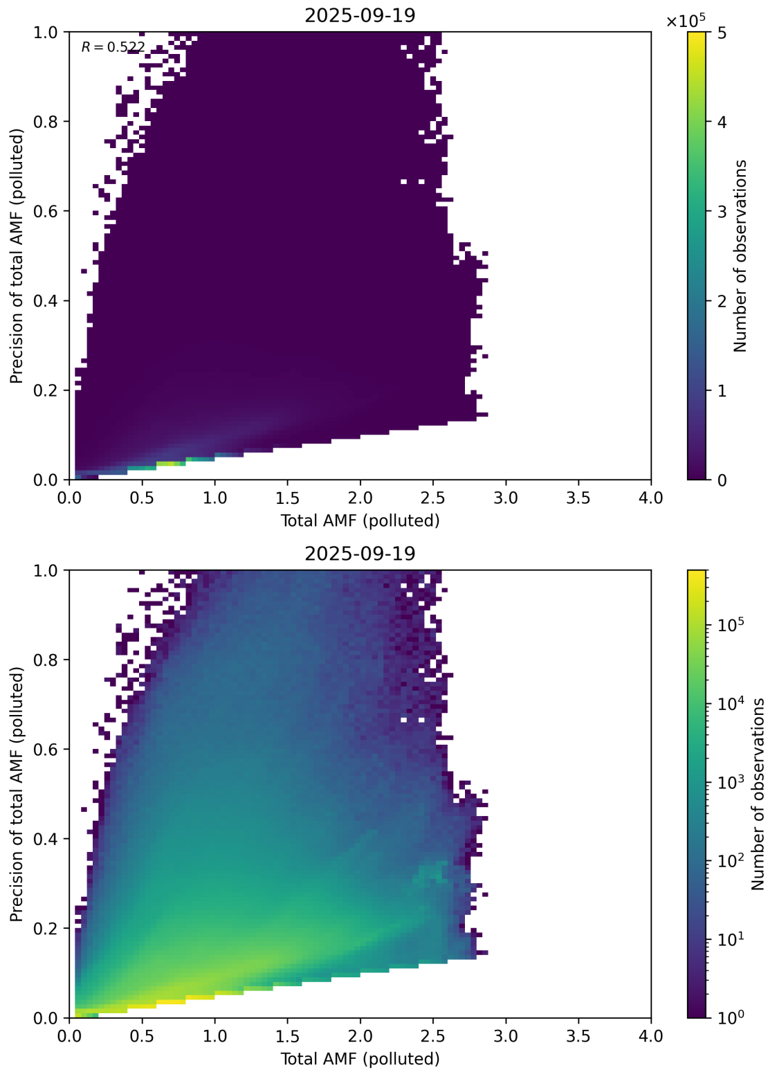
Figure 322: Scatter density plot of “Total AMF (polluted)” against “Precision of total AMF (polluted)” for 2025-09-18 to 2025-09-20.
