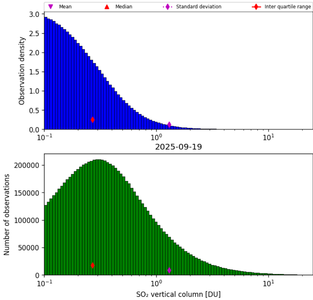
Figure 58: Histogram of “SO 2 vertical column” for 2025-09-18 to 2025-09-20
