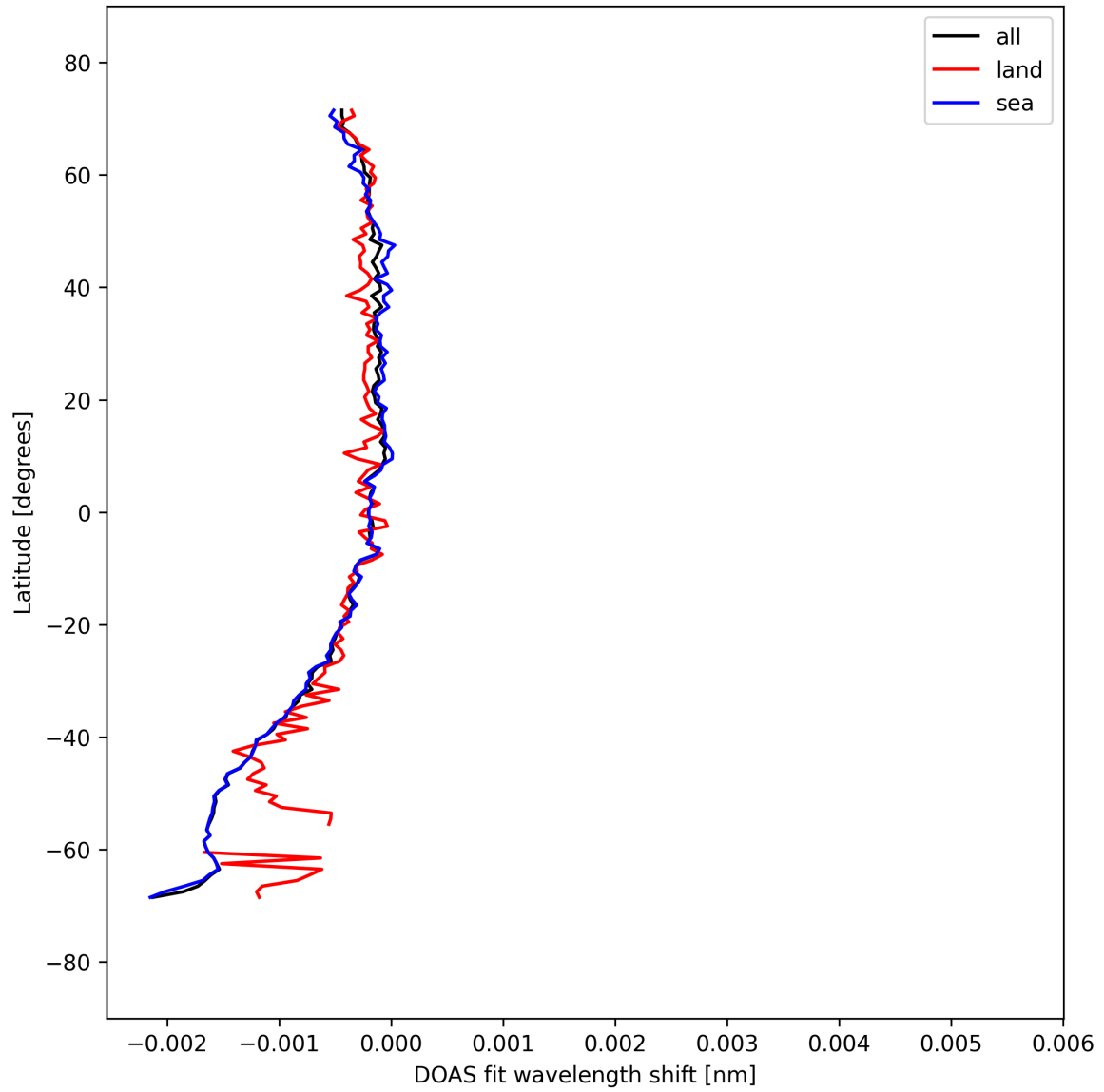
Figure 50: Zonal average of "DOAS fit wavelength shift" for 2025-09-18 to 2025-09-20.
