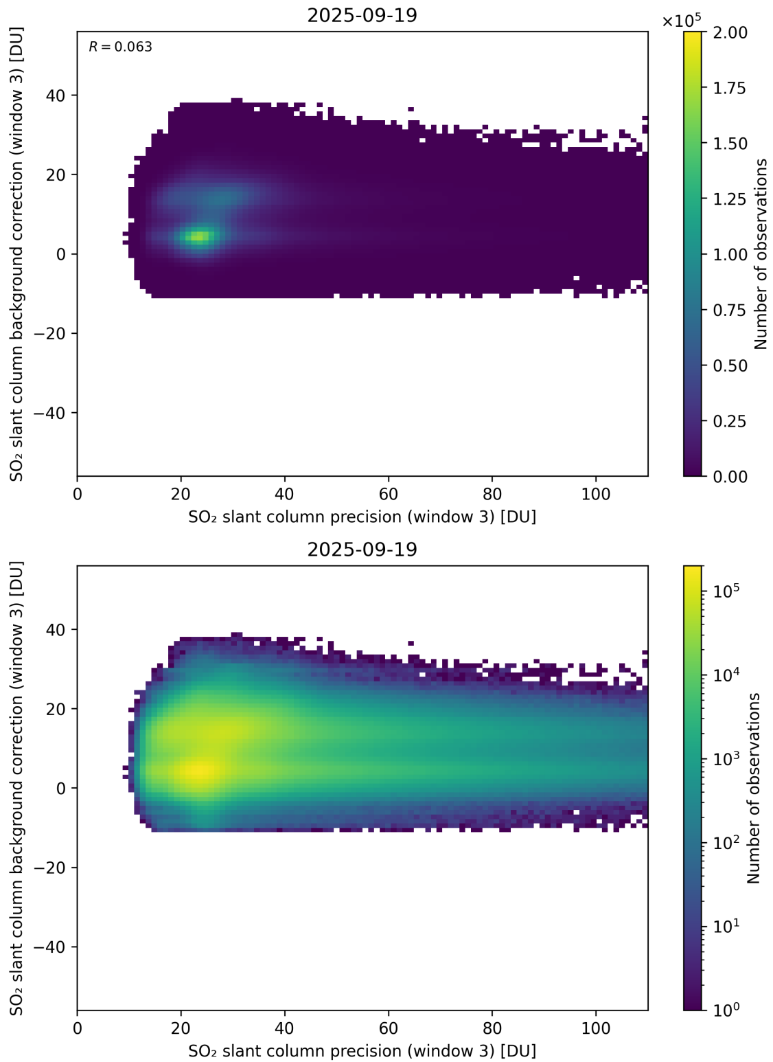
Figure 307: Scatter density plot of “SO 2 slant column precision (window 3)” against “SO 2 slant column background correction (window 3)” for 2025-09-18 to 2025-09-20.
