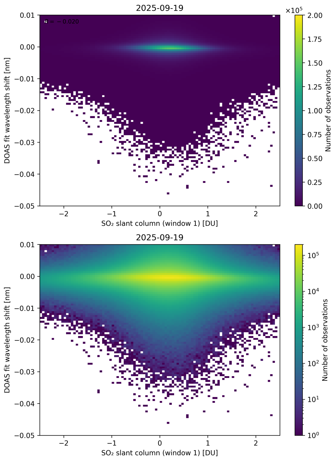
Figure 265: Scatter density plot of “SO 2 slant column (window 1)” against “DOAS fit wavelength shift” for 2025-09-18 to 2025-09-20.
