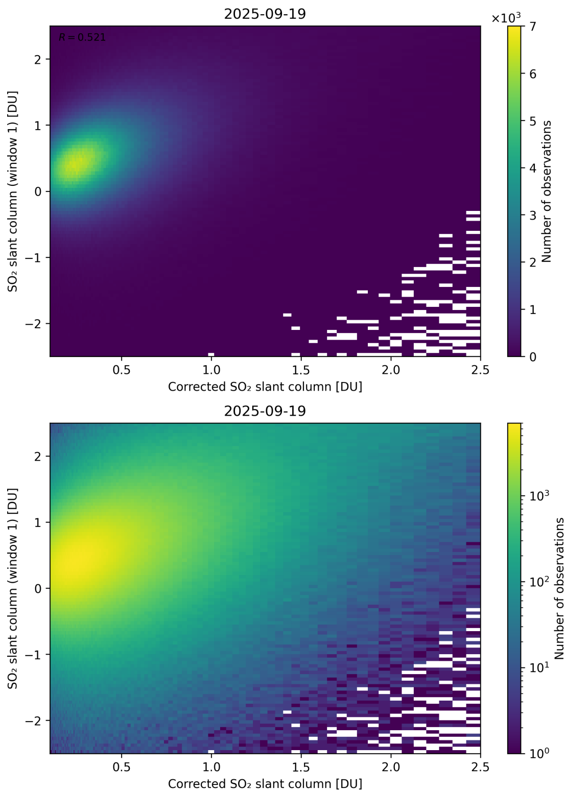
Figure 237: Scatter density plot of “Corrected SO 2 slant column” against “SO 2 slant column (window 1)” for 2025-09-18 to 2025-09-20.
