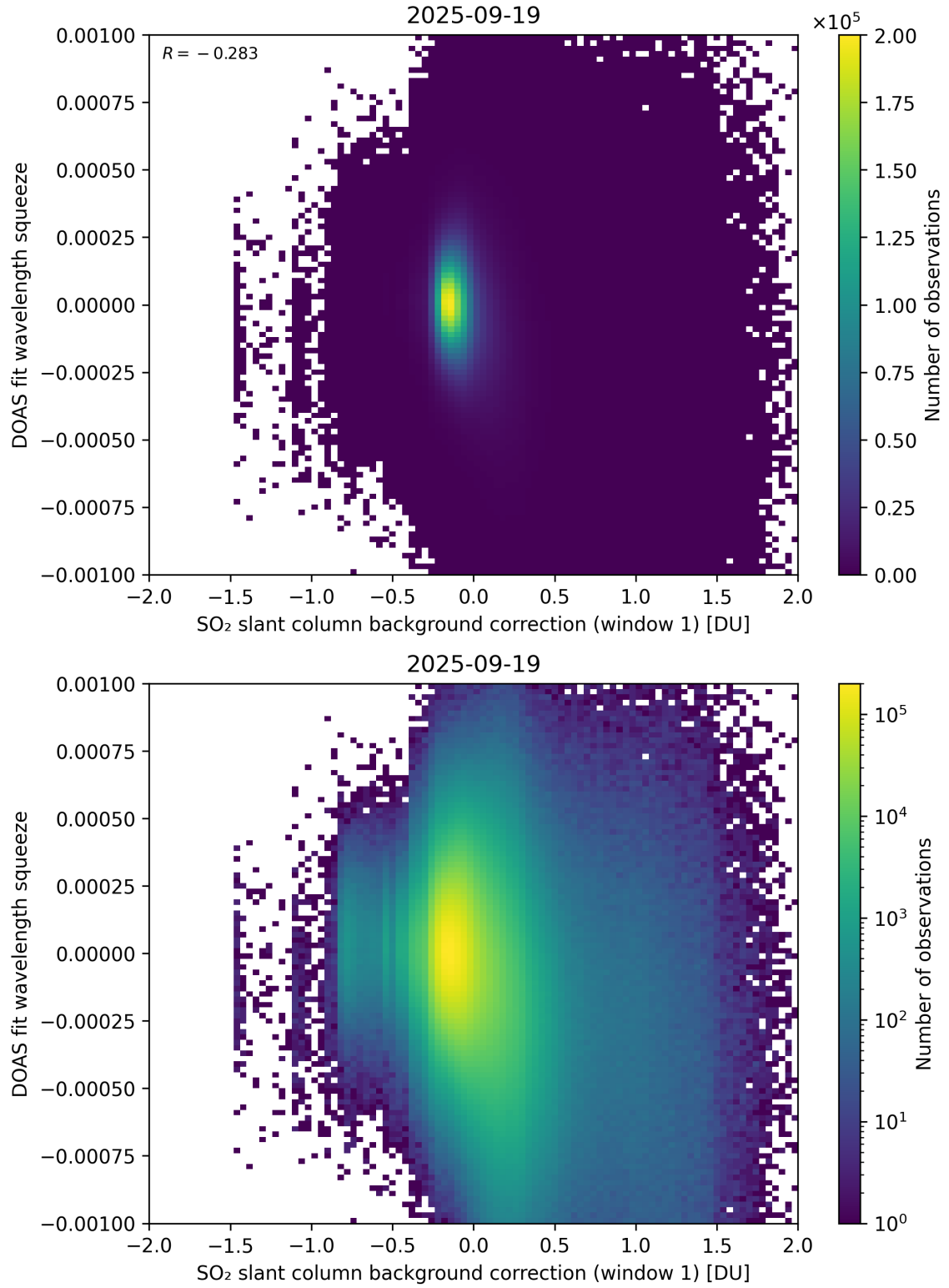
Figure 112: Scatter density plot of “SO 2 slant column background correction (window 1)” against “DOAS fit wavelength squeeze” for 2025-09-18 to 2025-09-20.
