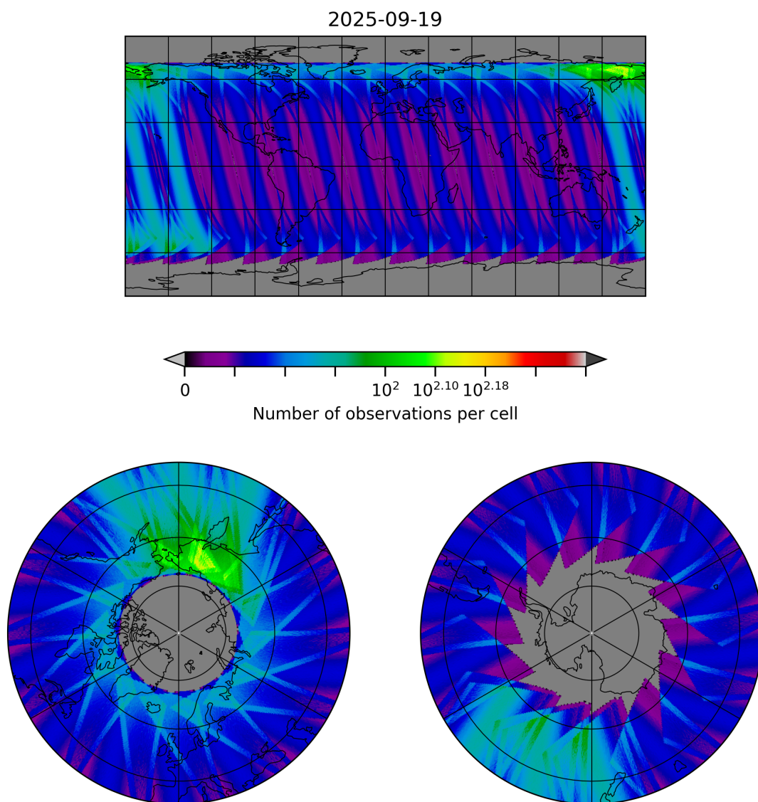
Figure 30: Map of the number of observations for 2025-09-18 to 2025-09-20
