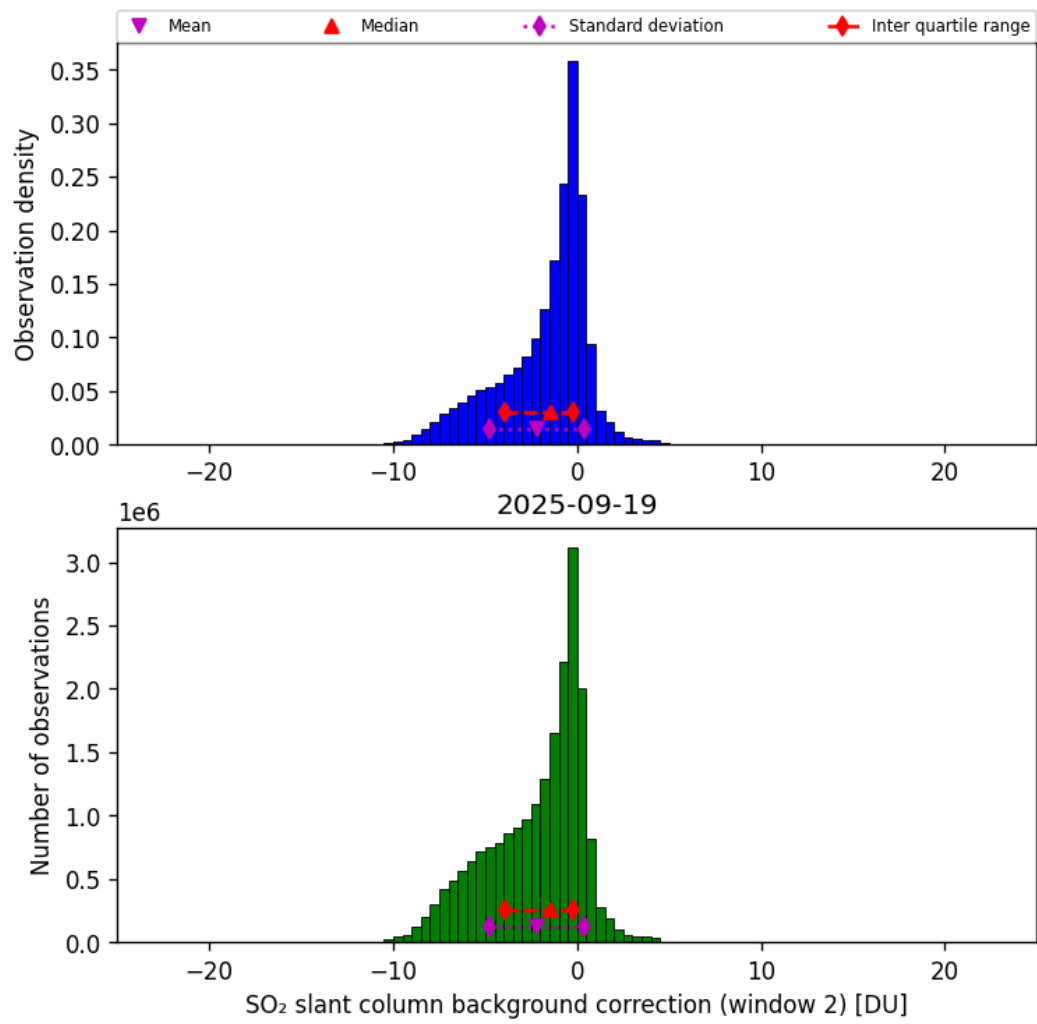
Figure 70: Histogram of “SO 2 slant column background correction (window 2)” for 2025-09-18 to 2025-09-20
