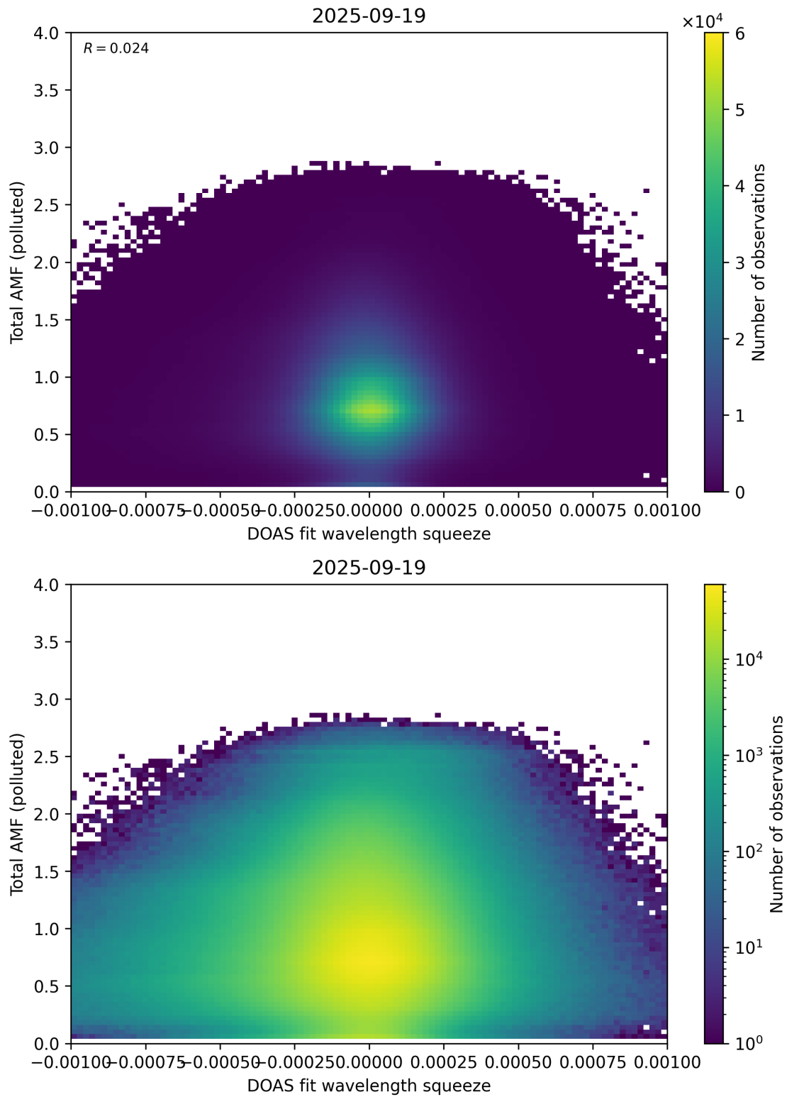
Figure 145: Scatter density plot of “DOAS fit wavelength squeeze” against “Total AMF (polluted)” for 2025-09-18 to 2025-09-20.
