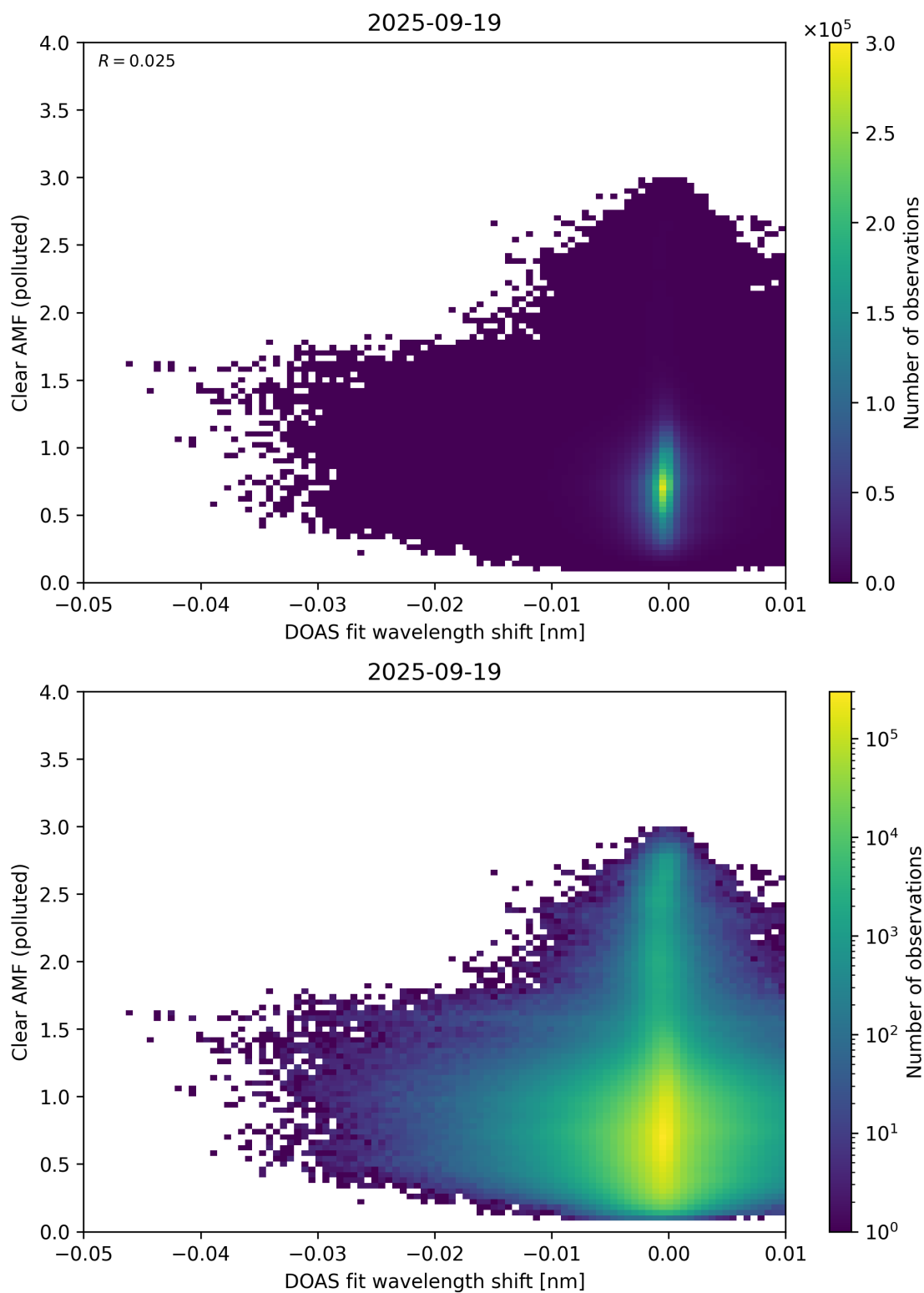
Figure 140: Scatter density plot of “DOAS fit wavelength shift” against “Clear AMF (polluted)” for 2025-09-18 to 2025-09-20.
