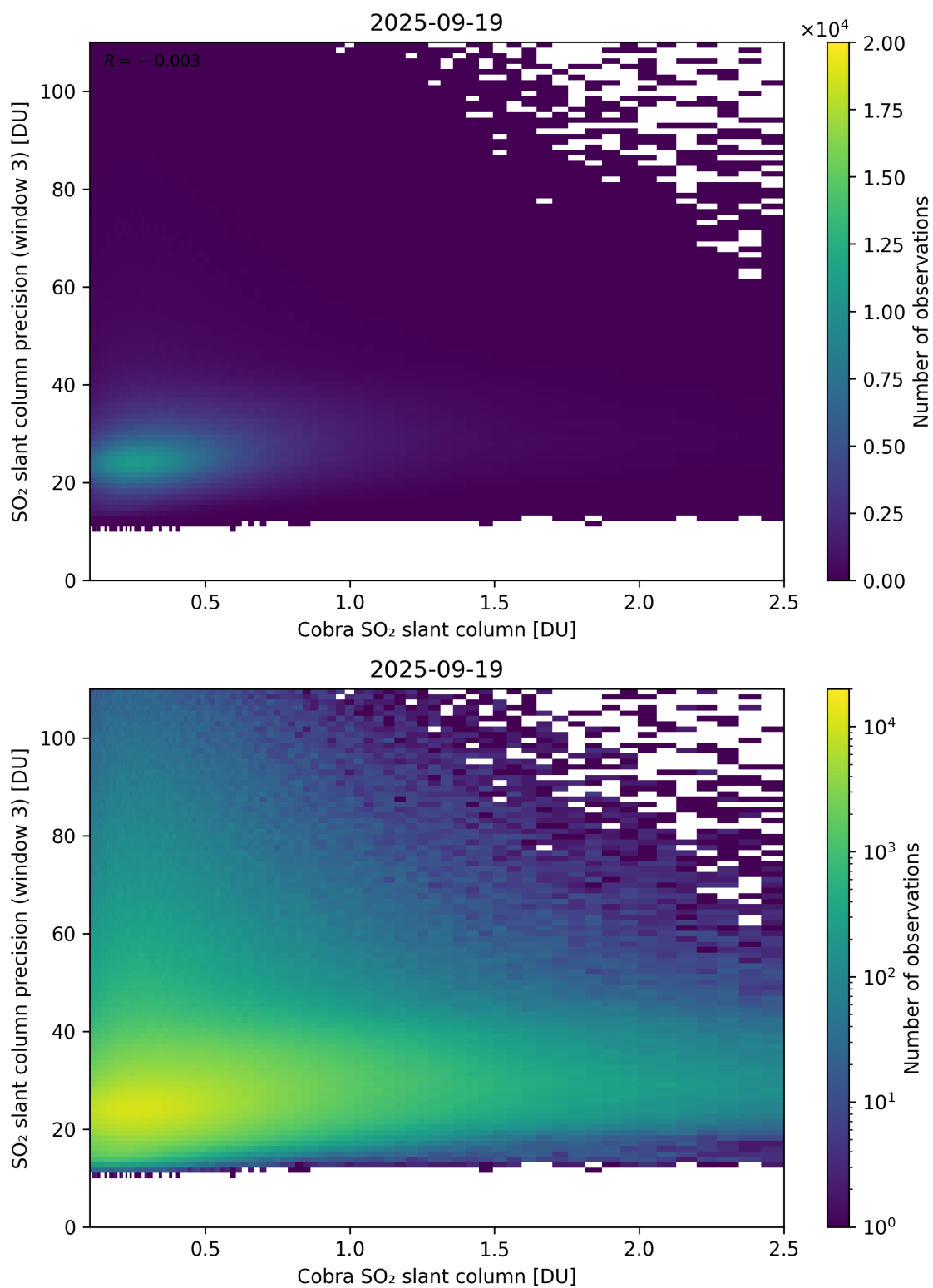
Figure 223: Scatter density plot of “Cobra SO 2 slant column” against “SO 2 slant column precision (window 3)” for 2025-09-18 to 2025-09-20.
