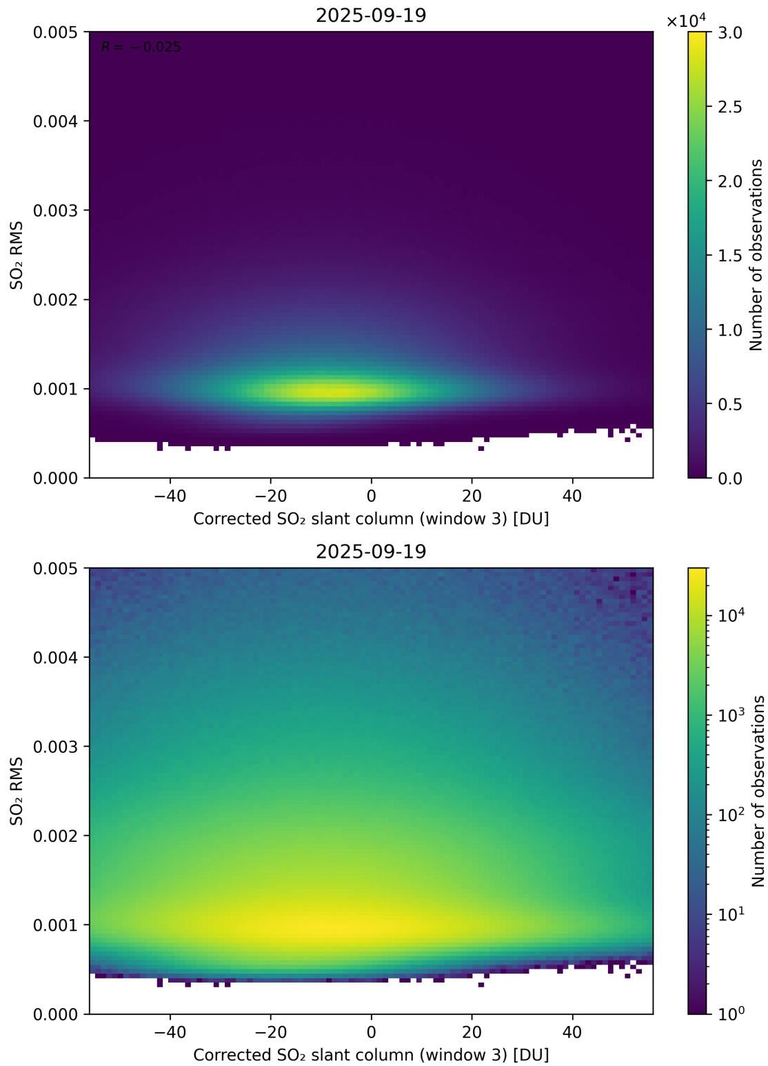
Figure 258: Scatter density plot of “Corrected SO 2 slant column (window 3)” against “SO 2 RMS” for 2025-09-18 to 2025-09-20.
