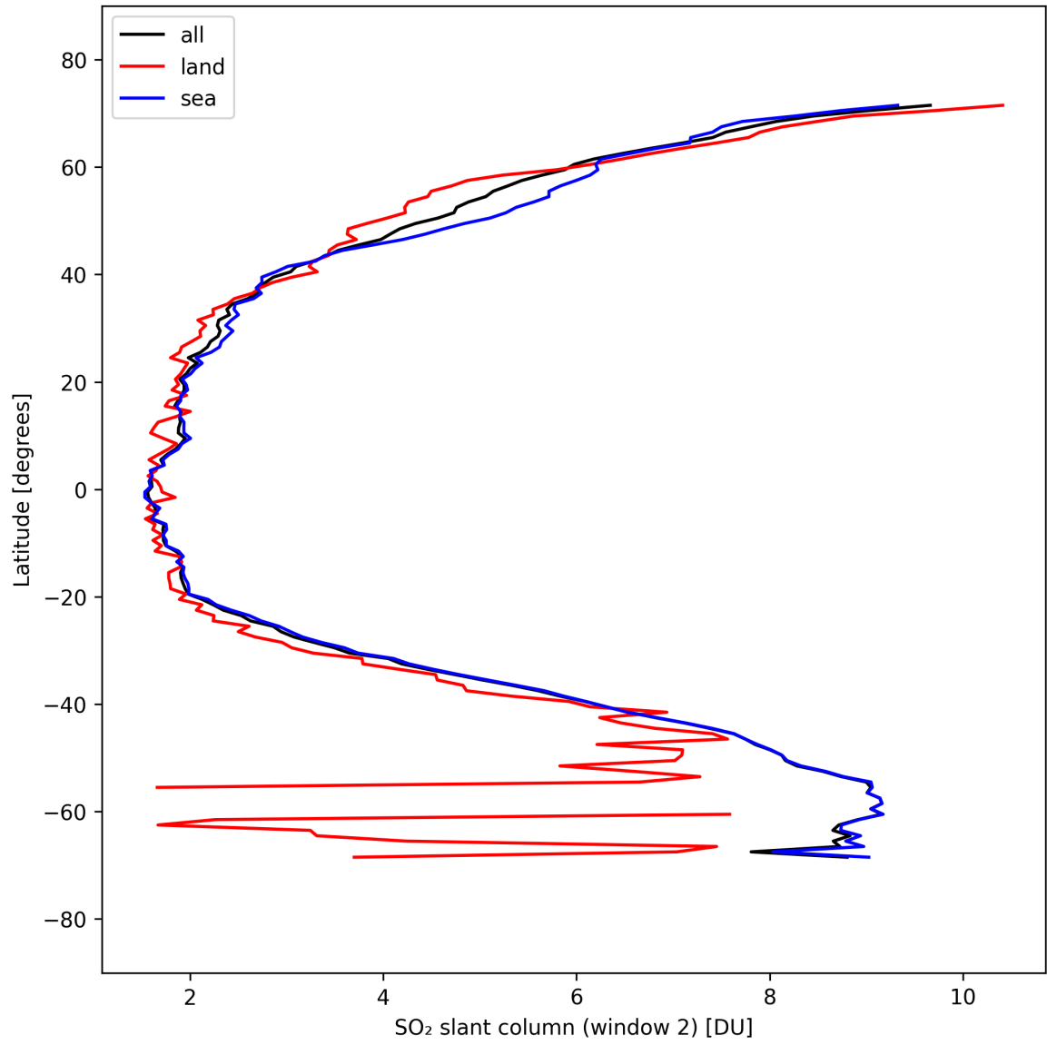
Figure 41: Zonal average of “SO 2 slant column (window 2)” for 2025-09-18 to 2025-09-20.
