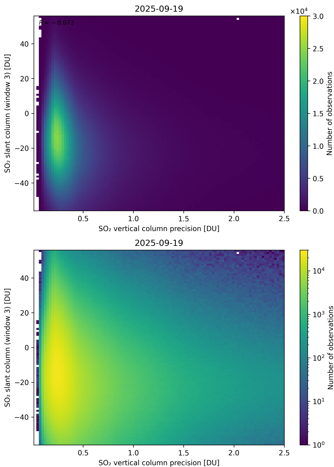
Figure 344: Scatter density plot of “SO 2 vertical column precision” against “SO 2 slant column (window 3)” for 2025-09-18 to 2025-09-20.
