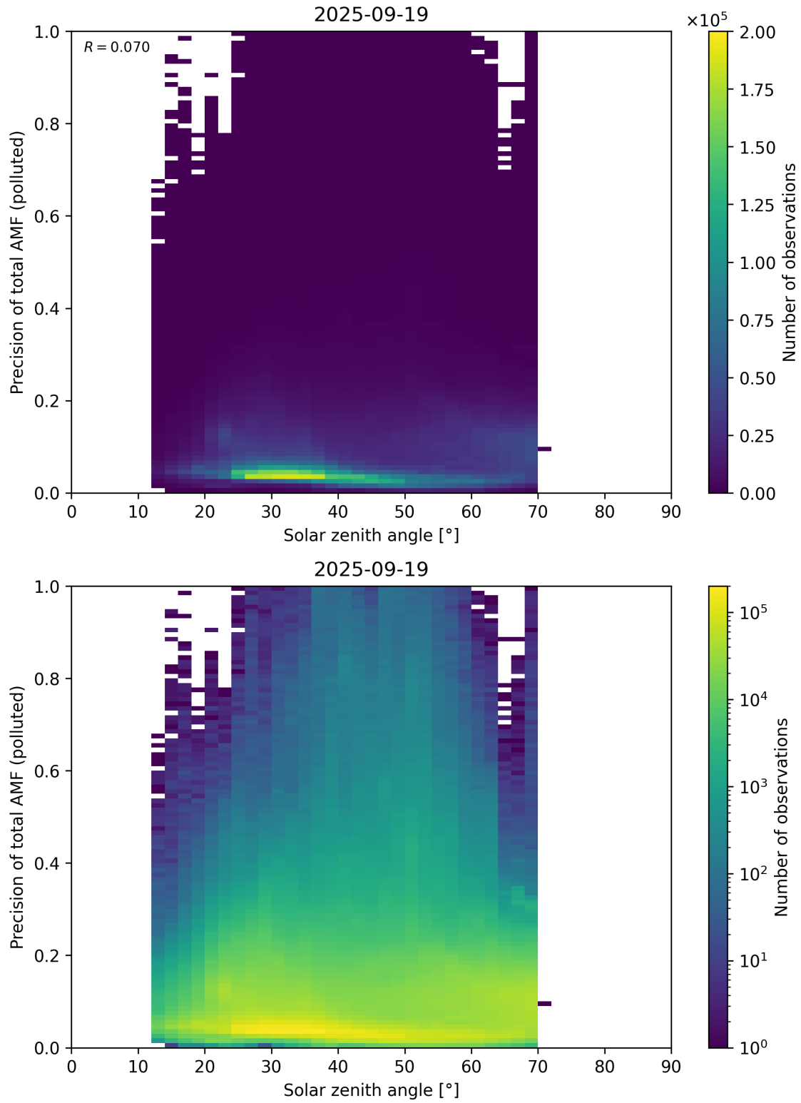
Figure 190: Scatter density plot of “Solar zenith angle” against “Precision of total AMF (polluted)” for 2025-09-18 to 2025-09-20.
