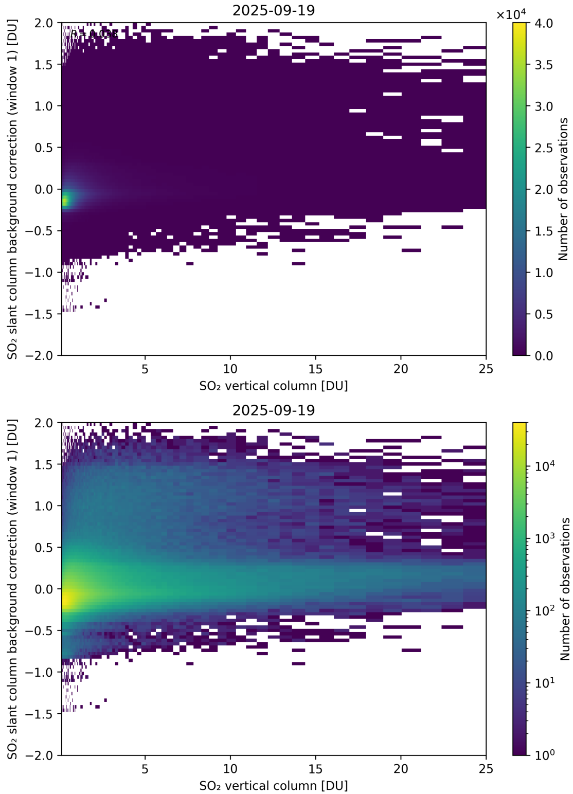
Figure 323: Scatter density plot of “SO 2 vertical column” against “SO 2 slant column background correction (window 1)” for 2025-09-18 to 2025-09-20.
