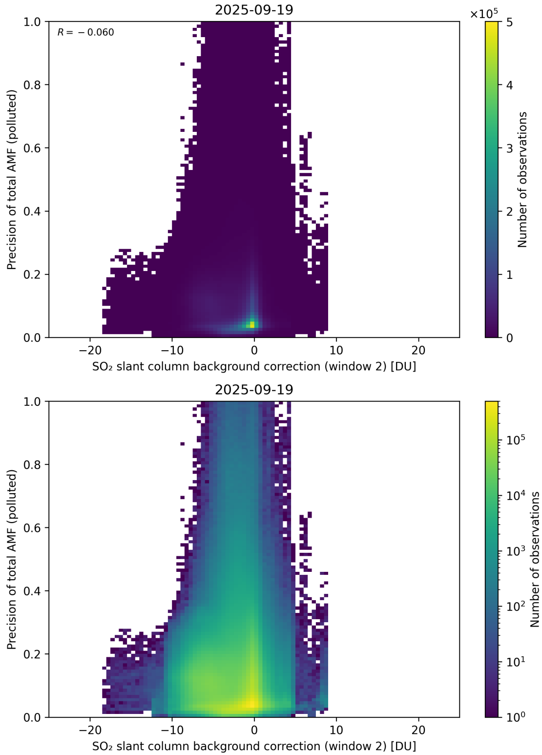
Figure 131: Scatter density plot of “SO 2 slant column background correction (window 2)” against “Precision of total AMF (polluted)” for 2025-09-18 to 2025-09-20.
