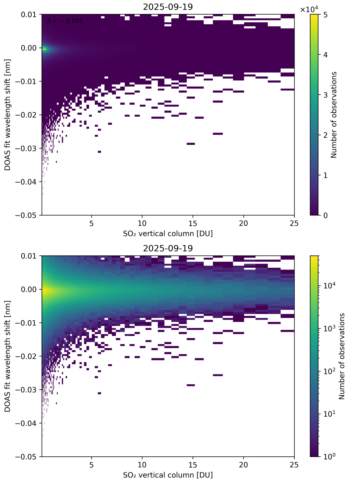
Figure 326: Scatter density plot of “SO 2 vertical column” against “DOAS fit wavelength shift” for 2025-09-18 to 2025-09-20.
