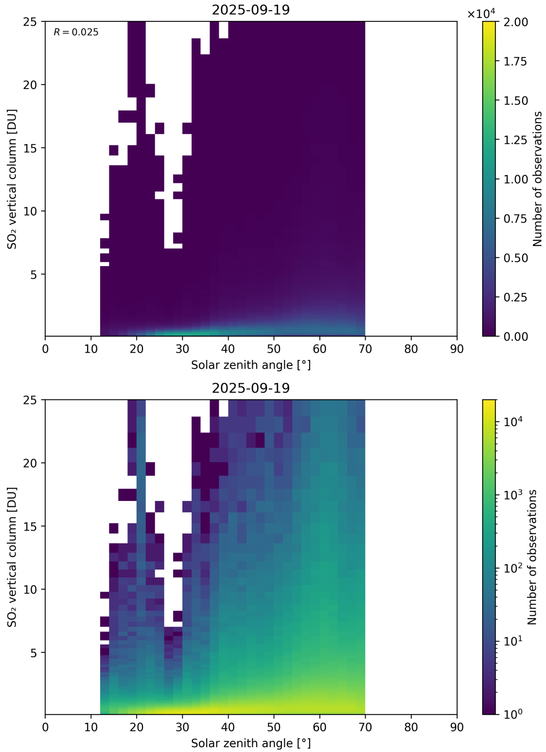
Figure 191: Scatter density plot of “Solar zenith angle” against “SO 2 vertical column” for 2025-09-18 to 2025-09-20.
