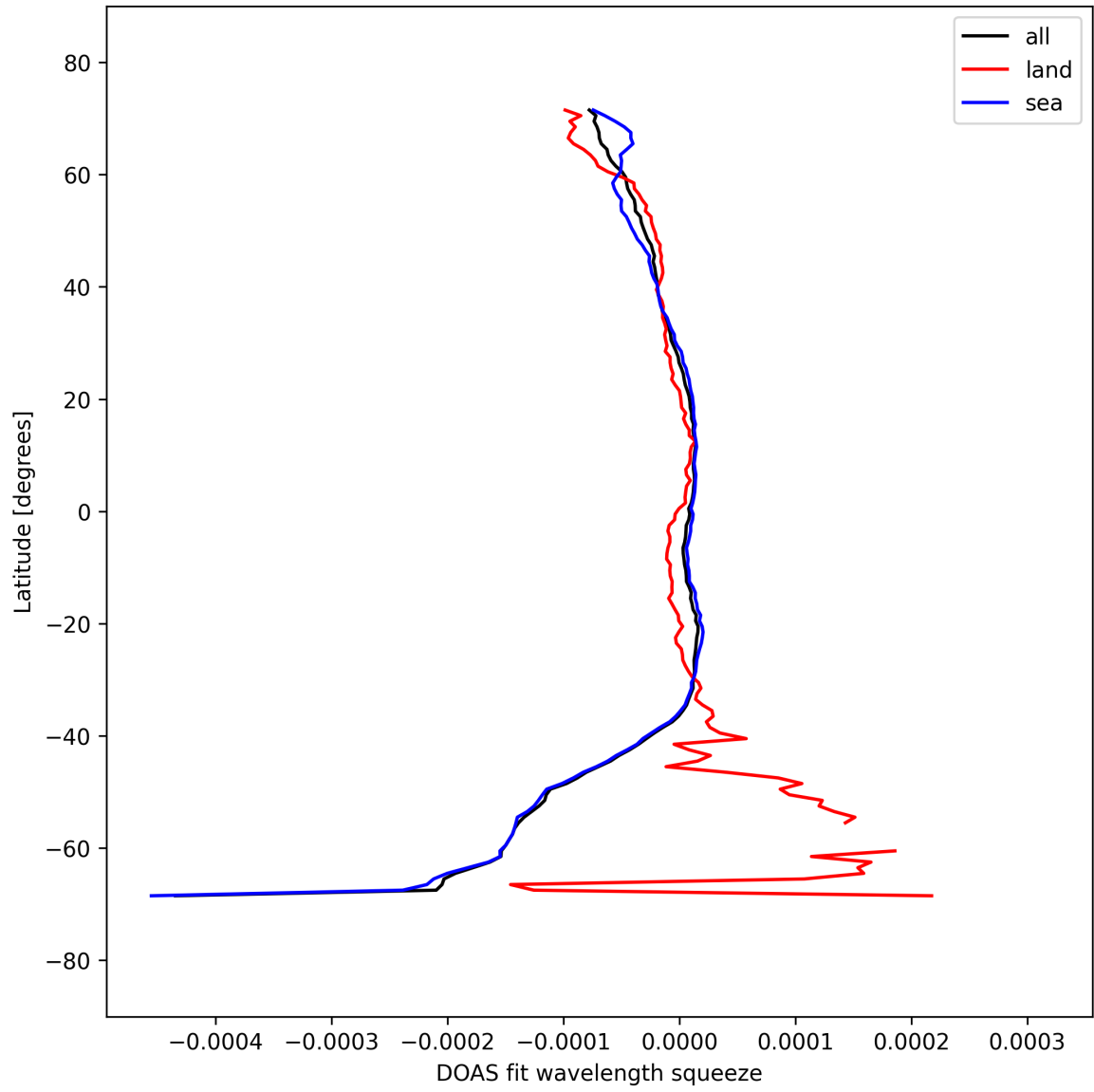
Figure 51: Zonal average of “DOAS fit wavelength squeeze” for 2025-09-18 to 2025-09-20.
