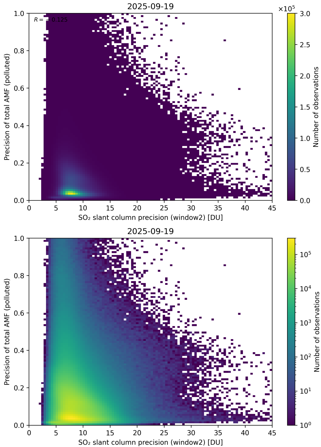
Figure 302: Scatter density plot of “SO 2 slant column precision (window2)” against “Precision of total AMF (polluted)” for 2025-09-18 to 2025-09-20.
