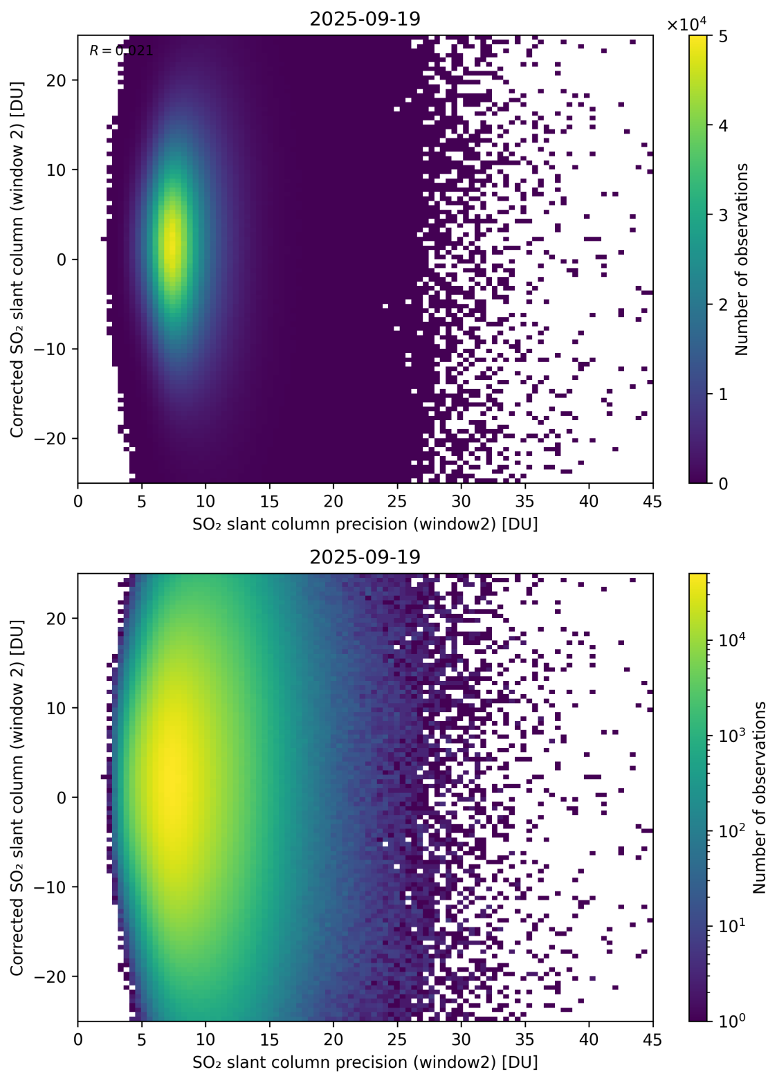
Figure 297: Scatter density plot of “SO 2 slant column precision (window2)” against “Corrected SO 2 slant column (window 2)” for 2025-09-18 to 2025-09-20.
