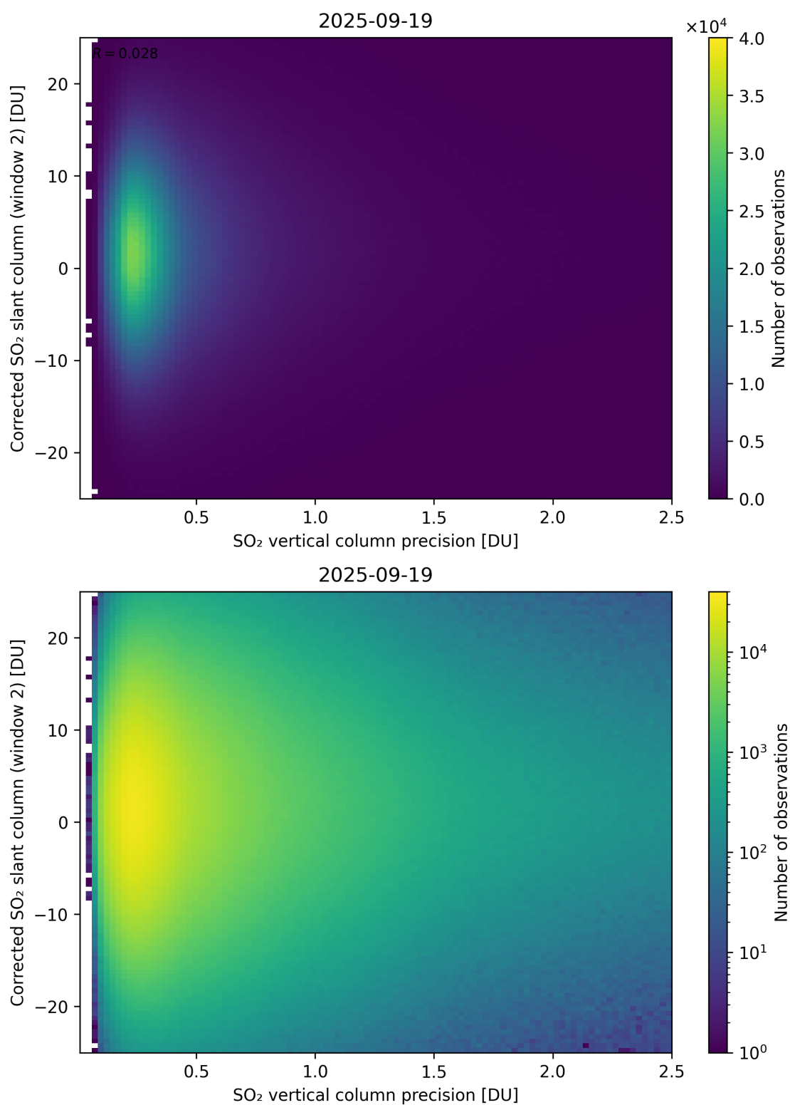
Figure 339: Scatter density plot of “SO 2 vertical column precision” against “Corrected SO 2 slant column (window 2)” for 2025-09-18 to 2025-09-20.
