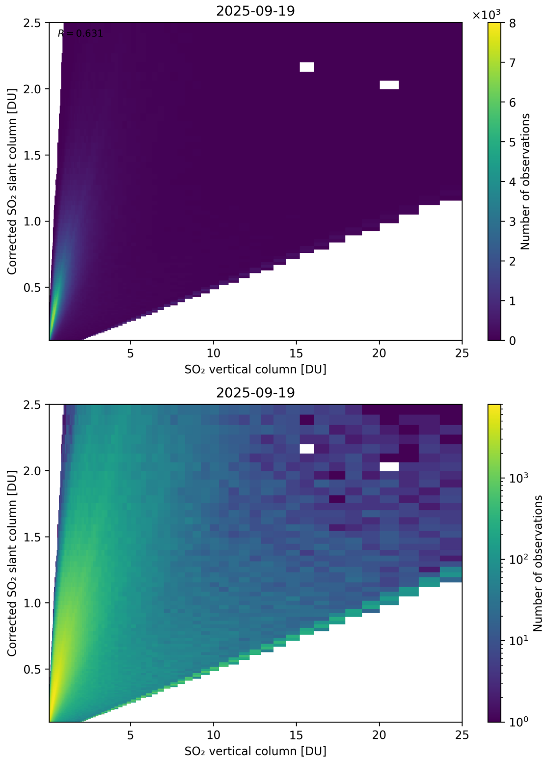
Figure 351: Scatter density plot of “SO 2 vertical column” against “Corrected SO 2 slant column” for 2025-09-18 to 2025-09-20.
