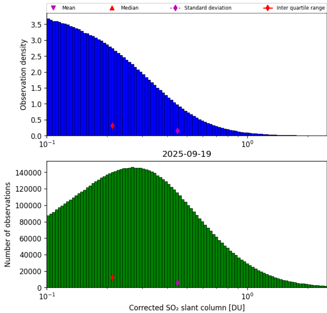
Figure 60: Histogram of "Corrected SO 2 slant column" for 2025-09-18 to 2025-09-20
