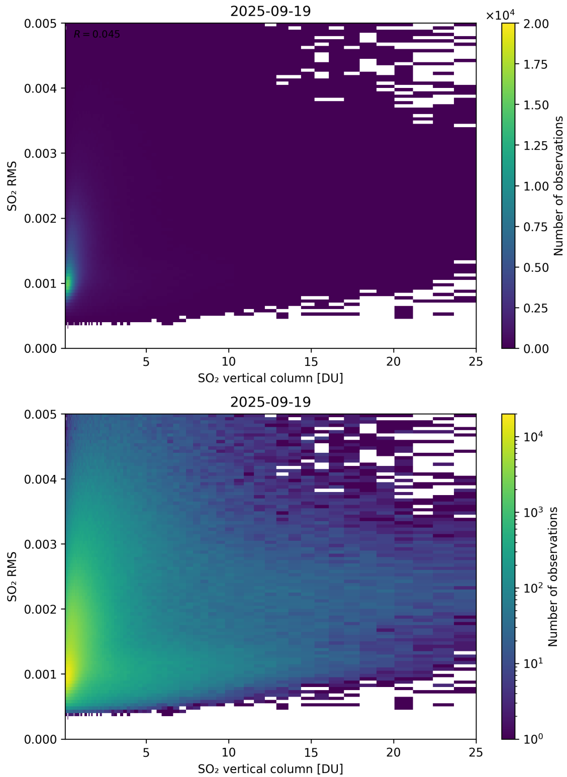
Figure 328: Scatter density plot of “SO 2 vertical column” against “SO 2 RMS” for 2025-09-18 to 2025-09-20.
