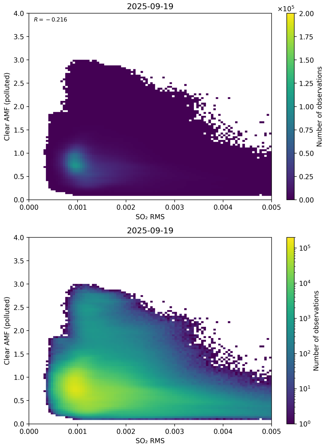
Figure 147: Scatter density plot of “SO 2 RMS” against “Clear AMF (polluted)” for 2025-09-18 to 2025-09-20.
