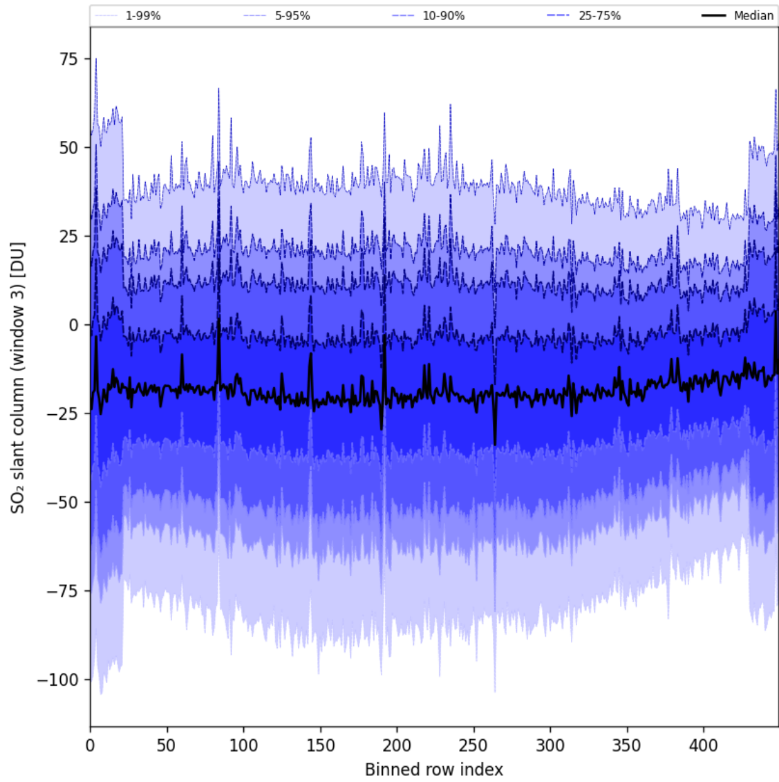
Figure 97: Along track statistics of “SO 2 slant column (window 3)” for 2025-09-18 to 2025-09-20
