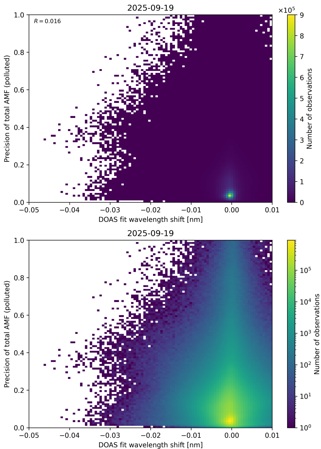
Figure 142: Scatter density plot of “DOAS fit wavelength shift” against “Precision of total AMF (polluted)” for 2025-09-18 to 2025-09-20.
