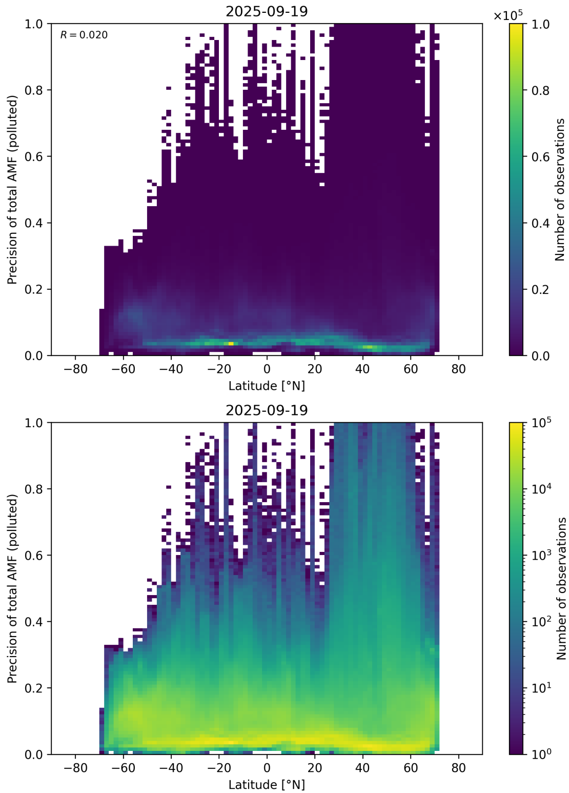
Figure 168: Scatter density plot of “Latitude” against “Precision of total AMF (polluted)” for 2025-09-18 to 2025-09-20.
