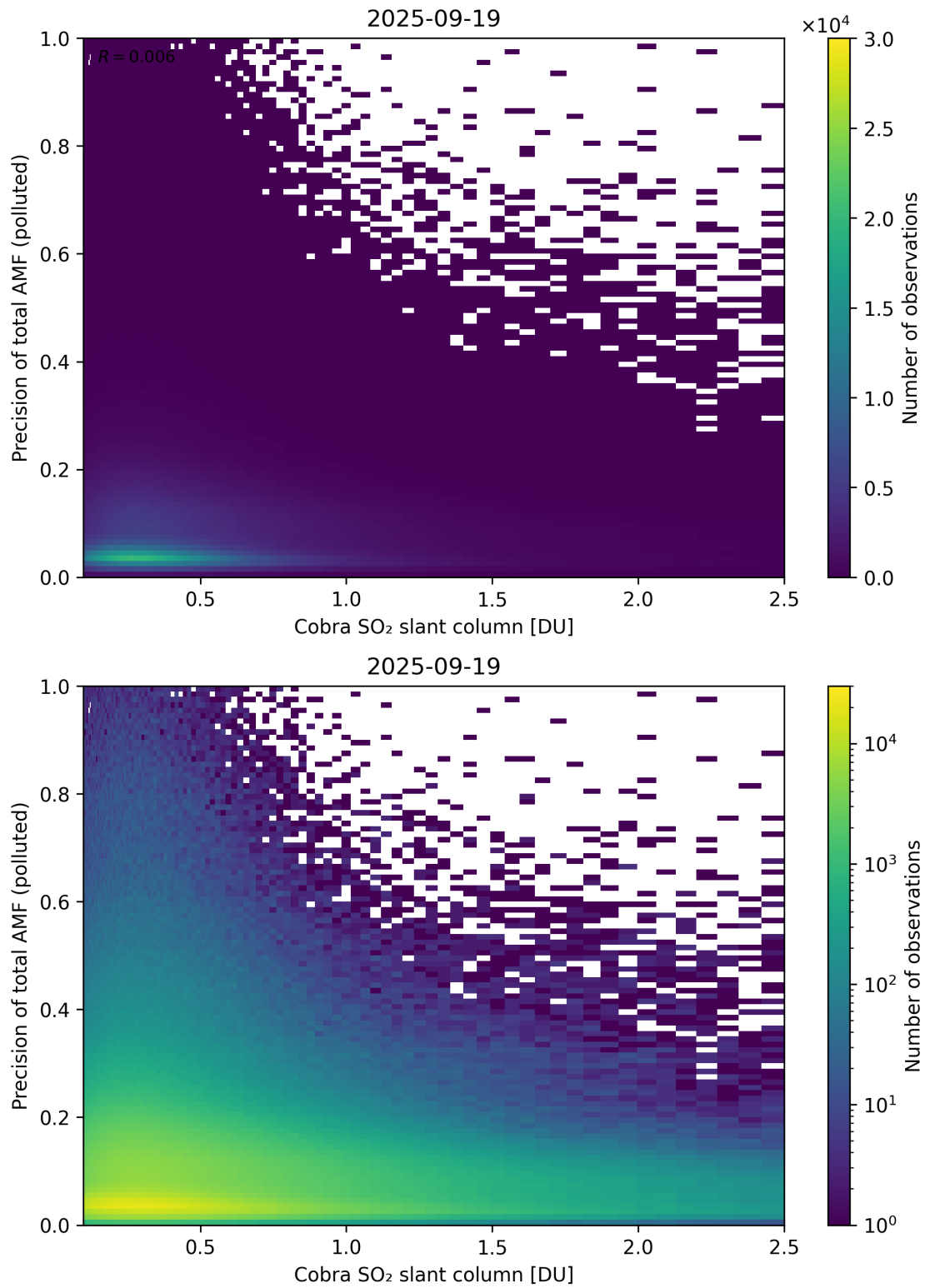
Figure 225: Scatter density plot of “Cobra SO 2 slant column” against “Precision of total AMF (polluted)” for 2025-09-18 to 2025-09-20.
