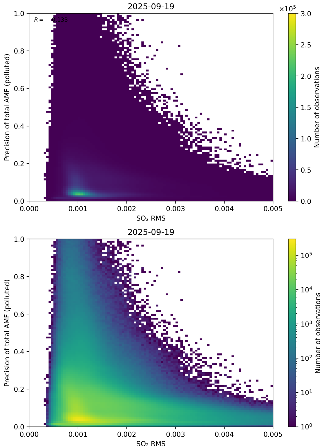
Figure 149: Scatter density plot of “SO 2 RMS” against “Precision of total AMF (polluted)” for 2025-09-18 to 2025-09-20.
