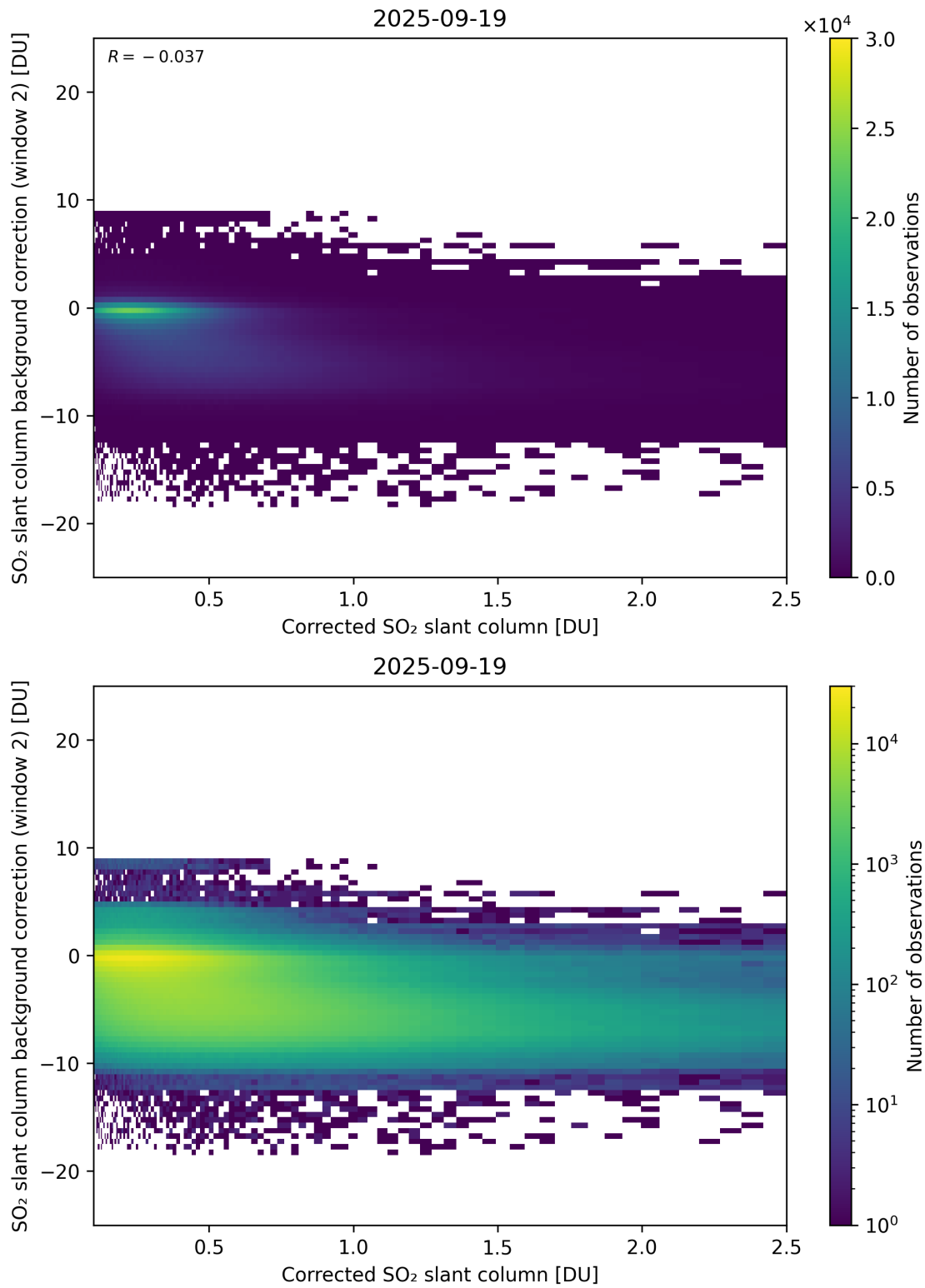
Figure 227: Scatter density plot of “Corrected SO 2 slant column” against “SO 2 slant column background correction (window 2)” for 2025-09-18 to 2025-09-20.
