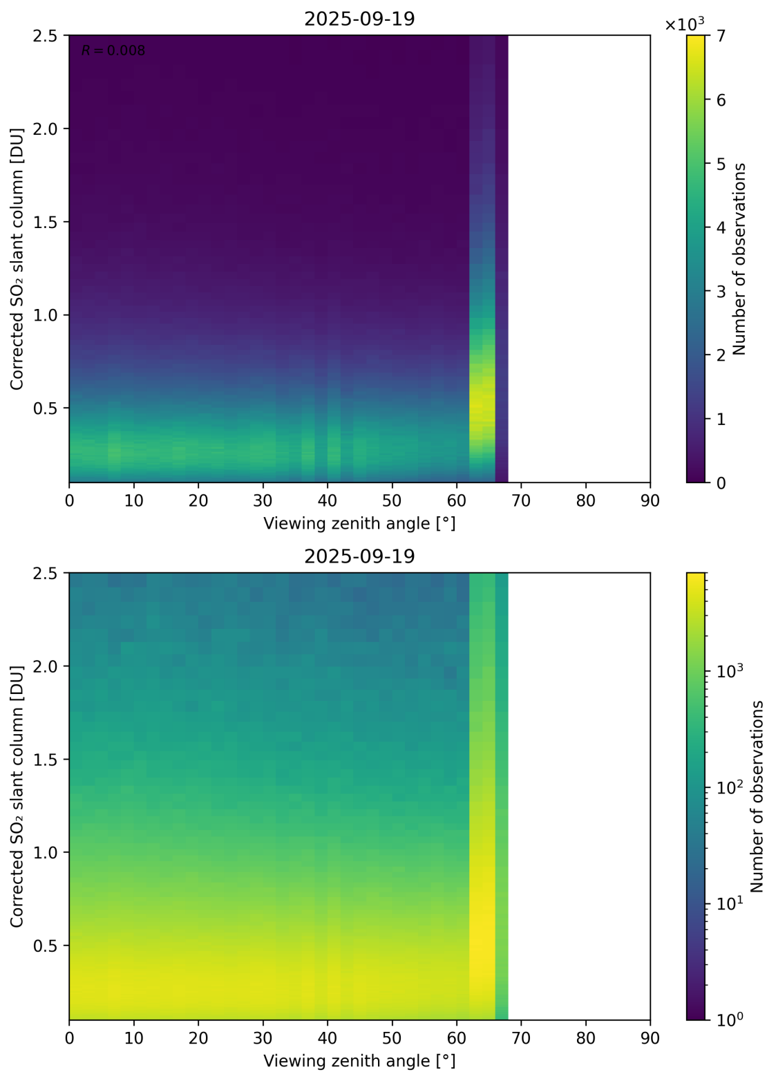
Figure 373: Scatter density plot of “Viewing zenith angle” against “Corrected SO 2 slant column” for 2025-09-18 to 2025-09-20.
