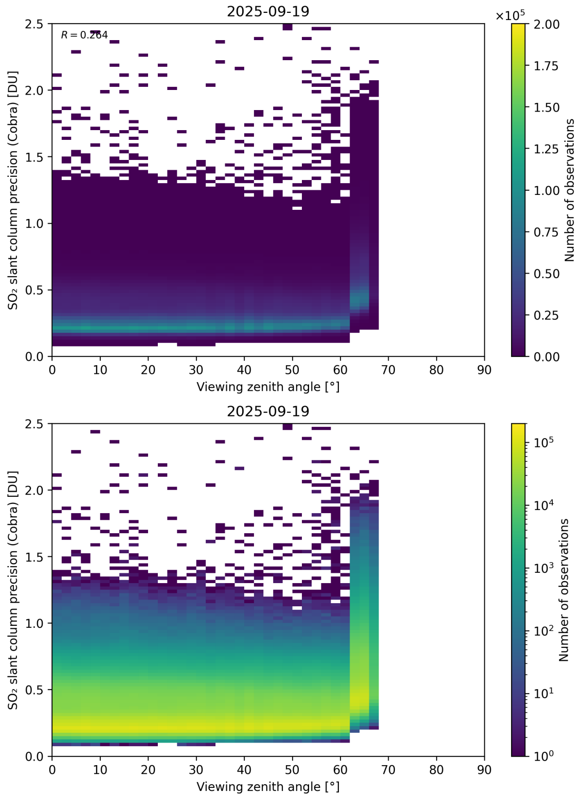
Figure 372: Scatter density plot of “Viewing zenith angle” against “SO 2 slant column precision (Cobra)” for 2025-09-18 to 2025-09-20.
