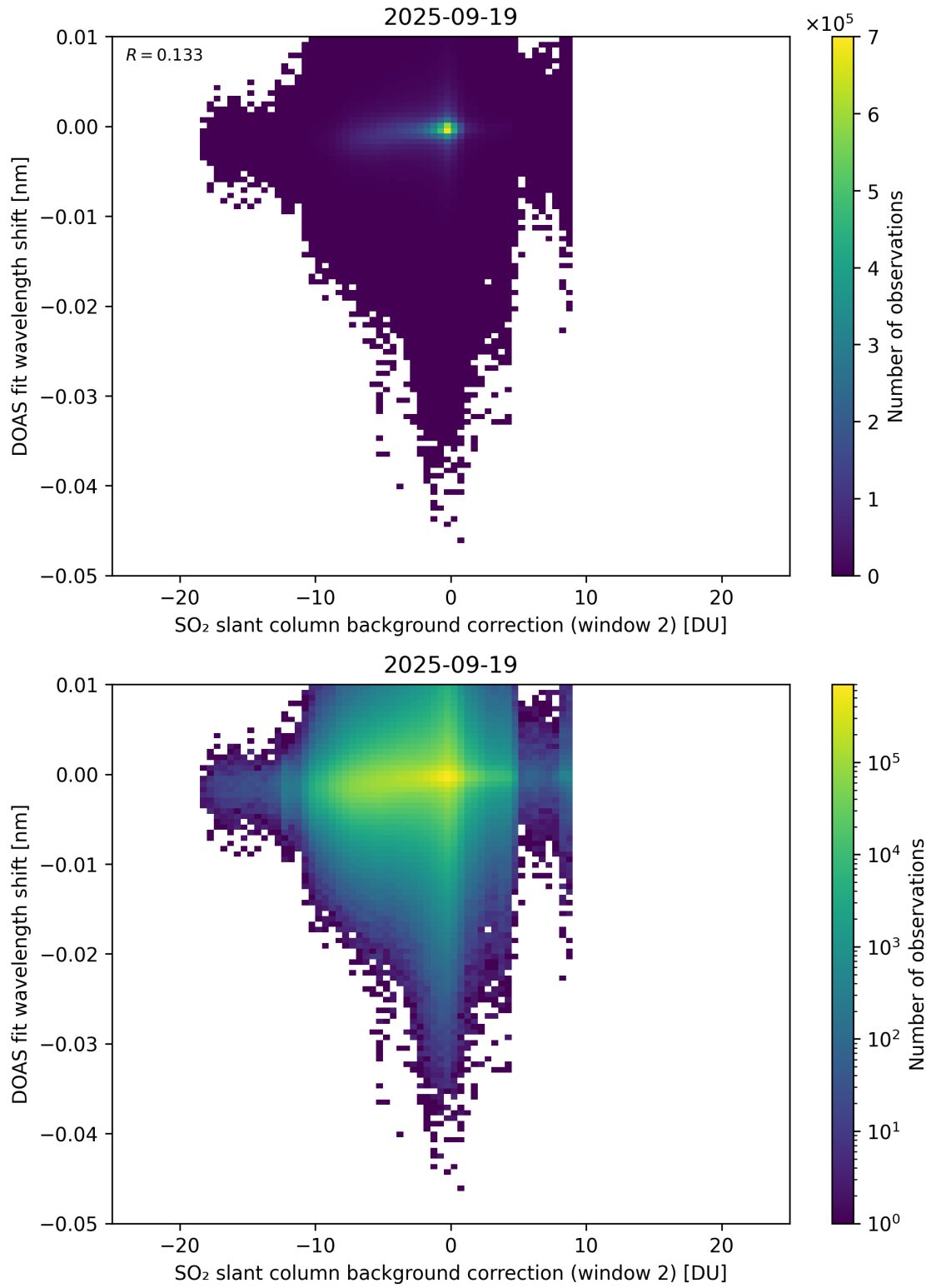
Figure 123: Scatter density plot of “SO 2 slant column background correction (window 2)” against “DOAS fit wavelength shift” for 2025-09-18 to 2025-09-20.
