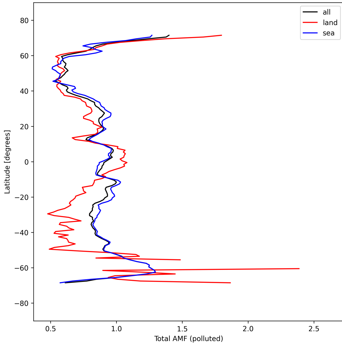
Figure 53: Zonal average of “Total AMF (polluted)” for 2025-09-18 to 2025-09-20.
