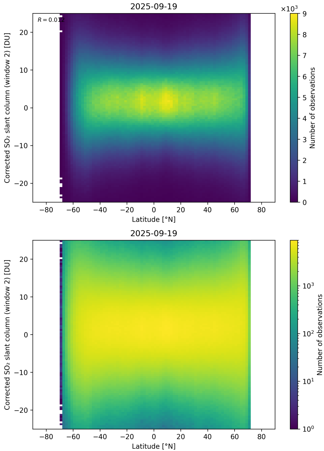
Figure 160: Scatter density plot of “Latitude” against “Corrected SO 2 slant column (window 2)” for 2025-09-18 to 2025-09-20.
