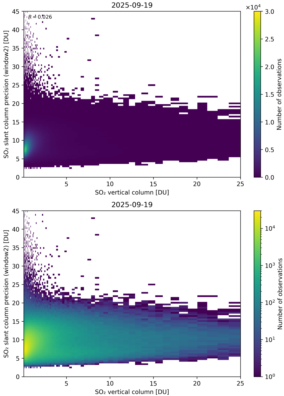
Figure 356: Scatter density plot of “SO 2 vertical column” against “SO 2 slant column precision (window2)” for 2025-09-18 to 2025-09-20.
