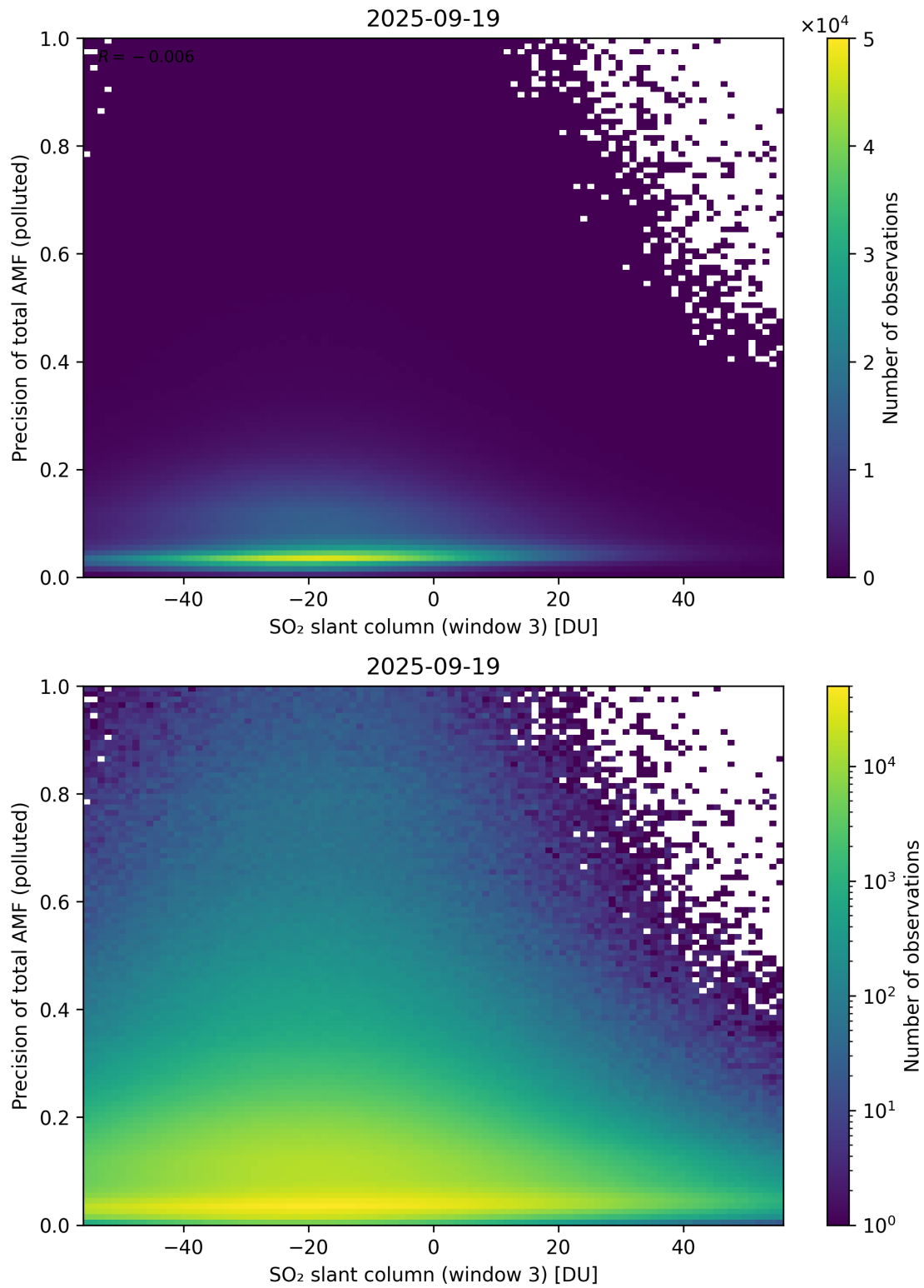
Figure 319: Scatter density plot of “SO 2 slant column (window 3)” against “Precision of total AMF (polluted)” for 2025-09-18 to 2025-09-20.
