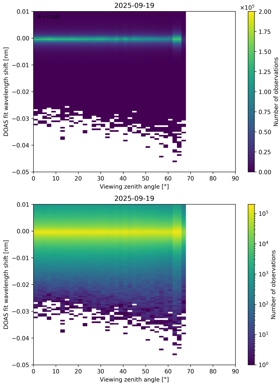
Figure 365: Scatter density plot of “Viewing zenith angle” against “DOAS fit wavelength shift” for 2025-09-18 to 2025-09-20.
