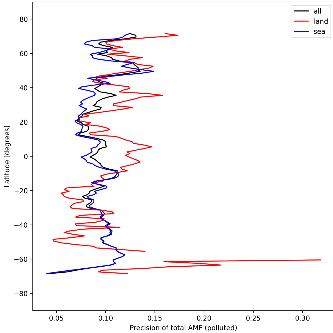
Figure 54: Zonal average of “Precision of total AMF (polluted)” for 2025-09-18 to 2025-09-20.
