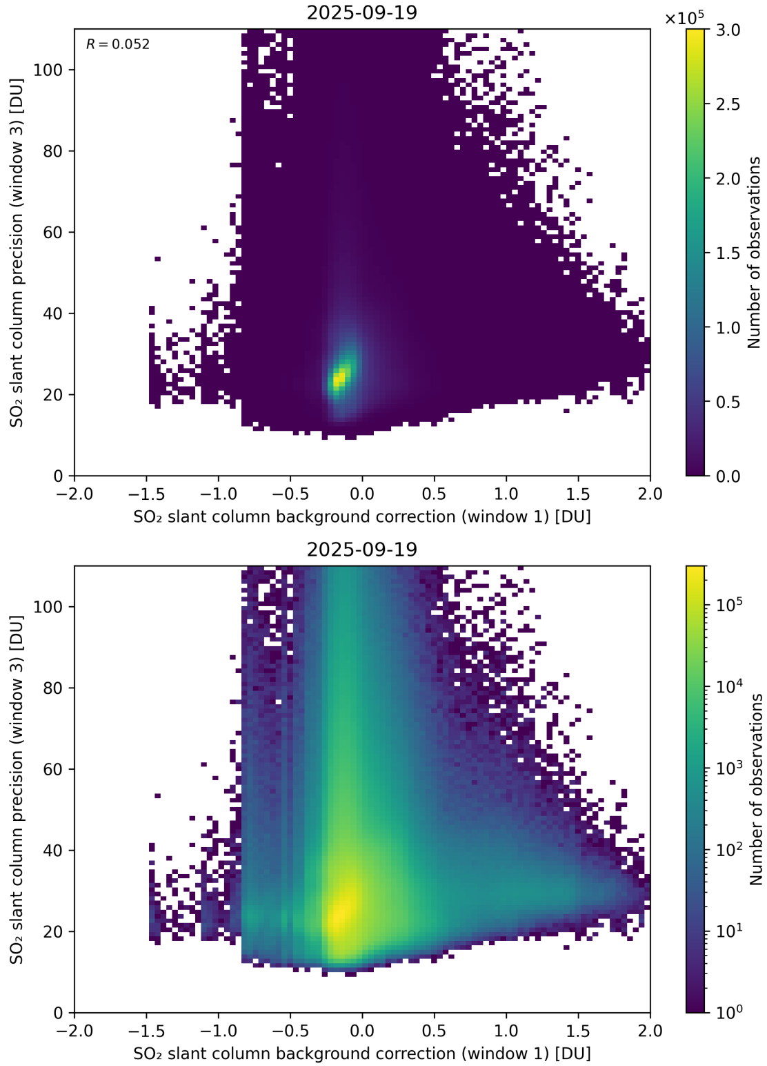
Figure 119: Scatter density plot of “SO 2 slant column background correction (window 1)” against “SO 2 slant column precision (window 3)” for 2025-09-18 to 2025-09-20.
