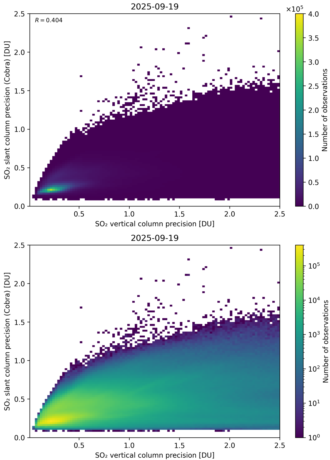
Figure 337: Scatter density plot of “SO 2 vertical column precision” against “SO 2 slant column precision (Cobra)” for 2025-09-18 to 2025-09-20.
