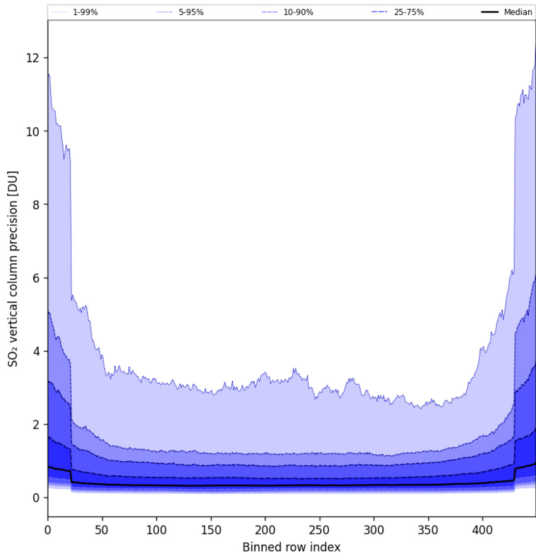
Figure 85: Along track statistics of “SO 2 vertical column precision” for 2025-09-18 to 2025-09-20
