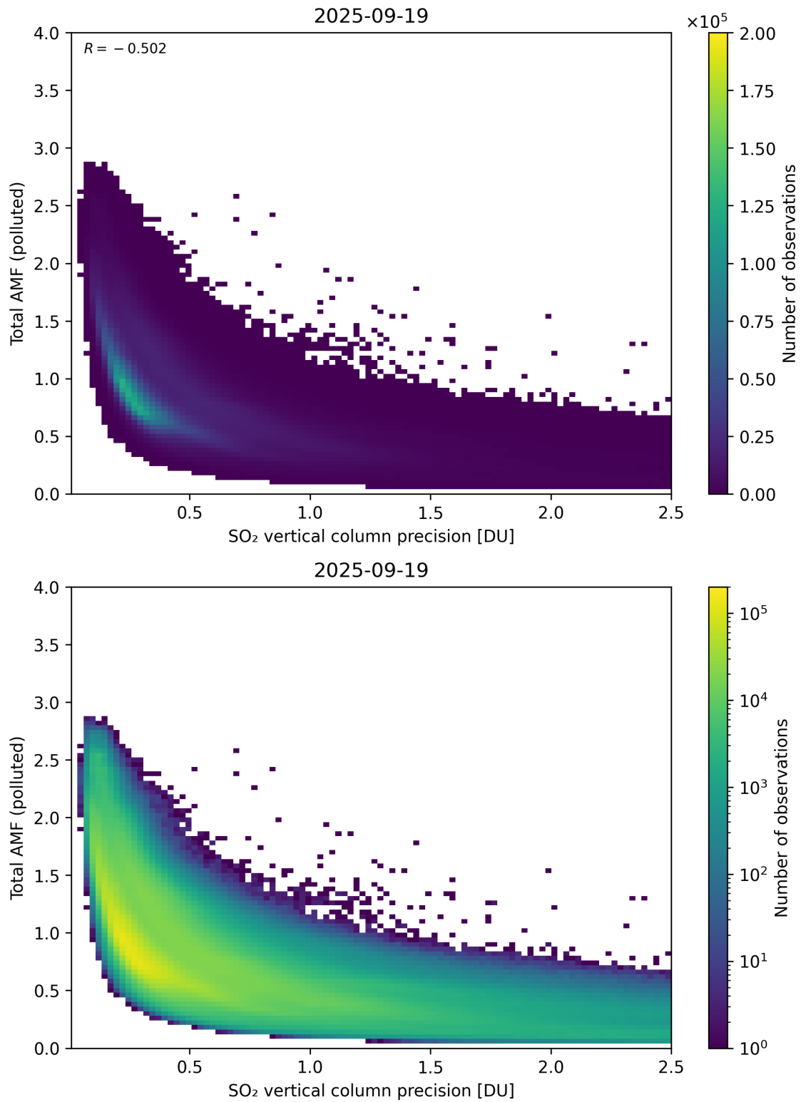
Figure 346: Scatter density plot of “SO 2 vertical column precision” against “Total AMF (polluted)” for 2025-09-18 to 2025-09-20.
