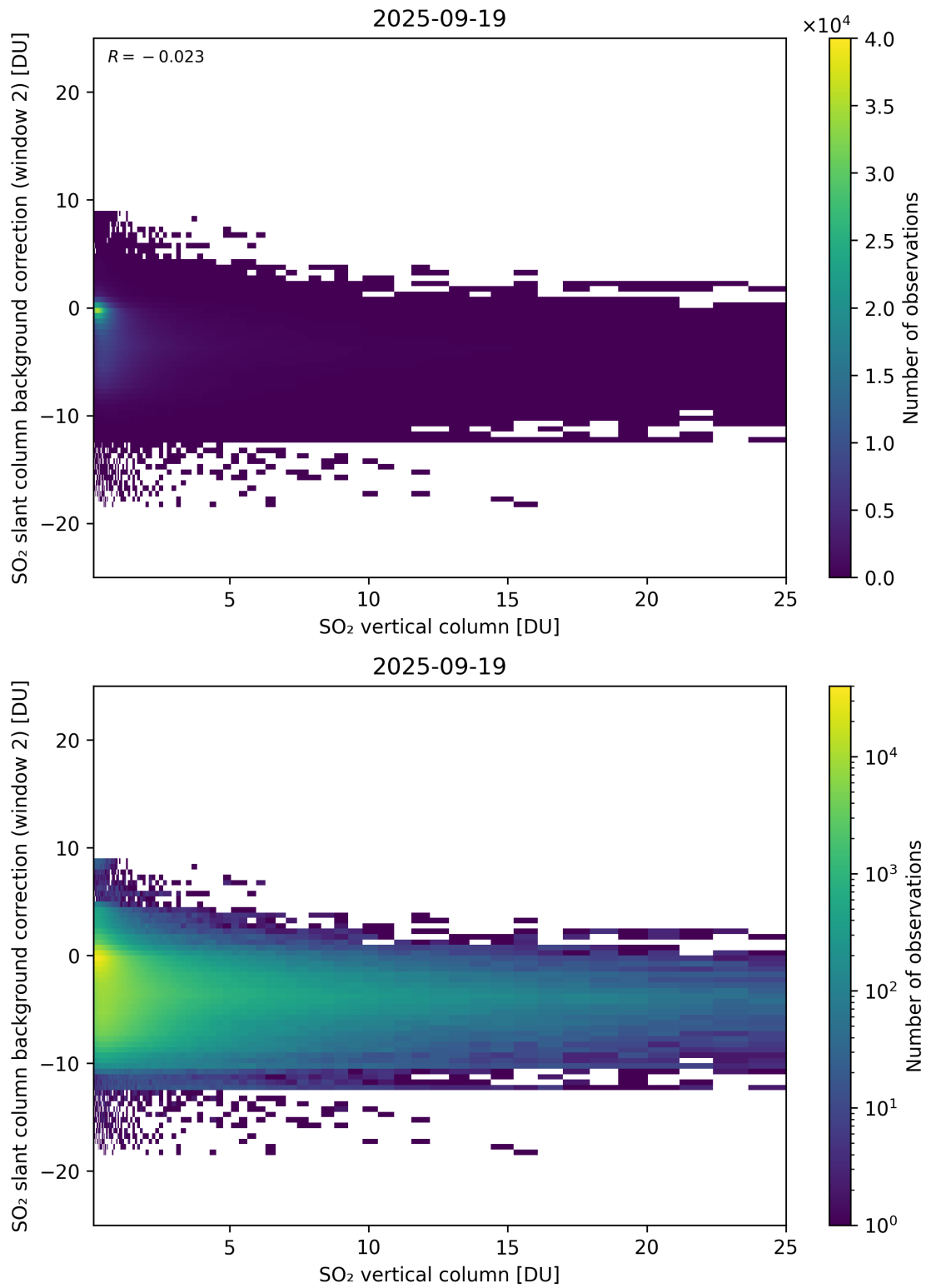
Figure 324: Scatter density plot of “SO 2 vertical column” against “SO 2 slant column background correction (window 2)” for 2025-09-18 to 2025-09-20.
