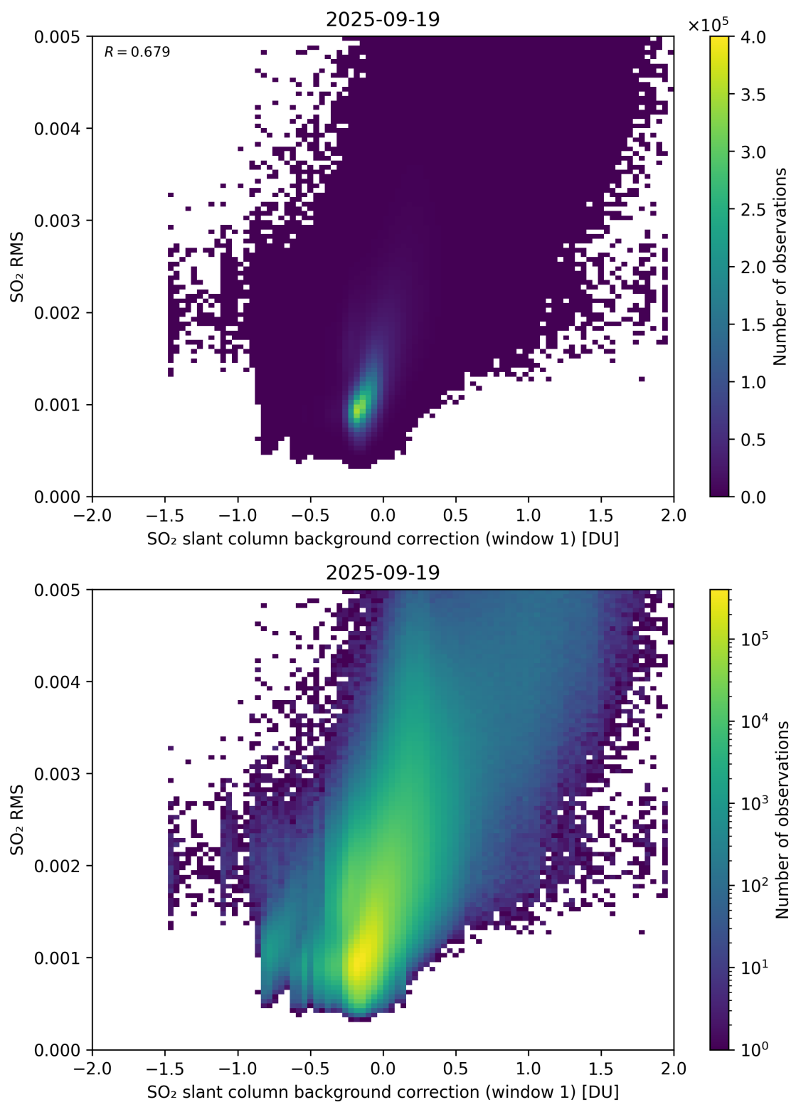
Figure 113: Scatter density plot of “SO 2 slant column background correction (window 1)” against “SO 2 RMS” for 2025-09-18 to 2025-09-20.
