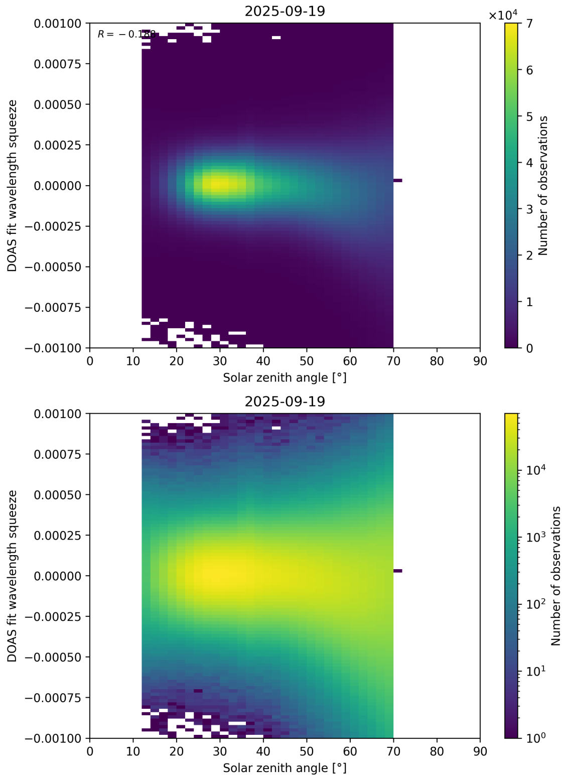
Figure 175: Scatter density plot of “Solar zenith angle” against “DOAS fit wavelength squeeze” for 2025-09-18 to 2025-09-20.
