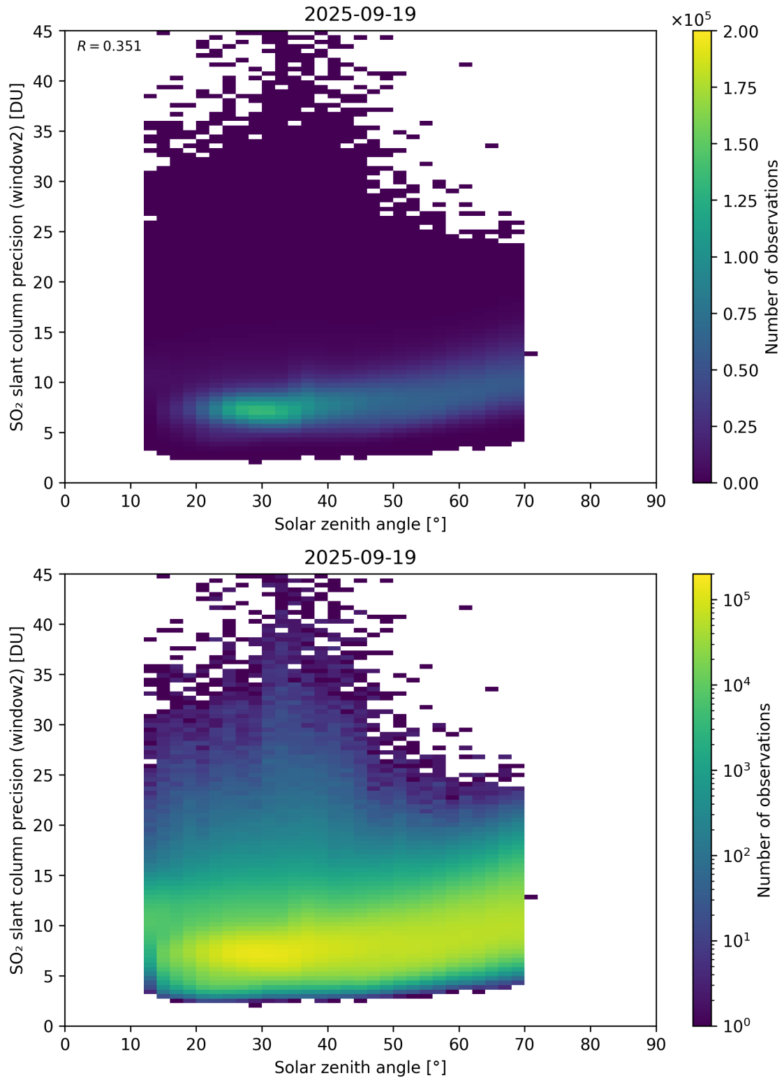
Figure 186: Scatter density plot of “Solar zenith angle” against “SO 2 slant column precision (window2)” for 2025-09-18 to 2025-09-20.
