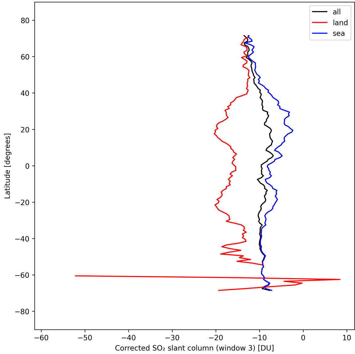
Figure 47: Zonal average of “Corrected SO 2 slant column (window 3)” for 2025-09-18 to 2025-09-20.
