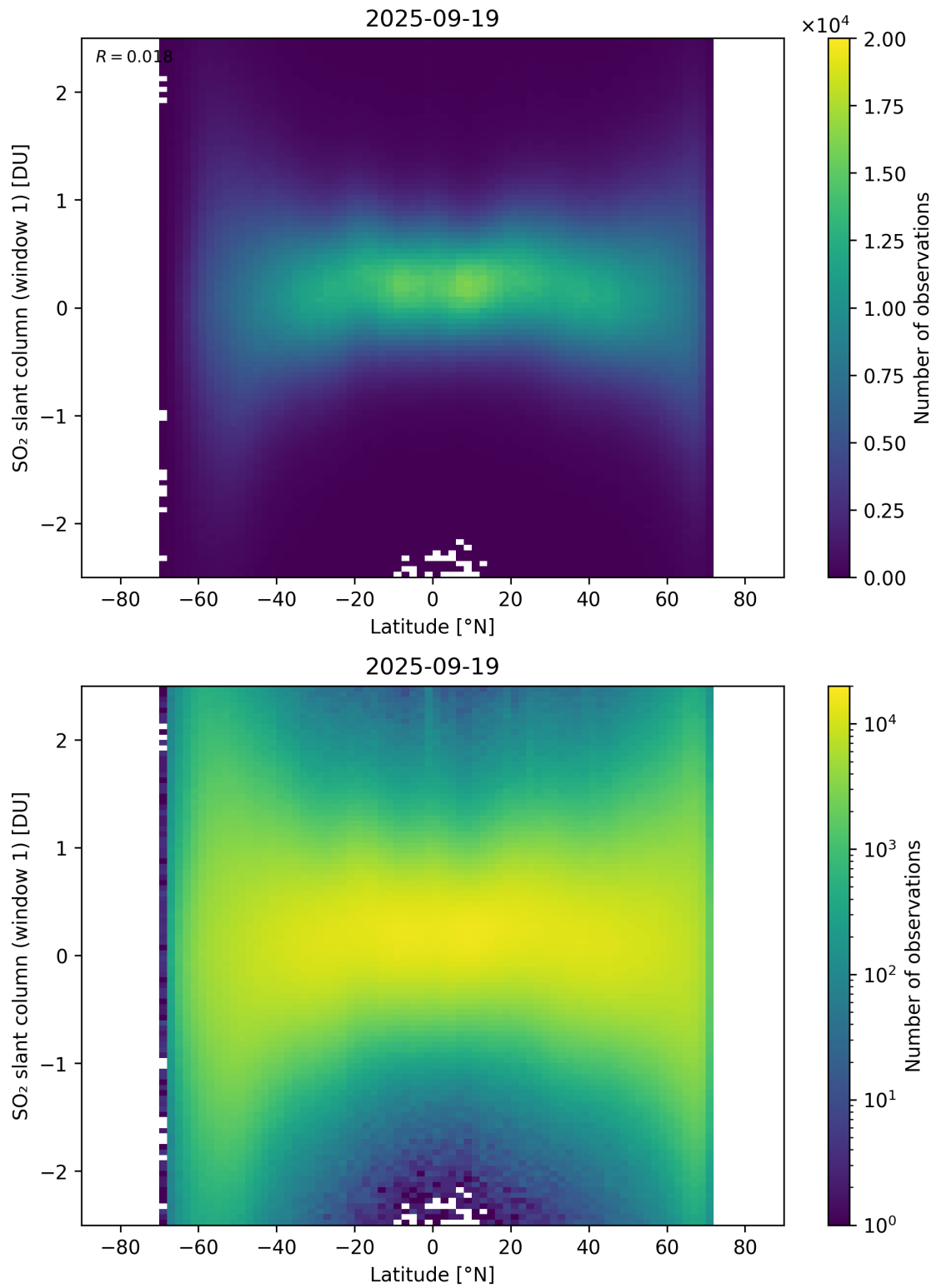
Figure 162: Scatter density plot of “Latitude” against “SO 2 slant column (window 1)” for 2025-09-18 to 2025-09-20.
