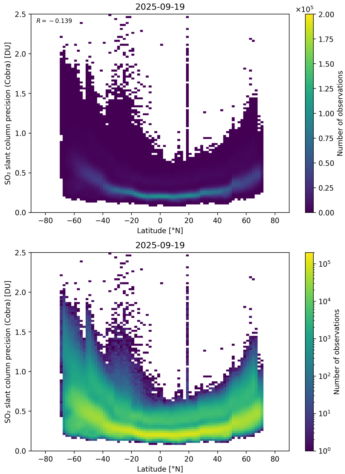
Figure 158: Scatter density plot of “Latitude” against “SO 2 slant column precision (Cobra)” for 2025-09-18 to 2025-09-20.
