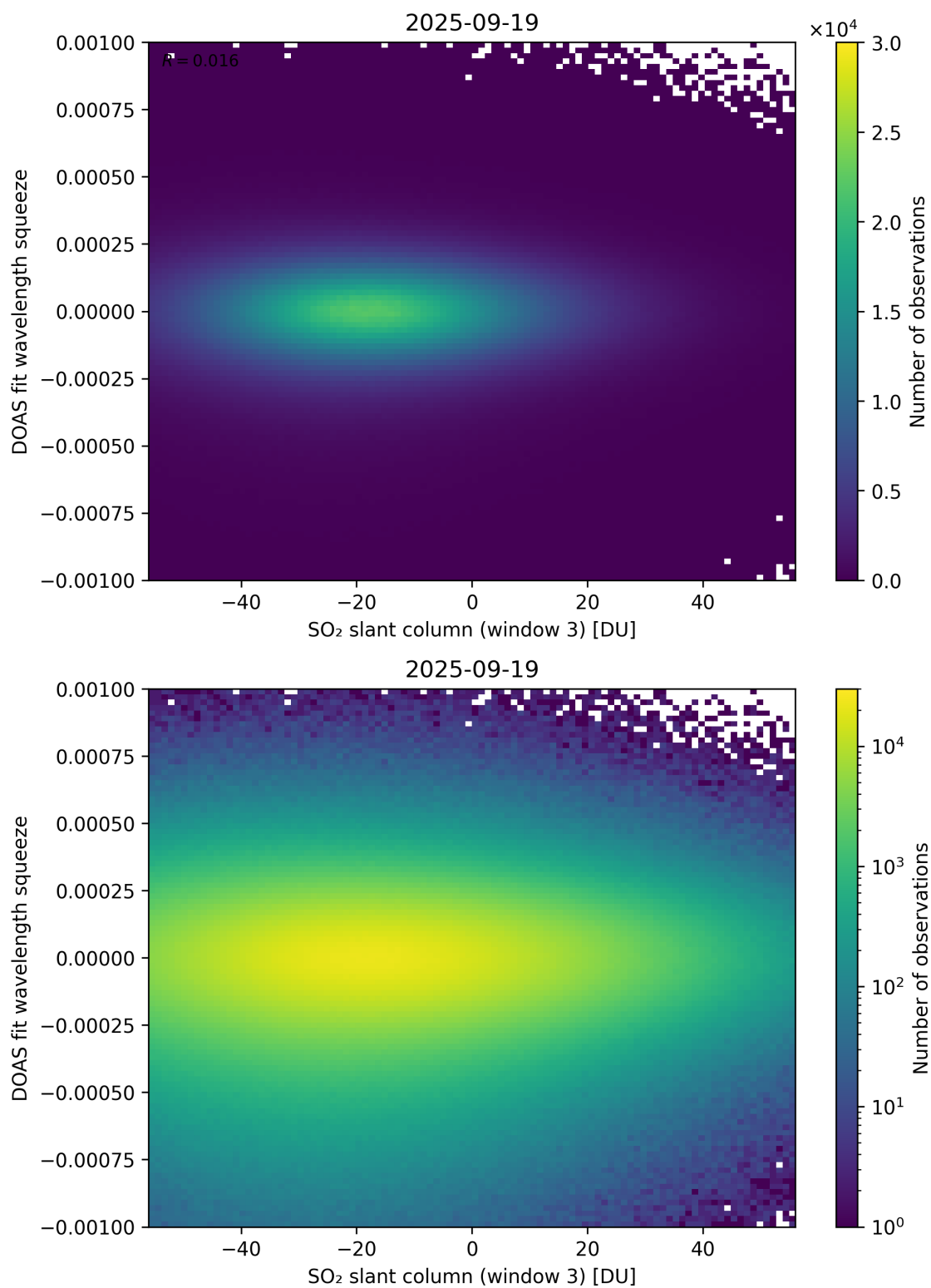
Figure 305: Scatter density plot of “SO 2 slant column (window 3)” against “DOAS fit wavelength squeeze” for 2025-09-18 to 2025-09-20.
