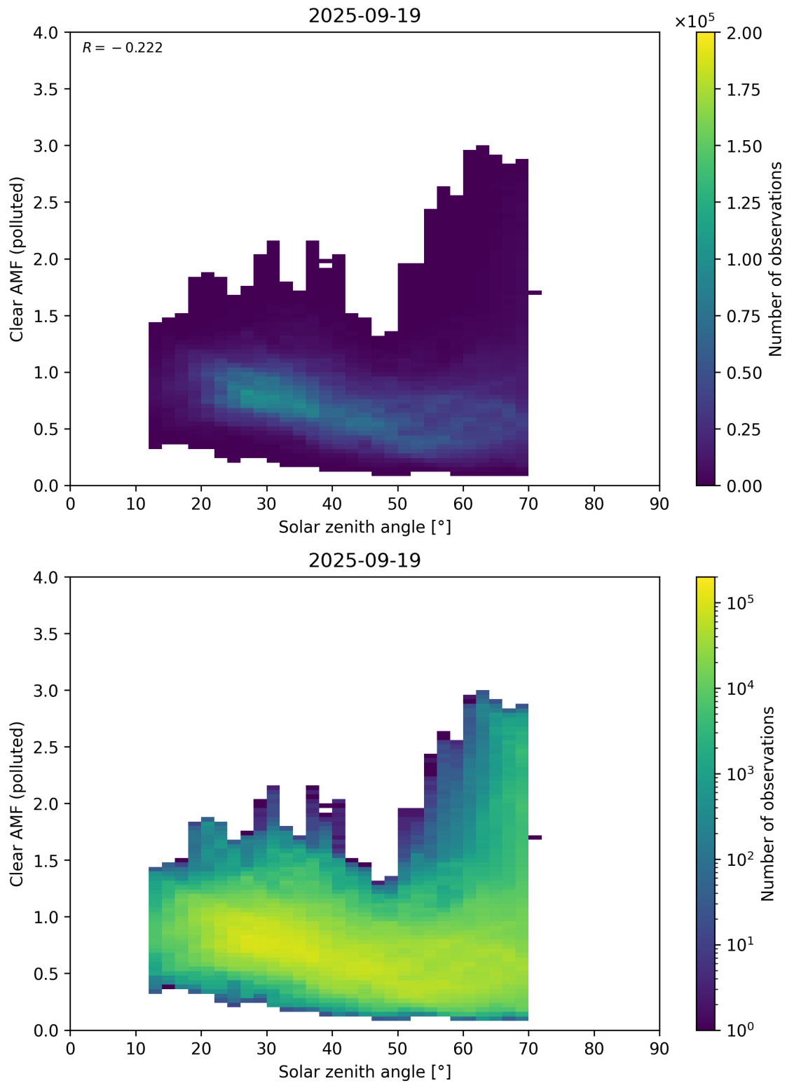
Figure 178: Scatter density plot of “Solar zenith angle” against “Clear AMF (polluted)” for 2025-09-18 to 2025-09-20.
