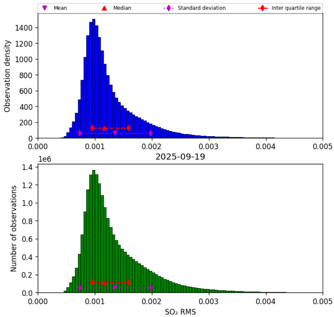
Figure 78: Histogram of “SO 2 RMS” for 2025-09-18 to 2025-09-20
