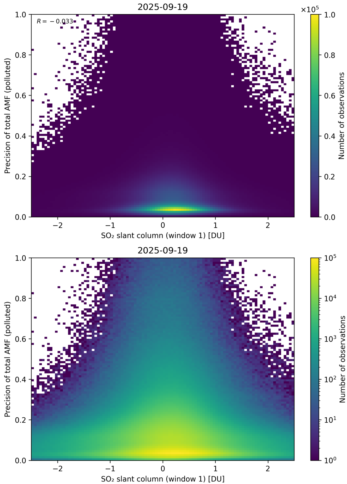
Figure 290: Scatter density plot of “SO 2 slant column (window 1)” against “Precision of total AMF (polluted)” for 2025-09-18 to 2025-09-20.
