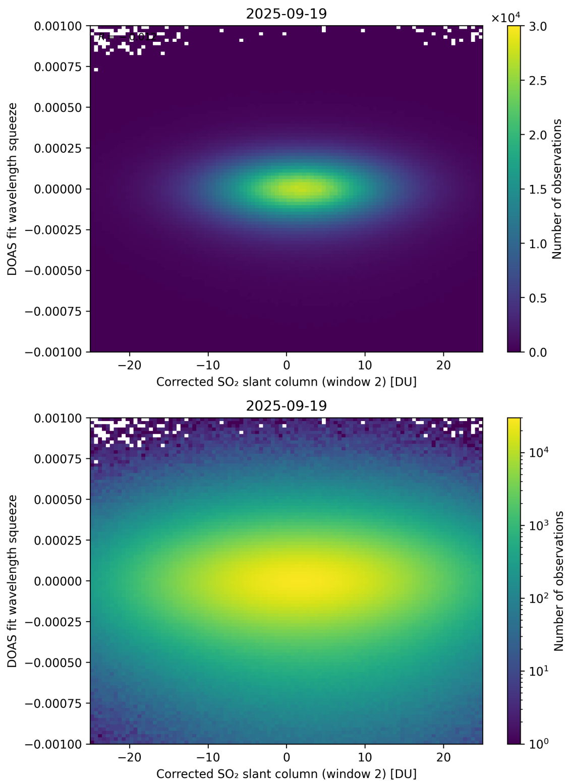
Figure 247: Scatter density plot of “Corrected SO 2 slant column (window 2)” against “DOAS fit wavelength squeeze” for 2025-09-18 to 2025-09-20.
