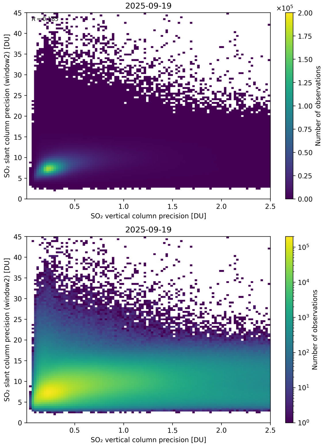
Figure 343: Scatter density plot of “SO 2 vertical column precision” against “SO 2 slant column precision (window2)” for 2025-09-18 to 2025-09-20.
