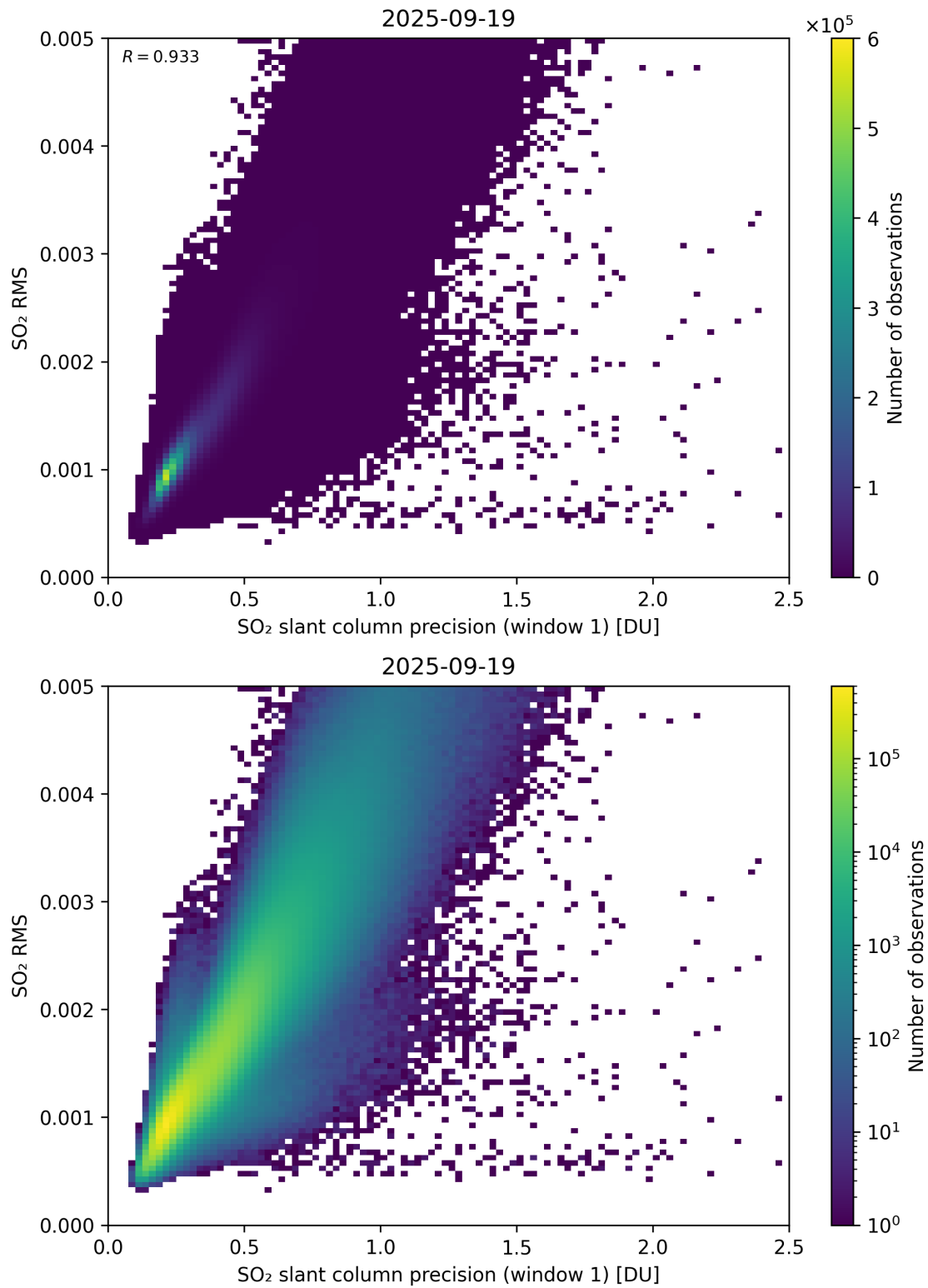
Figure 273: Scatter density plot of “SO 2 slant column precision (window 1)” against “SO 2 RMS” for 2025-09-18 to 2025-09-20.
