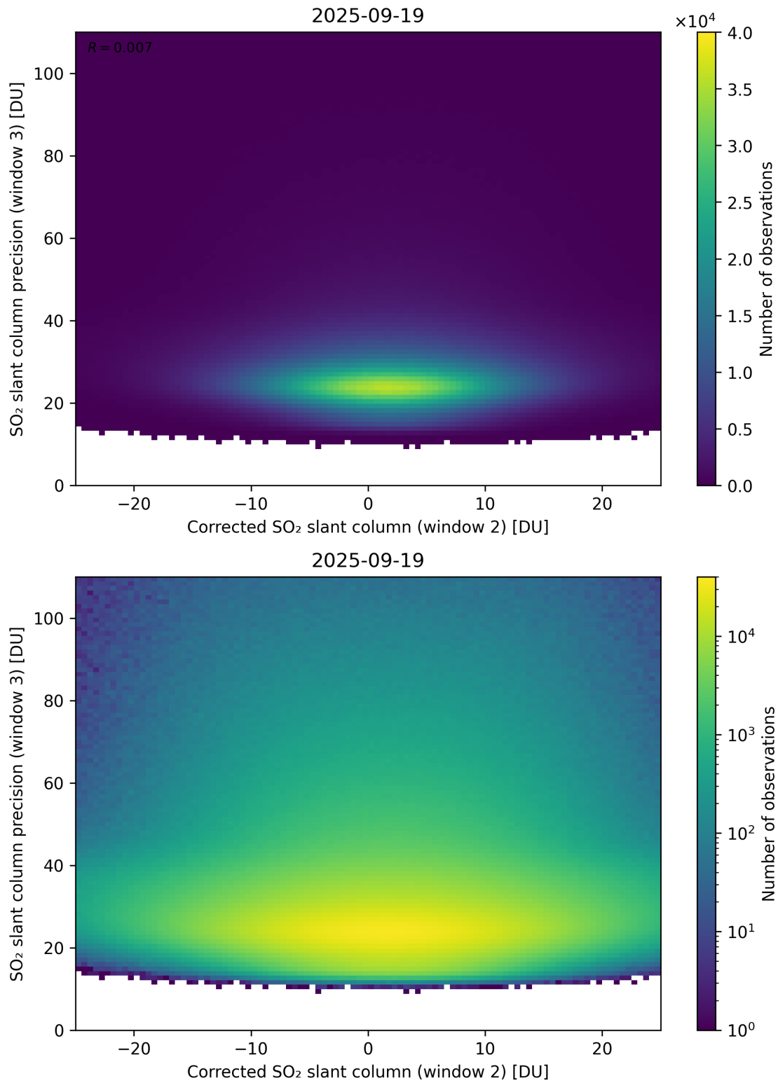
Figure 252: Scatter density plot of “Corrected SO 2 slant column (window 2)” against “SO 2 slant column precision (window 3)” for 2025-09-18 to 2025-09-20.
