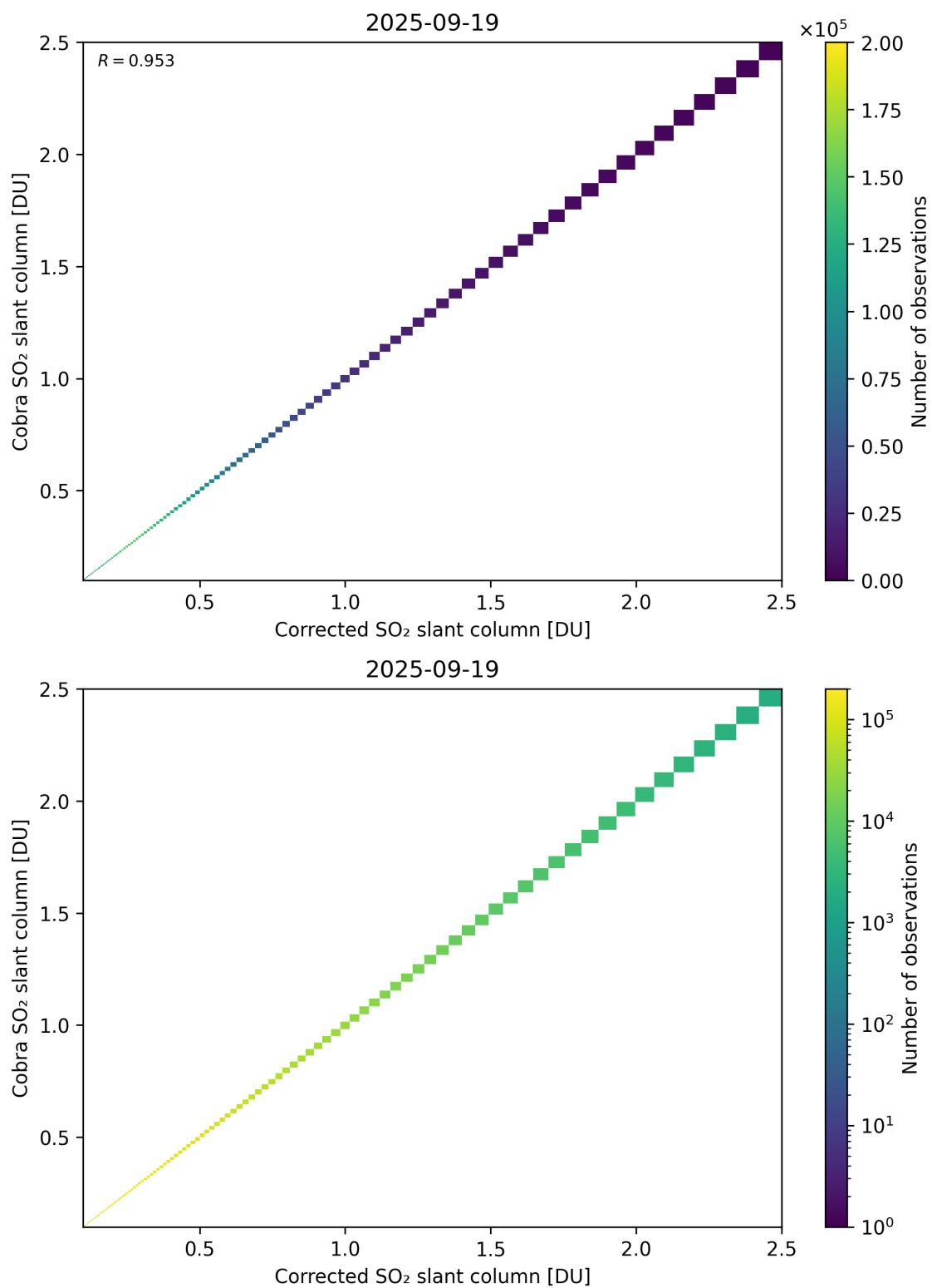
Figure 233: Scatter density plot of “Corrected SO 2 slant column” against “Cobra SO 2 slant column” for 2025-09-18 to 2025-09-20.
