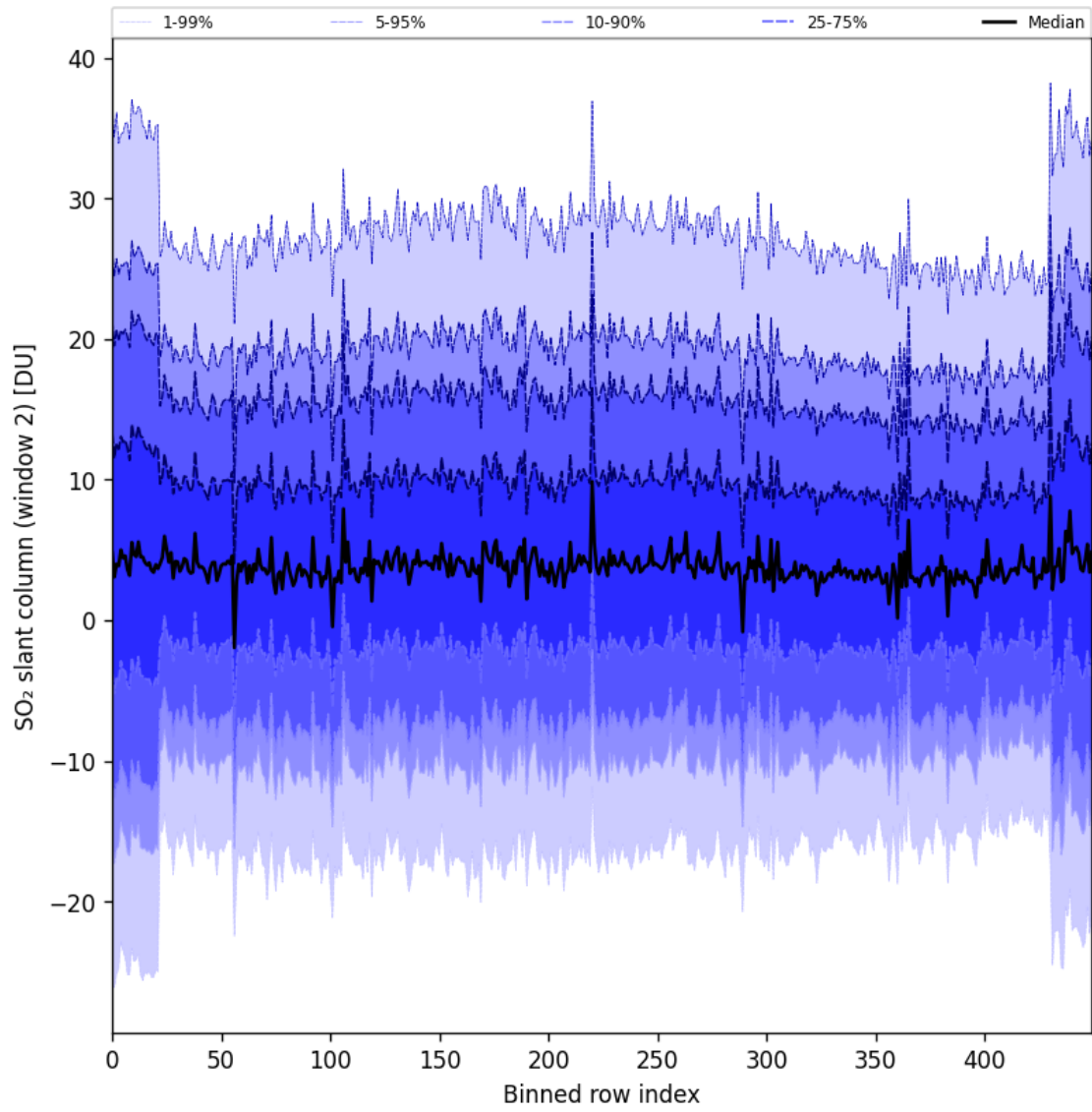
Figure 93: Along track statistics of “SO 2 slant column (window 2)” for 2025-09-18 to 2025-09-20
