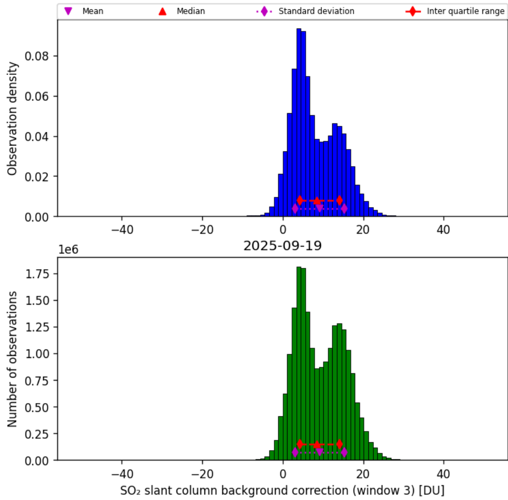
Figure 74: Histogram of “SO 2 slant column background correction (window 3)” for 2025-09-18 to 2025-09-20
