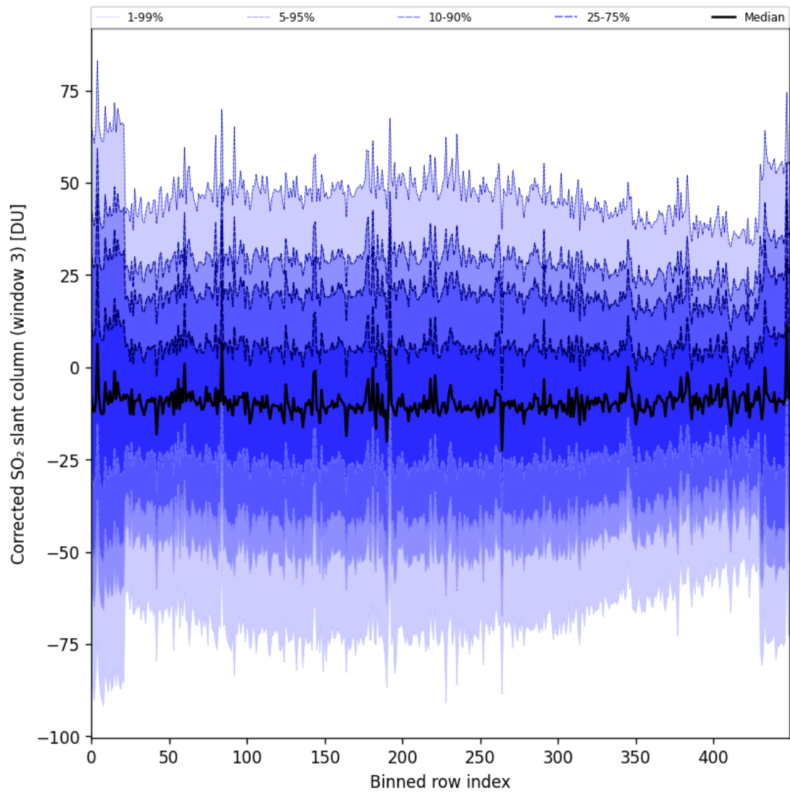
Figure 99: Along track statistics of “Corrected SO 2 slant column (window 3)” for 2025-09-18 to 2025-09-20
