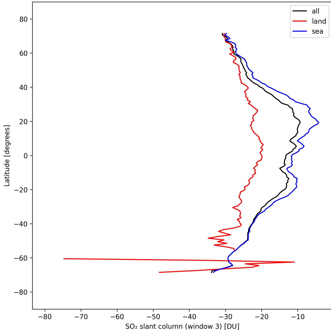
Figure 45: Zonal average of “SO 2 slant column (window 3)” for 2025-09-18 to 2025-09-20.
