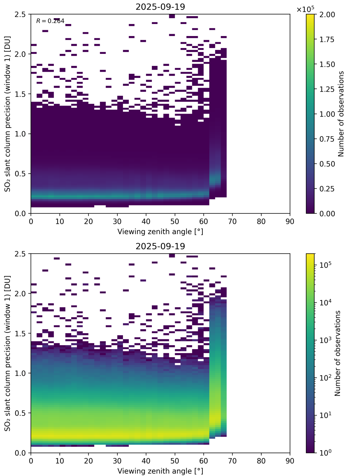
Figure 377: Scatter density plot of “Viewing zenith angle” against “SO 2 slant column precision (window 1)” for 2025-09-18 to 2025-09-20.
