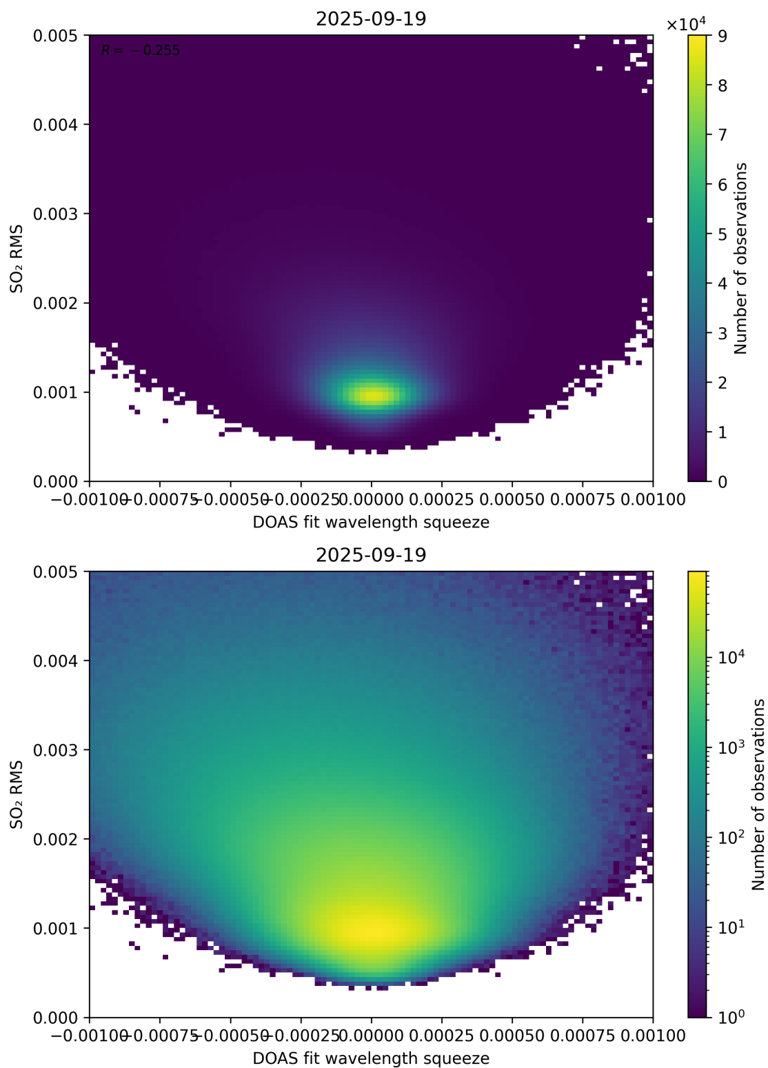
Figure 143: Scatter density plot of “DOAS fit wavelength squeeze” against “SO 2 RMS” for 2025-09-18 to 2025-09-20.
