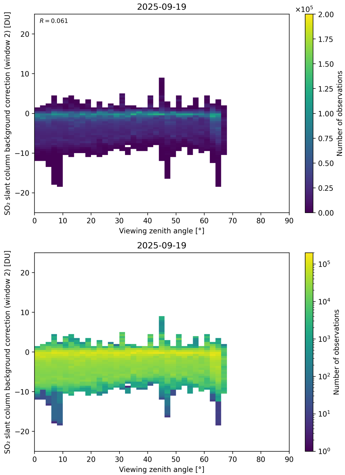
Figure 363: Scatter density plot of “Viewing zenith angle” against “SO 2 slant column background correction (window 2)” for 2025-09-18 to 2025-09-20.
