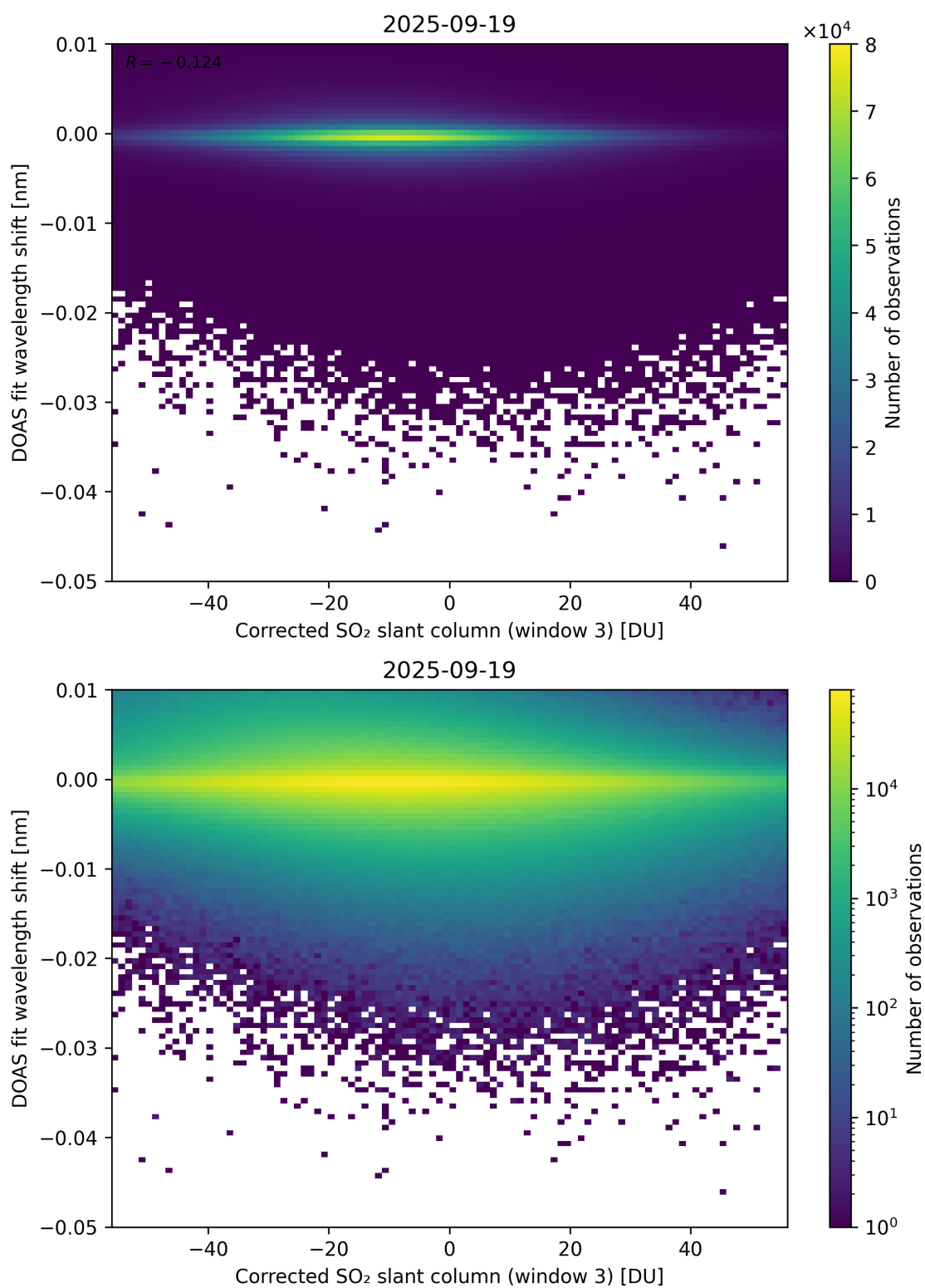
Figure 256: Scatter density plot of “Corrected SO 2 slant column (window 3)” against “DOAS fit wavelength shift” for 2025-09-18 to 2025-09-20.
