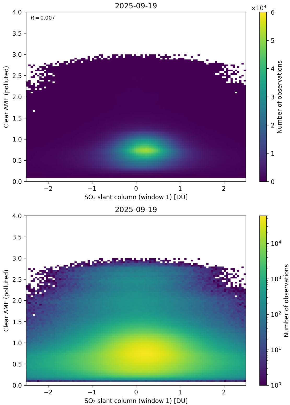
Figure 282: Scatter density plot of “SO 2 slant column (window 1)” against “Clear AMF (polluted)” for 2025-09-18 to 2025-09-20.
