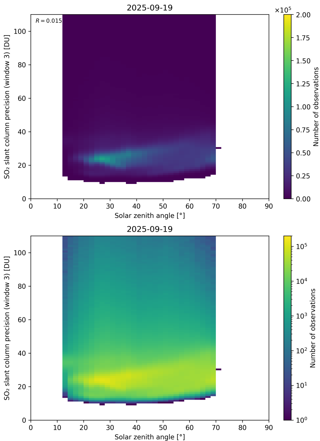
Figure 188: Scatter density plot of “Solar zenith angle” against “SO 2 slant column precision (window 3)” for 2025-09-18 to 2025-09-20.
