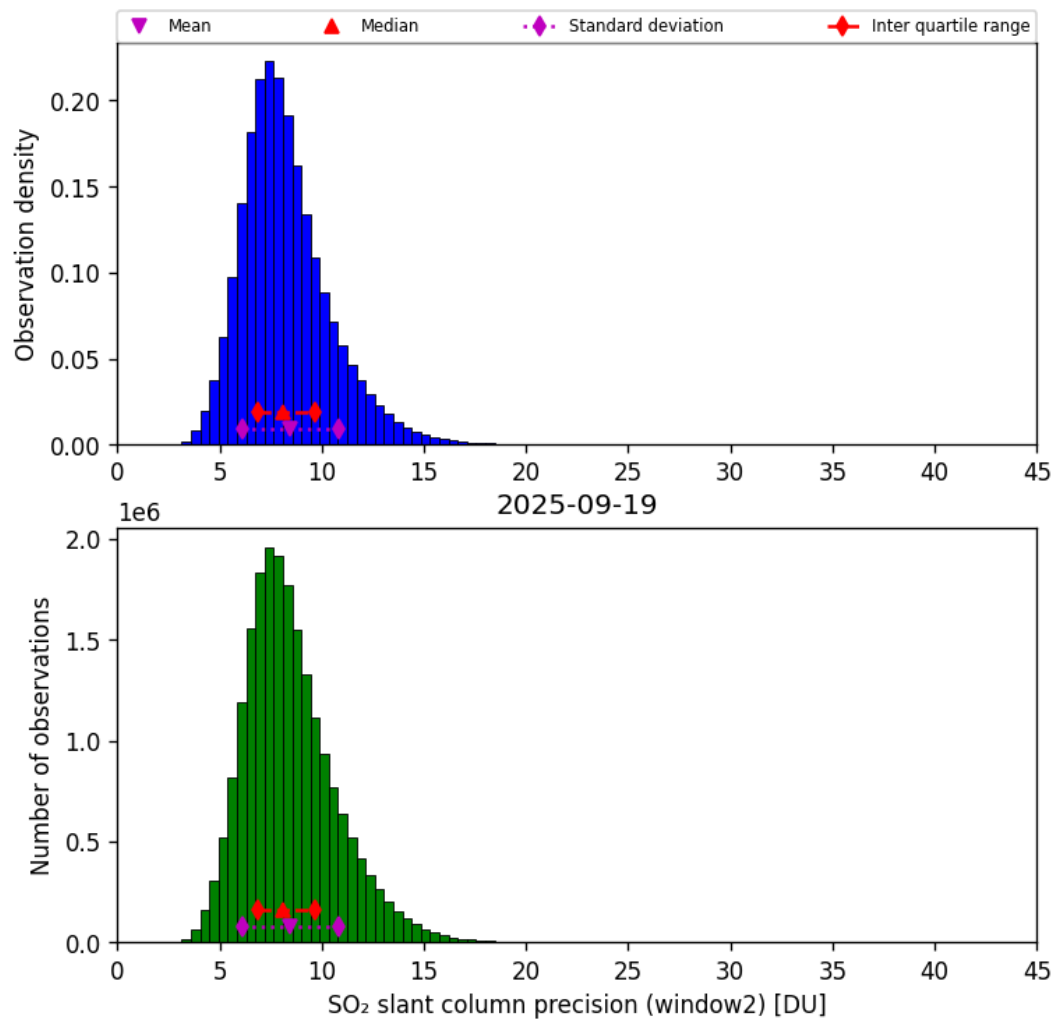
Figure 68: Histogram of “SO 2 slant column precision (window2)” for 2025-09-18 to 2025-09-20
