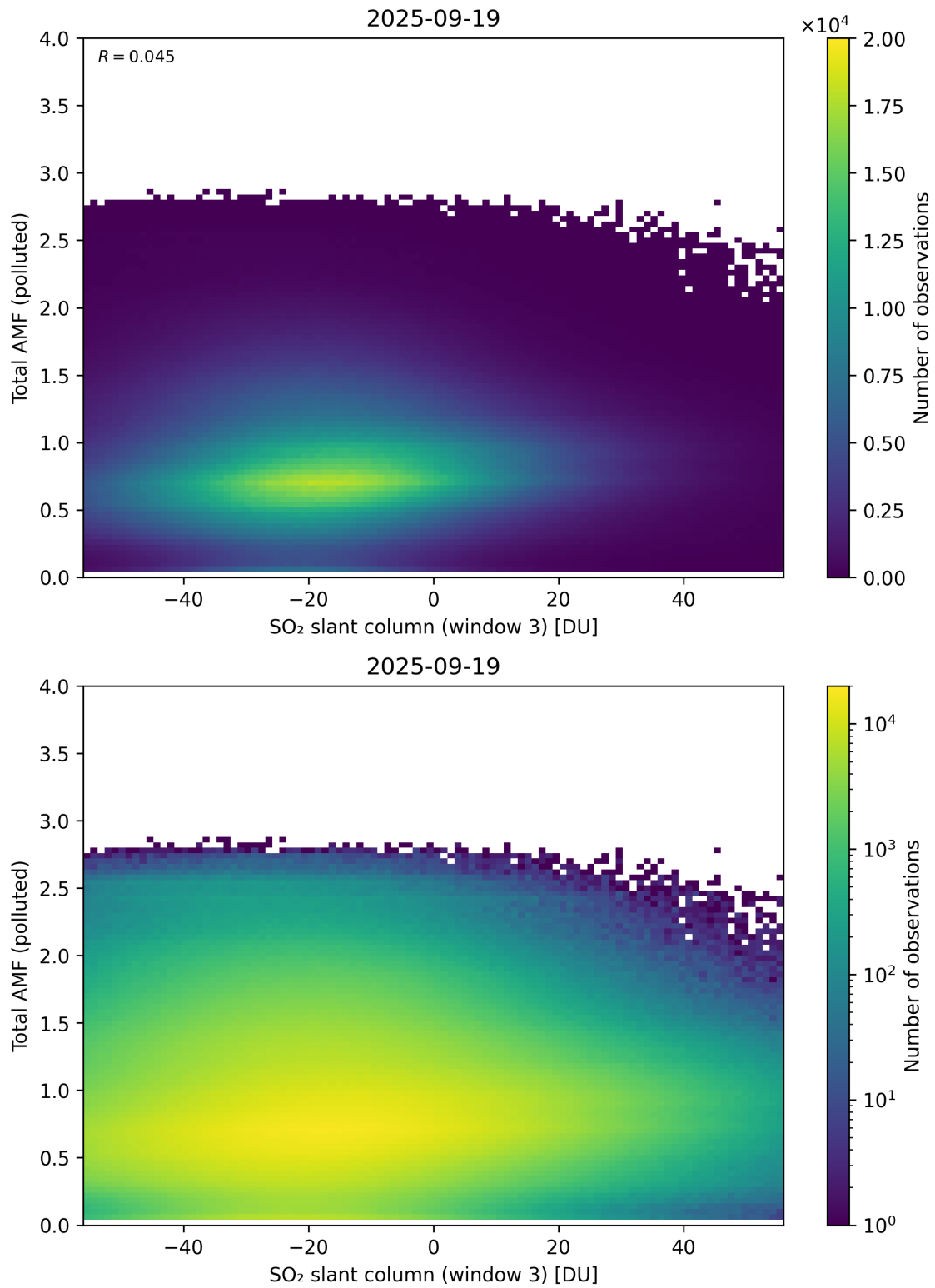
Figure 318: Scatter density plot of “SO 2 slant column (window 3)” against “Total AMF (polluted)” for 2025-09-18 to 2025-09-20.
