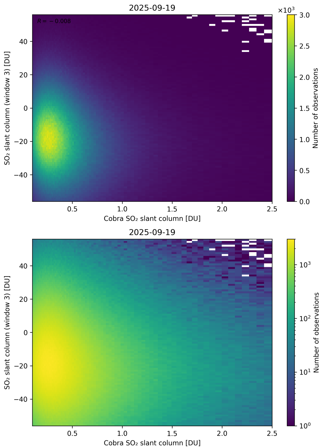
Figure 222: Scatter density plot of “Cobra SO 2 slant column” against “SO 2 slant column (window 3)” for 2025-09-18 to 2025-09-20.
