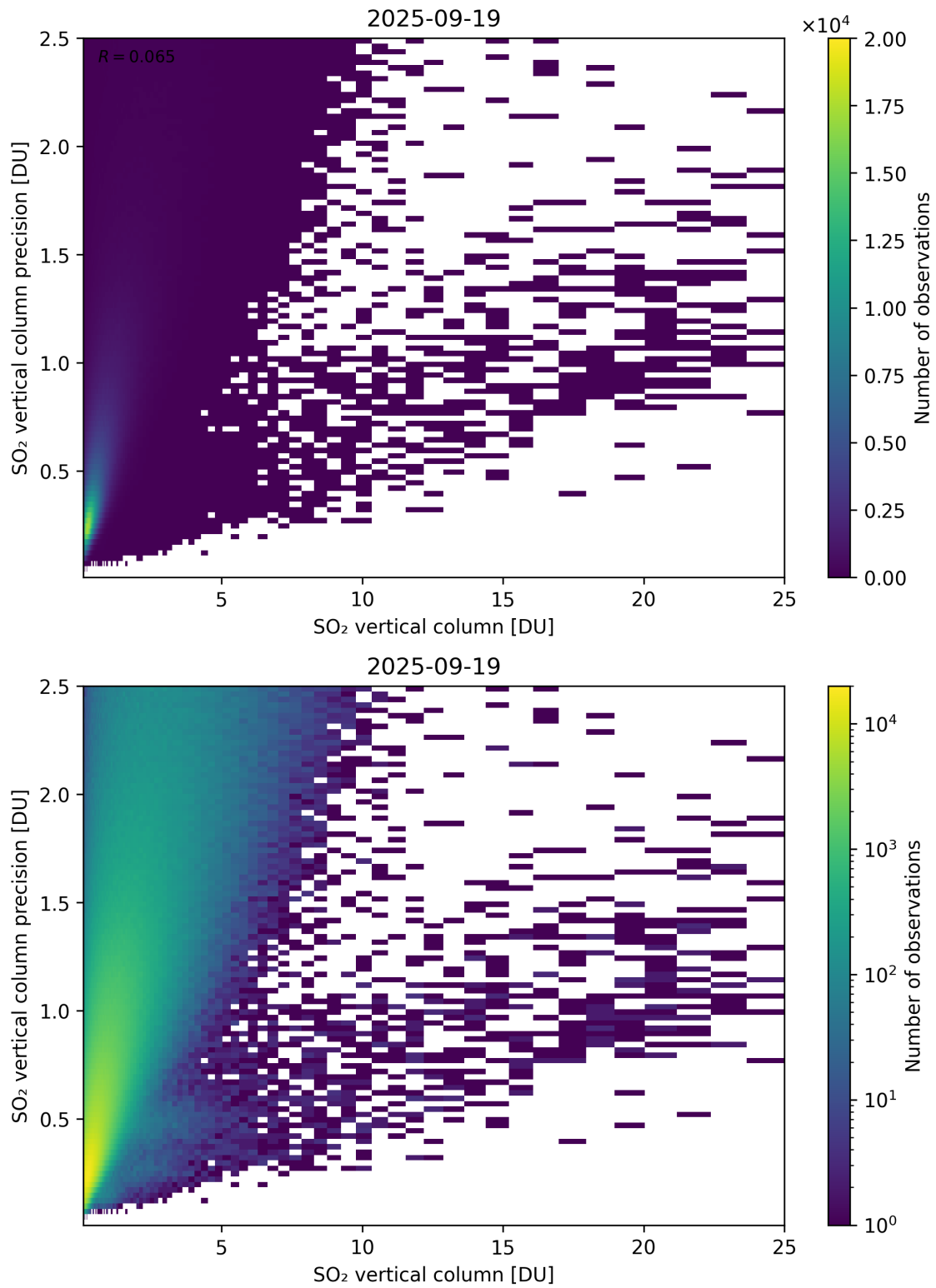
Figure 361: Scatter density plot of “SO 2 vertical column” against “SO 2 vertical column precision” for 2025-09-18 to 2025-09-20.
