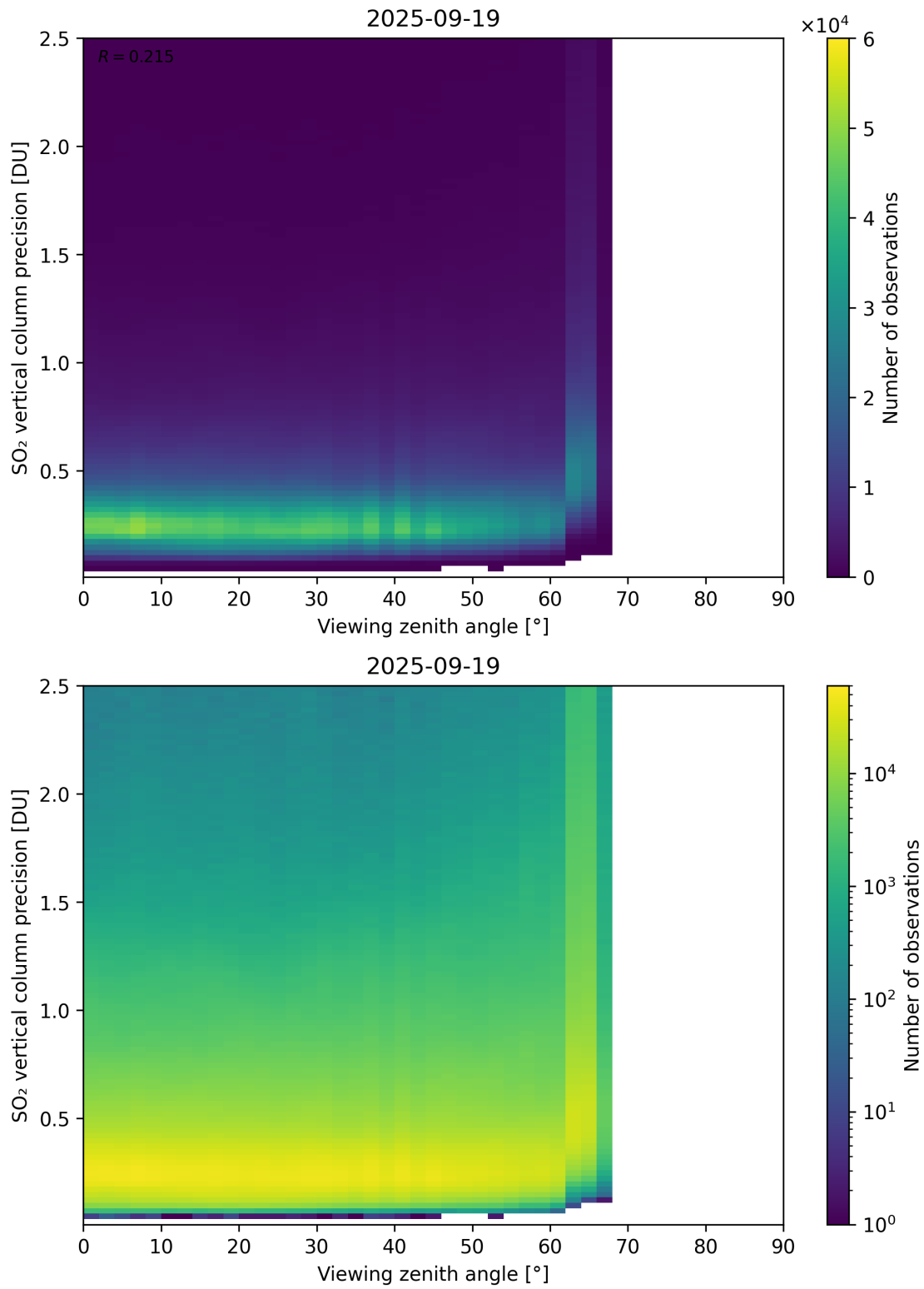
Figure 384: Scatter density plot of “Viewing zenith angle” against “SO 2 vertical column precision” for 2025-09-18 to 2025-09-20.
