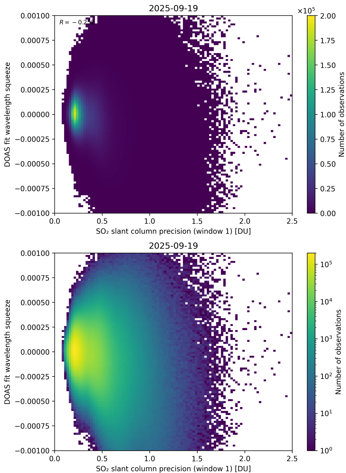
Figure 272: Scatter density plot of “SO 2 slant column precision (window 1)” against “DOAS fit wavelength squeeze” for 2025-09-18 to 2025-09-20.
