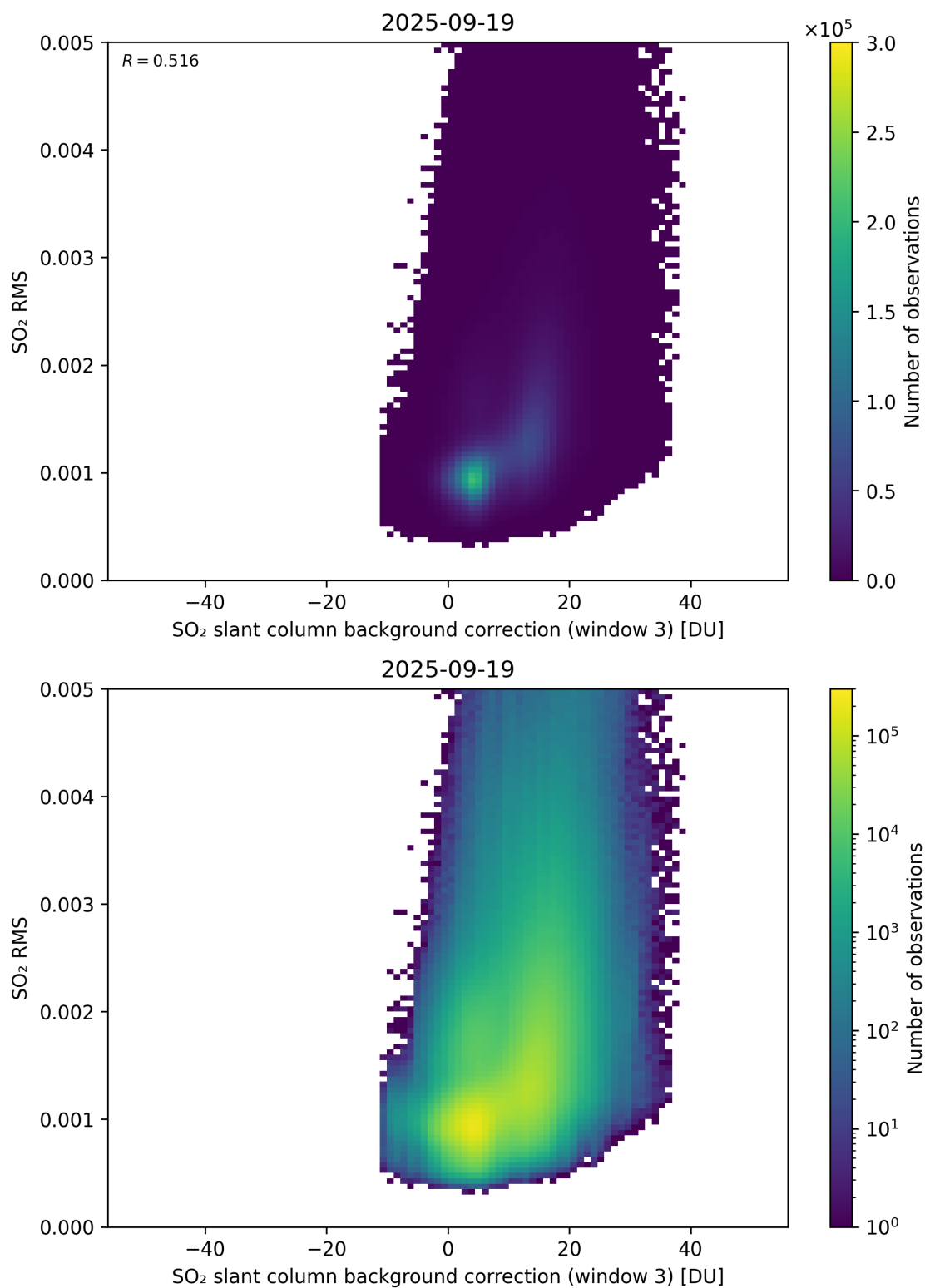
Figure 134: Scatter density plot of “SO 2 slant column background correction (window 3)” against “SO 2 RMS” for 2025-09-18 to 2025-09-20.
