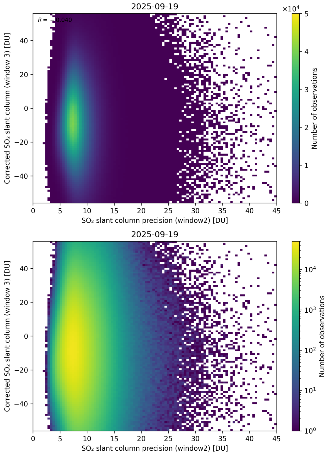
Figure 298: Scatter density plot of “SO 2 slant column precision (window2)” against “Corrected SO 2 slant column (window 3)” for 2025-09-18 to 2025-09-20.
