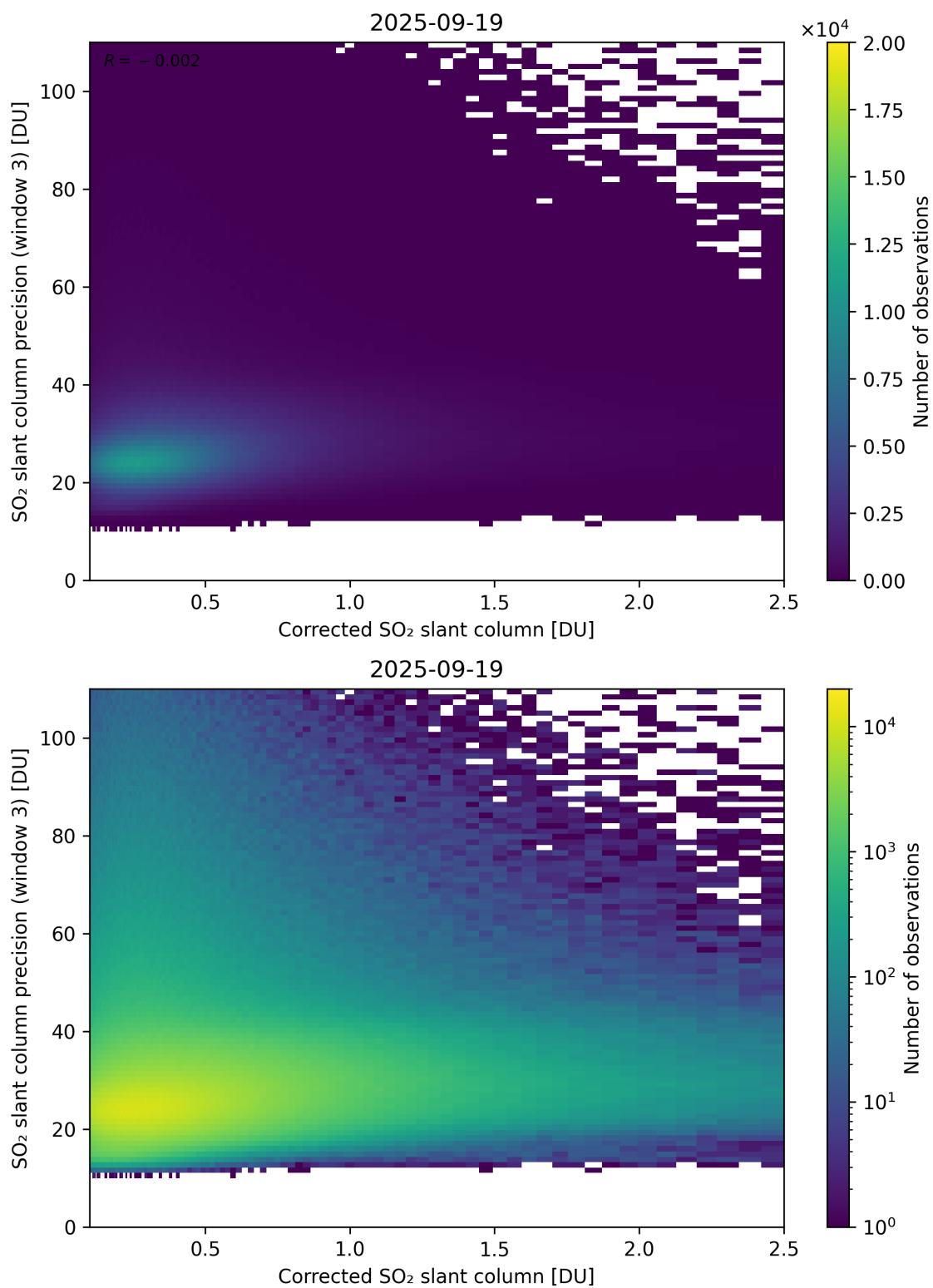
Figure 241: Scatter density plot of “Corrected SO 2 slant column” against “SO 2 slant column precision (window 3)” for 2025-09-18 to 2025-09-20.
