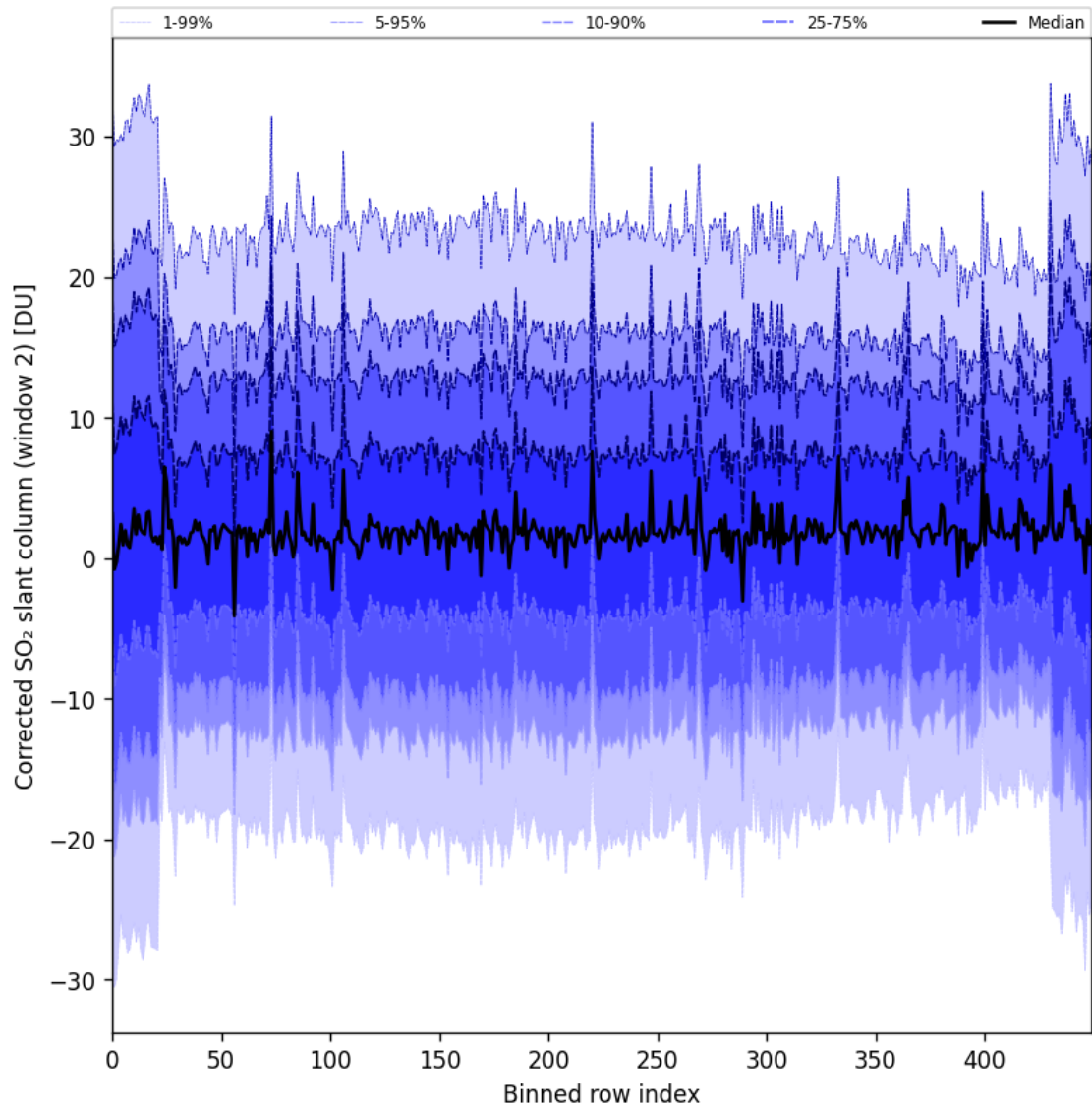
Figure 95: Along track statistics of “Corrected SO 2 slant column (window 2)” for 2025-09-18 to 2025-09-20
