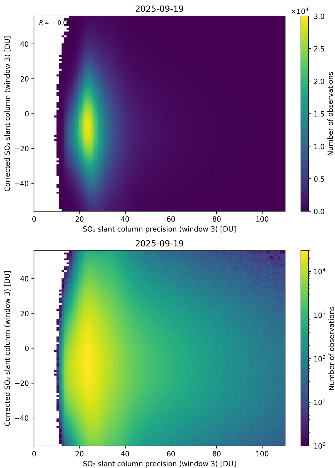
Figure 312: Scatter density plot of “SO 2 slant column precision (window 3)” against “Corrected SO 2 slant column (window 3)” for 2025-09-18 to 2025-09-20.
