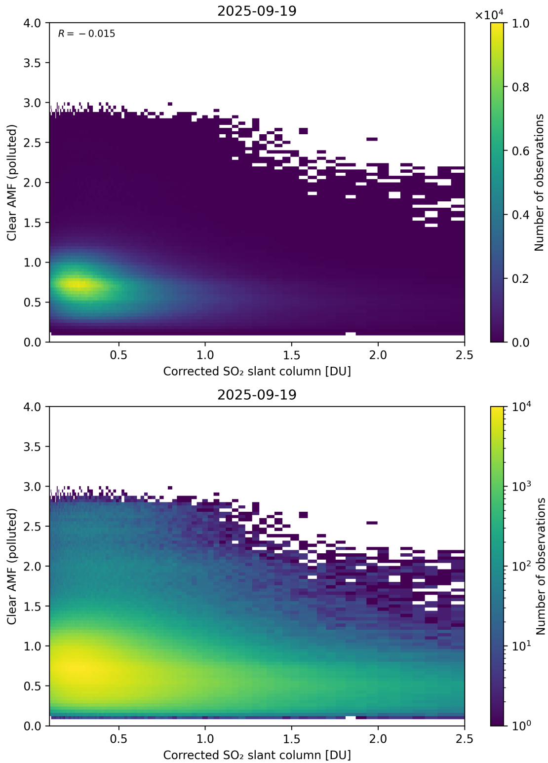
Figure 232: Scatter density plot of “Corrected SO 2 slant column” against “Clear AMF (polluted)” for 2025-09-18 to 2025-09-20.
