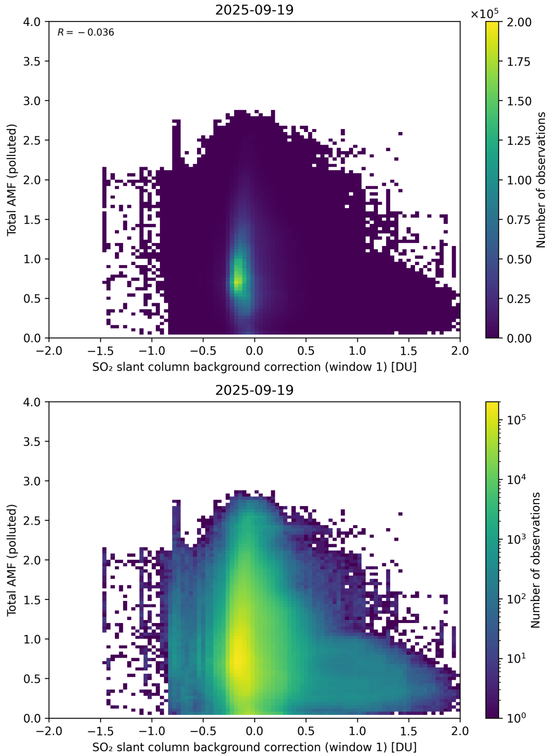
Figure 120: Scatter density plot of “SO 2 slant column background correction (window 1)” against “Total AMF (polluted)” for 2025-09-18 to 2025-09-20.
