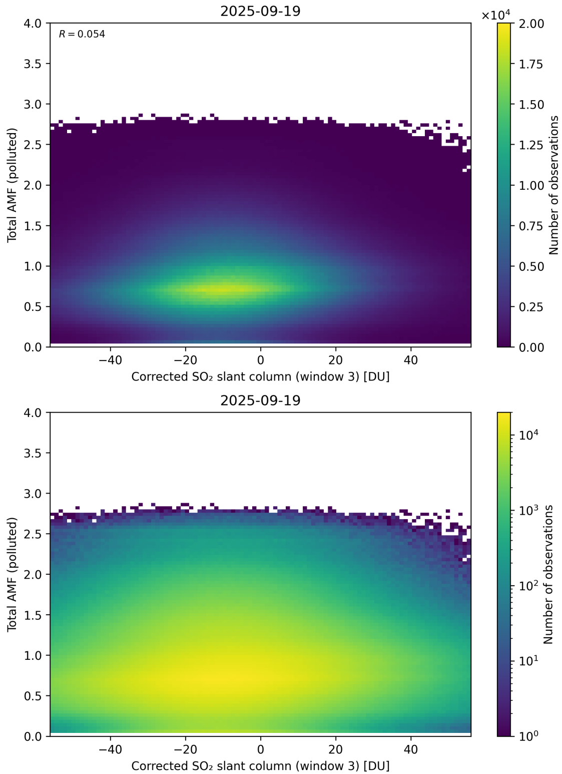
Figure 260: Scatter density plot of “Corrected SO 2 slant column (window 3)” against “Total AMF (polluted)” for 2025-09-18 to 2025-09-20.
