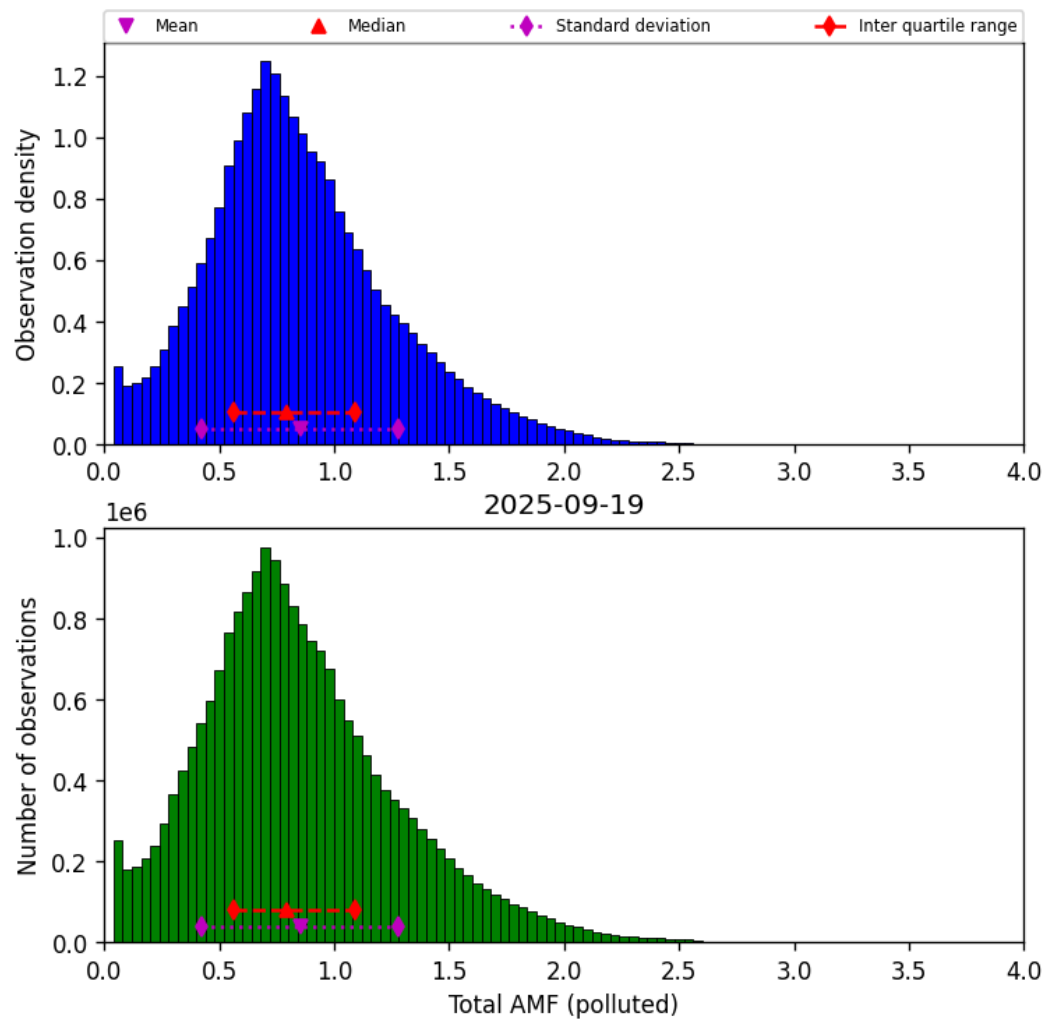
Figure 79: Histogram of “Total AMF (polluted)” for 2025-09-18 to 2025-09-20
