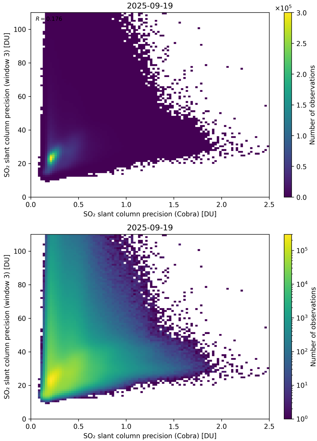
Figure 212: Scatter density plot of “SO 2 slant column precision (Cobra)” against “SO 2 slant column precision (window 3)” for 2025-09-18 to 2025-09-20.
