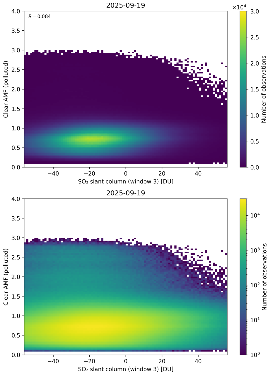
Figure 315: Scatter density plot of “SO 2 slant column (window 3)” against “Clear AMF (polluted)” for 2025-09-18 to 2025-09-20.
