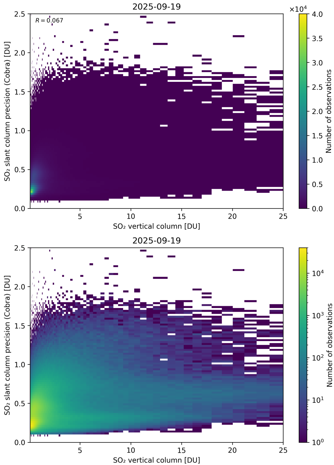
Figure 350: Scatter density plot of “SO 2 vertical column” against “SO 2 slant column precision (Cobra)” for 2025-09-18 to 2025-09-20.
