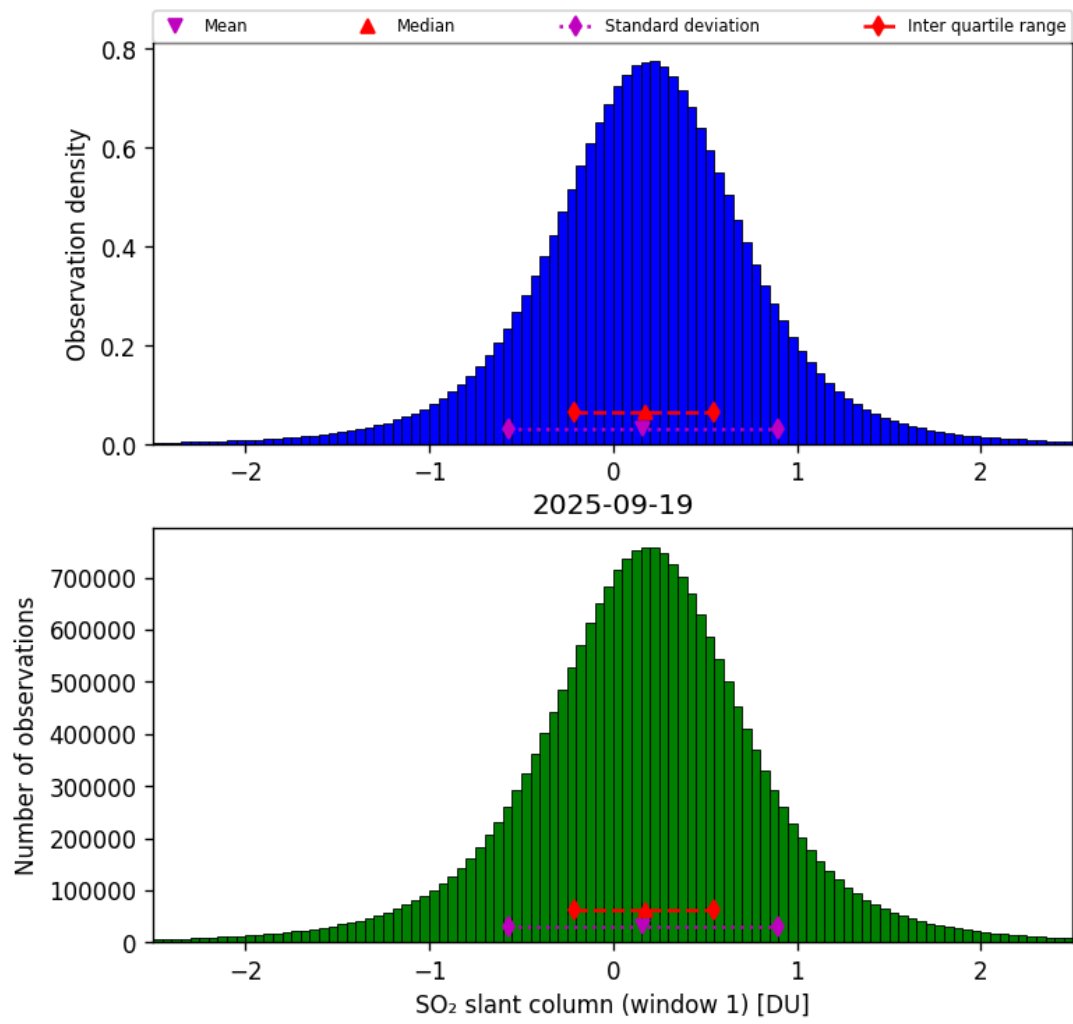
Figure 63: Histogram of “SO 2 slant column (window 1)” for 2025-09-18 to 2025-09-20
