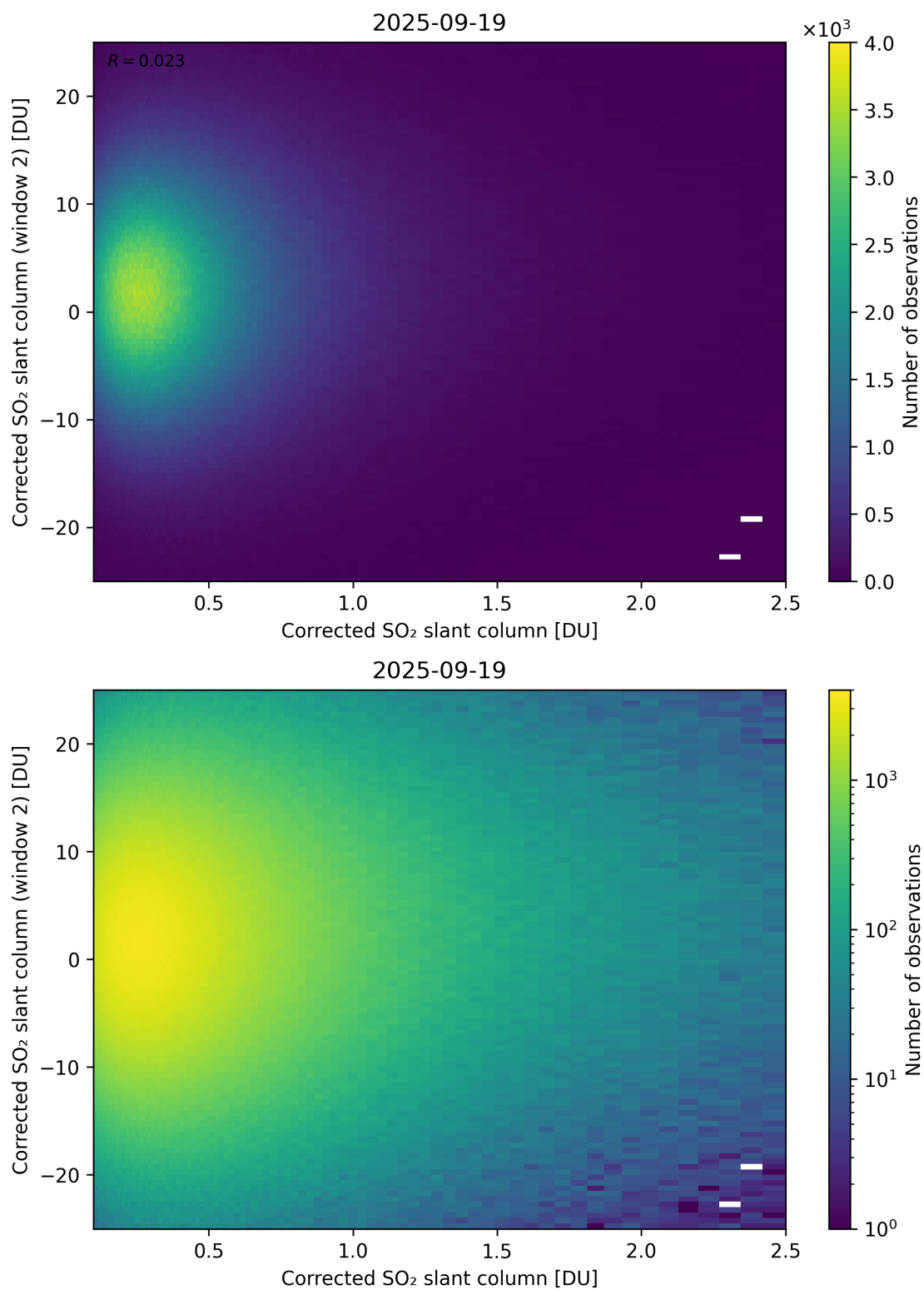
Figure 235: Scatter density plot of “Corrected SO 2 slant column” against “Corrected SO 2 slant column (window 2)” for 2025-09-18 to 2025-09-20.
