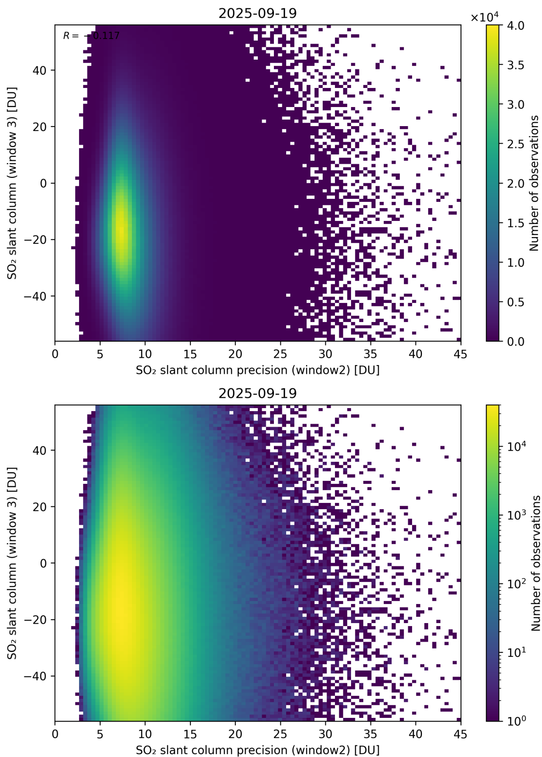
Figure 299: Scatter density plot of “SO 2 slant column precision (window2)” against “SO 2 slant column (window 3)” for 2025-09-18 to 2025-09-20.
