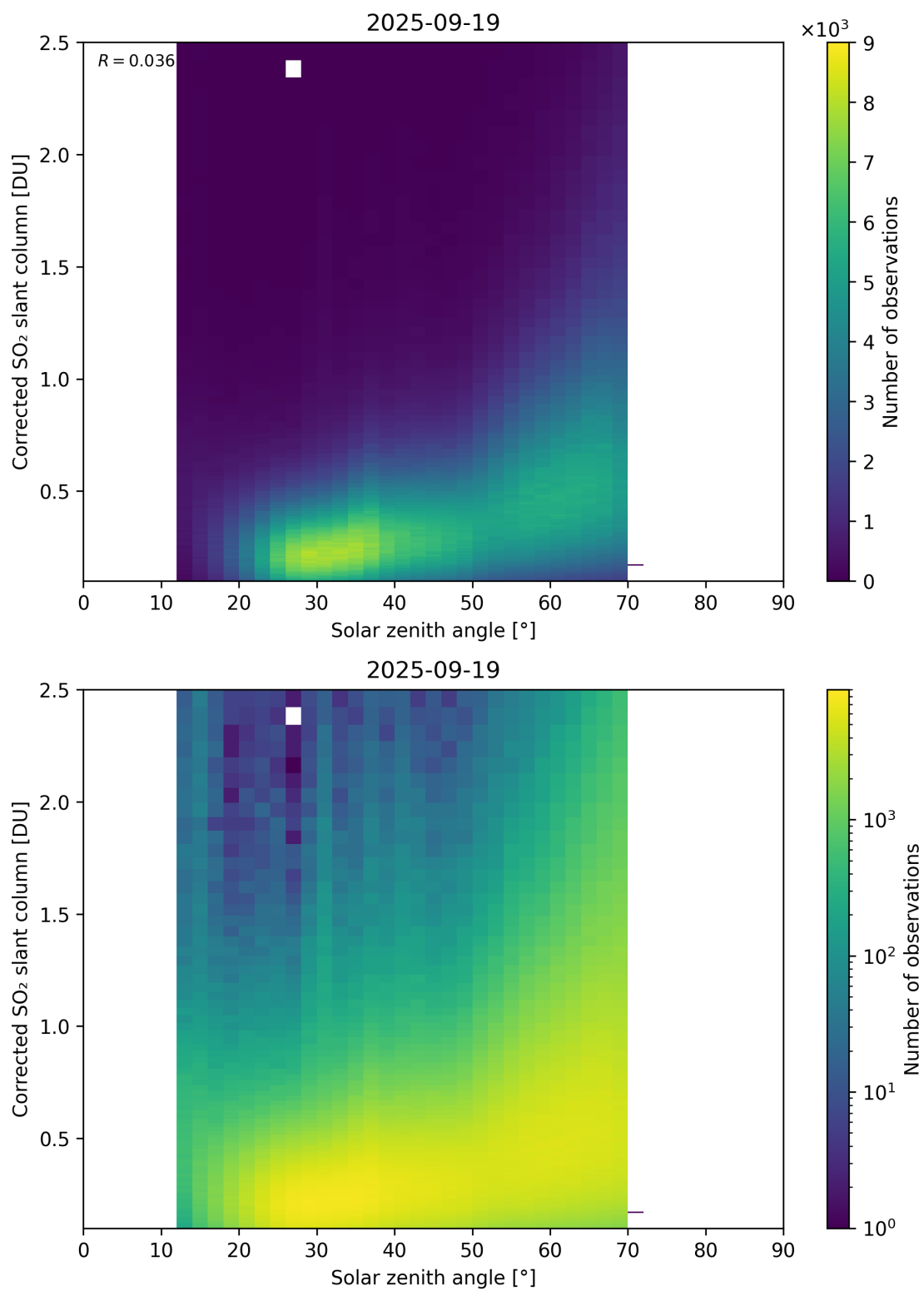
Figure 181: Scatter density plot of “Solar zenith angle” against “Corrected SO 2 slant column” for 2025-09-18 to 2025-09-20.
