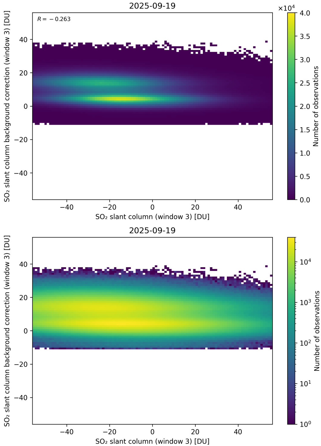
Figure 303: Scatter density plot of “SO 2 slant column (window 3)” against “SO 2 slant column background correction (window 3)” for 2025-09-18 to 2025-09-20.
