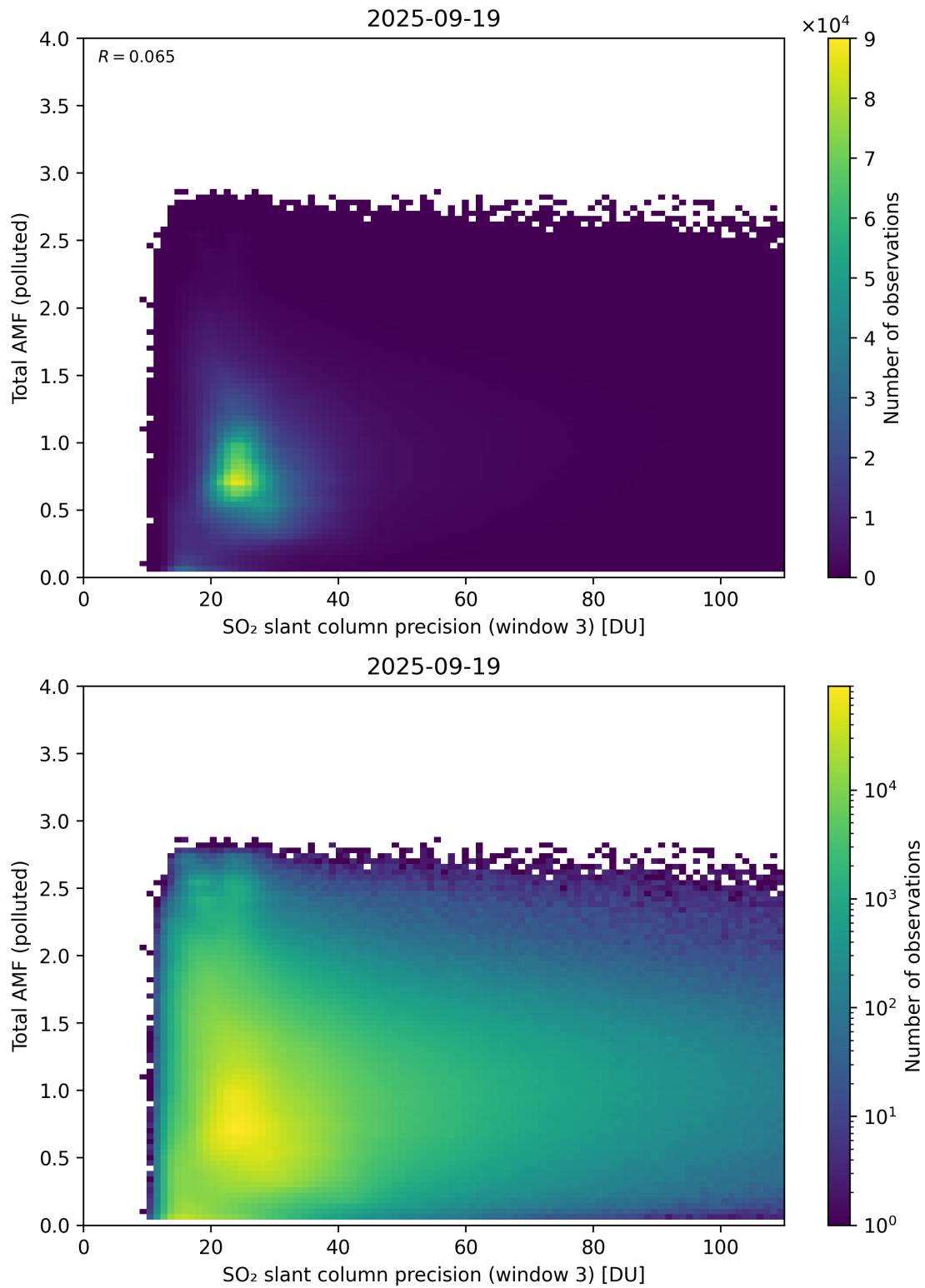
Figure 313: Scatter density plot of “SO 2 slant column precision (window 3)” against “Total AMF (polluted)” for 2025-09-18 to 2025-09-20.
