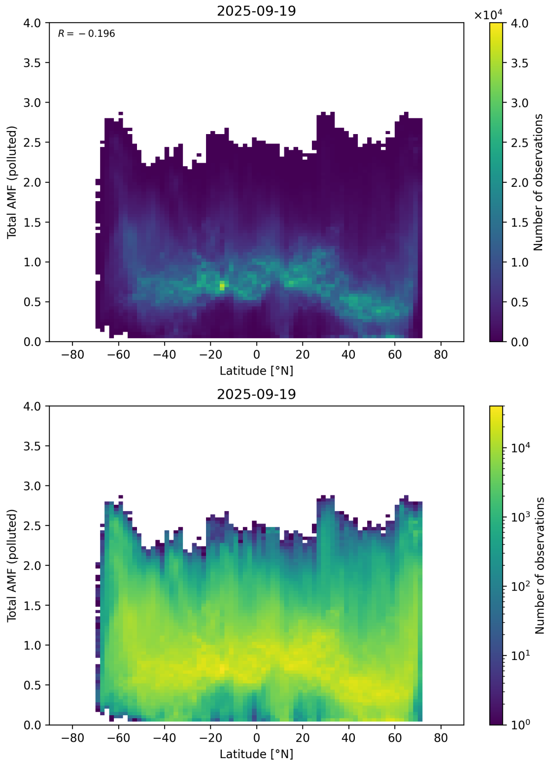
Figure 167: Scatter density plot of “Latitude” against “Total AMF (polluted)” for 2025-09-18 to 2025-09-20.
