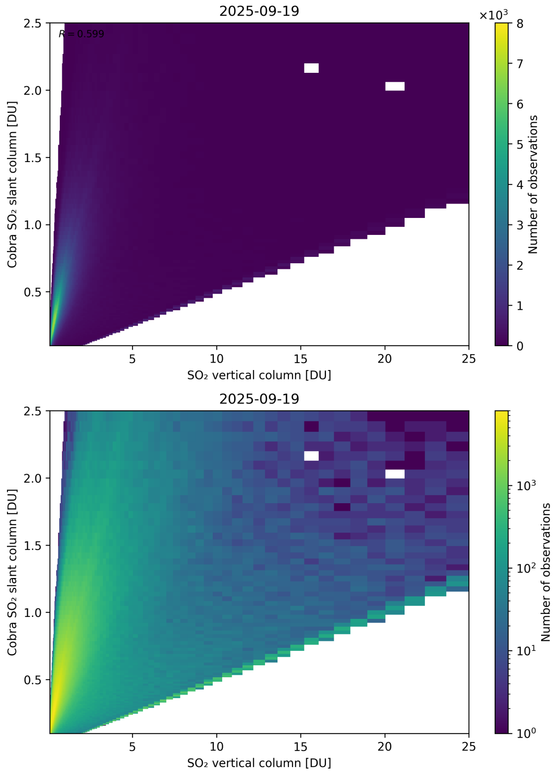
Figure 349: Scatter density plot of “SO 2 vertical column” against “Cobra SO 2 slant column” for 2025-09-18 to 2025-09-20.
