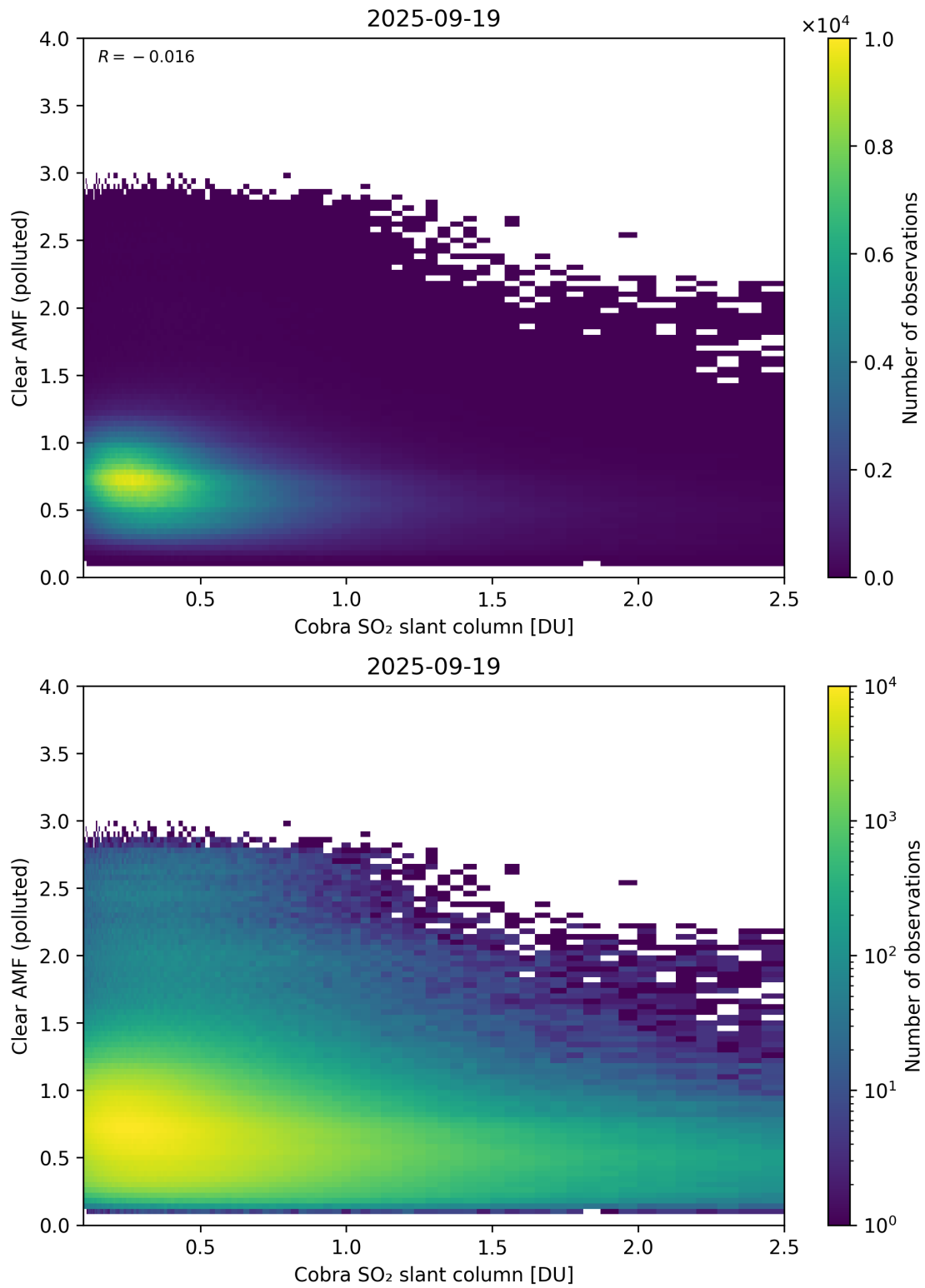
Figure 215: Scatter density plot of “Cobra SO 2 slant column” against “Clear AMF (polluted)” for 2025-09-18 to 2025-09-20.
