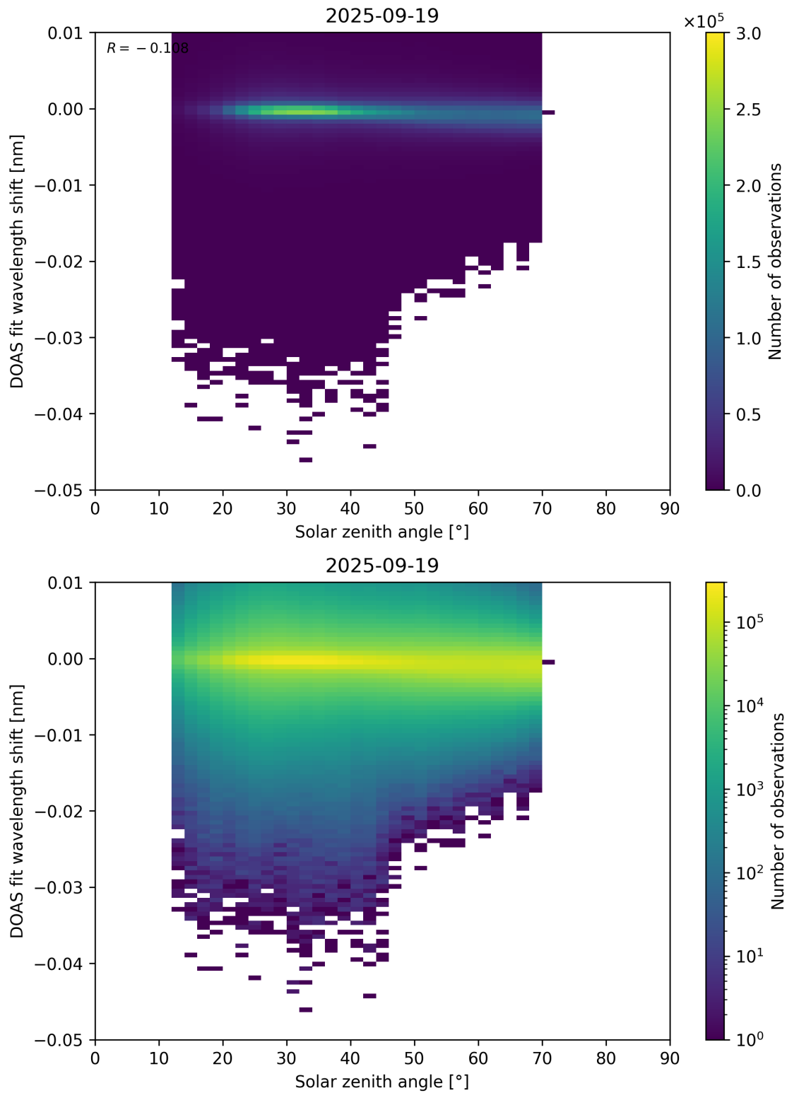
Figure 174: Scatter density plot of “Solar zenith angle” against “DOAS fit wavelength shift” for 2025-09-18 to 2025-09-20.
