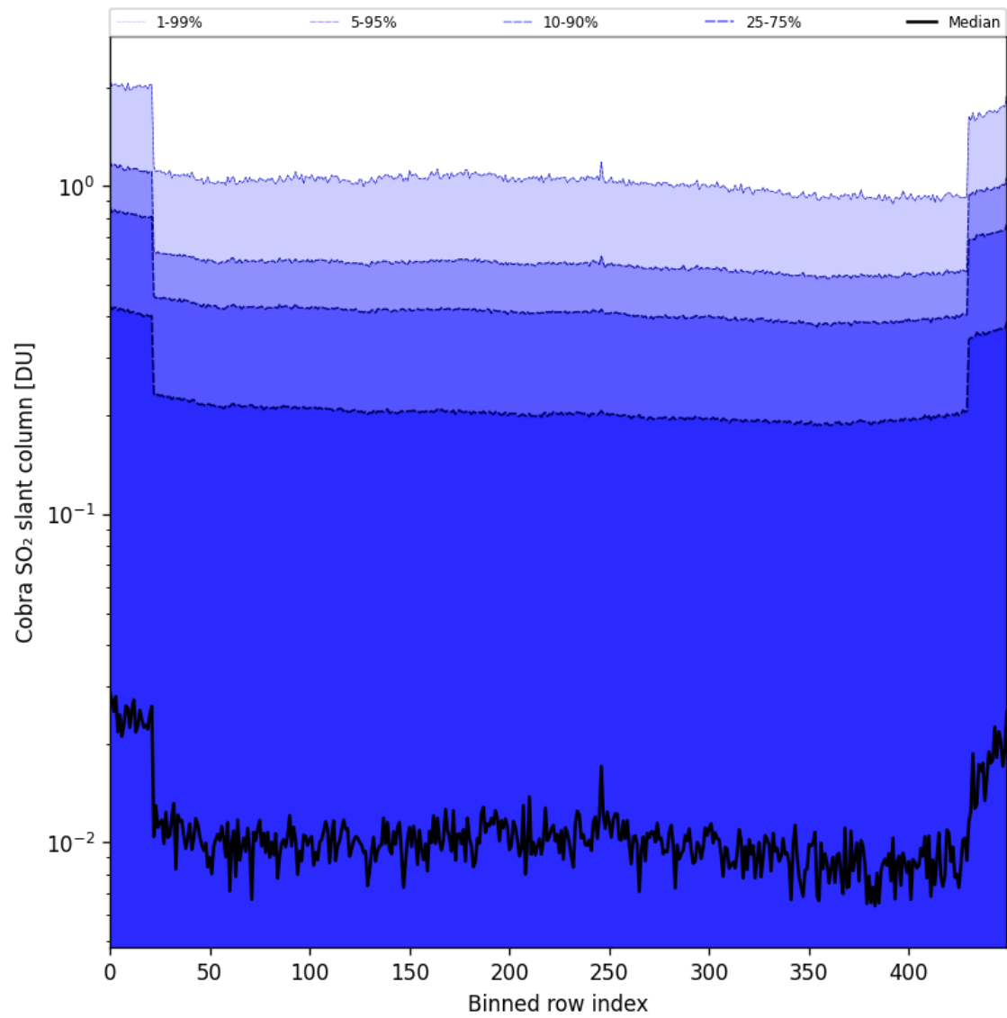
Figure 87: Along track statistics of “Cobra SO 2 slant column” for 2025-09-18 to 2025-09-20
