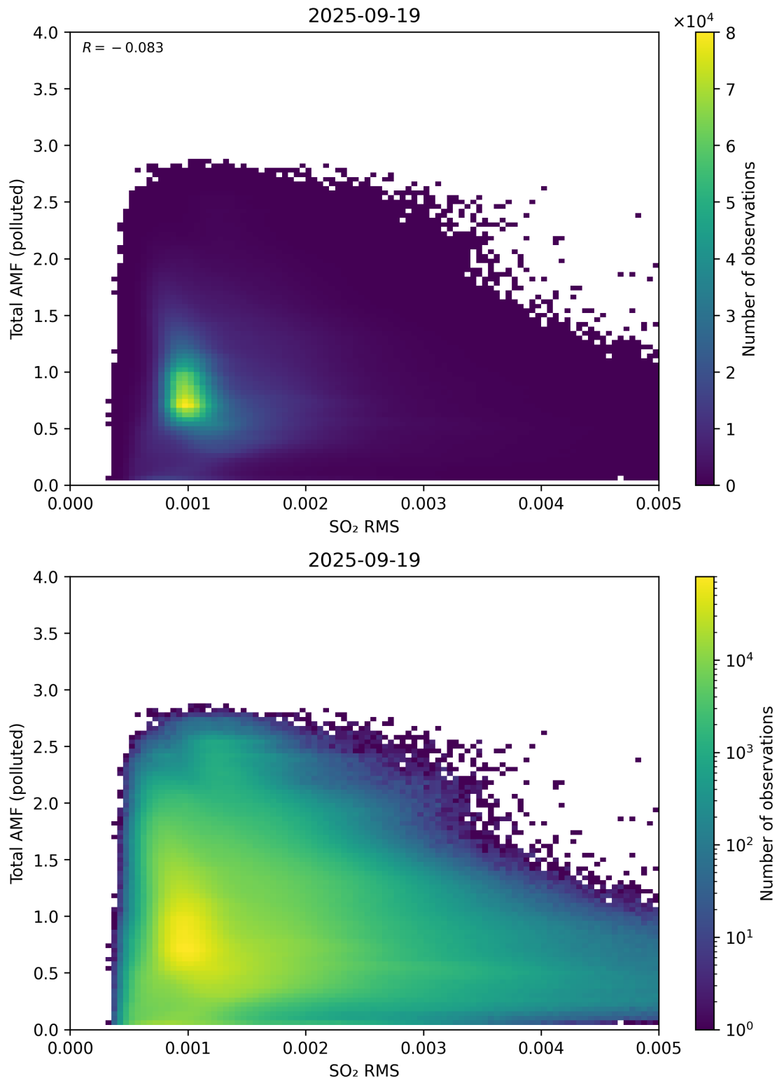
Figure 148: Scatter density plot of “SO 2 RMS” against “Total AMF (polluted)” for 2025-09-18 to 2025-09-20.
