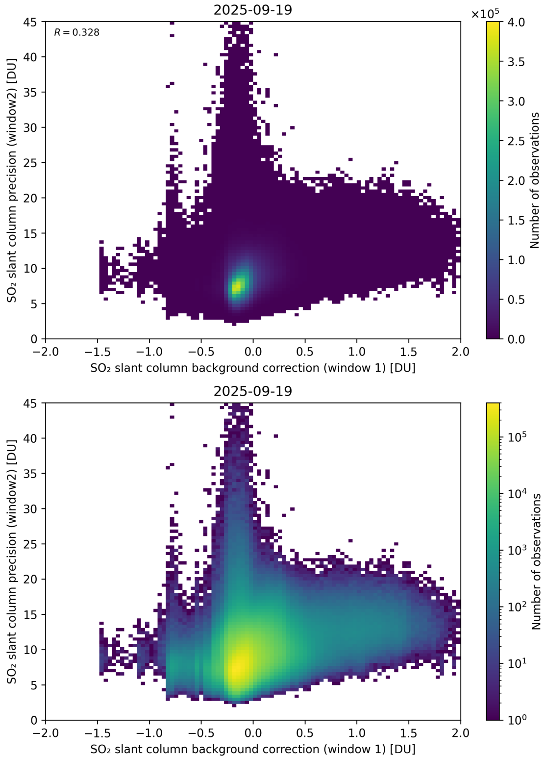
Figure 117: Scatter density plot of “SO 2 slant column background correction (window 1)” against “SO 2 slant column precision (window2)” for 2025-09-18 to 2025-09-20.
