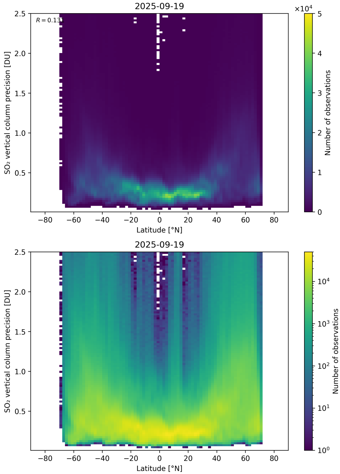
Figure 170: Scatter density plot of “Latitude” against “SO 2 vertical column precision” for 2025-09-18 to 2025-09-20.
