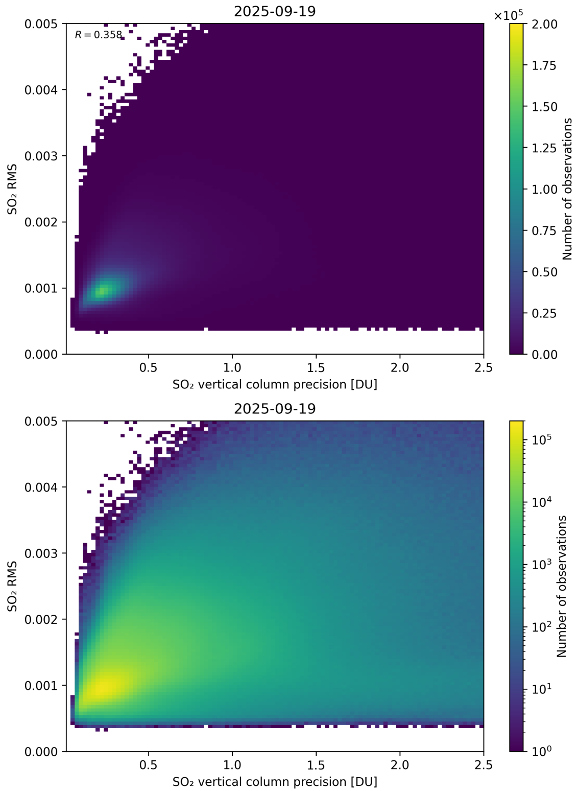
Figure 334: Scatter density plot of “SO 2 vertical column precision” against “SO 2 RMS” for 2025-09-18 to 2025-09-20.
