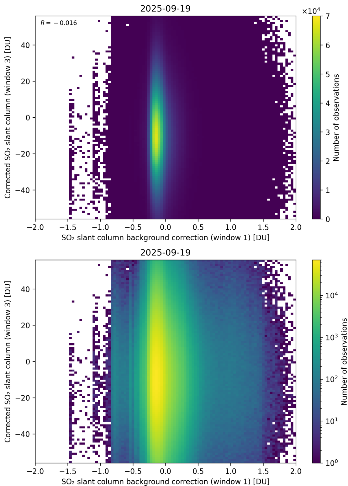
Figure 116: Scatter density plot of “SO 2 slant column background correction (window 1)” against “Corrected SO 2 slant column (window 3)” for 2025-09-18 to 2025-09-20.
