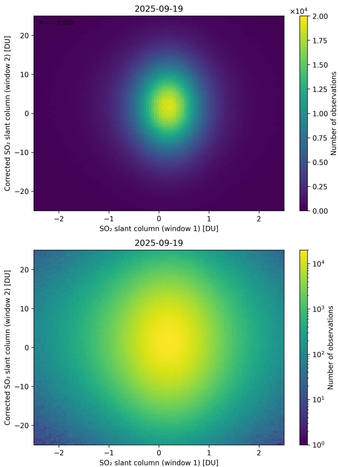
Figure 283: Scatter density plot of “SO 2 slant column (window 1)” against “Corrected SO 2 slant column (window 2)” for 2025-09-18 to 2025-09-20.
