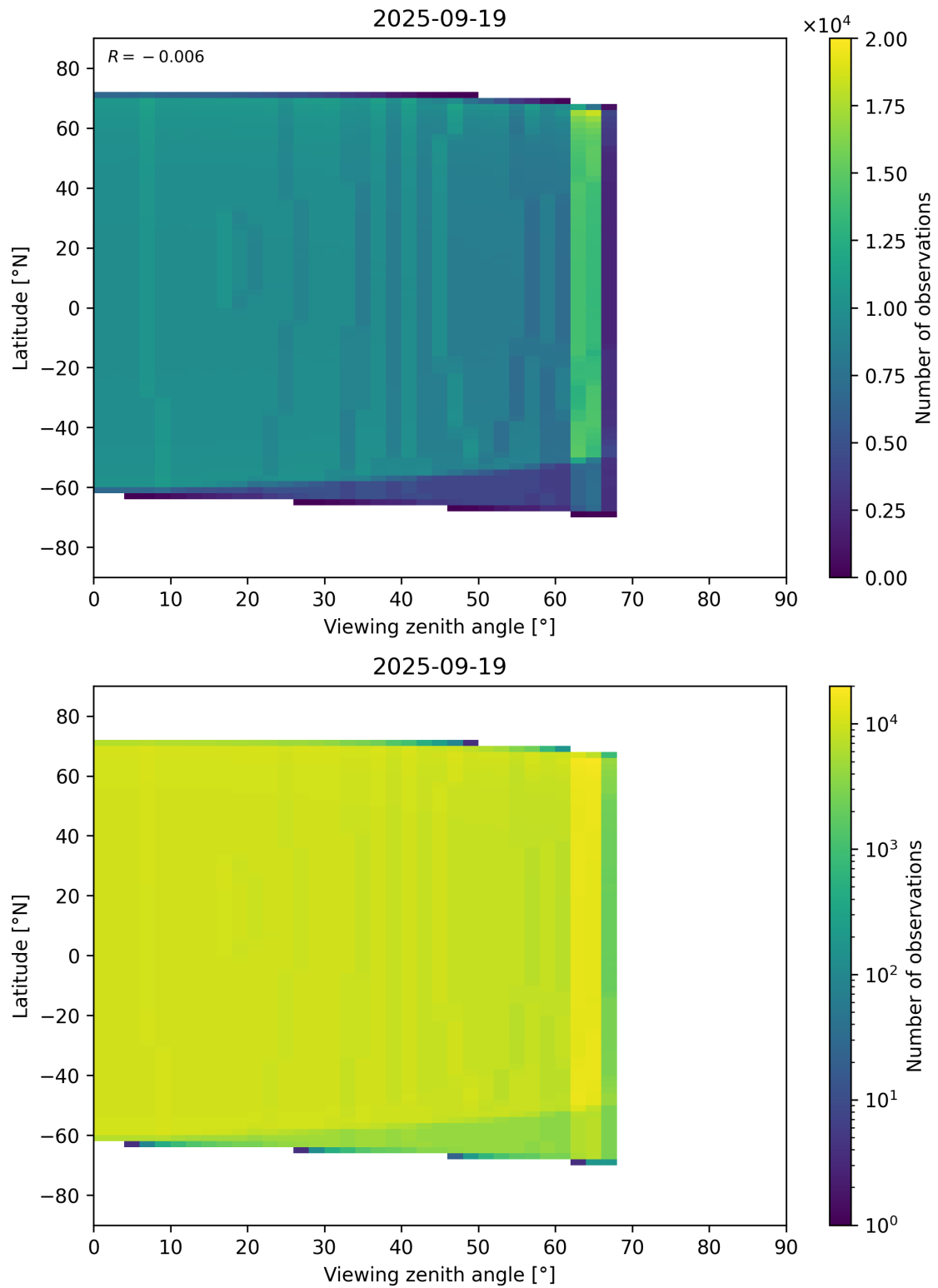
Figure 368: Scatter density plot of “Viewing zenith angle” against “Latitude” for 2025-09-18 to 2025-09-20.
