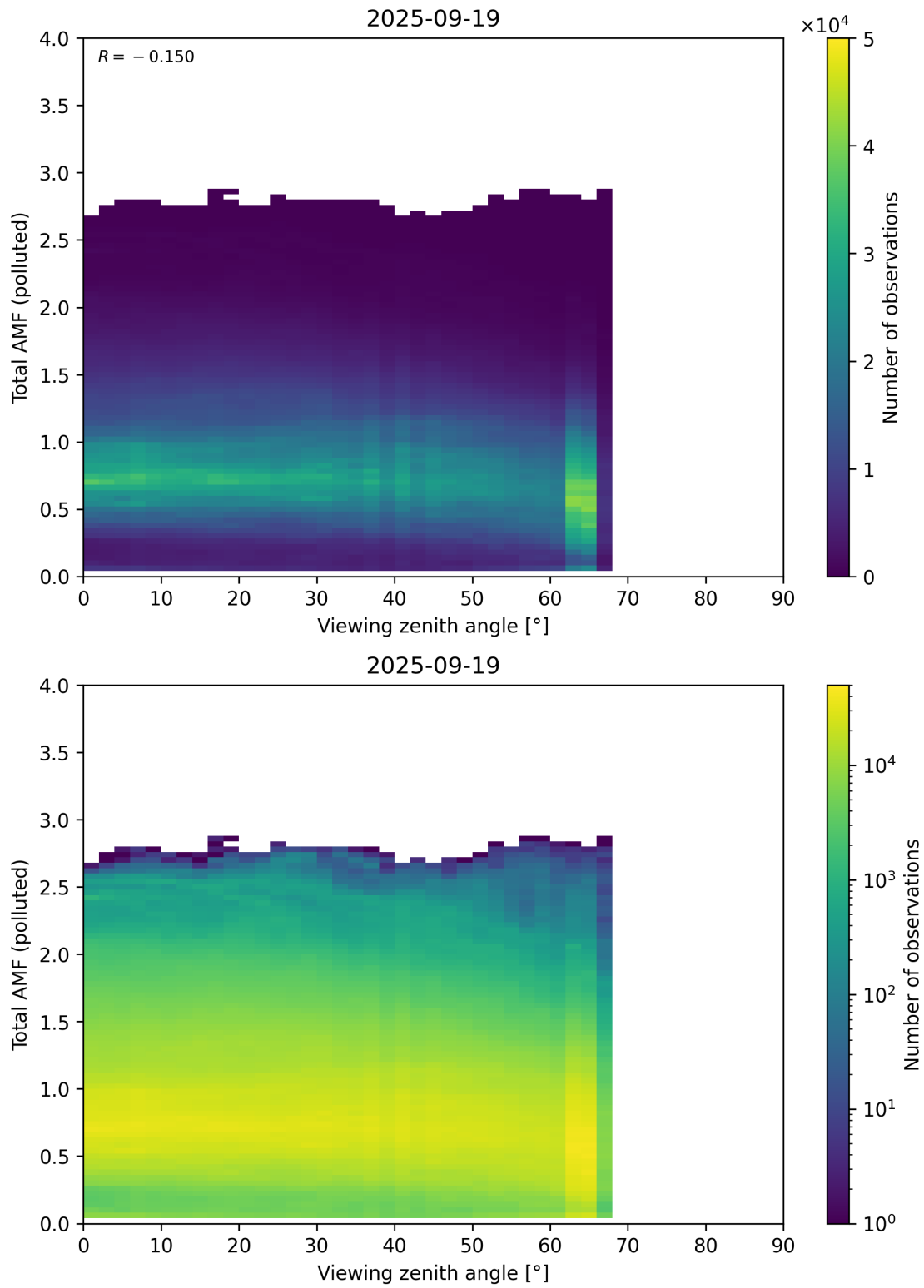
Figure 381: Scatter density plot of “Viewing zenith angle” against “Total AMF (polluted)” for 2025-09-18 to 2025-09-20.
