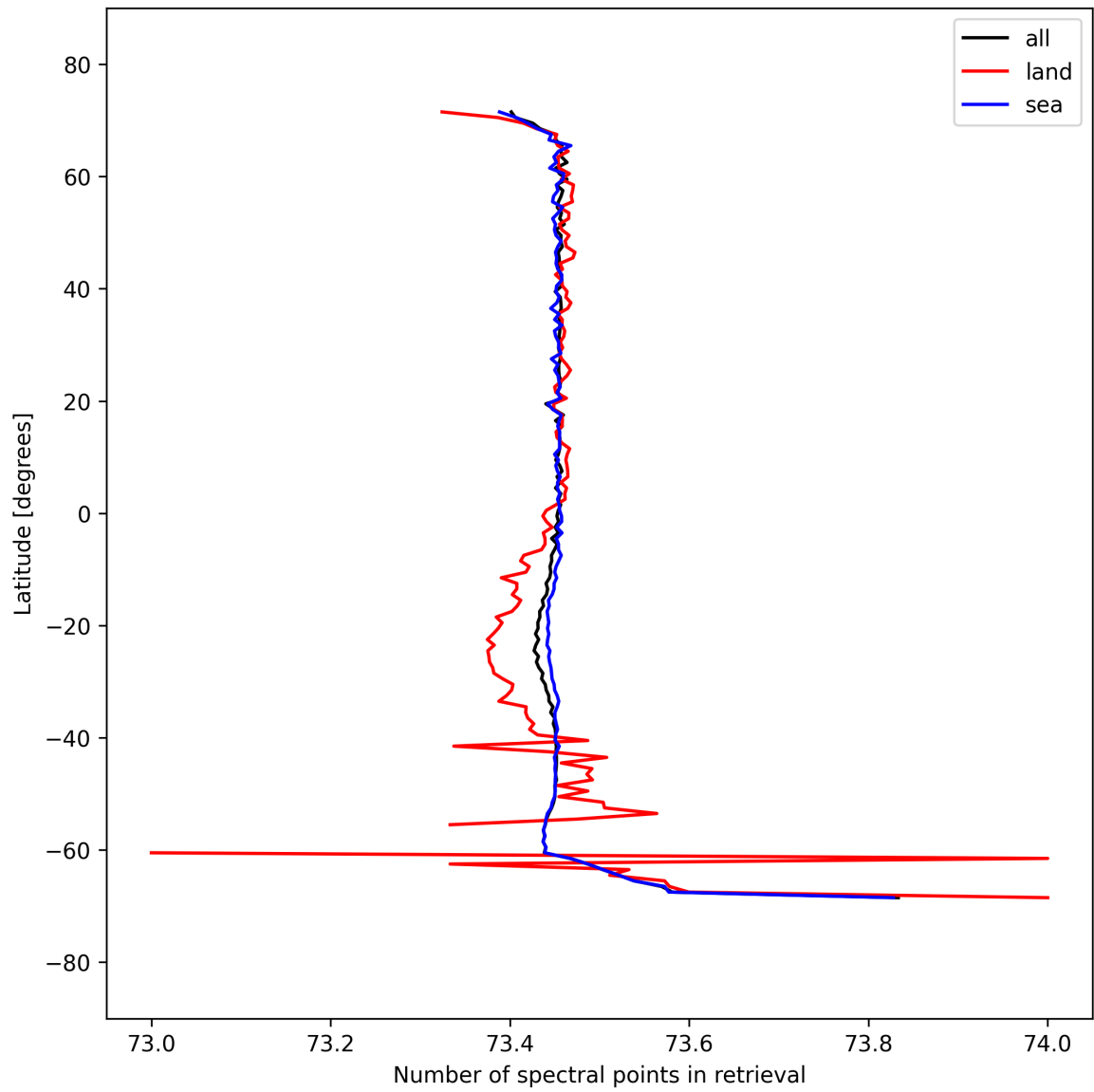
Figure 56: Zonal average of “Number of spectral points in retrieval” for 2025-09-18 to 2025-09-20.
