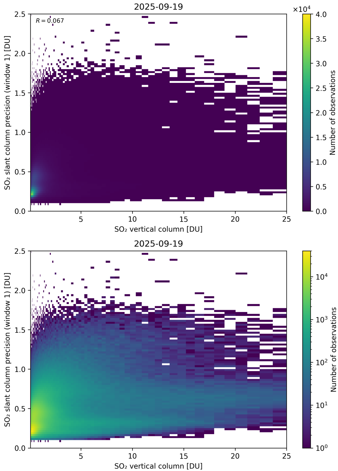
Figure 355: Scatter density plot of “SO 2 vertical column” against “SO 2 slant column precision (window 1)” for 2025-09-18 to 2025-09-20.
