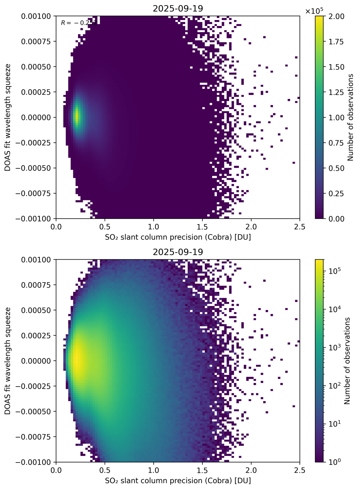
Figure 203: Scatter density plot of “SO 2 slant column precision (Cobra)” against “DOAS fit wavelength squeeze” for 2025-09-18 to 2025-09-20.
