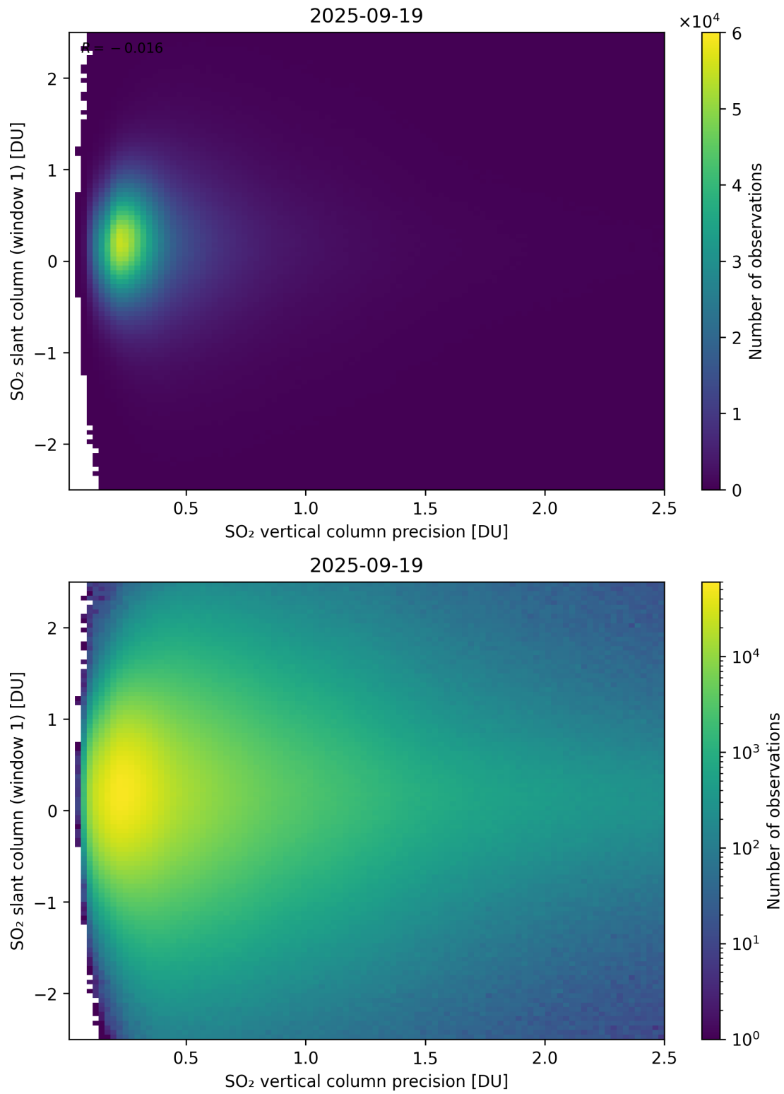
Figure 341: Scatter density plot of “SO 2 vertical column precision” against “SO 2 slant column (window 1)” for 2025-09-18 to 2025-09-20.
