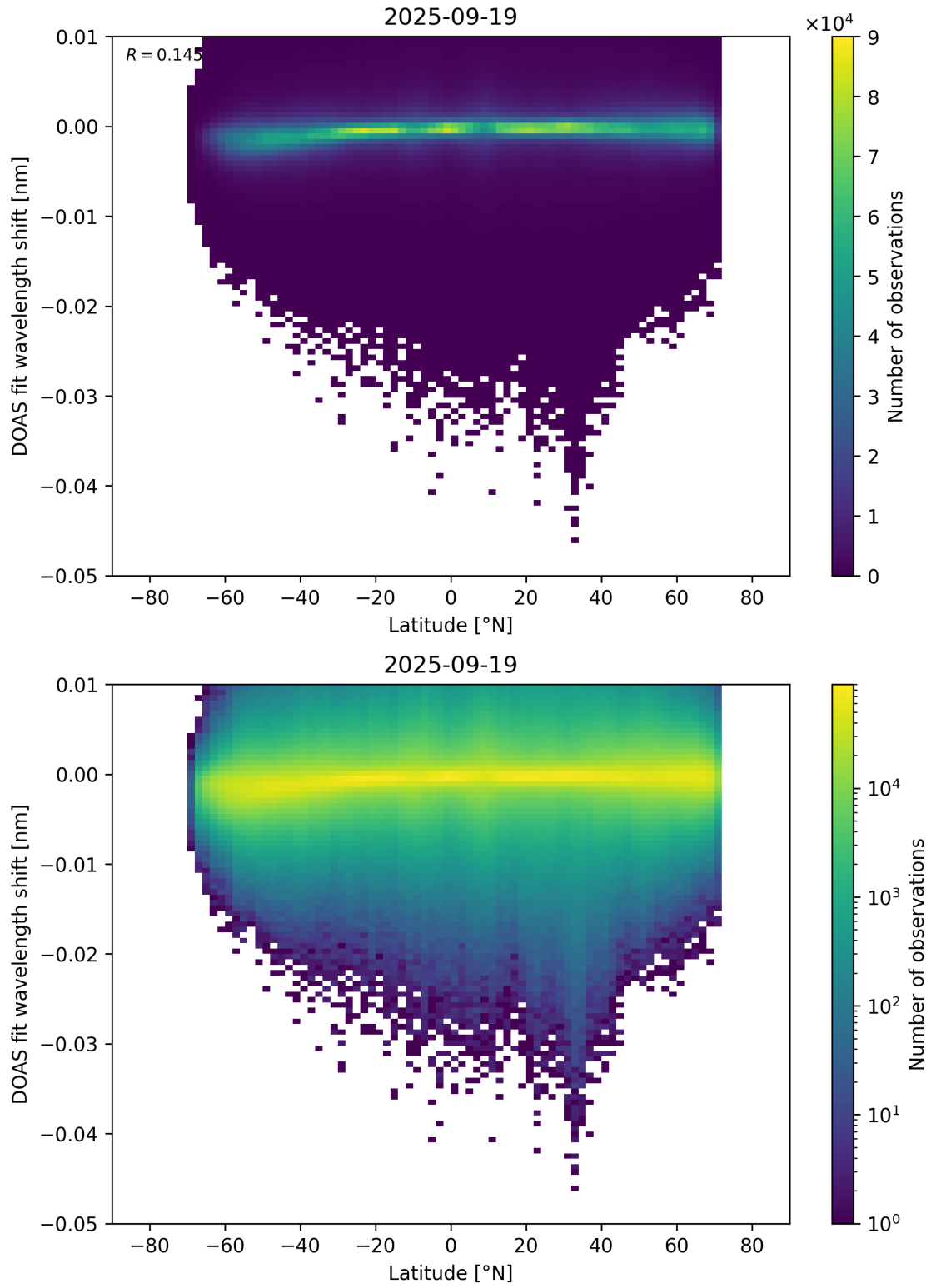
Figure 153: Scatter density plot of “Latitude” against “DOAS fit wavelength shift” for 2025-09-18 to 2025-09-20.
