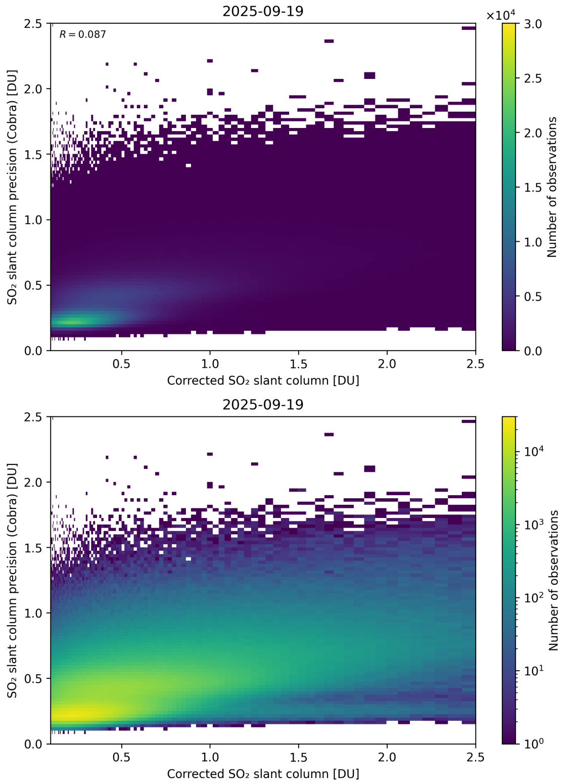
Figure 234: Scatter density plot of “Corrected SO 2 slant column” against “SO 2 slant column precision (Cobra)” for 2025-09-18 to 2025-09-20.
