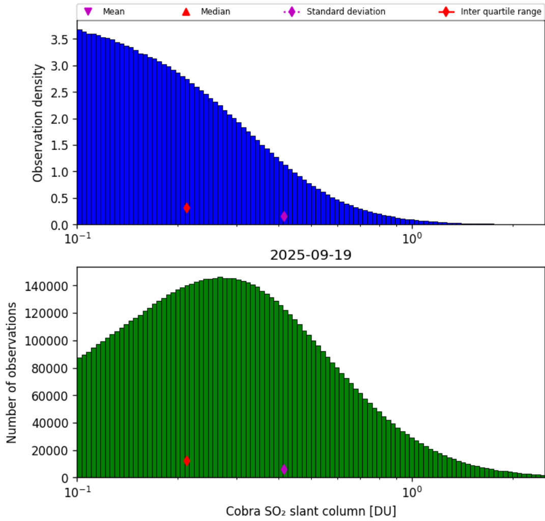
Figure 61: Histogram of “Cobra SO 2 slant column” for 2025-09-18 to 2025-09-20
