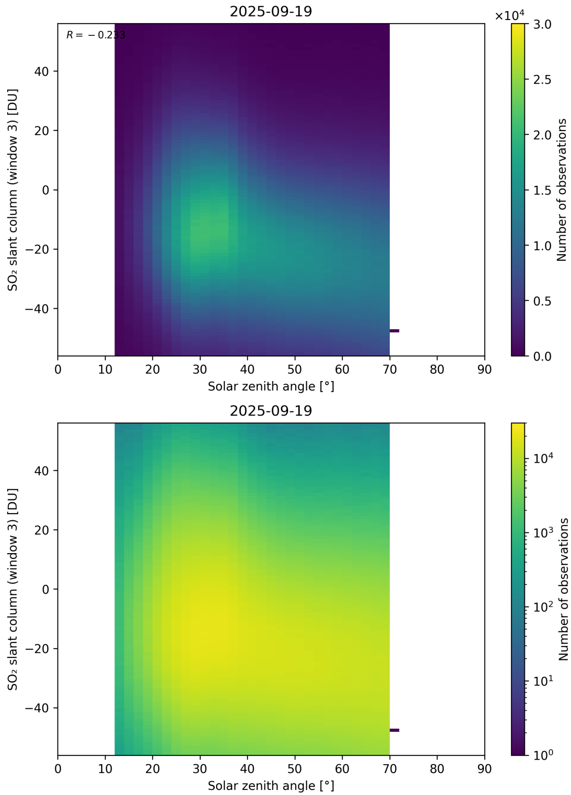
Figure 187: Scatter density plot of “Solar zenith angle” against “SO 2 slant column (window 3)” for 2025-09-18 to 2025-09-20.
