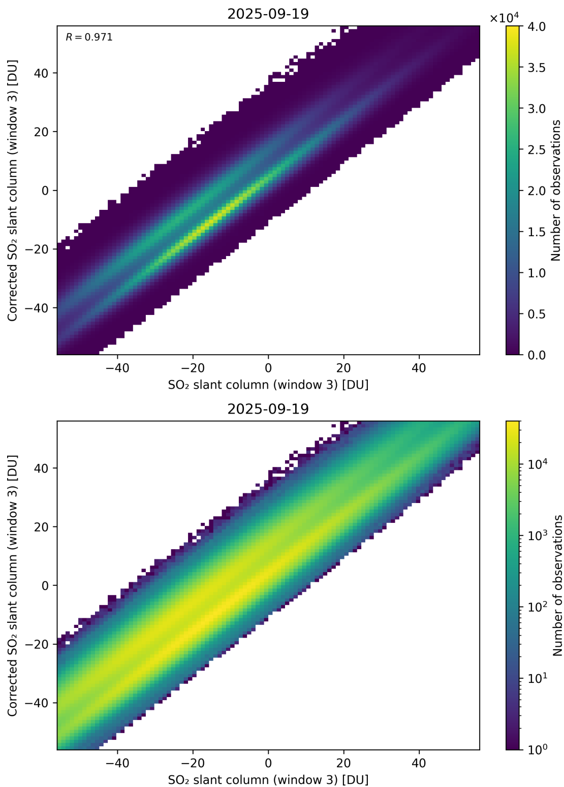
Figure 316: Scatter density plot of “SO 2 slant column (window 3)” against “Corrected SO 2 slant column (window 3)” for 2025-09-18 to 2025-09-20.
