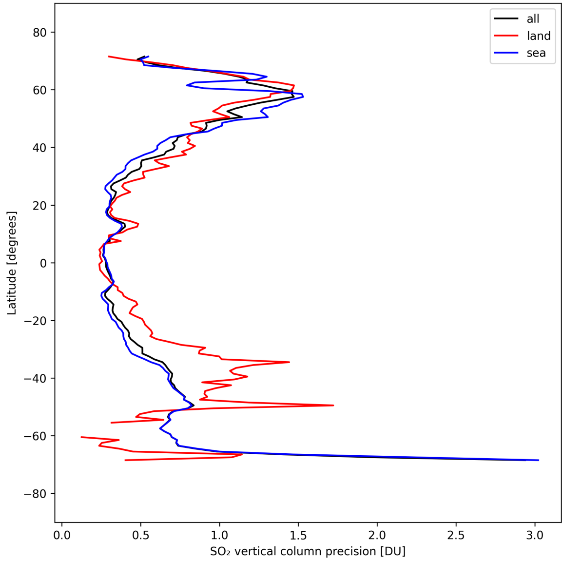
Figure 33: Zonal average of “SO 2 vertical column precision” for 2025-09-18 to 2025-09-20.
