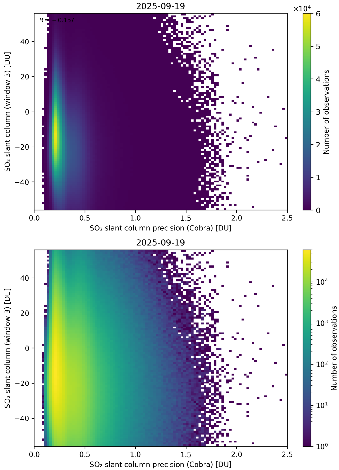
Figure 211: Scatter density plot of “SO 2 slant column precision (Cobra)” against “SO 2 slant column (window 3)” for 2025-09-18 to 2025-09-20.
