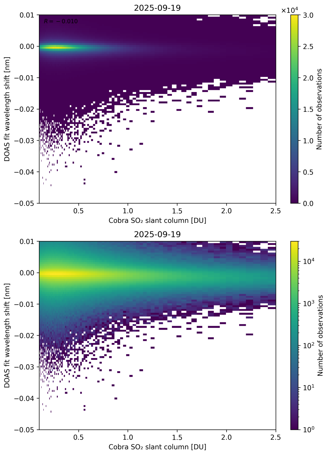
Figure 196: Scatter density plot of “Cobra SO 2 slant column” against “DOAS fit wavelength shift” for 2025-09-18 to 2025-09-20.
