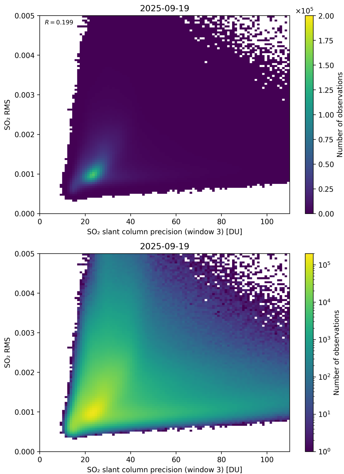
Figure 310: Scatter density plot of “SO 2 slant column precision (window 3)” against “SO 2 RMS” for 2025-09-18 to 2025-09-20.
