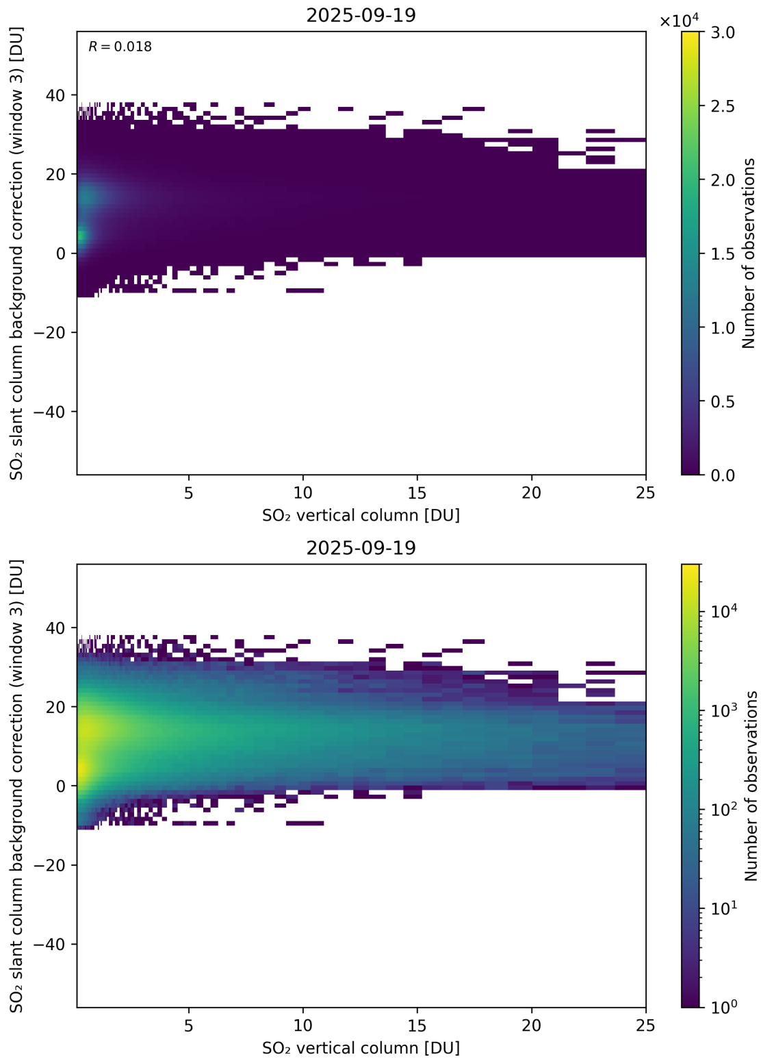
Figure 325: Scatter density plot of “SO 2 vertical column” against “SO 2 slant column background correction (window 3)” for 2025-09-18 to 2025-09-20.
