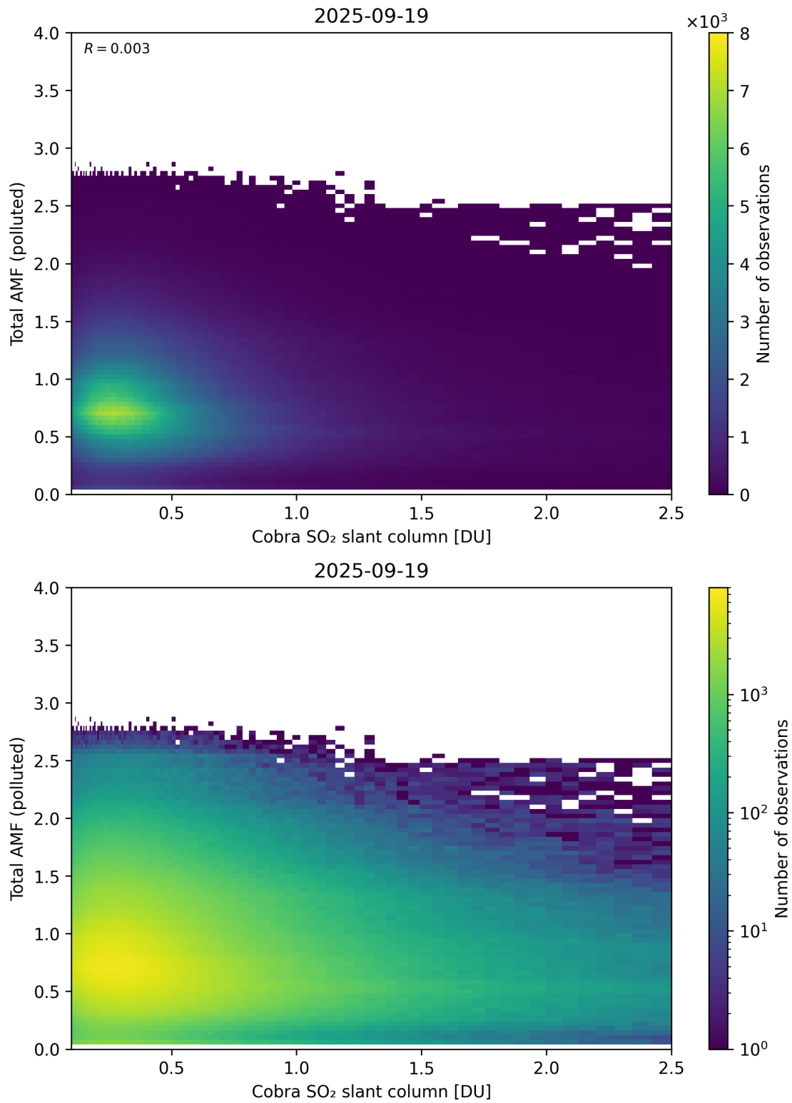
Figure 224: Scatter density plot of “Cobra SO 2 slant column” against “Total AMF (polluted)” for 2025-09-18 to 2025-09-20.
