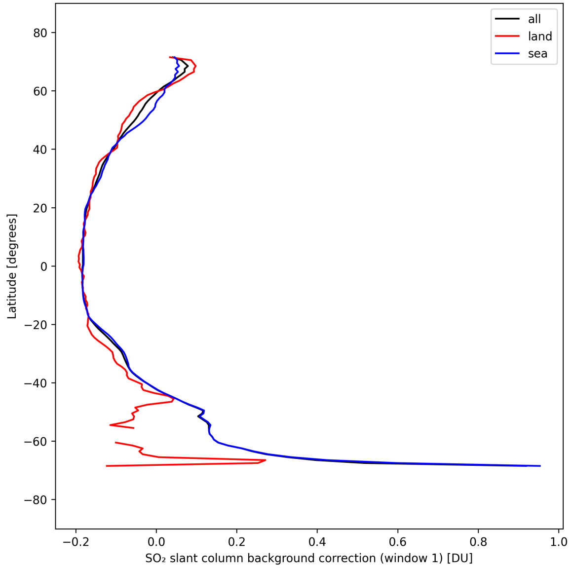
Figure 40: Zonal average of “SO 2 slant column background correction (window 1)” for 2025-09-18 to 2025-09-20.
