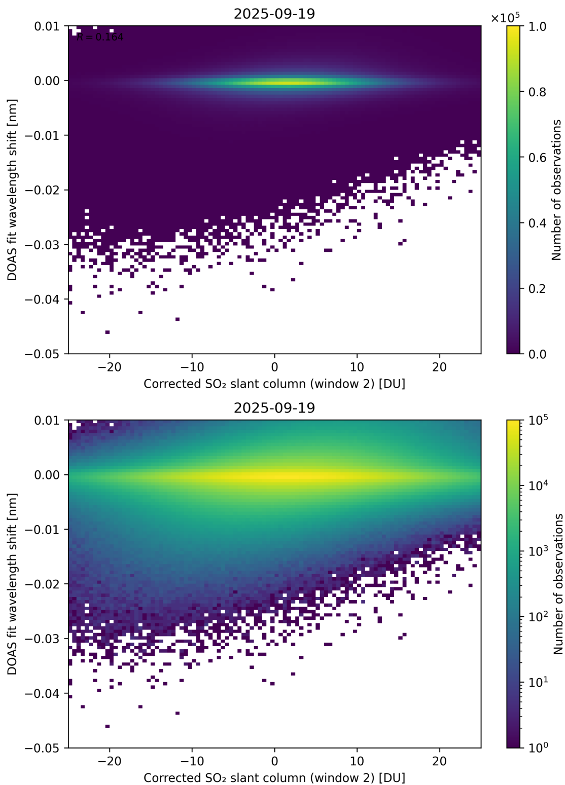
Figure 246: Scatter density plot of “Corrected SO 2 slant column (window 2)” against “DOAS fit wavelength shift” for 2025-09-18 to 2025-09-20.
