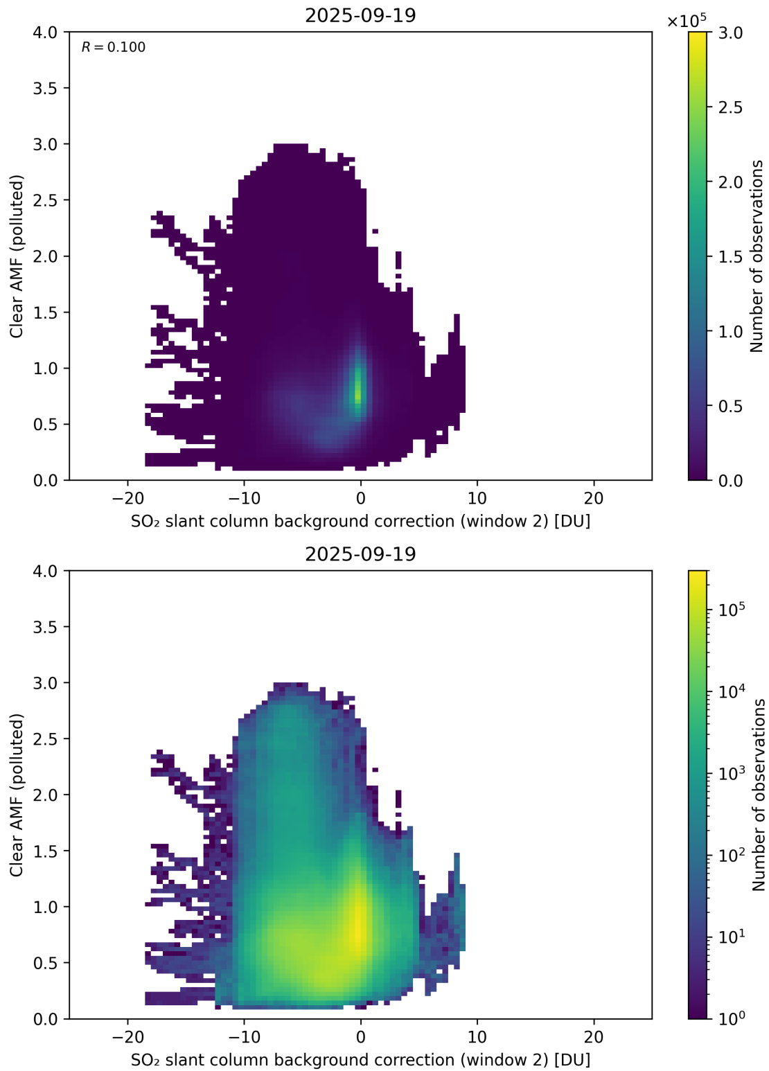
Figure 126: Scatter density plot of “SO 2 slant column background correction (window 2)” against “Clear AMF (polluted)” for 2025-09-18 to 2025-09-20.
