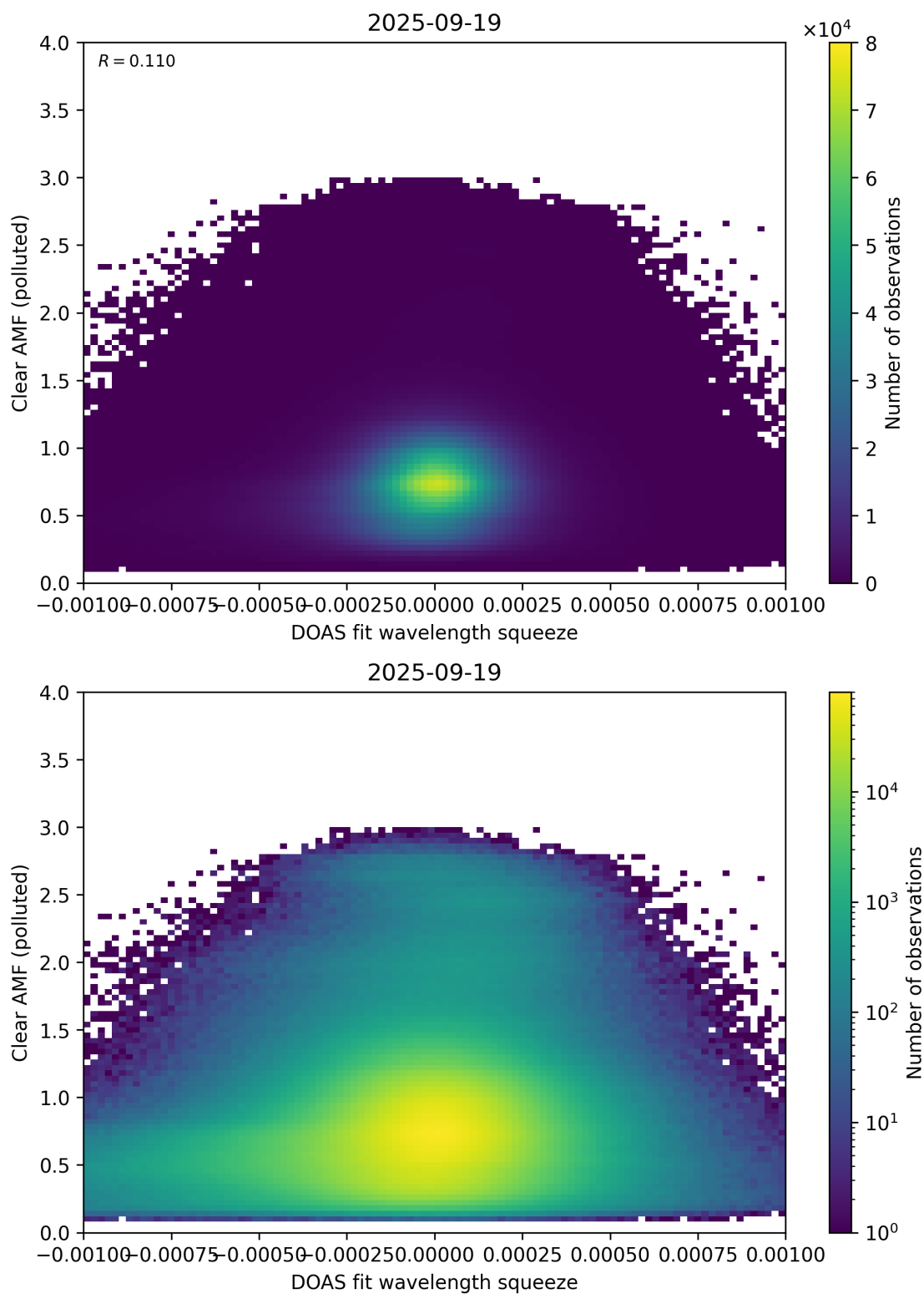
Figure 144: Scatter density plot of “DOAS fit wavelength squeeze” against “Clear AMF (polluted)” for 2025-09-18 to 2025-09-20.
