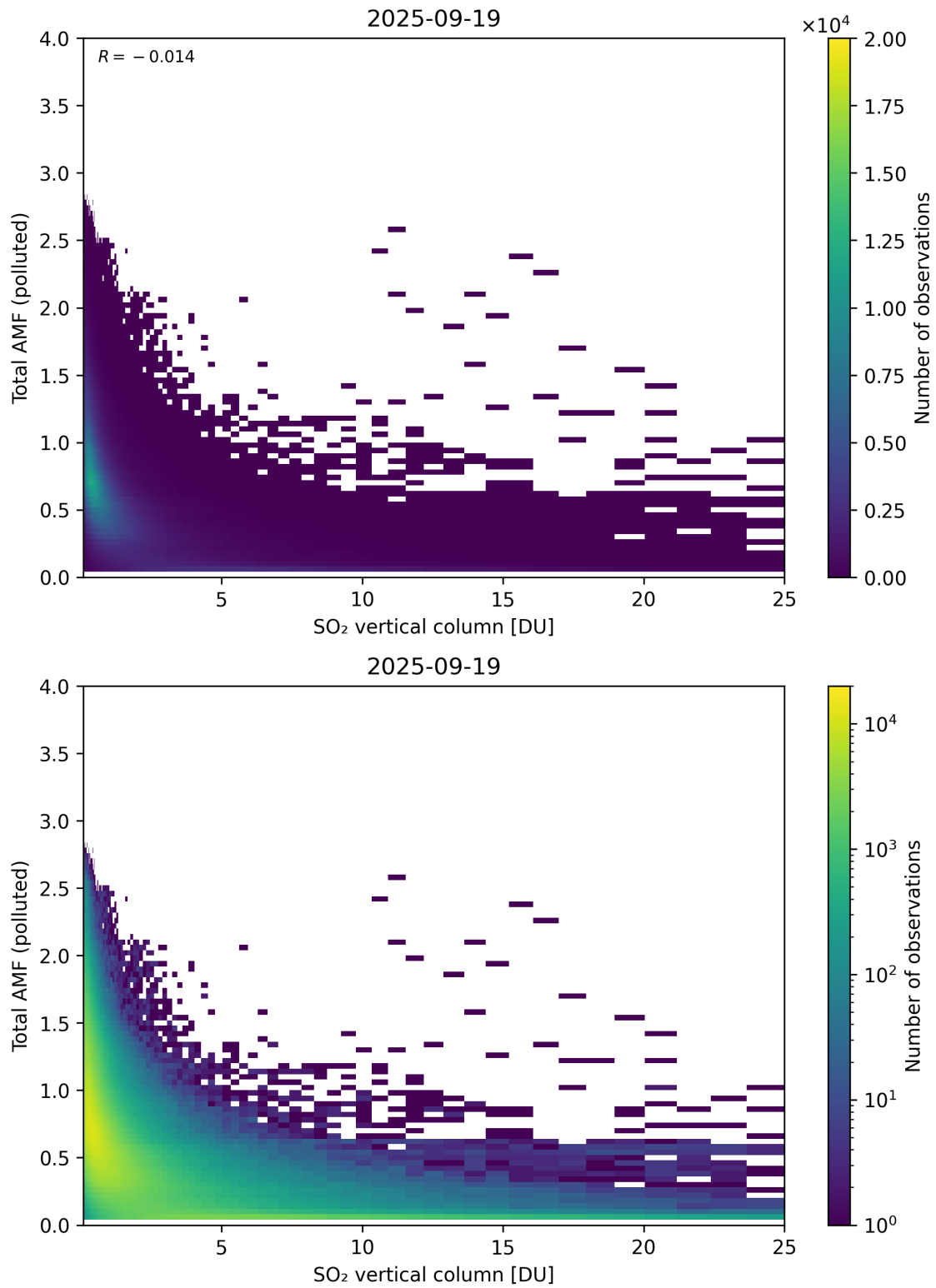
Figure 359: Scatter density plot of “SO 2 vertical column” against “Total AMF (polluted)” for 2025-09-18 to 2025-09-20.
