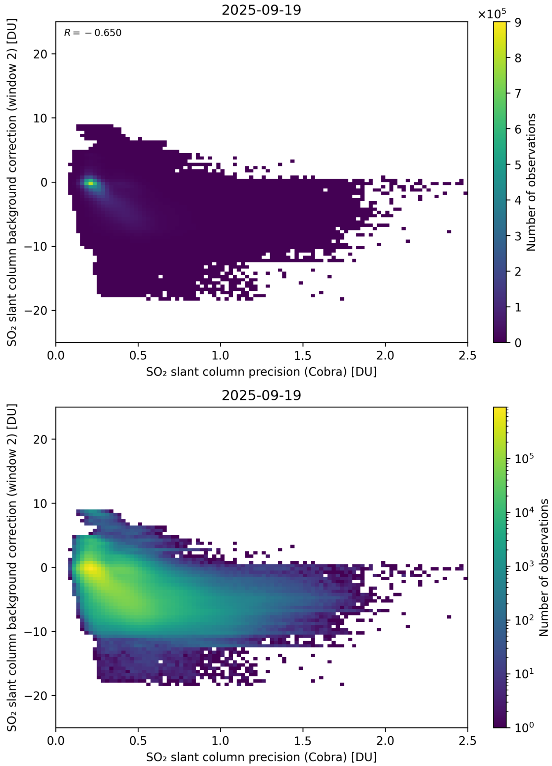
Figure 200: Scatter density plot of “SO 2 slant column precision (Cobra)” against “SO 2 slant column background correction (window 2)” for 2025-09-18 to 2025-09-20.
