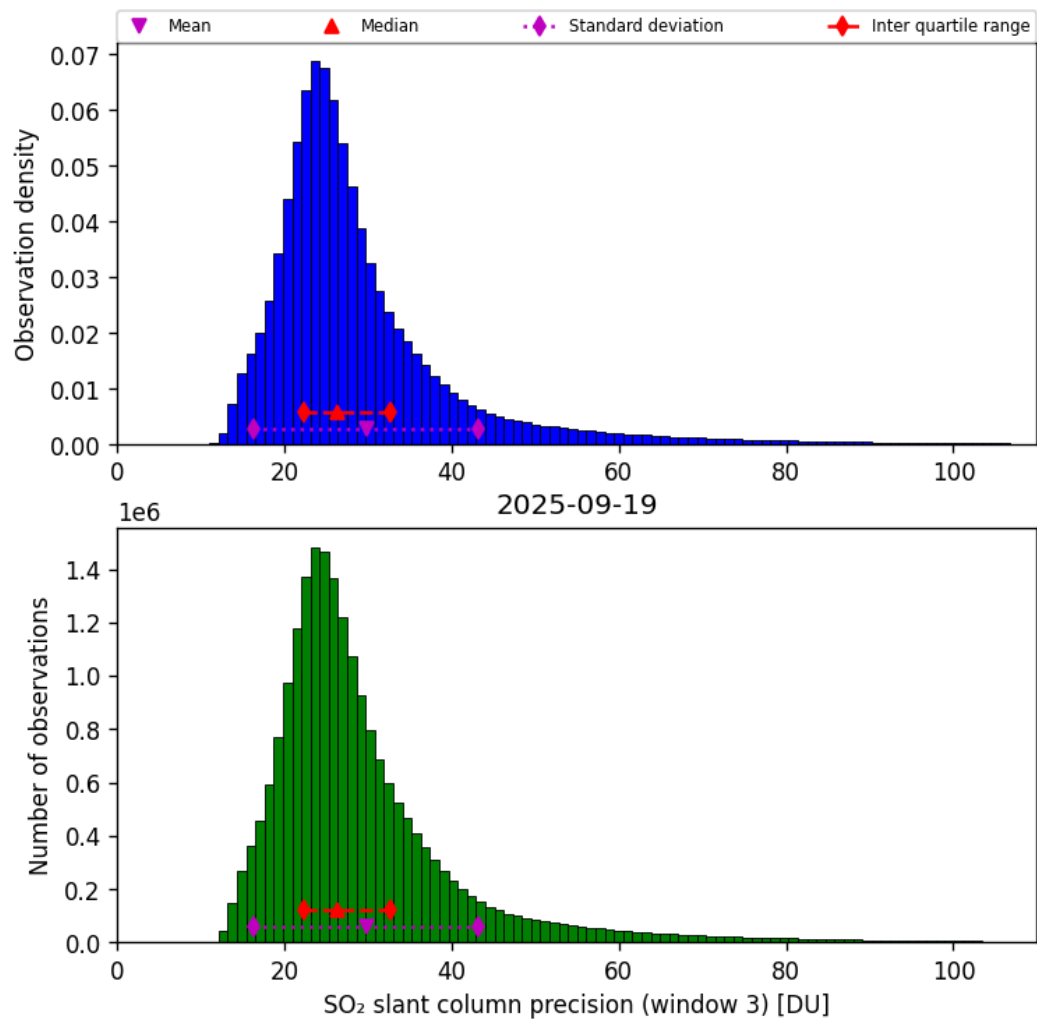
Figure 72: Histogram of “SO 2 slant column precision (window 3)” for 2025-09-18 to 2025-09-20
