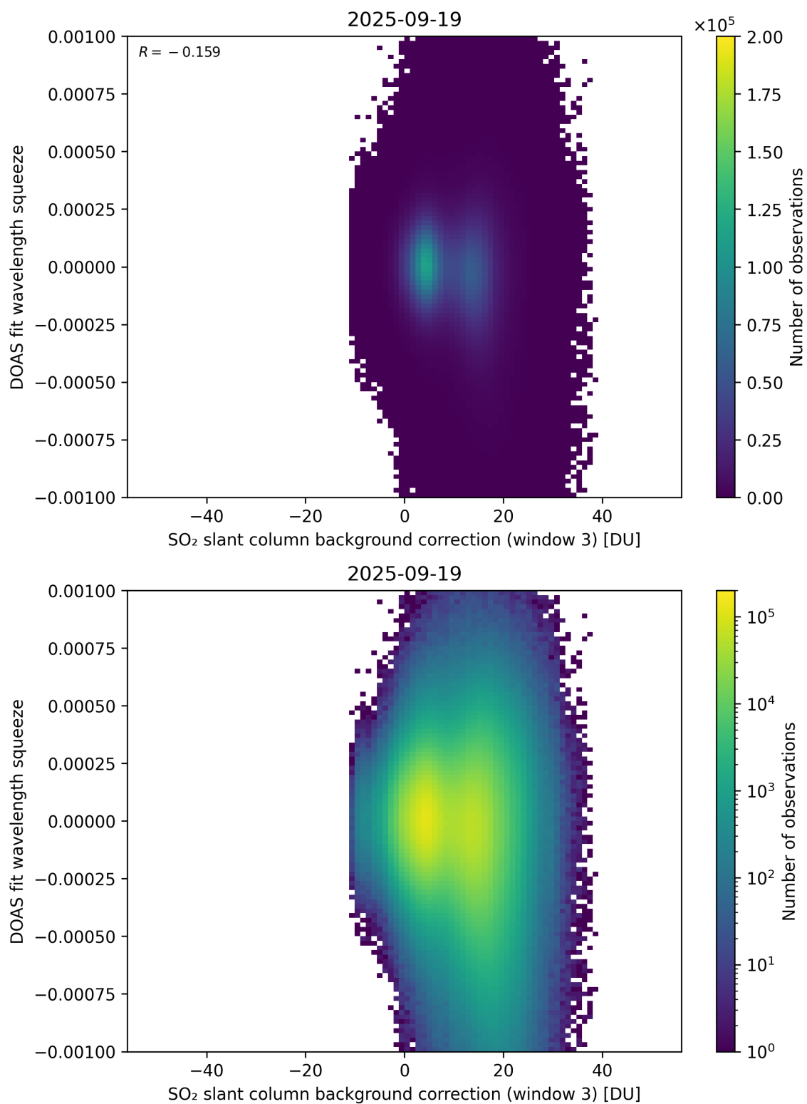
Figure 133: Scatter density plot of “SO 2 slant column background correction (window 3)” against “DOAS fit wavelength squeeze” for 2025-09-18 to 2025-09-20.
