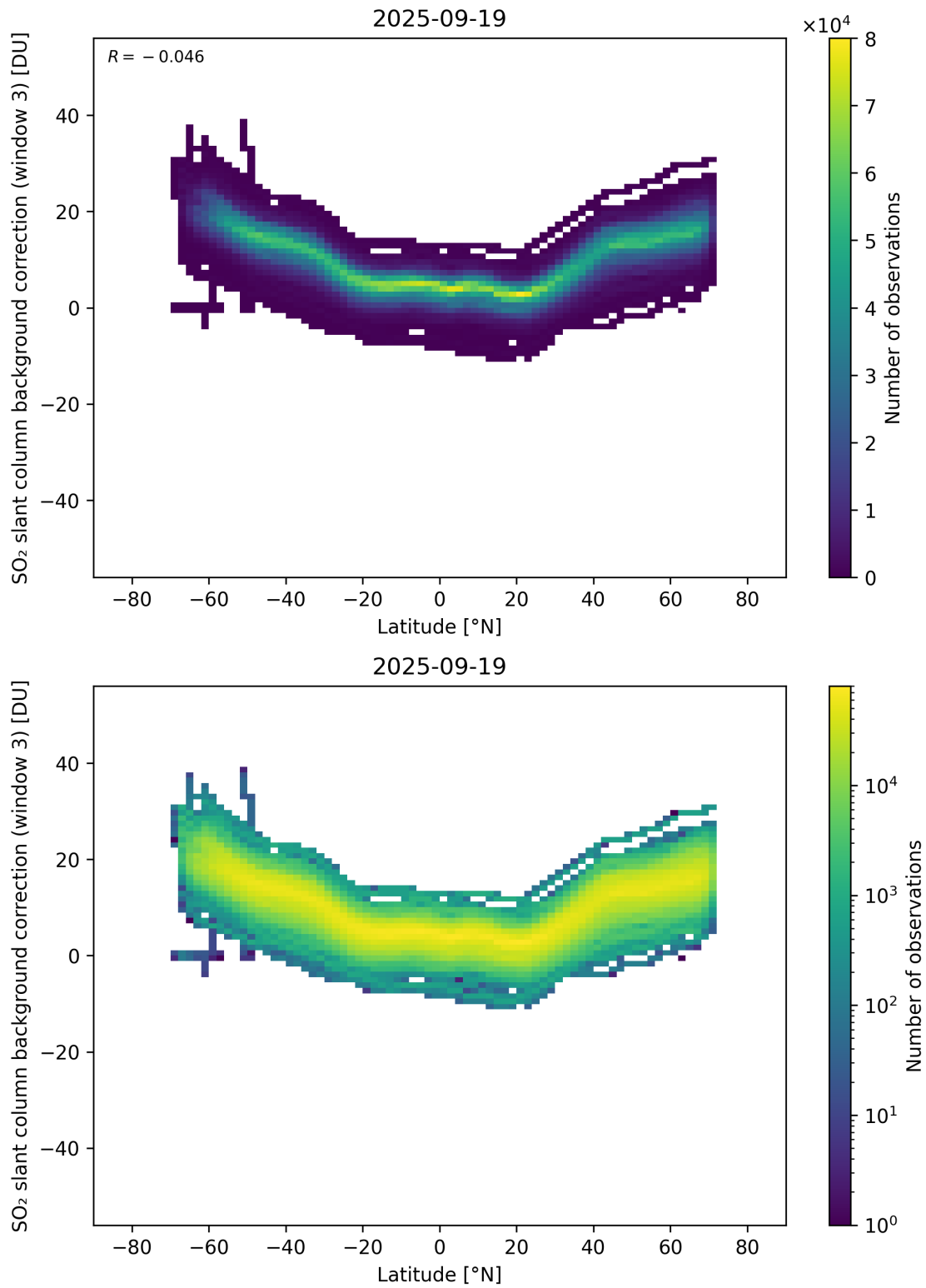
Figure 152: Scatter density plot of “Latitude” against “SO 2 slant column background correction (window 3)” for 2025-09-18 to 2025-09-20.
