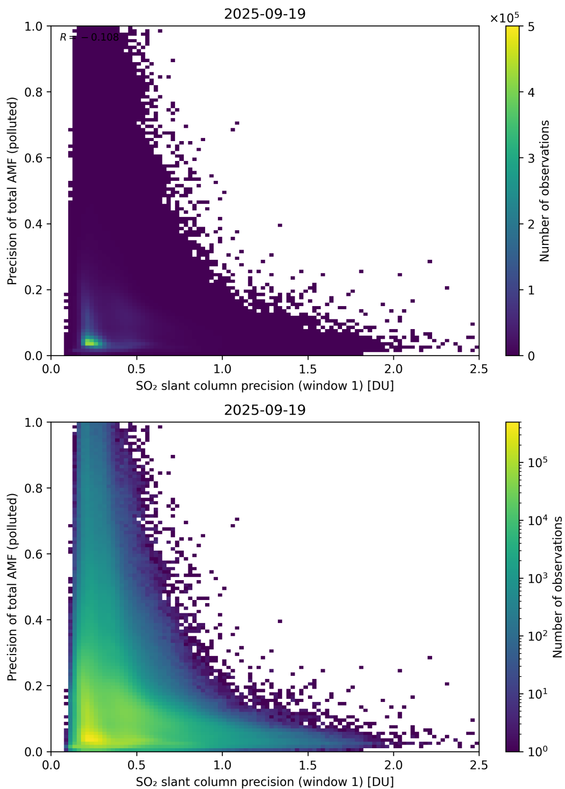
Figure 281: Scatter density plot of “SO 2 slant column precision (window 1)” against “Precision of total AMF (polluted)” for 2025-09-18 to 2025-09-20.
