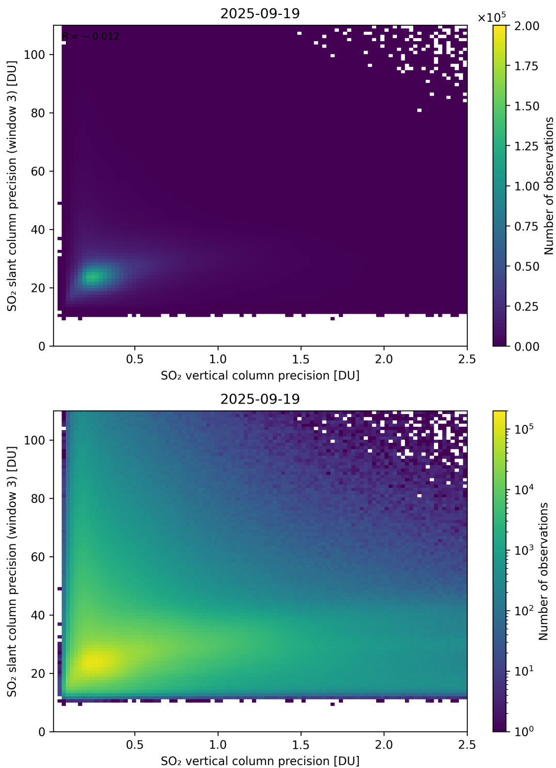
Figure 345: Scatter density plot of “SO 2 vertical column precision” against “SO 2 slant column precision (window 3)” for 2025-09-18 to 2025-09-20.
