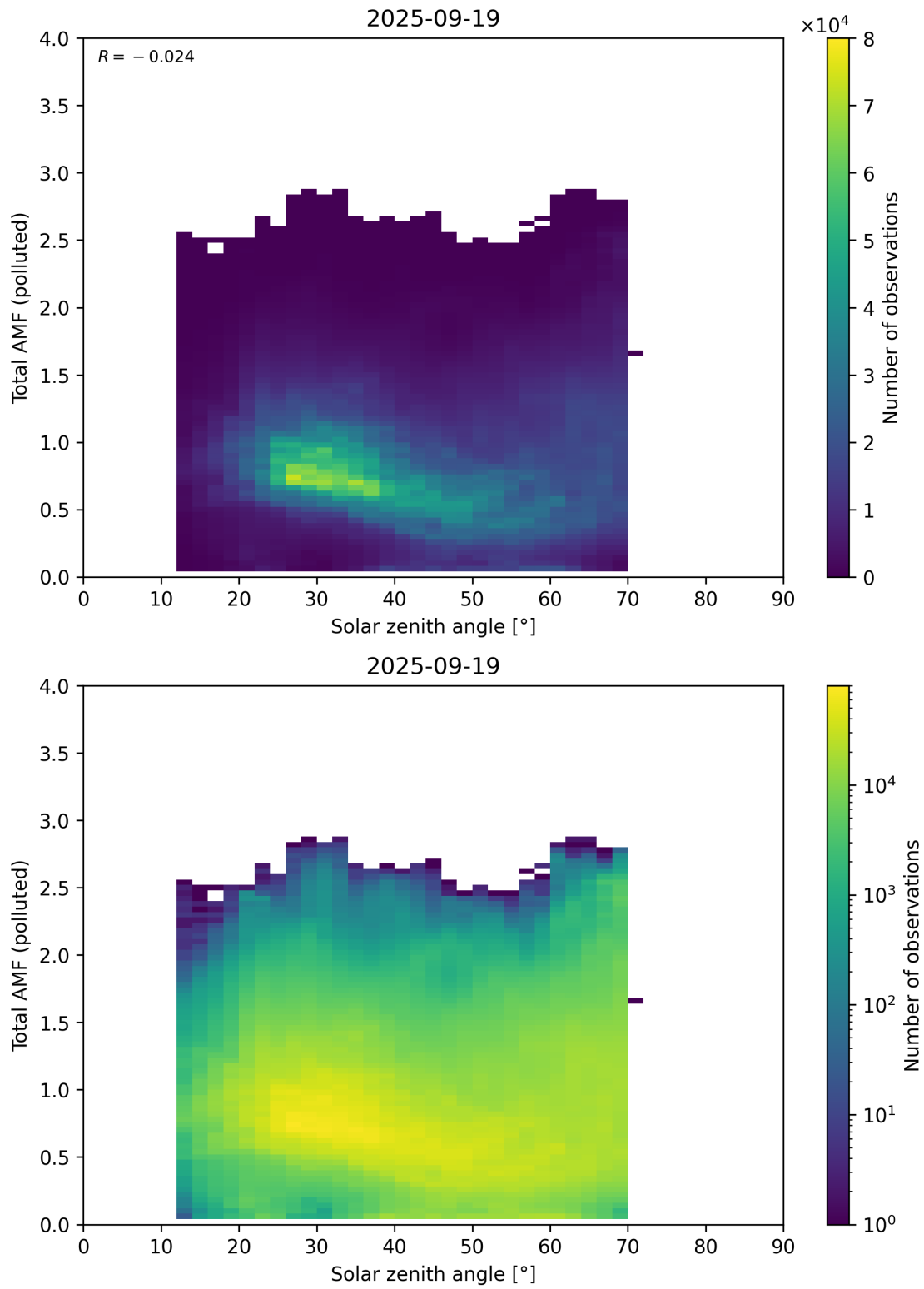
Figure 189: Scatter density plot of “Solar zenith angle” against “Total AMF (polluted)” for 2025-09-18 to 2025-09-20.
