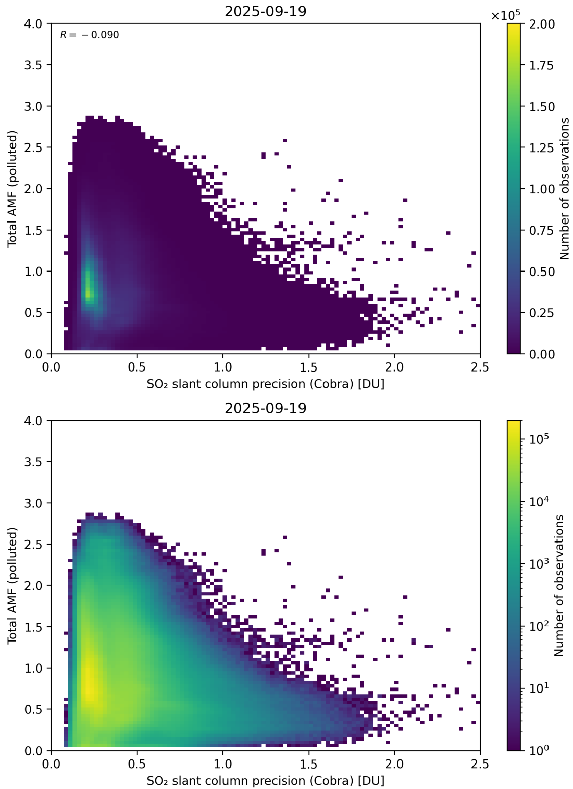
Figure 213: Scatter density plot of “SO 2 slant column precision (Cobra)” against “Total AMF (polluted)” for 2025-09-18 to 2025-09-20.
