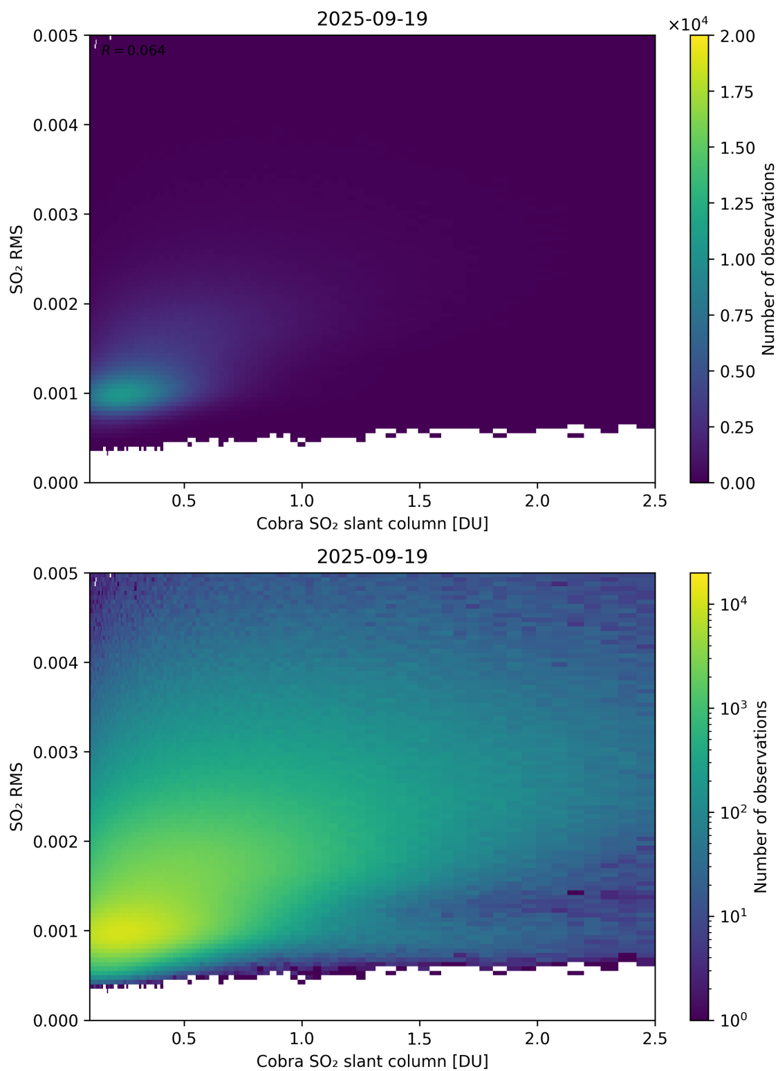
Figure 198: Scatter density plot of “Cobra SO 2 slant column” against “SO 2 RMS” for 2025-09-18 to 2025-09-20.
