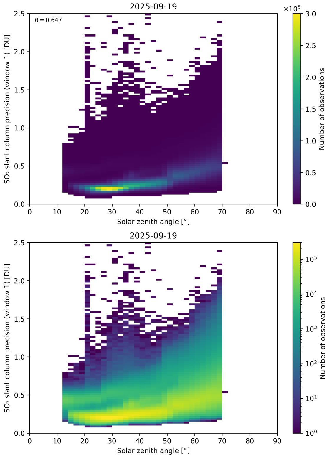
Figure 185: Scatter density plot of “Solar zenith angle” against “SO 2 slant column precision (window 1)” for 2025-09-18 to 2025-09-20.
