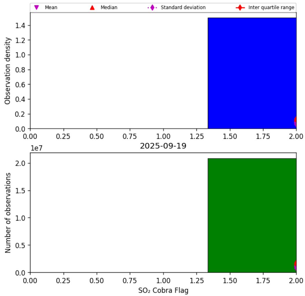
Figure 75: Histogram of “SO 2 Cobra Flag” for 2025-09-18 to 2025-09-20
