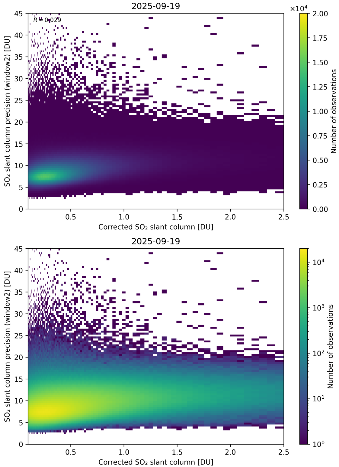
Figure 239: Scatter density plot of “Corrected SO 2 slant column” against “SO 2 slant column precision (window2)” for 2025-09-18 to 2025-09-20.
