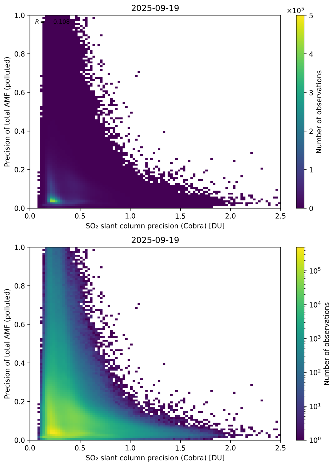
Figure 214: Scatter density plot of “SO 2 slant column precision (Cobra)” against “Precision of total AMF (polluted)” for 2025-09-18 to 2025-09-20.
