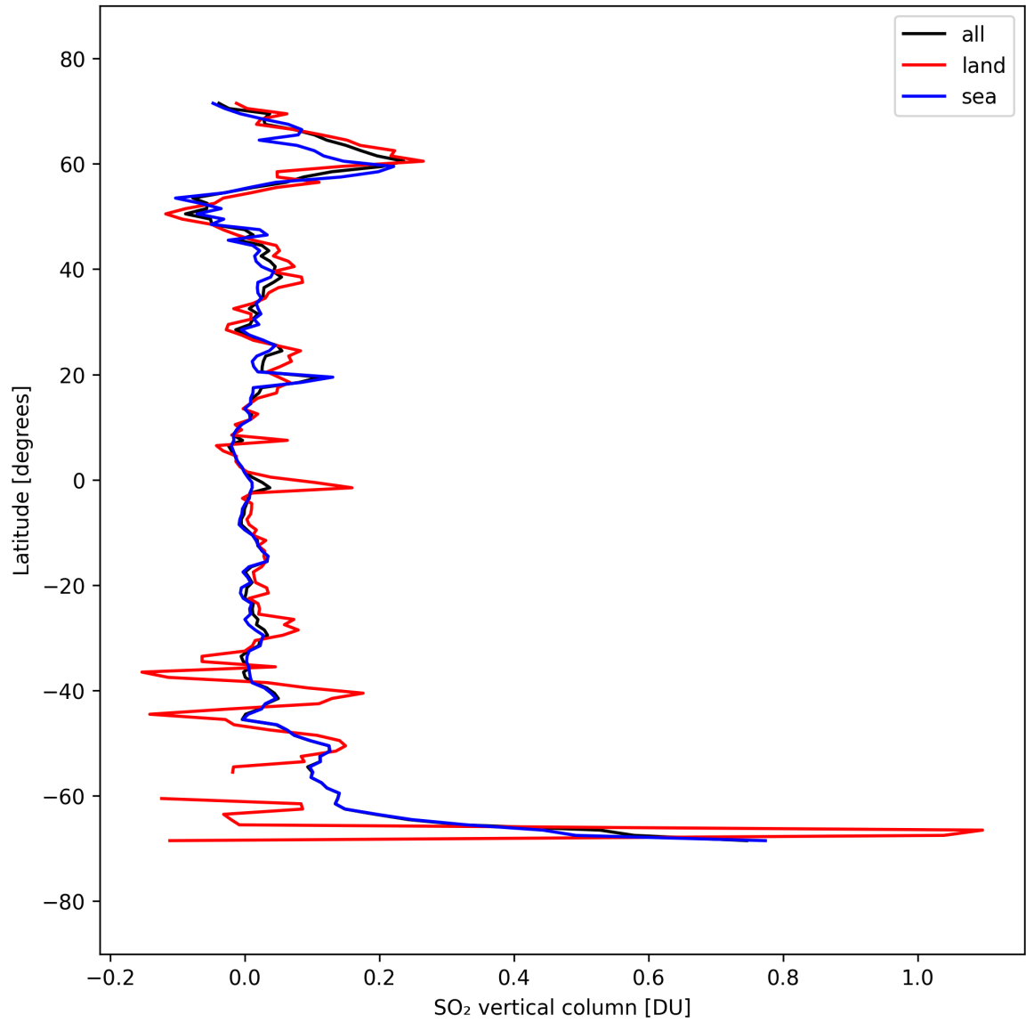
Figure 32: Zonal average of “SO 2 vertical column” for 2025-09-18 to 2025-09-20.
