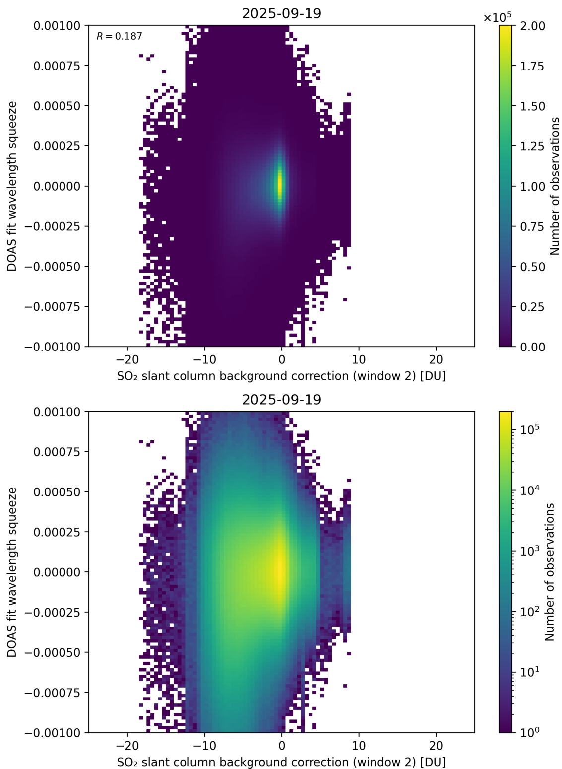
Figure 124: Scatter density plot of “SO 2 slant column background correction (window 2)” against “DOAS fit wavelength squeeze” for 2025-09-18 to 2025-09-20.
