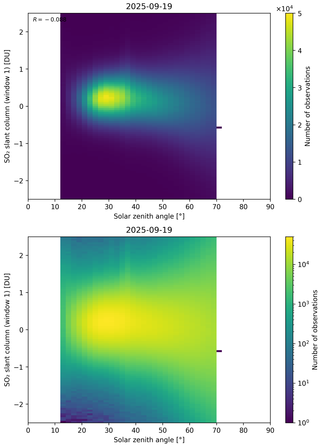
Figure 184: Scatter density plot of “Solar zenith angle” against “SO 2 slant column (window 1)” for 2025-09-18 to 2025-09-20.
