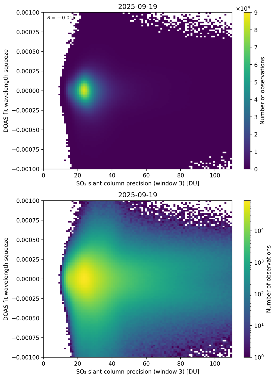
Figure 309: Scatter density plot of “SO 2 slant column precision (window 3)” against “DOAS fit wavelength squeeze” for 2025-09-18 to 2025-09-20.
