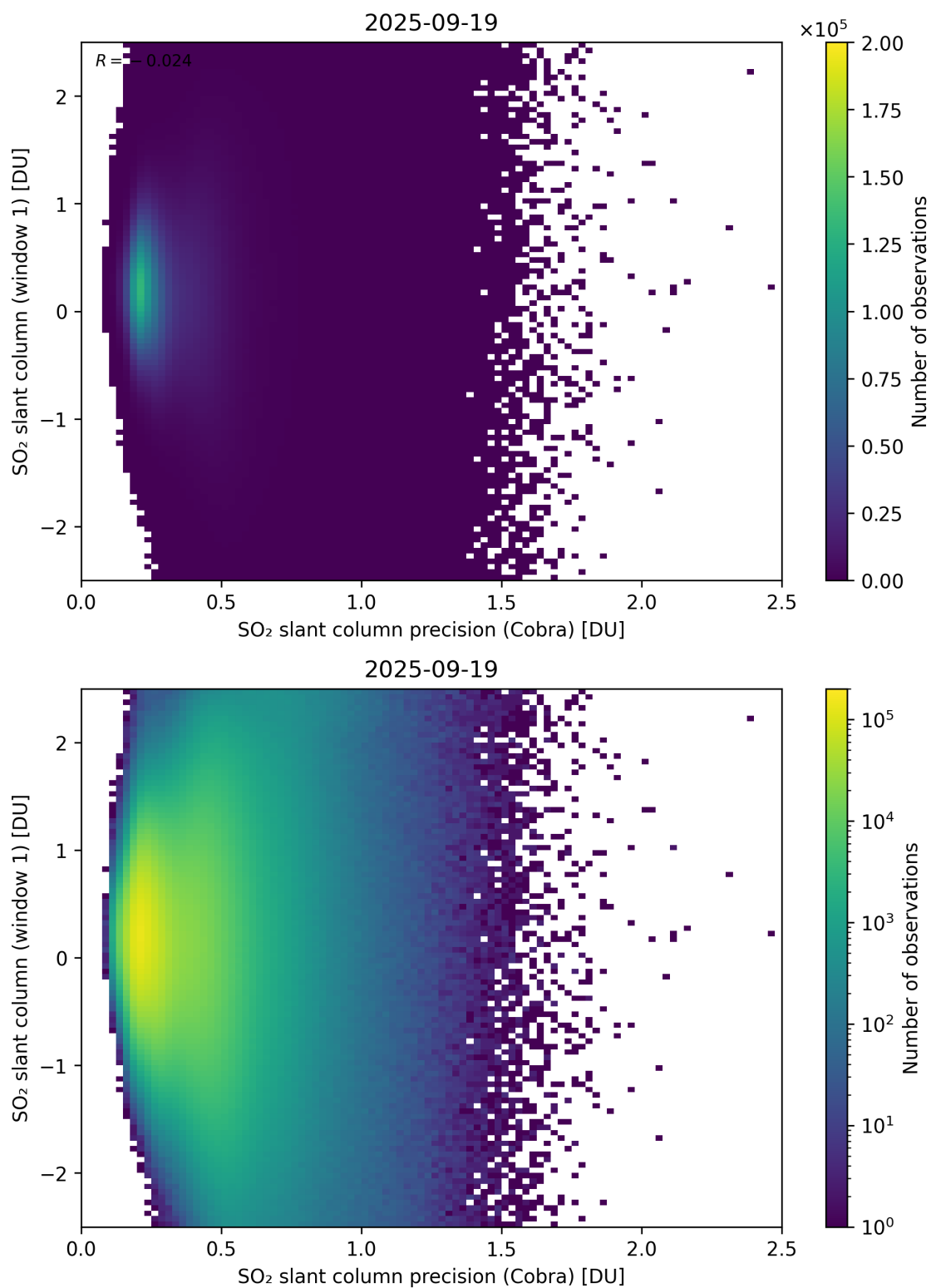
Figure 208: Scatter density plot of “SO 2 slant column precision (Cobra)” against “SO 2 slant column (window 1)” for 2025-09-18 to 2025-09-20.
