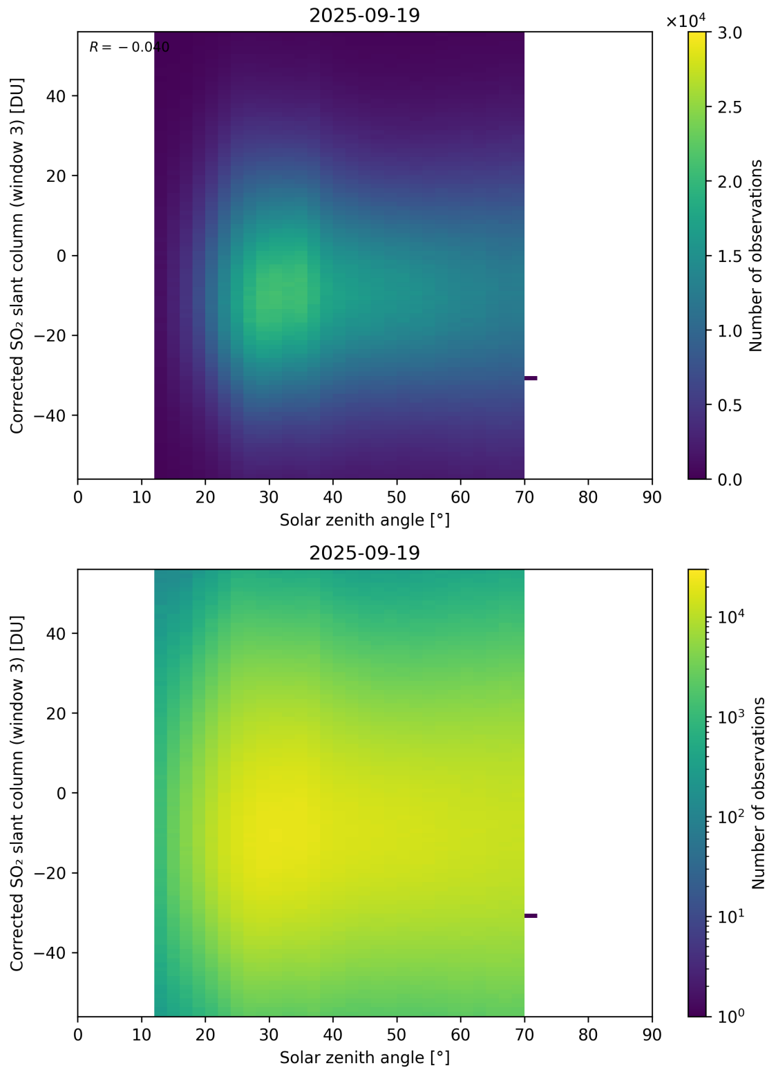
Figure 183: Scatter density plot of “Solar zenith angle” against “Corrected SO 2 slant column (window 3)” for 2025-09-18 to 2025-09-20.
