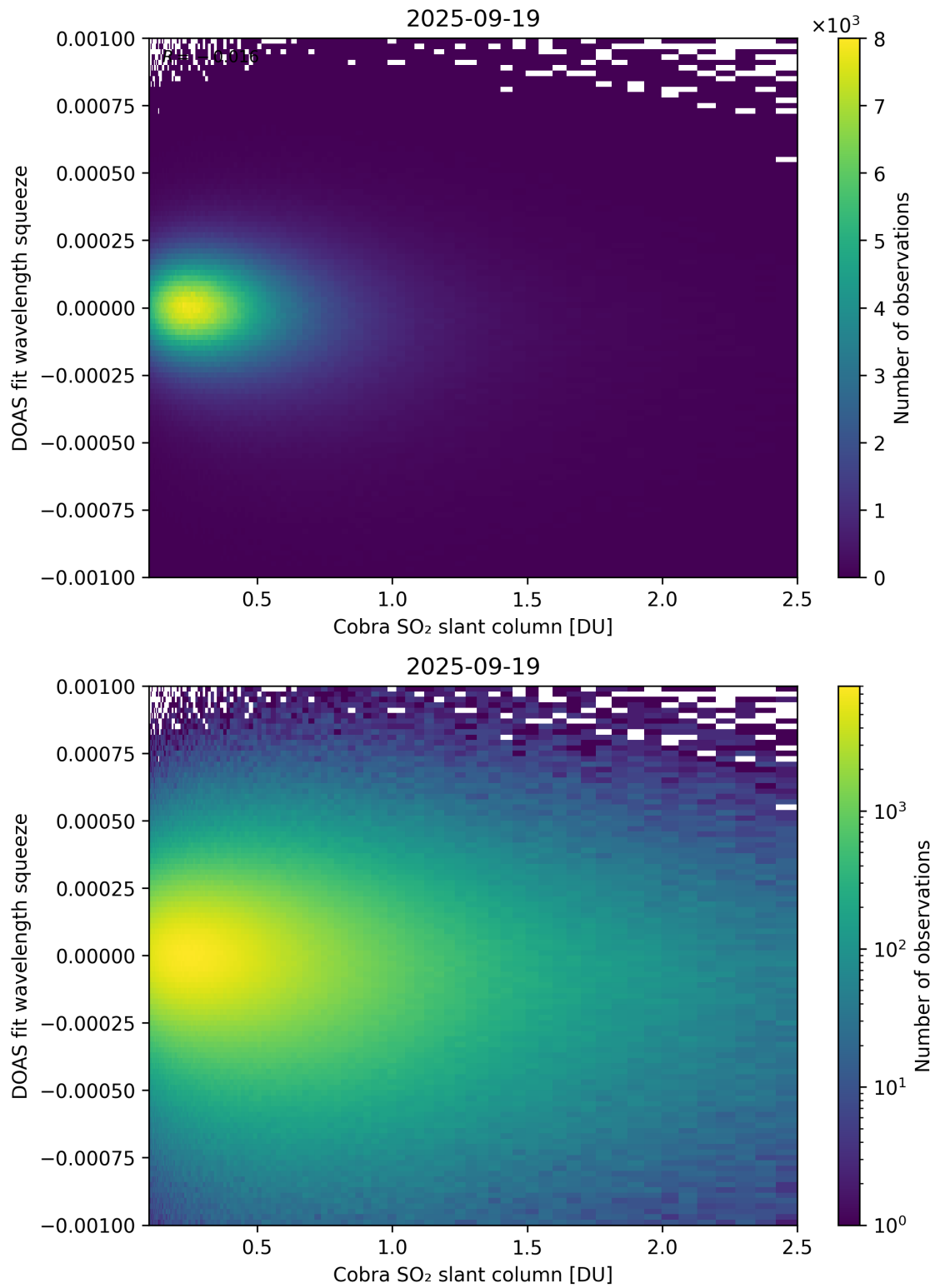
Figure 197: Scatter density plot of “Cobra SO 2 slant column” against “DOAS fit wavelength squeeze” for 2025-09-18 to 2025-09-20.
