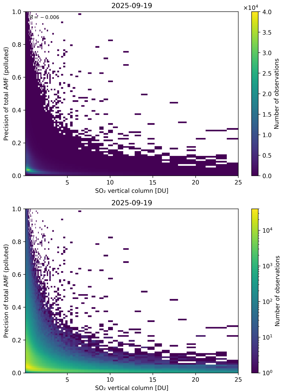
Figure 360: Scatter density plot of “SO 2 vertical column” against “Precision of total AMF (polluted)” for 2025-09-18 to 2025-09-20.
