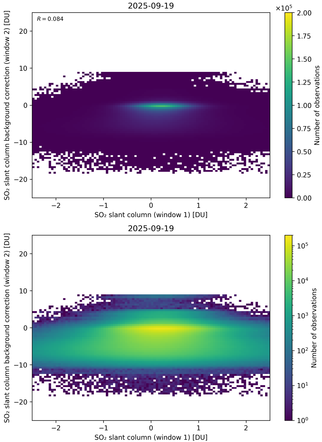
Figure 263: Scatter density plot of “SO 2 slant column (window 1)” against “SO 2 slant column background correction (window 2)” for 2025-09-18 to 2025-09-20.
