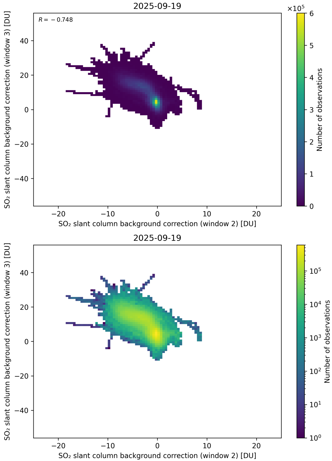
Figure 122: Scatter density plot of “SO 2 slant column background correction (window 2)” against “SO 2 slant column background correction (window 3)” for 2025-09-18 to 2025-09-20.
