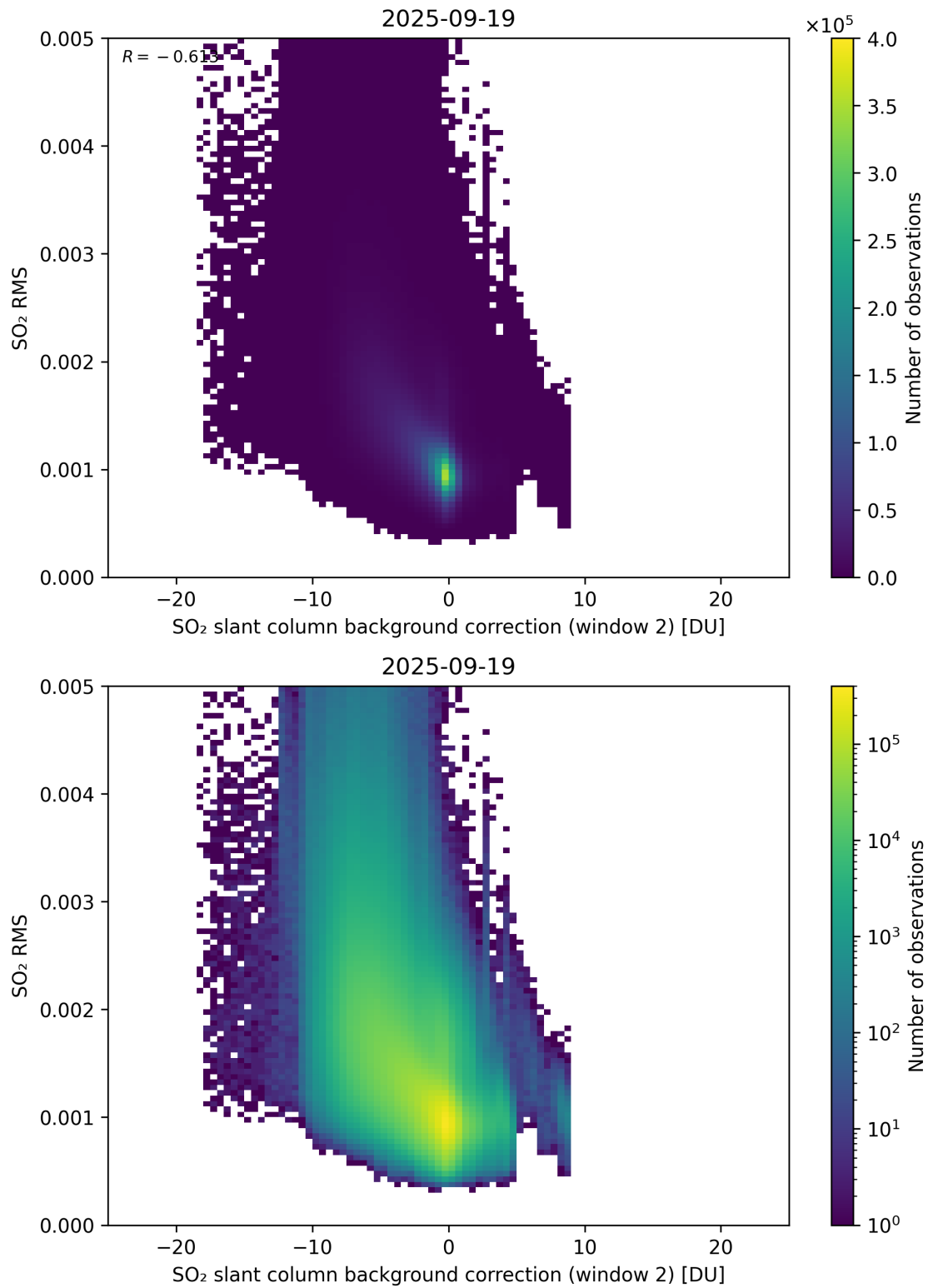
Figure 125: Scatter density plot of “SO 2 slant column background correction (window 2)” against “SO 2 RMS” for 2025-09-18 to 2025-09-20.
