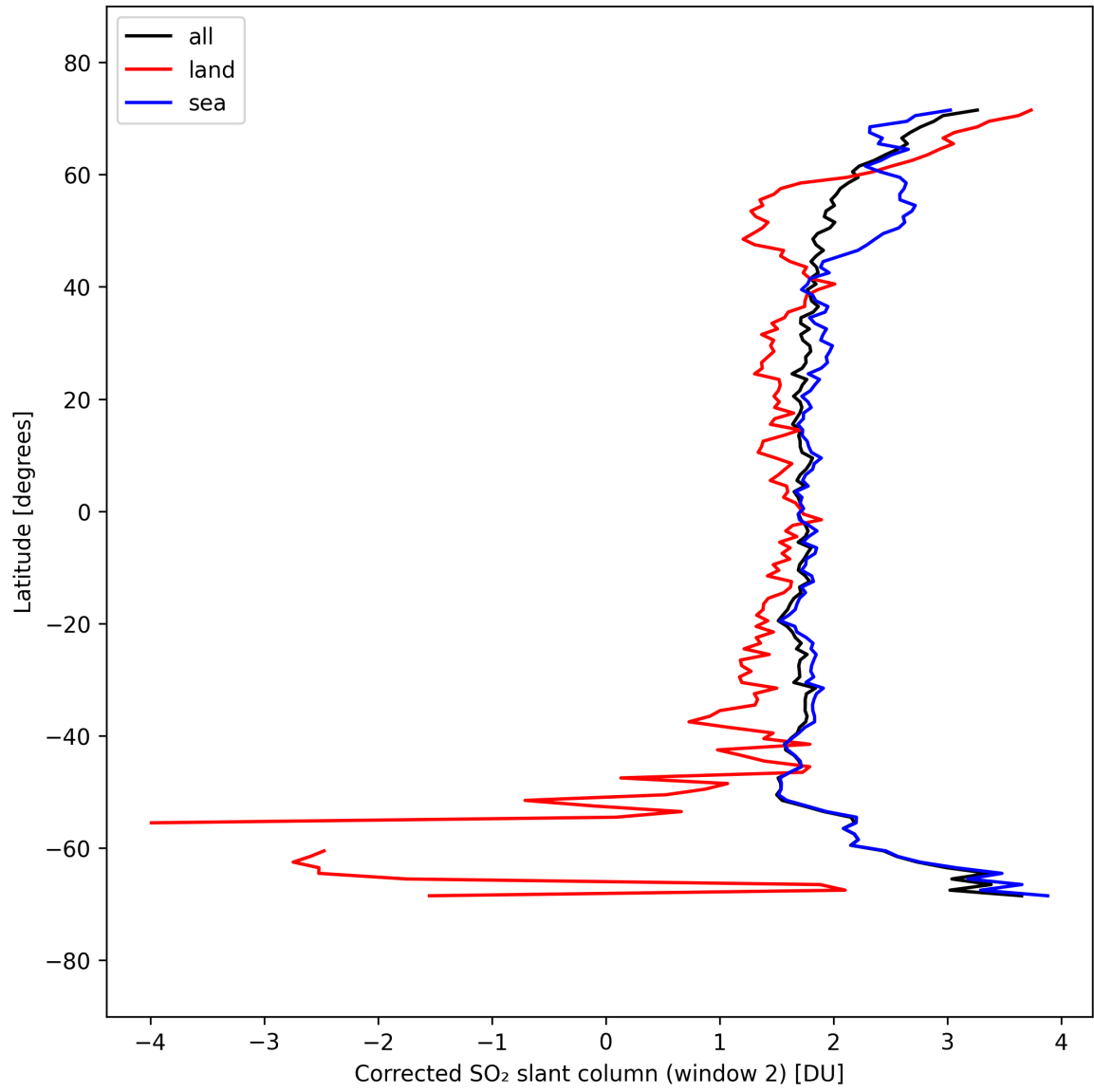
Figure 43: Zonal average of “Corrected SO 2 slant column (window 2)” for 2025-09-18 to 2025-09-20.
