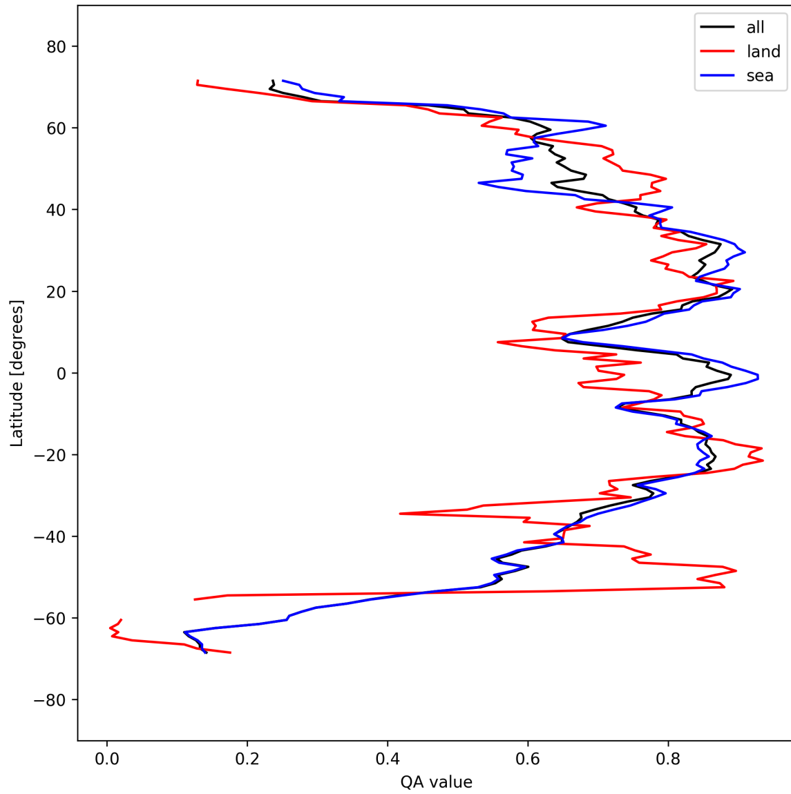
Figure 31: Zonal average of “QA value” for 2025-09-18 to 2025-09-20.
