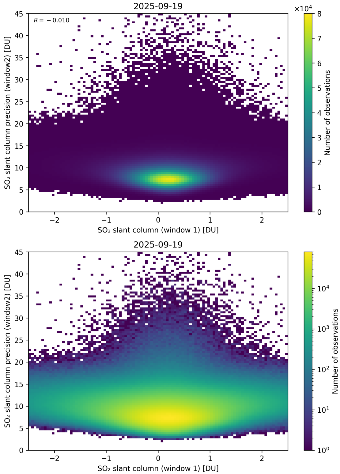
Figure 286: Scatter density plot of “SO 2 slant column (window 1)” against “SO 2 slant column precision (window2)” for 2025-09-18 to 2025-09-20.
