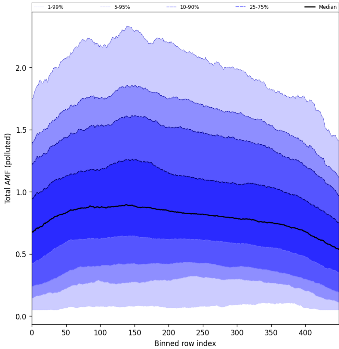
Figure 105: Along track statistics of “Total AMF (polluted)” for 2025-09-18 to 2025-09-20
