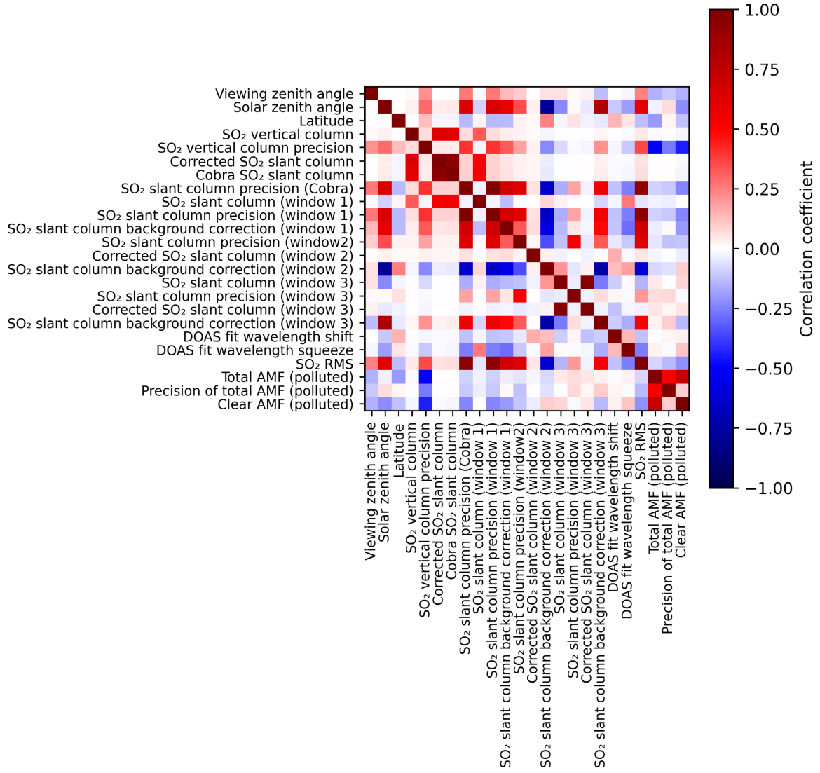
Figure 2: Map of correlation matrix for 2025-09-18 to 2025-09-20.
