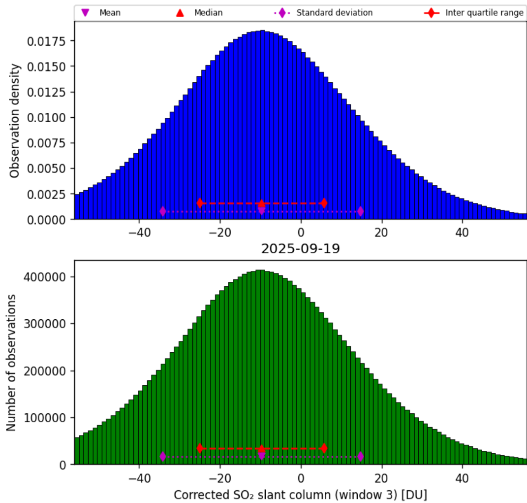
Figure 73: Histogram of “Corrected SO 2 slant column (window 3)” for 2025-09-18 to 2025-09-20
