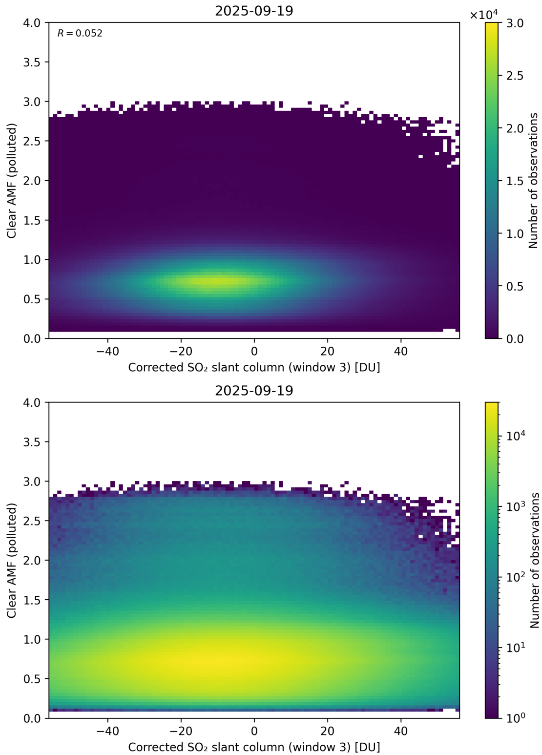
Figure 259: Scatter density plot of “Corrected SO 2 slant column (window 3)” against “Clear AMF (polluted)” for 2025-09-18 to 2025-09-20.
