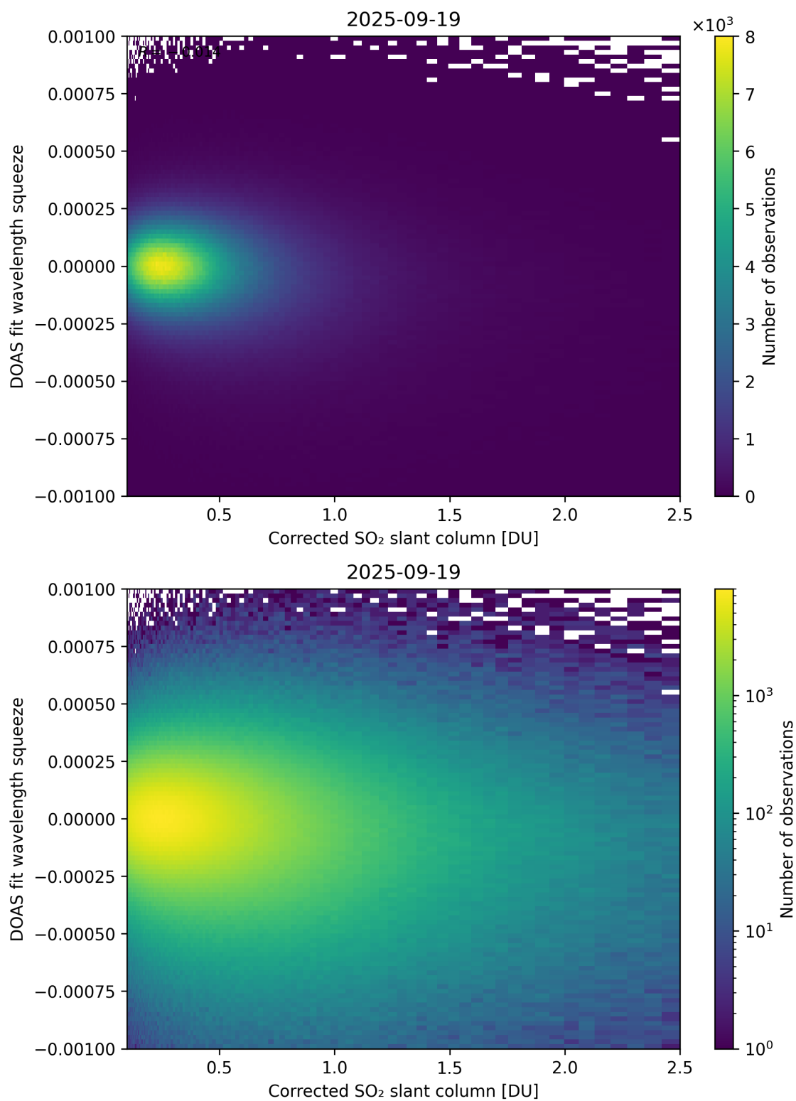
Figure 230: Scatter density plot of “Corrected SO 2 slant column” against “DOAS fit wavelength squeeze” for 2025-09-18 to 2025-09-20.
