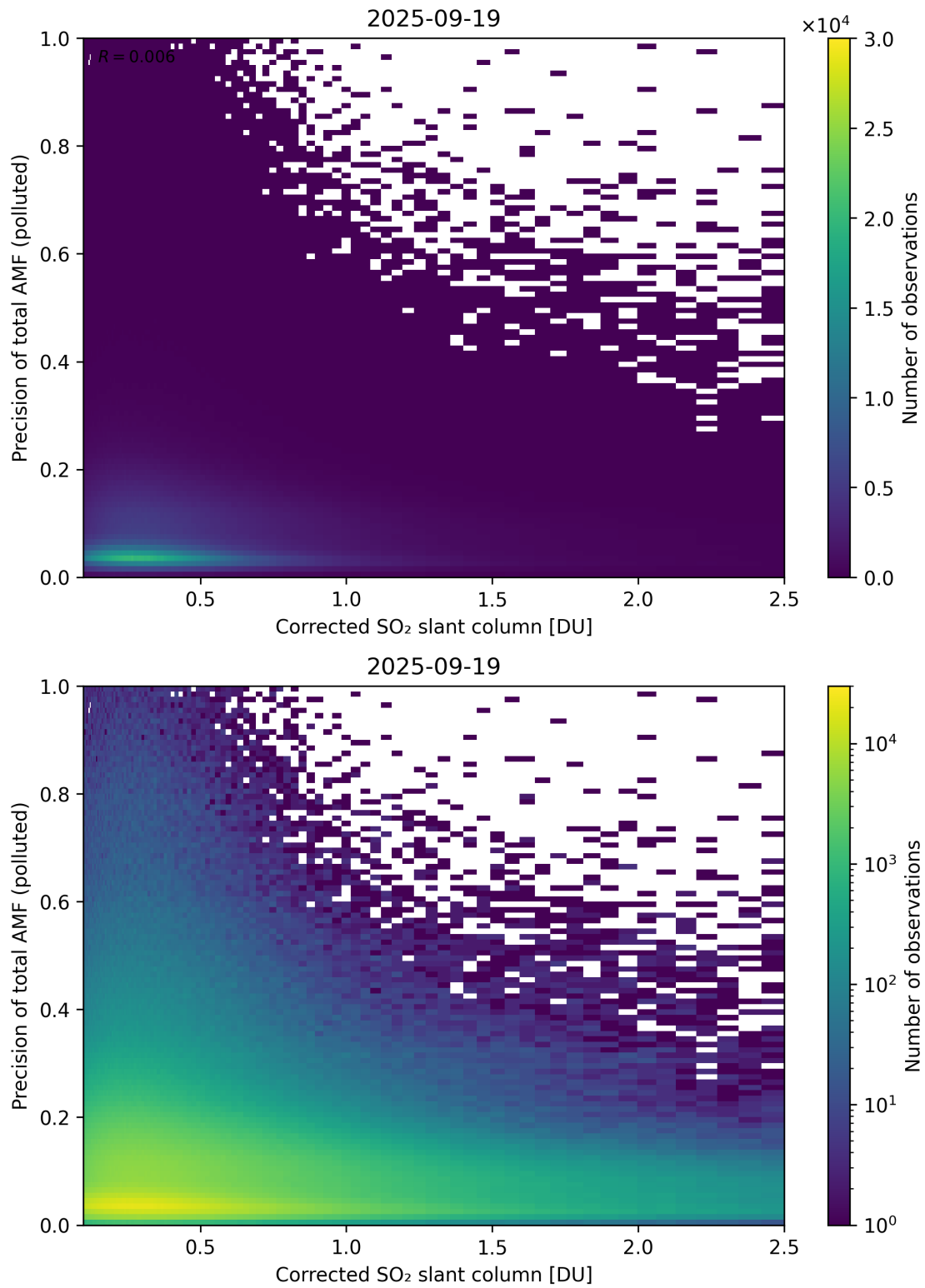
Figure 243: Scatter density plot of “Corrected SO 2 slant column” against “Precision of total AMF (polluted)” for 2025-09-18 to 2025-09-20.
