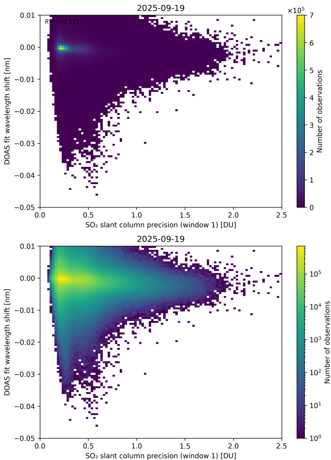
Figure 271: Scatter density plot of “SO 2 slant column precision (window 1)” against “DOAS fit wavelength shift” for 2025-09-18 to 2025-09-20.
