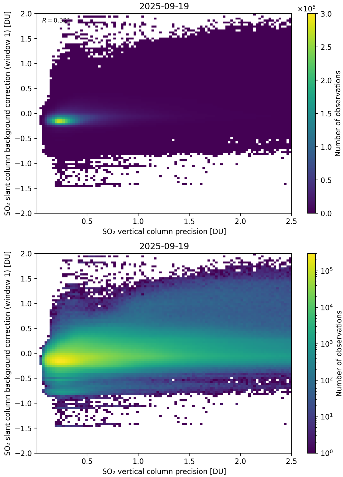
Figure 329: Scatter density plot of “SO 2 vertical column precision” against “SO 2 slant column background correction (window 1)” for 2025-09-18 to 2025-09-20.
