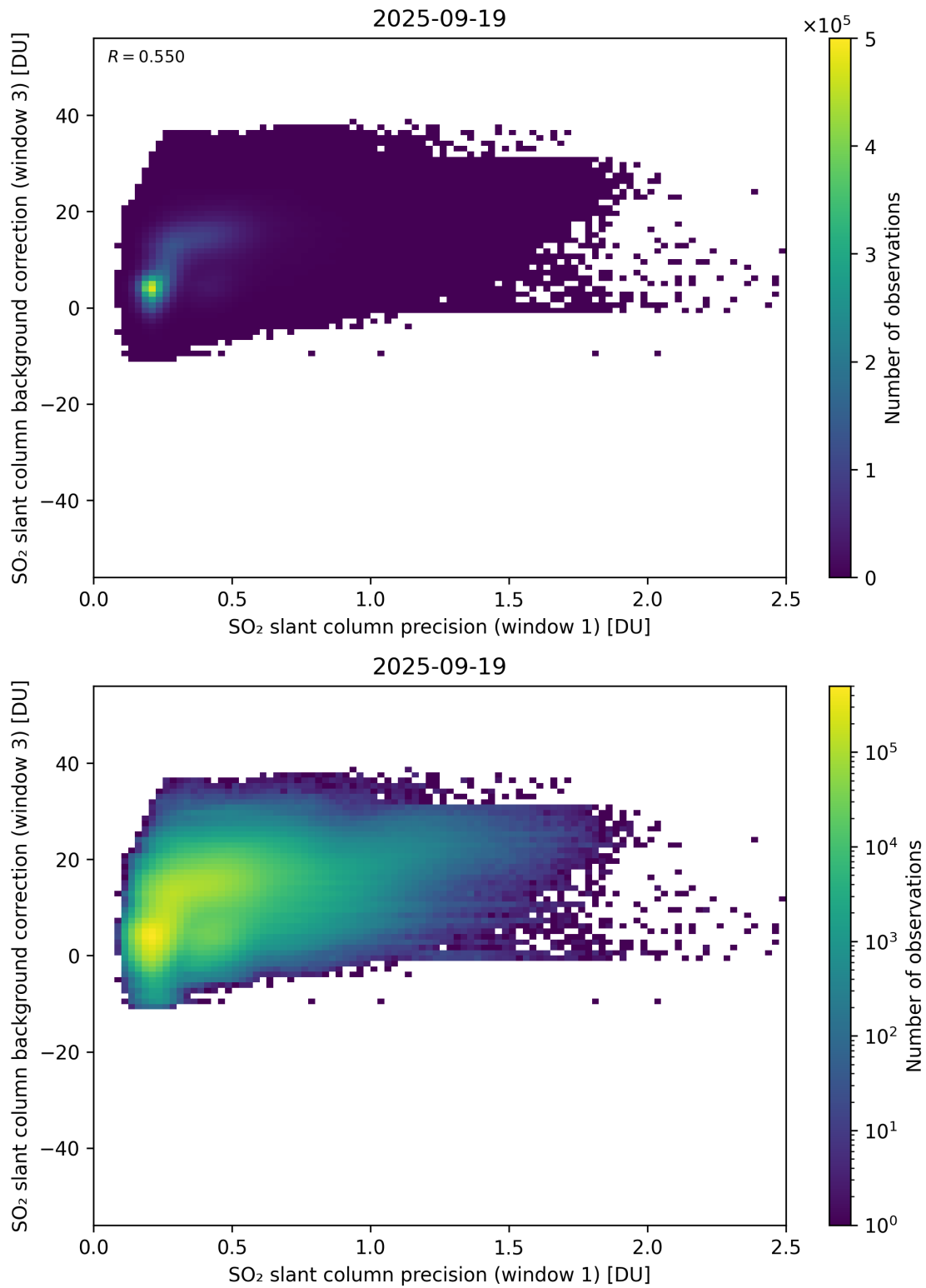
Figure 270: Scatter density plot of “SO 2 slant column precision (window 1)” against “SO 2 slant column background correction (window 3)” for 2025-09-18 to 2025-09-20.
