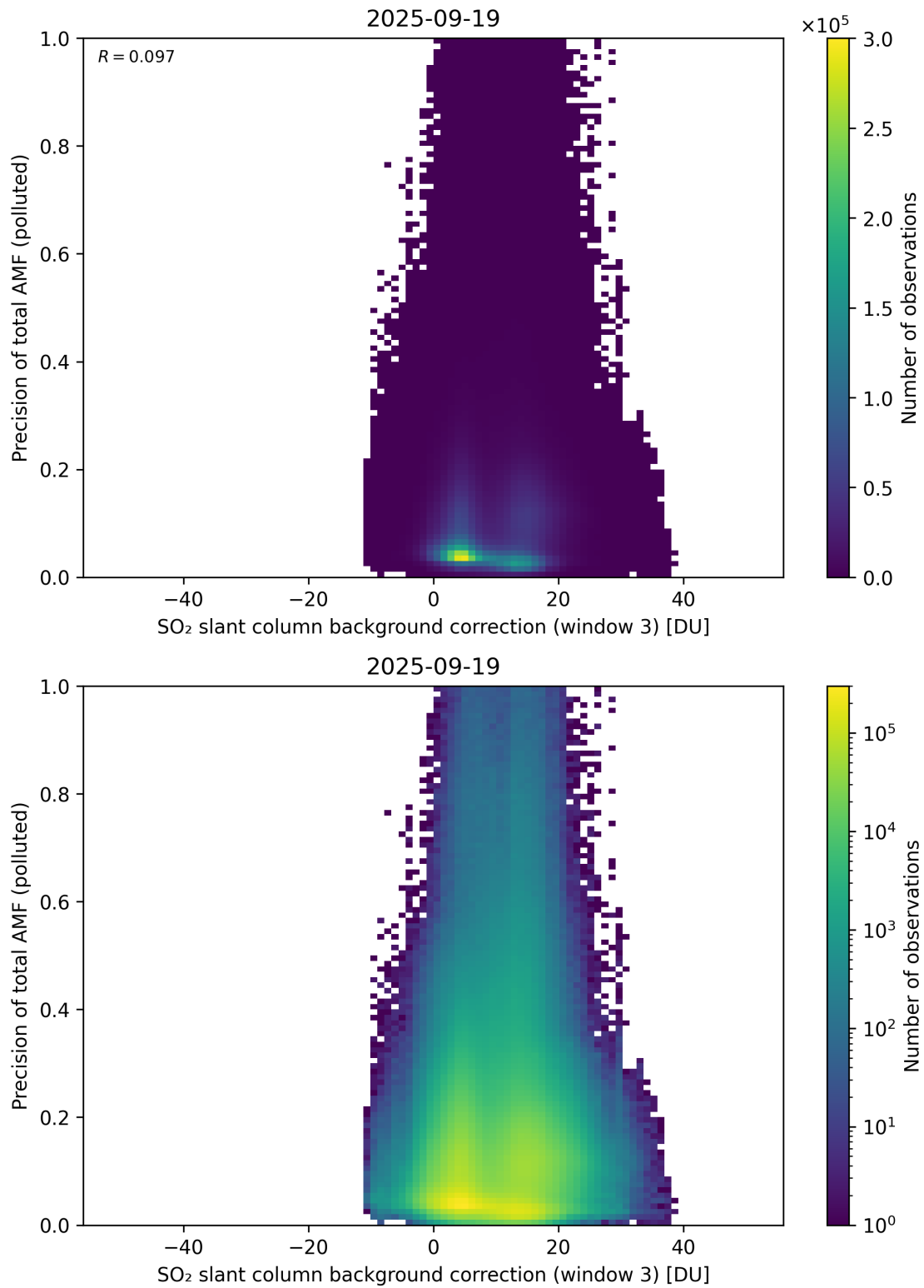
Figure 137: Scatter density plot of “SO 2 slant column background correction (window 3)” against “Precision of total AMF (polluted)” for 2025-09-18 to 2025-09-20.
