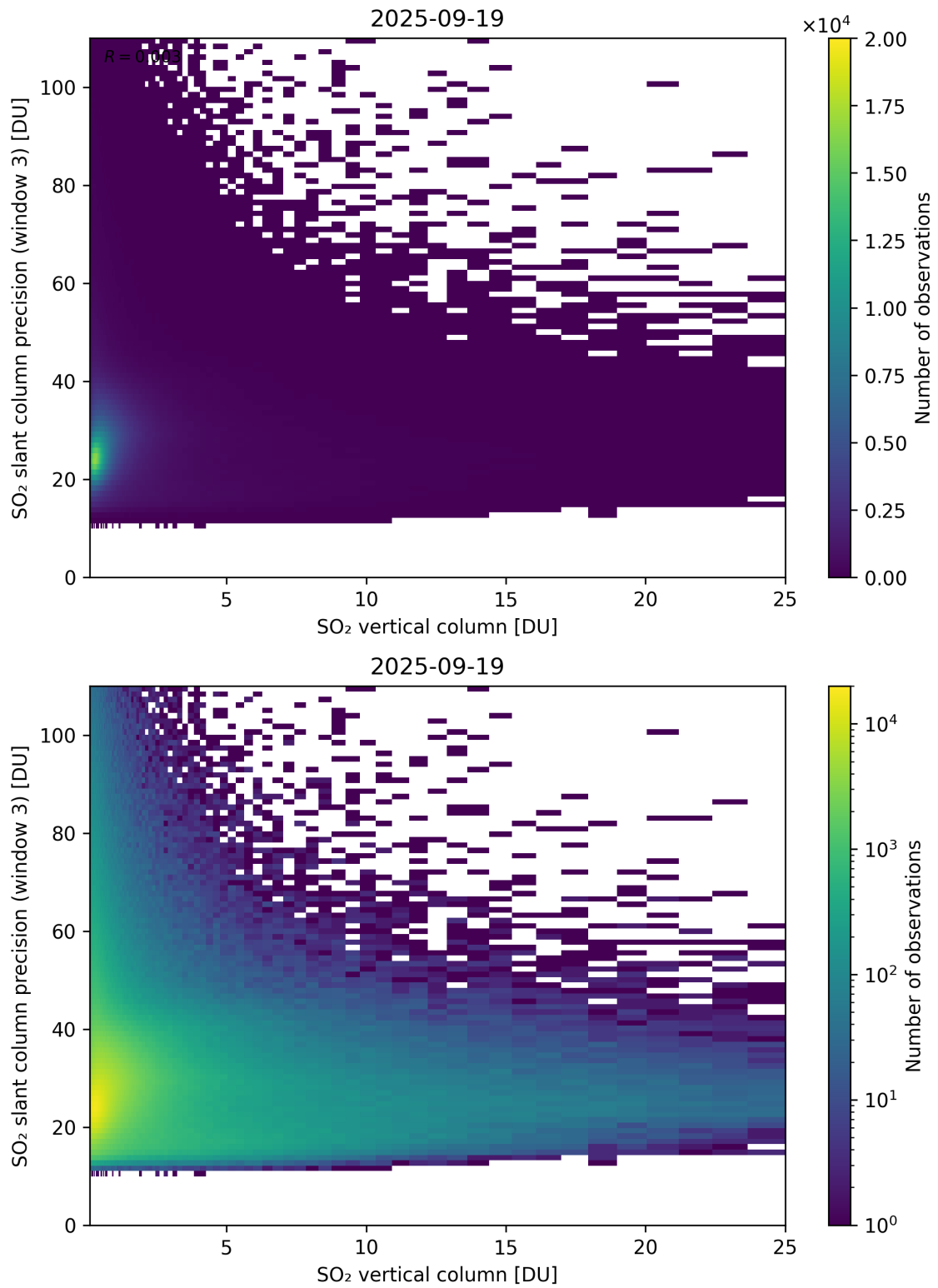
Figure 358: Scatter density plot of “SO 2 vertical column” against “SO 2 slant column precision (window 3)” for 2025-09-18 to 2025-09-20.
