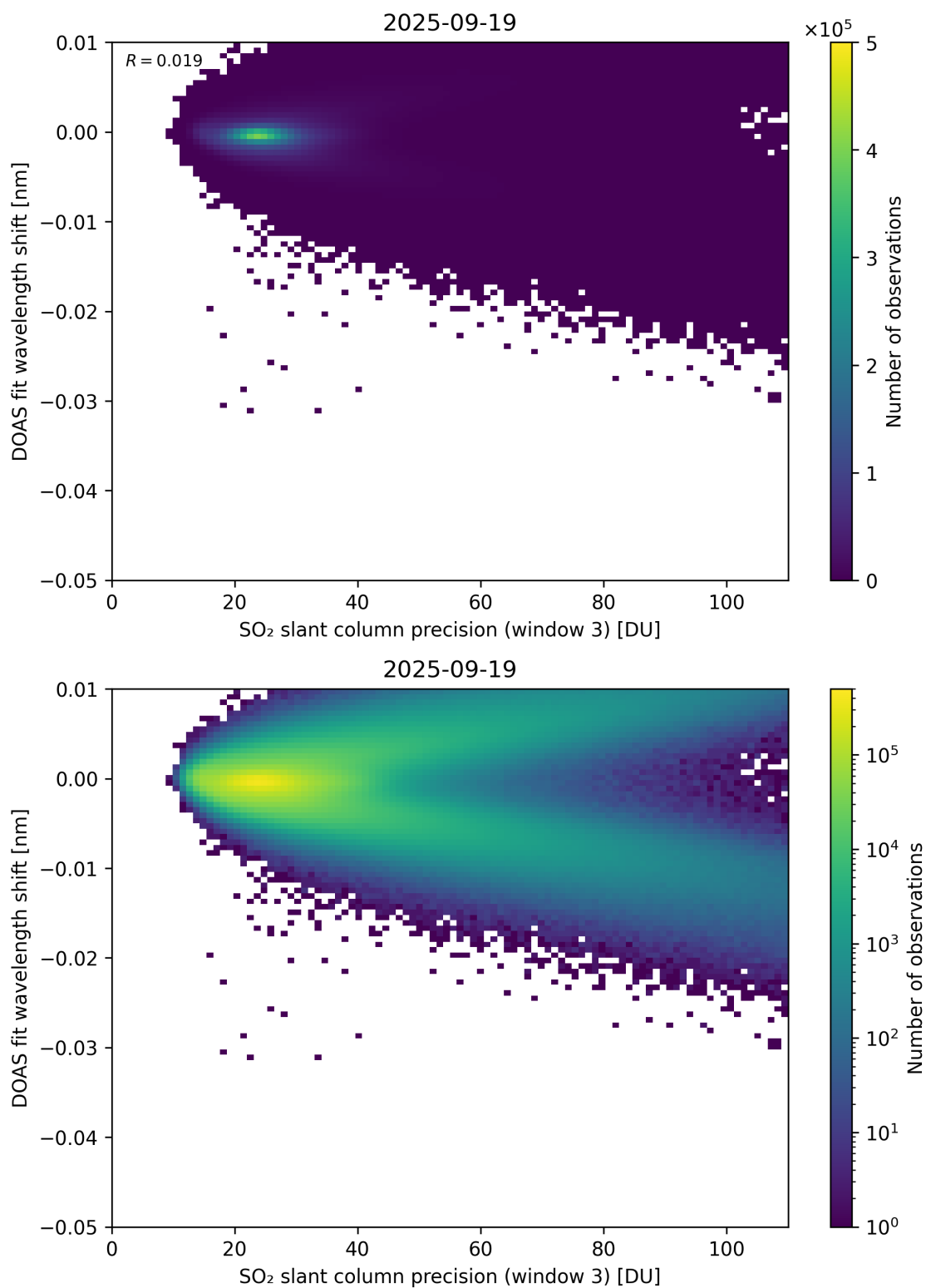
Figure 308: Scatter density plot of “SO 2 slant column precision (window 3)” against “DOAS fit wavelength shift” for 2025-09-18 to 2025-09-20.
