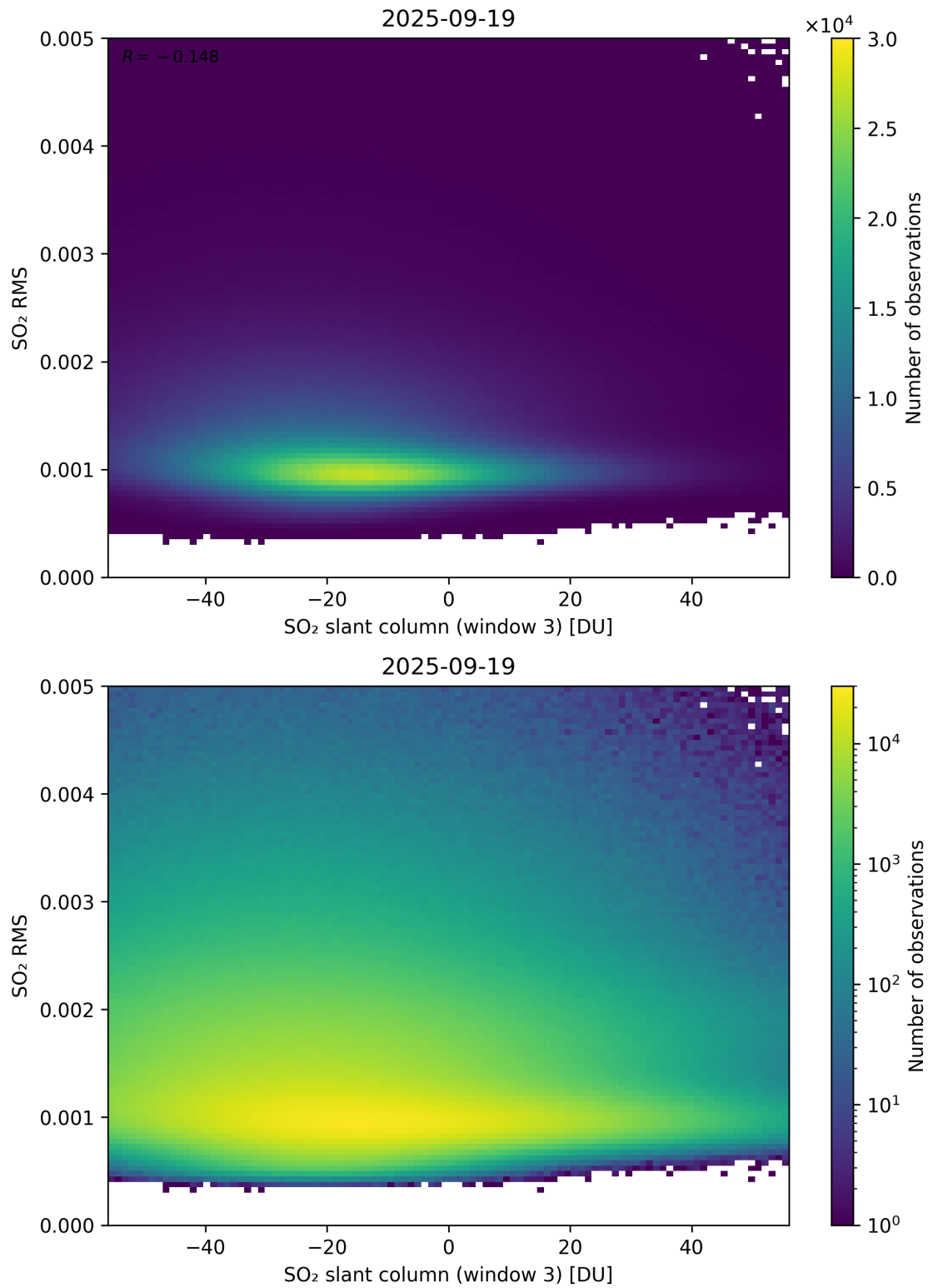
Figure 306: Scatter density plot of “SO 2 slant column (window 3)” against “SO 2 RMS” for 2025-09-18 to 2025-09-20.
