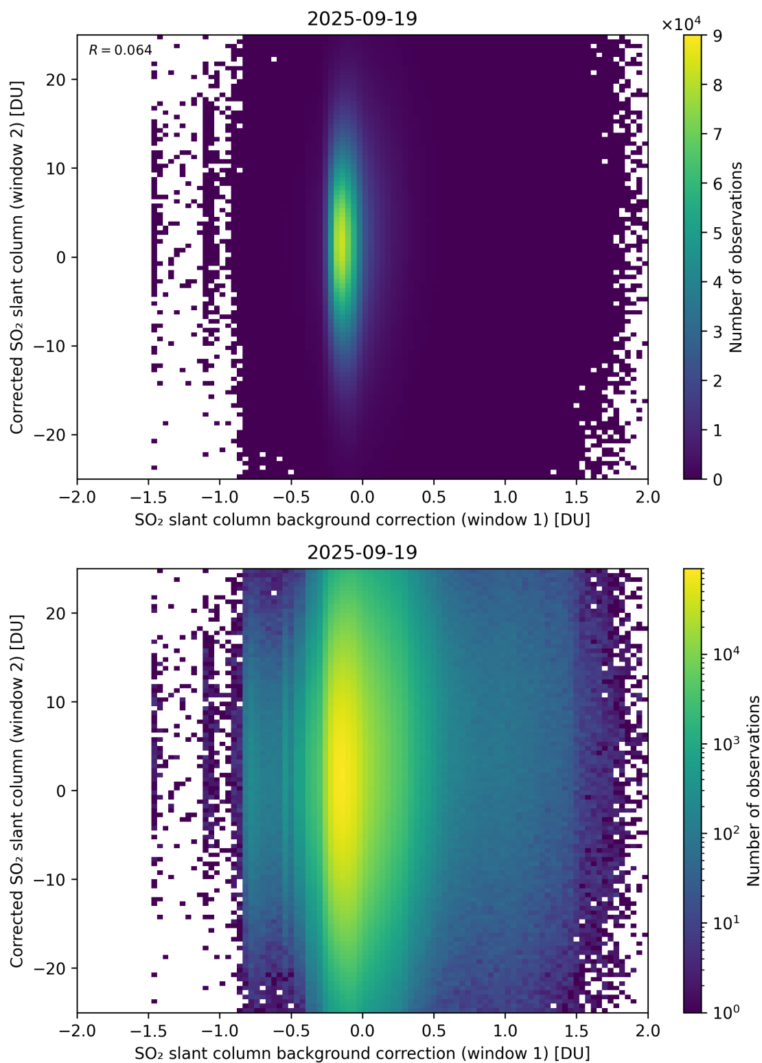
Figure 115: Scatter density plot of “SO 2 slant column background correction (window 1)” against “Corrected SO 2 slant column (window 2)” for 2025-09-18 to 2025-09-20.
