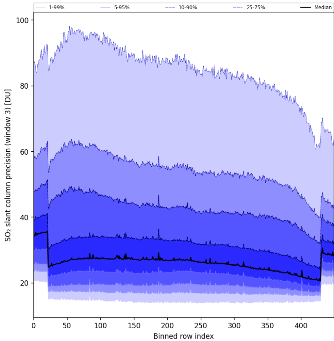
Figure 98: Along track statistics of “SO 2 slant column precision (window 3)” for 2025-09-18 to 2025-09-20
