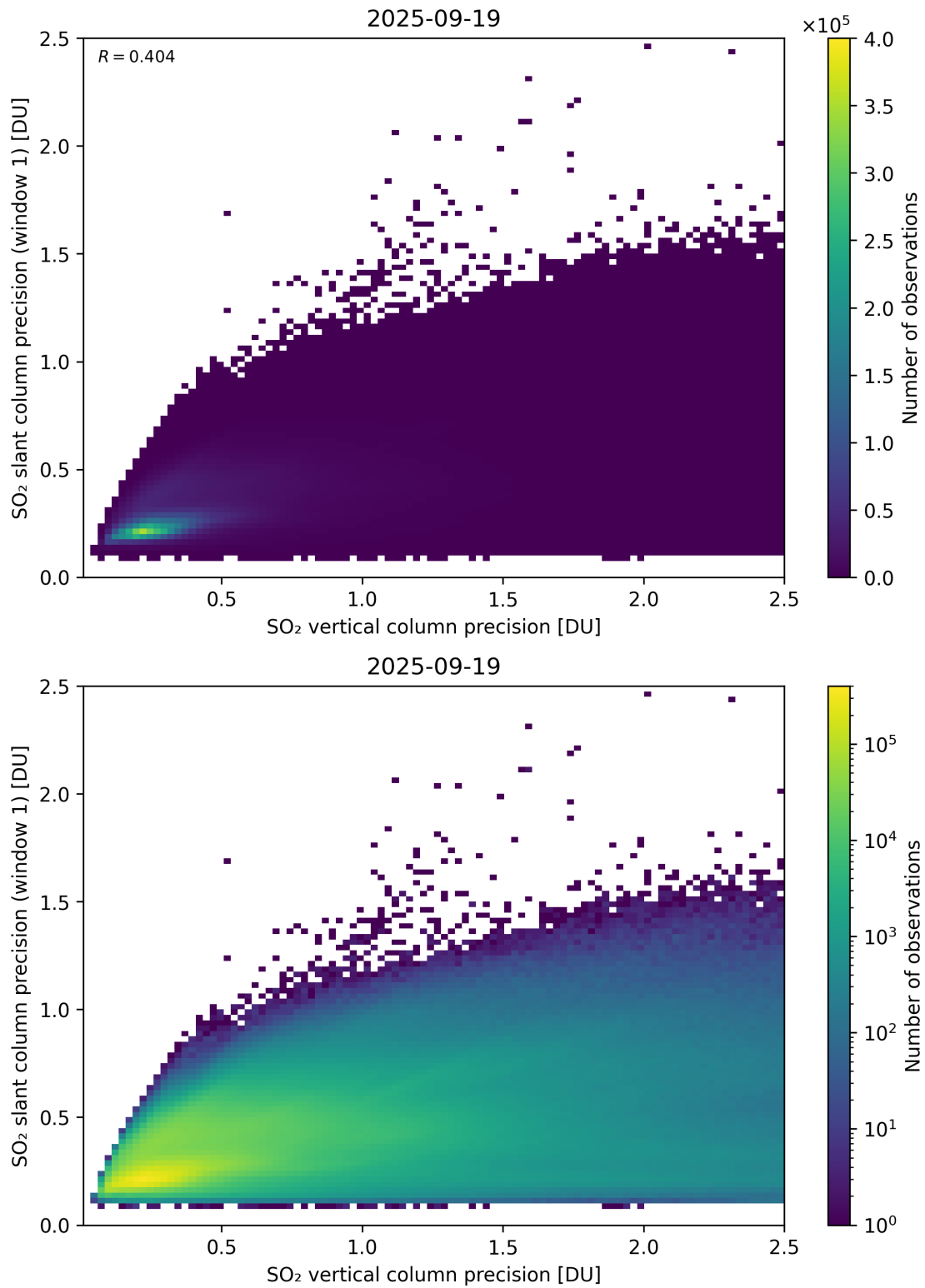
Figure 342: Scatter density plot of “SO 2 vertical column precision” against “SO 2 slant column precision (window 1)” for 2025-09-18 to 2025-09-20.
