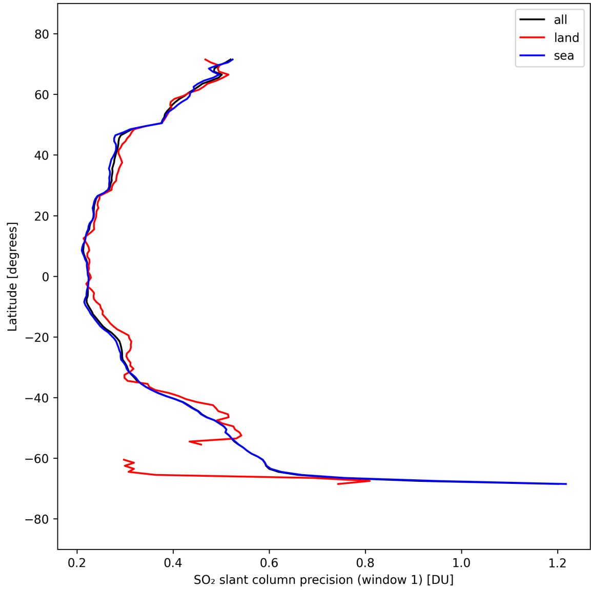
Figure 38: Zonal average of “SO 2 slant column precision (window 1)” for 2025-09-18 to 2025-09-20.
