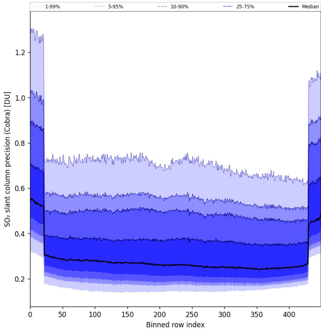
Figure 88: Along track statistics of “SO 2 slant column precision (Cobra)” for 2025-09-18 to 2025-09-20
