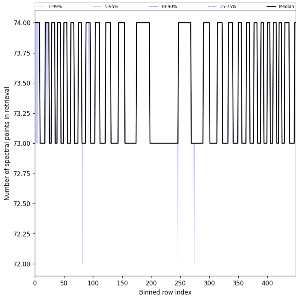
Figure 108: Along track statistics of “Number of spectral points in retrieval” for 2025-09-18 to 2025-09-20
