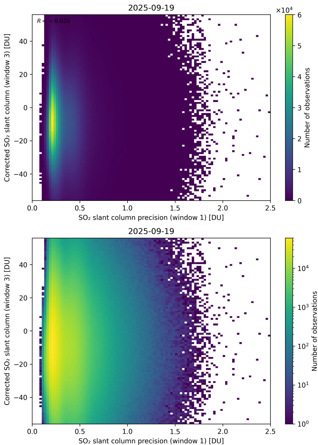
Figure 276: Scatter density plot of “SO 2 slant column precision (window 1)” against “Corrected SO 2 slant column (window 3)” for 2025-09-18 to 2025-09-20.
