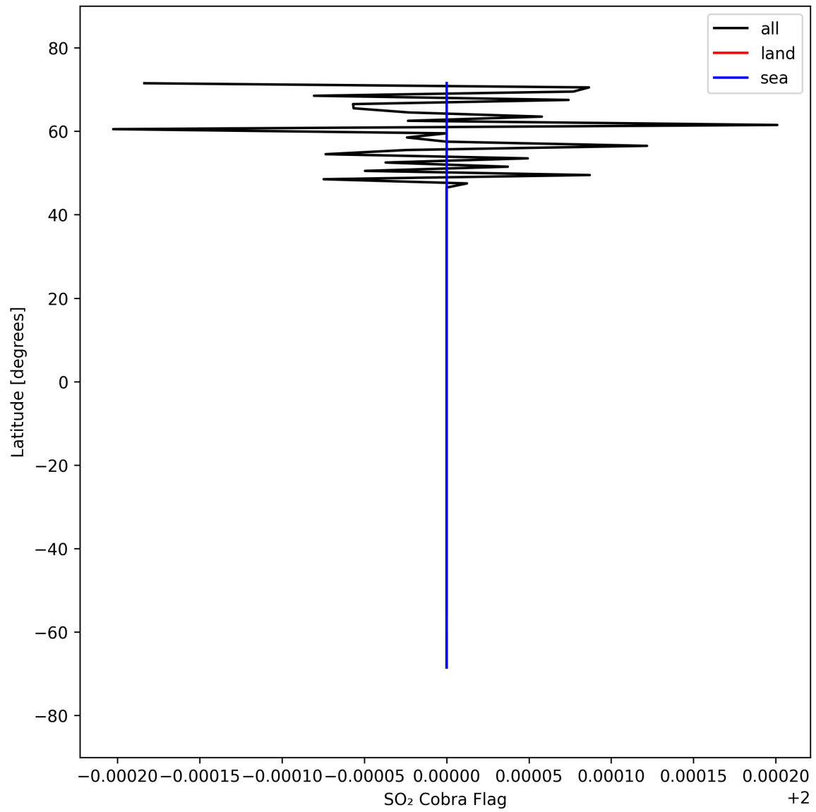
Figure 49: Zonal average of “SO 2 Cobra Flag” for 2025-09-18 to 2025-09-20.
