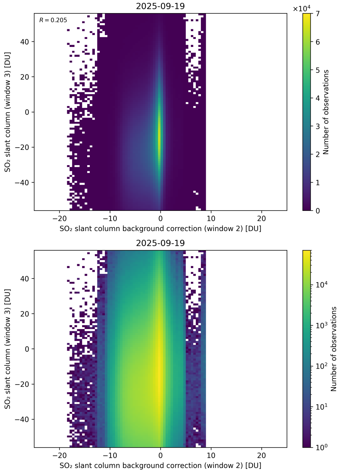
Figure 128: Scatter density plot of “SO 2 slant column background correction (window 2)” against “SO 2 slant column (window 3)” for 2025-09-18 to 2025-09-20.
