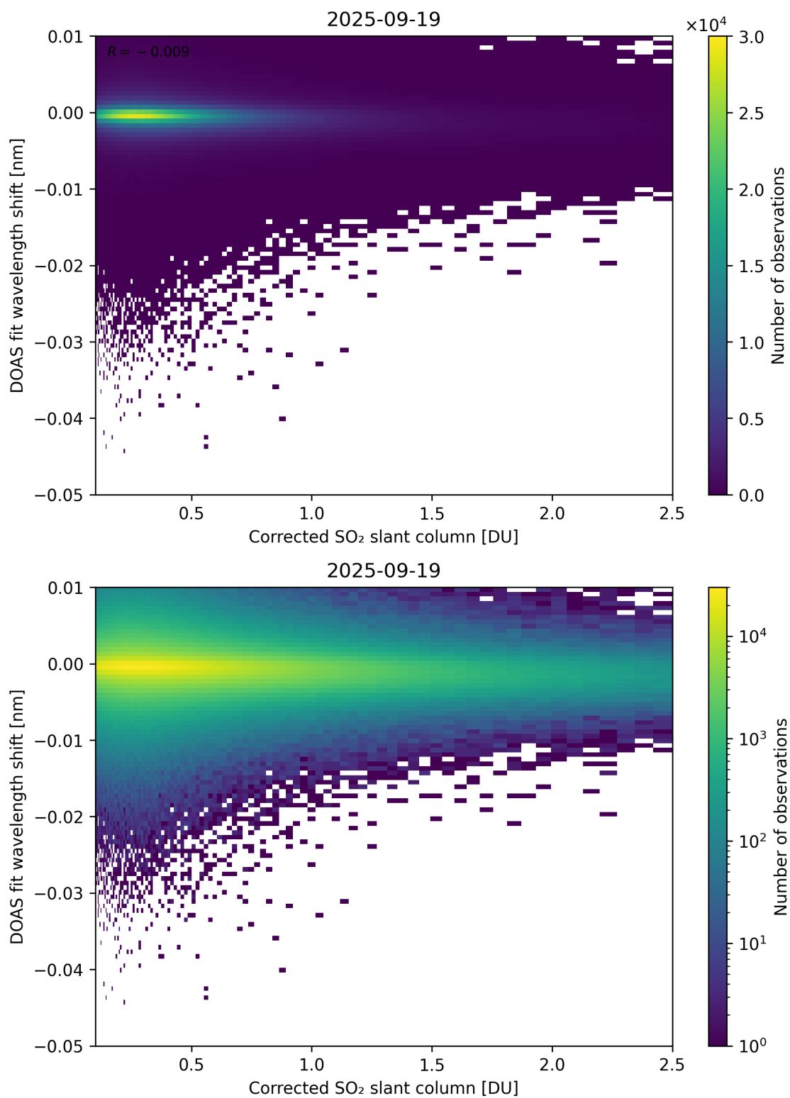
Figure 229: Scatter density plot of “Corrected SO 2 slant column” against “DOAS fit wavelength shift” for 2025-09-18 to 2025-09-20.
