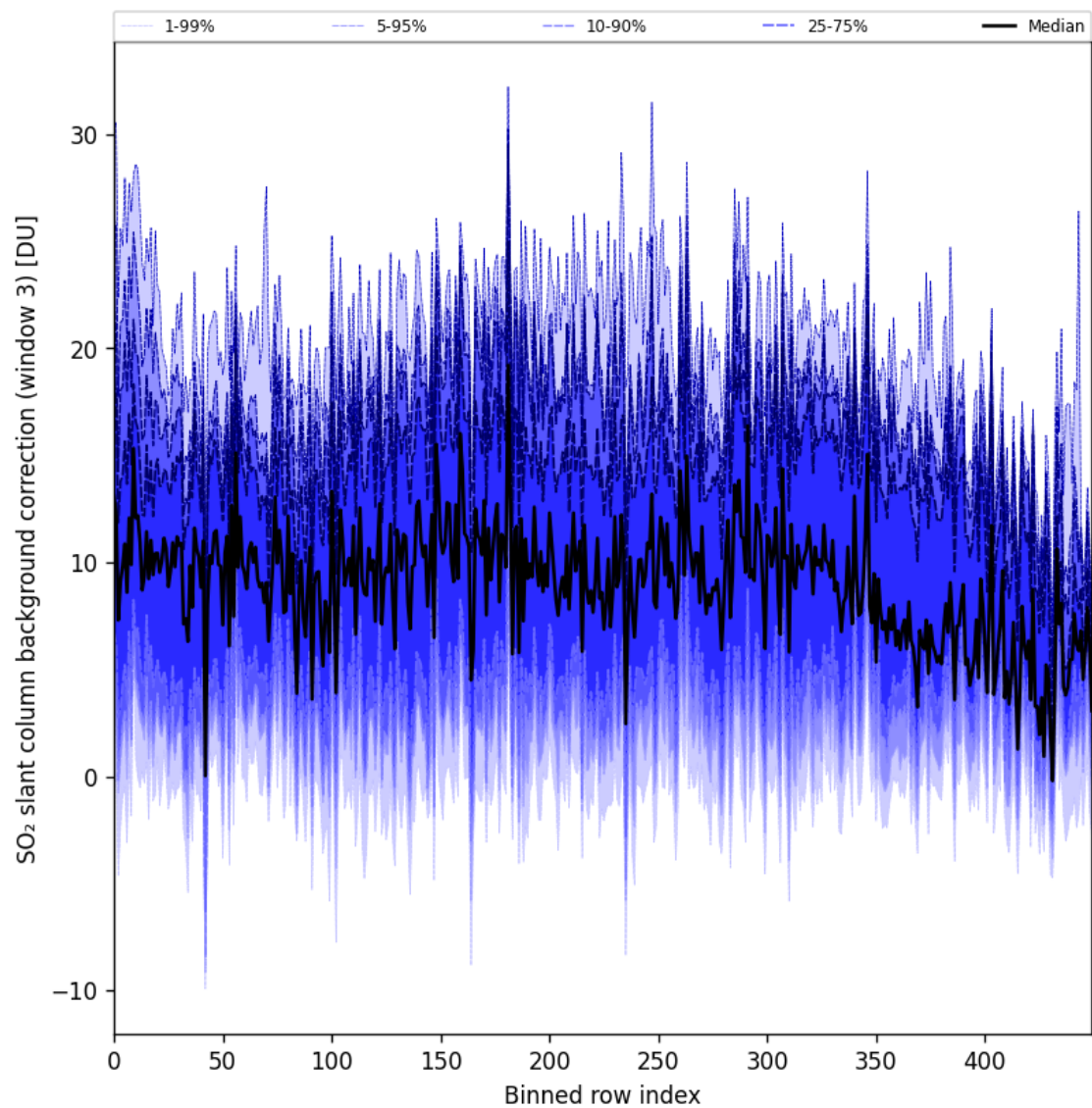
Figure 100: Along track statistics of “SO 2 slant column background correction (window 3)” for 2025-09-18 to 2025-09-20
