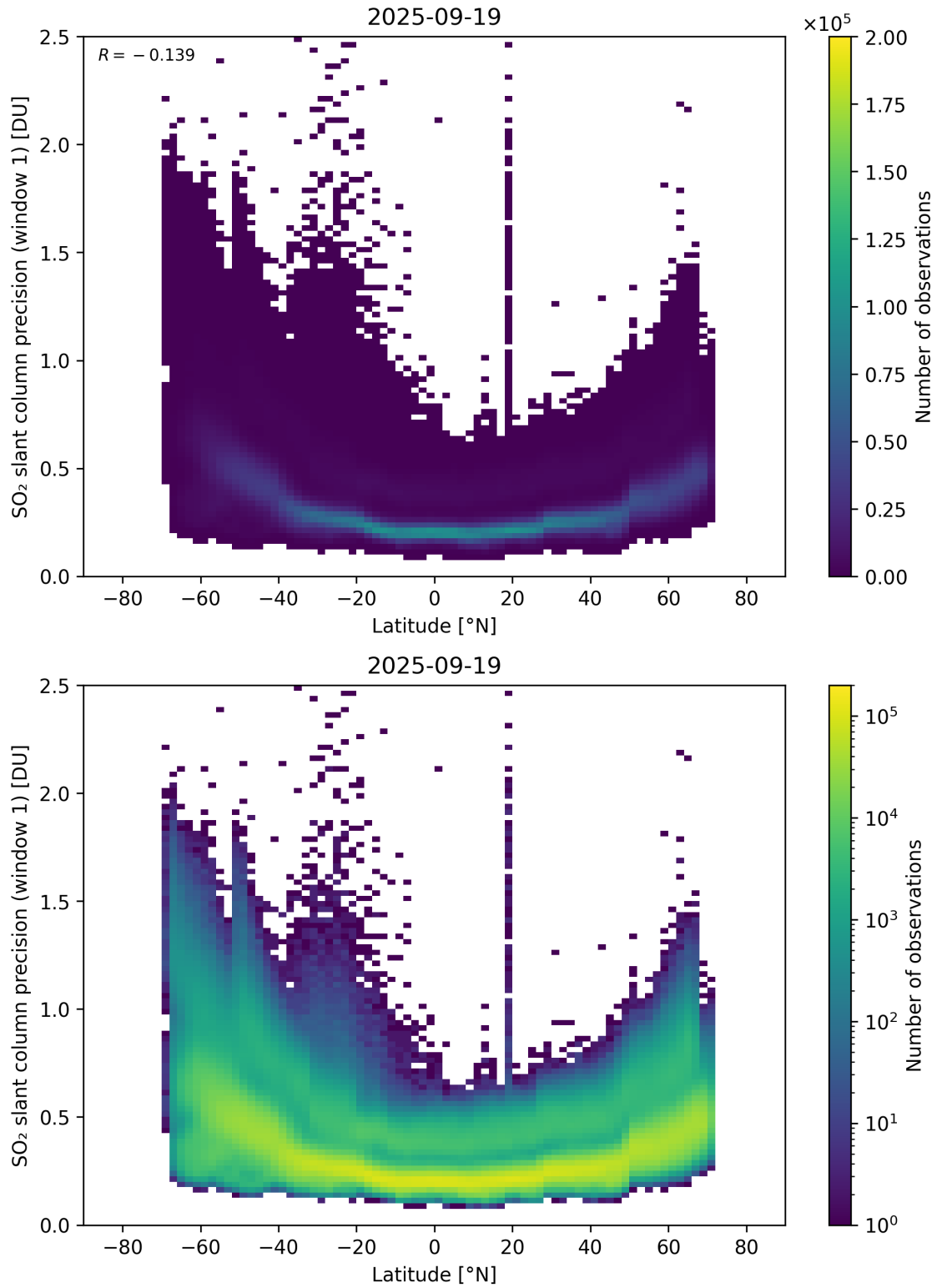
Figure 163: Scatter density plot of “Latitude” against “SO 2 slant column precision (window 1)” for 2025-09-18 to 2025-09-20.
