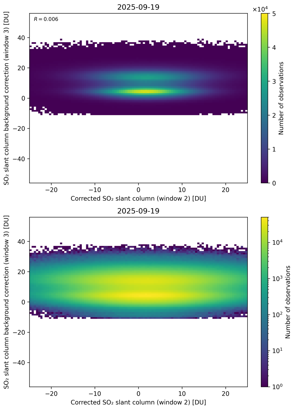
Figure 245: Scatter density plot of “Corrected SO 2 slant column (window 2)” against “SO 2 slant column background correction (window 3)” for 2025-09-18 to 2025-09-20.
