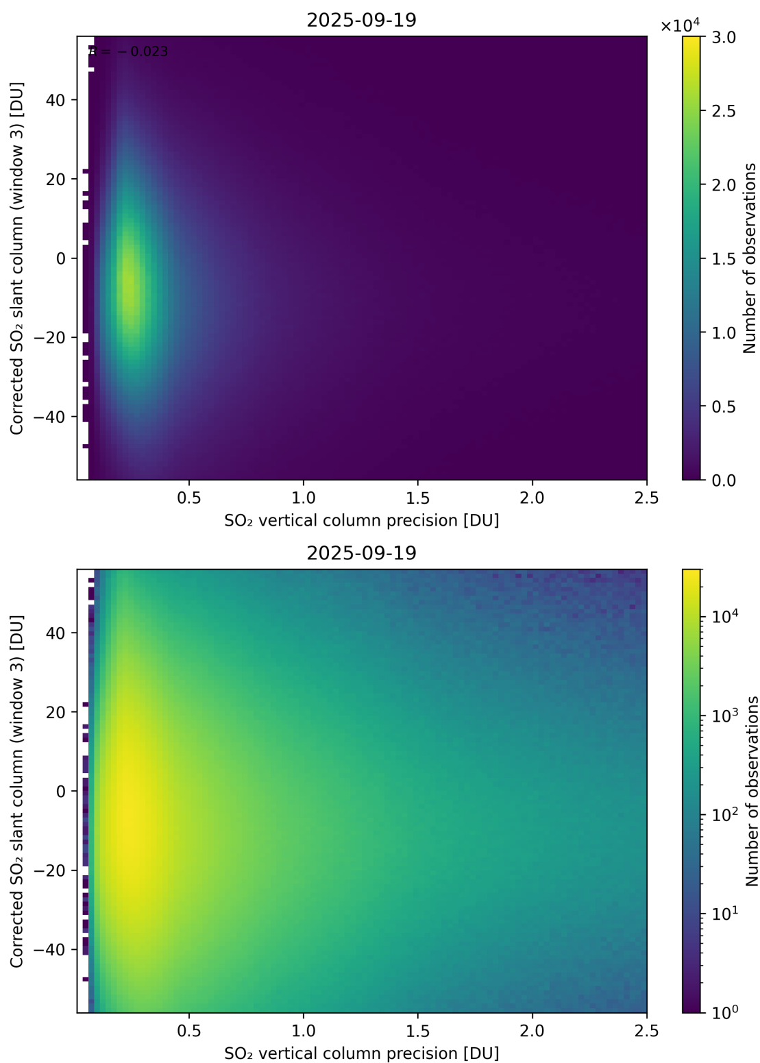
Figure 340: Scatter density plot of “SO 2 vertical column precision” against “Corrected SO 2 slant column (window 3)” for 2025-09-18 to 2025-09-20.
