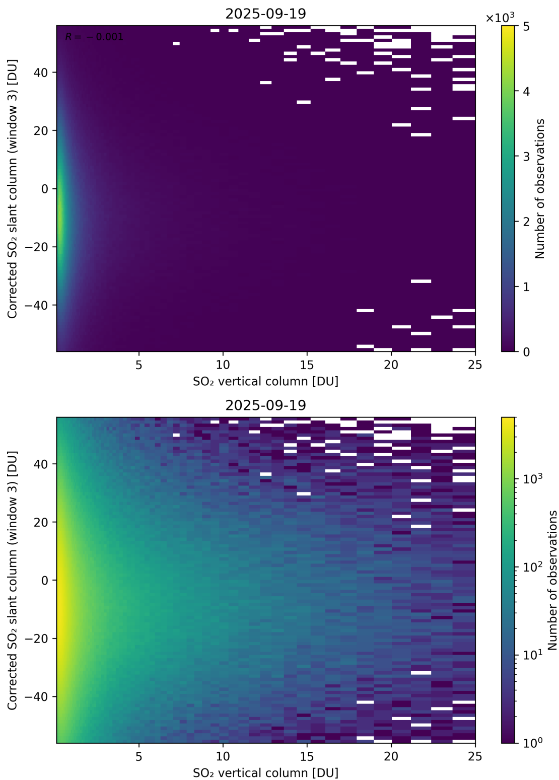
Figure 353: Scatter density plot of “SO 2 vertical column” against “Corrected SO 2 slant column (window 3)” for 2025-09-18 to 2025-09-20.
