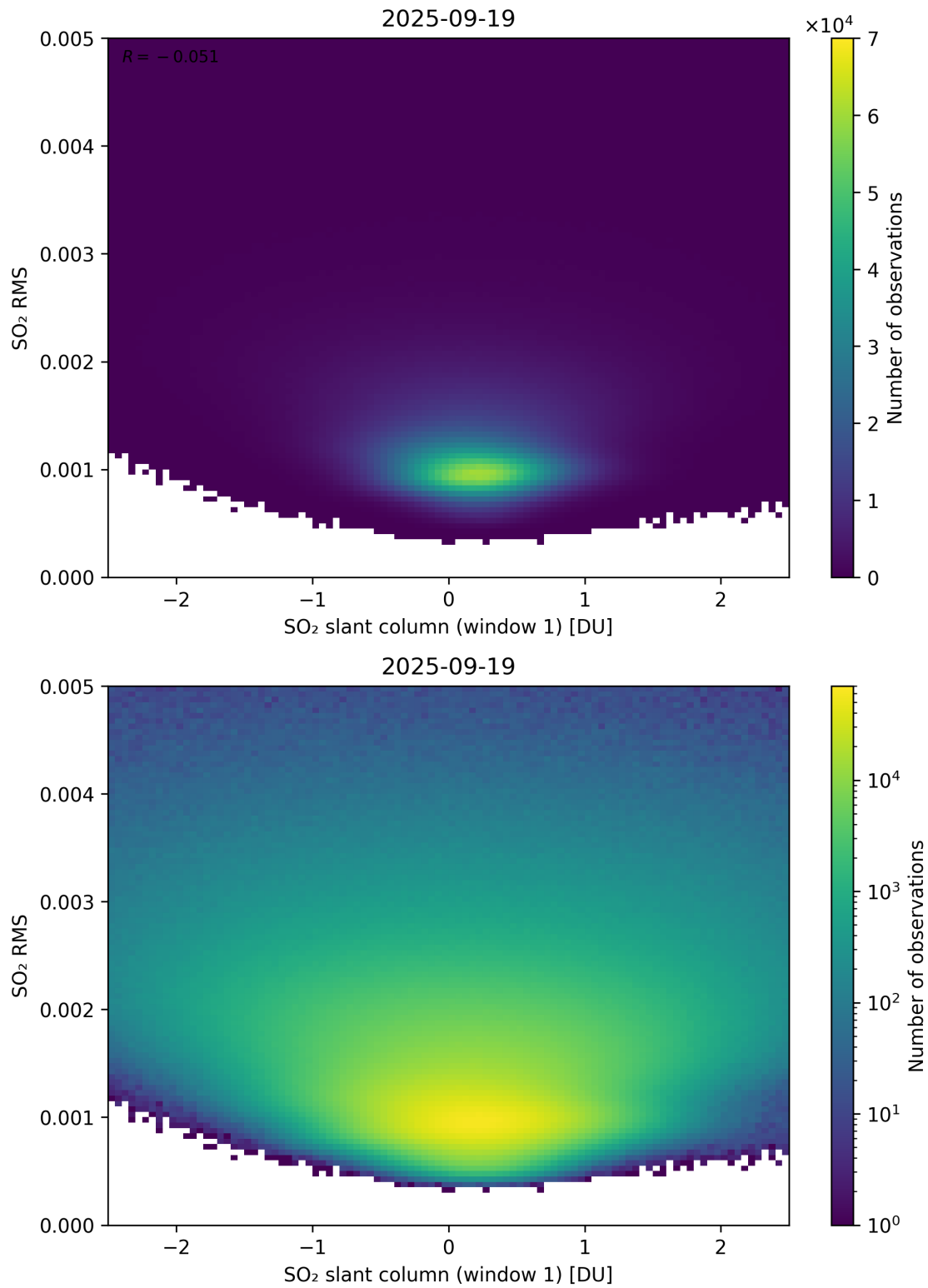
Figure 267: Scatter density plot of “SO 2 slant column (window 1)” against “SO 2 RMS” for 2025-09-18 to 2025-09-20.
