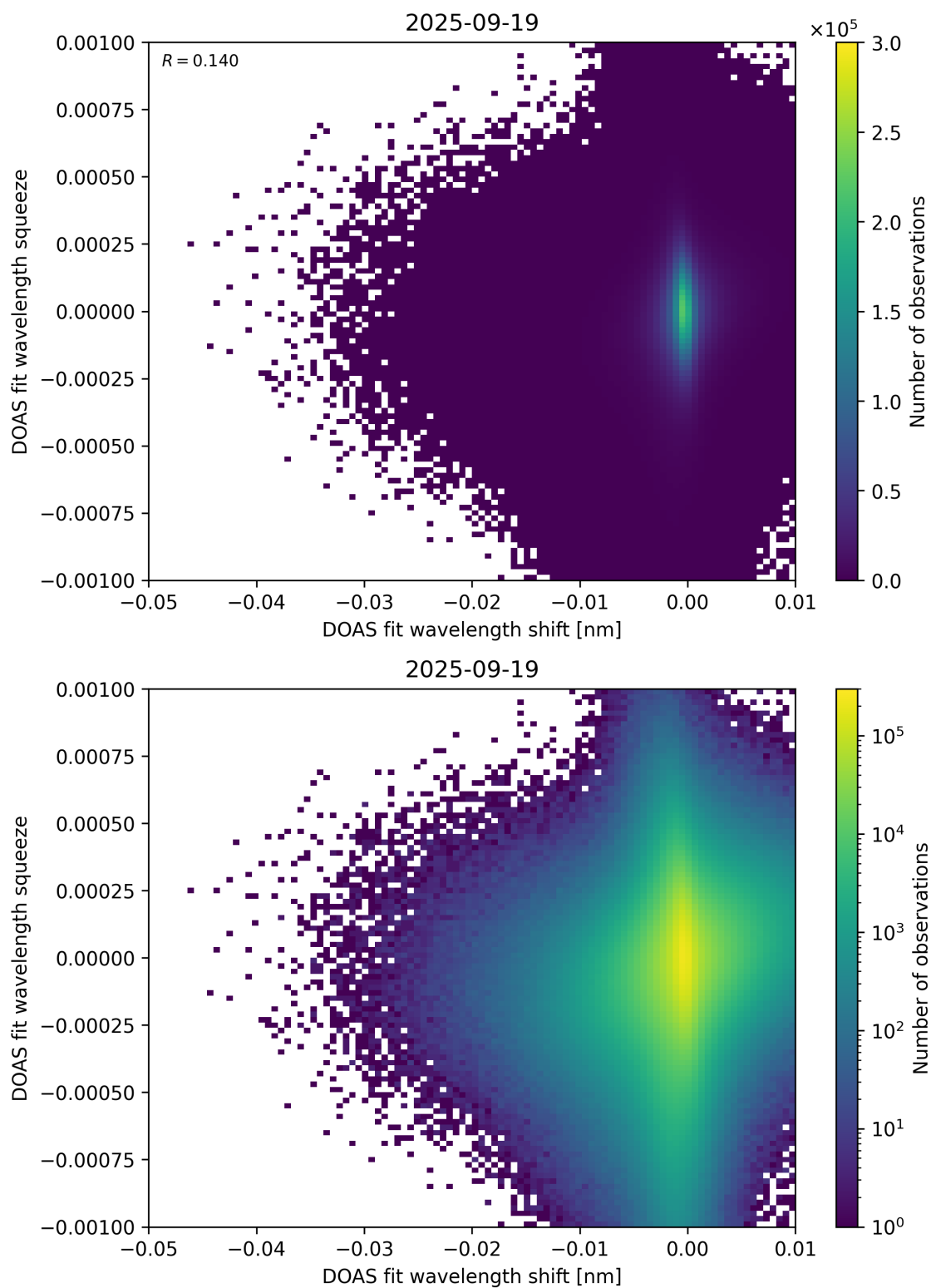
Figure 138: Scatter density plot of “DOAS fit wavelength shift” against “DOAS fit wavelength squeeze” for 2025-09-18 to 2025-09-20.
