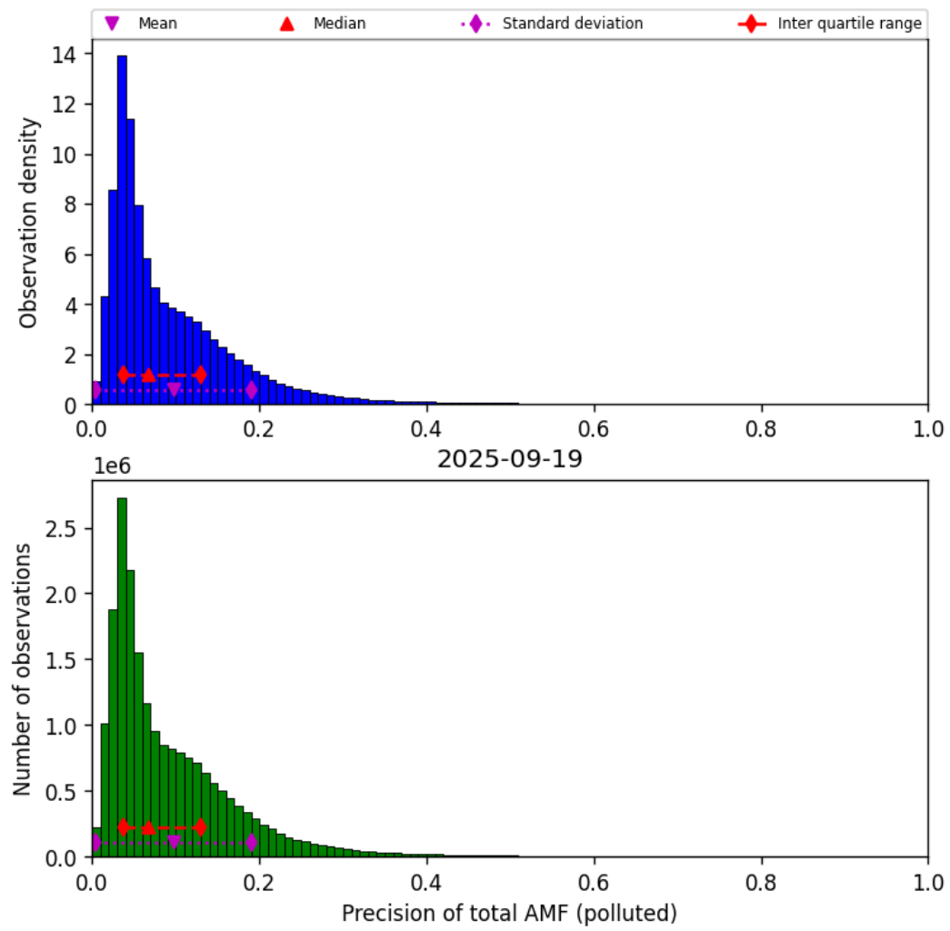
Figure 80: Histogram of “Precision of total AMF (polluted)” for 2025-09-18 to 2025-09-20
