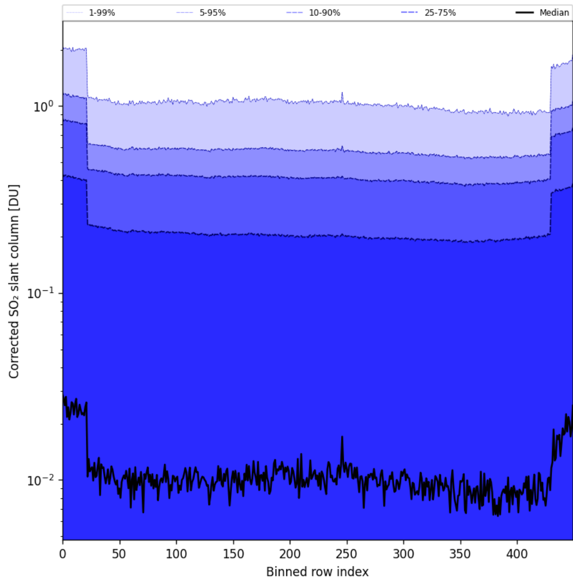
Figure 86: Along track statistics of “Corrected SO 2 slant column” for 2025-09-18 to 2025-09-20
