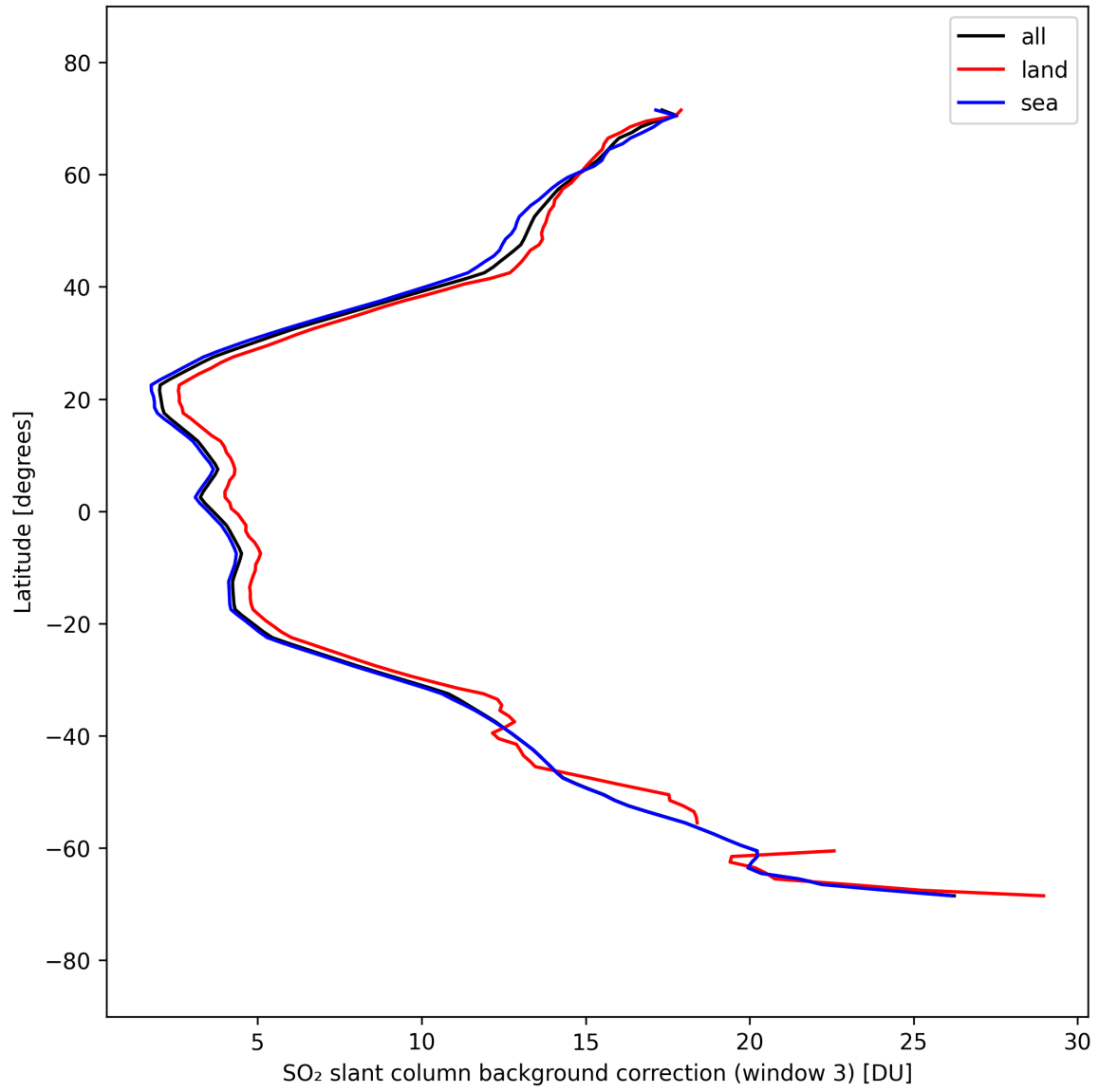
Figure 48: Zonal average of "SO 2 slant column background correction (window 3)" for 2025-09-18 to 2025-09-20.
