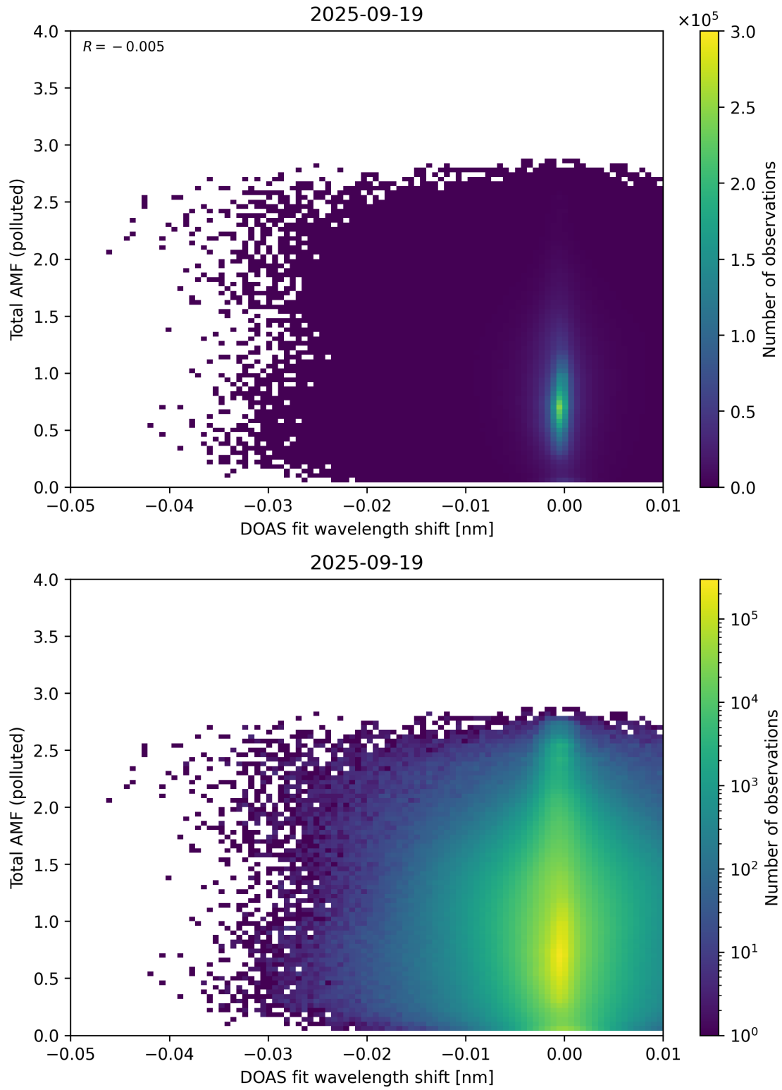
Figure 141: Scatter density plot of “DOAS fit wavelength shift” against “Total AMF (polluted)” for 2025-09-18 to 2025-09-20.
