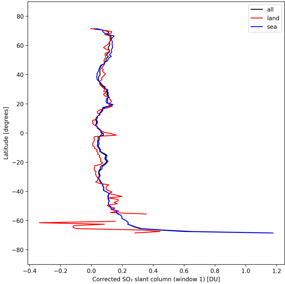
Figure 39: Zonal average of “Corrected SO 2 slant column (window 1)” for 2025-09-18 to 2025-09-20.
