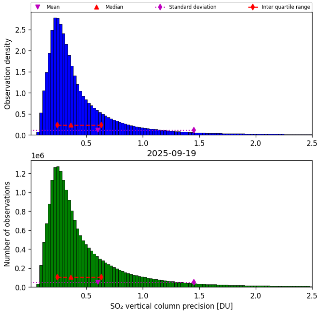
Figure 59: Histogram of “SO 2 vertical column precision” for 2025-09-18 to 2025-09-20
