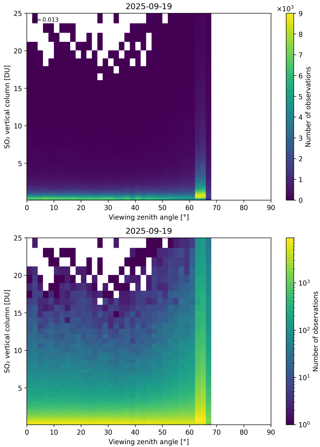
Figure 383: Scatter density plot of “Viewing zenith angle” against “SO 2 vertical column” for 2025-09-18 to 2025-09-20.
