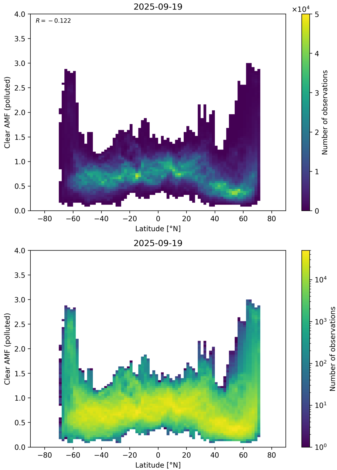
Figure 156: Scatter density plot of “Latitude” against “Clear AMF (polluted)” for 2025-09-18 to 2025-09-20.
