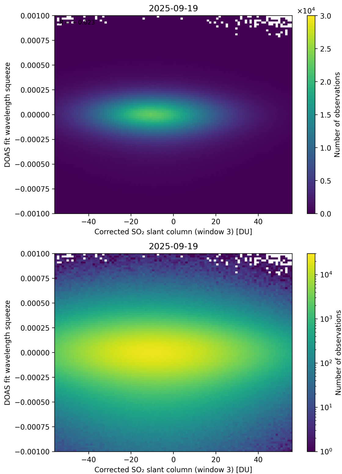
Figure 257: Scatter density plot of “Corrected SO 2 slant column (window 3)” against “DOAS fit wavelength squeeze” for 2025-09-18 to 2025-09-20.
