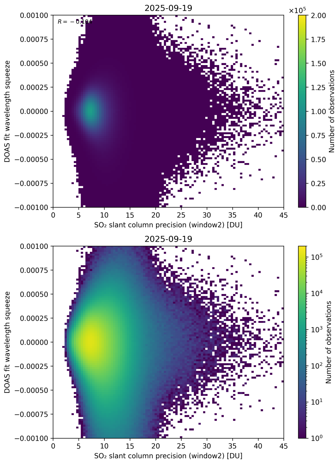
Figure 294: Scatter density plot of “SO 2 slant column precision (window2)” against “DOAS fit wavelength squeeze” for 2025-09-18 to 2025-09-20.
