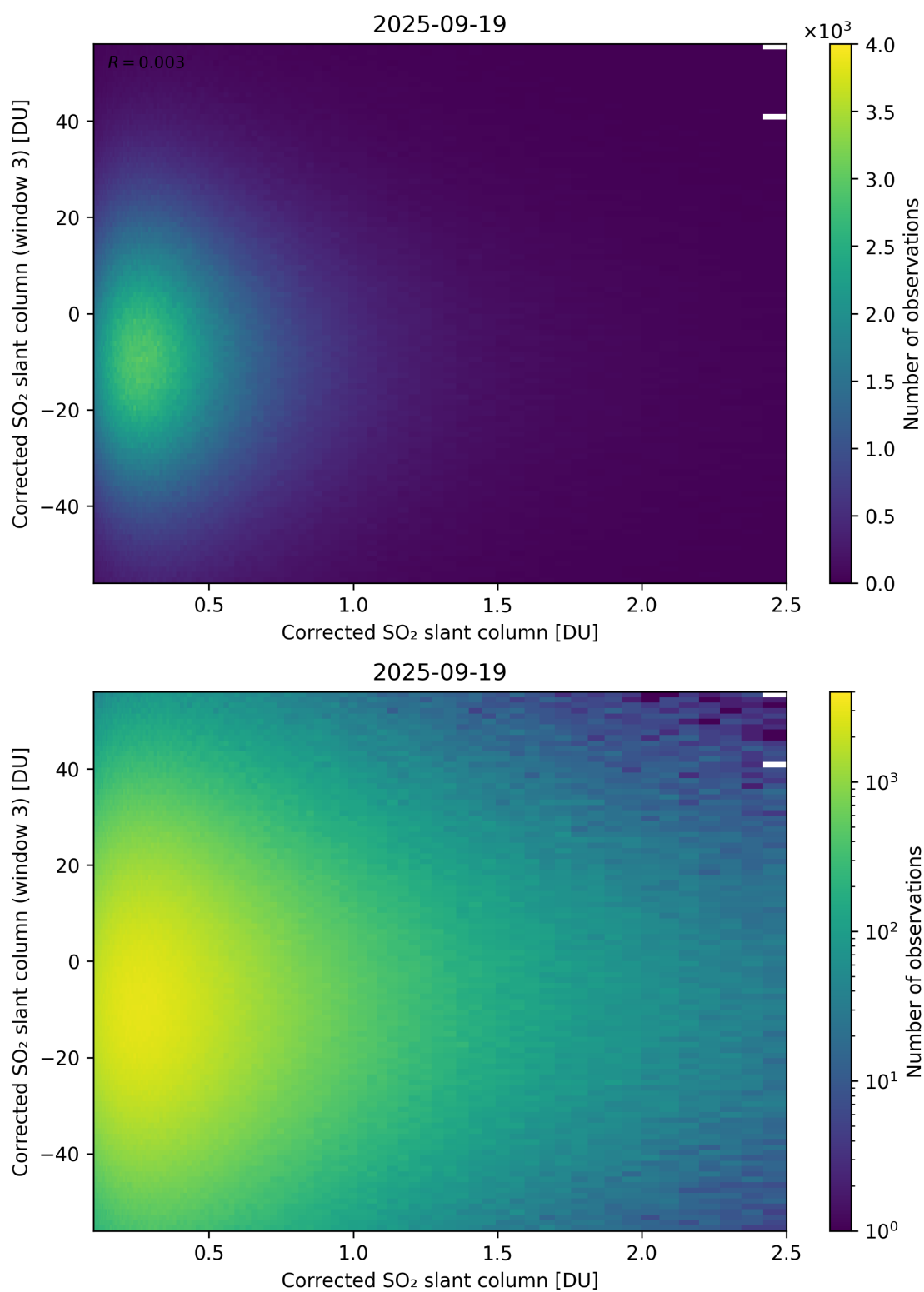
Figure 236: Scatter density plot of “Corrected SO 2 slant column” against “Corrected SO 2 slant column (window 3)” for 2025-09-18 to 2025-09-20.
