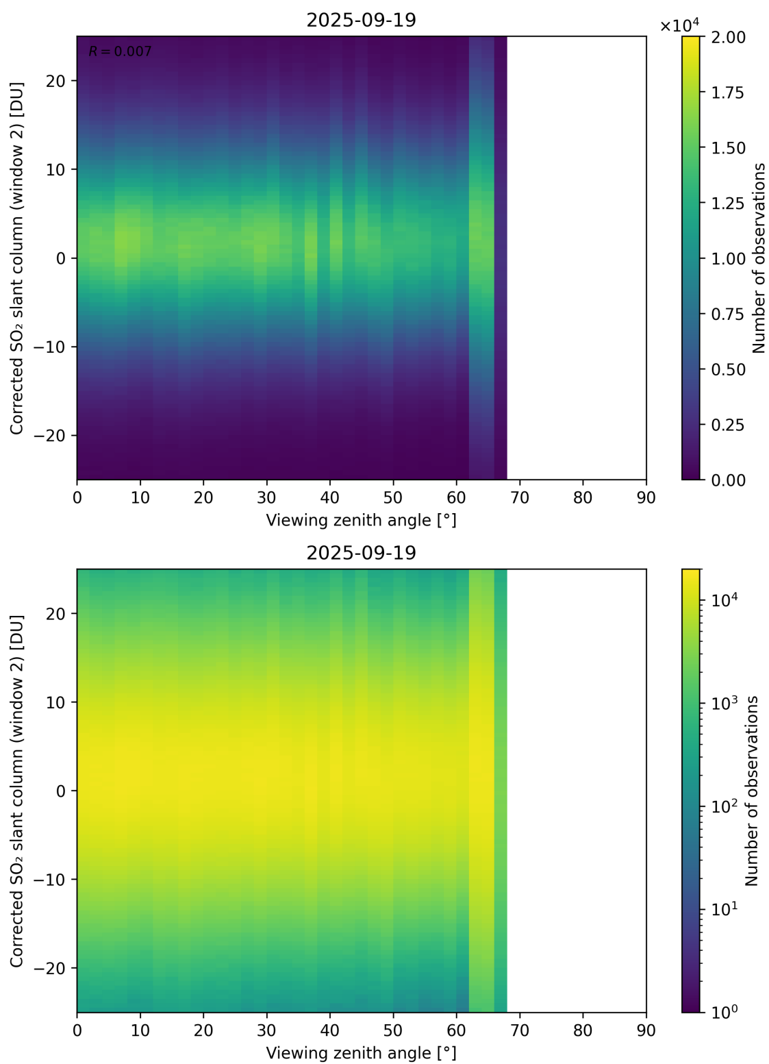
Figure 374: Scatter density plot of “Viewing zenith angle” against “Corrected SO 2 slant column (window 2)” for 2025-09-18 to 2025-09-20.
