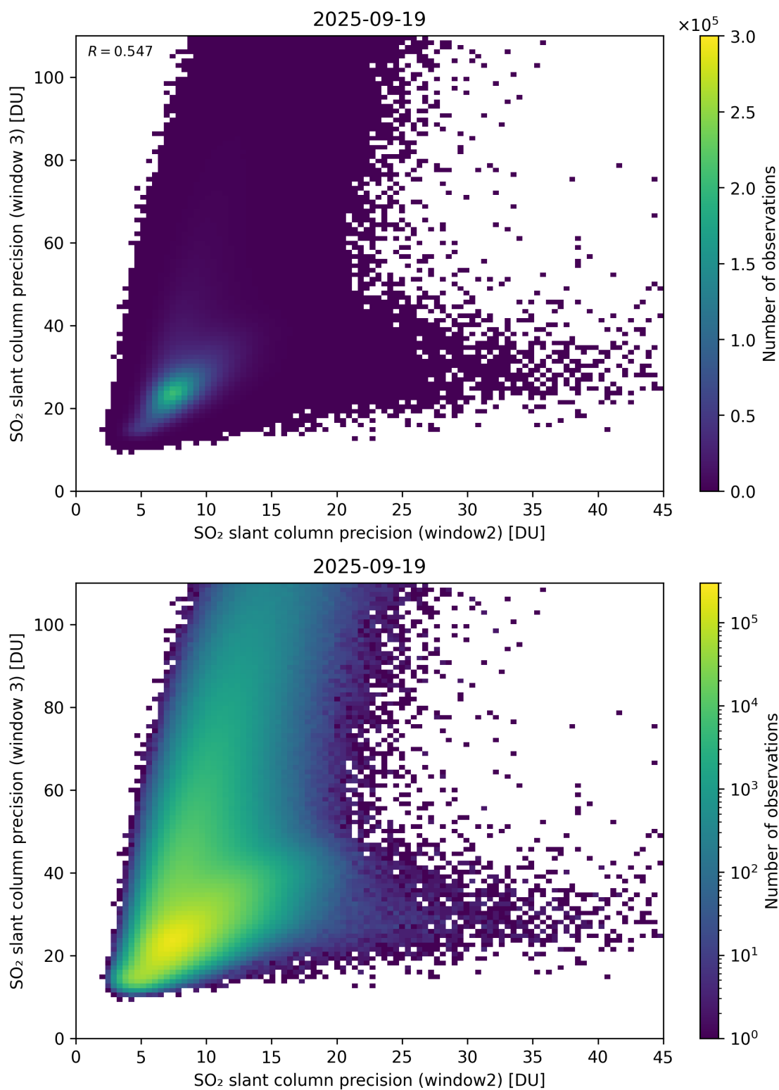
Figure 300: Scatter density plot of “SO 2 slant column precision (window2)” against “SO 2 slant column precision (window 3)” for 2025-09-18 to 2025-09-20.
