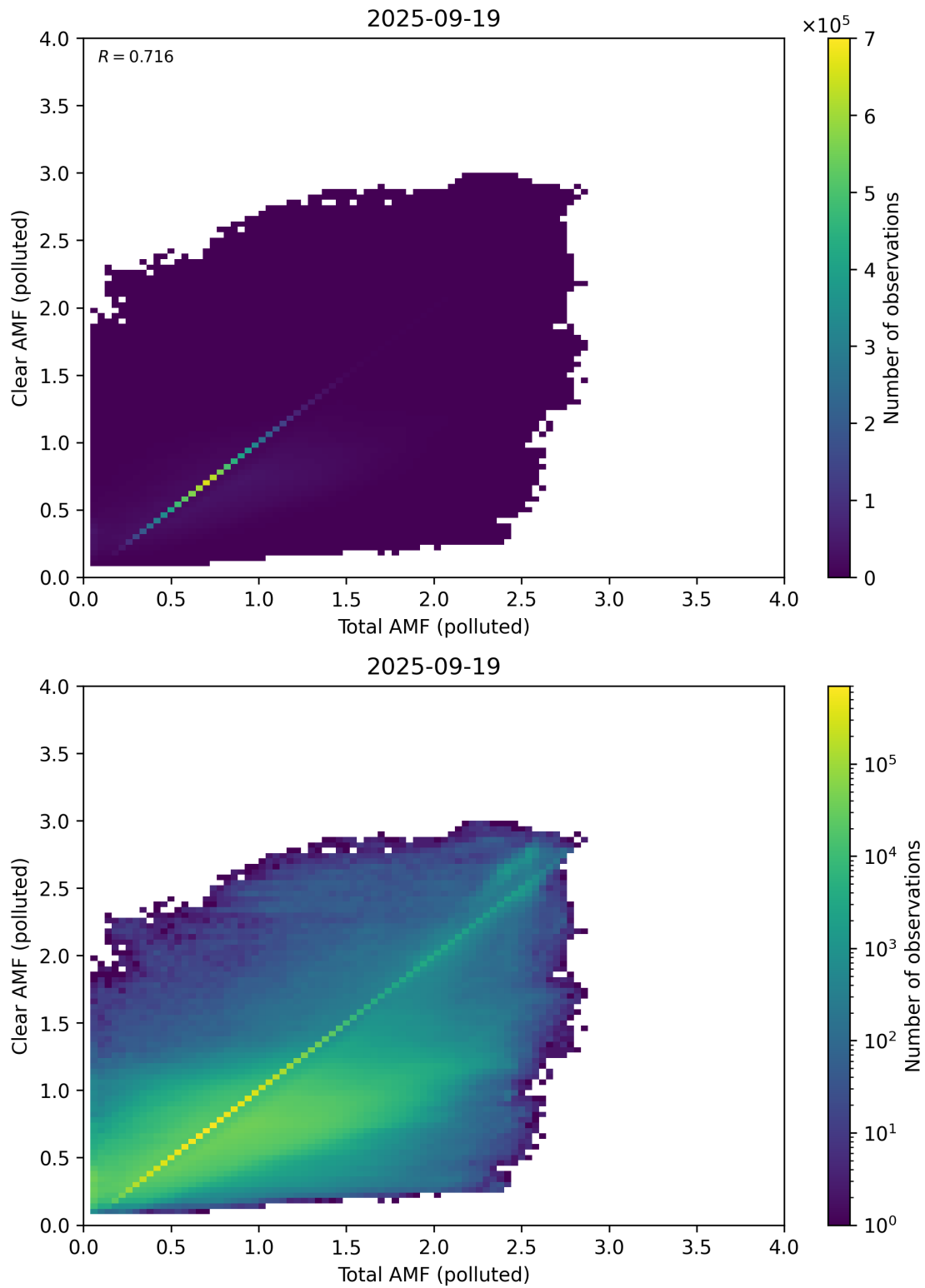
Figure 321: Scatter density plot of “Total AMF (polluted)” against “Clear AMF (polluted)” for 2025-09-18 to 2025-09-20.
