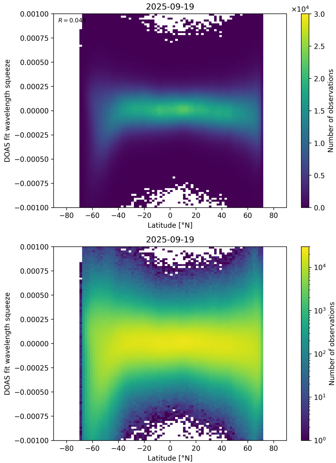
Figure 154: Scatter density plot of “Latitude” against “DOAS fit wavelength squeeze” for 2025-09-18 to 2025-09-20.
