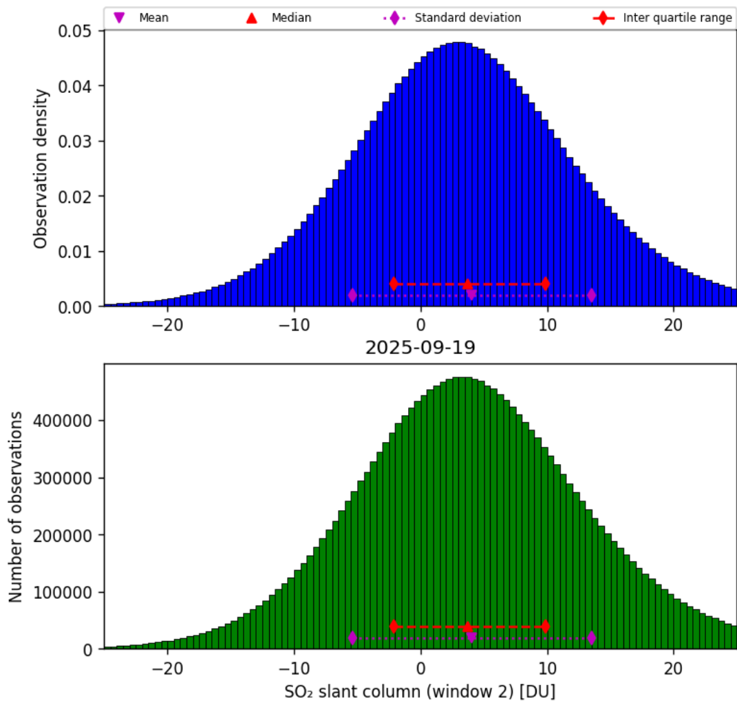
Figure 67: Histogram of “SO 2 slant column (window 2)” for 2025-09-18 to 2025-09-20
