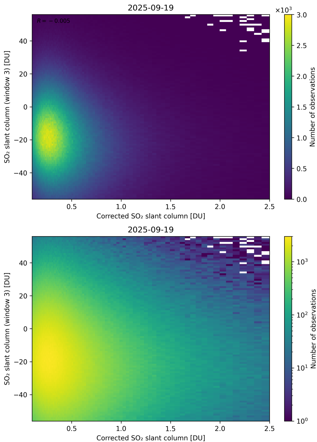
Figure 240: Scatter density plot of “Corrected SO 2 slant column” against “SO 2 slant column (window 3)” for 2025-09-18 to 2025-09-20.
