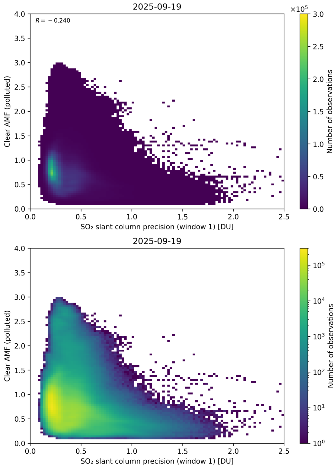
Figure 274: Scatter density plot of “SO 2 slant column precision (window 1)” against “Clear AMF (polluted)” for 2025-09-18 to 2025-09-20.
