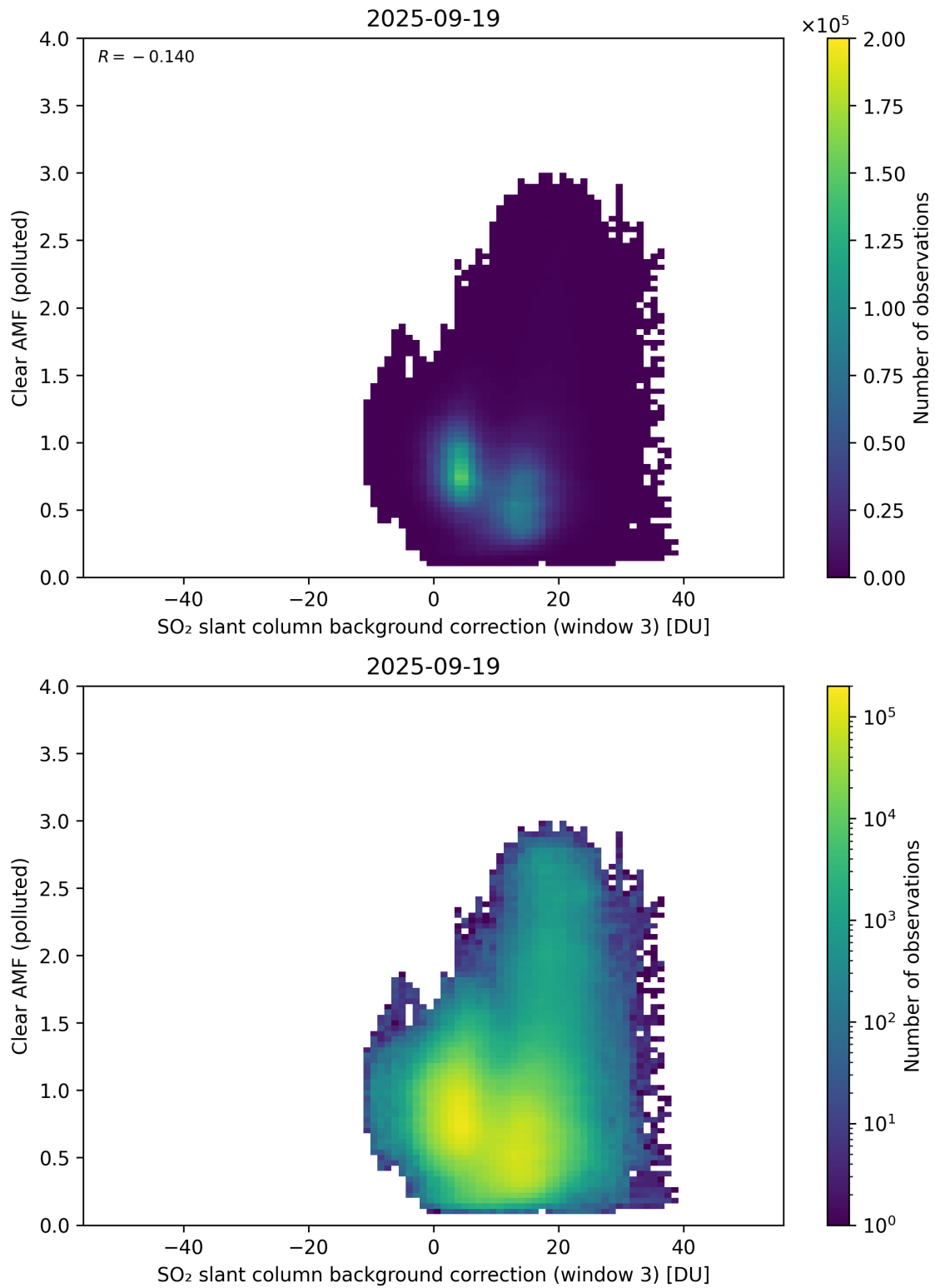
Figure 135: Scatter density plot of “SO 2 slant column background correction (window 3)” against “Clear AMF (polluted)” for 2025-09-18 to 2025-09-20.
