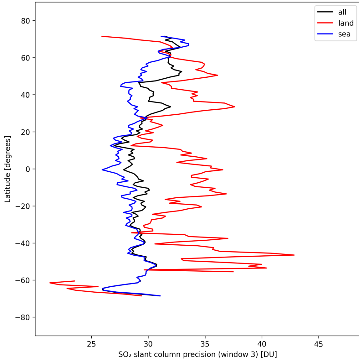
Figure 46: Zonal average of “SO 2 slant column precision (window 3)” for 2025-09-18 to 2025-09-20.
