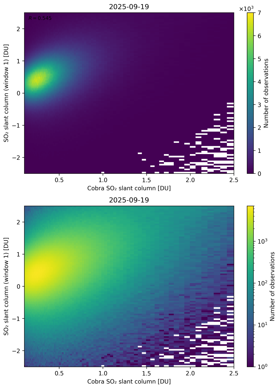
Figure 219: Scatter density plot of “Cobra SO 2 slant column” against “SO 2 slant column (window 1)” for 2025-09-18 to 2025-09-20.
