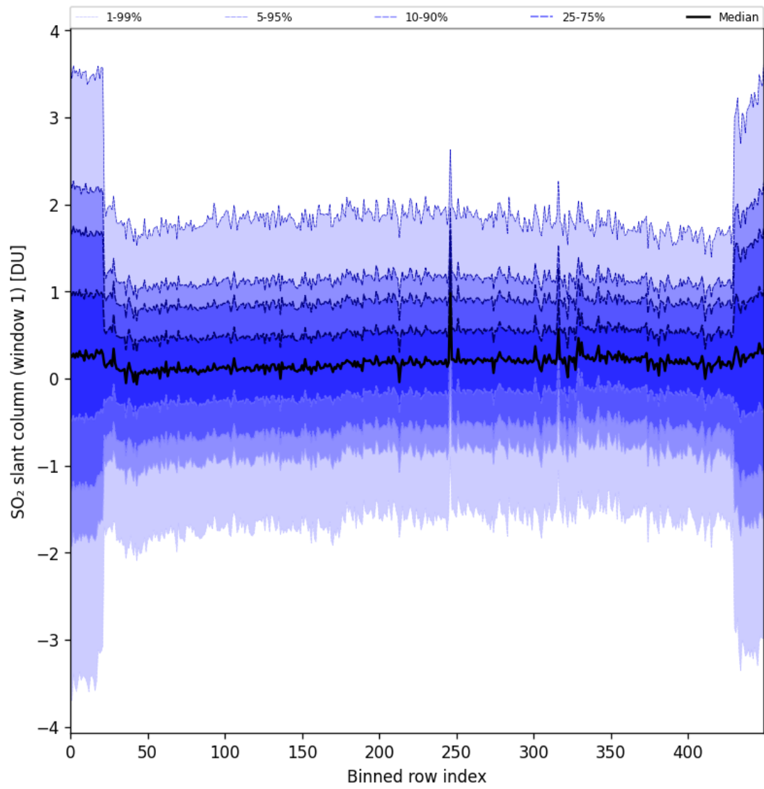
Figure 89: Along track statistics of “SO 2 slant column (window 1)” for 2025-09-18 to 2025-09-20
