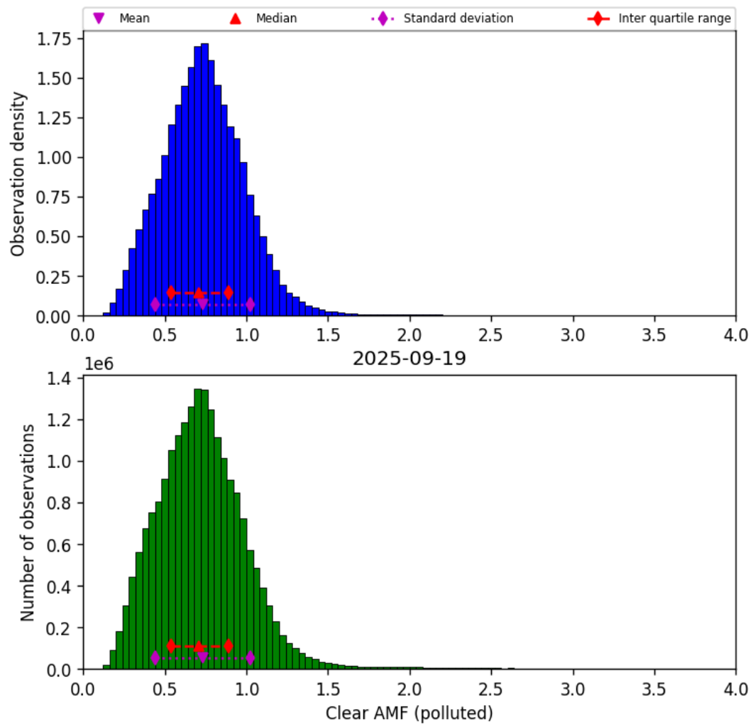
Figure 81: Histogram of “Clear AMF (polluted)” for 2025-09-18 to 2025-09-20
