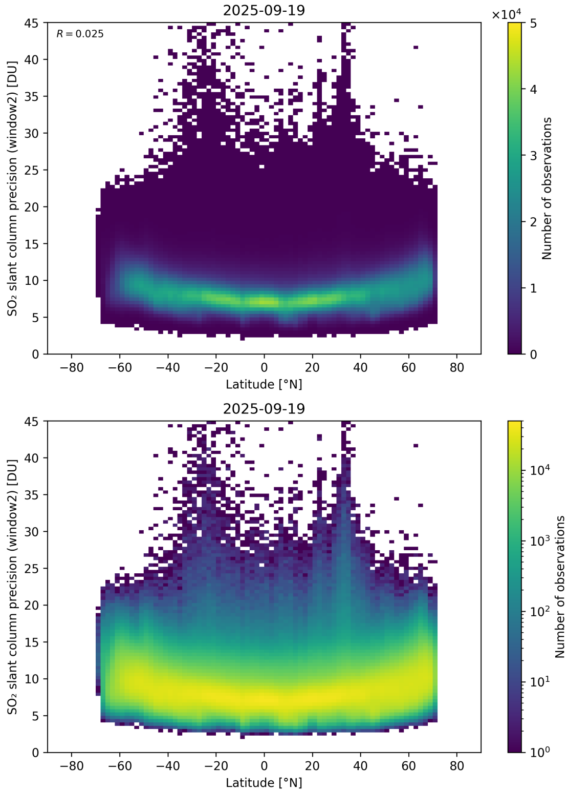
Figure 164: Scatter density plot of “Latitude” against “SO 2 slant column precision (window2)” for 2025-09-18 to 2025-09-20.
