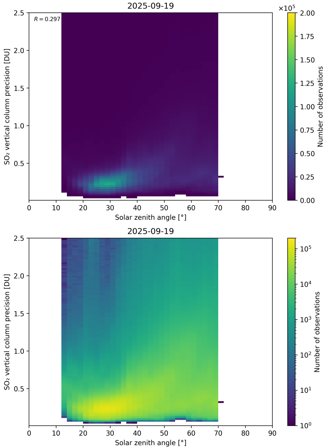
Figure 192: Scatter density plot of “Solar zenith angle” against “SO 2 vertical column precision” for 2025-09-18 to 2025-09-20.
