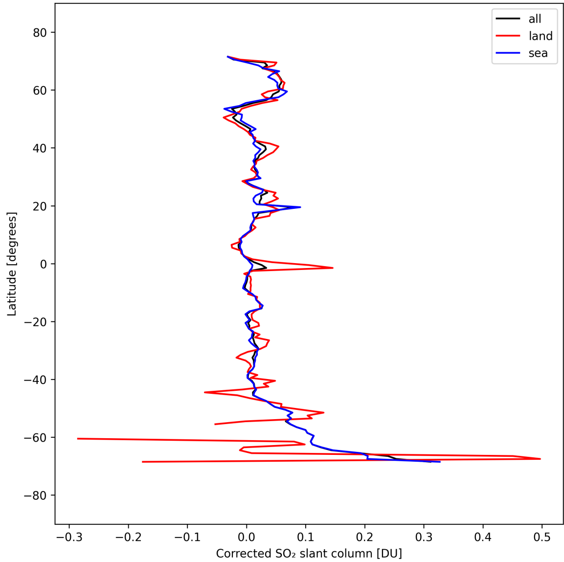
Figure 34: Zonal average of “Corrected SO 2 slant column” for 2025-09-18 to 2025-09-20.
