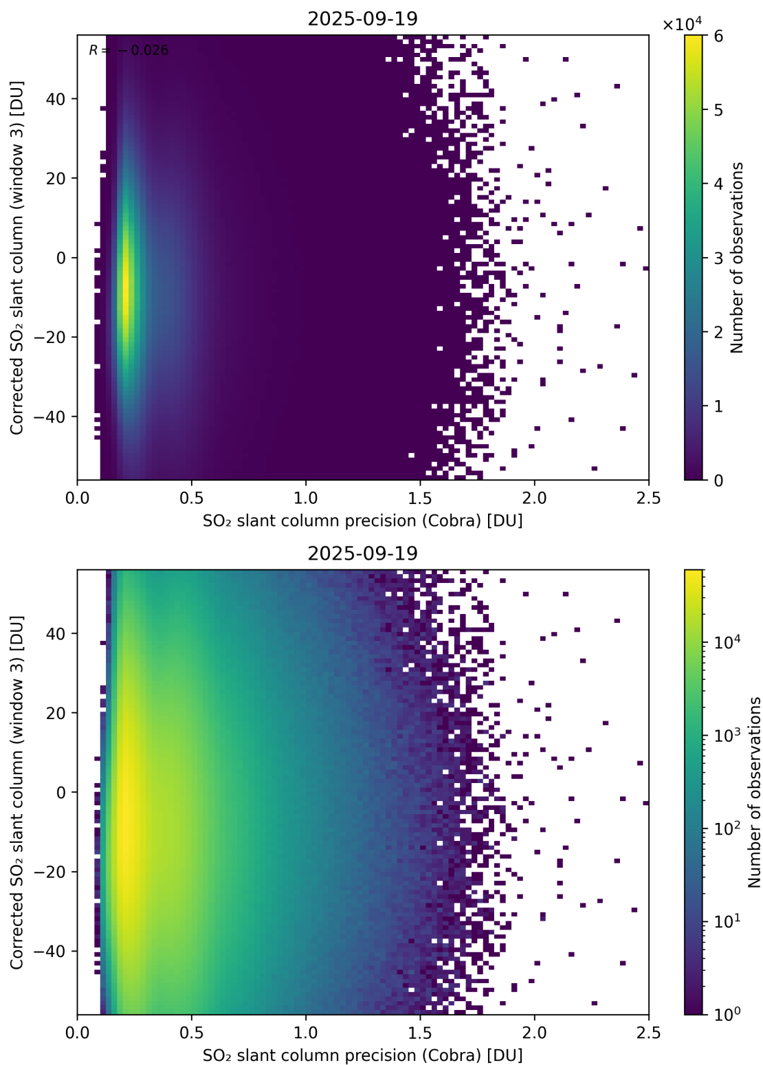
Figure 207: Scatter density plot of “SO 2 slant column precision (Cobra)” against “Corrected SO 2 slant column (window 3)” for 2025-09-18 to 2025-09-20.
