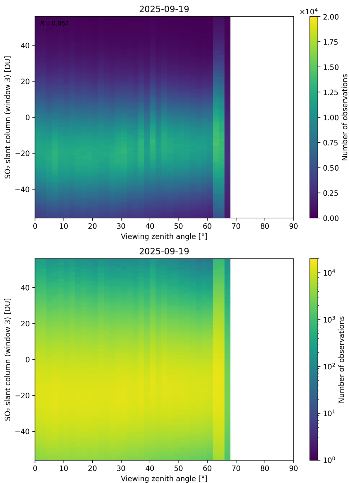
Figure 379: Scatter density plot of “Viewing zenith angle” against “SO 2 slant column (window 3)” for 2025-09-18 to 2025-09-20.
