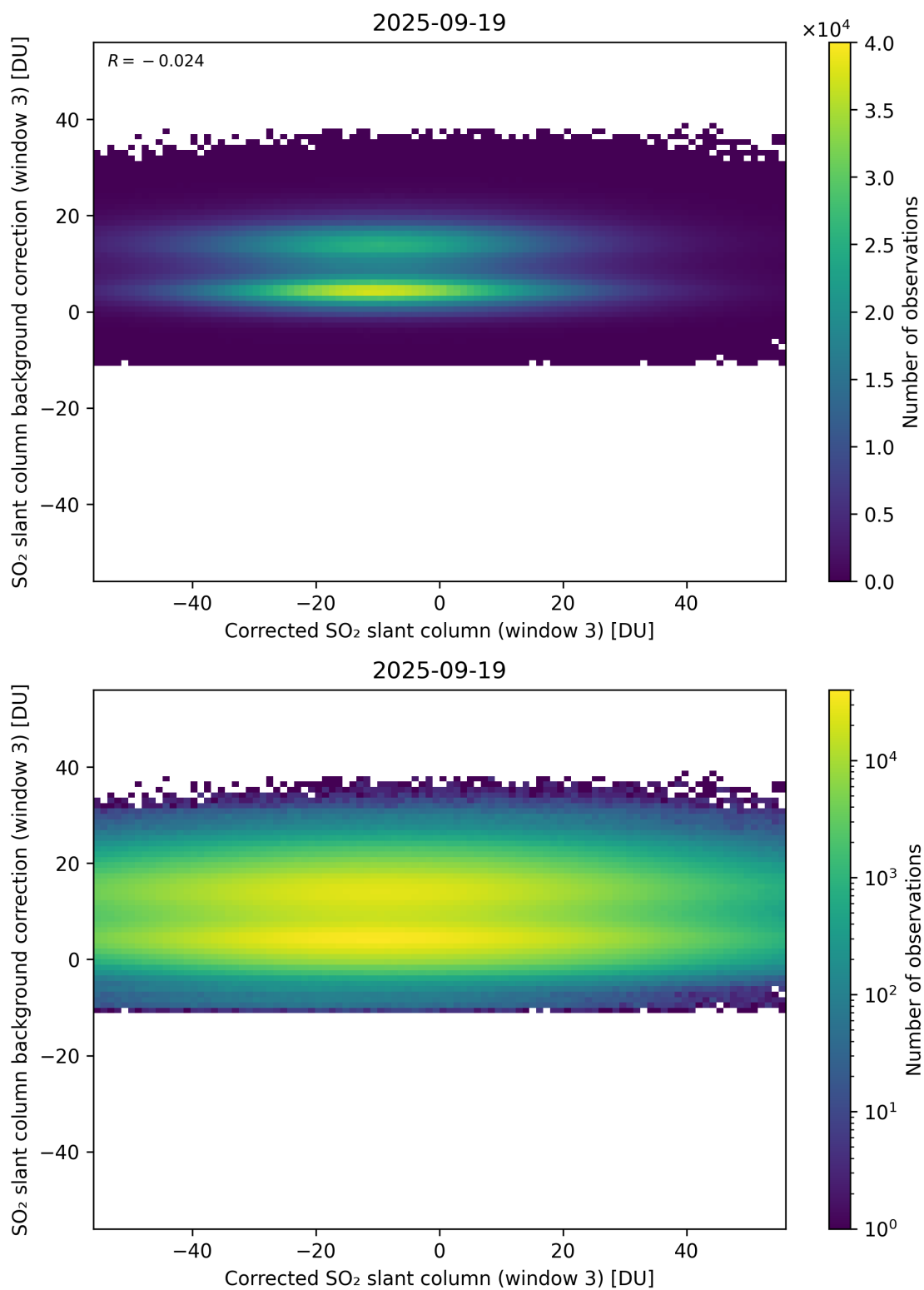
Figure 255: Scatter density plot of “Corrected SO 2 slant column (window 3)” against “SO 2 slant column background correction (window 3)” for 2025-09-18 to 2025-09-20.
