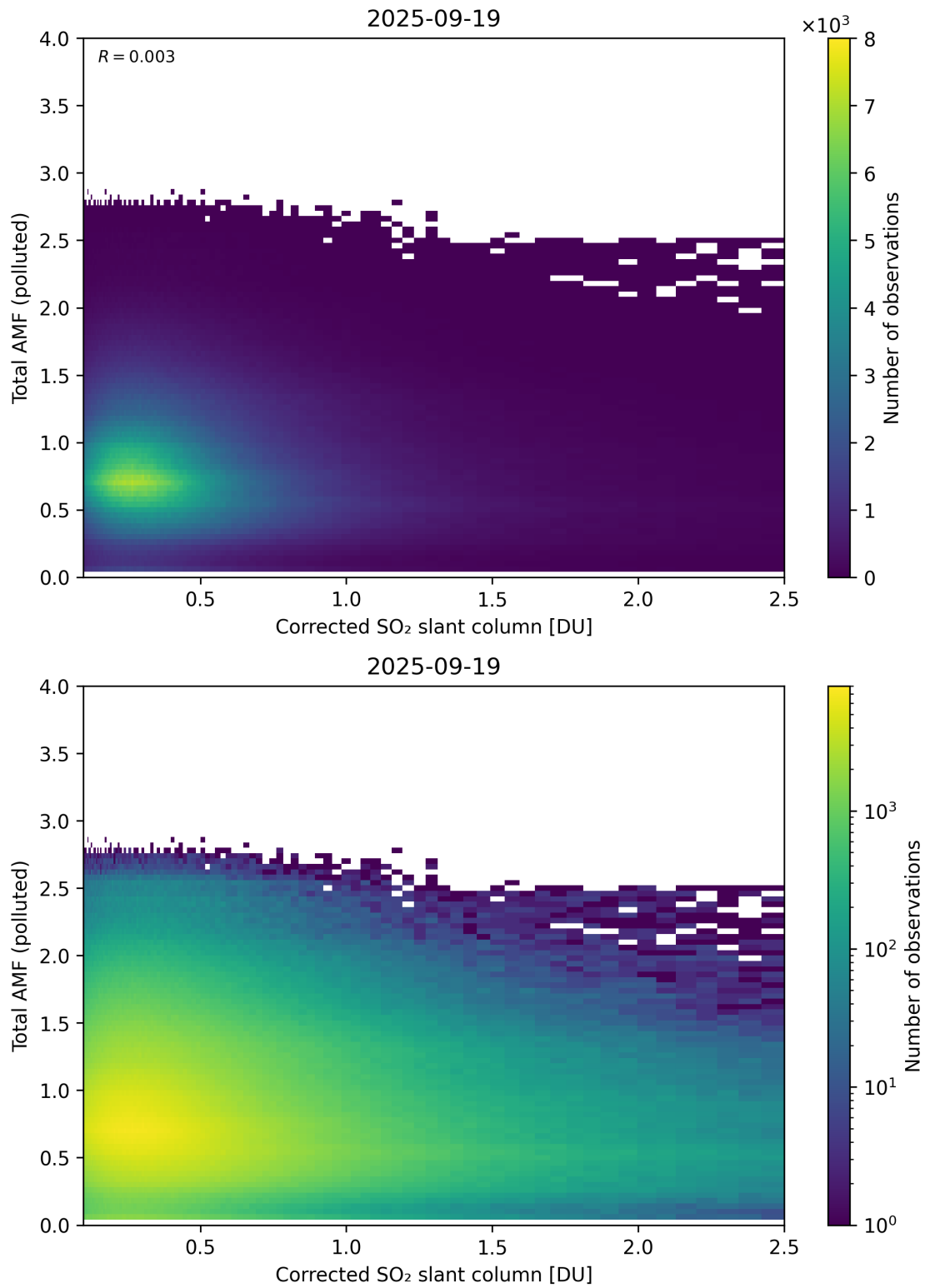
Figure 242: Scatter density plot of “Corrected SO 2 slant column” against “Total AMF (polluted)” for 2025-09-18 to 2025-09-20.
