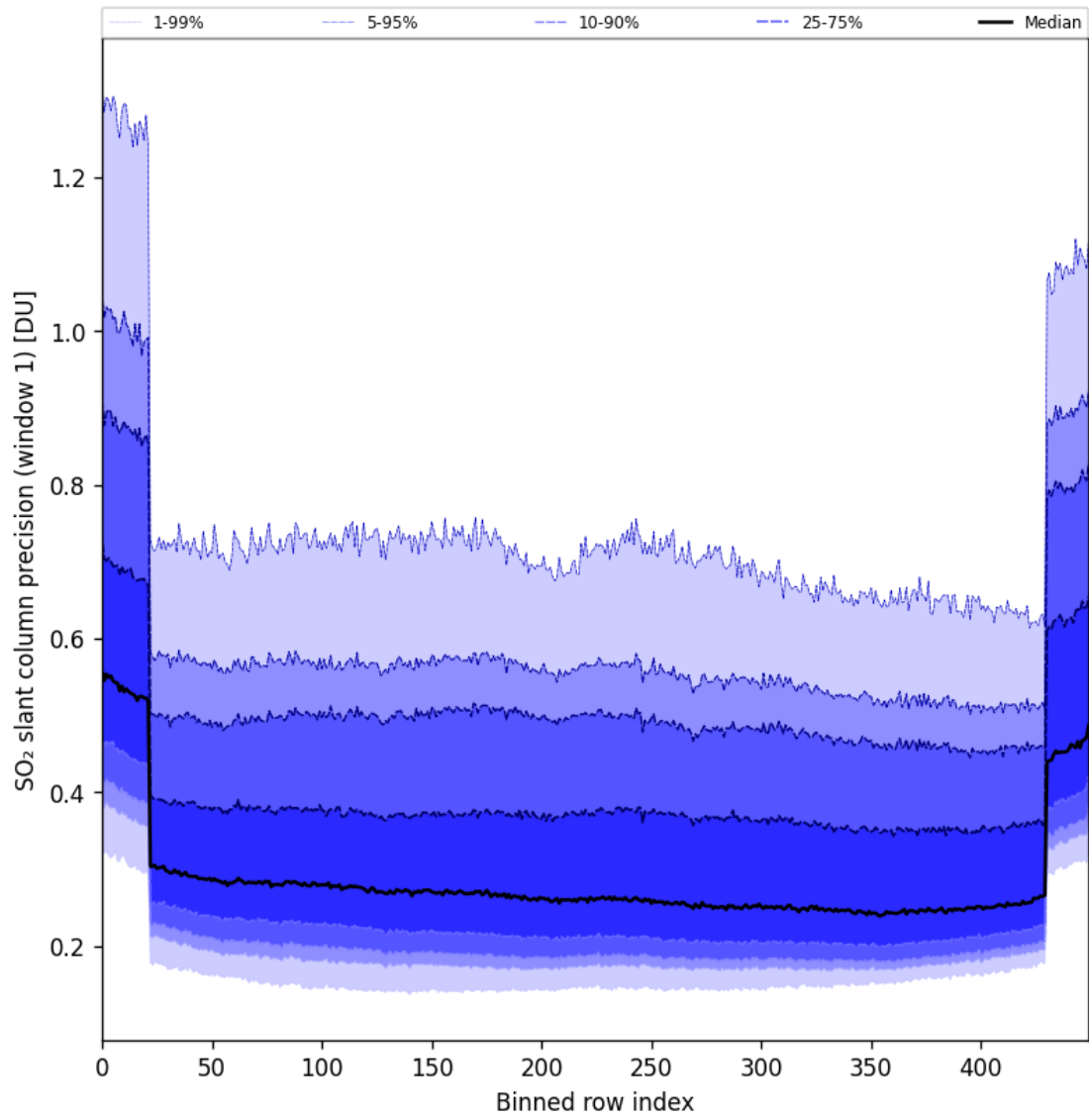
Figure 90: Along track statistics of “SO 2 slant column precision (window 1)” for 2025-09-18 to 2025-09-20
