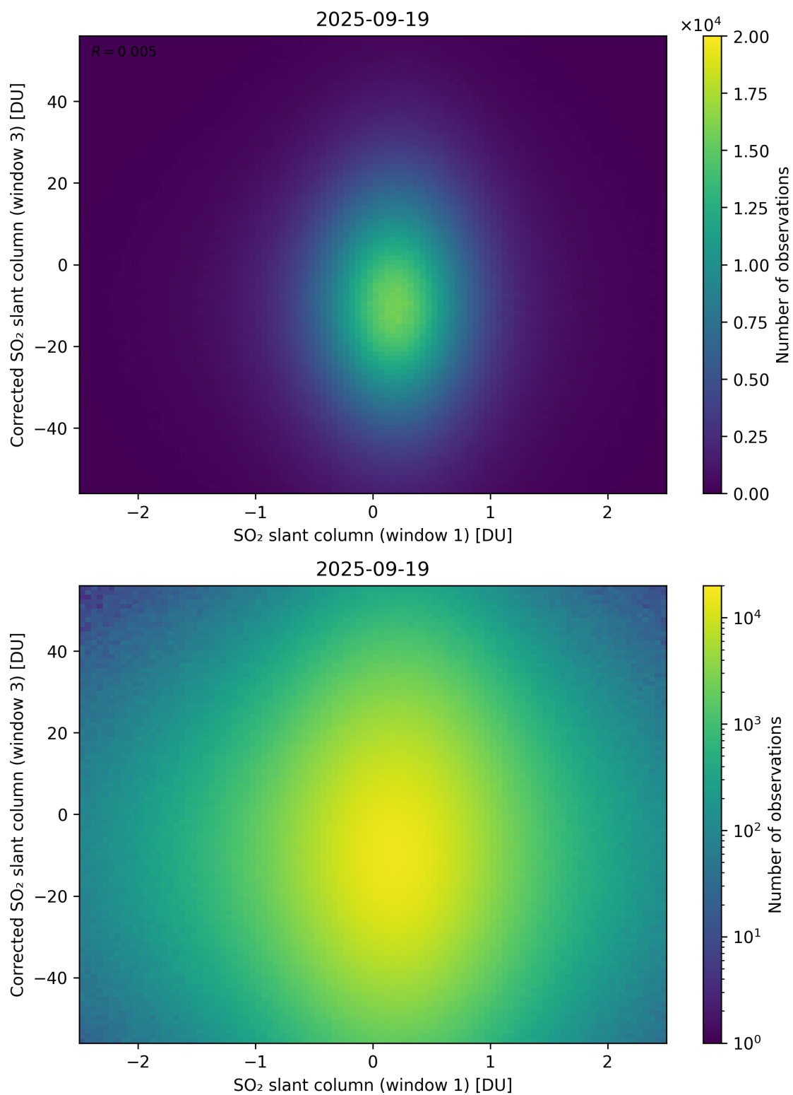
Figure 284: Scatter density plot of “SO 2 slant column (window 1)” against “Corrected SO 2 slant column (window 3)” for 2025-09-18 to 2025-09-20.
