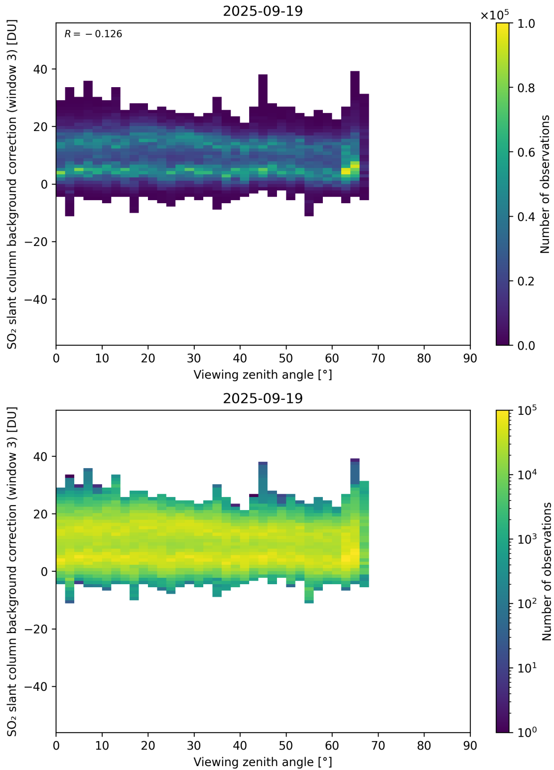
Figure 364: Scatter density plot of “Viewing zenith angle” against “SO 2 slant column background correction (window 3)” for 2025-09-18 to 2025-09-20.
