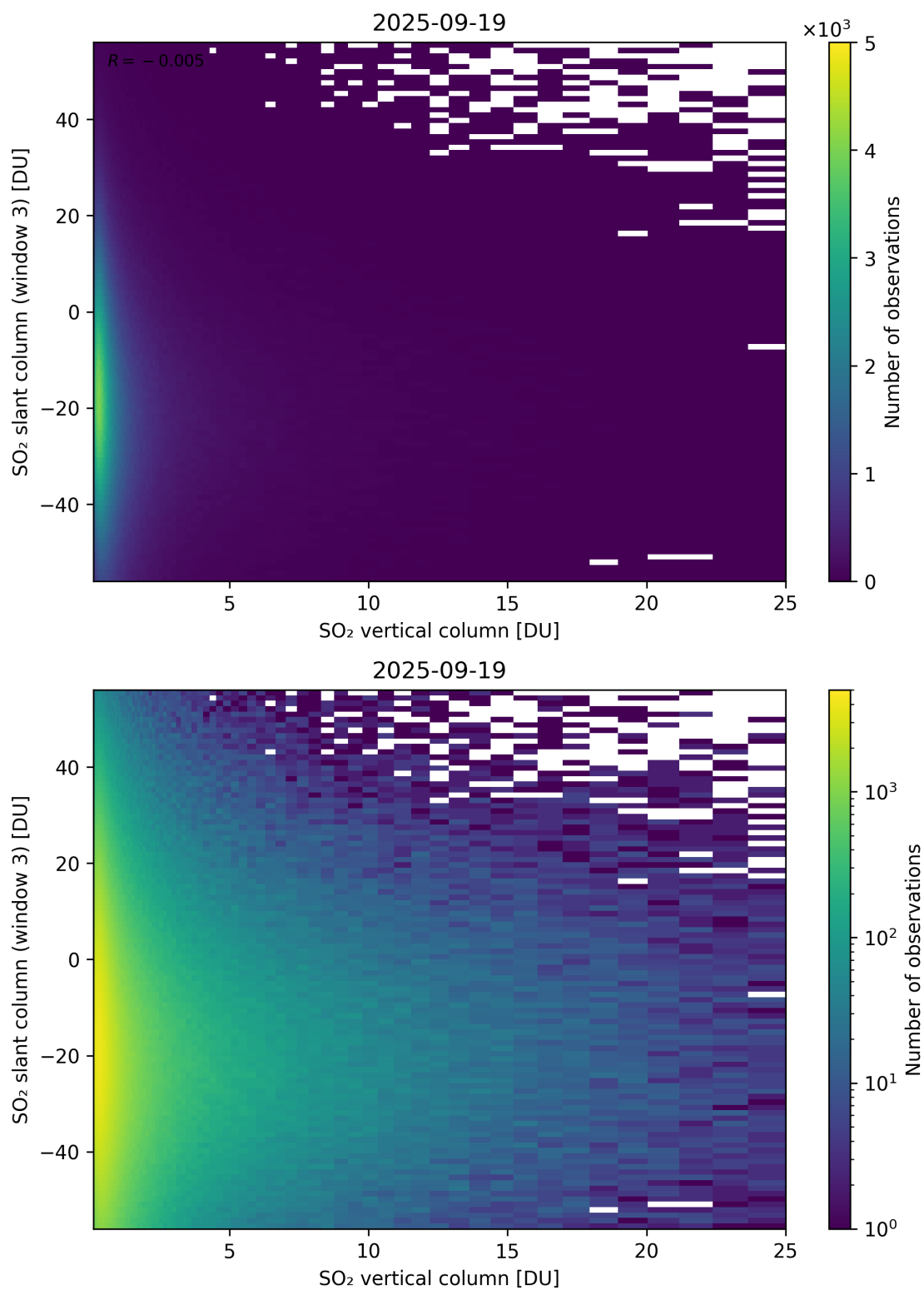
Figure 357: Scatter density plot of “SO 2 vertical column” against “SO 2 slant column (window 3)” for 2025-09-18 to 2025-09-20.
