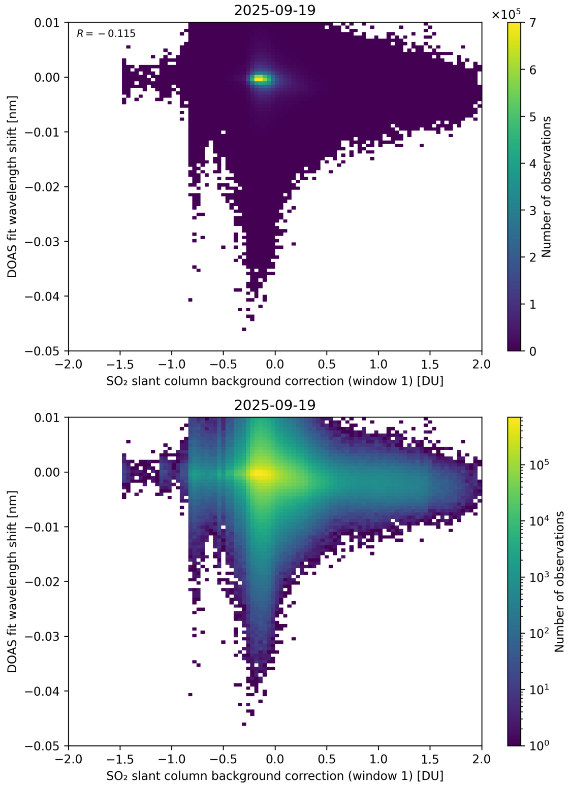
Figure 111: Scatter density plot of “SO 2 slant column background correction (window 1)” against “DOAS fit wavelength shift” for 2025-09-18 to 2025-09-20.
