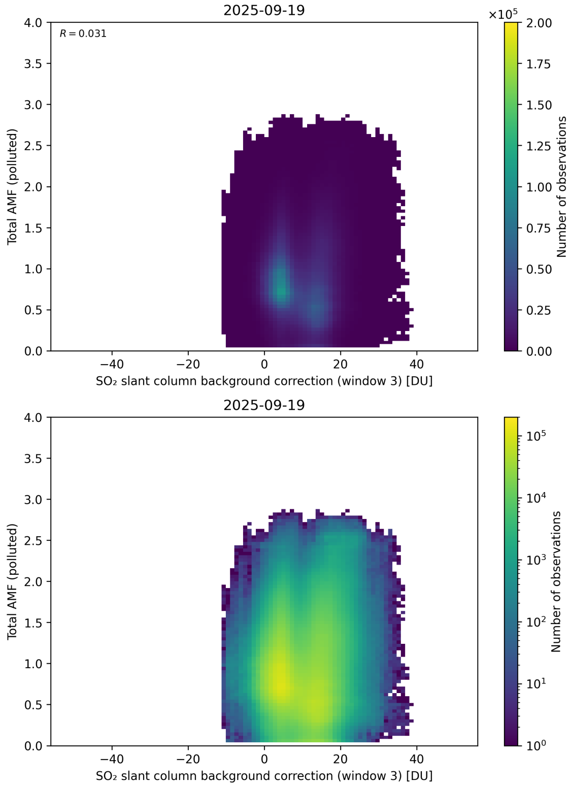
Figure 136: Scatter density plot of “SO 2 slant column background correction (window 3)” against “Total AMF (polluted)” for 2025-09-18 to 2025-09-20.
