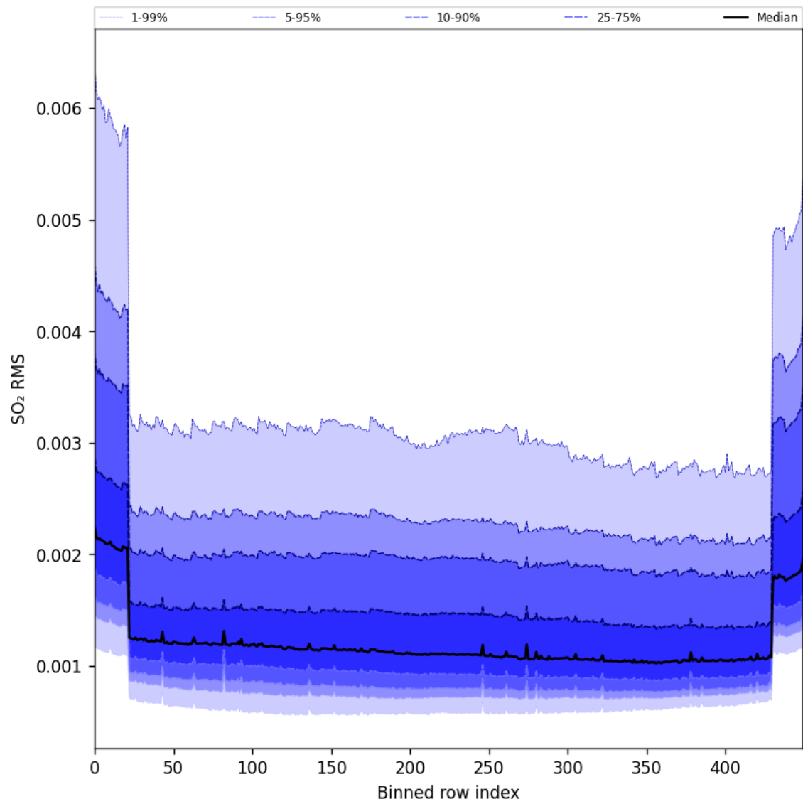
Figure 104: Along track statistics of “SO 2 RMS” for 2025-09-18 to 2025-09-20
