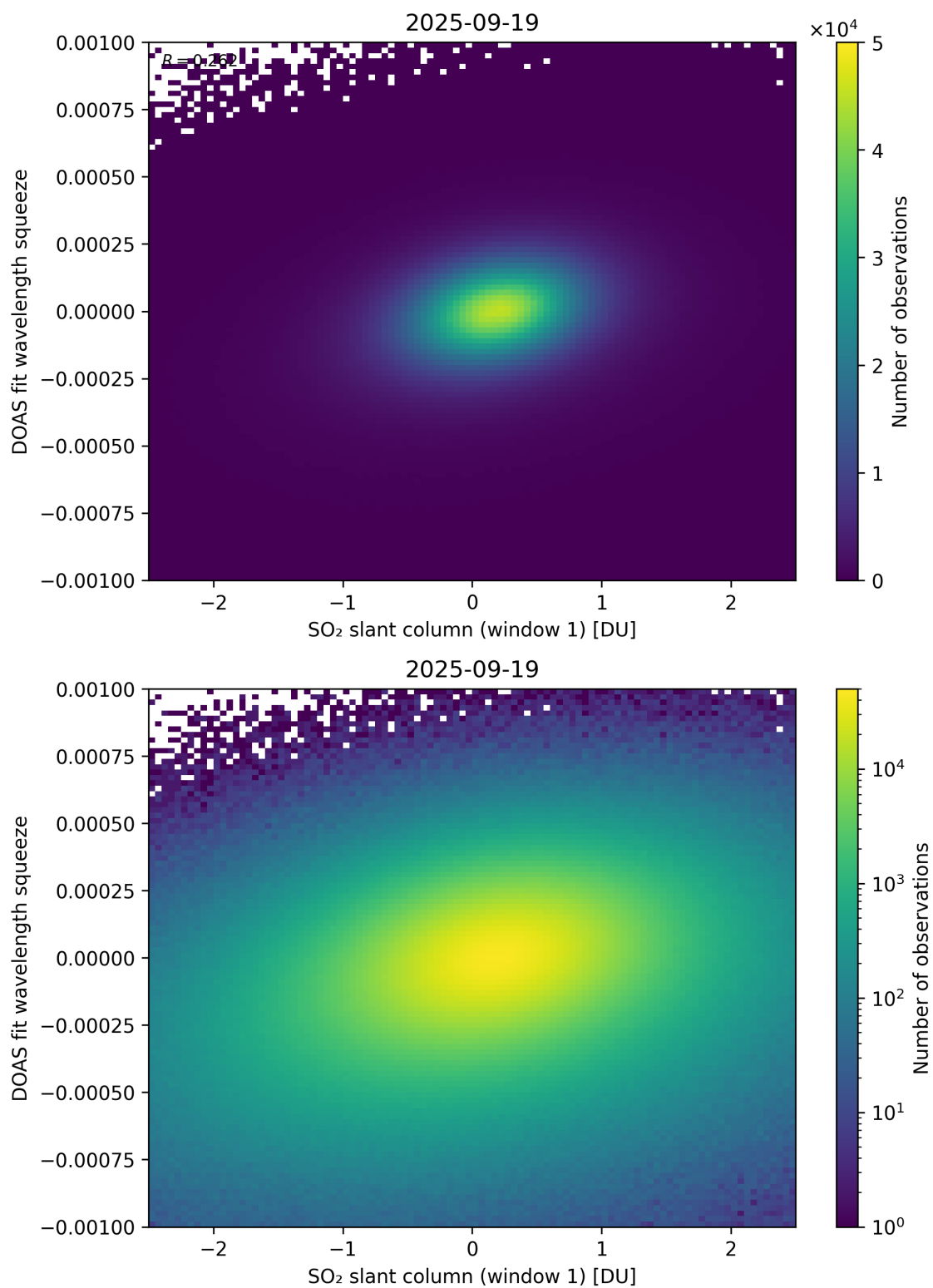
Figure 266: Scatter density plot of “SO 2 slant column (window 1)” against “DOAS fit wavelength squeeze” for 2025-09-18 to 2025-09-20.
