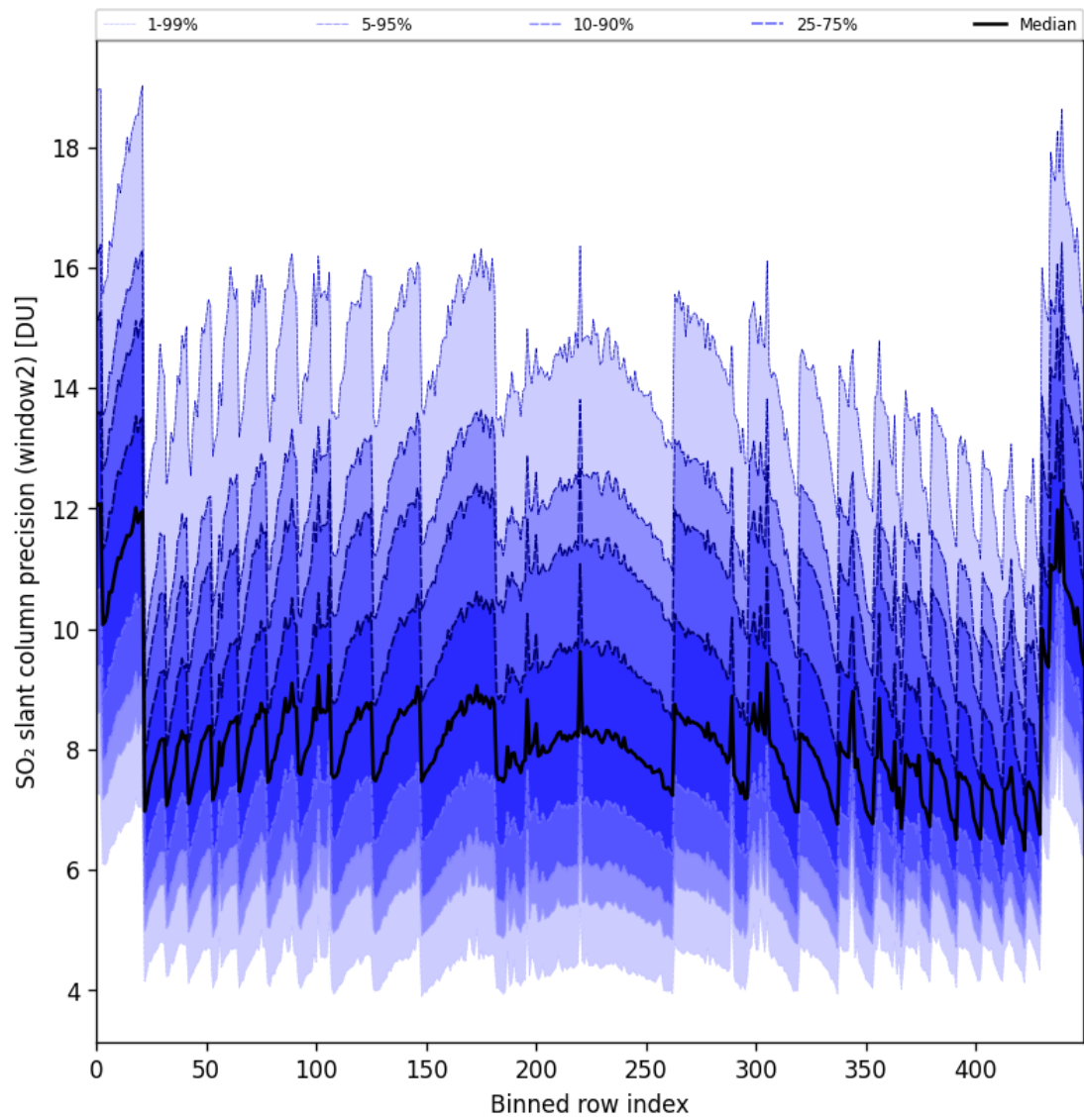
Figure 94: Along track statistics of “SO 2 slant column precision (window2)” for 2025-09-18 to 2025-09-20
