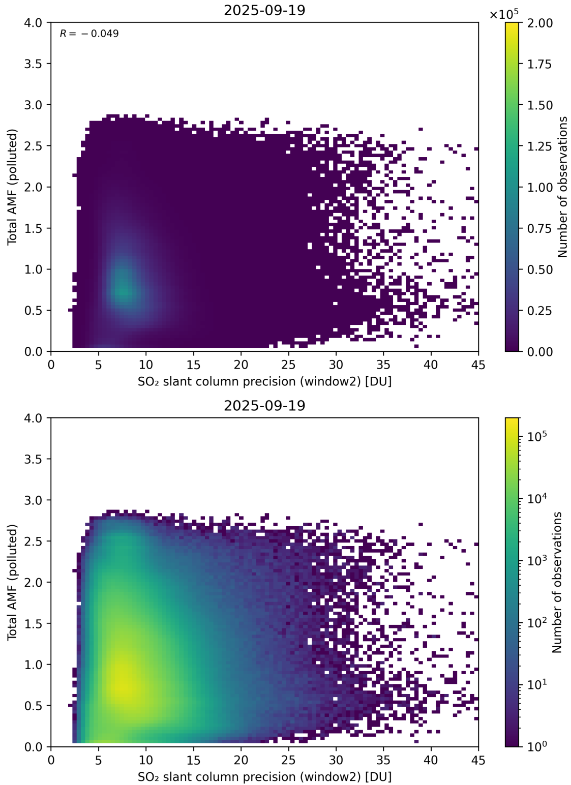
Figure 301: Scatter density plot of “SO 2 slant column precision (window2)” against “Total AMF (polluted)” for 2025-09-18 to 2025-09-20.
