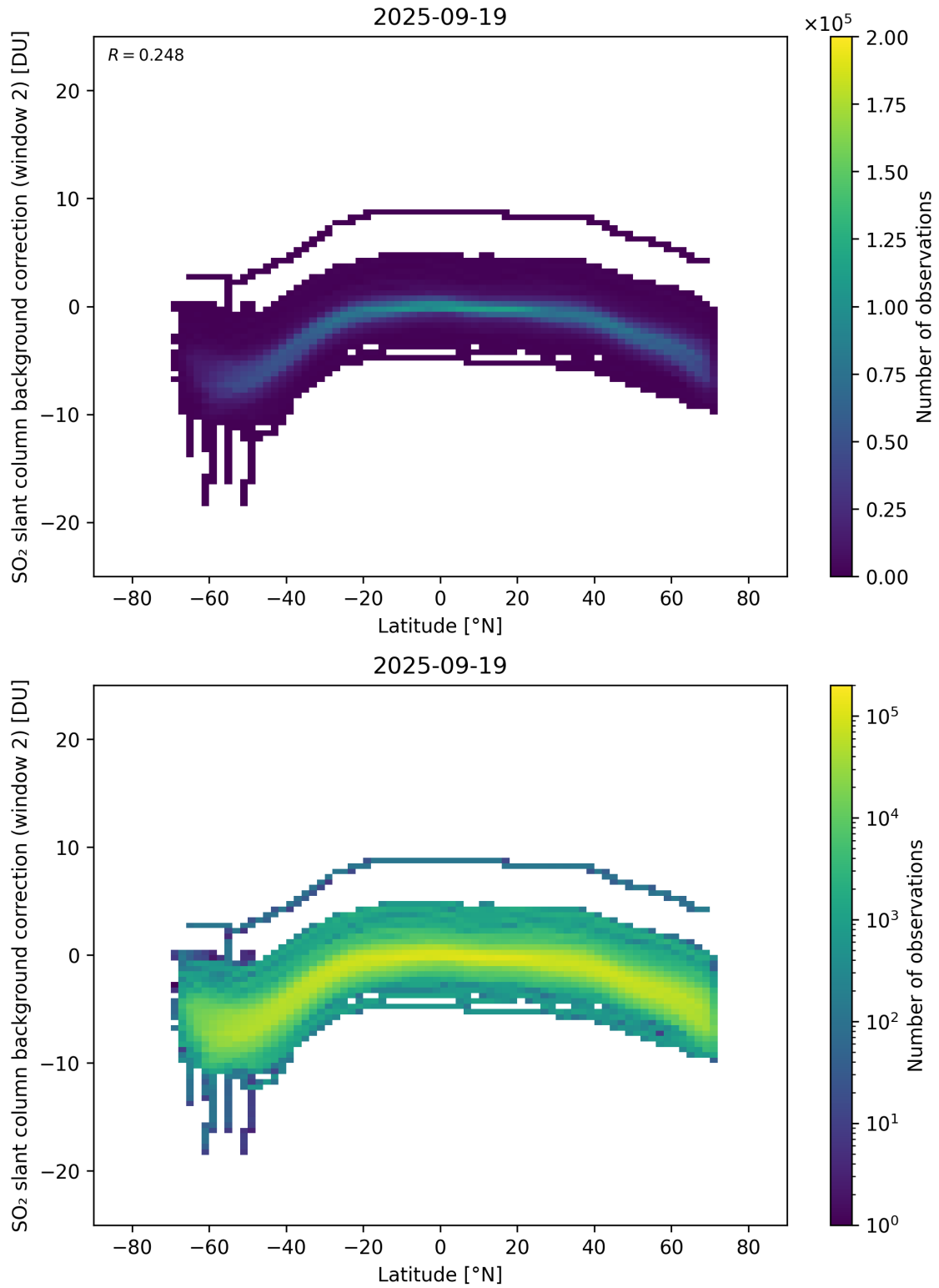
Figure 151: Scatter density plot of “Latitude” against “SO 2 slant column background correction (window 2)” for 2025-09-18 to 2025-09-20.
