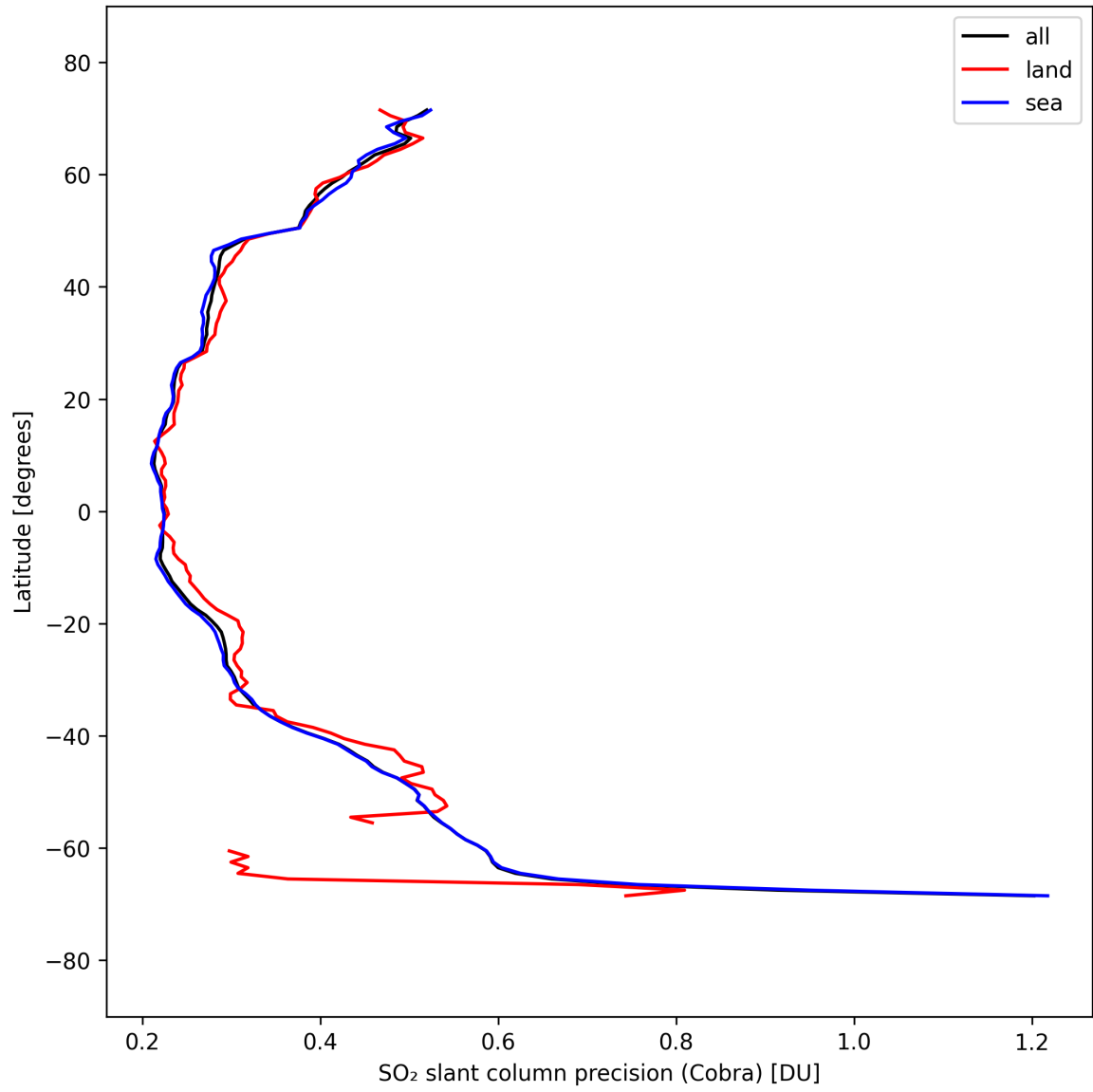
Figure 36: Zonal average of “SO 2 slant column precision (Cobra)” for 2025-09-18 to 2025-09-20.
