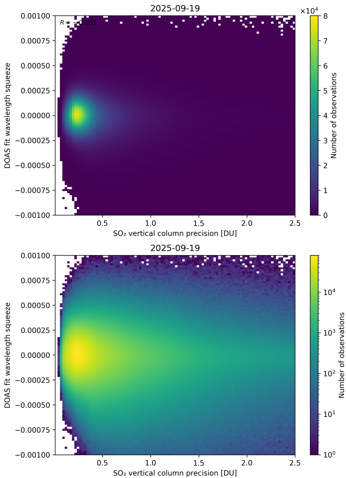
Figure 333: Scatter density plot of “SO 2 vertical column precision” against “DOAS fit wavelength squeeze” for 2025-09-18 to 2025-09-20.
