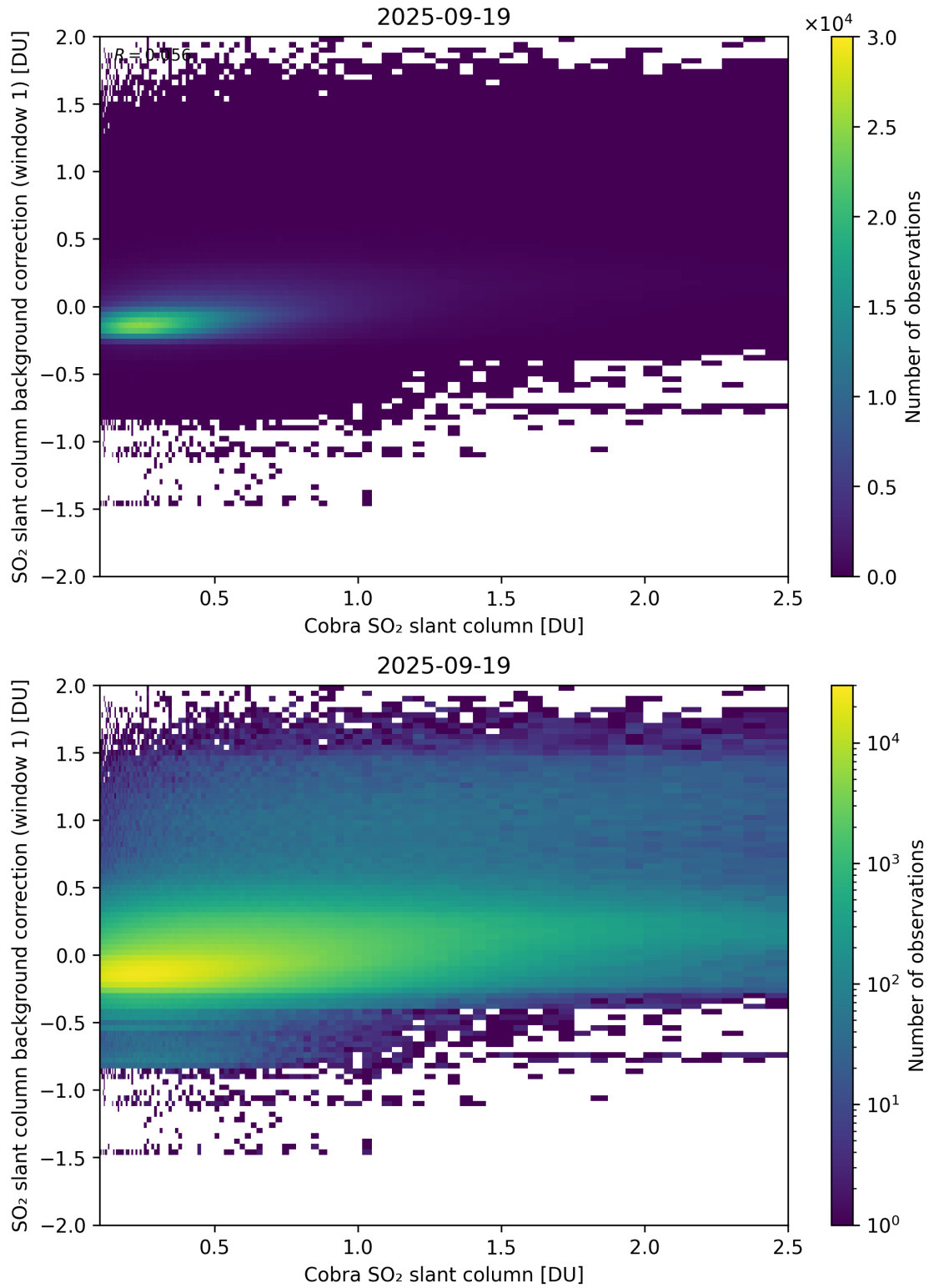
Figure 193: Scatter density plot of “Cobra SO 2 slant column” against “SO 2 slant column background correction (window 1)” for 2025-09-18 to 2025-09-20.
