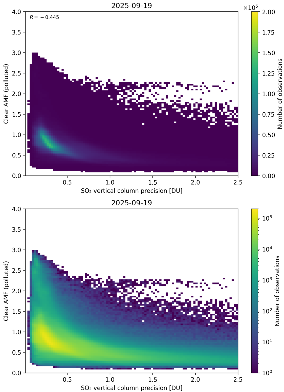
Figure 335: Scatter density plot of “SO 2 vertical column precision” against “Clear AMF (polluted)” for 2025-09-18 to 2025-09-20.
