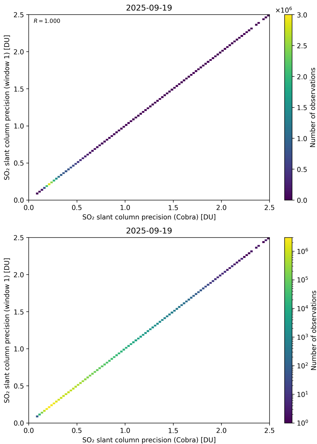
Figure 209: Scatter density plot of “SO 2 slant column precision (Cobra)” against “SO 2 slant column precision (window 1)” for 2025-09-18 to 2025-09-20.
