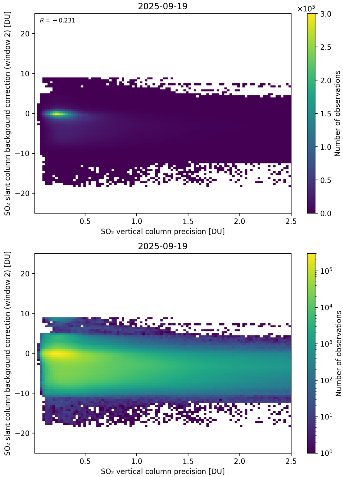
Figure 330: Scatter density plot of “SO 2 vertical column precision” against “SO 2 slant column background correction (window 2)” for 2025-09-18 to 2025-09-20.
