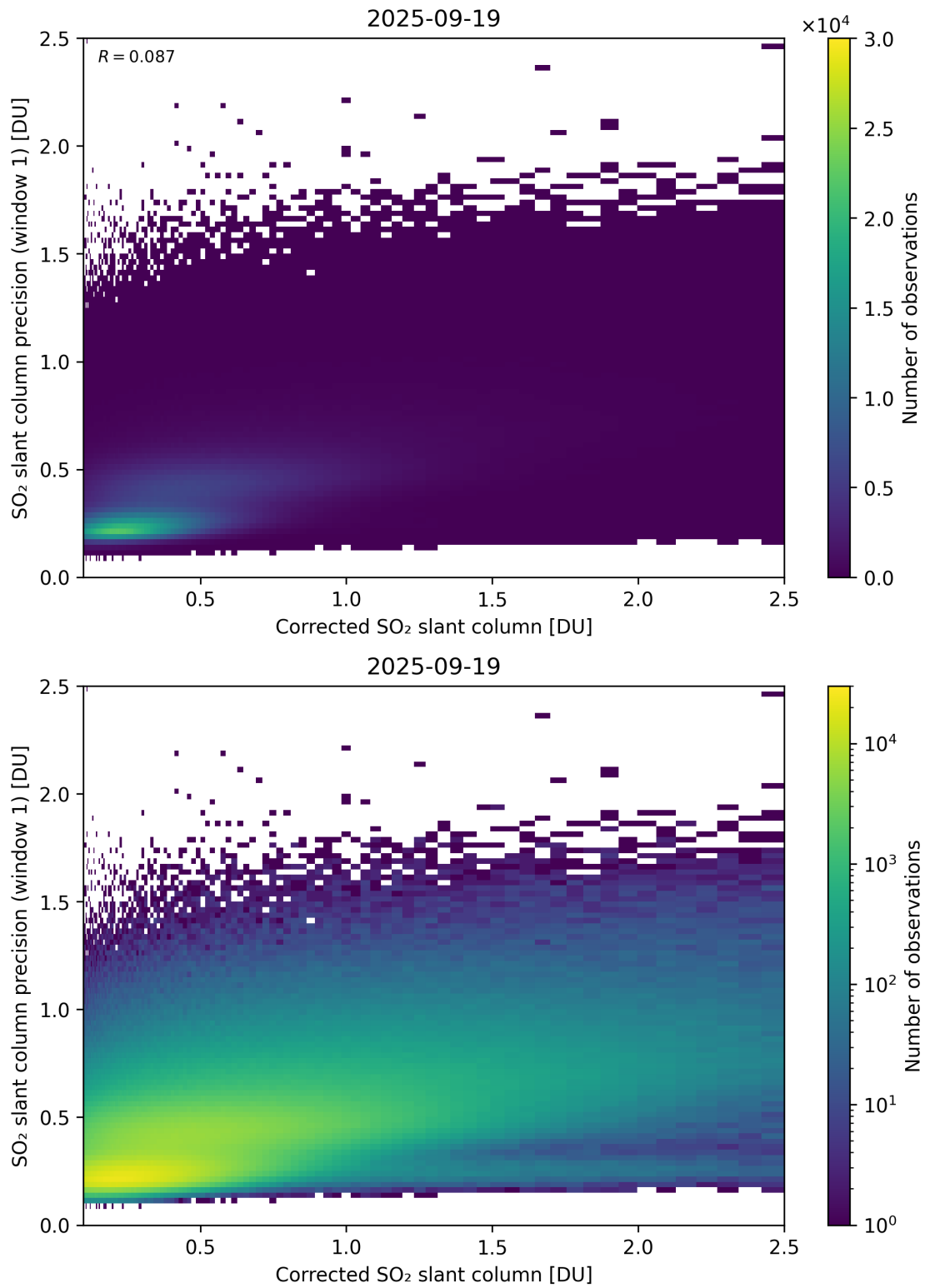
Figure 238: Scatter density plot of “Corrected SO 2 slant column” against “SO 2 slant column precision (window 1)” for 2025-09-18 to 2025-09-20.
