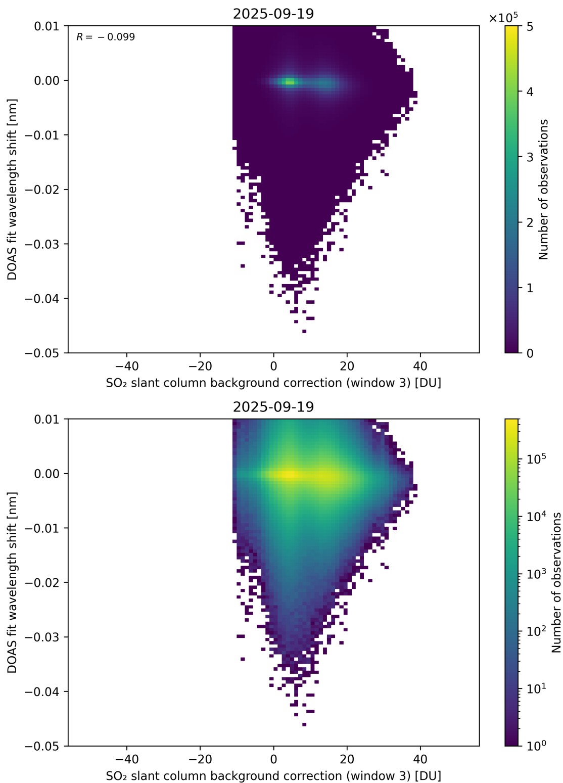
Figure 132: Scatter density plot of “SO 2 slant column background correction (window 3)” against “DOAS fit wavelength shift” for 2025-09-18 to 2025-09-20.
