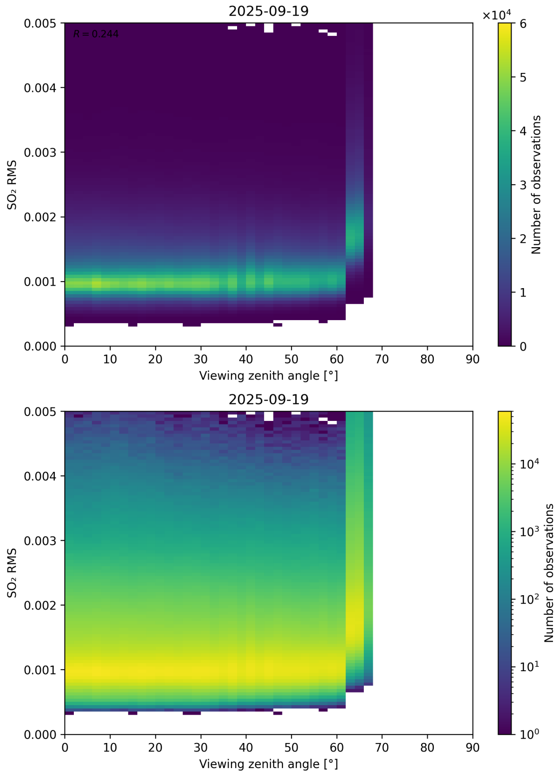
Figure 367: Scatter density plot of “Viewing zenith angle” against “SO 2 RMS” for 2025-09-18 to 2025-09-20.
