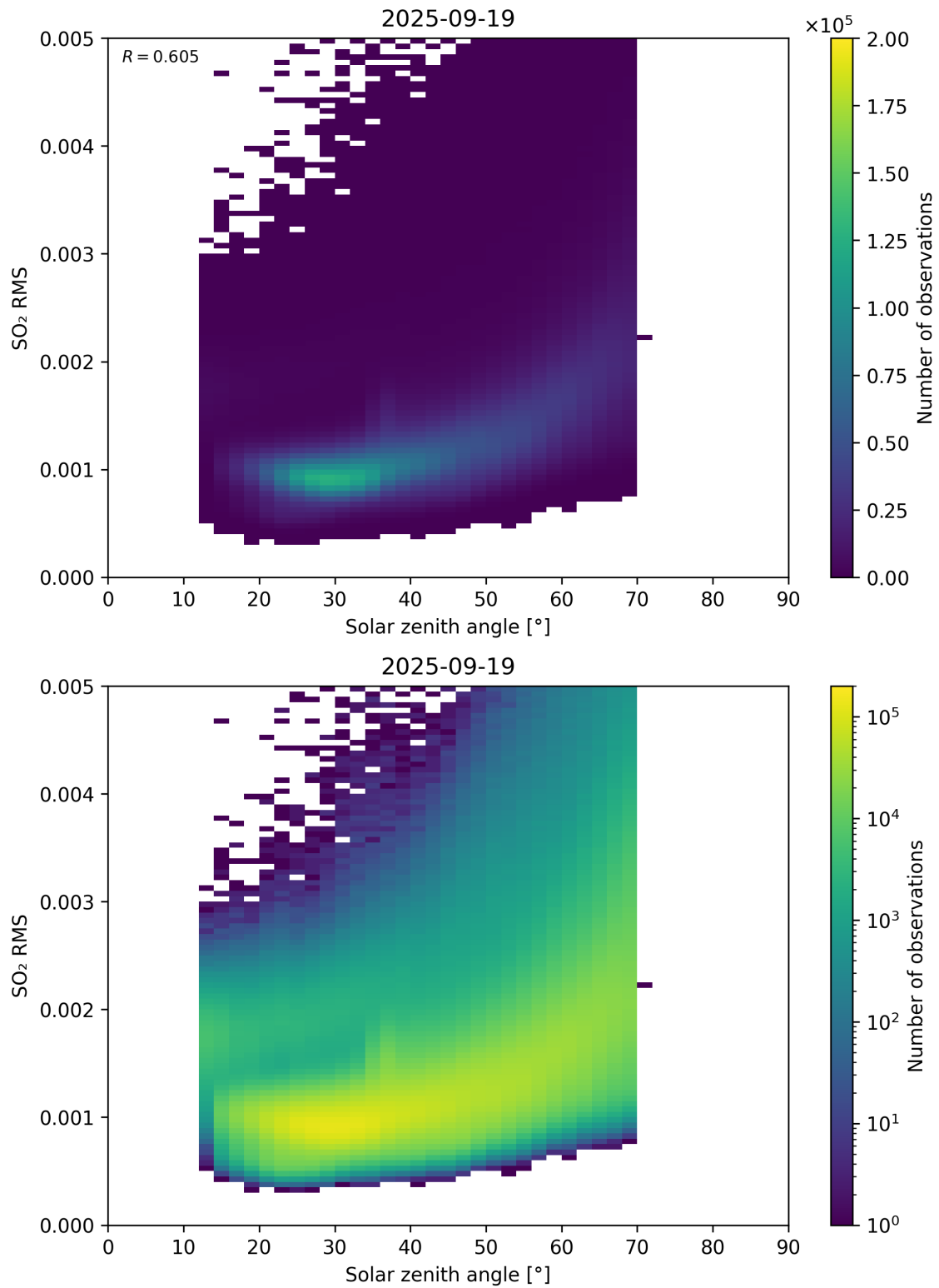
Figure 176: Scatter density plot of “Solar zenith angle” against “SO 2 RMS” for 2025-09-18 to 2025-09-20.
