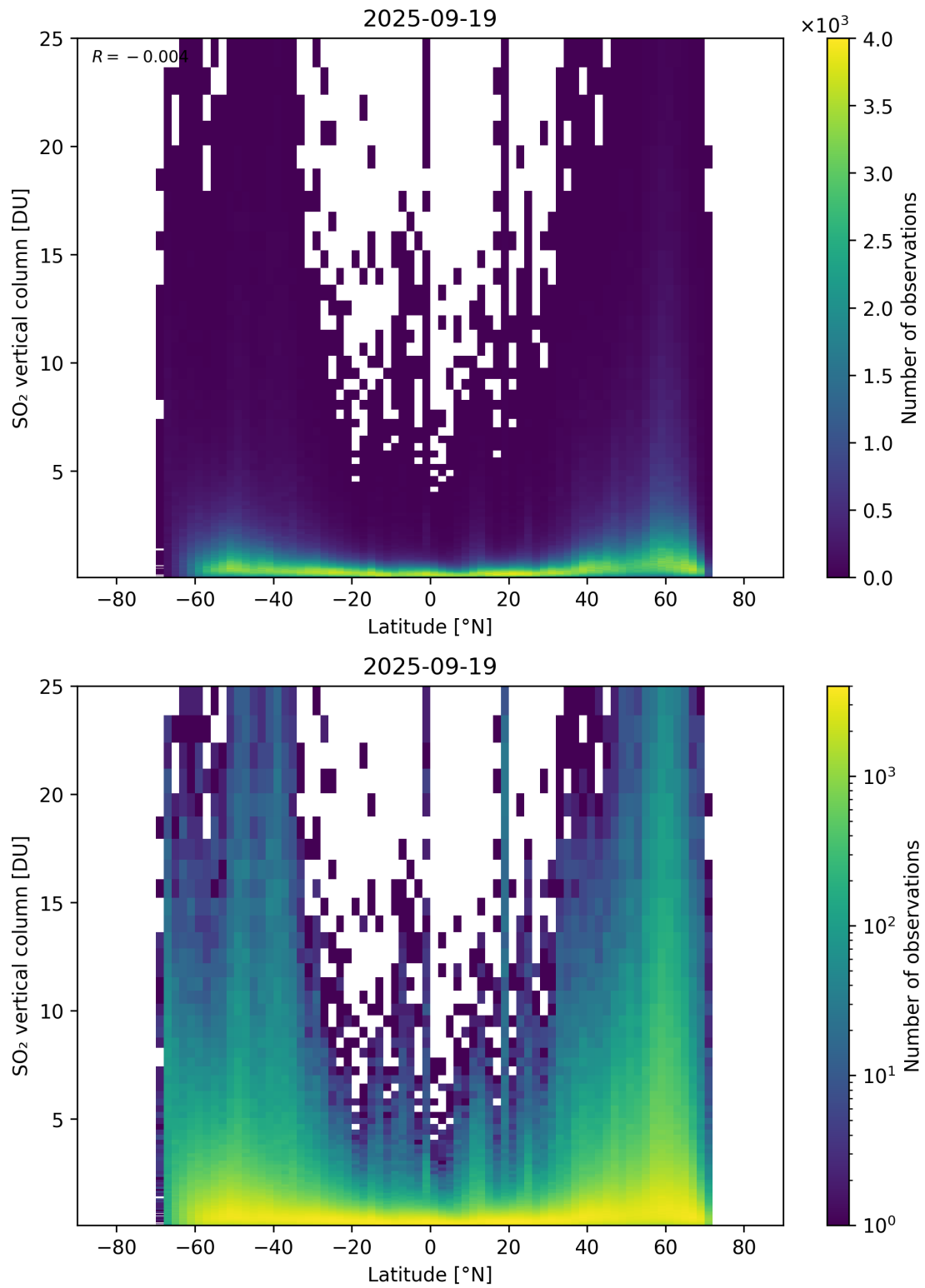
Figure 169: Scatter density plot of “Latitude” against “SO 2 vertical column” for 2025-09-18 to 2025-09-20.
