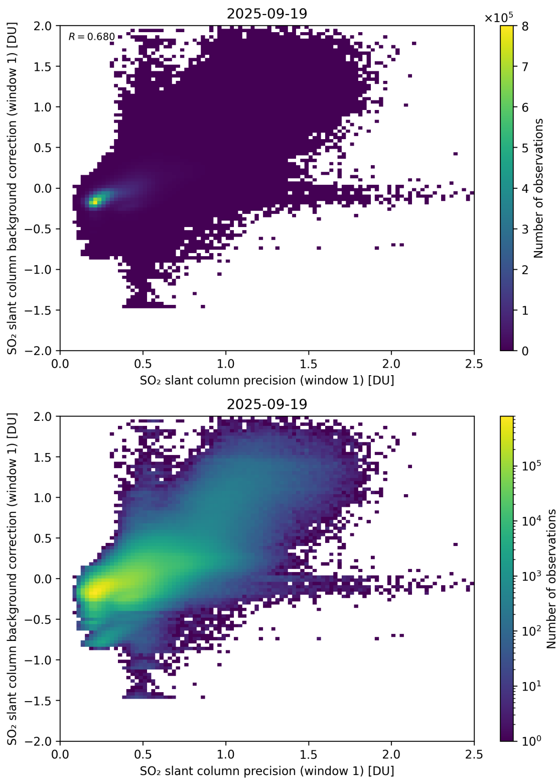
Figure 268: Scatter density plot of “SO 2 slant column precision (window 1)” against “SO 2 slant column background correction (window 1)” for 2025-09-18 to 2025-09-20.
