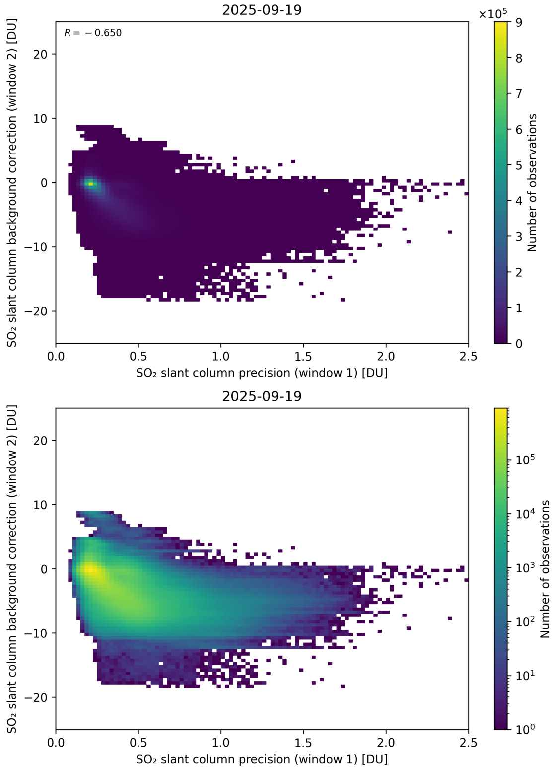
Figure 269: Scatter density plot of “SO 2 slant column precision (window 1)” against “SO 2 slant column background correction (window 2)” for 2025-09-18 to 2025-09-20.
