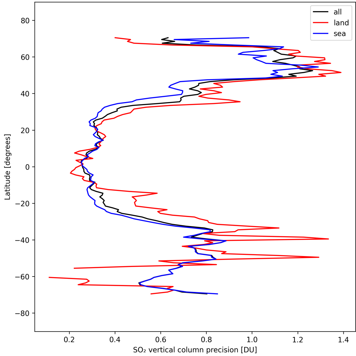
Figure 33: Zonal average of “SO 2 vertical column precision” for 2025-09-22 to 2025-09-23.
