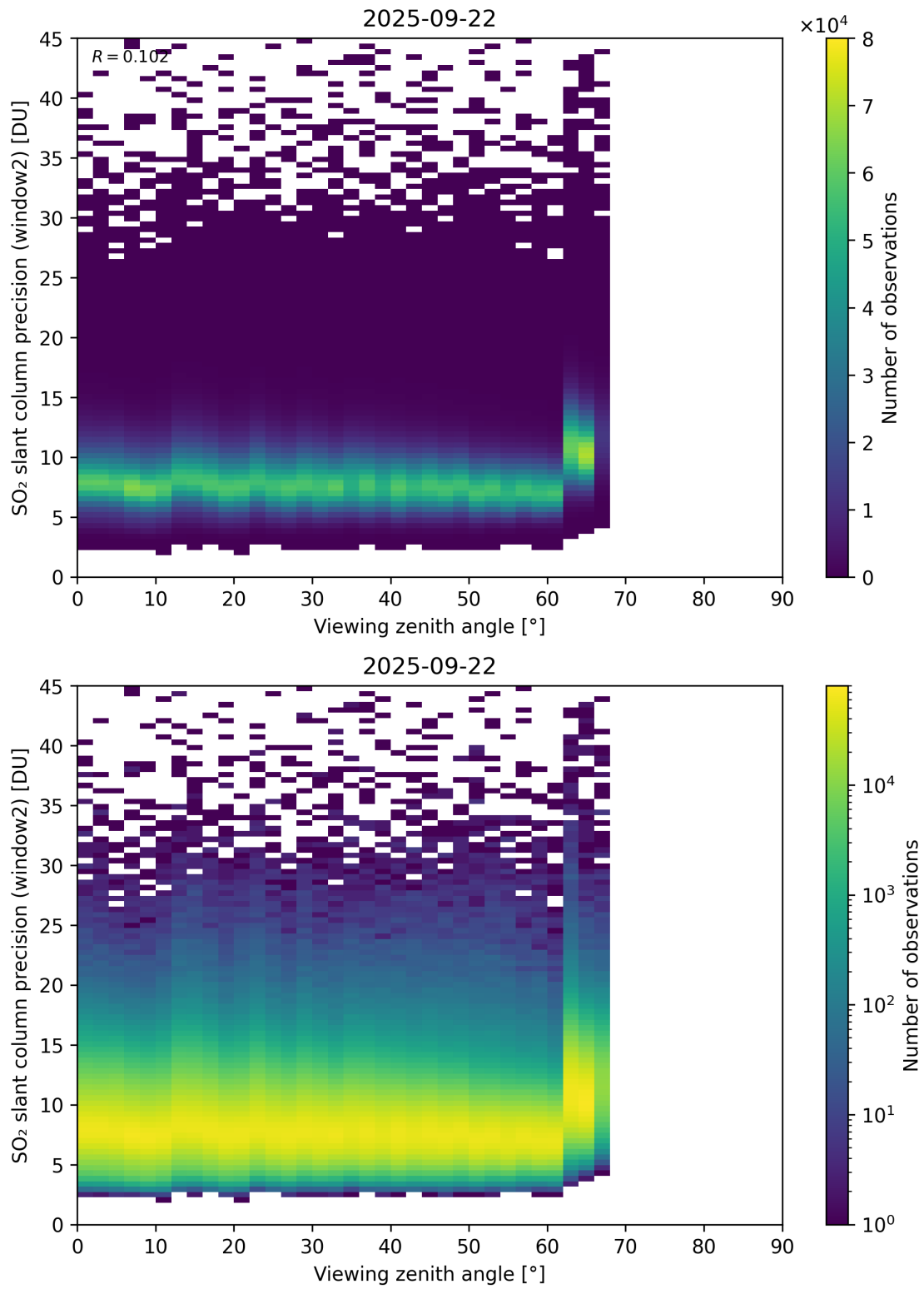
Figure 378: Scatter density plot of “Viewing zenith angle” against “SO 2 slant column precision (window2)” for 2025-09-22 to 2025-09-23.
