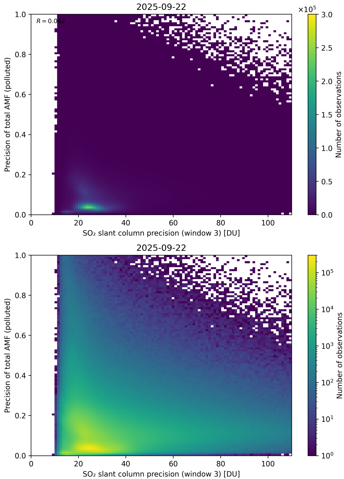
Figure 314: Scatter density plot of “SO 2 slant column precision (window 3)” against “Precision of total AMF (polluted)” for 2025-09-22 to 2025-09-23.
