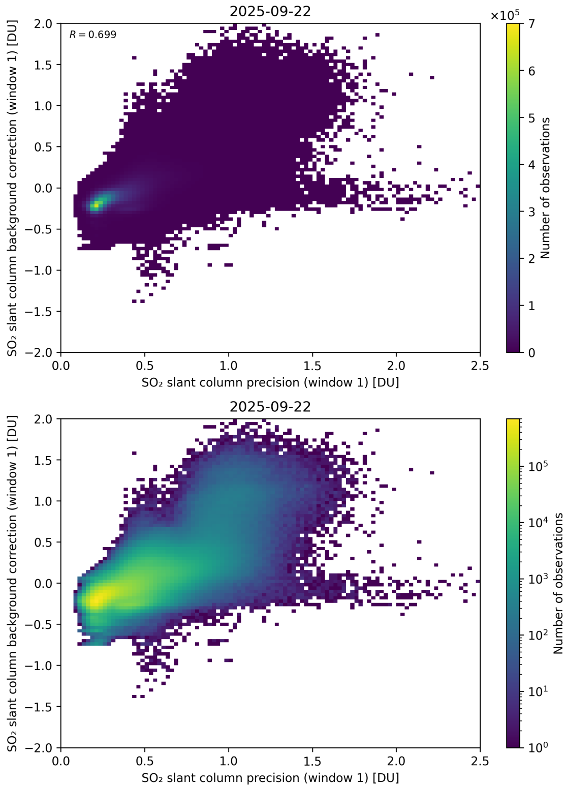
Figure 268: Scatter density plot of “SO 2 slant column precision (window 1)” against “SO 2 slant column background correction (window 1)” for 2025-09-22 to 2025-09-23.
