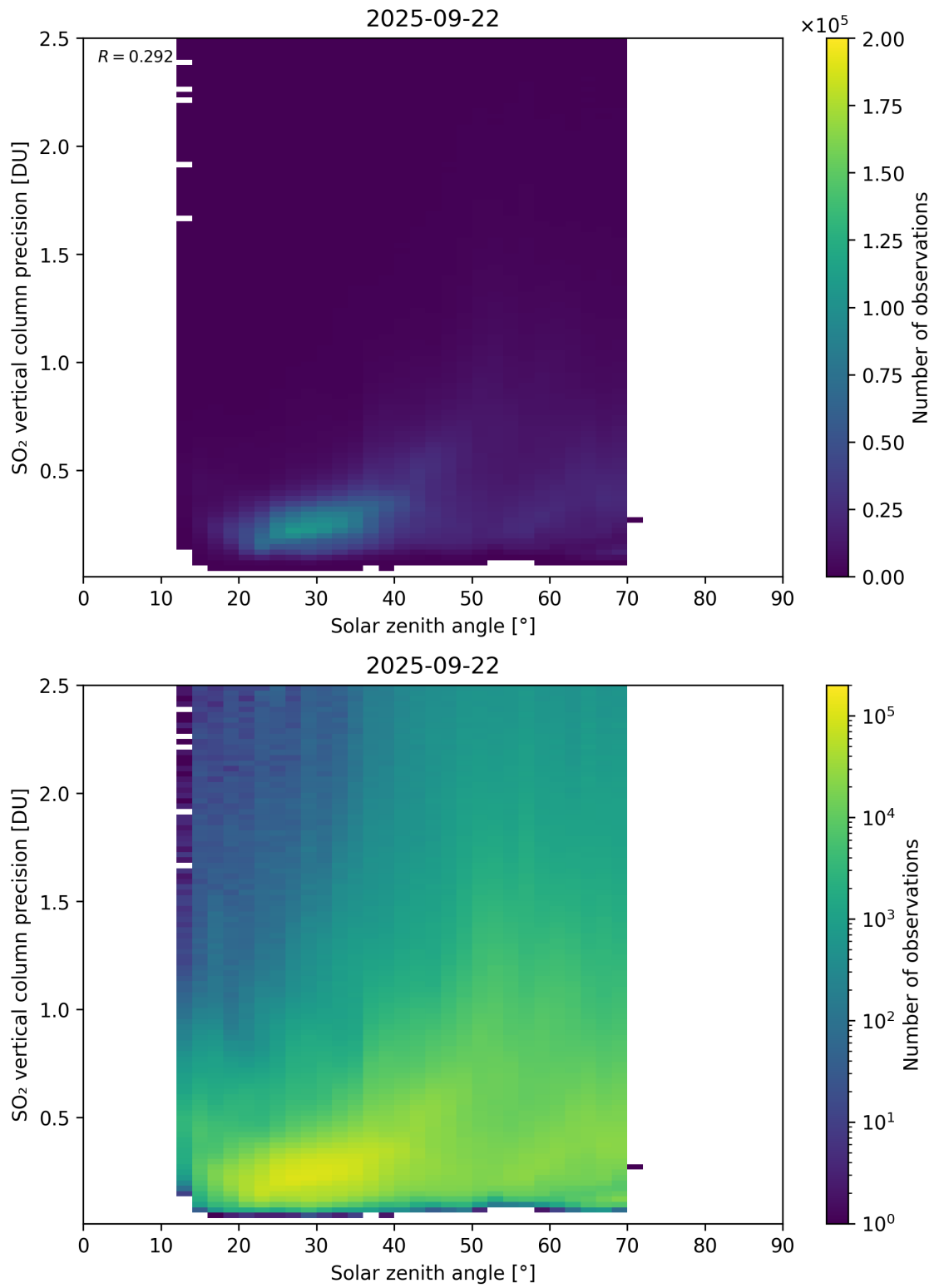
Figure 192: Scatter density plot of “Solar zenith angle” against “SO 2 vertical column precision” for 2025-09-22 to 2025-09-23.
