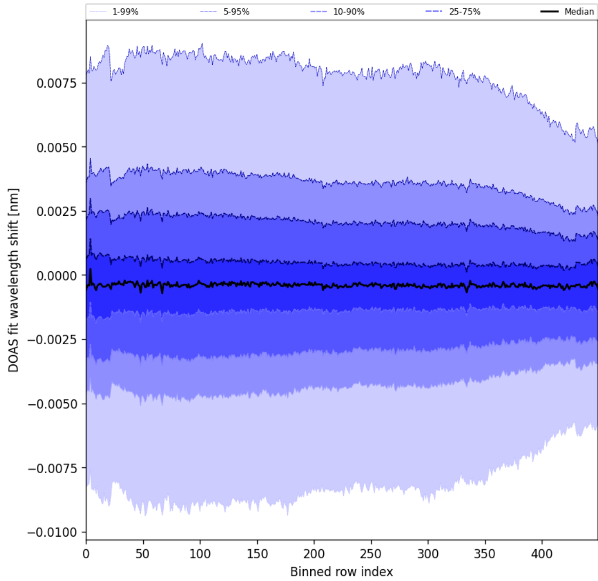
Figure 102: Along track statistics of “DOAS fit wavelength shift” for 2025-09-22 to 2025-09-23
