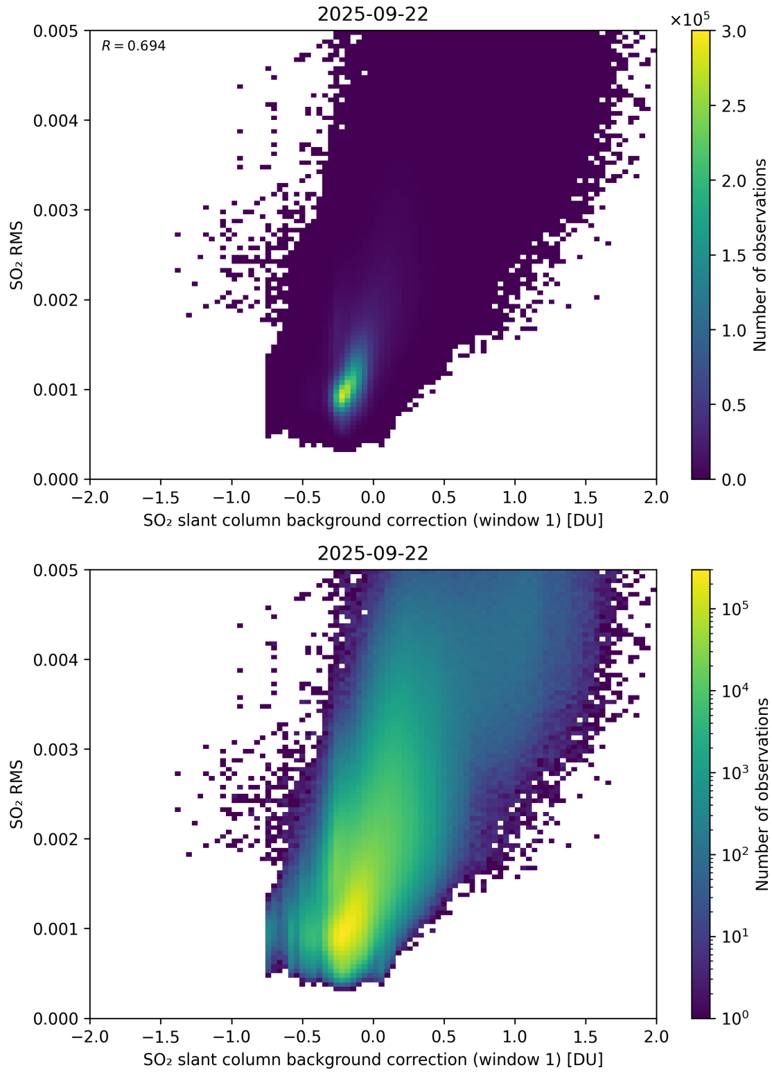
Figure 113: Scatter density plot of “SO 2 slant column background correction (window 1)” against “SO 2 RMS” for 2025-09-22 to 2025-09-23.
