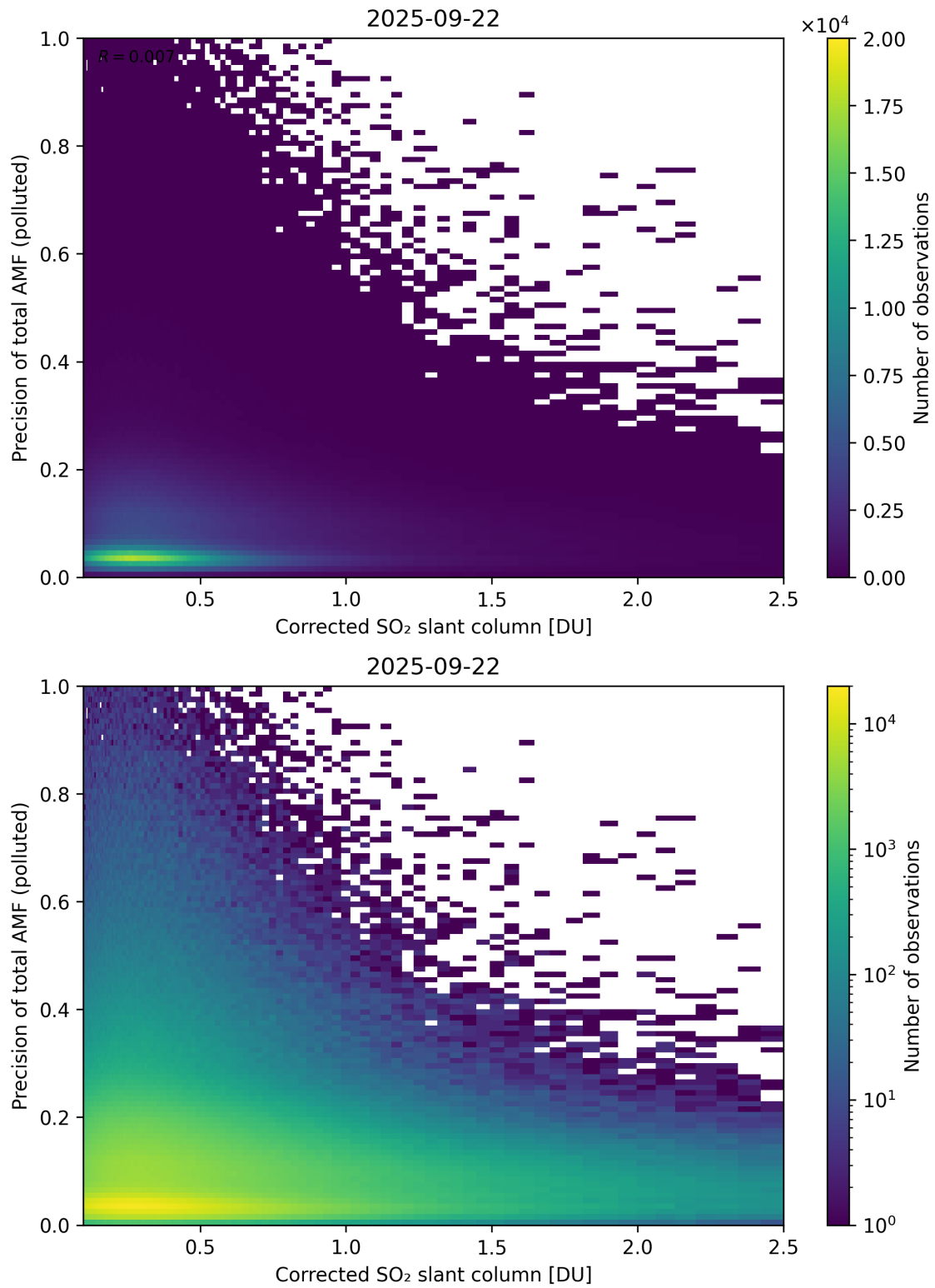
Figure 243: Scatter density plot of “Corrected SO 2 slant column” against “Precision of total AMF (polluted)” for 2025-09-22 to 2025-09-23.
