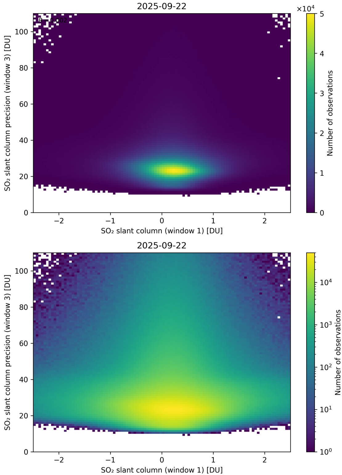
Figure 288: Scatter density plot of “SO 2 slant column (window 1)” against “SO 2 slant column precision (window 3)” for 2025-09-22 to 2025-09-23.
