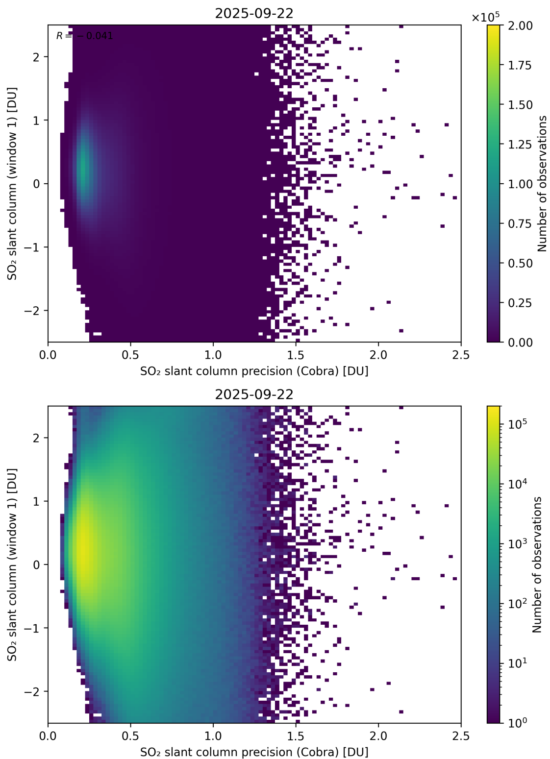
Figure 208: Scatter density plot of “SO 2 slant column precision (Cobra)” against “SO 2 slant column (window 1)” for 2025-09-22 to 2025-09-23.
