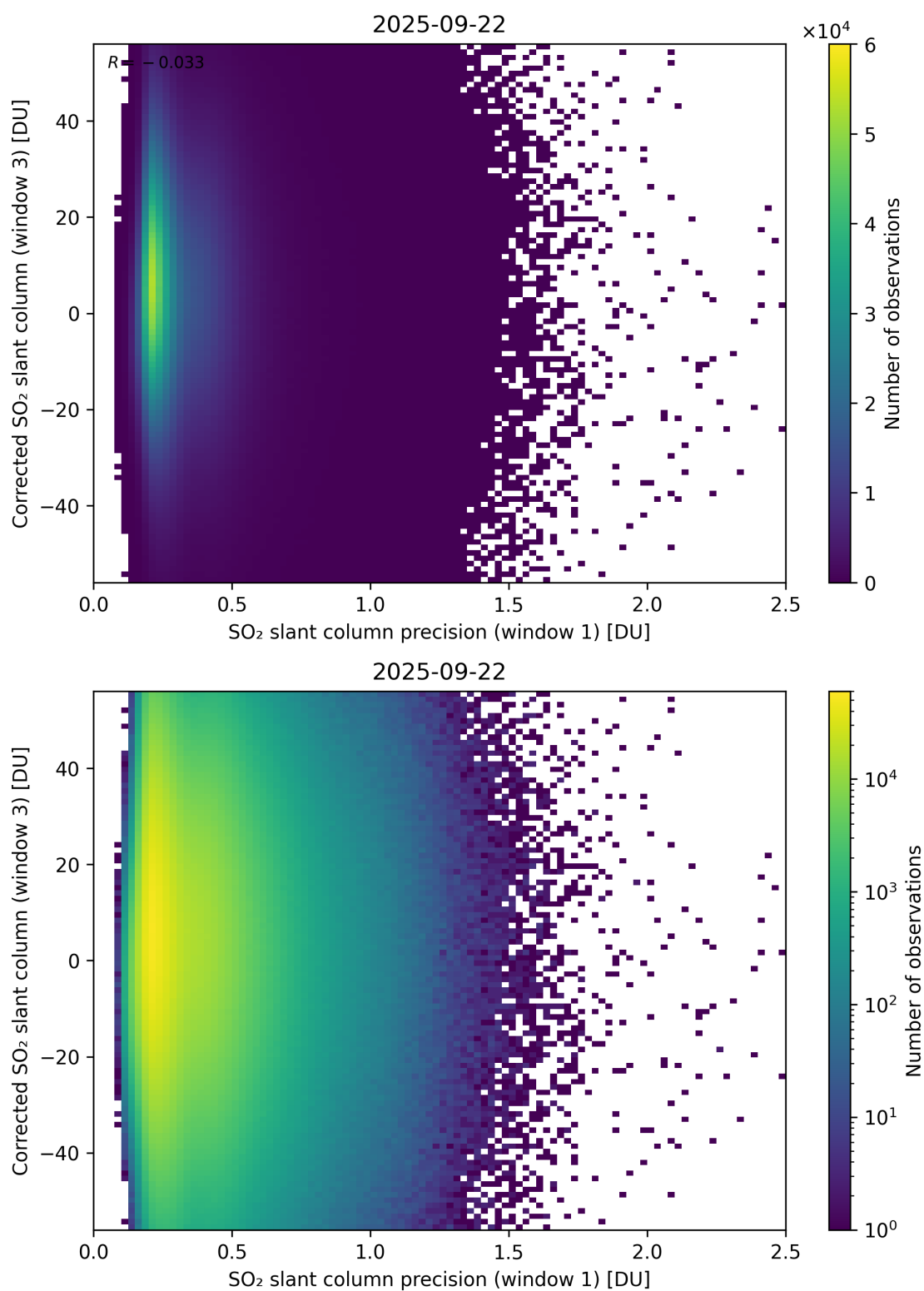
Figure 276: Scatter density plot of “SO 2 slant column precision (window 1)” against “Corrected SO 2 slant column (window 3)” for 2025-09-22 to 2025-09-23.
