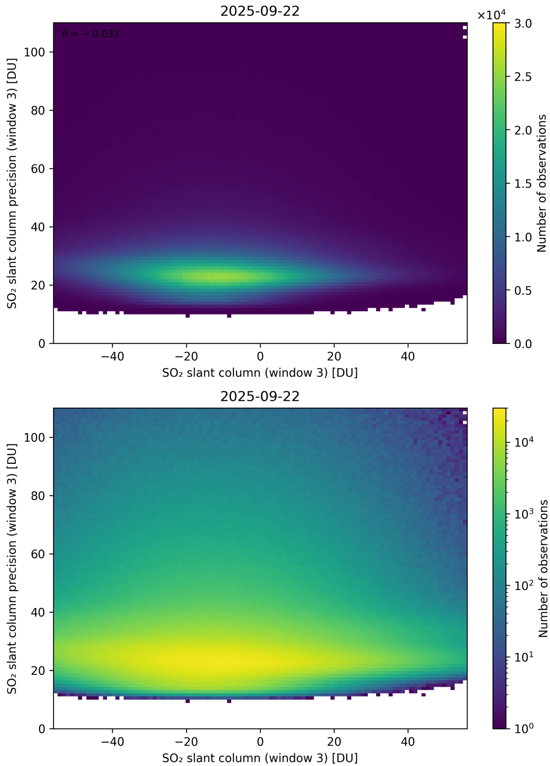
Figure 317: Scatter density plot of “SO 2 slant column (window 3)” against “SO 2 slant column precision (window 3)” for 2025-09-22 to 2025-09-23.
