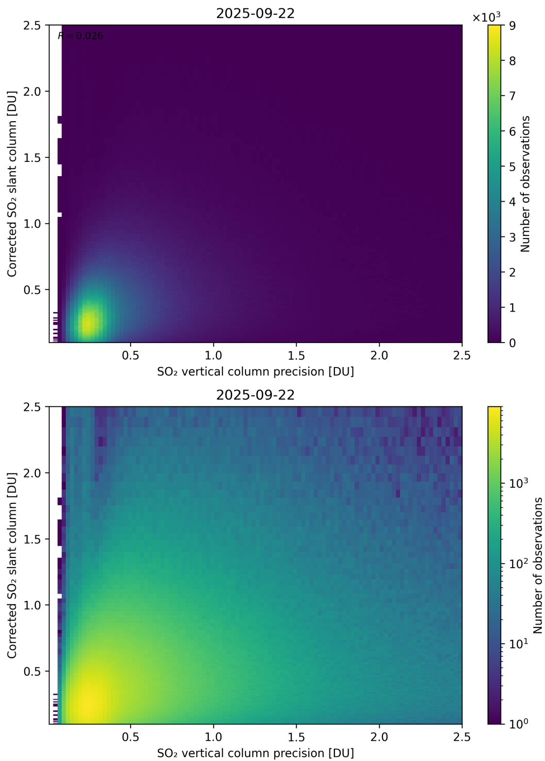
Figure 338: Scatter density plot of “SO 2 vertical column precision” against “Corrected SO 2 slant column” for 2025-09-22 to 2025-09-23.
