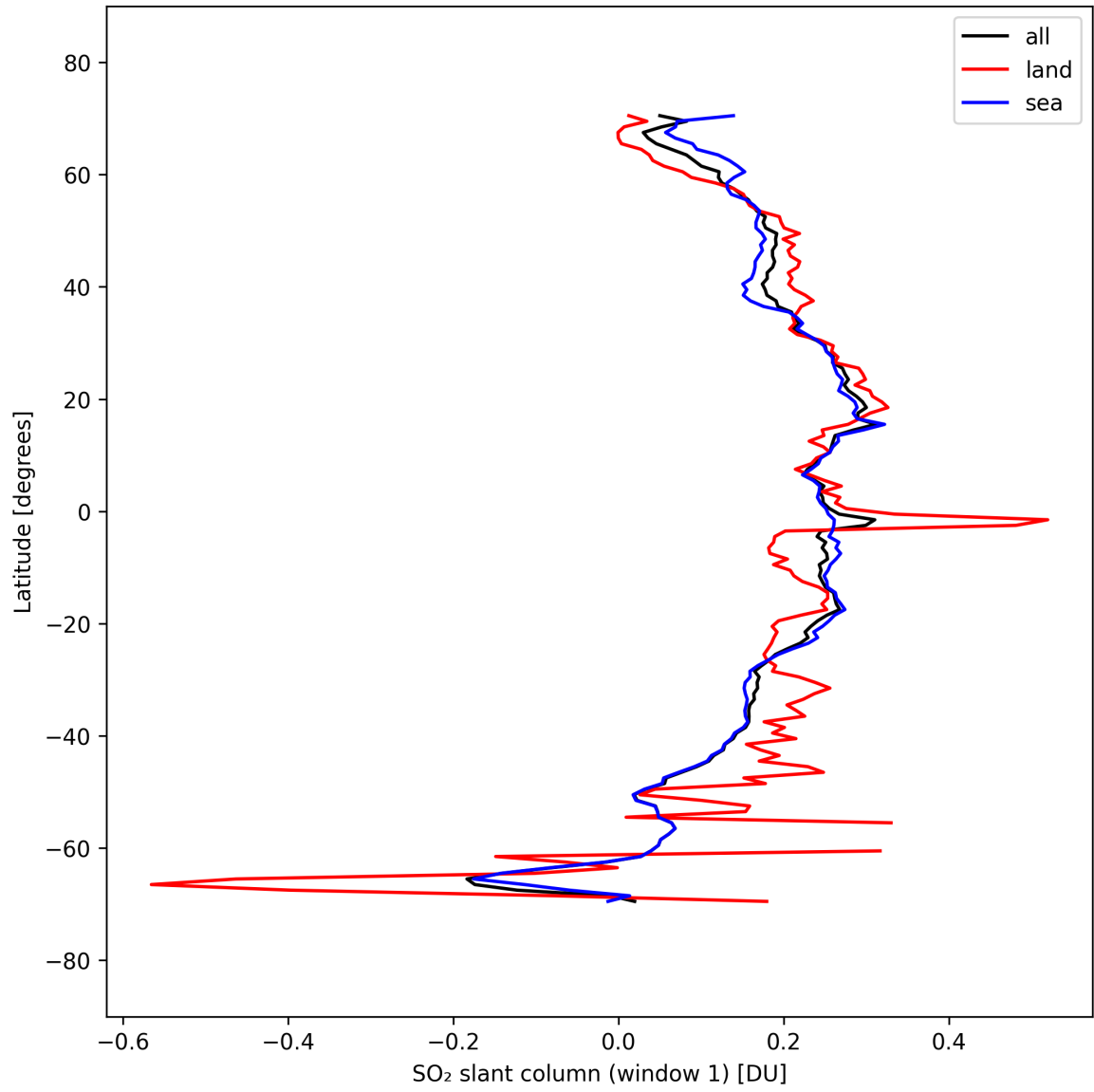
Figure 37: Zonal average of “SO 2 slant column (window 1)” for 2025-09-22 to 2025-09-23.
