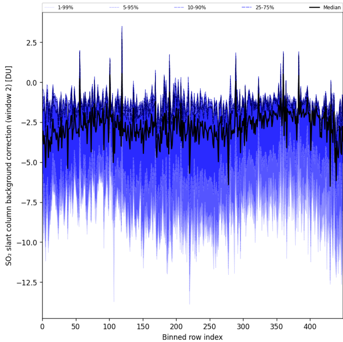
Figure 96: Along track statistics of “SO 2 slant column background correction (window 2)” for 2025-09-22 to 2025-09-23
