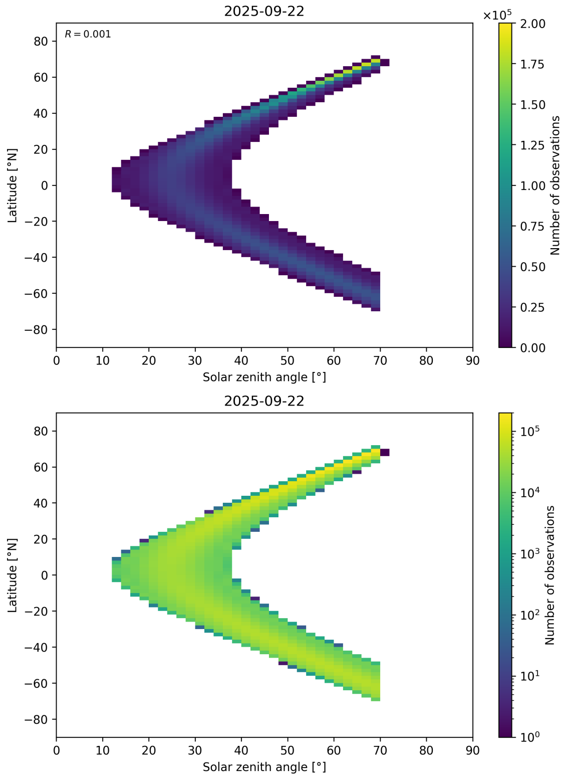
Figure 177: Scatter density plot of “Solar zenith angle” against “Latitude” for 2025-09-22 to 2025-09-23.
