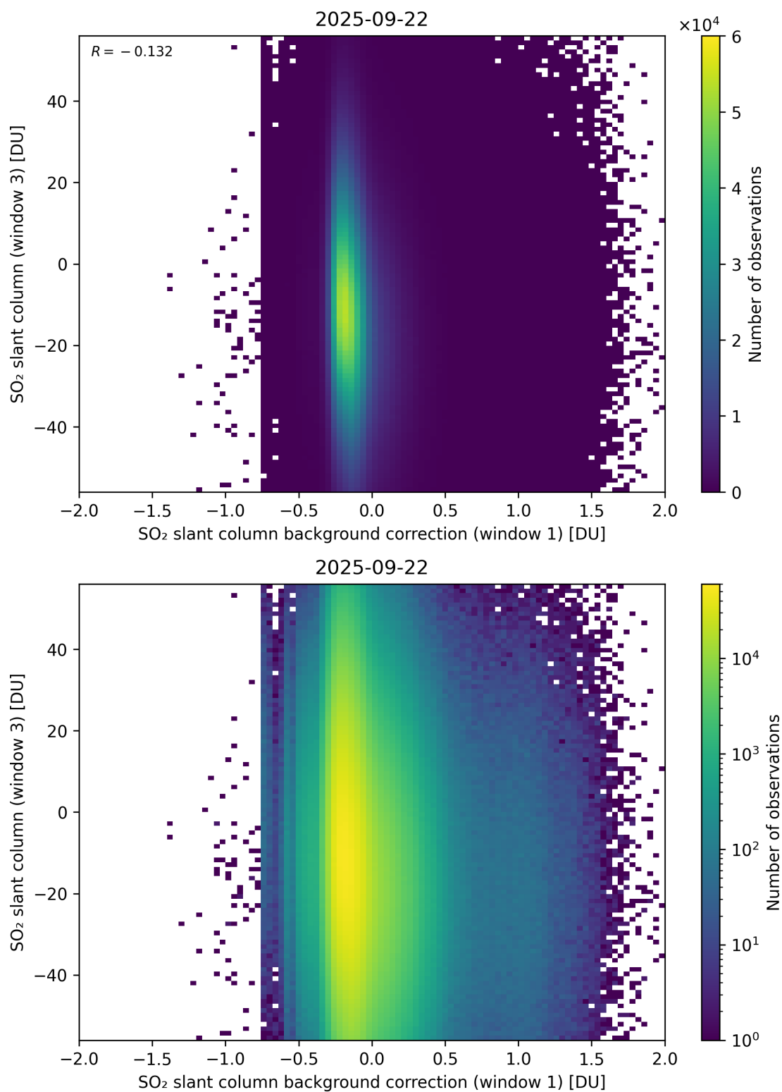
Figure 118: Scatter density plot of “SO 2 slant column background correction (window 1)” against “SO 2 slant column (window 3)” for 2025-09-22 to 2025-09-23.
