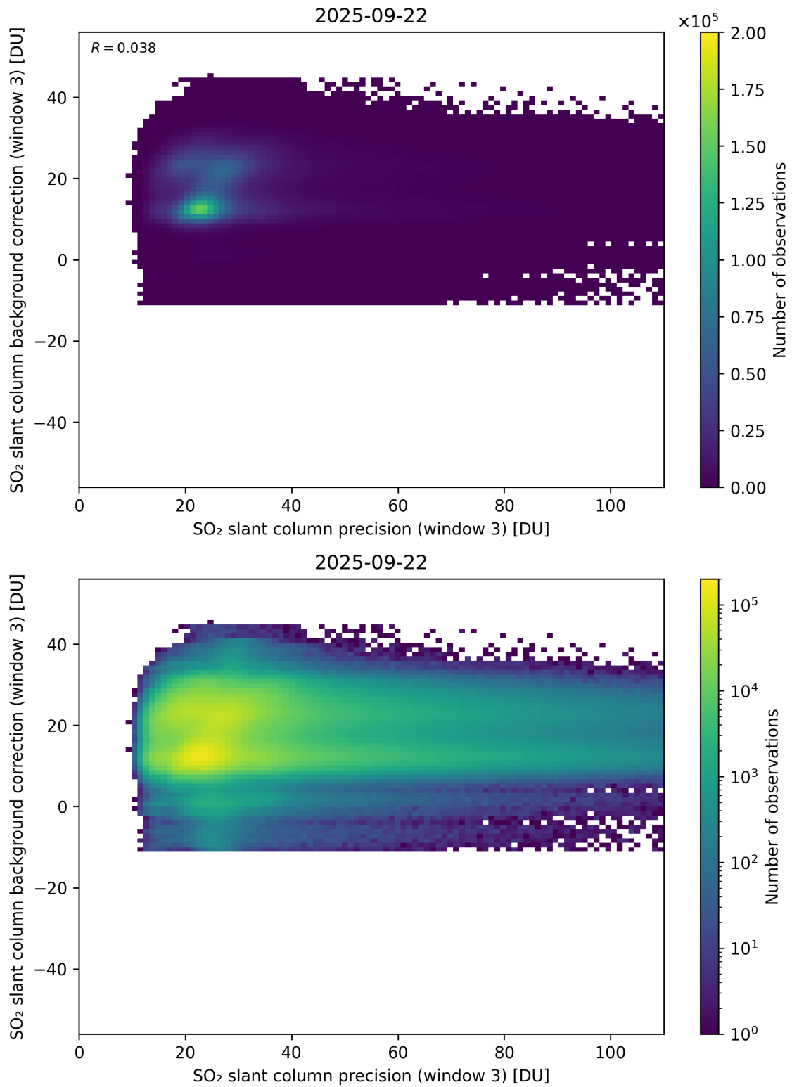
Figure 307: Scatter density plot of “SO 2 slant column precision (window 3)” against “SO 2 slant column background correction (window 3)” for 2025-09-22 to 2025-09-23.
