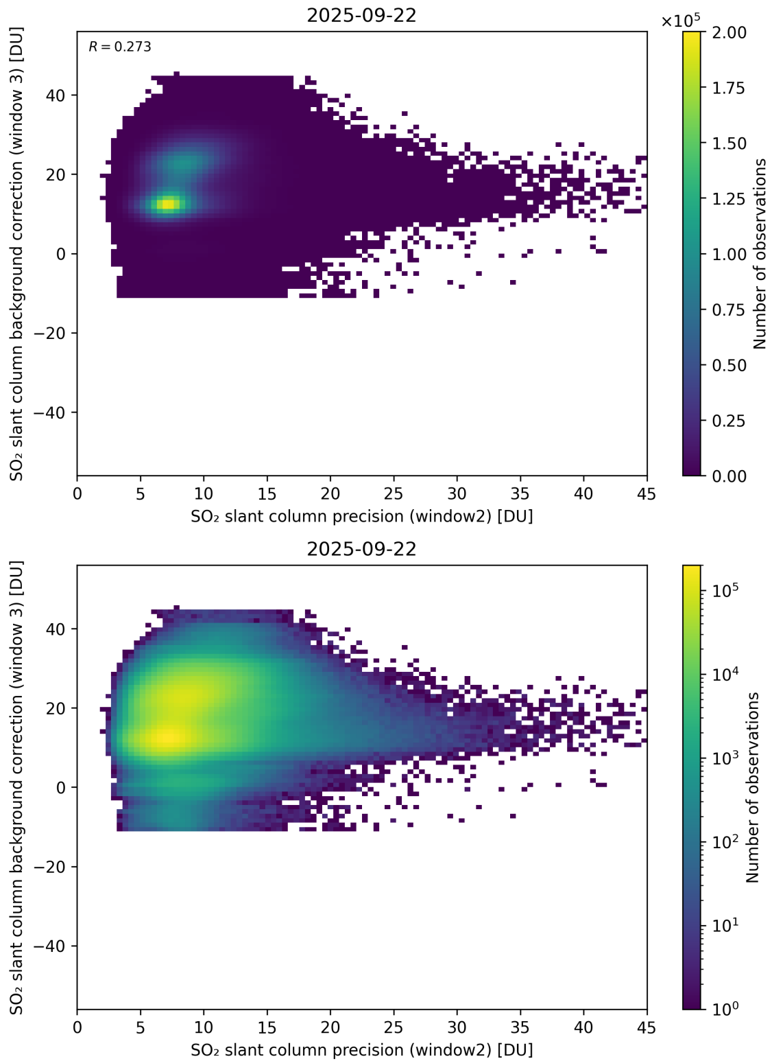
Figure 292: Scatter density plot of “SO 2 slant column precision (window2)” against “SO 2 slant column background correction (window 3)” for 2025-09-22 to 2025-09-23.
