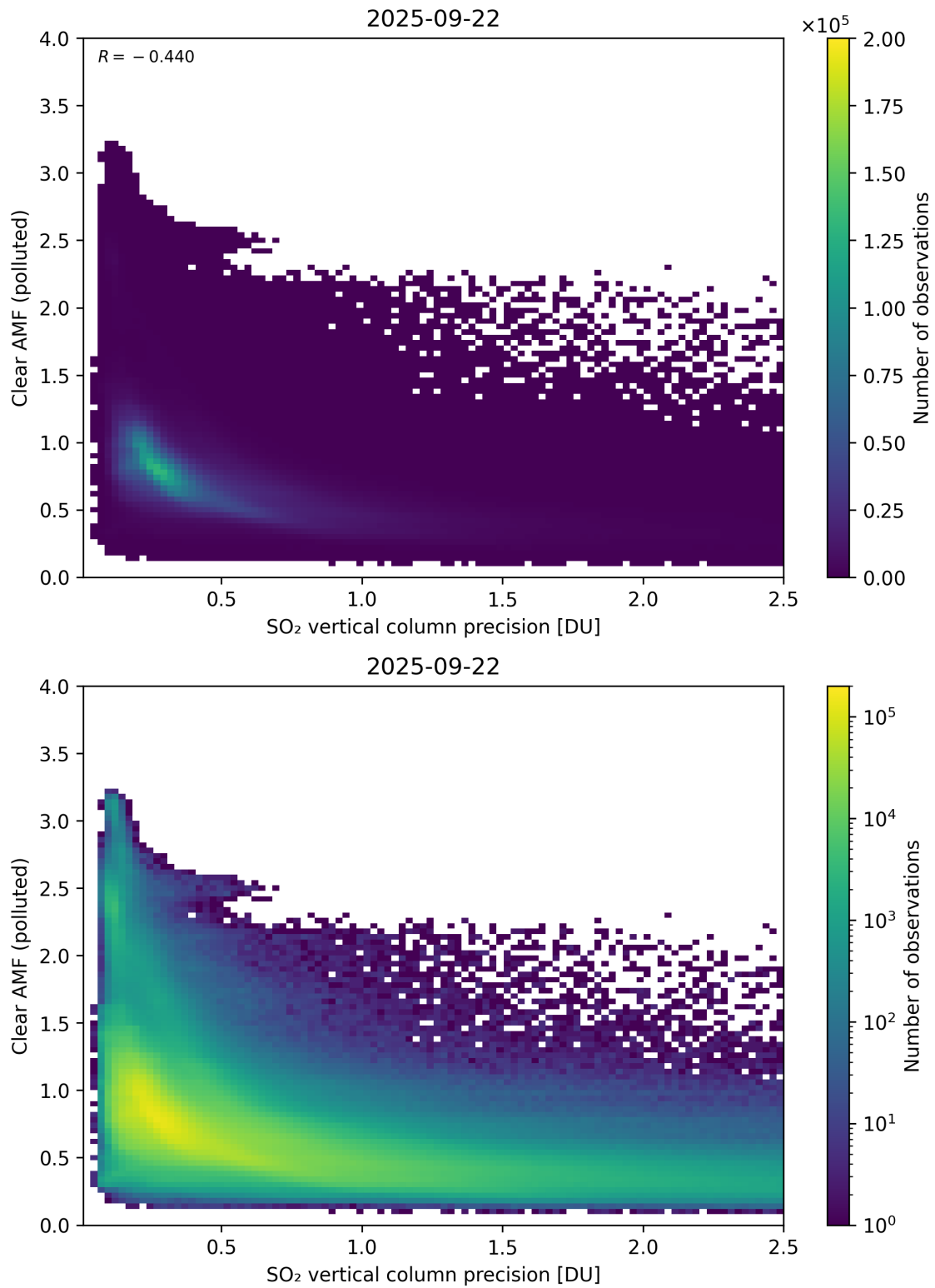
Figure 335: Scatter density plot of “SO 2 vertical column precision” against “Clear AMF (polluted)” for 2025-09-22 to 2025-09-23.
