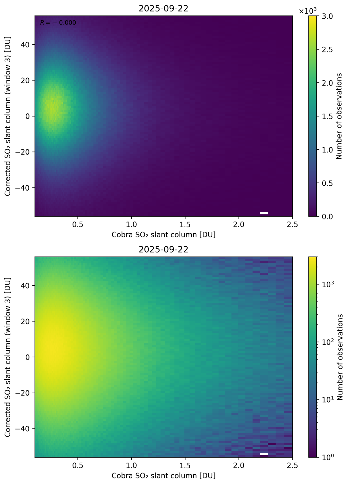
Figure 218: Scatter density plot of “Cobra SO 2 slant column” against “Corrected SO 2 slant column (window 3)” for 2025-09-22 to 2025-09-23.
