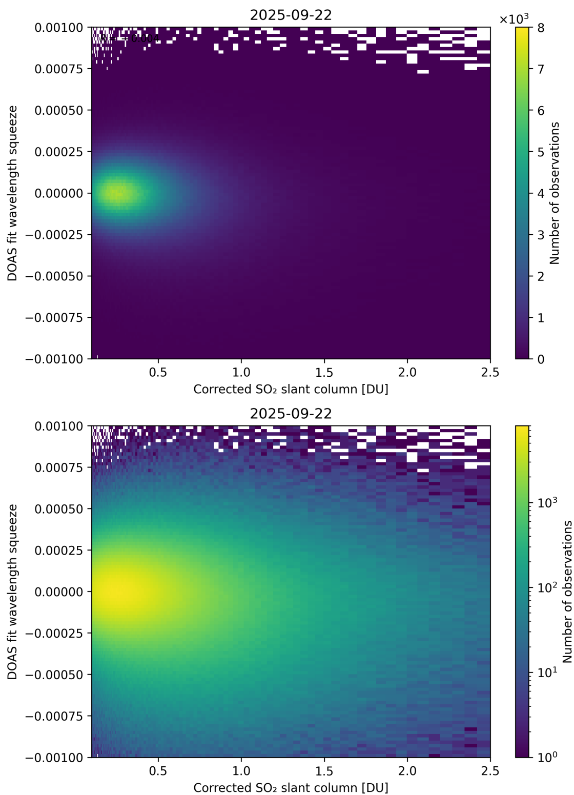
Figure 230: Scatter density plot of "Corrected SO 2 slant column" against "DOAS fit wavelength squeeze" for 2025-09-22 to 2025-09-23.
