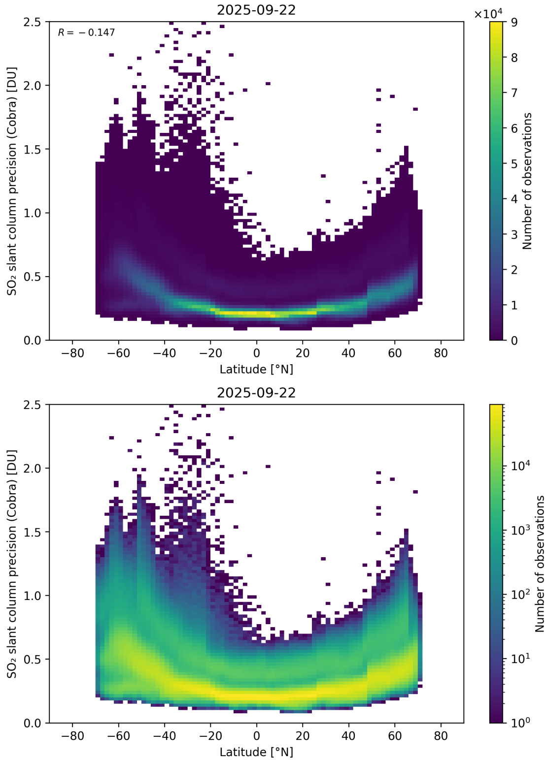
Figure 158: Scatter density plot of “Latitude” against “SO 2 slant column precision (Cobra)” for 2025-09-22 to 2025-09-23.
