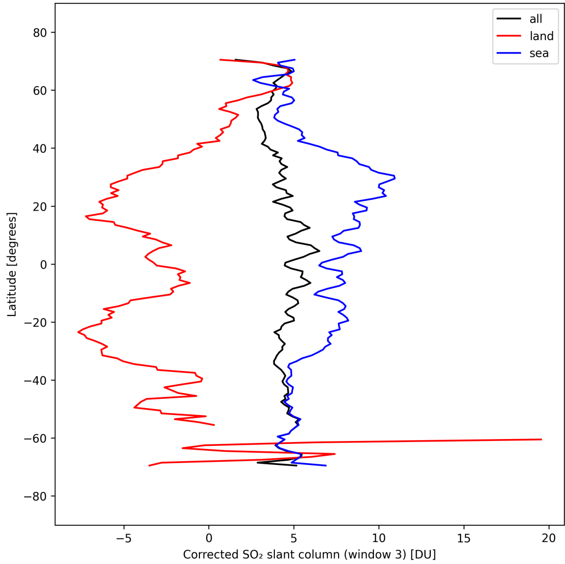
Figure 47: Zonal average of “Corrected SO 2 slant column (window 3)” for 2025-09-22 to 2025-09-23.
