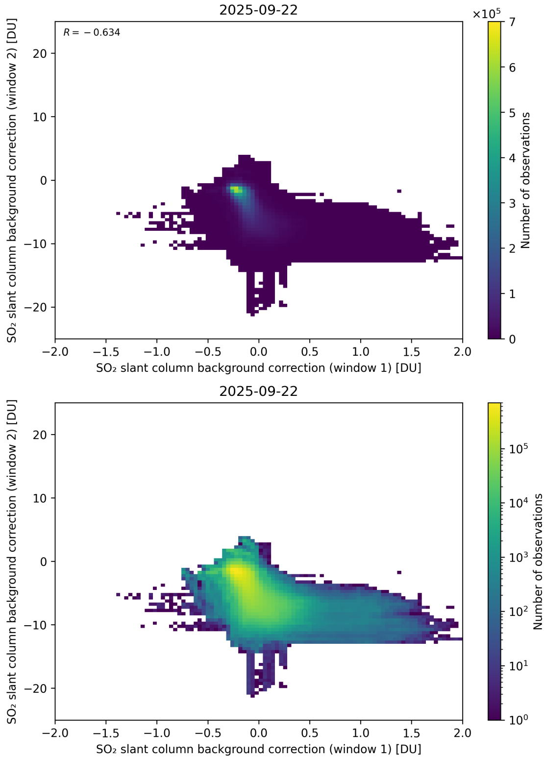
Figure 109: Scatter density plot of “SO 2 slant column background correction (window 1)” against “SO 2 slant column background correction (window 2)” for 2025-09-22 to 2025-09-23.
