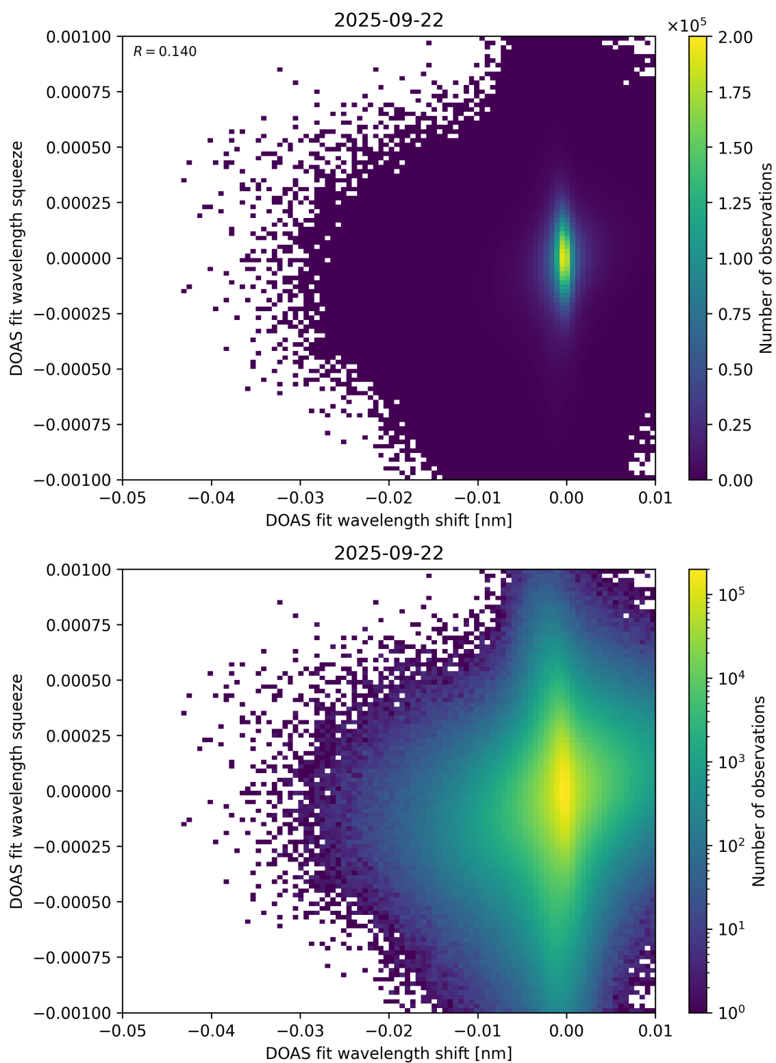
Figure 138: Scatter density plot of “DOAS fit wavelength shift” against “DOAS fit wavelength squeeze” for 2025-09-22 to 2025-09-23.
