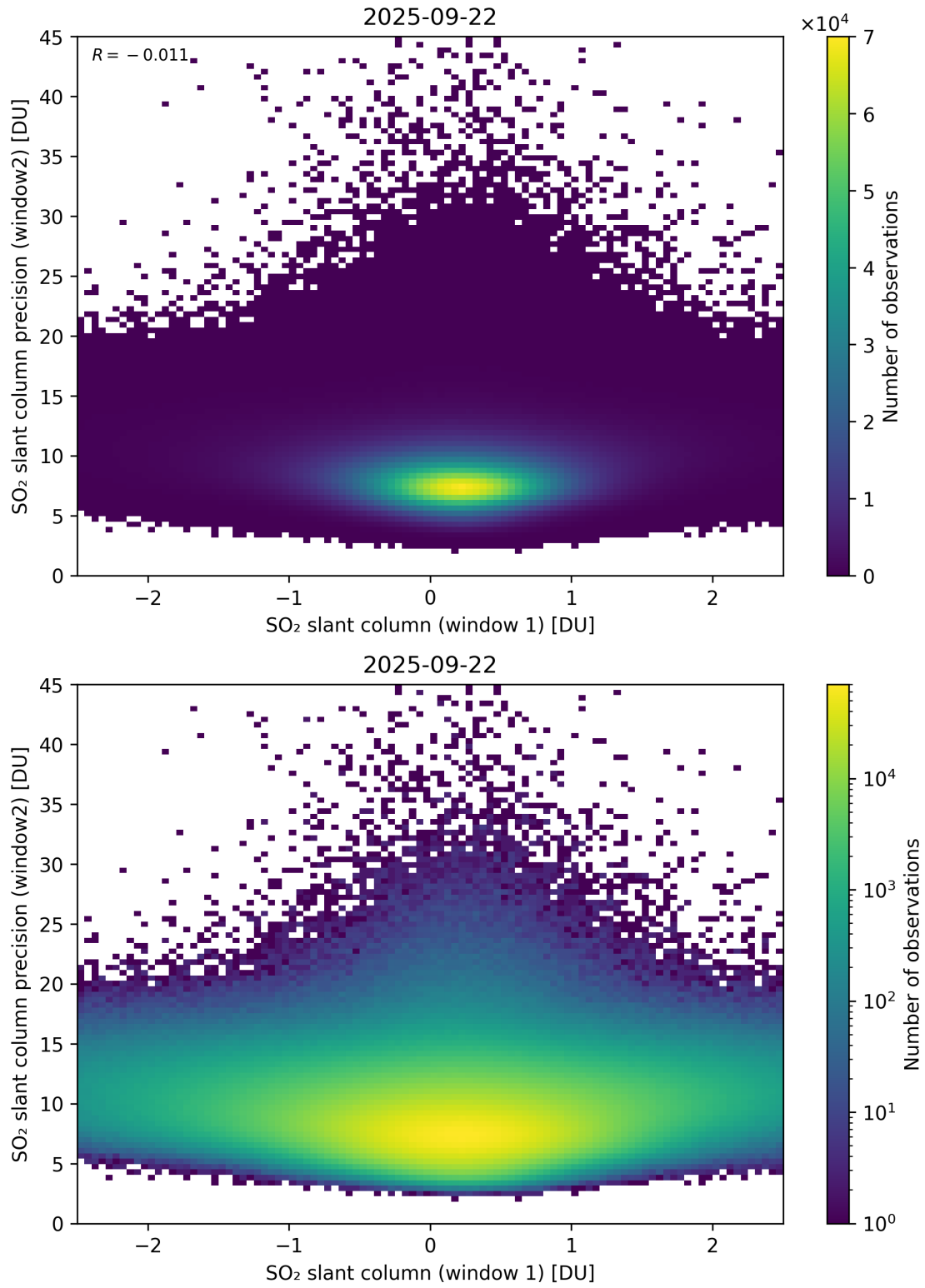
Figure 286: Scatter density plot of “SO 2 slant column (window 1)” against “SO 2 slant column precision (window2)” for 2025-09-22 to 2025-09-23.
