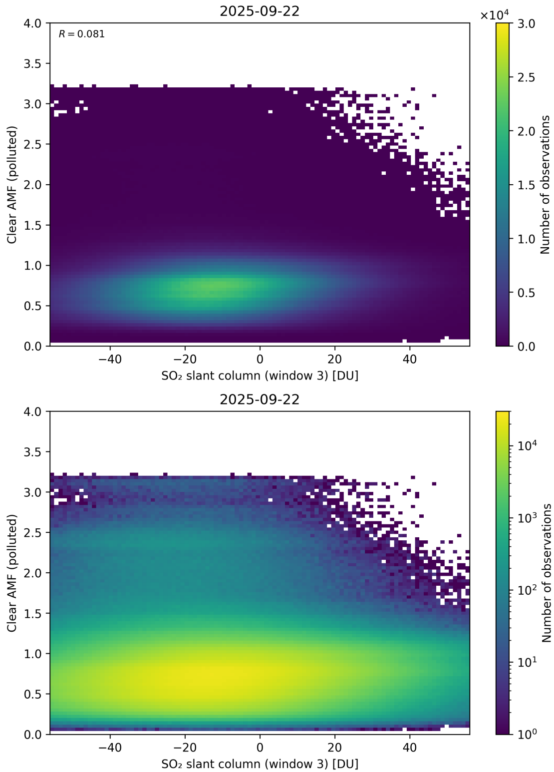
Figure 315: Scatter density plot of “SO 2 slant column (window 3)” against “Clear AMF (polluted)” for 2025-09-22 to 2025-09-23.
