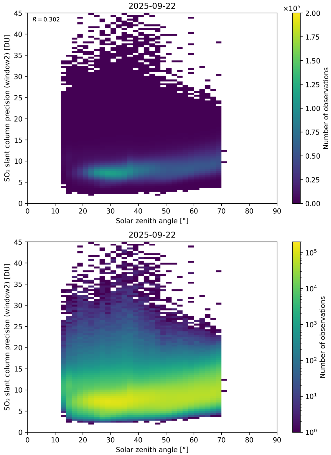
Figure 186: Scatter density plot of “Solar zenith angle” against “SO 2 slant column precision (window2)” for 2025-09-22 to 2025-09-23.
