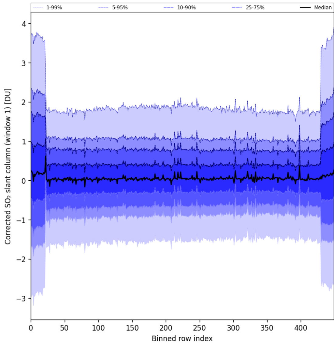
Figure 91: Along track statistics of “Corrected SO 2 slant column (window 1)” for 2025-09-22 to 2025-09-23
