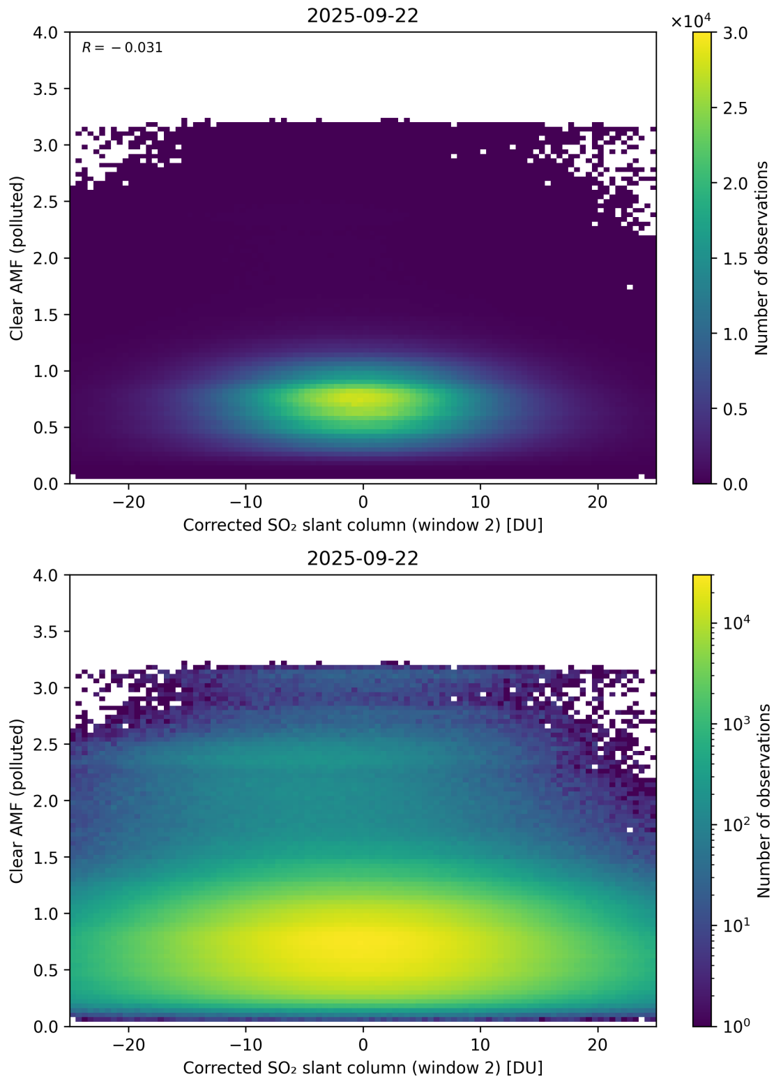
Figure 249: Scatter density plot of “Corrected SO 2 slant column (window 2)” against “Clear AMF (polluted)” for 2025-09-22 to 2025-09-23.
