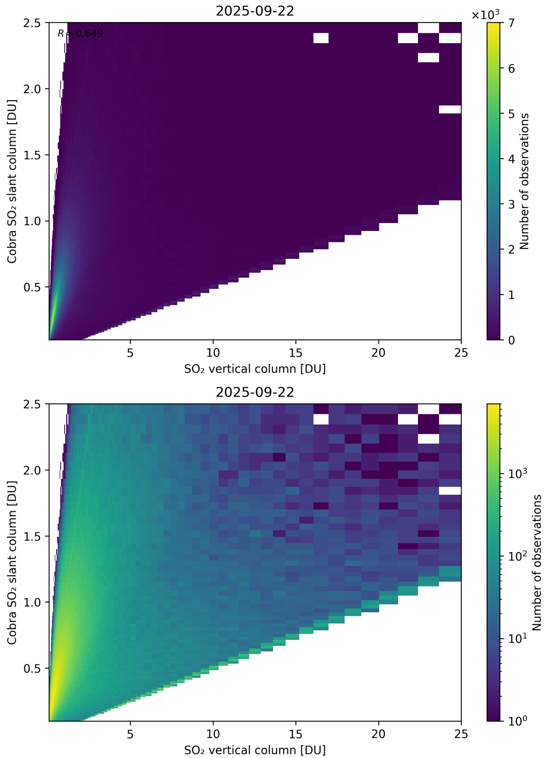
Figure 349: Scatter density plot of “SO 2 vertical column” against “Cobra SO 2 slant column” for 2025-09-22 to 2025-09-23.
