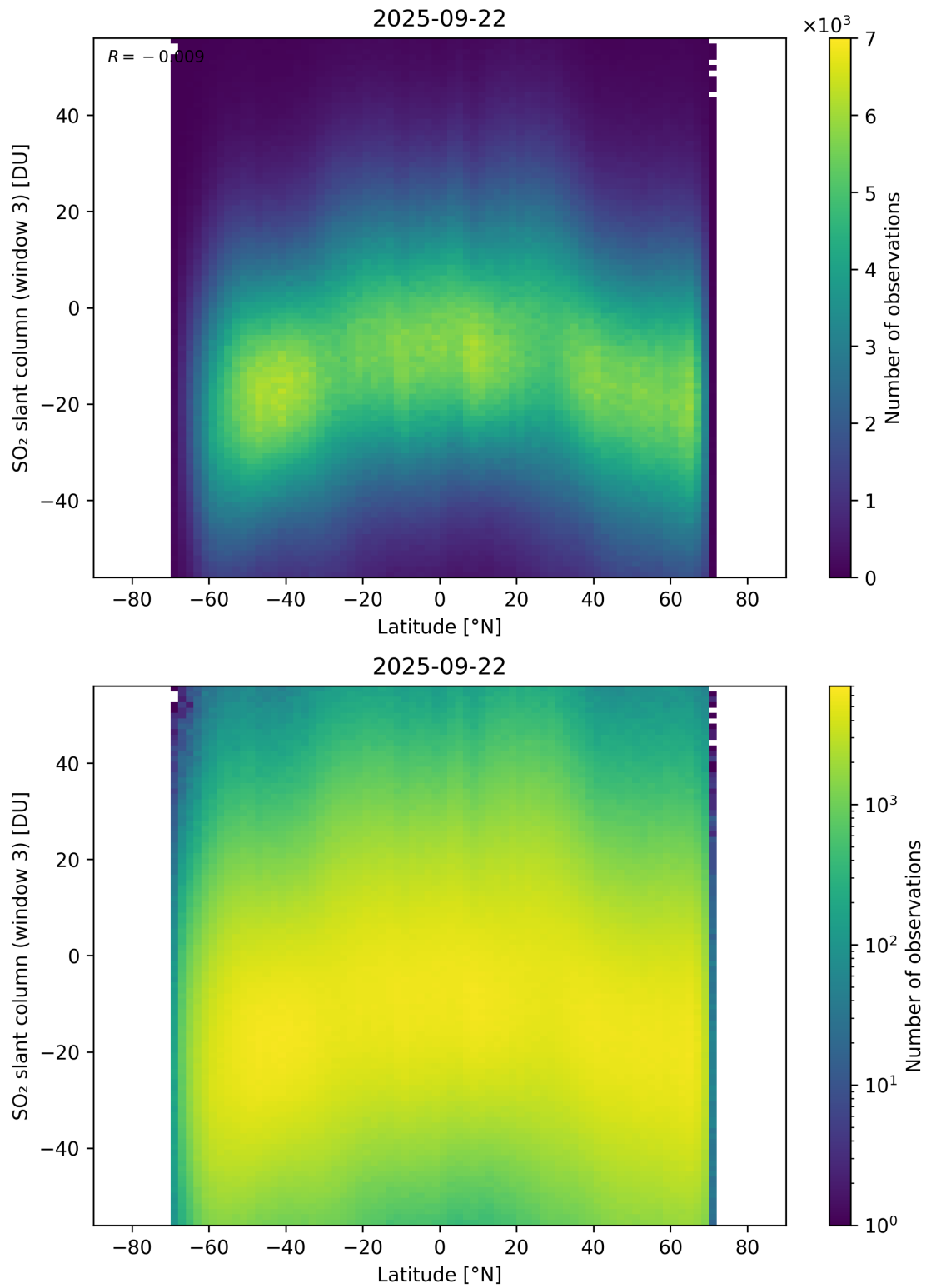
Figure 165: Scatter density plot of “Latitude” against “SO 2 slant column (window 3)” for 2025-09-22 to 2025-09-23.
