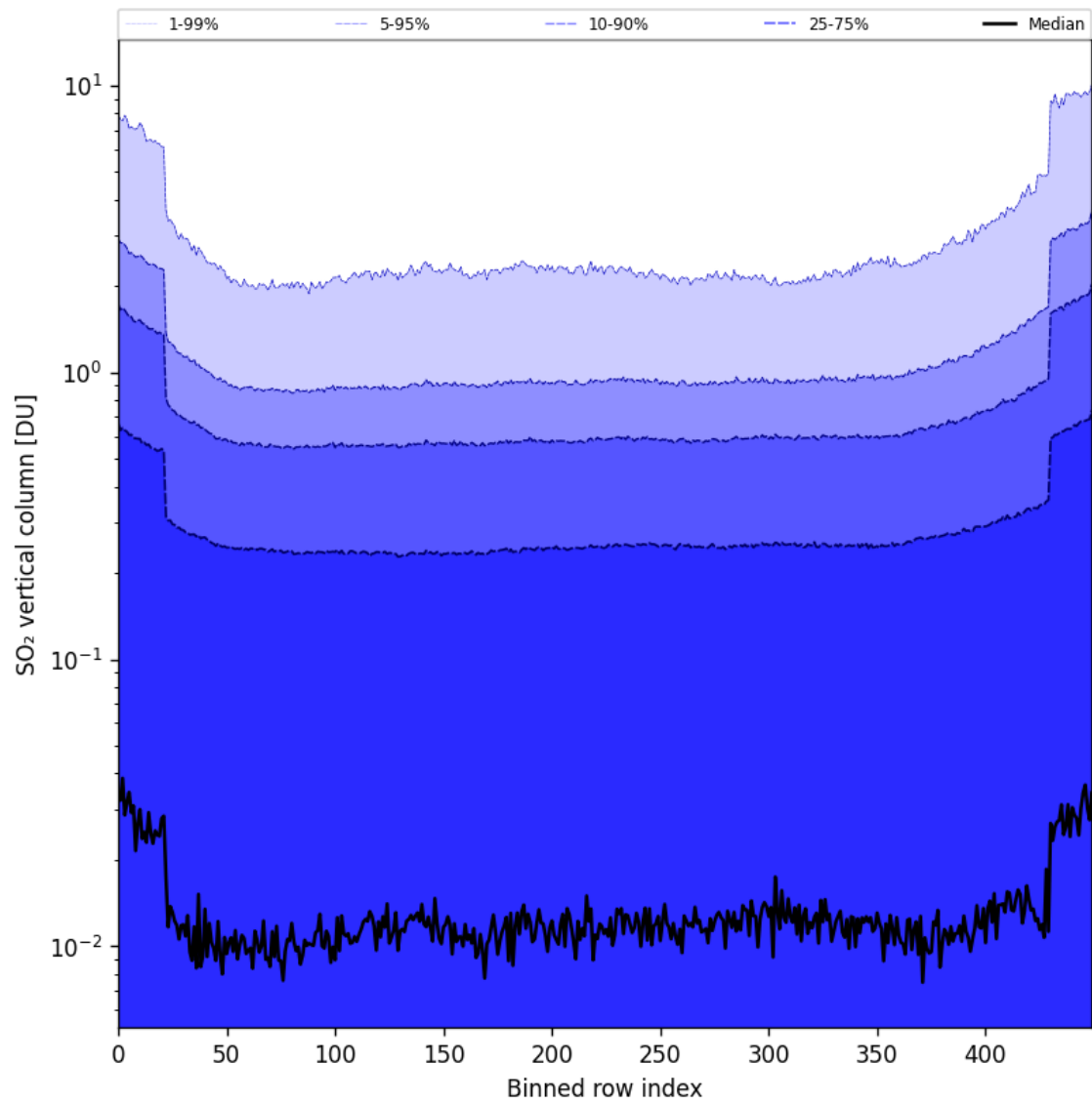
Figure 84: Along track statistics of “SO 2 vertical column” for 2025-09-22 to 2025-09-23
