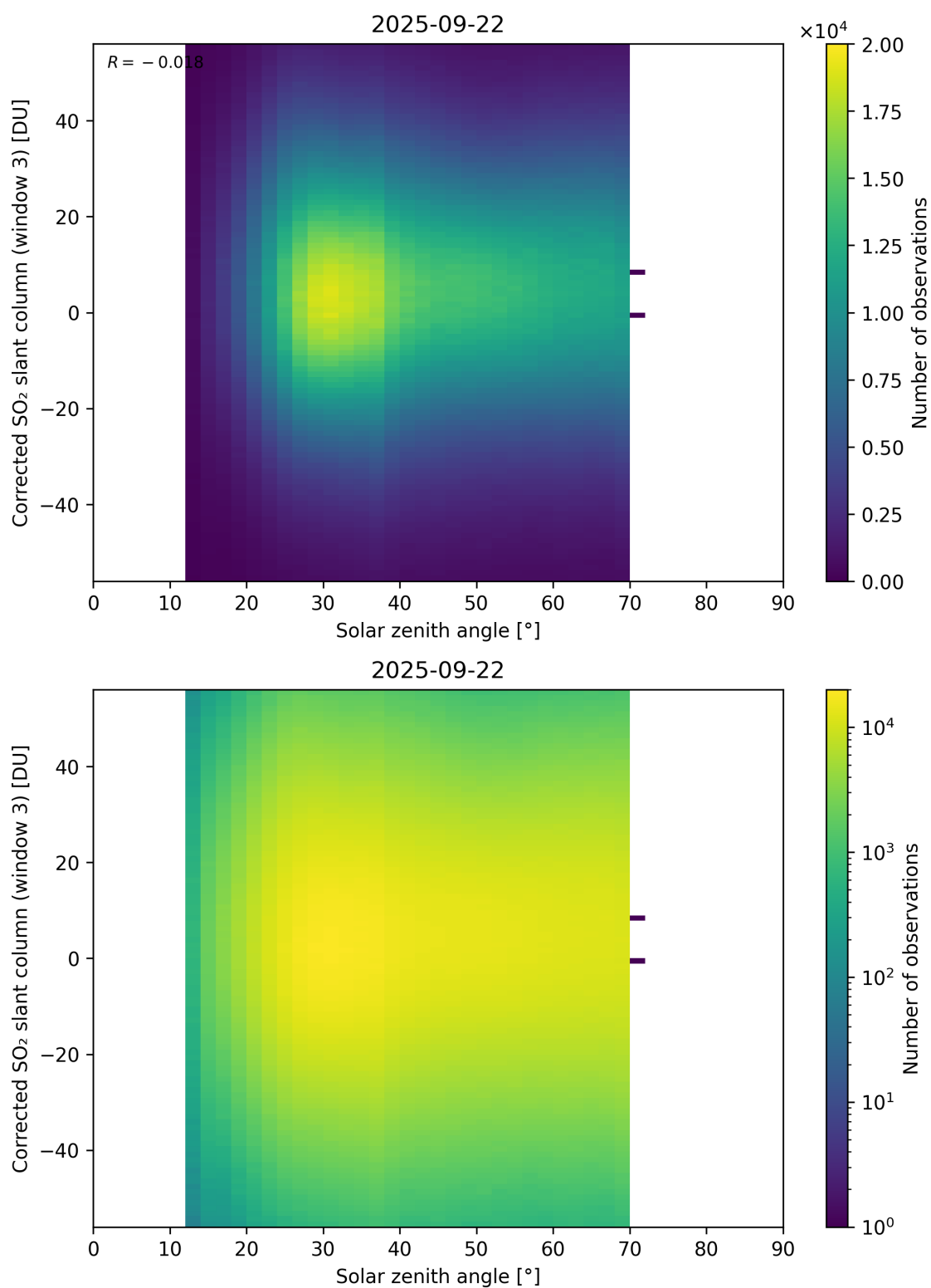
Figure 183: Scatter density plot of “Solar zenith angle” against “Corrected SO 2 slant column (window 3)” for 2025-09-22 to 2025-09-23.
