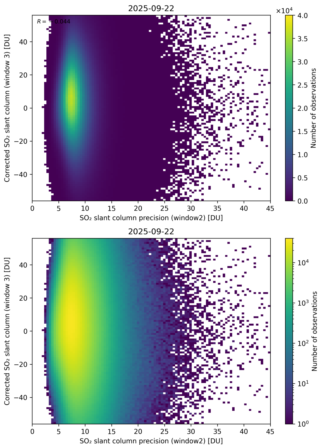
Figure 298: Scatter density plot of “SO 2 slant column precision (window2)” against “Corrected SO 2 slant column (window 3)” for 2025-09-22 to 2025-09-23.
