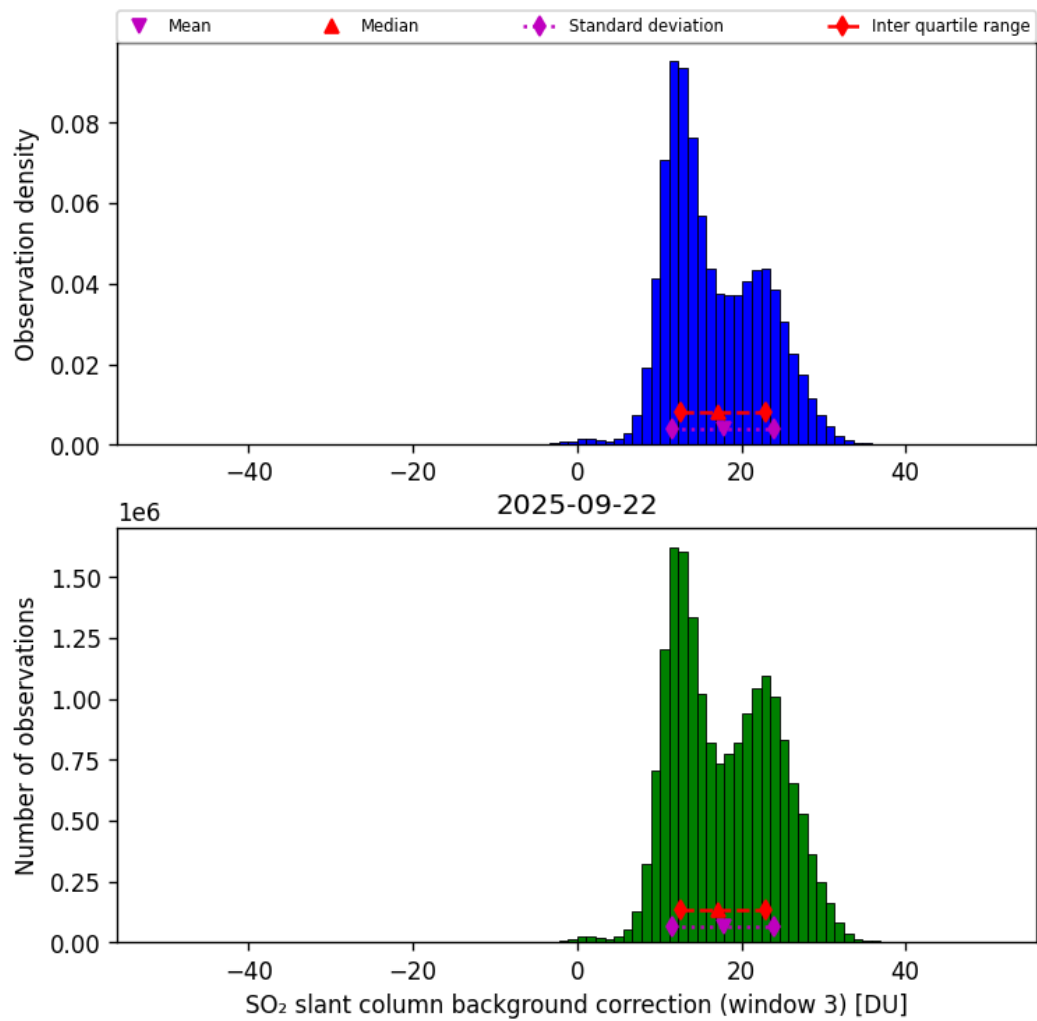
Figure 74: Histogram of “SO 2 slant column background correction (window 3)” for 2025-09-22 to 2025-09-23
