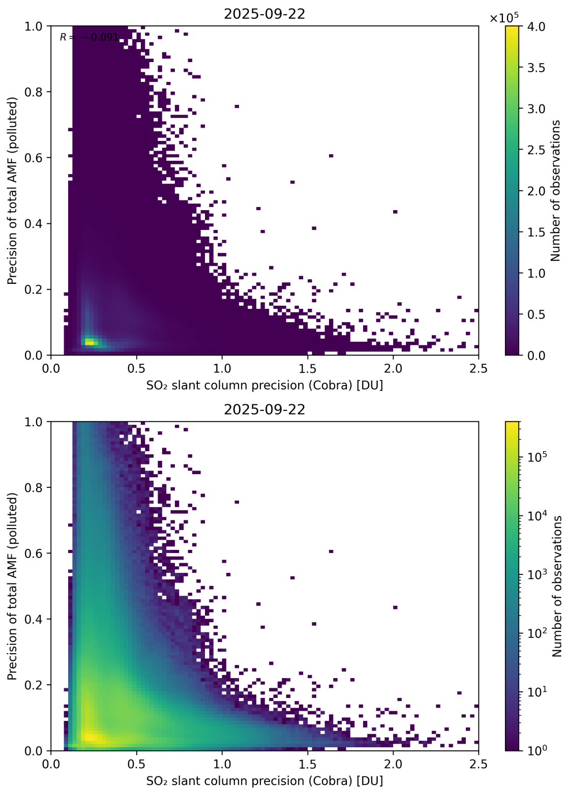
Figure 214: Scatter density plot of “SO 2 slant column precision (Cobra)” against “Precision of total AMF (polluted)” for 2025-09-22 to 2025-09-23.
