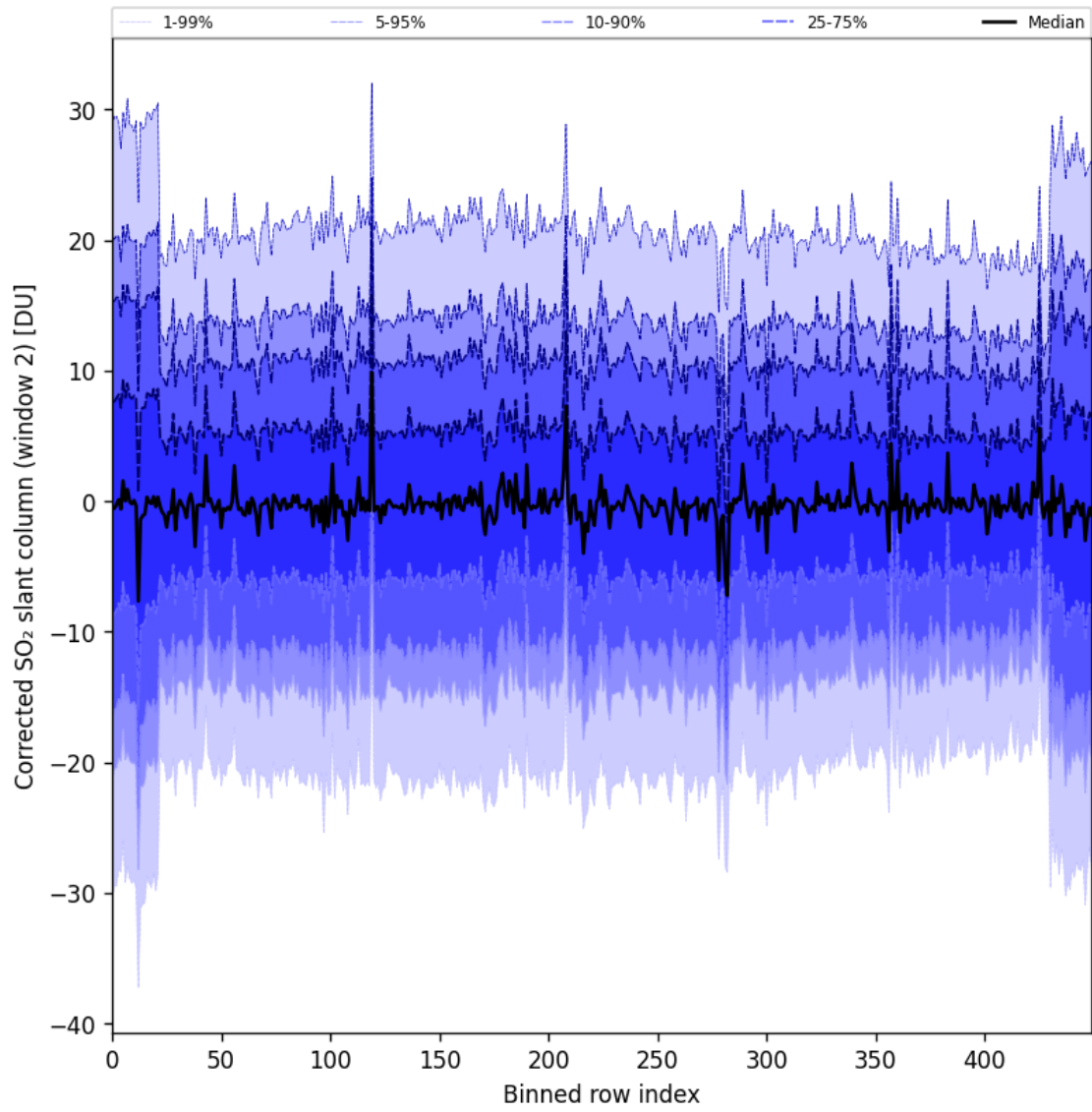
Figure 95: Along track statistics of “Corrected SO 2 slant column (window 2)” for 2025-09-22 to 2025-09-23
