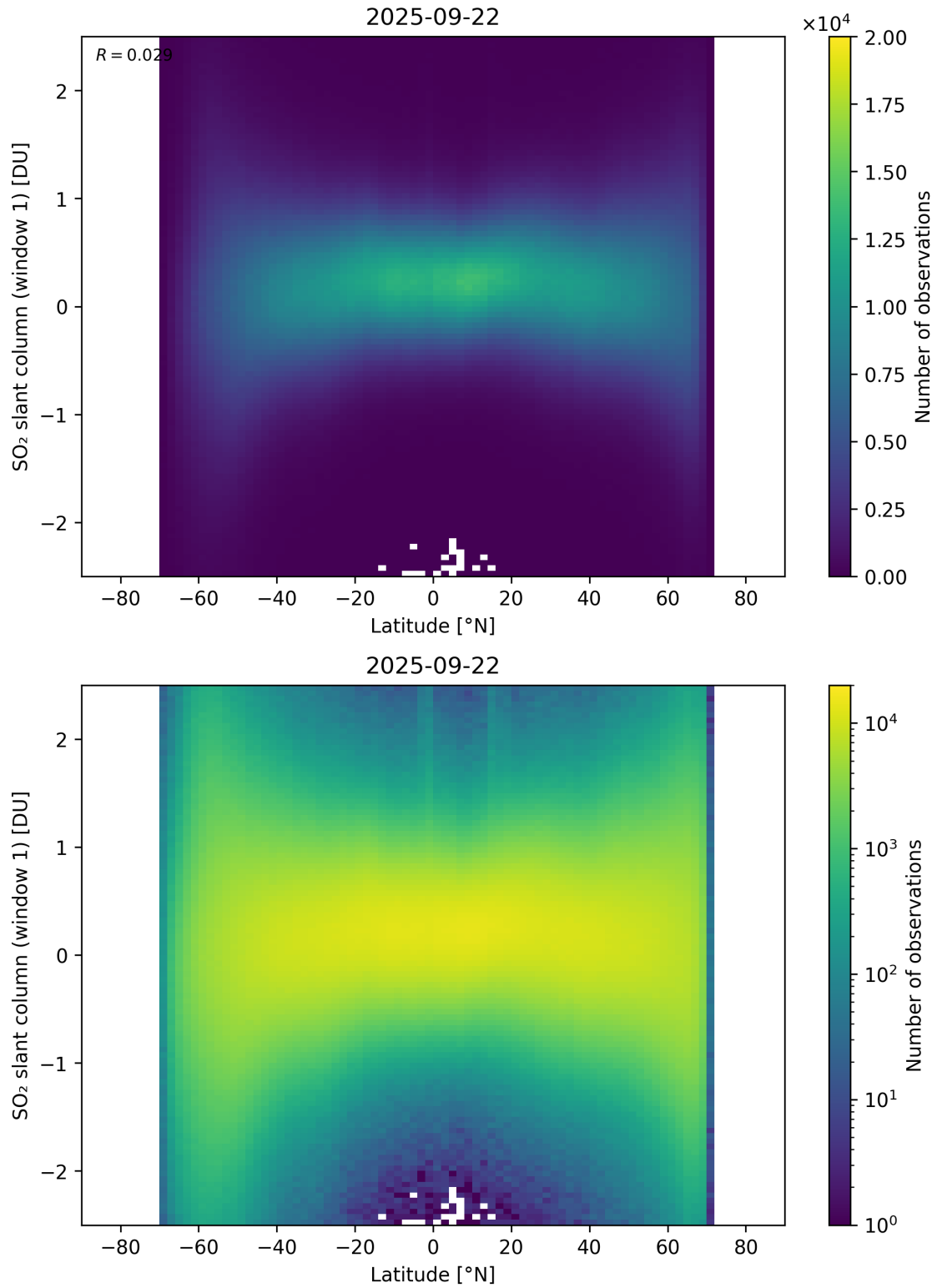
Figure 162: Scatter density plot of “Latitude” against “SO 2 slant column (window 1)” for 2025-09-22 to 2025-09-23.
