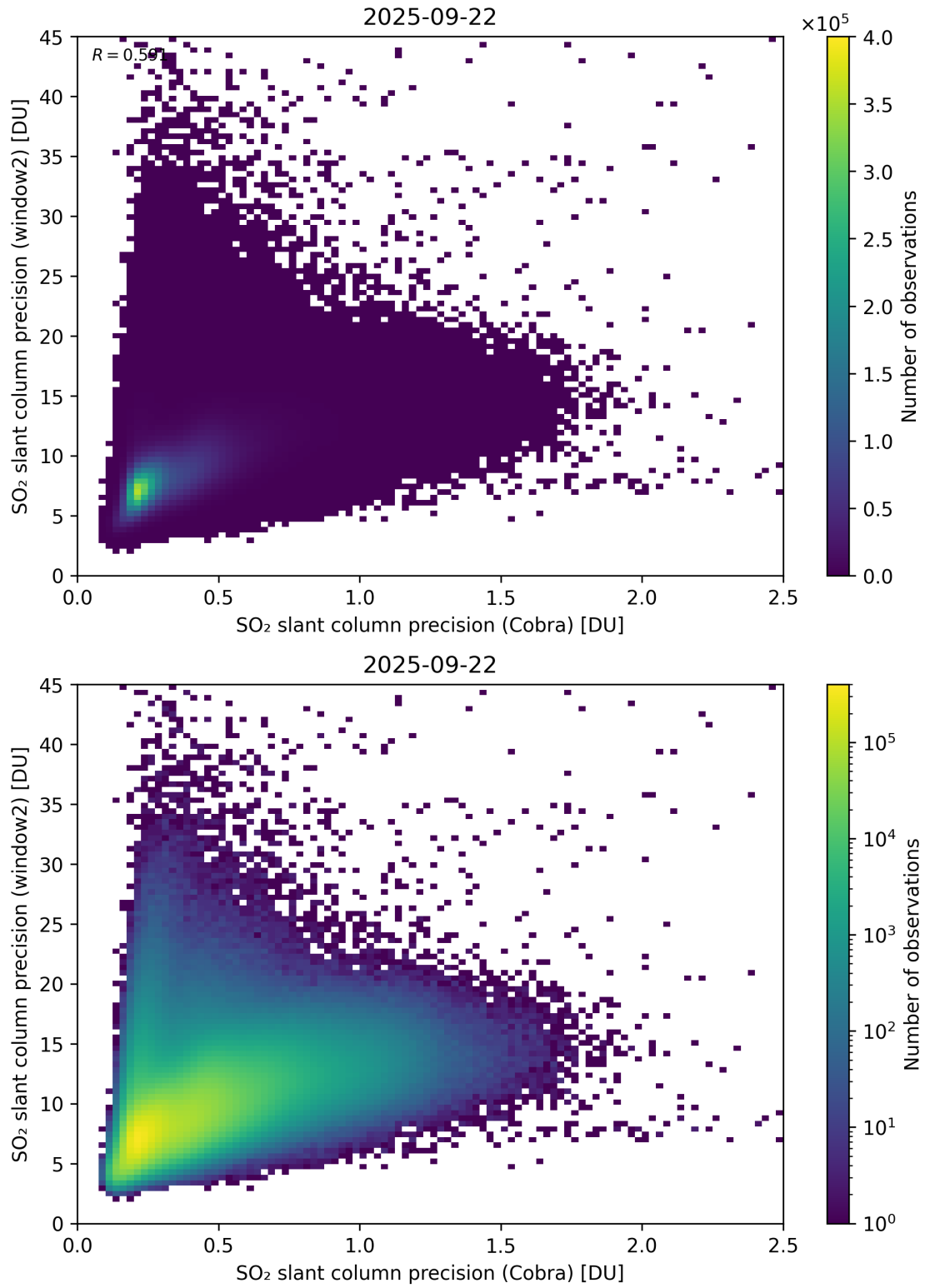
Figure 210: Scatter density plot of “SO 2 slant column precision (Cobra)” against “SO 2 slant column precision (window2)” for 2025-09-22 to 2025-09-23.
