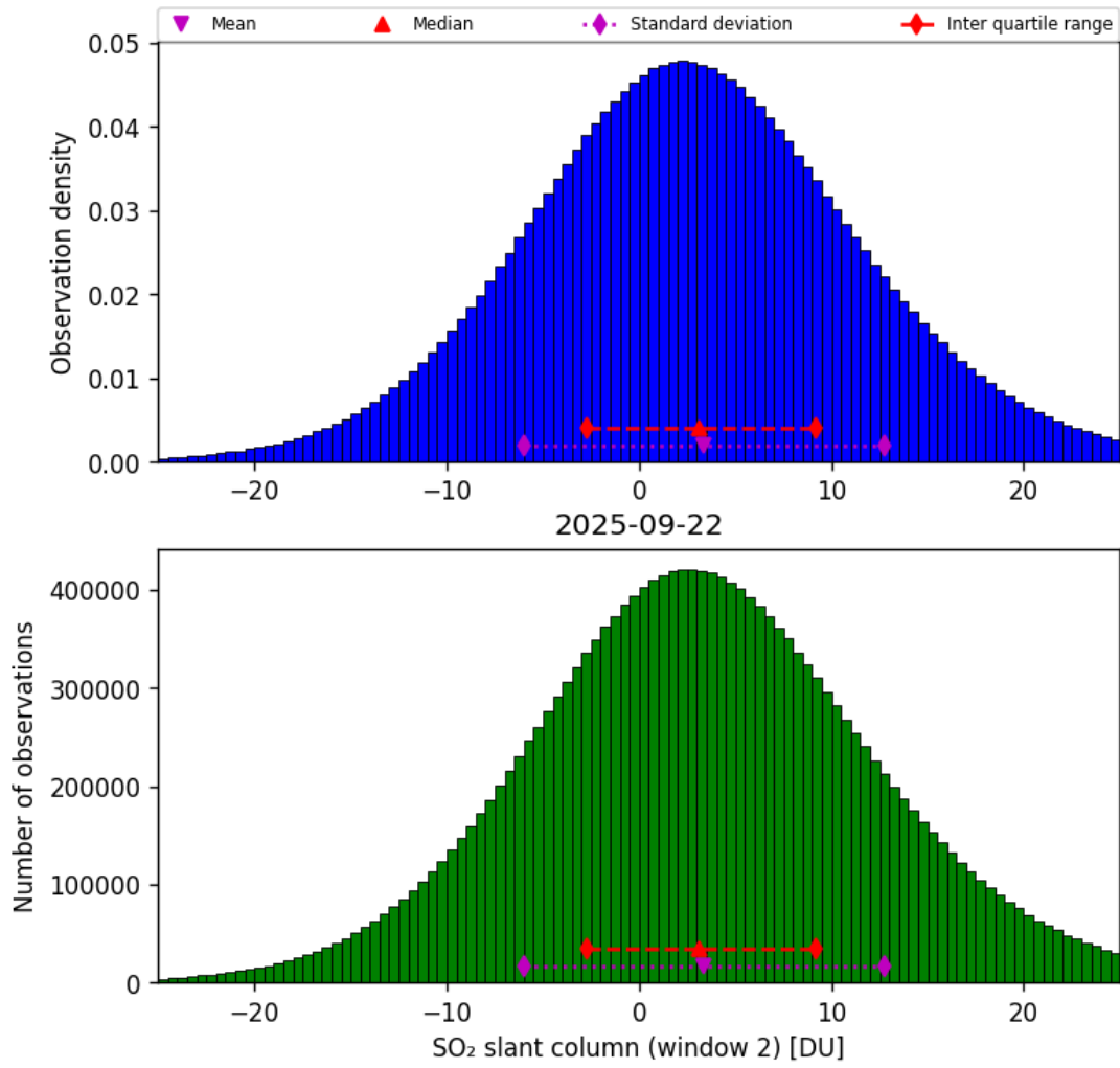
Figure 67: Histogram of “SO 2 slant column (window 2)” for 2025-09-22 to 2025-09-23
