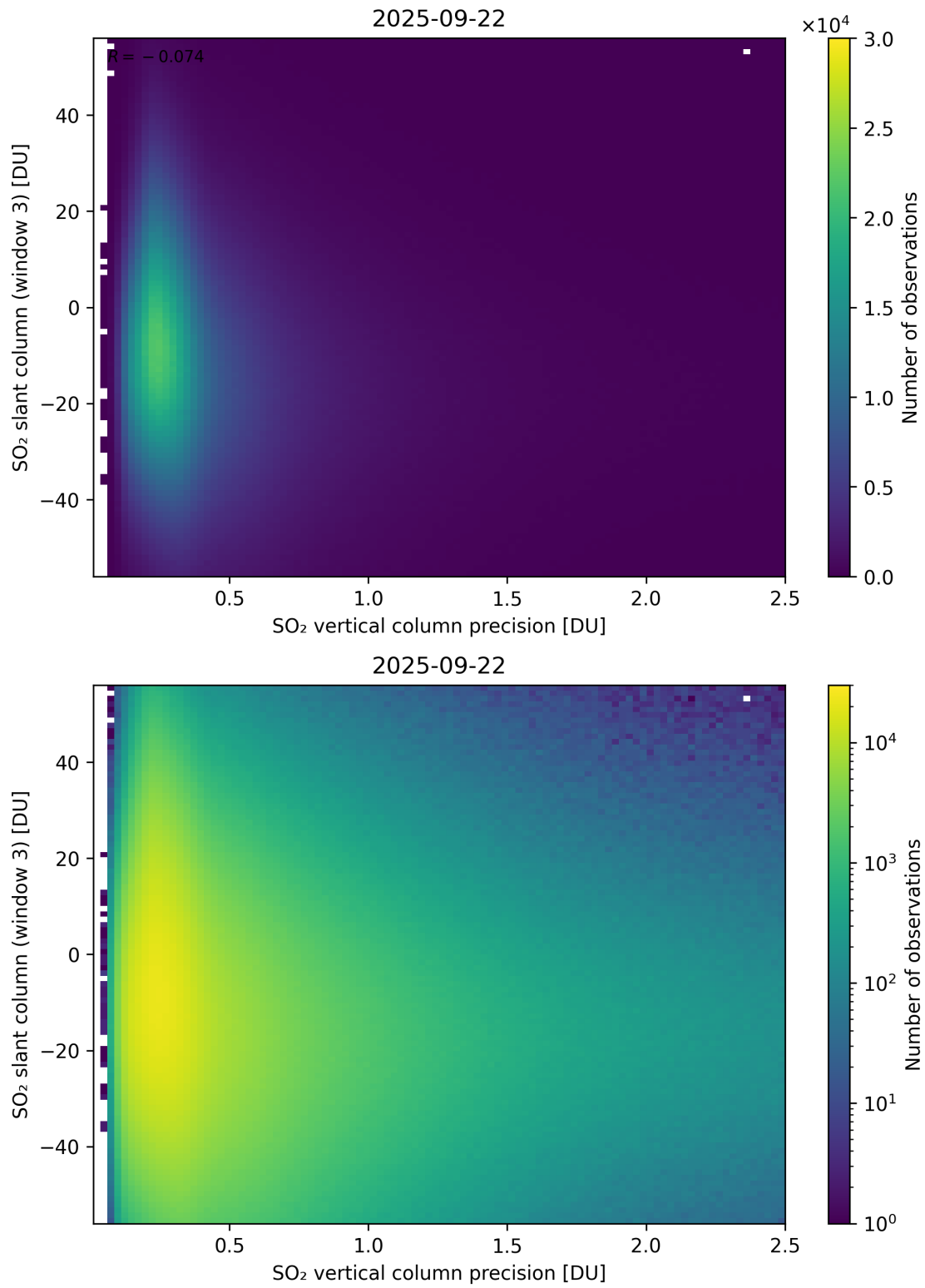
Figure 344: Scatter density plot of “SO 2 vertical column precision” against “SO 2 slant column (window 3)” for 2025-09-22 to 2025-09-23.
