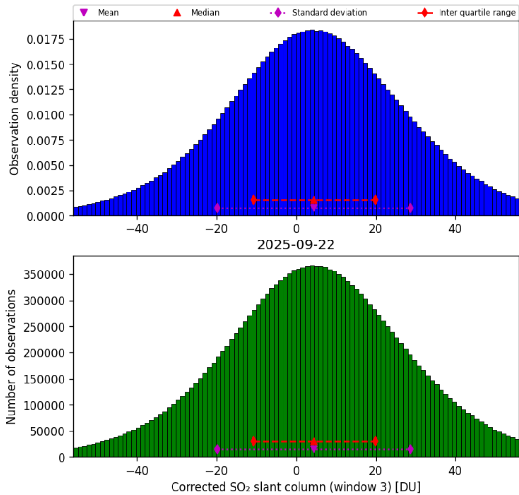
Figure 73: Histogram of “Corrected SO 2 slant column (window 3)” for 2025-09-22 to 2025-09-23
