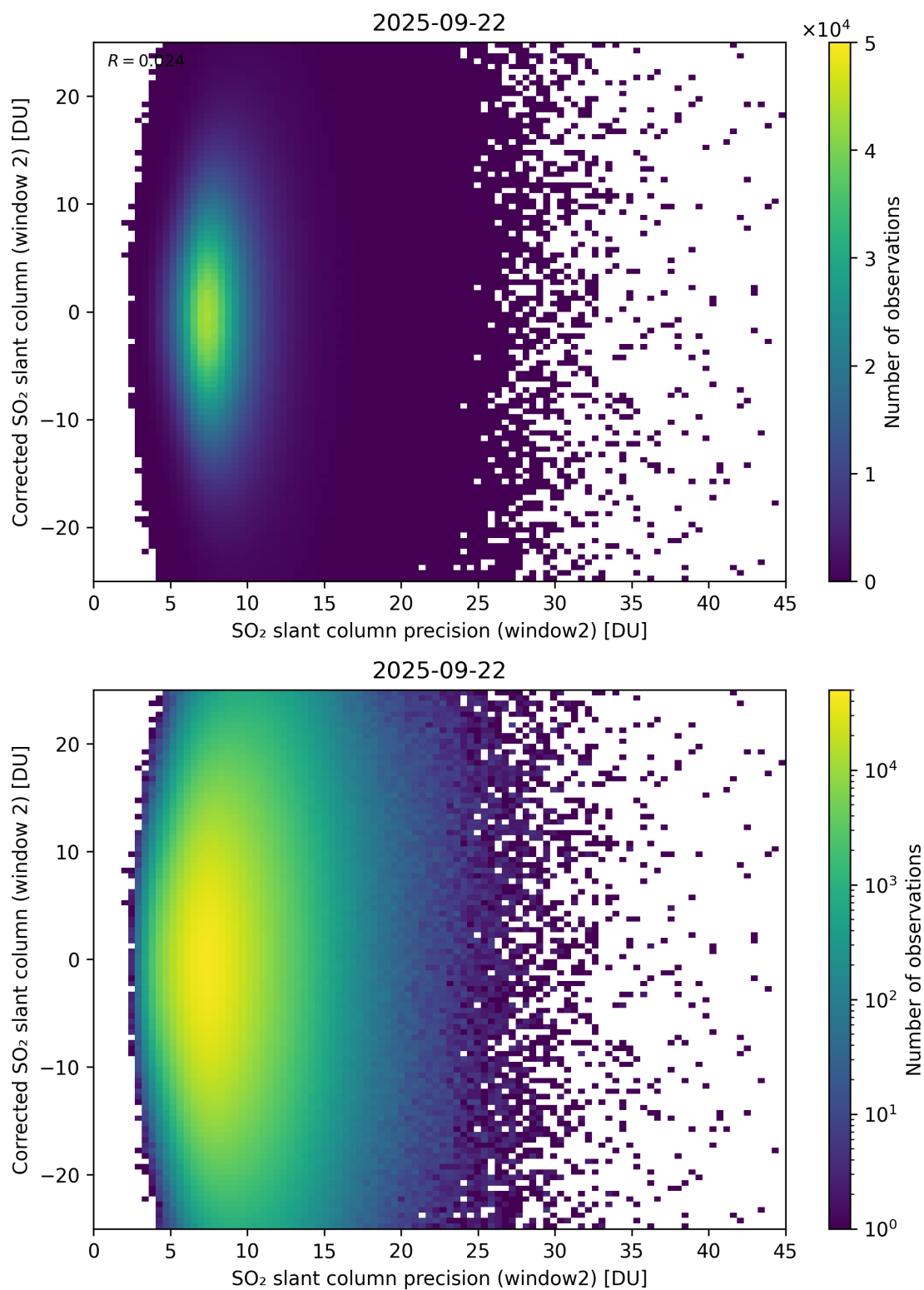
Figure 297: Scatter density plot of “SO 2 slant column precision (window2)” against “Corrected SO 2 slant column (window 2)” for 2025-09-22 to 2025-09-23.
