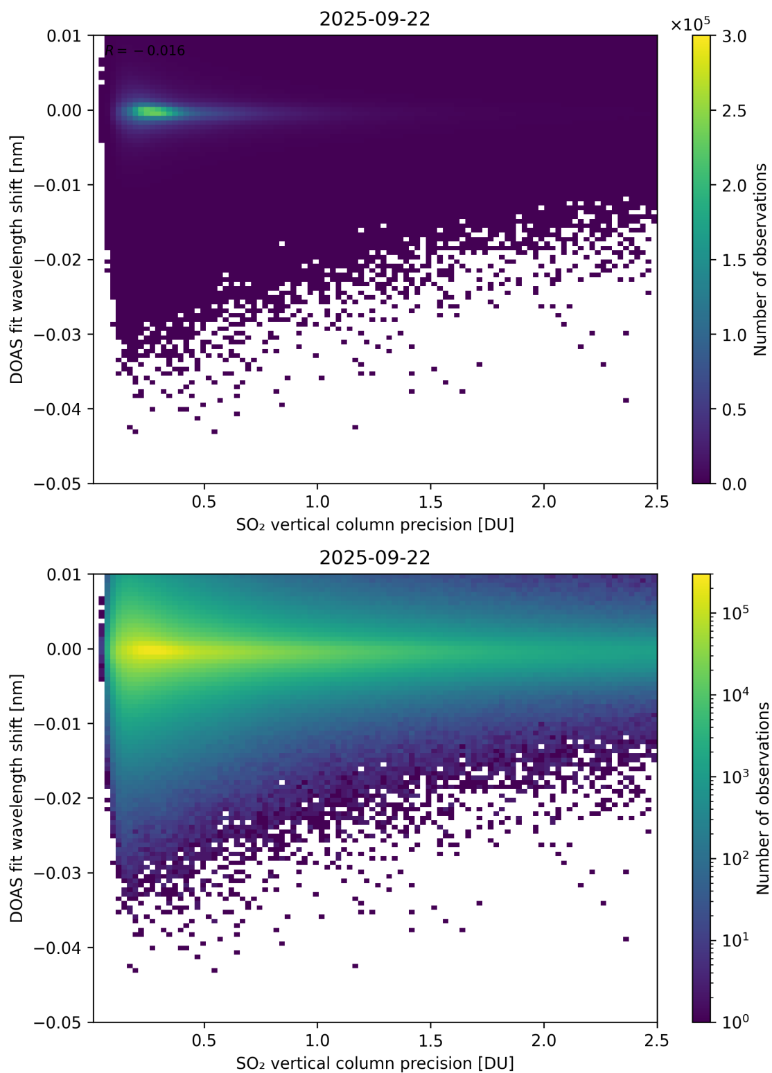
Figure 332: Scatter density plot of “SO 2 vertical column precision” against “DOAS fit wavelength shift” for 2025-09-22 to 2025-09-23.
