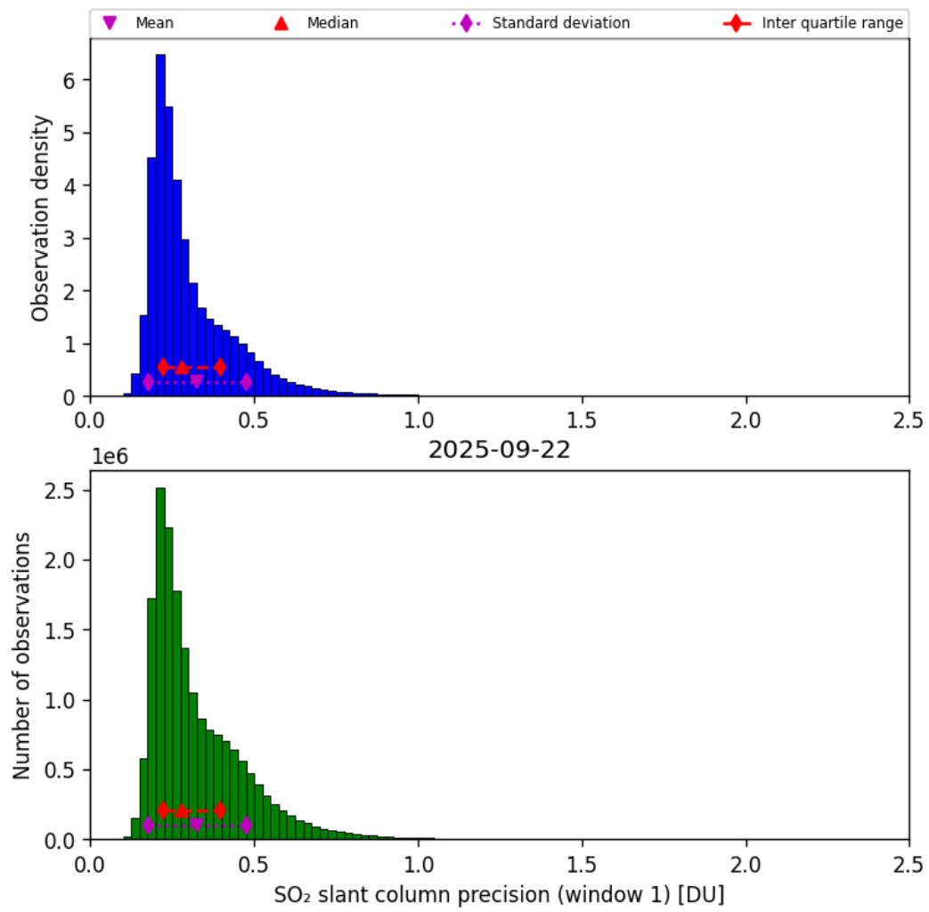
Figure 64: Histogram of “SO 2 slant column precision (window 1)” for 2025-09-22 to 2025-09-23
