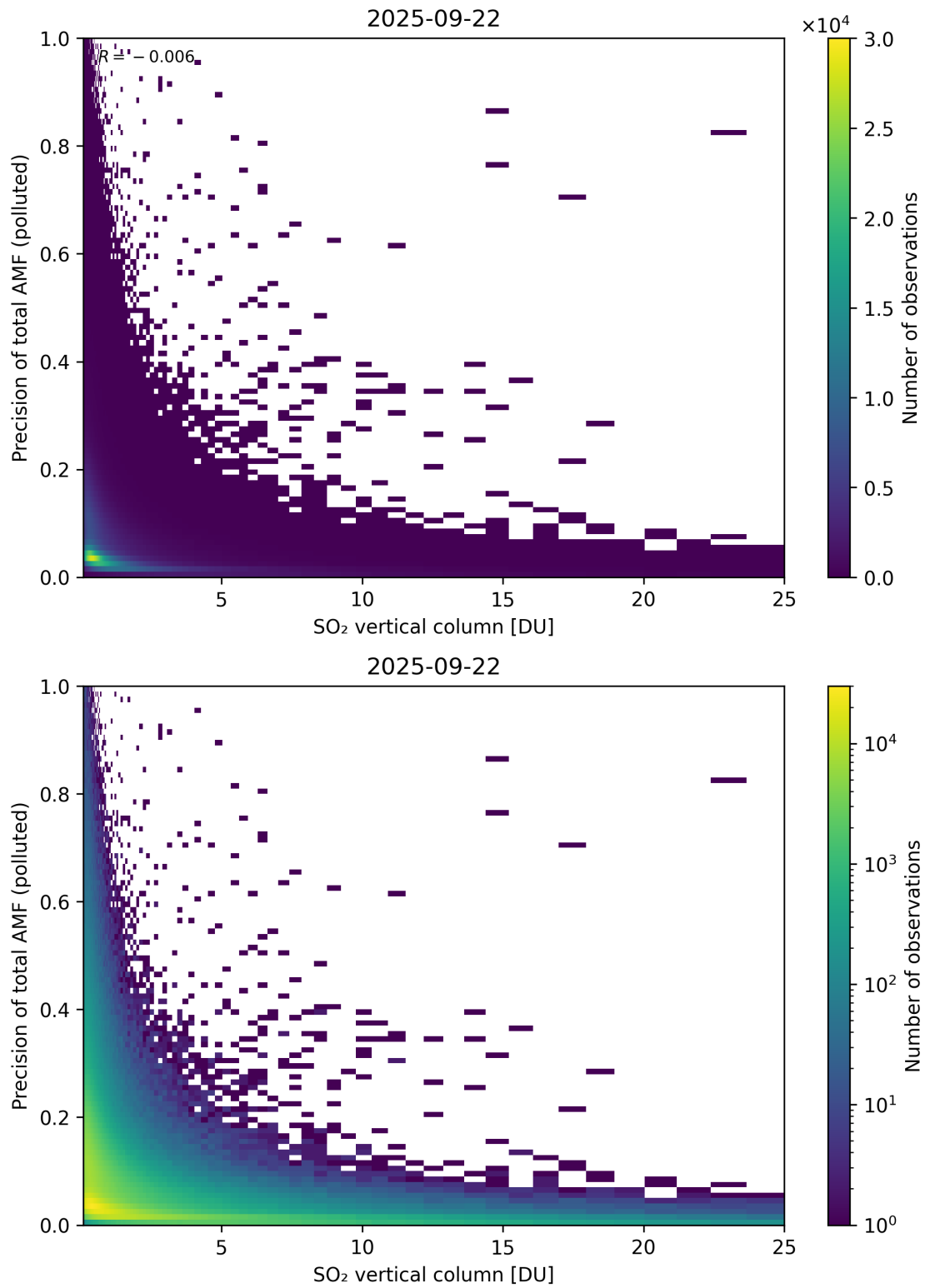
Figure 360: Scatter density plot of “SO 2 vertical column” against “Precision of total AMF (polluted)” for 2025-09-22 to 2025-09-23.
