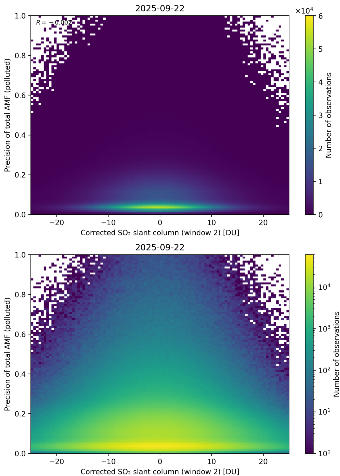
Figure 254: Scatter density plot of “Corrected SO 2 slant column (window 2)” against “Precision of total AMF (polluted)” for 2025-09-22 to 2025-09-23.
