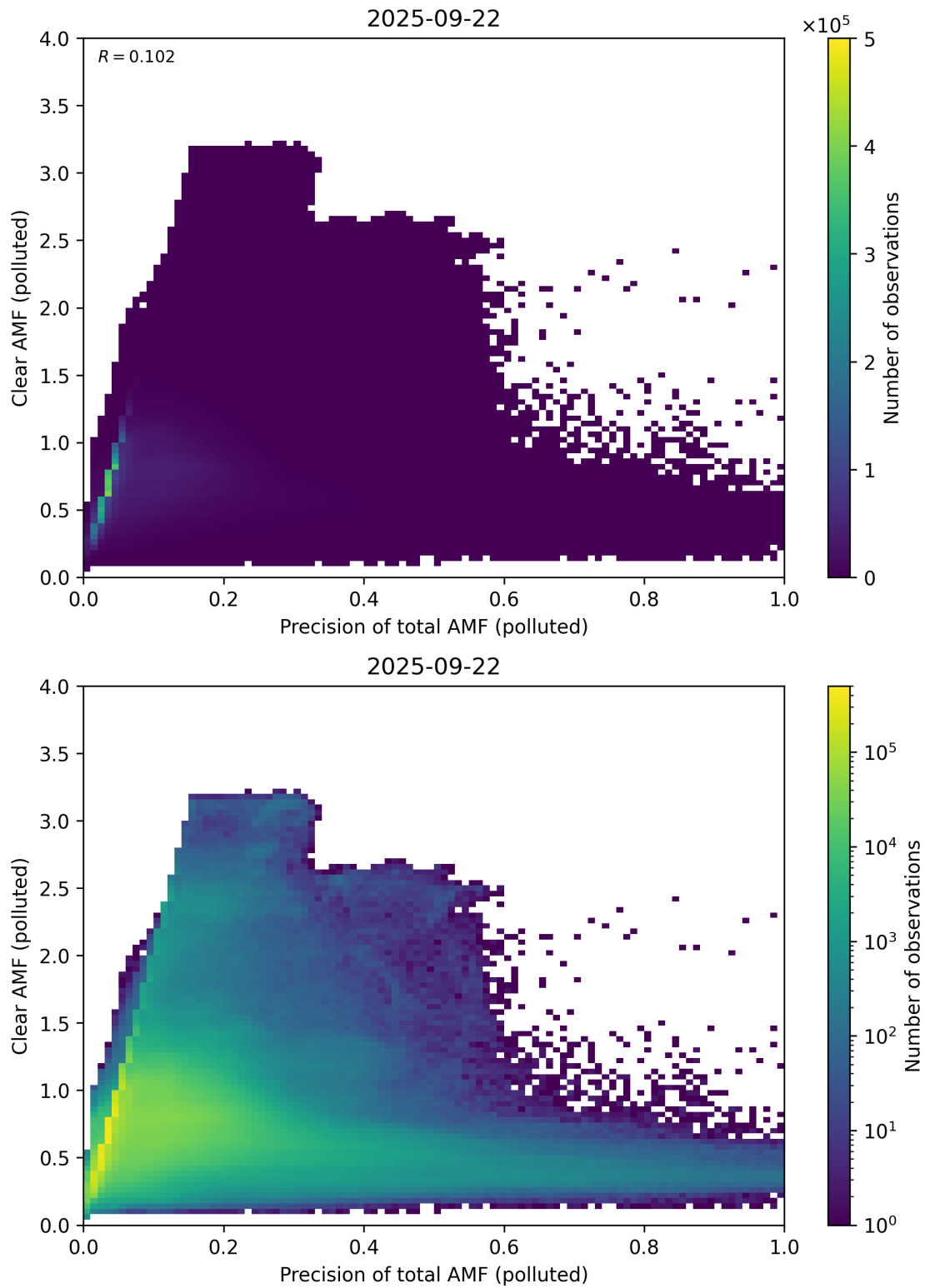
Figure 320: Scatter density plot of “Precision of total AMF (polluted)” against “Clear AMF (polluted)” for 2025-09-22 to 2025-09-23.
