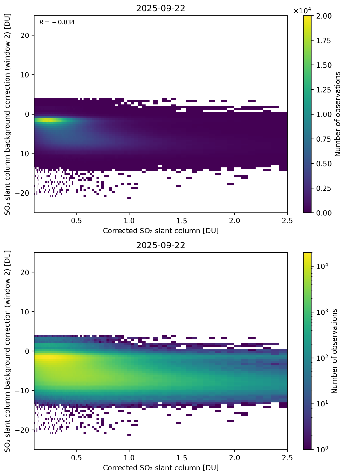
Figure 227: Scatter density plot of “Corrected SO 2 slant column” against “SO 2 slant column background correction (window 2)” for 2025-09-22 to 2025-09-23.
