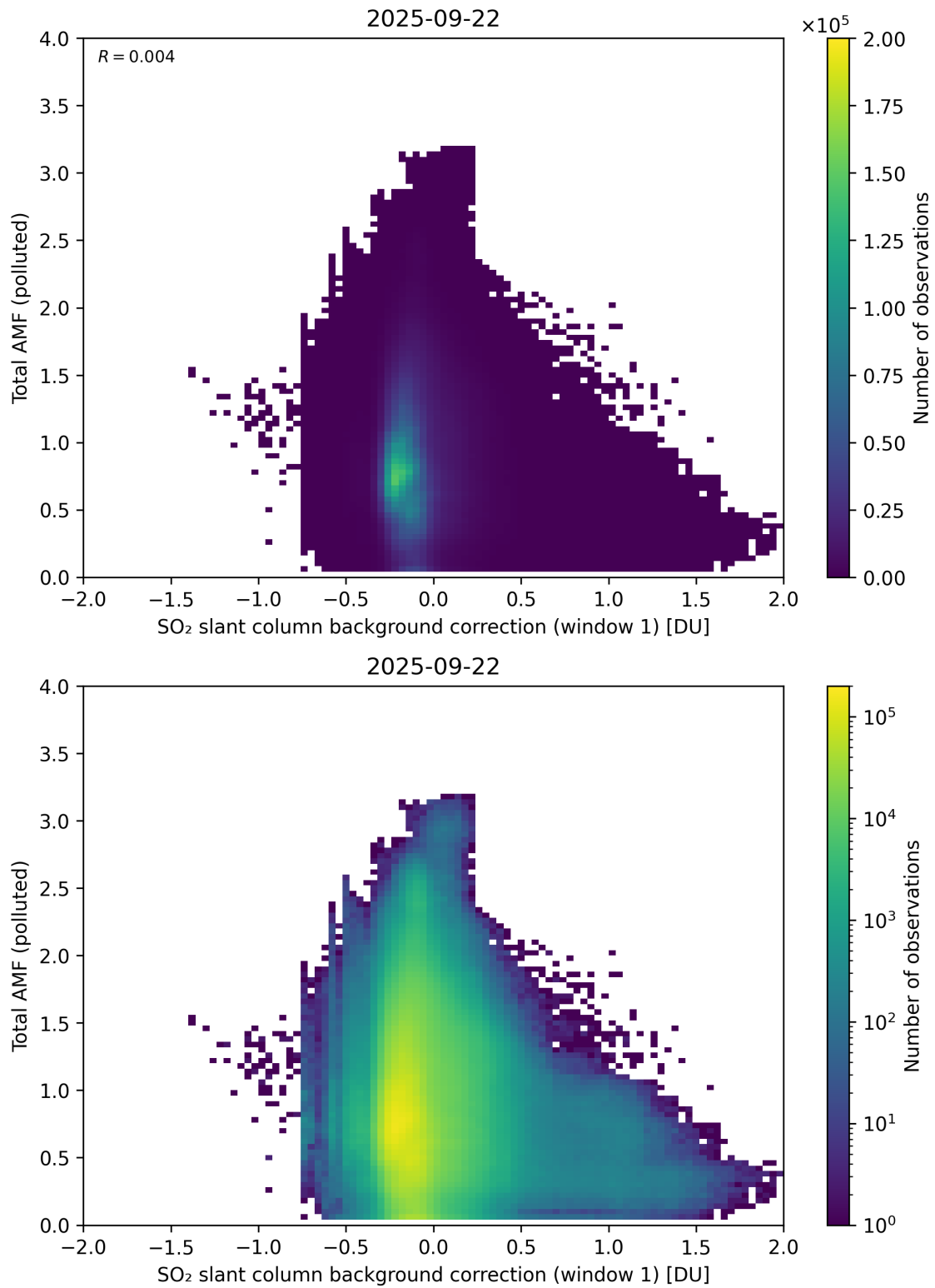
Figure 120: Scatter density plot of “SO 2 slant column background correction (window 1)” against “Total AMF (polluted)” for 2025-09-22 to 2025-09-23.
