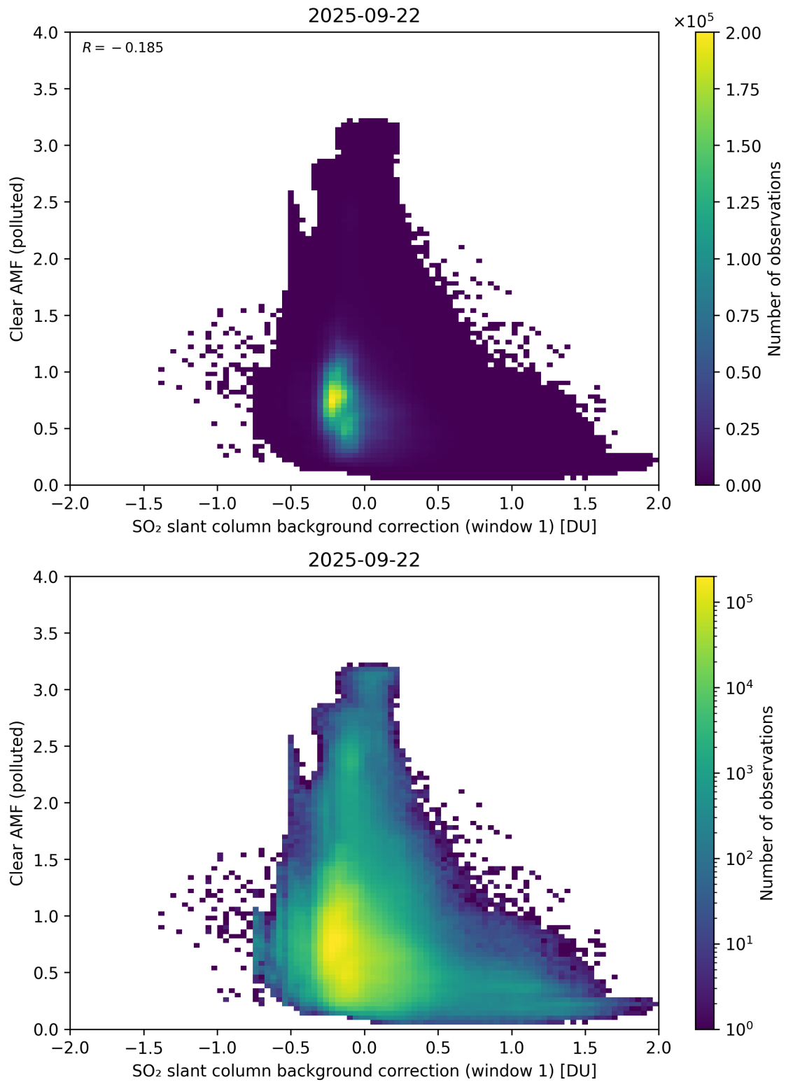
Figure 114: Scatter density plot of “SO 2 slant column background correction (window 1)” against “Clear AMF (polluted)” for 2025-09-22 to 2025-09-23.
