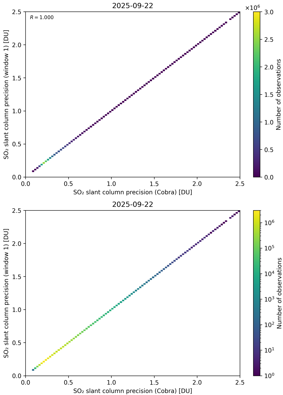
Figure 209: Scatter density plot of “SO 2 slant column precision (Cobra)” against “SO 2 slant column precision (window 1)” for 2025-09-22 to 2025-09-23.
