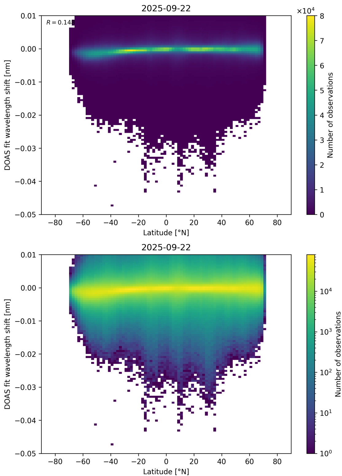
Figure 153: Scatter density plot of “Latitude” against “DOAS fit wavelength shift” for 2025-09-22 to 2025-09-23.
