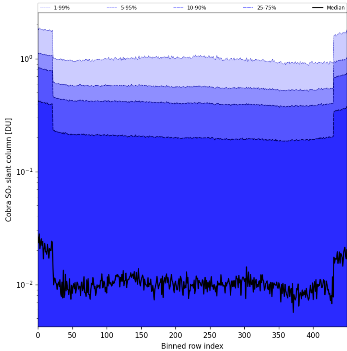
Figure 87: Along track statistics of “Cobra SO 2 slant column” for 2025-09-22 to 2025-09-23
