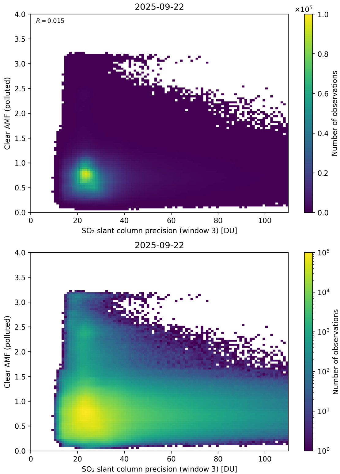
Figure 311: Scatter density plot of “SO 2 slant column precision (window 3)” against “Clear AMF (polluted)” for 2025-09-22 to 2025-09-23.
