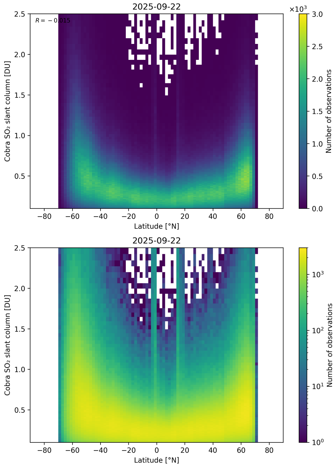
Figure 157: Scatter density plot of “Latitude” against “Cobra SO 2 slant column” for 2025-09-22 to 2025-09-23.
