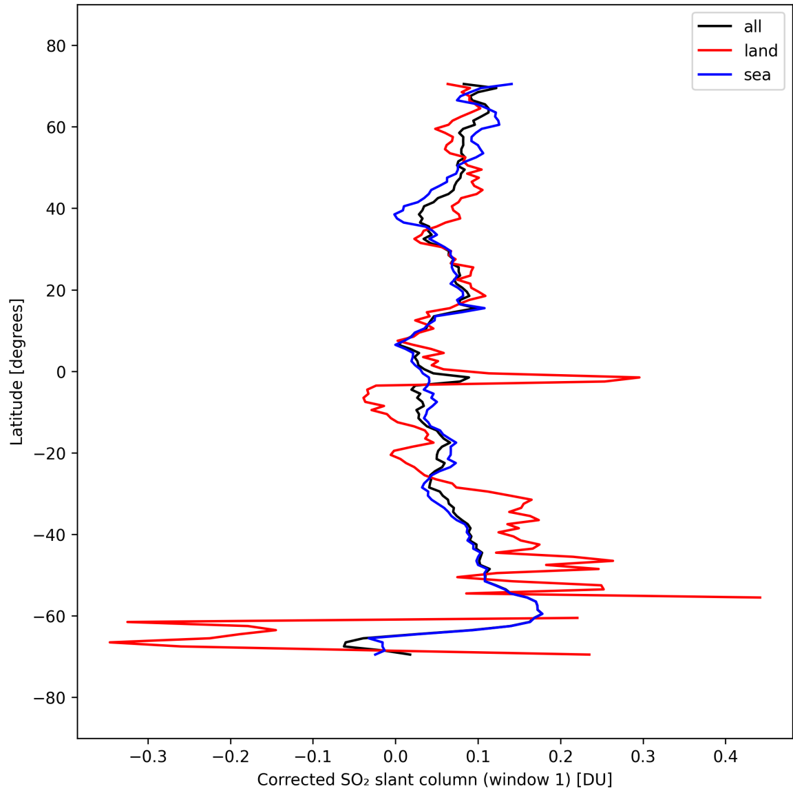
Figure 39: Zonal average of “Corrected SO 2 slant column (window 1)” for 2025-09-22 to 2025-09-23.
