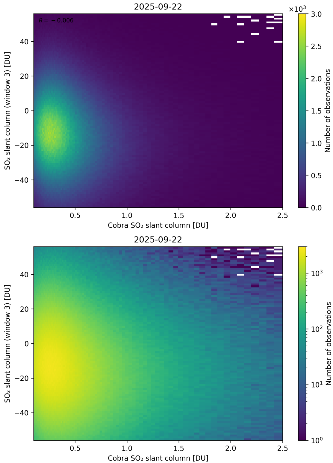
Figure 222: Scatter density plot of “Cobra SO 2 slant column” against “SO 2 slant column (window 3)” for 2025-09-22 to 2025-09-23.
