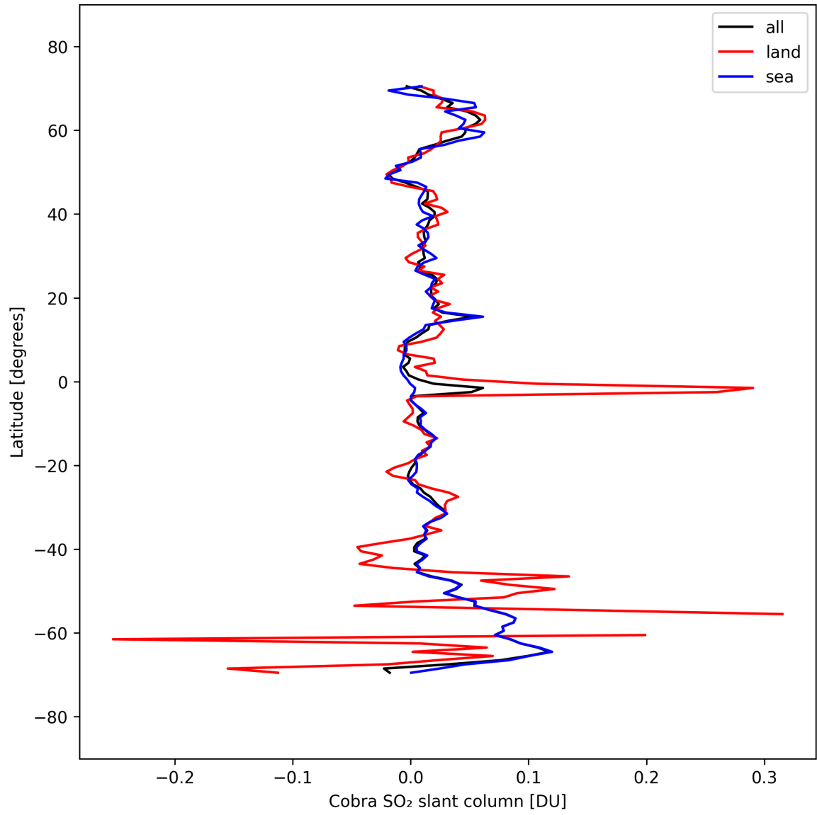
Figure 35: Zonal average of “Cobra SO 2 slant column” for 2025-09-22 to 2025-09-23.
