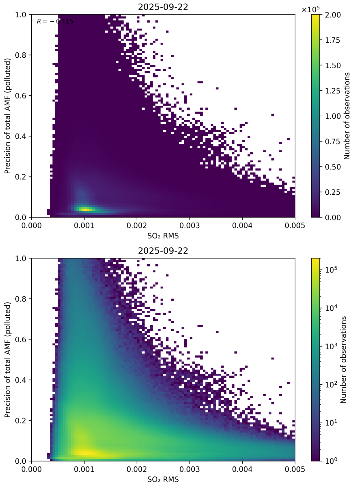
Figure 149: Scatter density plot of “SO 2 RMS” against “Precision of total AMF (polluted)” for 2025-09-22 to 2025-09-23.
