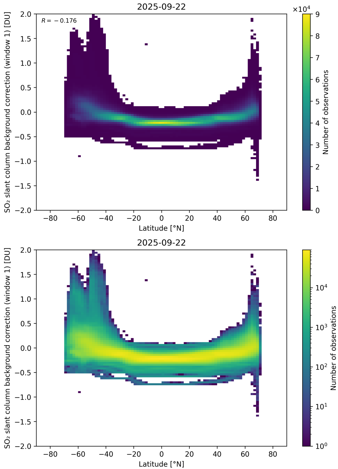
Figure 150: Scatter density plot of “Latitude” against “SO 2 slant column background correction (window 1)” for 2025-09-22 to 2025-09-23.
