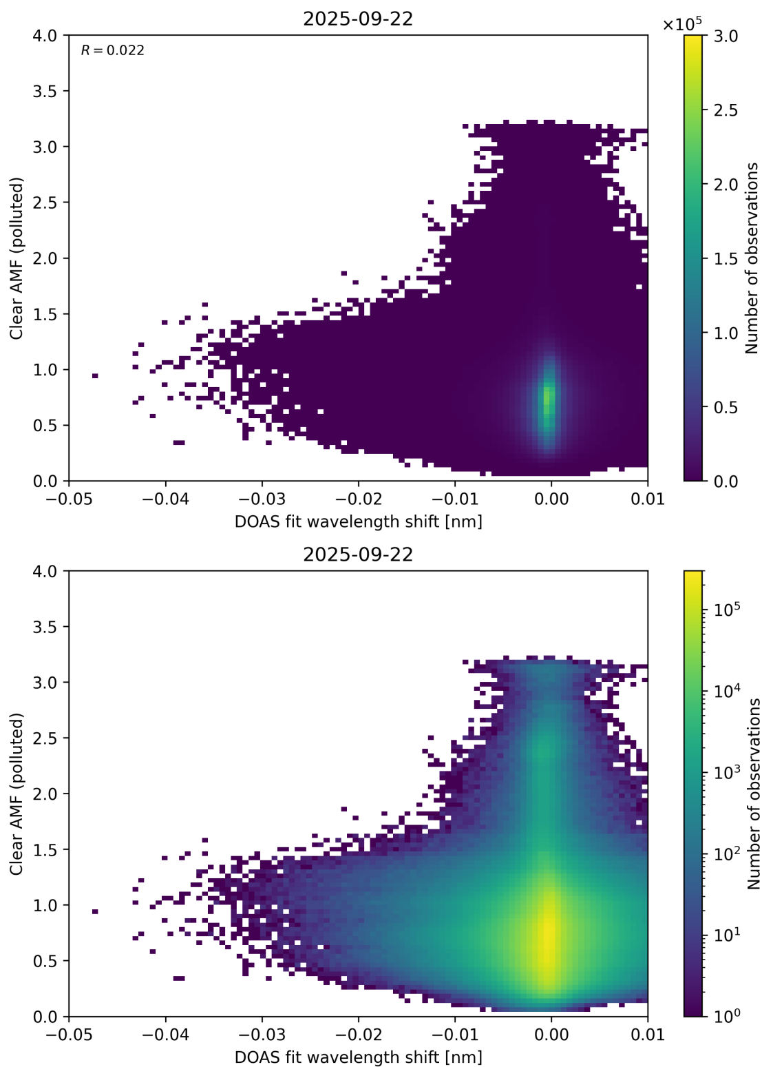
Figure 140: Scatter density plot of “DOAS fit wavelength shift” against “Clear AMF (polluted)” for 2025-09-22 to 2025-09-23.
