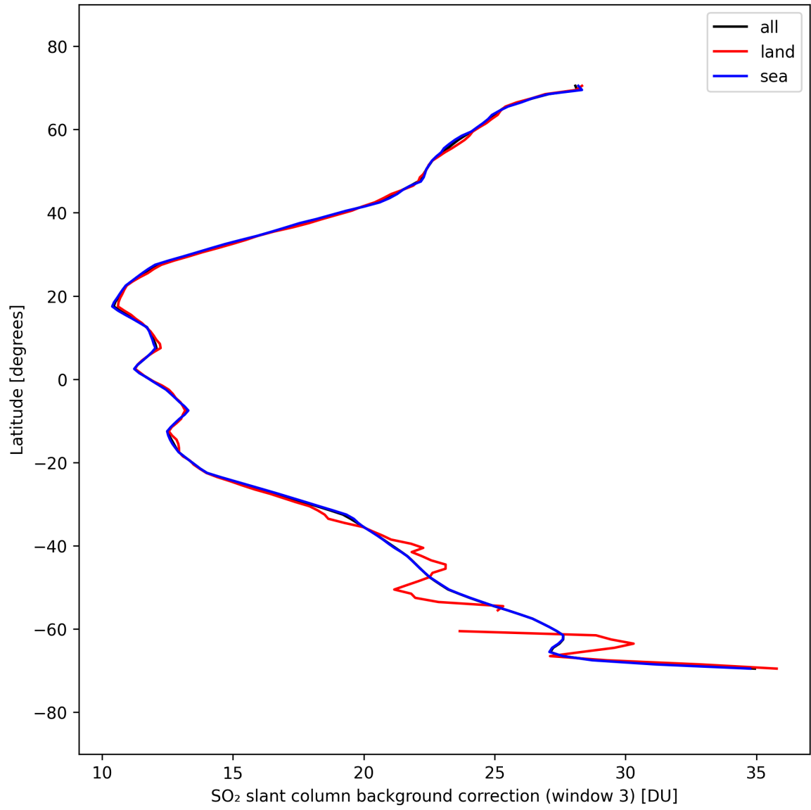
Figure 48: Zonal average of “SO 2 slant column background correction (window 3)” for 2025-09-22 to 2025-09-23.
