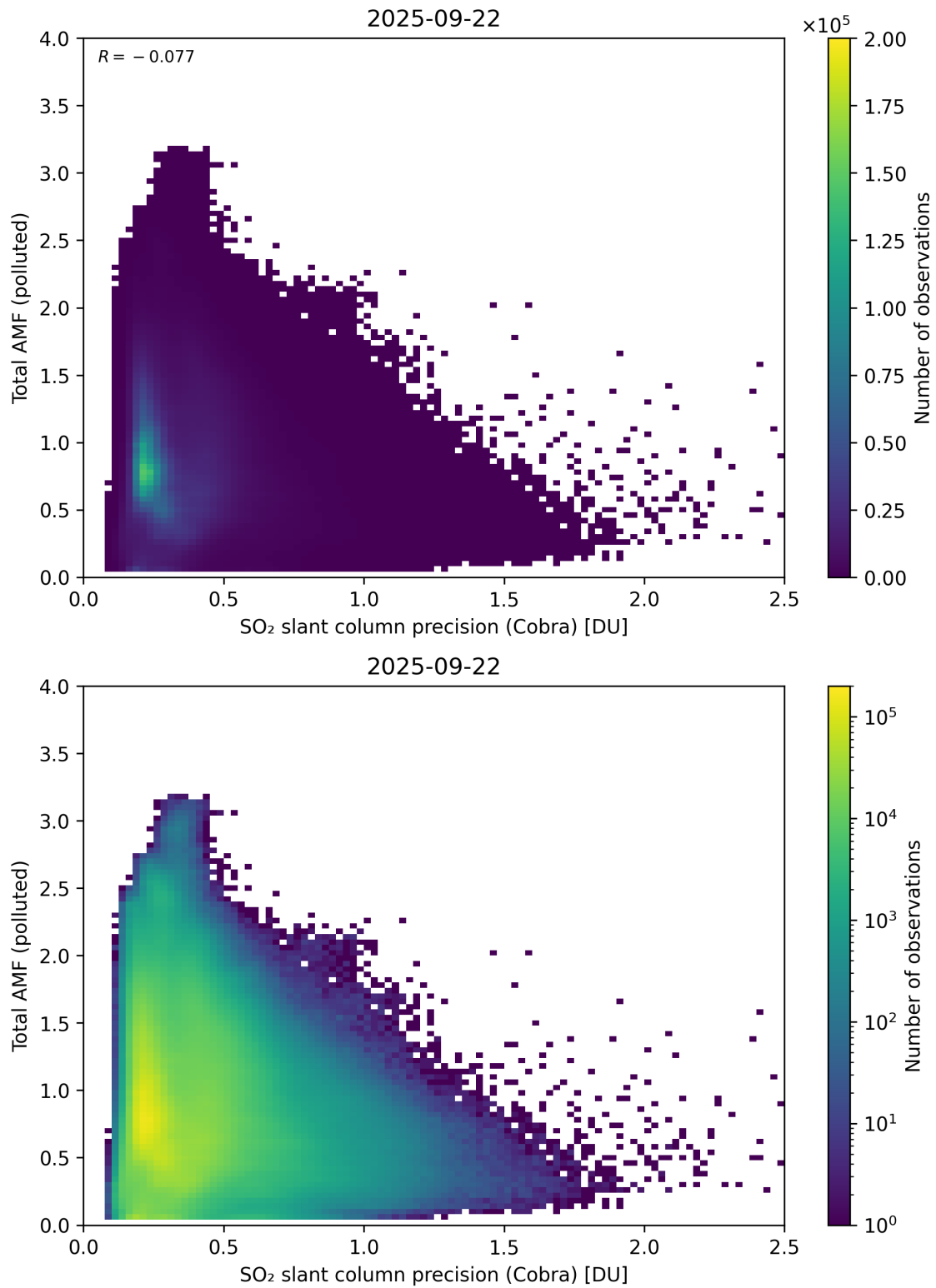
Figure 213: Scatter density plot of “SO 2 slant column precision (Cobra)” against “Total AMF (polluted)” for 2025-09-22 to 2025-09-23.
