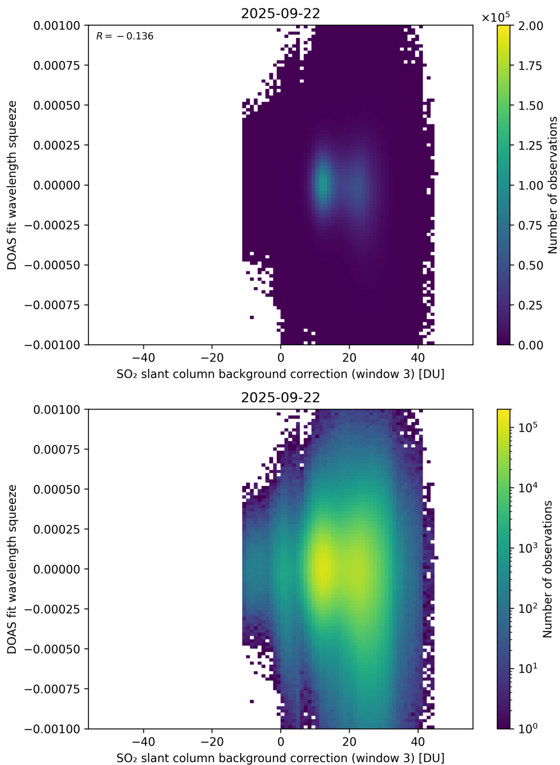
Figure 133: Scatter density plot of “SO 2 slant column background correction (window 3)” against “DOAS fit wavelength squeeze” for 2025-09-22 to 2025-09-23.
