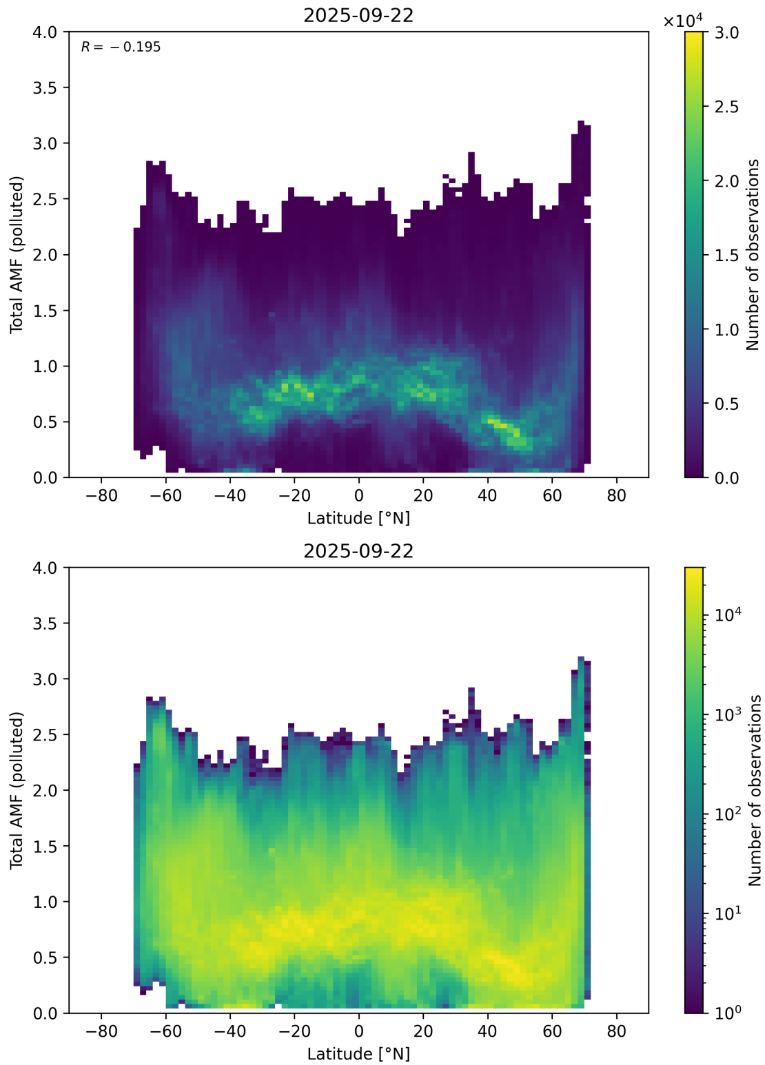
Figure 167: Scatter density plot of “Latitude” against “Total AMF (polluted)” for 2025-09-22 to 2025-09-23.
