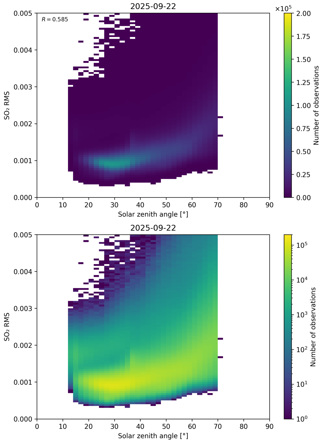
Figure 176: Scatter density plot of “Solar zenith angle” against “SO 2 RMS” for 2025-09-22 to 2025-09-23.
