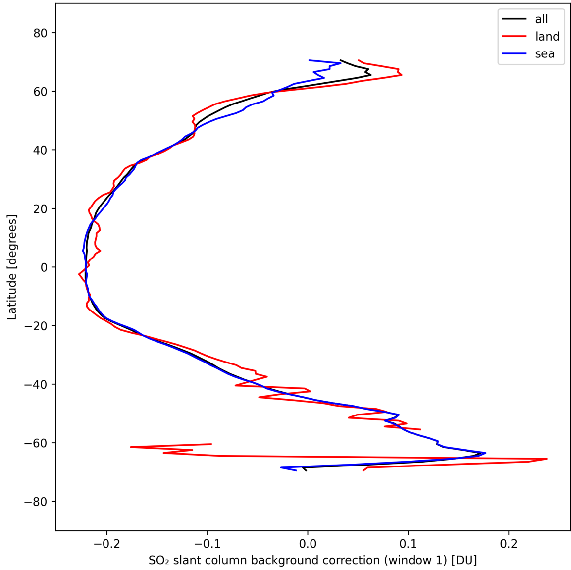
Figure 40: Zonal average of “SO 2 slant column background correction (window 1)” for 2025-09-22 to 2025-09-23.
