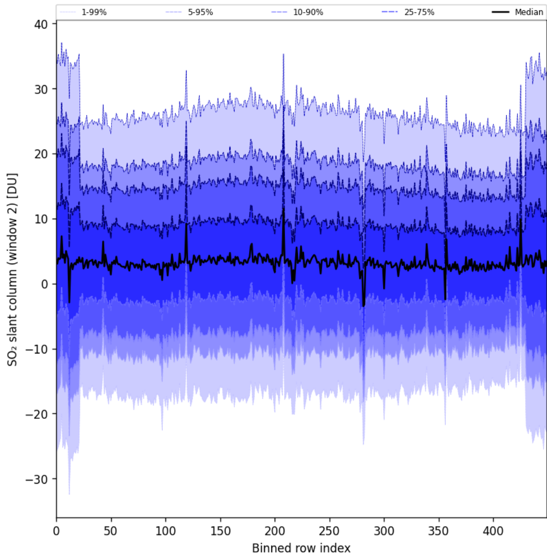
Figure 93: Along track statistics of “SO 2 slant column (window 2)” for 2025-09-22 to 2025-09-23
