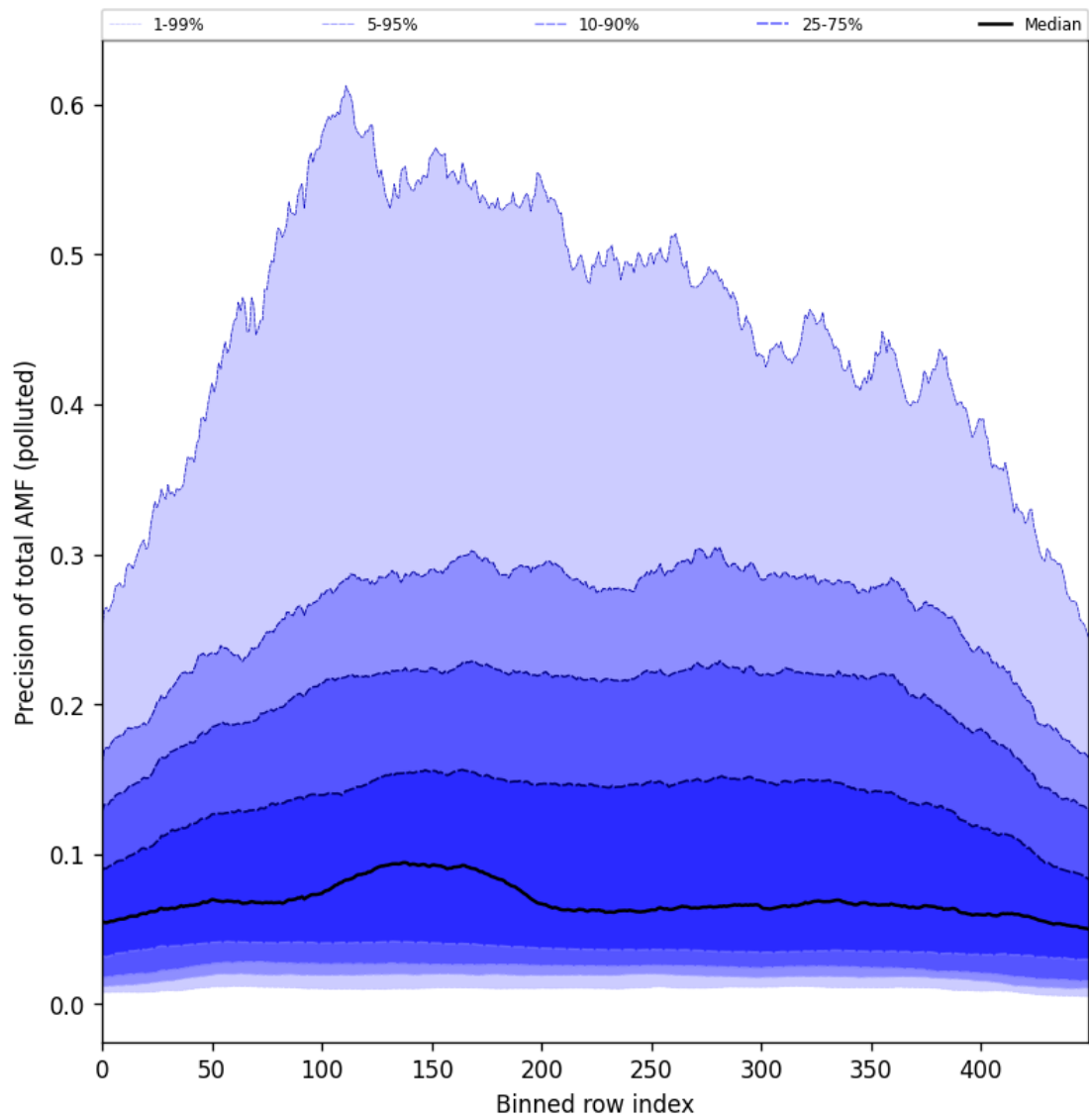
Figure 106: Along track statistics of “Precision of total AMF (polluted)” for 2025-09-22 to 2025-09-23
