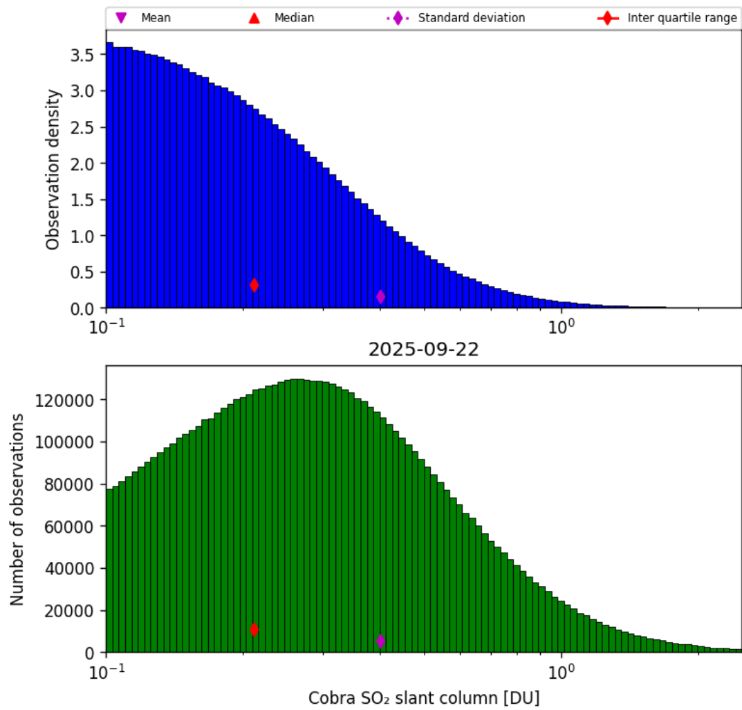
Figure 61: Histogram of “Cobra SO 2 slant column” for 2025-09-22 to 2025-09-23
