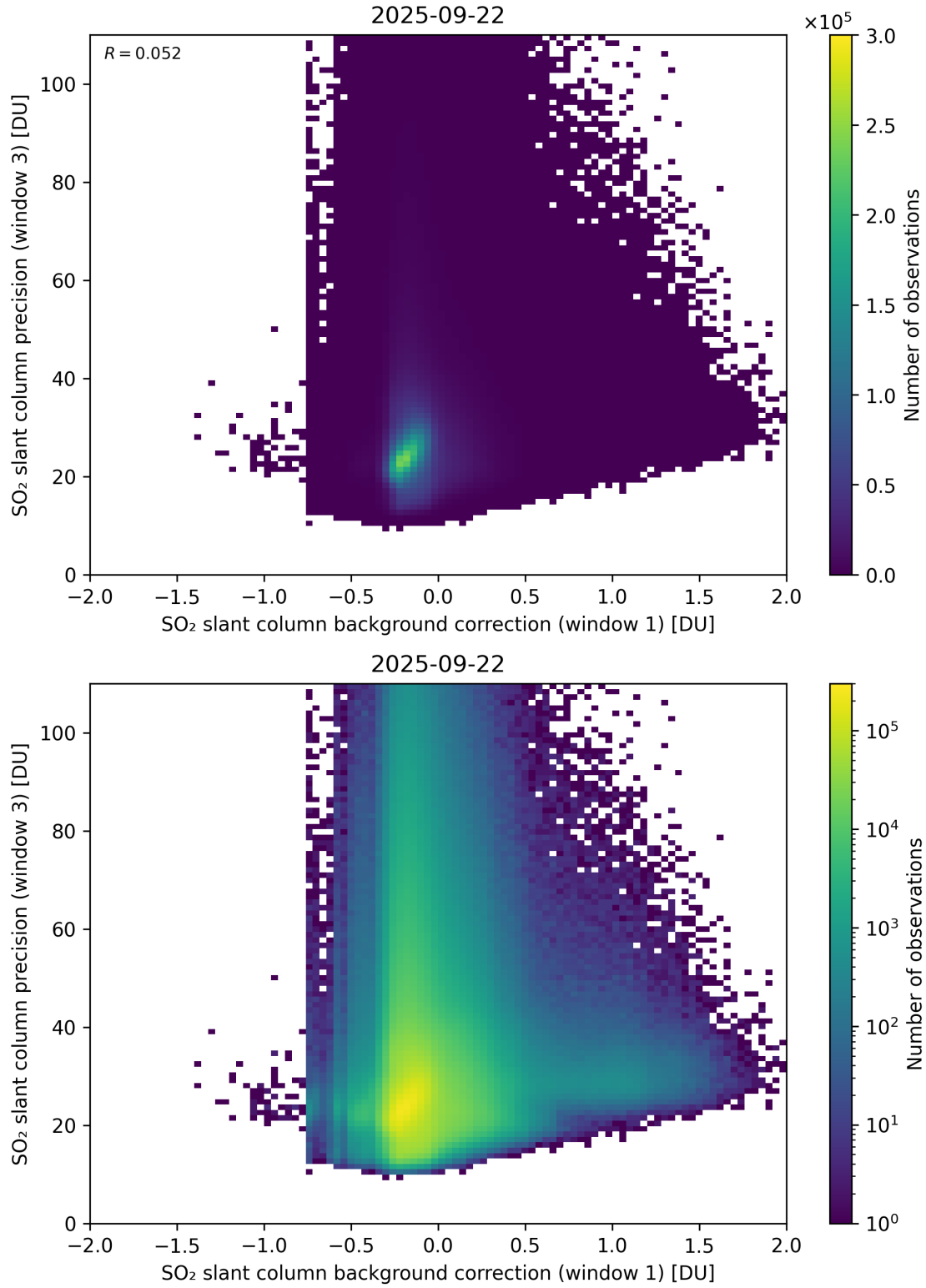
Figure 119: Scatter density plot of “SO 2 slant column background correction (window 1)” against “SO 2 slant column precision (window 3)” for 2025-09-22 to 2025-09-23.
