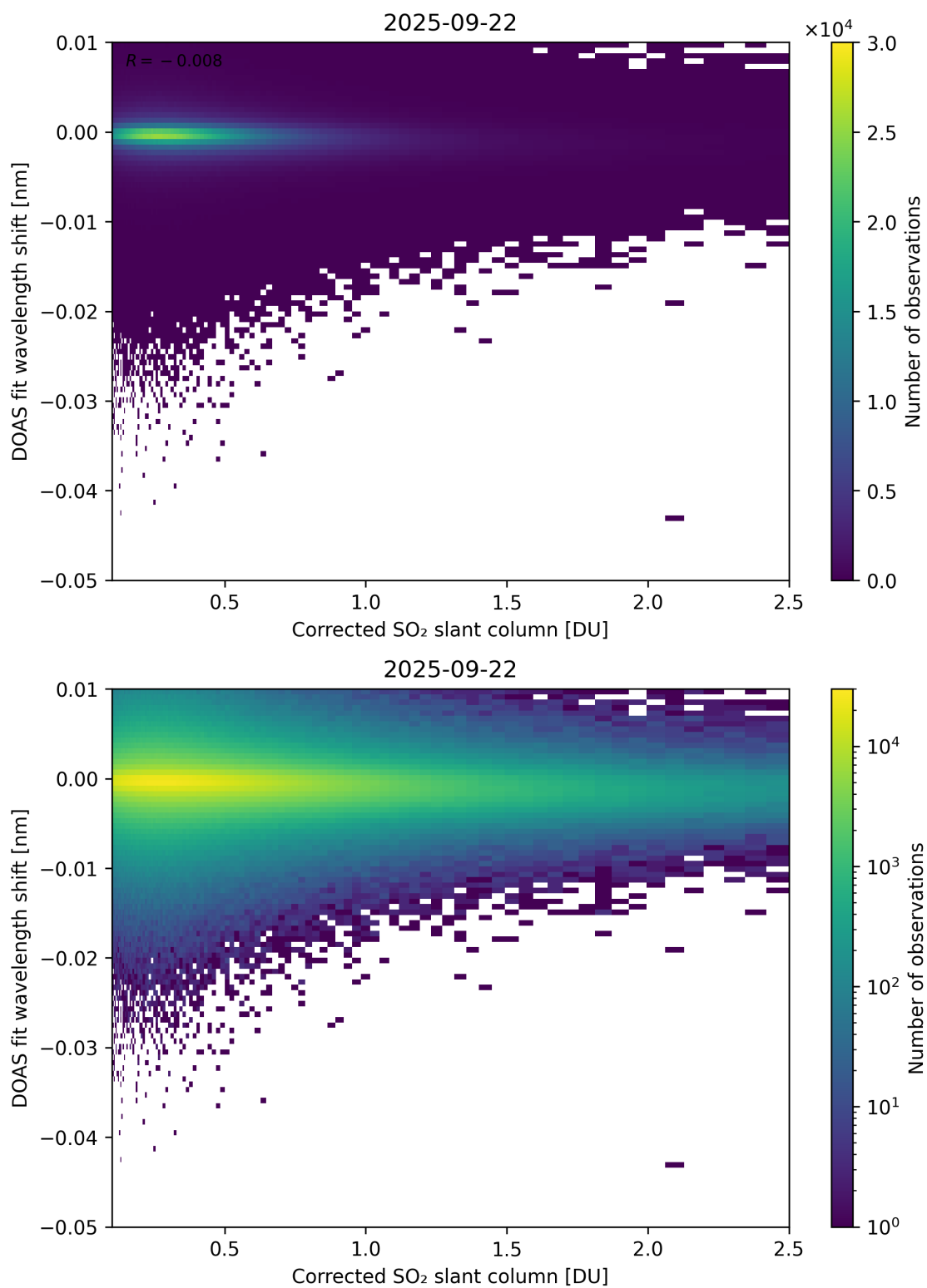
Figure 229: Scatter density plot of “Corrected SO 2 slant column” against “DOAS fit wavelength shift” for 2025-09-22 to 2025-09-23.
