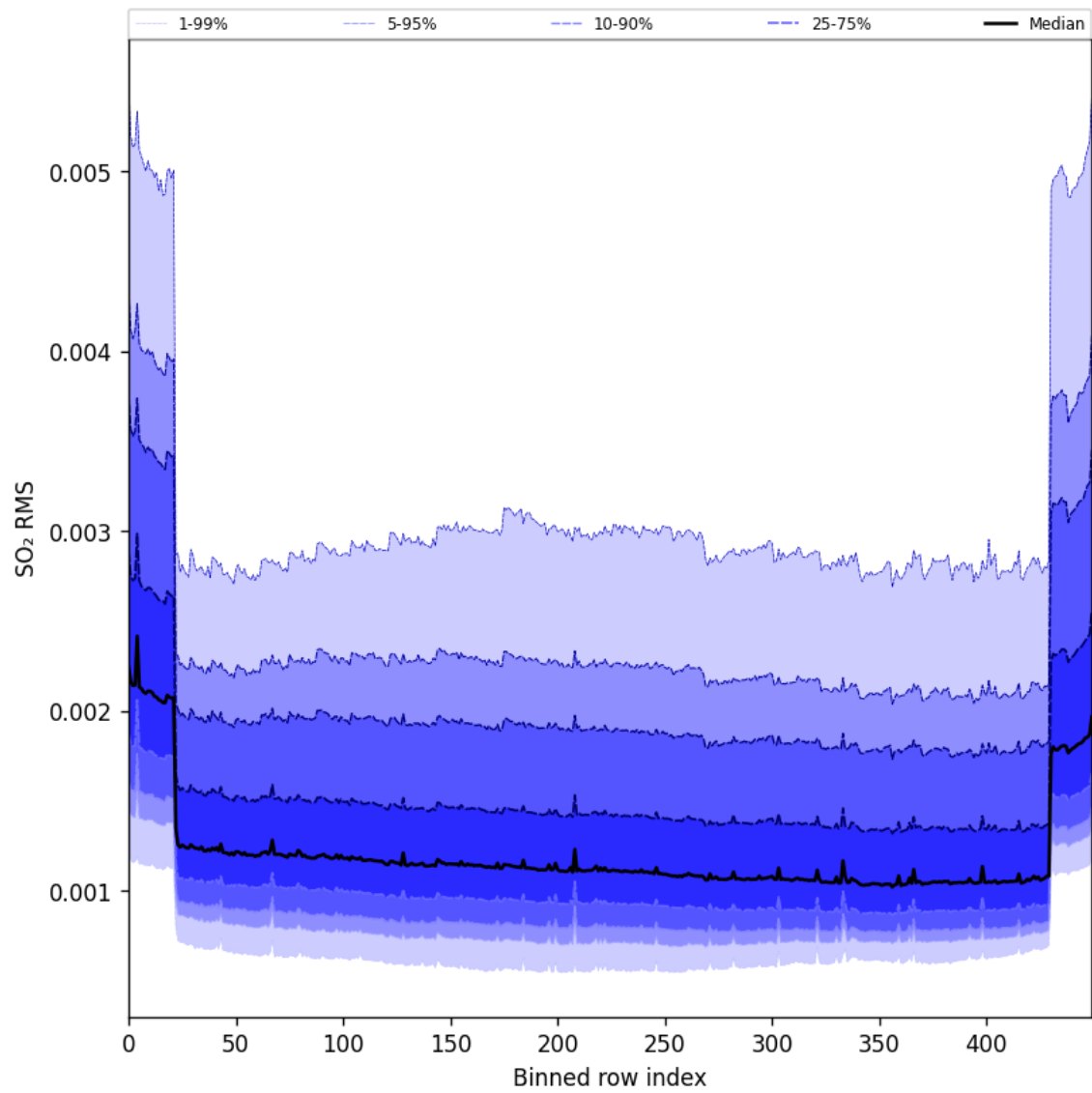
Figure 104: Along track statistics of “SO 2 RMS” for 2025-09-22 to 2025-09-23
