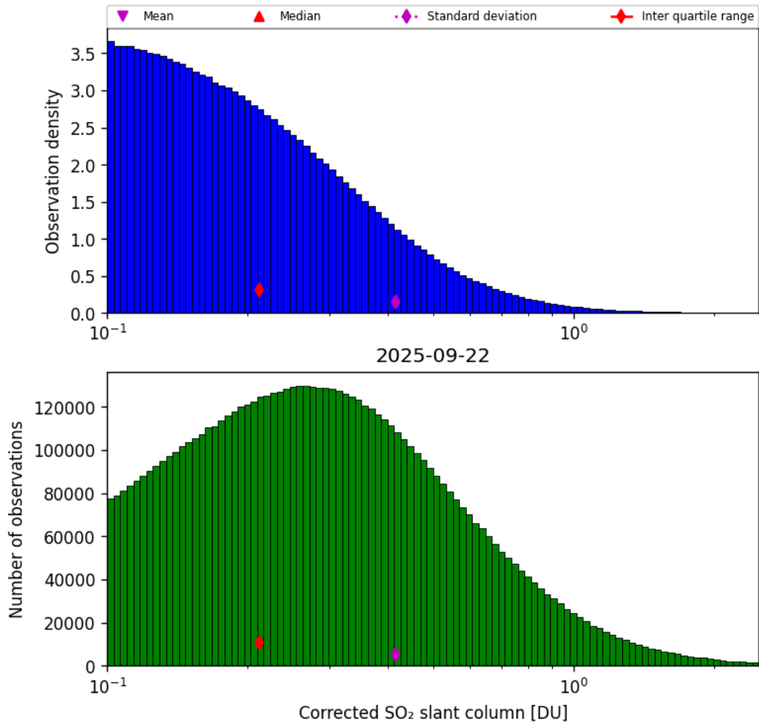
Figure 60: Histogram of “Corrected SO 2 slant column” for 2025-09-22 to 2025-09-23
