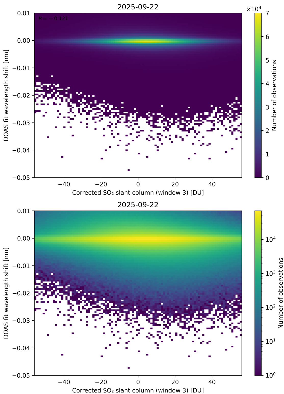
Figure 256: Scatter density plot of “Corrected SO 2 slant column (window 3)” against “DOAS fit wavelength shift” for 2025-09-22 to 2025-09-23.
