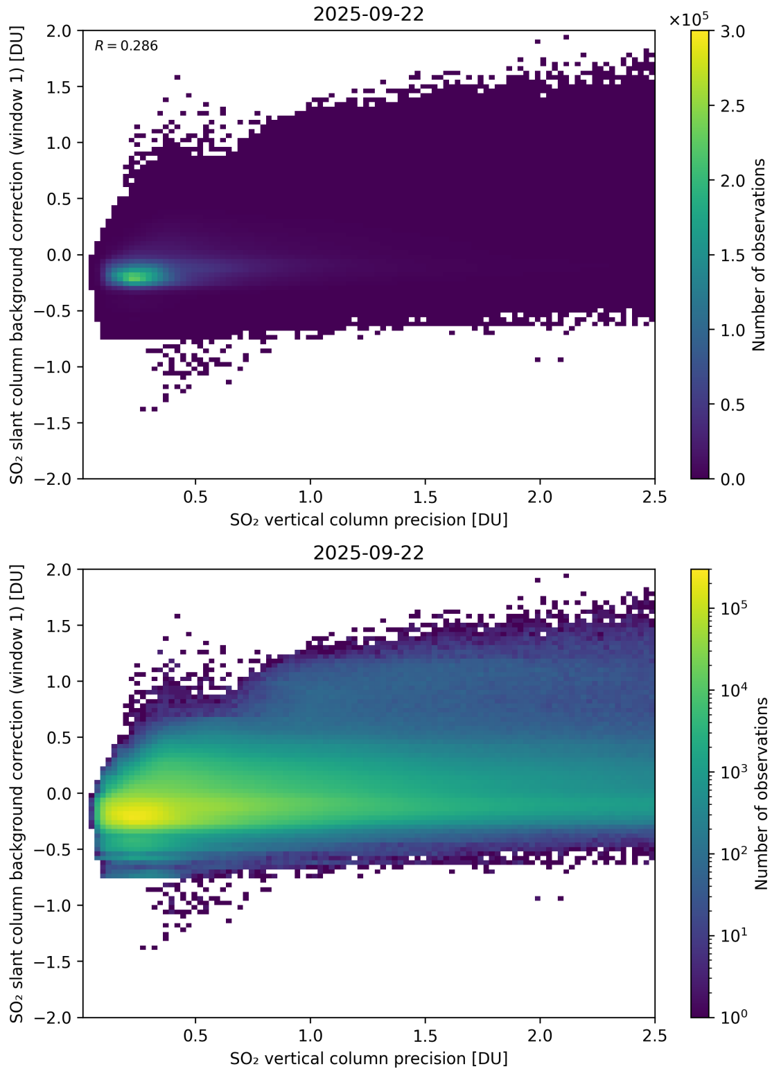
Figure 329: Scatter density plot of “SO 2 vertical column precision” against “SO 2 slant column background correction (window 1)” for 2025-09-22 to 2025-09-23.
