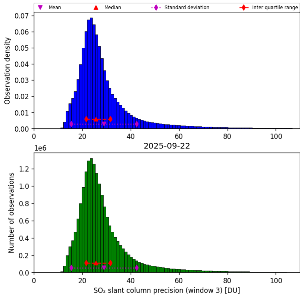
Figure 72: Histogram of “SO 2 slant column precision (window 3)” for 2025-09-22 to 2025-09-23
