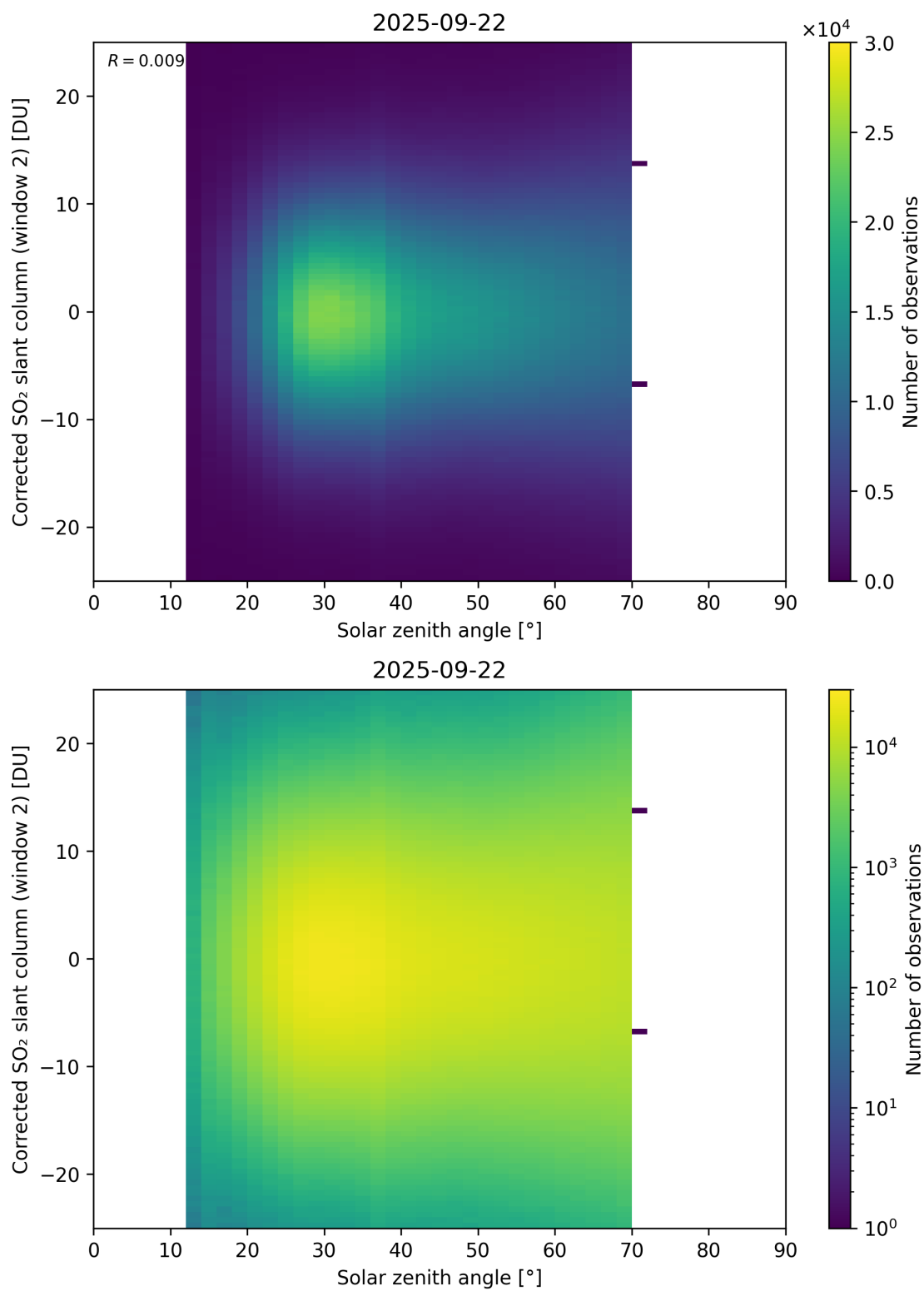
Figure 182: Scatter density plot of “Solar zenith angle” against “Corrected SO 2 slant column (window 2)” for 2025-09-22 to 2025-09-23.
