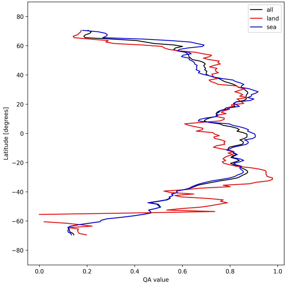
Figure 31: Zonal average of “QA value” for 2025-09-22 to 2025-09-23.
