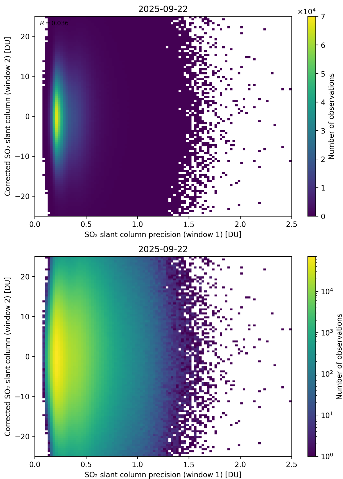
Figure 275: Scatter density plot of “SO 2 slant column precision (window 1)” against “Corrected SO 2 slant column (window 2)” for 2025-09-22 to 2025-09-23.
