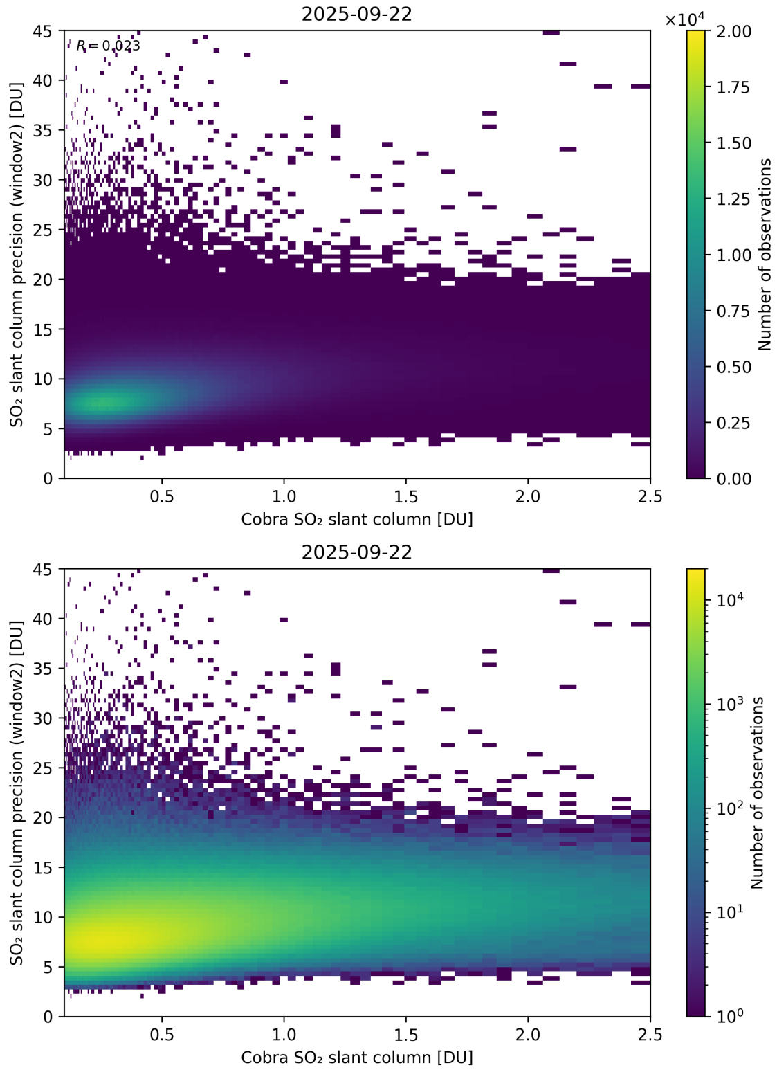
Figure 221: Scatter density plot of “Cobra SO 2 slant column” against “SO 2 slant column precision (window2)” for 2025-09-22 to 2025-09-23.
