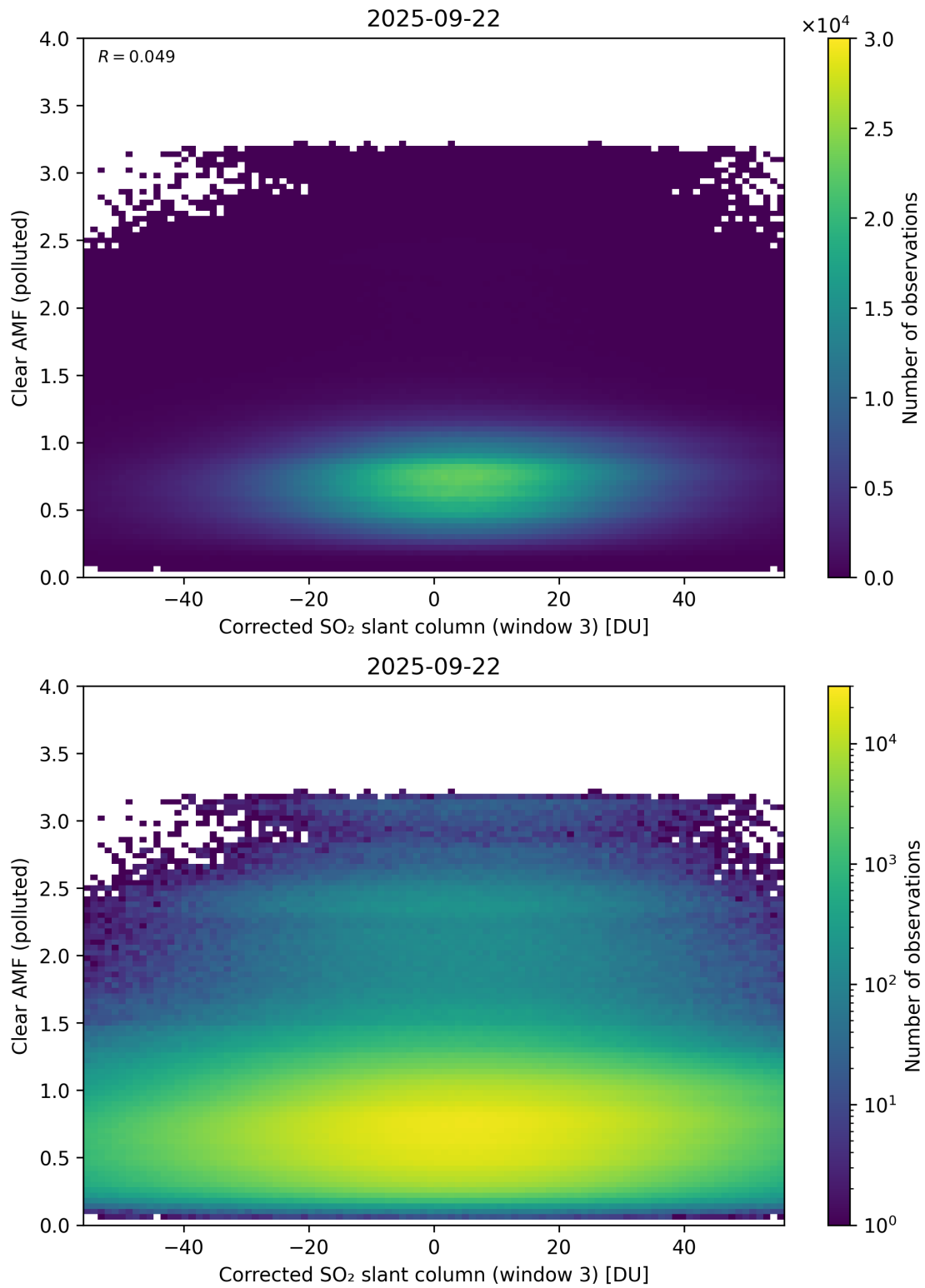
Figure 259: Scatter density plot of “Corrected SO 2 slant column (window 3)” against “Clear AMF (polluted)” for 2025-09-22 to 2025-09-23.
