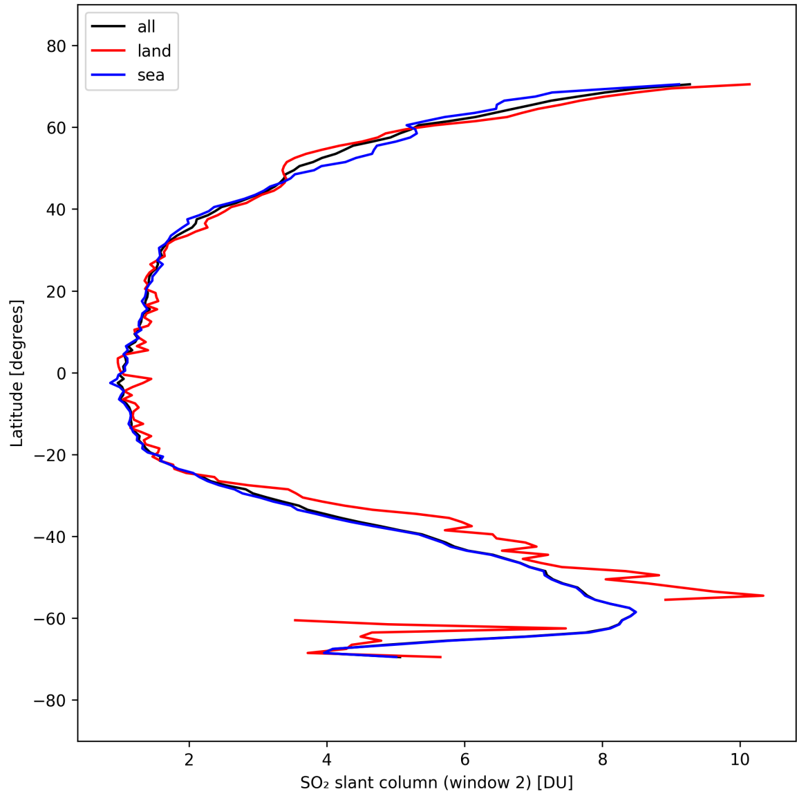
Figure 41: Zonal average of “SO 2 slant column (window 2)” for 2025-09-22 to 2025-09-23.
