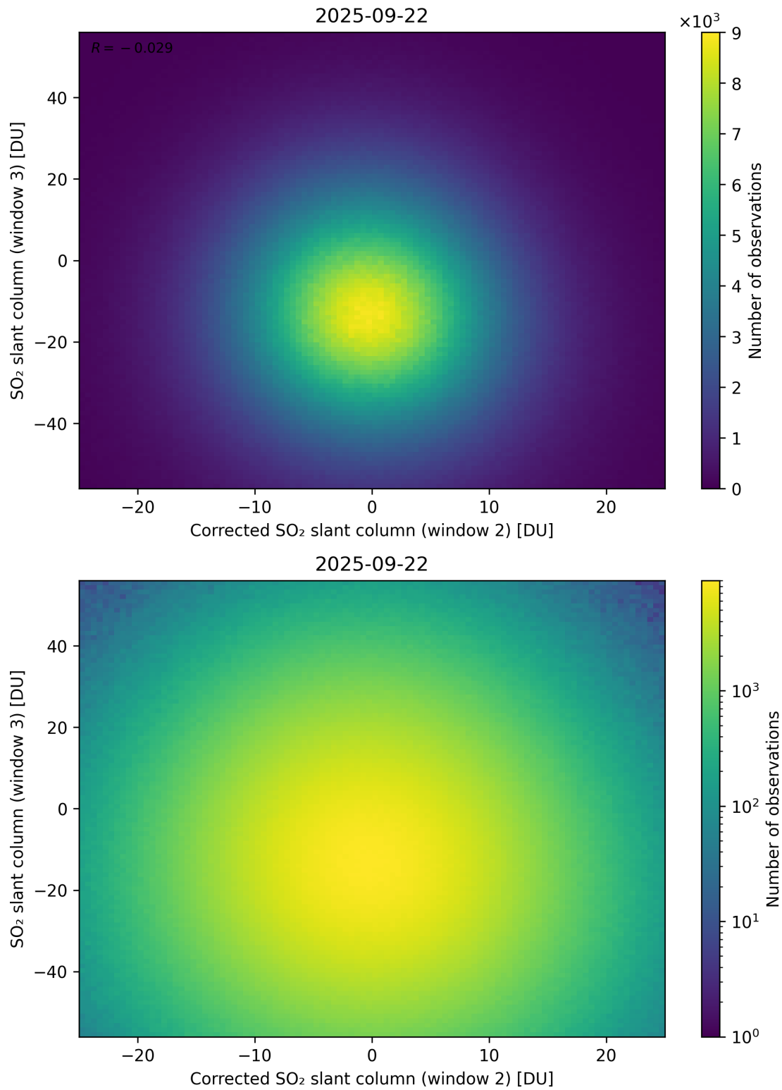
Figure 251: Scatter density plot of “Corrected SO 2 slant column (window 2)” against “SO 2 slant column (window 3)” for 2025-09-22 to 2025-09-23.
