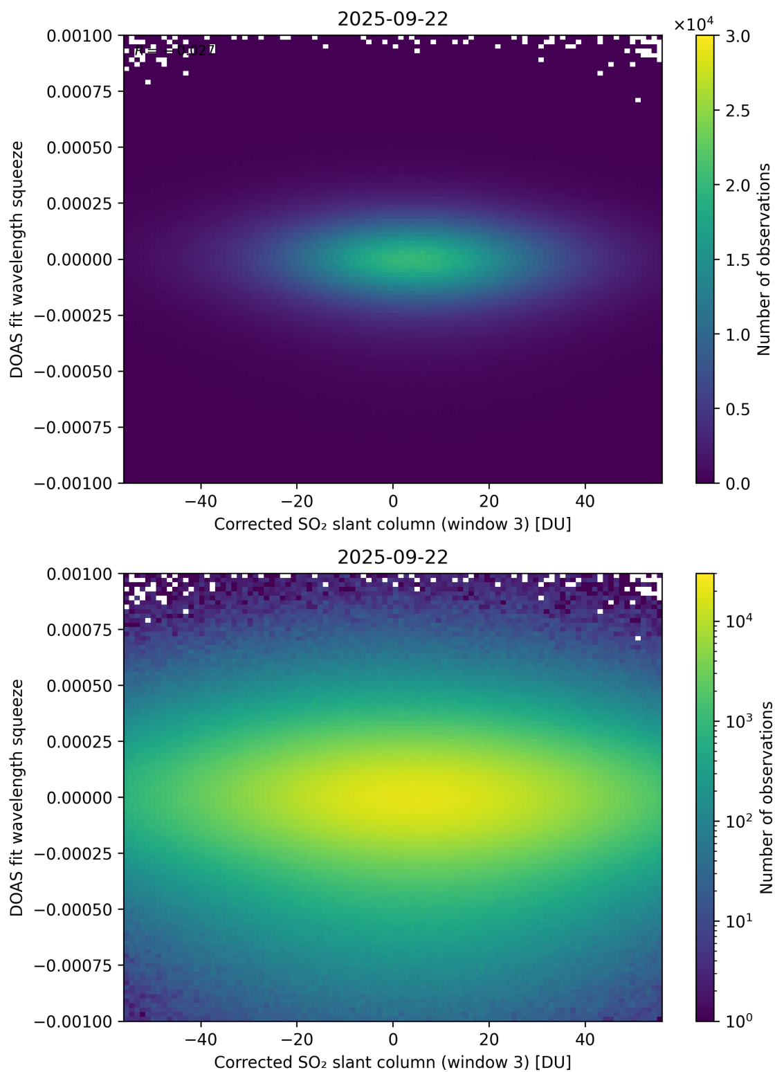
Figure 257: Scatter density plot of “Corrected SO 2 slant column (window 3)” against “DOAS fit wavelength squeeze” for 2025-09-22 to 2025-09-23.
