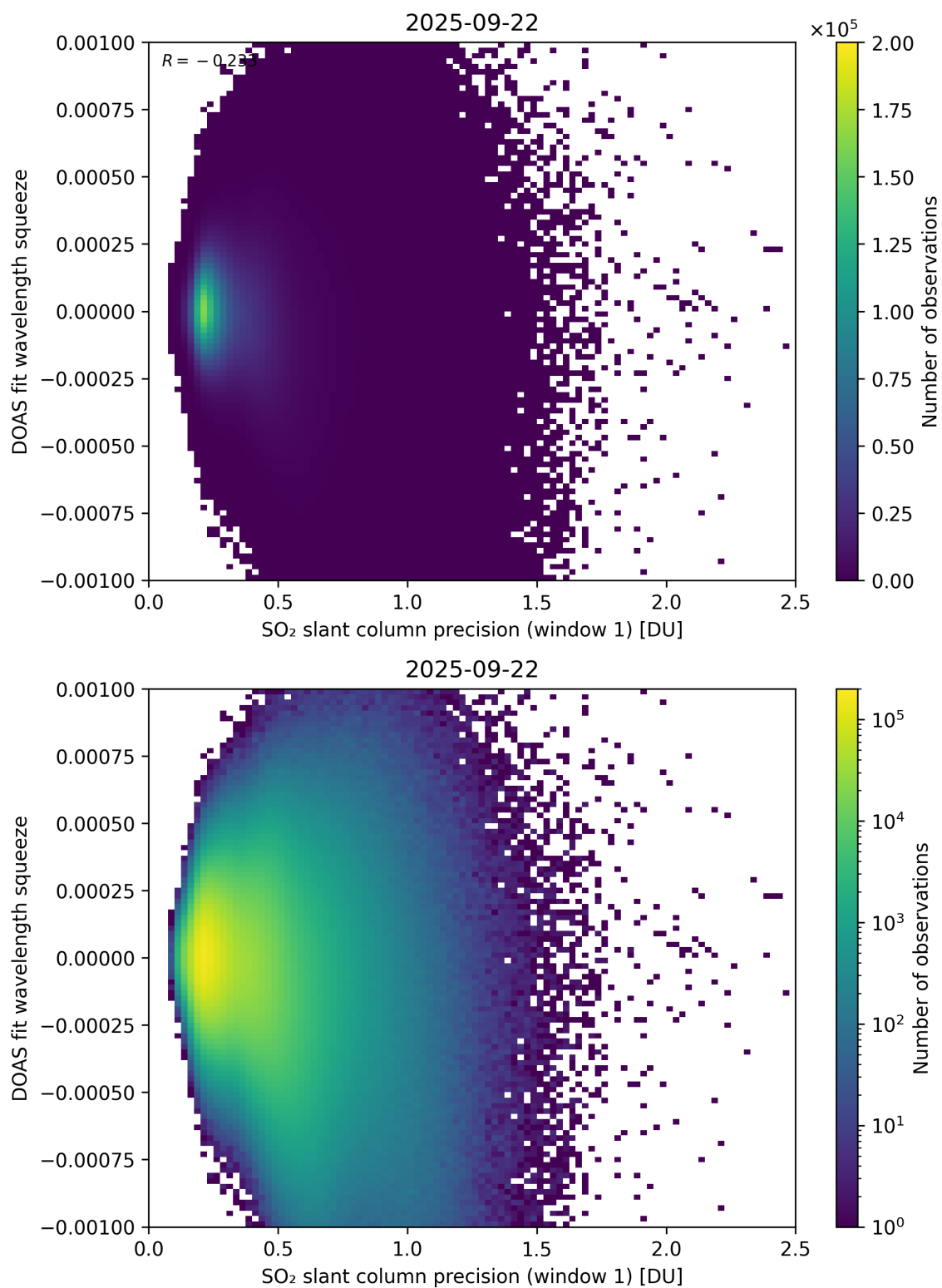
Figure 272: Scatter density plot of “SO 2 slant column precision (window 1)” against “DOAS fit wavelength squeeze” for 2025-09-22 to 2025-09-23.
