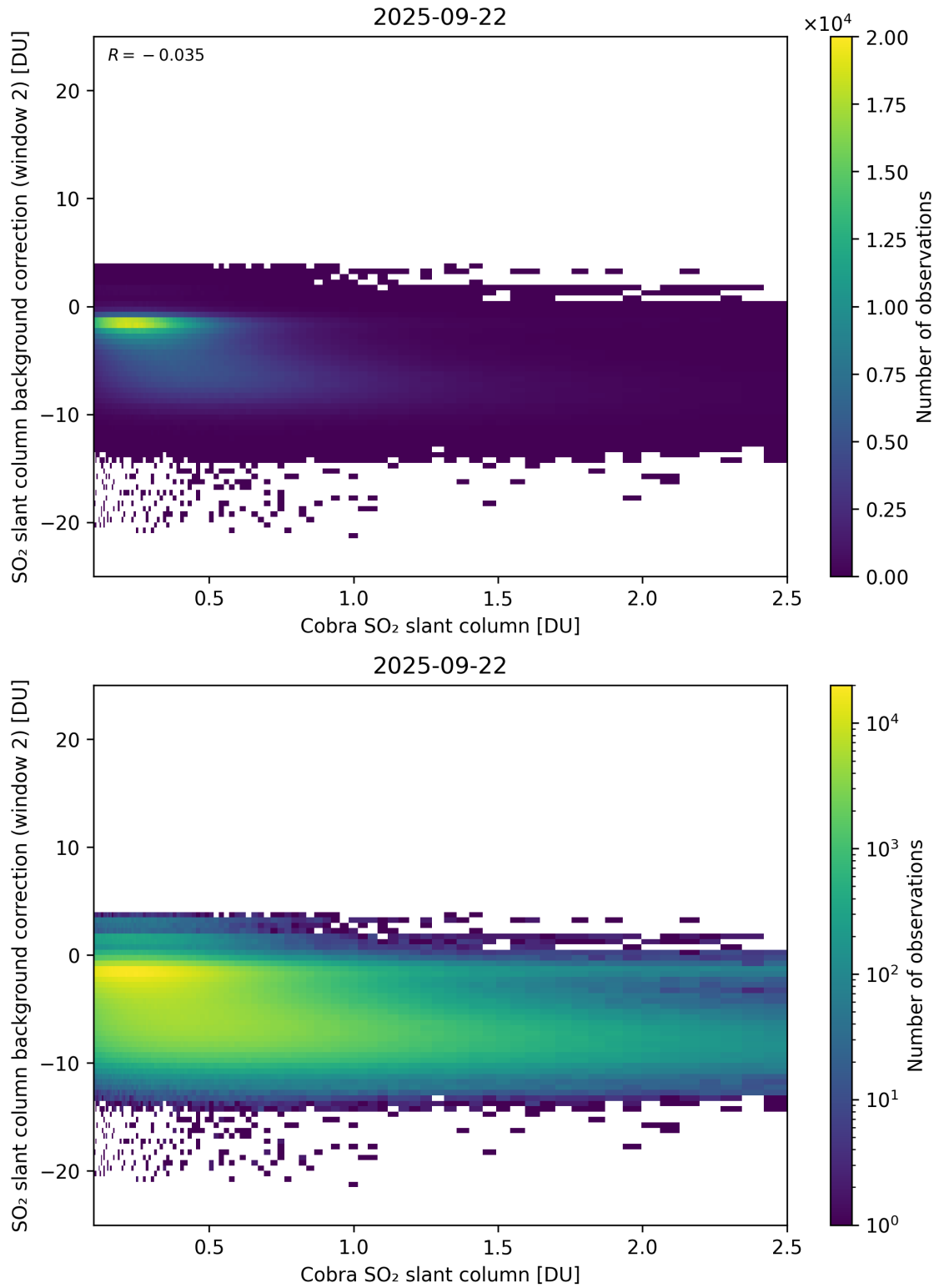
Figure 194: Scatter density plot of “Cobra SO 2 slant column” against “SO 2 slant column background correction (window 2)” for 2025-09-22 to 2025-09-23.
