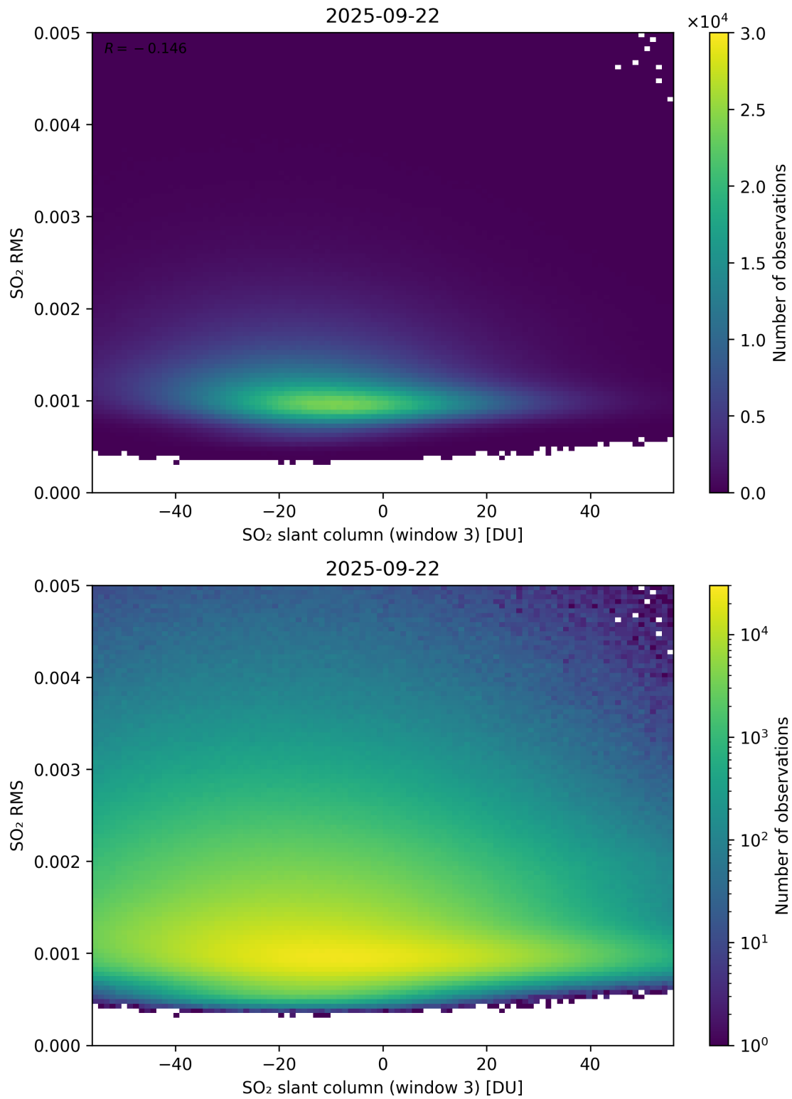
Figure 306: Scatter density plot of “SO 2 slant column (window 3)” against “SO 2 RMS” for 2025-09-22 to 2025-09-23.
