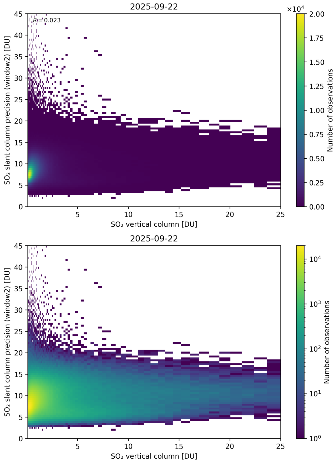
Figure 356: Scatter density plot of “SO 2 vertical column” against “SO 2 slant column precision (window2)” for 2025-09-22 to 2025-09-23.
