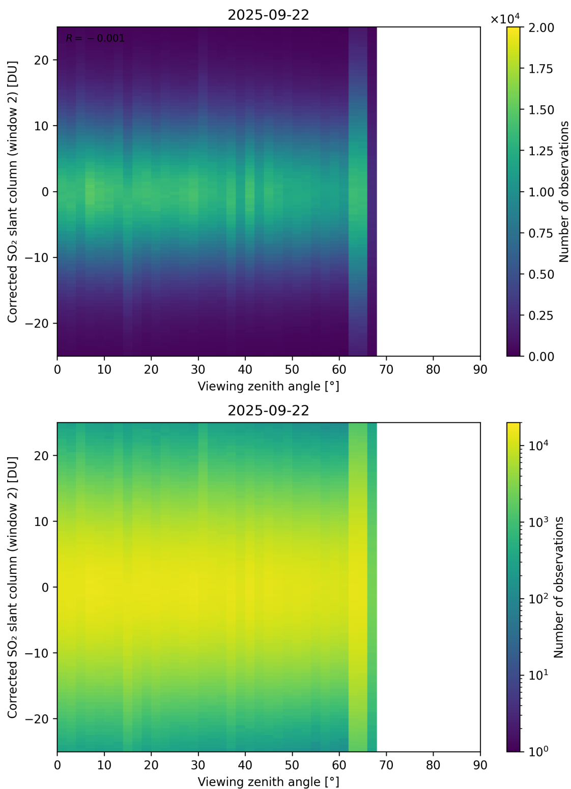
Figure 374: Scatter density plot of “Viewing zenith angle” against “Corrected SO 2 slant column (window 2)” for 2025-09-22 to 2025-09-23.
