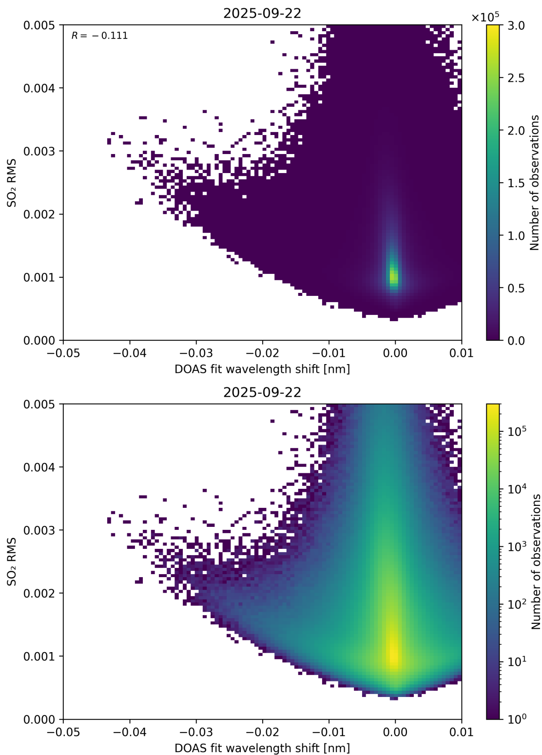
Figure 139: Scatter density plot of “DOAS fit wavelength shift” against “SO 2 RMS” for 2025-09-22 to 2025-09-23.
