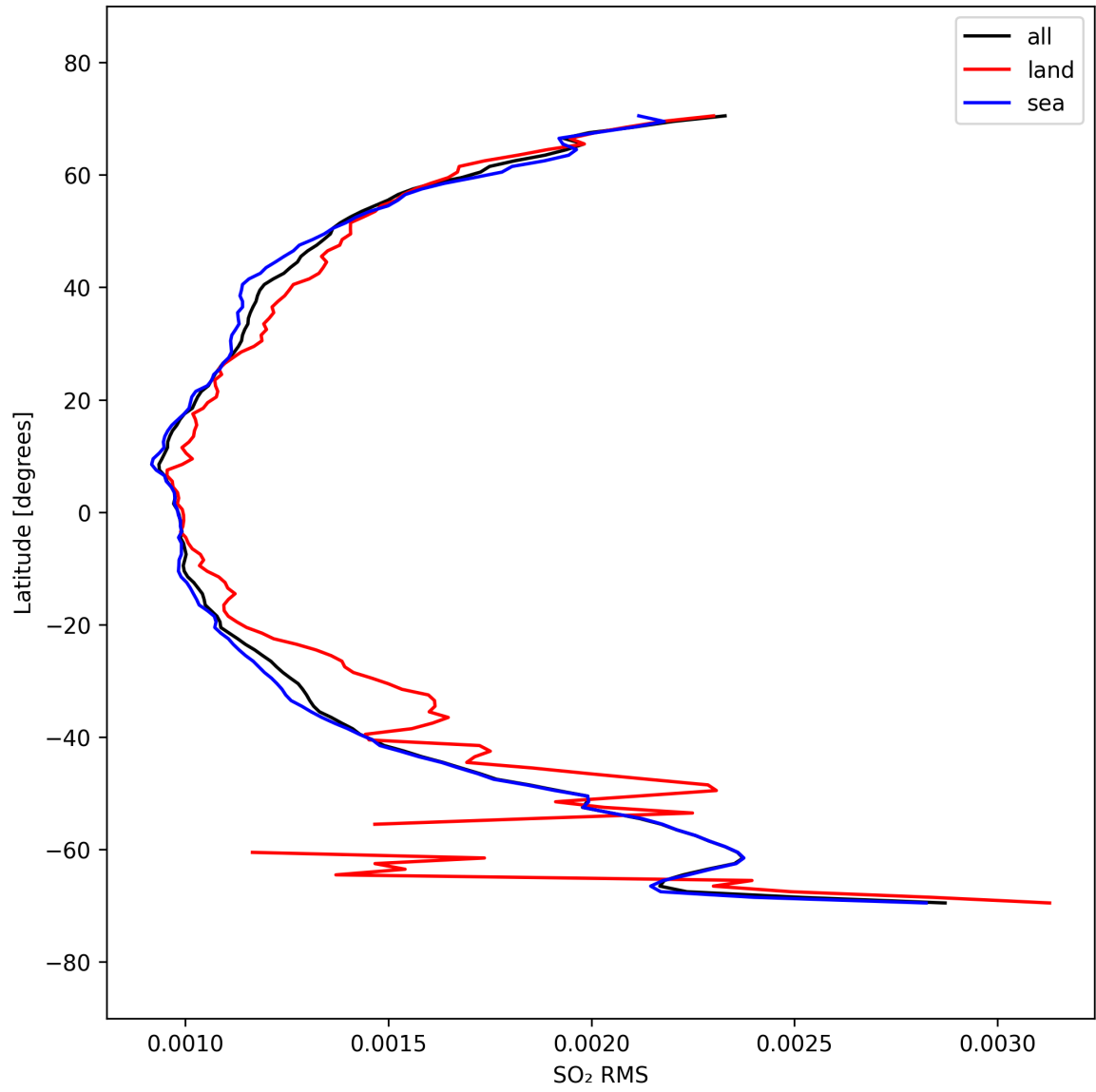
Figure 52: Zonal average of “SO 2 RMS” for 2025-09-22 to 2025-09-23.
