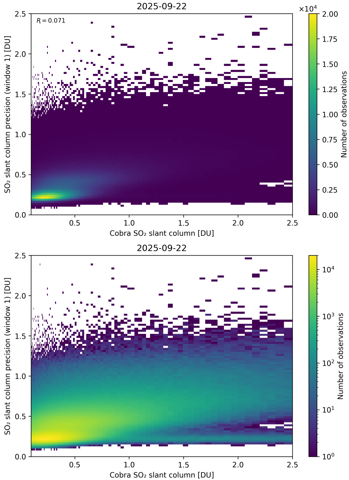
Figure 220: Scatter density plot of “Cobra SO 2 slant column” against “SO 2 slant column precision (window 1)” for 2025-09-22 to 2025-09-23.
