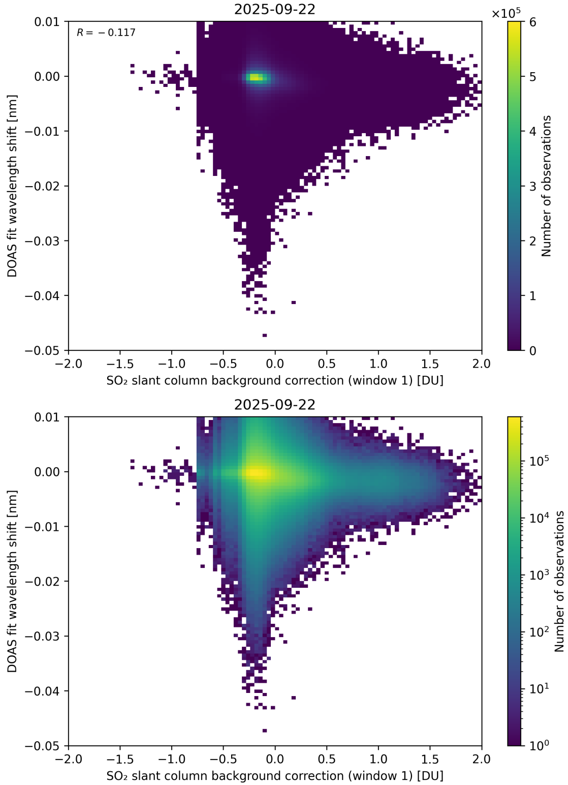
Figure 111: Scatter density plot of “SO 2 slant column background correction (window 1)” against “DOAS fit wavelength shift” for 2025-09-22 to 2025-09-23.
