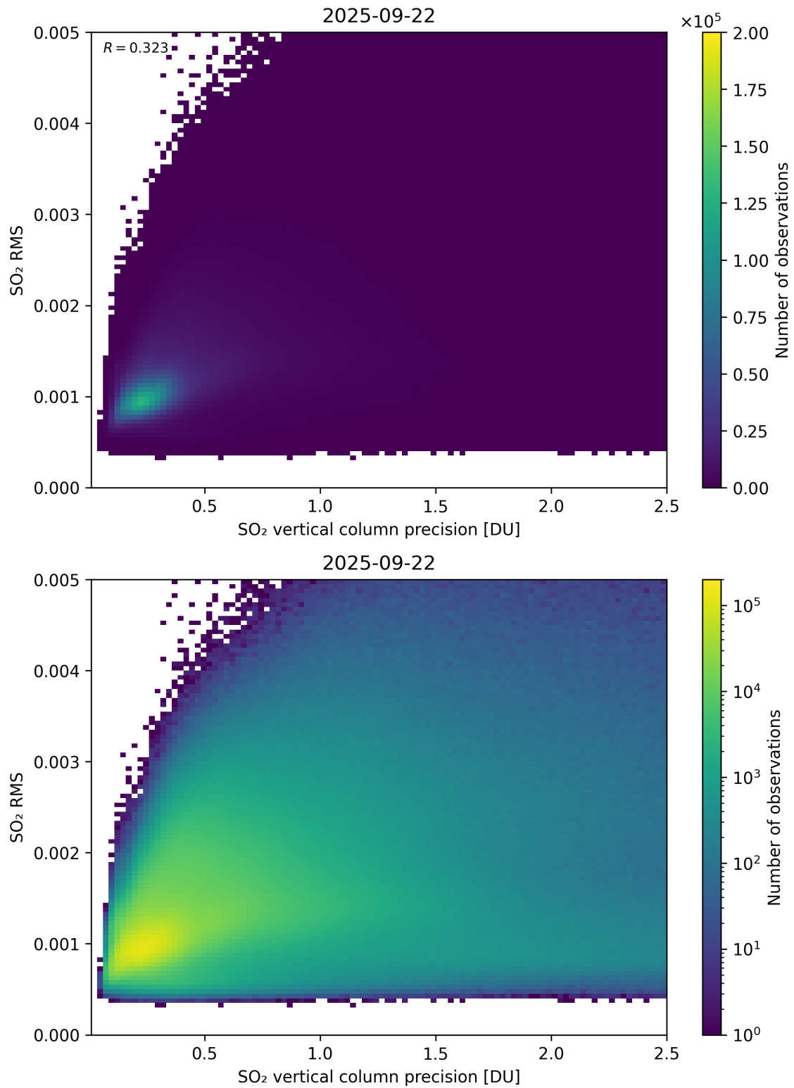
Figure 334: Scatter density plot of “SO 2 vertical column precision” against “SO 2 RMS” for 2025-09-22 to 2025-09-23.
