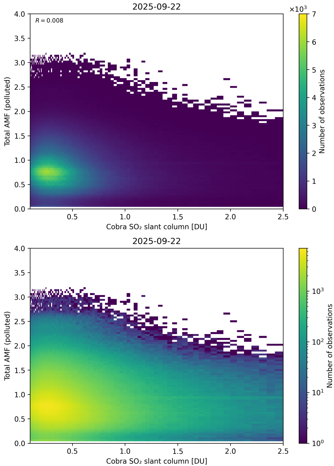
Figure 224: Scatter density plot of “Cobra SO 2 slant column” against “Total AMF (polluted)” for 2025-09-22 to 2025-09-23.
