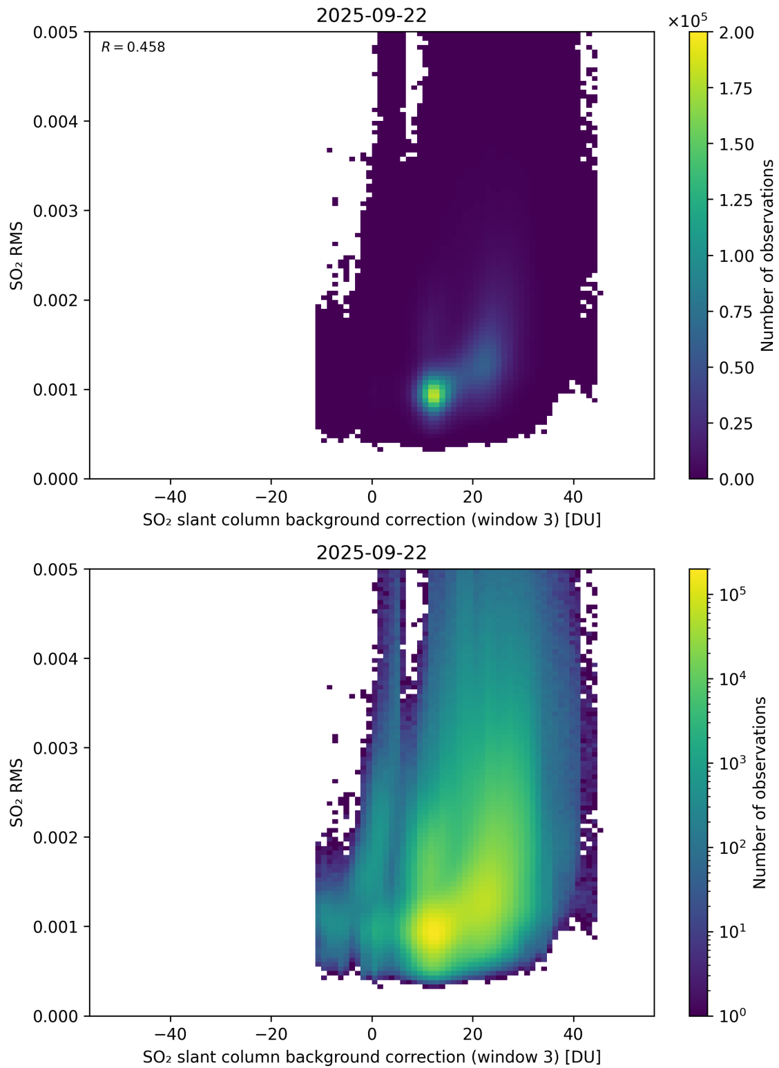
Figure 134: Scatter density plot of “SO 2 slant column background correction (window 3)” against “SO 2 RMS” for 2025-09-22 to 2025-09-23.
