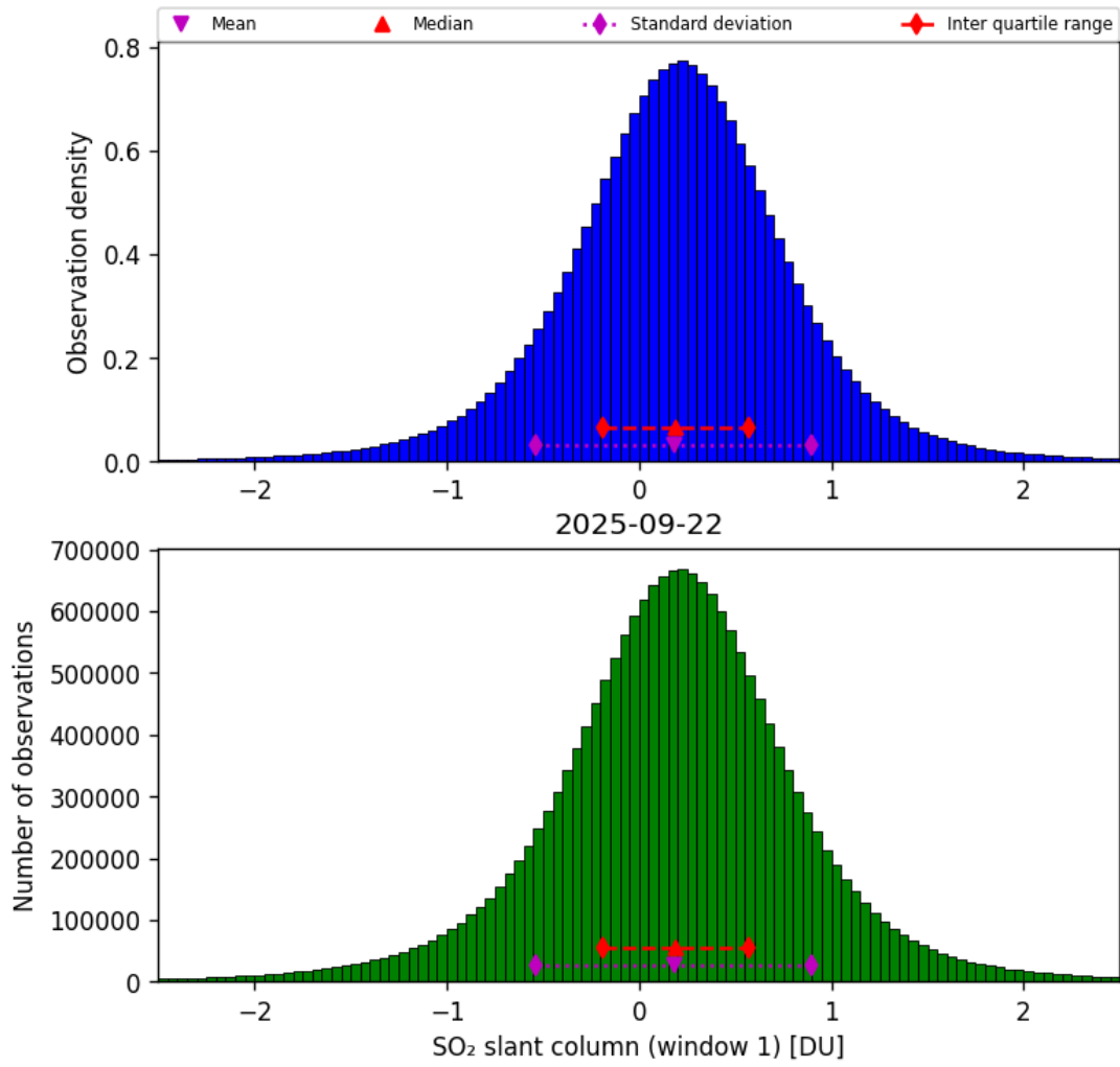
Figure 63: Histogram of “SO 2 slant column (window 1)” for 2025-09-22 to 2025-09-23
