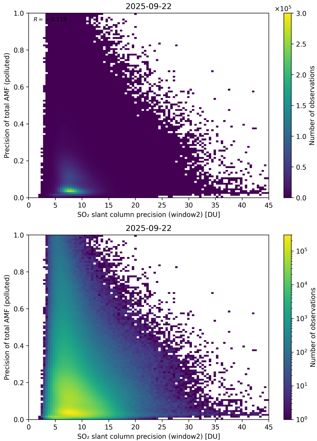
Figure 302: Scatter density plot of “SO 2 slant column precision (window2)” against “Precision of total AMF (polluted)” for 2025-09-22 to 2025-09-23.
