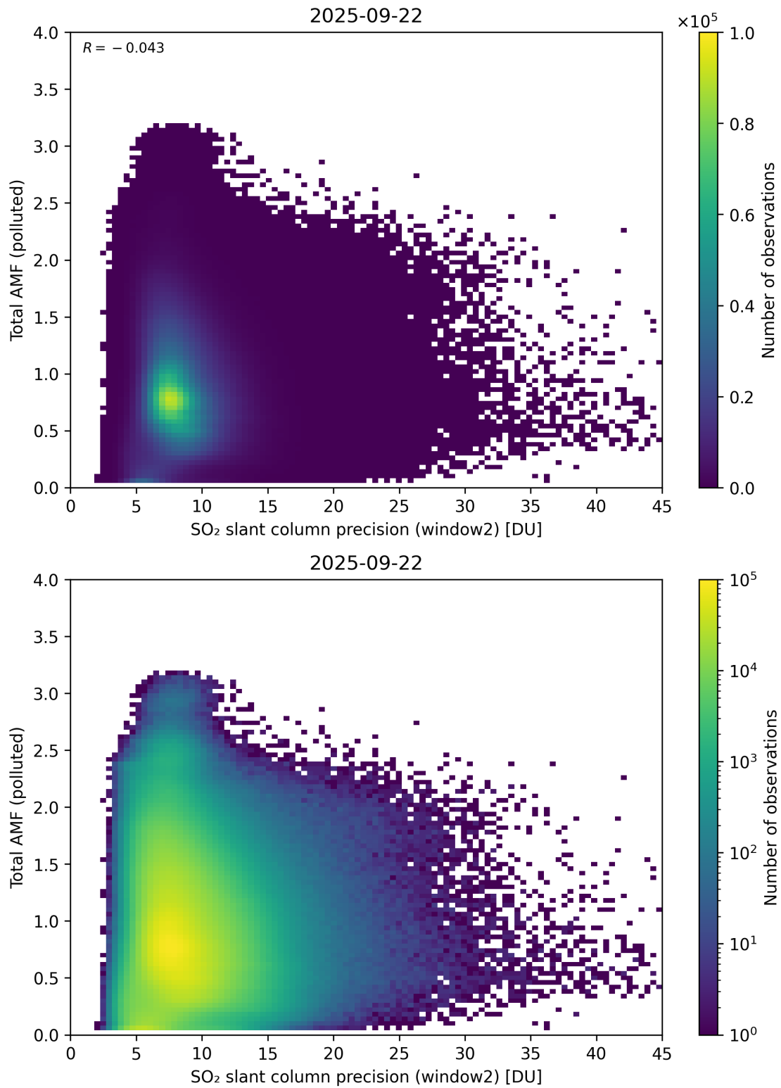
Figure 301: Scatter density plot of “SO 2 slant column precision (window2)” against “Total AMF (polluted)” for 2025-09-22 to 2025-09-23.
