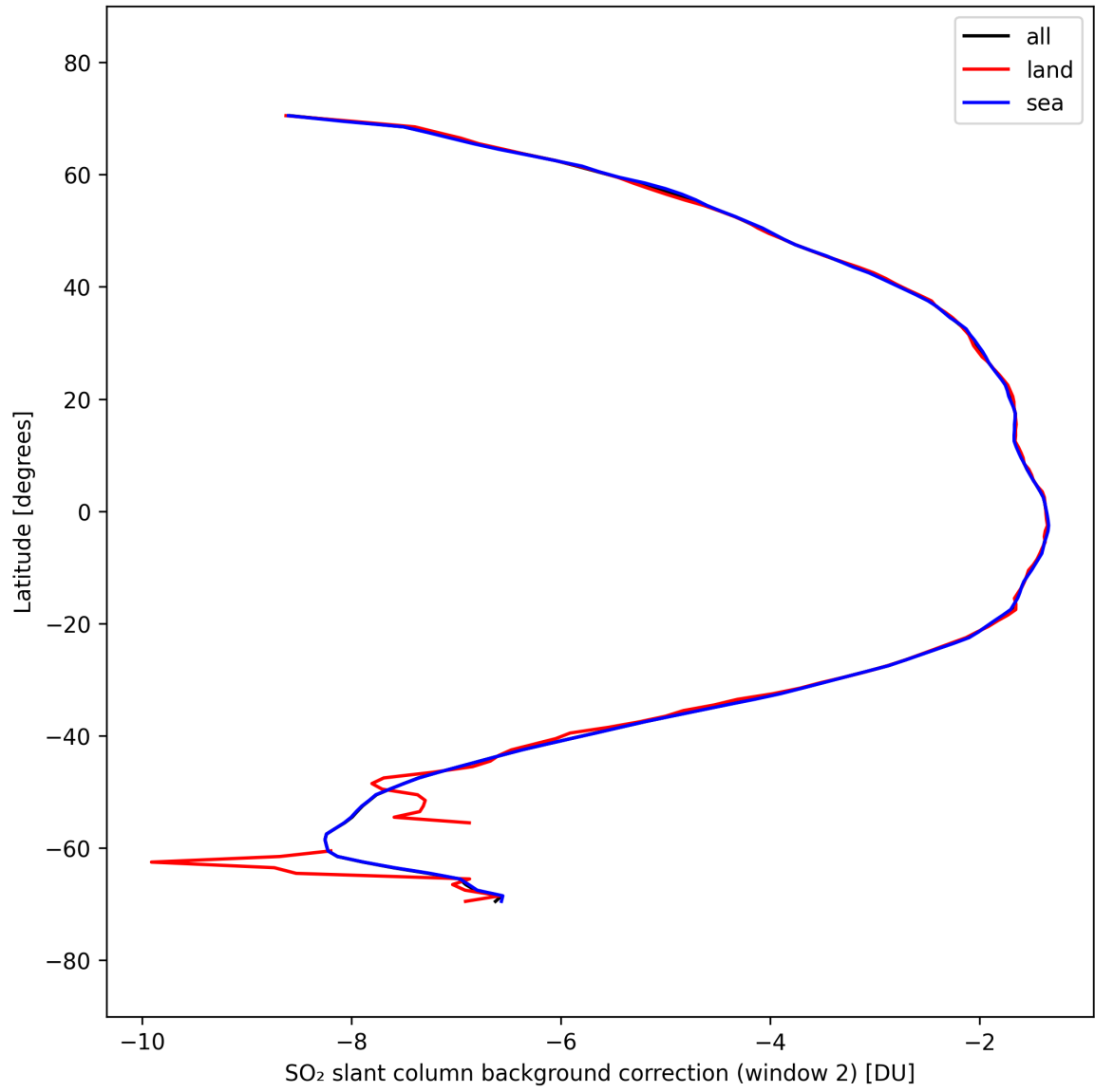
Figure 44: Zonal average of “SO 2 slant column background correction (window 2)” for 2025-09-22 to 2025-09-23.
