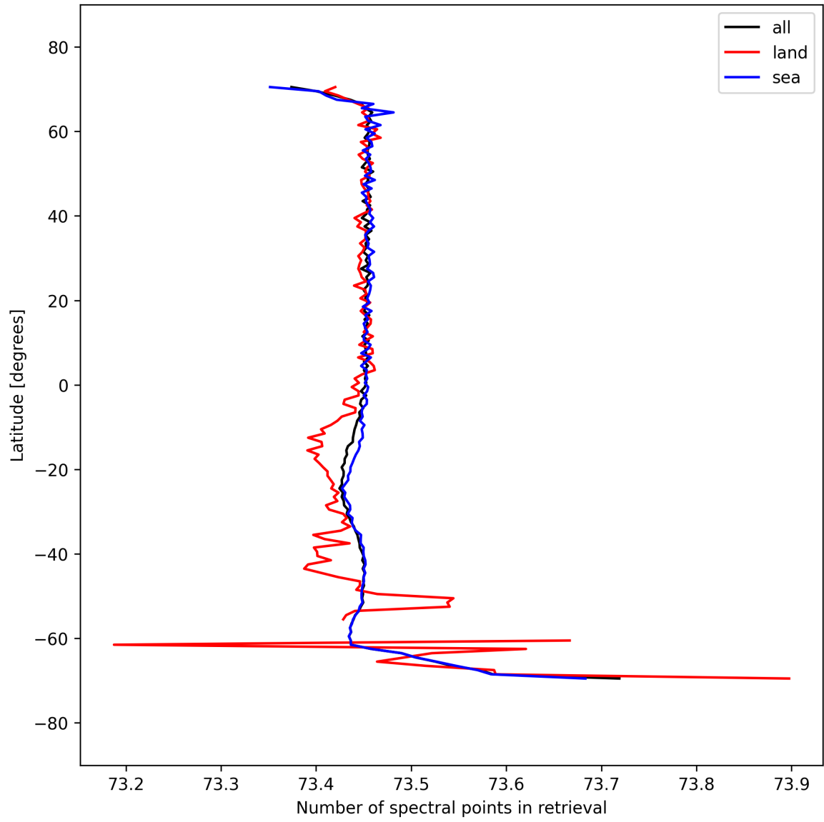
Figure 56: Zonal average of “Number of spectral points in retrieval” for 2025-09-22 to 2025-09-23.
