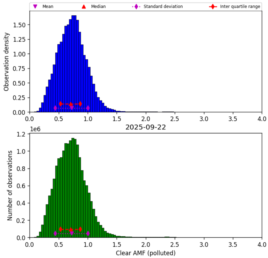
Figure 81: Histogram of “Clear AMF (polluted)” for 2025-09-22 to 2025-09-23
