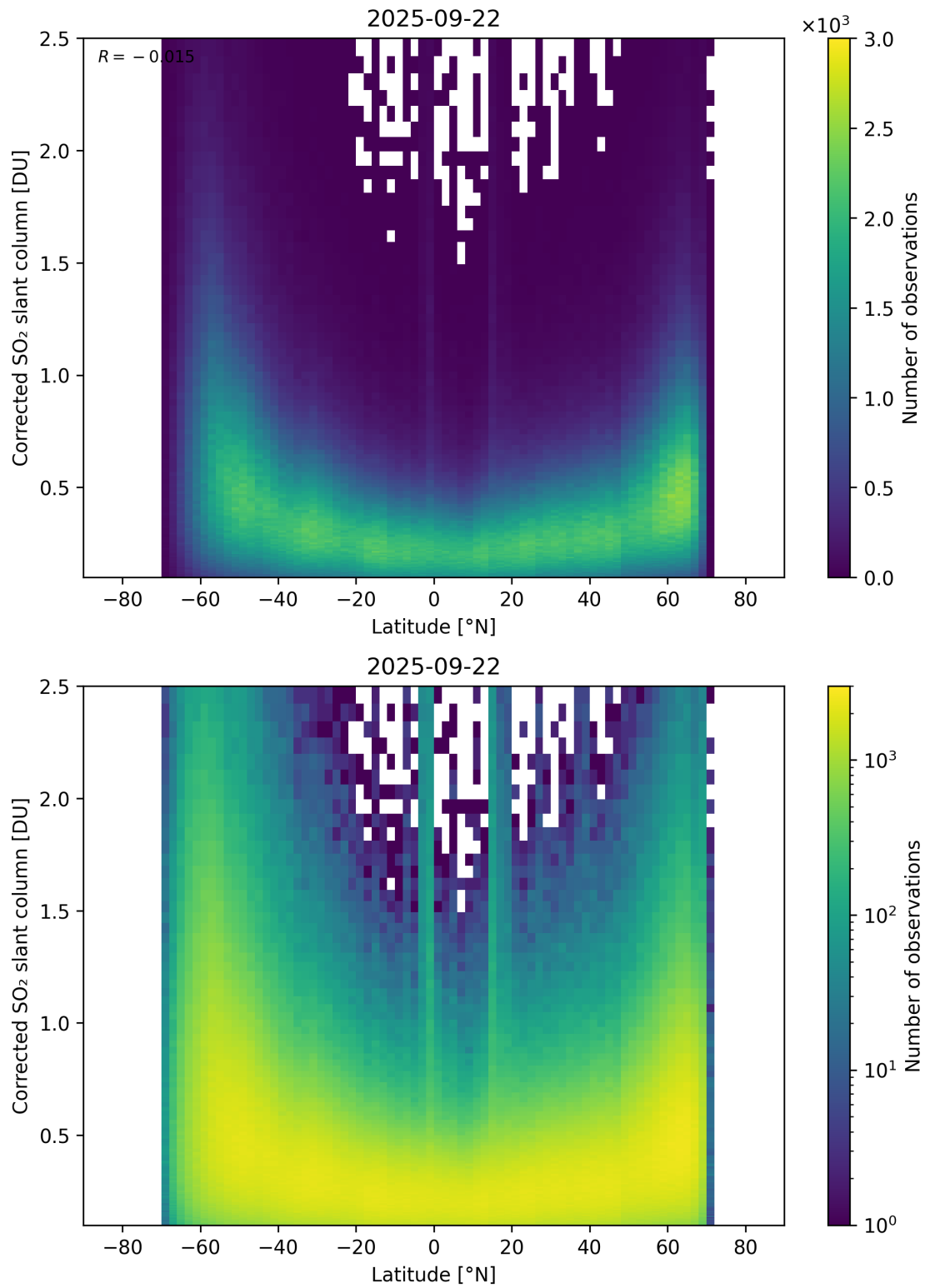
Figure 159: Scatter density plot of “Latitude” against “Corrected SO 2 slant column” for 2025-09-22 to 2025-09-23.
