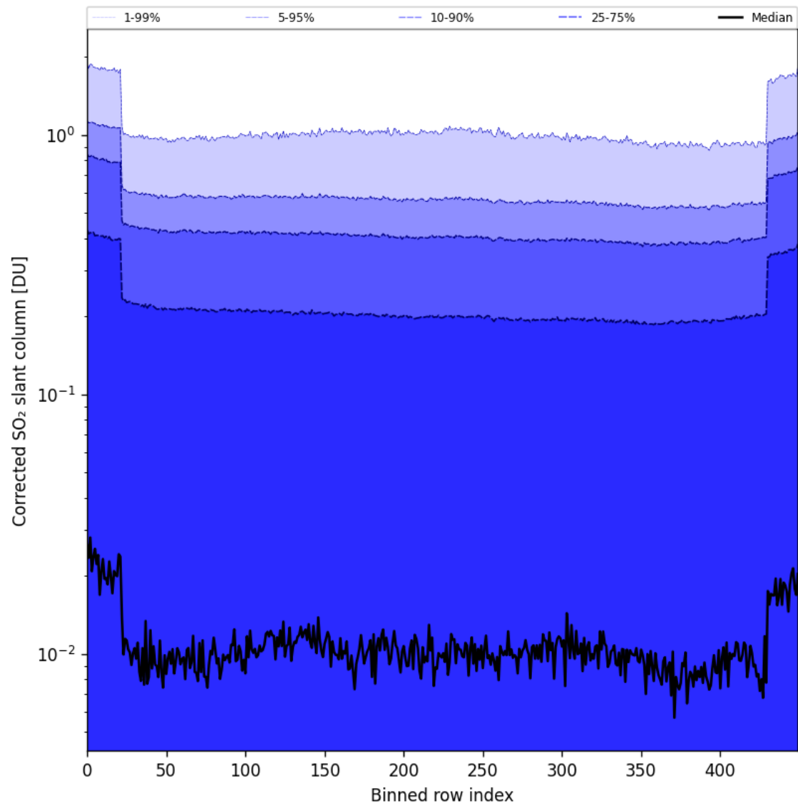
Figure 86: Along track statistics of “Corrected SO 2 slant column” for 2025-09-22 to 2025-09-23
