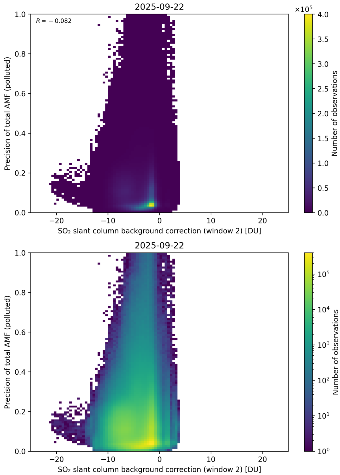
Figure 131: Scatter density plot of “SO 2 slant column background correction (window 2)” against “Precision of total AMF (polluted)” for 2025-09-22 to 2025-09-23.
