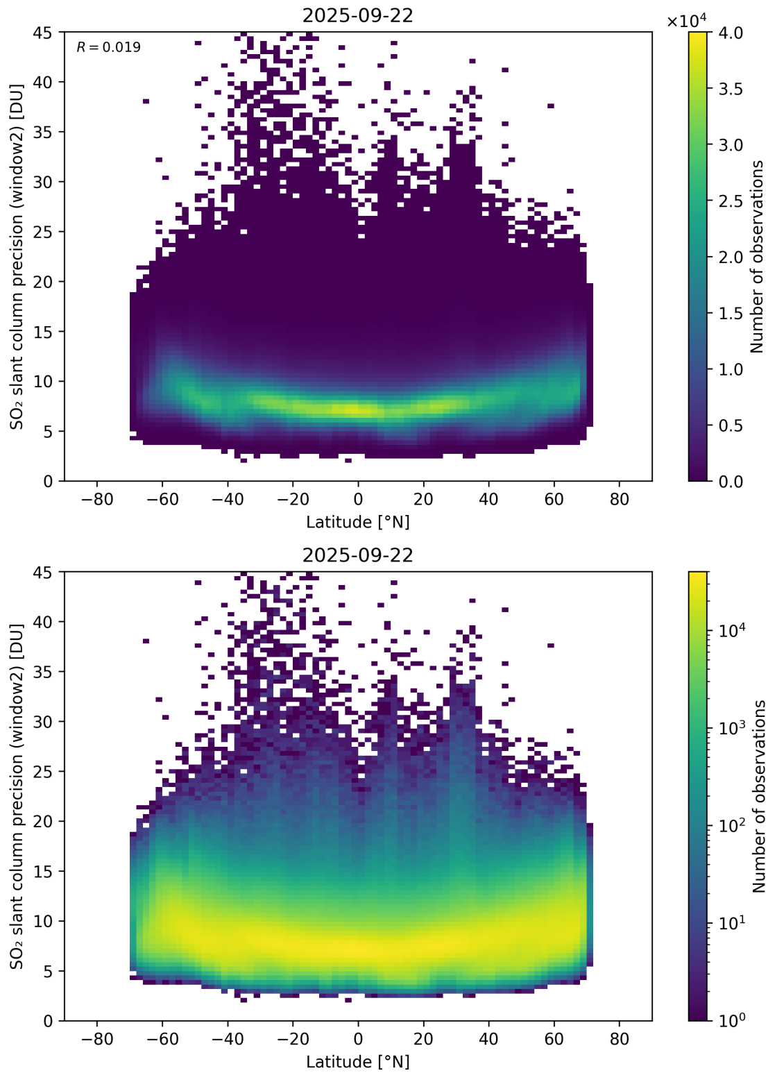
Figure 164: Scatter density plot of “Latitude” against “SO 2 slant column precision (window2)” for 2025-09-22 to 2025-09-23.
