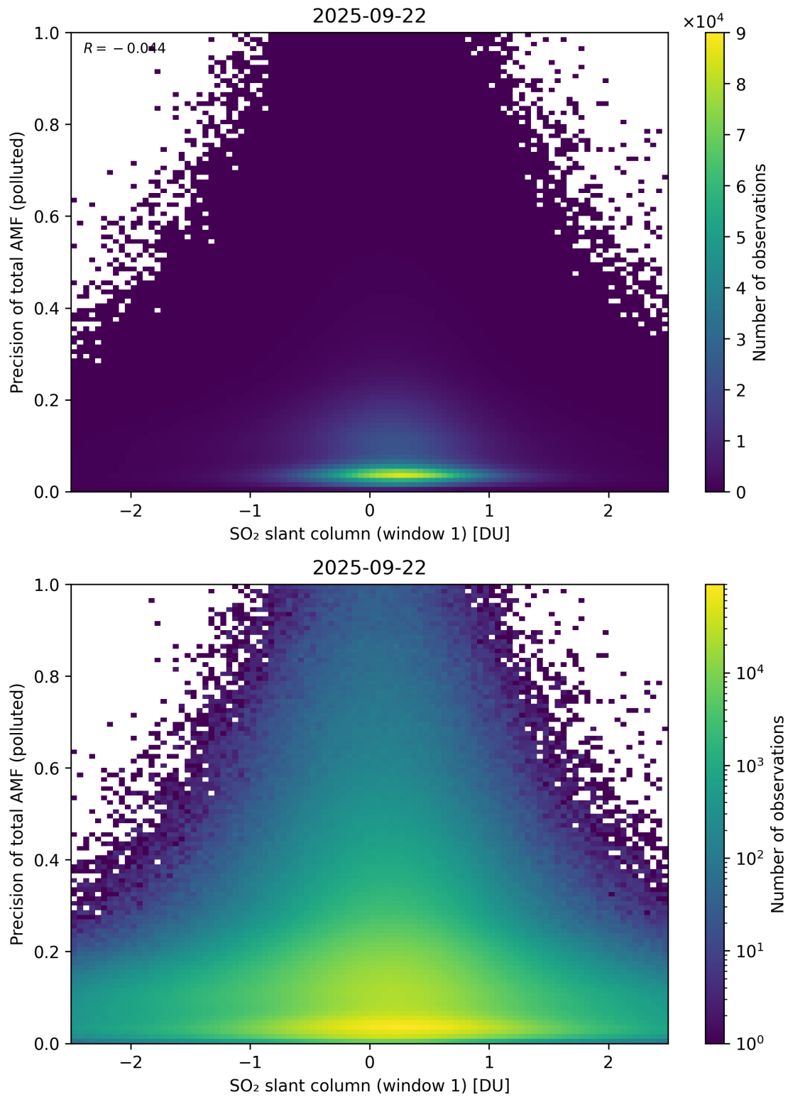
Figure 290: Scatter density plot of “SO 2 slant column (window 1)” against “Precision of total AMF (polluted)” for 2025-09-22 to 2025-09-23.
