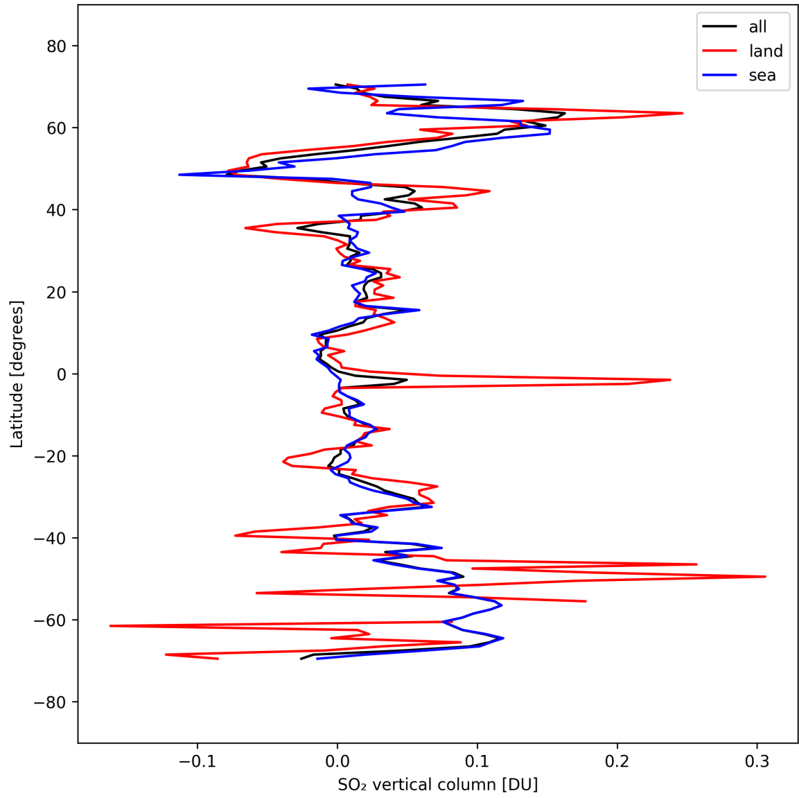
Figure 32: Zonal average of “SO 2 vertical column” for 2025-09-22 to 2025-09-23.
