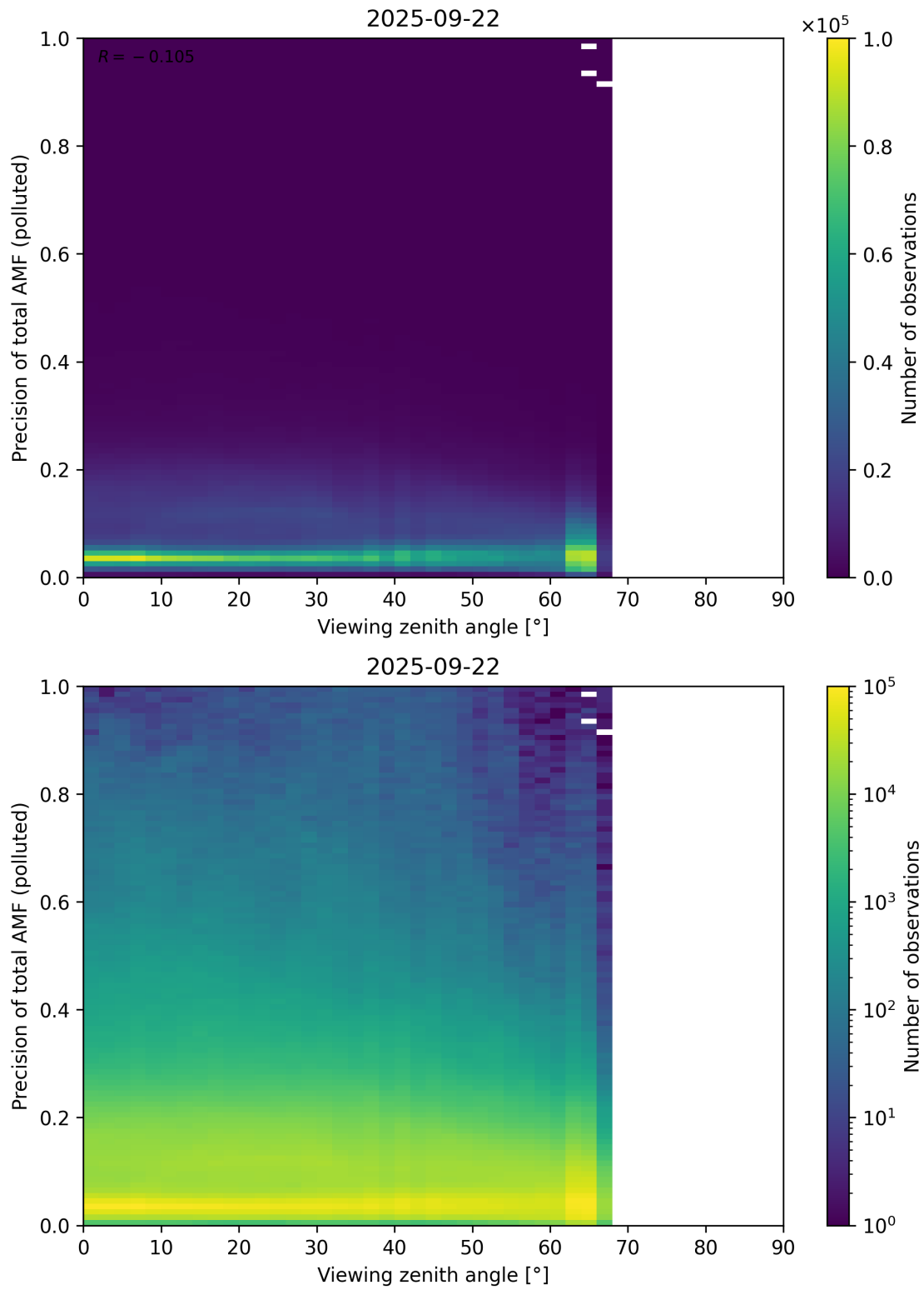
Figure 382: Scatter density plot of “Viewing zenith angle” against “Precision of total AMF (polluted)” for 2025-09-22 to 2025-09-23.
