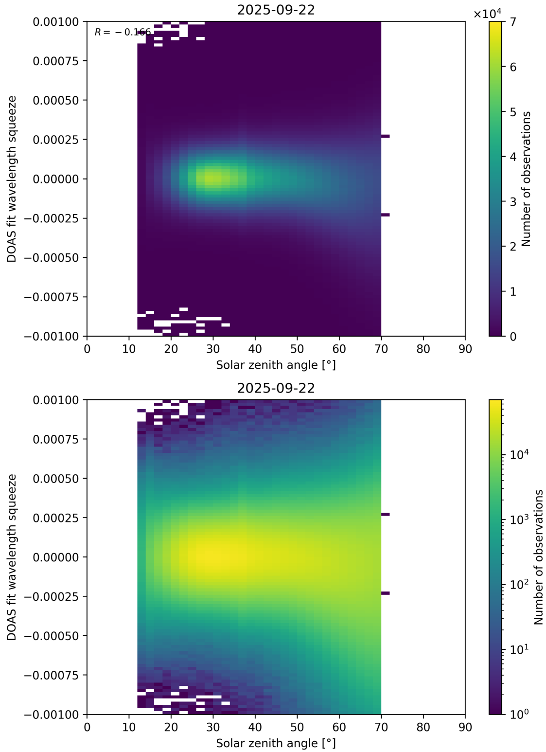
Figure 175: Scatter density plot of “Solar zenith angle” against “DOAS fit wavelength squeeze” for 2025-09-22 to 2025-09-23.
