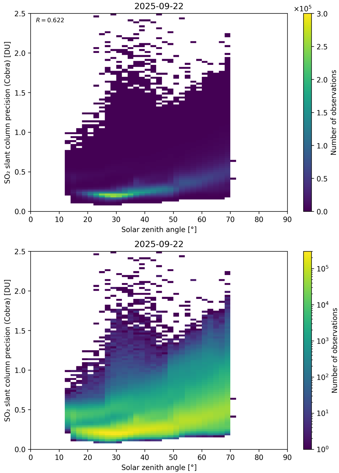
Figure 180: Scatter density plot of “Solar zenith angle” against “SO 2 slant column precision (Cobra)” for 2025-09-22 to 2025-09-23.
