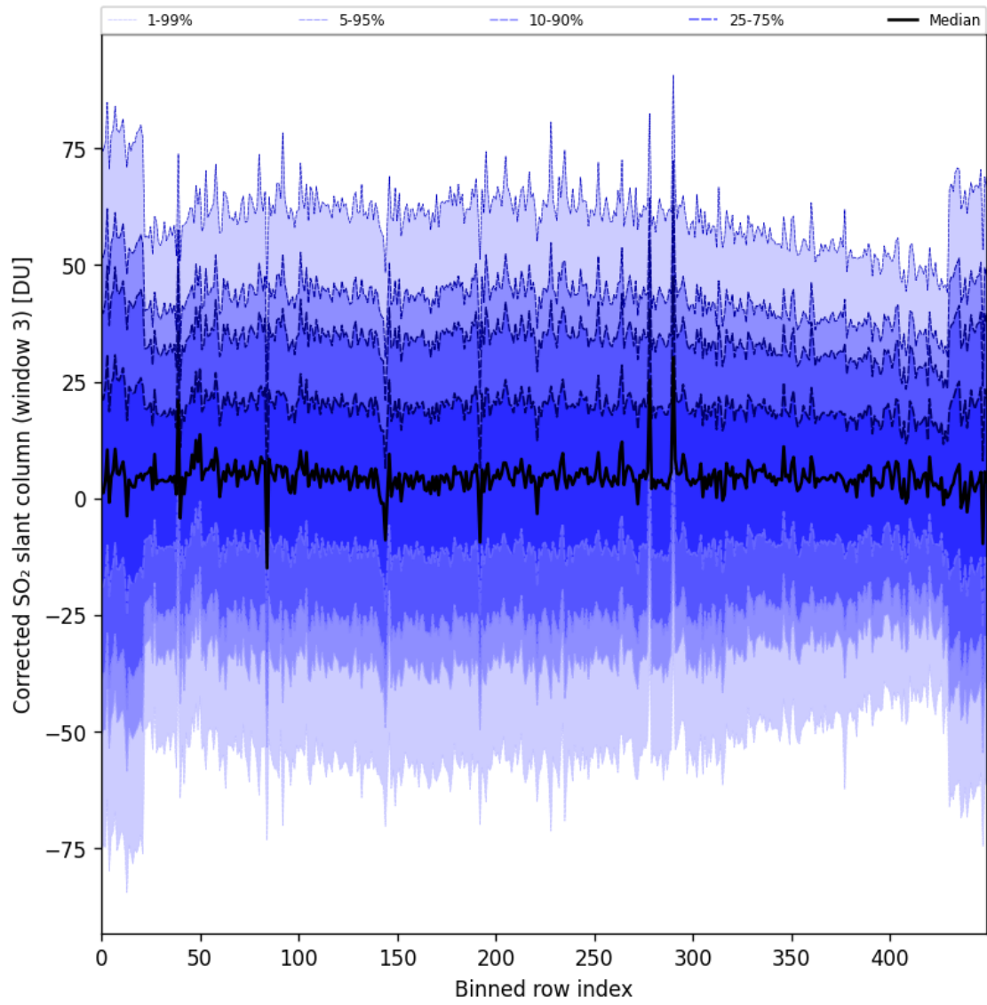
Figure 99: Along track statistics of “Corrected SO 2 slant column (window 3)” for 2025-09-22 to 2025-09-23
