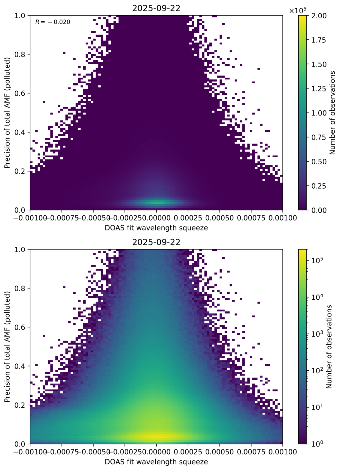
Figure 146: Scatter density plot of “DOAS fit wavelength squeeze” against “Precision of total AMF (polluted)” for 2025-09-22 to 2025-09-23.
