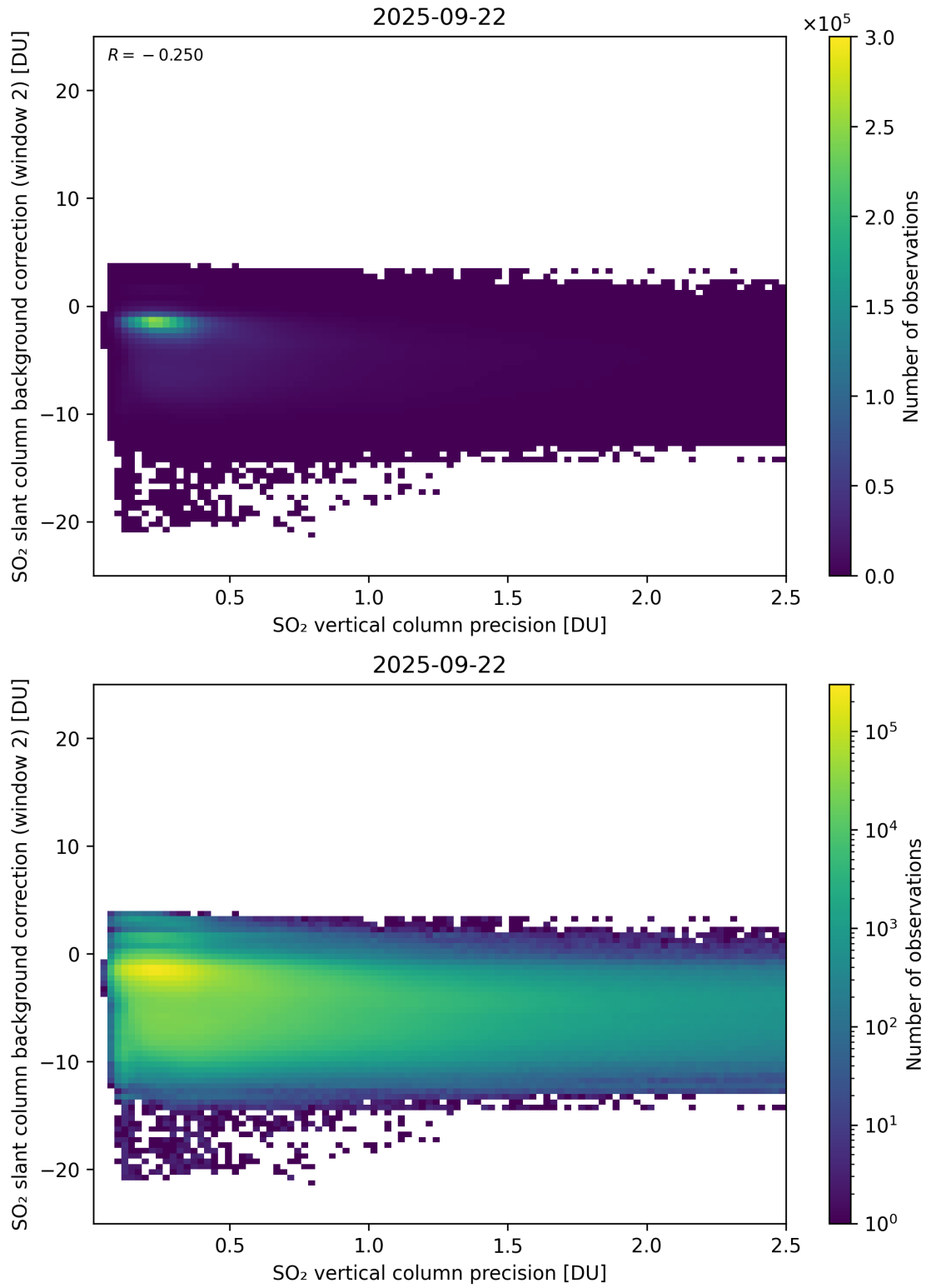
Figure 330: Scatter density plot of “SO 2 vertical column precision” against “SO 2 slant column background correction (window 2)” for 2025-09-22 to 2025-09-23.
