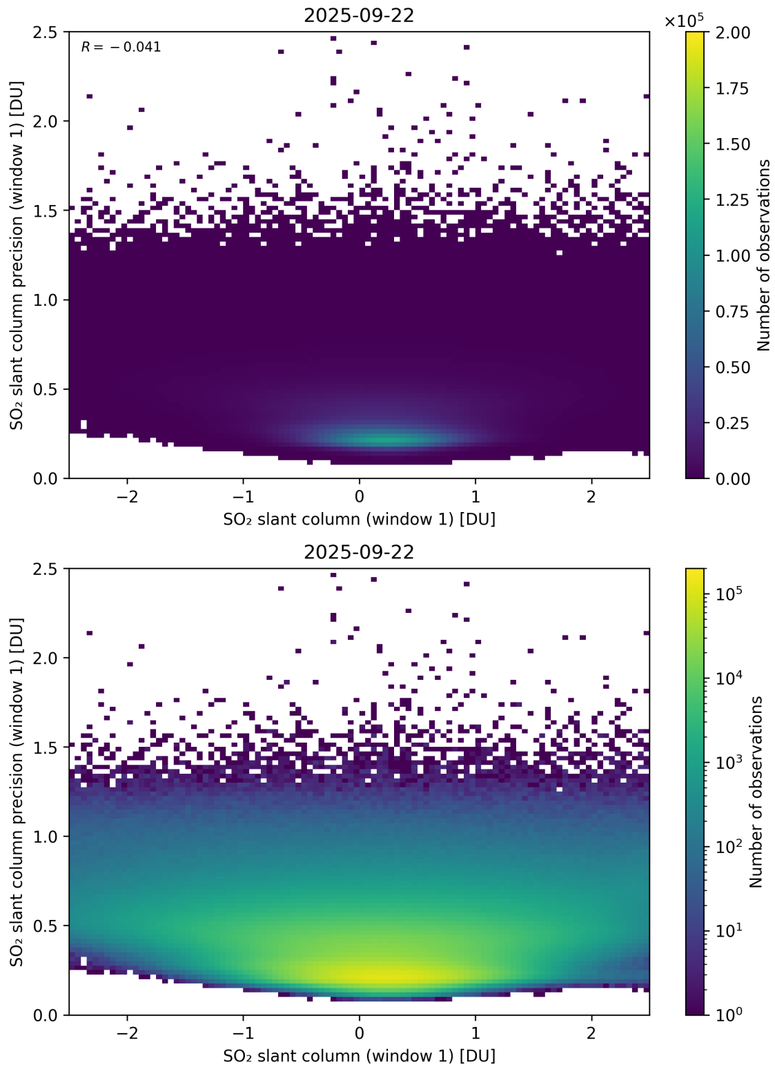
Figure 285: Scatter density plot of “SO 2 slant column (window 1)” against “SO 2 slant column precision (window 1)” for 2025-09-22 to 2025-09-23.
