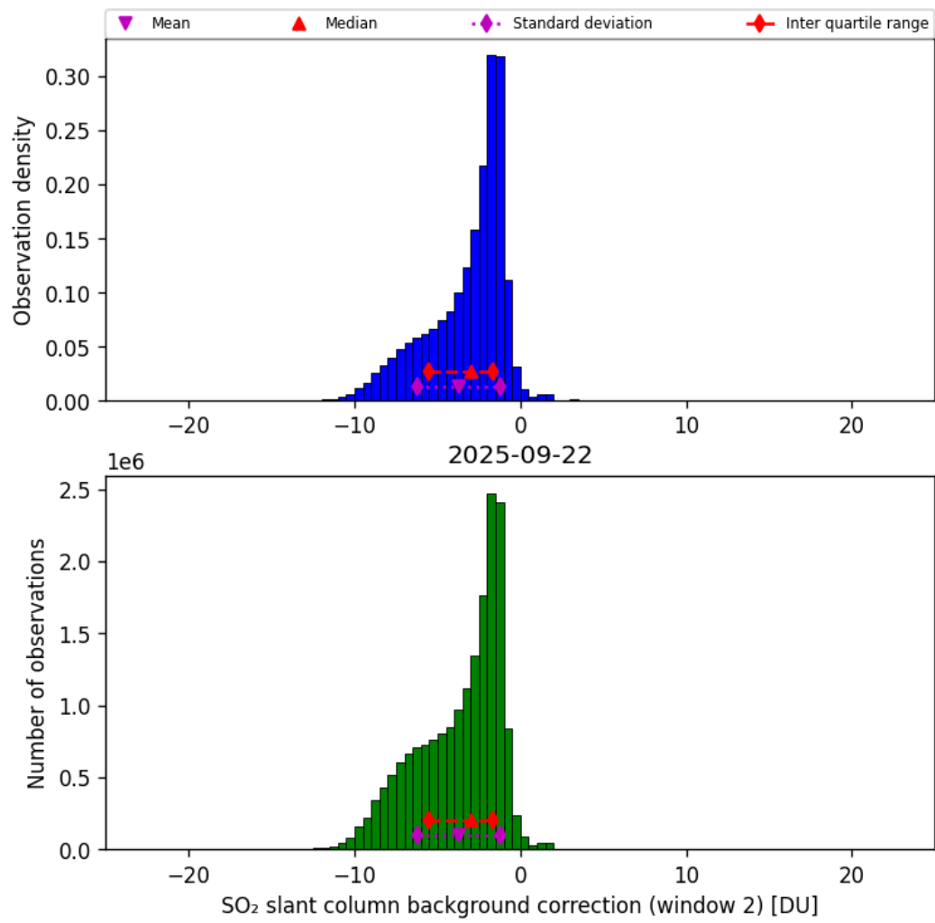
Figure 70: Histogram of “SO 2 slant column background correction (window 2)” for 2025-09-22 to 2025-09-23
