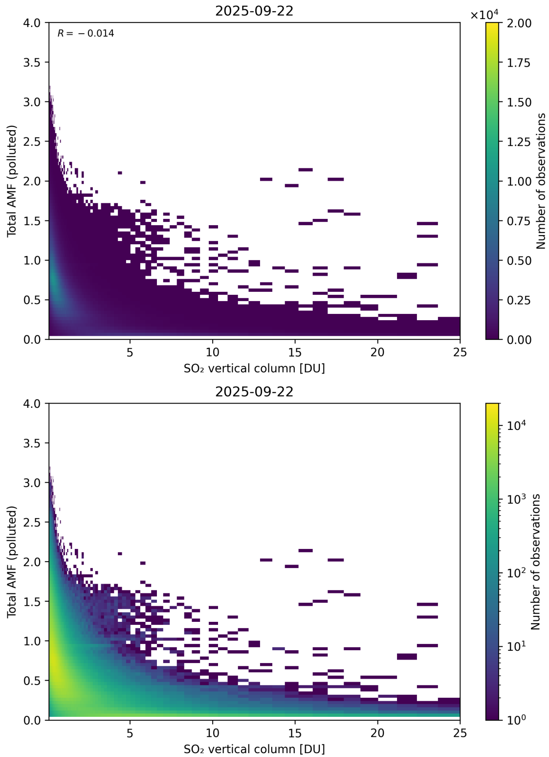
Figure 359: Scatter density plot of “SO 2 vertical column” against “Total AMF (polluted)” for 2025-09-22 to 2025-09-23.
