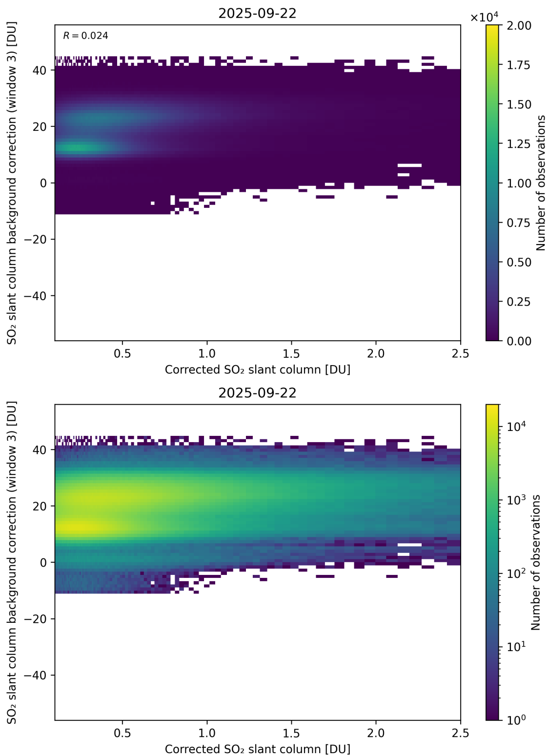
Figure 228: Scatter density plot of “Corrected SO 2 slant column” against “SO 2 slant column background correction (window 3)” for 2025-09-22 to 2025-09-23.
