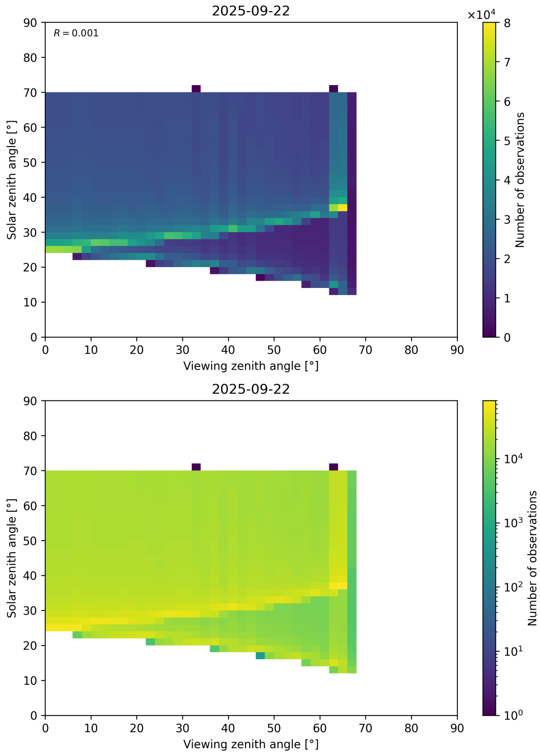
Figure 369: Scatter density plot of “Viewing zenith angle” against “Solar zenith angle” for 2025-09-22 to 2025-09-23.
