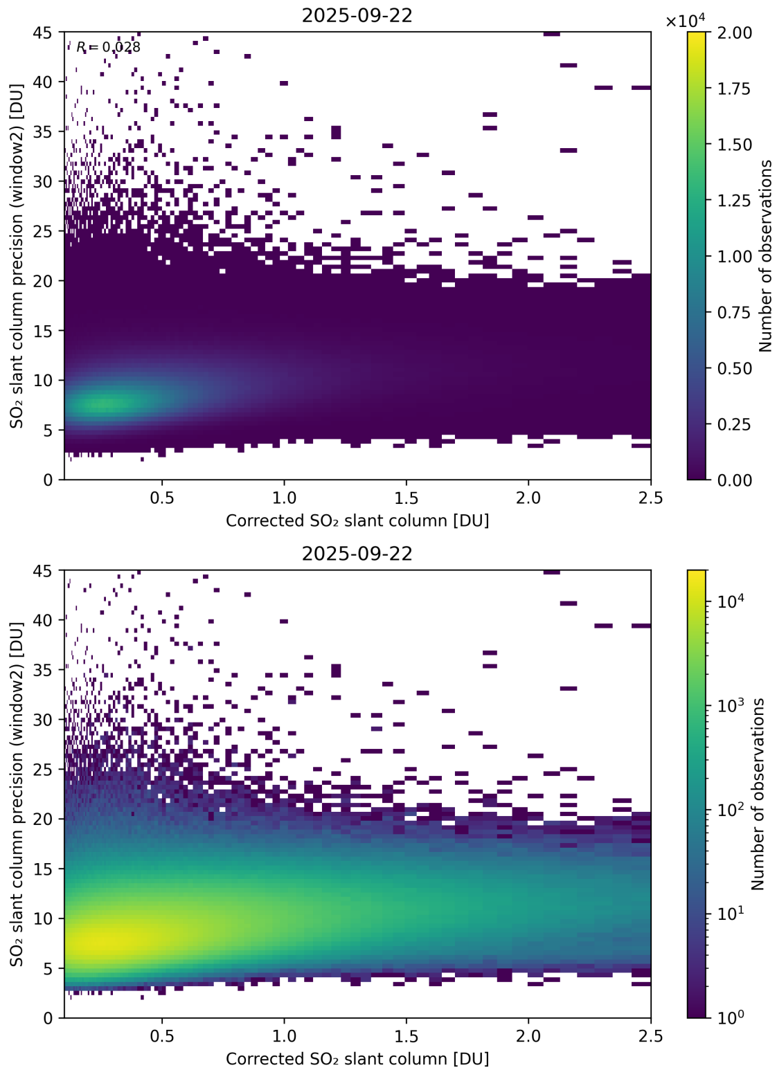
Figure 239: Scatter density plot of “Corrected SO 2 slant column” against “SO 2 slant column precision (window2)” for 2025-09-22 to 2025-09-23.
