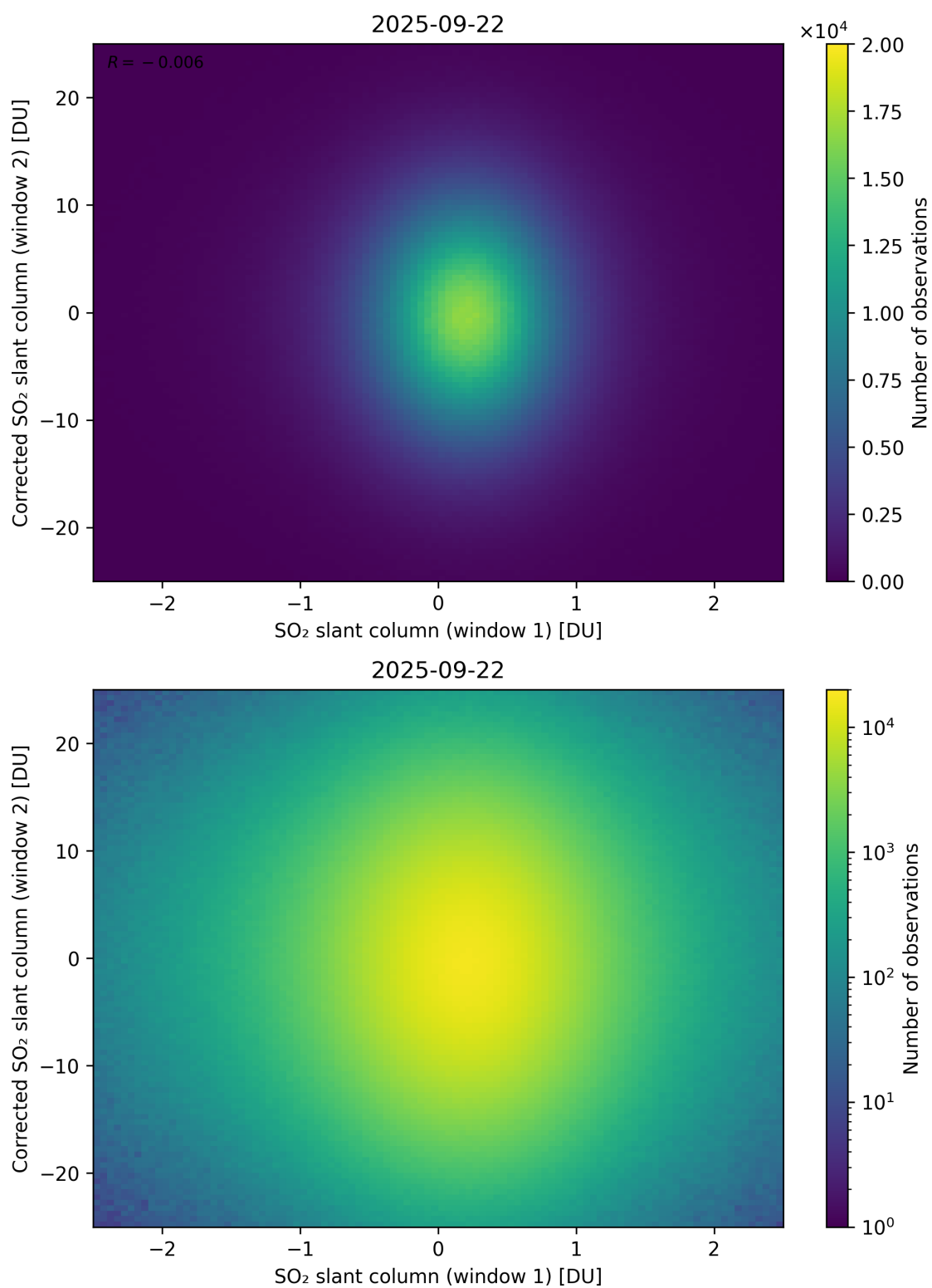
Figure 283: Scatter density plot of “SO 2 slant column (window 1)” against “Corrected SO 2 slant column (window 2)” for 2025-09-22 to 2025-09-23.
