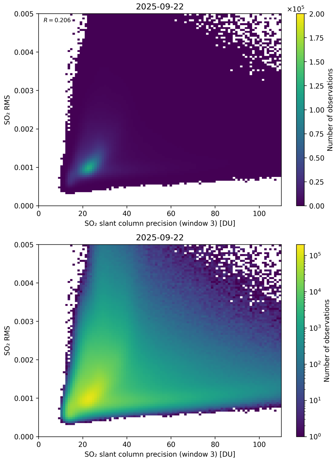
Figure 310: Scatter density plot of “SO 2 slant column precision (window 3)” against “SO 2 RMS” for 2025-09-22 to 2025-09-23.
