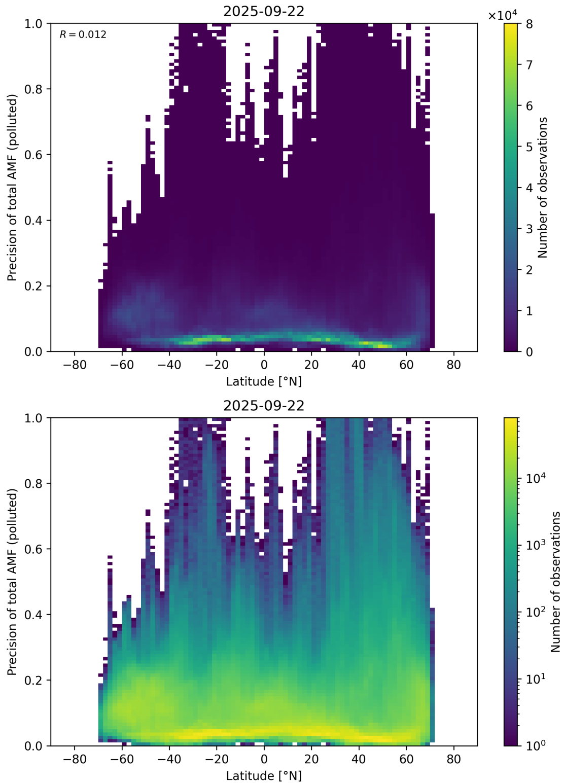
Figure 168: Scatter density plot of “Latitude” against “Precision of total AMF (polluted)” for 2025-09-22 to 2025-09-23.
