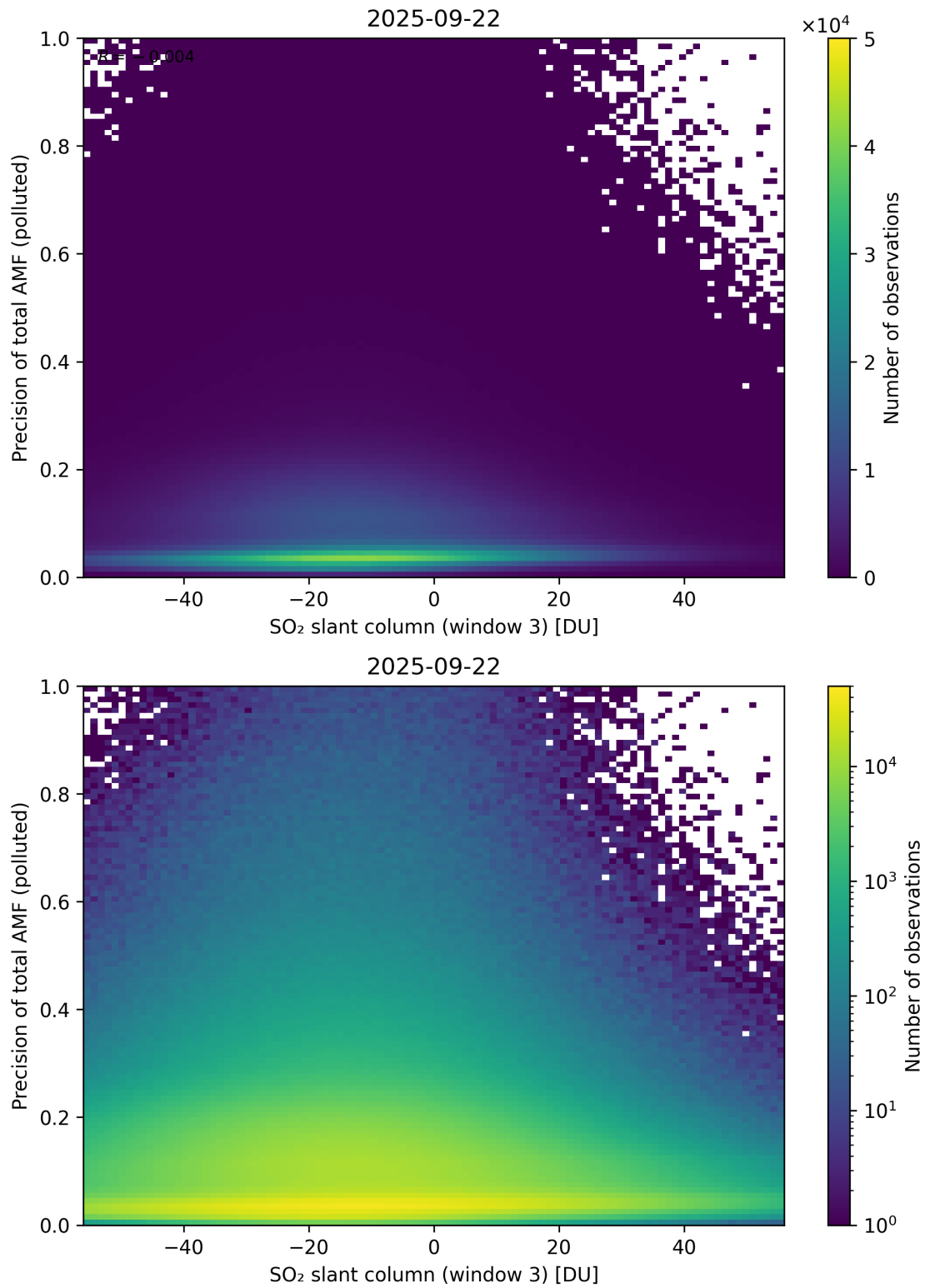
Figure 319: Scatter density plot of “SO 2 slant column (window 3)” against “Precision of total AMF (polluted)” for 2025-09-22 to 2025-09-23.
