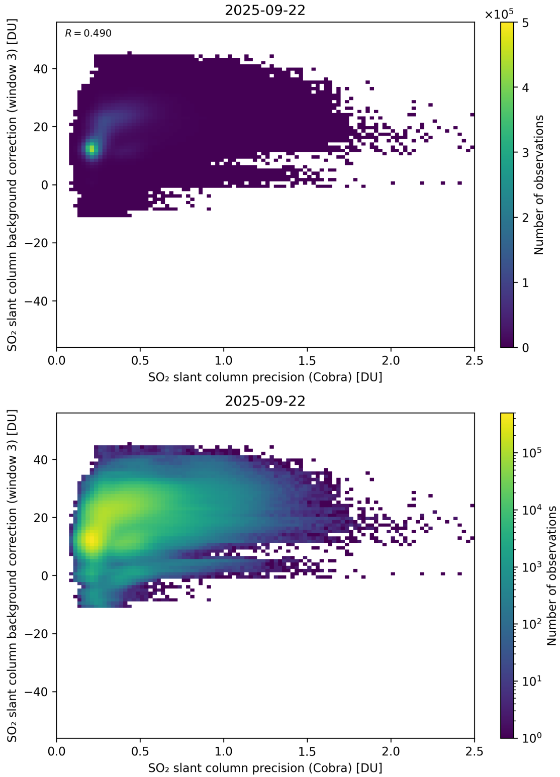
Figure 201: Scatter density plot of “SO 2 slant column precision (Cobra)” against “SO 2 slant column background correction (window 3)” for 2025-09-22 to 2025-09-23.
