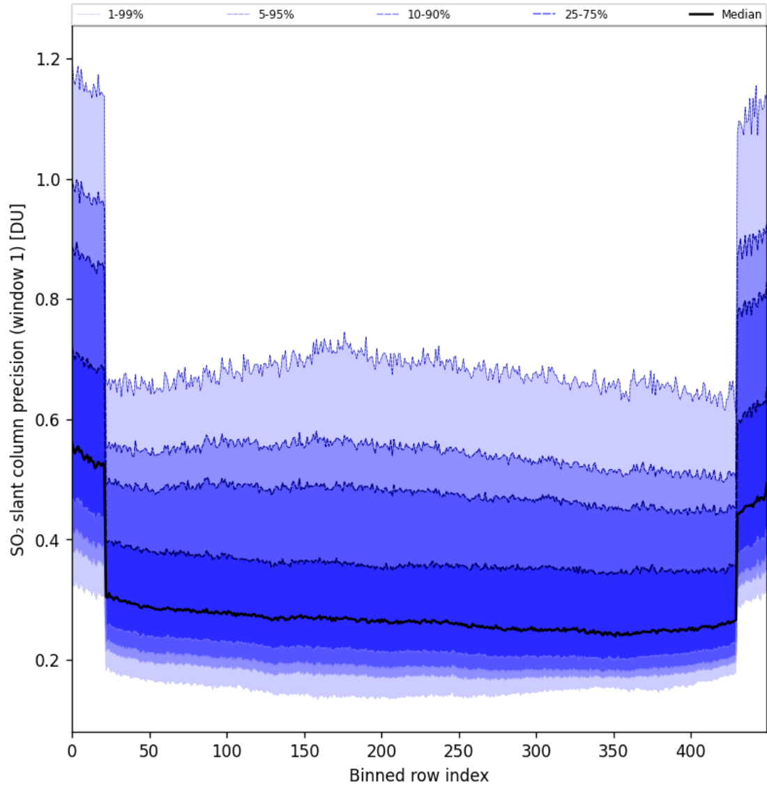
Figure 90: Along track statistics of “SO 2 slant column precision (window 1)” for 2025-09-22 to 2025-09-23
