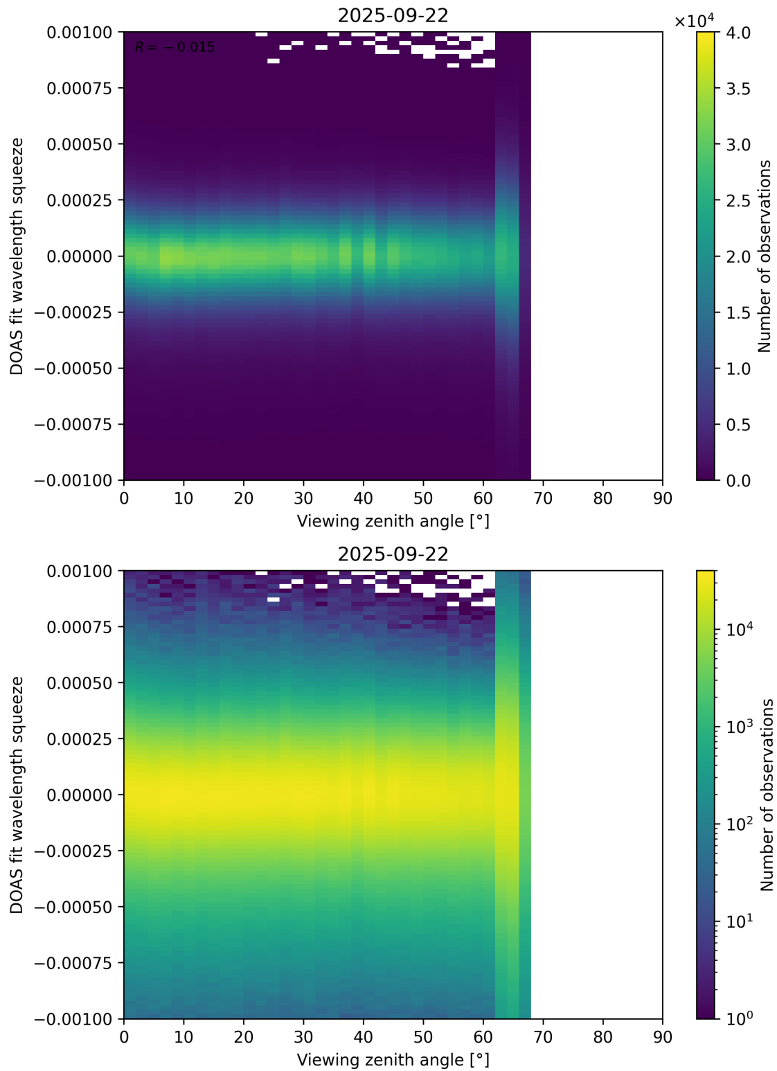
Figure 366: Scatter density plot of “Viewing zenith angle” against “DOAS fit wavelength squeeze” for 2025-09-22 to 2025-09-23.
