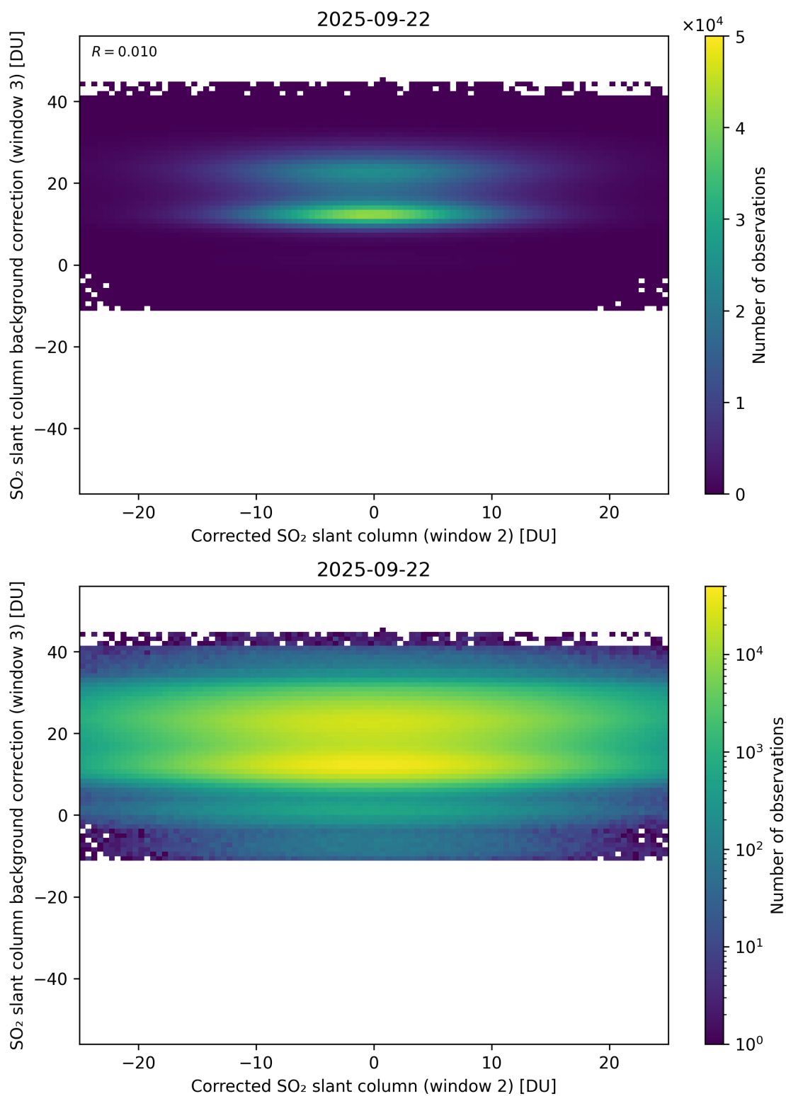
Figure 245: Scatter density plot of “Corrected SO 2 slant column (window 2)” against “SO 2 slant column background correction (window 3)” for 2025-09-22 to 2025-09-23.
