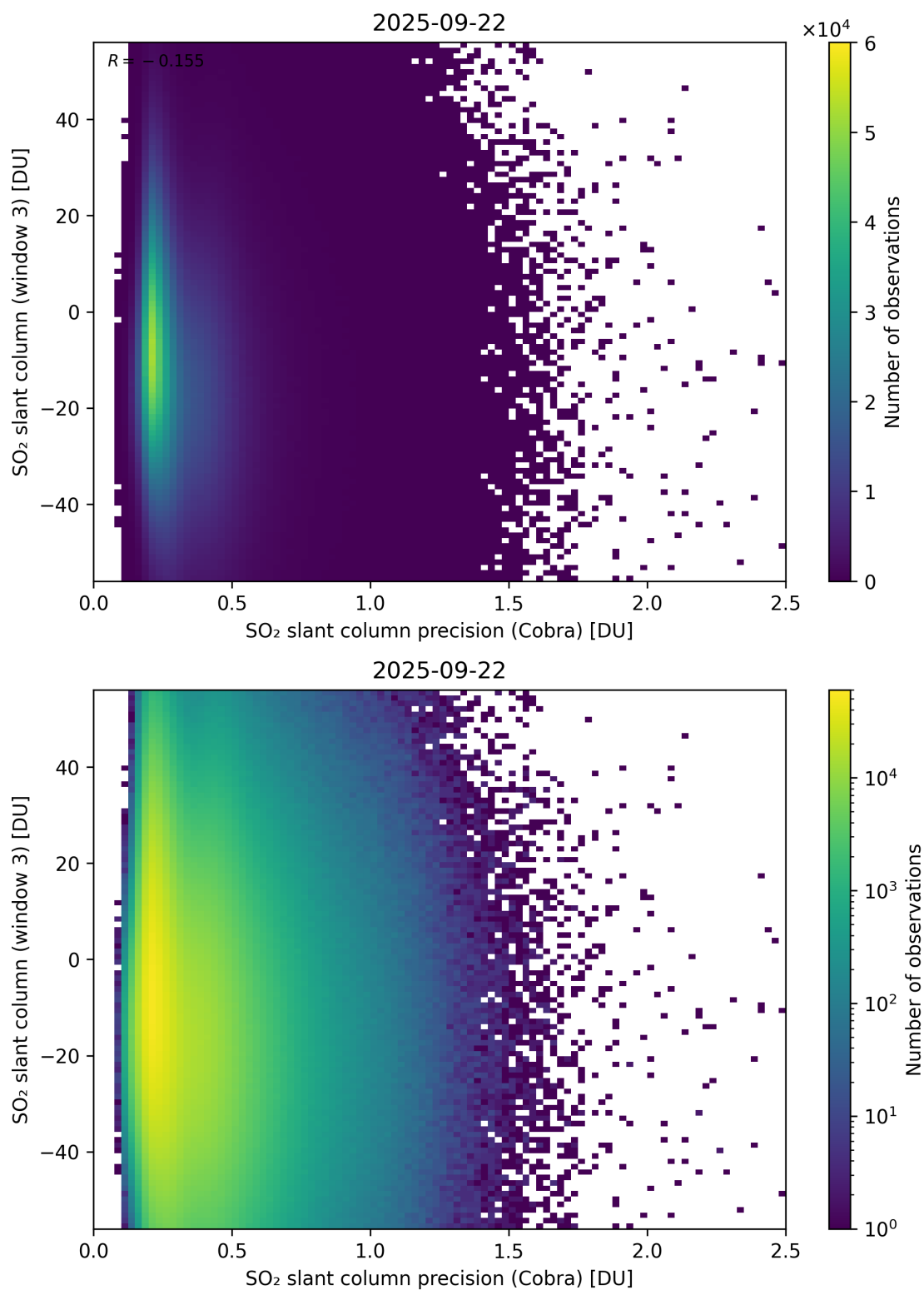
Figure 211: Scatter density plot of “SO 2 slant column precision (Cobra)” against “SO 2 slant column (window 3)” for 2025-09-22 to 2025-09-23.
