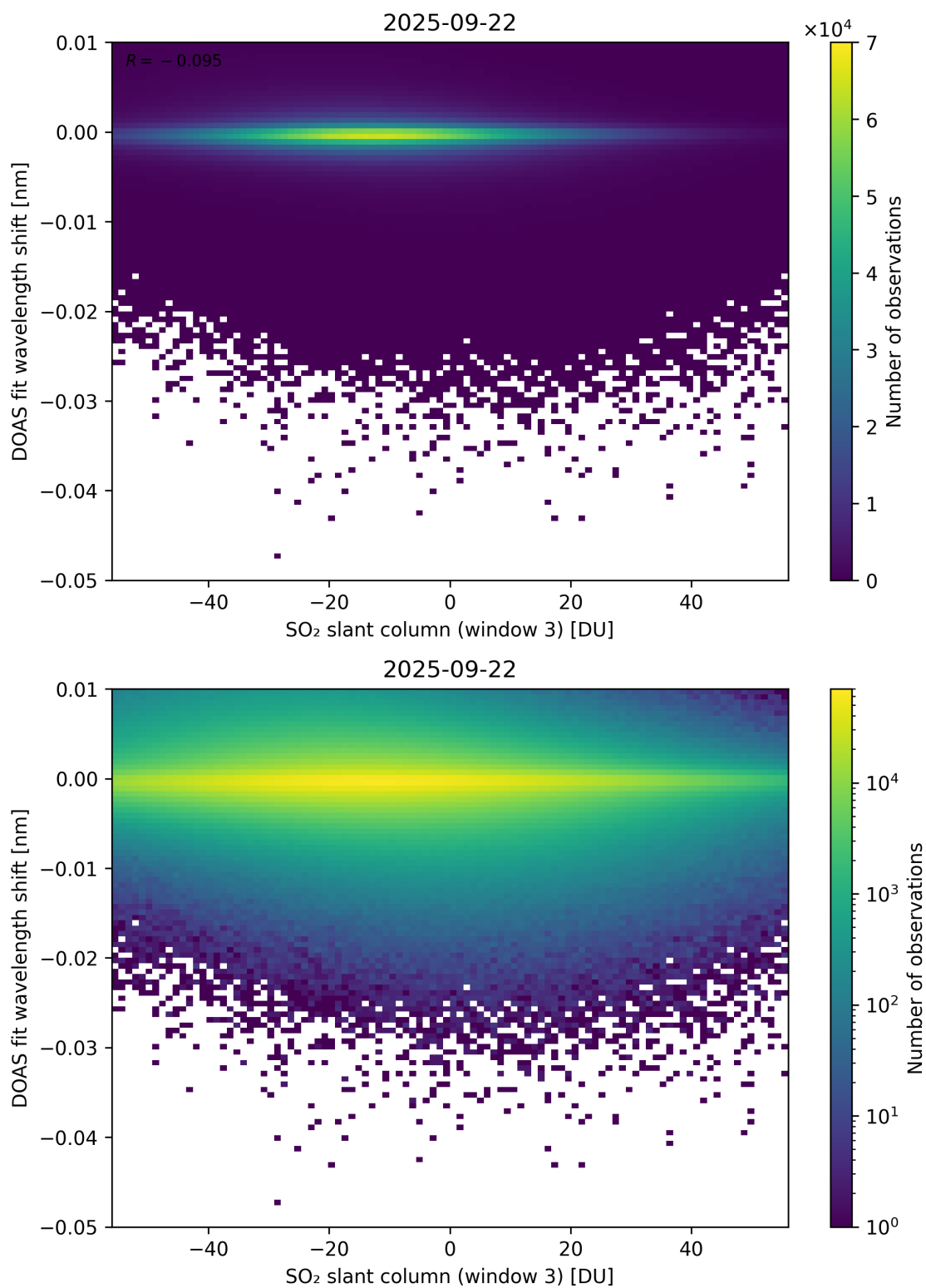
Figure 304: Scatter density plot of “SO 2 slant column (window 3)” against “DOAS fit wavelength shift” for 2025-09-22 to 2025-09-23.
