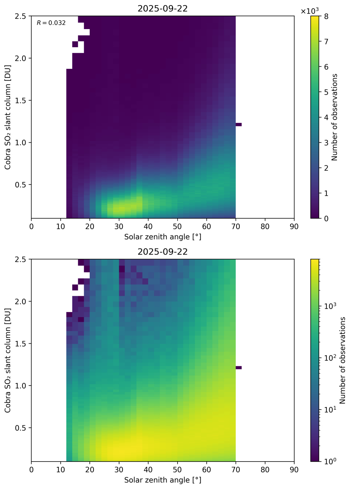
Figure 179: Scatter density plot of “Solar zenith angle” against “Cobra SO 2 slant column” for 2025-09-22 to 2025-09-23.
