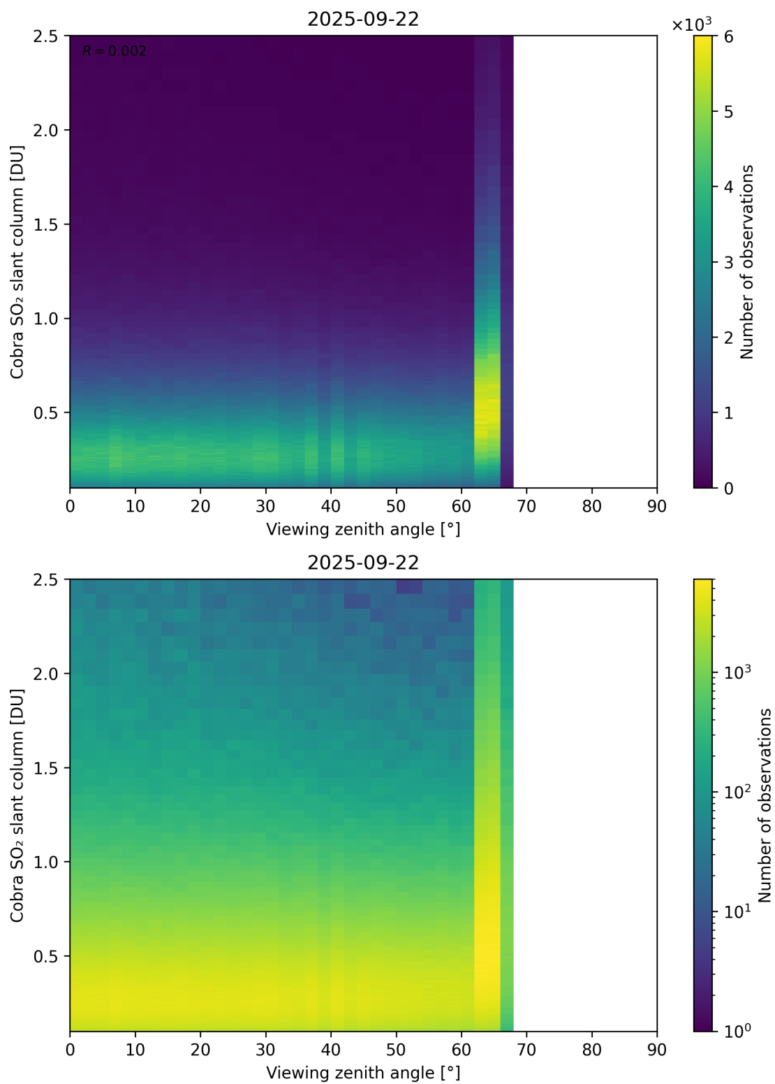
Figure 371: Scatter density plot of “Viewing zenith angle” against “Cobra SO 2 slant column” for 2025-09-22 to 2025-09-23.
