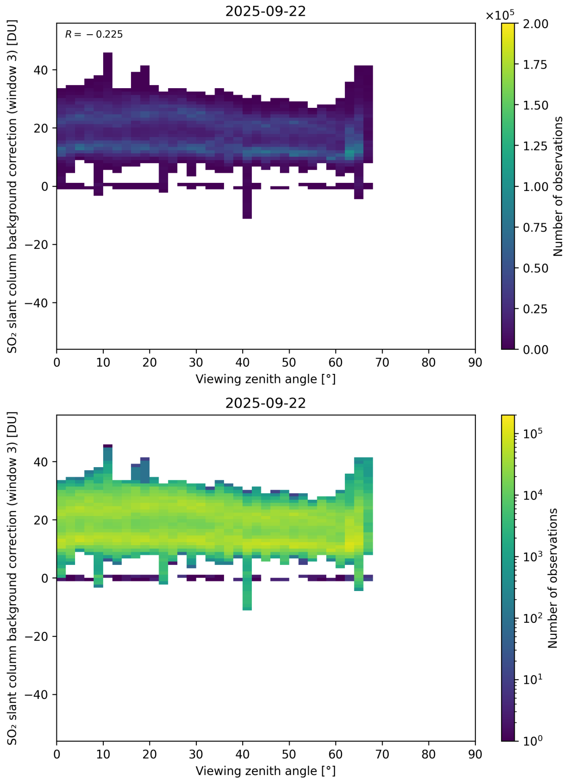
Figure 364: Scatter density plot of “Viewing zenith angle” against “SO 2 slant column background correction (window 3)” for 2025-09-22 to 2025-09-23.
