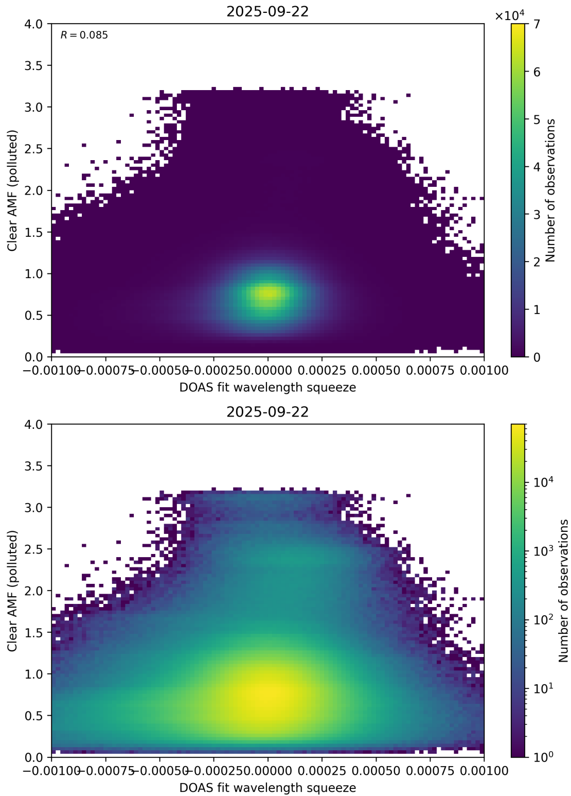
Figure 144: Scatter density plot of “DOAS fit wavelength squeeze” against “Clear AMF (polluted)” for 2025-09-22 to 2025-09-23.
