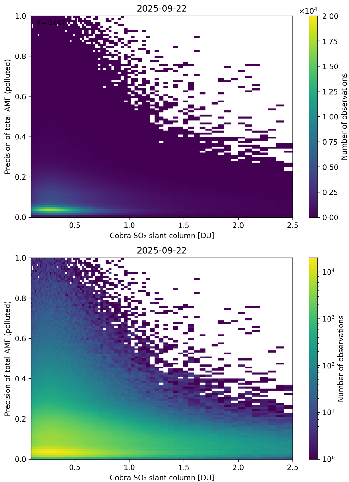
Figure 225: Scatter density plot of “Cobra SO 2 slant column” against “Precision of total AMF (polluted)” for 2025-09-22 to 2025-09-23.
