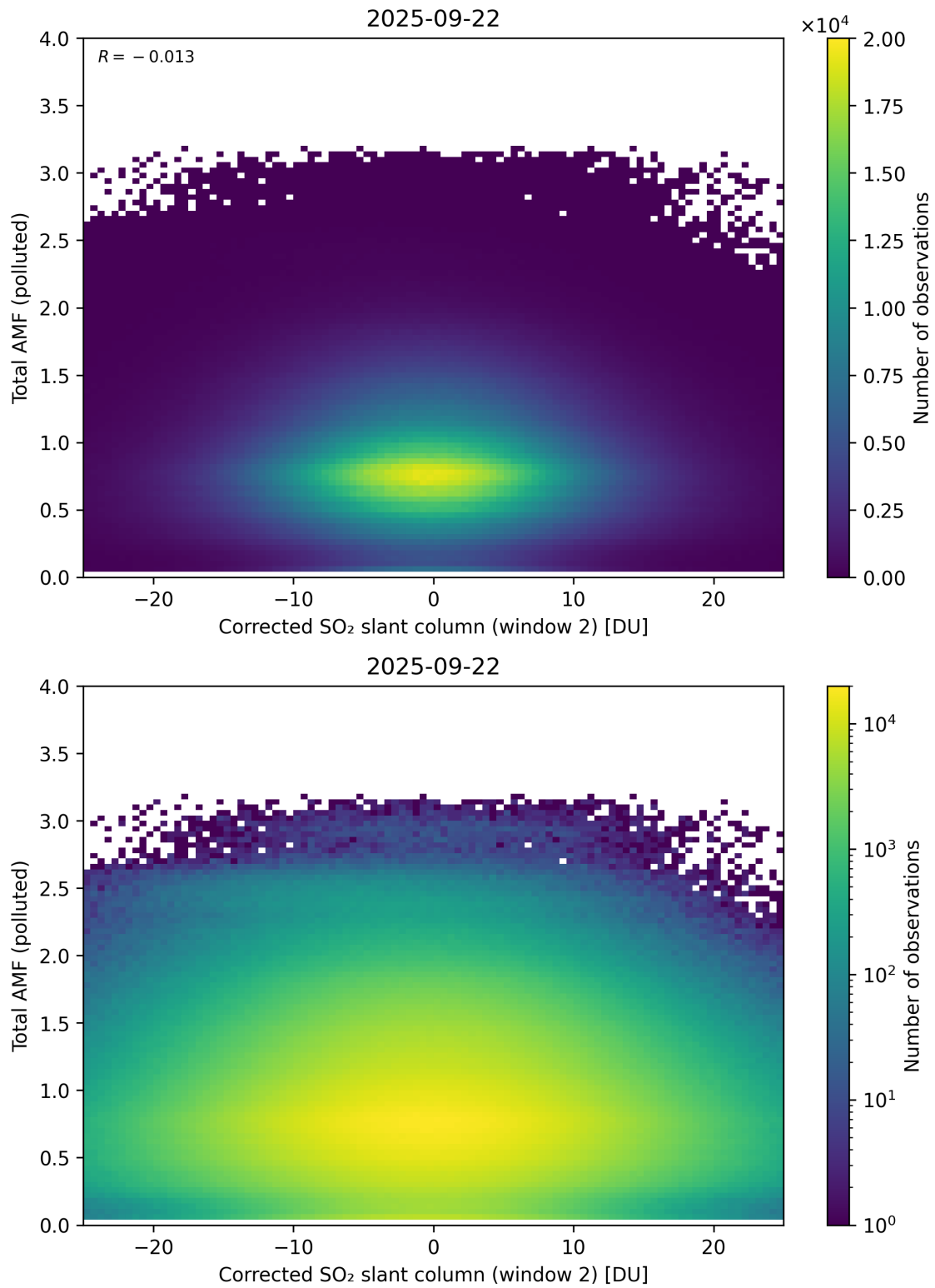
Figure 253: Scatter density plot of “Corrected SO 2 slant column (window 2)” against “Total AMF (polluted)” for 2025-09-22 to 2025-09-23.
