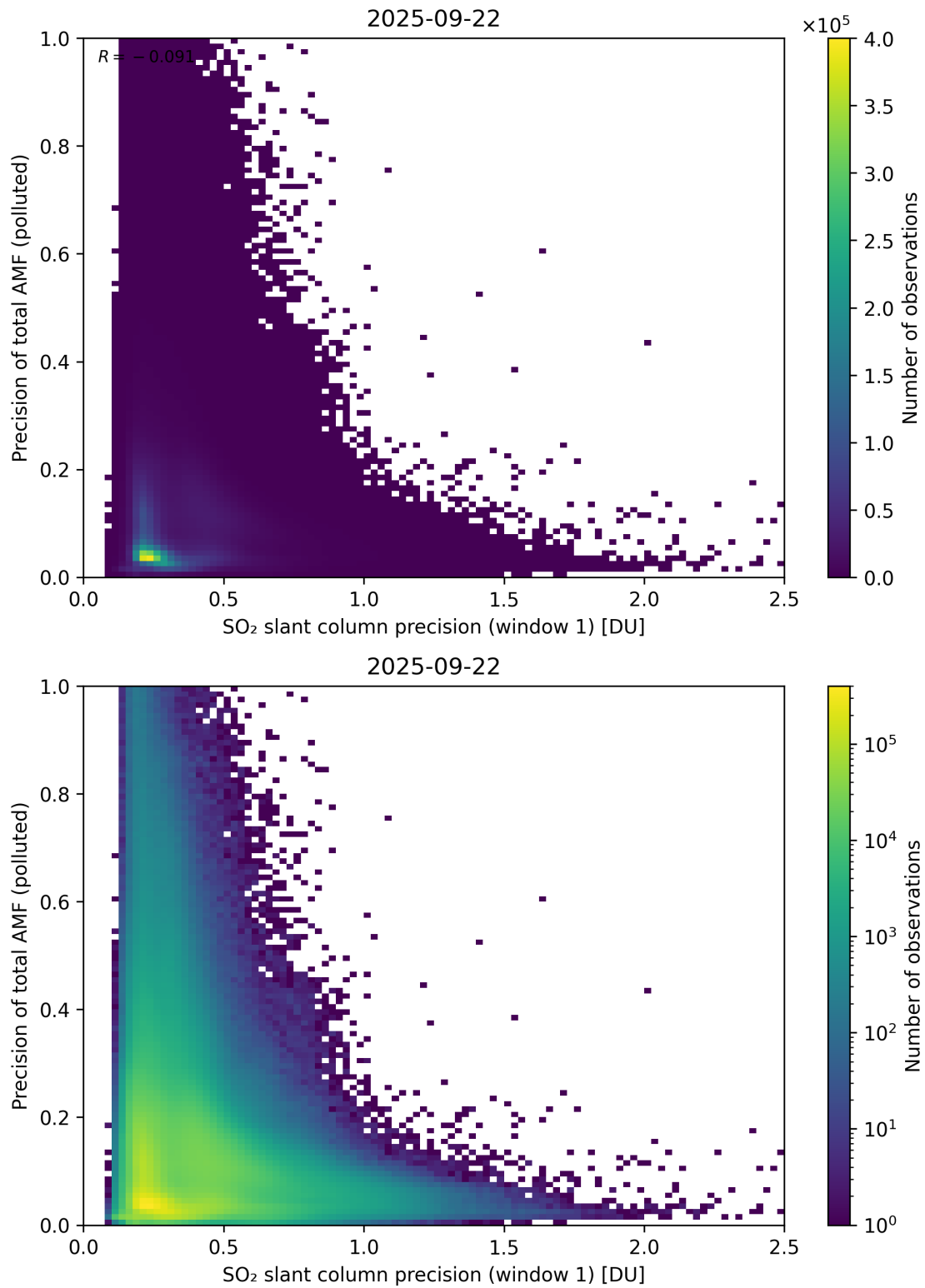
Figure 281: Scatter density plot of “SO 2 slant column precision (window 1)” against “Precision of total AMF (polluted)” for 2025-09-22 to 2025-09-23.
