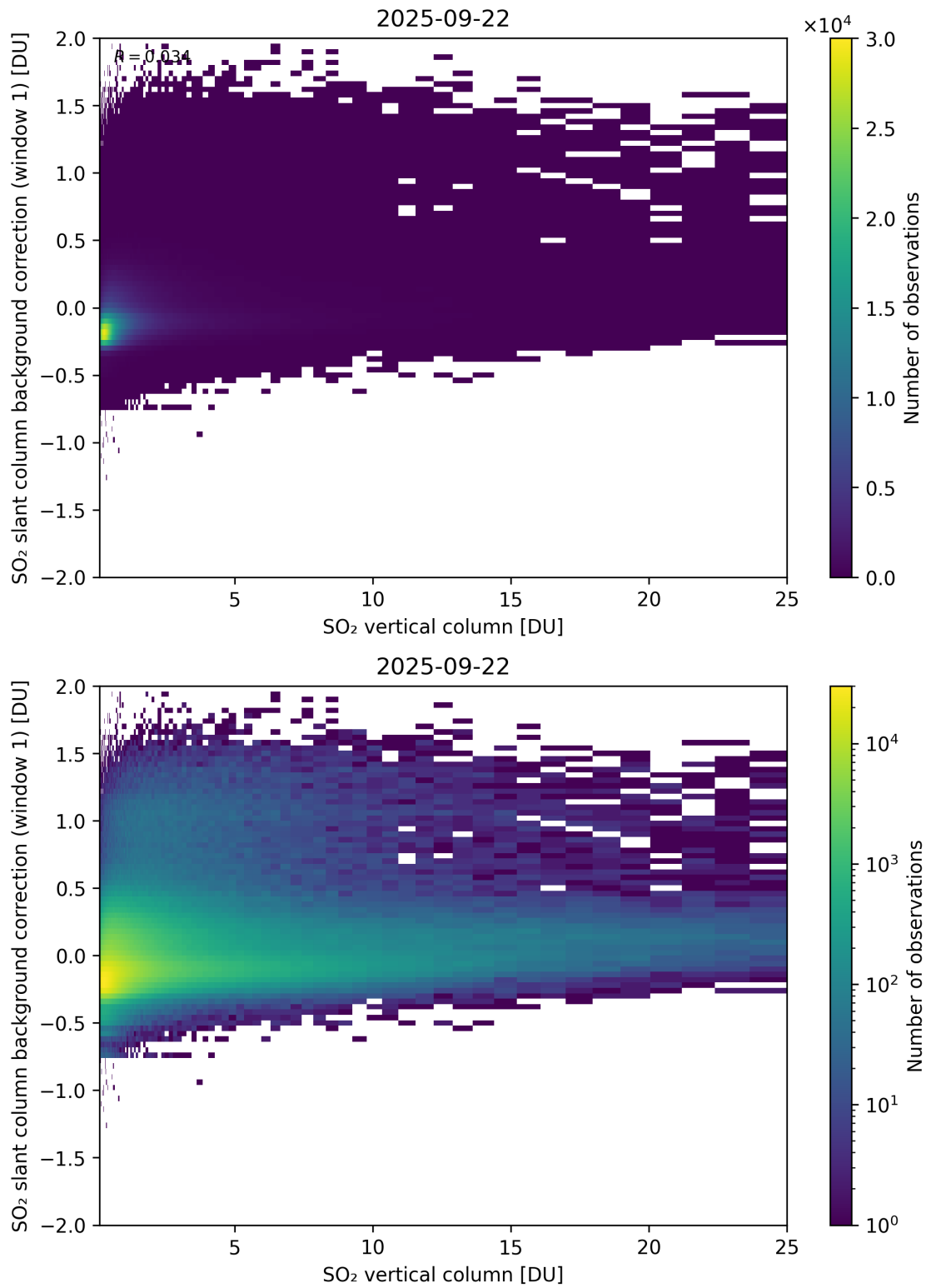
Figure 323: Scatter density plot of “SO 2 vertical column” against “SO 2 slant column background correction (window 1)” for 2025-09-22 to 2025-09-23.
