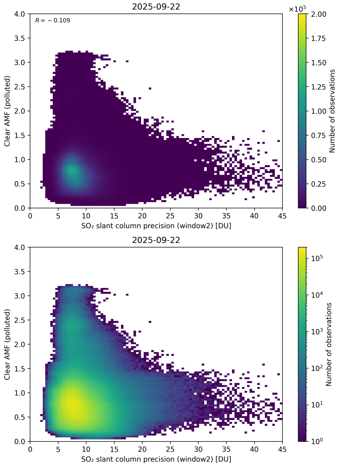
Figure 296: Scatter density plot of “SO 2 slant column precision (window2)” against “Clear AMF (polluted)” for 2025-09-22 to 2025-09-23.
