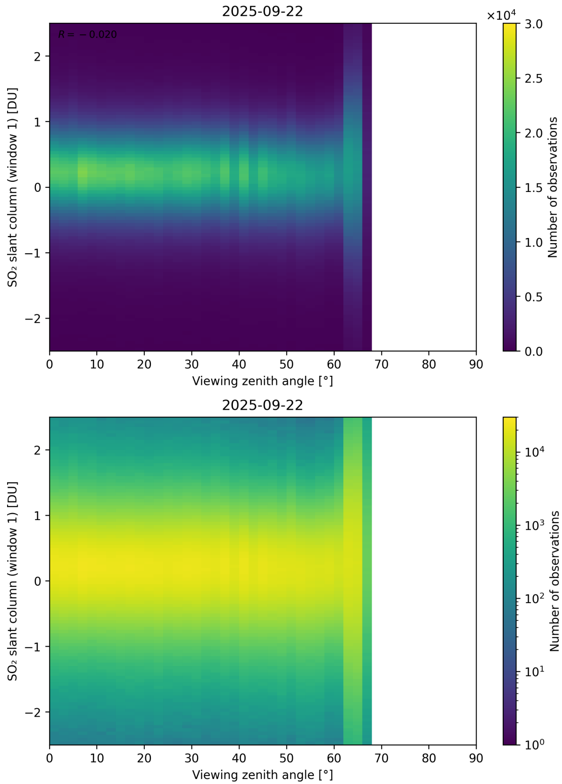
Figure 376: Scatter density plot of “Viewing zenith angle” against “SO 2 slant column (window 1)” for 2025-09-22 to 2025-09-23.
