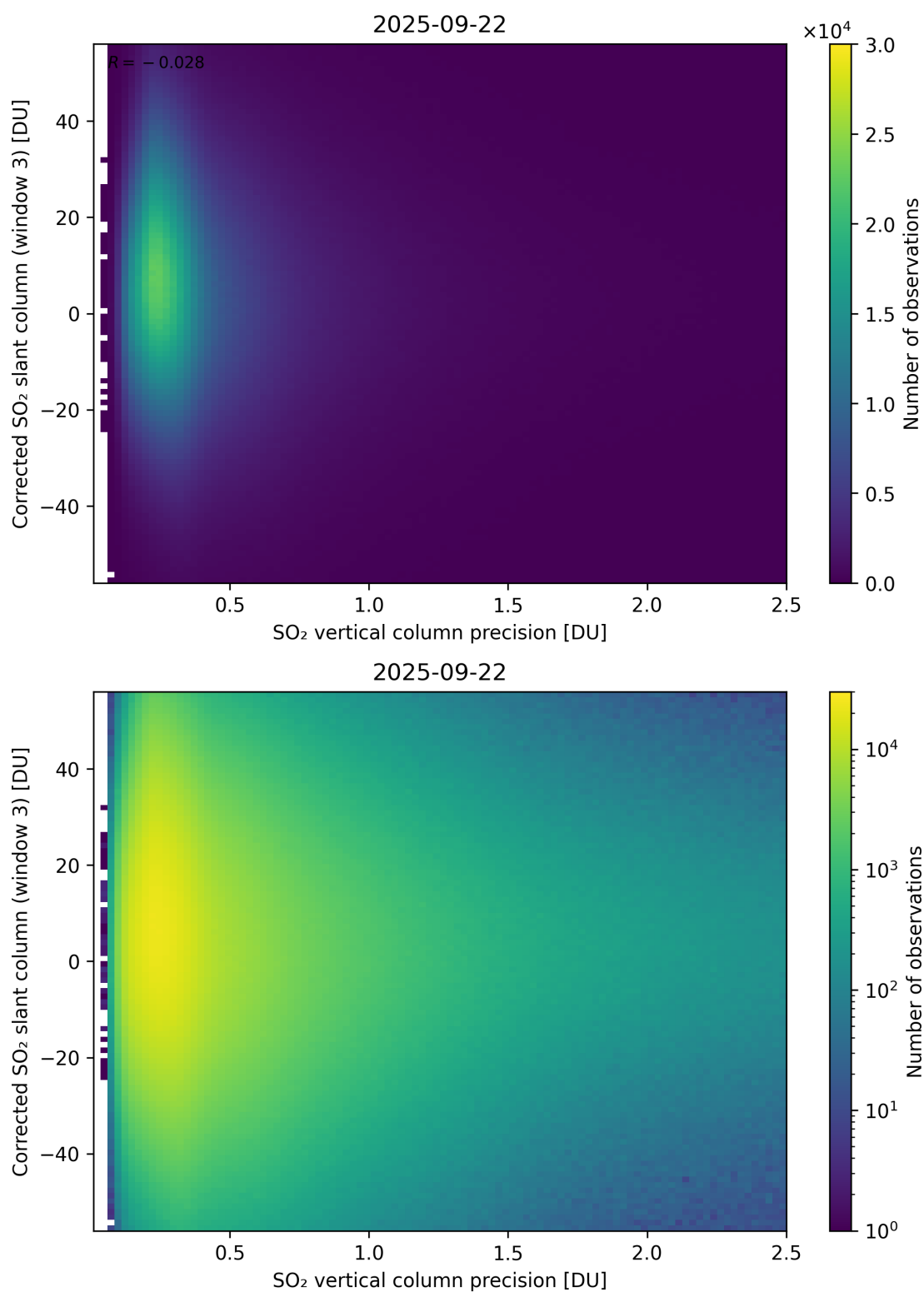
Figure 340: Scatter density plot of “SO 2 vertical column precision” against “Corrected SO 2 slant column (window 3)” for 2025-09-22 to 2025-09-23.
