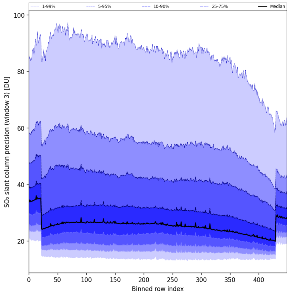
Figure 98: Along track statistics of “SO 2 slant column precision (window 3)” for 2025-09-22 to 2025-09-23
