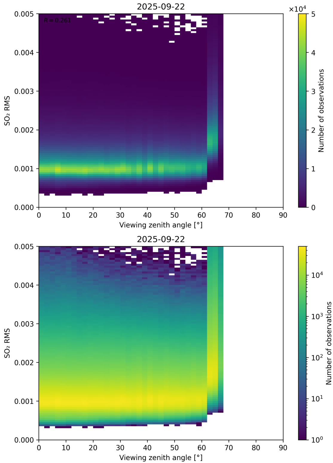
Figure 367: Scatter density plot of “Viewing zenith angle” against “SO 2 RMS” for 2025-09-22 to 2025-09-23.
