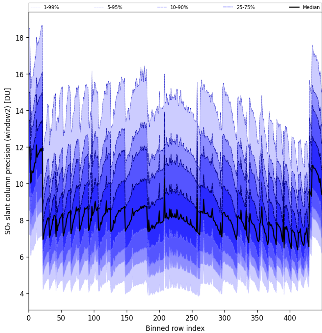
Figure 94: Along track statistics of “SO 2 slant column precision (window2)” for 2025-09-22 to 2025-09-23
