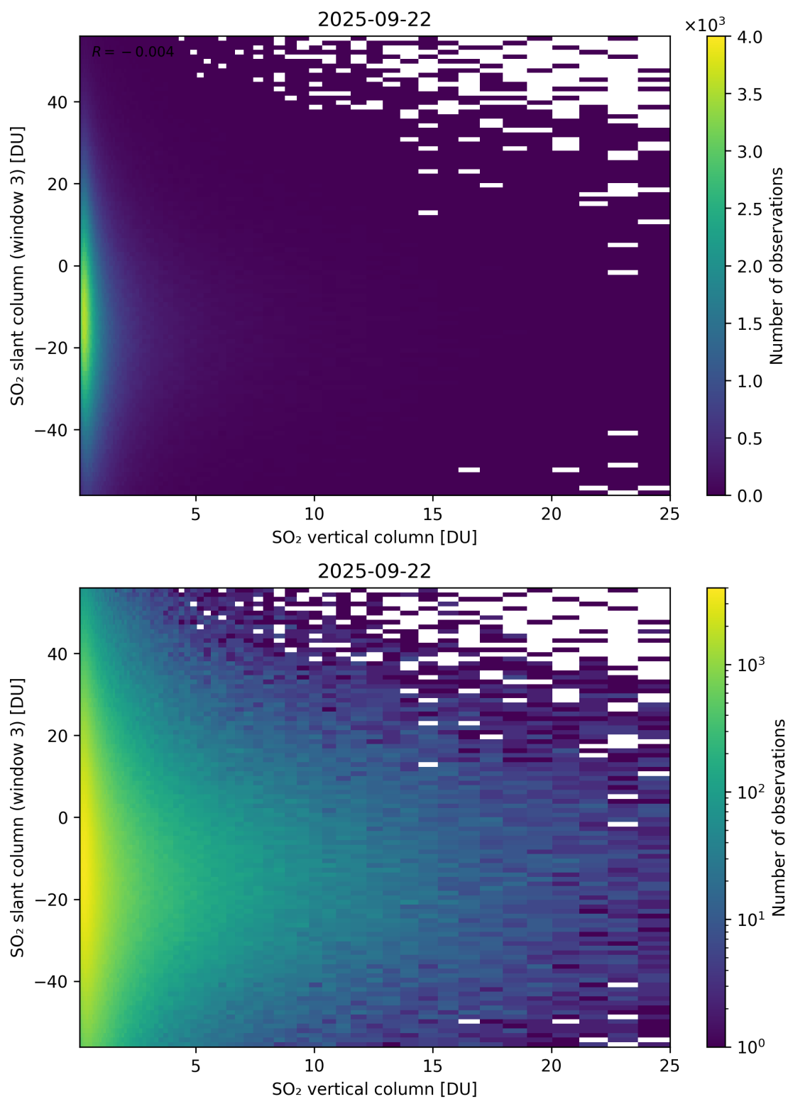
Figure 357: Scatter density plot of “SO 2 vertical column” against “SO 2 slant column (window 3)” for 2025-09-22 to 2025-09-23.
