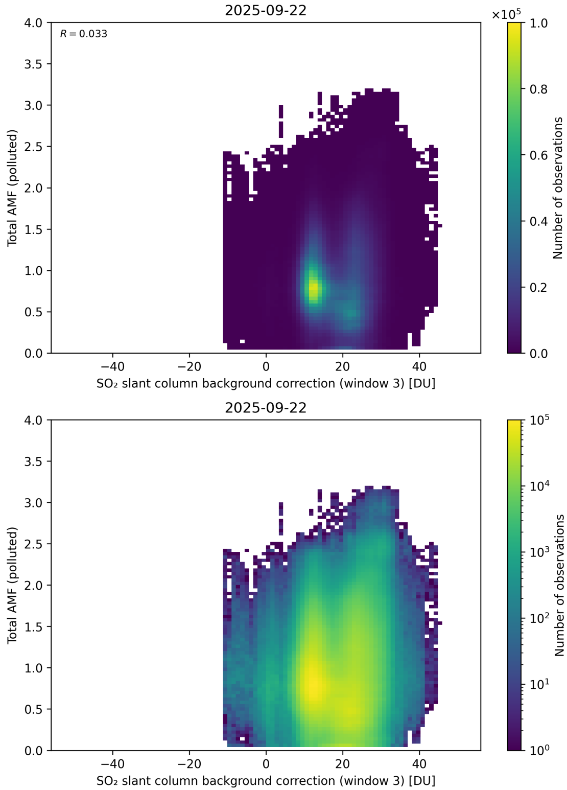
Figure 136: Scatter density plot of “SO 2 slant column background correction (window 3)” against “Total AMF (polluted)” for 2025-09-22 to 2025-09-23.
