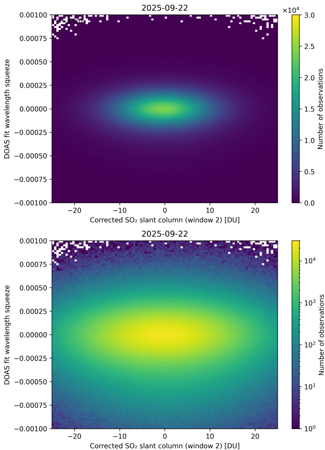
Figure 247: Scatter density plot of “Corrected SO 2 slant column (window 2)” against “DOAS fit wavelength squeeze” for 2025-09-22 to 2025-09-23.
