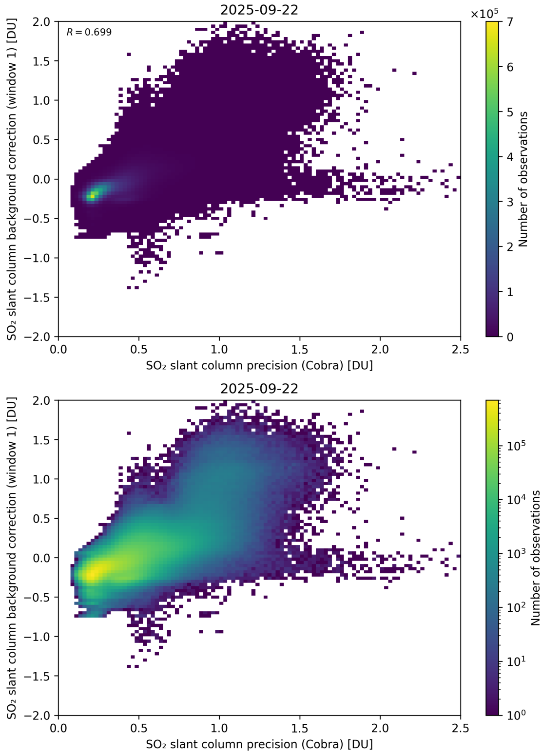
Figure 199: Scatter density plot of “SO 2 slant column precision (Cobra)” against “SO 2 slant column background correction (window 1)” for 2025-09-22 to 2025-09-23.
