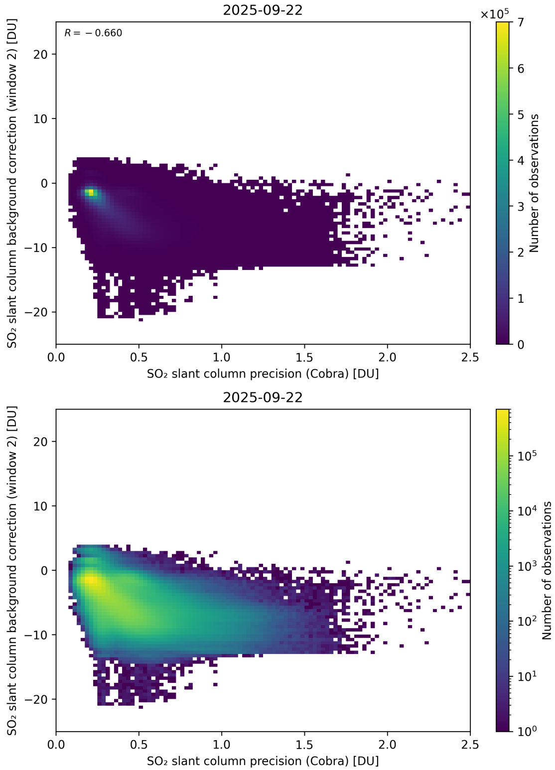
Figure 200: Scatter density plot of “SO 2 slant column precision (Cobra)” against “SO 2 slant column background correction (window 2)” for 2025-09-22 to 2025-09-23.
