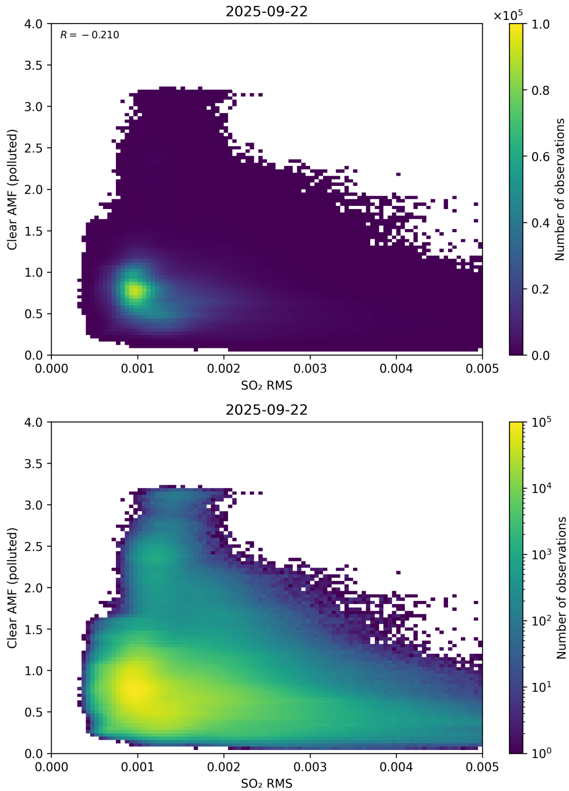
Figure 147: Scatter density plot of “SO 2 RMS” against “Clear AMF (polluted)” for 2025-09-22 to 2025-09-23.
