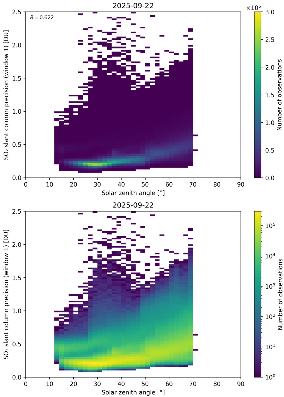
Figure 185: Scatter density plot of “Solar zenith angle” against “SO 2 slant column precision (window 1)” for 2025-09-22 to 2025-09-23.
