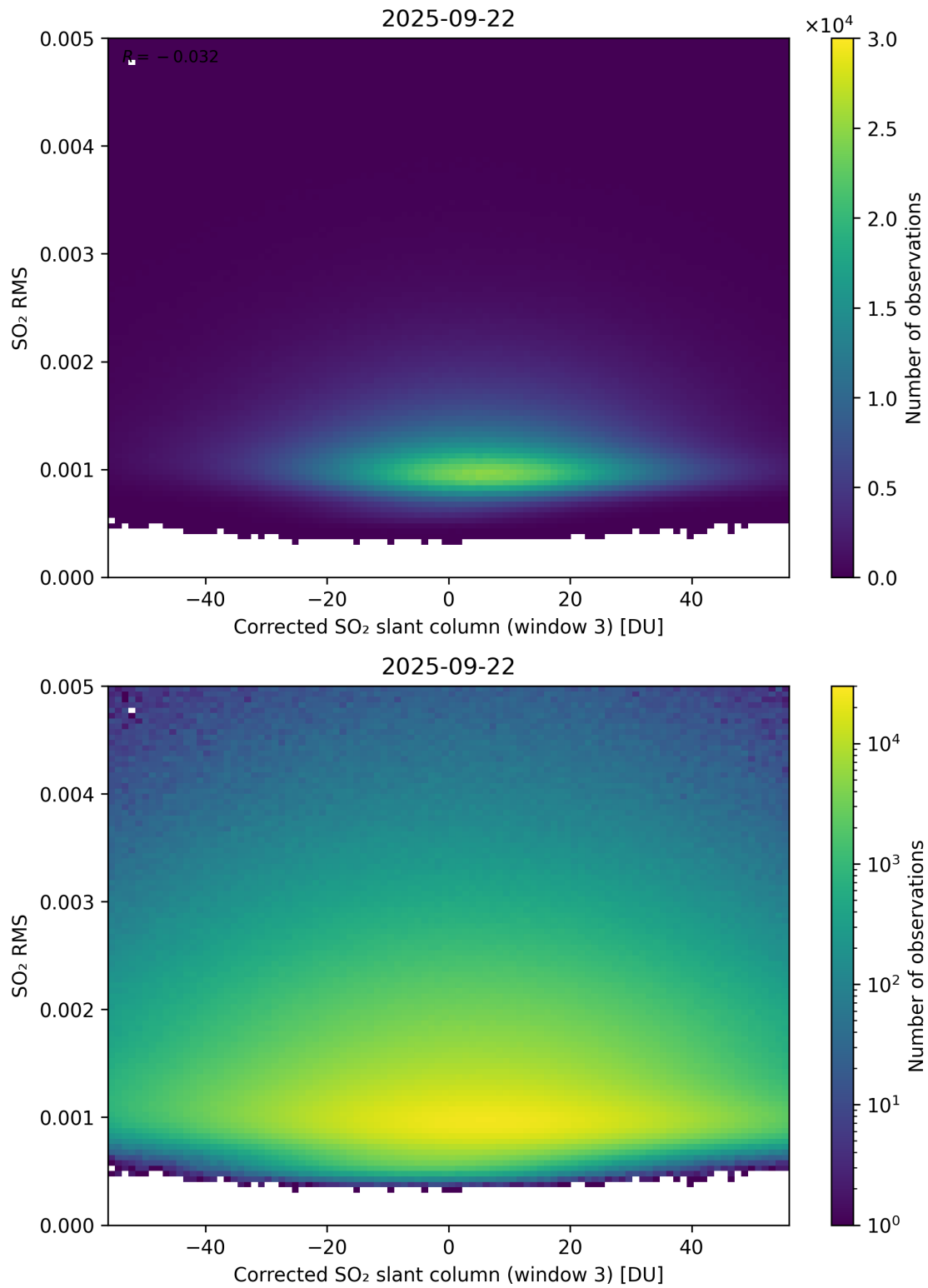
Figure 258: Scatter density plot of “Corrected SO 2 slant column (window 3)” against “SO 2 RMS” for 2025-09-22 to 2025-09-23.
