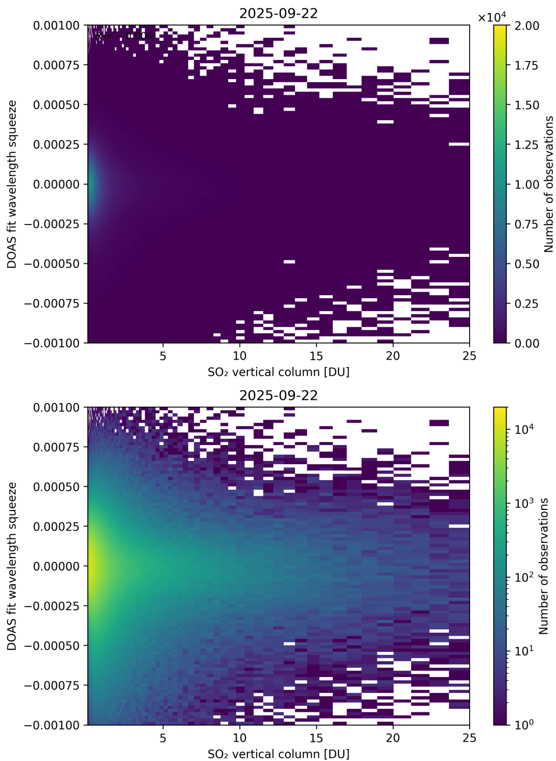
Figure 327: Scatter density plot of “SO 2 vertical column” against “DOAS fit wavelength squeeze” for 2025-09-22 to 2025-09-23.
