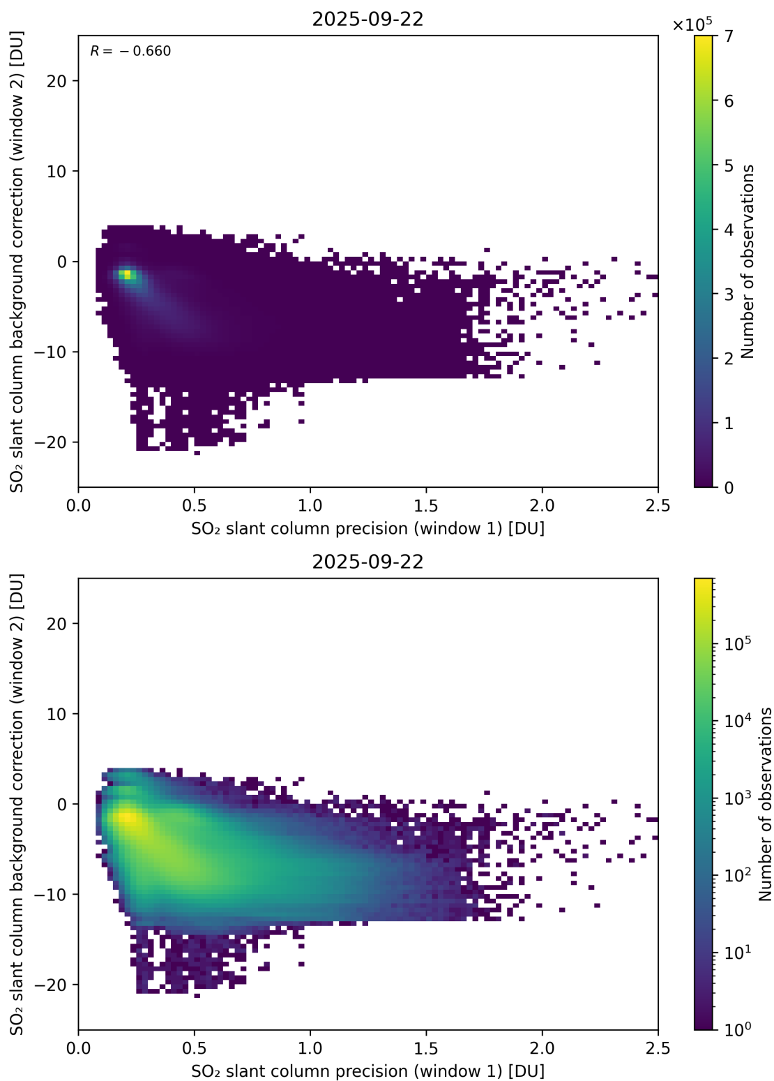
Figure 269: Scatter density plot of “SO 2 slant column precision (window 1)” against “SO 2 slant column background correction (window 2)” for 2025-09-22 to 2025-09-23.
