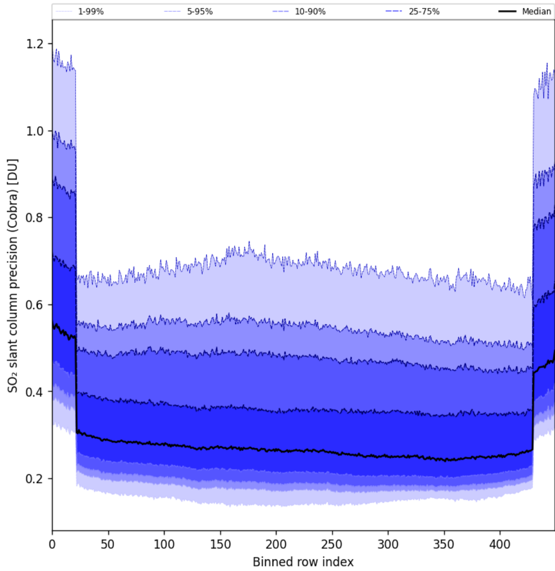
Figure 88: Along track statistics of “SO 2 slant column precision (Cobra)” for 2025-09-22 to 2025-09-23
