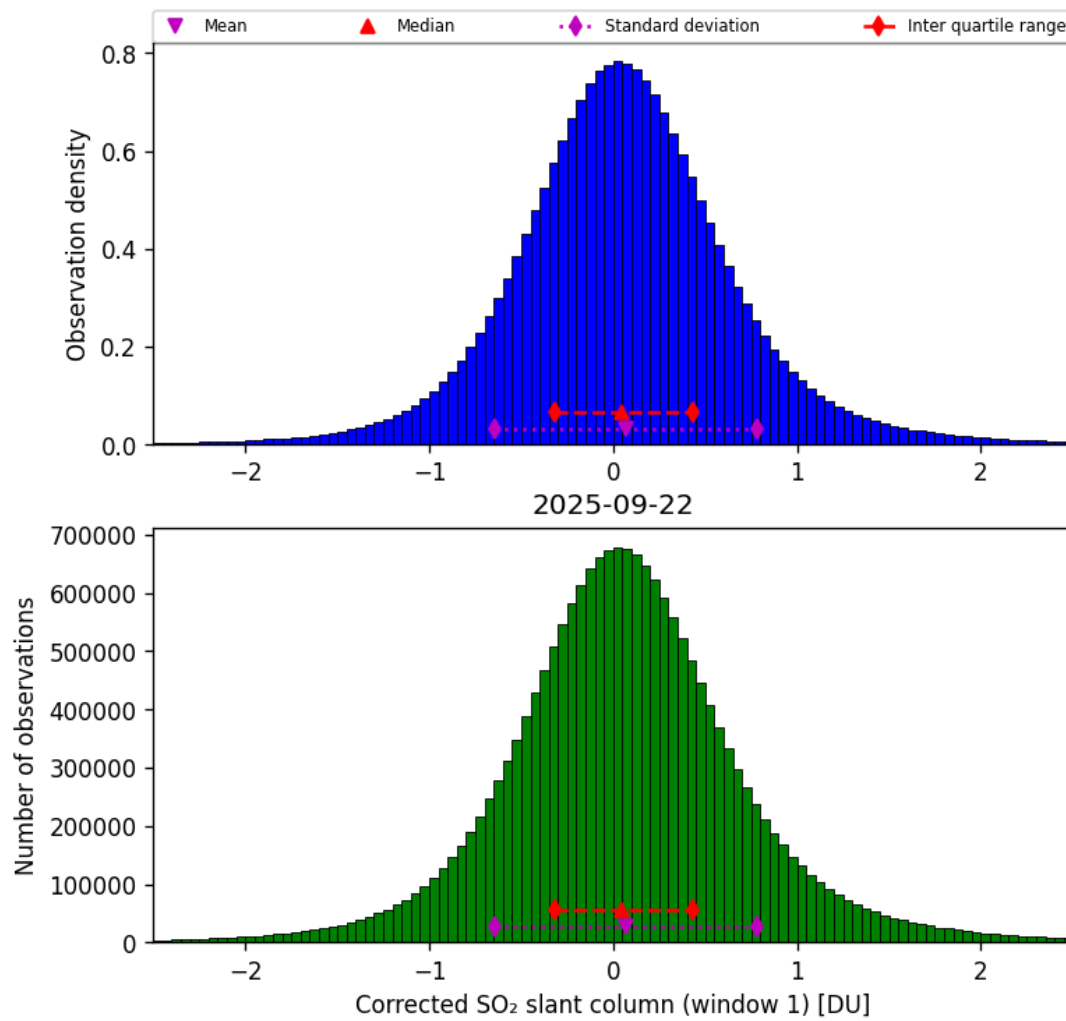
Figure 65: Histogram of “Corrected SO 2 slant column (window 1)” for 2025-09-22 to 2025-09-23
