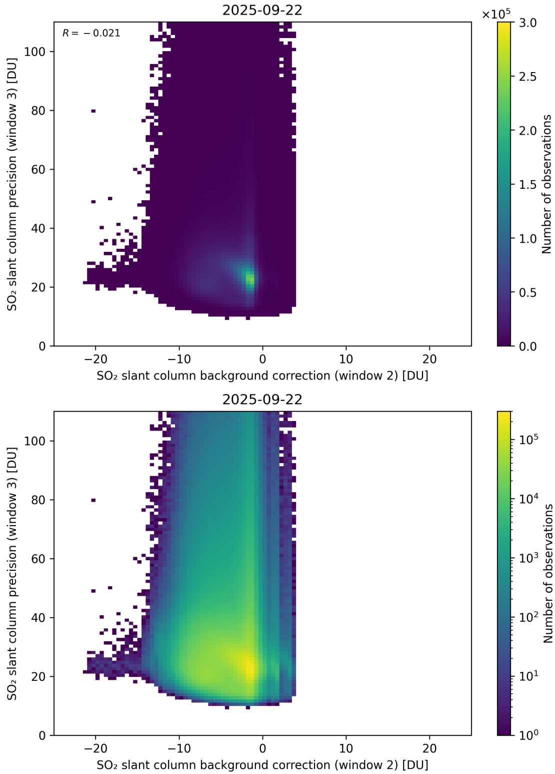
Figure 129: Scatter density plot of “SO 2 slant column background correction (window 2)” against “SO 2 slant column precision (window 3)” for 2025-09-22 to 2025-09-23.
