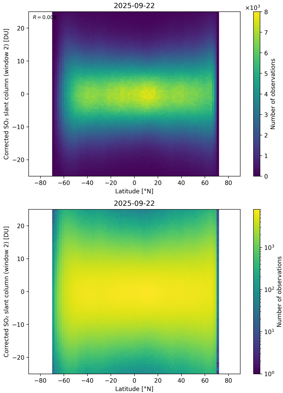
Figure 160: Scatter density plot of “Latitude” against “Corrected SO 2 slant column (window 2)” for 2025-09-22 to 2025-09-23.
