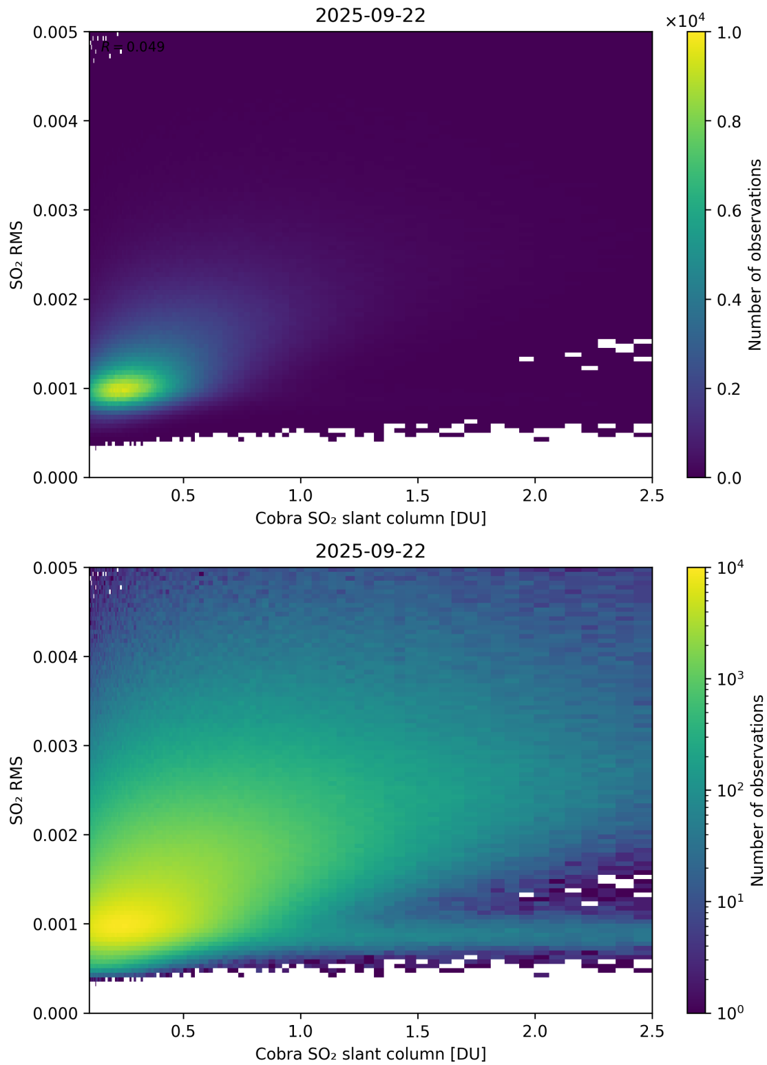
Figure 198: Scatter density plot of “Cobra SO 2 slant column” against “SO 2 RMS” for 2025-09-22 to 2025-09-23.
