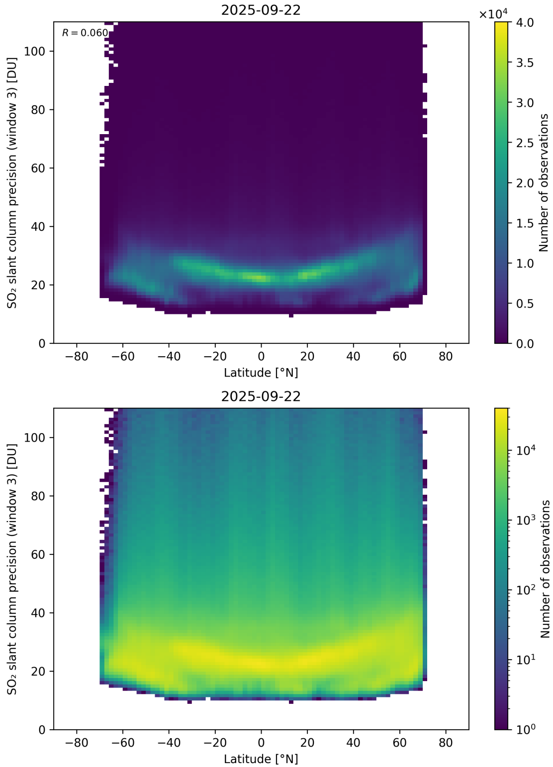
Figure 166: Scatter density plot of “Latitude” against “SO 2 slant column precision (window 3)” for 2025-09-22 to 2025-09-23.
