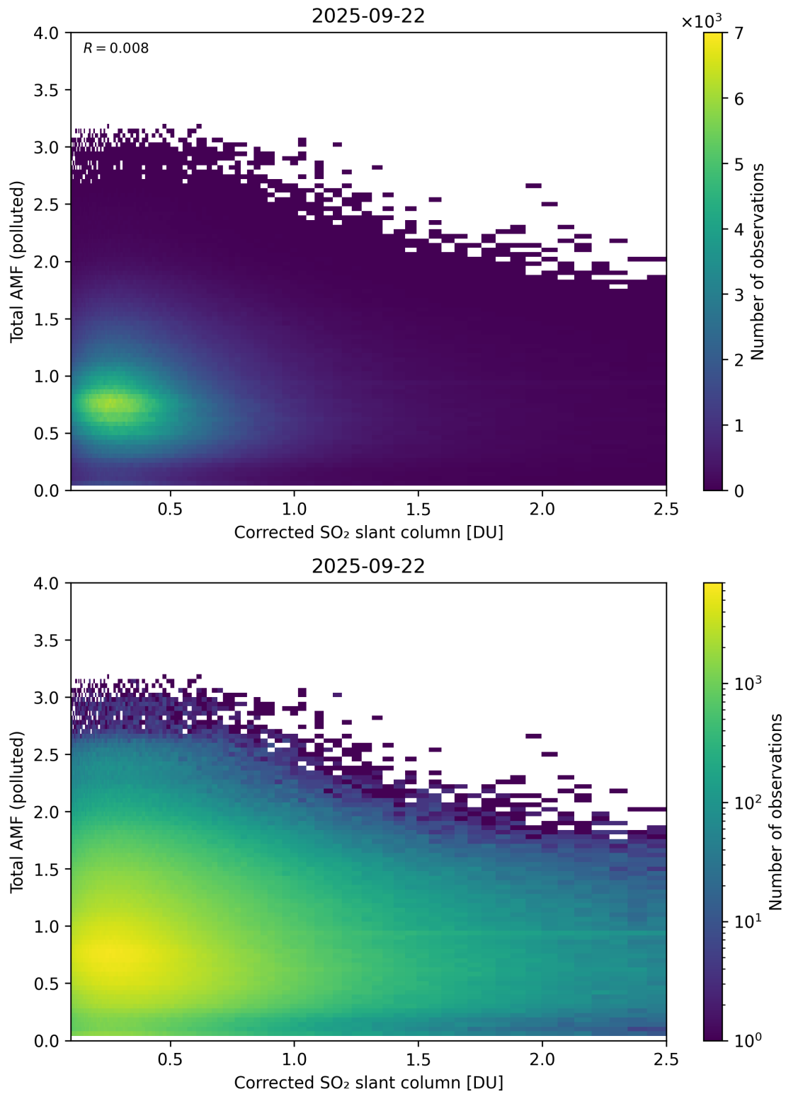
Figure 242: Scatter density plot of “Corrected SO 2 slant column” against “Total AMF (polluted)” for 2025-09-22 to 2025-09-23.
