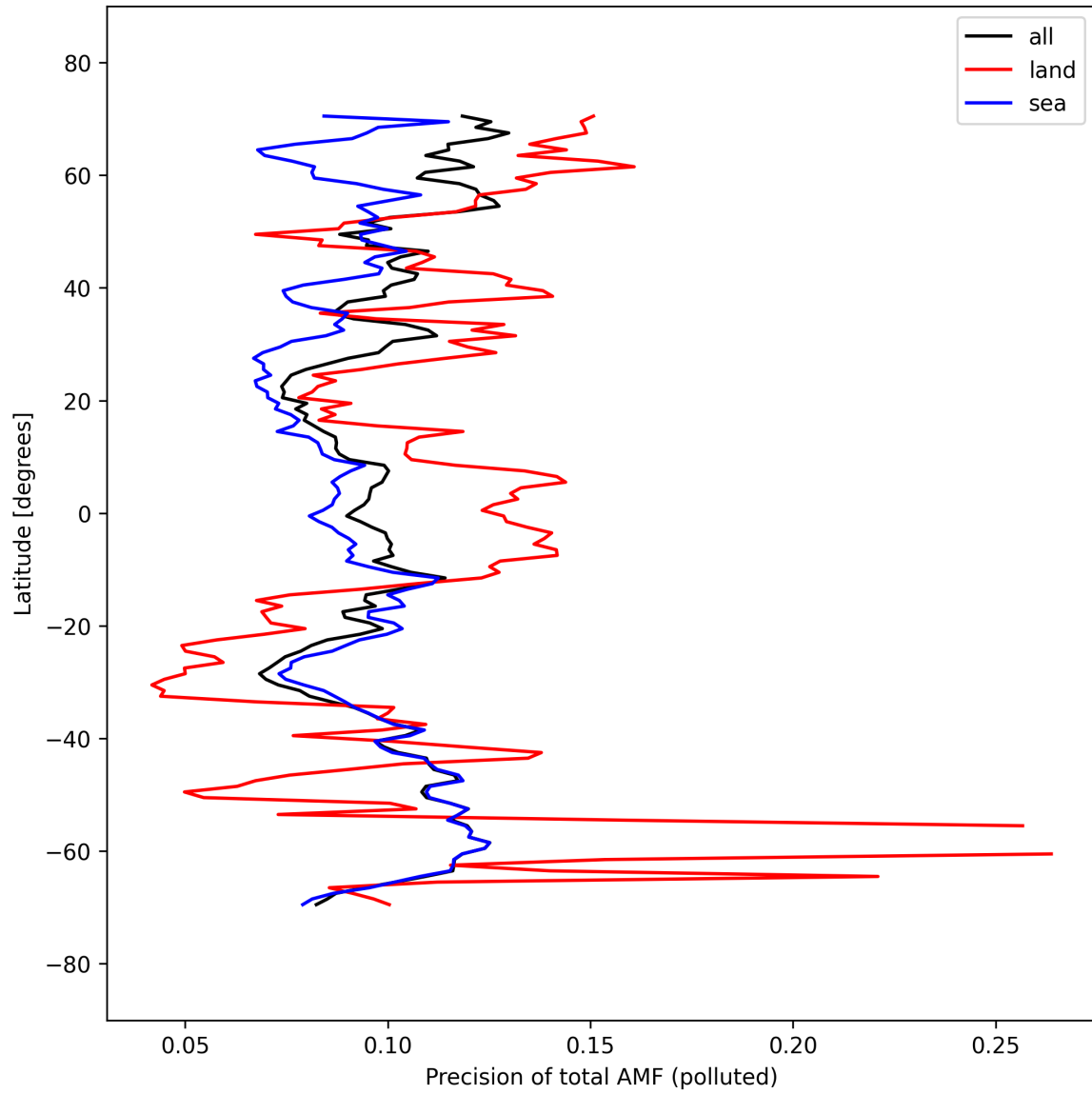
Figure 54: Zonal average of “Precision of total AMF (polluted)” for 2025-09-22 to 2025-09-23.
