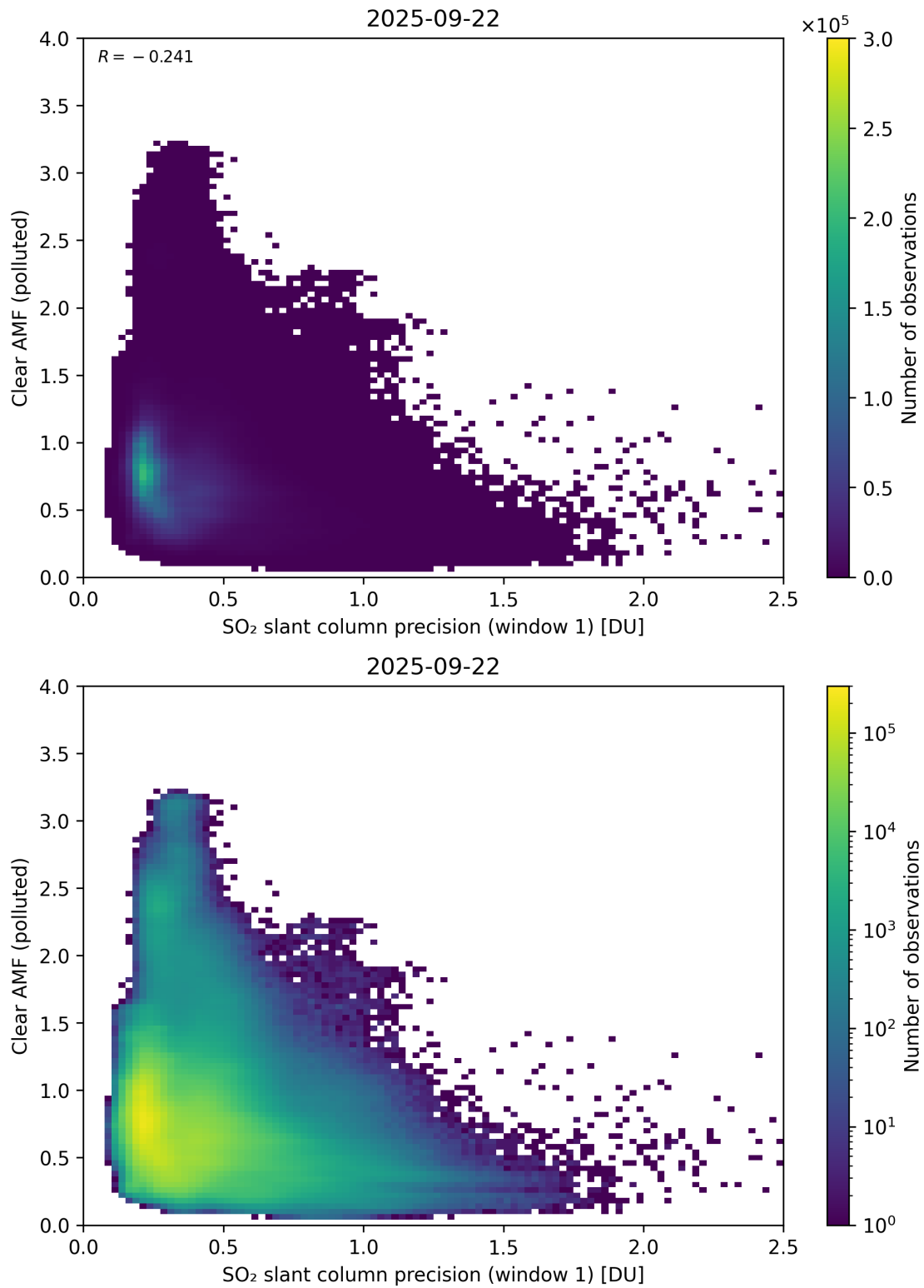
Figure 274: Scatter density plot of “SO 2 slant column precision (window 1)” against “Clear AMF (polluted)” for 2025-09-22 to 2025-09-23.
