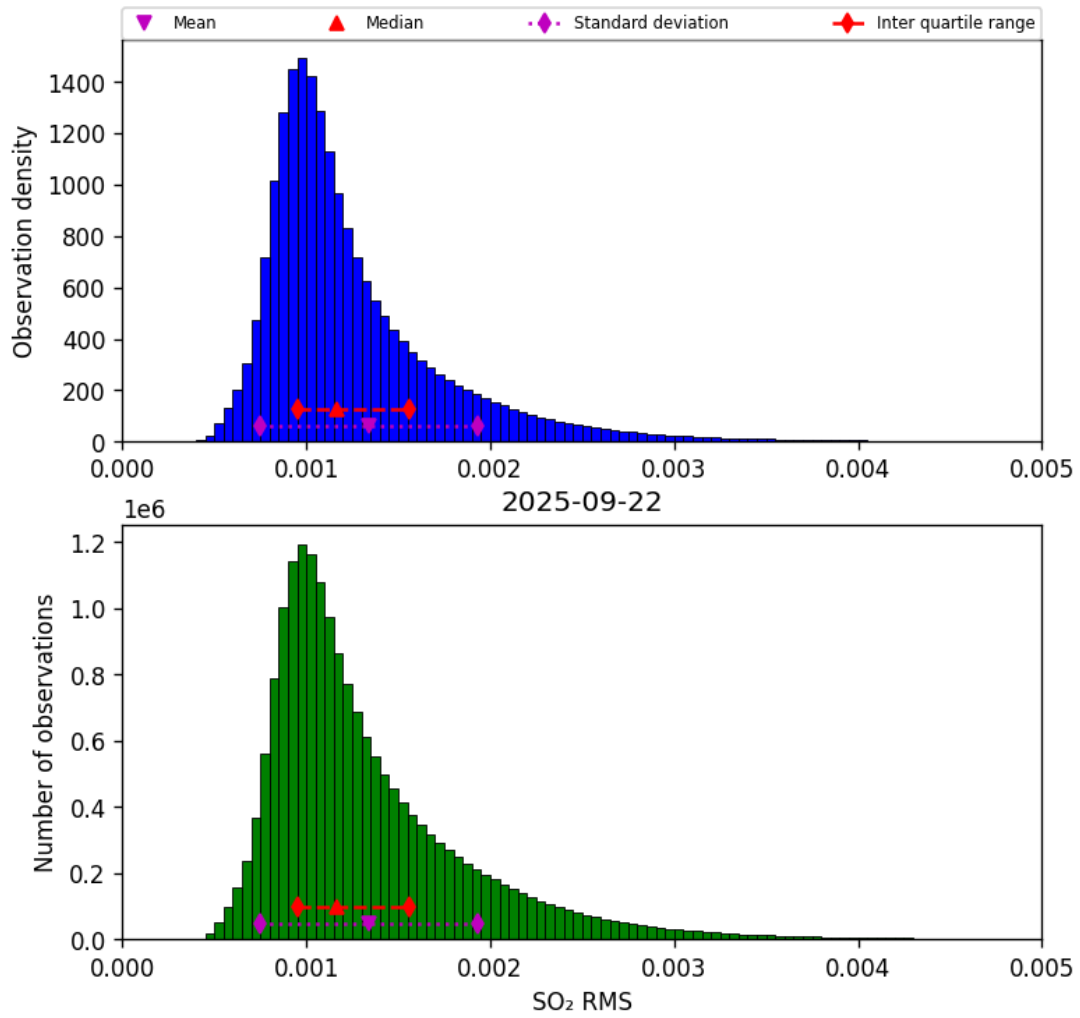
Figure 78: Histogram of “SO 2 RMS” for 2025-09-22 to 2025-09-23
