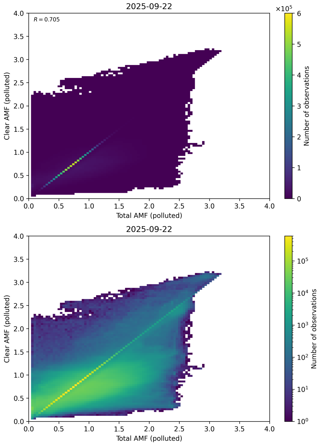
Figure 321: Scatter density plot of “Total AMF (polluted)” against “Clear AMF (polluted)” for 2025-09-22 to 2025-09-23.
