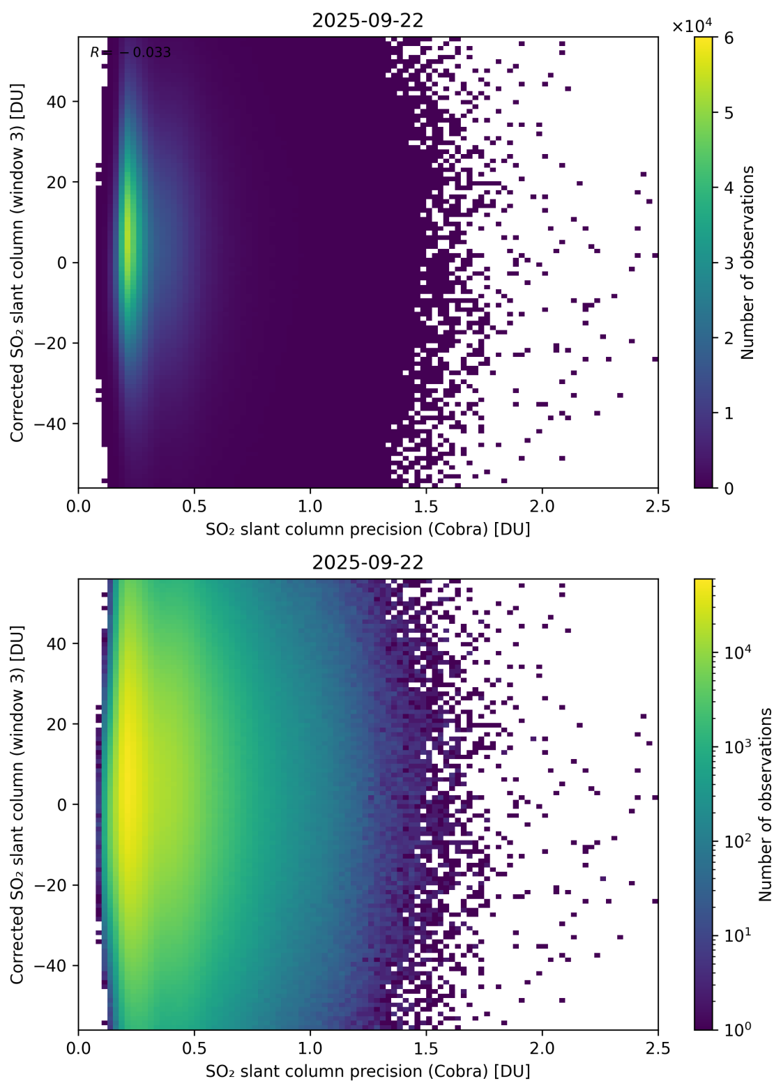
Figure 207: Scatter density plot of “SO 2 slant column precision (Cobra)” against “Corrected SO 2 slant column (window 3)” for 2025-09-22 to 2025-09-23.
