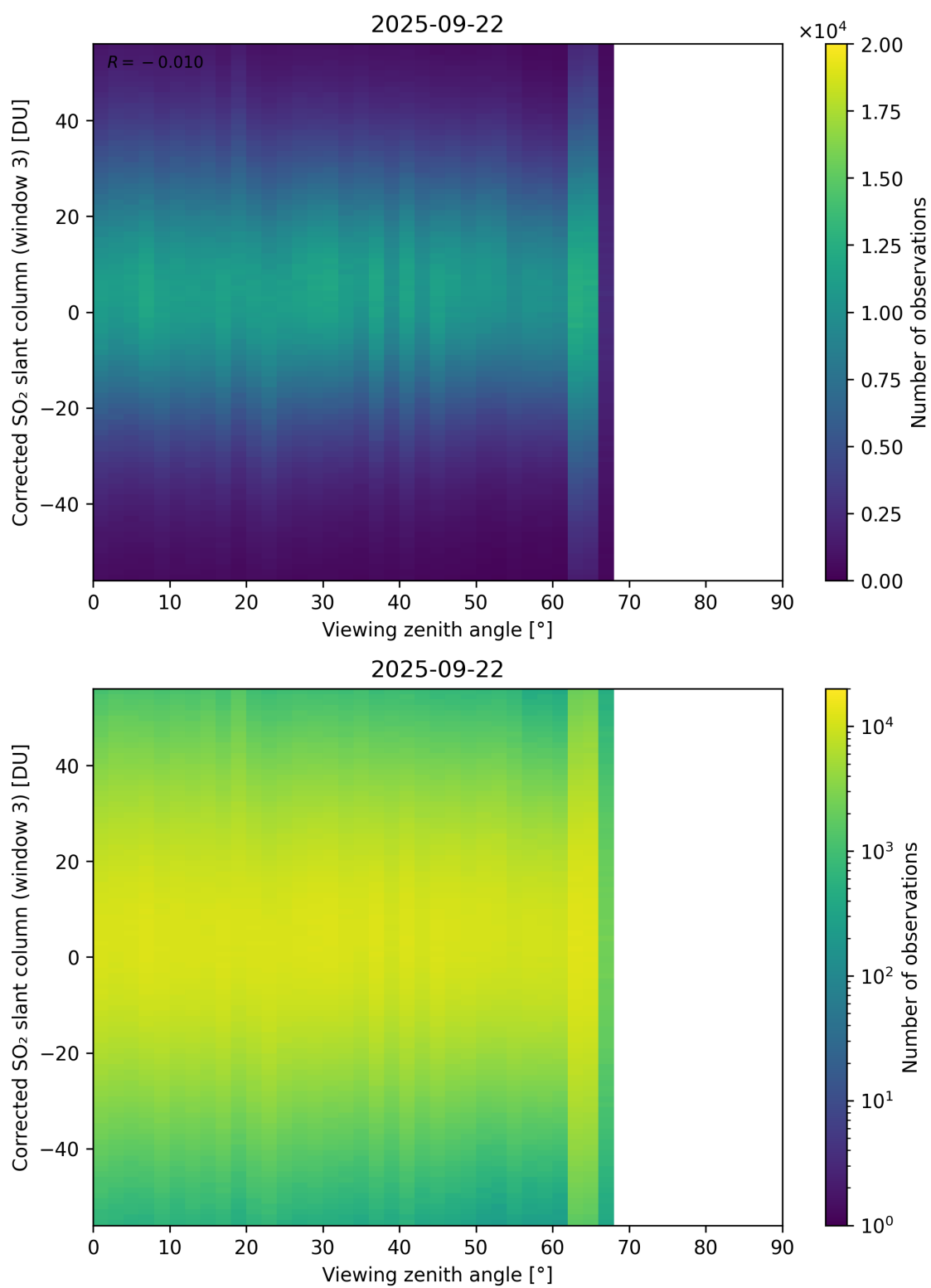
Figure 375: Scatter density plot of “Viewing zenith angle” against “Corrected SO 2 slant column (window 3)” for 2025-09-22 to 2025-09-23.
