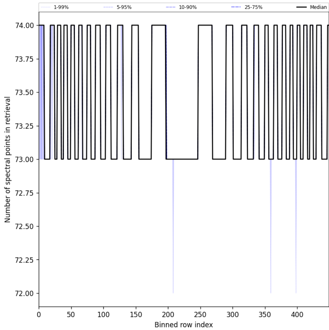
Figure 108: Along track statistics of “Number of spectral points in retrieval” for 2025-09-22 to 2025-09-23
