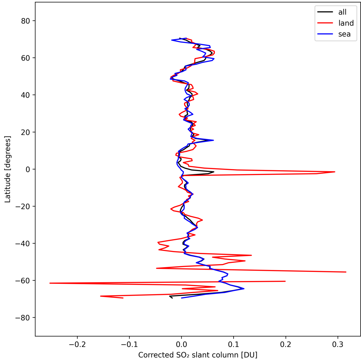
Figure 34: Zonal average of “Corrected SO 2 slant column” for 2025-09-22 to 2025-09-23.
