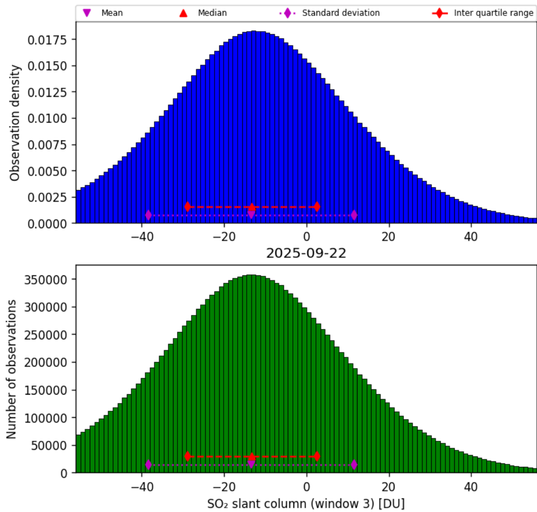
Figure 71: Histogram of “SO 2 slant column (window 3)” for 2025-09-22 to 2025-09-23
