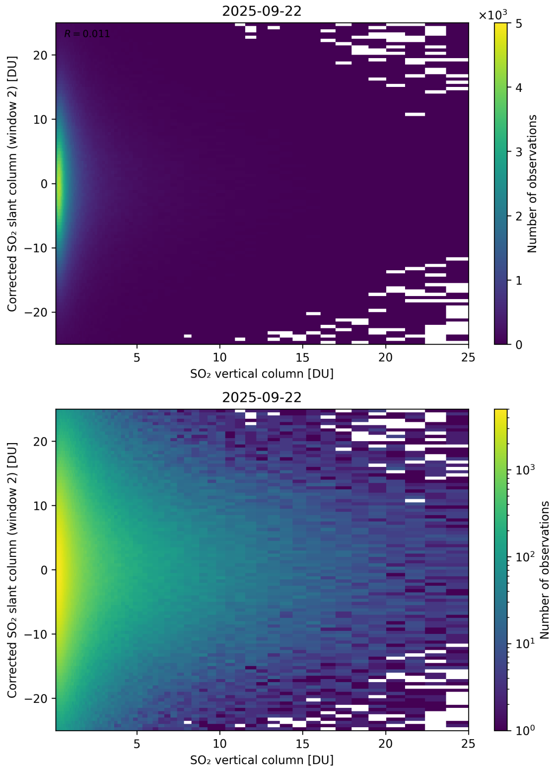
Figure 352: Scatter density plot of “SO 2 vertical column” against “Corrected SO 2 slant column (window 2)” for 2025-09-22 to 2025-09-23.
