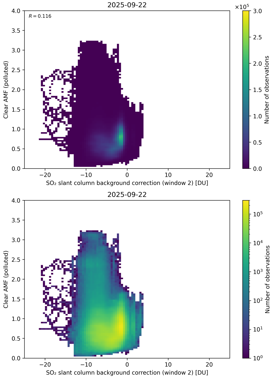
Figure 126: Scatter density plot of “SO 2 slant column background correction (window 2)” against “Clear AMF (polluted)” for 2025-09-22 to 2025-09-23.
