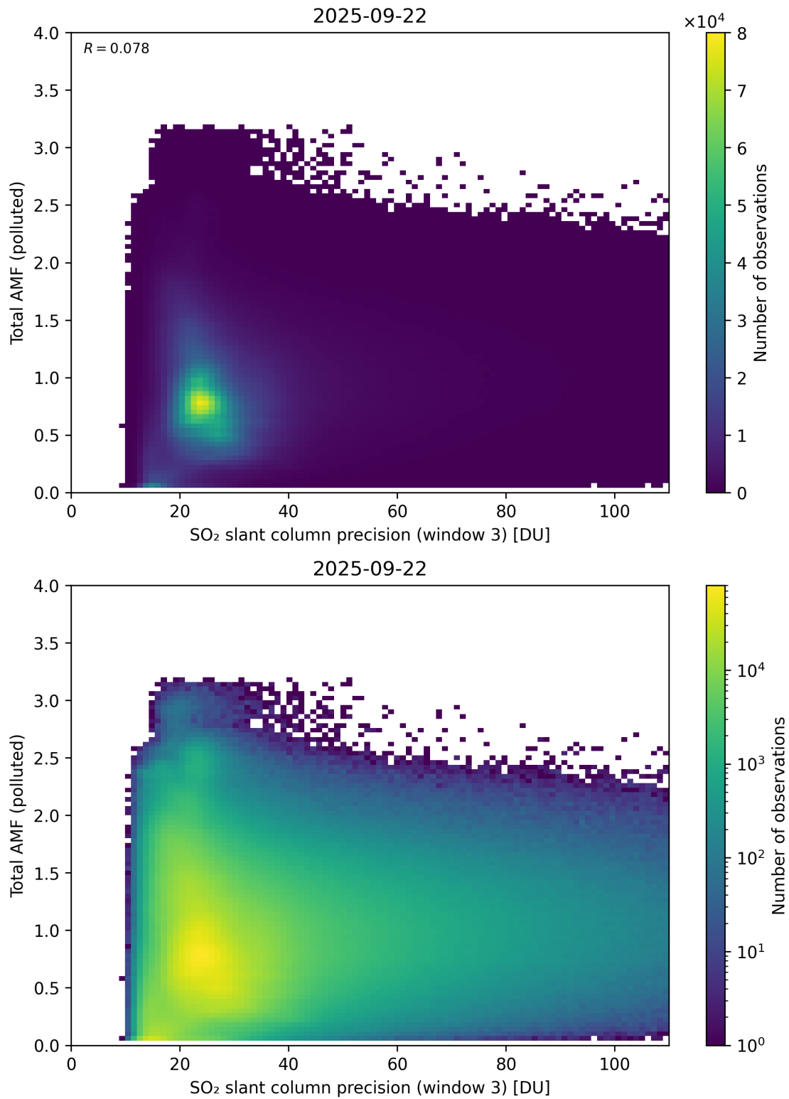
Figure 313: Scatter density plot of “SO 2 slant column precision (window 3)” against “Total AMF (polluted)” for 2025-09-22 to 2025-09-23.
