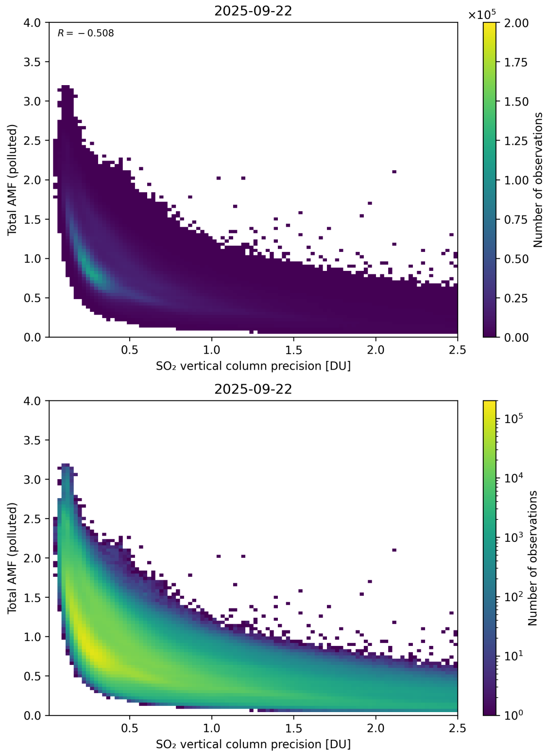
Figure 346: Scatter density plot of “SO 2 vertical column precision” against “Total AMF (polluted)” for 2025-09-22 to 2025-09-23.
