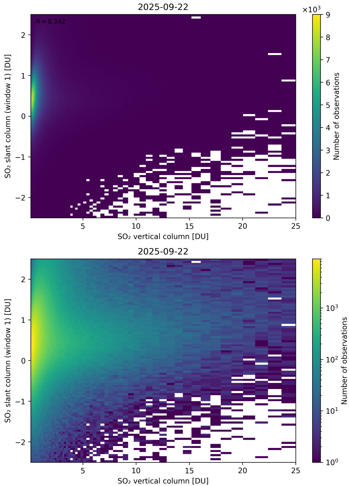
Figure 354: Scatter density plot of “SO 2 vertical column” against “SO 2 slant column (window 1)” for 2025-09-22 to 2025-09-23.
