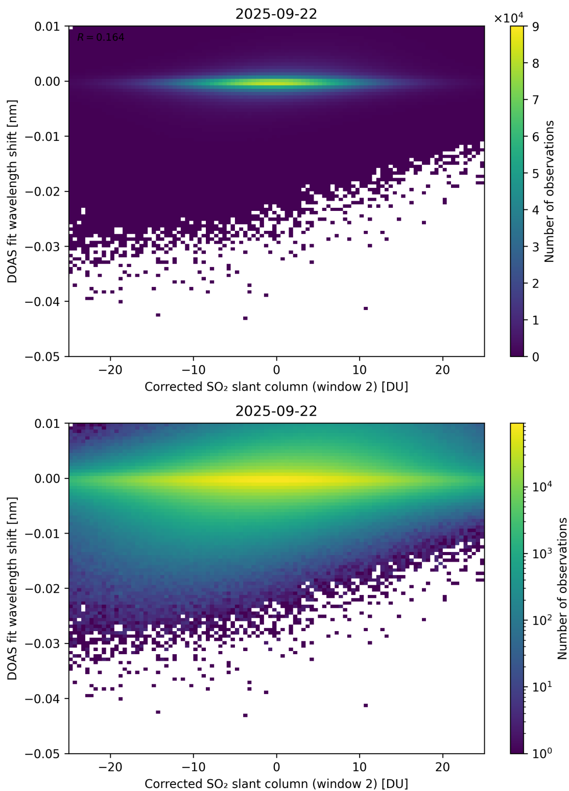
Figure 246: Scatter density plot of “Corrected SO 2 slant column (window 2)” against “DOAS fit wavelength shift” for 2025-09-22 to 2025-09-23.
