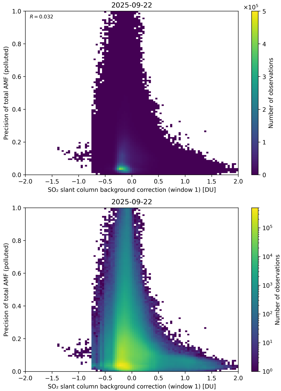
Figure 121: Scatter density plot of “SO 2 slant column background correction (window 1)” against “Precision of total AMF (polluted)” for 2025-09-22 to 2025-09-23.
