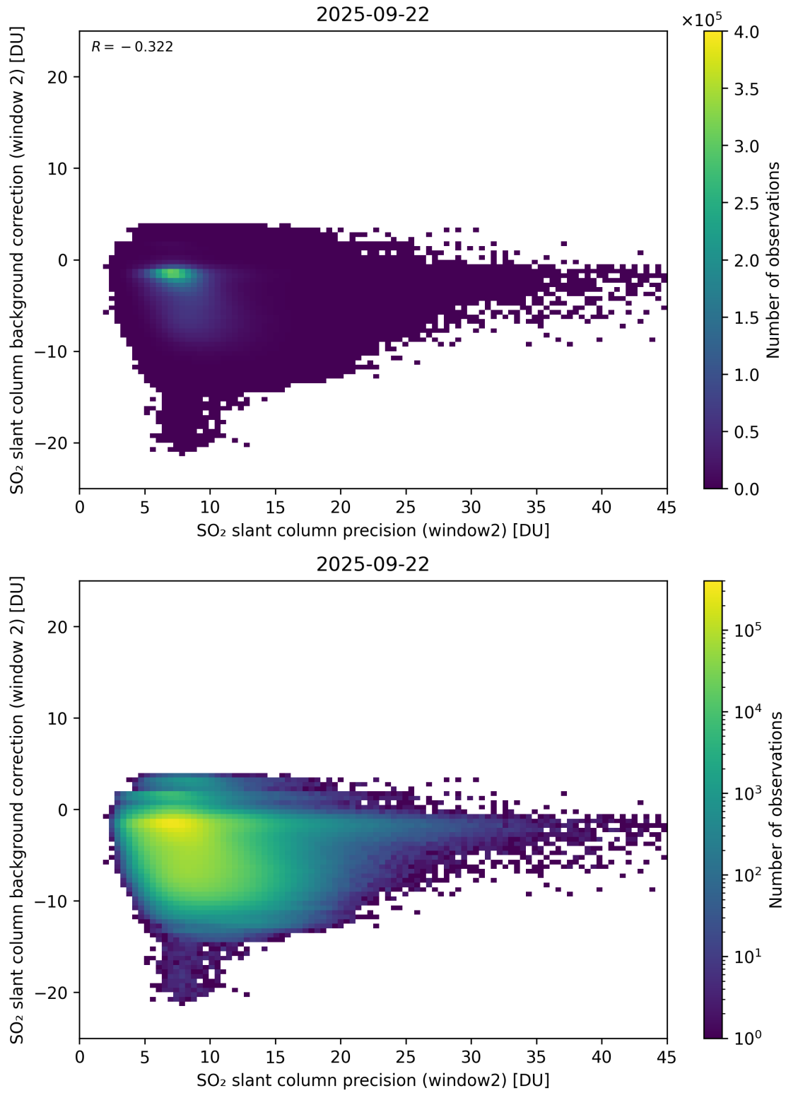
Figure 291: Scatter density plot of “SO 2 slant column precision (window2)” against “SO 2 slant column background correction (window 2)” for 2025-09-22 to 2025-09-23.
