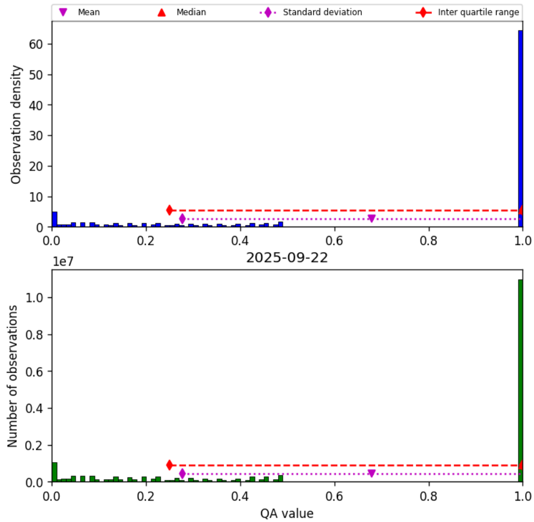
Figure 57: Histogram of “QA value” for 2025-09-22 to 2025-09-23
