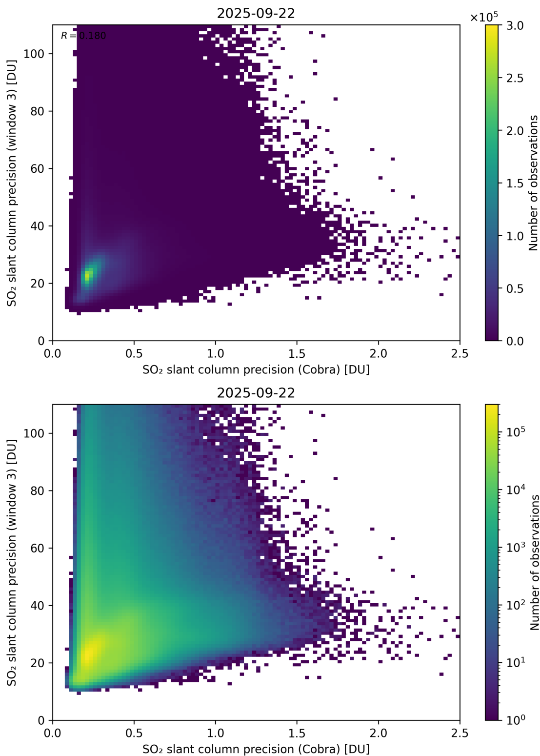
Figure 212: Scatter density plot of “SO 2 slant column precision (Cobra)” against “SO 2 slant column precision (window 3)” for 2025-09-22 to 2025-09-23.
