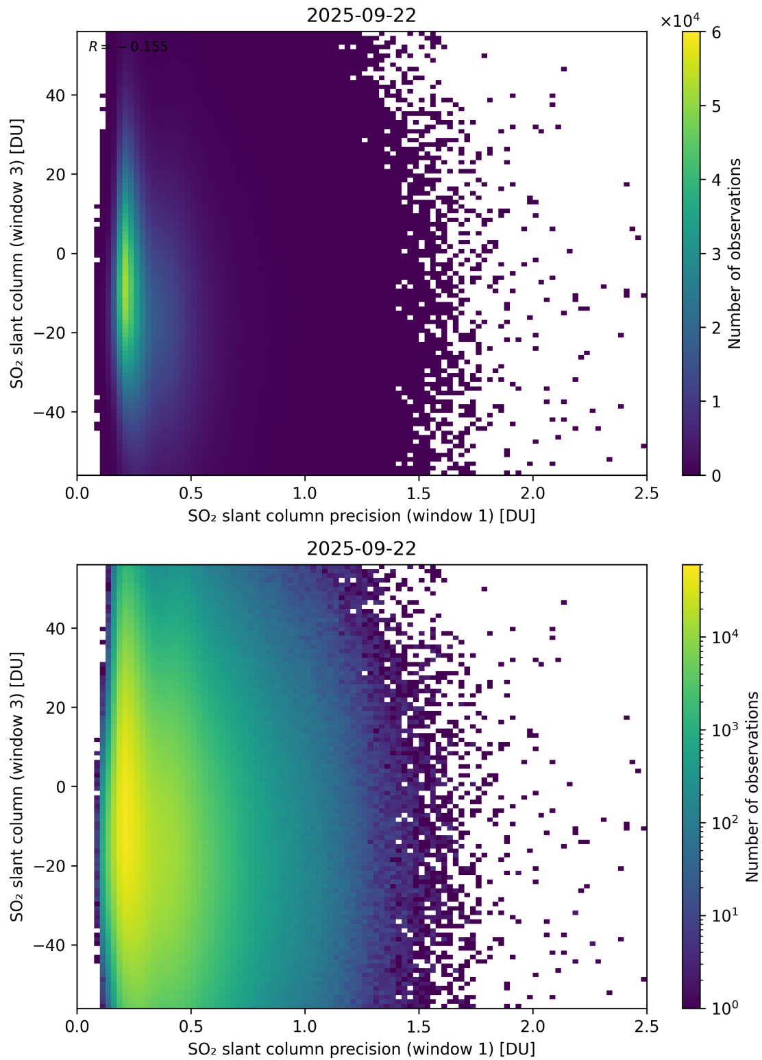
Figure 278: Scatter density plot of “SO 2 slant column precision (window 1)” against “SO 2 slant column (window 3)” for 2025-09-22 to 2025-09-23.
