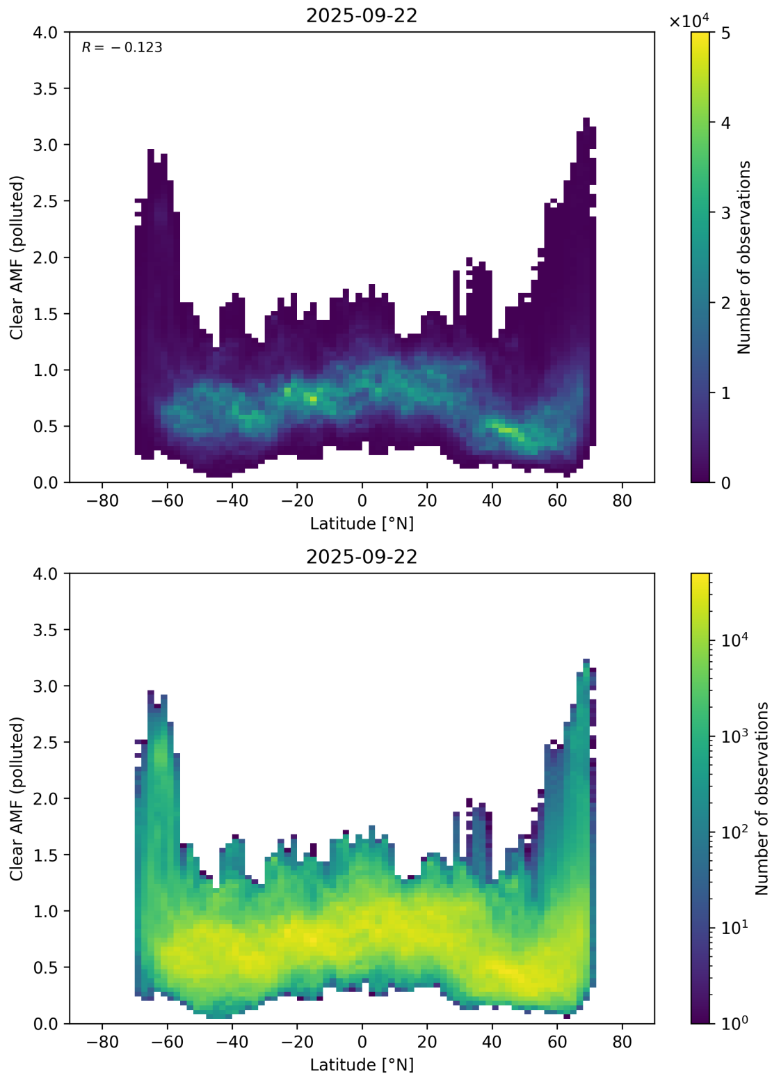
Figure 156: Scatter density plot of “Latitude” against “Clear AMF (polluted)” for 2025-09-22 to 2025-09-23.
