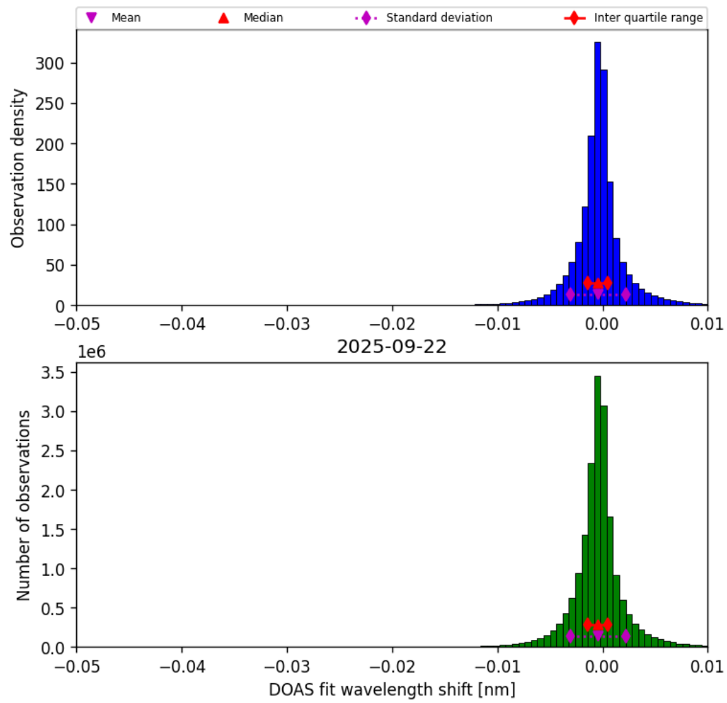
Figure 76: Histogram of “DOAS fit wavelength shift” for 2025-09-22 to 2025-09-23
