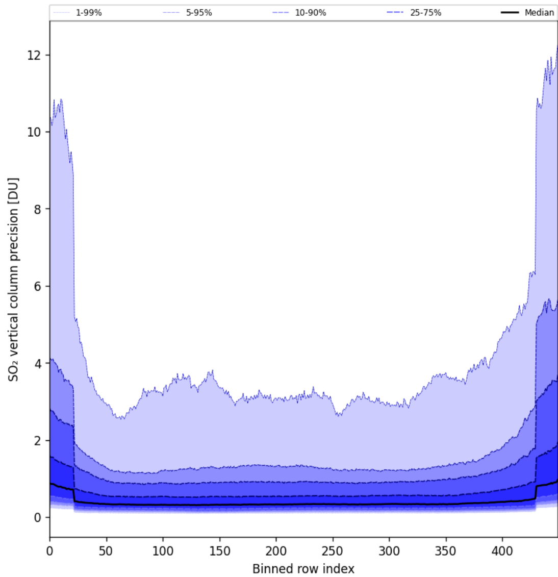
Figure 85: Along track statistics of “SO 2 vertical column precision” for 2025-09-22 to 2025-09-23
