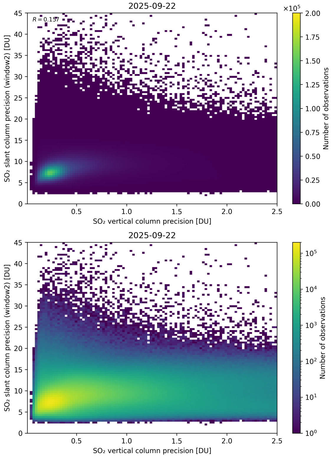
Figure 343: Scatter density plot of “SO 2 vertical column precision” against “SO 2 slant column precision (window2)” for 2025-09-22 to 2025-09-23.
