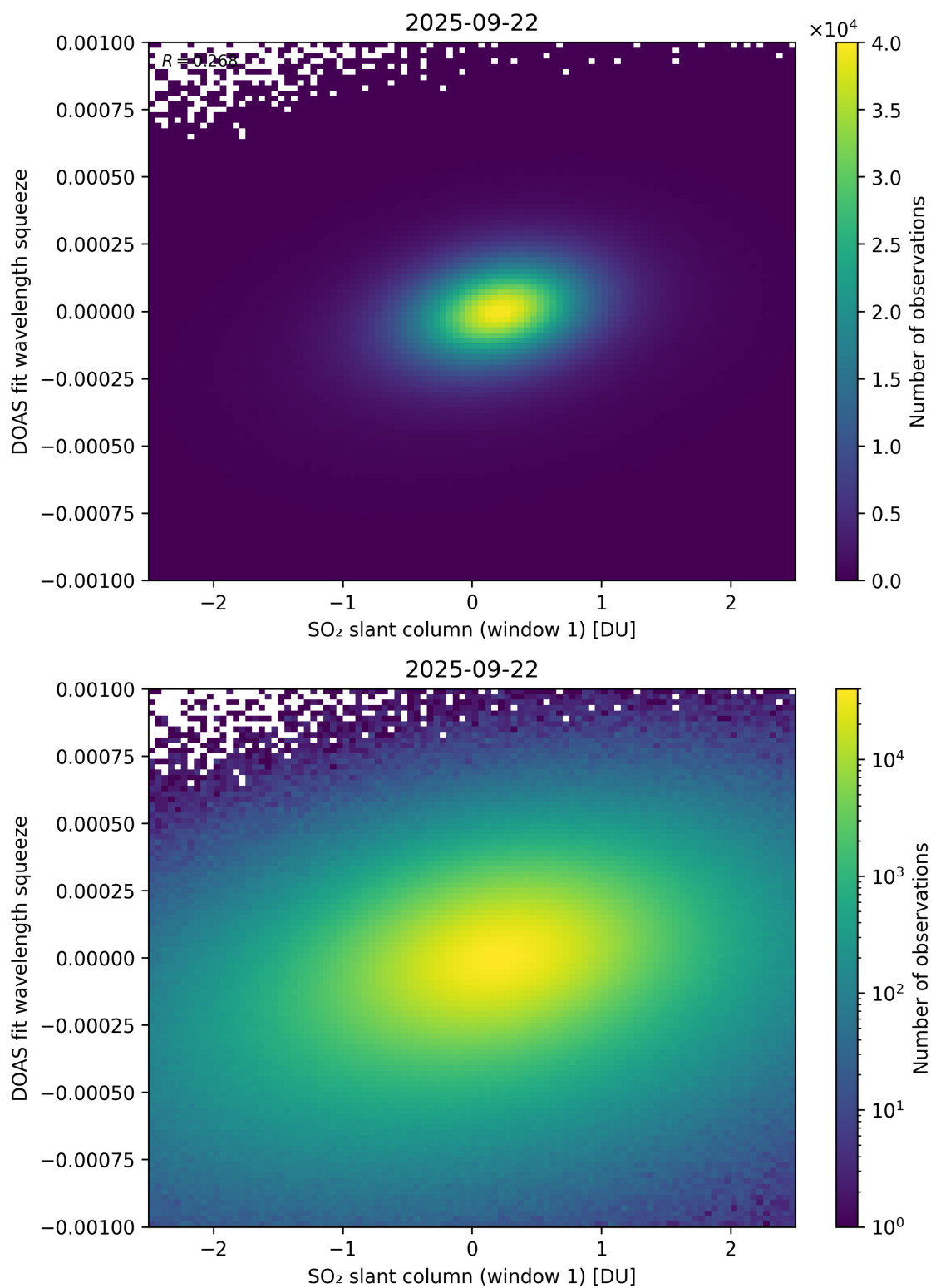
Figure 266: Scatter density plot of “SO 2 slant column (window 1)” against “DOAS fit wavelength squeeze” for 2025-09-22 to 2025-09-23.
