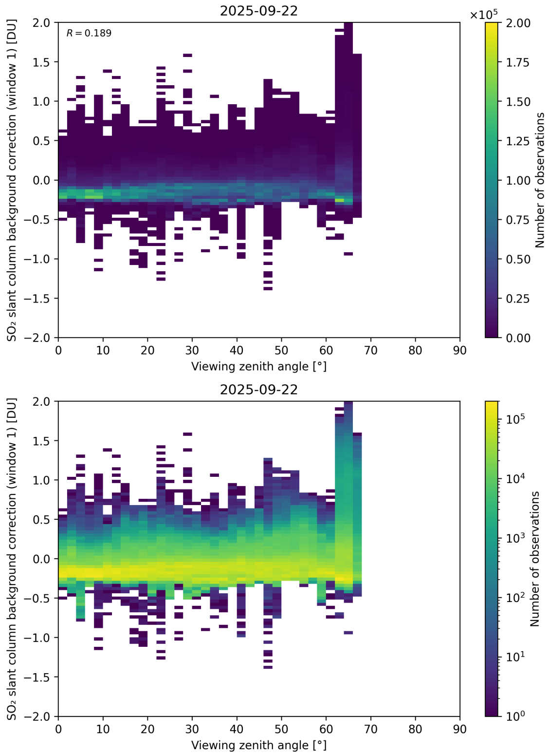
Figure 362: Scatter density plot of “Viewing zenith angle” against “SO 2 slant column background correction (window 1)” for 2025-09-22 to 2025-09-23.
