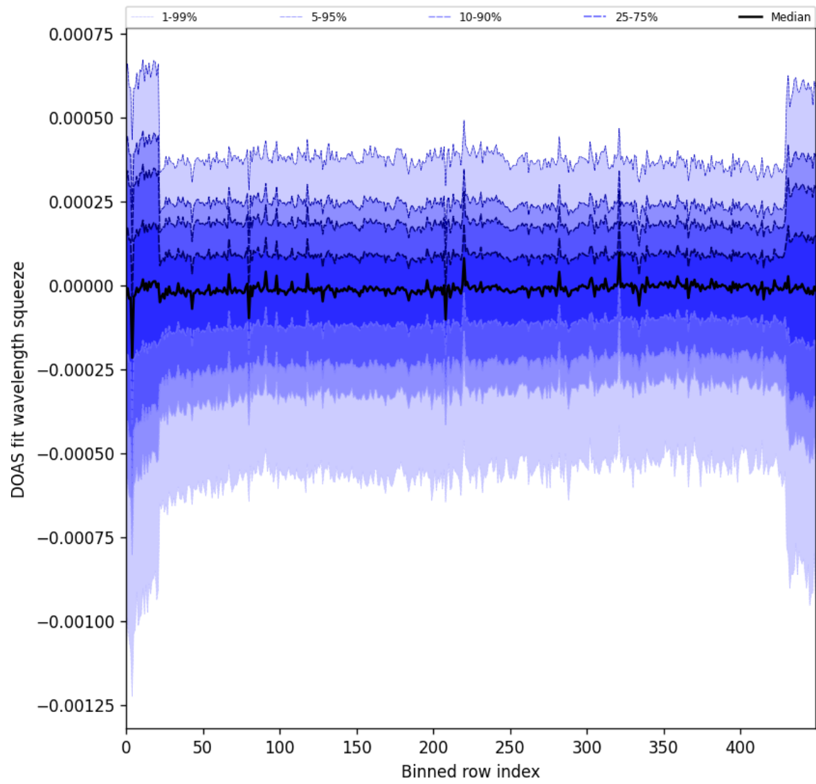
Figure 103: Along track statistics of “DOAS fit wavelength squeeze” for 2025-09-22 to 2025-09-23
