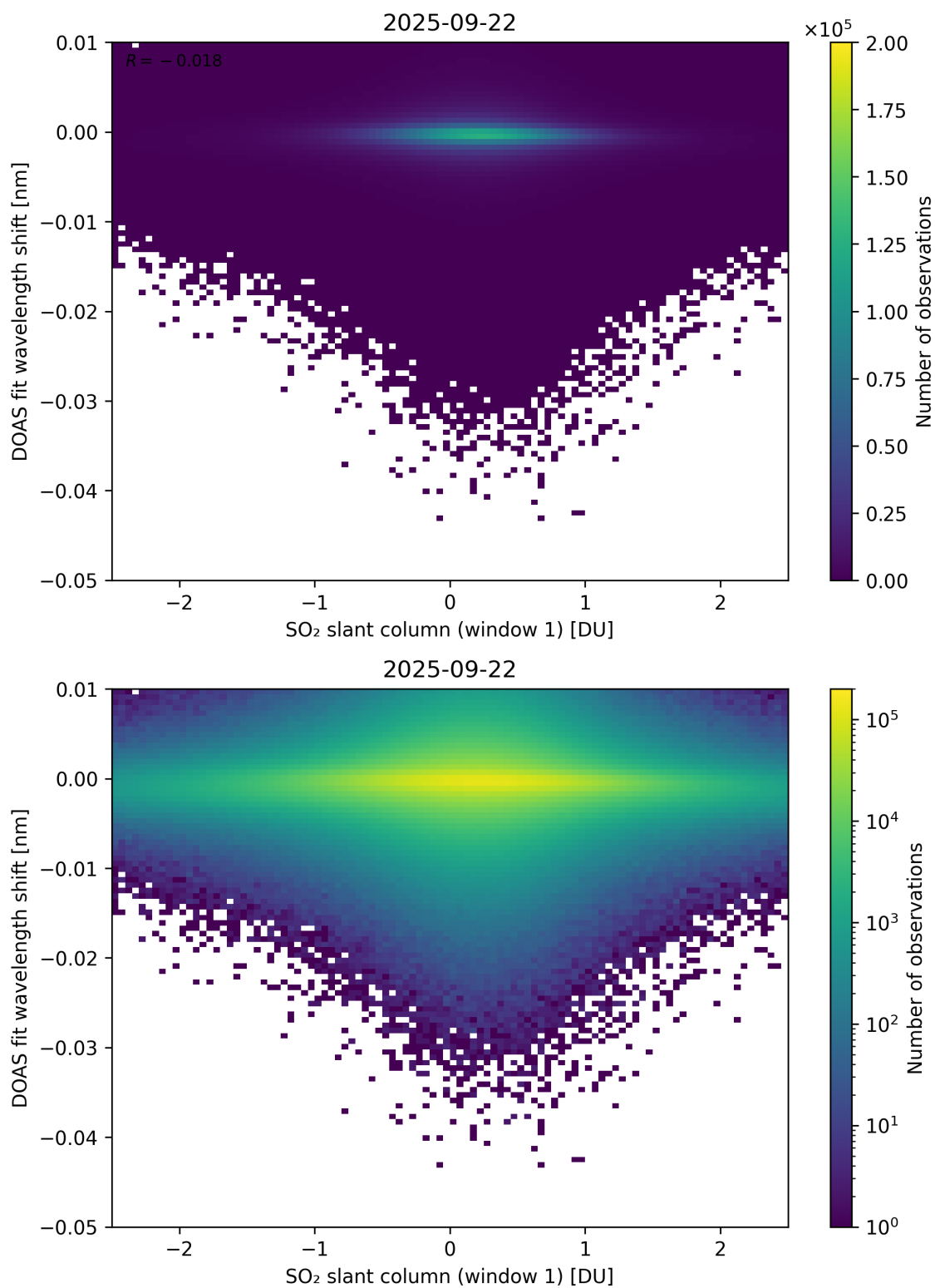
Figure 265: Scatter density plot of “SO 2 slant column (window 1)” against “DOAS fit wavelength shift” for 2025-09-22 to 2025-09-23.
