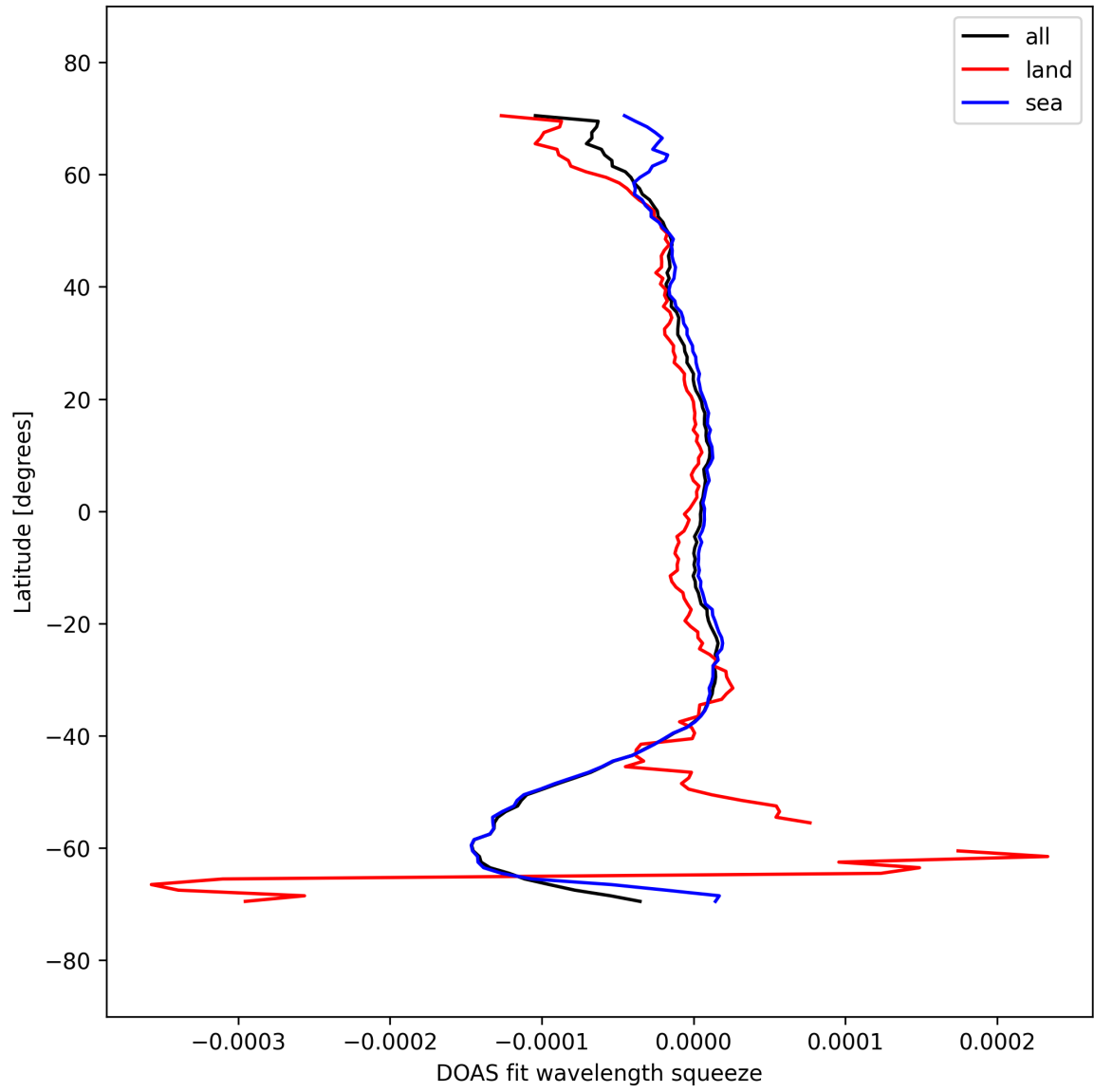
Figure 51: Zonal average of “DOAS fit wavelength squeeze” for 2025-09-22 to 2025-09-23.
