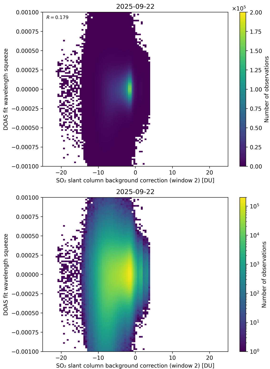
Figure 124: Scatter density plot of “SO 2 slant column background correction (window 2)” against “DOAS fit wavelength squeeze” for 2025-09-22 to 2025-09-23.
