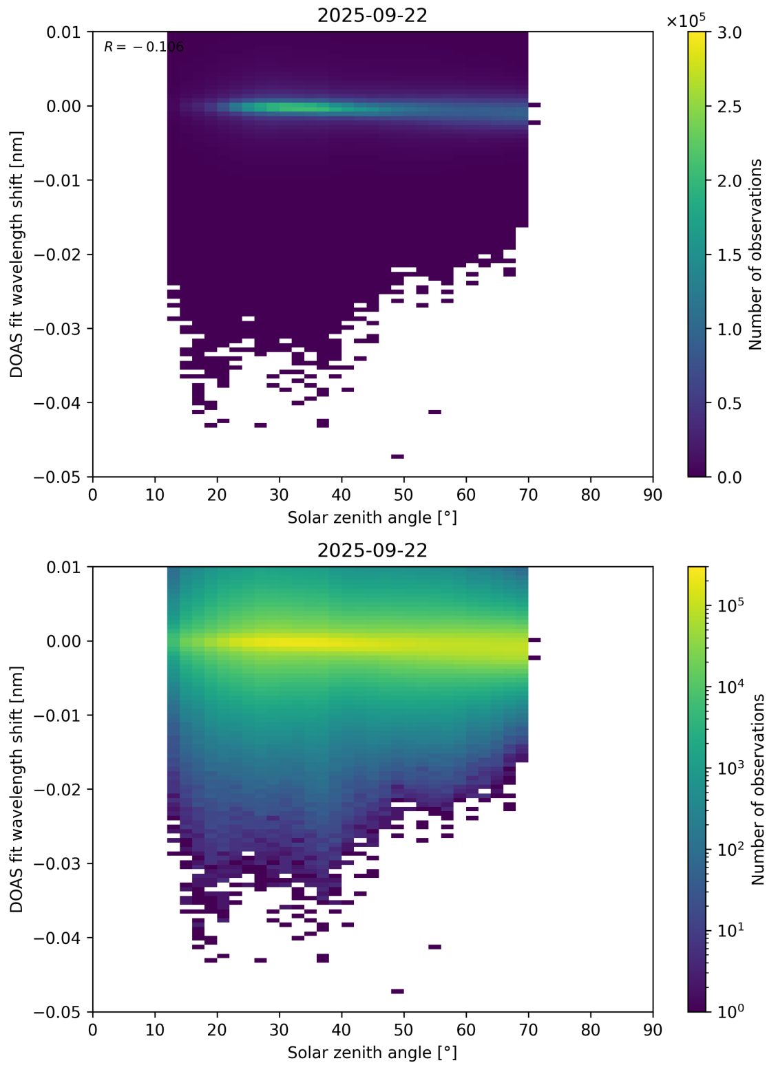
Figure 174: Scatter density plot of “Solar zenith angle” against “DOAS fit wavelength shift” for 2025-09-22 to 2025-09-23.
