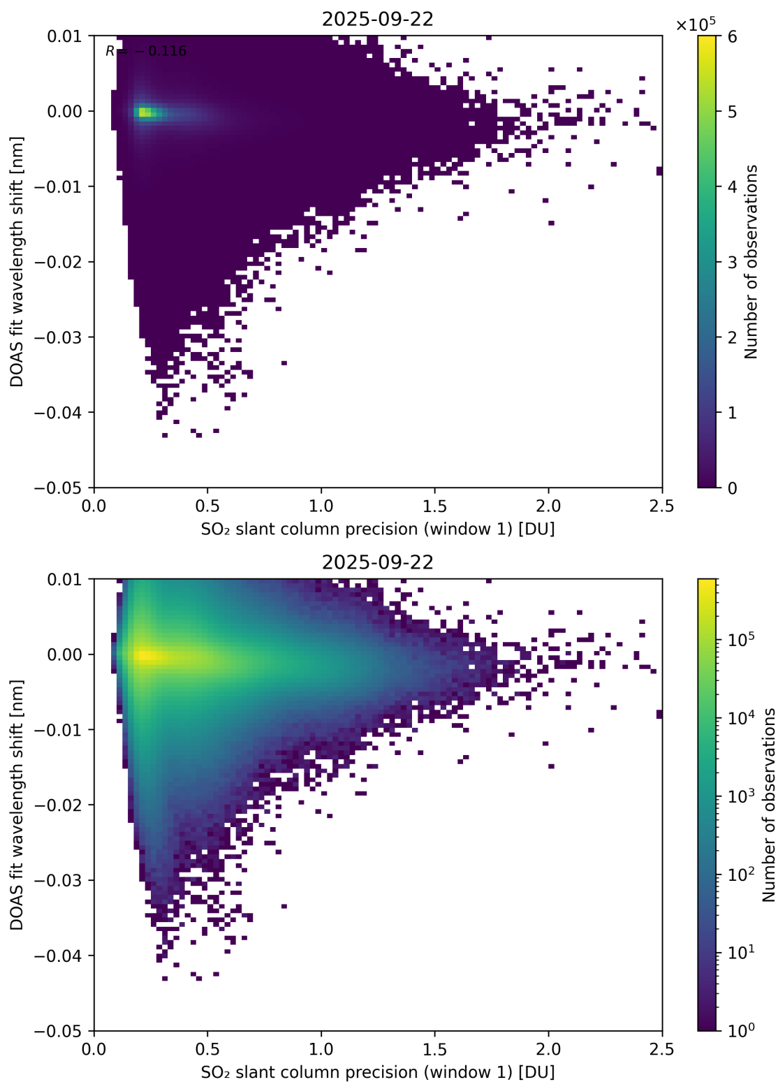
Figure 271: Scatter density plot of “SO 2 slant column precision (window 1)” against “DOAS fit wavelength shift” for 2025-09-22 to 2025-09-23.
