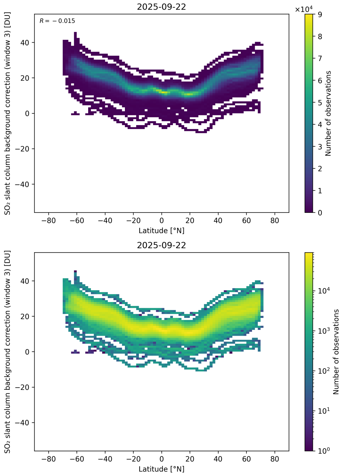
Figure 152: Scatter density plot of “Latitude” against “SO 2 slant column background correction (window 3)” for 2025-09-22 to 2025-09-23.
