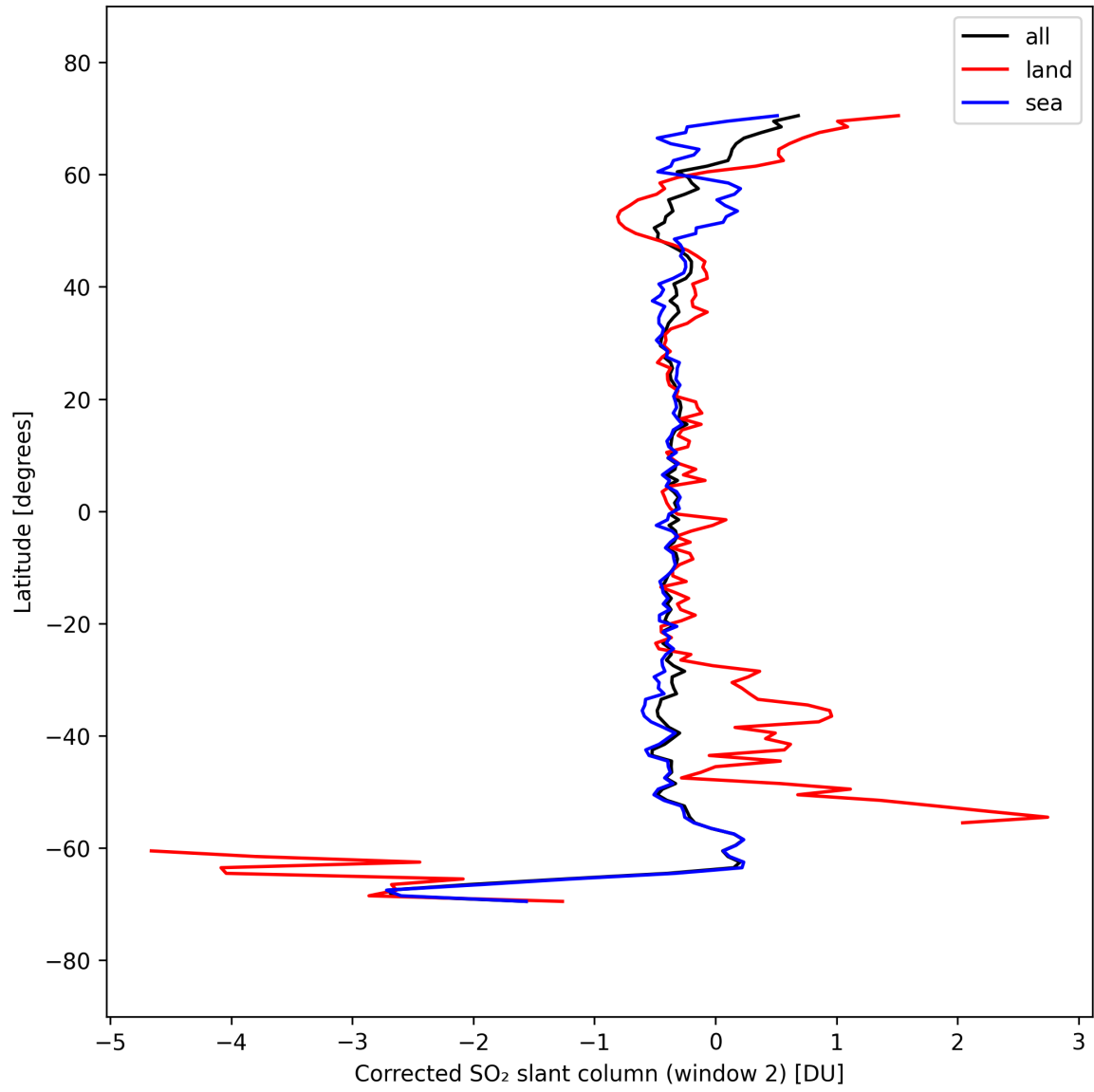
Figure 43: Zonal average of “Corrected SO 2 slant column (window 2)” for 2025-09-22 to 2025-09-23.
