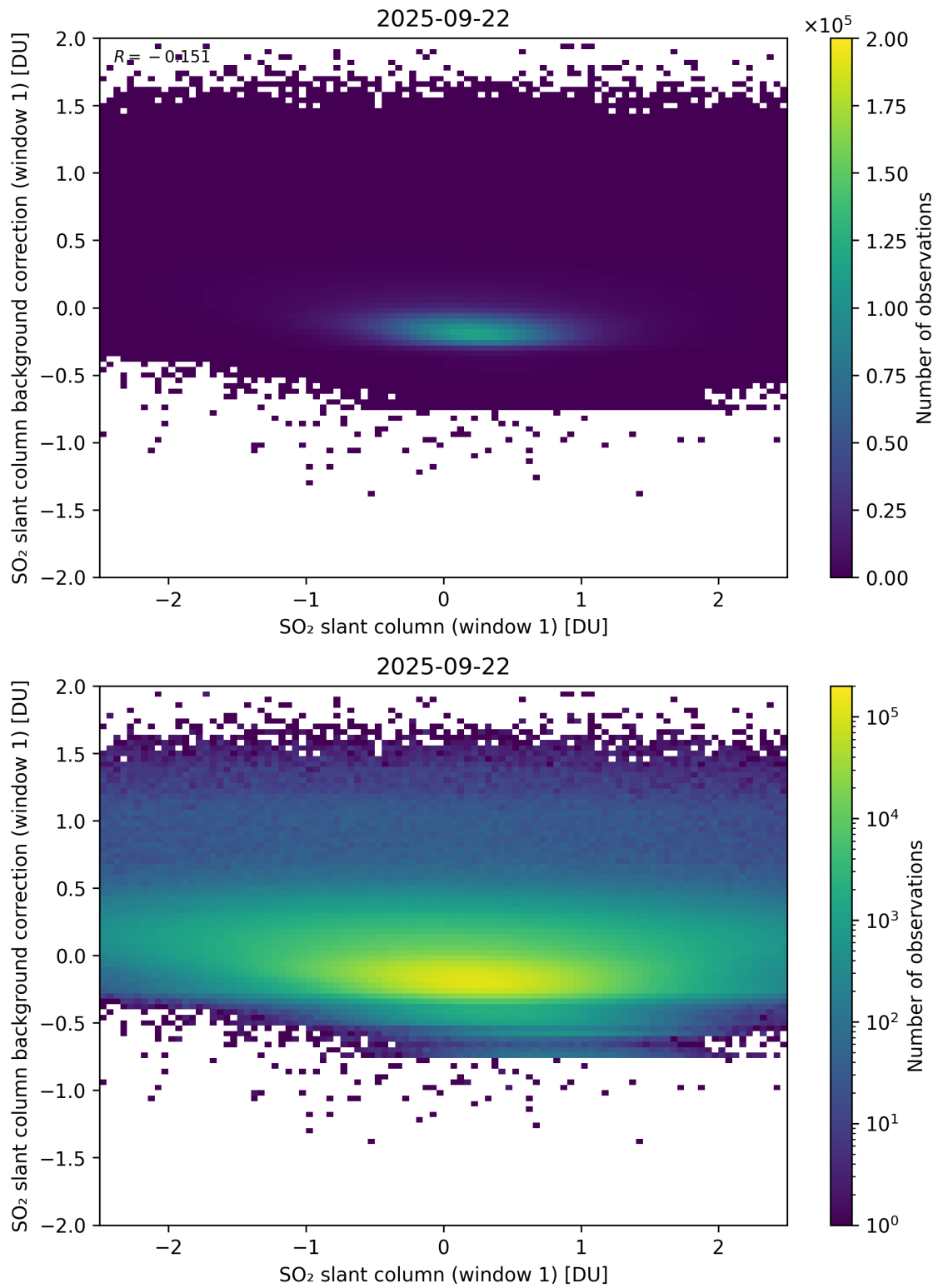
Figure 262: Scatter density plot of “SO 2 slant column (window 1)” against “SO 2 slant column background correction (window 1)” for 2025-09-22 to 2025-09-23.
