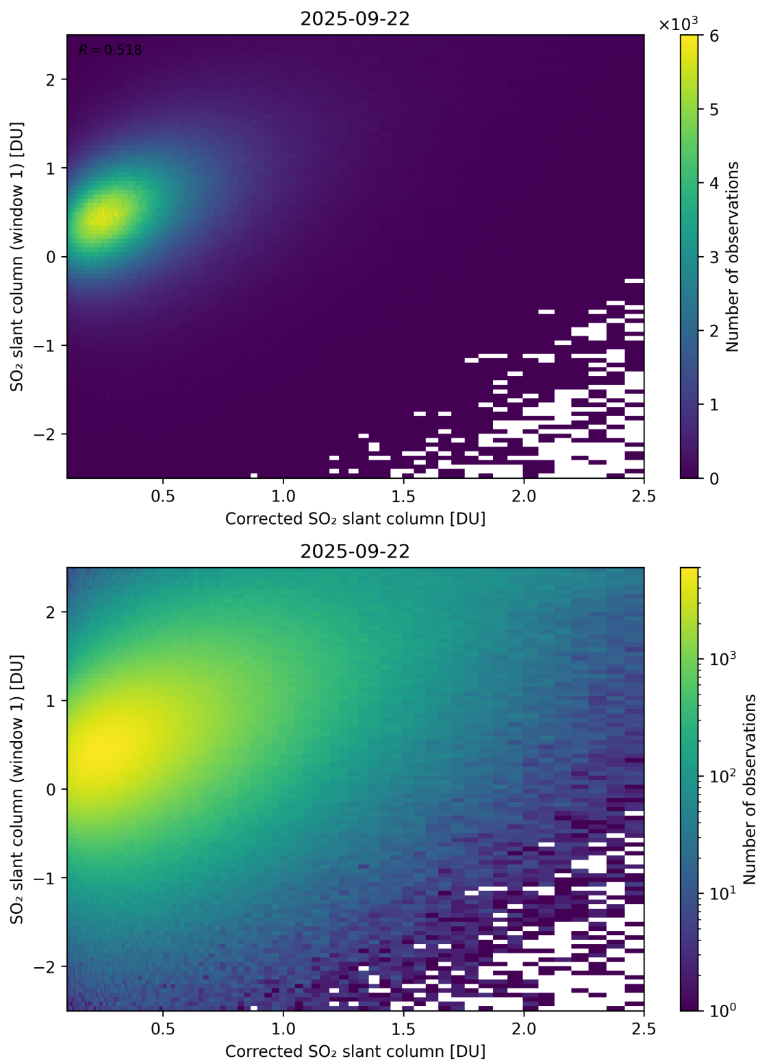
Figure 237: Scatter density plot of “Corrected SO 2 slant column” against “SO 2 slant column (window 1)” for 2025-09-22 to 2025-09-23.
