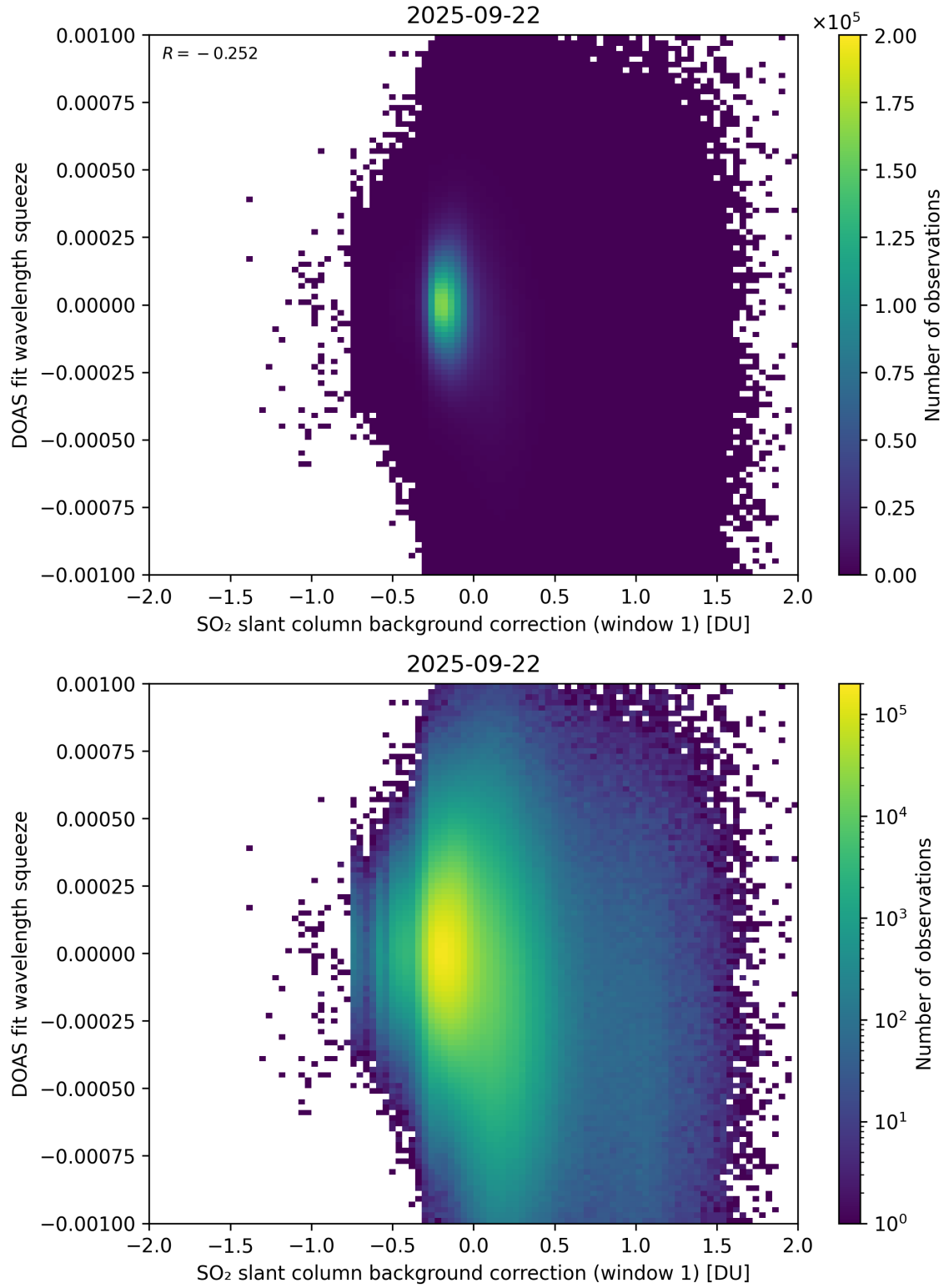
Figure 112: Scatter density plot of “SO 2 slant column background correction (window 1)” against “DOAS fit wavelength squeeze” for 2025-09-22 to 2025-09-23.
