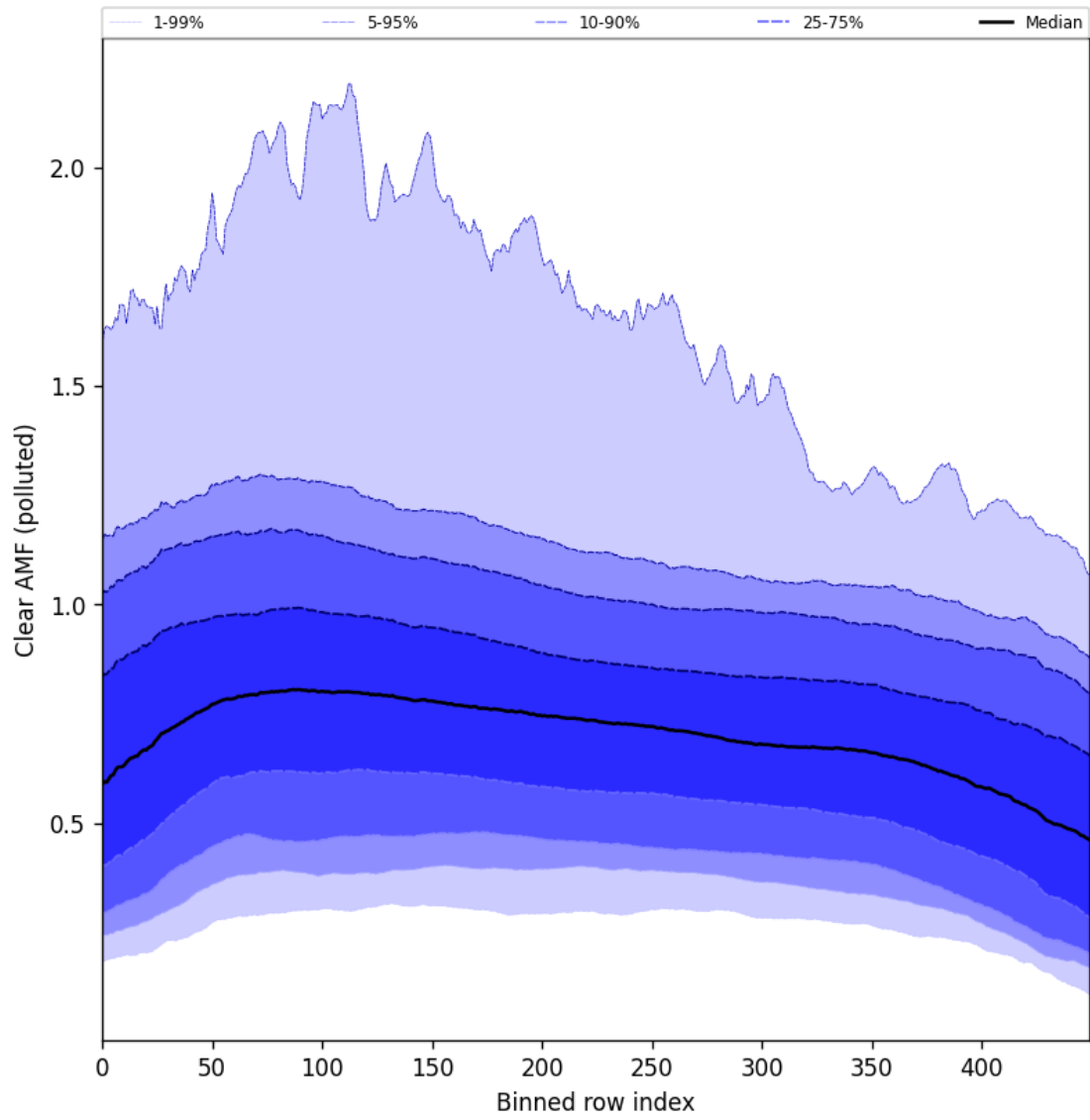
Figure 107: Along track statistics of “Clear AMF (polluted)” for 2025-09-22 to 2025-09-23
