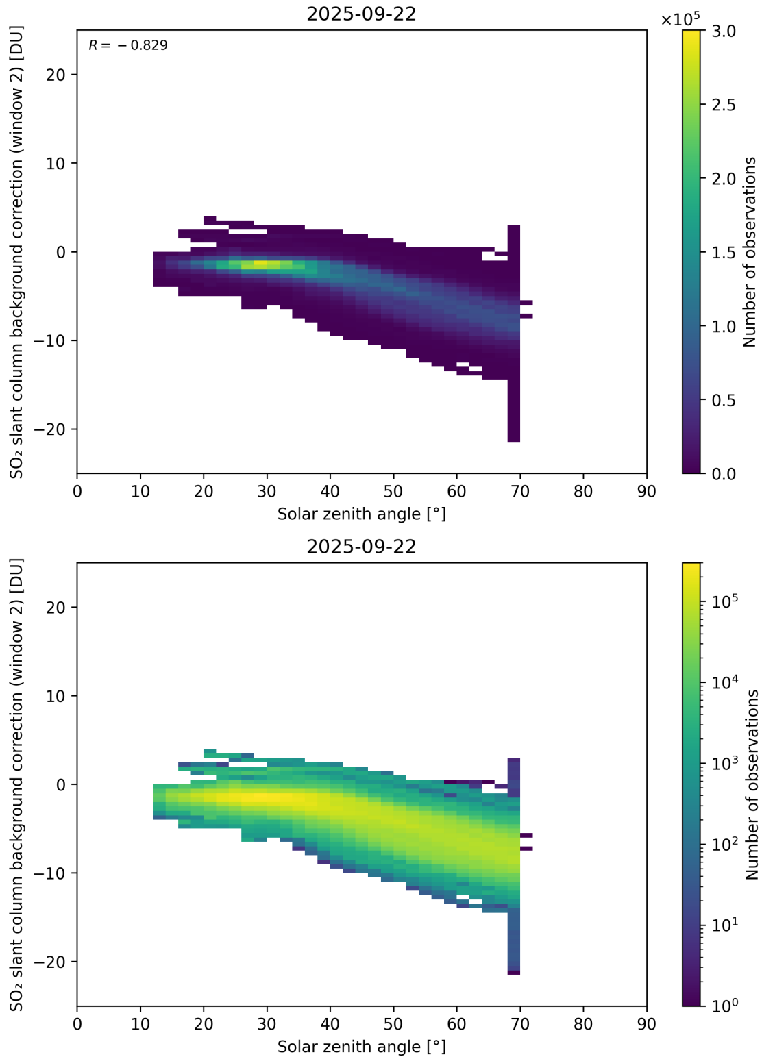
Figure 172: Scatter density plot of “Solar zenith angle” against “SO 2 slant column background correction (window 2)” for 2025-09-22 to 2025-09-23.
