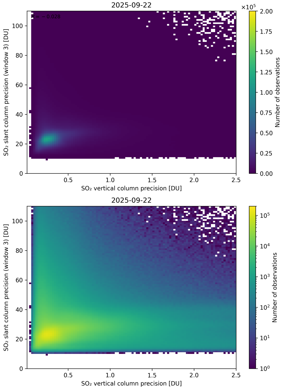
Figure 345: Scatter density plot of “SO 2 vertical column precision” against “SO 2 slant column precision (window 3)” for 2025-09-22 to 2025-09-23.
