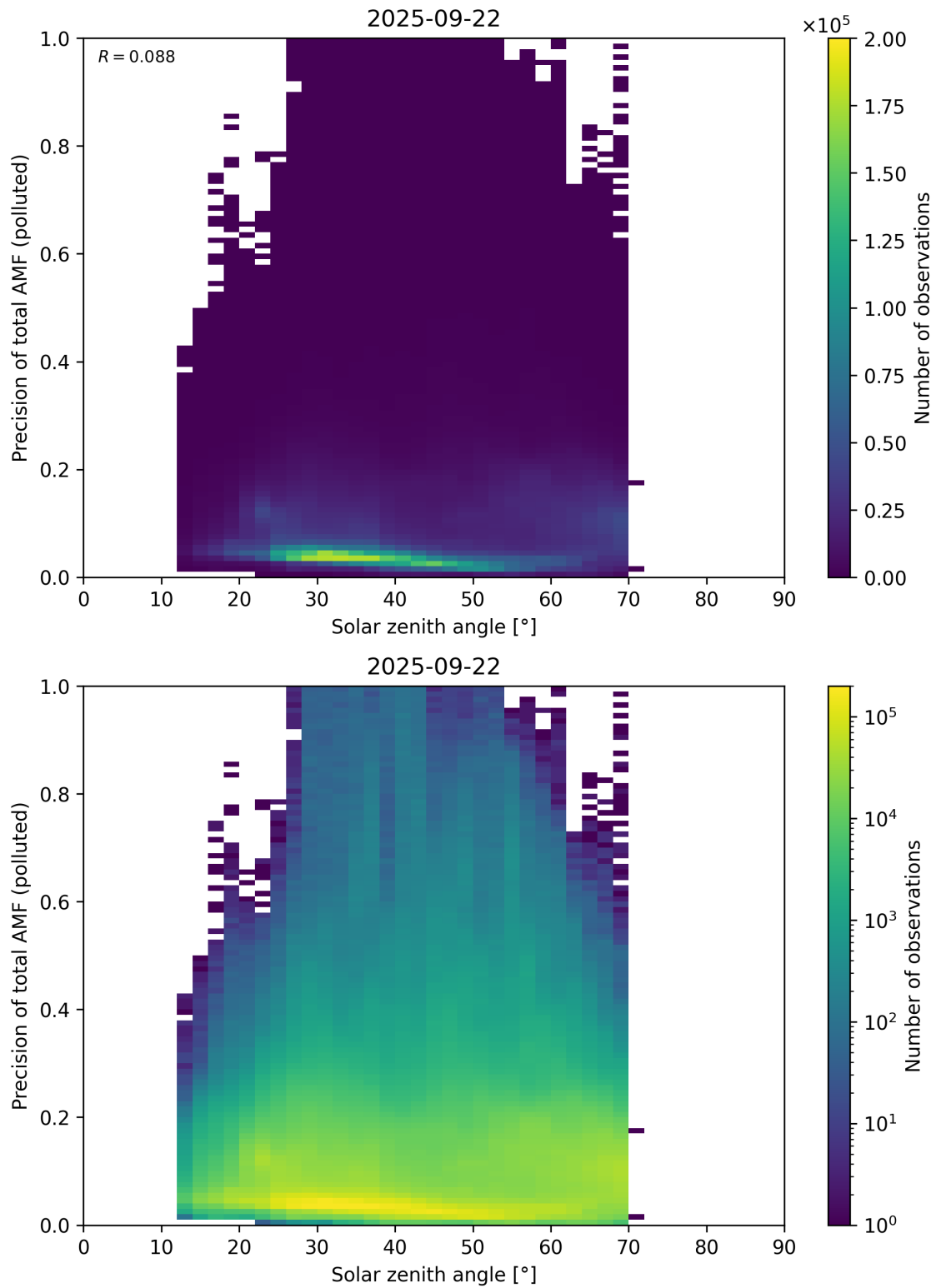
Figure 190: Scatter density plot of “Solar zenith angle” against “Precision of total AMF (polluted)” for 2025-09-22 to 2025-09-23.
