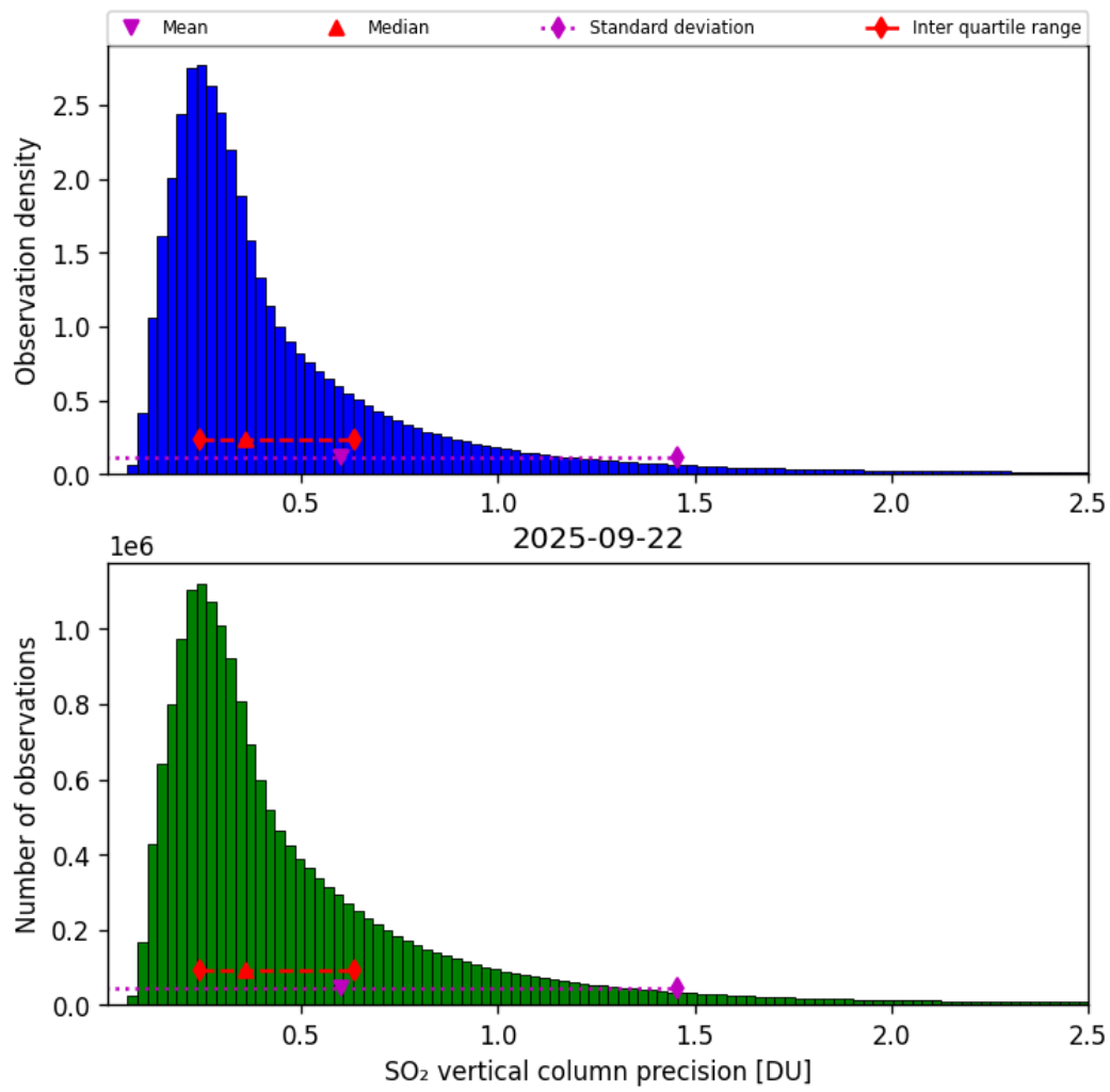
Figure 59: Histogram of “SO 2 vertical column precision” for 2025-09-22 to 2025-09-23
