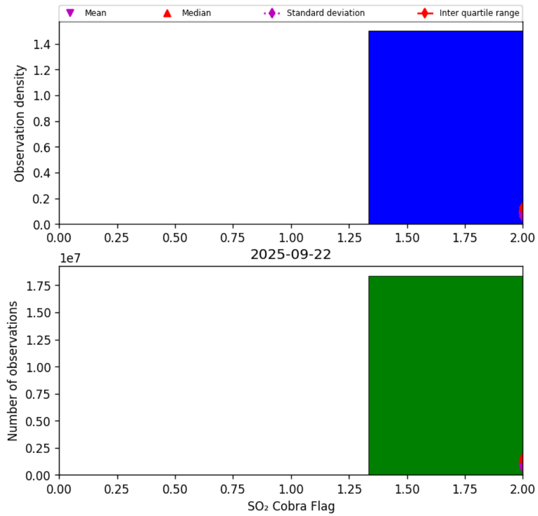
Figure 75: Histogram of “SO 2 Cobra Flag” for 2025-09-22 to 2025-09-23
