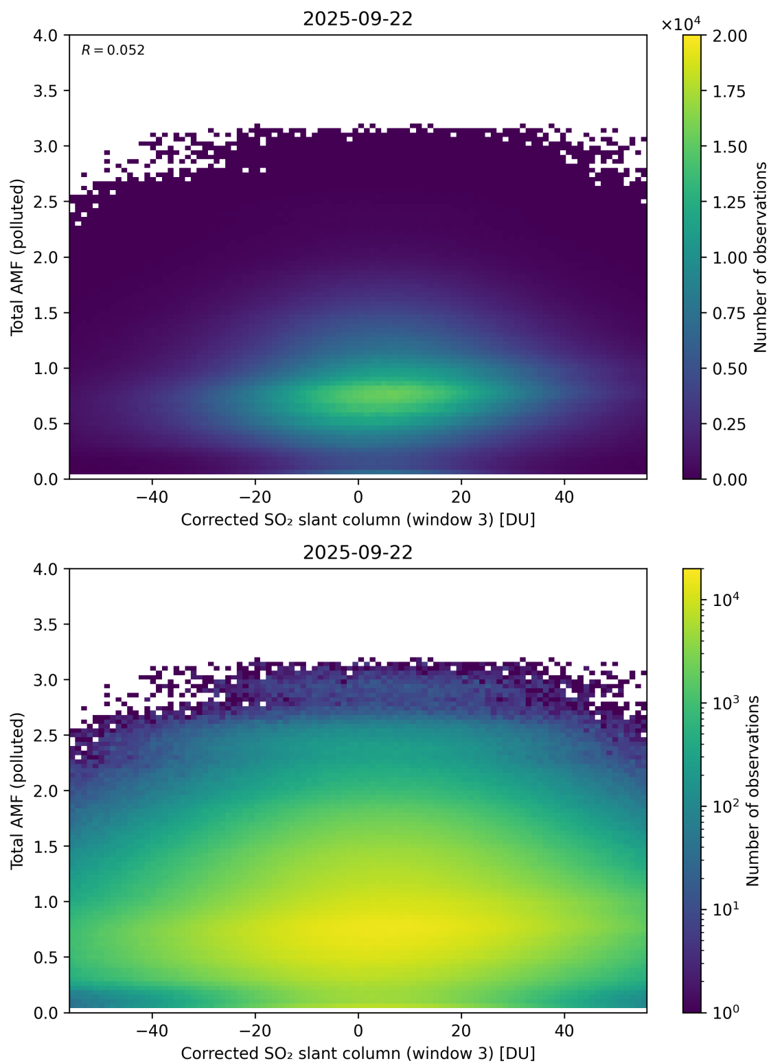
Figure 260: Scatter density plot of “Corrected SO 2 slant column (window 3)” against “Total AMF (polluted)” for 2025-09-22 to 2025-09-23.
