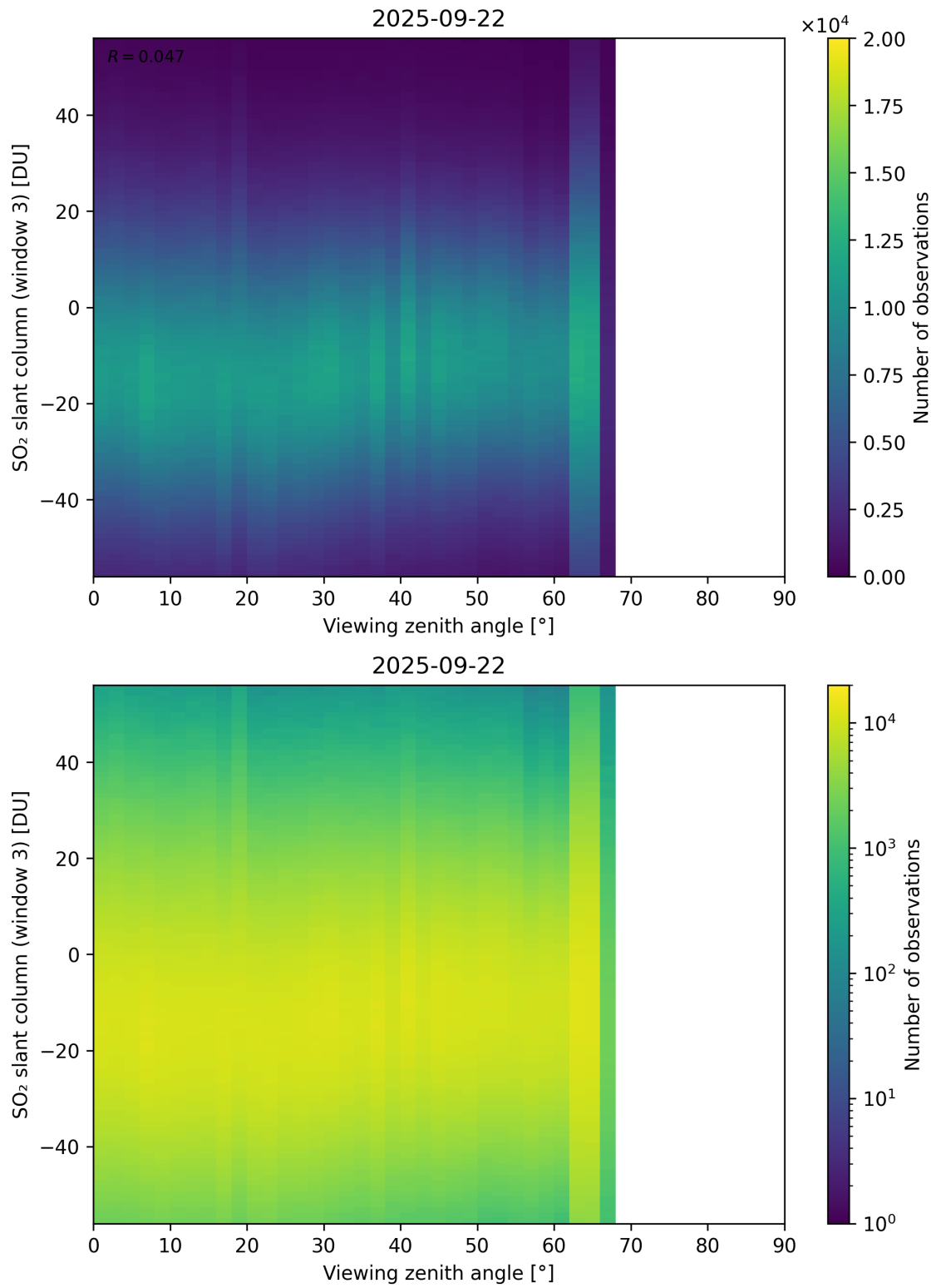
Figure 379: Scatter density plot of “Viewing zenith angle” against “SO 2 slant column (window 3)” for 2025-09-22 to 2025-09-23.
