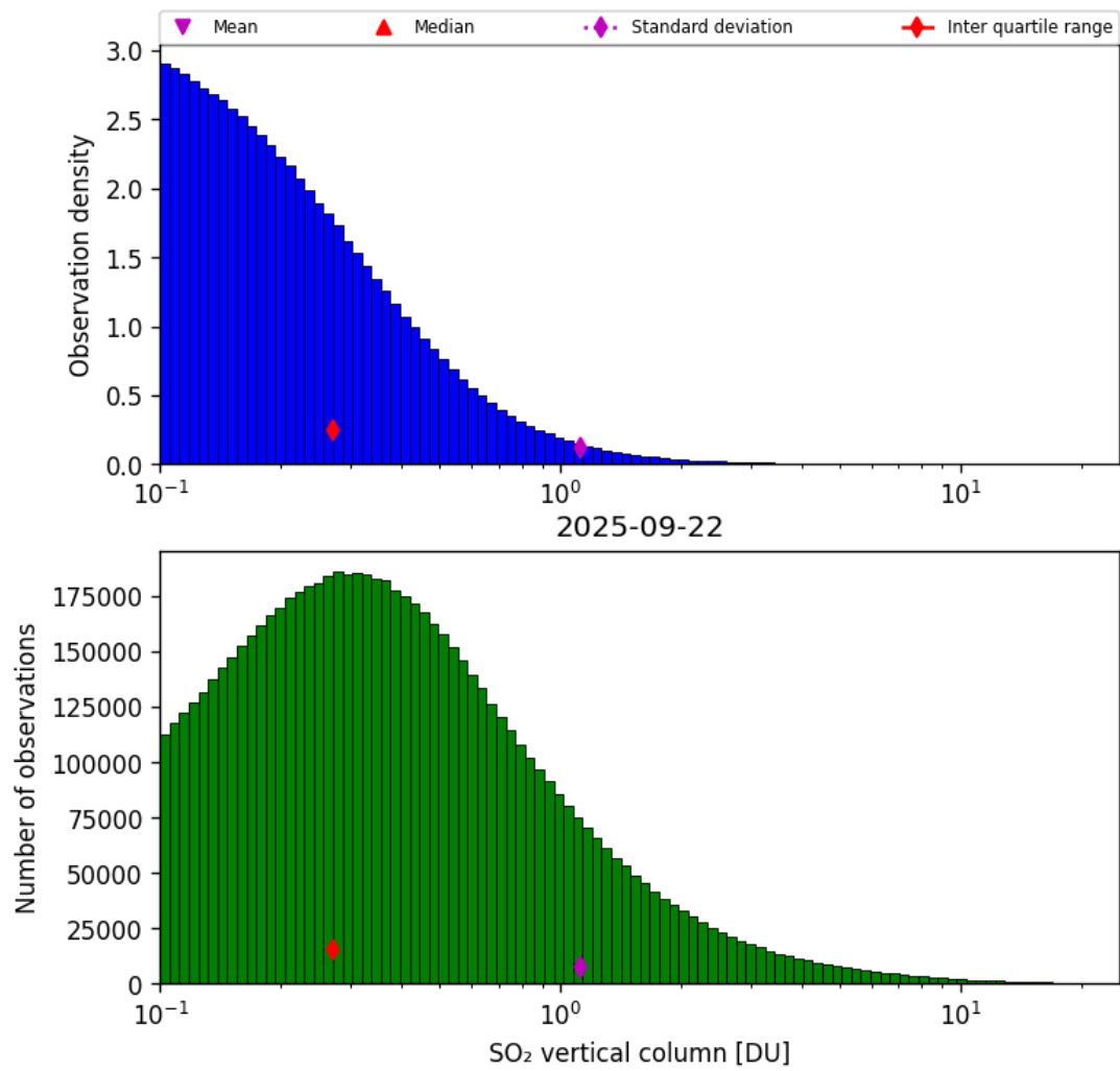
Figure 58: Histogram of “SO 2 vertical column” for 2025-09-22 to 2025-09-23
