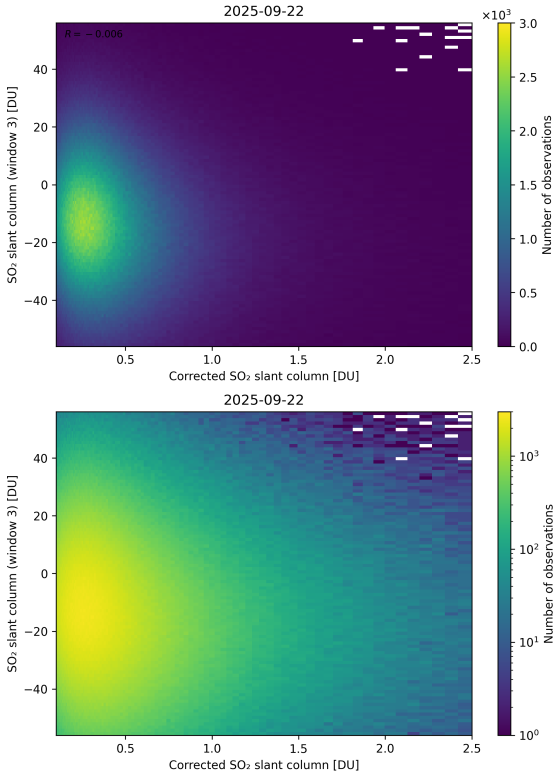
Figure 240: Scatter density plot of “Corrected SO 2 slant column” against “SO 2 slant column (window 3)” for 2025-09-22 to 2025-09-23.
