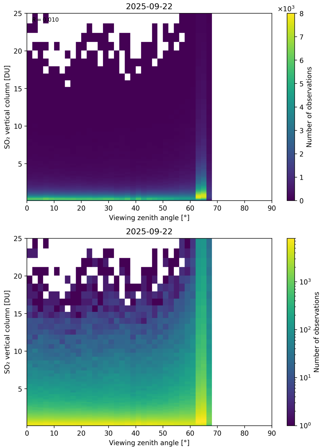
Figure 383: Scatter density plot of “Viewing zenith angle” against “SO 2 vertical column” for 2025-09-22 to 2025-09-23.
