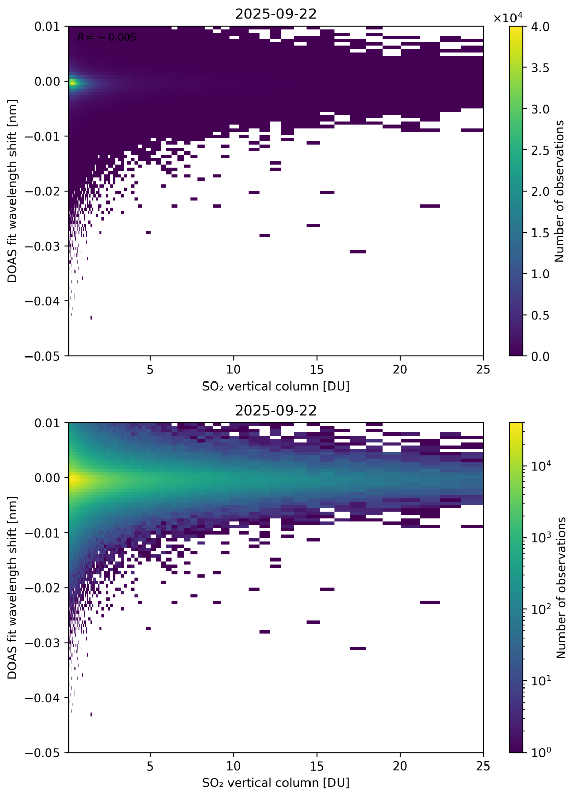
Figure 326: Scatter density plot of “SO 2 vertical column” against “DOAS fit wavelength shift” for 2025-09-22 to 2025-09-23.
