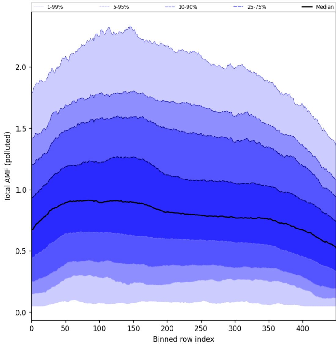
Figure 105: Along track statistics of “Total AMF (polluted)” for 2025-09-22 to 2025-09-23
