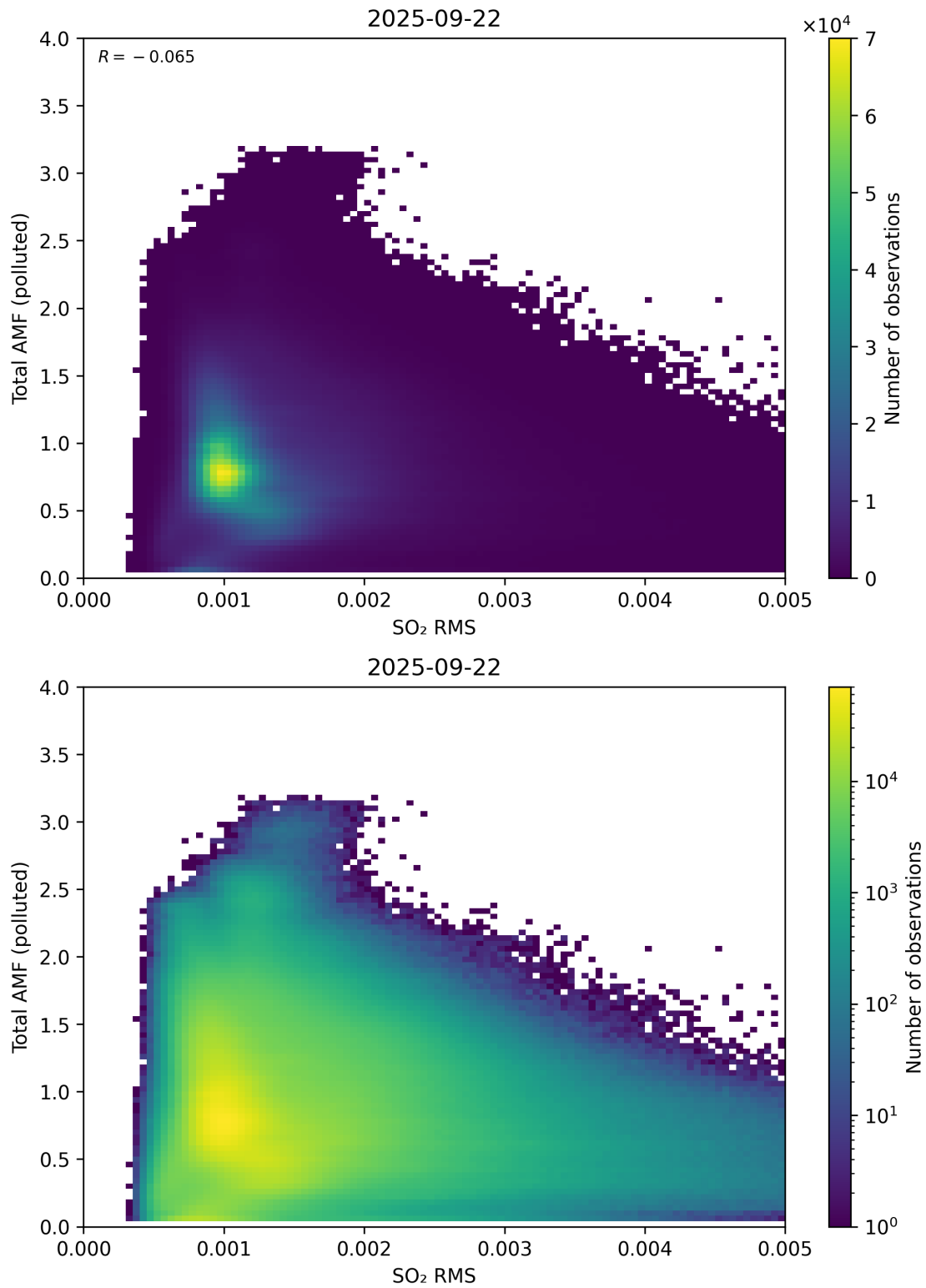
Figure 148: Scatter density plot of “SO 2 RMS” against “Total AMF (polluted)” for 2025-09-22 to 2025-09-23.
