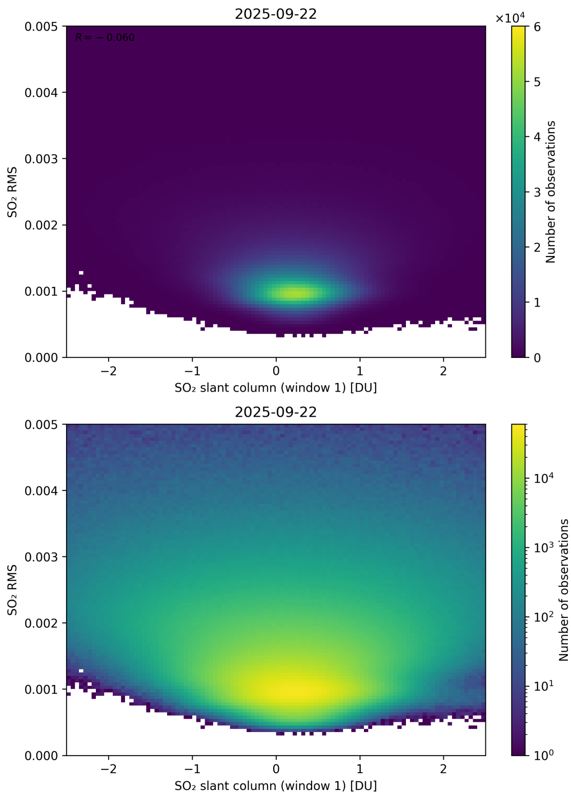
Figure 267: Scatter density plot of “SO 2 slant column (window 1)” against “SO 2 RMS” for 2025-09-22 to 2025-09-23.
