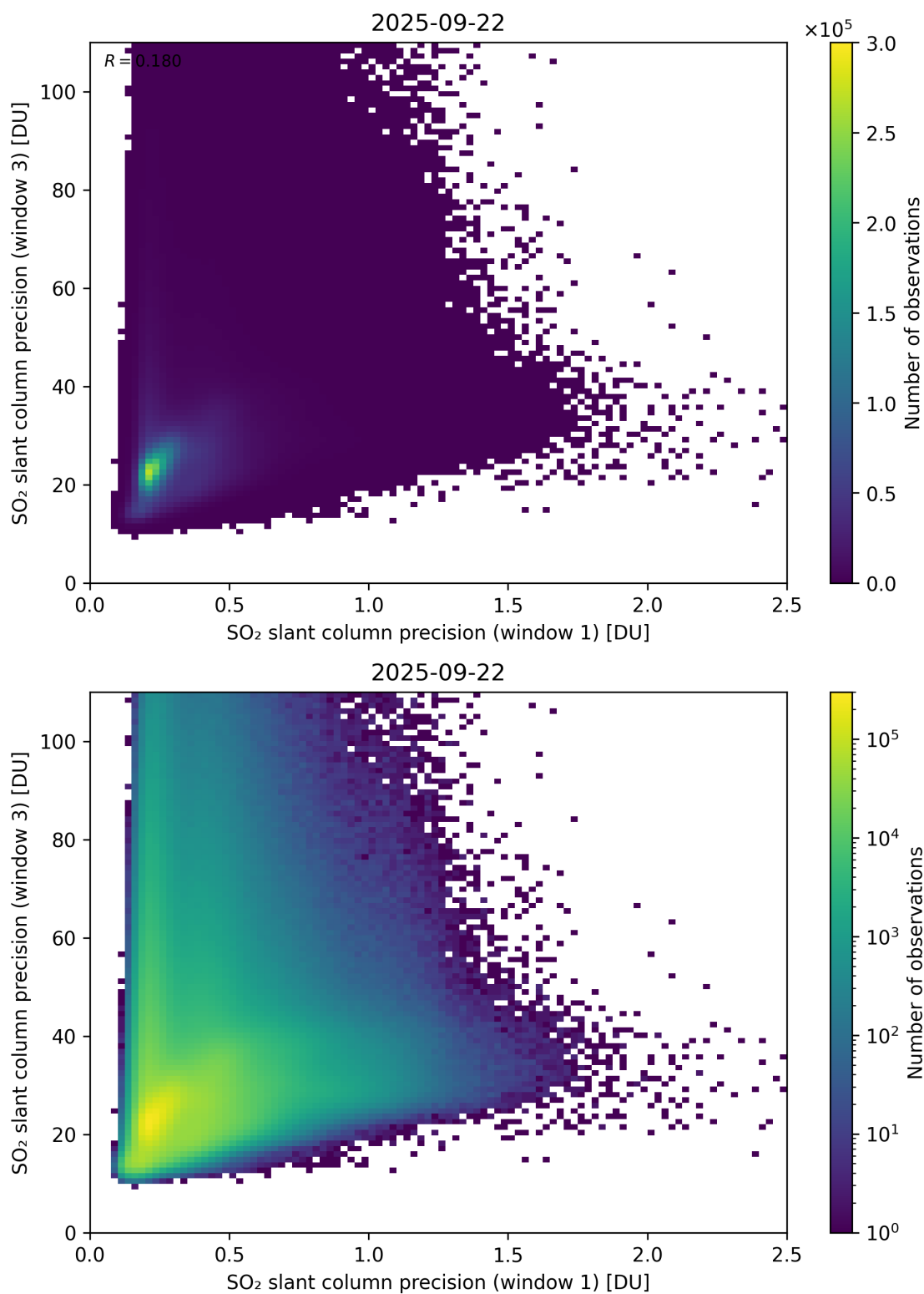
Figure 279: Scatter density plot of “SO 2 slant column precision (window 1)” against “SO 2 slant column precision (window 3)” for 2025-09-22 to 2025-09-23.
