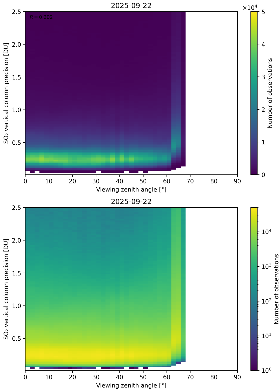
Figure 384: Scatter density plot of “Viewing zenith angle” against “SO 2 vertical column precision” for 2025-09-22 to 2025-09-23.
