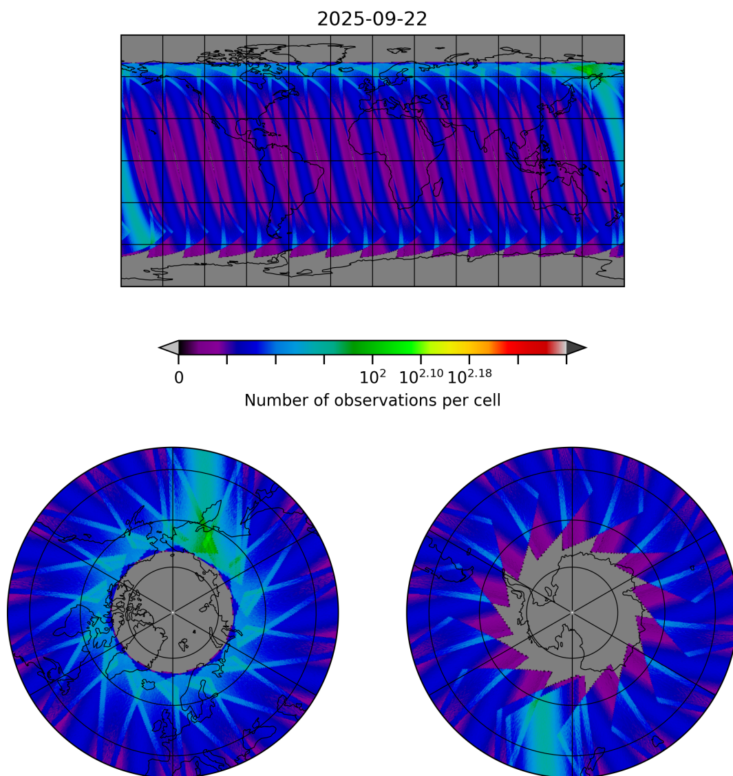
Figure 30: Map of the number of observations for 2025-09-22 to 2025-09-23
