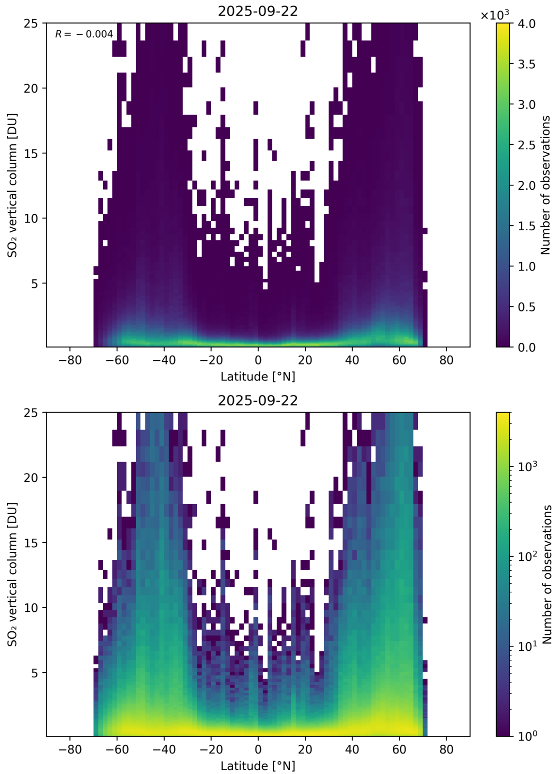
Figure 169: Scatter density plot of “Latitude” against “SO 2 vertical column” for 2025-09-22 to 2025-09-23.
