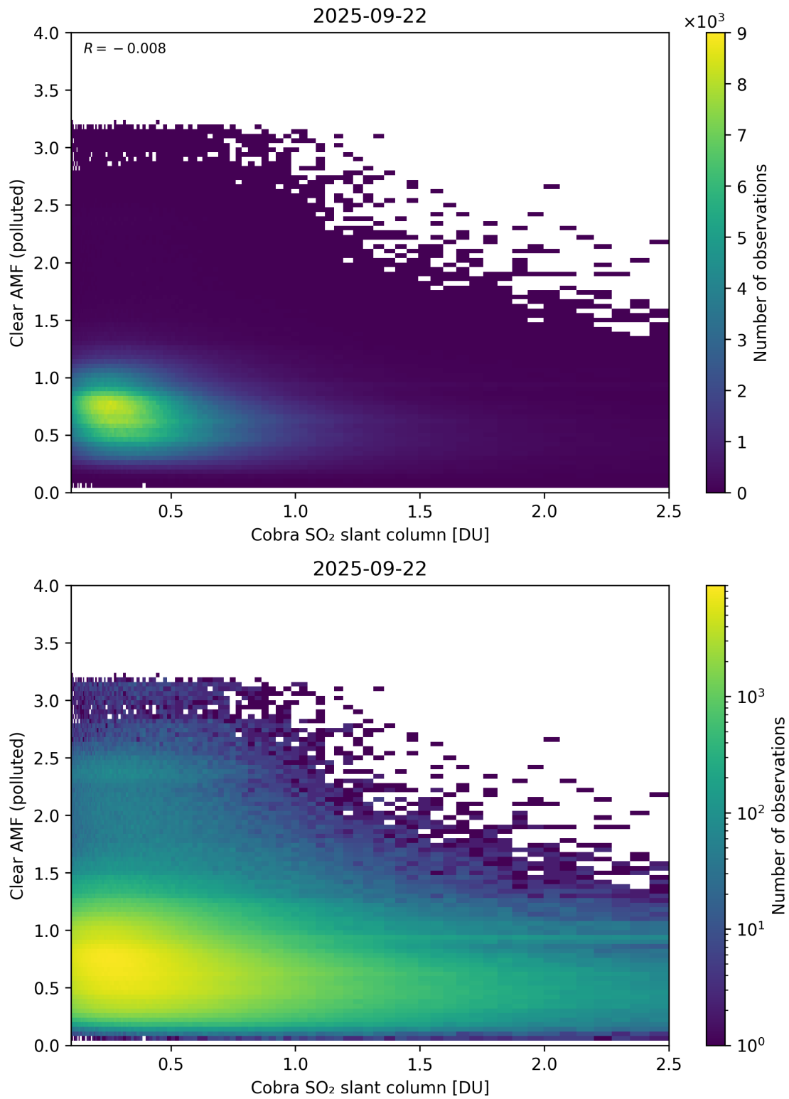
Figure 215: Scatter density plot of “Cobra SO 2 slant column” against “Clear AMF (polluted)” for 2025-09-22 to 2025-09-23.
