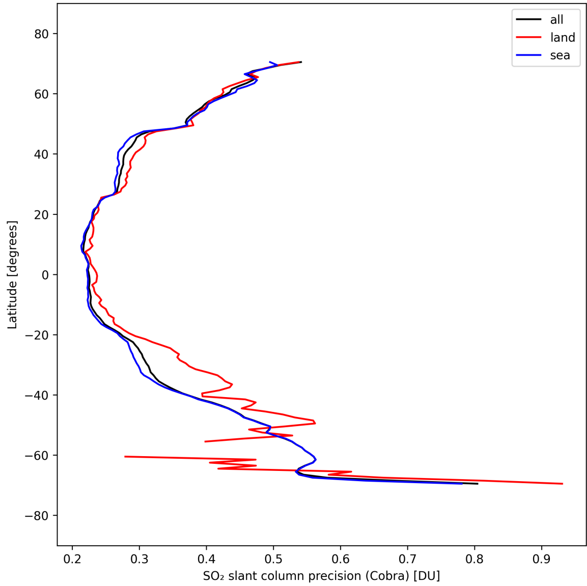
Figure 36: Zonal average of “SO 2 slant column precision (Cobra)” for 2025-09-22 to 2025-09-23.
