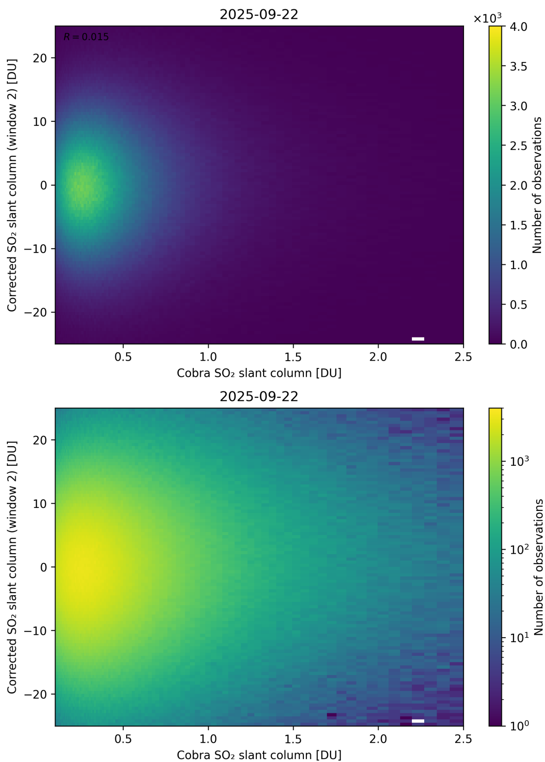
Figure 217: Scatter density plot of “Cobra SO 2 slant column” against “Corrected SO 2 slant column (window 2)” for 2025-09-22 to 2025-09-23.
