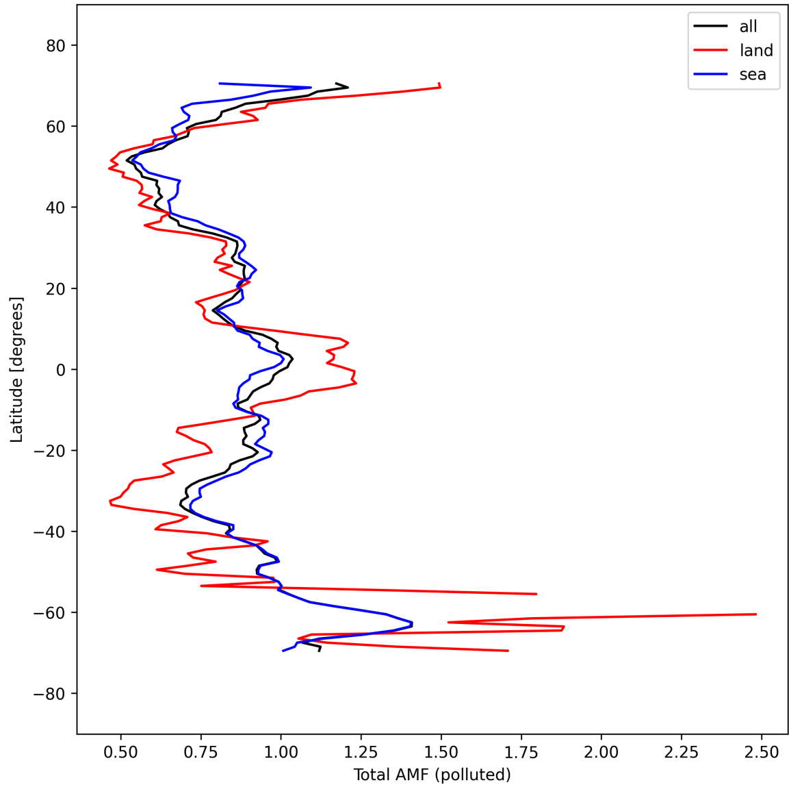
Figure 53: Zonal average of “Total AMF (polluted)” for 2025-09-22 to 2025-09-23.
