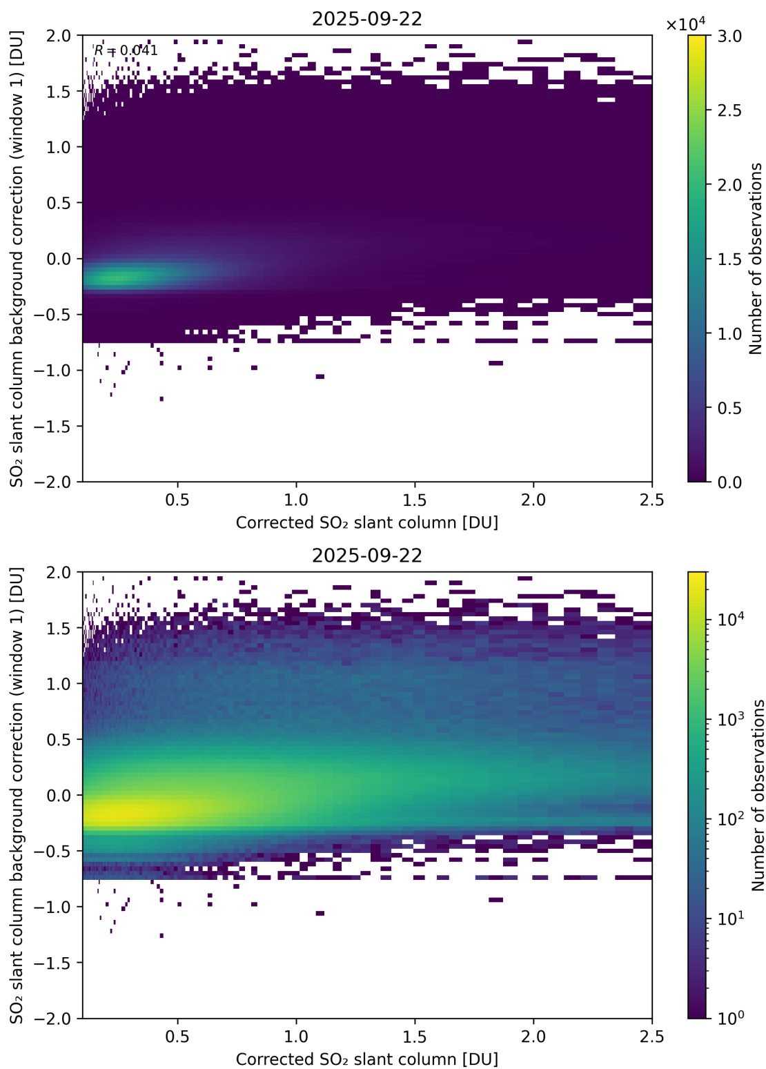
Figure 226: Scatter density plot of “Corrected SO 2 slant column” against “SO 2 slant column background correction (window 1)” for 2025-09-22 to 2025-09-23.
