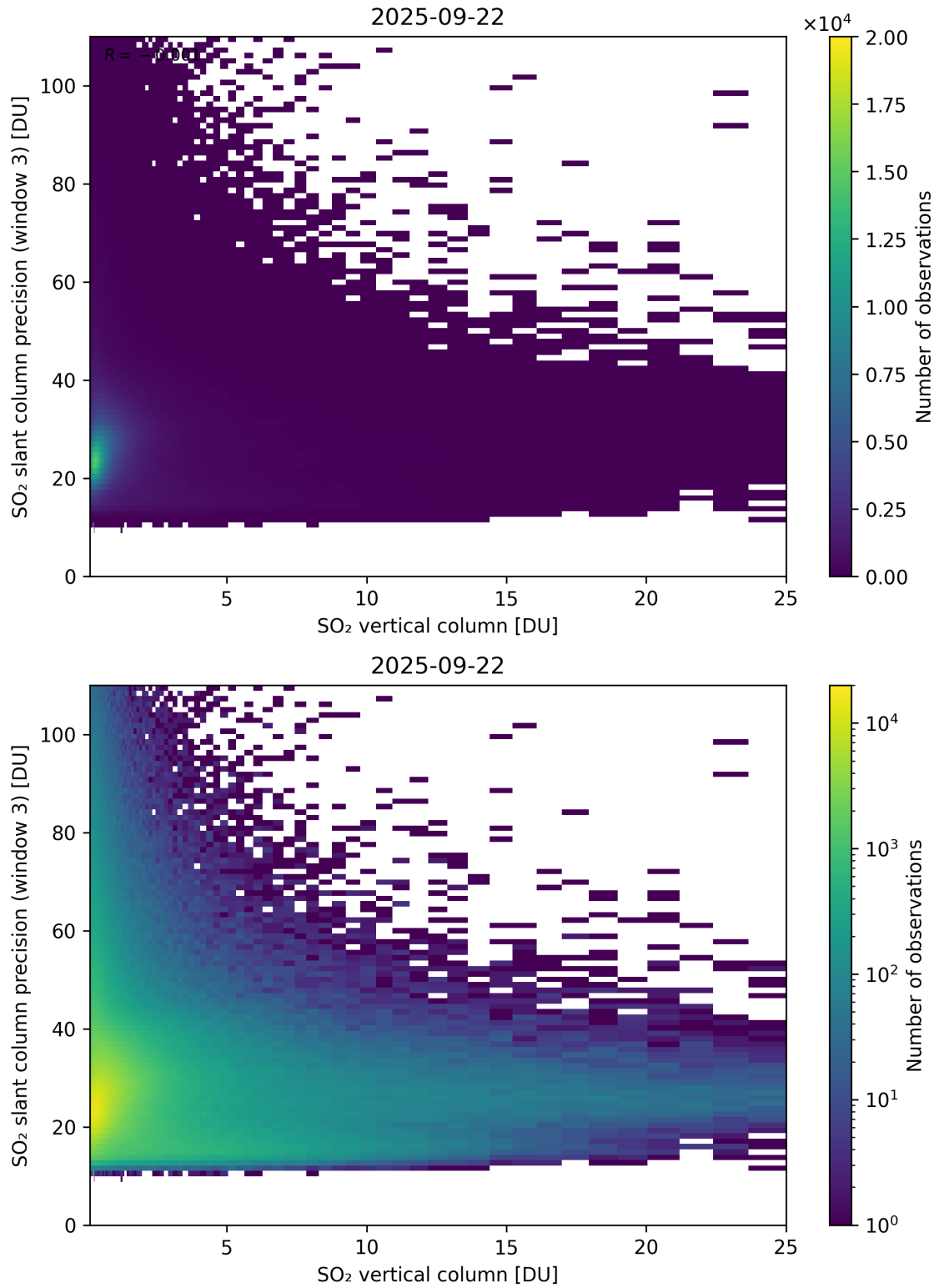
Figure 358: Scatter density plot of “SO 2 vertical column” against “SO 2 slant column precision (window 3)” for 2025-09-22 to 2025-09-23.
