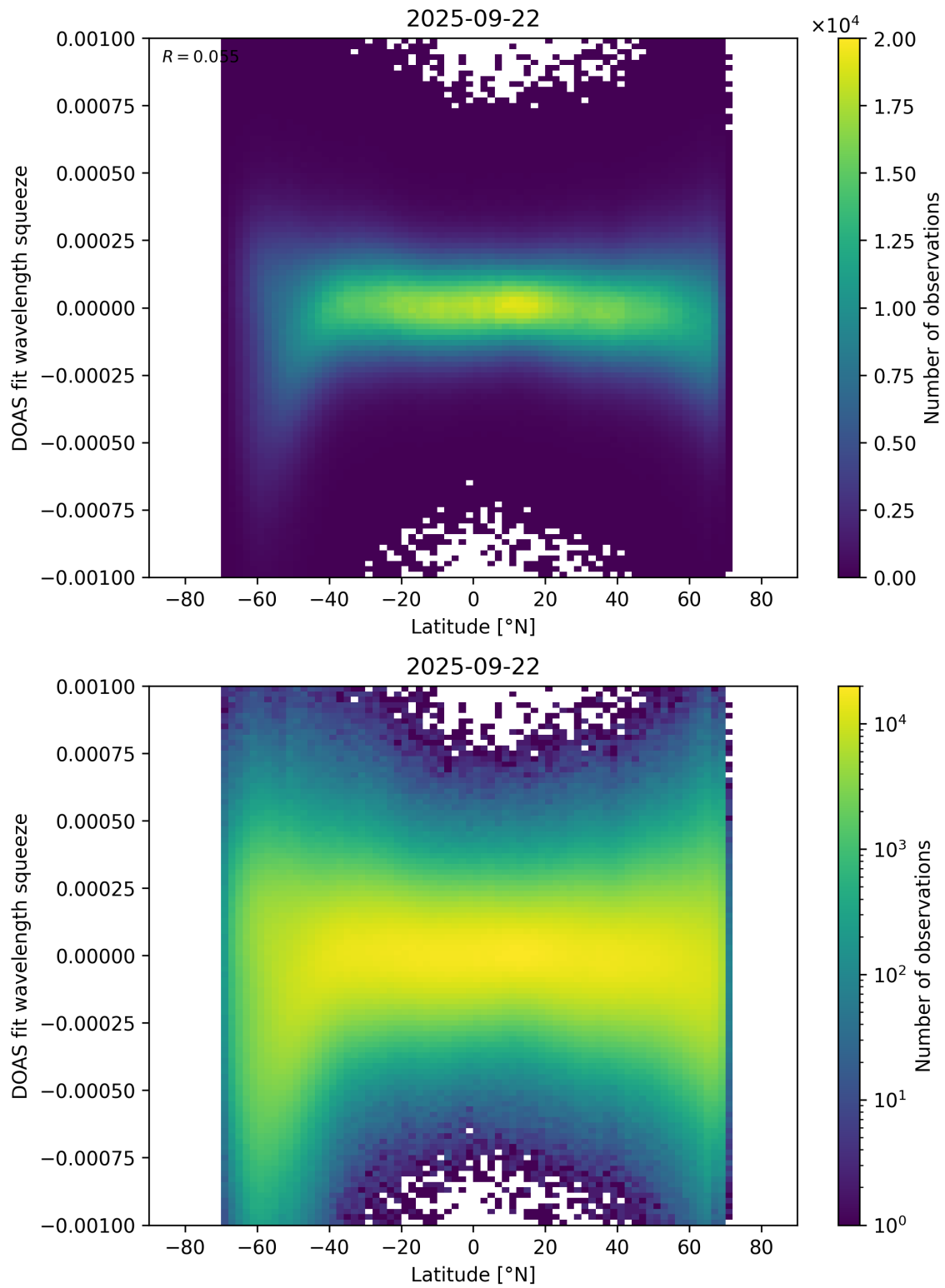
Figure 154: Scatter density plot of “Latitude” against “DOAS fit wavelength squeeze” for 2025-09-22 to 2025-09-23.
