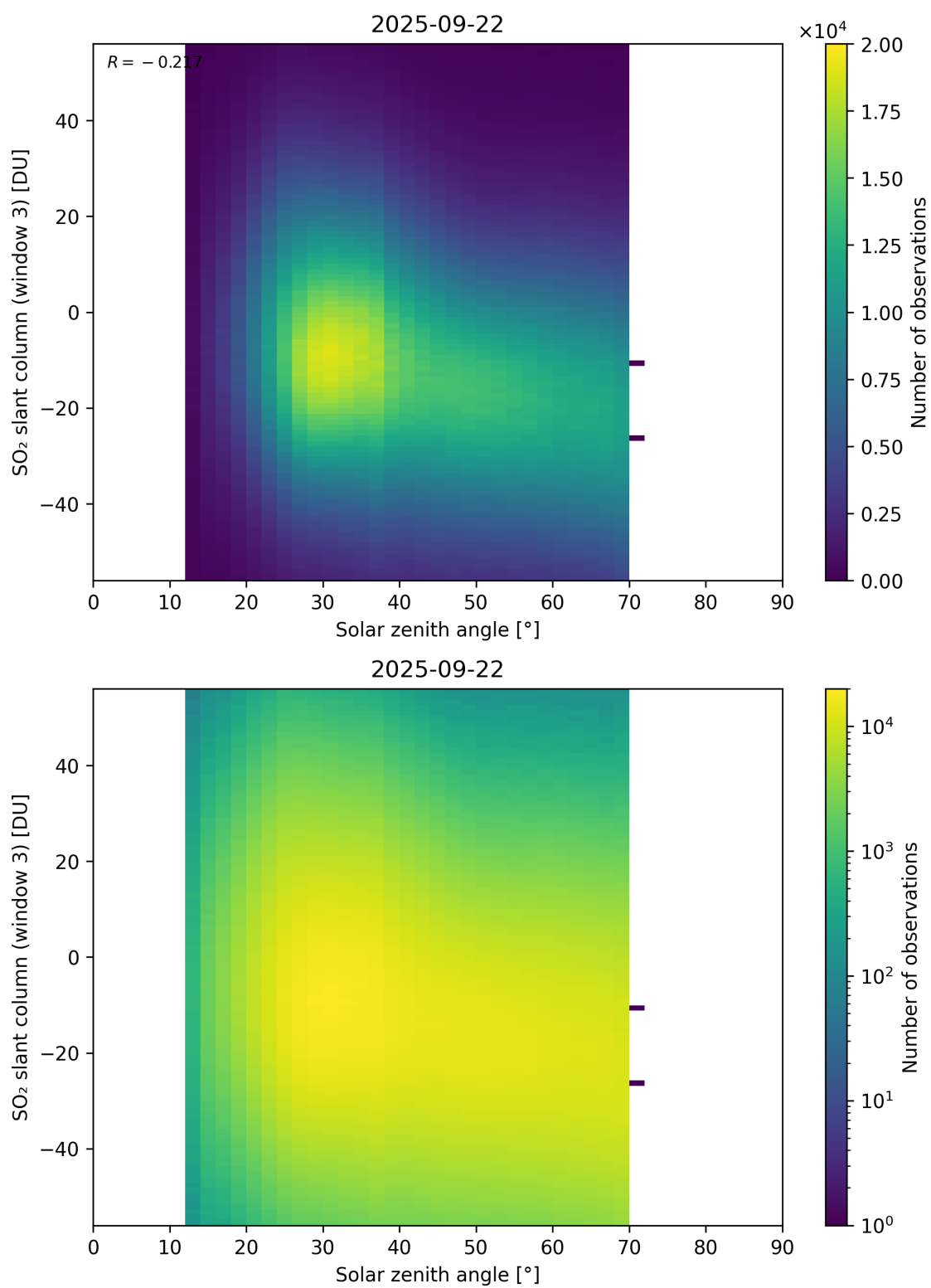
Figure 187: Scatter density plot of “Solar zenith angle” against “SO 2 slant column (window 3)” for 2025-09-22 to 2025-09-23.
