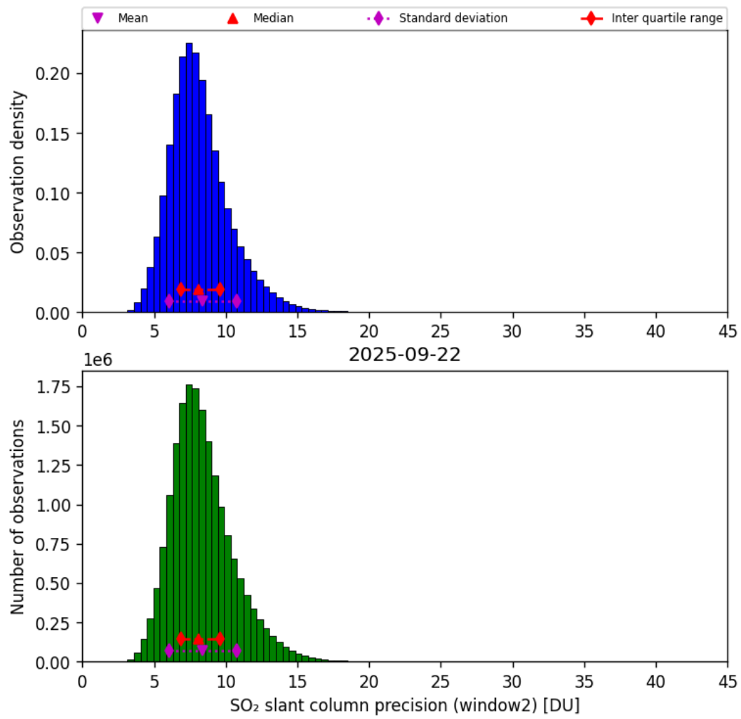
Figure 68: Histogram of “SO 2 slant column precision (window2)” for 2025-09-22 to 2025-09-23
