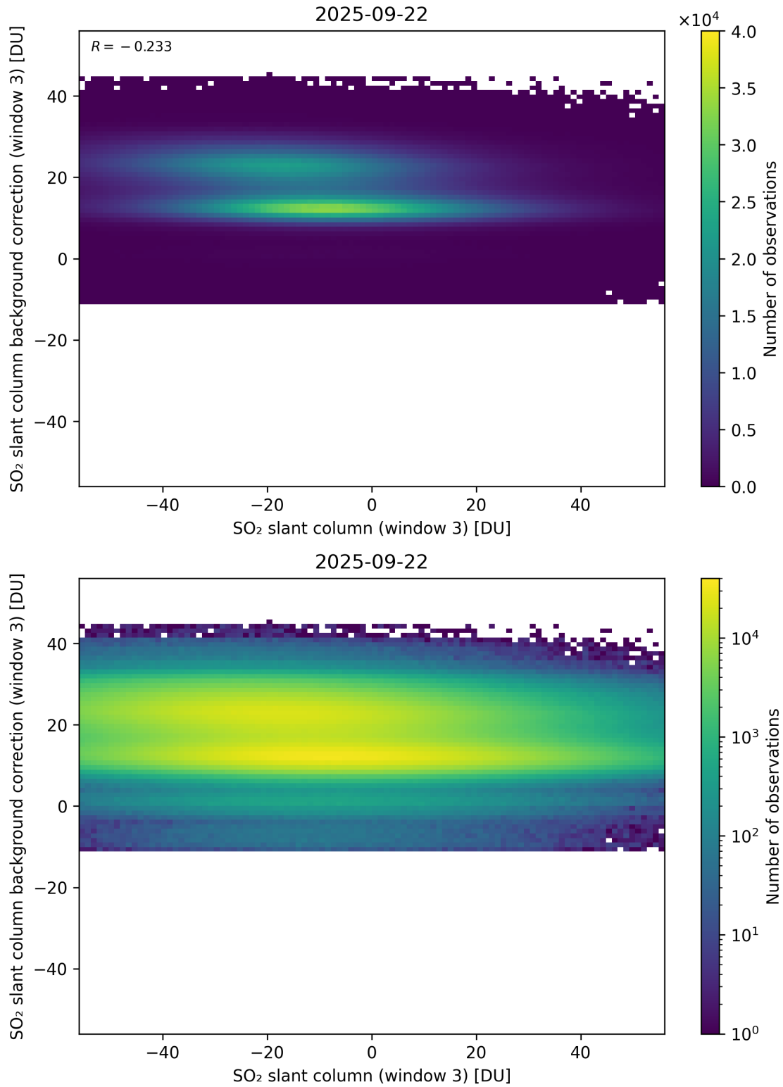
Figure 303: Scatter density plot of “SO 2 slant column (window 3)” against “SO 2 slant column background correction (window 3)” for 2025-09-22 to 2025-09-23.
