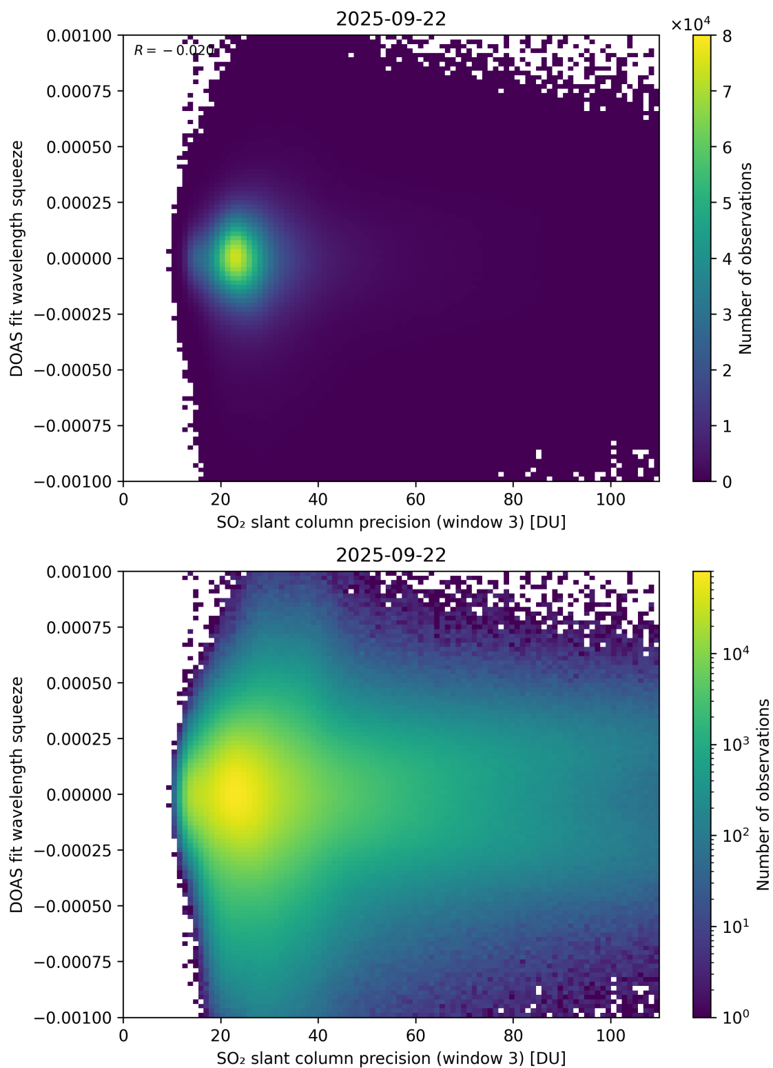
Figure 309: Scatter density plot of “SO 2 slant column precision (window 3)” against “DOAS fit wavelength squeeze” for 2025-09-22 to 2025-09-23.
