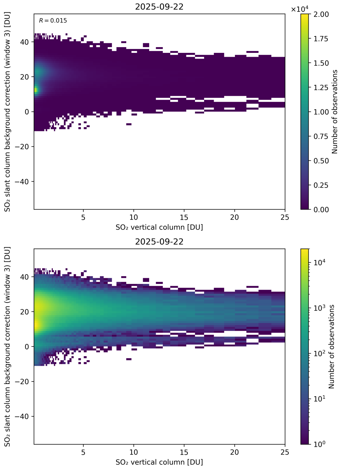
Figure 325: Scatter density plot of “SO 2 vertical column” against “SO 2 slant column background correction (window 3)” for 2025-09-22 to 2025-09-23.
