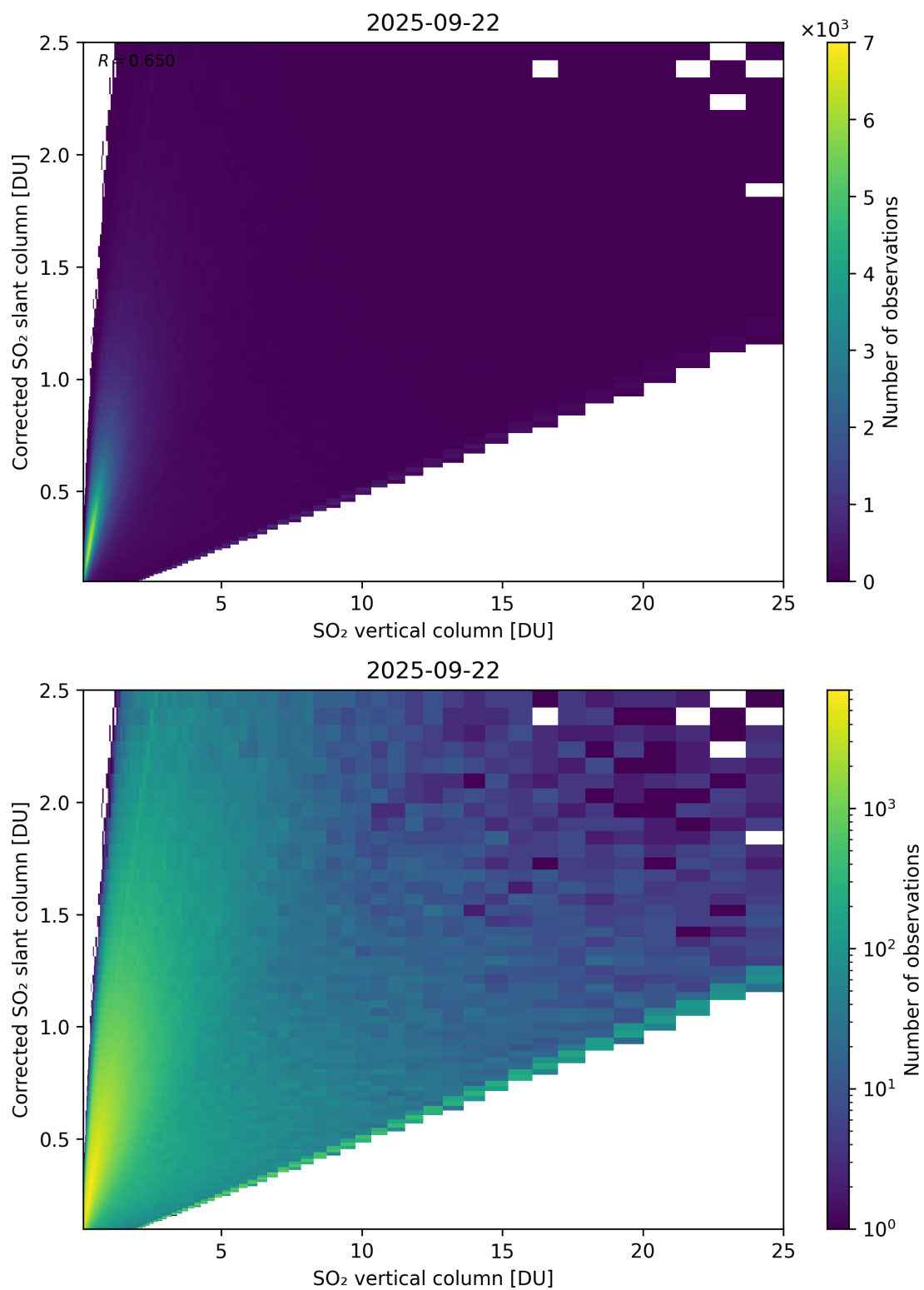
Figure 351: Scatter density plot of “SO 2 vertical column” against “Corrected SO 2 slant column” for 2025-09-22 to 2025-09-23.
