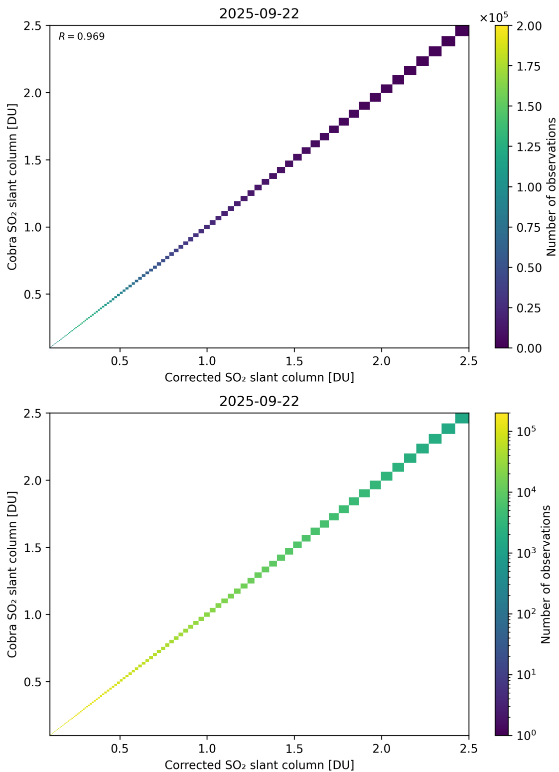
Figure 233: Scatter density plot of “Corrected SO 2 slant column” against “Cobra SO 2 slant column” for 2025-09-22 to 2025-09-23.
