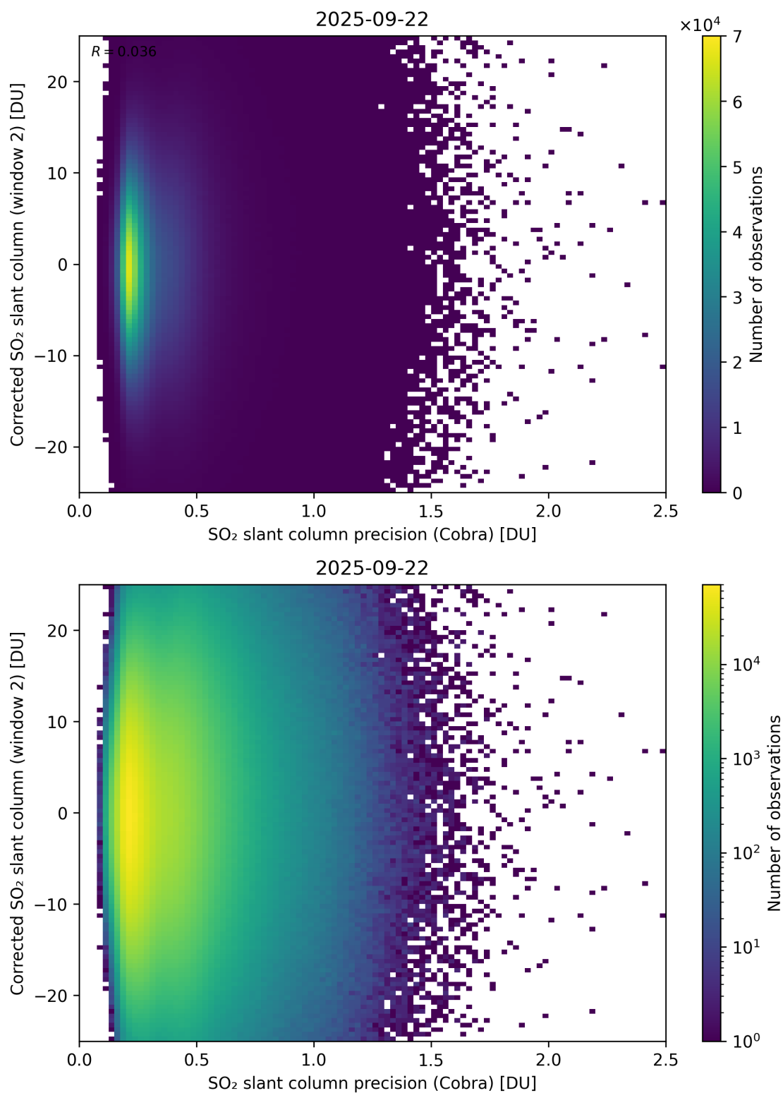
Figure 206: Scatter density plot of “SO 2 slant column precision (Cobra)” against “Corrected SO 2 slant column (window 2)” for 2025-09-22 to 2025-09-23.
