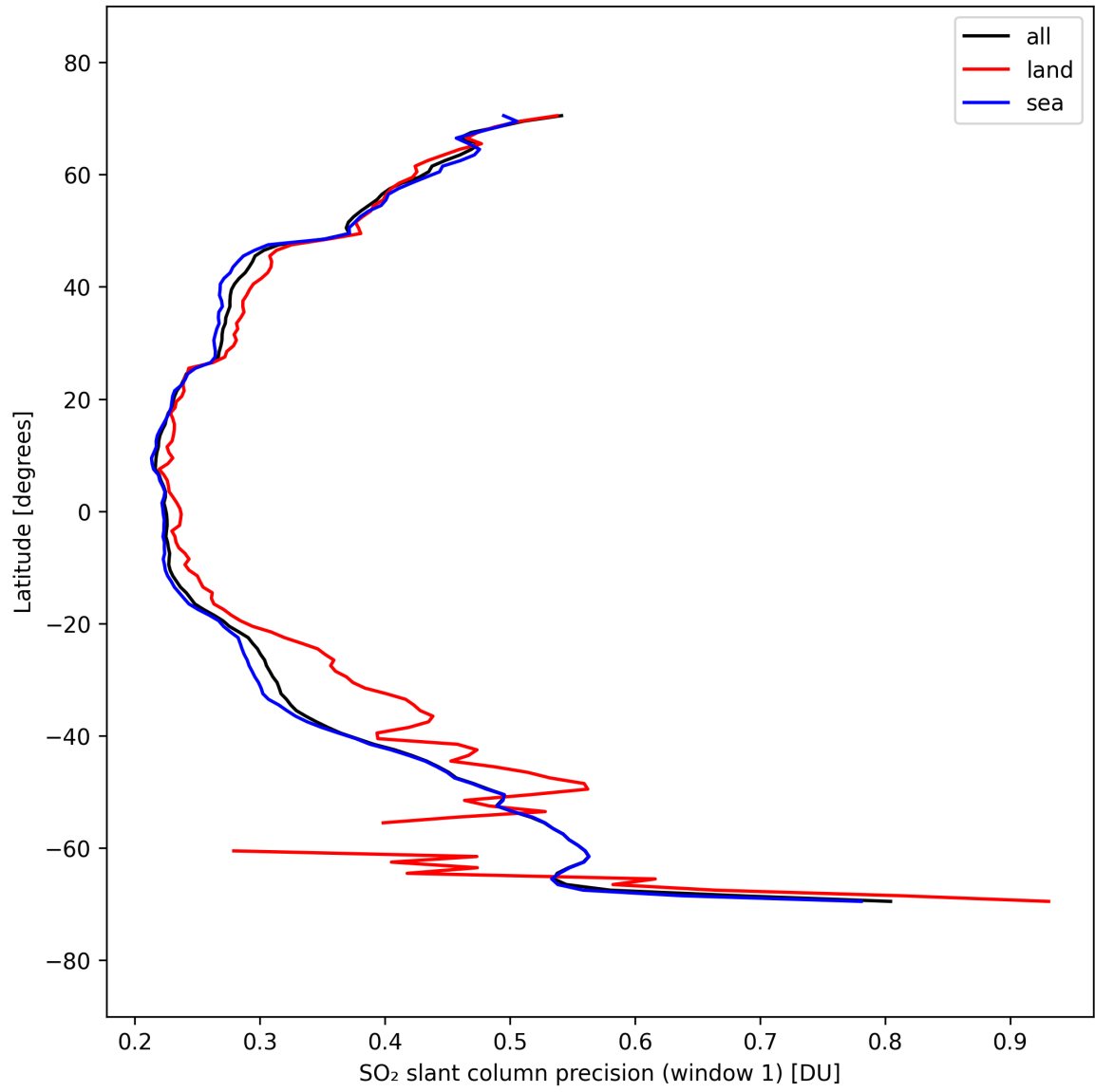
Figure 38: Zonal average of "SO 2 slant column precision (window 1)" for 2025-09-22 to 2025-09-23.
