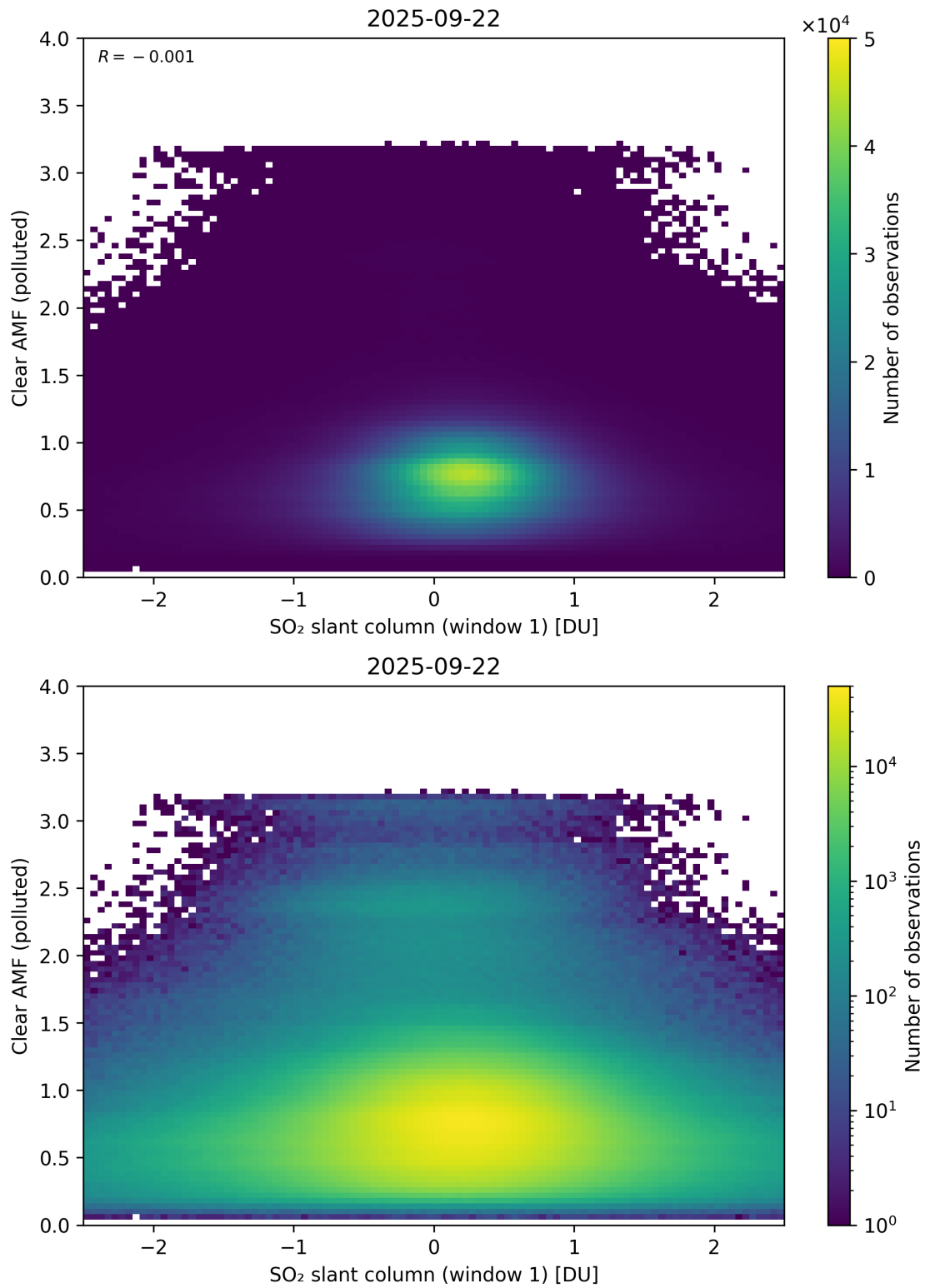
Figure 282: Scatter density plot of “SO 2 slant column (window 1)” against “Clear AMF (polluted)” for 2025-09-22 to 2025-09-23.
