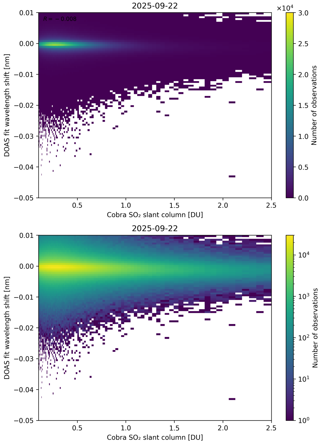
Figure 196: Scatter density plot of “Cobra SO 2 slant column” against “DOAS fit wavelength shift” for 2025-09-22 to 2025-09-23.
