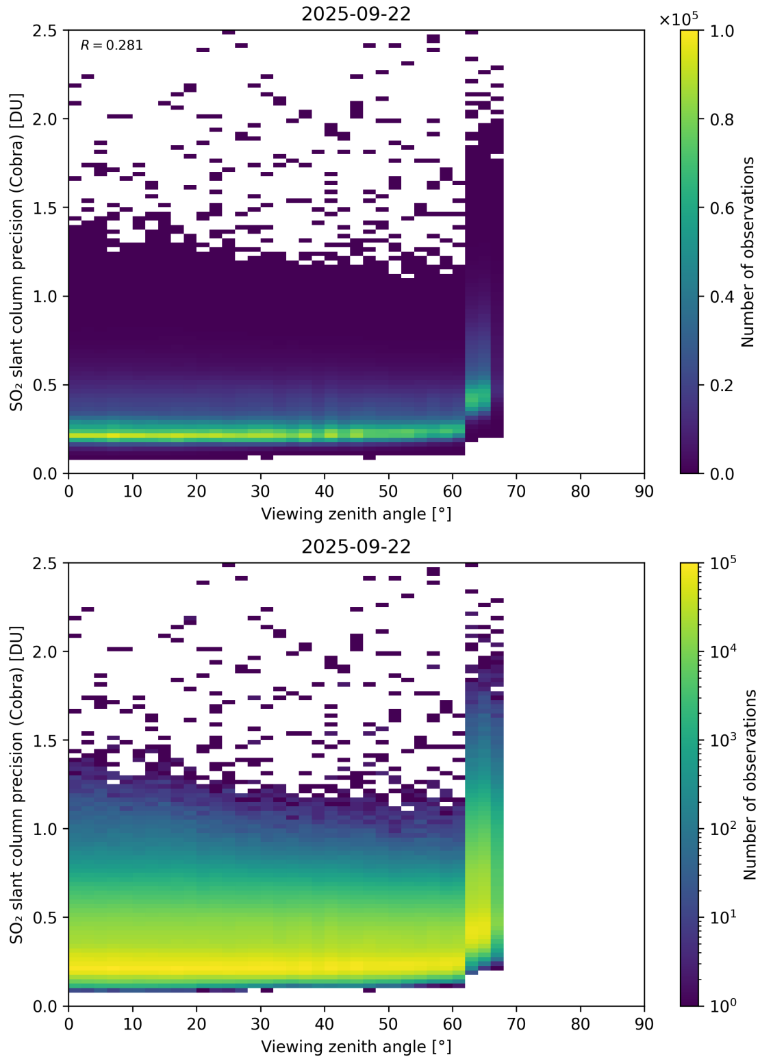
Figure 372: Scatter density plot of “Viewing zenith angle” against “SO 2 slant column precision (Cobra)” for 2025-09-22 to 2025-09-23.
