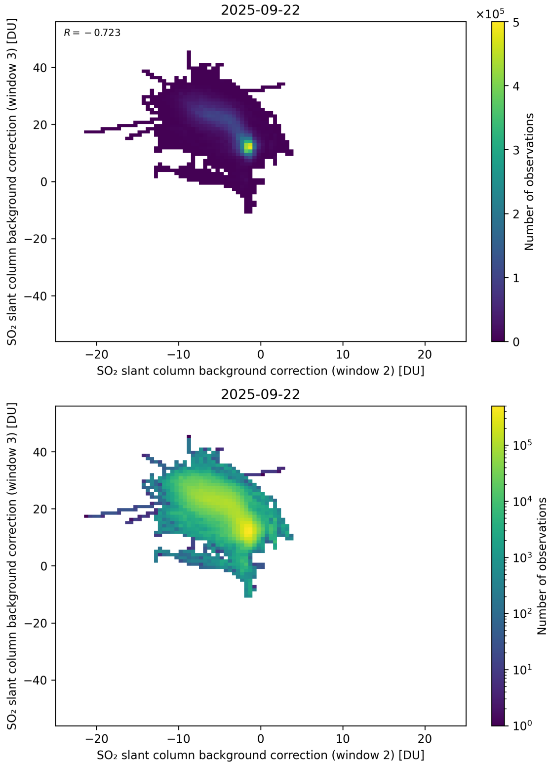
Figure 122: Scatter density plot of “SO 2 slant column background correction (window 2)” against “SO 2 slant column background correction (window 3)” for 2025-09-22 to 2025-09-23.
