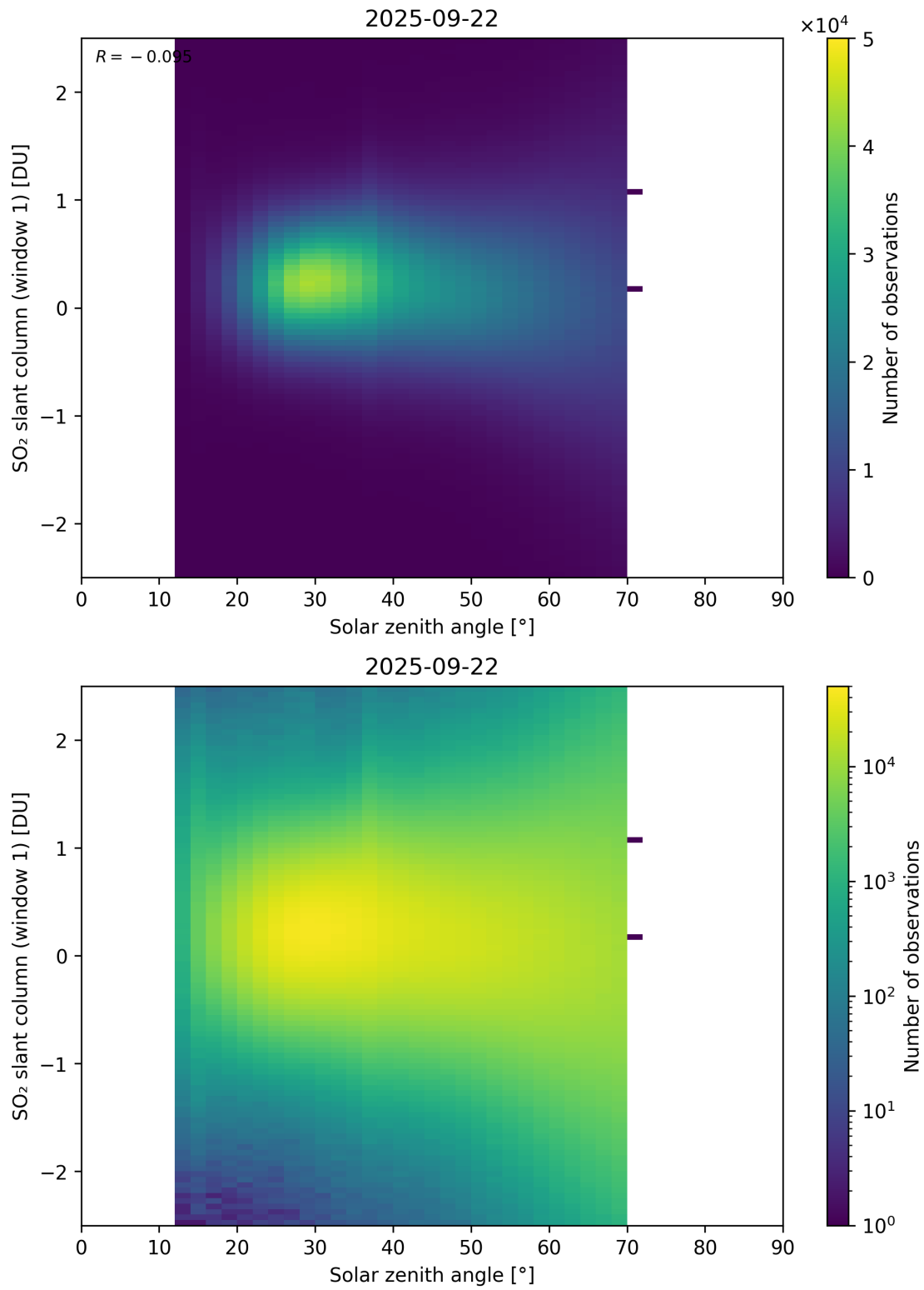
Figure 184: Scatter density plot of “Solar zenith angle” against “SO 2 slant column (window 1)” for 2025-09-22 to 2025-09-23.
