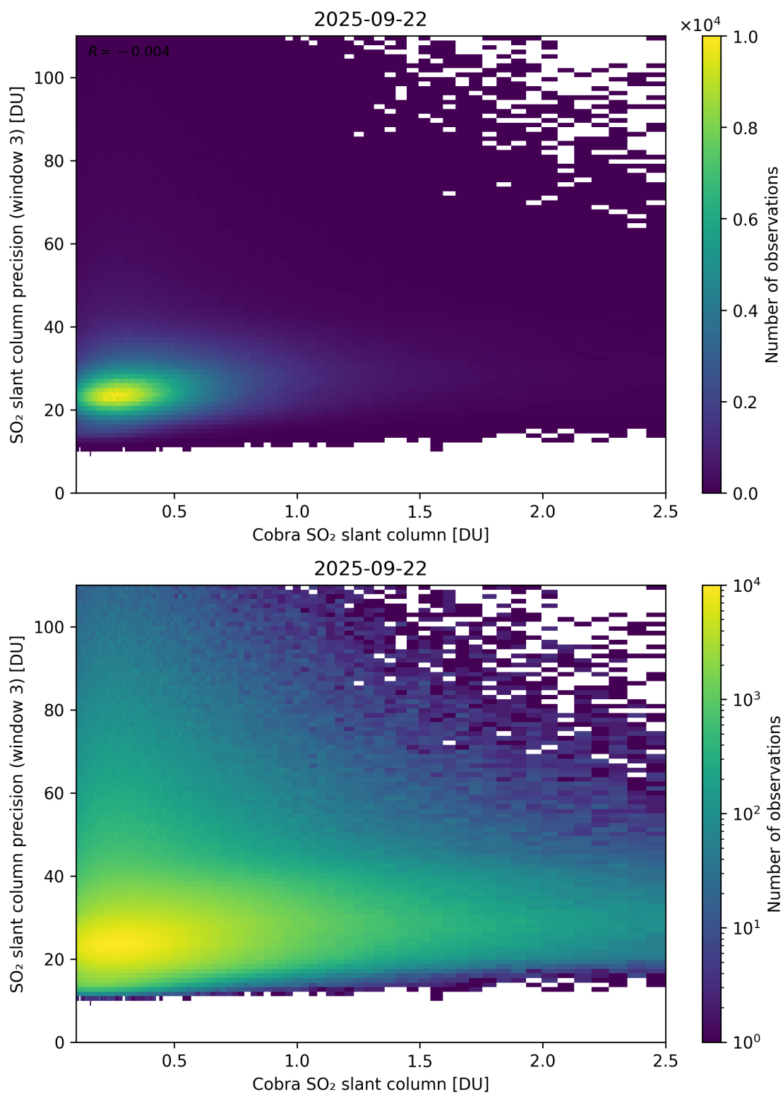
Figure 223: Scatter density plot of “Cobra SO 2 slant column” against “SO 2 slant column precision (window 3)” for 2025-09-22 to 2025-09-23.
