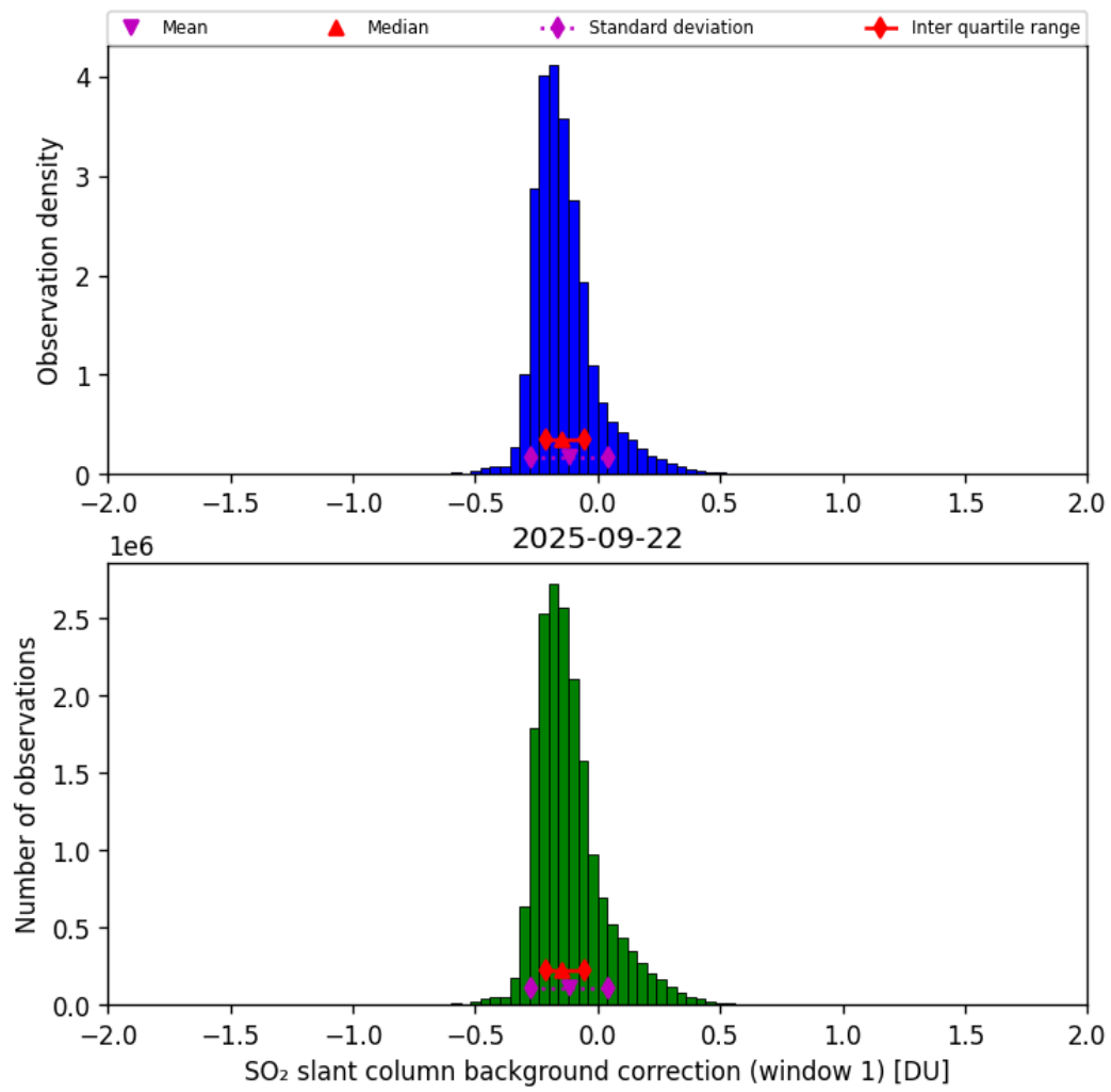
Figure 66: Histogram of “SO 2 slant column background correction (window 1)” for 2025-09-22 to 2025-09-23
