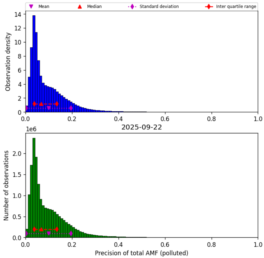
Figure 80: Histogram of “Precision of total AMF (polluted)” for 2025-09-22 to 2025-09-23
