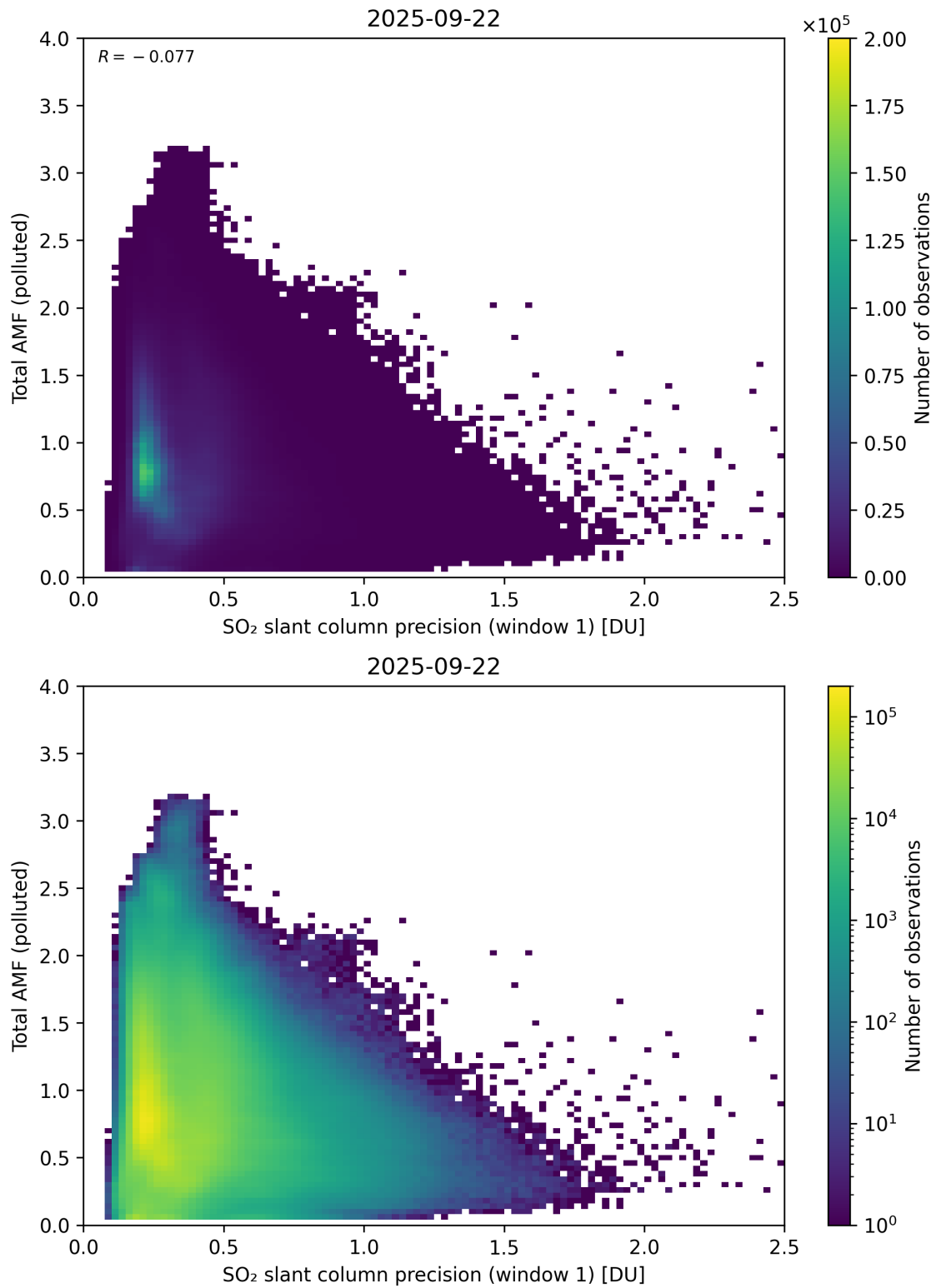
Figure 280: Scatter density plot of “SO 2 slant column precision (window 1)” against “Total AMF (polluted)” for 2025-09-22 to 2025-09-23.
