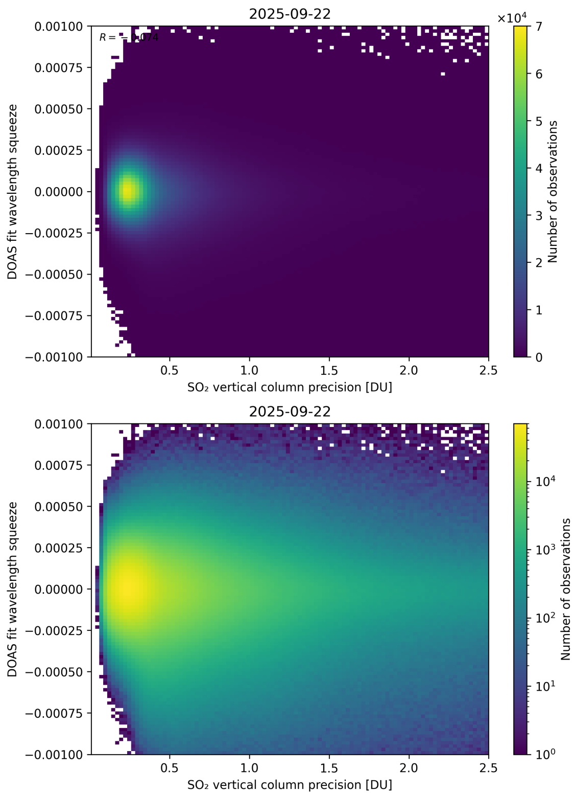
Figure 333: Scatter density plot of “SO 2 vertical column precision” against “DOAS fit wavelength squeeze” for 2025-09-22 to 2025-09-23.
