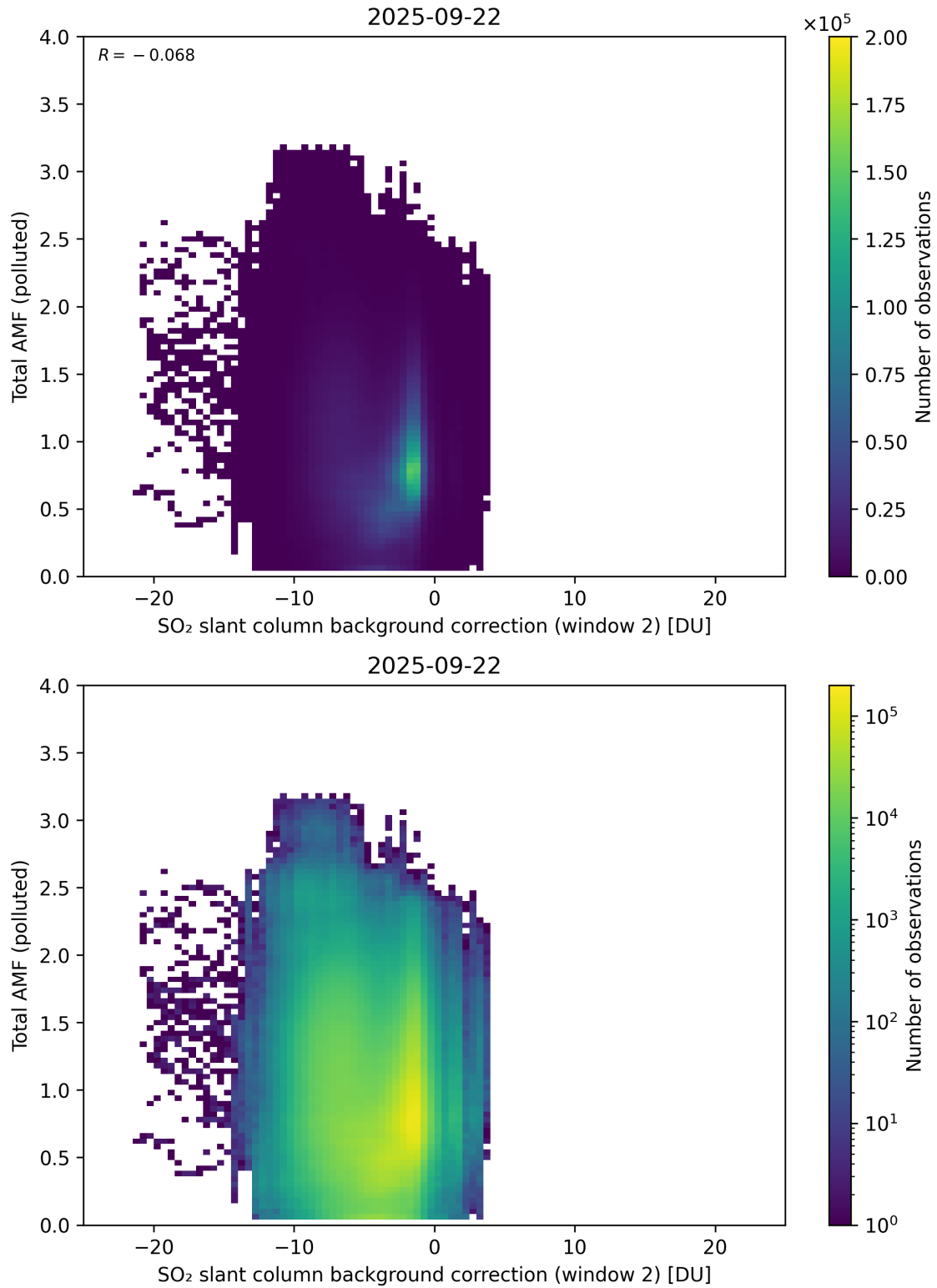
Figure 130: Scatter density plot of “SO 2 slant column background correction (window 2)” against “Total AMF (polluted)” for 2025-09-22 to 2025-09-23.
