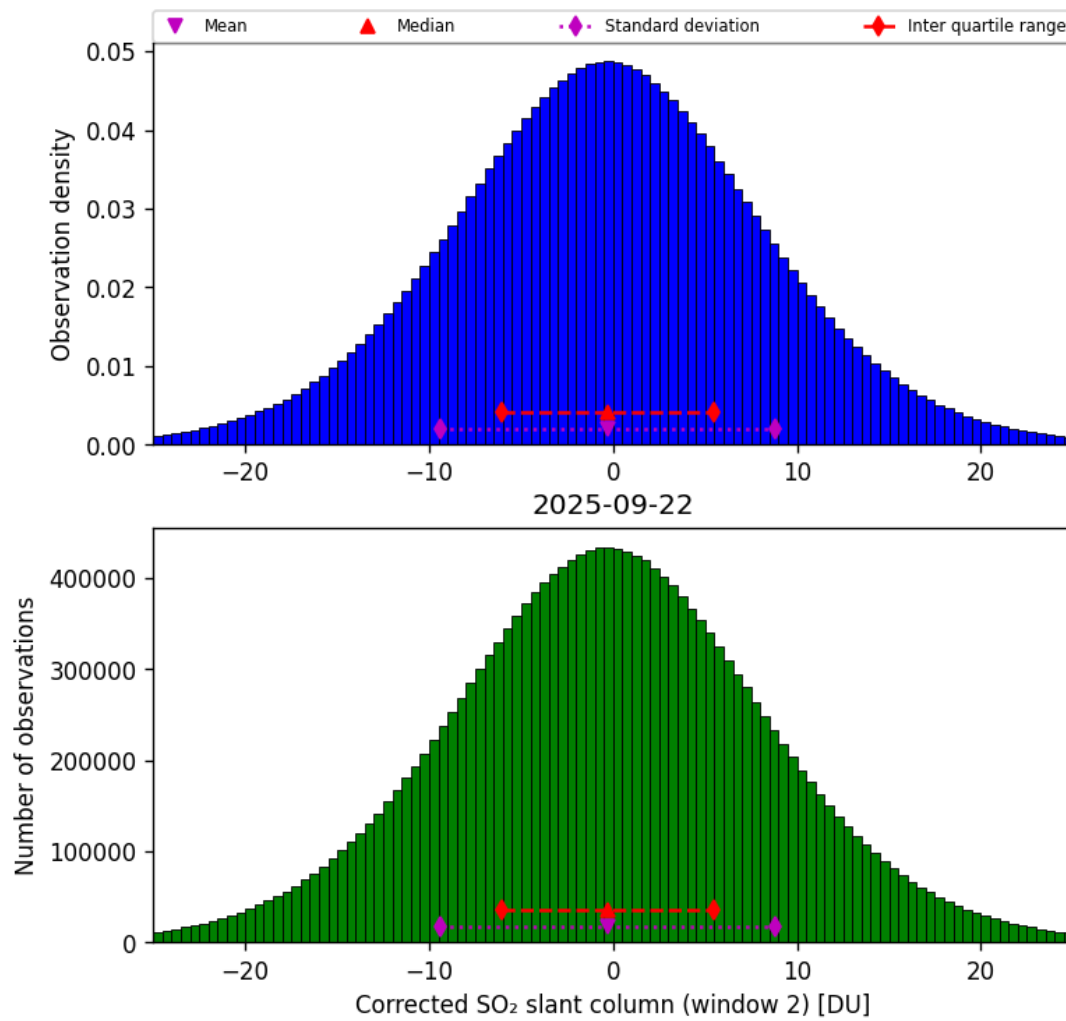
Figure 69: Histogram of “Corrected SO 2 slant column (window 2)” for 2025-09-22 to 2025-09-23
