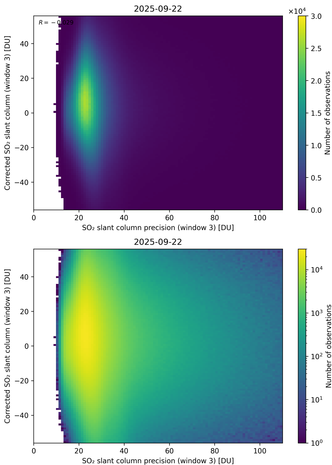
Figure 312: Scatter density plot of “SO 2 slant column precision (window 3)” against “Corrected SO 2 slant column (window 3)” for 2025-09-22 to 2025-09-23.
