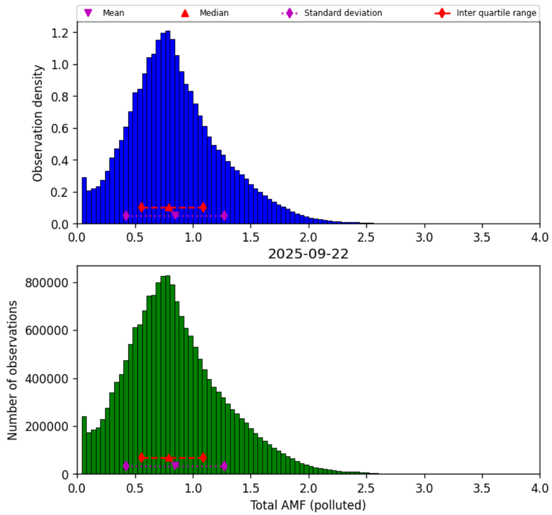
Figure 79: Histogram of “Total AMF (polluted)” for 2025-09-22 to 2025-09-23
