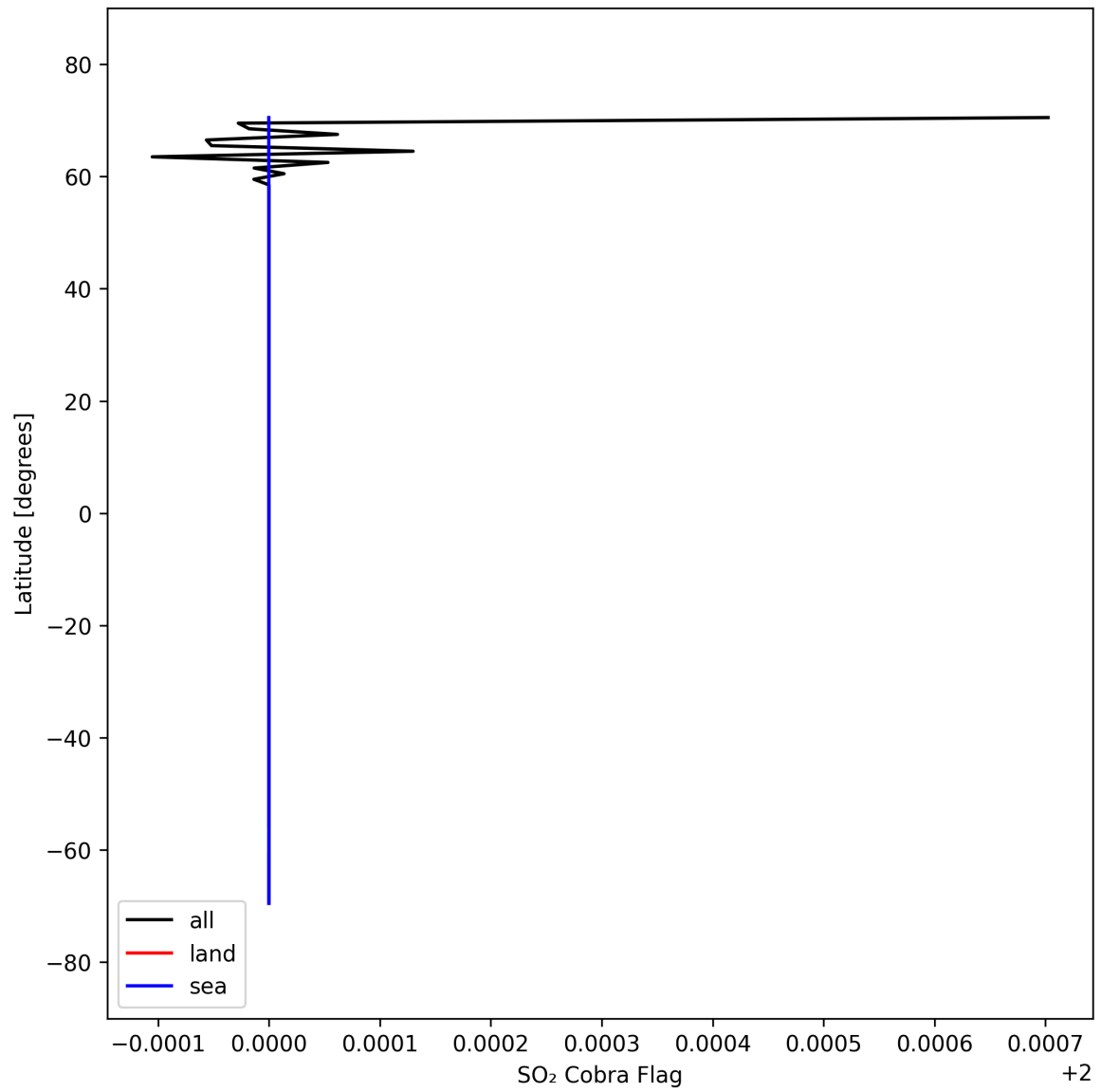
Figure 49: Zonal average of "SO 2 Cobra Flag" for 2025-09-22 to 2025-09-23.
