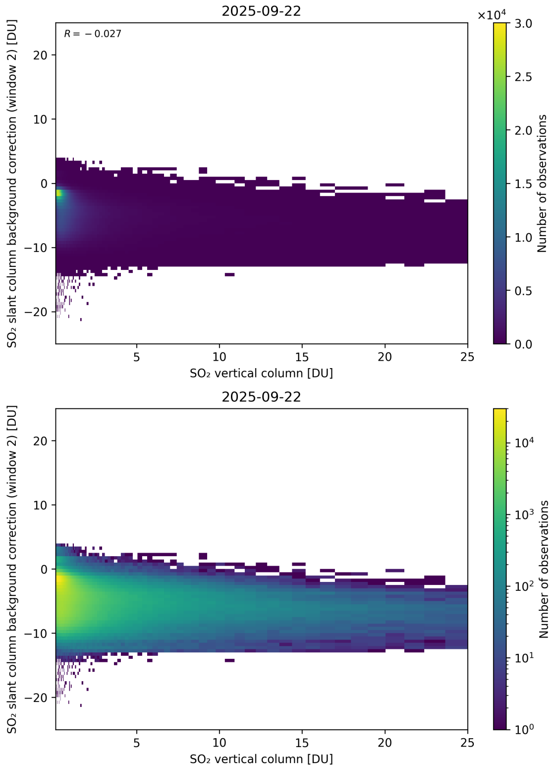
Figure 324: Scatter density plot of “SO 2 vertical column” against “SO 2 slant column background correction (window 2)” for 2025-09-22 to 2025-09-23.
