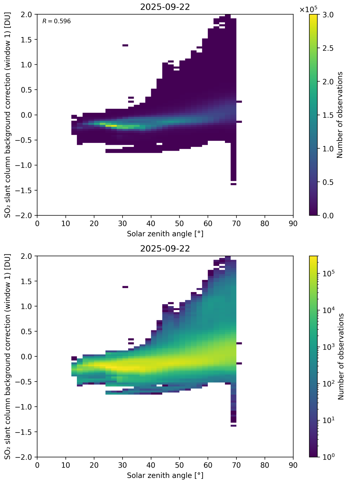
Figure 171: Scatter density plot of “Solar zenith angle” against “SO 2 slant column background correction (window 1)” for 2025-09-22 to 2025-09-23.
