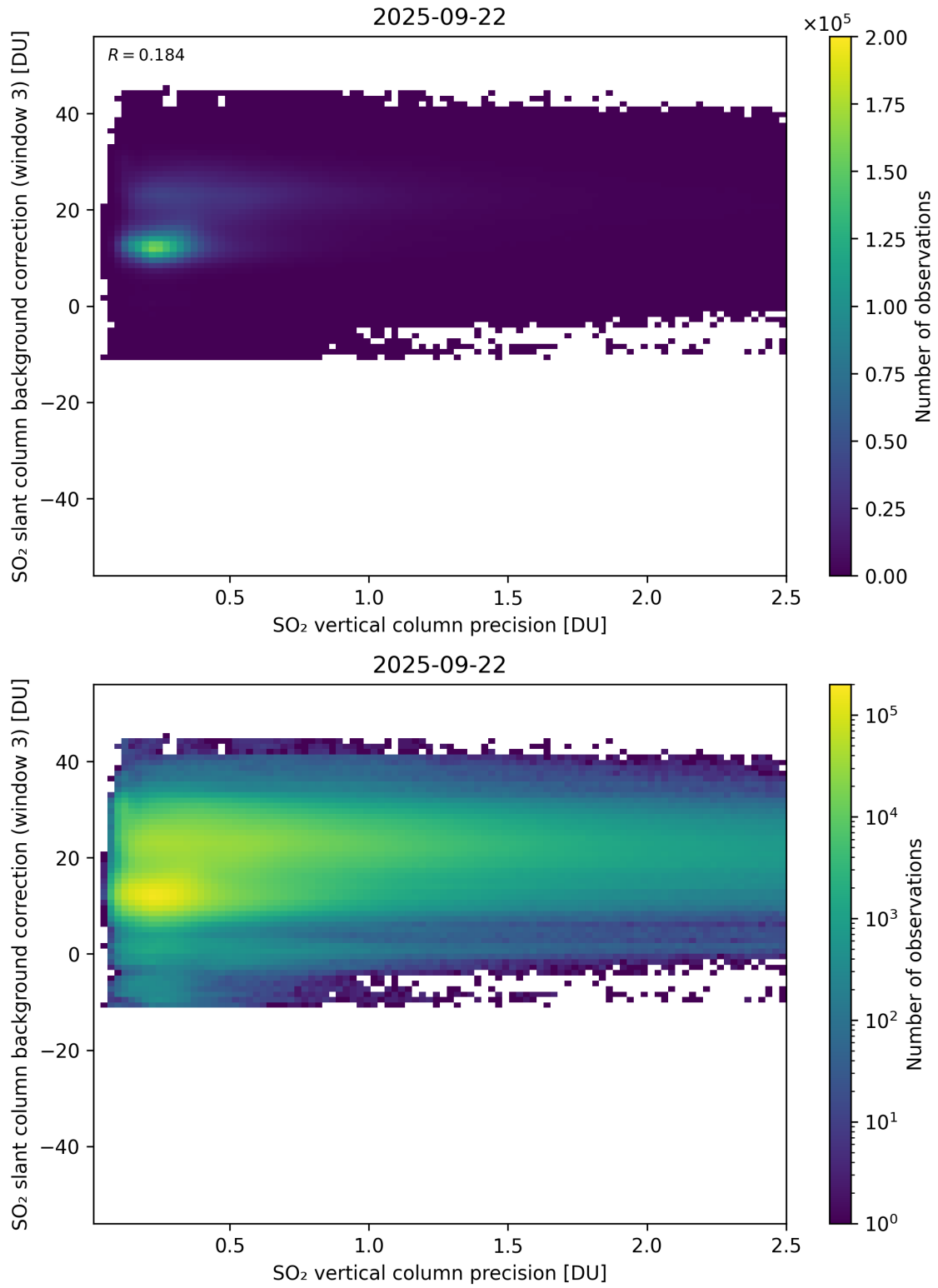
Figure 331: Scatter density plot of “SO 2 vertical column precision” against “SO 2 slant column background correction (window 3)” for 2025-09-22 to 2025-09-23.
