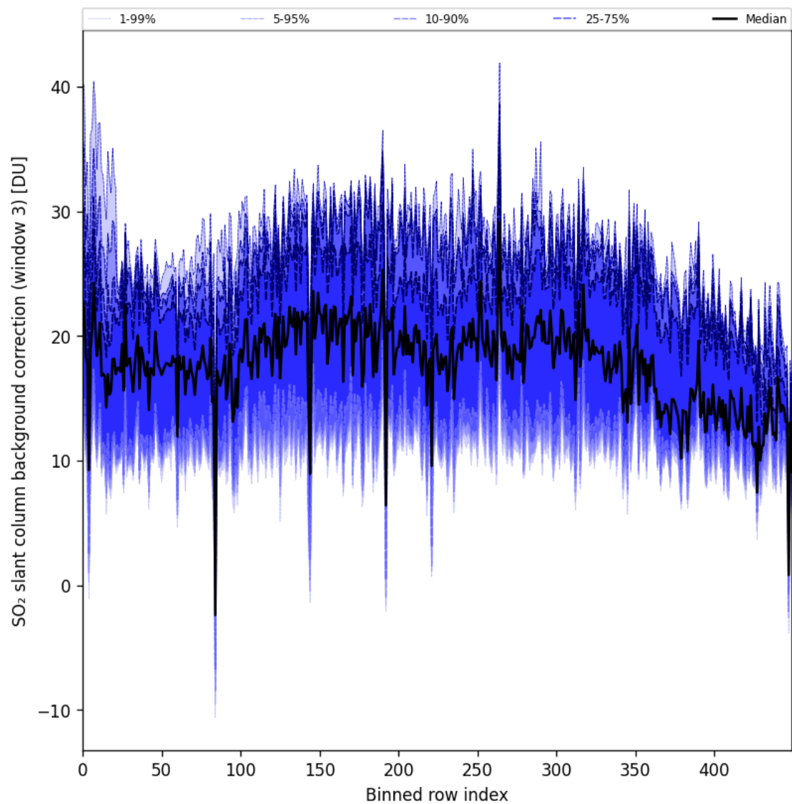
Figure 100: Along track statistics of “SO 2 slant column background correction (window 3)” for 2025-09-22 to 2025-09-23
