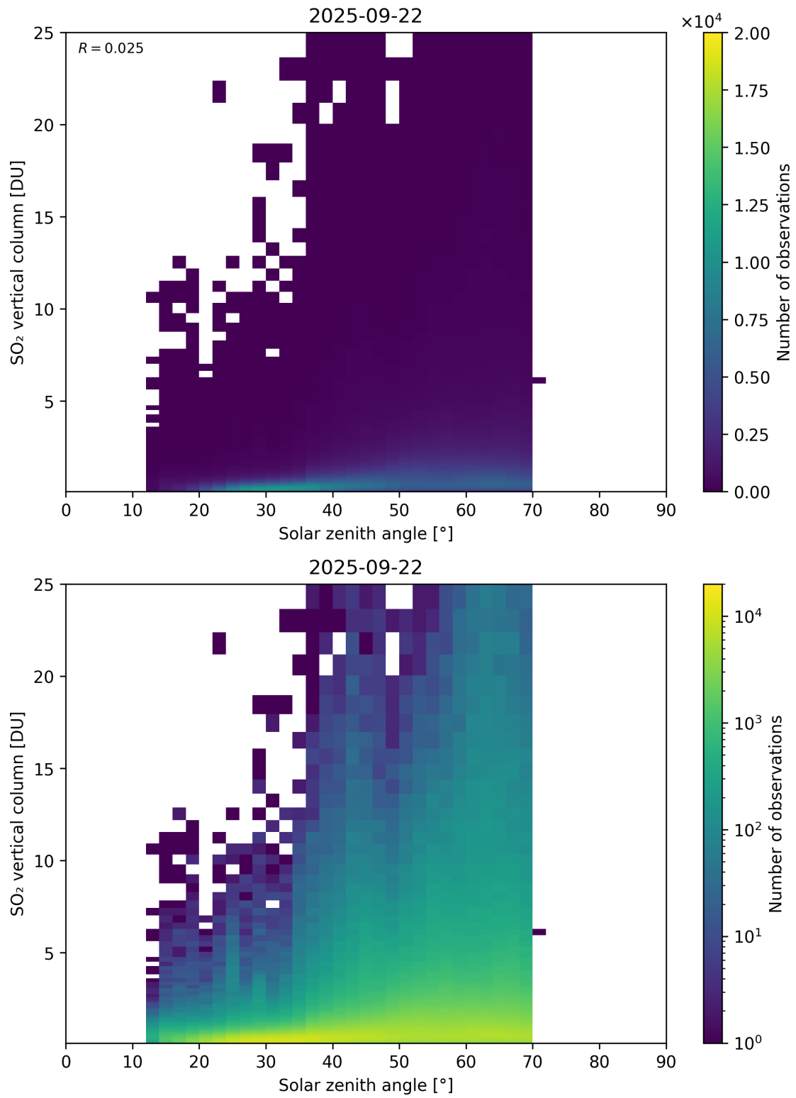
Figure 191: Scatter density plot of “Solar zenith angle” against “SO 2 vertical column” for 2025-09-22 to 2025-09-23.
