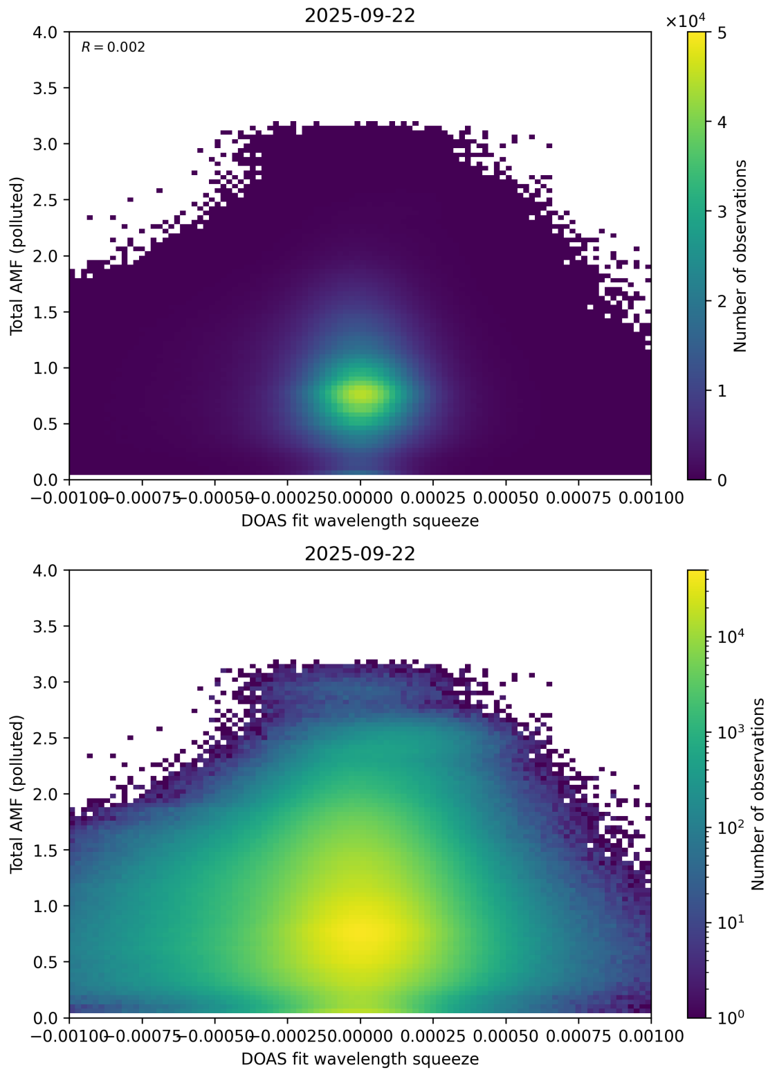
Figure 145: Scatter density plot of “DOAS fit wavelength squeeze” against “Total AMF (polluted)” for 2025-09-22 to 2025-09-23.
