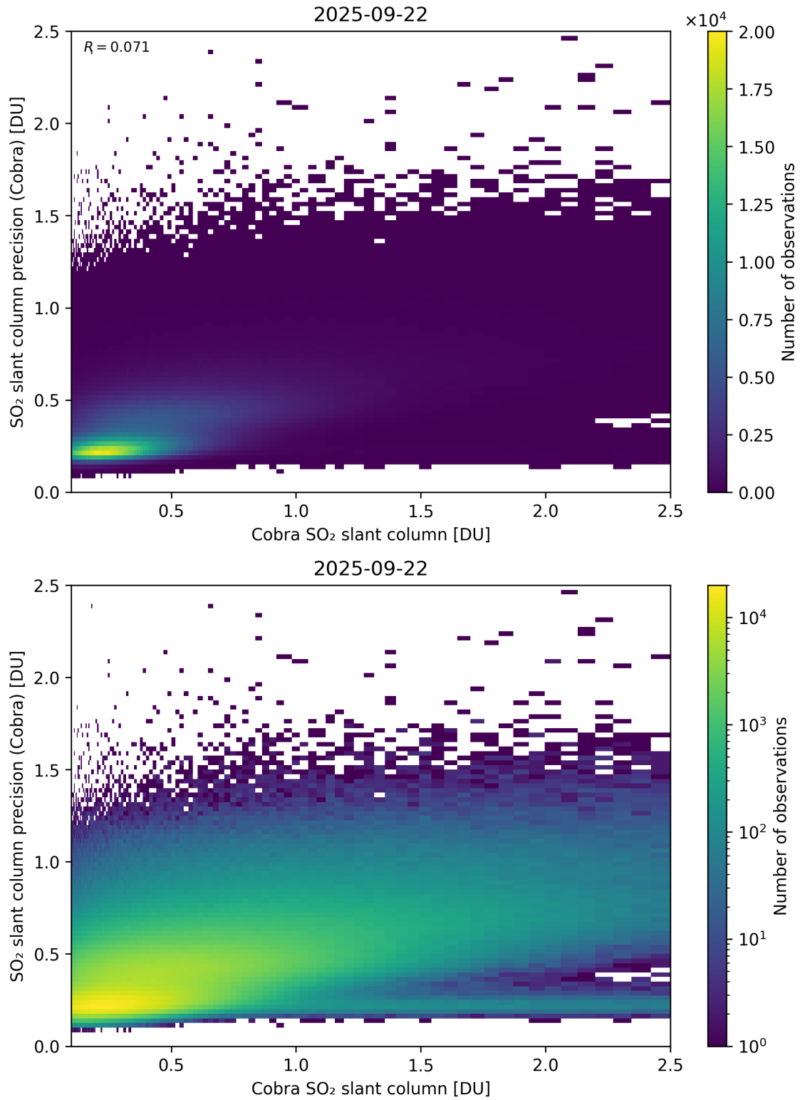
Figure 216: Scatter density plot of “Cobra SO 2 slant column” against “SO 2 slant column precision (Cobra)” for 2025-09-22 to 2025-09-23.
