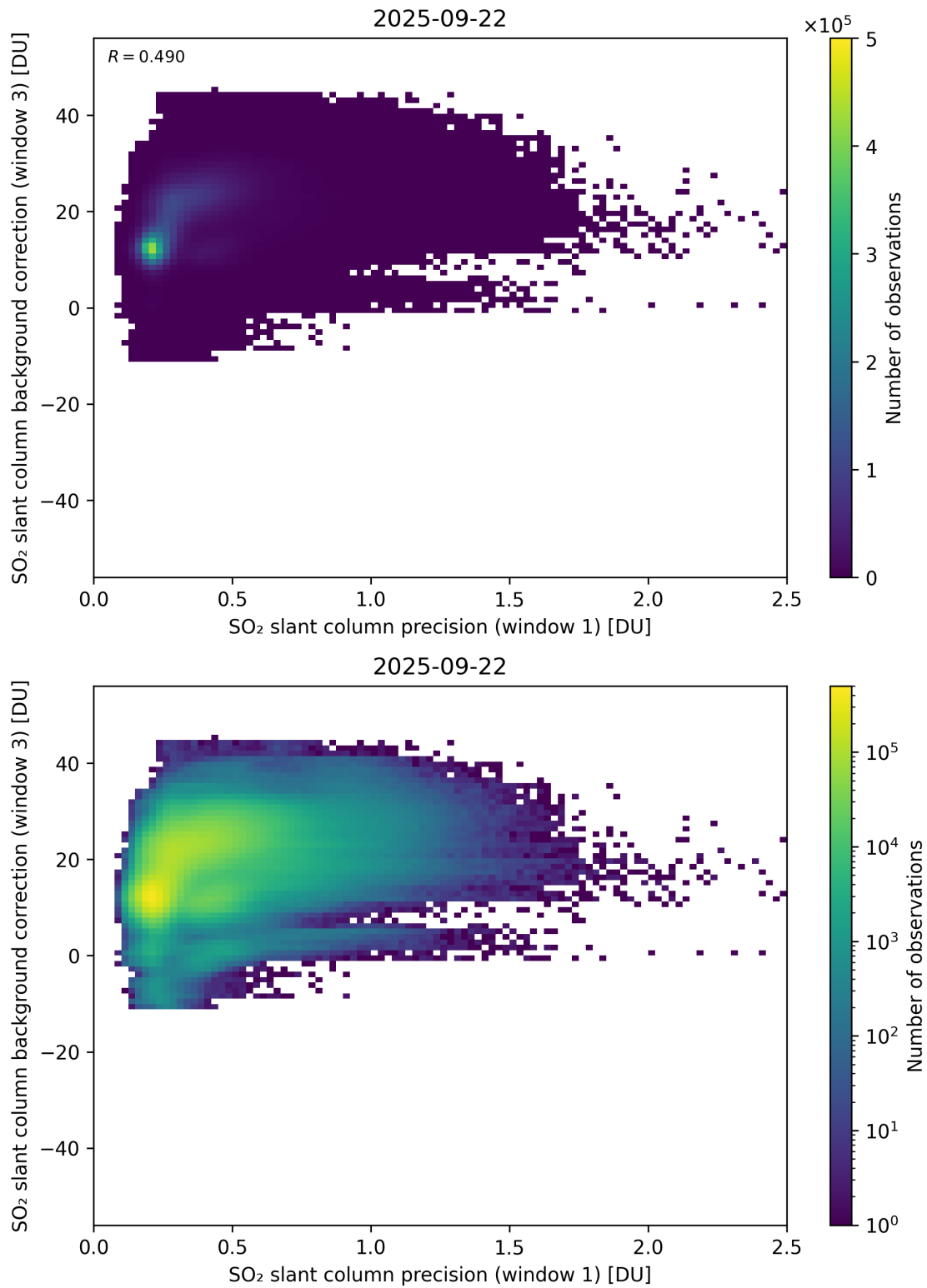
Figure 270: Scatter density plot of “SO 2 slant column precision (window 1)” against “SO 2 slant column background correction (window 3)” for 2025-09-22 to 2025-09-23.
