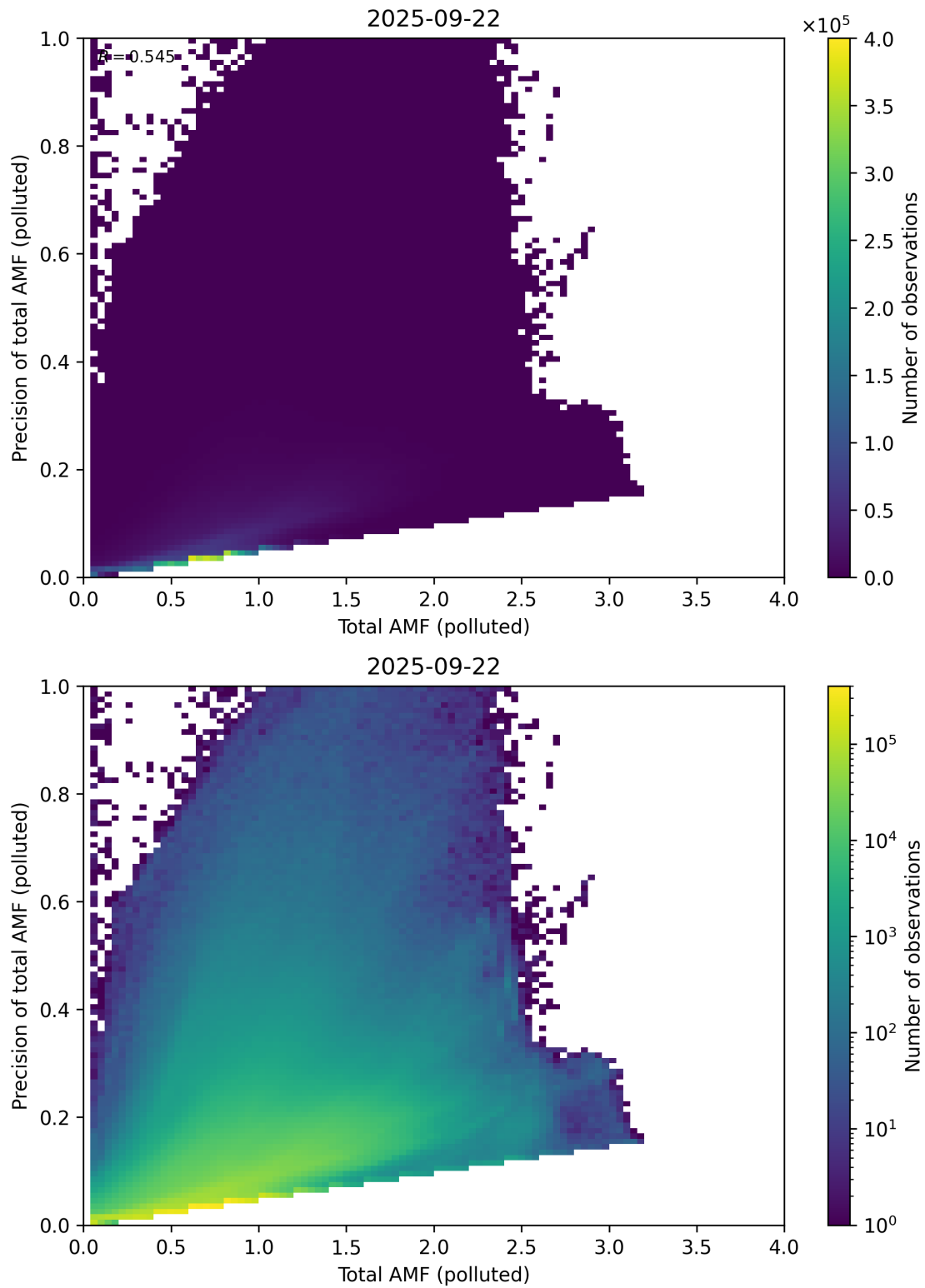
Figure 322: Scatter density plot of “Total AMF (polluted)” against “Precision of total AMF (polluted)” for 2025-09-22 to 2025-09-23.
