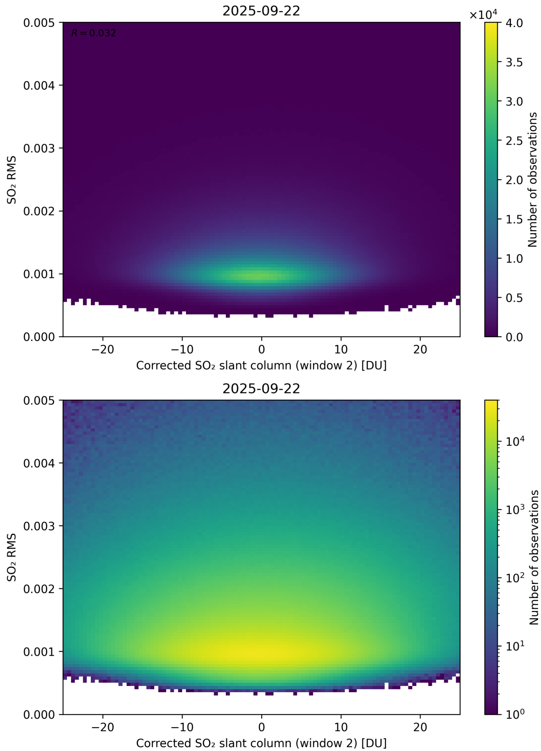
Figure 248: Scatter density plot of “Corrected SO 2 slant column (window 2)” against “SO 2 RMS” for 2025-09-22 to 2025-09-23.
