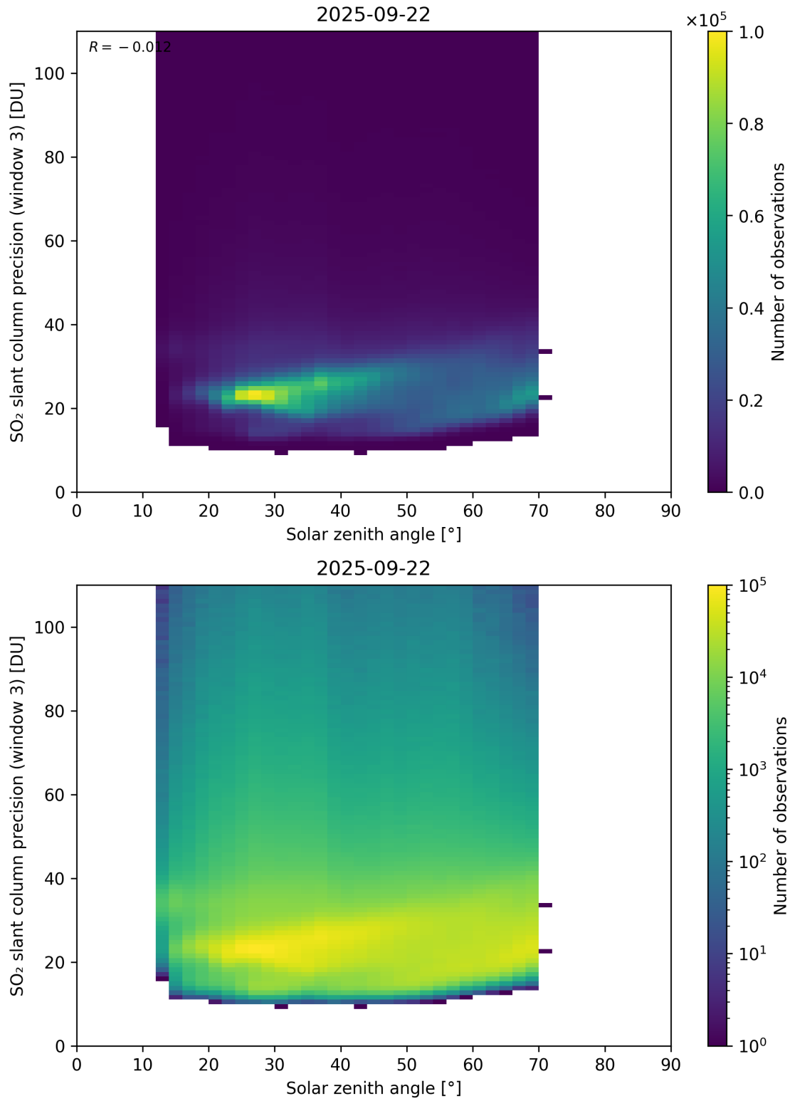
Figure 188: Scatter density plot of “Solar zenith angle” against “SO 2 slant column precision (window 3)” for 2025-09-22 to 2025-09-23.
