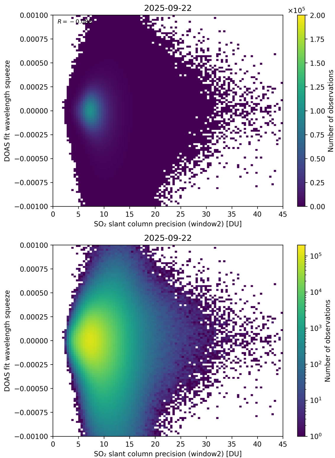
Figure 294: Scatter density plot of “SO 2 slant column precision (window2)” against “DOAS fit wavelength squeeze” for 2025-09-22 to 2025-09-23.
