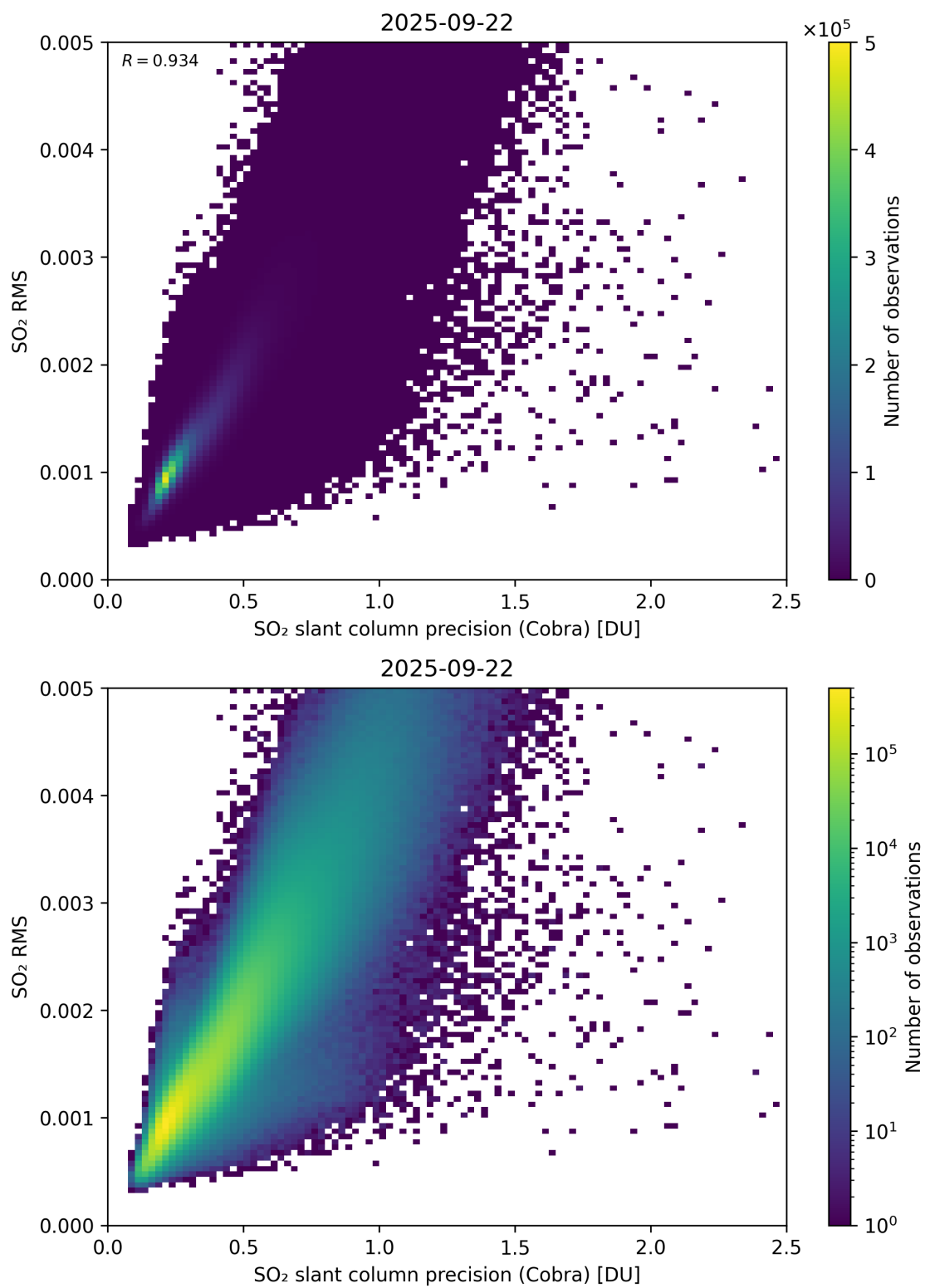
Figure 204: Scatter density plot of “SO 2 slant column precision (Cobra)” against “SO 2 RMS” for 2025-09-22 to 2025-09-23.
