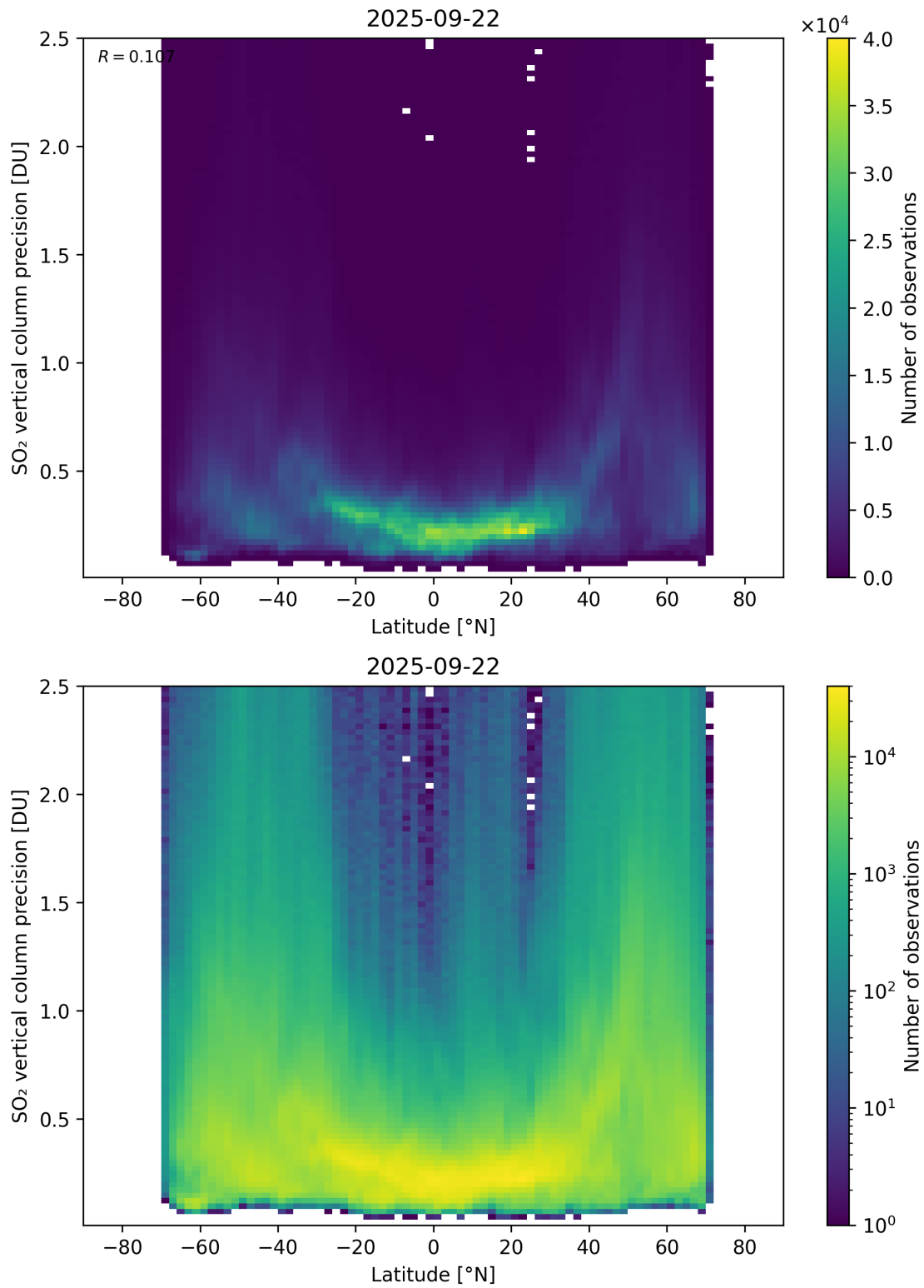
Figure 170: Scatter density plot of “Latitude” against “SO 2 vertical column precision” for 2025-09-22 to 2025-09-23.
