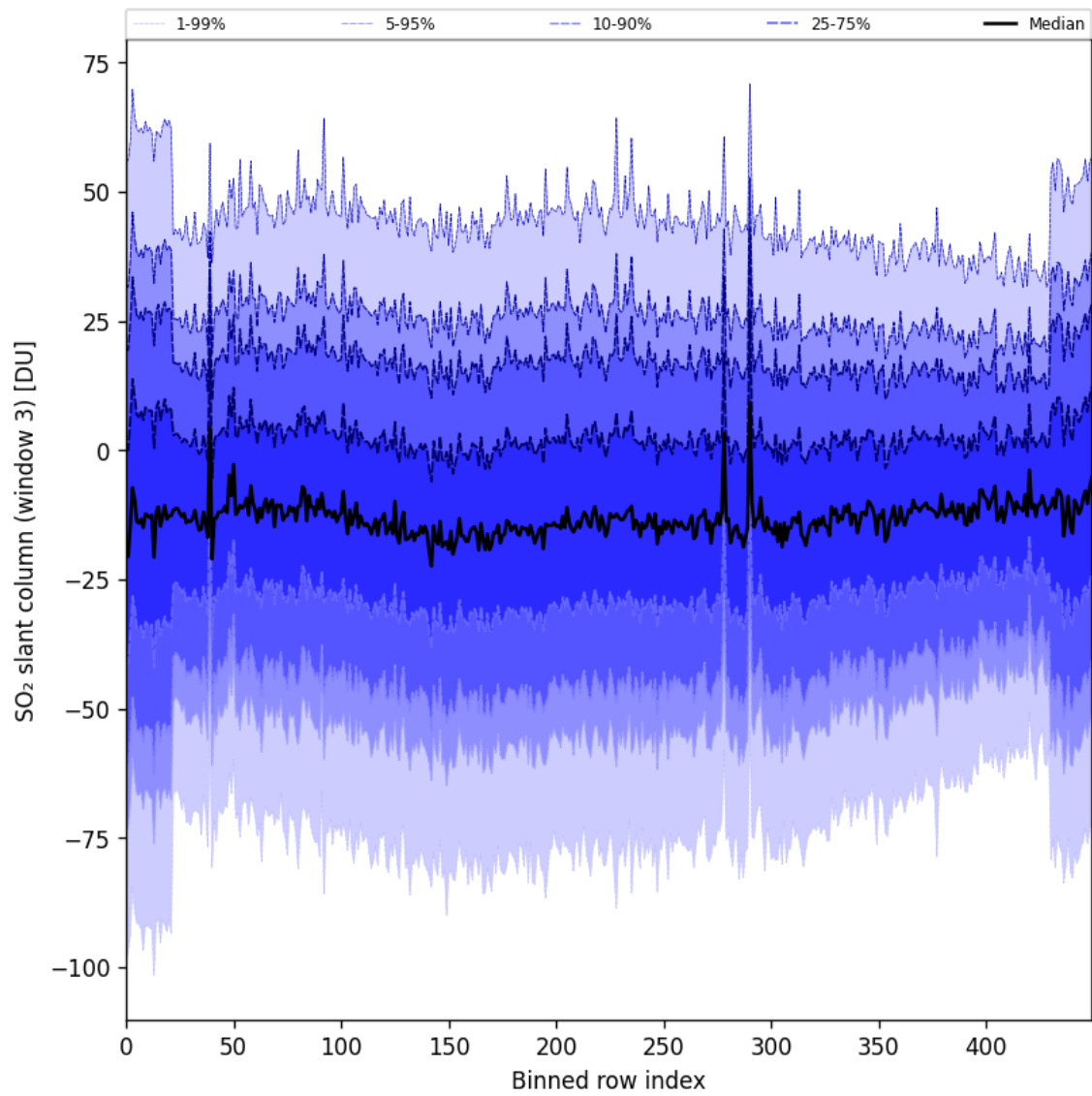
Figure 97: Along track statistics of “SO 2 slant column (window 3)” for 2025-09-22 to 2025-09-23
