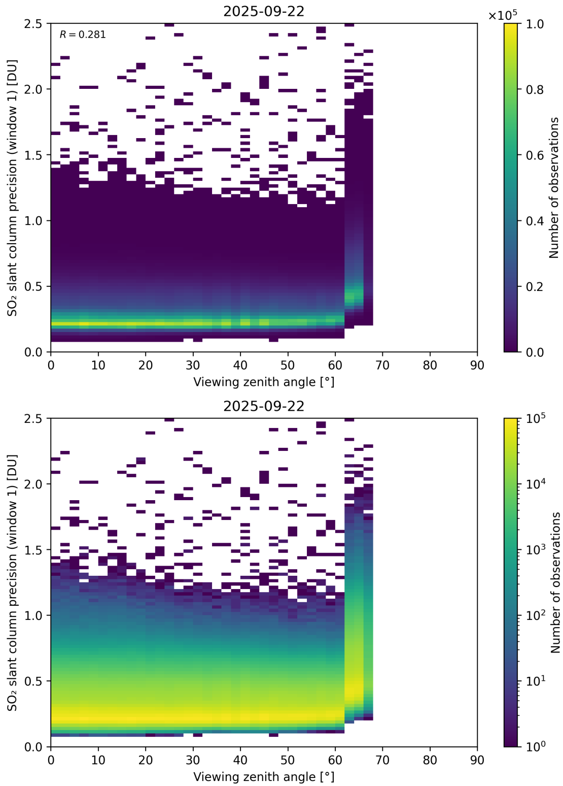
Figure 377: Scatter density plot of “Viewing zenith angle” against “SO 2 slant column precision (window 1)” for 2025-09-22 to 2025-09-23.
