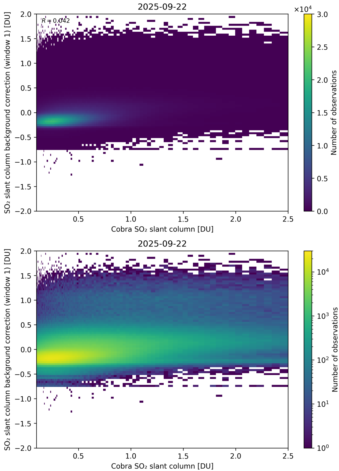
Figure 193: Scatter density plot of “Cobra SO 2 slant column” against “SO 2 slant column background correction (window 1)” for 2025-09-22 to 2025-09-23.
