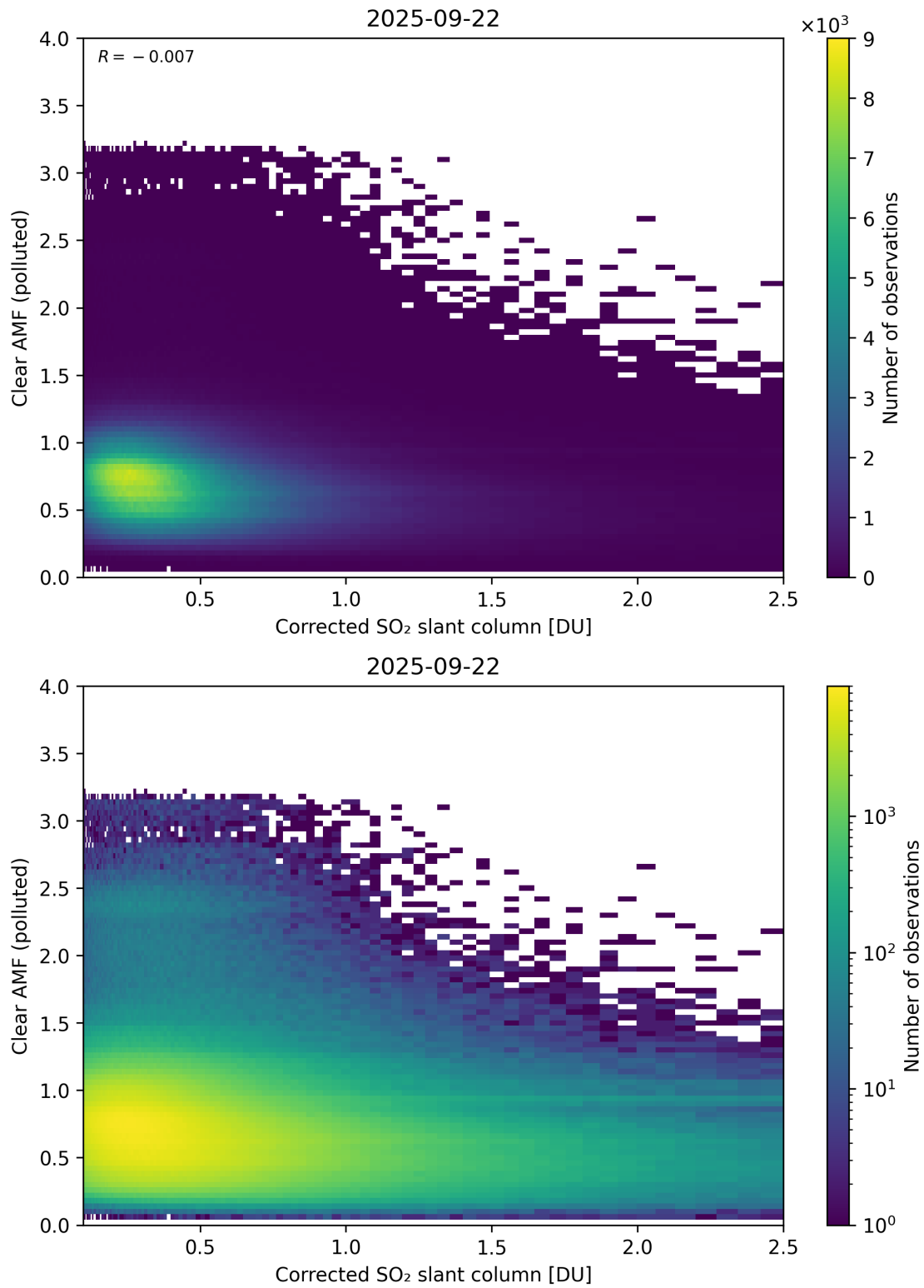
Figure 232: Scatter density plot of “Corrected SO 2 slant column” against “Clear AMF (polluted)” for 2025-09-22 to 2025-09-23.
