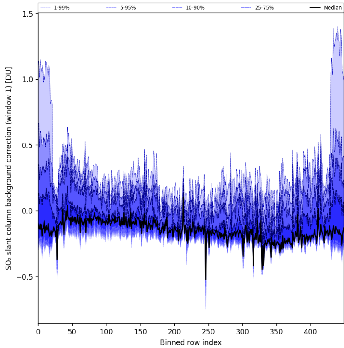
Figure 92: Along track statistics of “SO 2 slant column background correction (window 1)” for 2025-09-22 to 2025-09-23
