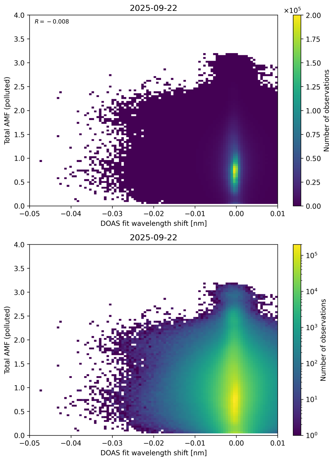
Figure 141: Scatter density plot of “DOAS fit wavelength shift” against “Total AMF (polluted)” for 2025-09-22 to 2025-09-23.
