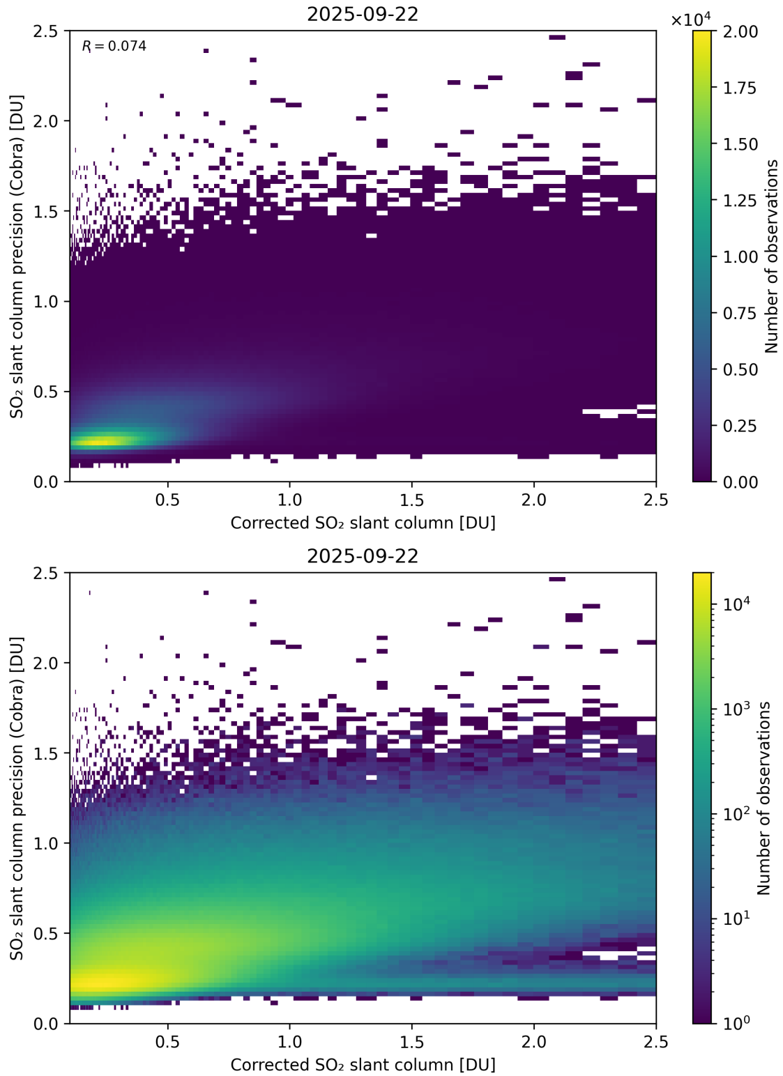
Figure 234: Scatter density plot of “Corrected SO 2 slant column” against “SO 2 slant column precision (Cobra)” for 2025-09-22 to 2025-09-23.
