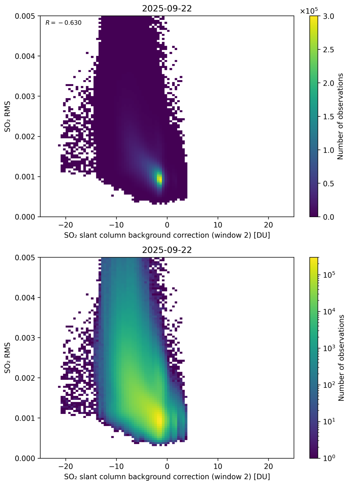
Figure 125: Scatter density plot of “SO 2 slant column background correction (window 2)” against “SO 2 RMS” for 2025-09-22 to 2025-09-23.
