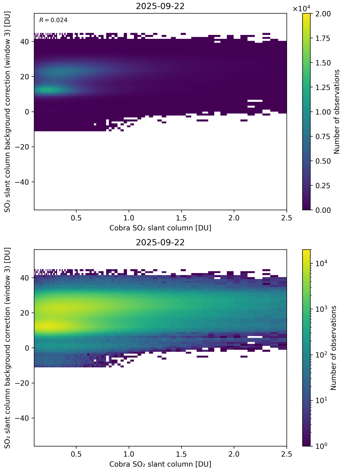
Figure 195: Scatter density plot of “Cobra SO 2 slant column” against “SO 2 slant column background correction (window 3)” for 2025-09-22 to 2025-09-23.
