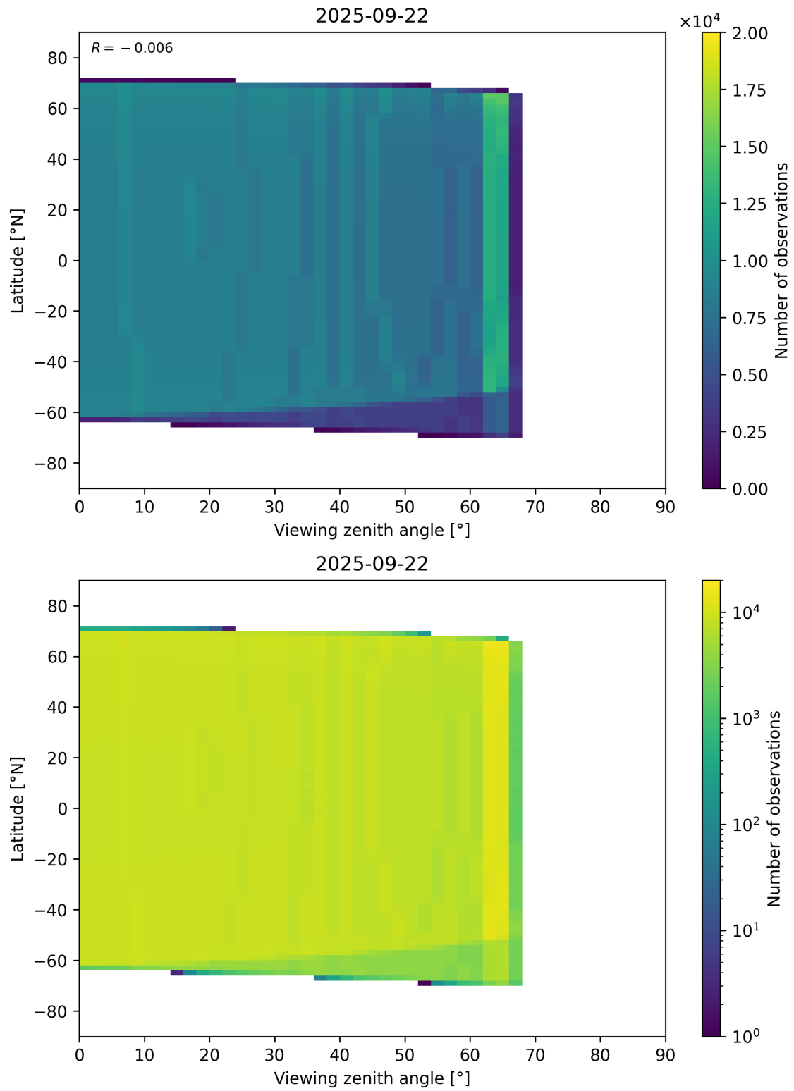
Figure 368: Scatter density plot of “Viewing zenith angle” against “Latitude” for 2025-09-22 to 2025-09-23.
