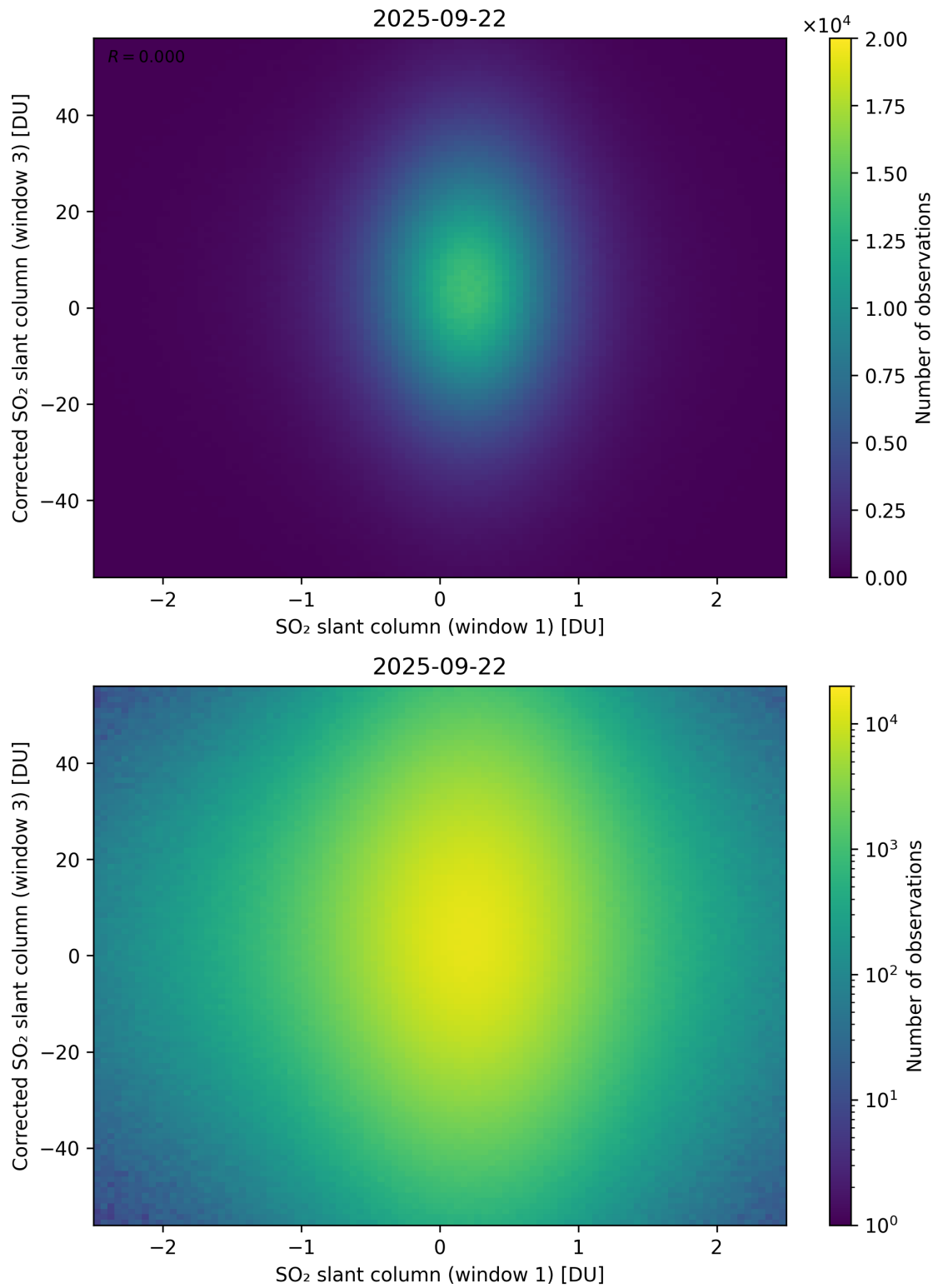
Figure 284: Scatter density plot of “SO 2 slant column (window 1)” against “Corrected SO 2 slant column (window 3)” for 2025-09-22 to 2025-09-23.
