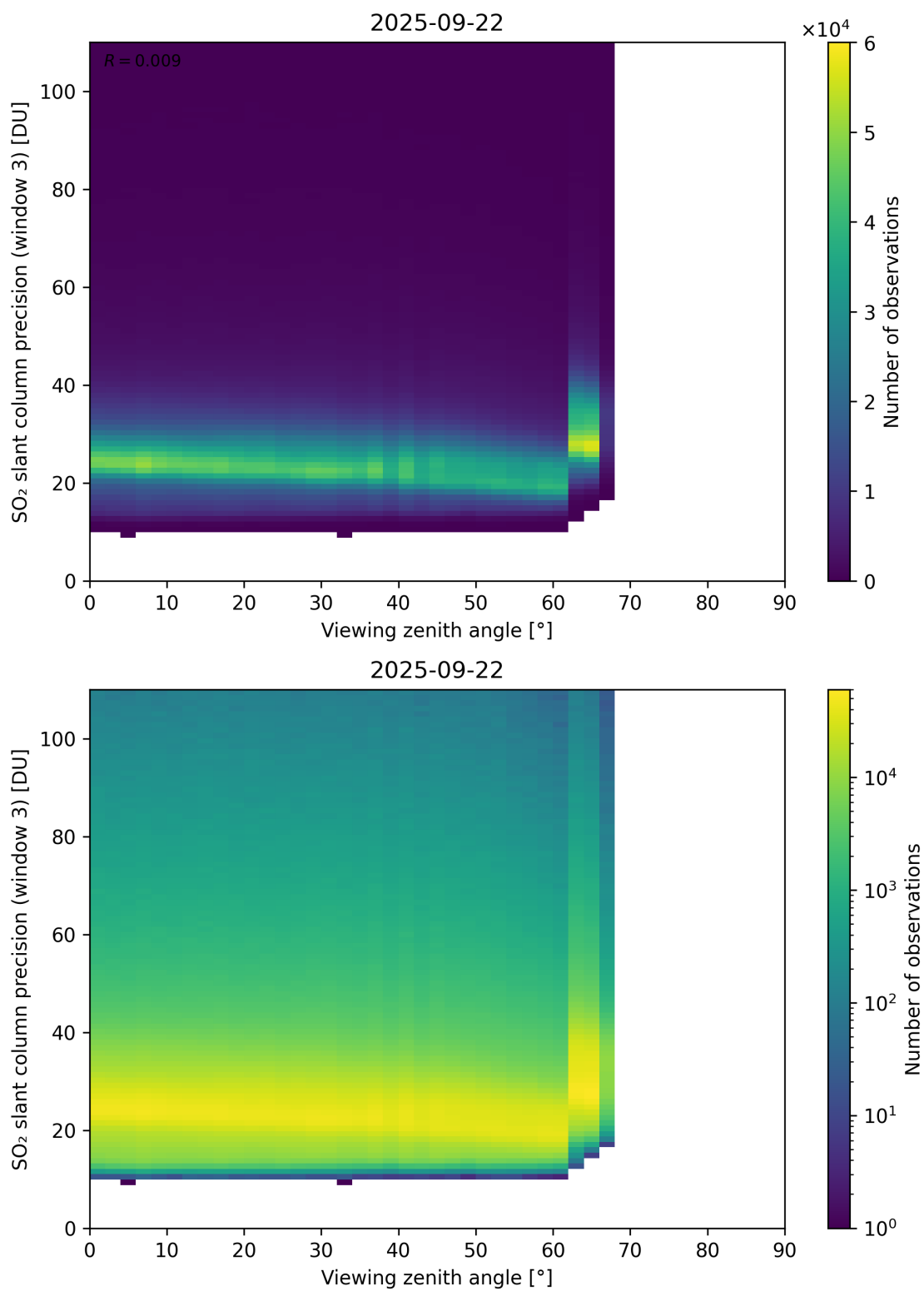
Figure 380: Scatter density plot of “Viewing zenith angle” against “SO 2 slant column precision (window 3)” for 2025-09-22 to 2025-09-23.
