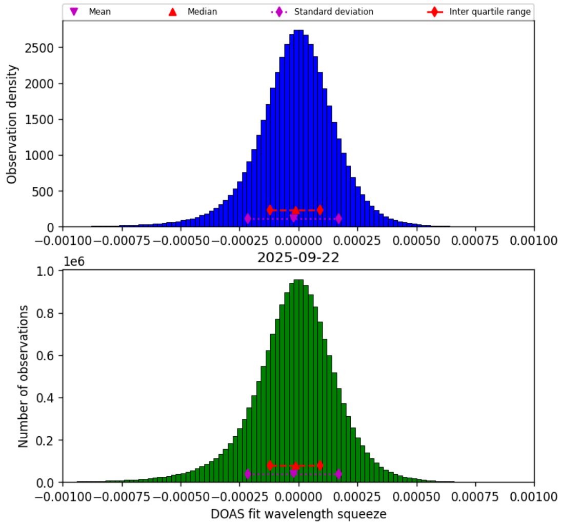
Figure 77: Histogram of “DOAS fit wavelength squeeze” for 2025-09-22 to 2025-09-23
