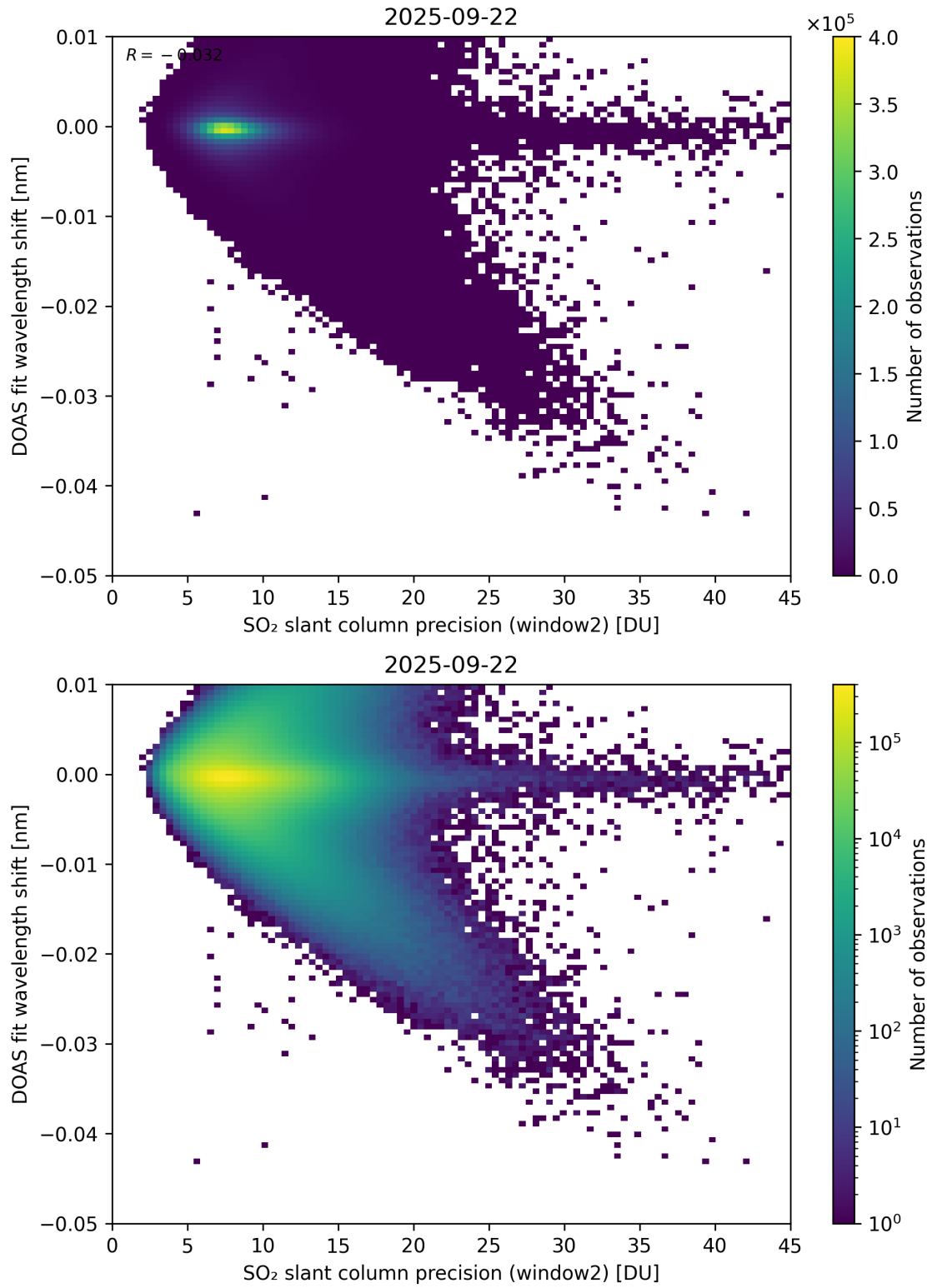
Figure 293: Scatter density plot of “SO 2 slant column precision (window2)” against “DOAS fit wavelength shift” for 2025-09-22 to 2025-09-23.
