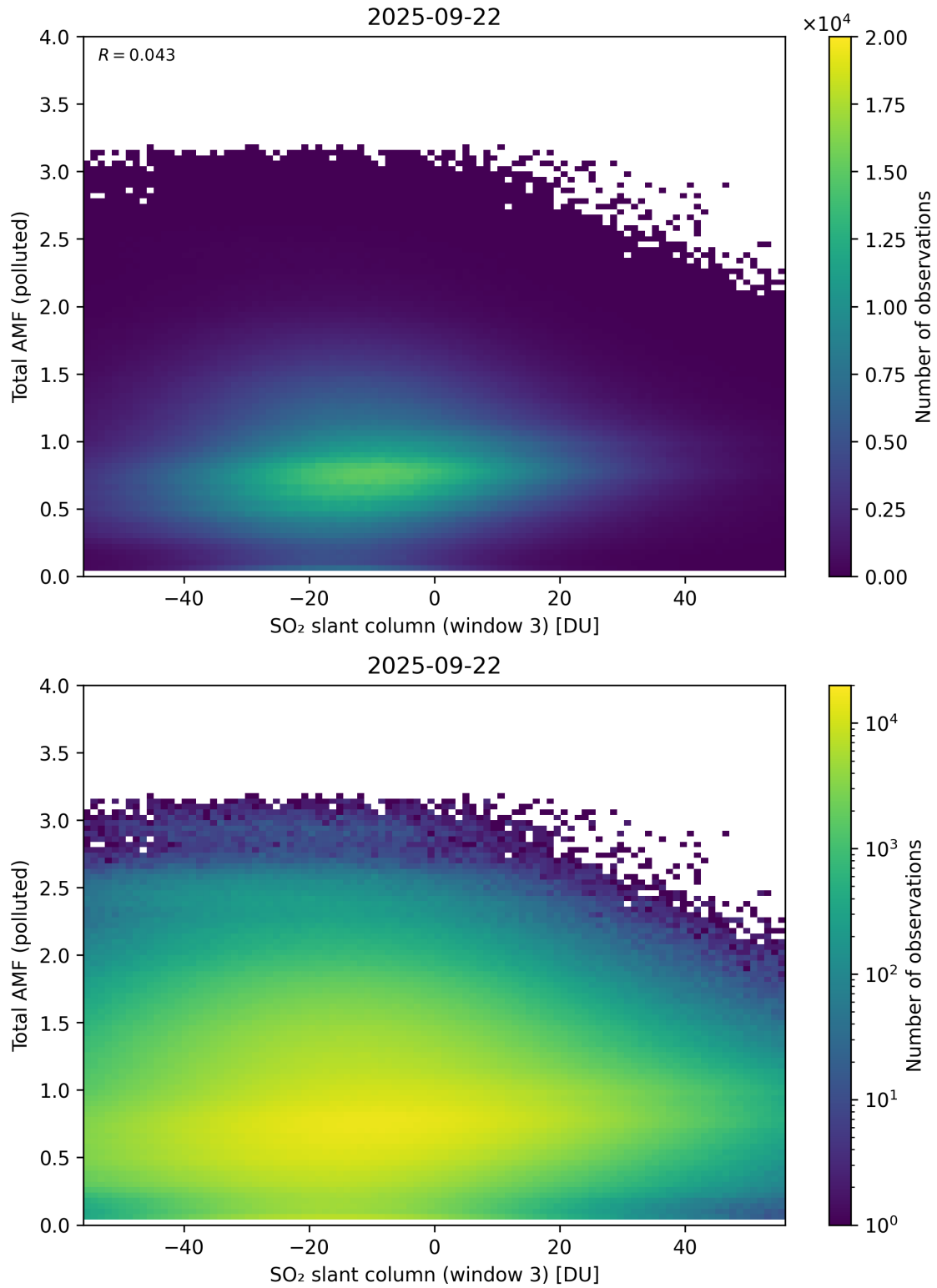
Figure 318: Scatter density plot of “SO 2 slant column (window 3)” against “Total AMF (polluted)” for 2025-09-22 to 2025-09-23.
