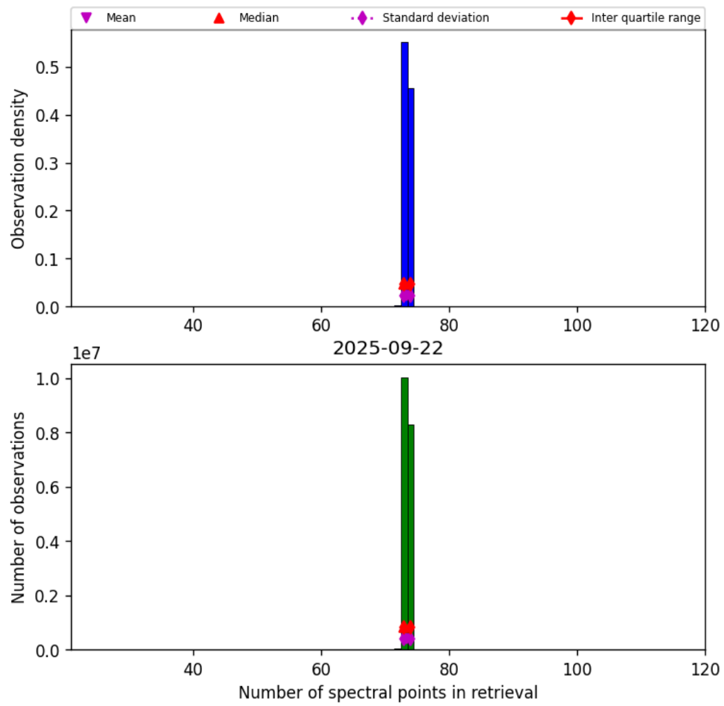
Figure 82: Histogram of “Number of spectral points in retrieval” for 2025-09-22 to 2025-09-23
