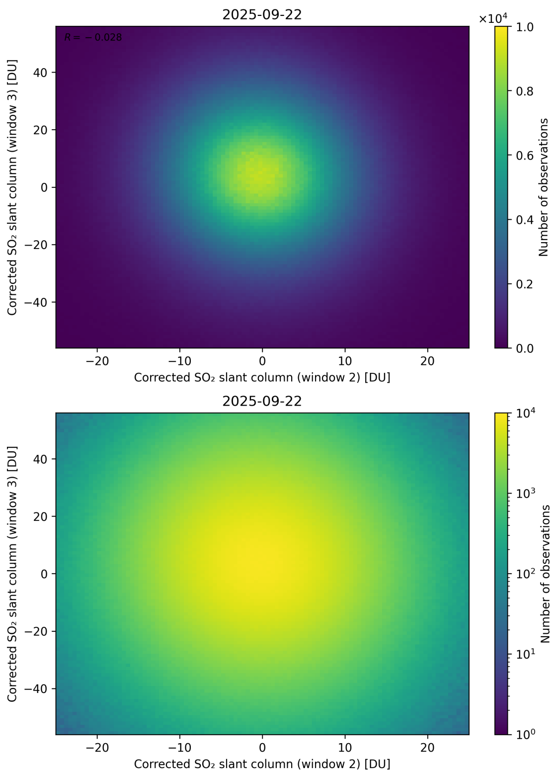
Figure 250: Scatter density plot of “Corrected SO 2 slant column (window 2)” against “Corrected SO 2 slant column (window 3)” for 2025-09-22 to 2025-09-23.
