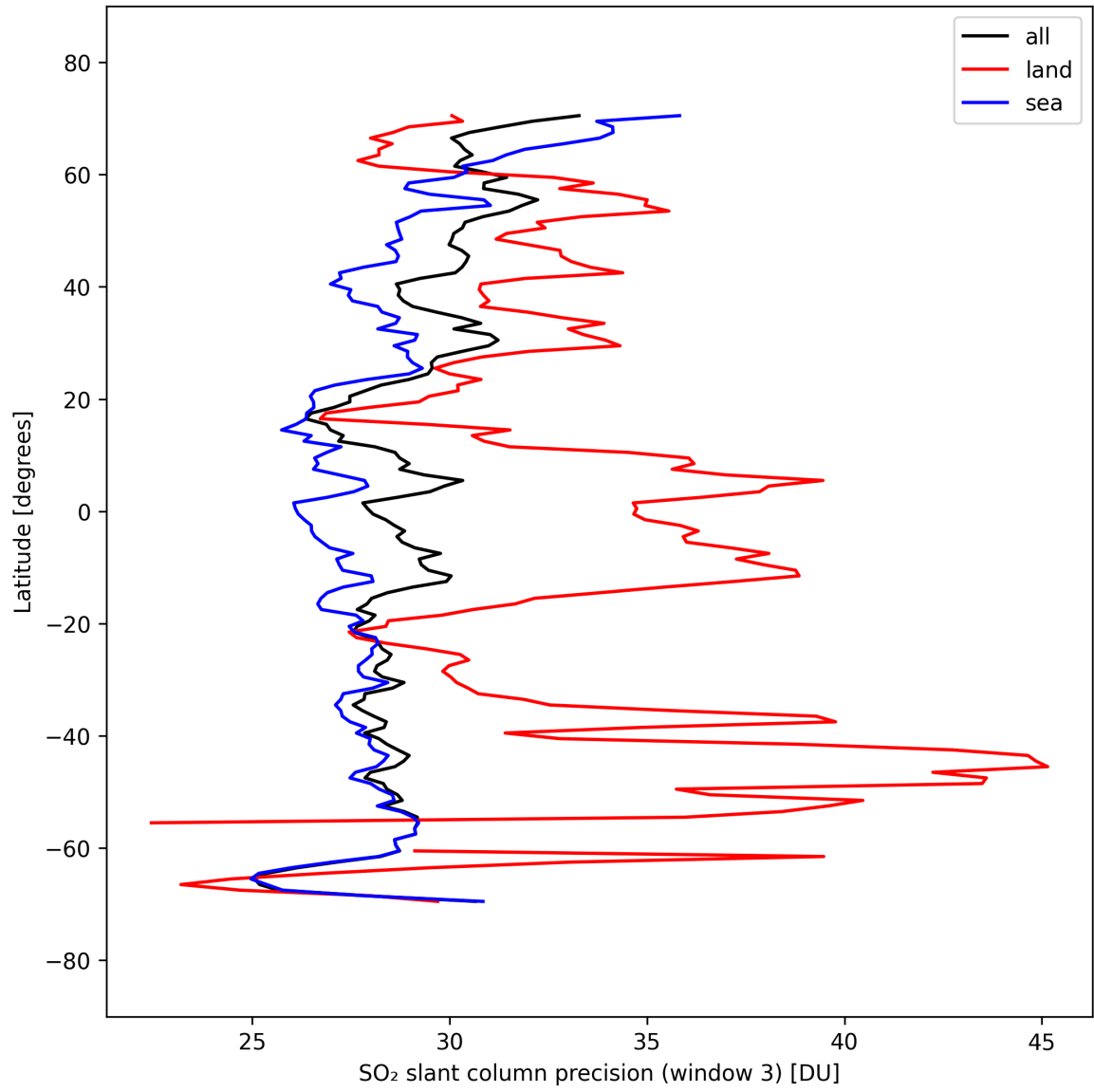
Figure 46: Zonal average of “SO 2 slant column precision (window 3)” for 2025-09-22 to 2025-09-23.
