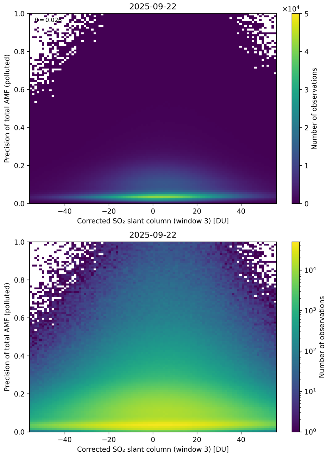
Figure 261: Scatter density plot of “Corrected SO 2 slant column (window 3)” against “Precision of total AMF (polluted)” for 2025-09-22 to 2025-09-23.
