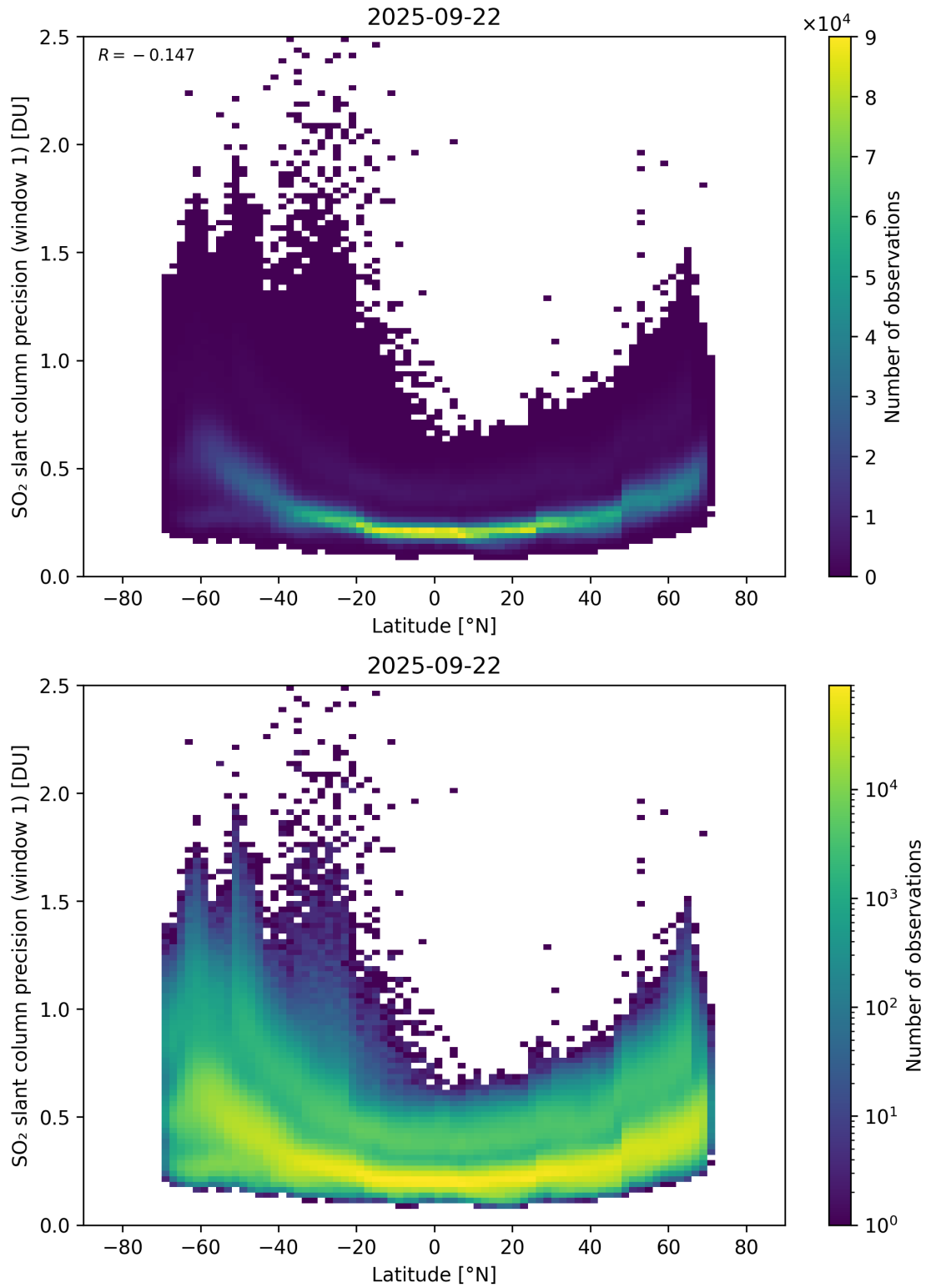
Figure 163: Scatter density plot of “Latitude” against “SO 2 slant column precision (window 1)” for 2025-09-22 to 2025-09-23.
