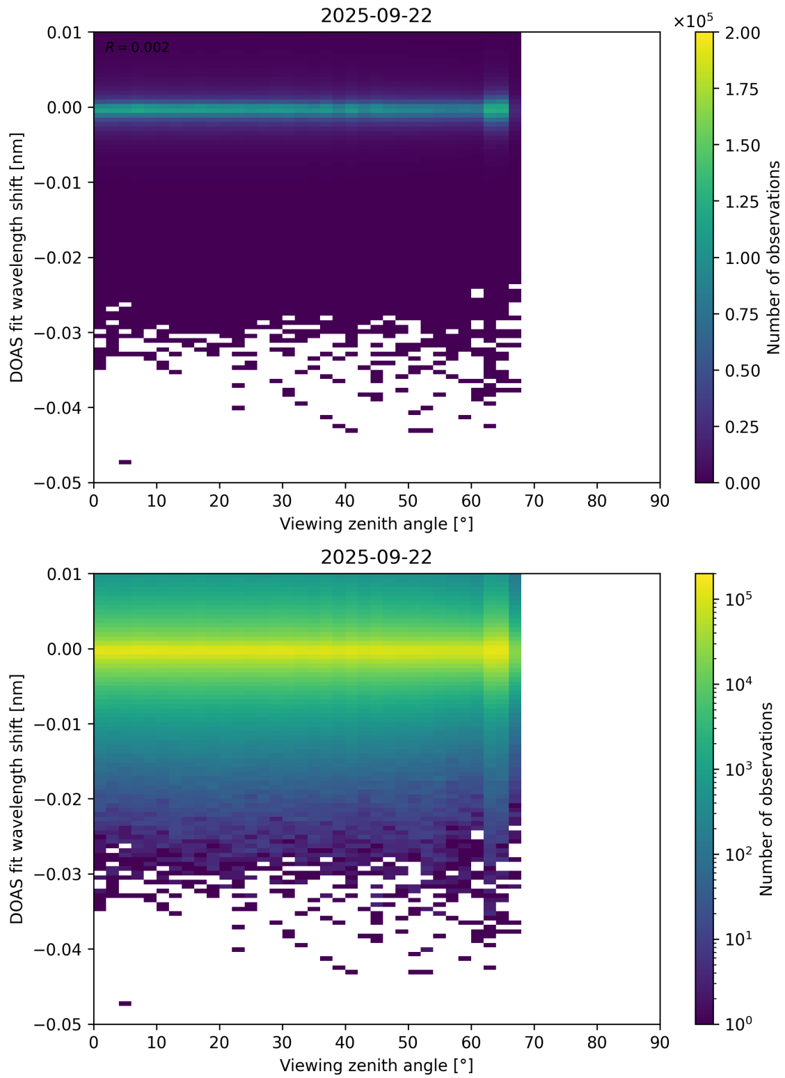
Figure 365: Scatter density plot of “Viewing zenith angle” against “DOAS fit wavelength shift” for 2025-09-22 to 2025-09-23.
