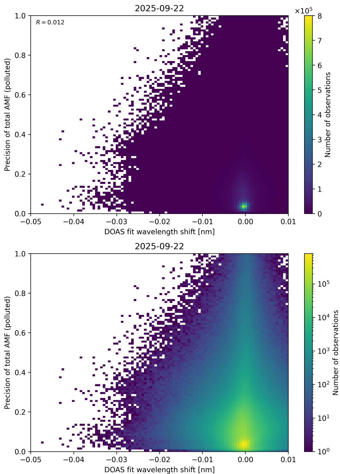
Figure 142: Scatter density plot of “DOAS fit wavelength shift” against “Precision of total AMF (polluted)” for 2025-09-22 to 2025-09-23.
