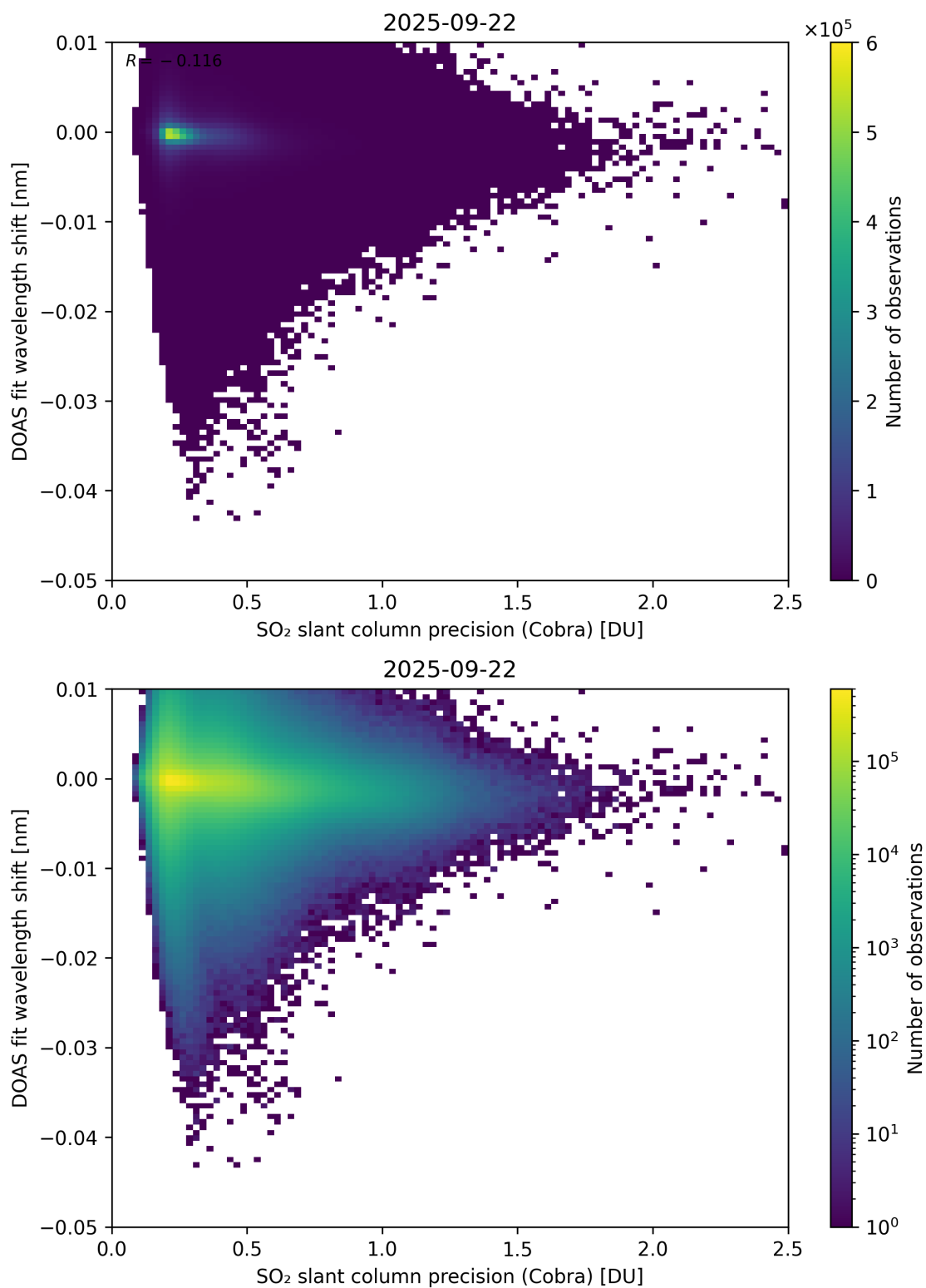
Figure 202: Scatter density plot of “SO 2 slant column precision (Cobra)” against “DOAS fit wavelength shift” for 2025-09-22 to 2025-09-23.
