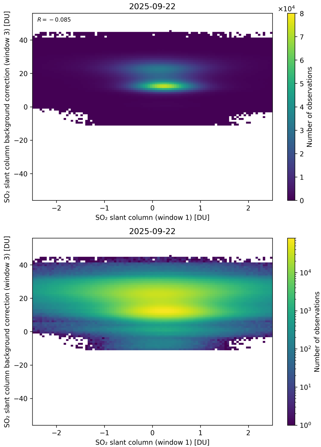
Figure 264: Scatter density plot of “SO 2 slant column (window 1)” against “SO 2 slant column background correction (window 3)” for 2025-09-22 to 2025-09-23.
