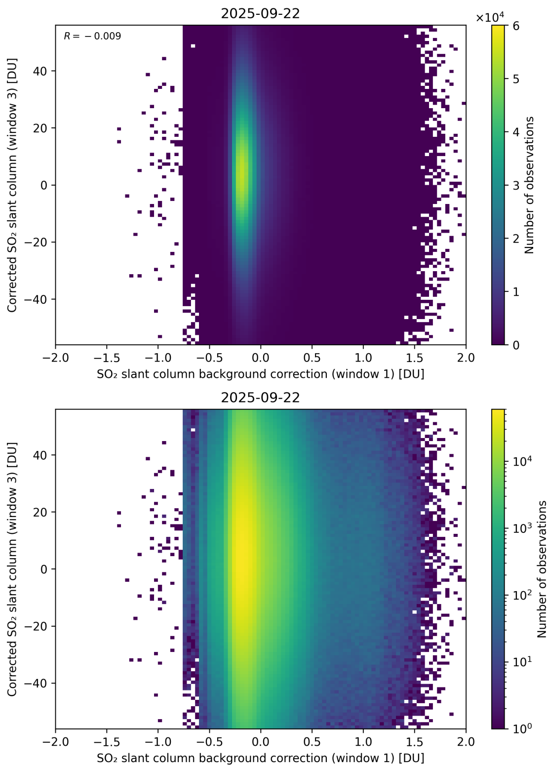
Figure 116: Scatter density plot of “SO 2 slant column background correction (window 1)” against “Corrected SO 2 slant column (window 3)” for 2025-09-22 to 2025-09-23.
