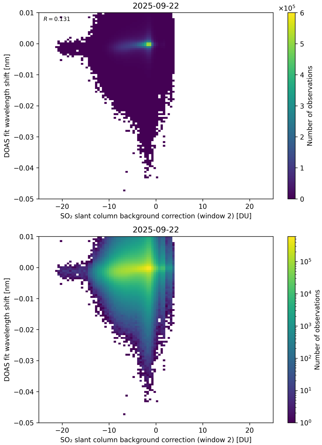
Figure 123: Scatter density plot of “SO 2 slant column background correction (window 2)” against “DOAS fit wavelength shift” for 2025-09-22 to 2025-09-23.
