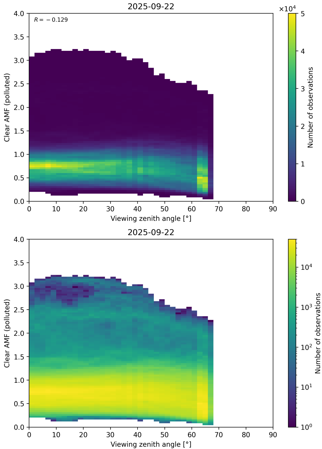
Figure 370: Scatter density plot of “Viewing zenith angle” against “Clear AMF (polluted)” for 2025-09-22 to 2025-09-23.
