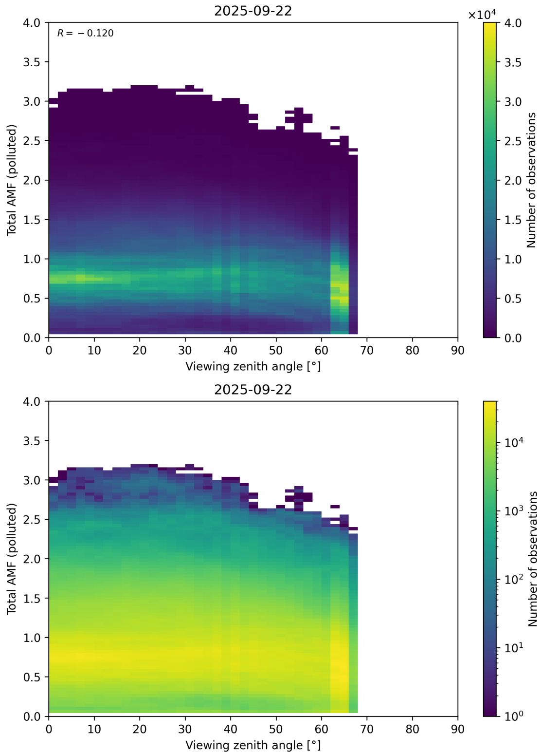
Figure 381: Scatter density plot of “Viewing zenith angle” against “Total AMF (polluted)” for 2025-09-22 to 2025-09-23.
