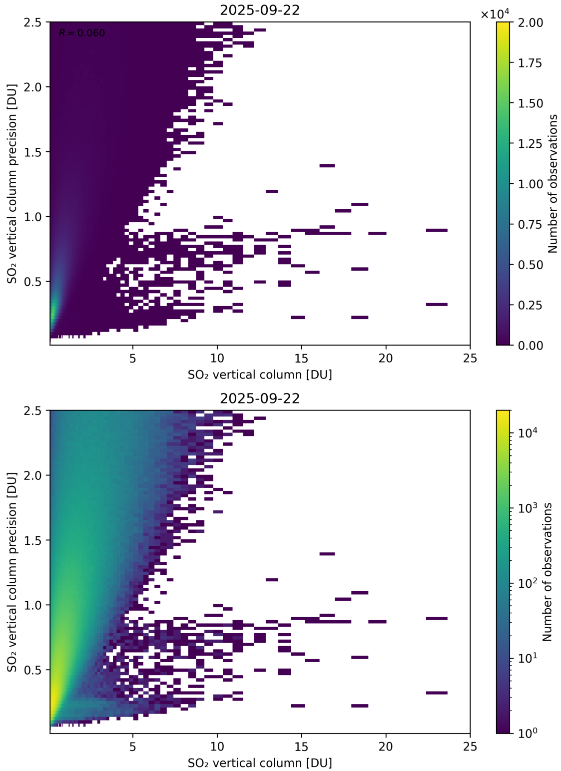
Figure 361: Scatter density plot of “SO 2 vertical column” against “SO 2 vertical column precision” for 2025-09-22 to 2025-09-23.
