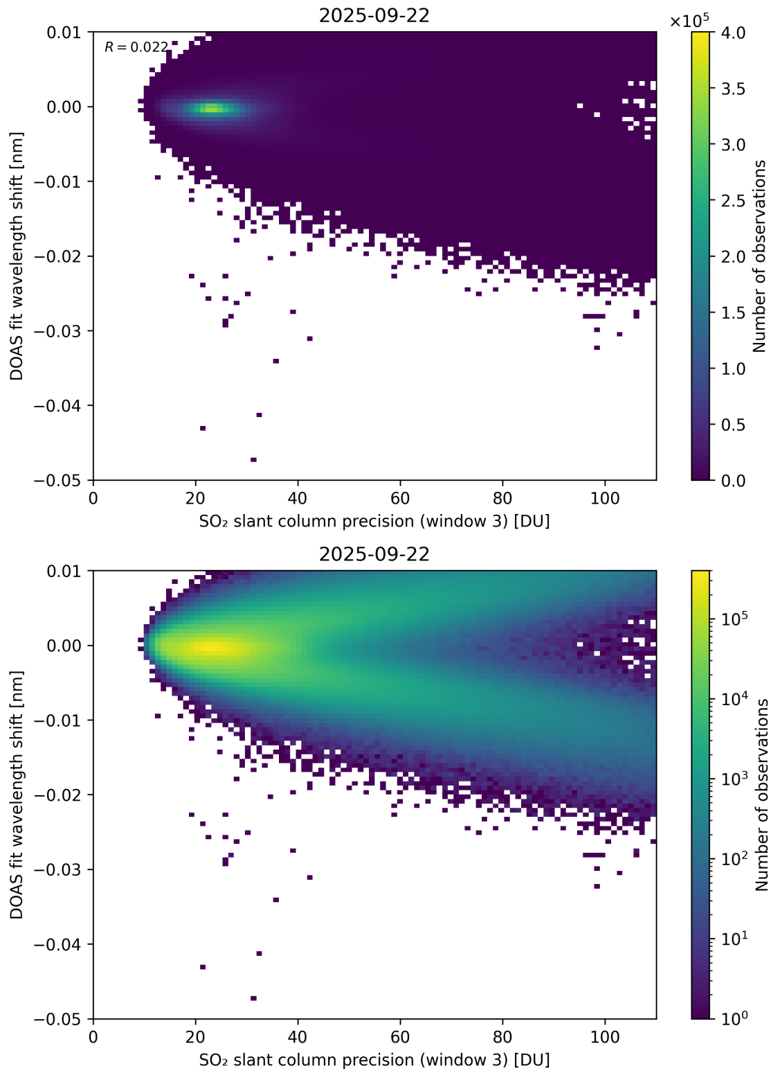
Figure 308: Scatter density plot of “SO 2 slant column precision (window 3)” against “DOAS fit wavelength shift” for 2025-09-22 to 2025-09-23.
