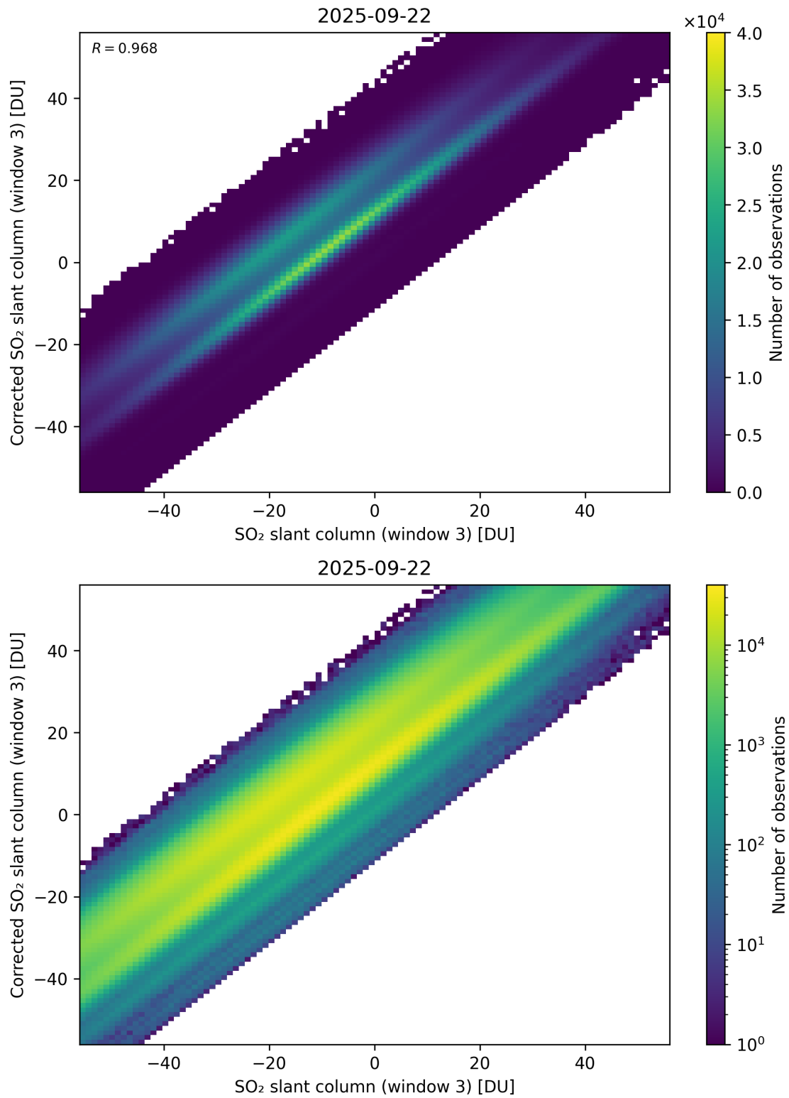
Figure 316: Scatter density plot of “SO 2 slant column (window 3)” against “Corrected SO 2 slant column (window 3)” for 2025-09-22 to 2025-09-23.
