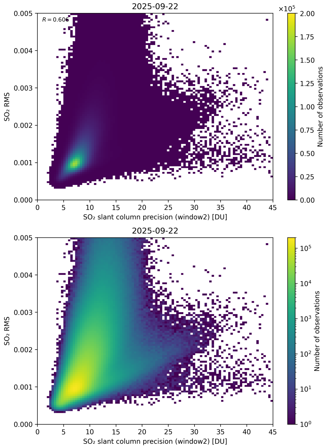
Figure 295: Scatter density plot of “SO 2 slant column precision (window2)” against “SO 2 RMS” for 2025-09-22 to 2025-09-23.
