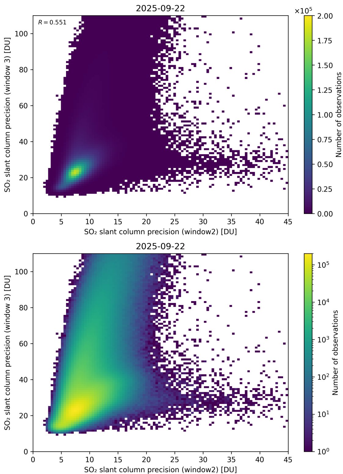
Figure 300: Scatter density plot of “SO 2 slant column precision (window2)” against “SO 2 slant column precision (window 3)” for 2025-09-22 to 2025-09-23.
