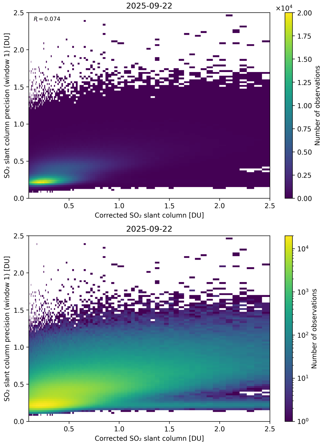
Figure 238: Scatter density plot of “Corrected SO 2 slant column” against “SO 2 slant column precision (window 1)” for 2025-09-22 to 2025-09-23.
