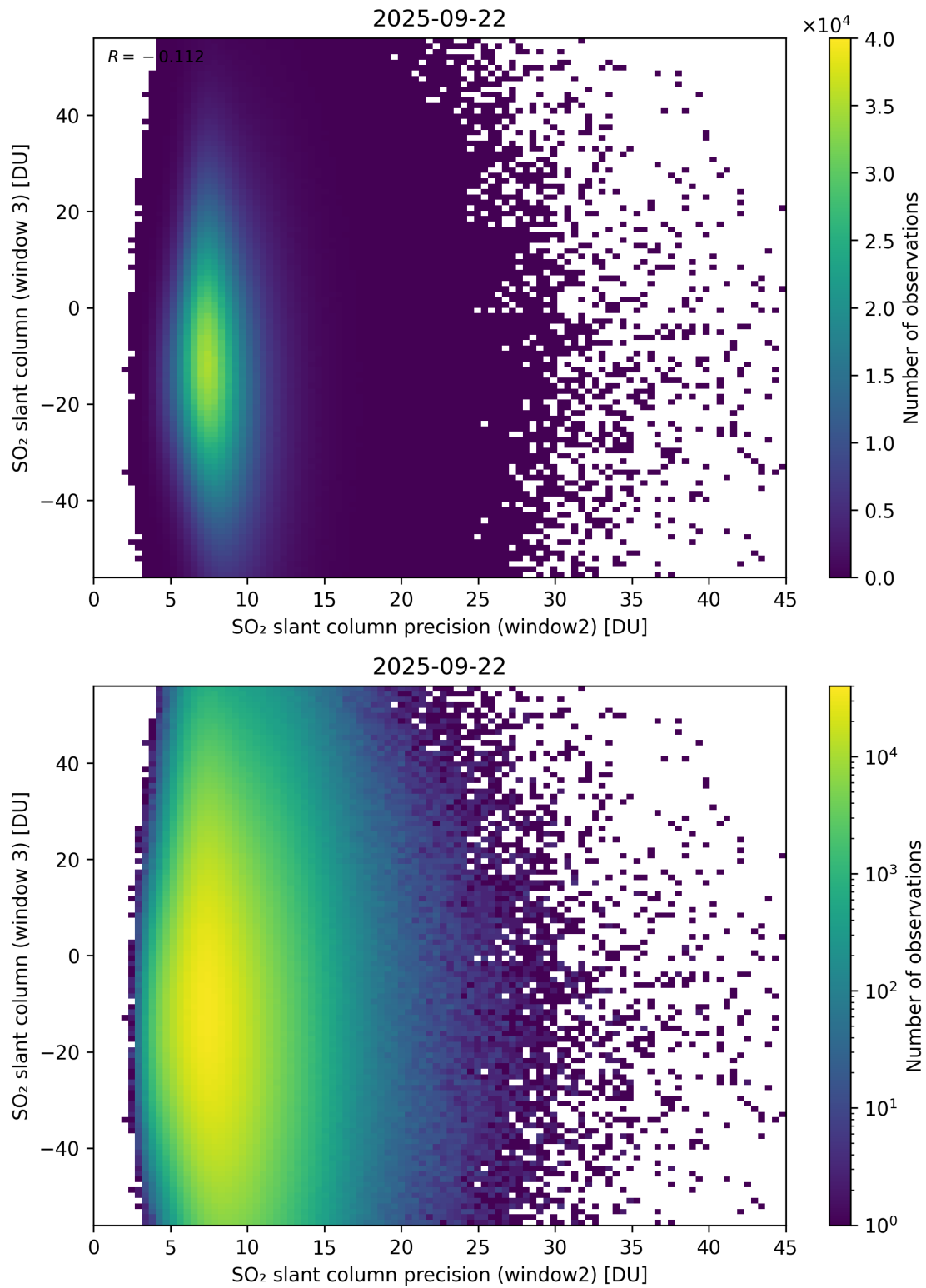
Figure 299: Scatter density plot of “SO 2 slant column precision (window2)” against “SO 2 slant column (window 3)” for 2025-09-22 to 2025-09-23.
