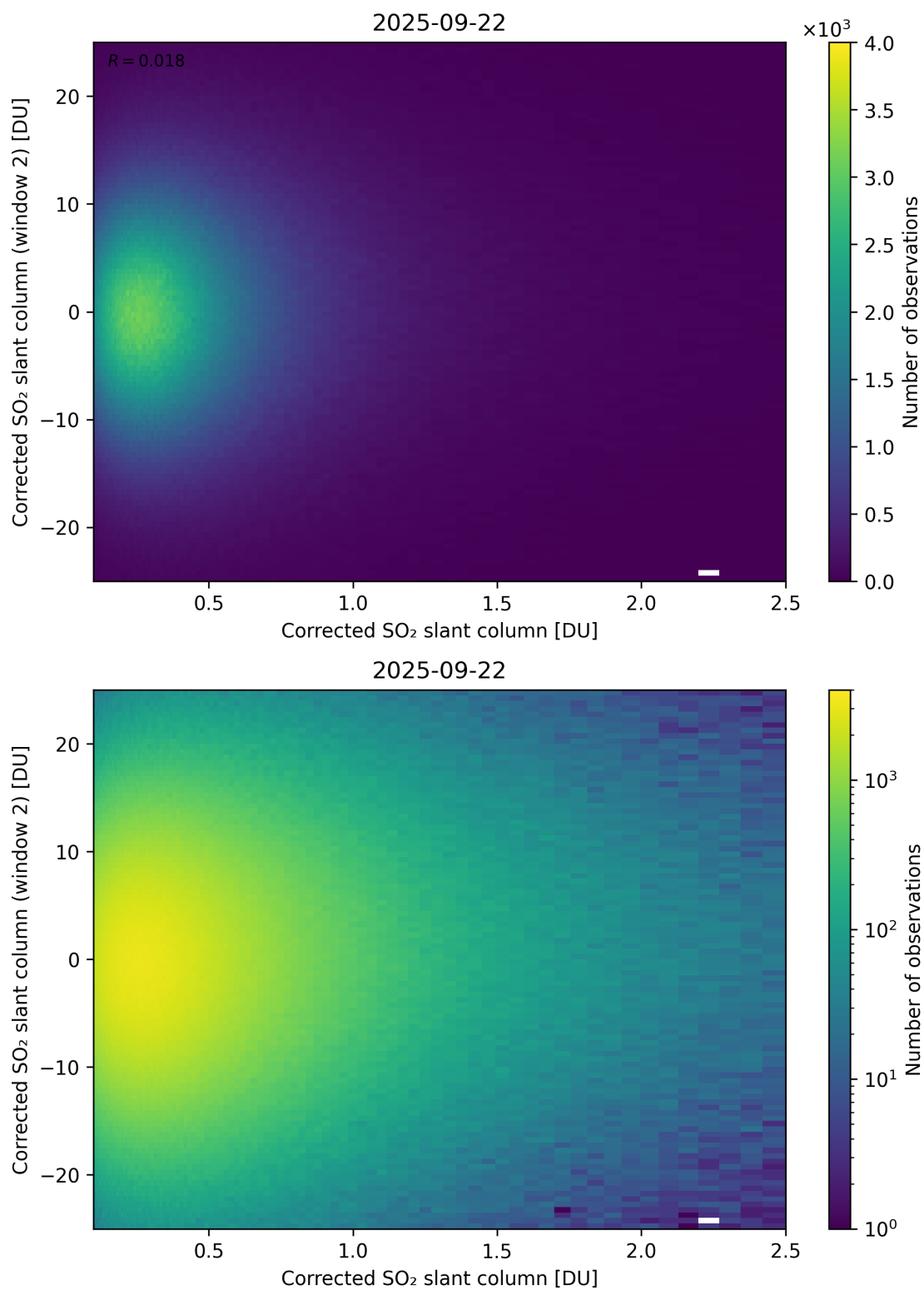
Figure 235: Scatter density plot of “Corrected SO 2 slant column” against “Corrected SO 2 slant column (window 2)” for 2025-09-22 to 2025-09-23.
