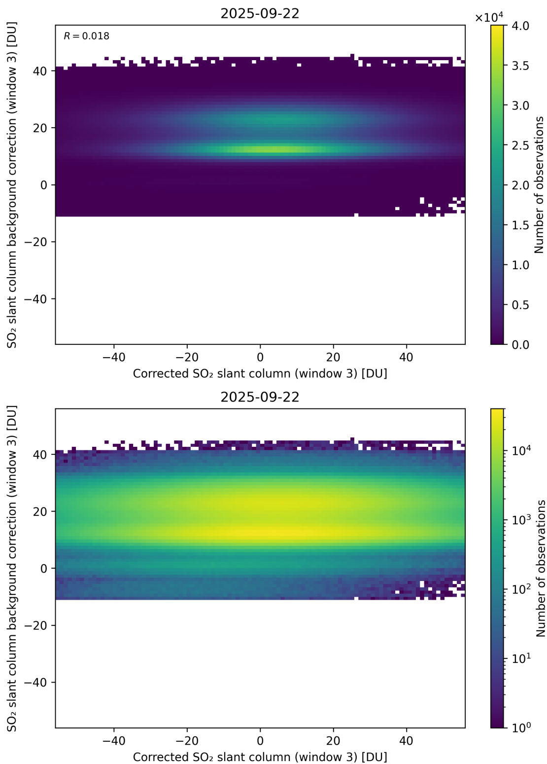
Figure 255: Scatter density plot of “Corrected SO 2 slant column (window 3)” against “SO 2 slant column background correction (window 3)” for 2025-09-22 to 2025-09-23.
