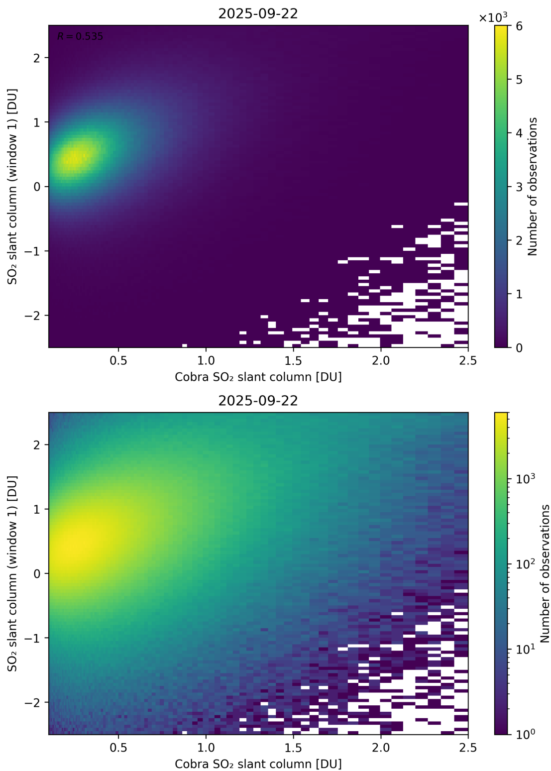
Figure 219: Scatter density plot of “Cobra SO 2 slant column” against “SO 2 slant column (window 1)” for 2025-09-22 to 2025-09-23.
