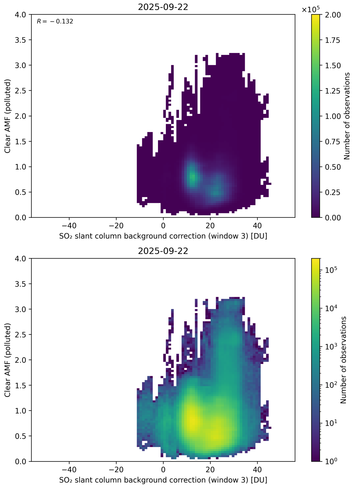
Figure 135: Scatter density plot of “SO 2 slant column background correction (window 3)” against “Clear AMF (polluted)” for 2025-09-22 to 2025-09-23.
