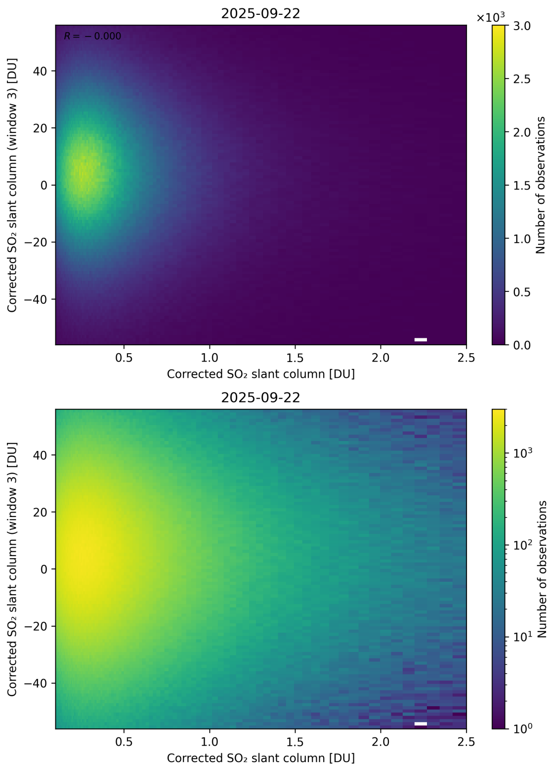
Figure 236: Scatter density plot of “Corrected SO 2 slant column” against “Corrected SO 2 slant column (window 3)” for 2025-09-22 to 2025-09-23.
