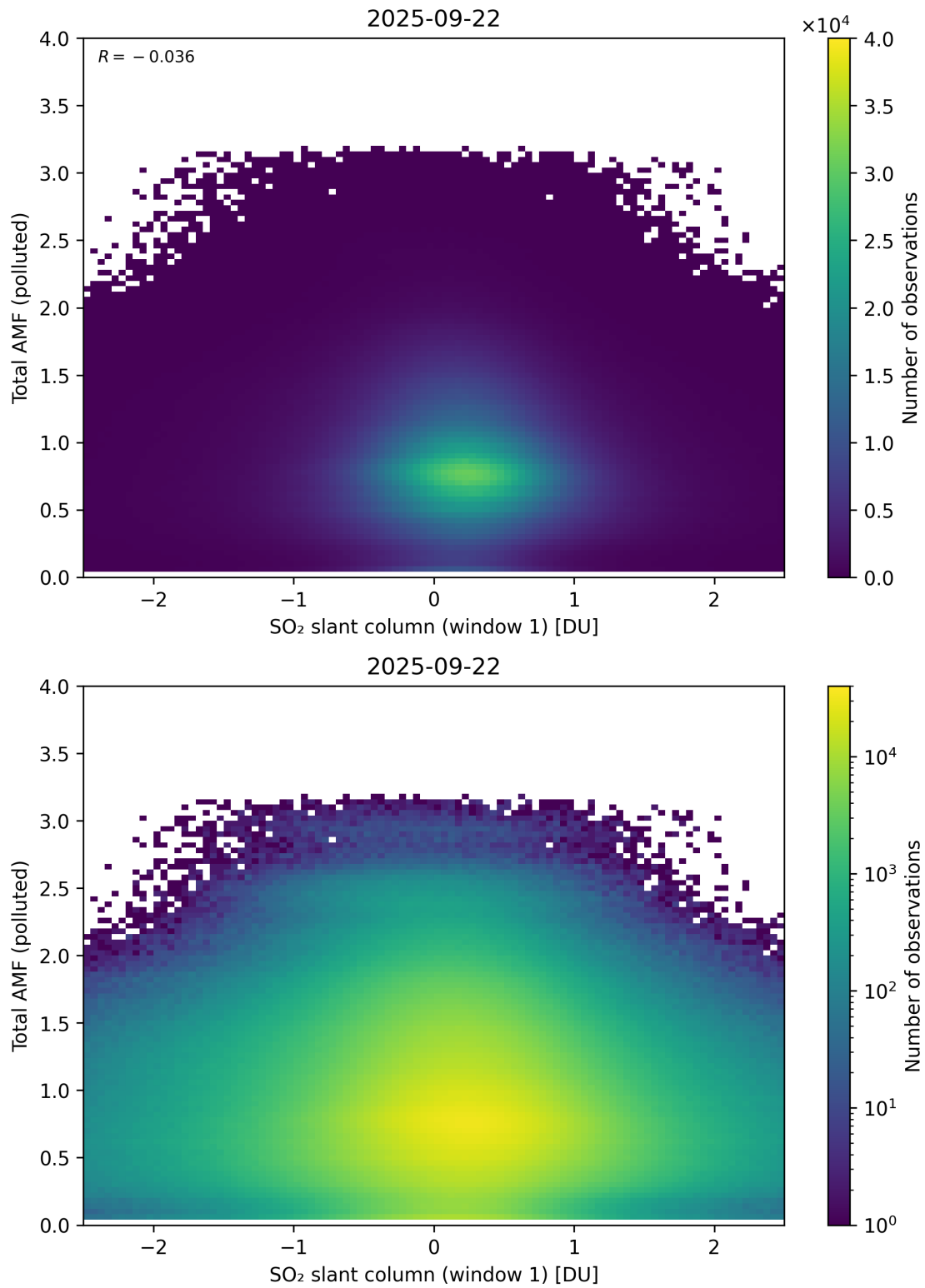
Figure 289: Scatter density plot of “SO 2 slant column (window 1)” against “Total AMF (polluted)” for 2025-09-22 to 2025-09-23.
