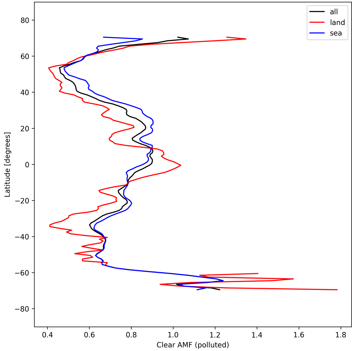
Figure 55: Zonal average of “Clear AMF (polluted)” for 2025-09-22 to 2025-09-23.
