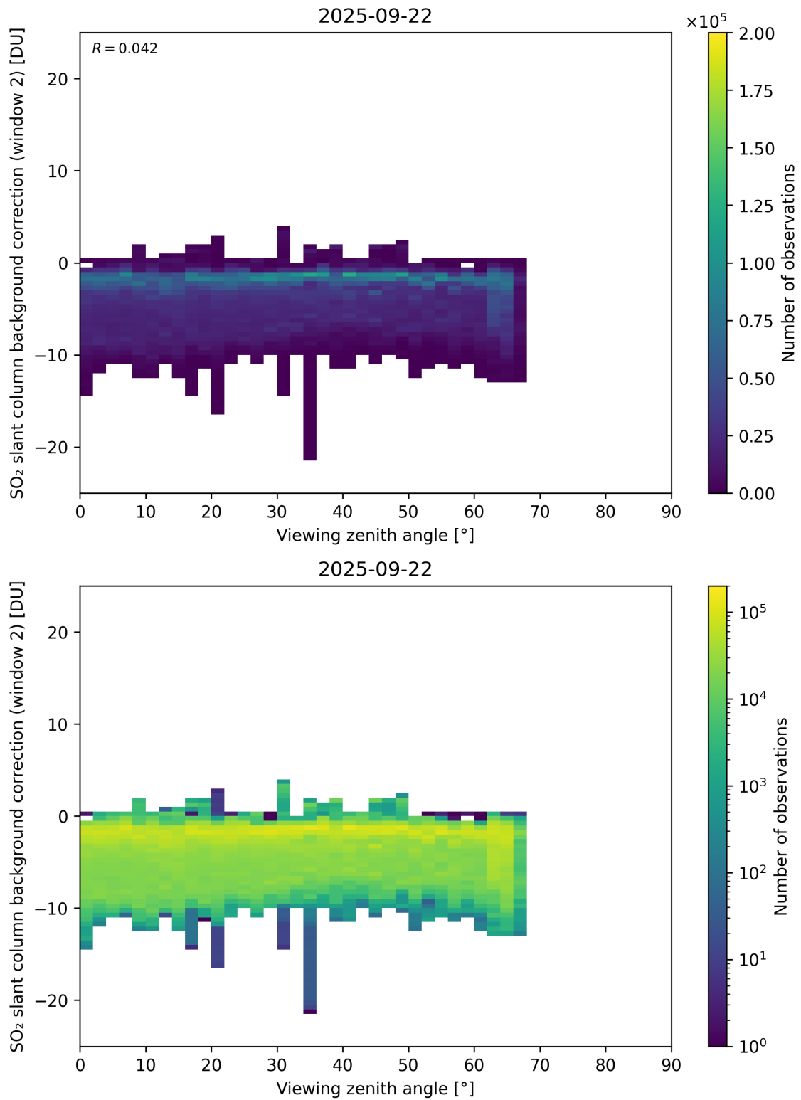
Figure 363: Scatter density plot of “Viewing zenith angle” against “SO 2 slant column background correction (window 2)” for 2025-09-22 to 2025-09-23.
