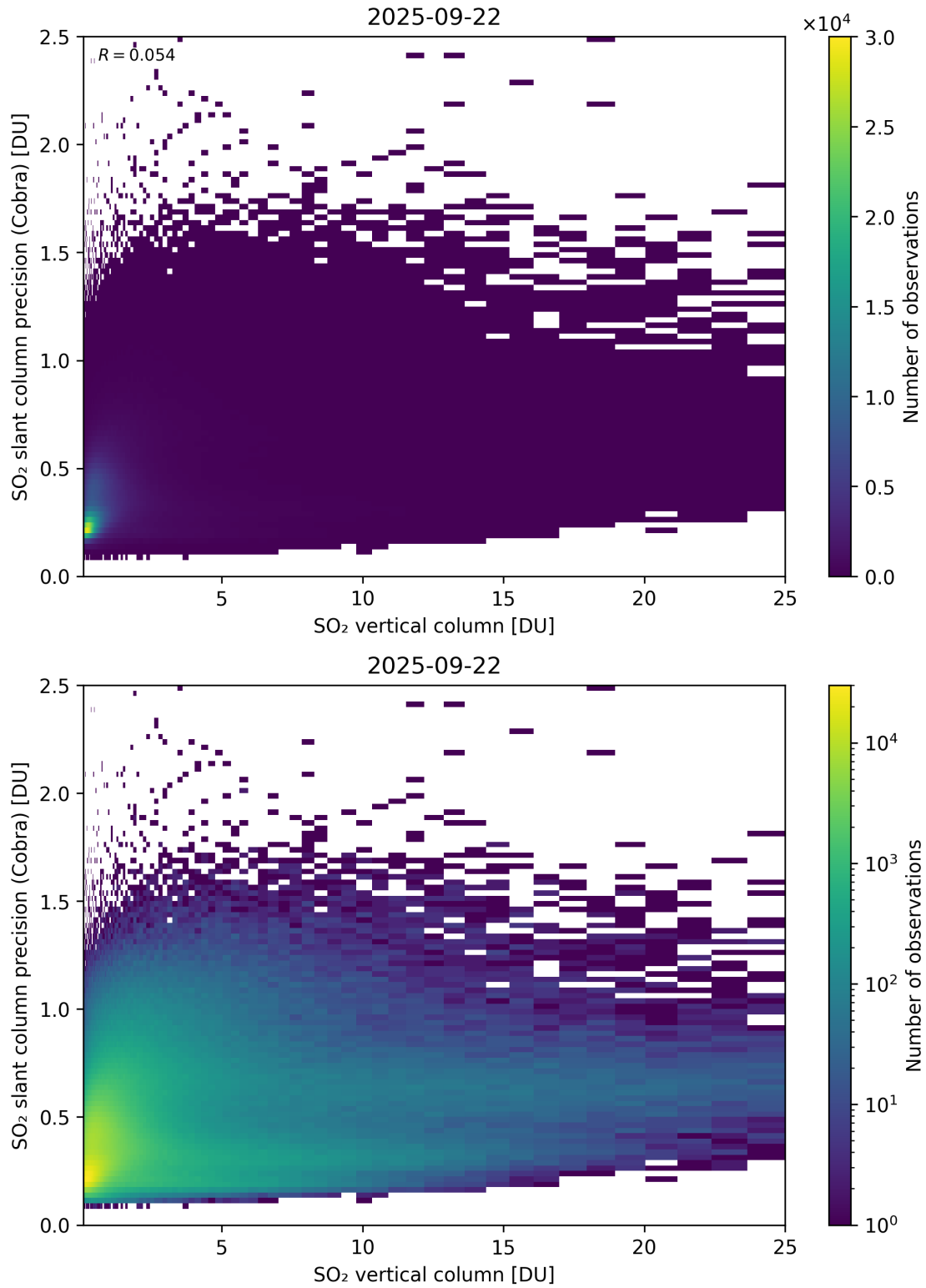
Figure 350: Scatter density plot of “SO 2 vertical column” against “SO 2 slant column precision (Cobra)” for 2025-09-22 to 2025-09-23.
