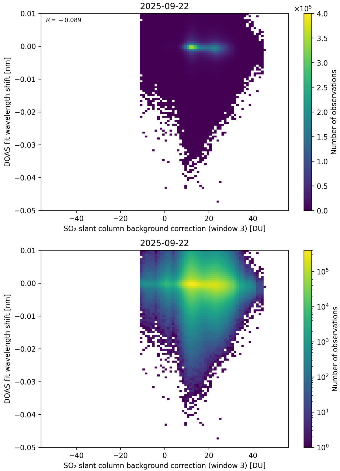
Figure 132: Scatter density plot of “SO 2 slant column background correction (window 3)” against “DOAS fit wavelength shift” for 2025-09-22 to 2025-09-23.
