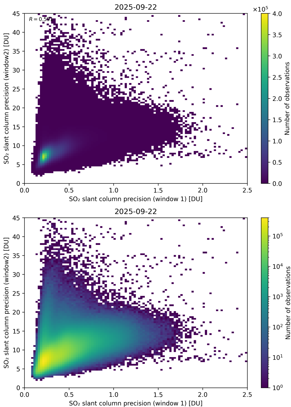
Figure 277: Scatter density plot of “SO 2 slant column precision (window 1)” against “SO 2 slant column precision (window2)” for 2025-09-22 to 2025-09-23.
