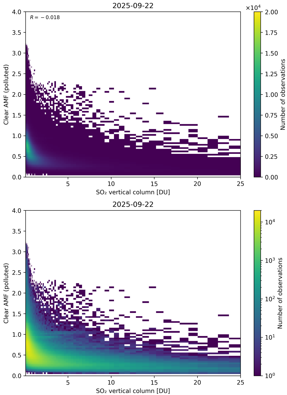
Figure 348: Scatter density plot of “SO 2 vertical column” against “Clear AMF (polluted)” for 2025-09-22 to 2025-09-23.
