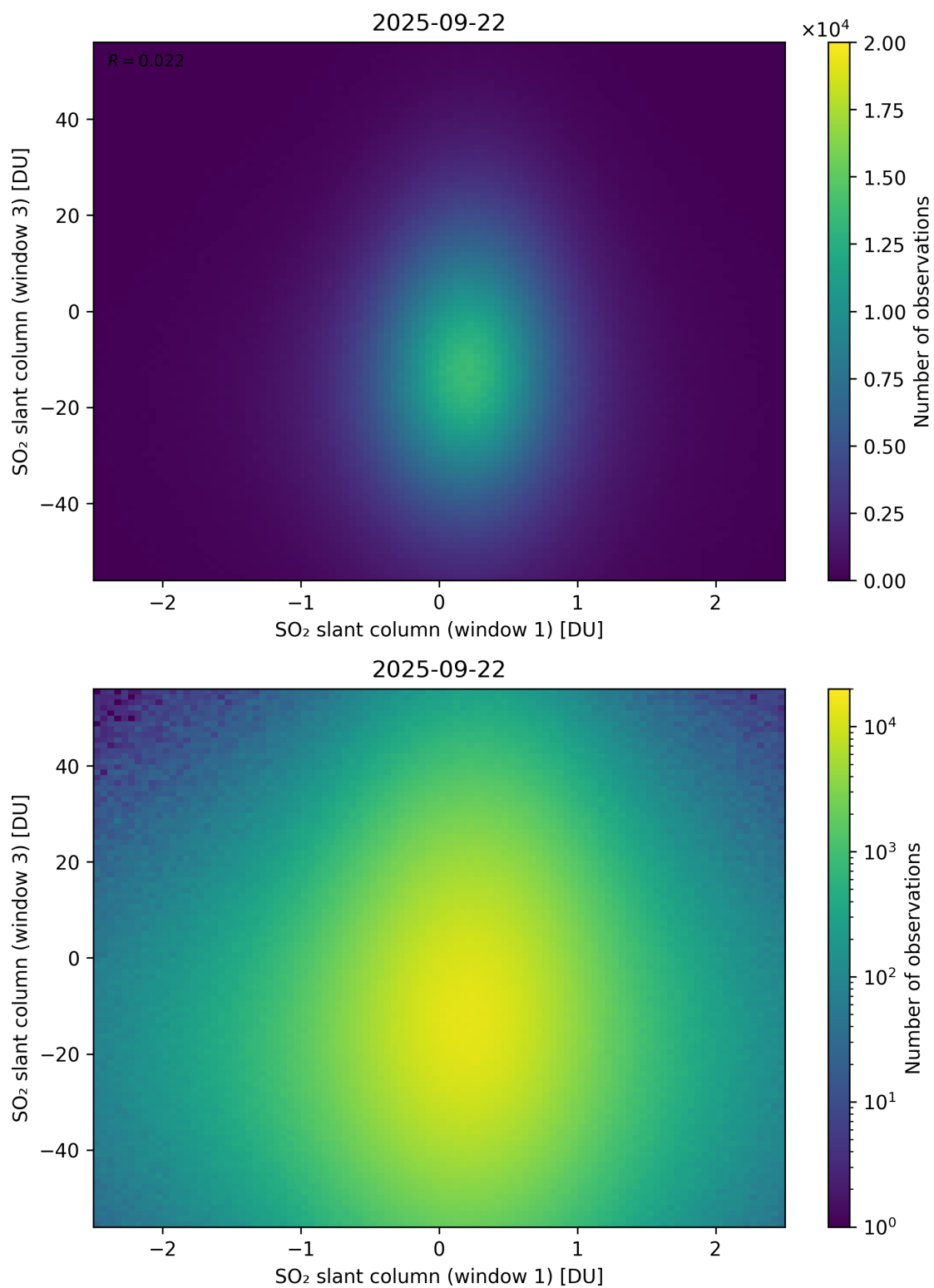
Figure 287: Scatter density plot of “SO 2 slant column (window 1)” against “SO 2 slant column (window 3)” for 2025-09-22 to 2025-09-23.
