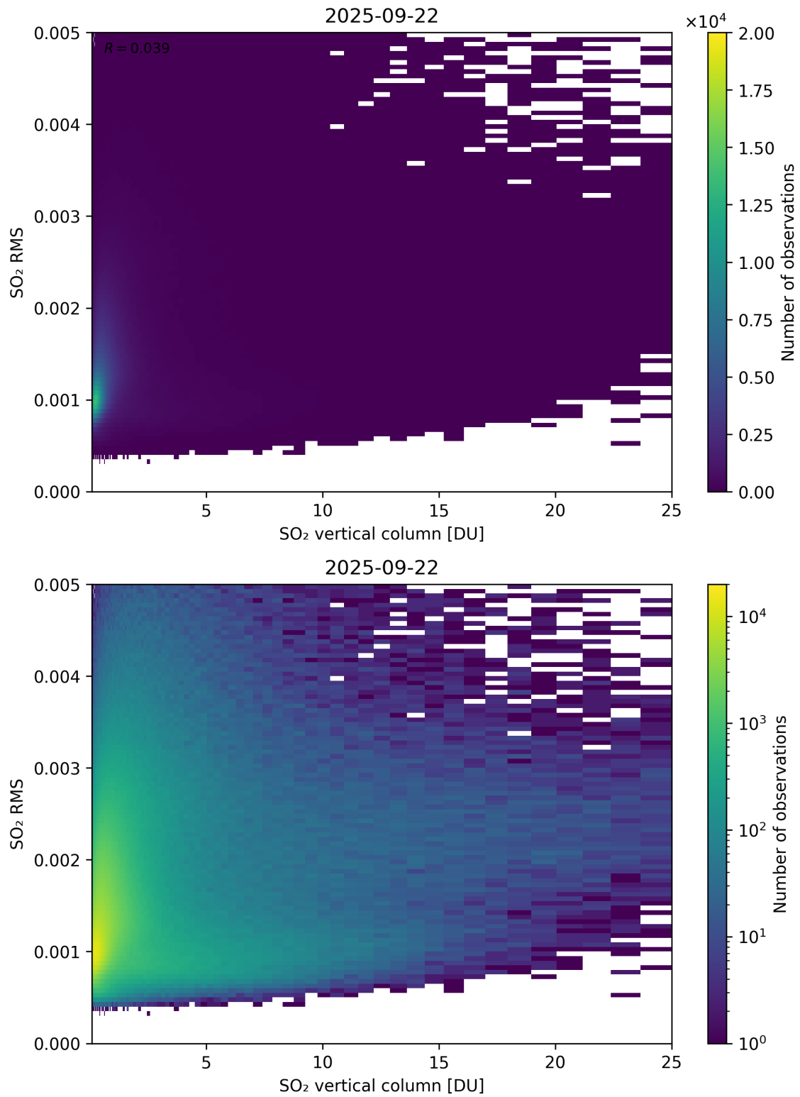
Figure 328: Scatter density plot of “SO 2 vertical column” against “SO 2 RMS” for 2025-09-22 to 2025-09-23.
