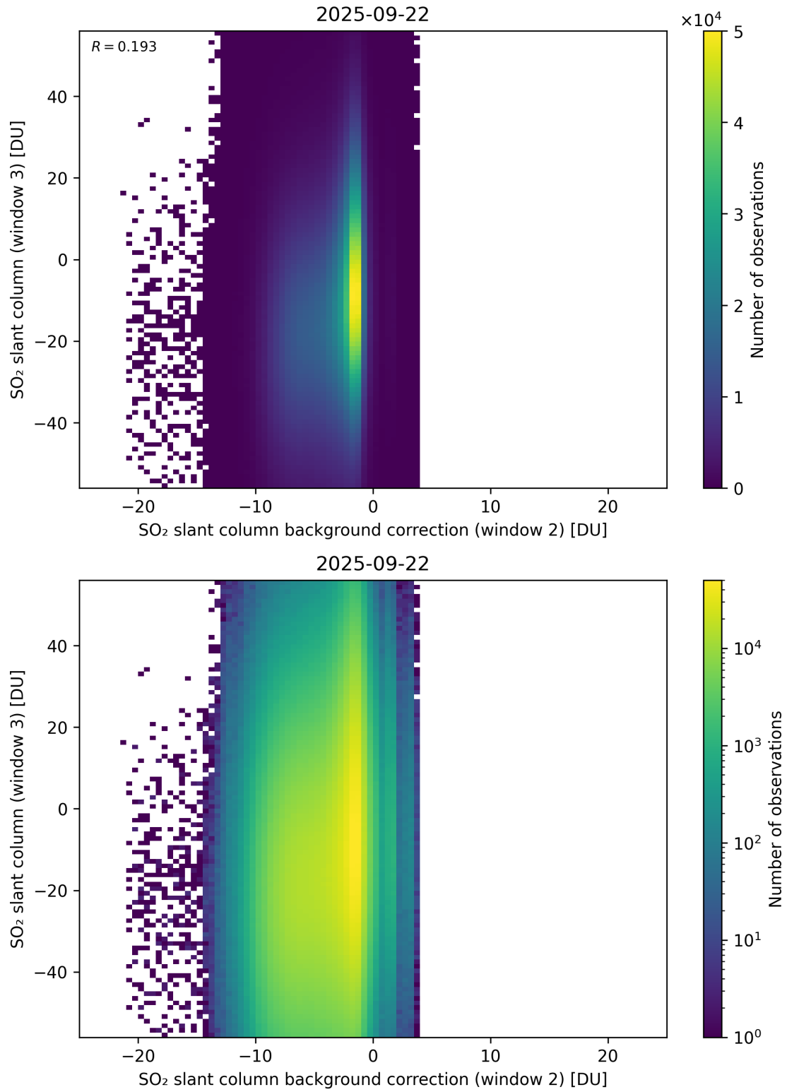
Figure 128: Scatter density plot of “SO 2 slant column background correction (window 2)” against “SO 2 slant column (window 3)” for 2025-09-22 to 2025-09-23.
