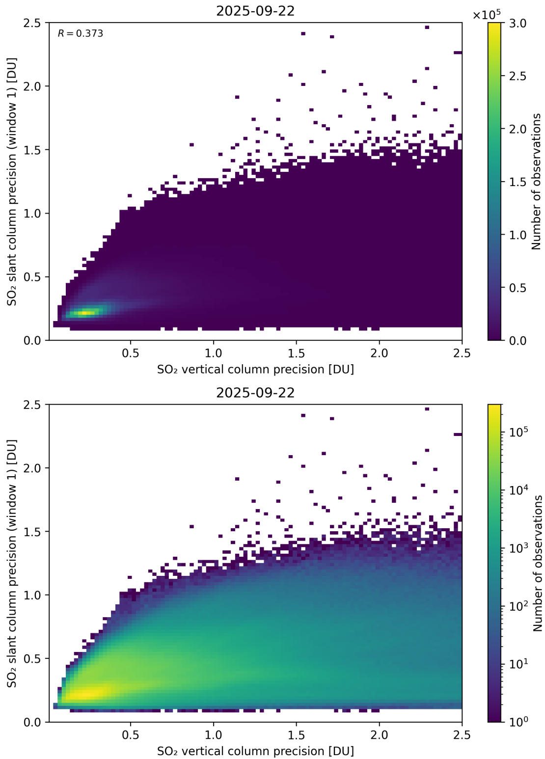
Figure 342: Scatter density plot of “SO 2 vertical column precision” against “SO 2 slant column precision (window 1)” for 2025-09-22 to 2025-09-23.
