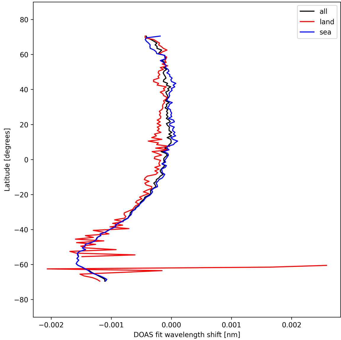
Figure 50: Zonal average of “DOAS fit wavelength shift” for 2025-09-22 to 2025-09-23.
