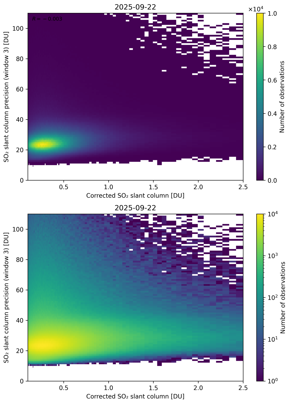
Figure 241: Scatter density plot of “Corrected SO 2 slant column” against “SO 2 slant column precision (window 3)” for 2025-09-22 to 2025-09-23.
