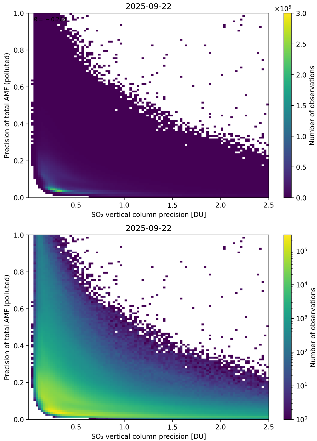
Figure 347: Scatter density plot of “SO 2 vertical column precision” against “Precision of total AMF (polluted)” for 2025-09-22 to 2025-09-23.
