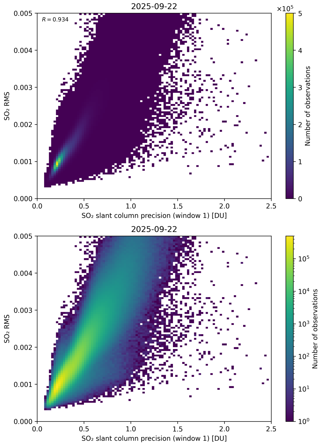
Figure 273: Scatter density plot of “SO 2 slant column precision (window 1)” against “SO 2 RMS” for 2025-09-22 to 2025-09-23.
