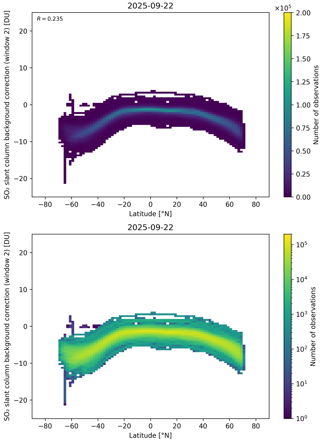
Figure 151: Scatter density plot of “Latitude” against “SO 2 slant column background correction (window 2)” for 2025-09-22 to 2025-09-23.
