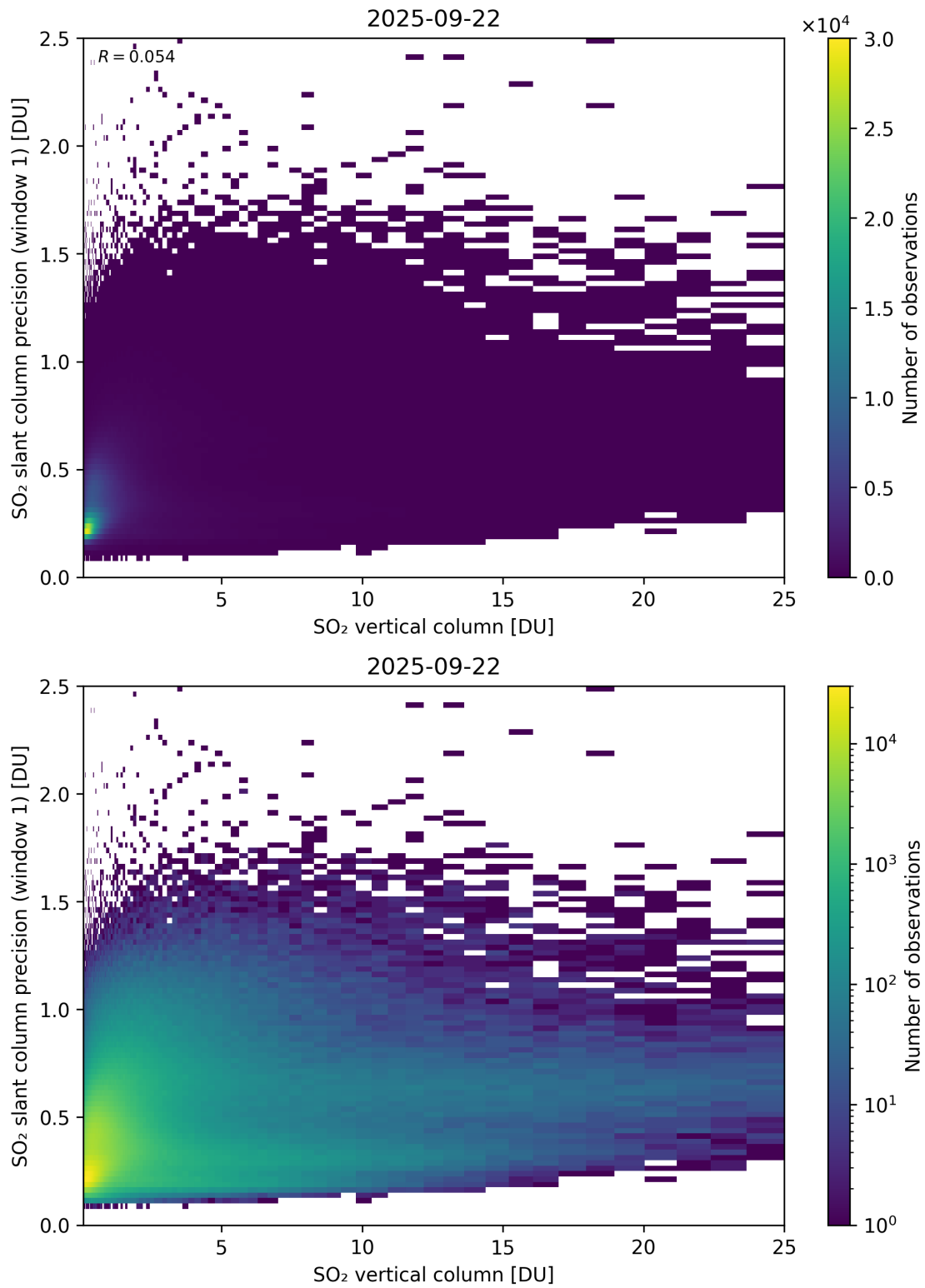
Figure 355: Scatter density plot of “SO 2 vertical column” against “SO 2 slant column precision (window 1)” for 2025-09-22 to 2025-09-23.
