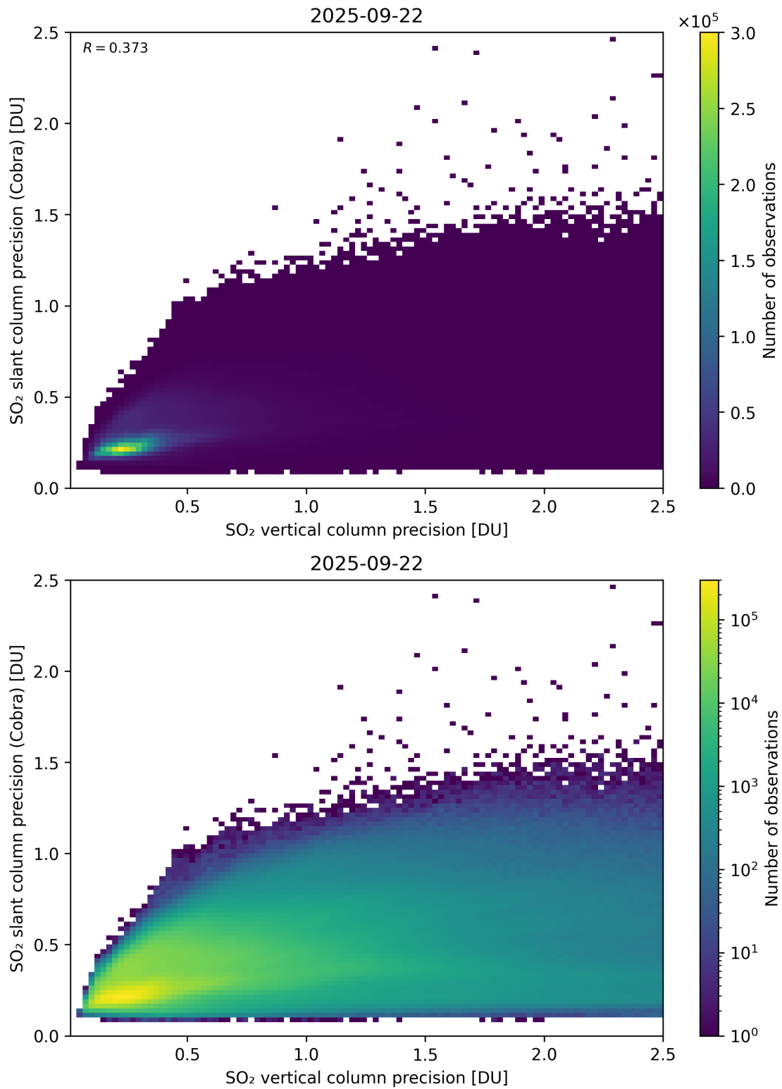
Figure 337: Scatter density plot of “SO 2 vertical column precision” against “SO 2 slant column precision (Cobra)” for 2025-09-22 to 2025-09-23.
