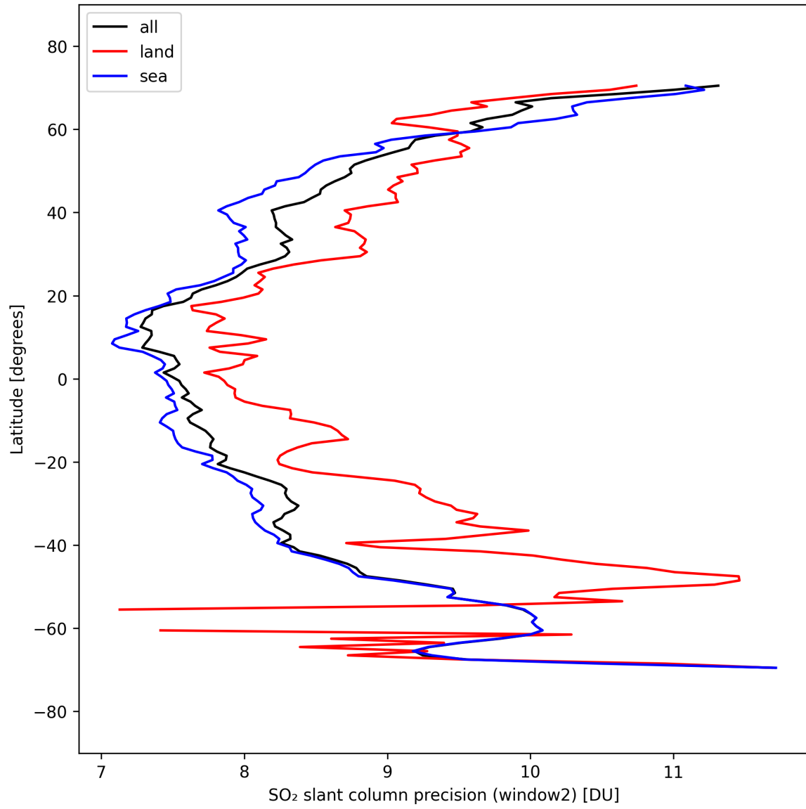
Figure 42: Zonal average of “SO 2 slant column precision (window2)” for 2025-09-22 to 2025-09-23.
