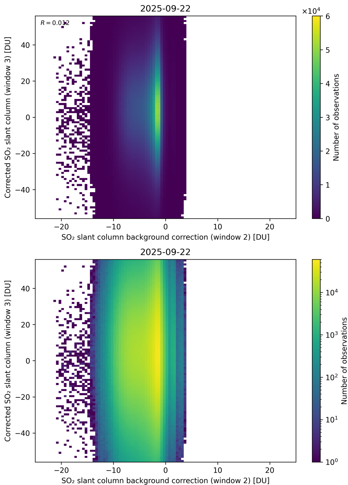
Figure 127: Scatter density plot of “SO 2 slant column background correction (window 2)” against “Corrected SO 2 slant column (window 3)” for 2025-09-22 to 2025-09-23.
