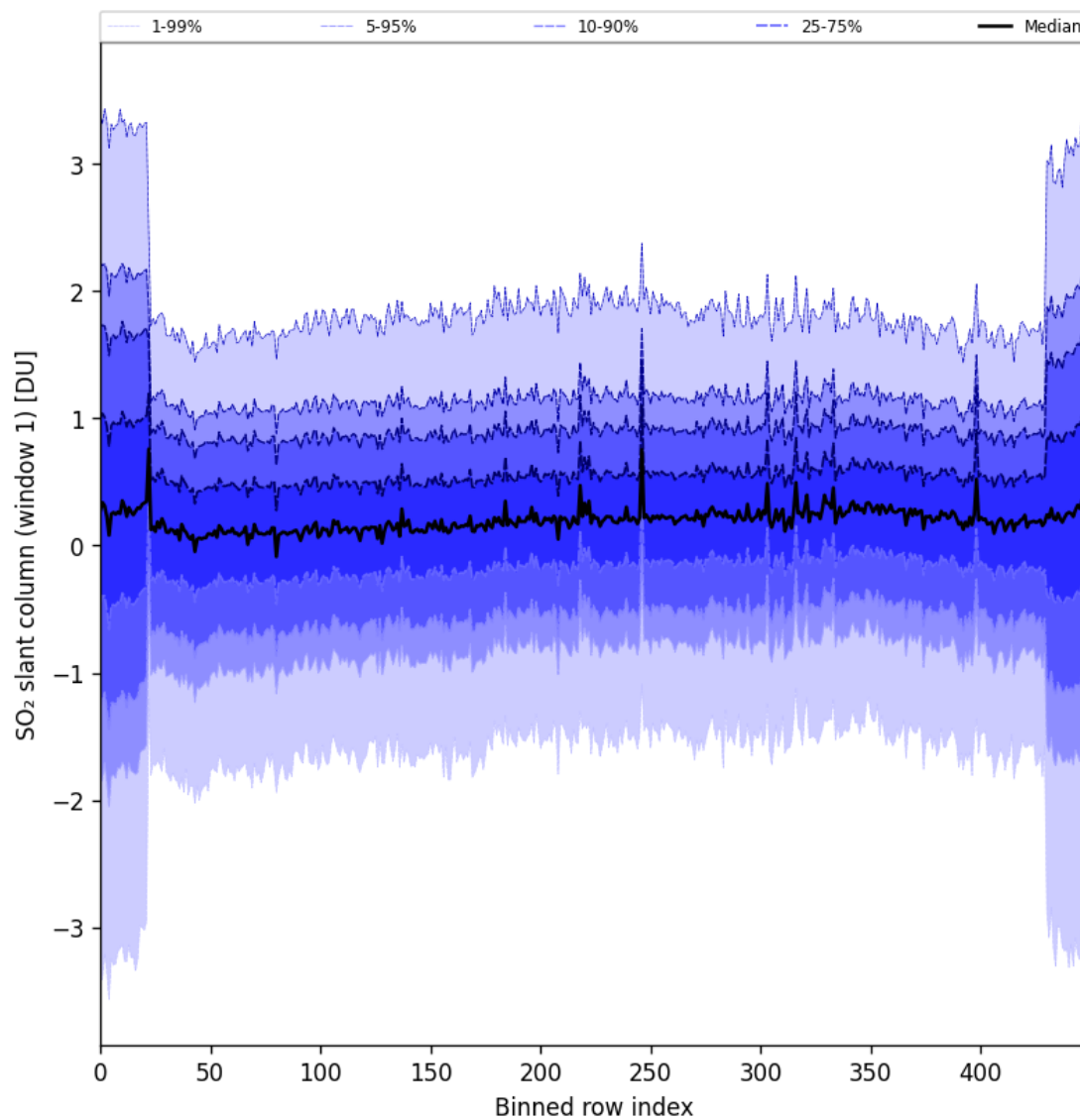
Figure 89: Along track statistics of “SO 2 slant column (window 1)” for 2025-09-22 to 2025-09-23
