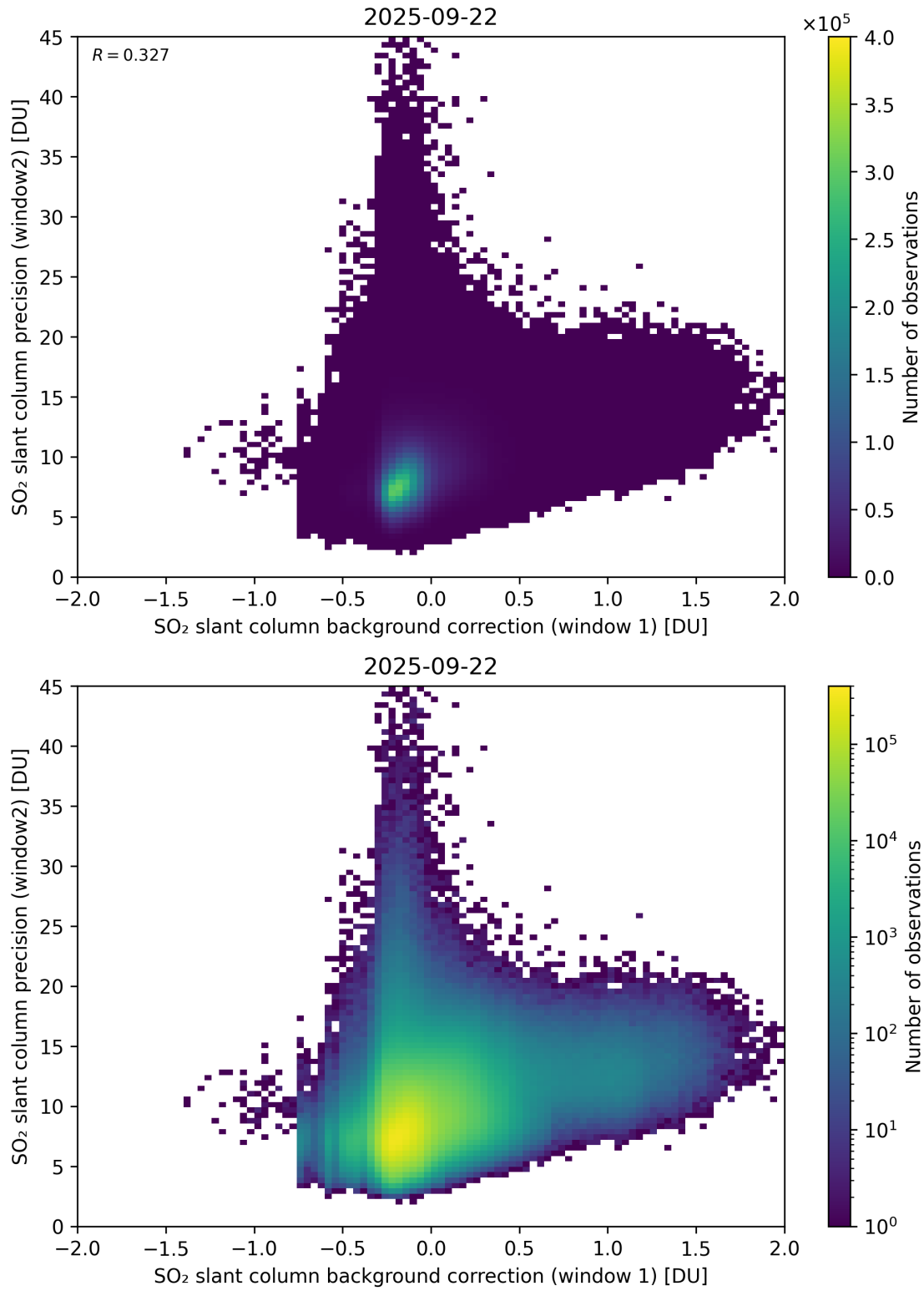
Figure 117: Scatter density plot of “SO 2 slant column background correction (window 1)” against “SO 2 slant column precision (window2)” for 2025-09-22 to 2025-09-23.
