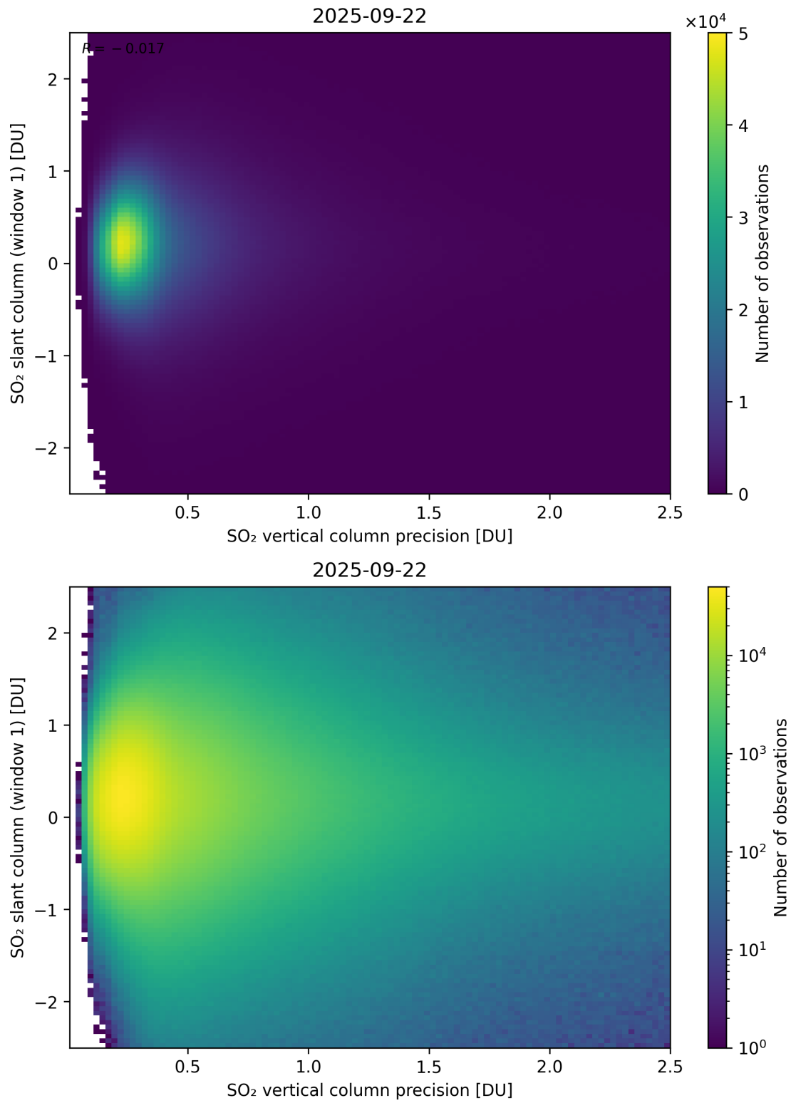
Figure 341: Scatter density plot of “SO 2 vertical column precision” against “SO 2 slant column (window 1)” for 2025-09-22 to 2025-09-23.
