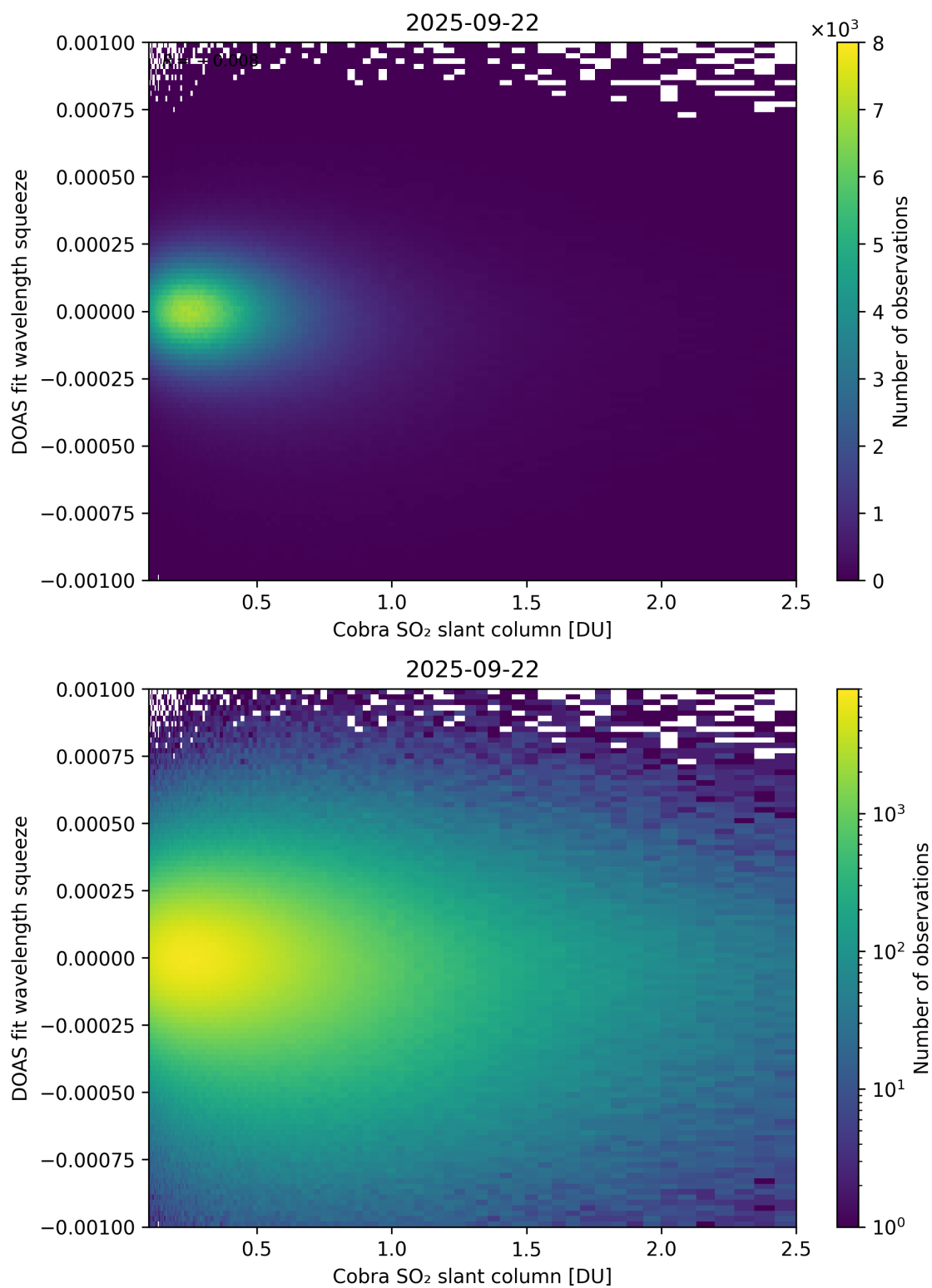
Figure 197: Scatter density plot of “Cobra SO 2 slant column” against “DOAS fit wavelength squeeze” for 2025-09-22 to 2025-09-23.
