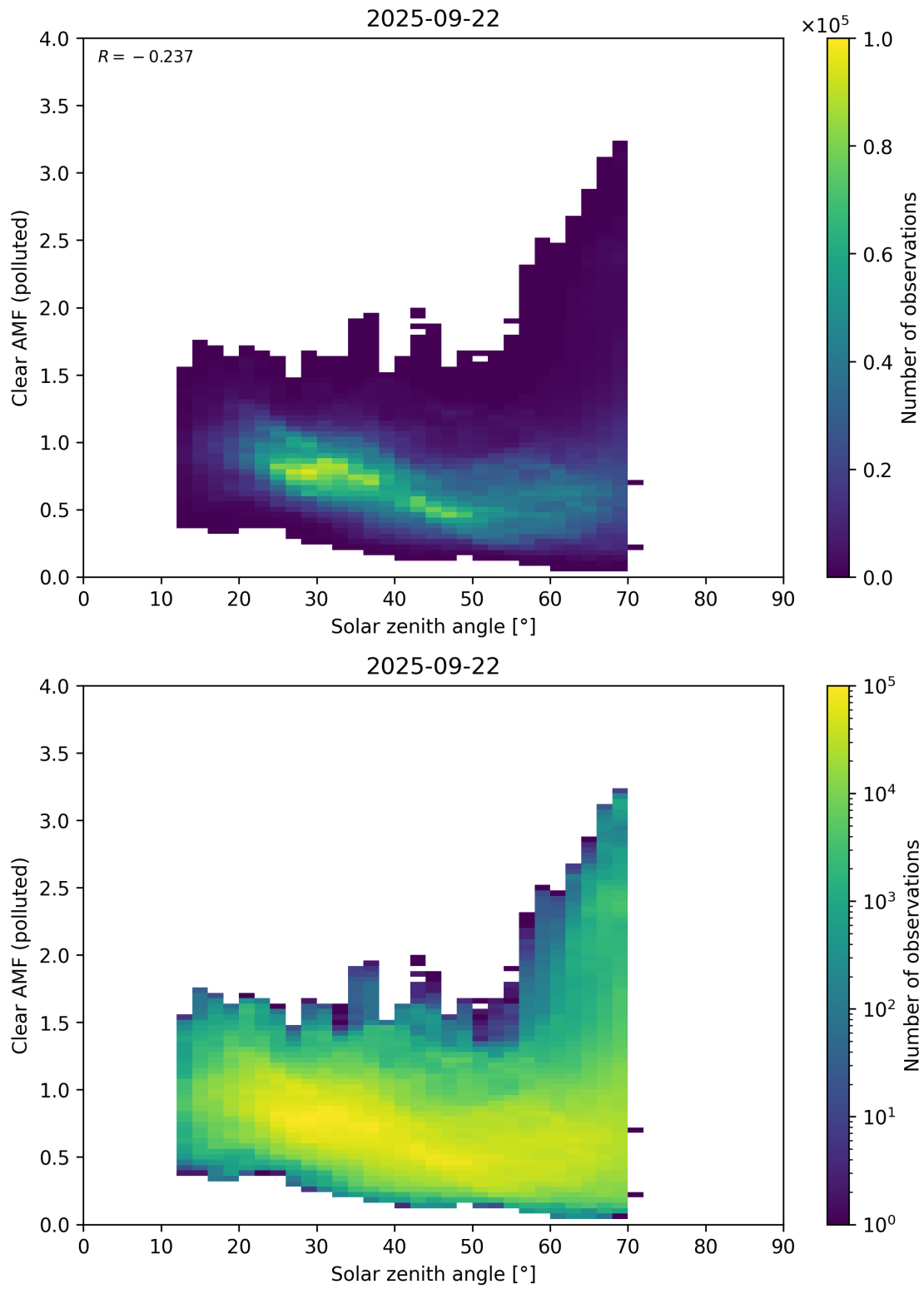
Figure 178: Scatter density plot of “Solar zenith angle” against “Clear AMF (polluted)” for 2025-09-22 to 2025-09-23.
