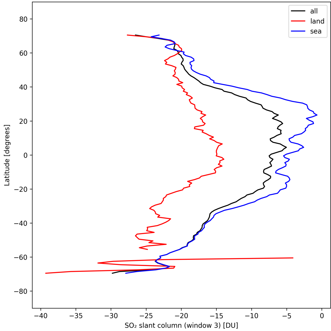
Figure 45: Zonal average of “SO 2 slant column (window 3)” for 2025-09-22 to 2025-09-23.
