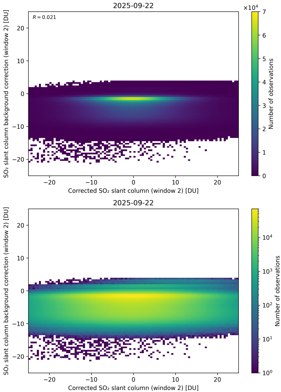
Figure 244: Scatter density plot of “Corrected SO 2 slant column (window 2)” against “SO 2 slant column background correction (window 2)” for 2025-09-22 to 2025-09-23.
