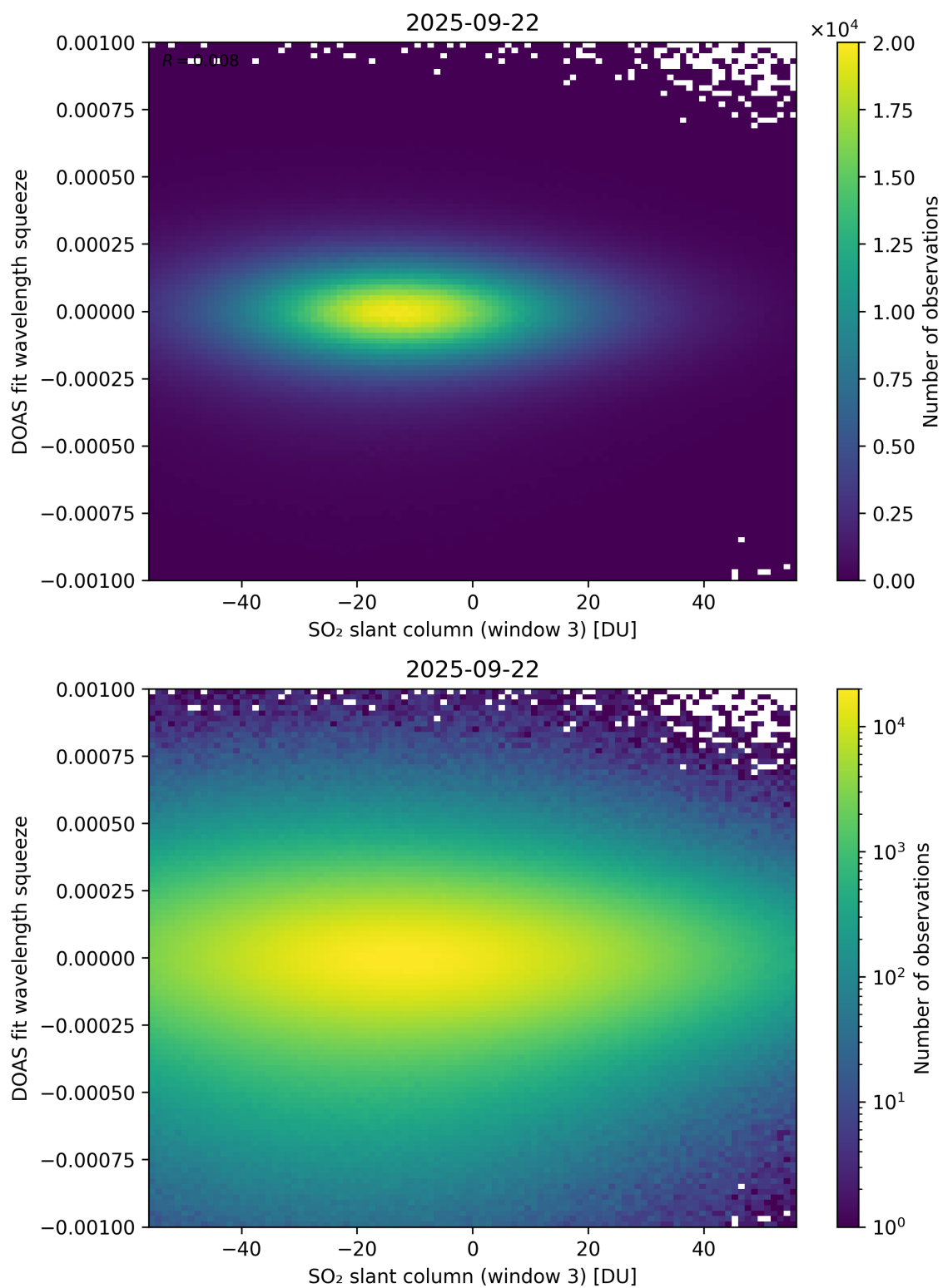
Figure 305: Scatter density plot of “SO 2 slant column (window 3)” against “DOAS fit wavelength squeeze” for 2025-09-22 to 2025-09-23.
