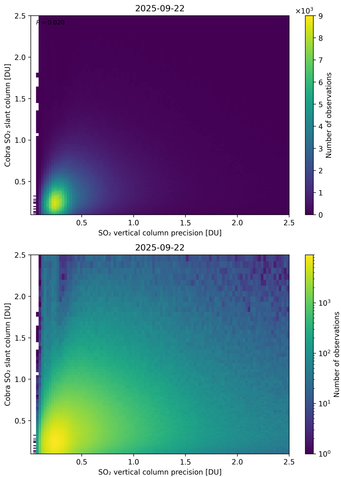
Figure 336: Scatter density plot of “SO 2 vertical column precision” against “Cobra SO 2 slant column” for 2025-09-22 to 2025-09-23.
