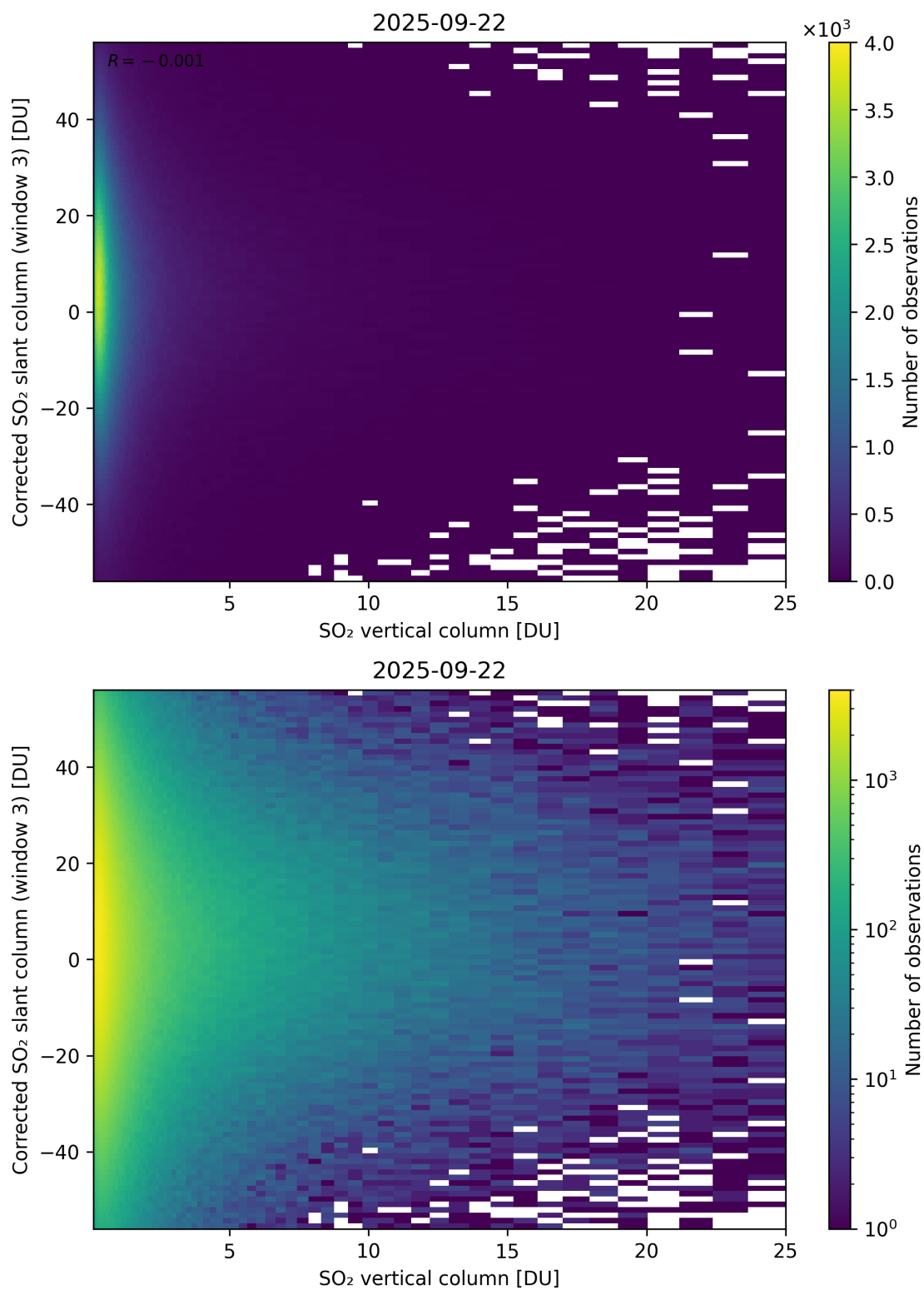
Figure 353: Scatter density plot of “SO 2 vertical column” against “Corrected SO 2 slant column (window 3)” for 2025-09-22 to 2025-09-23.
