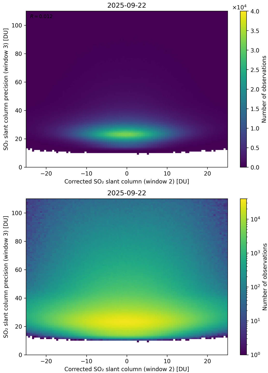
Figure 252: Scatter density plot of “Corrected SO 2 slant column (window 2)” against “SO 2 slant column precision (window 3)” for 2025-09-22 to 2025-09-23.
