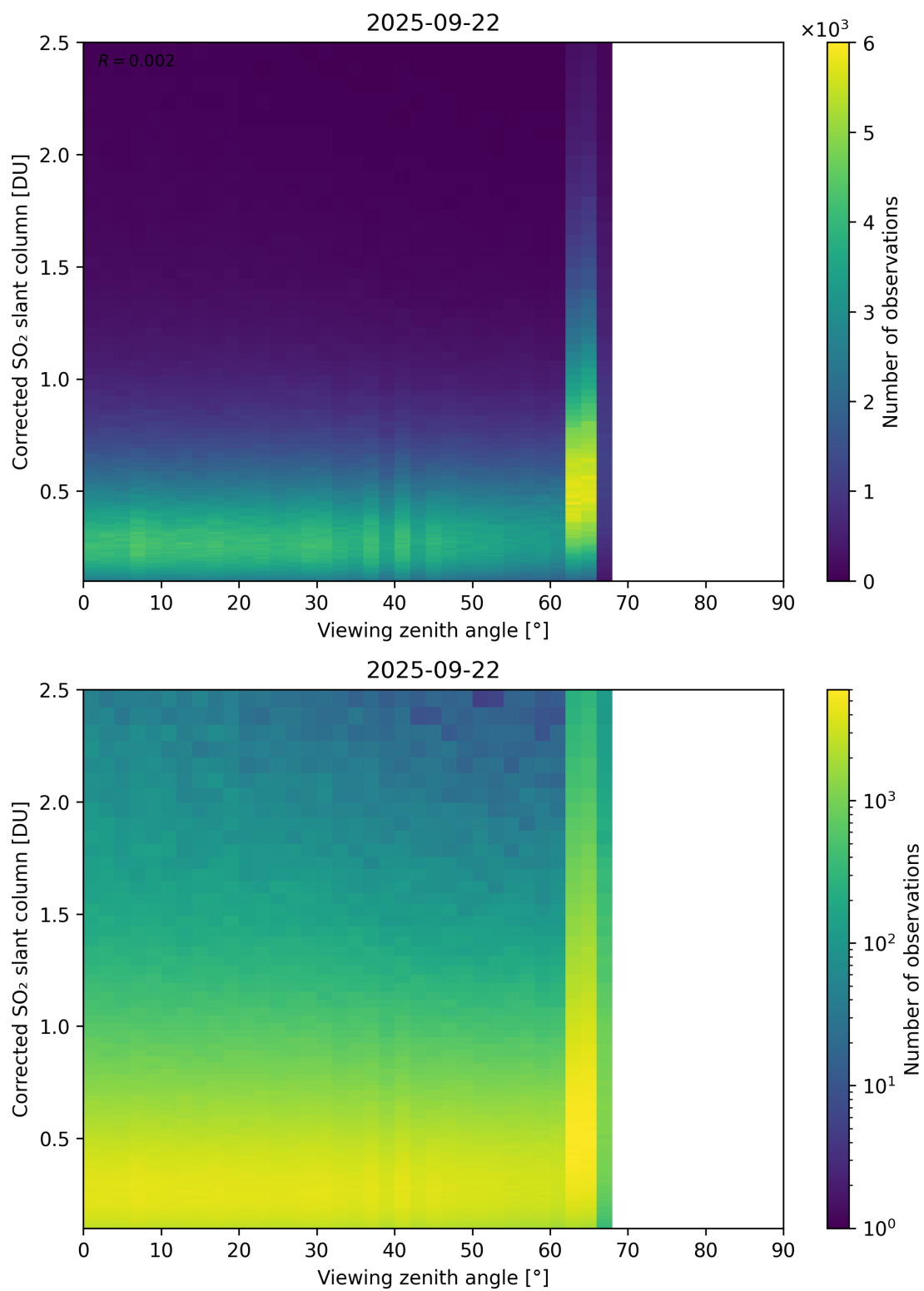
Figure 373: Scatter density plot of “Viewing zenith angle” against “Corrected SO 2 slant column” for 2025-09-22 to 2025-09-23.
