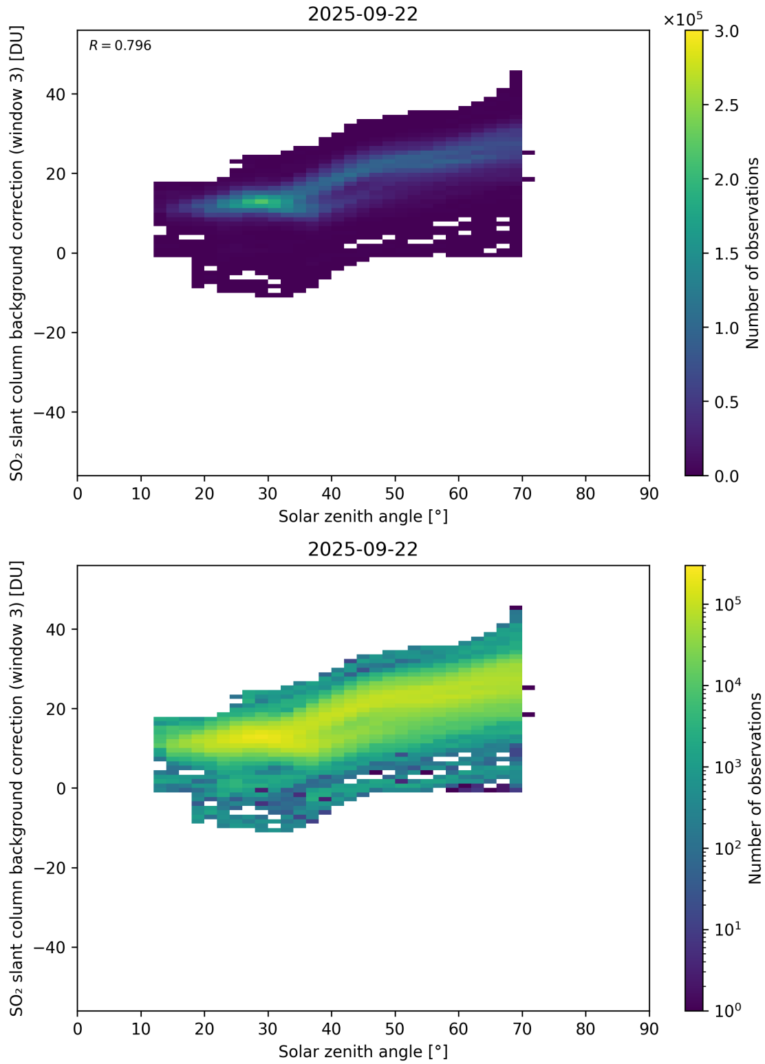
Figure 173: Scatter density plot of “Solar zenith angle” against “SO 2 slant column background correction (window 3)” for 2025-09-22 to 2025-09-23.
