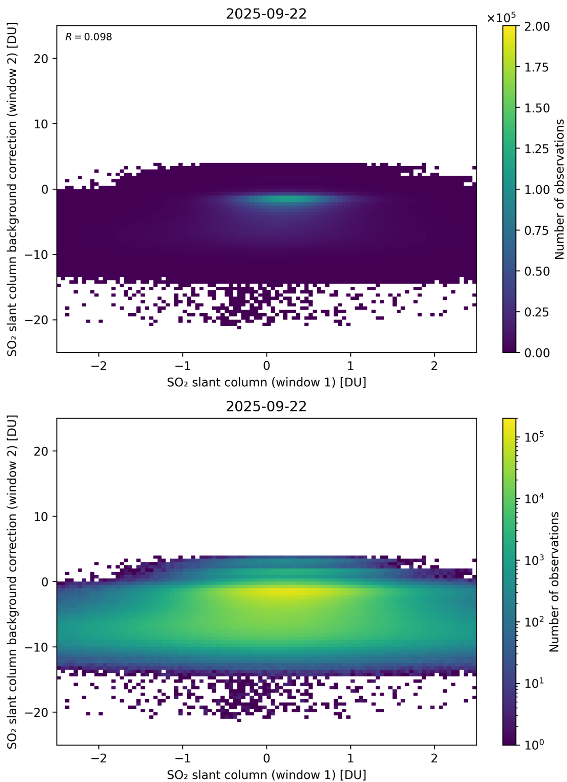
Figure 263: Scatter density plot of “SO 2 slant column (window 1)” against “SO 2 slant column background correction (window 2)” for 2025-09-22 to 2025-09-23.
