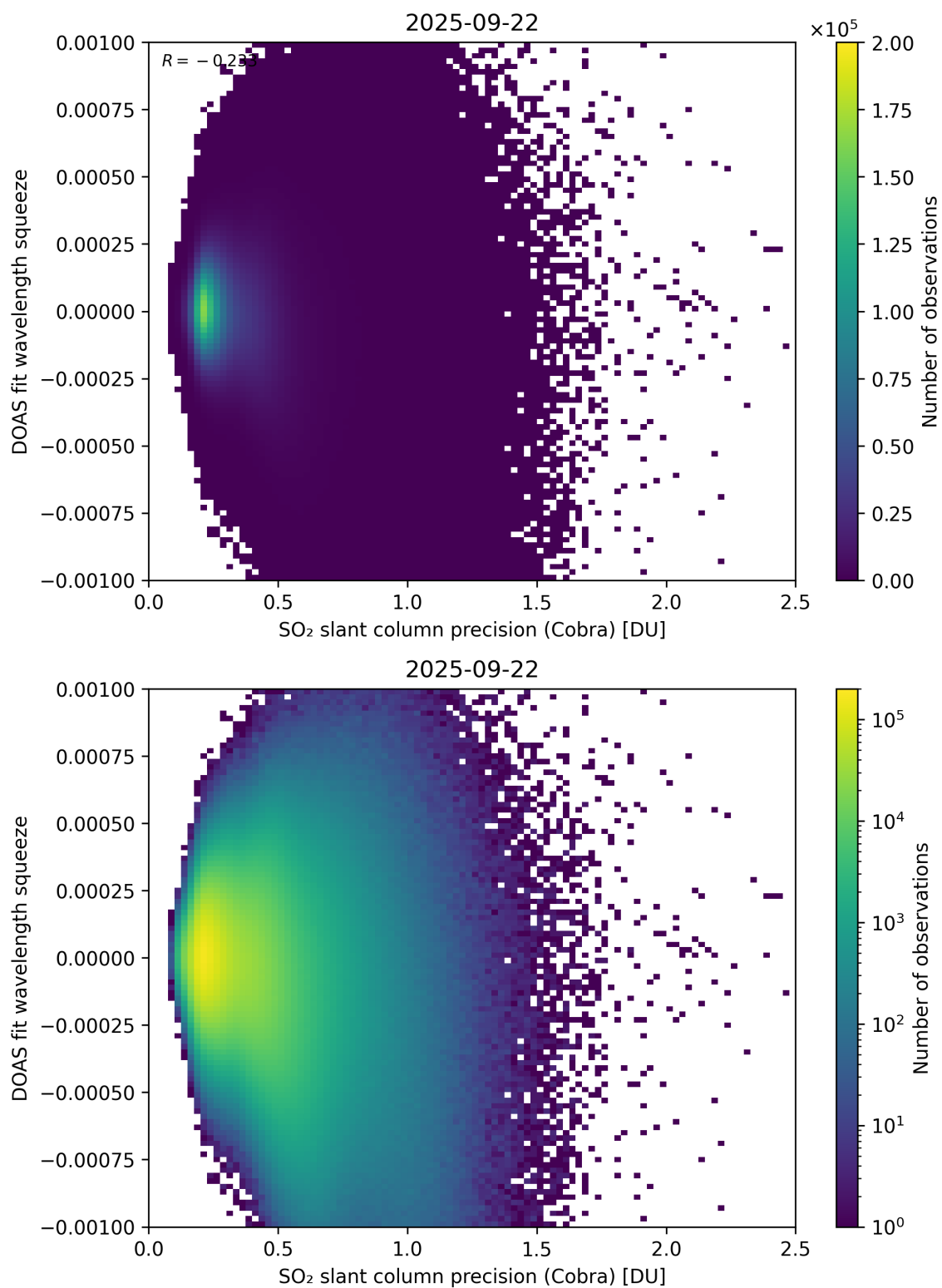
Figure 203: Scatter density plot of “SO 2 slant column precision (Cobra)” against “DOAS fit wavelength squeeze” for 2025-09-22 to 2025-09-23.
