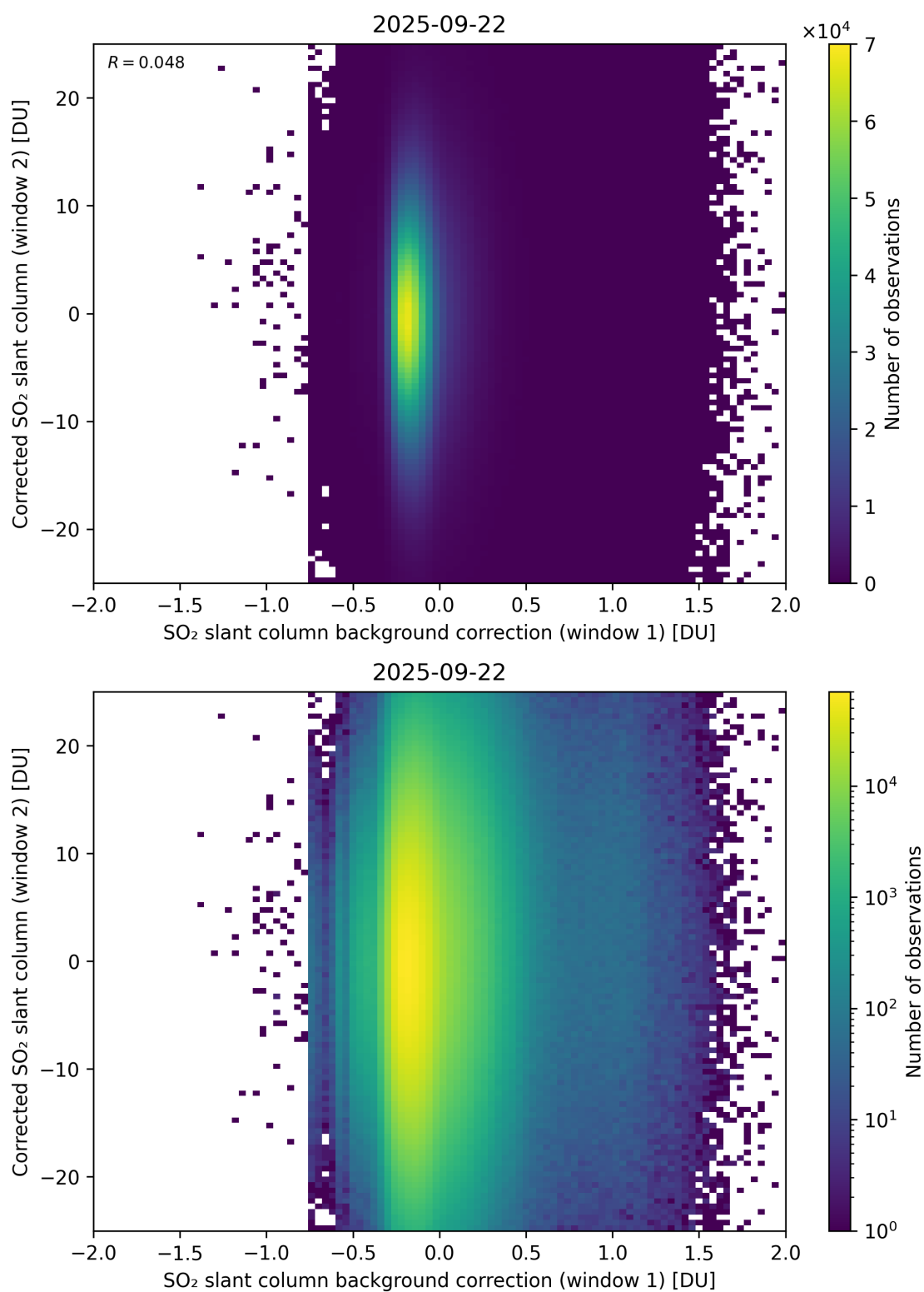
Figure 115: Scatter density plot of “SO 2 slant column background correction (window 1)” against “Corrected SO 2 slant column (window 2)” for 2025-09-22 to 2025-09-23.
