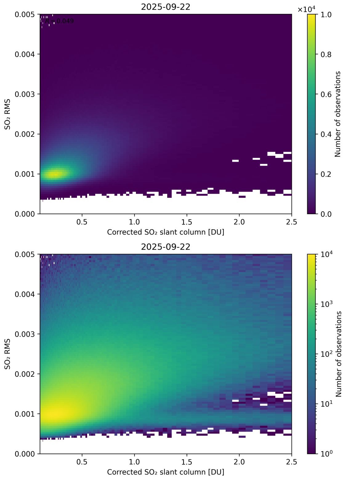
Figure 231: Scatter density plot of “Corrected SO 2 slant column” against “SO 2 RMS” for 2025-09-22 to 2025-09-23.
