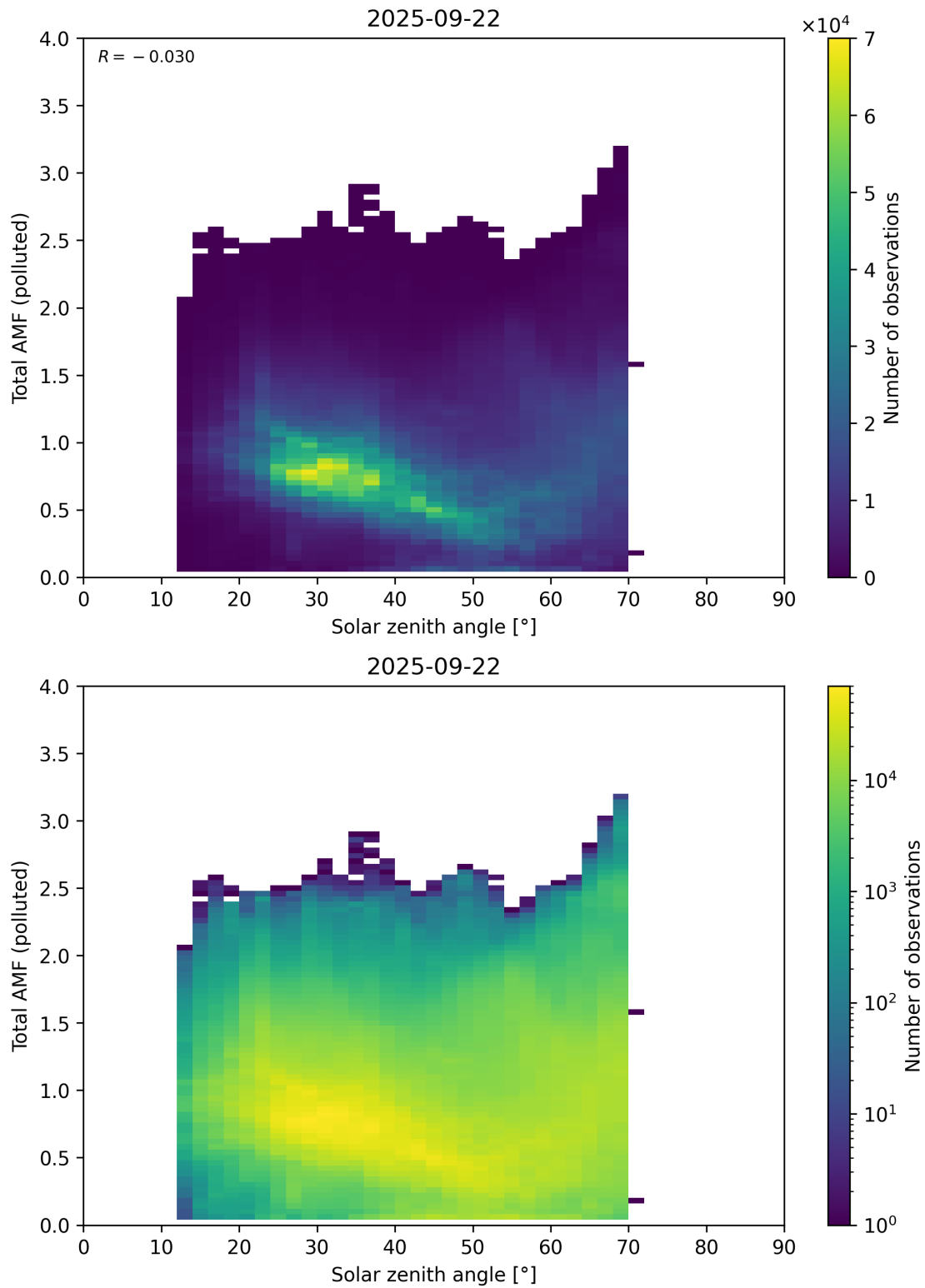
Figure 189: Scatter density plot of “Solar zenith angle” against “Total AMF (polluted)” for 2025-09-22 to 2025-09-23.
