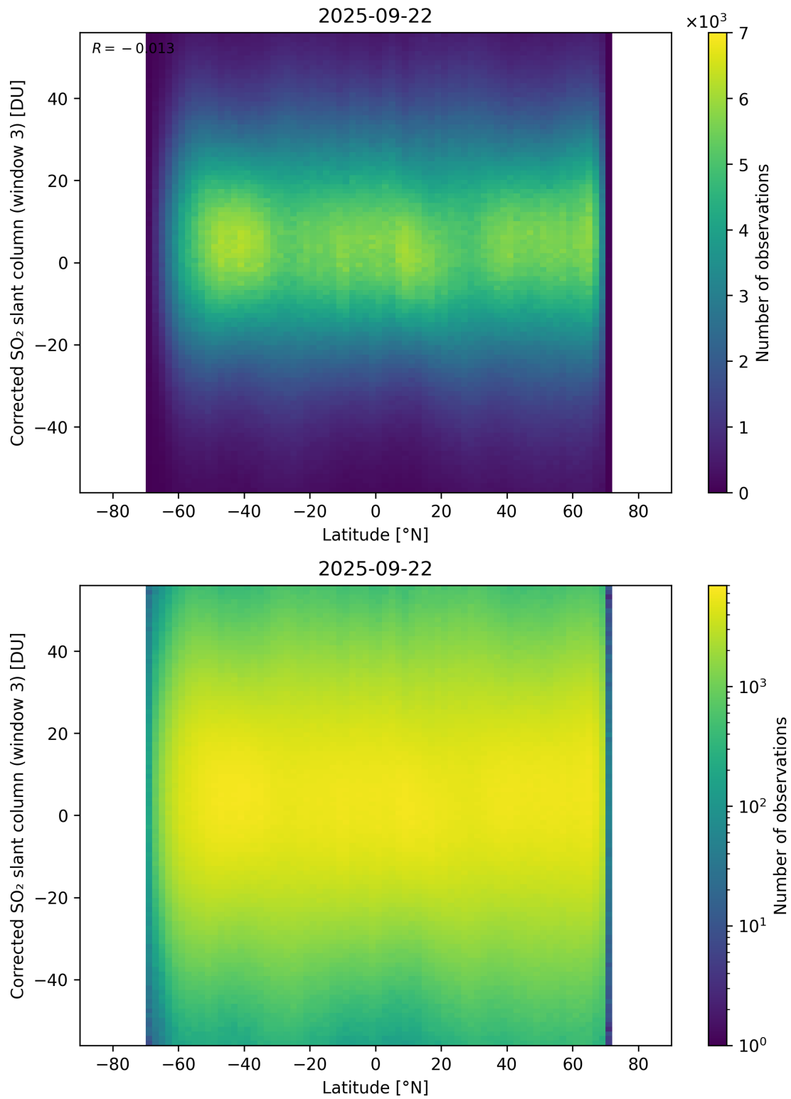
Figure 161: Scatter density plot of “Latitude” against “Corrected SO 2 slant column (window 3)” for 2025-09-22 to 2025-09-23.
