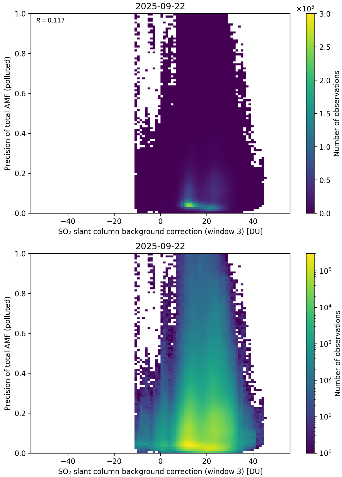
Figure 137: Scatter density plot of “SO 2 slant column background correction (window 3)” against “Precision of total AMF (polluted)” for 2025-09-22 to 2025-09-23.
