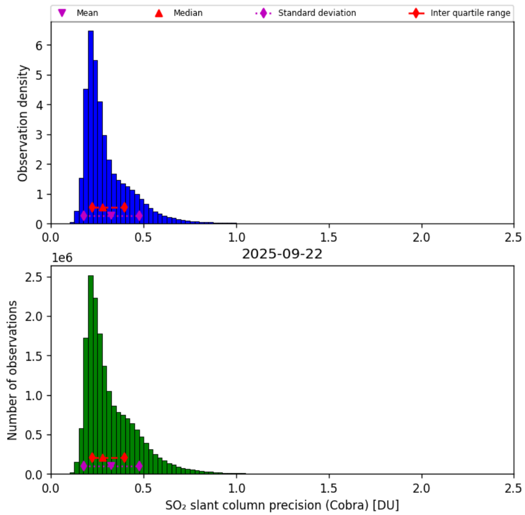
Figure 62: Histogram of “SO 2 slant column precision (Cobra)” for 2025-09-22 to 2025-09-23
