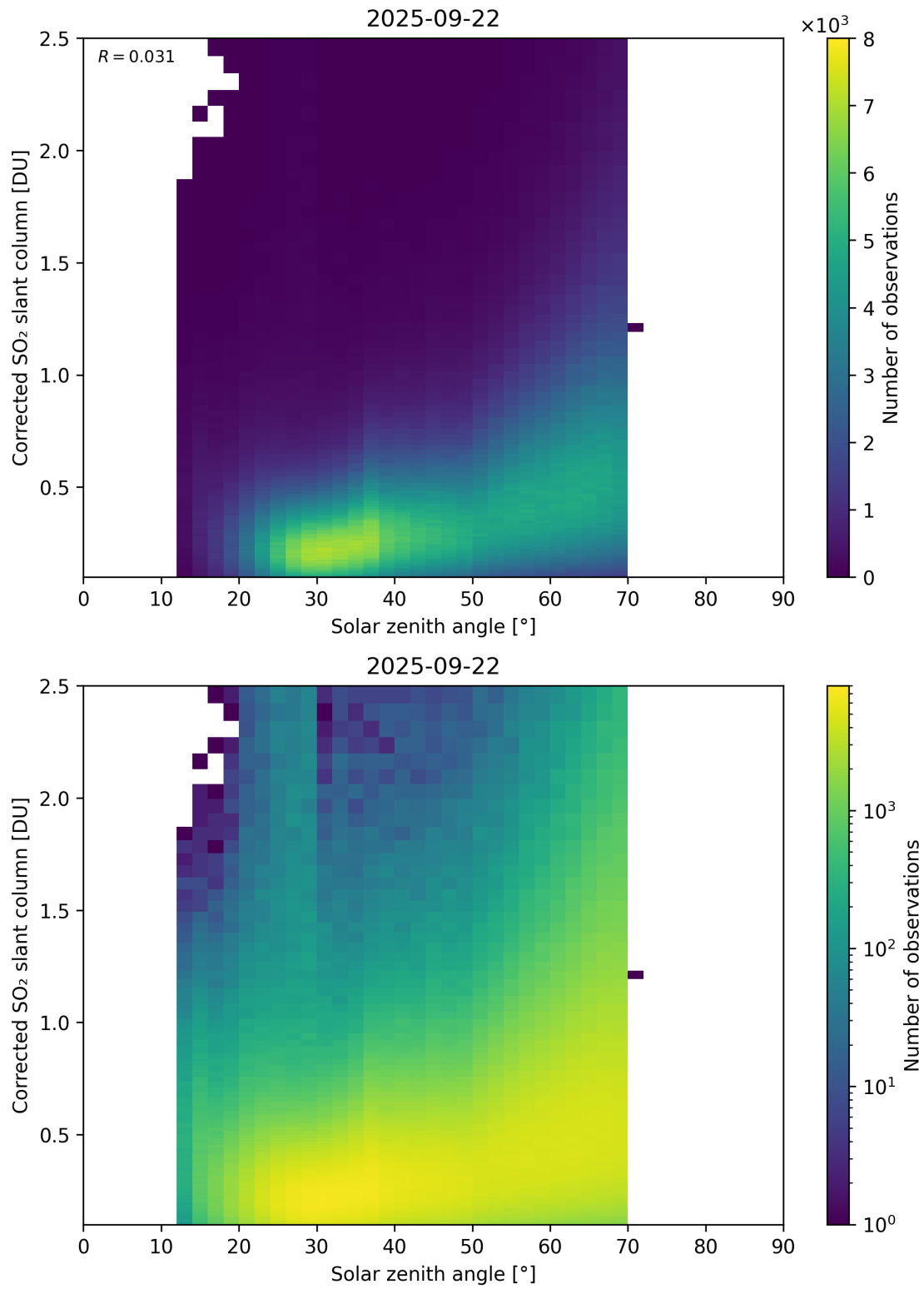
Figure 181: Scatter density plot of “Solar zenith angle” against “Corrected SO 2 slant column” for 2025-09-22 to 2025-09-23.
