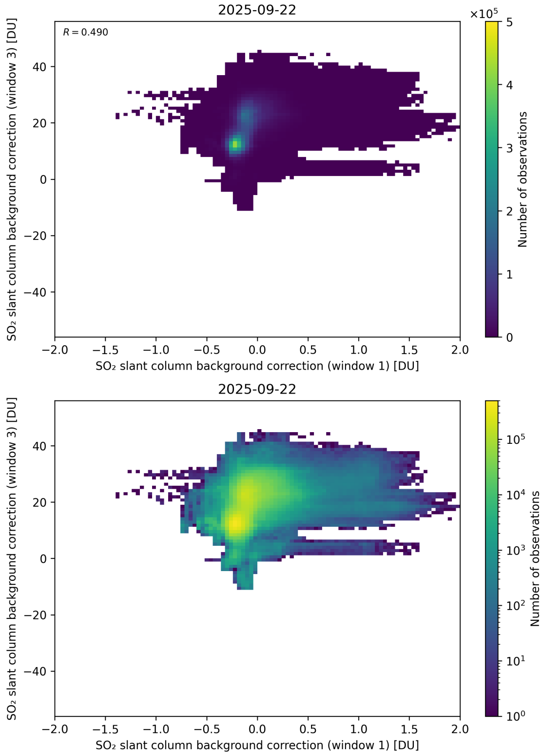
Figure 110: Scatter density plot of “SO 2 slant column background correction (window 1)” against “SO 2 slant column background correction (window 3)” for 2025-09-22 to 2025-09-23.
