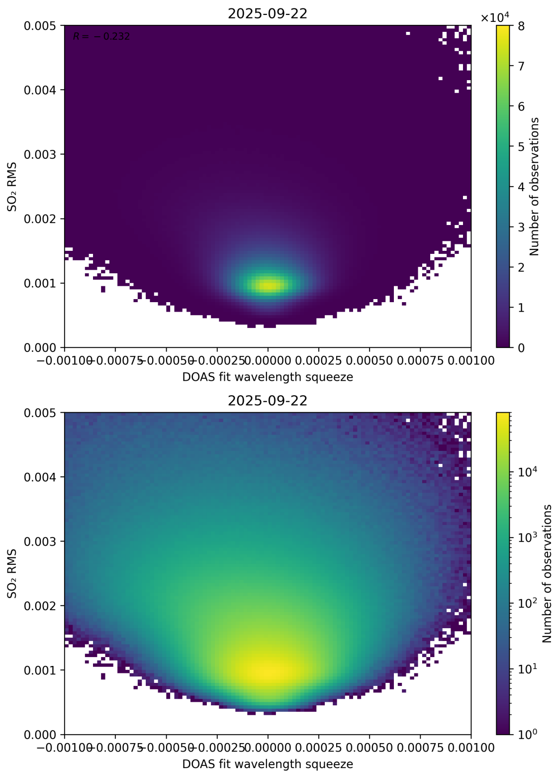
Figure 143: Scatter density plot of “DOAS fit wavelength squeeze” against “SO 2 RMS” for 2025-09-22 to 2025-09-23.
