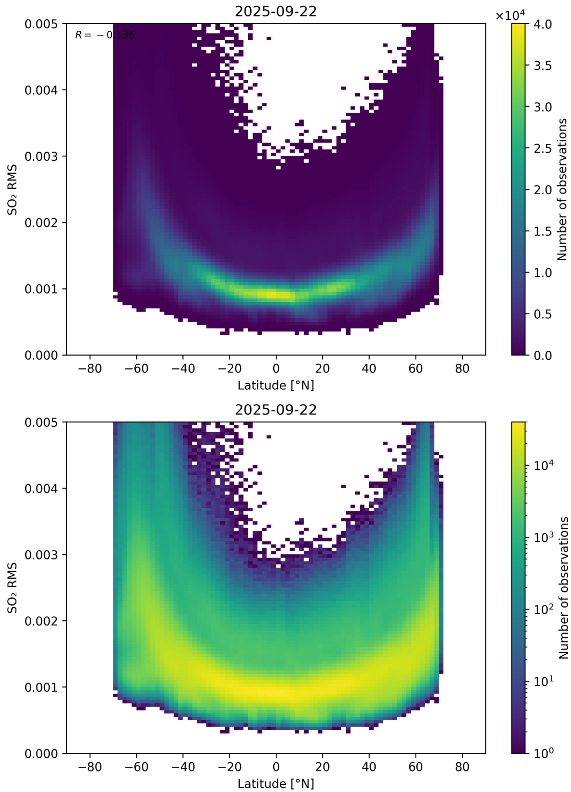
Figure 155: Scatter density plot of “Latitude” against “SO 2 RMS” for 2025-09-22 to 2025-09-23.
