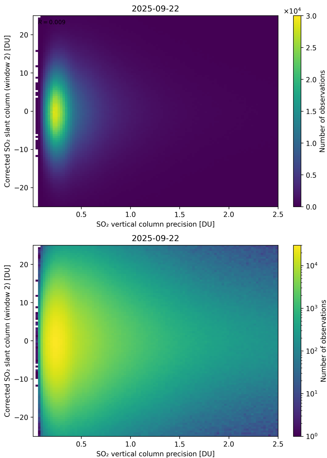
Figure 339: Scatter density plot of “SO 2 vertical column precision” against “Corrected SO 2 slant column (window 2)” for 2025-09-22 to 2025-09-23.
