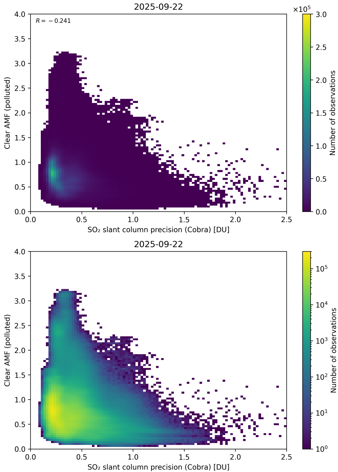
Figure 205: Scatter density plot of “SO 2 slant column precision (Cobra)” against “Clear AMF (polluted)” for 2025-09-22 to 2025-09-23.
