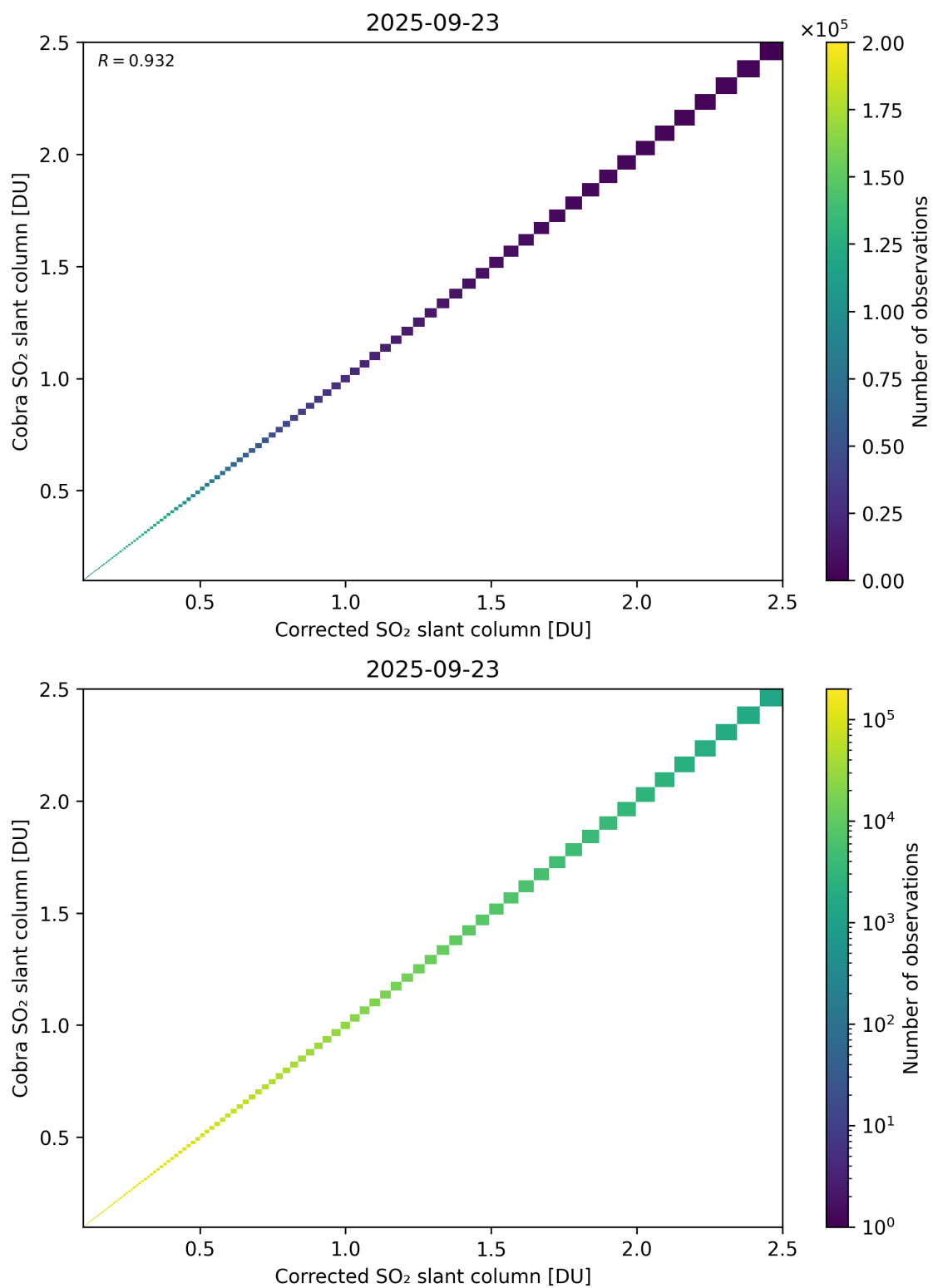
Figure 233: Scatter density plot of “Corrected SO 2 slant column” against “Cobra SO 2 slant column” for 2025-09-22 to 2025-09-24.
