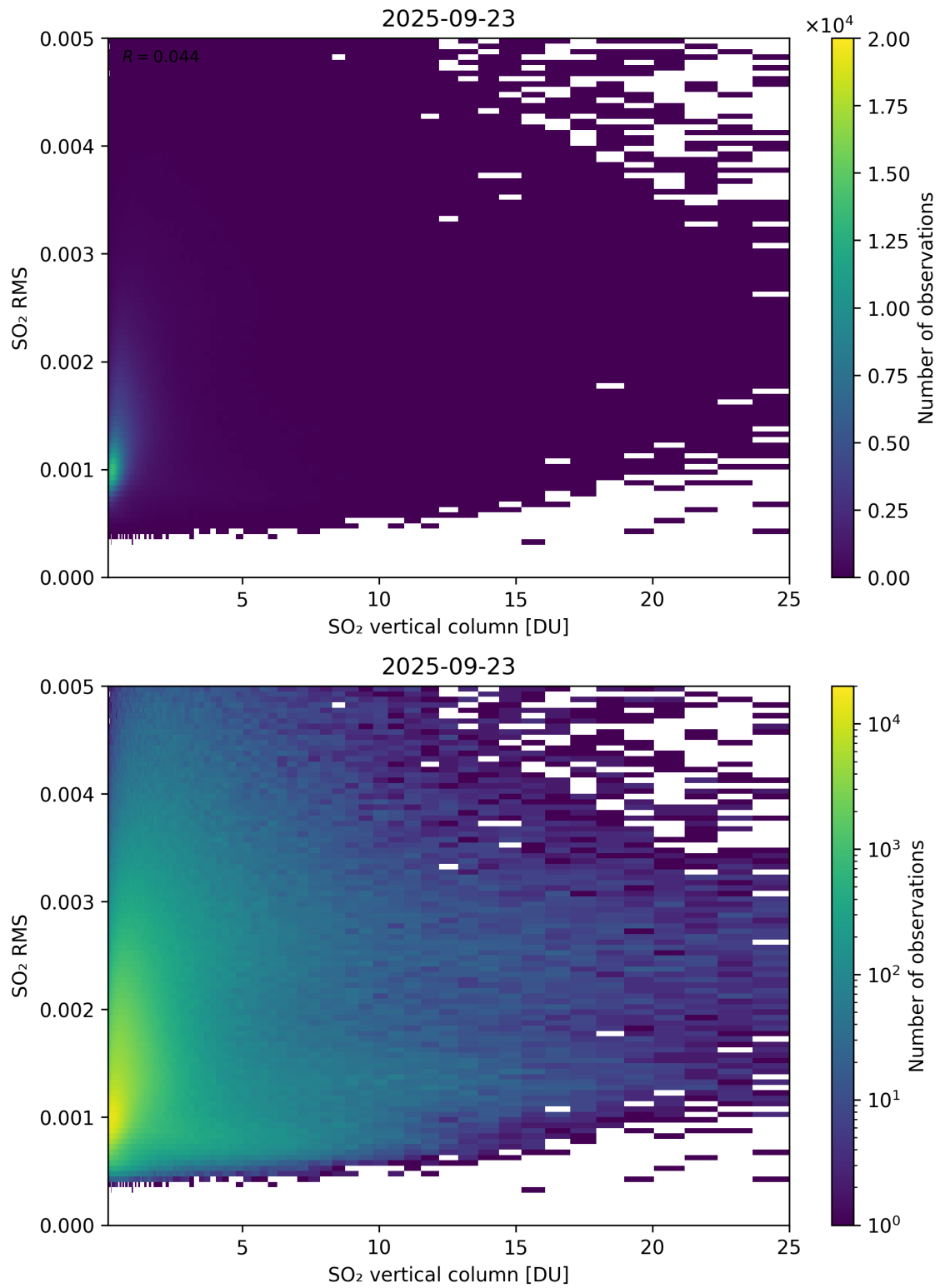
Figure 328: Scatter density plot of “SO 2 vertical column” against “SO 2 RMS” for 2025-09-22 to 2025-09-24.
