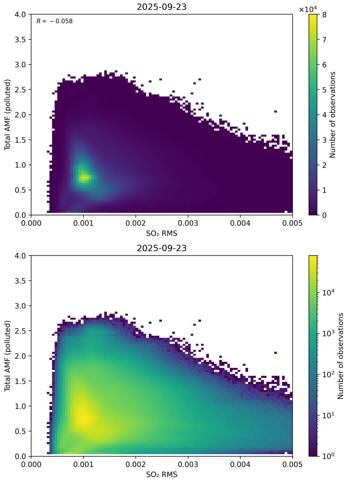
Figure 148: Scatter density plot of “SO 2 RMS” against “Total AMF (polluted)” for 2025-09-22 to 2025-09-24.
