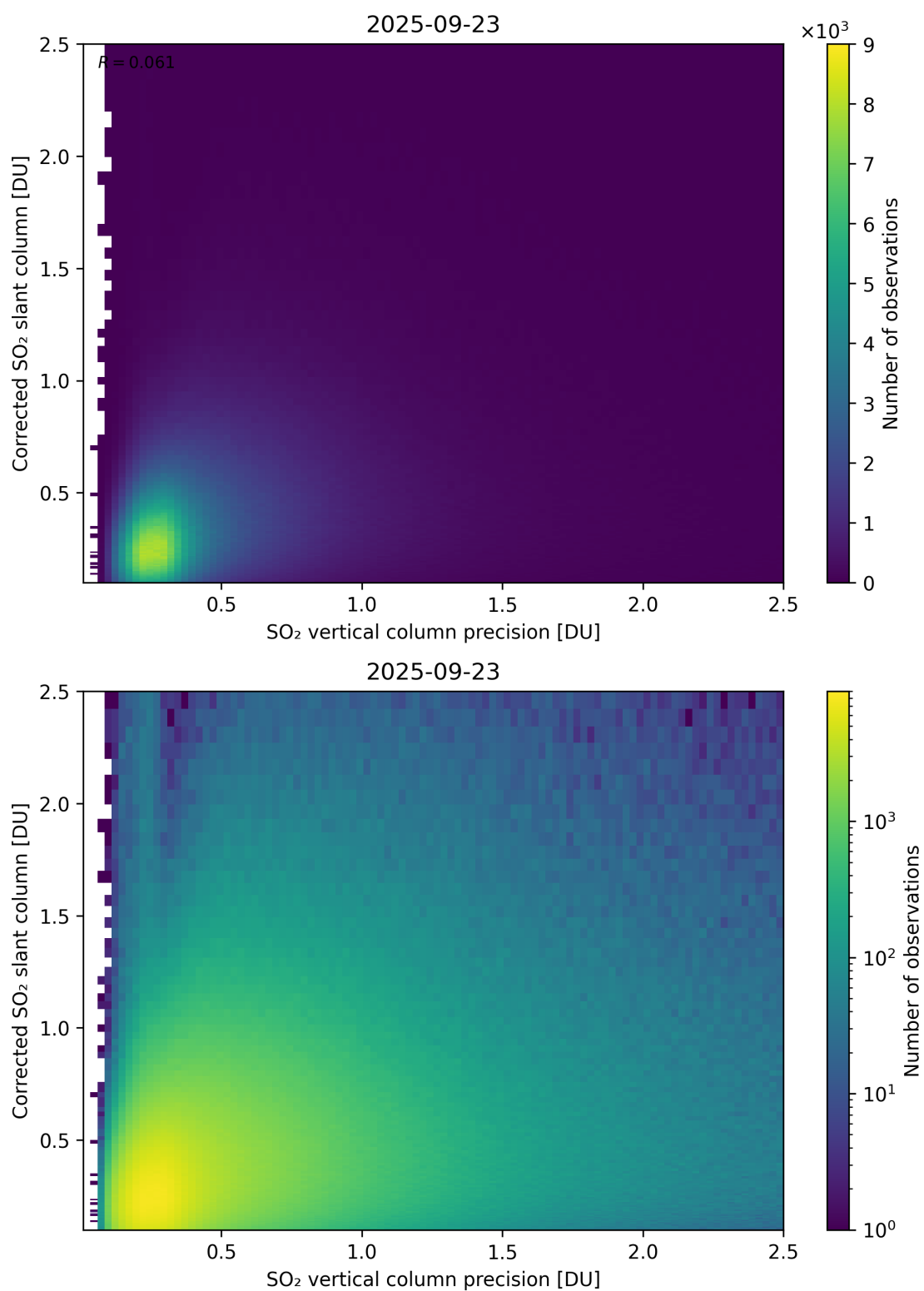
Figure 338: Scatter density plot of “SO 2 vertical column precision” against “Corrected SO 2 slant column” for 2025-09-22 to 2025-09-24.
