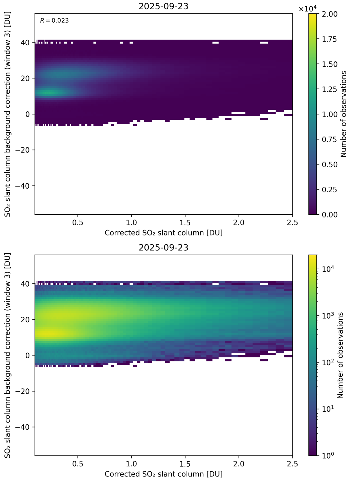
Figure 228: Scatter density plot of “Corrected SO 2 slant column” against “SO 2 slant column background correction (window 3)” for 2025-09-22 to 2025-09-24.
