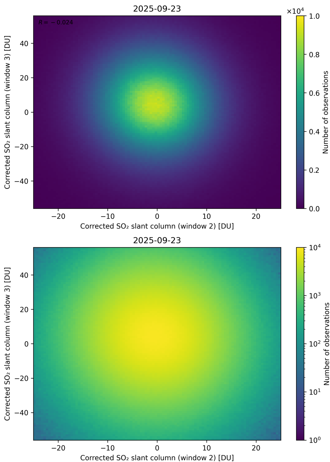
Figure 250: Scatter density plot of “Corrected SO 2 slant column (window 2)” against “Corrected SO 2 slant column (window 3)” for 2025-09-22 to 2025-09-24.
