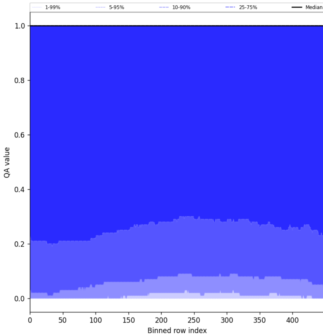
Figure 83: Along track statistics of “QA value” for 2025-09-22 to 2025-09-24
