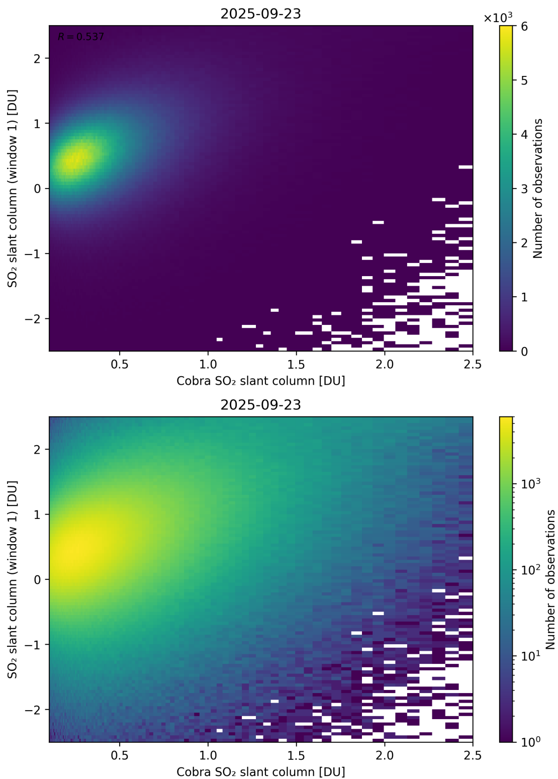
Figure 219: Scatter density plot of “Cobra SO 2 slant column” against “SO 2 slant column (window 1)” for 2025-09-22 to 2025-09-24.
