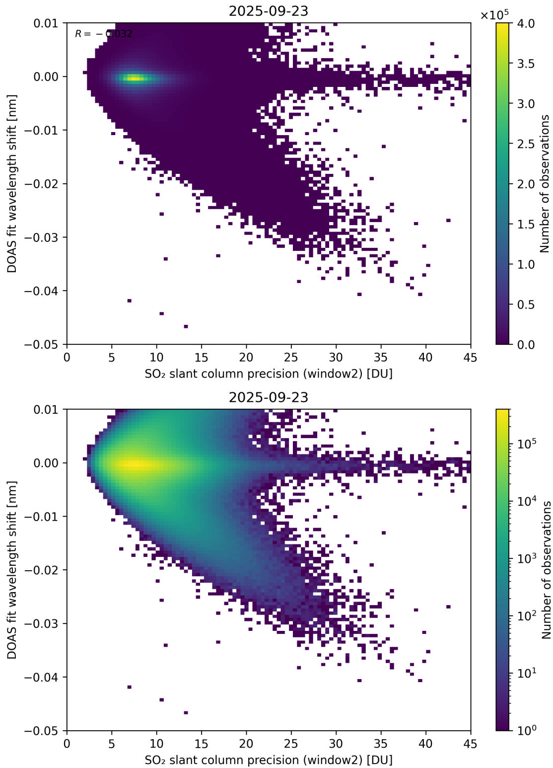
Figure 293: Scatter density plot of “SO 2 slant column precision (window2)” against “DOAS fit wavelength shift” for 2025-09-22 to 2025-09-24.
