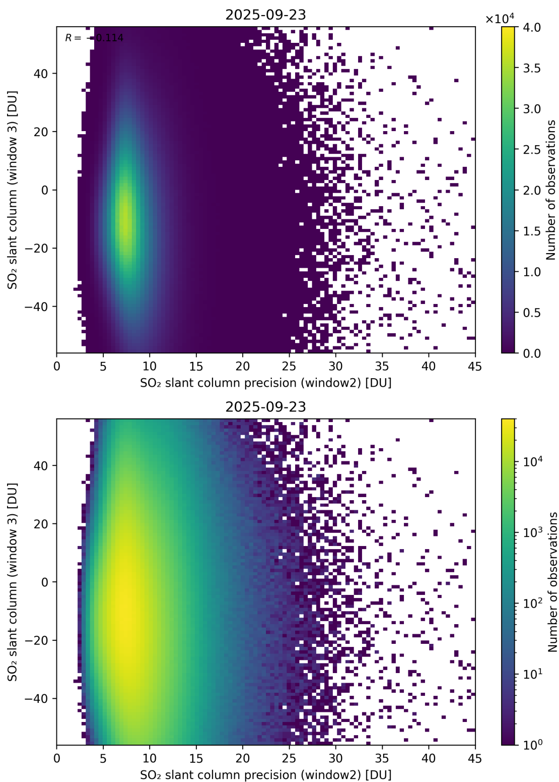
Figure 299: Scatter density plot of “SO 2 slant column precision (window2)” against “SO 2 slant column (window 3)” for 2025-09-22 to 2025-09-24.
