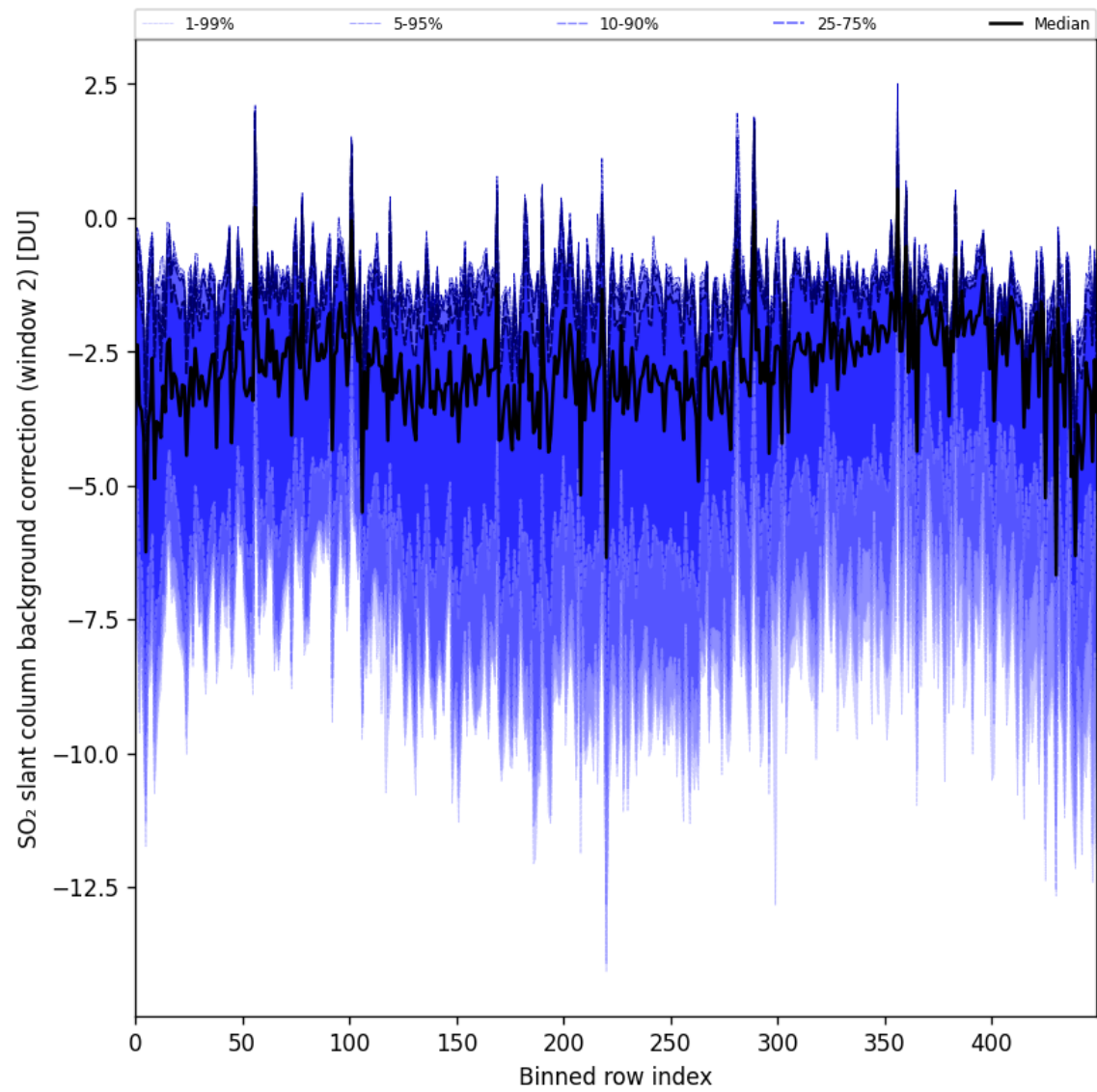
Figure 96: Along track statistics of “SO 2 slant column background correction (window 2)” for 2025-09-22 to 2025-09-24
