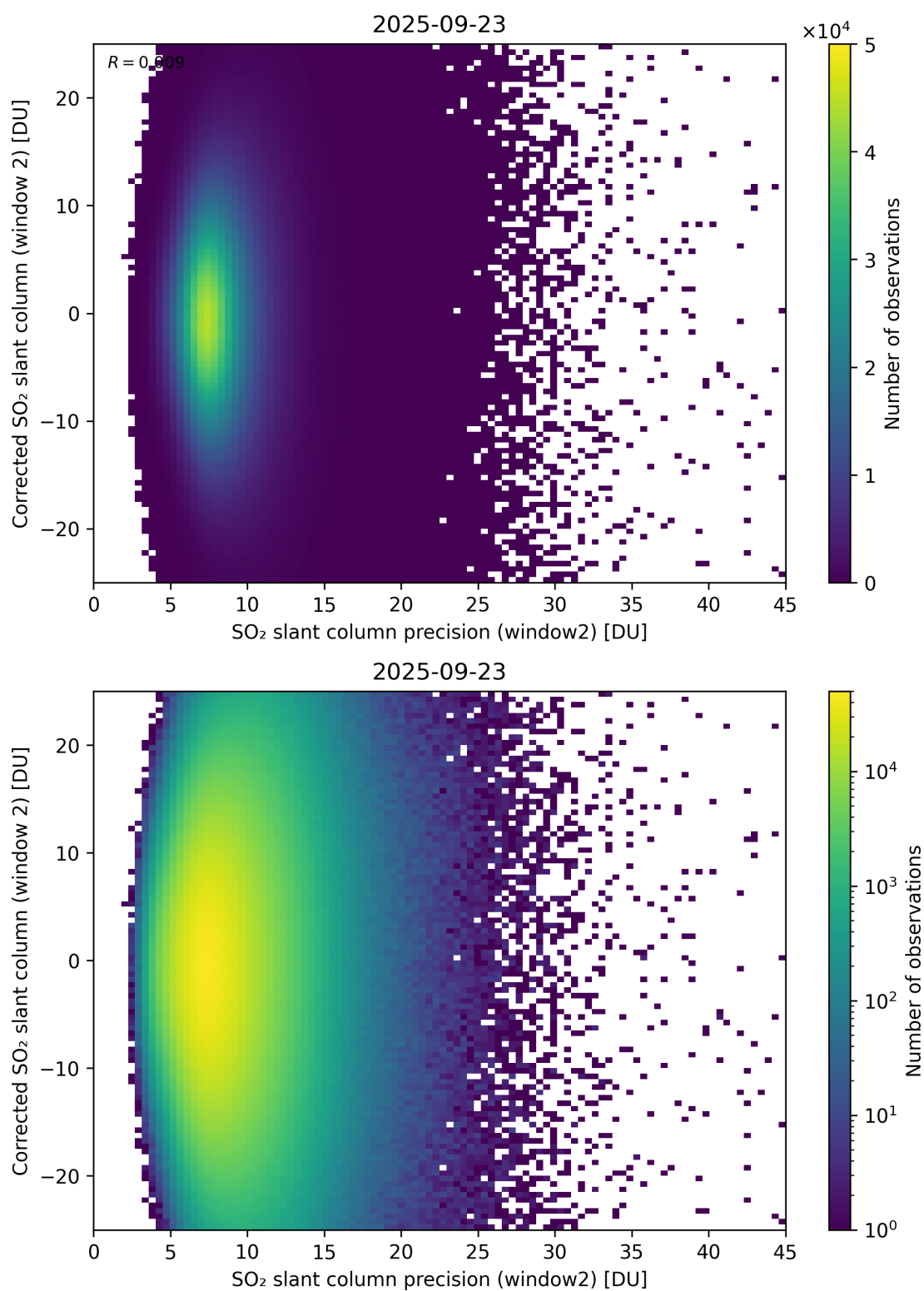
Figure 297: Scatter density plot of “SO 2 slant column precision (window2)” against “Corrected SO 2 slant column (window 2)” for 2025-09-22 to 2025-09-24.
