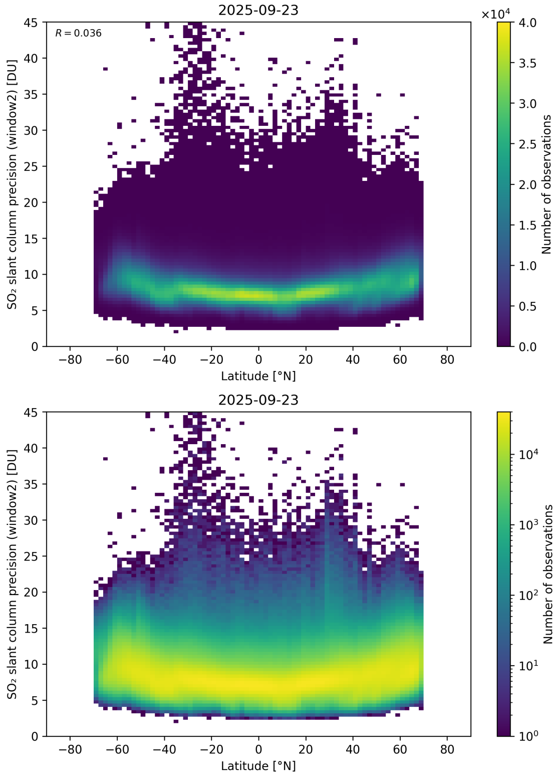
Figure 164: Scatter density plot of “Latitude” against “SO 2 slant column precision (window2)” for 2025-09-22 to 2025-09-24.
