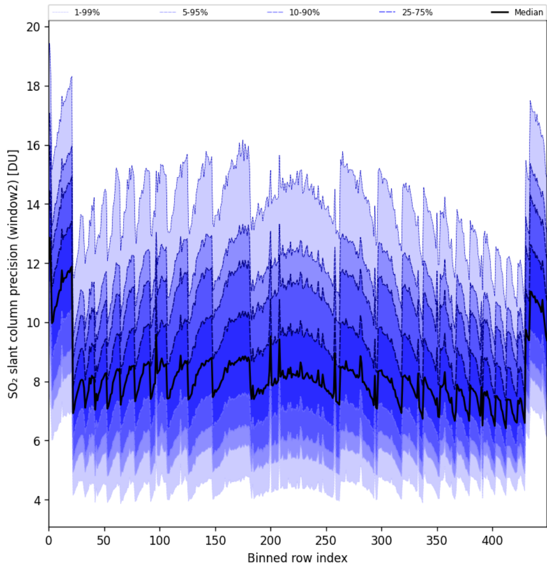
Figure 94: Along track statistics of “SO 2 slant column precision (window2)” for 2025-09-22 to 2025-09-24
