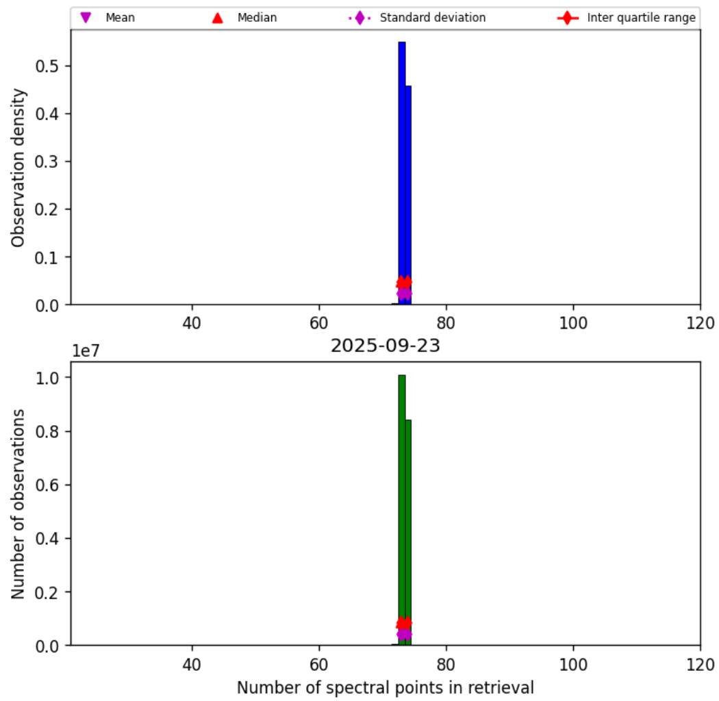
Figure 82: Histogram of “Number of spectral points in retrieval” for 2025-09-22 to 2025-09-24
