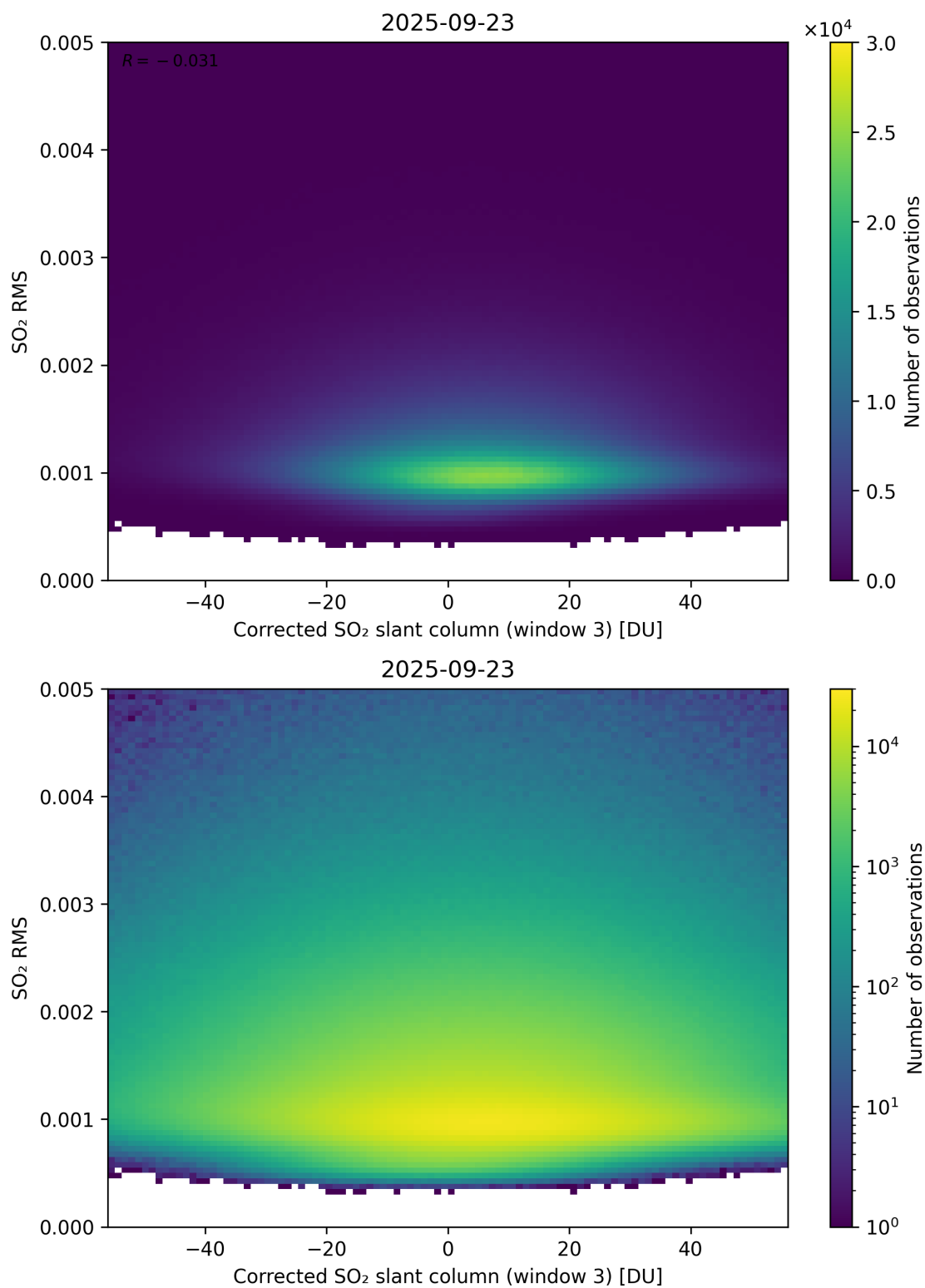
Figure 258: Scatter density plot of “Corrected SO 2 slant column (window 3)” against “SO 2 RMS” for 2025-09-22 to 2025-09-24.
