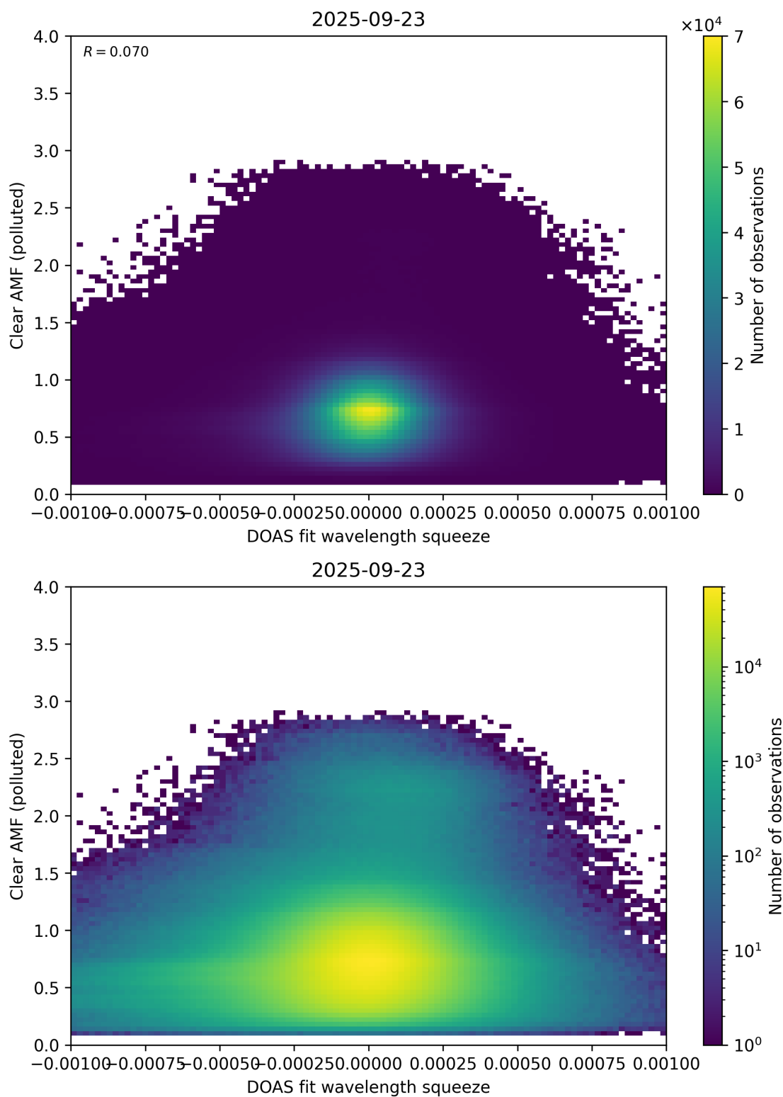
Figure 144: Scatter density plot of “DOAS fit wavelength squeeze” against “Clear AMF (polluted)” for 2025-09-22 to 2025-09-24.
