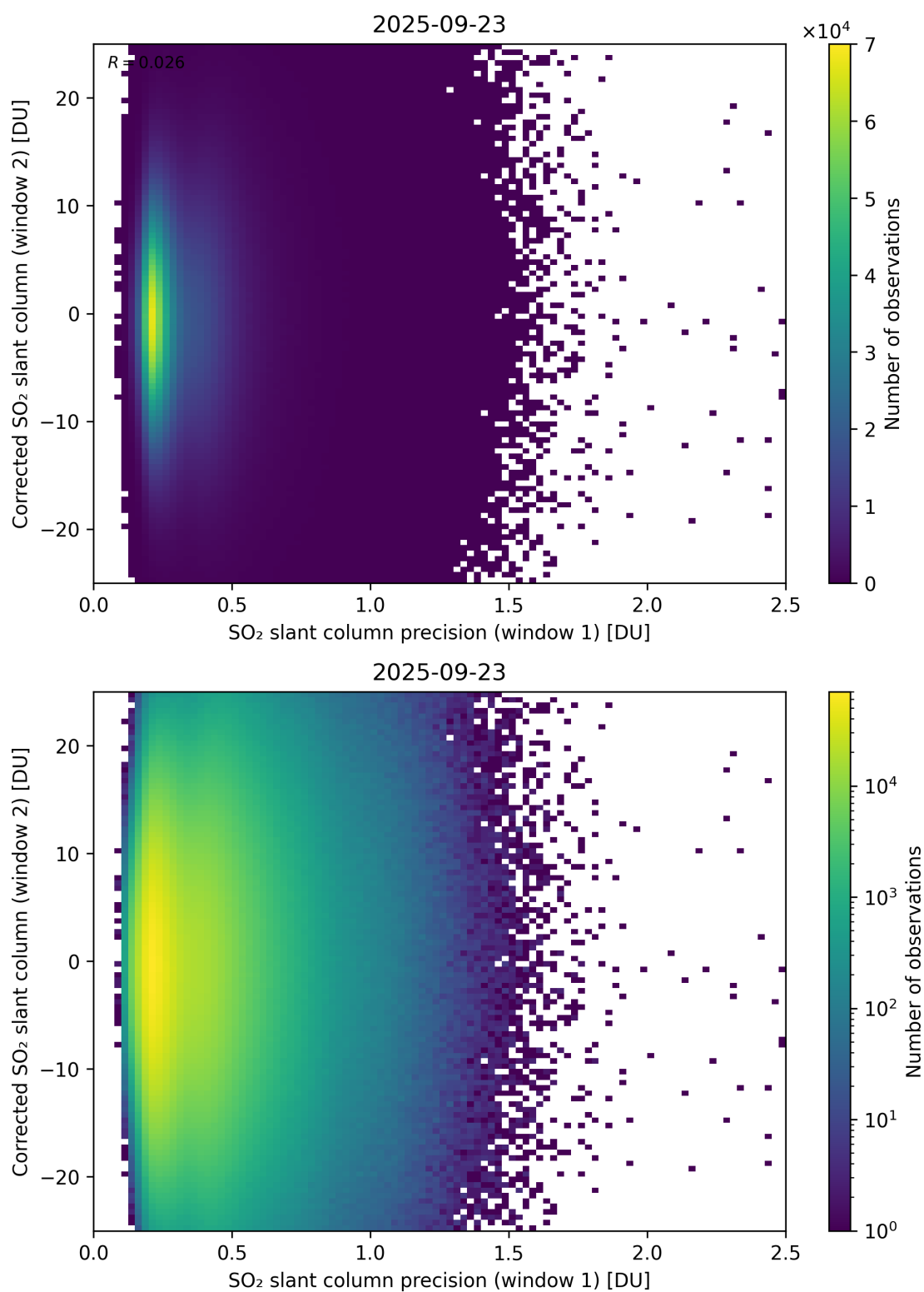
Figure 275: Scatter density plot of “SO 2 slant column precision (window 1)” against “Corrected SO 2 slant column (window 2)” for 2025-09-22 to 2025-09-24.
