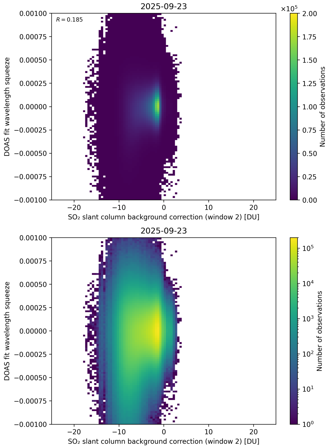
Figure 124: Scatter density plot of “SO 2 slant column background correction (window 2)” against “DOAS fit wavelength squeeze” for 2025-09-22 to 2025-09-24.
