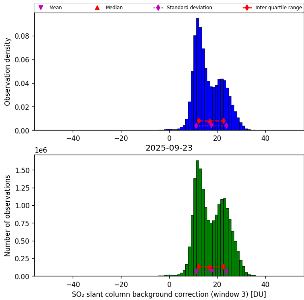
Figure 74: Histogram of “SO 2 slant column background correction (window 3)” for 2025-09-22 to 2025-09-24
