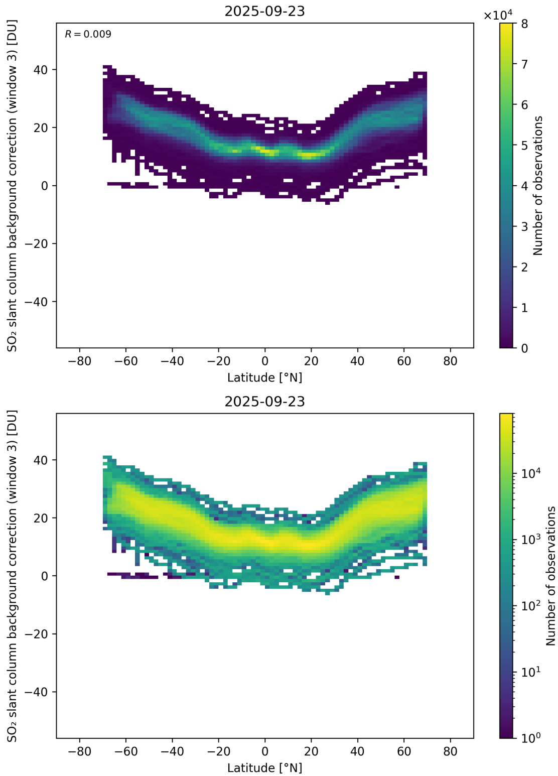
Figure 152: Scatter density plot of “Latitude” against “SO 2 slant column background correction (window 3)” for 2025-09-22 to 2025-09-24.
