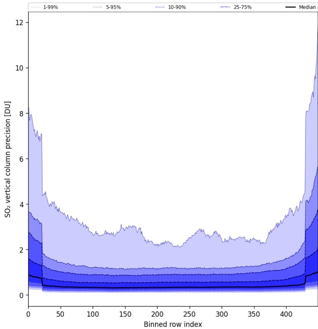
Figure 85: Along track statistics of “SO 2 vertical column precision” for 2025-09-22 to 2025-09-24
