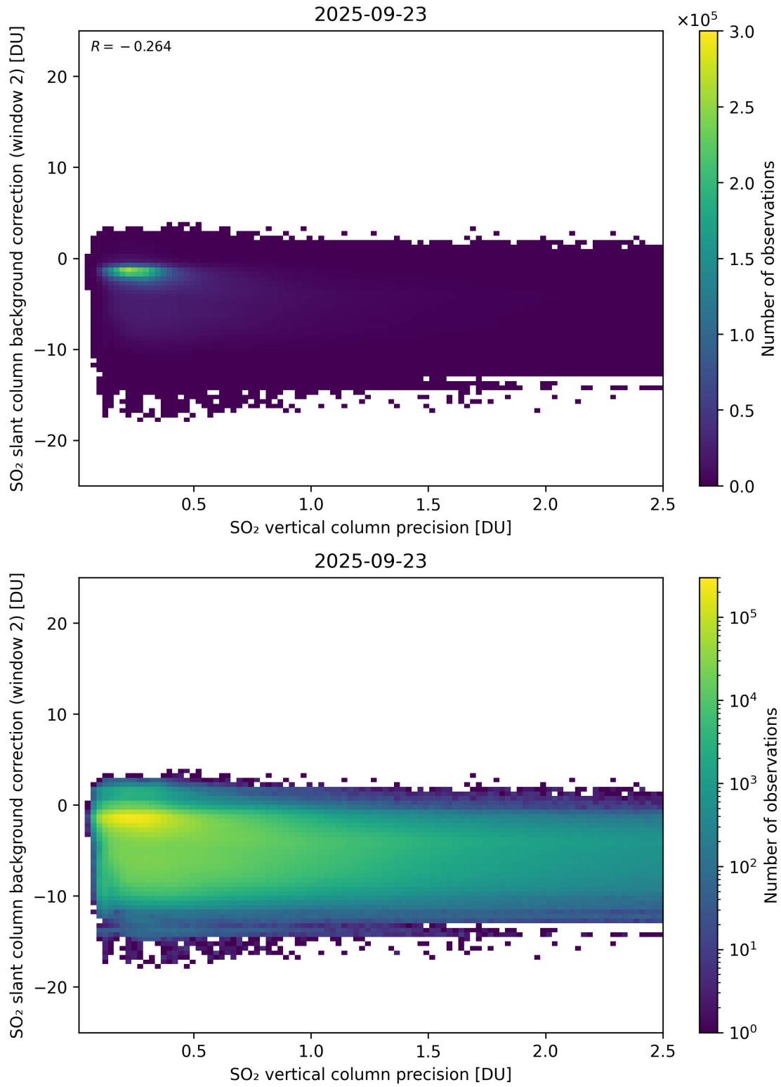
Figure 330: Scatter density plot of “SO 2 vertical column precision” against “SO 2 slant column background correction (window 2)” for 2025-09-22 to 2025-09-24.
