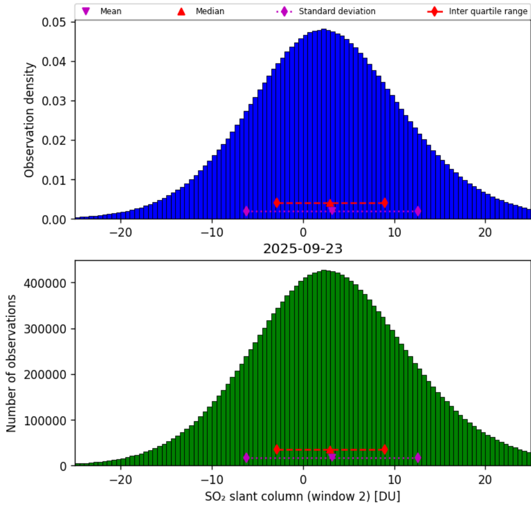
Figure 67: Histogram of “SO 2 slant column (window 2)” for 2025-09-22 to 2025-09-24
