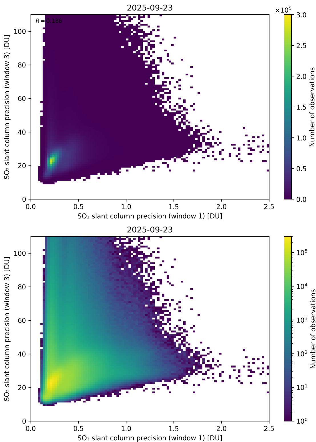
Figure 279: Scatter density plot of “SO 2 slant column precision (window 1)” against “SO 2 slant column precision (window 3)” for 2025-09-22 to 2025-09-24.
