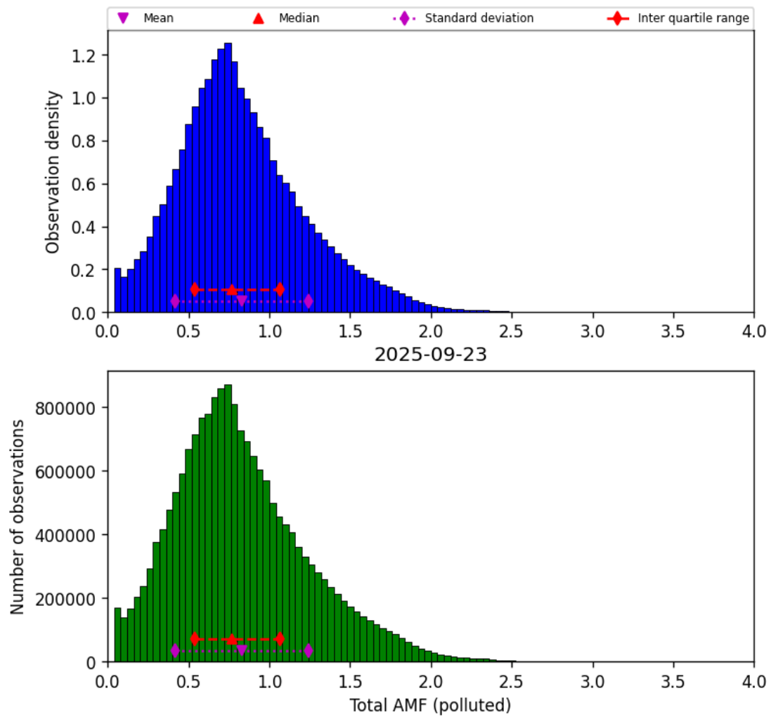
Figure 79: Histogram of “Total AMF (polluted)” for 2025-09-22 to 2025-09-24
