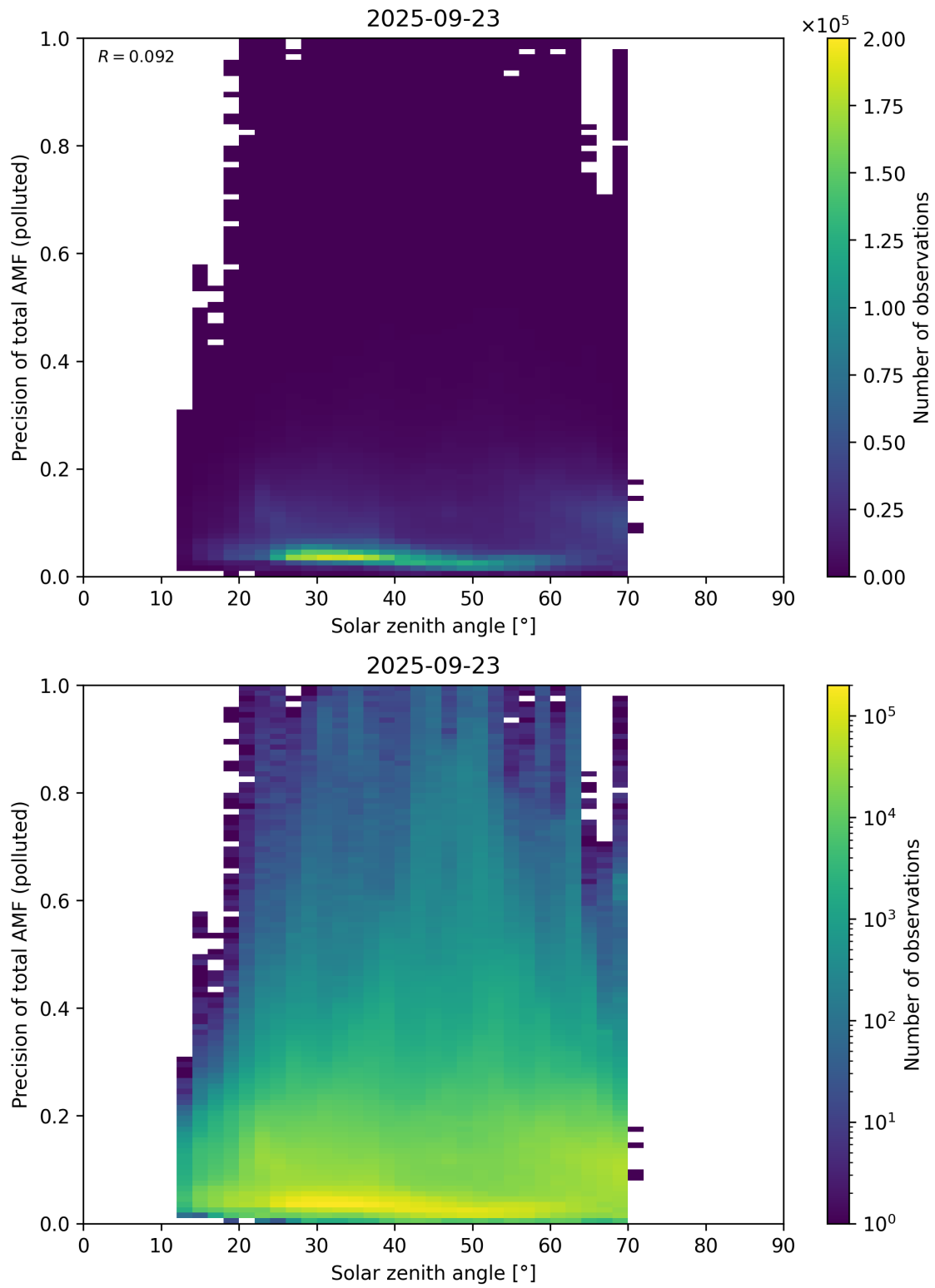
Figure 190: Scatter density plot of “Solar zenith angle” against “Precision of total AMF (polluted)” for 2025-09-22 to 2025-09-24.
