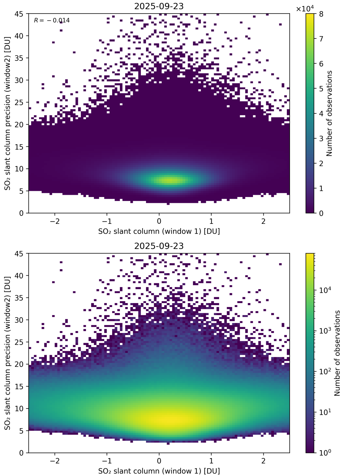
Figure 286: Scatter density plot of “SO 2 slant column (window 1)” against “SO 2 slant column precision (window2)” for 2025-09-22 to 2025-09-24.
