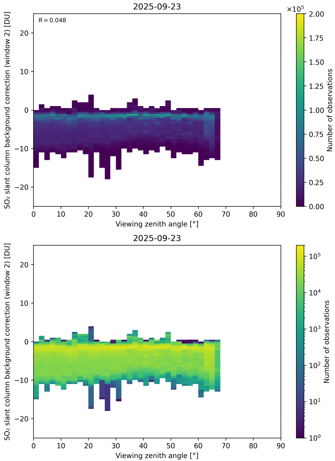
Figure 363: Scatter density plot of “Viewing zenith angle” against “SO 2 slant column background correction (window 2)” for 2025-09-22 to 2025-09-24.
