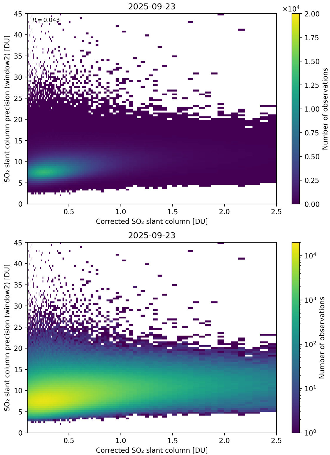
Figure 239: Scatter density plot of “Corrected SO 2 slant column” against “SO 2 slant column precision (window2)” for 2025-09-22 to 2025-09-24.
