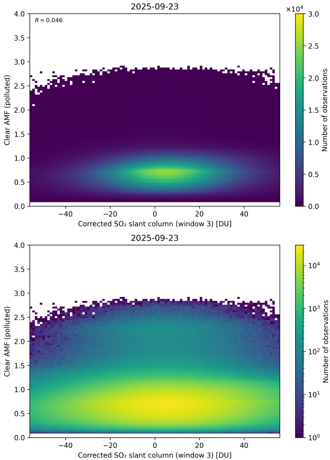
Figure 259: Scatter density plot of “Corrected SO 2 slant column (window 3)” against “Clear AMF (polluted)” for 2025-09-22 to 2025-09-24.
