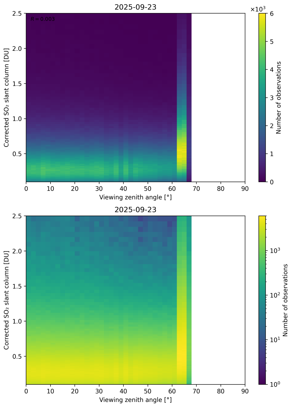
Figure 373: Scatter density plot of “Viewing zenith angle” against “Corrected SO 2 slant column” for 2025-09-22 to 2025-09-24.
