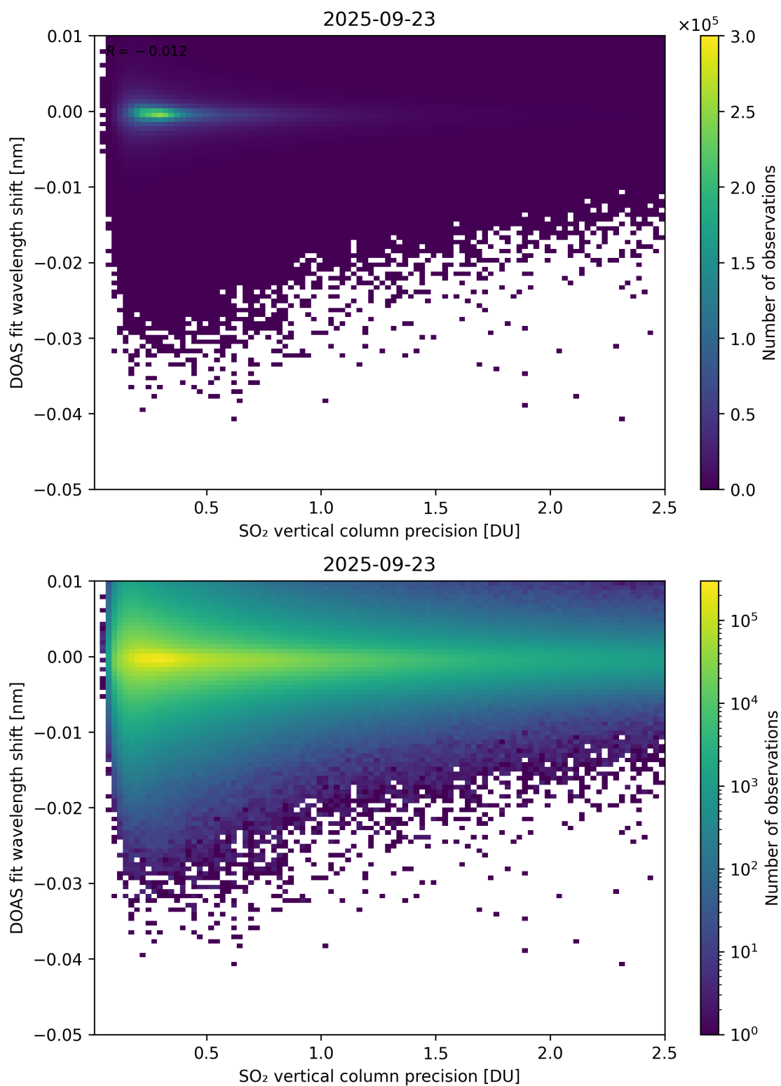
Figure 332: Scatter density plot of “SO 2 vertical column precision” against “DOAS fit wavelength shift” for 2025-09-22 to 2025-09-24.
