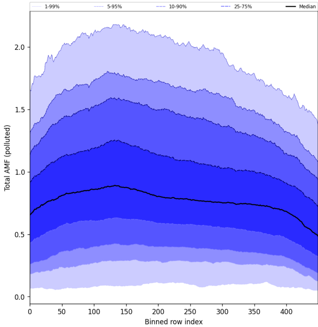
Figure 105: Along track statistics of “Total AMF (polluted)” for 2025-09-22 to 2025-09-24
