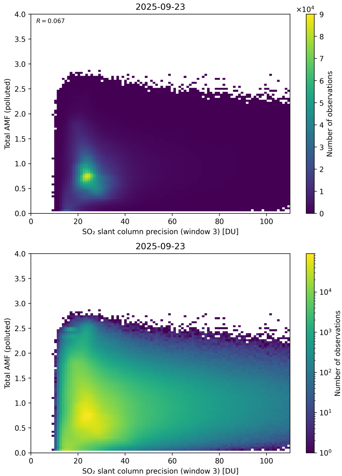
Figure 313: Scatter density plot of “SO 2 slant column precision (window 3)” against “Total AMF (polluted)” for 2025-09-22 to 2025-09-24.
