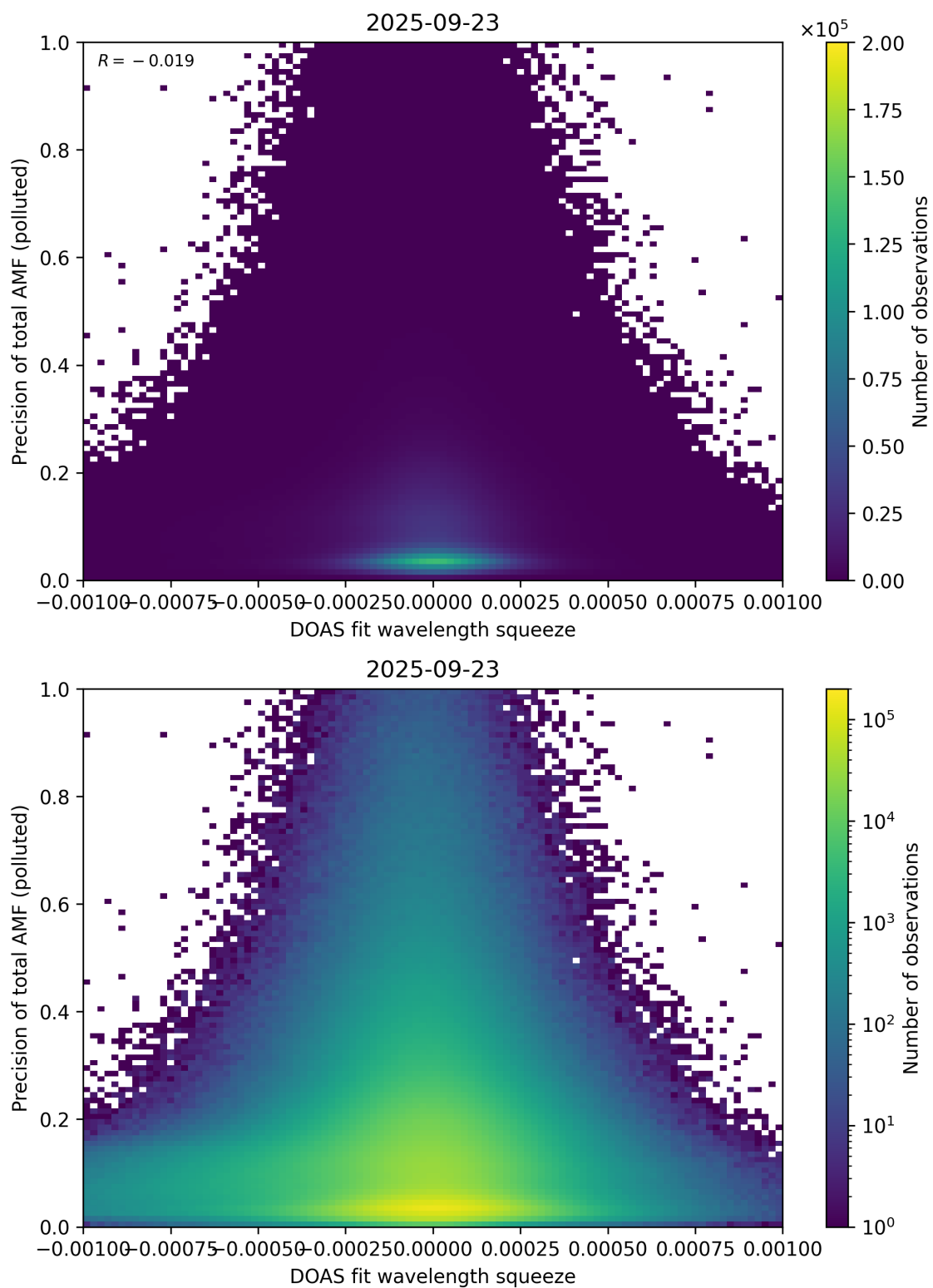
Figure 146: Scatter density plot of “DOAS fit wavelength squeeze” against “Precision of total AMF (polluted)” for 2025-09-22 to 2025-09-24.
