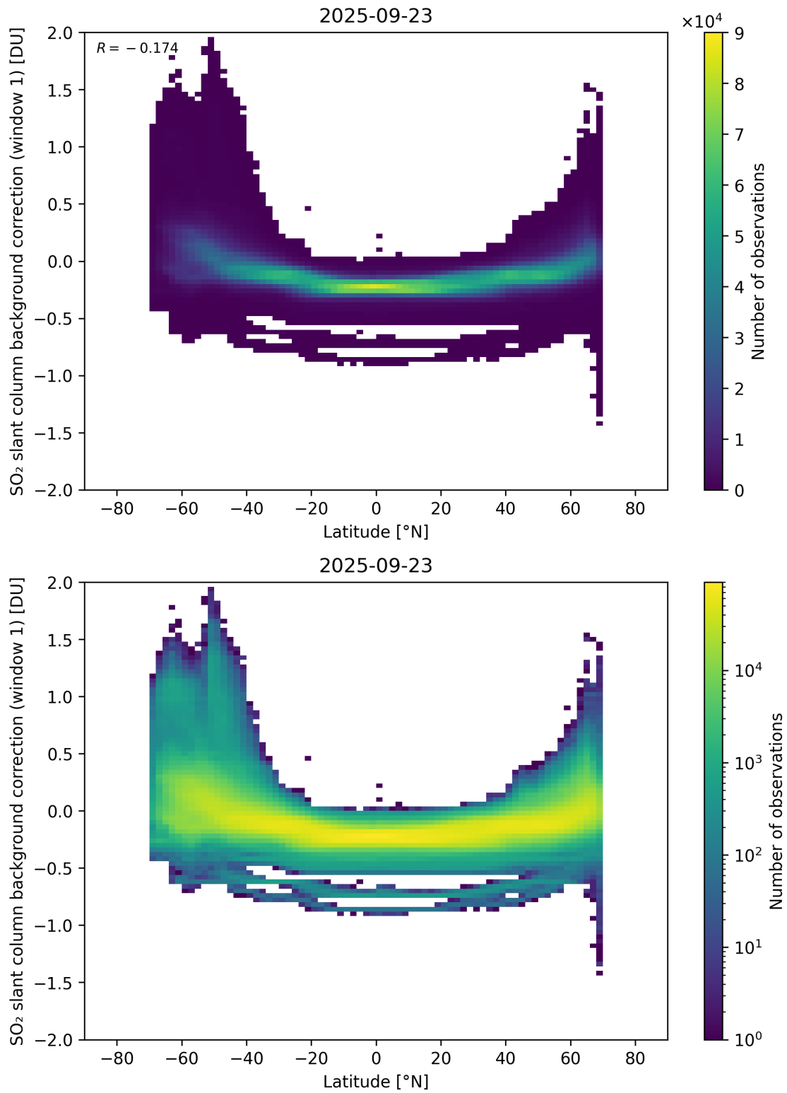
Figure 150: Scatter density plot of “Latitude” against “SO 2 slant column background correction (window 1)” for 2025-09-22 to 2025-09-24.
