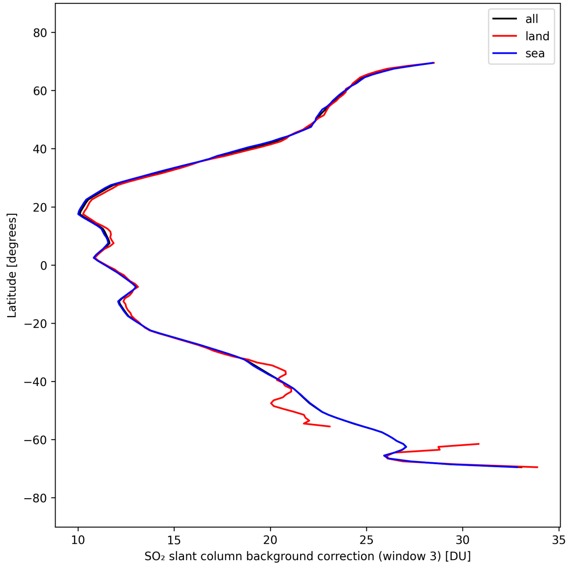
Figure 48: Zonal average of “SO 2 slant column background correction (window 3)” for 2025-09-22 to 2025-09-24.
