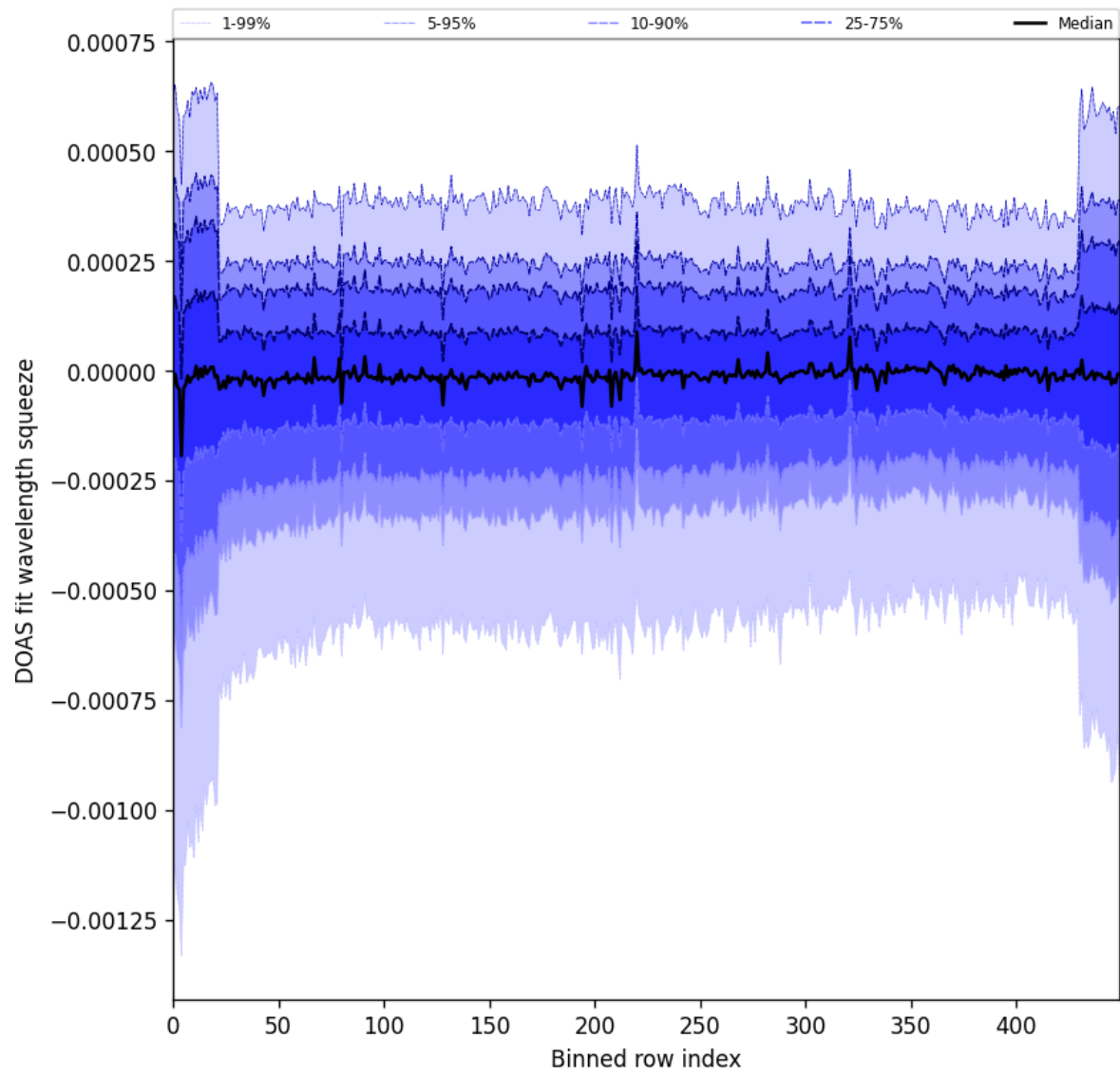
Figure 103: Along track statistics of “DOAS fit wavelength squeeze” for 2025-09-22 to 2025-09-24
