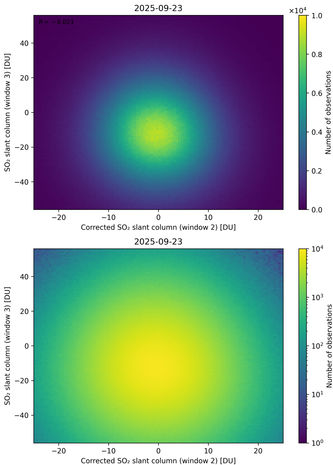
Figure 251: Scatter density plot of “Corrected SO 2 slant column (window 2)” against “SO 2 slant column (window 3)” for 2025-09-22 to 2025-09-24.
