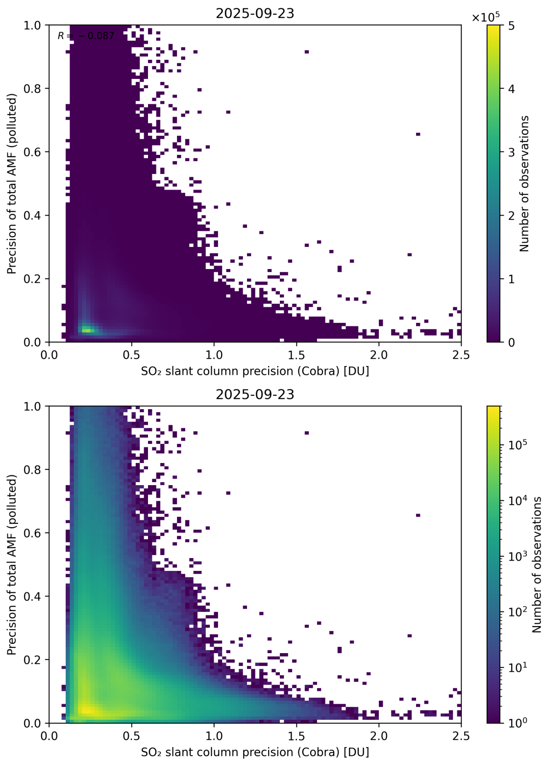
Figure 214: Scatter density plot of “SO 2 slant column precision (Cobra)” against “Precision of total AMF (polluted)” for 2025-09-22 to 2025-09-24.
