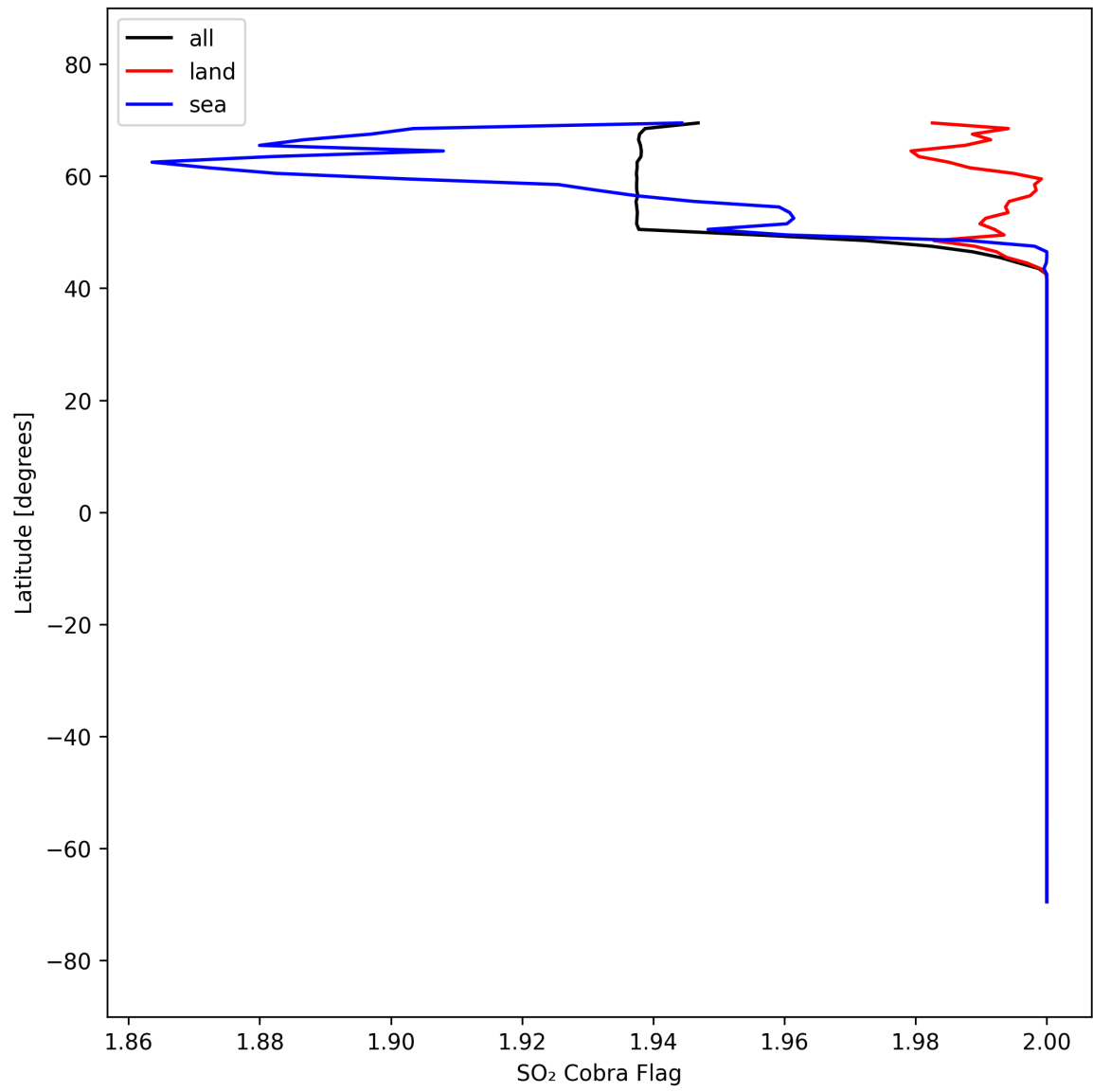
Figure 49: Zonal average of "SO 2 Cobra Flag" for 2025-09-22 to 2025-09-24.
