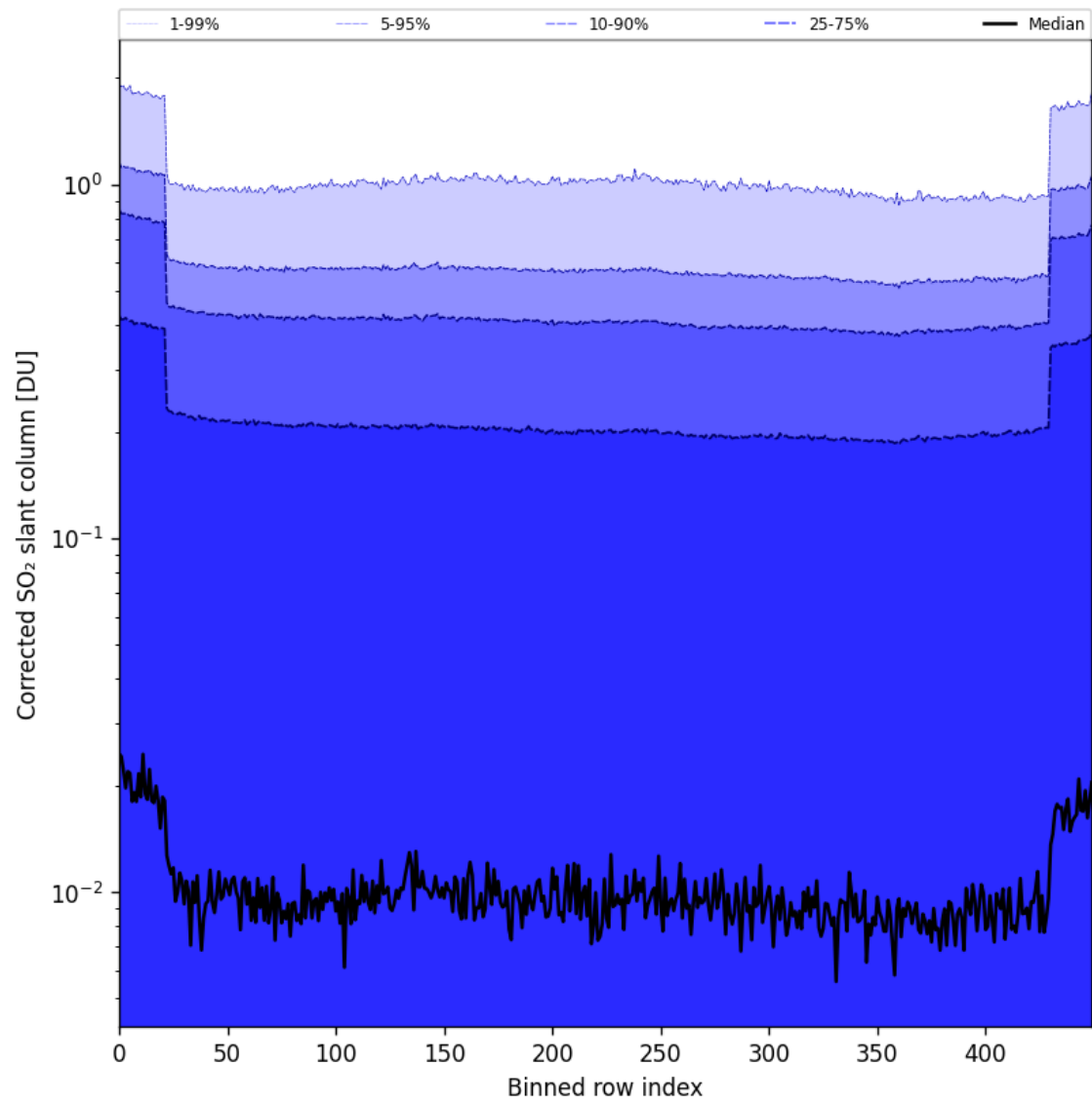
Figure 86: Along track statistics of “Corrected SO 2 slant column” for 2025-09-22 to 2025-09-24
