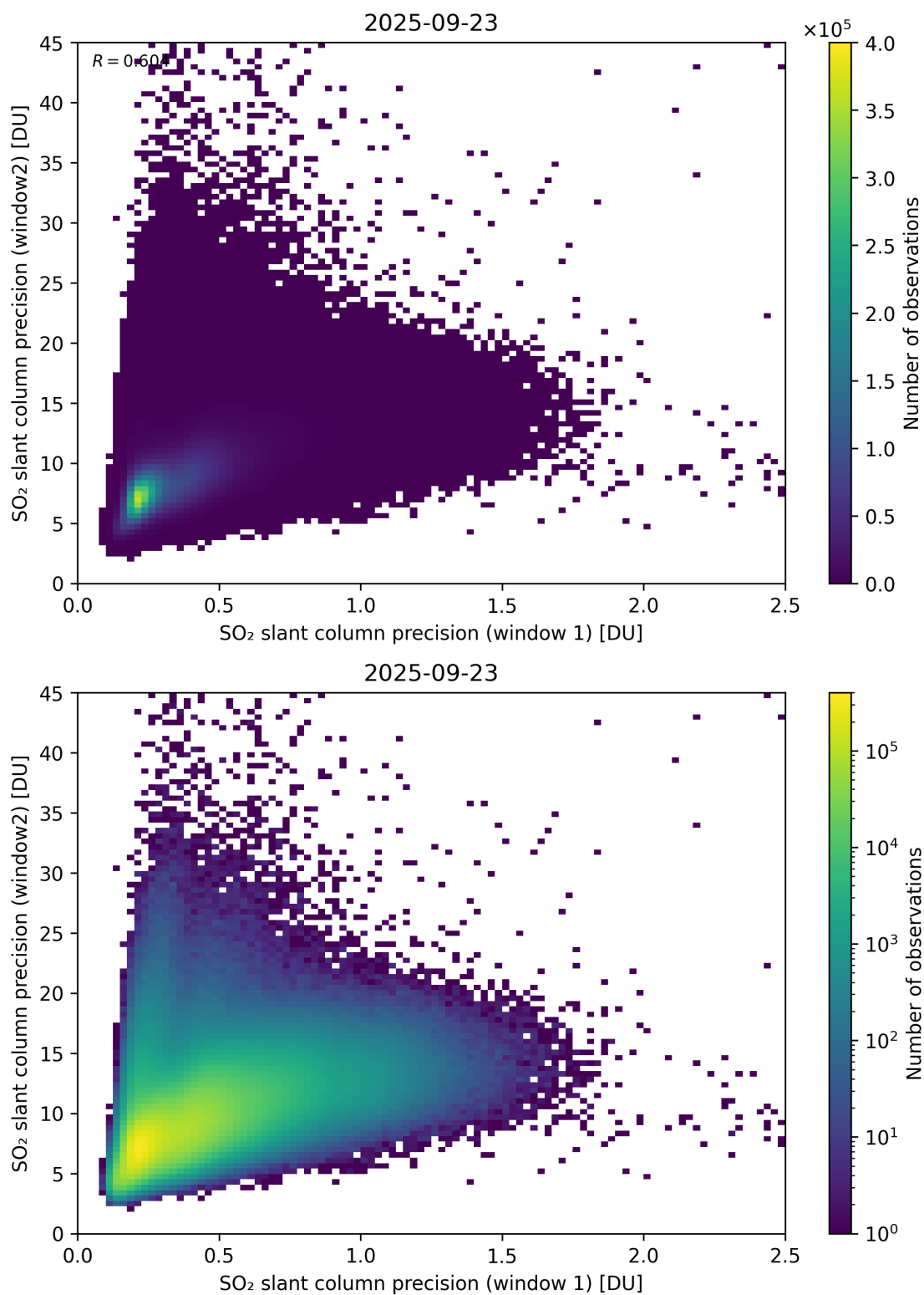
Figure 277: Scatter density plot of “SO 2 slant column precision (window 1)” against “SO 2 slant column precision (window2)” for 2025-09-22 to 2025-09-24.
