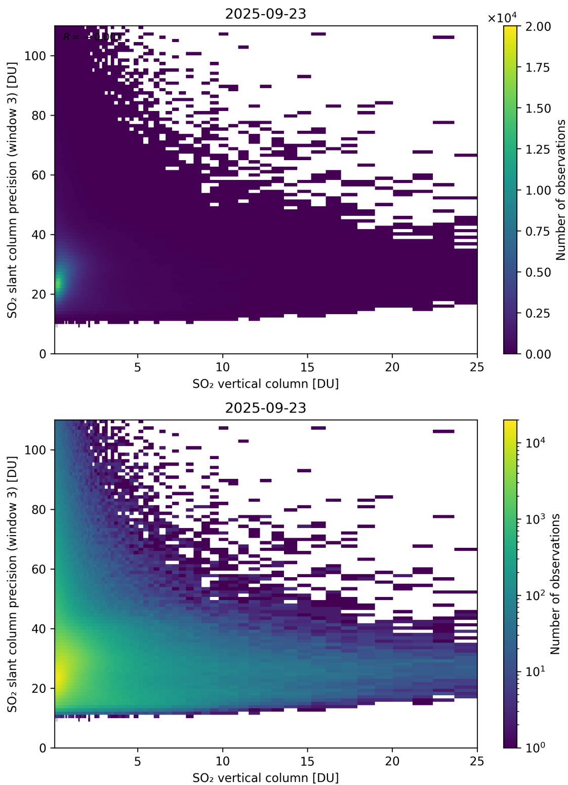
Figure 358: Scatter density plot of “SO 2 vertical column” against “SO 2 slant column precision (window 3)” for 2025-09-22 to 2025-09-24.
