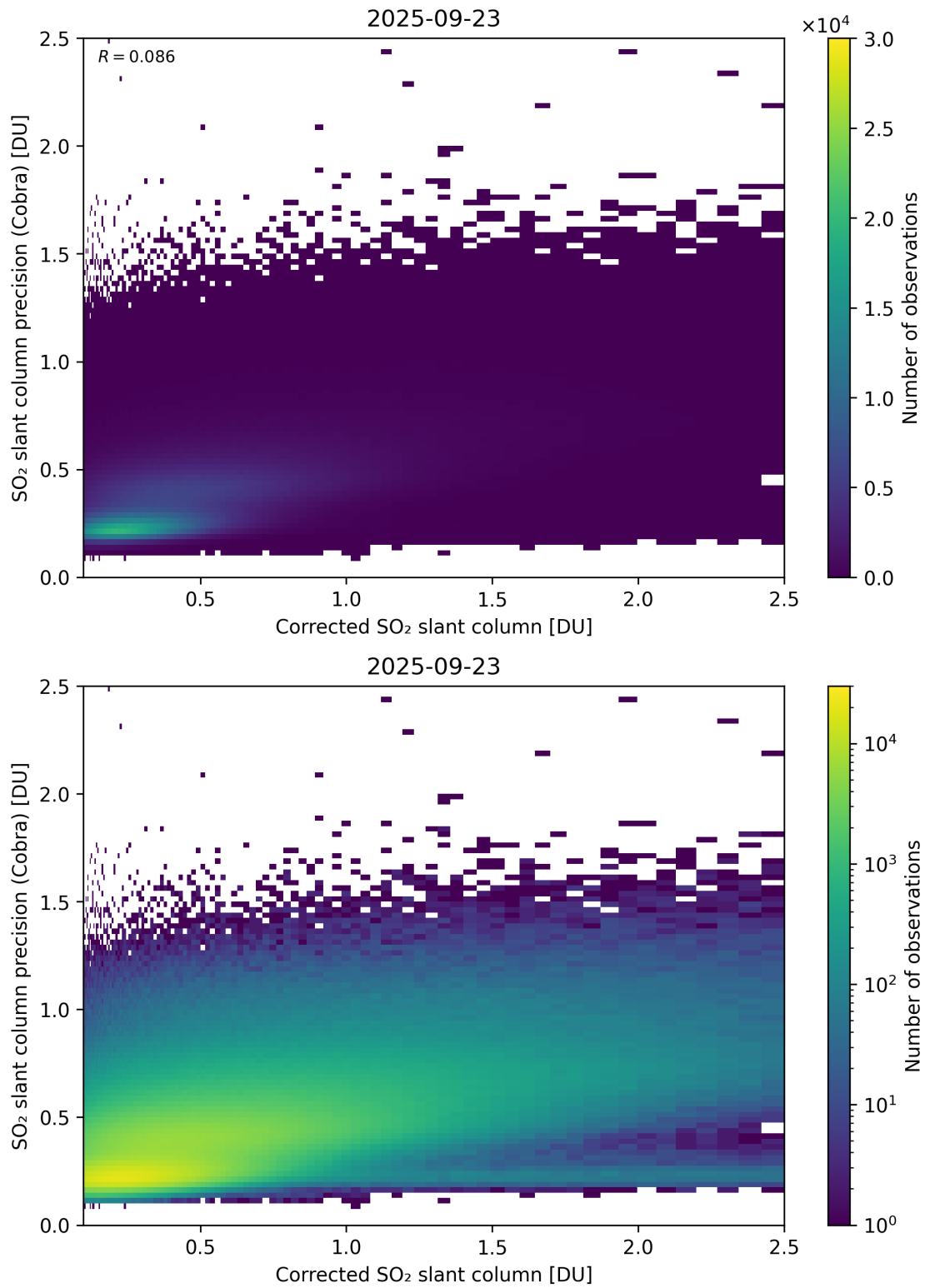
Figure 234: Scatter density plot of “Corrected SO 2 slant column” against “SO 2 slant column precision (Cobra)” for 2025-09-22 to 2025-09-24.
