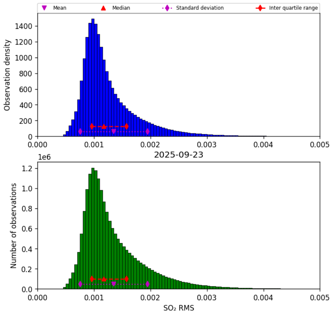
Figure 78: Histogram of “SO 2 RMS” for 2025-09-22 to 2025-09-24
