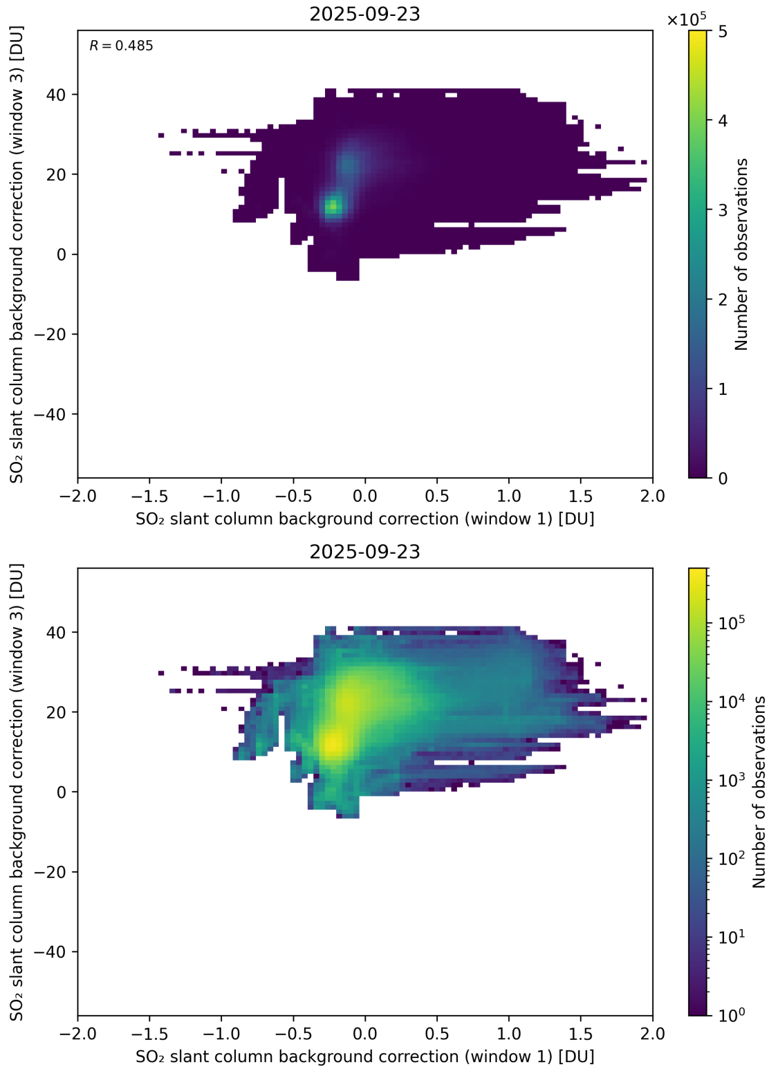
Figure 110: Scatter density plot of “SO 2 slant column background correction (window 1)” against “SO 2 slant column background correction (window 3)” for 2025-09-22 to 2025-09-24.
