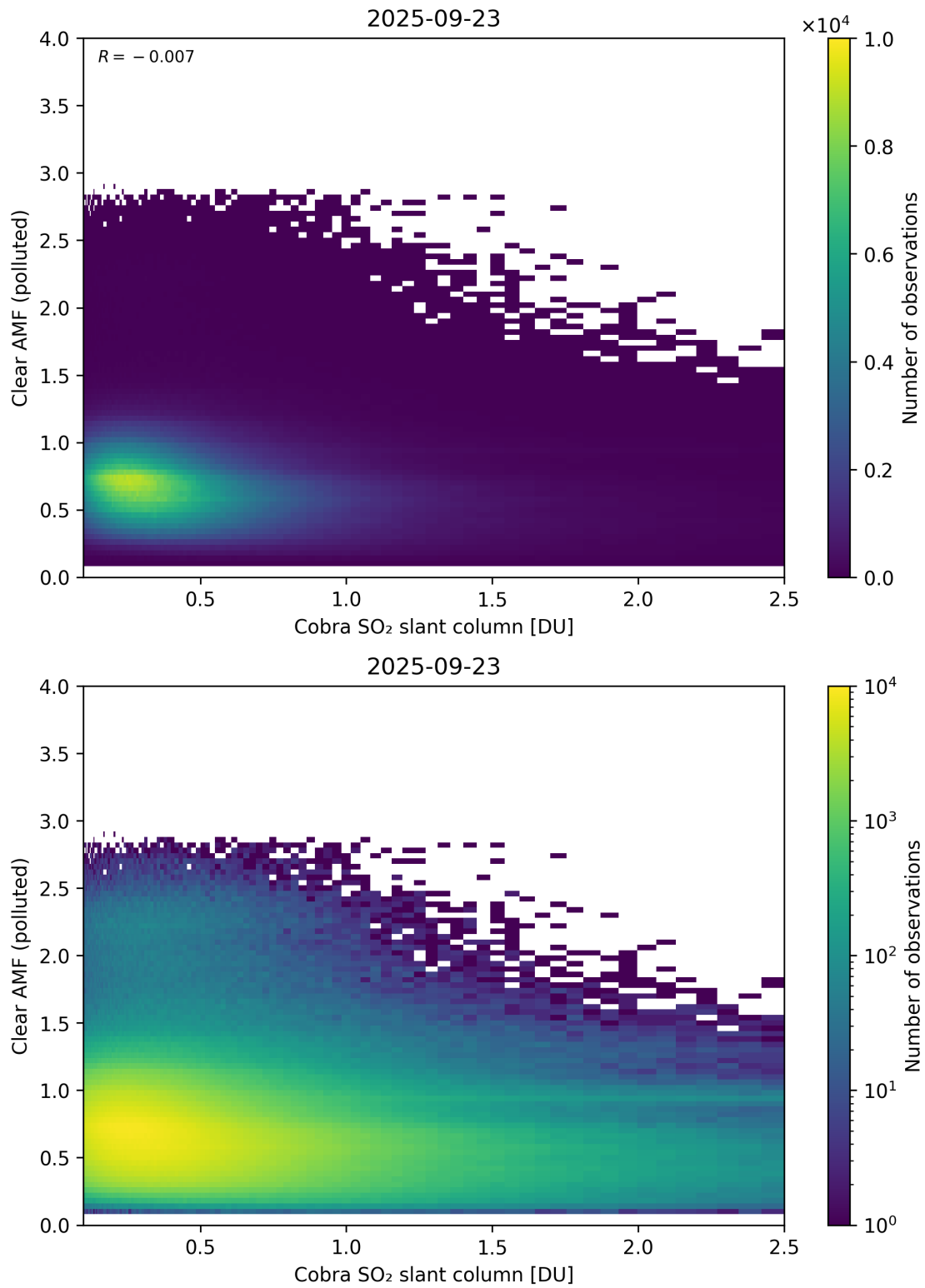
Figure 215: Scatter density plot of “Cobra SO 2 slant column” against “Clear AMF (polluted)” for 2025-09-22 to 2025-09-24.
