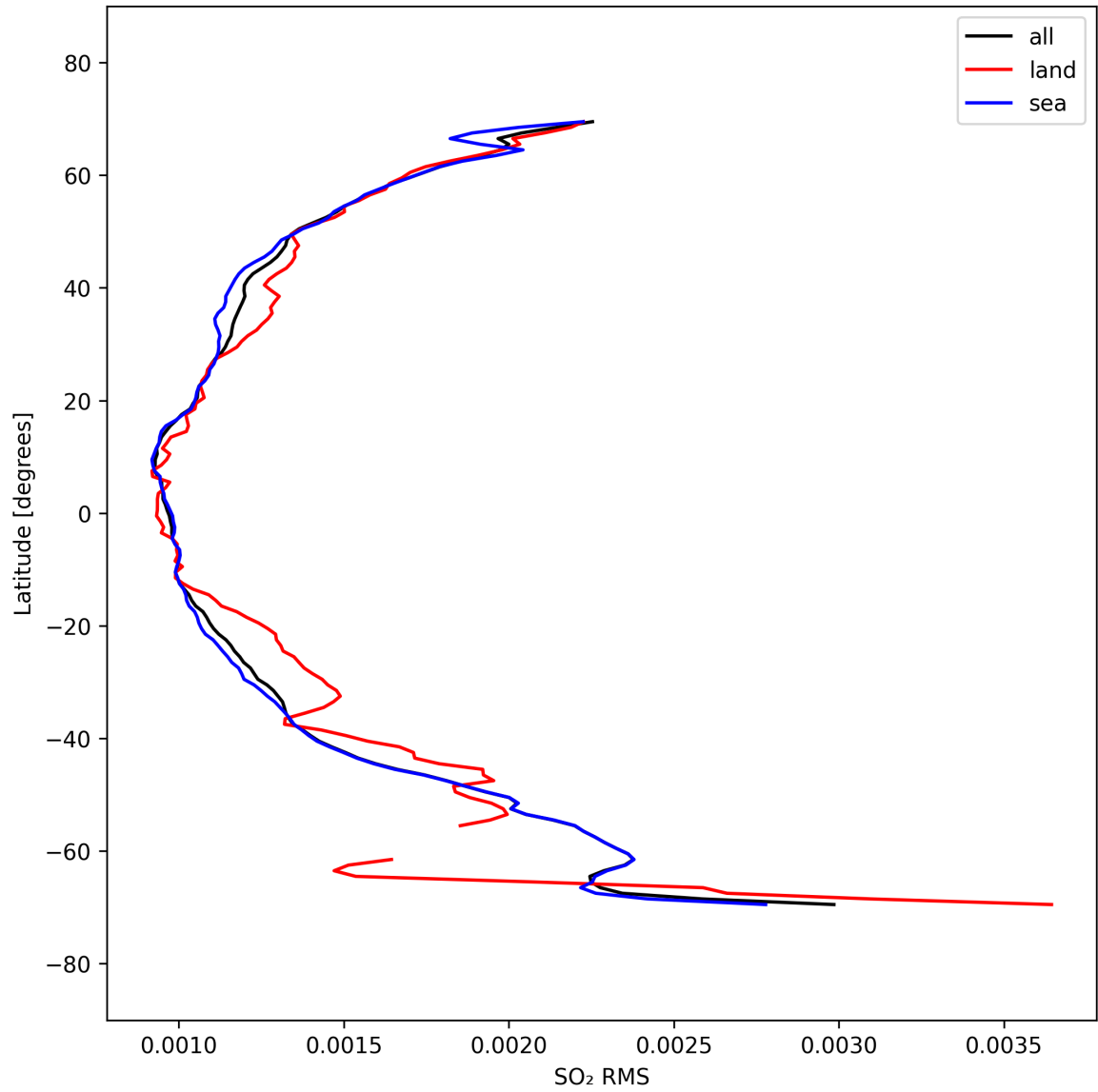
Figure 52: Zonal average of “SO 2 RMS” for 2025-09-22 to 2025-09-24.
