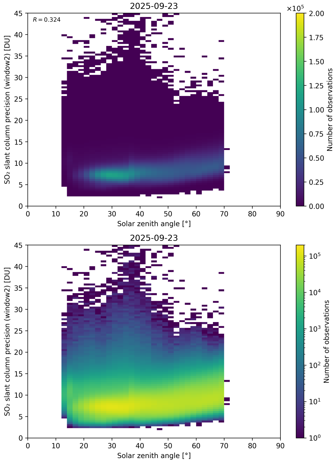
Figure 186: Scatter density plot of “Solar zenith angle” against “SO 2 slant column precision (window2)” for 2025-09-22 to 2025-09-24.
