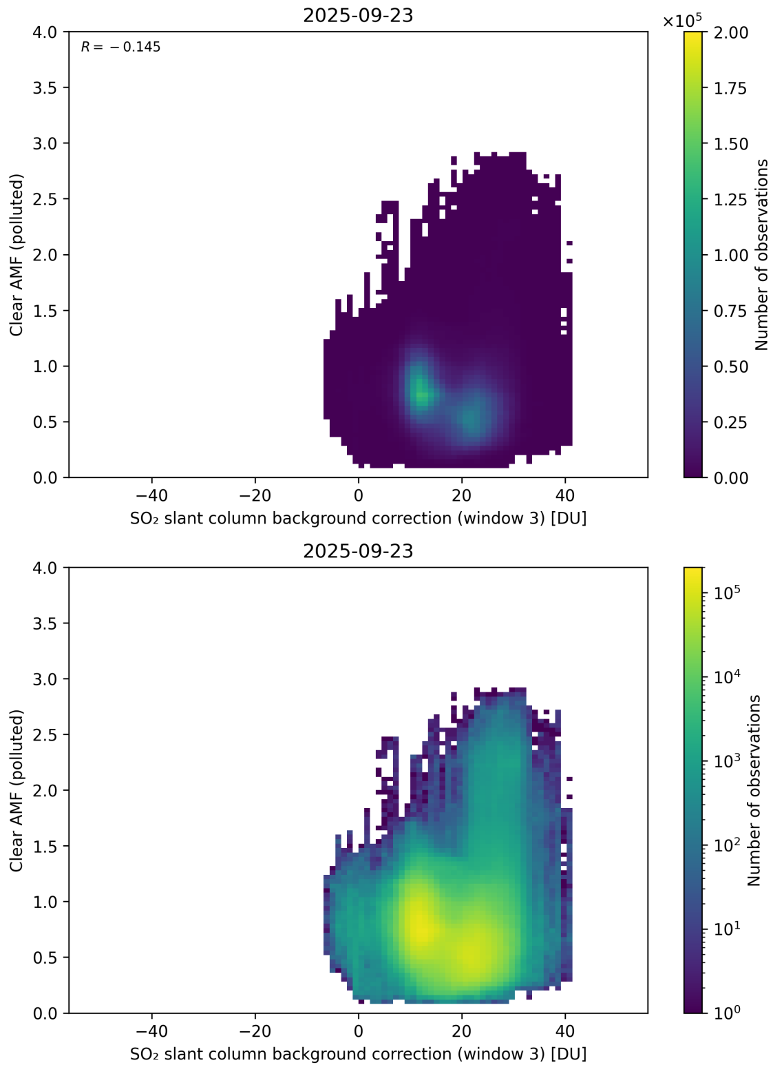
Figure 135: Scatter density plot of “SO 2 slant column background correction (window 3)” against “Clear AMF (polluted)” for 2025-09-22 to 2025-09-24.
