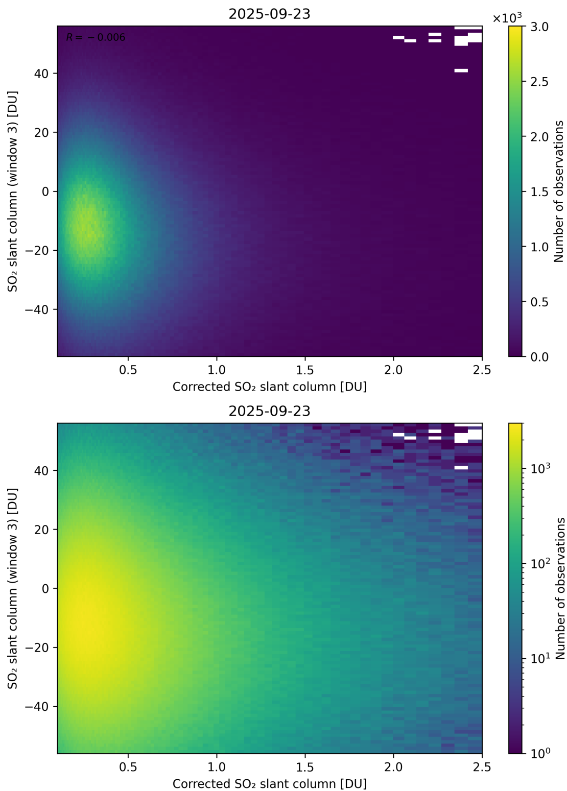
Figure 240: Scatter density plot of “Corrected SO 2 slant column” against “SO 2 slant column (window 3)” for 2025-09-22 to 2025-09-24.
