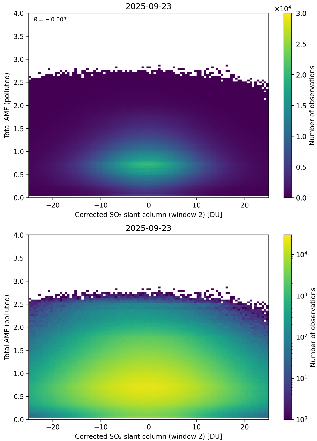
Figure 253: Scatter density plot of “Corrected SO 2 slant column (window 2)” against “Total AMF (polluted)” for 2025-09-22 to 2025-09-24.
