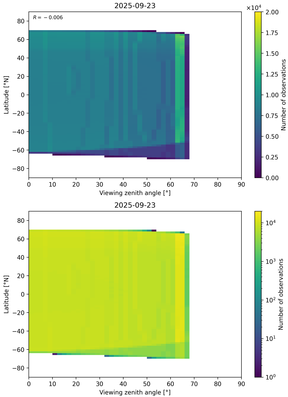
Figure 368: Scatter density plot of “Viewing zenith angle” against “Latitude” for 2025-09-22 to 2025-09-24.
