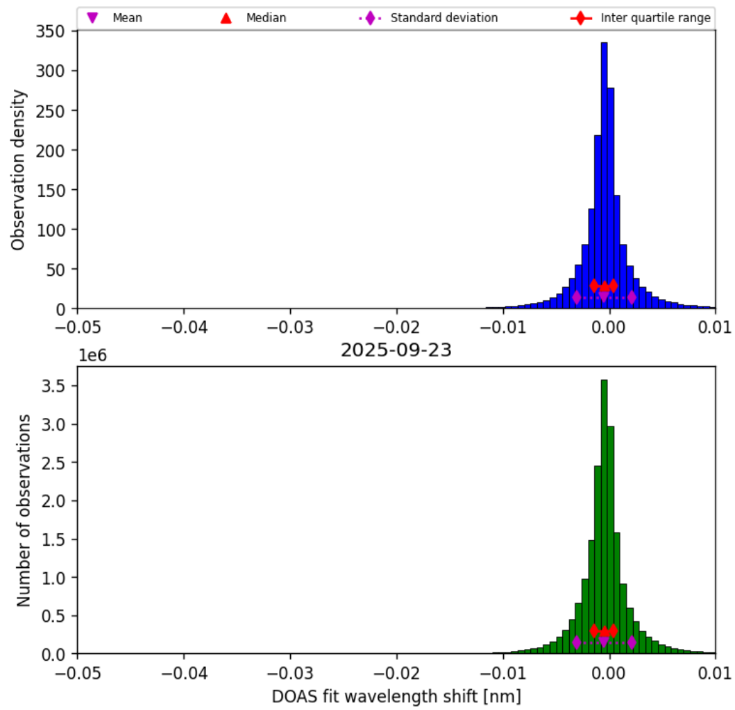
Figure 76: Histogram of “DOAS fit wavelength shift” for 2025-09-22 to 2025-09-24
