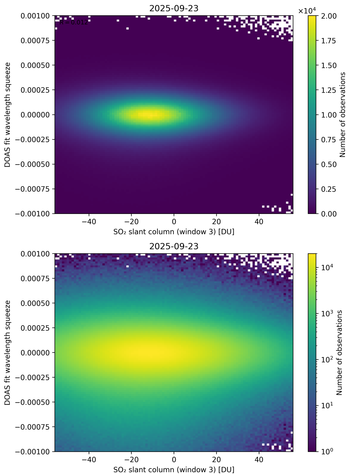
Figure 305: Scatter density plot of “SO 2 slant column (window 3)” against “DOAS fit wavelength squeeze” for 2025-09-22 to 2025-09-24.
