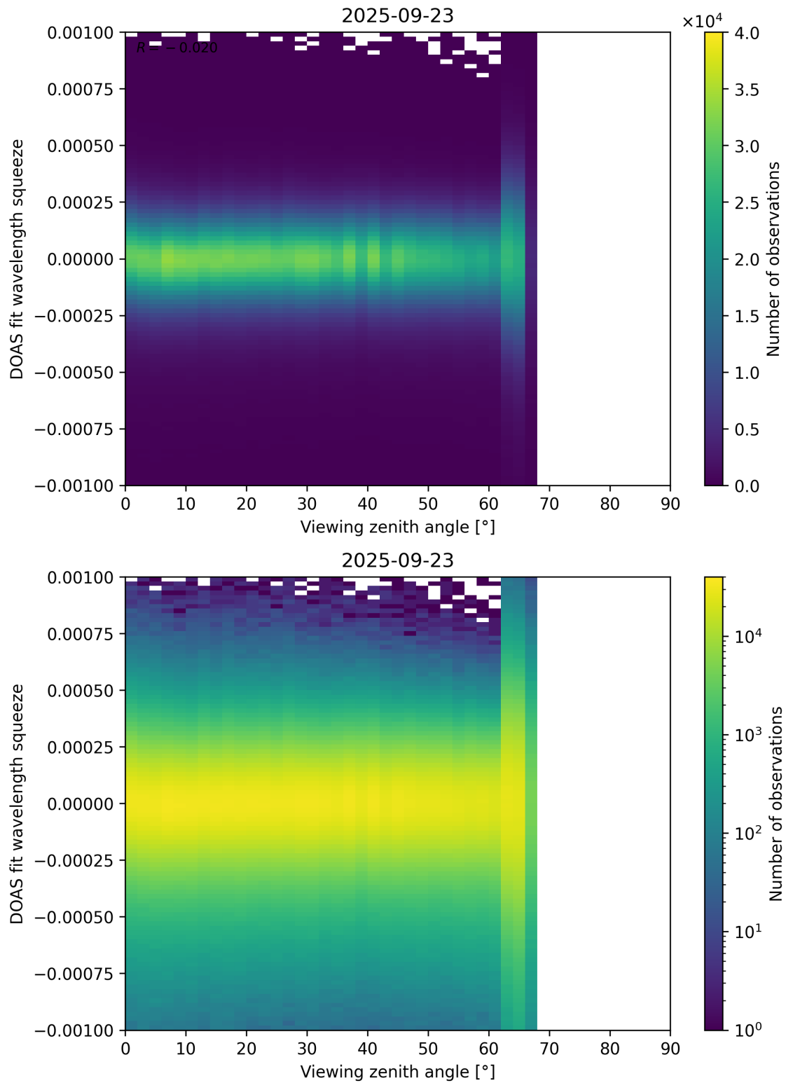
Figure 366: Scatter density plot of “Viewing zenith angle” against “DOAS fit wavelength squeeze” for 2025-09-22 to 2025-09-24.
