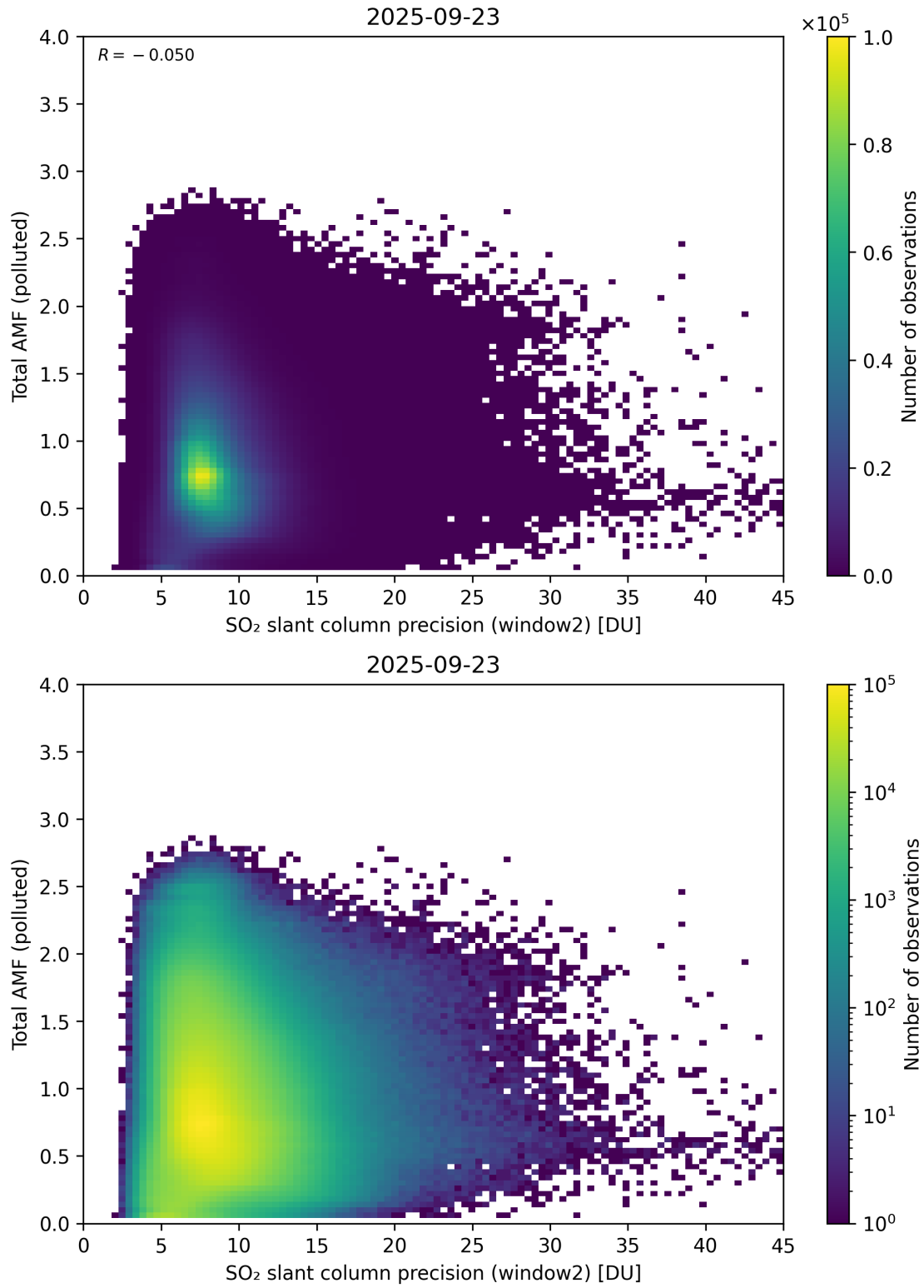
Figure 301: Scatter density plot of “SO 2 slant column precision (window2)” against “Total AMF (polluted)” for 2025-09-22 to 2025-09-24.
