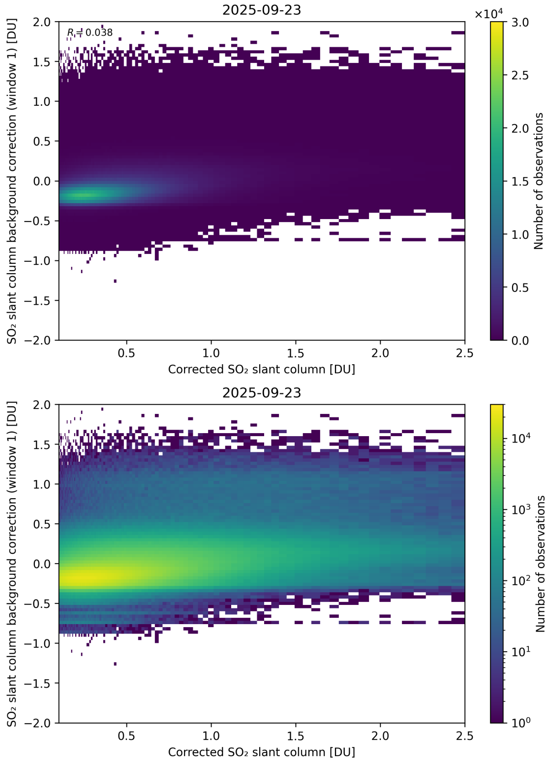
Figure 226: Scatter density plot of “Corrected SO 2 slant column” against “SO 2 slant column background correction (window 1)” for 2025-09-22 to 2025-09-24.
