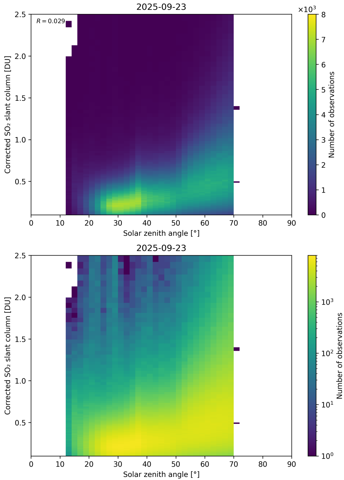
Figure 181: Scatter density plot of “Solar zenith angle” against “Corrected SO 2 slant column” for 2025-09-22 to 2025-09-24.
