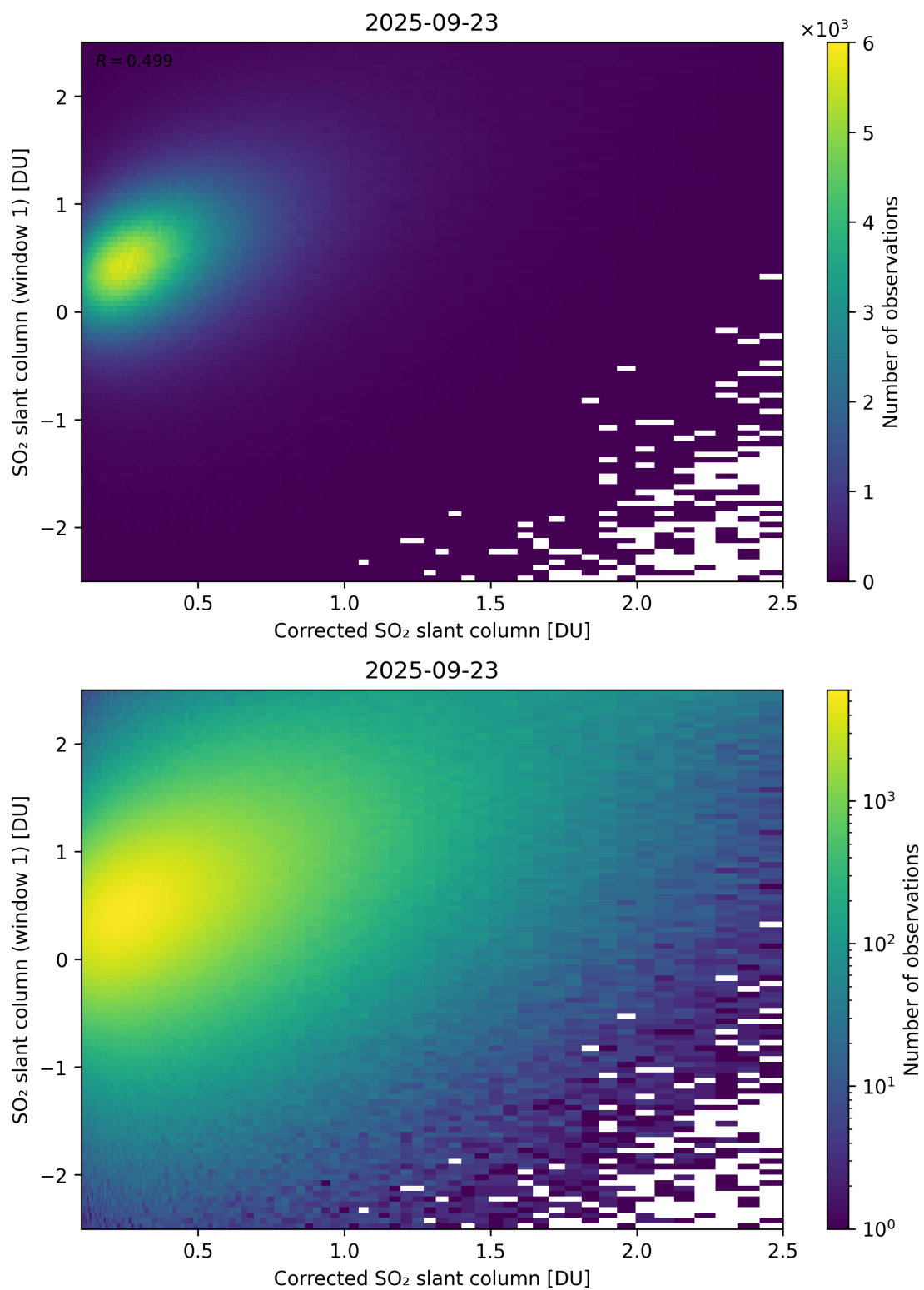
Figure 237: Scatter density plot of “Corrected SO 2 slant column” against “SO 2 slant column (window 1)” for 2025-09-22 to 2025-09-24.
