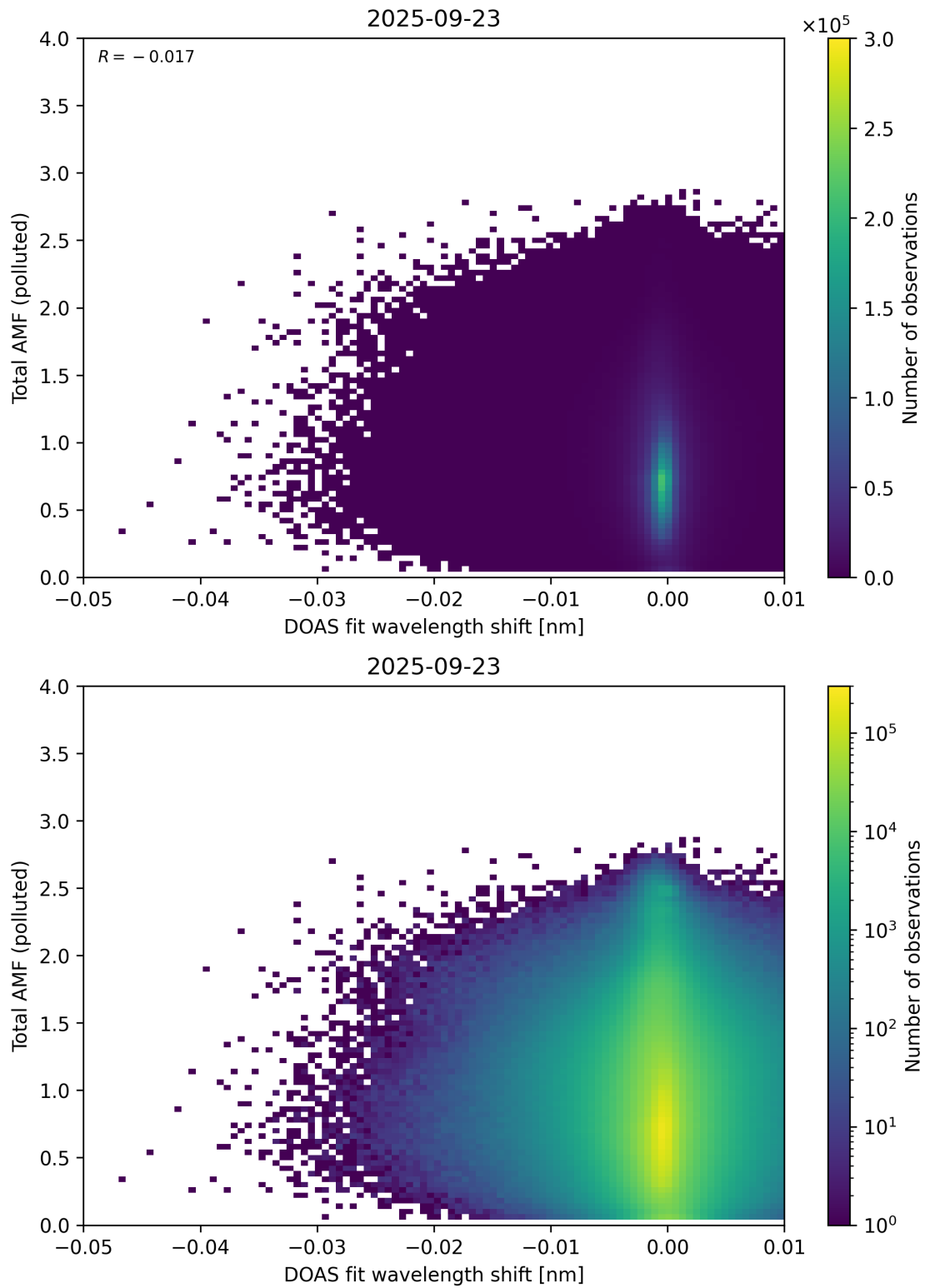
Figure 141: Scatter density plot of “DOAS fit wavelength shift” against “Total AMF (polluted)” for 2025-09-22 to 2025-09-24.
