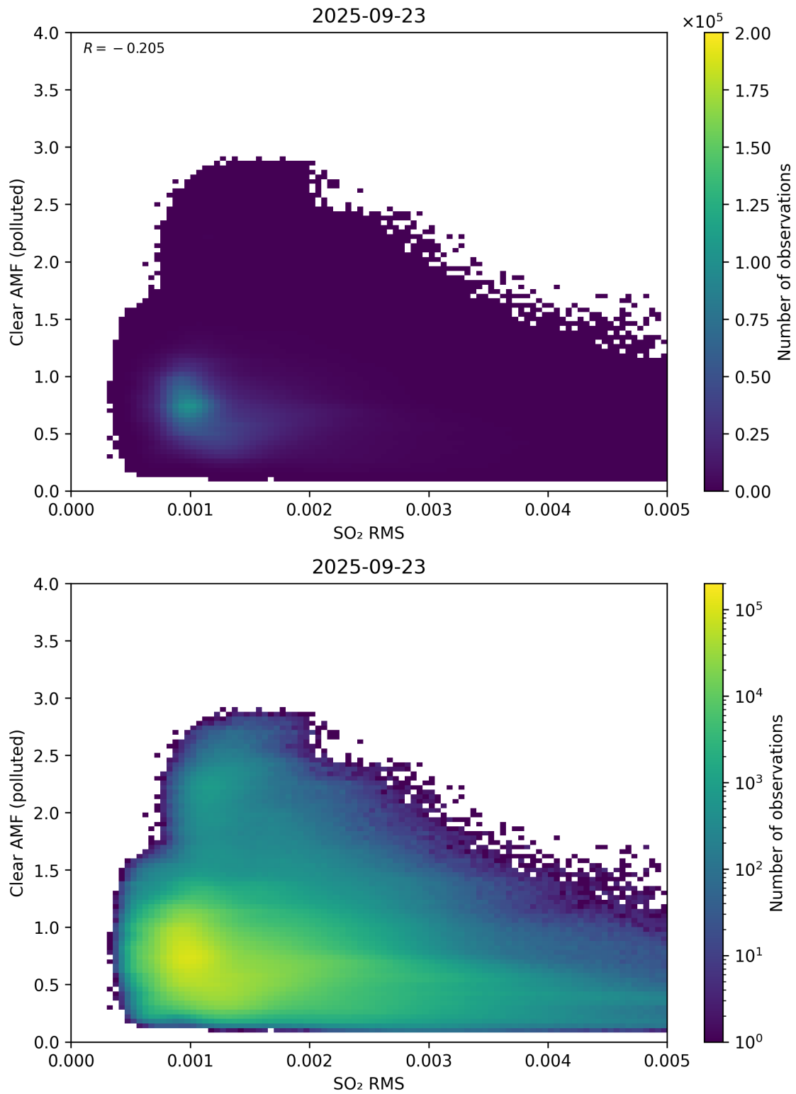
Figure 147: Scatter density plot of “SO 2 RMS” against “Clear AMF (polluted)” for 2025-09-22 to 2025-09-24.
