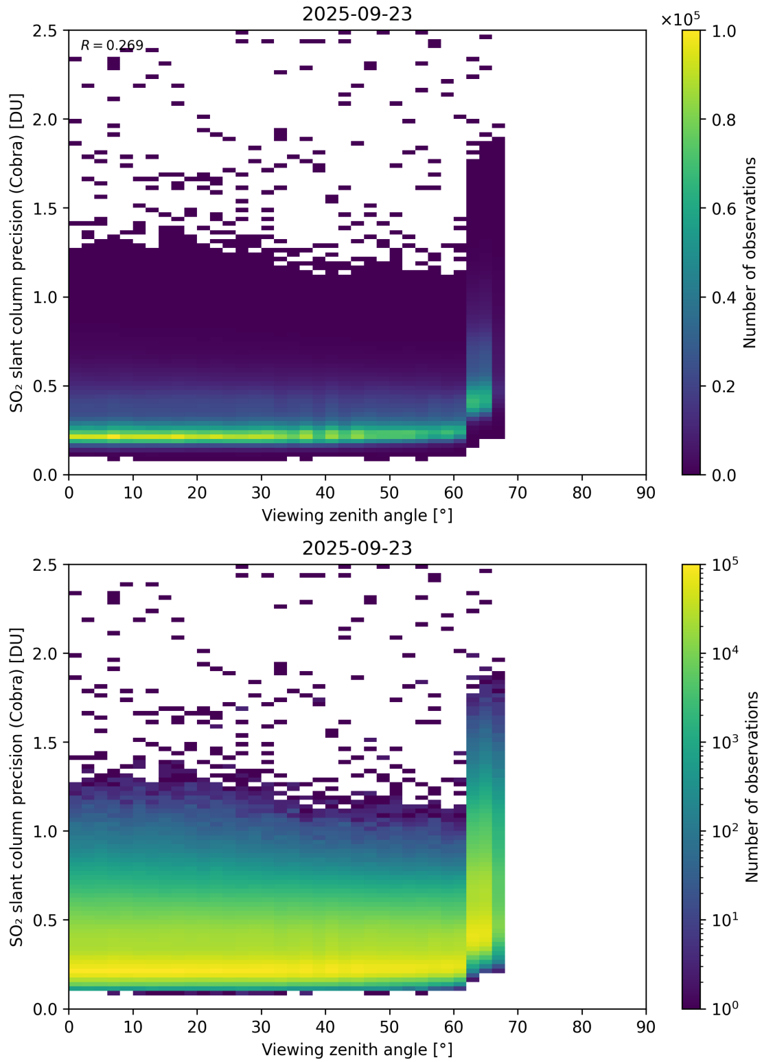
Figure 372: Scatter density plot of “Viewing zenith angle” against “SO 2 slant column precision (Cobra)” for 2025-09-22 to 2025-09-24.
