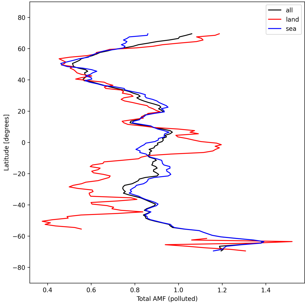
Figure 53: Zonal average of “Total AMF (polluted)” for 2025-09-22 to 2025-09-24.
