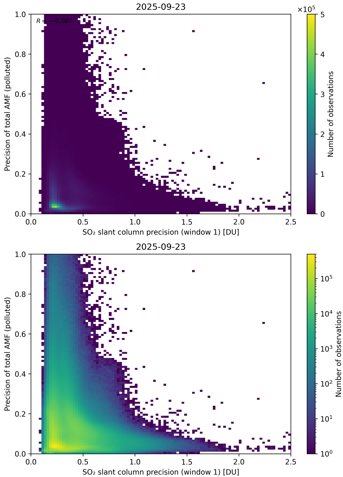
Figure 281: Scatter density plot of “SO 2 slant column precision (window 1)” against “Precision of total AMF (polluted)” for 2025-09-22 to 2025-09-24.
