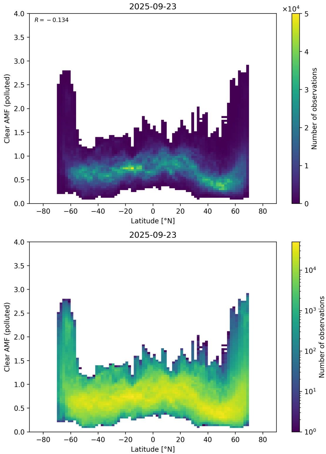
Figure 156: Scatter density plot of “Latitude” against “Clear AMF (polluted)” for 2025-09-22 to 2025-09-24.
