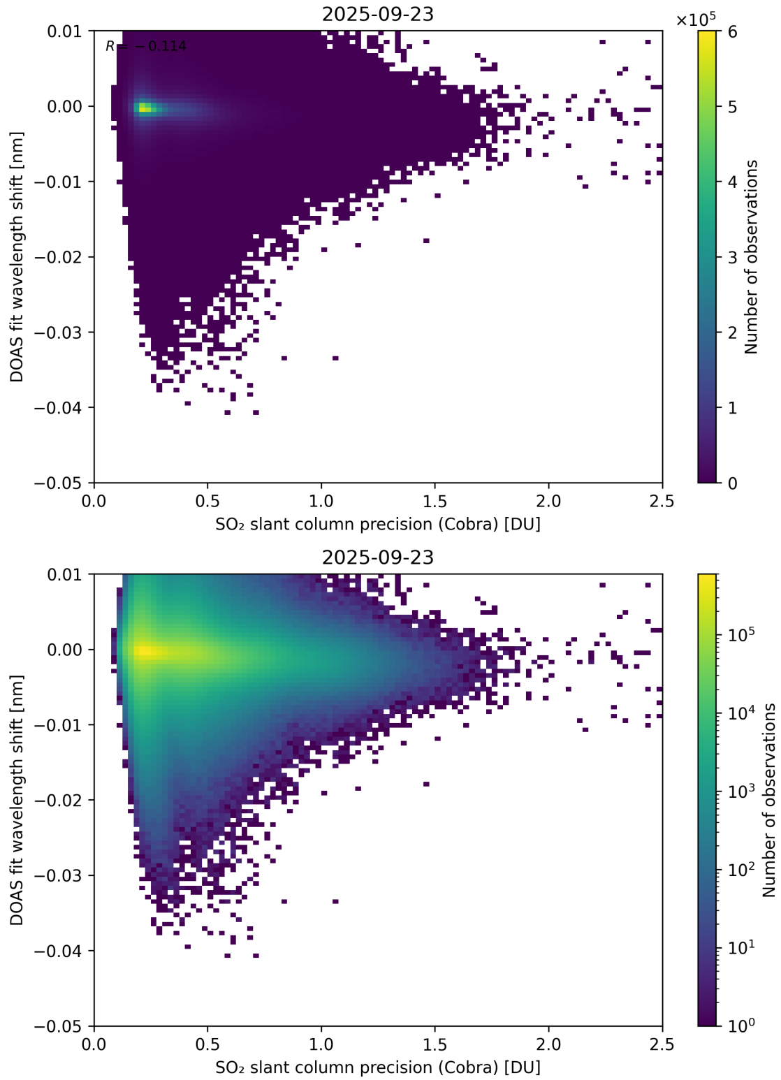
Figure 202: Scatter density plot of “SO 2 slant column precision (Cobra)” against “DOAS fit wavelength shift” for 2025-09-22 to 2025-09-24.
