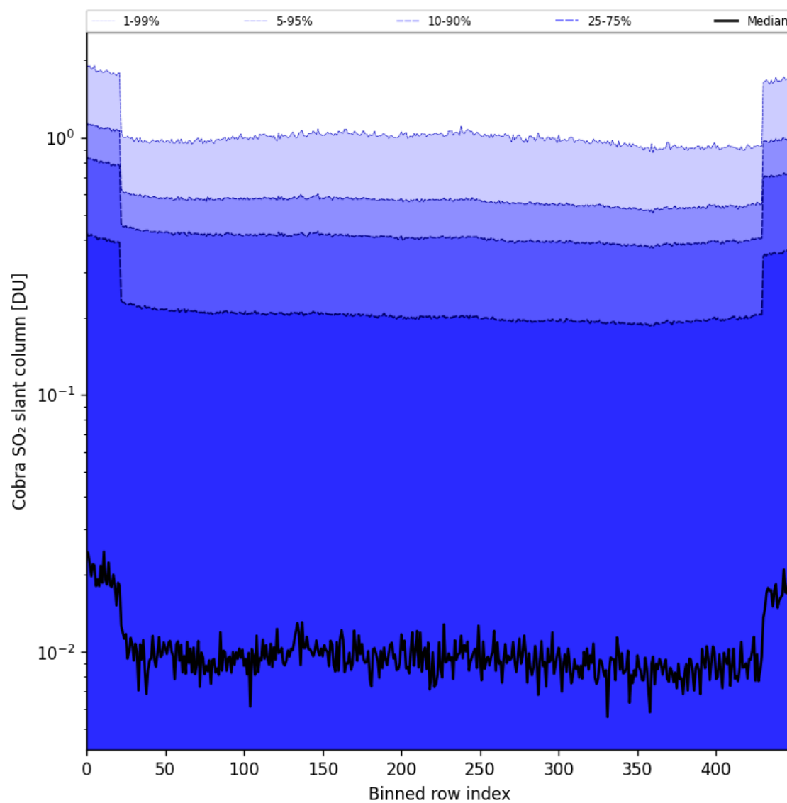
Figure 87: Along track statistics of “Cobra SO 2 slant column” for 2025-09-22 to 2025-09-24
