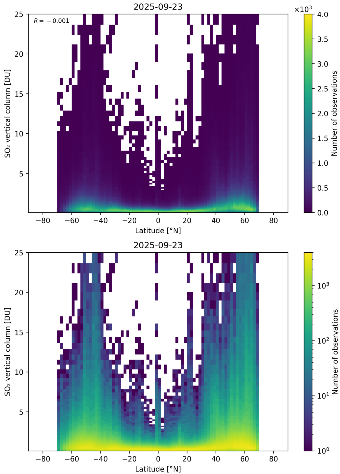
Figure 169: Scatter density plot of “Latitude” against “SO 2 vertical column” for 2025-09-22 to 2025-09-24.
