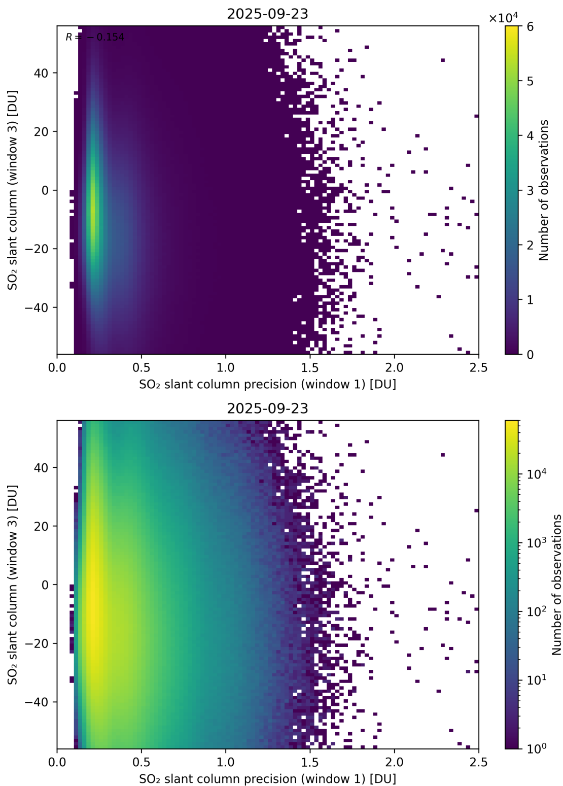
Figure 278: Scatter density plot of “SO 2 slant column precision (window 1)” against “SO 2 slant column (window 3)” for 2025-09-22 to 2025-09-24.
