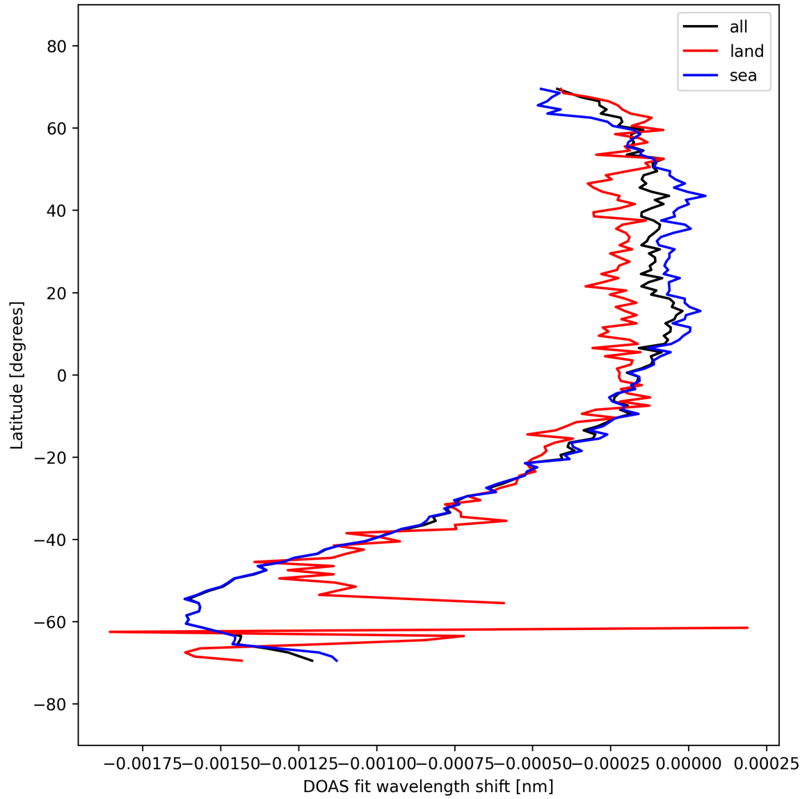
Figure 50: Zonal average of “DOAS fit wavelength shift” for 2025-09-22 to 2025-09-24.
