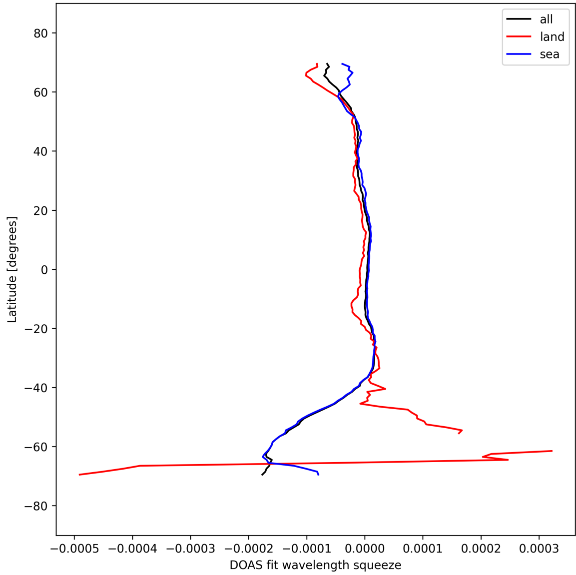
Figure 51: Zonal average of “DOAS fit wavelength squeeze” for 2025-09-22 to 2025-09-24.
