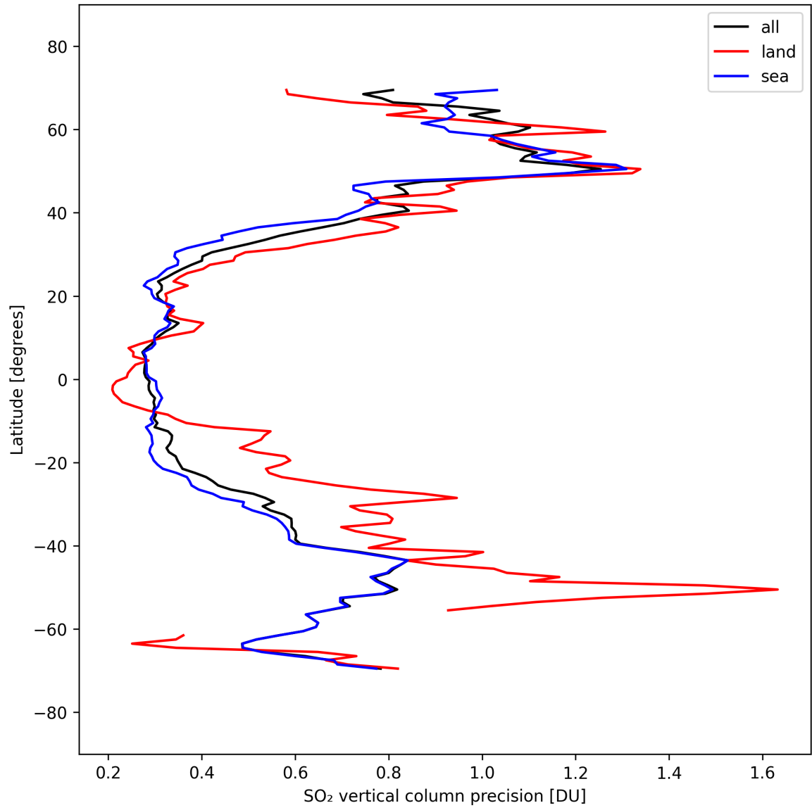
Figure 33: Zonal average of “SO 2 vertical column precision” for 2025-09-22 to 2025-09-24.
