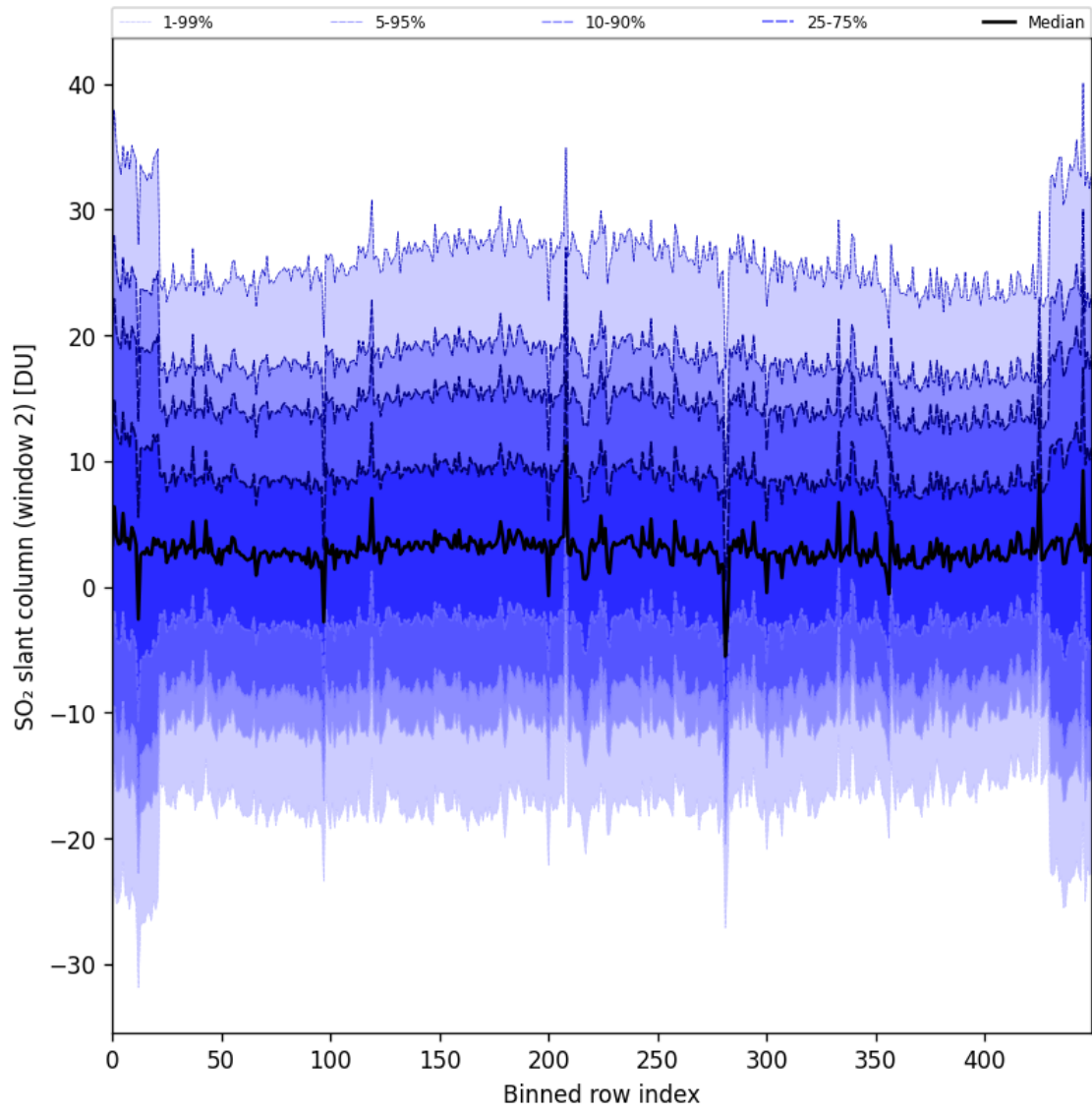
Figure 93: Along track statistics of “SO 2 slant column (window 2)” for 2025-09-22 to 2025-09-24
