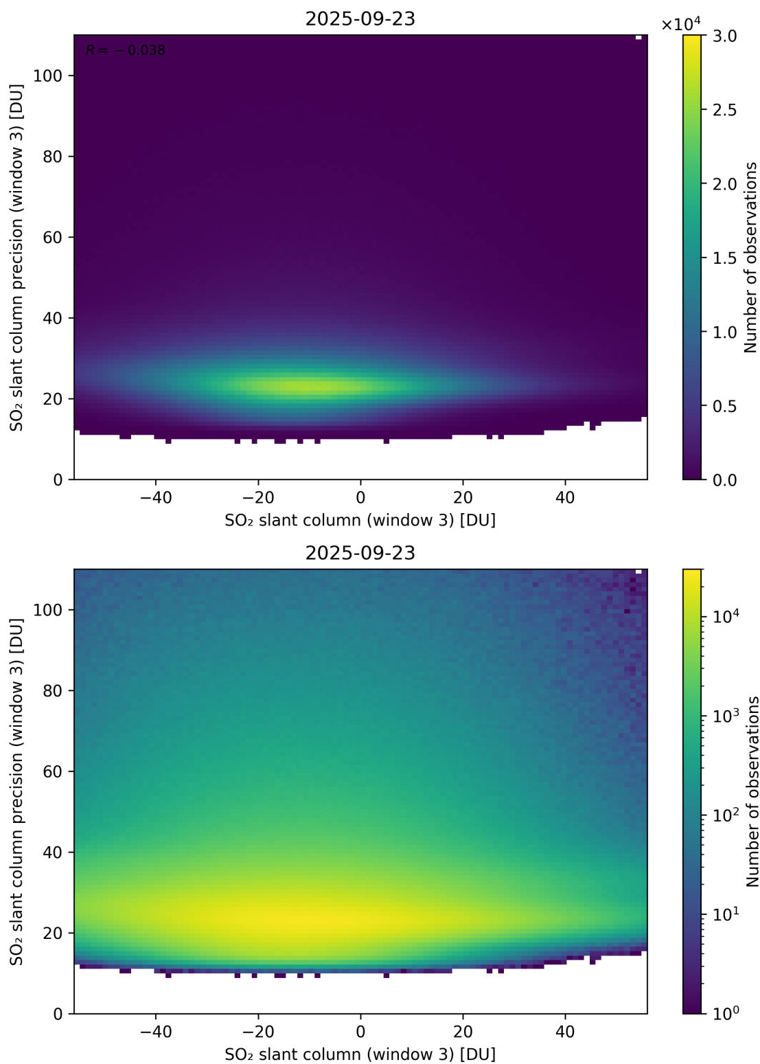
Figure 317: Scatter density plot of “SO 2 slant column (window 3)” against “SO 2 slant column precision (window 3)” for 2025-09-22 to 2025-09-24.
