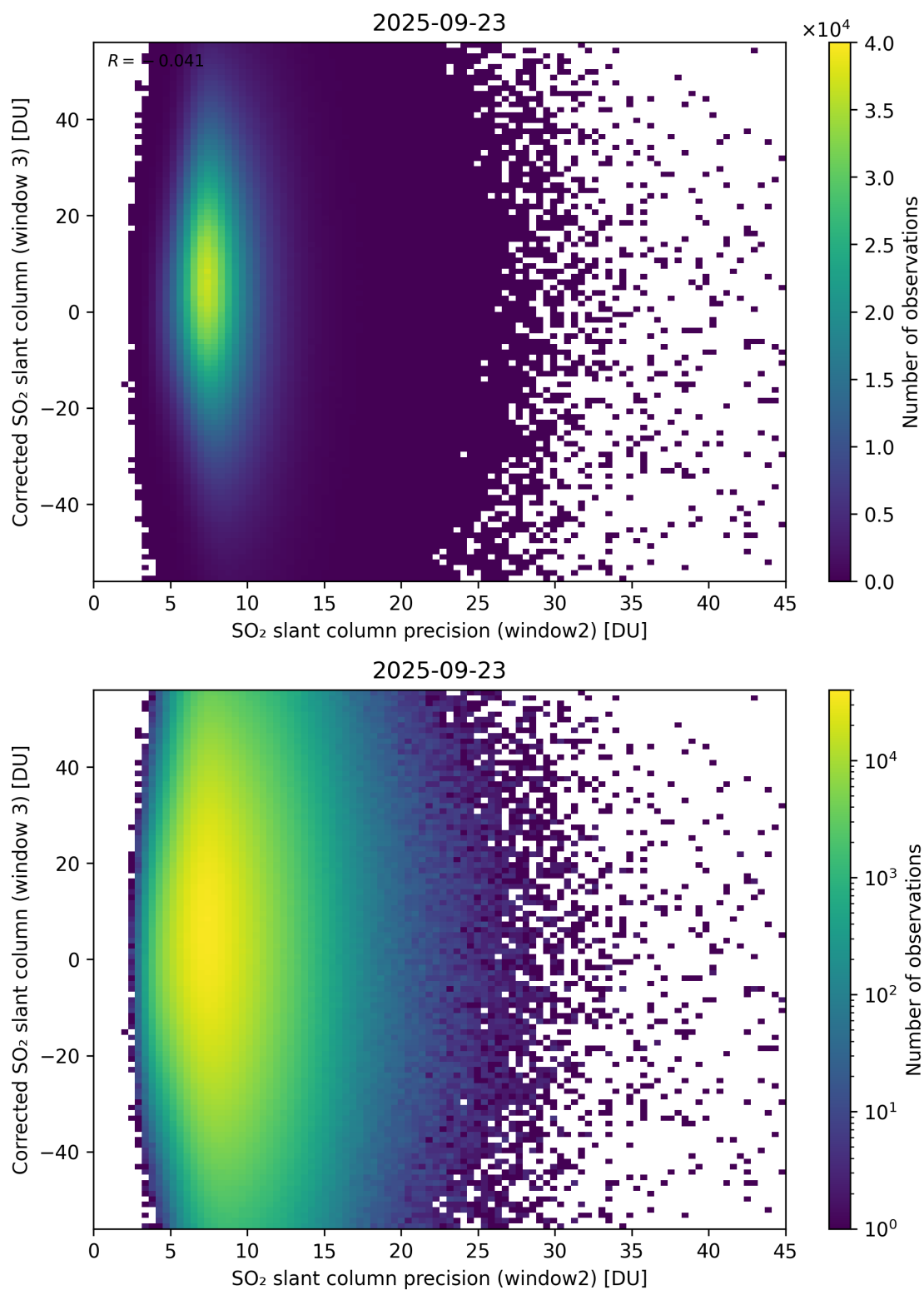
Figure 298: Scatter density plot of “SO 2 slant column precision (window2)” against “Corrected SO 2 slant column (window 3)” for 2025-09-22 to 2025-09-24.
