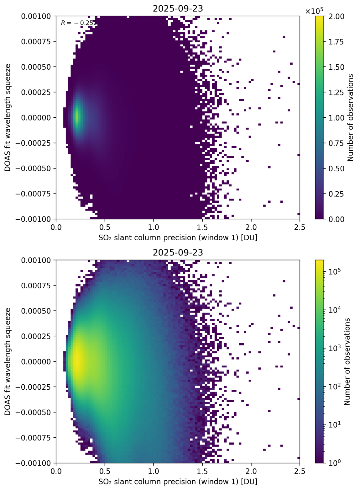
Figure 272: Scatter density plot of “SO 2 slant column precision (window 1)” against “DOAS fit wavelength squeeze” for 2025-09-22 to 2025-09-24.
