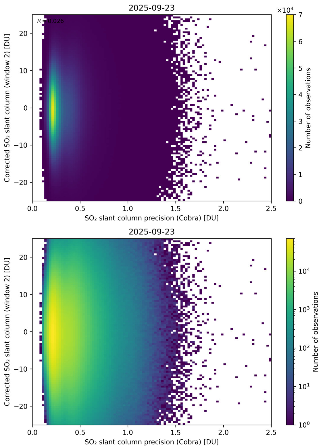
Figure 206: Scatter density plot of “SO 2 slant column precision (Cobra)” against “Corrected SO 2 slant column (window 2)” for 2025-09-22 to 2025-09-24.
