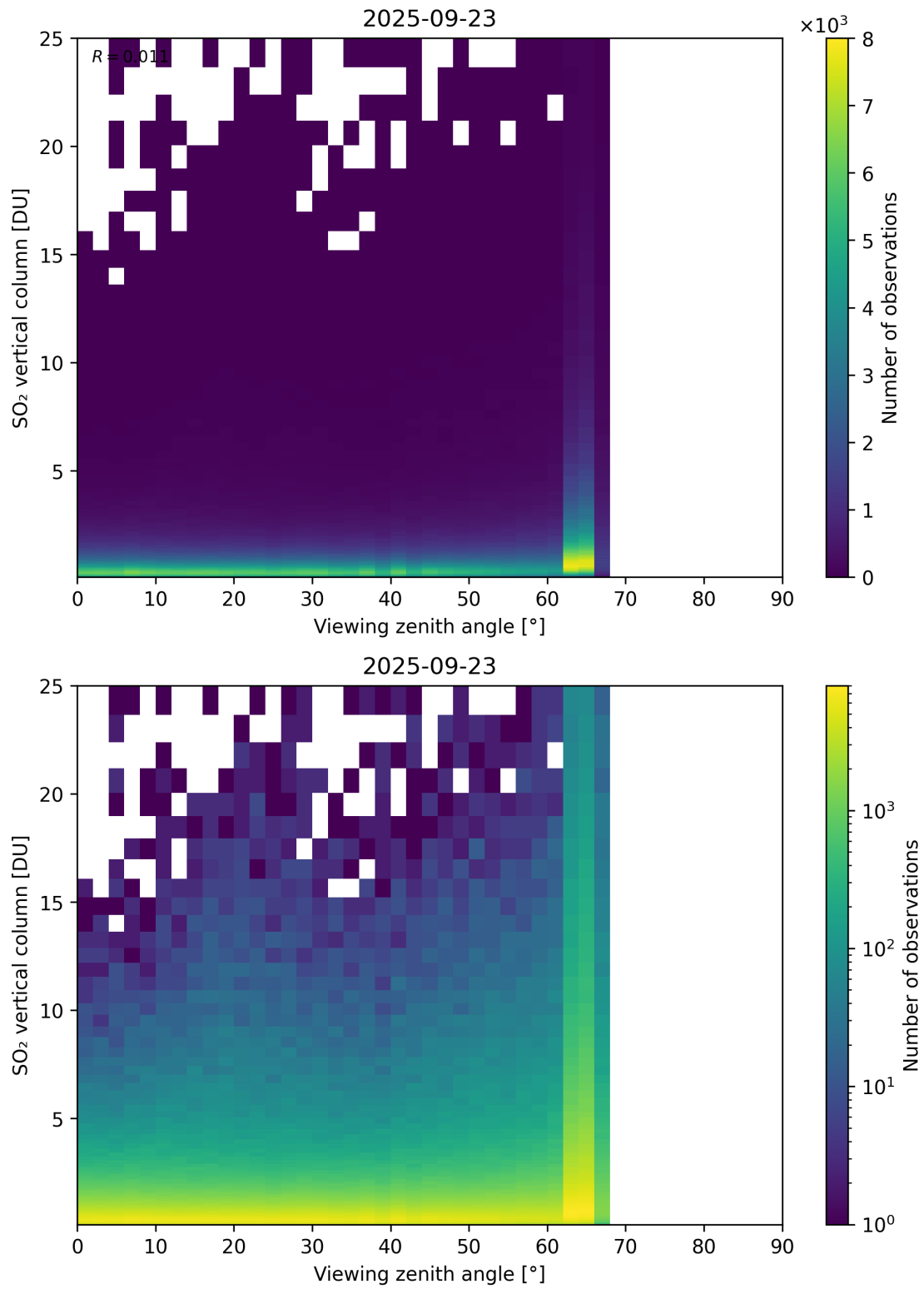
Figure 383: Scatter density plot of “Viewing zenith angle” against “SO 2 vertical column” for 2025-09-22 to 2025-09-24.
