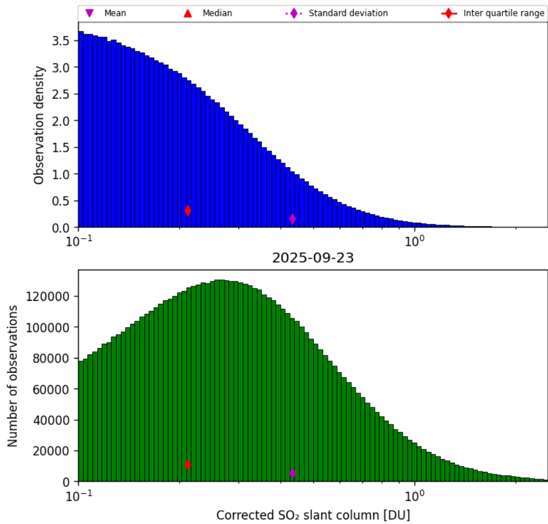
Figure 60: Histogram of "Corrected SO 2 slant column" for 2025-09-22 to 2025-09-24
