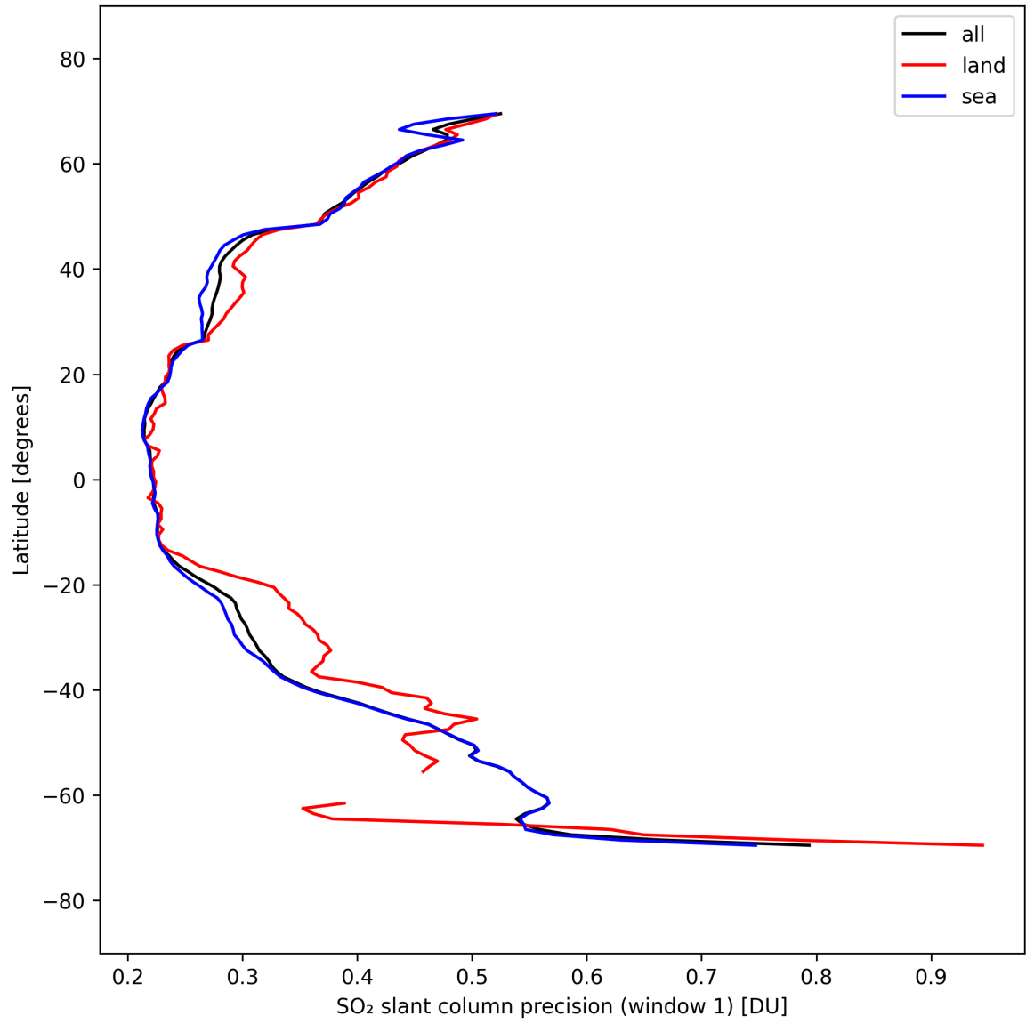
Figure 38: Zonal average of “SO 2 slant column precision (window 1)” for 2025-09-22 to 2025-09-24.
