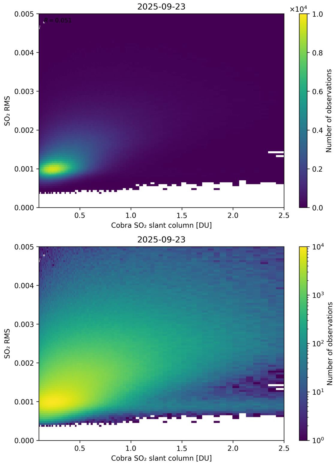
Figure 198: Scatter density plot of “Cobra SO 2 slant column” against “SO 2 RMS” for 2025-09-22 to 2025-09-24.
