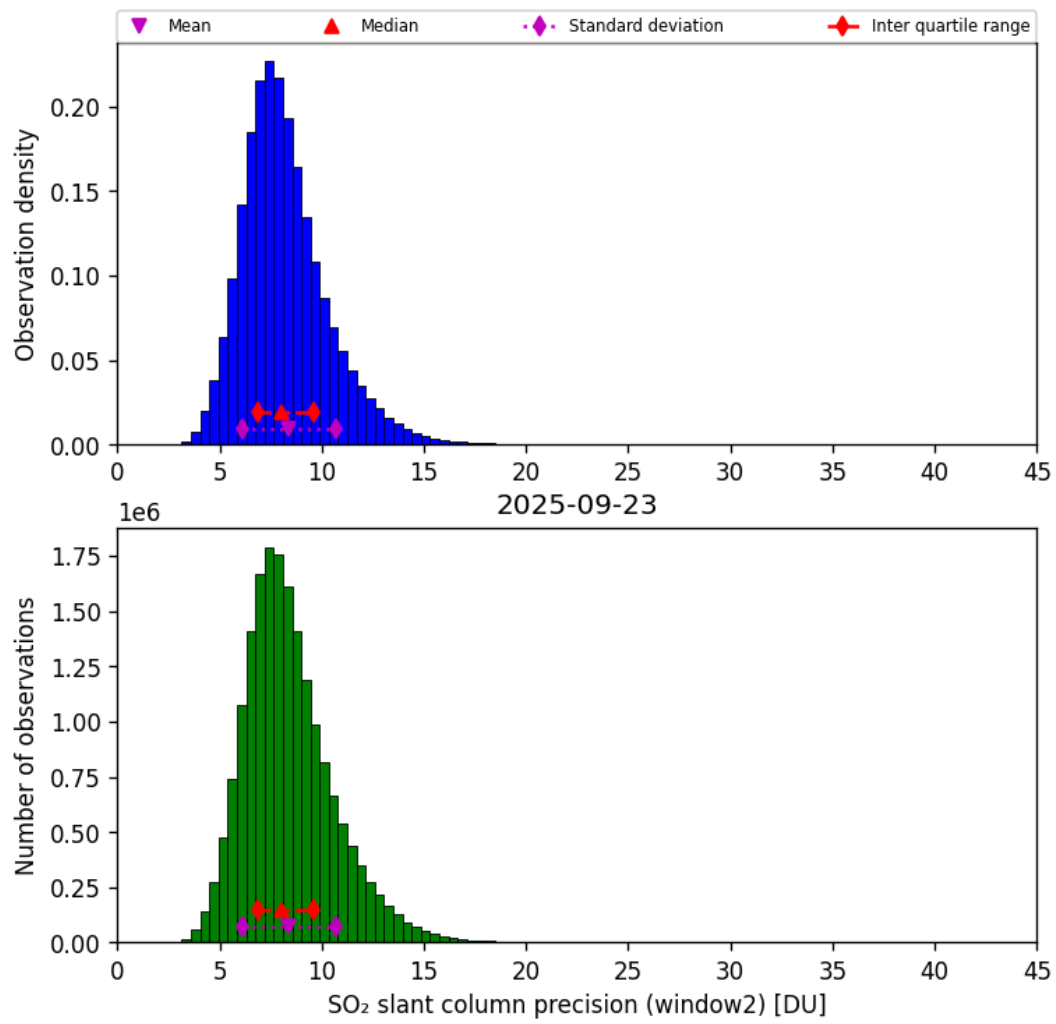
Figure 68: Histogram of “SO 2 slant column precision (window2)” for 2025-09-22 to 2025-09-24
