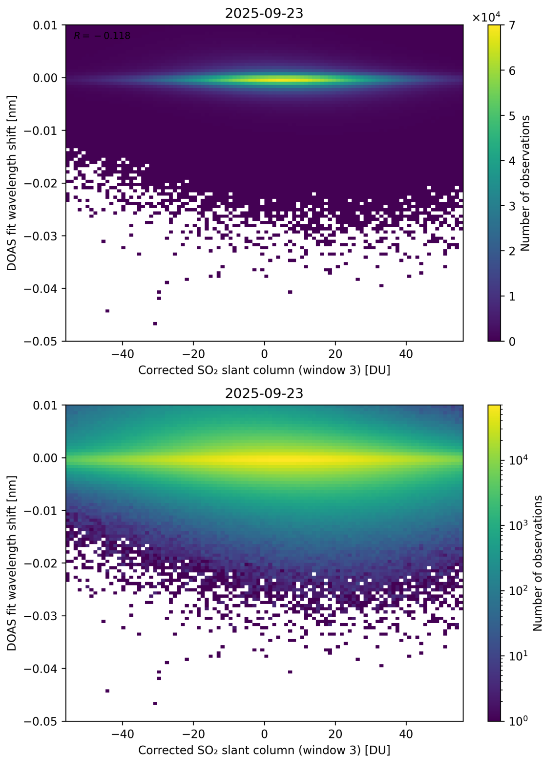
Figure 256: Scatter density plot of “Corrected SO 2 slant column (window 3)” against “DOAS fit wavelength shift” for 2025-09-22 to 2025-09-24.
