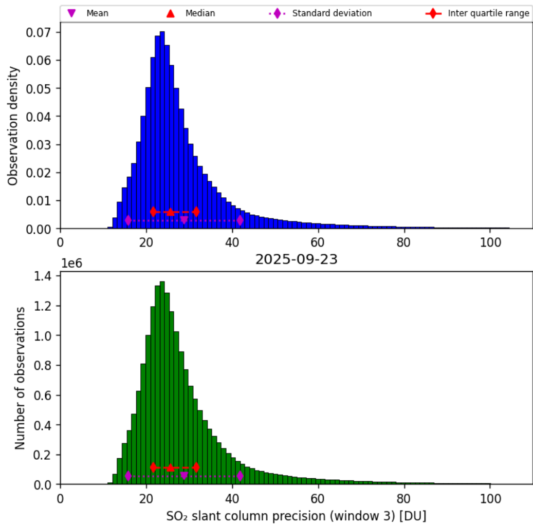
Figure 72: Histogram of “SO 2 slant column precision (window 3)” for 2025-09-22 to 2025-09-24
