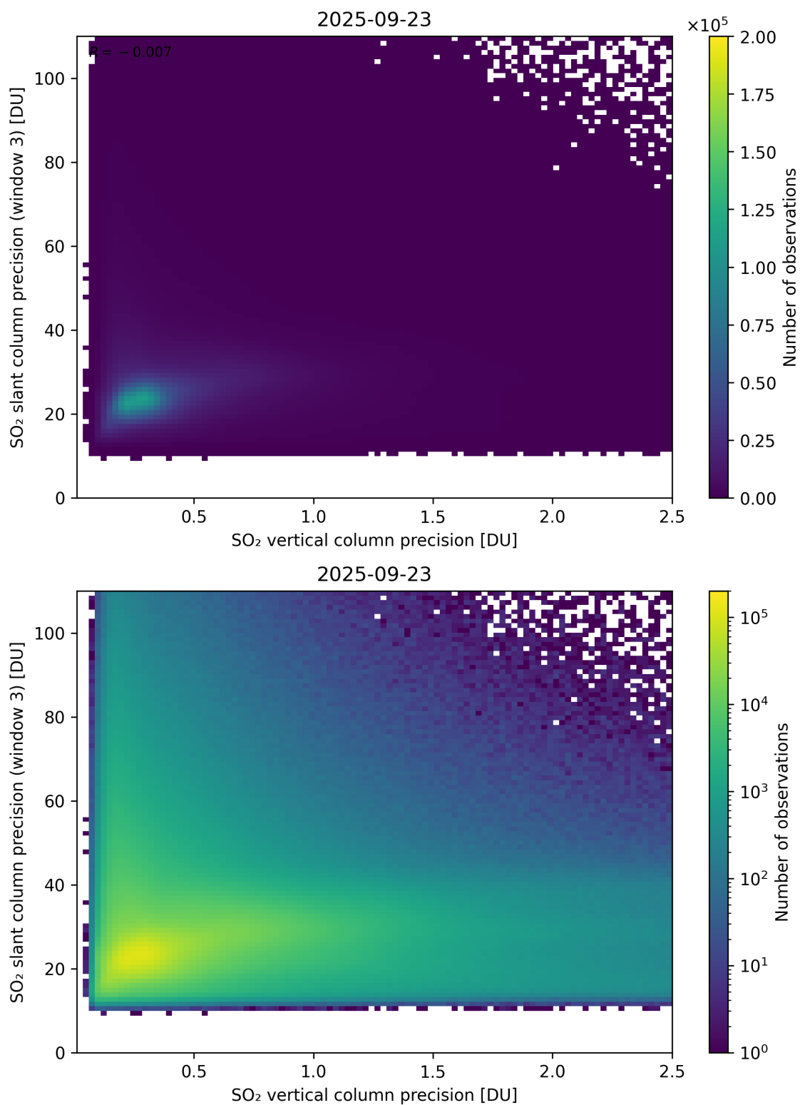
Figure 345: Scatter density plot of “SO 2 vertical column precision” against “SO 2 slant column precision (window 3)” for 2025-09-22 to 2025-09-24.
