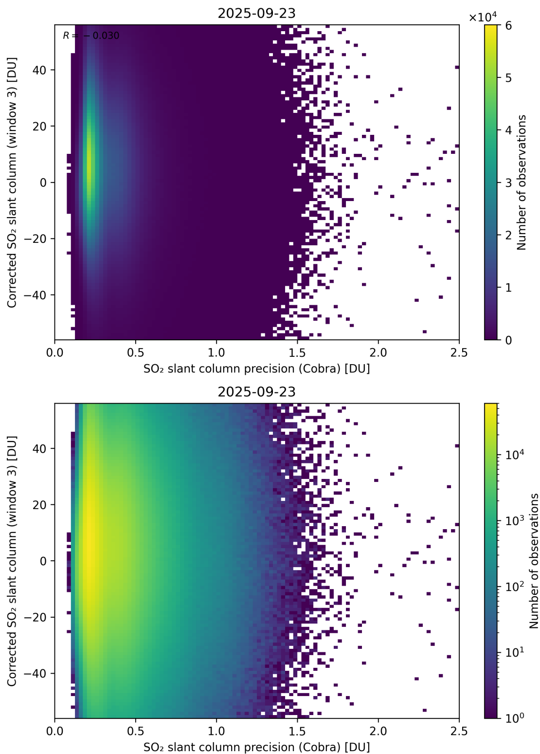
Figure 207: Scatter density plot of “SO 2 slant column precision (Cobra)” against “Corrected SO 2 slant column (window 3)” for 2025-09-22 to 2025-09-24.
