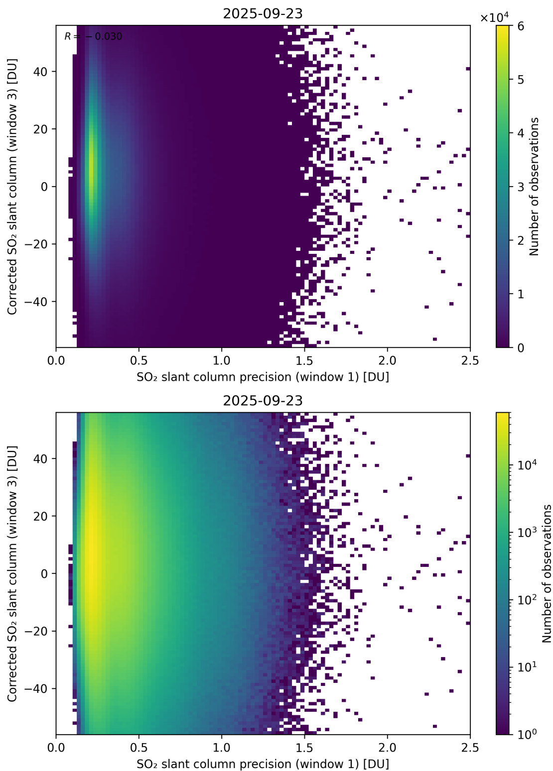
Figure 276: Scatter density plot of “SO 2 slant column precision (window 1)” against “Corrected SO 2 slant column (window 3)” for 2025-09-22 to 2025-09-24.
