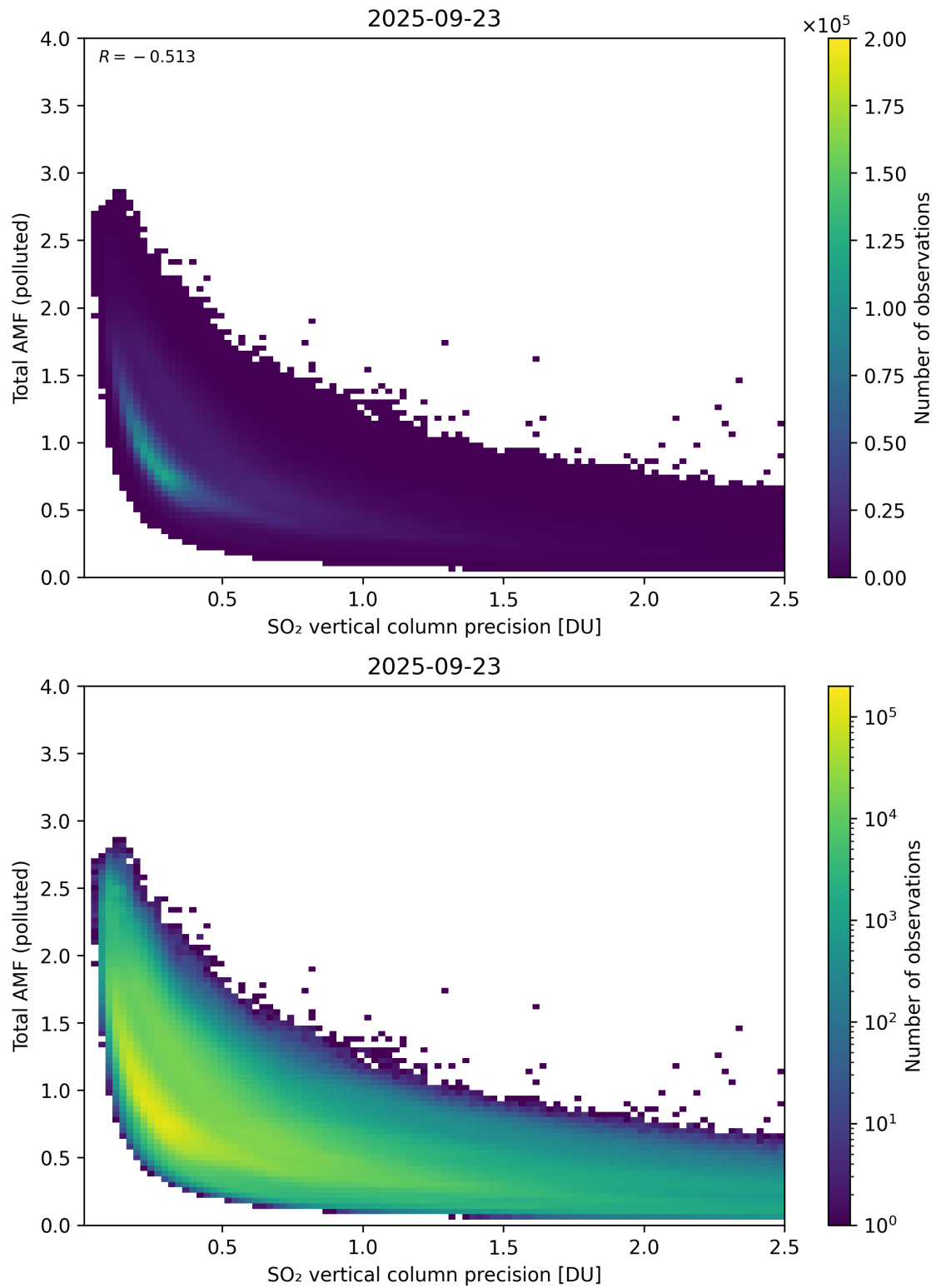
Figure 346: Scatter density plot of “SO 2 vertical column precision” against “Total AMF (polluted)” for 2025-09-22 to 2025-09-24.
