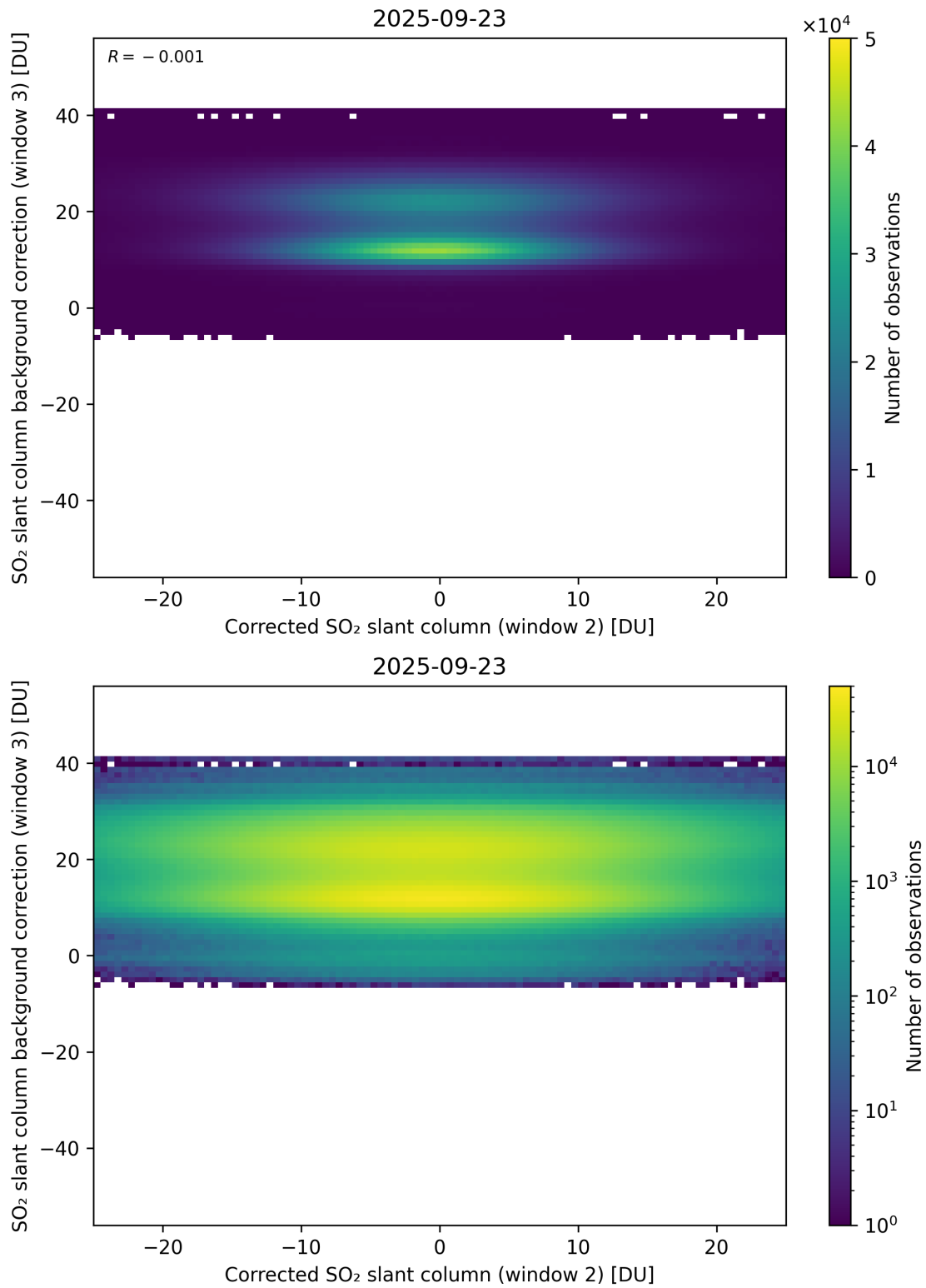
Figure 245: Scatter density plot of “Corrected SO 2 slant column (window 2)” against “SO 2 slant column background correction (window 3)” for 2025-09-22 to 2025-09-24.
