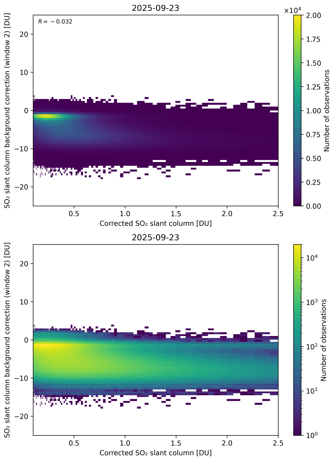
Figure 227: Scatter density plot of “Corrected SO 2 slant column” against “SO 2 slant column background correction (window 2)” for 2025-09-22 to 2025-09-24.
