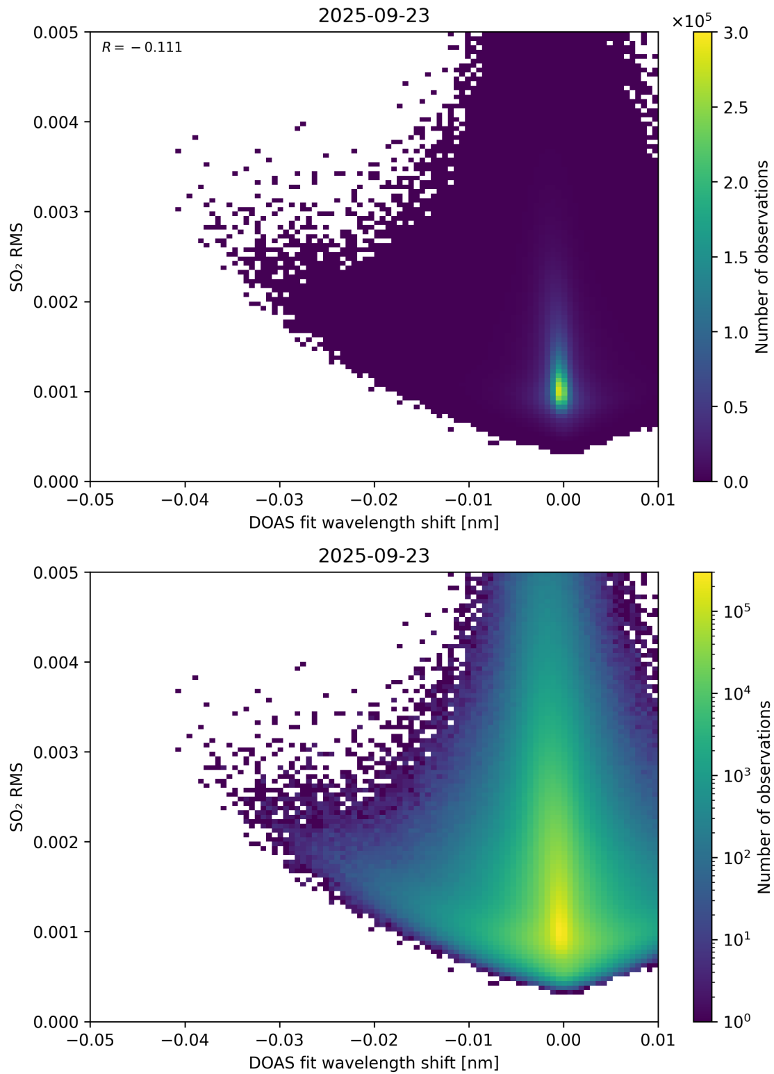
Figure 139: Scatter density plot of “DOAS fit wavelength shift” against “SO 2 RMS” for 2025-09-22 to 2025-09-24.
