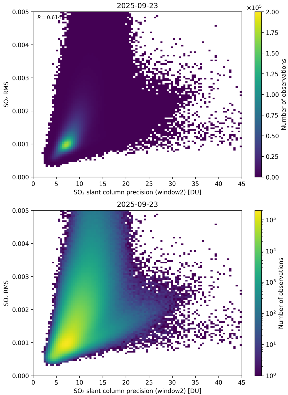
Figure 295: Scatter density plot of “SO 2 slant column precision (window2)” against “SO 2 RMS” for 2025-09-22 to 2025-09-24.
