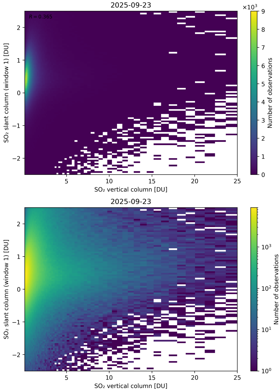
Figure 354: Scatter density plot of “SO 2 vertical column” against “SO 2 slant column (window 1)” for 2025-09-22 to 2025-09-24.
