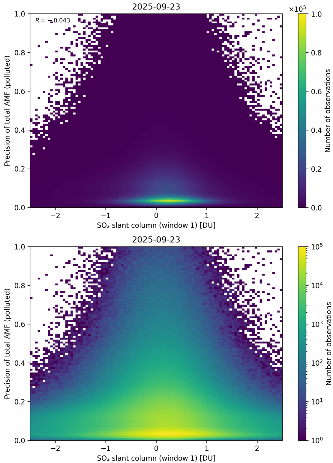
Figure 290: Scatter density plot of “SO 2 slant column (window 1)” against “Precision of total AMF (polluted)” for 2025-09-22 to 2025-09-24.
