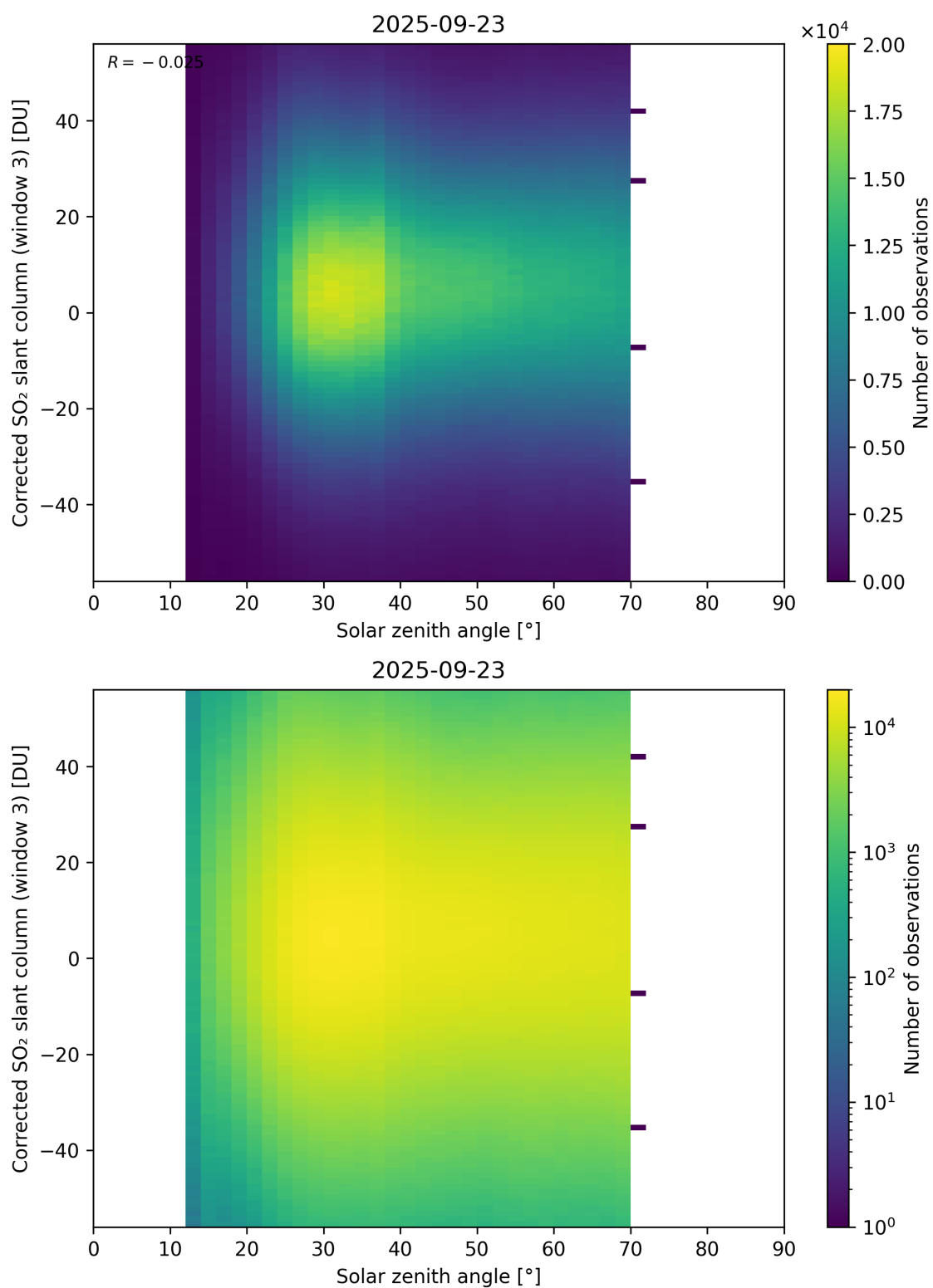
Figure 183: Scatter density plot of “Solar zenith angle” against “Corrected SO 2 slant column (window 3)” for 2025-09-22 to 2025-09-24.
