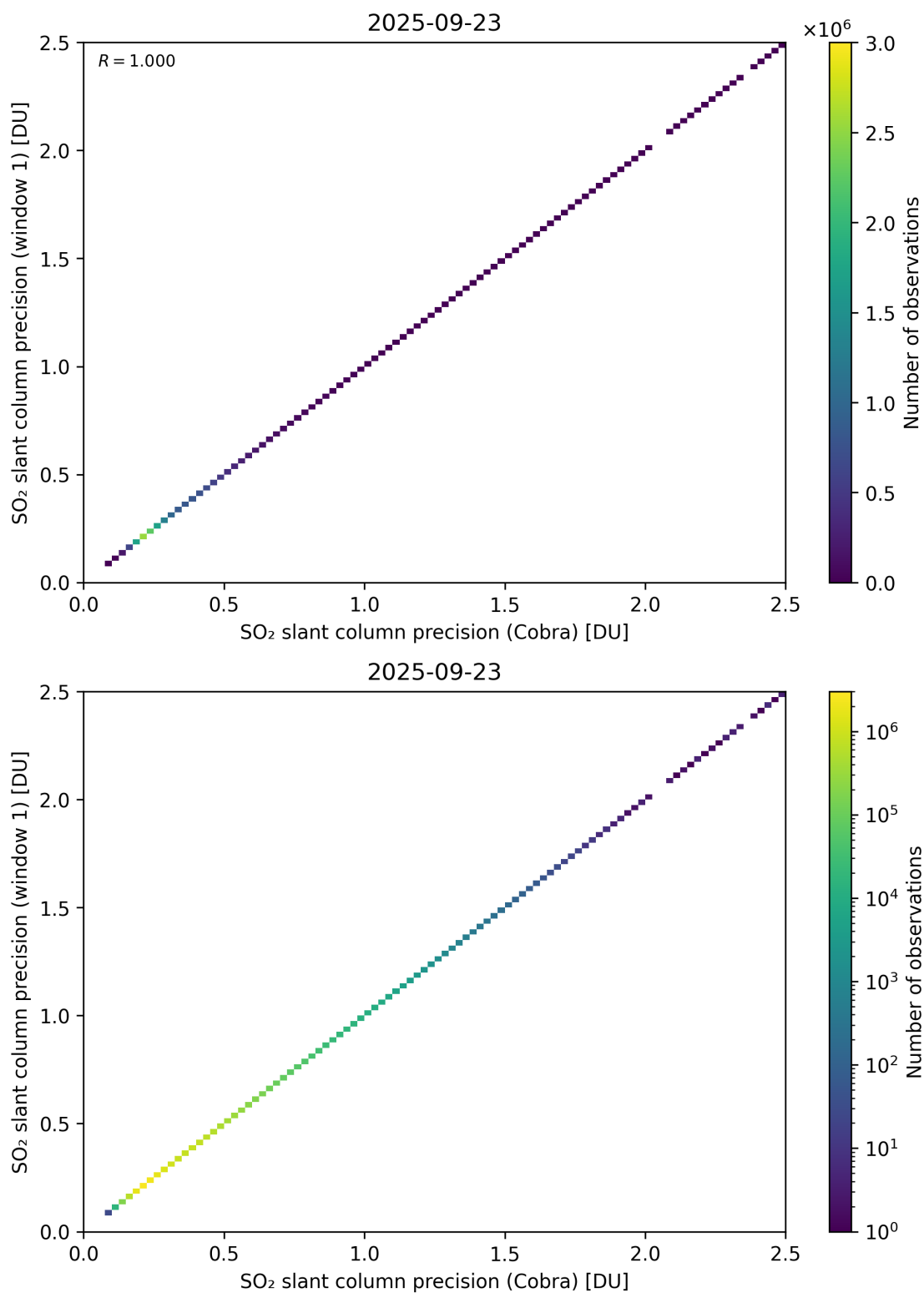
Figure 209: Scatter density plot of “SO 2 slant column precision (Cobra)” against “SO 2 slant column precision (window 1)” for 2025-09-22 to 2025-09-24.
