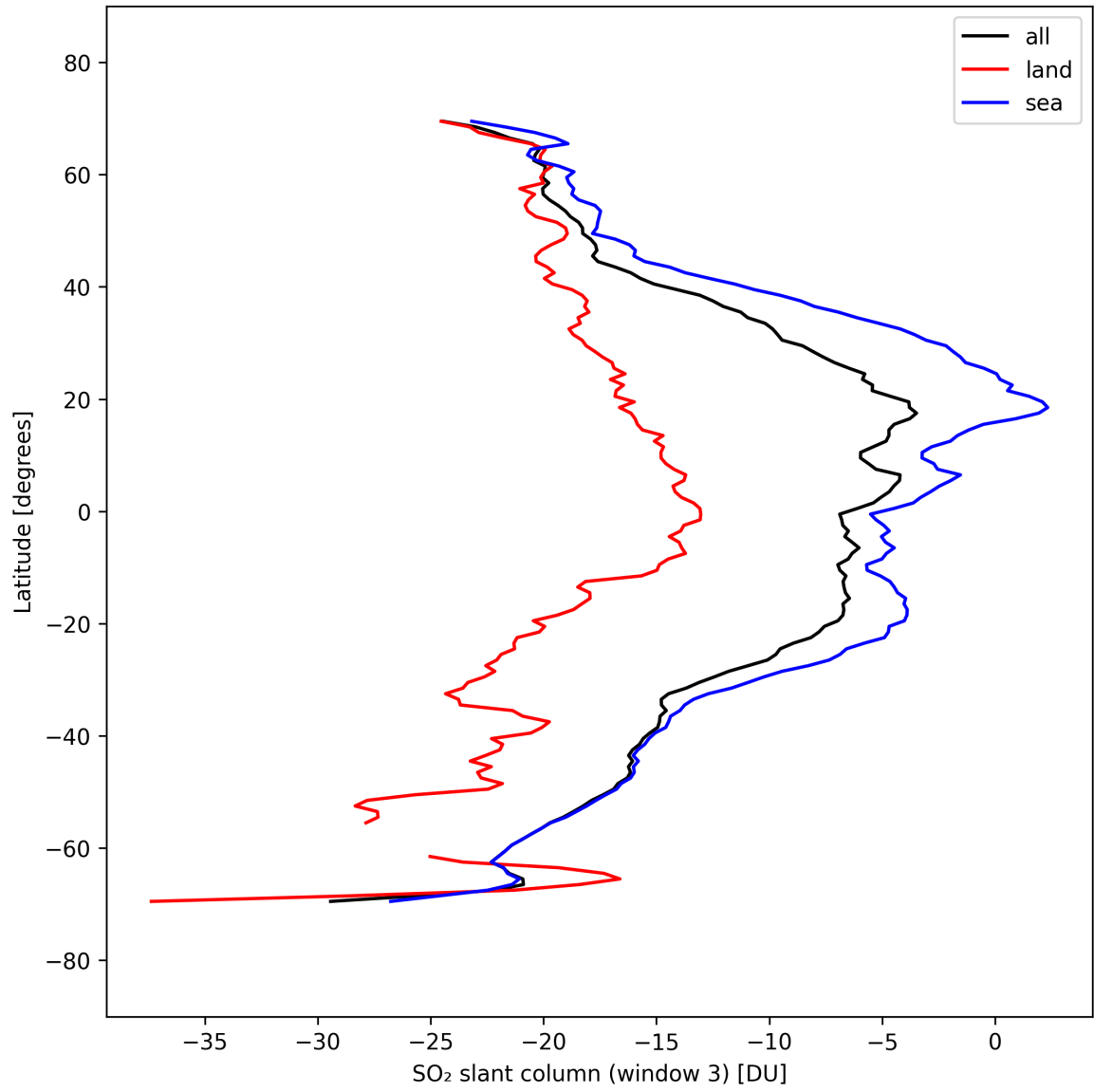
Figure 45: Zonal average of “SO 2 slant column (window 3)” for 2025-09-22 to 2025-09-24.
