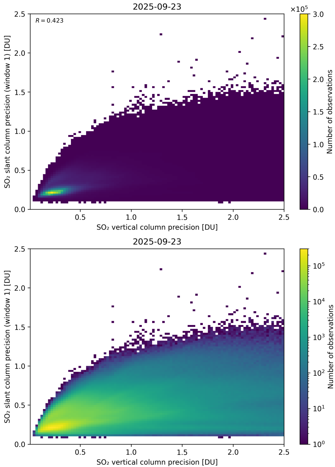
Figure 342: Scatter density plot of “SO 2 vertical column precision” against “SO 2 slant column precision (window 1)” for 2025-09-22 to 2025-09-24.
