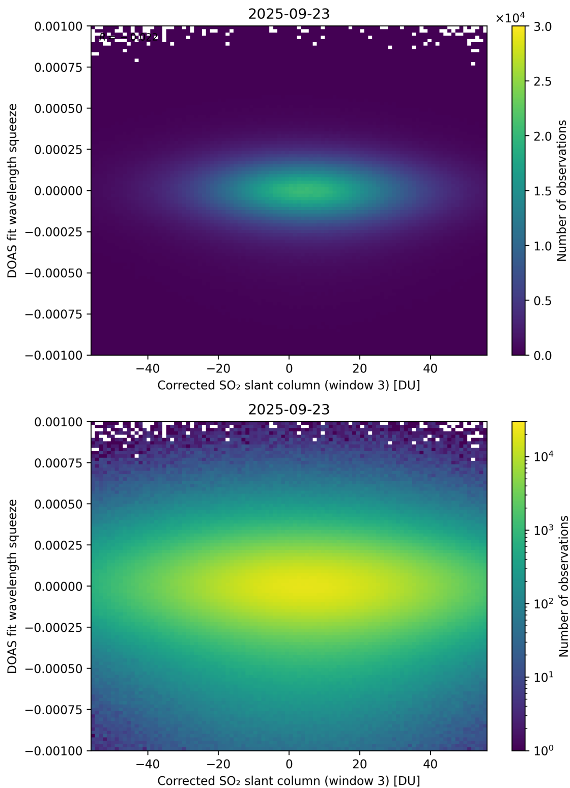
Figure 257: Scatter density plot of “Corrected SO 2 slant column (window 3)” against “DOAS fit wavelength squeeze” for 2025-09-22 to 2025-09-24.
