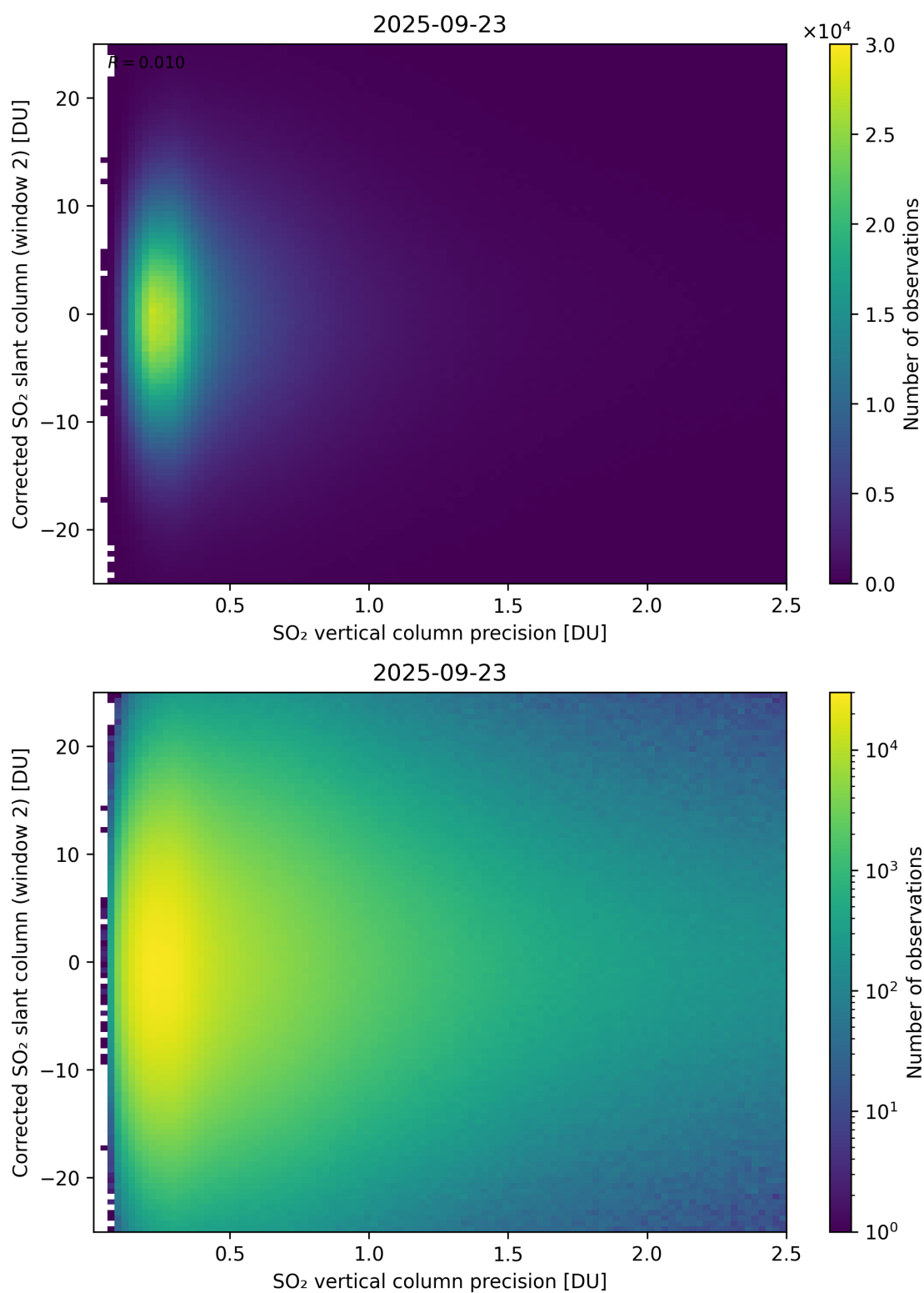
Figure 339: Scatter density plot of “SO 2 vertical column precision” against “Corrected SO 2 slant column (window 2)” for 2025-09-22 to 2025-09-24.
