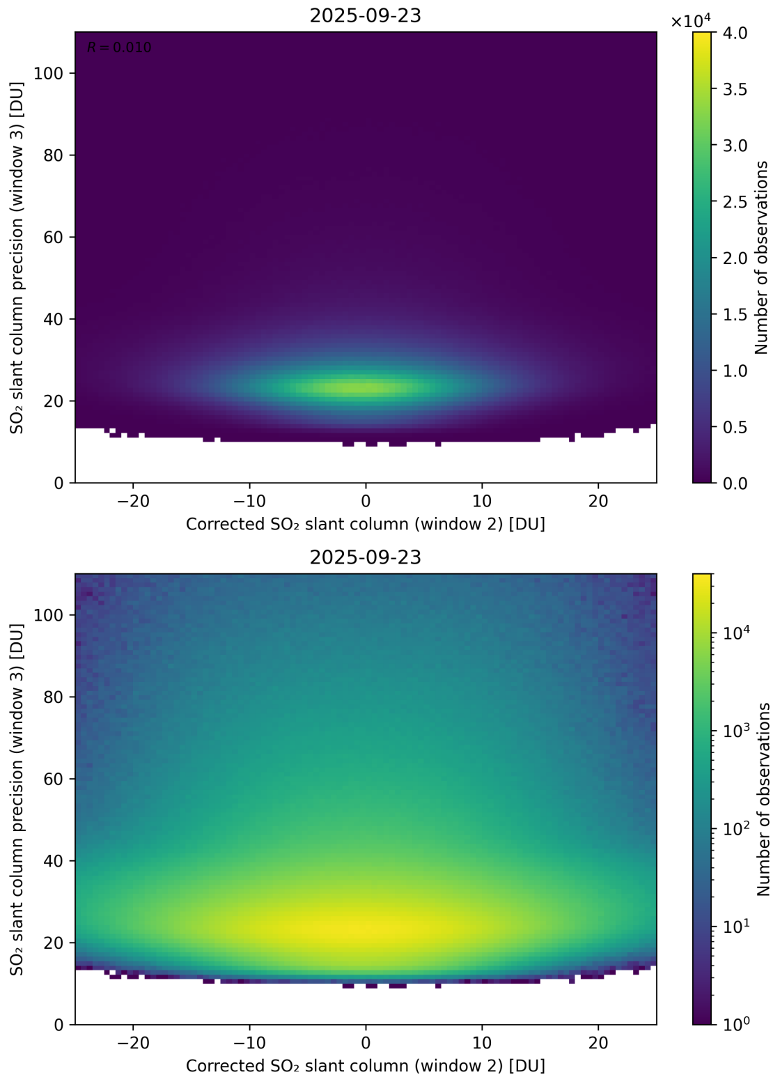
Figure 252: Scatter density plot of “Corrected SO 2 slant column (window 2)” against “SO 2 slant column precision (window 3)” for 2025-09-22 to 2025-09-24.
