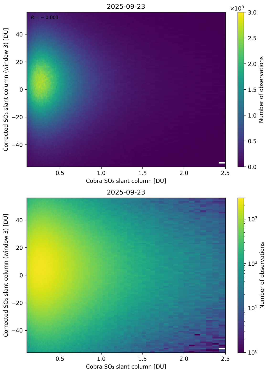
Figure 218: Scatter density plot of “Cobra SO 2 slant column” against “Corrected SO 2 slant column (window 3)” for 2025-09-22 to 2025-09-24.
