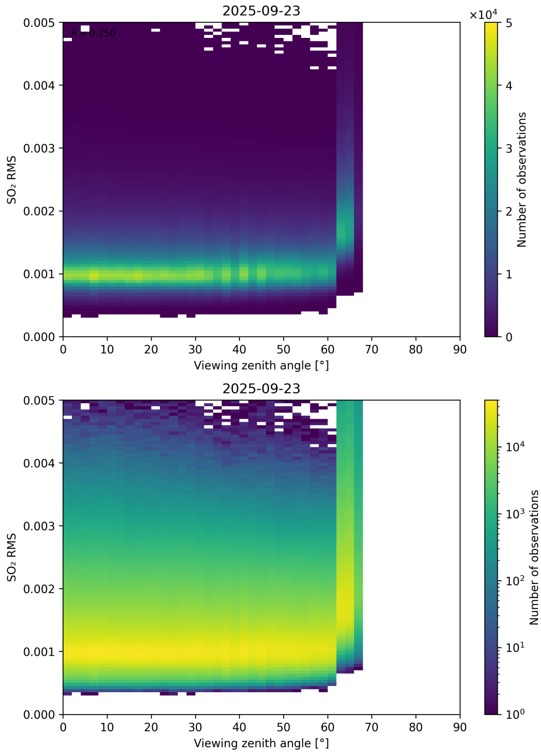
Figure 367: Scatter density plot of “Viewing zenith angle” against “SO 2 RMS” for 2025-09-22 to 2025-09-24.
