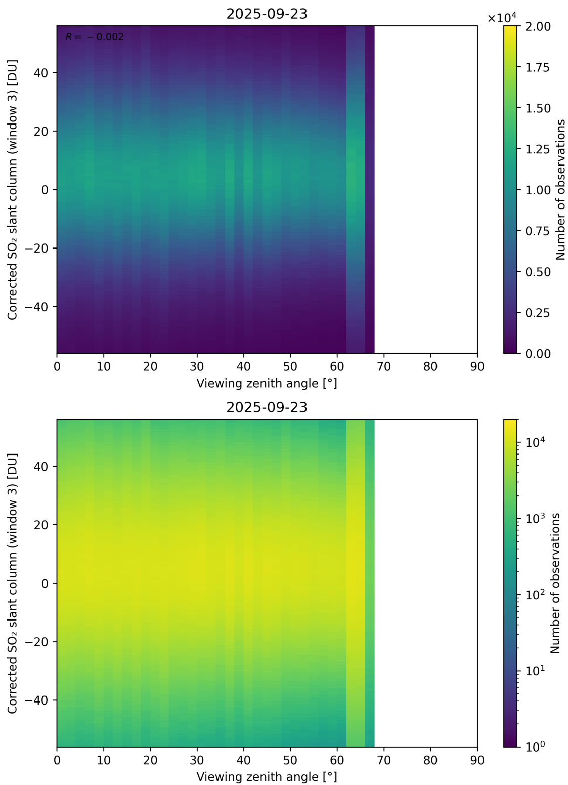
Figure 375: Scatter density plot of “Viewing zenith angle” against “Corrected SO 2 slant column (window 3)” for 2025-09-22 to 2025-09-24.
