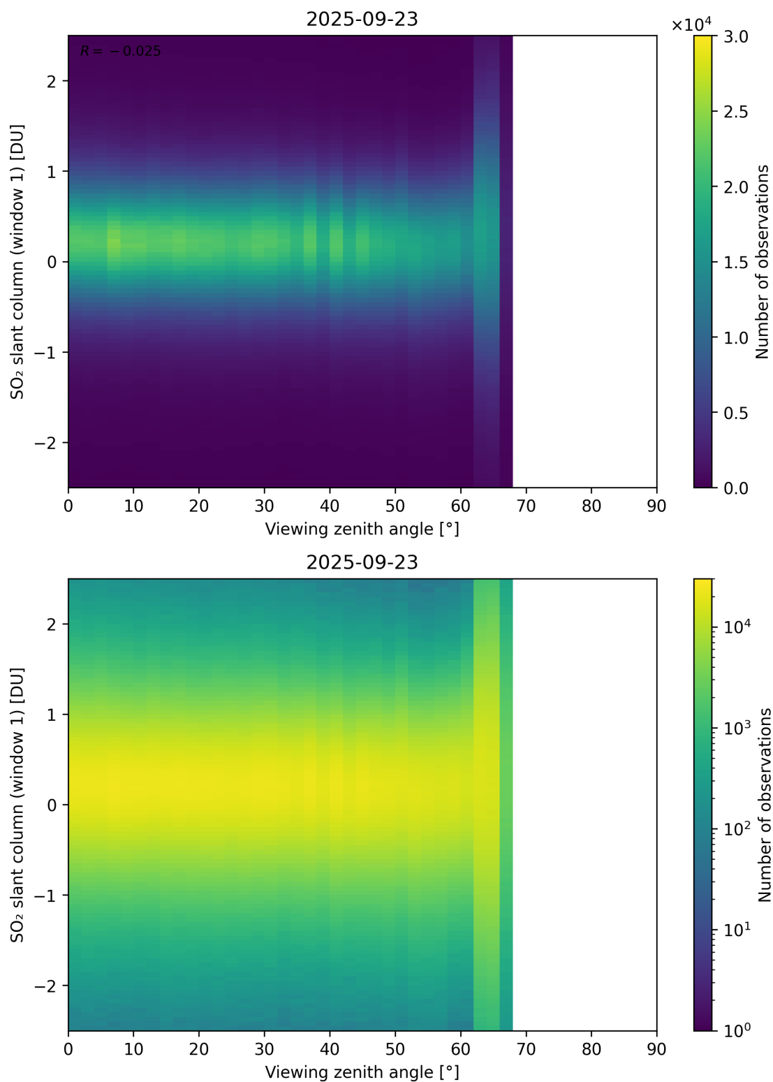
Figure 376: Scatter density plot of “Viewing zenith angle” against “SO 2 slant column (window 1)” for 2025-09-22 to 2025-09-24.
