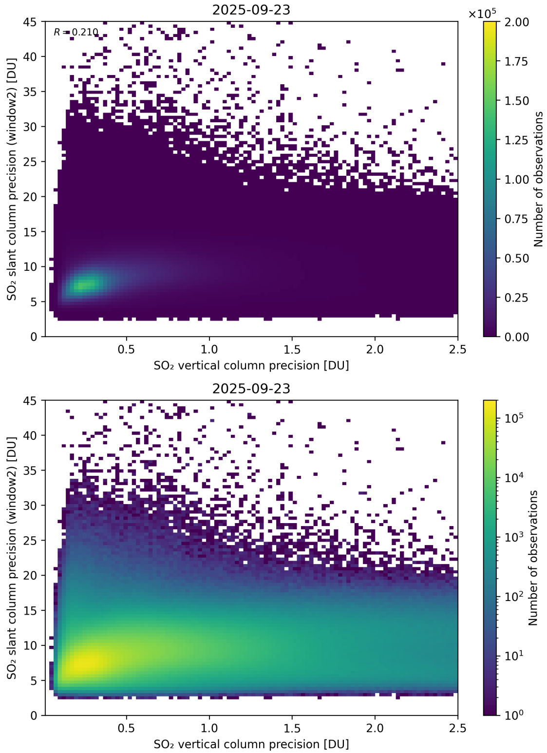
Figure 343: Scatter density plot of “SO 2 vertical column precision” against “SO 2 slant column precision (window2)” for 2025-09-22 to 2025-09-24.
