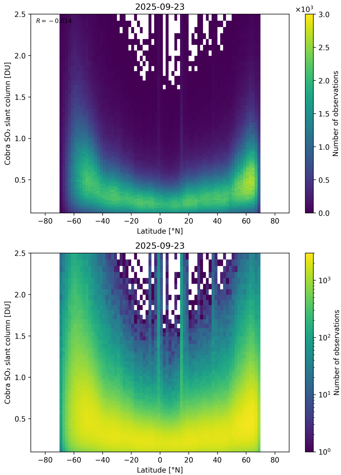
Figure 157: Scatter density plot of “Latitude” against “Cobra SO 2 slant column” for 2025-09-22 to 2025-09-24.
