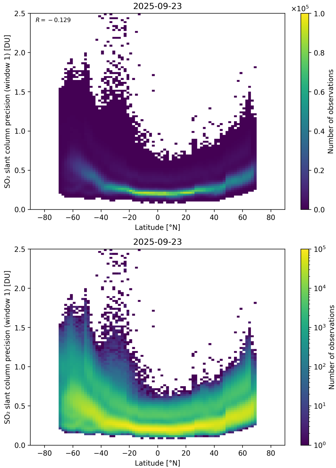
Figure 163: Scatter density plot of “Latitude” against “SO 2 slant column precision (window 1)” for 2025-09-22 to 2025-09-24.
