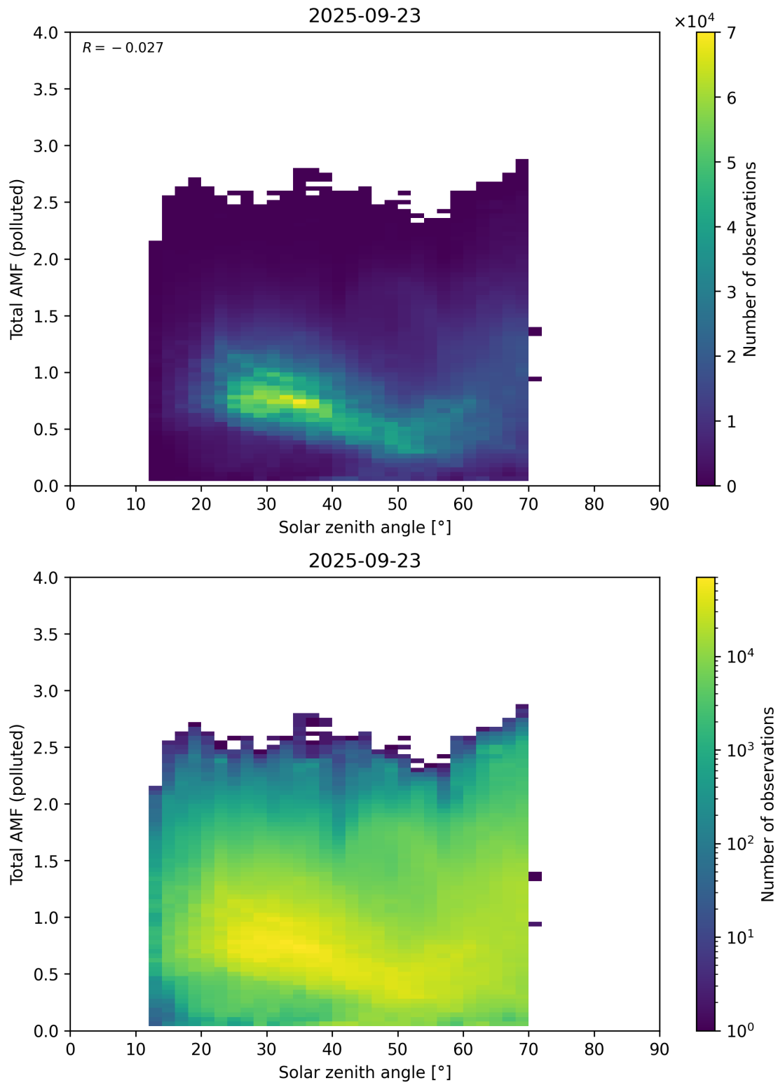
Figure 189: Scatter density plot of “Solar zenith angle” against “Total AMF (polluted)” for 2025-09-22 to 2025-09-24.
