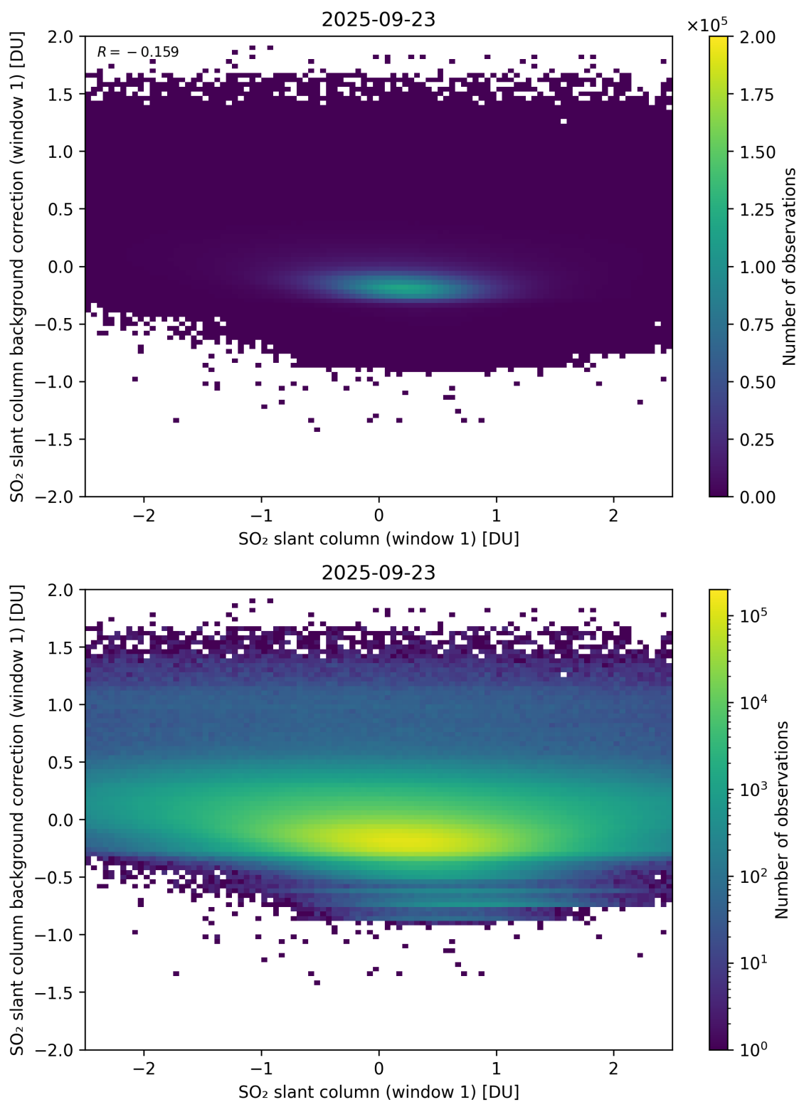
Figure 262: Scatter density plot of “SO 2 slant column (window 1)” against “SO 2 slant column background correction (window 1)” for 2025-09-22 to 2025-09-24.
