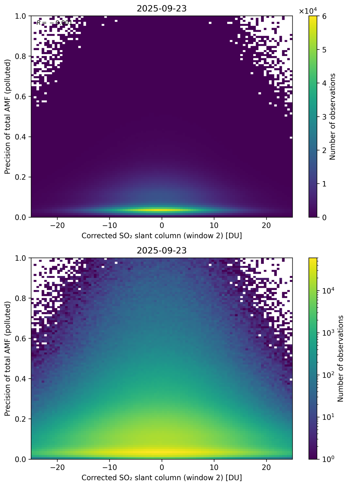
Figure 254: Scatter density plot of “Corrected SO 2 slant column (window 2)” against “Precision of total AMF (polluted)” for 2025-09-22 to 2025-09-24.
