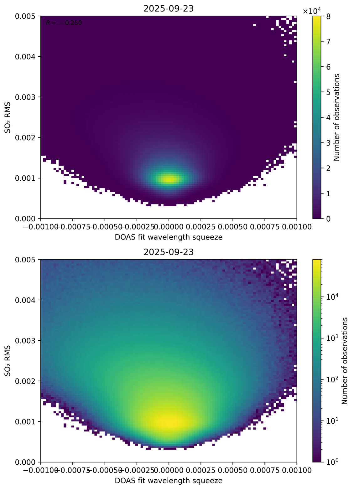
Figure 143: Scatter density plot of “DOAS fit wavelength squeeze” against “SO 2 RMS” for 2025-09-22 to 2025-09-24.
