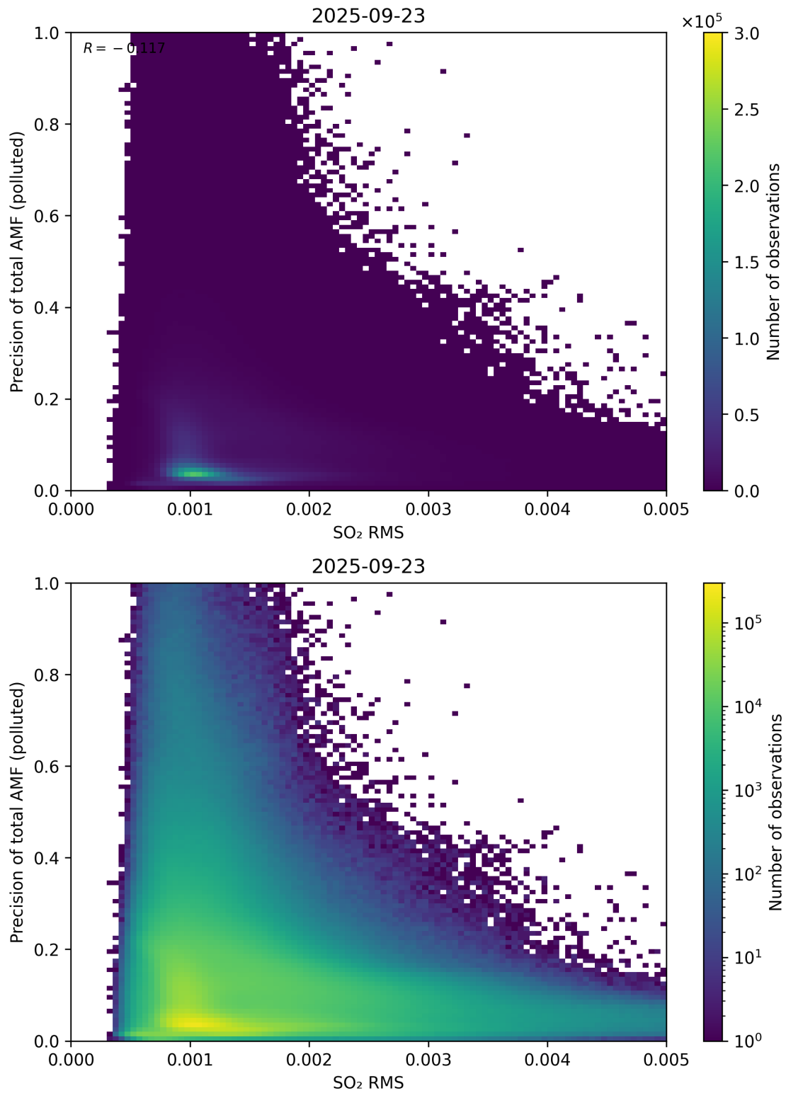
Figure 149: Scatter density plot of “SO 2 RMS” against “Precision of total AMF (polluted)” for 2025-09-22 to 2025-09-24.
