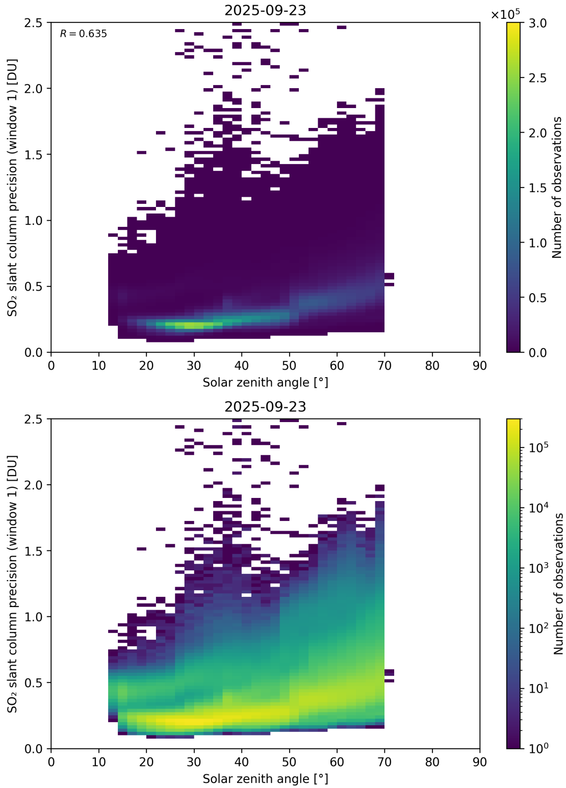
Figure 185: Scatter density plot of “Solar zenith angle” against “SO 2 slant column precision (window 1)” for 2025-09-22 to 2025-09-24.
