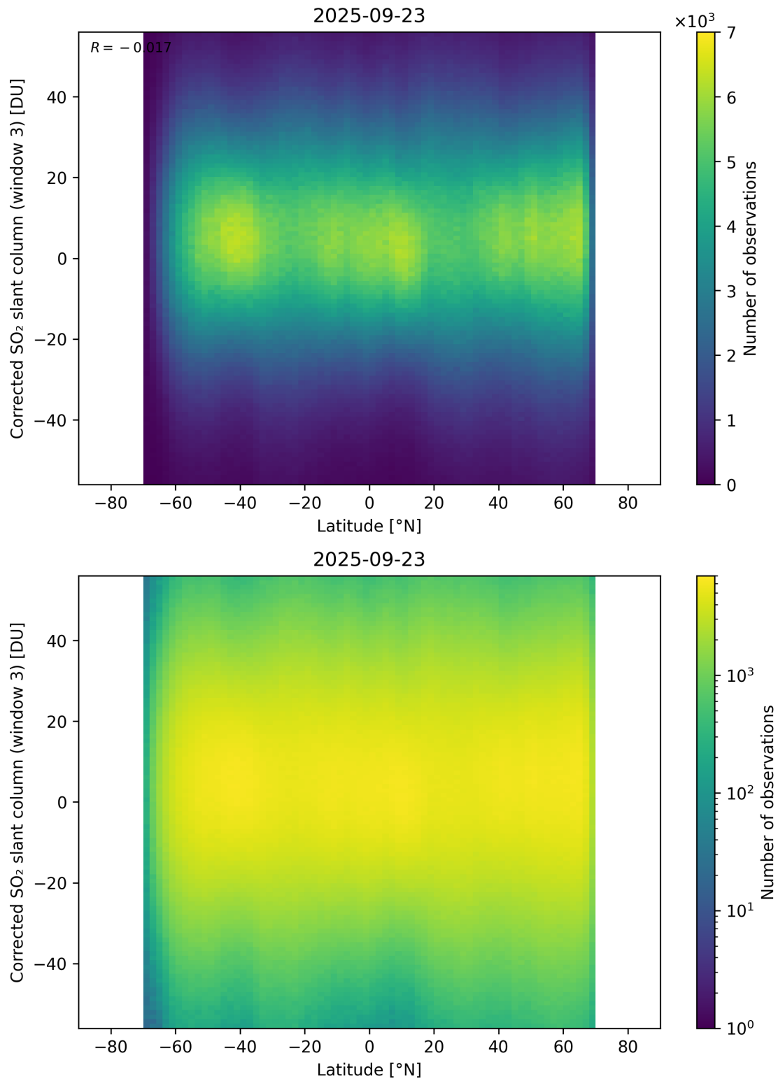
Figure 161: Scatter density plot of “Latitude” against “Corrected SO 2 slant column (window 3)” for 2025-09-22 to 2025-09-24.
