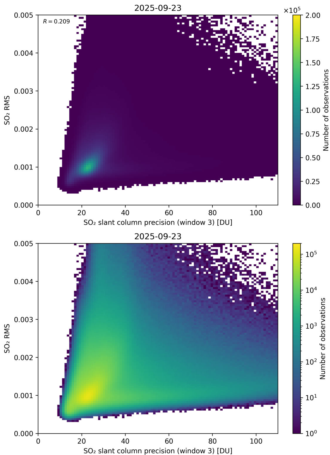
Figure 310: Scatter density plot of “SO 2 slant column precision (window 3)” against “SO 2 RMS” for 2025-09-22 to 2025-09-24.
