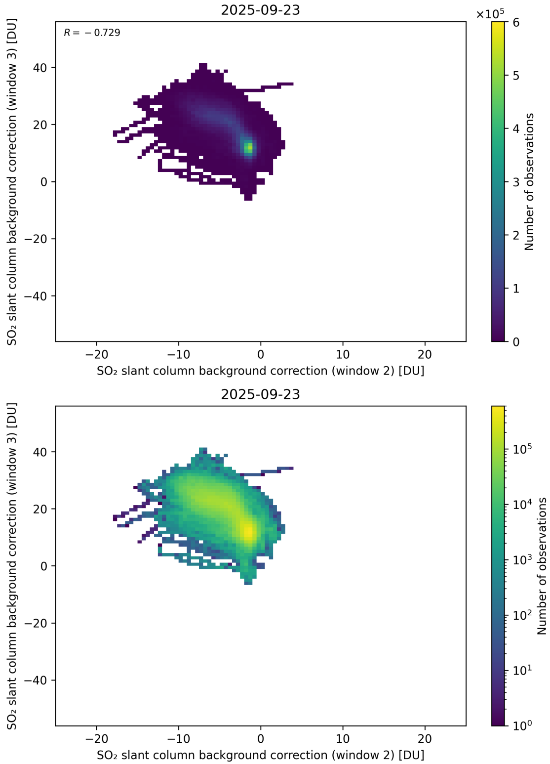
Figure 122: Scatter density plot of “SO 2 slant column background correction (window 2)” against “SO 2 slant column background correction (window 3)” for 2025-09-22 to 2025-09-24.
