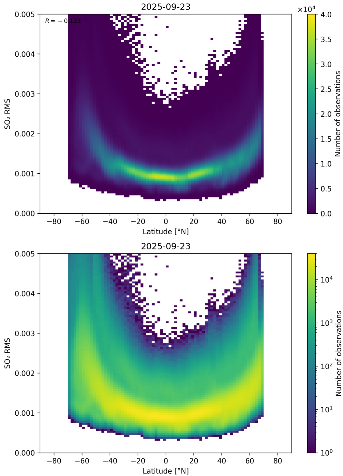
Figure 155: Scatter density plot of “Latitude” against “SO 2 RMS” for 2025-09-22 to 2025-09-24.
