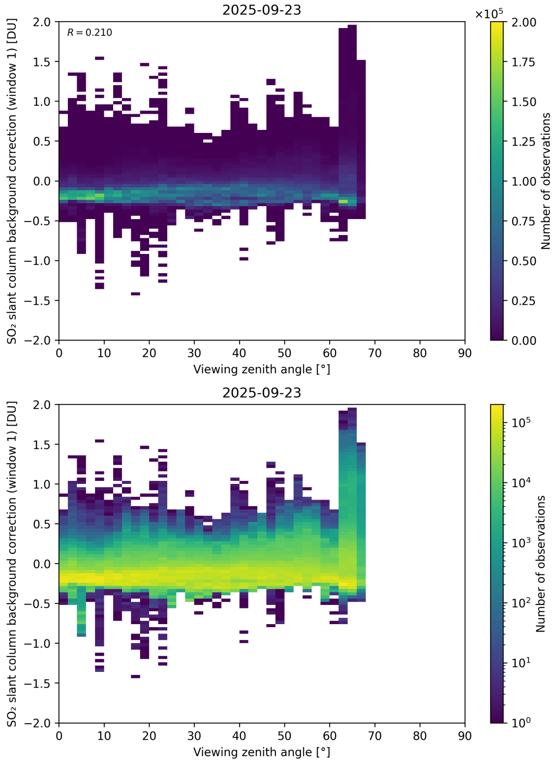
Figure 362: Scatter density plot of “Viewing zenith angle” against “SO 2 slant column background correction (window 1)” for 2025-09-22 to 2025-09-24.
