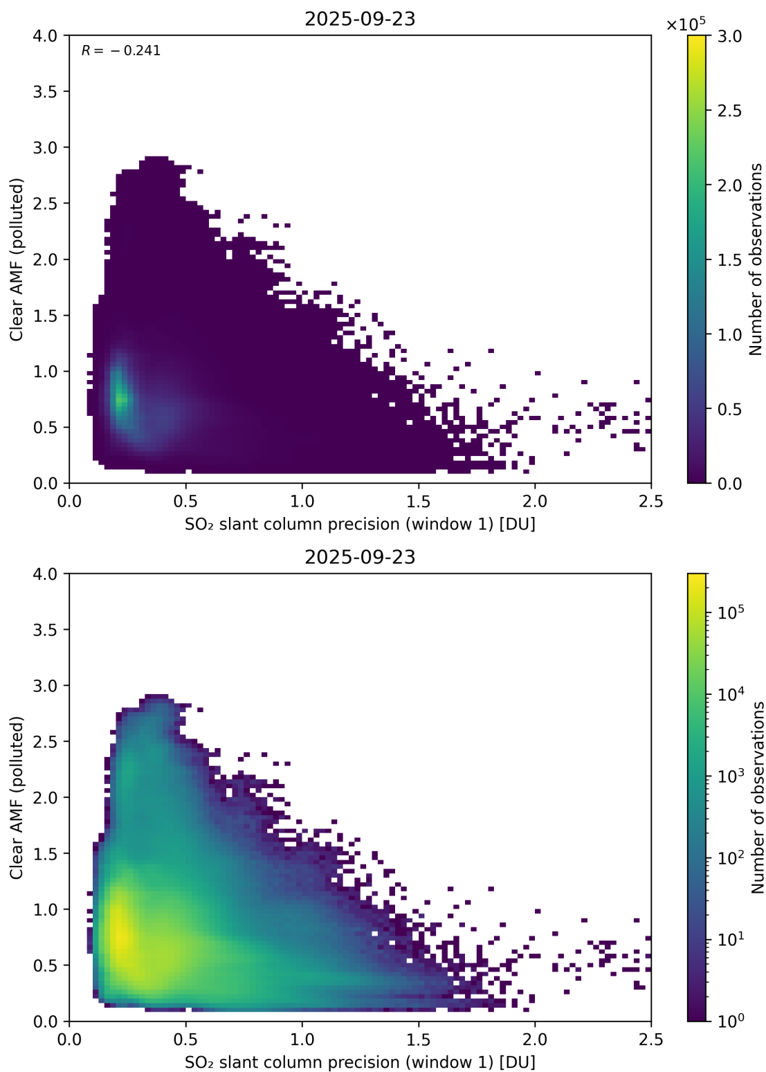
Figure 274: Scatter density plot of “SO 2 slant column precision (window 1)” against “Clear AMF (polluted)” for 2025-09-22 to 2025-09-24.
