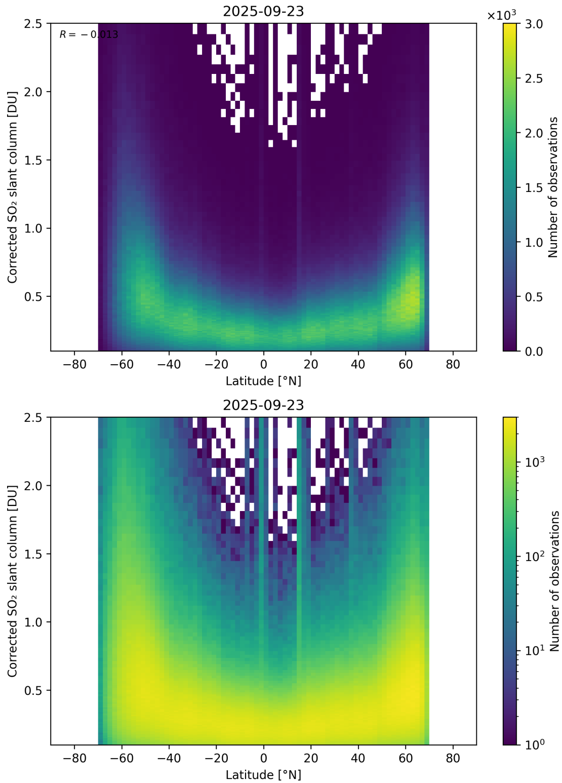
Figure 159: Scatter density plot of “Latitude” against “Corrected SO 2 slant column” for 2025-09-22 to 2025-09-24.
