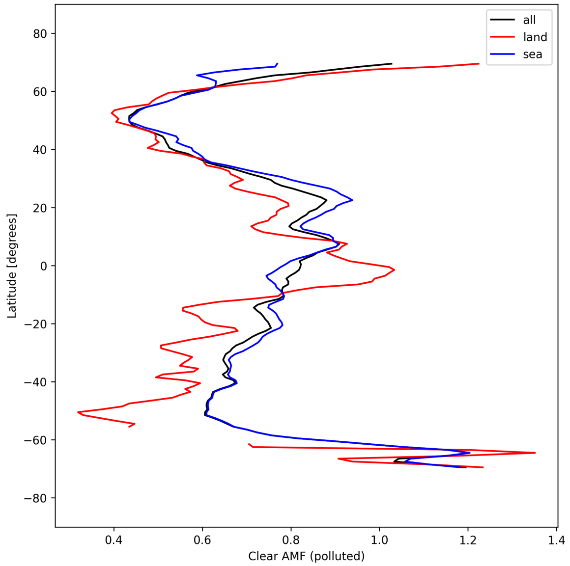
Figure 55: Zonal average of “Clear AMF (polluted)” for 2025-09-22 to 2025-09-24.
