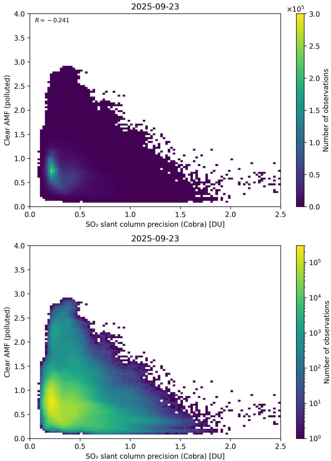
Figure 205: Scatter density plot of “SO 2 slant column precision (Cobra)” against “Clear AMF (polluted)” for 2025-09-22 to 2025-09-24.
