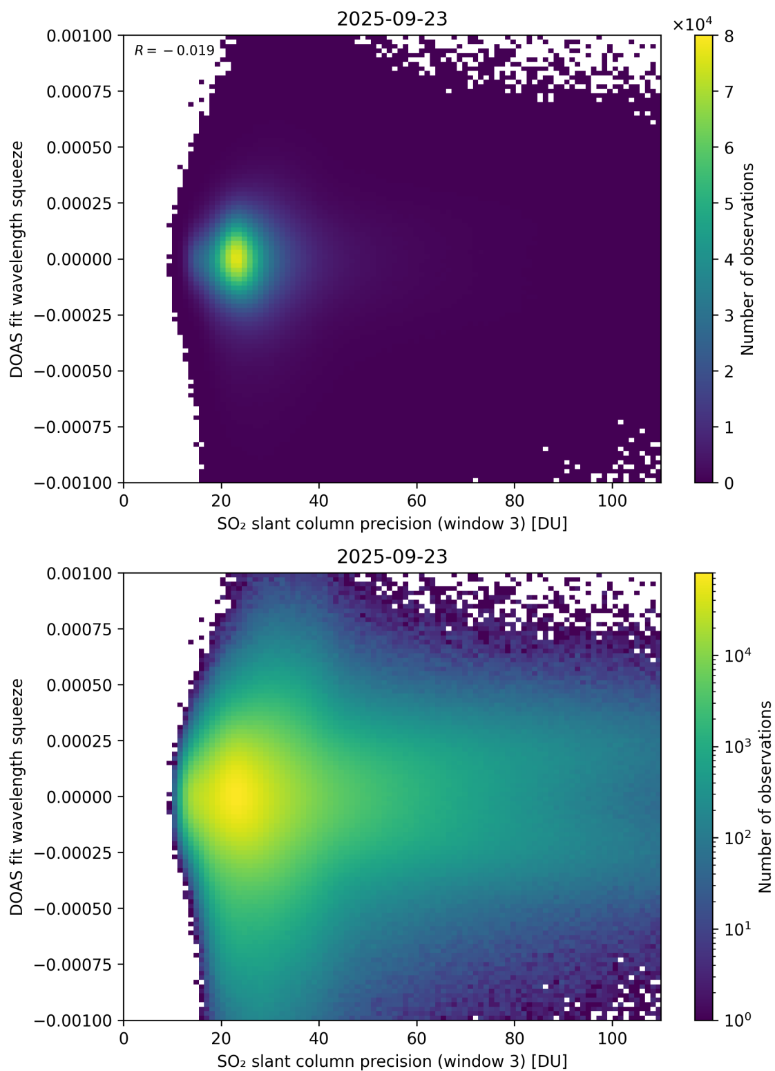
Figure 309: Scatter density plot of “SO 2 slant column precision (window 3)” against “DOAS fit wavelength squeeze” for 2025-09-22 to 2025-09-24.
