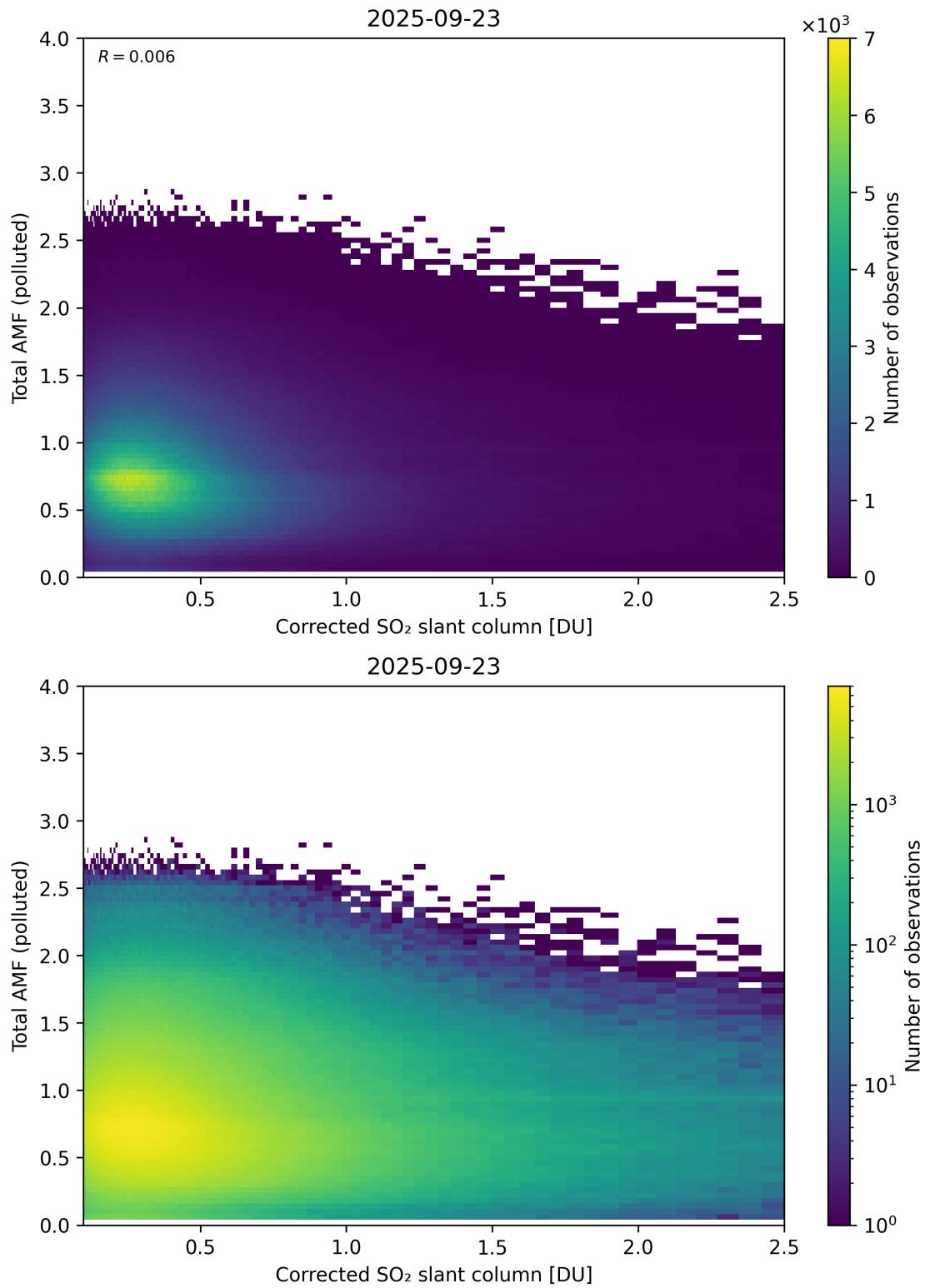
Figure 242: Scatter density plot of “Corrected SO 2 slant column” against “Total AMF (polluted)” for 2025-09-22 to 2025-09-24.
