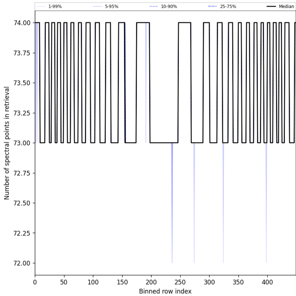
Figure 108: Along track statistics of “Number of spectral points in retrieval” for 2025-09-22 to 2025-09-24
