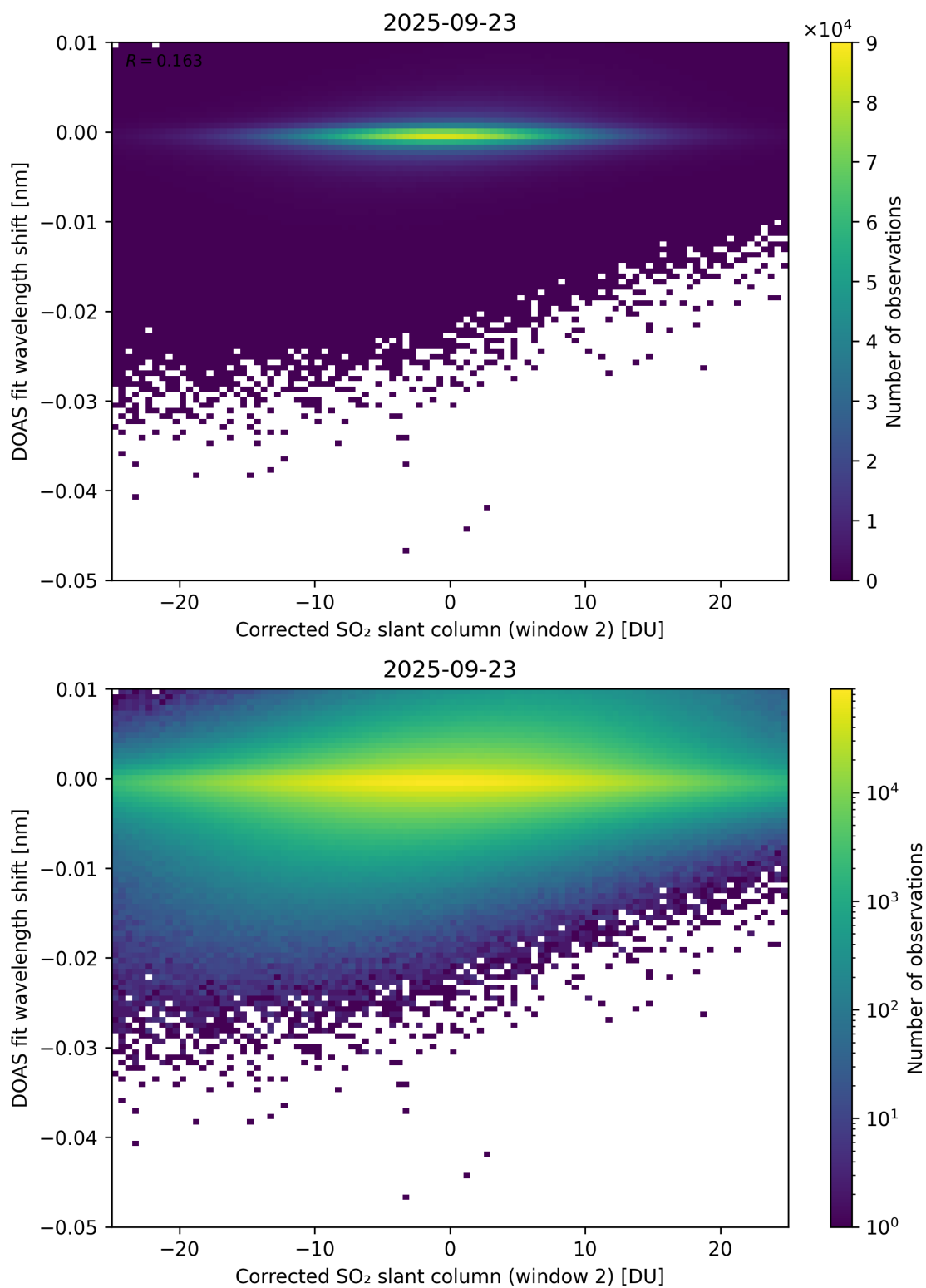
Figure 246: Scatter density plot of “Corrected SO 2 slant column (window 2)” against “DOAS fit wavelength shift” for 2025-09-22 to 2025-09-24.
