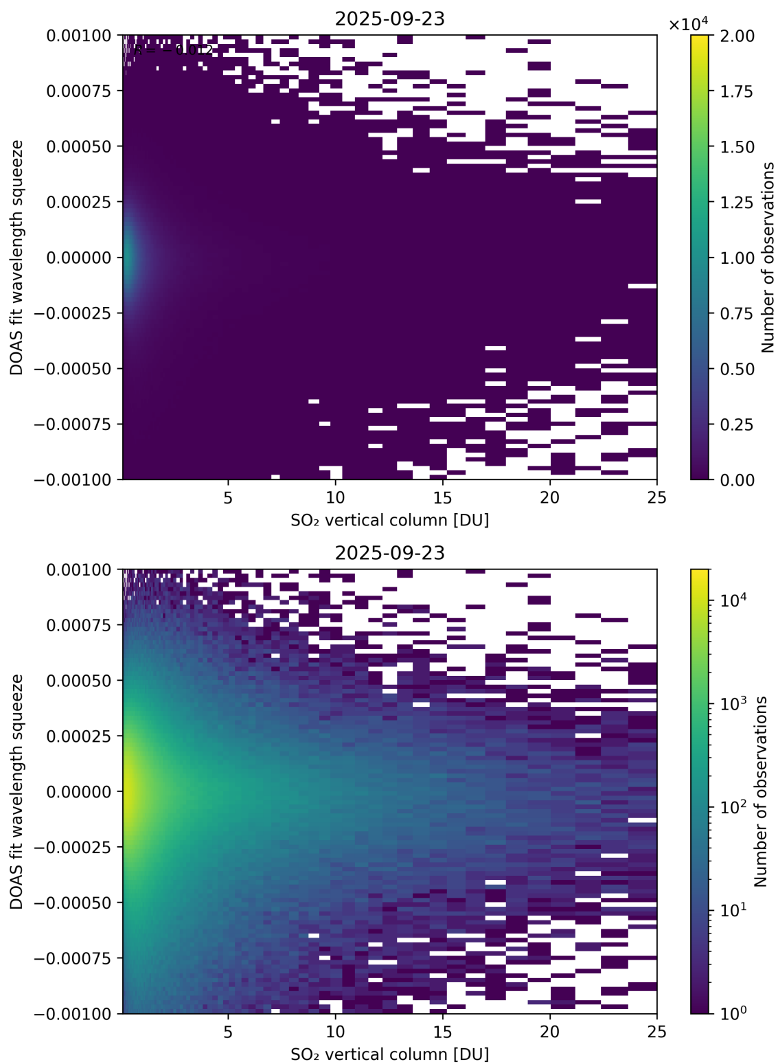
Figure 327: Scatter density plot of “SO 2 vertical column” against “DOAS fit wavelength squeeze” for 2025-09-22 to 2025-09-24.
