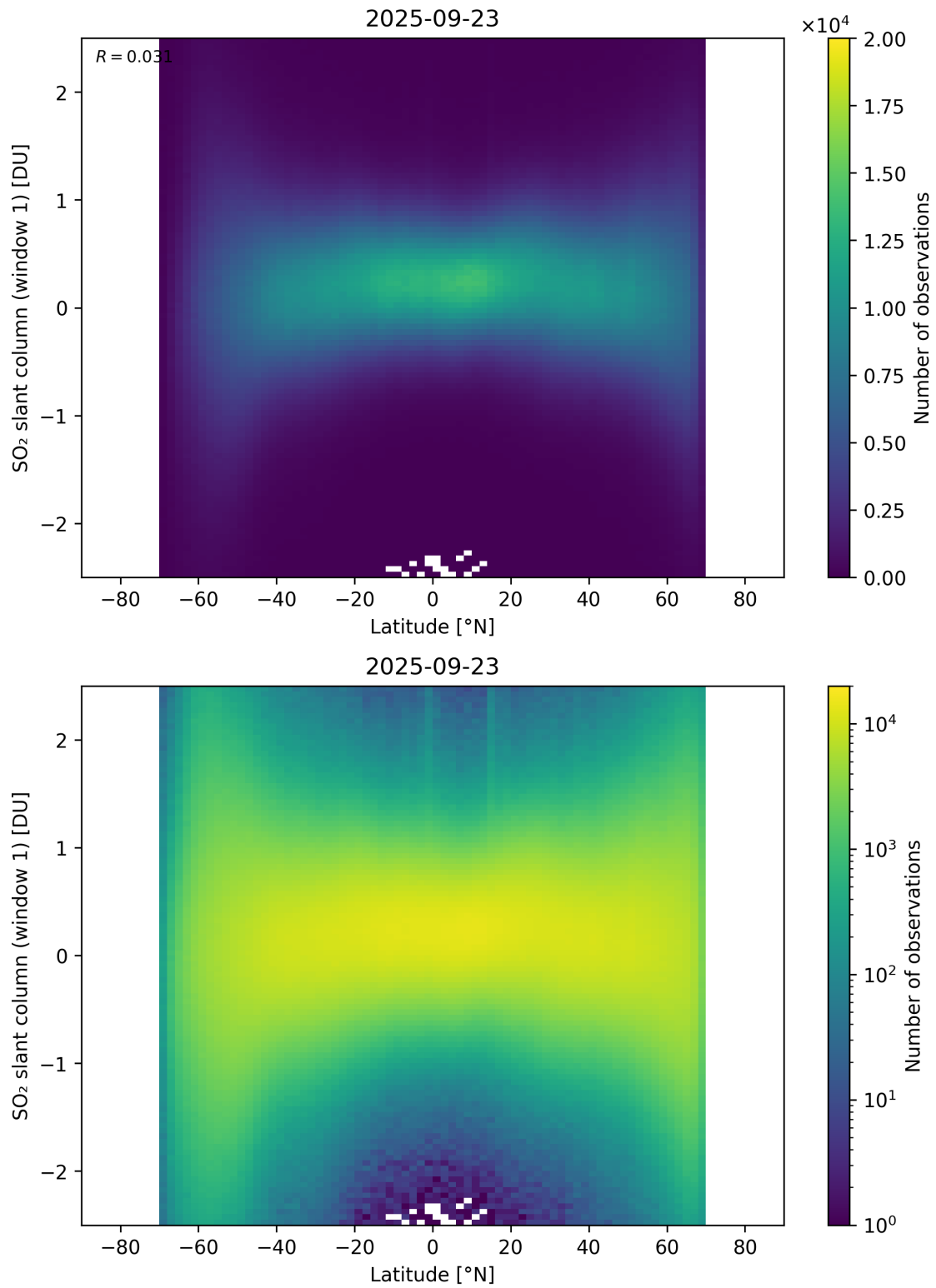
Figure 162: Scatter density plot of “Latitude” against “SO 2 slant column (window 1)” for 2025-09-22 to 2025-09-24.
