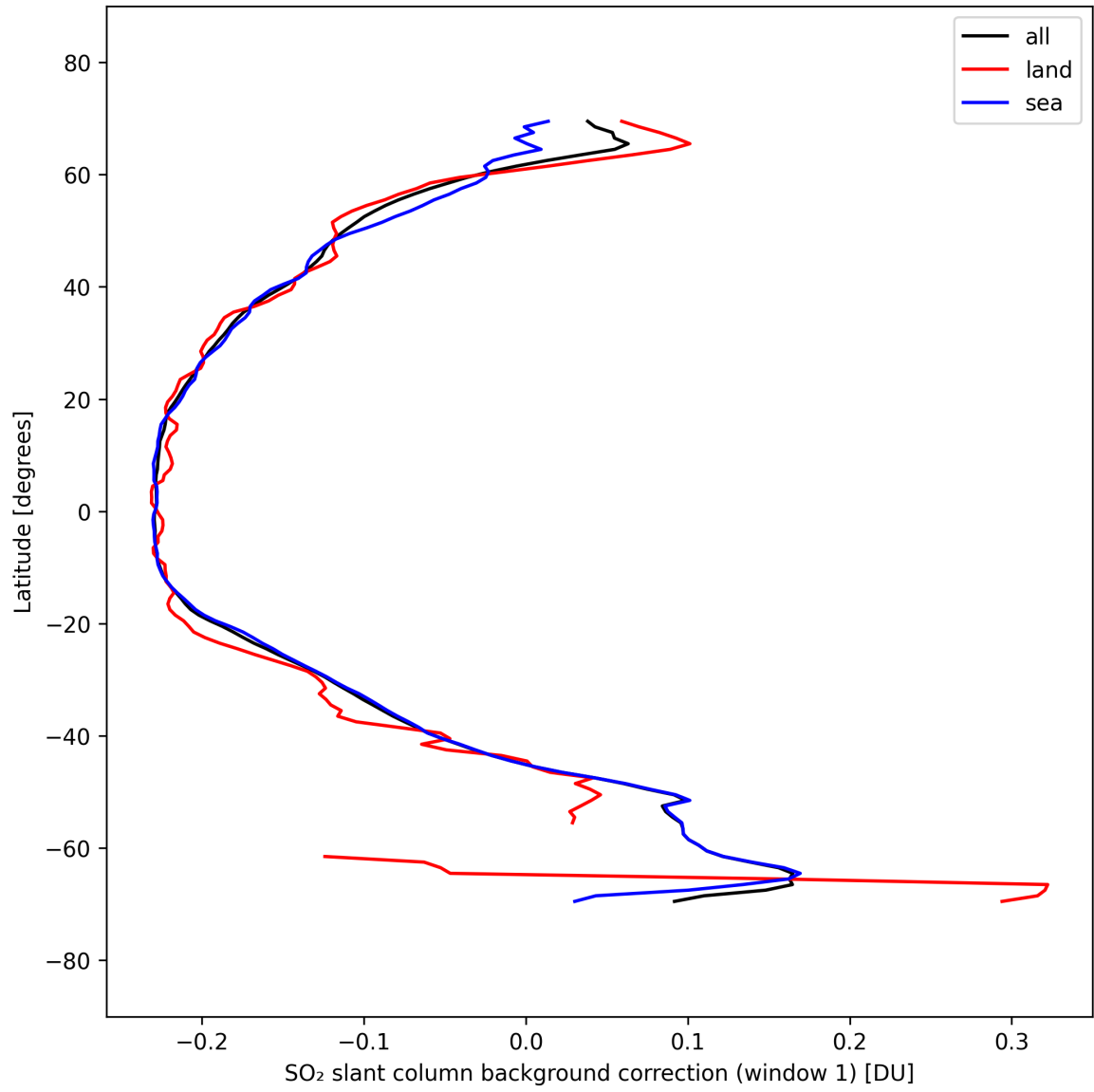
Figure 40: Zonal average of “SO 2 slant column background correction (window 1)” for 2025-09-22 to 2025-09-24.
