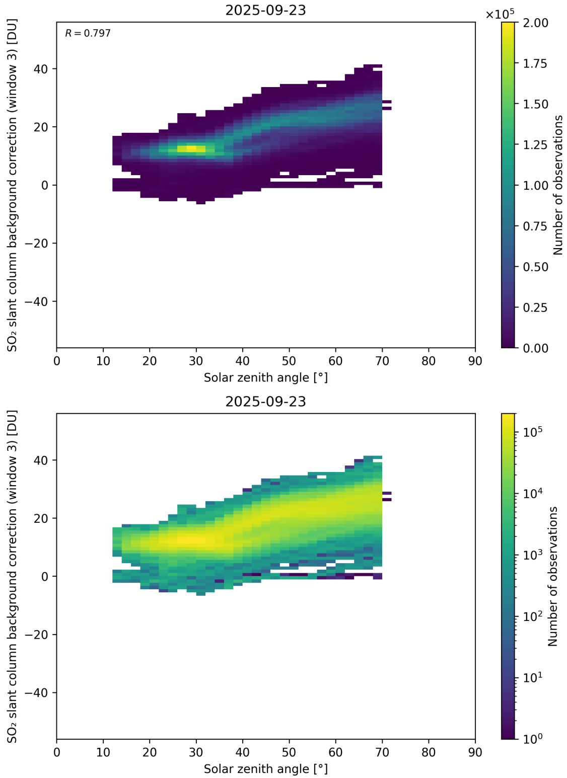
Figure 173: Scatter density plot of “Solar zenith angle” against “SO 2 slant column background correction (window 3)” for 2025-09-22 to 2025-09-24.
