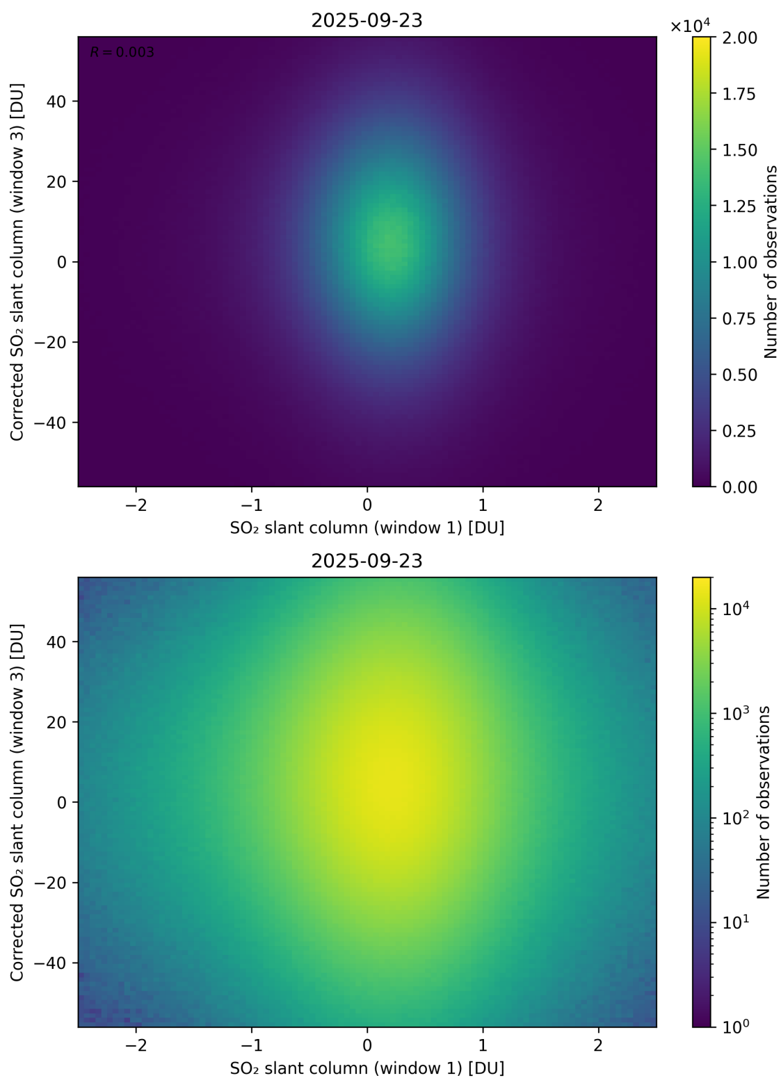
Figure 284: Scatter density plot of “SO 2 slant column (window 1)” against “Corrected SO 2 slant column (window 3)” for 2025-09-22 to 2025-09-24.
