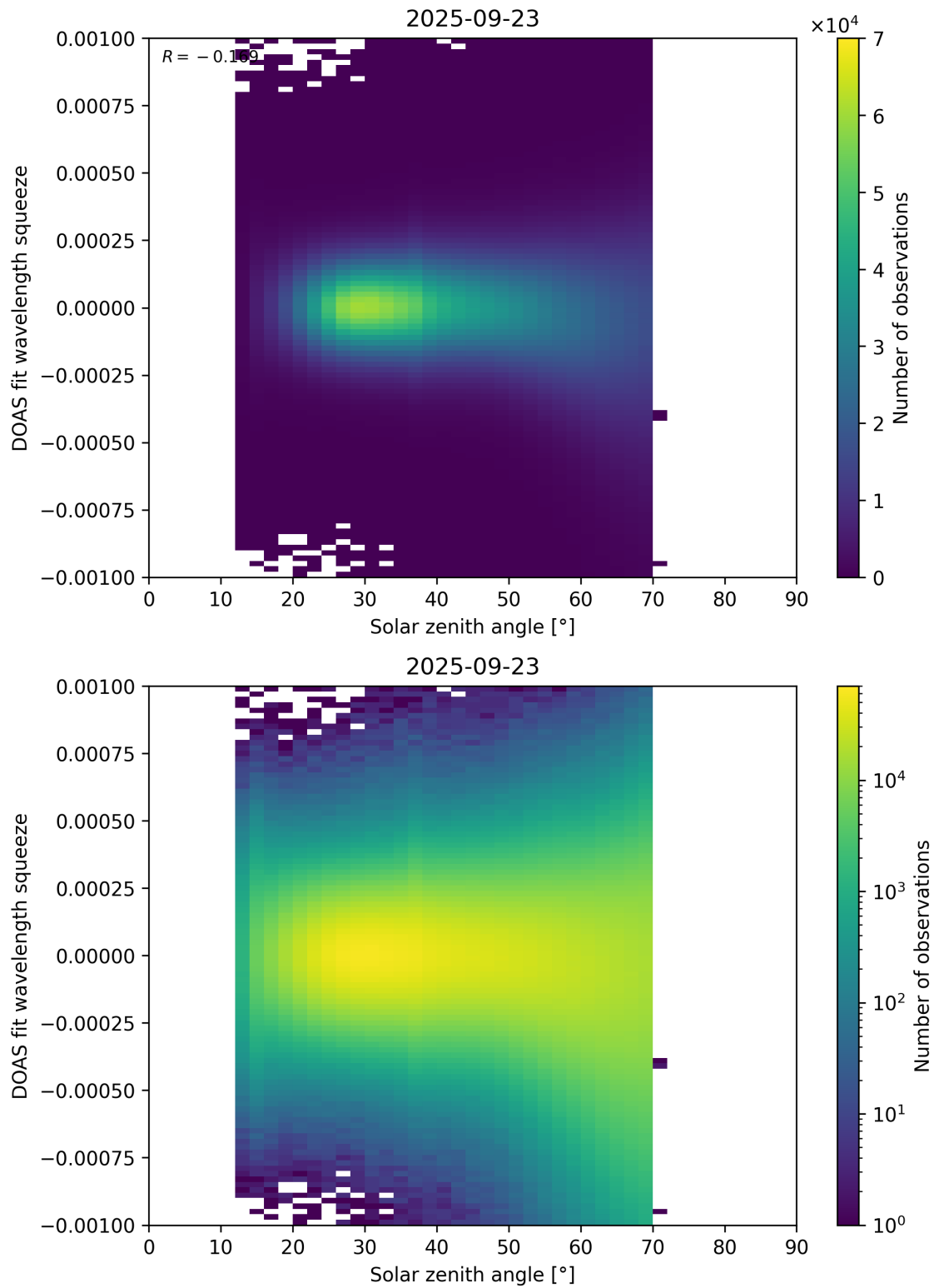
Figure 175: Scatter density plot of “Solar zenith angle” against “DOAS fit wavelength squeeze” for 2025-09-22 to 2025-09-24.
