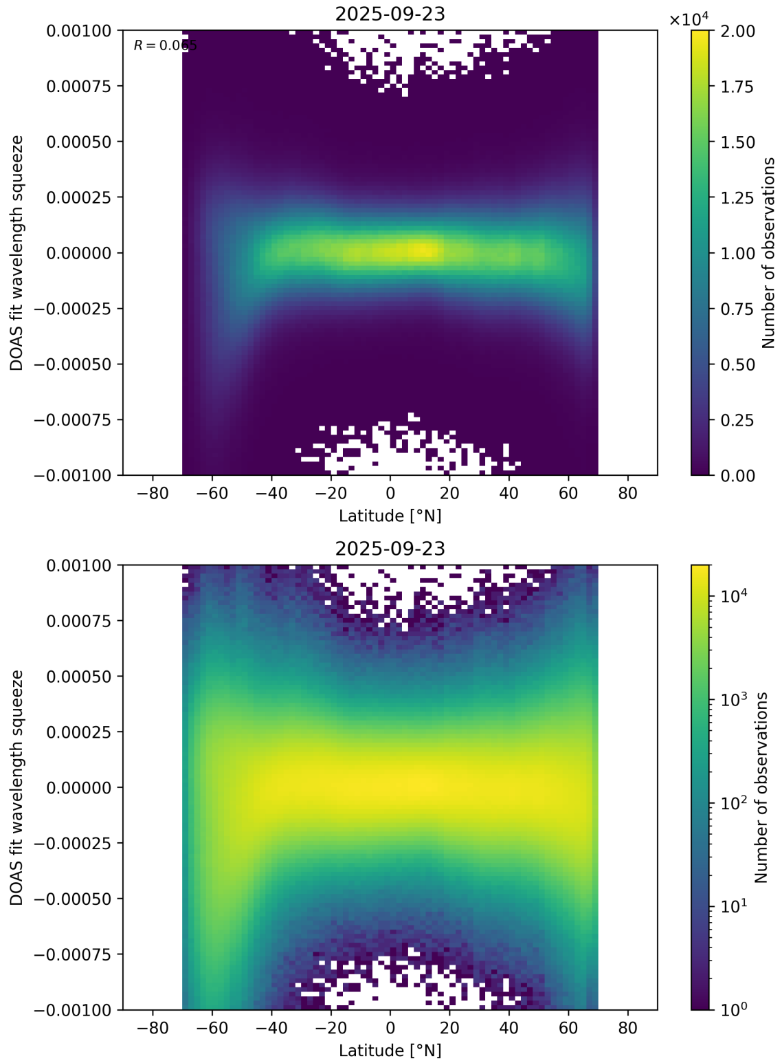
Figure 154: Scatter density plot of “Latitude” against “DOAS fit wavelength squeeze” for 2025-09-22 to 2025-09-24.
