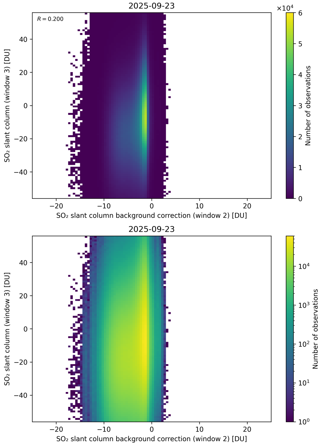
Figure 128: Scatter density plot of “SO 2 slant column background correction (window 2)” against “SO 2 slant column (window 3)” for 2025-09-22 to 2025-09-24.
