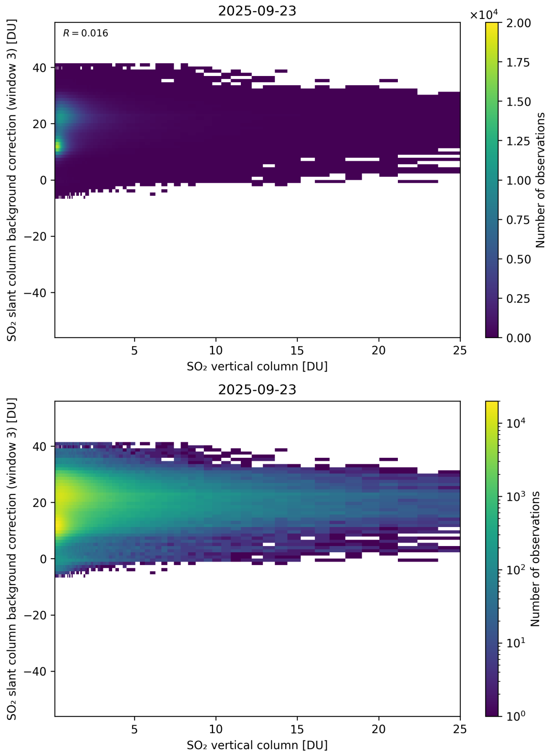
Figure 325: Scatter density plot of “SO 2 vertical column” against “SO 2 slant column background correction (window 3)” for 2025-09-22 to 2025-09-24.
