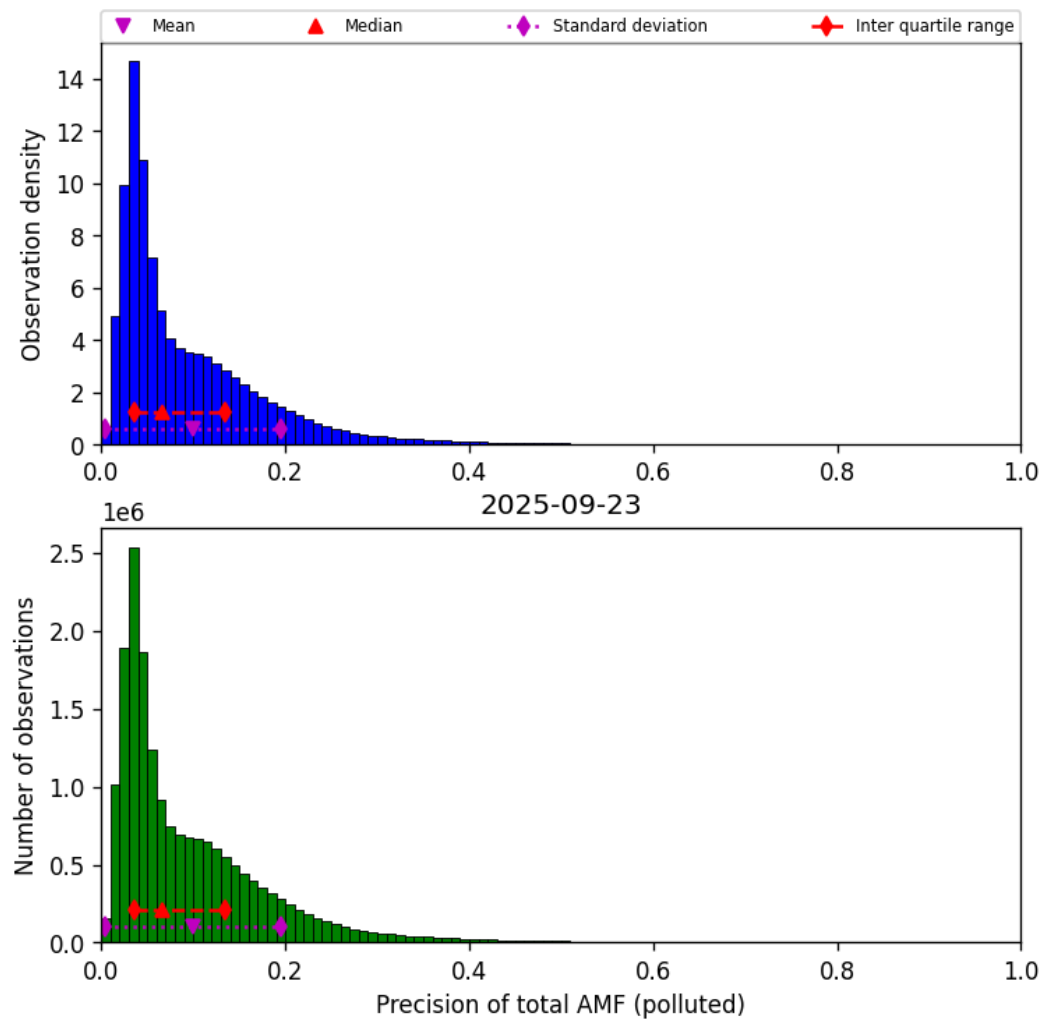
Figure 80: Histogram of “Precision of total AMF (polluted)” for 2025-09-22 to 2025-09-24
