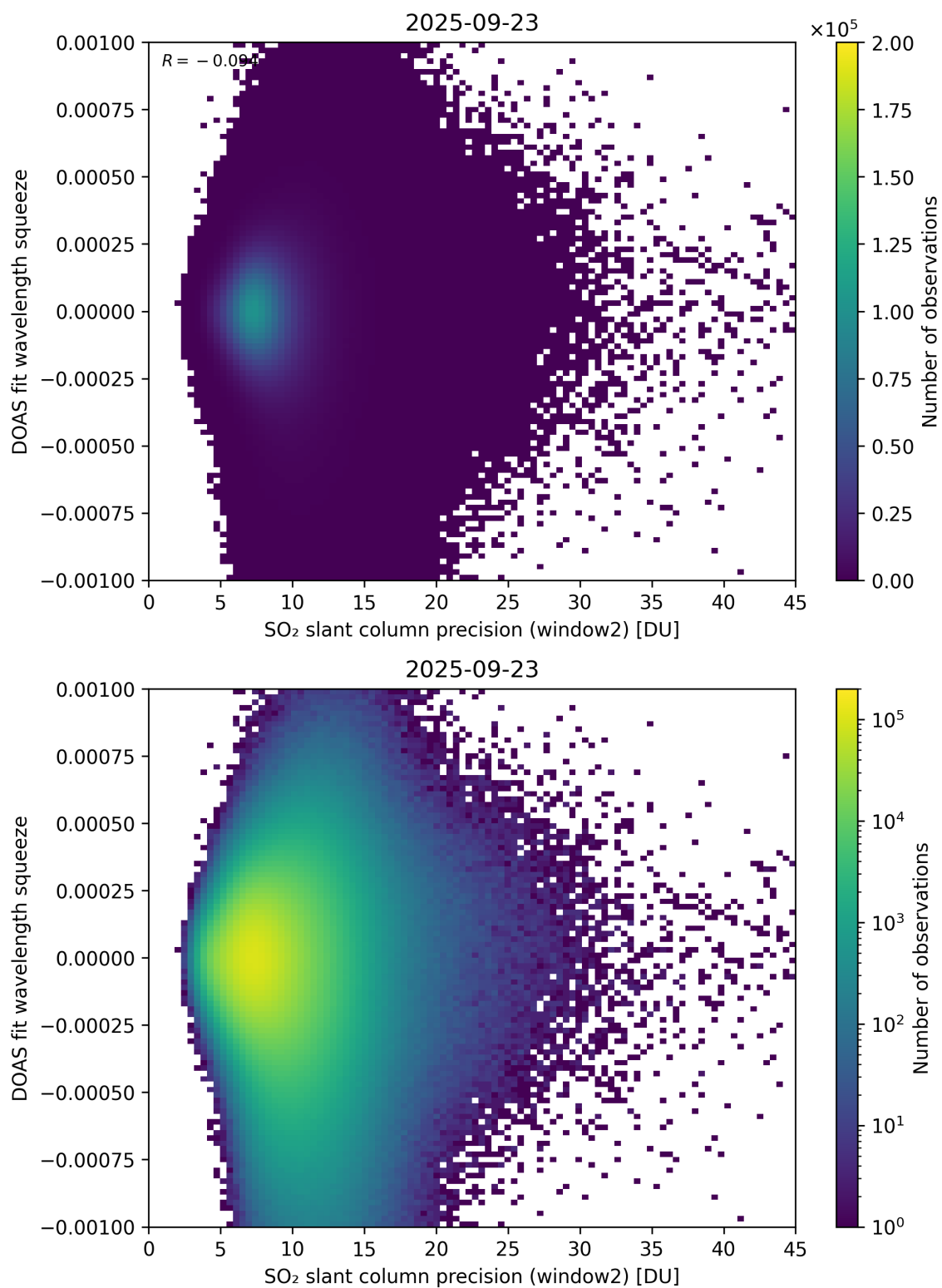
Figure 294: Scatter density plot of “SO 2 slant column precision (window2)” against “DOAS fit wavelength squeeze” for 2025-09-22 to 2025-09-24.
