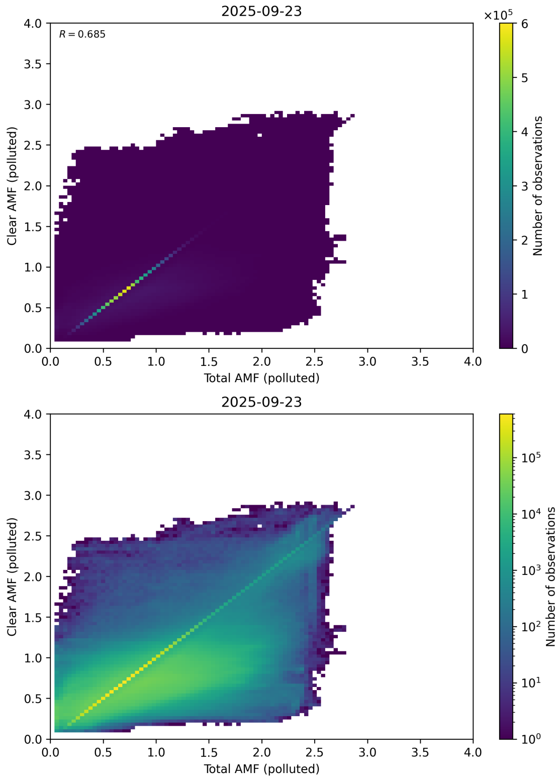
Figure 321: Scatter density plot of “Total AMF (polluted)” against “Clear AMF (polluted)” for 2025-09-22 to 2025-09-24.
