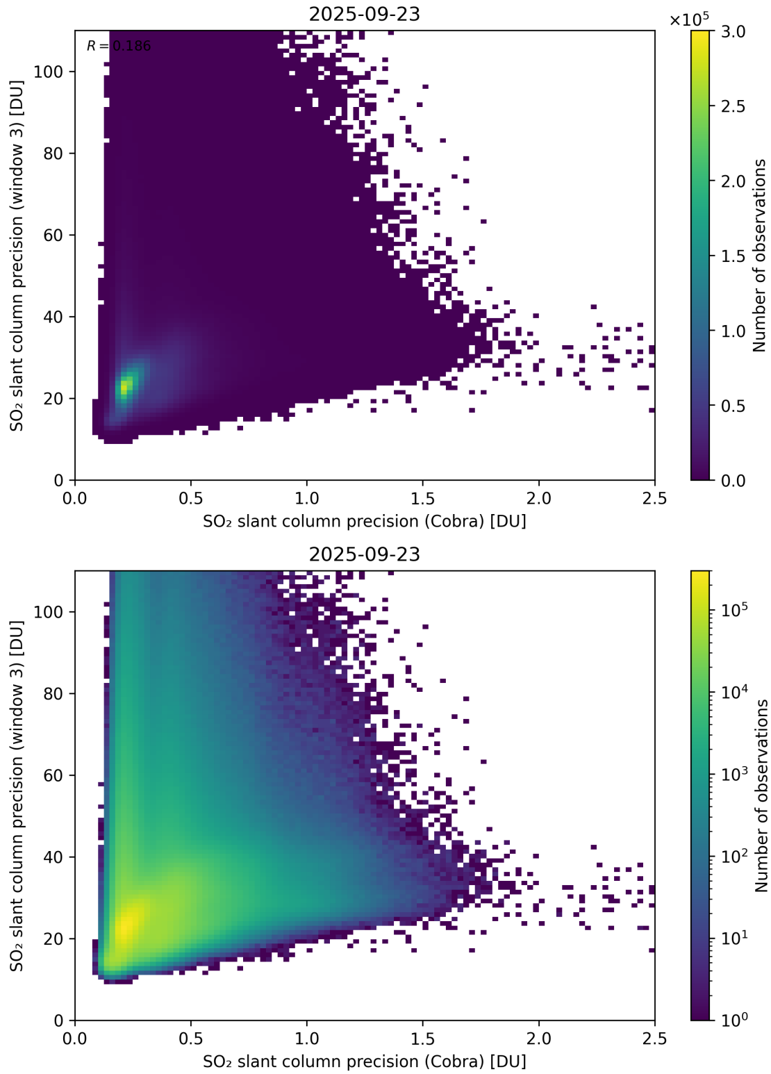
Figure 212: Scatter density plot of “SO 2 slant column precision (Cobra)” against “SO 2 slant column precision (window 3)” for 2025-09-22 to 2025-09-24.
