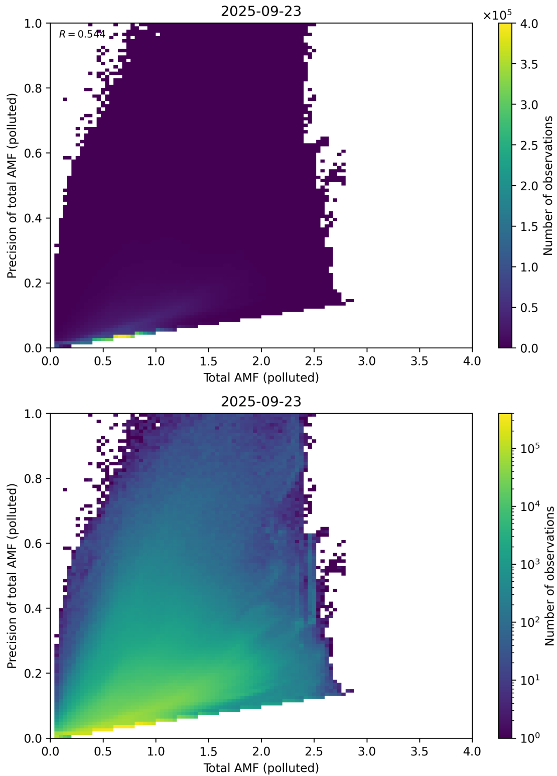
Figure 322: Scatter density plot of “Total AMF (polluted)” against “Precision of total AMF (polluted)” for 2025-09-22 to 2025-09-24.
