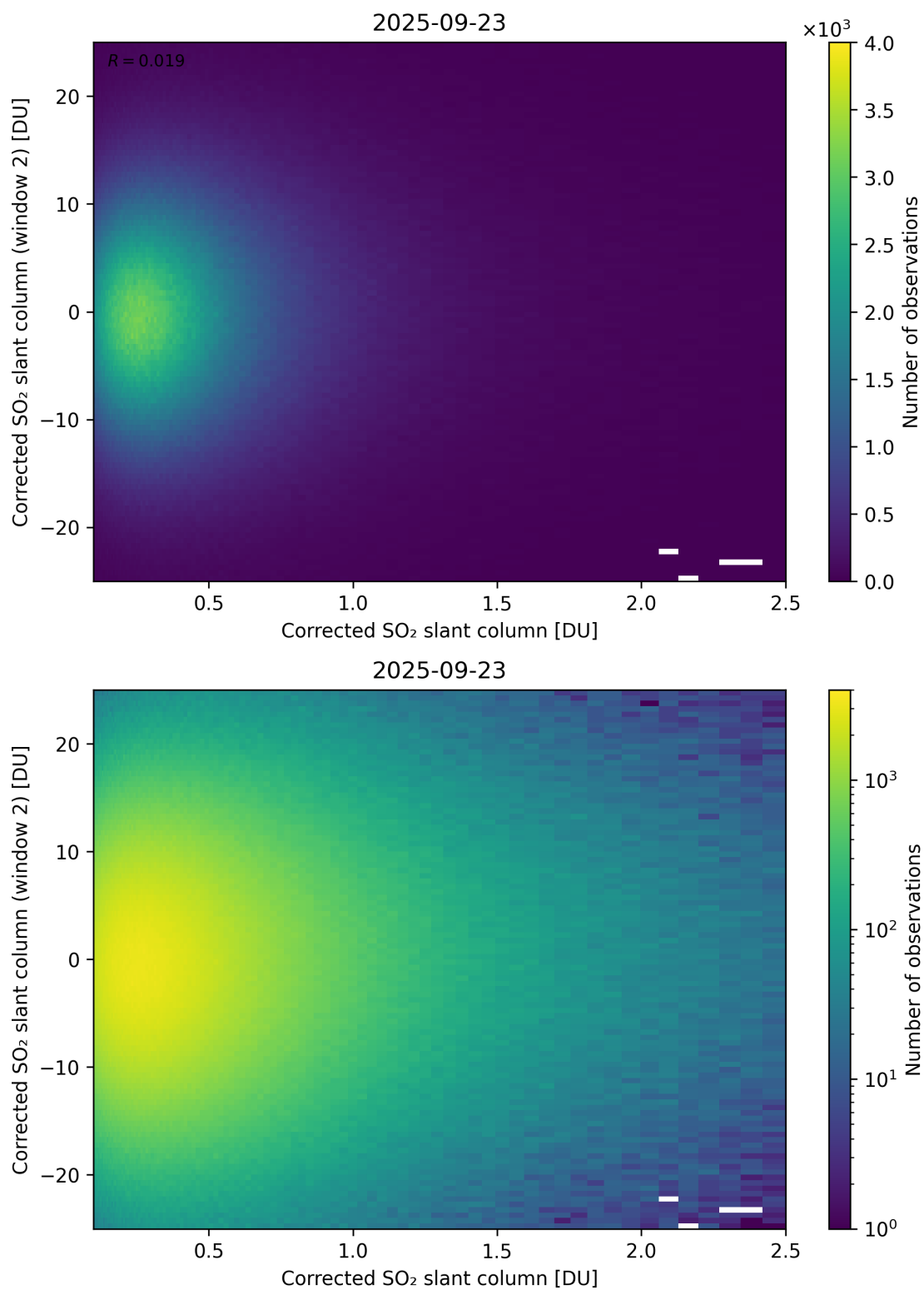
Figure 235: Scatter density plot of “Corrected SO 2 slant column” against “Corrected SO 2 slant column (window 2)” for 2025-09-22 to 2025-09-24.
