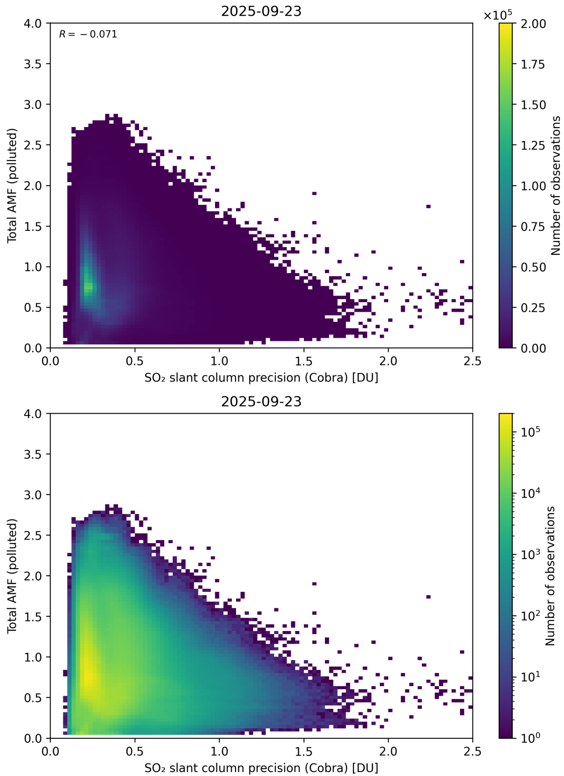
Figure 213: Scatter density plot of “SO 2 slant column precision (Cobra)” against “Total AMF (polluted)” for 2025-09-22 to 2025-09-24.
