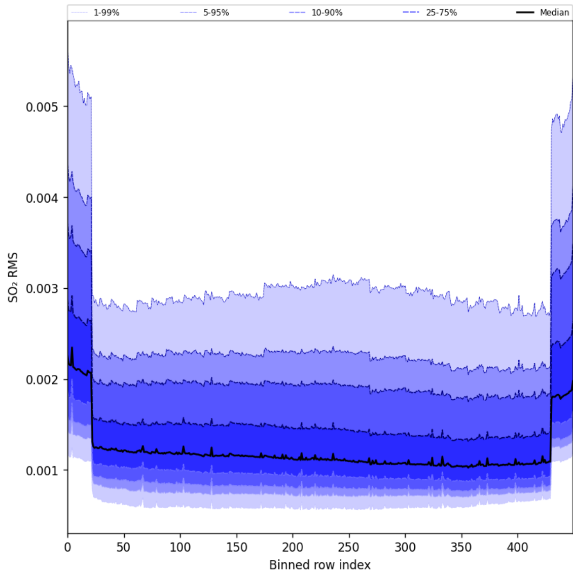
Figure 104: Along track statistics of “SO 2 RMS” for 2025-09-22 to 2025-09-24
