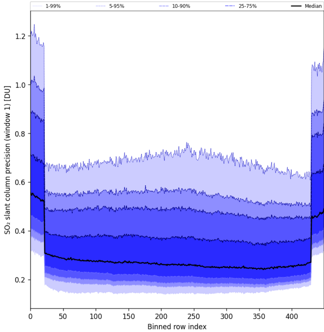
Figure 90: Along track statistics of “SO 2 slant column precision (window 1)” for 2025-09-22 to 2025-09-24
