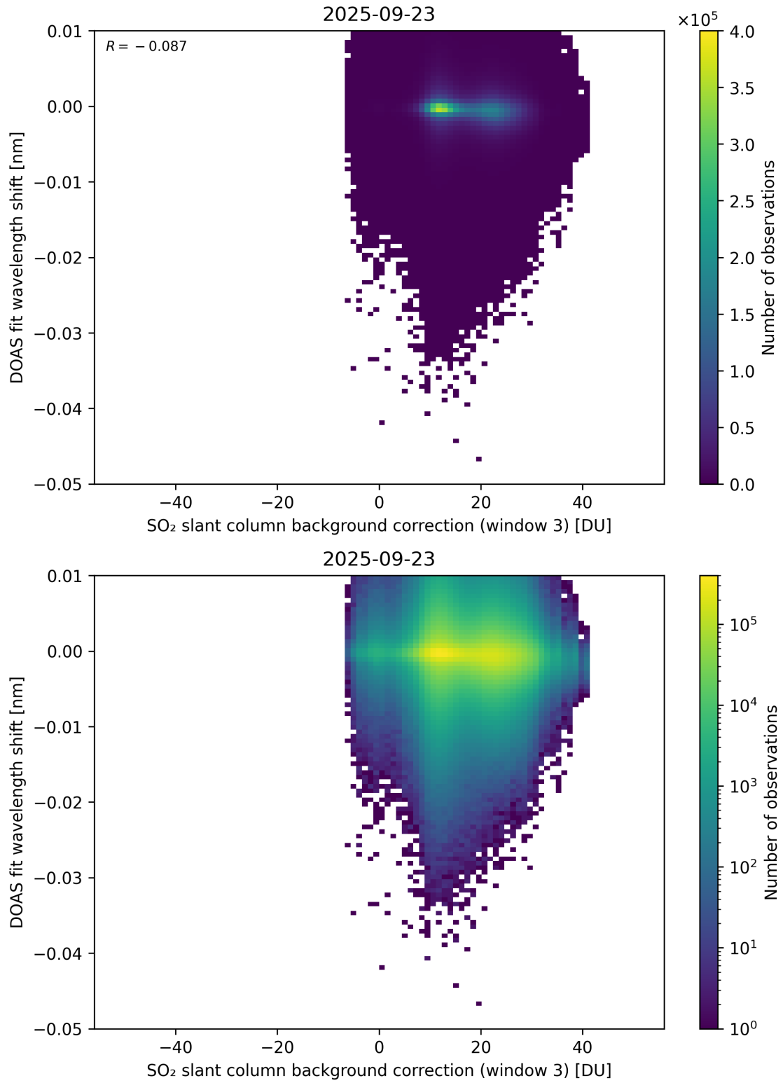
Figure 132: Scatter density plot of “SO 2 slant column background correction (window 3)” against “DOAS fit wavelength shift” for 2025-09-22 to 2025-09-24.
