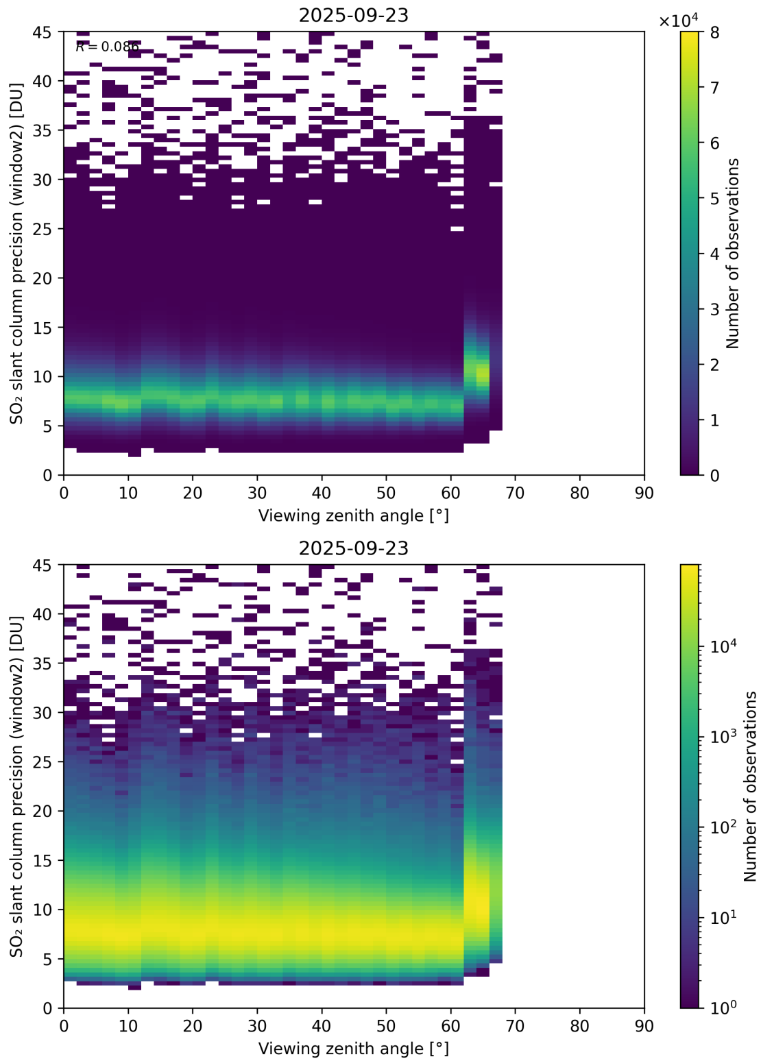
Figure 378: Scatter density plot of “Viewing zenith angle” against “SO 2 slant column precision (window2)” for 2025-09-22 to 2025-09-24.
