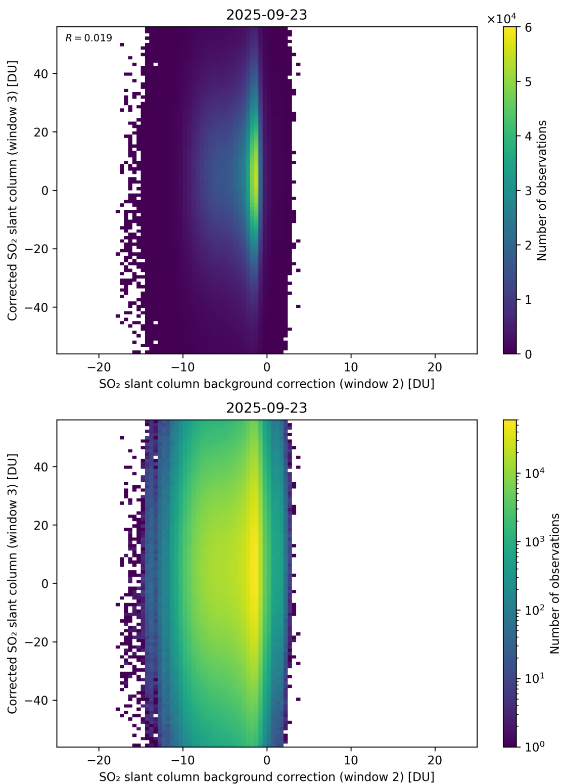
Figure 127: Scatter density plot of “SO 2 slant column background correction (window 2)” against “Corrected SO 2 slant column (window 3)” for 2025-09-22 to 2025-09-24.
