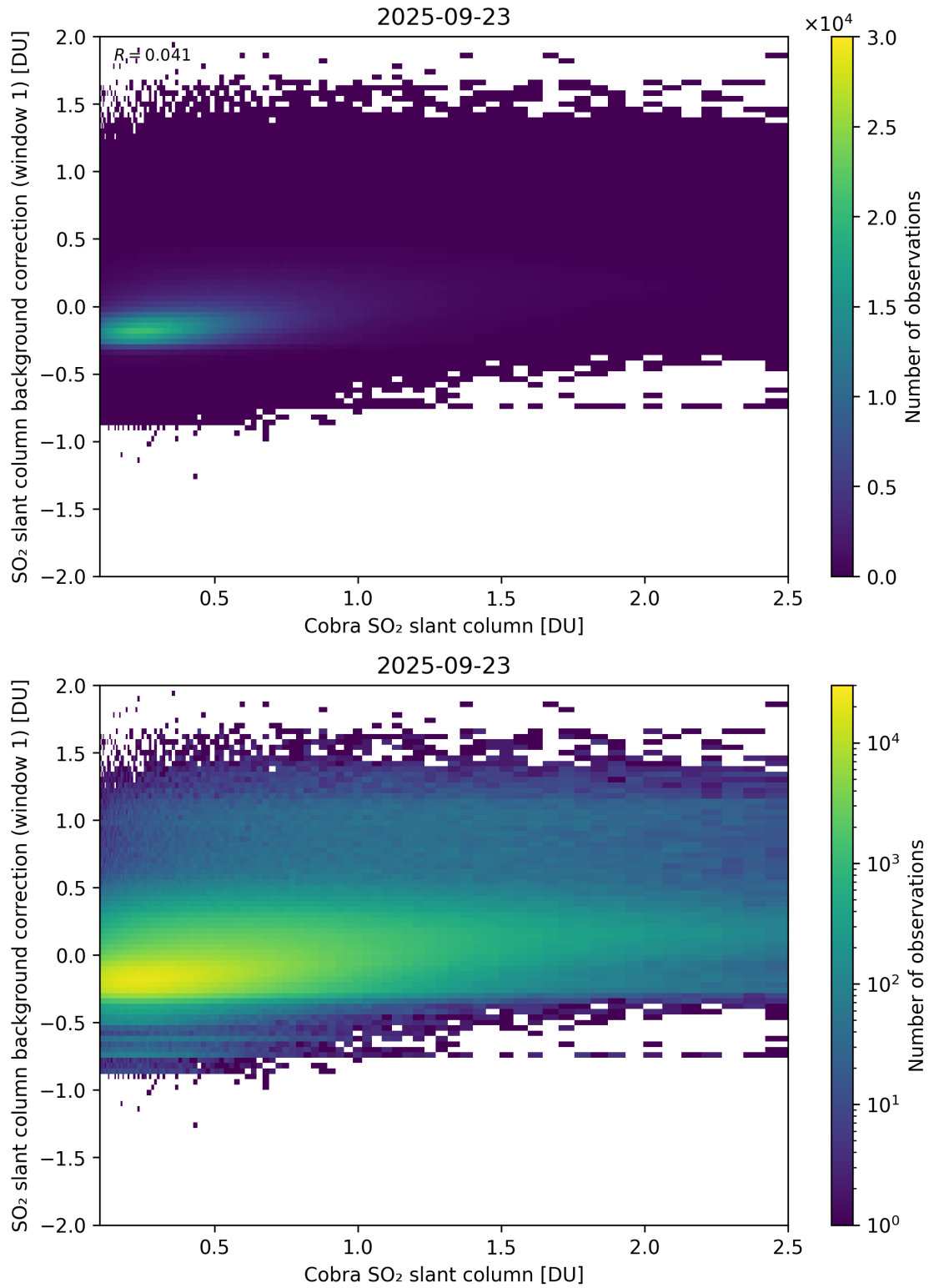
Figure 193: Scatter density plot of “Cobra SO 2 slant column” against “SO 2 slant column background correction (window 1)” for 2025-09-22 to 2025-09-24.
