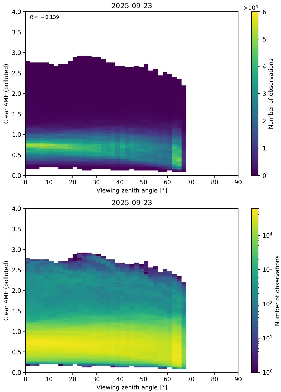
Figure 370: Scatter density plot of “Viewing zenith angle” against “Clear AMF (polluted)” for 2025-09-22 to 2025-09-24.
