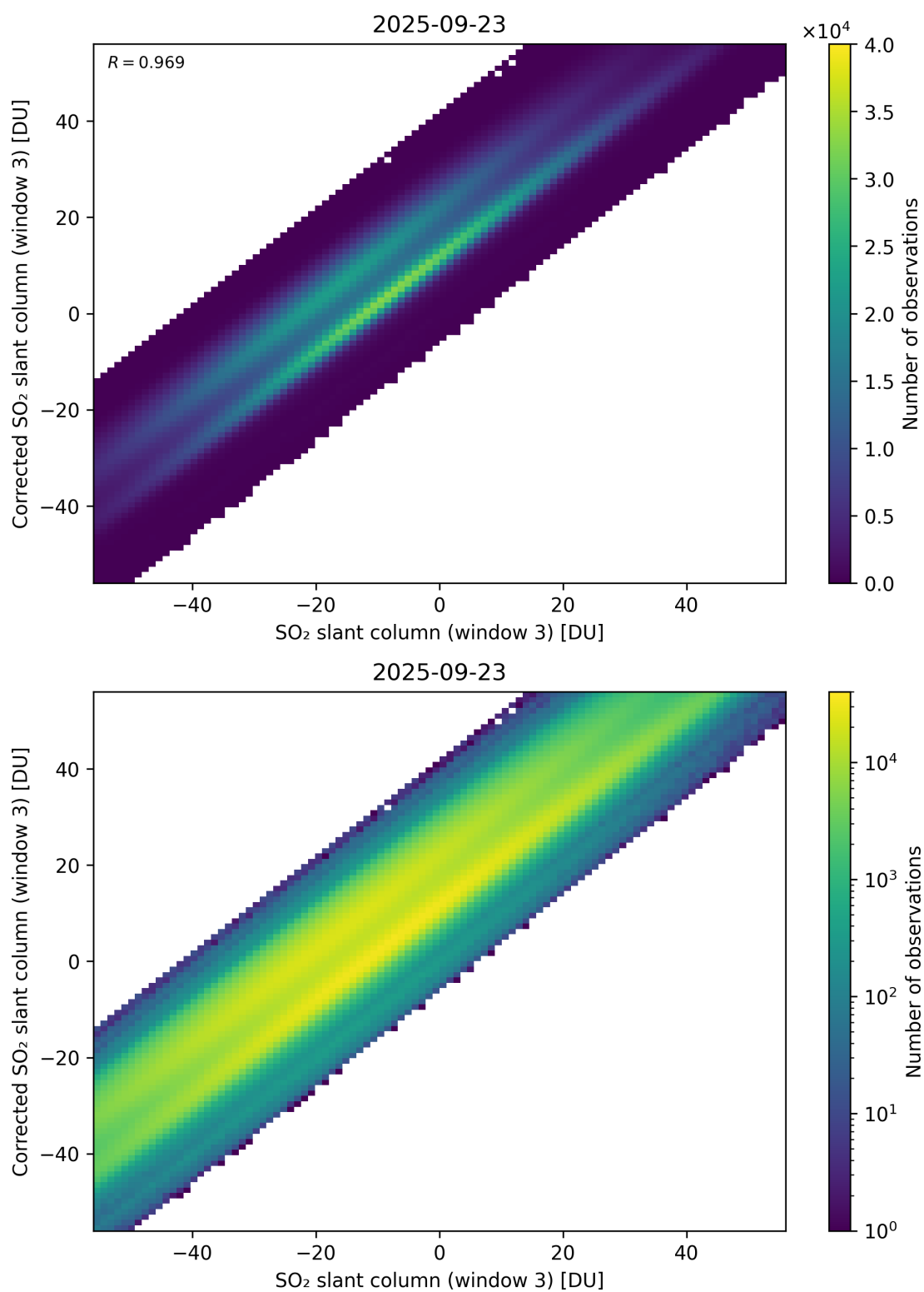
Figure 316: Scatter density plot of “SO 2 slant column (window 3)” against “Corrected SO 2 slant column (window 3)” for 2025-09-22 to 2025-09-24.
