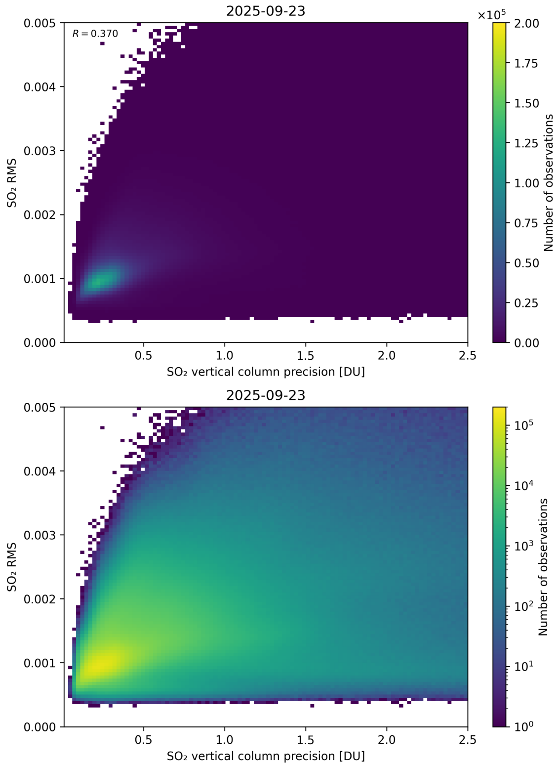
Figure 334: Scatter density plot of “SO 2 vertical column precision” against “SO 2 RMS” for 2025-09-22 to 2025-09-24.
