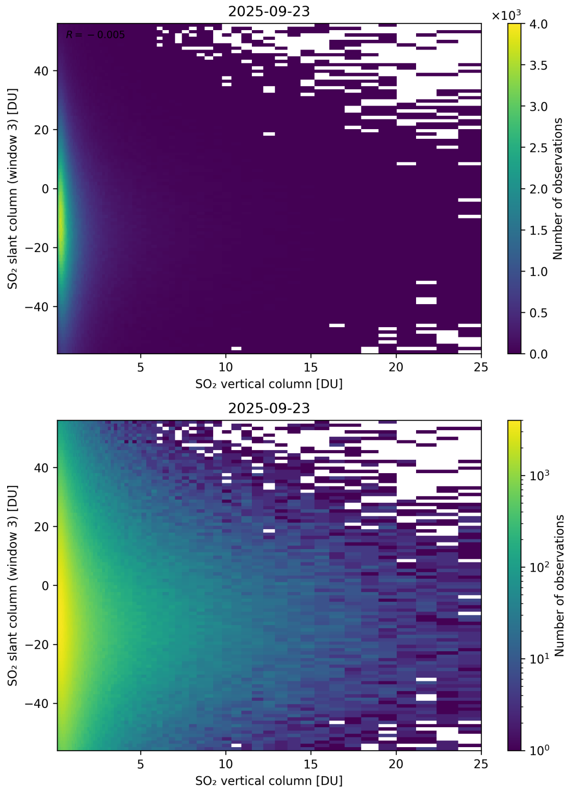
Figure 357: Scatter density plot of “SO 2 vertical column” against “SO 2 slant column (window 3)” for 2025-09-22 to 2025-09-24.
