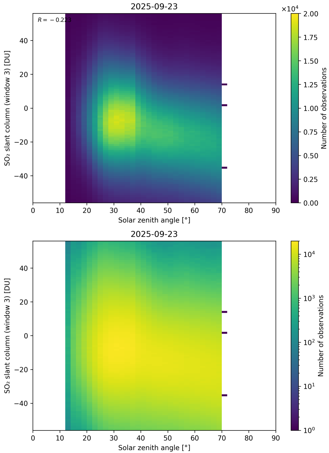
Figure 187: Scatter density plot of “Solar zenith angle” against “SO 2 slant column (window 3)” for 2025-09-22 to 2025-09-24.
