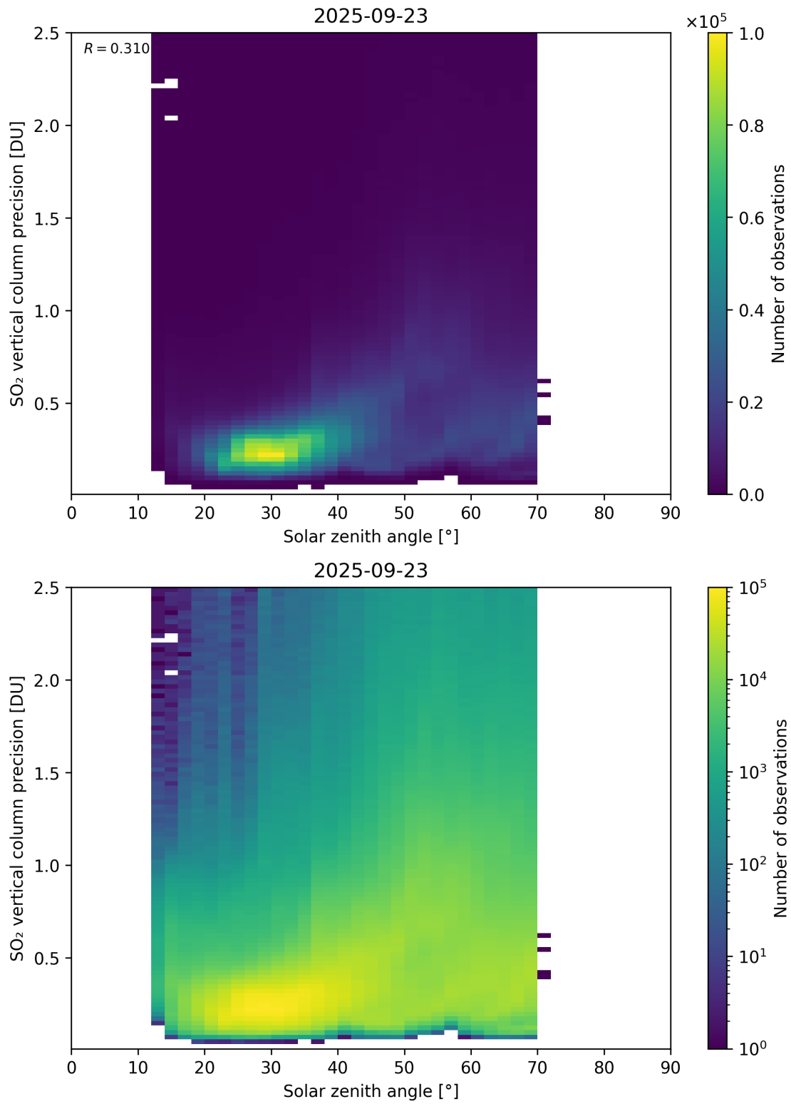
Figure 192: Scatter density plot of “Solar zenith angle” against “SO 2 vertical column precision” for 2025-09-22 to 2025-09-24.
