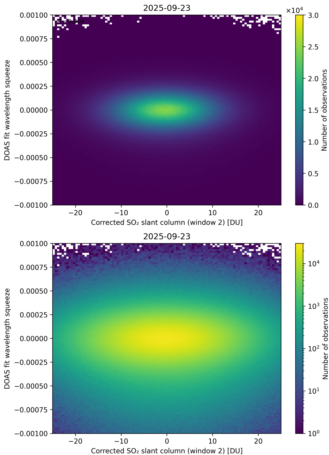
Figure 247: Scatter density plot of “Corrected SO 2 slant column (window 2)” against “DOAS fit wavelength squeeze” for 2025-09-22 to 2025-09-24.
