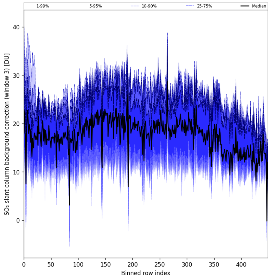
Figure 100: Along track statistics of “SO 2 slant column background correction (window 3)” for 2025-09-22 to 2025-09-24
