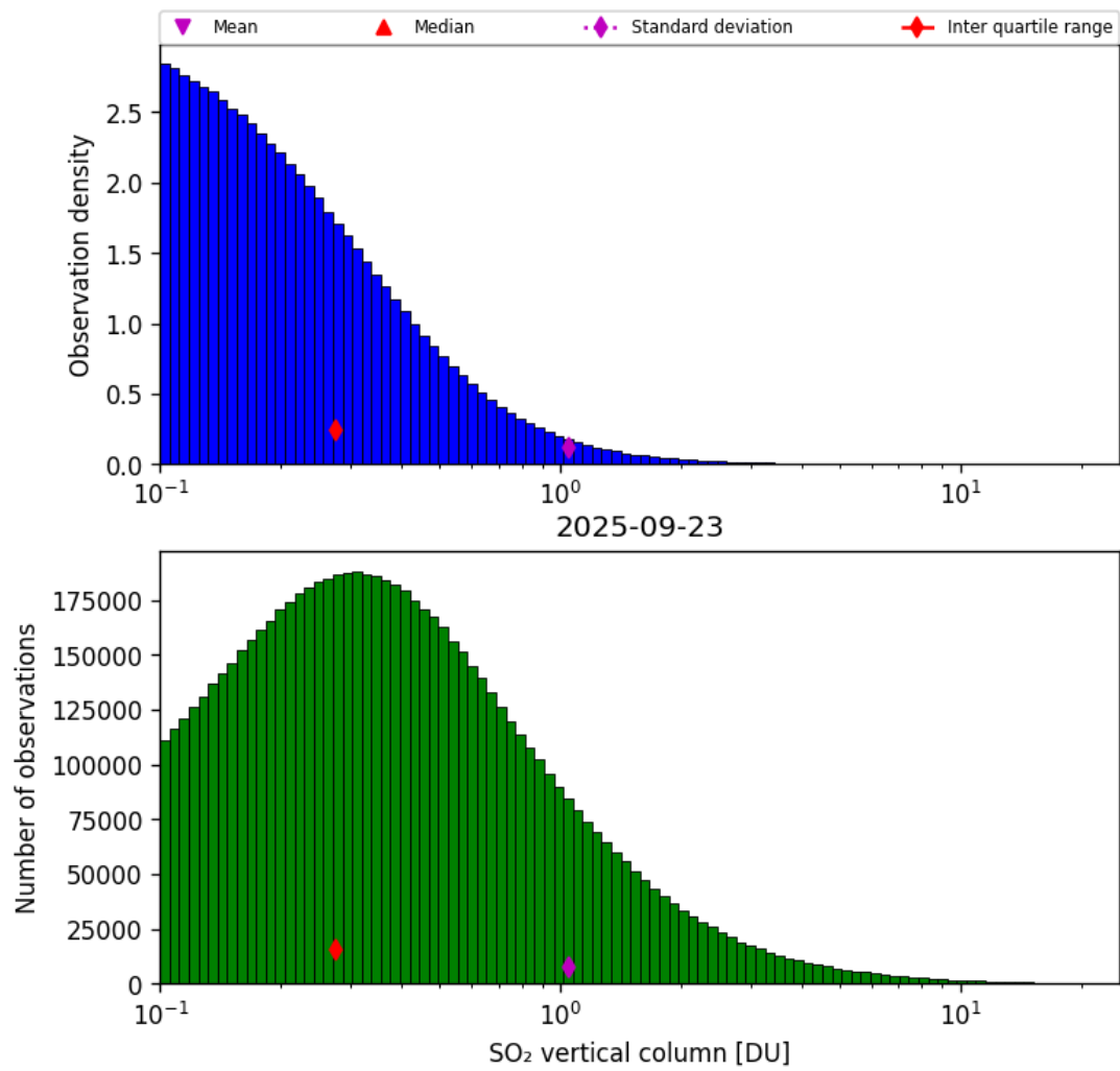
Figure 58: Histogram of "SO 2 vertical column" for 2025-09-22 to 2025-09-24
