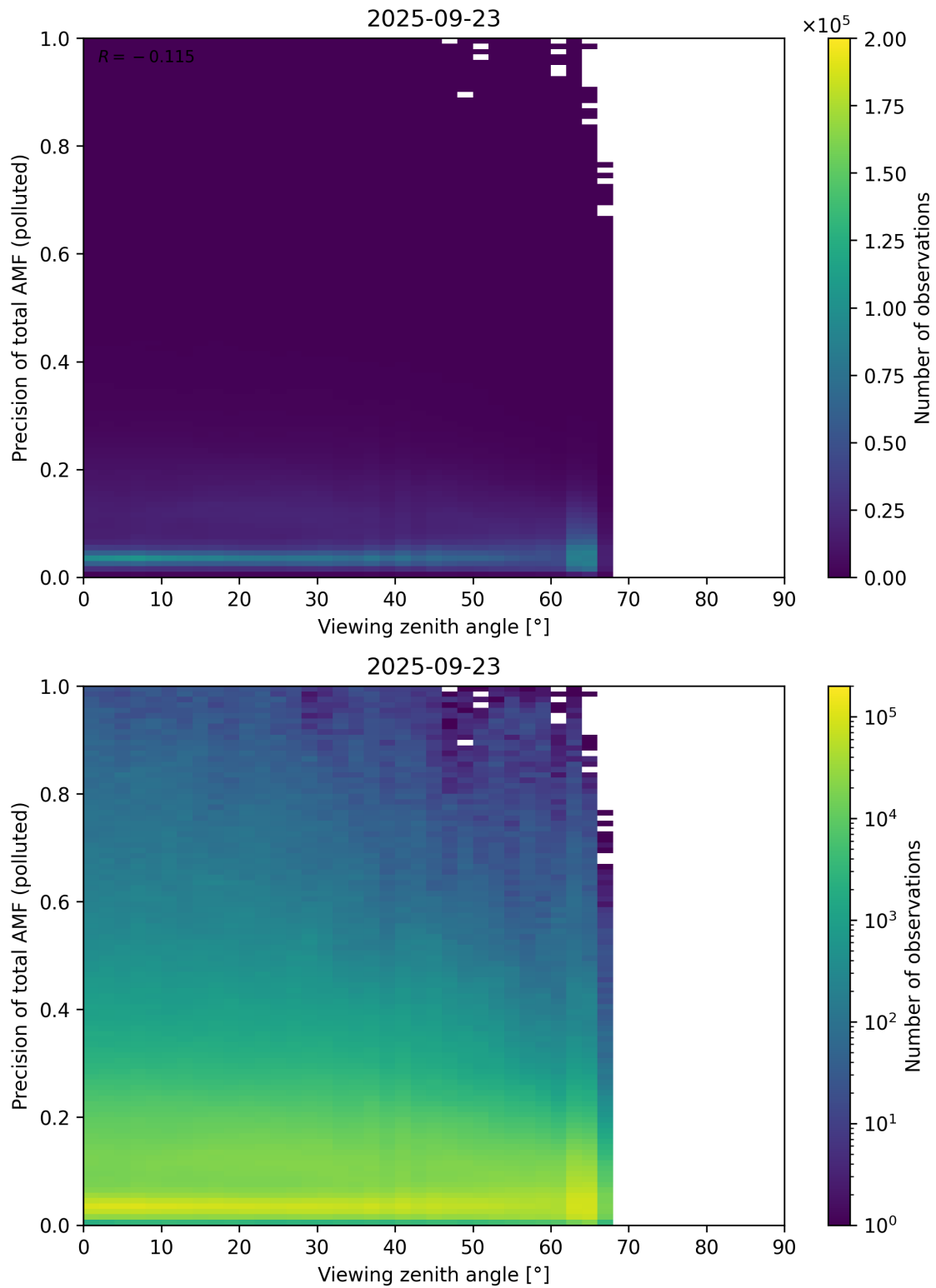
Figure 382: Scatter density plot of “Viewing zenith angle” against “Precision of total AMF (polluted)” for 2025-09-22 to 2025-09-24.
