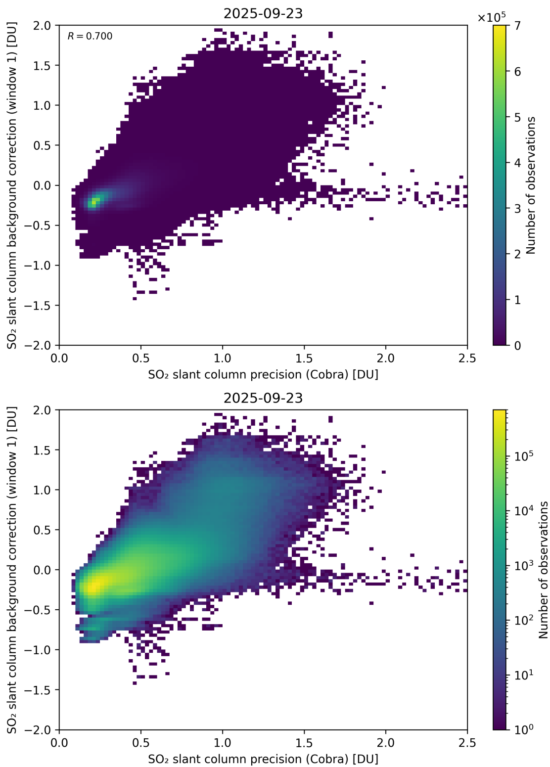
Figure 199: Scatter density plot of “SO 2 slant column precision (Cobra)” against “SO 2 slant column background correction (window 1)” for 2025-09-22 to 2025-09-24.
