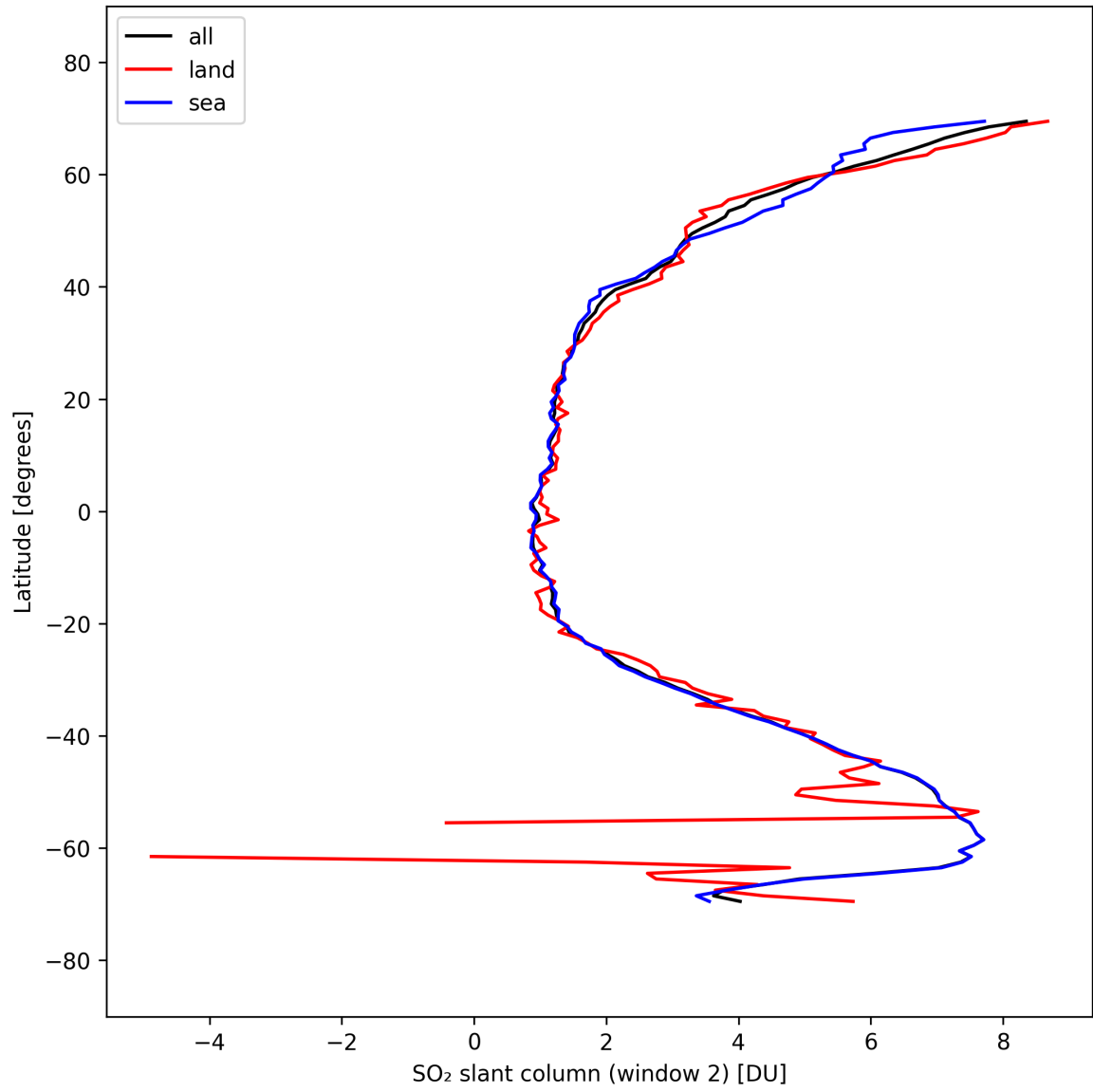
Figure 41: Zonal average of “SO 2 slant column (window 2)” for 2025-09-22 to 2025-09-24.
