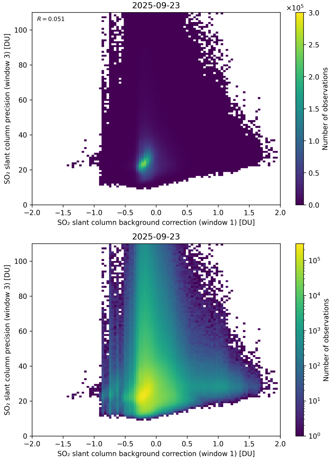
Figure 119: Scatter density plot of “SO 2 slant column background correction (window 1)” against “SO 2 slant column precision (window 3)” for 2025-09-22 to 2025-09-24.
