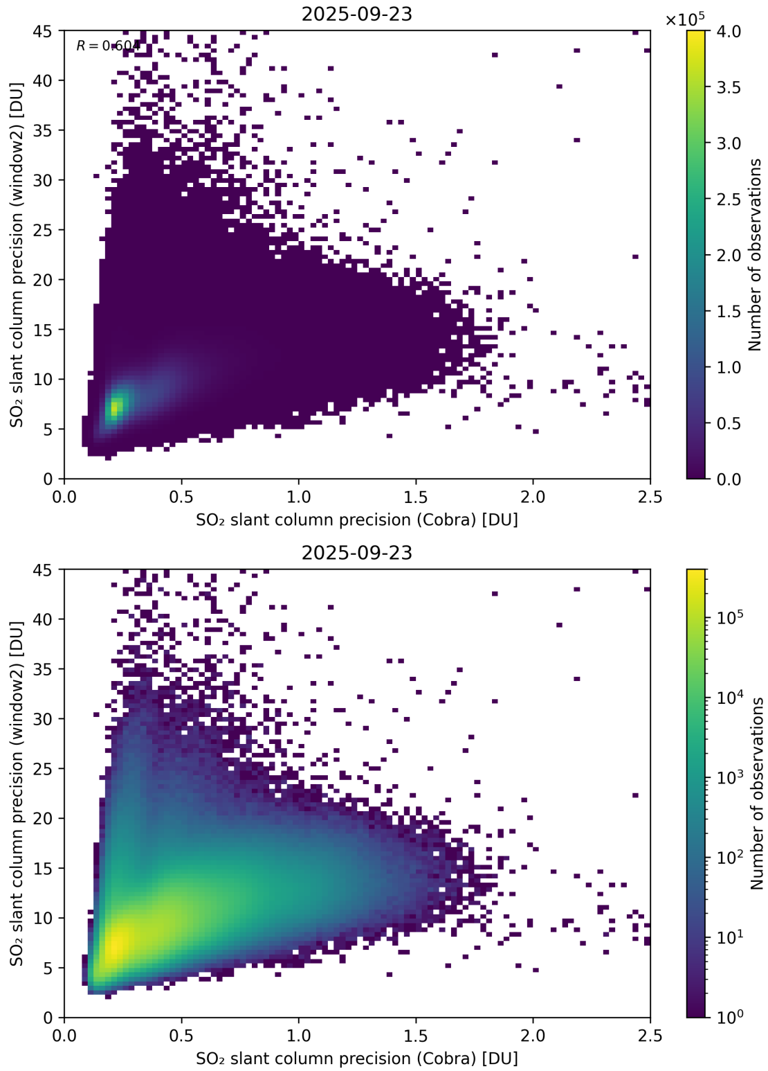
Figure 210: Scatter density plot of “SO 2 slant column precision (Cobra)” against “SO 2 slant column precision (window2)” for 2025-09-22 to 2025-09-24.
