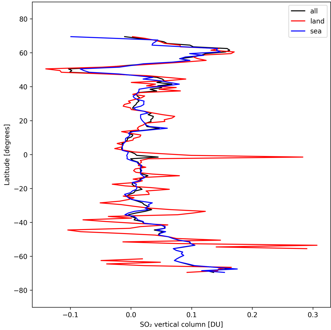
Figure 32: Zonal average of “SO 2 vertical column” for 2025-09-22 to 2025-09-24.
