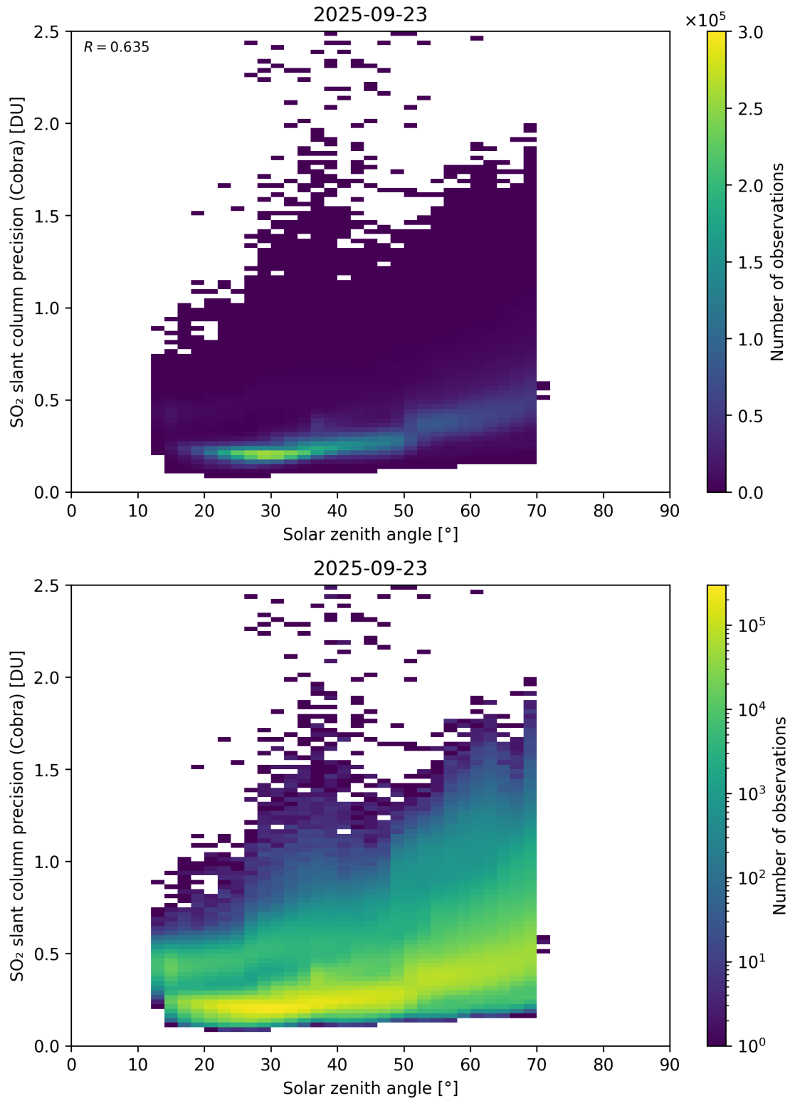
Figure 180: Scatter density plot of “Solar zenith angle” against “SO 2 slant column precision (Cobra)” for 2025-09-22 to 2025-09-24.
