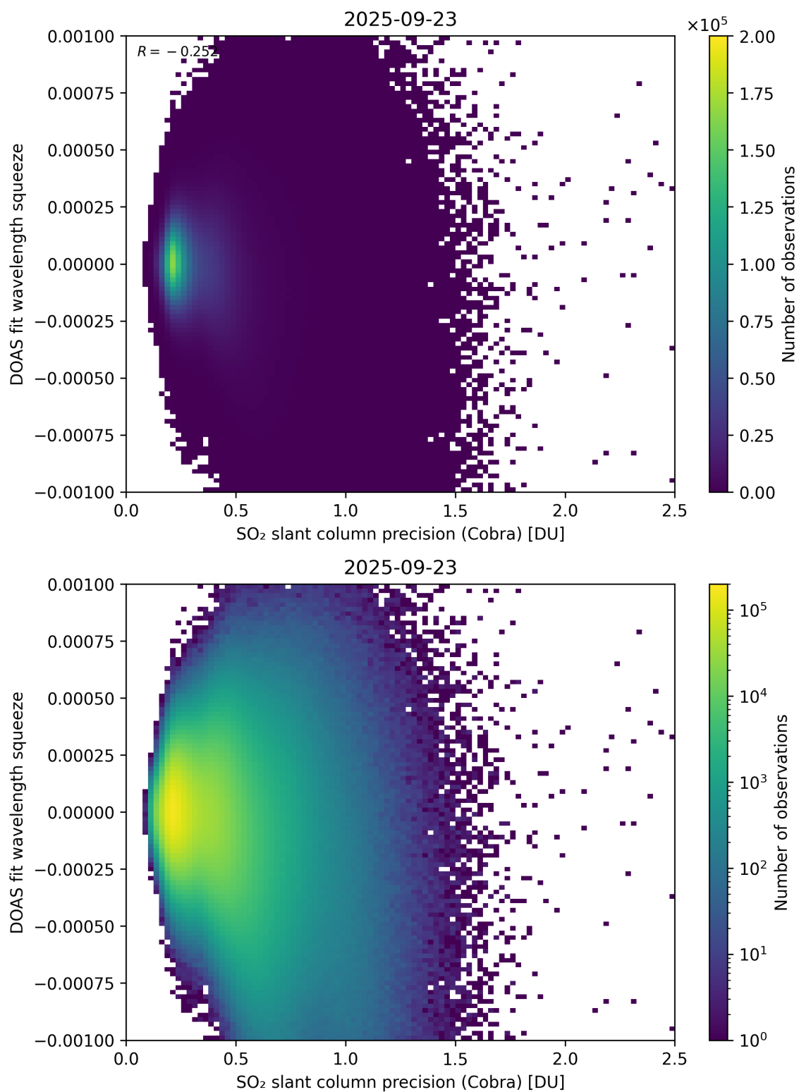
Figure 203: Scatter density plot of “SO 2 slant column precision (Cobra)” against “DOAS fit wavelength squeeze” for 2025-09-22 to 2025-09-24.
