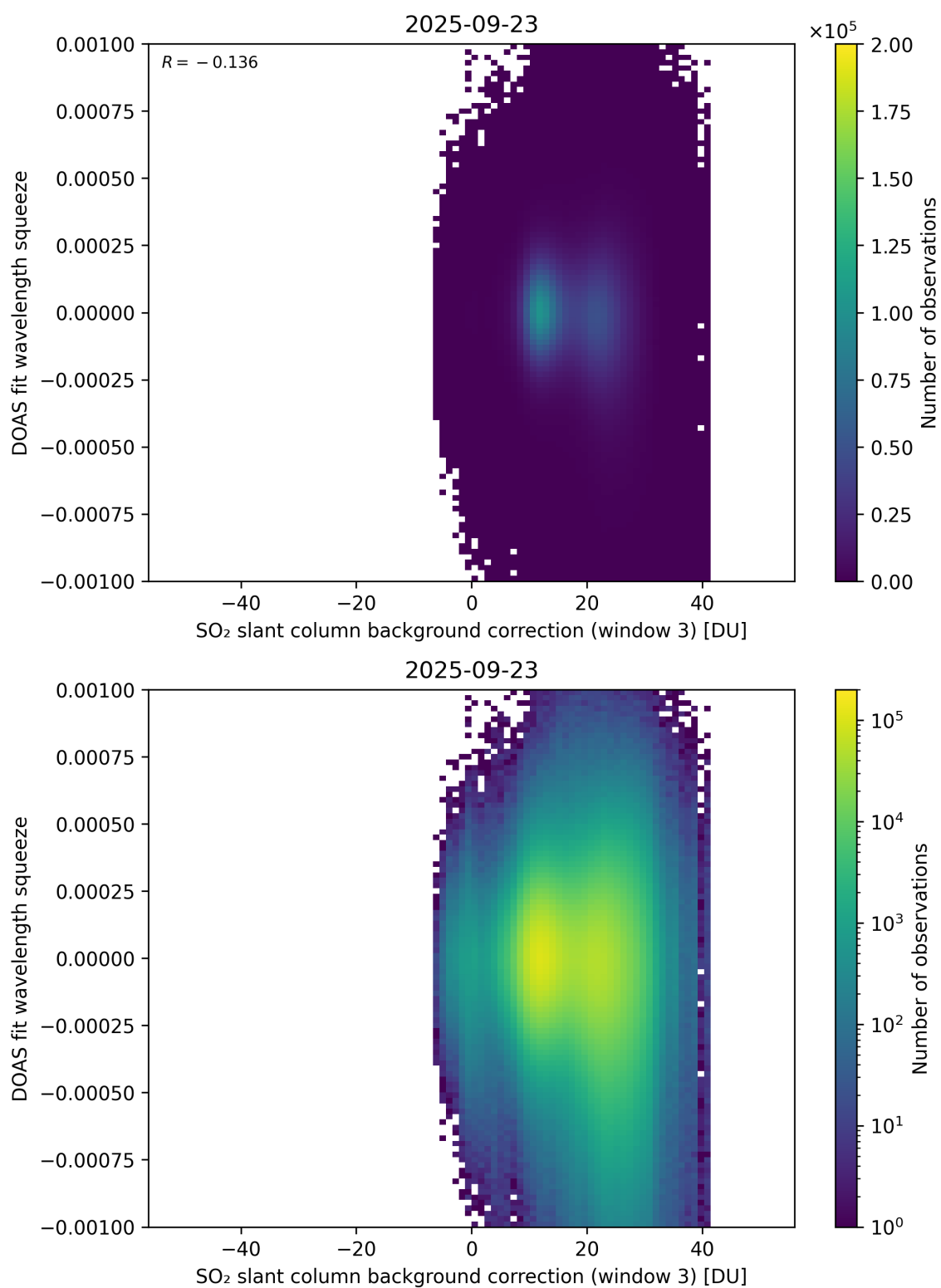
Figure 133: Scatter density plot of “SO 2 slant column background correction (window 3)” against “DOAS fit wavelength squeeze” for 2025-09-22 to 2025-09-24.
