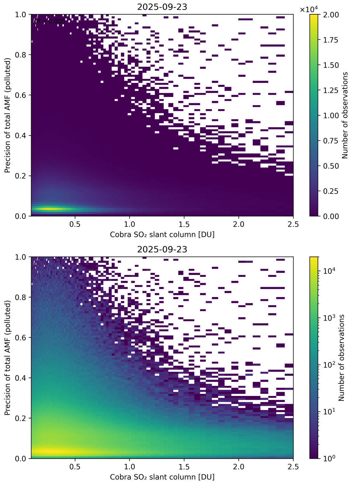
Figure 225: Scatter density plot of “Cobra SO 2 slant column” against “Precision of total AMF (polluted)” for 2025-09-22 to 2025-09-24.
