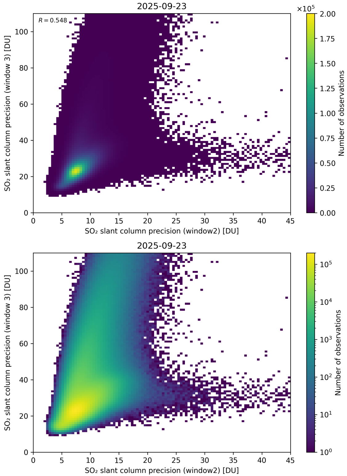
Figure 300: Scatter density plot of “SO 2 slant column precision (window2)” against “SO 2 slant column precision (window 3)” for 2025-09-22 to 2025-09-24.
