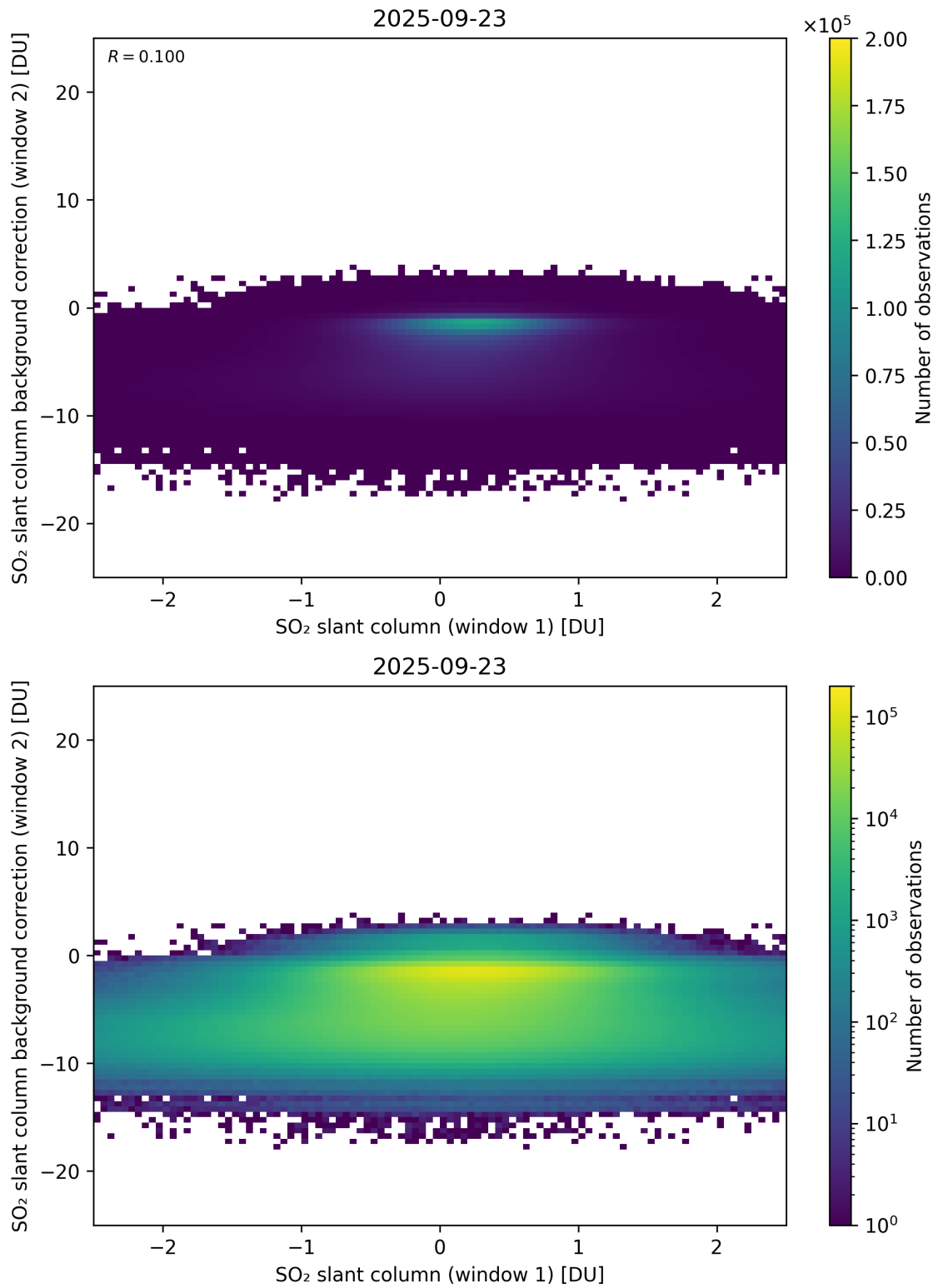
Figure 263: Scatter density plot of “SO 2 slant column (window 1)” against “SO 2 slant column background correction (window 2)” for 2025-09-22 to 2025-09-24.
