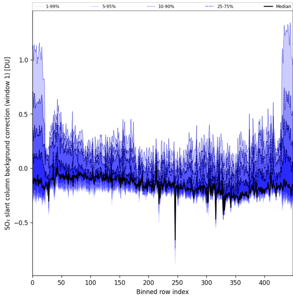
Figure 92: Along track statistics of “SO 2 slant column background correction (window 1)” for 2025-09-22 to 2025-09-24
