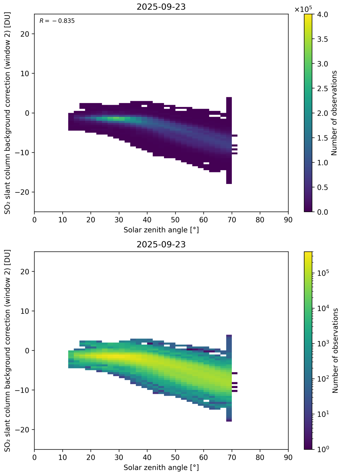
Figure 172: Scatter density plot of “Solar zenith angle” against “SO 2 slant column background correction (window 2)” for 2025-09-22 to 2025-09-24.
