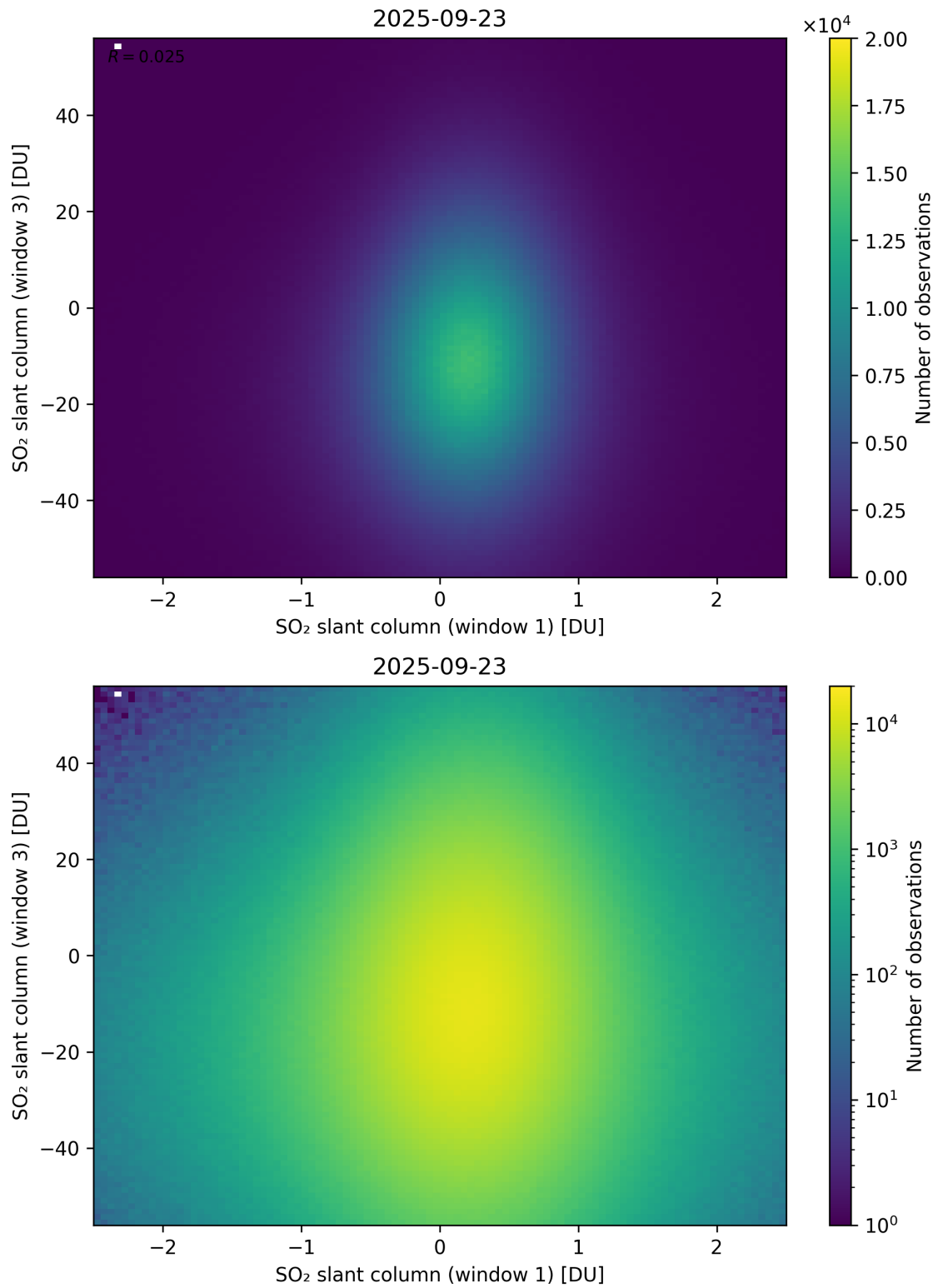
Figure 287: Scatter density plot of “SO 2 slant column (window 1)” against “SO 2 slant column (window 3)” for 2025-09-22 to 2025-09-24.
