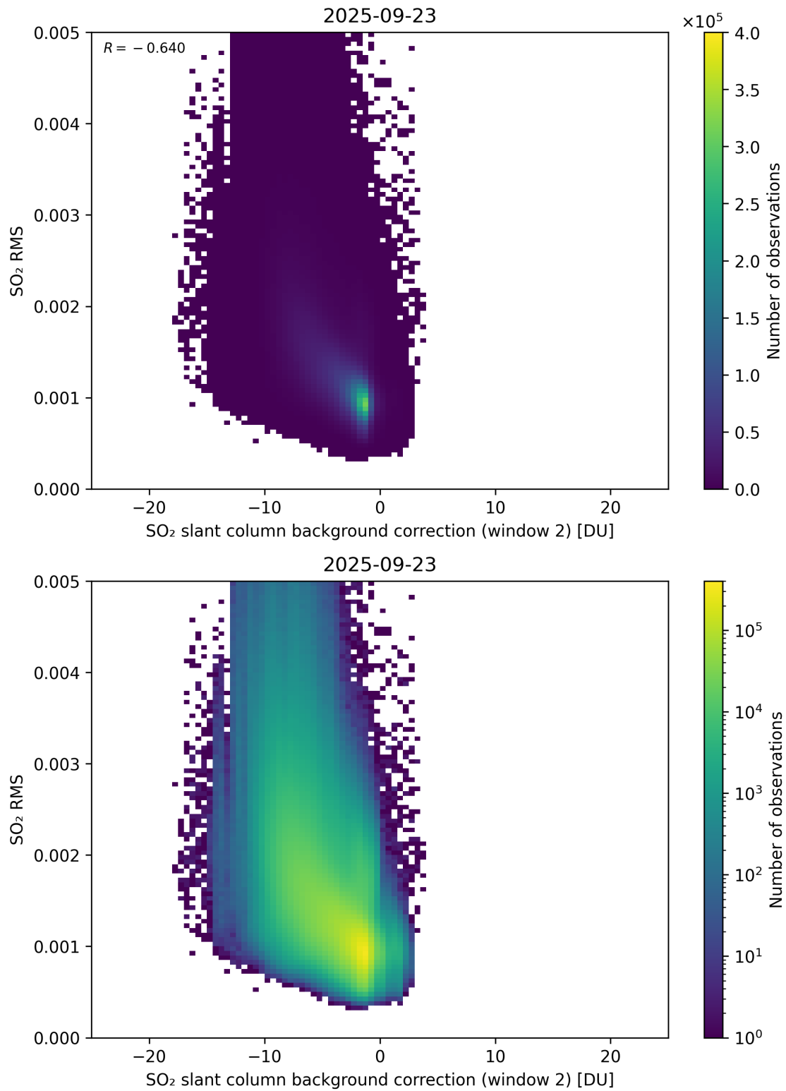
Figure 125: Scatter density plot of “SO 2 slant column background correction (window 2)” against “SO 2 RMS” for 2025-09-22 to 2025-09-24.
