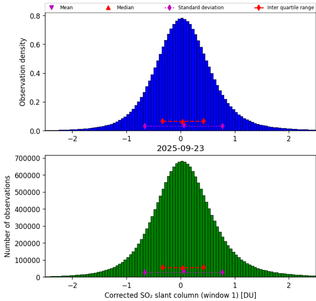
Figure 65: Histogram of “Corrected SO 2 slant column (window 1)” for 2025-09-22 to 2025-09-24
