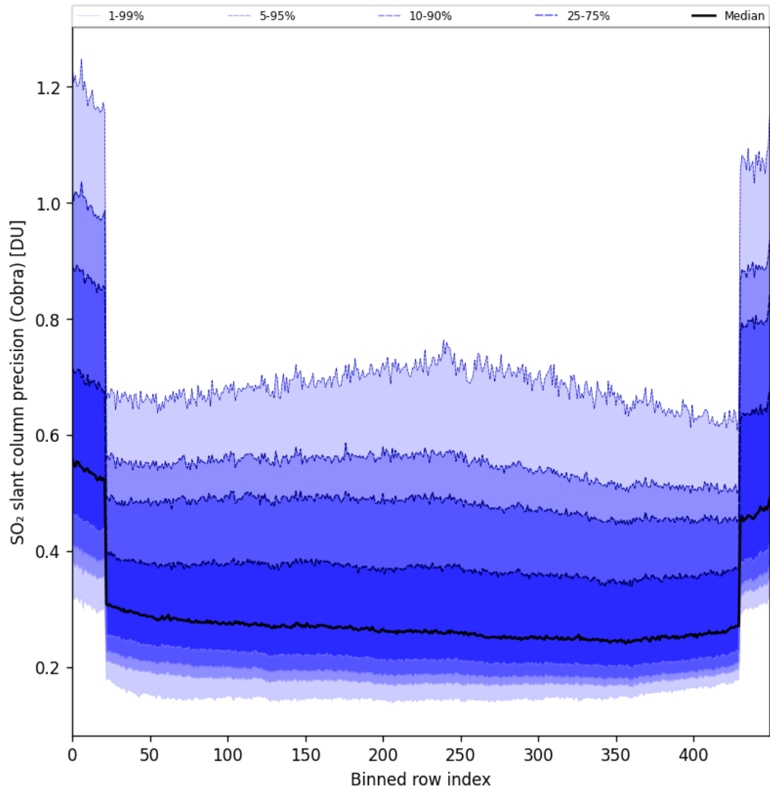
Figure 88: Along track statistics of “SO 2 slant column precision (Cobra)” for 2025-09-22 to 2025-09-24
