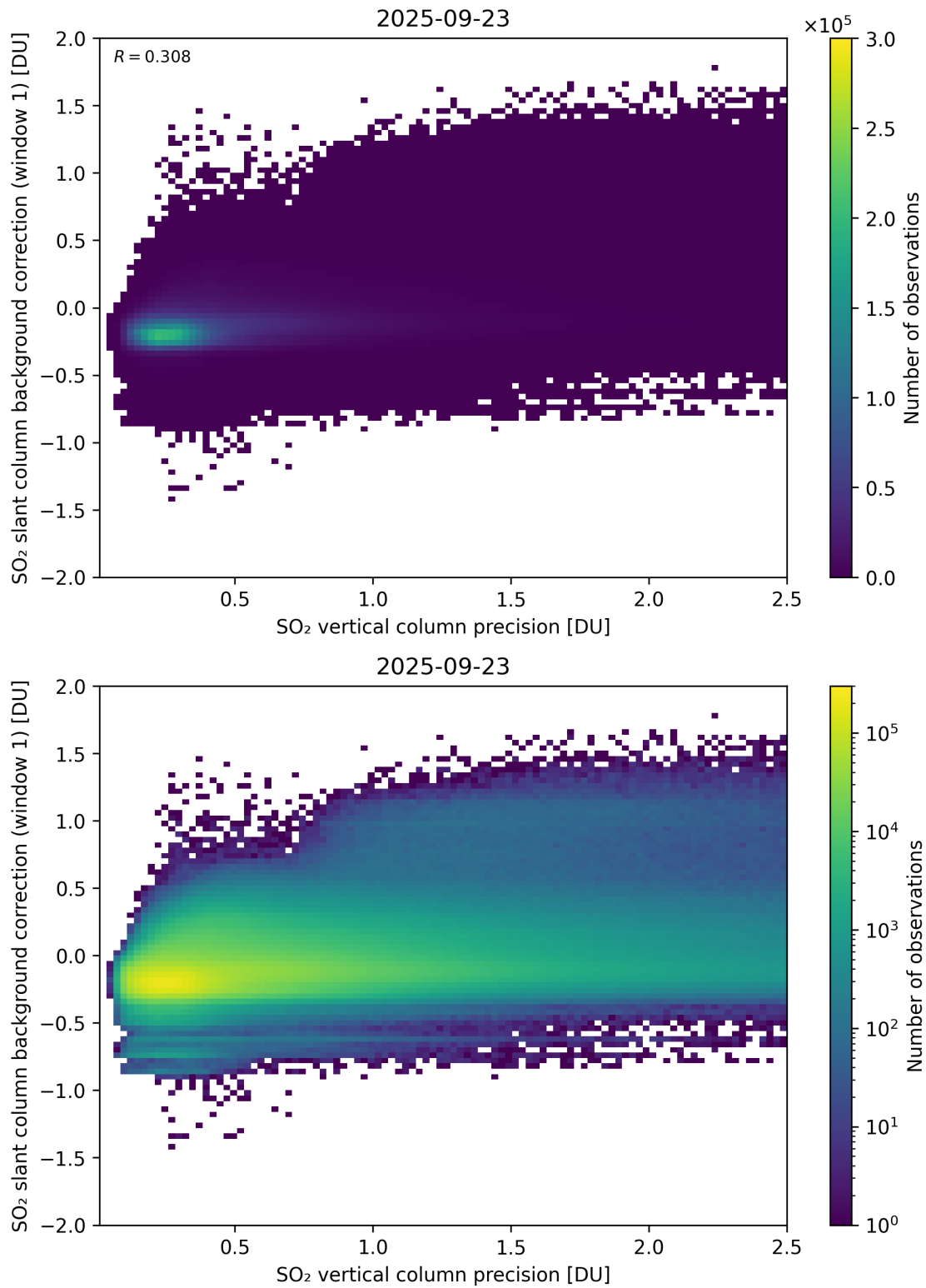
Figure 329: Scatter density plot of “SO 2 vertical column precision” against “SO 2 slant column background correction (window 1)” for 2025-09-22 to 2025-09-24.
