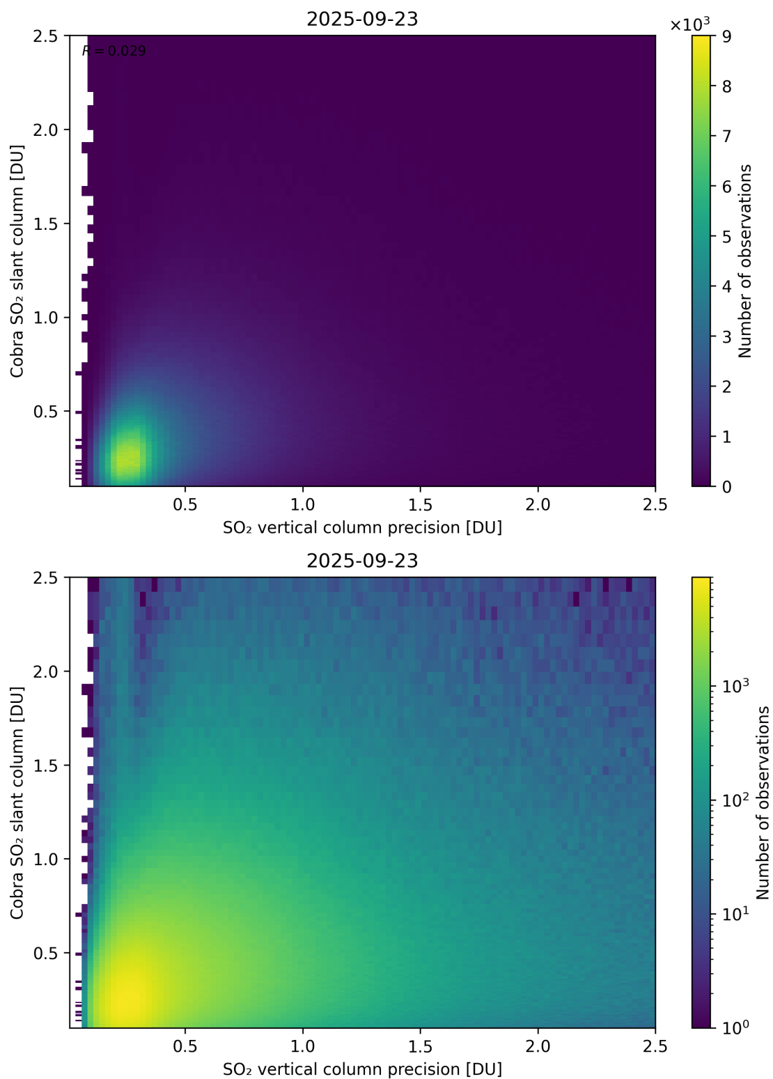
Figure 336: Scatter density plot of “SO 2 vertical column precision” against “Cobra SO 2 slant column” for 2025-09-22 to 2025-09-24.
