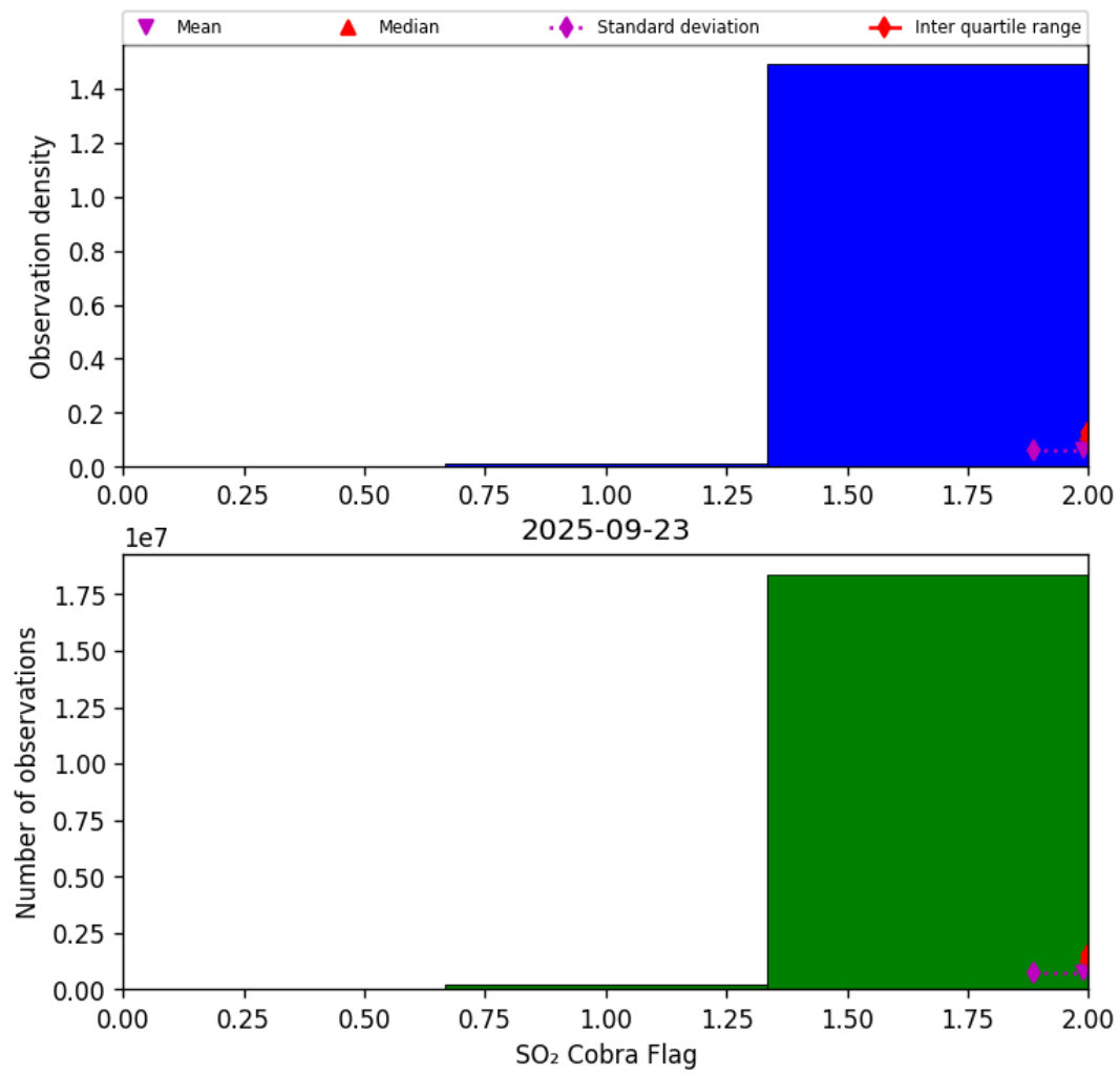
Figure 75: Histogram of “SO 2 Cobra Flag” for 2025-09-22 to 2025-09-24
