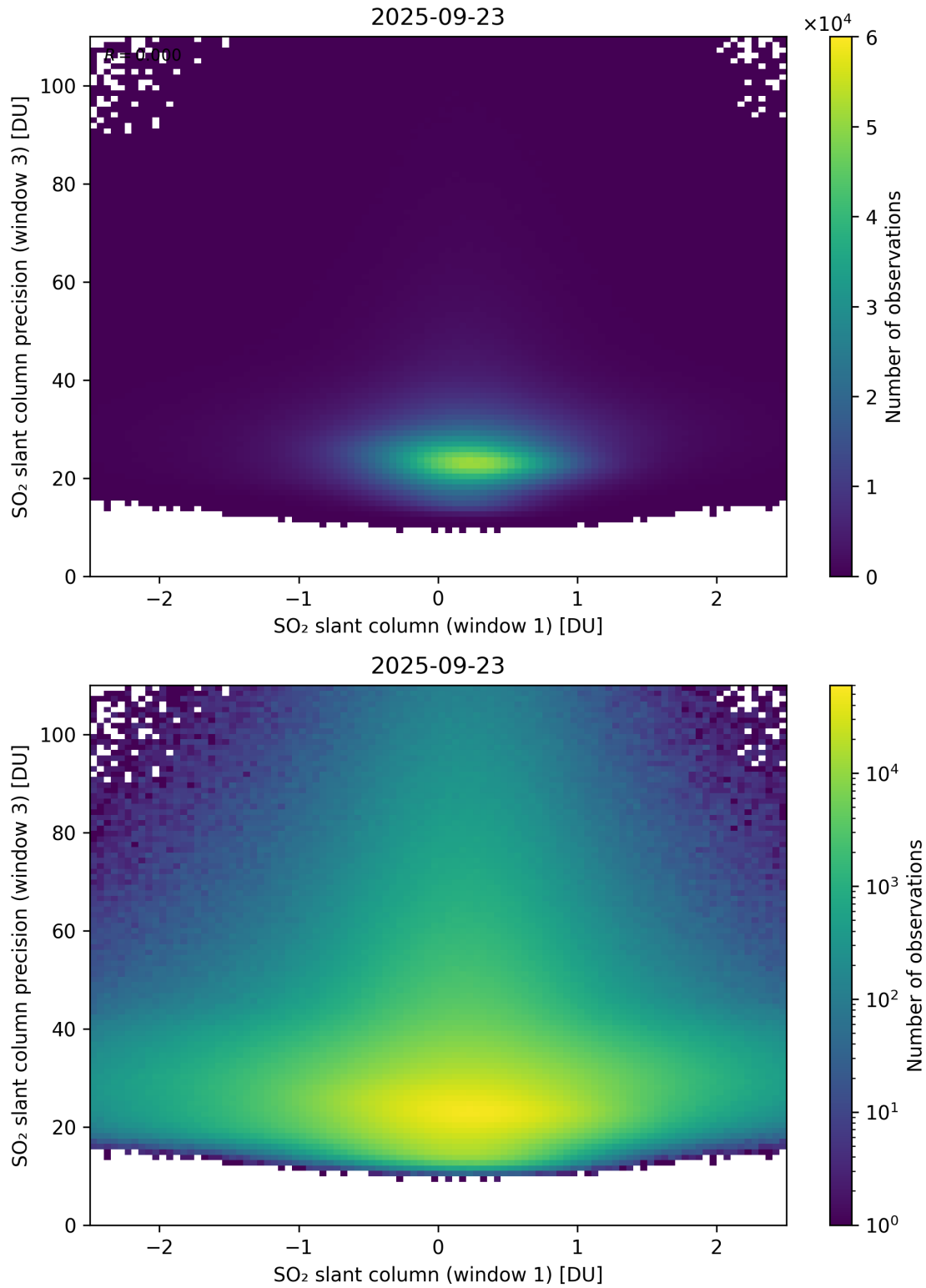
Figure 288: Scatter density plot of “SO 2 slant column (window 1)” against “SO 2 slant column precision (window 3)” for 2025-09-22 to 2025-09-24.
