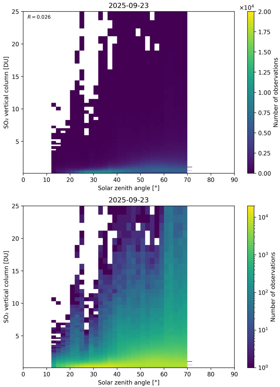
Figure 191: Scatter density plot of “Solar zenith angle” against “SO 2 vertical column” for 2025-09-22 to 2025-09-24.
