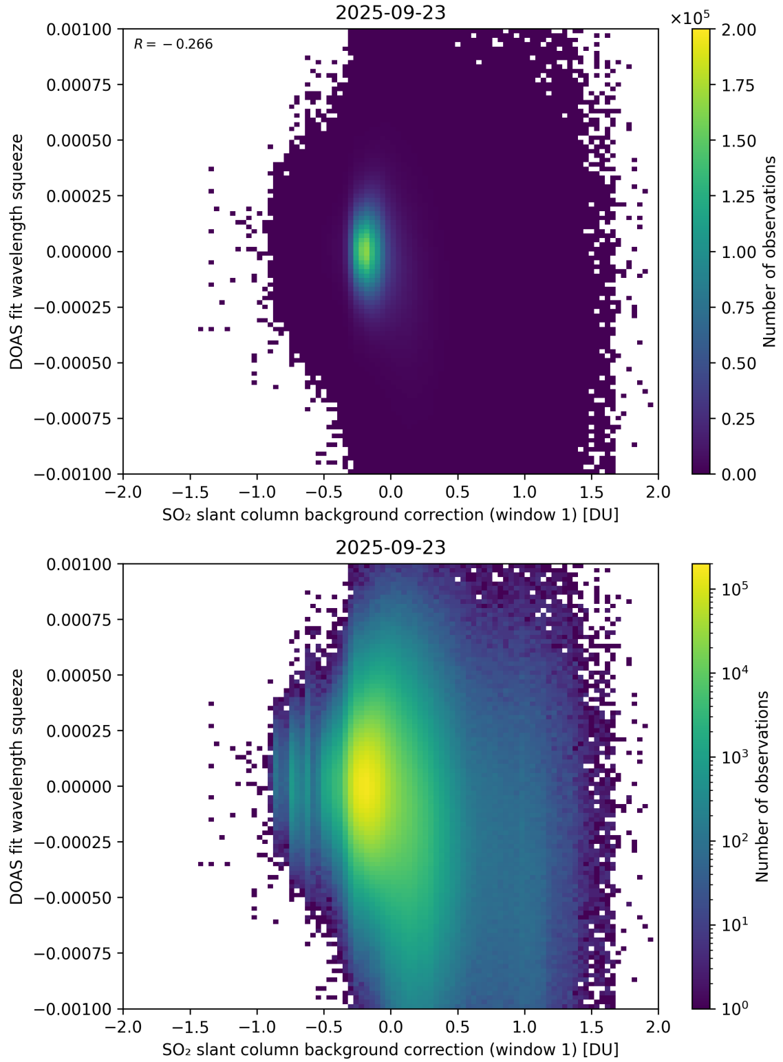
Figure 112: Scatter density plot of “SO 2 slant column background correction (window 1)” against “DOAS fit wavelength squeeze” for 2025-09-22 to 2025-09-24.
