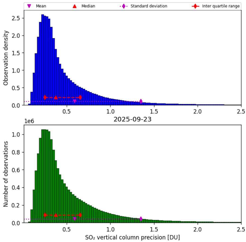
Figure 59: Histogram of “SO 2 vertical column precision” for 2025-09-22 to 2025-09-24
