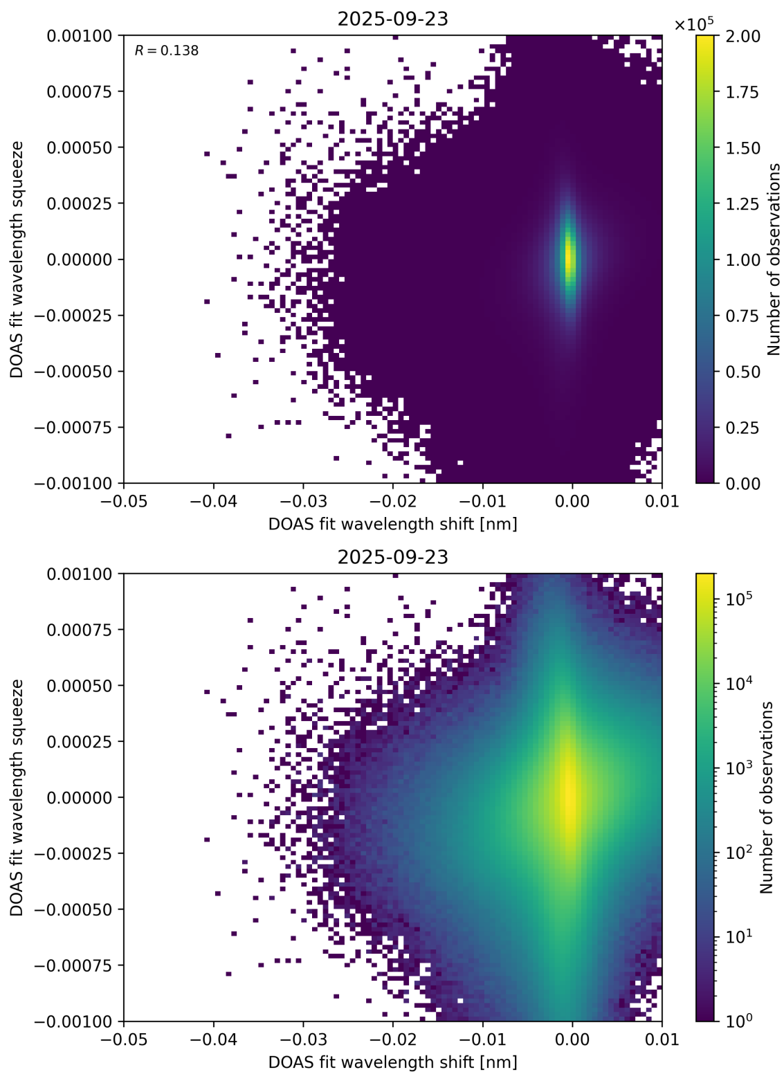
Figure 138: Scatter density plot of “DOAS fit wavelength shift” against “DOAS fit wavelength squeeze” for 2025-09-22 to 2025-09-24.
