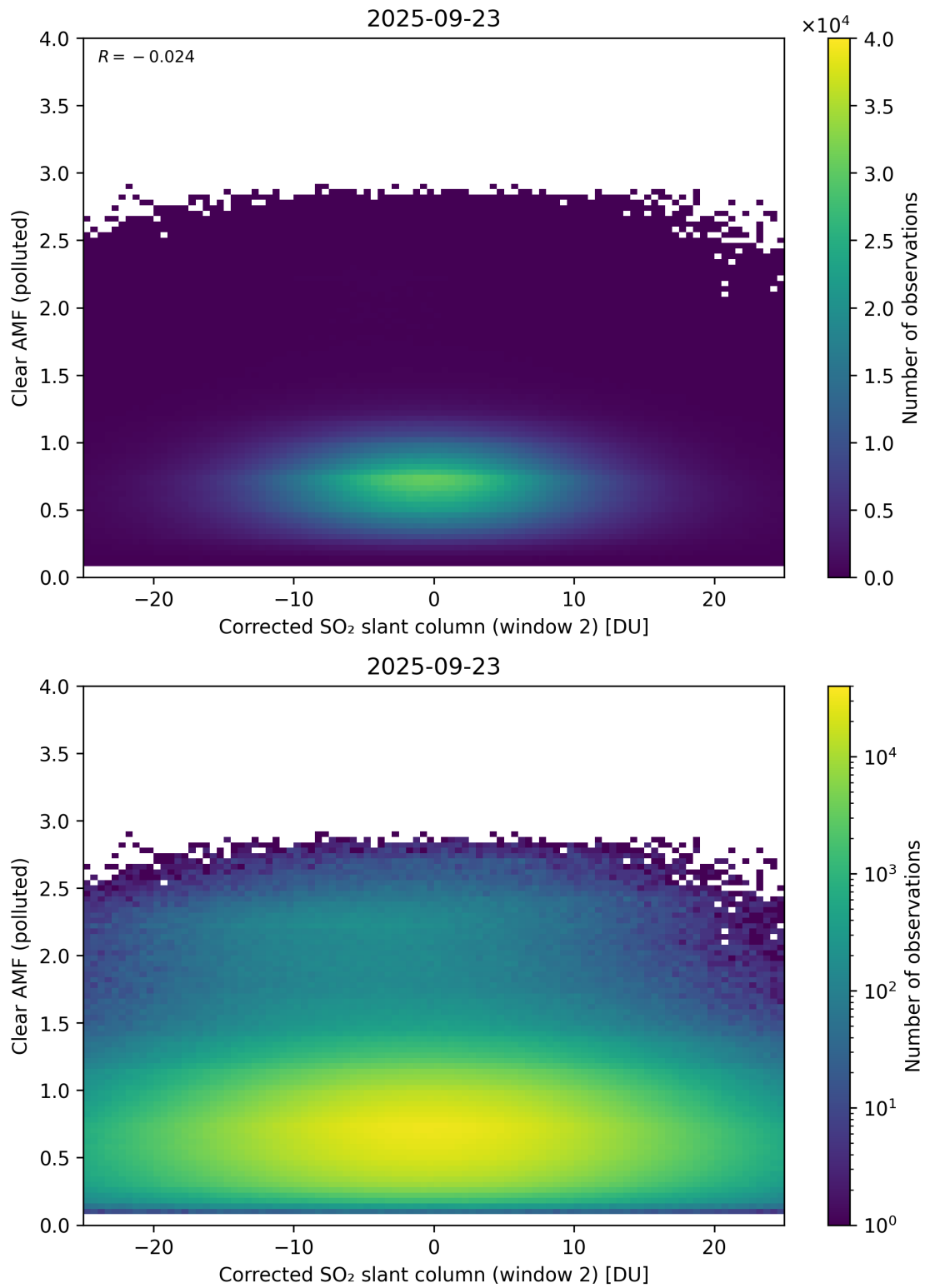
Figure 249: Scatter density plot of “Corrected SO 2 slant column (window 2)” against “Clear AMF (polluted)” for 2025-09-22 to 2025-09-24.
