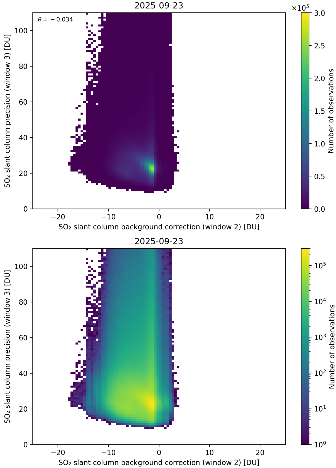
Figure 129: Scatter density plot of “SO 2 slant column background correction (window 2)” against “SO 2 slant column precision (window 3)” for 2025-09-22 to 2025-09-24.
