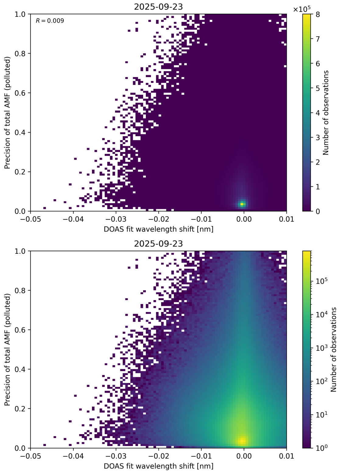
Figure 142: Scatter density plot of “DOAS fit wavelength shift” against “Precision of total AMF (polluted)” for 2025-09-22 to 2025-09-24.
