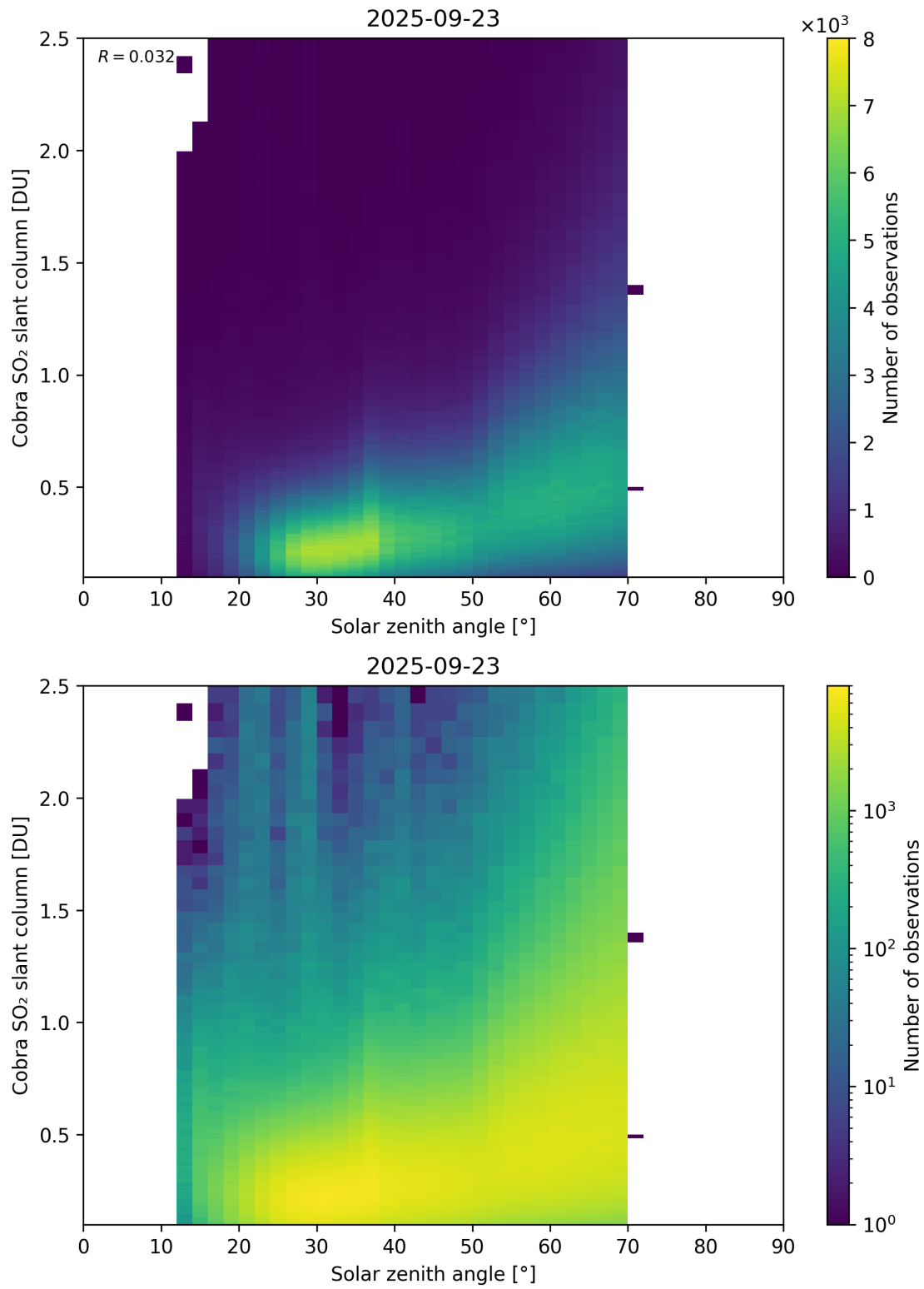
Figure 179: Scatter density plot of “Solar zenith angle” against “Cobra SO 2 slant column” for 2025-09-22 to 2025-09-24.
