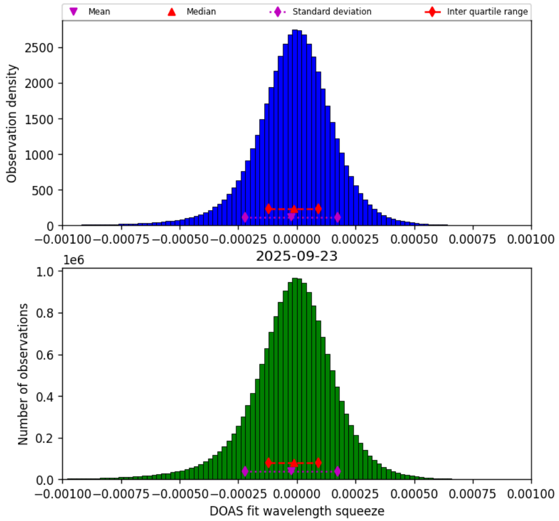
Figure 77: Histogram of “DOAS fit wavelength squeeze” for 2025-09-22 to 2025-09-24
