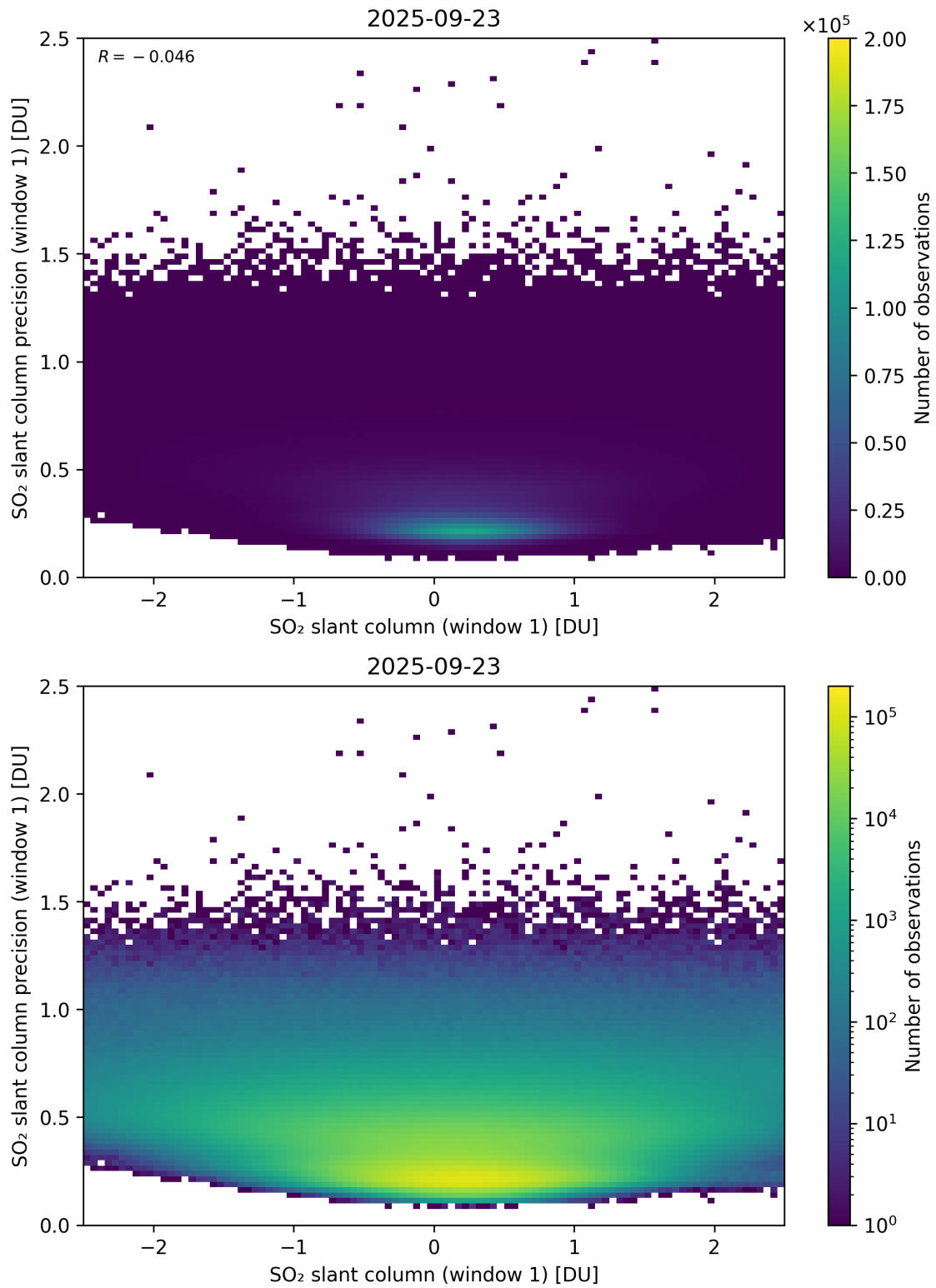
Figure 285: Scatter density plot of “SO 2 slant column (window 1)” against “SO 2 slant column precision (window 1)” for 2025-09-22 to 2025-09-24.
