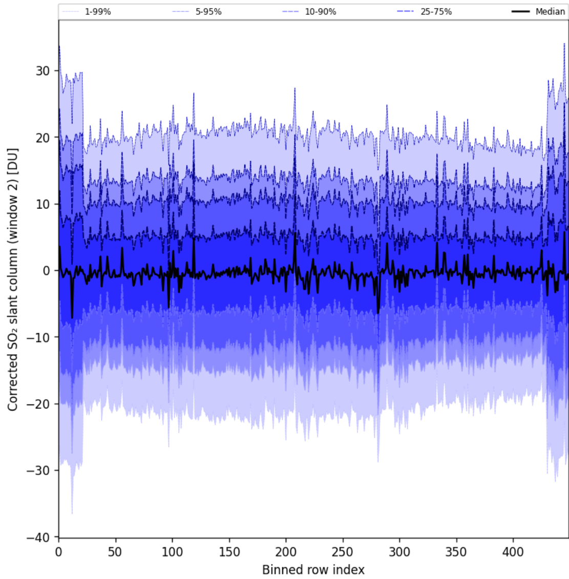
Figure 95: Along track statistics of “Corrected SO 2 slant column (window 2)” for 2025-09-22 to 2025-09-24
