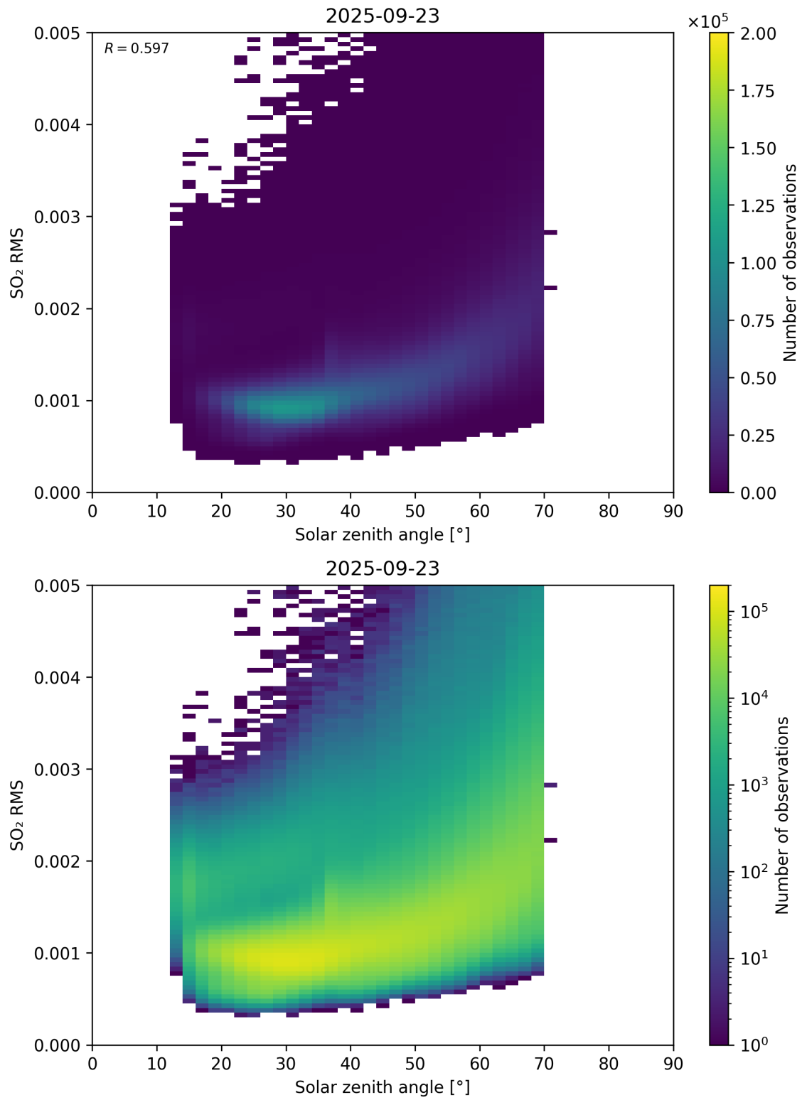
Figure 176: Scatter density plot of “Solar zenith angle” against “SO 2 RMS” for 2025-09-22 to 2025-09-24.
