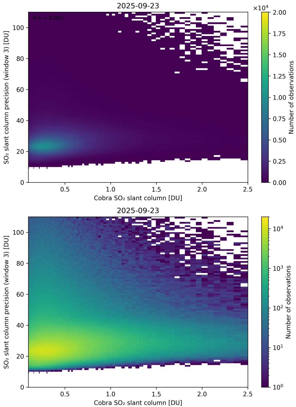
Figure 223: Scatter density plot of “Cobra SO 2 slant column” against “SO 2 slant column precision (window 3)” for 2025-09-22 to 2025-09-24.
