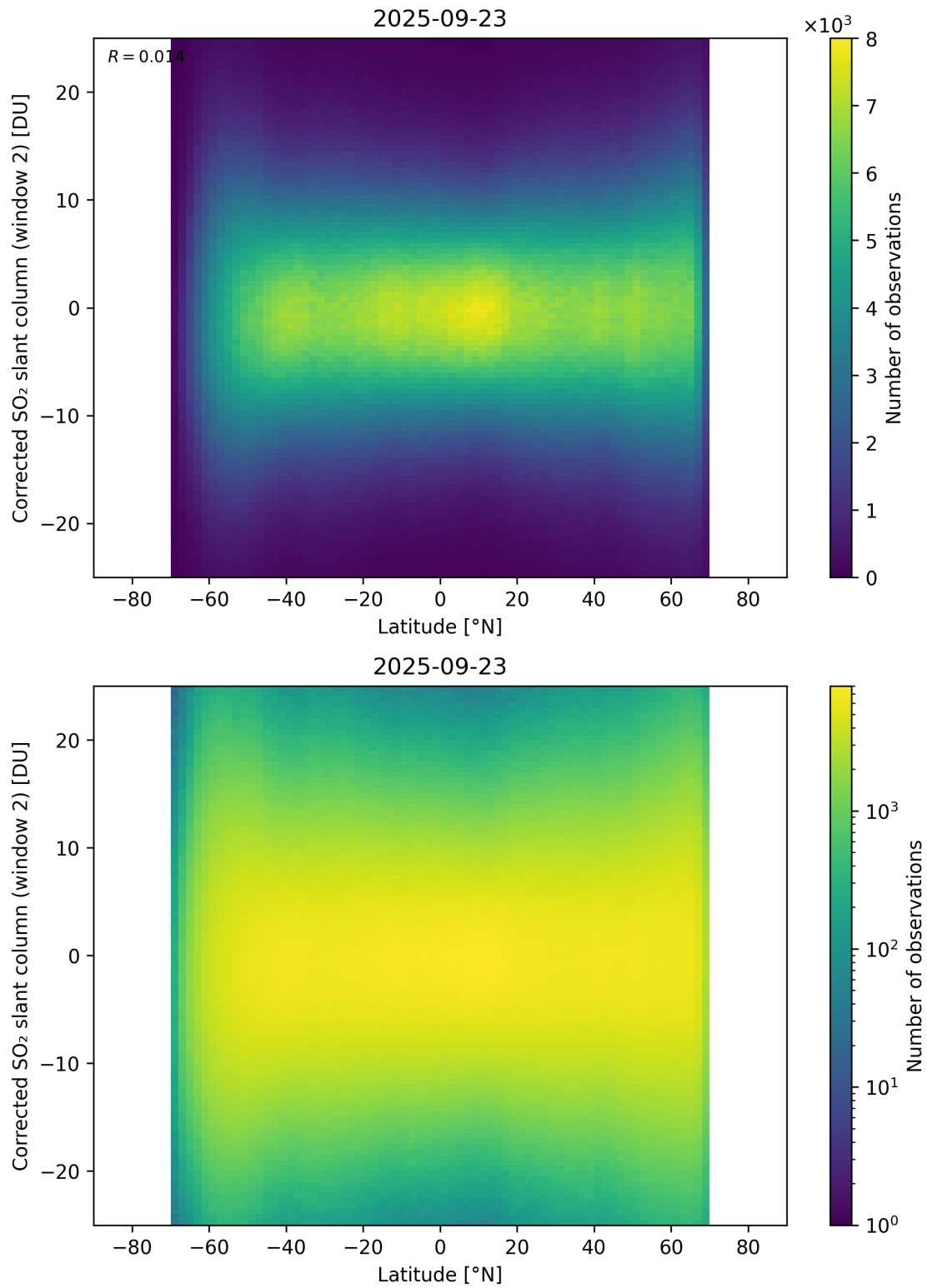
Figure 160: Scatter density plot of “Latitude” against “Corrected SO 2 slant column (window 2)” for 2025-09-22 to 2025-09-24.
