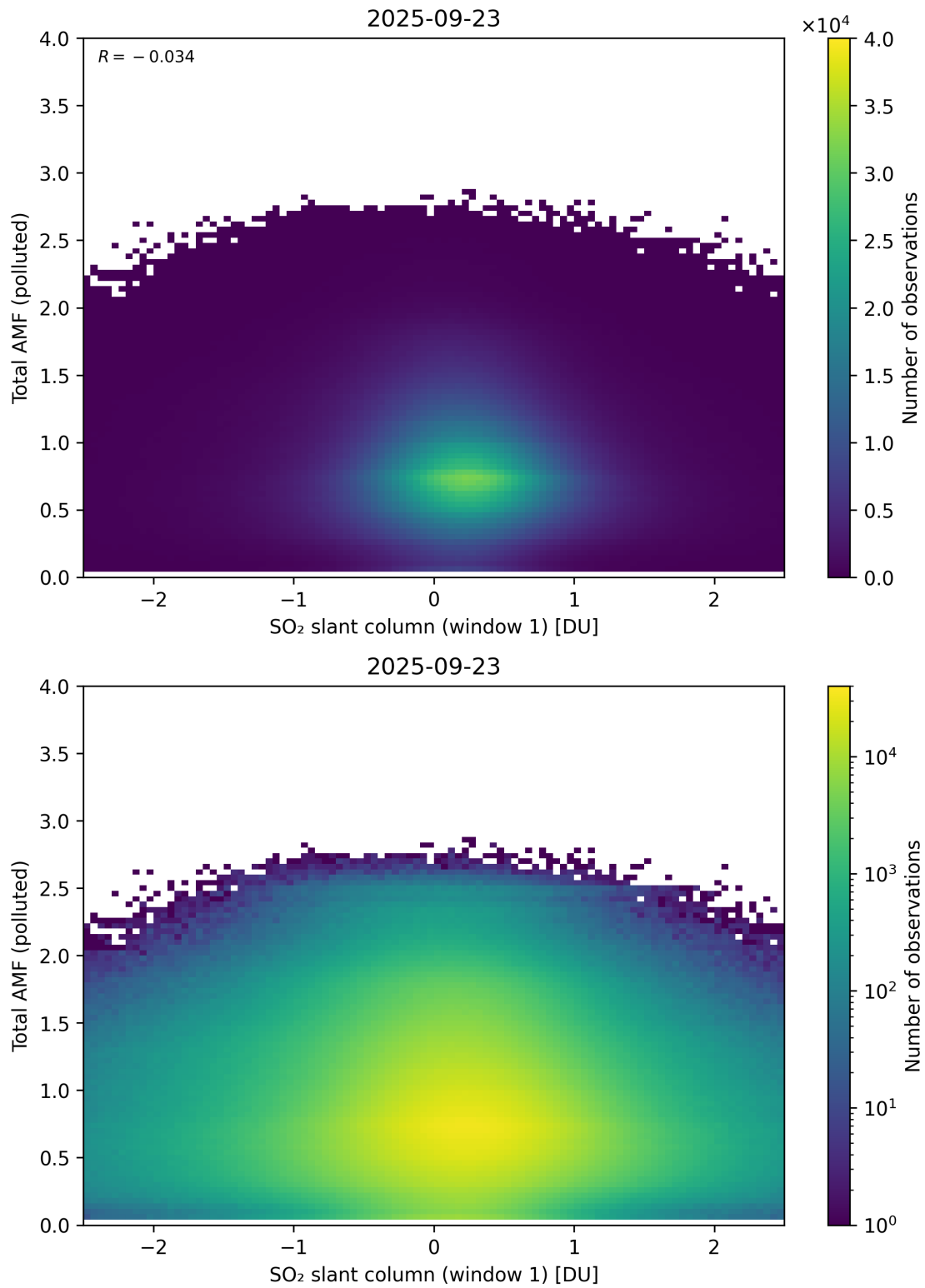
Figure 289: Scatter density plot of “SO 2 slant column (window 1)” against “Total AMF (polluted)” for 2025-09-22 to 2025-09-24.
