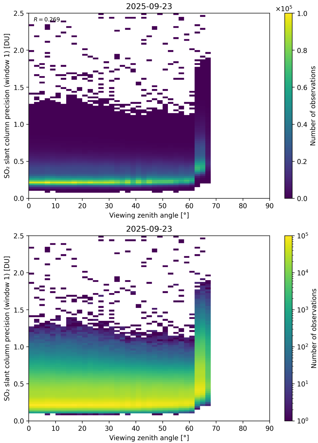
Figure 377: Scatter density plot of “Viewing zenith angle” against “SO 2 slant column precision (window 1)” for 2025-09-22 to 2025-09-24.
