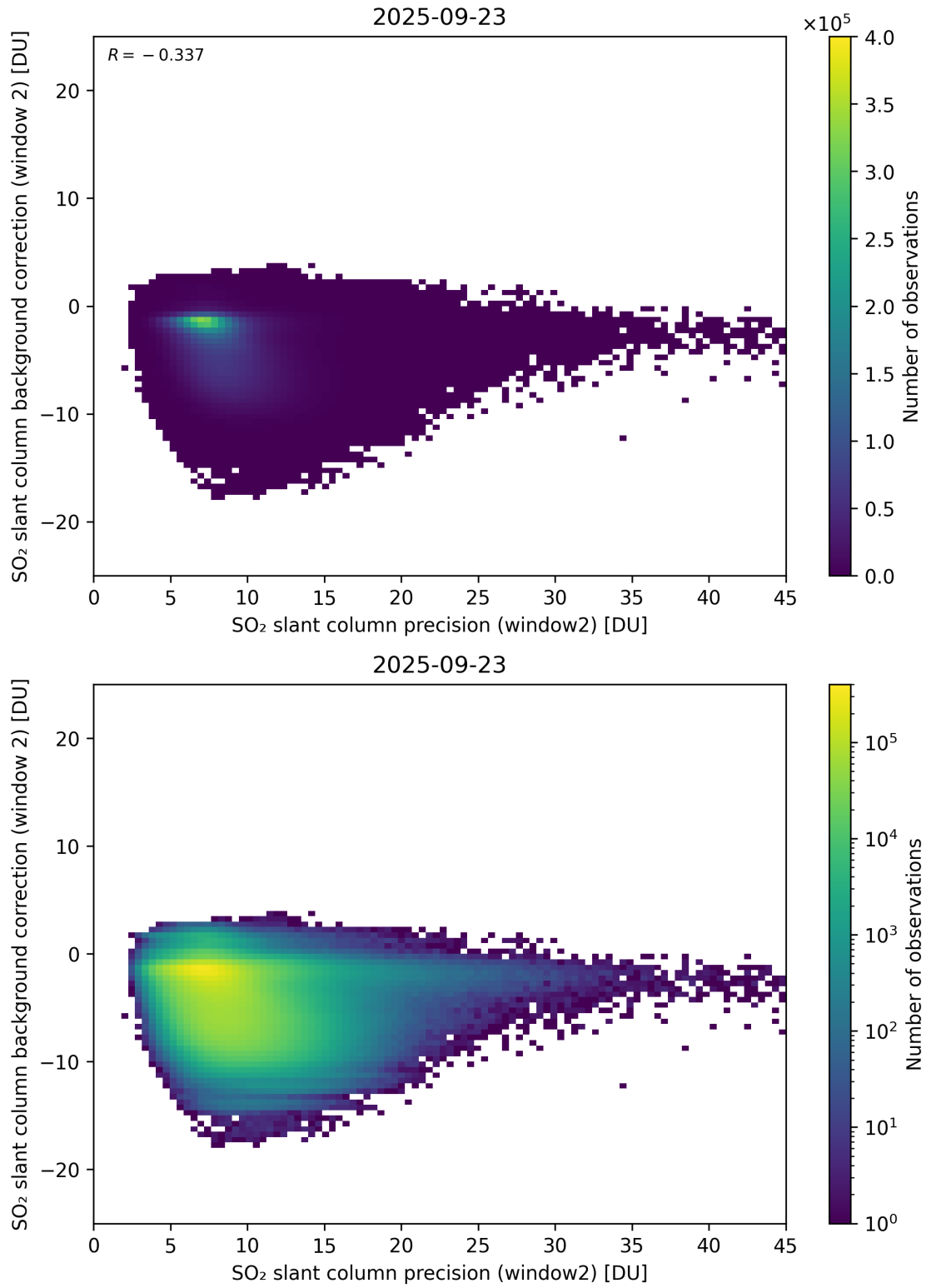
Figure 291: Scatter density plot of “SO 2 slant column precision (window2)” against “SO 2 slant column background correction (window 2)” for 2025-09-22 to 2025-09-24.
