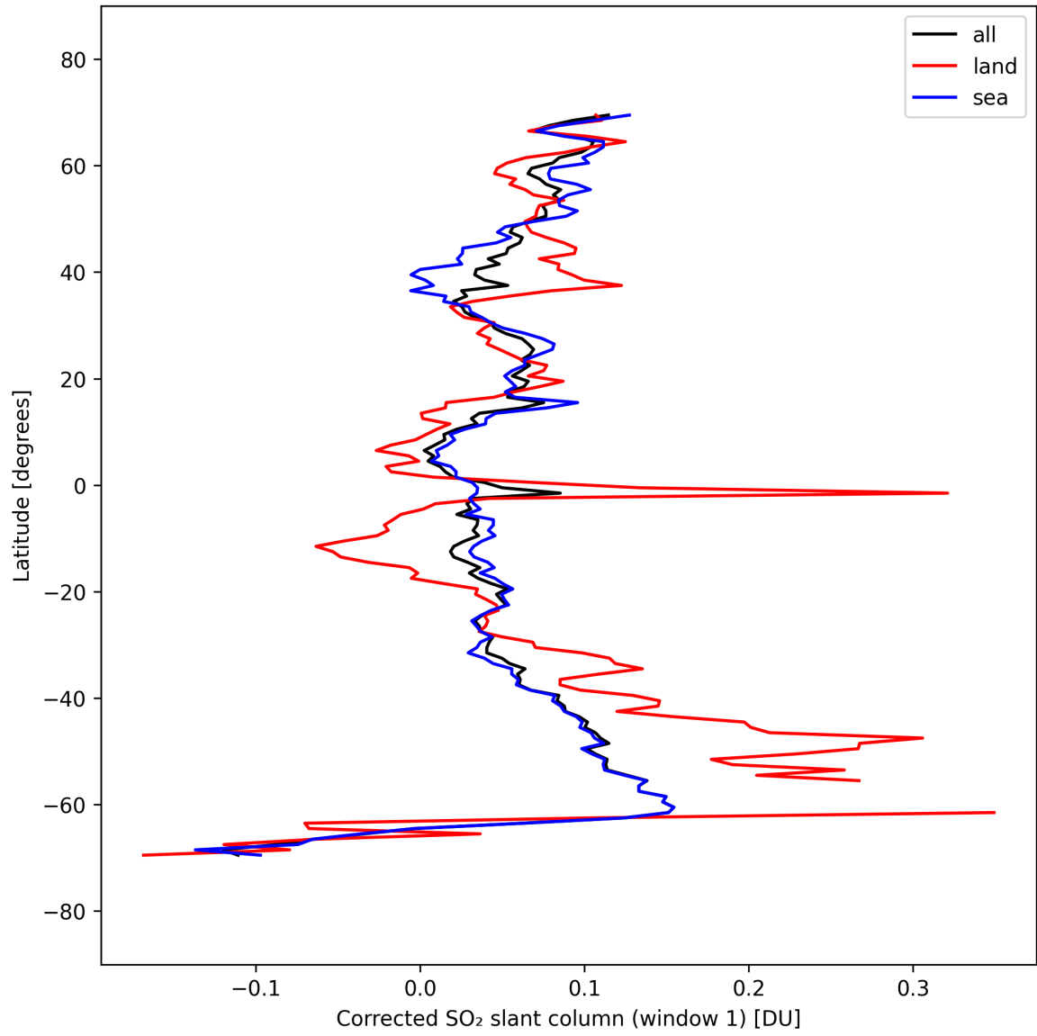
Figure 39: Zonal average of “Corrected SO 2 slant column (window 1)” for 2025-09-22 to 2025-09-24.
