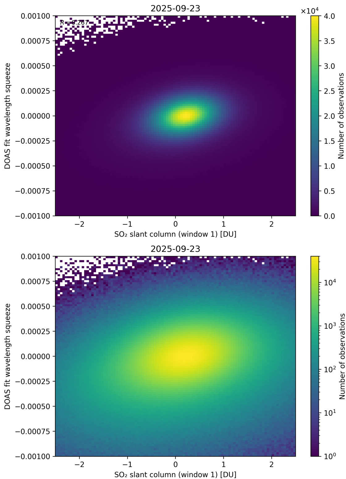
Figure 266: Scatter density plot of “SO 2 slant column (window 1)” against “DOAS fit wavelength squeeze” for 2025-09-22 to 2025-09-24.
