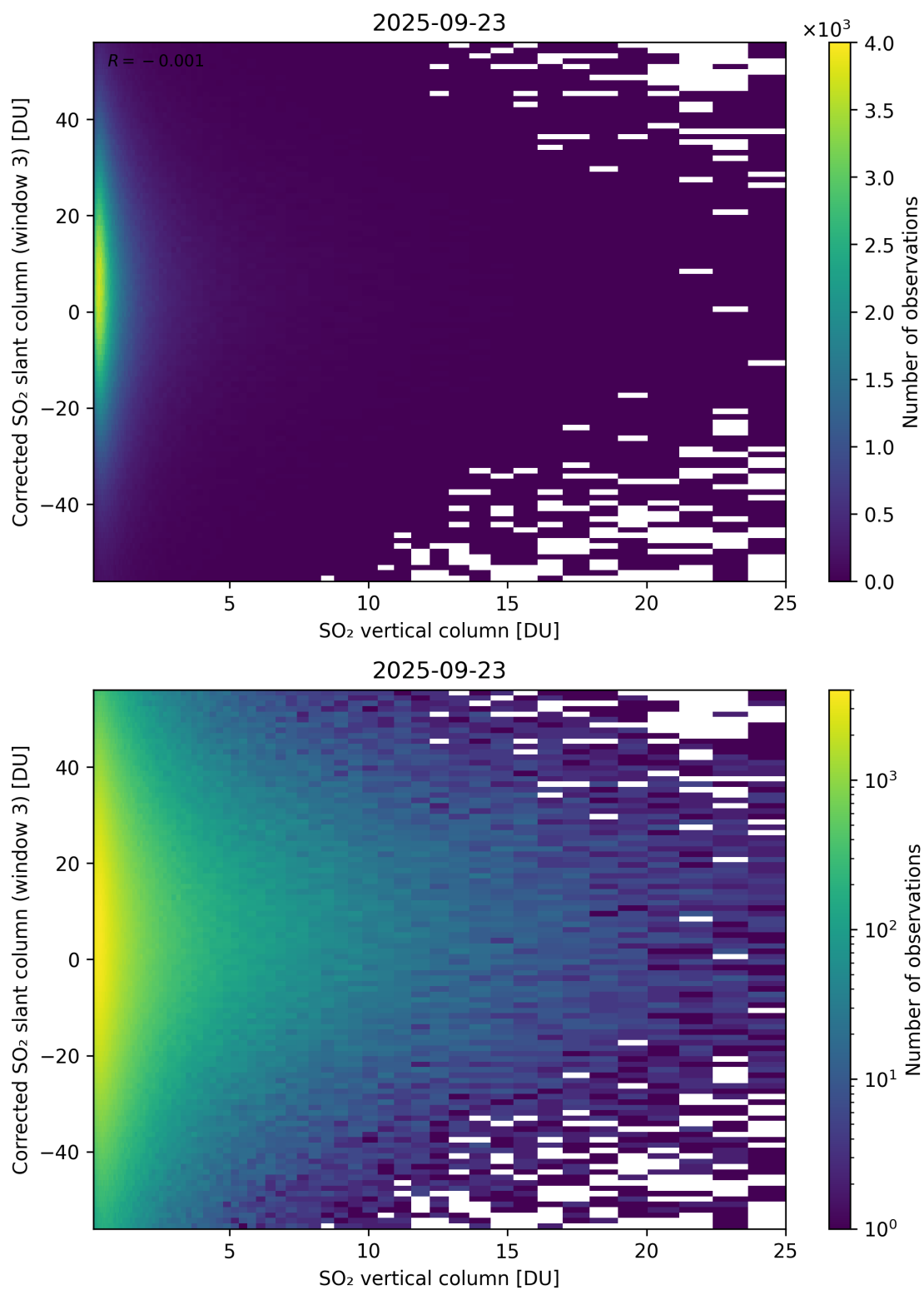
Figure 353: Scatter density plot of “SO 2 vertical column” against “Corrected SO 2 slant column (window 3)” for 2025-09-22 to 2025-09-24.
