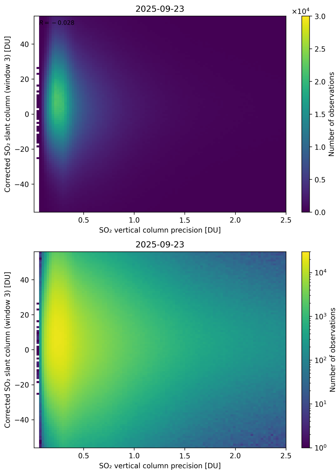
Figure 340: Scatter density plot of “SO 2 vertical column precision” against “Corrected SO 2 slant column (window 3)” for 2025-09-22 to 2025-09-24.
