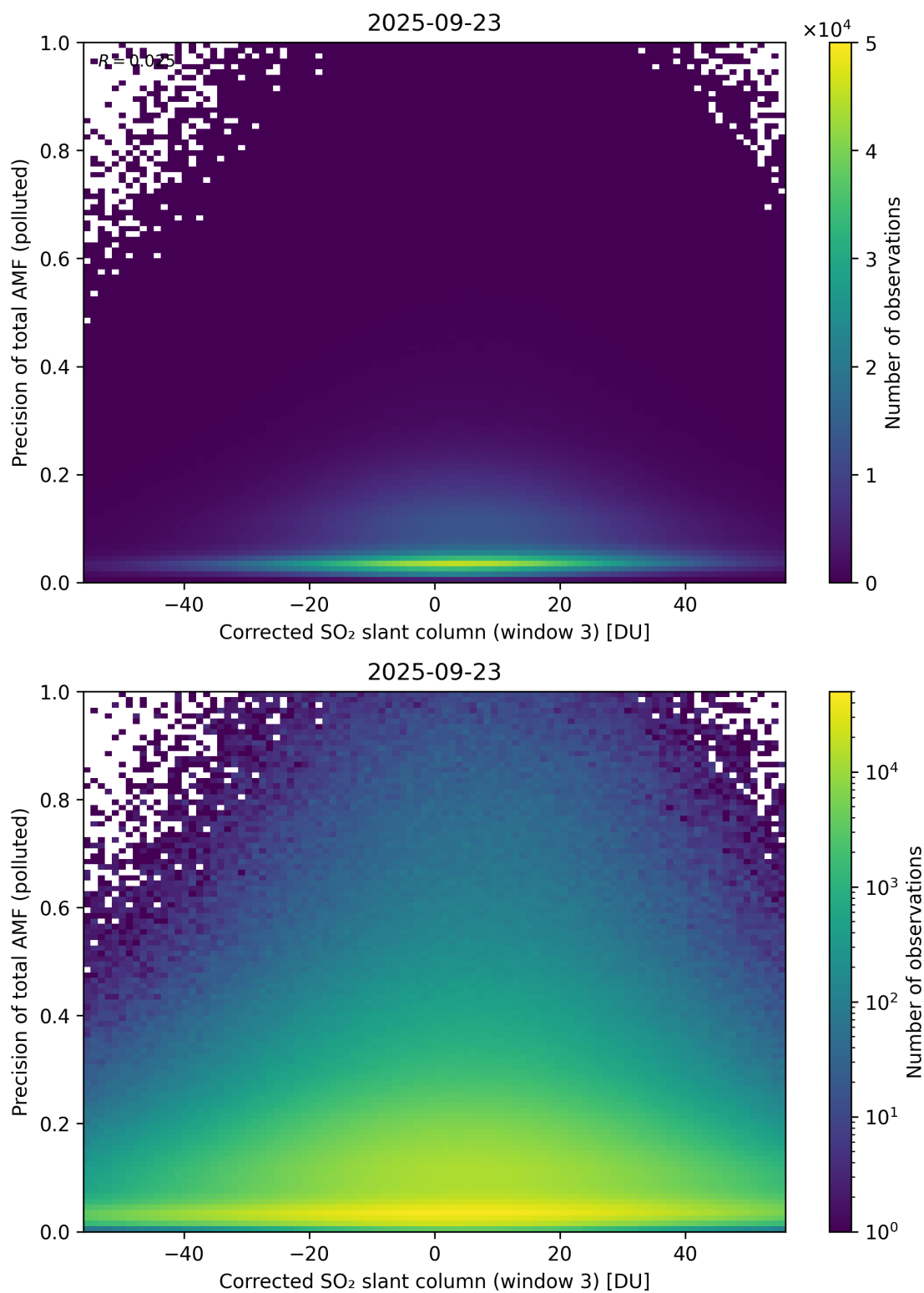
Figure 261: Scatter density plot of “Corrected SO 2 slant column (window 3)” against “Precision of total AMF (polluted)” for 2025-09-22 to 2025-09-24.
