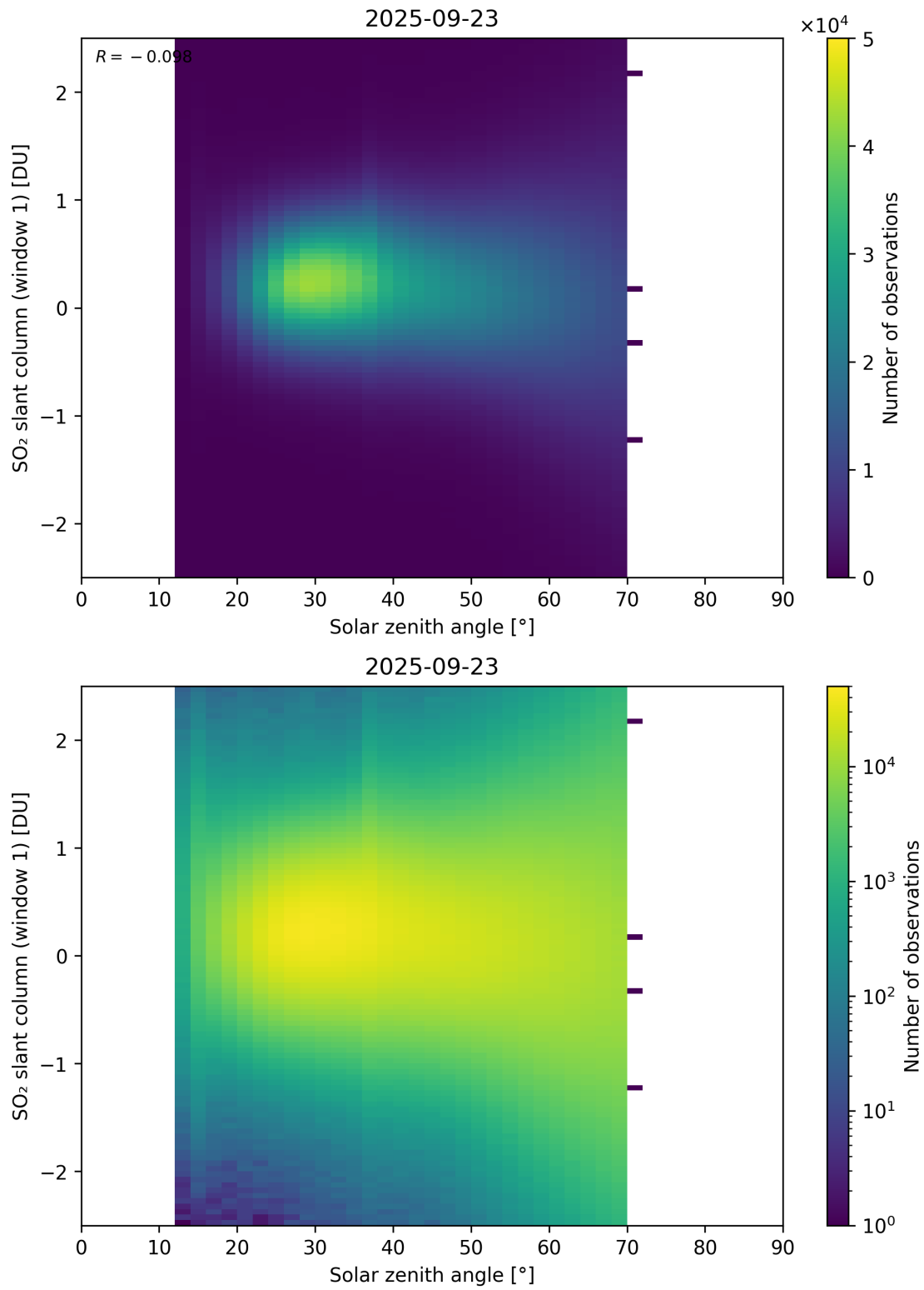
Figure 184: Scatter density plot of “Solar zenith angle” against “SO 2 slant column (window 1)” for 2025-09-22 to 2025-09-24.
