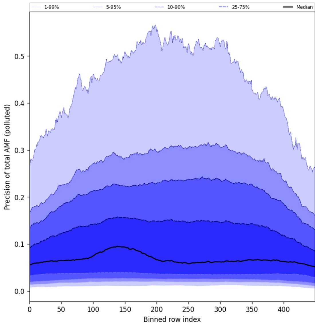
Figure 106: Along track statistics of “Precision of total AMF (polluted)” for 2025-09-22 to 2025-09-24
