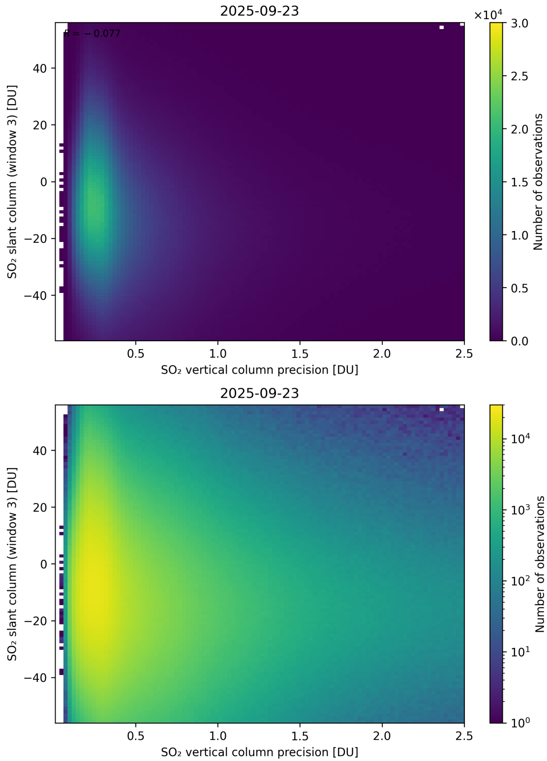
Figure 344: Scatter density plot of “SO 2 vertical column precision” against “SO 2 slant column (window 3)” for 2025-09-22 to 2025-09-24.
