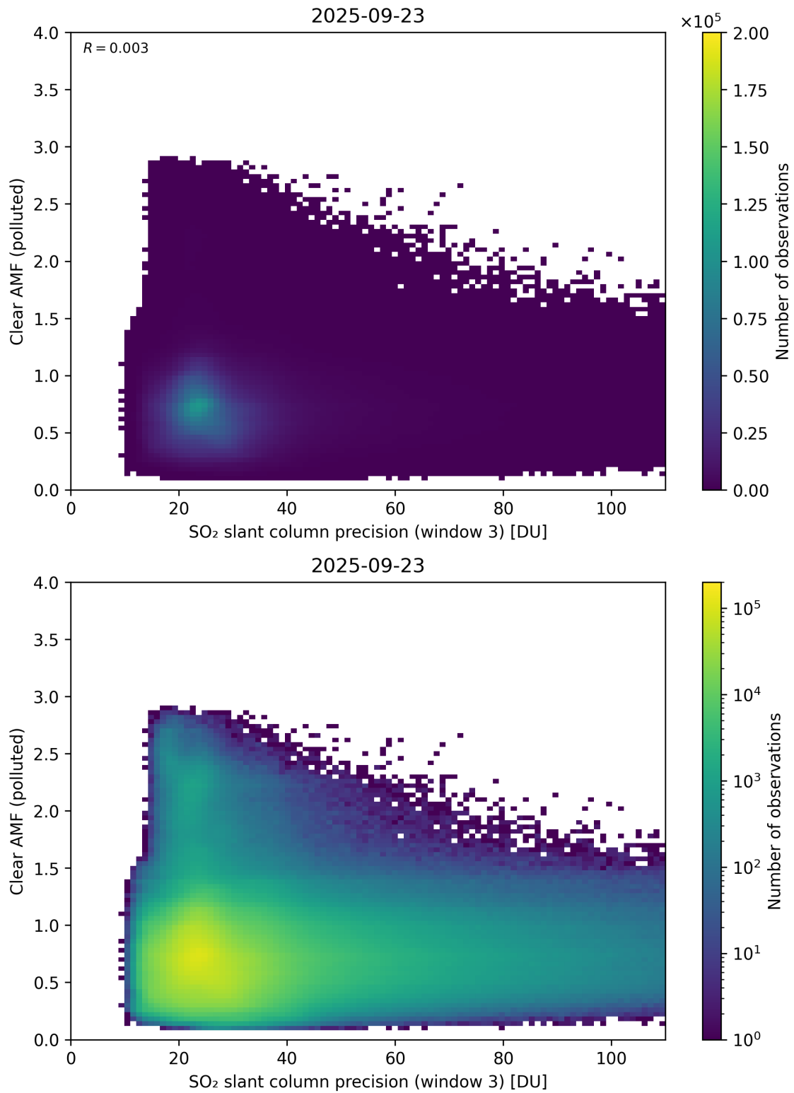
Figure 311: Scatter density plot of “SO 2 slant column precision (window 3)” against “Clear AMF (polluted)” for 2025-09-22 to 2025-09-24.
