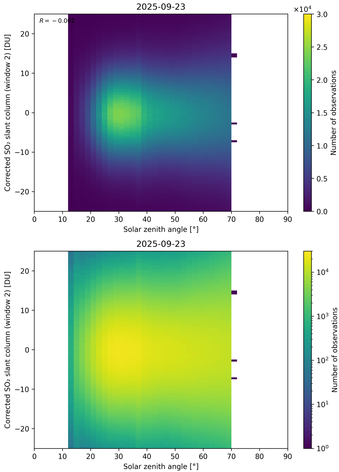
Figure 182: Scatter density plot of “Solar zenith angle” against “Corrected SO 2 slant column (window 2)” for 2025-09-22 to 2025-09-24.
