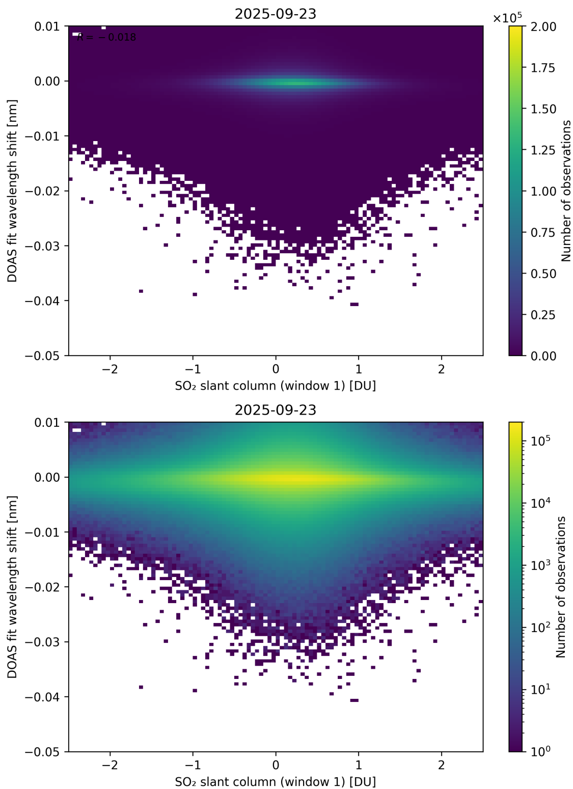
Figure 265: Scatter density plot of “SO 2 slant column (window 1)” against “DOAS fit wavelength shift” for 2025-09-22 to 2025-09-24.
