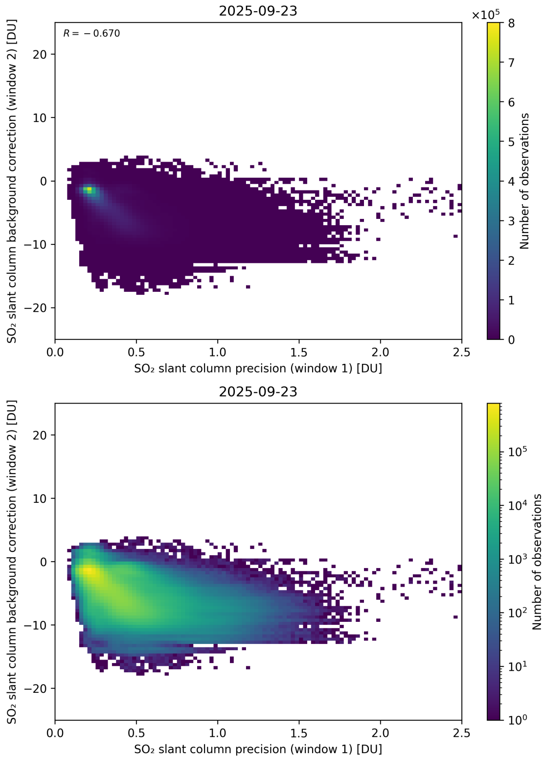
Figure 269: Scatter density plot of “SO 2 slant column precision (window 1)” against “SO 2 slant column background correction (window 2)” for 2025-09-22 to 2025-09-24.
