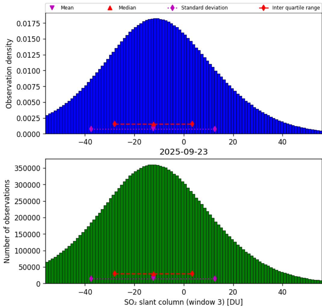
Figure 71: Histogram of “SO 2 slant column (window 3)” for 2025-09-22 to 2025-09-24
