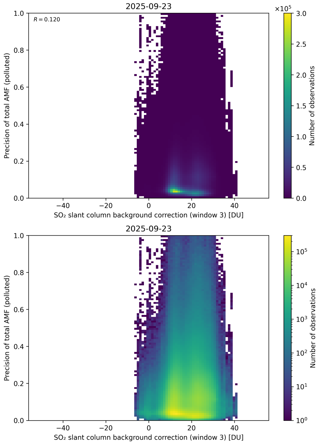
Figure 137: Scatter density plot of “SO 2 slant column background correction (window 3)” against “Precision of total AMF (polluted)” for 2025-09-22 to 2025-09-24.
