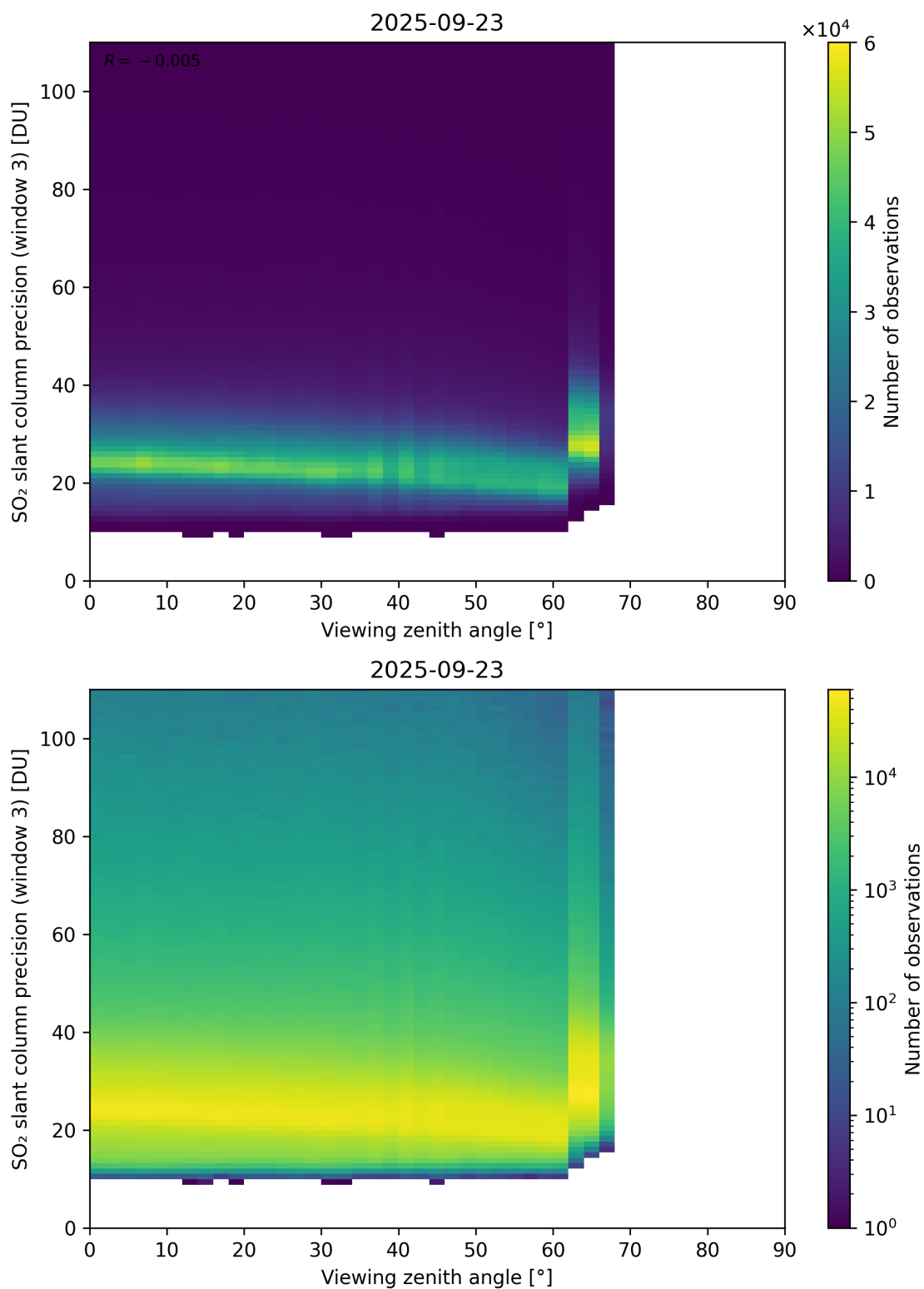
Figure 380: Scatter density plot of “Viewing zenith angle” against “SO 2 slant column precision (window 3)” for 2025-09-22 to 2025-09-24.
