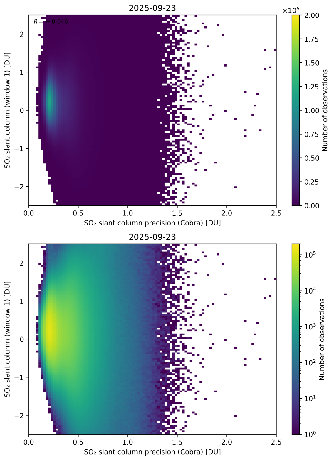
Figure 208: Scatter density plot of “SO 2 slant column precision (Cobra)” against “SO 2 slant column (window 1)” for 2025-09-22 to 2025-09-24.
