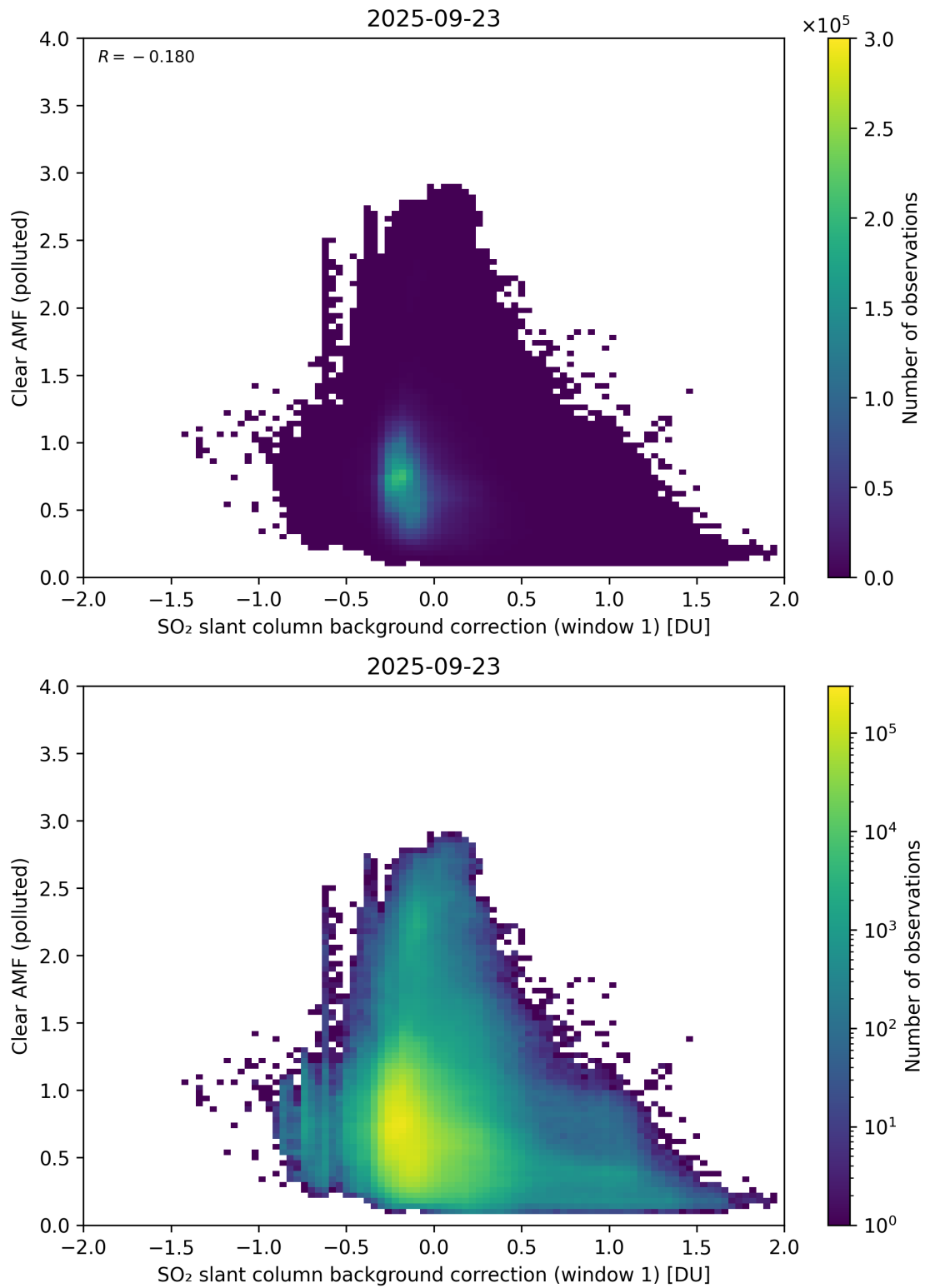
Figure 114: Scatter density plot of “SO 2 slant column background correction (window 1)” against “Clear AMF (polluted)” for 2025-09-22 to 2025-09-24.
