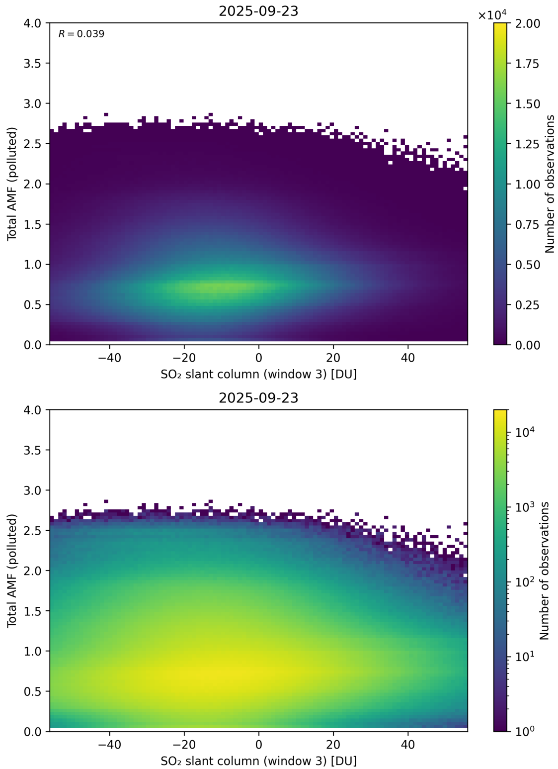
Figure 318: Scatter density plot of “SO 2 slant column (window 3)” against “Total AMF (polluted)” for 2025-09-22 to 2025-09-24.
