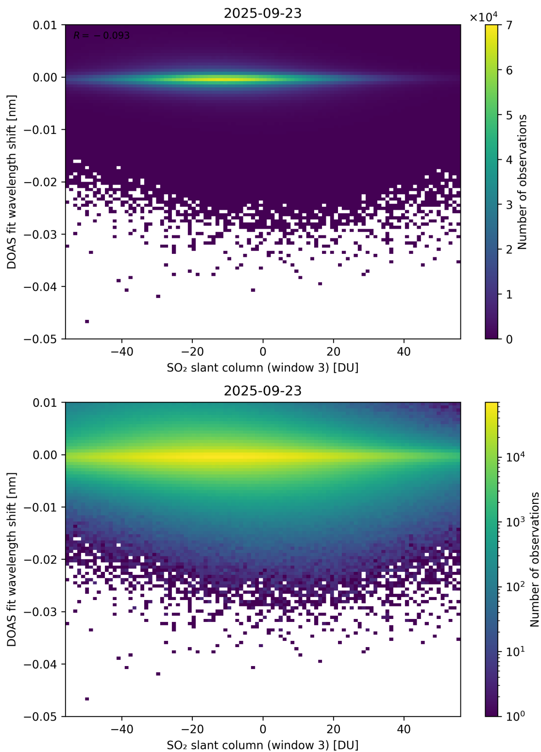
Figure 304: Scatter density plot of “SO 2 slant column (window 3)” against “DOAS fit wavelength shift” for 2025-09-22 to 2025-09-24.
