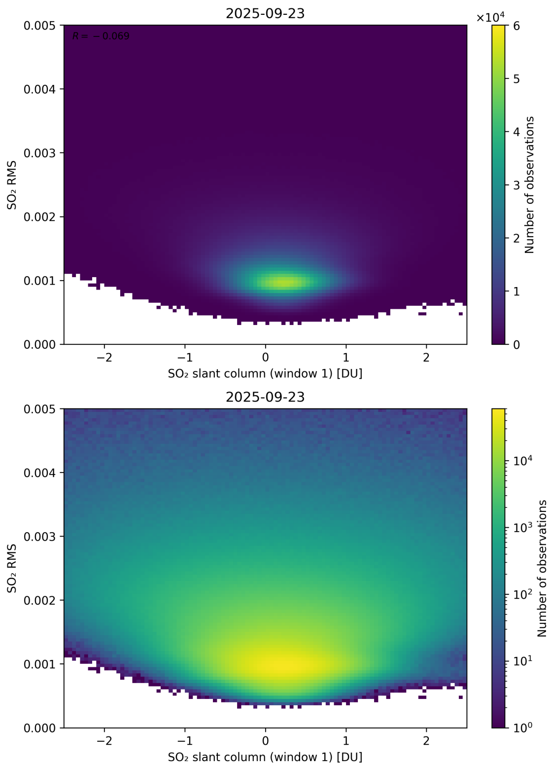
Figure 267: Scatter density plot of “SO 2 slant column (window 1)” against “SO 2 RMS” for 2025-09-22 to 2025-09-24.
