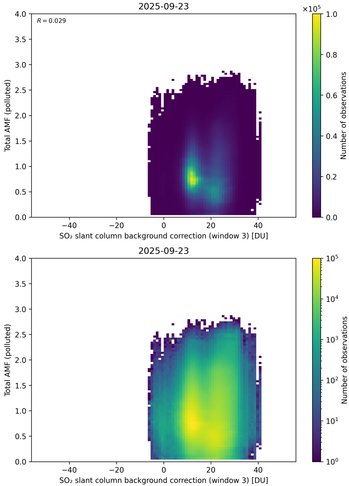
Figure 136: Scatter density plot of “SO 2 slant column background correction (window 3)” against “Total AMF (polluted)” for 2025-09-22 to 2025-09-24.
