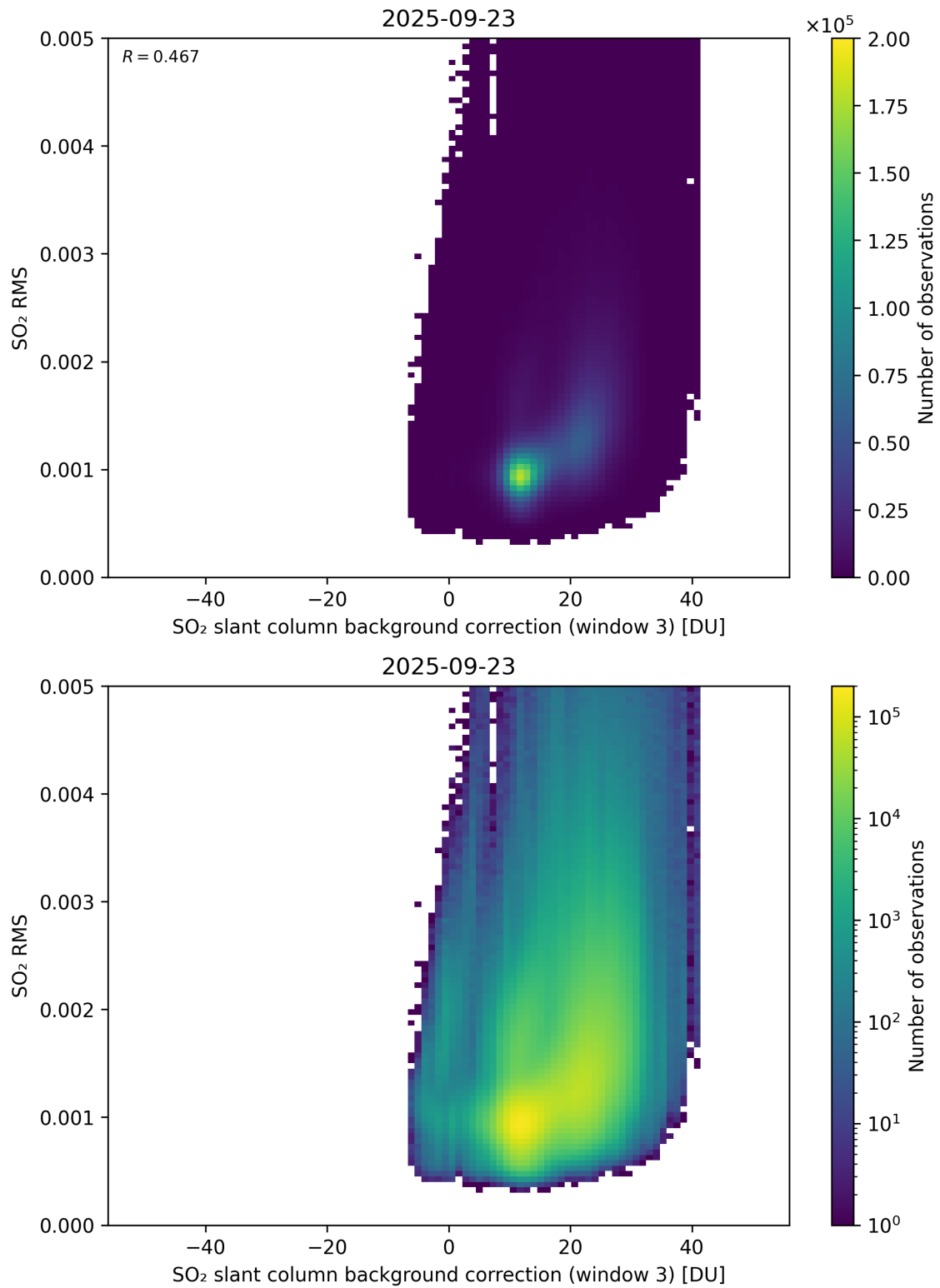
Figure 134: Scatter density plot of “SO 2 slant column background correction (window 3)” against “SO 2 RMS” for 2025-09-22 to 2025-09-24.
