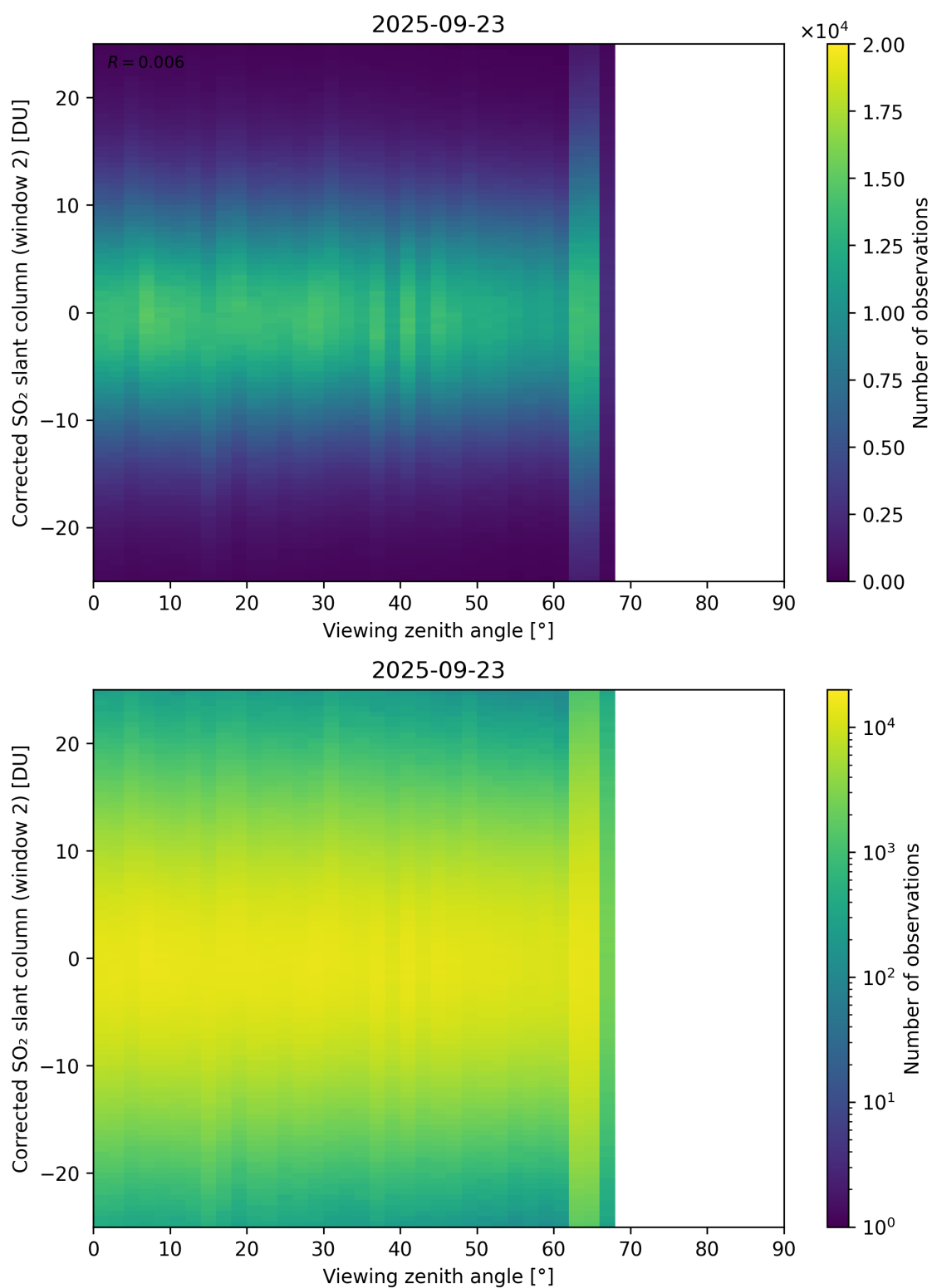
Figure 374: Scatter density plot of “Viewing zenith angle” against “Corrected SO 2 slant column (window 2)” for 2025-09-22 to 2025-09-24.
