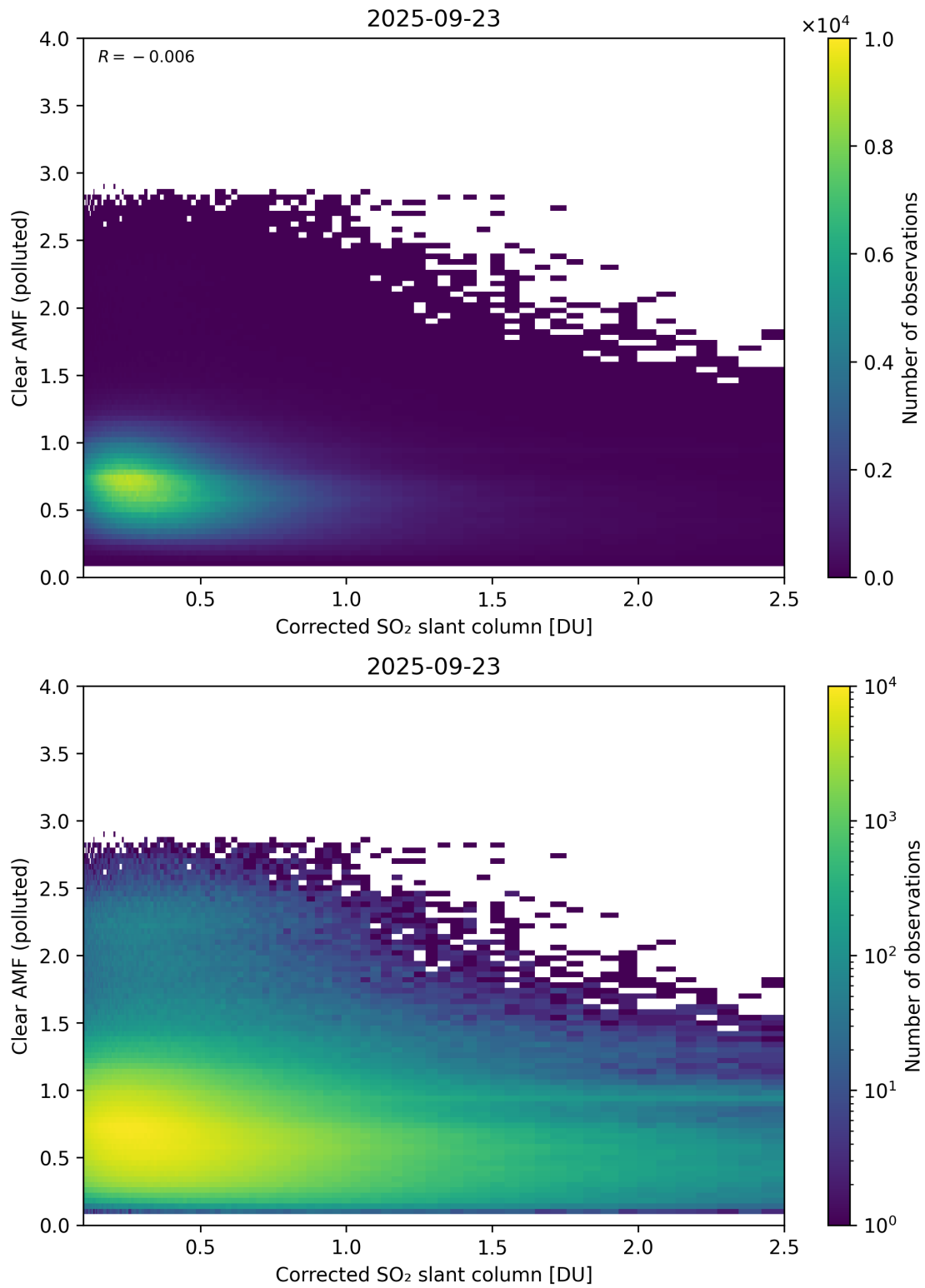
Figure 232: Scatter density plot of “Corrected SO 2 slant column” against “Clear AMF (polluted)” for 2025-09-22 to 2025-09-24.
