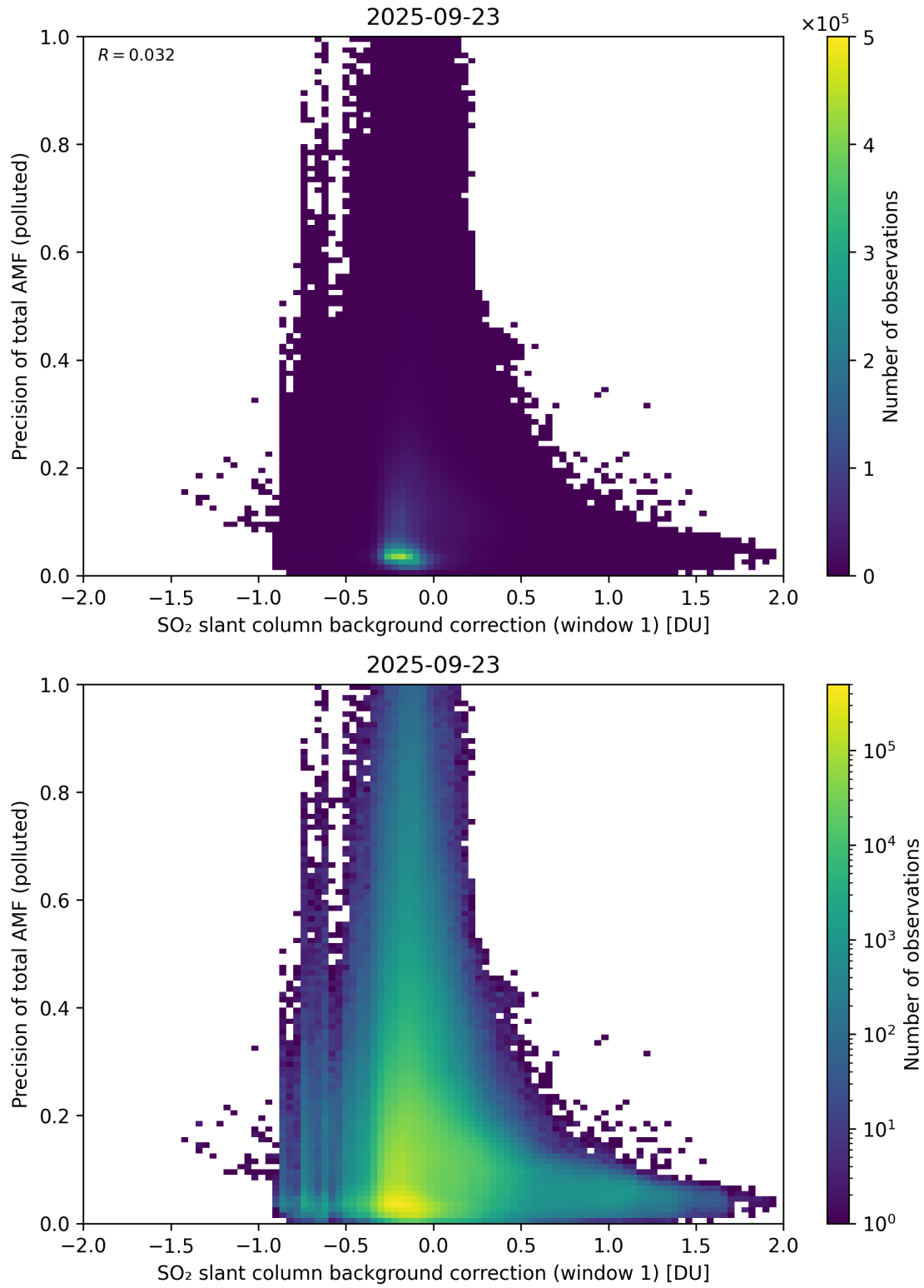
Figure 121: Scatter density plot of “SO 2 slant column background correction (window 1)” against “Precision of total AMF (polluted)” for 2025-09-22 to 2025-09-24.
