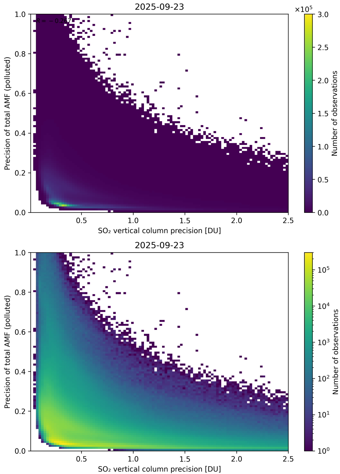
Figure 347: Scatter density plot of “SO 2 vertical column precision” against “Precision of total AMF (polluted)” for 2025-09-22 to 2025-09-24.
