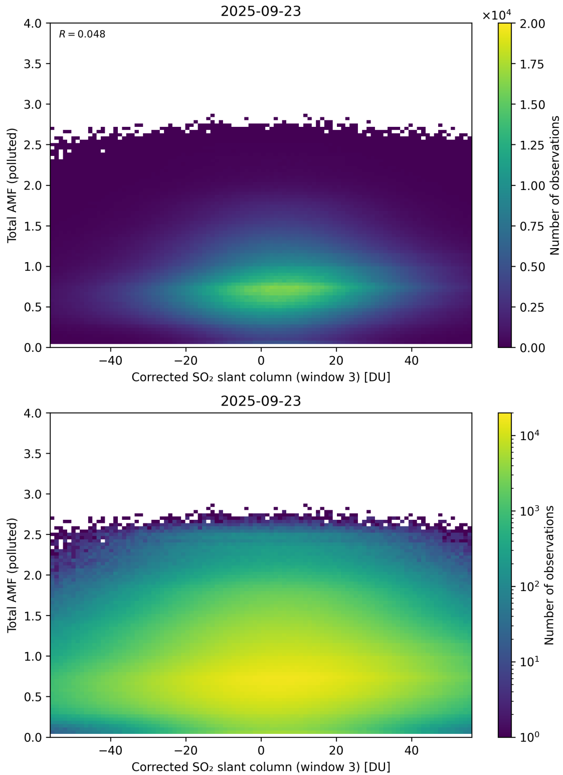
Figure 260: Scatter density plot of “Corrected SO 2 slant column (window 3)” against “Total AMF (polluted)” for 2025-09-22 to 2025-09-24.
