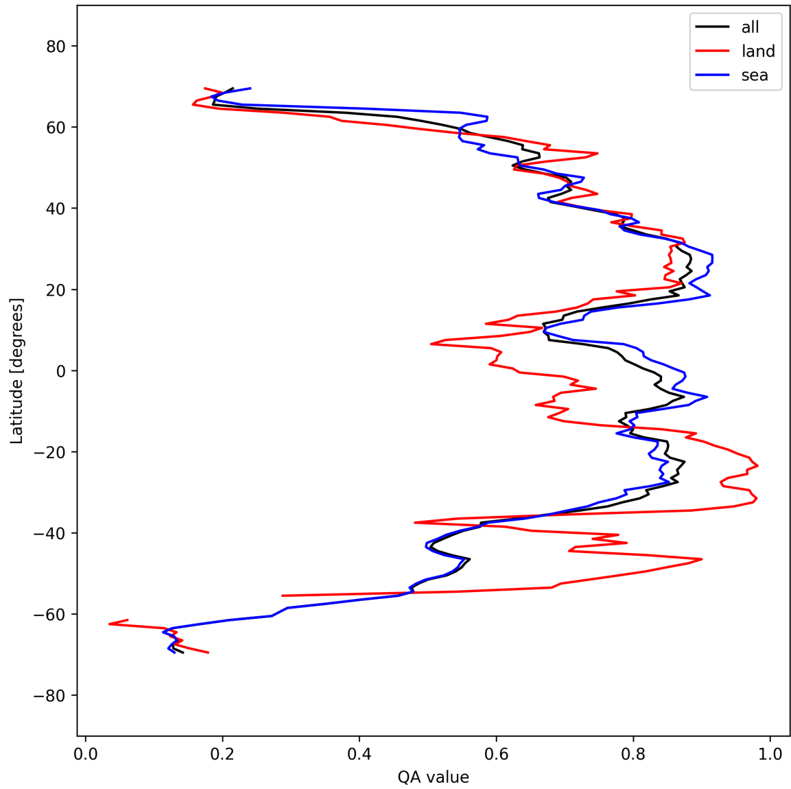
Figure 31: Zonal average of “QA value” for 2025-09-22 to 2025-09-24.
