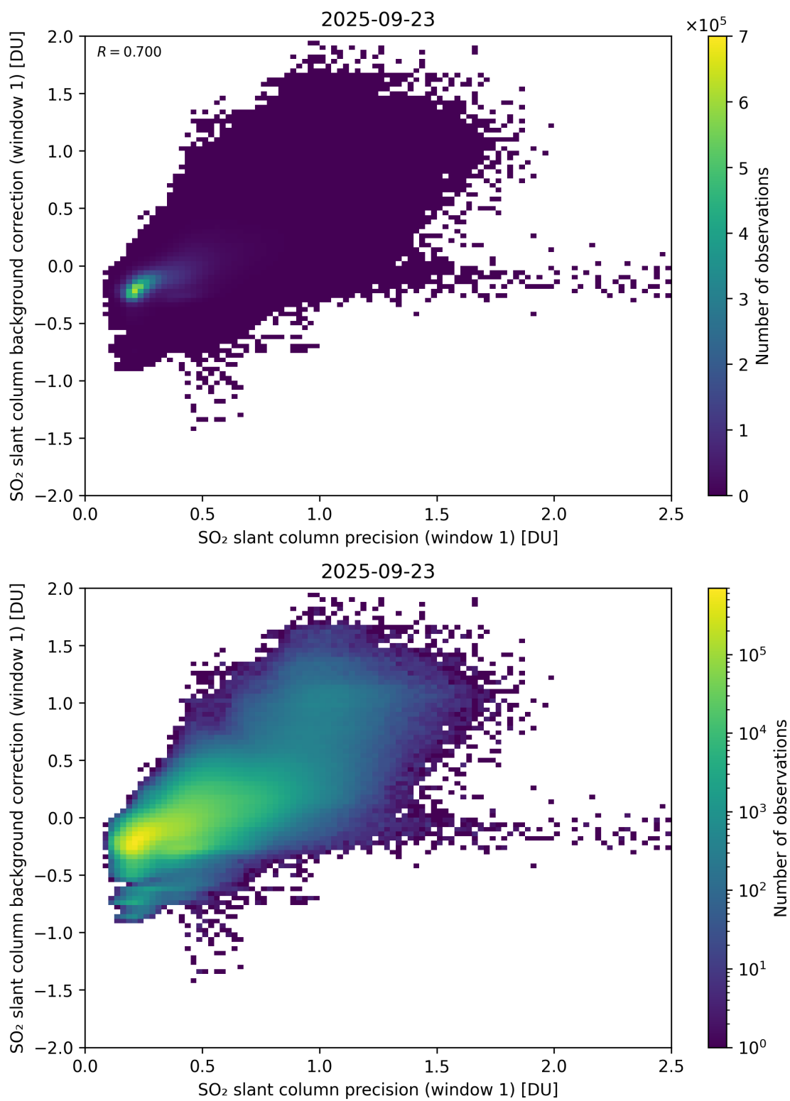
Figure 268: Scatter density plot of “SO 2 slant column precision (window 1)” against “SO 2 slant column background correction (window 1)” for 2025-09-22 to 2025-09-24.
