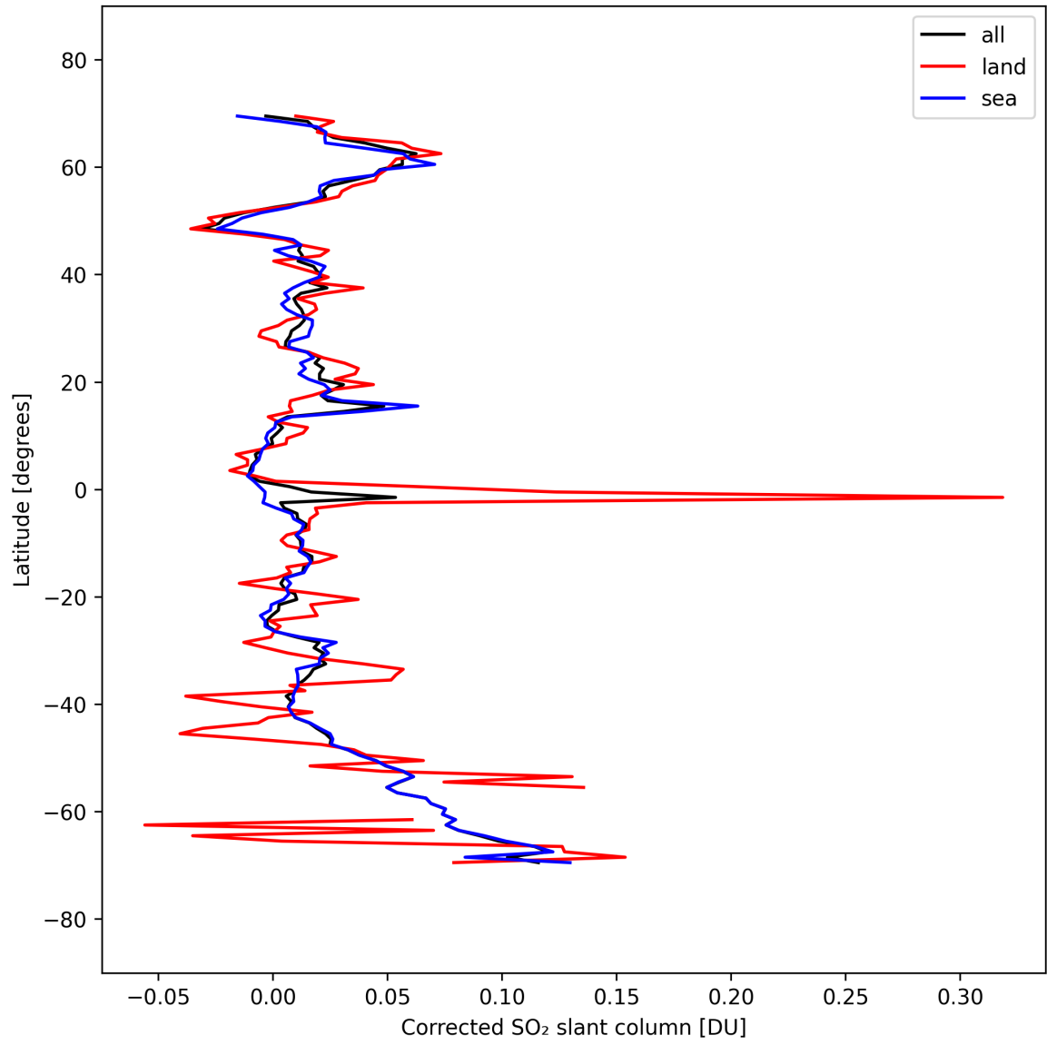
Figure 34: Zonal average of “Corrected SO 2 slant column” for 2025-09-22 to 2025-09-24.
