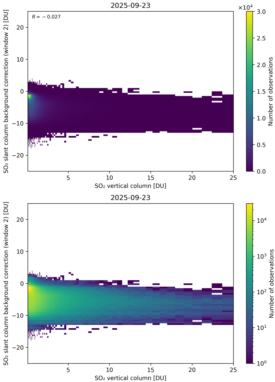
Figure 324: Scatter density plot of “SO 2 vertical column” against “SO 2 slant column background correction (window 2)” for 2025-09-22 to 2025-09-24.
