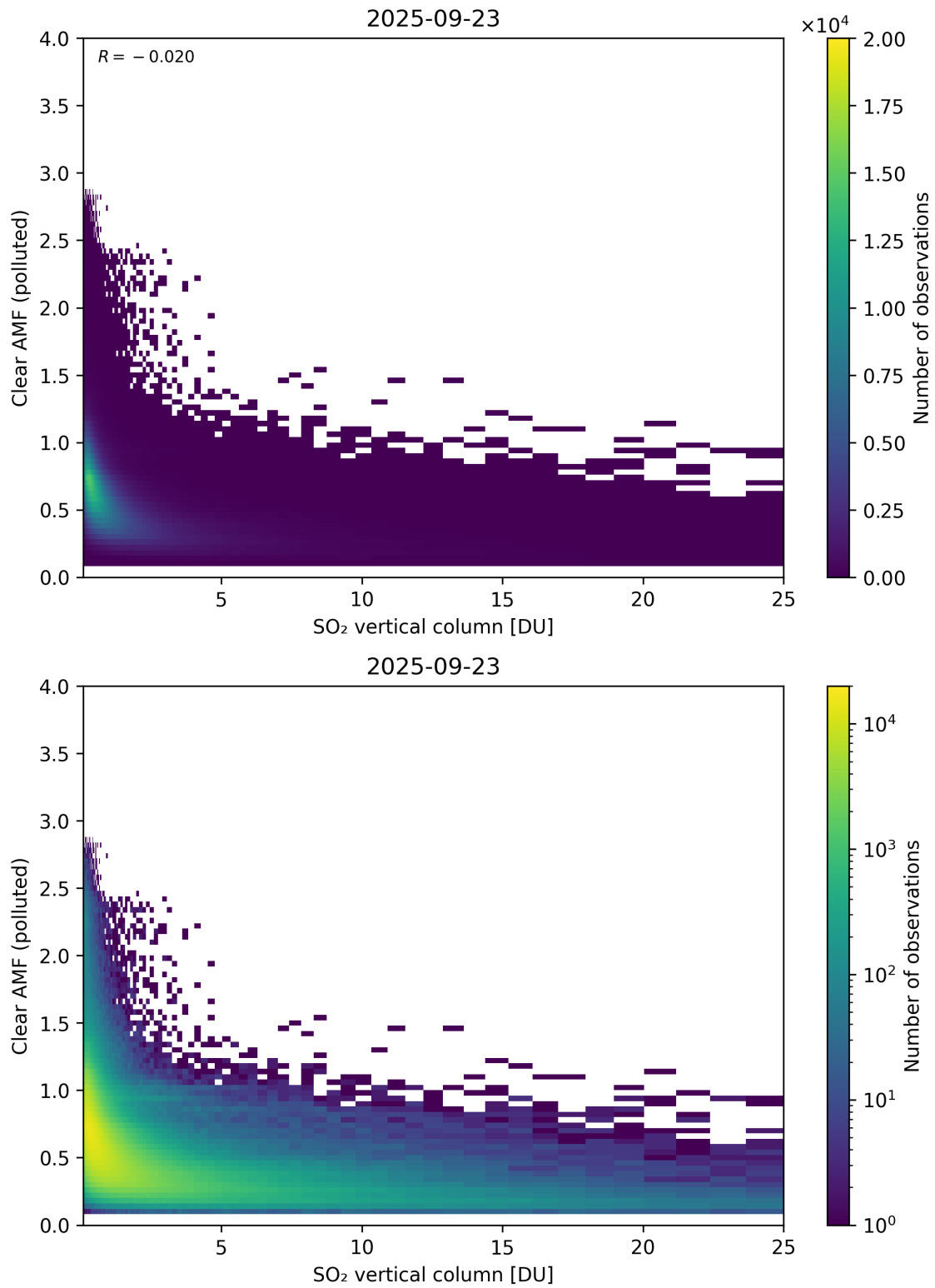
Figure 348: Scatter density plot of “SO 2 vertical column” against “Clear AMF (polluted)” for 2025-09-22 to 2025-09-24.
