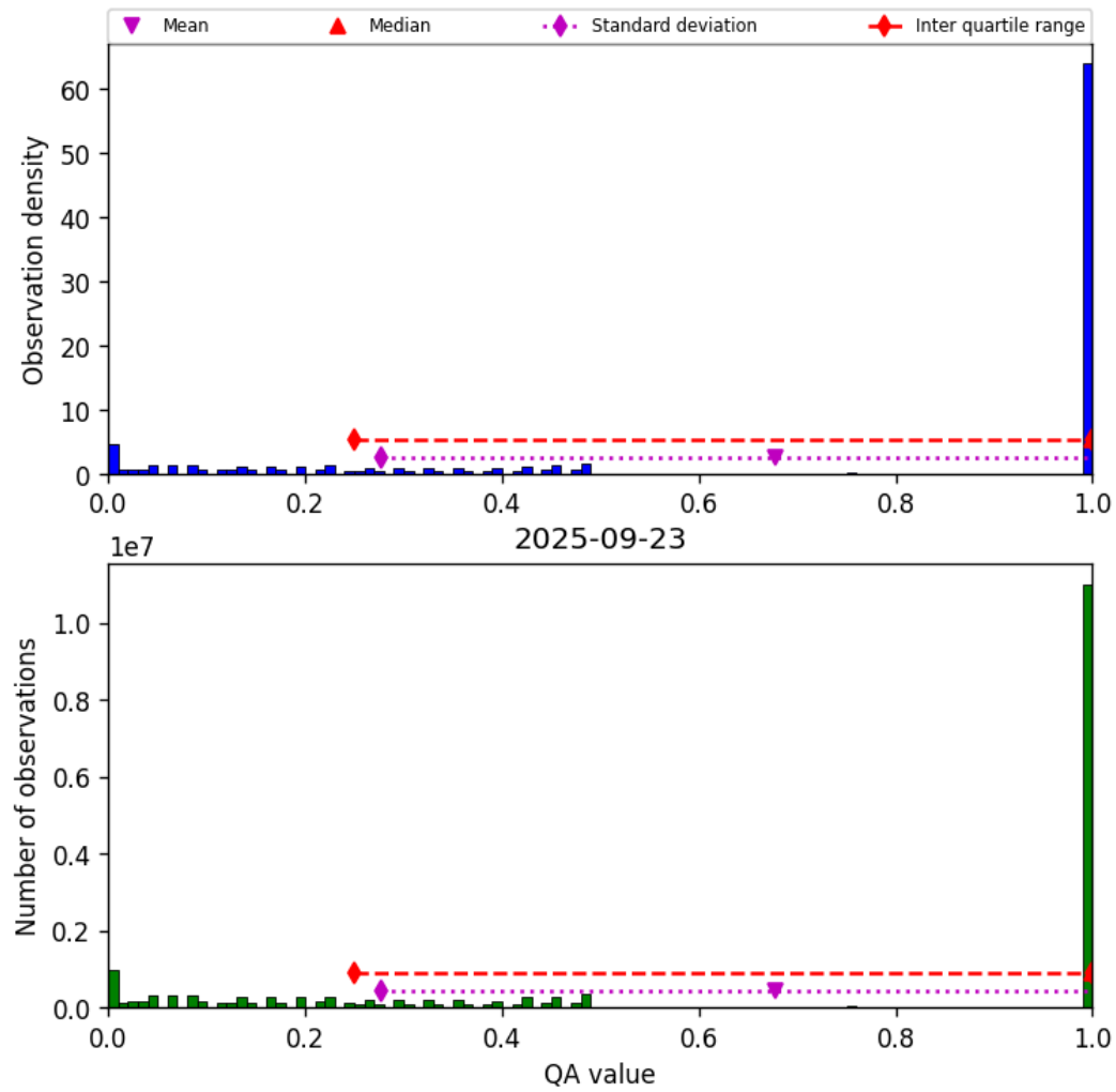
Figure 57: Histogram of “QA value” for 2025-09-22 to 2025-09-24
