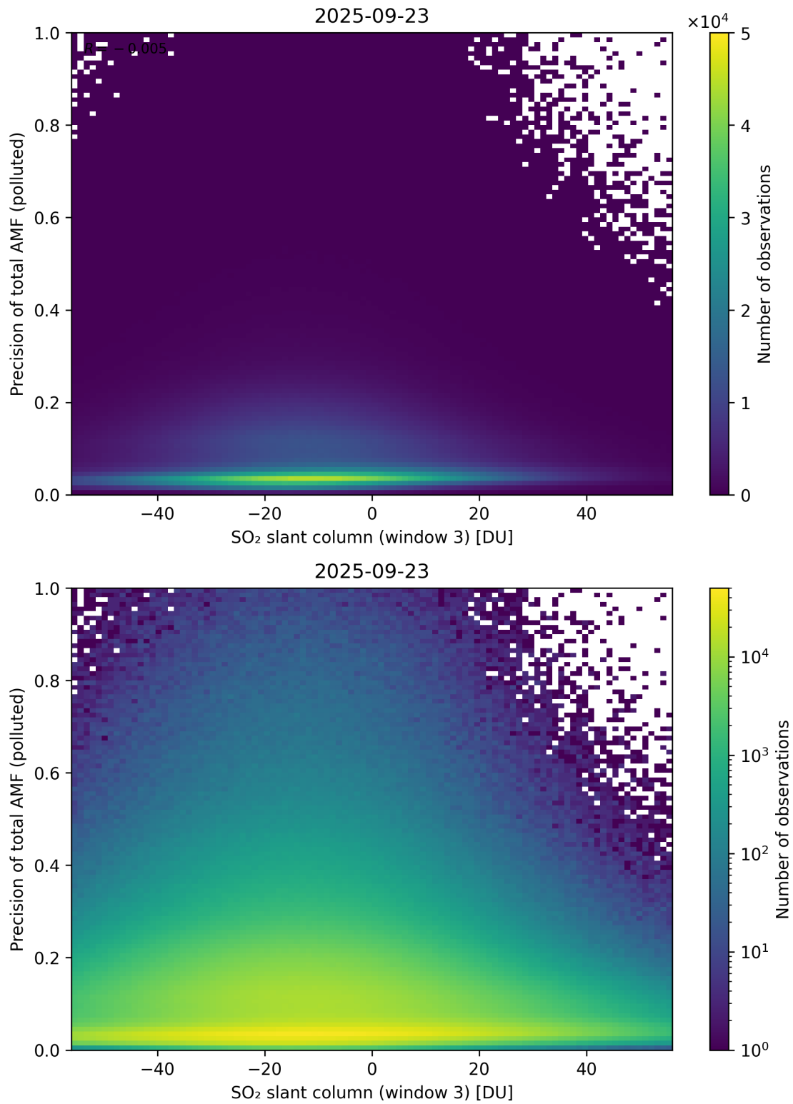
Figure 319: Scatter density plot of “SO 2 slant column (window 3)” against “Precision of total AMF (polluted)” for 2025-09-22 to 2025-09-24.
