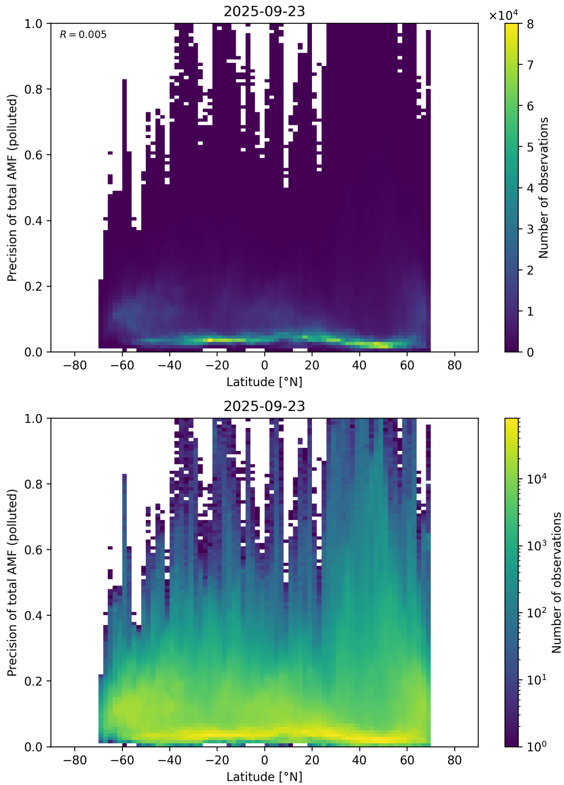
Figure 168: Scatter density plot of “Latitude” against “Precision of total AMF (polluted)” for 2025-09-22 to 2025-09-24.
