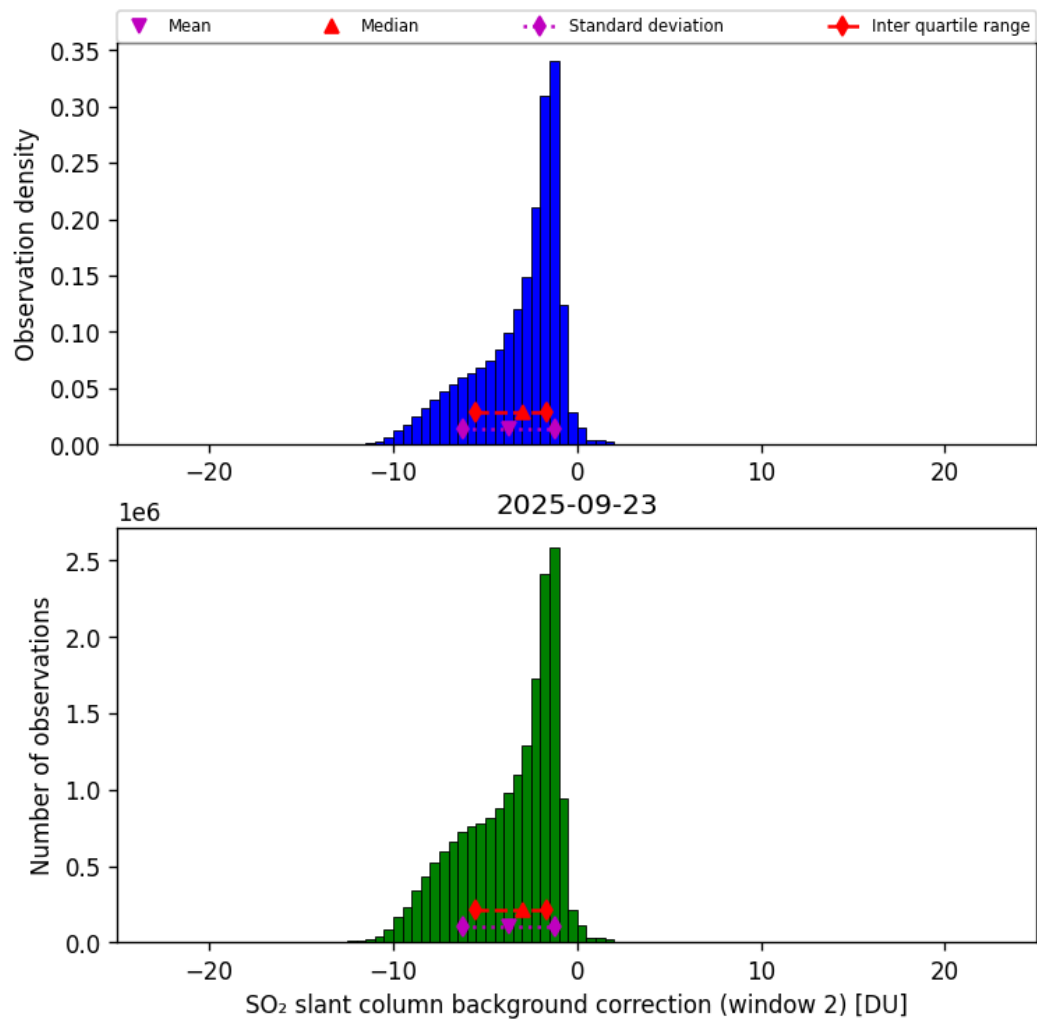
Figure 70: Histogram of “SO 2 slant column background correction (window 2)” for 2025-09-22 to 2025-09-24
