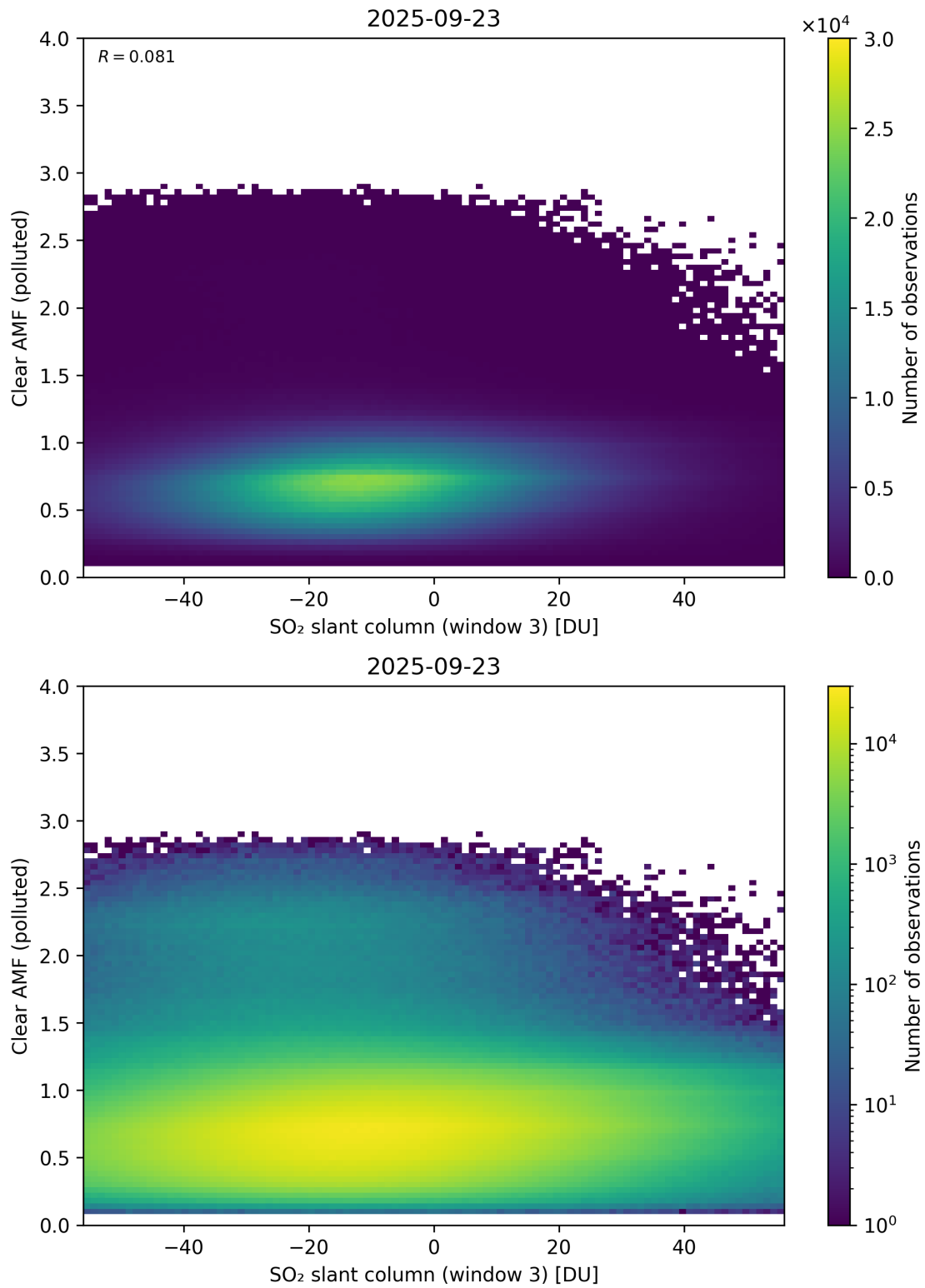
Figure 315: Scatter density plot of “SO 2 slant column (window 3)” against “Clear AMF (polluted)” for 2025-09-22 to 2025-09-24.
