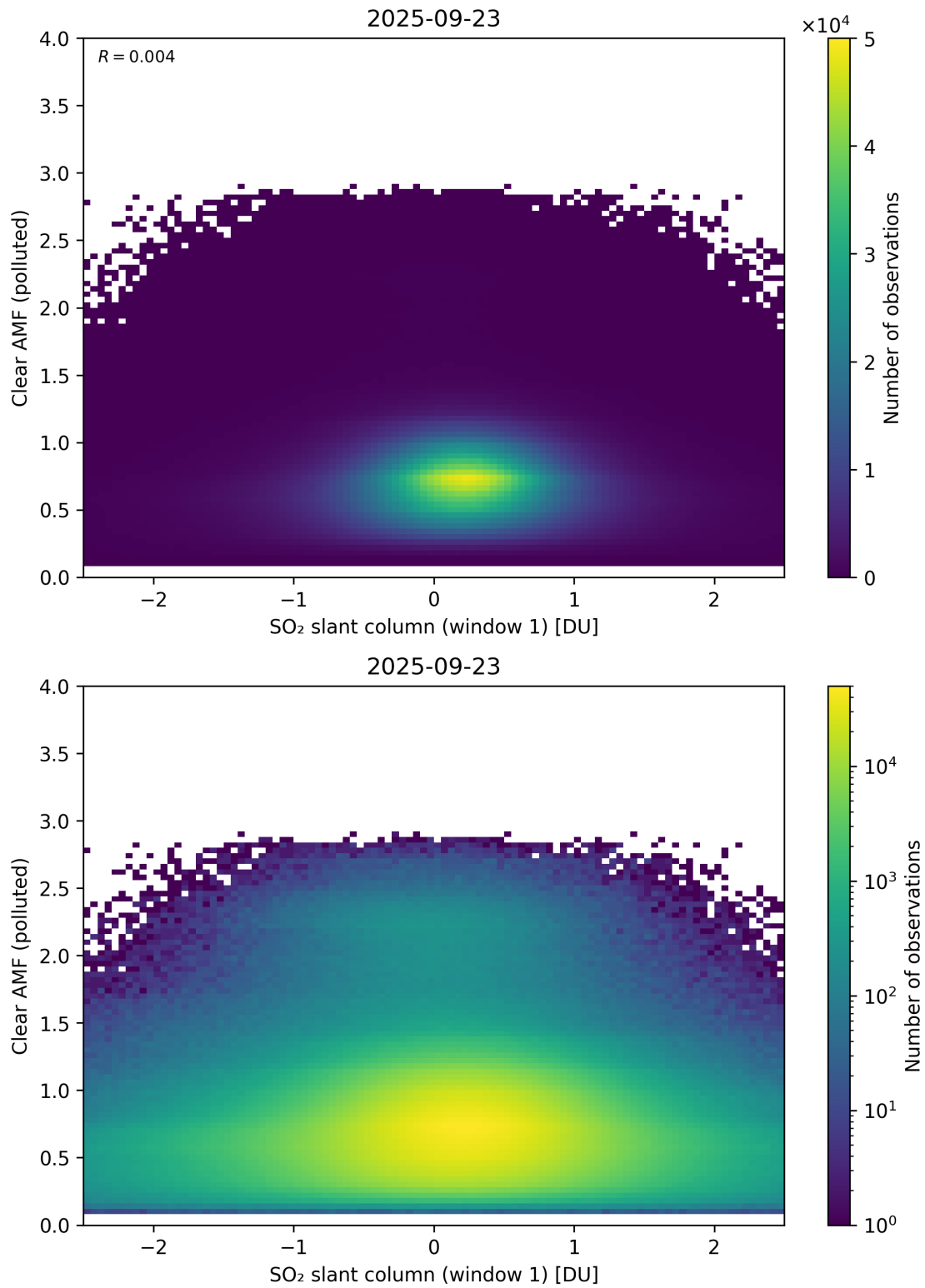
Figure 282: Scatter density plot of “SO 2 slant column (window 1)” against “Clear AMF (polluted)” for 2025-09-22 to 2025-09-24.
