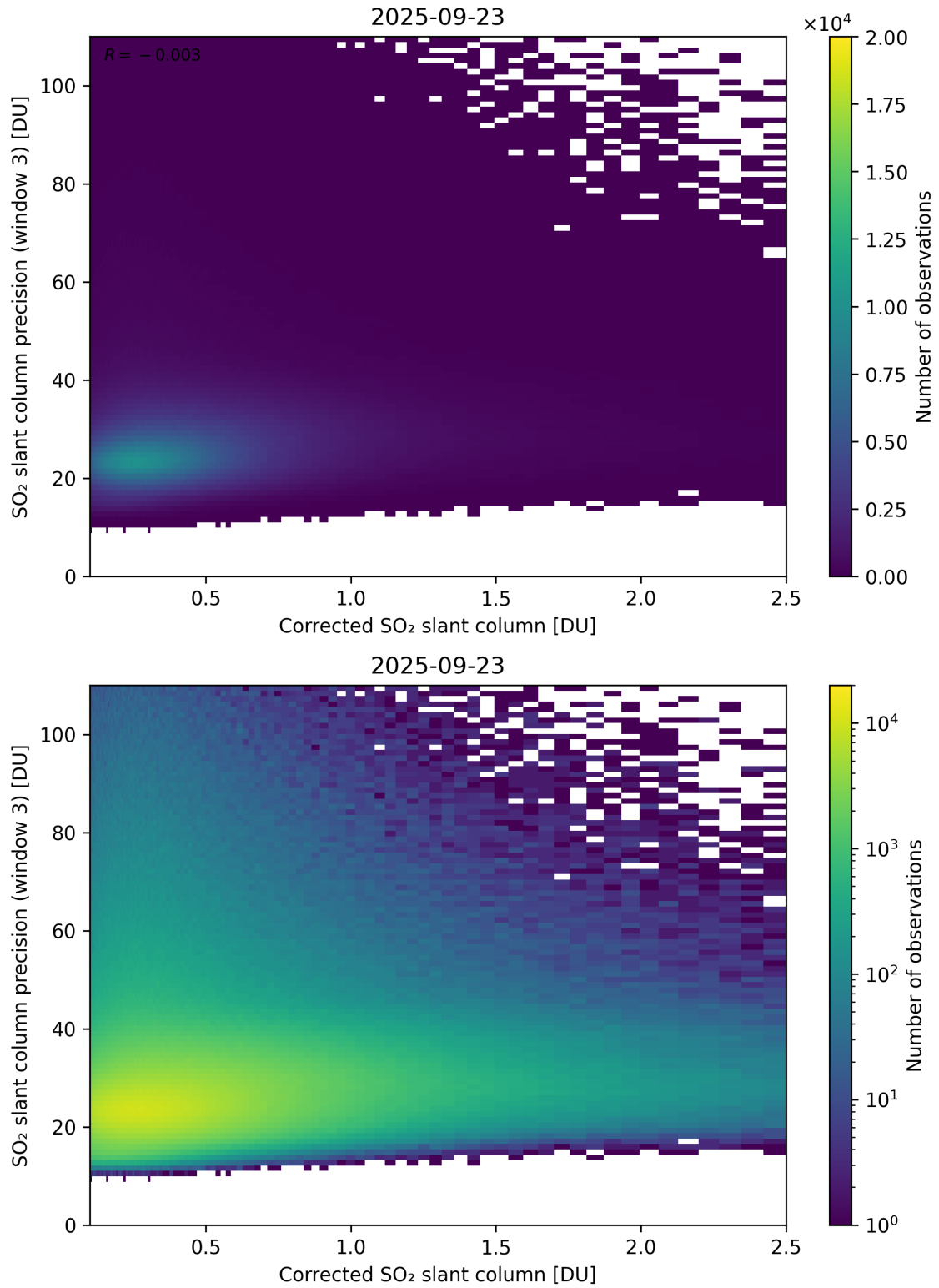
Figure 241: Scatter density plot of “Corrected SO 2 slant column” against “SO 2 slant column precision (window 3)” for 2025-09-22 to 2025-09-24.
