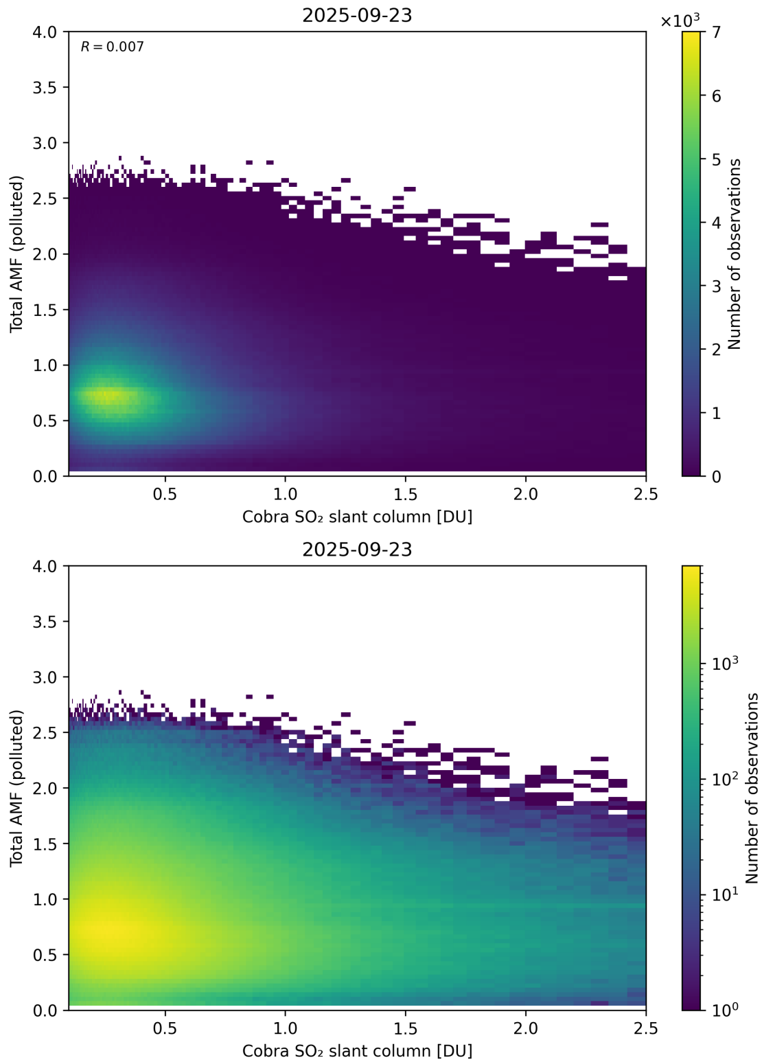
Figure 224: Scatter density plot of “Cobra SO 2 slant column” against “Total AMF (polluted)” for 2025-09-22 to 2025-09-24.
