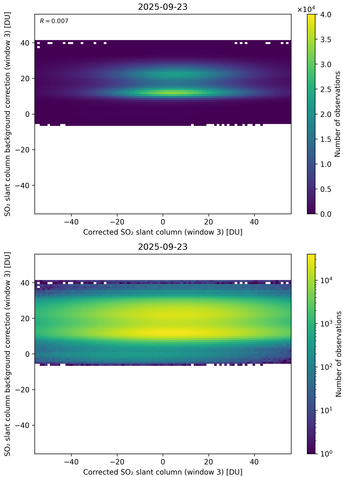
Figure 255: Scatter density plot of “Corrected SO 2 slant column (window 3)” against “SO 2 slant column background correction (window 3)” for 2025-09-22 to 2025-09-24.
