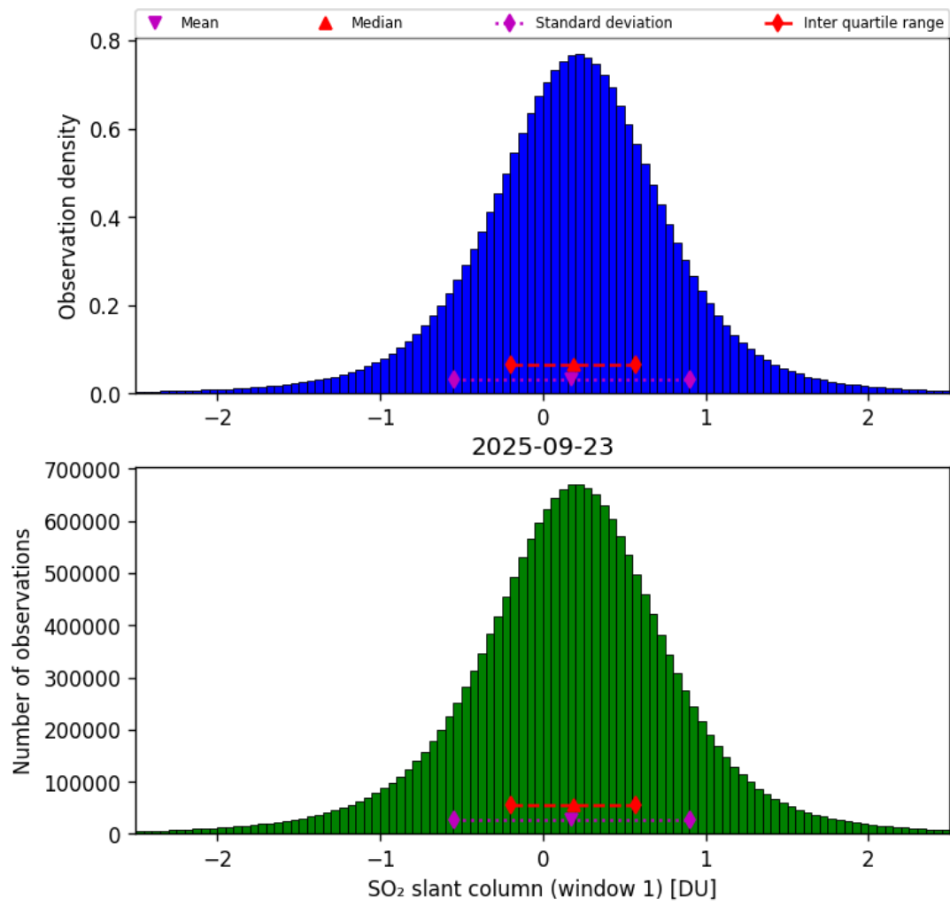
Figure 63: Histogram of “SO 2 slant column (window 1)” for 2025-09-22 to 2025-09-24
