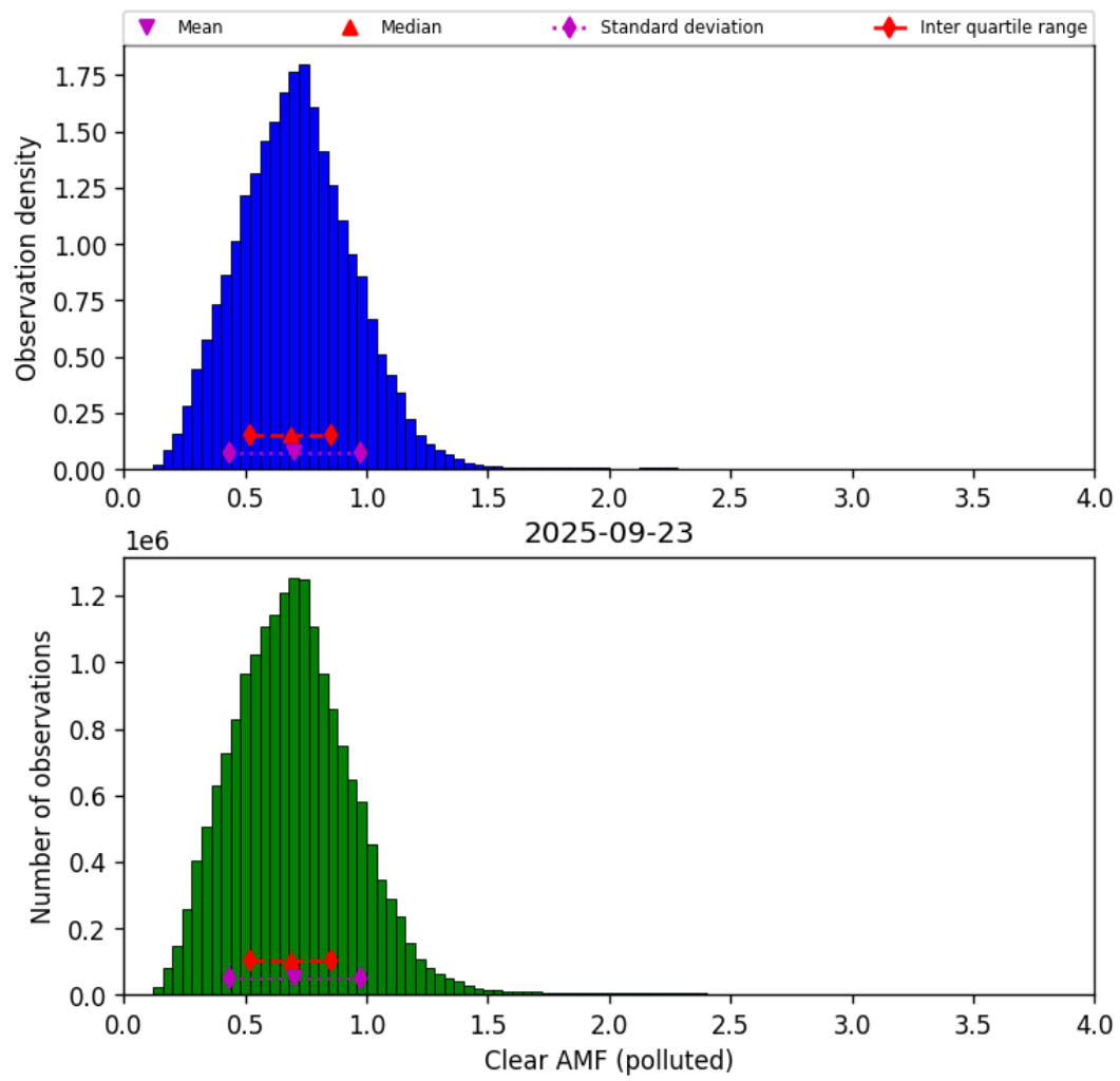
Figure 81: Histogram of “Clear AMF (polluted)” for 2025-09-22 to 2025-09-24
