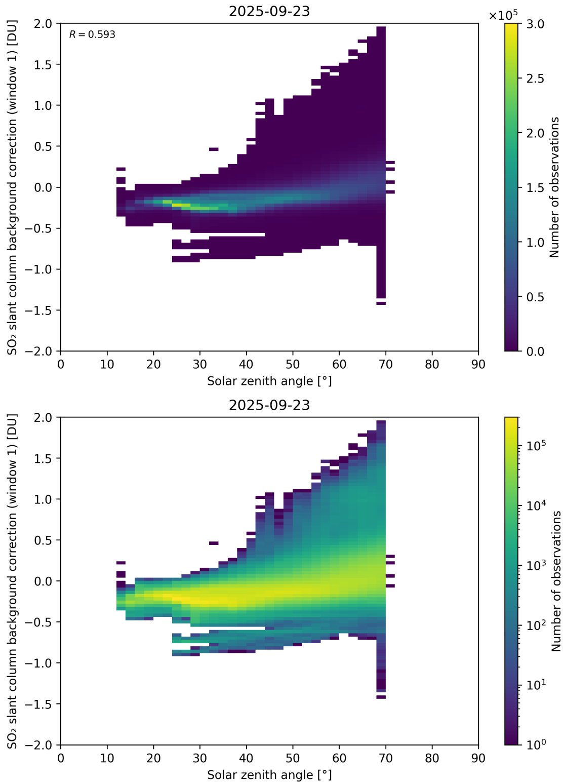
Figure 171: Scatter density plot of “Solar zenith angle” against “SO 2 slant column background correction (window 1)” for 2025-09-22 to 2025-09-24.
