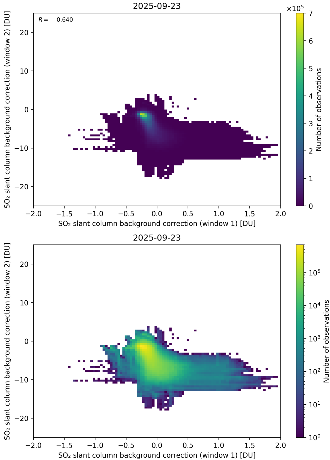
Figure 109: Scatter density plot of “SO 2 slant column background correction (window 1)” against “SO 2 slant column background correction (window 2)” for 2025-09-22 to 2025-09-24.
