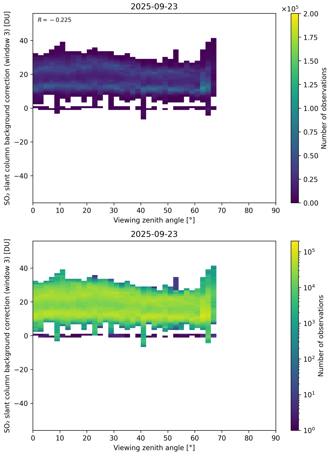
Figure 364: Scatter density plot of “Viewing zenith angle” against “SO 2 slant column background correction (window 3)” for 2025-09-22 to 2025-09-24.
