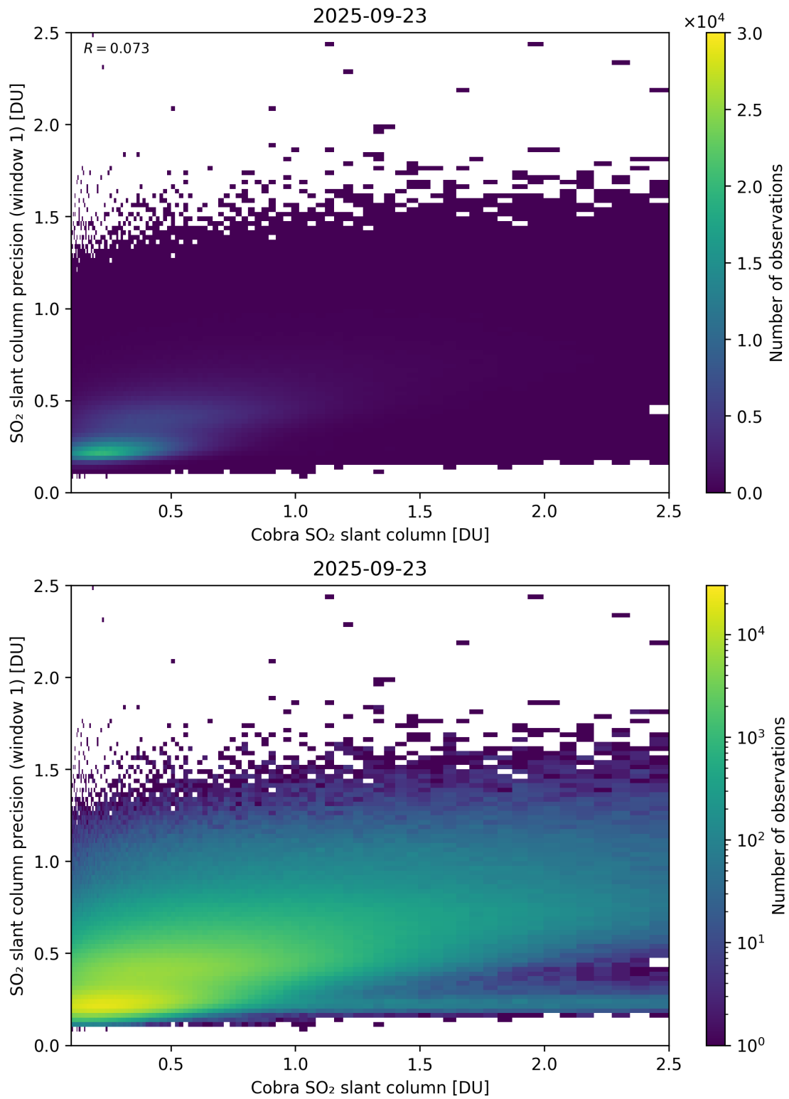
Figure 220: Scatter density plot of “Cobra SO 2 slant column” against “SO 2 slant column precision (window 1)” for 2025-09-22 to 2025-09-24.
