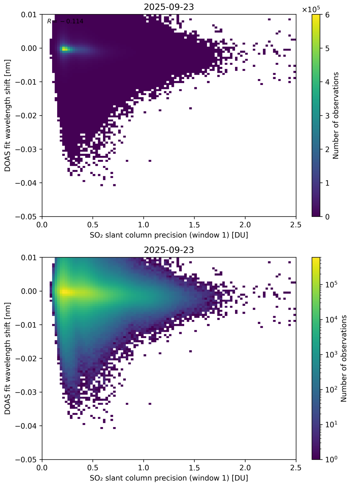
Figure 271: Scatter density plot of “SO 2 slant column precision (window 1)” against “DOAS fit wavelength shift” for 2025-09-22 to 2025-09-24.
