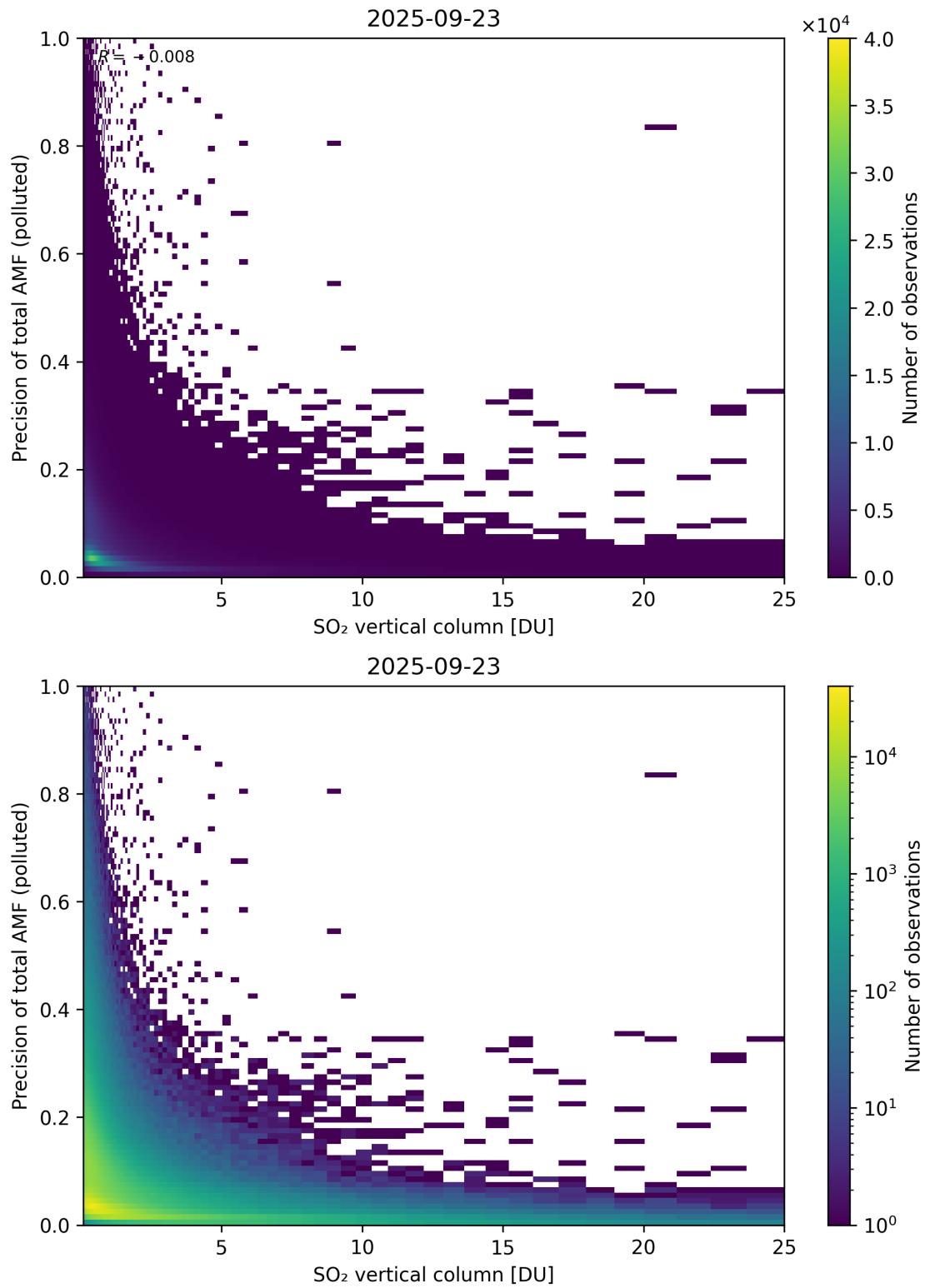
Figure 360: Scatter density plot of “SO 2 vertical column” against “Precision of total AMF (polluted)” for 2025-09-22 to 2025-09-24.
