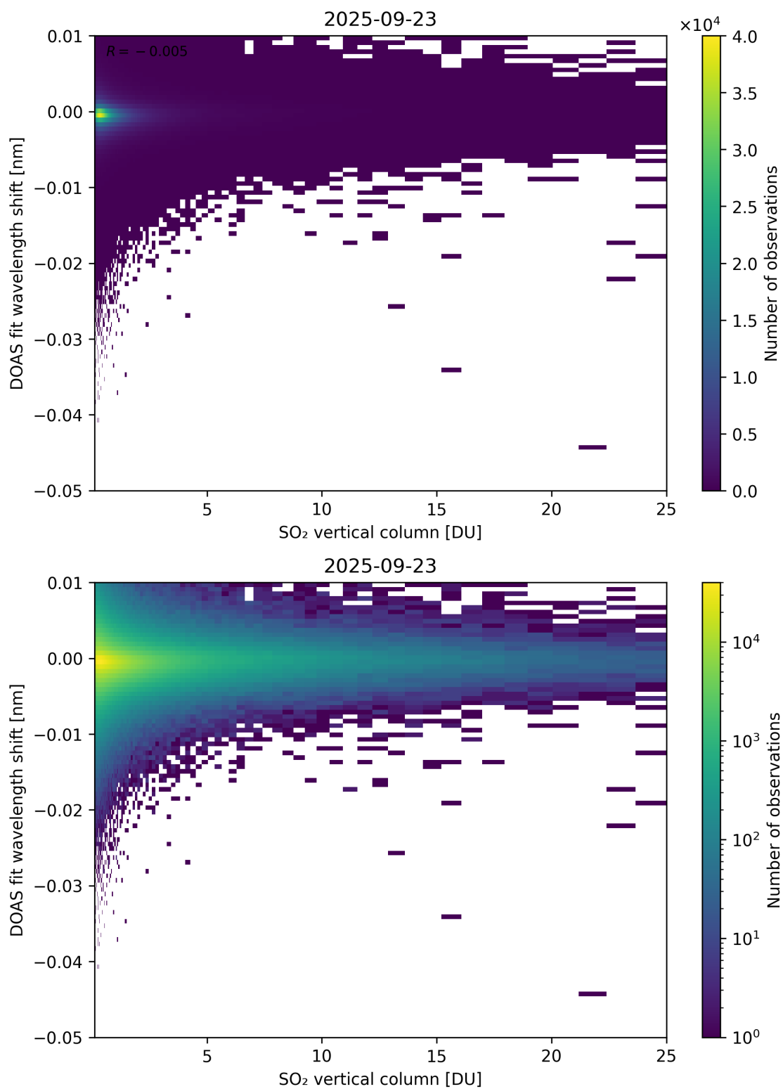
Figure 326: Scatter density plot of “SO 2 vertical column” against “DOAS fit wavelength shift” for 2025-09-22 to 2025-09-24.
