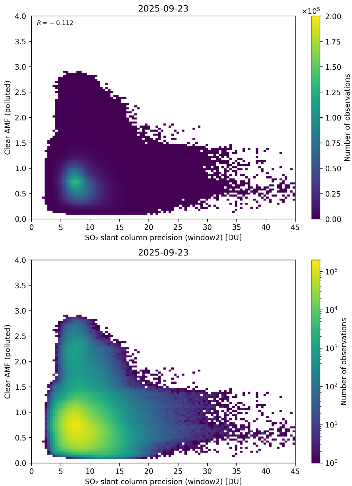
Figure 296: Scatter density plot of “SO 2 slant column precision (window2)” against “Clear AMF (polluted)” for 2025-09-22 to 2025-09-24.
