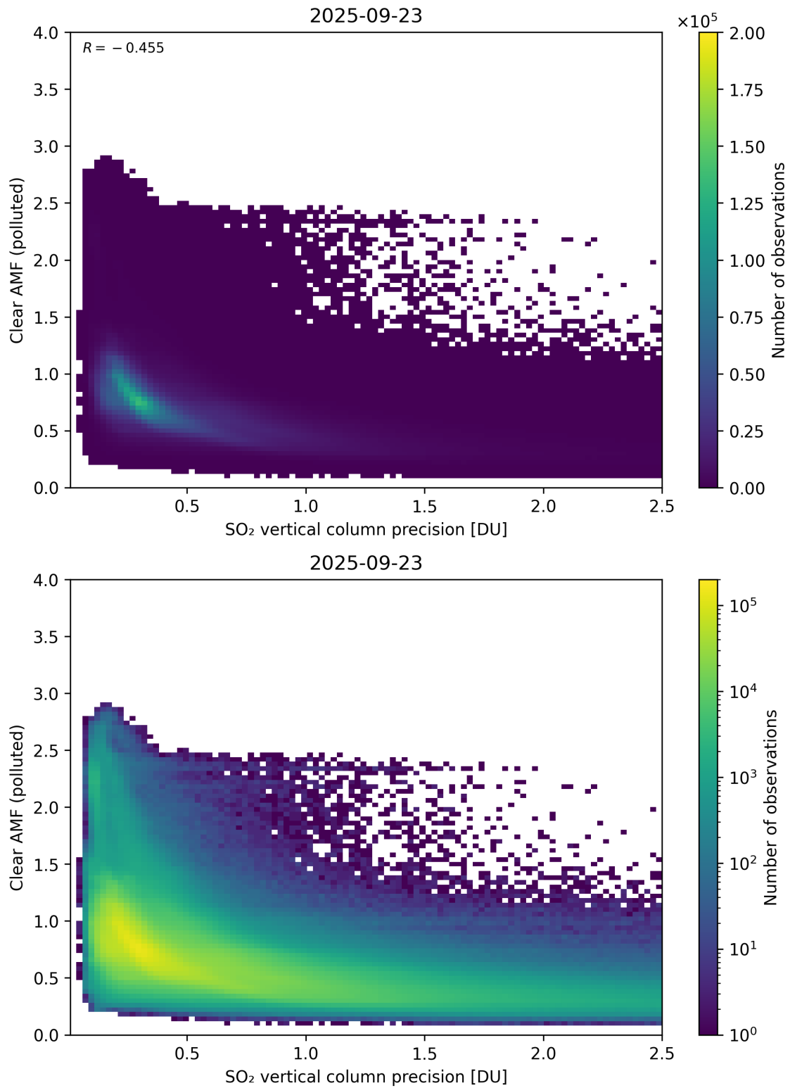
Figure 335: Scatter density plot of “SO 2 vertical column precision” against “Clear AMF (polluted)” for 2025-09-22 to 2025-09-24.
