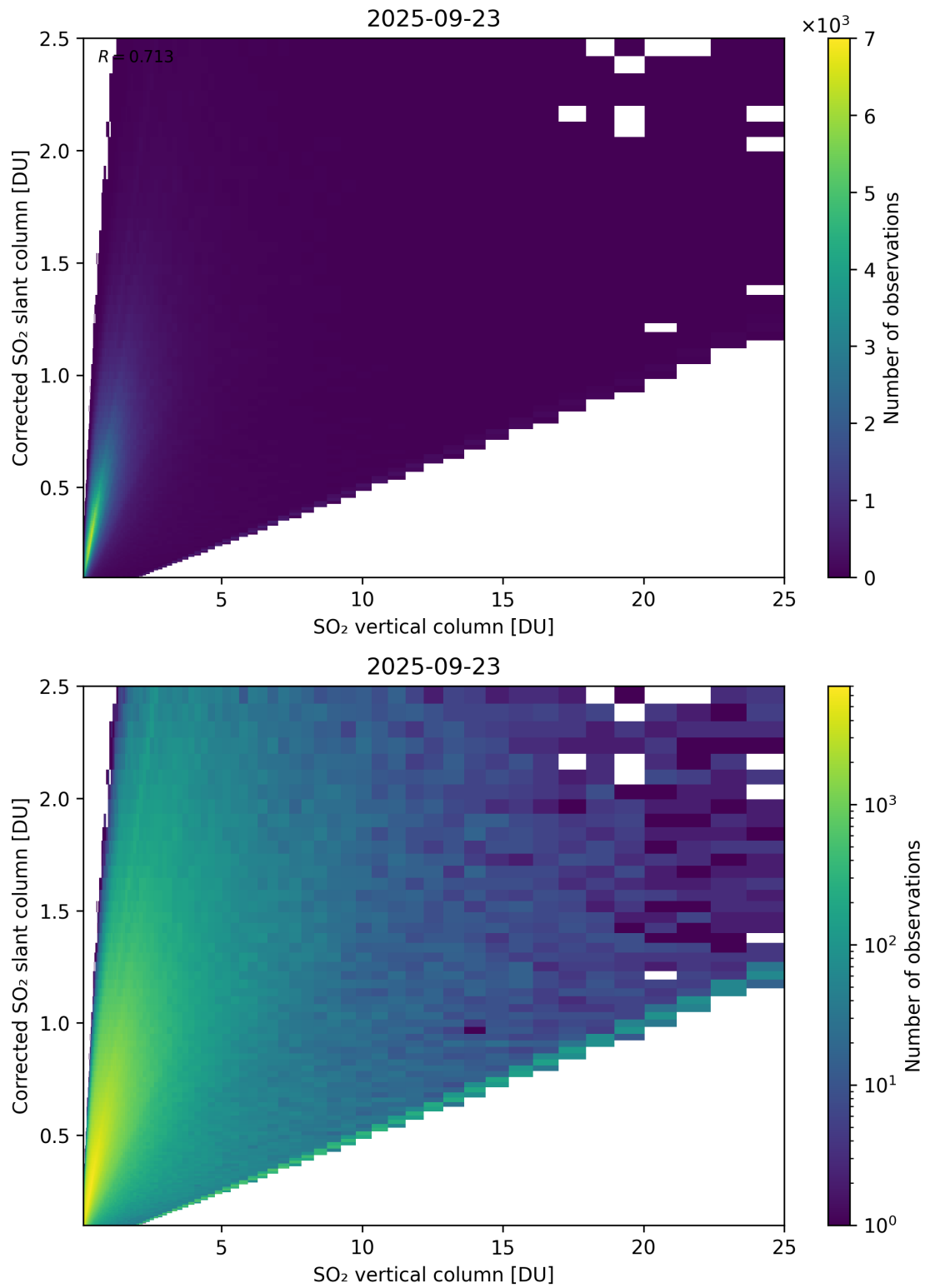
Figure 351: Scatter density plot of “SO 2 vertical column” against “Corrected SO 2 slant column” for 2025-09-22 to 2025-09-24.
