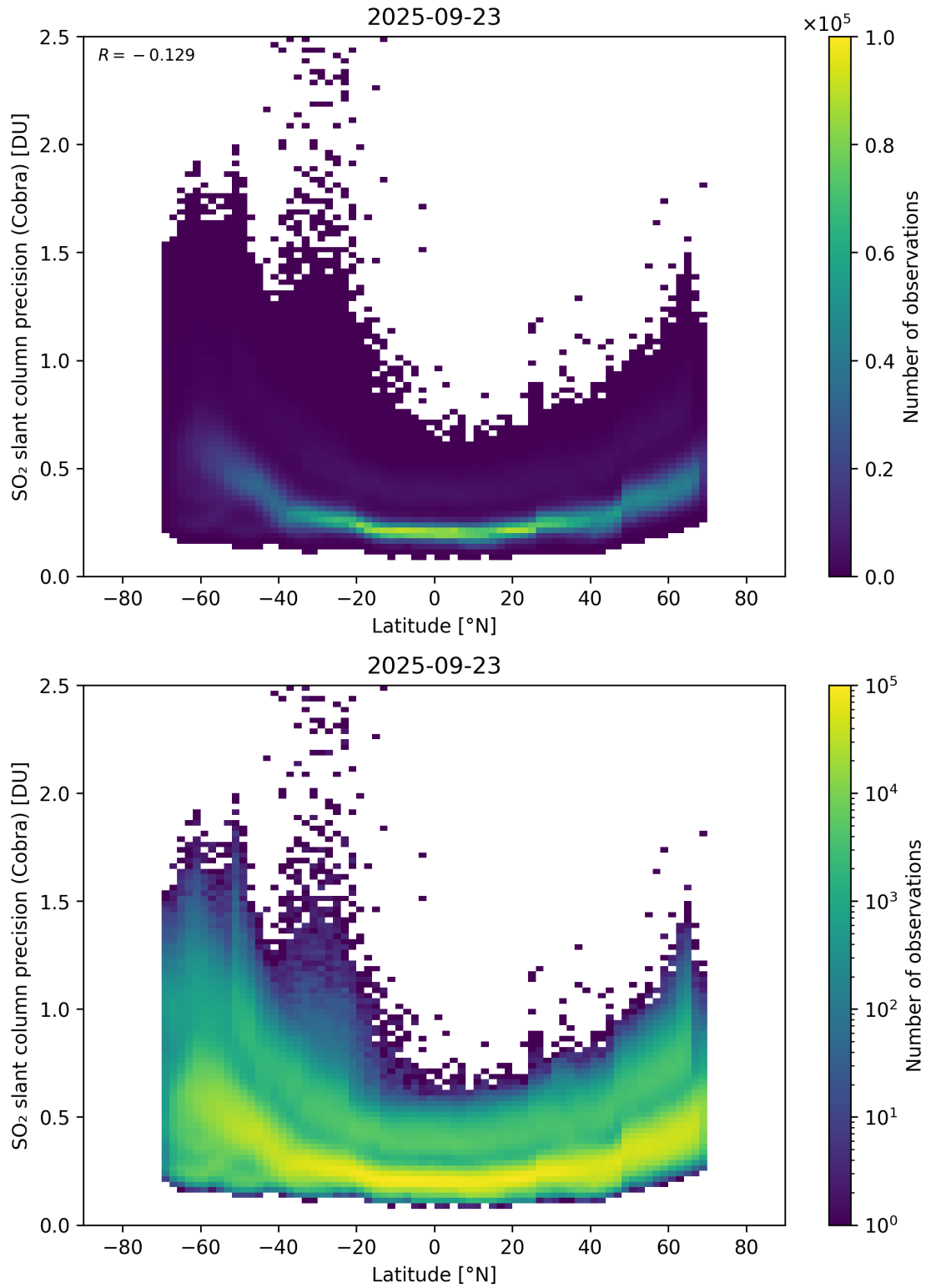
Figure 158: Scatter density plot of “Latitude” against “SO 2 slant column precision (Cobra)” for 2025-09-22 to 2025-09-24.
