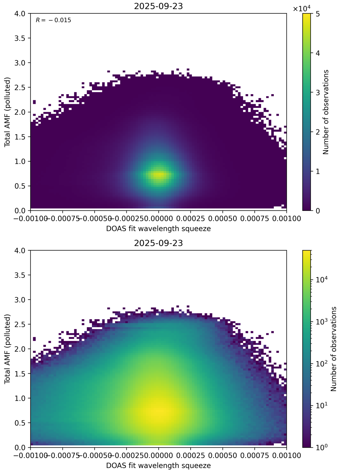
Figure 145: Scatter density plot of “DOAS fit wavelength squeeze” against “Total AMF (polluted)” for 2025-09-22 to 2025-09-24.
