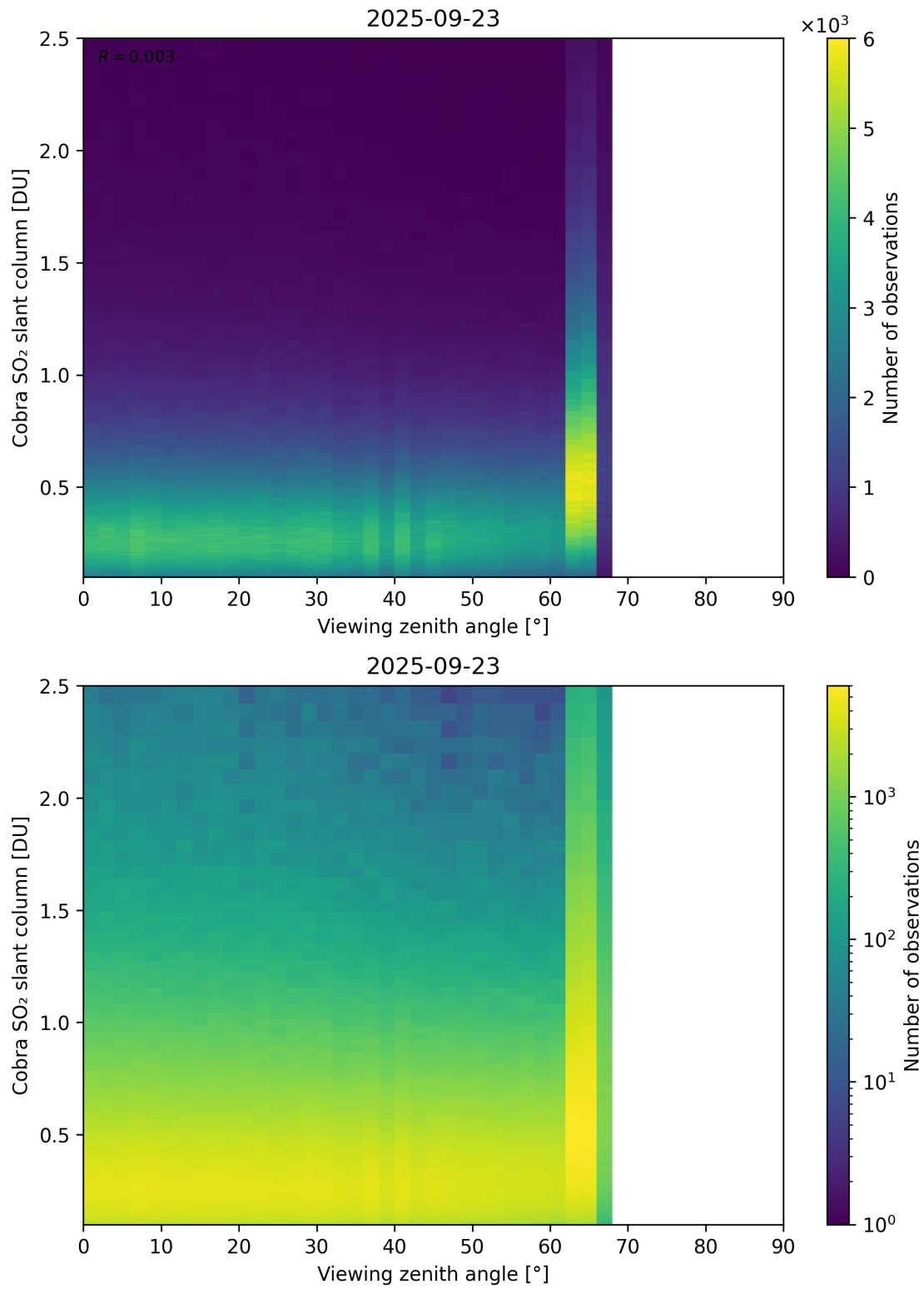
Figure 371: Scatter density plot of “Viewing zenith angle” against “Cobra SO 2 slant column” for 2025-09-22 to 2025-09-24.
