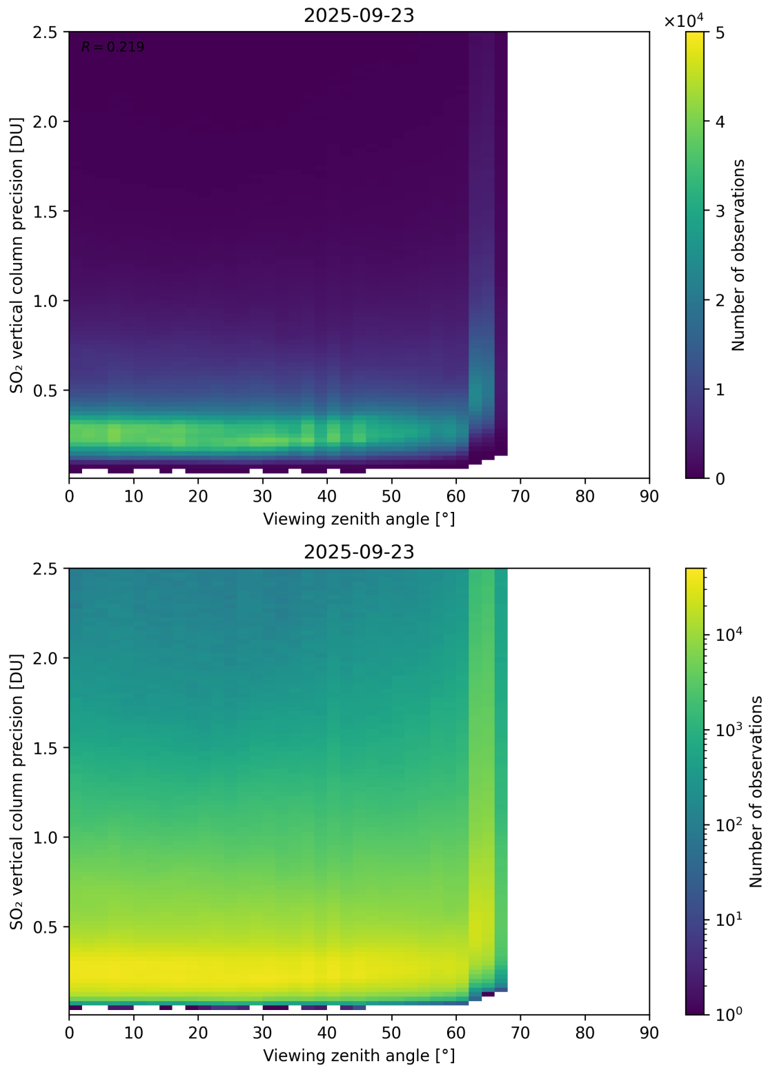
Figure 384: Scatter density plot of “Viewing zenith angle” against “SO 2 vertical column precision” for 2025-09-22 to 2025-09-24.
