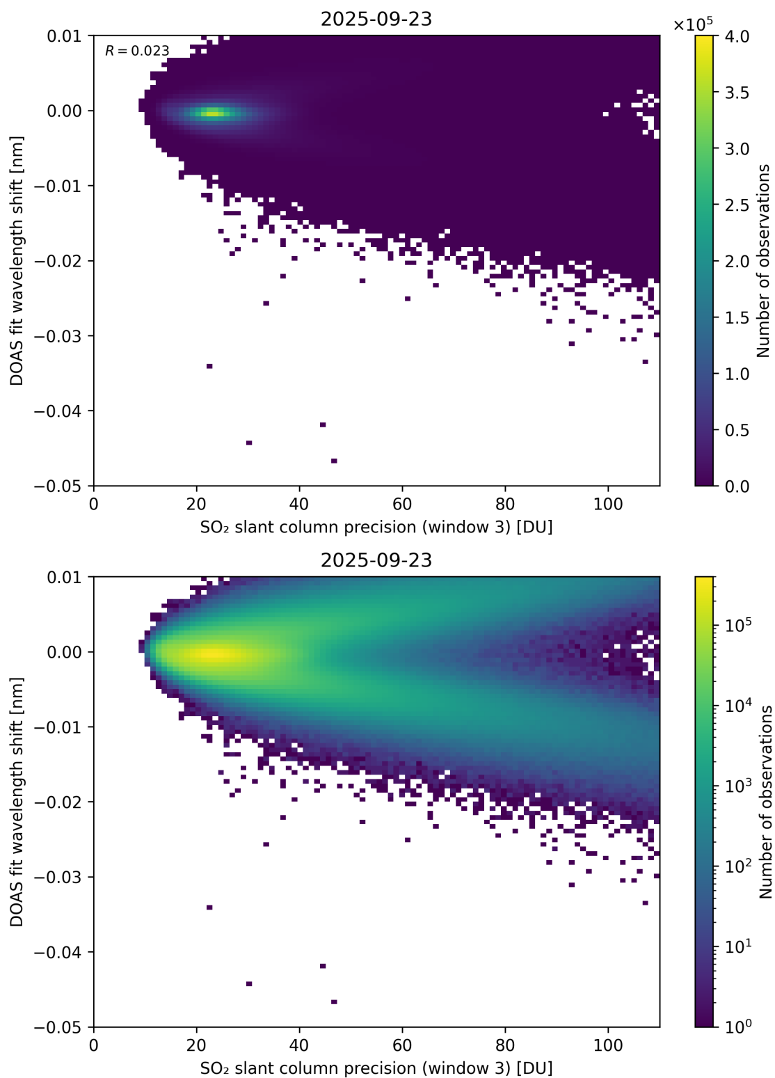
Figure 308: Scatter density plot of “SO 2 slant column precision (window 3)” against “DOAS fit wavelength shift” for 2025-09-22 to 2025-09-24.
