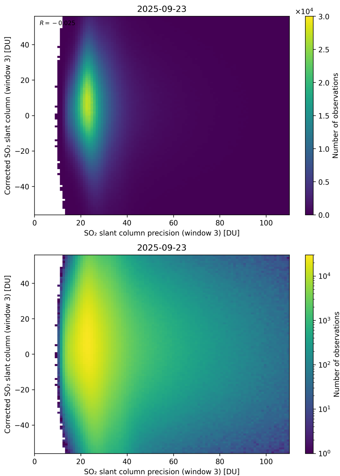
Figure 312: Scatter density plot of “SO 2 slant column precision (window 3)” against “Corrected SO 2 slant column (window 3)” for 2025-09-22 to 2025-09-24.
