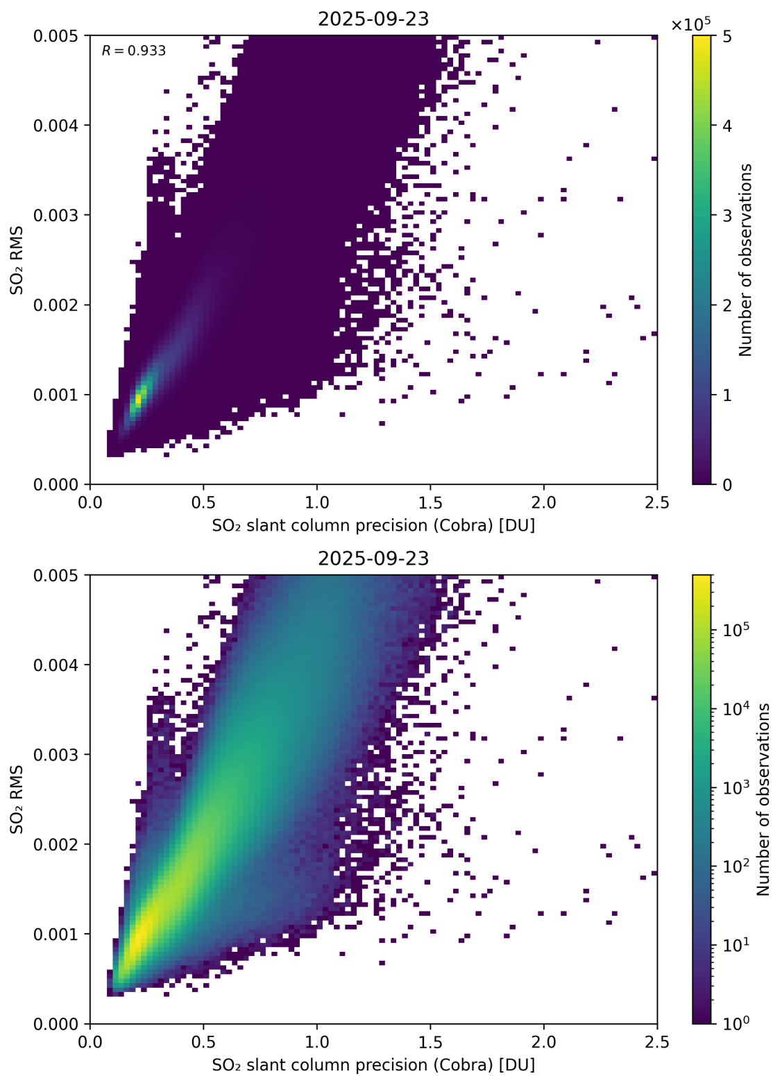
Figure 204: Scatter density plot of “SO 2 slant column precision (Cobra)” against “SO 2 RMS” for 2025-09-22 to 2025-09-24.
