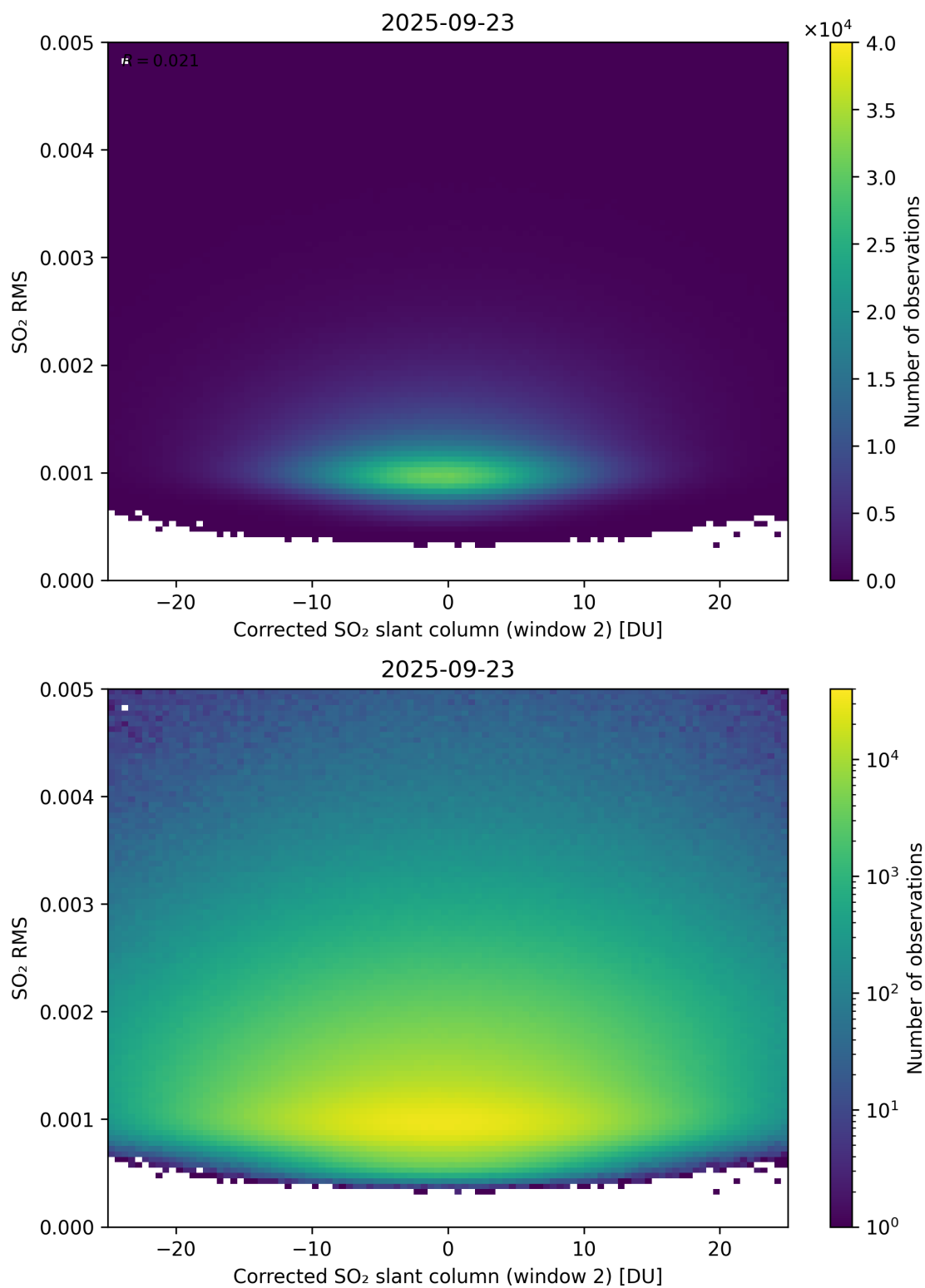
Figure 248: Scatter density plot of “Corrected SO 2 slant column (window 2)” against “SO 2 RMS” for 2025-09-22 to 2025-09-24.
