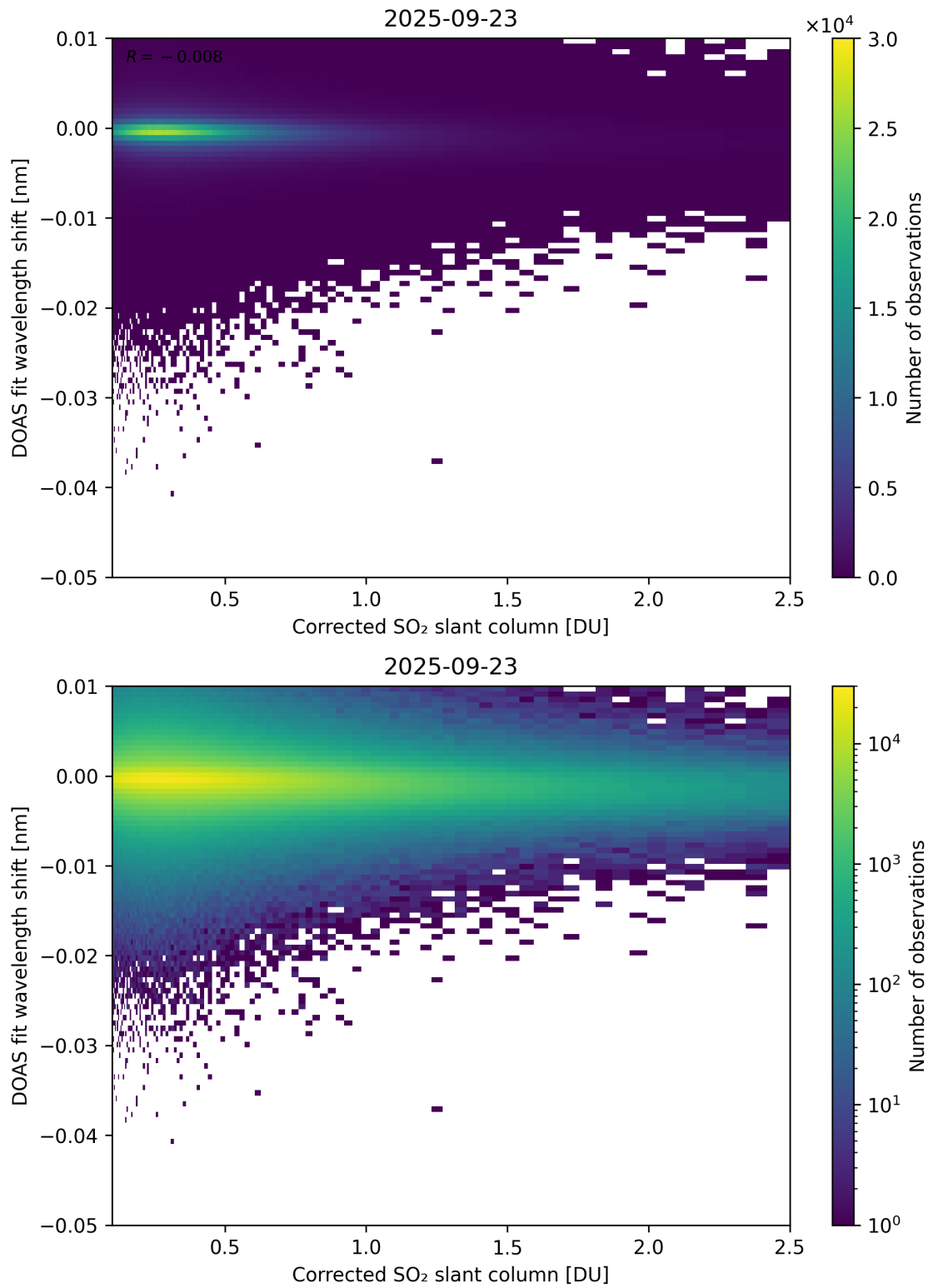
Figure 229: Scatter density plot of “Corrected SO 2 slant column” against “DOAS fit wavelength shift” for 2025-09-22 to 2025-09-24.
