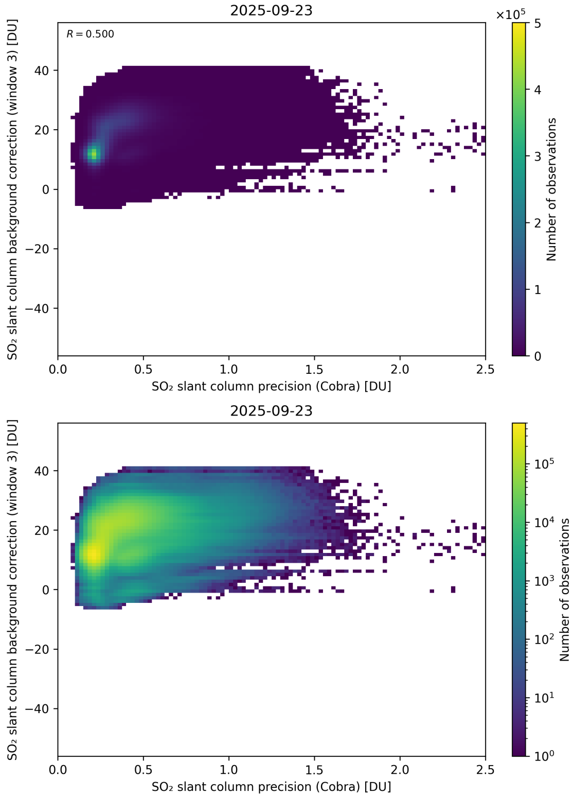
Figure 201: Scatter density plot of “SO 2 slant column precision (Cobra)” against “SO 2 slant column background correction (window 3)” for 2025-09-22 to 2025-09-24.
