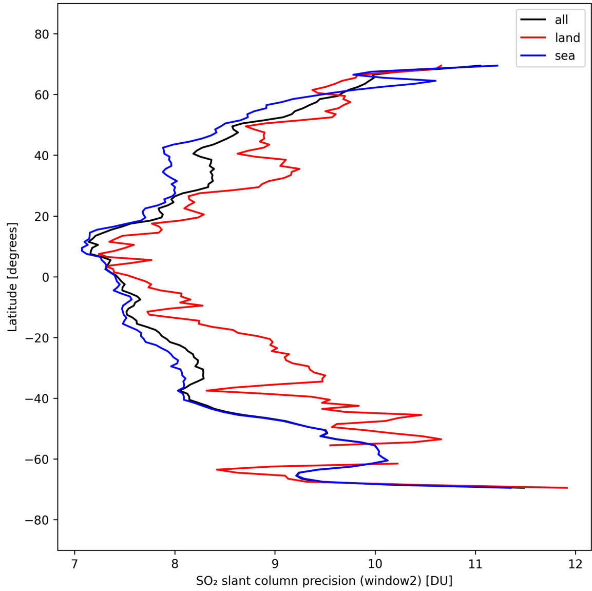
Figure 42: Zonal average of “SO 2 slant column precision (window2)” for 2025-09-22 to 2025-09-24.
