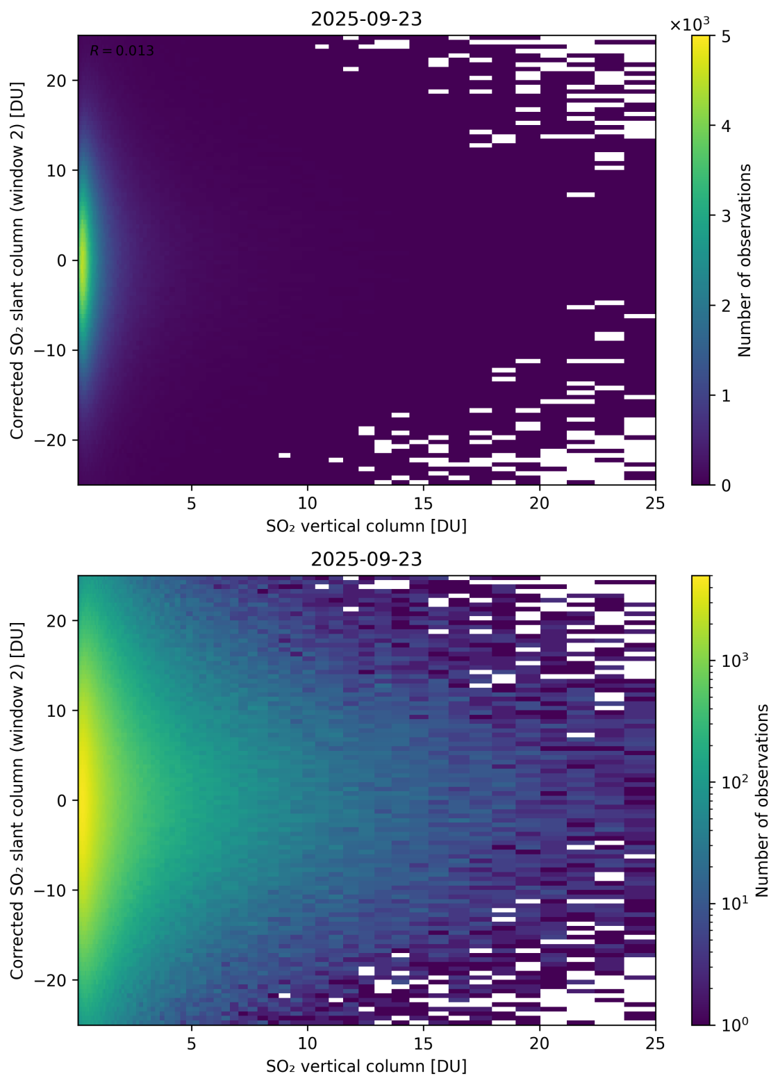
Figure 352: Scatter density plot of “SO 2 vertical column” against “Corrected SO 2 slant column (window 2)” for 2025-09-22 to 2025-09-24.
