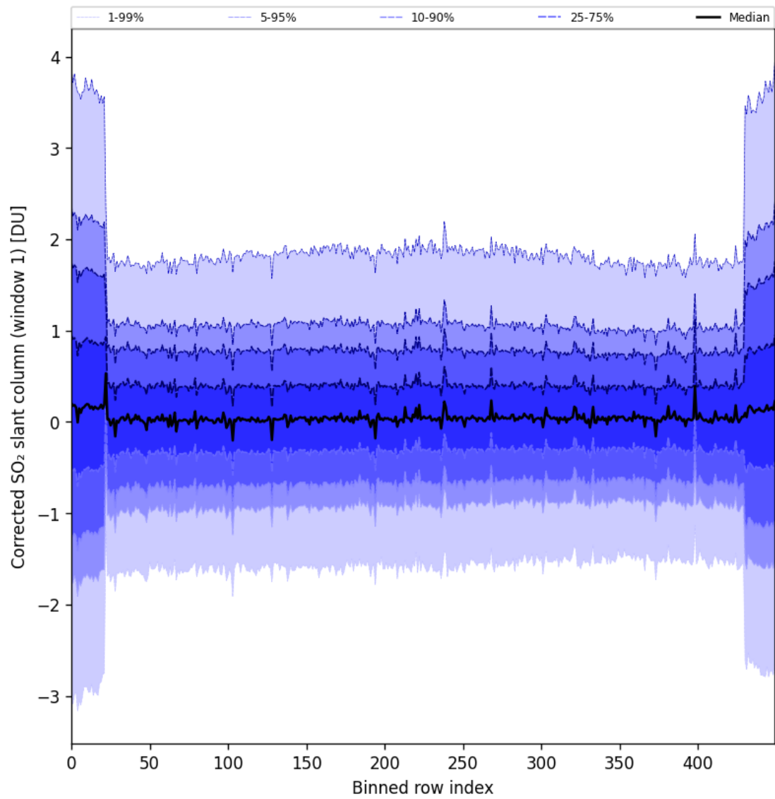
Figure 91: Along track statistics of “Corrected SO 2 slant column (window 1)” for 2025-09-22 to 2025-09-24
