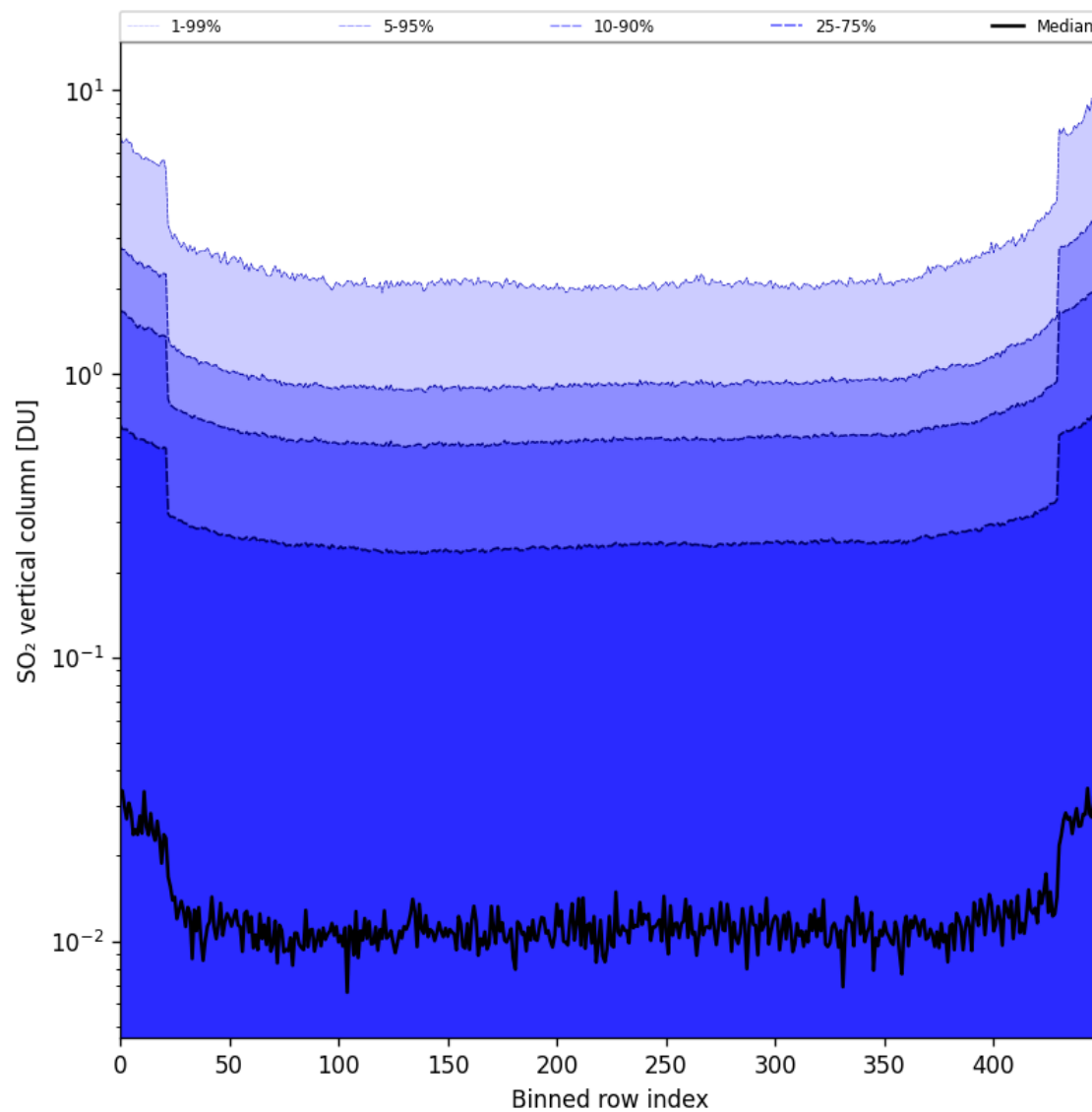
Figure 84: Along track statistics of “SO 2 vertical column” for 2025-09-22 to 2025-09-24
