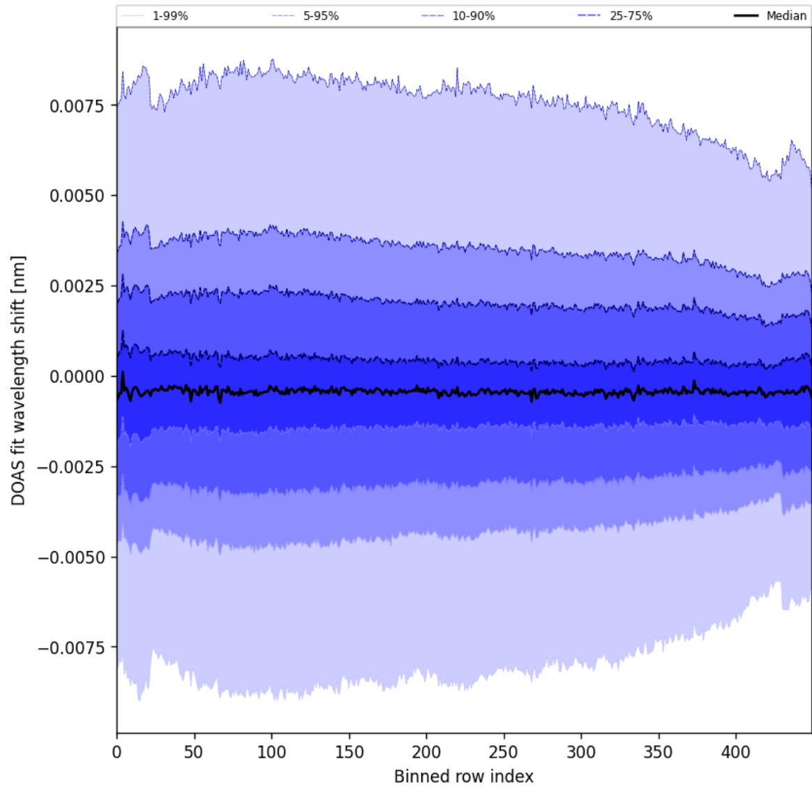
Figure 102: Along track statistics of “DOAS fit wavelength shift” for 2025-09-22 to 2025-09-24
