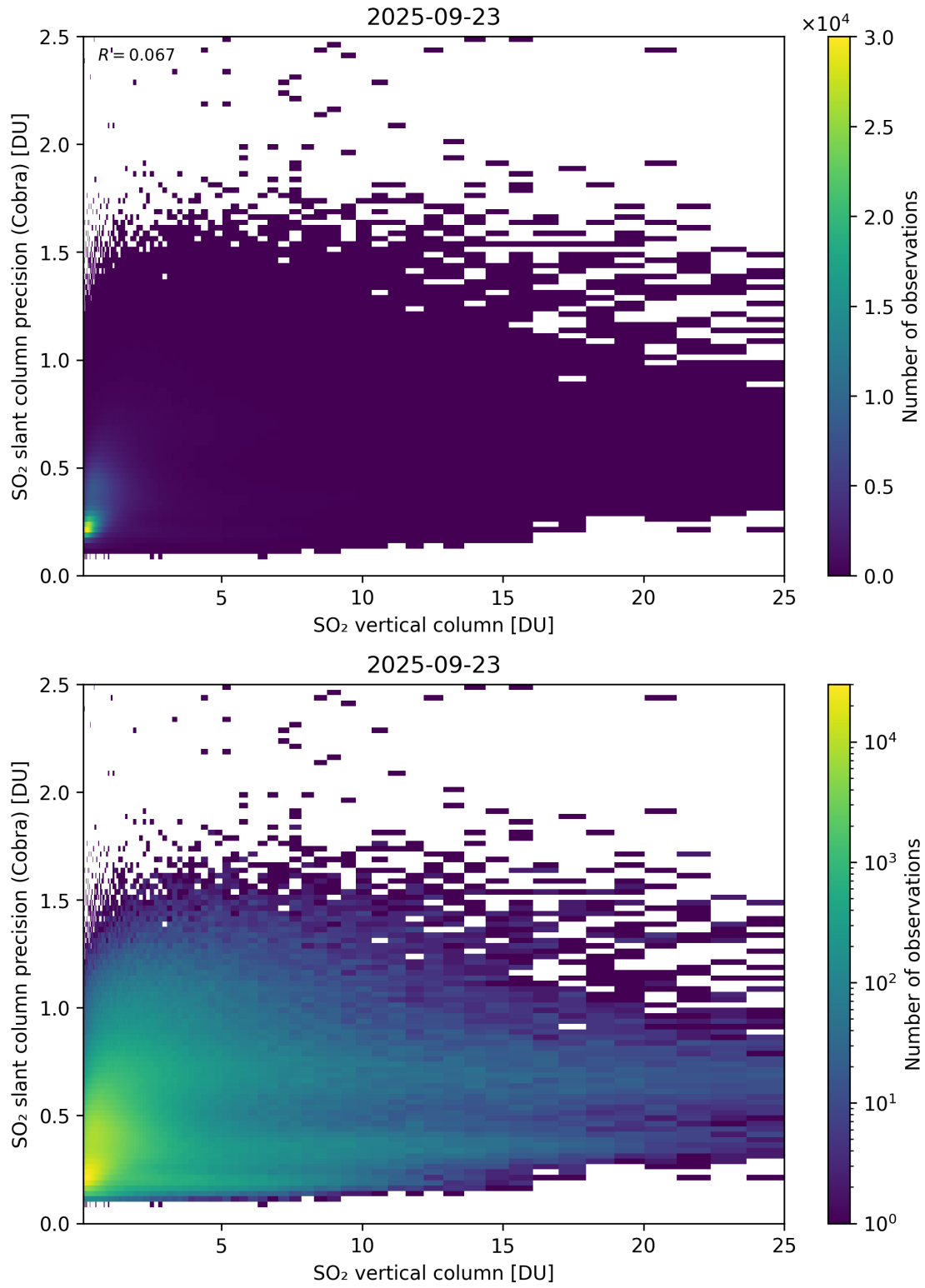
Figure 350: Scatter density plot of “SO 2 vertical column” against “SO 2 slant column precision (Cobra)” for 2025-09-22 to 2025-09-24.
