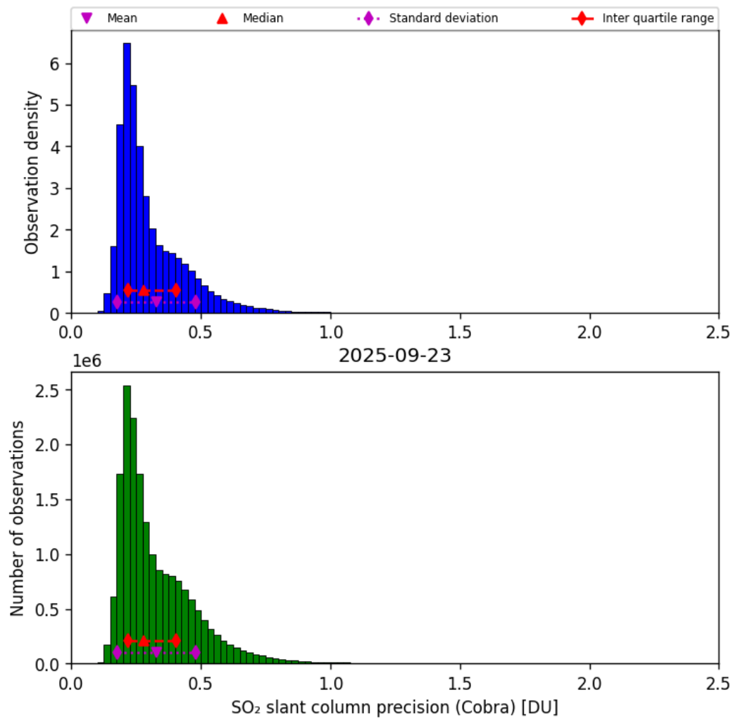
Figure 62: Histogram of “SO 2 slant column precision (Cobra)” for 2025-09-22 to 2025-09-24
