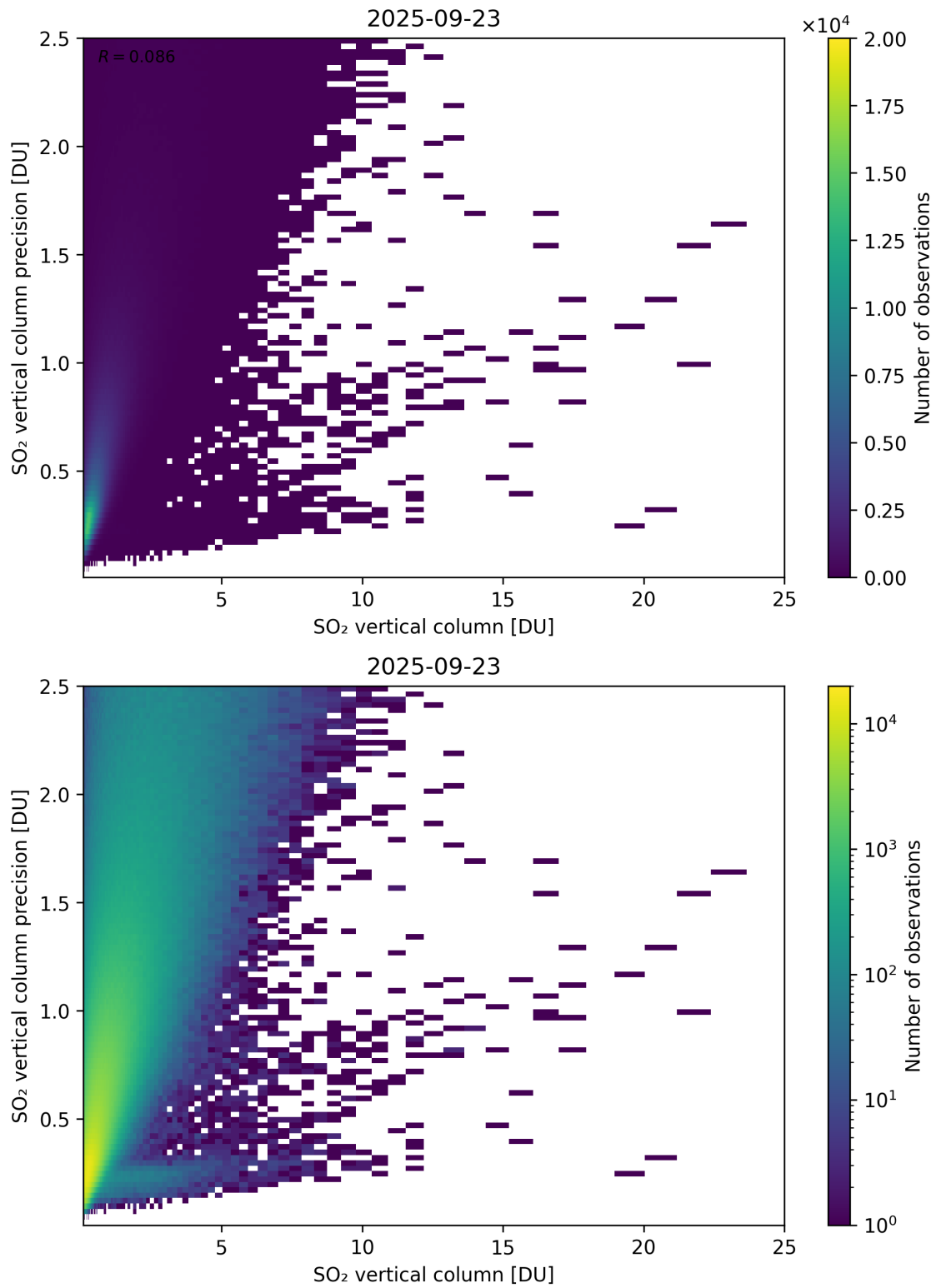
Figure 361: Scatter density plot of “SO 2 vertical column” against “SO 2 vertical column precision” for 2025-09-22 to 2025-09-24.
