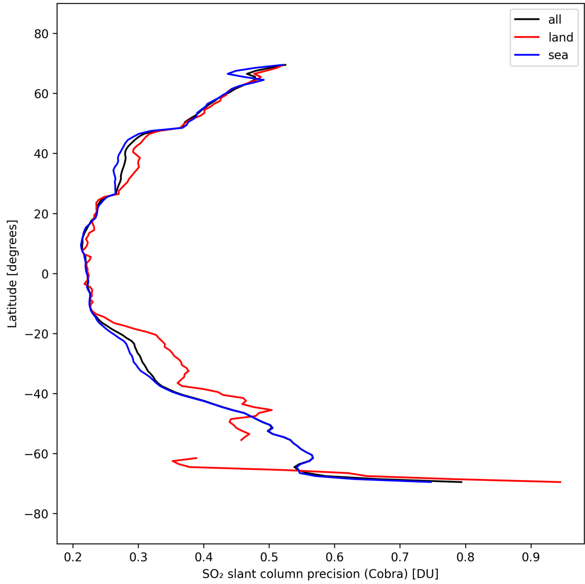
Figure 36: Zonal average of “SO 2 slant column precision (Cobra)” for 2025-09-22 to 2025-09-24.
