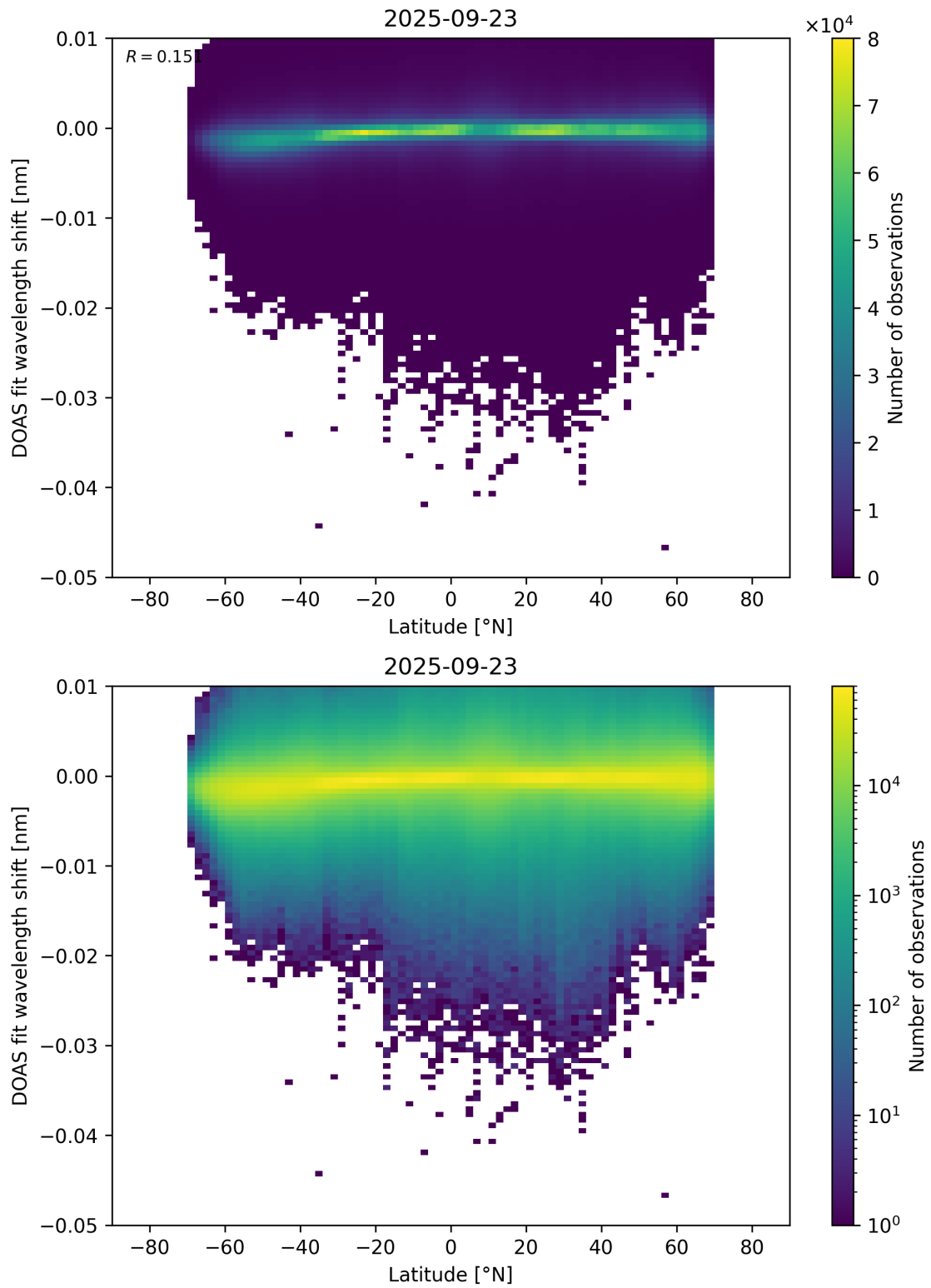
Figure 153: Scatter density plot of “Latitude” against “DOAS fit wavelength shift” for 2025-09-22 to 2025-09-24.
