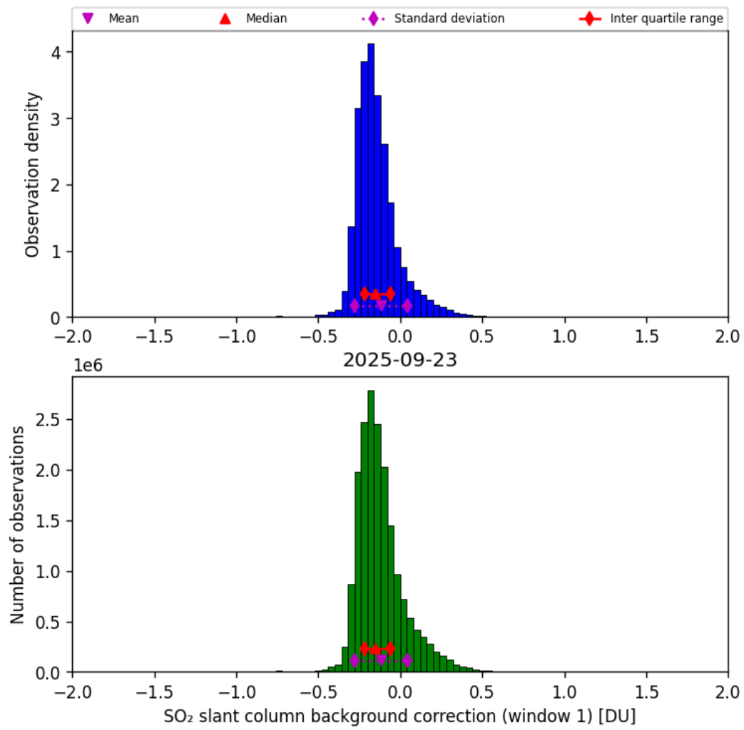
Figure 66: Histogram of “SO 2 slant column background correction (window 1)” for 2025-09-22 to 2025-09-24
