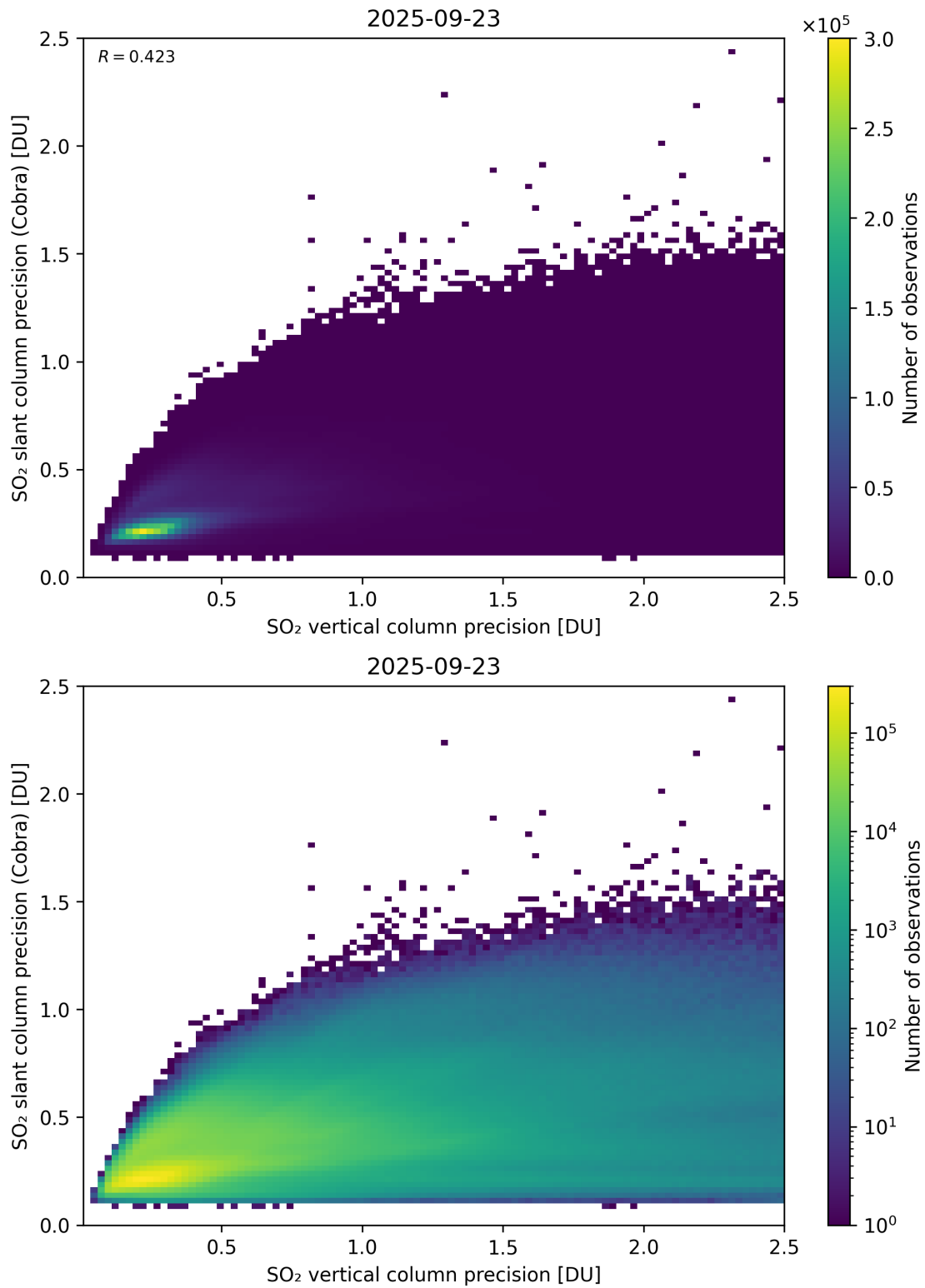
Figure 337: Scatter density plot of “SO 2 vertical column precision” against “SO 2 slant column precision (Cobra)” for 2025-09-22 to 2025-09-24.
