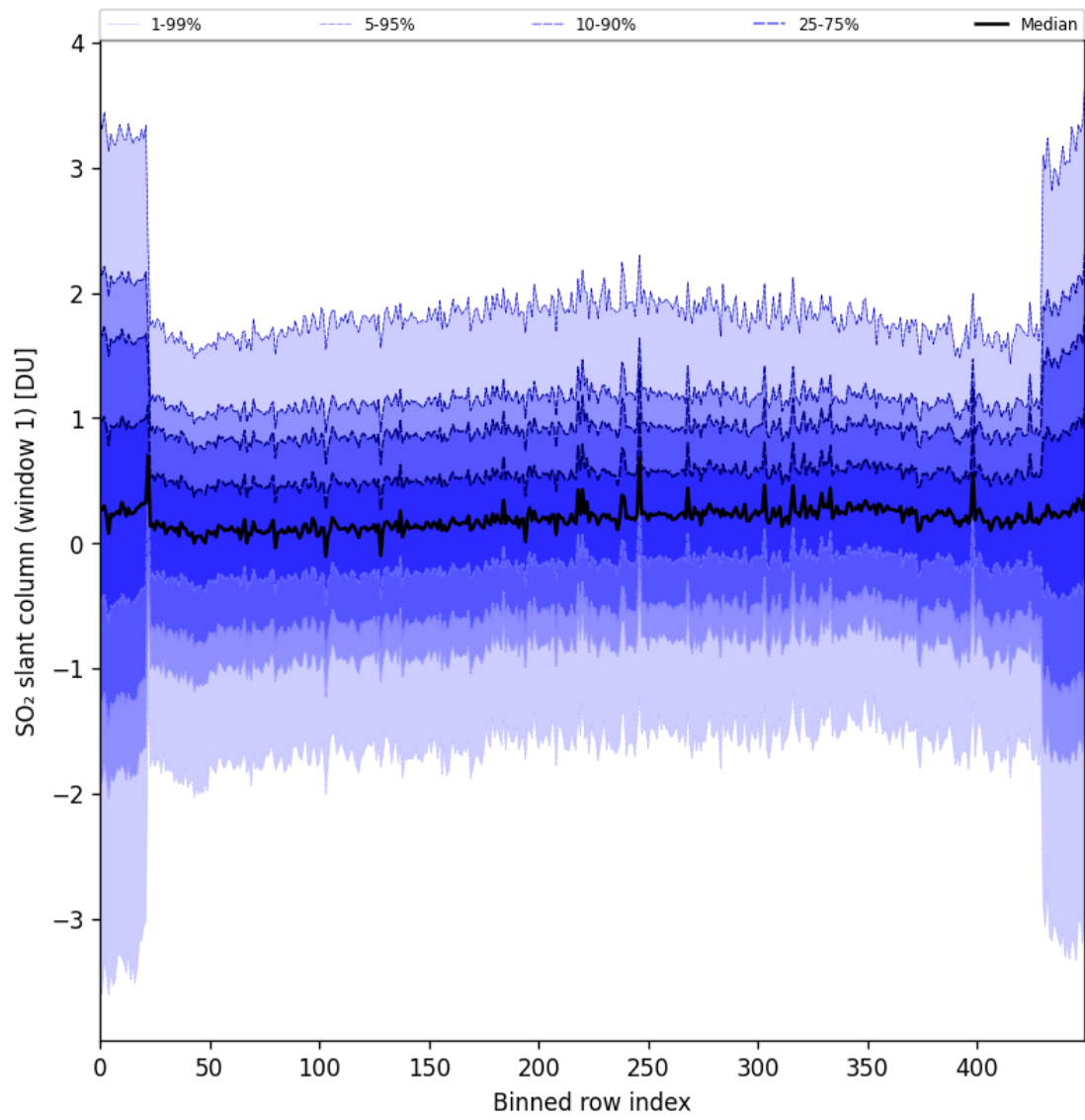
Figure 89: Along track statistics of "SO 2 slant column (window 1)" for 2025-09-22 to 2025-09-24
