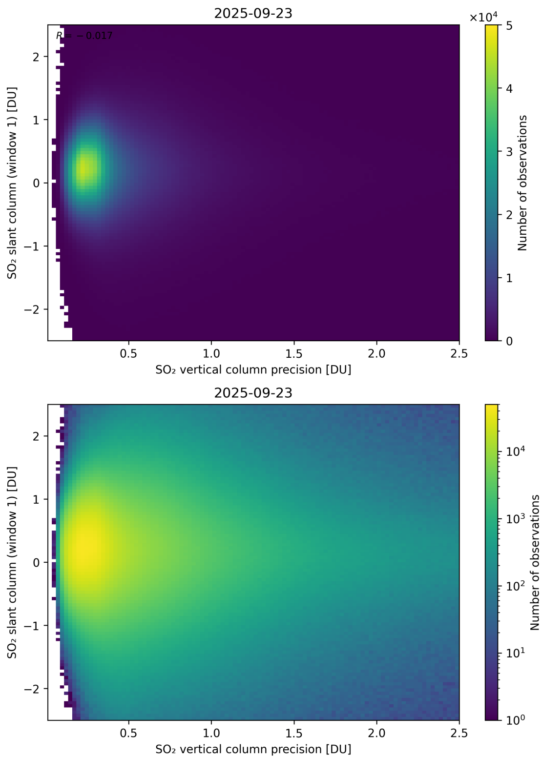
Figure 341: Scatter density plot of “SO 2 vertical column precision” against “SO 2 slant column (window 1)” for 2025-09-22 to 2025-09-24.
