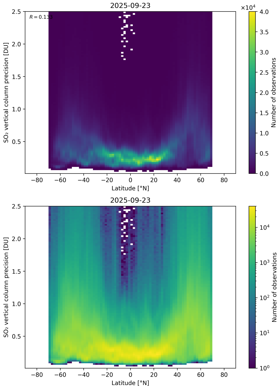
Figure 170: Scatter density plot of “Latitude” against “SO 2 vertical column precision” for 2025-09-22 to 2025-09-24.
