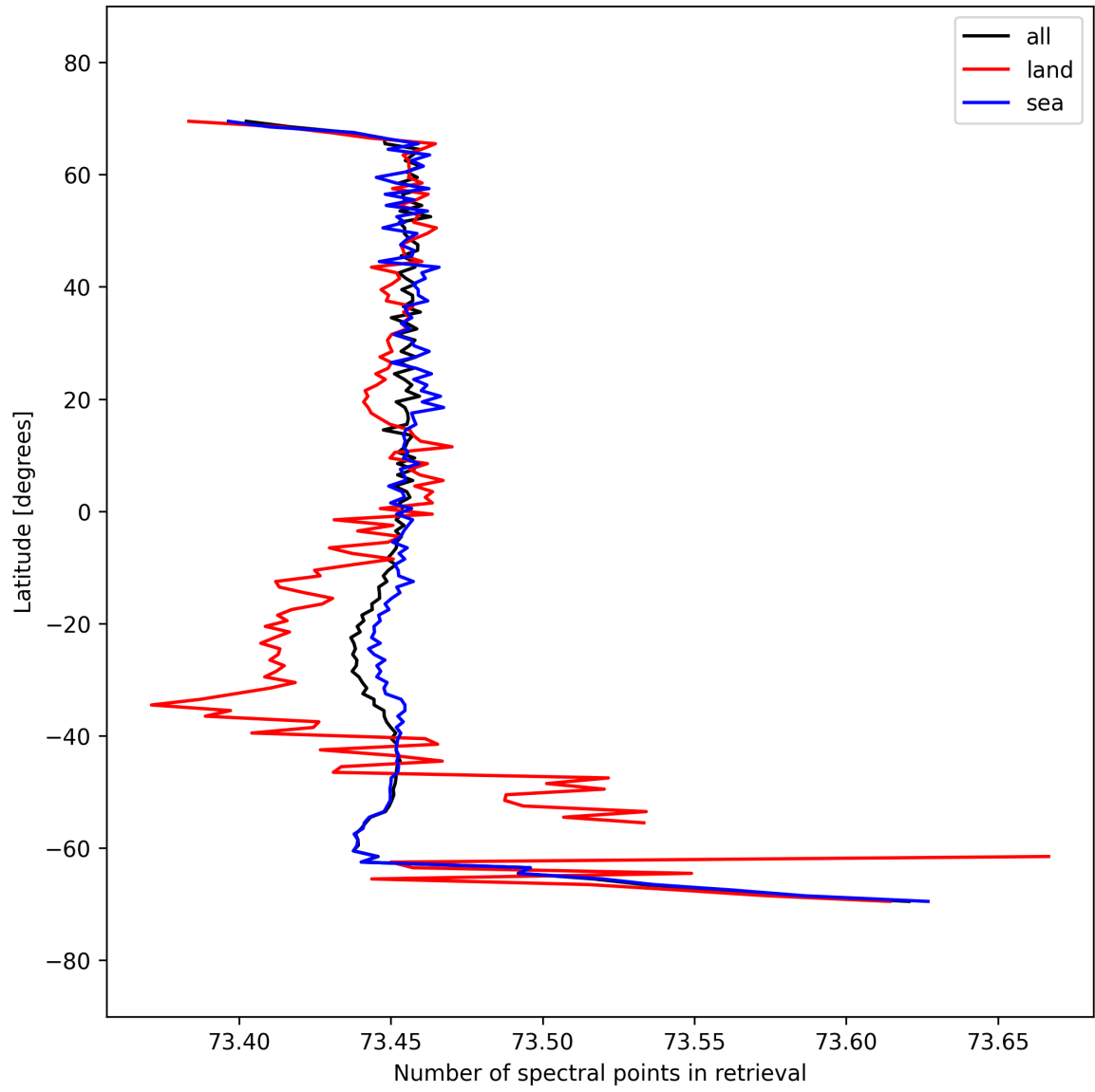
Figure 56: Zonal average of “Number of spectral points in retrieval” for 2025-09-22 to 2025-09-24.
