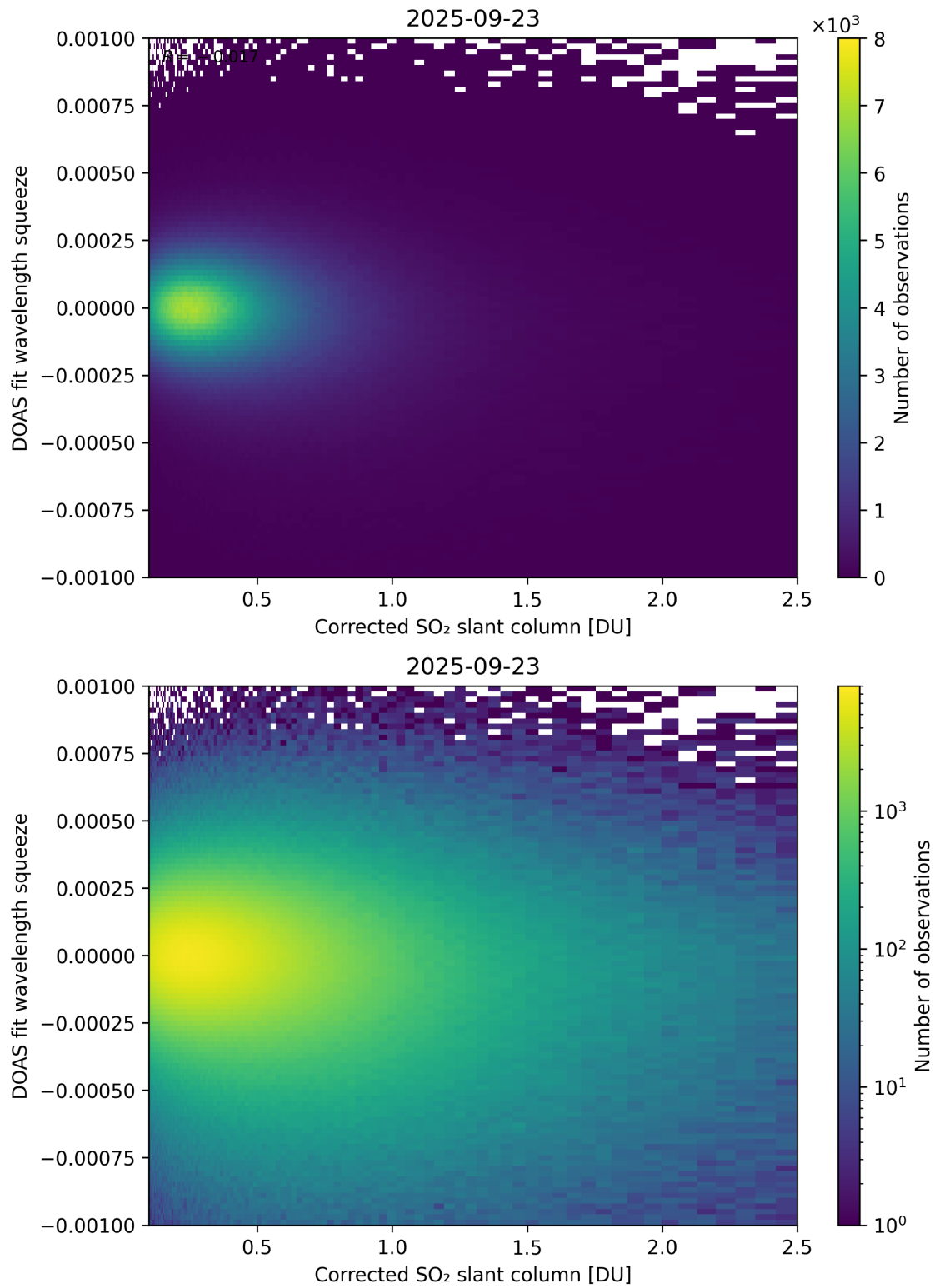
Figure 230: Scatter density plot of “Corrected SO 2 slant column” against “DOAS fit wavelength squeeze” for 2025-09-22 to 2025-09-24.
