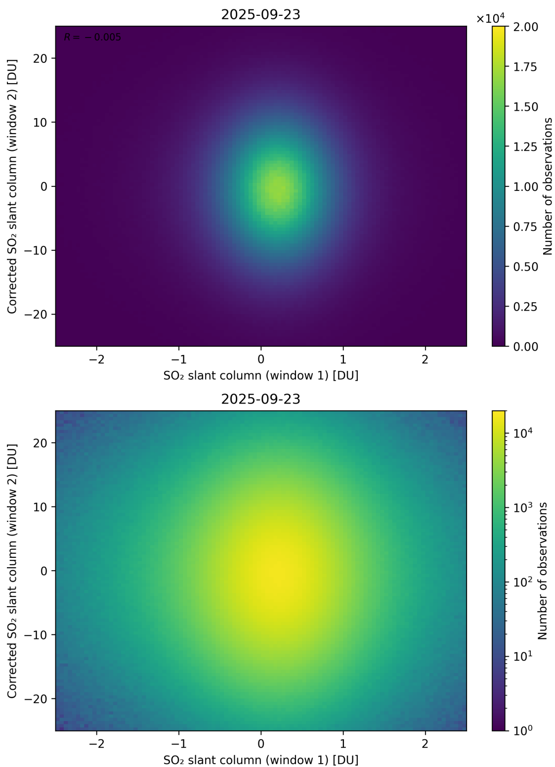
Figure 283: Scatter density plot of “SO 2 slant column (window 1)” against “Corrected SO 2 slant column (window 2)” for 2025-09-22 to 2025-09-24.
