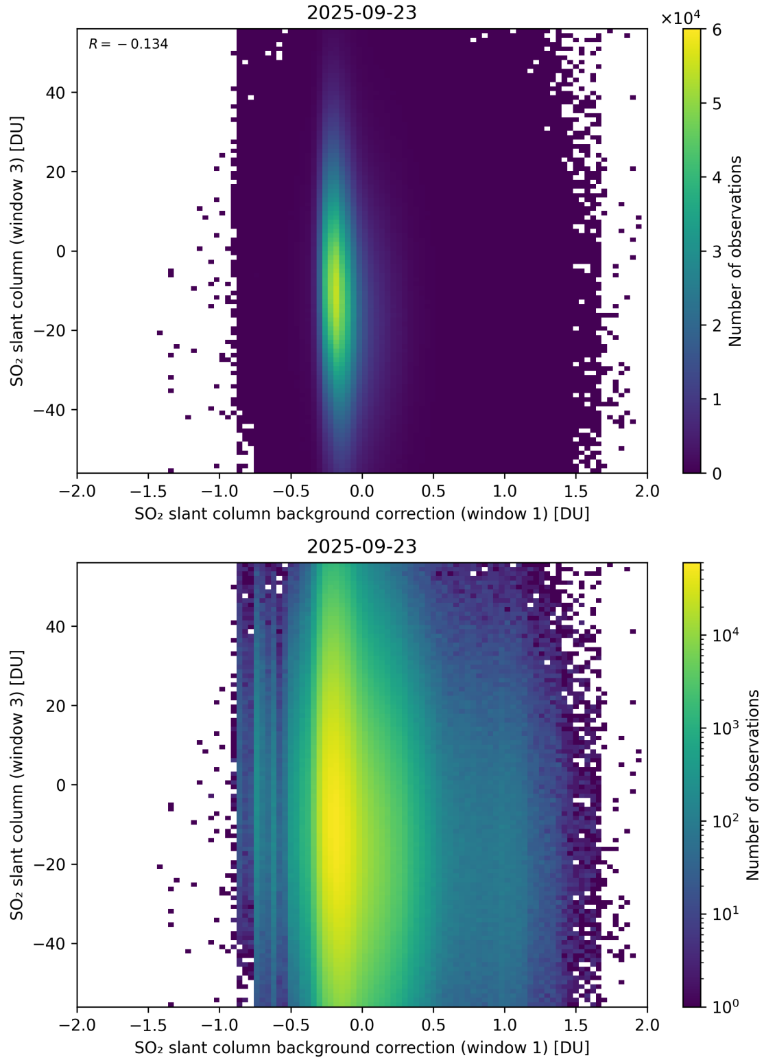
Figure 118: Scatter density plot of “SO 2 slant column background correction (window 1)” against “SO 2 slant column (window 3)” for 2025-09-22 to 2025-09-24.
