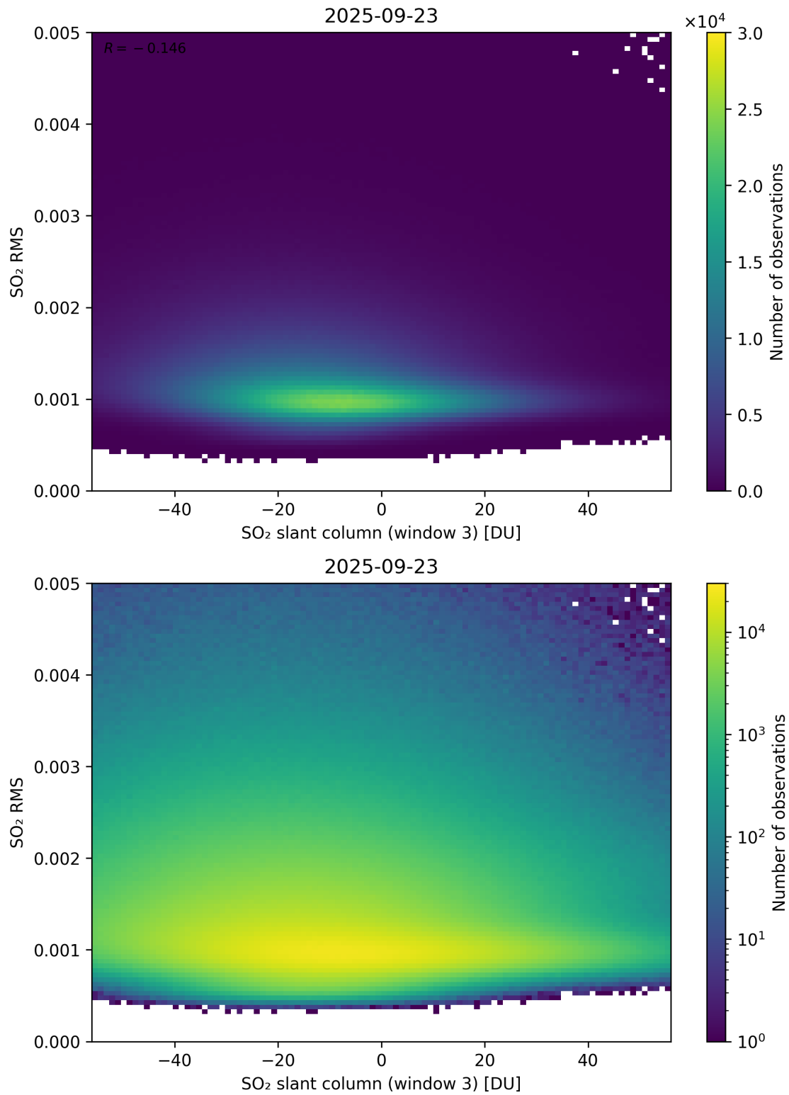
Figure 306: Scatter density plot of “SO 2 slant column (window 3)” against “SO 2 RMS” for 2025-09-22 to 2025-09-24.
