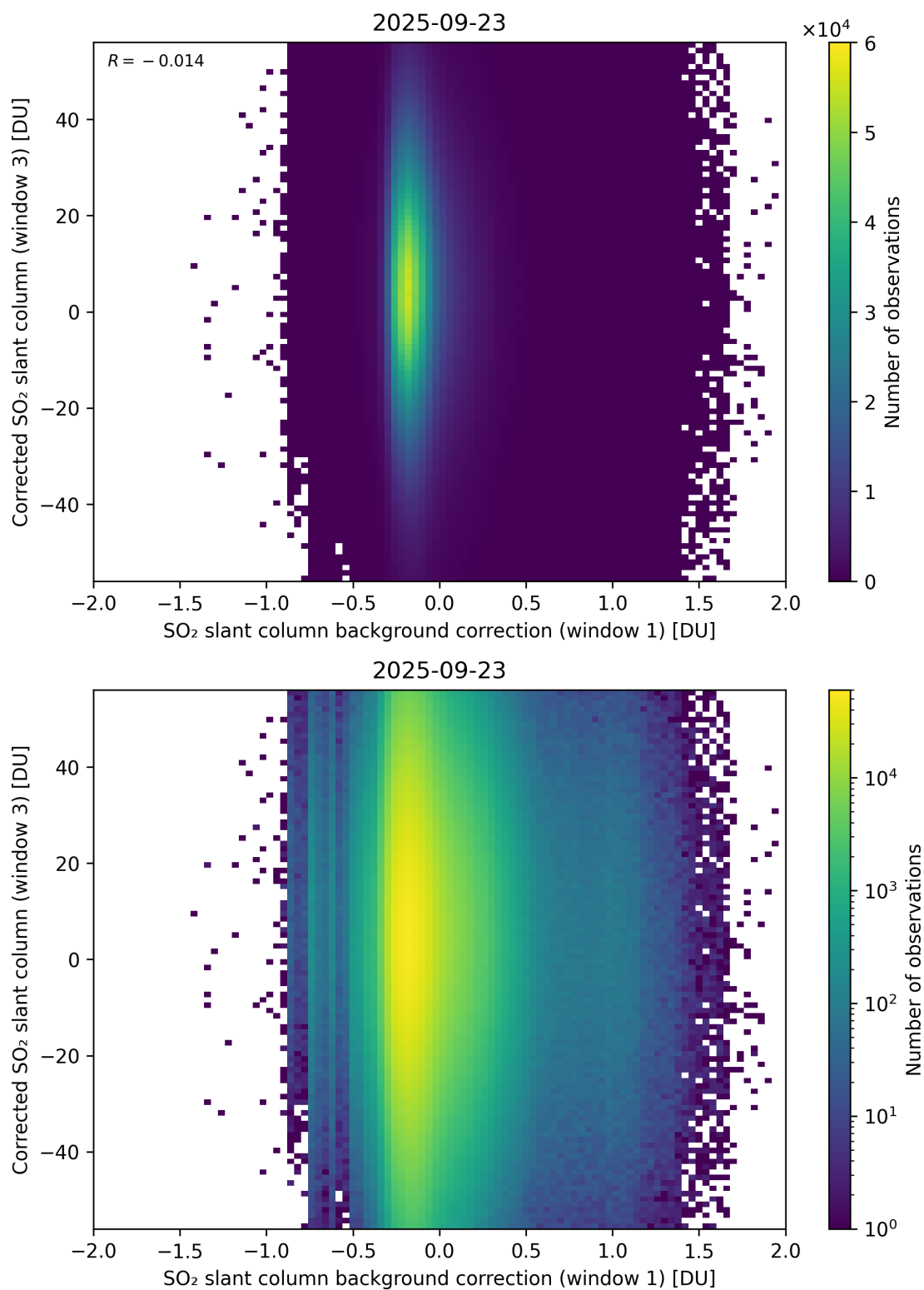
Figure 116: Scatter density plot of “SO 2 slant column background correction (window 1)” against “Corrected SO 2 slant column (window 3)” for 2025-09-22 to 2025-09-24.
