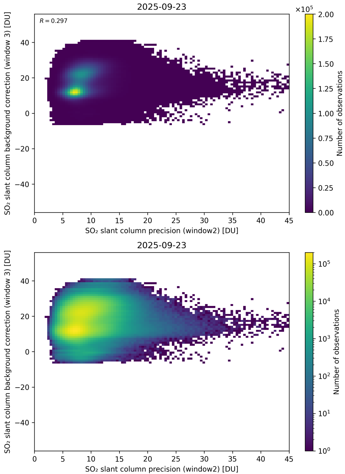
Figure 292: Scatter density plot of “SO 2 slant column precision (window2)” against “SO 2 slant column background correction (window 3)” for 2025-09-22 to 2025-09-24.
