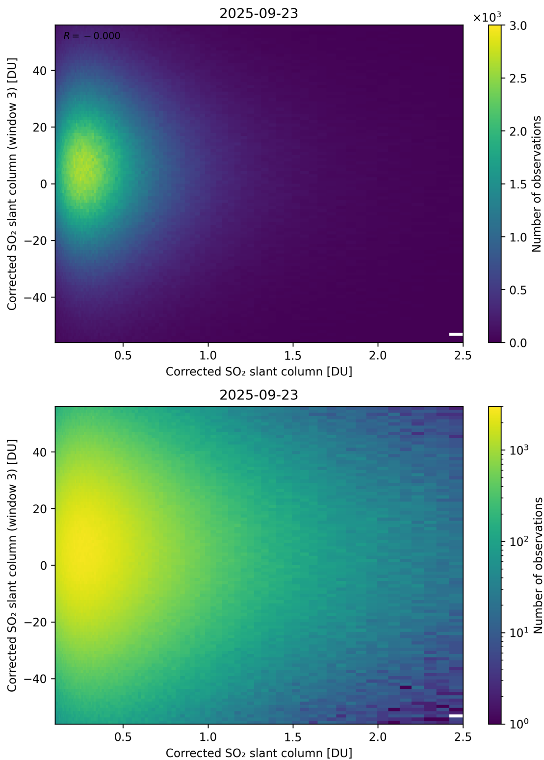
Figure 236: Scatter density plot of “Corrected SO 2 slant column” against “Corrected SO 2 slant column (window 3)” for 2025-09-22 to 2025-09-24.
