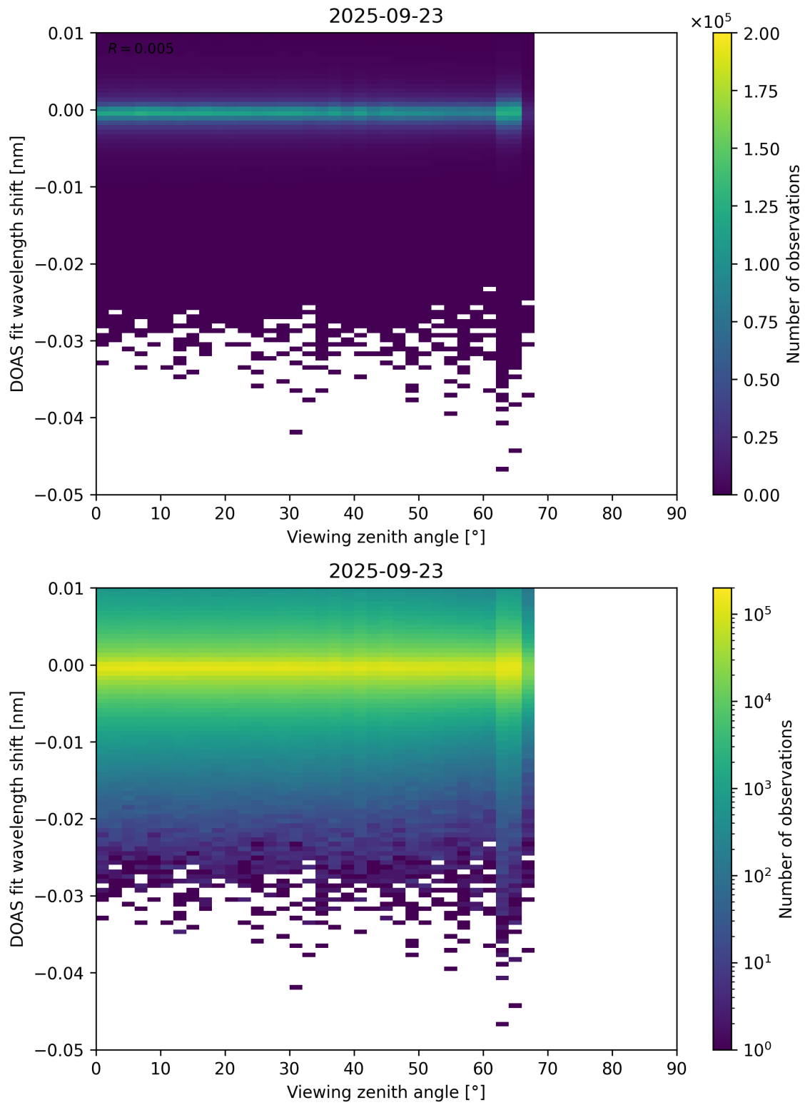
Figure 365: Scatter density plot of “Viewing zenith angle” against “DOAS fit wavelength shift” for 2025-09-22 to 2025-09-24.
