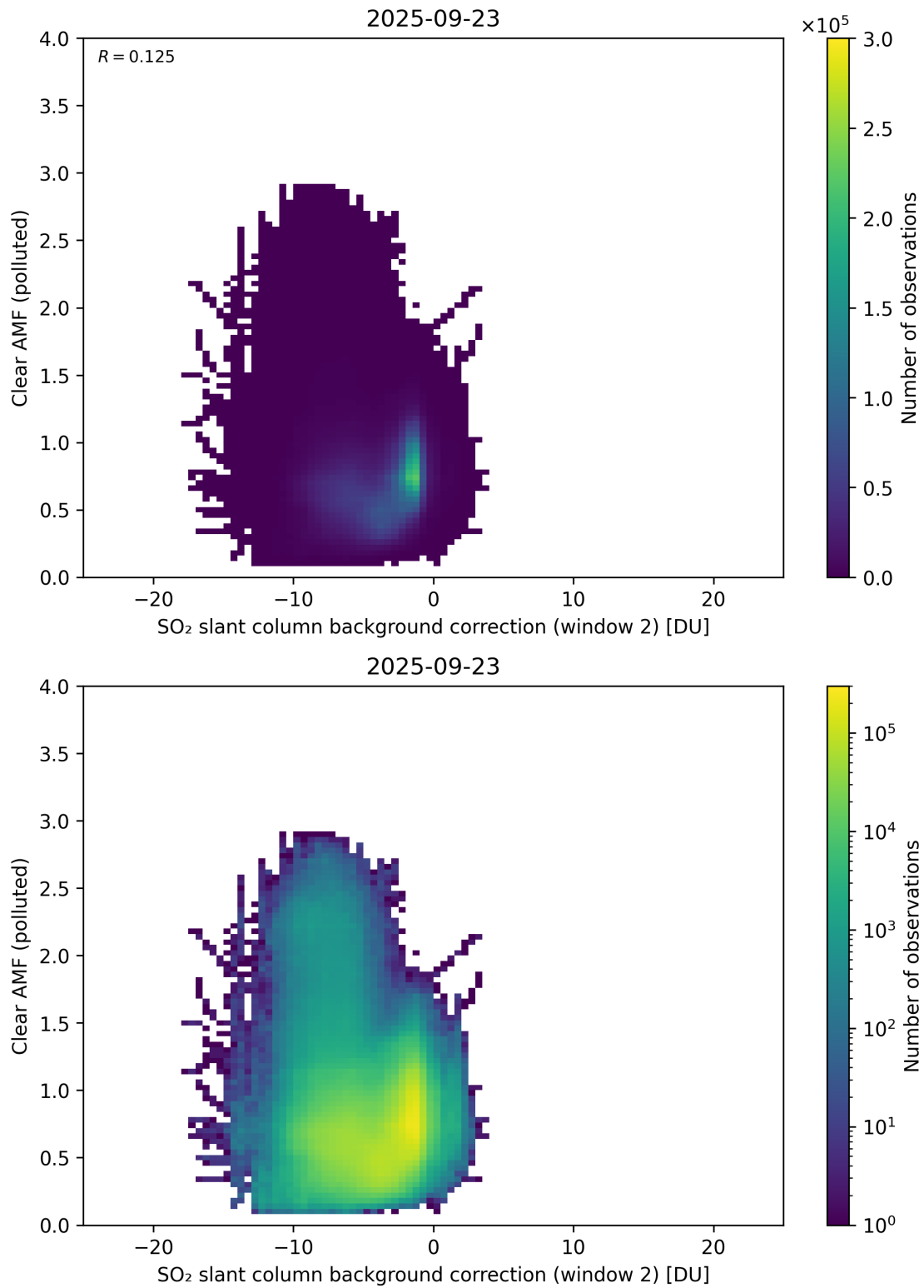
Figure 126: Scatter density plot of “SO 2 slant column background correction (window 2)” against “Clear AMF (polluted)” for 2025-09-22 to 2025-09-24.
