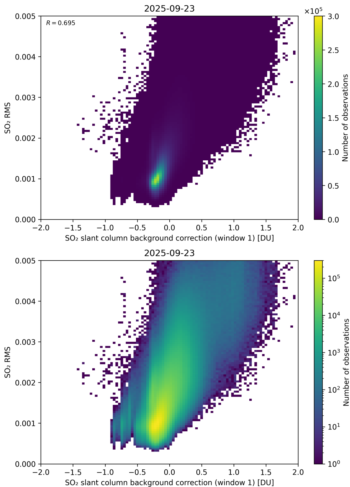
Figure 113: Scatter density plot of “SO 2 slant column background correction (window 1)” against “SO 2 RMS” for 2025-09-22 to 2025-09-24.
