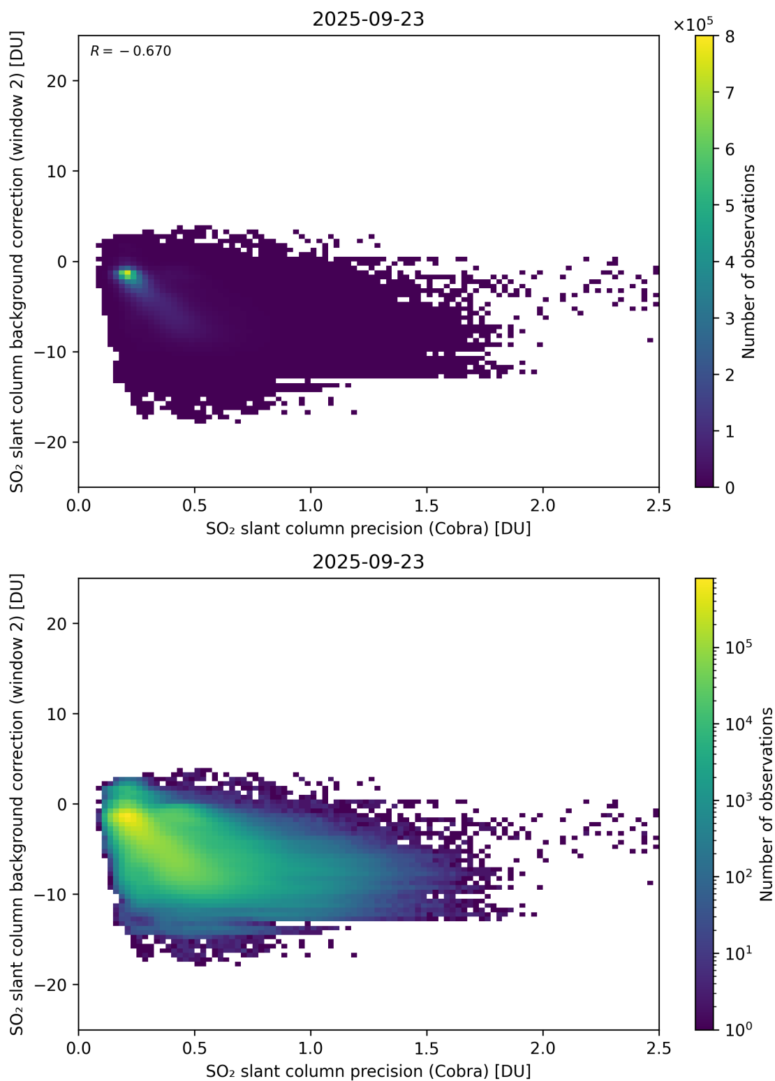
Figure 200: Scatter density plot of “SO 2 slant column precision (Cobra)” against “SO 2 slant column background correction (window 2)” for 2025-09-22 to 2025-09-24.
