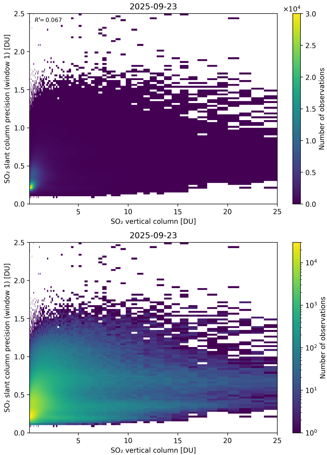
Figure 355: Scatter density plot of “SO 2 vertical column” against “SO 2 slant column precision (window 1)” for 2025-09-22 to 2025-09-24.
