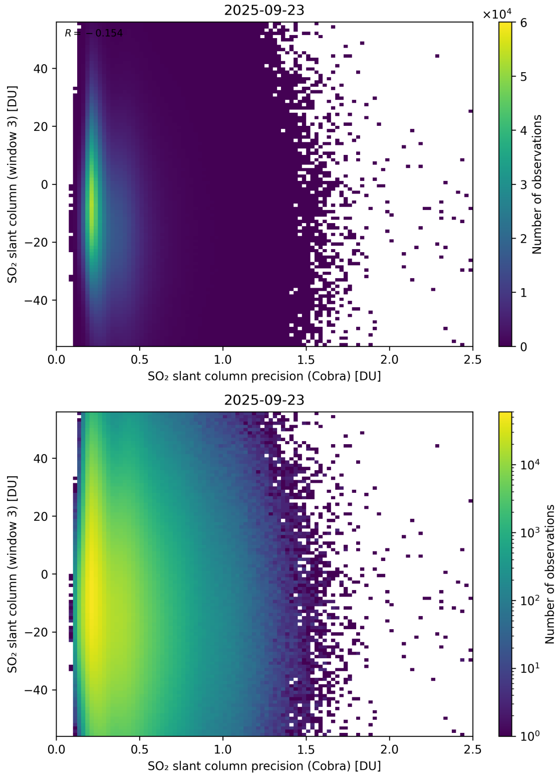
Figure 211: Scatter density plot of “SO 2 slant column precision (Cobra)” against “SO 2 slant column (window 3)” for 2025-09-22 to 2025-09-24.
