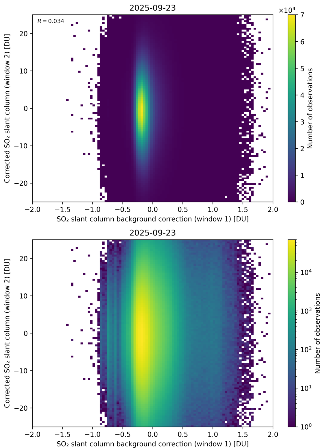
Figure 115: Scatter density plot of “SO 2 slant column background correction (window 1)” against “Corrected SO 2 slant column (window 2)” for 2025-09-22 to 2025-09-24.
