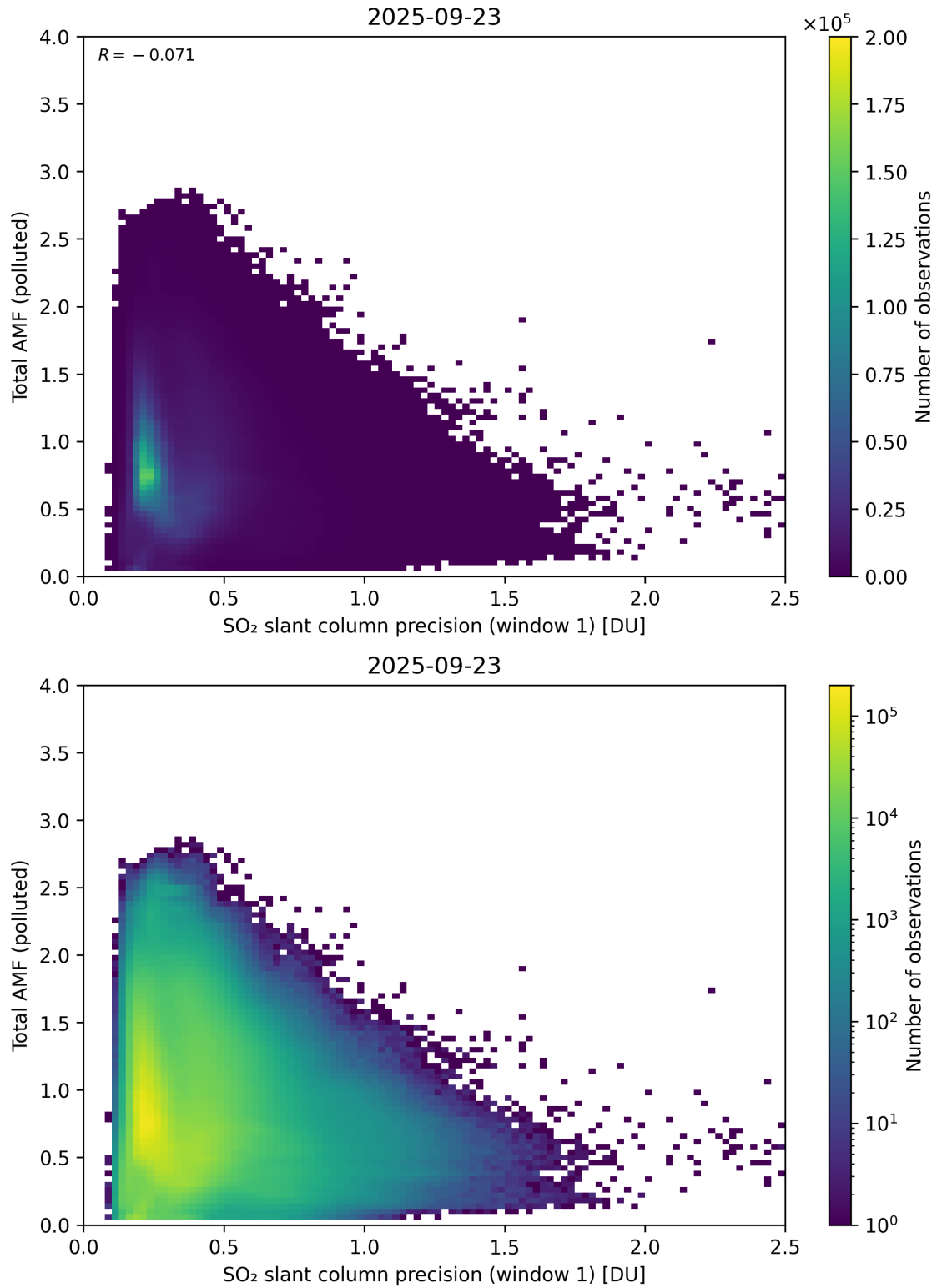
Figure 280: Scatter density plot of “SO 2 slant column precision (window 1)” against “Total AMF (polluted)” for 2025-09-22 to 2025-09-24.
