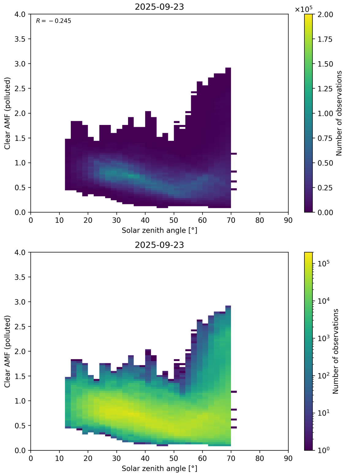
Figure 178: Scatter density plot of “Solar zenith angle” against “Clear AMF (polluted)” for 2025-09-22 to 2025-09-24.
