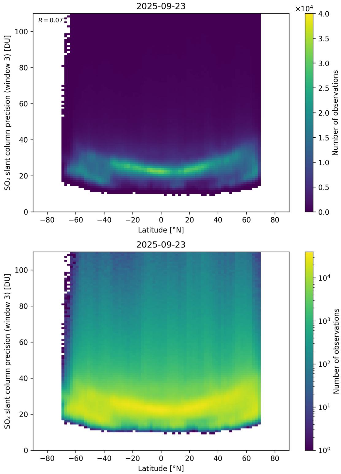
Figure 166: Scatter density plot of “Latitude” against “SO 2 slant column precision (window 3)” for 2025-09-22 to 2025-09-24.
