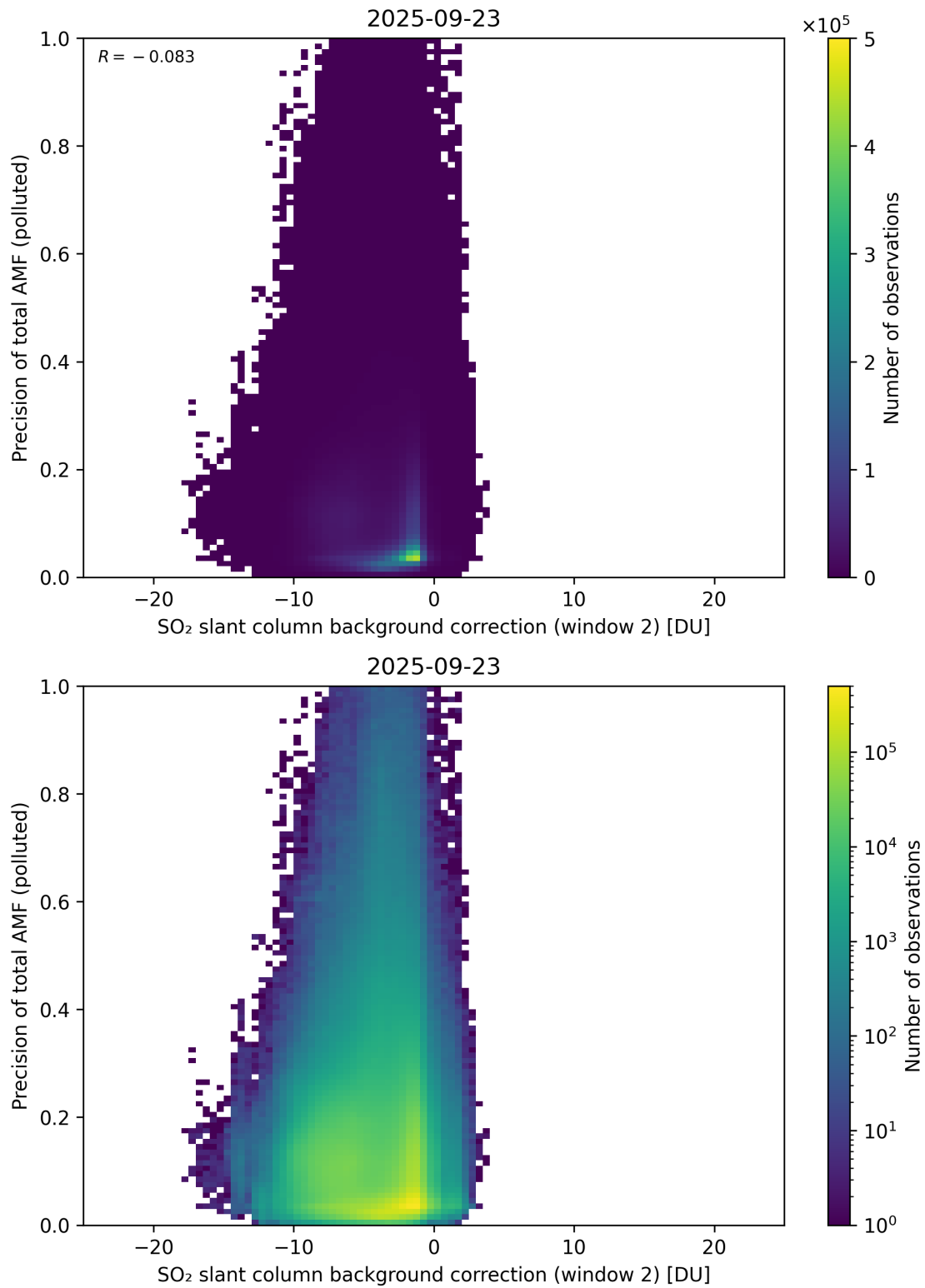
Figure 131: Scatter density plot of “SO 2 slant column background correction (window 2)” against “Precision of total AMF (polluted)” for 2025-09-22 to 2025-09-24.
