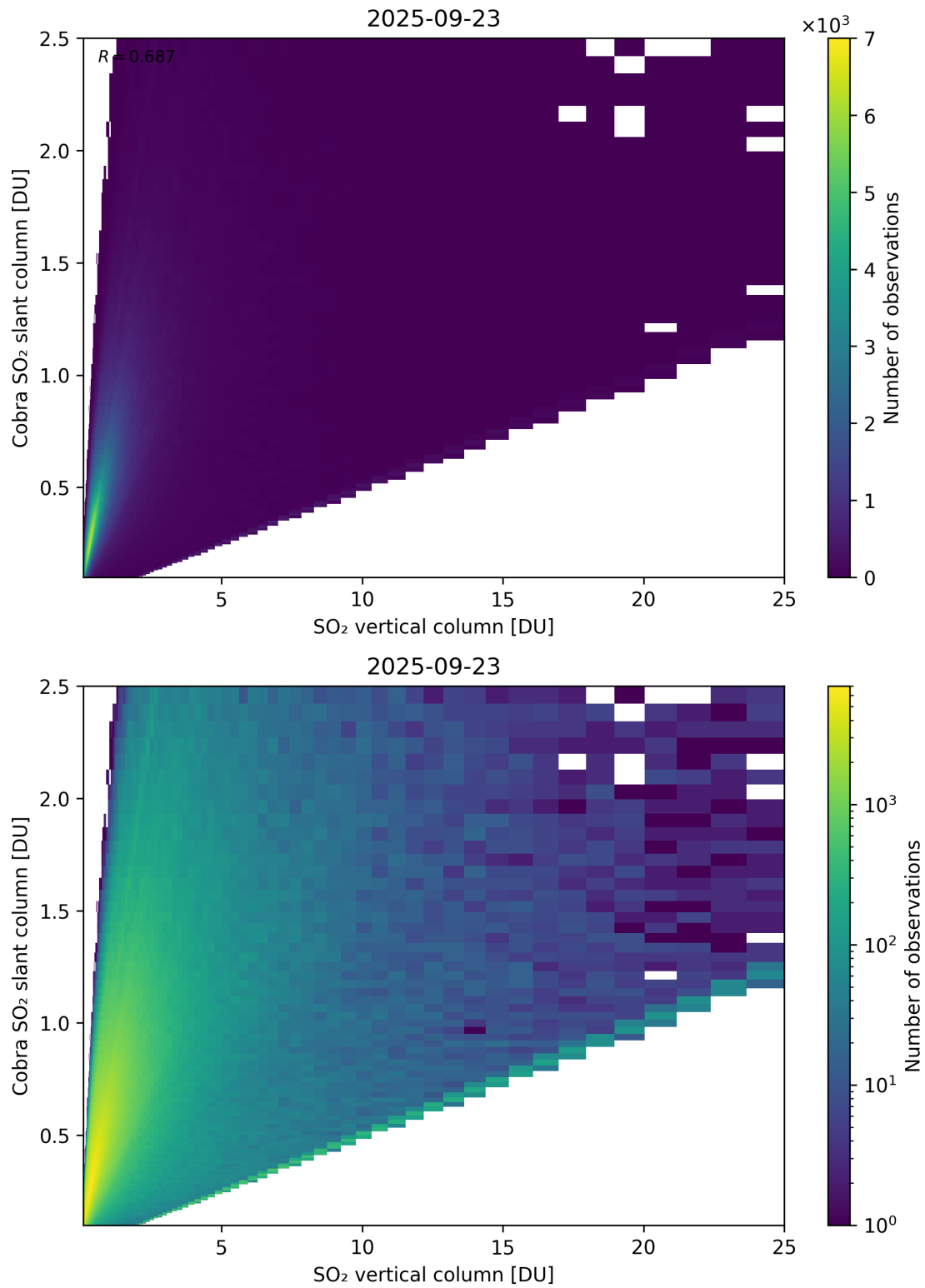
Figure 349: Scatter density plot of “SO 2 vertical column” against “Cobra SO 2 slant column” for 2025-09-22 to 2025-09-24.
