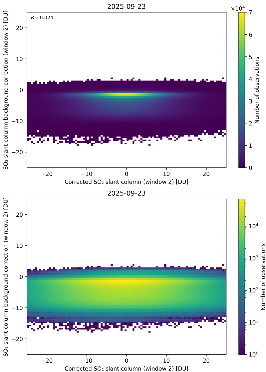
Figure 244: Scatter density plot of “Corrected SO 2 slant column (window 2)” against “SO 2 slant column background correction (window 2)” for 2025-09-22 to 2025-09-24.
