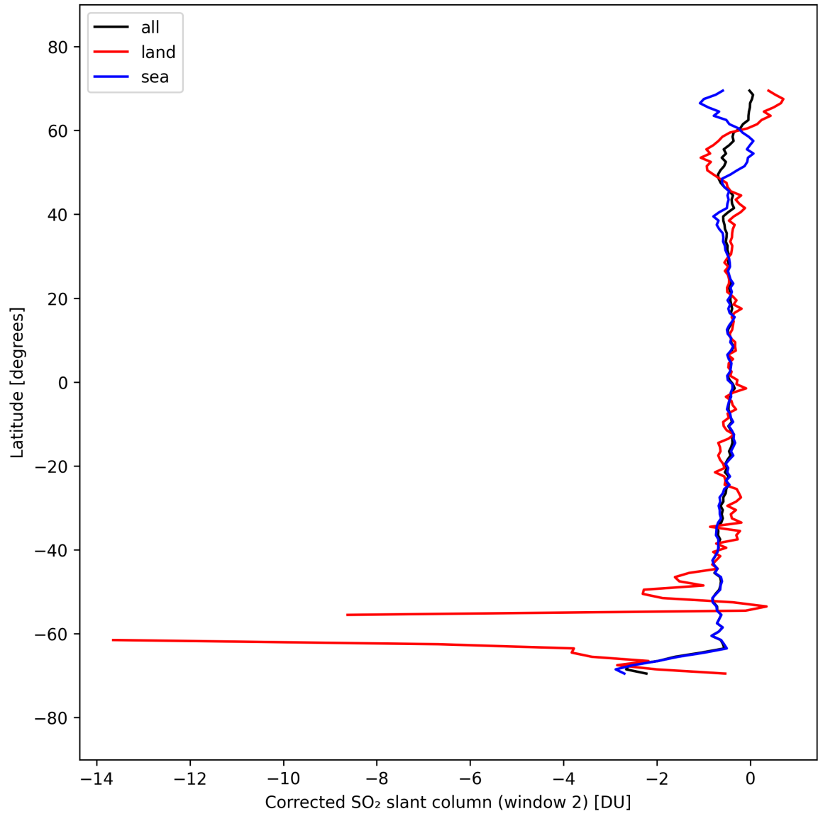
Figure 43: Zonal average of “Corrected SO 2 slant column (window 2)” for 2025-09-22 to 2025-09-24.
