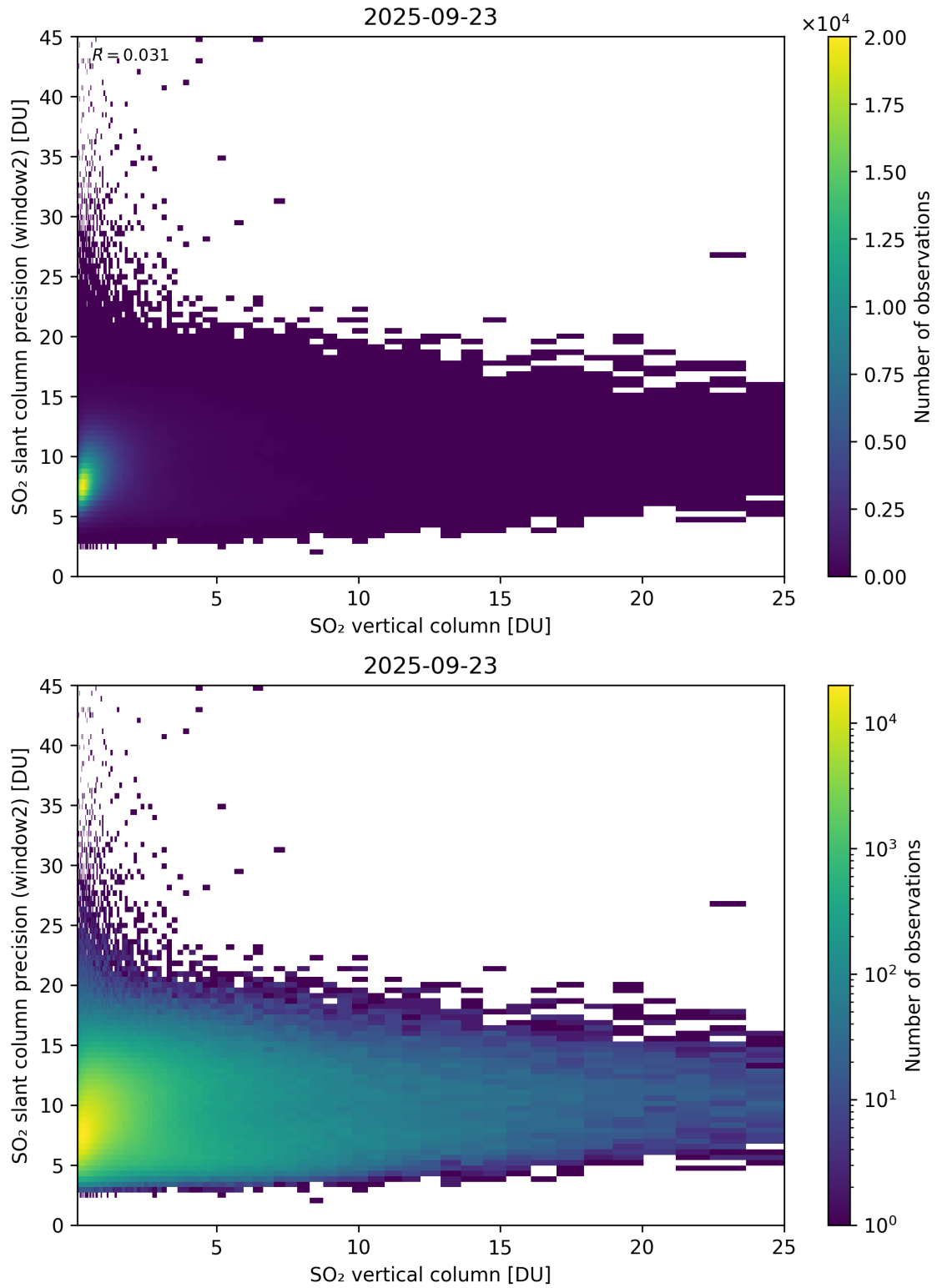
Figure 356: Scatter density plot of “SO 2 vertical column” against “SO 2 slant column precision (window2)” for 2025-09-22 to 2025-09-24.
