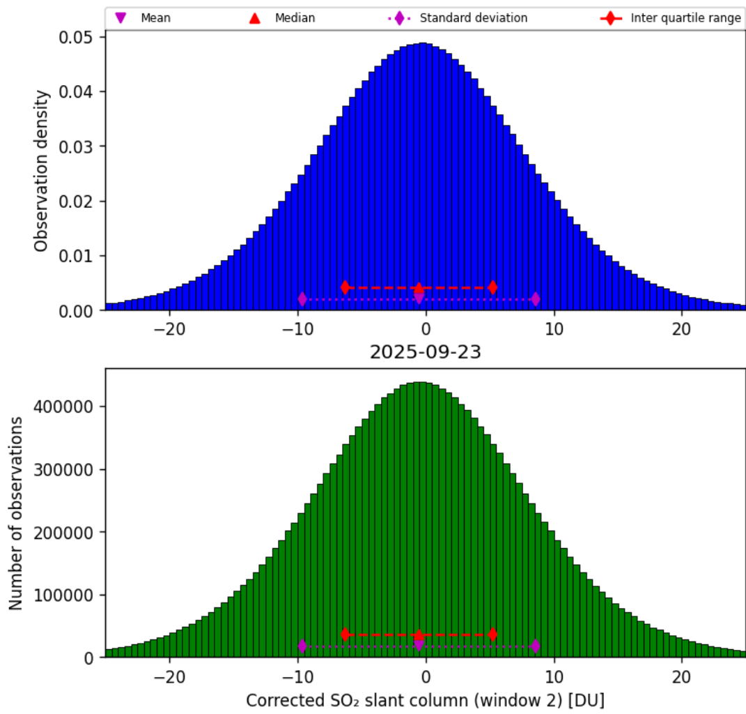
Figure 69: Histogram of “Corrected SO 2 slant column (window 2)” for 2025-09-22 to 2025-09-24
