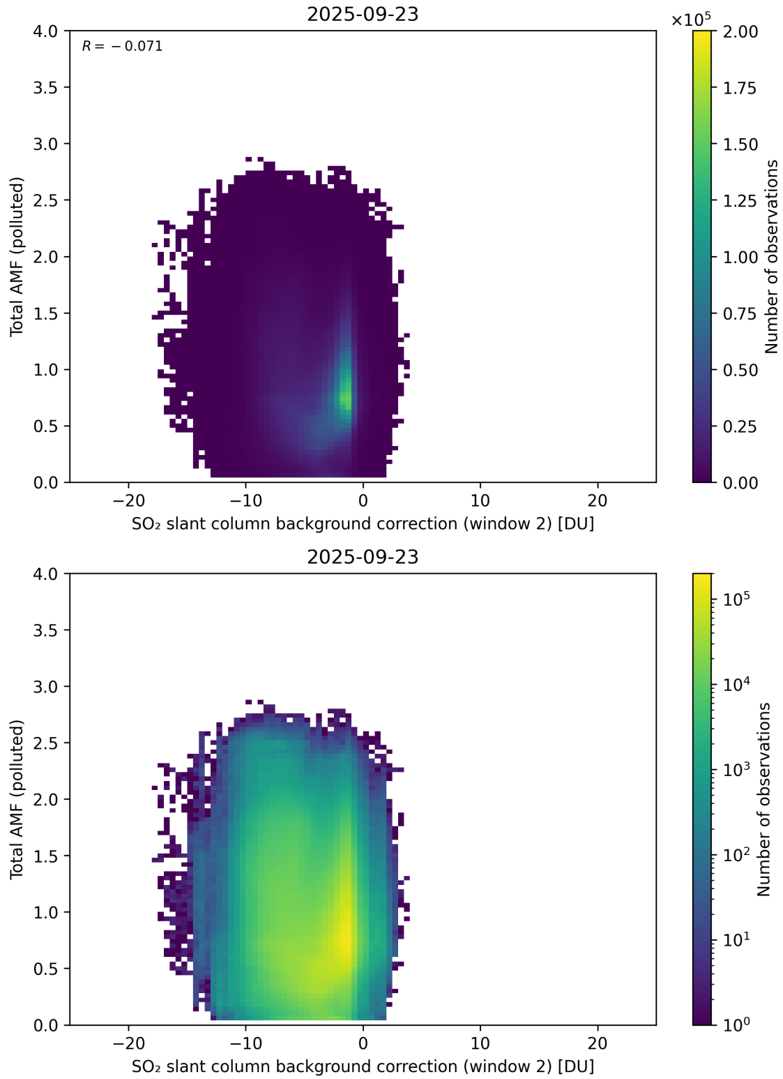
Figure 130: Scatter density plot of “SO 2 slant column background correction (window 2)” against “Total AMF (polluted)” for 2025-09-22 to 2025-09-24.
