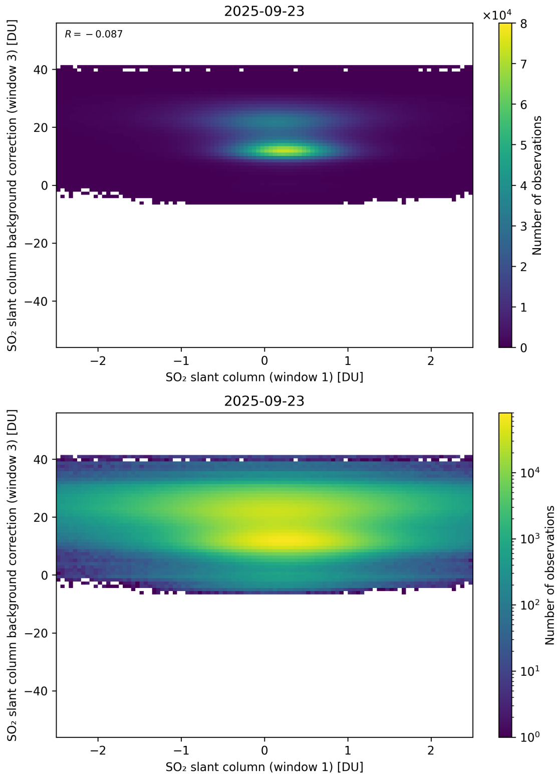
Figure 264: Scatter density plot of “SO 2 slant column (window 1)” against “SO 2 slant column background correction (window 3)” for 2025-09-22 to 2025-09-24.
