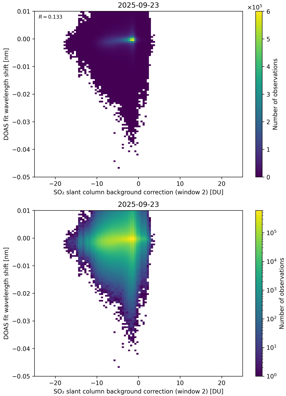
Figure 123: Scatter density plot of “SO 2 slant column background correction (window 2)” against “DOAS fit wavelength shift” for 2025-09-22 to 2025-09-24.
