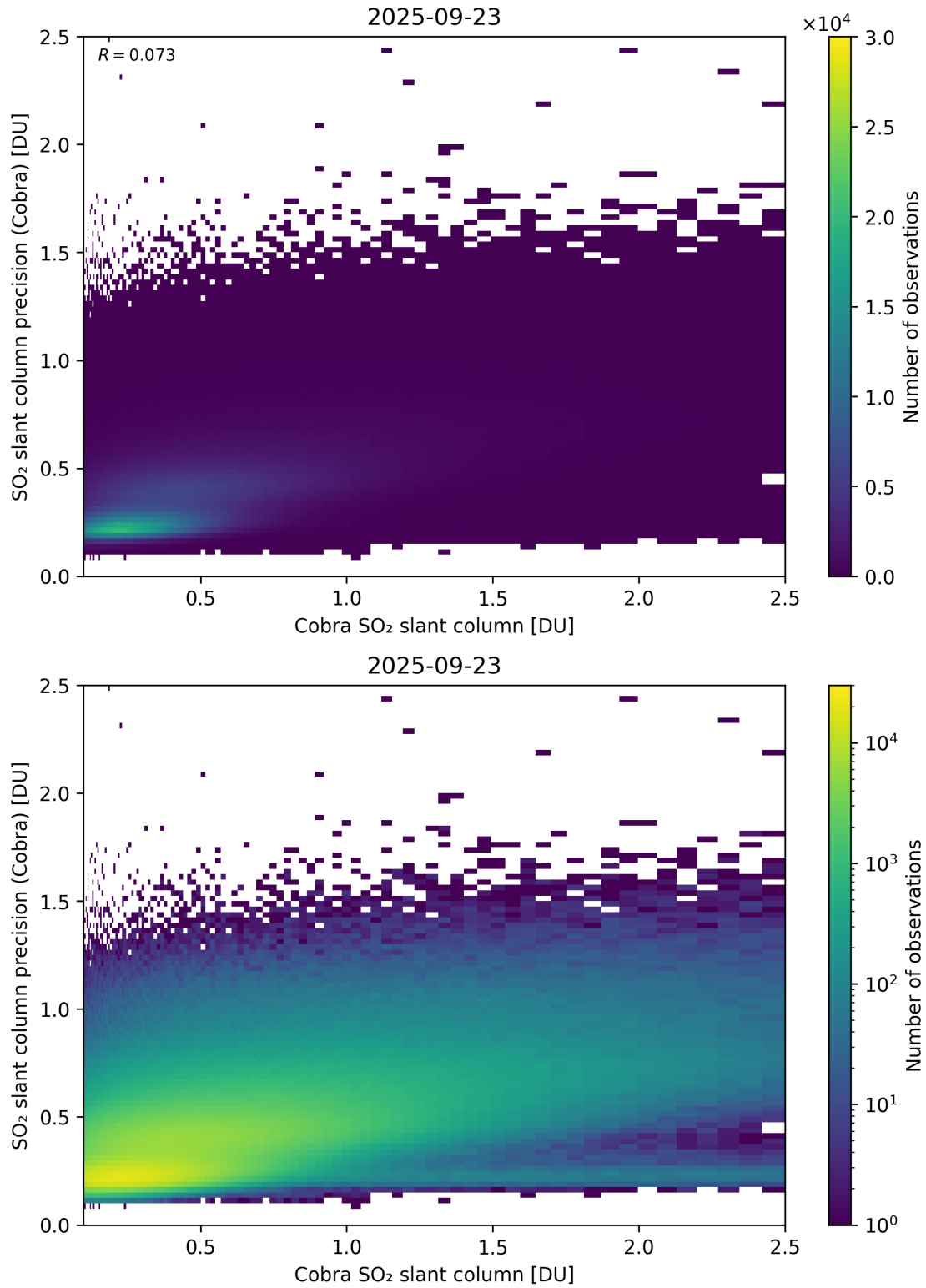
Figure 216: Scatter density plot of “Cobra SO 2 slant column” against “SO 2 slant column precision (Cobra)” for 2025-09-22 to 2025-09-24.
