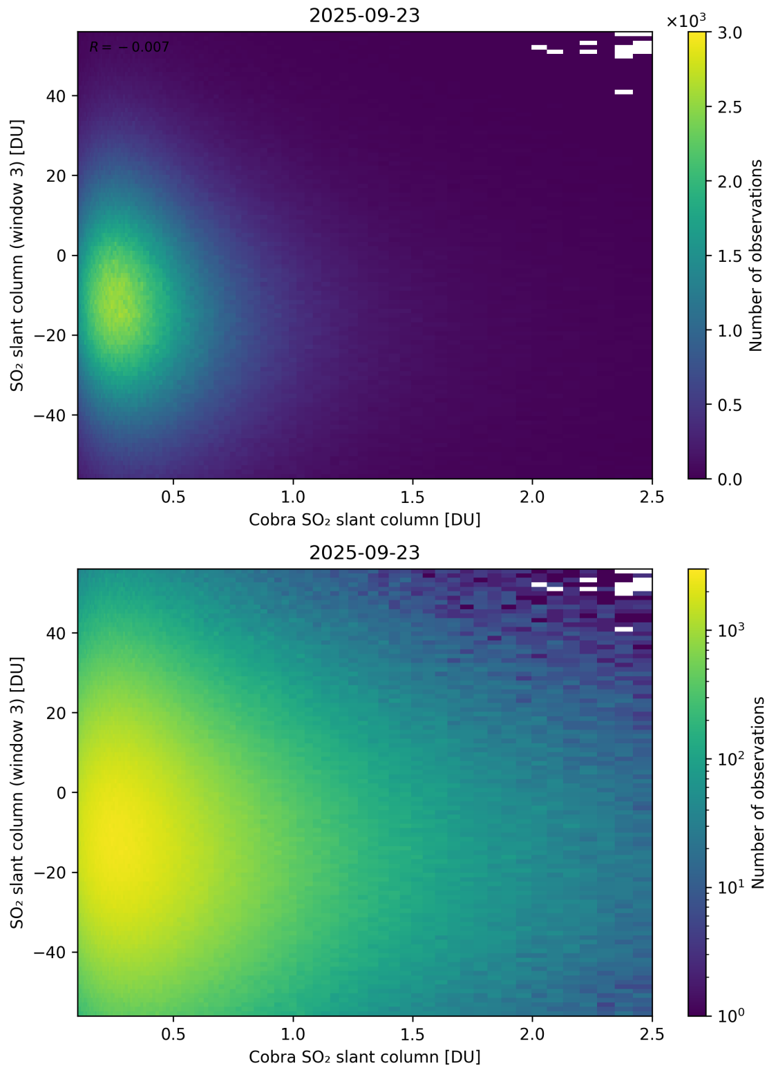
Figure 222: Scatter density plot of “Cobra SO 2 slant column” against “SO 2 slant column (window 3)” for 2025-09-22 to 2025-09-24.
