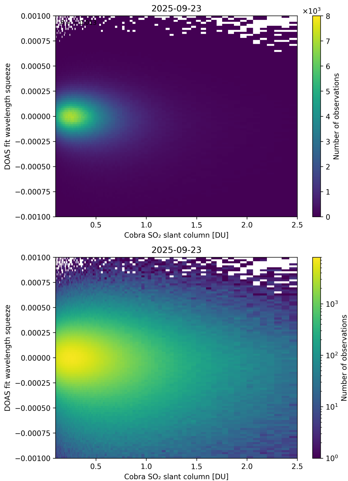
Figure 197: Scatter density plot of “Cobra SO 2 slant column” against “DOAS fit wavelength squeeze” for 2025-09-22 to 2025-09-24.
