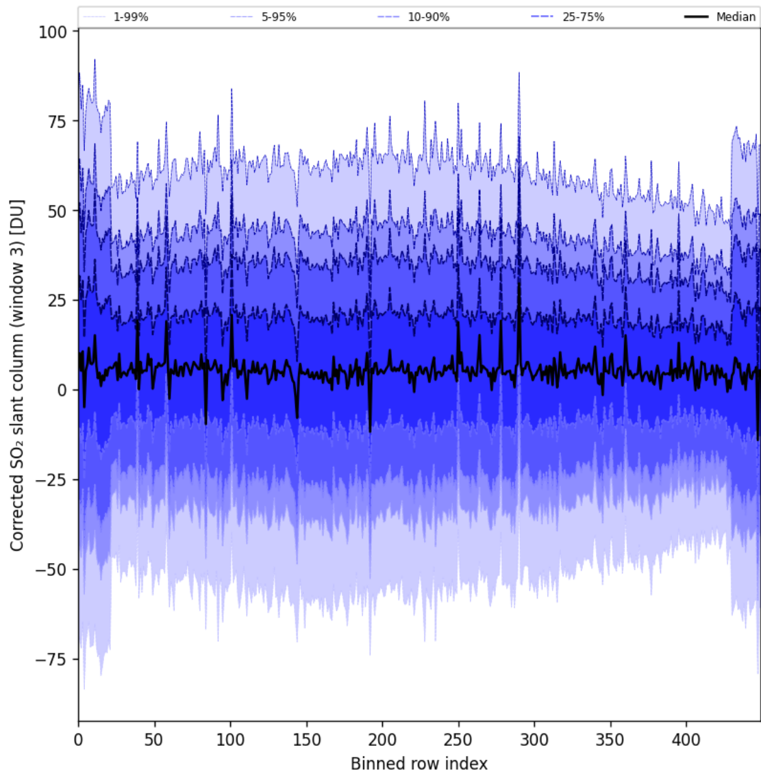
Figure 99: Along track statistics of “Corrected SO 2 slant column (window 3)” for 2025-09-22 to 2025-09-24
