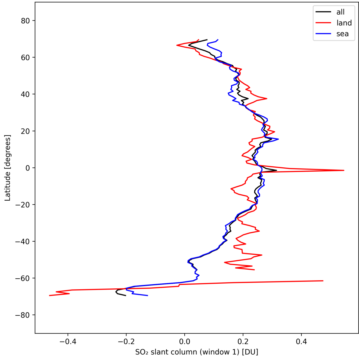
Figure 37: Zonal average of “SO 2 slant column (window 1)” for 2025-09-22 to 2025-09-24.
