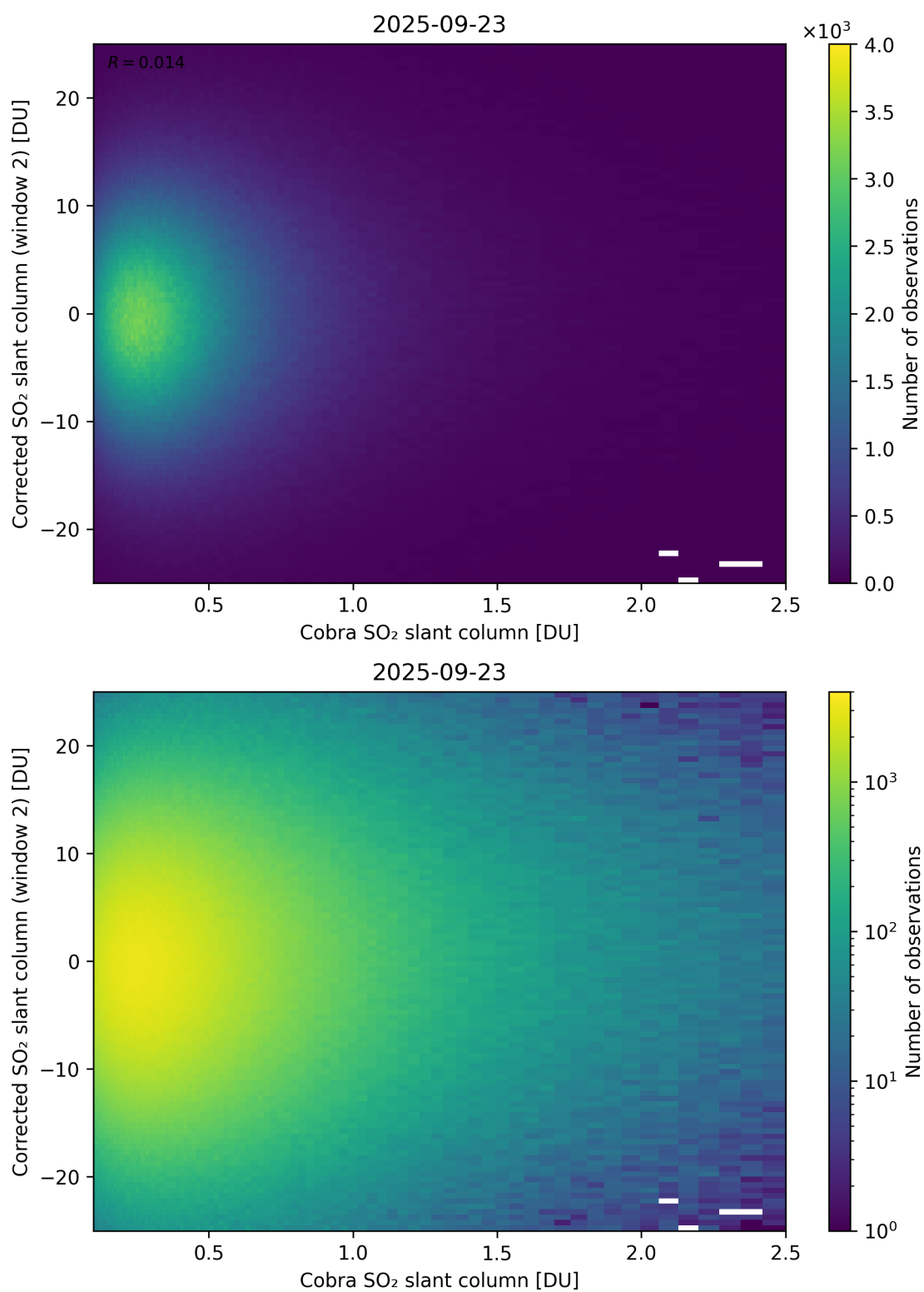
Figure 217: Scatter density plot of “Cobra SO 2 slant column” against “Corrected SO 2 slant column (window 2)” for 2025-09-22 to 2025-09-24.
