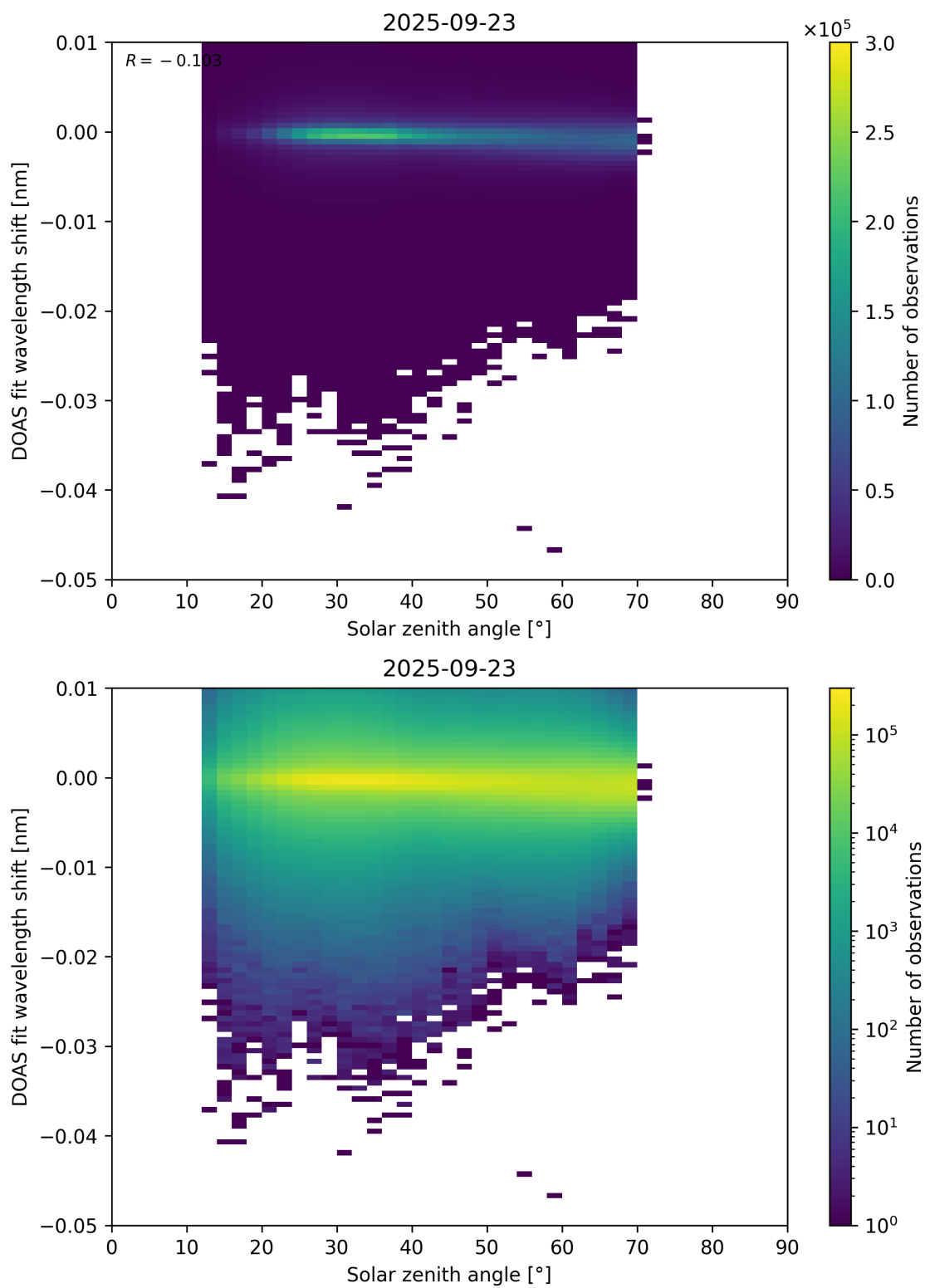
Figure 174: Scatter density plot of “Solar zenith angle” against “DOAS fit wavelength shift” for 2025-09-22 to 2025-09-24.
