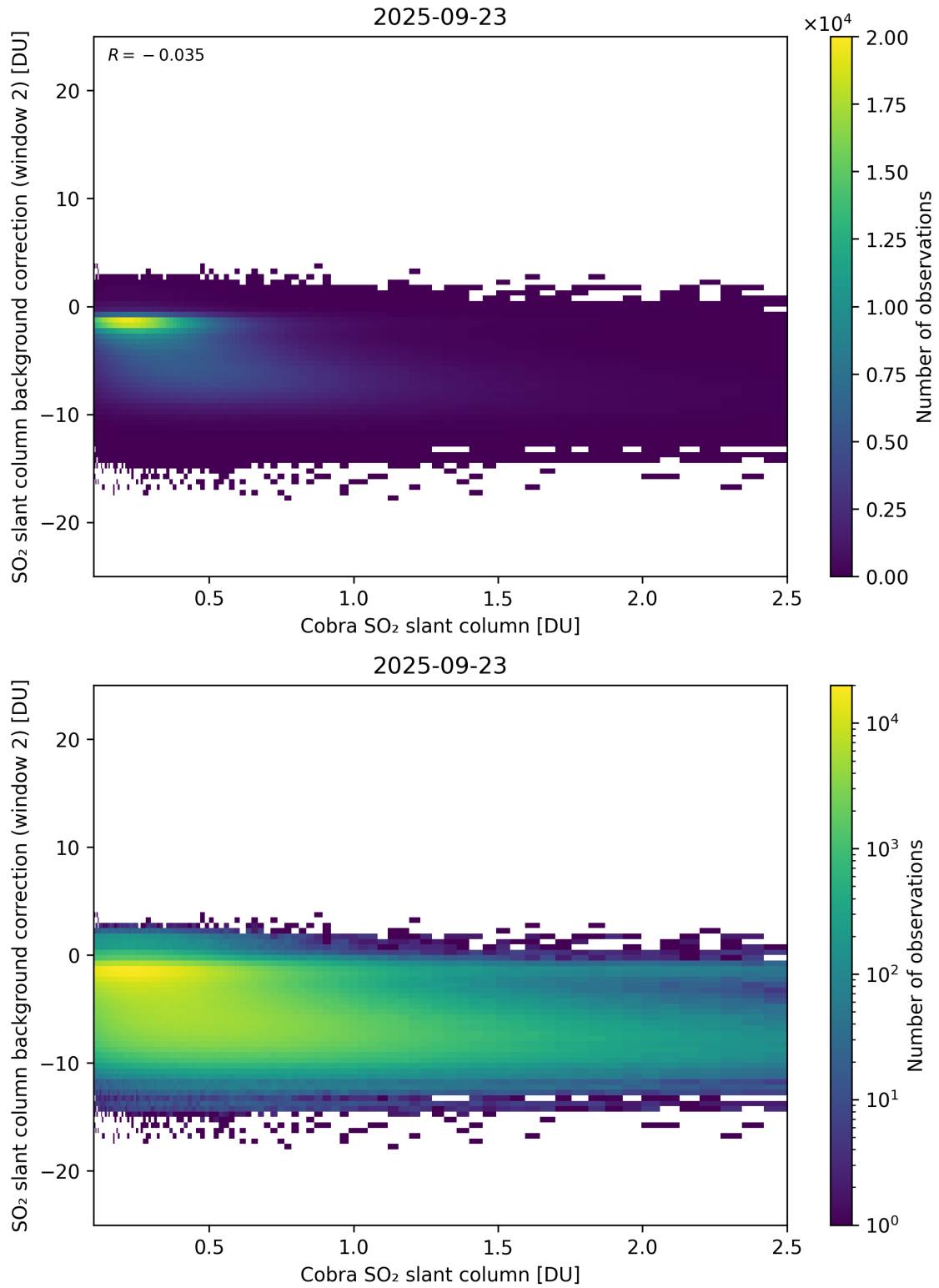
Figure 194: Scatter density plot of “Cobra SO 2 slant column” against “SO 2 slant column background correction (window 2)” for 2025-09-22 to 2025-09-24.
