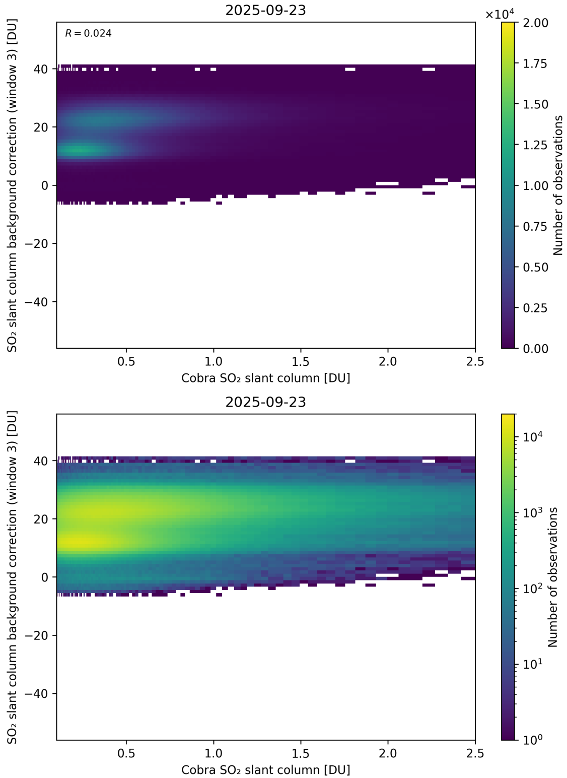
Figure 195: Scatter density plot of “Cobra SO 2 slant column” against “SO 2 slant column background correction (window 3)” for 2025-09-22 to 2025-09-24.
