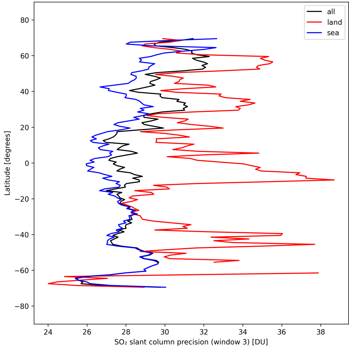
Figure 46: Zonal average of “SO 2 slant column precision (window 3)” for 2025-09-22 to 2025-09-24.
