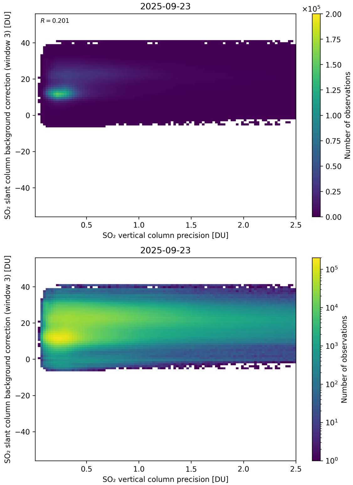
Figure 331: Scatter density plot of “SO 2 vertical column precision” against “SO 2 slant column background correction (window 3)” for 2025-09-22 to 2025-09-24.
