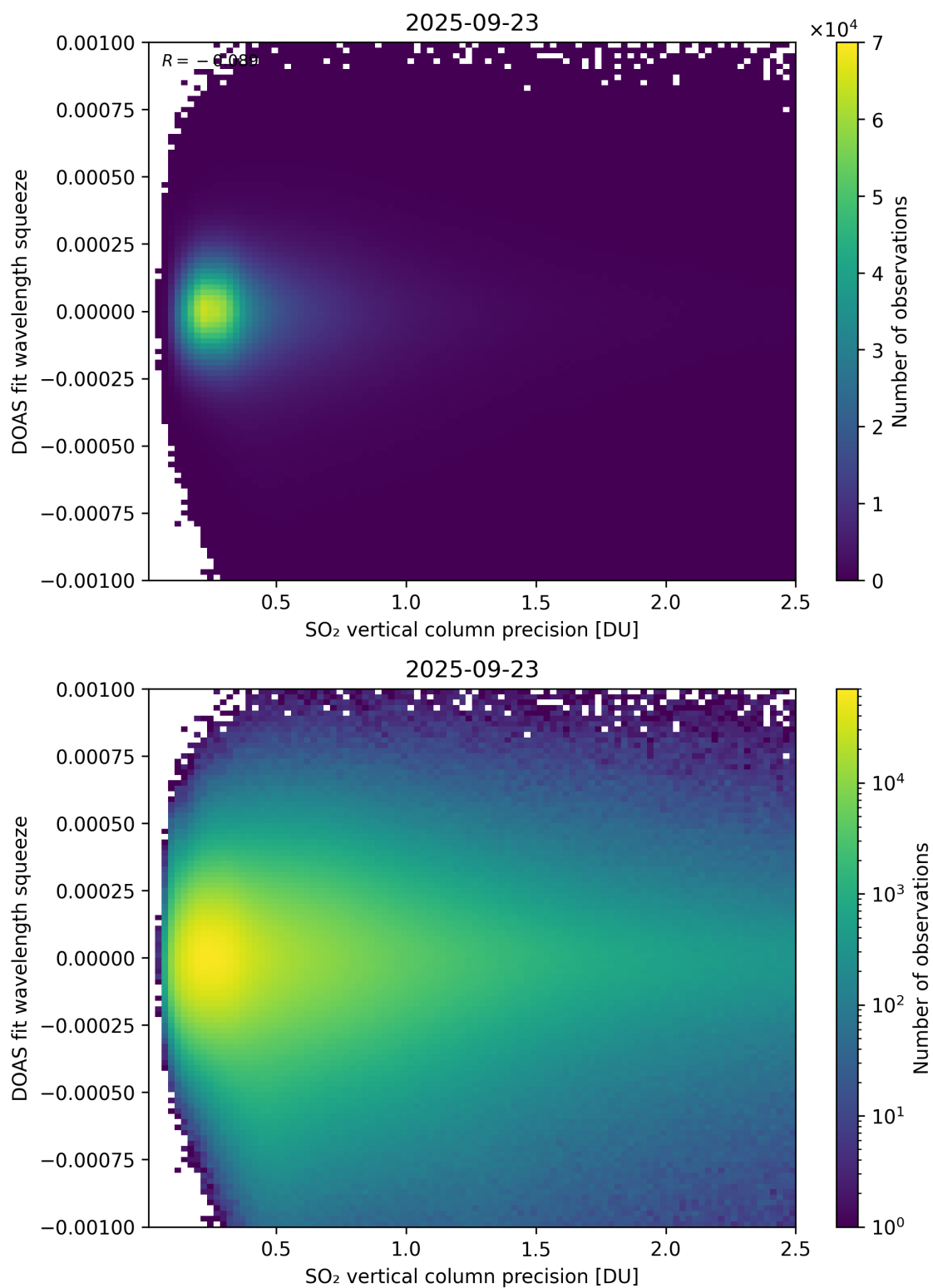
Figure 333: Scatter density plot of “SO 2 vertical column precision” against “DOAS fit wavelength squeeze” for 2025-09-22 to 2025-09-24.
