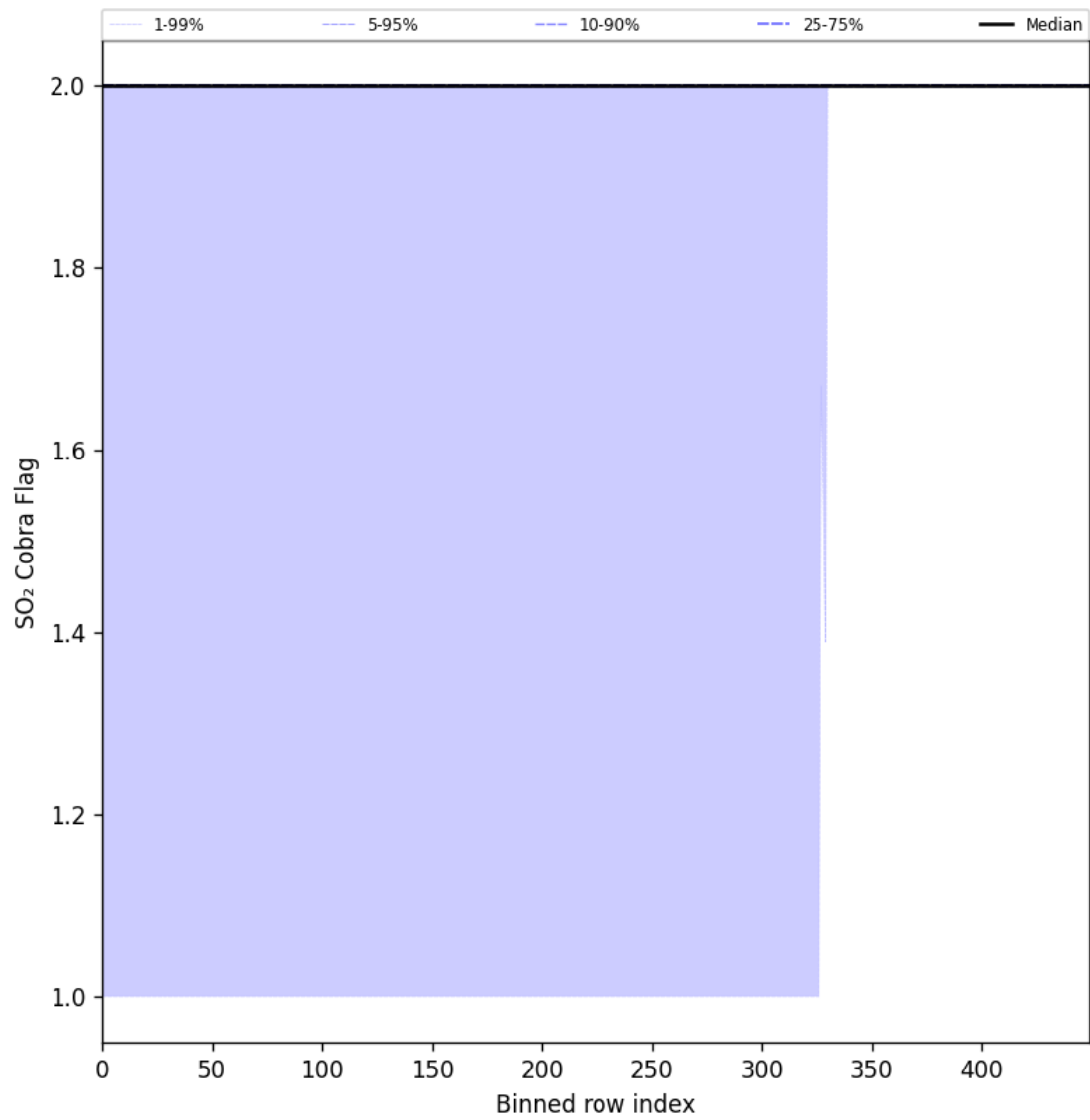
Figure 101: Along track statistics of “SO 2 Cobra Flag” for 2025-09-22 to 2025-09-24
