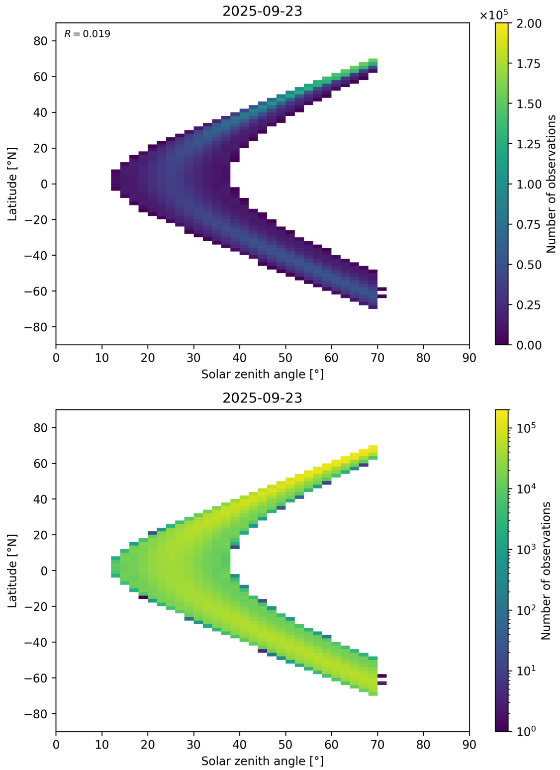
Figure 177: Scatter density plot of “Solar zenith angle” against “Latitude” for 2025-09-22 to 2025-09-24.
