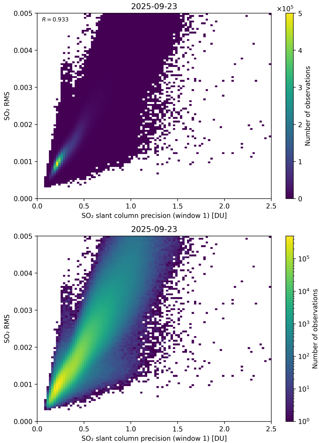
Figure 273: Scatter density plot of “SO 2 slant column precision (window 1)” against “SO 2 RMS” for 2025-09-22 to 2025-09-24.
