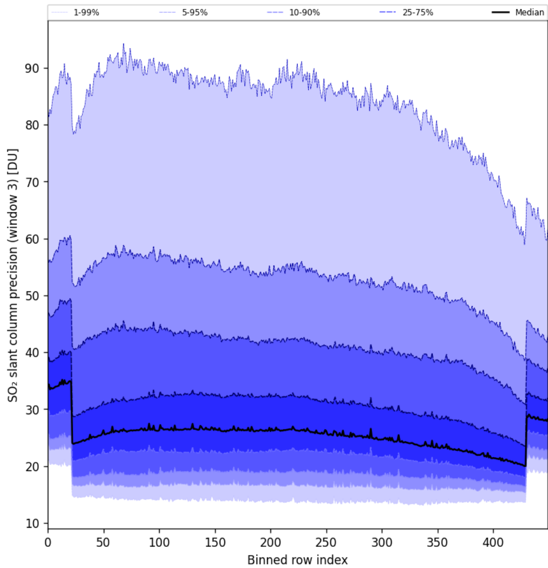
Figure 98: Along track statistics of “SO 2 slant column precision (window 3)” for 2025-09-22 to 2025-09-24
