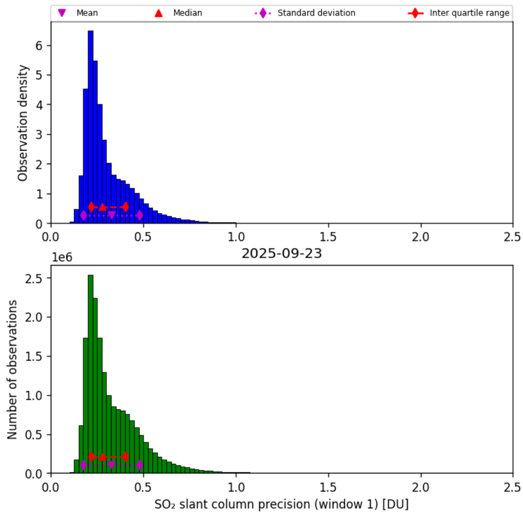
Figure 64: Histogram of “SO 2 slant column precision (window 1)” for 2025-09-22 to 2025-09-24
