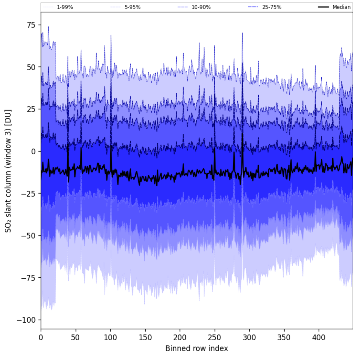
Figure 97: Along track statistics of “SO 2 slant column (window 3)” for 2025-09-22 to 2025-09-24
