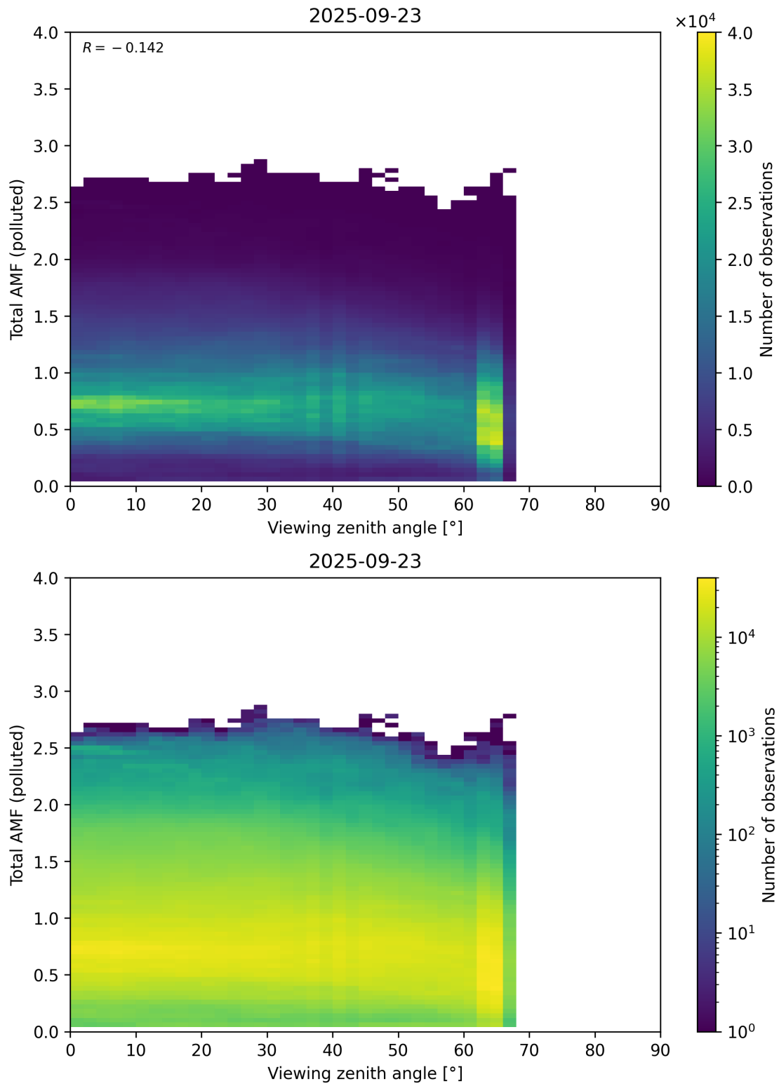
Figure 381: Scatter density plot of “Viewing zenith angle” against “Total AMF (polluted)” for 2025-09-22 to 2025-09-24.
