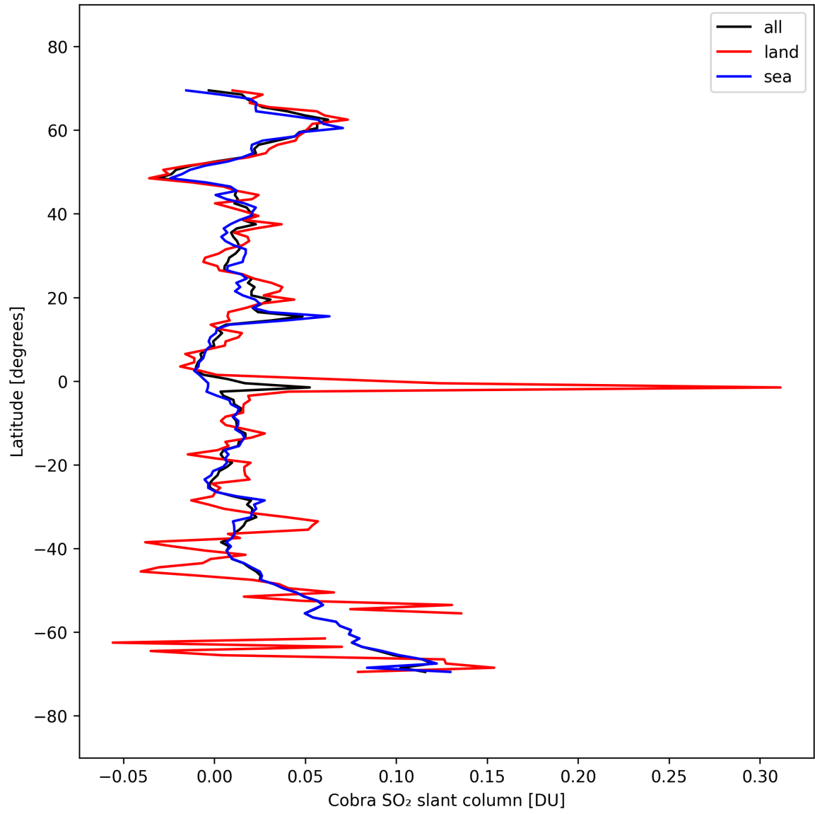
Figure 35: Zonal average of “Cobra SO 2 slant column” for 2025-09-22 to 2025-09-24.
