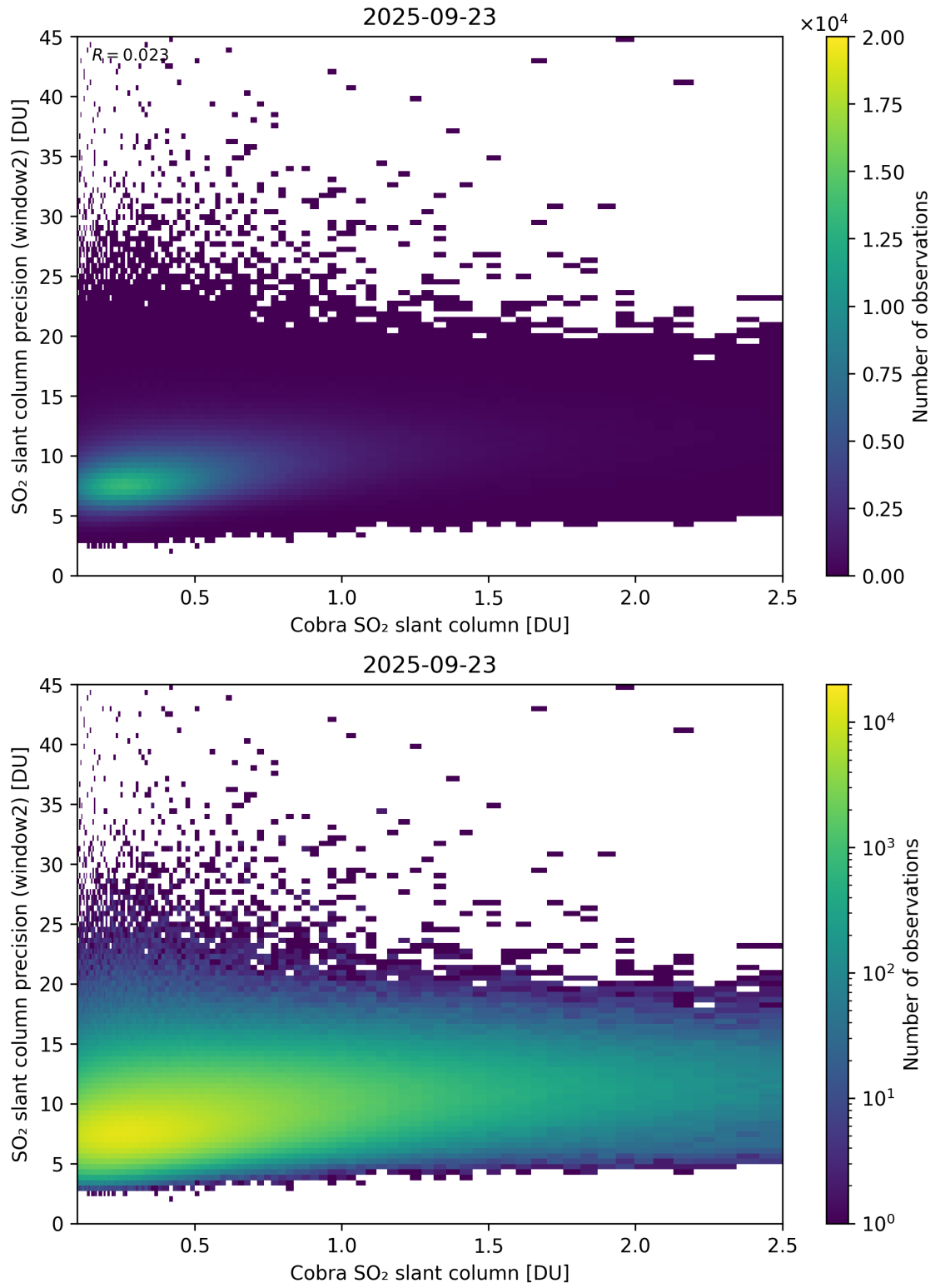
Figure 221: Scatter density plot of “Cobra SO 2 slant column” against “SO 2 slant column precision (window2)” for 2025-09-22 to 2025-09-24.
