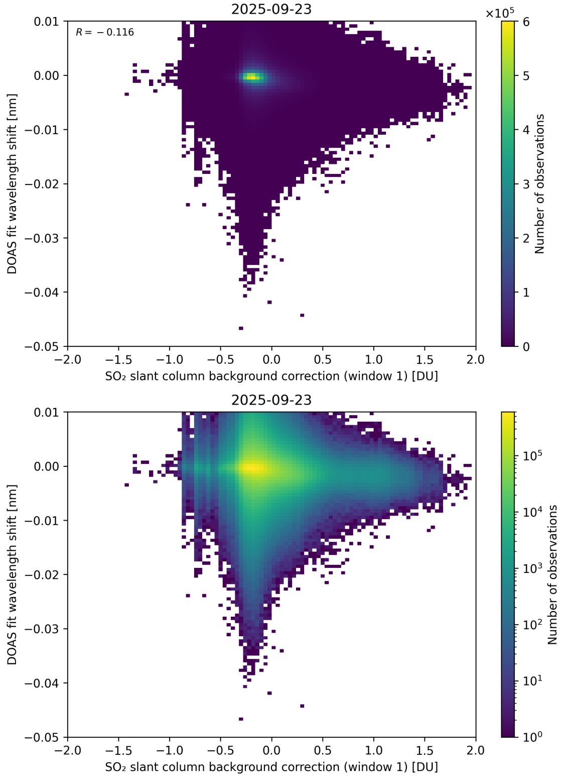
Figure 111: Scatter density plot of “SO 2 slant column background correction (window 1)” against “DOAS fit wavelength shift” for 2025-09-22 to 2025-09-24.
