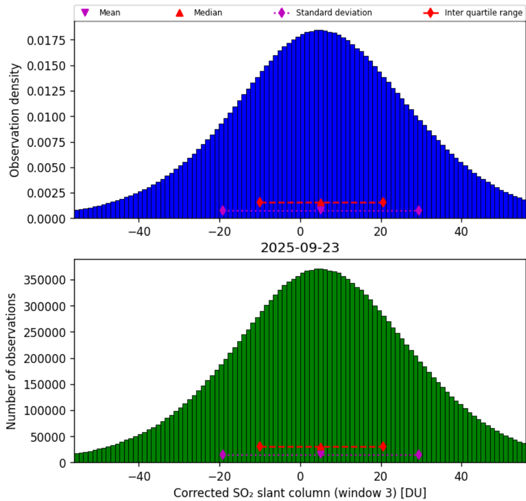
Figure 73: Histogram of “Corrected SO 2 slant column (window 3)” for 2025-09-22 to 2025-09-24
