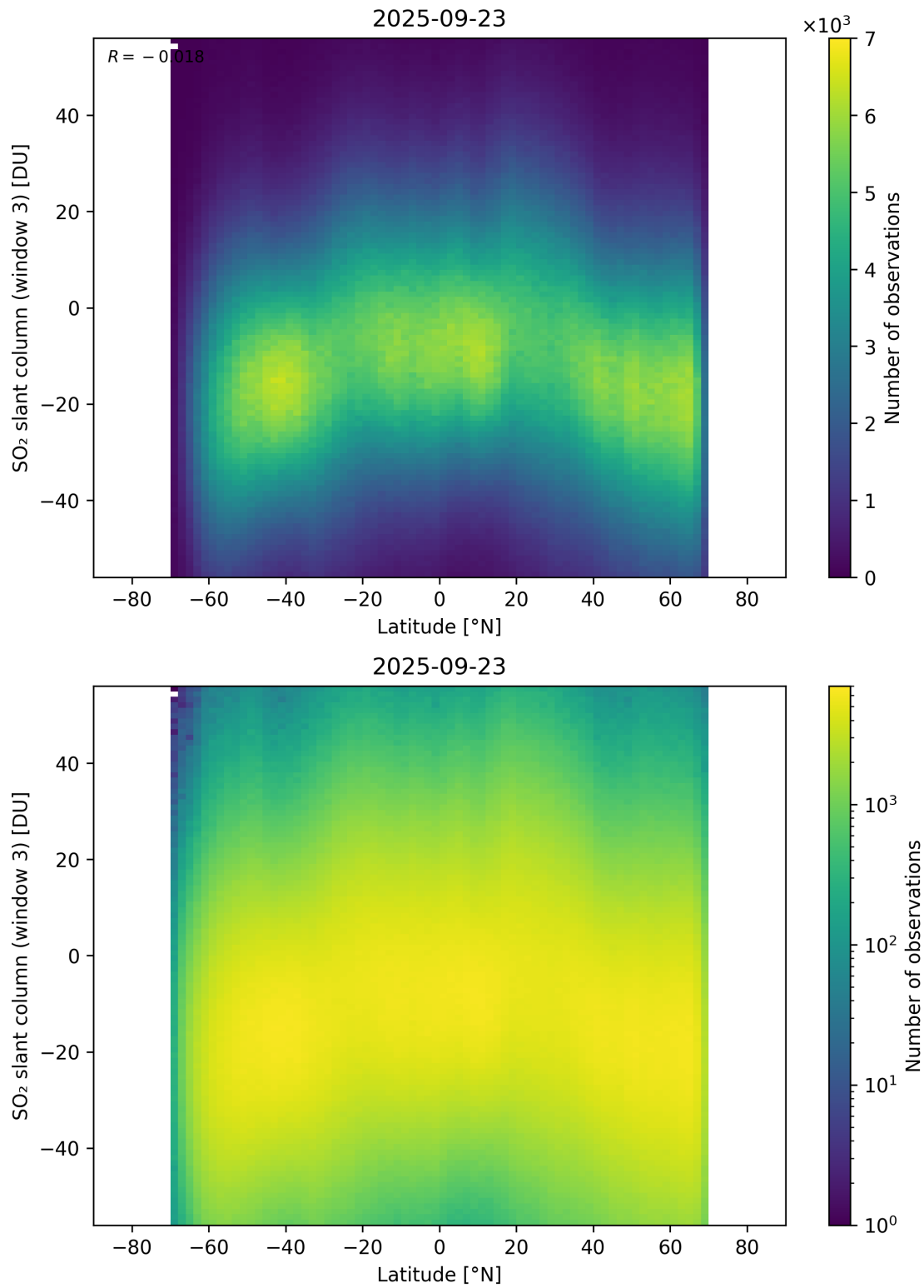
Figure 165: Scatter density plot of “Latitude” against “SO 2 slant column (window 3)” for 2025-09-22 to 2025-09-24.
