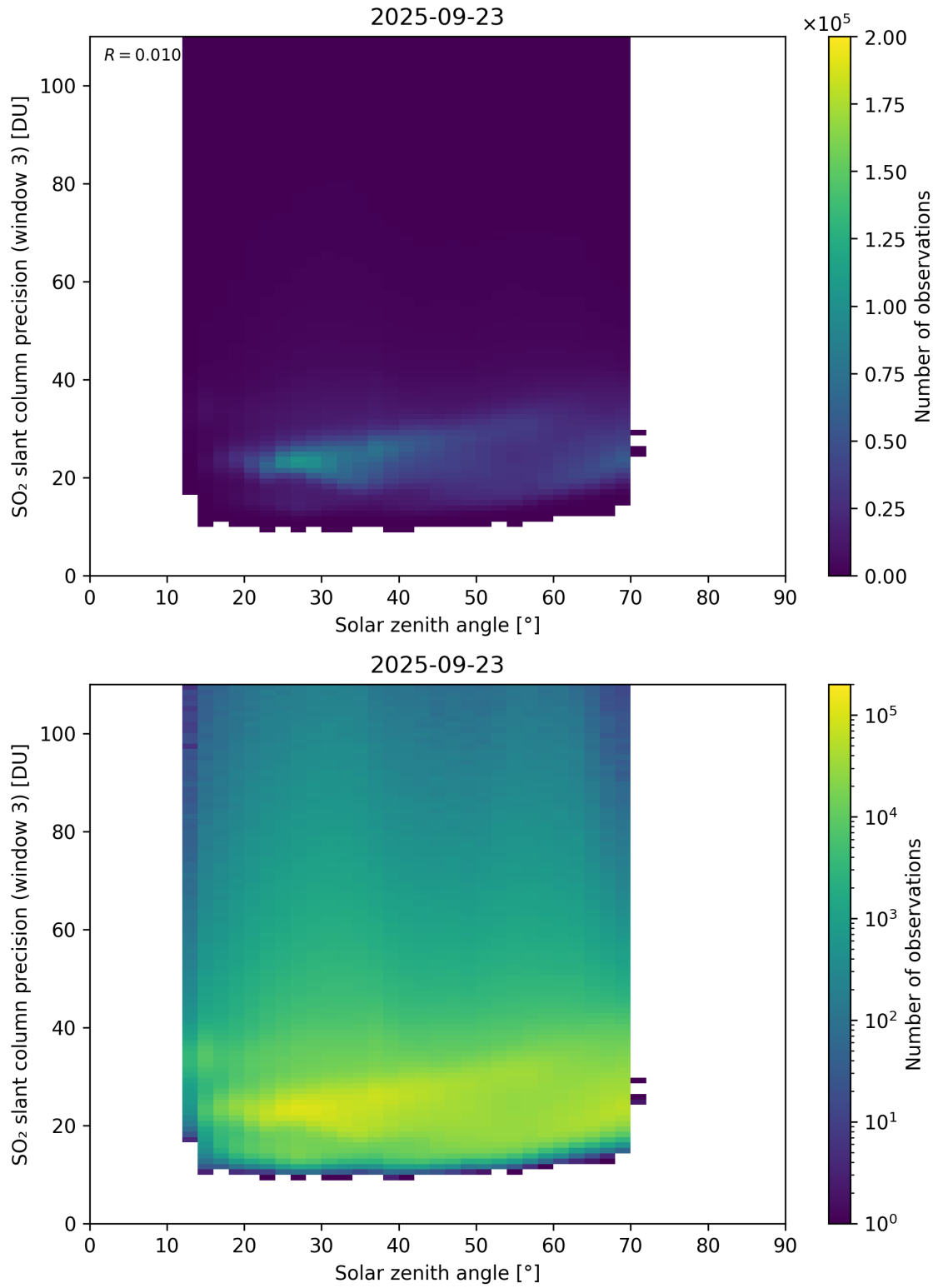
Figure 188: Scatter density plot of “Solar zenith angle” against “SO 2 slant column precision (window 3)” for 2025-09-22 to 2025-09-24.
