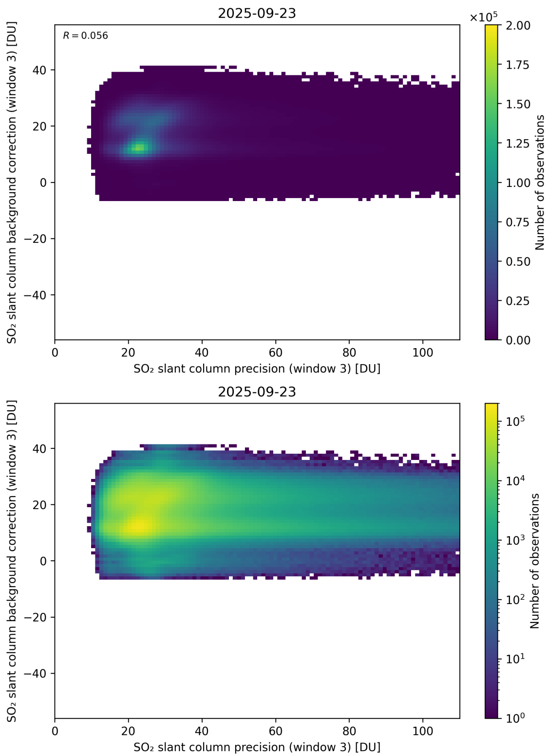
Figure 307: Scatter density plot of “SO 2 slant column precision (window 3)” against “SO 2 slant column background correction (window 3)” for 2025-09-22 to 2025-09-24.
