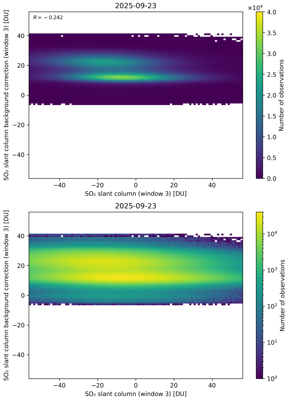
Figure 303: Scatter density plot of “SO 2 slant column (window 3)” against “SO 2 slant column background correction (window 3)” for 2025-09-22 to 2025-09-24.
