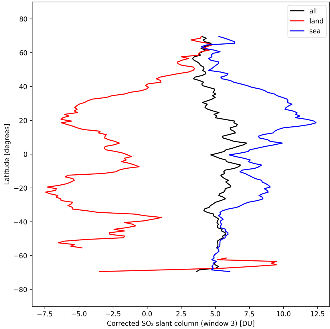
Figure 47: Zonal average of “Corrected SO 2 slant column (window 3)” for 2025-09-22 to 2025-09-24.
