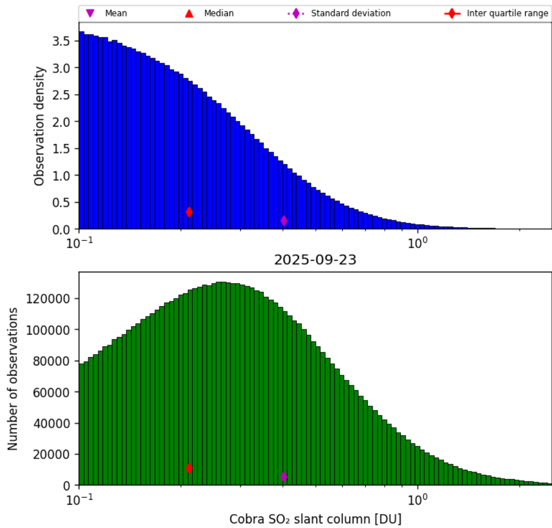
Figure 61: Histogram of “Cobra SO 2 slant column” for 2025-09-22 to 2025-09-24
