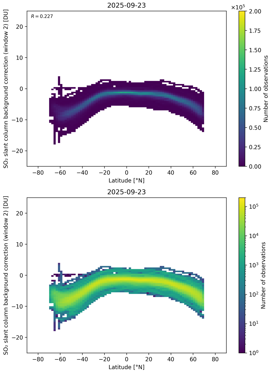
Figure 151: Scatter density plot of “Latitude” against “SO 2 slant column background correction (window 2)” for 2025-09-22 to 2025-09-24.
