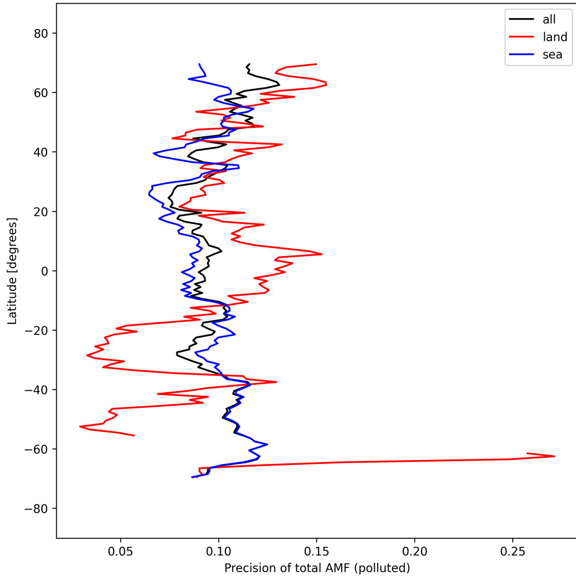
Figure 54: Zonal average of “Precision of total AMF (polluted)” for 2025-09-22 to 2025-09-24.
