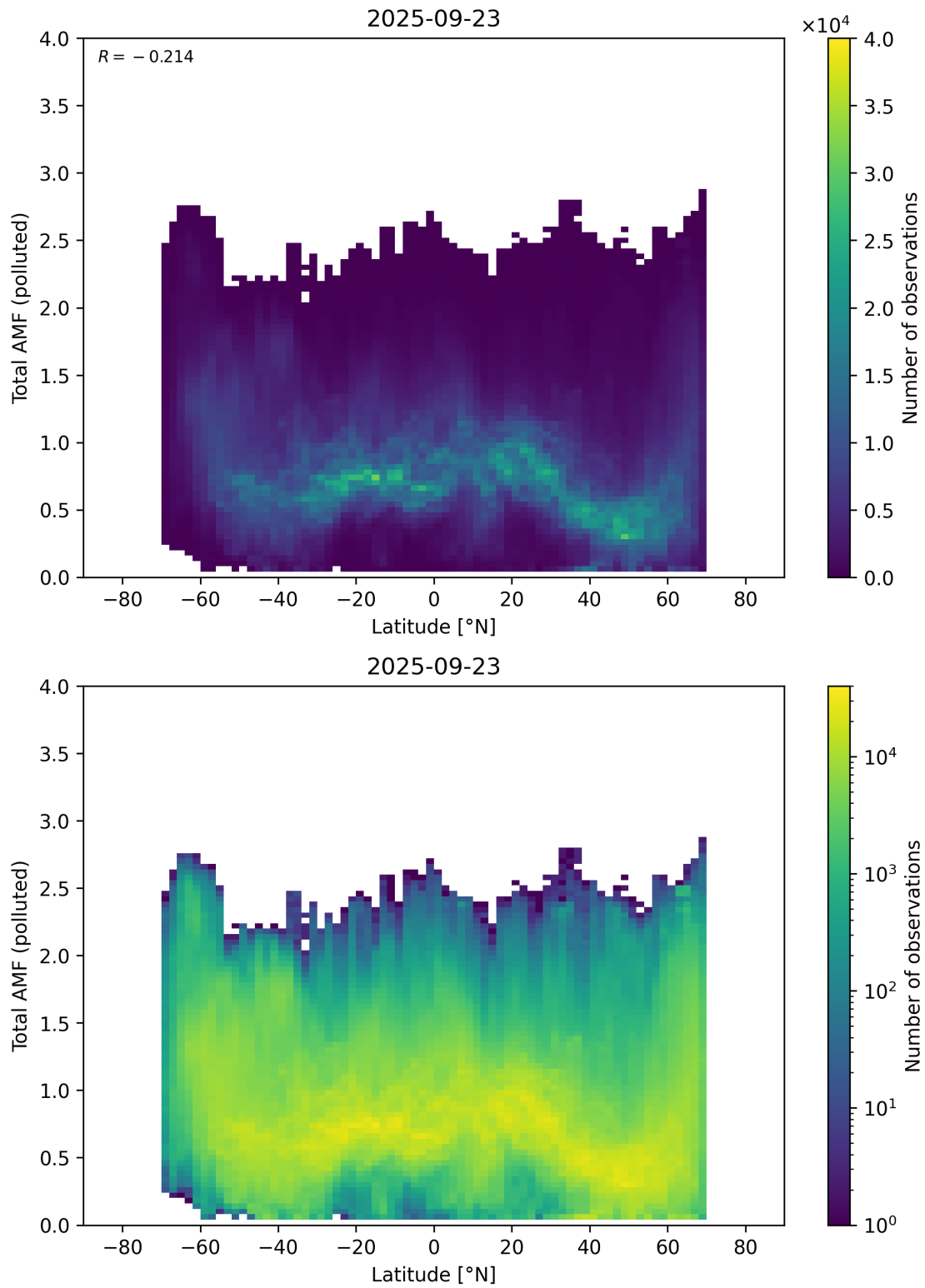
Figure 167: Scatter density plot of “Latitude” against “Total AMF (polluted)” for 2025-09-22 to 2025-09-24.
