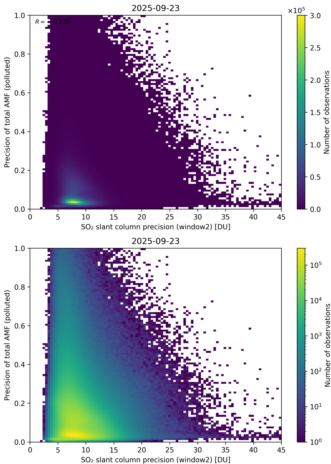
Figure 302: Scatter density plot of “SO 2 slant column precision (window2)” against “Precision of total AMF (polluted)” for 2025-09-22 to 2025-09-24.
