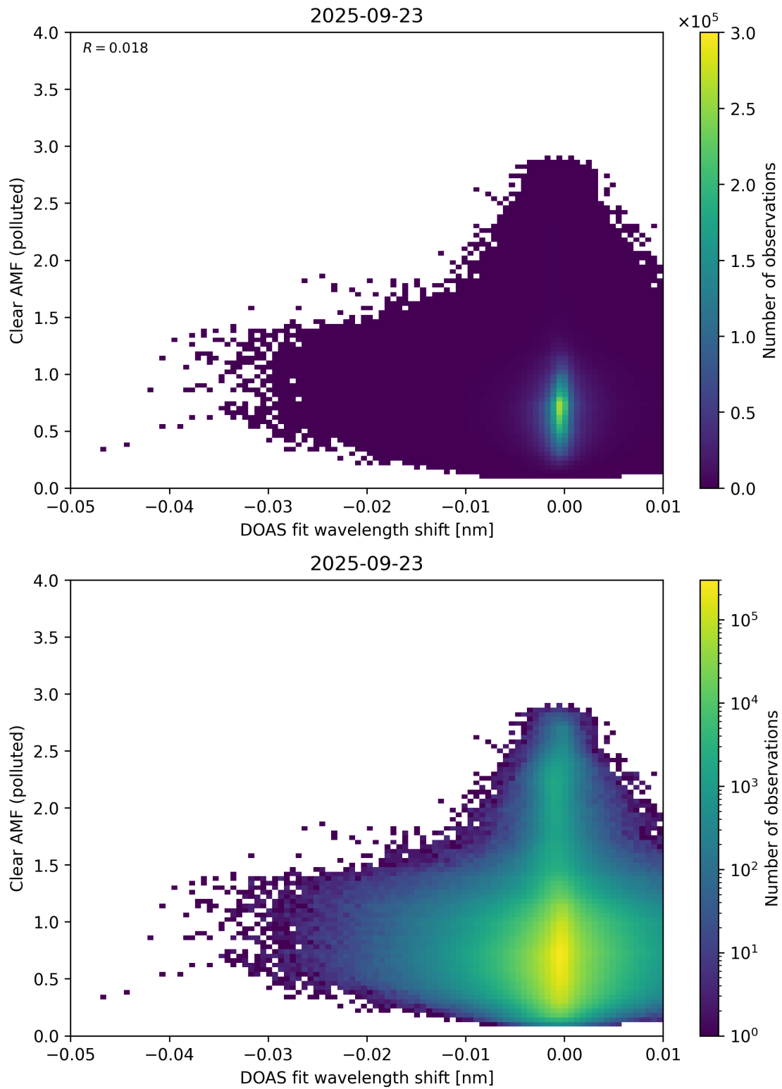
Figure 140: Scatter density plot of “DOAS fit wavelength shift” against “Clear AMF (polluted)” for 2025-09-22 to 2025-09-24.
