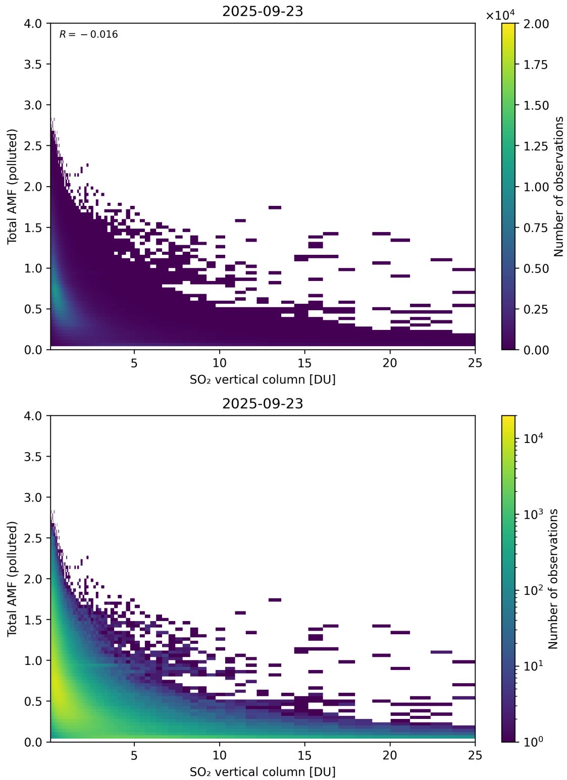
Figure 359: Scatter density plot of “SO 2 vertical column” against “Total AMF (polluted)” for 2025-09-22 to 2025-09-24.
