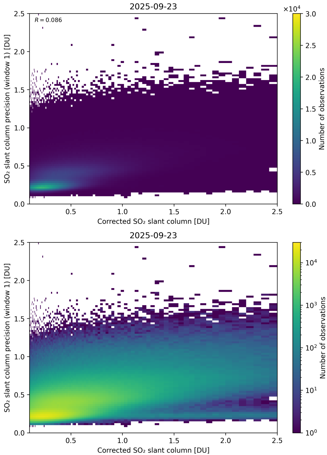
Figure 238: Scatter density plot of “Corrected SO 2 slant column” against “SO 2 slant column precision (window 1)” for 2025-09-22 to 2025-09-24.
