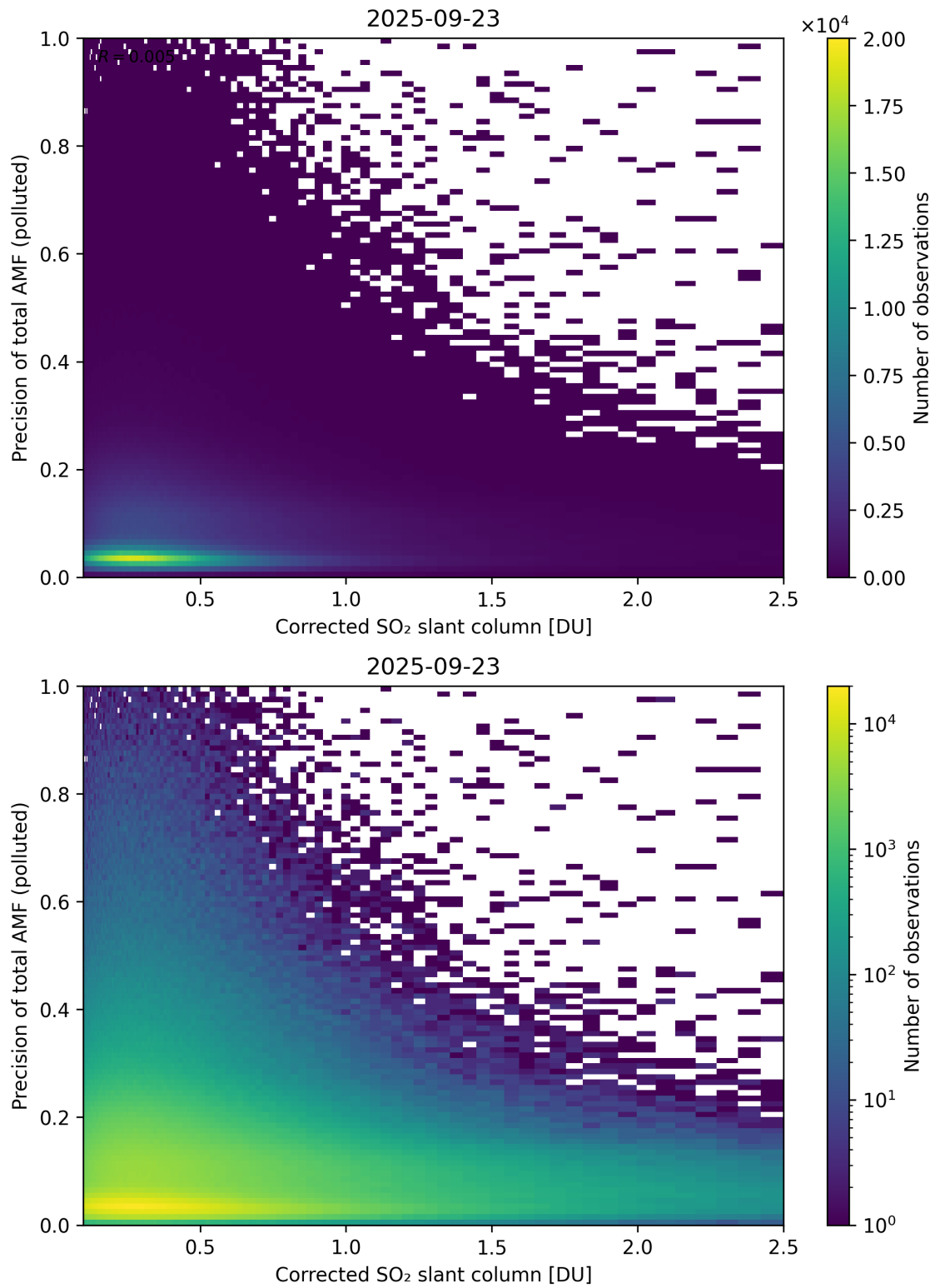
Figure 243: Scatter density plot of “Corrected SO 2 slant column” against “Precision of total AMF (polluted)” for 2025-09-22 to 2025-09-24.
