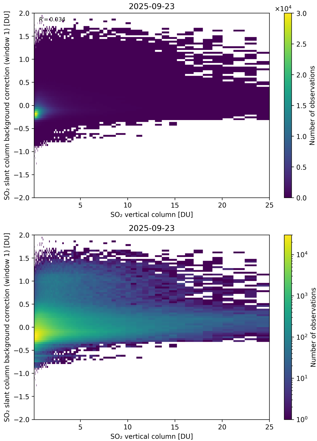
Figure 323: Scatter density plot of “SO 2 vertical column” against “SO 2 slant column background correction (window 1)” for 2025-09-22 to 2025-09-24.
