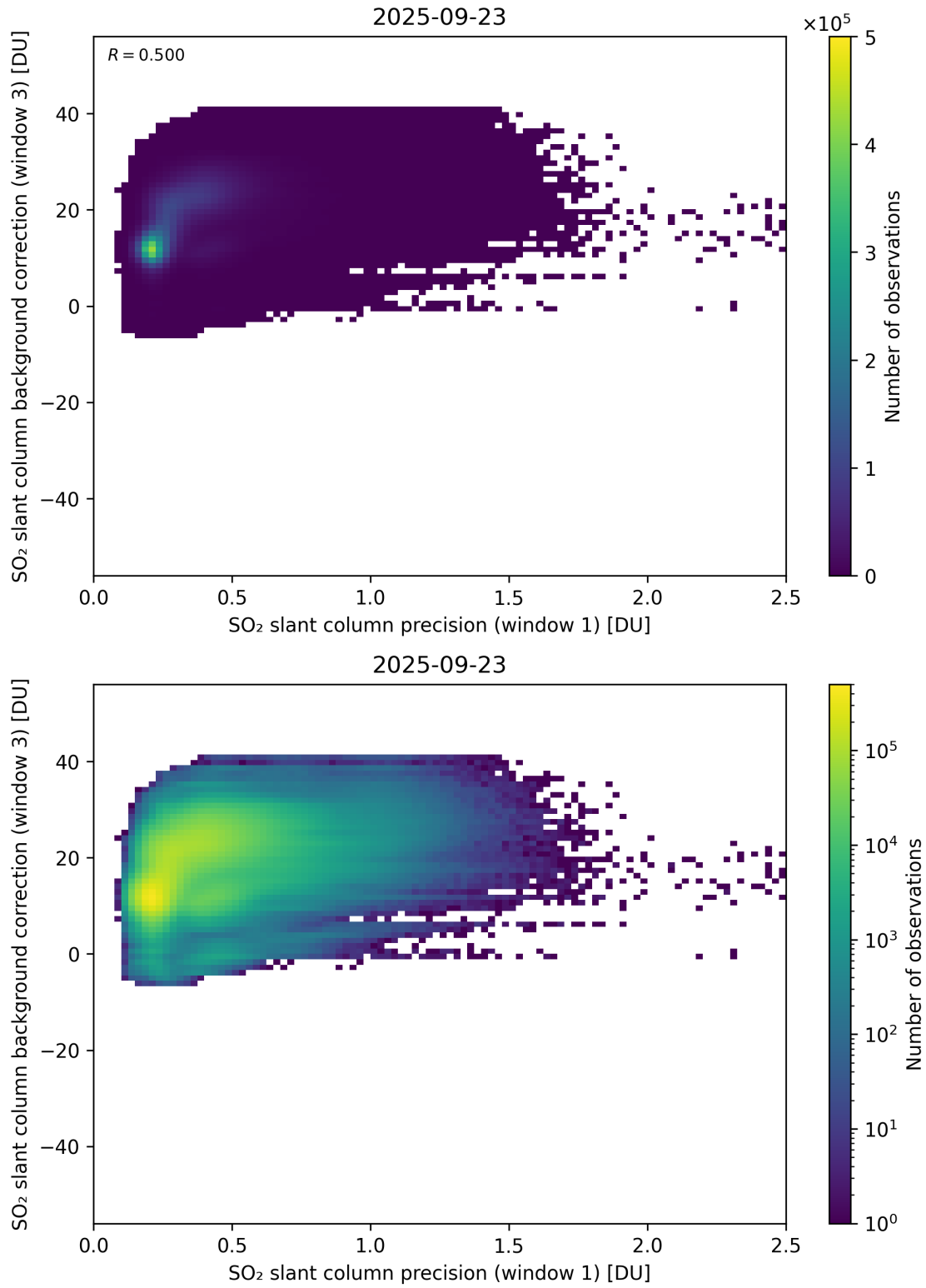
Figure 270: Scatter density plot of “SO 2 slant column precision (window 1)” against “SO 2 slant column background correction (window 3)” for 2025-09-22 to 2025-09-24.
