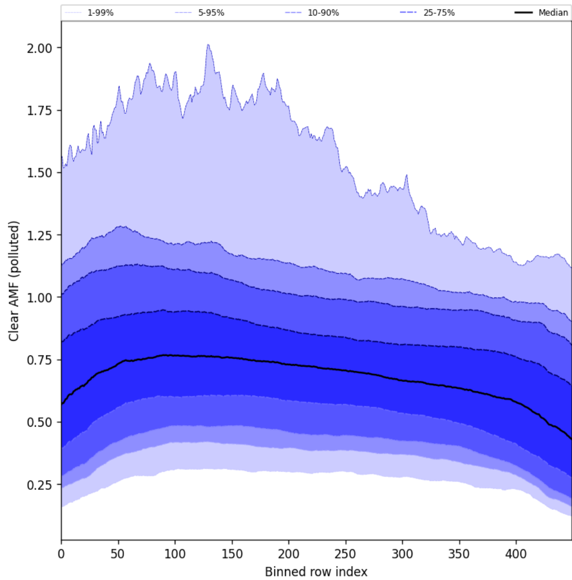
Figure 107: Along track statistics of “Clear AMF (polluted)” for 2025-09-22 to 2025-09-24
