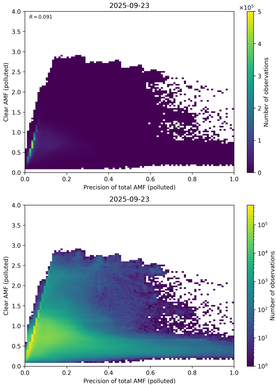
Figure 320: Scatter density plot of “Precision of total AMF (polluted)” against “Clear AMF (polluted)” for 2025-09-22 to 2025-09-24.
