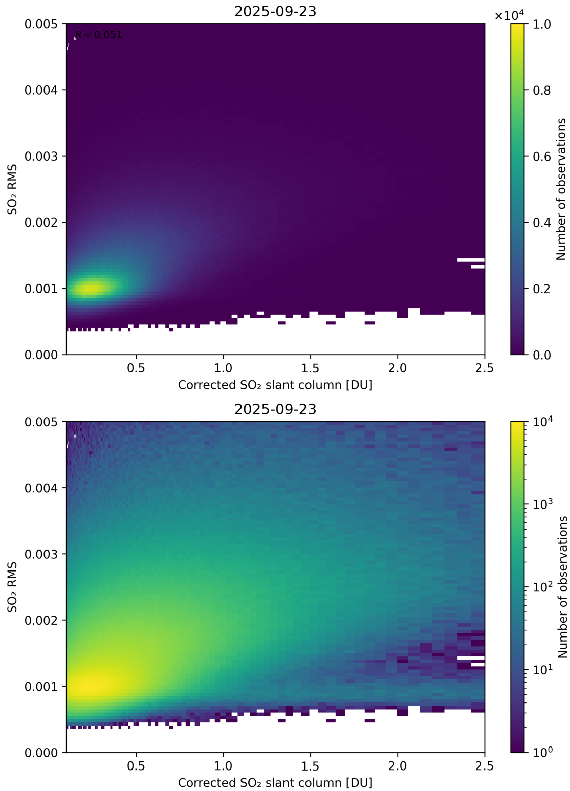
Figure 231: Scatter density plot of “Corrected SO 2 slant column” against “SO 2 RMS” for 2025-09-22 to 2025-09-24.
