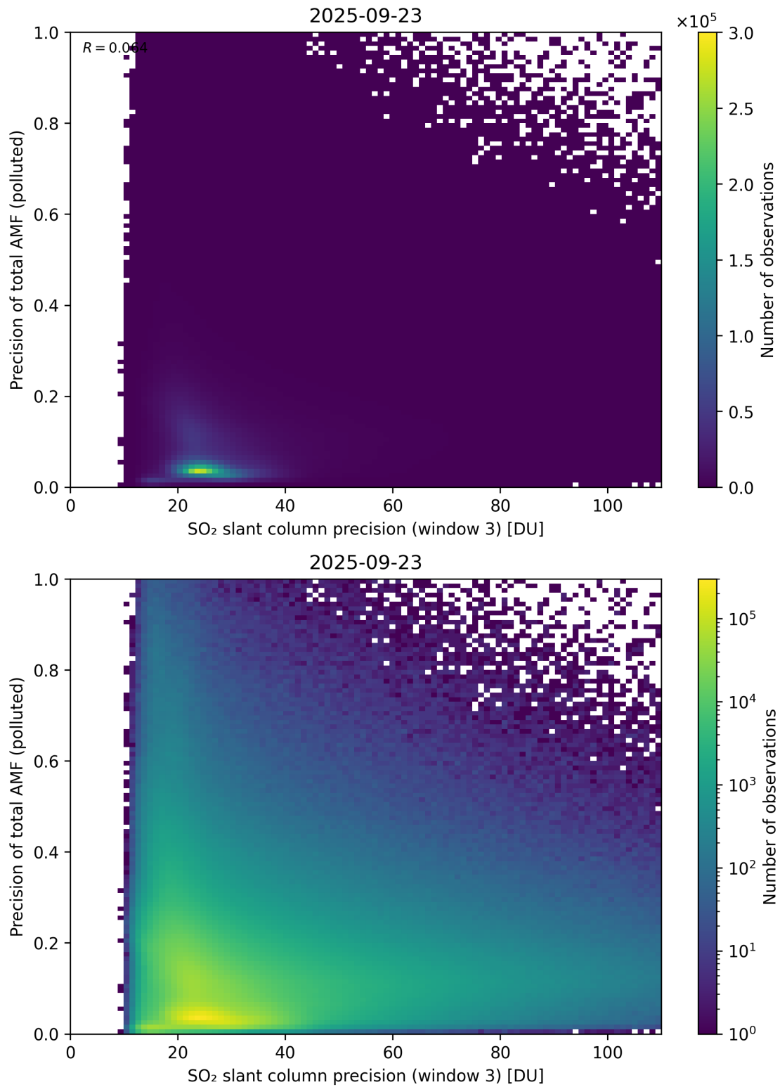
Figure 314: Scatter density plot of “SO 2 slant column precision (window 3)” against “Precision of total AMF (polluted)” for 2025-09-22 to 2025-09-24.
