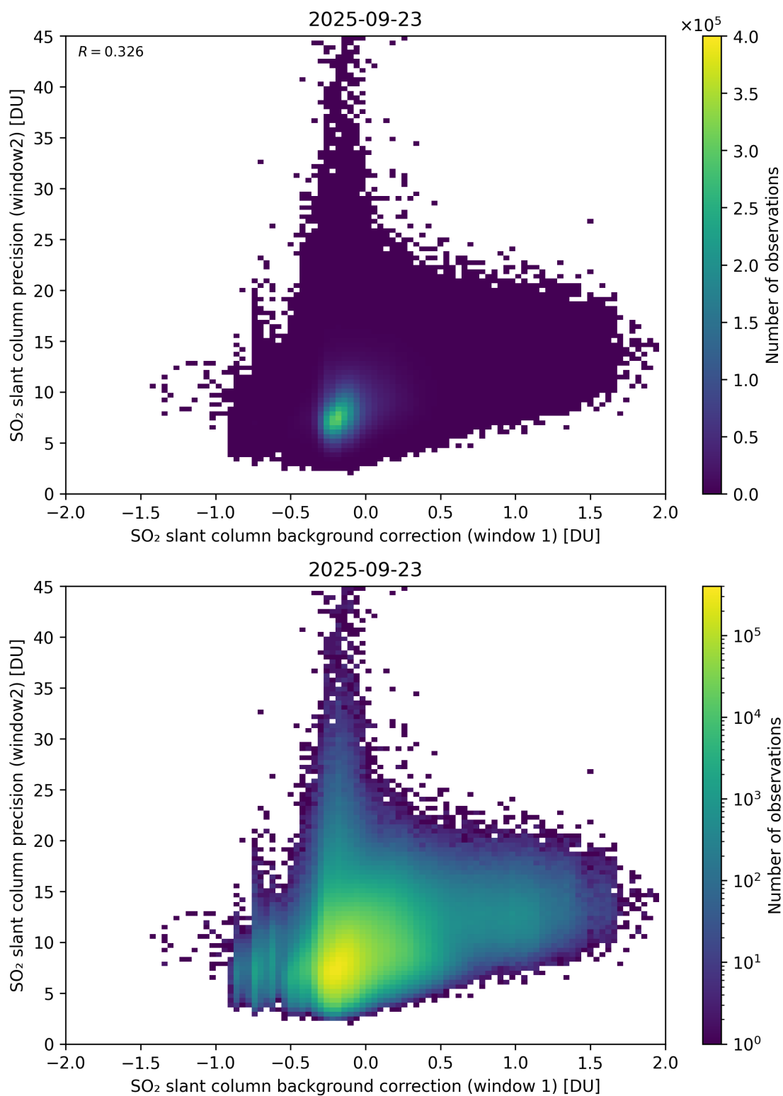
Figure 117: Scatter density plot of “SO 2 slant column background correction (window 1)” against “SO 2 slant column precision (window2)” for 2025-09-22 to 2025-09-24.
