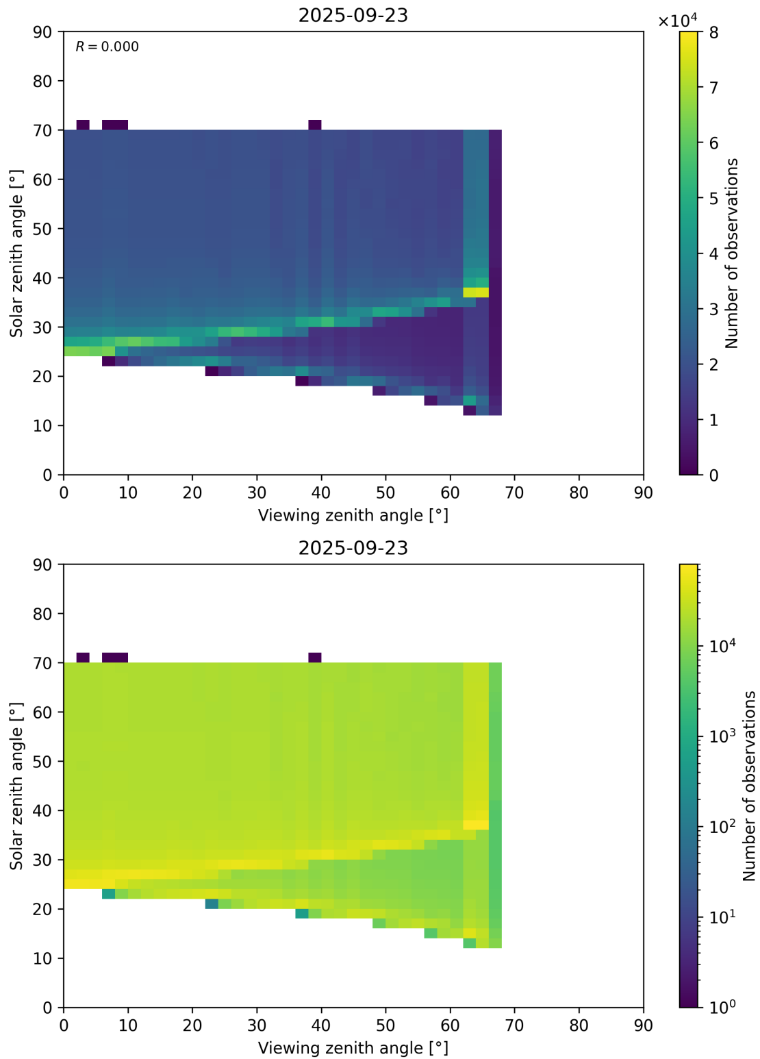
Figure 369: Scatter density plot of “Viewing zenith angle” against “Solar zenith angle” for 2025-09-22 to 2025-09-24.
