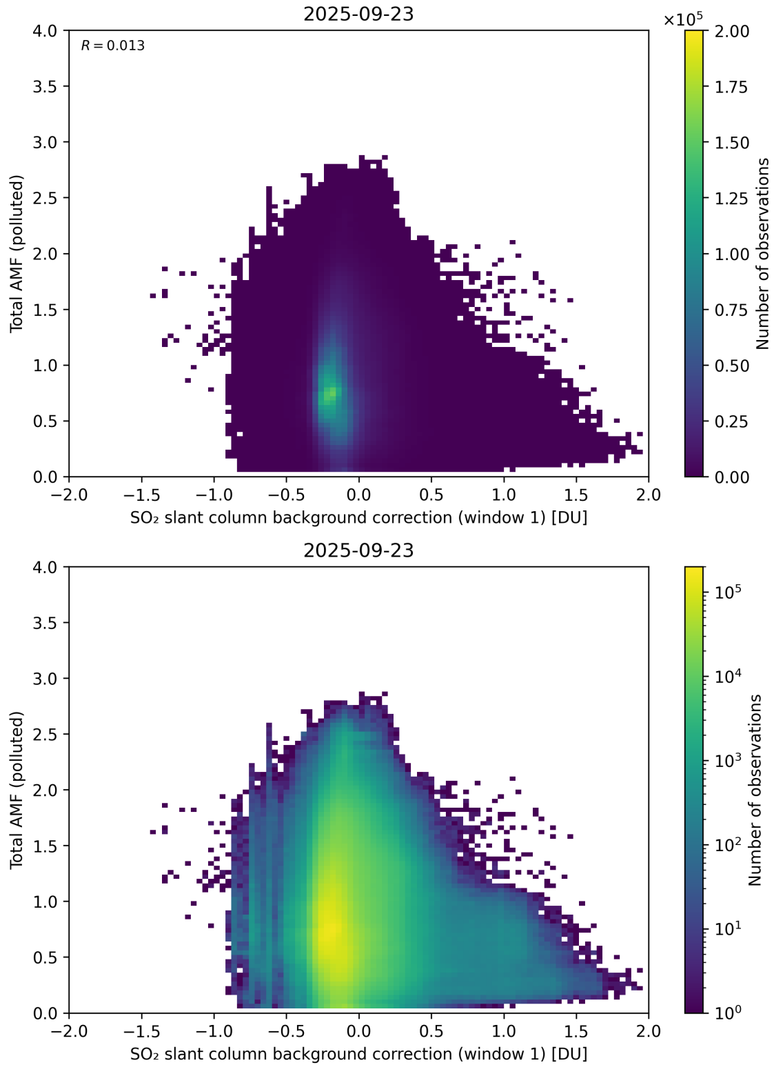
Figure 120: Scatter density plot of “SO 2 slant column background correction (window 1)” against “Total AMF (polluted)” for 2025-09-22 to 2025-09-24.
