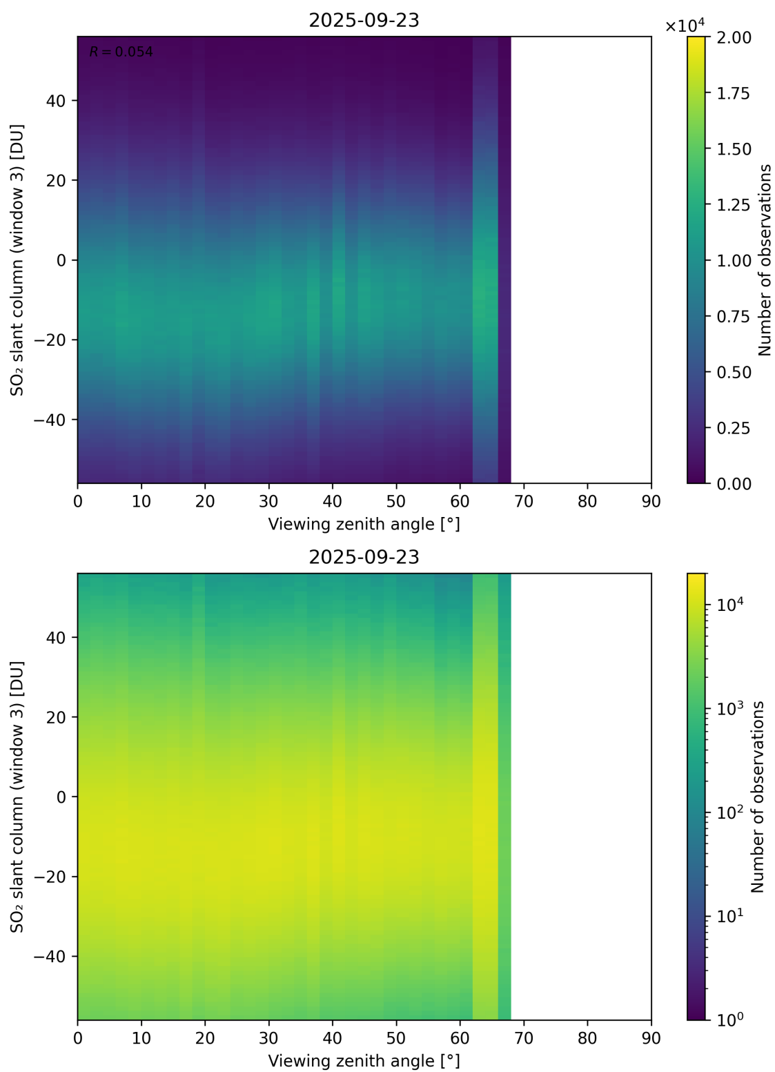
Figure 379: Scatter density plot of “Viewing zenith angle” against “SO 2 slant column (window 3)” for 2025-09-22 to 2025-09-24.
