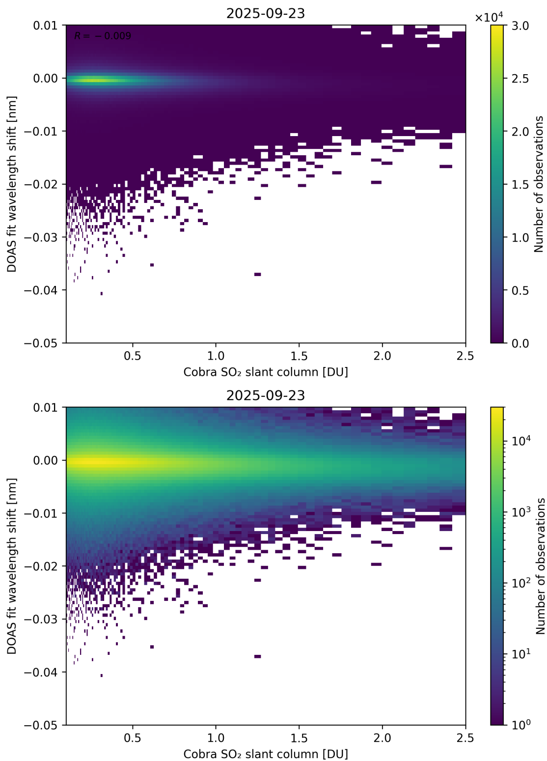
Figure 196: Scatter density plot of “Cobra SO 2 slant column” against “DOAS fit wavelength shift” for 2025-09-22 to 2025-09-24.
