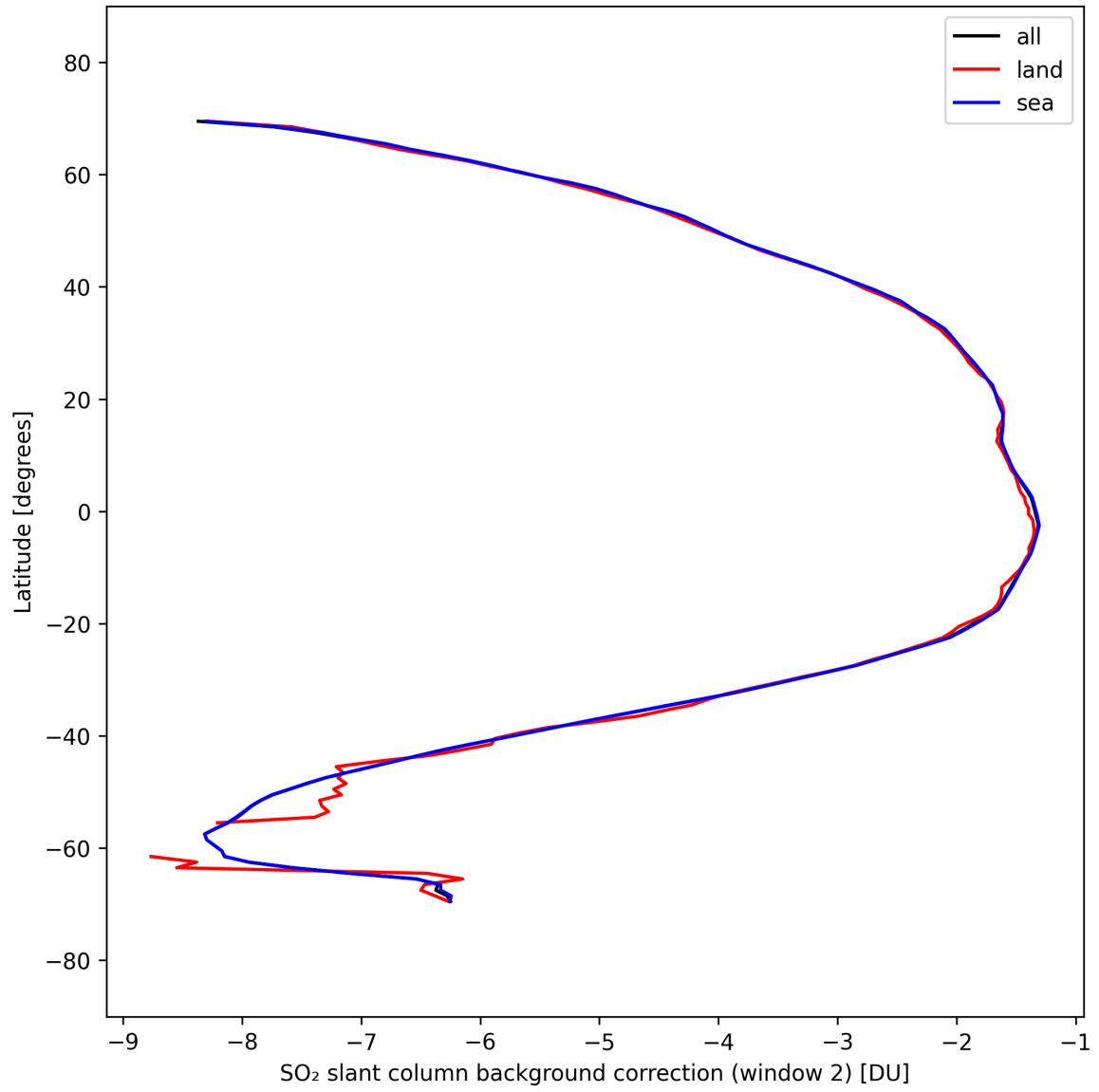
Figure 44: Zonal average of “SO 2 slant column background correction (window 2)” for 2025-09-22 to 2025-09-24.
