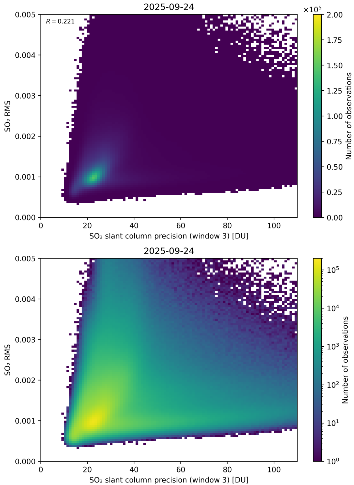
Figure 310: Scatter density plot of “SO 2 slant column precision (window 3)” against “SO 2 RMS” for 2025-09-23 to 2025-09-25.
