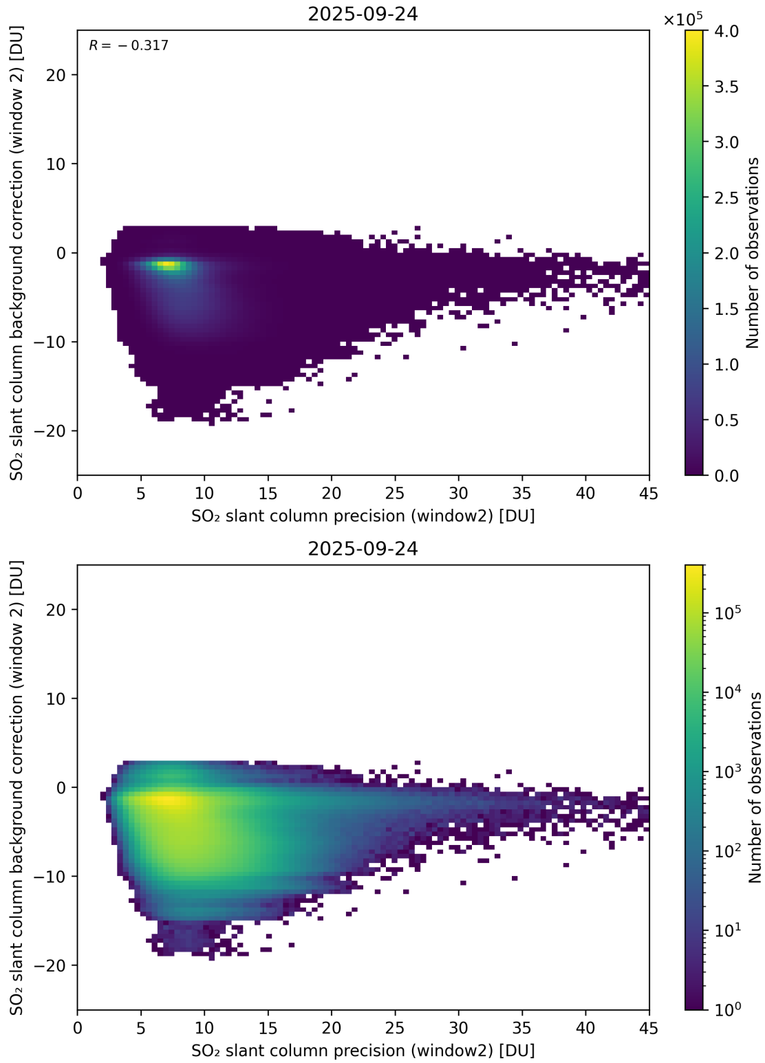
Figure 291: Scatter density plot of “SO 2 slant column precision (window2)” against “SO 2 slant column background correction (window 2)” for 2025-09-23 to 2025-09-25.
