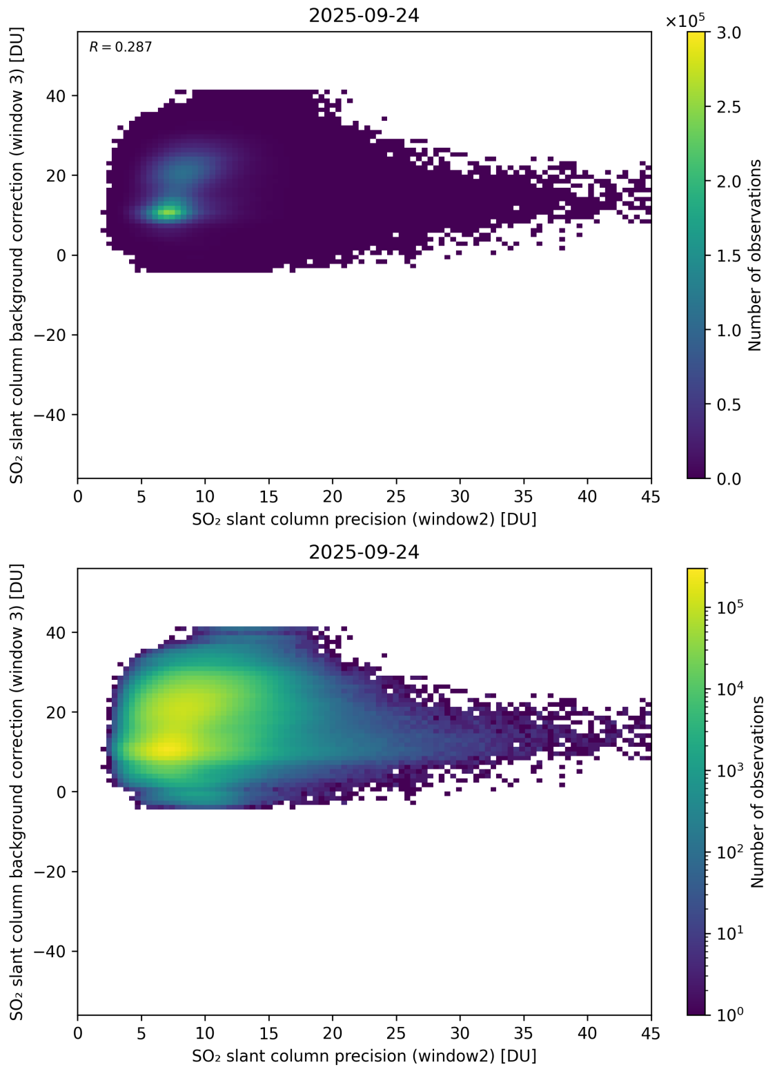
Figure 292: Scatter density plot of “SO 2 slant column precision (window2)” against “SO 2 slant column background correction (window 3)” for 2025-09-23 to 2025-09-25.
