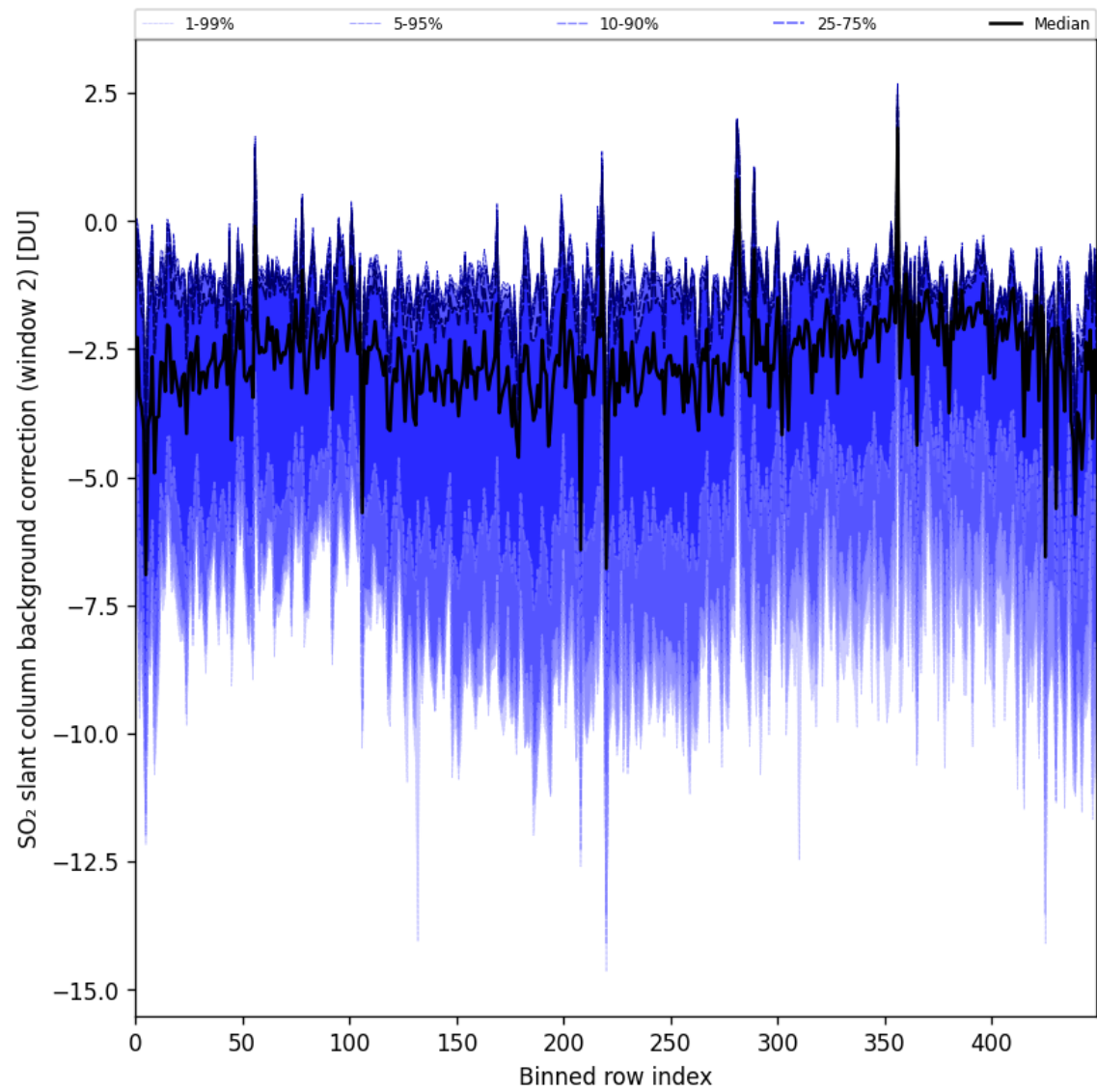
Figure 96: Along track statistics of “SO 2 slant column background correction (window 2)” for 2025-09-23 to 2025-09-25
