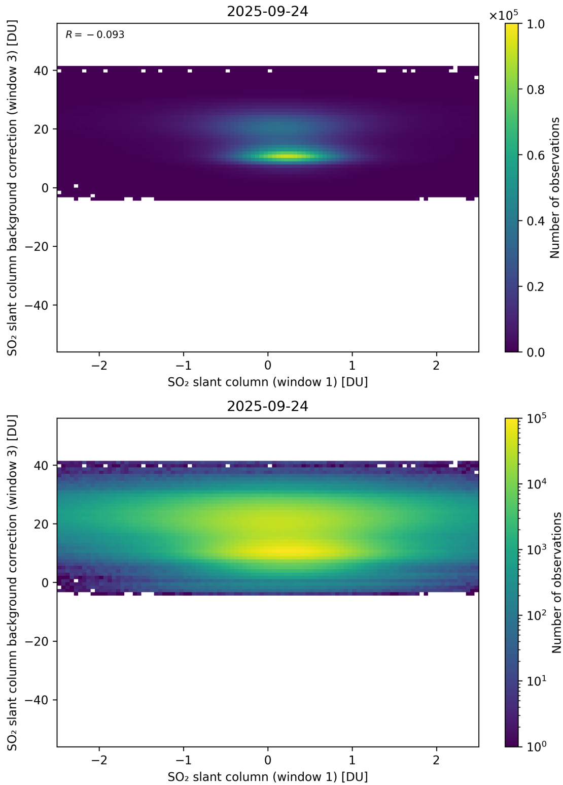
Figure 264: Scatter density plot of “SO 2 slant column (window 1)” against “SO 2 slant column background correction (window 3)” for 2025-09-23 to 2025-09-25.
