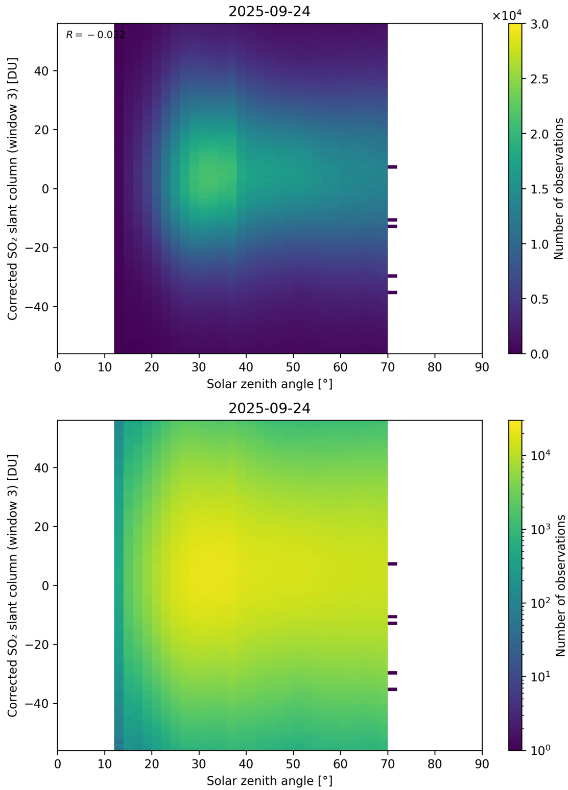
Figure 183: Scatter density plot of “Solar zenith angle” against “Corrected SO 2 slant column (window 3)” for 2025-09-23 to 2025-09-25.
