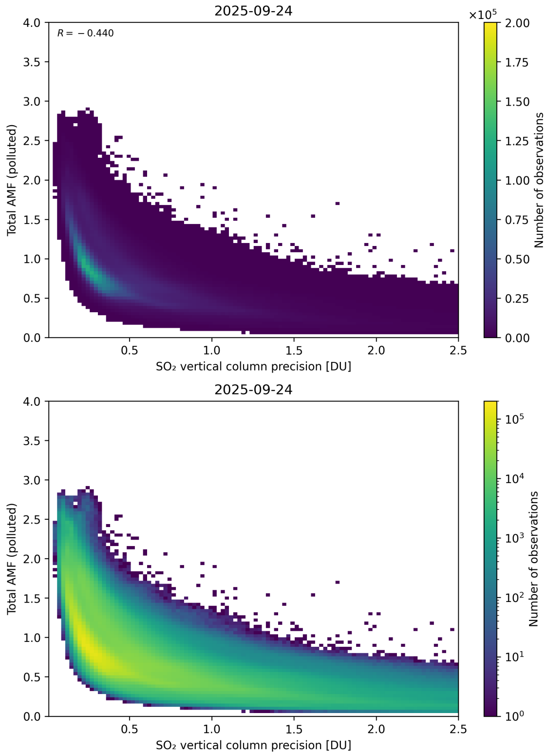
Figure 346: Scatter density plot of “SO 2 vertical column precision” against “Total AMF (polluted)” for 2025-09-23 to 2025-09-25.
