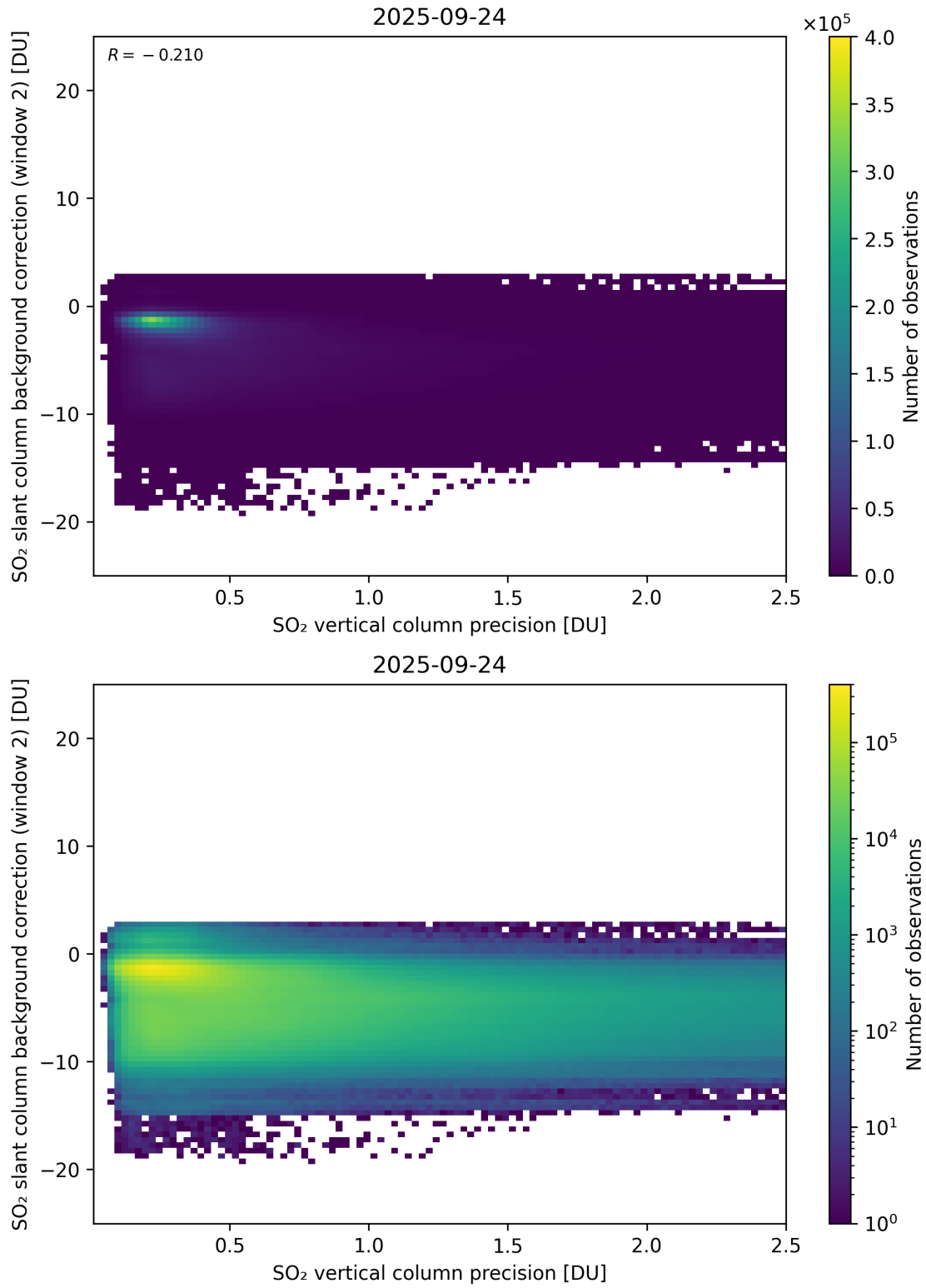
Figure 330: Scatter density plot of “SO 2 vertical column precision” against “SO 2 slant column background correction (window 2)” for 2025-09-23 to 2025-09-25.
