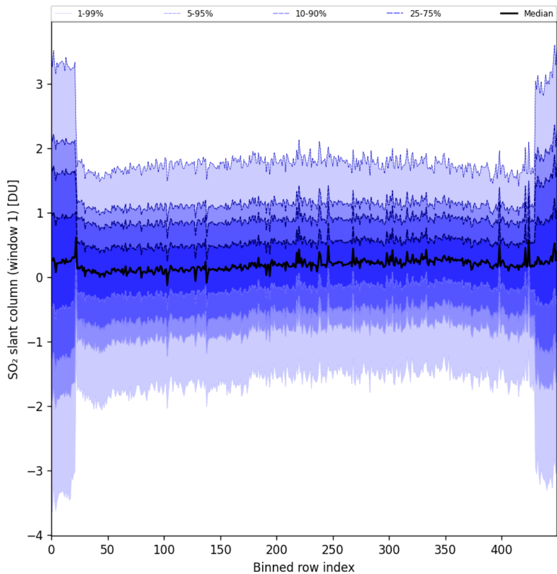
Figure 89: Along track statistics of “SO 2 slant column (window 1)” for 2025-09-23 to 2025-09-25
