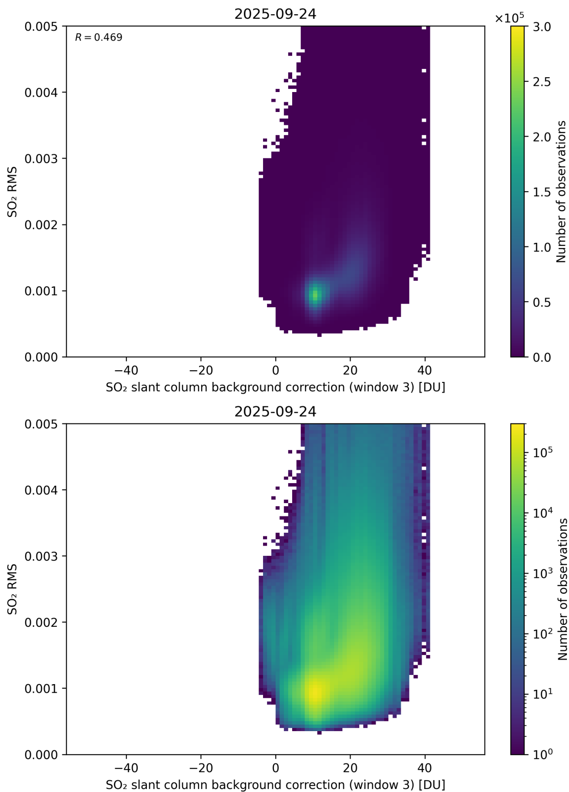
Figure 134: Scatter density plot of “SO 2 slant column background correction (window 3)” against “SO 2 RMS” for 2025-09-23 to 2025-09-25.
