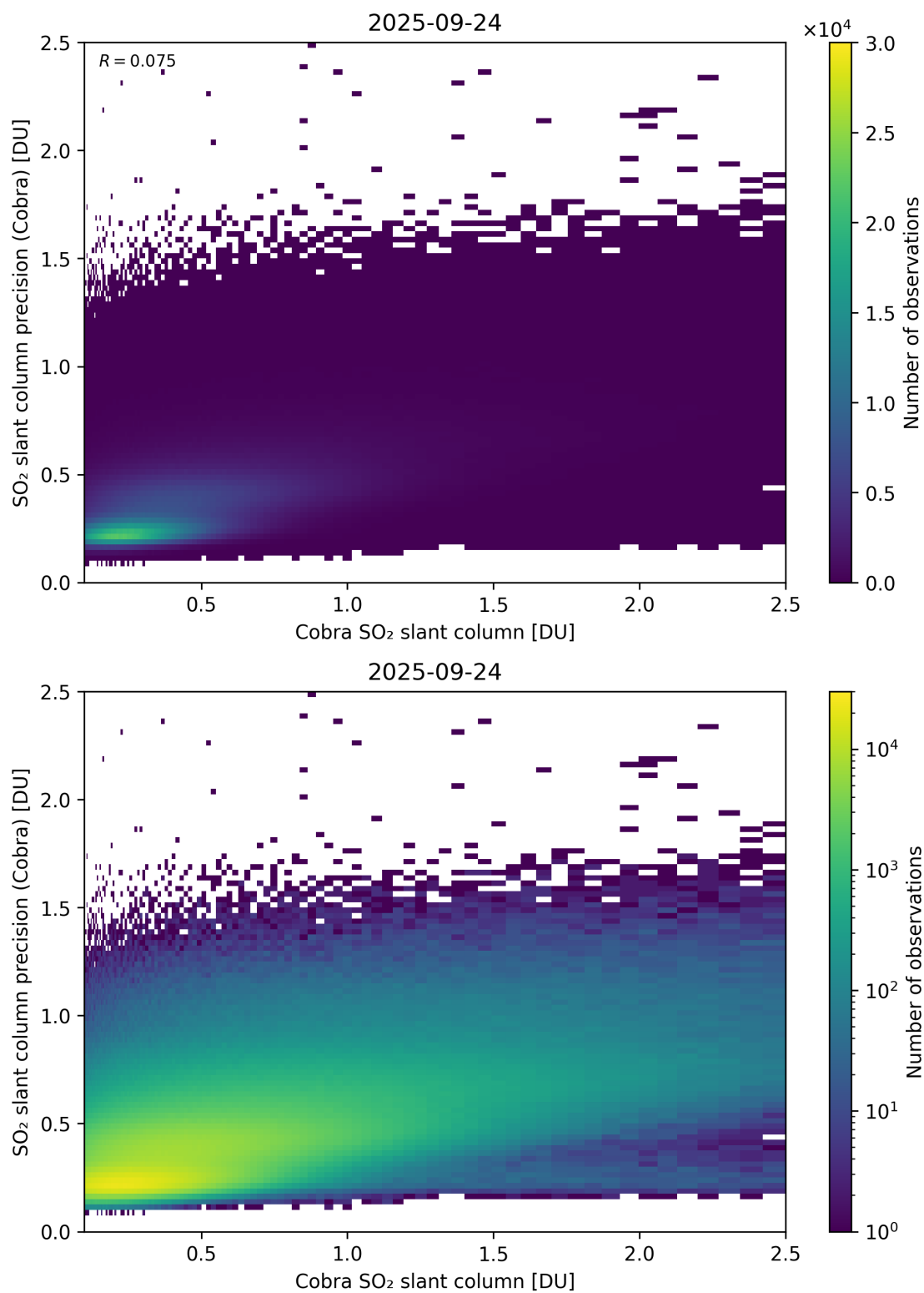
Figure 216: Scatter density plot of “Cobra SO 2 slant column” against “SO 2 slant column precision (Cobra)” for 2025-09-23 to 2025-09-25.
