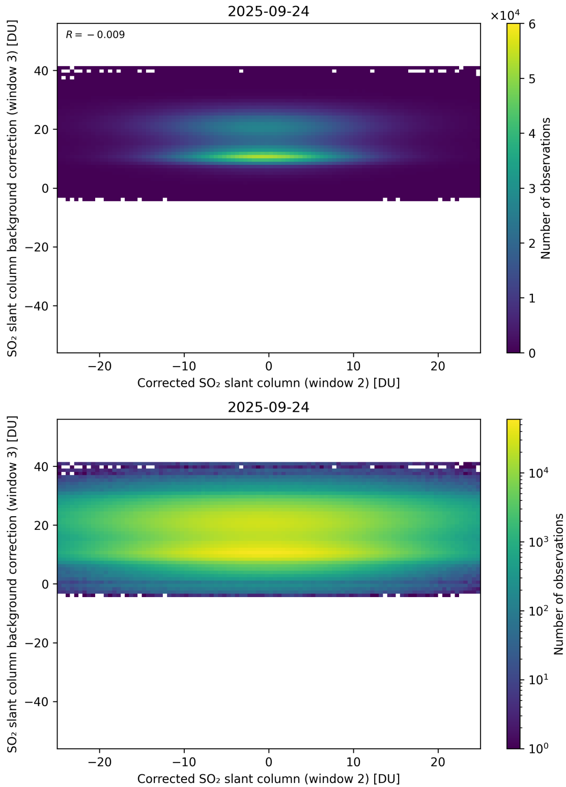
Figure 245: Scatter density plot of “Corrected SO 2 slant column (window 2)” against “SO 2 slant column background correction (window 3)” for 2025-09-23 to 2025-09-25.
