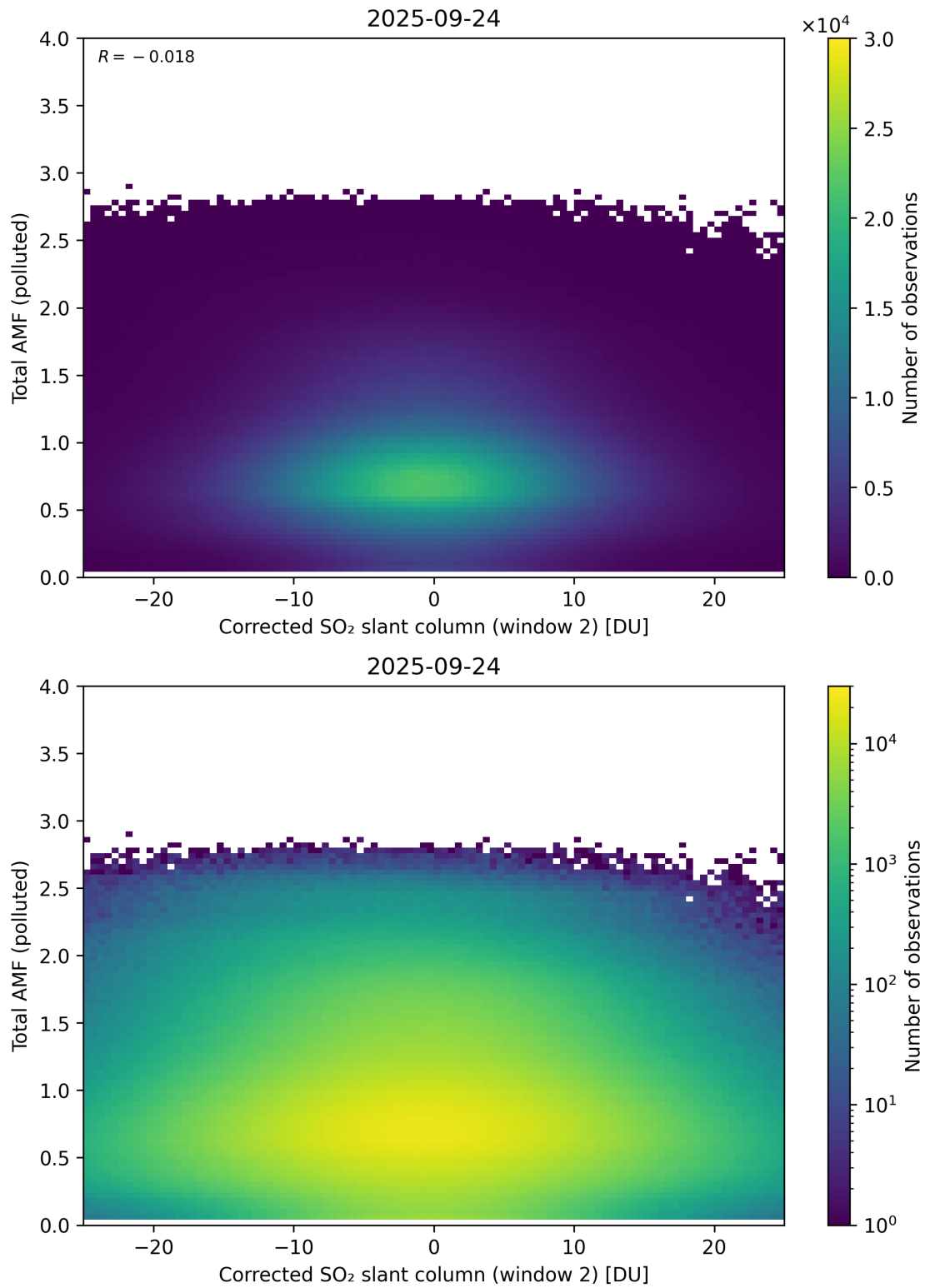
Figure 253: Scatter density plot of “Corrected SO 2 slant column (window 2)” against “Total AMF (polluted)” for 2025-09-23 to 2025-09-25.
