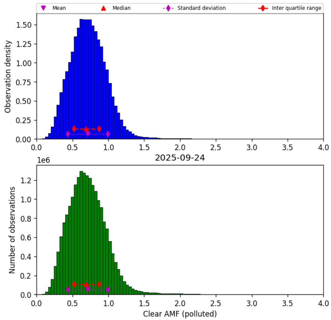
Figure 81: Histogram of “Clear AMF (polluted)” for 2025-09-23 to 2025-09-25
