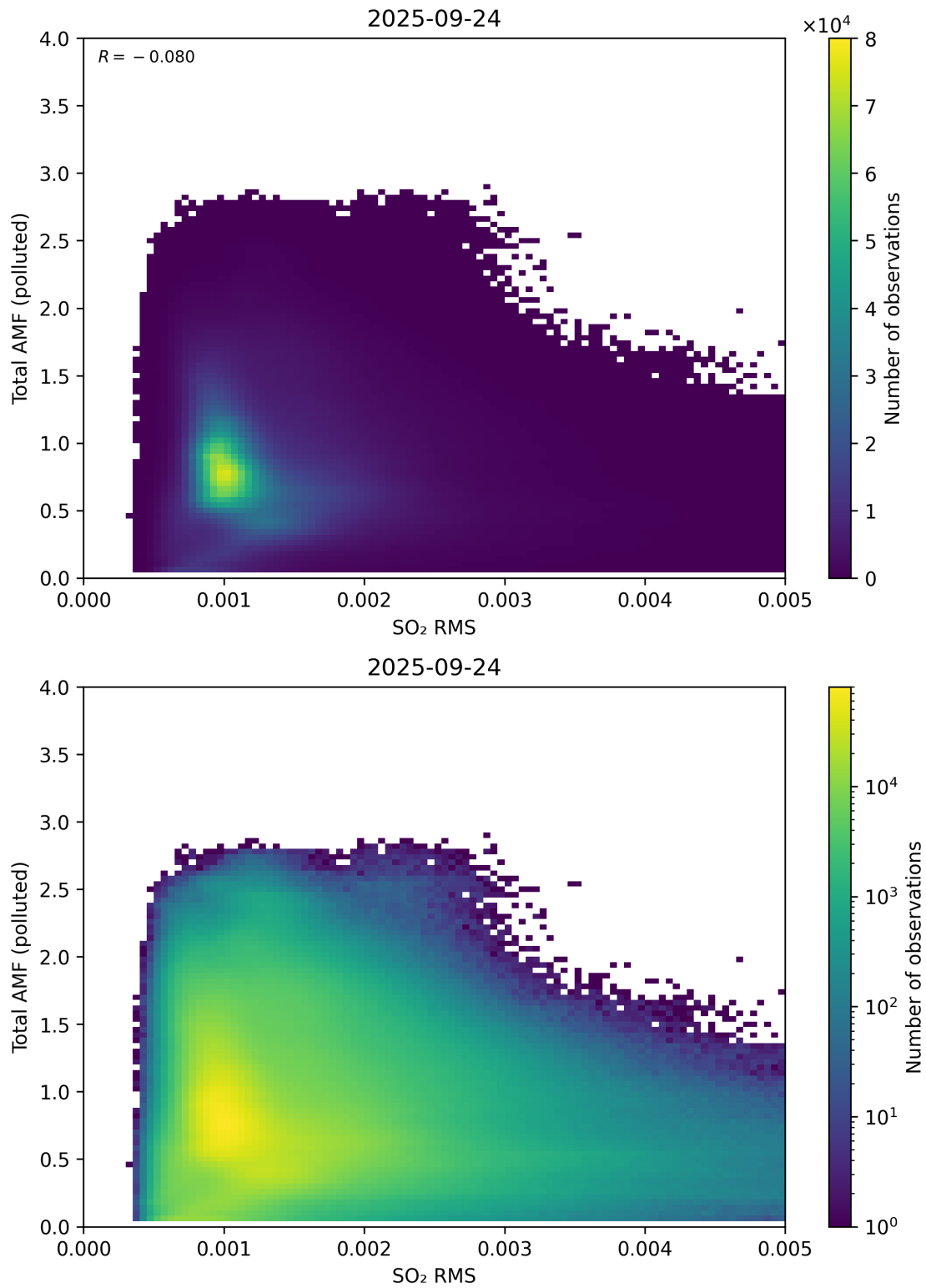
Figure 148: Scatter density plot of “SO 2 RMS” against “Total AMF (polluted)” for 2025-09-23 to 2025-09-25.
