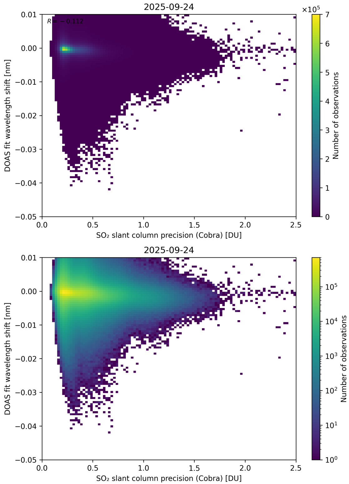
Figure 202: Scatter density plot of “SO 2 slant column precision (Cobra)” against “DOAS fit wavelength shift” for 2025-09-23 to 2025-09-25.
