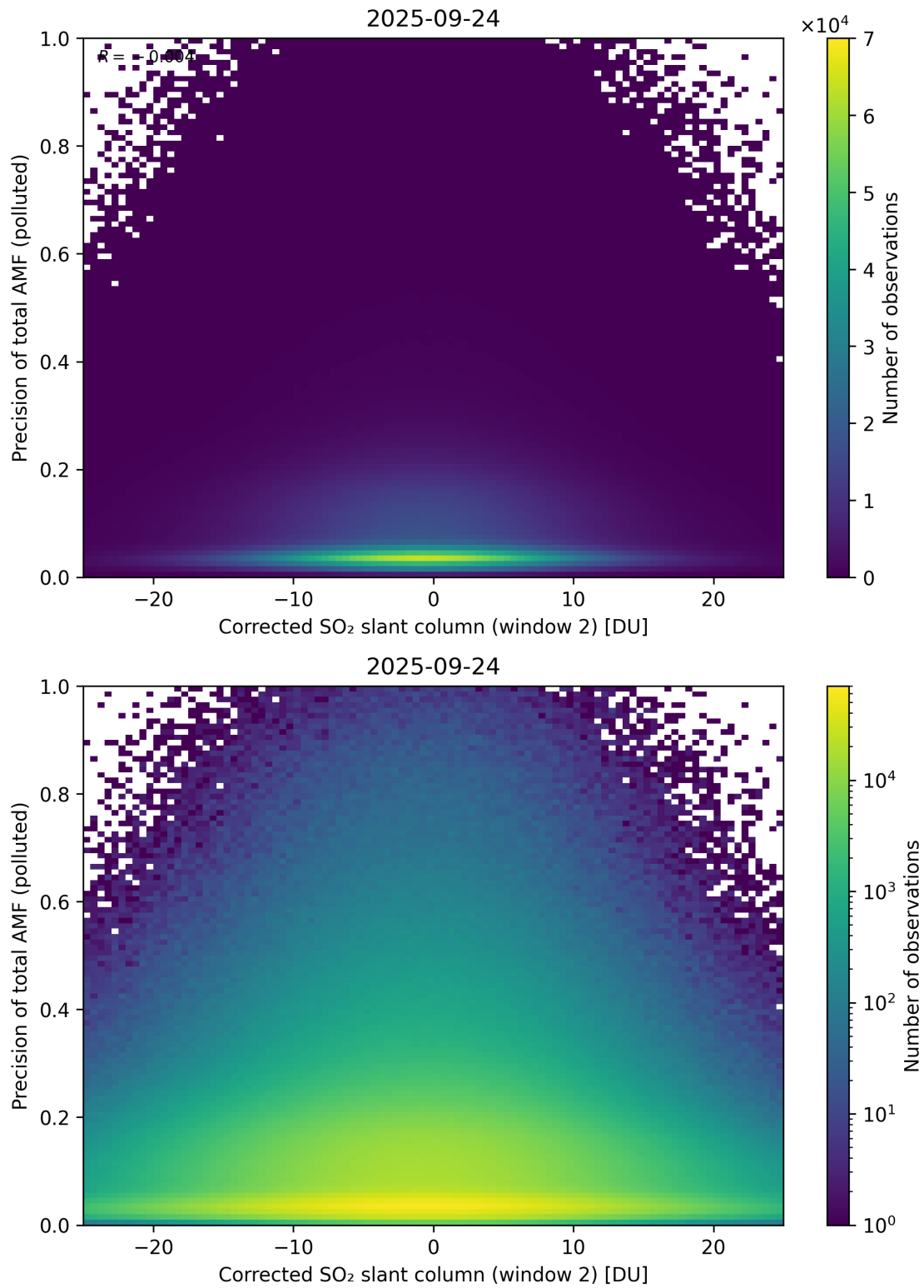
Figure 254: Scatter density plot of “Corrected SO 2 slant column (window 2)” against “Precision of total AMF (polluted)” for 2025-09-23 to 2025-09-25.
