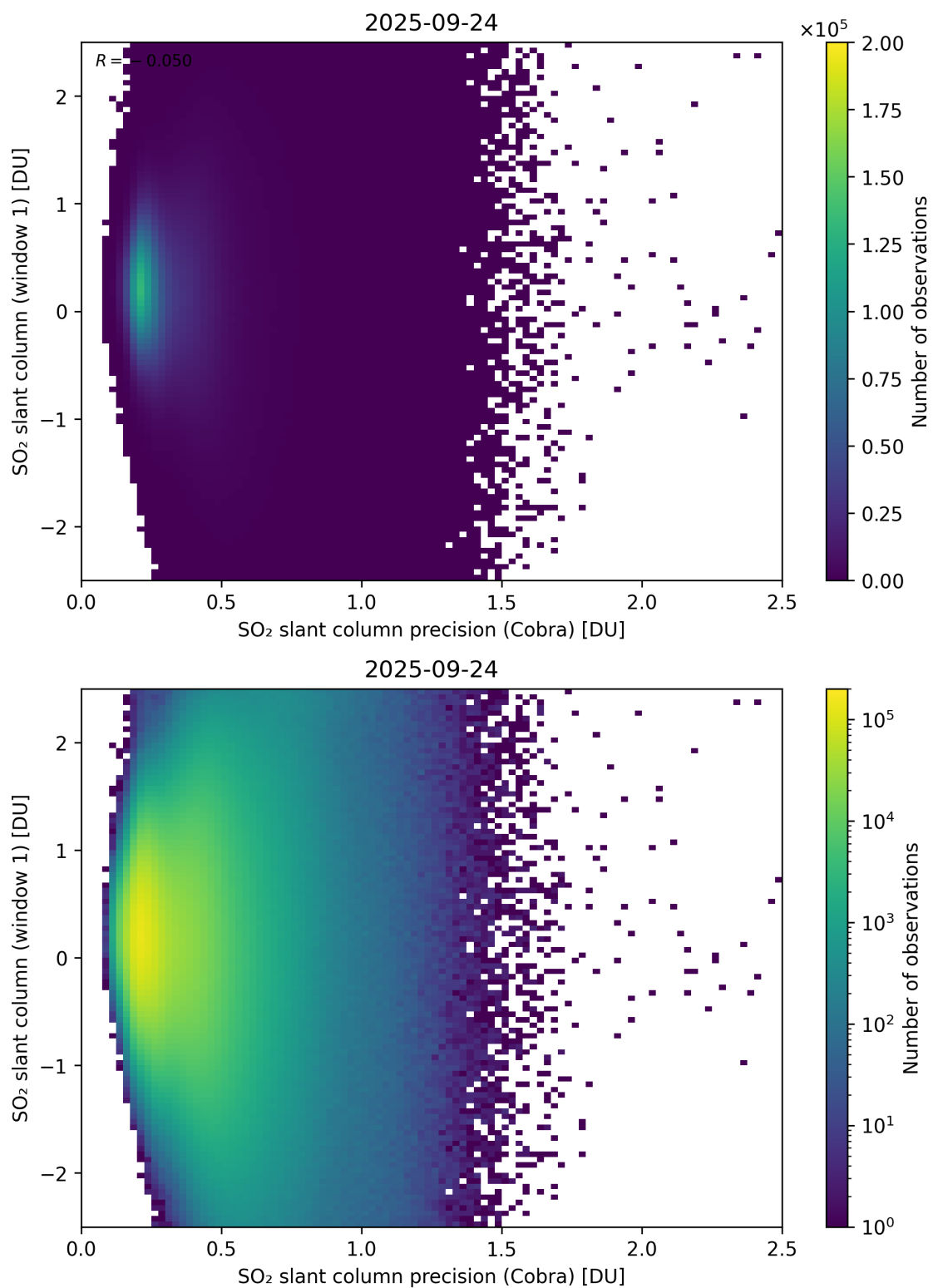
Figure 208: Scatter density plot of “SO 2 slant column precision (Cobra)” against “SO 2 slant column (window 1)” for 2025-09-23 to 2025-09-25.
