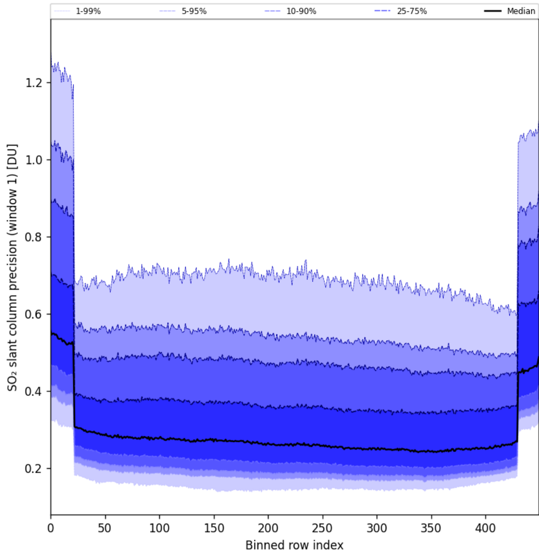
Figure 90: Along track statistics of “SO 2 slant column precision (window 1)” for 2025-09-23 to 2025-09-25
