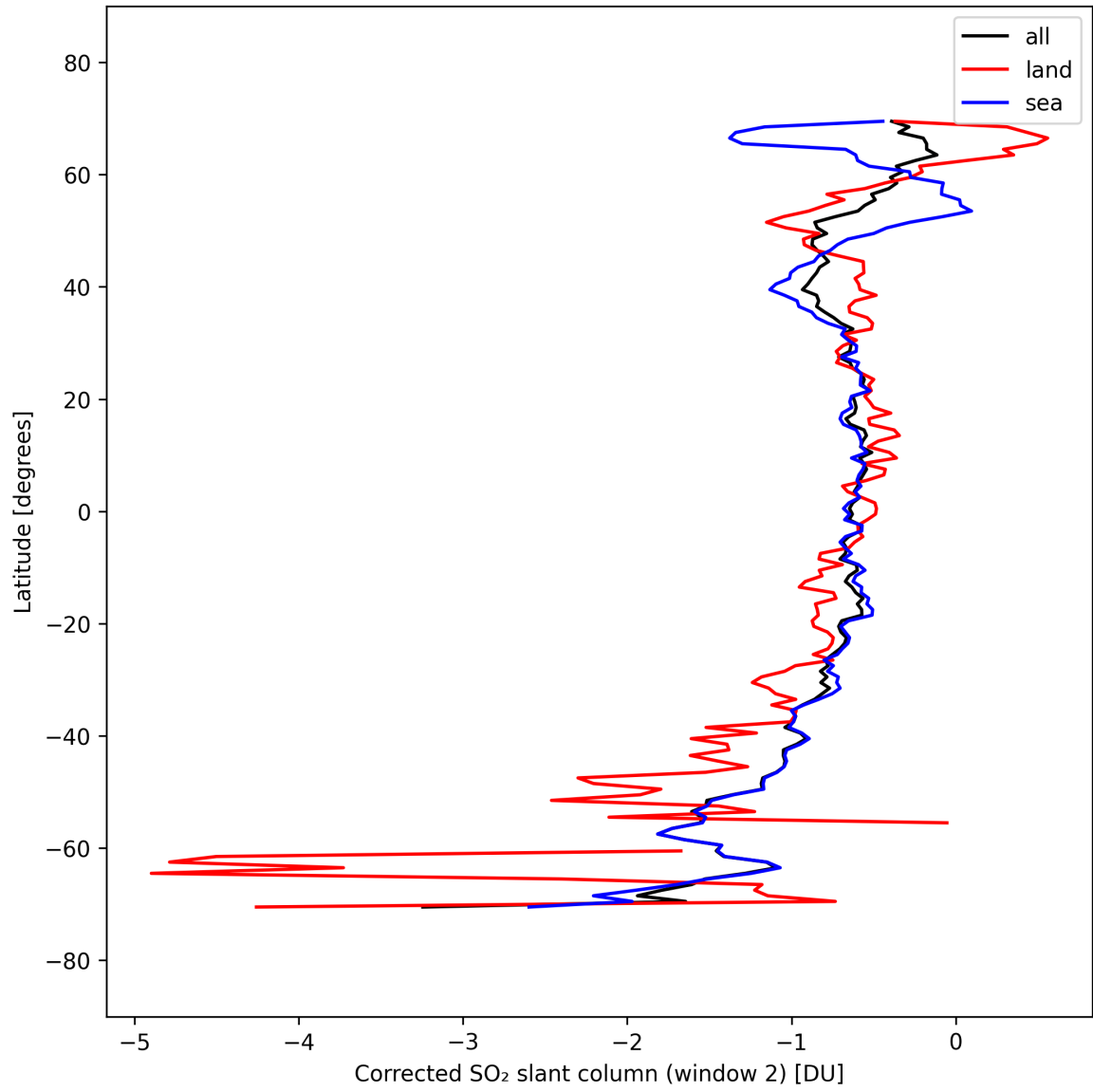
Figure 43: Zonal average of “Corrected SO 2 slant column (window 2)” for 2025-09-23 to 2025-09-25.
