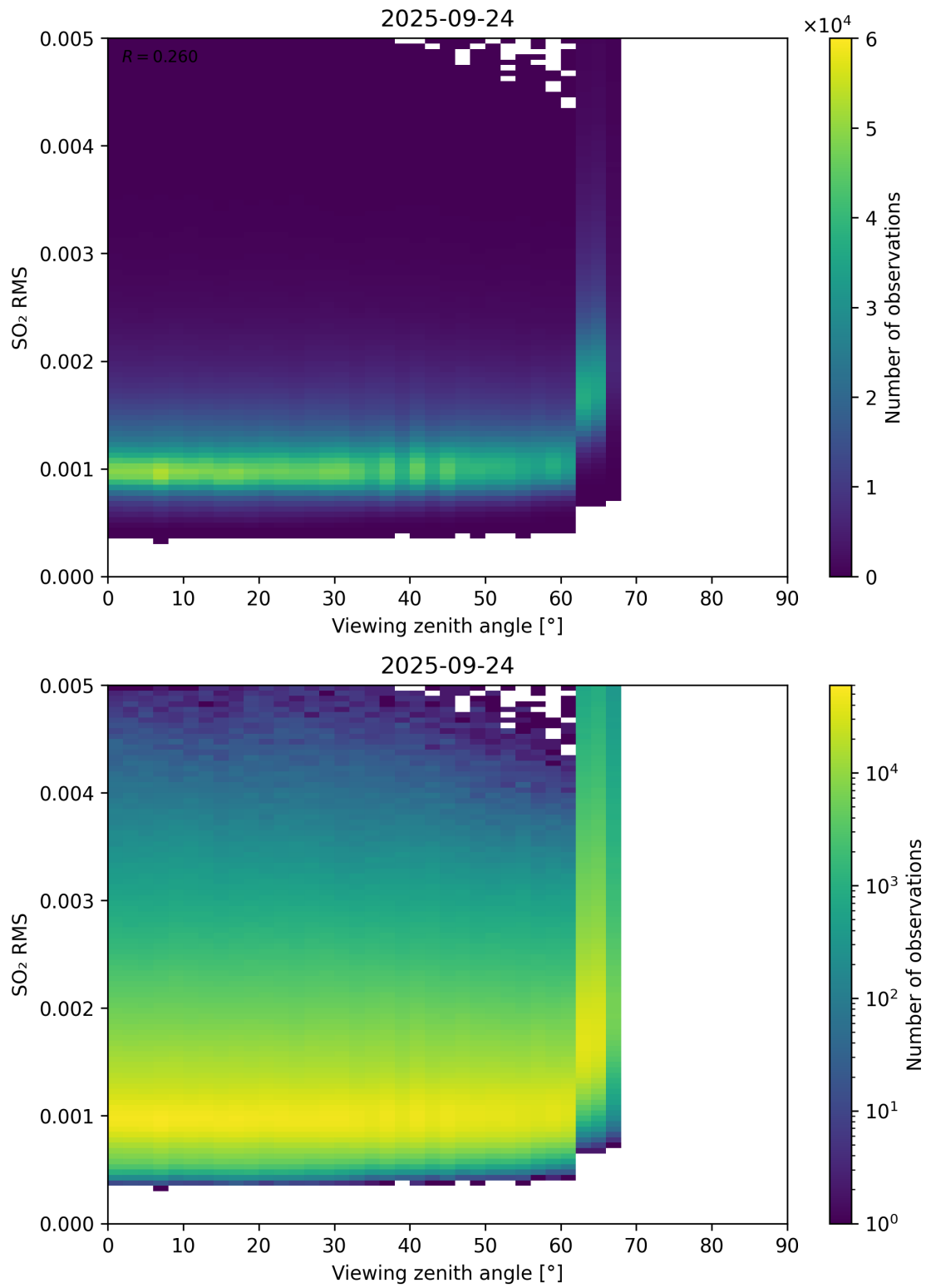
Figure 367: Scatter density plot of “Viewing zenith angle” against “SO 2 RMS” for 2025-09-23 to 2025-09-25.
