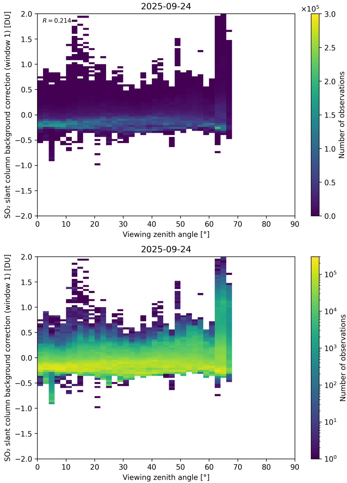
Figure 362: Scatter density plot of “Viewing zenith angle” against “SO 2 slant column background correction (window 1)” for 2025-09-23 to 2025-09-25.
