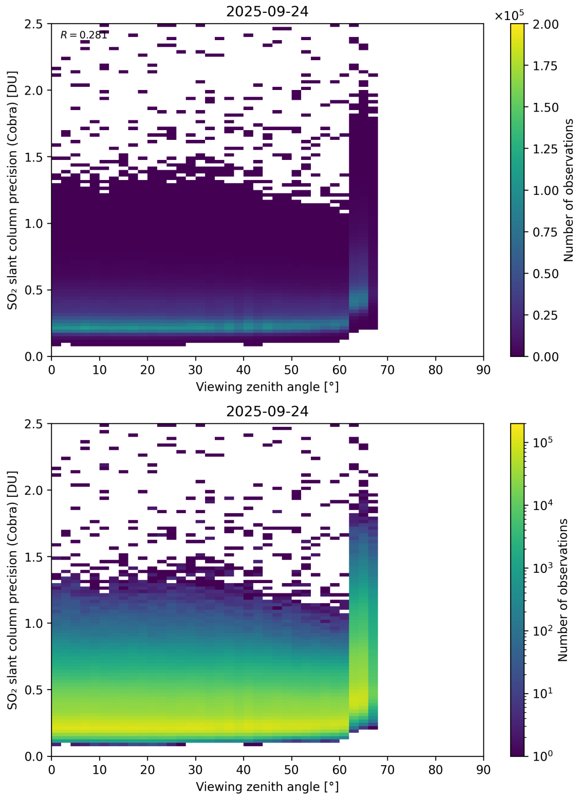
Figure 372: Scatter density plot of “Viewing zenith angle” against “SO 2 slant column precision (Cobra)” for 2025-09-23 to 2025-09-25.
