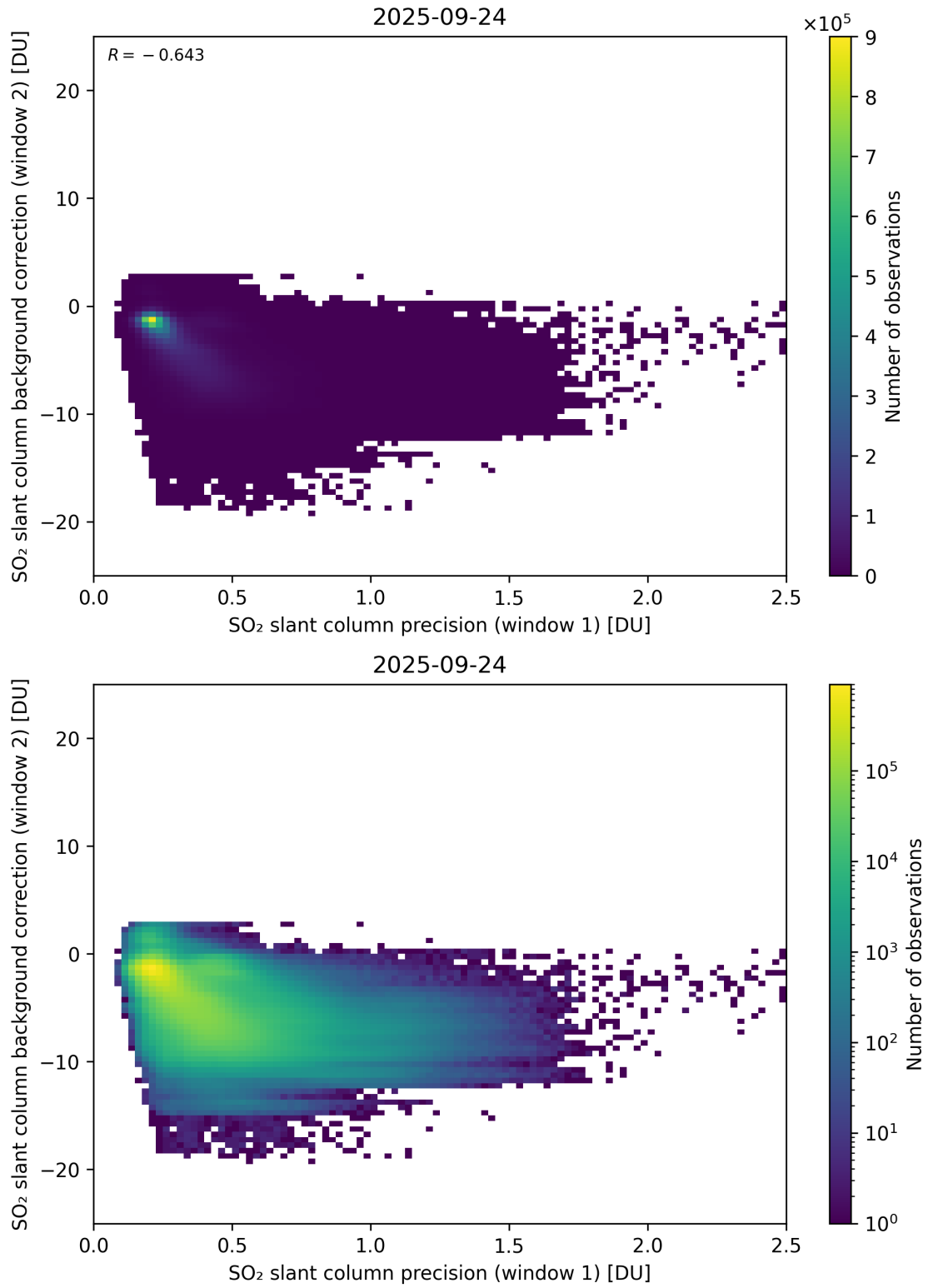
Figure 269: Scatter density plot of “SO 2 slant column precision (window 1)” against “SO 2 slant column background correction (window 2)” for 2025-09-23 to 2025-09-25.
