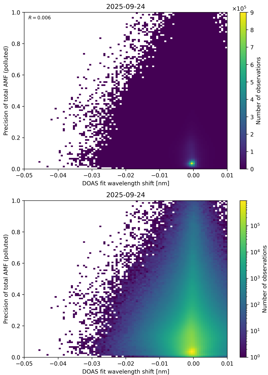
Figure 142: Scatter density plot of “DOAS fit wavelength shift” against “Precision of total AMF (polluted)” for 2025-09-23 to 2025-09-25.
