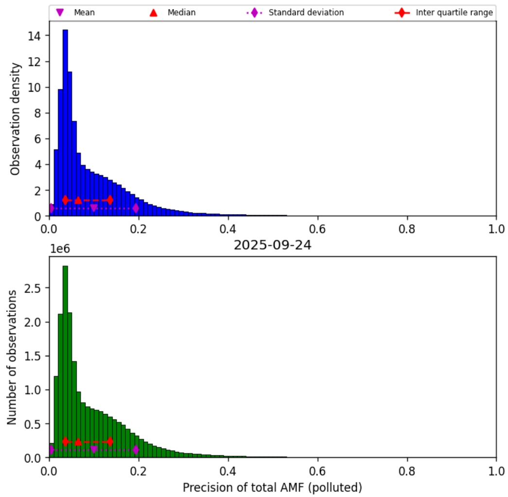
Figure 80: Histogram of “Precision of total AMF (polluted)” for 2025-09-23 to 2025-09-25
