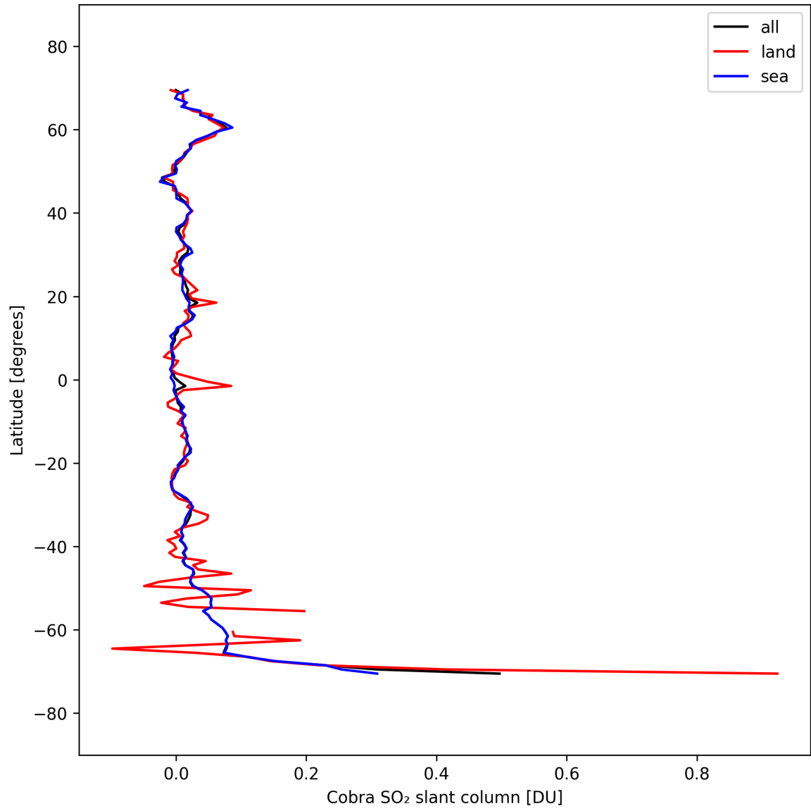
Figure 35: Zonal average of “Cobra SO 2 slant column” for 2025-09-23 to 2025-09-25.
