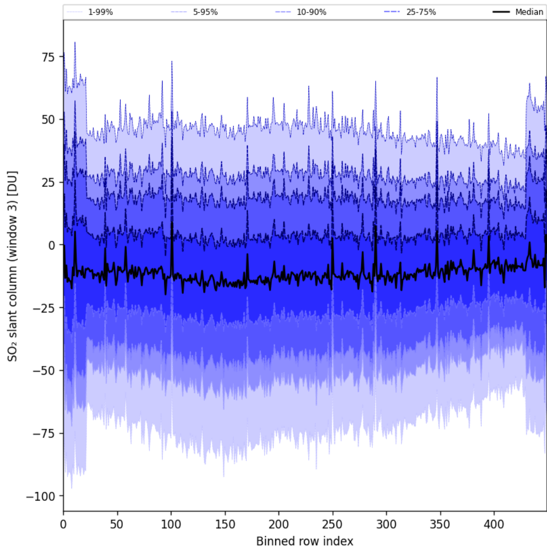
Figure 97: Along track statistics of “SO 2 slant column (window 3)” for 2025-09-23 to 2025-09-25
