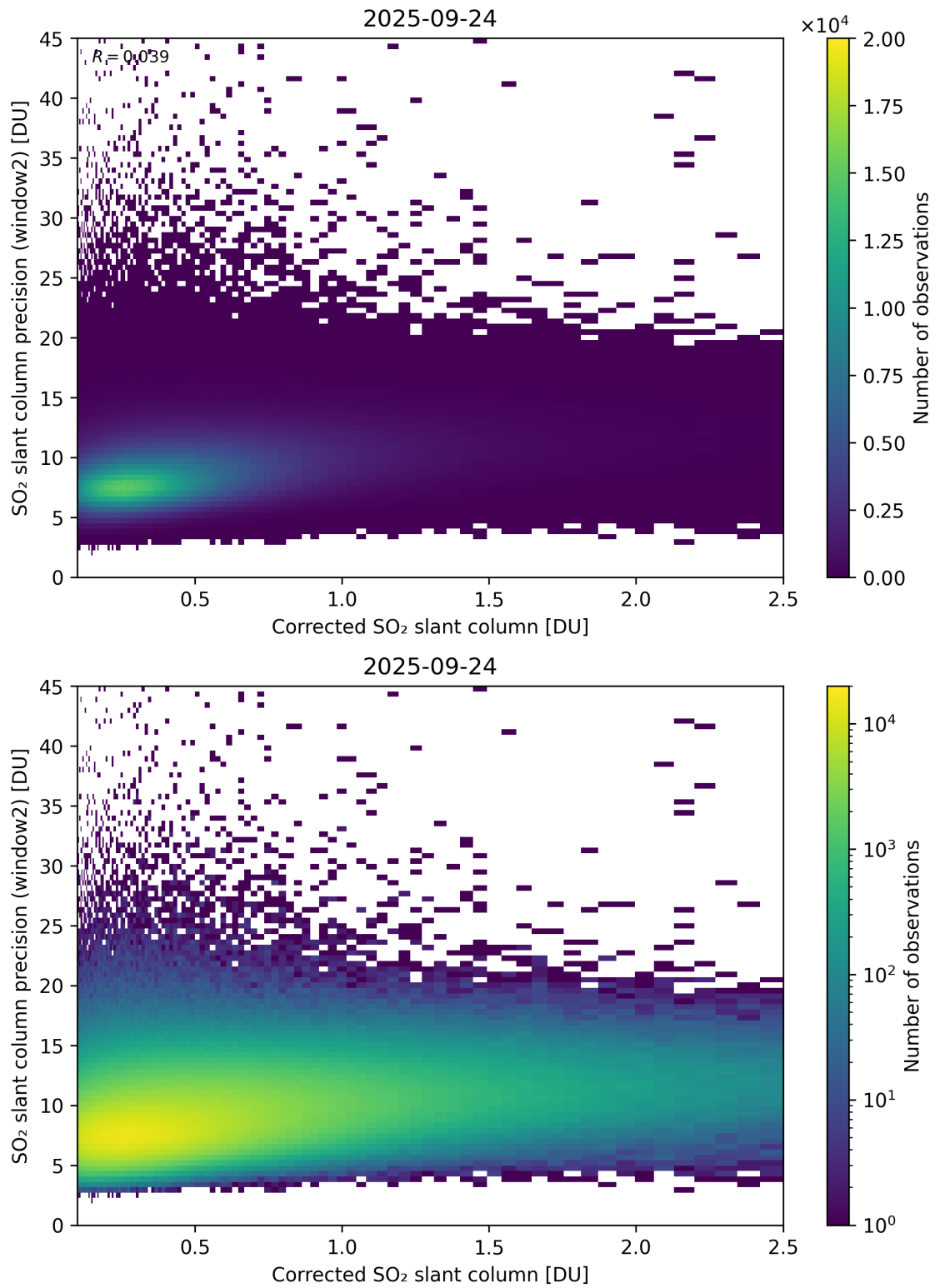
Figure 239: Scatter density plot of “Corrected SO 2 slant column” against “SO 2 slant column precision (window2)” for 2025-09-23 to 2025-09-25.
