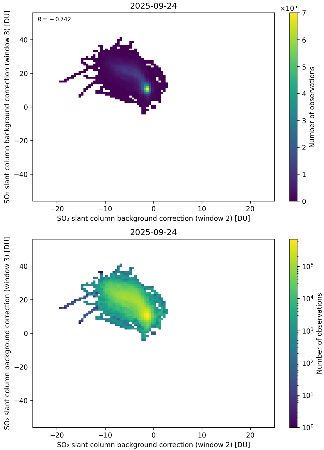
Figure 122: Scatter density plot of “SO 2 slant column background correction (window 2)” against “SO 2 slant column background correction (window 3)” for 2025-09-23 to 2025-09-25.
