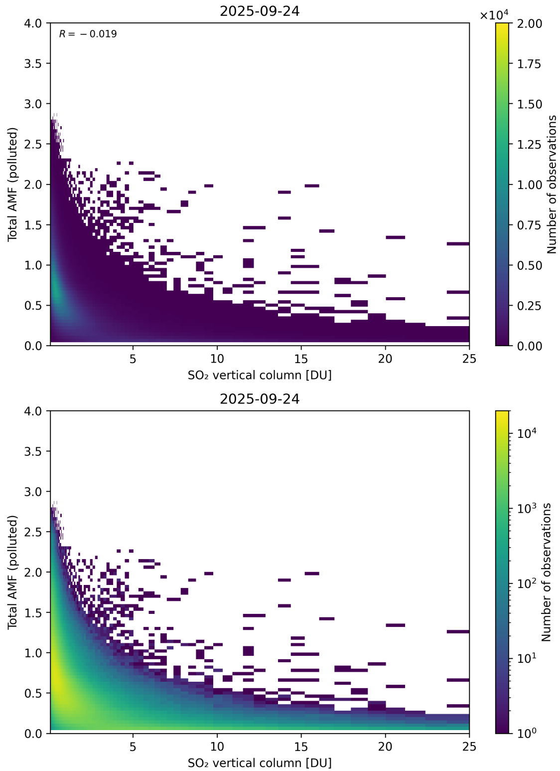
Figure 359: Scatter density plot of “SO 2 vertical column” against “Total AMF (polluted)” for 2025-09-23 to 2025-09-25.
