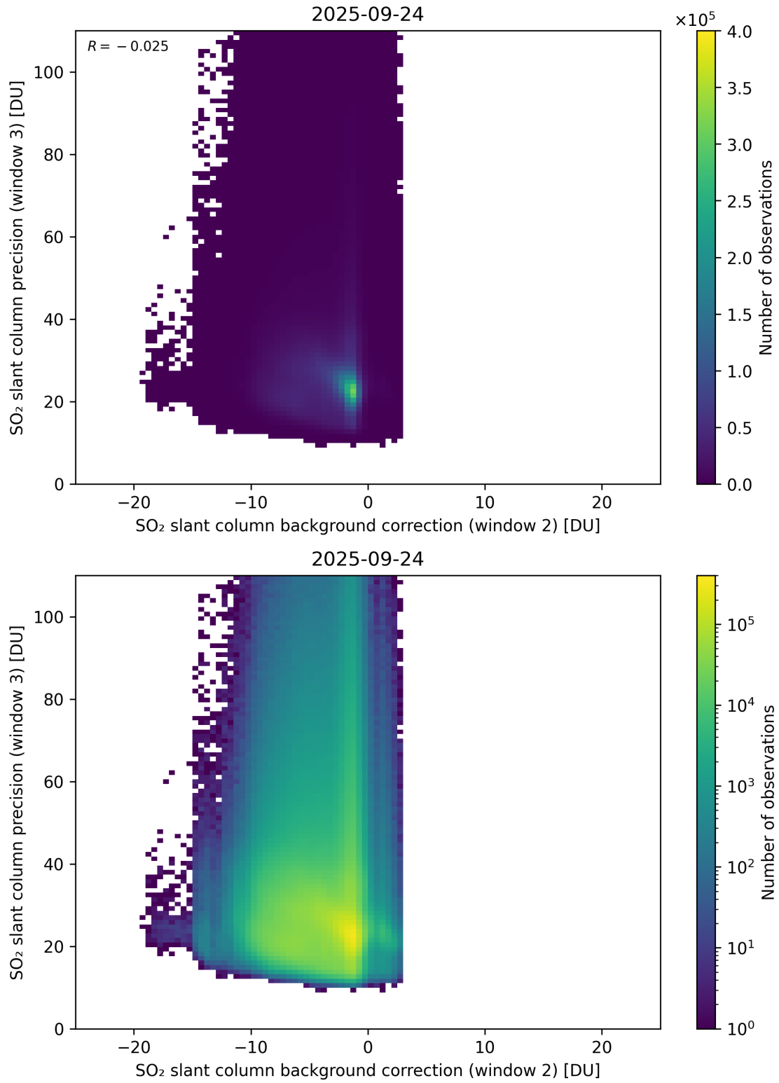
Figure 129: Scatter density plot of “SO 2 slant column background correction (window 2)” against “SO 2 slant column precision (window 3)” for 2025-09-23 to 2025-09-25.
