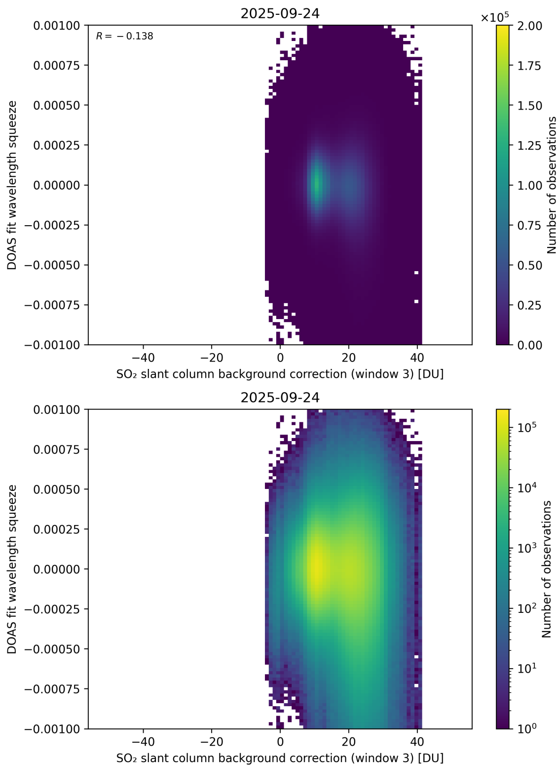
Figure 133: Scatter density plot of “SO 2 slant column background correction (window 3)” against “DOAS fit wavelength squeeze” for 2025-09-23 to 2025-09-25.
