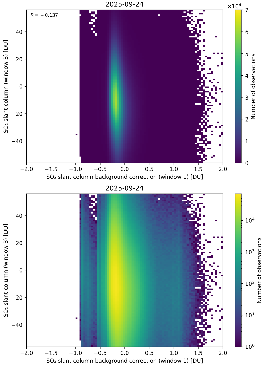
Figure 118: Scatter density plot of “SO 2 slant column background correction (window 1)” against “SO 2 slant column (window 3)” for 2025-09-23 to 2025-09-25.
