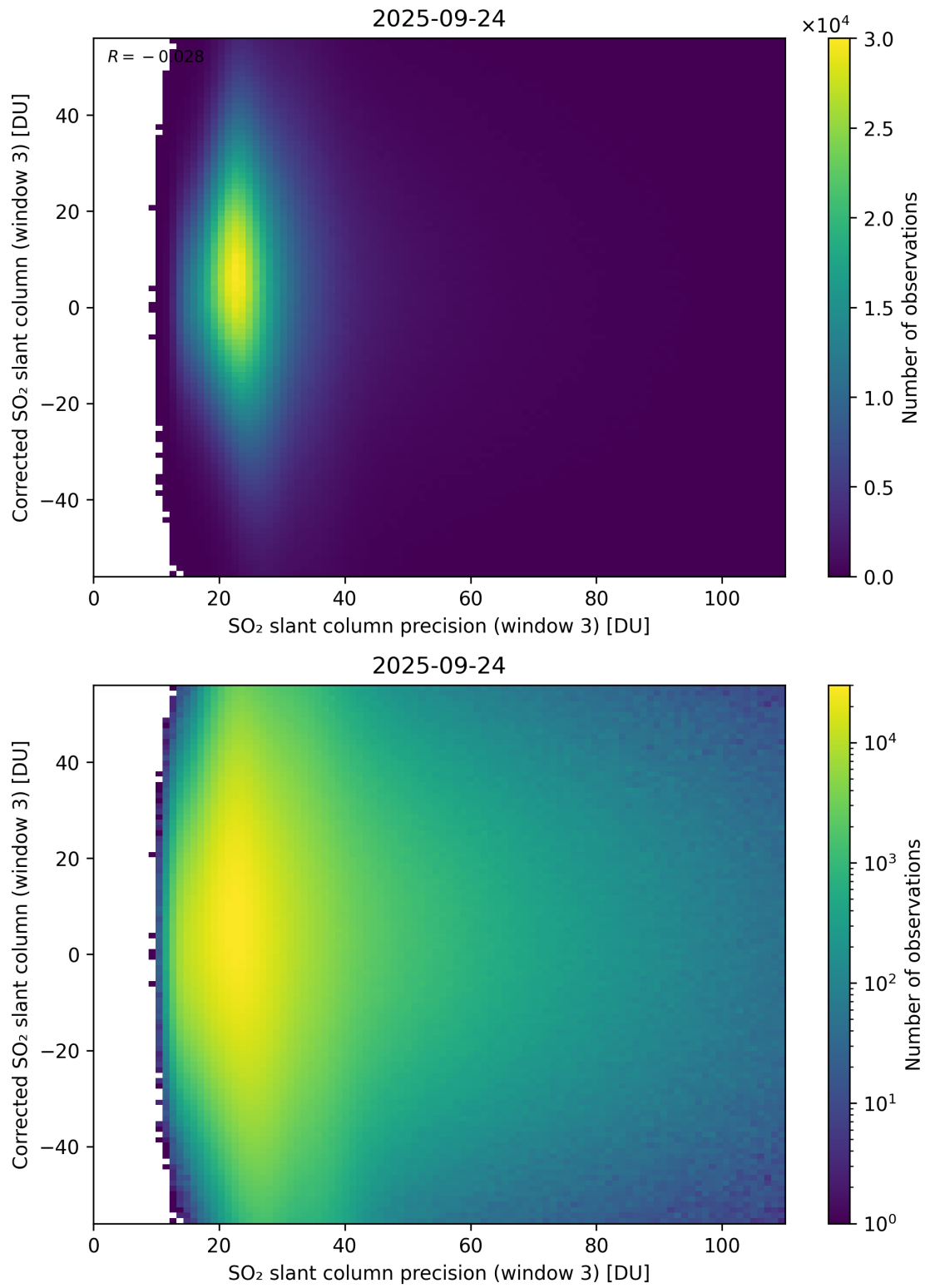
Figure 312: Scatter density plot of “SO 2 slant column precision (window 3)” against “Corrected SO 2 slant column (window 3)” for 2025-09-23 to 2025-09-25.
