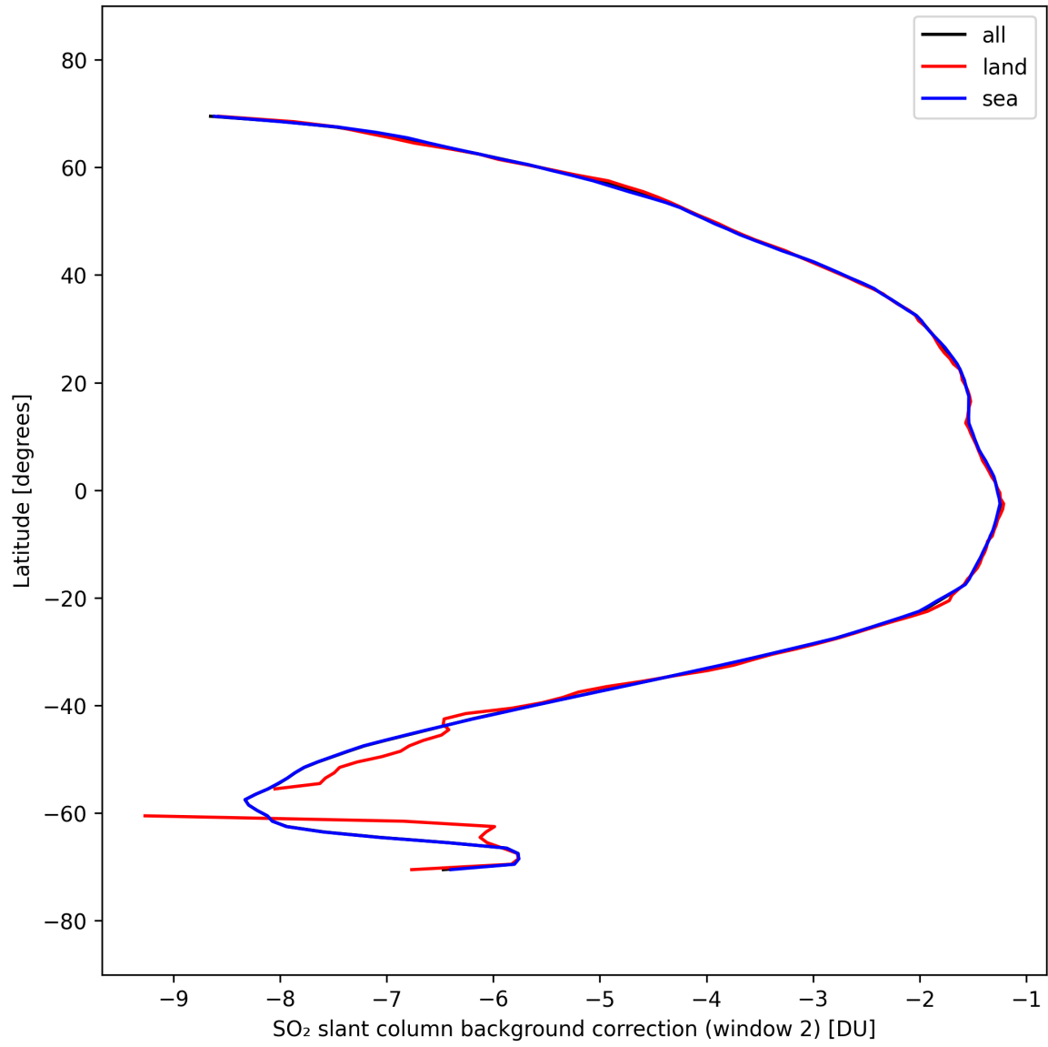
Figure 44: Zonal average of “SO 2 slant column background correction (window 2)” for 2025-09-23 to 2025-09-25.
