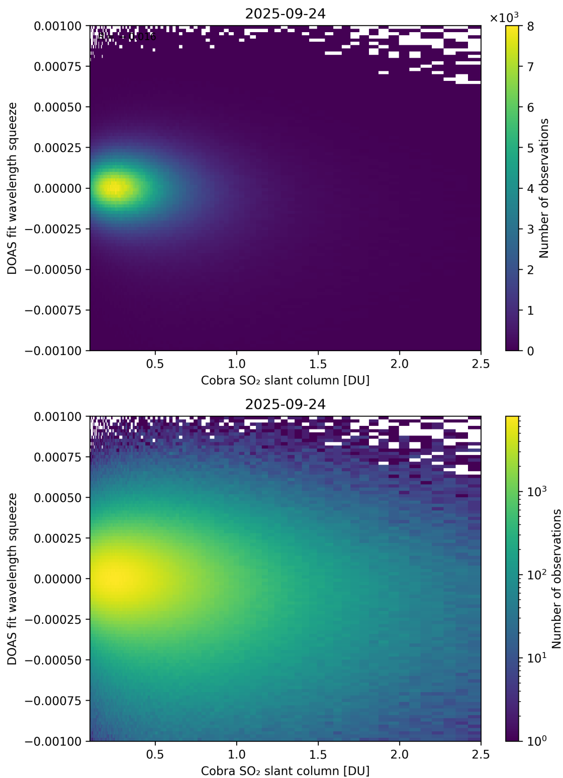
Figure 197: Scatter density plot of “Cobra SO 2 slant column” against “DOAS fit wavelength squeeze” for 2025-09-23 to 2025-09-25.
