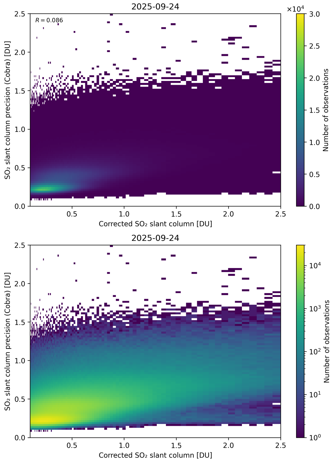
Figure 234: Scatter density plot of “Corrected SO 2 slant column” against “SO 2 slant column precision (Cobra)” for 2025-09-23 to 2025-09-25.
