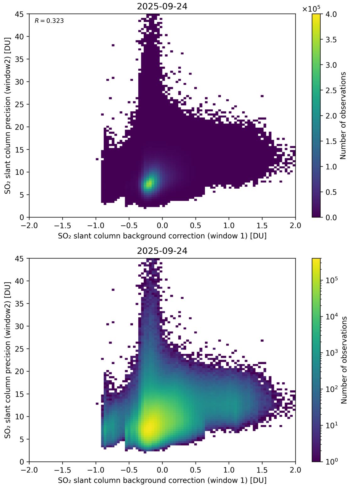
Figure 117: Scatter density plot of “SO 2 slant column background correction (window 1)” against “SO 2 slant column precision (window2)” for 2025-09-23 to 2025-09-25.
