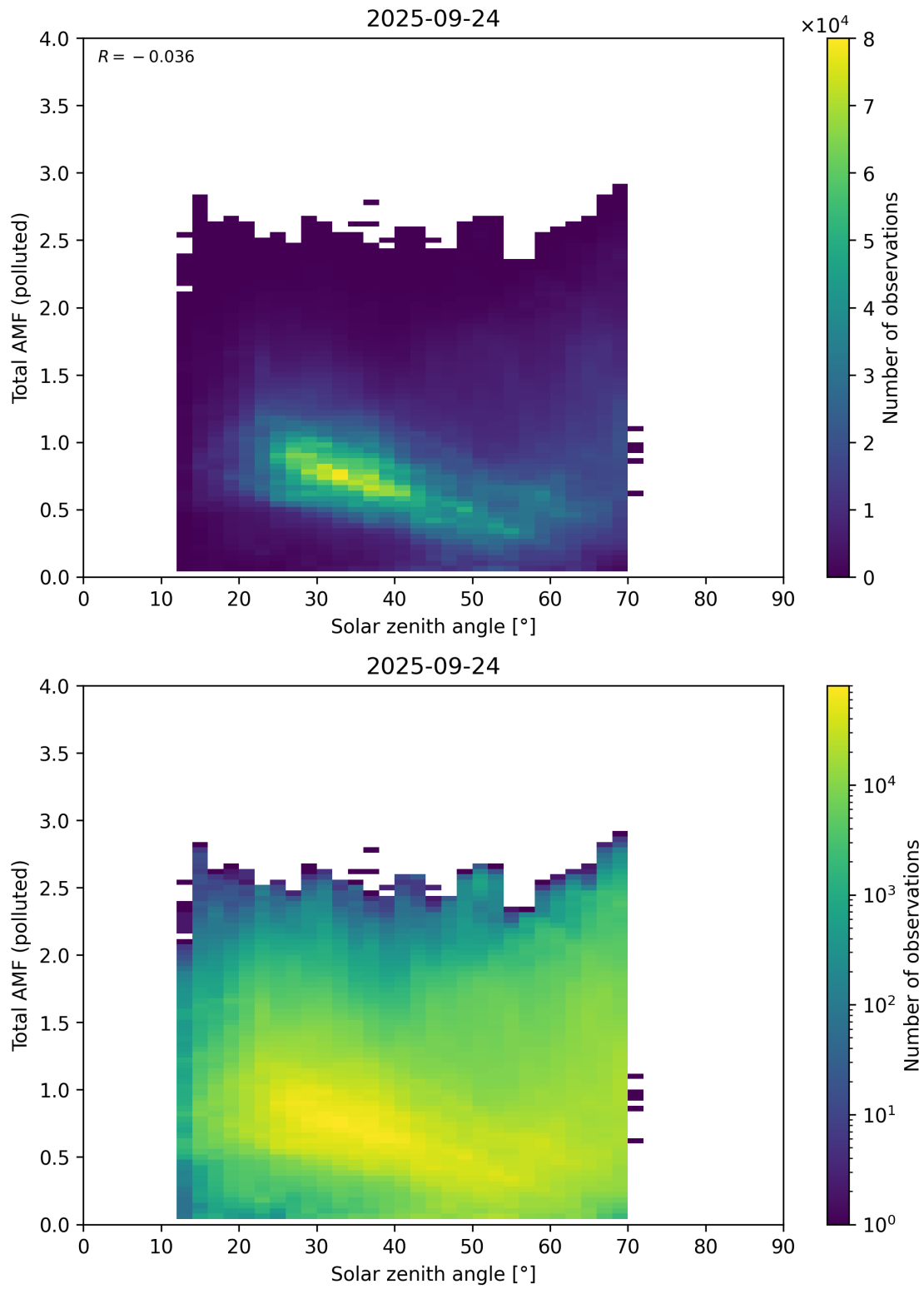
Figure 189: Scatter density plot of “Solar zenith angle” against “Total AMF (polluted)” for 2025-09-23 to 2025-09-25.
