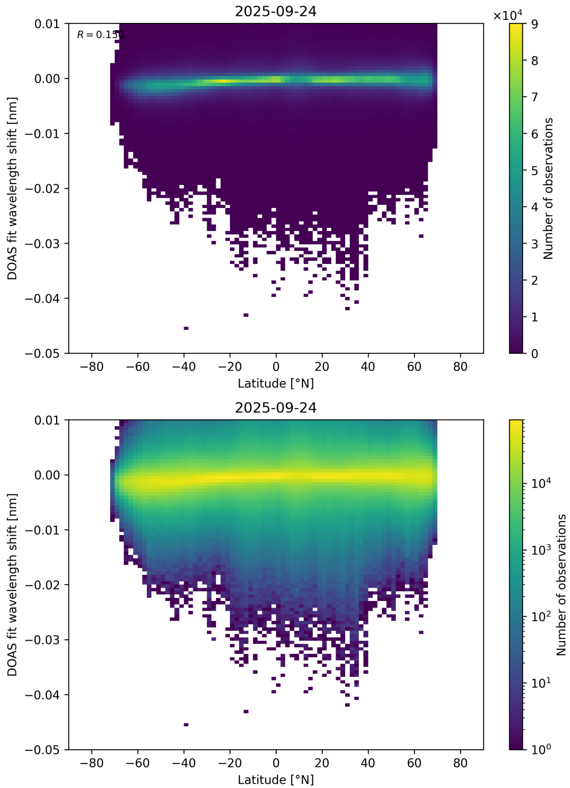
Figure 153: Scatter density plot of “Latitude” against “DOAS fit wavelength shift” for 2025-09-23 to 2025-09-25.
