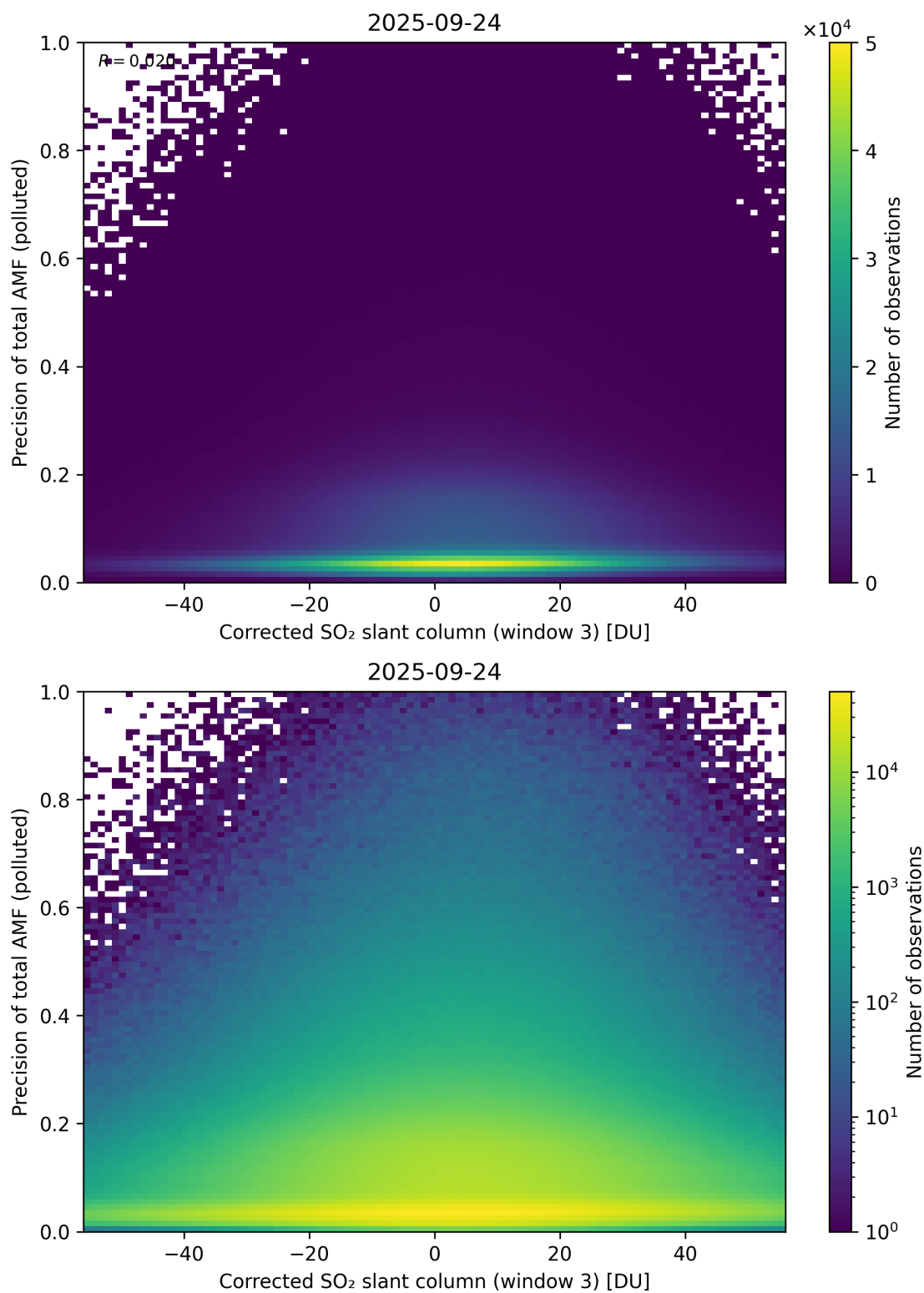
Figure 261: Scatter density plot of “Corrected SO 2 slant column (window 3)” against “Precision of total AMF (polluted)” for 2025-09-23 to 2025-09-25.
