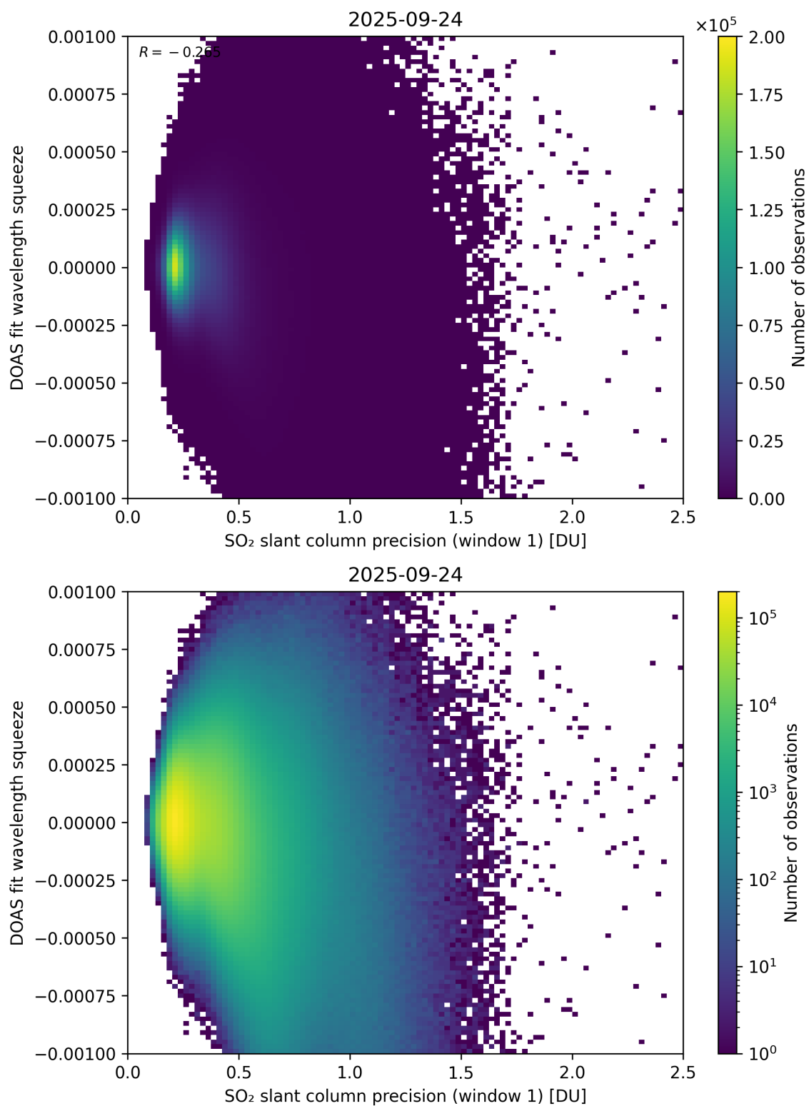
Figure 272: Scatter density plot of “SO 2 slant column precision (window 1)” against “DOAS fit wavelength squeeze” for 2025-09-23 to 2025-09-25.
