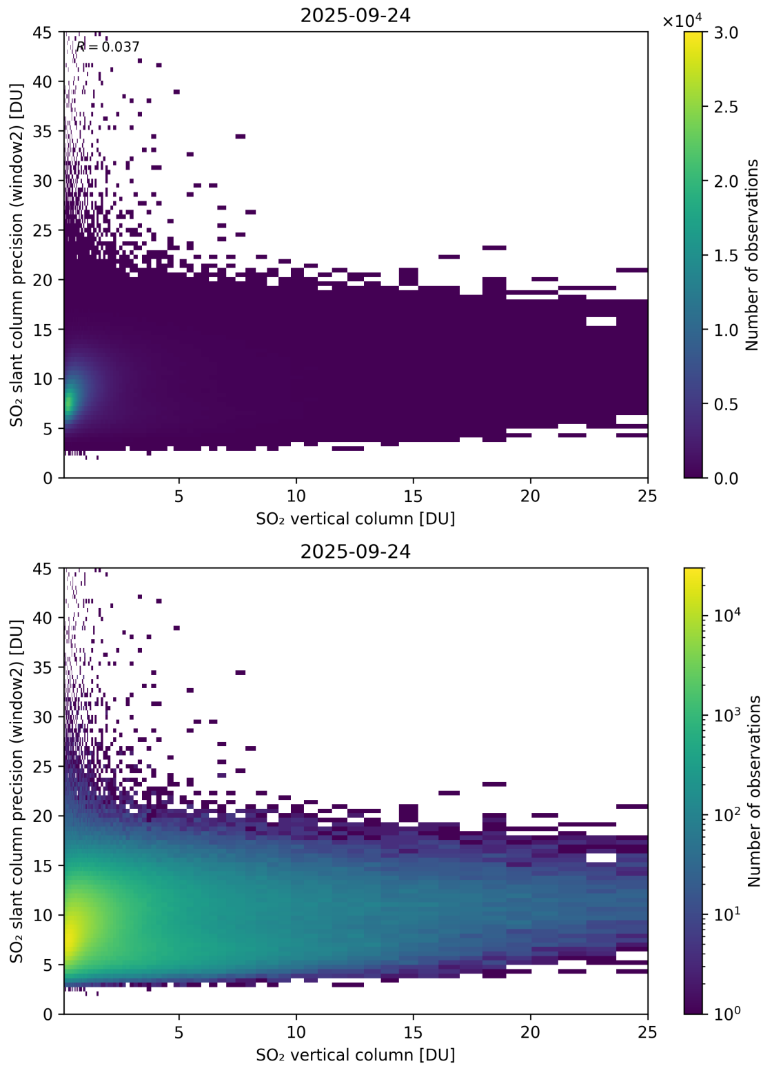
Figure 356: Scatter density plot of “SO 2 vertical column” against “SO 2 slant column precision (window2)” for 2025-09-23 to 2025-09-25.
