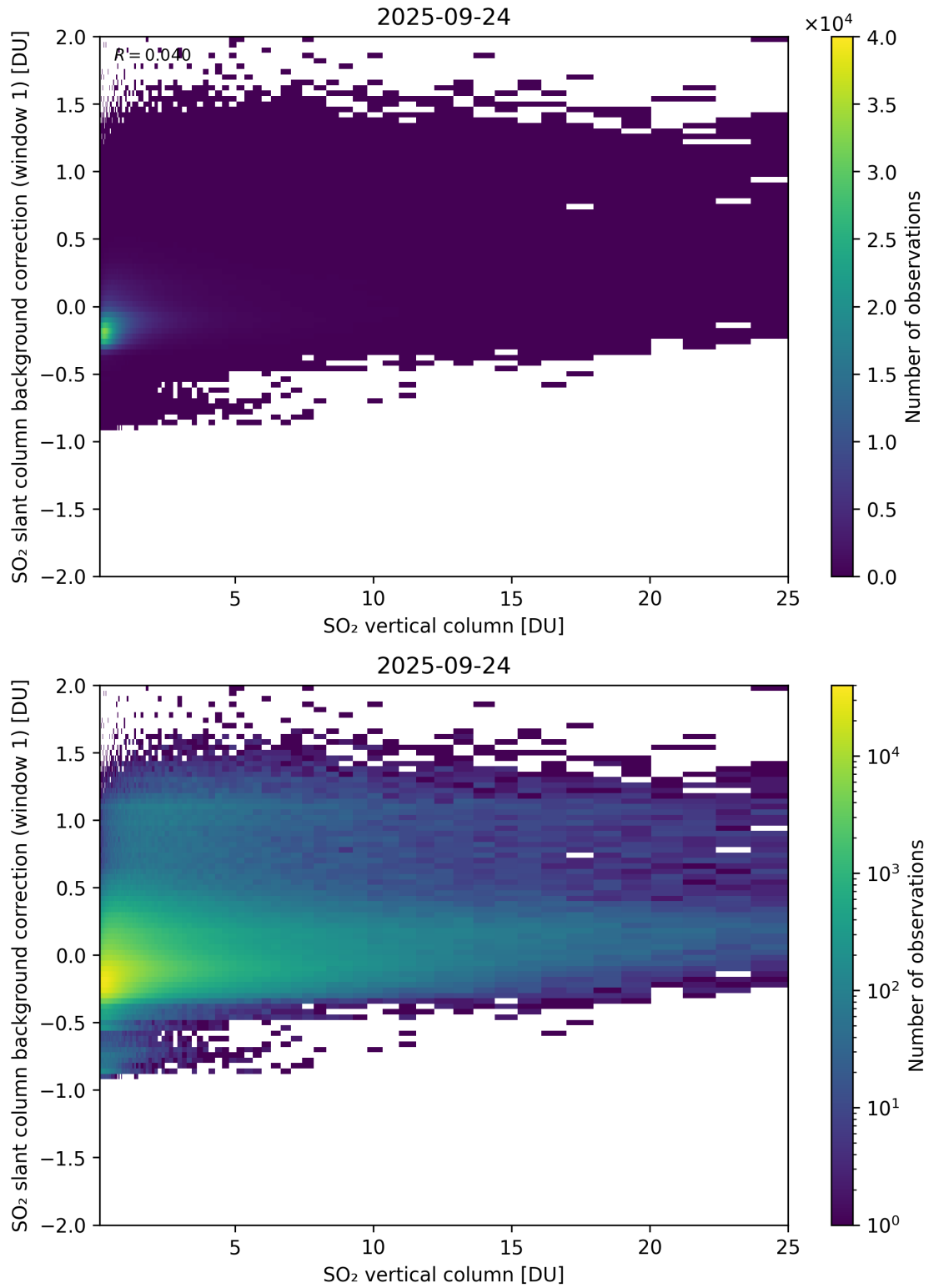
Figure 323: Scatter density plot of “SO 2 vertical column” against “SO 2 slant column background correction (window 1)” for 2025-09-23 to 2025-09-25.
