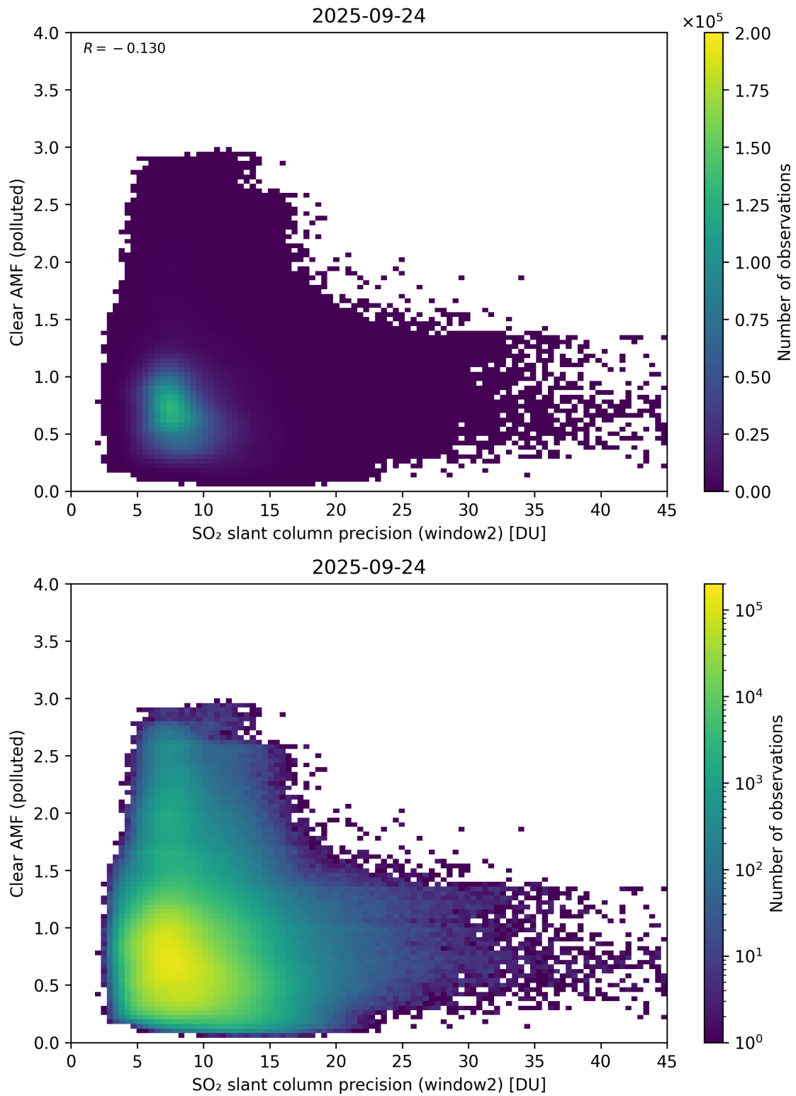
Figure 296: Scatter density plot of “SO 2 slant column precision (window2)” against “Clear AMF (polluted)” for 2025-09-23 to 2025-09-25.
