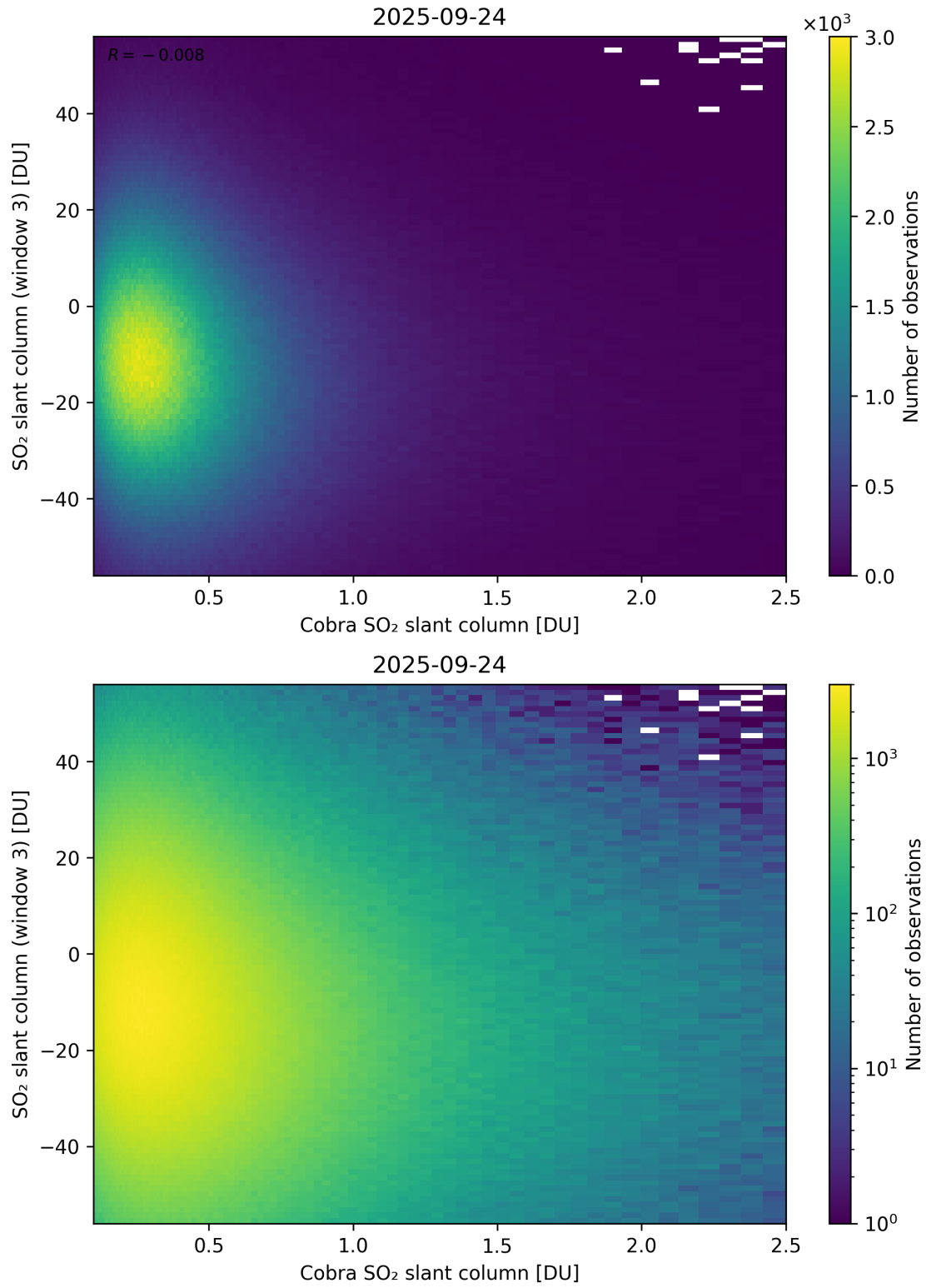
Figure 222: Scatter density plot of “Cobra SO 2 slant column” against “SO 2 slant column (window 3)” for 2025-09-23 to 2025-09-25.
