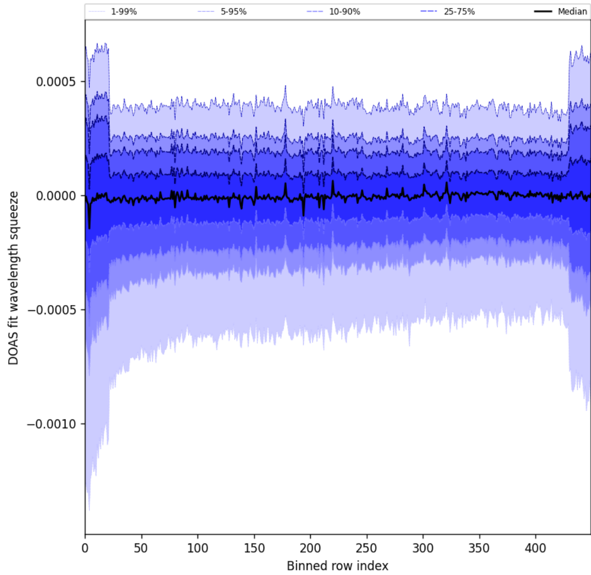
Figure 103: Along track statistics of “DOAS fit wavelength squeeze” for 2025-09-23 to 2025-09-25
