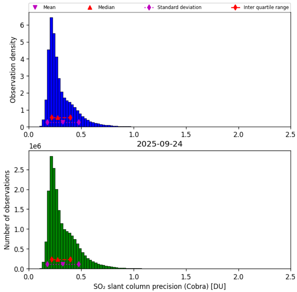
Figure 62: Histogram of “SO 2 slant column precision (Cobra)” for 2025-09-23 to 2025-09-25
