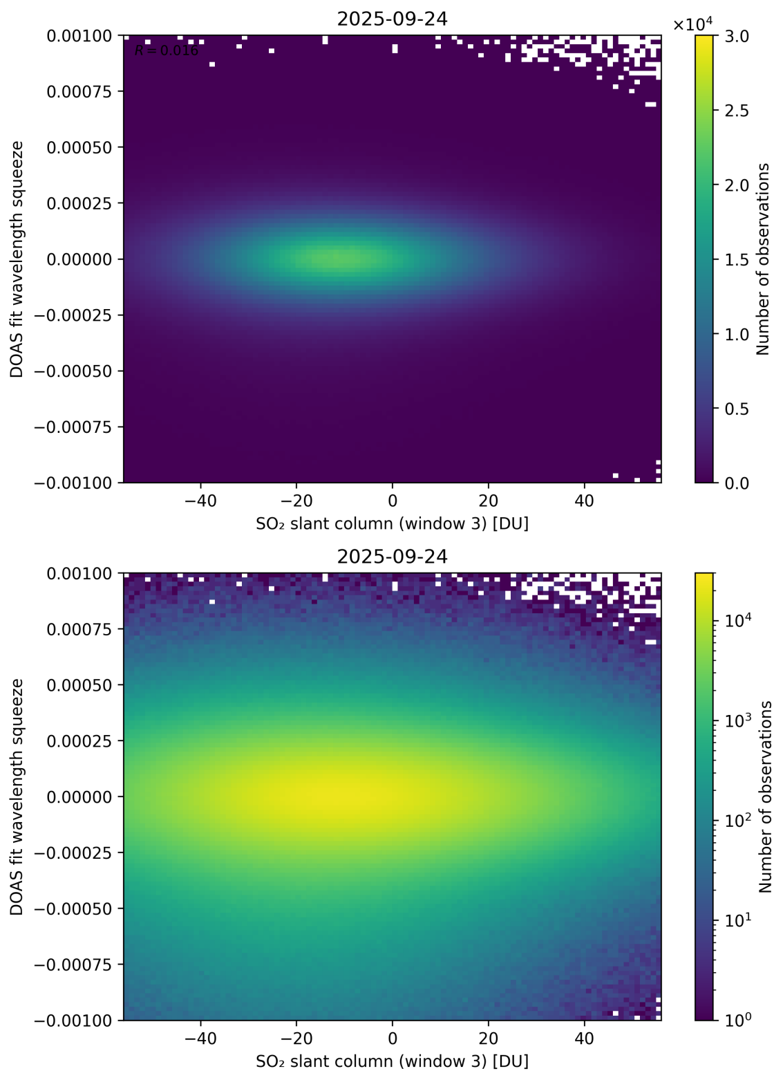
Figure 305: Scatter density plot of “SO 2 slant column (window 3)” against “DOAS fit wavelength squeeze” for 2025-09-23 to 2025-09-25.
