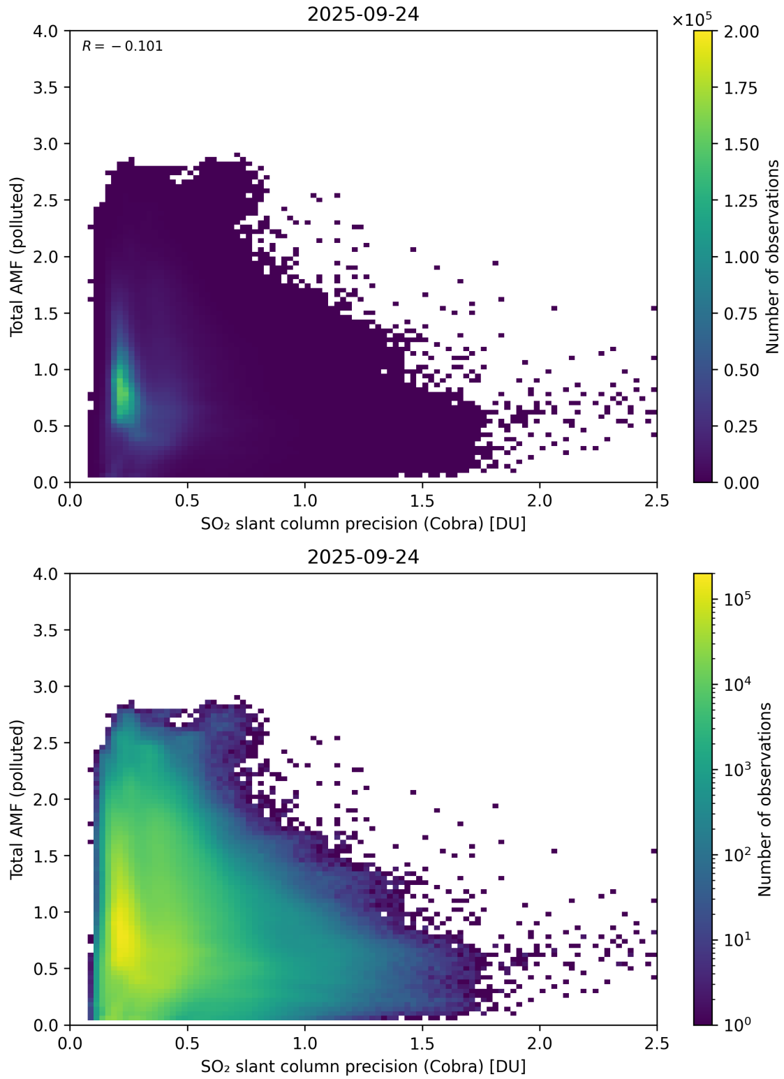
Figure 213: Scatter density plot of “SO 2 slant column precision (Cobra)” against “Total AMF (polluted)” for 2025-09-23 to 2025-09-25.
