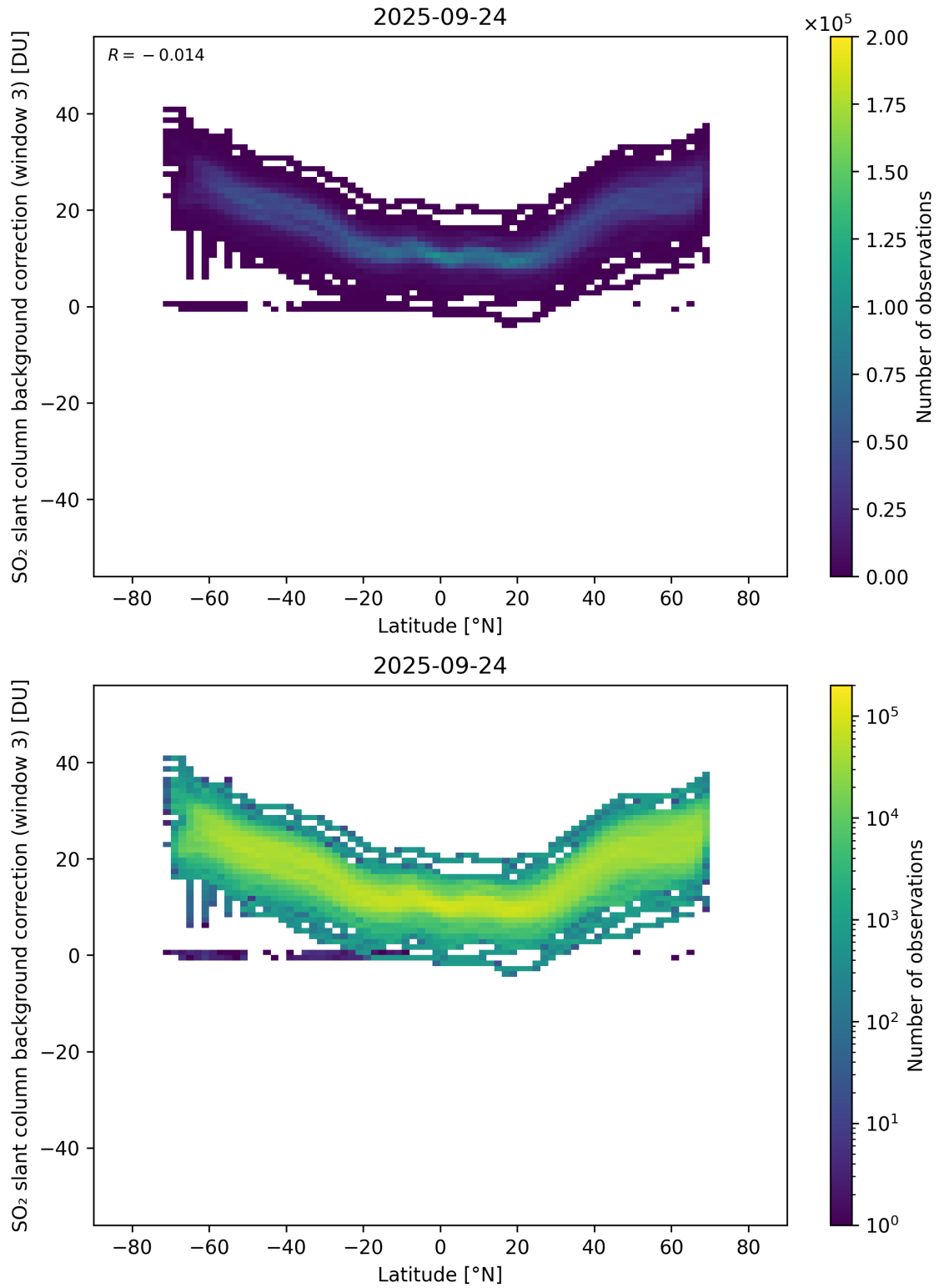
Figure 152: Scatter density plot of “Latitude” against “SO 2 slant column background correction (window 3)” for 2025-09-23 to 2025-09-25.
