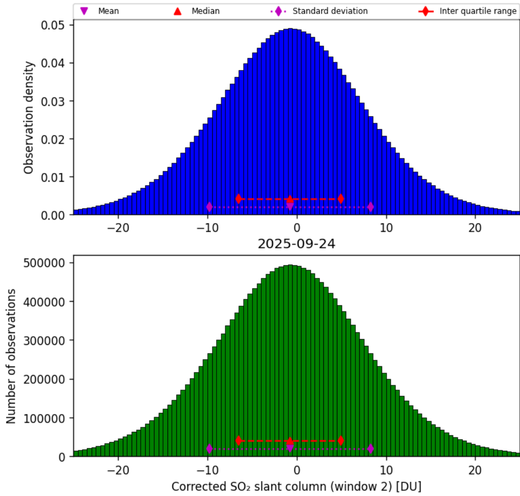
Figure 69: Histogram of “Corrected SO 2 slant column (window 2)” for 2025-09-23 to 2025-09-25
