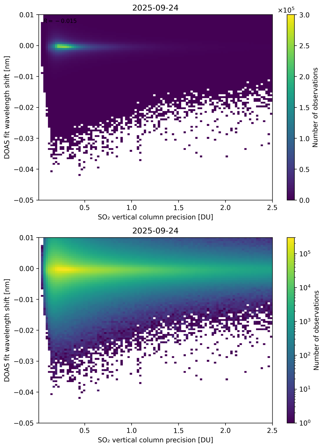
Figure 332: Scatter density plot of “SO 2 vertical column precision” against “DOAS fit wavelength shift” for 2025-09-23 to 2025-09-25.
