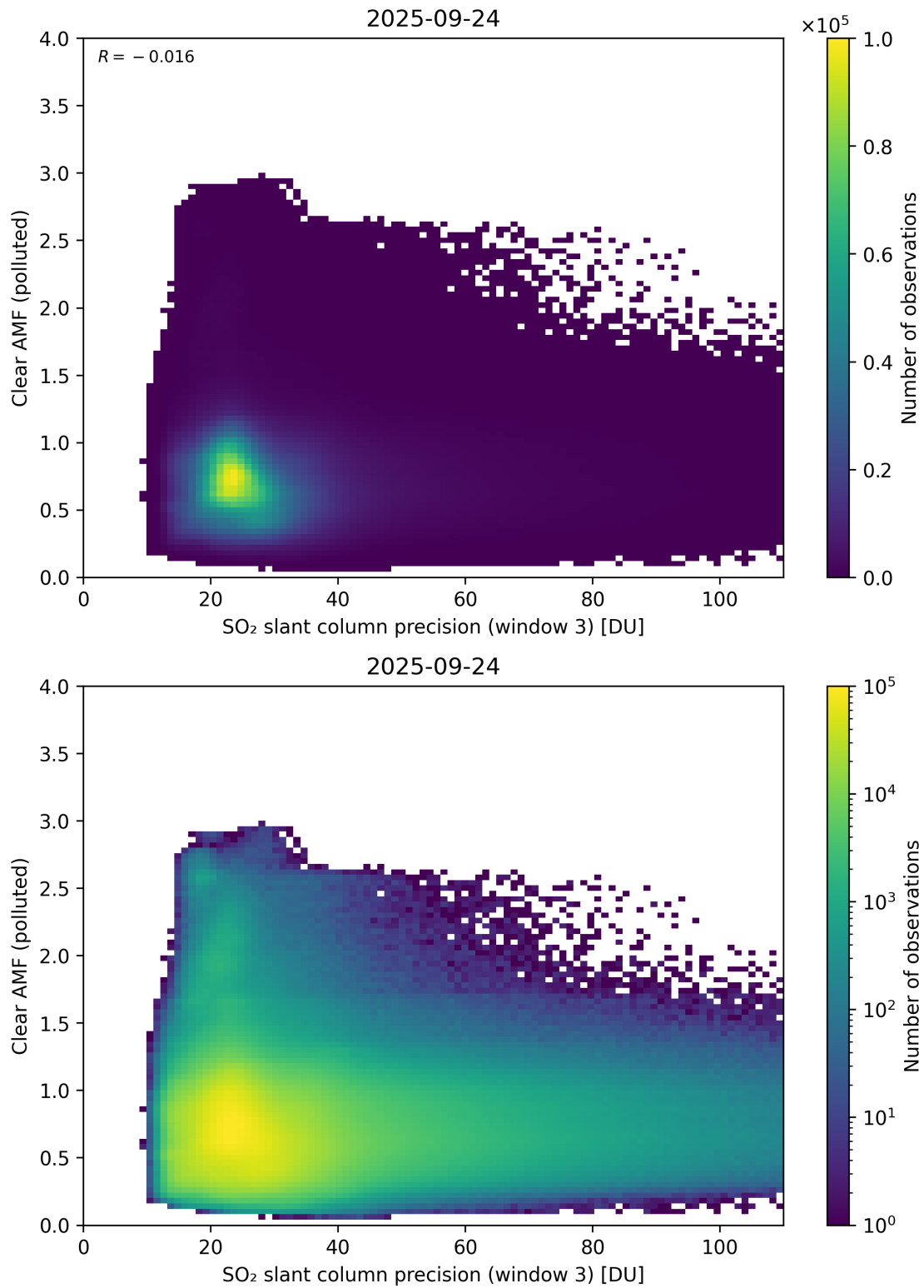
Figure 311: Scatter density plot of “SO 2 slant column precision (window 3)” against “Clear AMF (polluted)” for 2025-09-23 to 2025-09-25.
