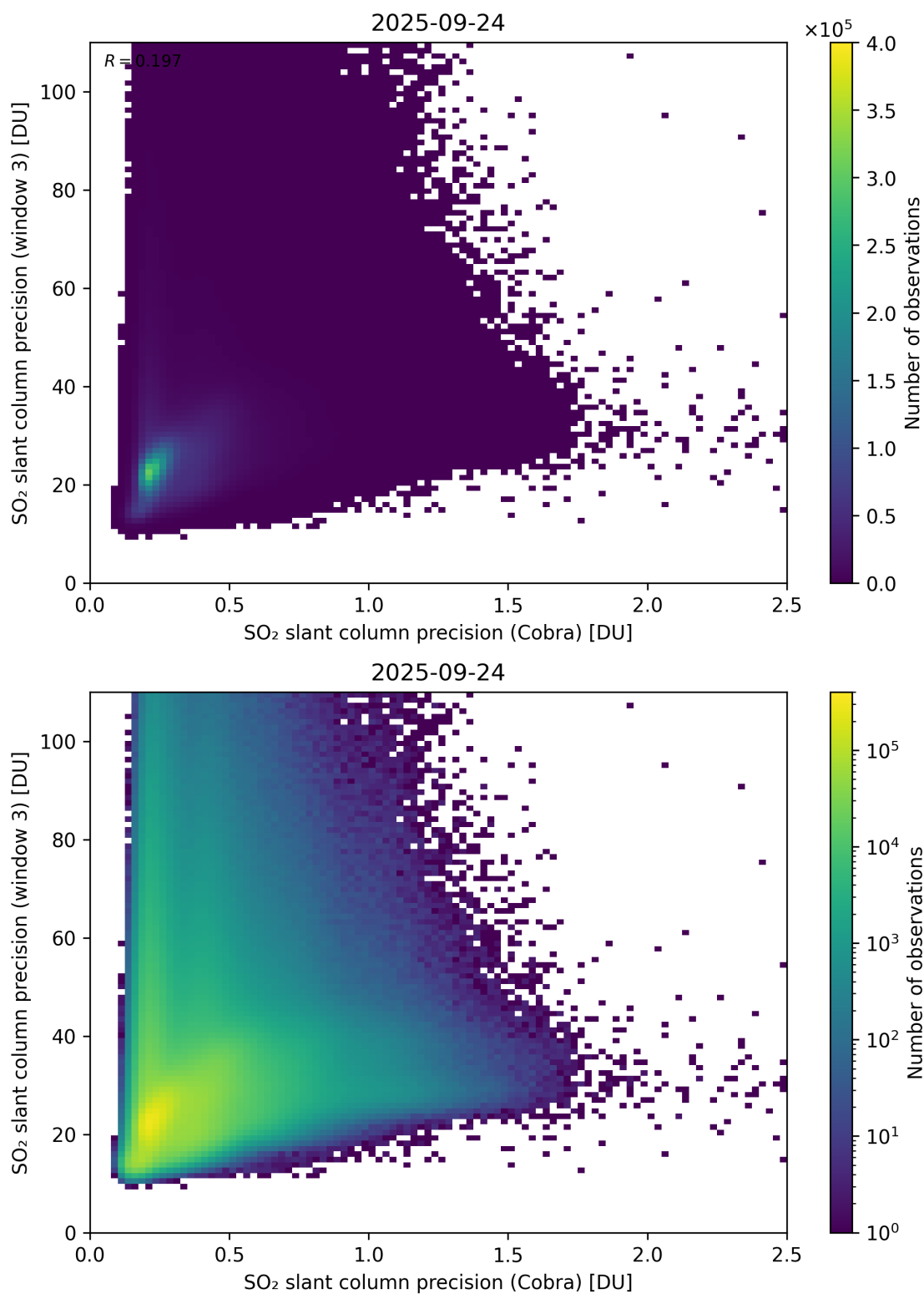
Figure 212: Scatter density plot of “SO 2 slant column precision (Cobra)” against “SO 2 slant column precision (window 3)” for 2025-09-23 to 2025-09-25.
