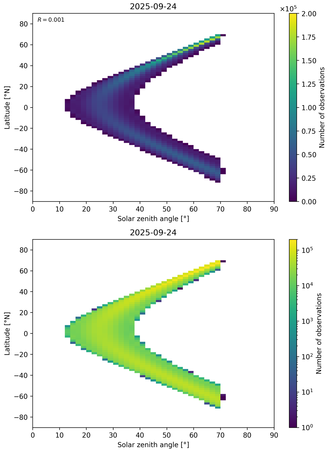
Figure 177: Scatter density plot of “Solar zenith angle” against “Latitude” for 2025-09-23 to 2025-09-25.
