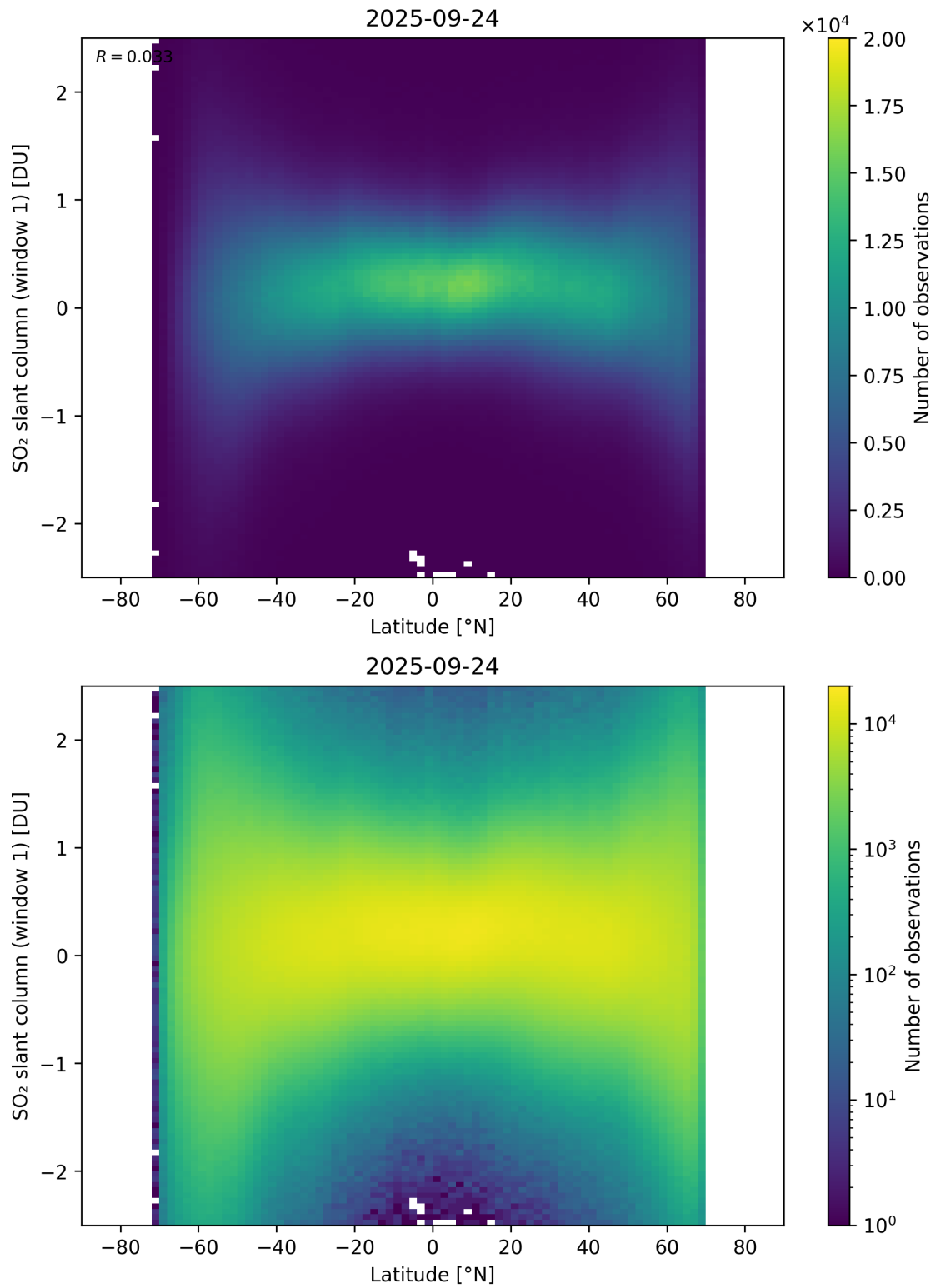
Figure 162: Scatter density plot of “Latitude” against “SO 2 slant column (window 1)” for 2025-09-23 to 2025-09-25.
