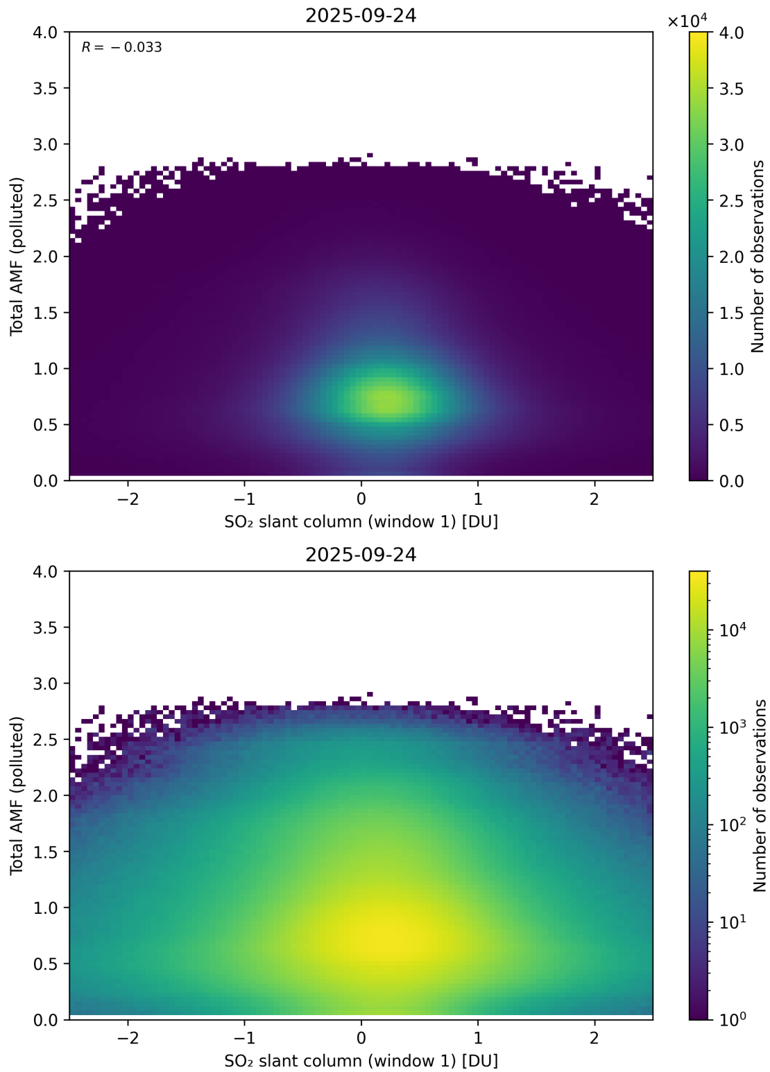
Figure 289: Scatter density plot of “SO 2 slant column (window 1)” against “Total AMF (polluted)” for 2025-09-23 to 2025-09-25.
