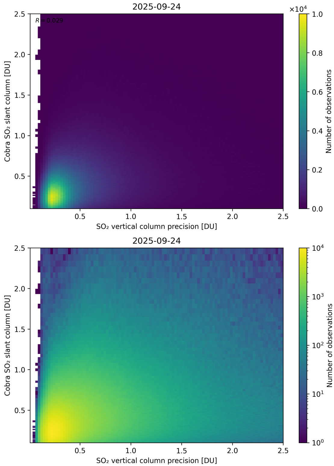
Figure 336: Scatter density plot of “SO 2 vertical column precision” against “Cobra SO 2 slant column” for 2025-09-23 to 2025-09-25.
