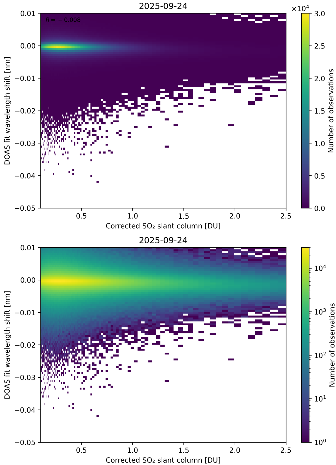
Figure 229: Scatter density plot of “Corrected SO 2 slant column” against “DOAS fit wavelength shift” for 2025-09-23 to 2025-09-25.
