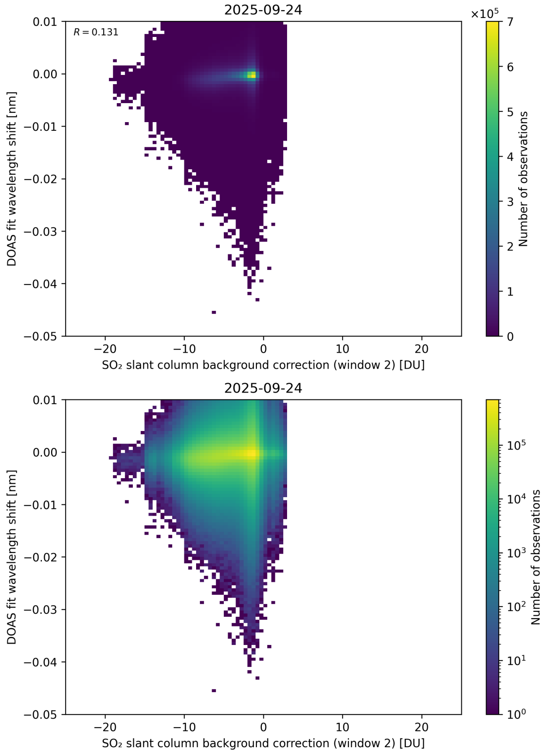
Figure 123: Scatter density plot of “SO 2 slant column background correction (window 2)” against “DOAS fit wavelength shift” for 2025-09-23 to 2025-09-25.
