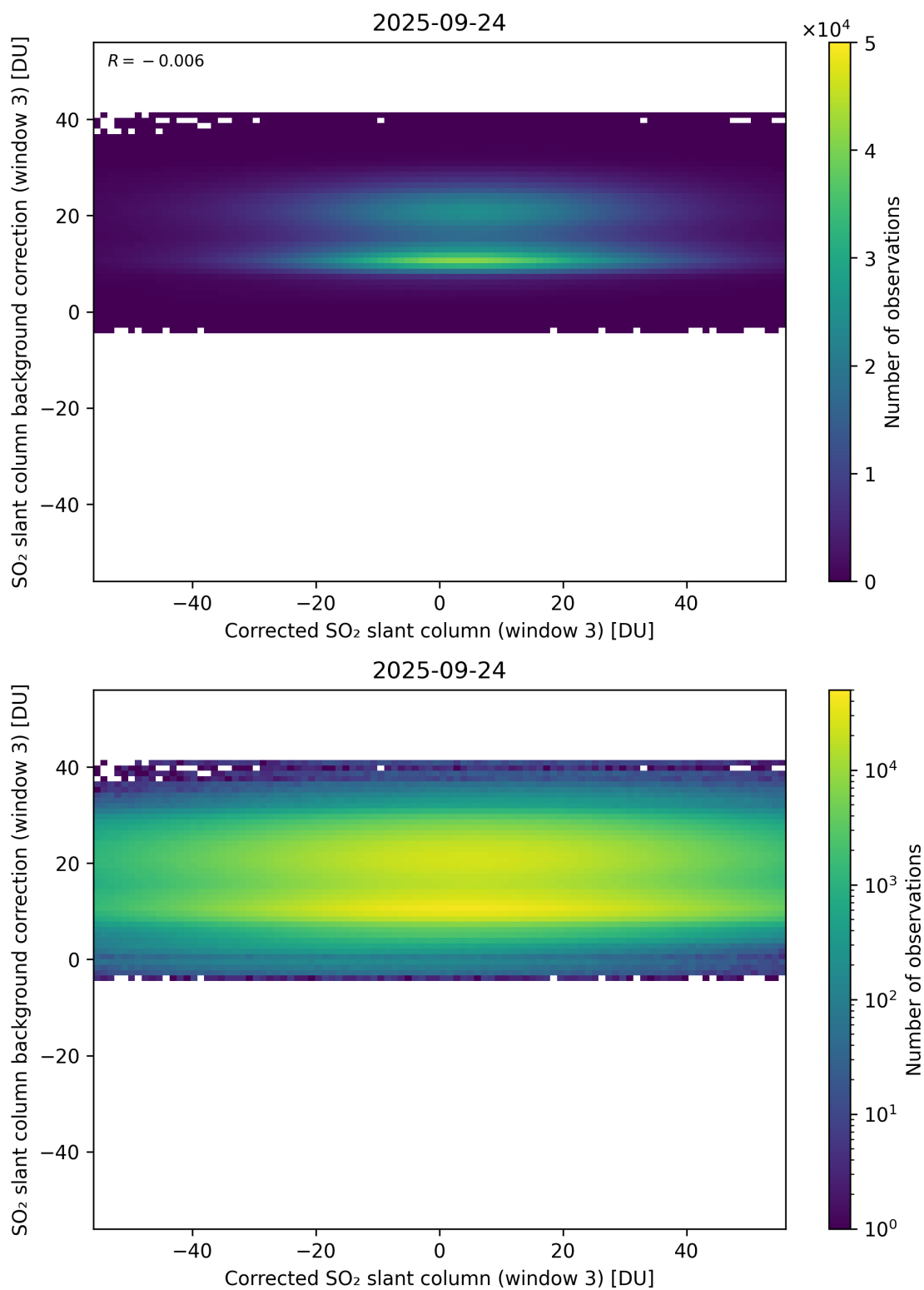
Figure 255: Scatter density plot of “Corrected SO 2 slant column (window 3)” against “SO 2 slant column background correction (window 3)” for 2025-09-23 to 2025-09-25.
