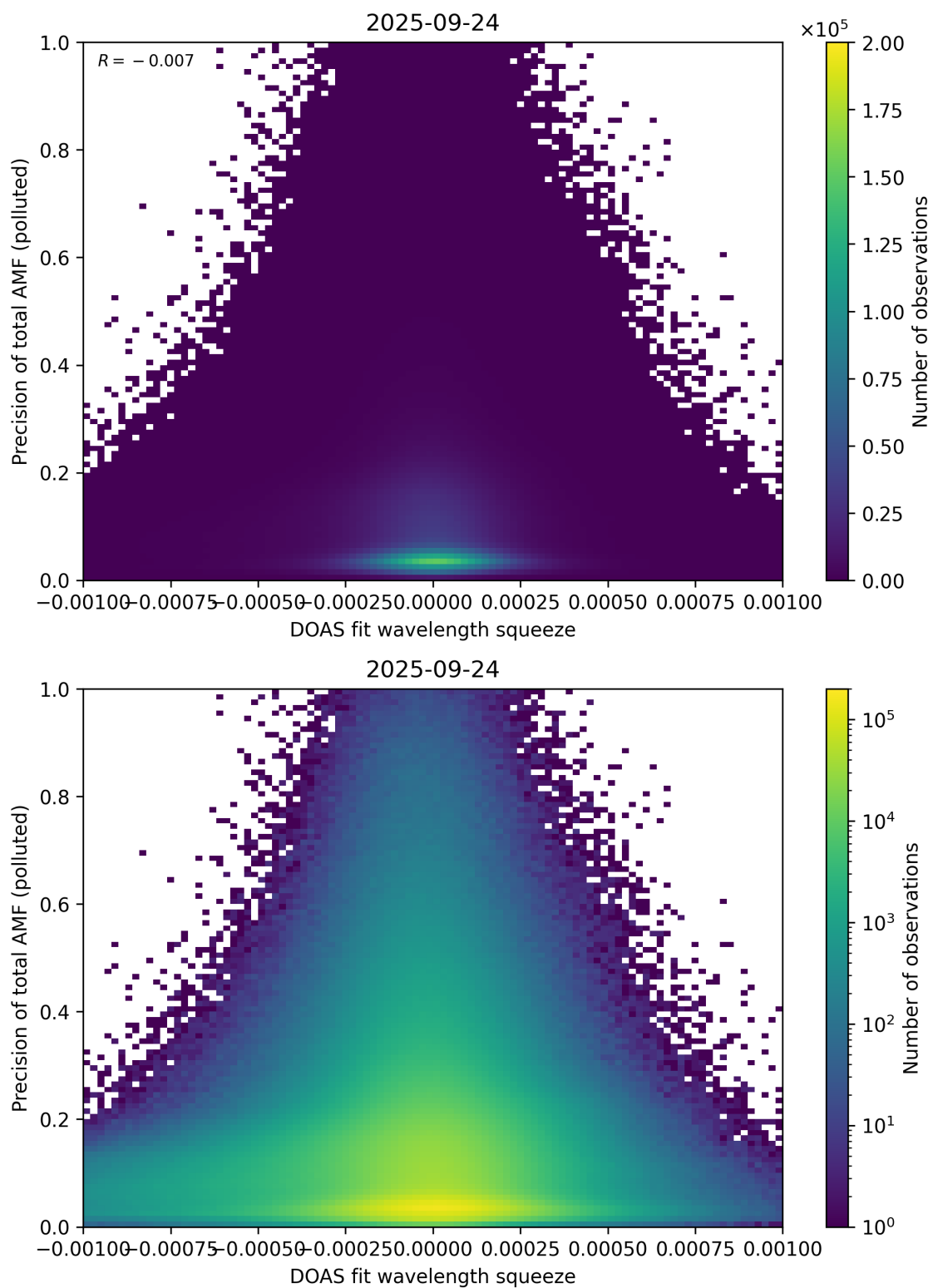
Figure 146: Scatter density plot of “DOAS fit wavelength squeeze” against “Precision of total AMF (polluted)” for 2025-09-23 to 2025-09-25.
