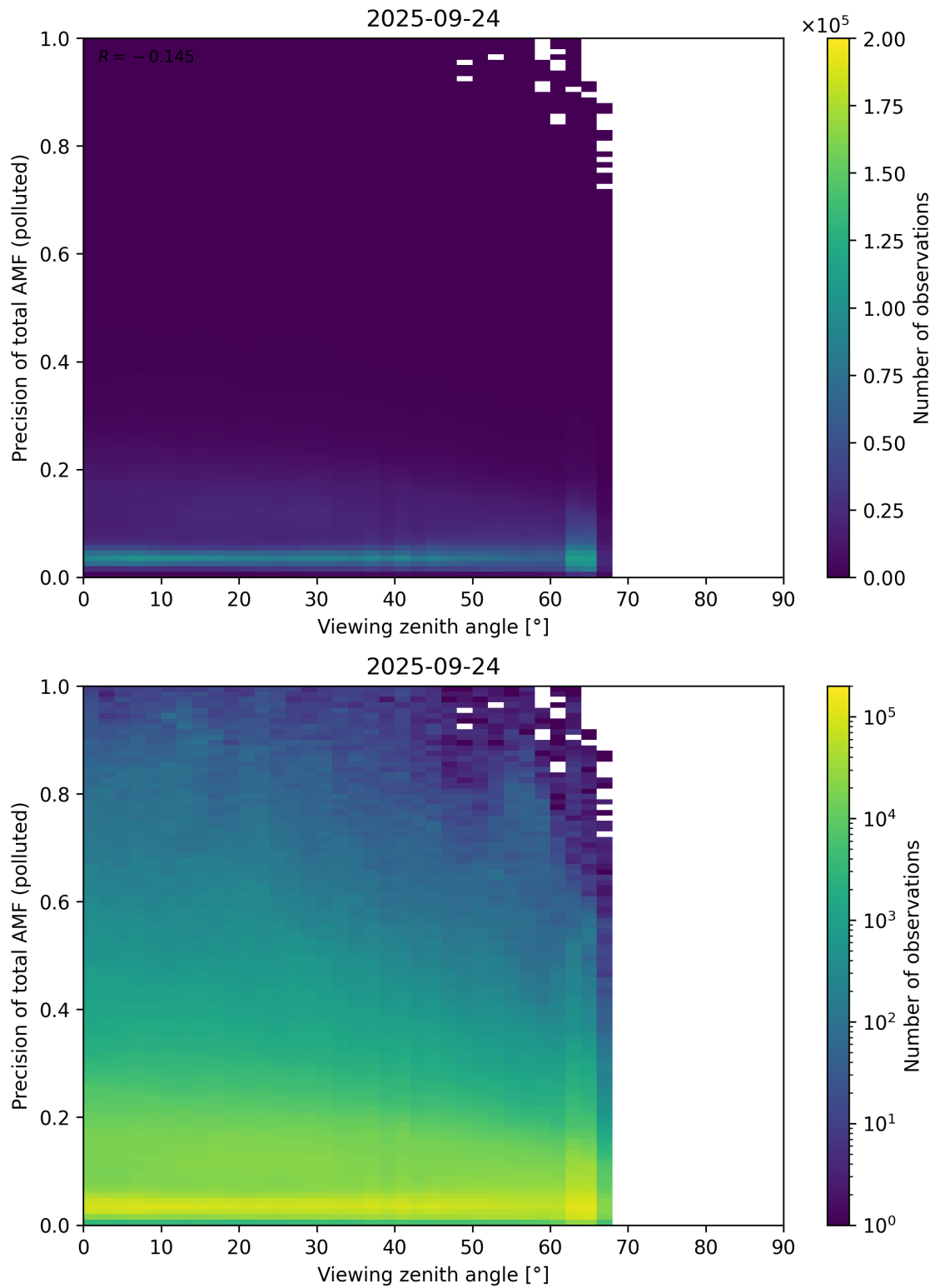
Figure 382: Scatter density plot of “Viewing zenith angle” against “Precision of total AMF (polluted)” for 2025-09-23 to 2025-09-25.
