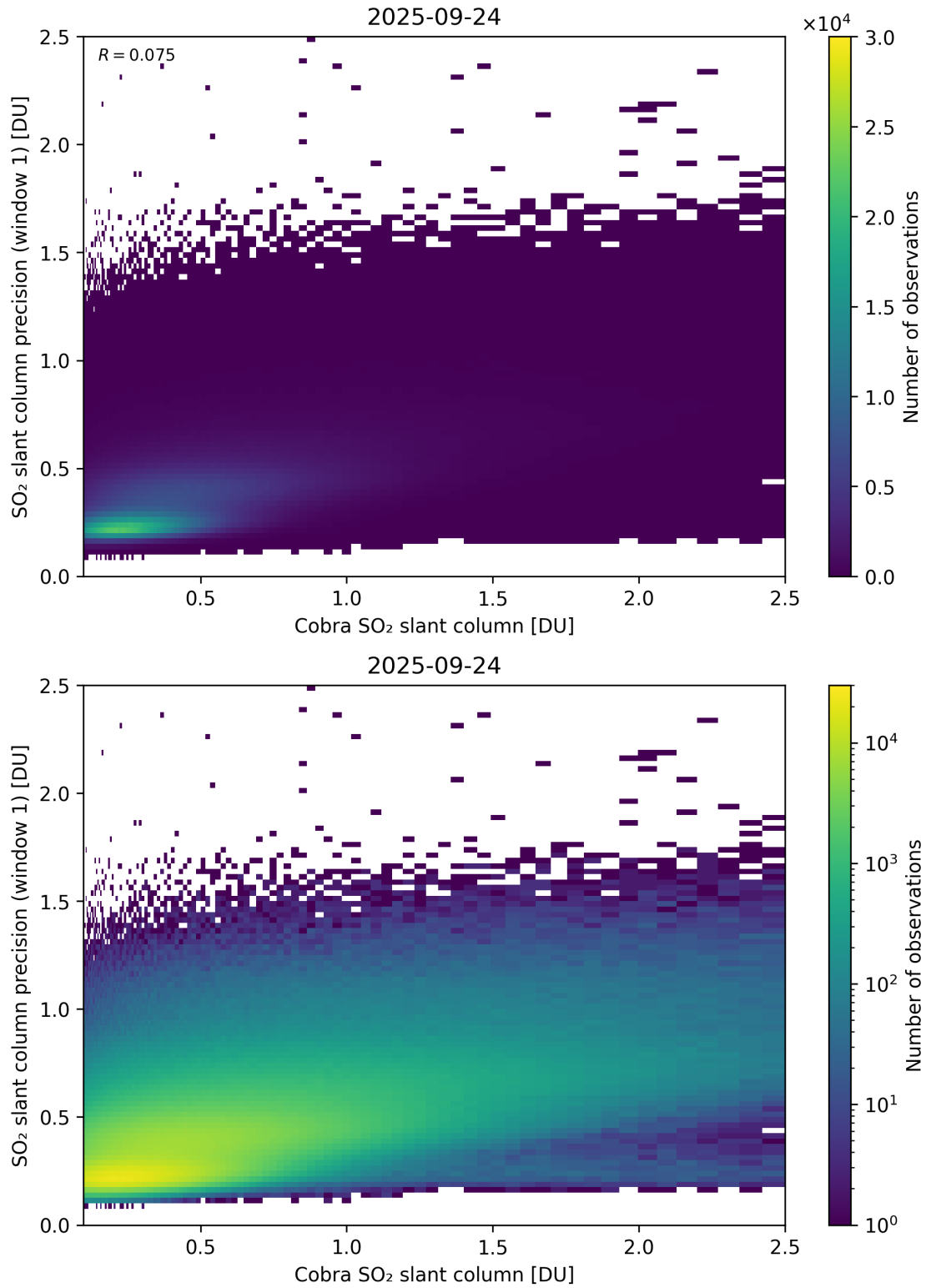
Figure 220: Scatter density plot of “Cobra SO 2 slant column” against “SO 2 slant column precision (window 1)” for 2025-09-23 to 2025-09-25.
