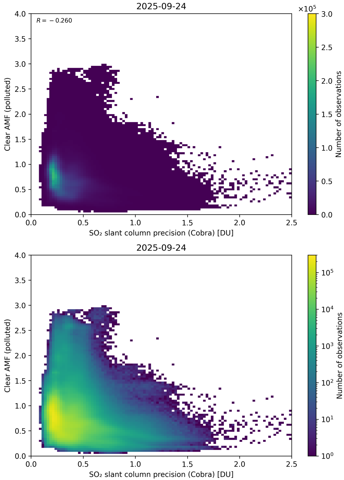
Figure 205: Scatter density plot of “SO 2 slant column precision (Cobra)” against “Clear AMF (polluted)” for 2025-09-23 to 2025-09-25.
