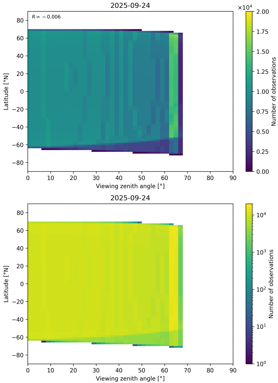
Figure 368: Scatter density plot of “Viewing zenith angle” against “Latitude” for 2025-09-23 to 2025-09-25.
