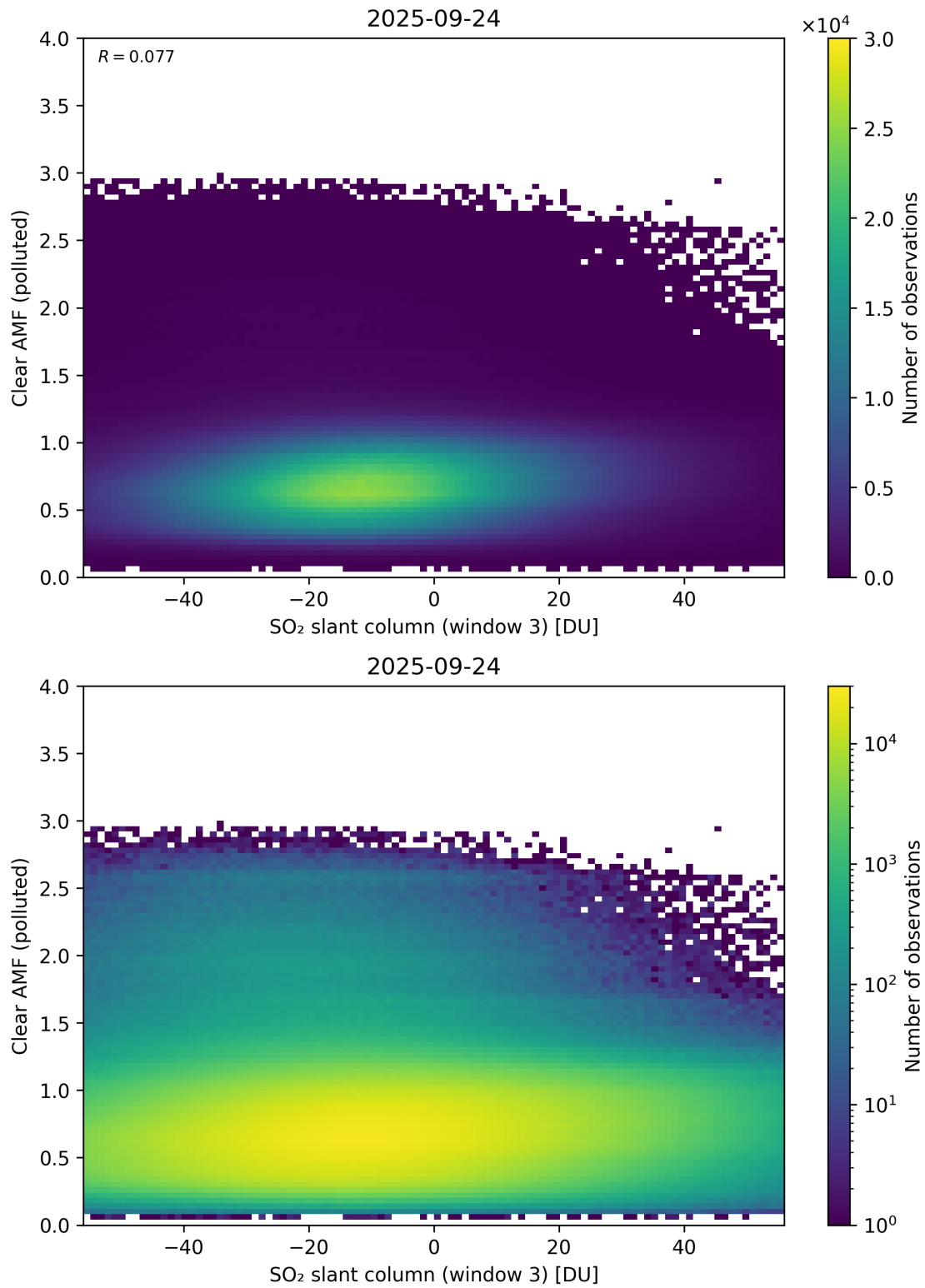
Figure 315: Scatter density plot of “SO 2 slant column (window 3)” against “Clear AMF (polluted)” for 2025-09-23 to 2025-09-25.
