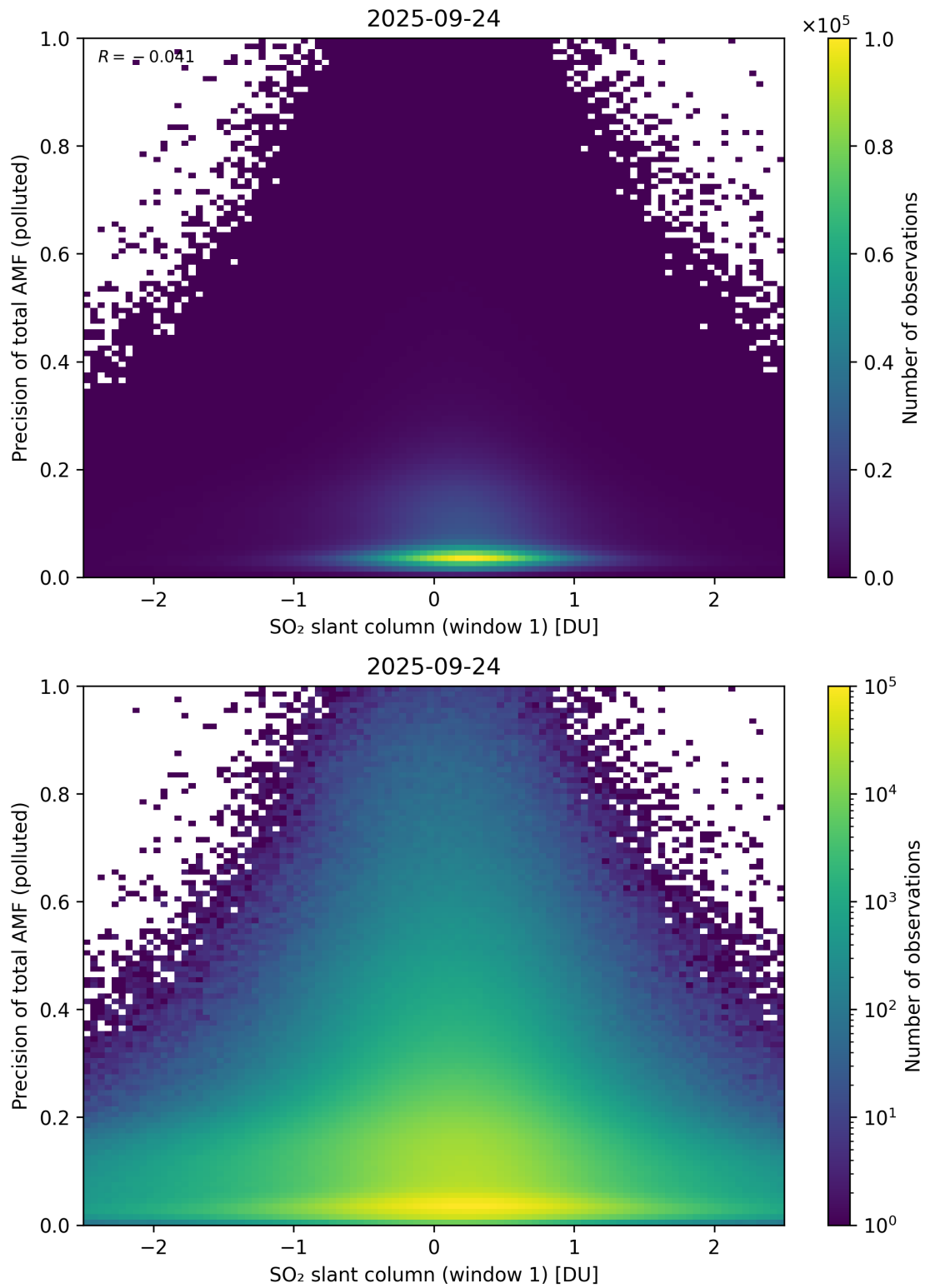
Figure 290: Scatter density plot of “SO 2 slant column (window 1)” against “Precision of total AMF (polluted)” for 2025-09-23 to 2025-09-25.
