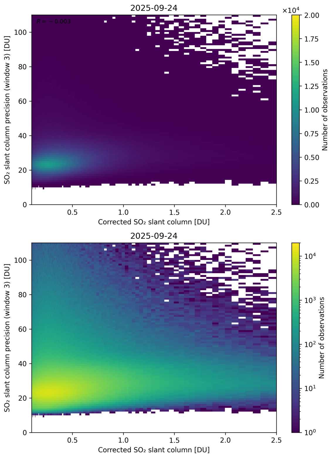
Figure 241: Scatter density plot of “Corrected SO 2 slant column” against “SO 2 slant column precision (window 3)” for 2025-09-23 to 2025-09-25.
