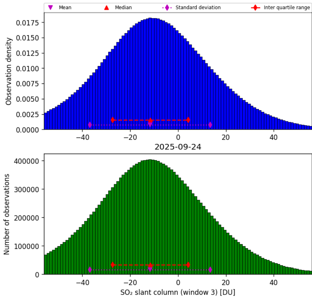
Figure 71: Histogram of “SO 2 slant column (window 3)” for 2025-09-23 to 2025-09-25
