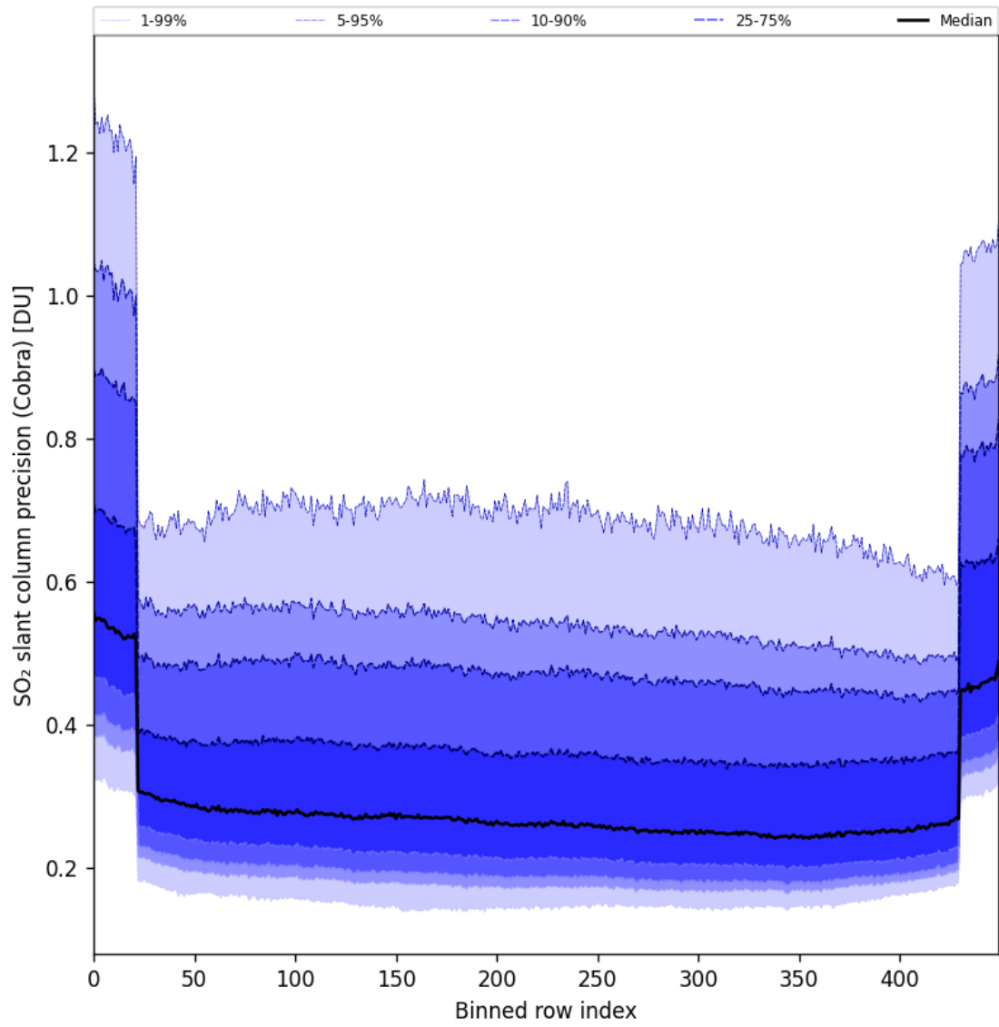
Figure 88: Along track statistics of “SO 2 slant column precision (Cobra)” for 2025-09-23 to 2025-09-25
