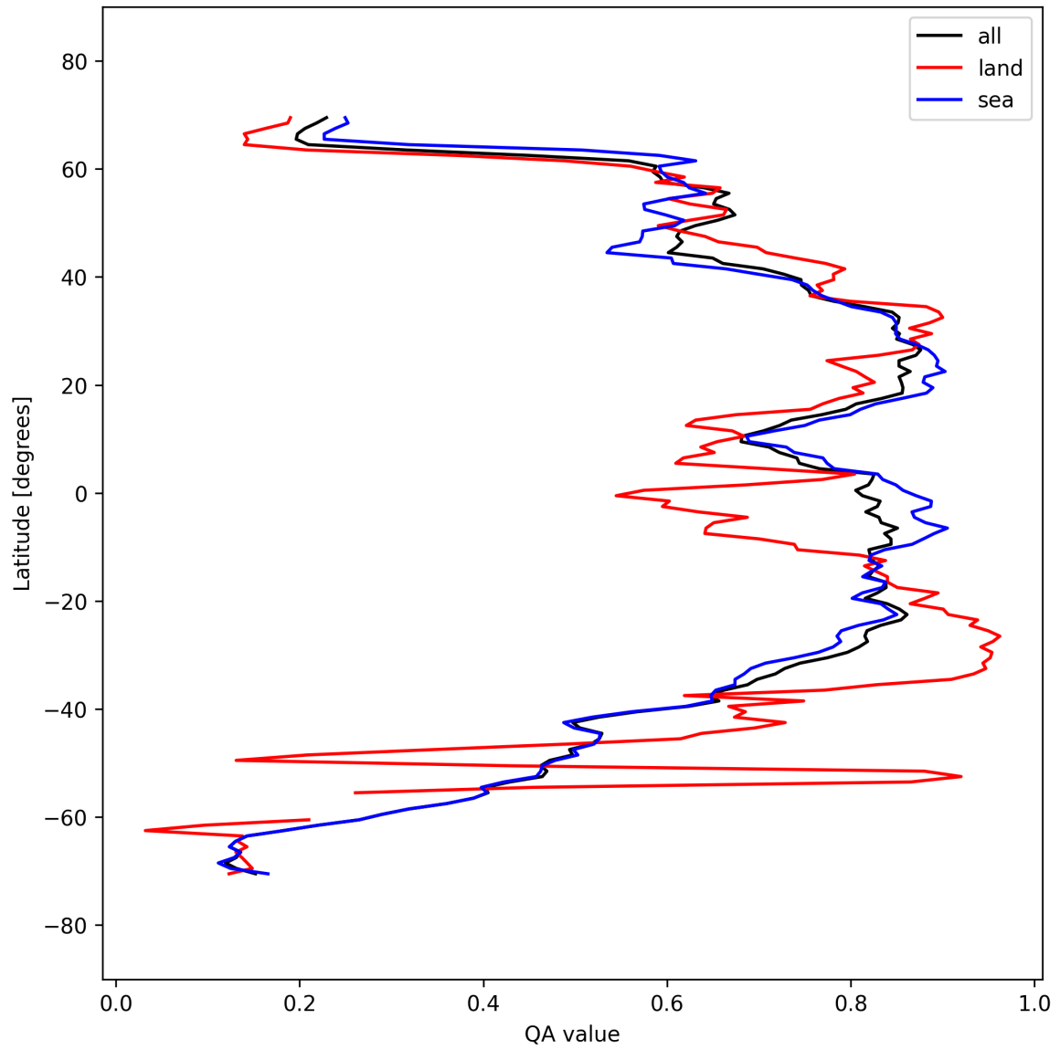
Figure 31: Zonal average of “QA value” for 2025-09-23 to 2025-09-25.
