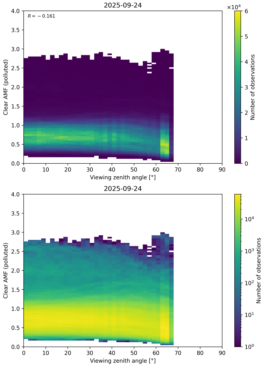
Figure 370: Scatter density plot of “Viewing zenith angle” against “Clear AMF (polluted)” for 2025-09-23 to 2025-09-25.
