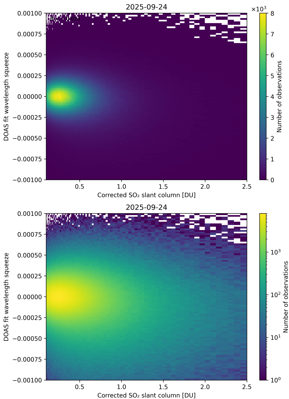
Figure 230: Scatter density plot of “Corrected SO 2 slant column” against “DOAS fit wavelength squeeze” for 2025-09-23 to 2025-09-25.
