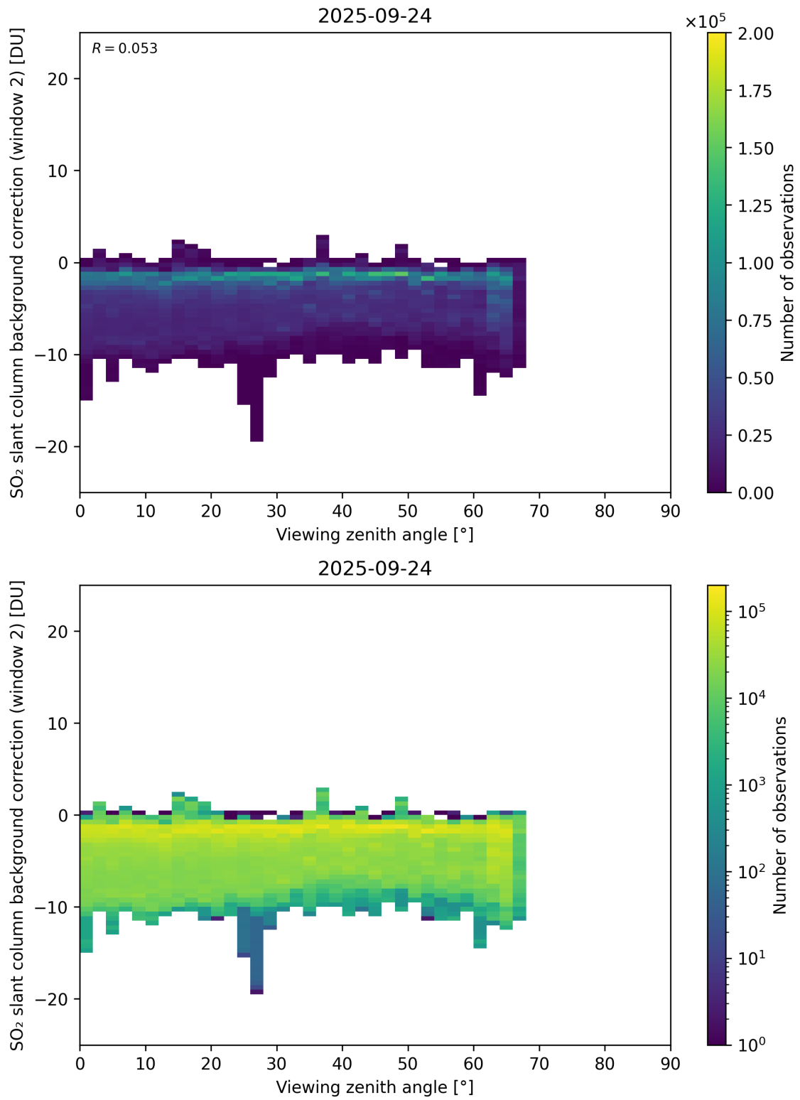
Figure 363: Scatter density plot of “Viewing zenith angle” against “SO 2 slant column background correction (window 2)” for 2025-09-23 to 2025-09-25.
