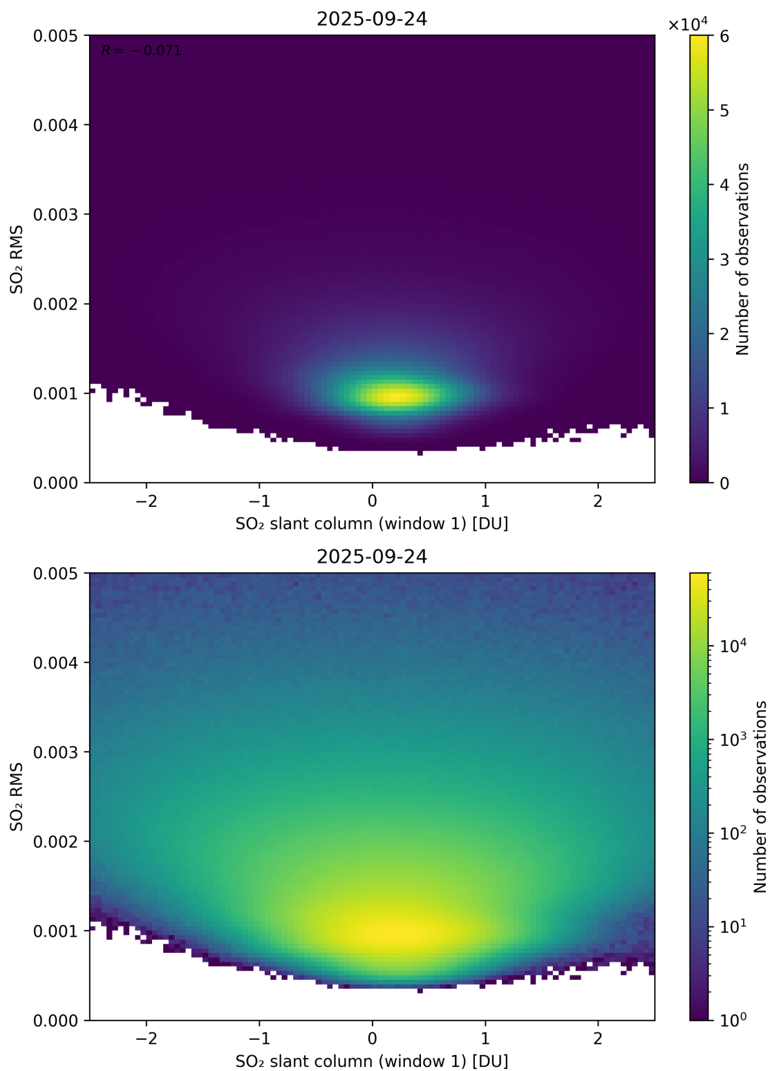
Figure 267: Scatter density plot of “SO 2 slant column (window 1)” against “SO 2 RMS” for 2025-09-23 to 2025-09-25.
