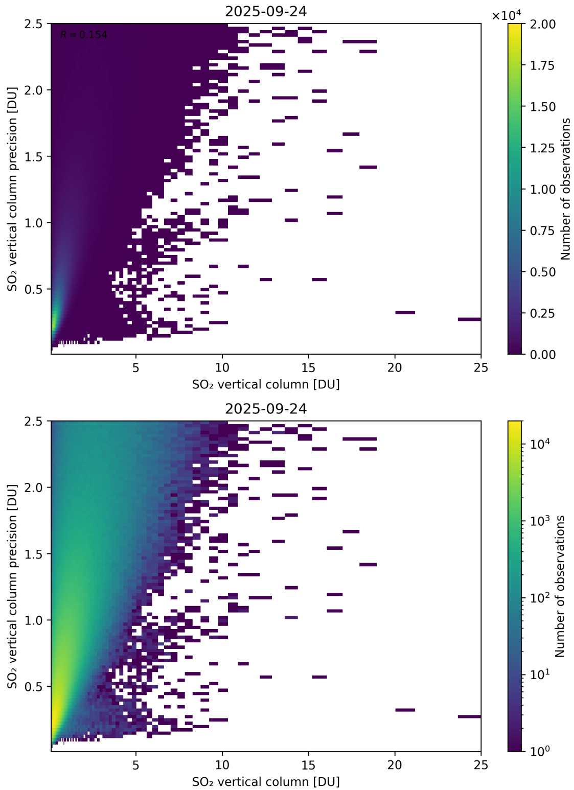
Figure 361: Scatter density plot of “SO 2 vertical column” against “SO 2 vertical column precision” for 2025-09-23 to 2025-09-25.
