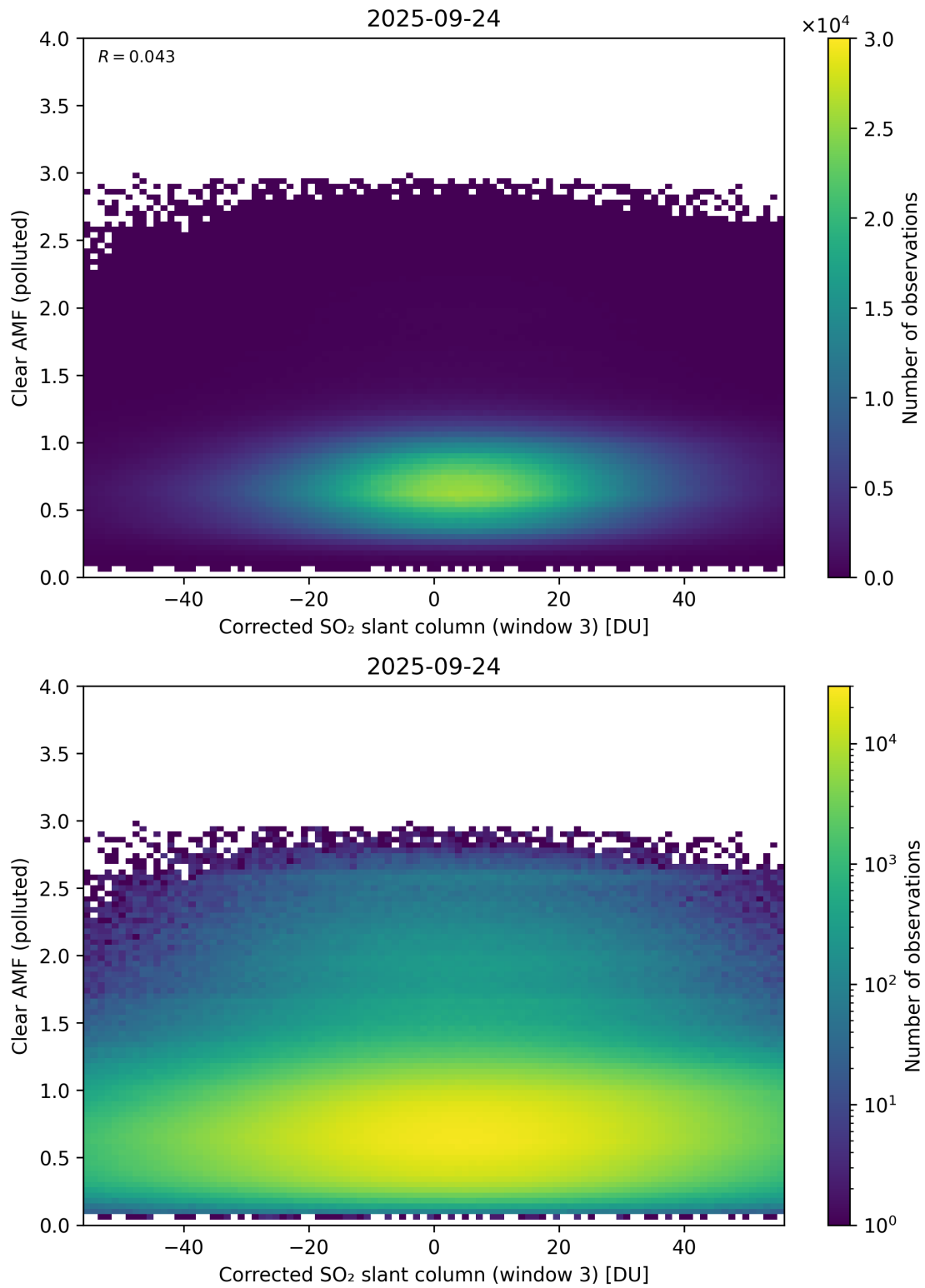
Figure 259: Scatter density plot of “Corrected SO 2 slant column (window 3)” against “Clear AMF (polluted)” for 2025-09-23 to 2025-09-25.
