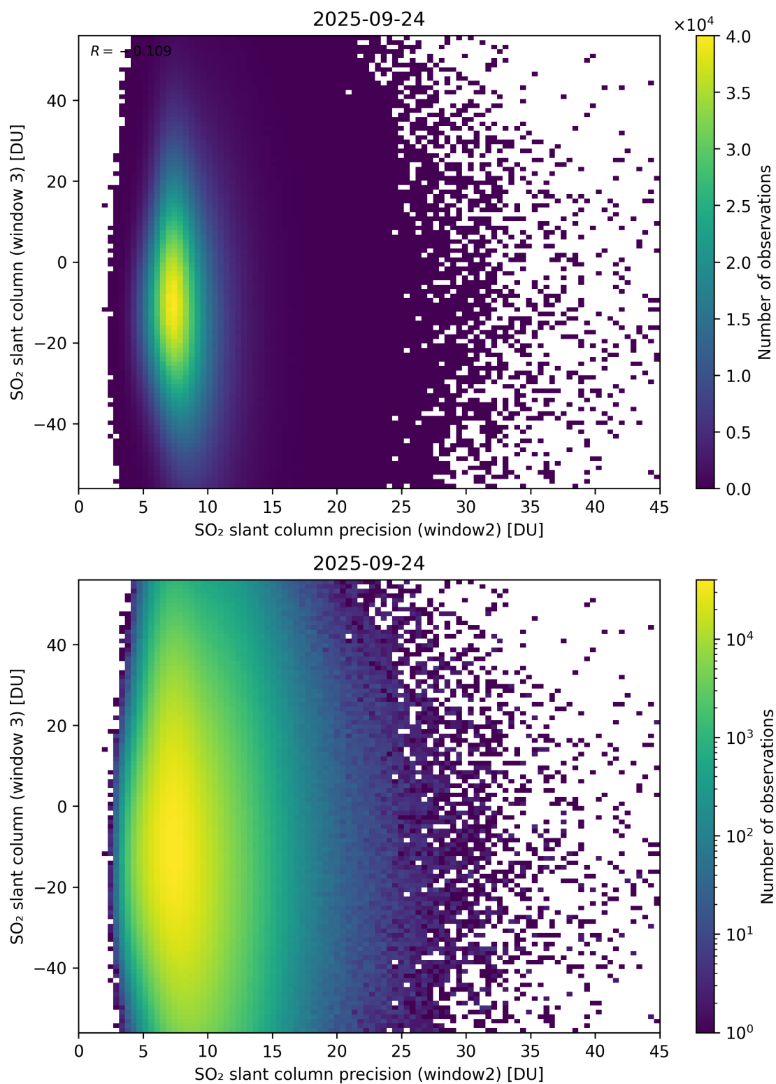
Figure 299: Scatter density plot of “SO 2 slant column precision (window2)” against “SO 2 slant column (window 3)” for 2025-09-23 to 2025-09-25.
