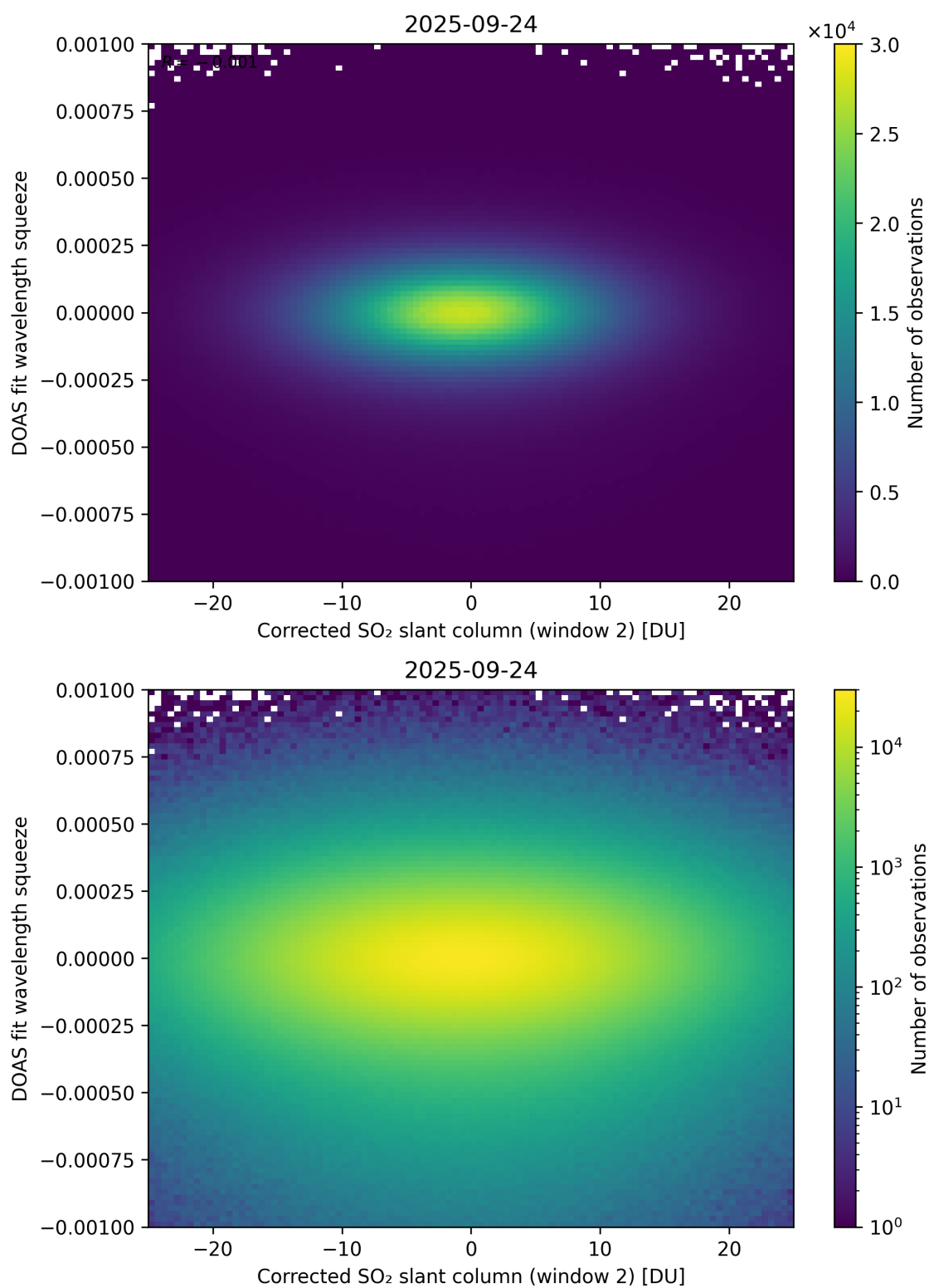
Figure 247: Scatter density plot of “Corrected SO 2 slant column (window 2)” against “DOAS fit wavelength squeeze” for 2025-09-23 to 2025-09-25.
