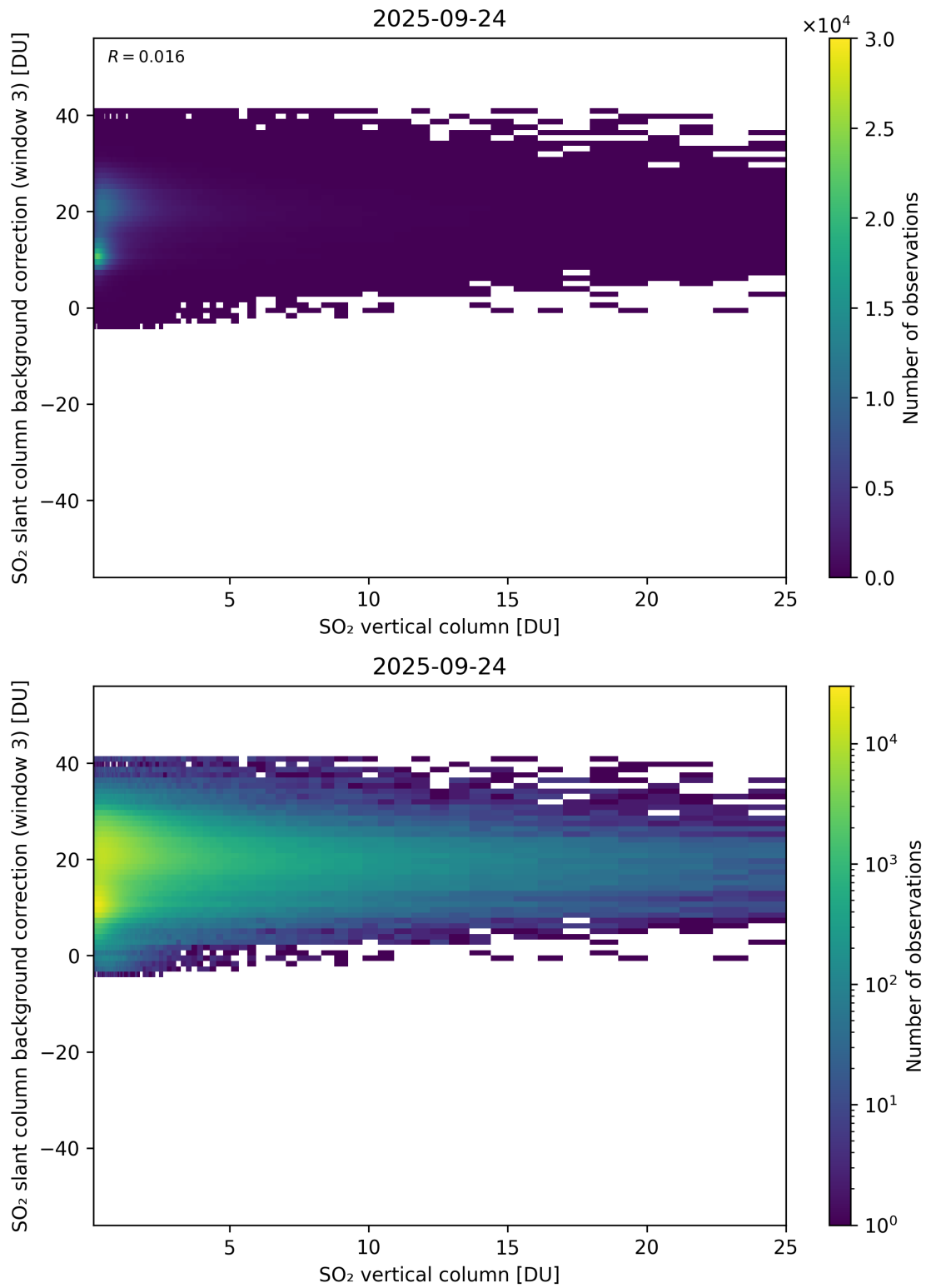
Figure 325: Scatter density plot of “SO 2 vertical column” against “SO 2 slant column background correction (window 3)” for 2025-09-23 to 2025-09-25.
