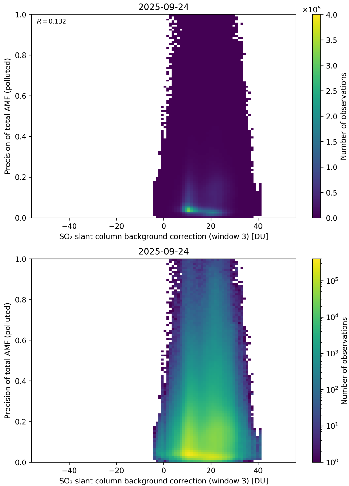
Figure 137: Scatter density plot of “SO 2 slant column background correction (window 3)” against “Precision of total AMF (polluted)” for 2025-09-23 to 2025-09-25.
