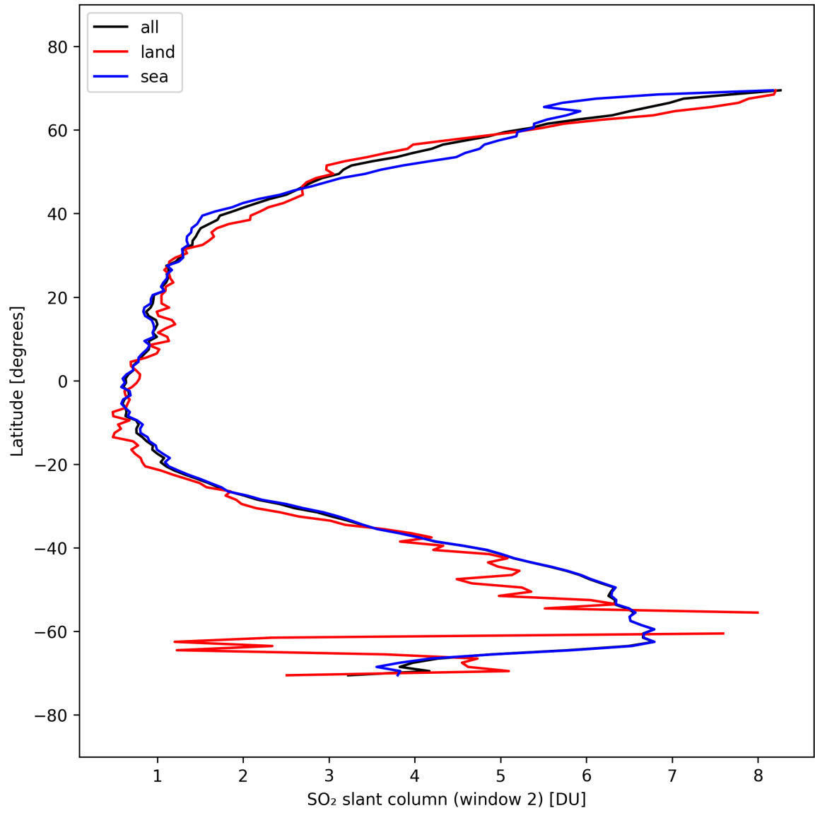
Figure 41: Zonal average of “SO 2 slant column (window 2)” for 2025-09-23 to 2025-09-25.
