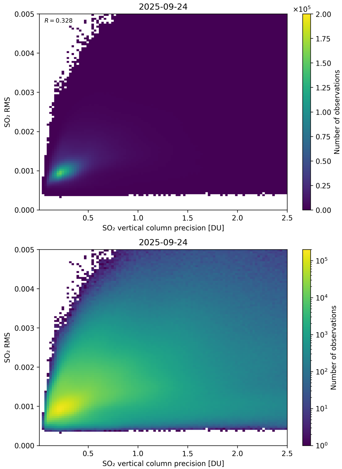
Figure 334: Scatter density plot of “SO 2 vertical column precision” against “SO 2 RMS” for 2025-09-23 to 2025-09-25.
