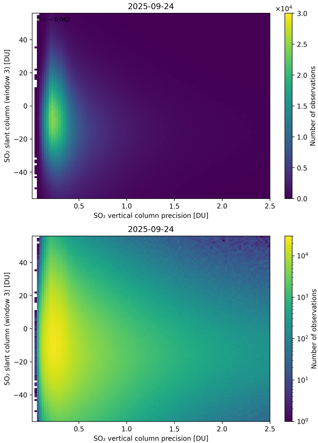
Figure 344: Scatter density plot of “SO 2 vertical column precision” against “SO 2 slant column (window 3)” for 2025-09-23 to 2025-09-25.
