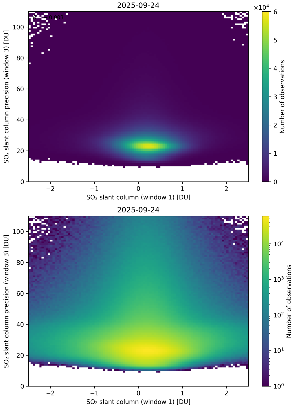
Figure 288: Scatter density plot of “SO 2 slant column (window 1)” against “SO 2 slant column precision (window 3)” for 2025-09-23 to 2025-09-25.
