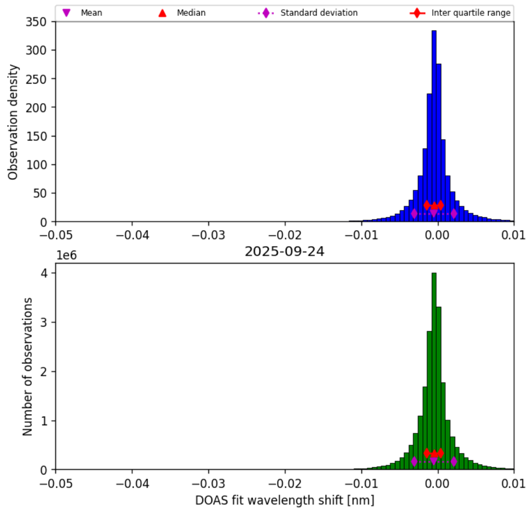
Figure 76: Histogram of “DOAS fit wavelength shift” for 2025-09-23 to 2025-09-25
