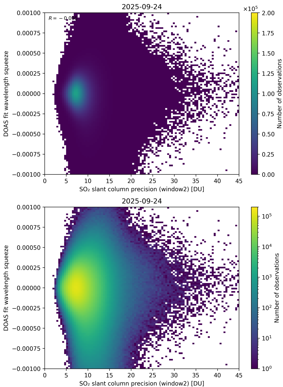
Figure 294: Scatter density plot of “SO 2 slant column precision (window2)” against “DOAS fit wavelength squeeze” for 2025-09-23 to 2025-09-25.
