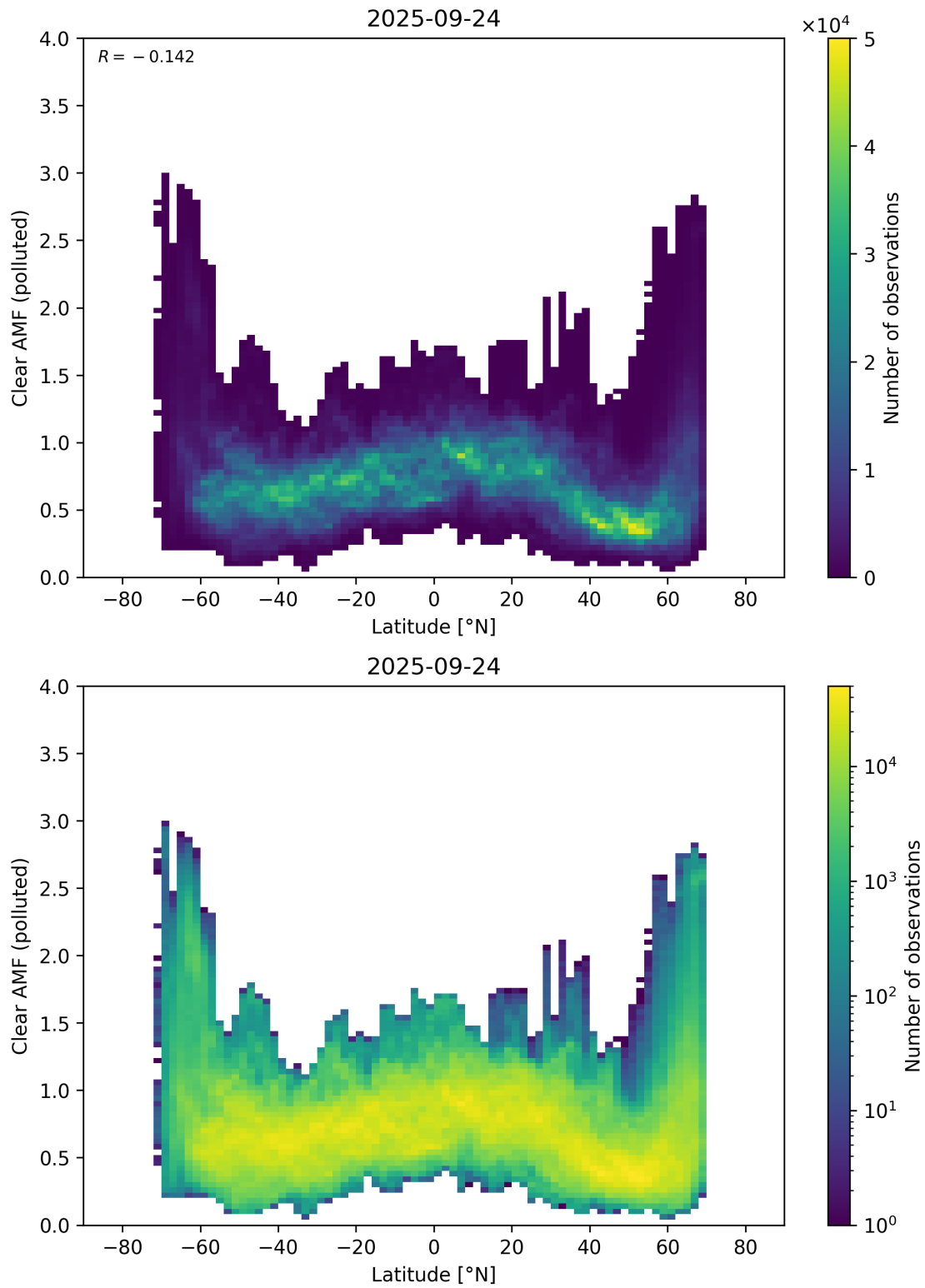
Figure 156: Scatter density plot of “Latitude” against “Clear AMF (polluted)” for 2025-09-23 to 2025-09-25.
