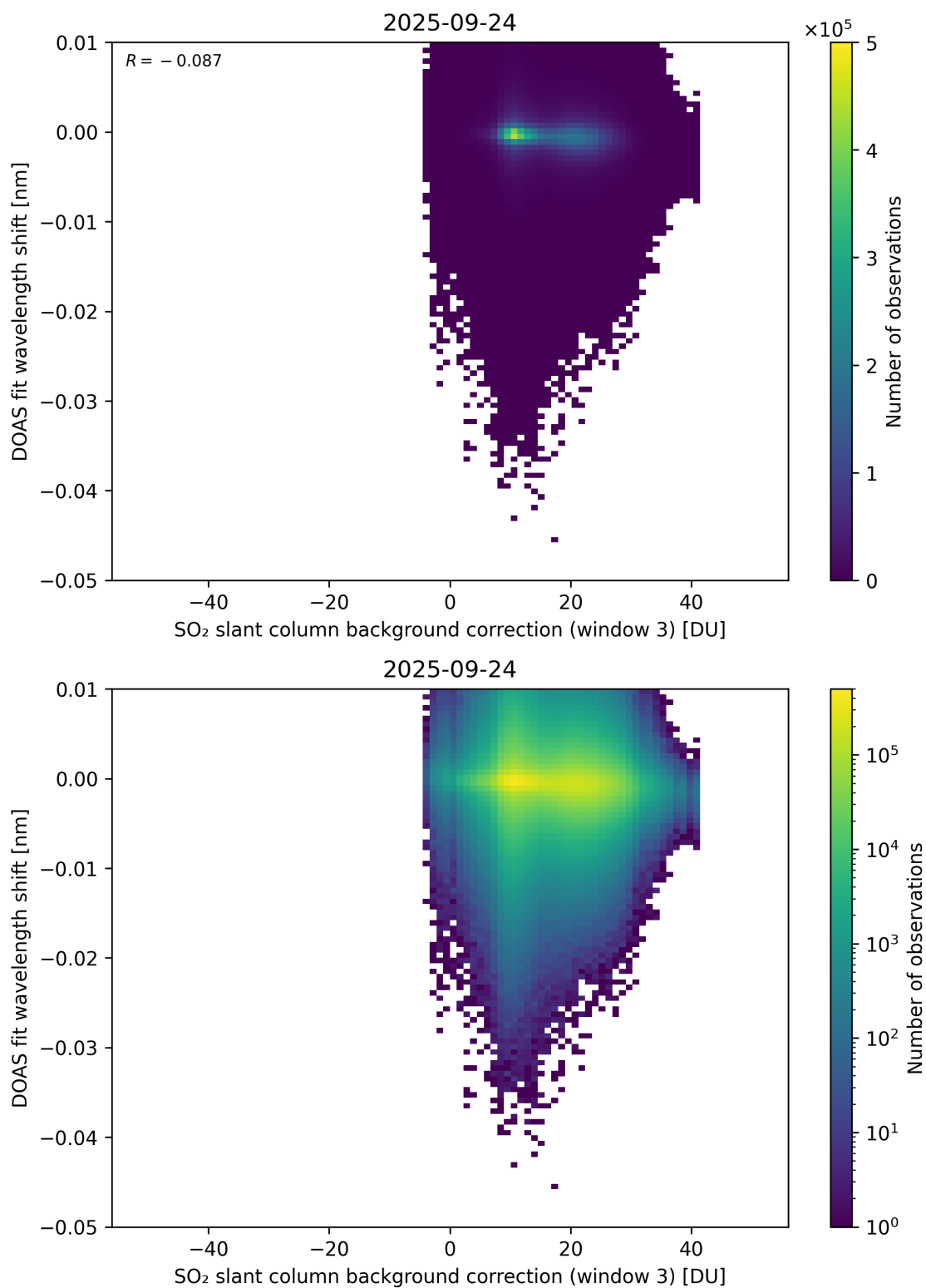
Figure 132: Scatter density plot of “SO 2 slant column background correction (window 3)” against “DOAS fit wavelength shift” for 2025-09-23 to 2025-09-25.
