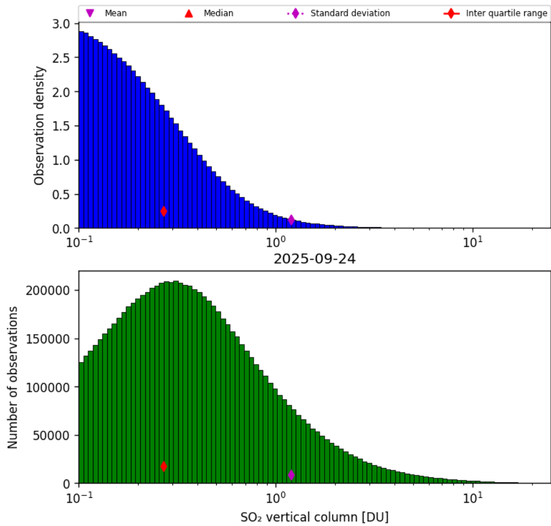
Figure 58: Histogram of “SO 2 vertical column” for 2025-09-23 to 2025-09-25
