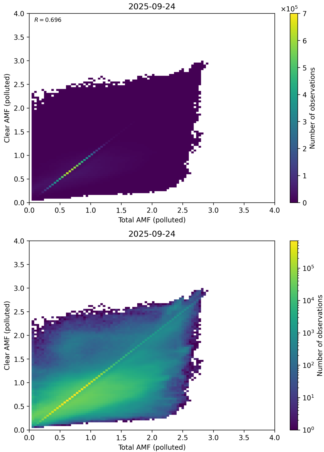
Figure 321: Scatter density plot of “Total AMF (polluted)” against “Clear AMF (polluted)” for 2025-09-23 to 2025-09-25.
