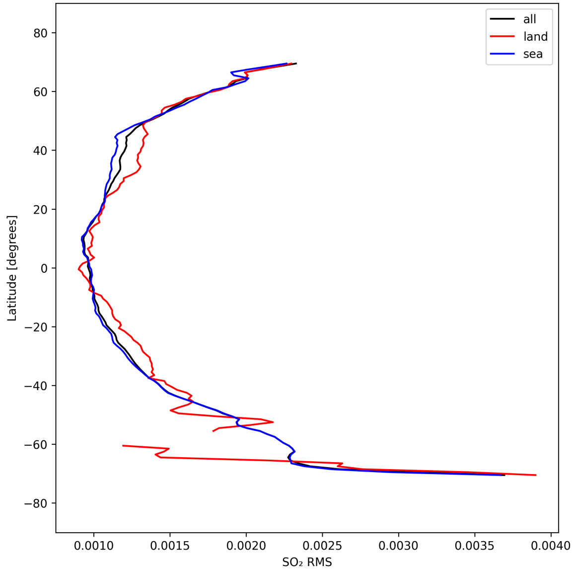
Figure 52: Zonal average of “SO 2 RMS” for 2025-09-23 to 2025-09-25.
