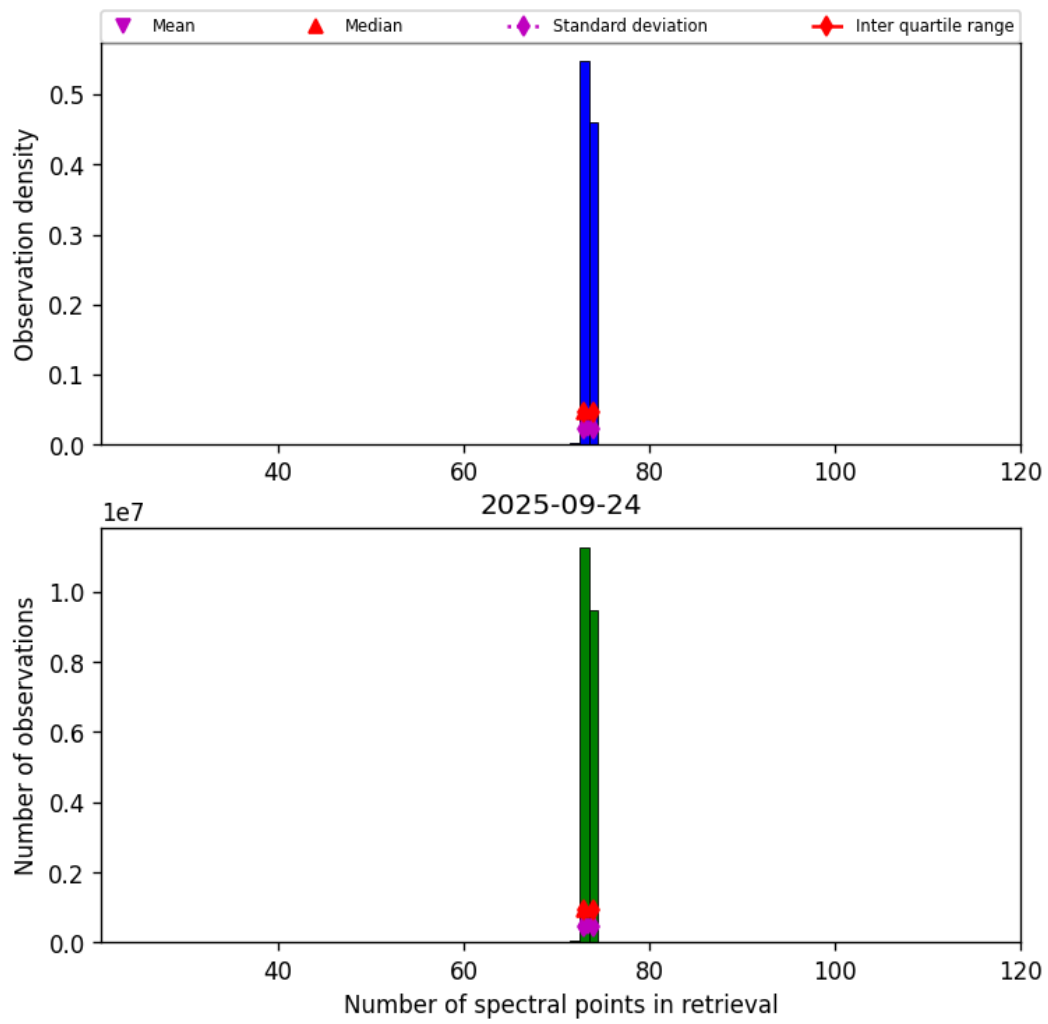
Figure 82: Histogram of “Number of spectral points in retrieval” for 2025-09-23 to 2025-09-25
