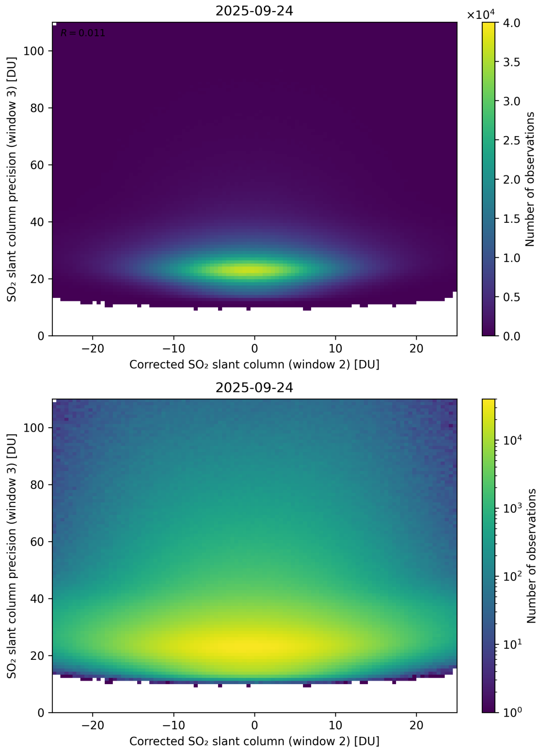
Figure 252: Scatter density plot of “Corrected SO 2 slant column (window 2)” against “SO 2 slant column precision (window 3)” for 2025-09-23 to 2025-09-25.
