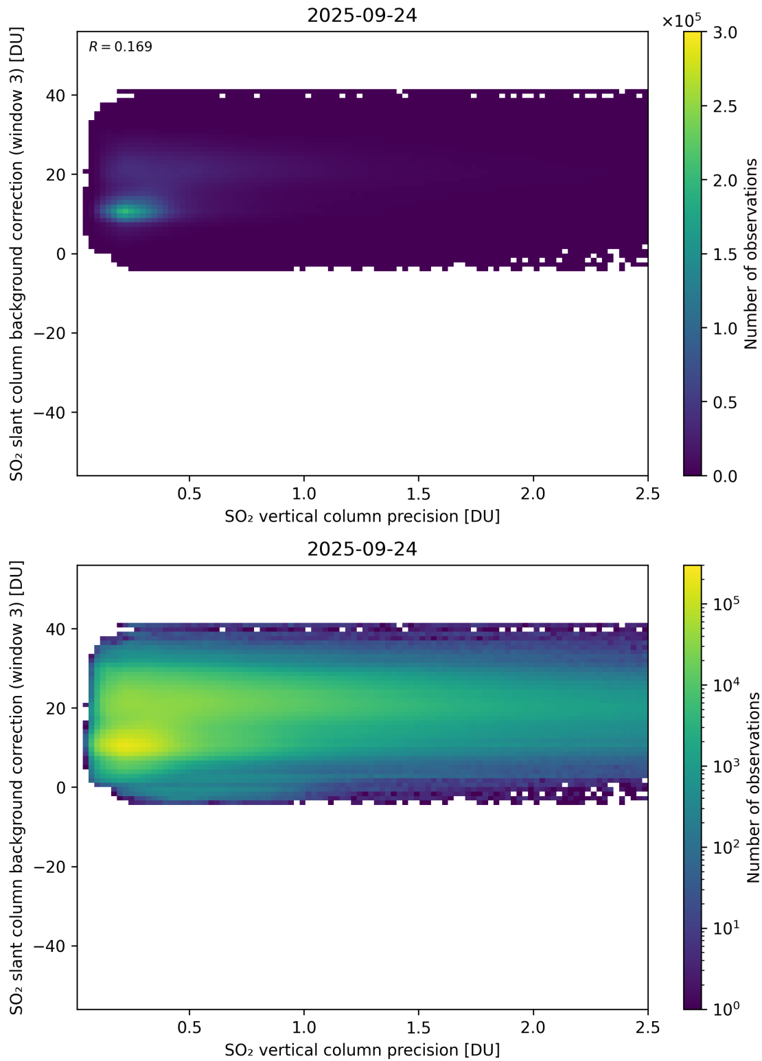
Figure 331: Scatter density plot of “SO 2 vertical column precision” against “SO 2 slant column background correction (window 3)” for 2025-09-23 to 2025-09-25.
