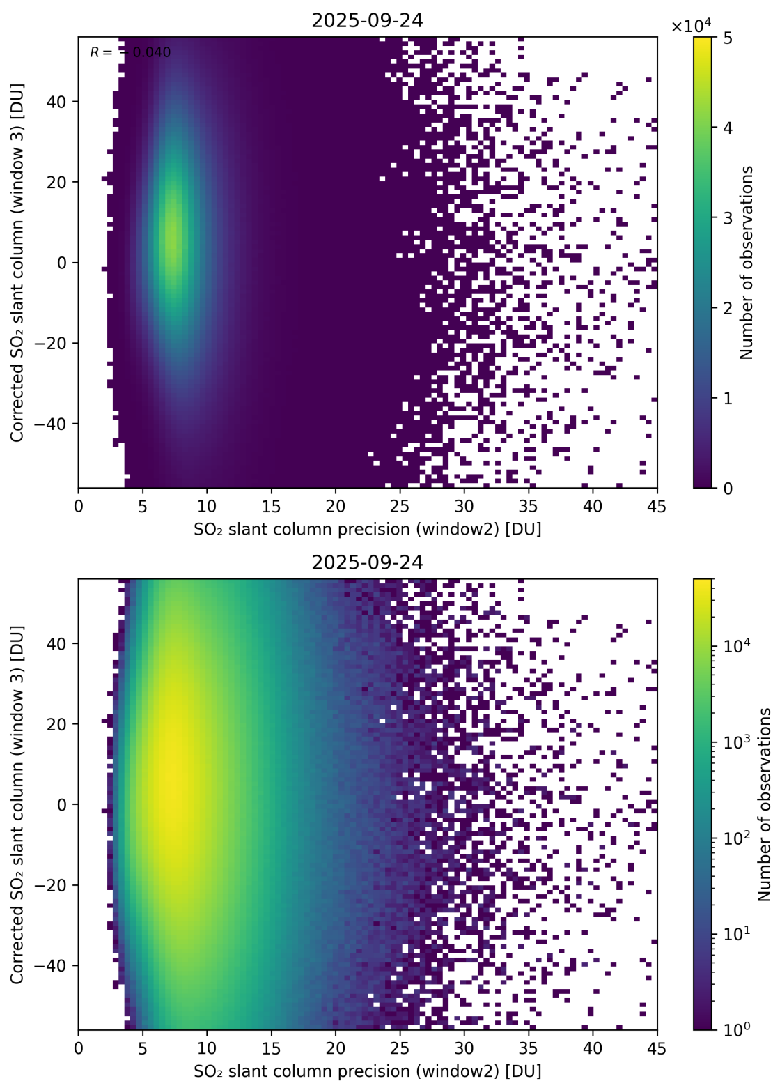
Figure 298: Scatter density plot of “SO 2 slant column precision (window2)” against “Corrected SO 2 slant column (window 3)” for 2025-09-23 to 2025-09-25.
