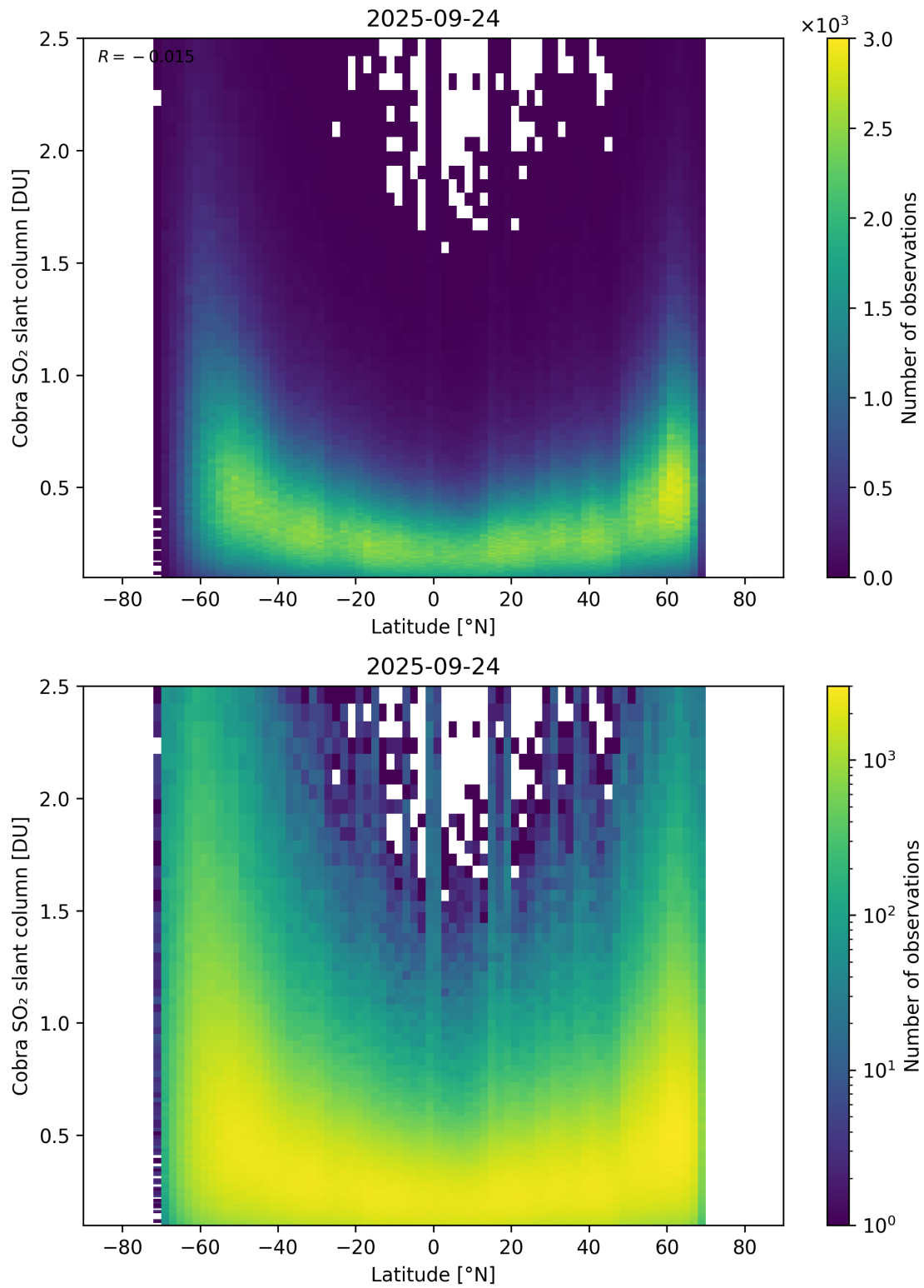
Figure 157: Scatter density plot of “Latitude” against “Cobra SO 2 slant column” for 2025-09-23 to 2025-09-25.
