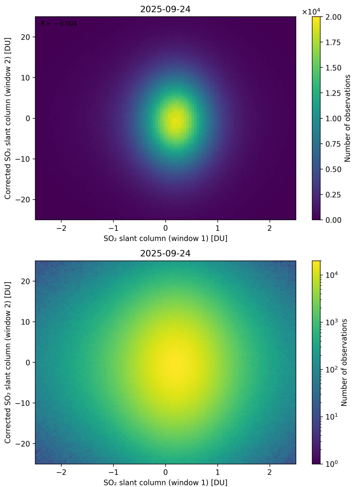
Figure 283: Scatter density plot of “SO 2 slant column (window 1)” against “Corrected SO 2 slant column (window 2)” for 2025-09-23 to 2025-09-25.
