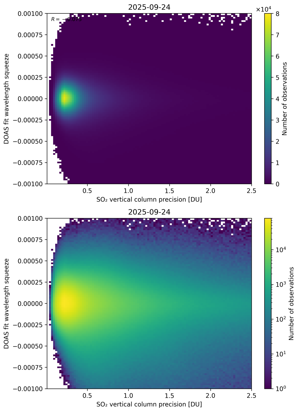
Figure 333: Scatter density plot of “SO 2 vertical column precision” against “DOAS fit wavelength squeeze” for 2025-09-23 to 2025-09-25.
