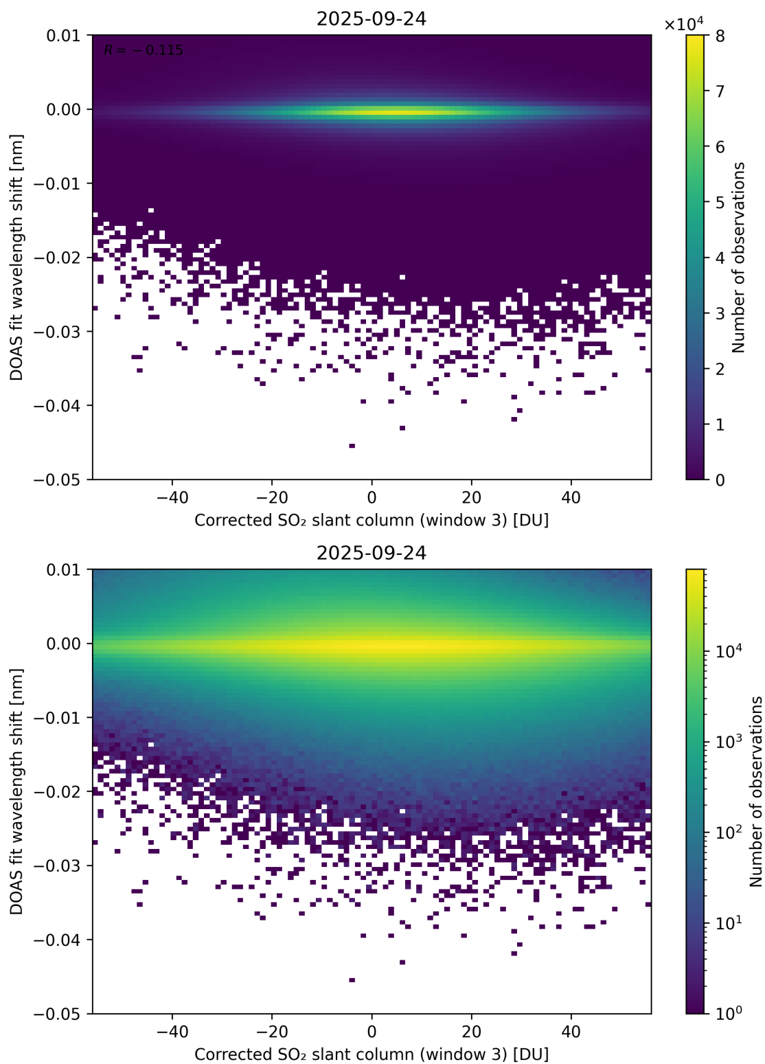
Figure 256: Scatter density plot of “Corrected SO 2 slant column (window 3)” against “DOAS fit wavelength shift” for 2025-09-23 to 2025-09-25.
