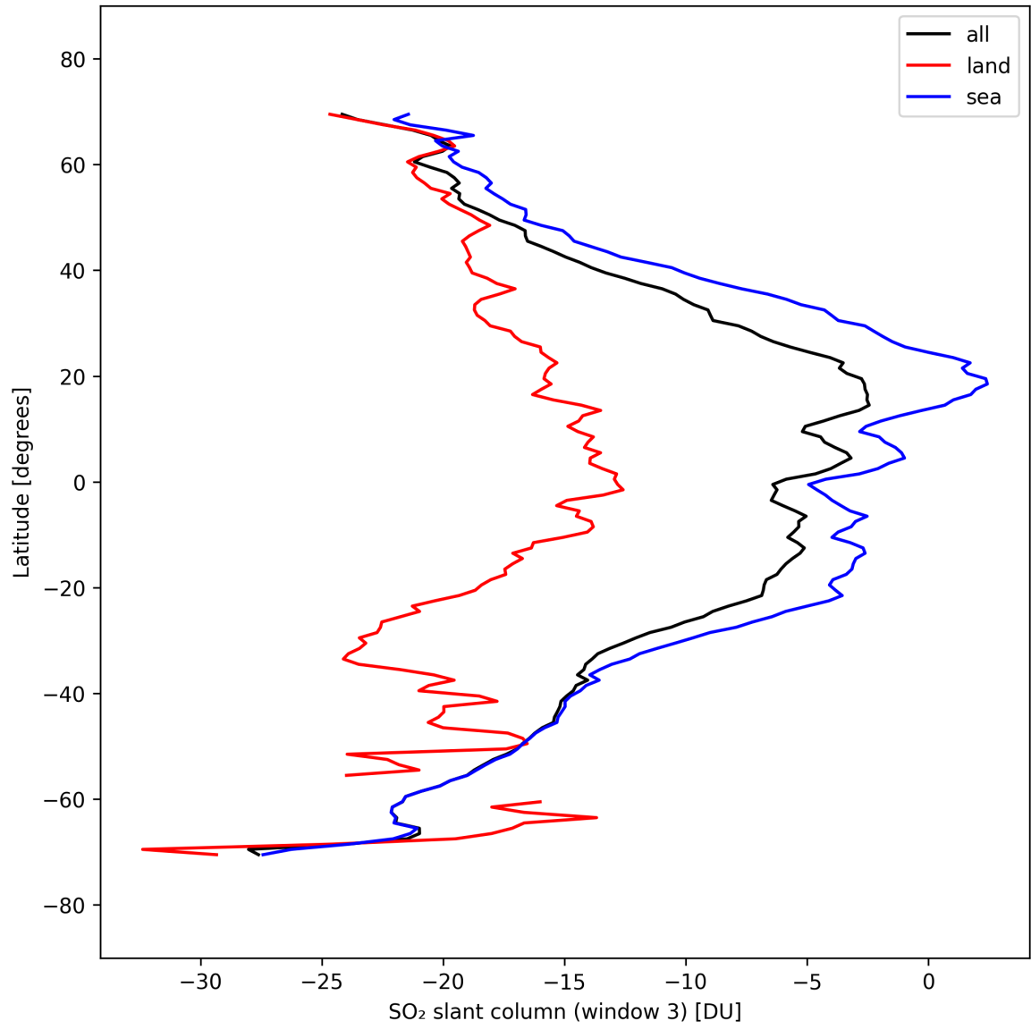
Figure 45: Zonal average of “SO 2 slant column (window 3)” for 2025-09-23 to 2025-09-25.
