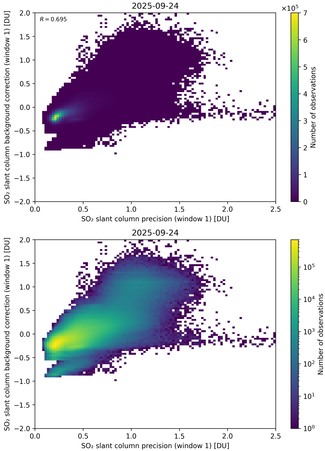
Figure 268: Scatter density plot of “SO 2 slant column precision (window 1)” against “SO 2 slant column background correction (window 1)” for 2025-09-23 to 2025-09-25.
