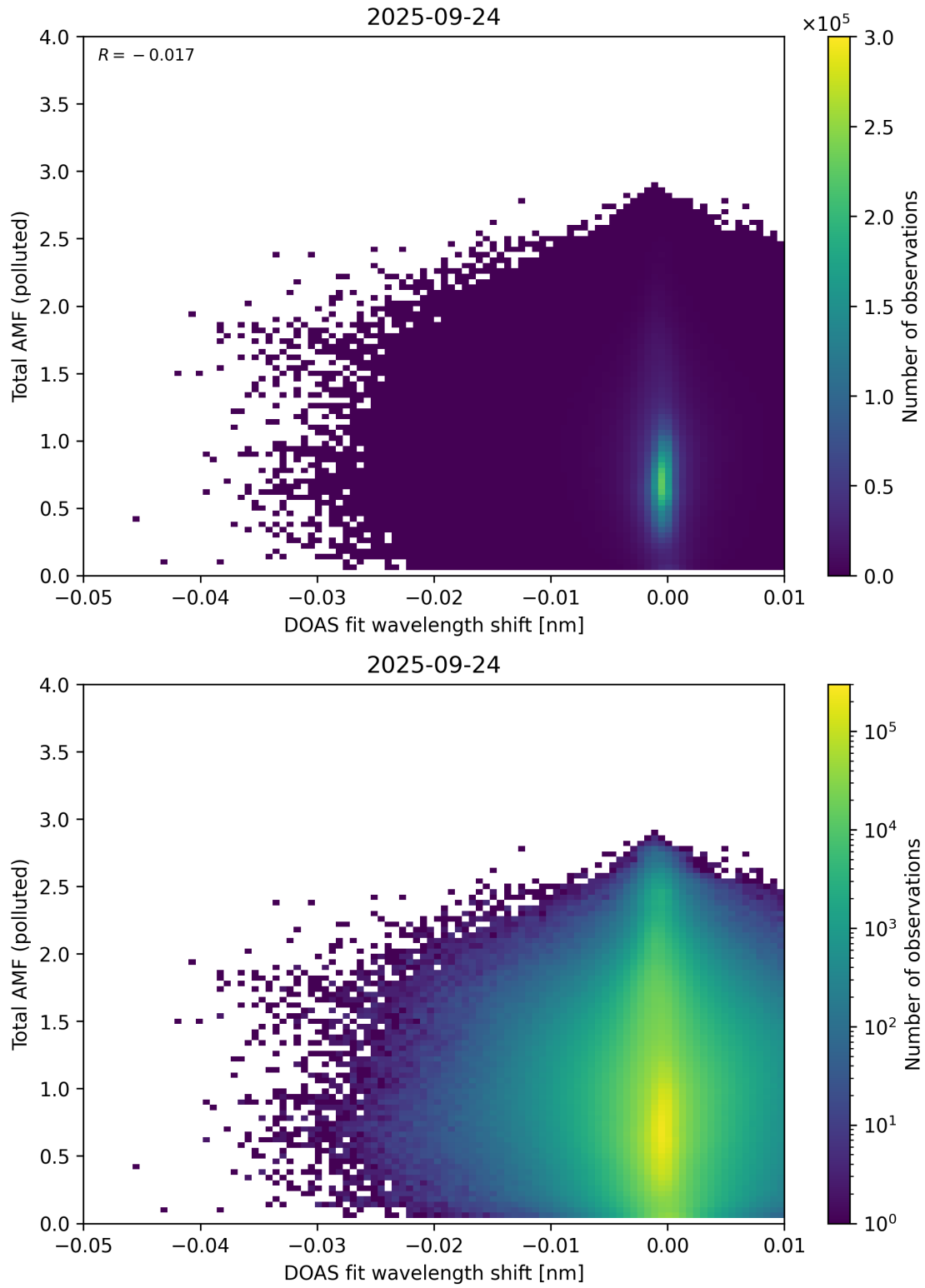
Figure 141: Scatter density plot of “DOAS fit wavelength shift” against “Total AMF (polluted)” for 2025-09-23 to 2025-09-25.
