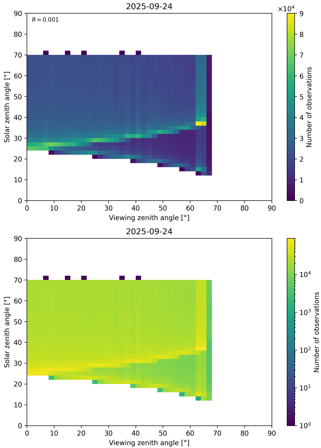
Figure 369: Scatter density plot of “Viewing zenith angle” against “Solar zenith angle” for 2025-09-23 to 2025-09-25.
