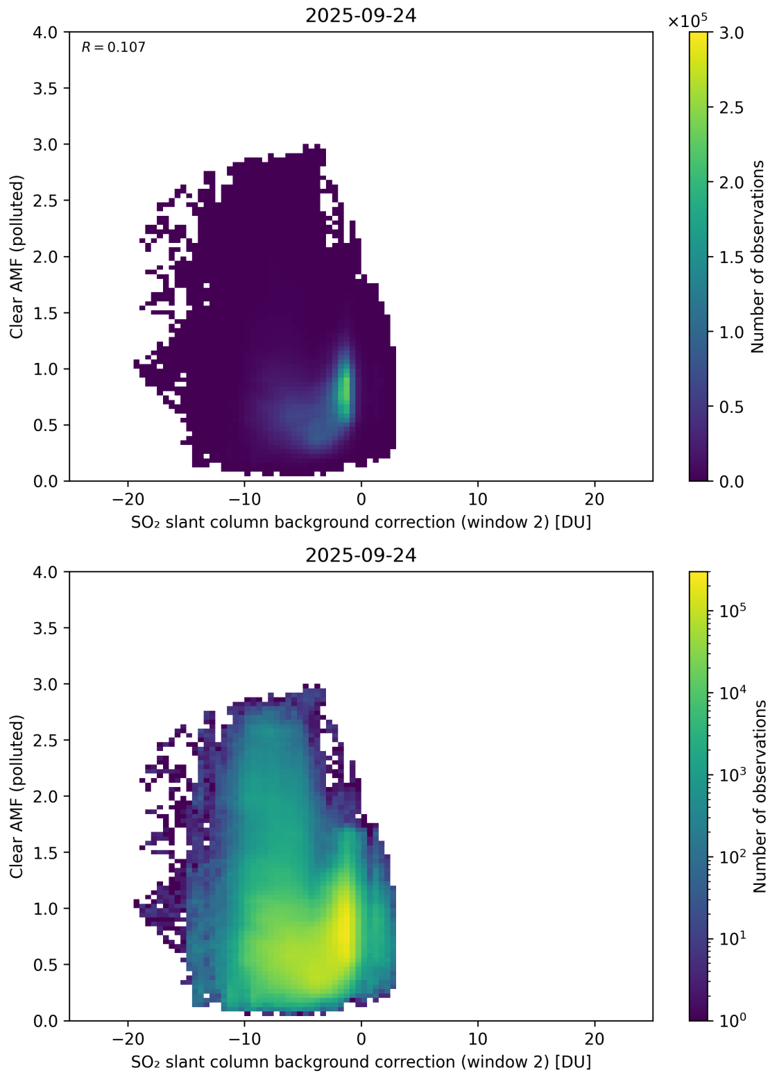
Figure 126: Scatter density plot of “SO 2 slant column background correction (window 2)” against “Clear AMF (polluted)” for 2025-09-23 to 2025-09-25.
