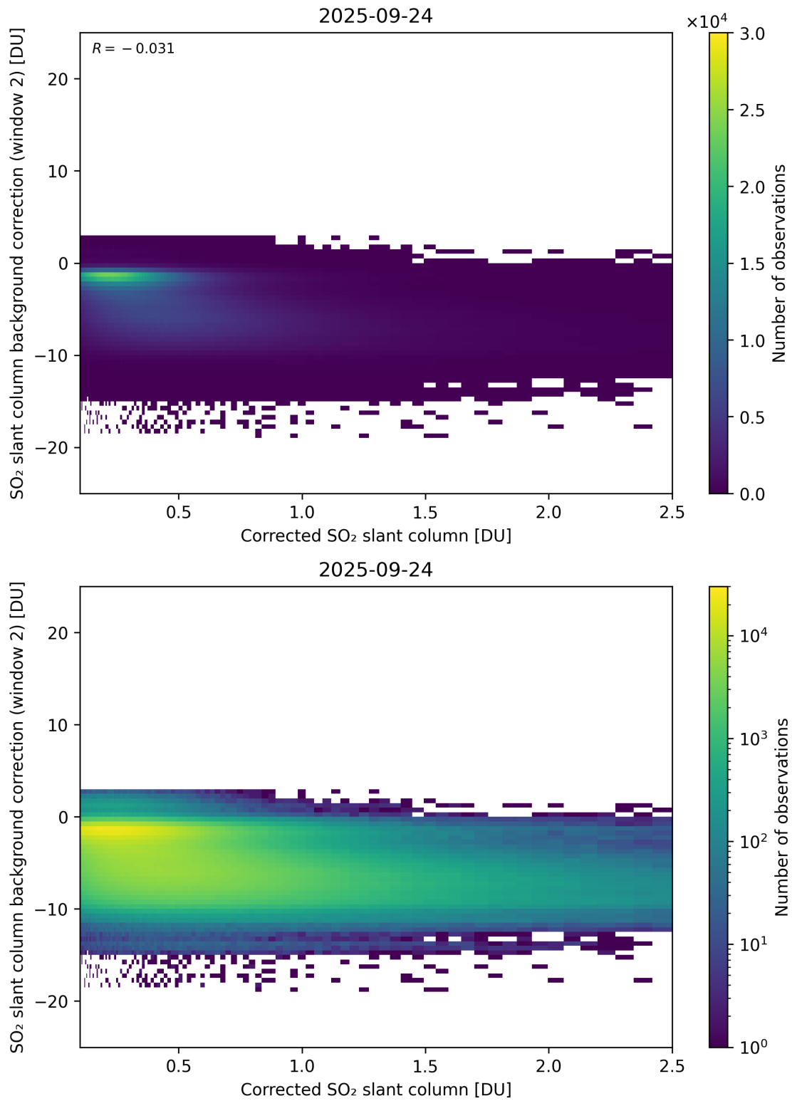
Figure 227: Scatter density plot of “Corrected SO 2 slant column” against “SO 2 slant column background correction (window 2)” for 2025-09-23 to 2025-09-25.
