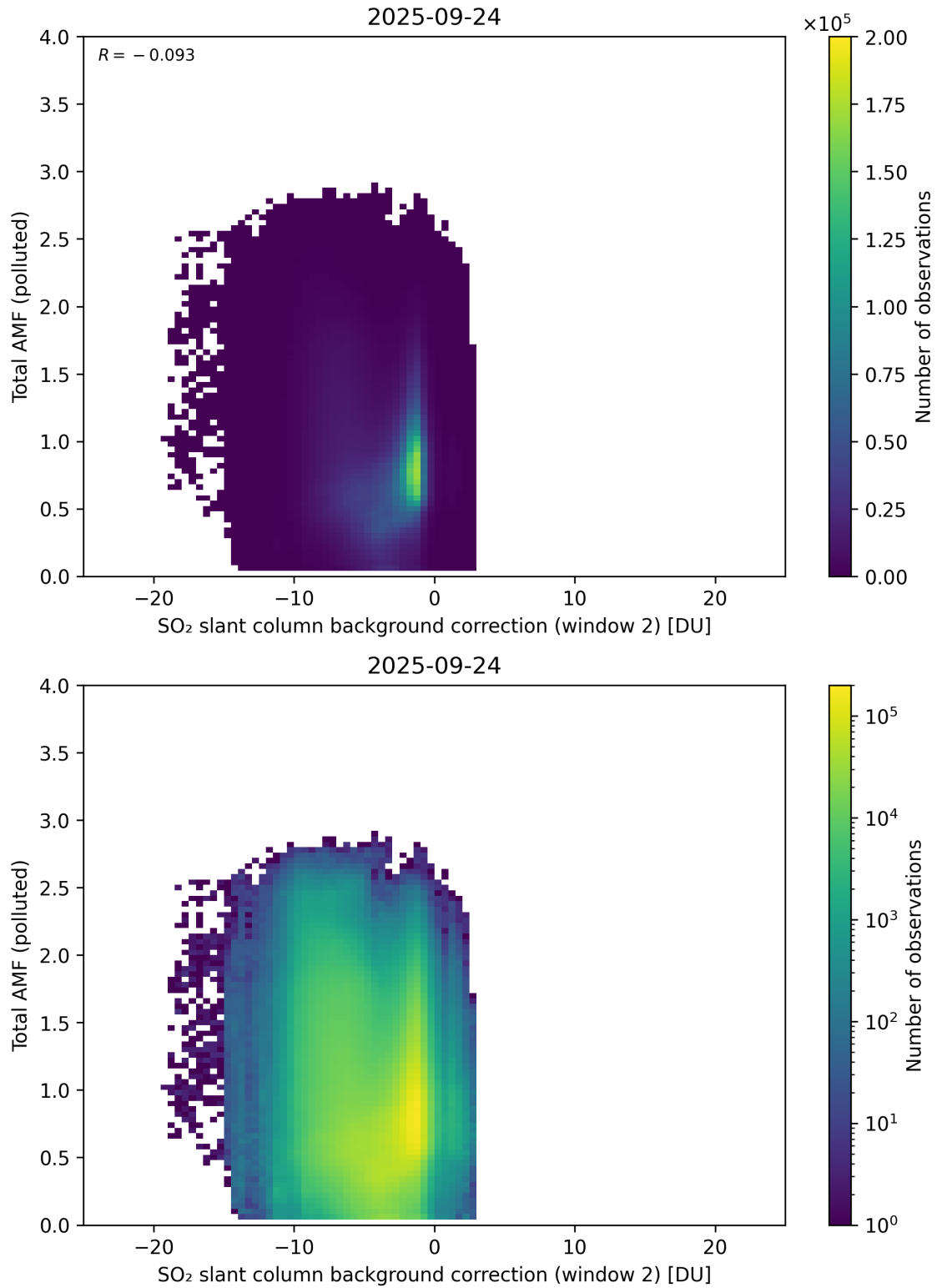
Figure 130: Scatter density plot of “SO 2 slant column background correction (window 2)” against “Total AMF (polluted)” for 2025-09-23 to 2025-09-25.
