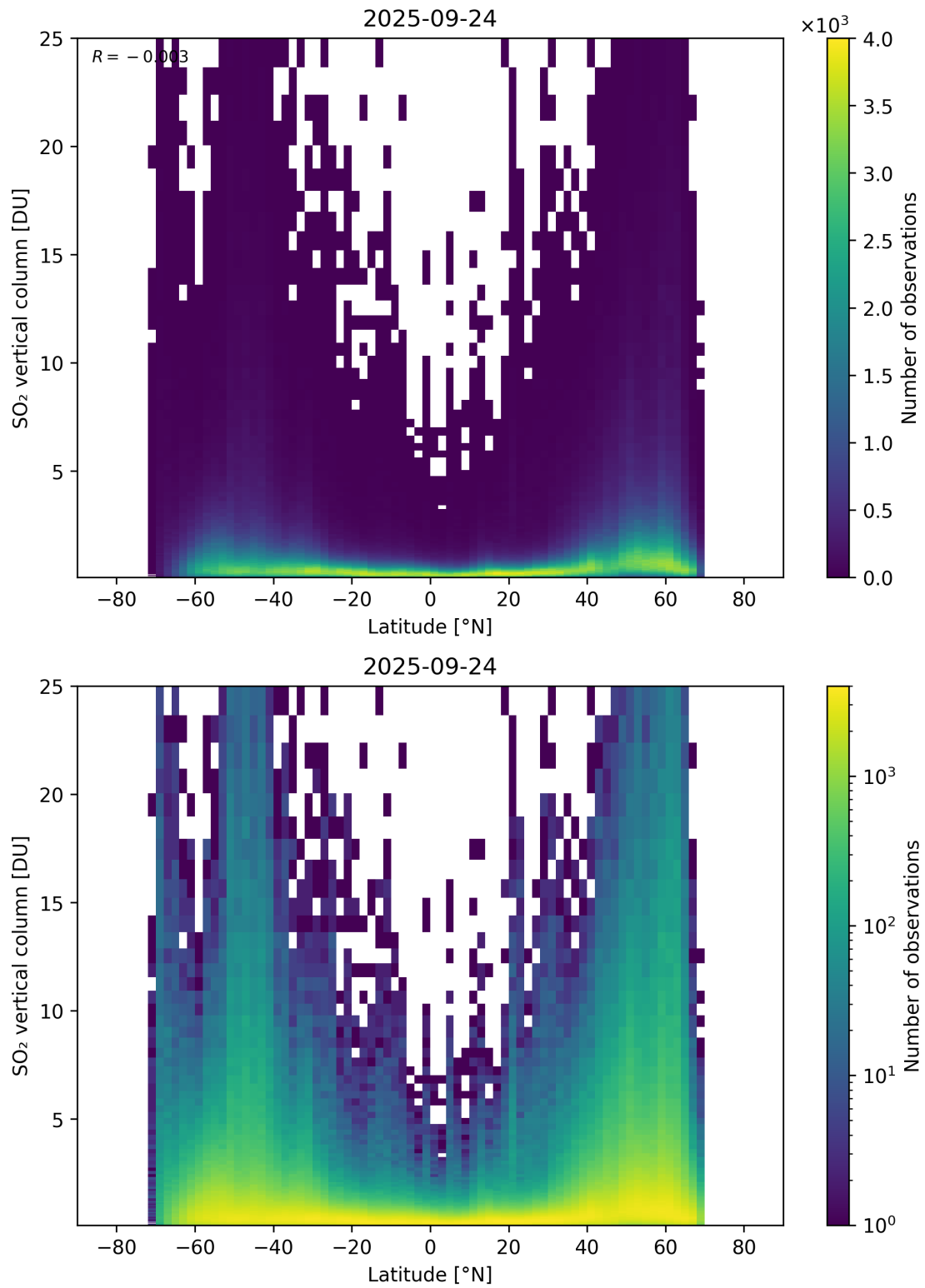
Figure 169: Scatter density plot of “Latitude” against “SO 2 vertical column” for 2025-09-23 to 2025-09-25.
