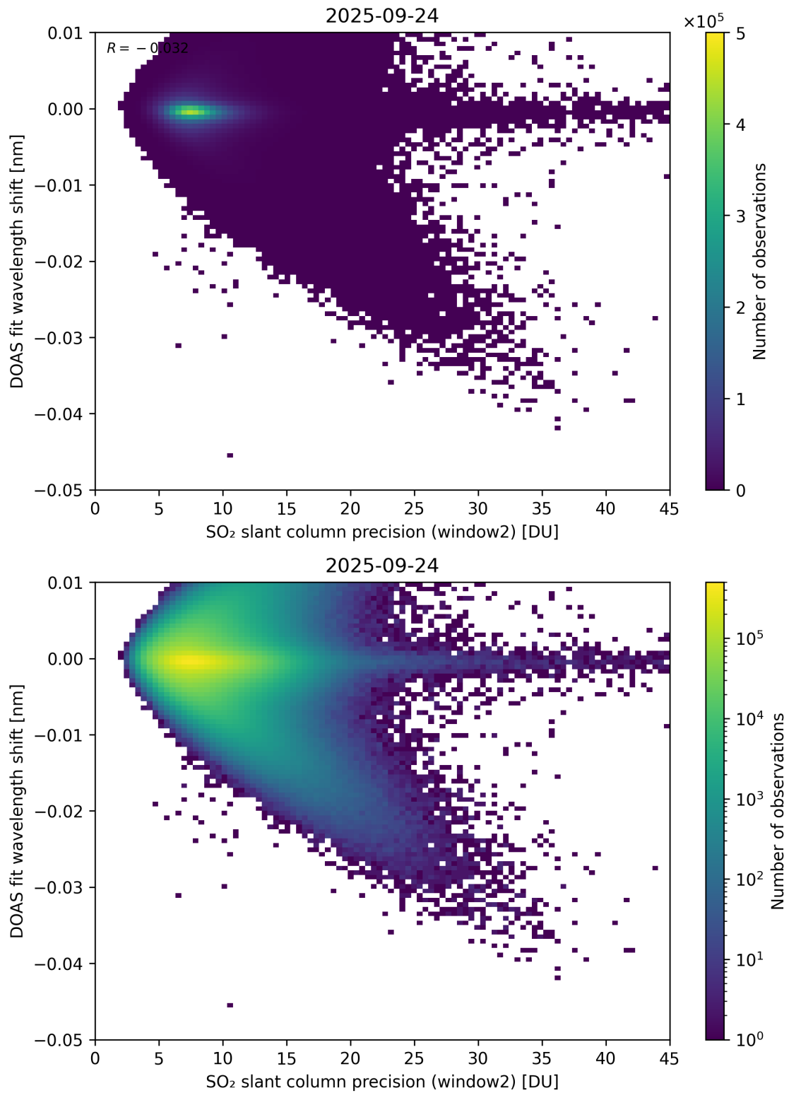
Figure 293: Scatter density plot of “SO 2 slant column precision (window2)” against “DOAS fit wavelength shift” for 2025-09-23 to 2025-09-25.
