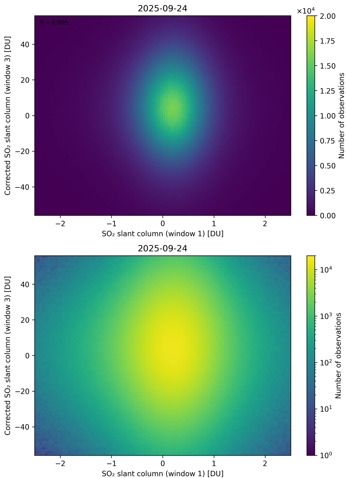
Figure 284: Scatter density plot of “SO 2 slant column (window 1)” against “Corrected SO 2 slant column (window 3)” for 2025-09-23 to 2025-09-25.
