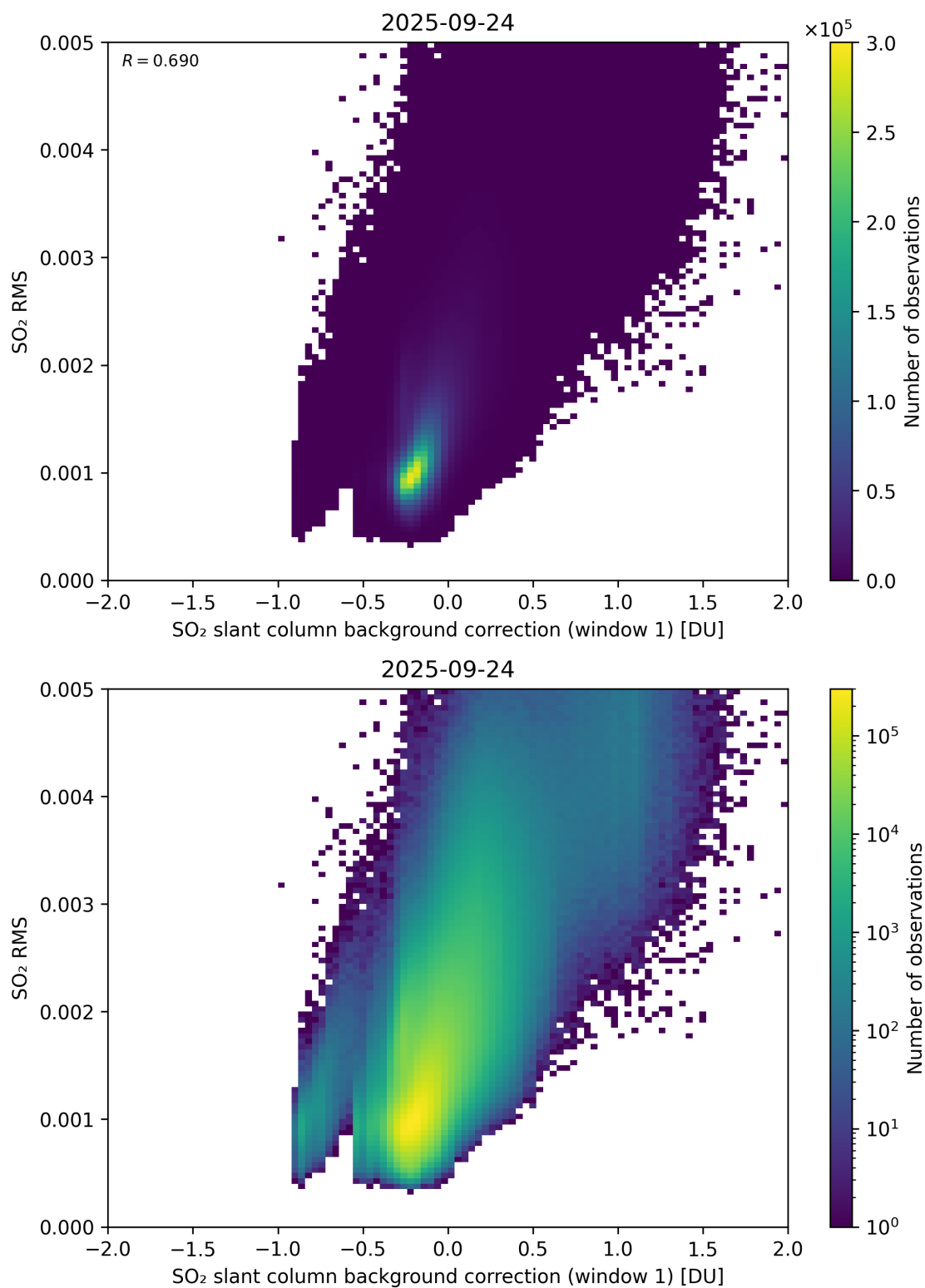
Figure 113: Scatter density plot of “SO 2 slant column background correction (window 1)” against “SO 2 RMS” for 2025-09-23 to 2025-09-25.
