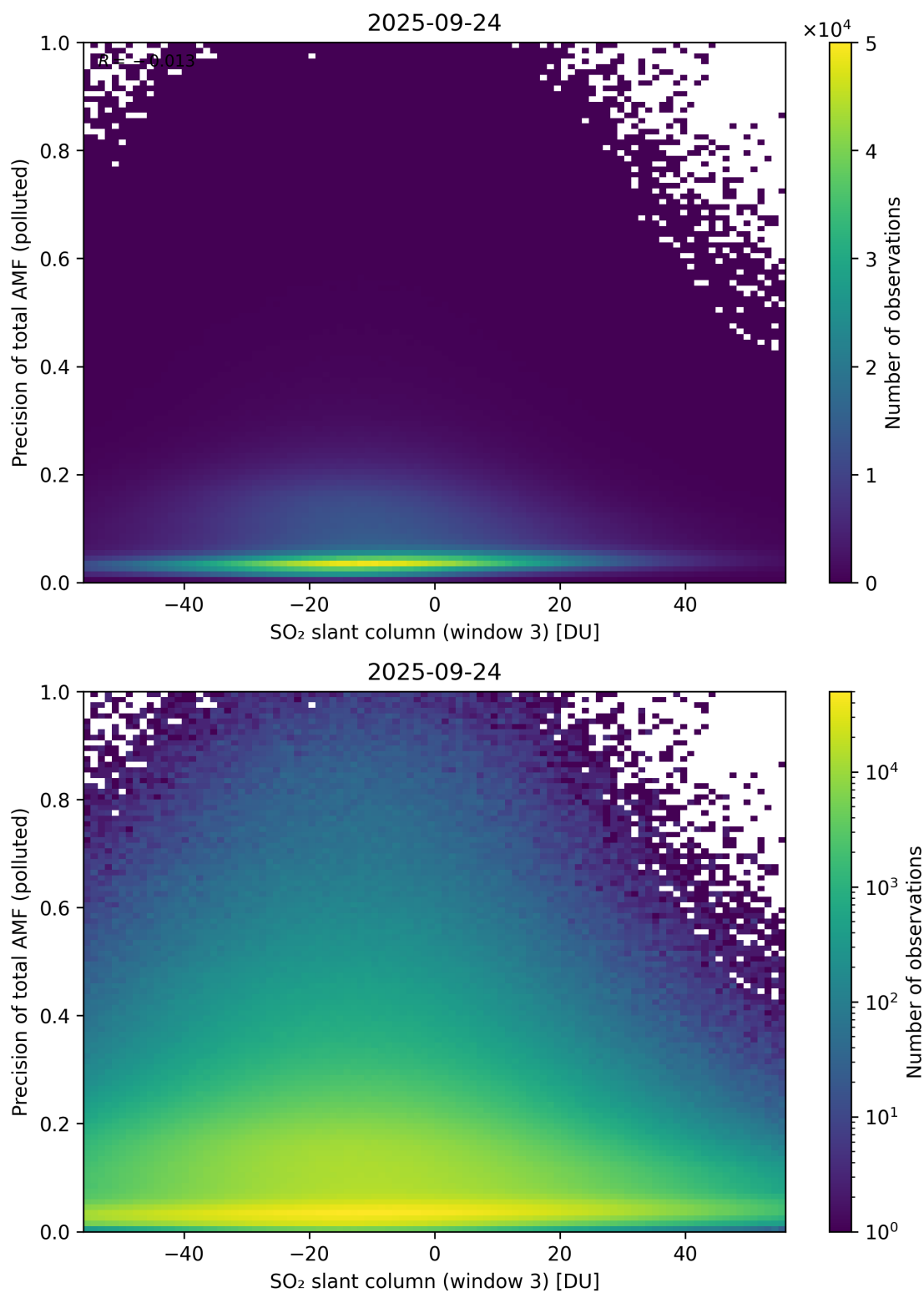
Figure 319: Scatter density plot of “SO 2 slant column (window 3)” against “Precision of total AMF (polluted)” for 2025-09-23 to 2025-09-25.
