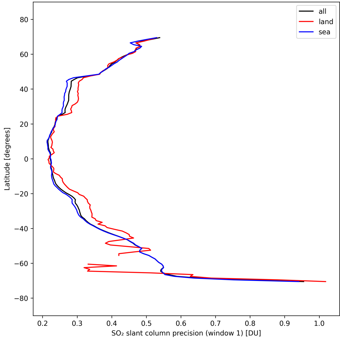
Figure 38: Zonal average of “SO 2 slant column precision (window 1)” for 2025-09-23 to 2025-09-25.
