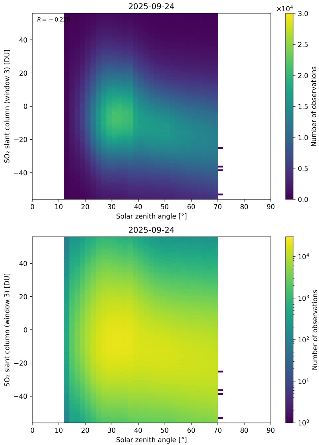
Figure 187: Scatter density plot of “Solar zenith angle” against “SO 2 slant column (window 3)” for 2025-09-23 to 2025-09-25.
