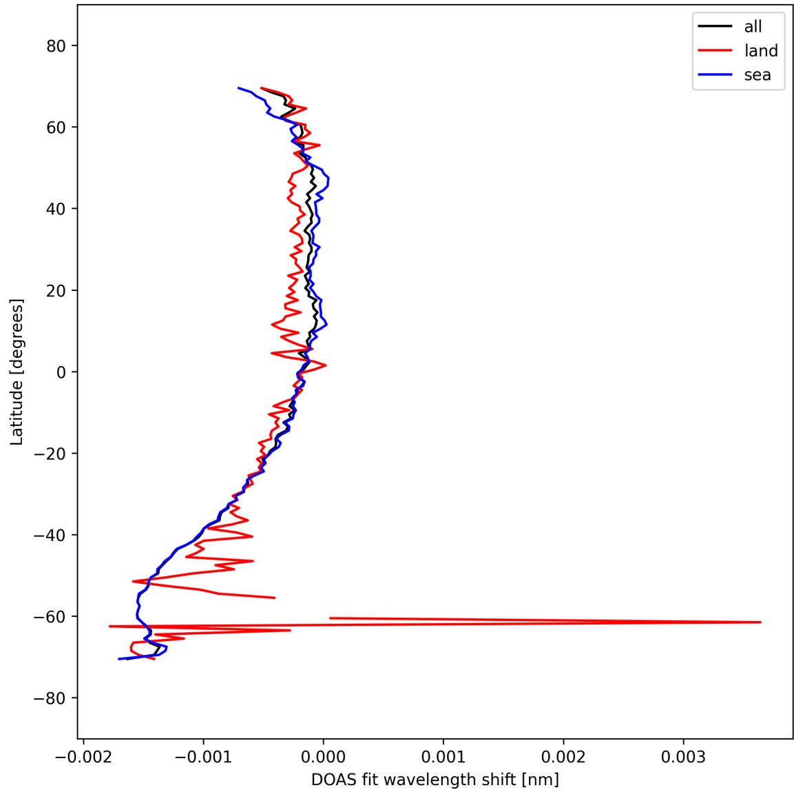
Figure 50: Zonal average of “DOAS fit wavelength shift” for 2025-09-23 to 2025-09-25.
