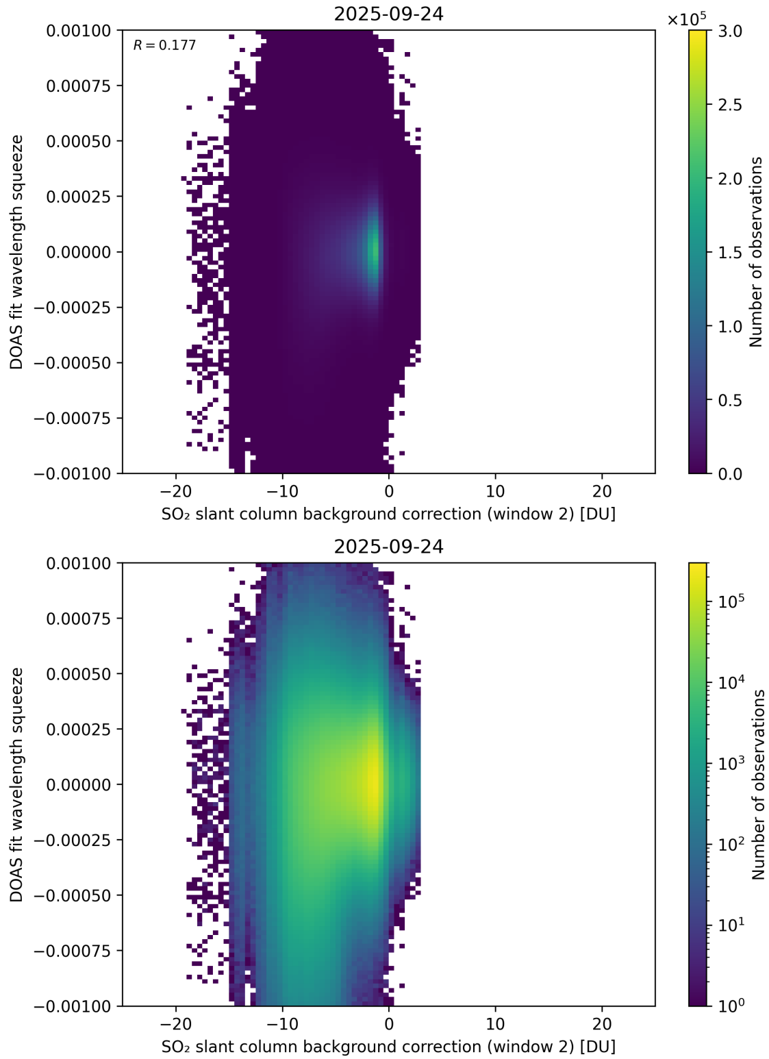
Figure 124: Scatter density plot of “SO 2 slant column background correction (window 2)” against “DOAS fit wavelength squeeze” for 2025-09-23 to 2025-09-25.
