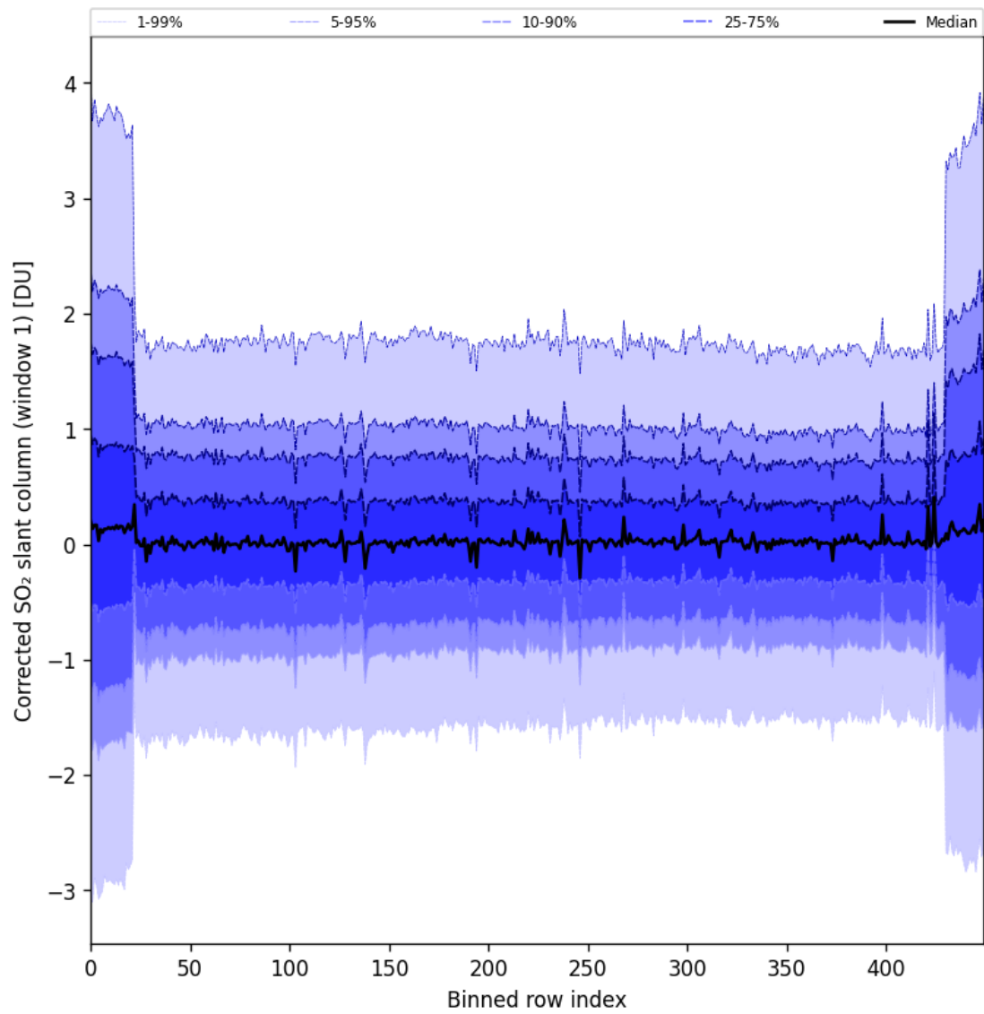
Figure 91: Along track statistics of “Corrected SO 2 slant column (window 1)” for 2025-09-23 to 2025-09-25
