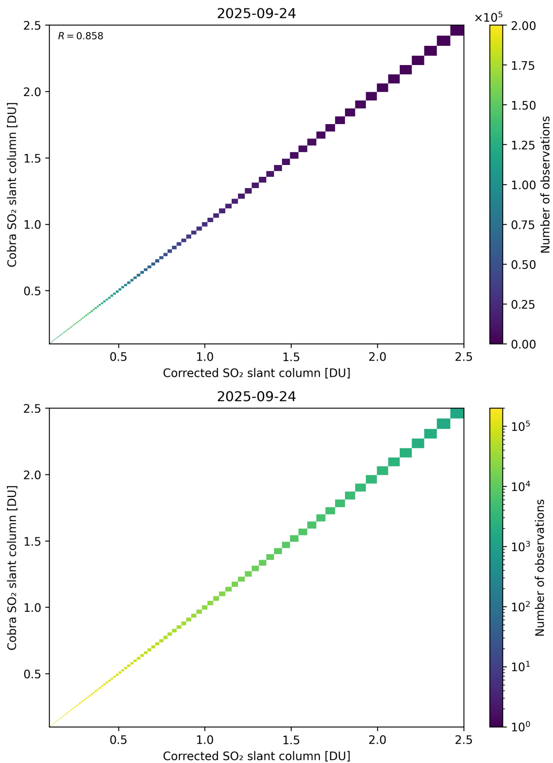
Figure 233: Scatter density plot of “Corrected SO 2 slant column” against “Cobra SO 2 slant column” for 2025-09-23 to 2025-09-25.
