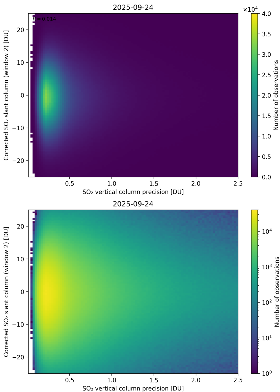
Figure 339: Scatter density plot of “SO 2 vertical column precision” against “Corrected SO 2 slant column (window 2)” for 2025-09-23 to 2025-09-25.
