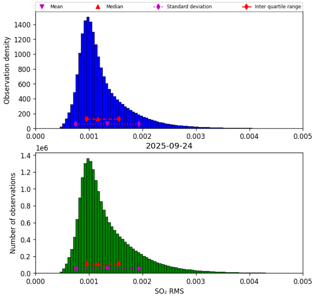
Figure 78: Histogram of “SO 2 RMS” for 2025-09-23 to 2025-09-25
