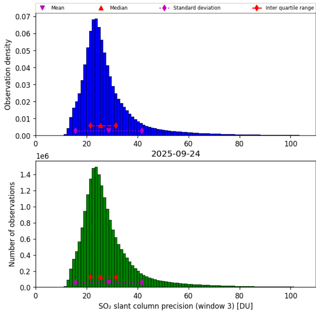
Figure 72: Histogram of “SO 2 slant column precision (window 3)” for 2025-09-23 to 2025-09-25
