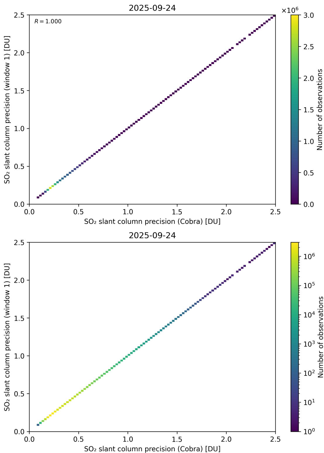
Figure 209: Scatter density plot of “SO 2 slant column precision (Cobra)” against “SO 2 slant column precision (window 1)” for 2025-09-23 to 2025-09-25.
