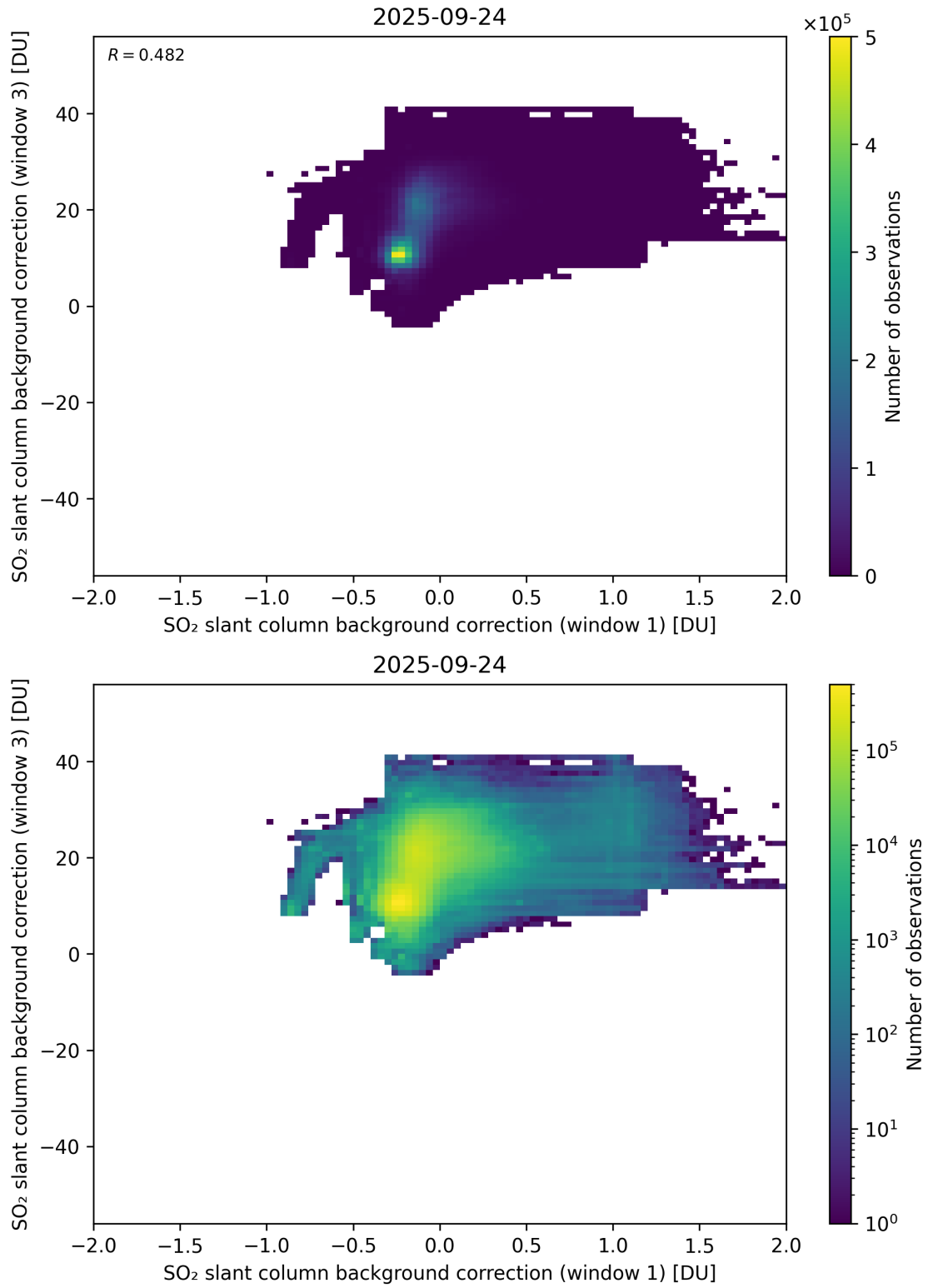
Figure 110: Scatter density plot of “SO 2 slant column background correction (window 1)” against “SO 2 slant column background correction (window 3)” for 2025-09-23 to 2025-09-25.
