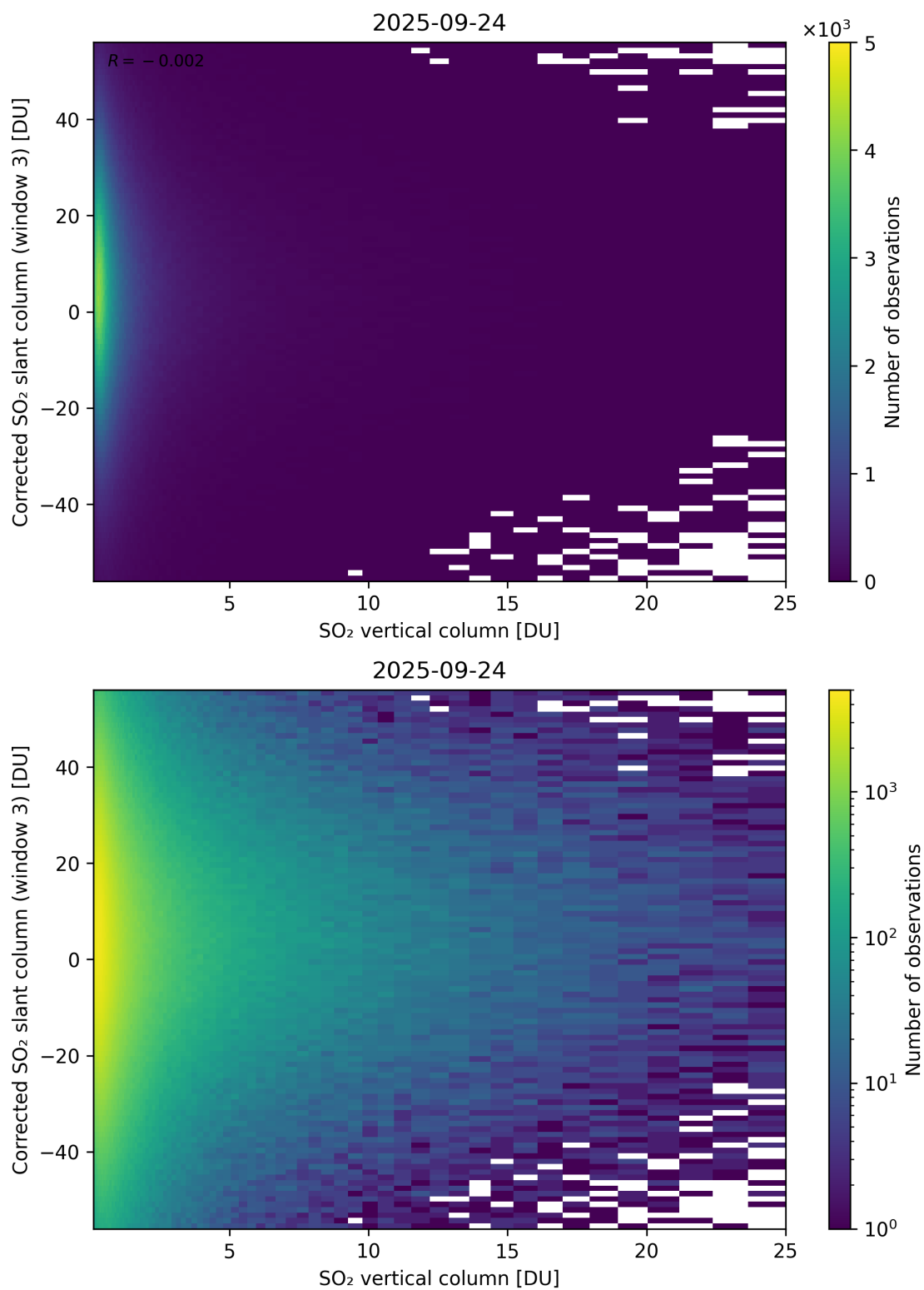
Figure 353: Scatter density plot of “SO 2 vertical column” against “Corrected SO 2 slant column (window 3)” for 2025-09-23 to 2025-09-25.
