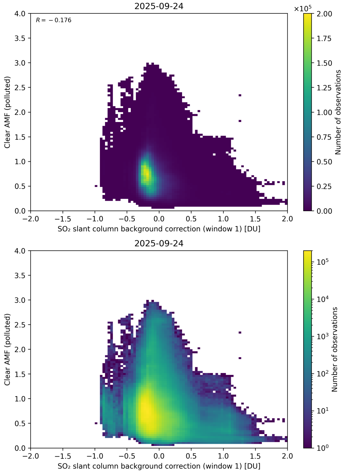
Figure 114: Scatter density plot of “SO 2 slant column background correction (window 1)” against “Clear AMF (polluted)” for 2025-09-23 to 2025-09-25.
