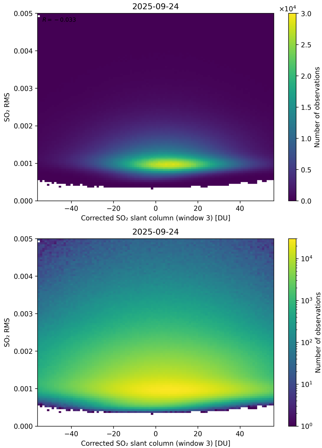
Figure 258: Scatter density plot of “Corrected SO 2 slant column (window 3)” against “SO 2 RMS” for 2025-09-23 to 2025-09-25.
