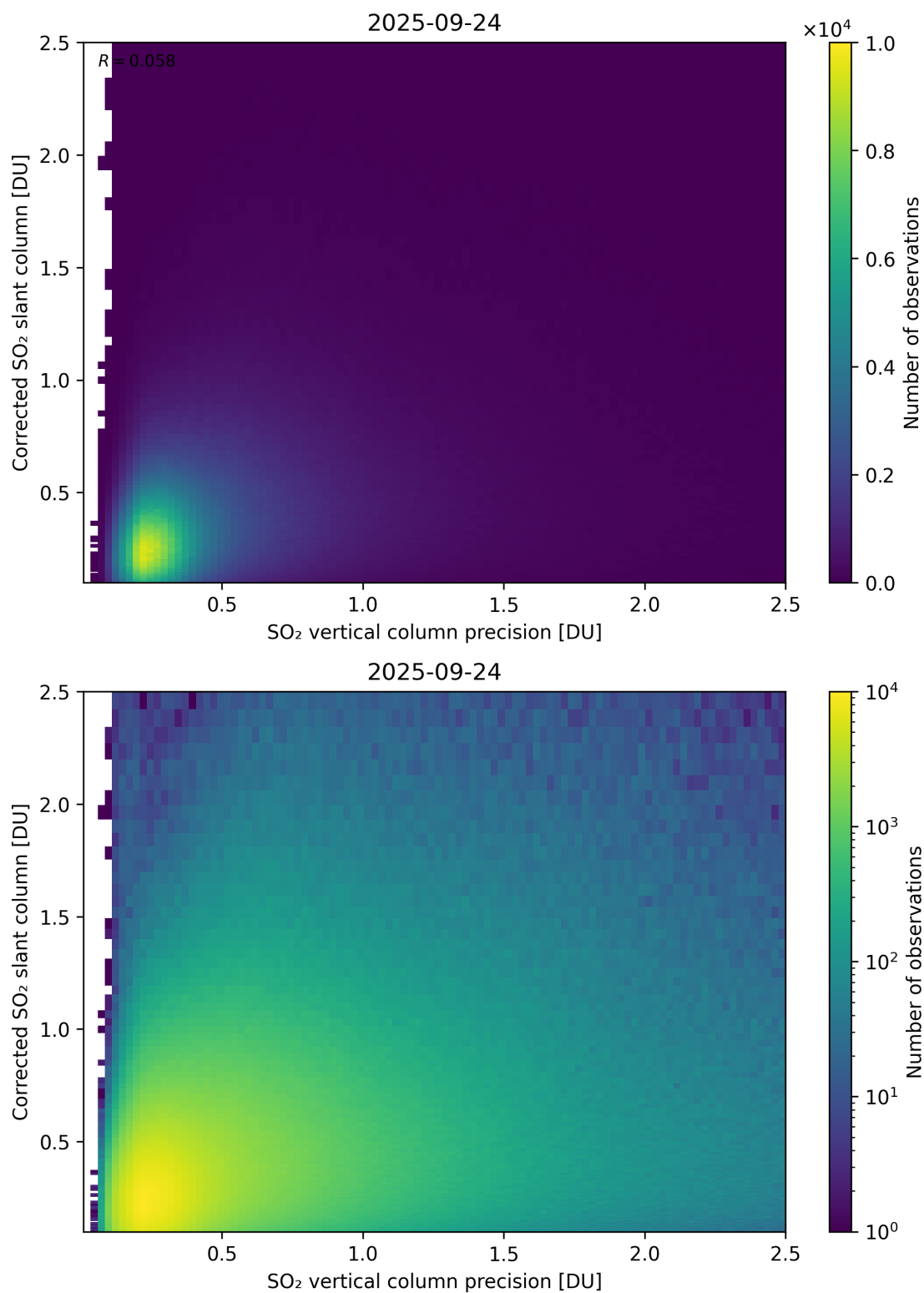
Figure 338: Scatter density plot of “SO 2 vertical column precision” against “Corrected SO 2 slant column” for 2025-09-23 to 2025-09-25.
