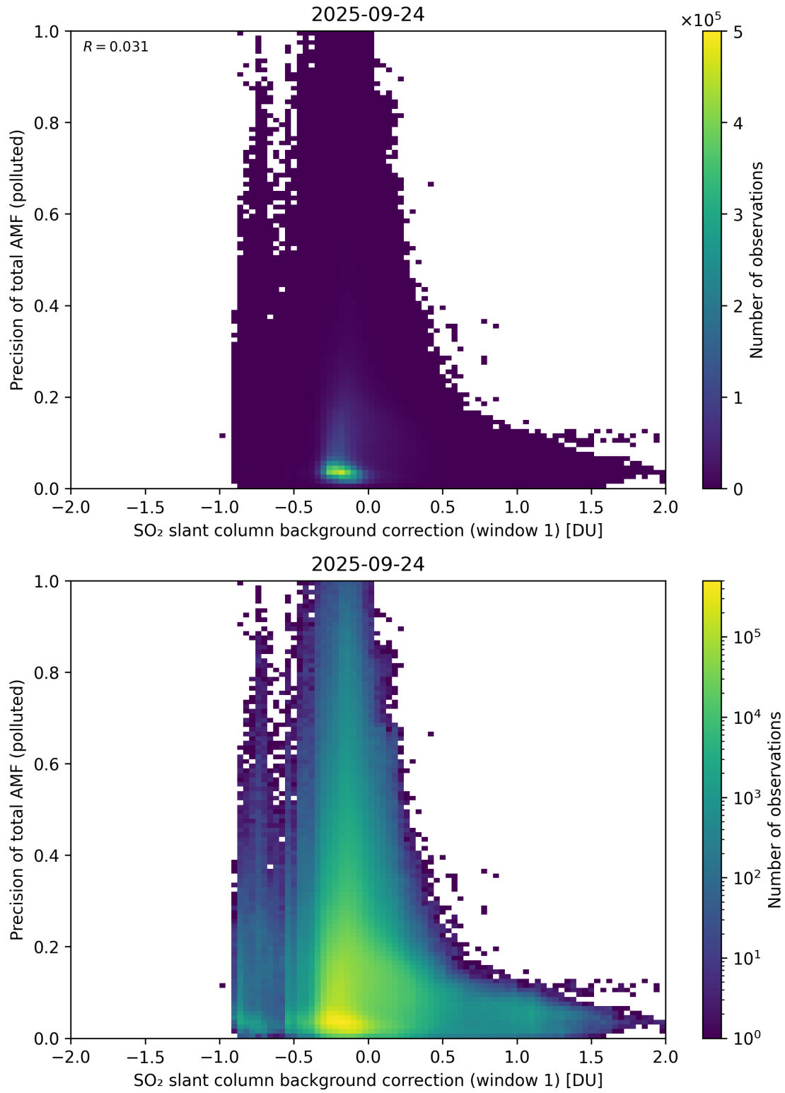
Figure 121: Scatter density plot of “SO 2 slant column background correction (window 1)” against “Precision of total AMF (polluted)” for 2025-09-23 to 2025-09-25.
