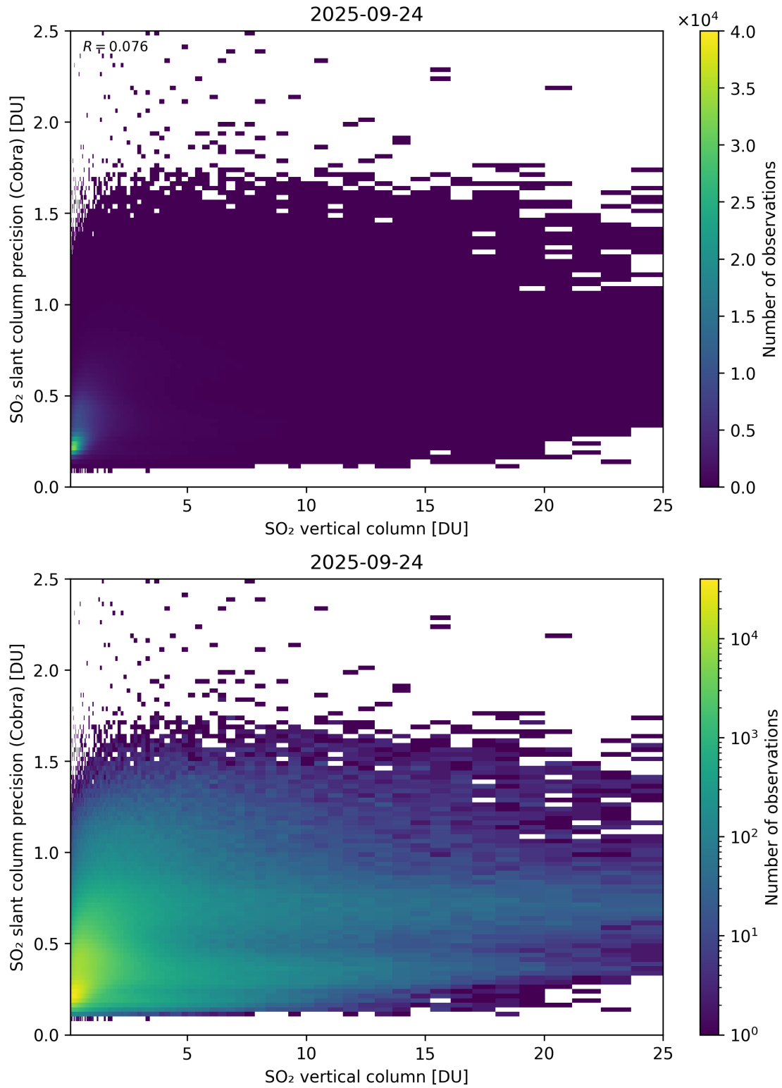
Figure 350: Scatter density plot of “SO 2 vertical column” against “SO 2 slant column precision (Cobra)” for 2025-09-23 to 2025-09-25.
