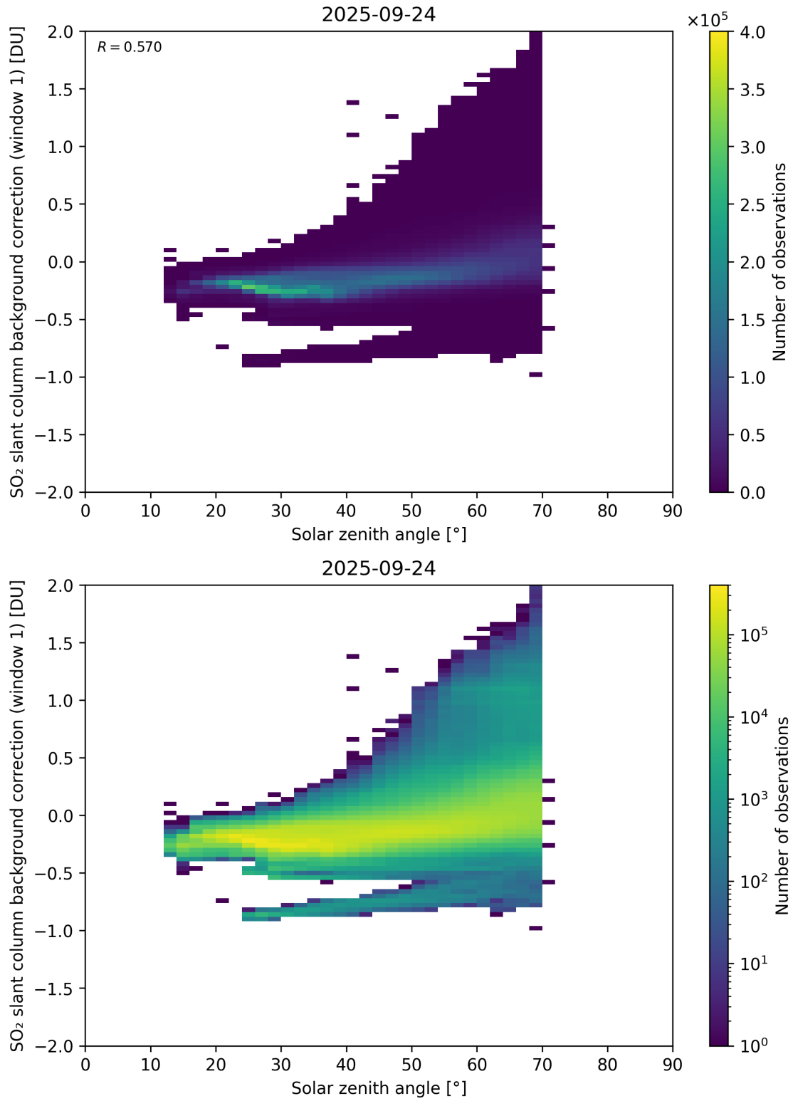
Figure 171: Scatter density plot of “Solar zenith angle” against “SO 2 slant column background correction (window 1)” for 2025-09-23 to 2025-09-25.
