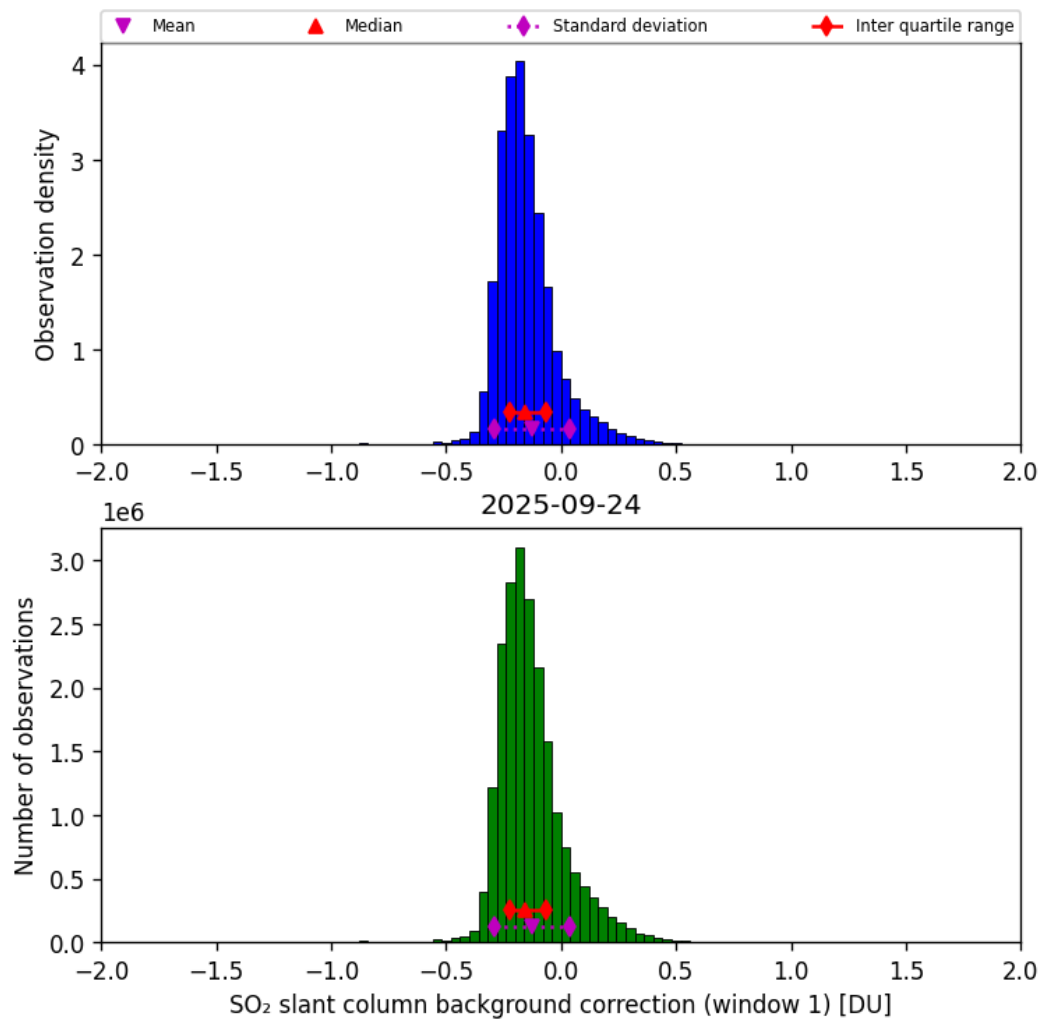
Figure 66: Histogram of “SO 2 slant column background correction (window 1)” for 2025-09-23 to 2025-09-25
