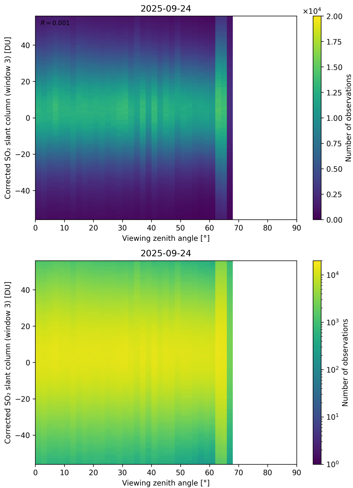
Figure 375: Scatter density plot of “Viewing zenith angle” against “Corrected SO 2 slant column (window 3)” for 2025-09-23 to 2025-09-25.
