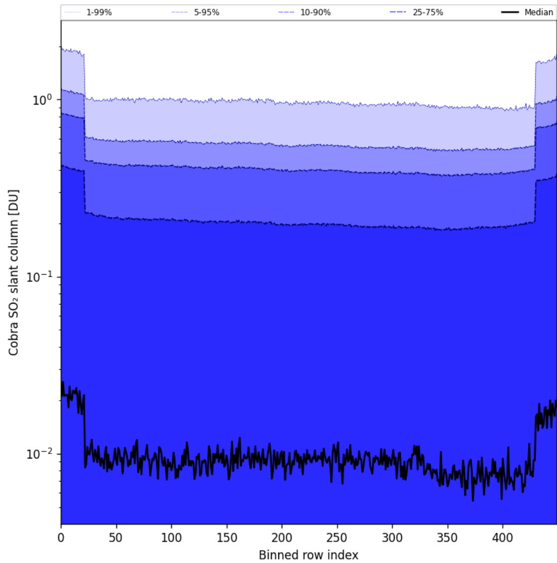
Figure 87: Along track statistics of "Cobra SO 2 slant column" for 2025-09-23 to 2025-09-25
