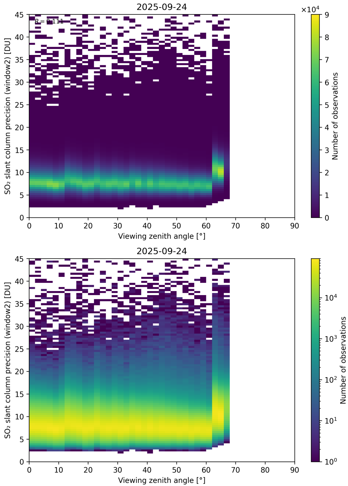
Figure 378: Scatter density plot of “Viewing zenith angle” against “SO 2 slant column precision (window2)” for 2025-09-23 to 2025-09-25.
