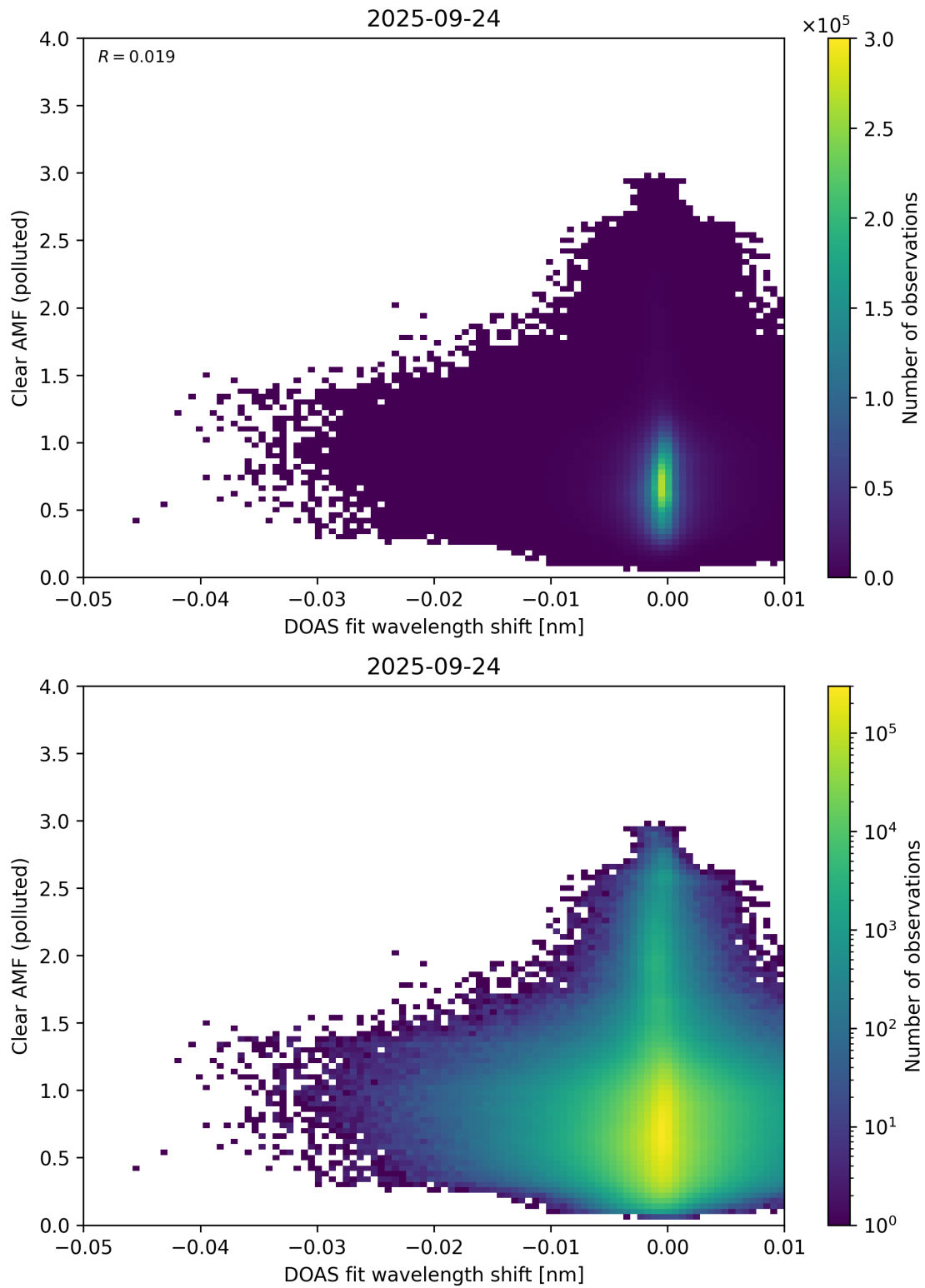
Figure 140: Scatter density plot of “DOAS fit wavelength shift” against “Clear AMF (polluted)” for 2025-09-23 to 2025-09-25.
