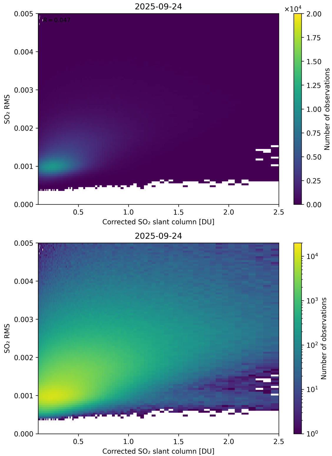
Figure 231: Scatter density plot of “Corrected SO 2 slant column” against “SO 2 RMS” for 2025-09-23 to 2025-09-25.
