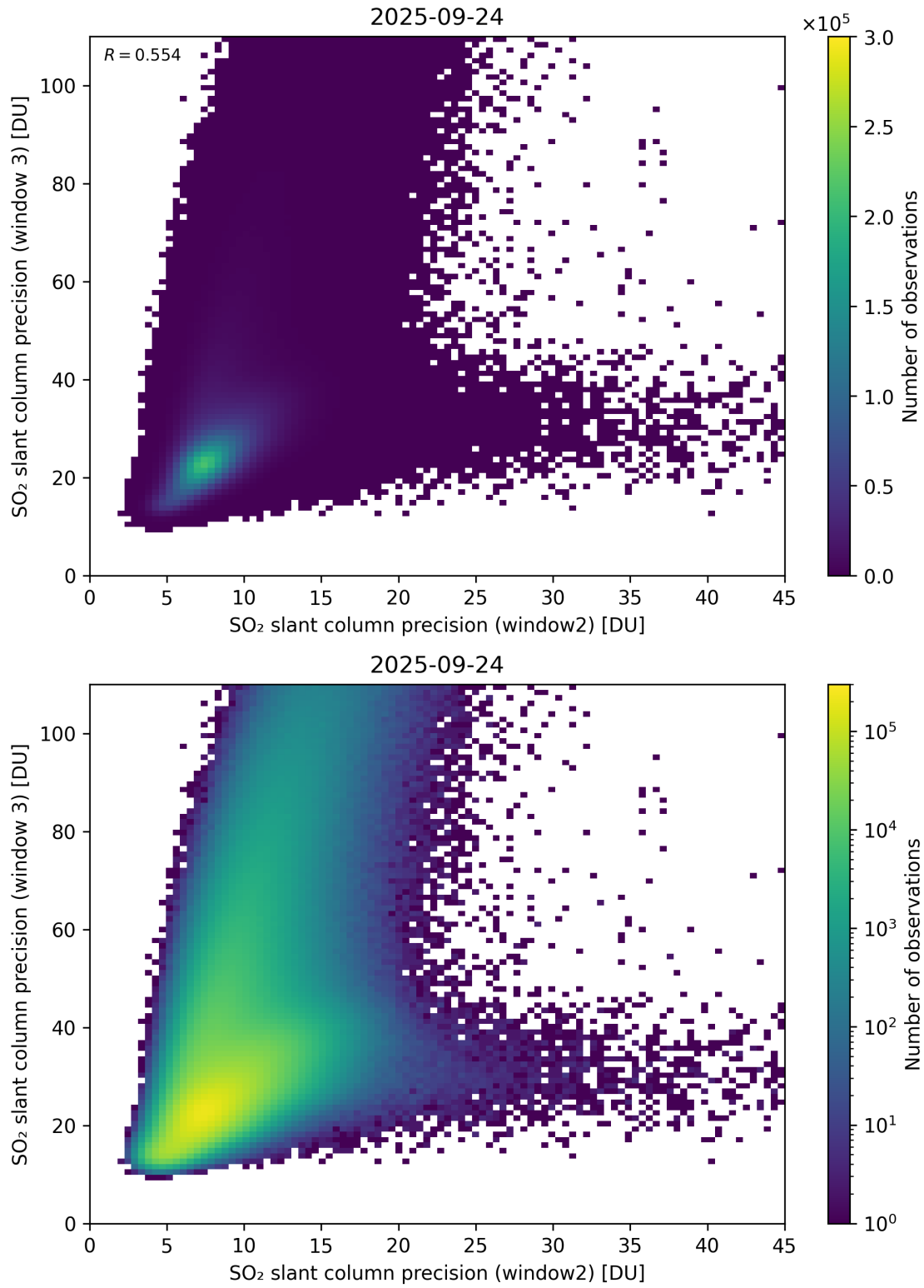
Figure 300: Scatter density plot of “SO 2 slant column precision (window2)” against “SO 2 slant column precision (window 3)” for 2025-09-23 to 2025-09-25.
