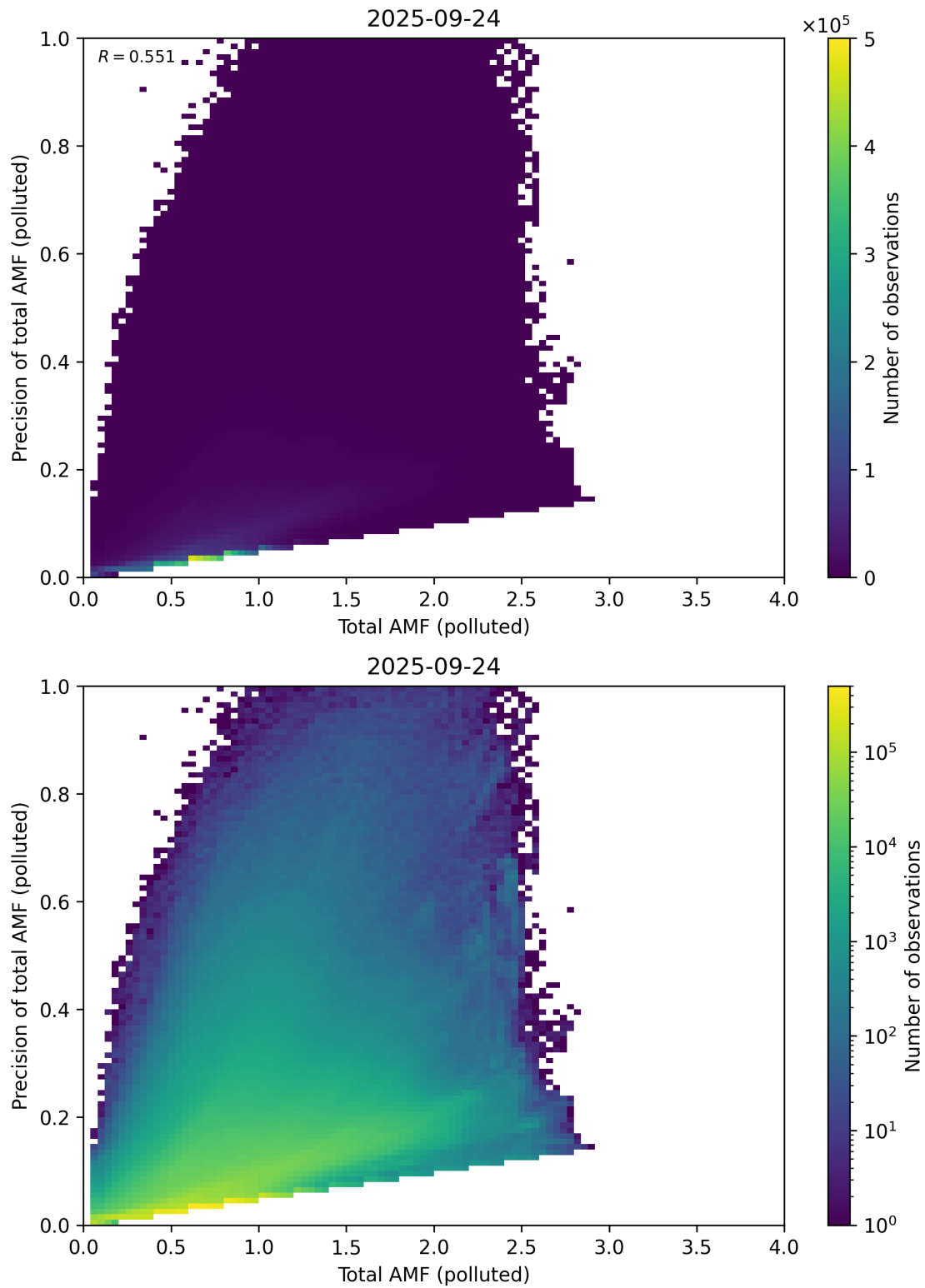
Figure 322: Scatter density plot of “Total AMF (polluted)” against “Precision of total AMF (polluted)” for 2025-09-23 to 2025-09-25.
