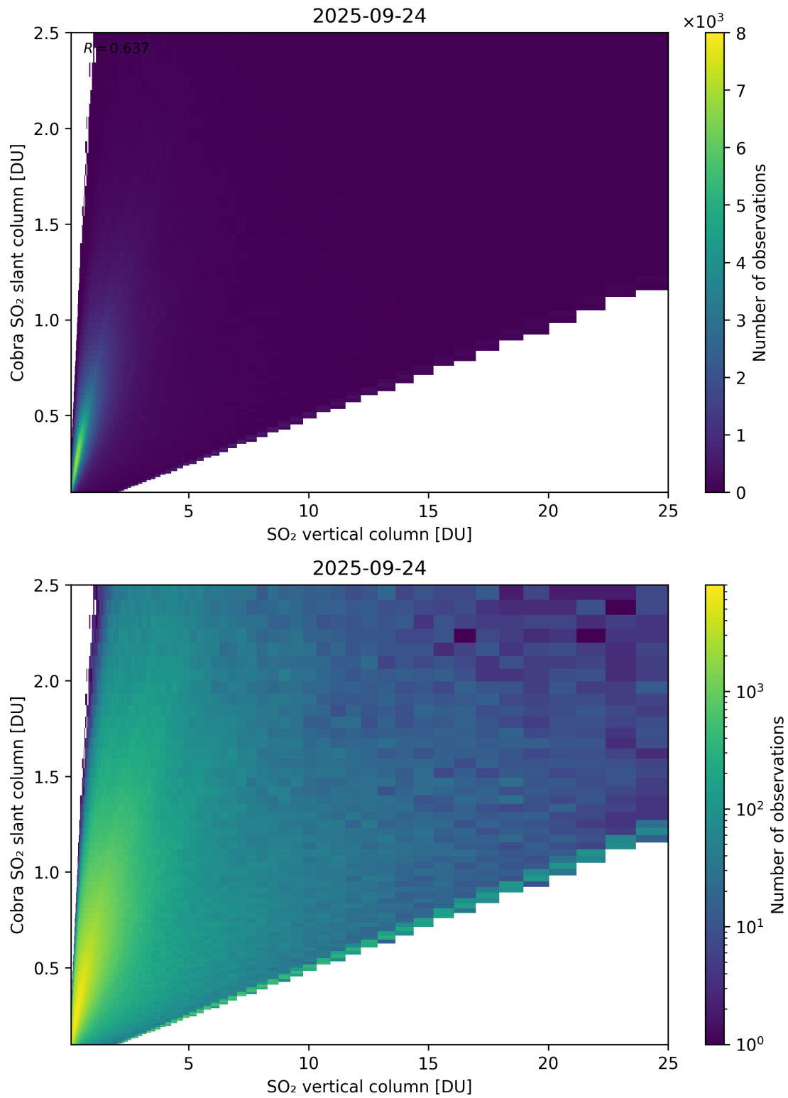
Figure 349: Scatter density plot of “SO 2 vertical column” against “Cobra SO 2 slant column” for 2025-09-23 to 2025-09-25.
