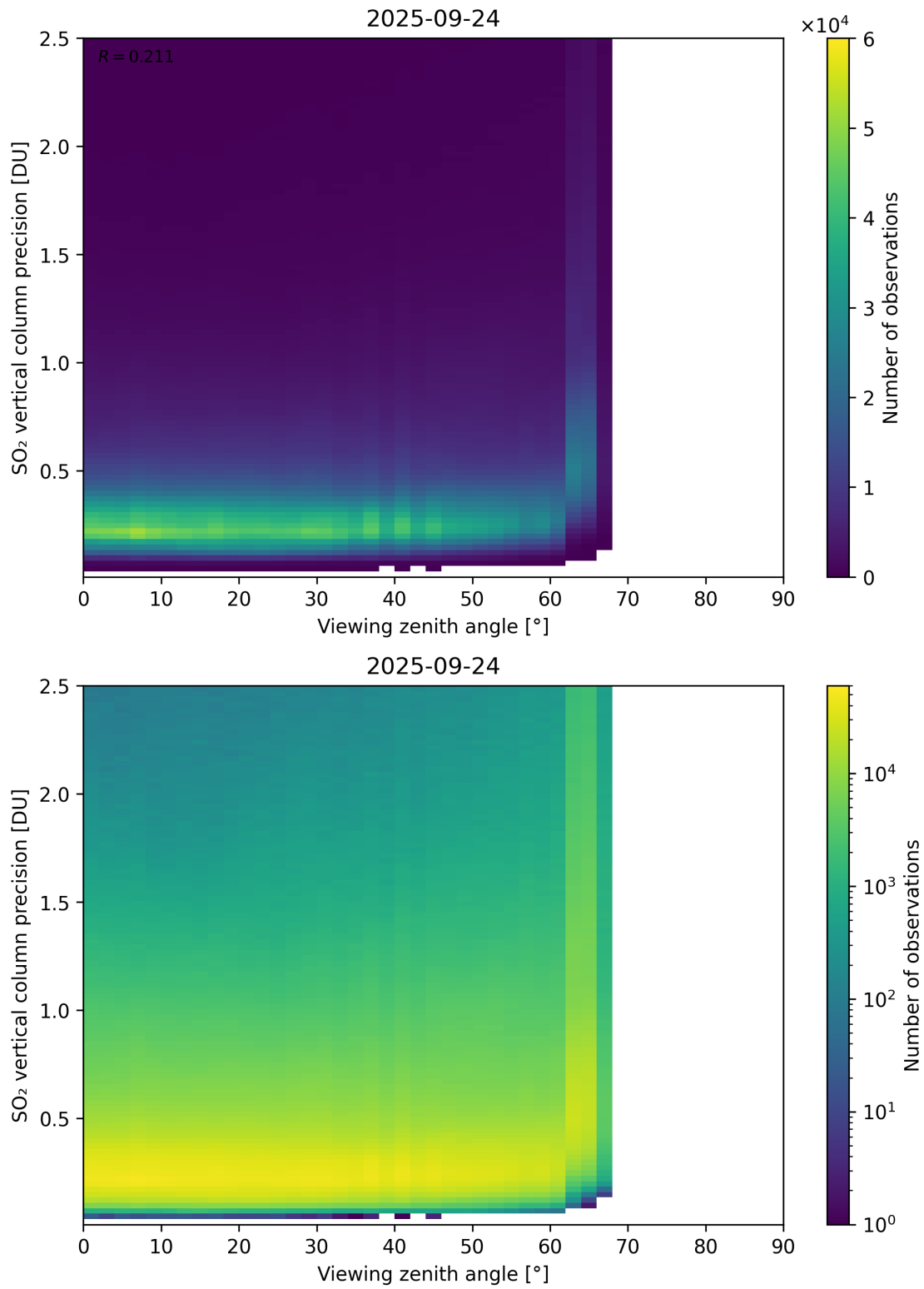
Figure 384: Scatter density plot of “Viewing zenith angle” against “SO 2 vertical column precision” for 2025-09-23 to 2025-09-25.
