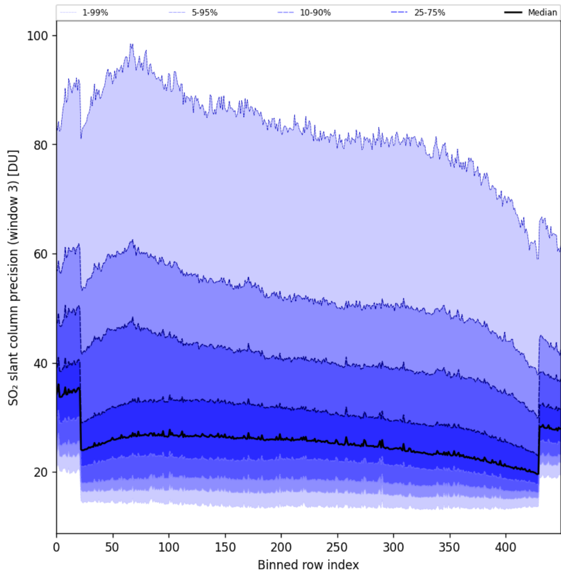
Figure 98: Along track statistics of “SO 2 slant column precision (window 3)” for 2025-09-23 to 2025-09-25
