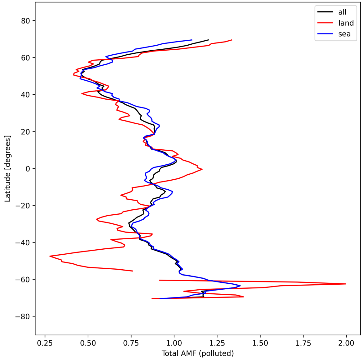
Figure 53: Zonal average of “Total AMF (polluted)” for 2025-09-23 to 2025-09-25.
