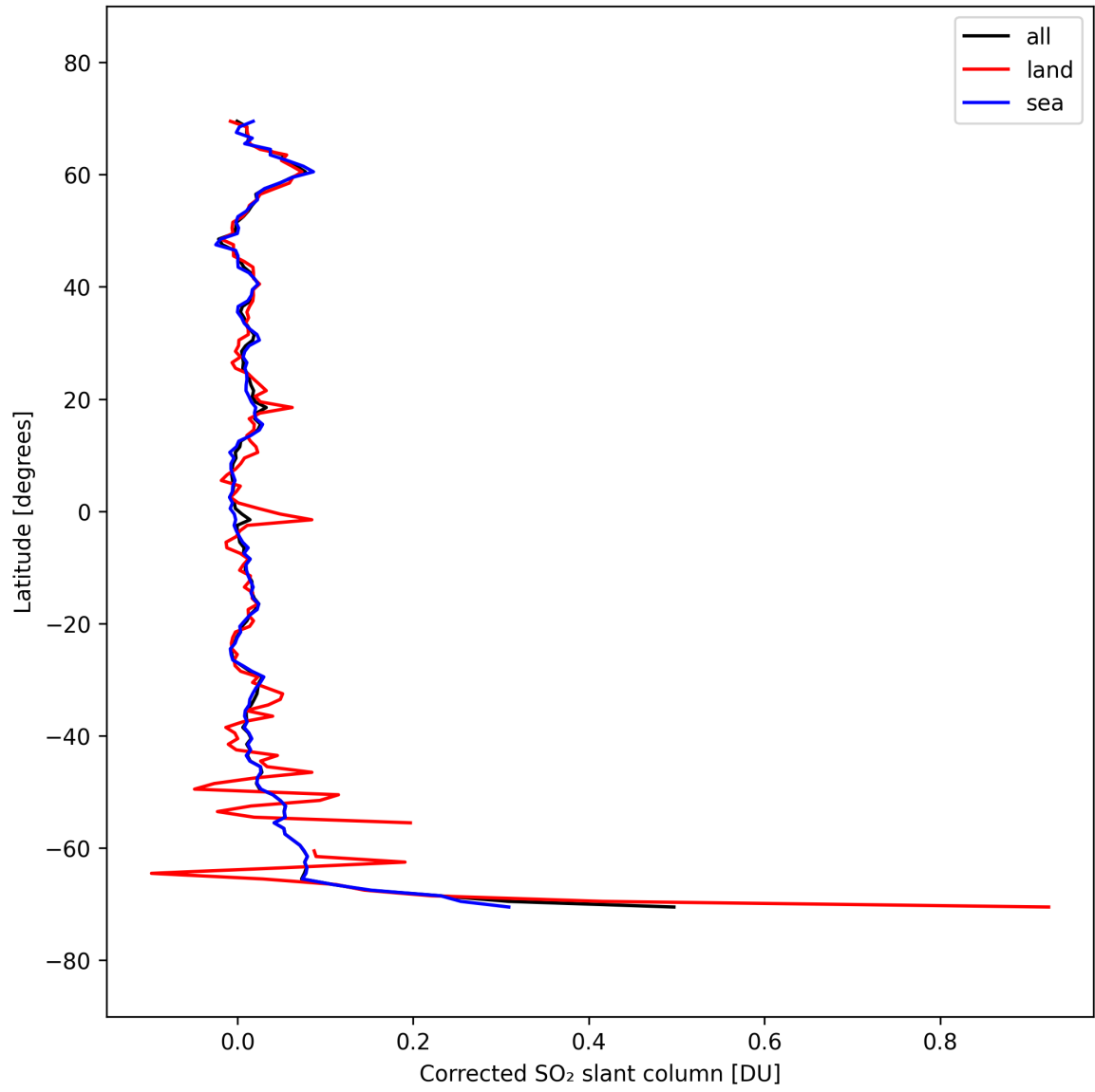
Figure 34: Zonal average of “Corrected SO 2 slant column” for 2025-09-23 to 2025-09-25.
