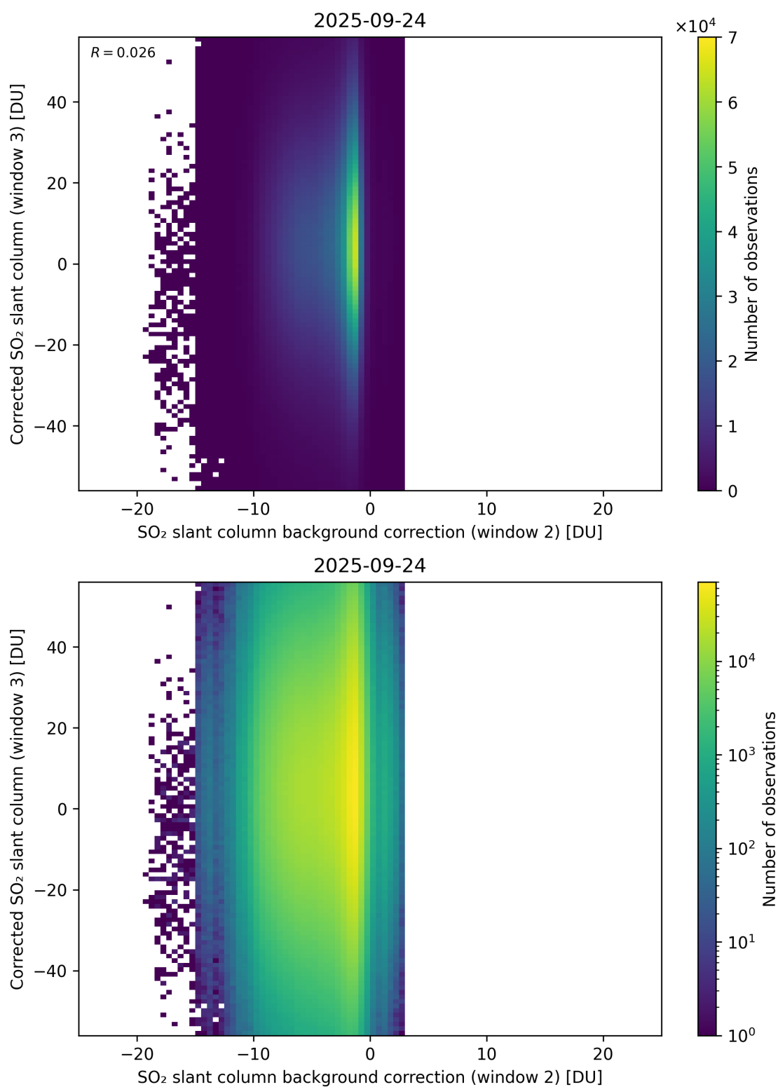
Figure 127: Scatter density plot of “SO 2 slant column background correction (window 2)” against “Corrected SO 2 slant column (window 3)” for 2025-09-23 to 2025-09-25.
