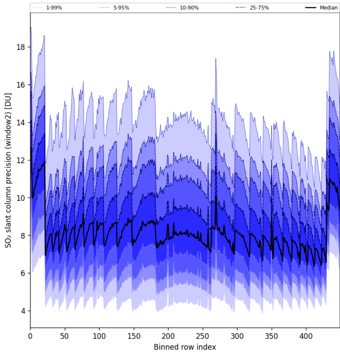
Figure 94: Along track statistics of “SO 2 slant column precision (window2)” for 2025-09-23 to 2025-09-25
