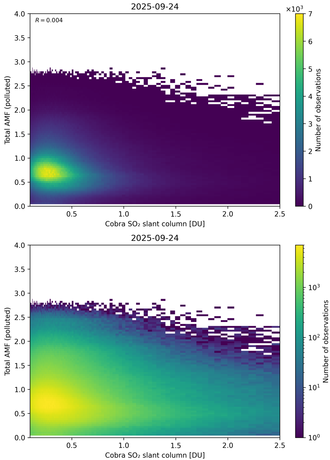
Figure 224: Scatter density plot of “Cobra SO 2 slant column” against “Total AMF (polluted)” for 2025-09-23 to 2025-09-25.
