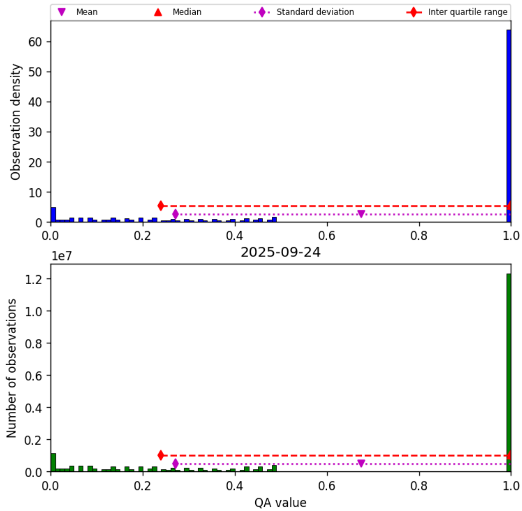
Figure 57: Histogram of “QA value” for 2025-09-23 to 2025-09-25
