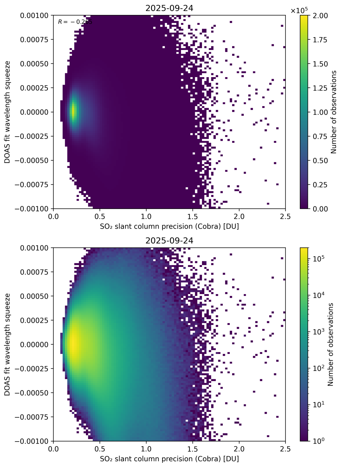
Figure 203: Scatter density plot of “SO 2 slant column precision (Cobra)” against “DOAS fit wavelength squeeze” for 2025-09-23 to 2025-09-25.
