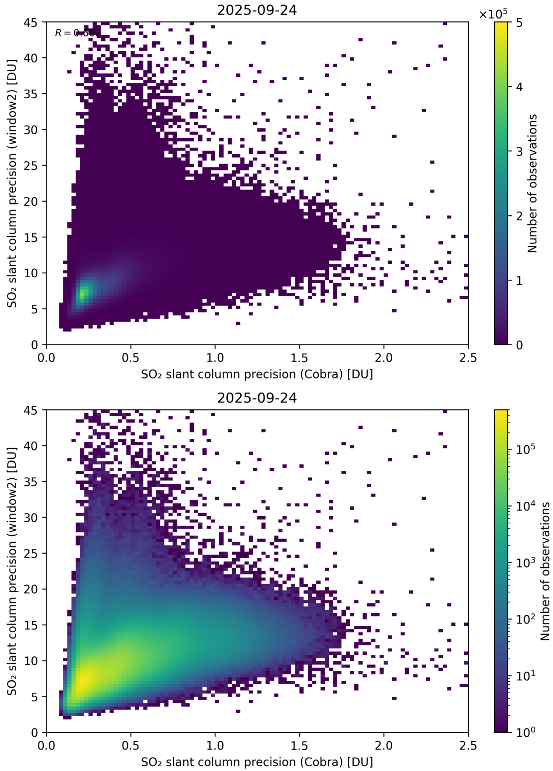
Figure 210: Scatter density plot of “SO 2 slant column precision (Cobra)” against “SO 2 slant column precision (window2)” for 2025-09-23 to 2025-09-25.
