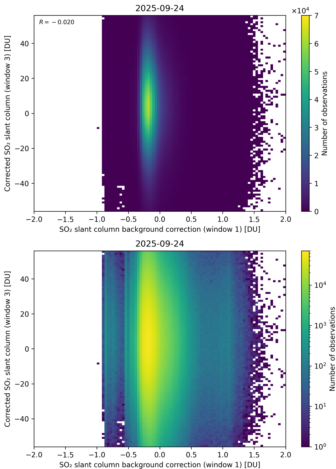
Figure 116: Scatter density plot of “SO 2 slant column background correction (window 1)” against “Corrected SO 2 slant column (window 3)” for 2025-09-23 to 2025-09-25.
