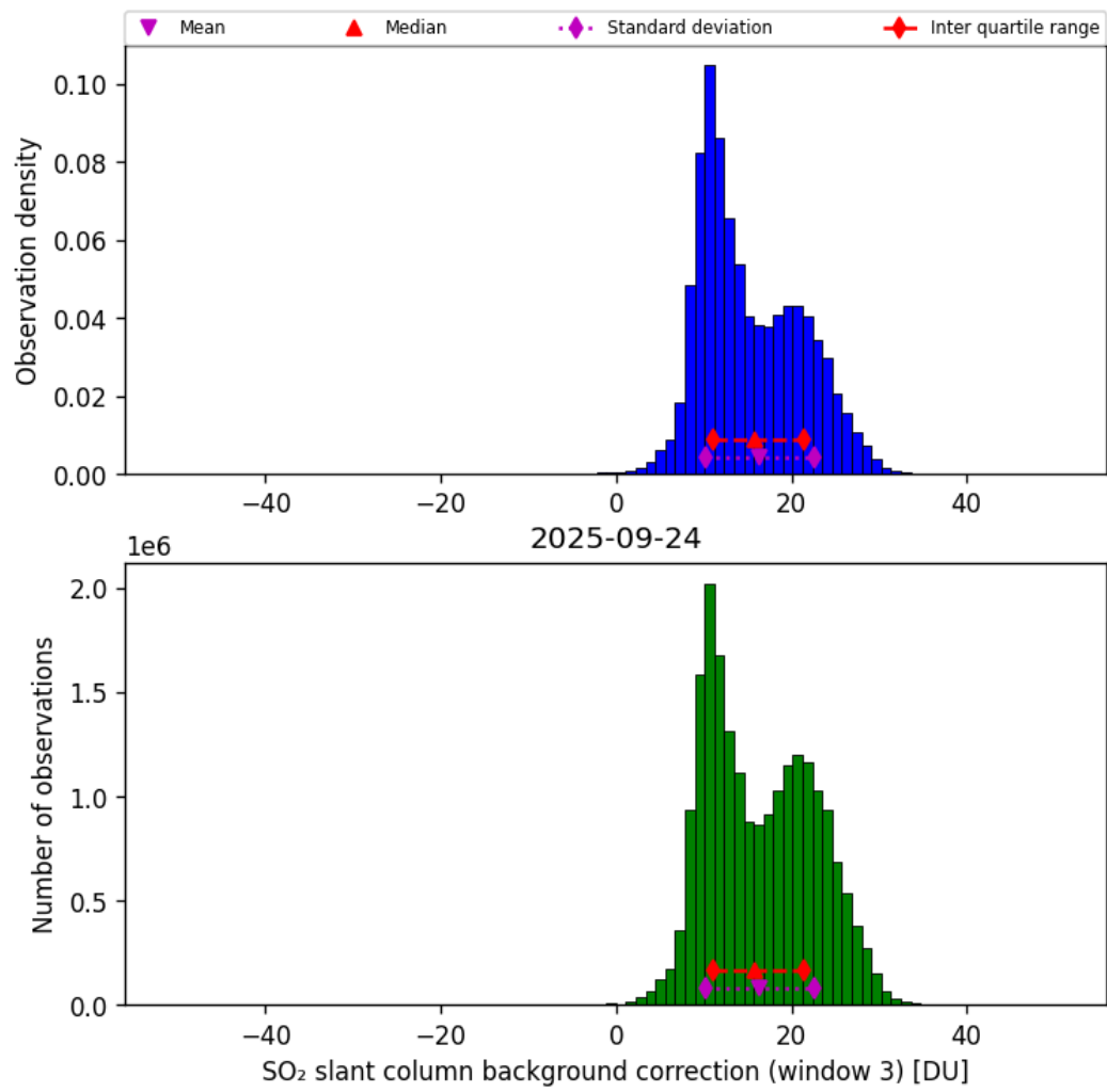
Figure 74: Histogram of “SO 2 slant column background correction (window 3)” for 2025-09-23 to 2025-09-25
