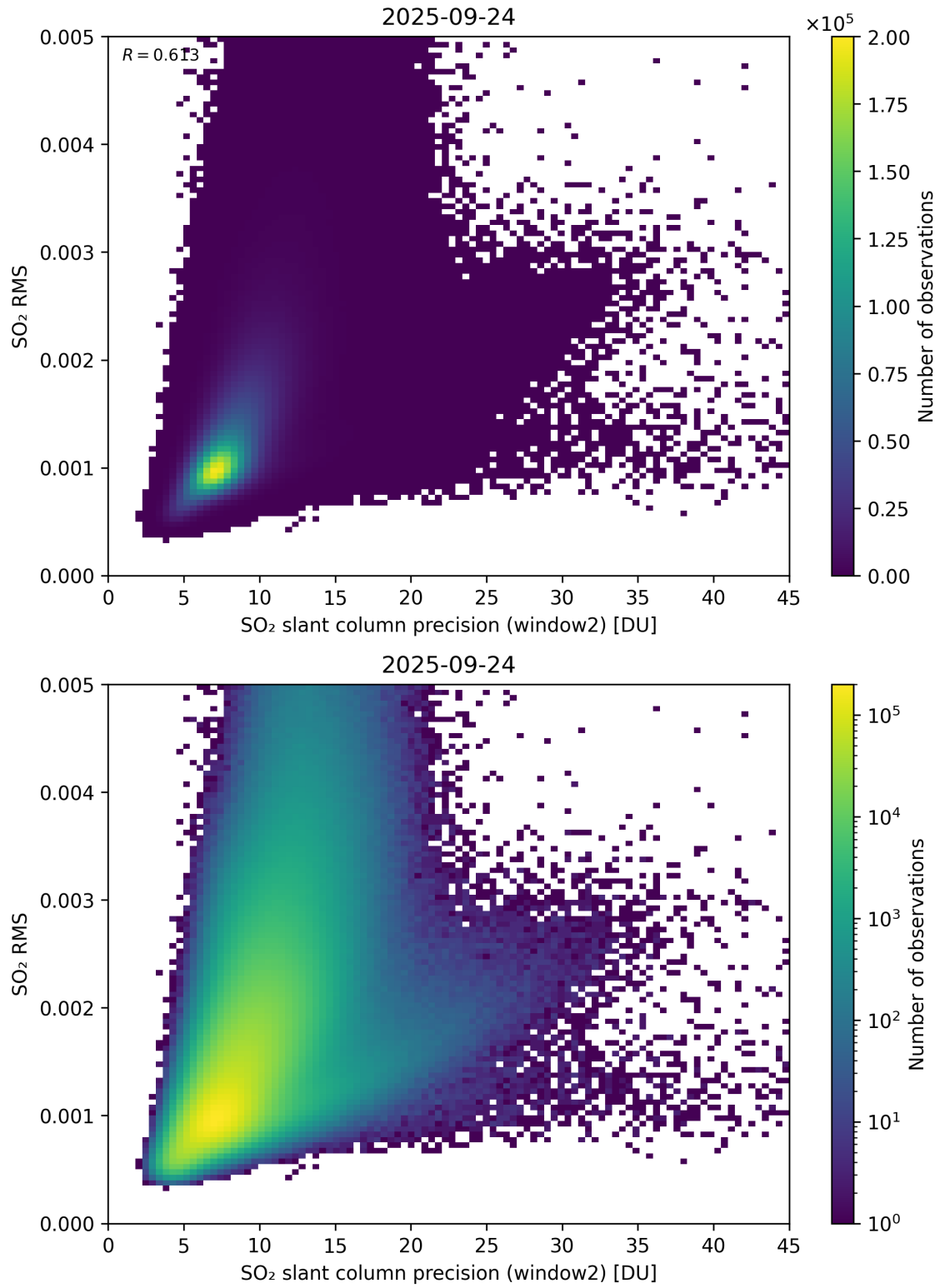
Figure 295: Scatter density plot of “SO 2 slant column precision (window2)” against “SO 2 RMS” for 2025-09-23 to 2025-09-25.
