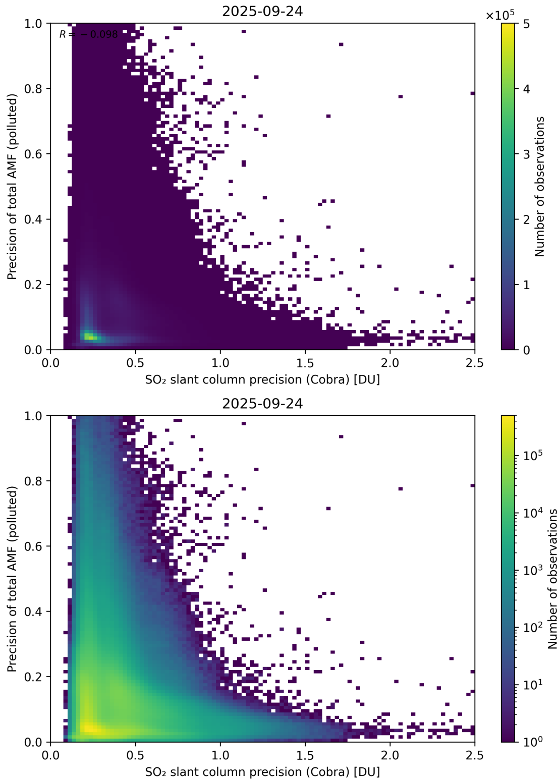
Figure 214: Scatter density plot of “SO 2 slant column precision (Cobra)” against “Precision of total AMF (polluted)” for 2025-09-23 to 2025-09-25.
