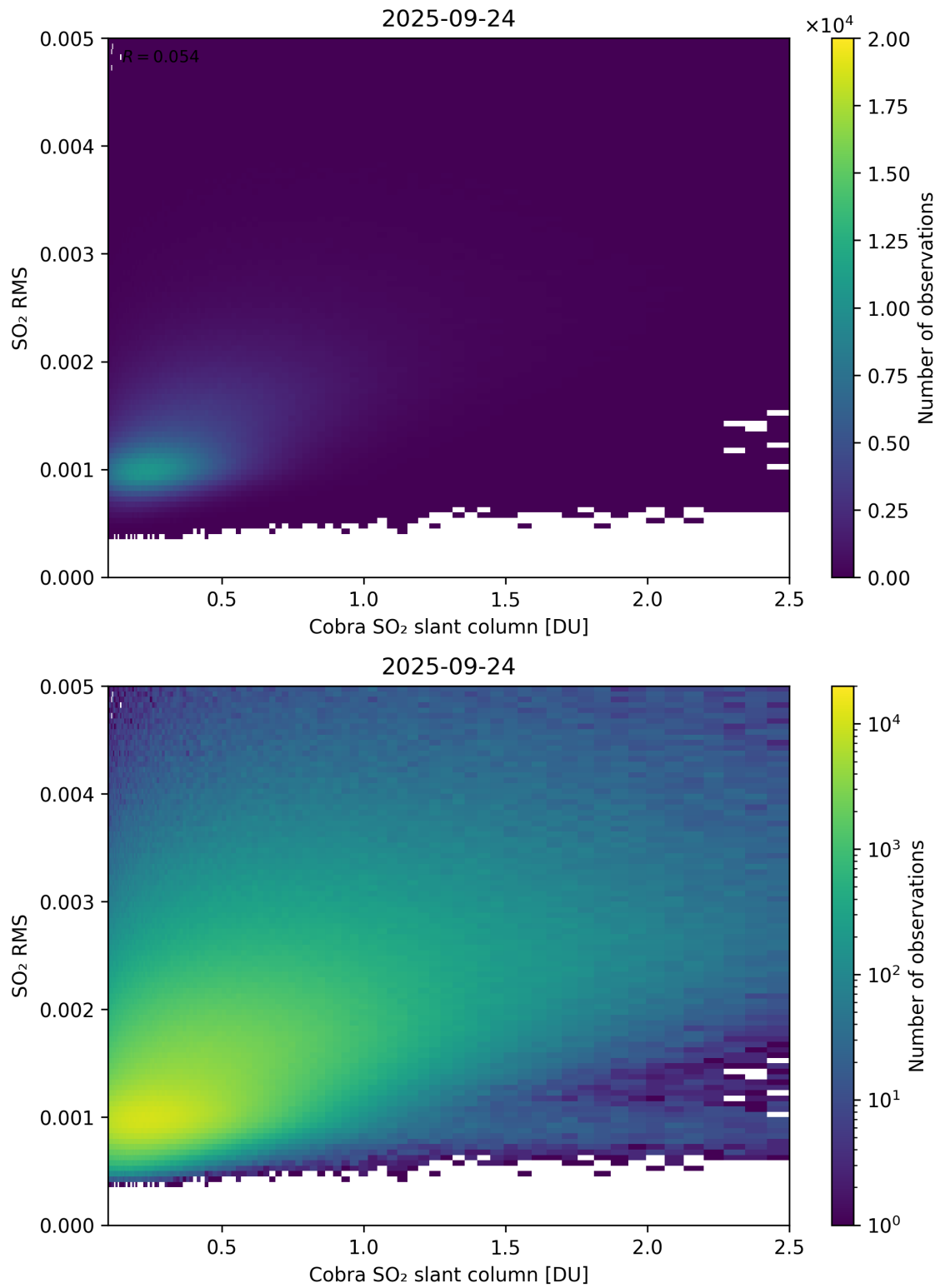
Figure 198: Scatter density plot of “Cobra SO 2 slant column” against “SO 2 RMS” for 2025-09-23 to 2025-09-25.
