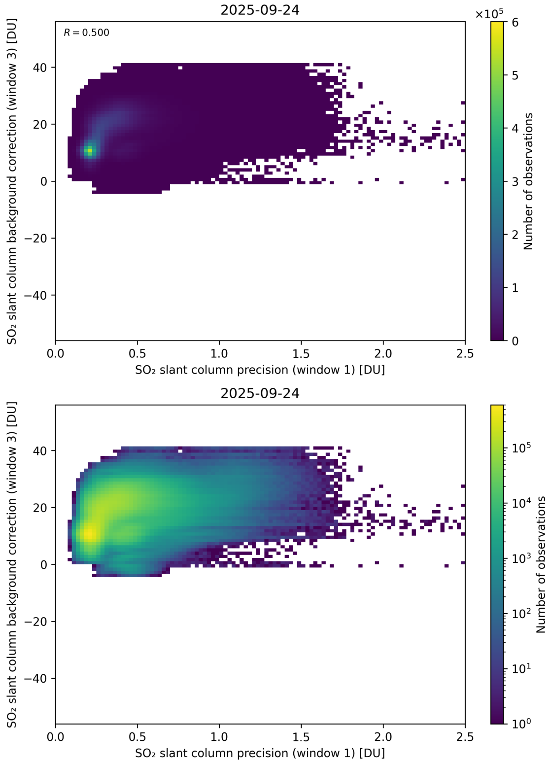
Figure 270: Scatter density plot of “SO 2 slant column precision (window 1)” against “SO 2 slant column background correction (window 3)” for 2025-09-23 to 2025-09-25.
