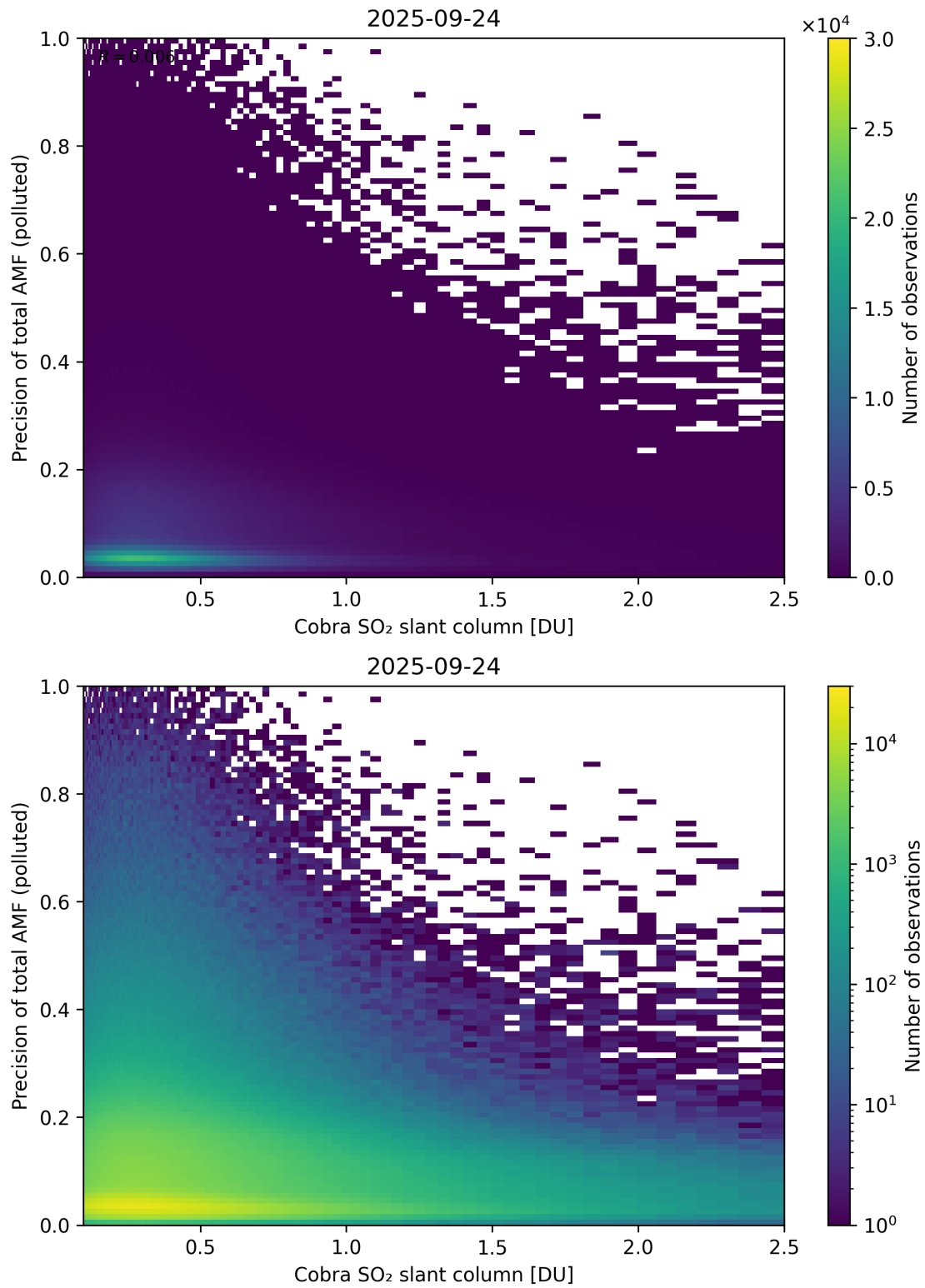
Figure 225: Scatter density plot of “Cobra SO 2 slant column” against “Precision of total AMF (polluted)” for 2025-09-23 to 2025-09-25.
