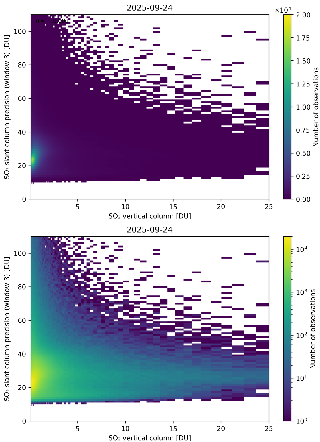
Figure 358: Scatter density plot of “SO 2 vertical column” against “SO 2 slant column precision (window 3)” for 2025-09-23 to 2025-09-25.
