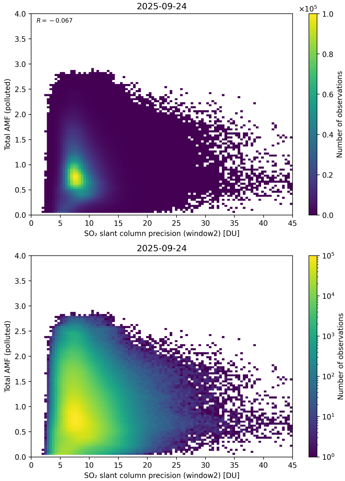
Figure 301: Scatter density plot of “SO 2 slant column precision (window2)” against “Total AMF (polluted)” for 2025-09-23 to 2025-09-25.
