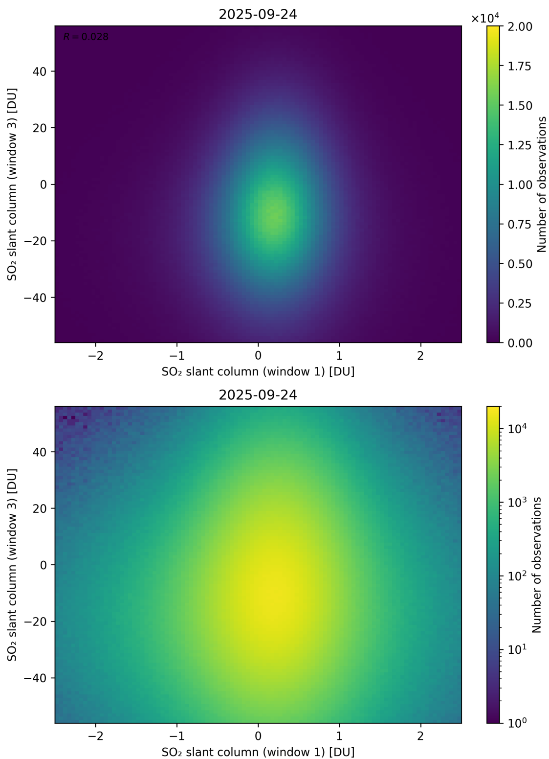
Figure 287: Scatter density plot of “SO 2 slant column (window 1)” against “SO 2 slant column (window 3)” for 2025-09-23 to 2025-09-25.
