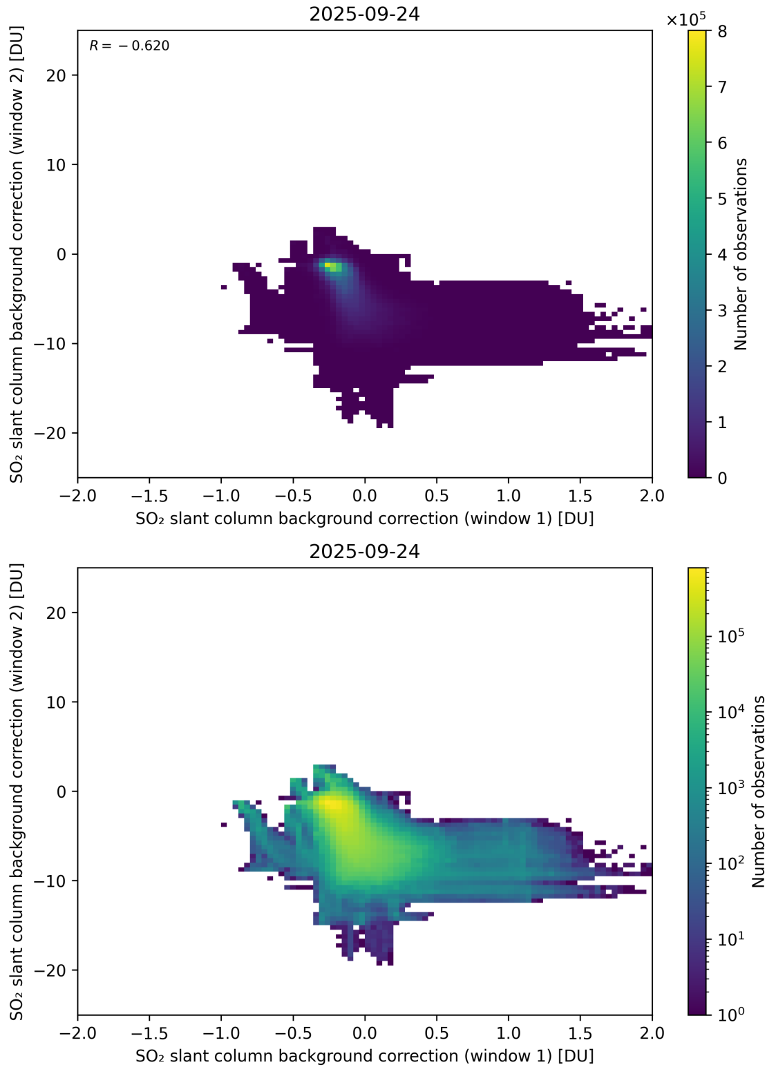
Figure 109: Scatter density plot of “SO 2 slant column background correction (window 1)” against “SO 2 slant column background correction (window 2)” for 2025-09-23 to 2025-09-25.
