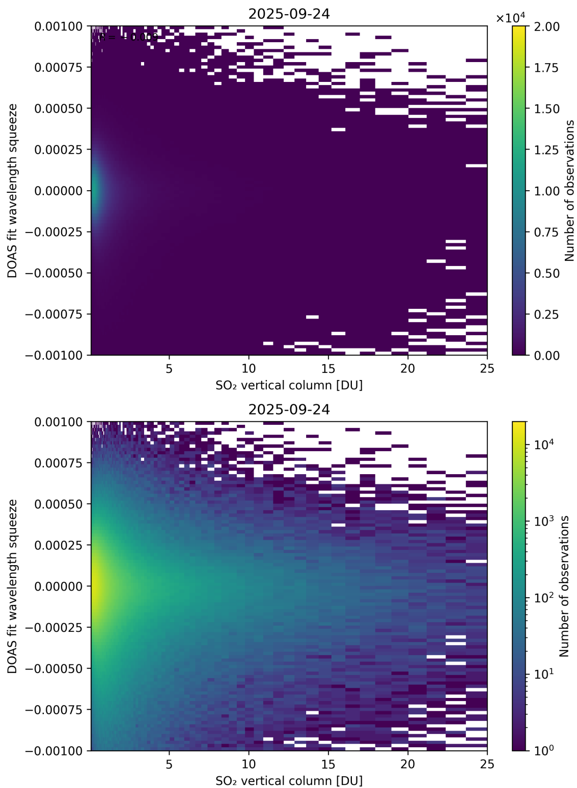
Figure 327: Scatter density plot of “SO 2 vertical column” against “DOAS fit wavelength squeeze” for 2025-09-23 to 2025-09-25.
