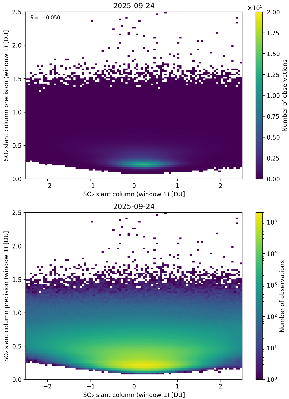
Figure 285: Scatter density plot of “SO 2 slant column (window 1)” against “SO 2 slant column precision (window 1)” for 2025-09-23 to 2025-09-25.
