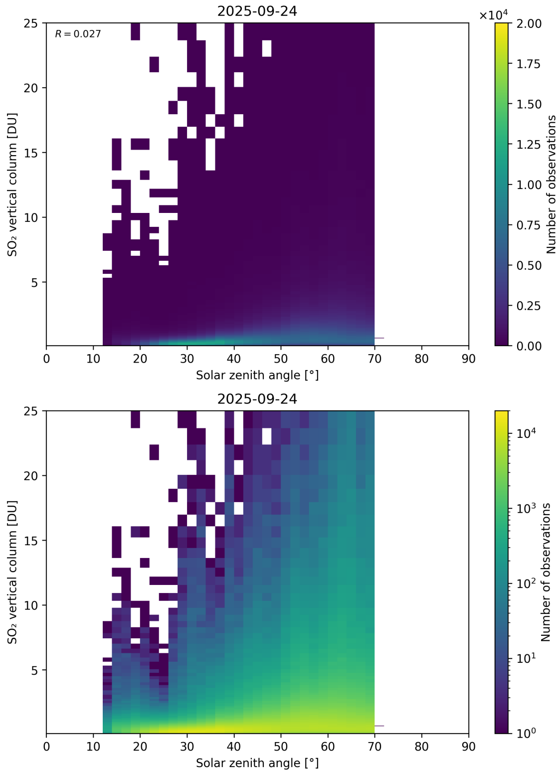
Figure 191: Scatter density plot of “Solar zenith angle” against “SO 2 vertical column” for 2025-09-23 to 2025-09-25.
