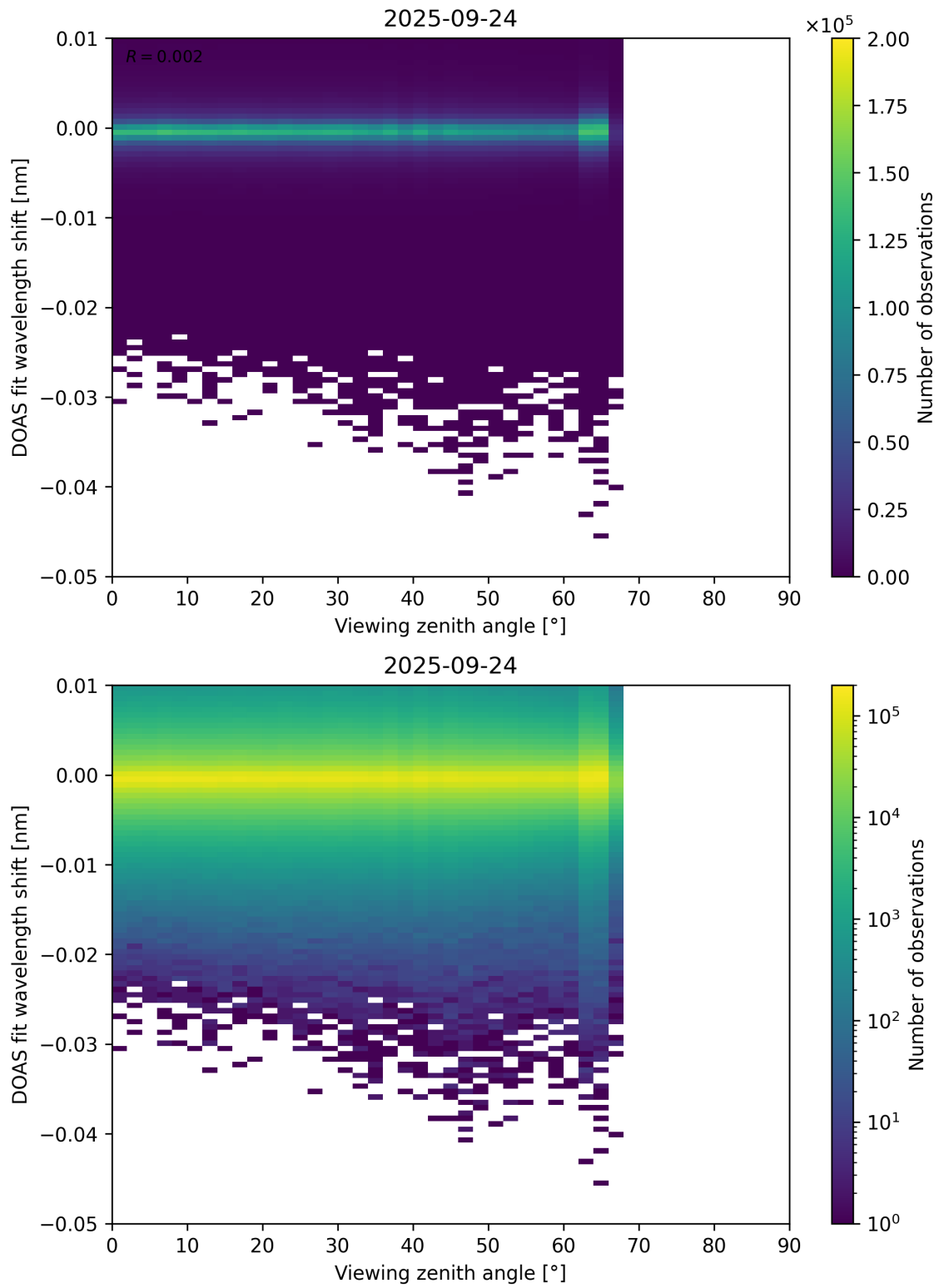
Figure 365: Scatter density plot of “Viewing zenith angle” against “DOAS fit wavelength shift” for 2025-09-23 to 2025-09-25.
