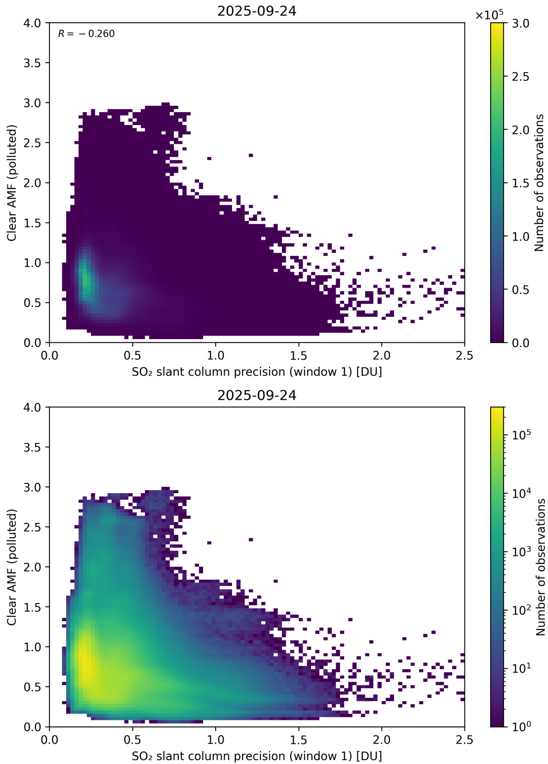
Figure 274: Scatter density plot of “SO 2 slant column precision (window 1)” against “Clear AMF (polluted)” for 2025-09-23 to 2025-09-25.
