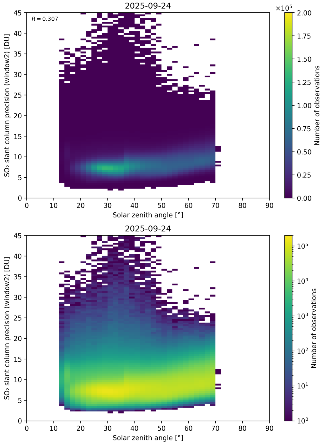
Figure 186: Scatter density plot of “Solar zenith angle” against “SO 2 slant column precision (window2)” for 2025-09-23 to 2025-09-25.
