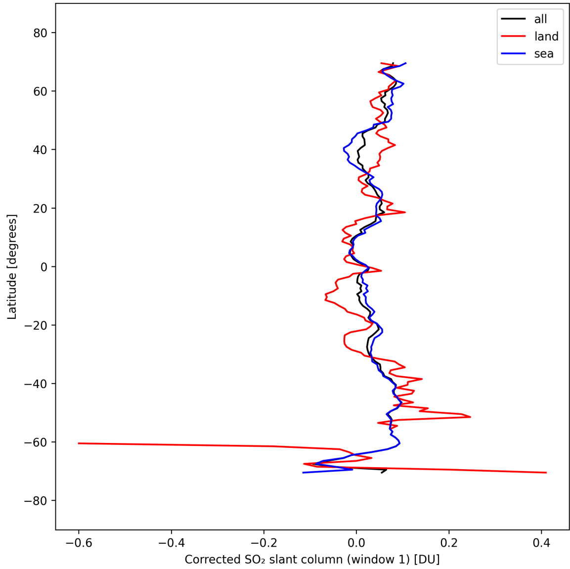
Figure 39: Zonal average of “Corrected SO 2 slant column (window 1)” for 2025-09-23 to 2025-09-25.
