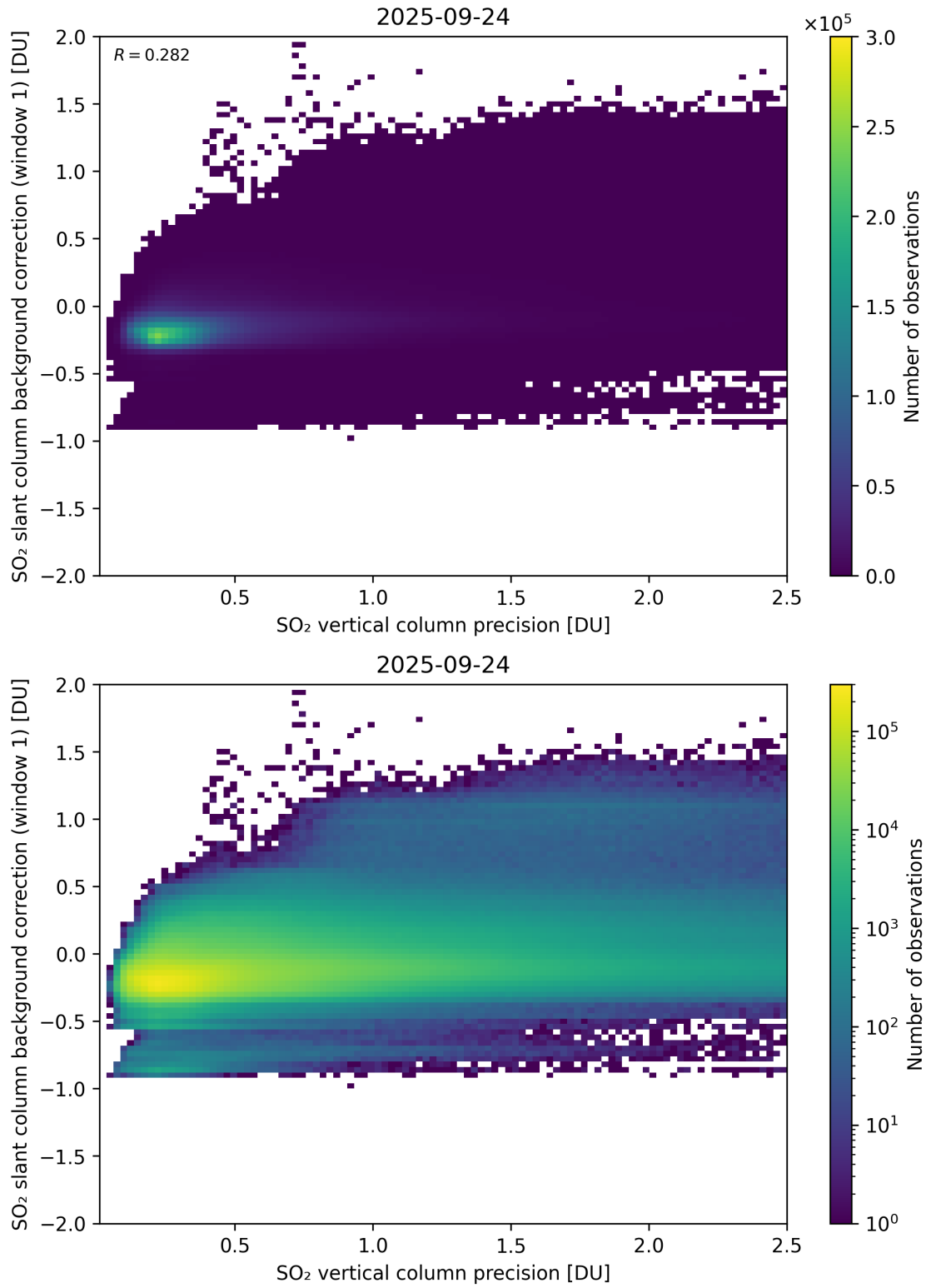
Figure 329: Scatter density plot of “SO 2 vertical column precision” against “SO 2 slant column background correction (window 1)” for 2025-09-23 to 2025-09-25.
