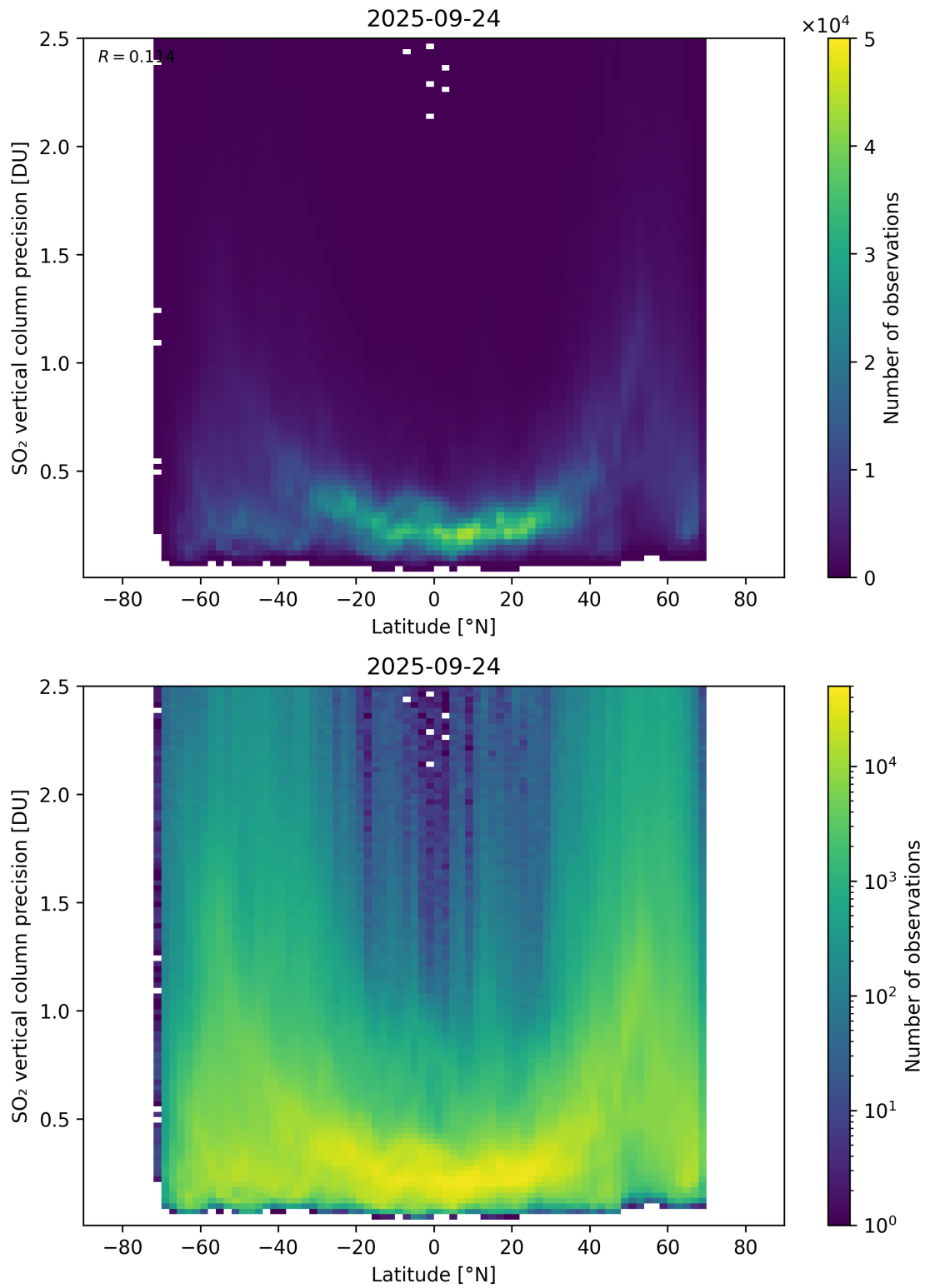
Figure 170: Scatter density plot of “Latitude” against “SO 2 vertical column precision” for 2025-09-23 to 2025-09-25.
