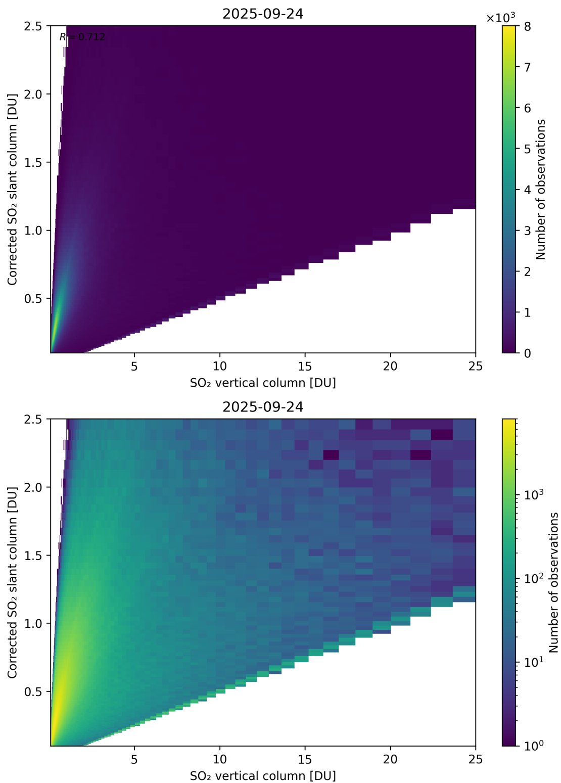
Figure 351: Scatter density plot of “SO 2 vertical column” against “Corrected SO 2 slant column” for 2025-09-23 to 2025-09-25.
