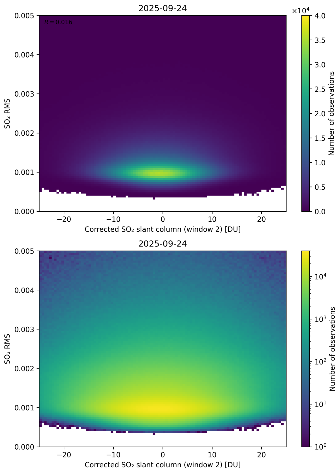
Figure 248: Scatter density plot of “Corrected SO 2 slant column (window 2)” against “SO 2 RMS” for 2025-09-23 to 2025-09-25.
