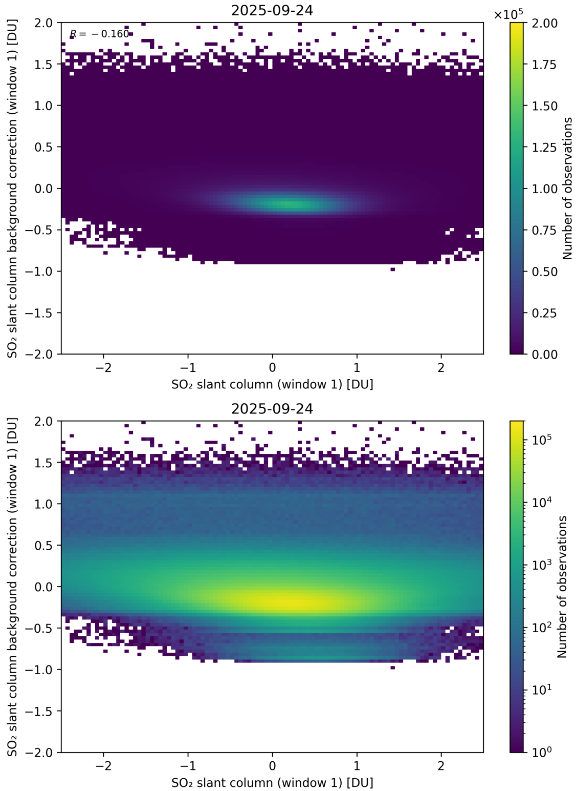
Figure 262: Scatter density plot of “SO 2 slant column (window 1)” against “SO 2 slant column background correction (window 1)” for 2025-09-23 to 2025-09-25.
