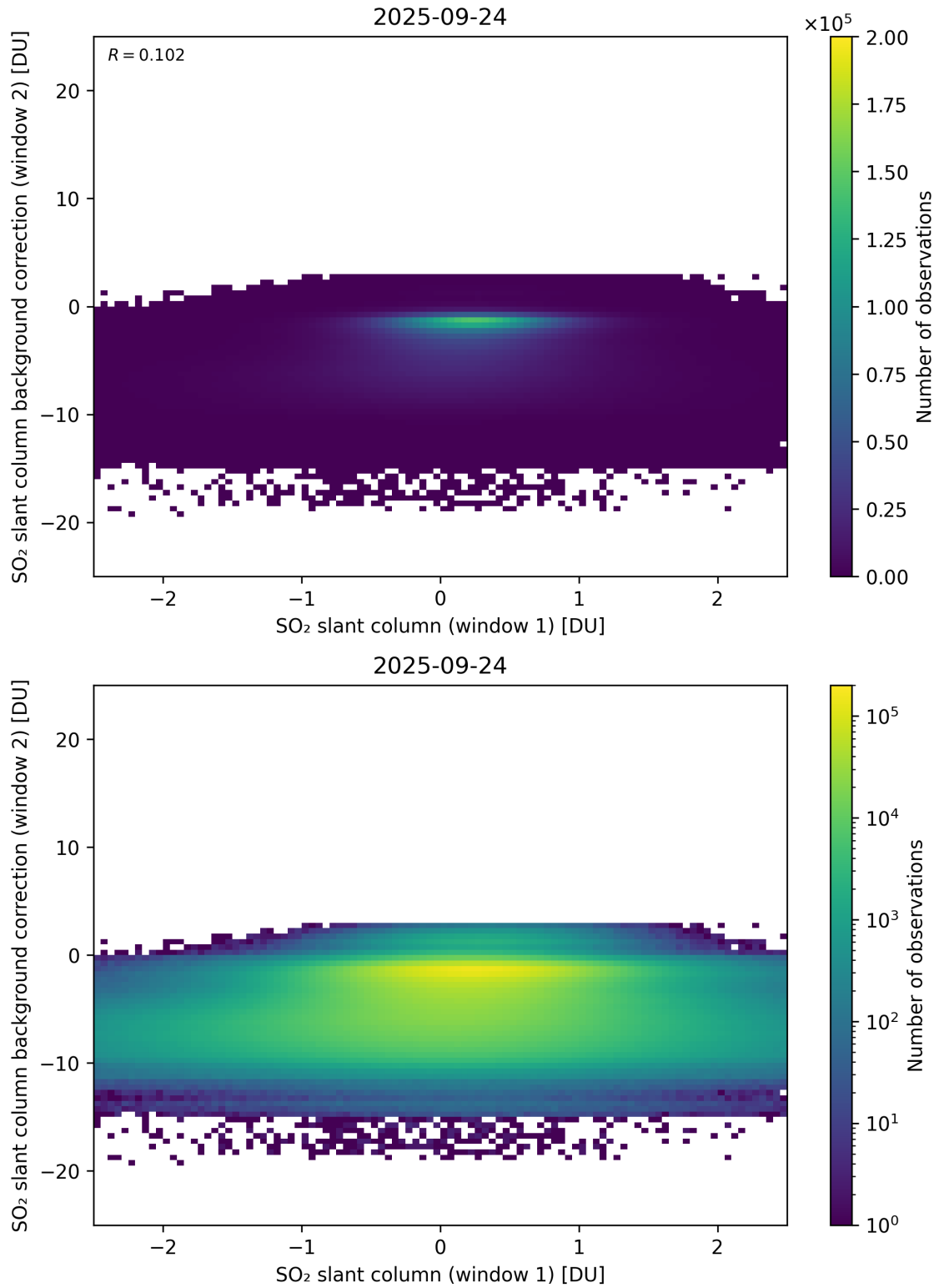
Figure 263: Scatter density plot of “SO 2 slant column (window 1)” against “SO 2 slant column background correction (window 2)” for 2025-09-23 to 2025-09-25.
