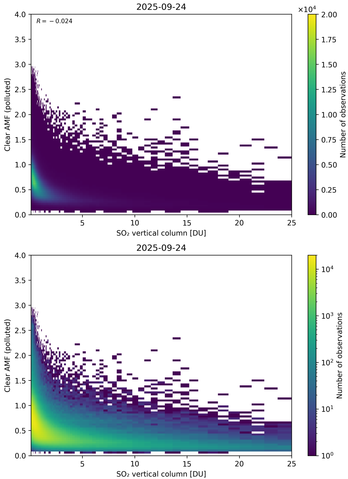
Figure 348: Scatter density plot of “SO 2 vertical column” against “Clear AMF (polluted)” for 2025-09-23 to 2025-09-25.
