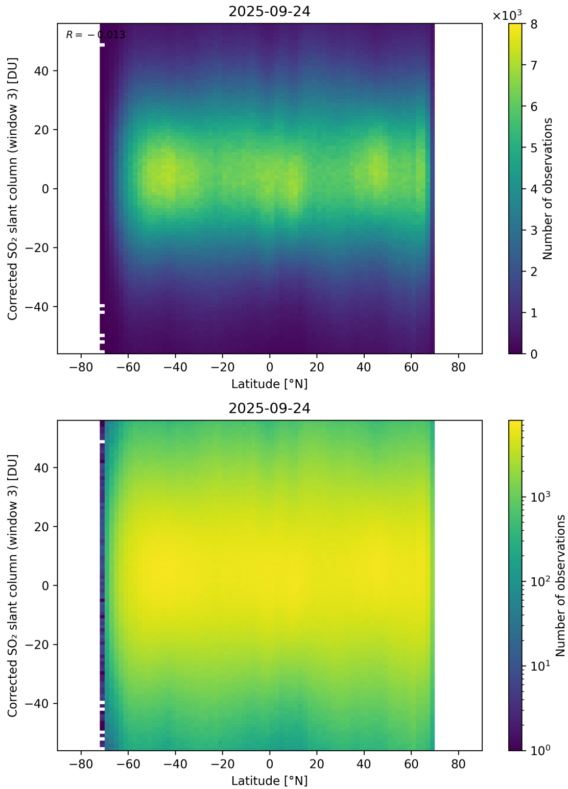
Figure 161: Scatter density plot of “Latitude” against “Corrected SO 2 slant column (window 3)” for 2025-09-23 to 2025-09-25.
