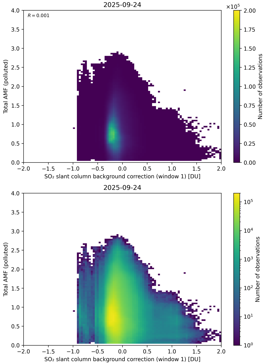
Figure 120: Scatter density plot of “SO 2 slant column background correction (window 1)” against “Total AMF (polluted)” for 2025-09-23 to 2025-09-25.
