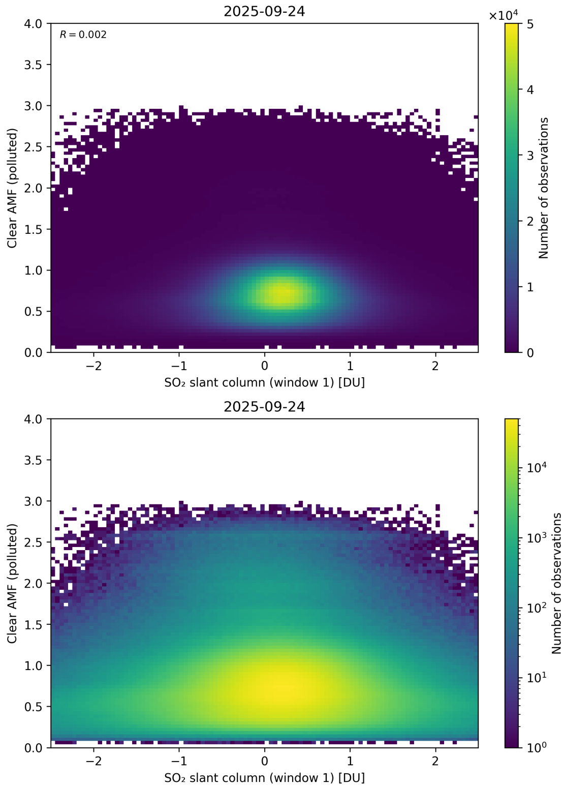
Figure 282: Scatter density plot of “SO 2 slant column (window 1)” against “Clear AMF (polluted)” for 2025-09-23 to 2025-09-25.
