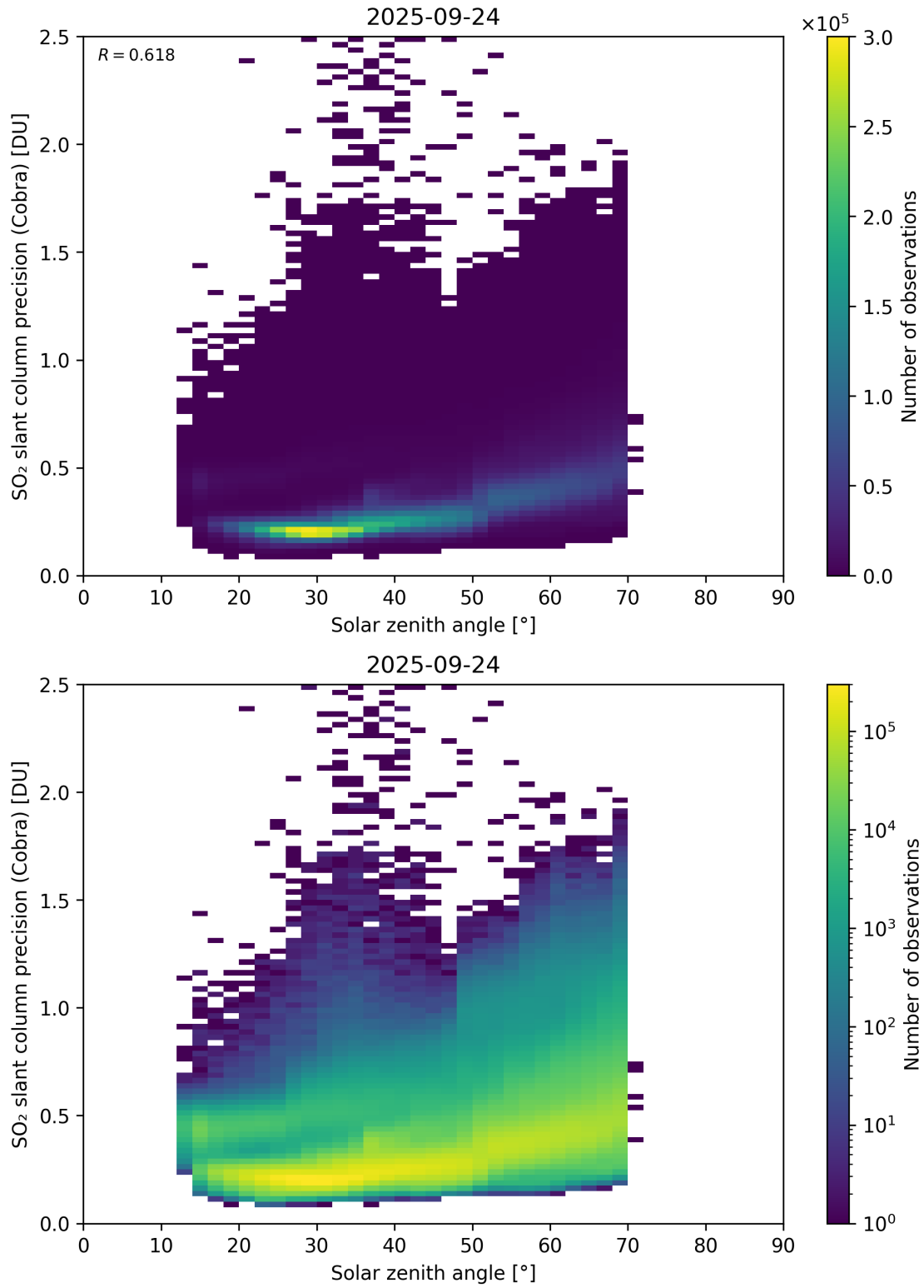
Figure 180: Scatter density plot of “Solar zenith angle” against “SO 2 slant column precision (Cobra)” for 2025-09-23 to 2025-09-25.
