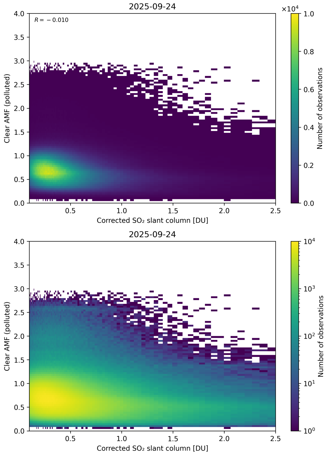
Figure 232: Scatter density plot of “Corrected SO 2 slant column” against “Clear AMF (polluted)” for 2025-09-23 to 2025-09-25.
