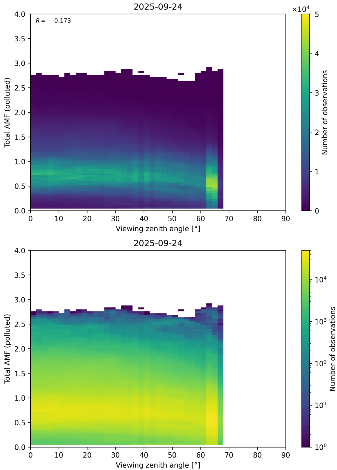
Figure 381: Scatter density plot of “Viewing zenith angle” against “Total AMF (polluted)” for 2025-09-23 to 2025-09-25.
