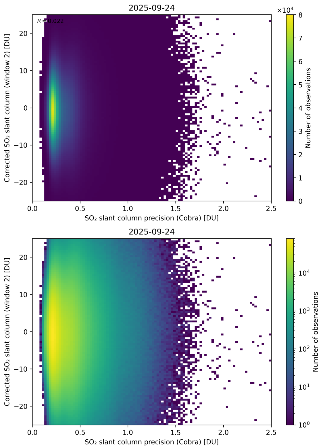
Figure 206: Scatter density plot of “SO 2 slant column precision (Cobra)” against “Corrected SO 2 slant column (window 2)” for 2025-09-23 to 2025-09-25.
