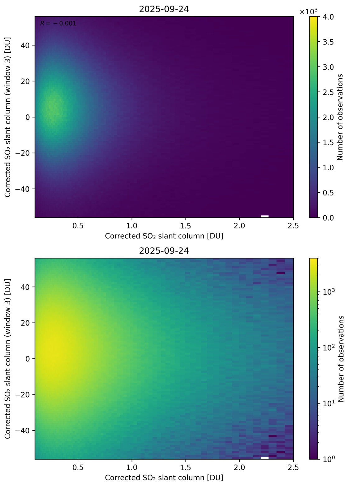
Figure 236: Scatter density plot of “Corrected SO 2 slant column” against “Corrected SO 2 slant column (window 3)” for 2025-09-23 to 2025-09-25.
