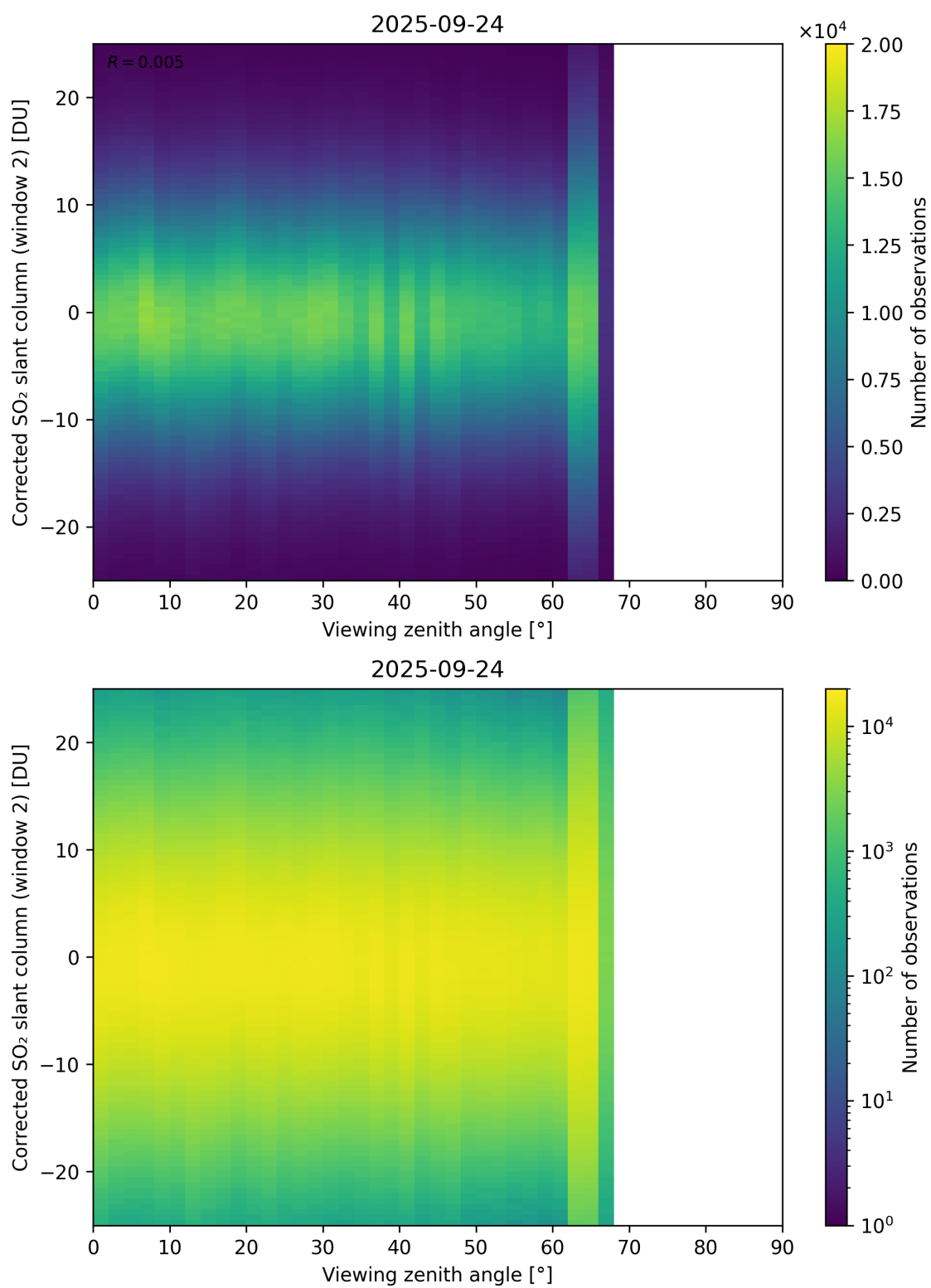
Figure 374: Scatter density plot of “Viewing zenith angle” against “Corrected SO 2 slant column (window 2)” for 2025-09-23 to 2025-09-25.
