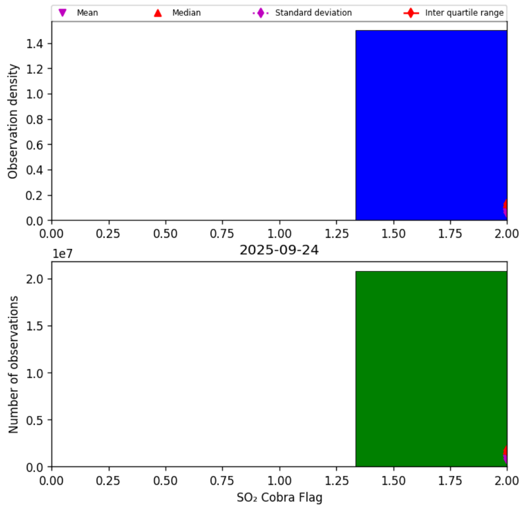
Figure 75: Histogram of “SO 2 Cobra Flag” for 2025-09-23 to 2025-09-25
