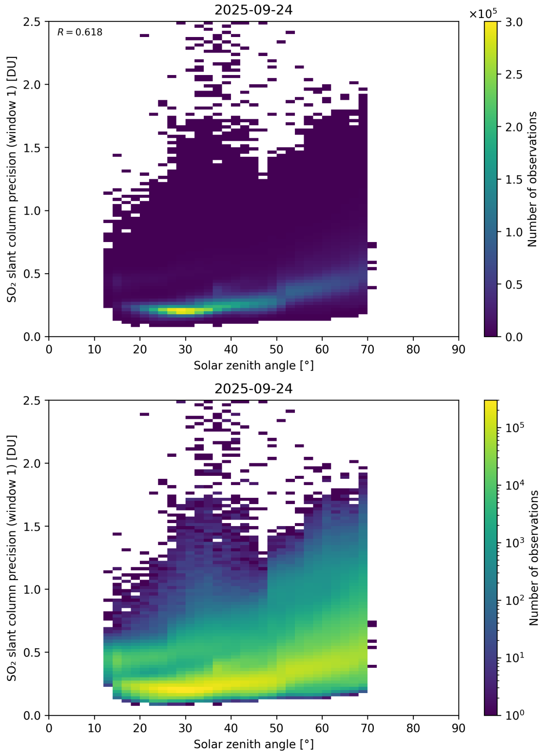
Figure 185: Scatter density plot of “Solar zenith angle” against “SO 2 slant column precision (window 1)” for 2025-09-23 to 2025-09-25.
