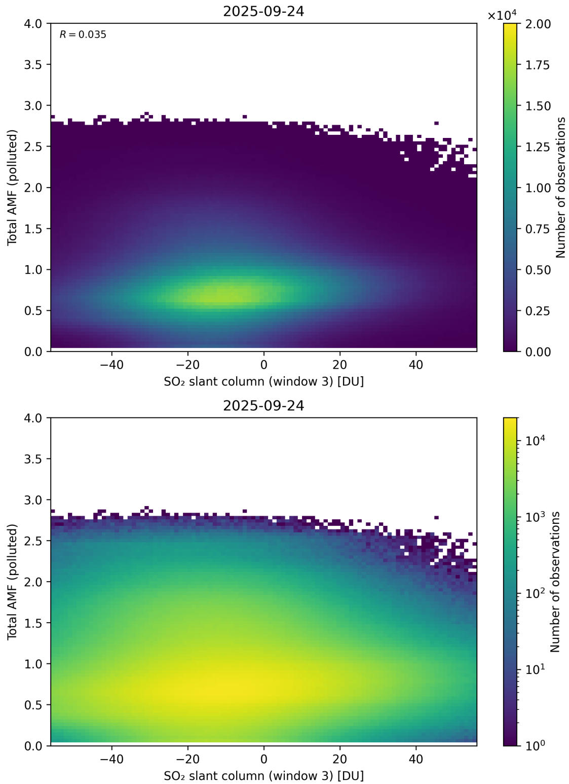
Figure 318: Scatter density plot of “SO 2 slant column (window 3)” against “Total AMF (polluted)” for 2025-09-23 to 2025-09-25.
