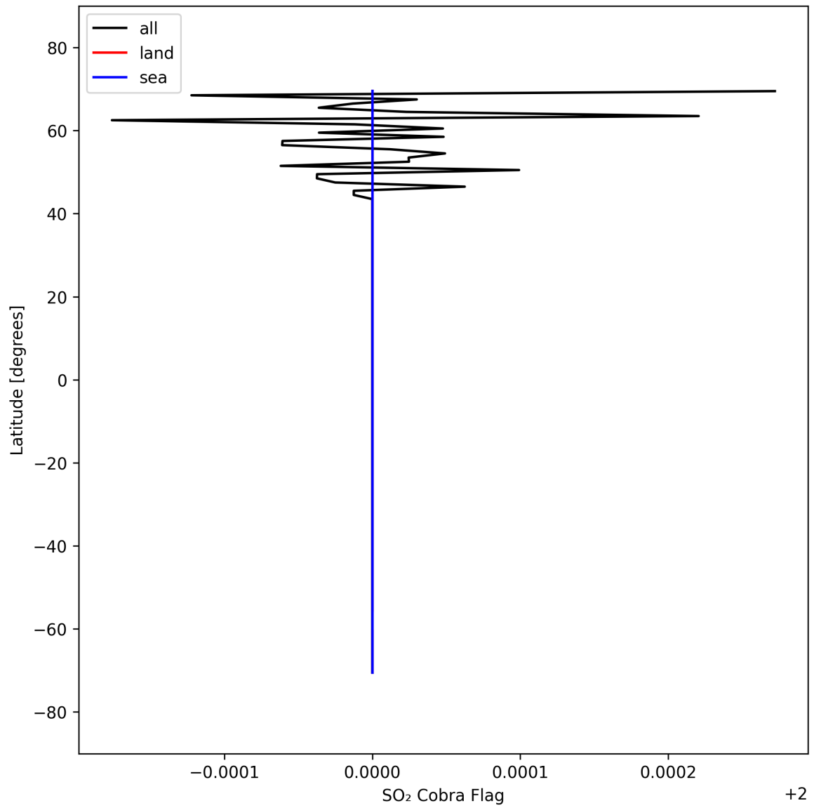
Figure 49: Zonal average of “SO 2 Cobra Flag” for 2025-09-23 to 2025-09-25.
