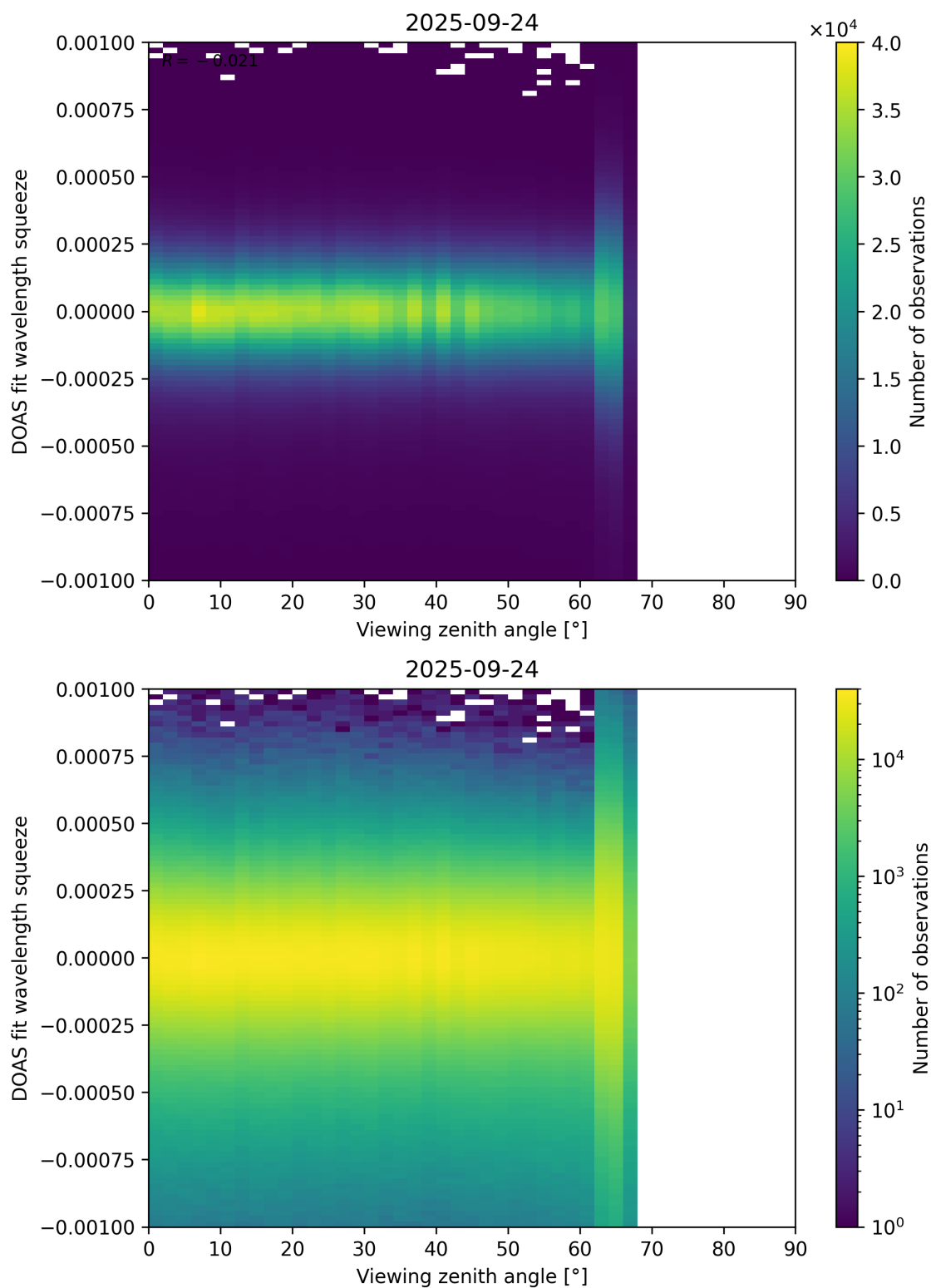
Figure 366: Scatter density plot of “Viewing zenith angle” against “DOAS fit wavelength squeeze” for 2025-09-23 to 2025-09-25.
