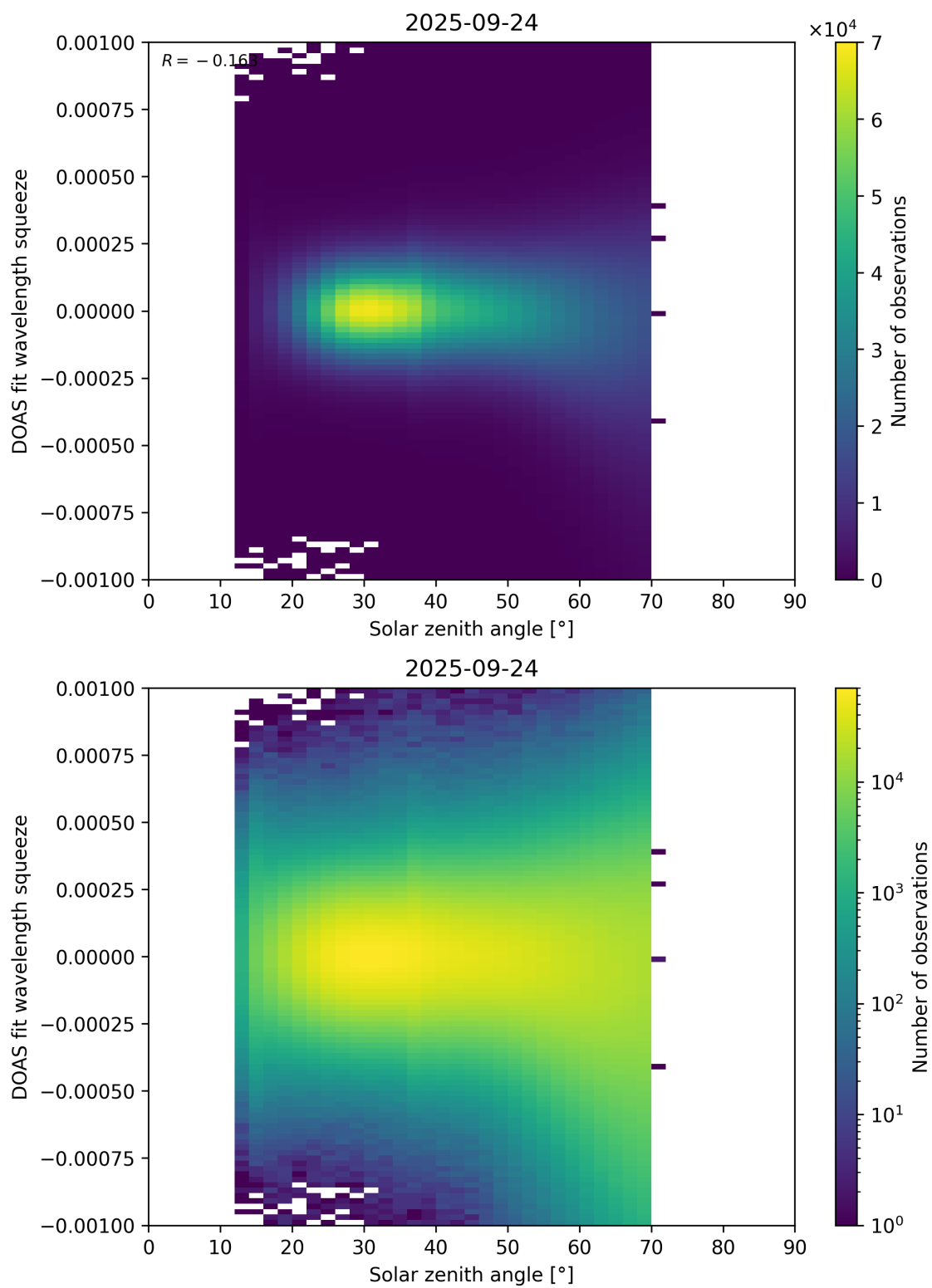
Figure 175: Scatter density plot of “Solar zenith angle” against “DOAS fit wavelength squeeze” for 2025-09-23 to 2025-09-25.
