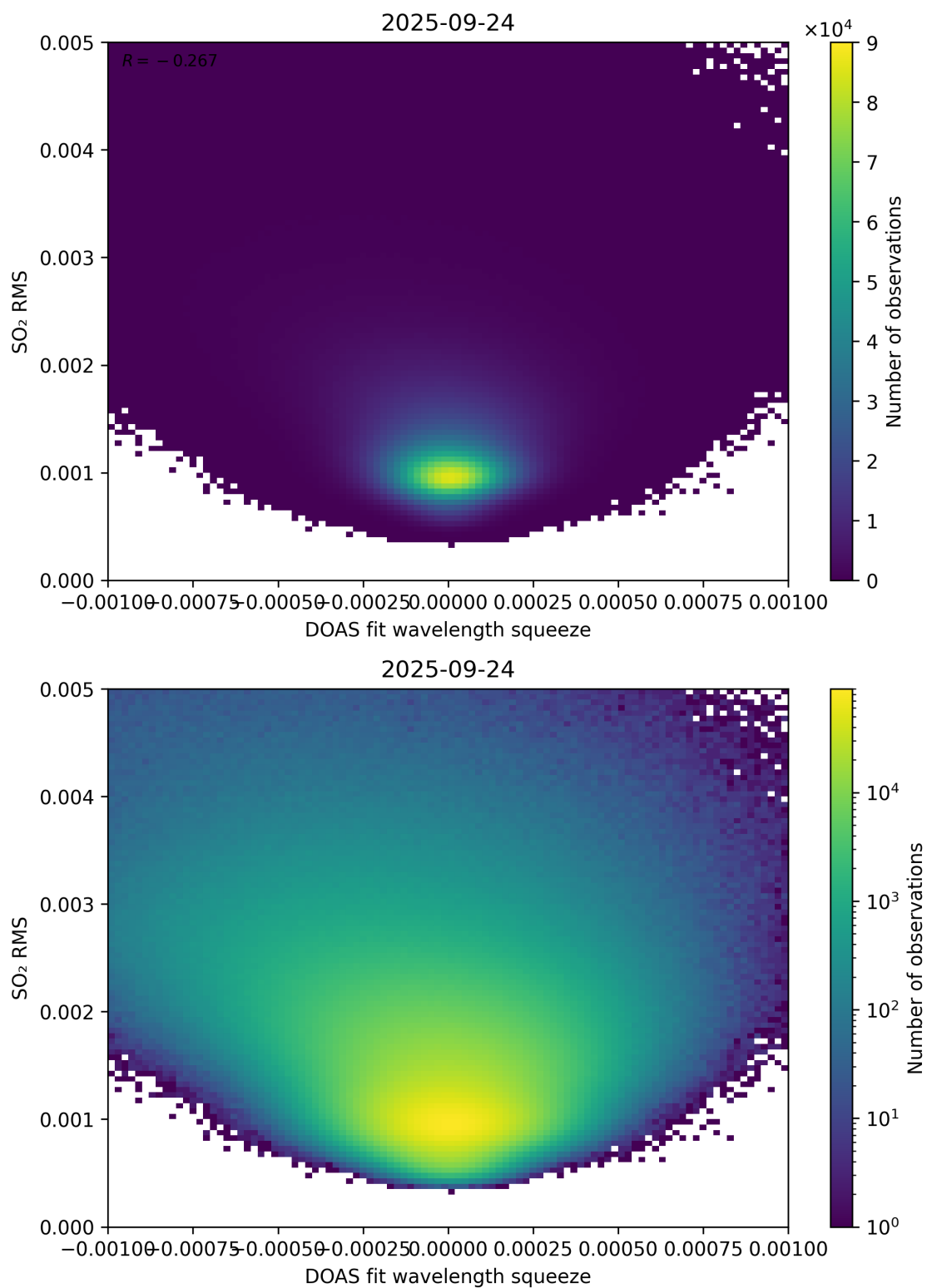
Figure 143: Scatter density plot of “DOAS fit wavelength squeeze” against “SO 2 RMS” for 2025-09-23 to 2025-09-25.
