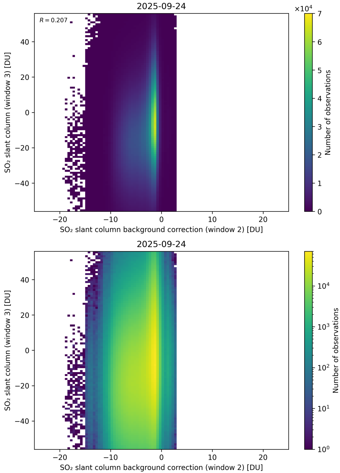
Figure 128: Scatter density plot of “SO 2 slant column background correction (window 2)” against “SO 2 slant column (window 3)” for 2025-09-23 to 2025-09-25.
