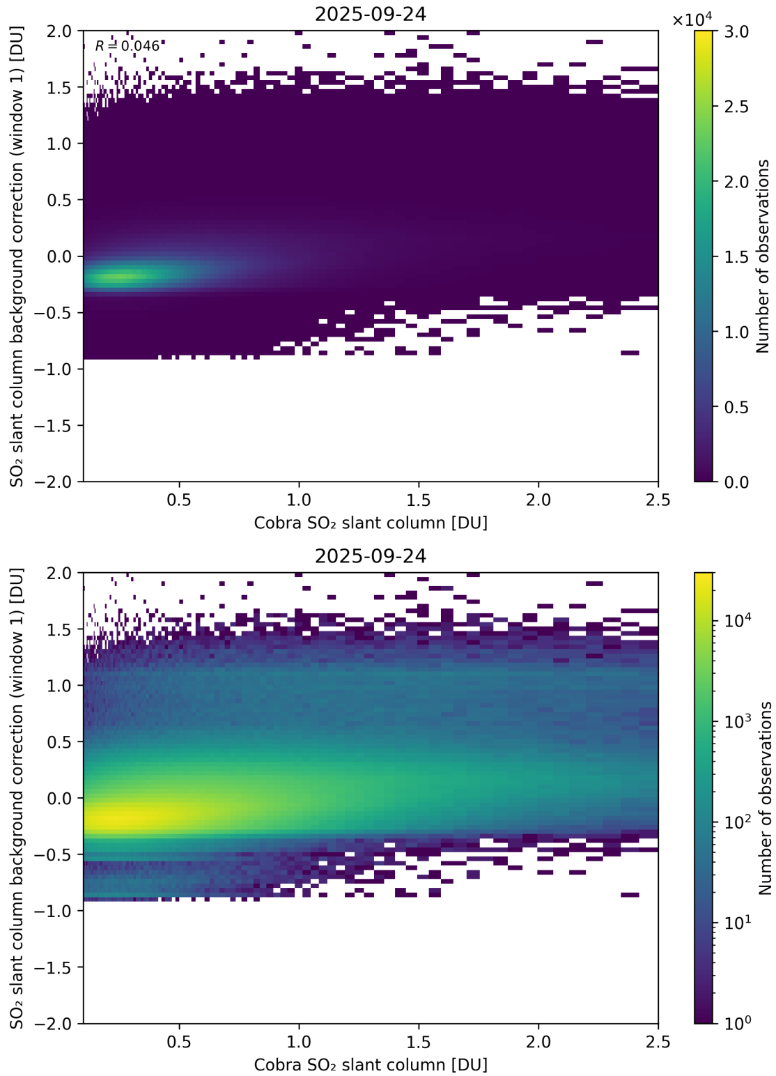
Figure 193: Scatter density plot of “Cobra SO 2 slant column” against “SO 2 slant column background correction (window 1)” for 2025-09-23 to 2025-09-25.
