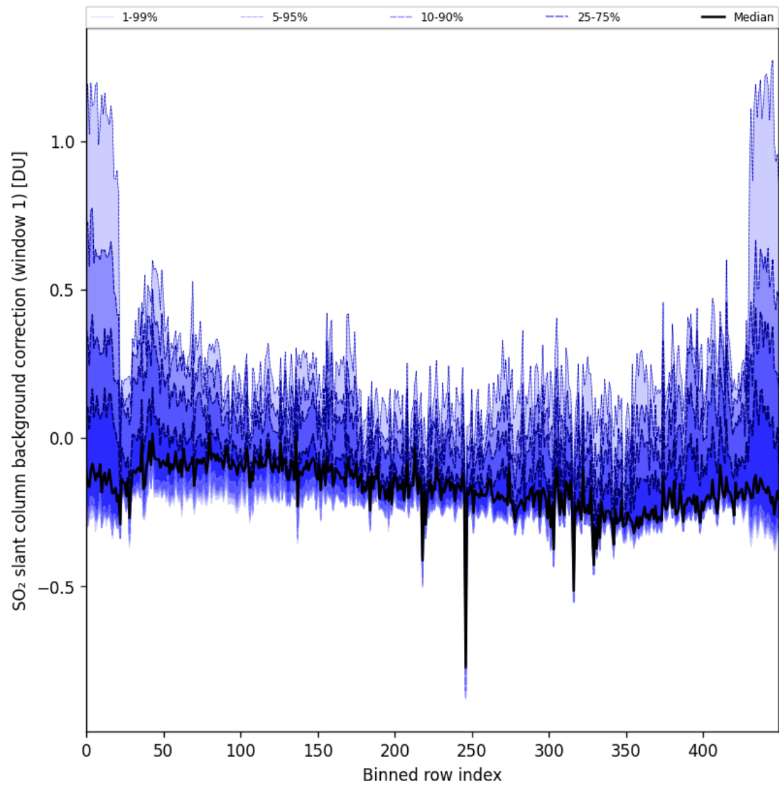
Figure 92: Along track statistics of “SO 2 slant column background correction (window 1)” for 2025-09-23 to 2025-09-25
