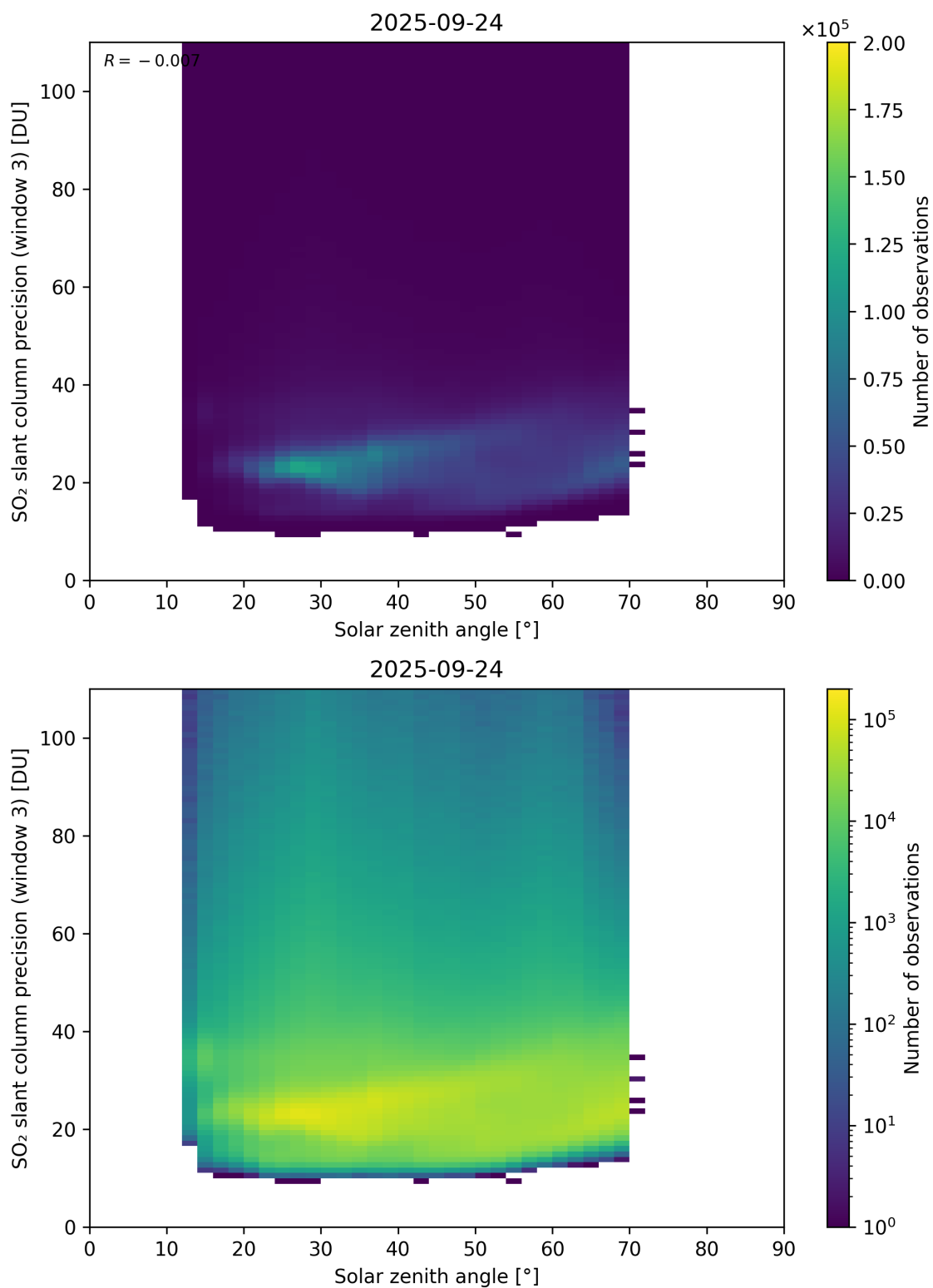
Figure 188: Scatter density plot of “Solar zenith angle” against “SO 2 slant column precision (window 3)” for 2025-09-23 to 2025-09-25.
