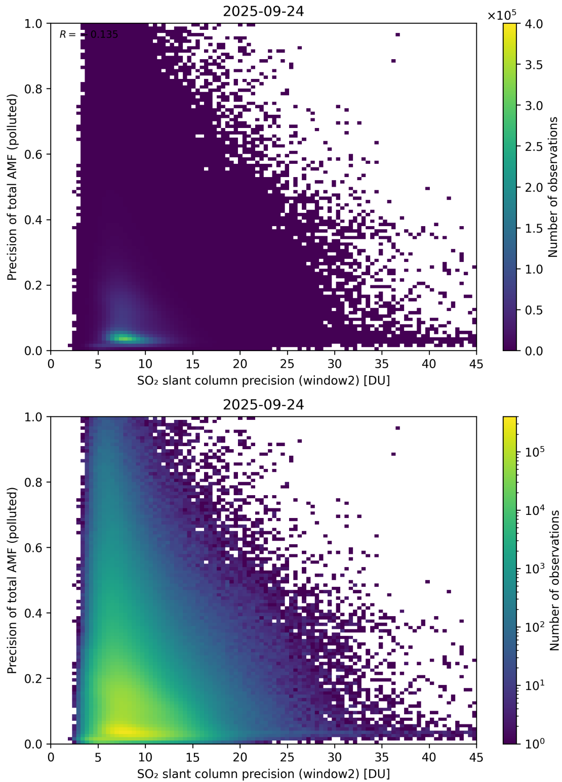
Figure 302: Scatter density plot of “SO 2 slant column precision (window2)” against “Precision of total AMF (polluted)” for 2025-09-23 to 2025-09-25.
