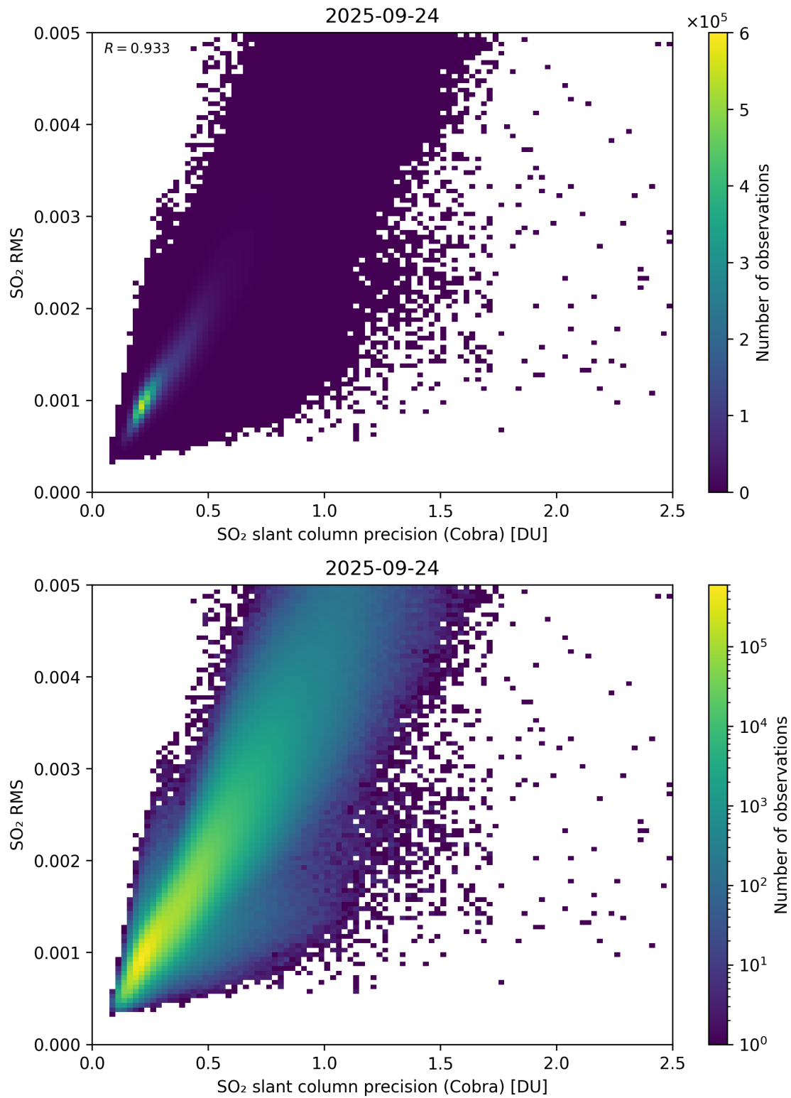
Figure 204: Scatter density plot of “SO 2 slant column precision (Cobra)” against “SO 2 RMS” for 2025-09-23 to 2025-09-25.
