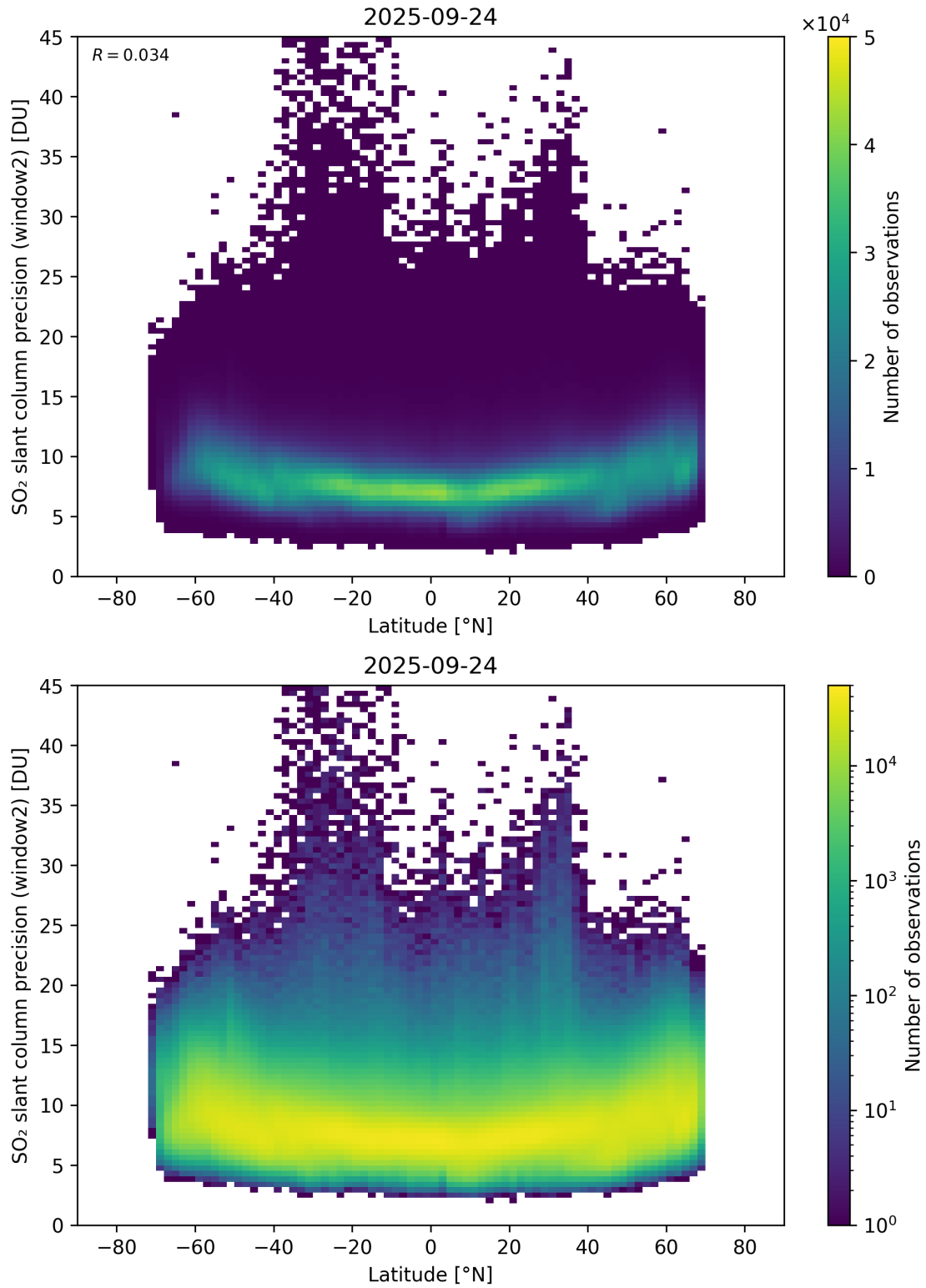
Figure 164: Scatter density plot of “Latitude” against “SO 2 slant column precision (window2)” for 2025-09-23 to 2025-09-25.
