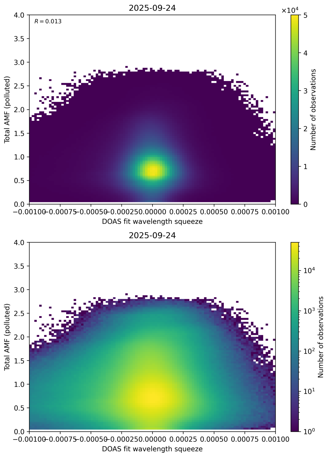
Figure 145: Scatter density plot of “DOAS fit wavelength squeeze” against “Total AMF (polluted)” for 2025-09-23 to 2025-09-25.
