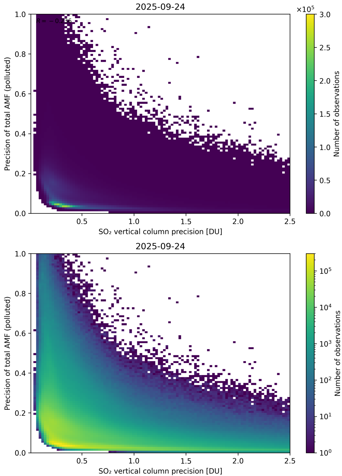
Figure 347: Scatter density plot of “SO 2 vertical column precision” against “Precision of total AMF (polluted)” for 2025-09-23 to 2025-09-25.
