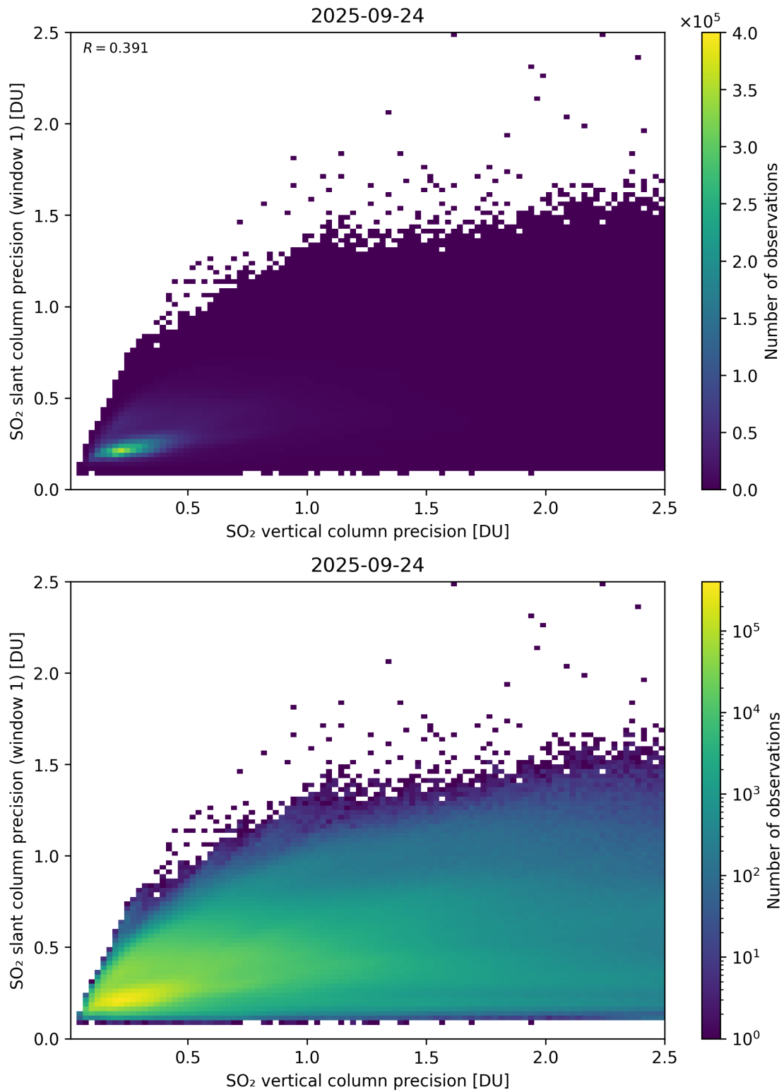
Figure 342: Scatter density plot of “SO 2 vertical column precision” against “SO 2 slant column precision (window 1)” for 2025-09-23 to 2025-09-25.
