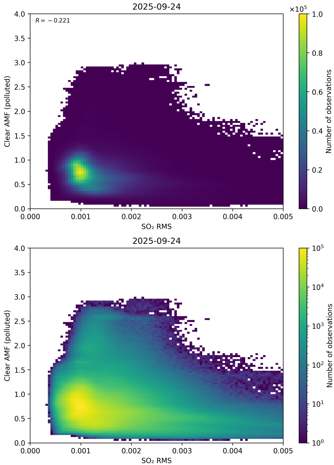
Figure 147: Scatter density plot of “SO 2 RMS” against “Clear AMF (polluted)” for 2025-09-23 to 2025-09-25.
