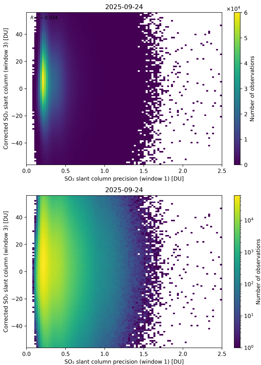
Figure 276: Scatter density plot of “SO 2 slant column precision (window 1)” against “Corrected SO 2 slant column (window 3)” for 2025-09-23 to 2025-09-25.
