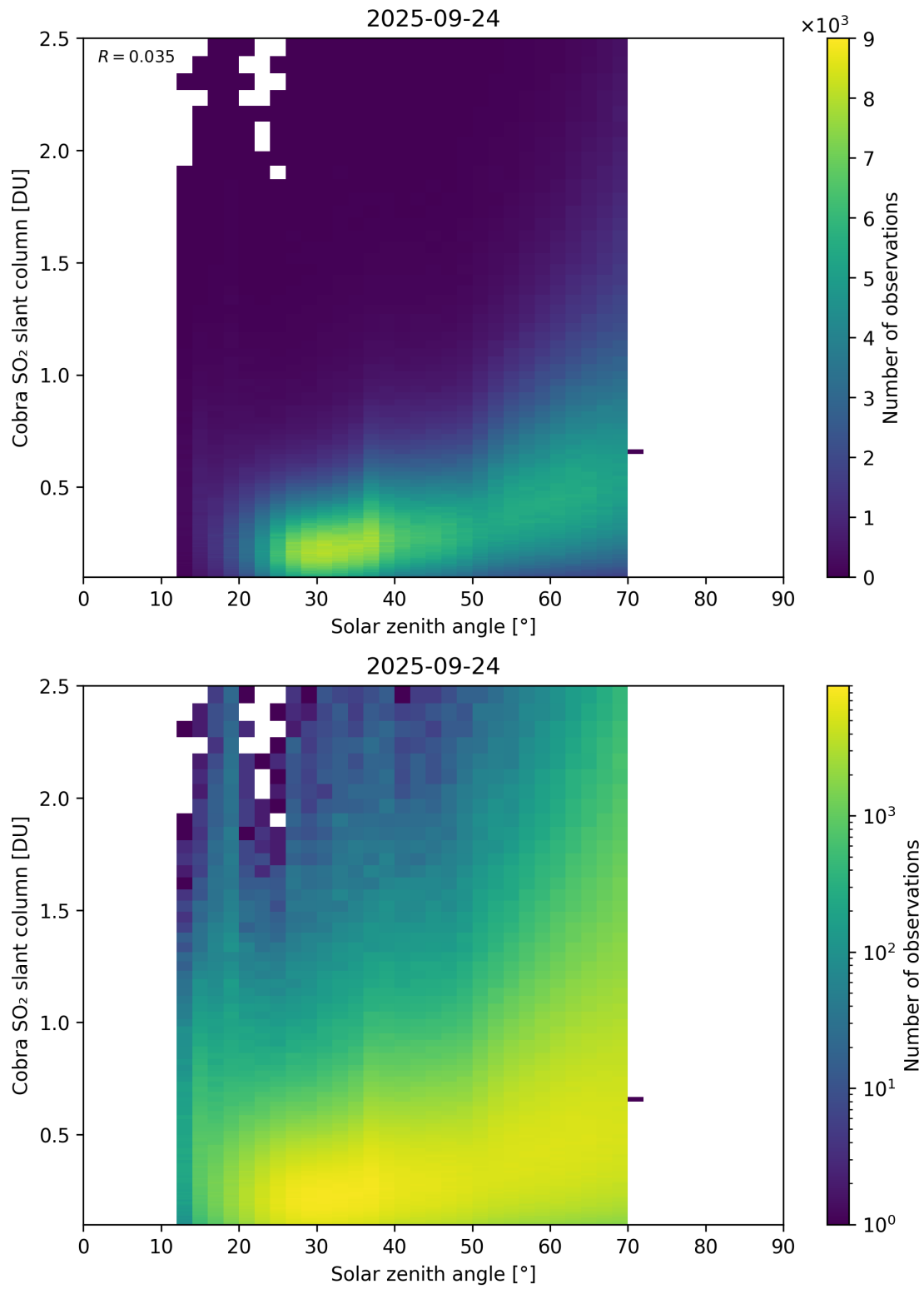
Figure 179: Scatter density plot of “Solar zenith angle” against “Cobra SO 2 slant column” for 2025-09-23 to 2025-09-25.
