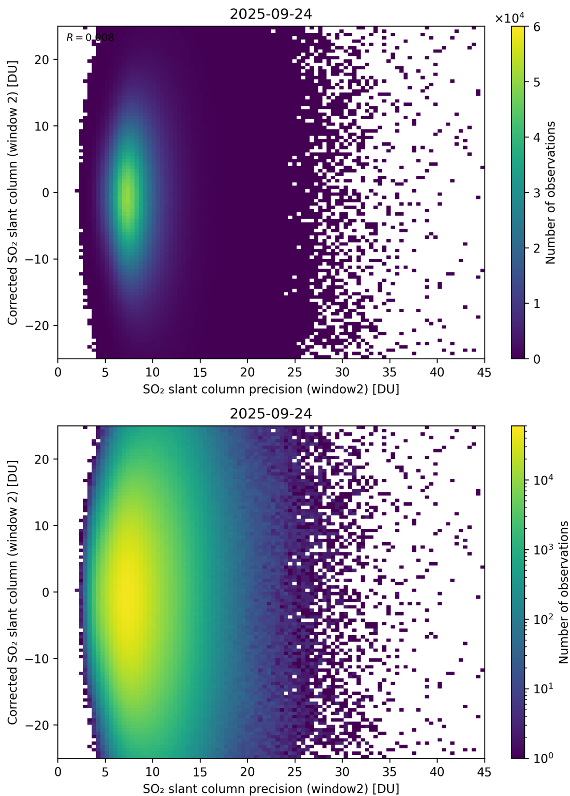
Figure 297: Scatter density plot of “SO 2 slant column precision (window2)” against “Corrected SO 2 slant column (window 2)” for 2025-09-23 to 2025-09-25.
