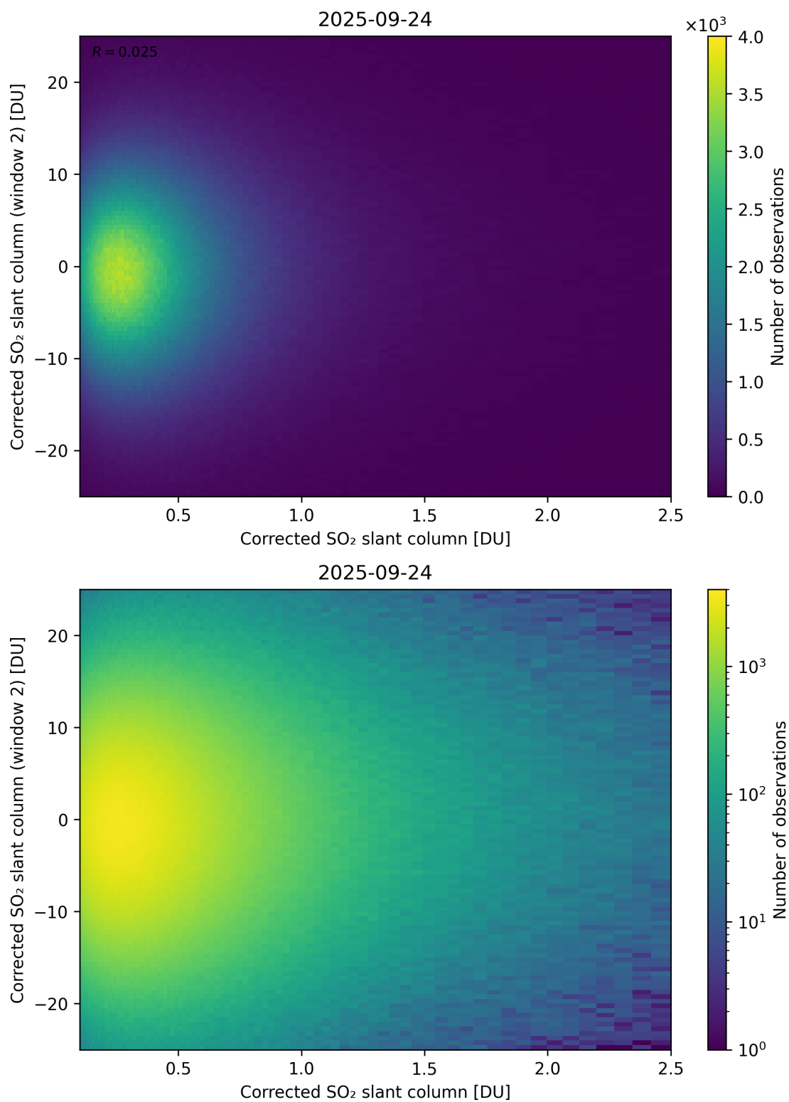
Figure 235: Scatter density plot of “Corrected SO 2 slant column” against “Corrected SO 2 slant column (window 2)” for 2025-09-23 to 2025-09-25.
