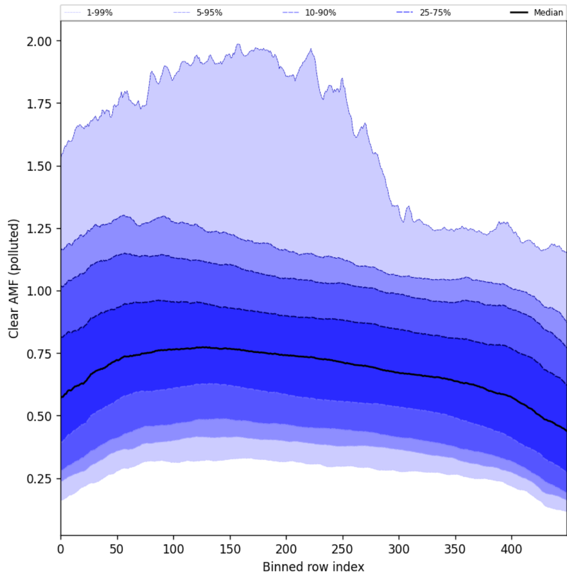
Figure 107: Along track statistics of “Clear AMF (polluted)” for 2025-09-23 to 2025-09-25
