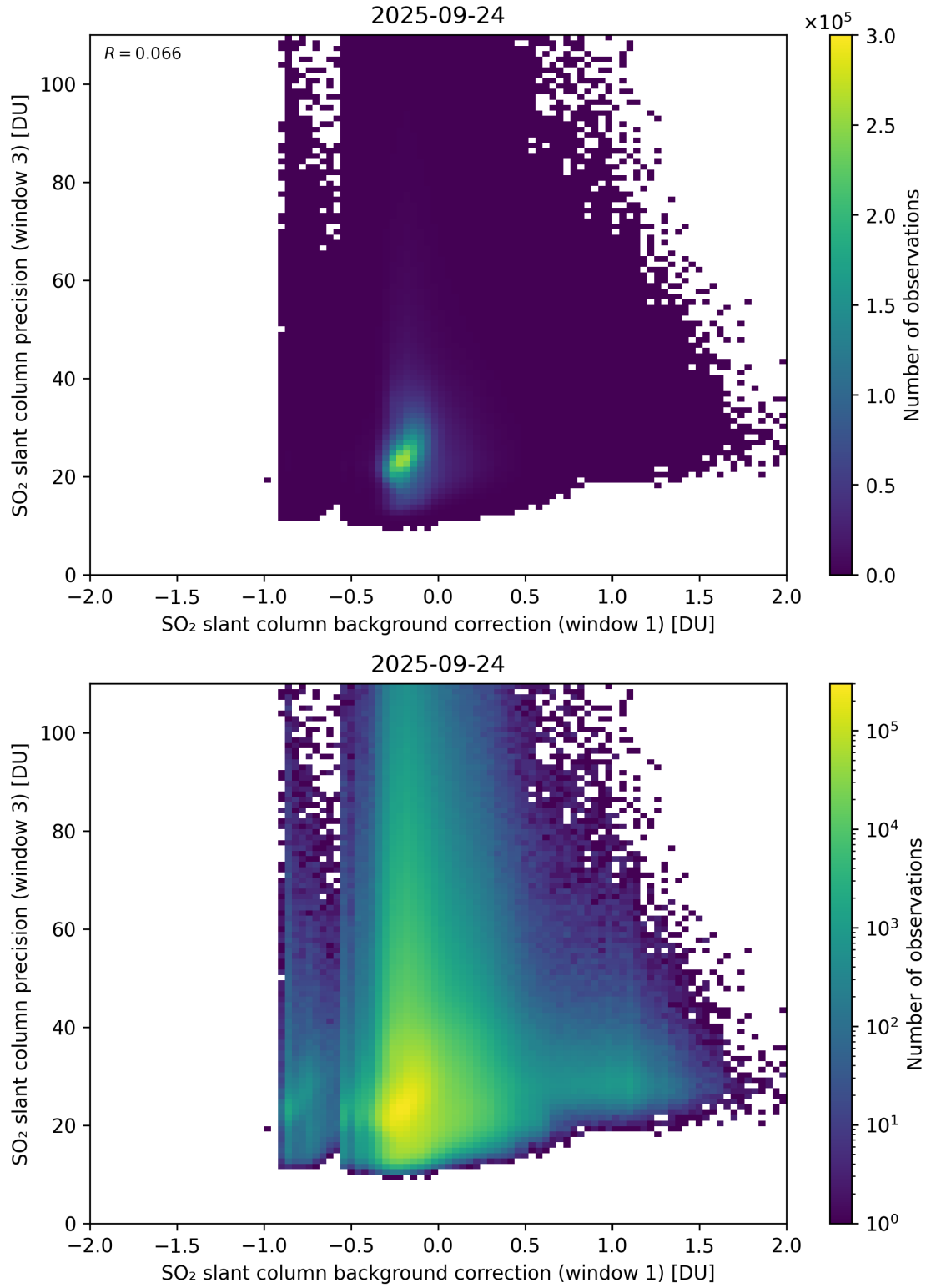
Figure 119: Scatter density plot of “SO 2 slant column background correction (window 1)” against “SO 2 slant column precision (window 3)” for 2025-09-23 to 2025-09-25.
