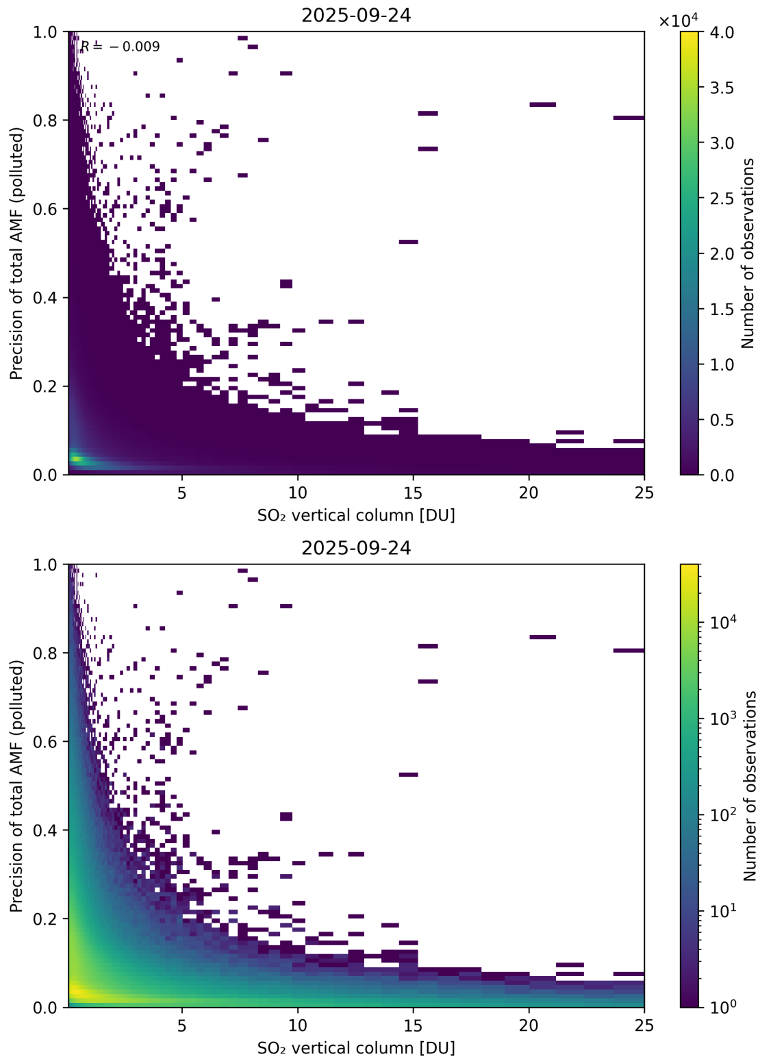
Figure 360: Scatter density plot of “SO 2 vertical column” against “Precision of total AMF (polluted)” for 2025-09-23 to 2025-09-25.
