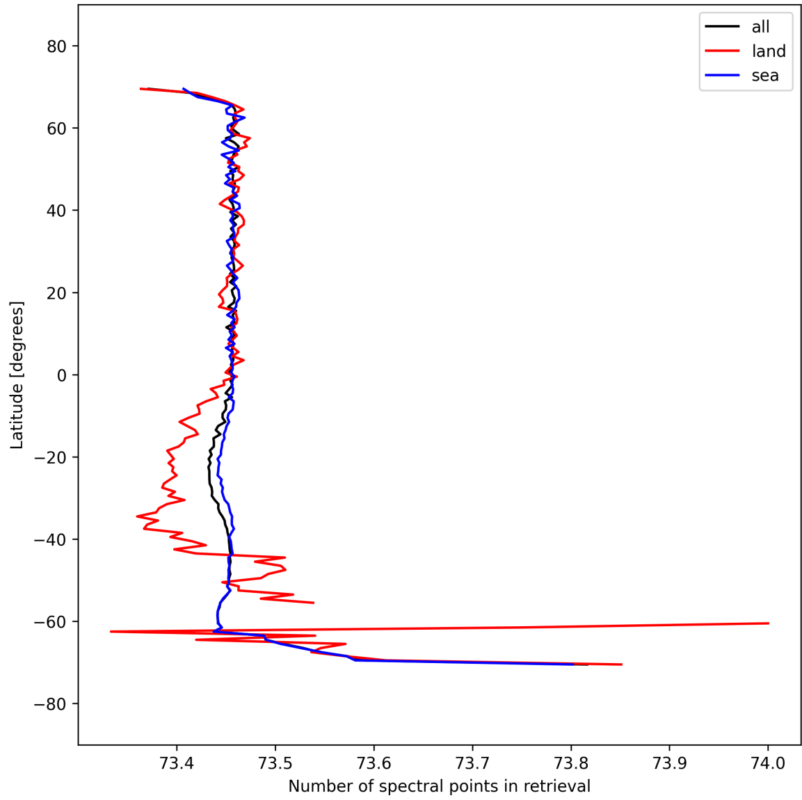
Figure 56: Zonal average of “Number of spectral points in retrieval” for 2025-09-23 to 2025-09-25.
