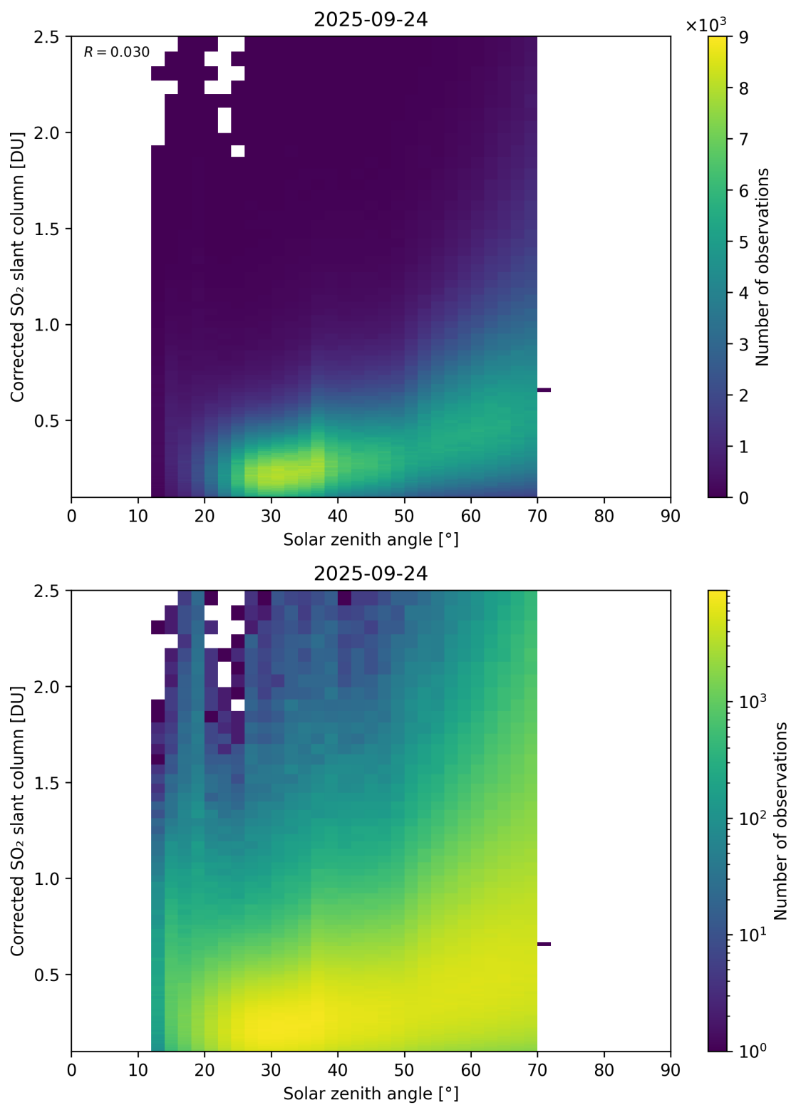
Figure 181: Scatter density plot of “Solar zenith angle” against “Corrected SO 2 slant column” for 2025-09-23 to 2025-09-25.
