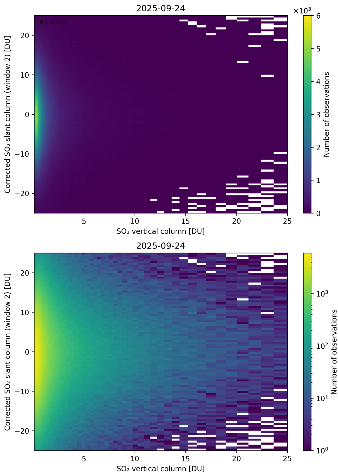
Figure 352: Scatter density plot of “SO 2 vertical column” against “Corrected SO 2 slant column (window 2)” for 2025-09-23 to 2025-09-25.
