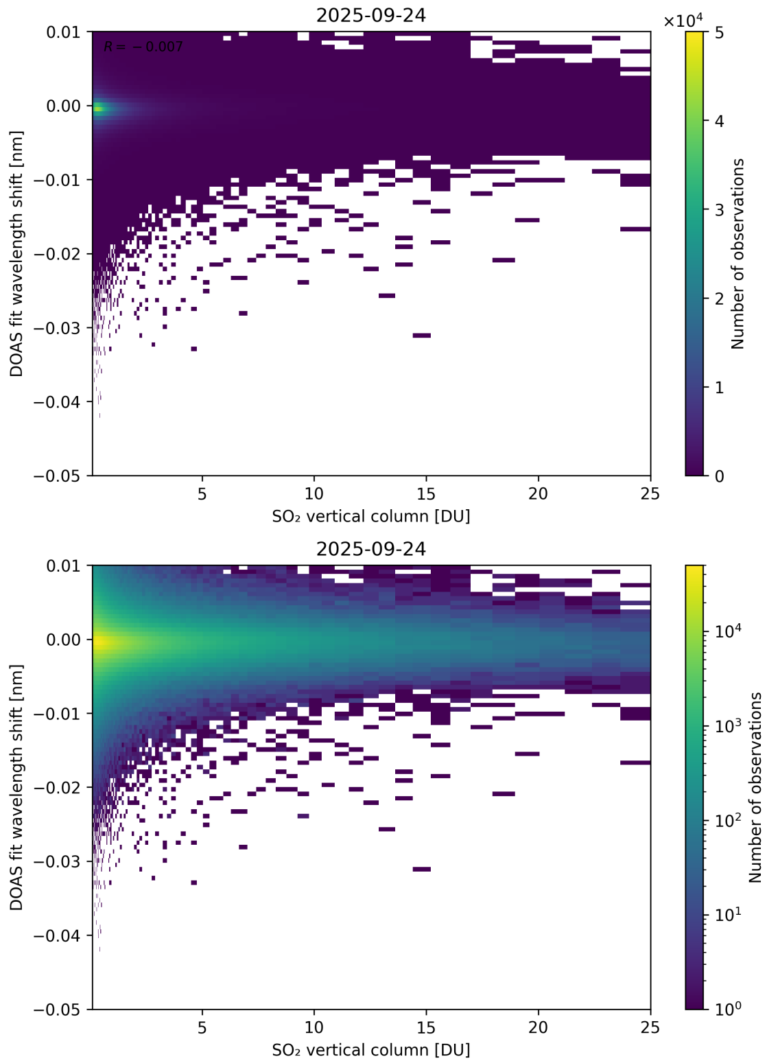
Figure 326: Scatter density plot of “SO 2 vertical column” against “DOAS fit wavelength shift” for 2025-09-23 to 2025-09-25.
