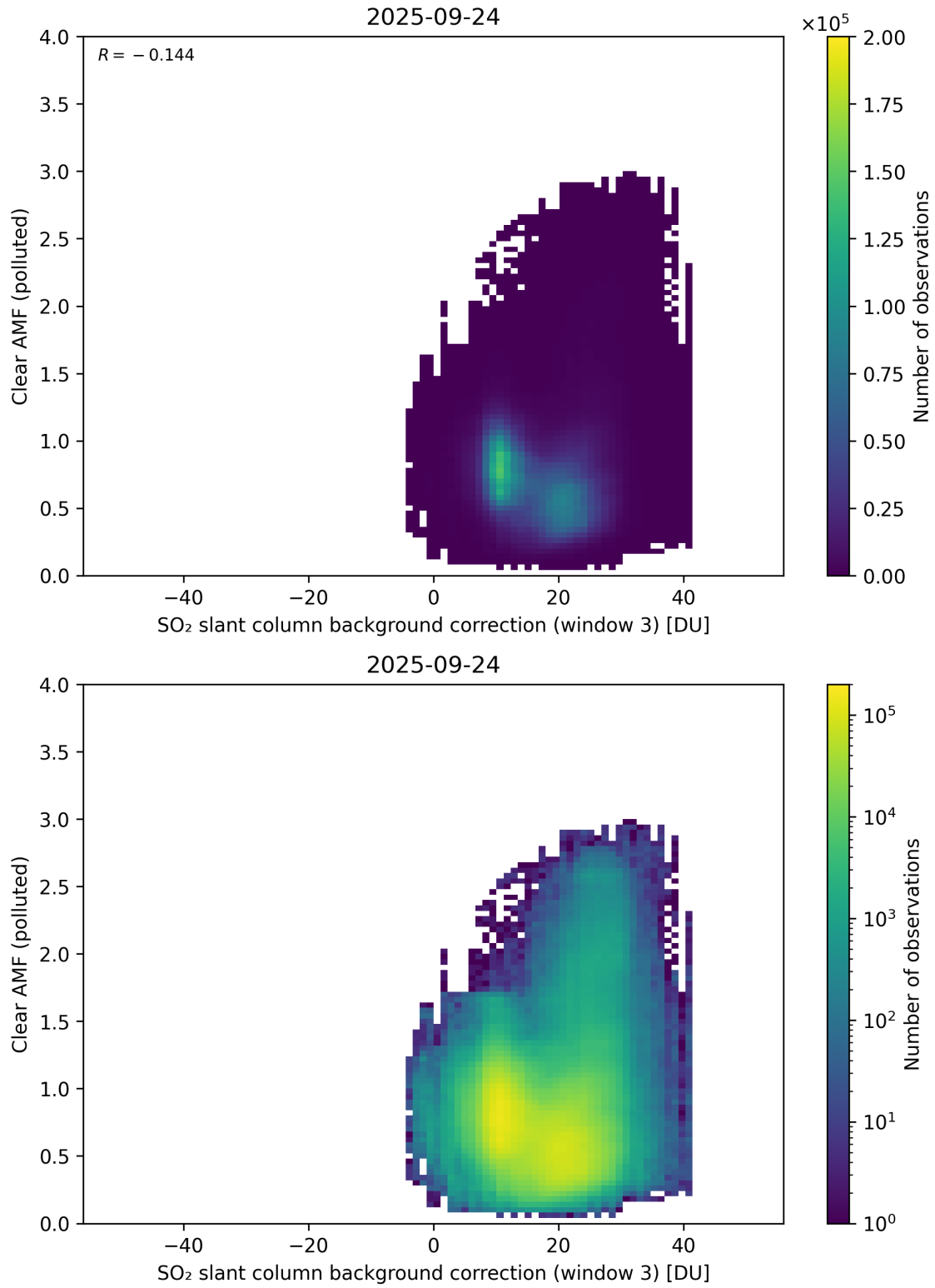
Figure 135: Scatter density plot of “SO 2 slant column background correction (window 3)” against “Clear AMF (polluted)” for 2025-09-23 to 2025-09-25.
