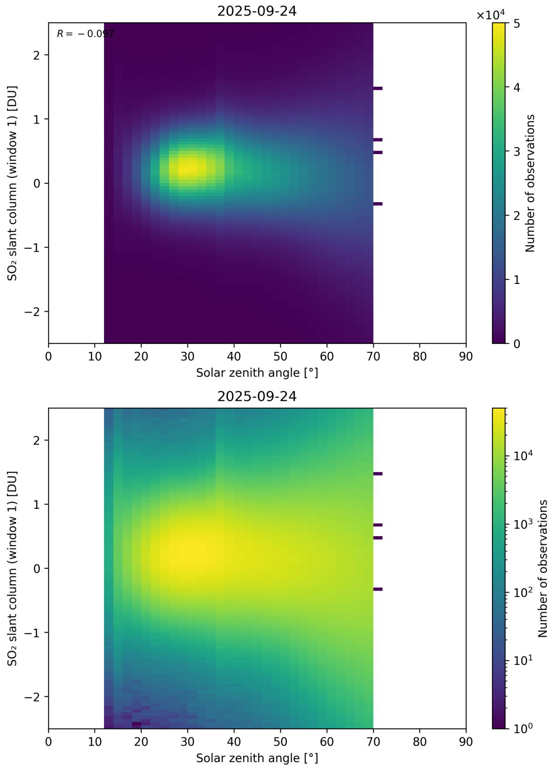
Figure 184: Scatter density plot of “Solar zenith angle” against “SO 2 slant column (window 1)” for 2025-09-23 to 2025-09-25.
