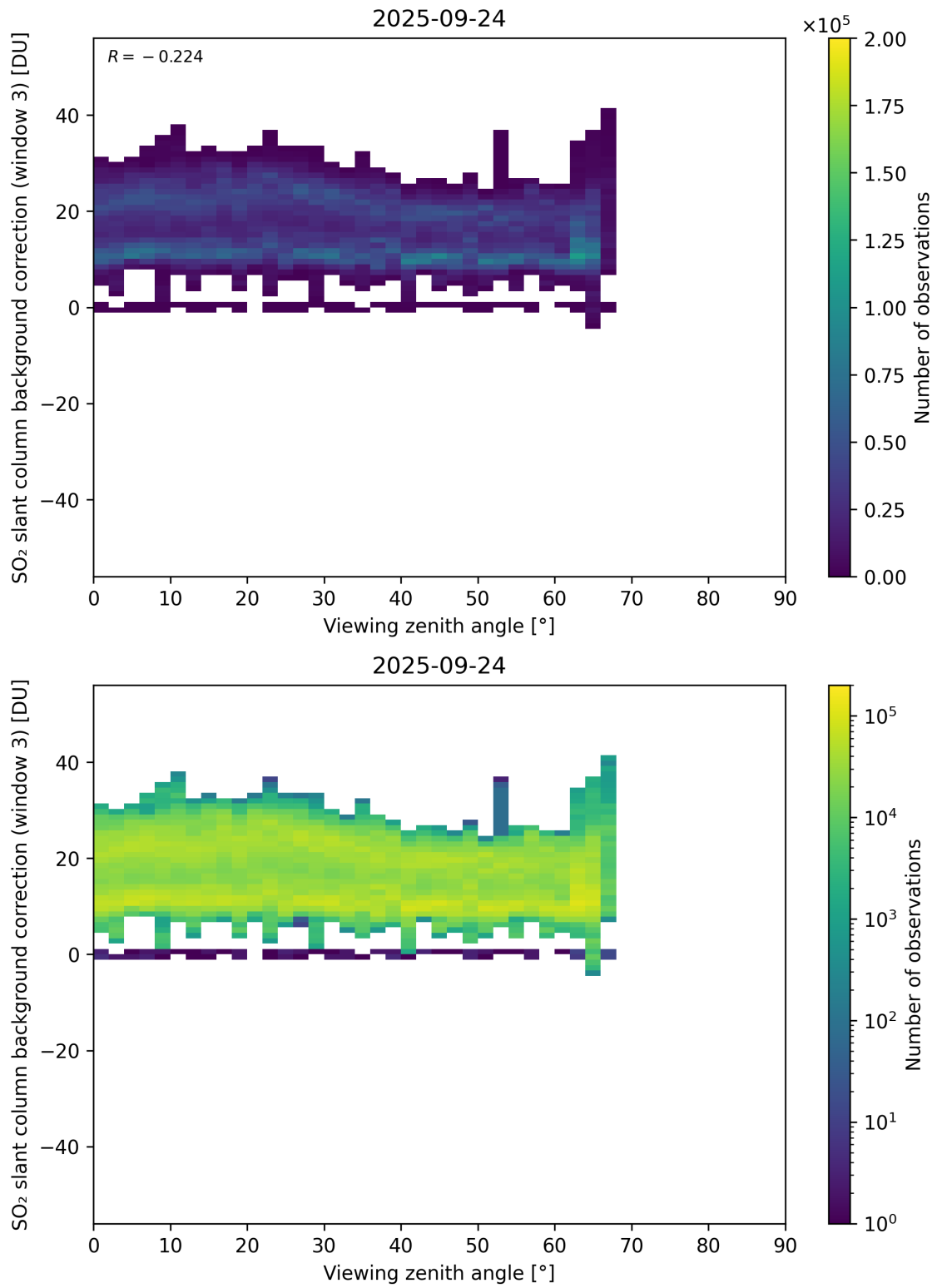
Figure 364: Scatter density plot of “Viewing zenith angle” against “SO 2 slant column background correction (window 3)” for 2025-09-23 to 2025-09-25.
