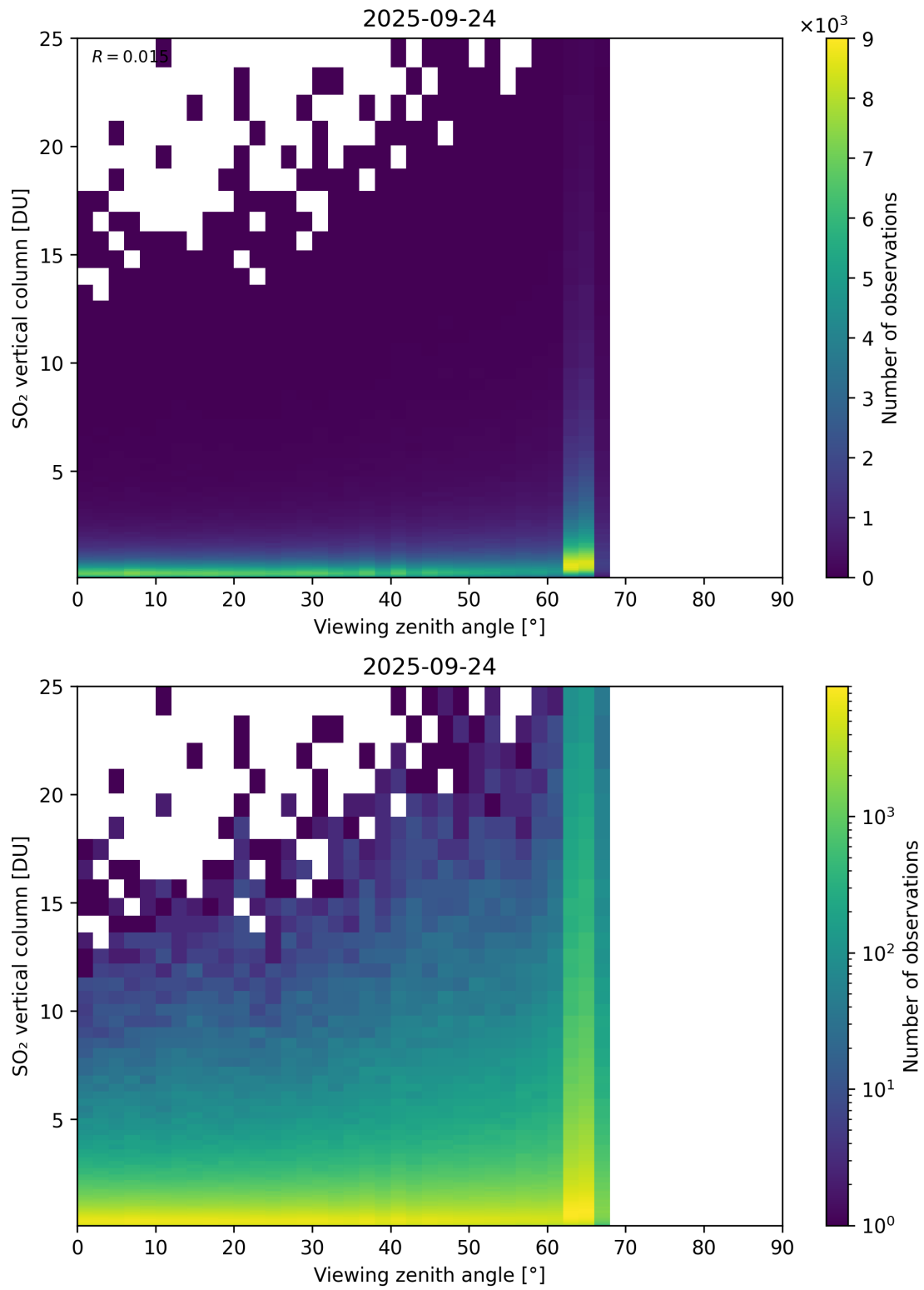
Figure 383: Scatter density plot of “Viewing zenith angle” against “SO 2 vertical column” for 2025-09-23 to 2025-09-25.
