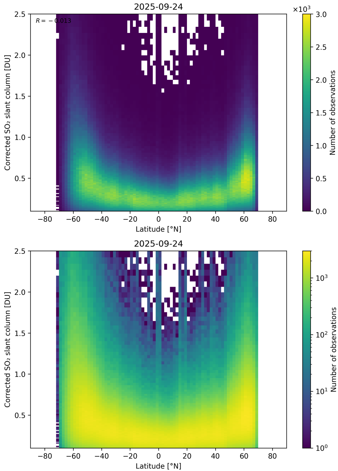
Figure 159: Scatter density plot of “Latitude” against “Corrected SO 2 slant column” for 2025-09-23 to 2025-09-25.
