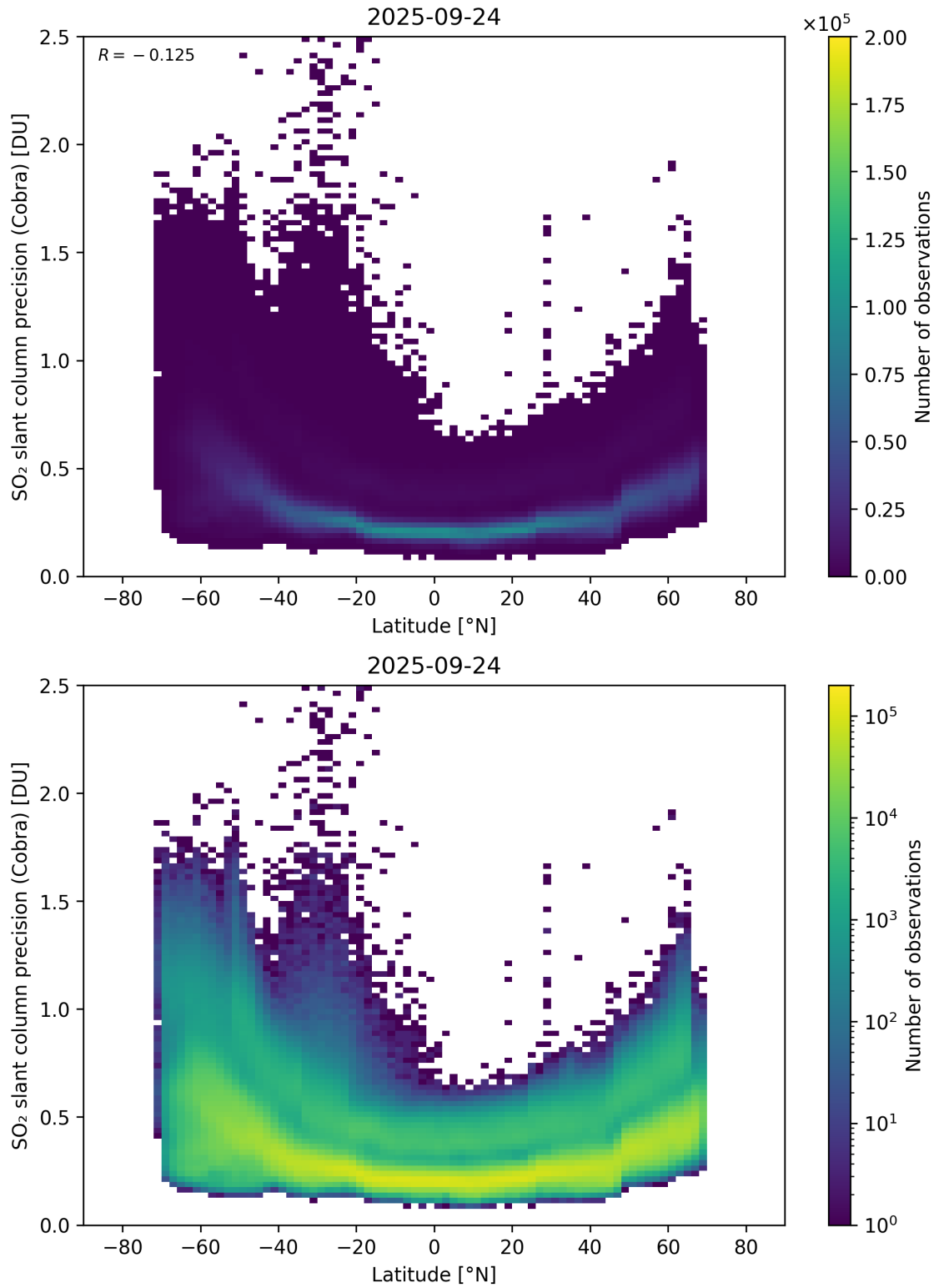
Figure 158: Scatter density plot of “Latitude” against “SO 2 slant column precision (Cobra)” for 2025-09-23 to 2025-09-25.
