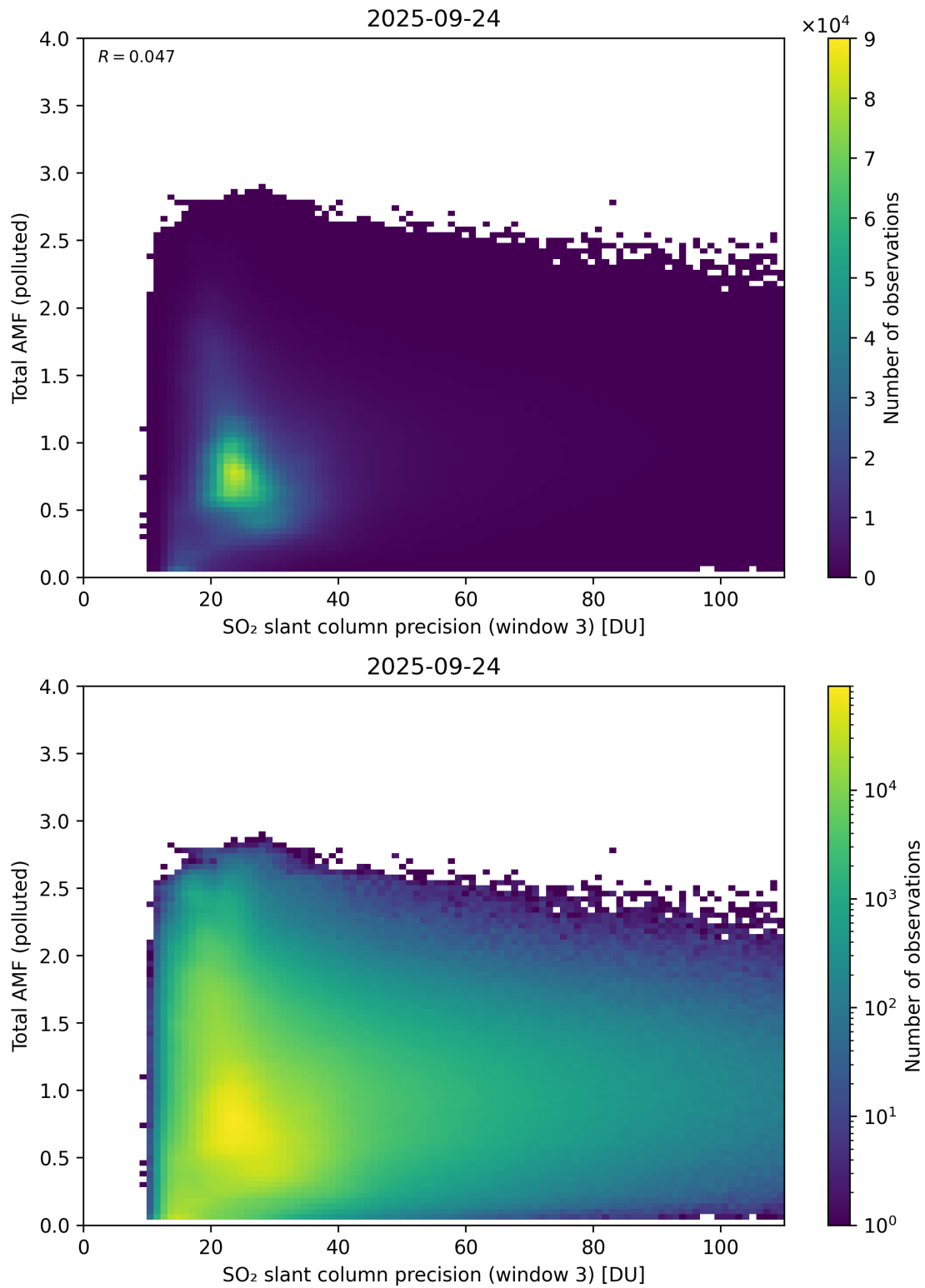
Figure 313: Scatter density plot of “SO 2 slant column precision (window 3)” against “Total AMF (polluted)” for 2025-09-23 to 2025-09-25.
