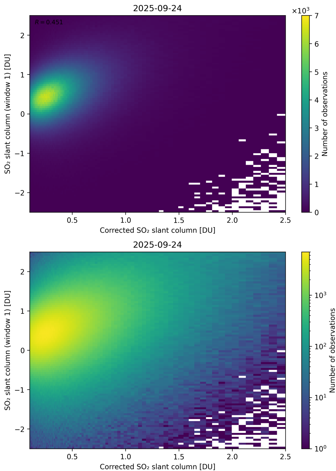
Figure 237: Scatter density plot of “Corrected SO 2 slant column” against “SO 2 slant column (window 1)” for 2025-09-23 to 2025-09-25.
