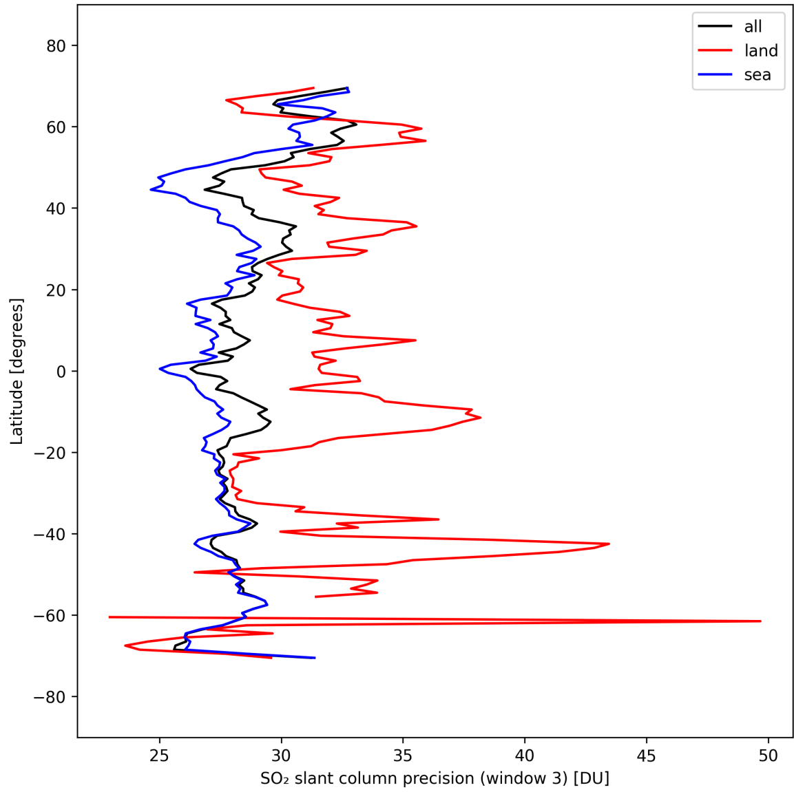
Figure 46: Zonal average of “SO 2 slant column precision (window 3)” for 2025-09-23 to 2025-09-25.
