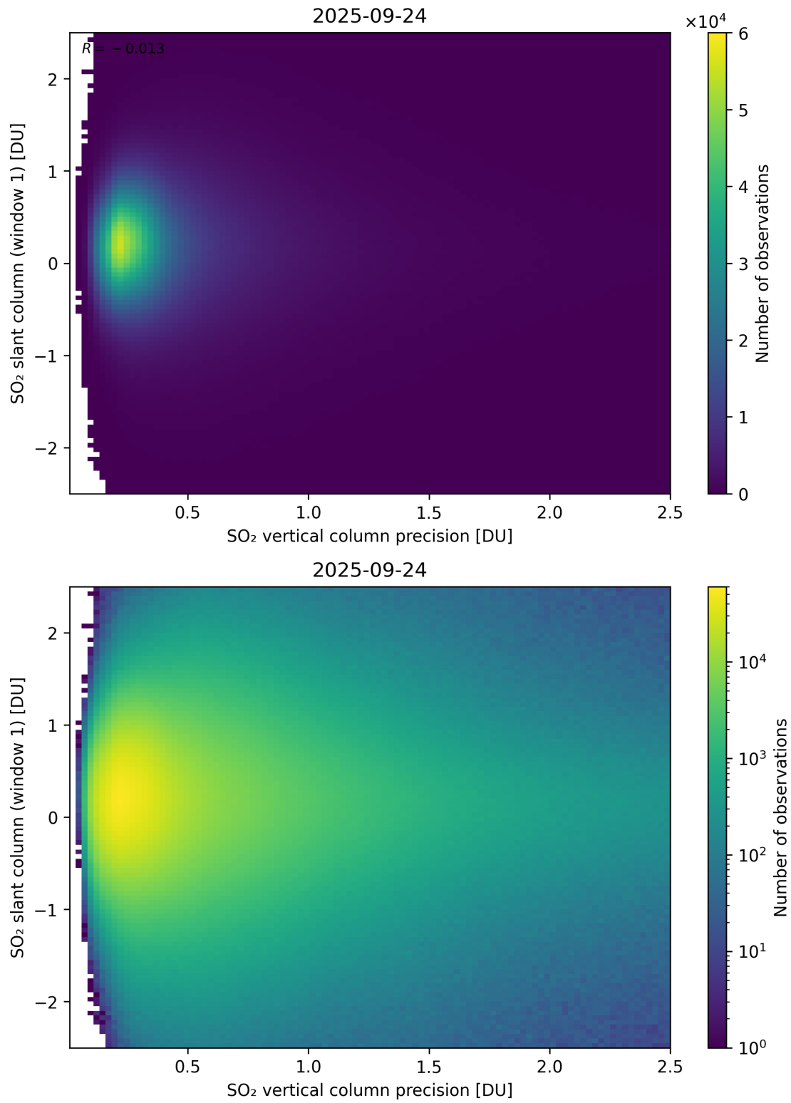
Figure 341: Scatter density plot of “SO 2 vertical column precision” against “SO 2 slant column (window 1)” for 2025-09-23 to 2025-09-25.
