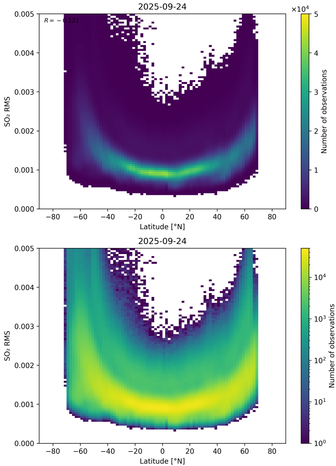
Figure 155: Scatter density plot of “Latitude” against “SO 2 RMS” for 2025-09-23 to 2025-09-25.
