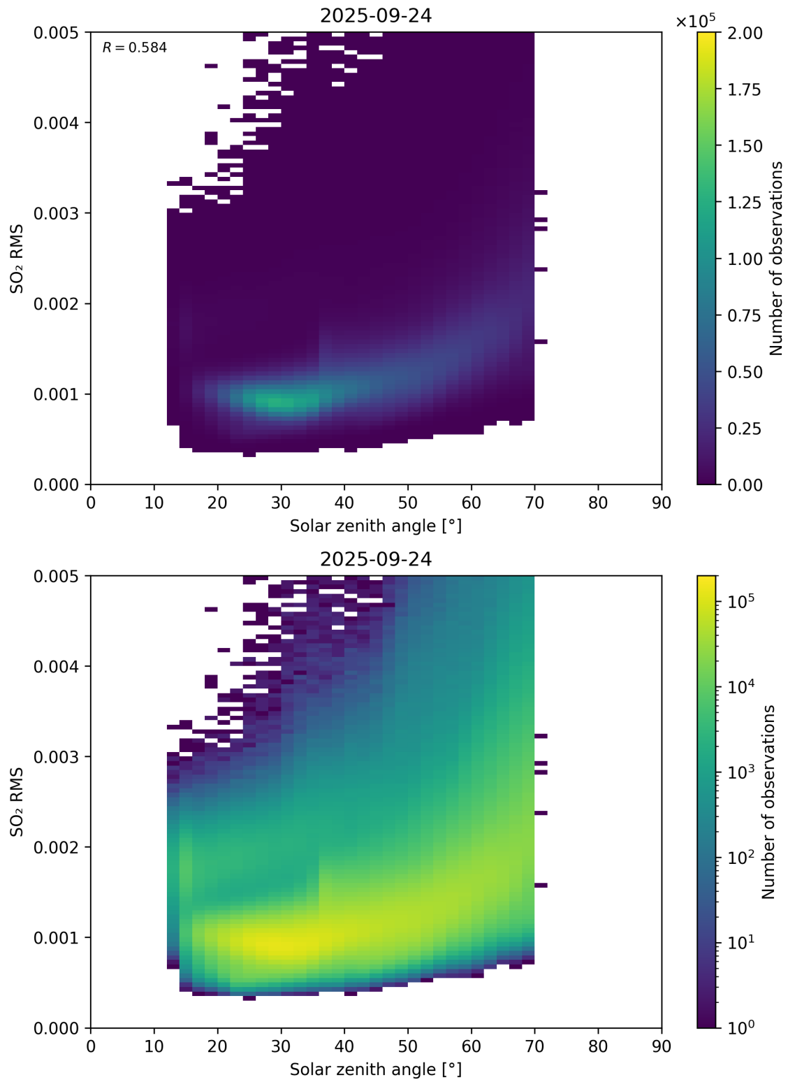
Figure 176: Scatter density plot of “Solar zenith angle” against “SO 2 RMS” for 2025-09-23 to 2025-09-25.
