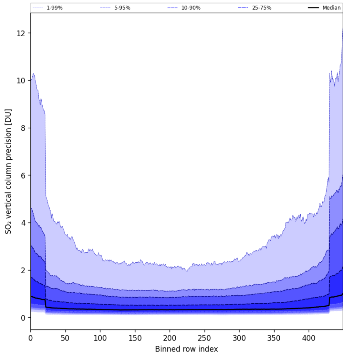
Figure 85: Along track statistics of “SO 2 vertical column precision” for 2025-09-23 to 2025-09-25
