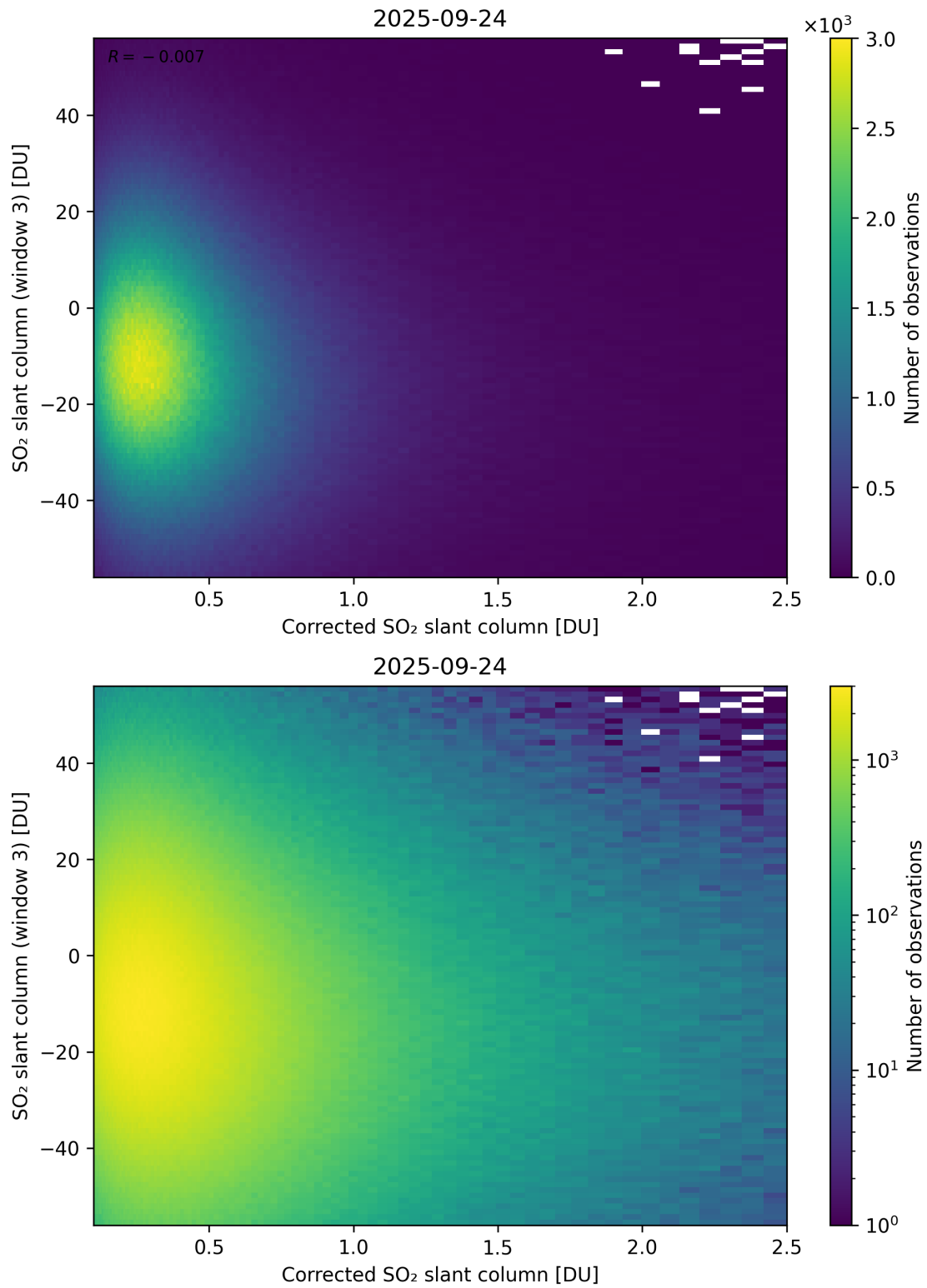
Figure 240: Scatter density plot of “Corrected SO 2 slant column” against “SO 2 slant column (window 3)” for 2025-09-23 to 2025-09-25.
