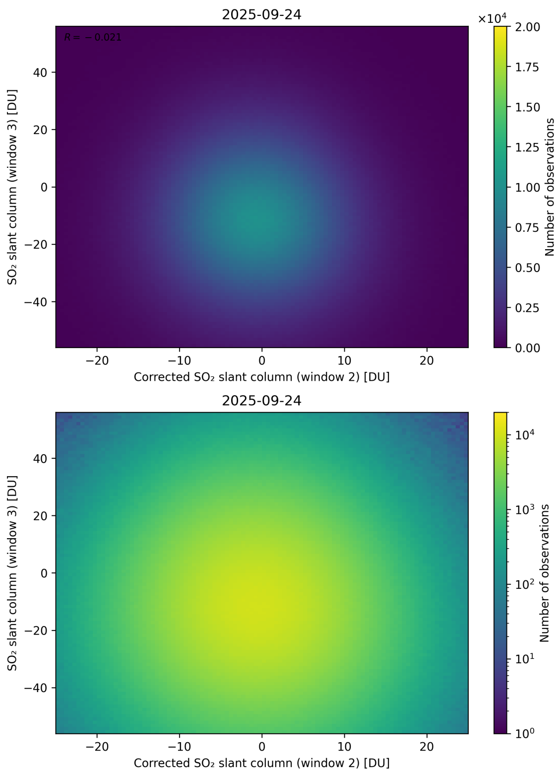
Figure 251: Scatter density plot of “Corrected SO 2 slant column (window 2)” against “SO 2 slant column (window 3)” for 2025-09-23 to 2025-09-25.
