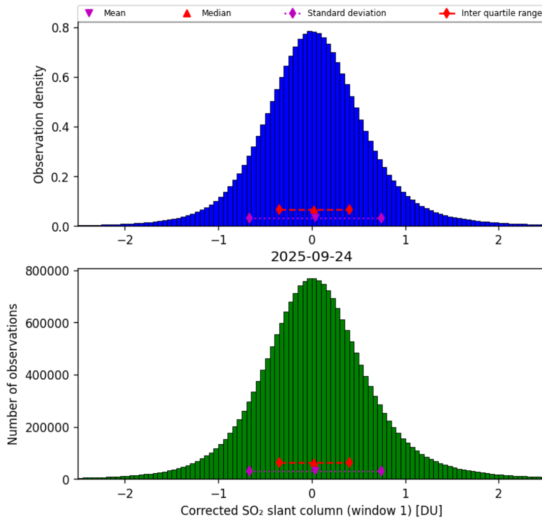
Figure 65: Histogram of “Corrected SO 2 slant column (window 1)” for 2025-09-23 to 2025-09-25
