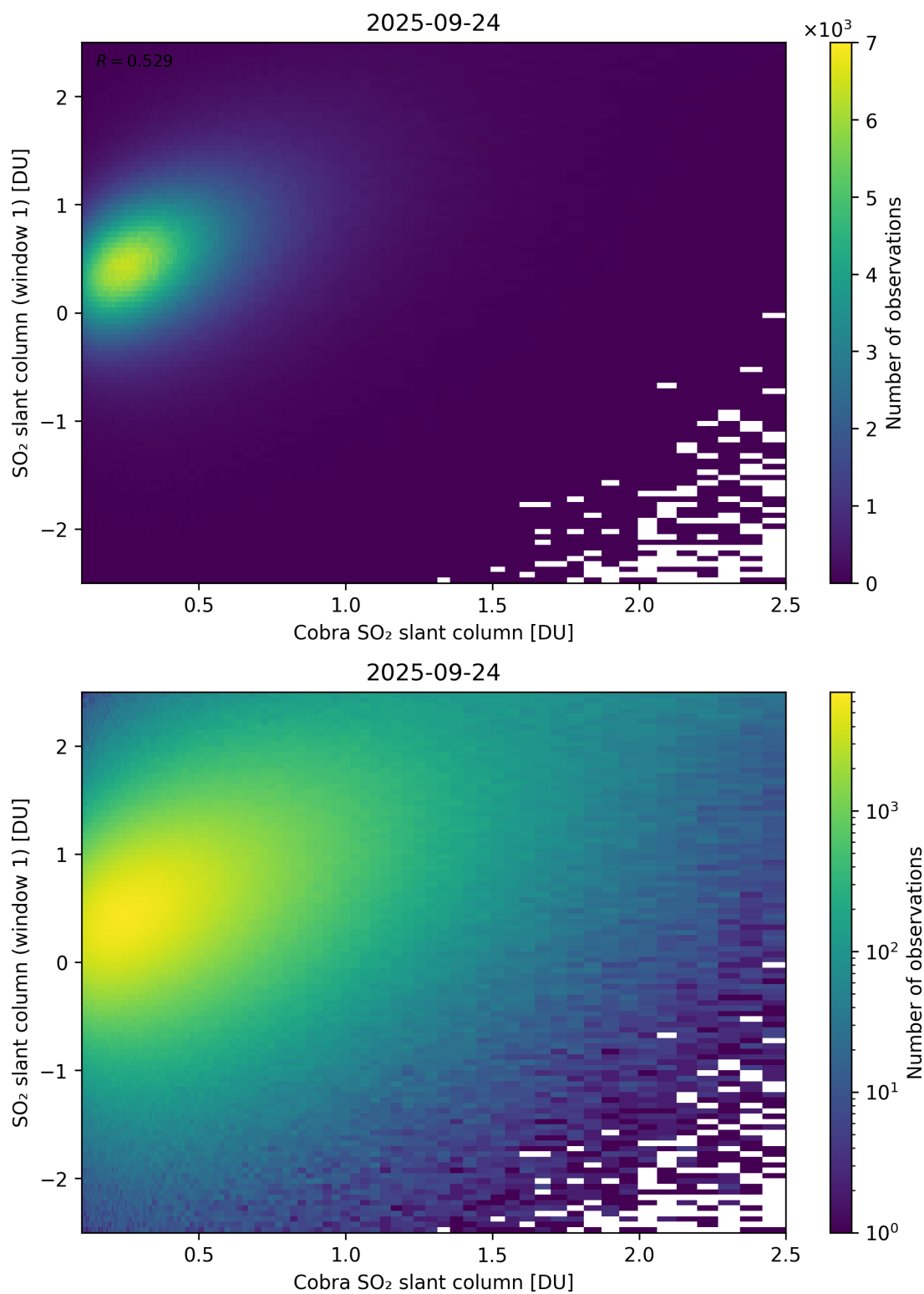
Figure 219: Scatter density plot of “Cobra SO 2 slant column” against “SO 2 slant column (window 1)” for 2025-09-23 to 2025-09-25.
