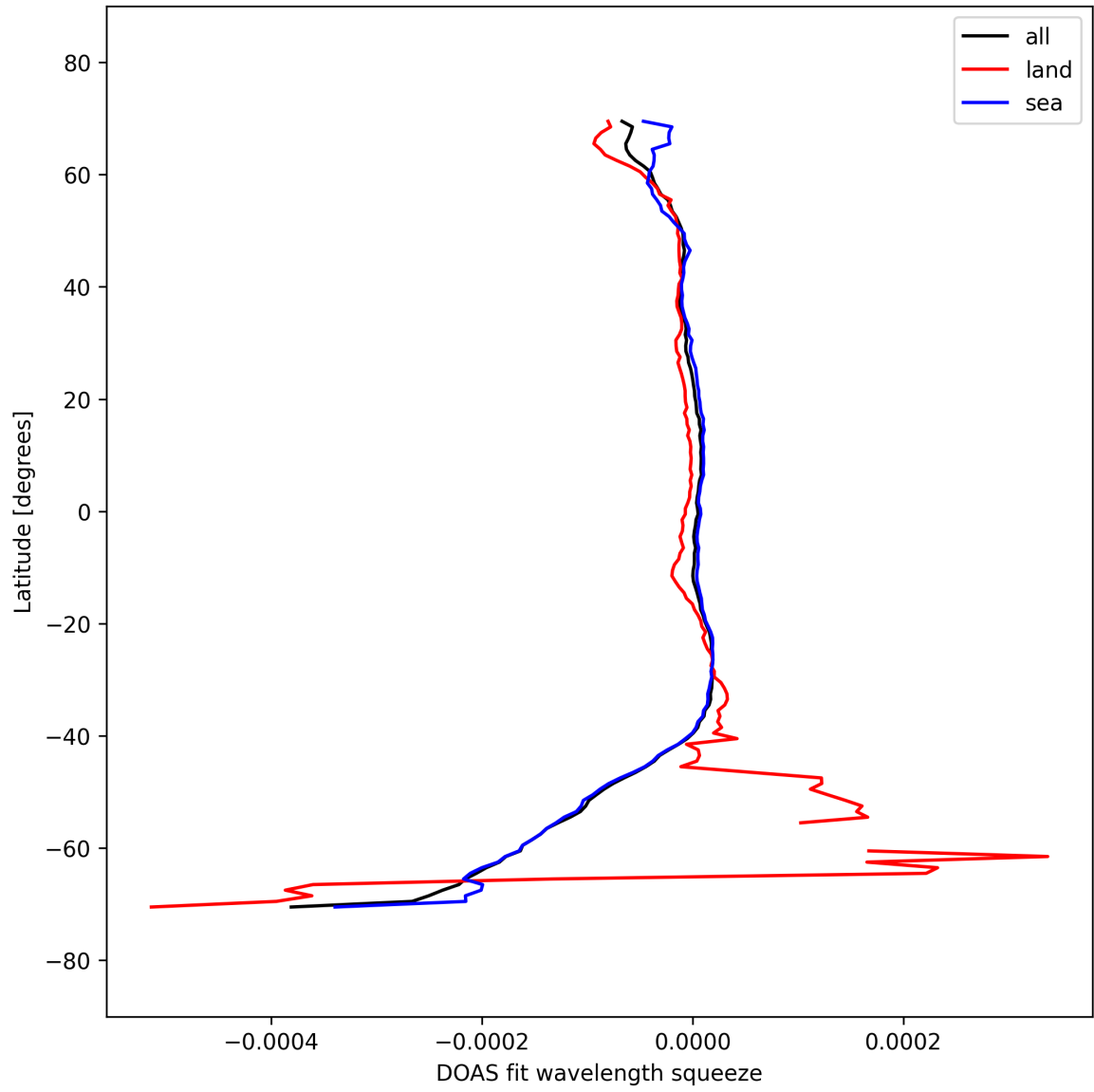
Figure 51: Zonal average of “DOAS fit wavelength squeeze” for 2025-09-23 to 2025-09-25.
