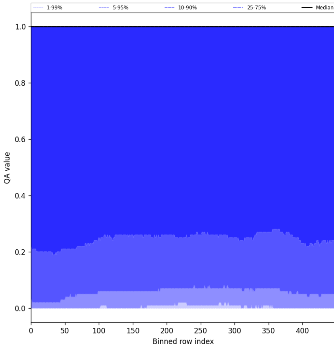
Figure 83: Along track statistics of “QA value” for 2025-09-23 to 2025-09-25
