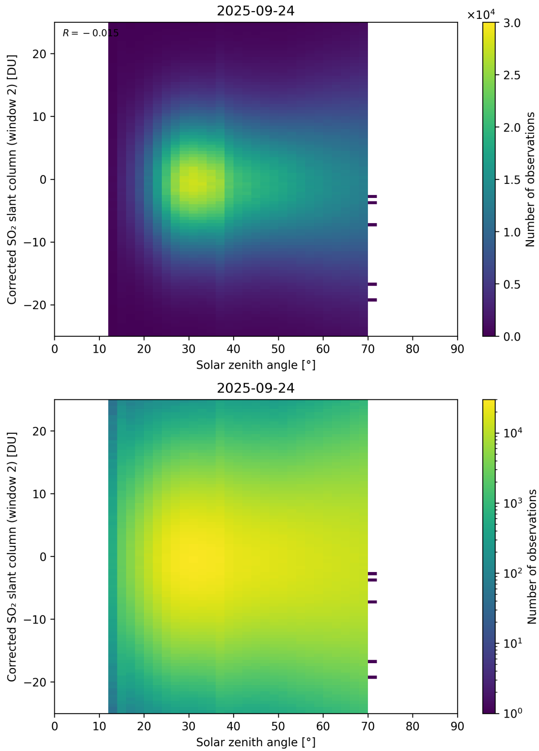
Figure 182: Scatter density plot of “Solar zenith angle” against “Corrected SO 2 slant column (window 2)” for 2025-09-23 to 2025-09-25.
