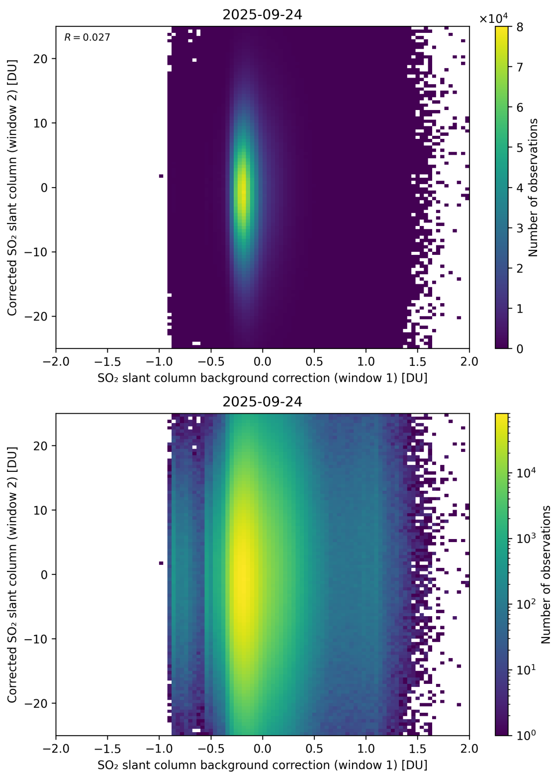
Figure 115: Scatter density plot of “SO 2 slant column background correction (window 1)” against “Corrected SO 2 slant column (window 2)” for 2025-09-23 to 2025-09-25.
