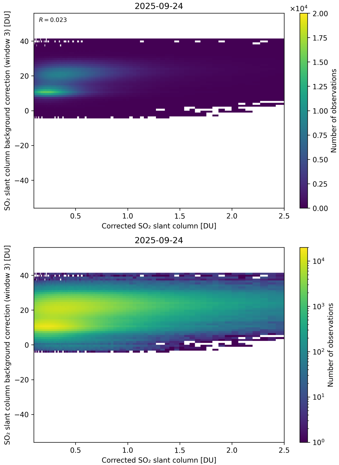
Figure 228: Scatter density plot of “Corrected SO 2 slant column” against “SO 2 slant column background correction (window 3)” for 2025-09-23 to 2025-09-25.
