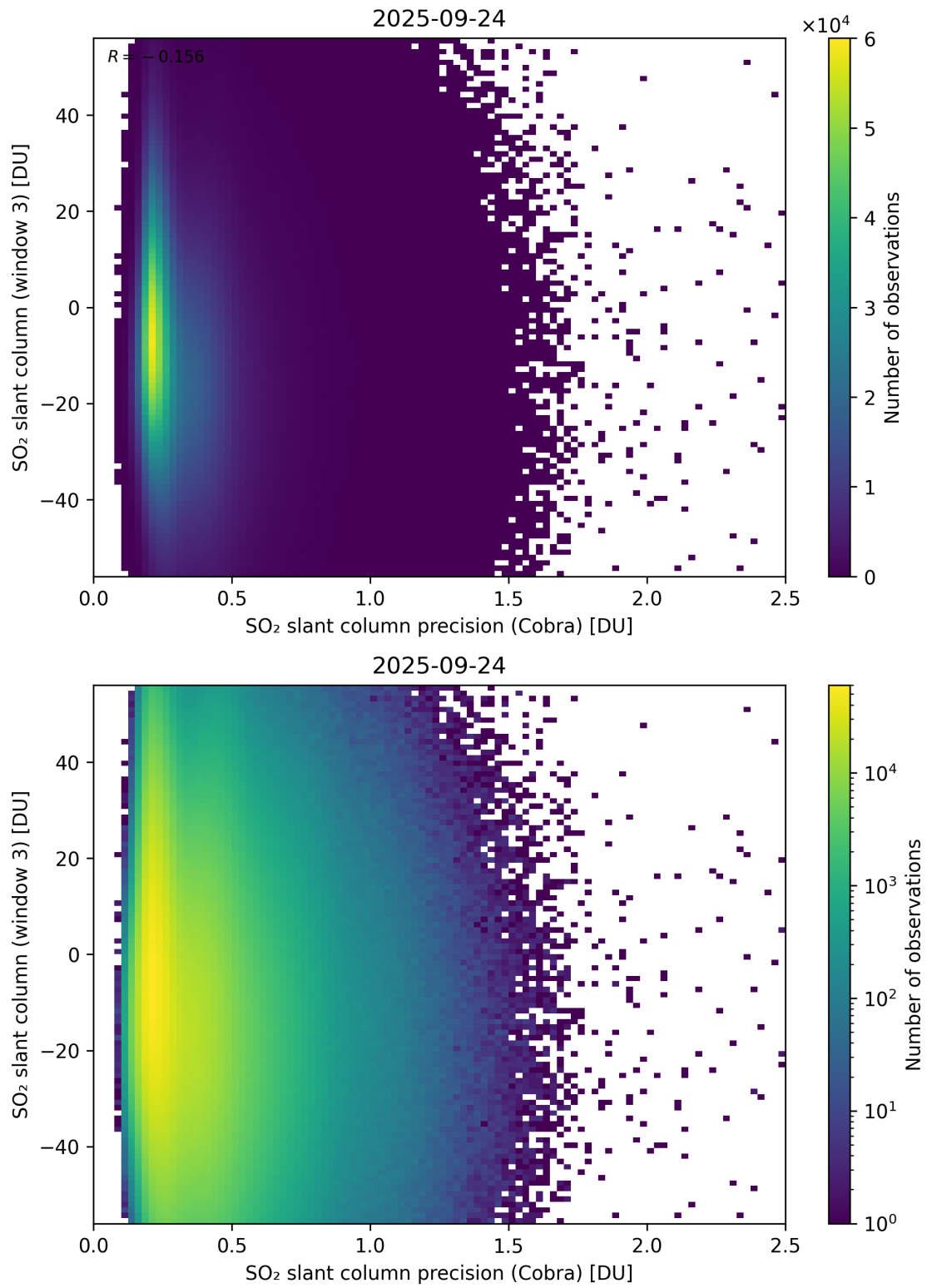
Figure 211: Scatter density plot of “SO 2 slant column precision (Cobra)” against “SO 2 slant column (window 3)” for 2025-09-23 to 2025-09-25.
