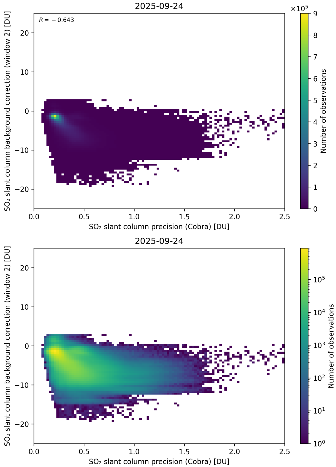
Figure 200: Scatter density plot of “SO 2 slant column precision (Cobra)” against “SO 2 slant column background correction (window 2)” for 2025-09-23 to 2025-09-25.
