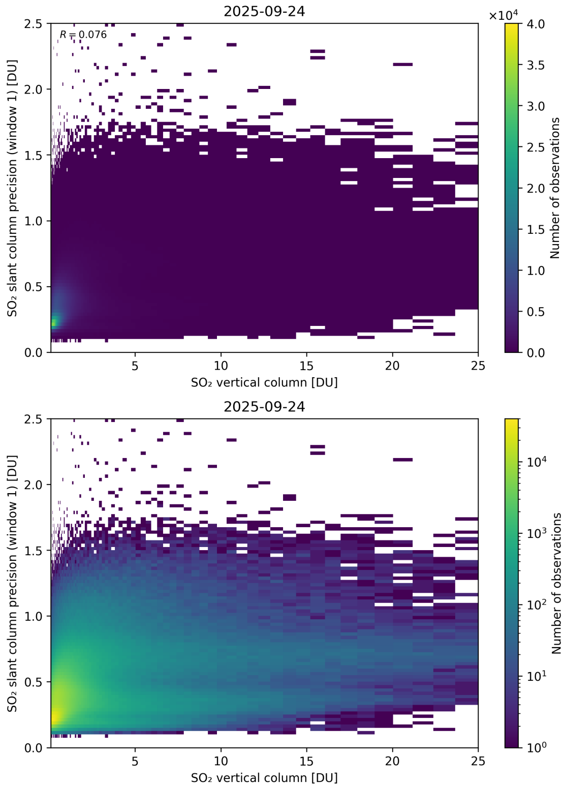
Figure 355: Scatter density plot of “SO 2 vertical column” against “SO 2 slant column precision (window 1)” for 2025-09-23 to 2025-09-25.
