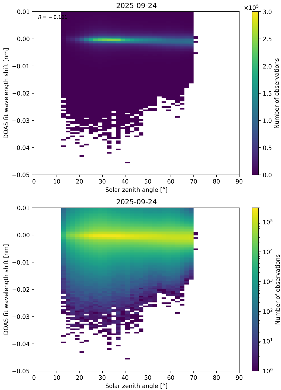
Figure 174: Scatter density plot of “Solar zenith angle” against “DOAS fit wavelength shift” for 2025-09-23 to 2025-09-25.
