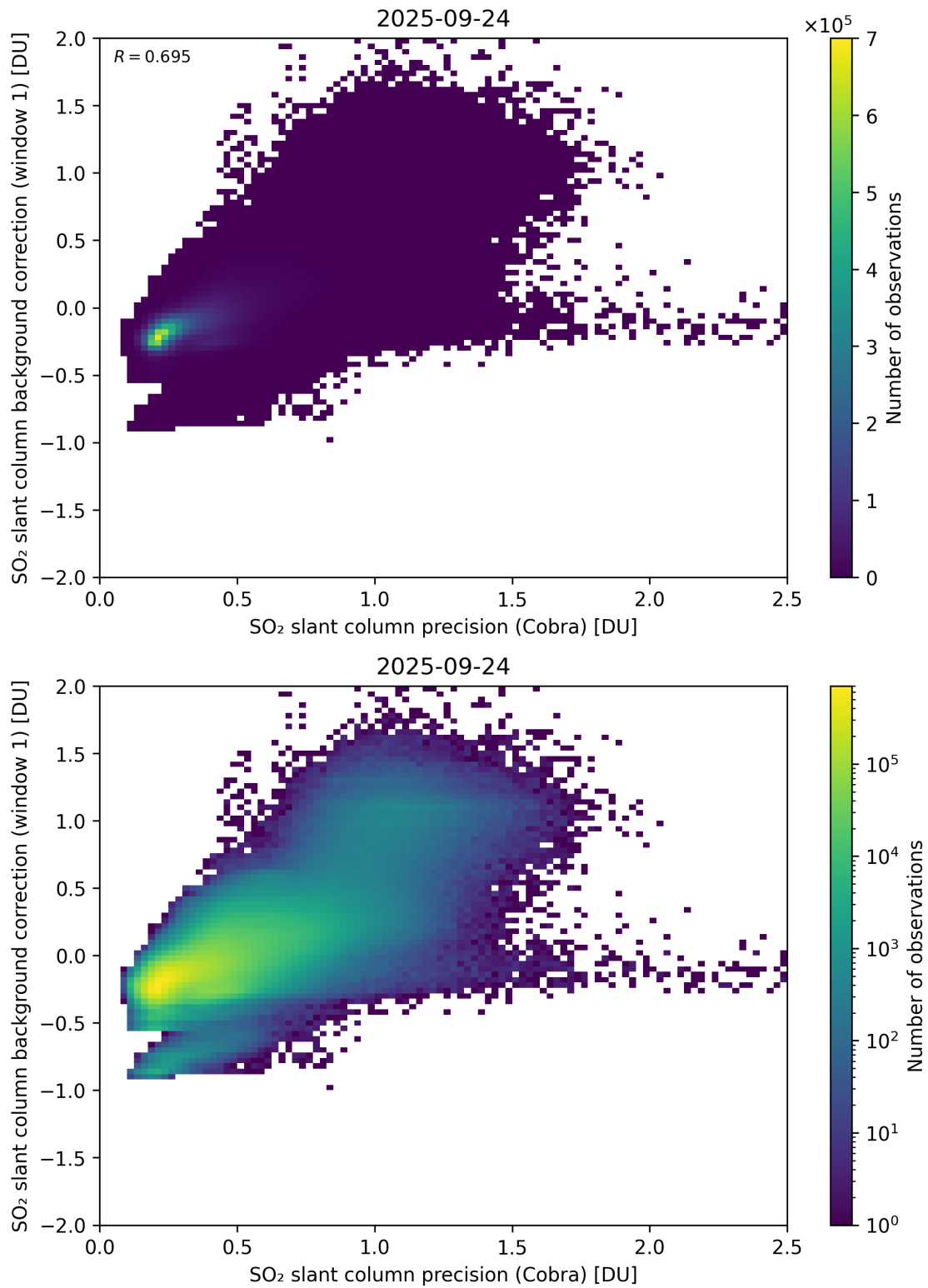
Figure 199: Scatter density plot of “SO 2 slant column precision (Cobra)” against “SO 2 slant column background correction (window 1)” for 2025-09-23 to 2025-09-25.
