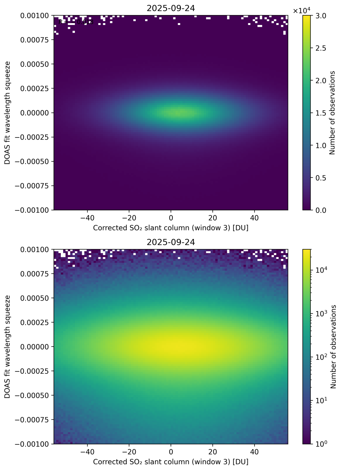
Figure 257: Scatter density plot of “Corrected SO 2 slant column (window 3)” against “DOAS fit wavelength squeeze” for 2025-09-23 to 2025-09-25.
