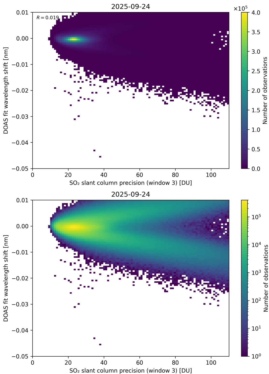
Figure 308: Scatter density plot of “SO 2 slant column precision (window 3)” against “DOAS fit wavelength shift” for 2025-09-23 to 2025-09-25.
