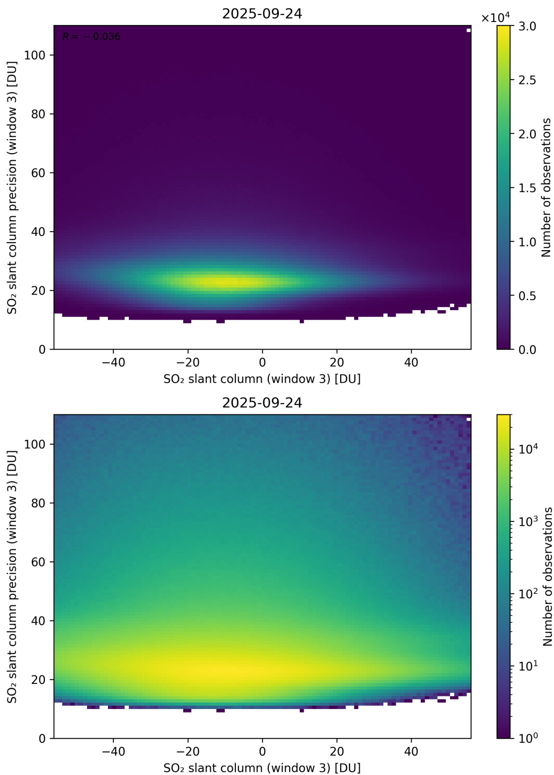
Figure 317: Scatter density plot of “SO 2 slant column (window 3)” against “SO 2 slant column precision (window 3)” for 2025-09-23 to 2025-09-25.
