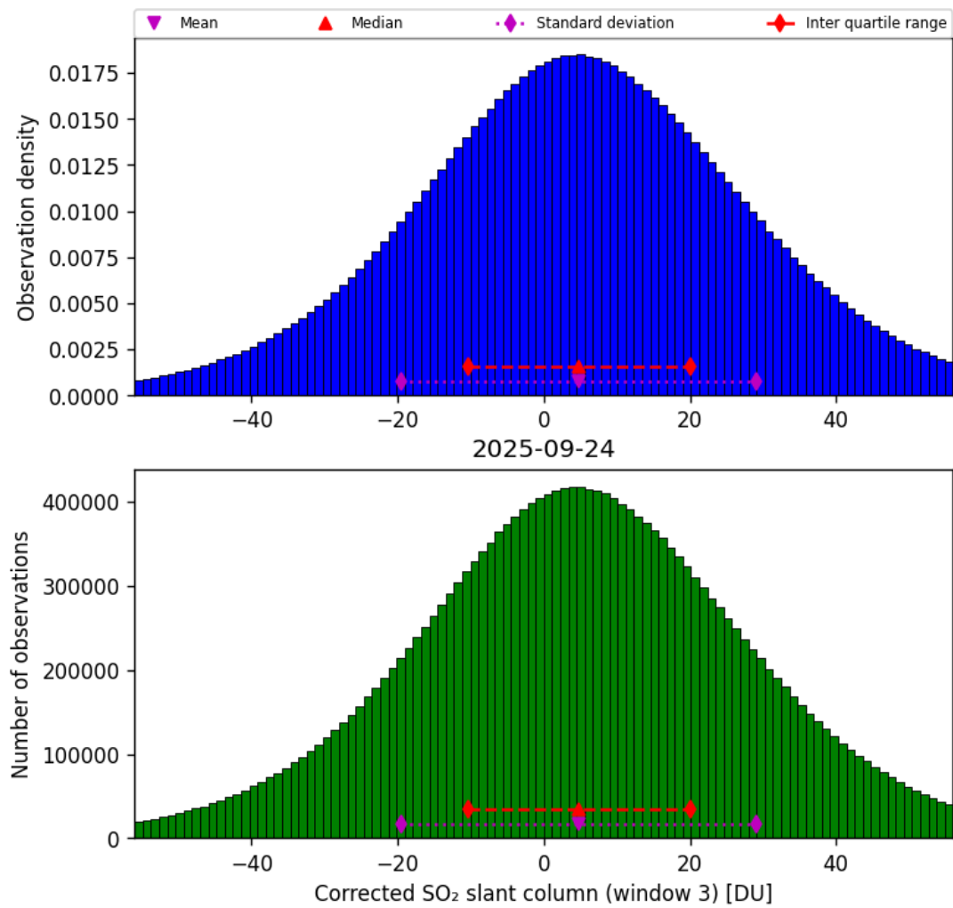
Figure 73: Histogram of “Corrected SO 2 slant column (window 3)” for 2025-09-23 to 2025-09-25
