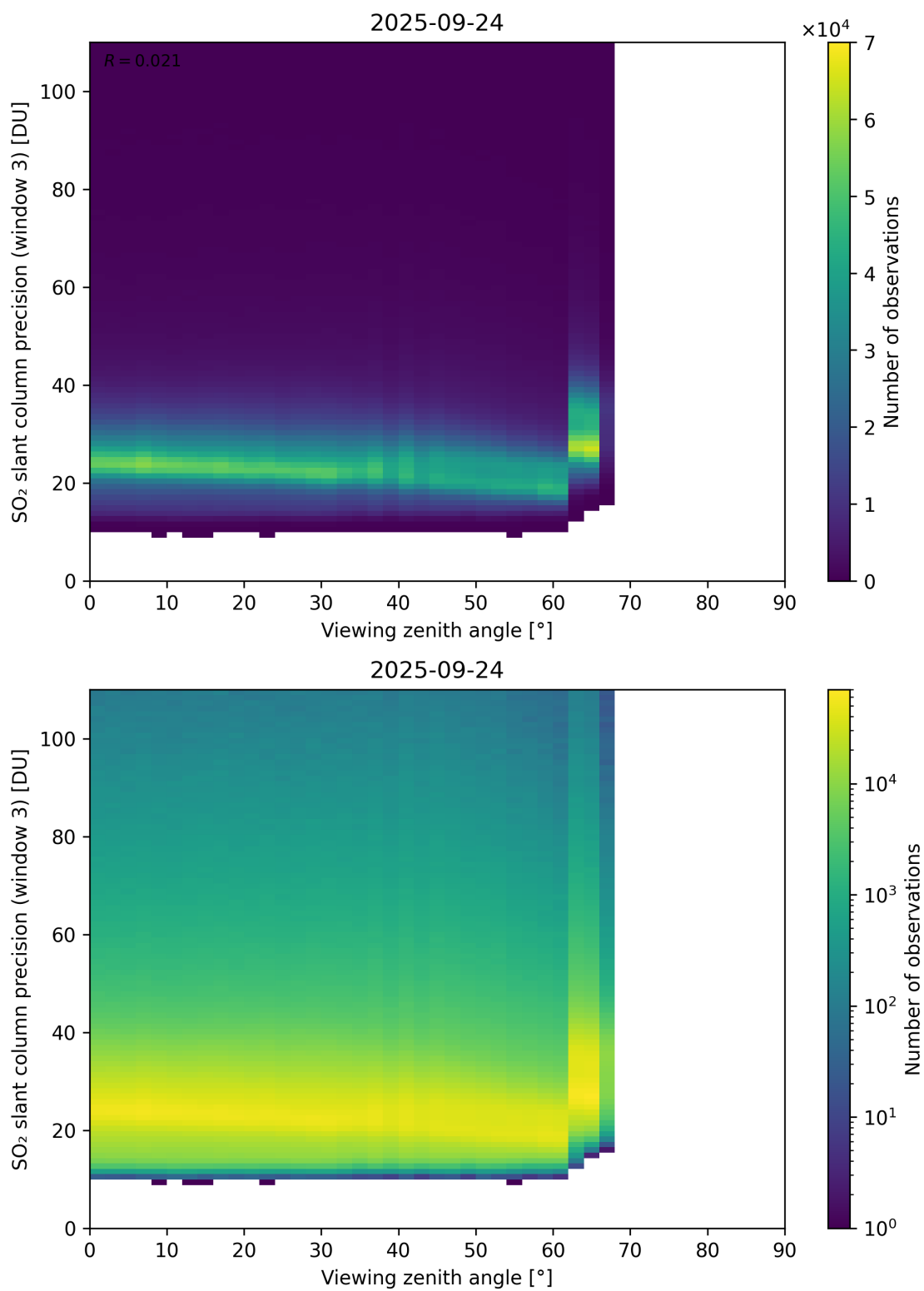
Figure 380: Scatter density plot of “Viewing zenith angle” against “SO 2 slant column precision (window 3)” for 2025-09-23 to 2025-09-25.
