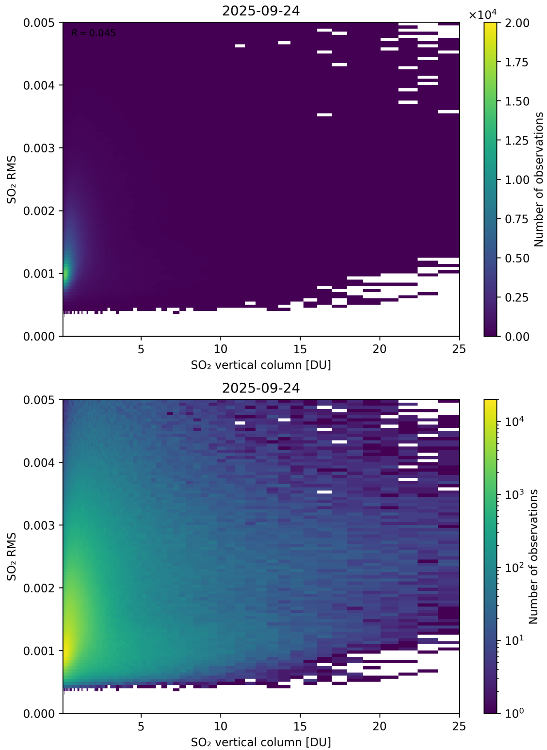
Figure 328: Scatter density plot of “SO 2 vertical column” against “SO 2 RMS” for 2025-09-23 to 2025-09-25.
