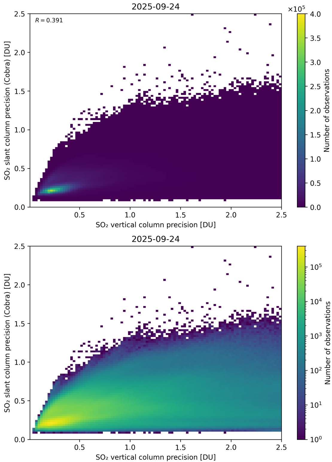
Figure 337: Scatter density plot of “SO 2 vertical column precision” against “SO 2 slant column precision (Cobra)” for 2025-09-23 to 2025-09-25.
