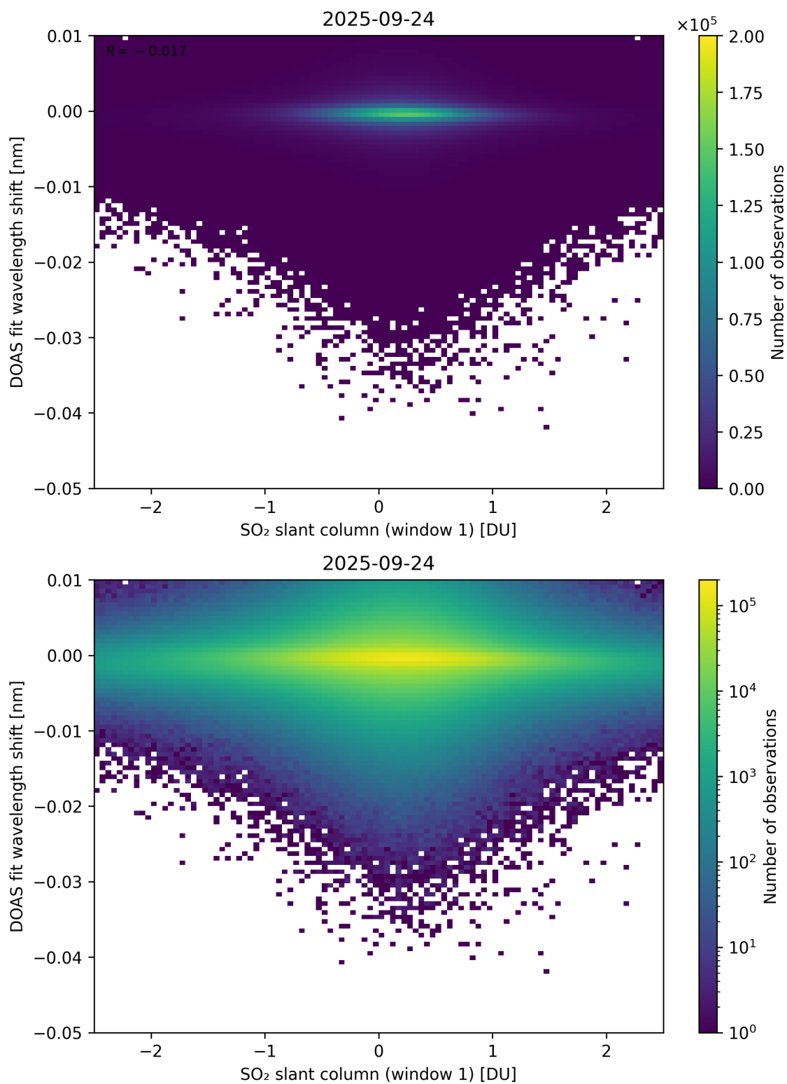
Figure 265: Scatter density plot of “SO 2 slant column (window 1)” against “DOAS fit wavelength shift” for 2025-09-23 to 2025-09-25.
