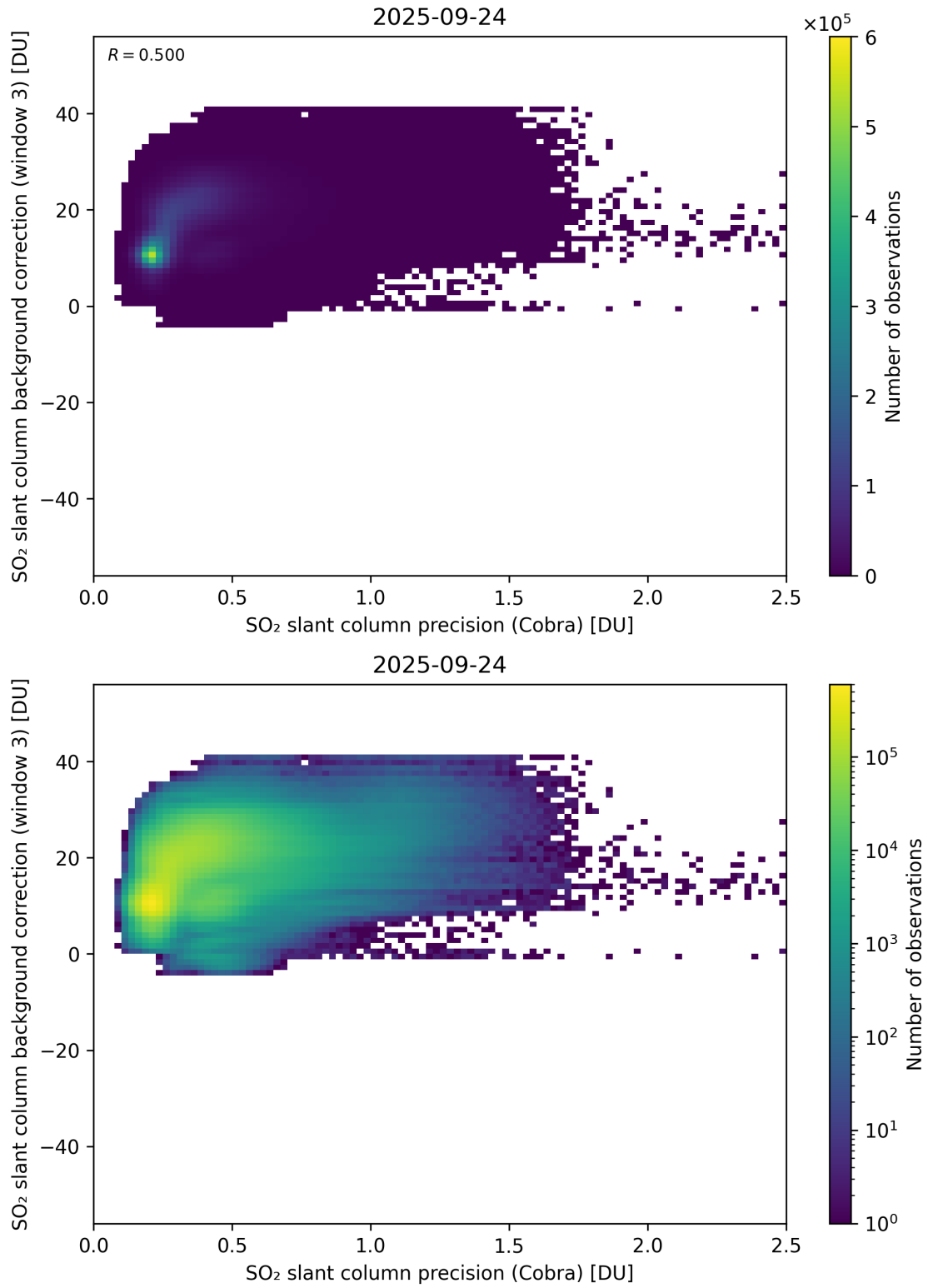
Figure 201: Scatter density plot of “SO 2 slant column precision (Cobra)” against “SO 2 slant column background correction (window 3)” for 2025-09-23 to 2025-09-25.
