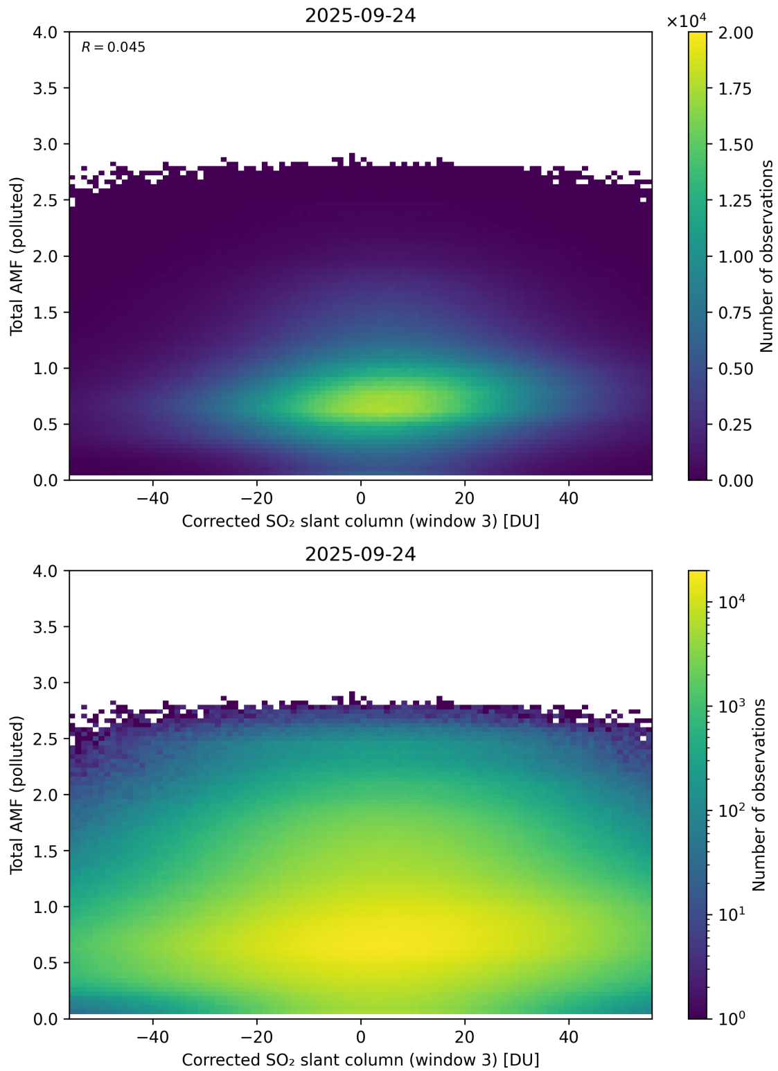
Figure 260: Scatter density plot of “Corrected SO 2 slant column (window 3)” against “Total AMF (polluted)” for 2025-09-23 to 2025-09-25.
