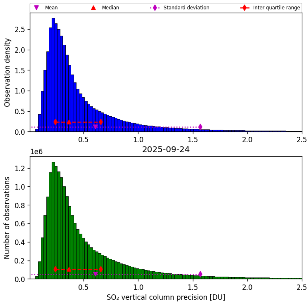
Figure 59: Histogram of “SO 2 vertical column precision” for 2025-09-23 to 2025-09-25
