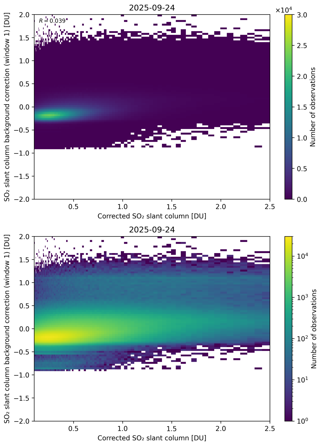
Figure 226: Scatter density plot of “Corrected SO 2 slant column” against “SO 2 slant column background correction (window 1)” for 2025-09-23 to 2025-09-25.
