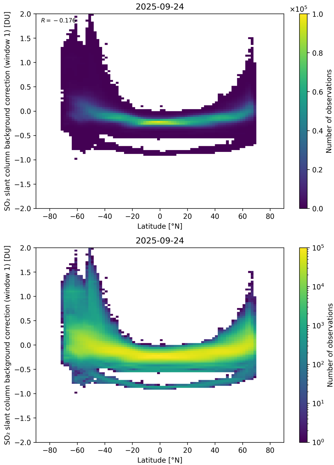
Figure 150: Scatter density plot of “Latitude” against “SO 2 slant column background correction (window 1)” for 2025-09-23 to 2025-09-25.
