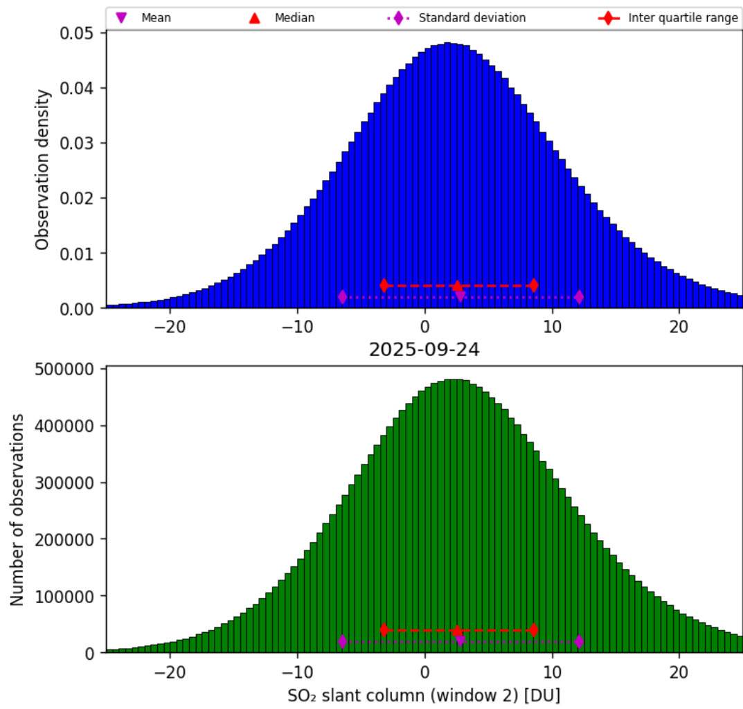
Figure 67: Histogram of “SO 2 slant column (window 2)” for 2025-09-23 to 2025-09-25
