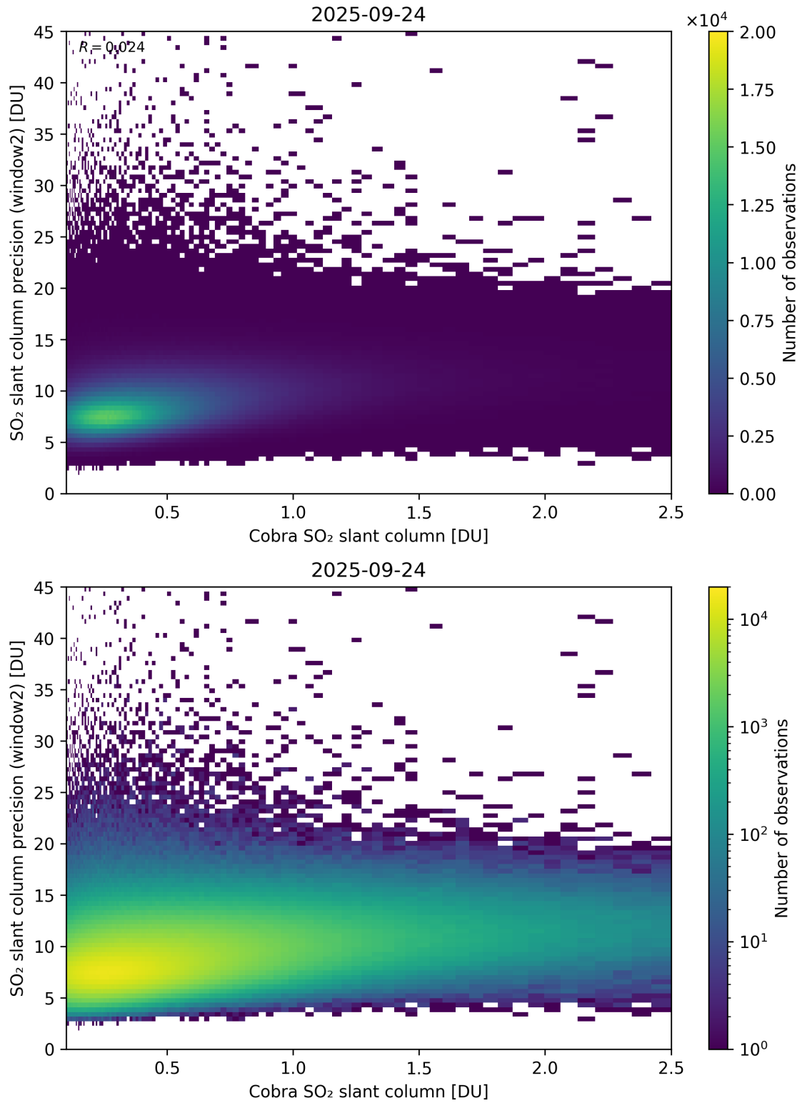
Figure 221: Scatter density plot of “Cobra SO 2 slant column” against “SO 2 slant column precision (window2)” for 2025-09-23 to 2025-09-25.
