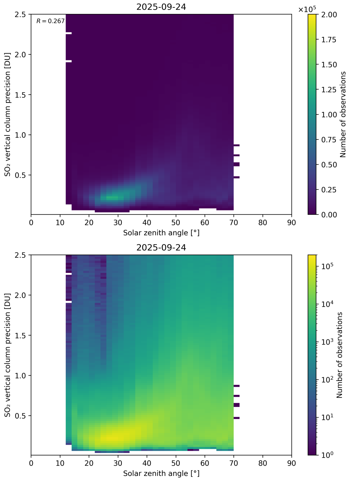
Figure 192: Scatter density plot of “Solar zenith angle” against “SO 2 vertical column precision” for 2025-09-23 to 2025-09-25.
