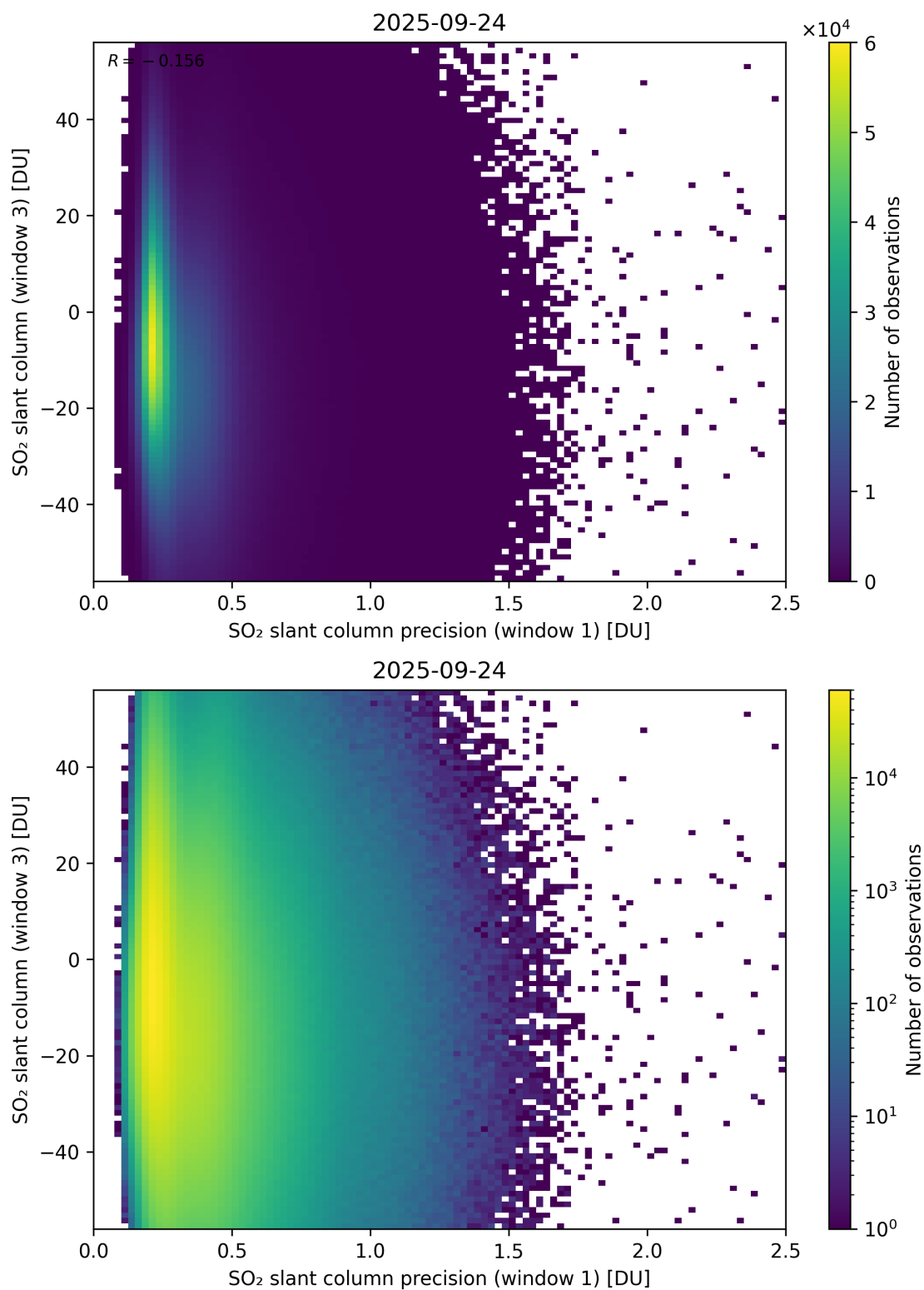
Figure 278: Scatter density plot of “SO 2 slant column precision (window 1)” against “SO 2 slant column (window 3)” for 2025-09-23 to 2025-09-25.
