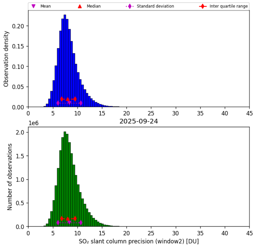
Figure 68: Histogram of “SO 2 slant column precision (window2)” for 2025-09-23 to 2025-09-25
