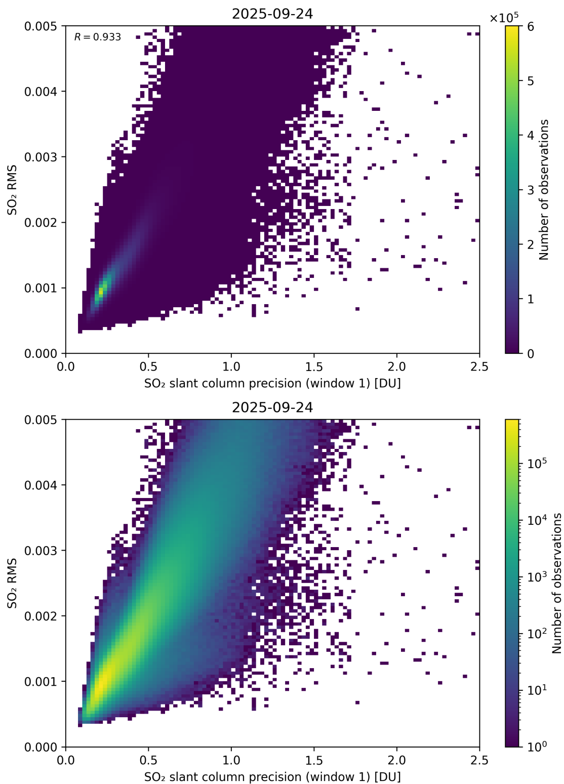
Figure 273: Scatter density plot of “SO 2 slant column precision (window 1)” against “SO 2 RMS” for 2025-09-23 to 2025-09-25.
