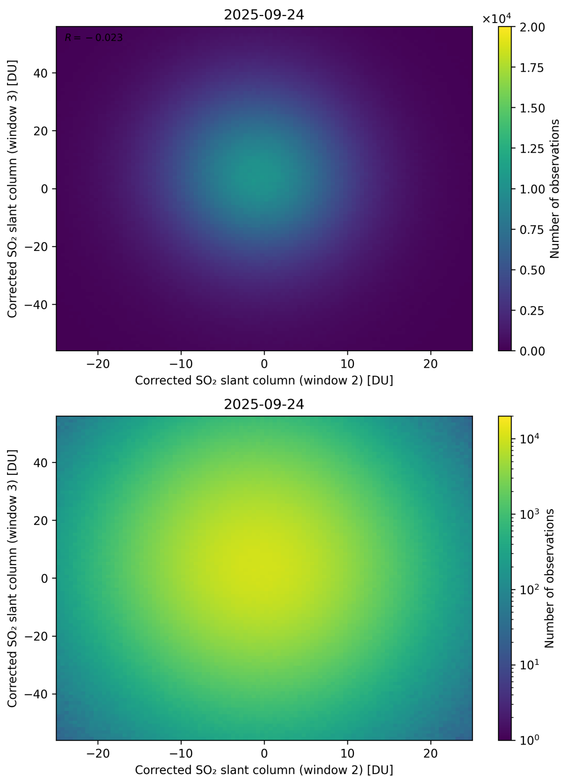
Figure 250: Scatter density plot of “Corrected SO 2 slant column (window 2)” against “Corrected SO 2 slant column (window 3)” for 2025-09-23 to 2025-09-25.
