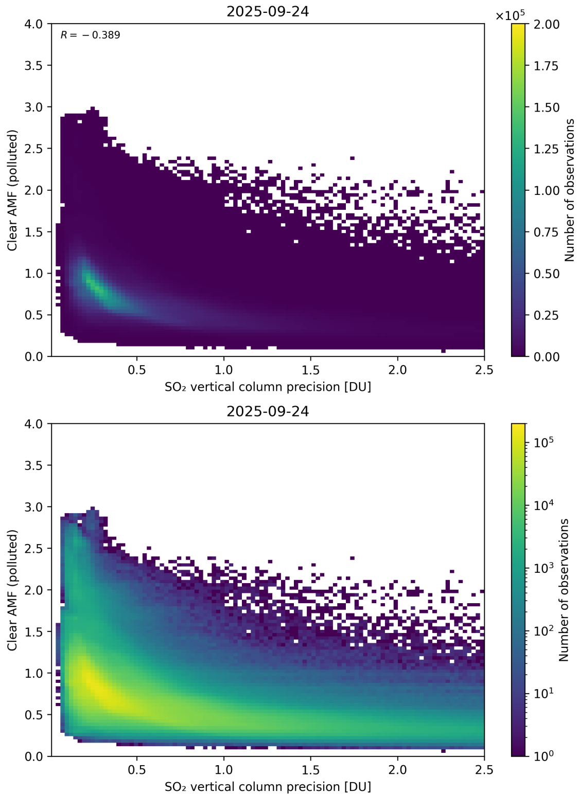
Figure 335: Scatter density plot of “SO 2 vertical column precision” against “Clear AMF (polluted)” for 2025-09-23 to 2025-09-25.
