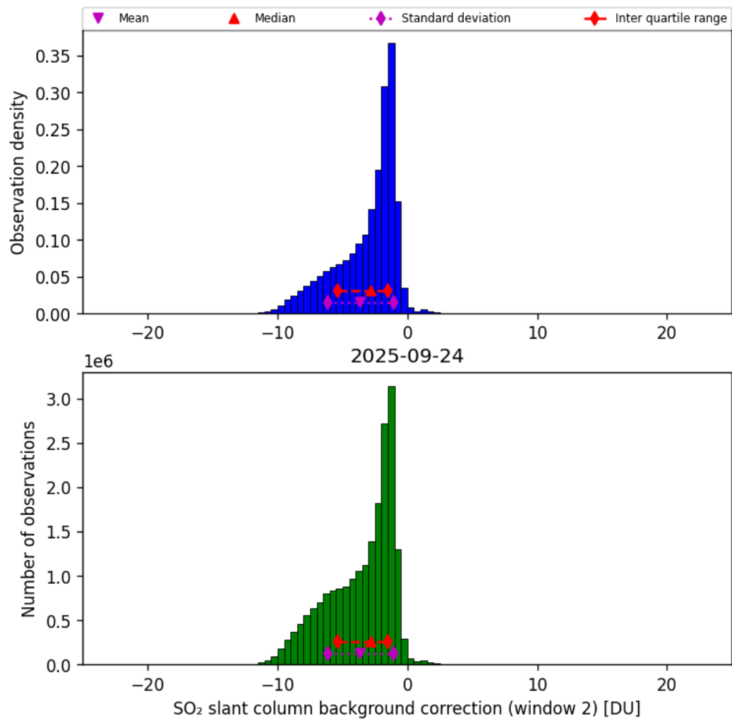
Figure 70: Histogram of “SO 2 slant column background correction (window 2)” for 2025-09-23 to 2025-09-25
