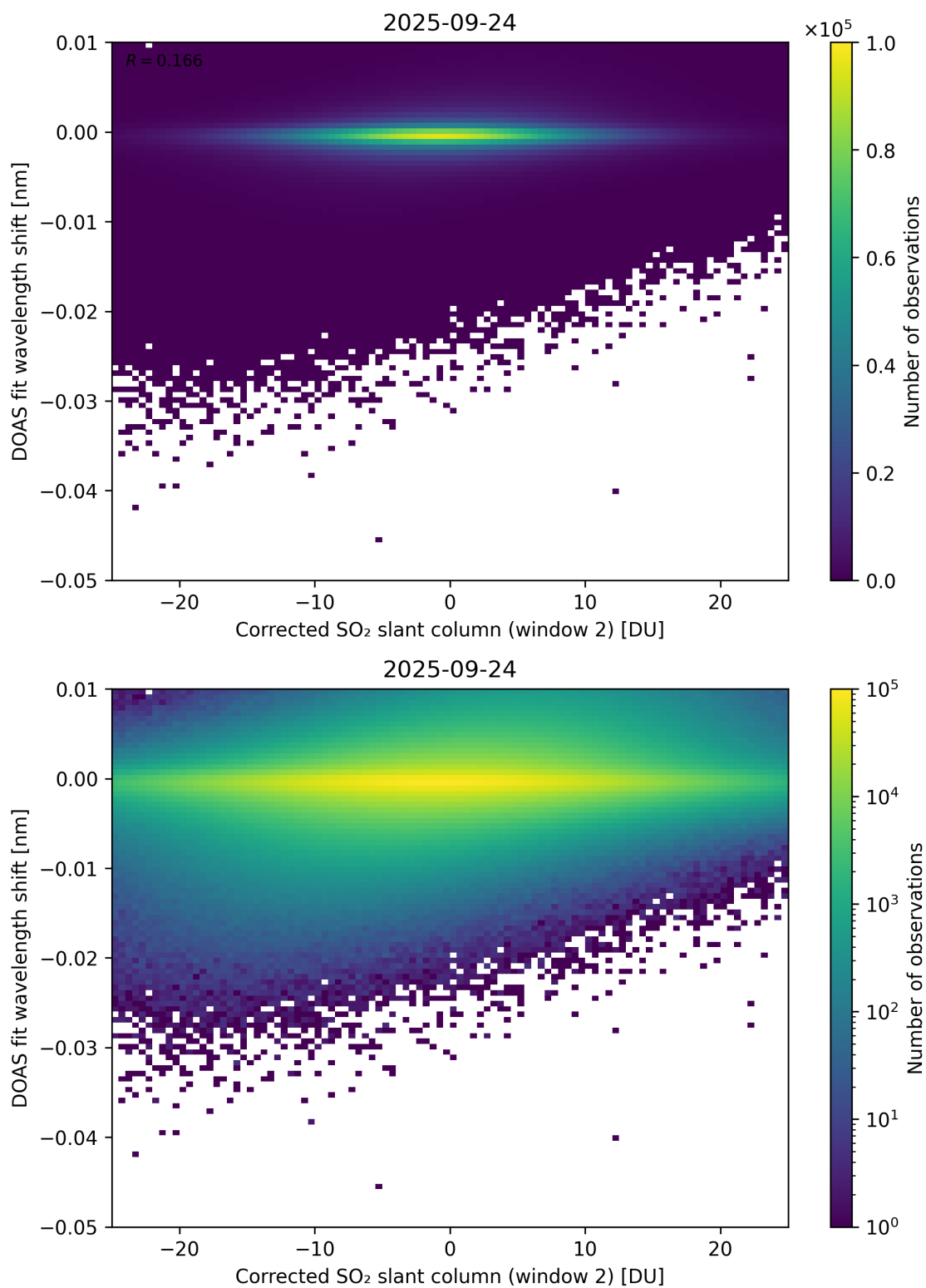
Figure 246: Scatter density plot of “Corrected SO 2 slant column (window 2)” against “DOAS fit wavelength shift” for 2025-09-23 to 2025-09-25.
