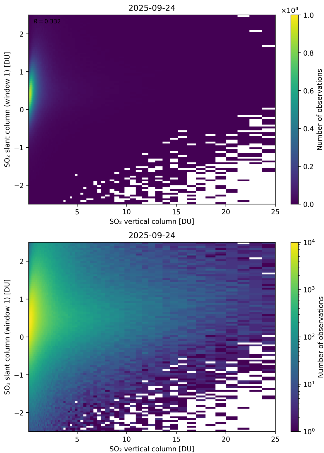
Figure 354: Scatter density plot of “SO 2 vertical column” against “SO 2 slant column (window 1)” for 2025-09-23 to 2025-09-25.
