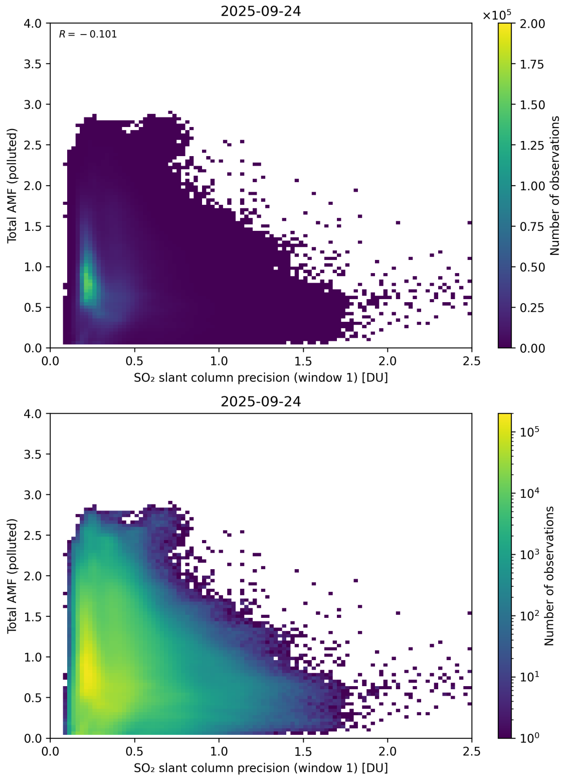
Figure 280: Scatter density plot of “SO 2 slant column precision (window 1)” against “Total AMF (polluted)” for 2025-09-23 to 2025-09-25.
