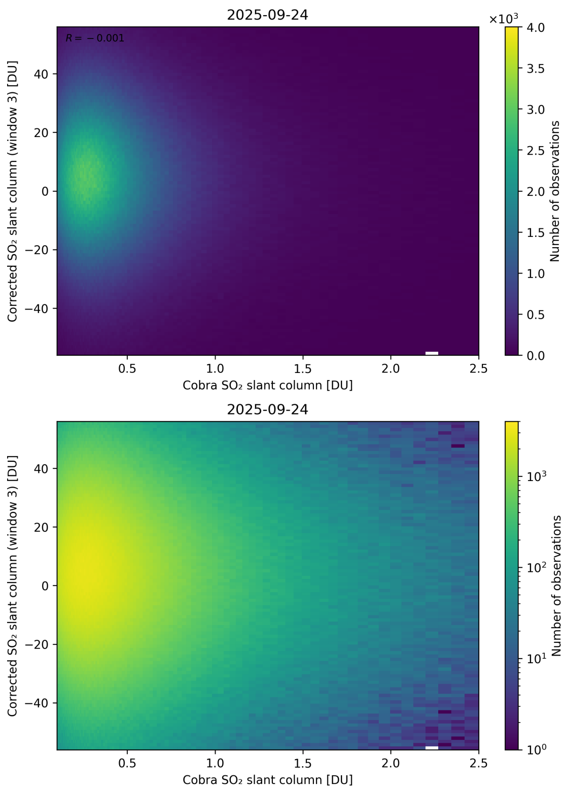
Figure 218: Scatter density plot of “Cobra SO 2 slant column” against “Corrected SO 2 slant column (window 3)” for 2025-09-23 to 2025-09-25.
