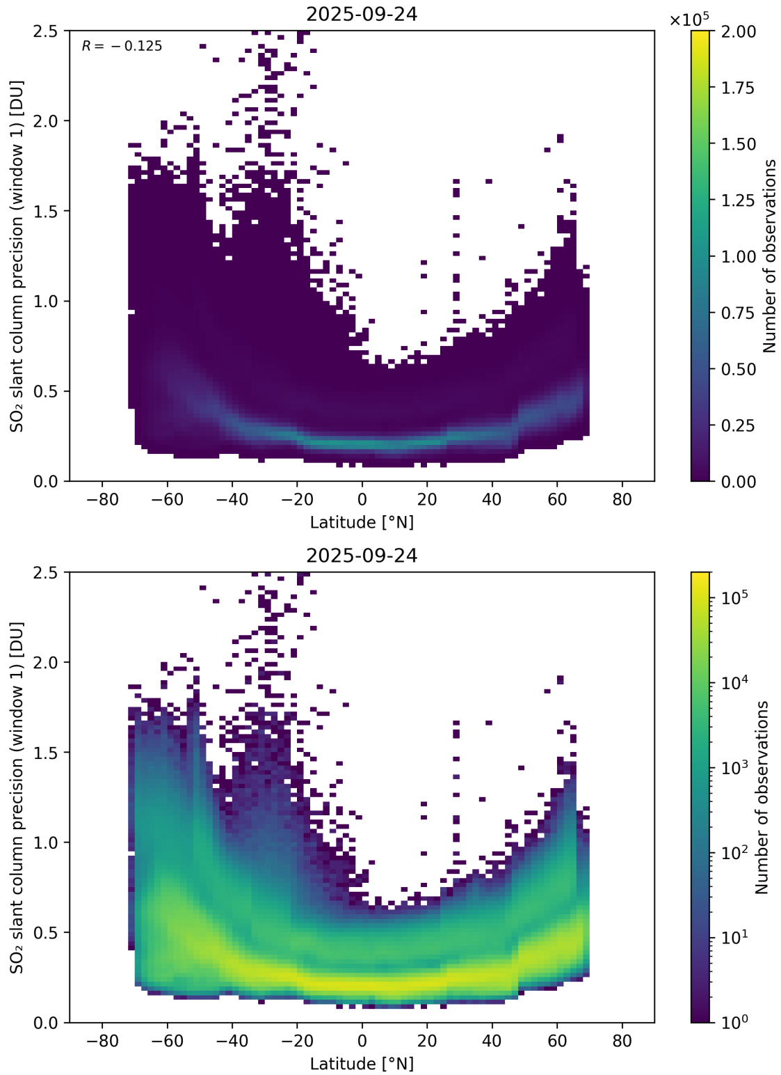
Figure 163: Scatter density plot of “Latitude” against “SO 2 slant column precision (window 1)” for 2025-09-23 to 2025-09-25.
