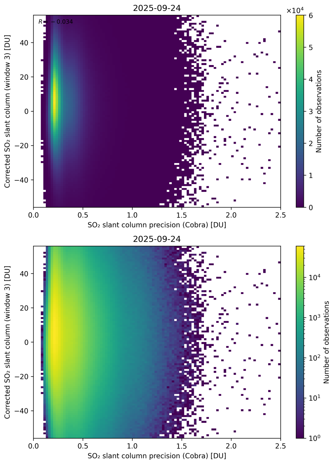
Figure 207: Scatter density plot of “SO 2 slant column precision (Cobra)” against “Corrected SO 2 slant column (window 3)” for 2025-09-23 to 2025-09-25.
