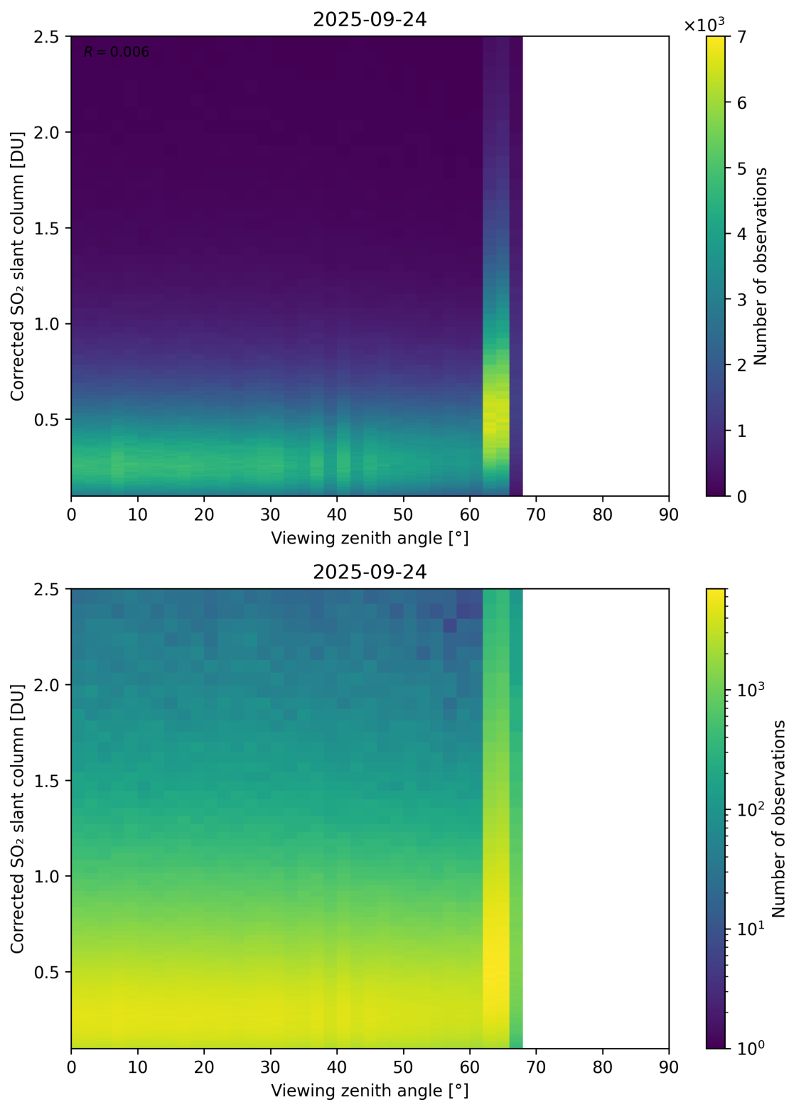
Figure 373: Scatter density plot of “Viewing zenith angle” against “Corrected SO 2 slant column” for 2025-09-23 to 2025-09-25.
