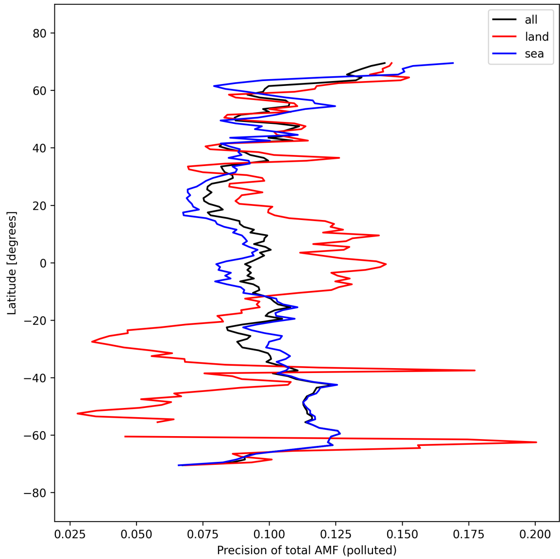
Figure 54: Zonal average of “Precision of total AMF (polluted)” for 2025-09-23 to 2025-09-25.
