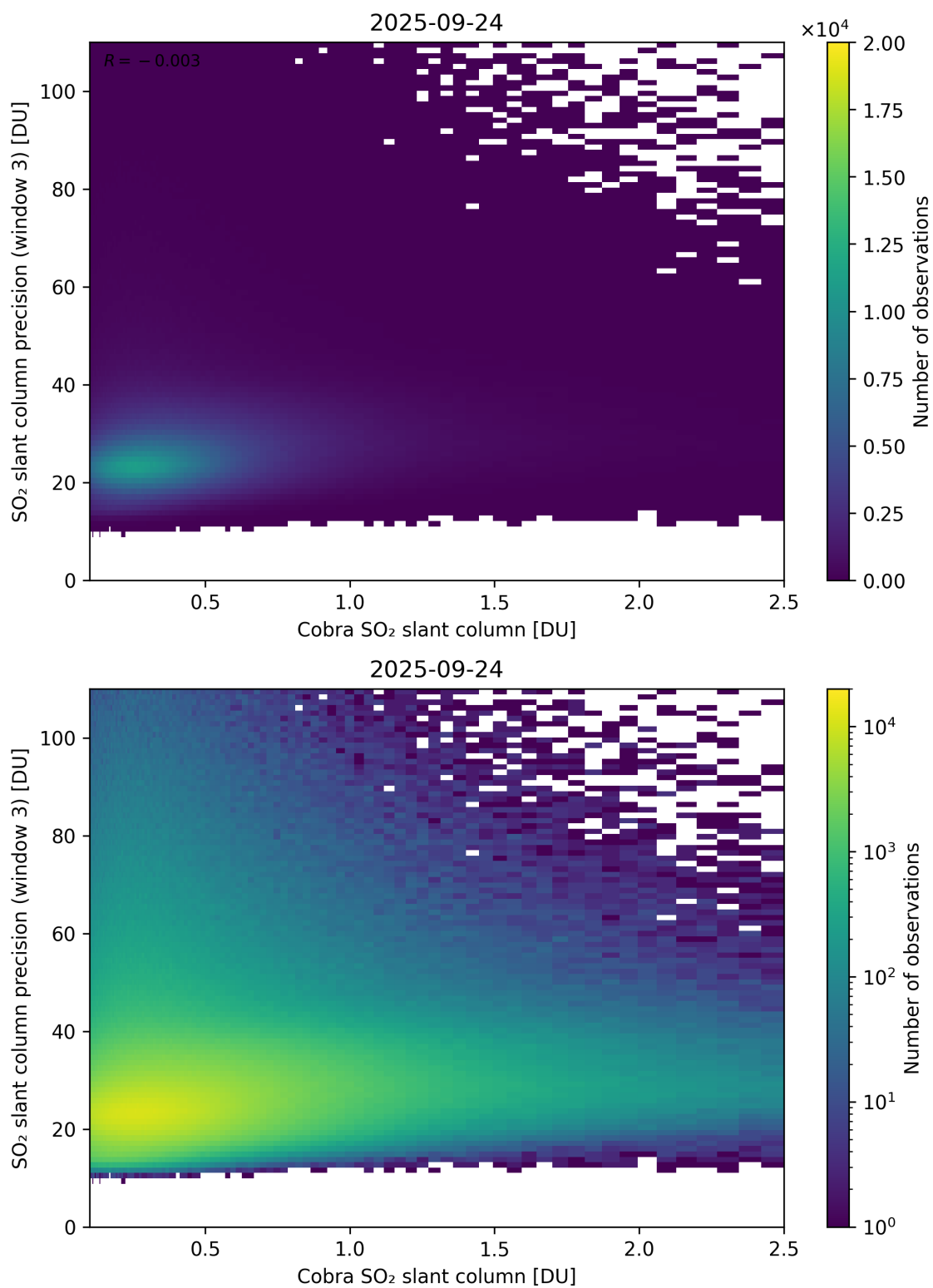
Figure 223: Scatter density plot of “Cobra SO 2 slant column” against “SO 2 slant column precision (window 3)” for 2025-09-23 to 2025-09-25.
