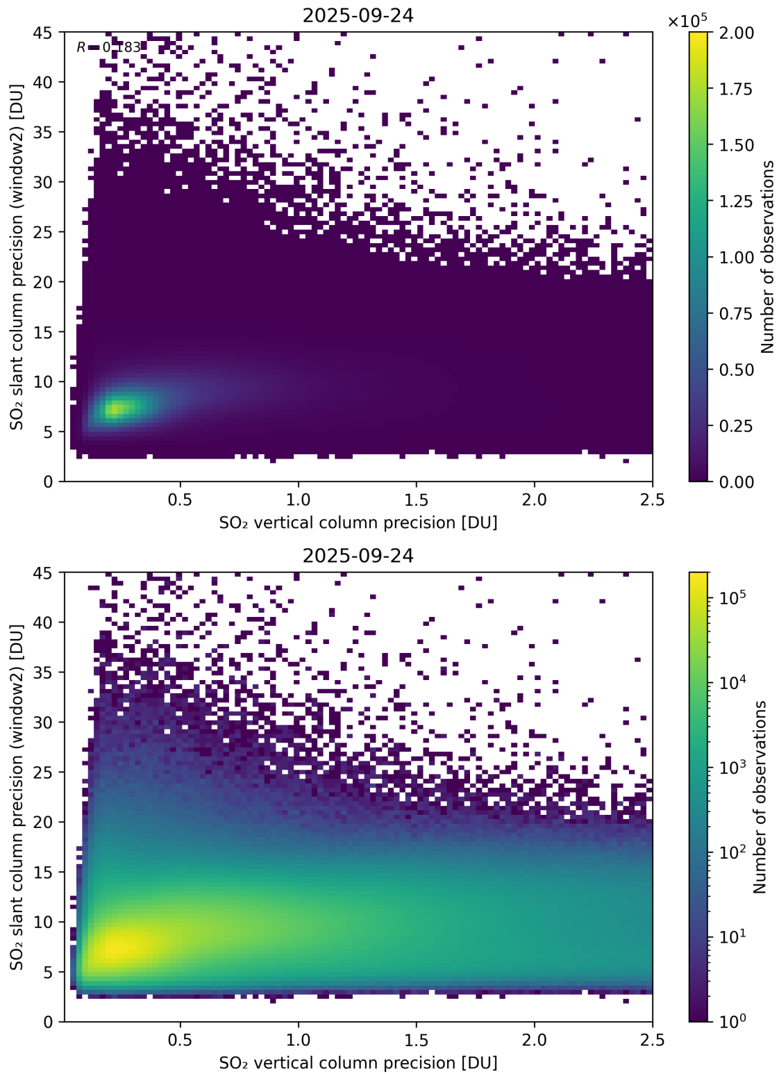
Figure 343: Scatter density plot of “SO 2 vertical column precision” against “SO 2 slant column precision (window2)” for 2025-09-23 to 2025-09-25.
