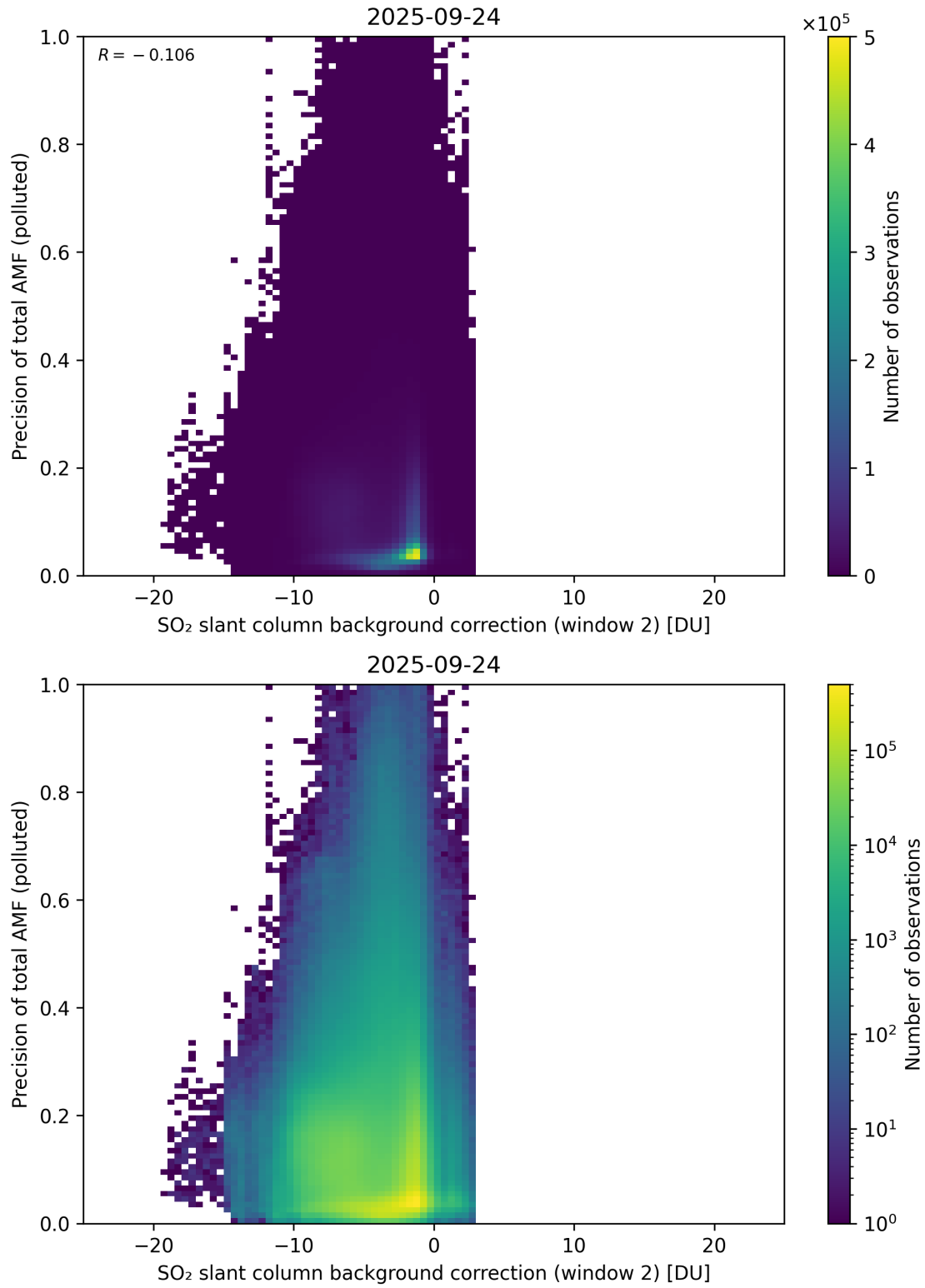
Figure 131: Scatter density plot of “SO 2 slant column background correction (window 2)” against “Precision of total AMF (polluted)” for 2025-09-23 to 2025-09-25.
