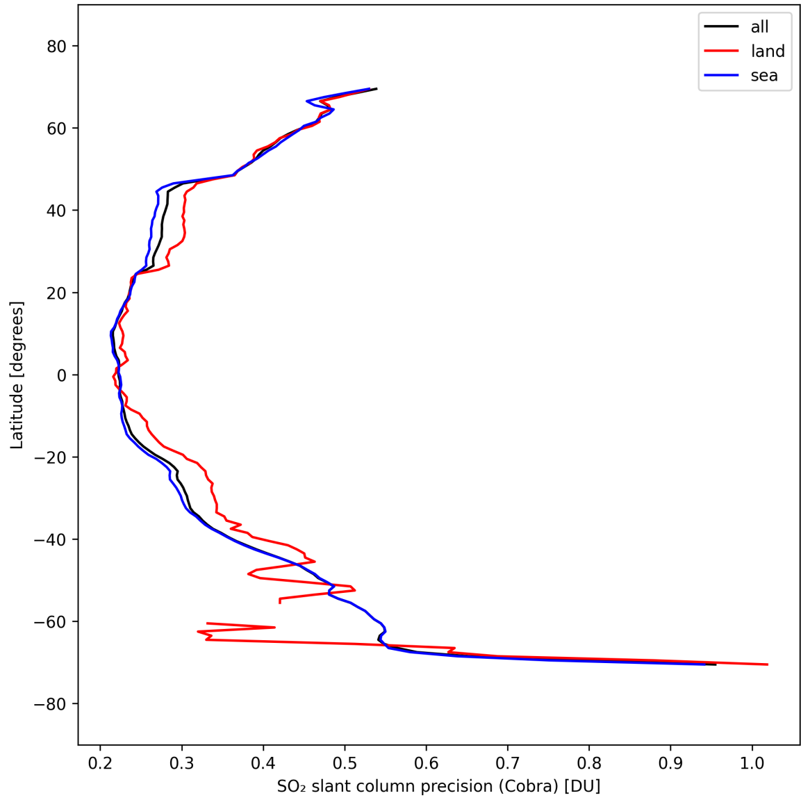
Figure 36: Zonal average of "SO 2 slant column precision (Cobra)" for 2025-09-23 to 2025-09-25.
