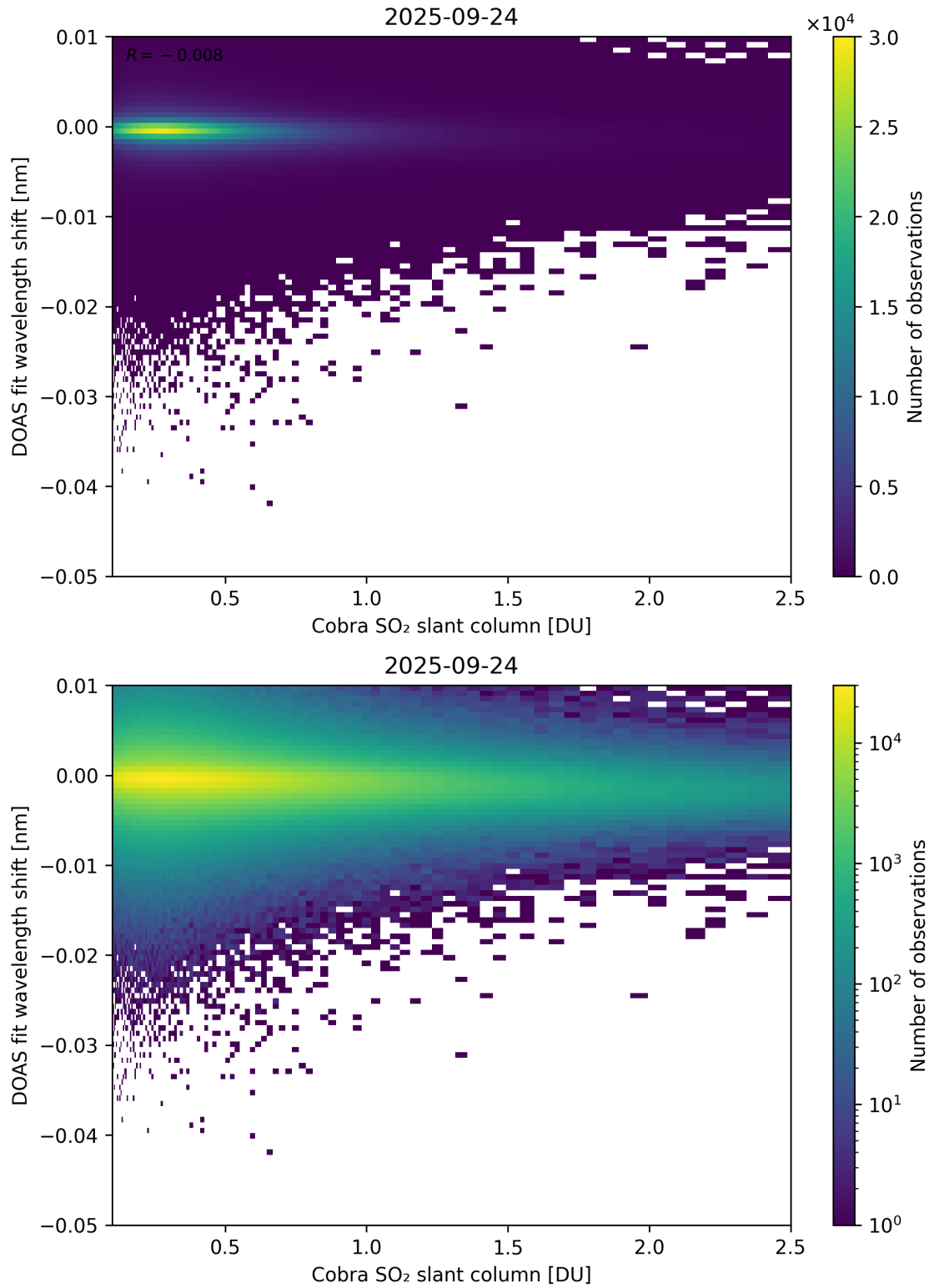
Figure 196: Scatter density plot of “Cobra SO 2 slant column” against “DOAS fit wavelength shift” for 2025-09-23 to 2025-09-25.
