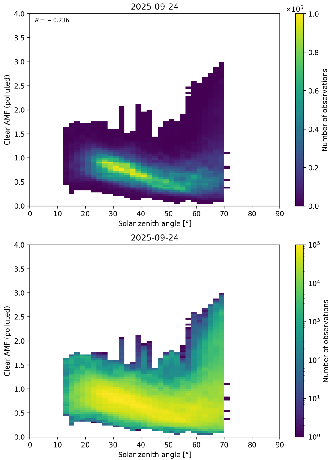
Figure 178: Scatter density plot of “Solar zenith angle” against “Clear AMF (polluted)” for 2025-09-23 to 2025-09-25.
