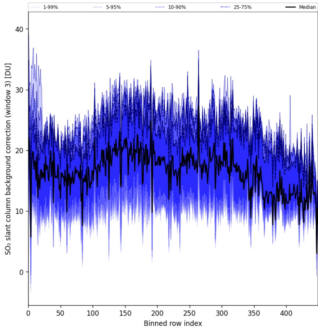
Figure 100: Along track statistics of “SO 2 slant column background correction (window 3)” for 2025-09-23 to 2025-09-25
