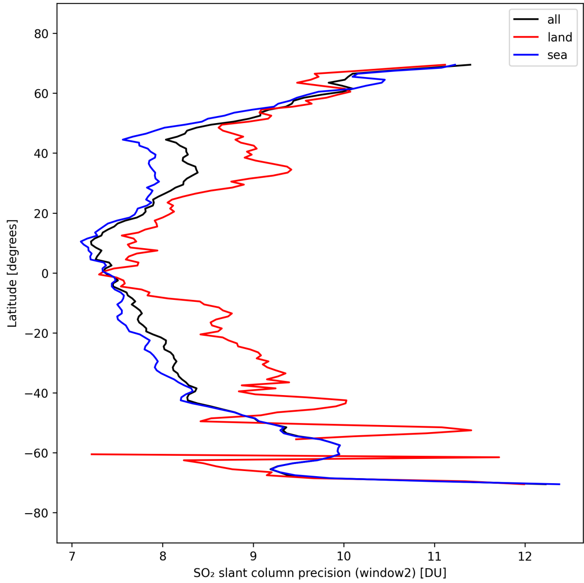
Figure 42: Zonal average of “SO 2 slant column precision (window2)” for 2025-09-23 to 2025-09-25.
