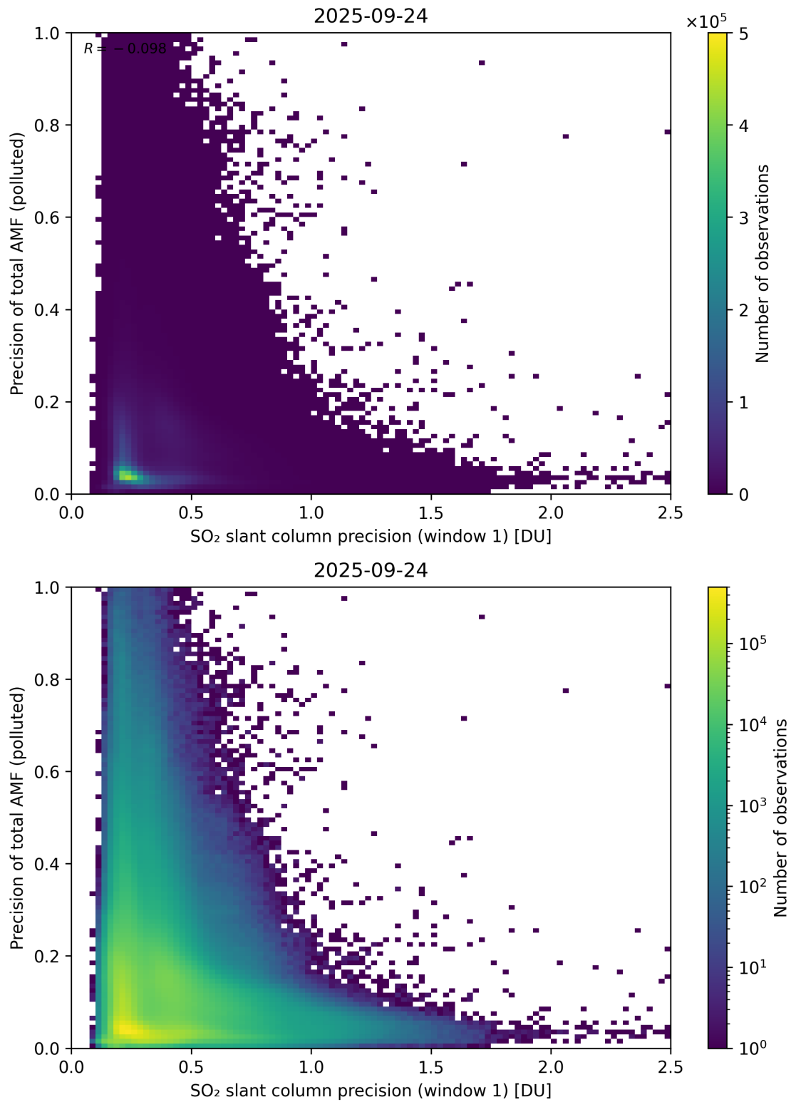
Figure 281: Scatter density plot of “SO 2 slant column precision (window 1)” against “Precision of total AMF (polluted)” for 2025-09-23 to 2025-09-25.
