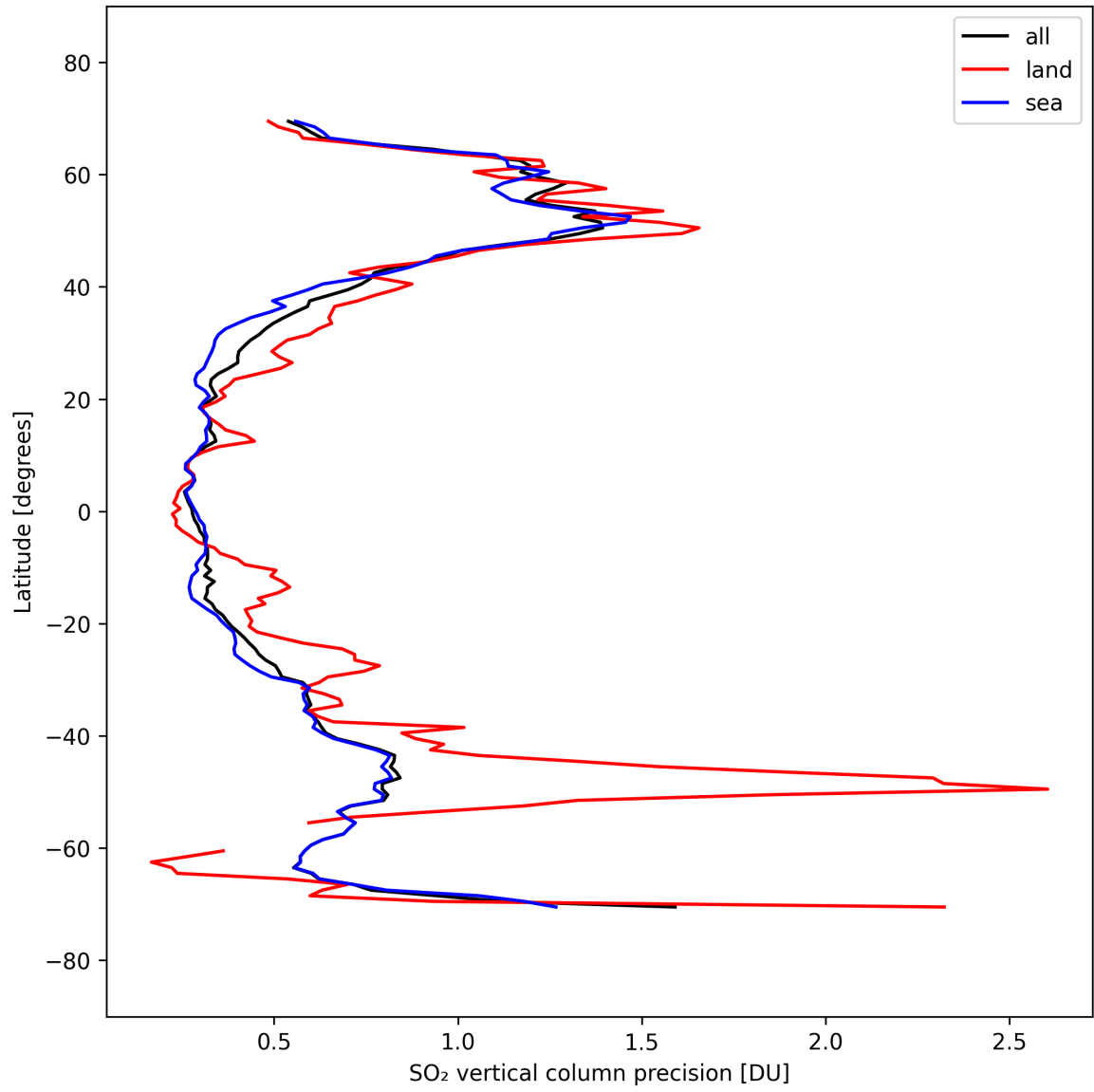
Figure 33: Zonal average of “SO 2 vertical column precision” for 2025-09-23 to 2025-09-25.
