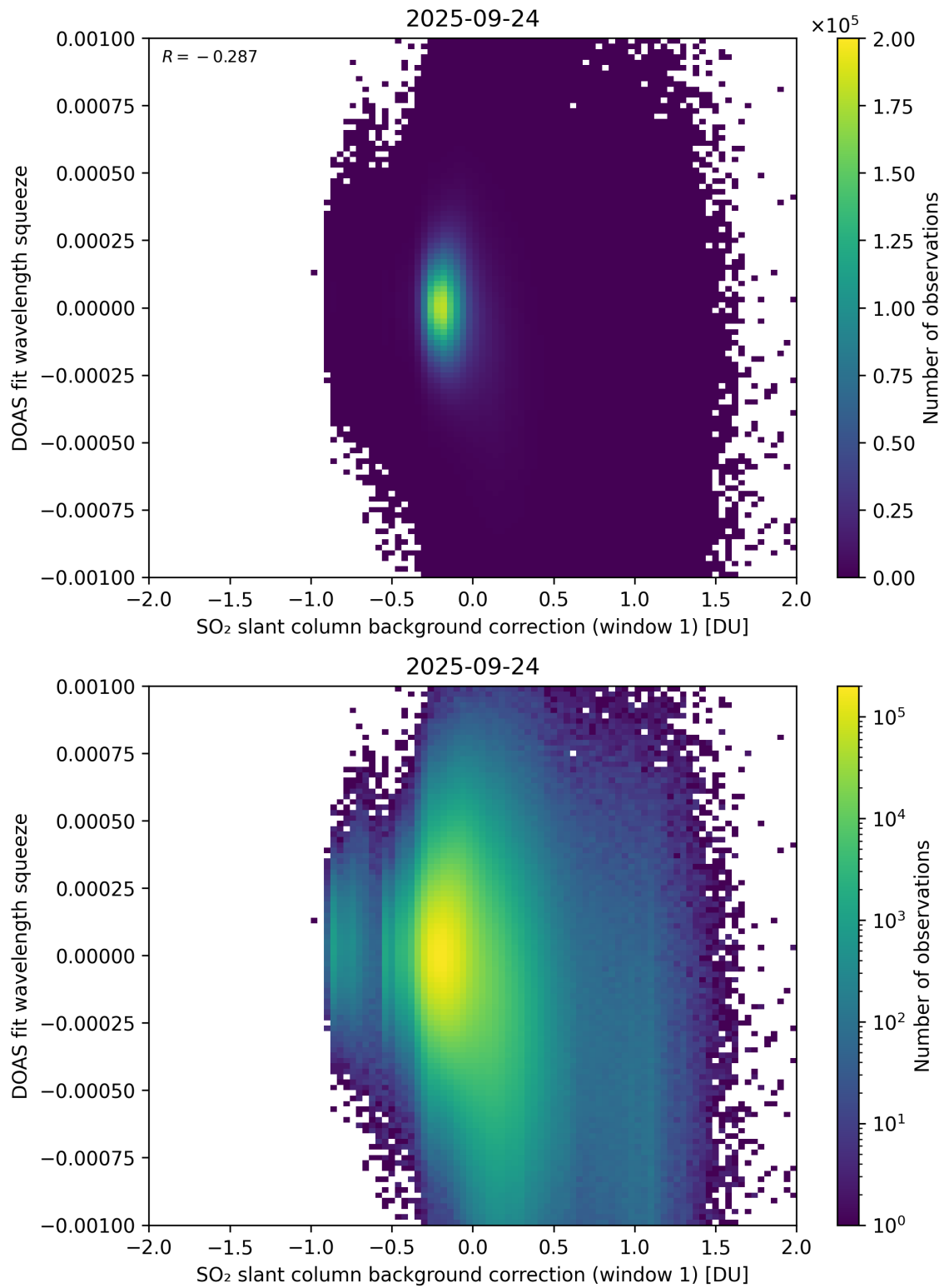
Figure 112: Scatter density plot of “SO 2 slant column background correction (window 1)” against “DOAS fit wavelength squeeze” for 2025-09-23 to 2025-09-25.
