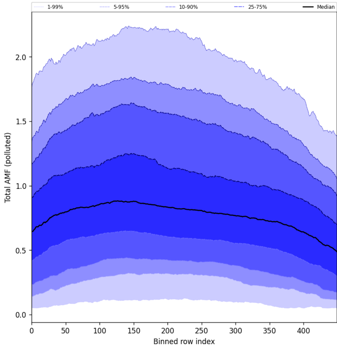
Figure 105: Along track statistics of “Total AMF (polluted)” for 2025-09-23 to 2025-09-25
