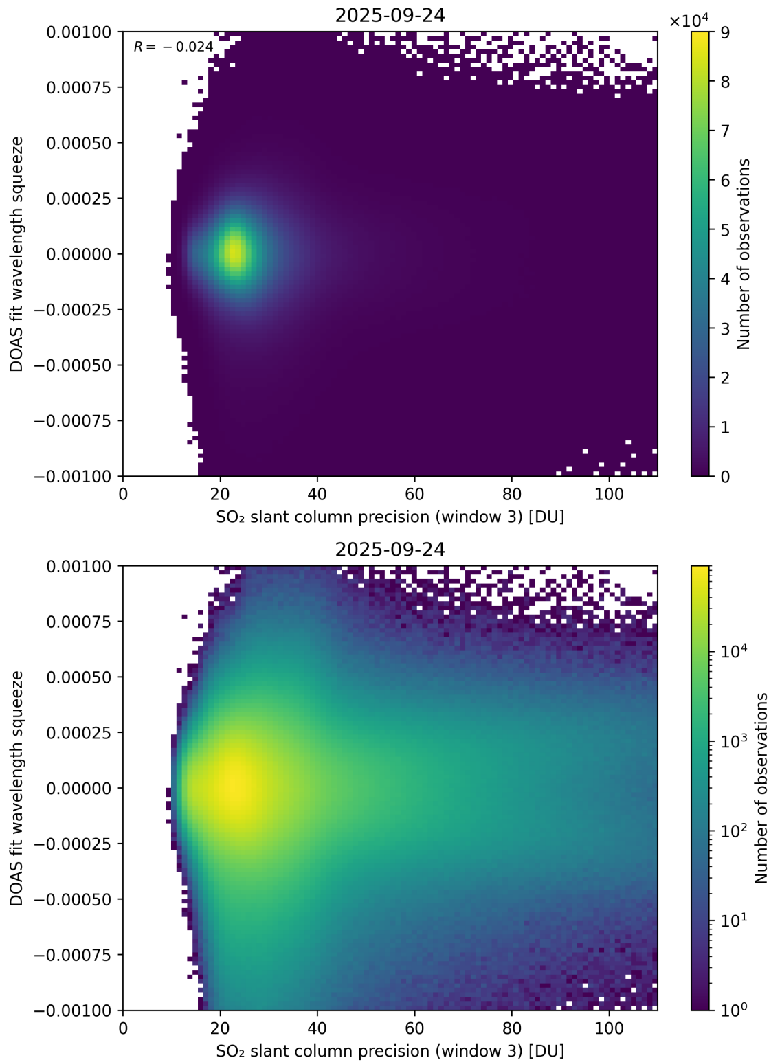
Figure 309: Scatter density plot of “SO 2 slant column precision (window 3)” against “DOAS fit wavelength squeeze” for 2025-09-23 to 2025-09-25.
