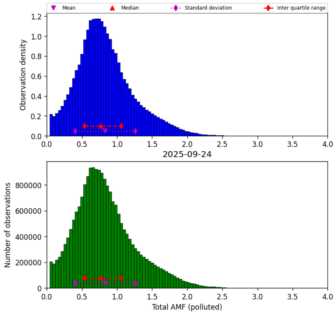
Figure 79: Histogram of “Total AMF (polluted)” for 2025-09-23 to 2025-09-25
