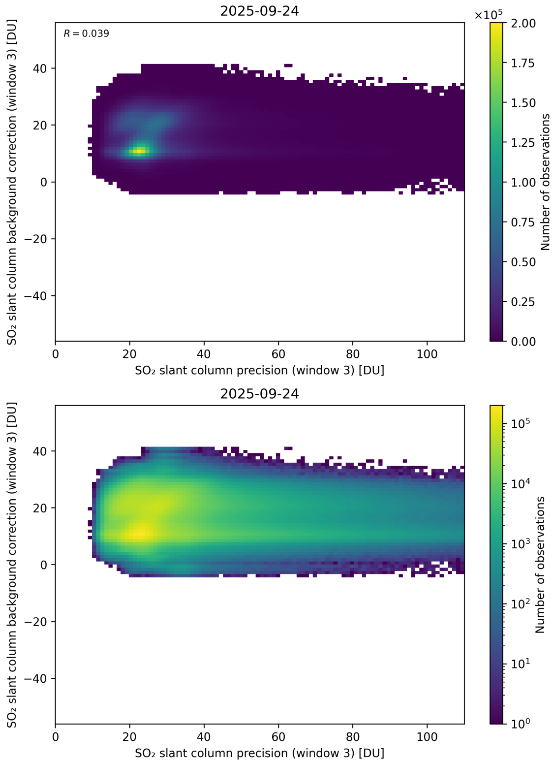
Figure 307: Scatter density plot of “SO 2 slant column precision (window 3)” against “SO 2 slant column background correction (window 3)” for 2025-09-23 to 2025-09-25.
