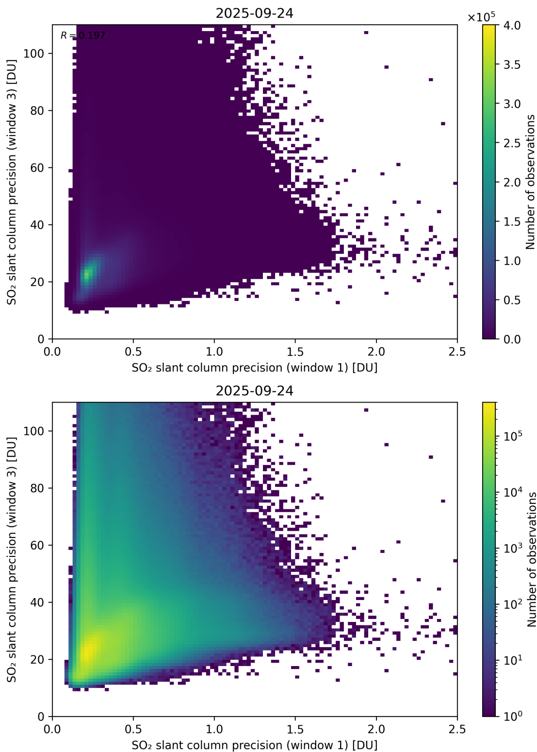
Figure 279: Scatter density plot of “SO 2 slant column precision (window 1)” against “SO 2 slant column precision (window 3)” for 2025-09-23 to 2025-09-25.
