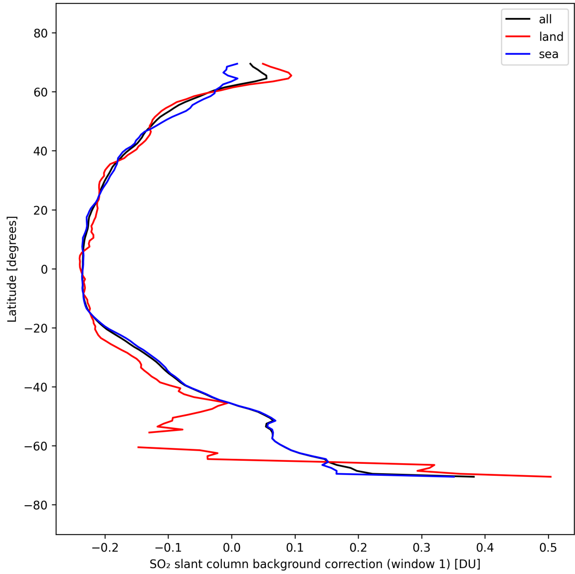
Figure 40: Zonal average of “SO 2 slant column background correction (window 1)” for 2025-09-23 to 2025-09-25.
