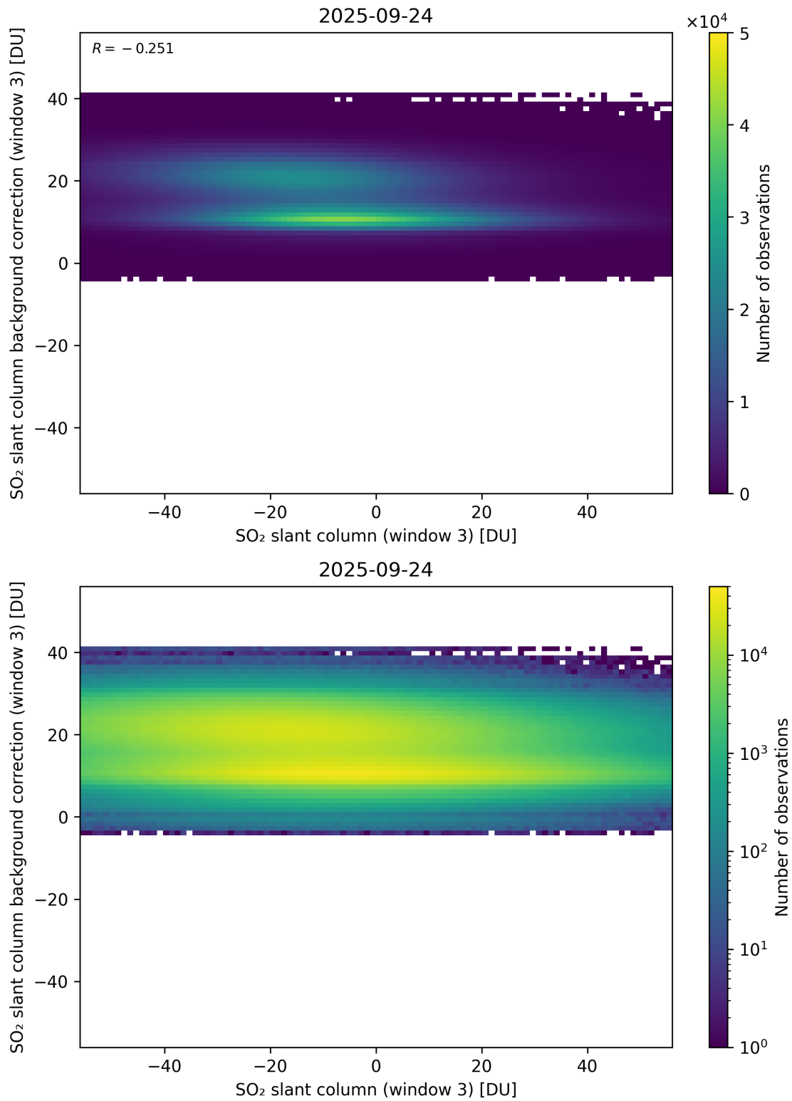
Figure 303: Scatter density plot of “SO 2 slant column (window 3)” against “SO 2 slant column background correction (window 3)” for 2025-09-23 to 2025-09-25.
