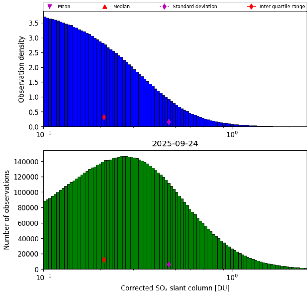
Figure 60: Histogram of “Corrected SO 2 slant column” for 2025-09-23 to 2025-09-25
