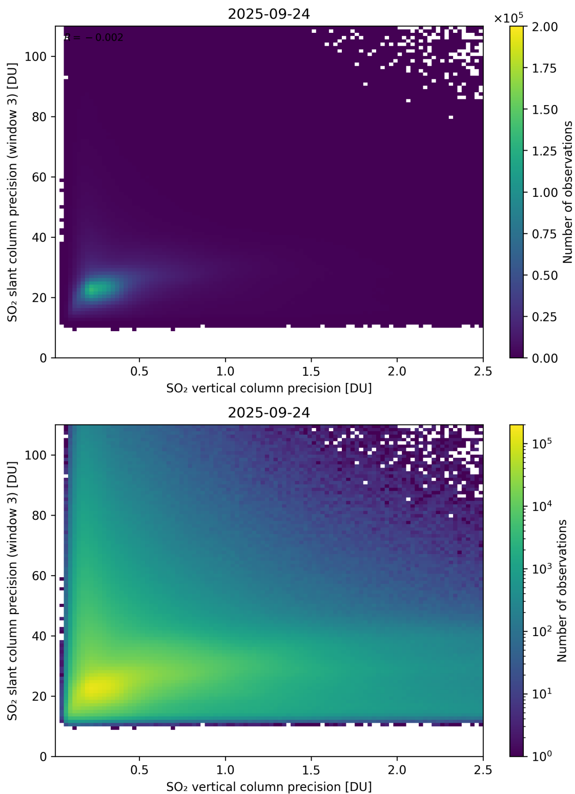
Figure 345: Scatter density plot of “SO 2 vertical column precision” against “SO 2 slant column precision (window 3)” for 2025-09-23 to 2025-09-25.
