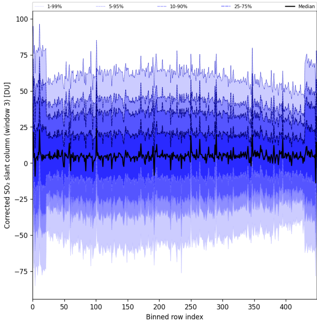
Figure 99: Along track statistics of “Corrected SO 2 slant column (window 3)” for 2025-09-23 to 2025-09-25
