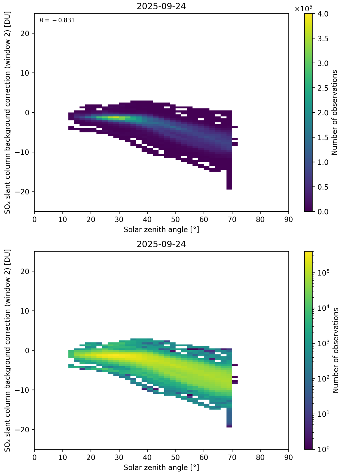
Figure 172: Scatter density plot of “Solar zenith angle” against “SO 2 slant column background correction (window 2)” for 2025-09-23 to 2025-09-25.
