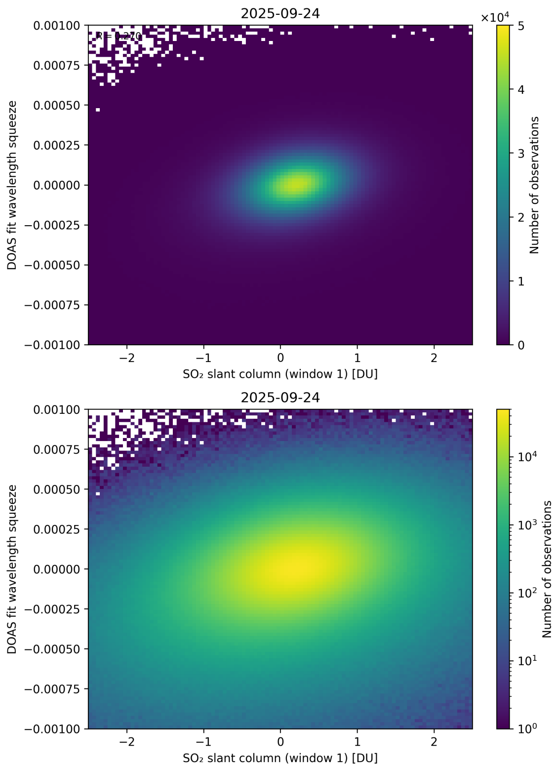
Figure 266: Scatter density plot of “SO 2 slant column (window 1)” against “DOAS fit wavelength squeeze” for 2025-09-23 to 2025-09-25.
