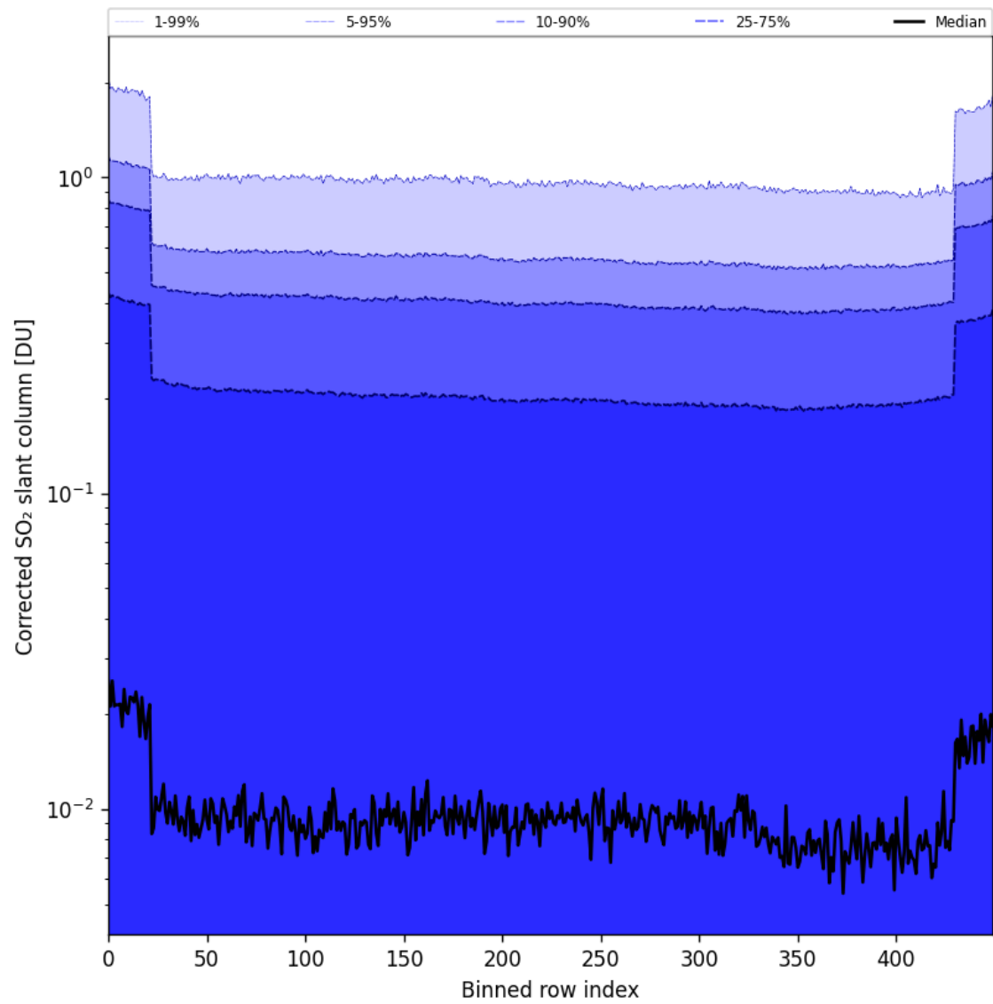
Figure 86: Along track statistics of “Corrected SO 2 slant column” for 2025-09-23 to 2025-09-25
