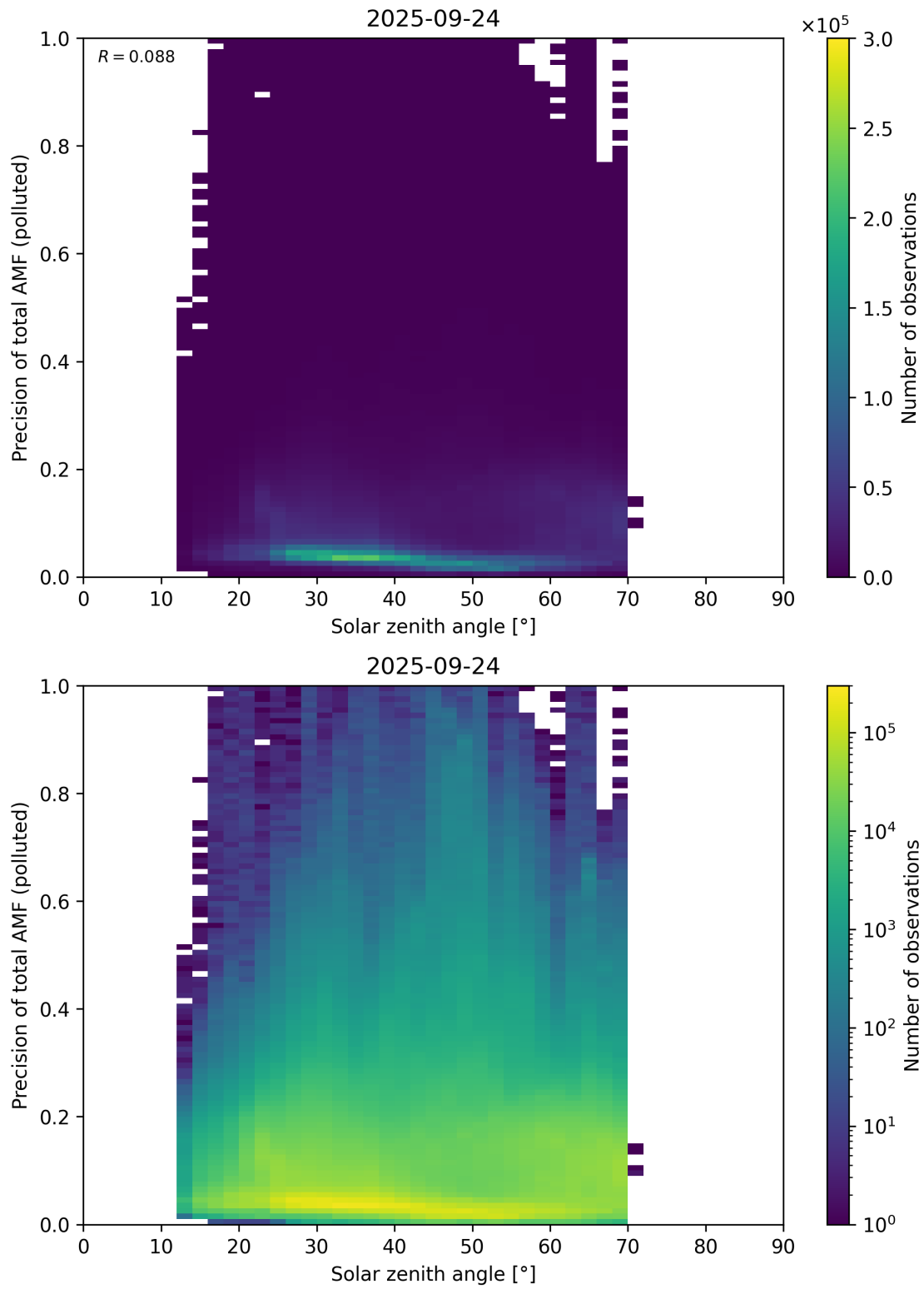
Figure 190: Scatter density plot of “Solar zenith angle” against “Precision of total AMF (polluted)” for 2025-09-23 to 2025-09-25.
