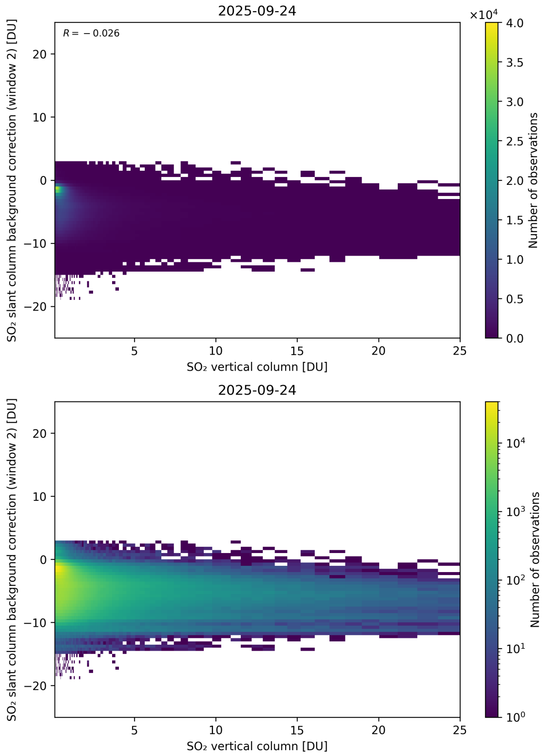
Figure 324: Scatter density plot of “SO 2 vertical column” against “SO 2 slant column background correction (window 2)” for 2025-09-23 to 2025-09-25.
