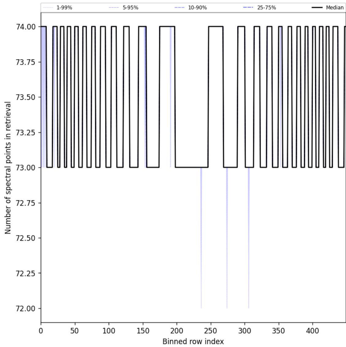
Figure 108: Along track statistics of “Number of spectral points in retrieval” for 2025-09-23 to 2025-09-25
