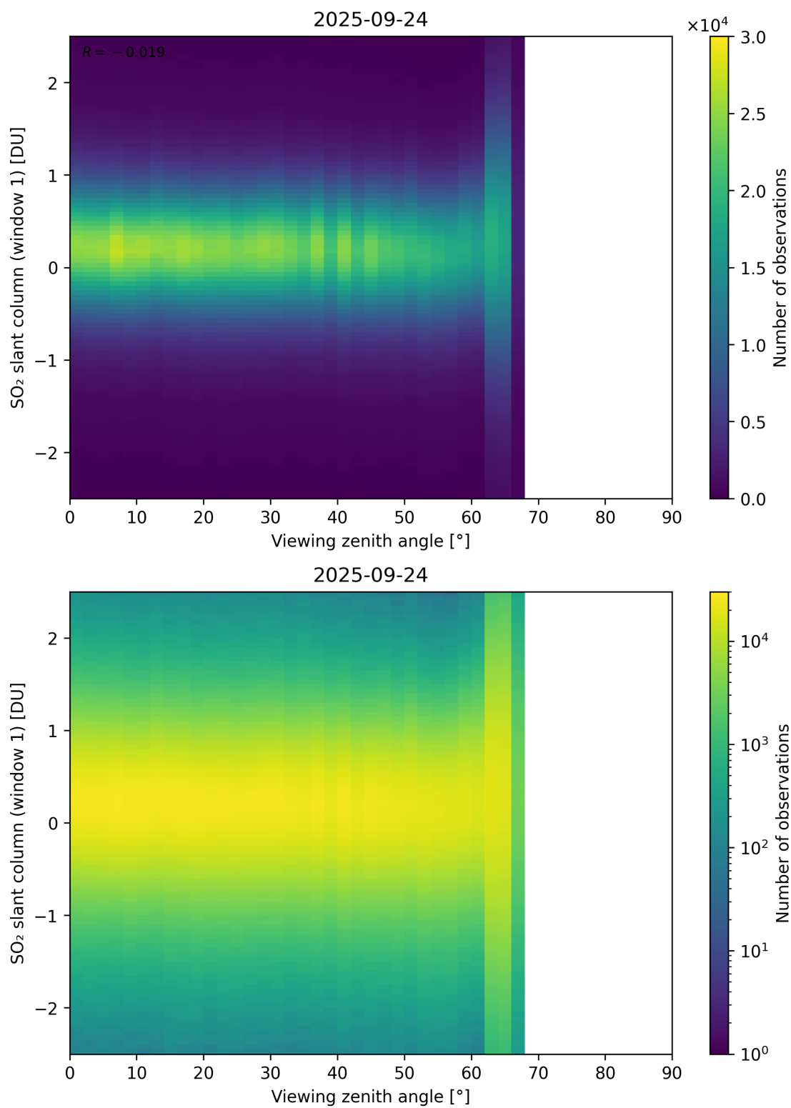
Figure 376: Scatter density plot of “Viewing zenith angle” against “SO 2 slant column (window 1)” for 2025-09-23 to 2025-09-25.
