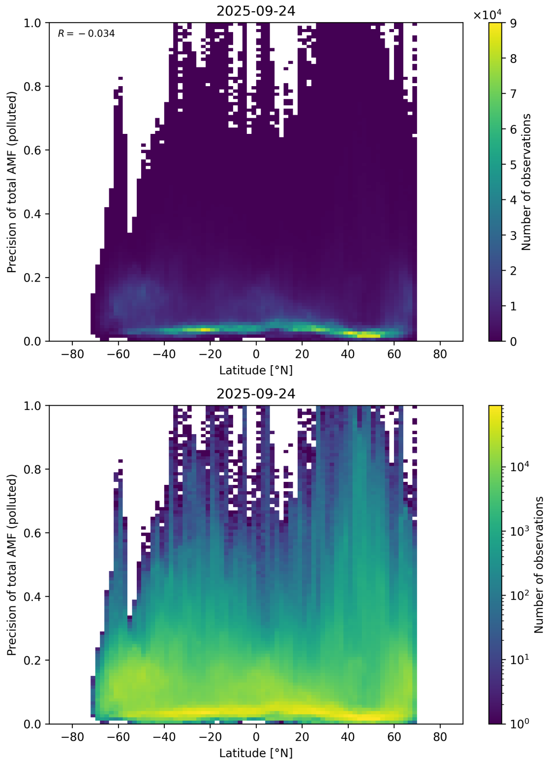
Figure 168: Scatter density plot of “Latitude” against “Precision of total AMF (polluted)” for 2025-09-23 to 2025-09-25.
