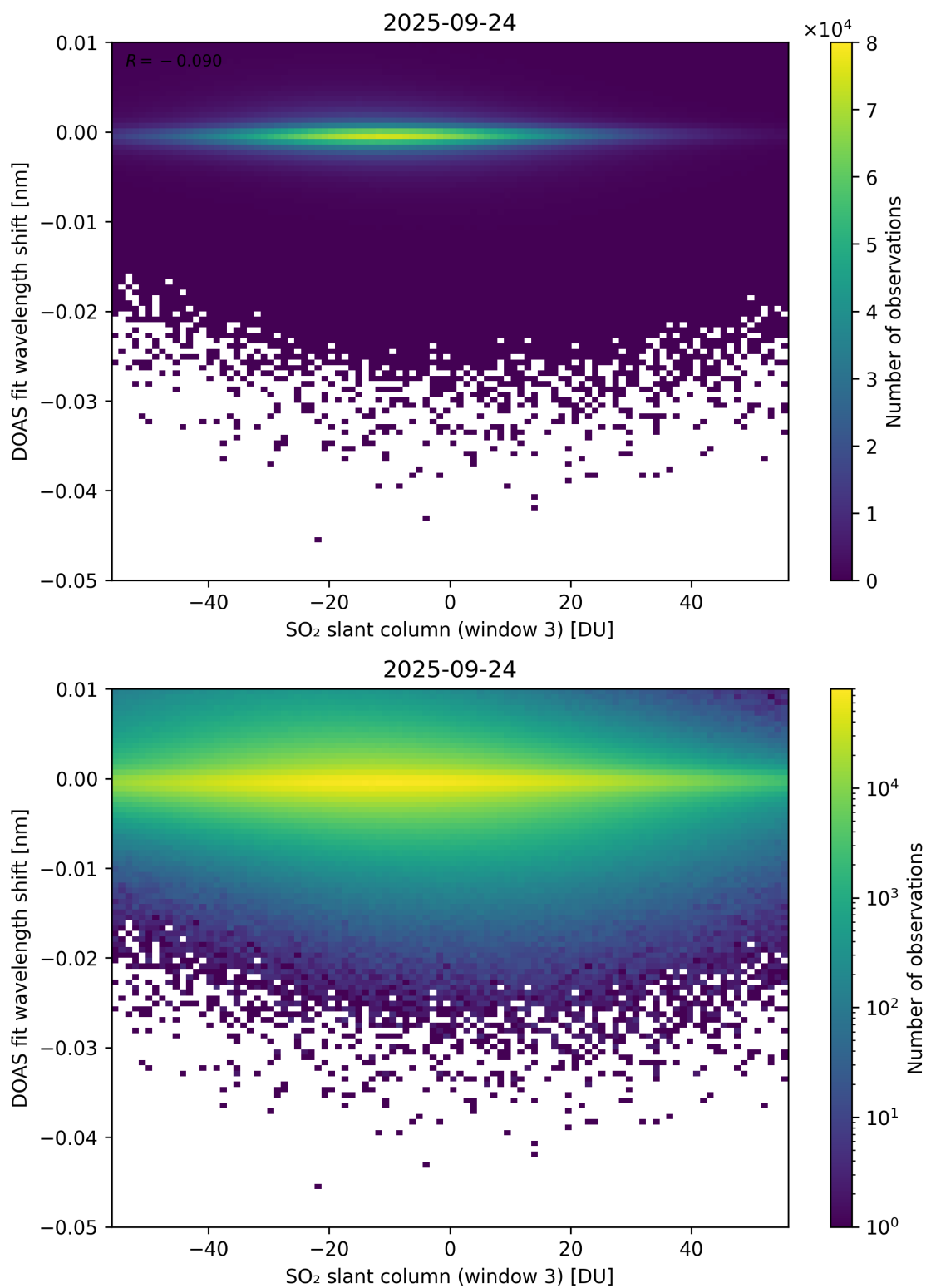
Figure 304: Scatter density plot of “SO 2 slant column (window 3)” against “DOAS fit wavelength shift” for 2025-09-23 to 2025-09-25.
