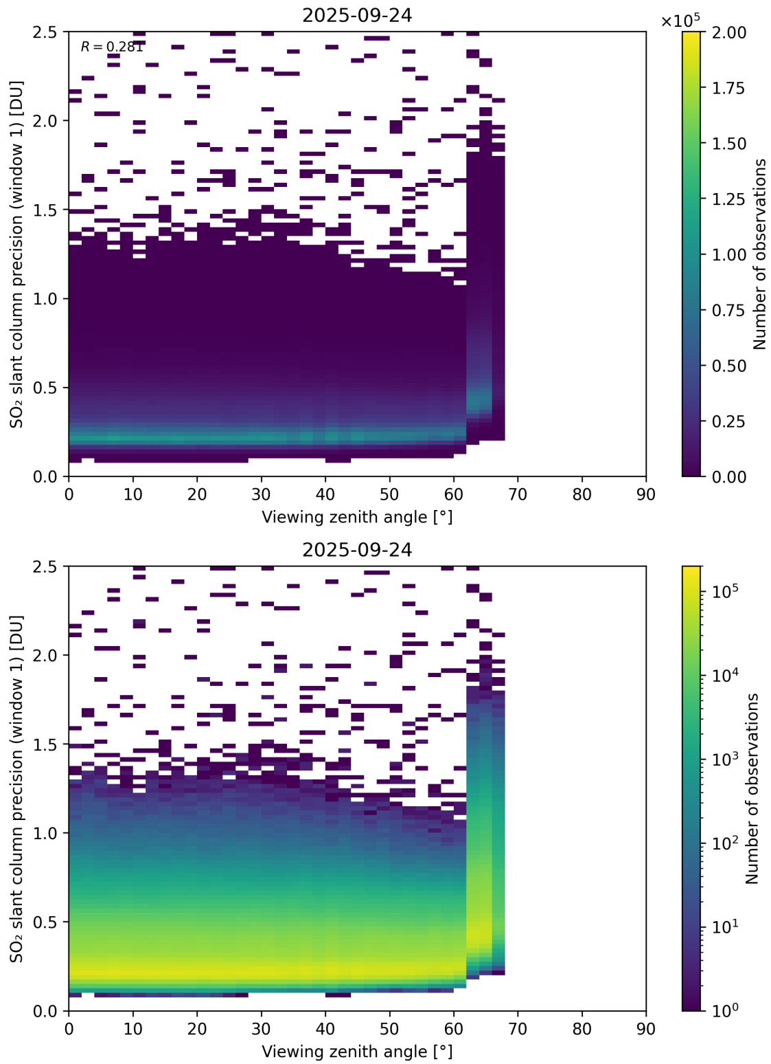
Figure 377: Scatter density plot of “Viewing zenith angle” against “SO 2 slant column precision (window 1)” for 2025-09-23 to 2025-09-25.
