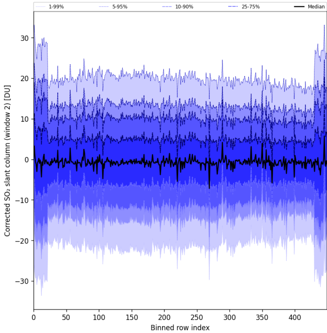
Figure 95: Along track statistics of “Corrected SO 2 slant column (window 2)” for 2025-09-23 to 2025-09-25
