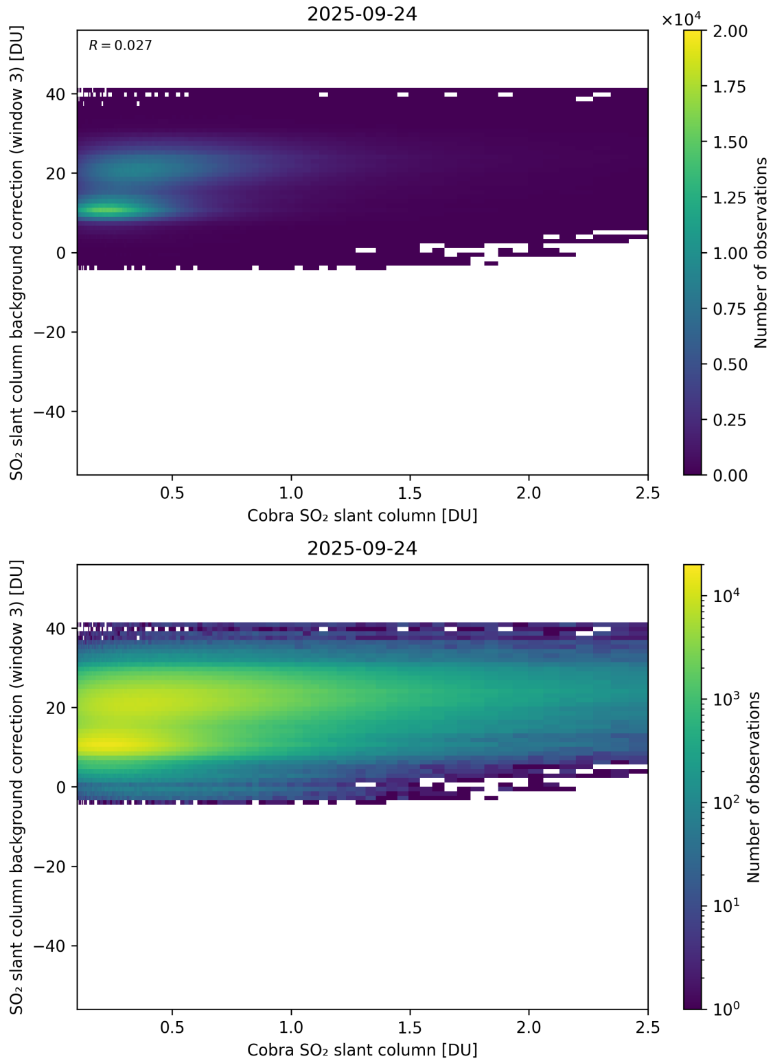
Figure 195: Scatter density plot of “Cobra SO 2 slant column” against “SO 2 slant column background correction (window 3)” for 2025-09-23 to 2025-09-25.
