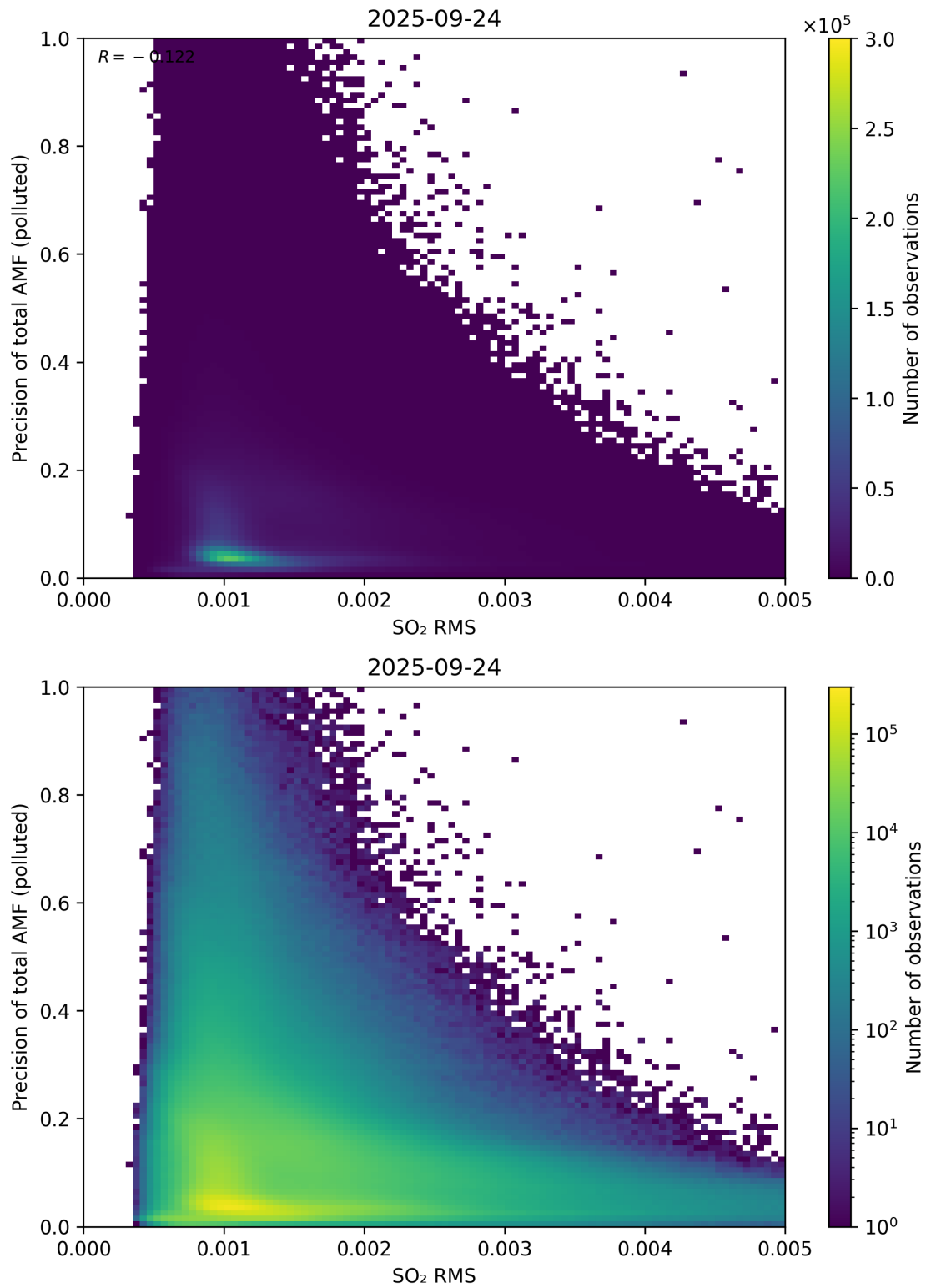
Figure 149: Scatter density plot of “SO 2 RMS” against “Precision of total AMF (polluted)” for 2025-09-23 to 2025-09-25.
