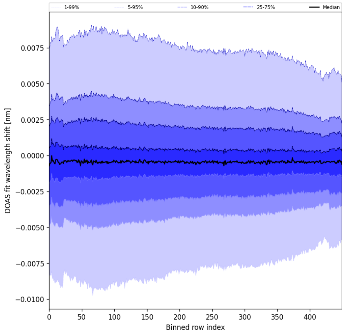
Figure 102: Along track statistics of “DOAS fit wavelength shift” for 2025-09-23 to 2025-09-25
