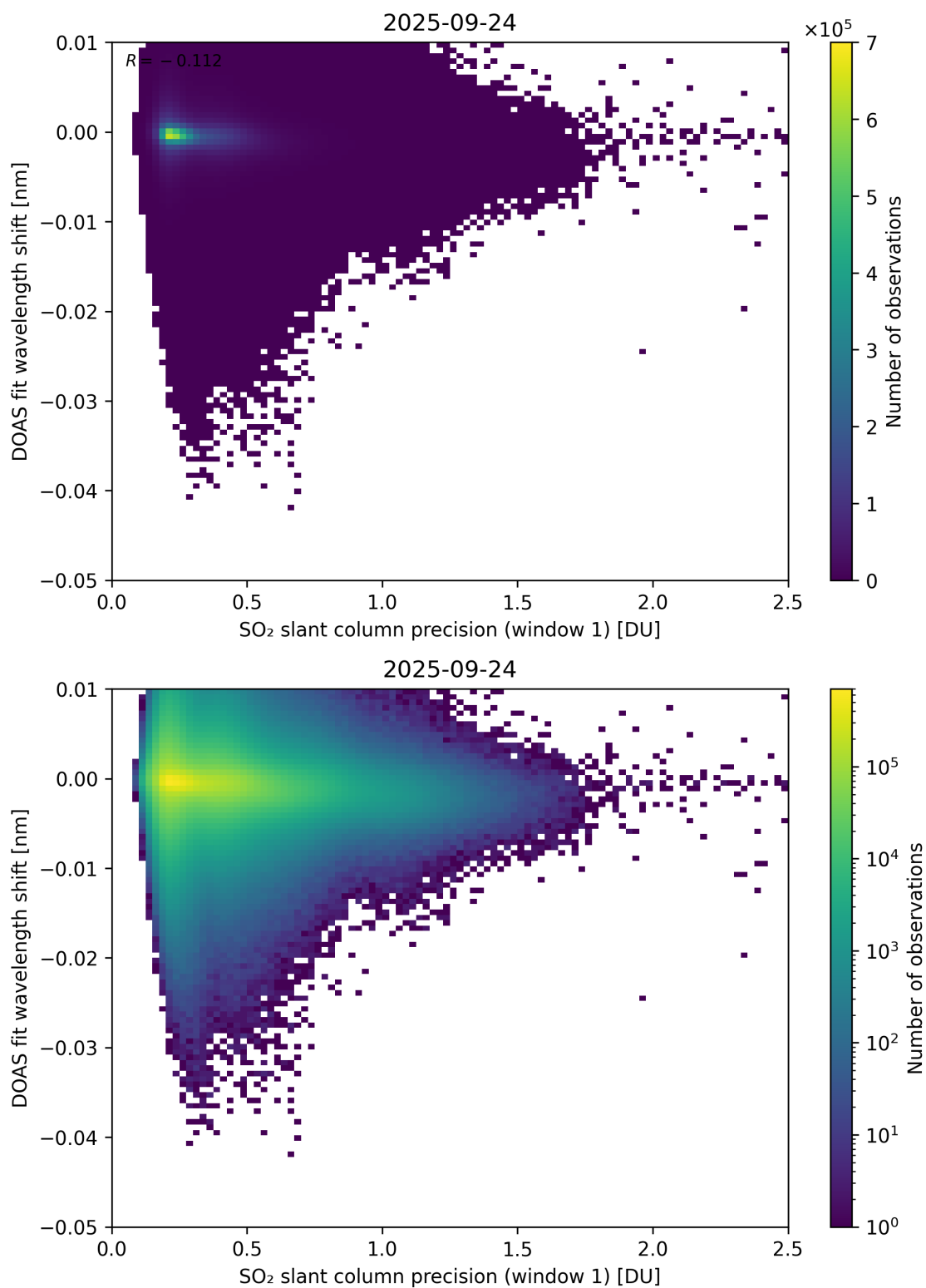
Figure 271: Scatter density plot of “SO 2 slant column precision (window 1)” against “DOAS fit wavelength shift” for 2025-09-23 to 2025-09-25.
