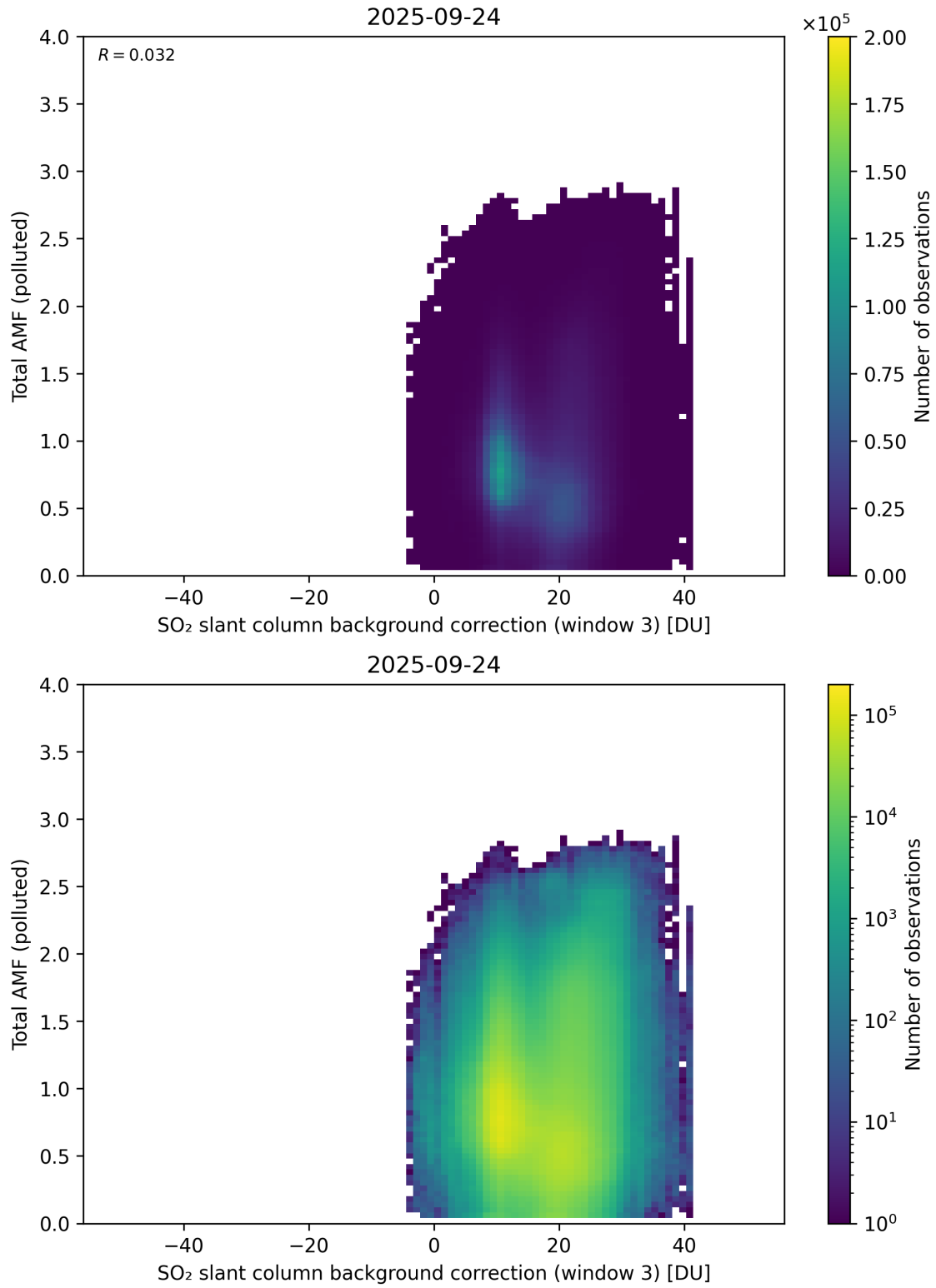
Figure 136: Scatter density plot of “SO 2 slant column background correction (window 3)” against “Total AMF (polluted)” for 2025-09-23 to 2025-09-25.
