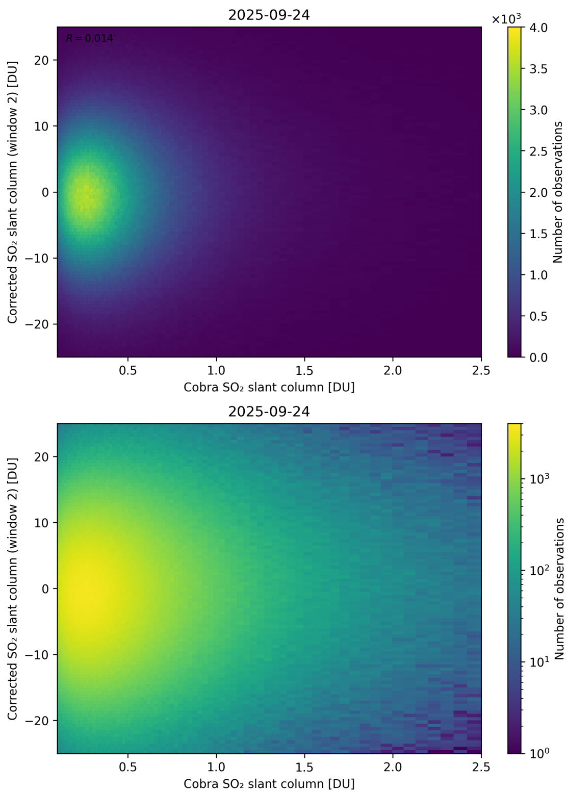
Figure 217: Scatter density plot of “Cobra SO 2 slant column” against “Corrected SO 2 slant column (window 2)” for 2025-09-23 to 2025-09-25.
