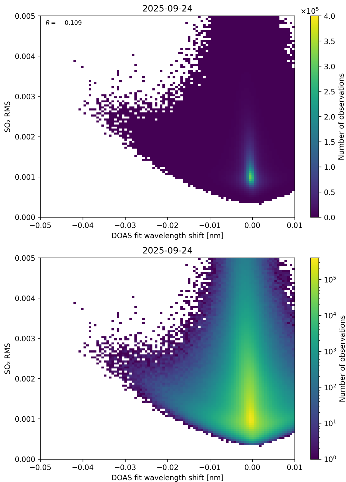
Figure 139: Scatter density plot of “DOAS fit wavelength shift” against “SO 2 RMS” for 2025-09-23 to 2025-09-25.
