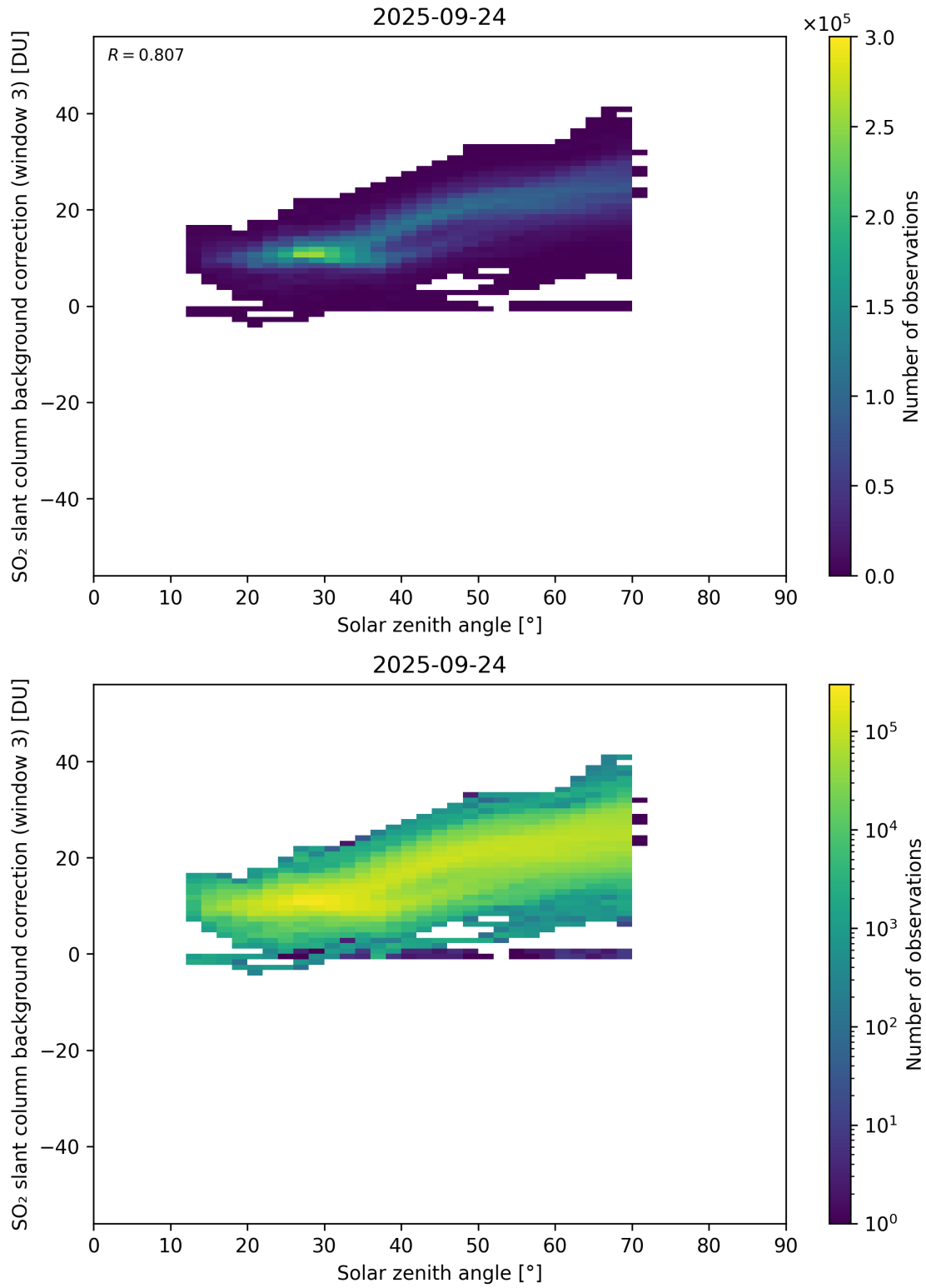
Figure 173: Scatter density plot of “Solar zenith angle” against “SO 2 slant column background correction (window 3)” for 2025-09-23 to 2025-09-25.
