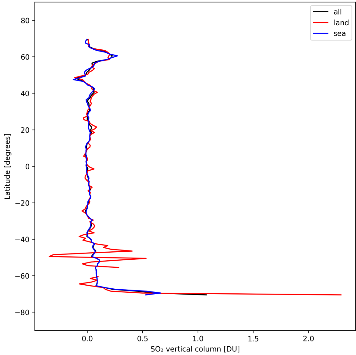
Figure 32: Zonal average of “SO 2 vertical column” for 2025-09-23 to 2025-09-25.
