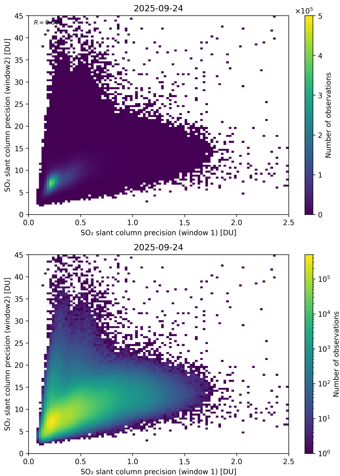
Figure 277: Scatter density plot of “SO 2 slant column precision (window 1)” against “SO 2 slant column precision (window2)” for 2025-09-23 to 2025-09-25.
