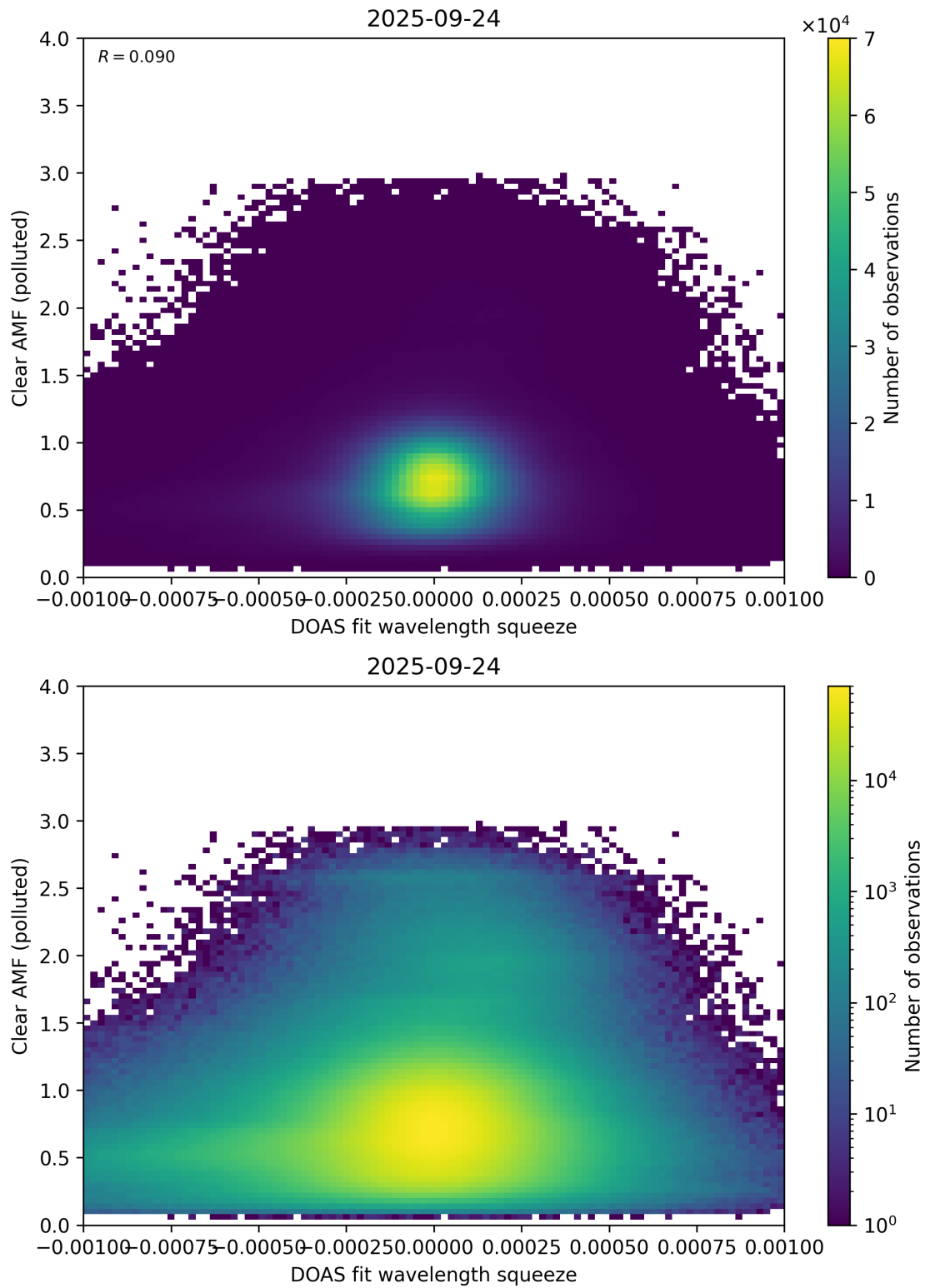
Figure 144: Scatter density plot of “DOAS fit wavelength squeeze” against “Clear AMF (polluted)” for 2025-09-23 to 2025-09-25.
