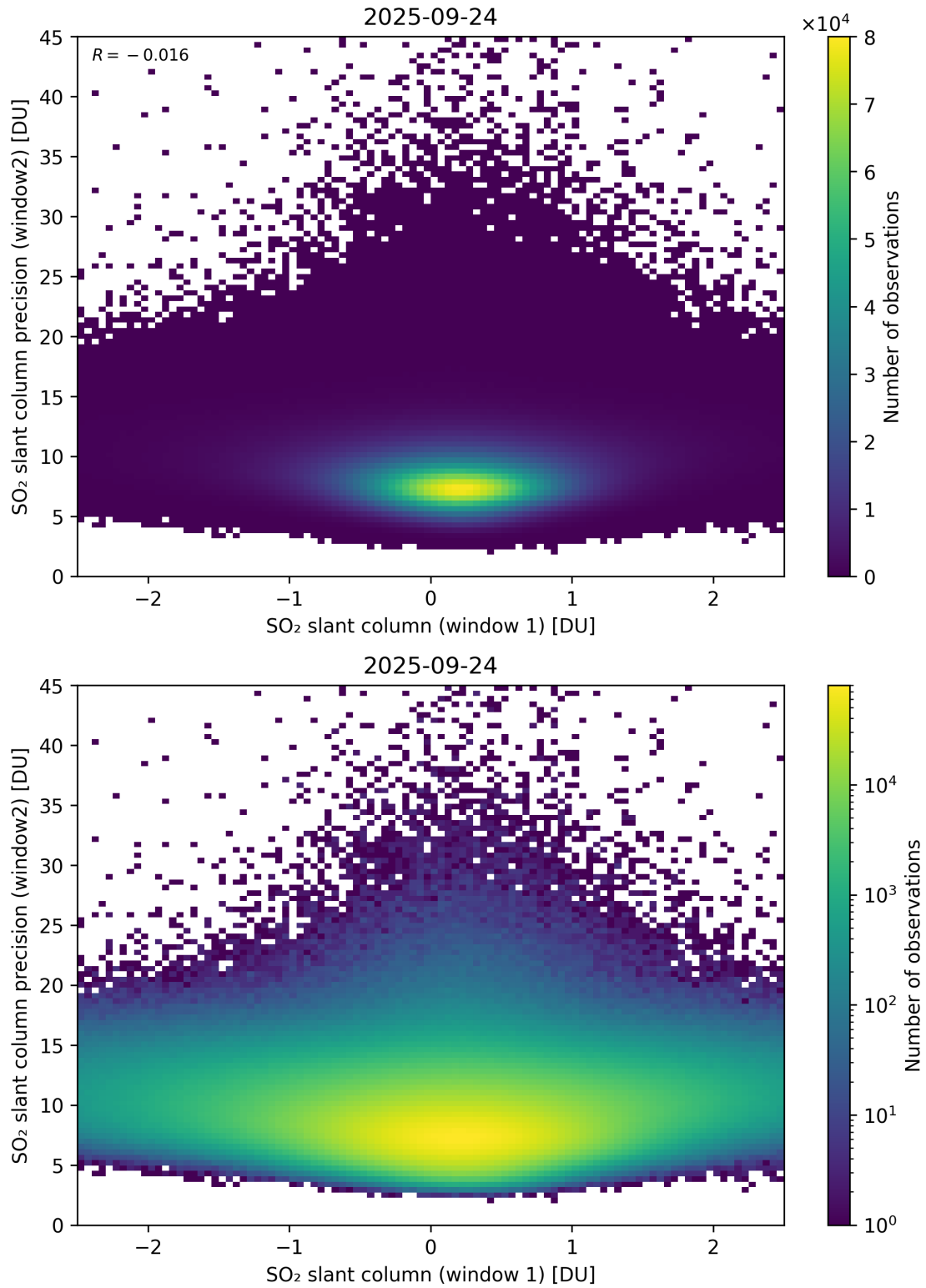
Figure 286: Scatter density plot of “SO 2 slant column (window 1)” against “SO 2 slant column precision (window2)” for 2025-09-23 to 2025-09-25.
