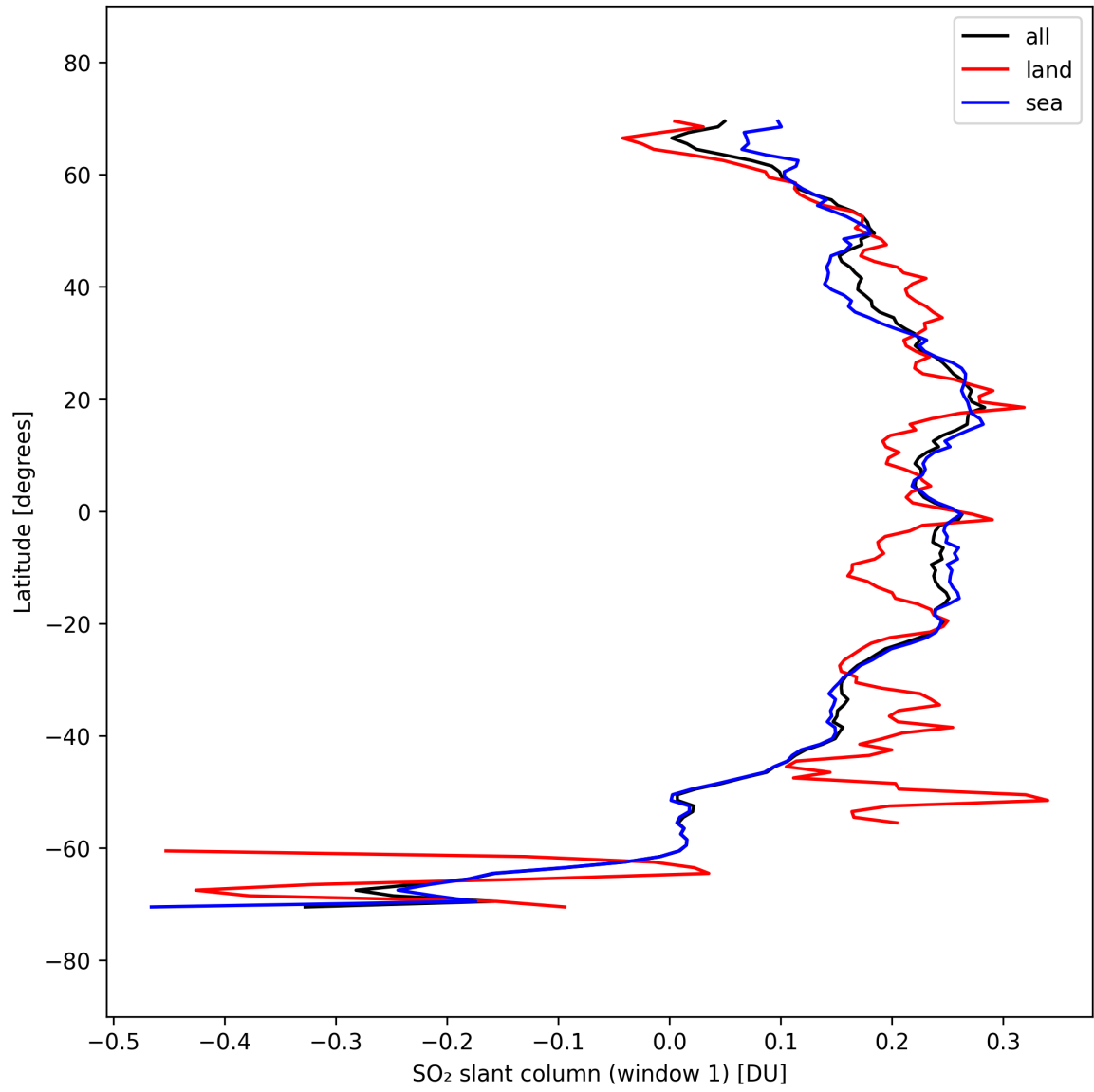
Figure 37: Zonal average of “SO 2 slant column (window 1)” for 2025-09-23 to 2025-09-25.
