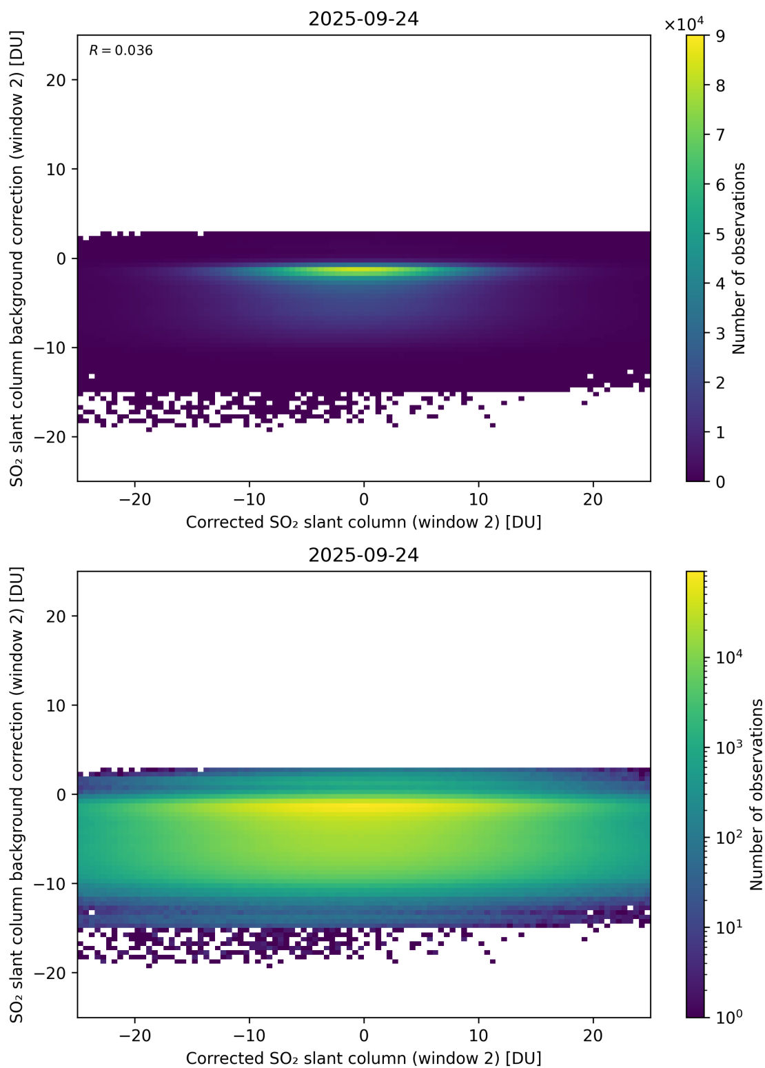
Figure 244: Scatter density plot of “Corrected SO 2 slant column (window 2)” against “SO 2 slant column background correction (window 2)” for 2025-09-23 to 2025-09-25.
