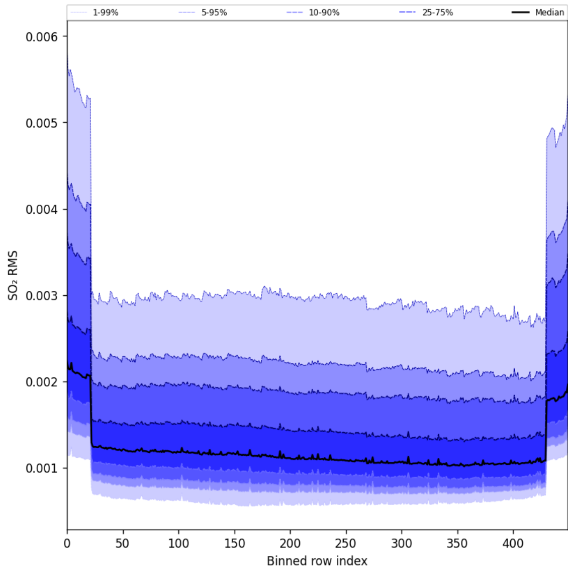
Figure 104: Along track statistics of “SO 2 RMS” for 2025-09-23 to 2025-09-25
