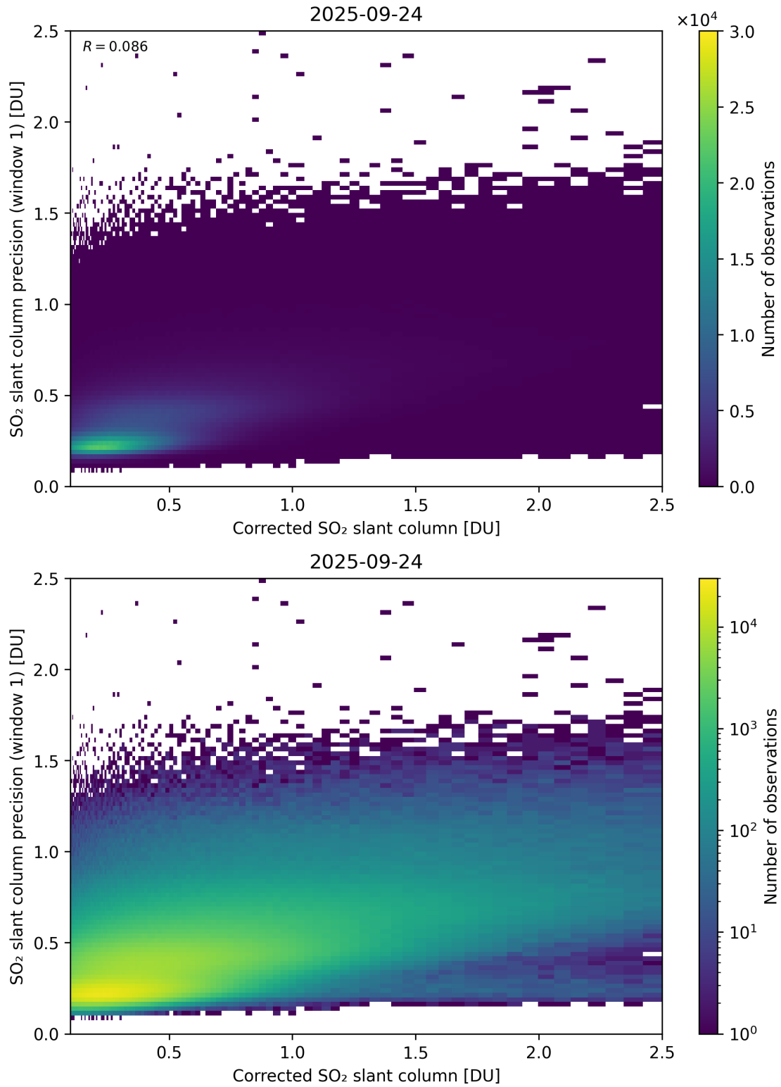
Figure 238: Scatter density plot of “Corrected SO 2 slant column” against “SO 2 slant column precision (window 1)” for 2025-09-23 to 2025-09-25.
