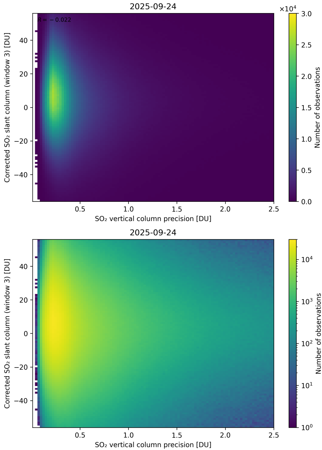
Figure 340: Scatter density plot of “SO 2 vertical column precision” against “Corrected SO 2 slant column (window 3)” for 2025-09-23 to 2025-09-25.
