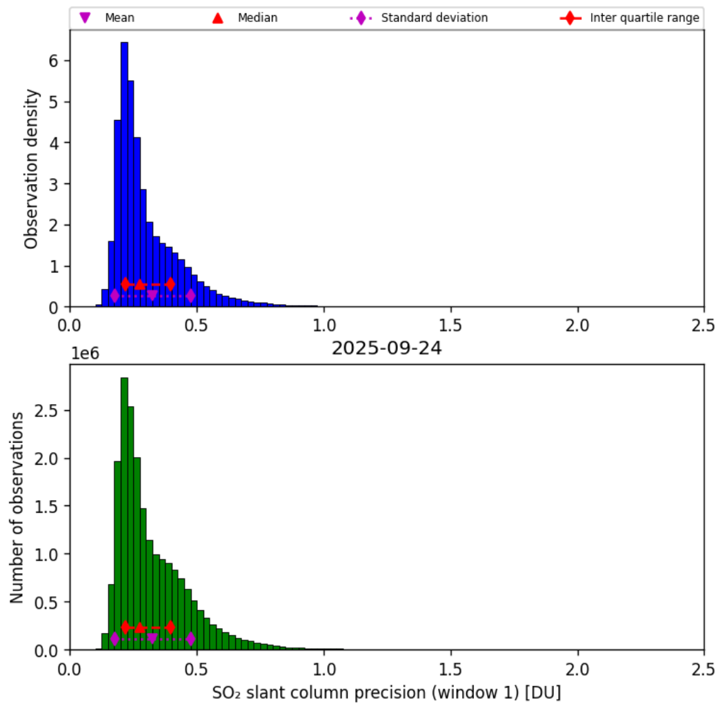
Figure 64: Histogram of “SO 2 slant column precision (window 1)” for 2025-09-23 to 2025-09-25
