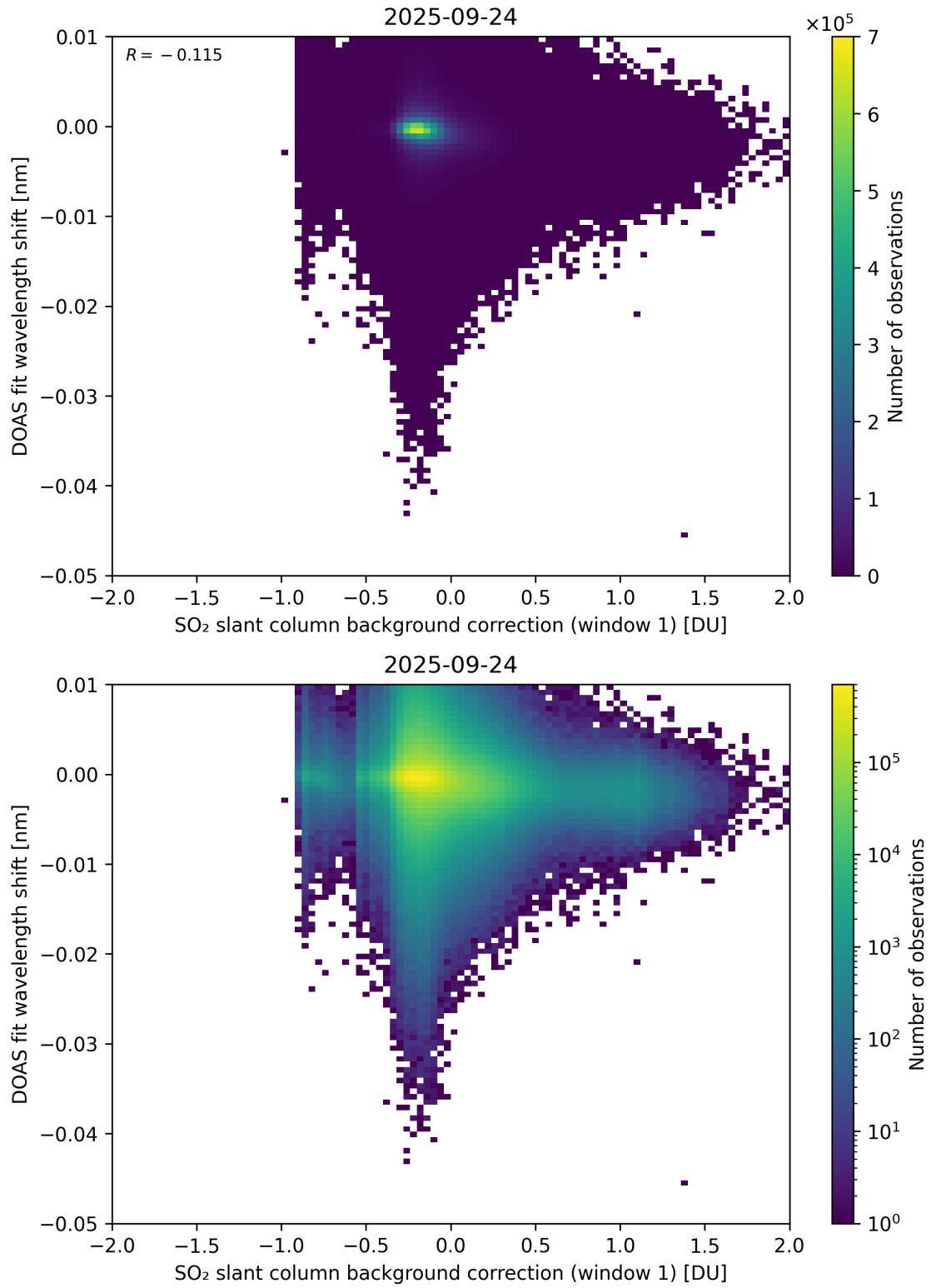
Figure 111: Scatter density plot of “SO 2 slant column background correction (window 1)” against “DOAS fit wavelength shift” for 2025-09-23 to 2025-09-25.
