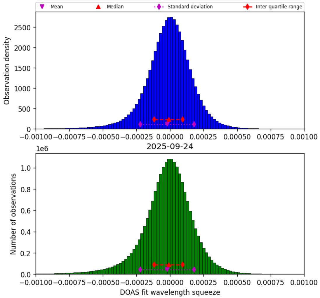
Figure 77: Histogram of “DOAS fit wavelength squeeze” for 2025-09-23 to 2025-09-25
