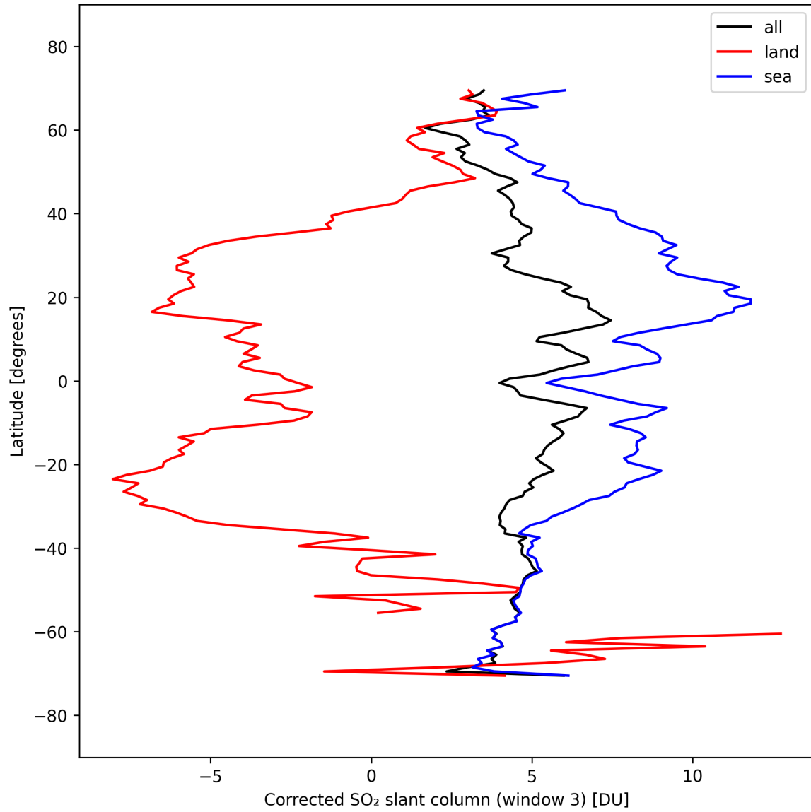
Figure 47: Zonal average of “Corrected SO 2 slant column (window 3)” for 2025-09-23 to 2025-09-25.
