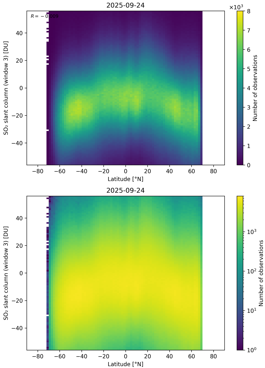
Figure 165: Scatter density plot of “Latitude” against “SO 2 slant column (window 3)” for 2025-09-23 to 2025-09-25.
