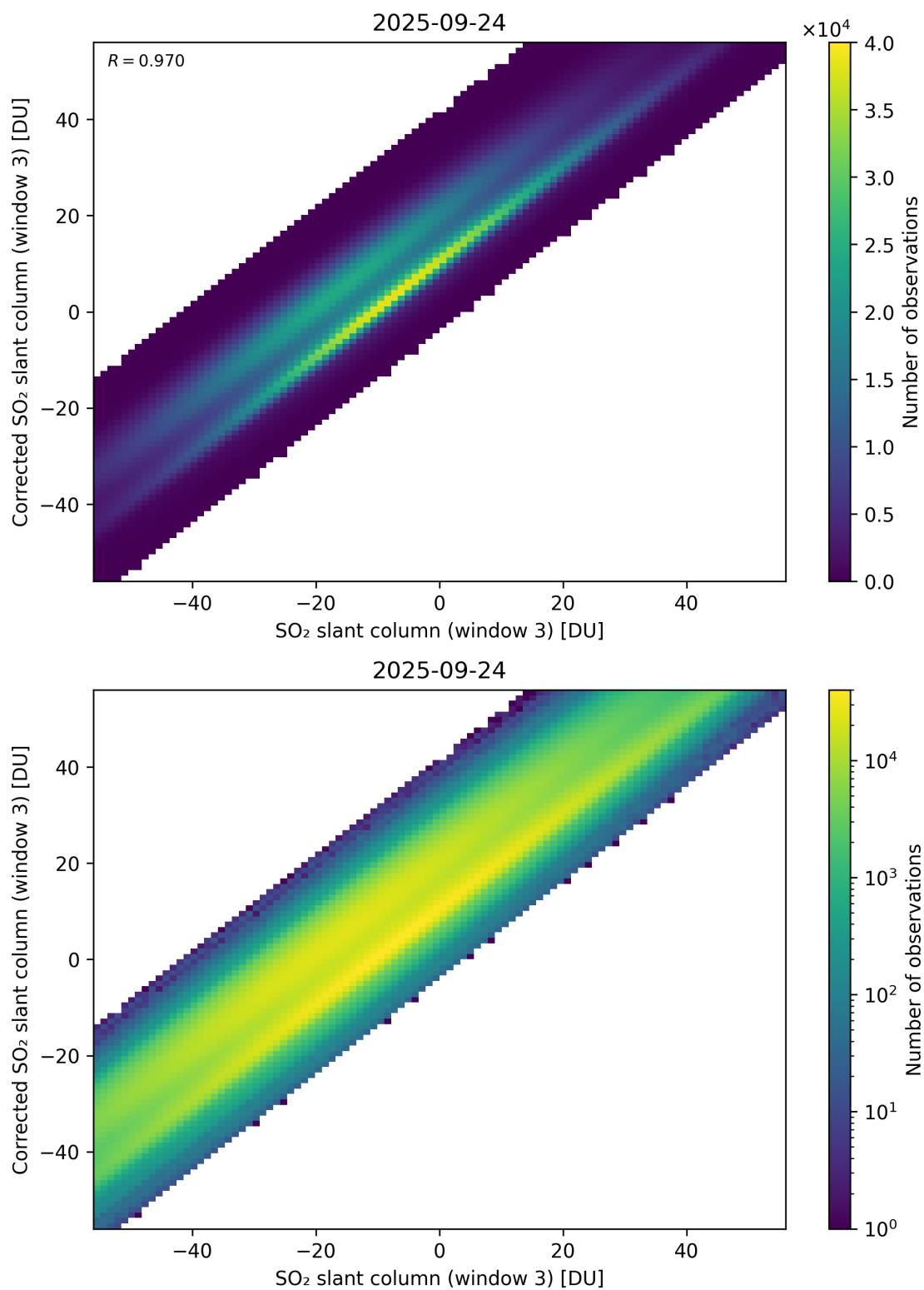
Figure 316: Scatter density plot of “SO 2 slant column (window 3)” against “Corrected SO 2 slant column (window 3)” for 2025-09-23 to 2025-09-25.
