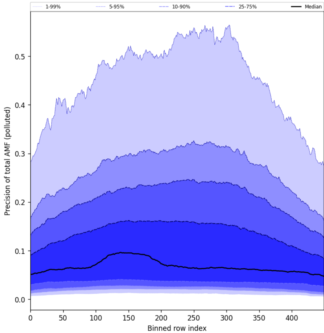
Figure 106: Along track statistics of “Precision of total AMF (polluted)” for 2025-09-23 to 2025-09-25
