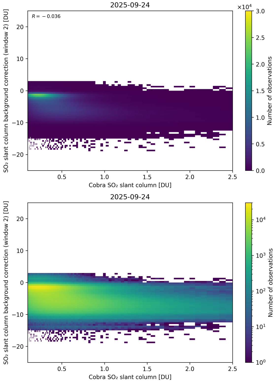
Figure 194: Scatter density plot of “Cobra SO 2 slant column” against “SO 2 slant column background correction (window 2)” for 2025-09-23 to 2025-09-25.
