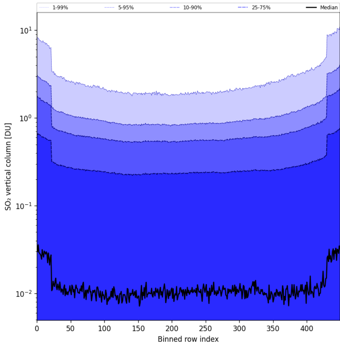
Figure 84: Along track statistics of “SO 2 vertical column” for 2025-09-23 to 2025-09-25
