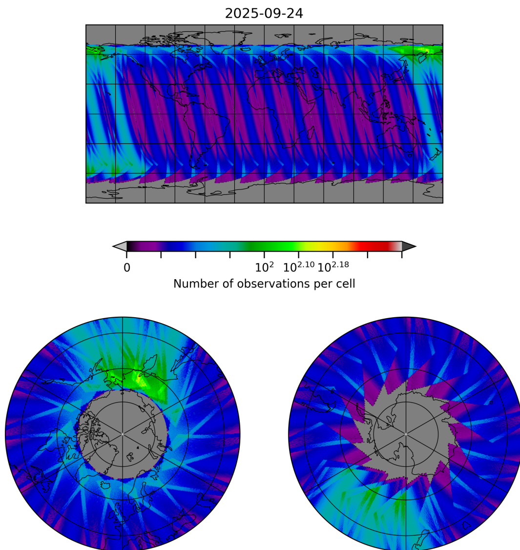
Figure 30: Map of the number of observations for 2025-09-23 to 2025-09-25
