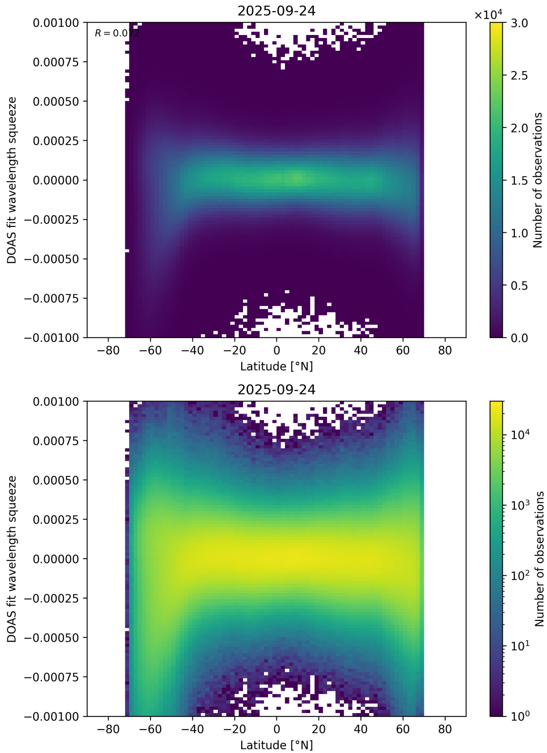
Figure 154: Scatter density plot of “Latitude” against “DOAS fit wavelength squeeze” for 2025-09-23 to 2025-09-25.
