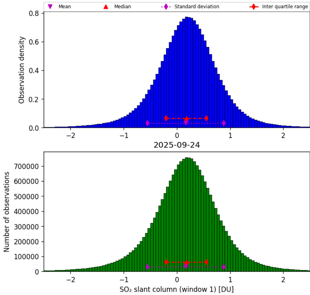
Figure 63: Histogram of “SO 2 slant column (window 1)” for 2025-09-23 to 2025-09-25
