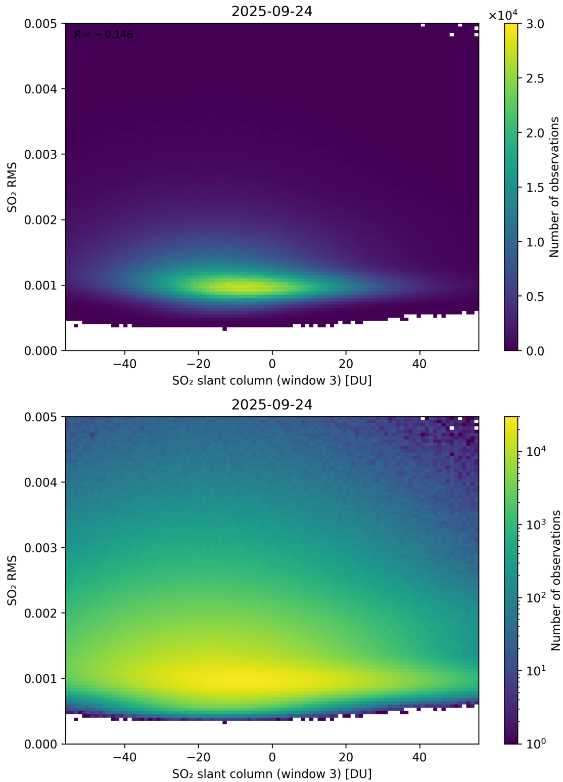
Figure 306: Scatter density plot of “SO 2 slant column (window 3)” against “SO 2 RMS” for 2025-09-23 to 2025-09-25.
