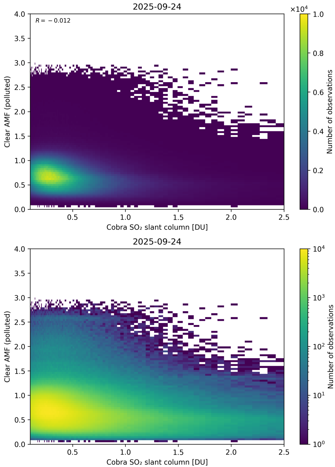
Figure 215: Scatter density plot of “Cobra SO 2 slant column” against “Clear AMF (polluted)” for 2025-09-23 to 2025-09-25.
