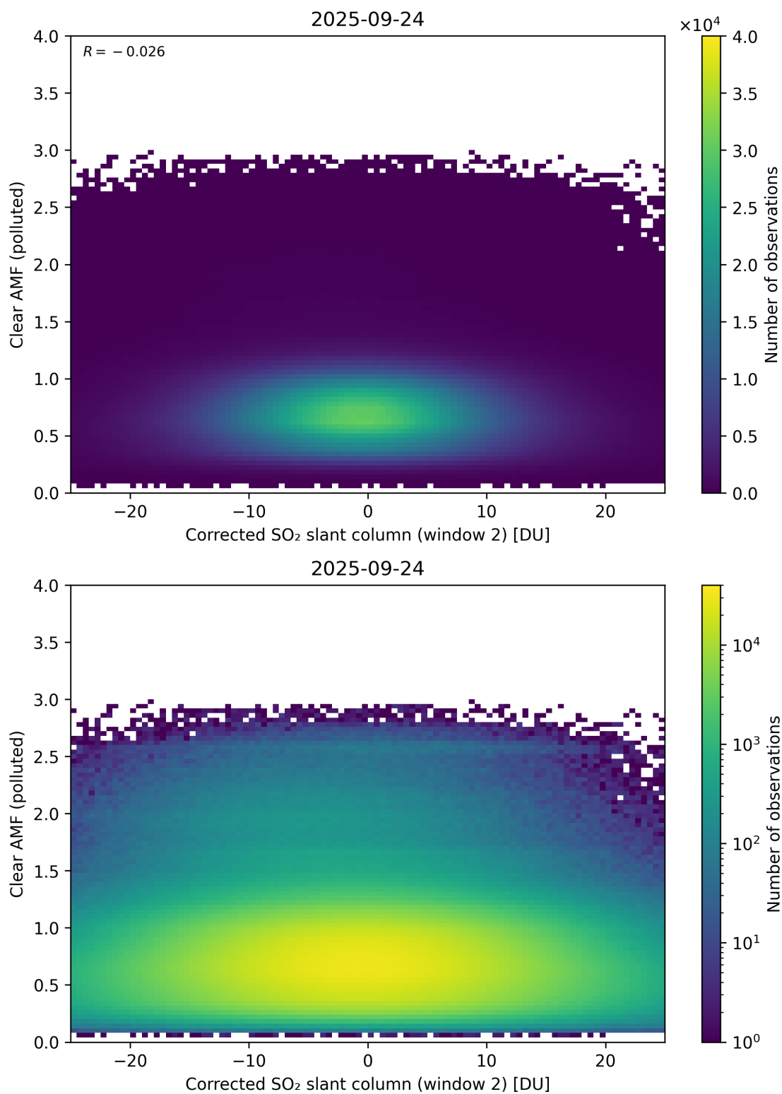
Figure 249: Scatter density plot of “Corrected SO 2 slant column (window 2)” against “Clear AMF (polluted)” for 2025-09-23 to 2025-09-25.
