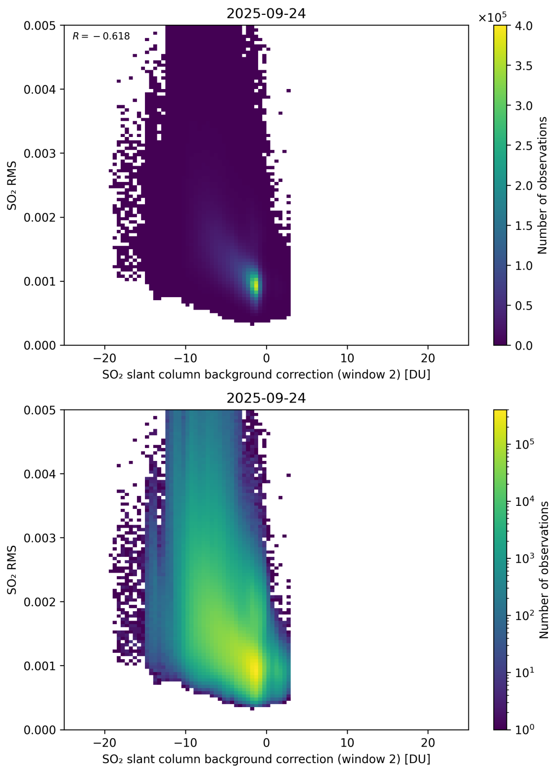
Figure 125: Scatter density plot of “SO 2 slant column background correction (window 2)” against “SO 2 RMS” for 2025-09-23 to 2025-09-25.
