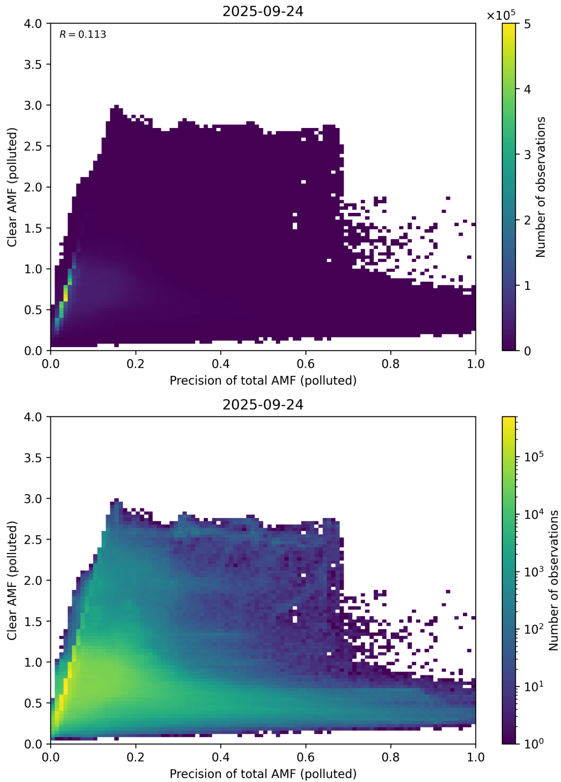
Figure 320: Scatter density plot of “Precision of total AMF (polluted)” against “Clear AMF (polluted)” for 2025-09-23 to 2025-09-25.
