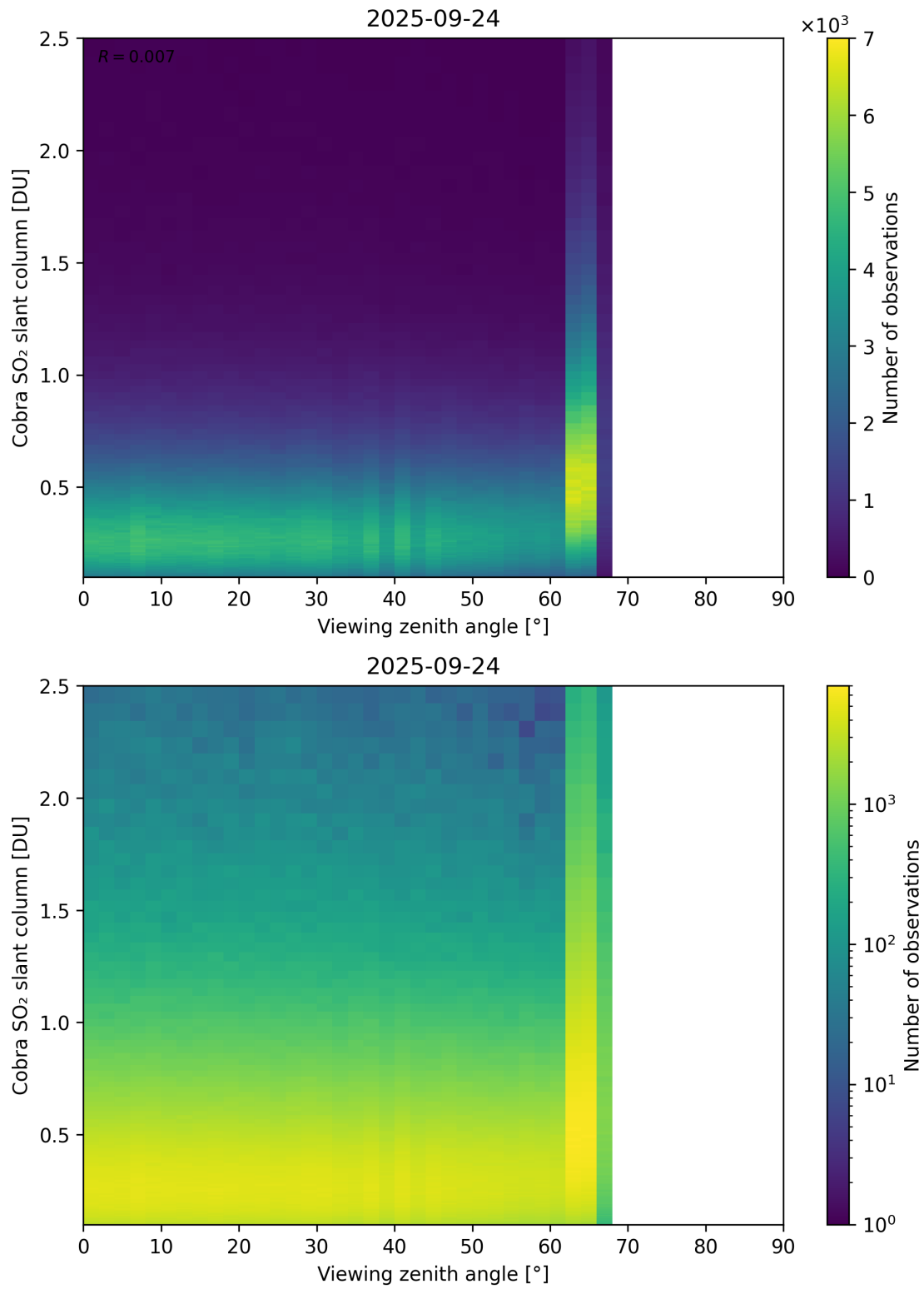
Figure 371: Scatter density plot of “Viewing zenith angle” against “Cobra SO 2 slant column” for 2025-09-23 to 2025-09-25.
