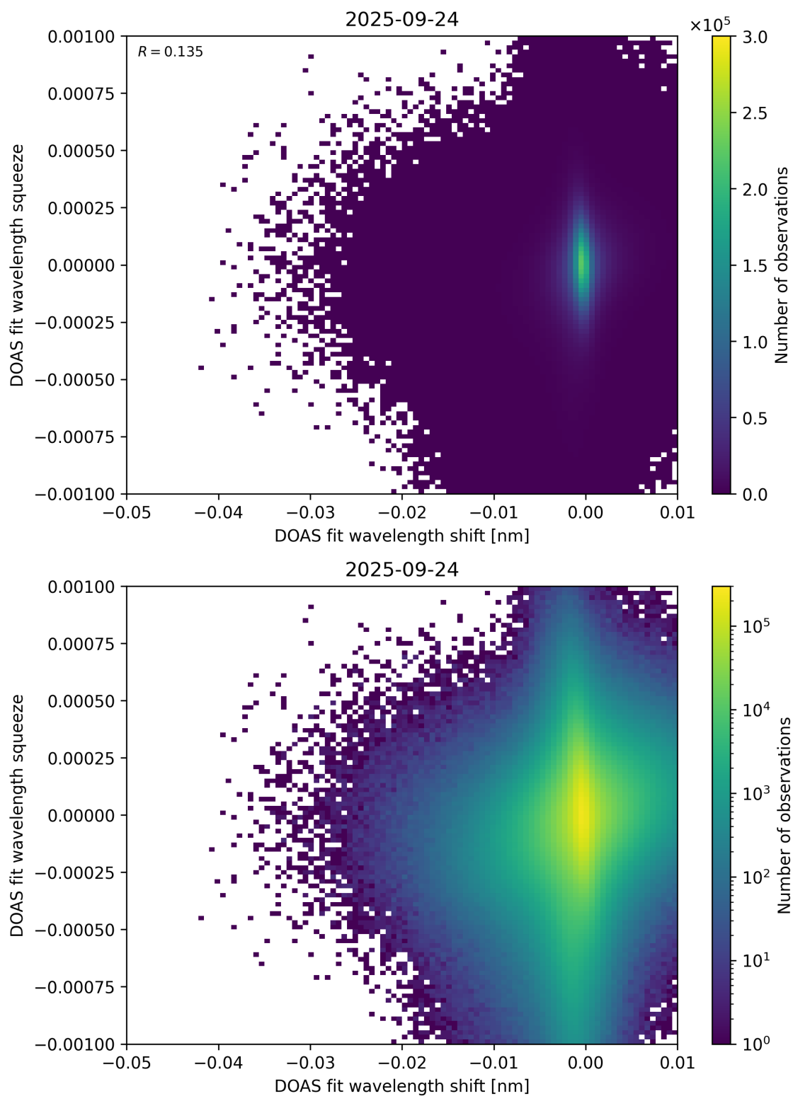
Figure 138: Scatter density plot of “DOAS fit wavelength shift” against “DOAS fit wavelength squeeze” for 2025-09-23 to 2025-09-25.
