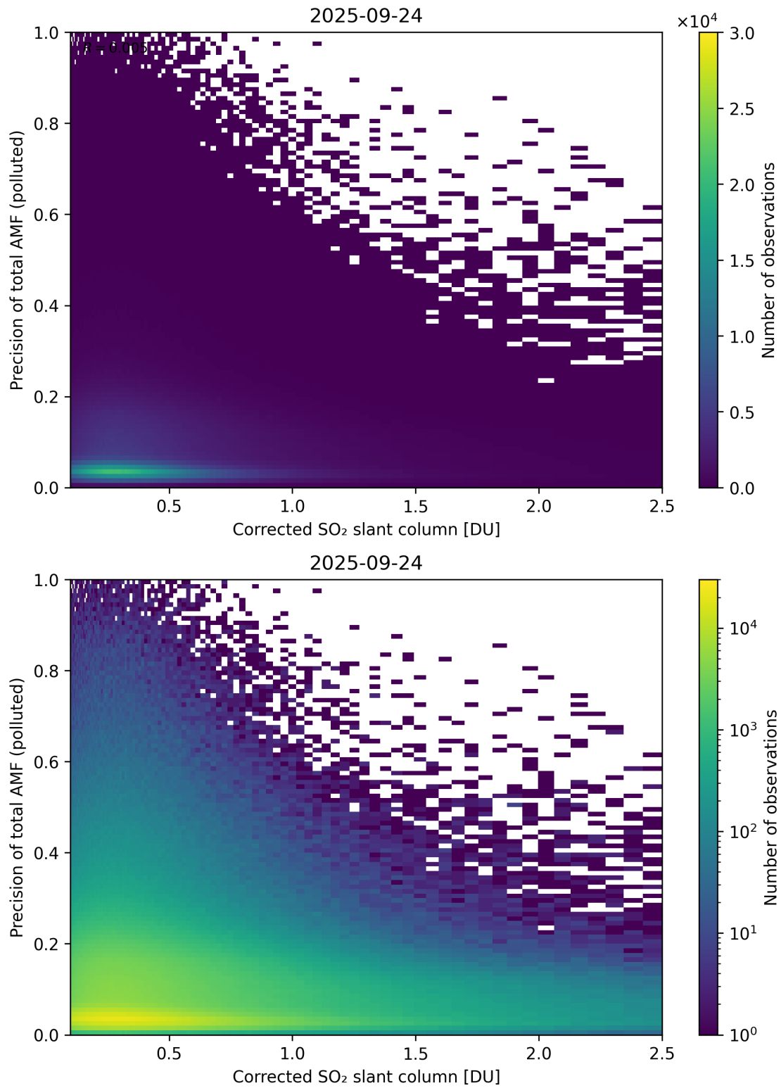
Figure 243: Scatter density plot of “Corrected SO 2 slant column” against “Precision of total AMF (polluted)” for 2025-09-23 to 2025-09-25.
