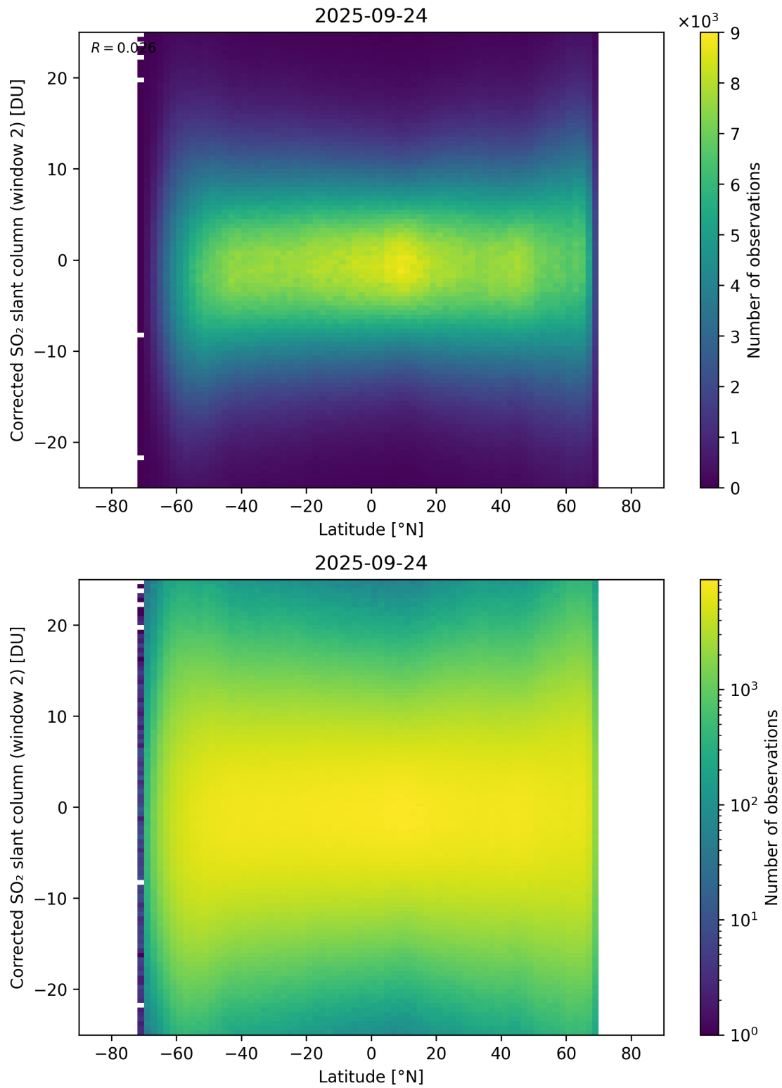
Figure 160: Scatter density plot of “Latitude” against “Corrected SO 2 slant column (window 2)” for 2025-09-23 to 2025-09-25.
