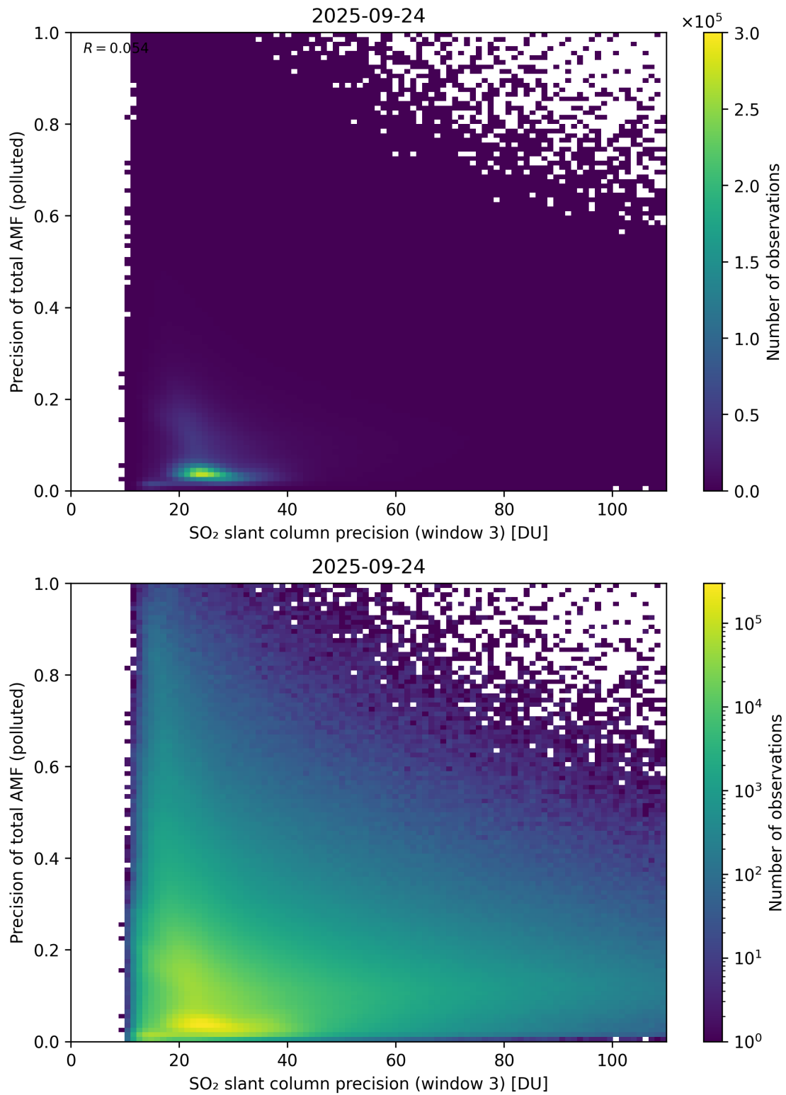
Figure 314: Scatter density plot of “SO 2 slant column precision (window 3)” against “Precision of total AMF (polluted)” for 2025-09-23 to 2025-09-25.
