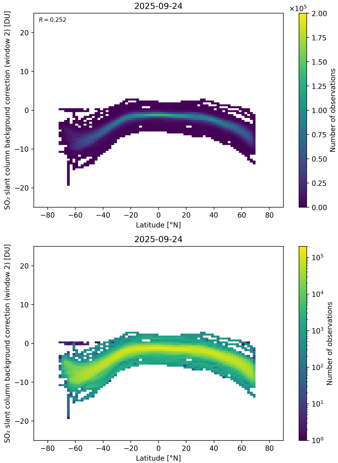
Figure 151: Scatter density plot of “Latitude” against “SO 2 slant column background correction (window 2)” for 2025-09-23 to 2025-09-25.
