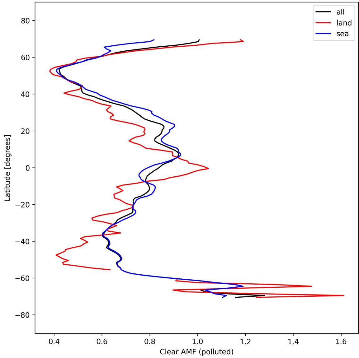
Figure 55: Zonal average of “Clear AMF (polluted)” for 2025-09-23 to 2025-09-25.
