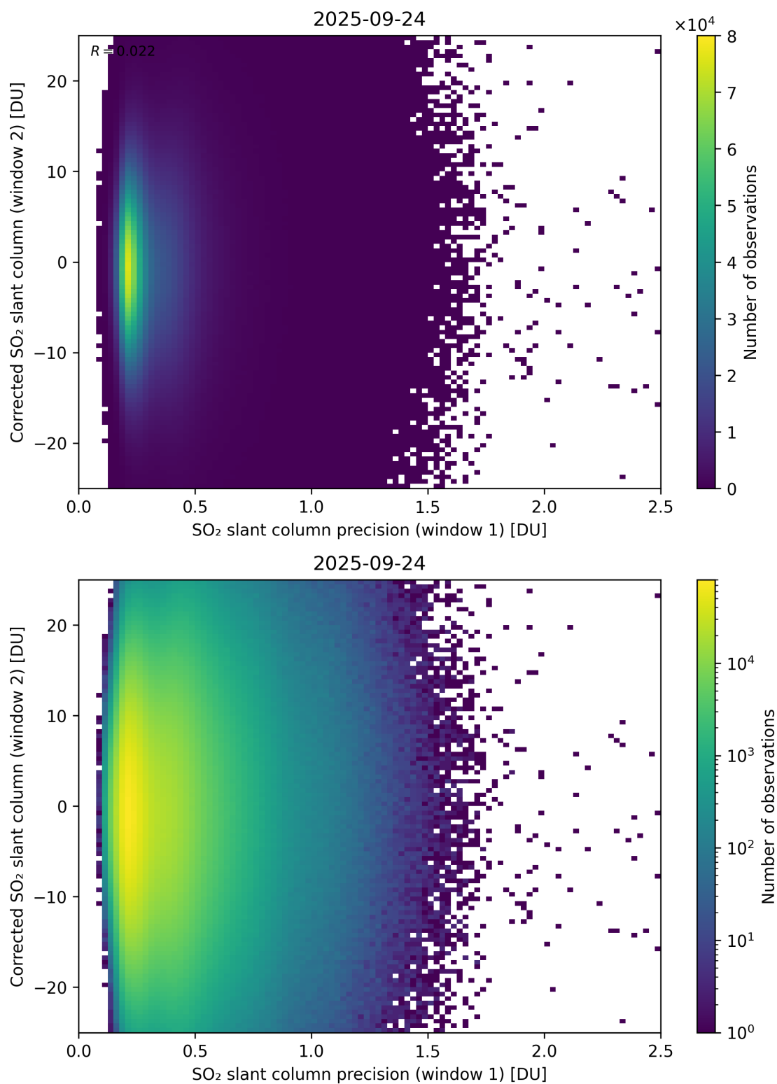
Figure 275: Scatter density plot of “SO 2 slant column precision (window 1)” against “Corrected SO 2 slant column (window 2)” for 2025-09-23 to 2025-09-25.
