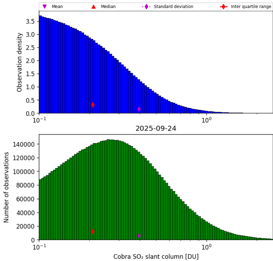
Figure 61: Histogram of “Cobra SO 2 slant column” for 2025-09-23 to 2025-09-25
