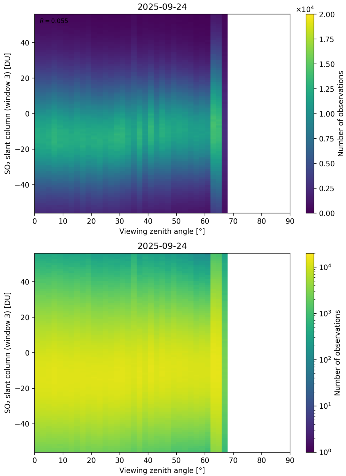
Figure 379: Scatter density plot of “Viewing zenith angle” against “SO 2 slant column (window 3)” for 2025-09-23 to 2025-09-25.
