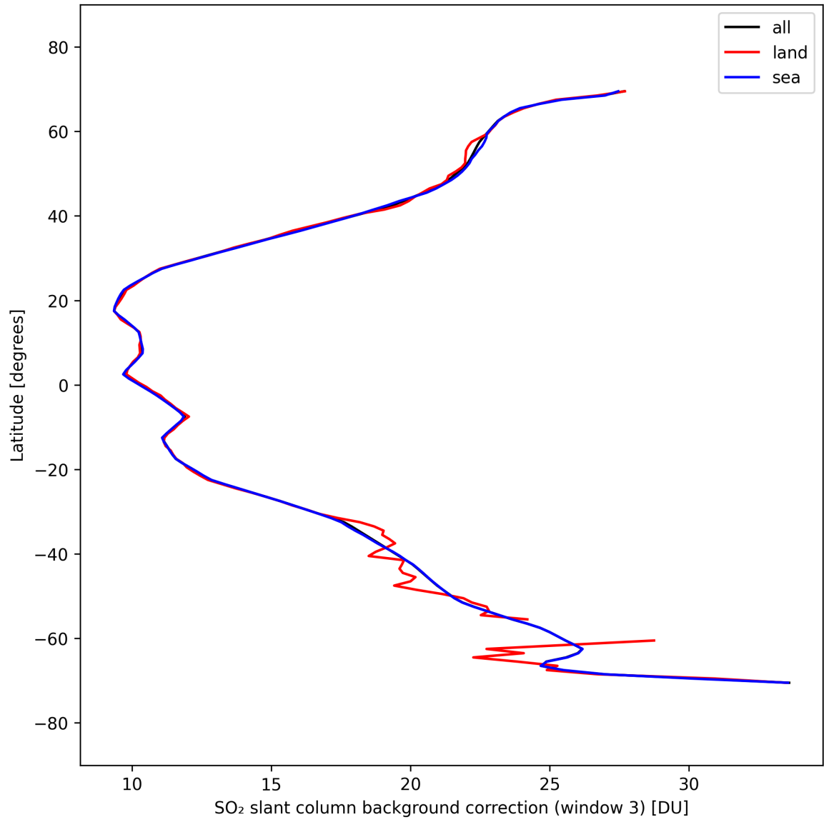
Figure 48: Zonal average of “SO 2 slant column background correction (window 3)” for 2025-09-23 to 2025-09-25.
