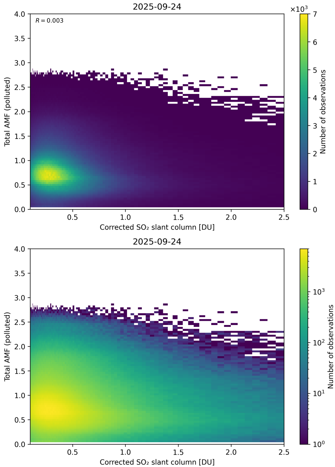
Figure 242: Scatter density plot of “Corrected SO 2 slant column” against “Total AMF (polluted)” for 2025-09-23 to 2025-09-25.
