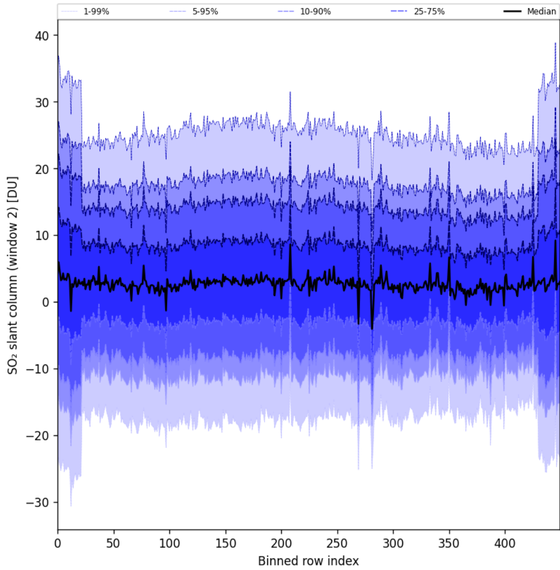
Figure 93: Along track statistics of “SO 2 slant column (window 2)” for 2025-09-23 to 2025-09-25
