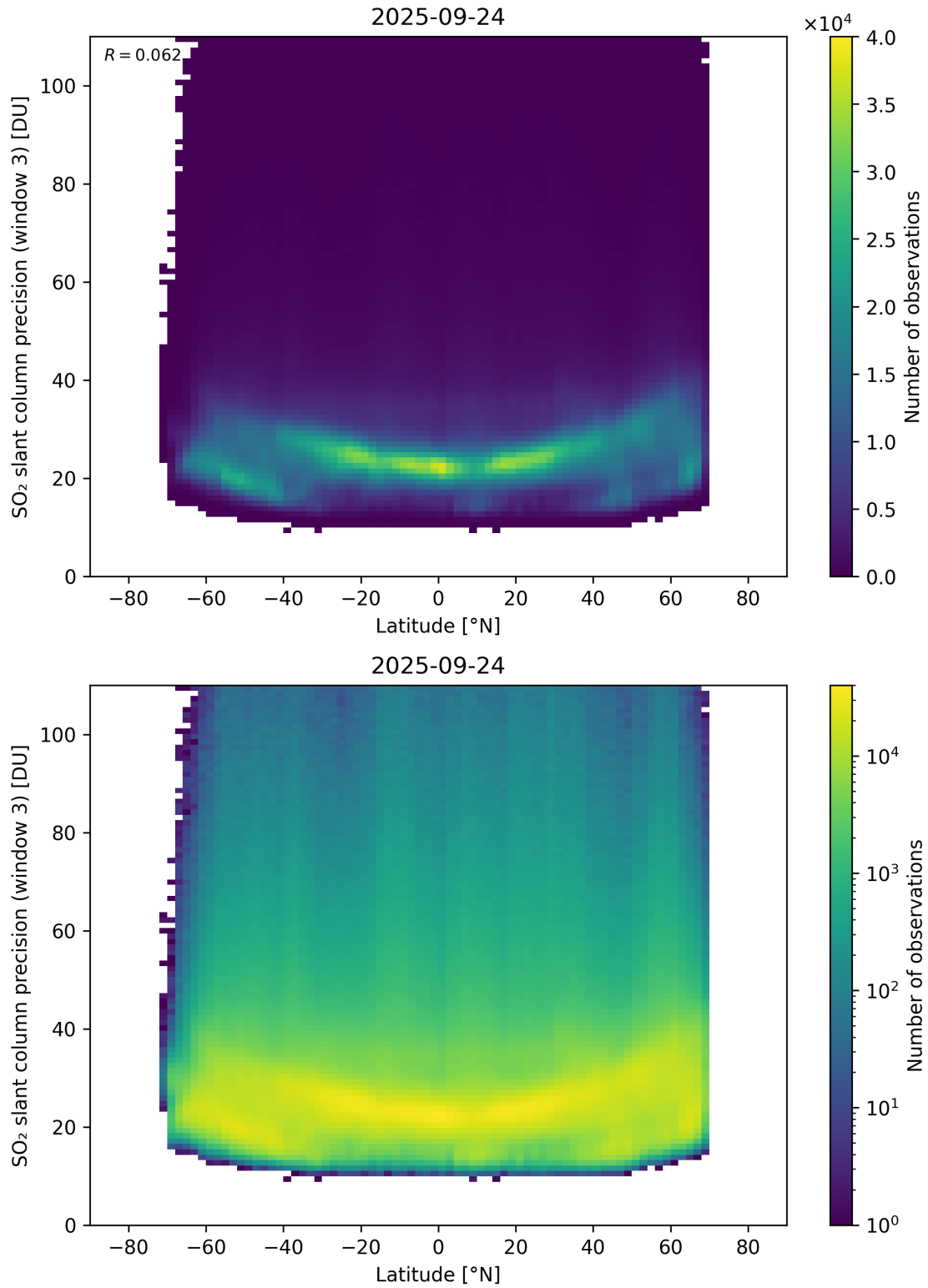
Figure 166: Scatter density plot of “Latitude” against “SO 2 slant column precision (window 3)” for 2025-09-23 to 2025-09-25.
