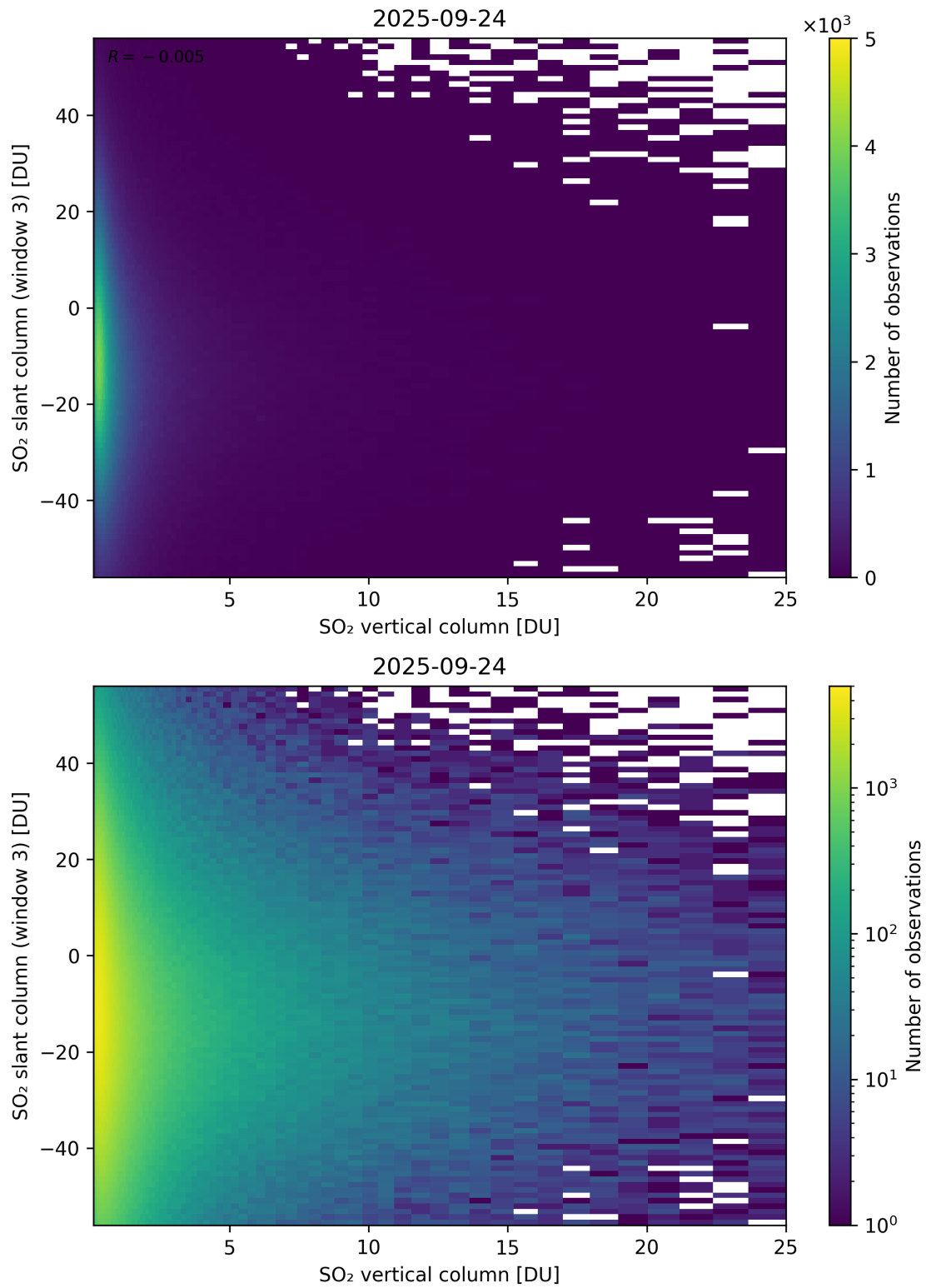
Figure 357: Scatter density plot of “SO 2 vertical column” against “SO 2 slant column (window 3)” for 2025-09-23 to 2025-09-25.
