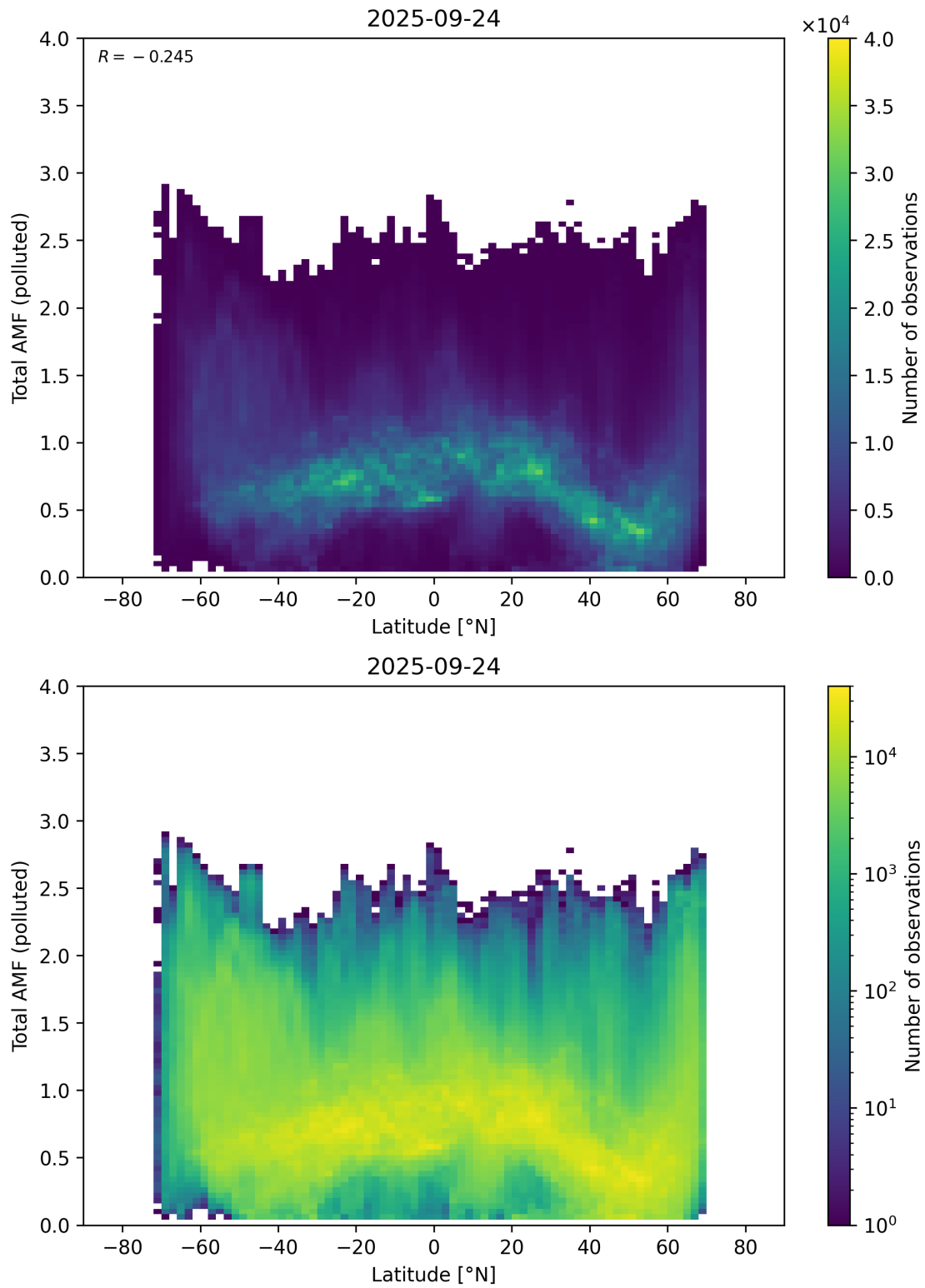
Figure 167: Scatter density plot of “Latitude” against “Total AMF (polluted)” for 2025-09-23 to 2025-09-25.
