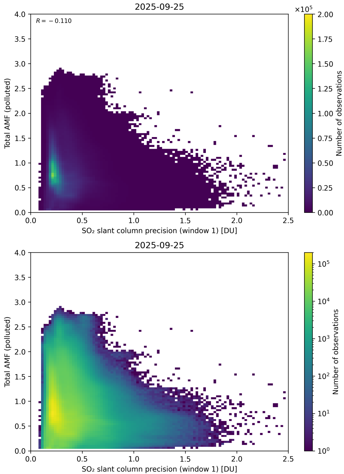
Figure 280: Scatter density plot of “SO 2 slant column precision (window 1)” against “Total AMF (polluted)” for 2025-09-25 to 2025-09-26.
