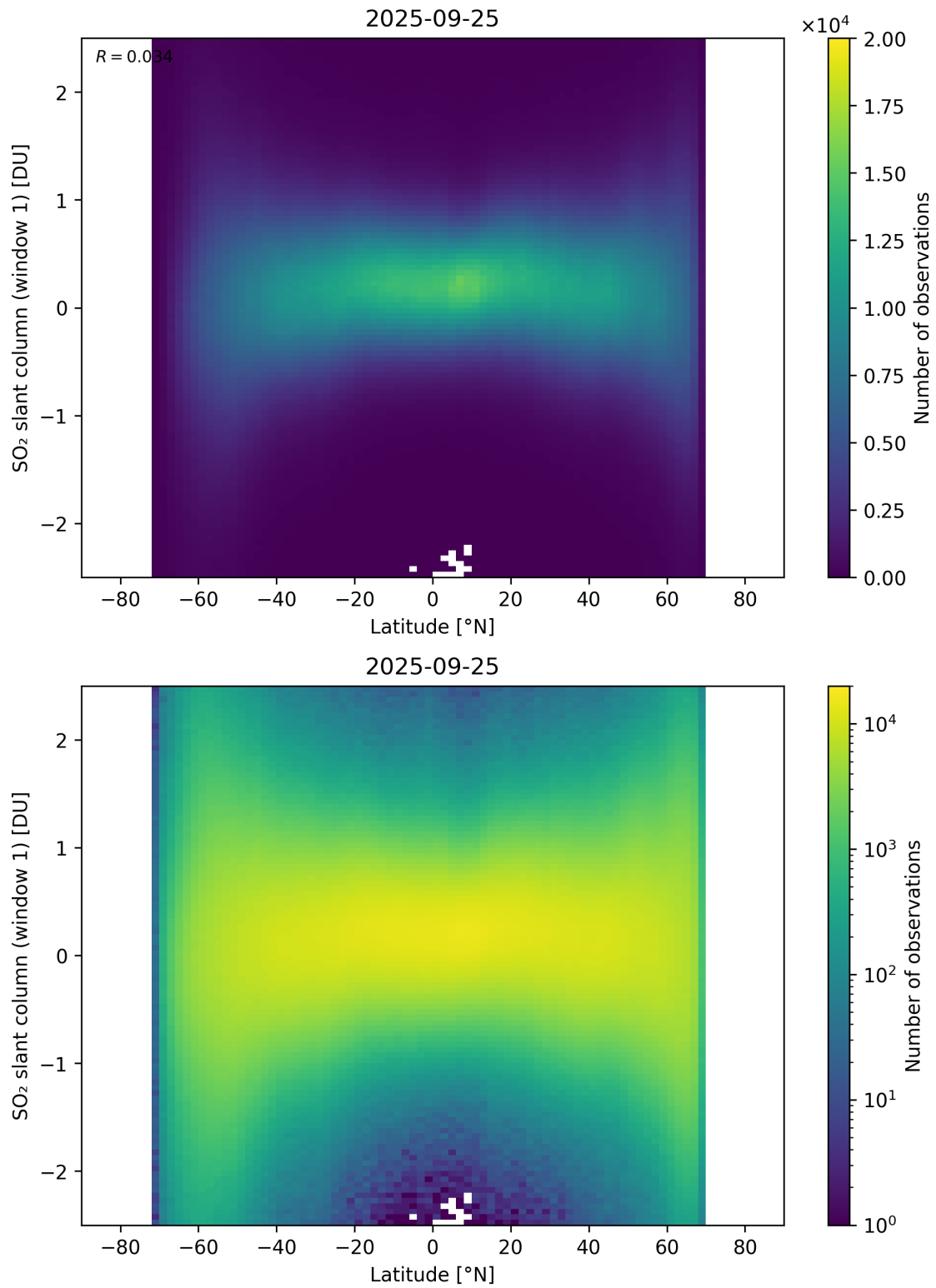
Figure 162: Scatter density plot of “Latitude” against “SO 2 slant column (window 1)” for 2025-09-25 to 2025-09-26.
