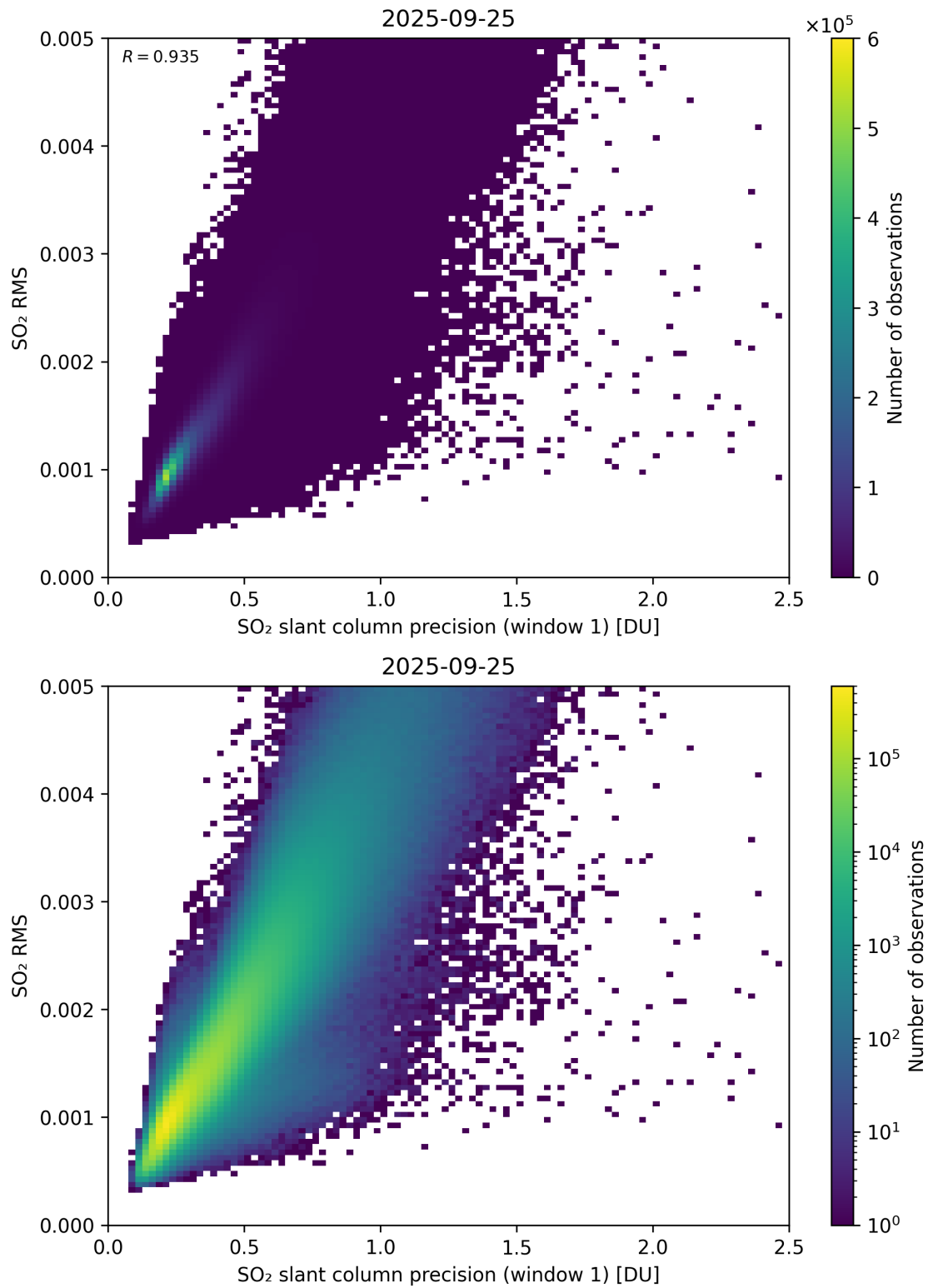
Figure 273: Scatter density plot of “SO 2 slant column precision (window 1)” against “SO 2 RMS” for 2025-09-25 to 2025-09-26.
