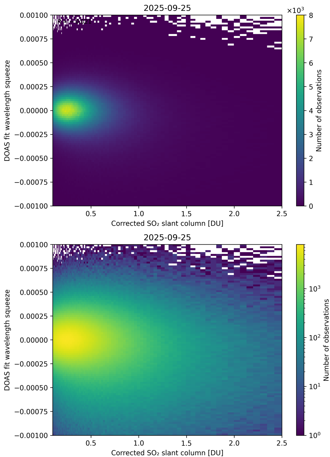
Figure 230: Scatter density plot of “Corrected SO 2 slant column” against “DOAS fit wavelength squeeze” for 2025-09-25 to 2025-09-26.
