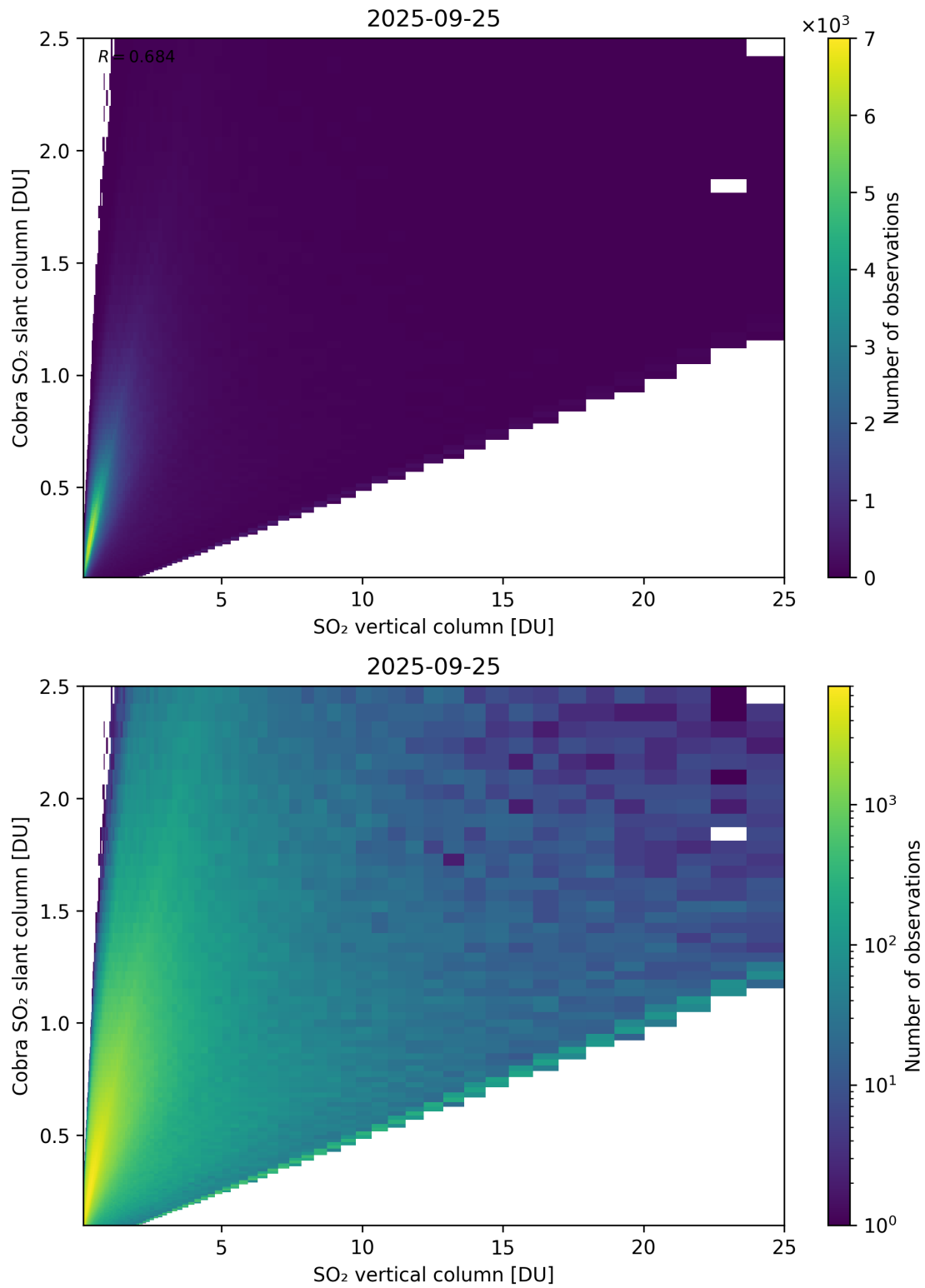
Figure 349: Scatter density plot of “SO 2 vertical column” against “Cobra SO 2 slant column” for 2025-09-25 to 2025-09-26.
