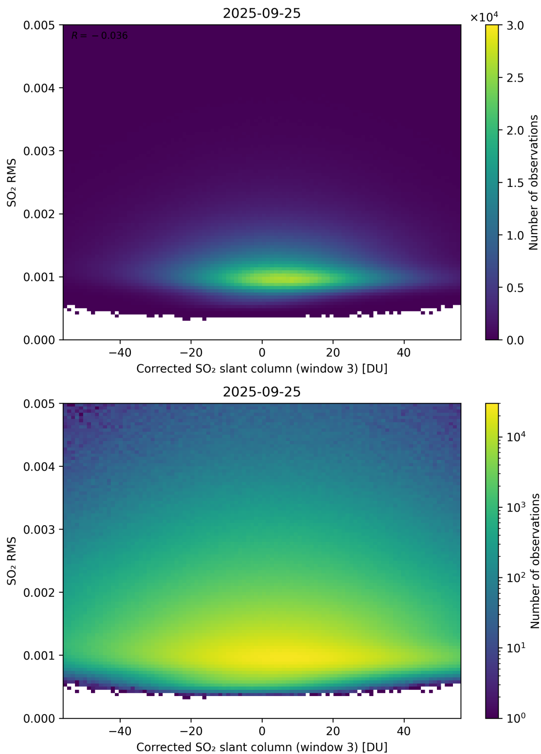
Figure 258: Scatter density plot of “Corrected SO 2 slant column (window 3)” against “SO 2 RMS” for 2025-09-25 to 2025-09-26.
