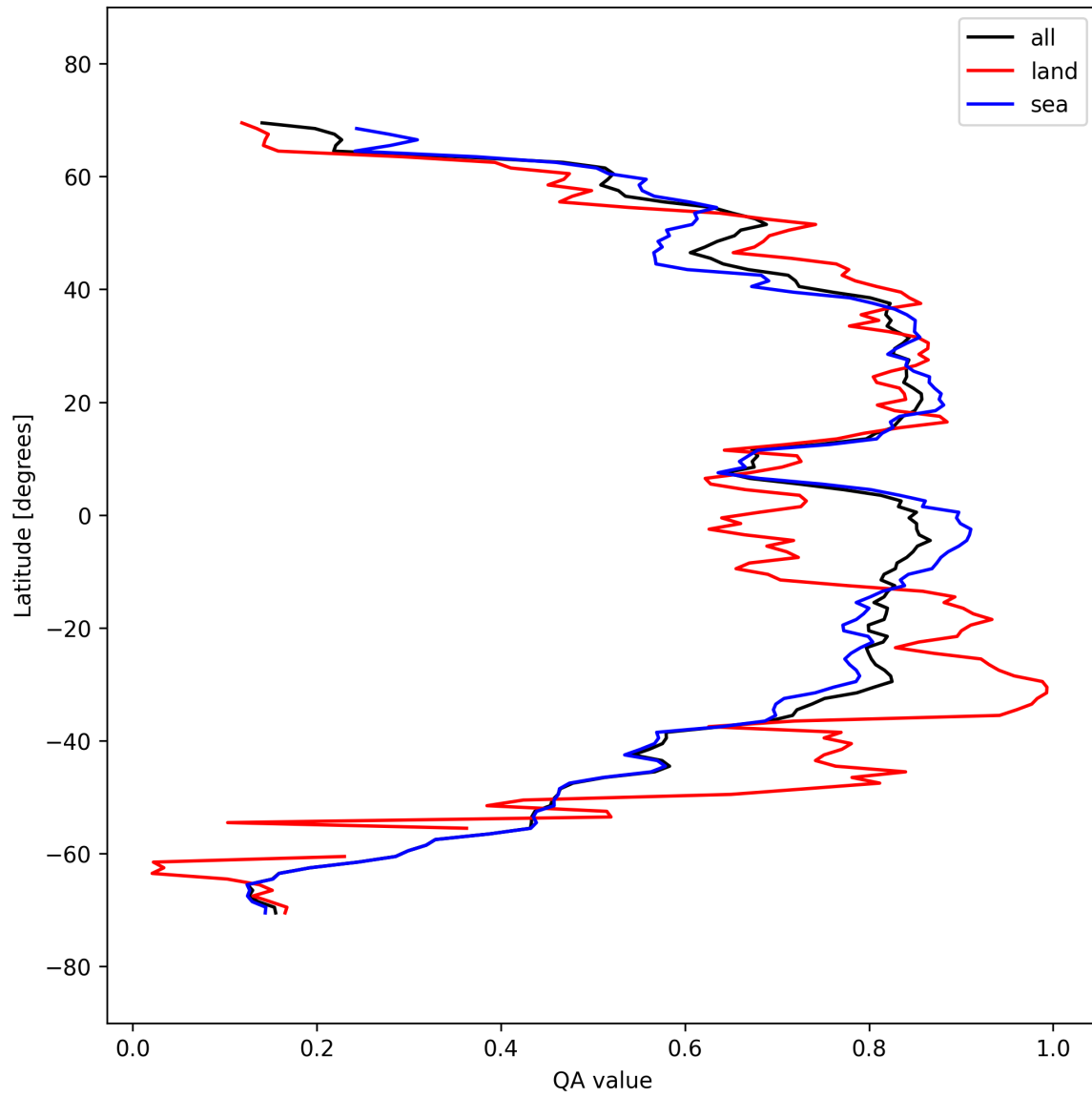
Figure 31: Zonal average of “QA value” for 2025-09-25 to 2025-09-26.
