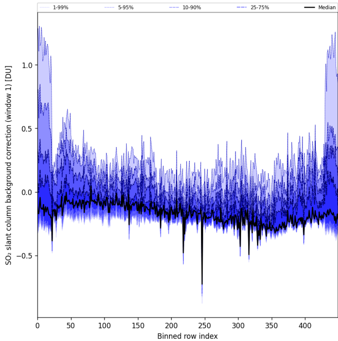
Figure 92: Along track statistics of “SO 2 slant column background correction (window 1)” for 2025-09-25 to 2025-09-26
