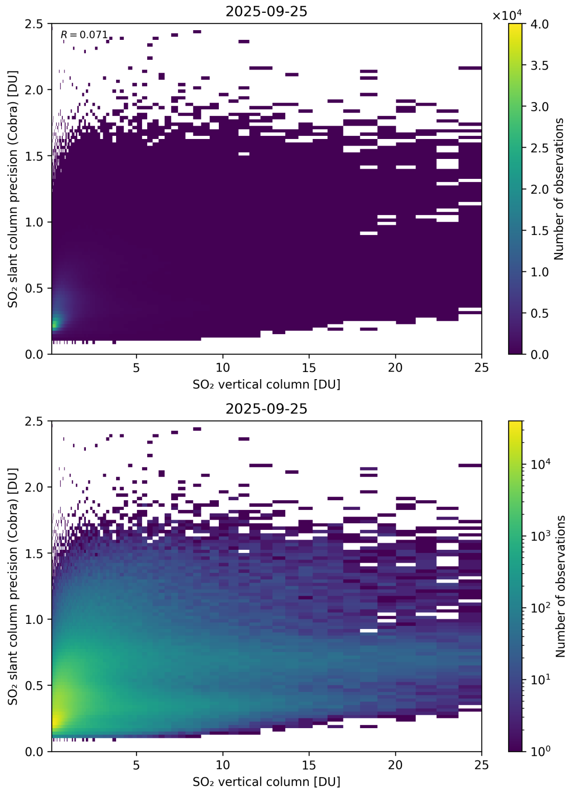
Figure 350: Scatter density plot of “SO 2 vertical column” against “SO 2 slant column precision (Cobra)” for 2025-09-25 to 2025-09-26.
