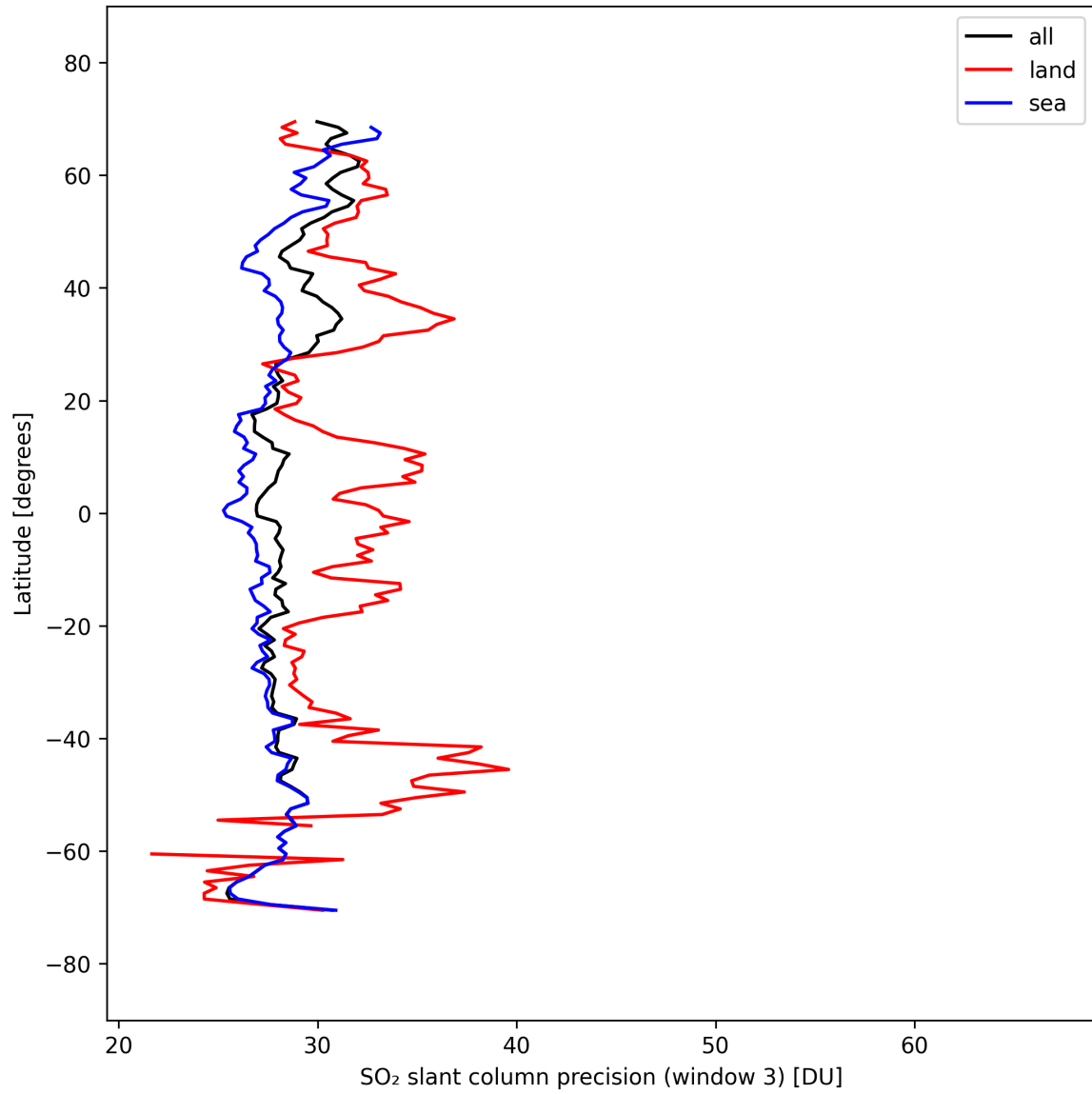
Figure 46: Zonal average of “SO 2 slant column precision (window 3)” for 2025-09-25 to 2025-09-26.
