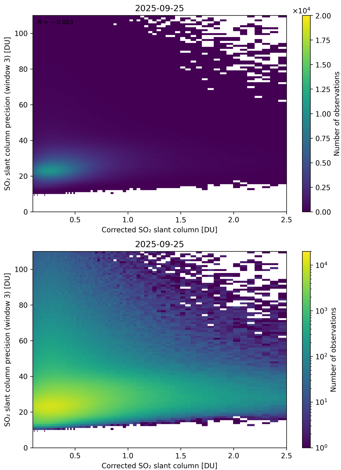
Figure 241: Scatter density plot of “Corrected SO 2 slant column” against “SO 2 slant column precision (window 3)” for 2025-09-25 to 2025-09-26.
