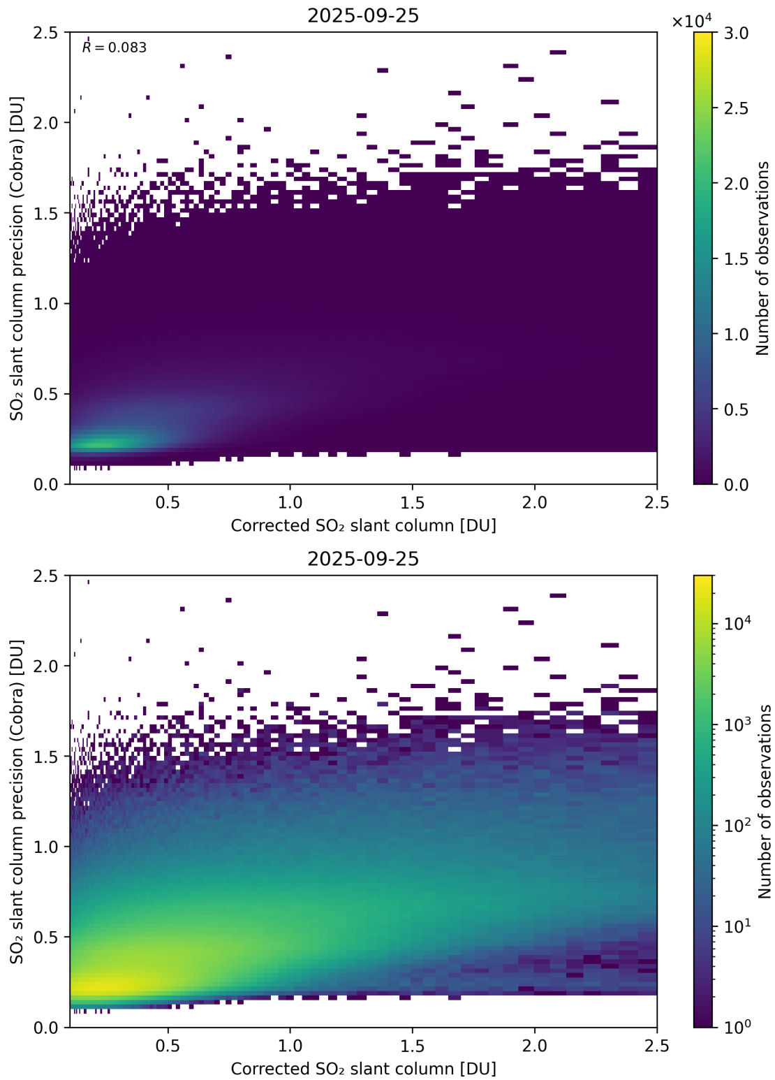
Figure 234: Scatter density plot of “Corrected SO 2 slant column” against “SO 2 slant column precision (Cobra)” for 2025-09-25 to 2025-09-26.
