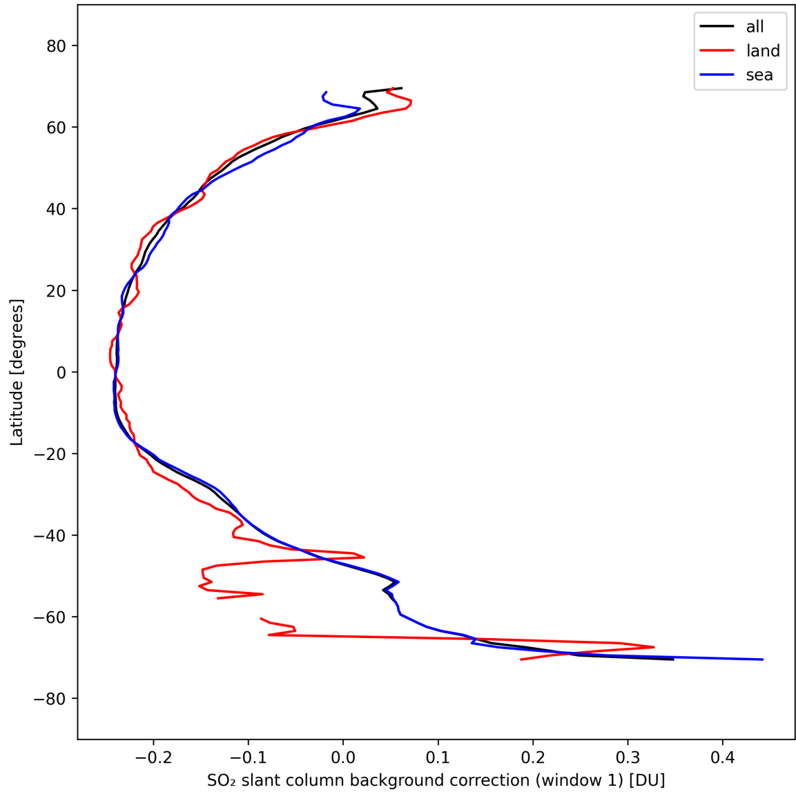
Figure 40: Zonal average of “SO 2 slant column background correction (window 1)” for 2025-09-25 to 2025-09-26.
