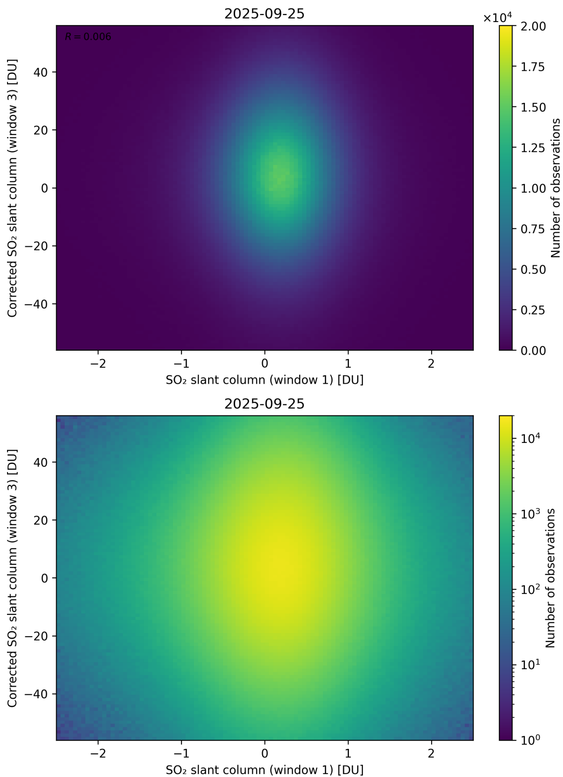
Figure 284: Scatter density plot of “SO 2 slant column (window 1)” against “Corrected SO 2 slant column (window 3)” for 2025-09-25 to 2025-09-26.
