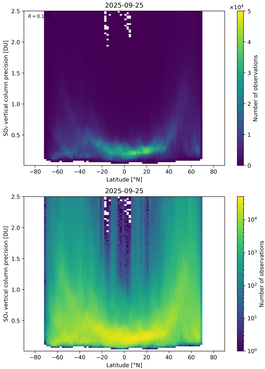
Figure 170: Scatter density plot of “Latitude” against “SO 2 vertical column precision” for 2025-09-25 to 2025-09-26.
