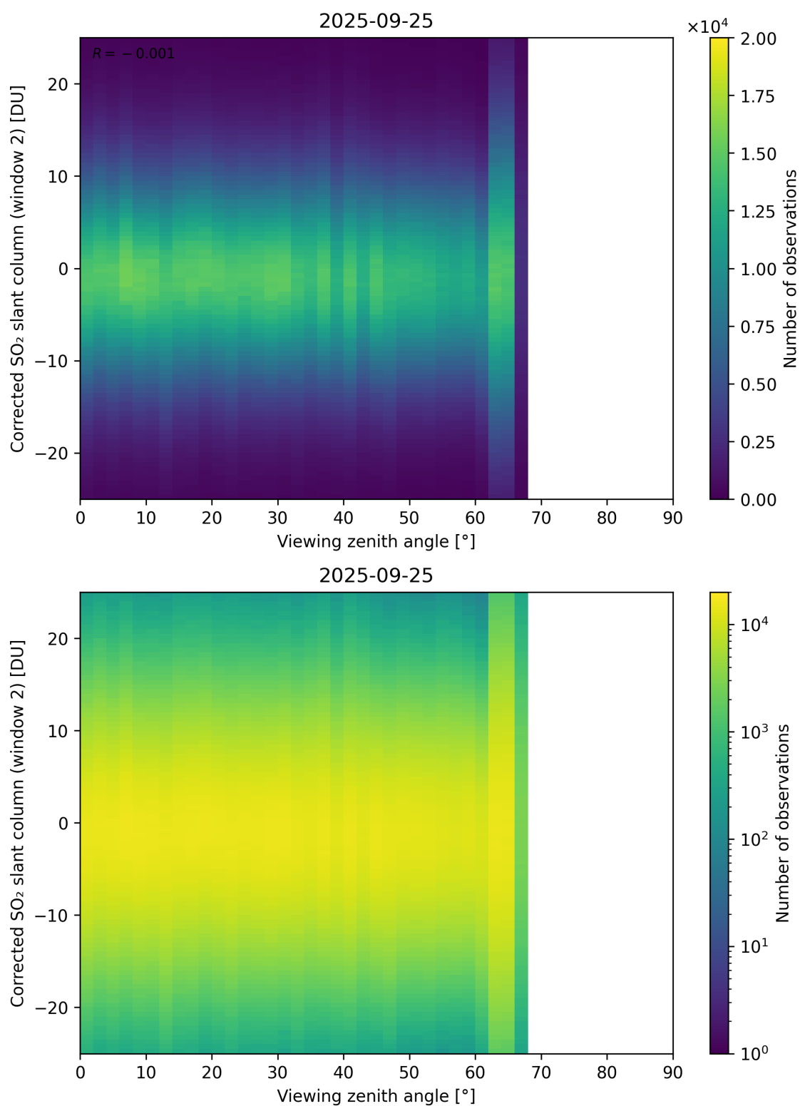
Figure 374: Scatter density plot of “Viewing zenith angle” against “Corrected SO 2 slant column (window 2)” for 2025-09-25 to 2025-09-26.
