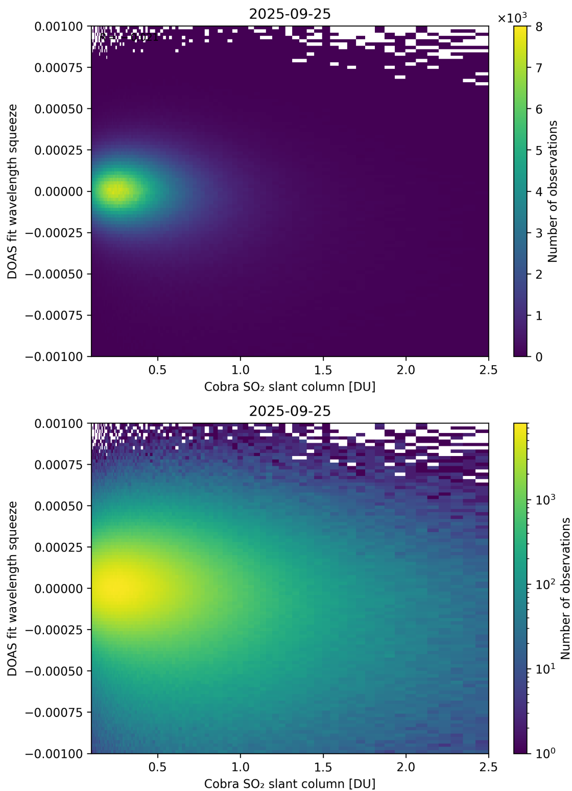
Figure 197: Scatter density plot of “Cobra SO 2 slant column” against “DOAS fit wavelength squeeze” for 2025-09-25 to 2025-09-26.
