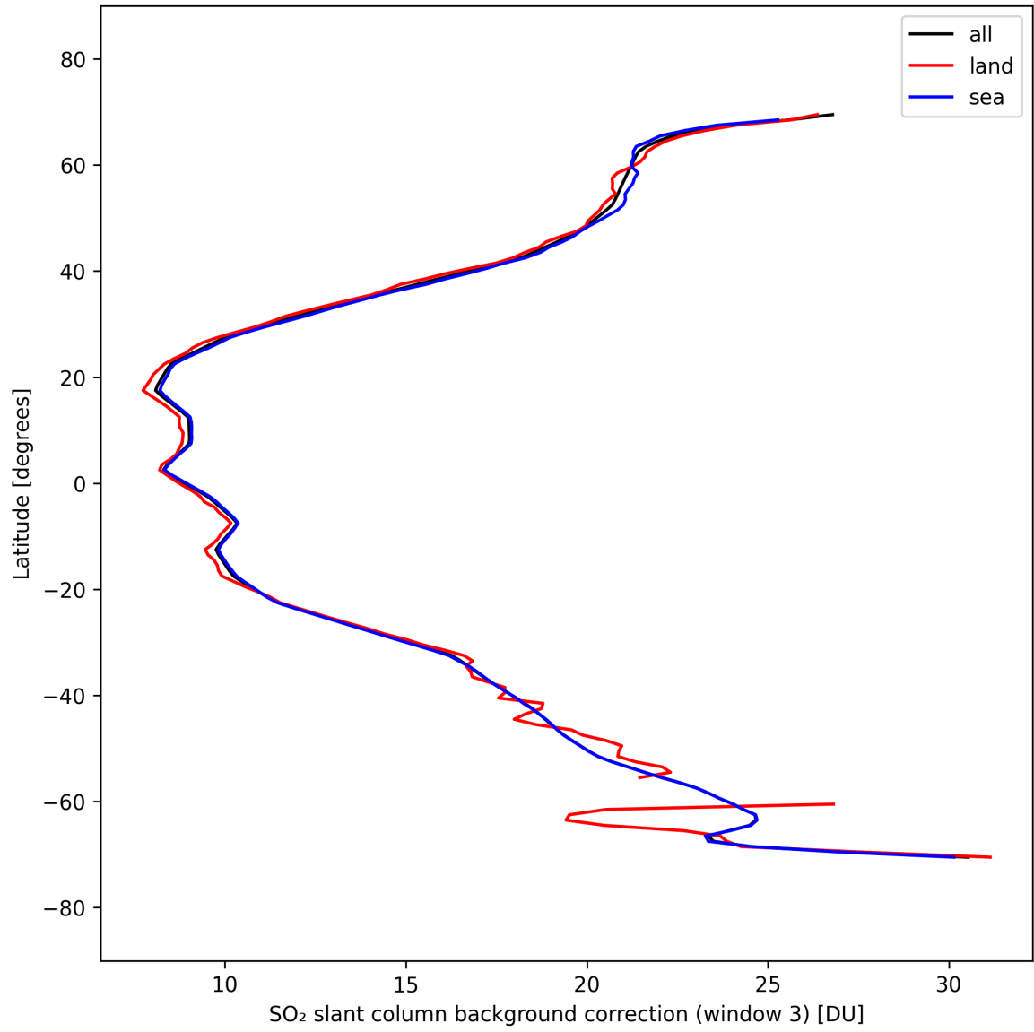
Figure 48: Zonal average of “SO 2 slant column background correction (window 3)” for 2025-09-25 to 2025-09-26.
