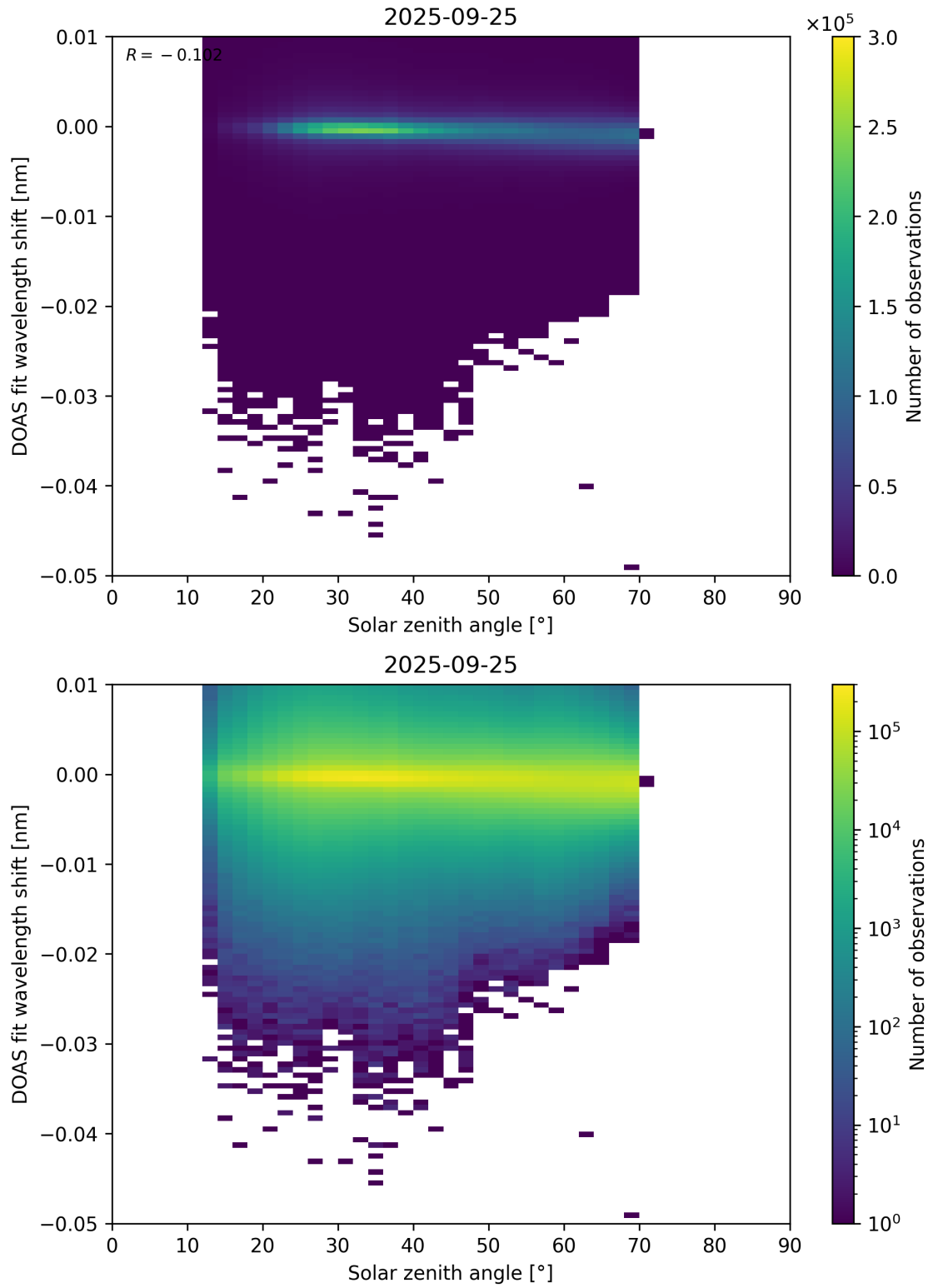
Figure 174: Scatter density plot of “Solar zenith angle” against “DOAS fit wavelength shift” for 2025-09-25 to 2025-09-26.
