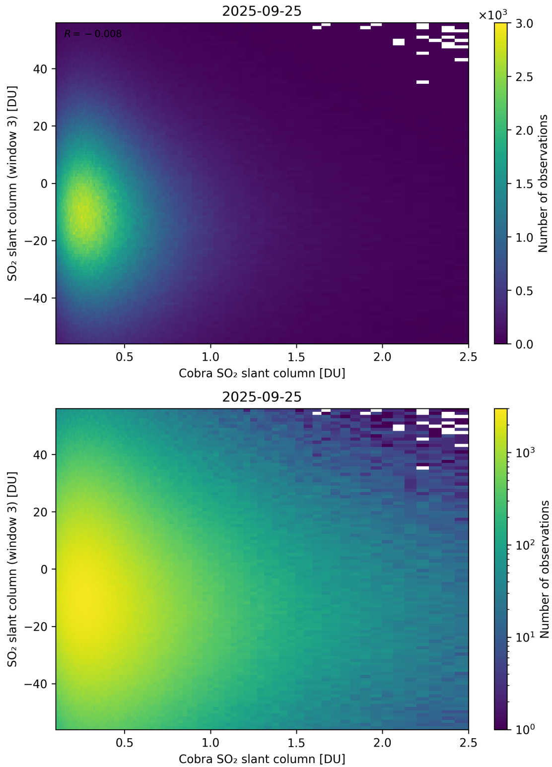
Figure 222: Scatter density plot of “Cobra SO 2 slant column” against “SO 2 slant column (window 3)” for 2025-09-25 to 2025-09-26.
