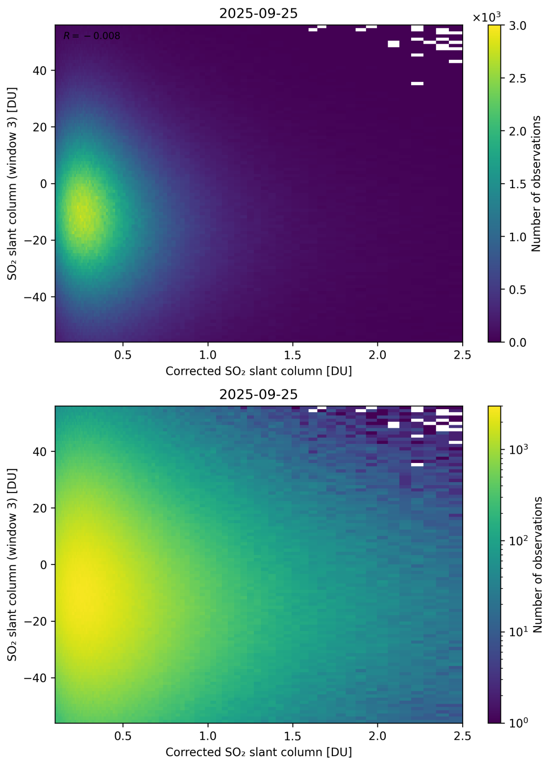
Figure 240: Scatter density plot of “Corrected SO 2 slant column” against “SO 2 slant column (window 3)” for 2025-09-25 to 2025-09-26.
