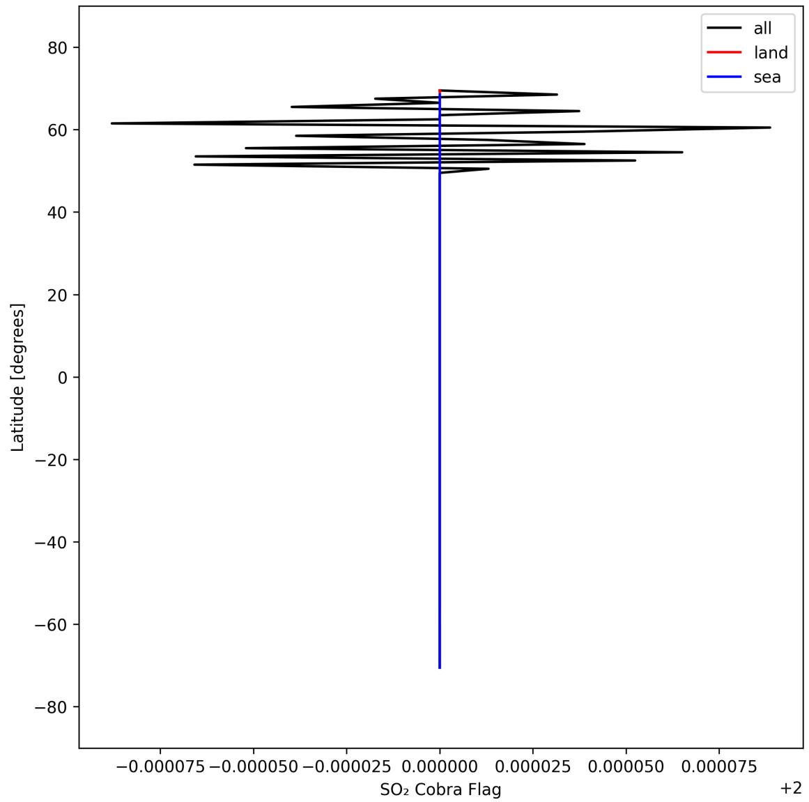
Figure 49: Zonal average of “SO 2 Cobra Flag” for 2025-09-25 to 2025-09-26.
