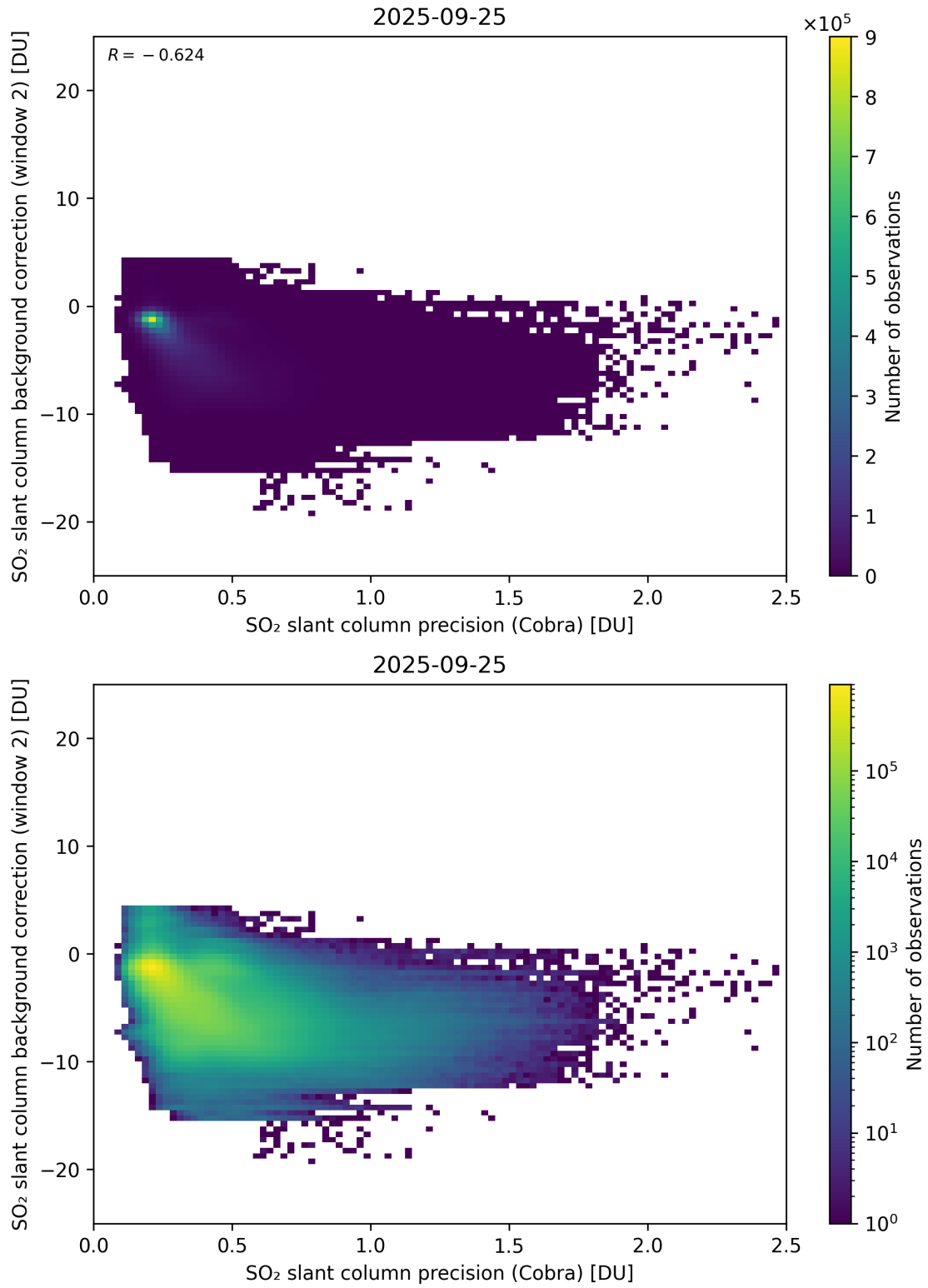
Figure 200: Scatter density plot of “SO 2 slant column precision (Cobra)” against “SO 2 slant column background correction (window 2)” for 2025-09-25 to 2025-09-26.
