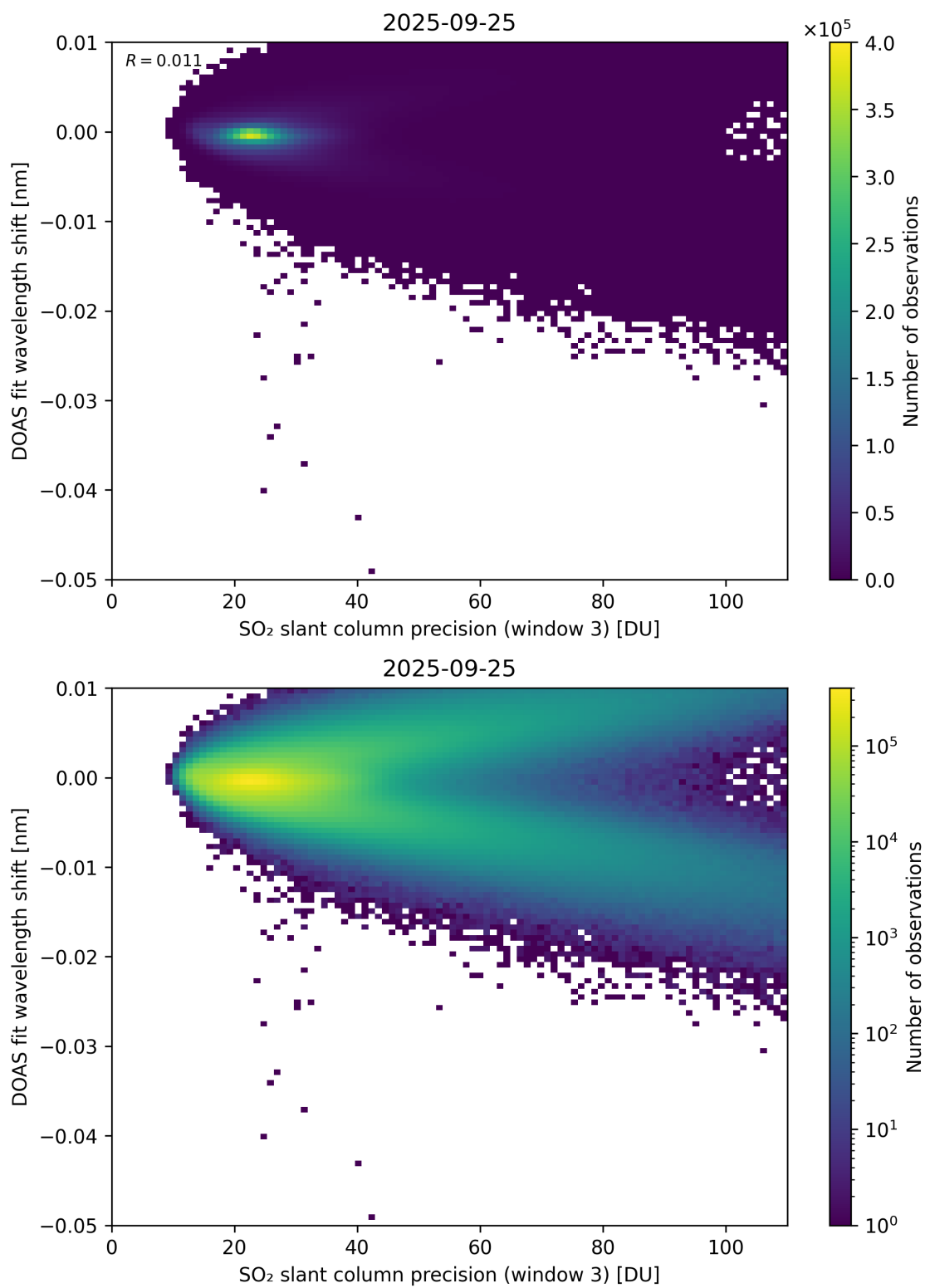
Figure 308: Scatter density plot of “SO 2 slant column precision (window 3)” against “DOAS fit wavelength shift” for 2025-09-25 to 2025-09-26.
