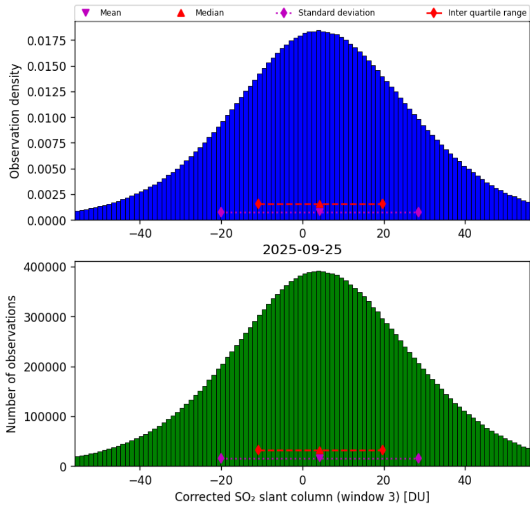
Figure 73: Histogram of "Corrected SO 2 slant column (window 3)" for 2025-09-25 to 2025-09-26
