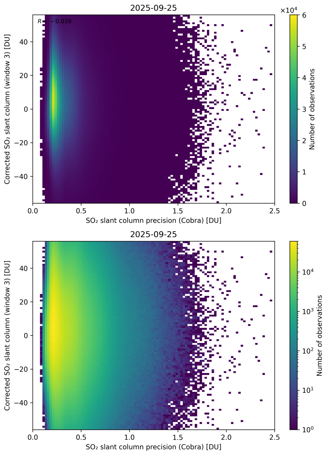
Figure 207: Scatter density plot of “SO 2 slant column precision (Cobra)” against “Corrected SO 2 slant column (window 3)” for 2025-09-25 to 2025-09-26.
