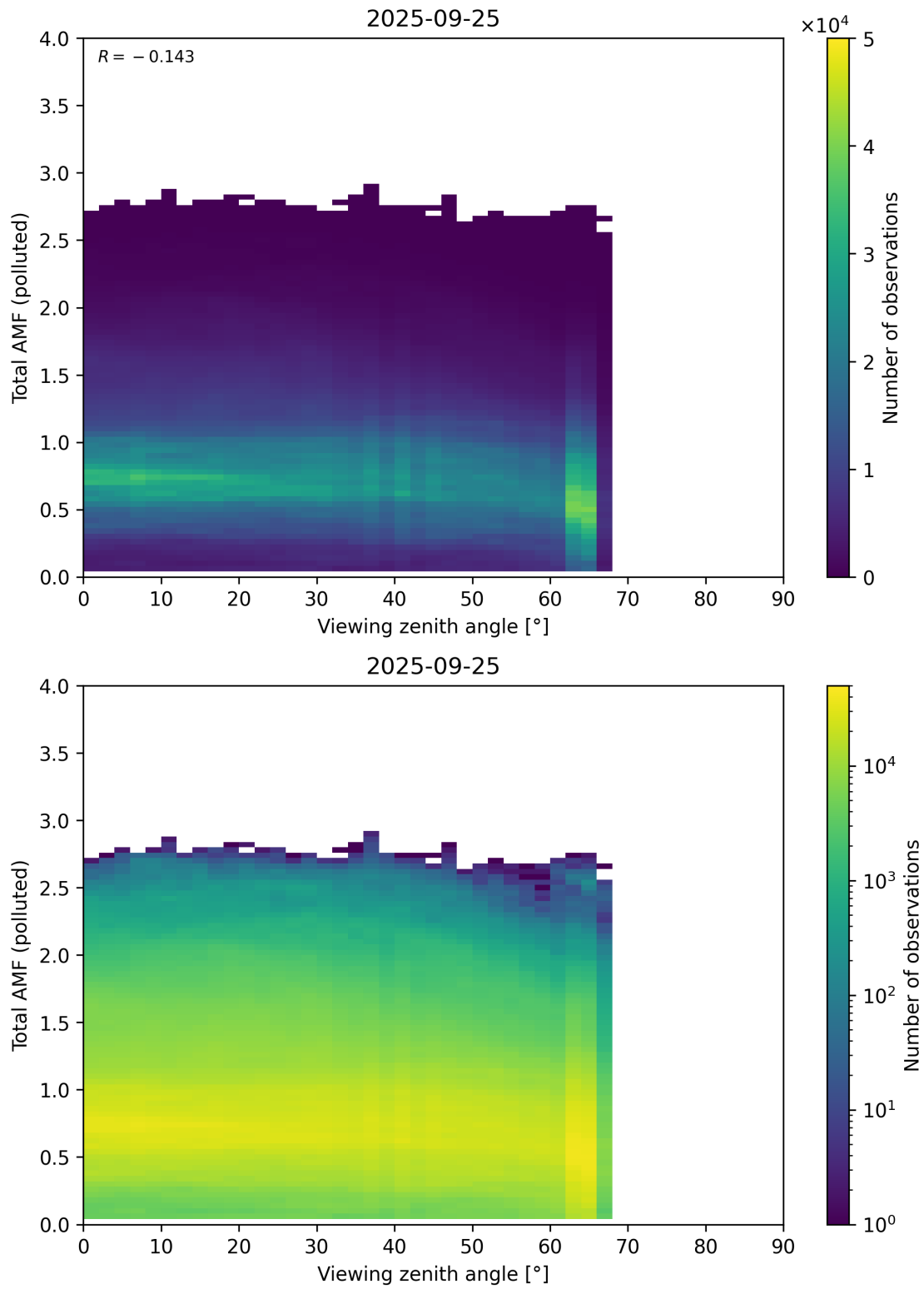
Figure 381: Scatter density plot of “Viewing zenith angle” against “Total AMF (polluted)” for 2025-09-25 to 2025-09-26.
