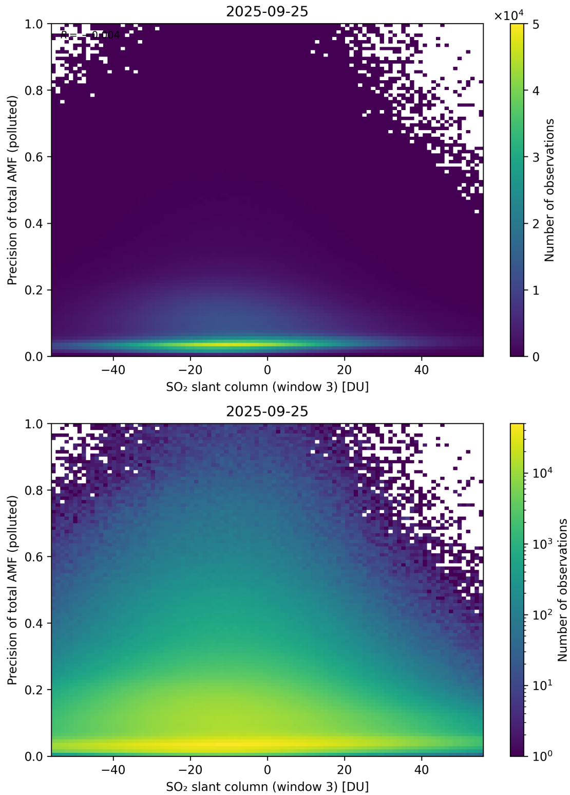
Figure 319: Scatter density plot of “SO 2 slant column (window 3)” against “Precision of total AMF (polluted)” for 2025-09-25 to 2025-09-26.
