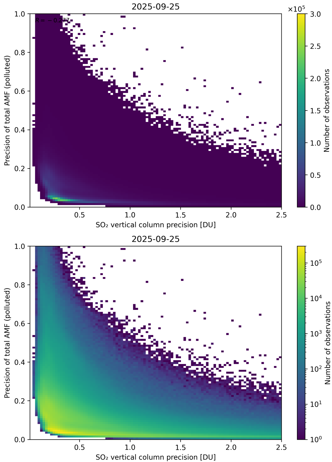
Figure 347: Scatter density plot of “SO 2 vertical column precision” against “Precision of total AMF (polluted)” for 2025-09-25 to 2025-09-26.
