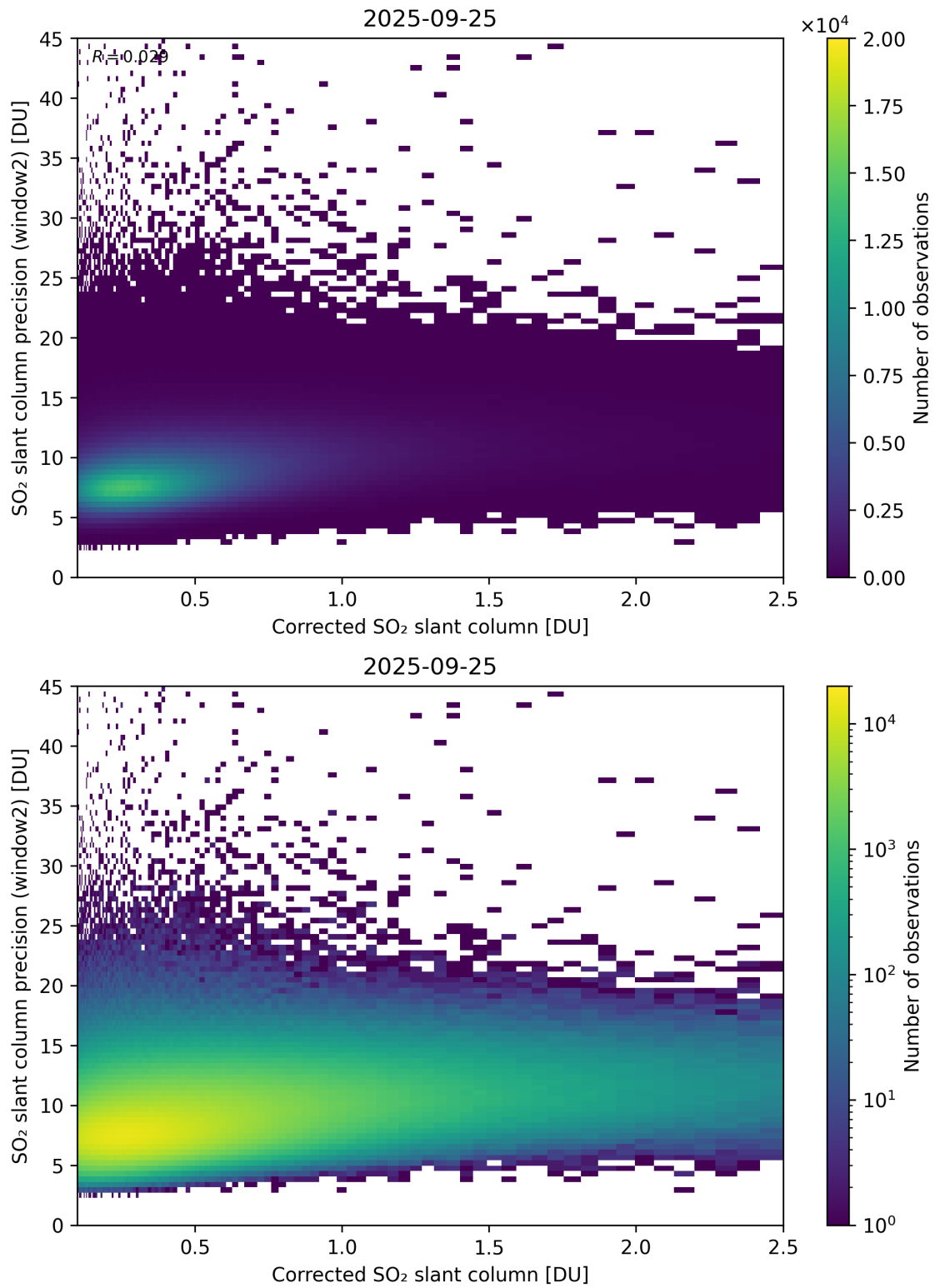
Figure 239: Scatter density plot of “Corrected SO 2 slant column” against “SO 2 slant column precision (window2)” for 2025-09-25 to 2025-09-26.
