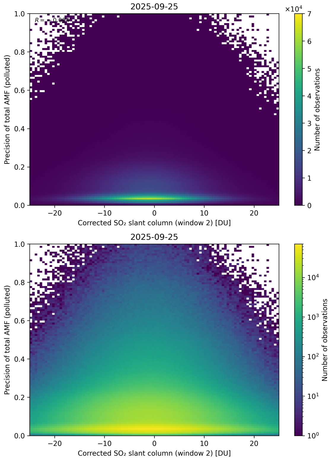
Figure 254: Scatter density plot of “Corrected SO 2 slant column (window 2)” against “Precision of total AMF (polluted)” for 2025-09-25 to 2025-09-26.
