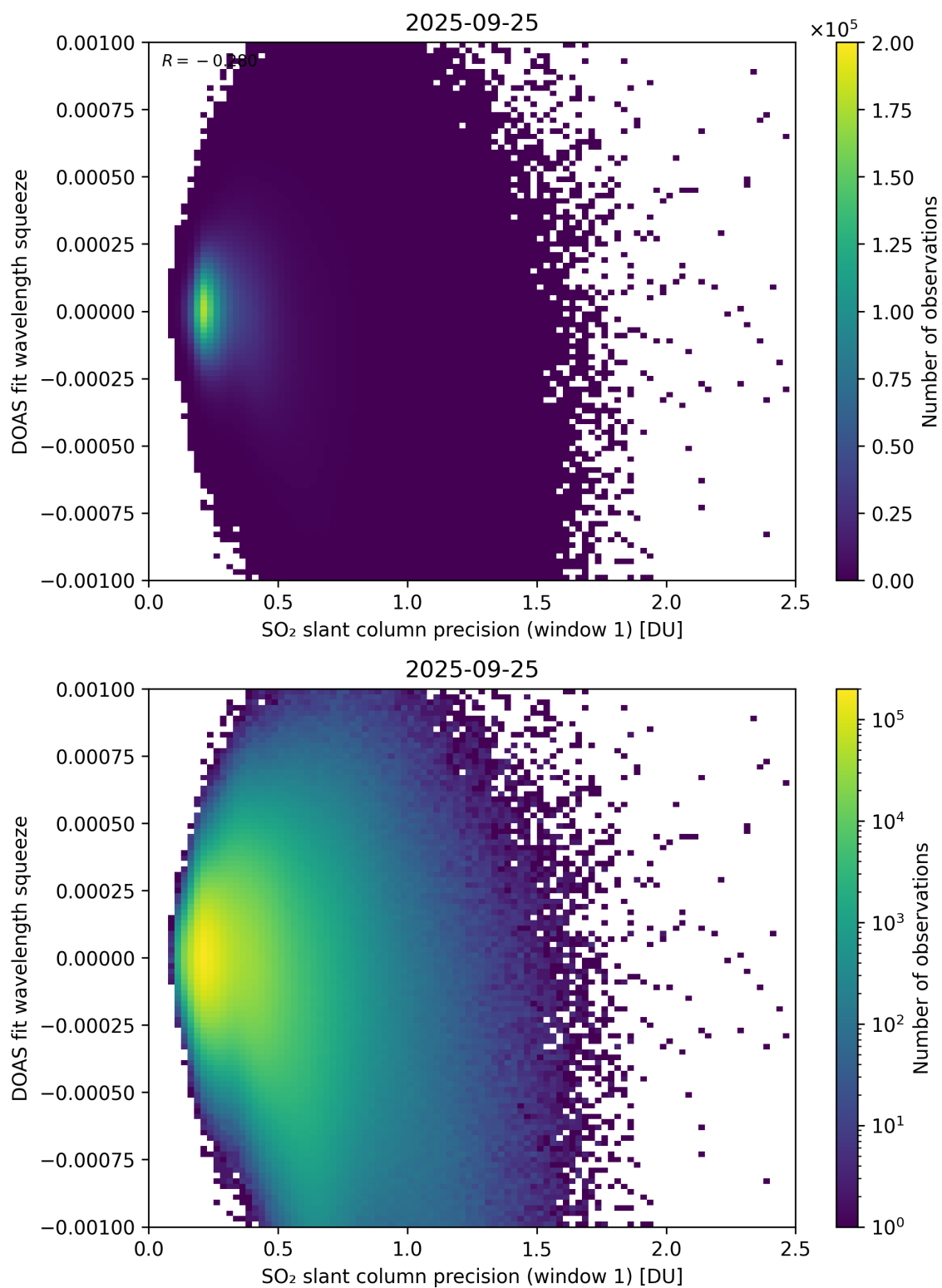
Figure 272: Scatter density plot of “SO 2 slant column precision (window 1)” against “DOAS fit wavelength squeeze” for 2025-09-25 to 2025-09-26.
