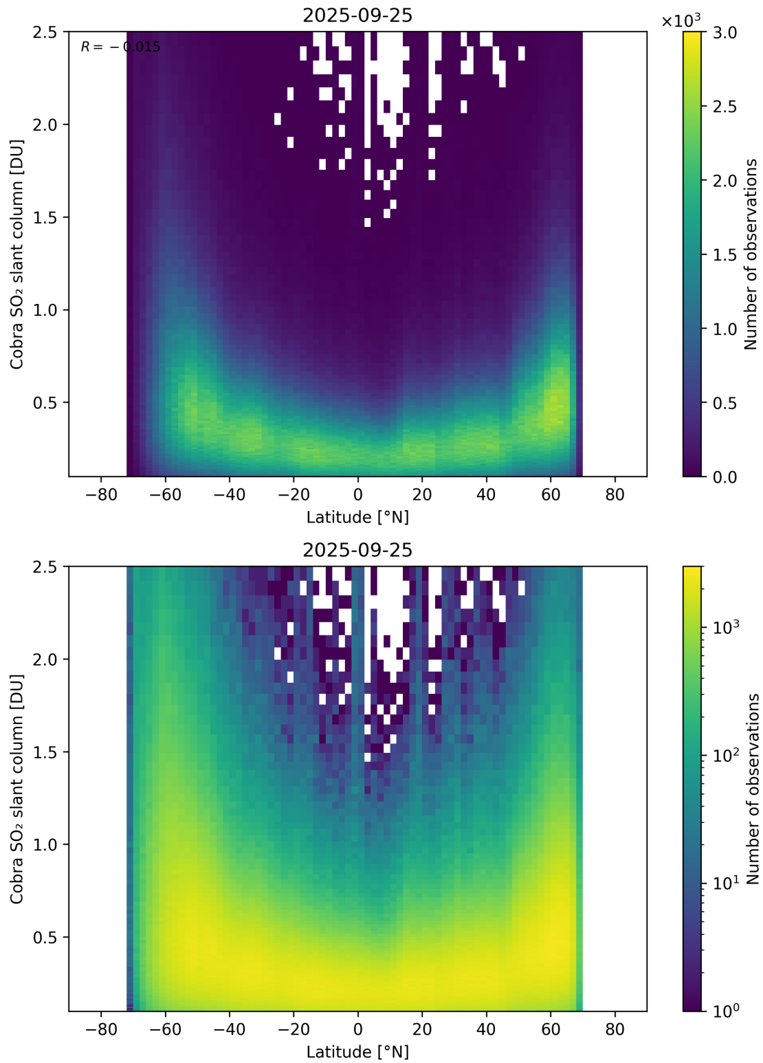
Figure 157: Scatter density plot of “Latitude” against “Cobra SO 2 slant column” for 2025-09-25 to 2025-09-26.
