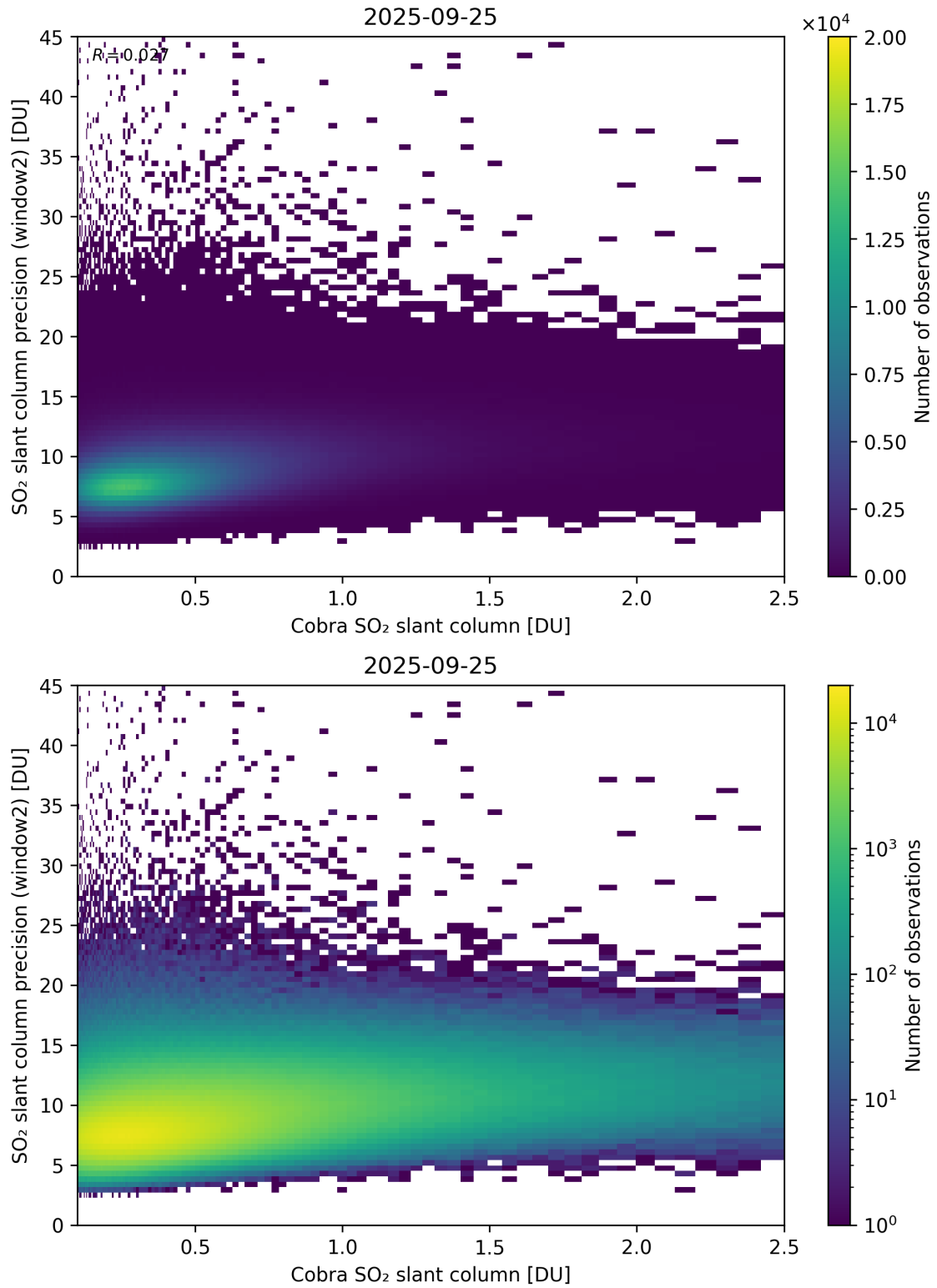
Figure 221: Scatter density plot of “Cobra SO 2 slant column” against “SO 2 slant column precision (window2)” for 2025-09-25 to 2025-09-26.
