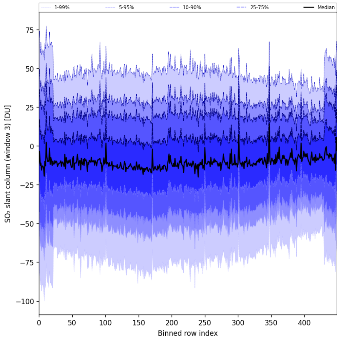
Figure 97: Along track statistics of “SO 2 slant column (window 3)” for 2025-09-25 to 2025-09-26
