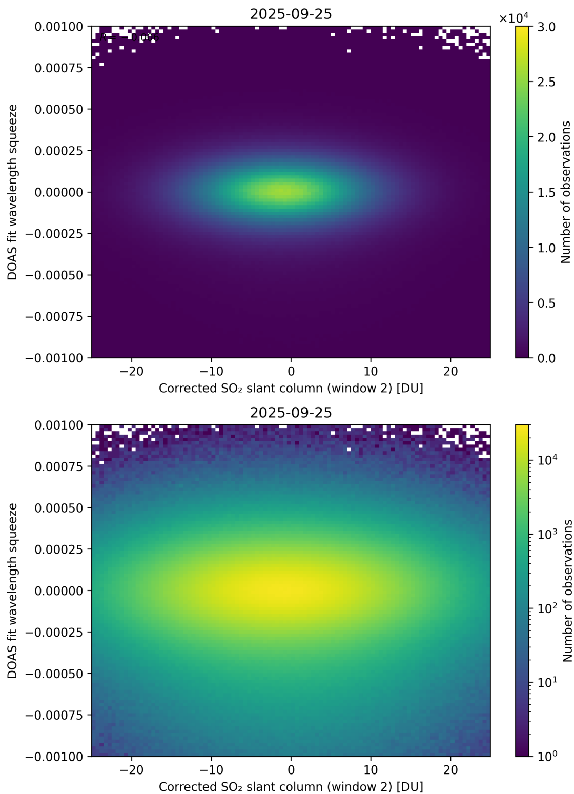
Figure 247: Scatter density plot of “Corrected SO 2 slant column (window 2)” against “DOAS fit wavelength squeeze” for 2025-09-25 to 2025-09-26.
