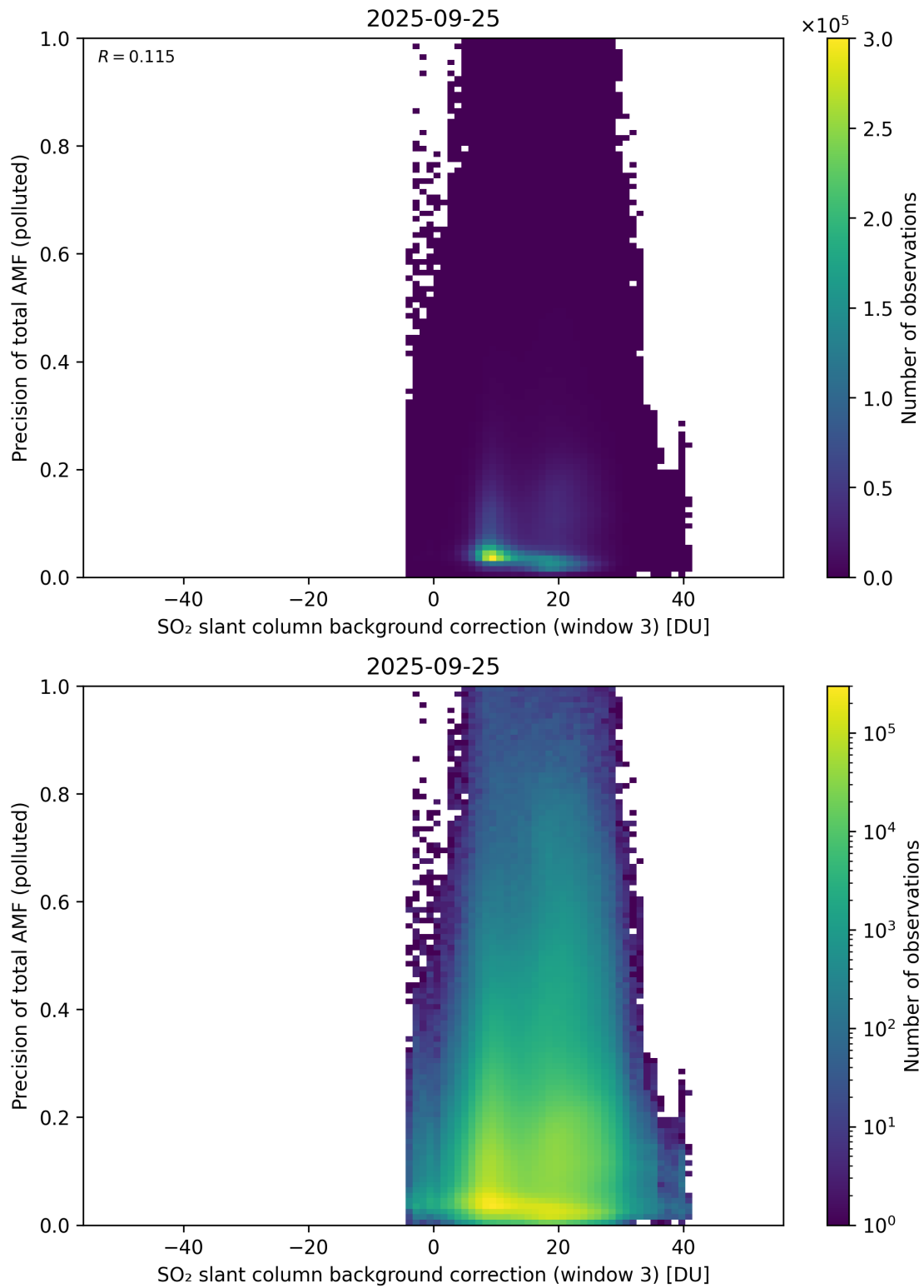
Figure 137: Scatter density plot of “SO 2 slant column background correction (window 3)” against “Precision of total AMF (polluted)” for 2025-09-25 to 2025-09-26.
