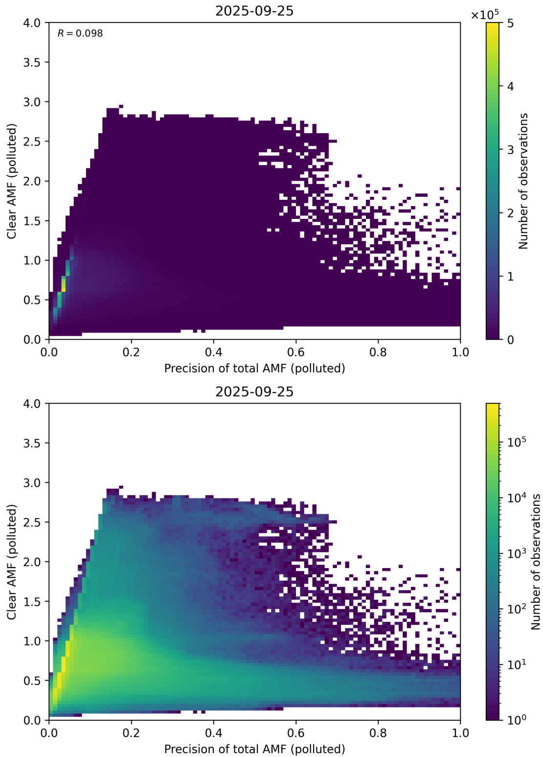
Figure 320: Scatter density plot of “Precision of total AMF (polluted)” against “Clear AMF (polluted)” for 2025-09-25 to 2025-09-26.
