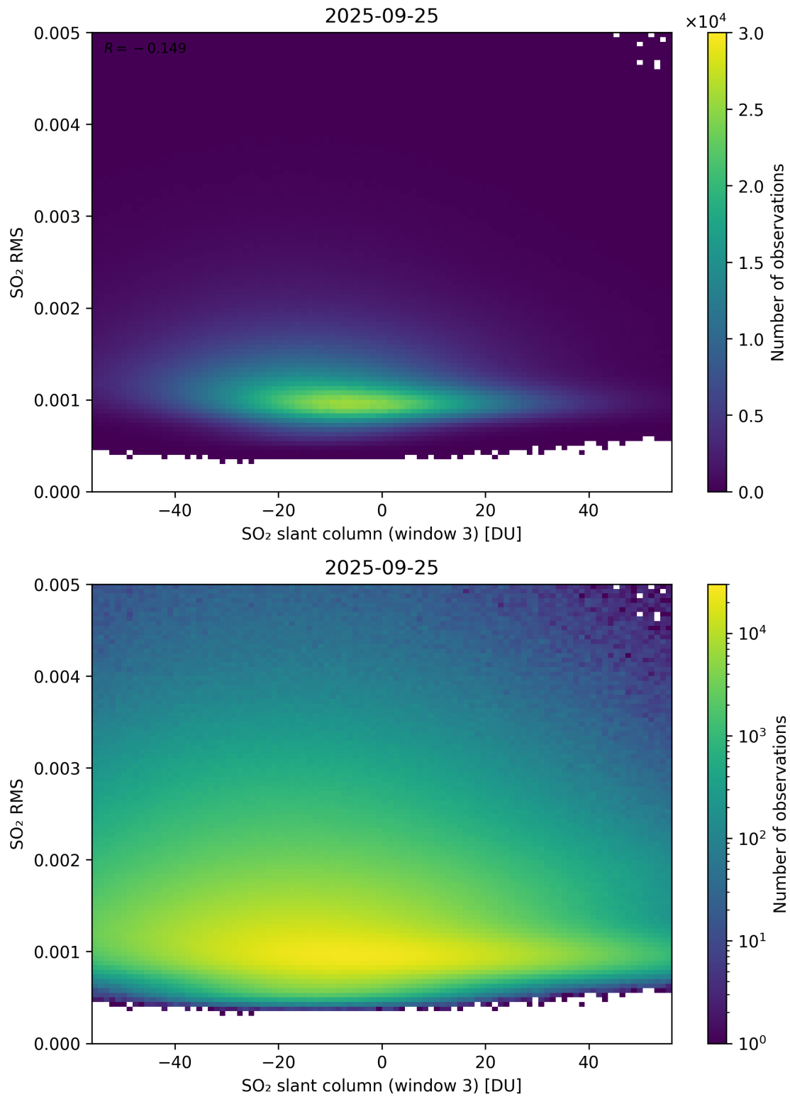
Figure 306: Scatter density plot of “SO 2 slant column (window 3)” against “SO 2 RMS” for 2025-09-25 to 2025-09-26.
