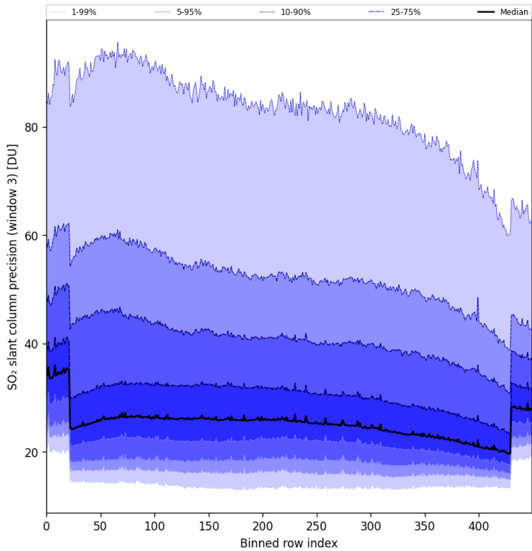
Figure 98: Along track statistics of “SO 2 slant column precision (window 3)” for 2025-09-25 to 2025-09-26
