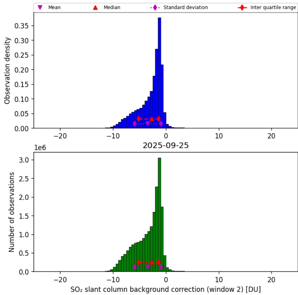
Figure 70: Histogram of “SO 2 slant column background correction (window 2)” for 2025-09-25 to 2025-09-26
