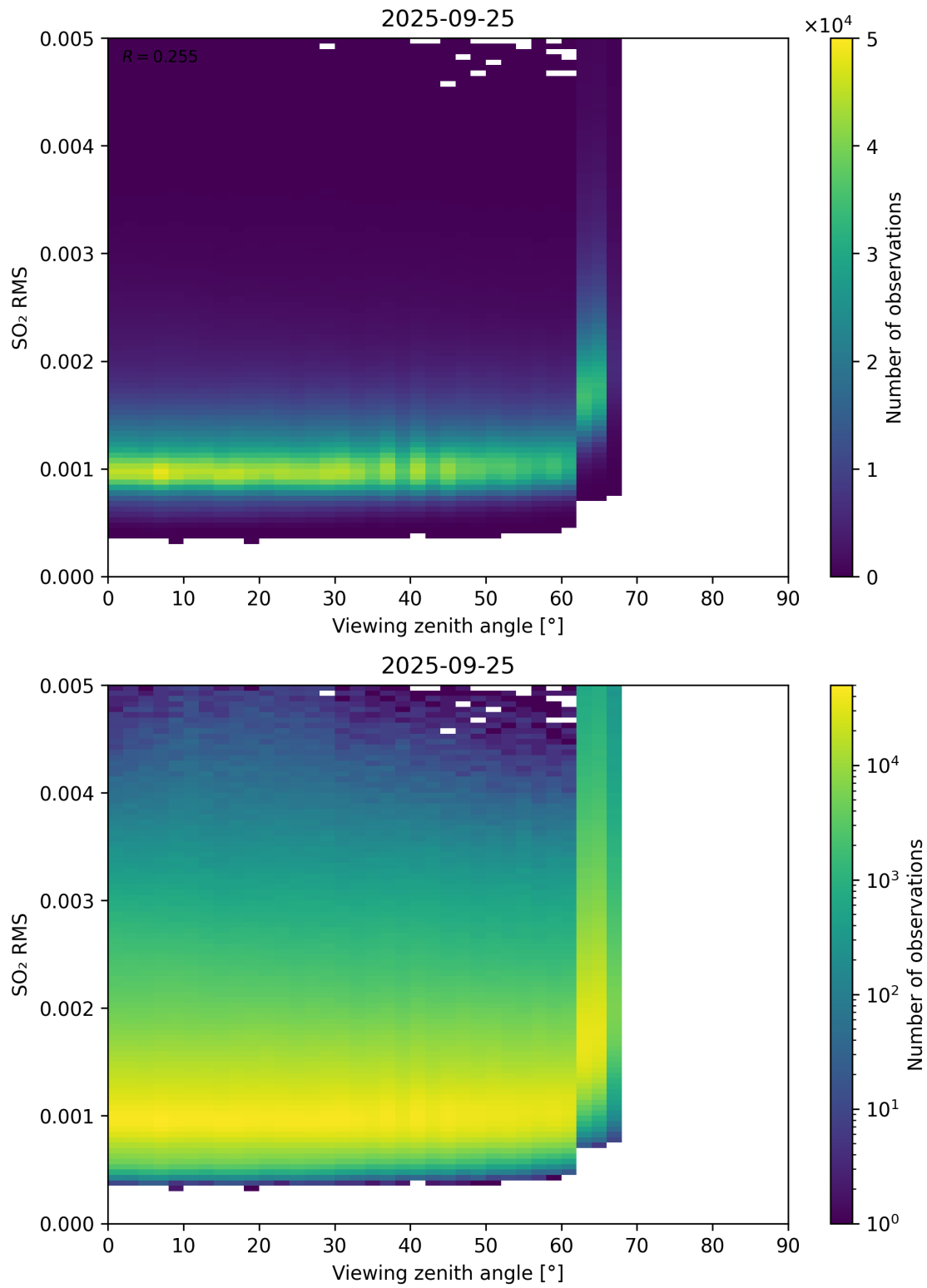
Figure 367: Scatter density plot of “Viewing zenith angle” against “SO 2 RMS” for 2025-09-25 to 2025-09-26.
