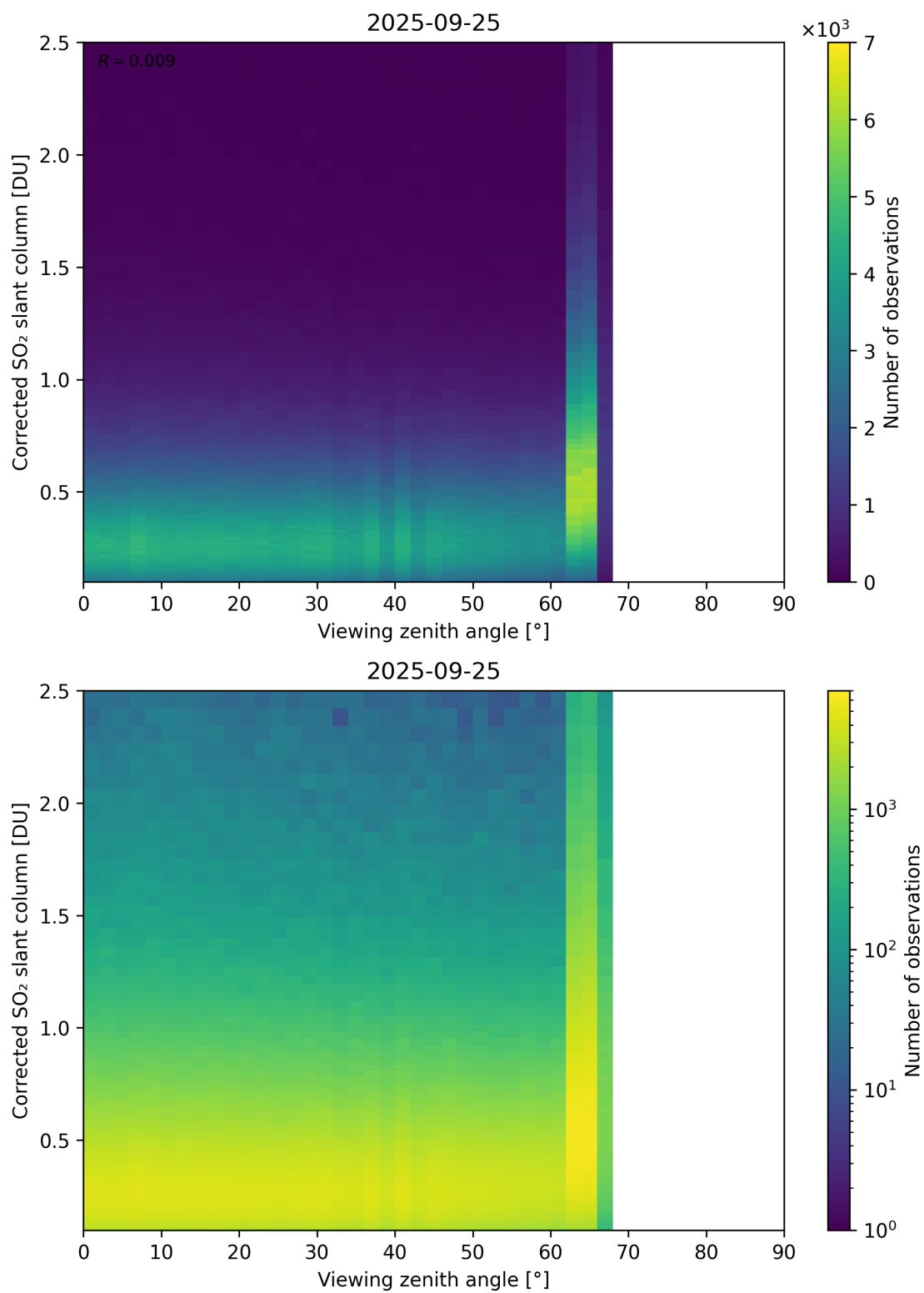
Figure 373: Scatter density plot of “Viewing zenith angle” against “Corrected SO 2 slant column” for 2025-09-25 to 2025-09-26.
