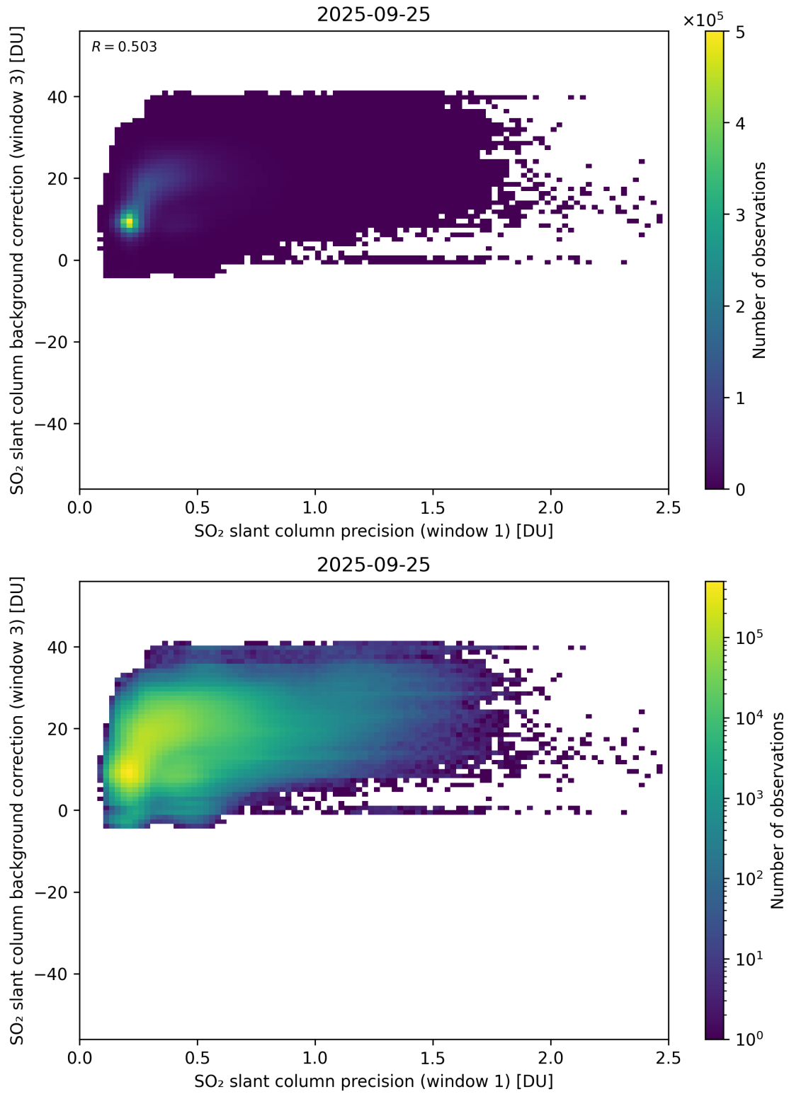
Figure 270: Scatter density plot of “SO 2 slant column precision (window 1)” against “SO 2 slant column background correction (window 3)” for 2025-09-25 to 2025-09-26.
