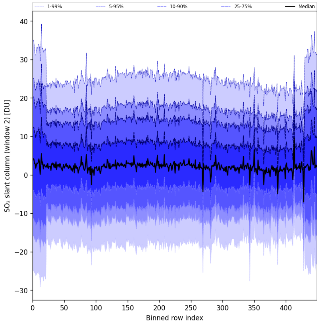
Figure 93: Along track statistics of “SO 2 slant column (window 2)” for 2025-09-25 to 2025-09-26
