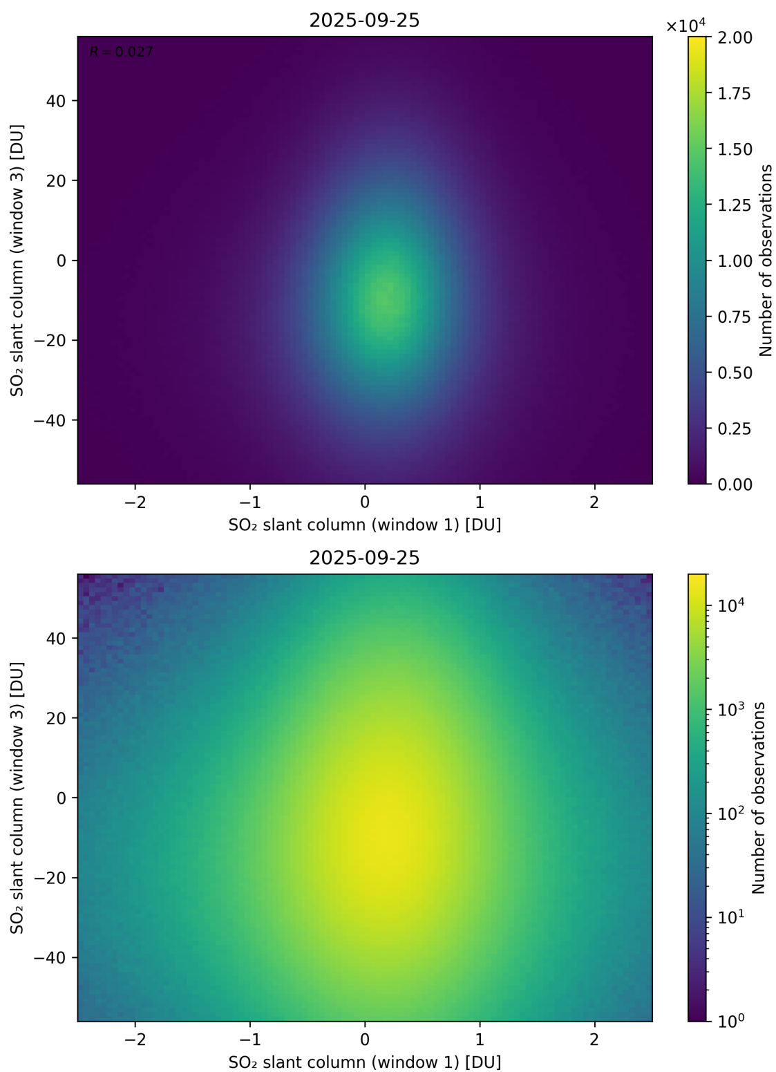
Figure 287: Scatter density plot of “SO 2 slant column (window 1)” against “SO 2 slant column (window 3)” for 2025-09-25 to 2025-09-26.
