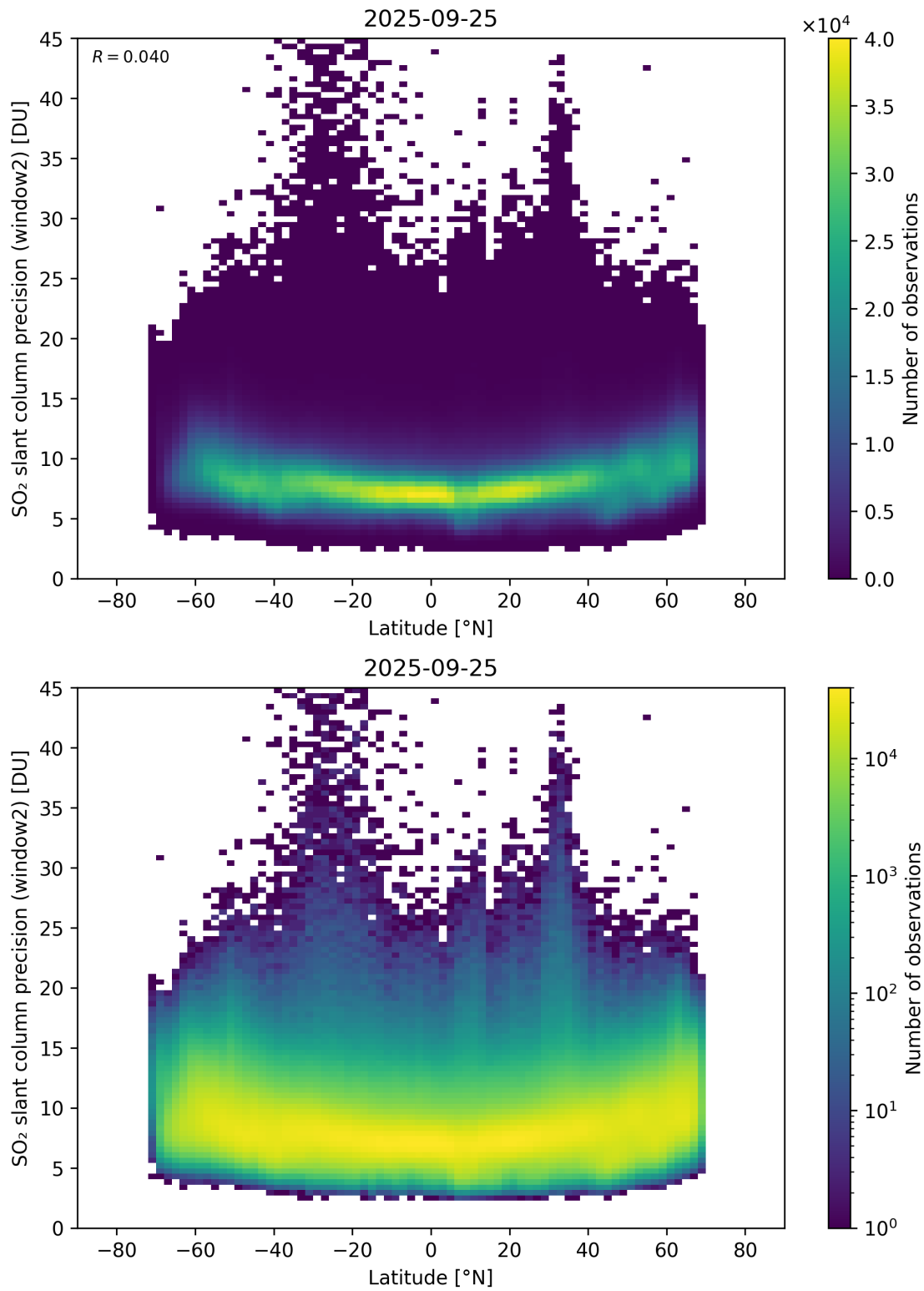
Figure 164: Scatter density plot of “Latitude” against “SO 2 slant column precision (window2)” for 2025-09-25 to 2025-09-26.
