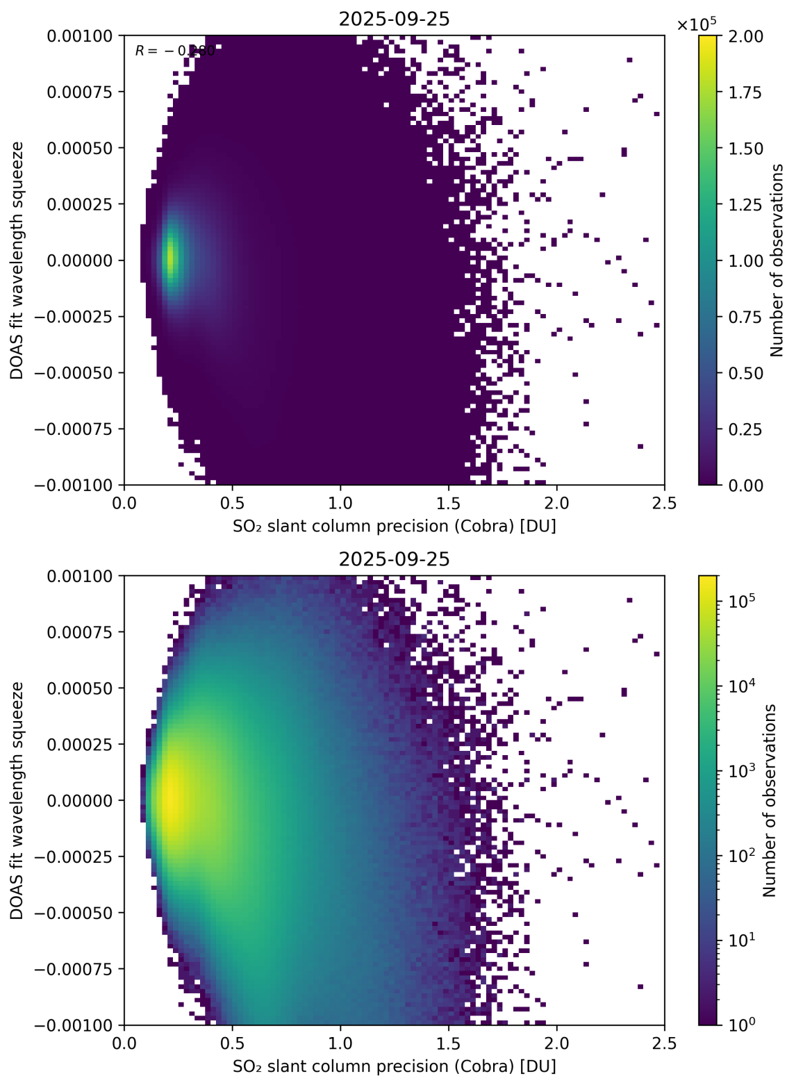
Figure 203: Scatter density plot of “SO 2 slant column precision (Cobra)” against “DOAS fit wavelength squeeze” for 2025-09-25 to 2025-09-26.
