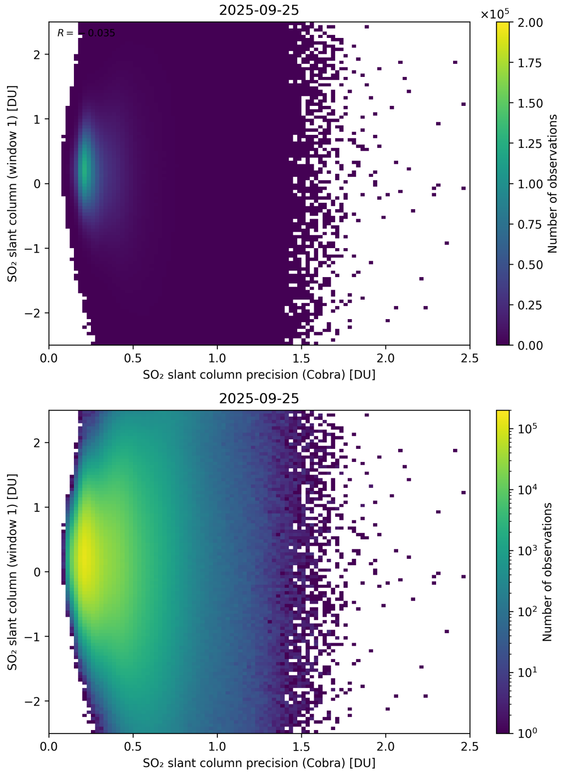
Figure 208: Scatter density plot of “SO 2 slant column precision (Cobra)” against “SO 2 slant column (window 1)” for 2025-09-25 to 2025-09-26.
