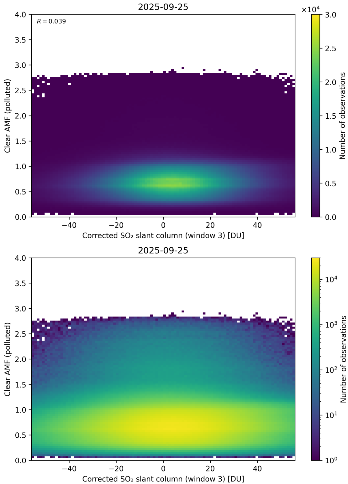
Figure 259: Scatter density plot of “Corrected SO 2 slant column (window 3)” against “Clear AMF (polluted)” for 2025-09-25 to 2025-09-26.
