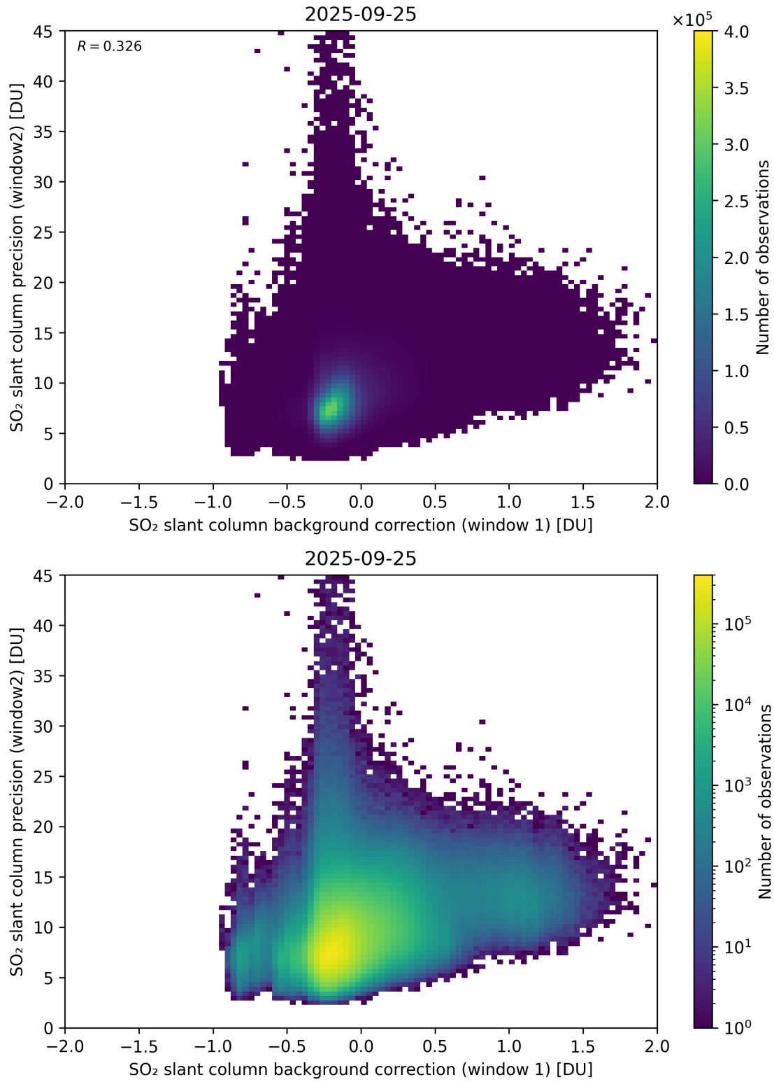
Figure 117: Scatter density plot of “SO 2 slant column background correction (window 1)” against “SO 2 slant column precision (window2)” for 2025-09-25 to 2025-09-26.
