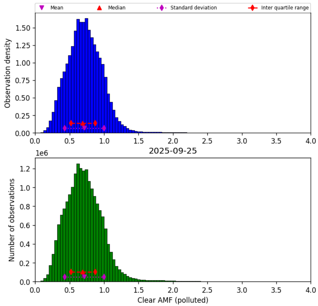
Figure 81: Histogram of “Clear AMF (polluted)” for 2025-09-25 to 2025-09-26
