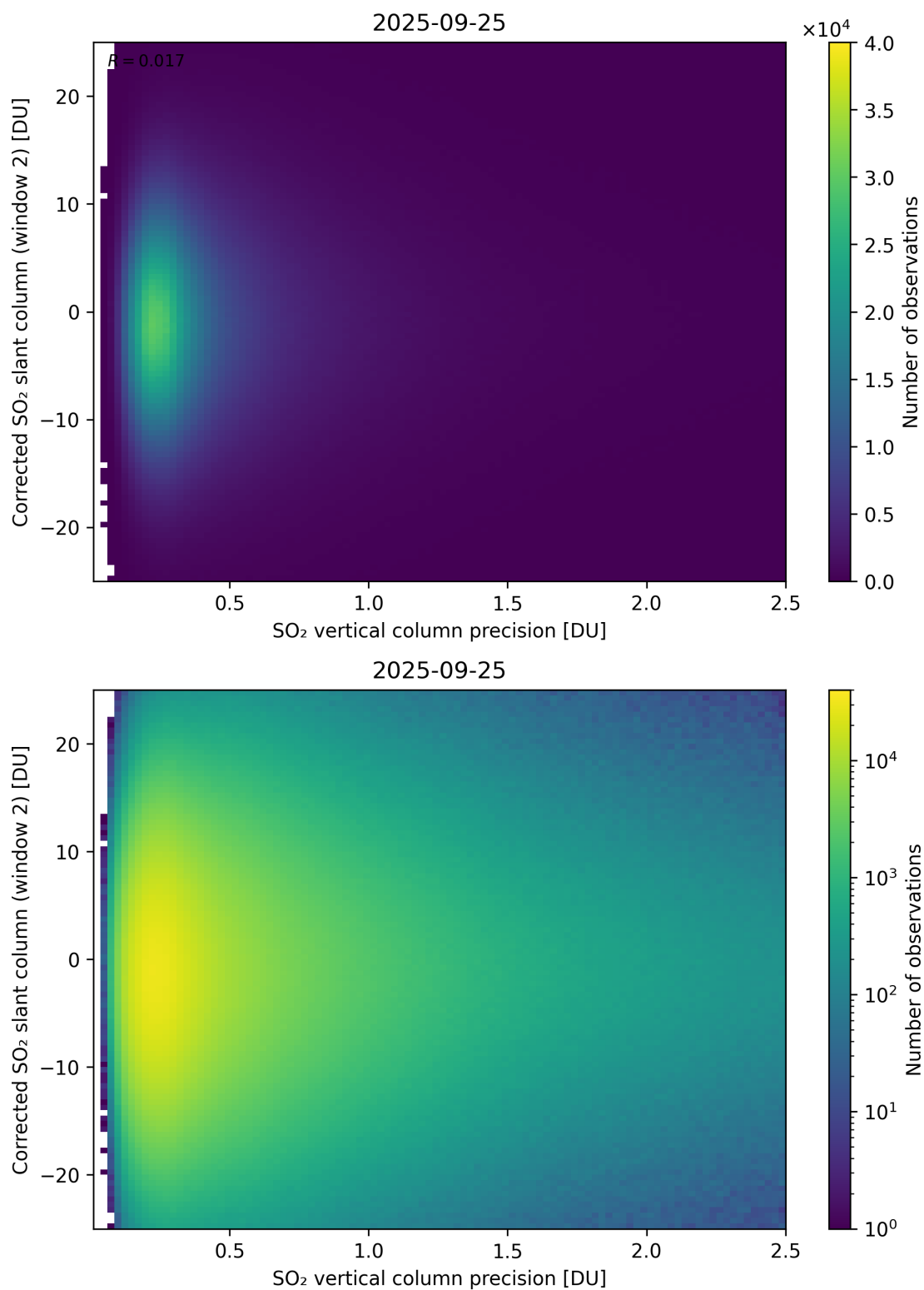
Figure 339: Scatter density plot of “SO 2 vertical column precision” against “Corrected SO 2 slant column (window 2)” for 2025-09-25 to 2025-09-26.
