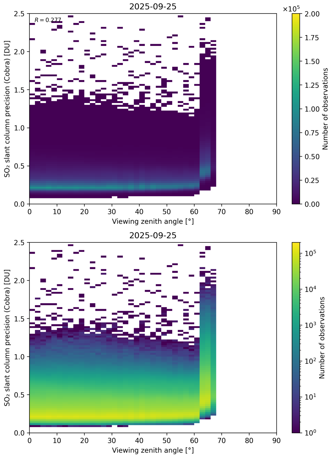
Figure 372: Scatter density plot of “Viewing zenith angle” against “SO 2 slant column precision (Cobra)” for 2025-09-25 to 2025-09-26.
