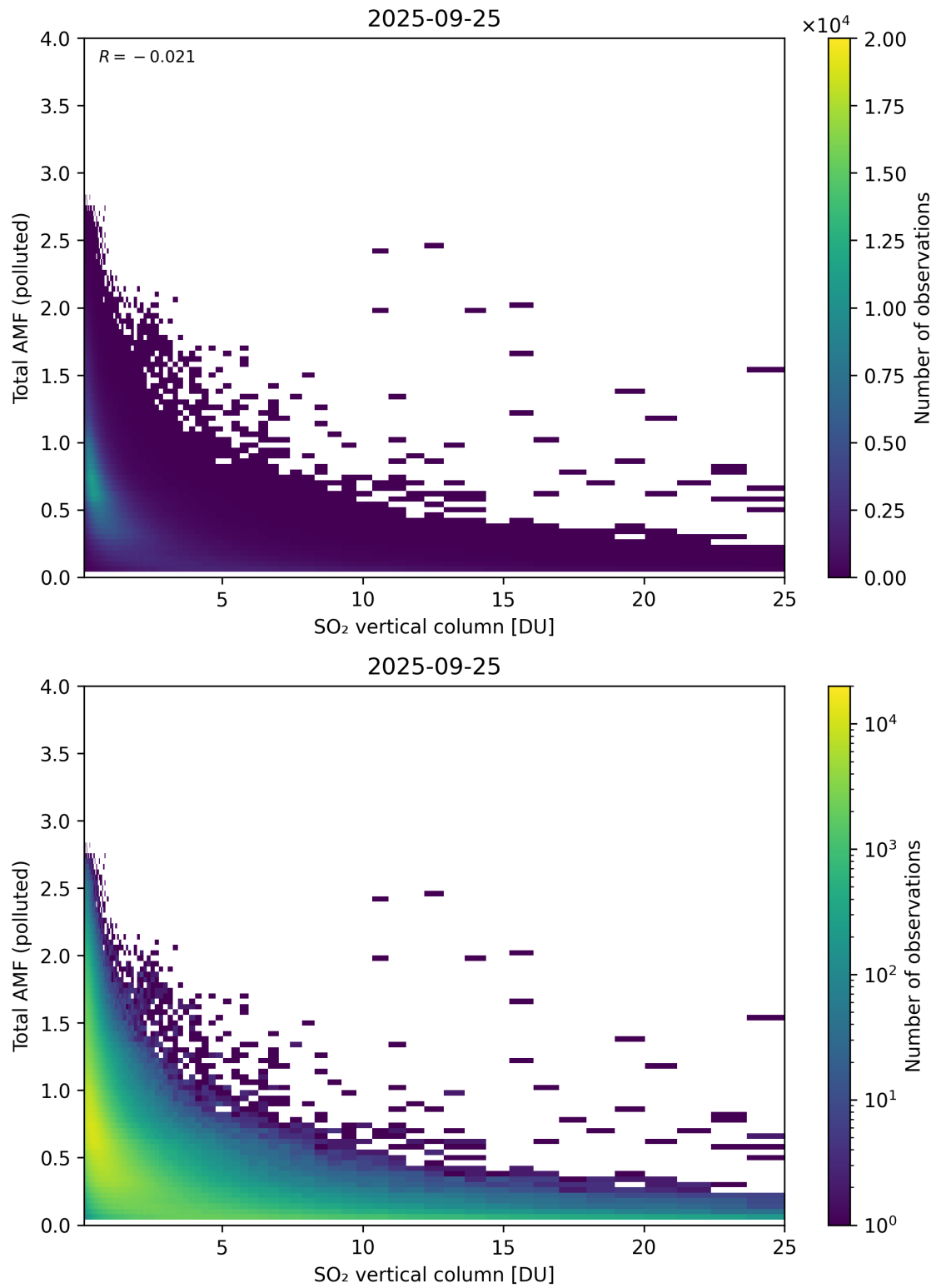
Figure 359: Scatter density plot of “SO 2 vertical column” against “Total AMF (polluted)” for 2025-09-25 to 2025-09-26.
