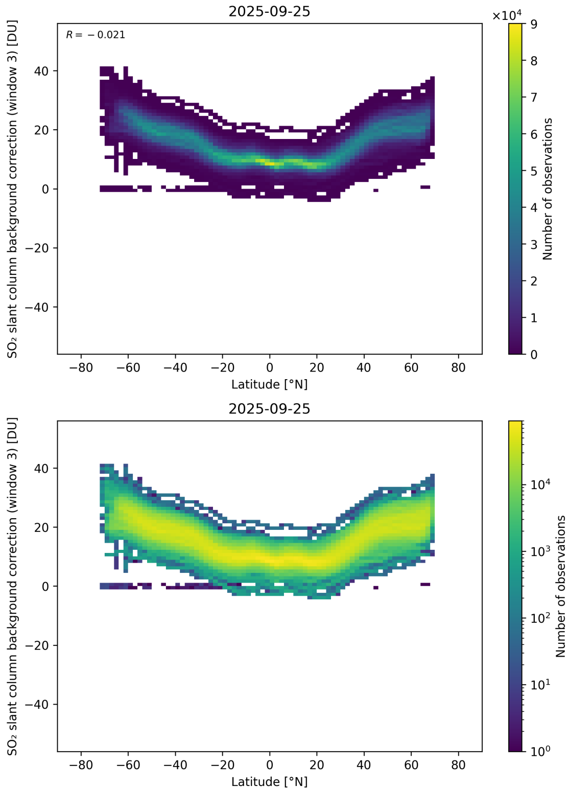
Figure 152: Scatter density plot of “Latitude” against “SO 2 slant column background correction (window 3)” for 2025-09-25 to 2025-09-26.
