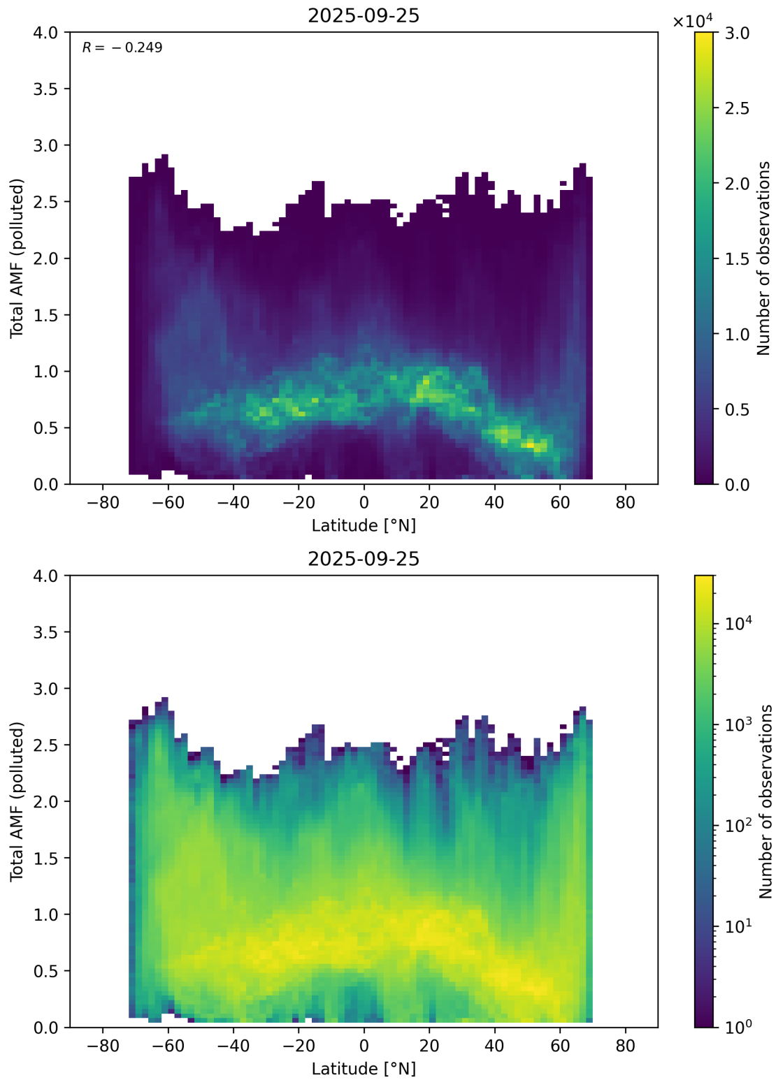
Figure 167: Scatter density plot of “Latitude” against “Total AMF (polluted)” for 2025-09-25 to 2025-09-26.
