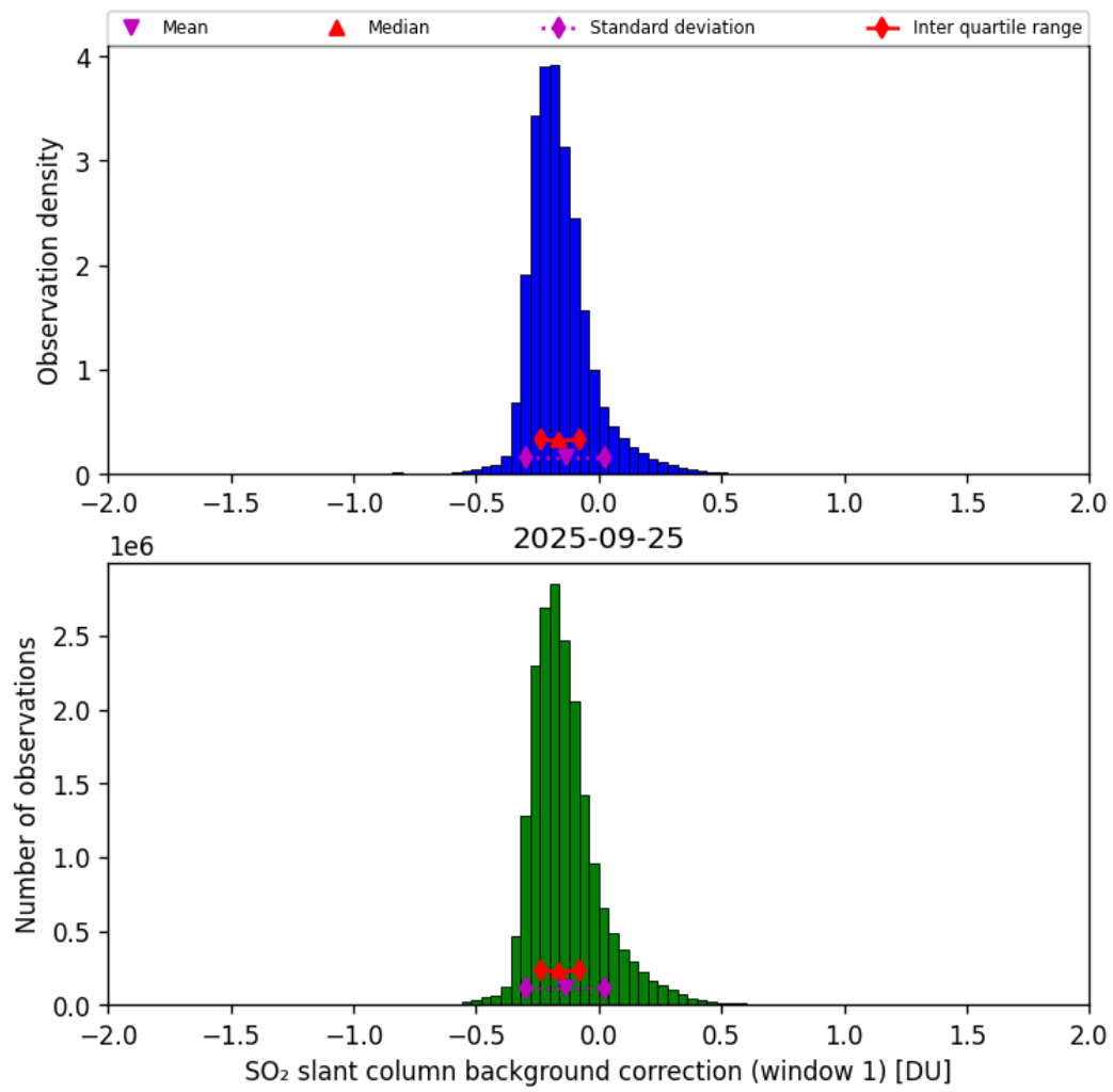
Figure 66: Histogram of “SO 2 slant column background correction (window 1)” for 2025-09-25 to 2025-09-26
