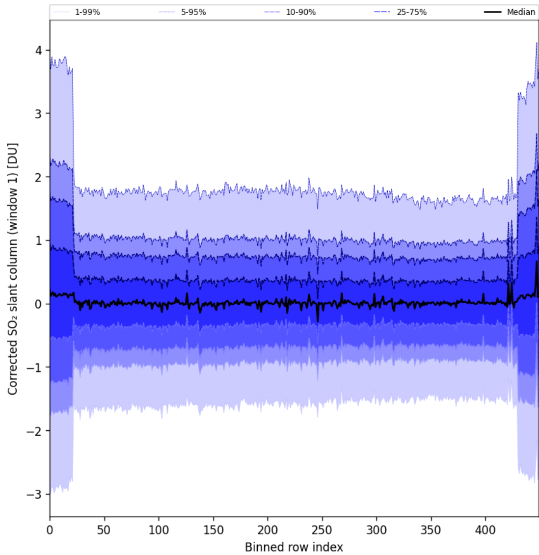
Figure 91: Along track statistics of “Corrected SO 2 slant column (window 1)” for 2025-09-25 to 2025-09-26
