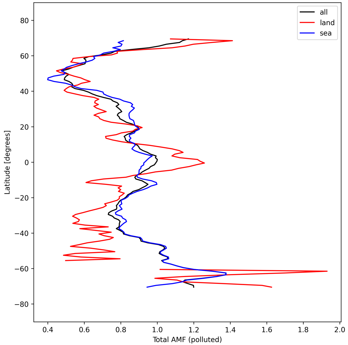
Figure 53: Zonal average of “Total AMF (polluted)” for 2025-09-25 to 2025-09-26.
