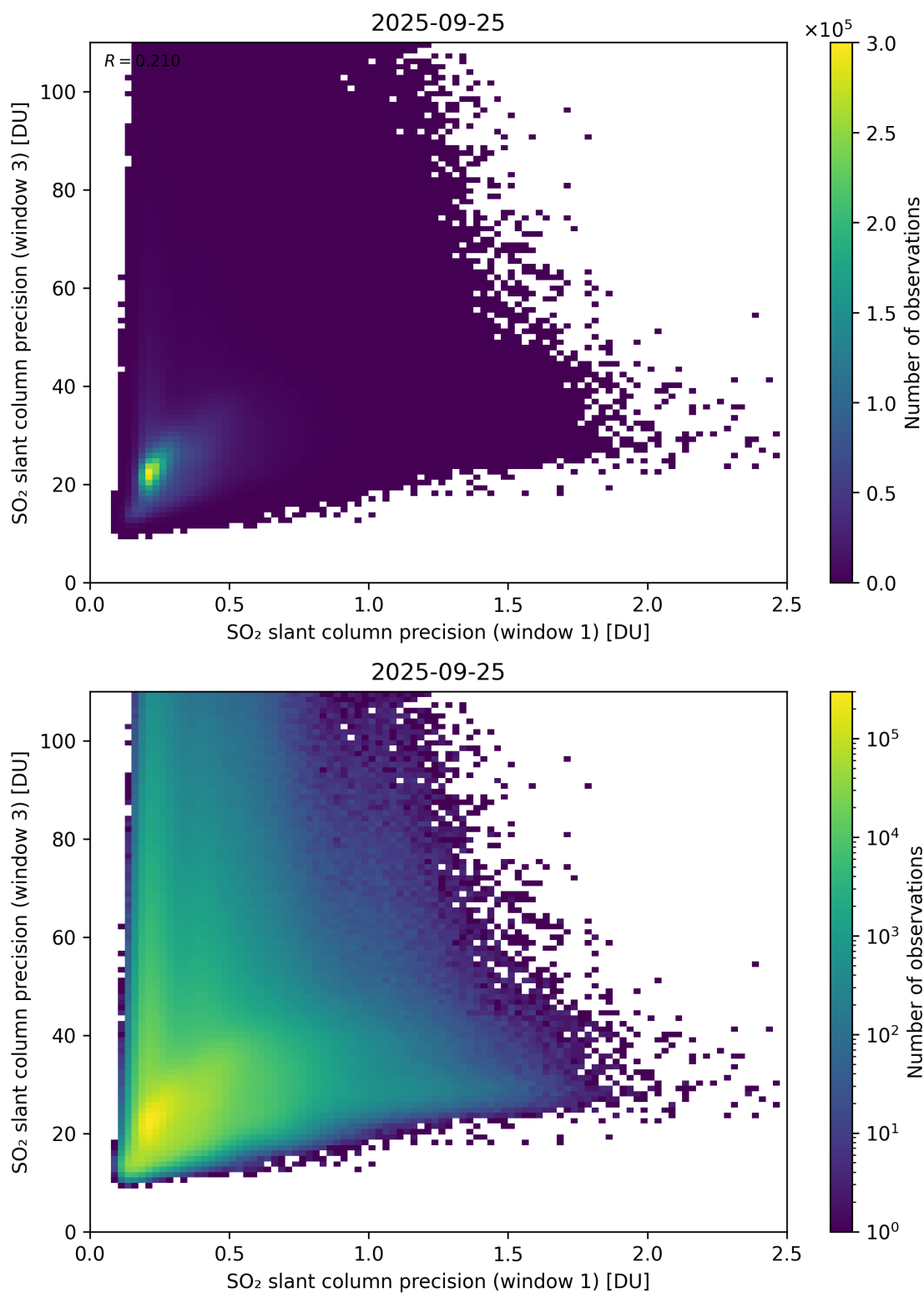
Figure 279: Scatter density plot of “SO 2 slant column precision (window 1)” against “SO 2 slant column precision (window 3)” for 2025-09-25 to 2025-09-26.
