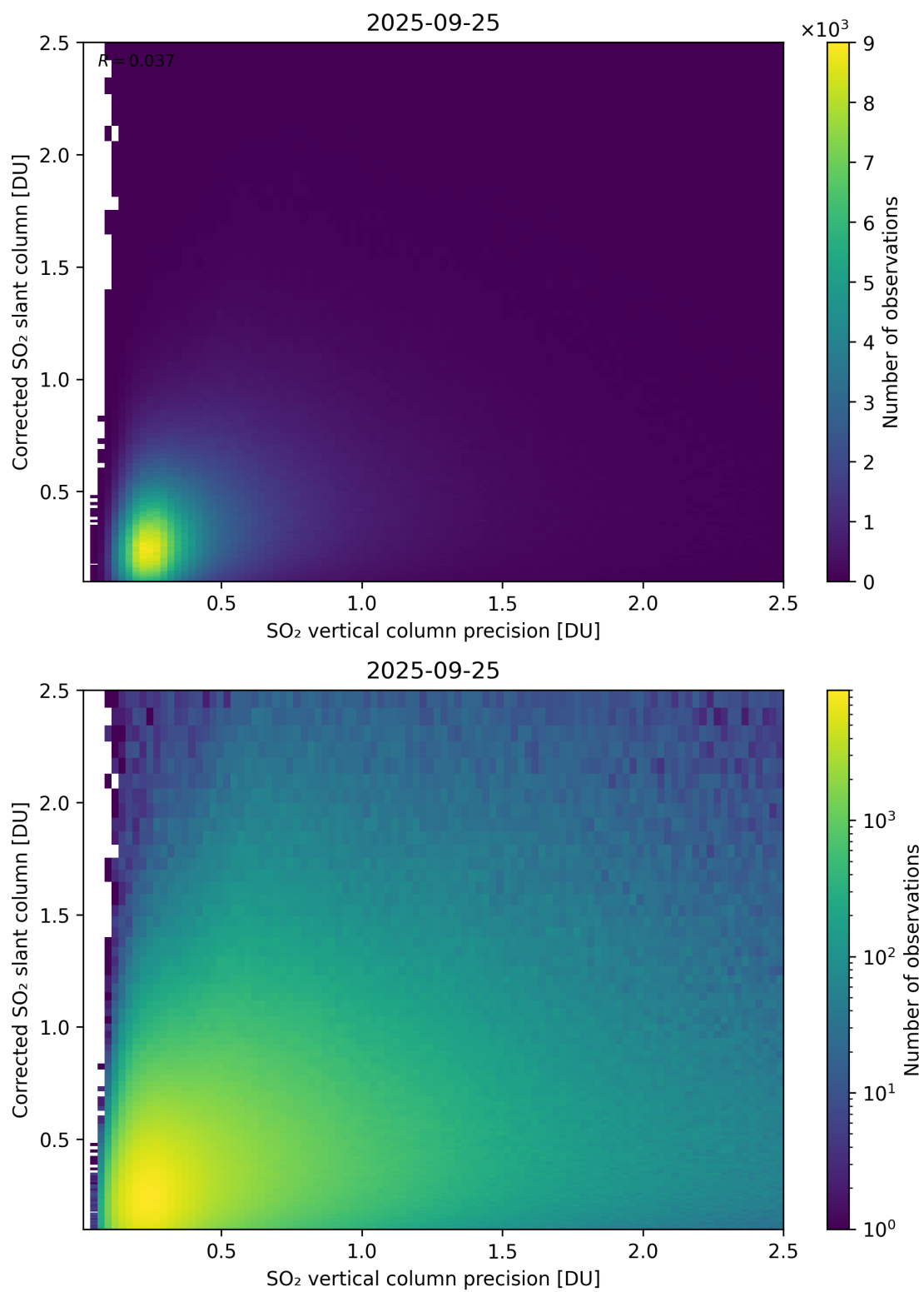
Figure 338: Scatter density plot of “SO 2 vertical column precision” against “Corrected SO 2 slant column” for 2025-09-25 to 2025-09-26.
