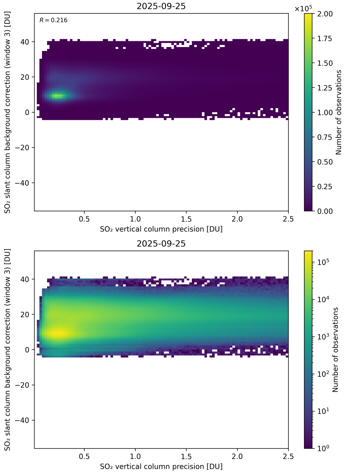
Figure 331: Scatter density plot of “SO 2 vertical column precision” against “SO 2 slant column background correction (window 3)” for 2025-09-25 to 2025-09-26.
