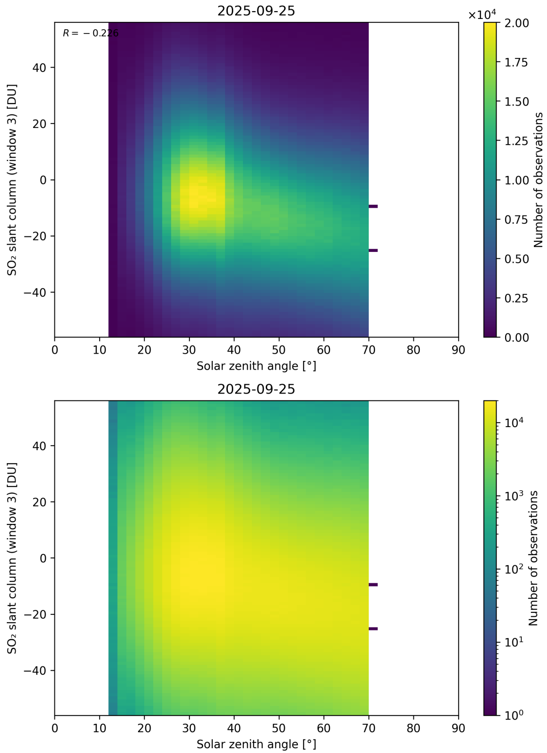
Figure 187: Scatter density plot of “Solar zenith angle” against “SO 2 slant column (window 3)” for 2025-09-25 to 2025-09-26.
