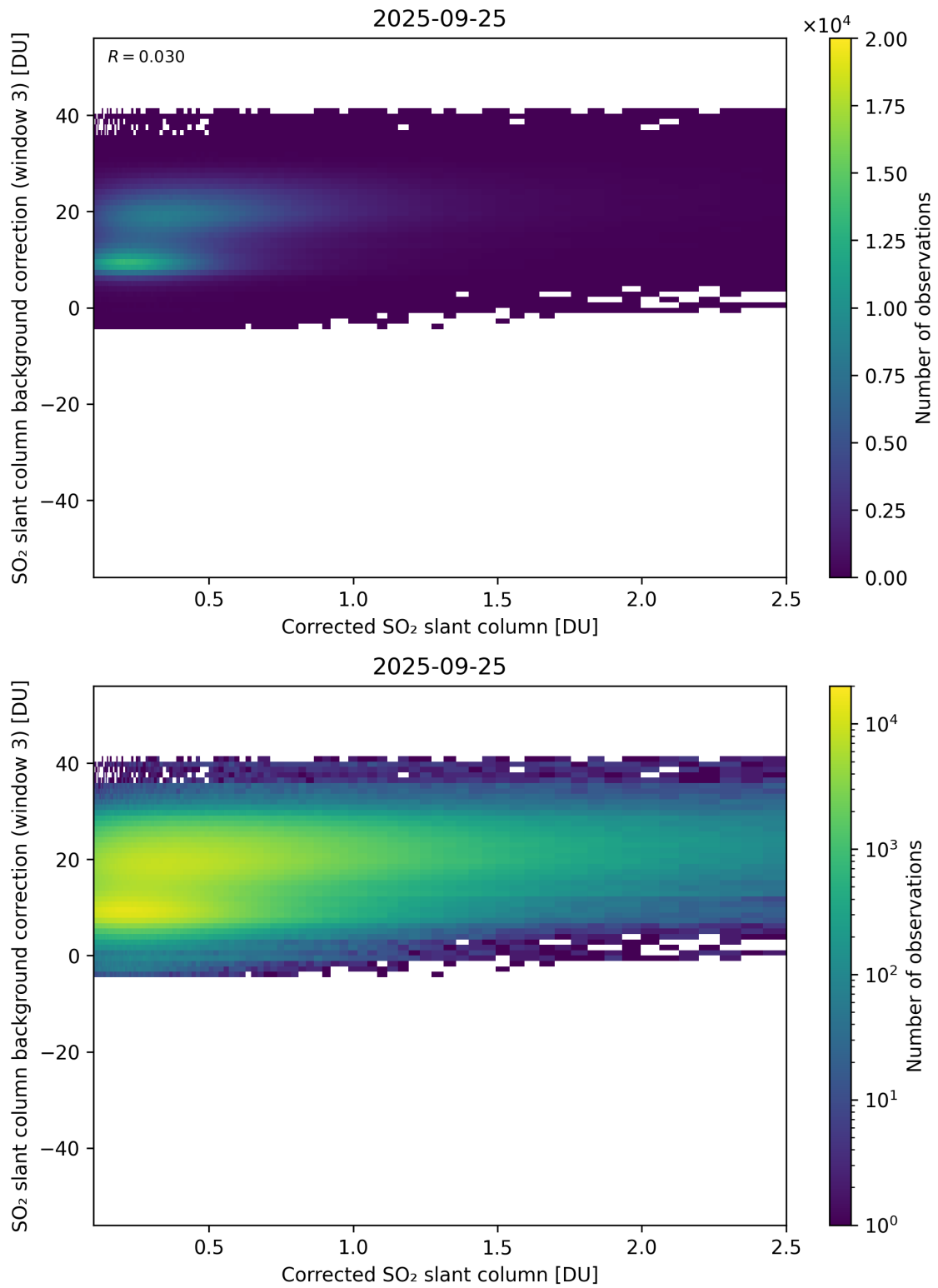
Figure 228: Scatter density plot of “Corrected SO 2 slant column” against “SO 2 slant column background correction (window 3)” for 2025-09-25 to 2025-09-26.
