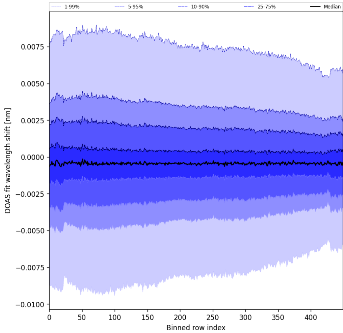
Figure 102: Along track statistics of “DOAS fit wavelength shift” for 2025-09-25 to 2025-09-26
