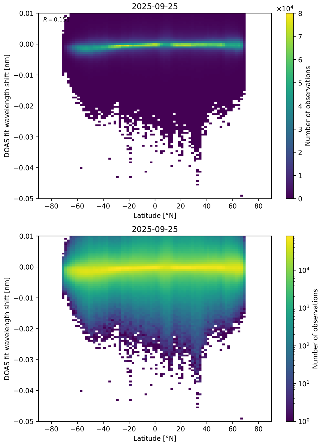
Figure 153: Scatter density plot of “Latitude” against “DOAS fit wavelength shift” for 2025-09-25 to 2025-09-26.
