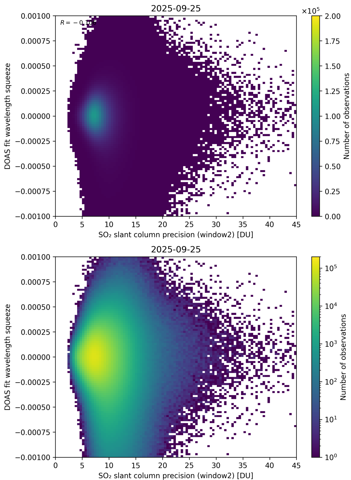
Figure 294: Scatter density plot of “SO 2 slant column precision (window2)” against “DOAS fit wavelength squeeze” for 2025-09-25 to 2025-09-26.
