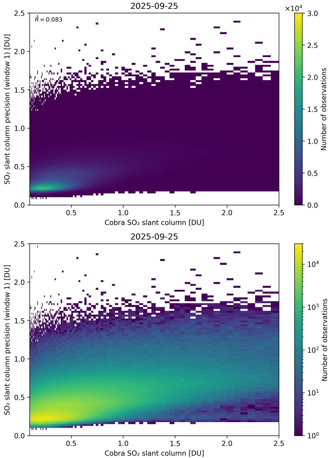
Figure 220: Scatter density plot of “Cobra SO 2 slant column” against “SO 2 slant column precision (window 1)” for 2025-09-25 to 2025-09-26.
