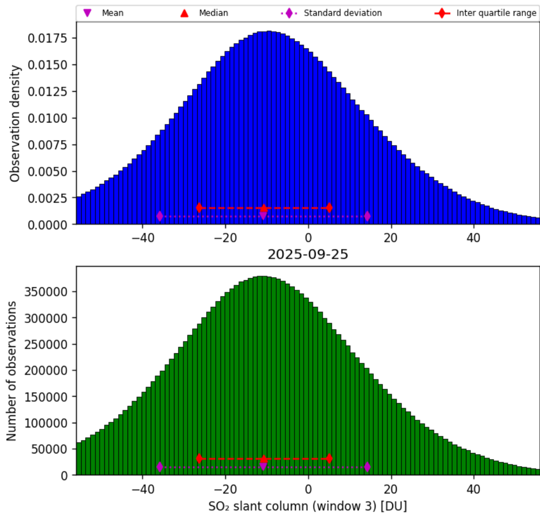
Figure 71: Histogram of “SO 2 slant column (window 3)” for 2025-09-25 to 2025-09-26
