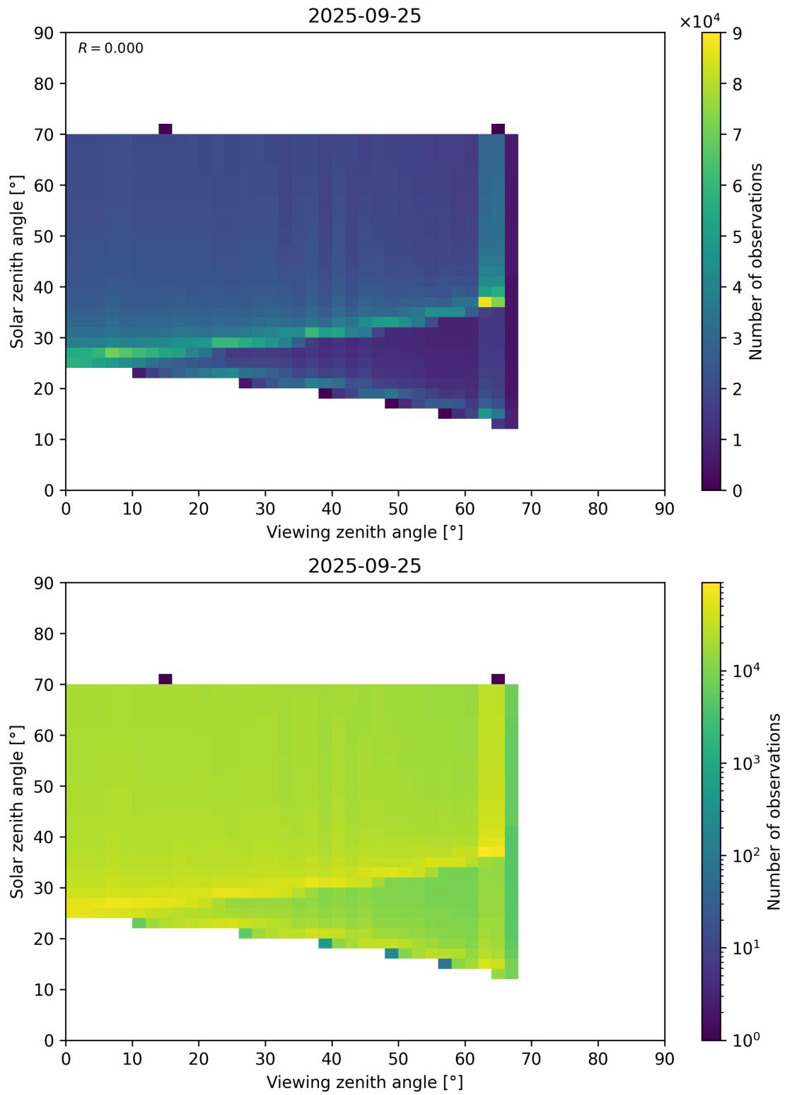
Figure 369: Scatter density plot of “Viewing zenith angle” against “Solar zenith angle” for 2025-09-25 to 2025-09-26.
