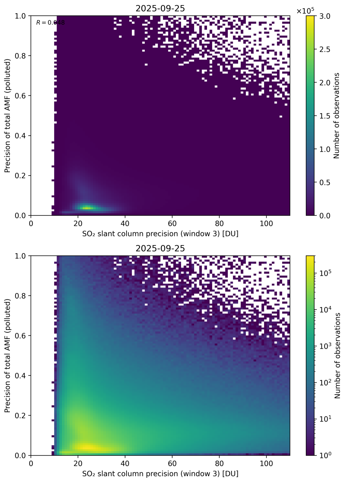
Figure 314: Scatter density plot of “SO 2 slant column precision (window 3)” against “Precision of total AMF (polluted)” for 2025-09-25 to 2025-09-26.
