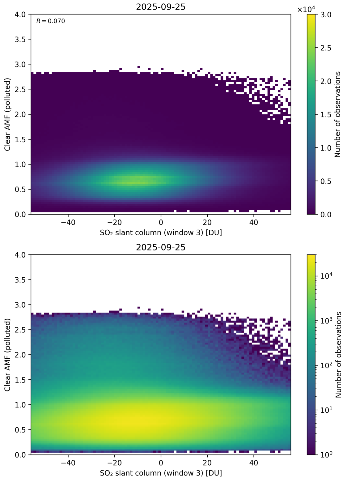
Figure 315: Scatter density plot of “SO 2 slant column (window 3)” against “Clear AMF (polluted)” for 2025-09-25 to 2025-09-26.
