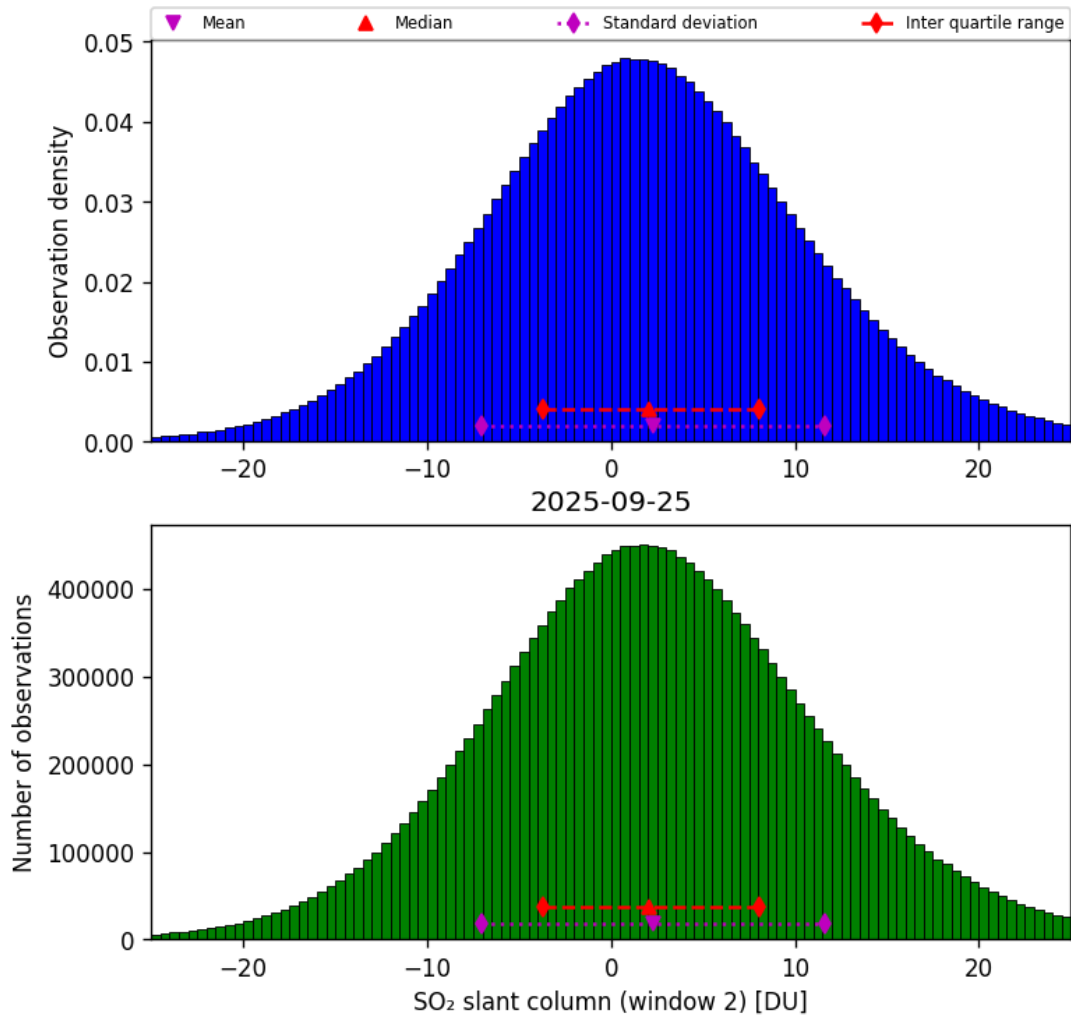
Figure 67: Histogram of “SO 2 slant column (window 2)” for 2025-09-25 to 2025-09-26
