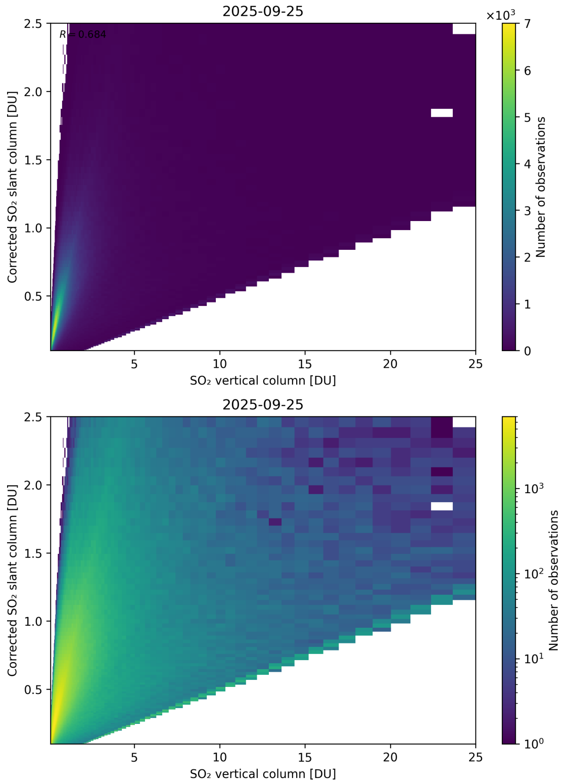
Figure 351: Scatter density plot of “SO 2 vertical column” against “Corrected SO 2 slant column” for 2025-09-25 to 2025-09-26.
