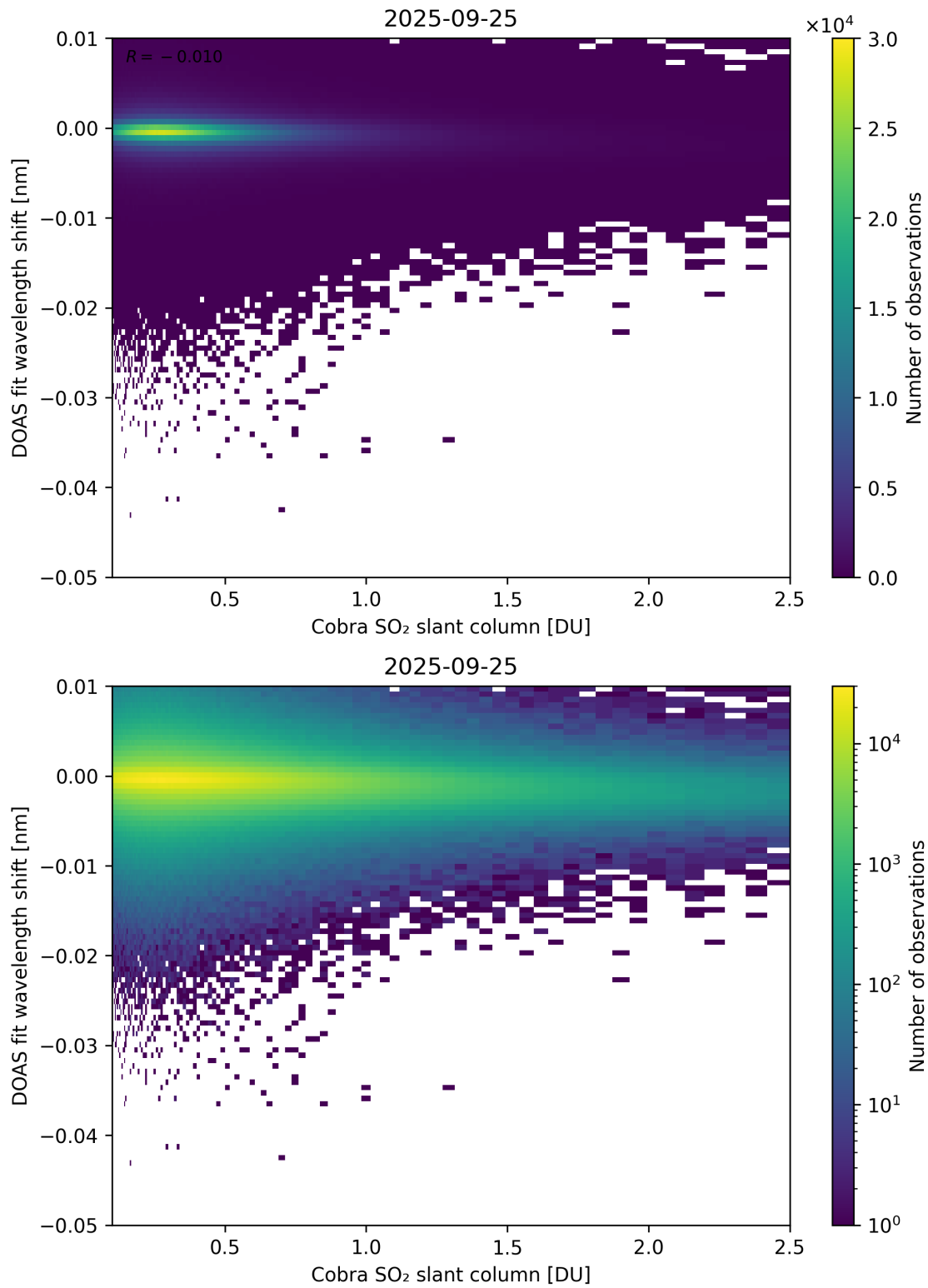
Figure 196: Scatter density plot of “Cobra SO 2 slant column” against “DOAS fit wavelength shift” for 2025-09-25 to 2025-09-26.
