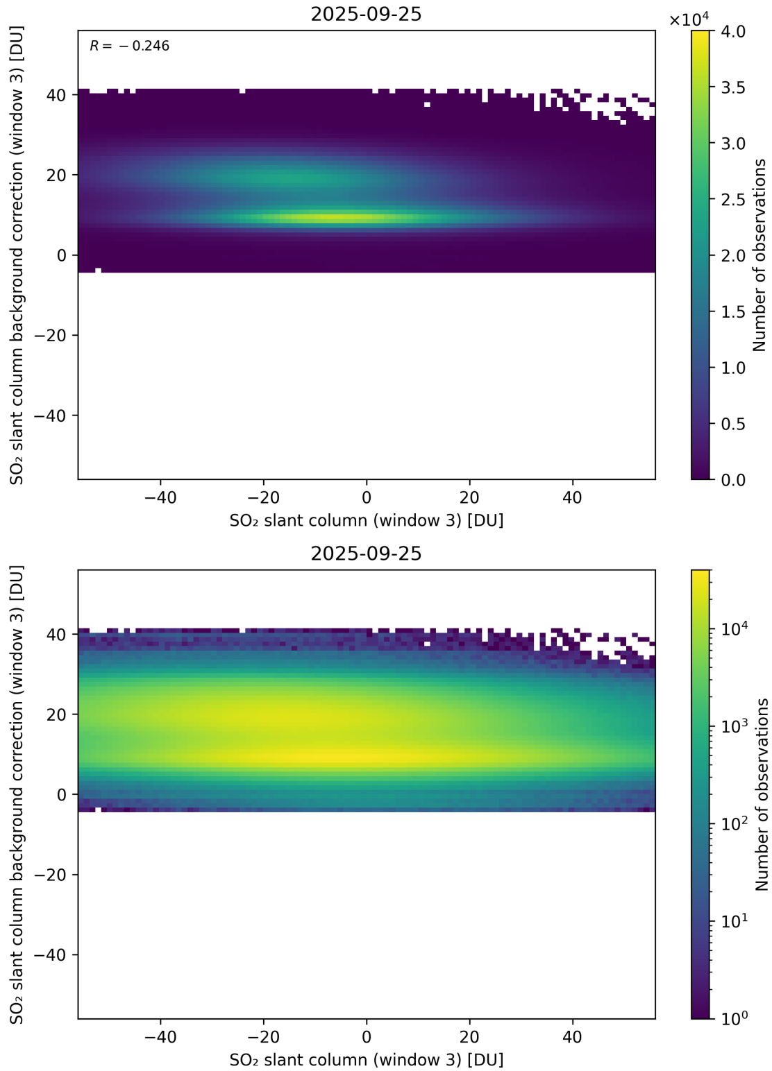
Figure 303: Scatter density plot of “SO 2 slant column (window 3)” against “SO 2 slant column background correction (window 3)” for 2025-09-25 to 2025-09-26.
