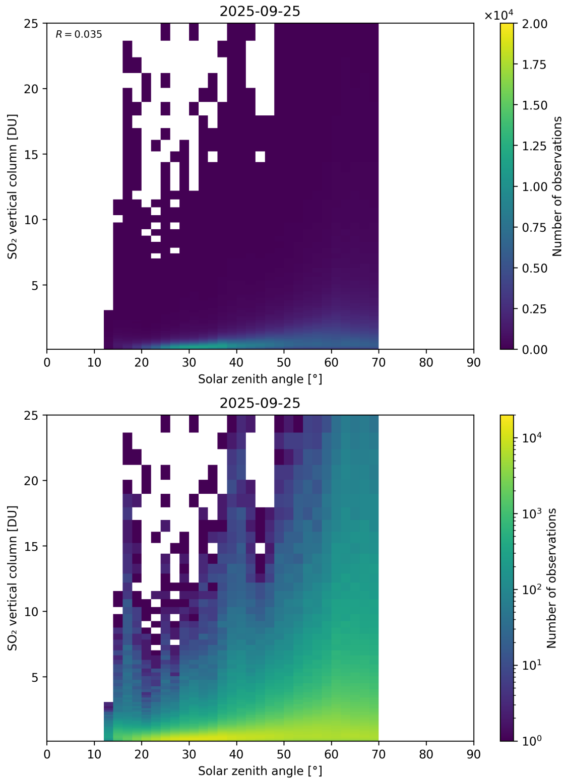
Figure 191: Scatter density plot of “Solar zenith angle” against “SO 2 vertical column” for 2025-09-25 to 2025-09-26.
