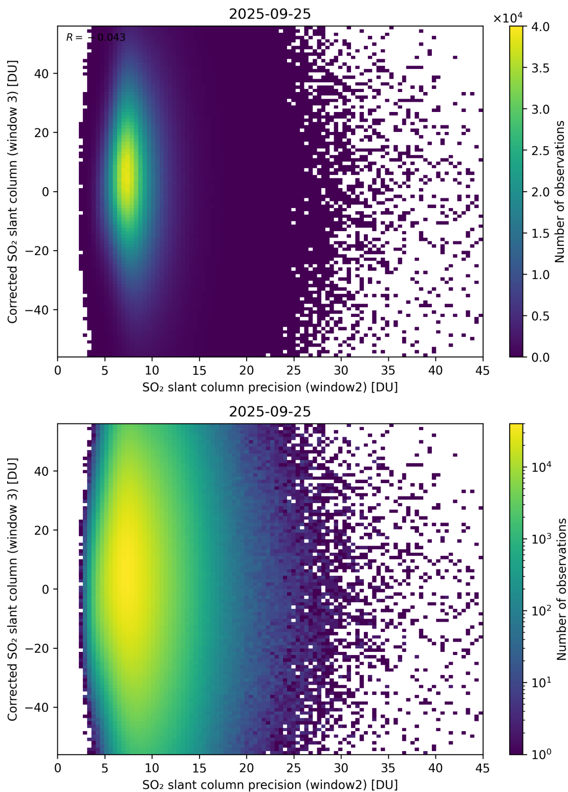
Figure 298: Scatter density plot of “SO 2 slant column precision (window2)” against “Corrected SO 2 slant column (window 3)” for 2025-09-25 to 2025-09-26.
