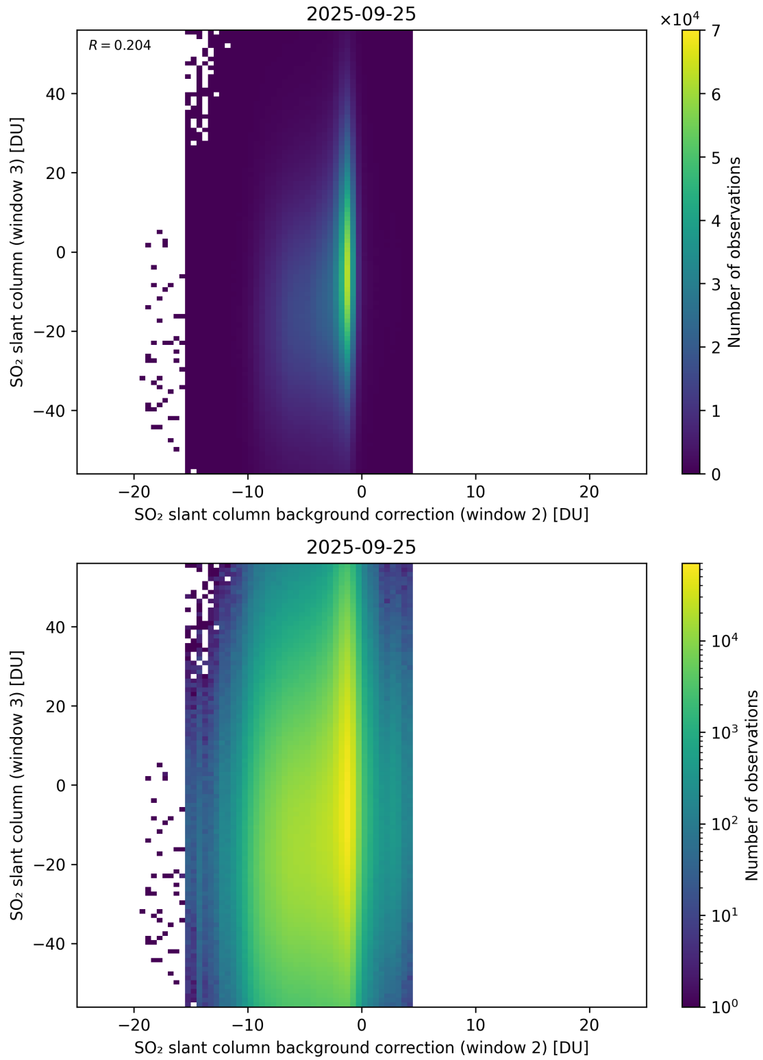
Figure 128: Scatter density plot of “SO 2 slant column background correction (window 2)” against “SO 2 slant column (window 3)” for 2025-09-25 to 2025-09-26.
