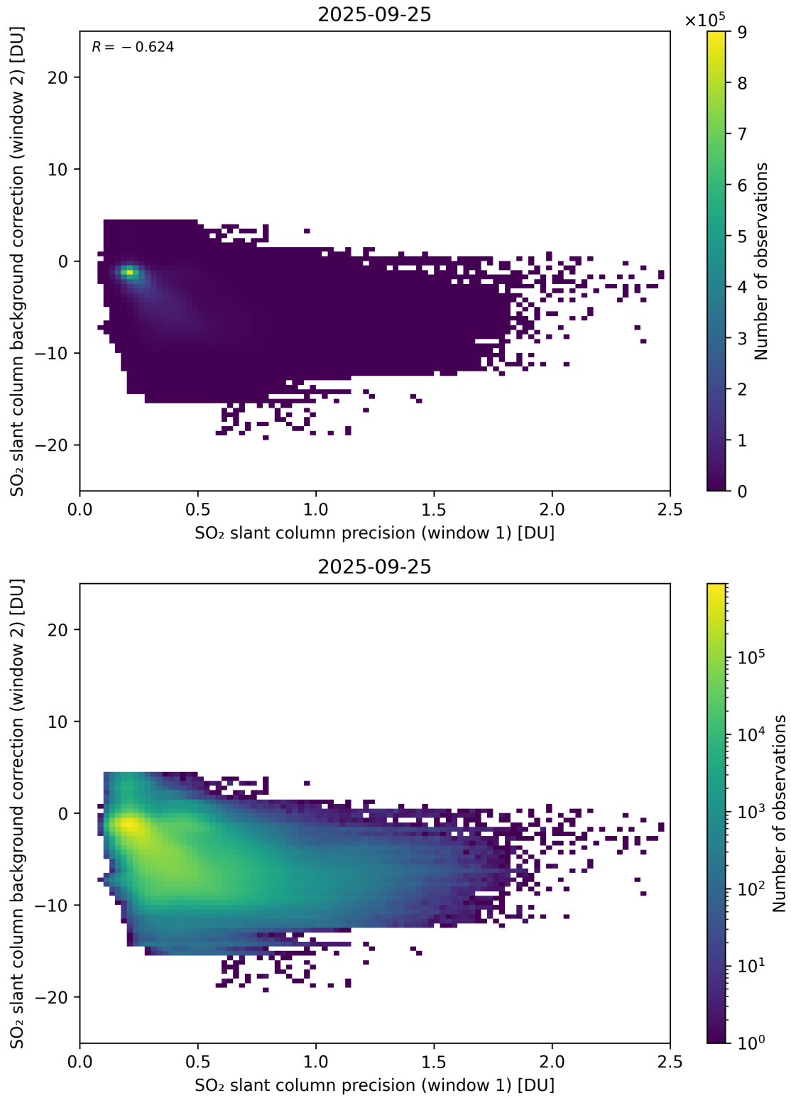
Figure 269: Scatter density plot of “SO 2 slant column precision (window 1)” against “SO 2 slant column background correction (window 2)” for 2025-09-25 to 2025-09-26.
