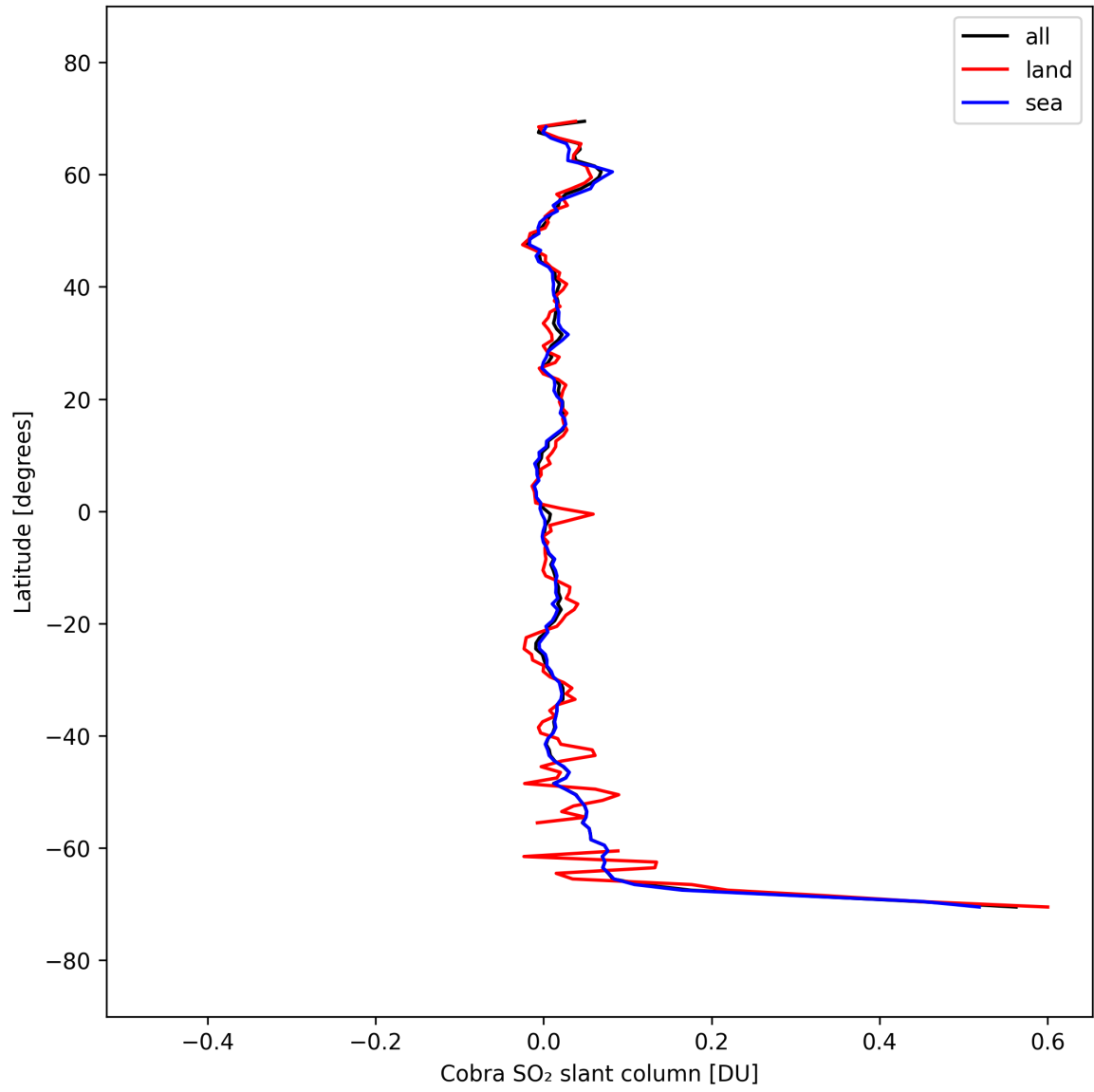
Figure 35: Zonal average of “Cobra SO 2 slant column” for 2025-09-25 to 2025-09-26.
