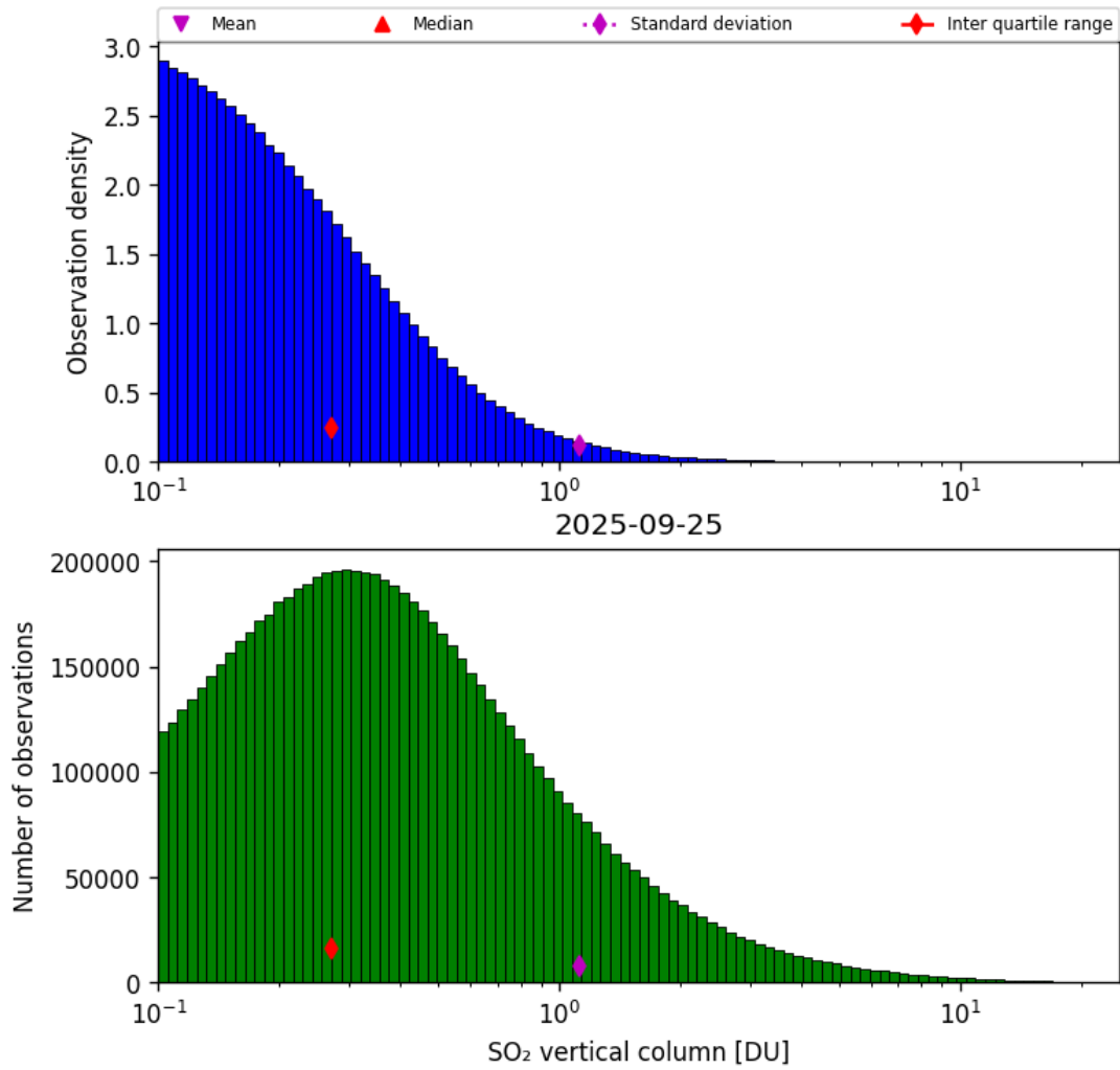
Figure 58: Histogram of “SO 2 vertical column” for 2025-09-25 to 2025-09-26
