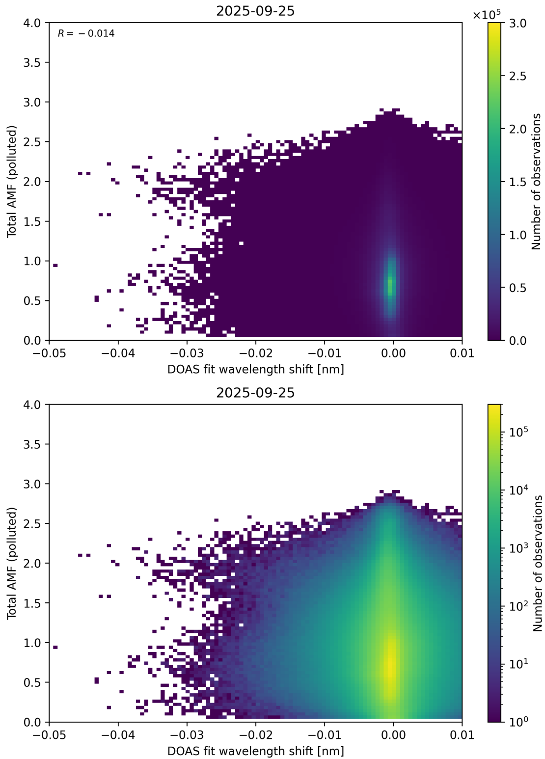
Figure 141: Scatter density plot of “DOAS fit wavelength shift” against “Total AMF (polluted)” for 2025-09-25 to 2025-09-26.
