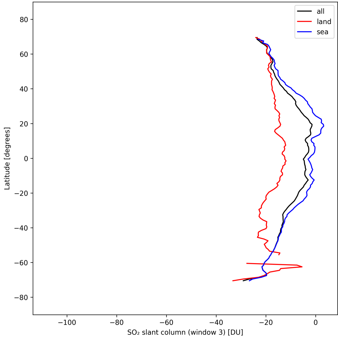
Figure 45: Zonal average of “SO 2 slant column (window 3)” for 2025-09-25 to 2025-09-26.
