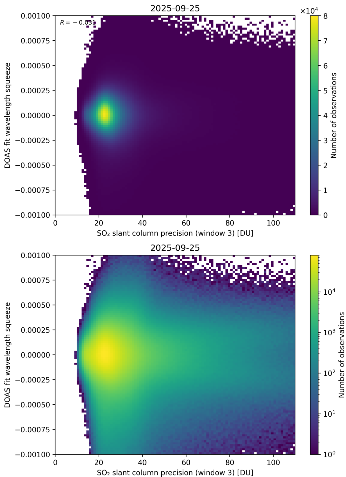
Figure 309: Scatter density plot of “SO 2 slant column precision (window 3)” against “DOAS fit wavelength squeeze” for 2025-09-25 to 2025-09-26.
