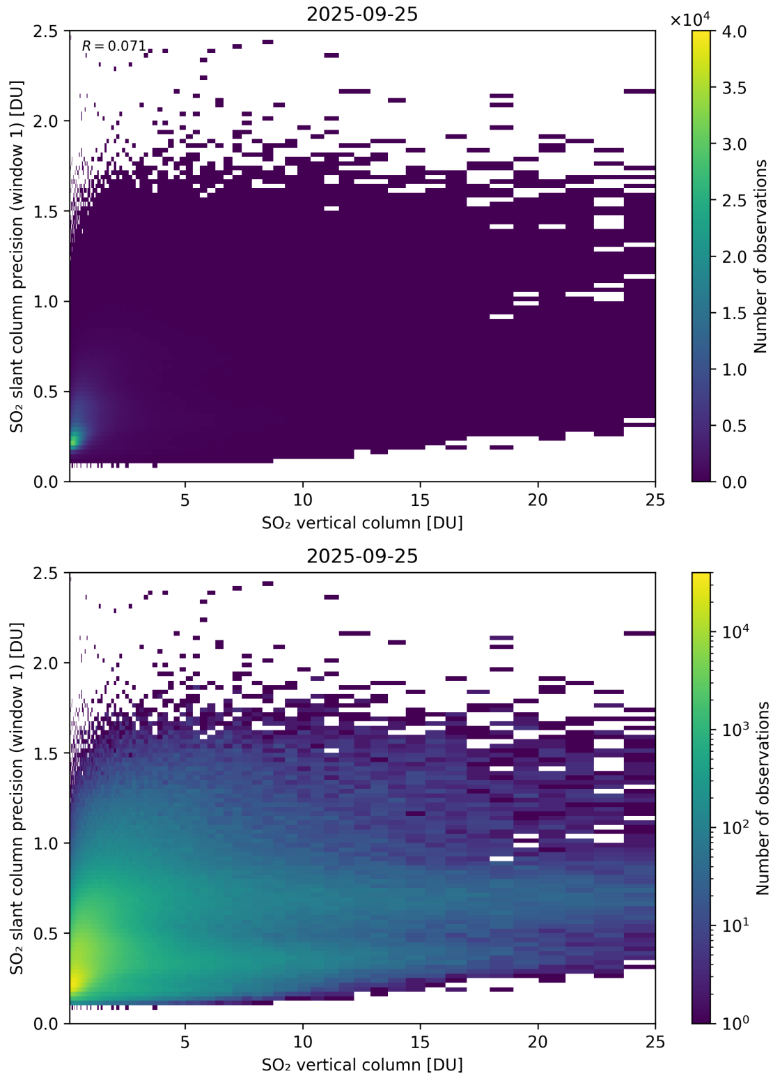
Figure 355: Scatter density plot of “SO 2 vertical column” against “SO 2 slant column precision (window 1)” for 2025-09-25 to 2025-09-26.
