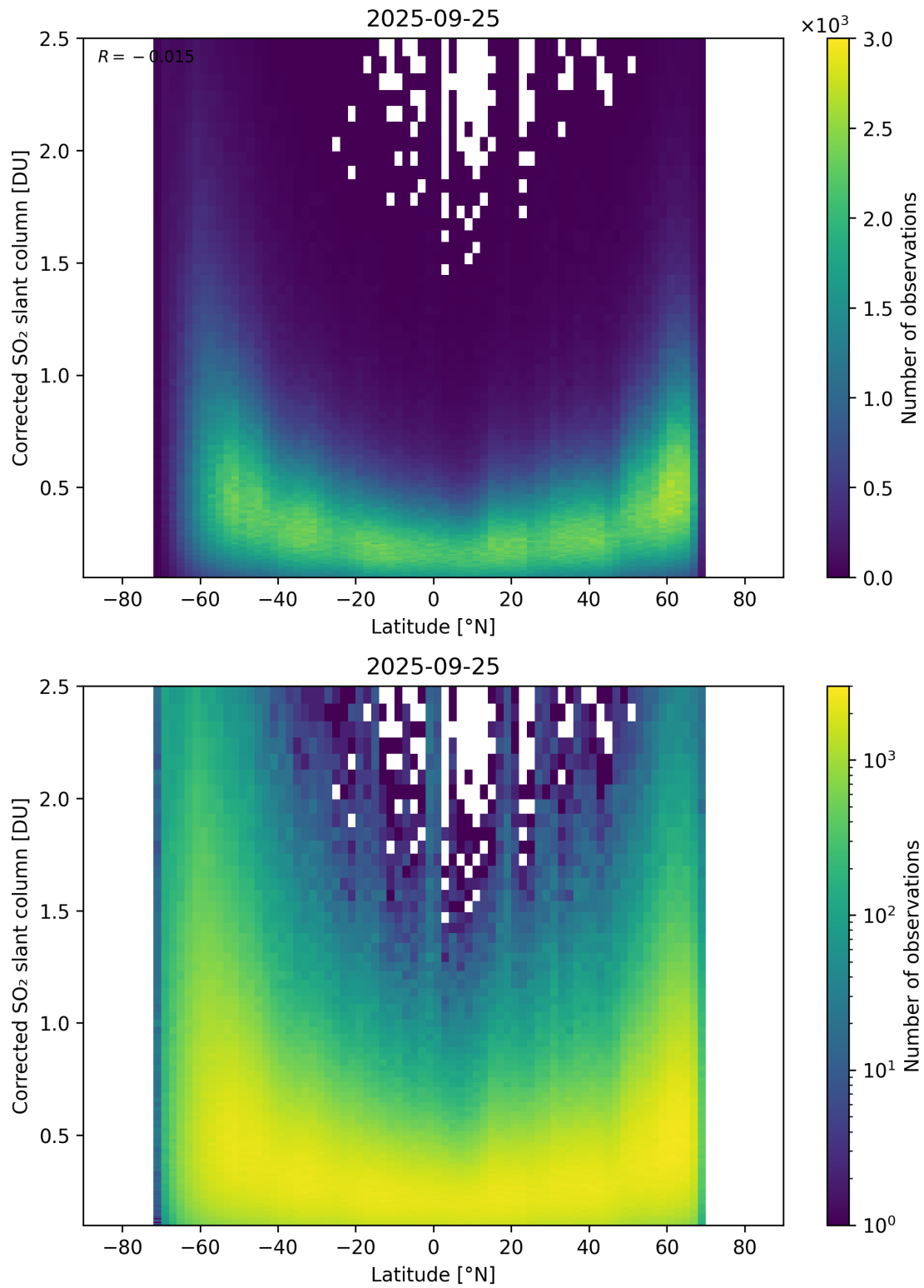
Figure 159: Scatter density plot of “Latitude” against “Corrected SO 2 slant column” for 2025-09-25 to 2025-09-26.
