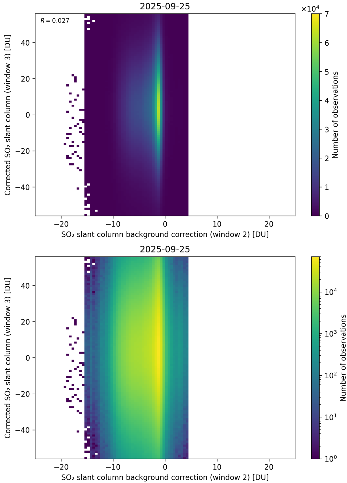
Figure 127: Scatter density plot of “SO 2 slant column background correction (window 2)” against “Corrected SO 2 slant column (window 3)” for 2025-09-25 to 2025-09-26.
