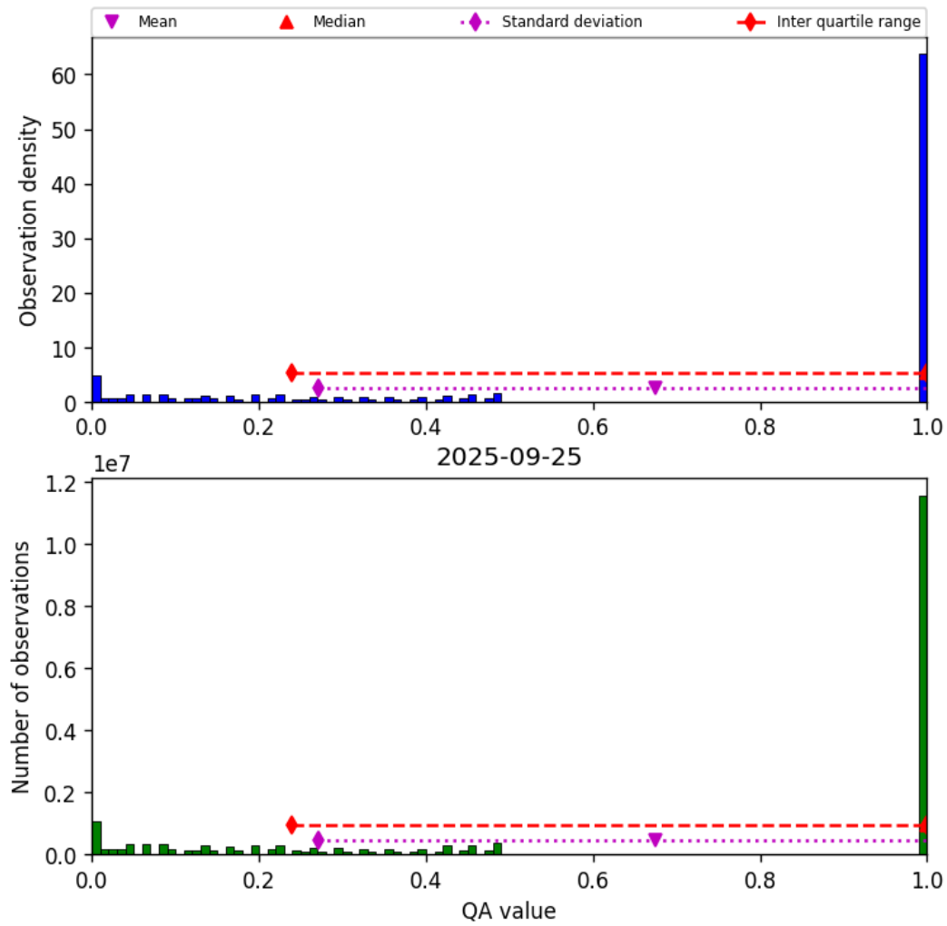
Figure 57: Histogram of “QA value” for 2025-09-25 to 2025-09-26
