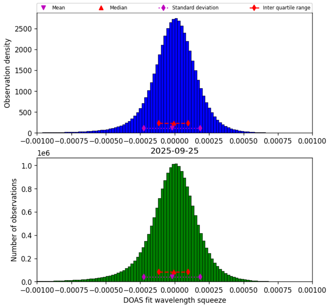
Figure 77: Histogram of “DOAS fit wavelength squeeze” for 2025-09-25 to 2025-09-26
