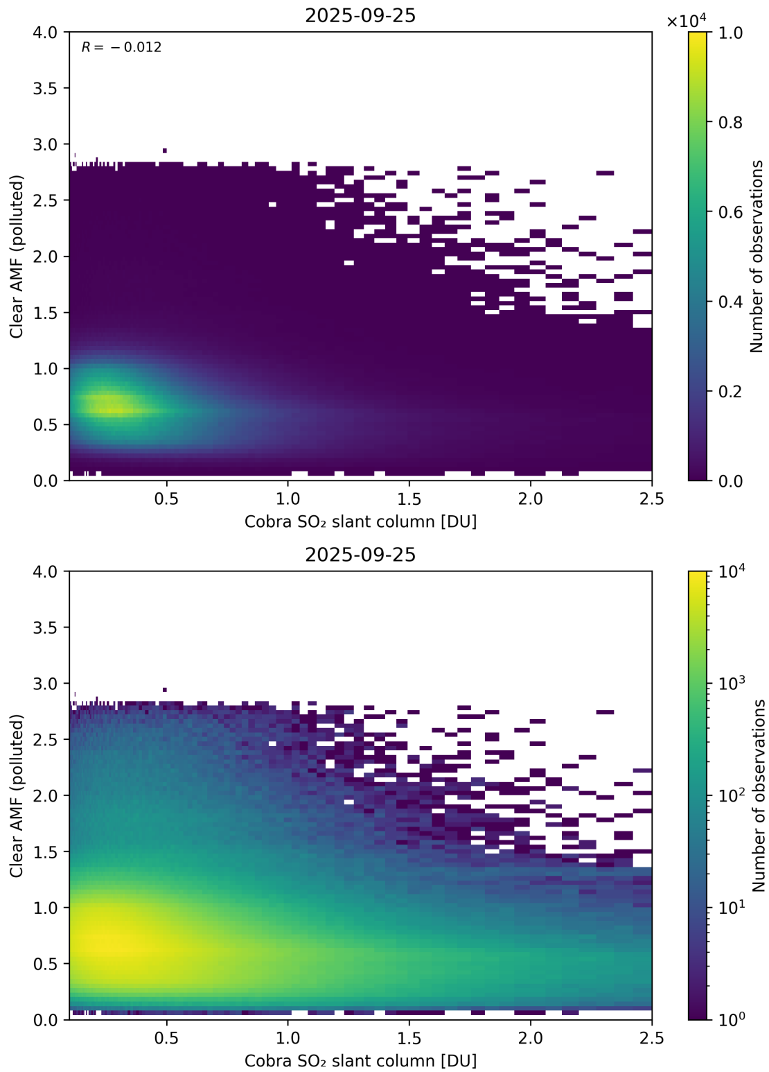
Figure 215: Scatter density plot of “Cobra SO 2 slant column” against “Clear AMF (polluted)” for 2025-09-25 to 2025-09-26.
