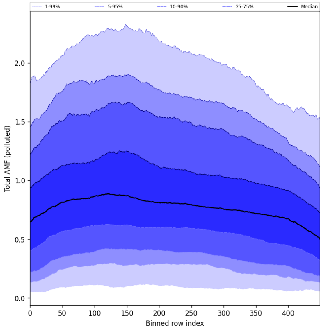
Figure 105: Along track statistics of “Total AMF (polluted)” for 2025-09-25 to 2025-09-26
