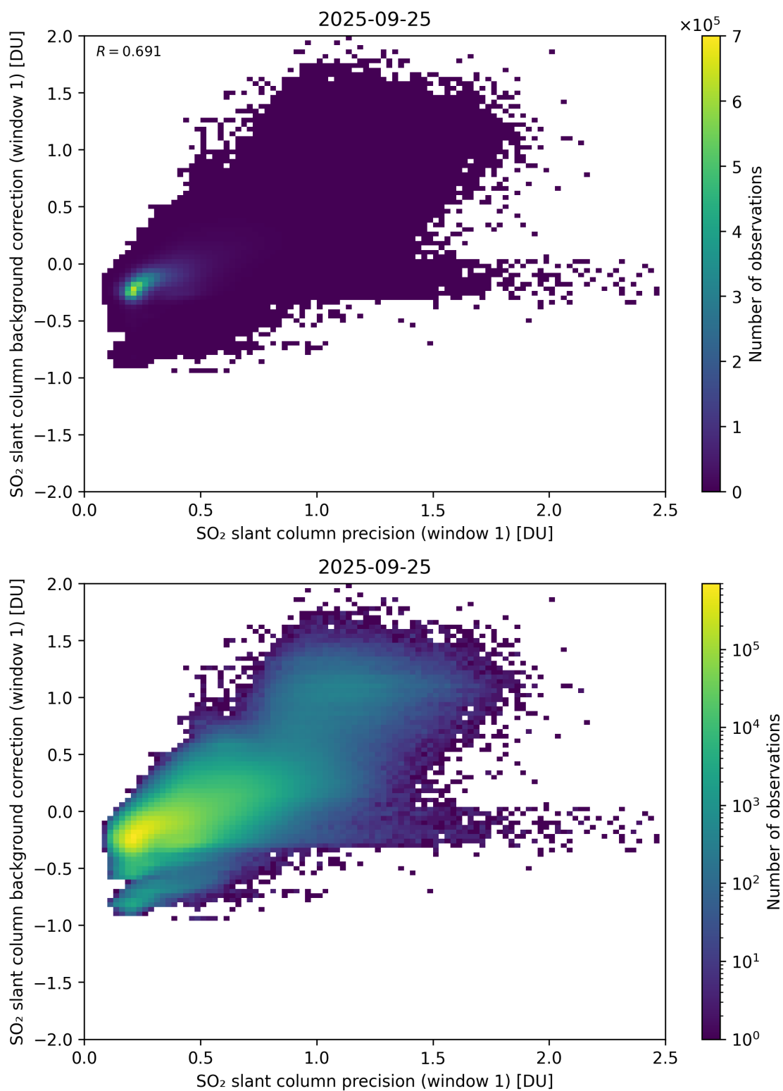
Figure 268: Scatter density plot of “SO 2 slant column precision (window 1)” against “SO 2 slant column background correction (window 1)” for 2025-09-25 to 2025-09-26.
