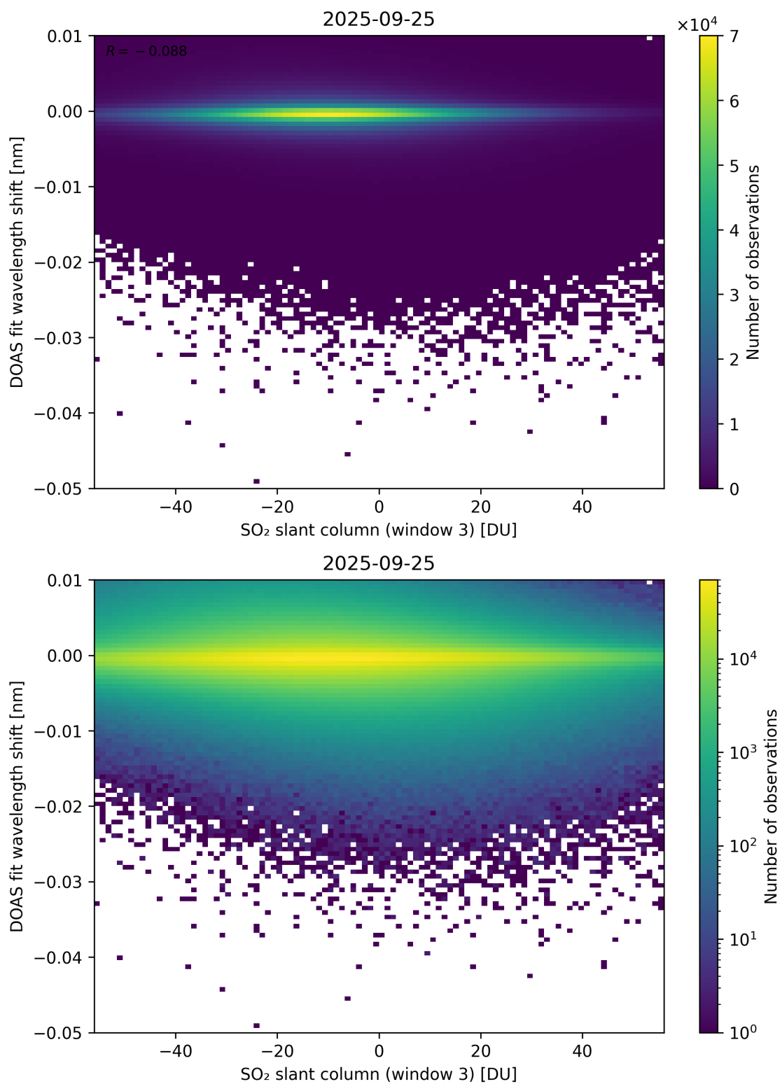
Figure 304: Scatter density plot of “SO 2 slant column (window 3)” against “DOAS fit wavelength shift” for 2025-09-25 to 2025-09-26.
