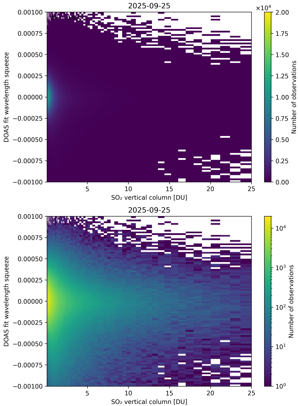
Figure 327: Scatter density plot of “SO 2 vertical column” against “DOAS fit wavelength squeeze” for 2025-09-25 to 2025-09-26.
