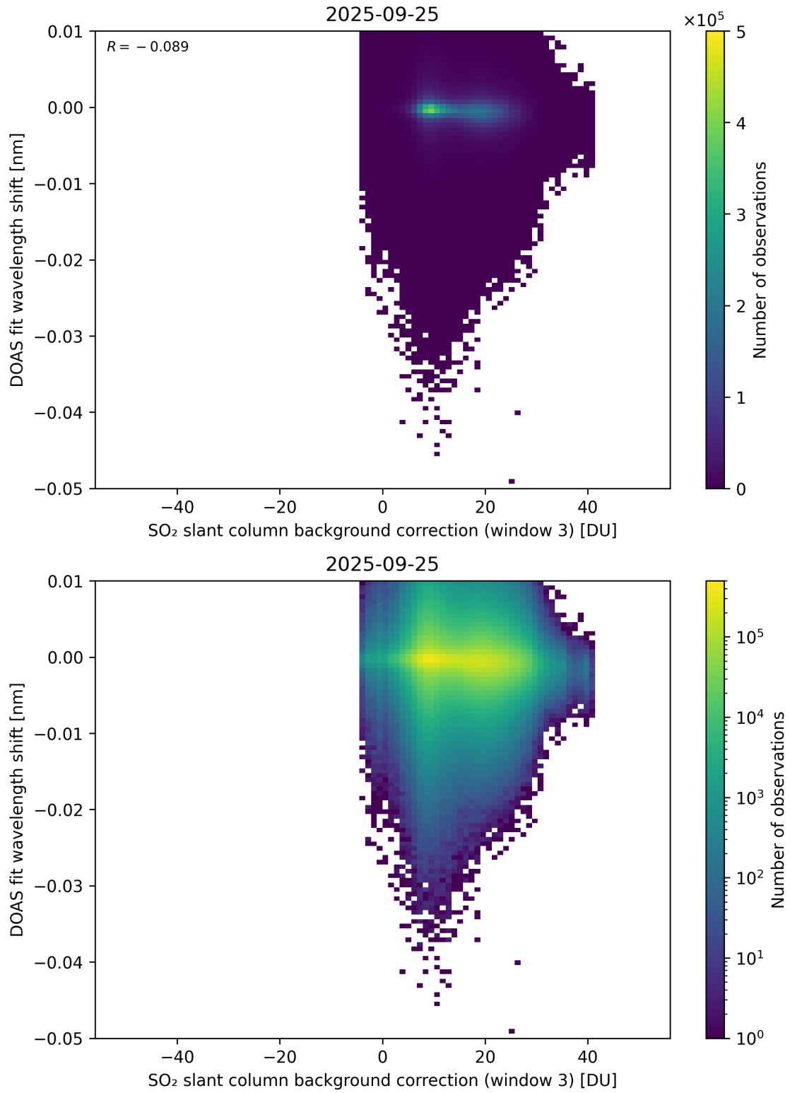
Figure 132: Scatter density plot of “SO 2 slant column background correction (window 3)” against “DOAS fit wavelength shift” for 2025-09-25 to 2025-09-26.
