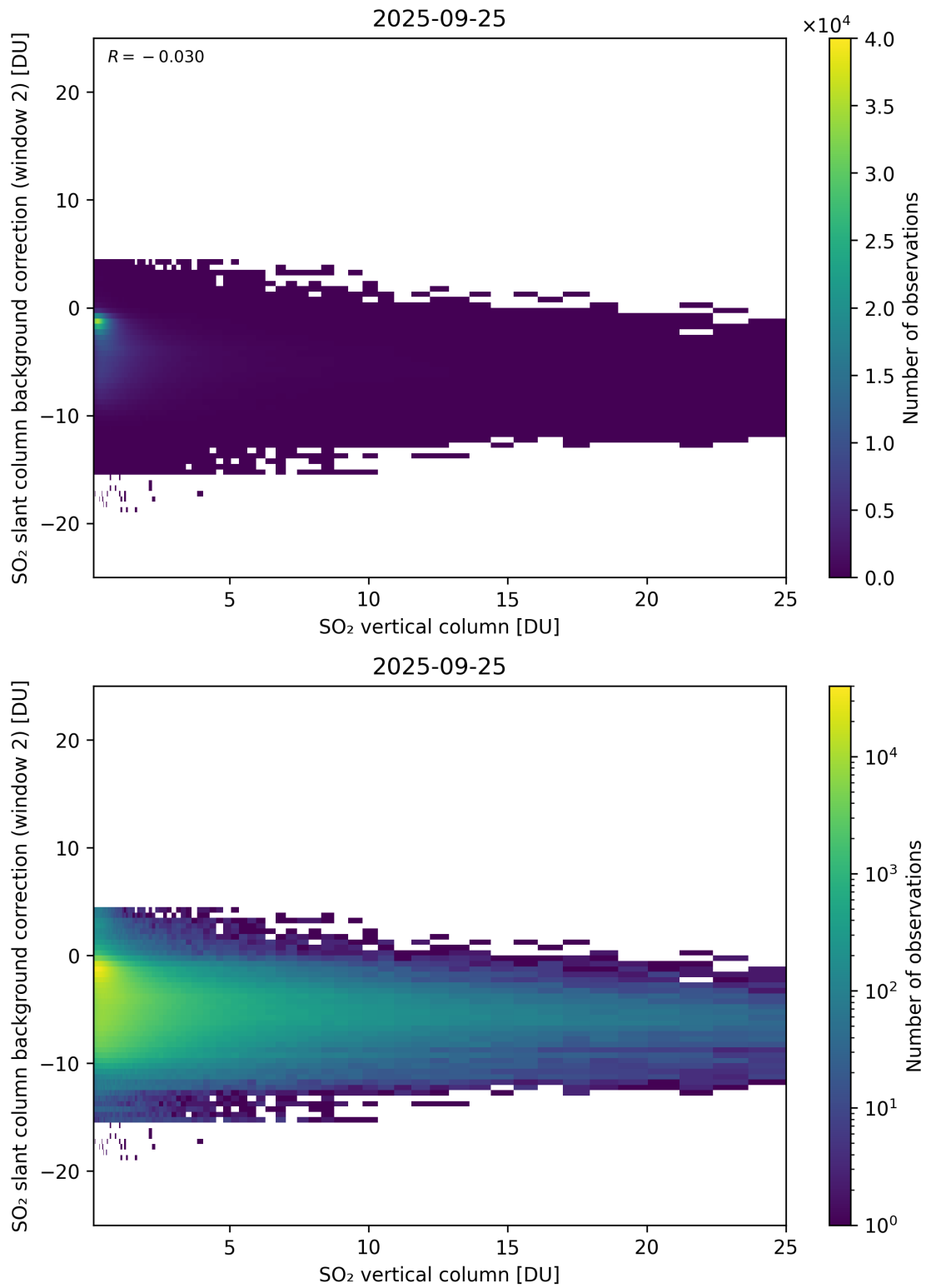
Figure 324: Scatter density plot of “SO 2 vertical column” against “SO 2 slant column background correction (window 2)” for 2025-09-25 to 2025-09-26.
