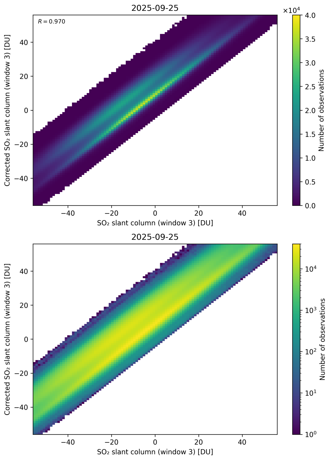
Figure 316: Scatter density plot of “SO 2 slant column (window 3)” against “Corrected SO 2 slant column (window 3)” for 2025-09-25 to 2025-09-26.
