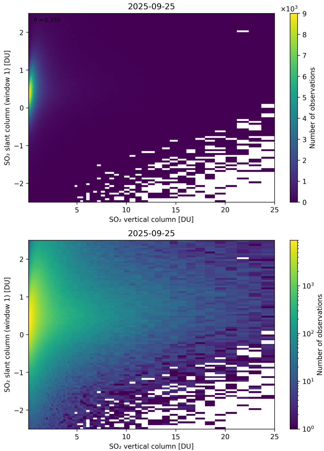
Figure 354: Scatter density plot of “SO 2 vertical column” against “SO 2 slant column (window 1)” for 2025-09-25 to 2025-09-26.
