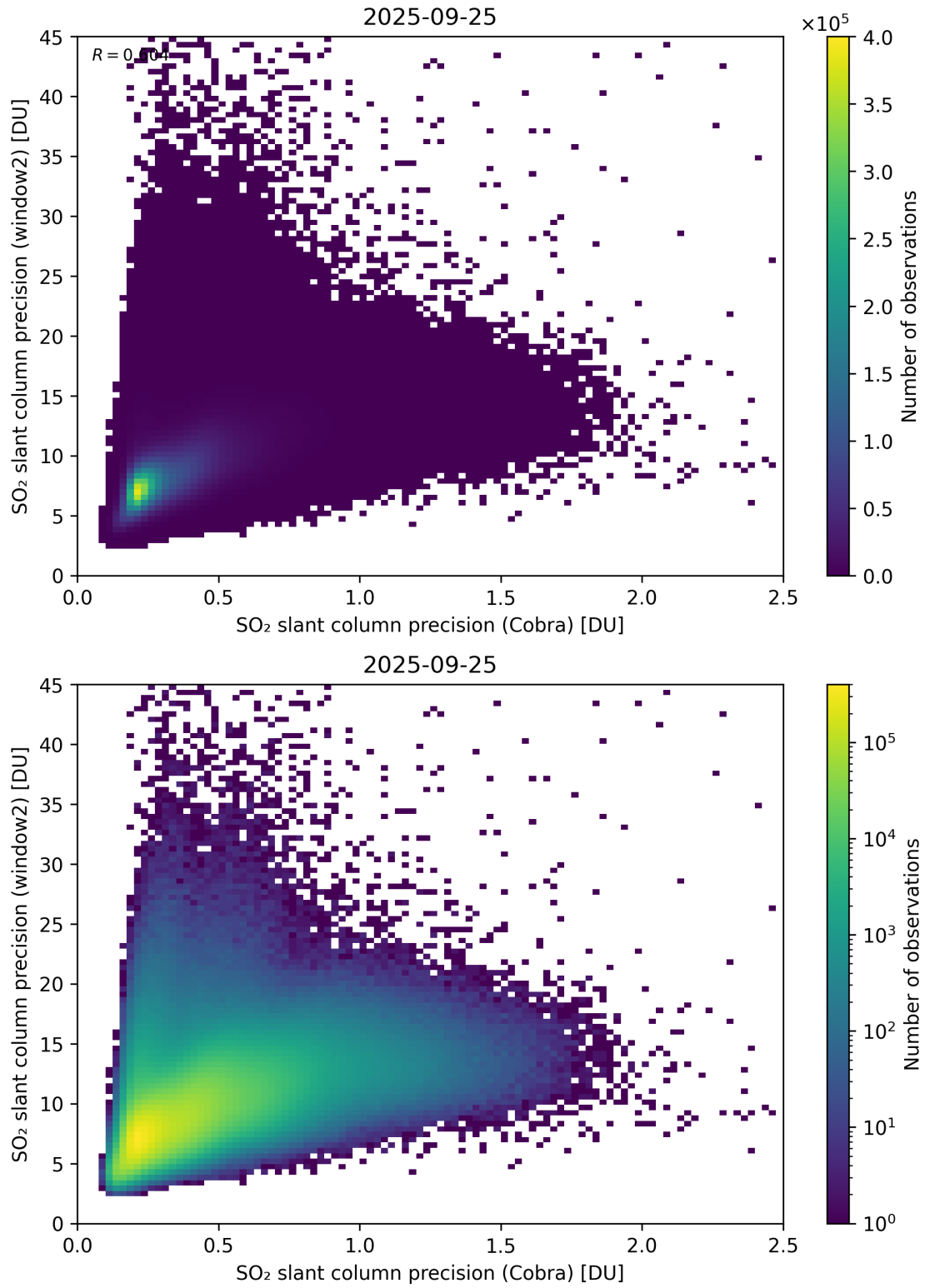
Figure 210: Scatter density plot of “SO 2 slant column precision (Cobra)” against “SO 2 slant column precision (window2)” for 2025-09-25 to 2025-09-26.
