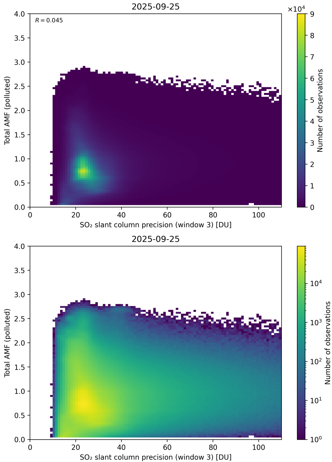
Figure 313: Scatter density plot of “SO 2 slant column precision (window 3)” against “Total AMF (polluted)” for 2025-09-25 to 2025-09-26.
