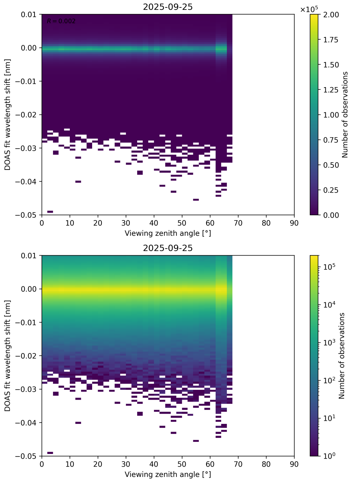
Figure 365: Scatter density plot of “Viewing zenith angle” against “DOAS fit wavelength shift” for 2025-09-25 to 2025-09-26.
