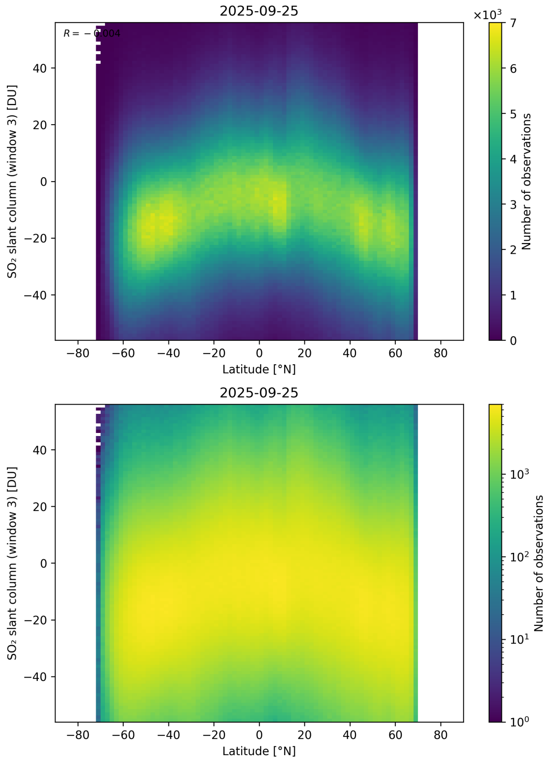
Figure 165: Scatter density plot of “Latitude” against “SO 2 slant column (window 3)” for 2025-09-25 to 2025-09-26.
