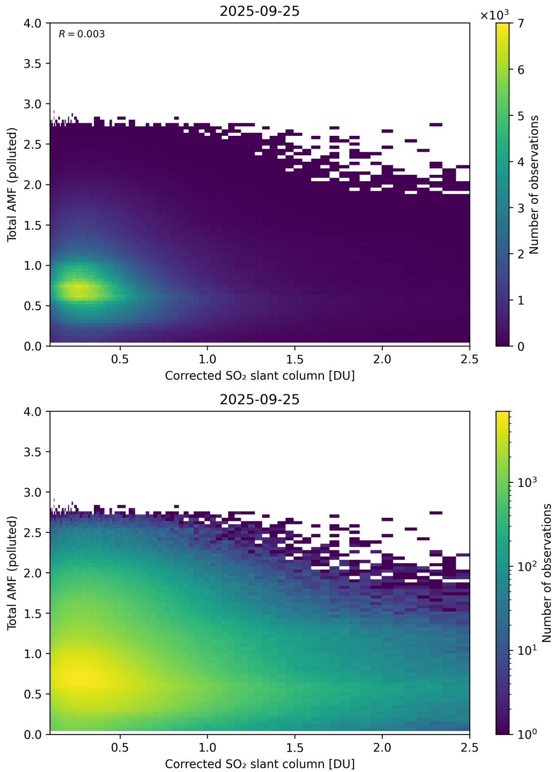
Figure 242: Scatter density plot of “Corrected SO 2 slant column” against “Total AMF (polluted)” for 2025-09-25 to 2025-09-26.
