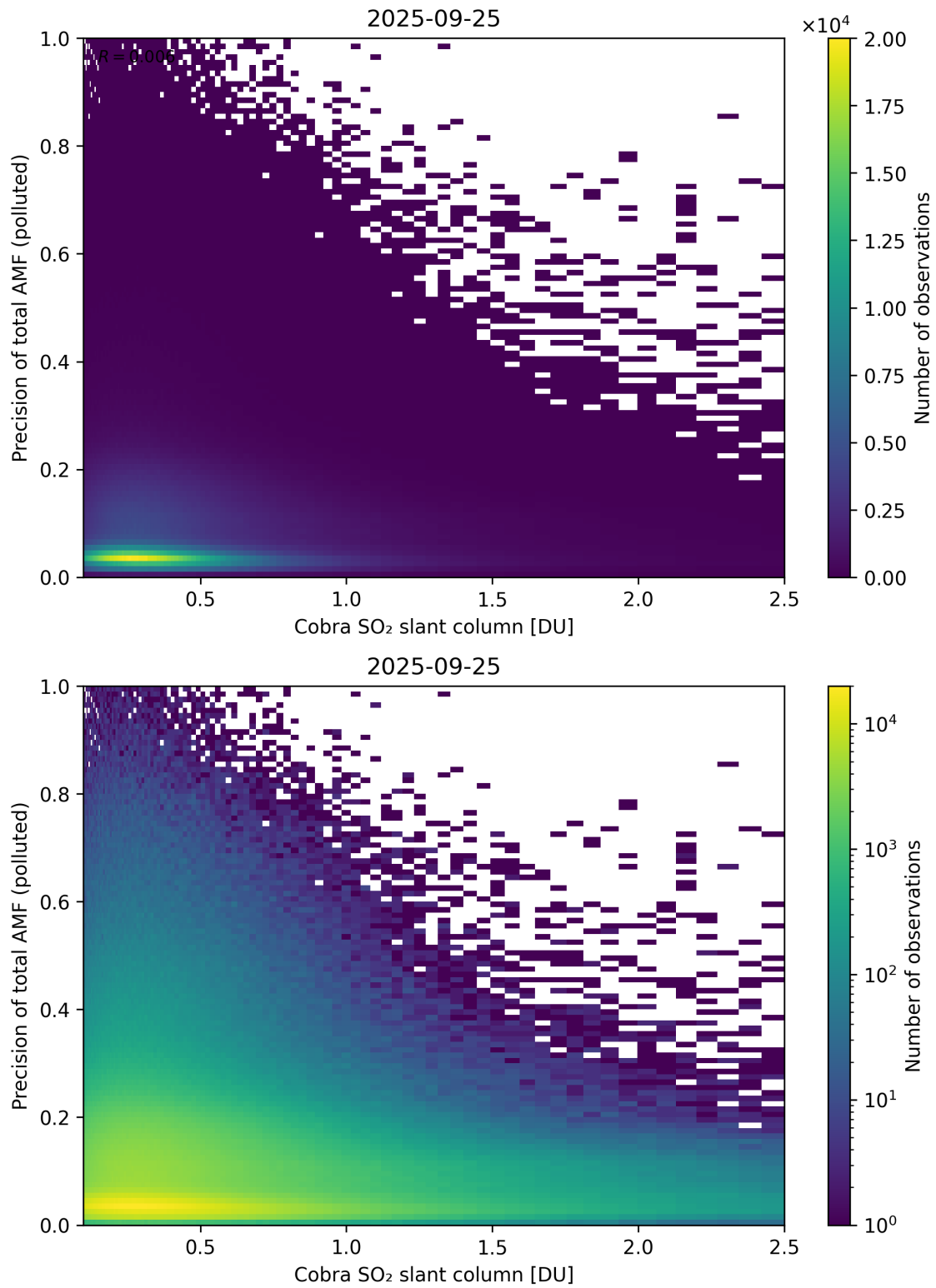
Figure 225: Scatter density plot of “Cobra SO 2 slant column” against “Precision of total AMF (polluted)” for 2025-09-25 to 2025-09-26.
