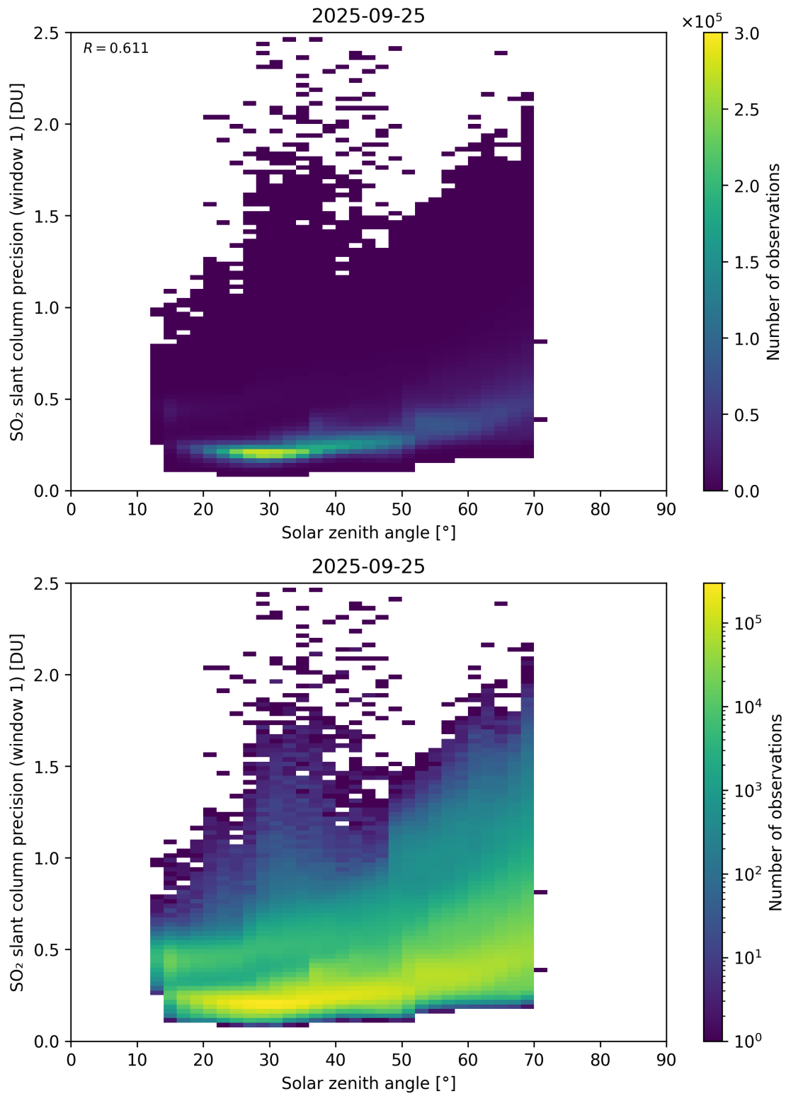
Figure 185: Scatter density plot of “Solar zenith angle” against “SO 2 slant column precision (window 1)” for 2025-09-25 to 2025-09-26.
