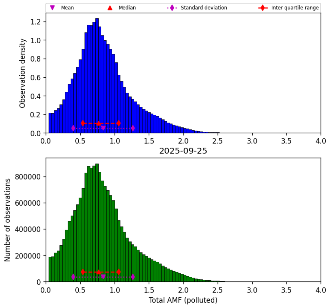
Figure 79: Histogram of “Total AMF (polluted)” for 2025-09-25 to 2025-09-26
