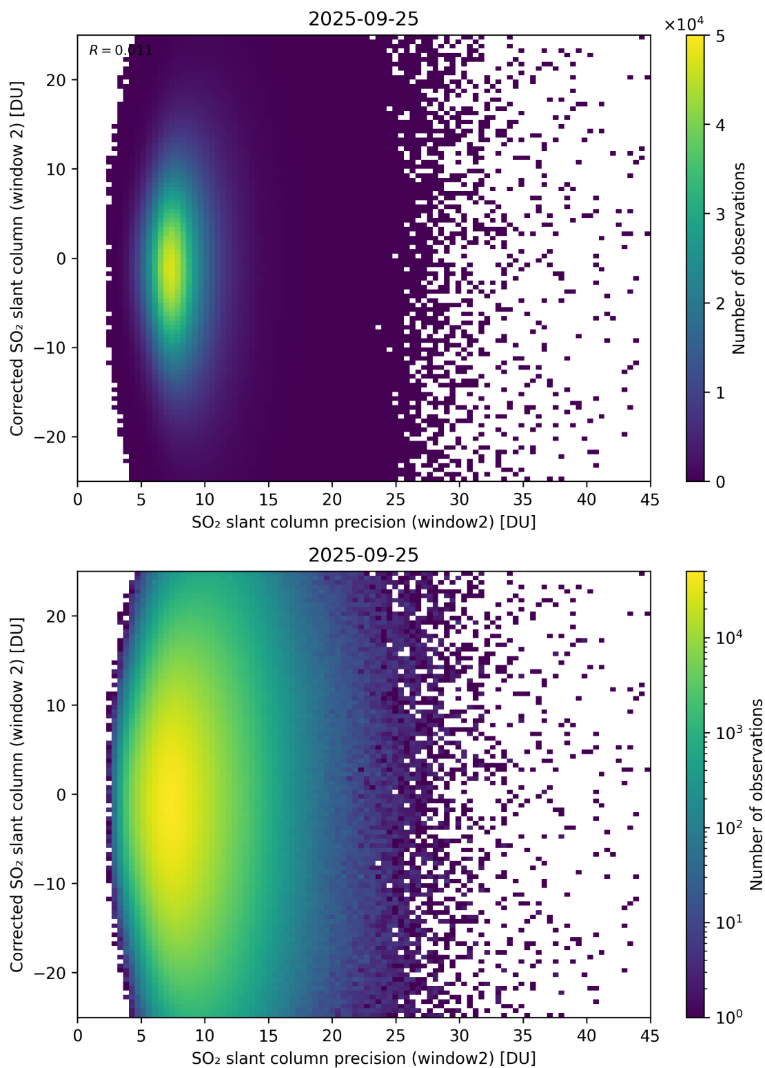
Figure 297: Scatter density plot of “SO 2 slant column precision (window2)” against “Corrected SO 2 slant column (window 2)” for 2025-09-25 to 2025-09-26.
