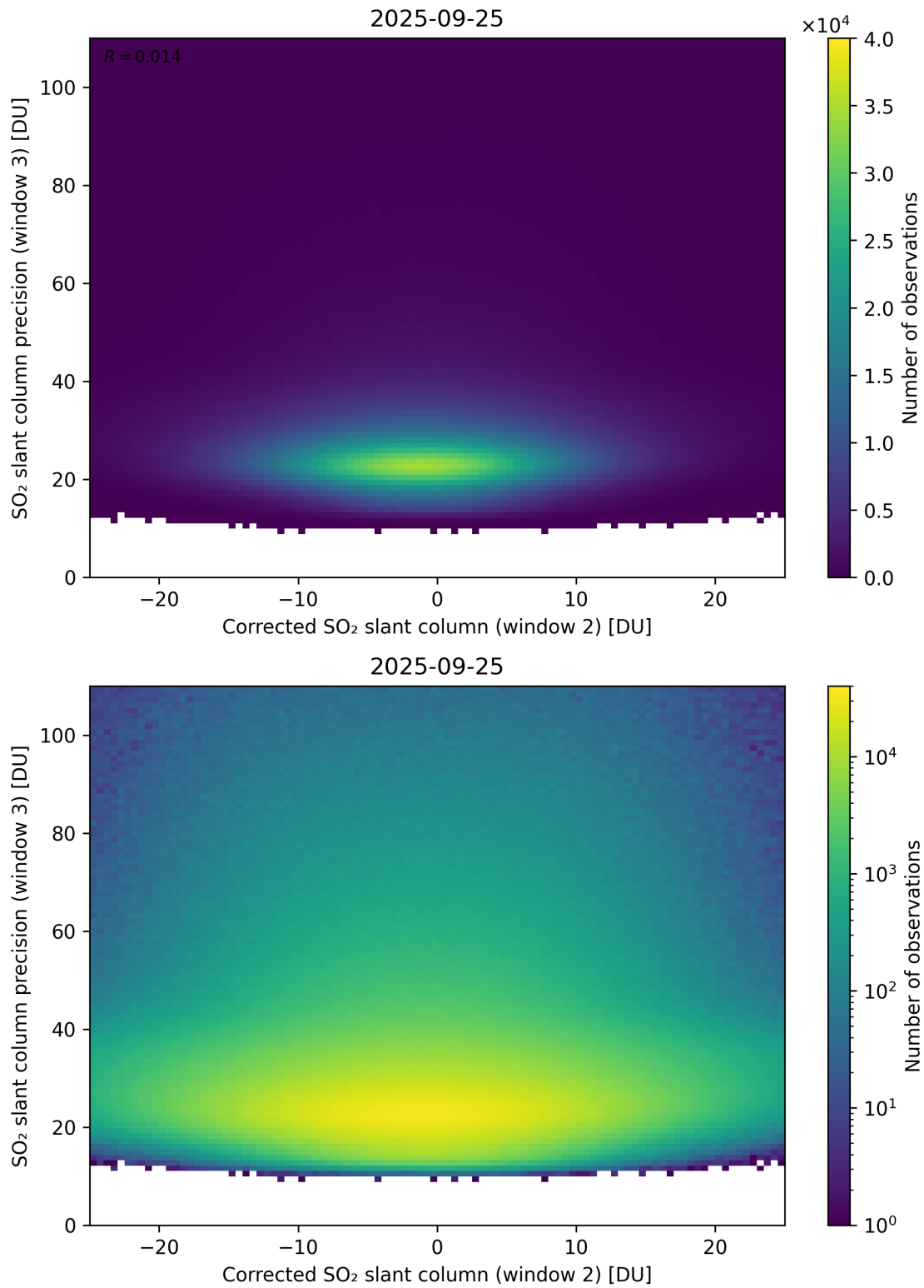
Figure 252: Scatter density plot of “Corrected SO 2 slant column (window 2)” against “SO 2 slant column precision (window 3)” for 2025-09-25 to 2025-09-26.
