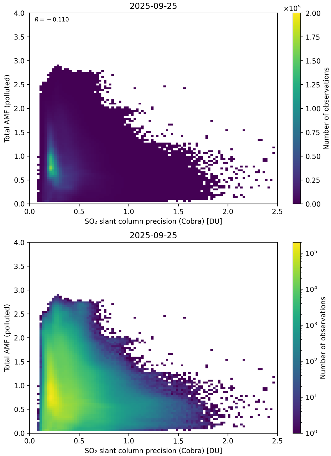
Figure 213: Scatter density plot of “SO 2 slant column precision (Cobra)” against “Total AMF (polluted)” for 2025-09-25 to 2025-09-26.
