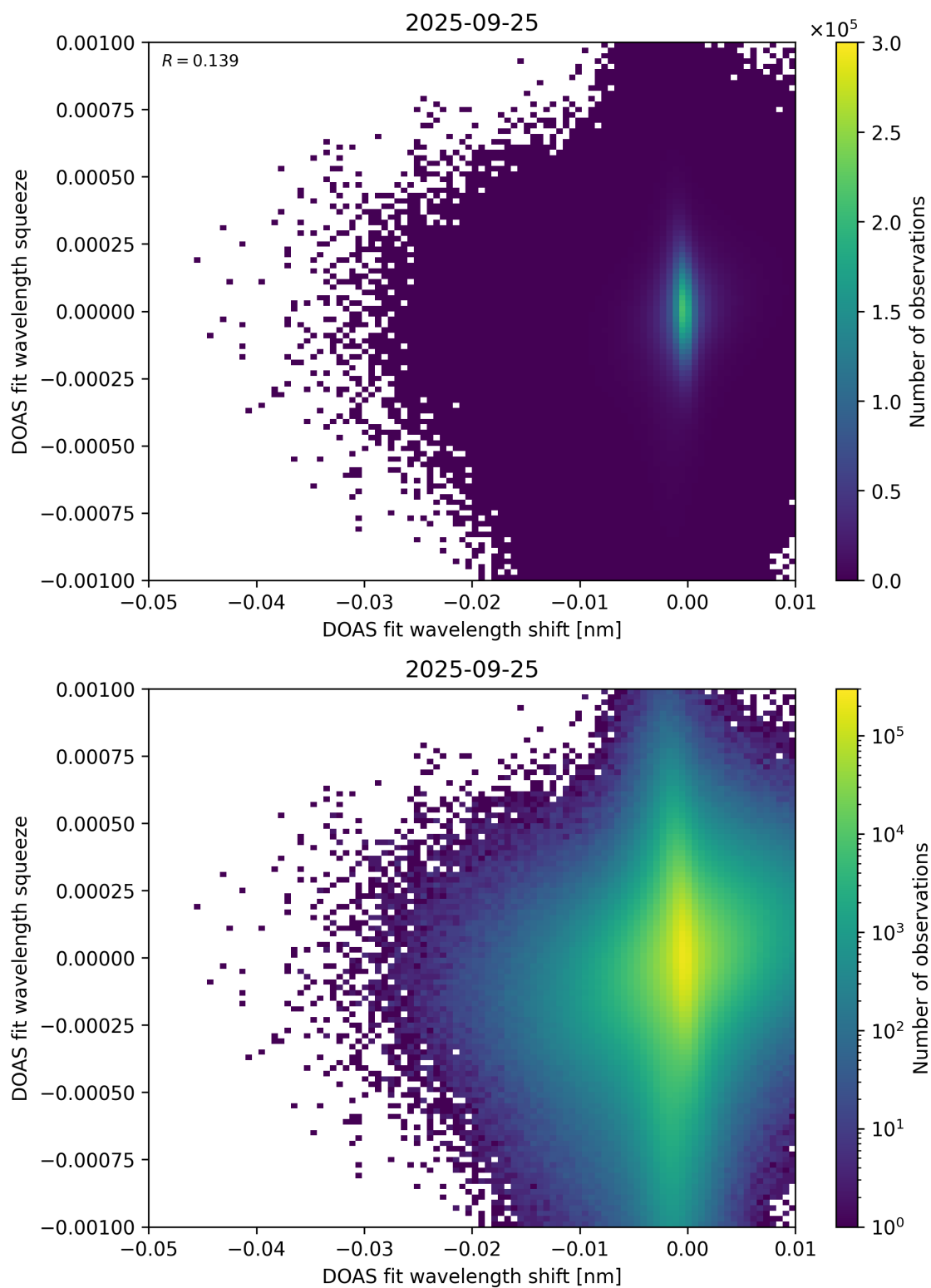
Figure 138: Scatter density plot of “DOAS fit wavelength shift” against “DOAS fit wavelength squeeze” for 2025-09-25 to 2025-09-26.
