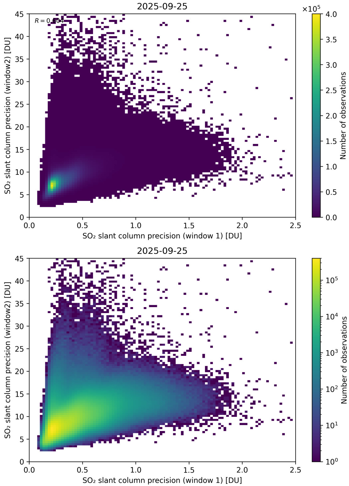
Figure 277: Scatter density plot of “SO 2 slant column precision (window 1)” against “SO 2 slant column precision (window2)” for 2025-09-25 to 2025-09-26.
