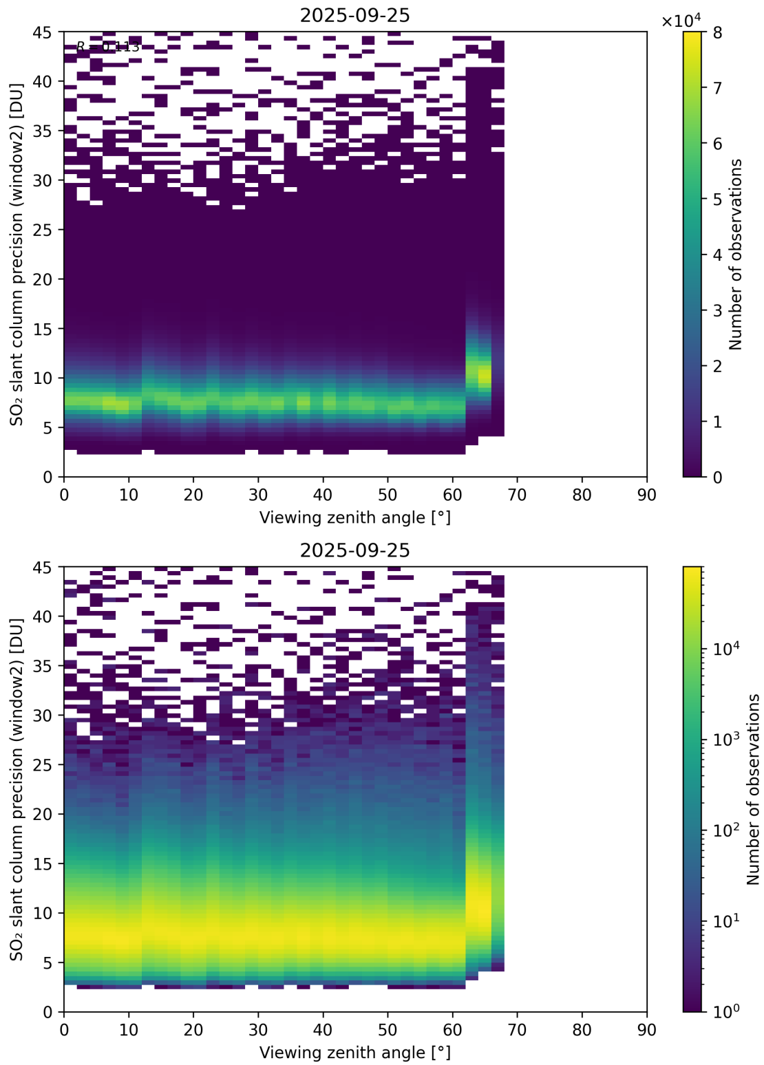
Figure 378: Scatter density plot of “Viewing zenith angle” against “SO 2 slant column precision (window2)” for 2025-09-25 to 2025-09-26.
