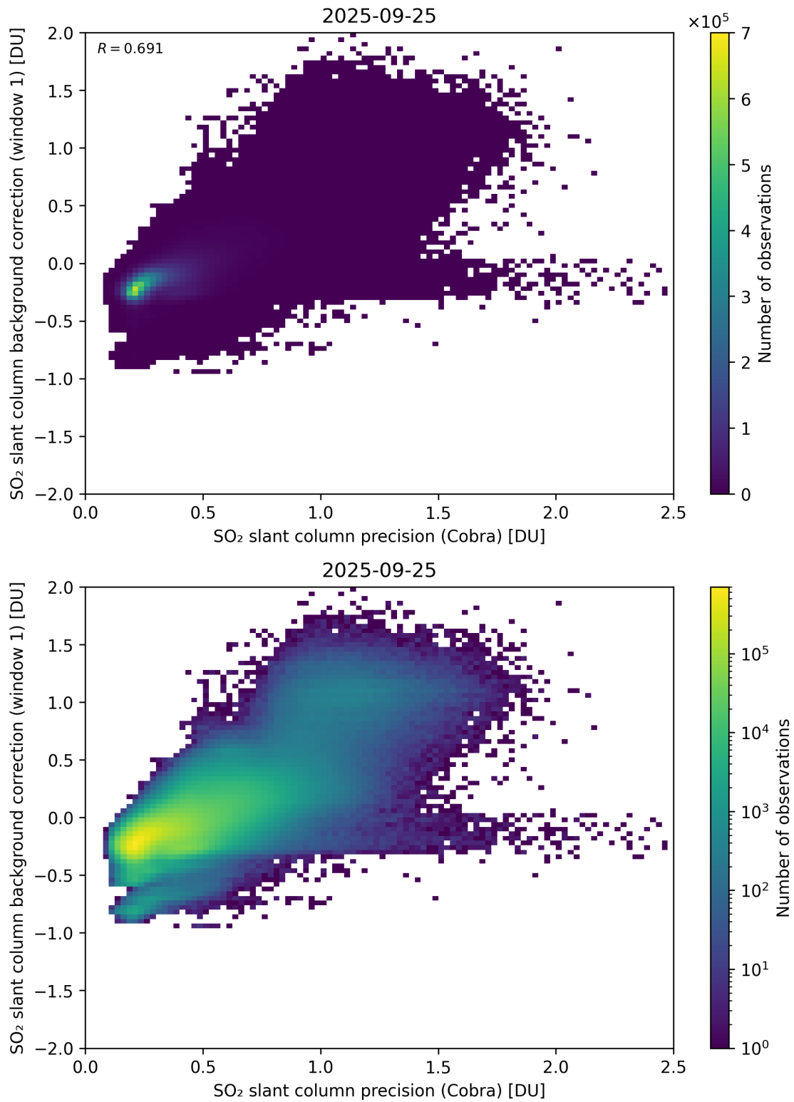
Figure 199: Scatter density plot of “SO 2 slant column precision (Cobra)” against “SO 2 slant column background correction (window 1)” for 2025-09-25 to 2025-09-26.
