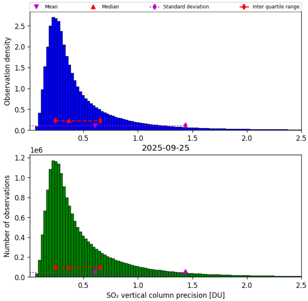
Figure 59: Histogram of “SO 2 vertical column precision” for 2025-09-25 to 2025-09-26
