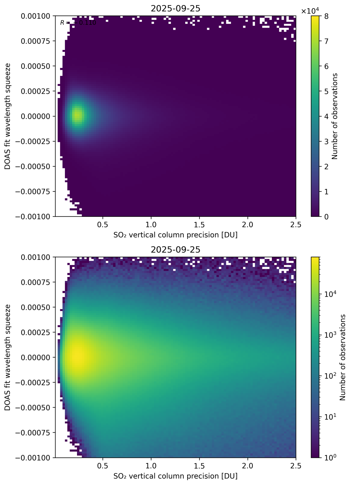
Figure 333: Scatter density plot of “SO 2 vertical column precision” against “DOAS fit wavelength squeeze” for 2025-09-25 to 2025-09-26.
