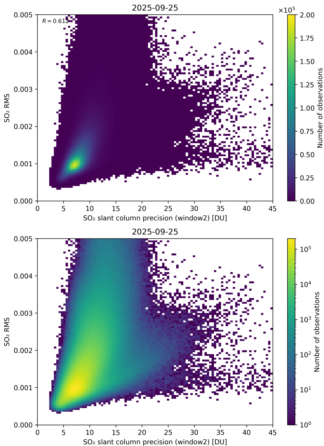
Figure 295: Scatter density plot of “SO 2 slant column precision (window2)” against “SO 2 RMS” for 2025-09-25 to 2025-09-26.
