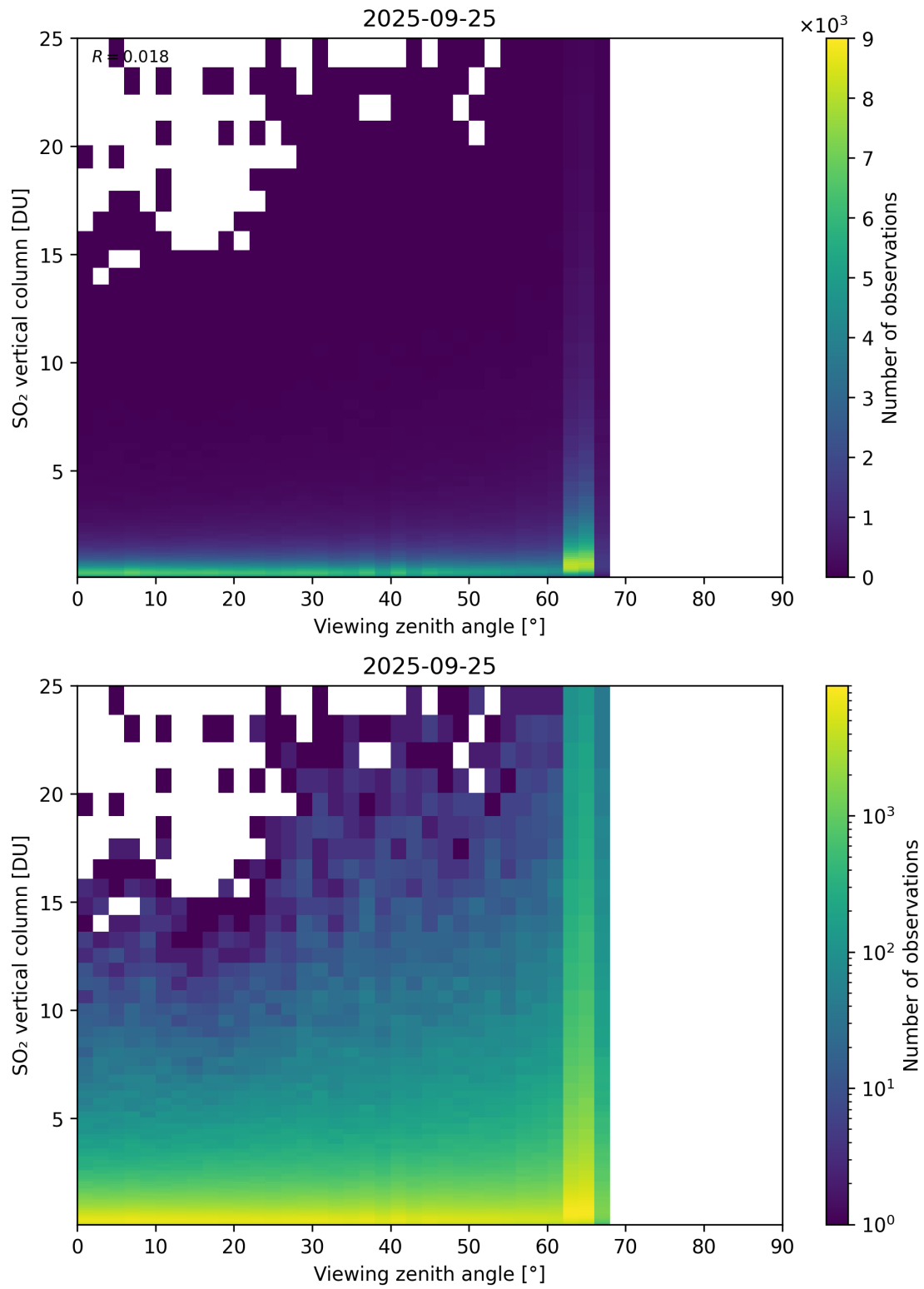
Figure 383: Scatter density plot of “Viewing zenith angle” against “SO 2 vertical column” for 2025-09-25 to 2025-09-26.
