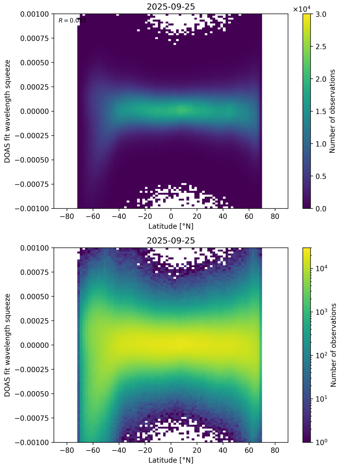
Figure 154: Scatter density plot of “Latitude” against “DOAS fit wavelength squeeze” for 2025-09-25 to 2025-09-26.
