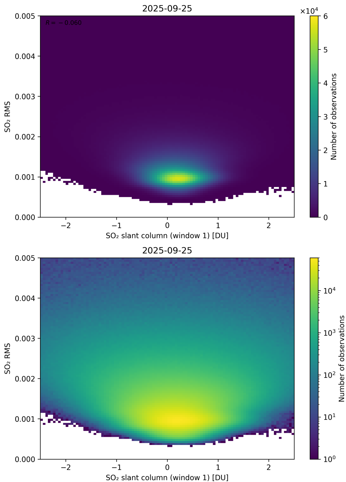
Figure 267: Scatter density plot of “SO 2 slant column (window 1)” against “SO 2 RMS” for 2025-09-25 to 2025-09-26.
