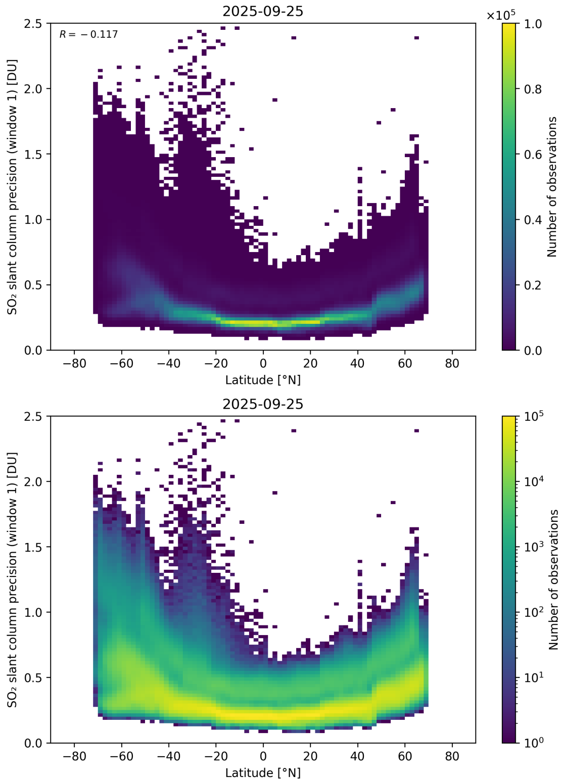
Figure 163: Scatter density plot of “Latitude” against “SO 2 slant column precision (window 1)” for 2025-09-25 to 2025-09-26.
