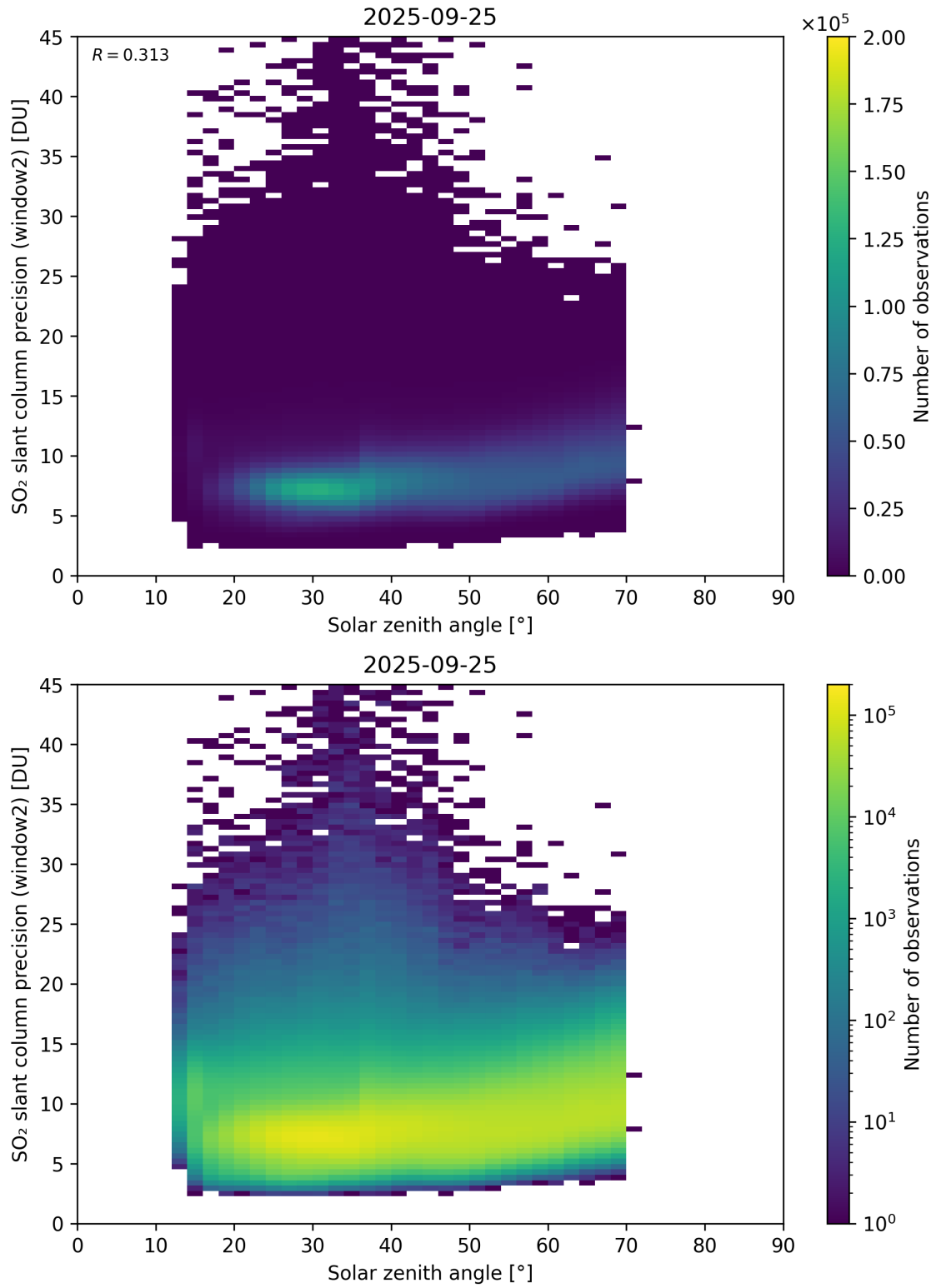
Figure 186: Scatter density plot of “Solar zenith angle” against “SO 2 slant column precision (window2)” for 2025-09-25 to 2025-09-26.
