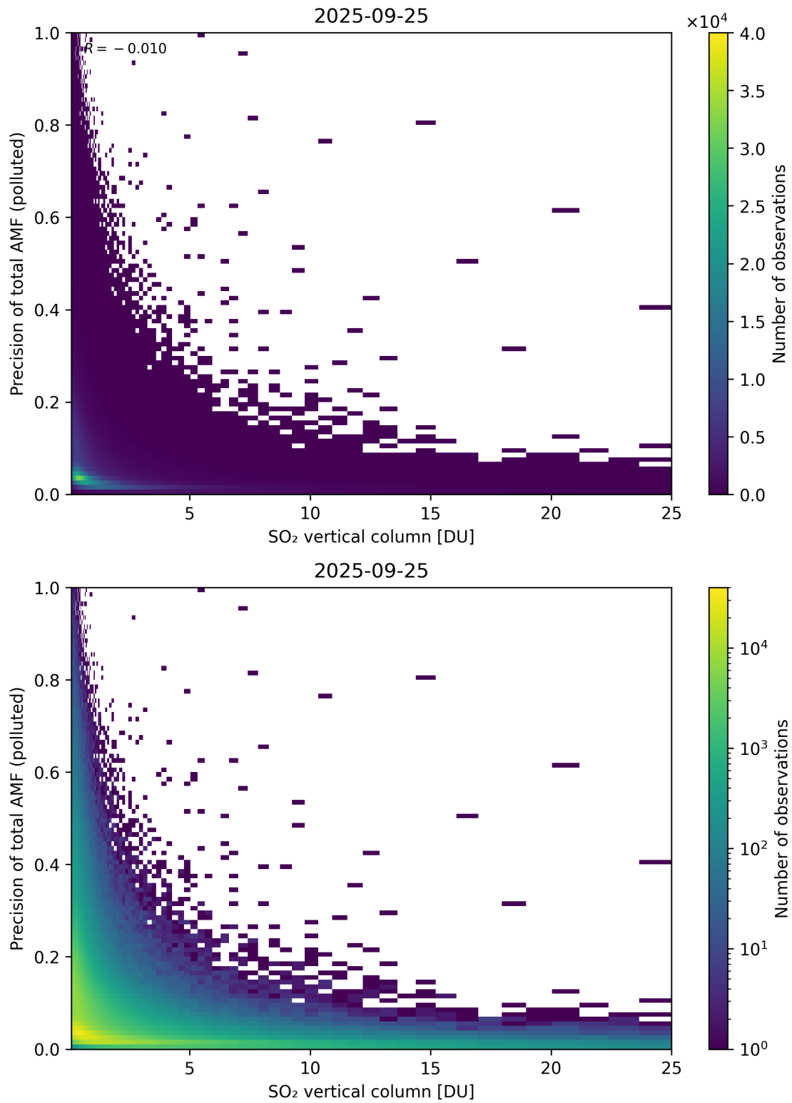
Figure 360: Scatter density plot of “SO 2 vertical column” against “Precision of total AMF (polluted)” for 2025-09-25 to 2025-09-26.
