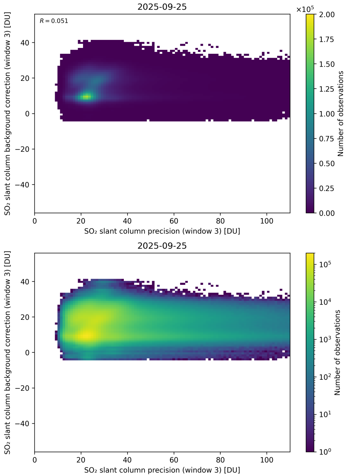
Figure 307: Scatter density plot of “SO 2 slant column precision (window 3)” against “SO 2 slant column background correction (window 3)” for 2025-09-25 to 2025-09-26.
