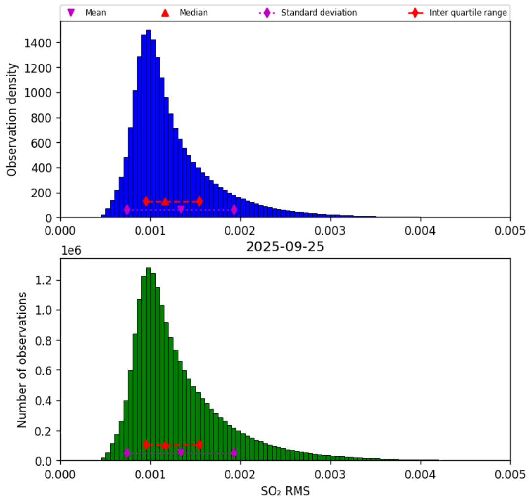
Figure 78: Histogram of “SO 2 RMS” for 2025-09-25 to 2025-09-26
