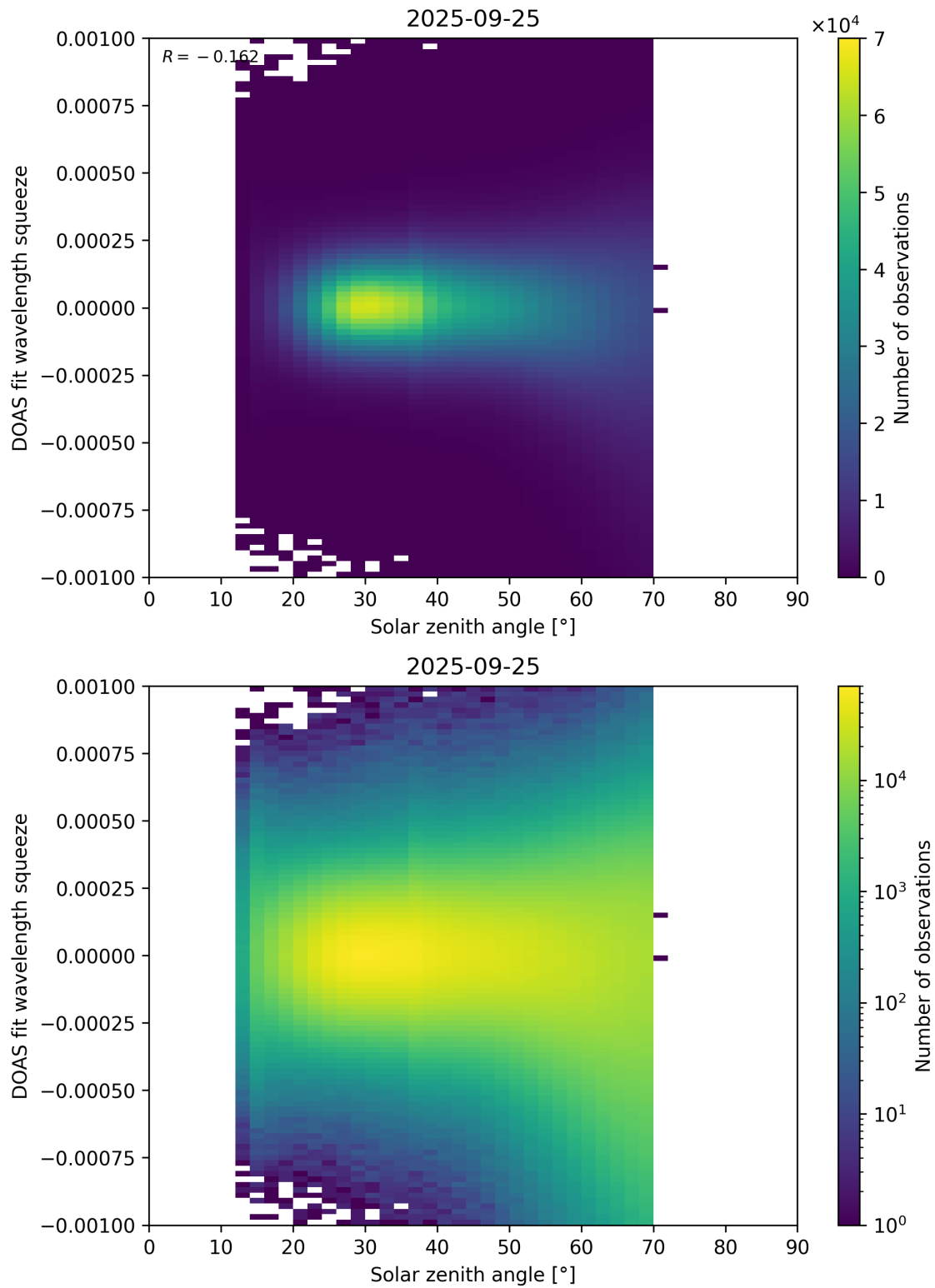
Figure 175: Scatter density plot of “Solar zenith angle” against “DOAS fit wavelength squeeze” for 2025-09-25 to 2025-09-26.
