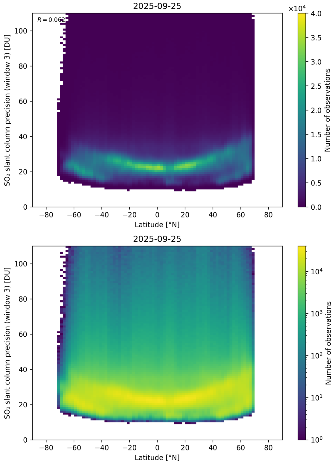
Figure 166: Scatter density plot of “Latitude” against “SO 2 slant column precision (window 3)” for 2025-09-25 to 2025-09-26.
