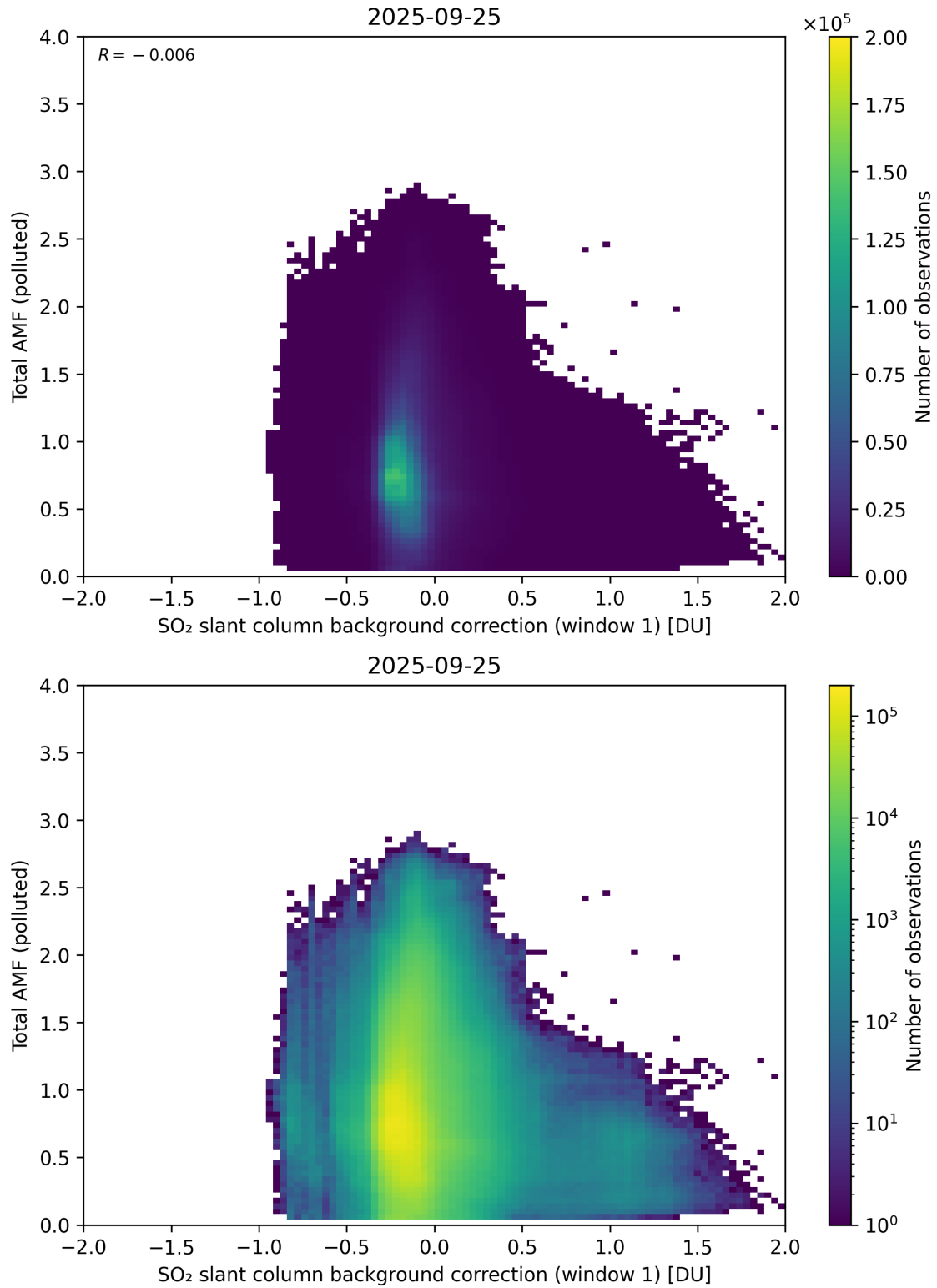
Figure 120: Scatter density plot of “SO 2 slant column background correction (window 1)” against “Total AMF (polluted)” for 2025-09-25 to 2025-09-26.
