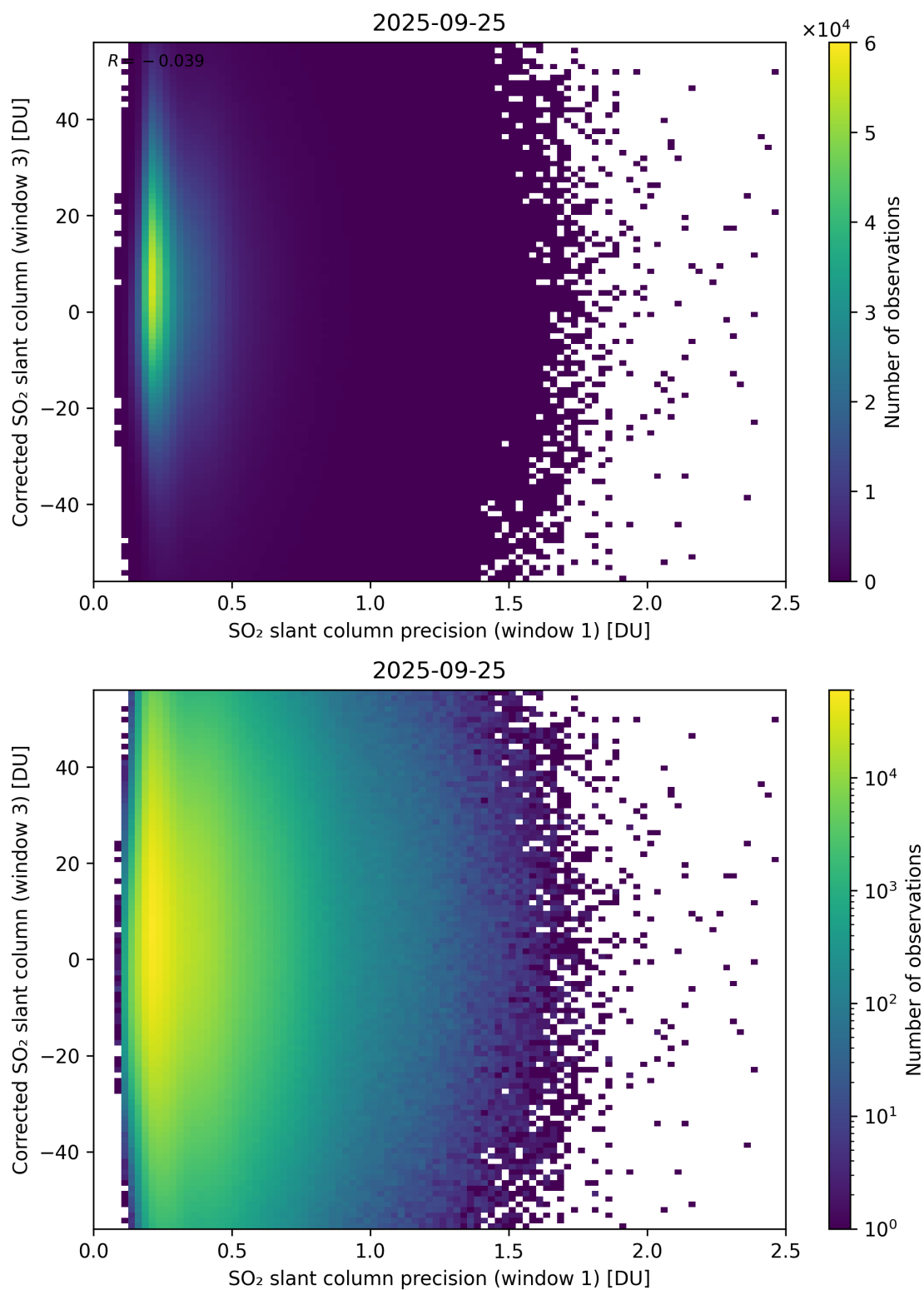
Figure 276: Scatter density plot of “SO 2 slant column precision (window 1)” against “Corrected SO 2 slant column (window 3)” for 2025-09-25 to 2025-09-26.
