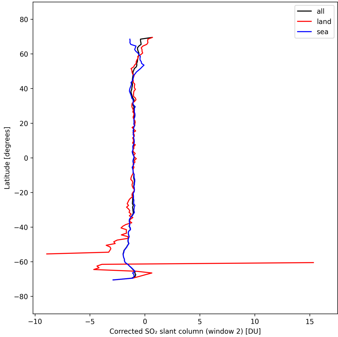
Figure 43: Zonal average of “Corrected SO 2 slant column (window 2)” for 2025-09-25 to 2025-09-26.
