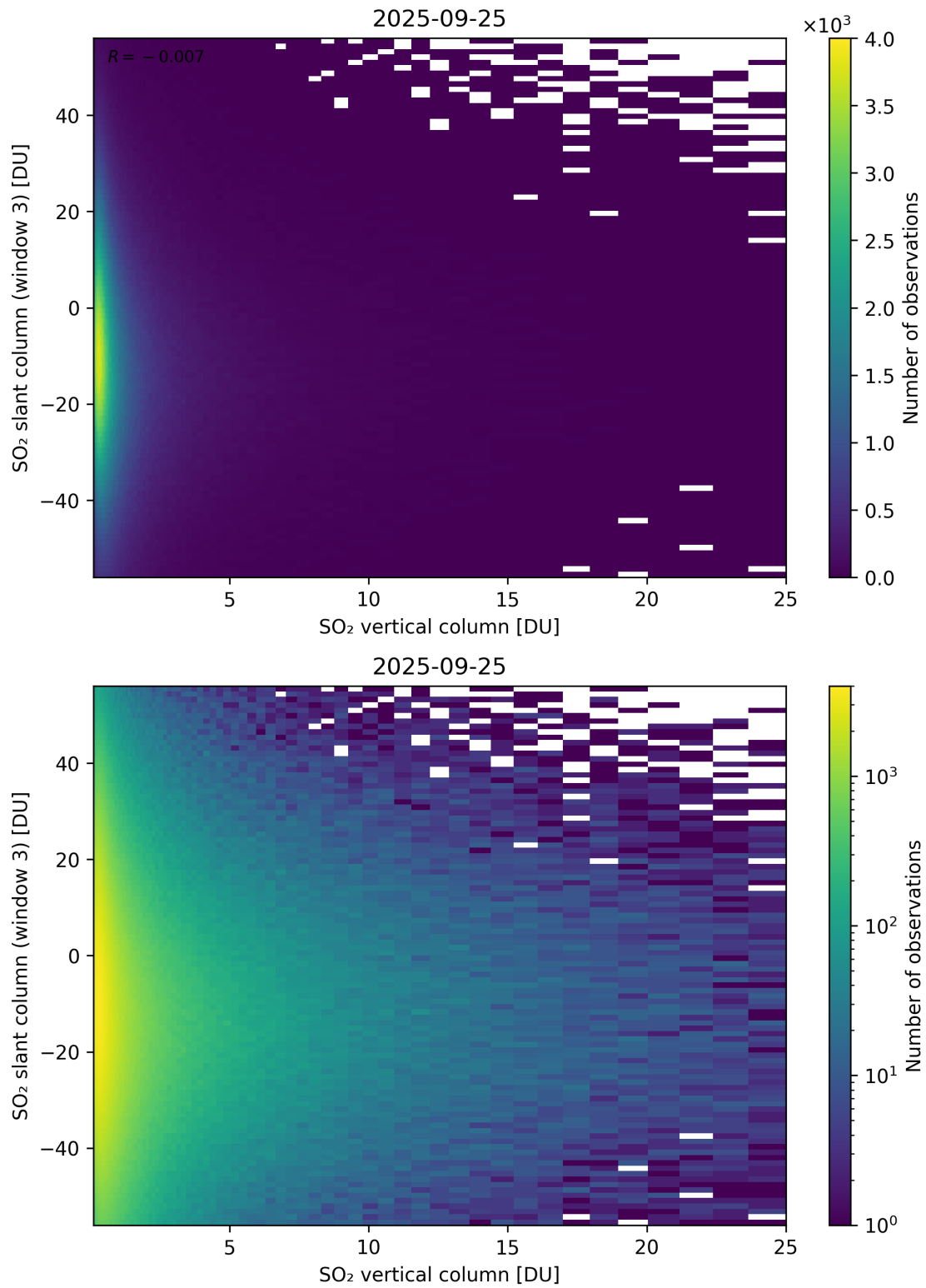
Figure 357: Scatter density plot of “SO 2 vertical column” against “SO 2 slant column (window 3)” for 2025-09-25 to 2025-09-26.
