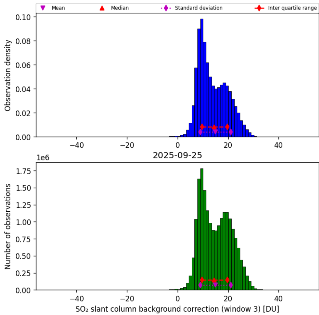
Figure 74: Histogram of “SO 2 slant column background correction (window 3)” for 2025-09-25 to 2025-09-26
