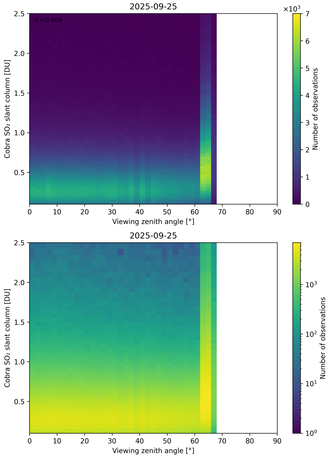
Figure 371: Scatter density plot of “Viewing zenith angle” against “Cobra SO 2 slant column” for 2025-09-25 to 2025-09-26.
