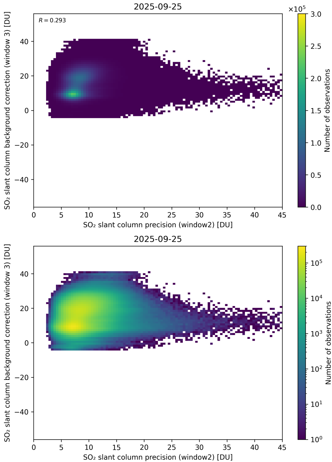
Figure 292: Scatter density plot of “SO 2 slant column precision (window2)” against “SO 2 slant column background correction (window 3)” for 2025-09-25 to 2025-09-26.
