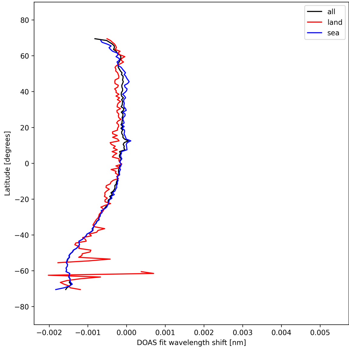
Figure 50: Zonal average of "DOAS fit wavelength shift" for 2025-09-25 to 2025-09-26.
