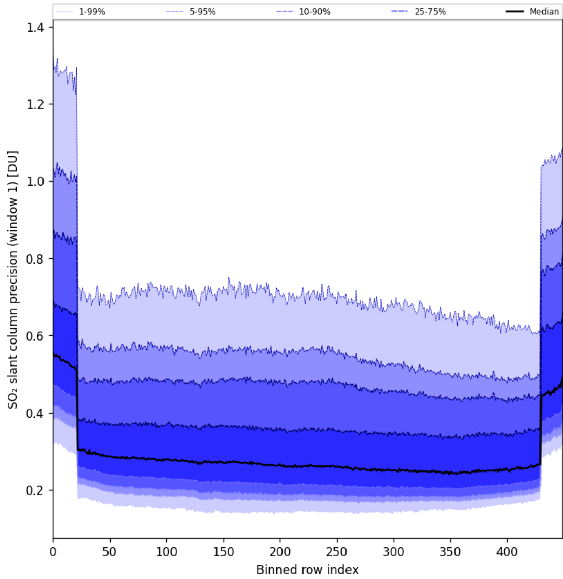
Figure 90: Along track statistics of “SO 2 slant column precision (window 1)” for 2025-09-25 to 2025-09-26
