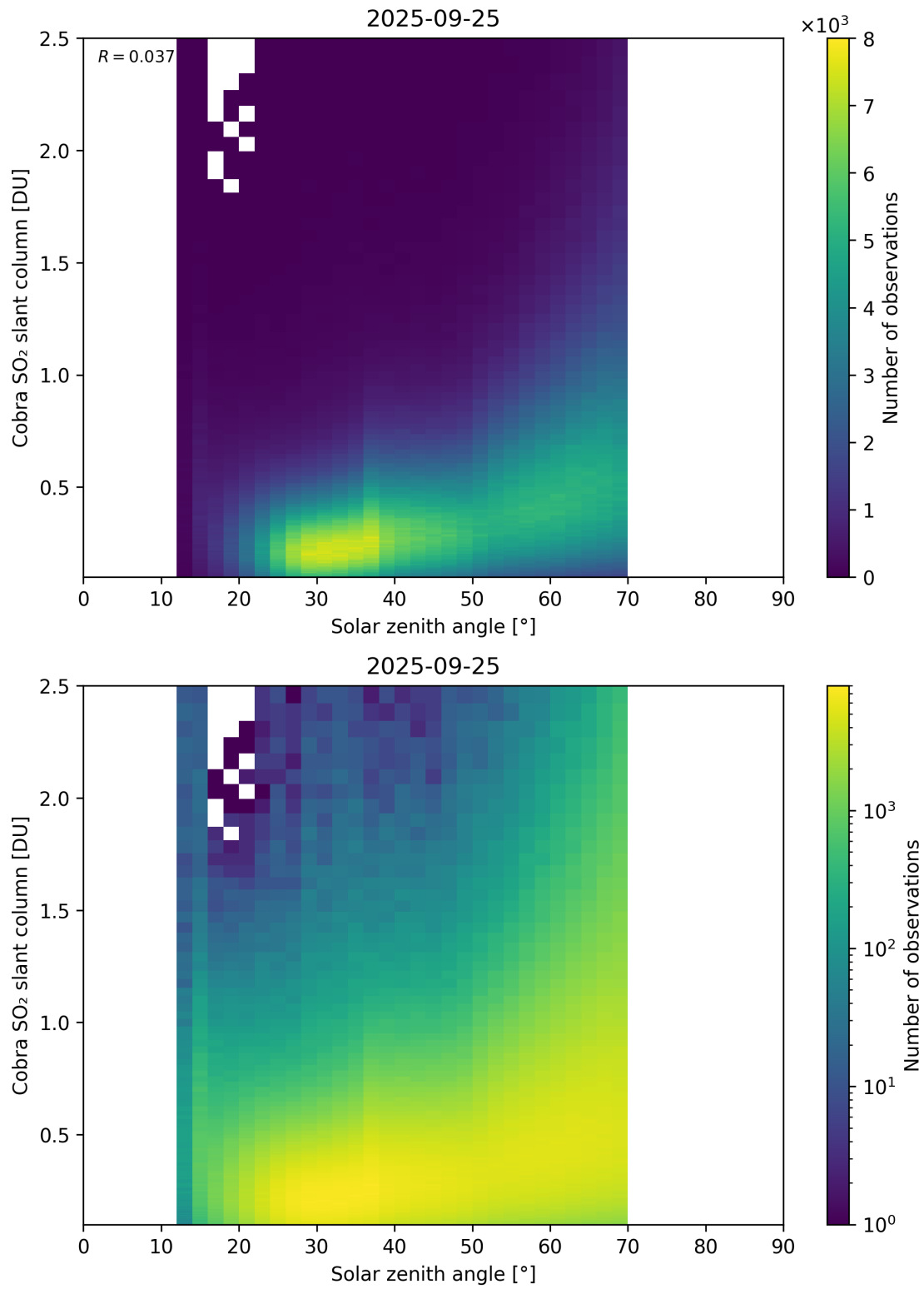
Figure 179: Scatter density plot of “Solar zenith angle” against “Cobra SO 2 slant column” for 2025-09-25 to 2025-09-26.
