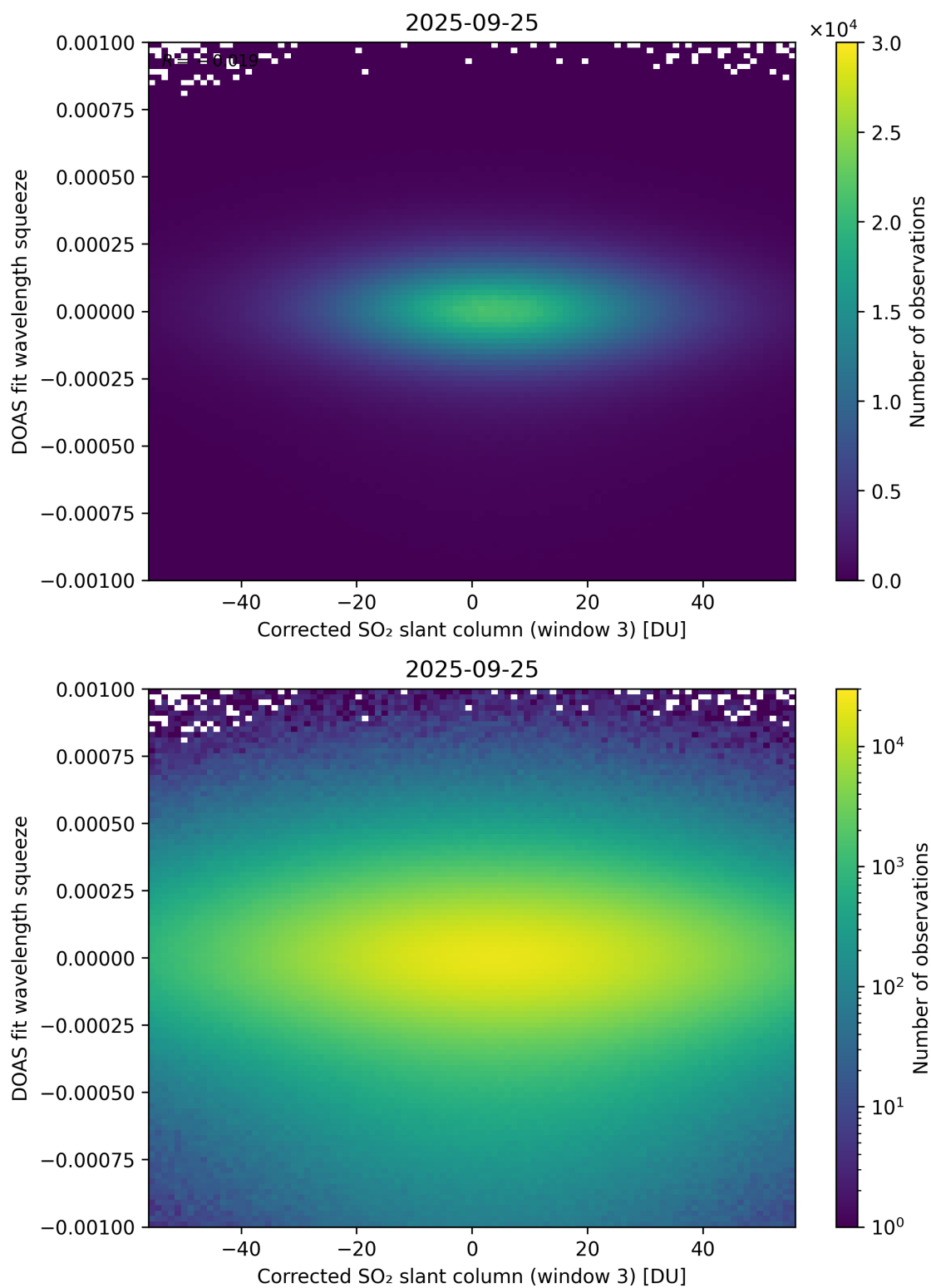
Figure 257: Scatter density plot of “Corrected SO 2 slant column (window 3)” against “DOAS fit wavelength squeeze” for 2025-09-25 to 2025-09-26.
