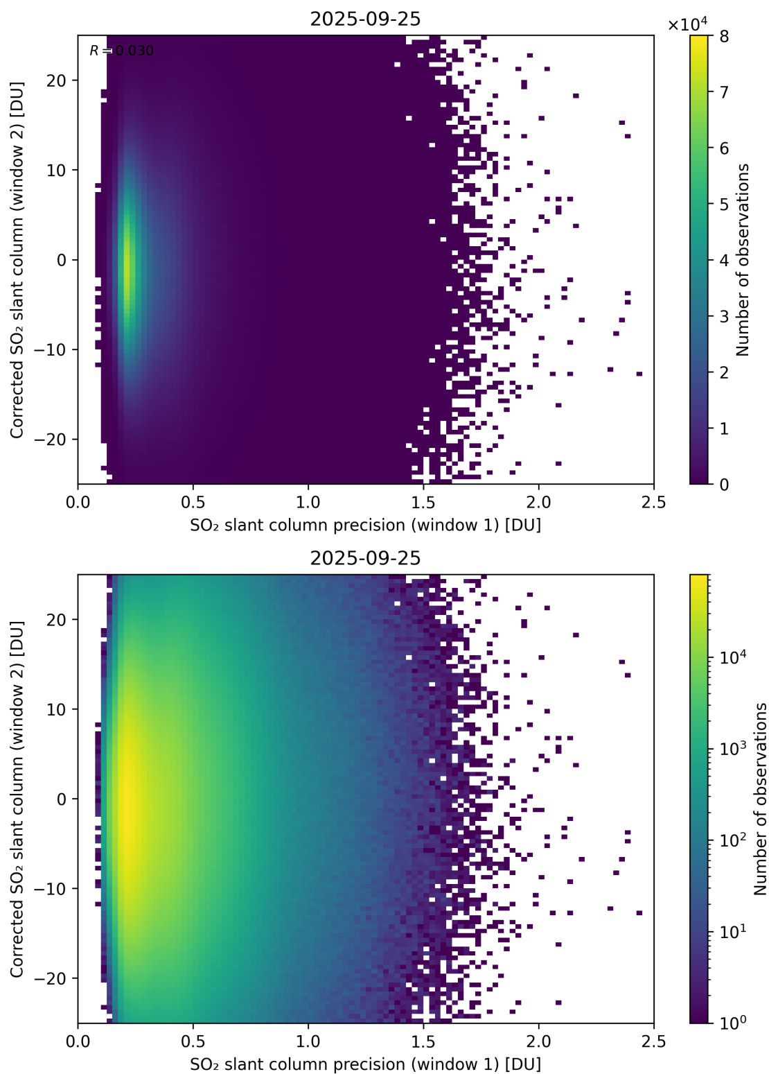
Figure 275: Scatter density plot of “SO 2 slant column precision (window 1)” against “Corrected SO 2 slant column (window 2)” for 2025-09-25 to 2025-09-26.
