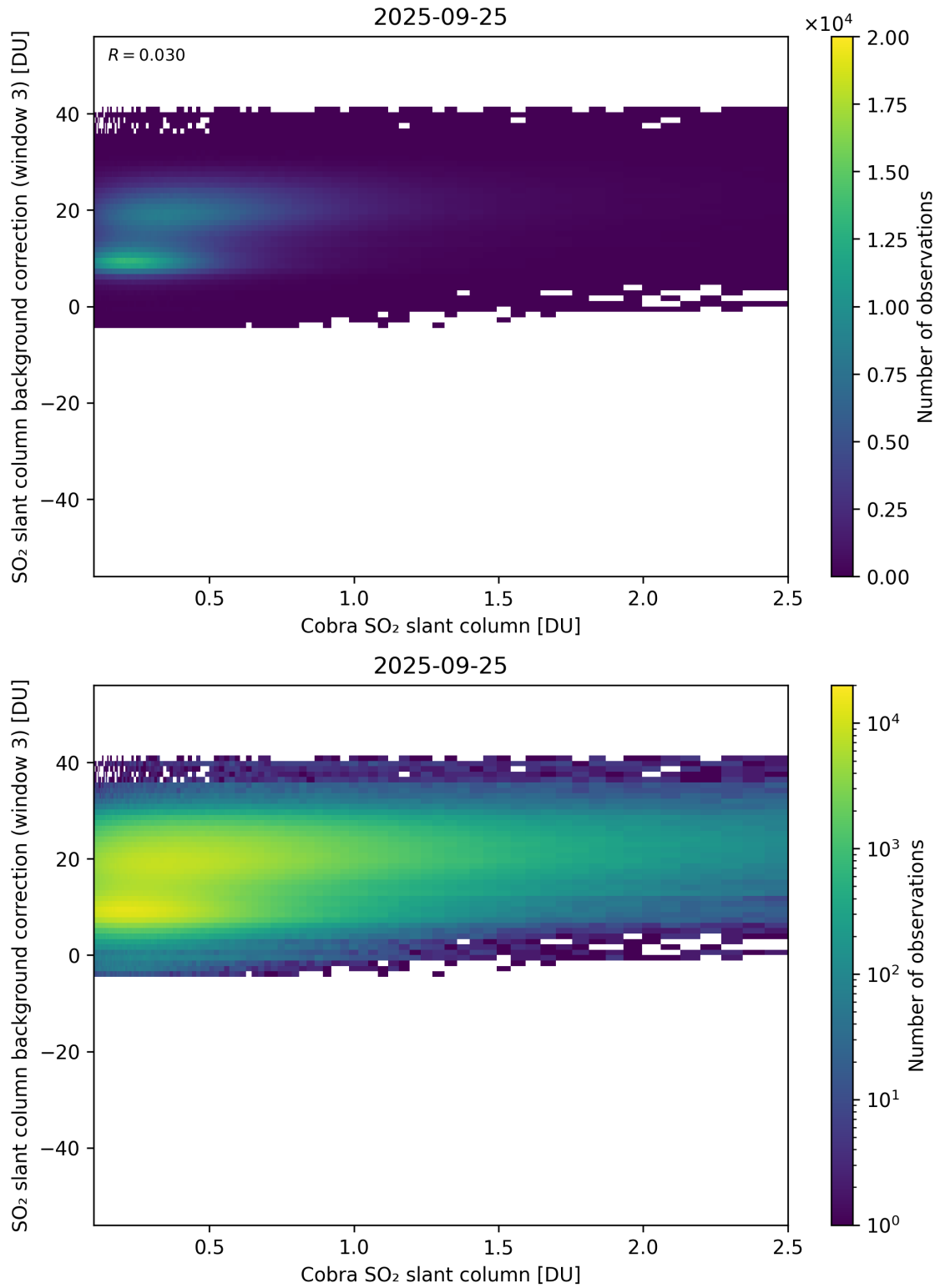
Figure 195: Scatter density plot of “Cobra SO 2 slant column” against “SO 2 slant column background correction (window 3)” for 2025-09-25 to 2025-09-26.
