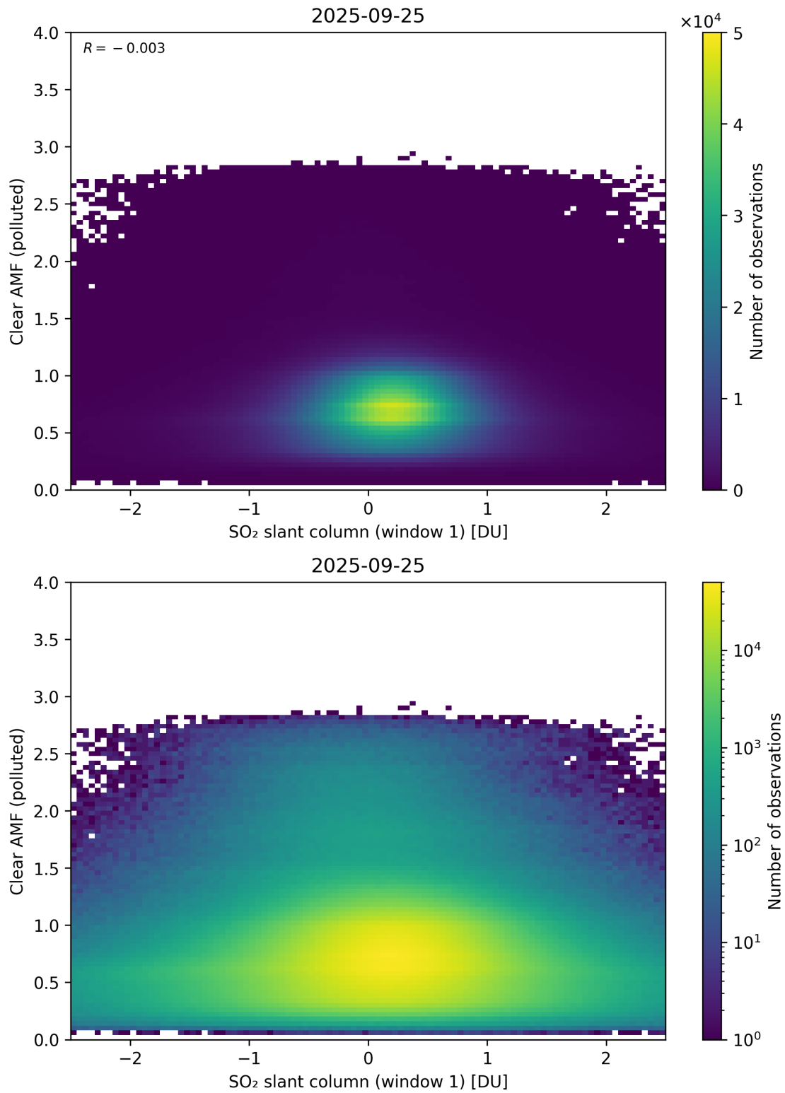
Figure 282: Scatter density plot of “SO 2 slant column (window 1)” against “Clear AMF (polluted)” for 2025-09-25 to 2025-09-26.
