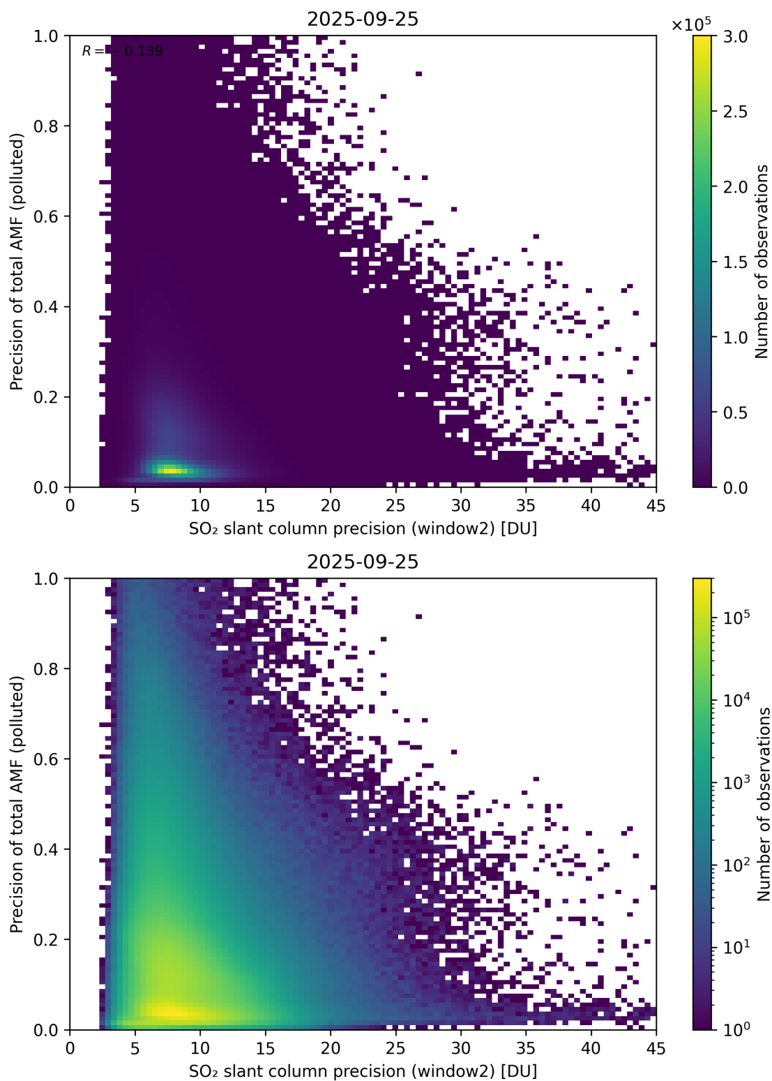
Figure 302: Scatter density plot of “SO 2 slant column precision (window2)” against “Precision of total AMF (polluted)” for 2025-09-25 to 2025-09-26.
