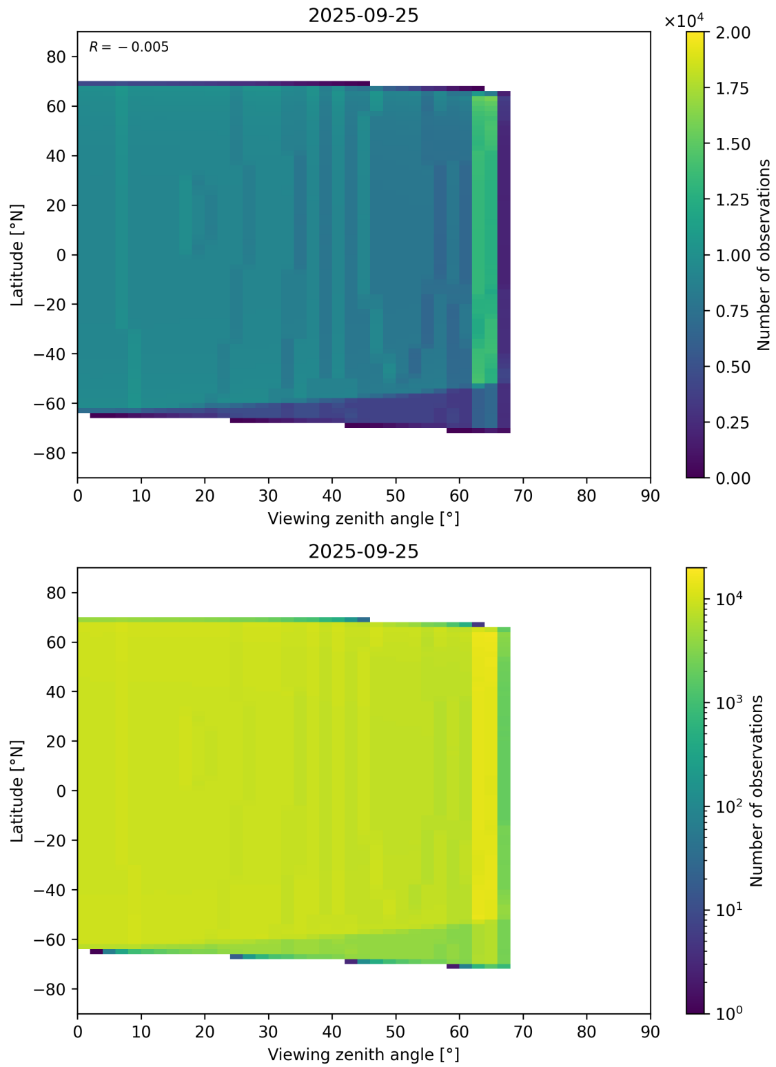
Figure 368: Scatter density plot of “Viewing zenith angle” against “Latitude” for 2025-09-25 to 2025-09-26.
