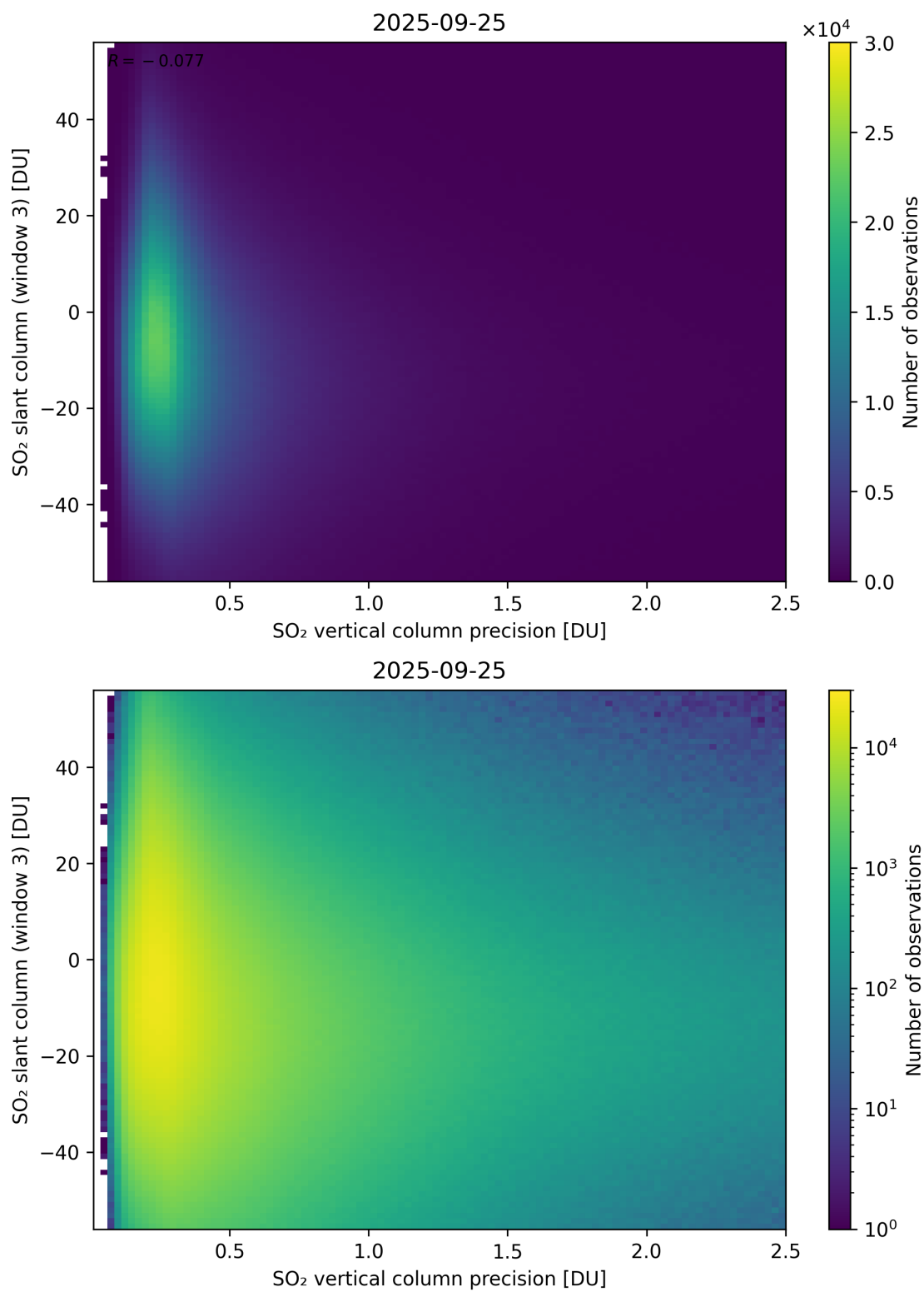
Figure 344: Scatter density plot of “SO 2 vertical column precision” against “SO 2 slant column (window 3)” for 2025-09-25 to 2025-09-26.
