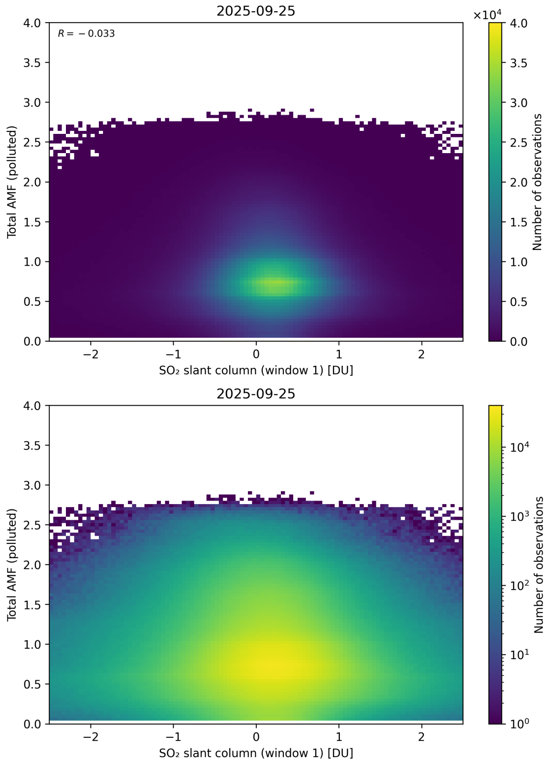
Figure 289: Scatter density plot of “SO 2 slant column (window 1)” against “Total AMF (polluted)” for 2025-09-25 to 2025-09-26.
