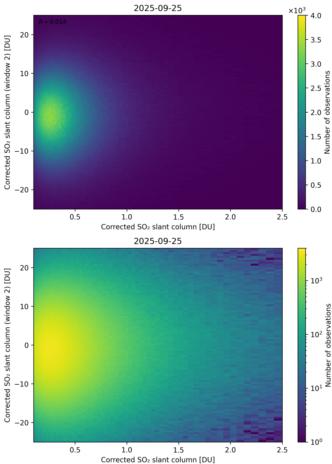
Figure 235: Scatter density plot of “Corrected SO 2 slant column” against “Corrected SO 2 slant column (window 2)” for 2025-09-25 to 2025-09-26.
