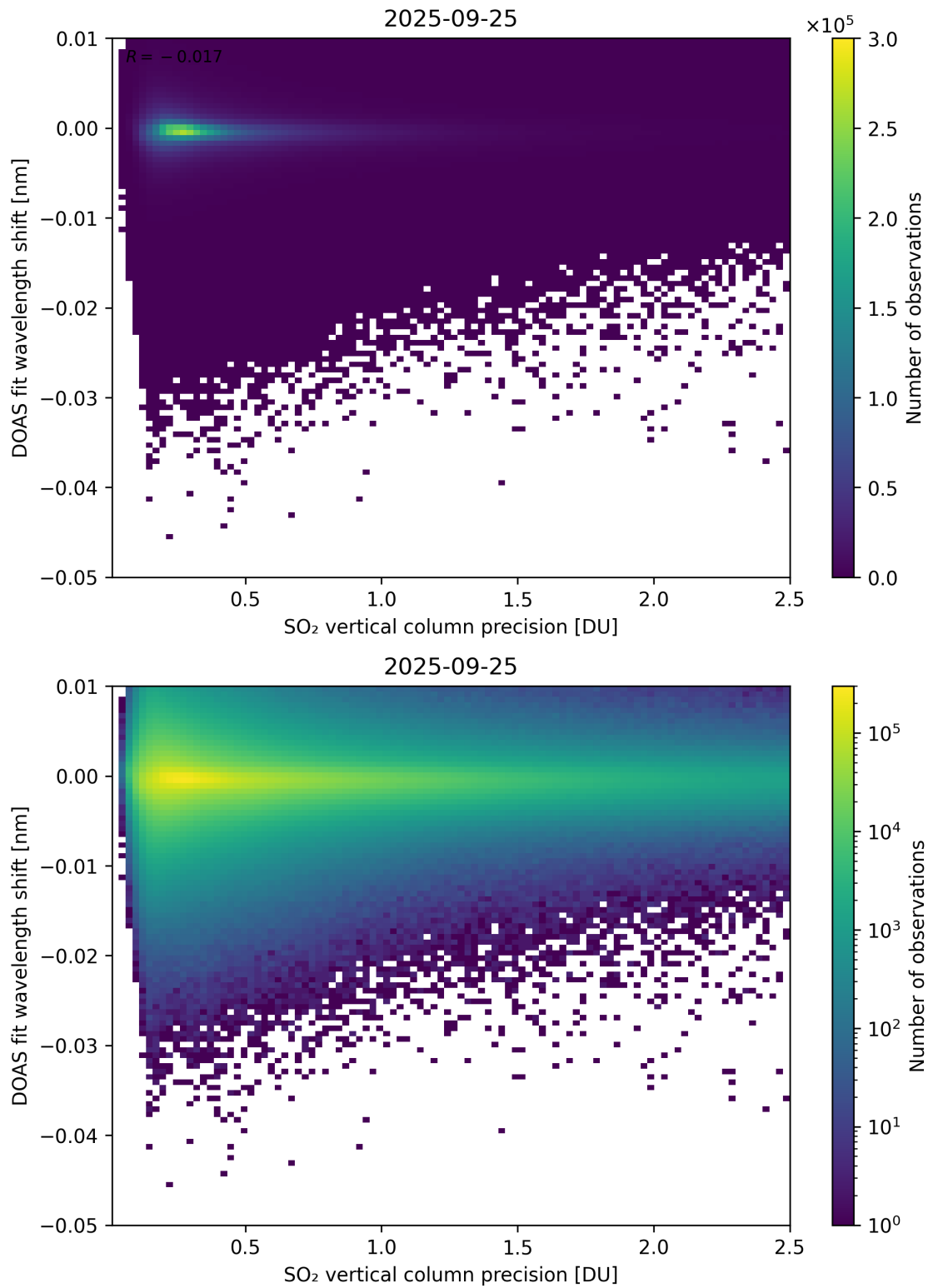
Figure 332: Scatter density plot of “SO 2 vertical column precision” against “DOAS fit wavelength shift” for 2025-09-25 to 2025-09-26.
