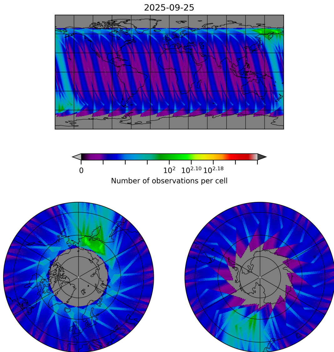
Figure 30: Map of the number of observations for 2025-09-25 to 2025-09-26
