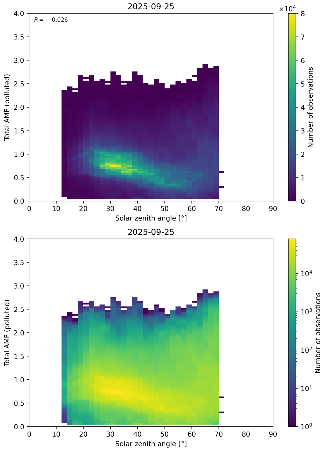
Figure 189: Scatter density plot of “Solar zenith angle” against “Total AMF (polluted)” for 2025-09-25 to 2025-09-26.
