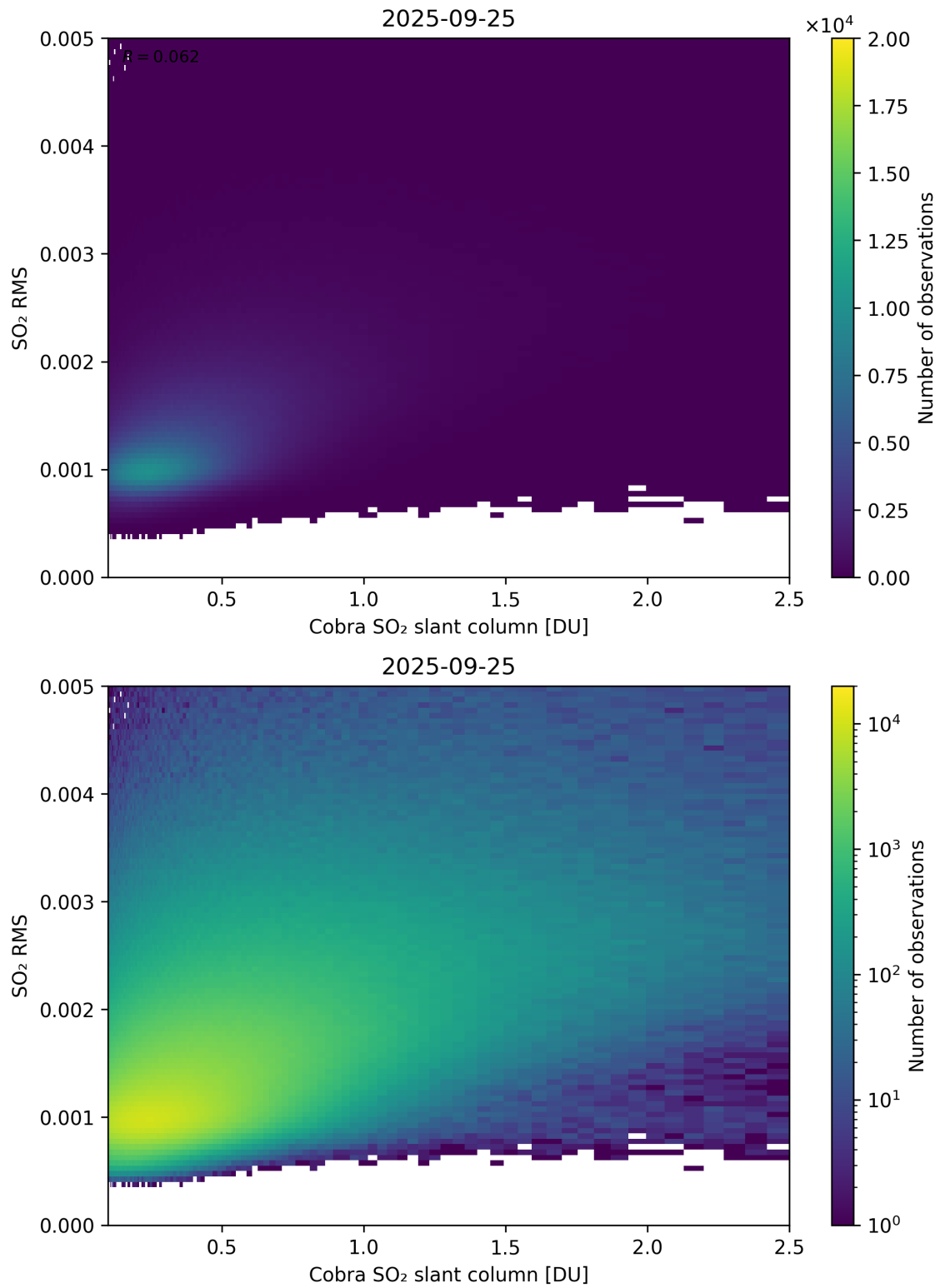
Figure 198: Scatter density plot of “Cobra SO 2 slant column” against “SO 2 RMS” for 2025-09-25 to 2025-09-26.
