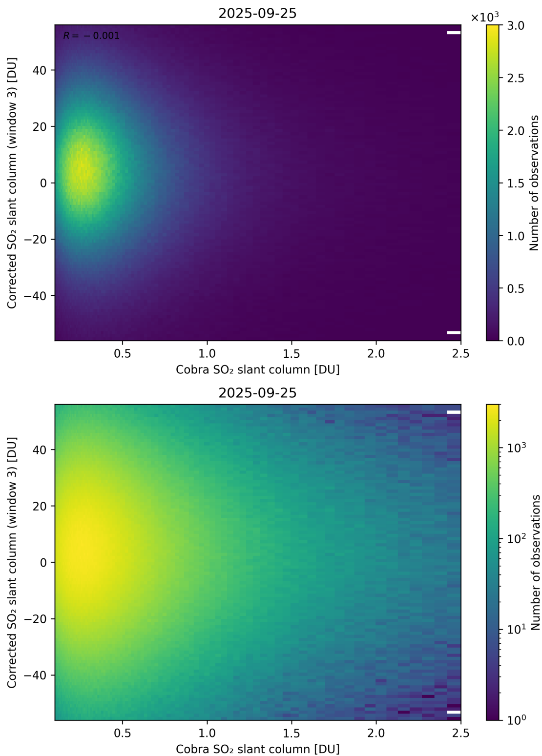
Figure 218: Scatter density plot of “Cobra SO 2 slant column” against “Corrected SO 2 slant column (window 3)” for 2025-09-25 to 2025-09-26.
