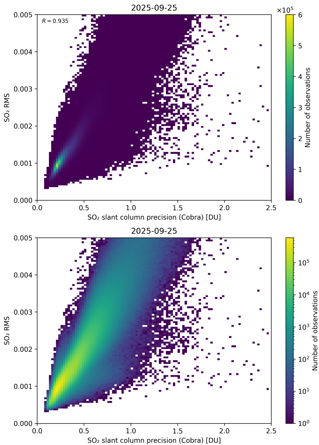
Figure 204: Scatter density plot of “SO 2 slant column precision (Cobra)” against “SO 2 RMS” for 2025-09-25 to 2025-09-26.
