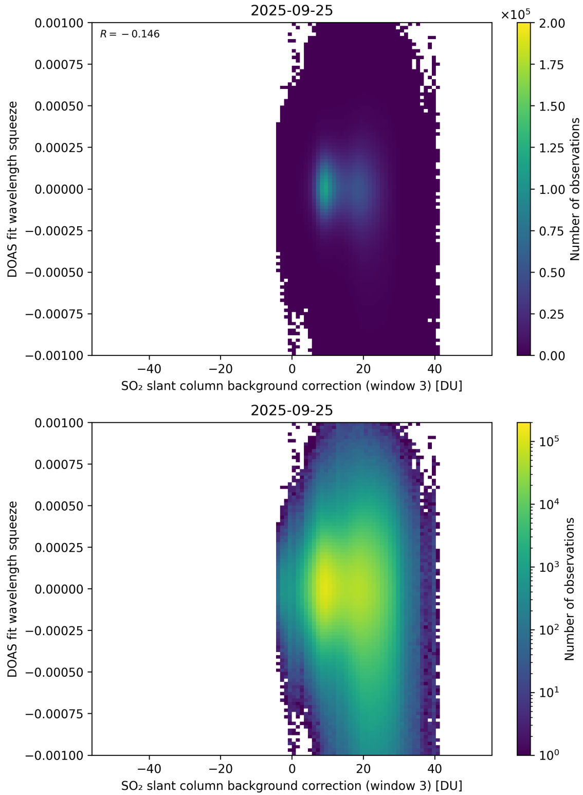
Figure 133: Scatter density plot of “SO 2 slant column background correction (window 3)” against “DOAS fit wavelength squeeze” for 2025-09-25 to 2025-09-26.
