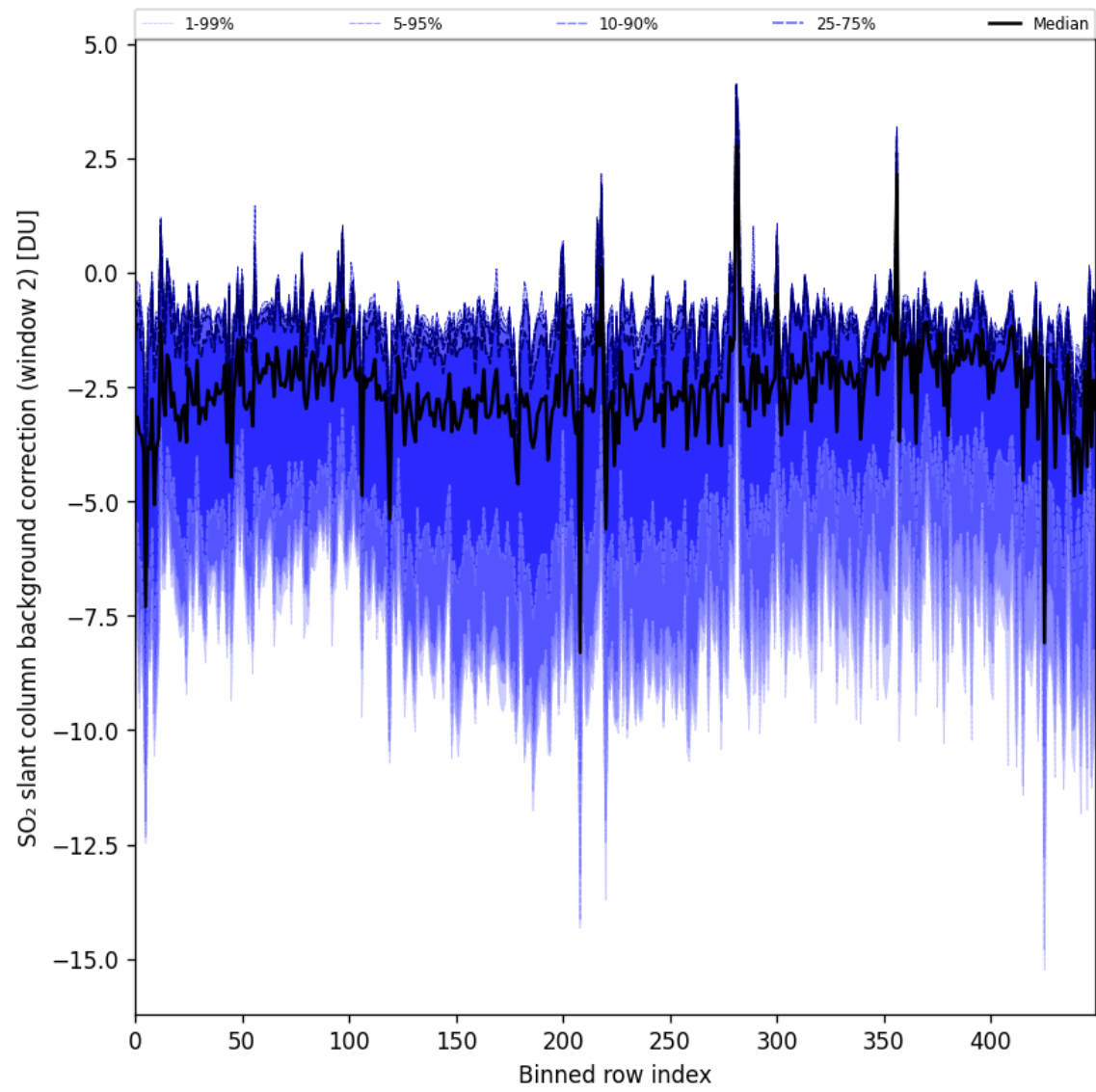
Figure 96: Along track statistics of “SO 2 slant column background correction (window 2)” for 2025-09-25 to 2025-09-26
