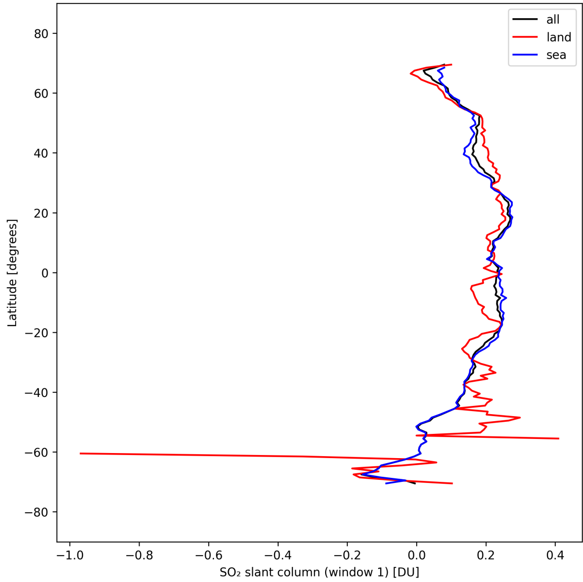
Figure 37: Zonal average of “SO 2 slant column (window 1)” for 2025-09-25 to 2025-09-26.
