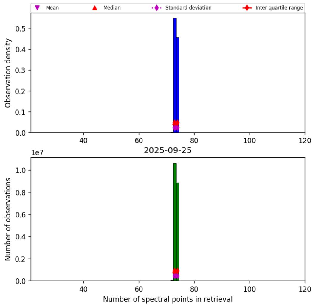
Figure 82: Histogram of “Number of spectral points in retrieval” for 2025-09-25 to 2025-09-26
