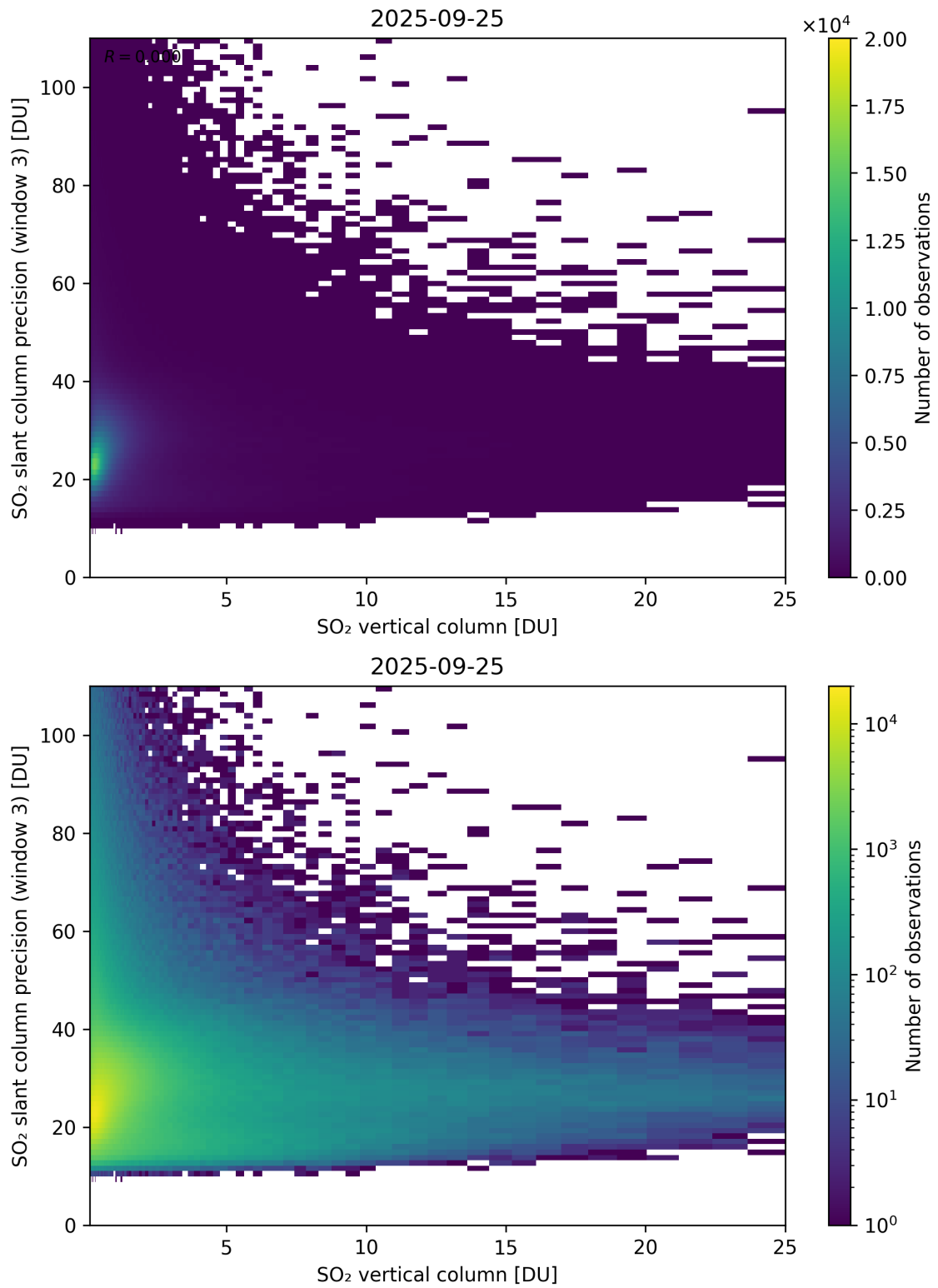
Figure 358: Scatter density plot of “SO 2 vertical column” against “SO 2 slant column precision (window 3)” for 2025-09-25 to 2025-09-26.
