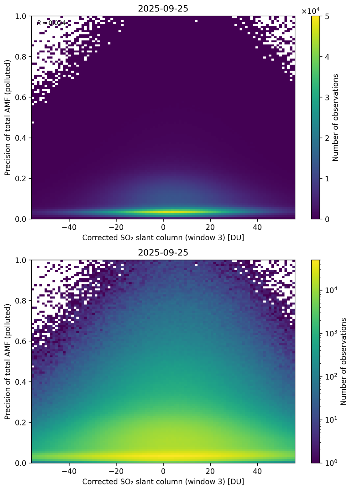
Figure 261: Scatter density plot of “Corrected SO 2 slant column (window 3)” against “Precision of total AMF (polluted)” for 2025-09-25 to 2025-09-26.
