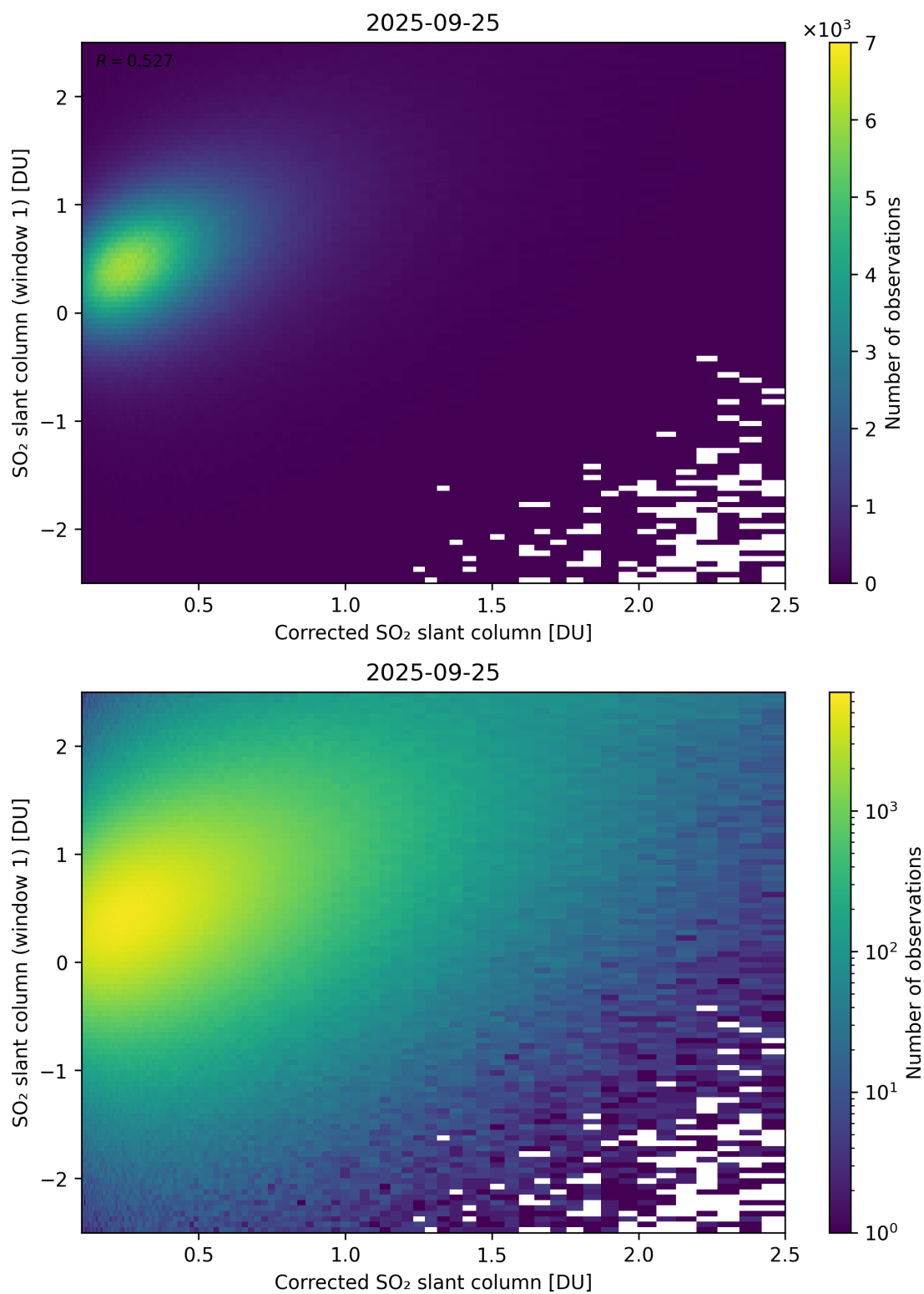
Figure 237: Scatter density plot of “Corrected SO 2 slant column” against “SO 2 slant column (window 1)” for 2025-09-25 to 2025-09-26.
