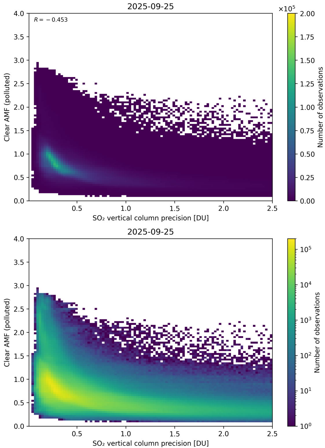
Figure 335: Scatter density plot of “SO 2 vertical column precision” against “Clear AMF (polluted)” for 2025-09-25 to 2025-09-26.
