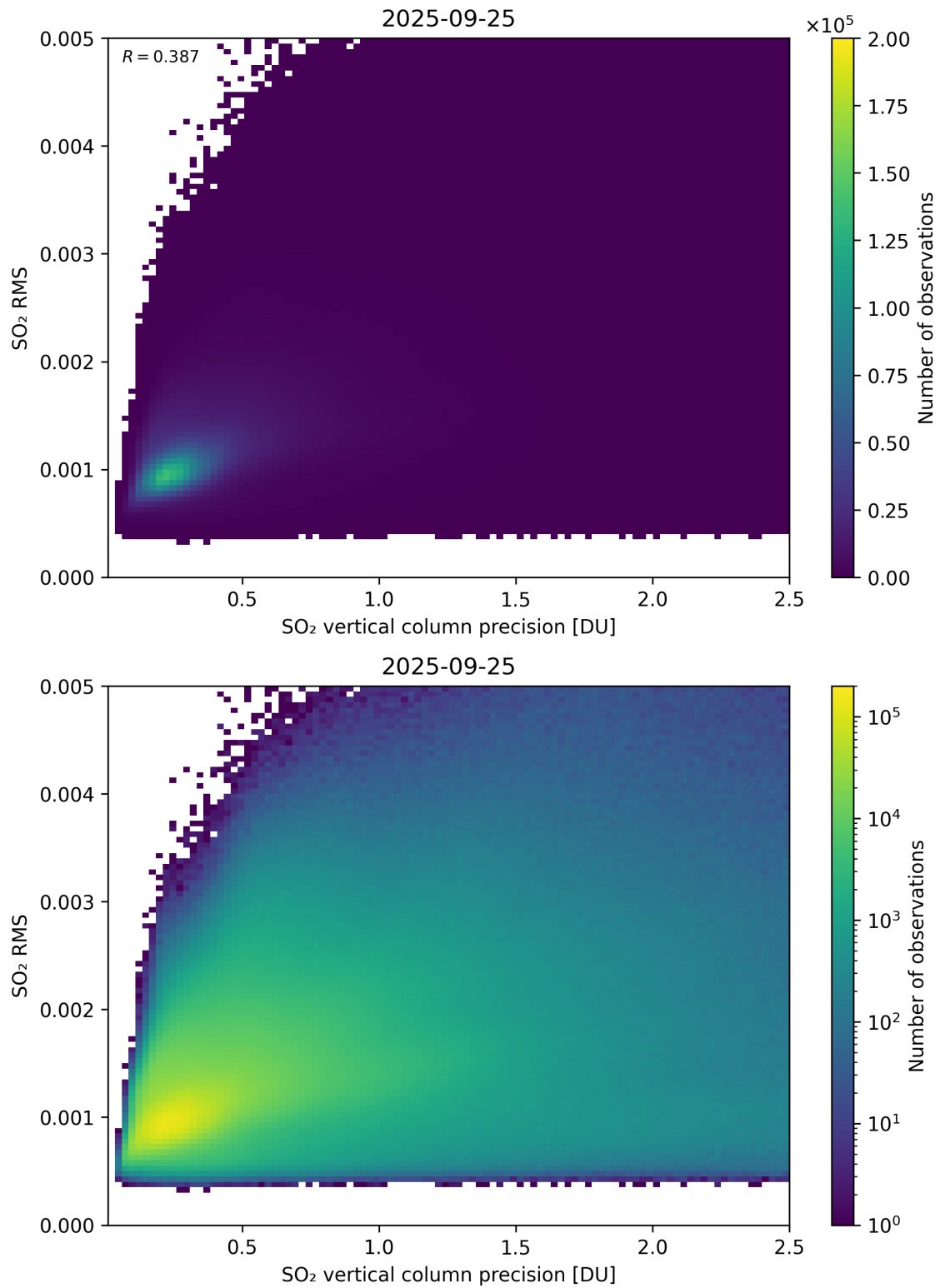
Figure 334: Scatter density plot of “SO 2 vertical column precision” against “SO 2 RMS” for 2025-09-25 to 2025-09-26.
