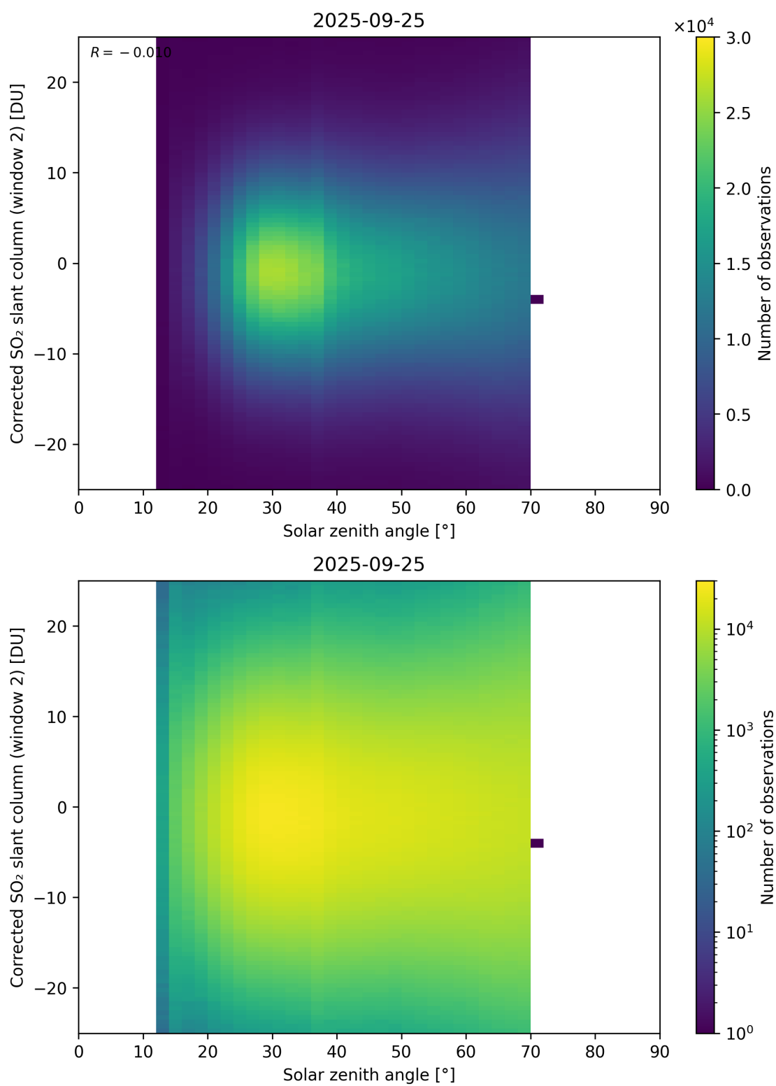
Figure 182: Scatter density plot of “Solar zenith angle” against “Corrected SO 2 slant column (window 2)” for 2025-09-25 to 2025-09-26.
