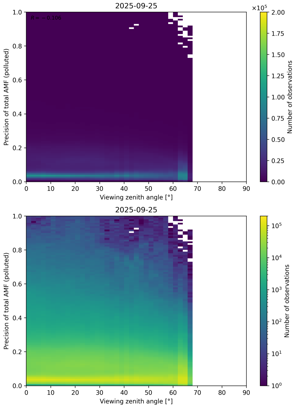
Figure 382: Scatter density plot of “Viewing zenith angle” against “Precision of total AMF (polluted)” for 2025-09-25 to 2025-09-26.
