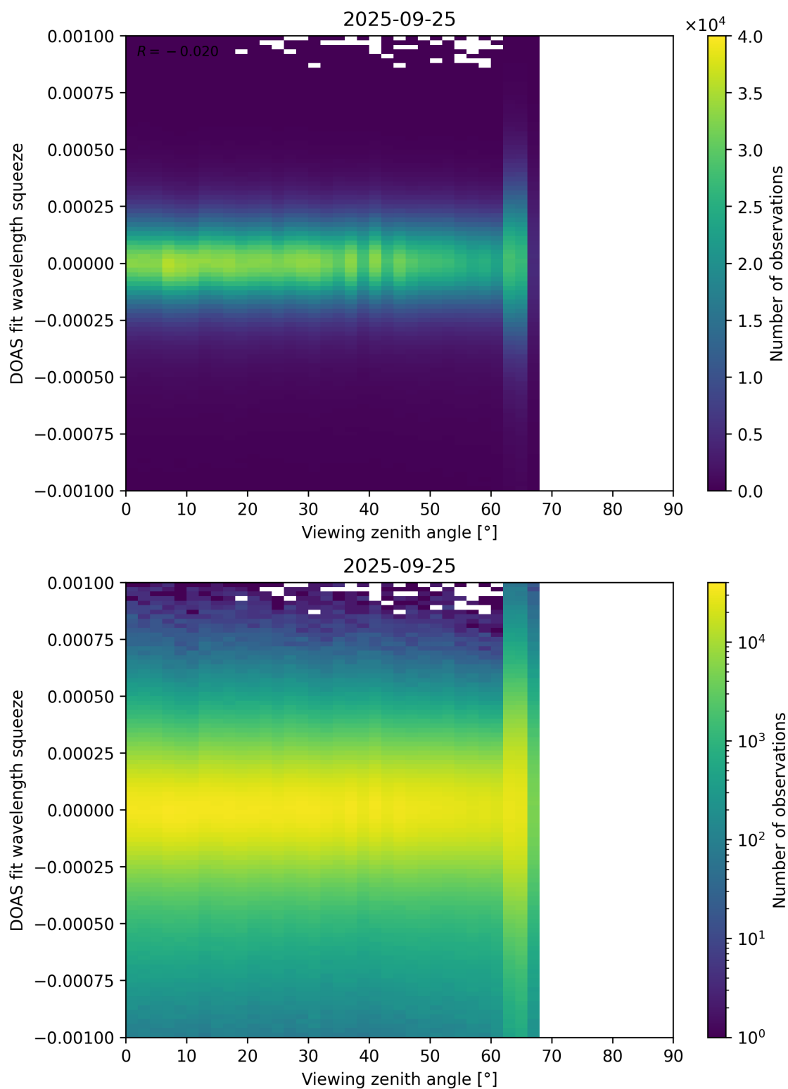
Figure 366: Scatter density plot of “Viewing zenith angle” against “DOAS fit wavelength squeeze” for 2025-09-25 to 2025-09-26.
