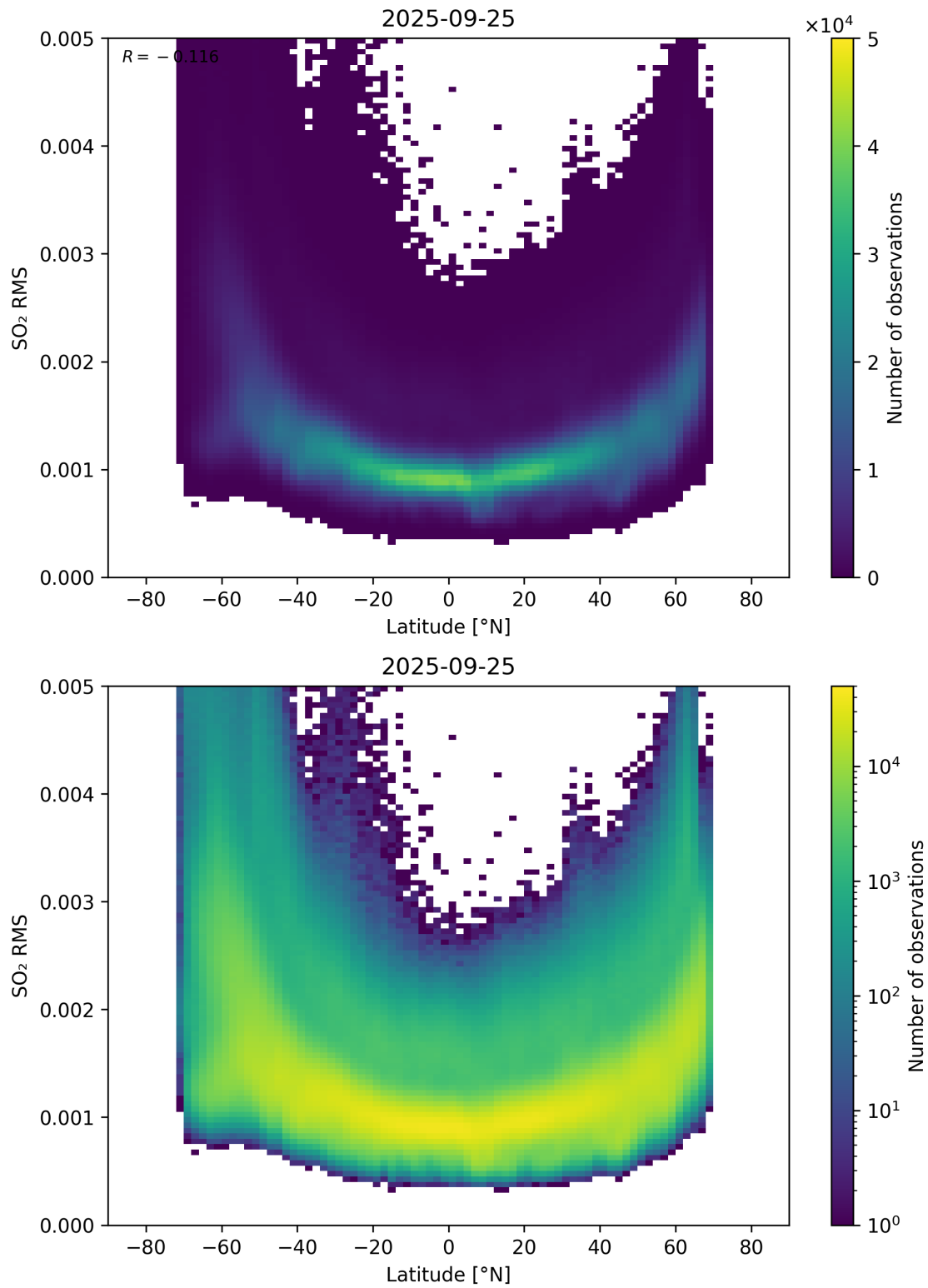
Figure 155: Scatter density plot of “Latitude” against “SO 2 RMS” for 2025-09-25 to 2025-09-26.
