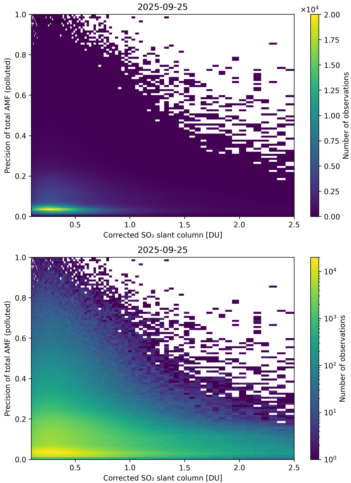
Figure 243: Scatter density plot of “Corrected SO 2 slant column” against “Precision of total AMF (polluted)” for 2025-09-25 to 2025-09-26.
