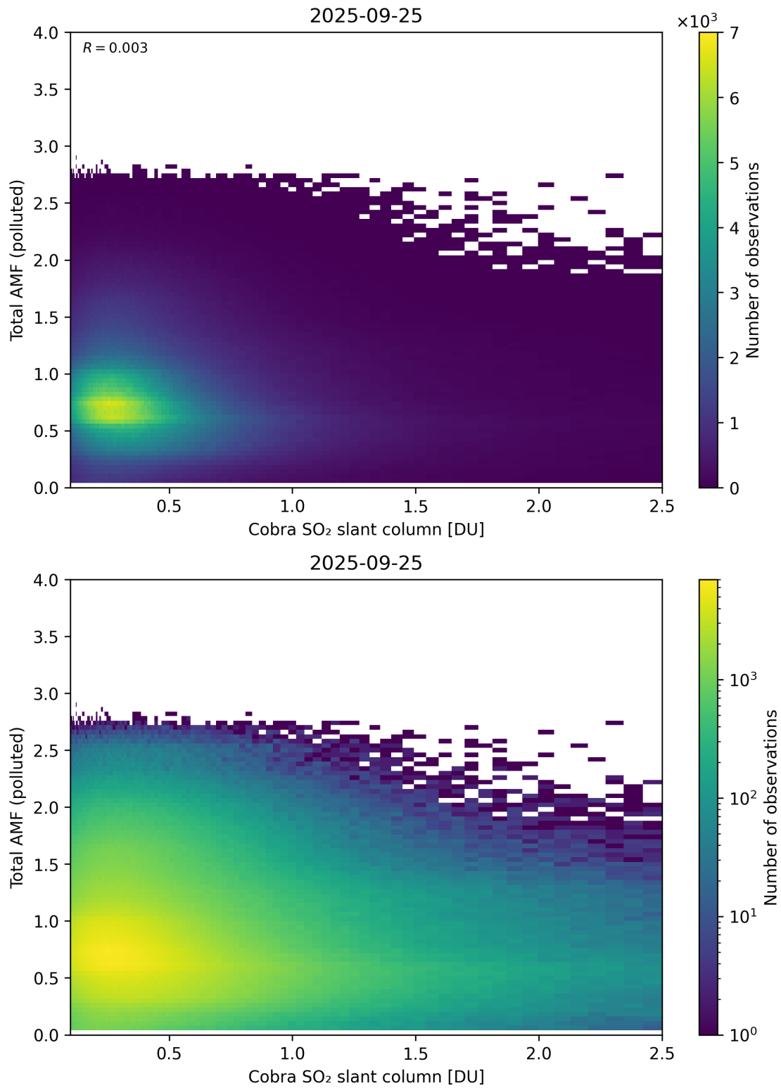
Figure 224: Scatter density plot of “Cobra SO 2 slant column” against “Total AMF (polluted)” for 2025-09-25 to 2025-09-26.
