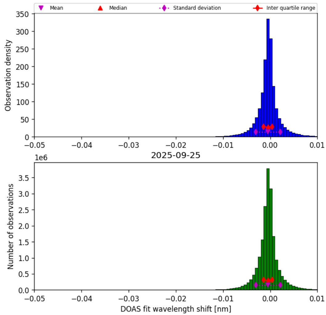
Figure 76: Histogram of “DOAS fit wavelength shift” for 2025-09-25 to 2025-09-26
