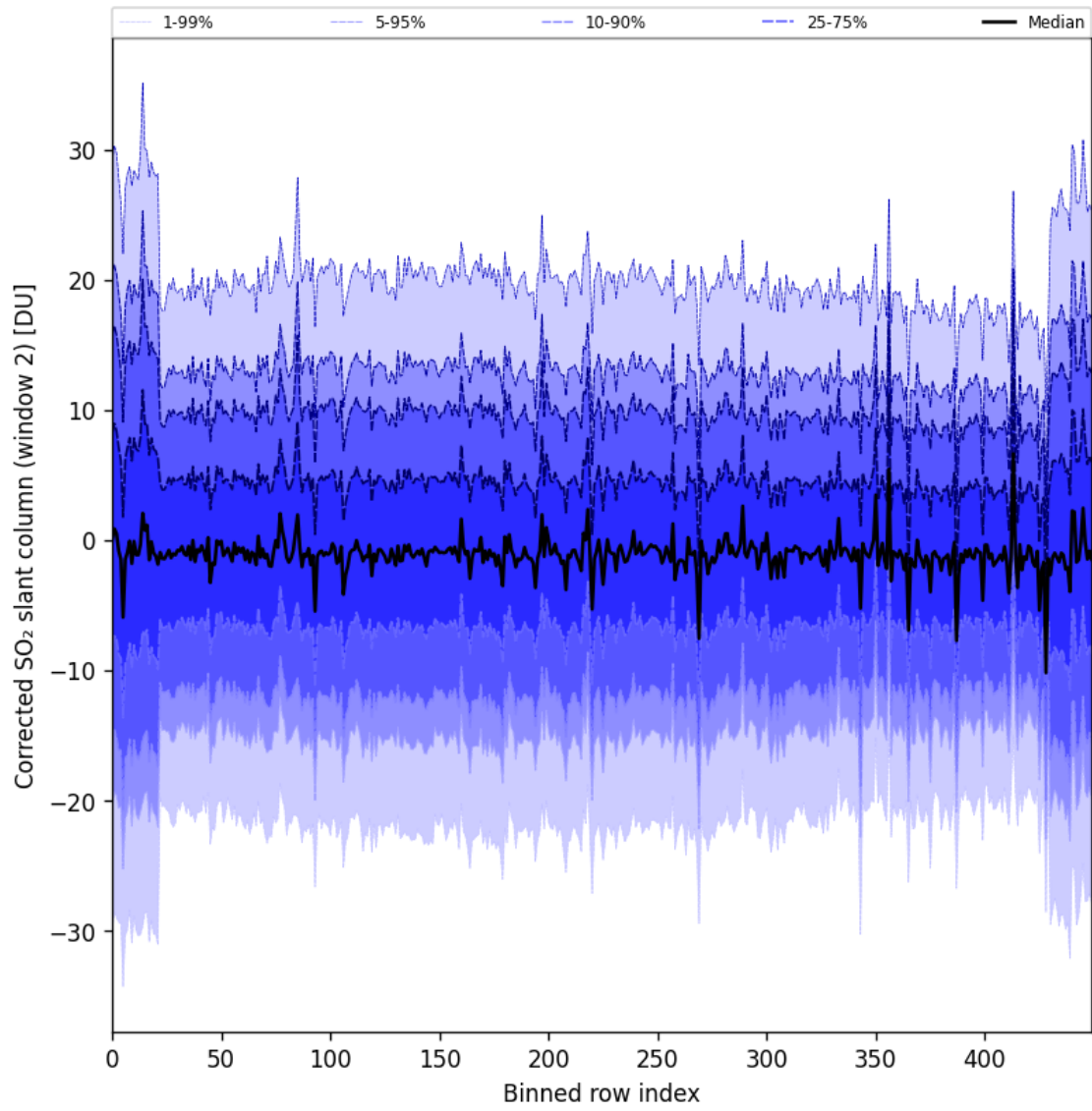
Figure 95: Along track statistics of “Corrected SO 2 slant column (window 2)” for 2025-09-25 to 2025-09-26
