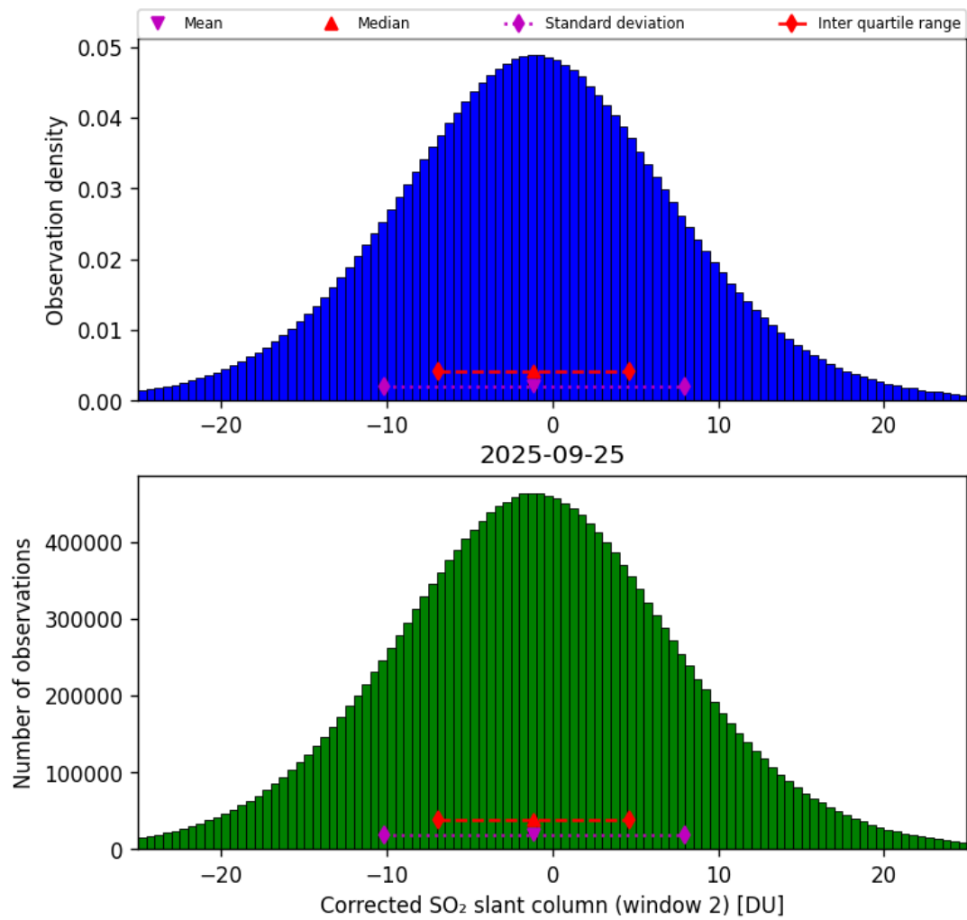
Figure 69: Histogram of “Corrected SO 2 slant column (window 2)” for 2025-09-25 to 2025-09-26
