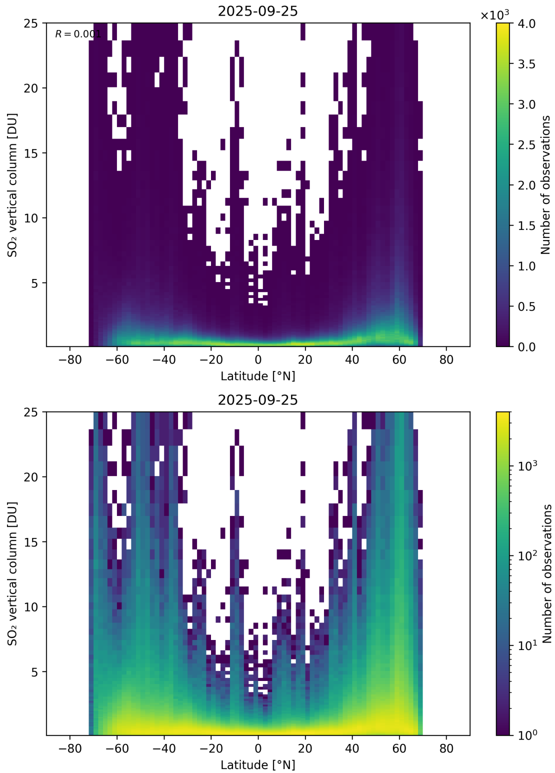
Figure 169: Scatter density plot of “Latitude” against “SO 2 vertical column” for 2025-09-25 to 2025-09-26.
