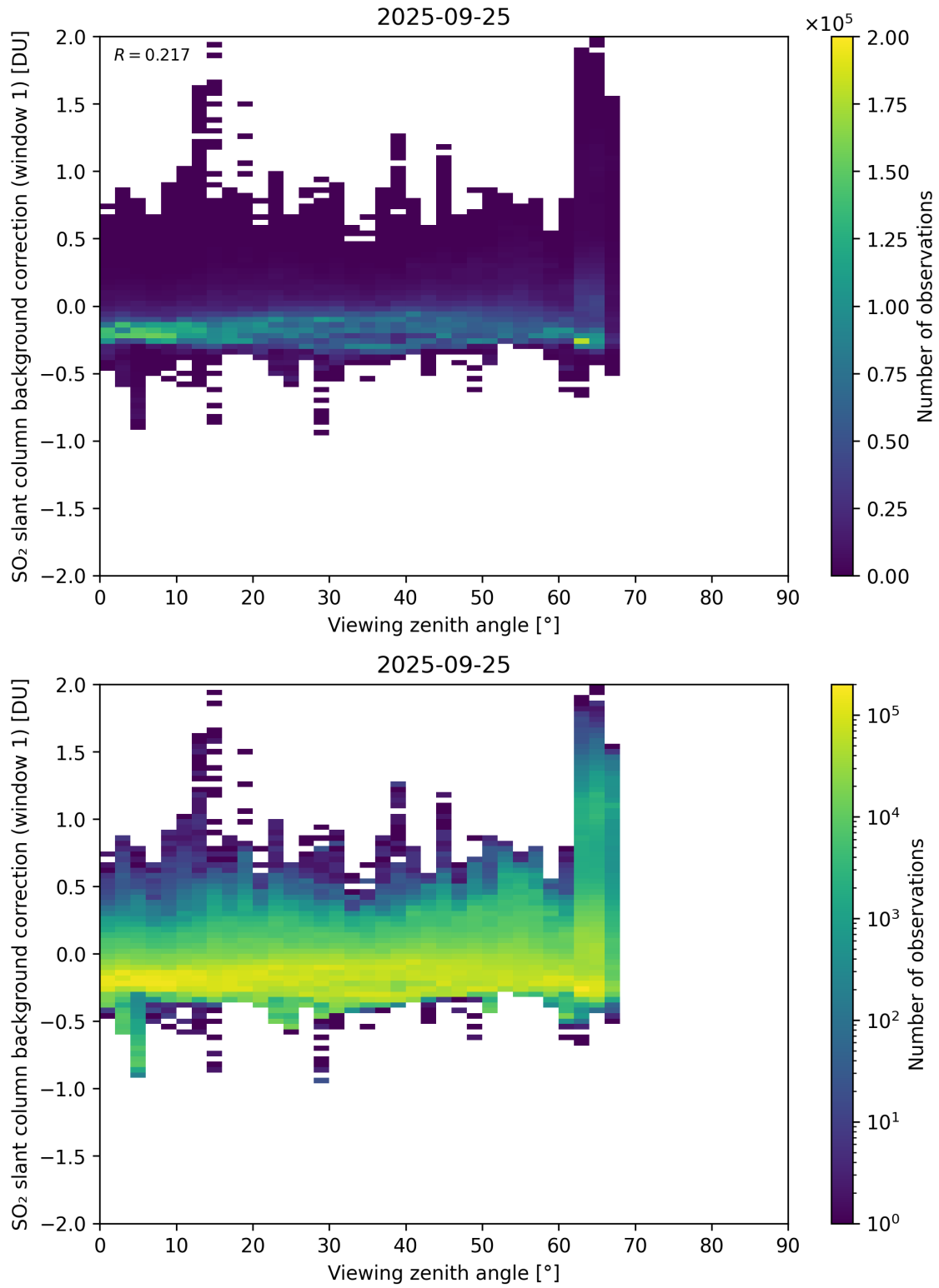
Figure 362: Scatter density plot of “Viewing zenith angle” against “SO 2 slant column background correction (window 1)” for 2025-09-25 to 2025-09-26.
