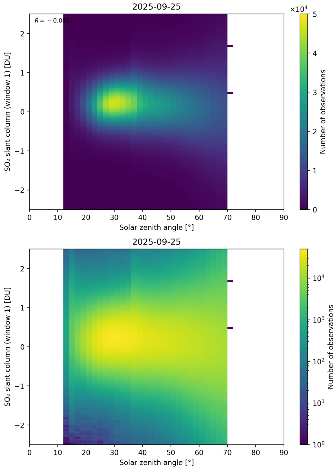
Figure 184: Scatter density plot of “Solar zenith angle” against “SO 2 slant column (window 1)” for 2025-09-25 to 2025-09-26.
