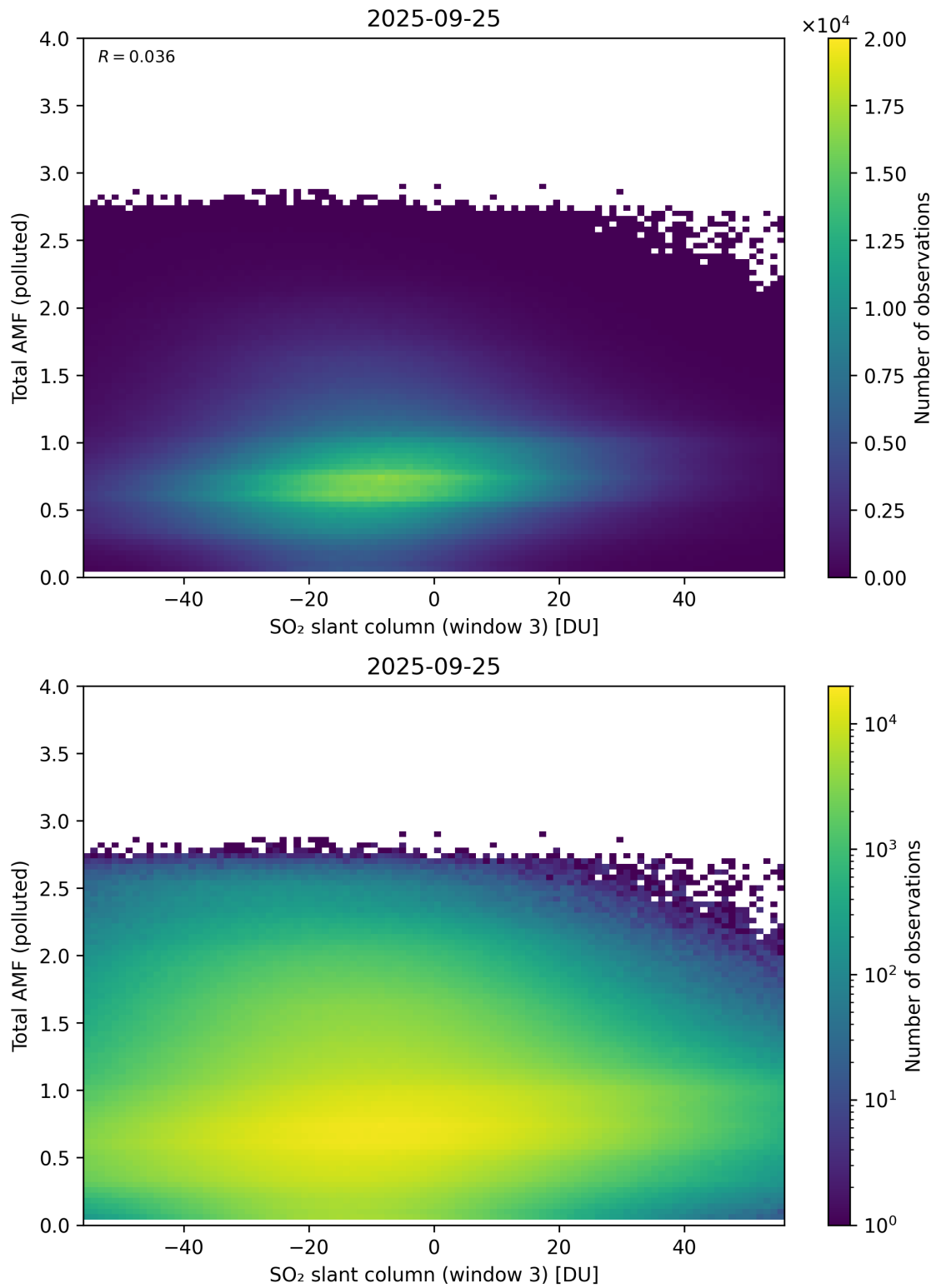
Figure 318: Scatter density plot of “SO 2 slant column (window 3)” against “Total AMF (polluted)” for 2025-09-25 to 2025-09-26.
