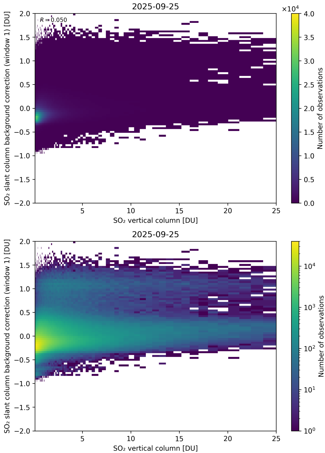
Figure 323: Scatter density plot of “SO 2 vertical column” against “SO 2 slant column background correction (window 1)” for 2025-09-25 to 2025-09-26.
