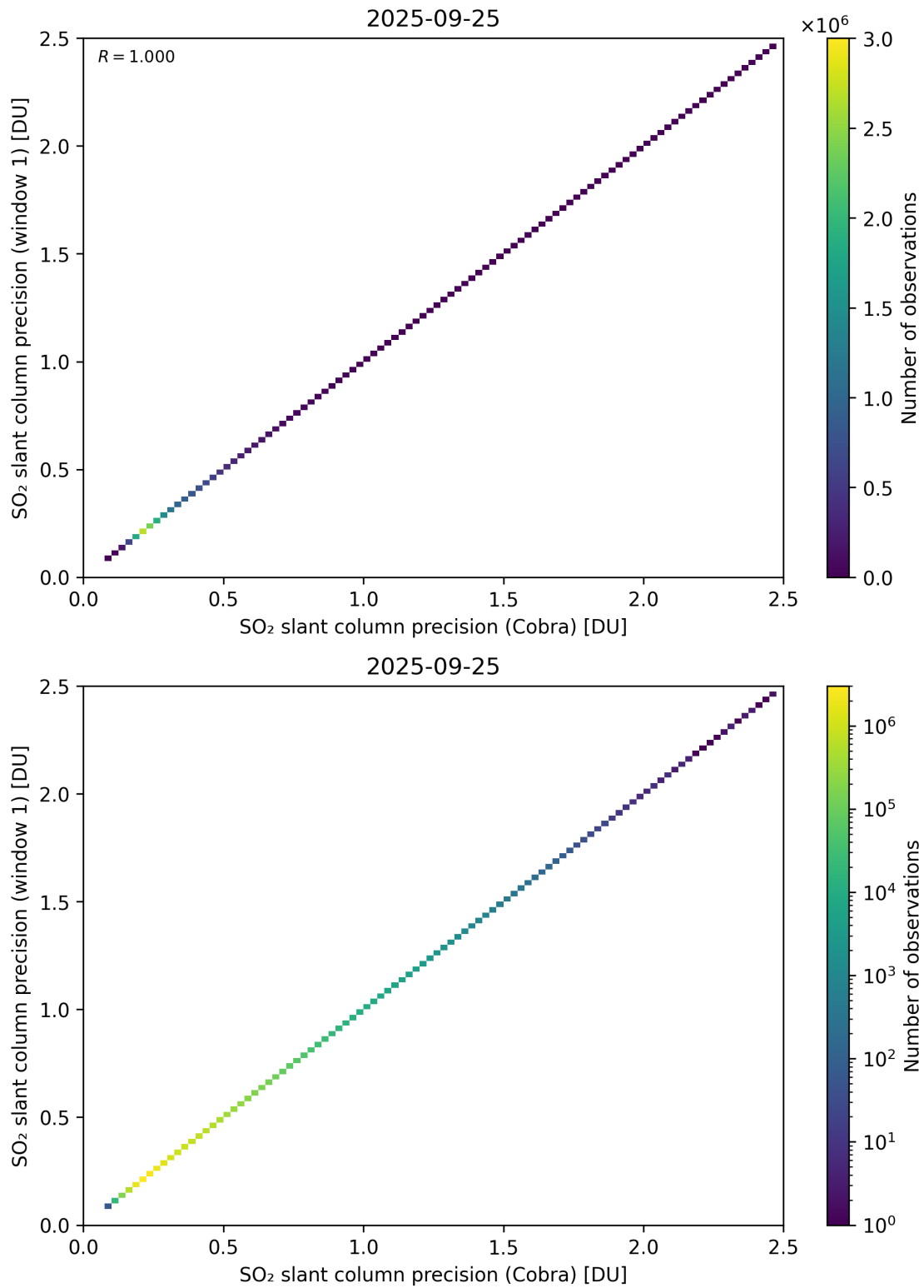
Figure 209: Scatter density plot of “SO 2 slant column precision (Cobra)” against “SO 2 slant column precision (window 1)” for 2025-09-25 to 2025-09-26.
