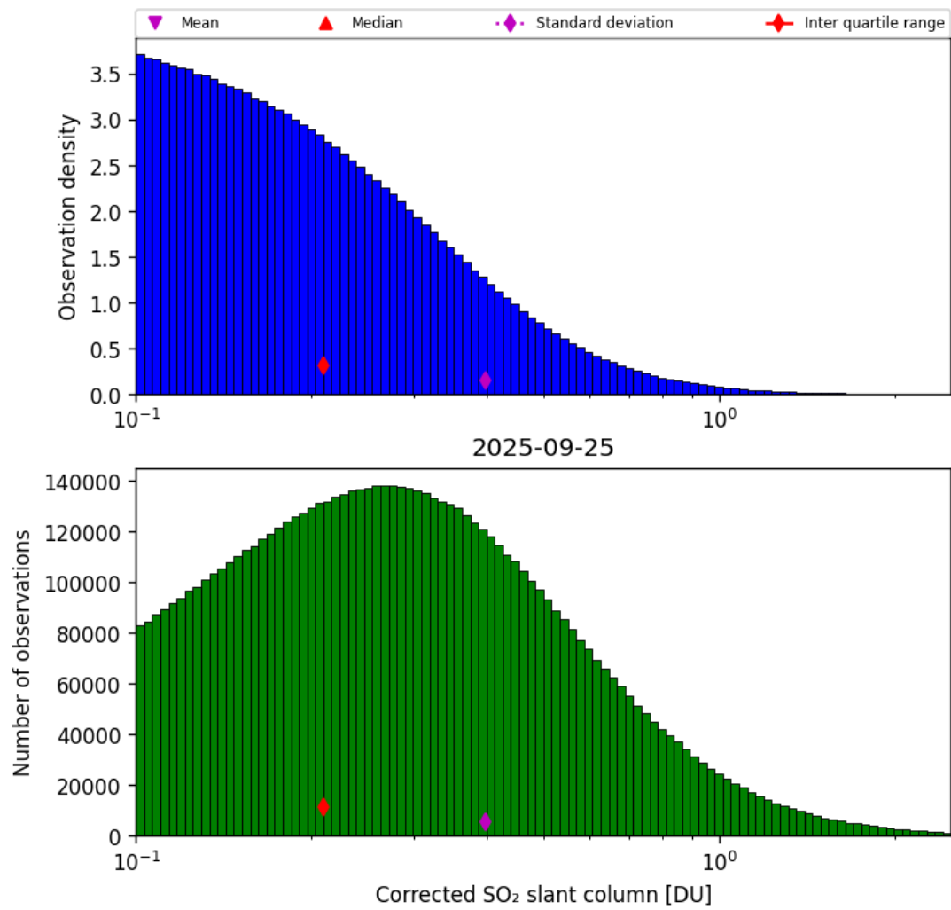
Figure 60: Histogram of “Corrected SO 2 slant column” for 2025-09-25 to 2025-09-26
