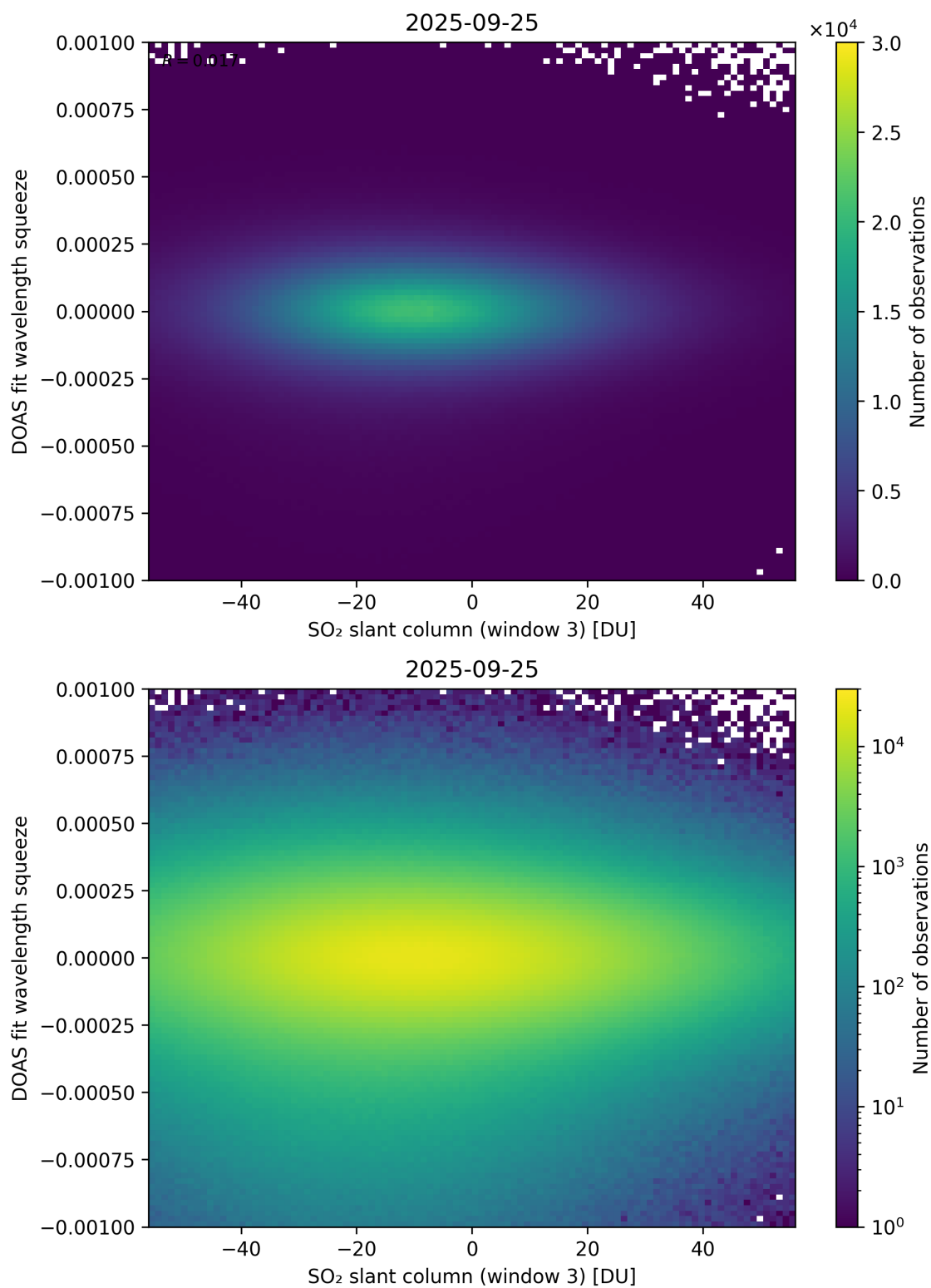
Figure 305: Scatter density plot of “SO 2 slant column (window 3)” against “DOAS fit wavelength squeeze” for 2025-09-25 to 2025-09-26.
