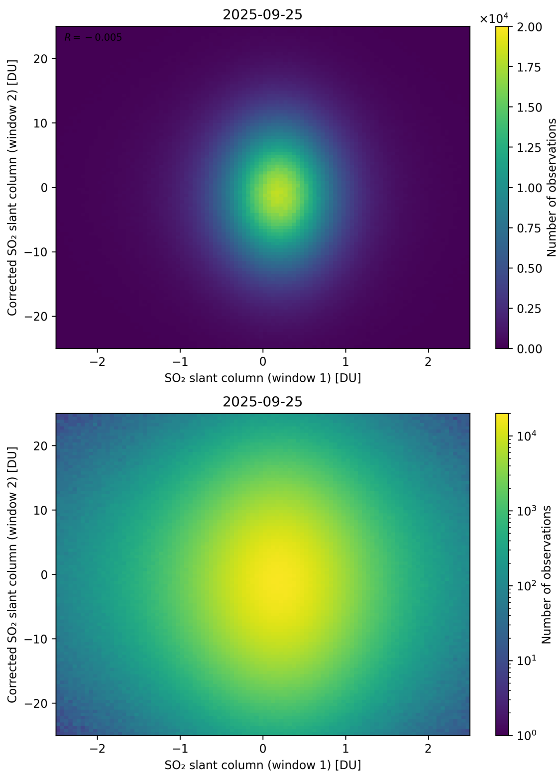
Figure 283: Scatter density plot of “SO 2 slant column (window 1)” against “Corrected SO 2 slant column (window 2)” for 2025-09-25 to 2025-09-26.
