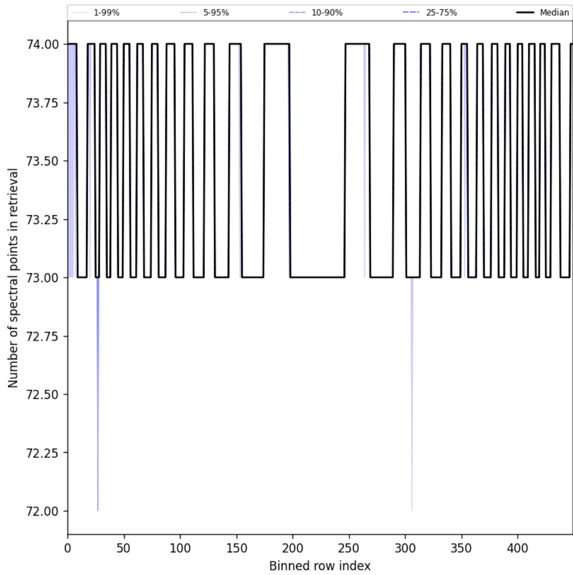
Figure 108: Along track statistics of “Number of spectral points in retrieval” for 2025-09-25 to 2025-09-26
