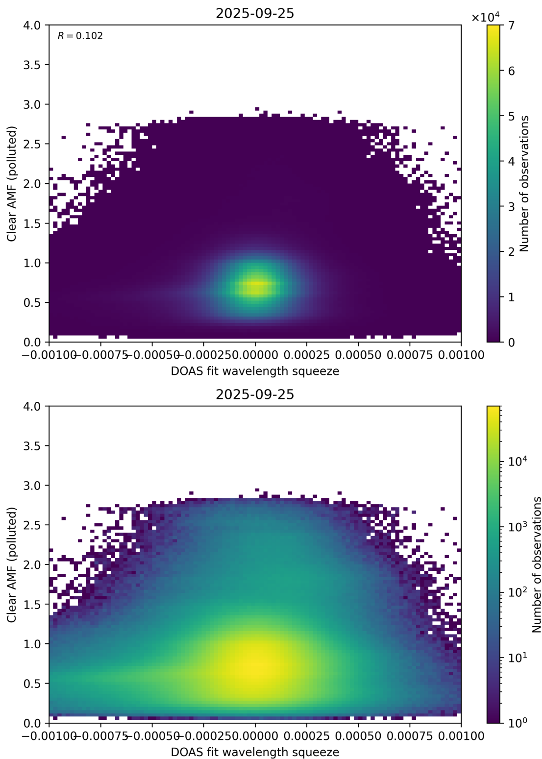
Figure 144: Scatter density plot of “DOAS fit wavelength squeeze” against “Clear AMF (polluted)” for 2025-09-25 to 2025-09-26.
