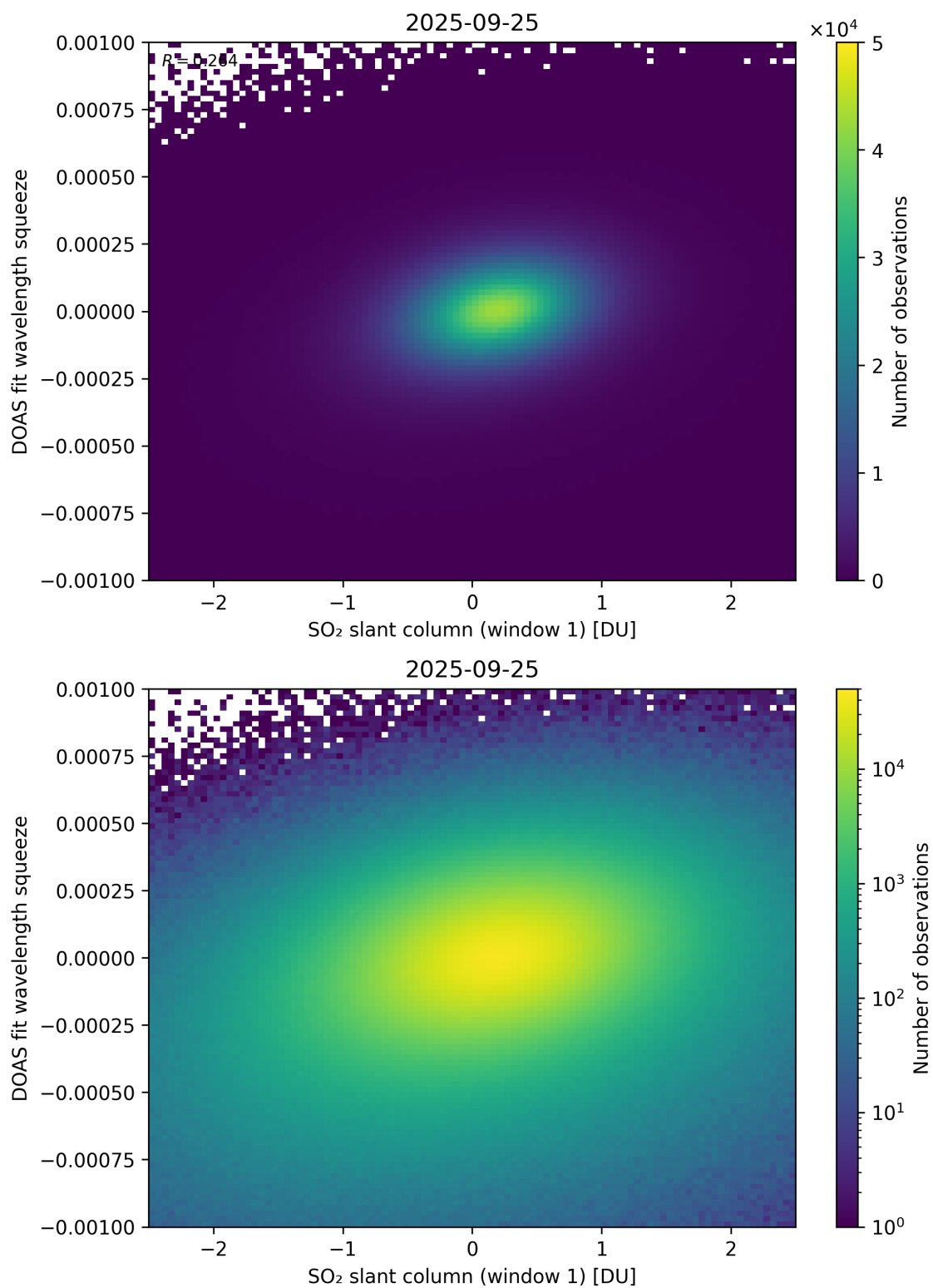
Figure 266: Scatter density plot of “SO 2 slant column (window 1)” against “DOAS fit wavelength squeeze” for 2025-09-25 to 2025-09-26.
