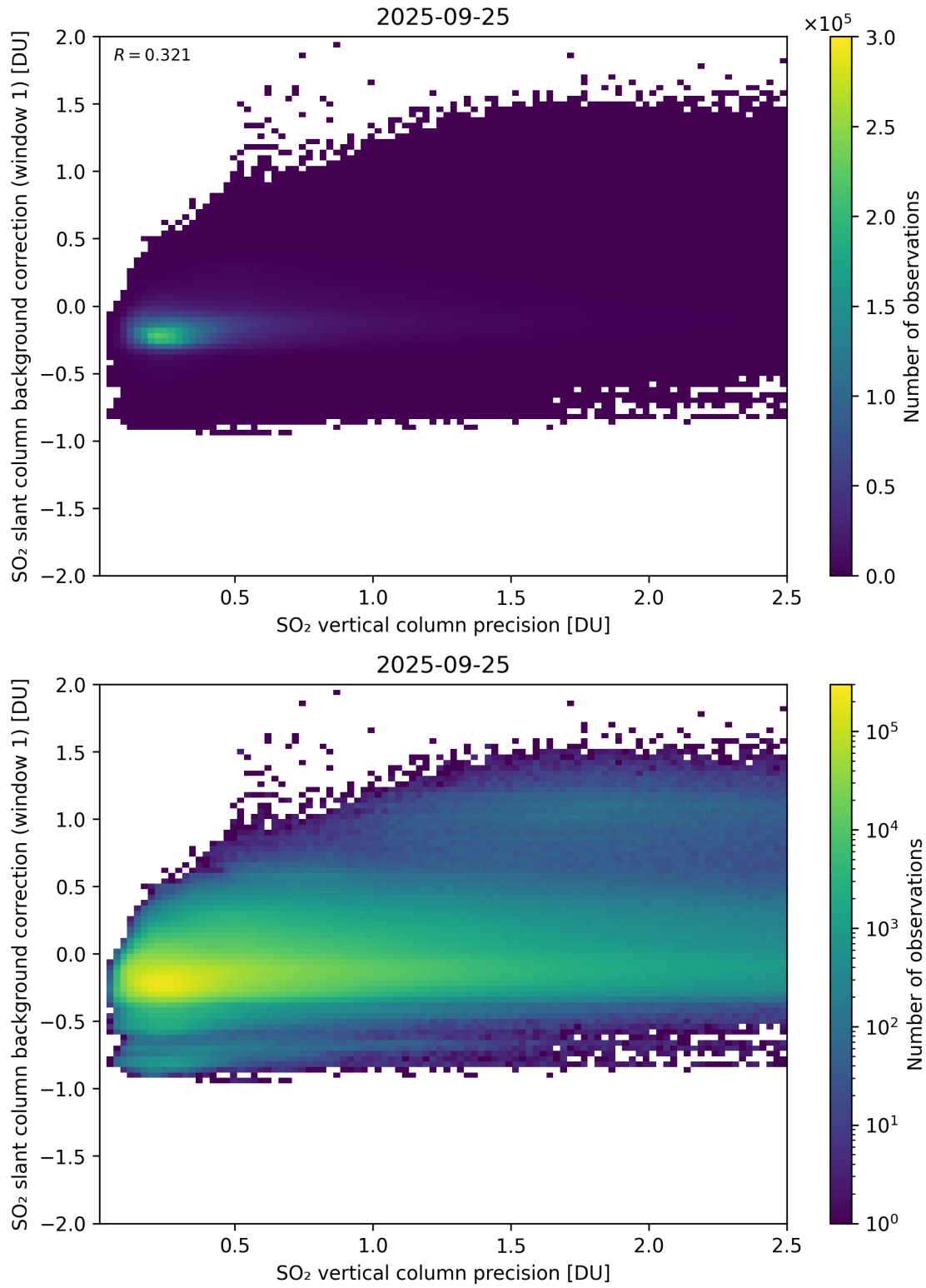
Figure 329: Scatter density plot of “SO 2 vertical column precision” against “SO 2 slant column background correction (window 1)” for 2025-09-25 to 2025-09-26.
