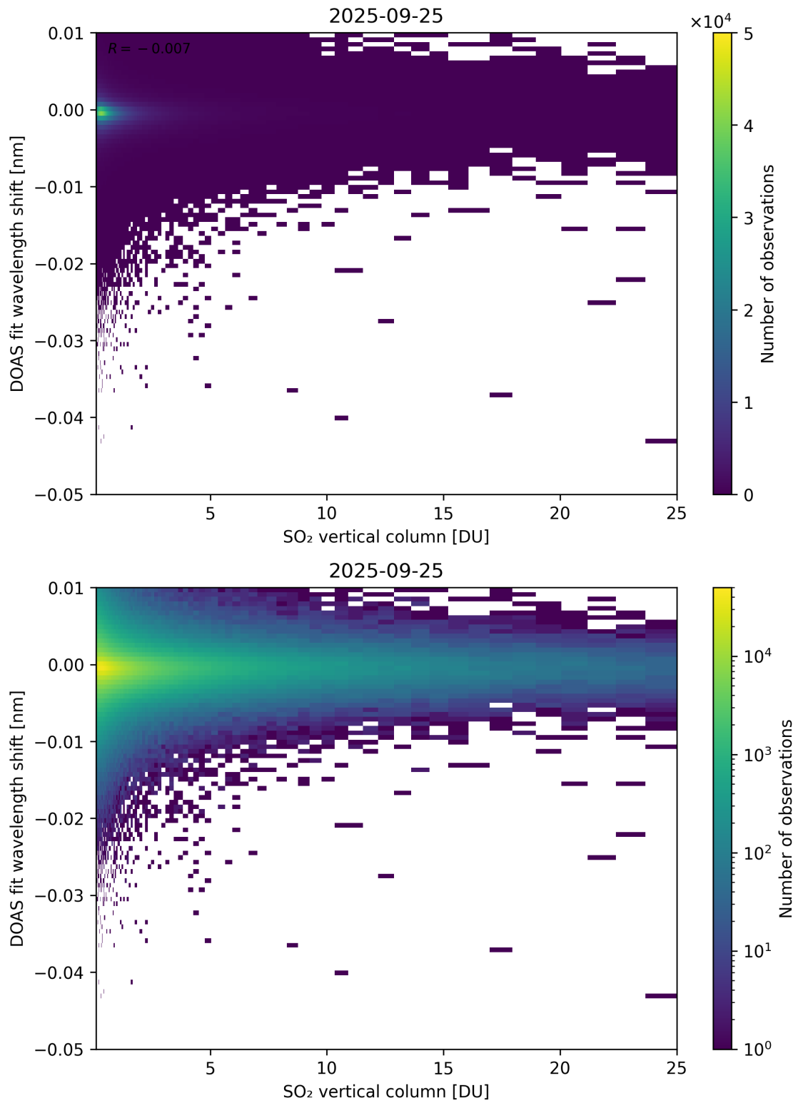
Figure 326: Scatter density plot of “SO 2 vertical column” against “DOAS fit wavelength shift” for 2025-09-25 to 2025-09-26.
