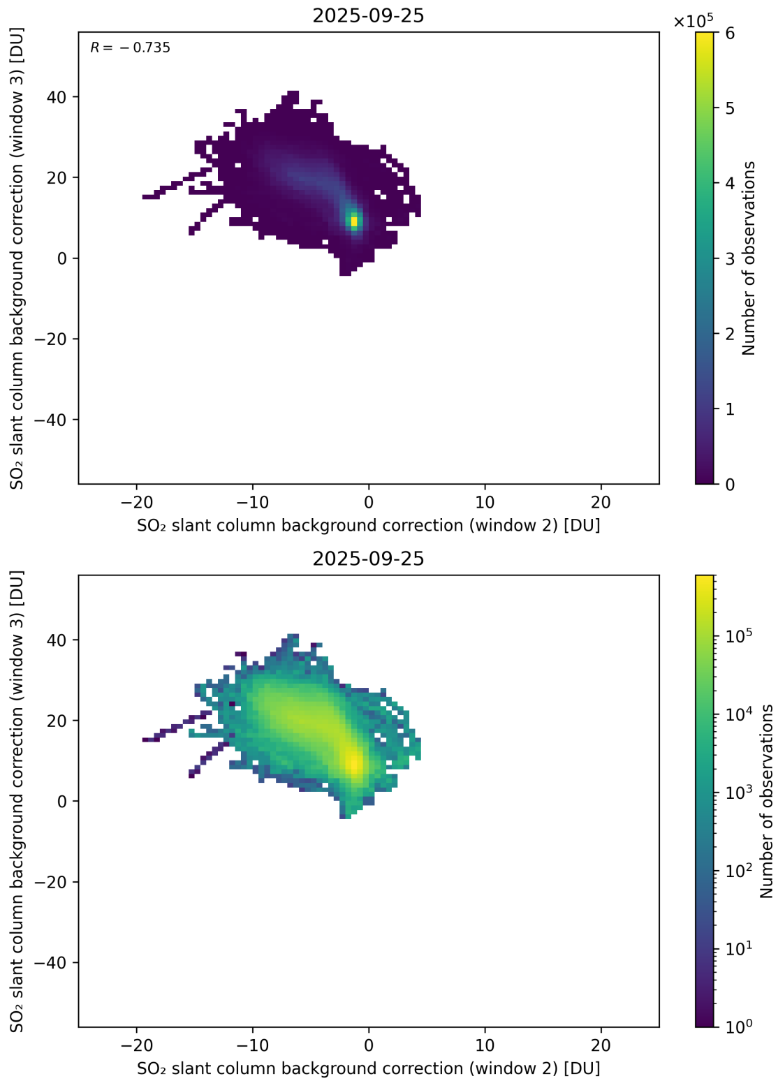
Figure 122: Scatter density plot of “SO 2 slant column background correction (window 2)” against “SO 2 slant column background correction (window 3)” for 2025-09-25 to 2025-09-26.
