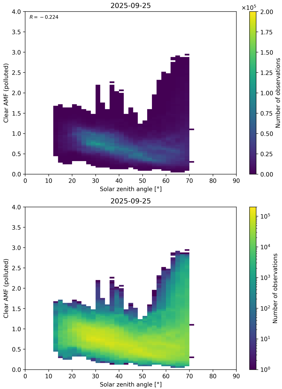
Figure 178: Scatter density plot of “Solar zenith angle” against “Clear AMF (polluted)” for 2025-09-25 to 2025-09-26.
