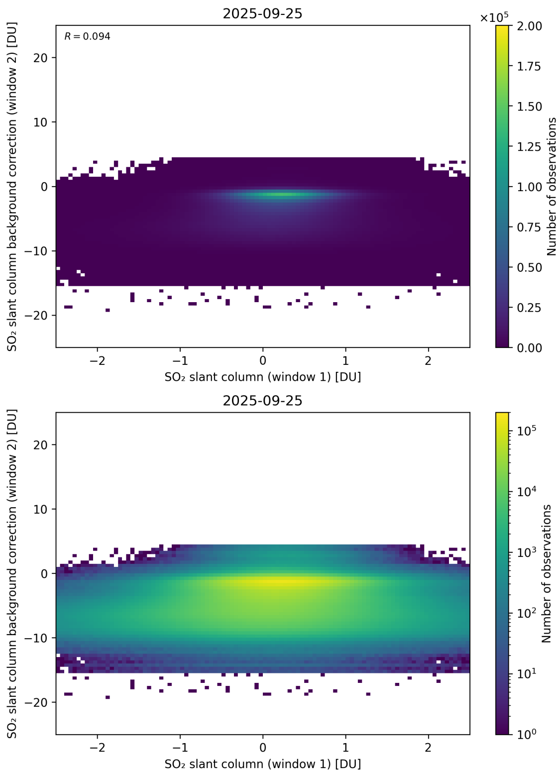
Figure 263: Scatter density plot of “SO 2 slant column (window 1)” against “SO 2 slant column background correction (window 2)” for 2025-09-25 to 2025-09-26.
