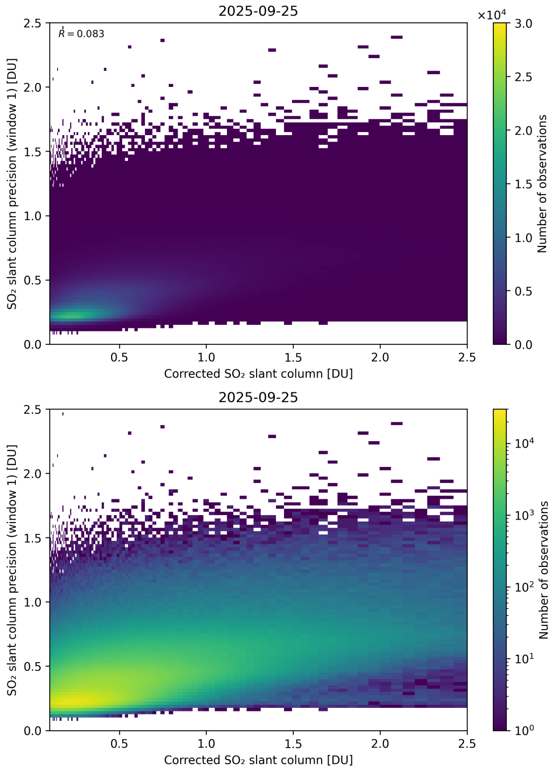
Figure 238: Scatter density plot of “Corrected SO 2 slant column” against “SO 2 slant column precision (window 1)” for 2025-09-25 to 2025-09-26.
