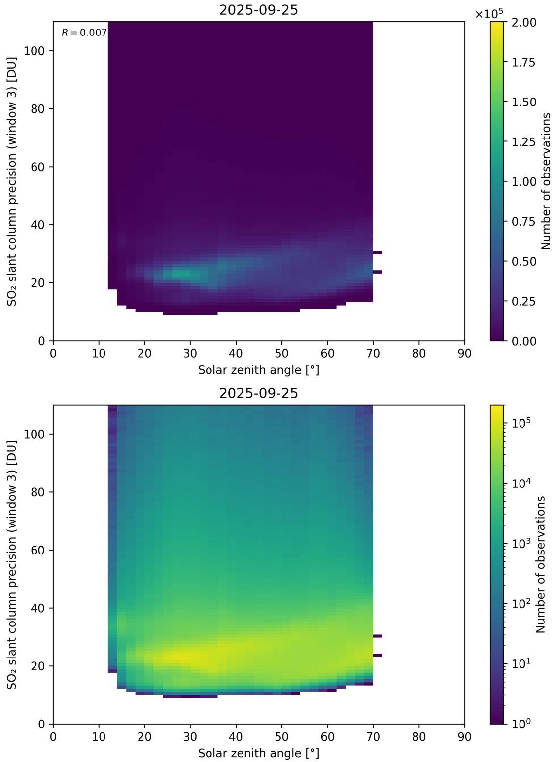
Figure 188: Scatter density plot of “Solar zenith angle” against “SO 2 slant column precision (window 3)” for 2025-09-25 to 2025-09-26.
