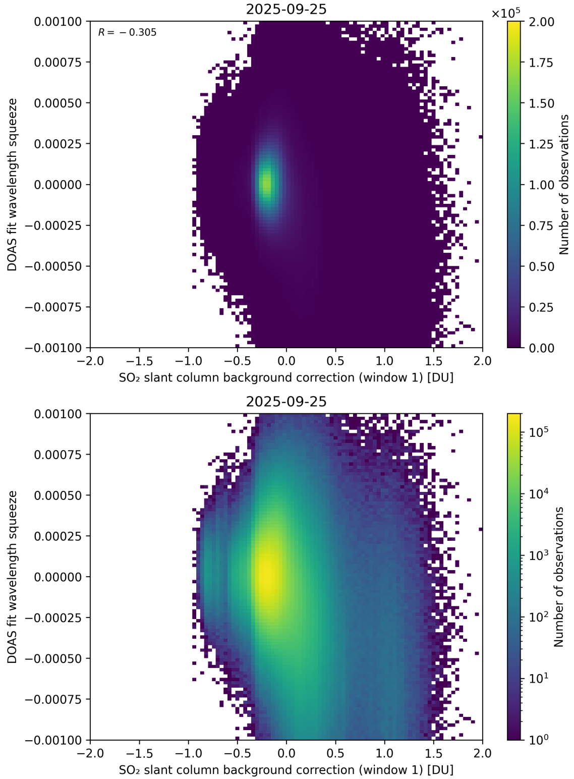
Figure 112: Scatter density plot of “SO 2 slant column background correction (window 1)” against “DOAS fit wavelength squeeze” for 2025-09-25 to 2025-09-26.
