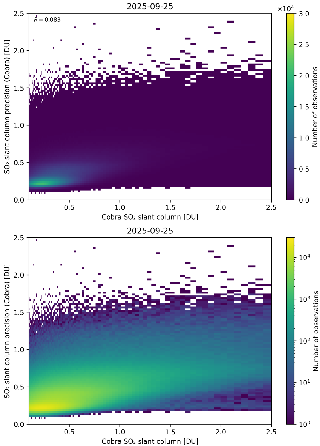
Figure 216: Scatter density plot of “Cobra SO 2 slant column” against “SO 2 slant column precision (Cobra)” for 2025-09-25 to 2025-09-26.
