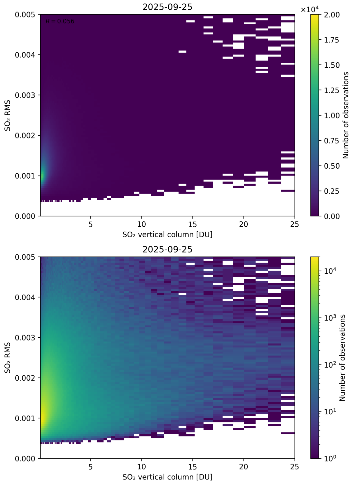
Figure 328: Scatter density plot of “SO 2 vertical column” against “SO 2 RMS” for 2025-09-25 to 2025-09-26.
