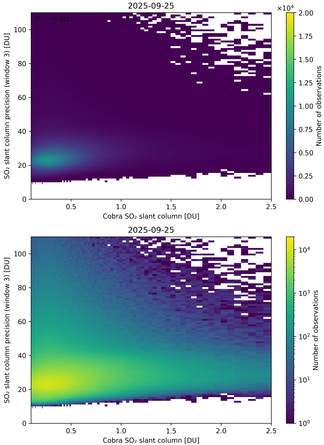
Figure 223: Scatter density plot of “Cobra SO 2 slant column” against “SO 2 slant column precision (window 3)” for 2025-09-25 to 2025-09-26.
