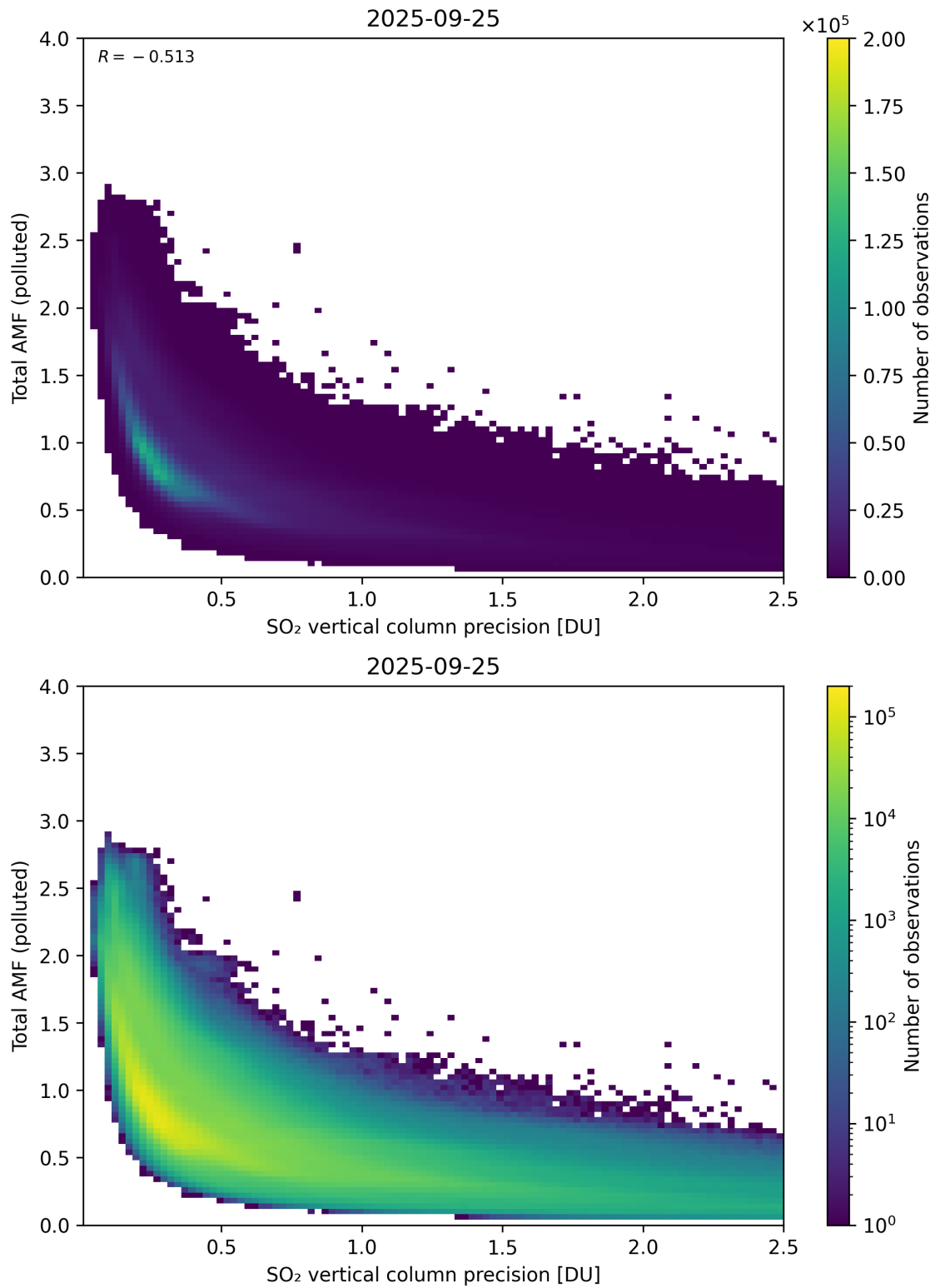
Figure 346: Scatter density plot of “SO 2 vertical column precision” against “Total AMF (polluted)” for 2025-09-25 to 2025-09-26.
