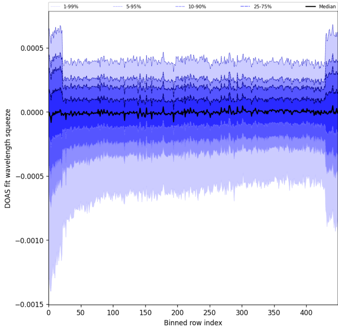
Figure 103: Along track statistics of “DOAS fit wavelength squeeze” for 2025-09-25 to 2025-09-26
