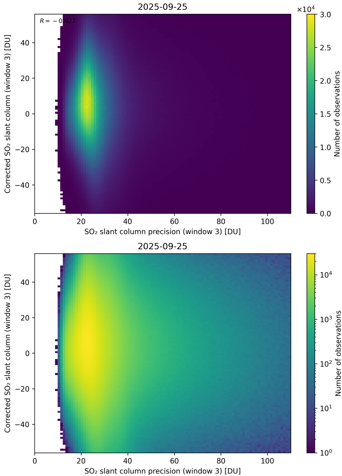
Figure 312: Scatter density plot of “SO 2 slant column precision (window 3)” against “Corrected SO 2 slant column (window 3)” for 2025-09-25 to 2025-09-26.
