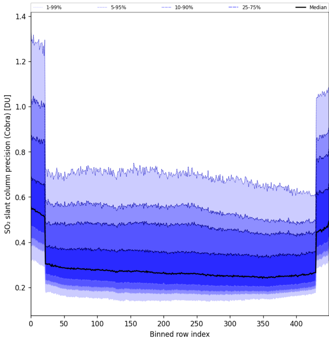
Figure 88: Along track statistics of “SO 2 slant column precision (Cobra)” for 2025-09-25 to 2025-09-26
