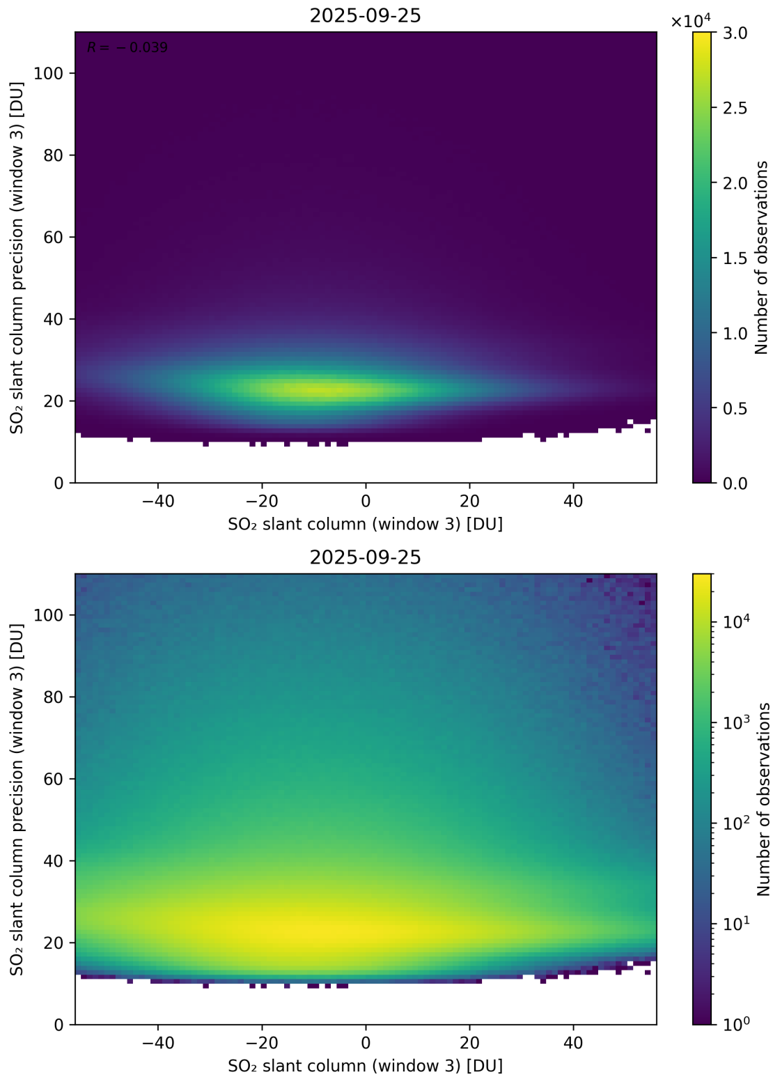
Figure 317: Scatter density plot of “SO 2 slant column (window 3)” against “SO 2 slant column precision (window 3)” for 2025-09-25 to 2025-09-26.
