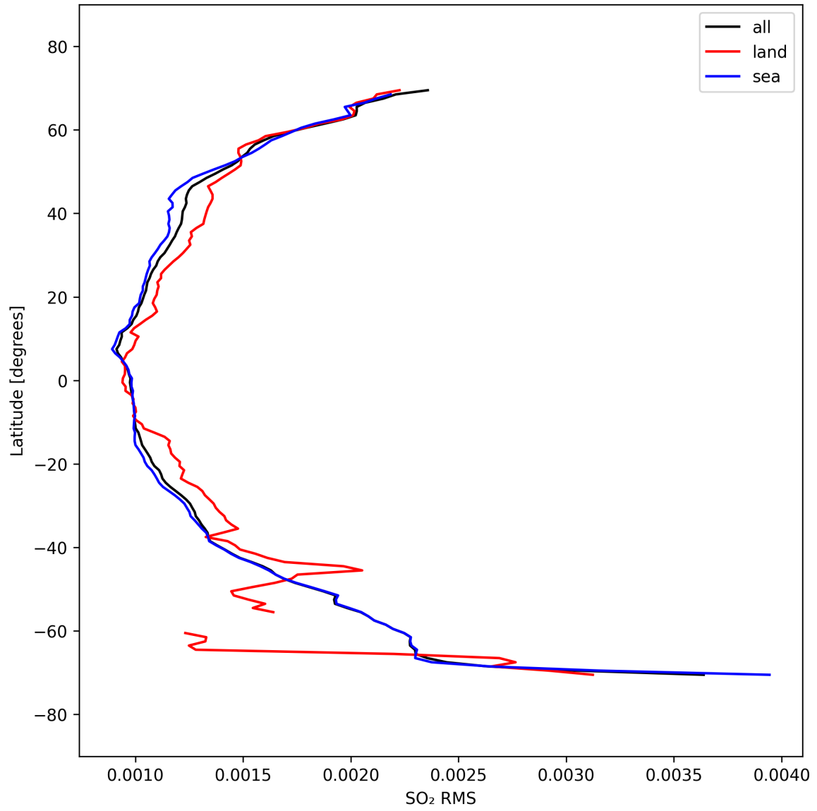
Figure 52: Zonal average of “SO 2 RMS” for 2025-09-25 to 2025-09-26.
