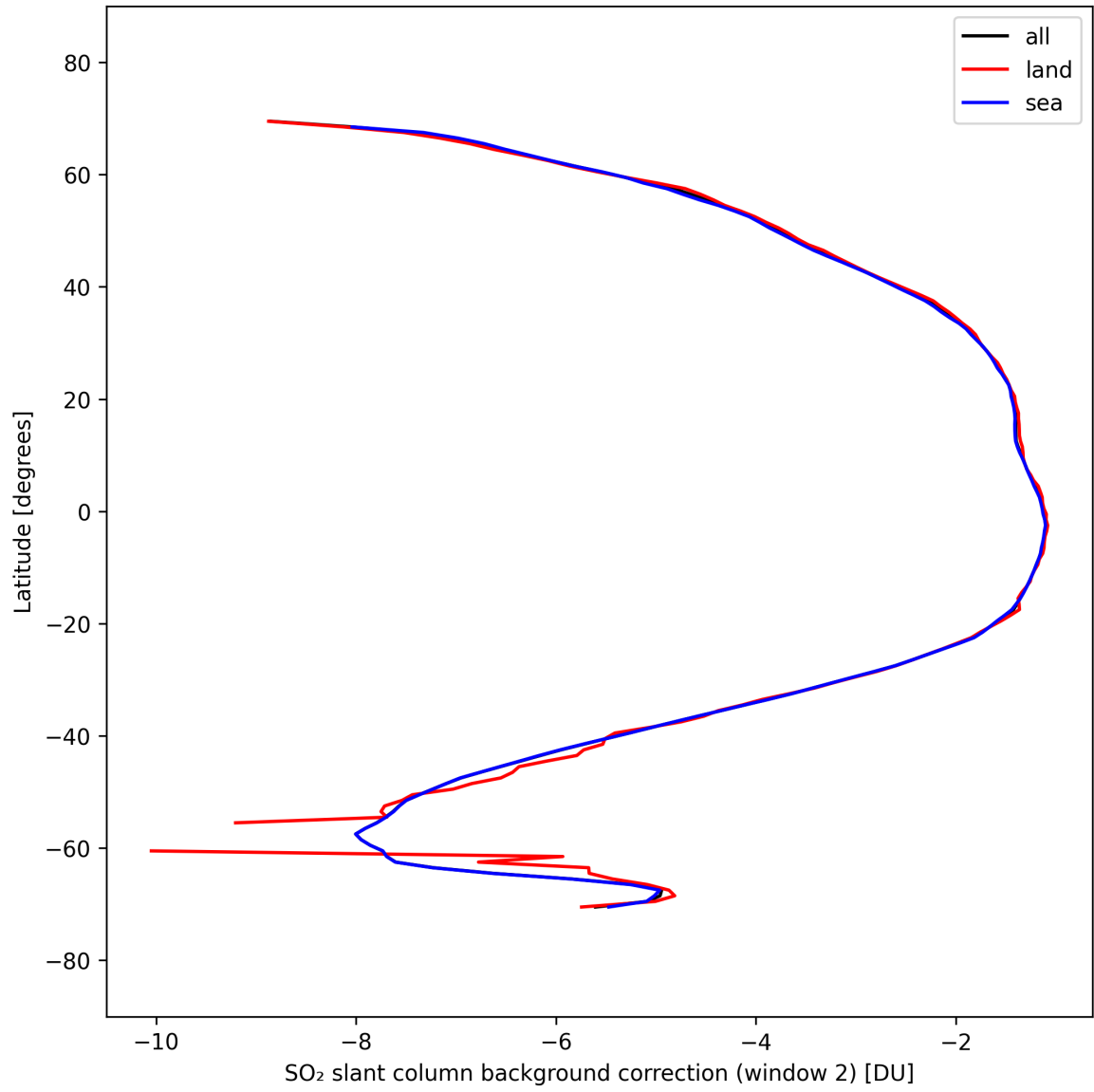
Figure 44: Zonal average of “SO 2 slant column background correction (window 2)” for 2025-09-25 to 2025-09-26.
