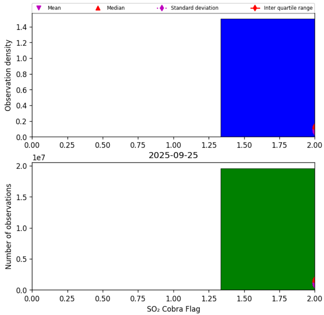
Figure 75: Histogram of “SO 2 Cobra Flag” for 2025-09-25 to 2025-09-26
