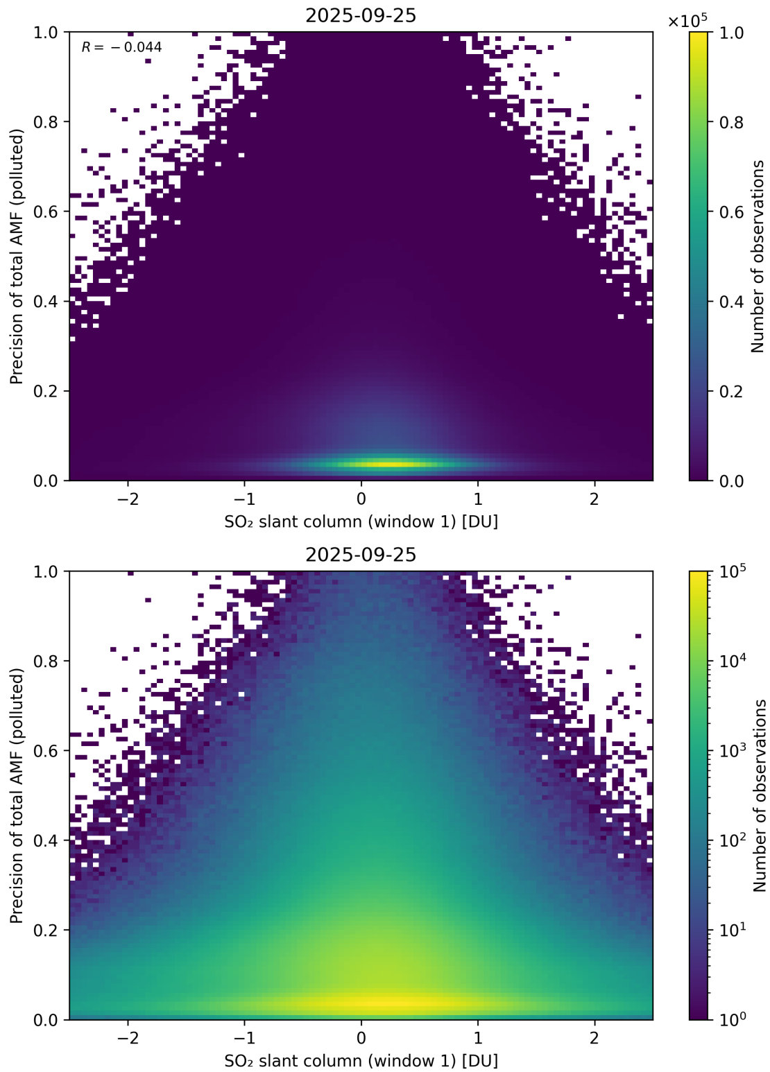
Figure 290: Scatter density plot of “SO 2 slant column (window 1)” against “Precision of total AMF (polluted)” for 2025-09-25 to 2025-09-26.
