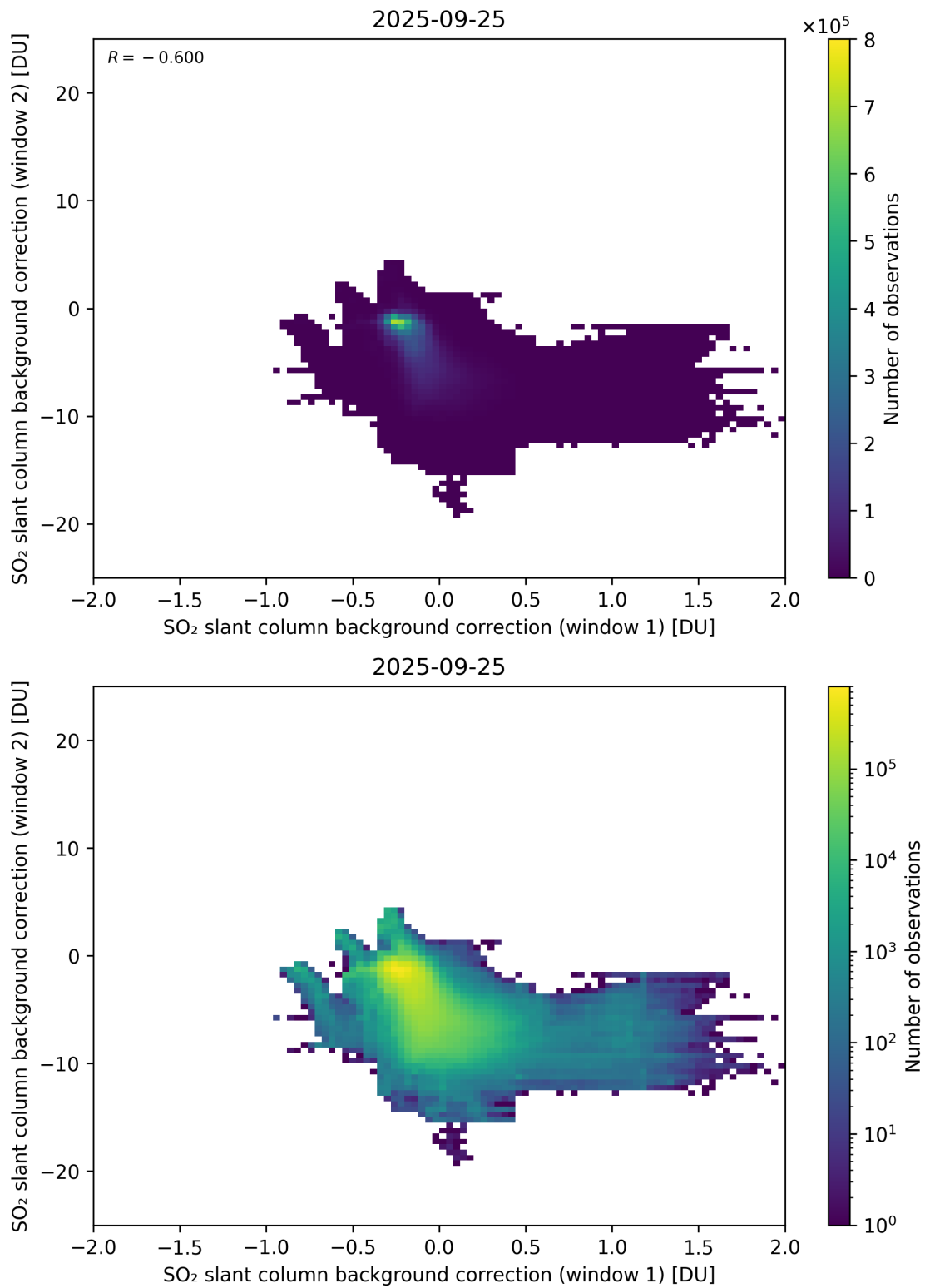
Figure 109: Scatter density plot of “SO 2 slant column background correction (window 1)” against “SO 2 slant column background correction (window 2)” for 2025-09-25 to 2025-09-26.
