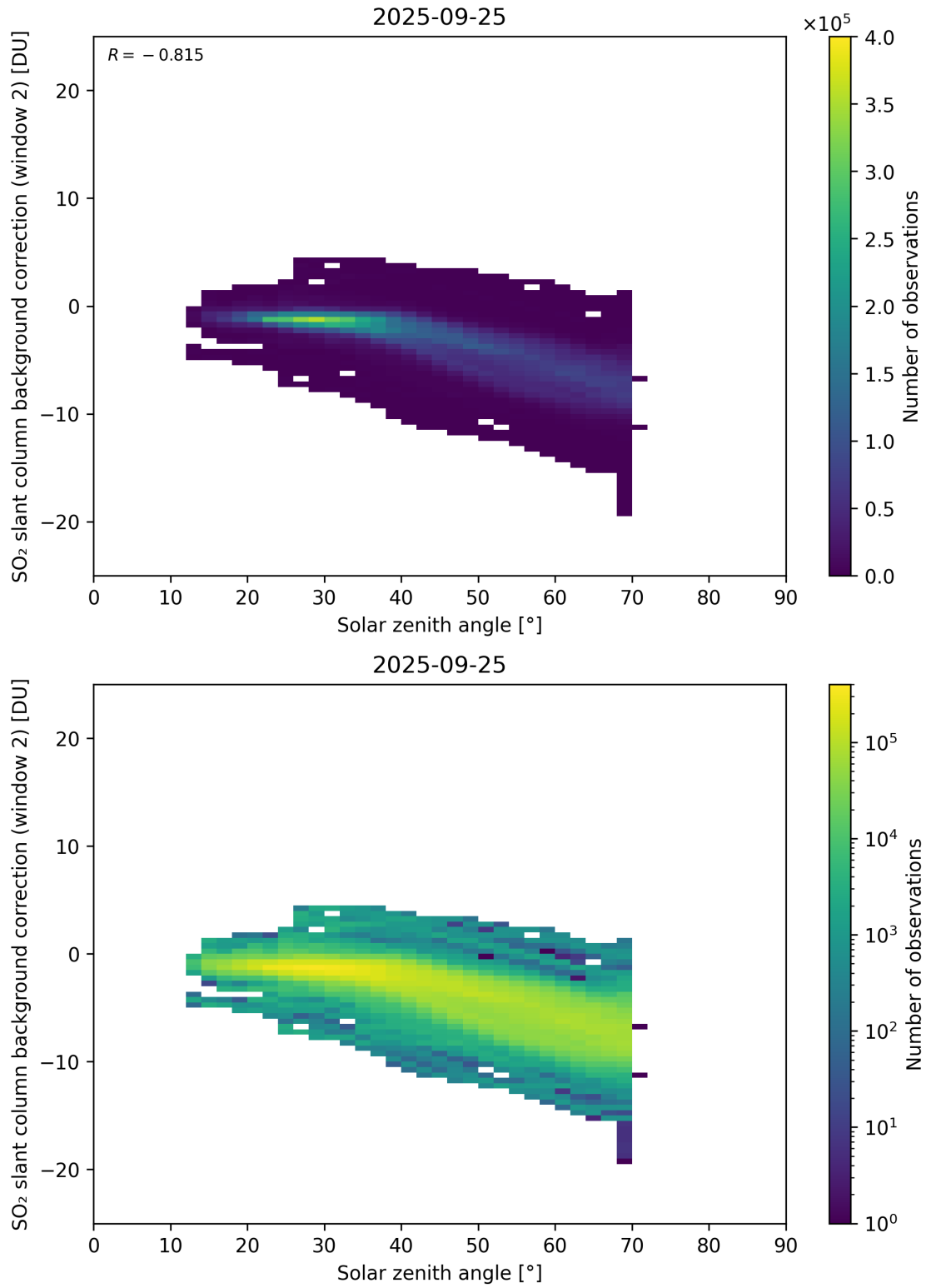
Figure 172: Scatter density plot of “Solar zenith angle” against “SO 2 slant column background correction (window 2)” for 2025-09-25 to 2025-09-26.
