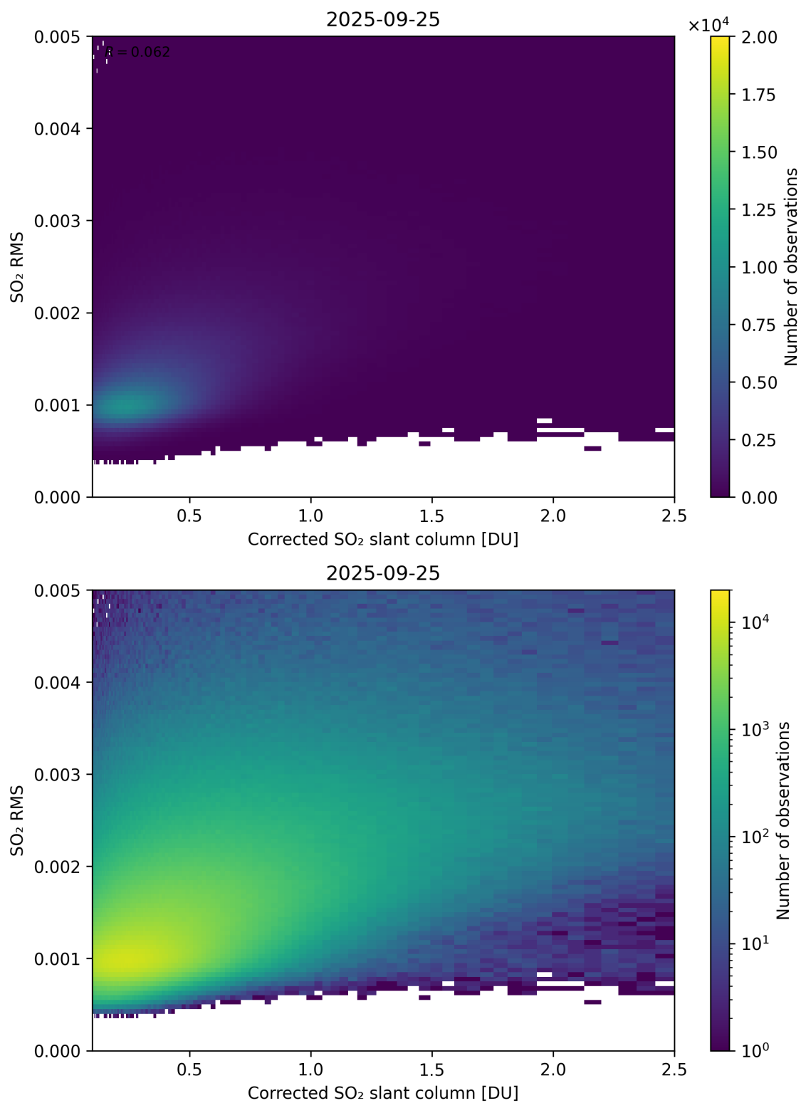
Figure 231: Scatter density plot of “Corrected SO 2 slant column” against “SO 2 RMS” for 2025-09-25 to 2025-09-26.
