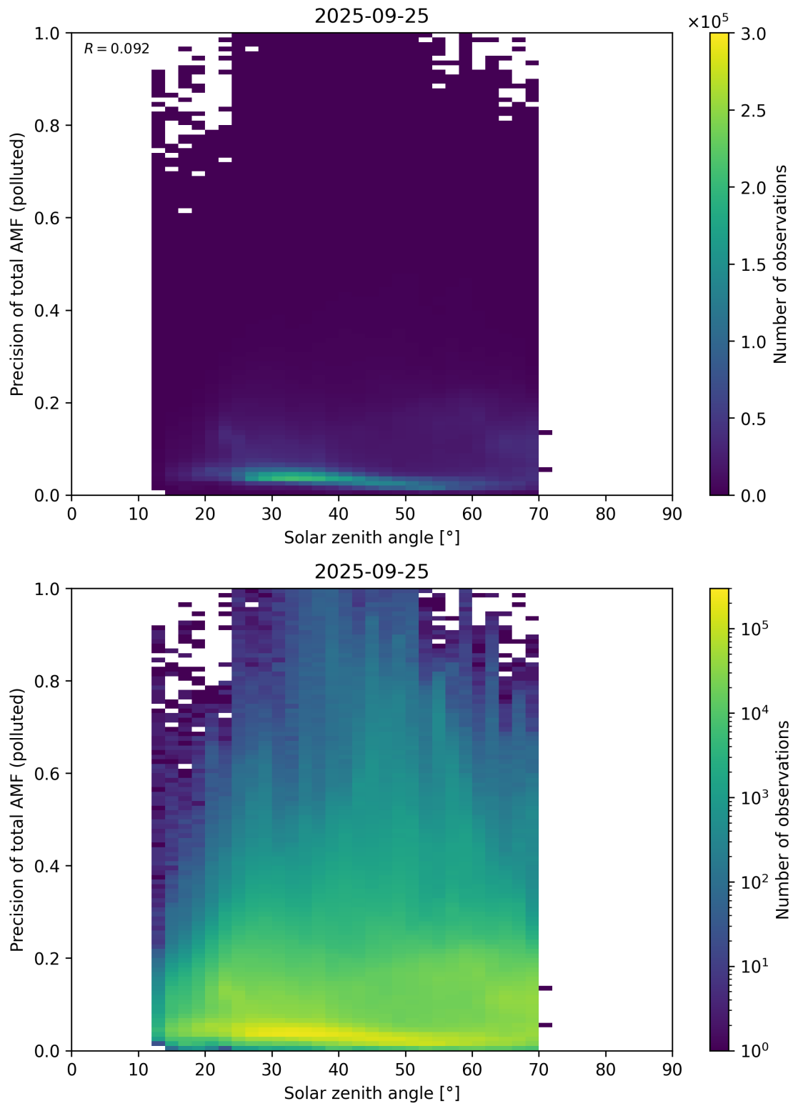
Figure 190: Scatter density plot of “Solar zenith angle” against “Precision of total AMF (polluted)” for 2025-09-25 to 2025-09-26.
