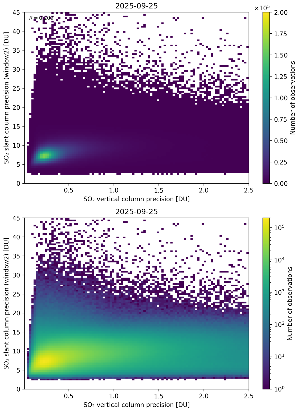
Figure 343: Scatter density plot of “SO 2 vertical column precision” against “SO 2 slant column precision (window2)” for 2025-09-25 to 2025-09-26.
