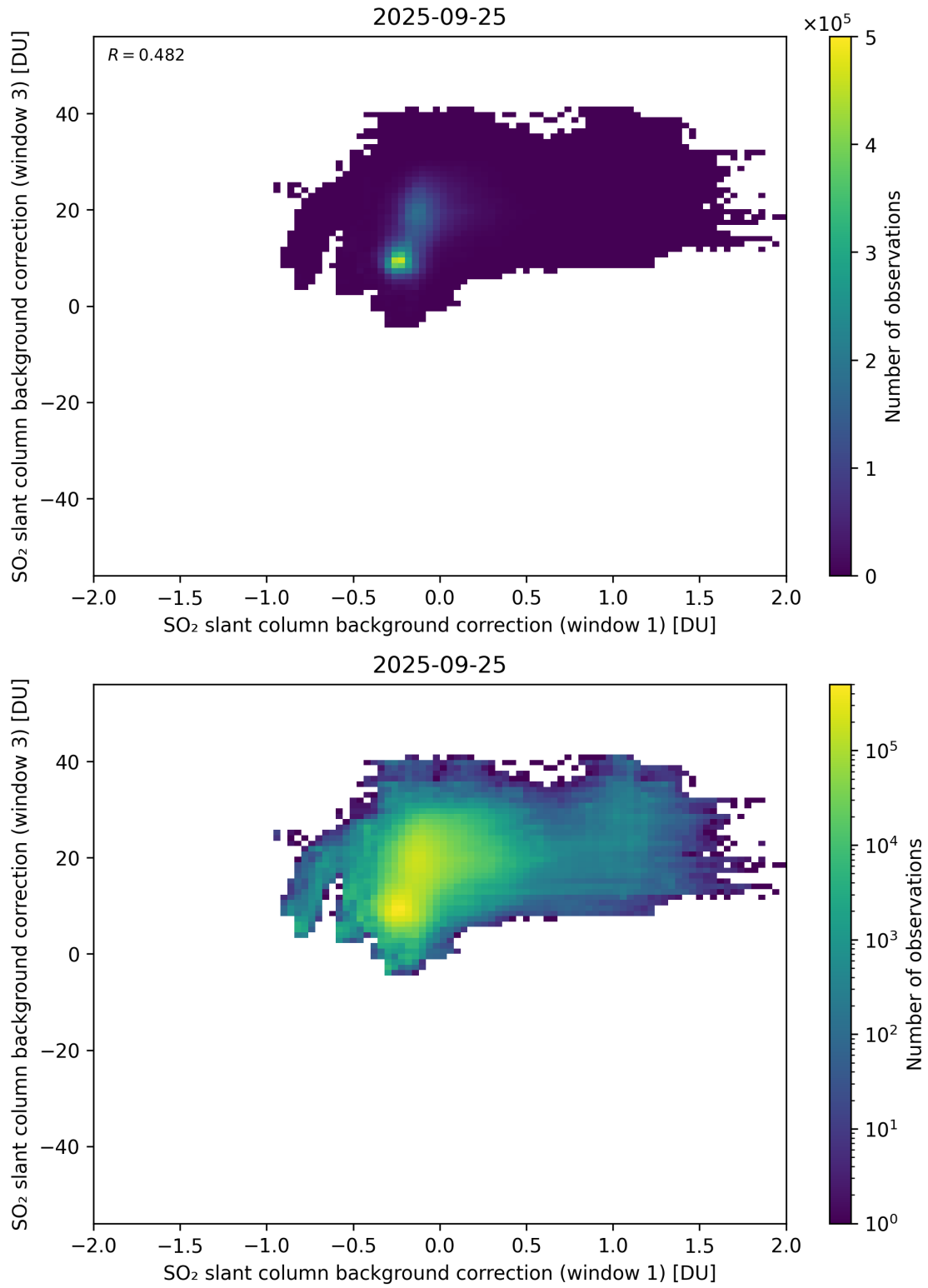
Figure 110: Scatter density plot of “SO 2 slant column background correction (window 1)” against “SO 2 slant column background correction (window 3)” for 2025-09-25 to 2025-09-26.
