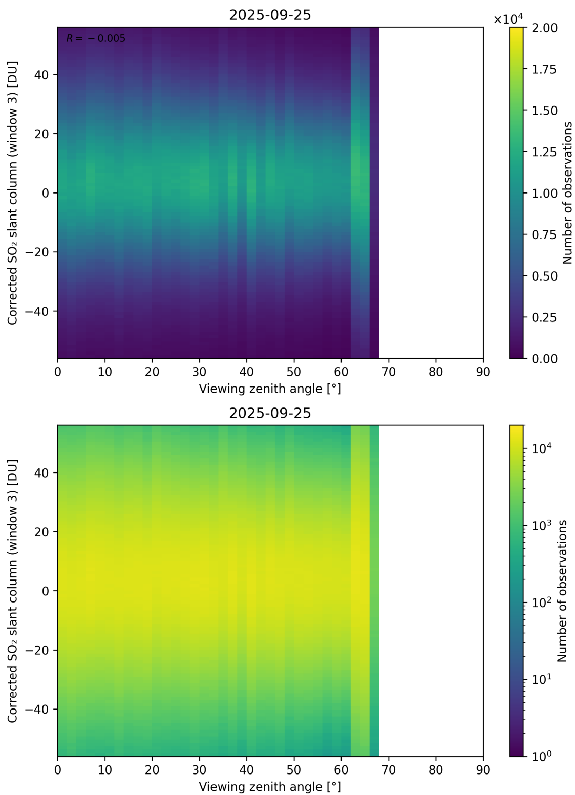
Figure 375: Scatter density plot of “Viewing zenith angle” against “Corrected SO 2 slant column (window 3)” for 2025-09-25 to 2025-09-26.
