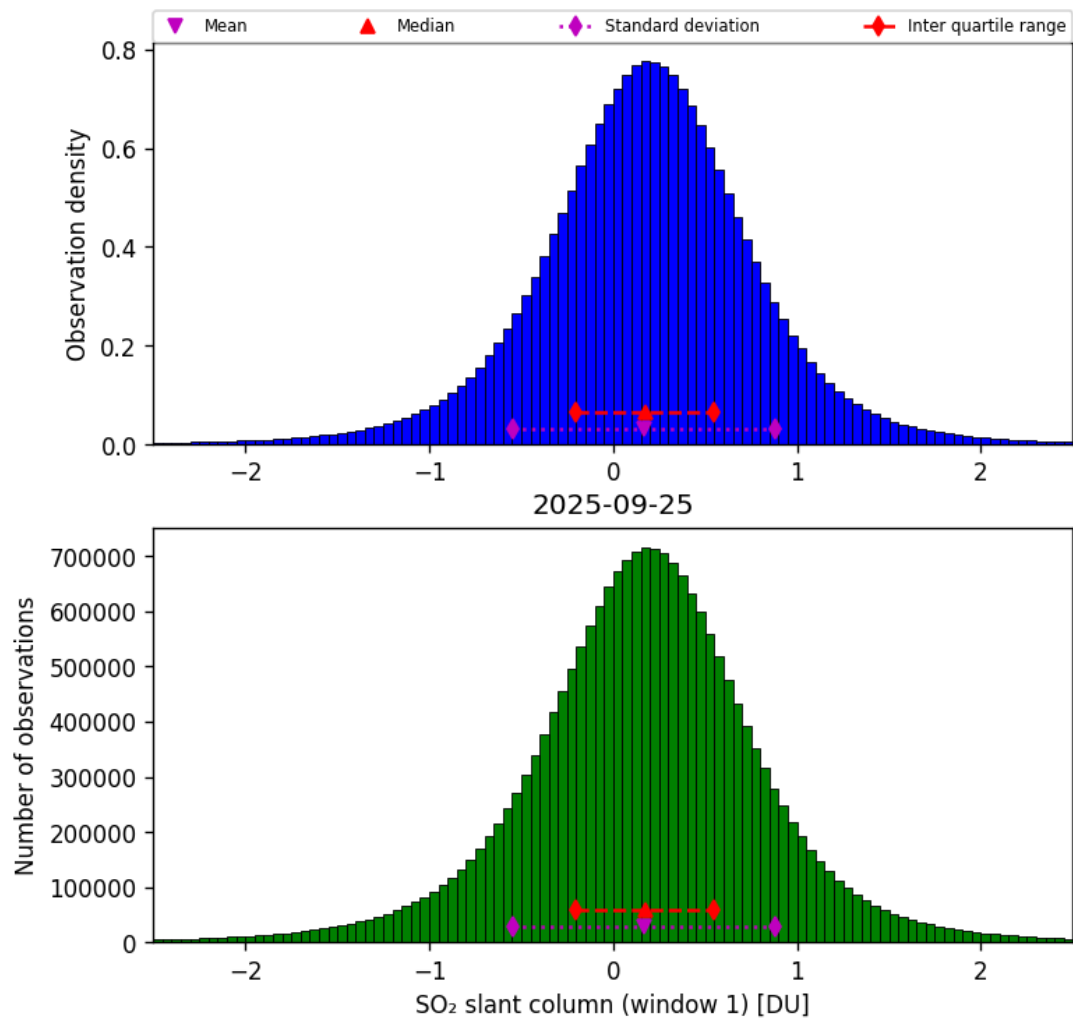
Figure 63: Histogram of “SO 2 slant column (window 1)” for 2025-09-25 to 2025-09-26
