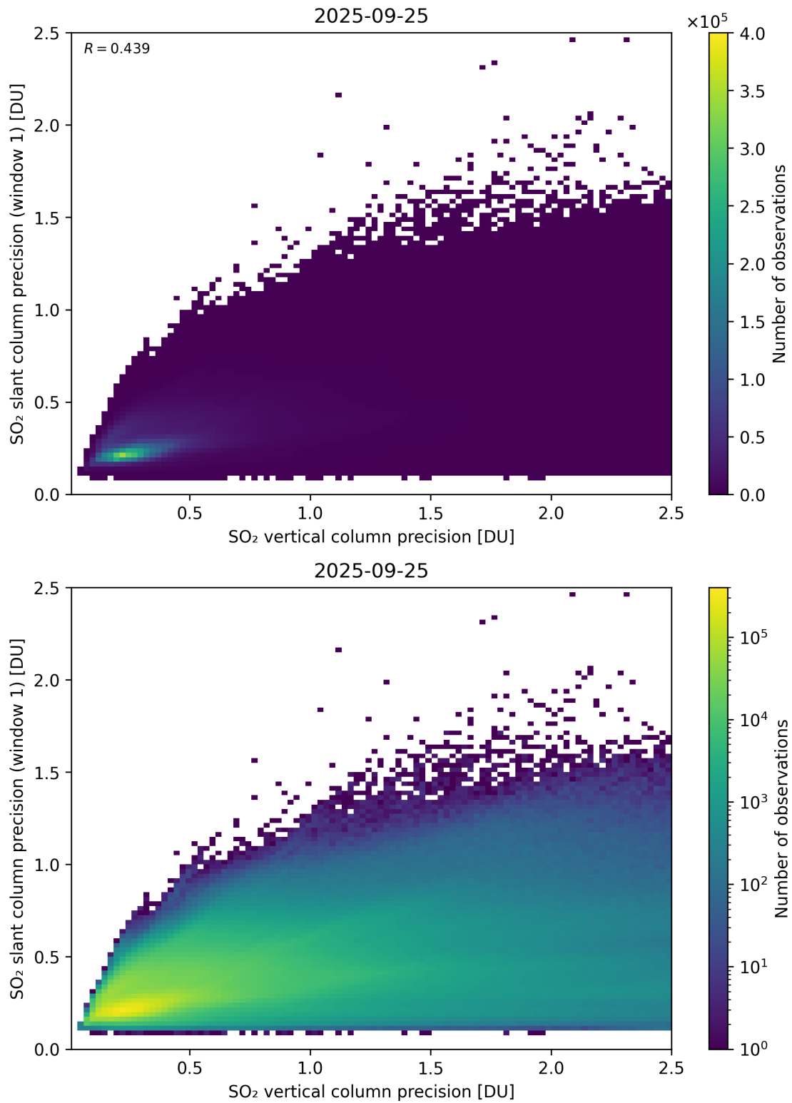
Figure 342: Scatter density plot of “SO 2 vertical column precision” against “SO 2 slant column precision (window 1)” for 2025-09-25 to 2025-09-26.
