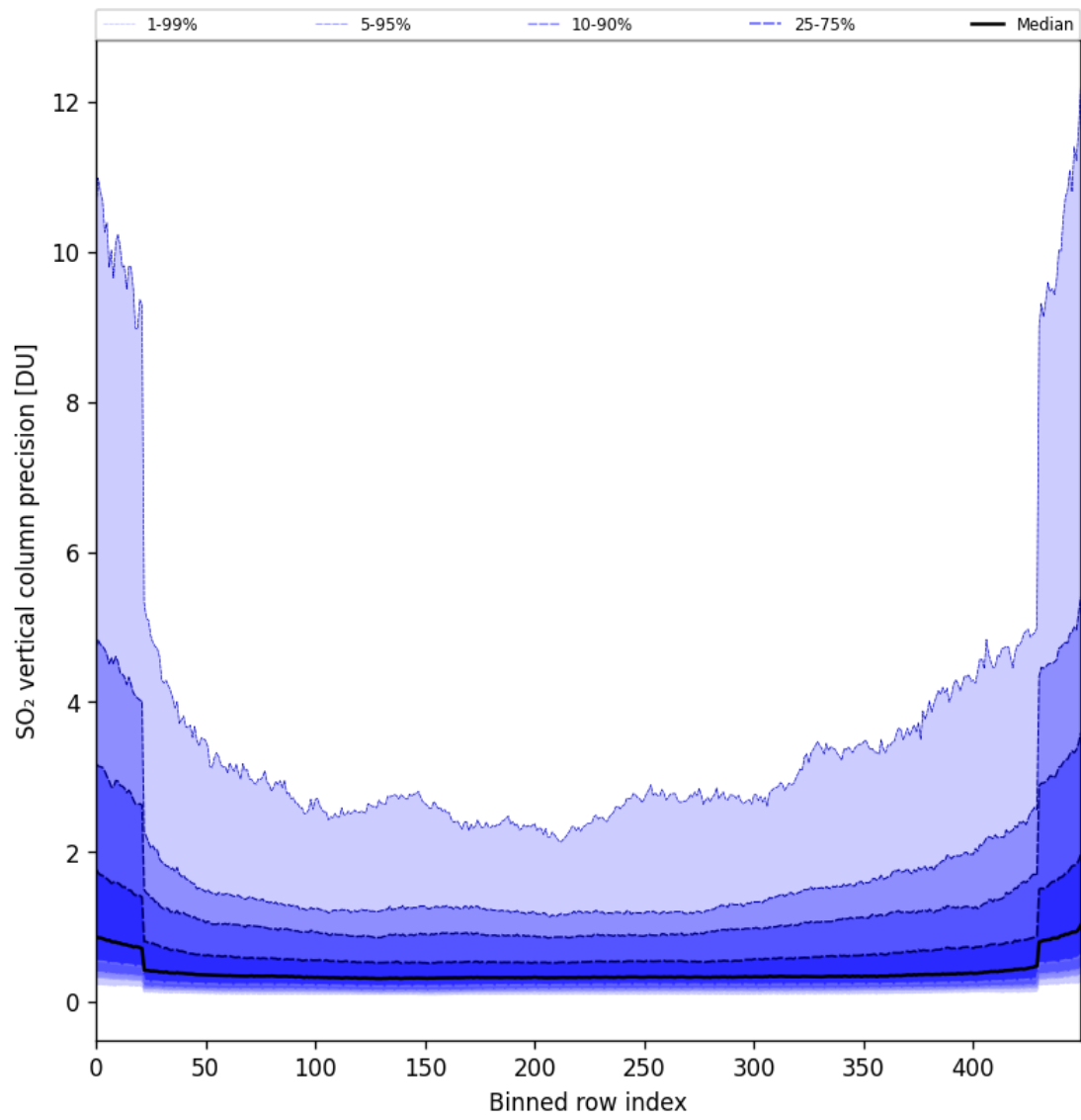
Figure 85: Along track statistics of “SO 2 vertical column precision” for 2025-09-25 to 2025-09-26
