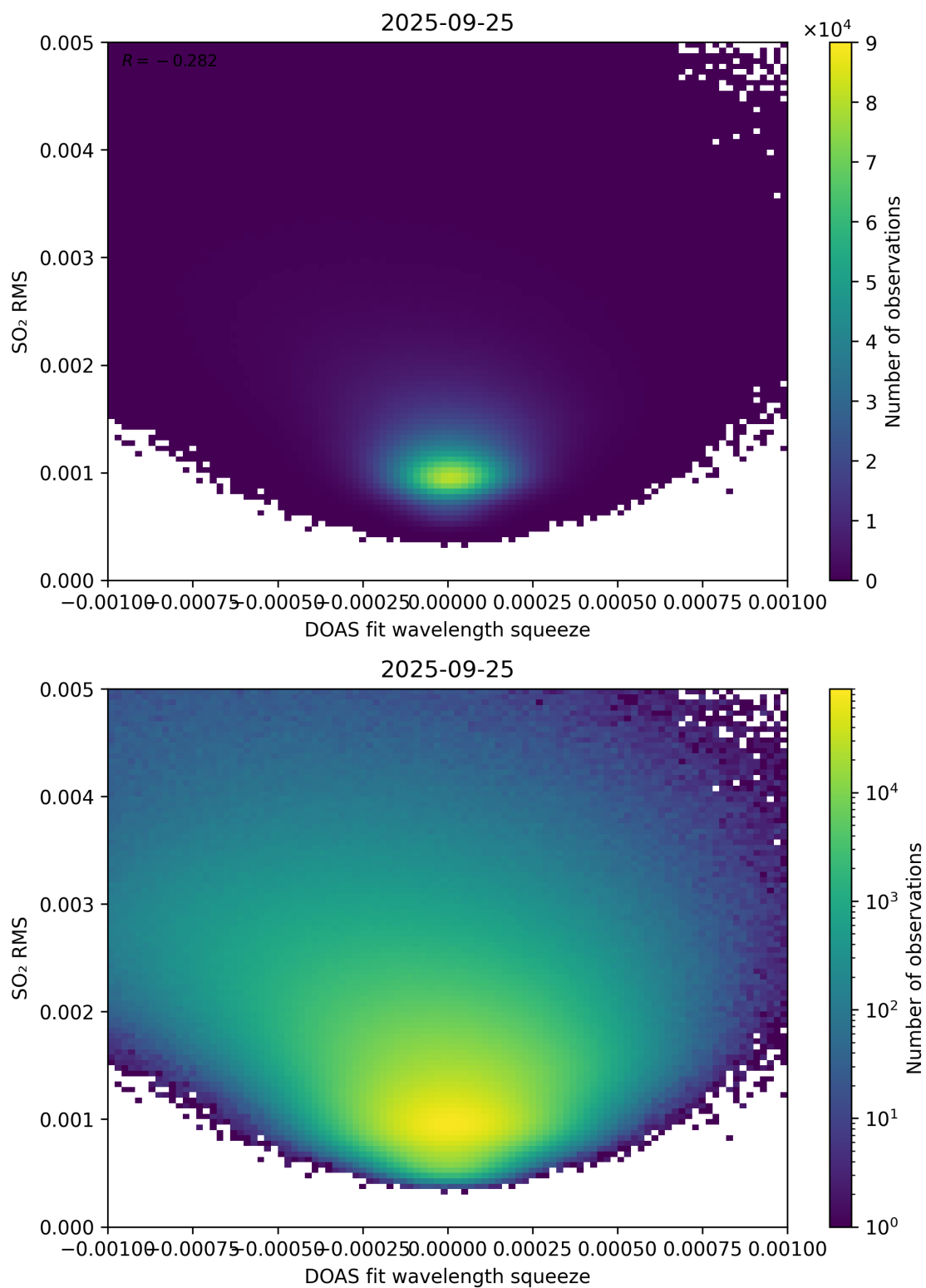
Figure 143: Scatter density plot of “DOAS fit wavelength squeeze” against “SO 2 RMS” for 2025-09-25 to 2025-09-26.
