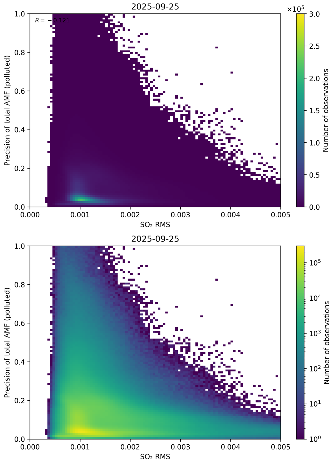
Figure 149: Scatter density plot of “SO 2 RMS” against “Precision of total AMF (polluted)” for 2025-09-25 to 2025-09-26.
