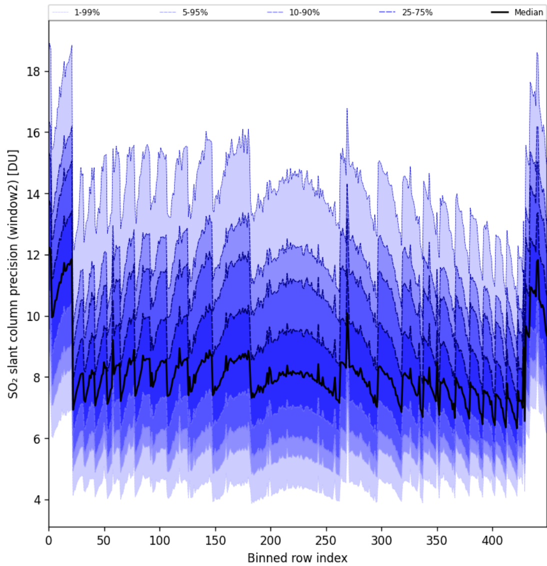
Figure 94: Along track statistics of “SO 2 slant column precision (window2)” for 2025-09-25 to 2025-09-26
