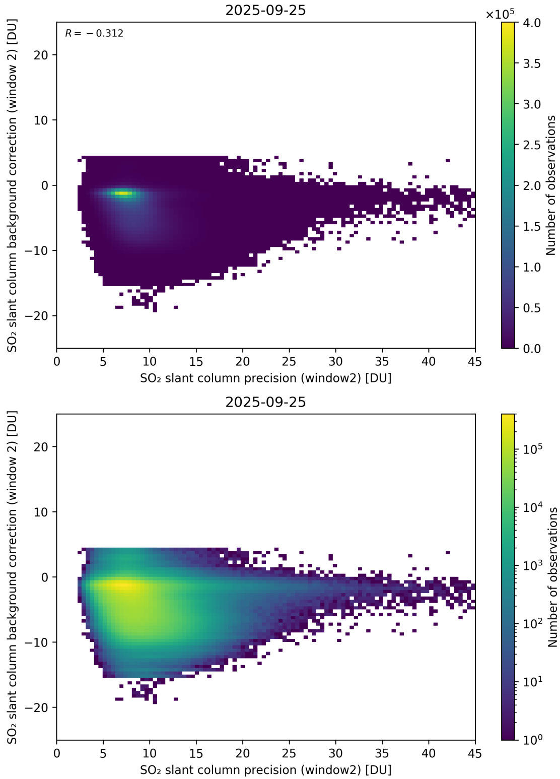
Figure 291: Scatter density plot of “SO 2 slant column precision (window2)” against “SO 2 slant column background correction (window 2)” for 2025-09-25 to 2025-09-26.
