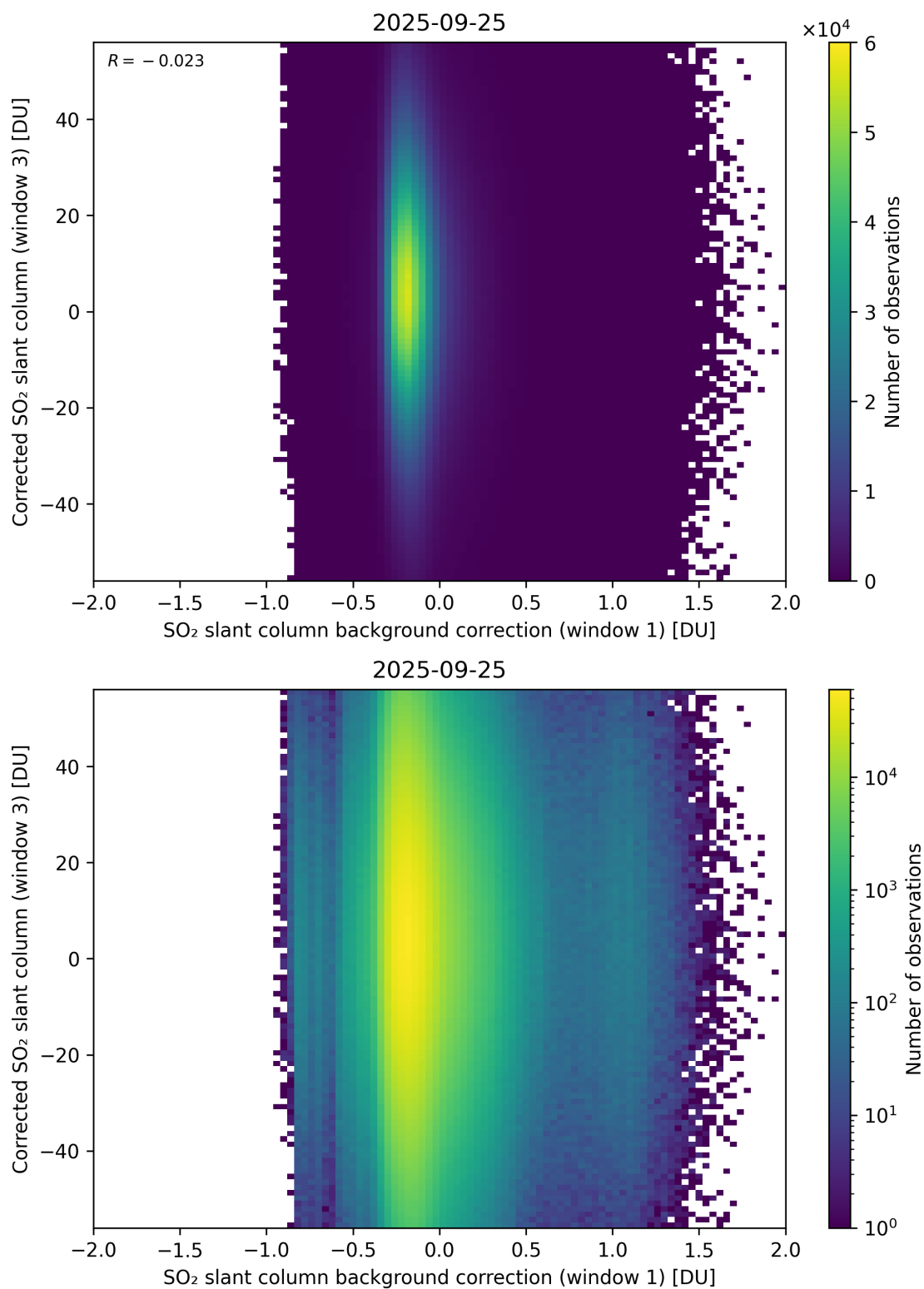
Figure 116: Scatter density plot of “SO 2 slant column background correction (window 1)” against “Corrected SO 2 slant column (window 3)” for 2025-09-25 to 2025-09-26.
