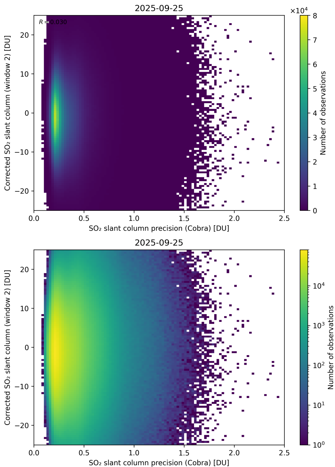
Figure 206: Scatter density plot of “SO 2 slant column precision (Cobra)” against “Corrected SO 2 slant column (window 2)” for 2025-09-25 to 2025-09-26.
