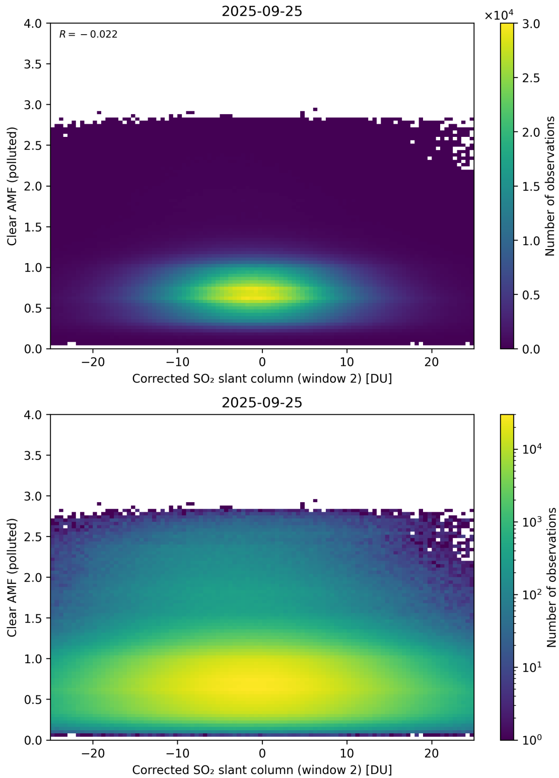
Figure 249: Scatter density plot of “Corrected SO 2 slant column (window 2)” against “Clear AMF (polluted)” for 2025-09-25 to 2025-09-26.
