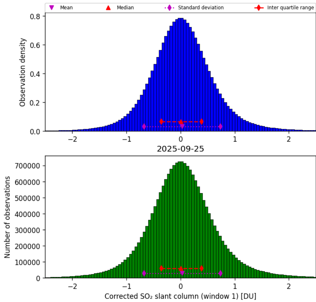
Figure 65: Histogram of “Corrected SO 2 slant column (window 1)” for 2025-09-25 to 2025-09-26
