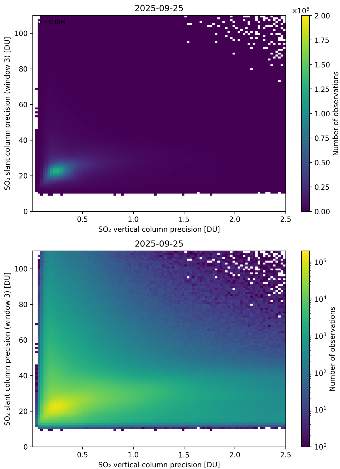
Figure 345: Scatter density plot of “SO 2 vertical column precision” against “SO 2 slant column precision (window 3)” for 2025-09-25 to 2025-09-26.
