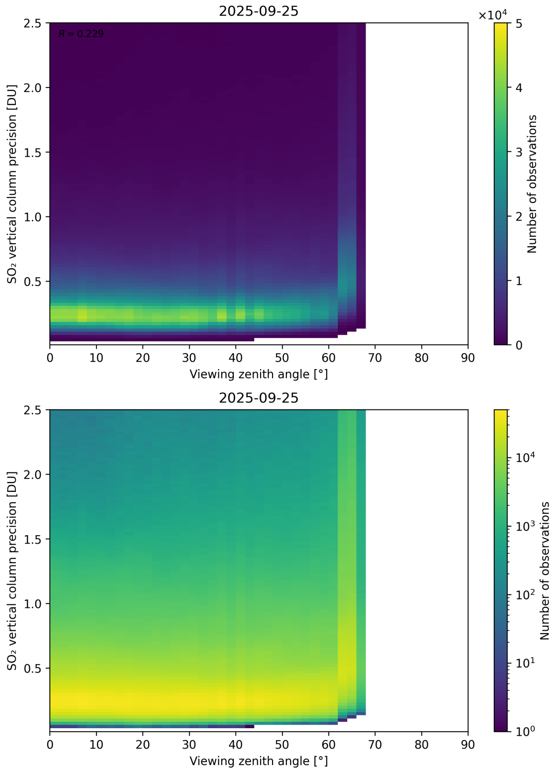
Figure 384: Scatter density plot of “Viewing zenith angle” against “SO 2 vertical column precision” for 2025-09-25 to 2025-09-26.
