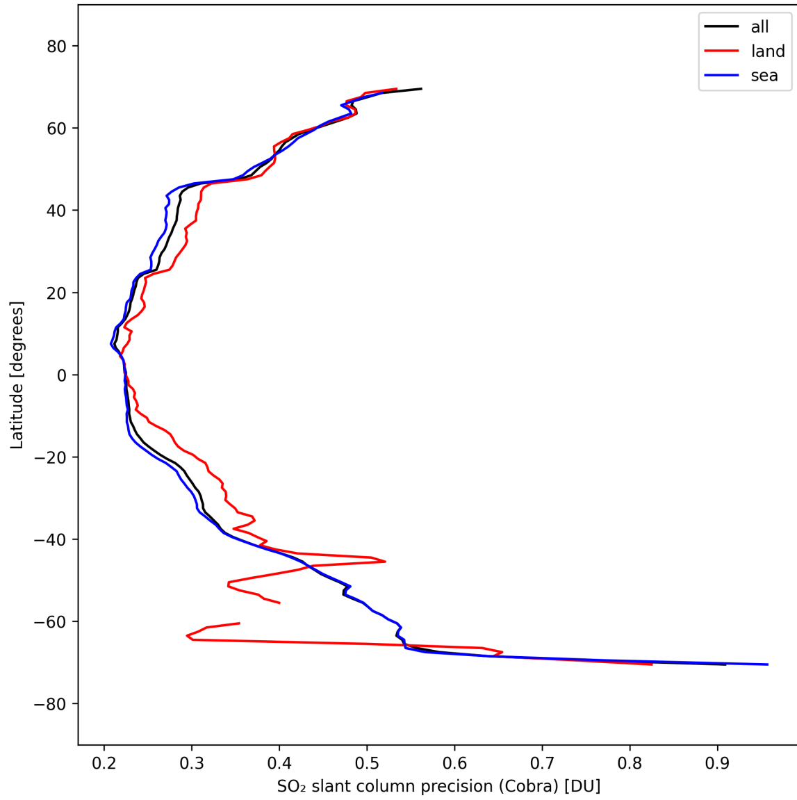
Figure 36: Zonal average of “SO 2 slant column precision (Cobra)” for 2025-09-25 to 2025-09-26.
