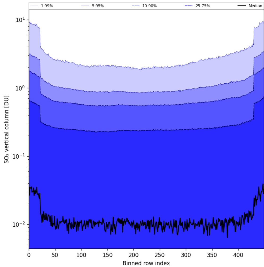
Figure 84: Along track statistics of “SO 2 vertical column” for 2025-09-25 to 2025-09-26
