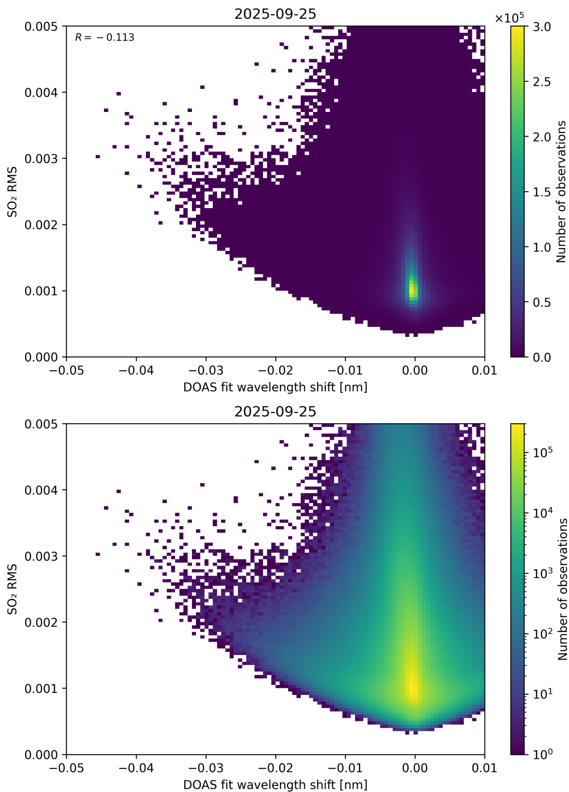
Figure 139: Scatter density plot of “DOAS fit wavelength shift” against “SO 2 RMS” for 2025-09-25 to 2025-09-26.
