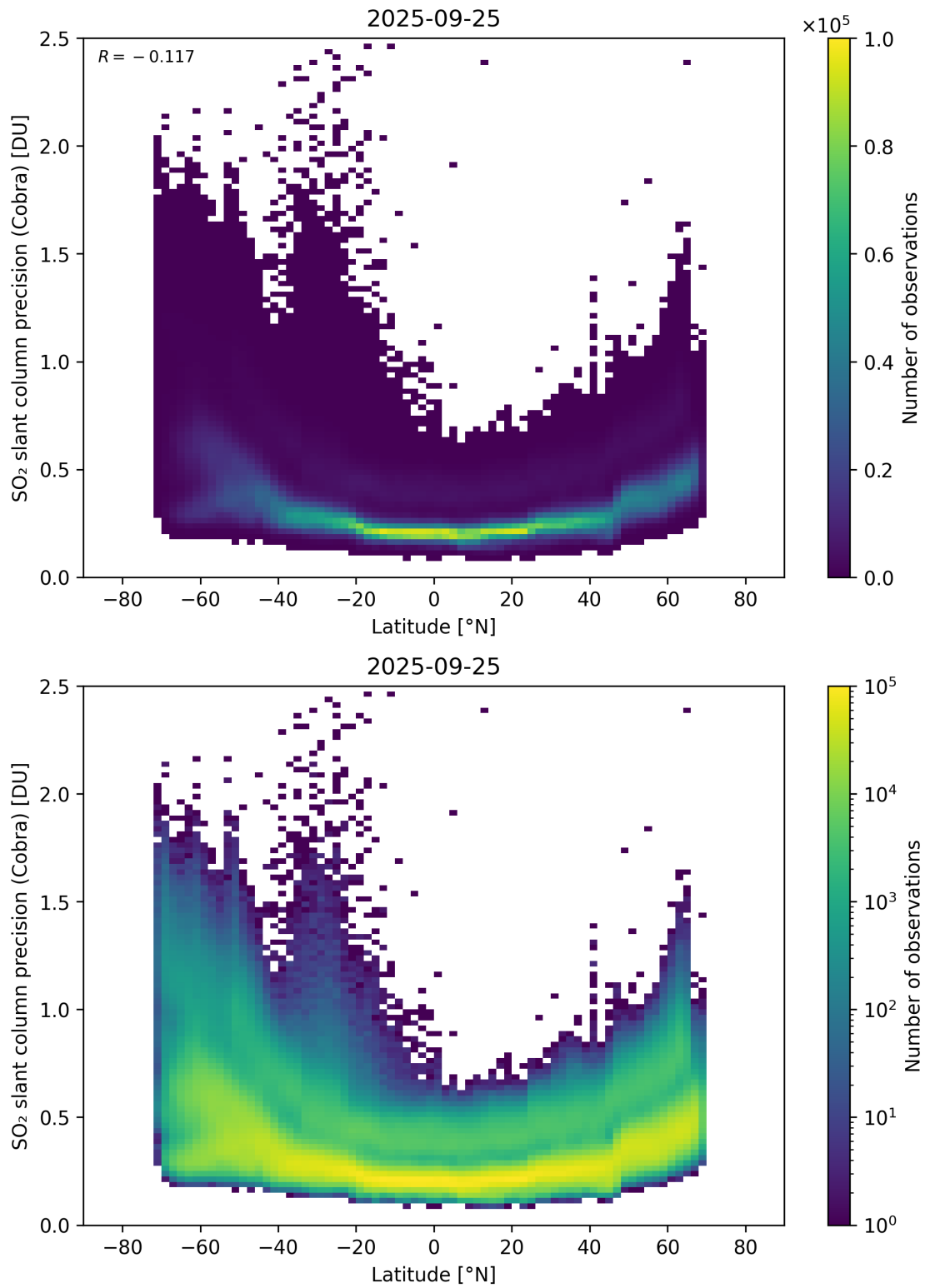
Figure 158: Scatter density plot of “Latitude” against “SO 2 slant column precision (Cobra)” for 2025-09-25 to 2025-09-26.
