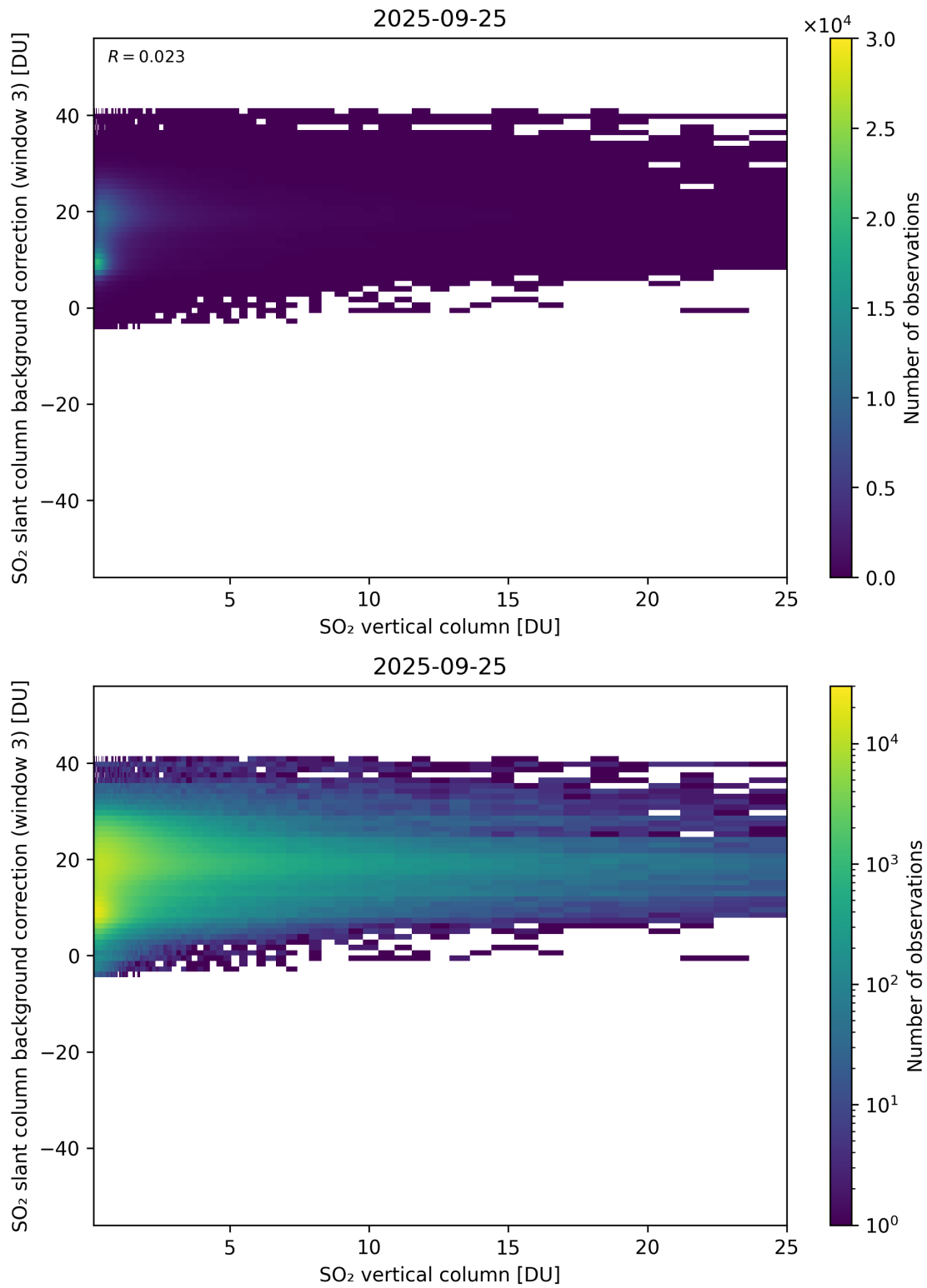
Figure 325: Scatter density plot of “SO 2 vertical column” against “SO 2 slant column background correction (window 3)” for 2025-09-25 to 2025-09-26.
