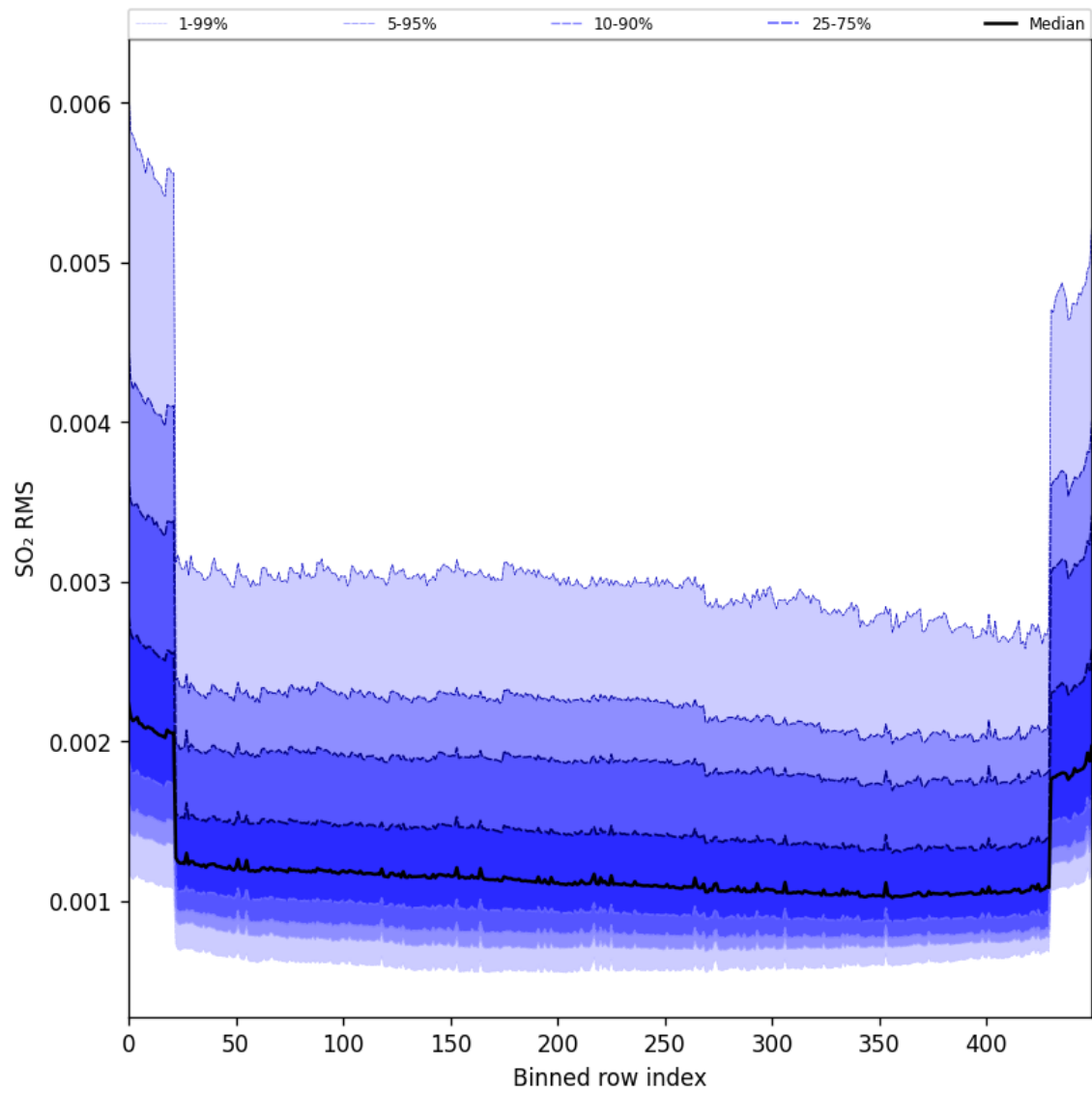
Figure 104: Along track statistics of “SO 2 RMS” for 2025-09-25 to 2025-09-26
