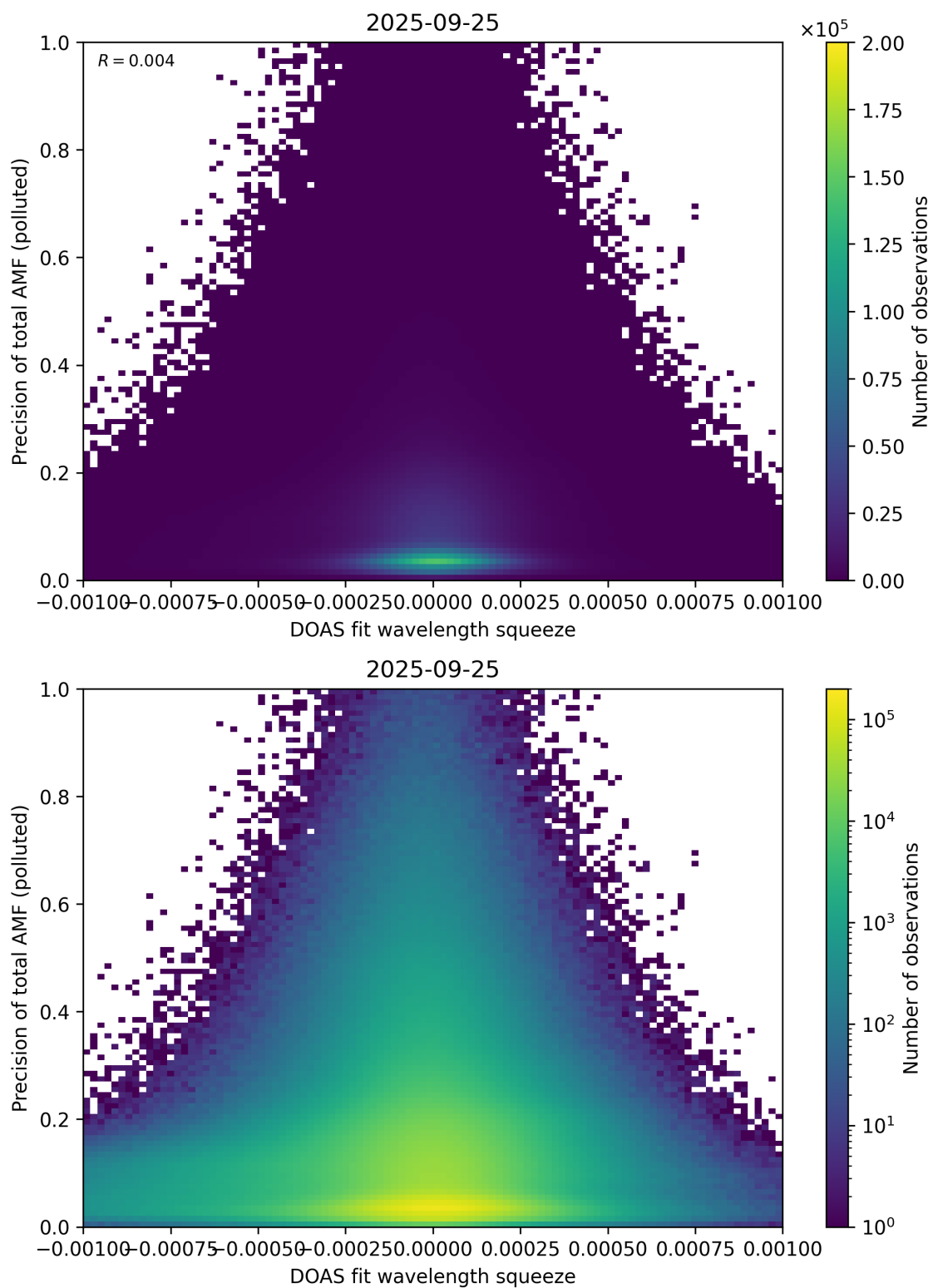
Figure 146: Scatter density plot of “DOAS fit wavelength squeeze” against “Precision of total AMF (polluted)” for 2025-09-25 to 2025-09-26.
