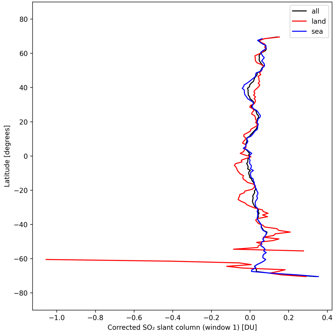
Figure 39: Zonal average of “Corrected SO 2 slant column (window 1)” for 2025-09-25 to 2025-09-26.
