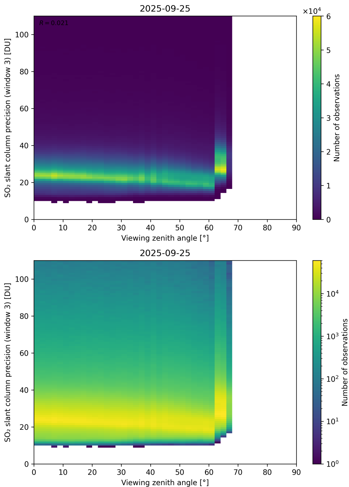
Figure 380: Scatter density plot of “Viewing zenith angle” against “SO 2 slant column precision (window 3)” for 2025-09-25 to 2025-09-26.
