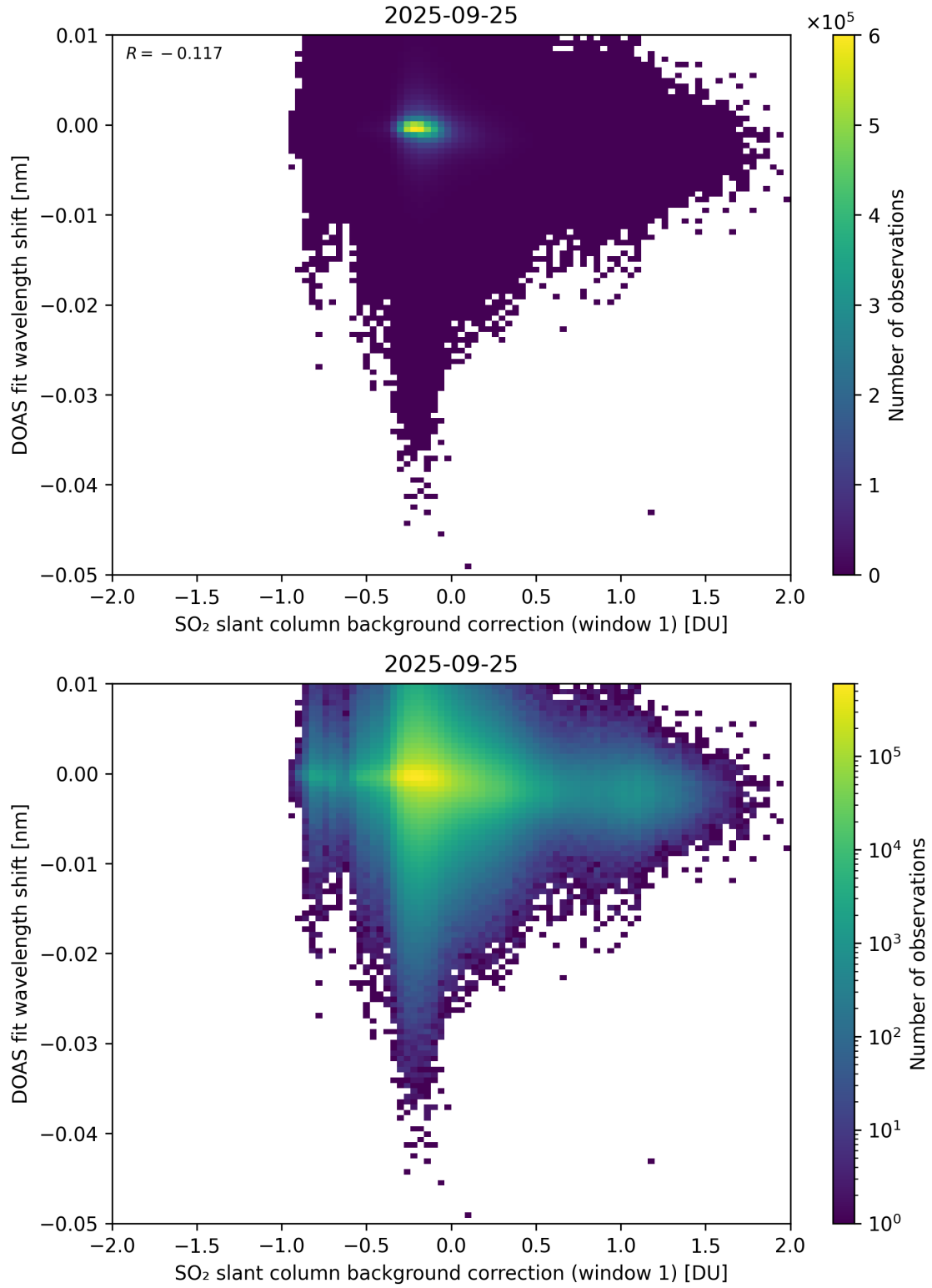
Figure 111: Scatter density plot of “SO 2 slant column background correction (window 1)” against “DOAS fit wavelength shift” for 2025-09-25 to 2025-09-26.
