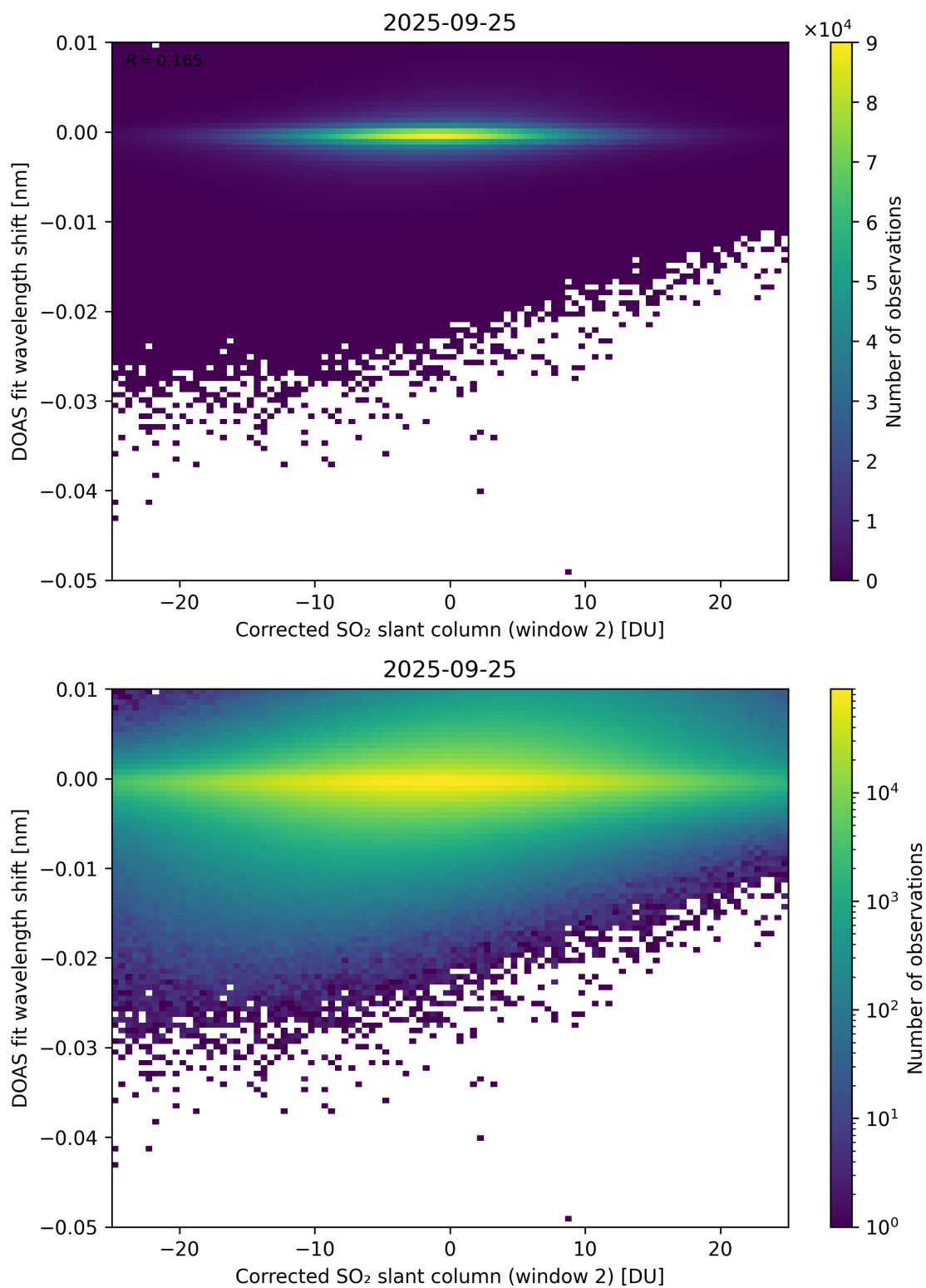
Figure 246: Scatter density plot of “Corrected SO 2 slant column (window 2)” against “DOAS fit wavelength shift” for 2025-09-25 to 2025-09-26.
