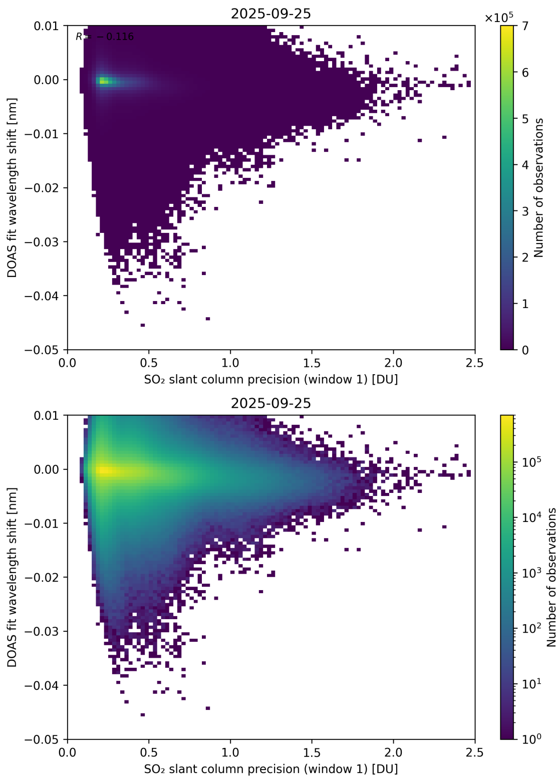
Figure 271: Scatter density plot of “SO 2 slant column precision (window 1)” against “DOAS fit wavelength shift” for 2025-09-25 to 2025-09-26.
