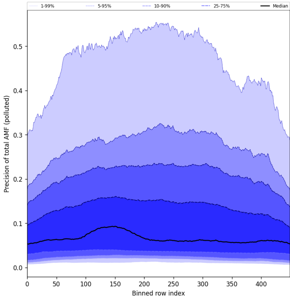
Figure 106: Along track statistics of “Precision of total AMF (polluted)” for 2025-09-25 to 2025-09-26
