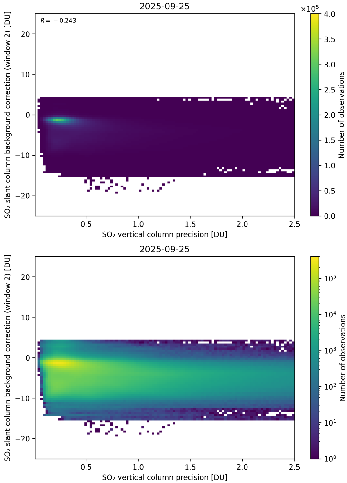
Figure 330: Scatter density plot of “SO 2 vertical column precision” against “SO 2 slant column background correction (window 2)” for 2025-09-25 to 2025-09-26.
