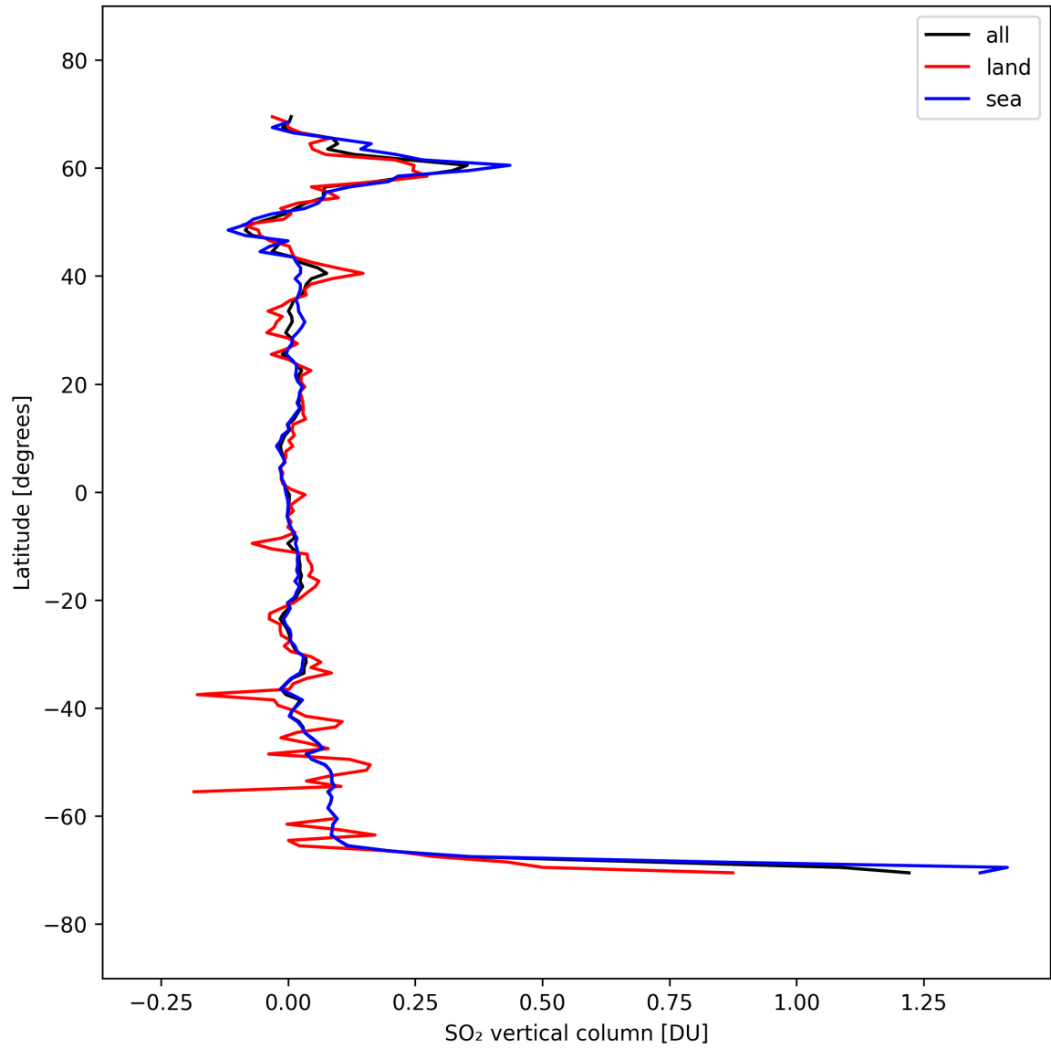
Figure 32: Zonal average of “SO 2 vertical column” for 2025-09-25 to 2025-09-26.
