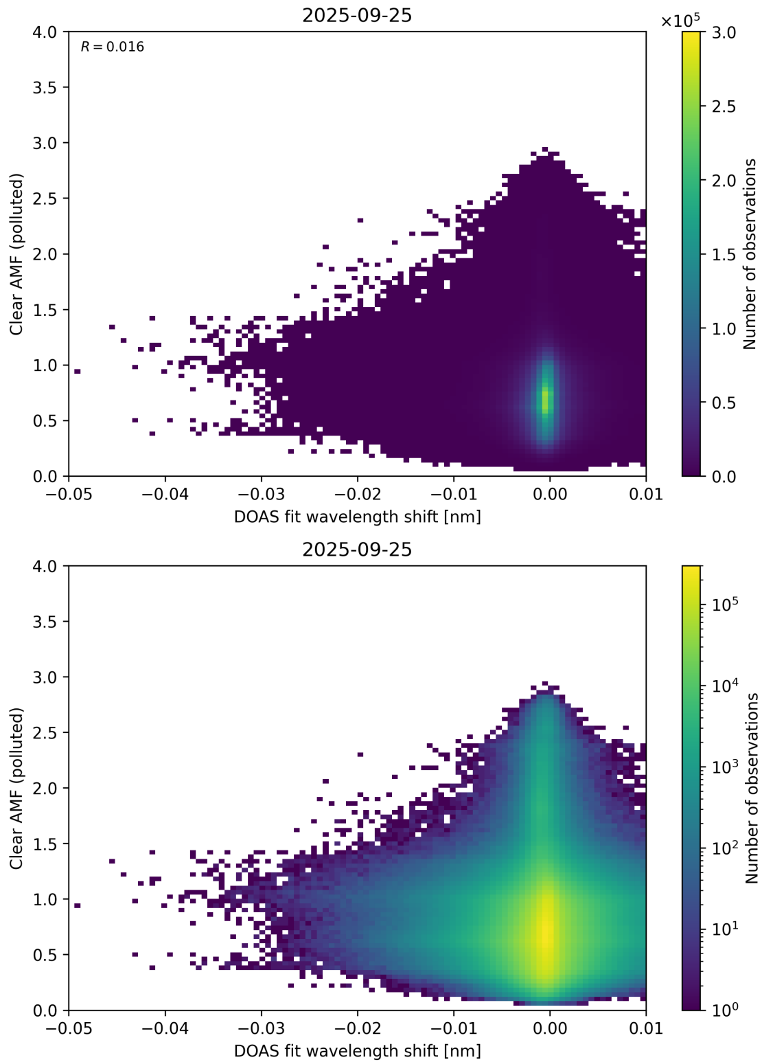
Figure 140: Scatter density plot of “DOAS fit wavelength shift” against “Clear AMF (polluted)” for 2025-09-25 to 2025-09-26.
