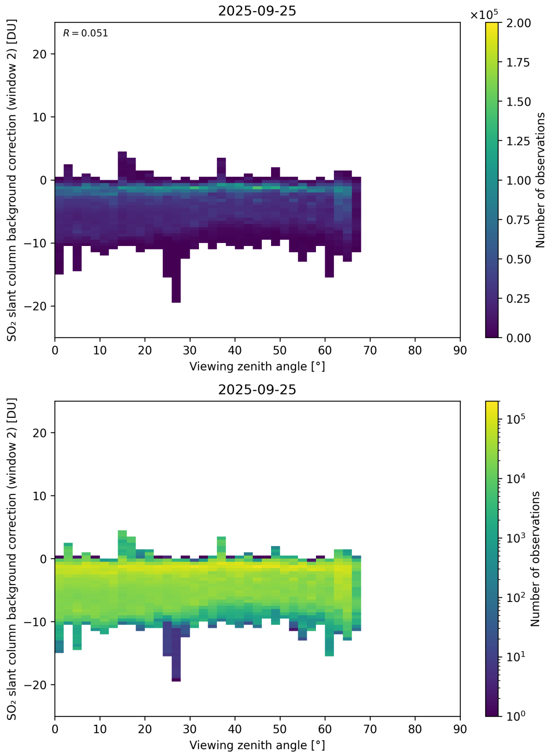
Figure 363: Scatter density plot of “Viewing zenith angle” against “SO 2 slant column background correction (window 2)” for 2025-09-25 to 2025-09-26.
