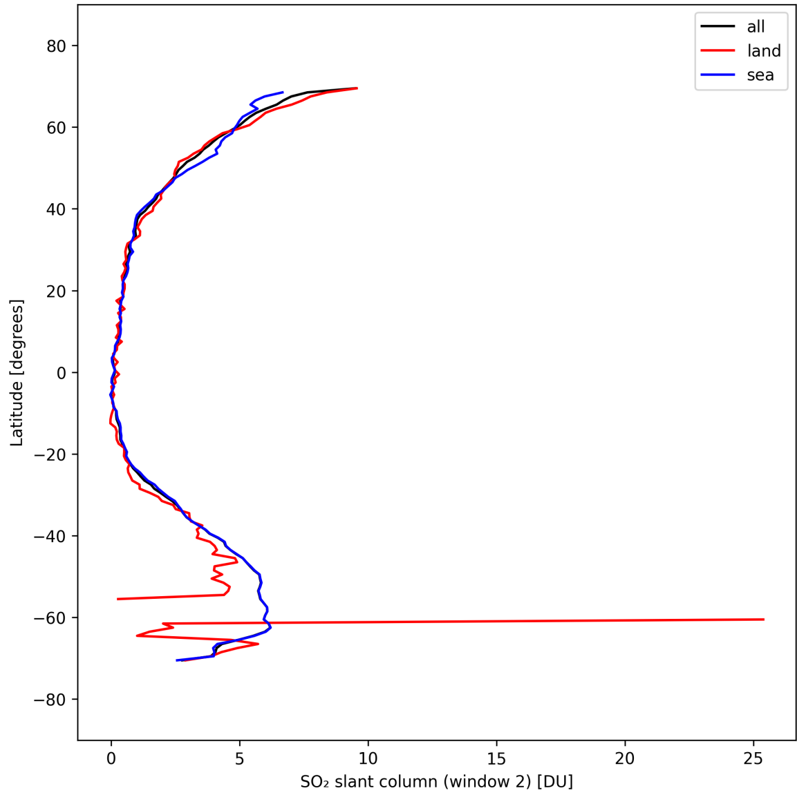
Figure 41: Zonal average of “SO 2 slant column (window 2)” for 2025-09-25 to 2025-09-26.
