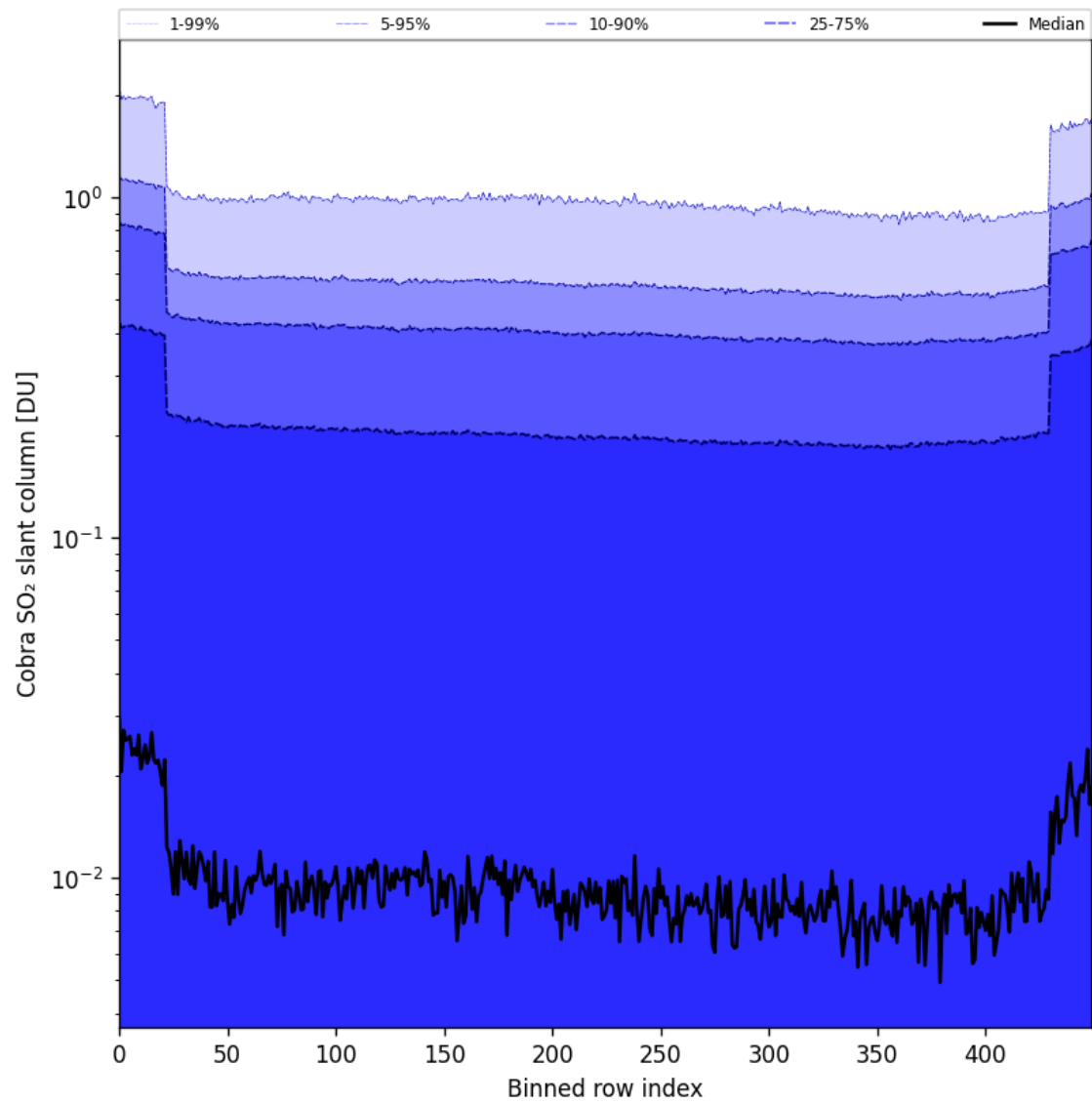
Figure 87: Along track statistics of “Cobra SO 2 slant column” for 2025-09-25 to 2025-09-26
