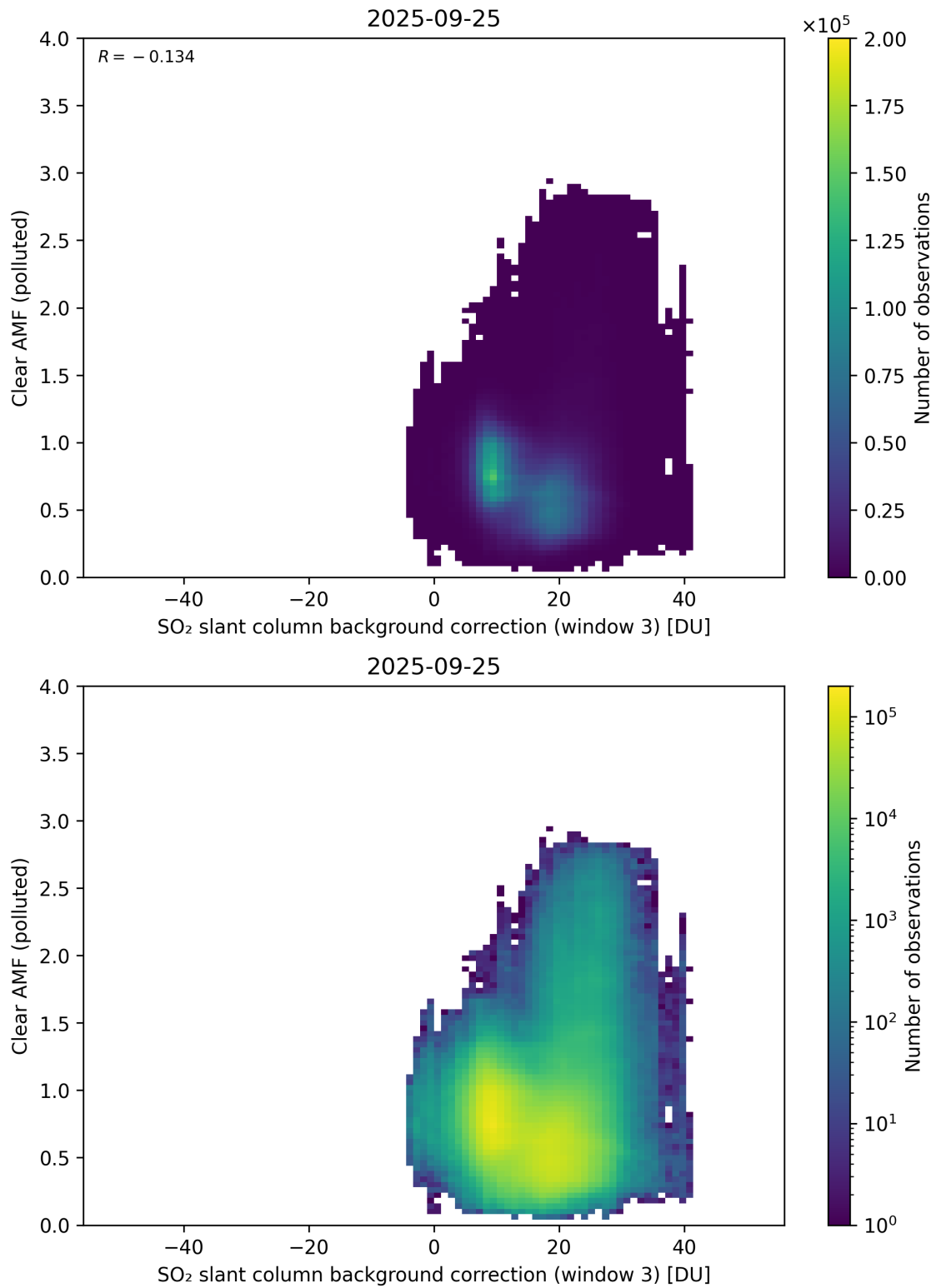
Figure 135: Scatter density plot of “SO 2 slant column background correction (window 3)” against “Clear AMF (polluted)” for 2025-09-25 to 2025-09-26.
