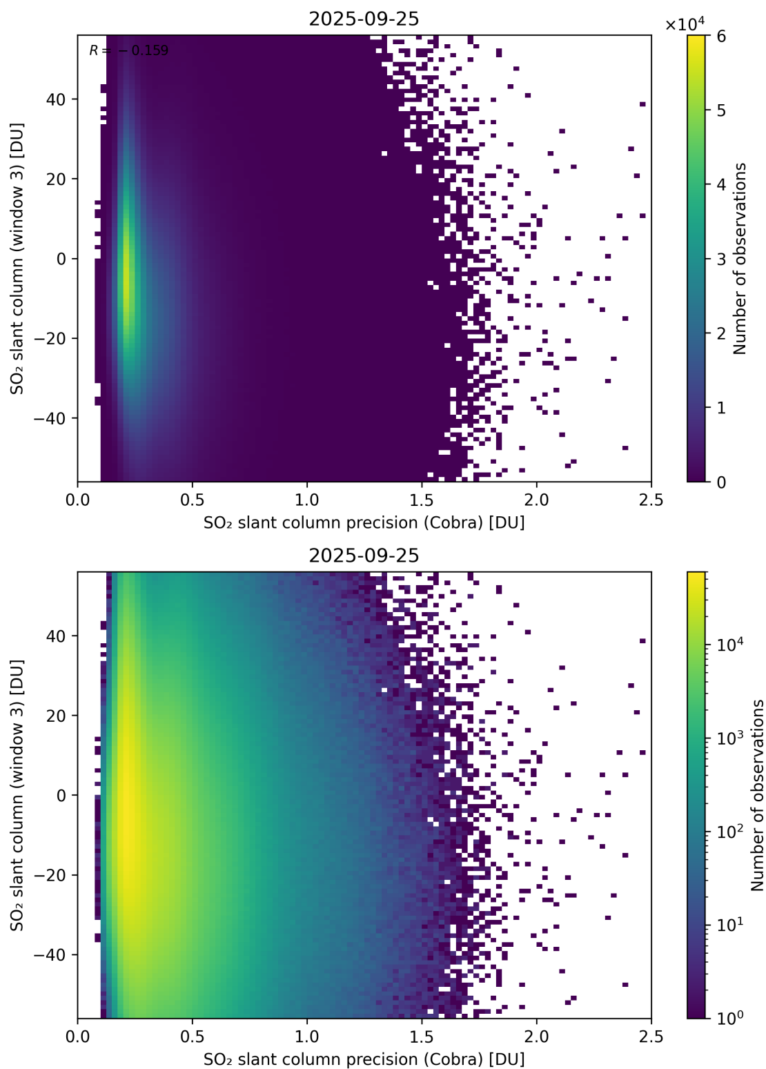
Figure 211: Scatter density plot of “SO 2 slant column precision (Cobra)” against “SO 2 slant column (window 3)” for 2025-09-25 to 2025-09-26.
