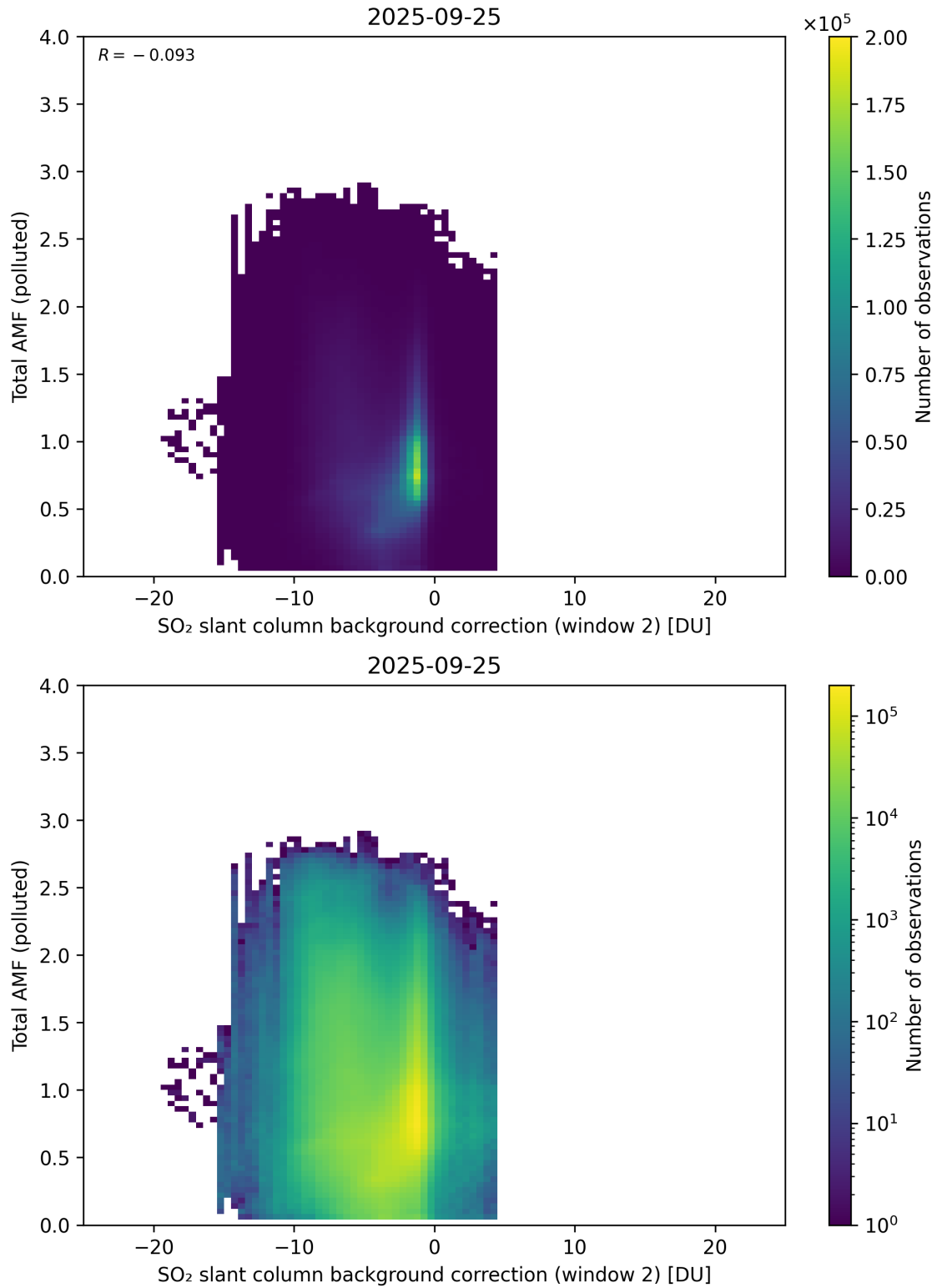
Figure 130: Scatter density plot of “SO 2 slant column background correction (window 2)” against “Total AMF (polluted)” for 2025-09-25 to 2025-09-26.
