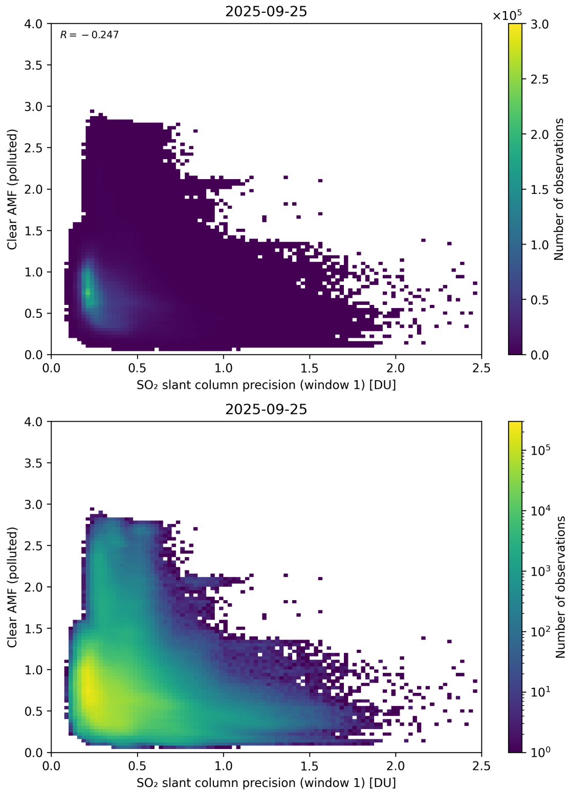
Figure 274: Scatter density plot of “SO 2 slant column precision (window 1)” against “Clear AMF (polluted)” for 2025-09-25 to 2025-09-26.
