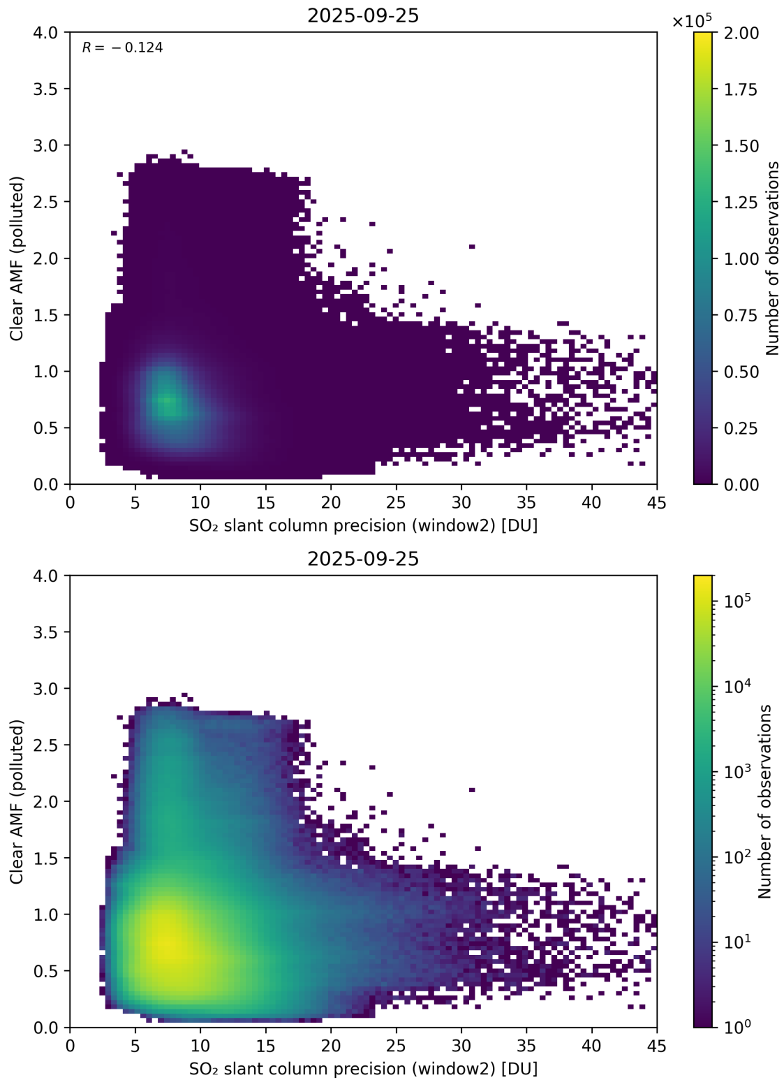
Figure 296: Scatter density plot of “SO 2 slant column precision (window2)” against “Clear AMF (polluted)” for 2025-09-25 to 2025-09-26.
