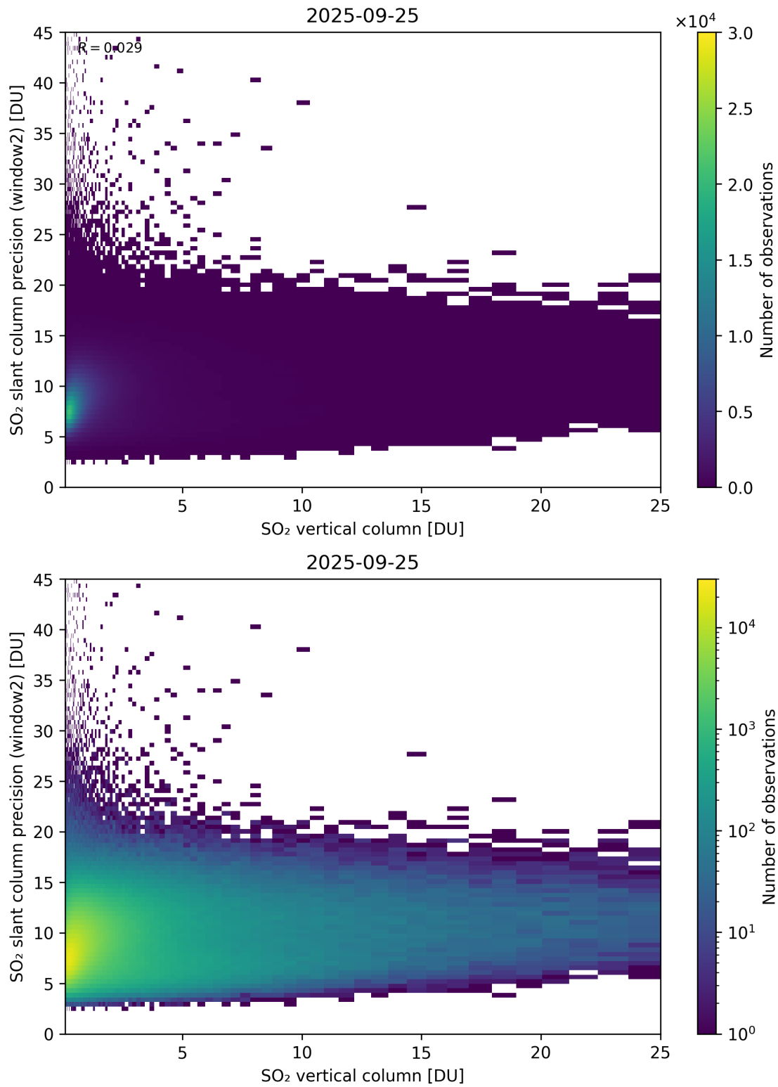
Figure 356: Scatter density plot of “SO 2 vertical column” against “SO 2 slant column precision (window2)” for 2025-09-25 to 2025-09-26.
