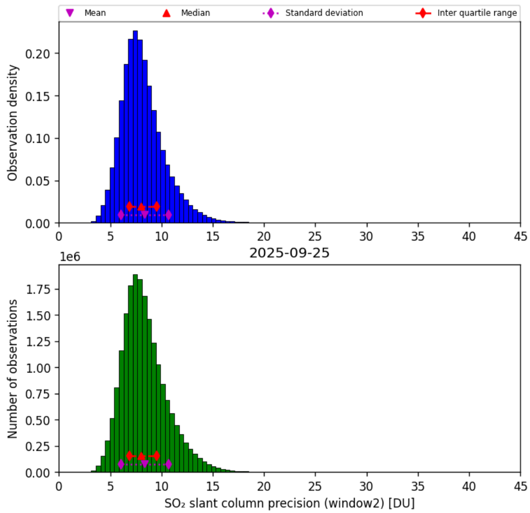
Figure 68: Histogram of “SO 2 slant column precision (window2)” for 2025-09-25 to 2025-09-26
