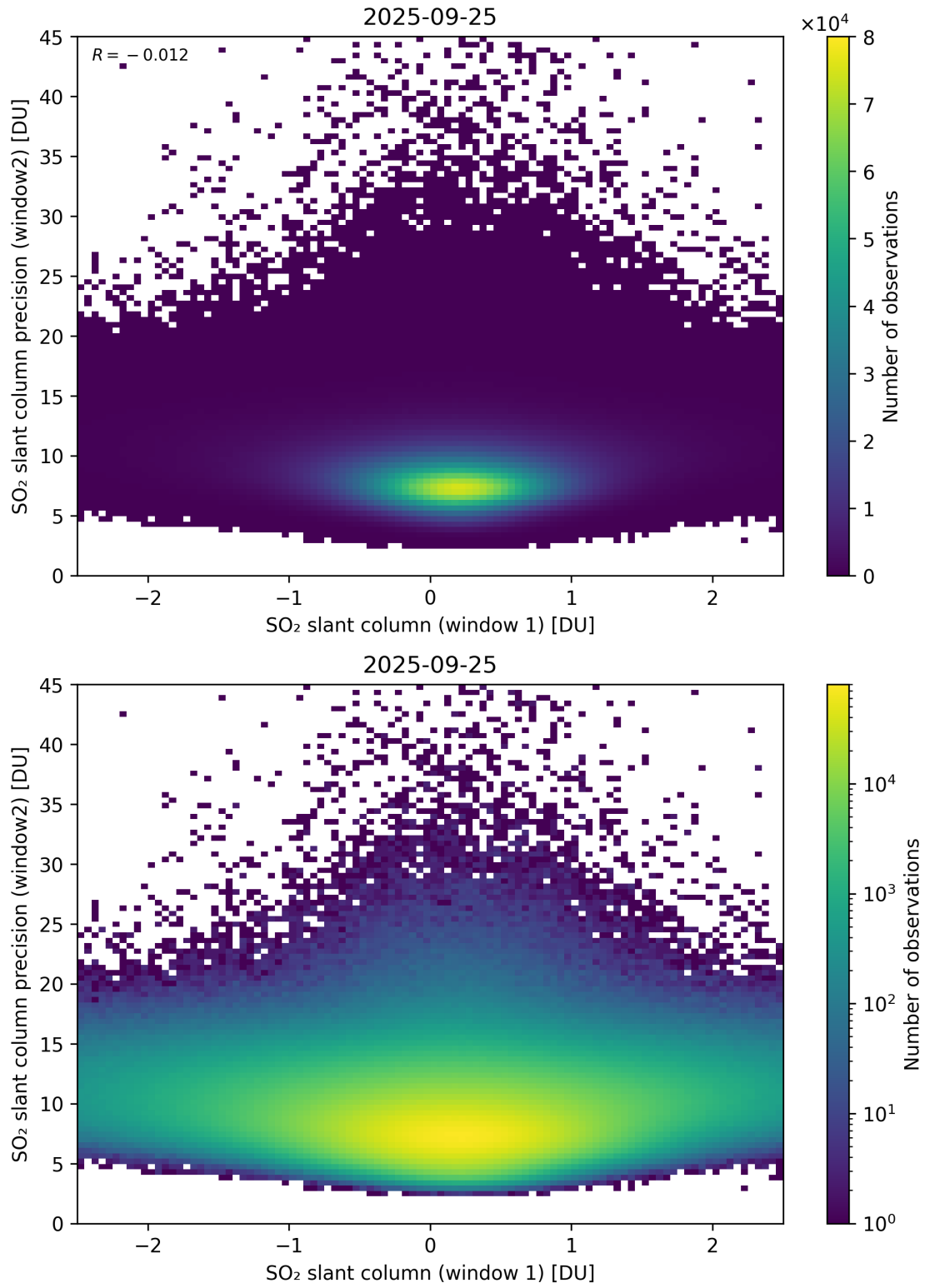
Figure 286: Scatter density plot of “SO 2 slant column (window 1)” against “SO 2 slant column precision (window2)” for 2025-09-25 to 2025-09-26.
