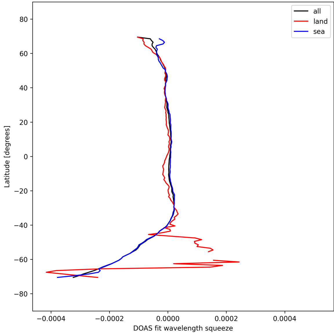
Figure 51: Zonal average of “DOAS fit wavelength squeeze” for 2025-09-25 to 2025-09-26.
