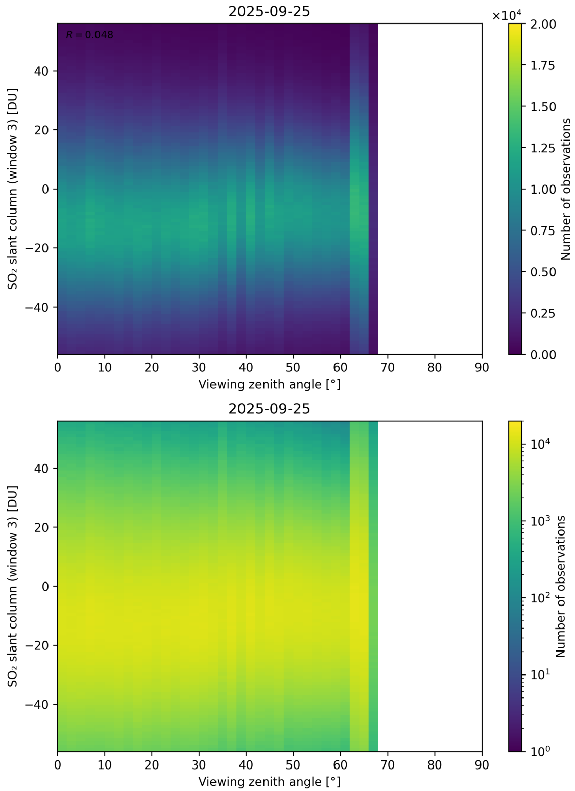
Figure 379: Scatter density plot of “Viewing zenith angle” against “SO 2 slant column (window 3)” for 2025-09-25 to 2025-09-26.
