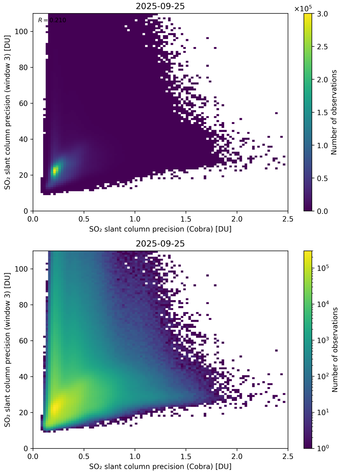
Figure 212: Scatter density plot of “SO 2 slant column precision (Cobra)” against “SO 2 slant column precision (window 3)” for 2025-09-25 to 2025-09-26.
