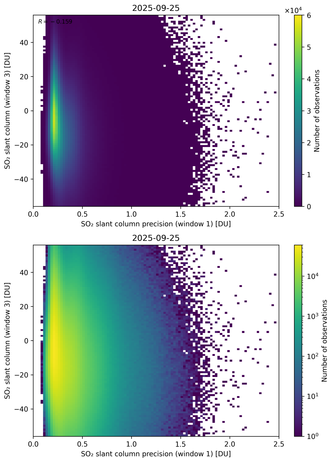
Figure 278: Scatter density plot of “SO 2 slant column precision (window 1)” against “SO 2 slant column (window 3)” for 2025-09-25 to 2025-09-26.
