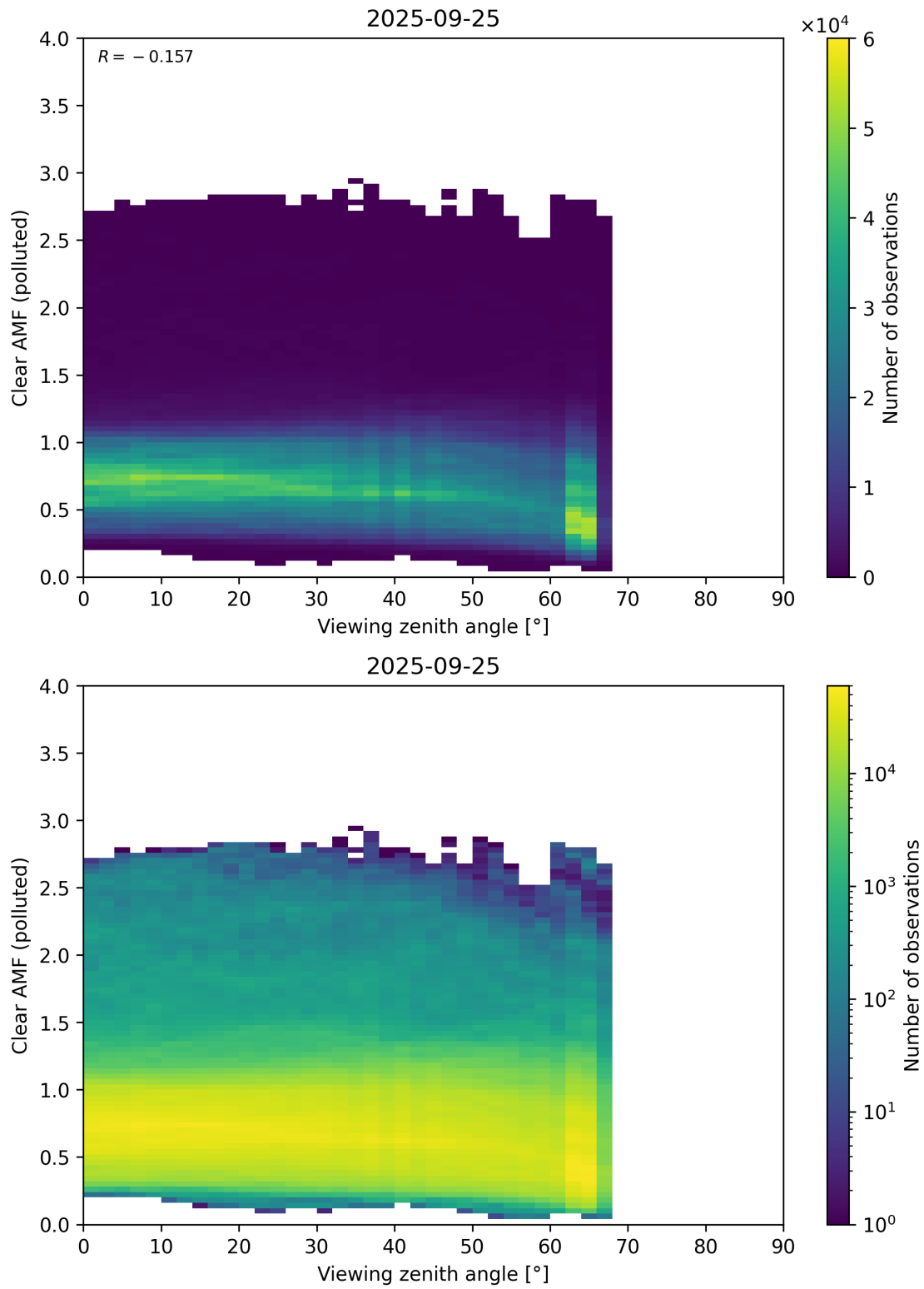
Figure 370: Scatter density plot of “Viewing zenith angle” against “Clear AMF (polluted)” for 2025-09-25 to 2025-09-26.
