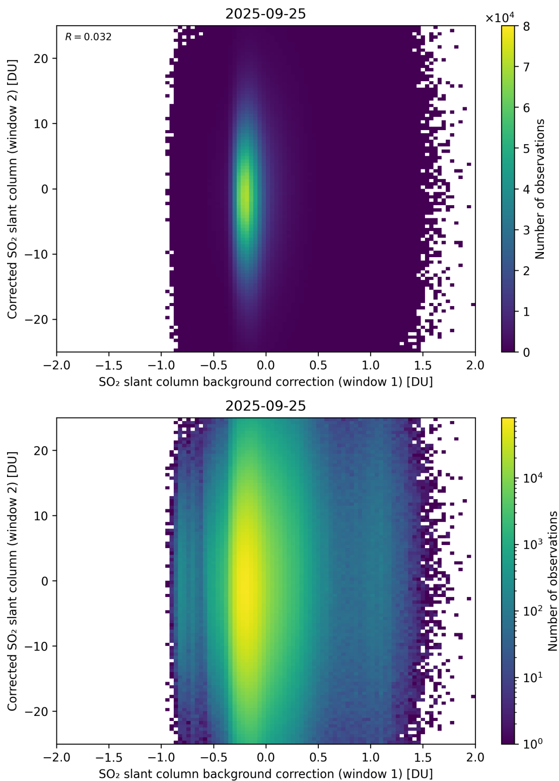
Figure 115: Scatter density plot of “SO 2 slant column background correction (window 1)” against “Corrected SO 2 slant column (window 2)” for 2025-09-25 to 2025-09-26.
