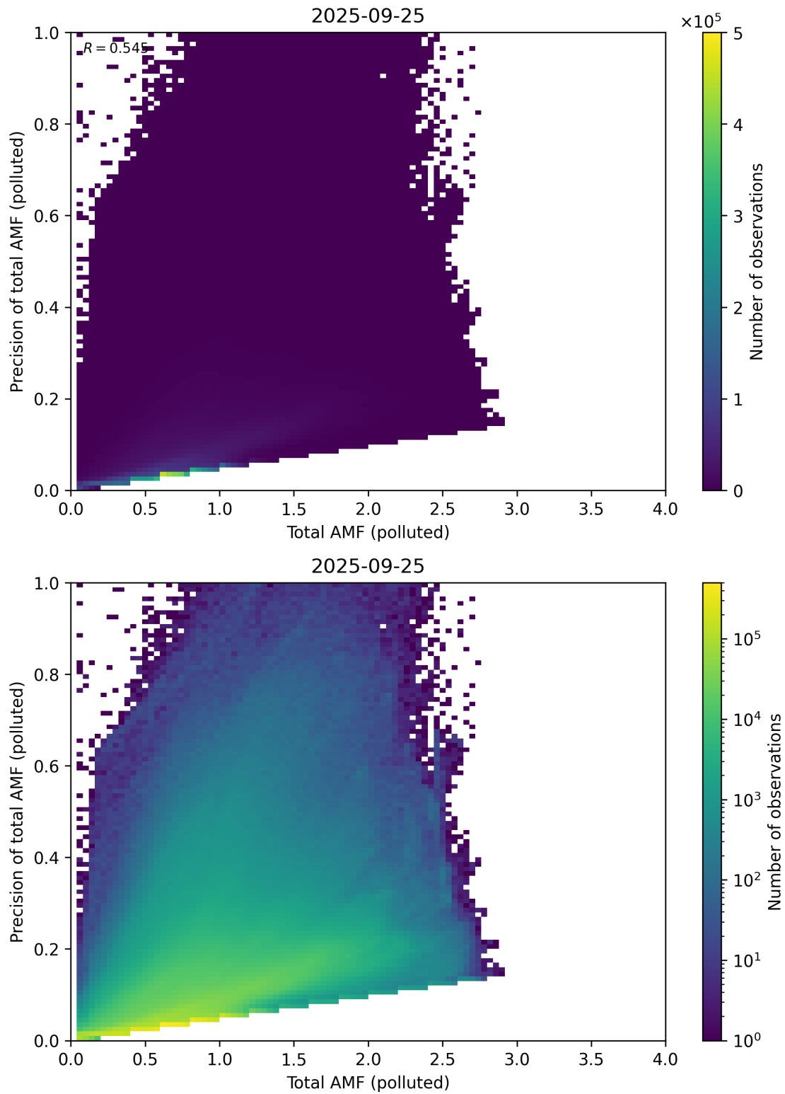
Figure 322: Scatter density plot of “Total AMF (polluted)” against “Precision of total AMF (polluted)” for 2025-09-25 to 2025-09-26.
