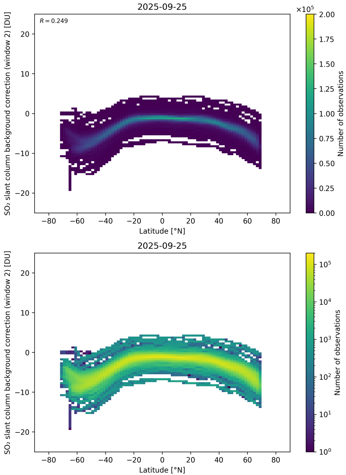
Figure 151: Scatter density plot of “Latitude” against “SO 2 slant column background correction (window 2)” for 2025-09-25 to 2025-09-26.
