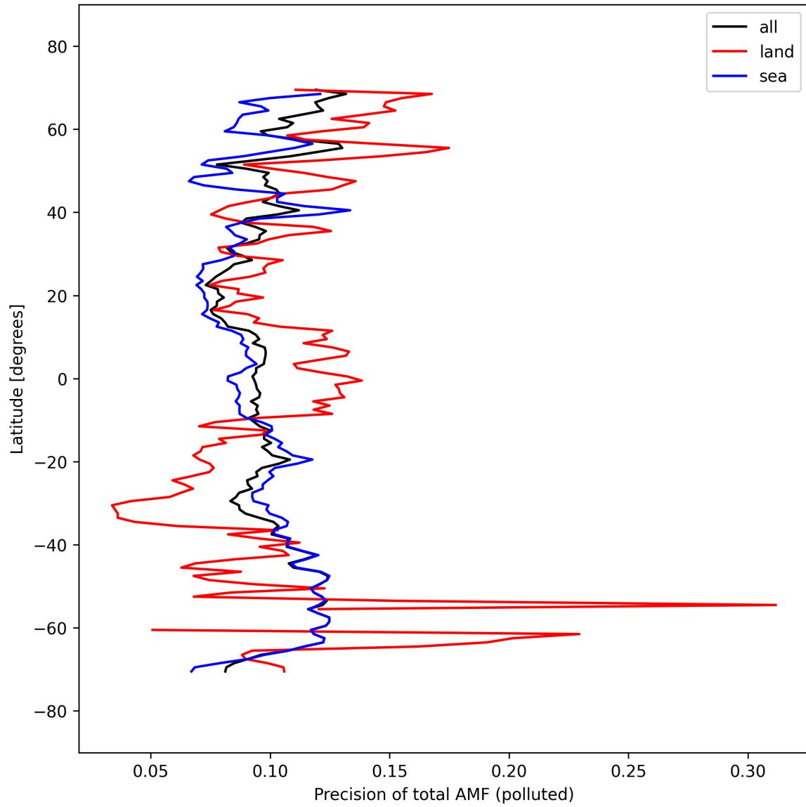
Figure 54: Zonal average of “Precision of total AMF (polluted)” for 2025-09-25 to 2025-09-26.
