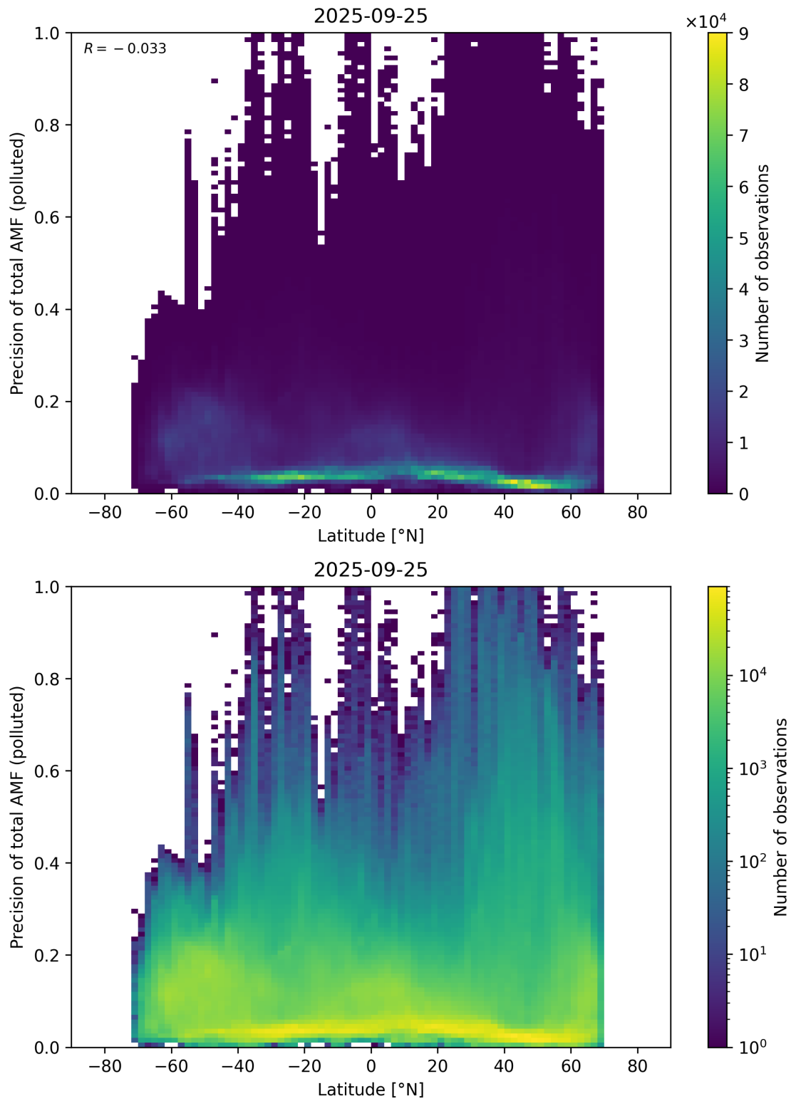
Figure 168: Scatter density plot of “Latitude” against “Precision of total AMF (polluted)” for 2025-09-25 to 2025-09-26.
