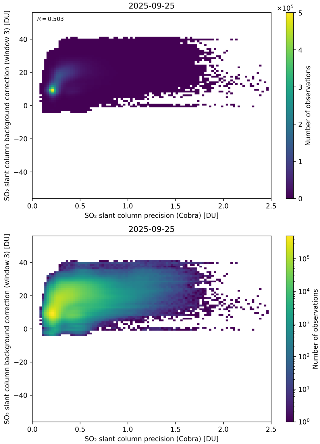
Figure 201: Scatter density plot of “SO 2 slant column precision (Cobra)” against “SO 2 slant column background correction (window 3)” for 2025-09-25 to 2025-09-26.
