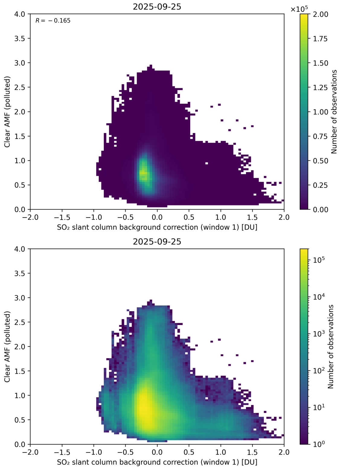
Figure 114: Scatter density plot of “SO 2 slant column background correction (window 1)” against “Clear AMF (polluted)” for 2025-09-25 to 2025-09-26.
