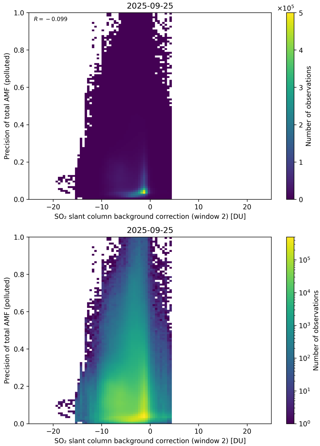
Figure 131: Scatter density plot of “SO 2 slant column background correction (window 2)” against “Precision of total AMF (polluted)” for 2025-09-25 to 2025-09-26.
