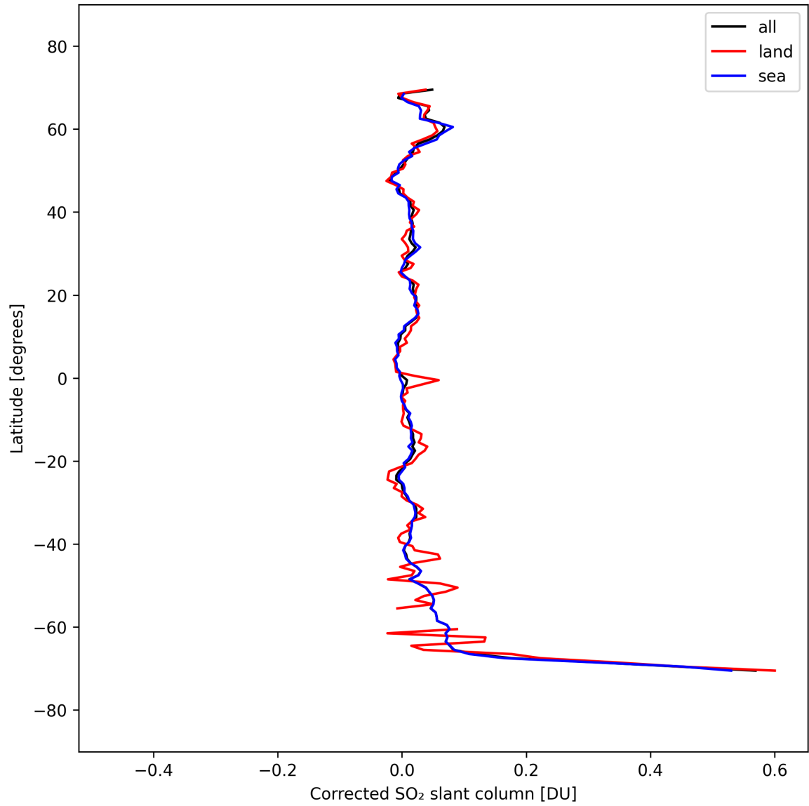
Figure 34: Zonal average of “Corrected SO 2 slant column” for 2025-09-25 to 2025-09-26.
