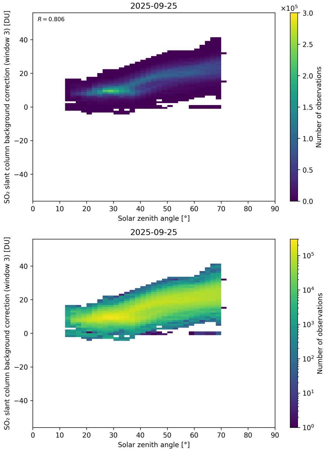
Figure 173: Scatter density plot of “Solar zenith angle” against “SO 2 slant column background correction (window 3)” for 2025-09-25 to 2025-09-26.
