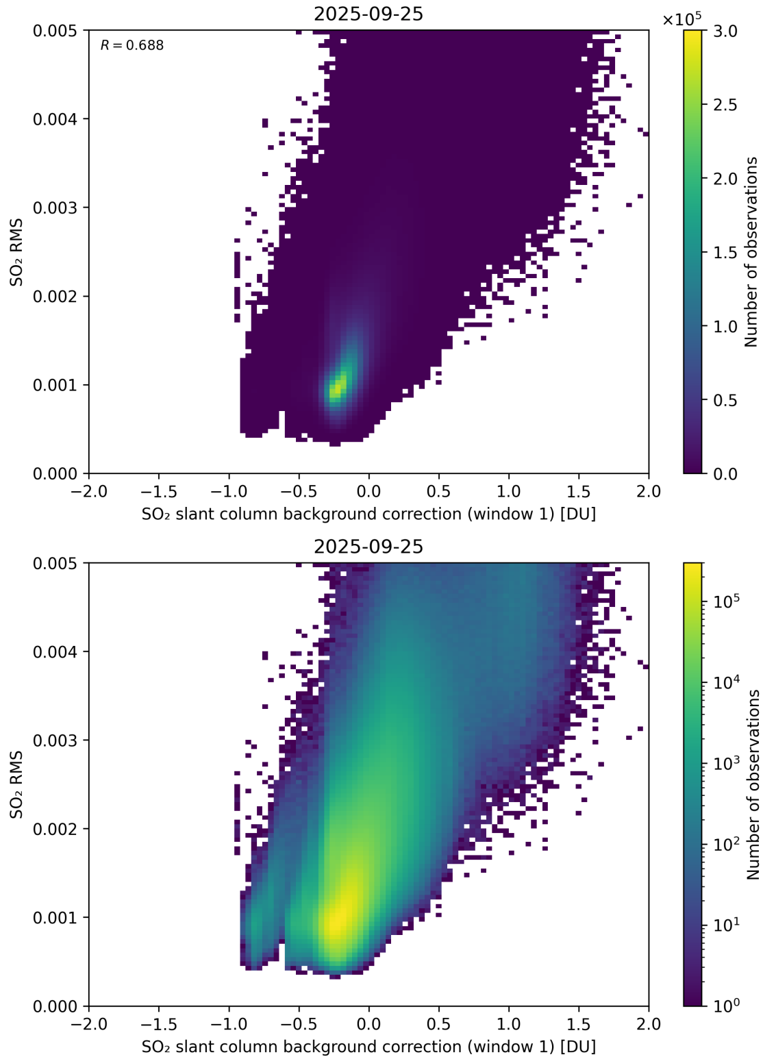
Figure 113: Scatter density plot of “SO 2 slant column background correction (window 1)” against “SO 2 RMS” for 2025-09-25 to 2025-09-26.
