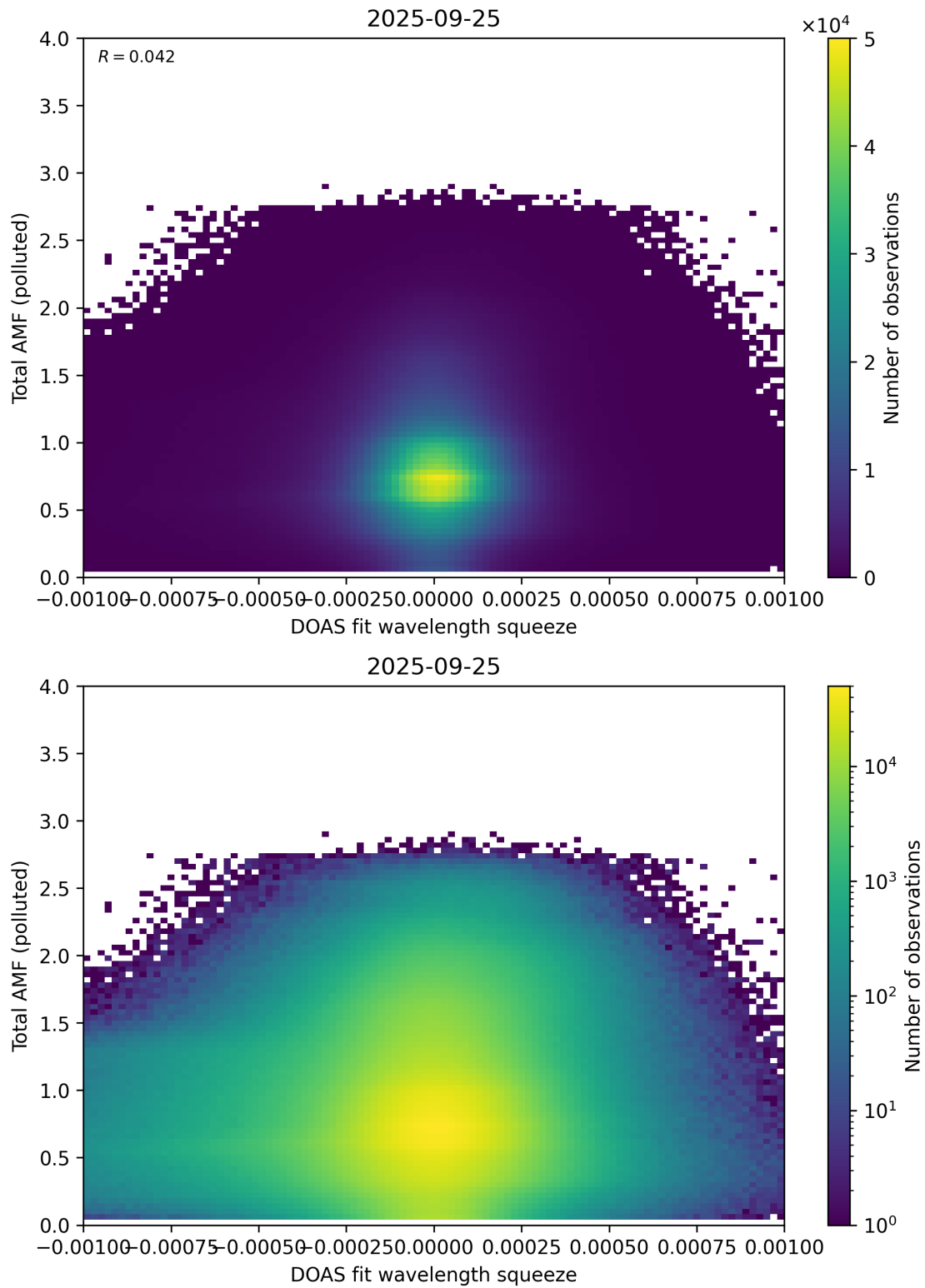
Figure 145: Scatter density plot of “DOAS fit wavelength squeeze” against “Total AMF (polluted)” for 2025-09-25 to 2025-09-26.
