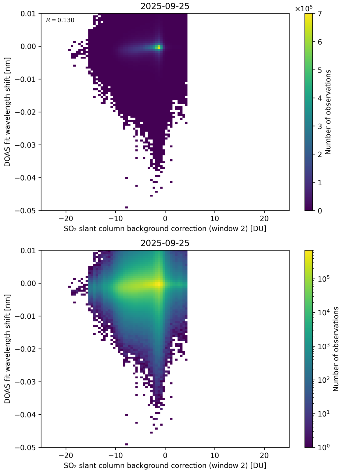
Figure 123: Scatter density plot of “SO 2 slant column background correction (window 2)” against “DOAS fit wavelength shift” for 2025-09-25 to 2025-09-26.
