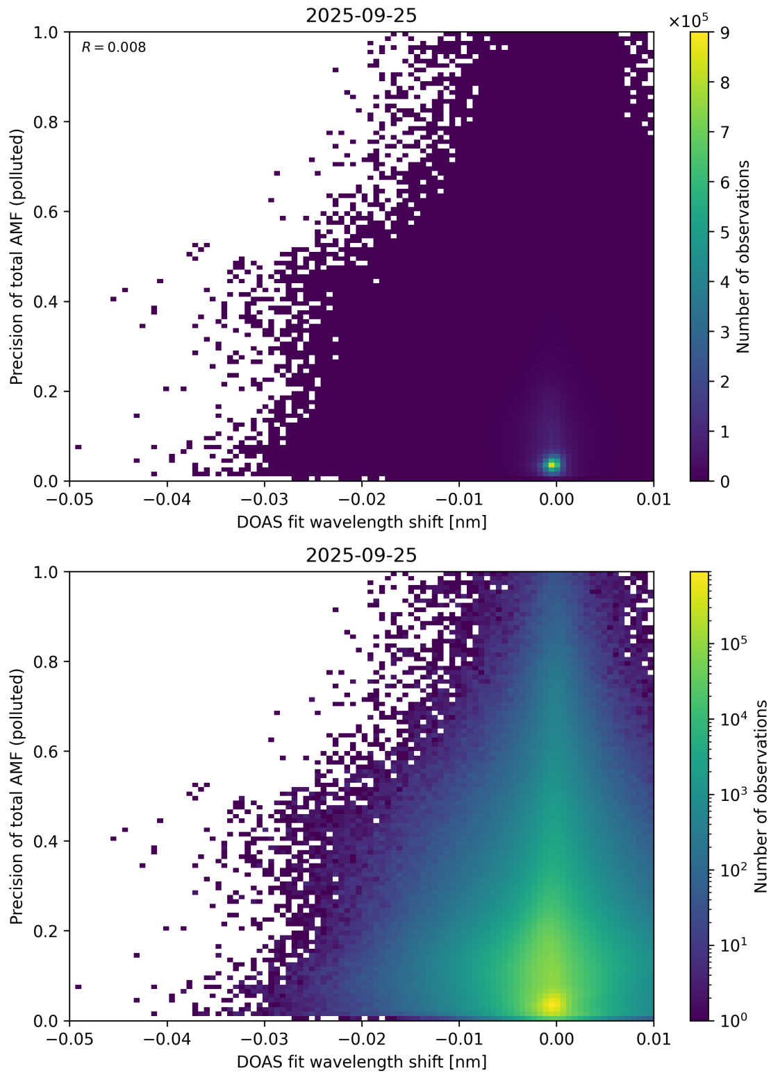
Figure 142: Scatter density plot of “DOAS fit wavelength shift” against “Precision of total AMF (polluted)” for 2025-09-25 to 2025-09-26.
