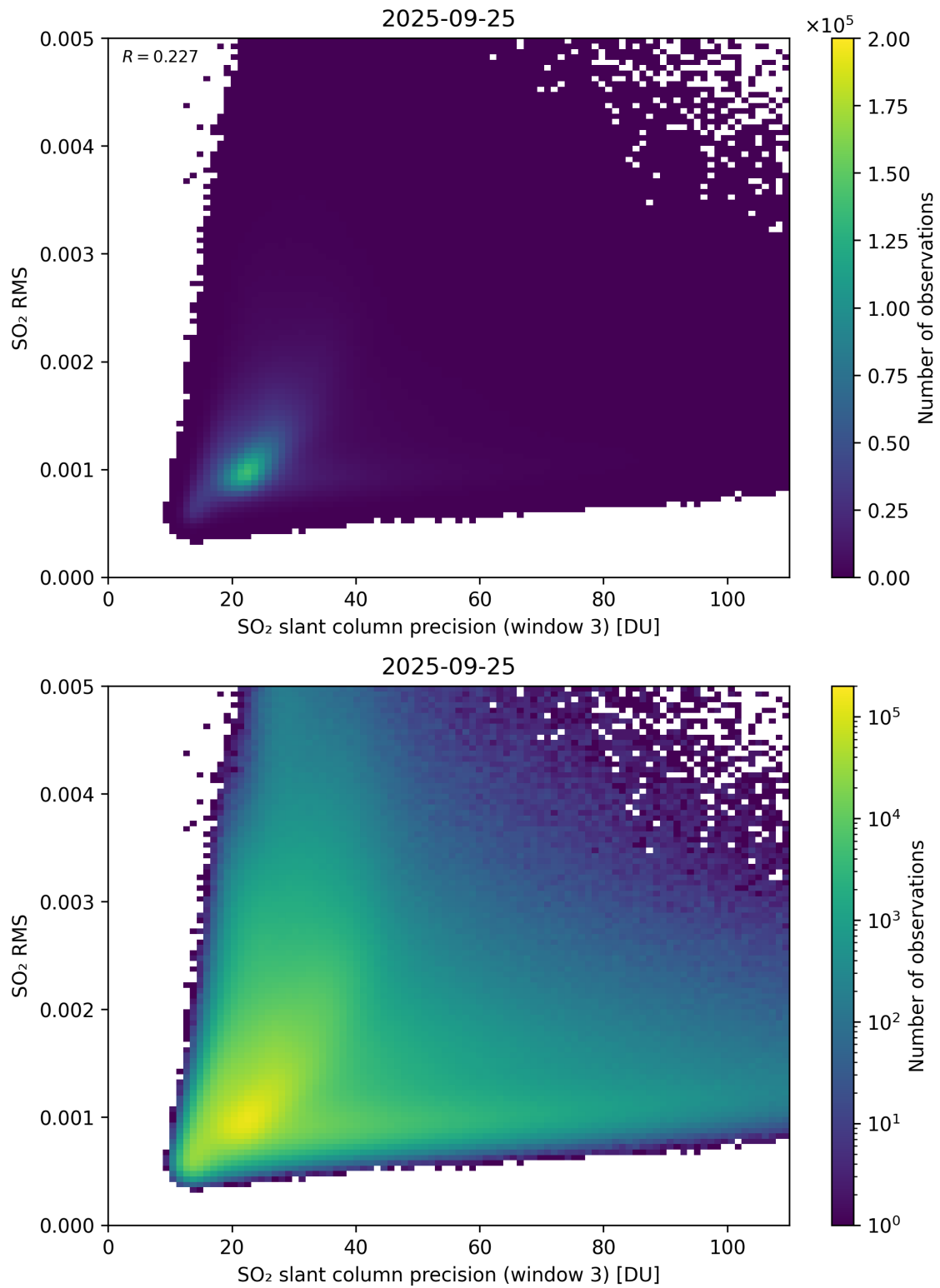
Figure 310: Scatter density plot of “SO 2 slant column precision (window 3)” against “SO 2 RMS” for 2025-09-25 to 2025-09-26.
