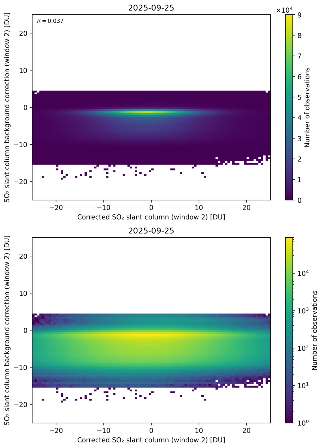
Figure 244: Scatter density plot of “Corrected SO 2 slant column (window 2)” against “SO 2 slant column background correction (window 2)” for 2025-09-25 to 2025-09-26.
