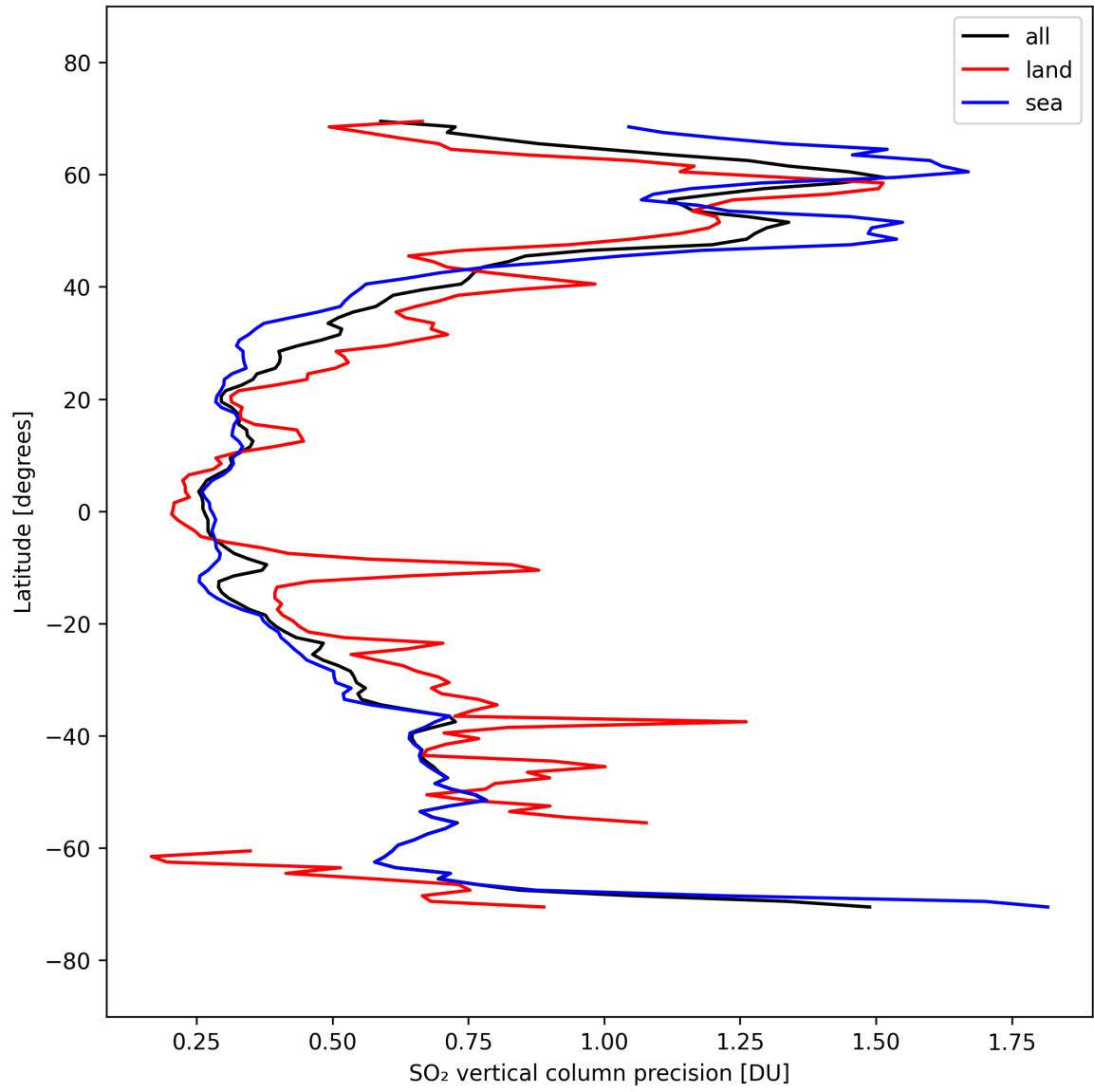
Figure 33: Zonal average of “SO 2 vertical column precision” for 2025-09-25 to 2025-09-26.
