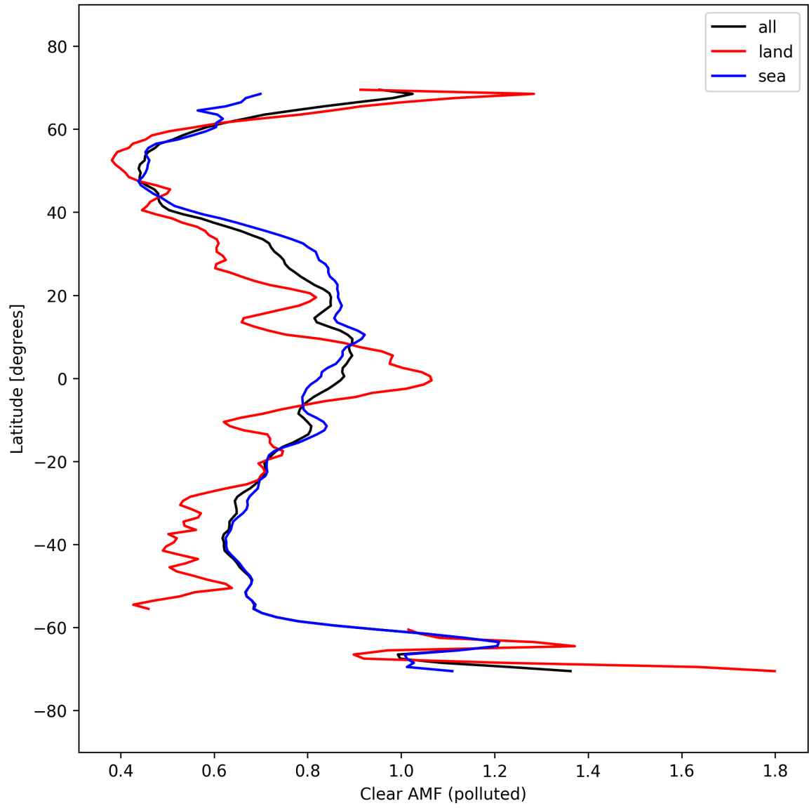
Figure 55: Zonal average of “Clear AMF (polluted)” for 2025-09-25 to 2025-09-26.
