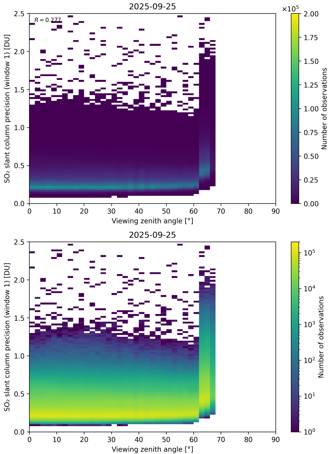
Figure 377: Scatter density plot of “Viewing zenith angle” against “SO 2 slant column precision (window 1)” for 2025-09-25 to 2025-09-26.
