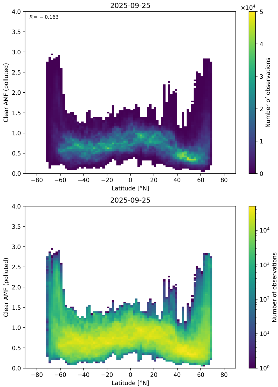
Figure 156: Scatter density plot of “Latitude” against “Clear AMF (polluted)” for 2025-09-25 to 2025-09-26.
