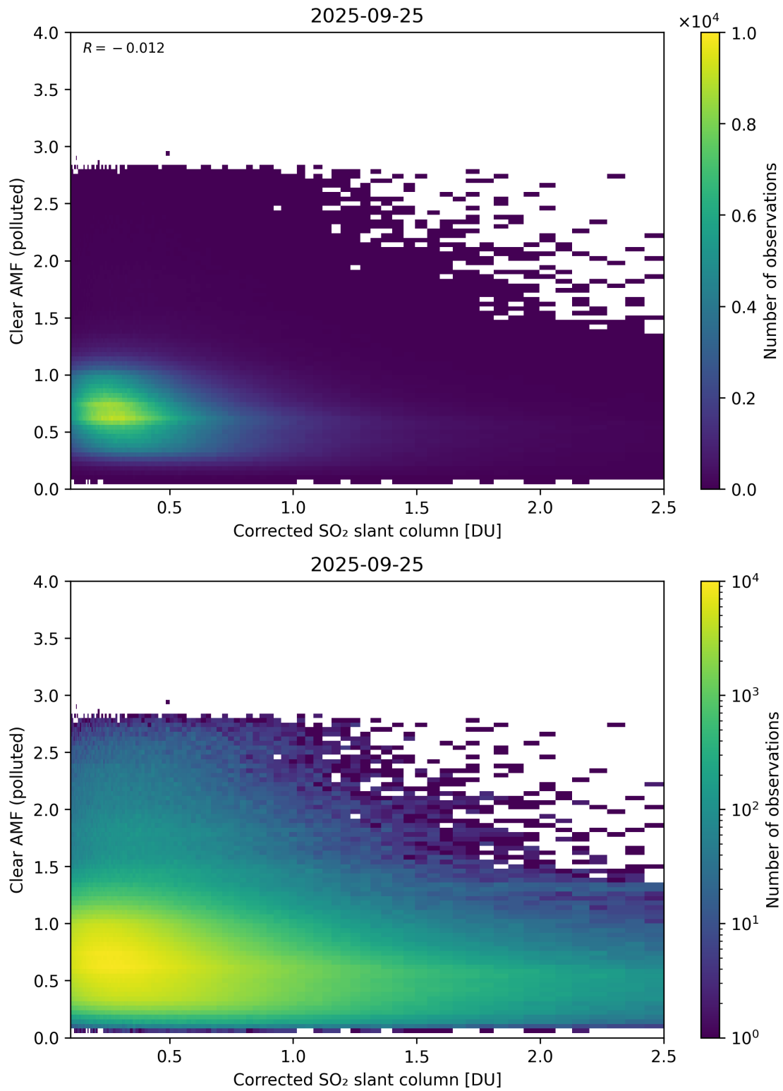
Figure 232: Scatter density plot of “Corrected SO 2 slant column” against “Clear AMF (polluted)” for 2025-09-25 to 2025-09-26.
