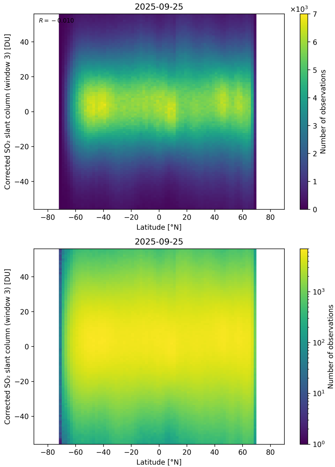
Figure 161: Scatter density plot of “Latitude” against “Corrected SO 2 slant column (window 3)” for 2025-09-25 to 2025-09-26.
