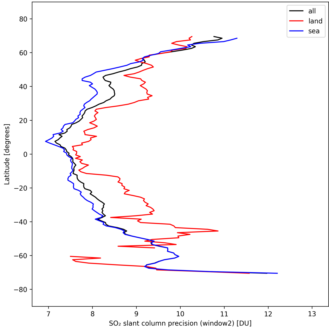
Figure 42: Zonal average of “SO 2 slant column precision (window2)” for 2025-09-25 to 2025-09-26.
