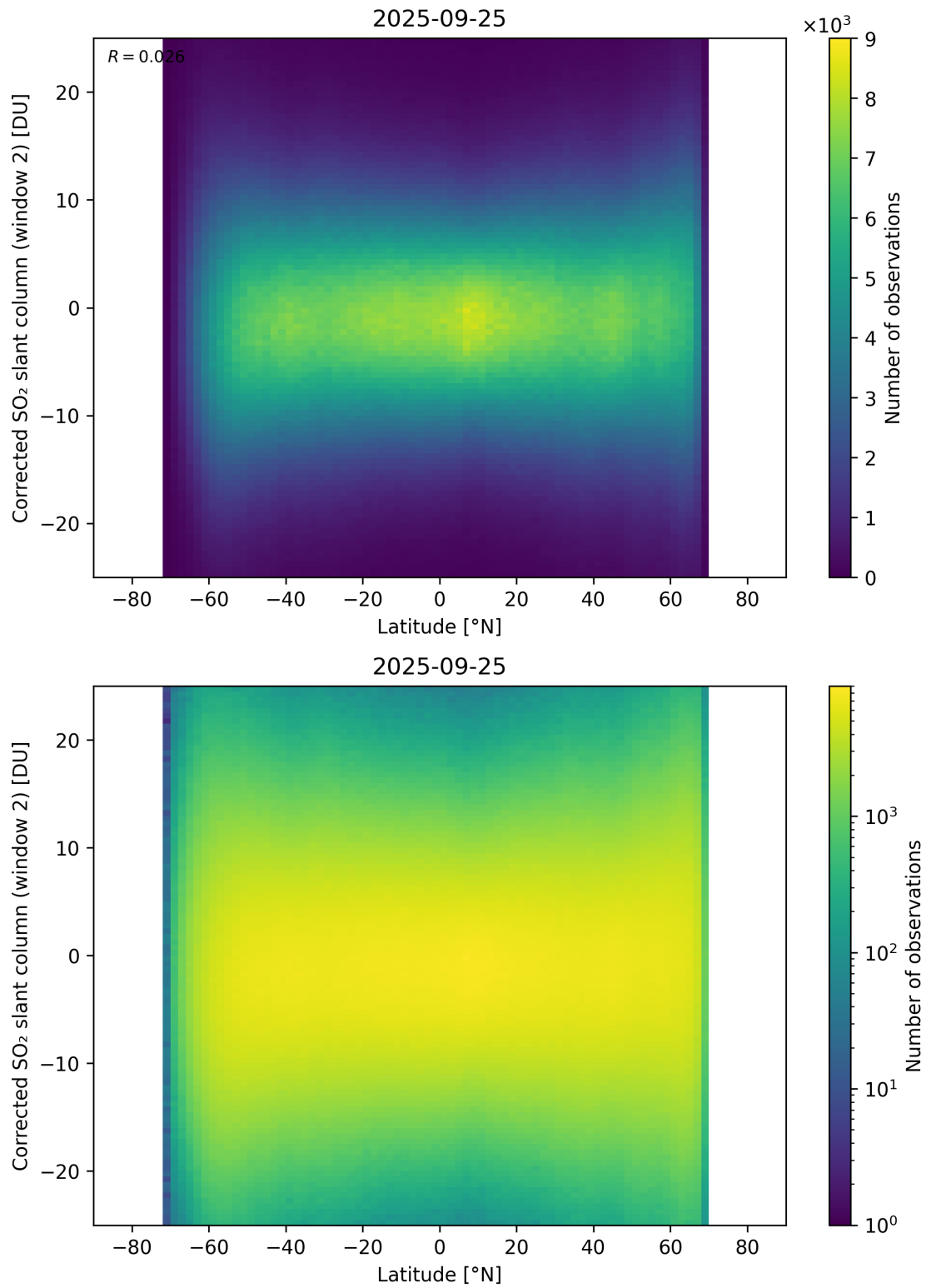
Figure 160: Scatter density plot of “Latitude” against “Corrected SO 2 slant column (window 2)” for 2025-09-25 to 2025-09-26.
