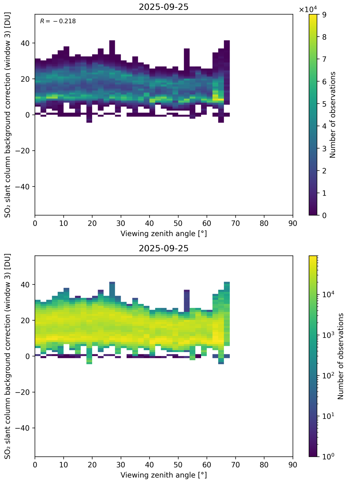
Figure 364: Scatter density plot of “Viewing zenith angle” against “SO 2 slant column background correction (window 3)” for 2025-09-25 to 2025-09-26.
