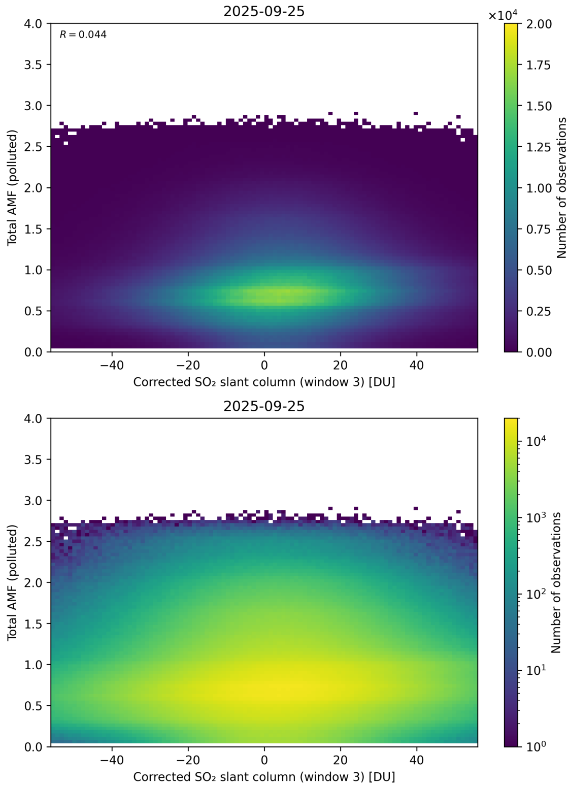
Figure 260: Scatter density plot of “Corrected SO 2 slant column (window 3)” against “Total AMF (polluted)” for 2025-09-25 to 2025-09-26.
