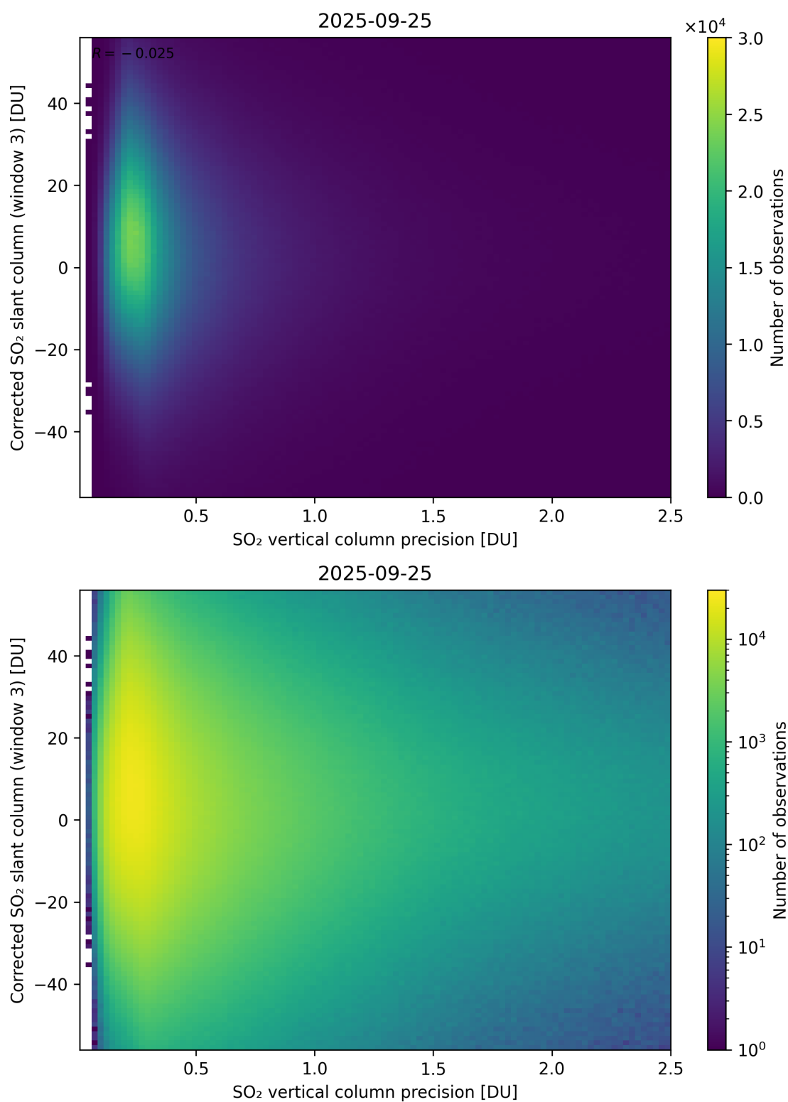
Figure 340: Scatter density plot of “SO 2 vertical column precision” against “Corrected SO 2 slant column (window 3)” for 2025-09-25 to 2025-09-26.
