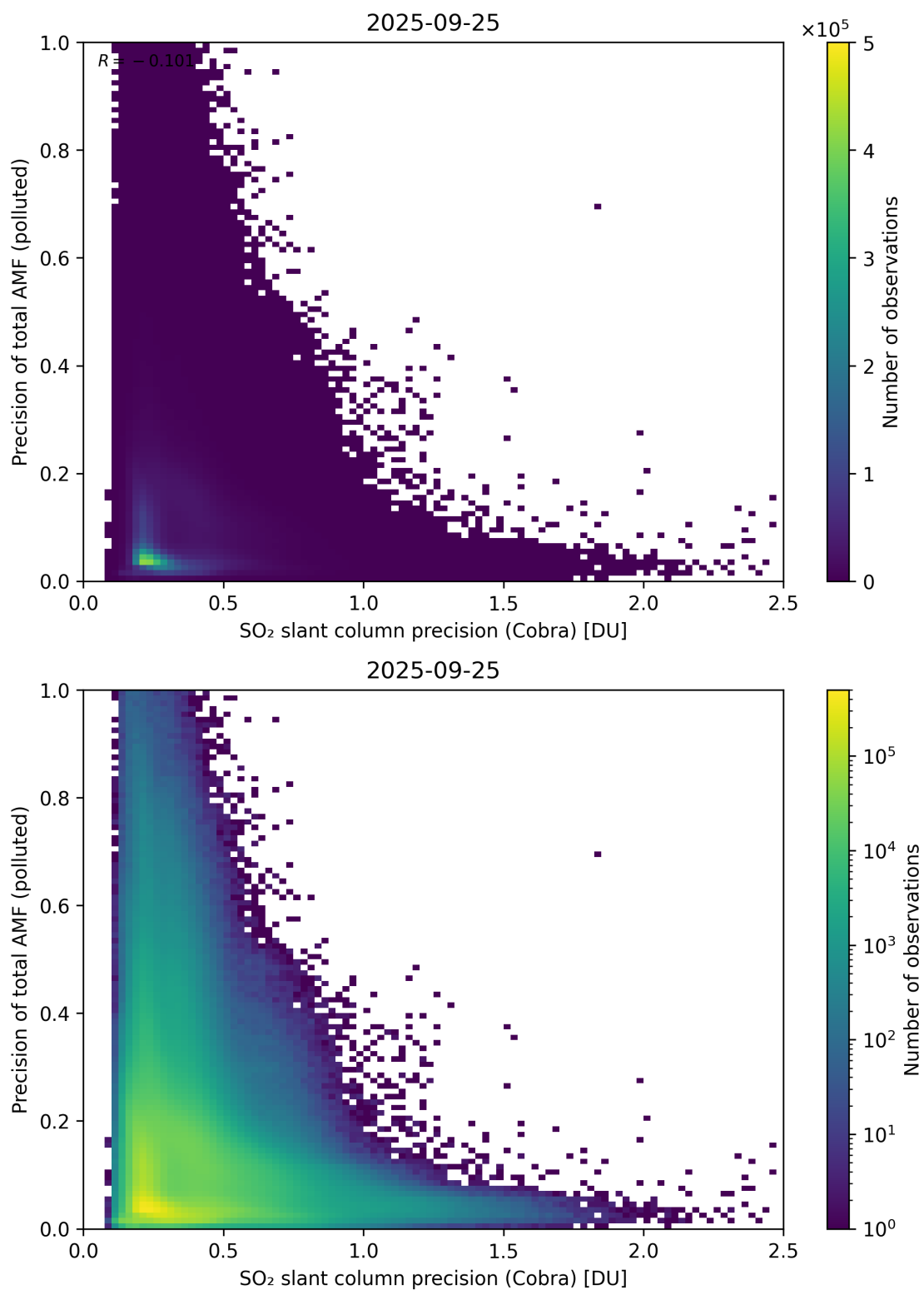
Figure 214: Scatter density plot of “SO 2 slant column precision (Cobra)” against “Precision of total AMF (polluted)” for 2025-09-25 to 2025-09-26.
