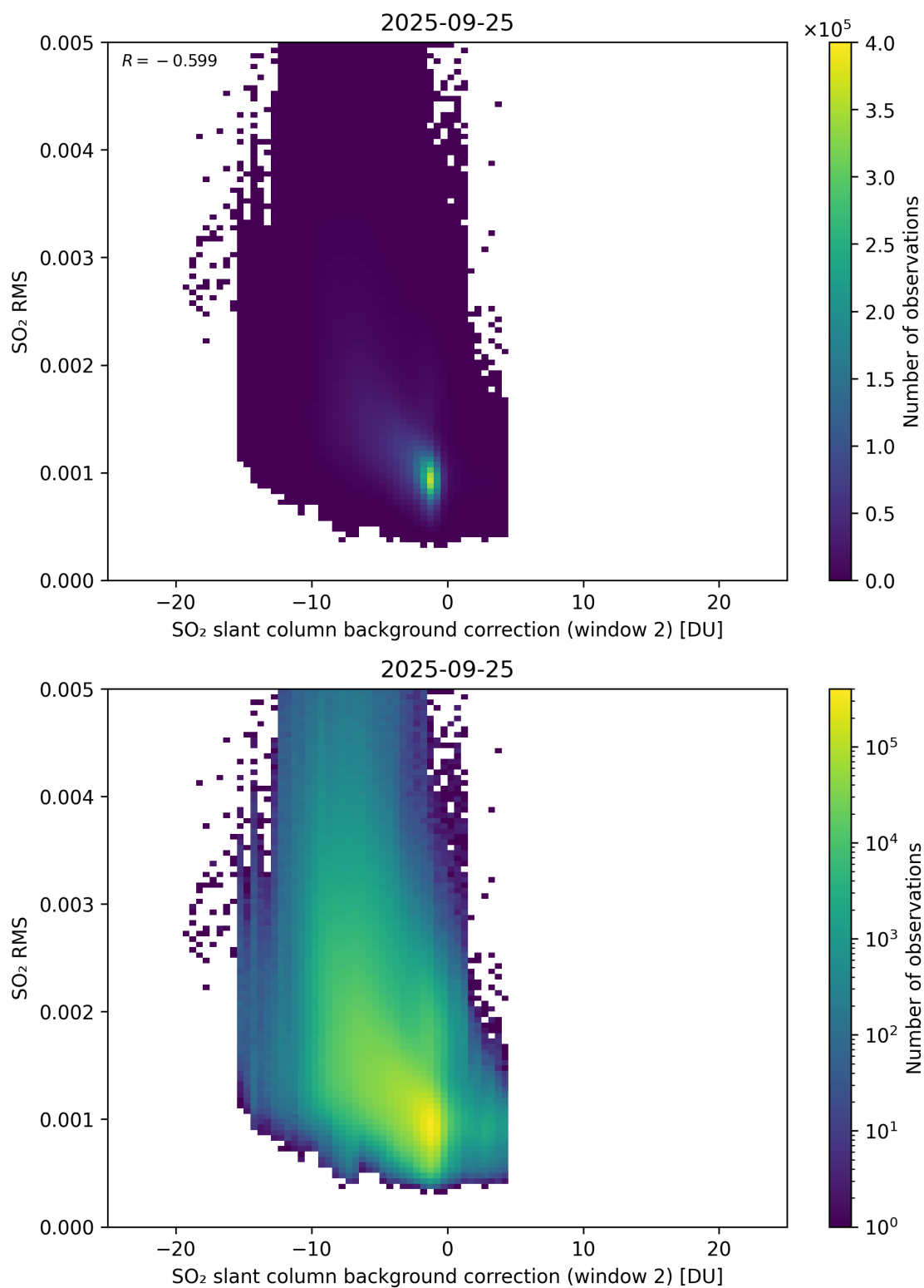
Figure 125: Scatter density plot of “SO 2 slant column background correction (window 2)” against “SO 2 RMS” for 2025-09-25 to 2025-09-26.
