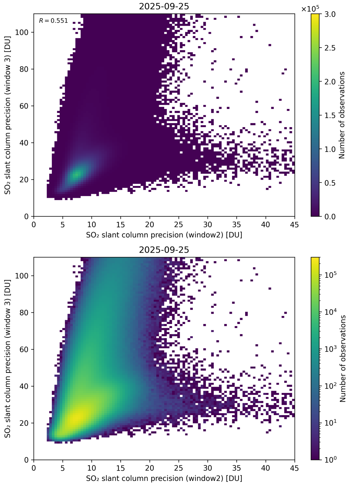
Figure 300: Scatter density plot of “SO 2 slant column precision (window2)” against “SO 2 slant column precision (window 3)” for 2025-09-25 to 2025-09-26.
