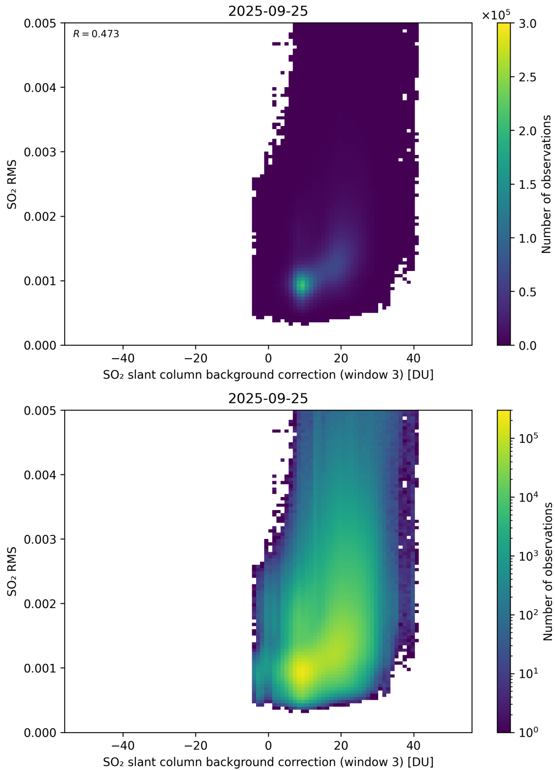
Figure 134: Scatter density plot of “SO 2 slant column background correction (window 3)” against “SO 2 RMS” for 2025-09-25 to 2025-09-26.
