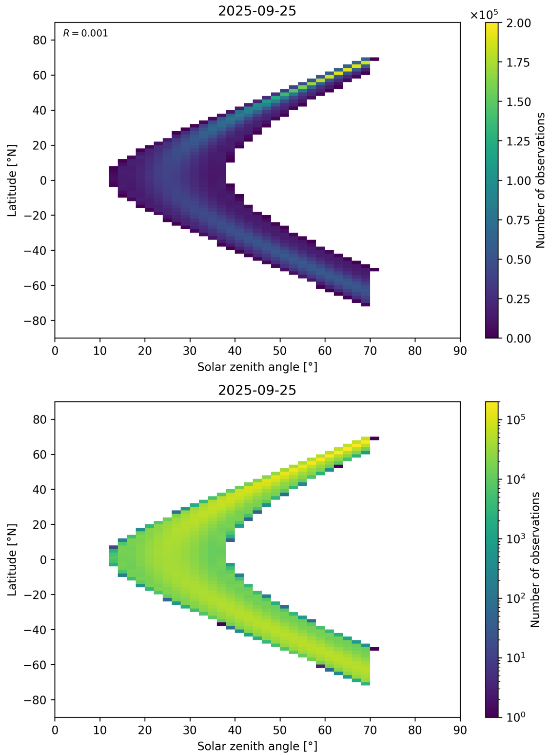
Figure 177: Scatter density plot of “Solar zenith angle” against “Latitude” for 2025-09-25 to 2025-09-26.
