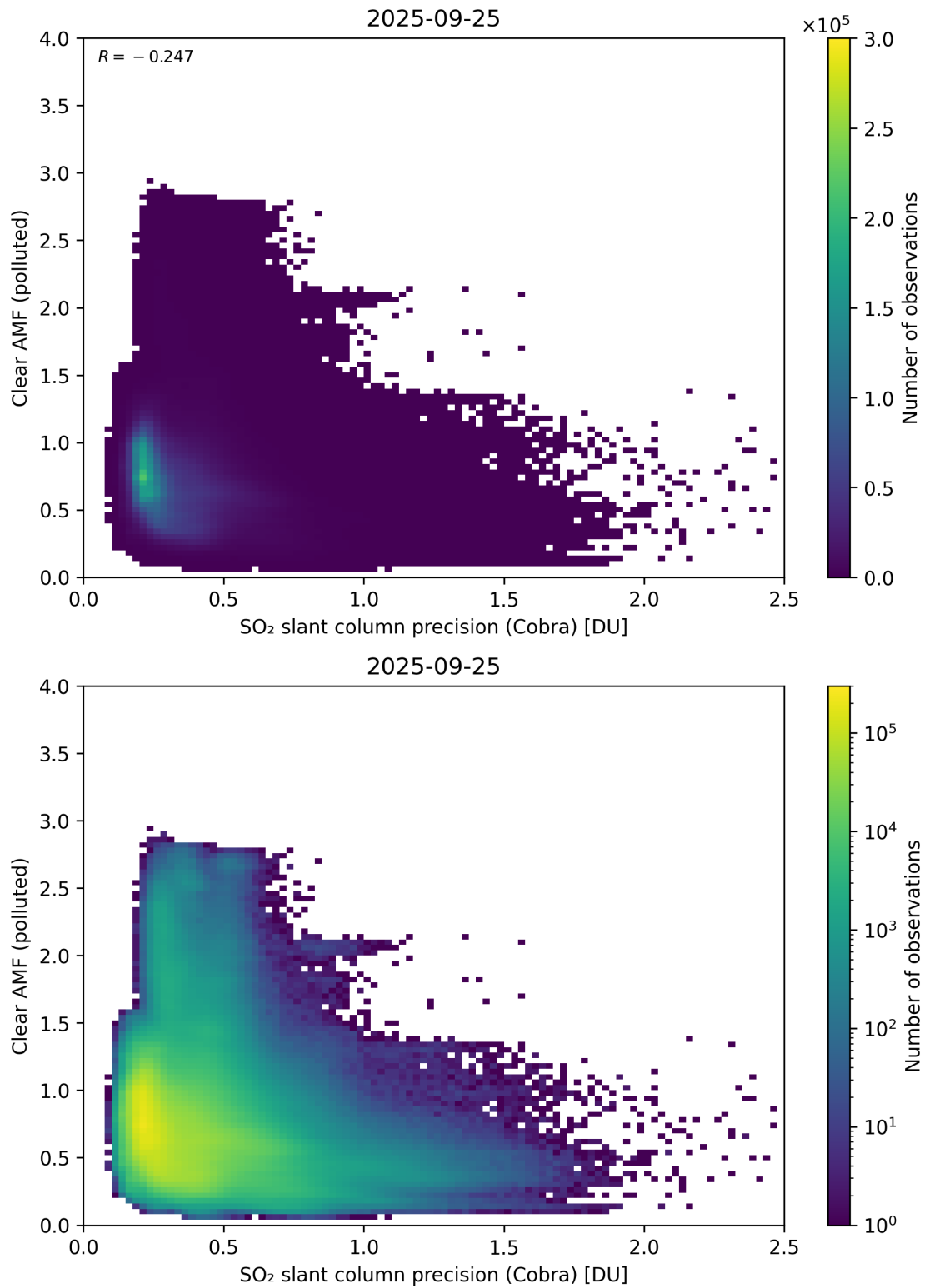
Figure 205: Scatter density plot of “SO 2 slant column precision (Cobra)” against “Clear AMF (polluted)” for 2025-09-25 to 2025-09-26.
