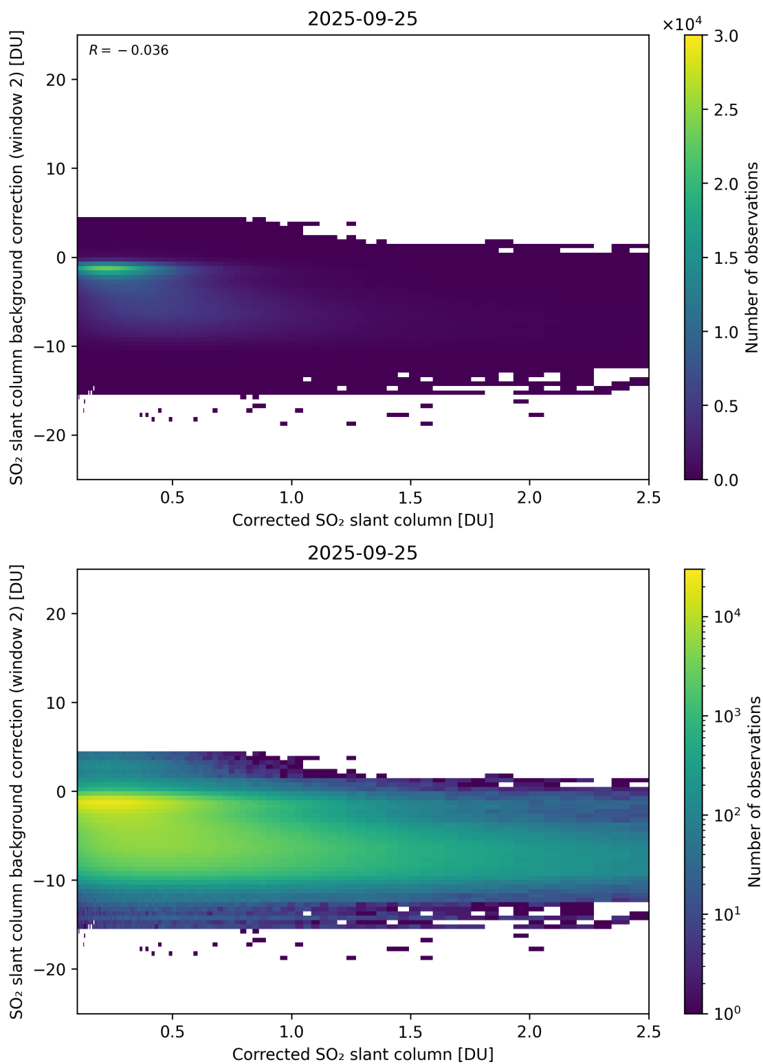
Figure 227: Scatter density plot of “Corrected SO 2 slant column” against “SO 2 slant column background correction (window 2)” for 2025-09-25 to 2025-09-26.
