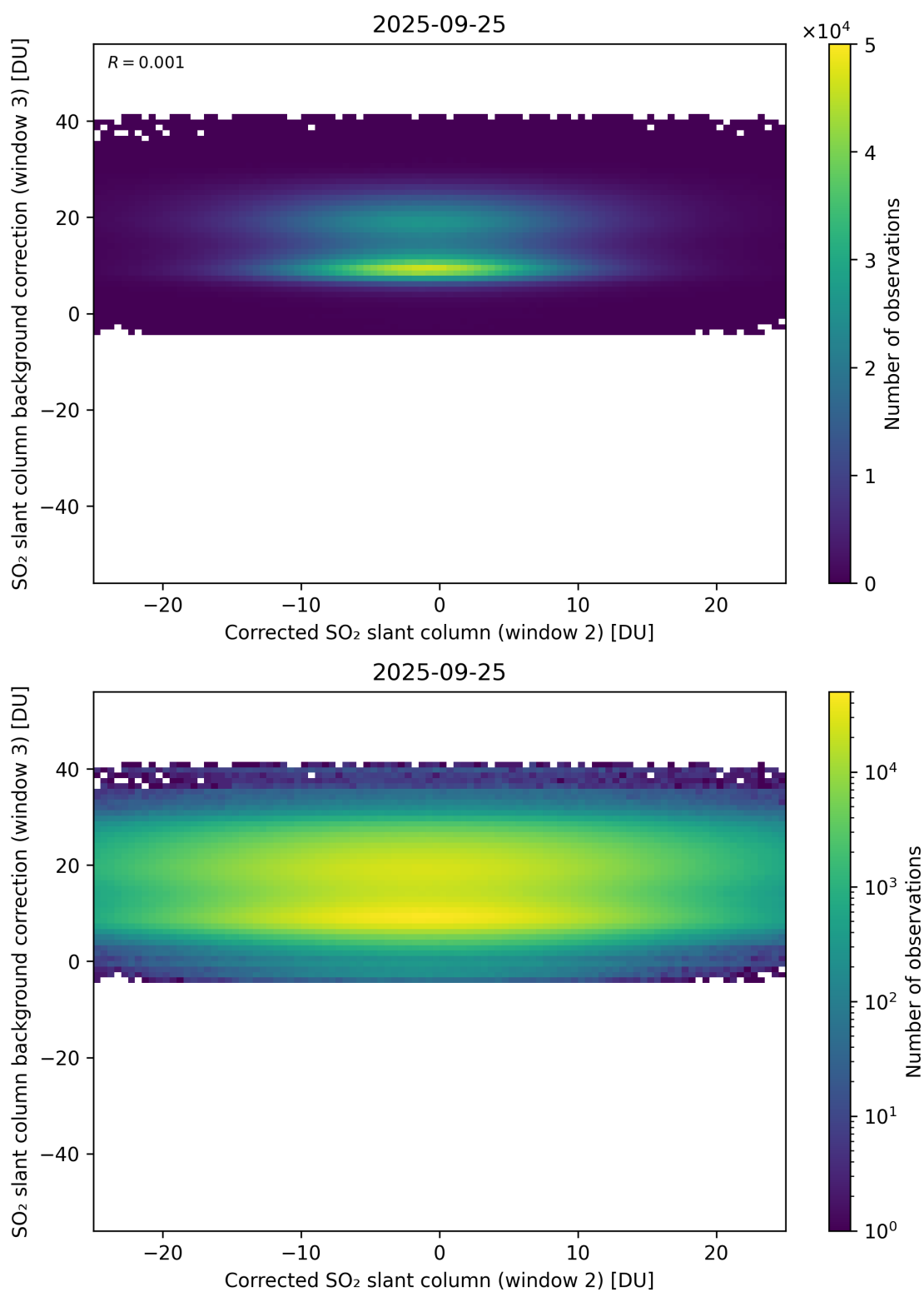
Figure 245: Scatter density plot of “Corrected SO 2 slant column (window 2)” against “SO 2 slant column background correction (window 3)” for 2025-09-25 to 2025-09-26.
