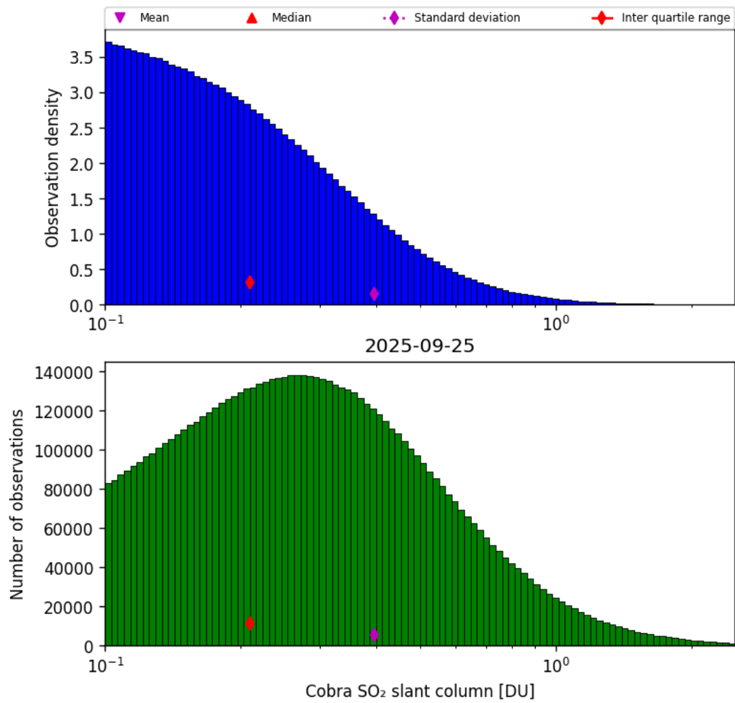
Figure 61: Histogram of “Cobra SO 2 slant column” for 2025-09-25 to 2025-09-26
