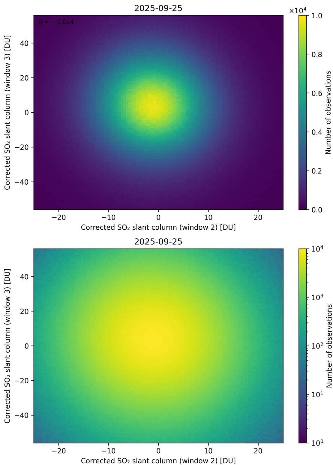
Figure 250: Scatter density plot of “Corrected SO 2 slant column (window 2)” against “Corrected SO 2 slant column (window 3)” for 2025-09-25 to 2025-09-26.
