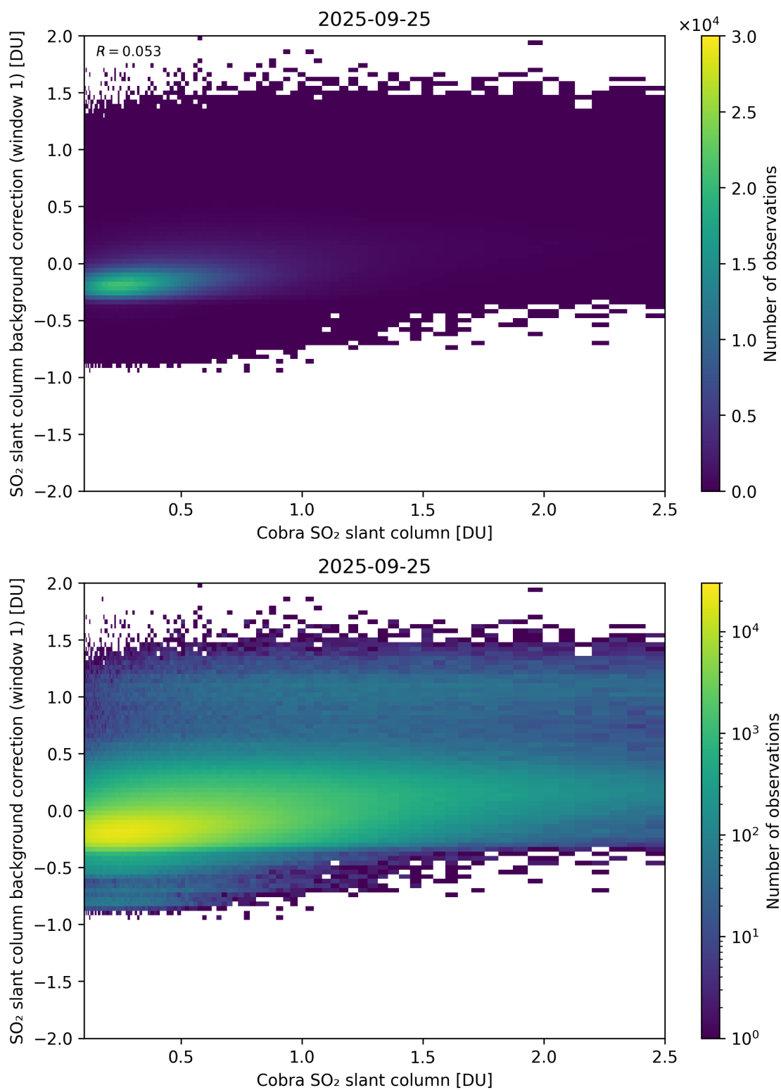
Figure 193: Scatter density plot of “Cobra SO 2 slant column” against “SO 2 slant column background correction (window 1)” for 2025-09-25 to 2025-09-26.
