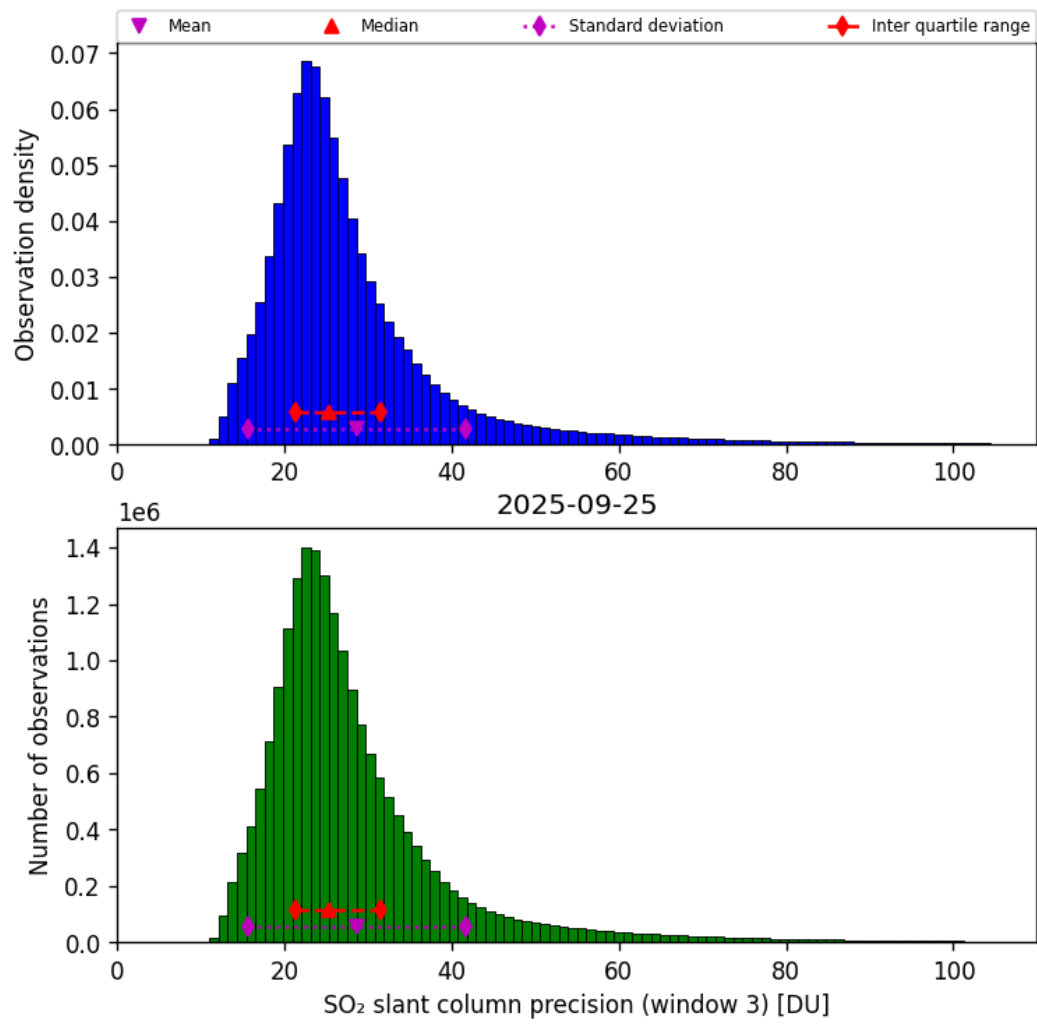
Figure 72: Histogram of “SO 2 slant column precision (window 3)” for 2025-09-25 to 2025-09-26
