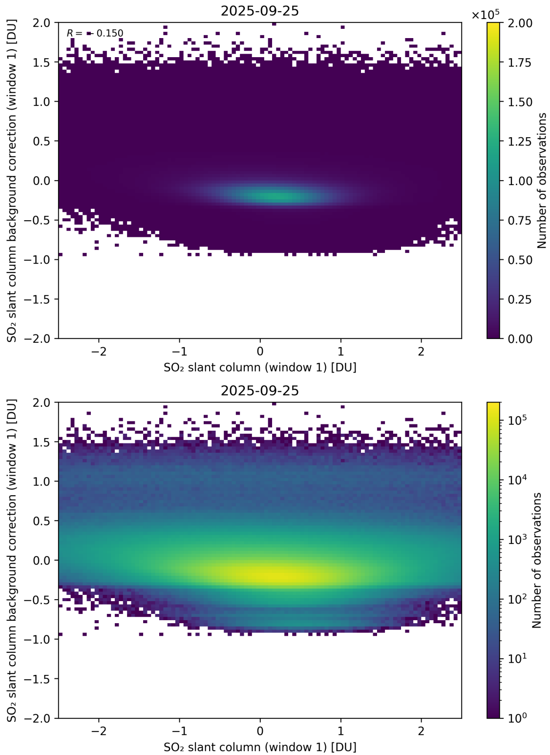
Figure 262: Scatter density plot of “SO 2 slant column (window 1)” against “SO 2 slant column background correction (window 1)” for 2025-09-25 to 2025-09-26.
