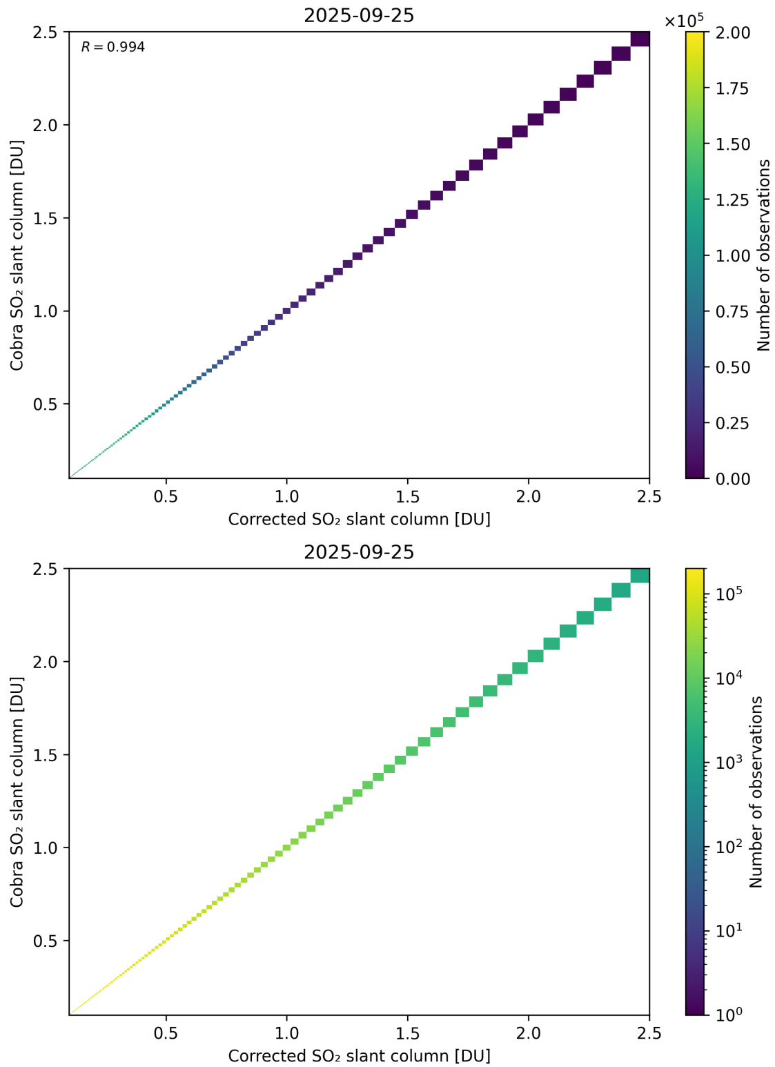
Figure 233: Scatter density plot of “Corrected SO 2 slant column” against “Cobra SO 2 slant column” for 2025-09-25 to 2025-09-26.
