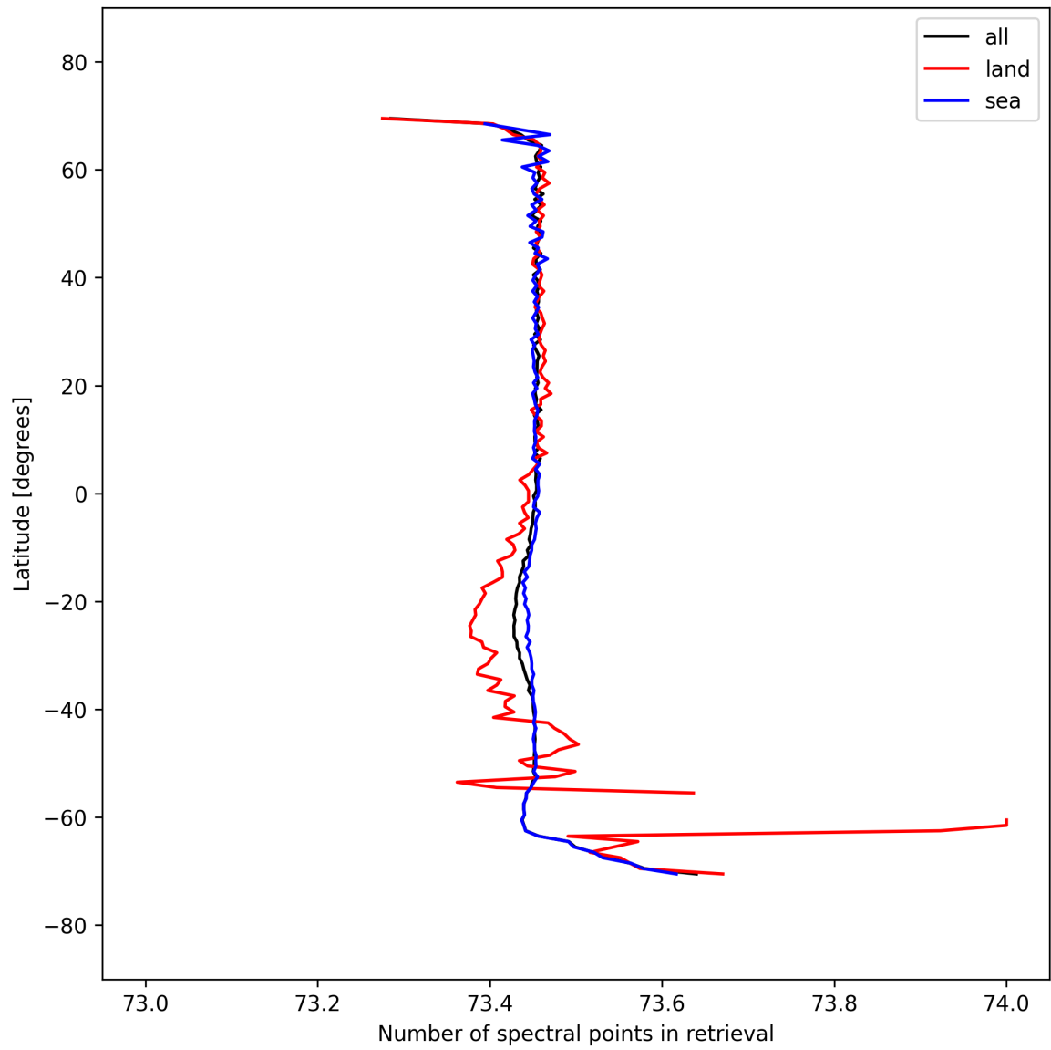
Figure 56: Zonal average of “Number of spectral points in retrieval” for 2025-09-25 to 2025-09-26.
