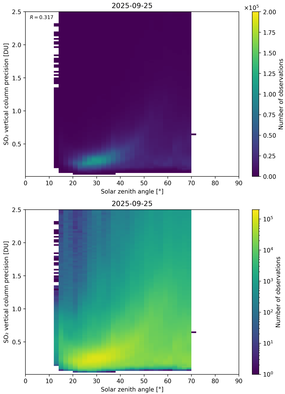
Figure 192: Scatter density plot of “Solar zenith angle” against “SO 2 vertical column precision” for 2025-09-25 to 2025-09-26.
