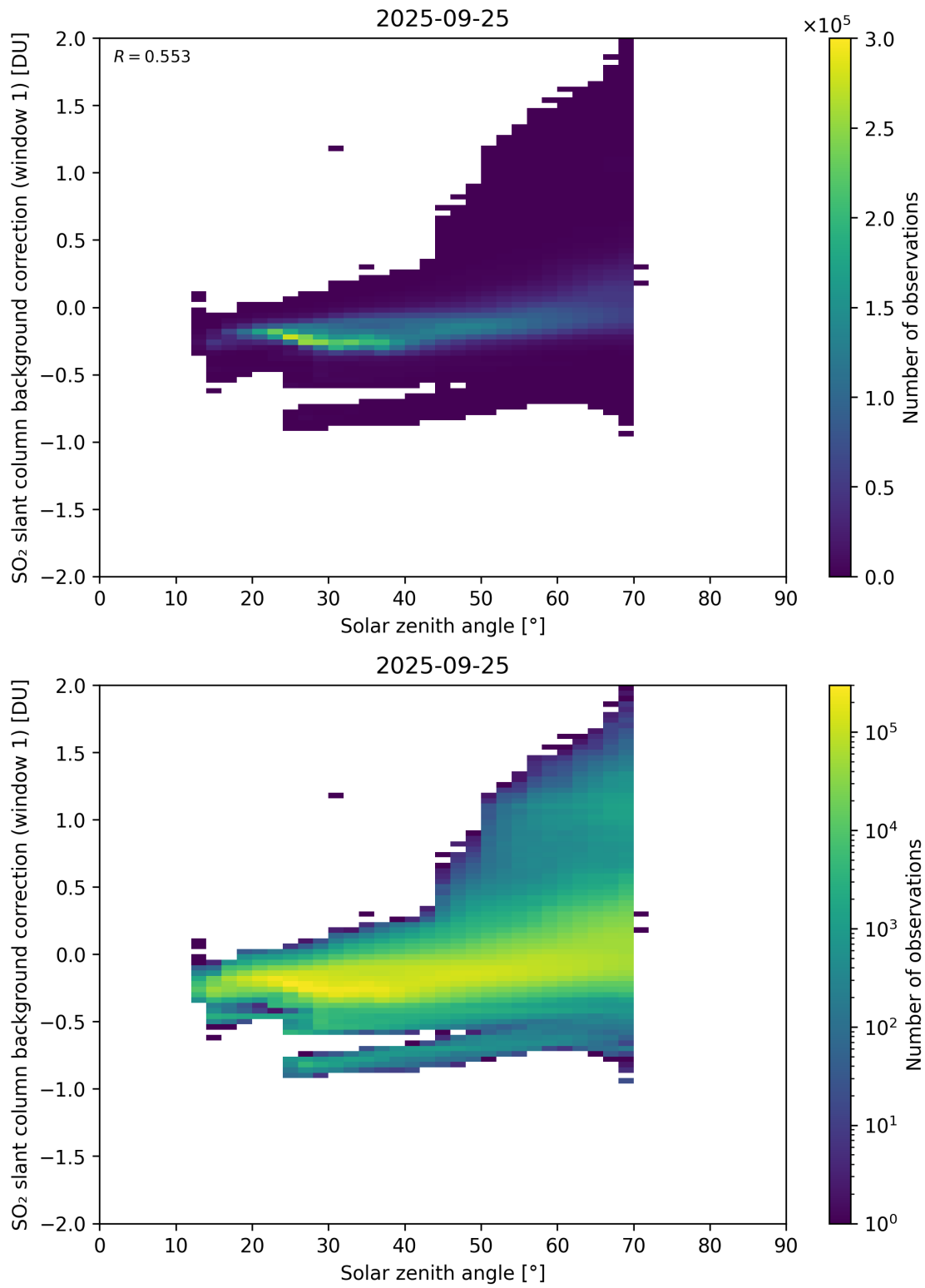
Figure 171: Scatter density plot of “Solar zenith angle” against “SO 2 slant column background correction (window 1)” for 2025-09-25 to 2025-09-26.
