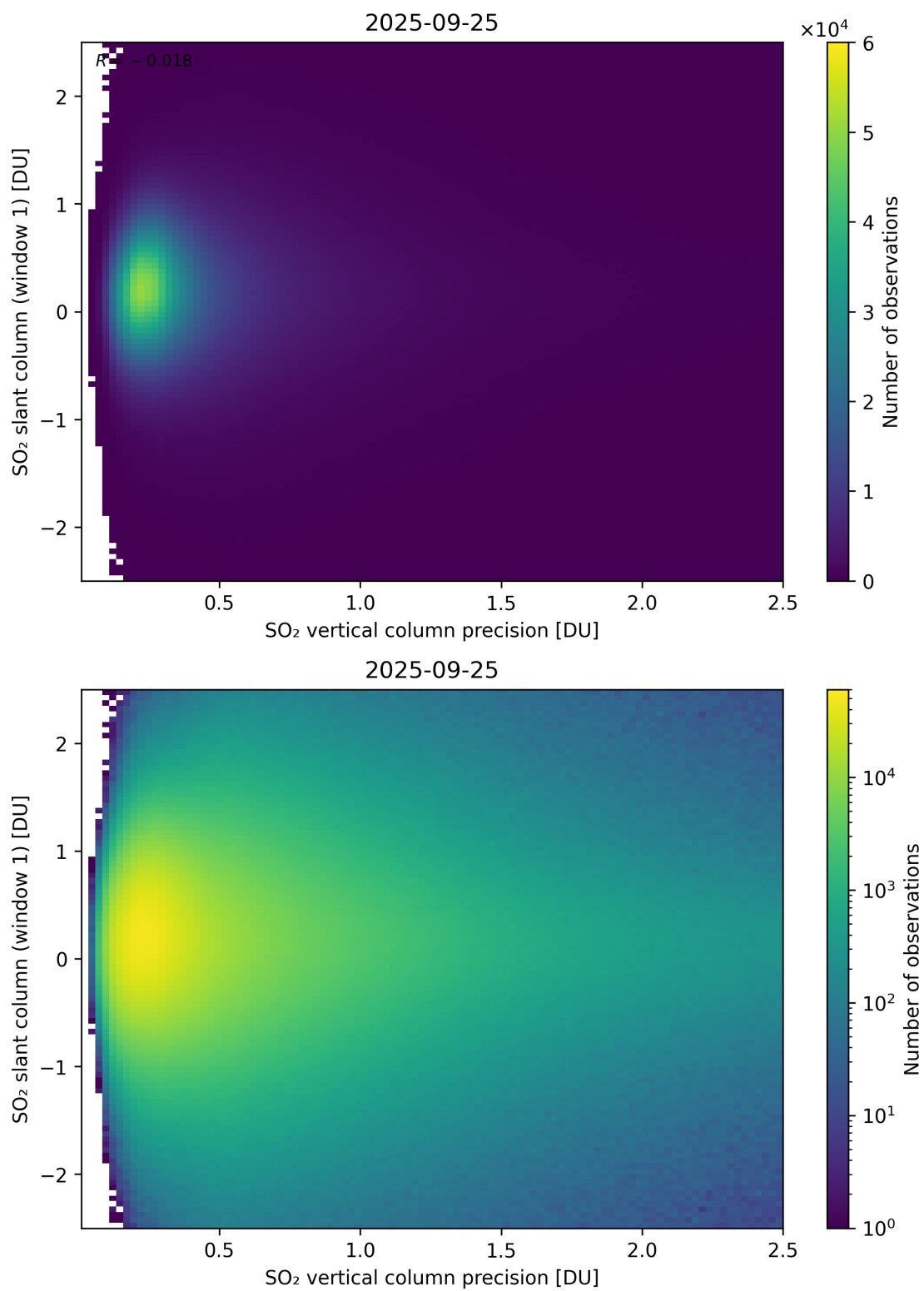
Figure 341: Scatter density plot of “SO 2 vertical column precision” against “SO 2 slant column (window 1)” for 2025-09-25 to 2025-09-26.
