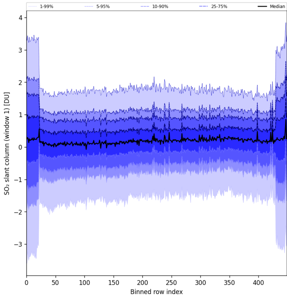
Figure 89: Along track statistics of “SO 2 slant column (window 1)” for 2025-09-25 to 2025-09-26
