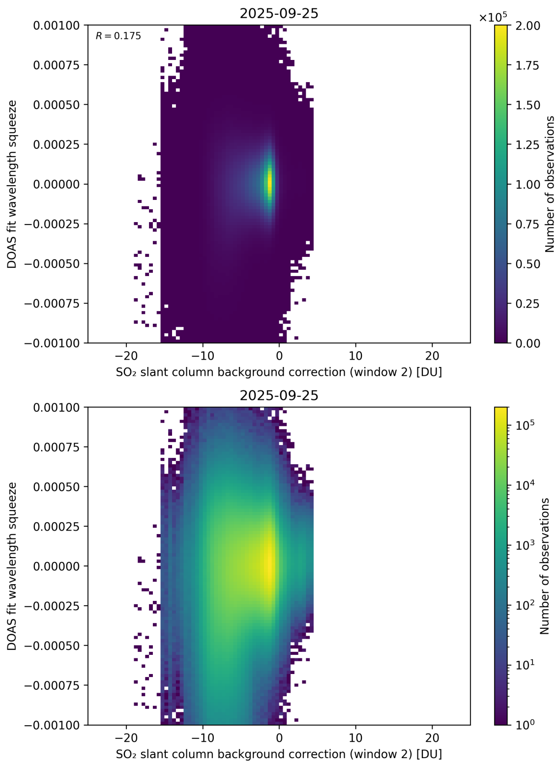
Figure 124: Scatter density plot of “SO 2 slant column background correction (window 2)” against “DOAS fit wavelength squeeze” for 2025-09-25 to 2025-09-26.
