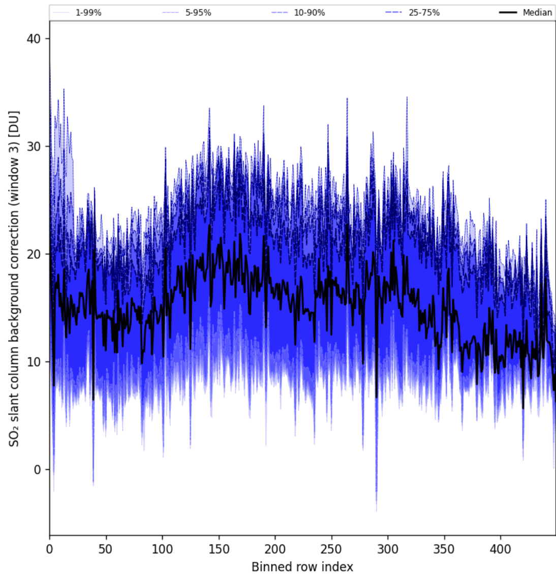
Figure 100: Along track statistics of “SO 2 slant column background correction (window 3)” for 2025-09-25 to 2025-09-26
