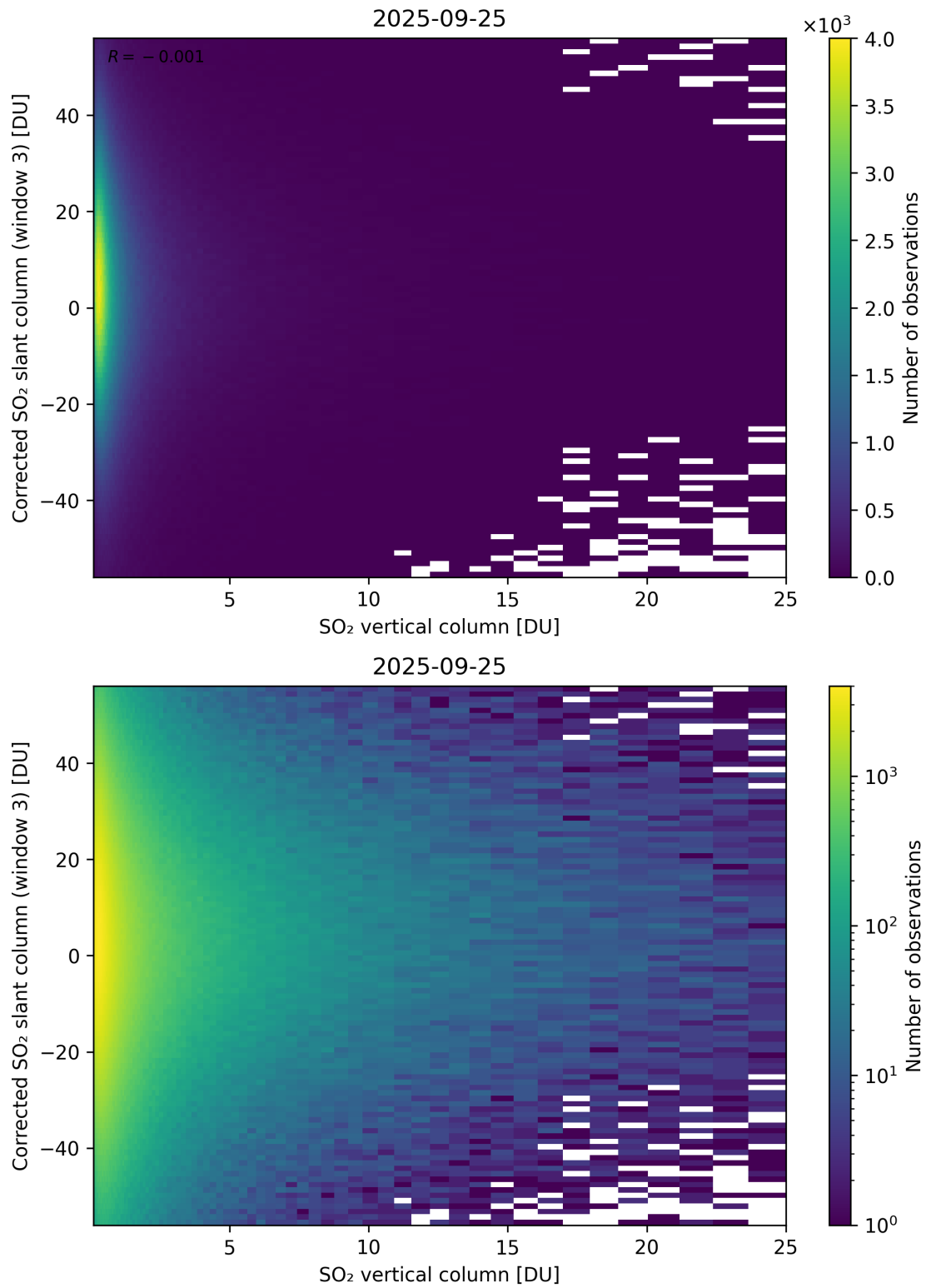
Figure 353: Scatter density plot of “SO 2 vertical column” against “Corrected SO 2 slant column (window 3)” for 2025-09-25 to 2025-09-26.
