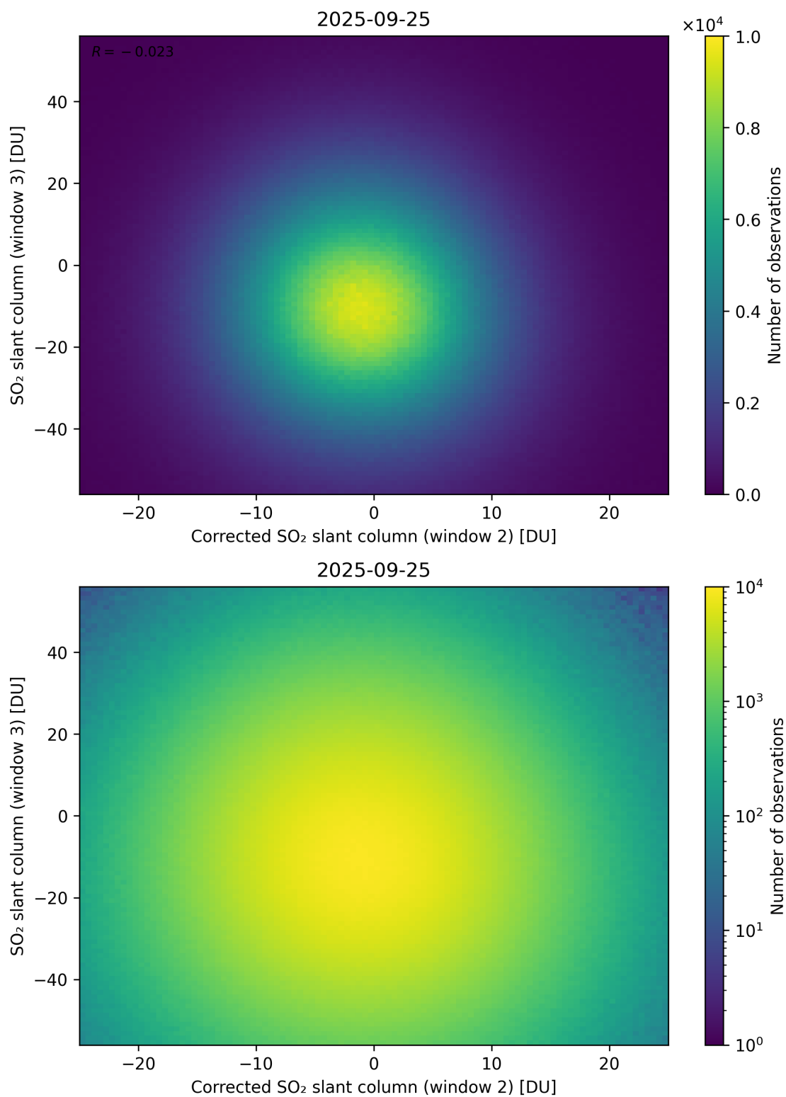
Figure 251: Scatter density plot of “Corrected SO 2 slant column (window 2)” against “SO 2 slant column (window 3)” for 2025-09-25 to 2025-09-26.
