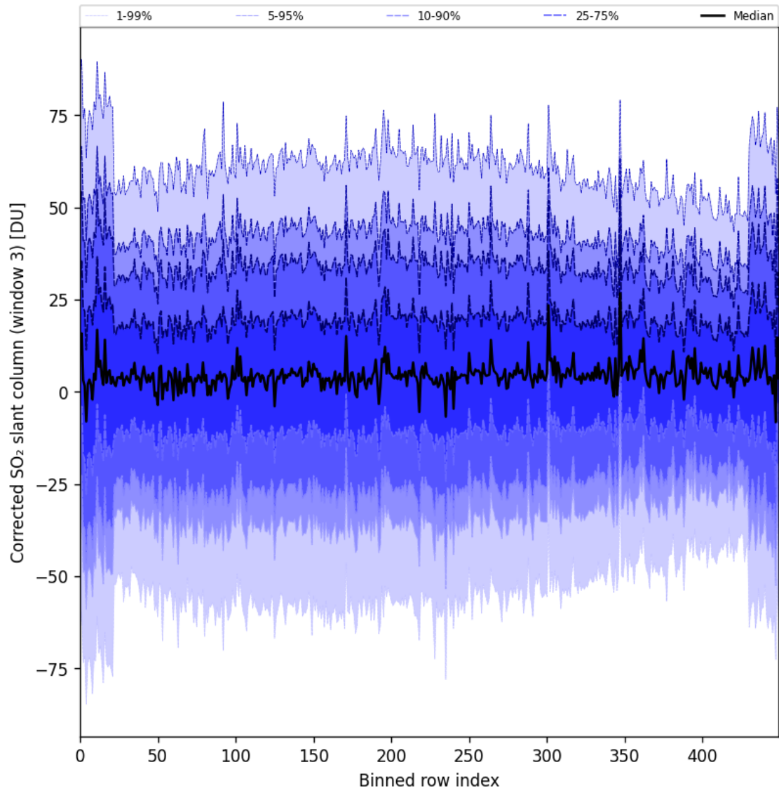
Figure 99: Along track statistics of “Corrected SO 2 slant column (window 3)” for 2025-09-25 to 2025-09-26
