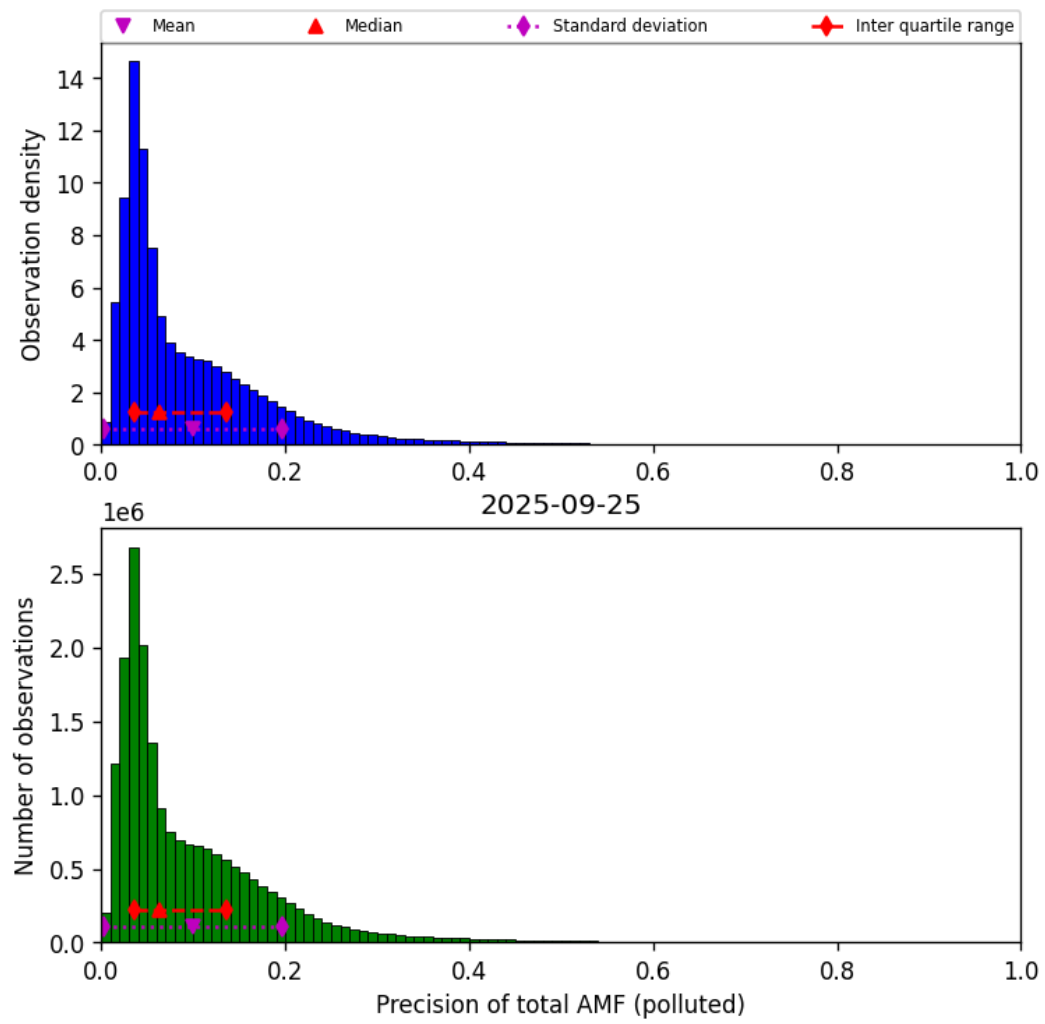
Figure 80: Histogram of “Precision of total AMF (polluted)” for 2025-09-25 to 2025-09-26
