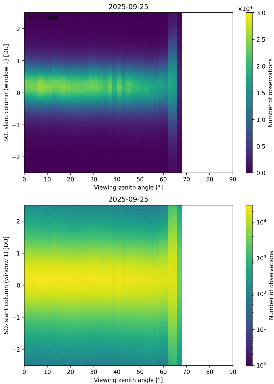
Figure 376: Scatter density plot of “Viewing zenith angle” against “SO 2 slant column (window 1)” for 2025-09-25 to 2025-09-26.
