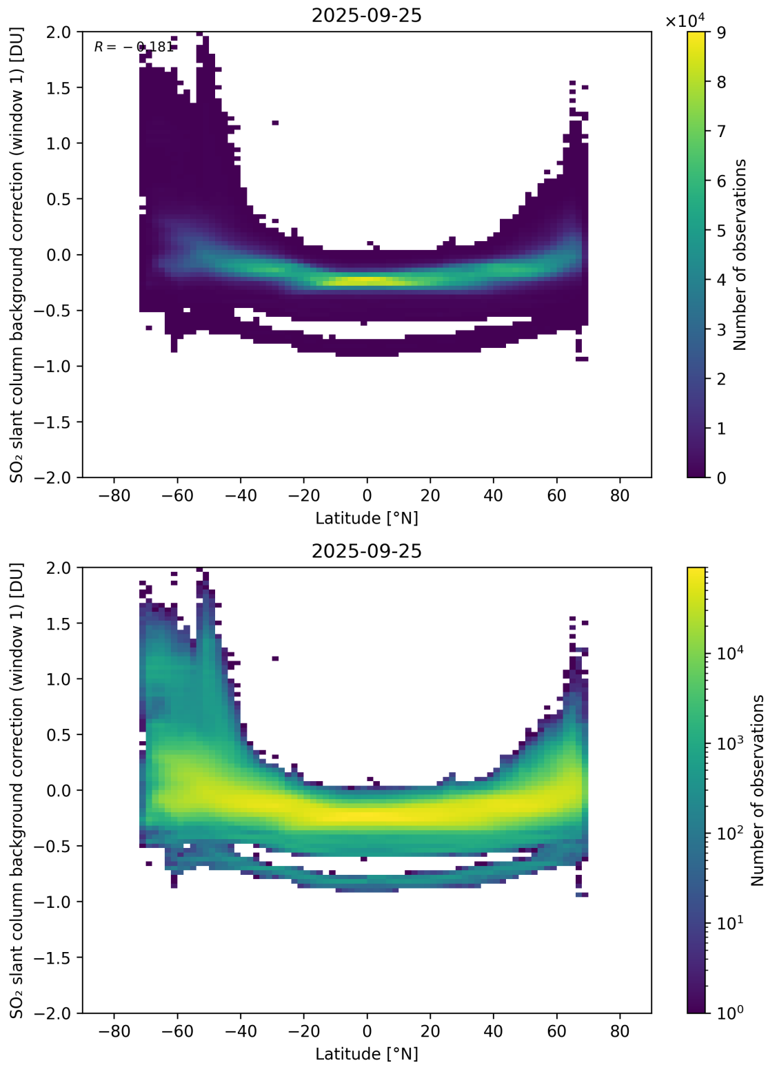
Figure 150: Scatter density plot of “Latitude” against “SO 2 slant column background correction (window 1)” for 2025-09-25 to 2025-09-26.
