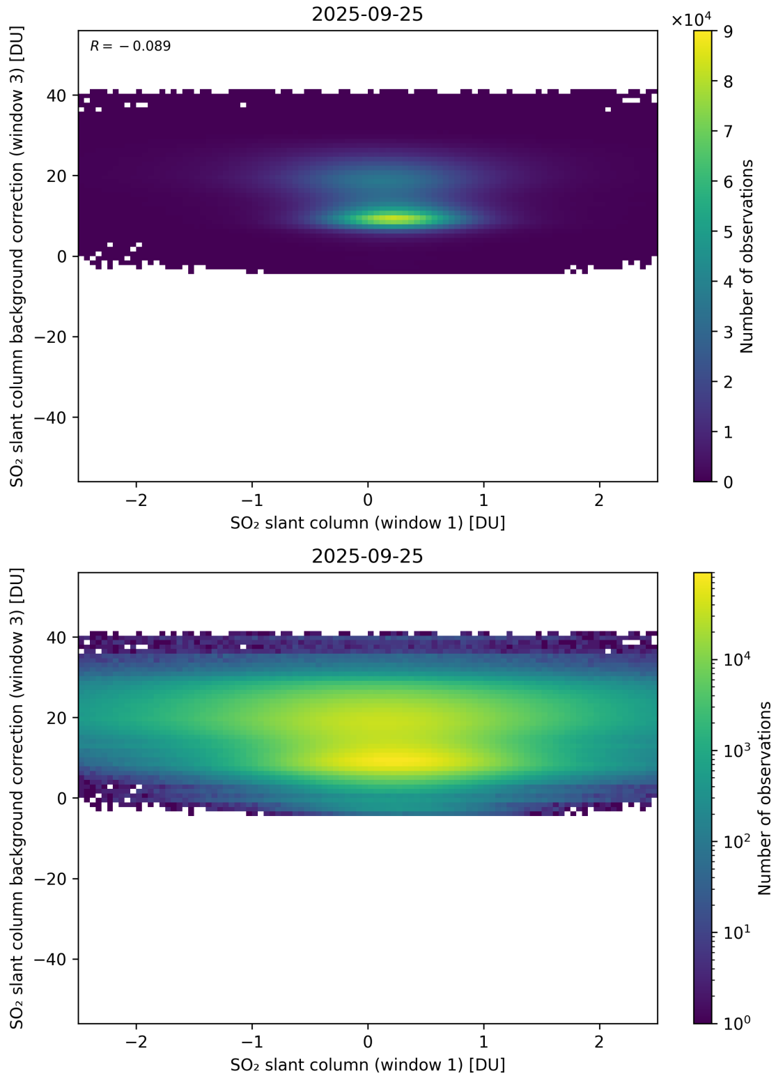
Figure 264: Scatter density plot of “SO 2 slant column (window 1)” against “SO 2 slant column background correction (window 3)” for 2025-09-25 to 2025-09-26.
