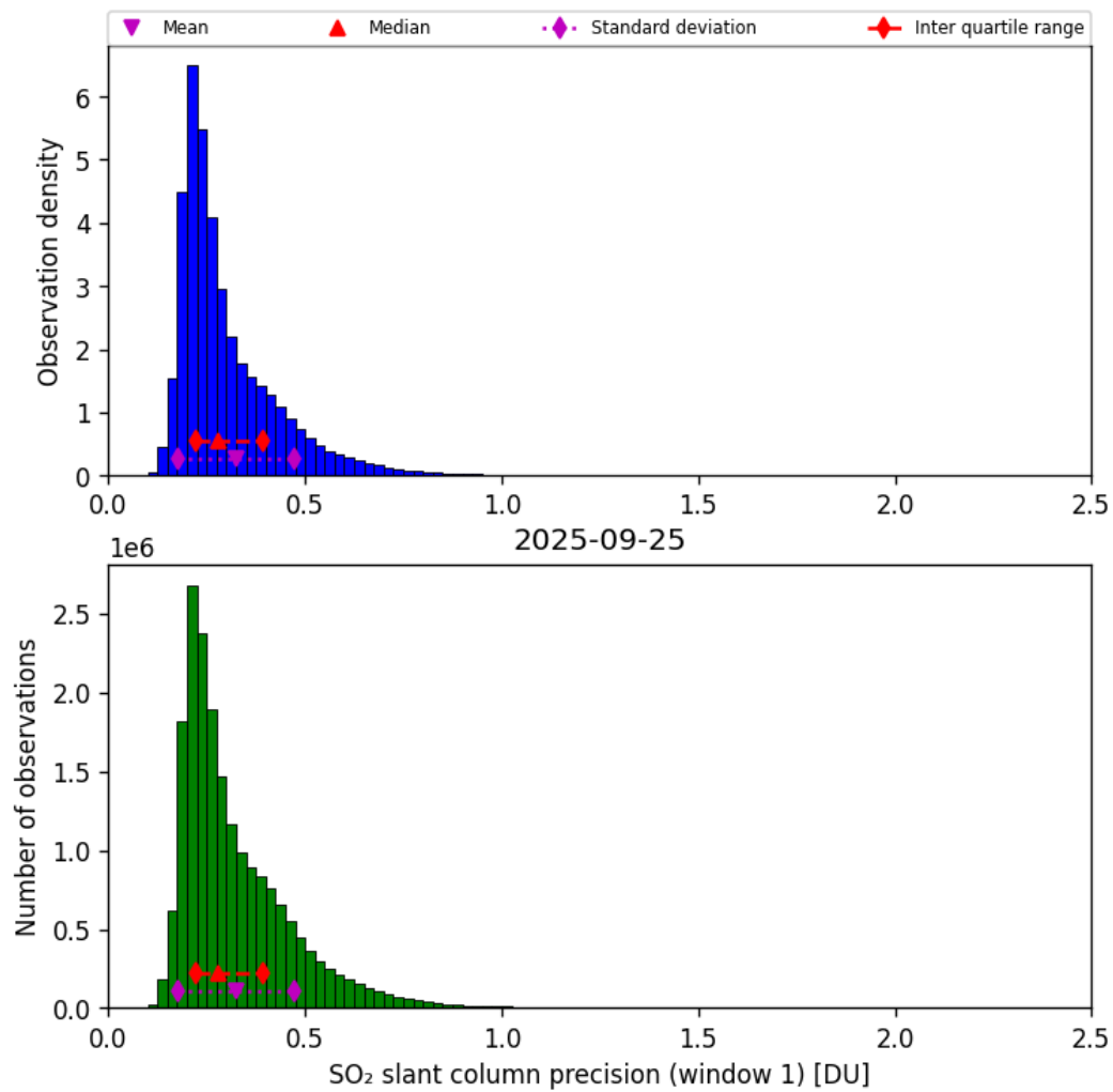
Figure 64: Histogram of “SO 2 slant column precision (window 1)” for 2025-09-25 to 2025-09-26
