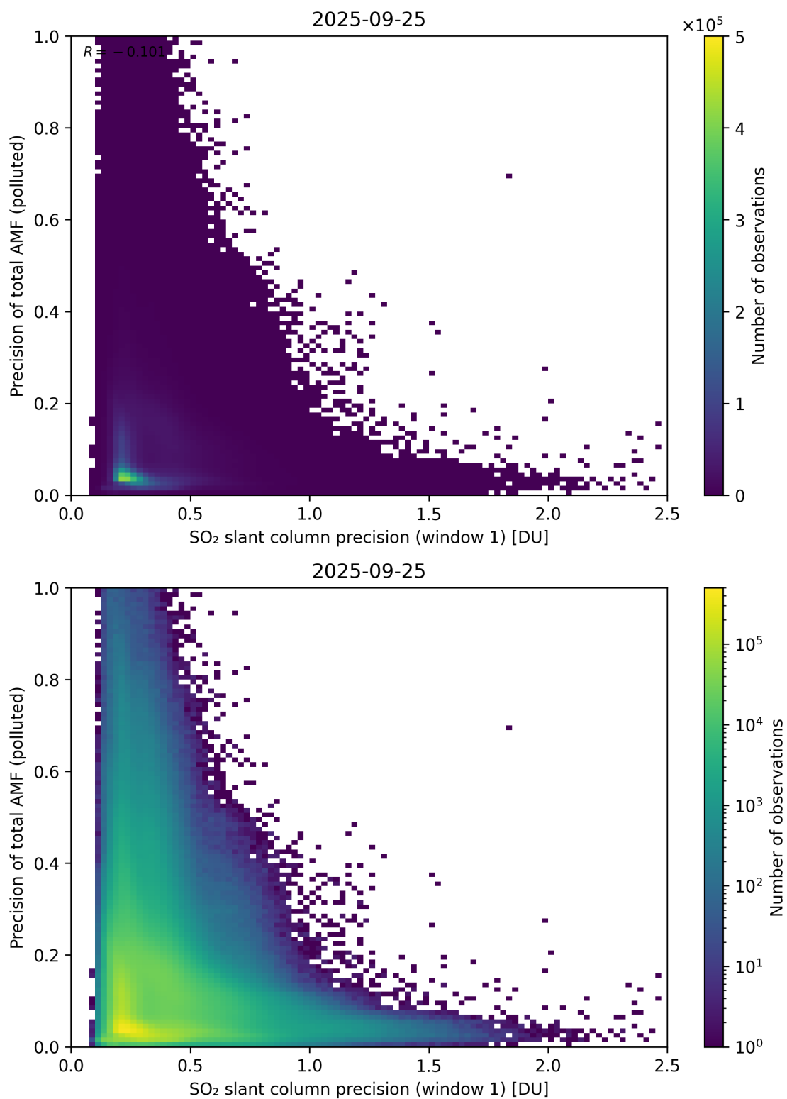
Figure 281: Scatter density plot of “SO 2 slant column precision (window 1)” against “Precision of total AMF (polluted)” for 2025-09-25 to 2025-09-26.
