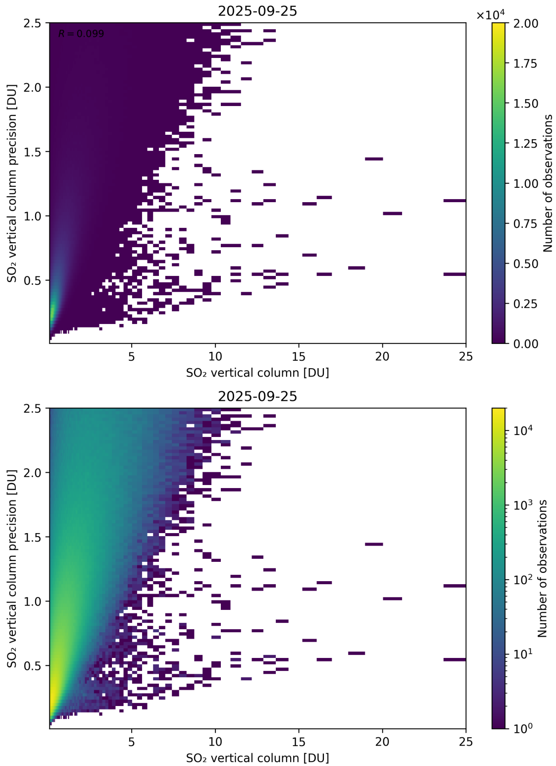
Figure 361: Scatter density plot of “SO 2 vertical column” against “SO 2 vertical column precision” for 2025-09-25 to 2025-09-26.
