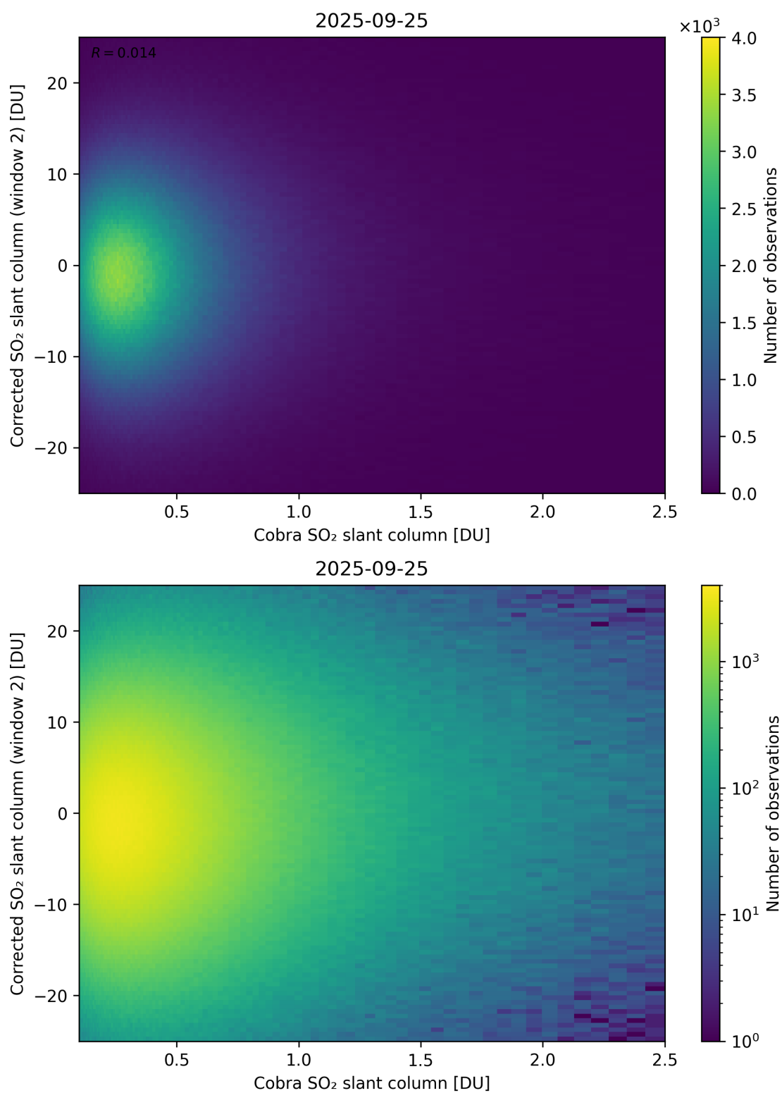
Figure 217: Scatter density plot of “Cobra SO 2 slant column” against “Corrected SO 2 slant column (window 2)” for 2025-09-25 to 2025-09-26.
