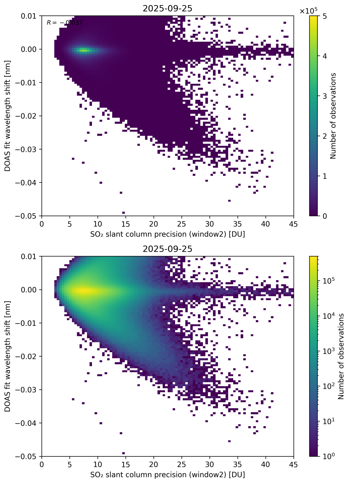
Figure 293: Scatter density plot of “SO 2 slant column precision (window2)” against “DOAS fit wavelength shift” for 2025-09-25 to 2025-09-26.
