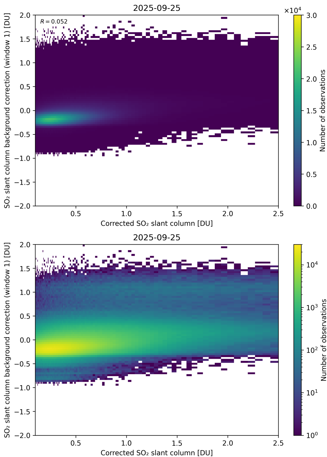
Figure 226: Scatter density plot of “Corrected SO 2 slant column” against “SO 2 slant column background correction (window 1)” for 2025-09-25 to 2025-09-26.
