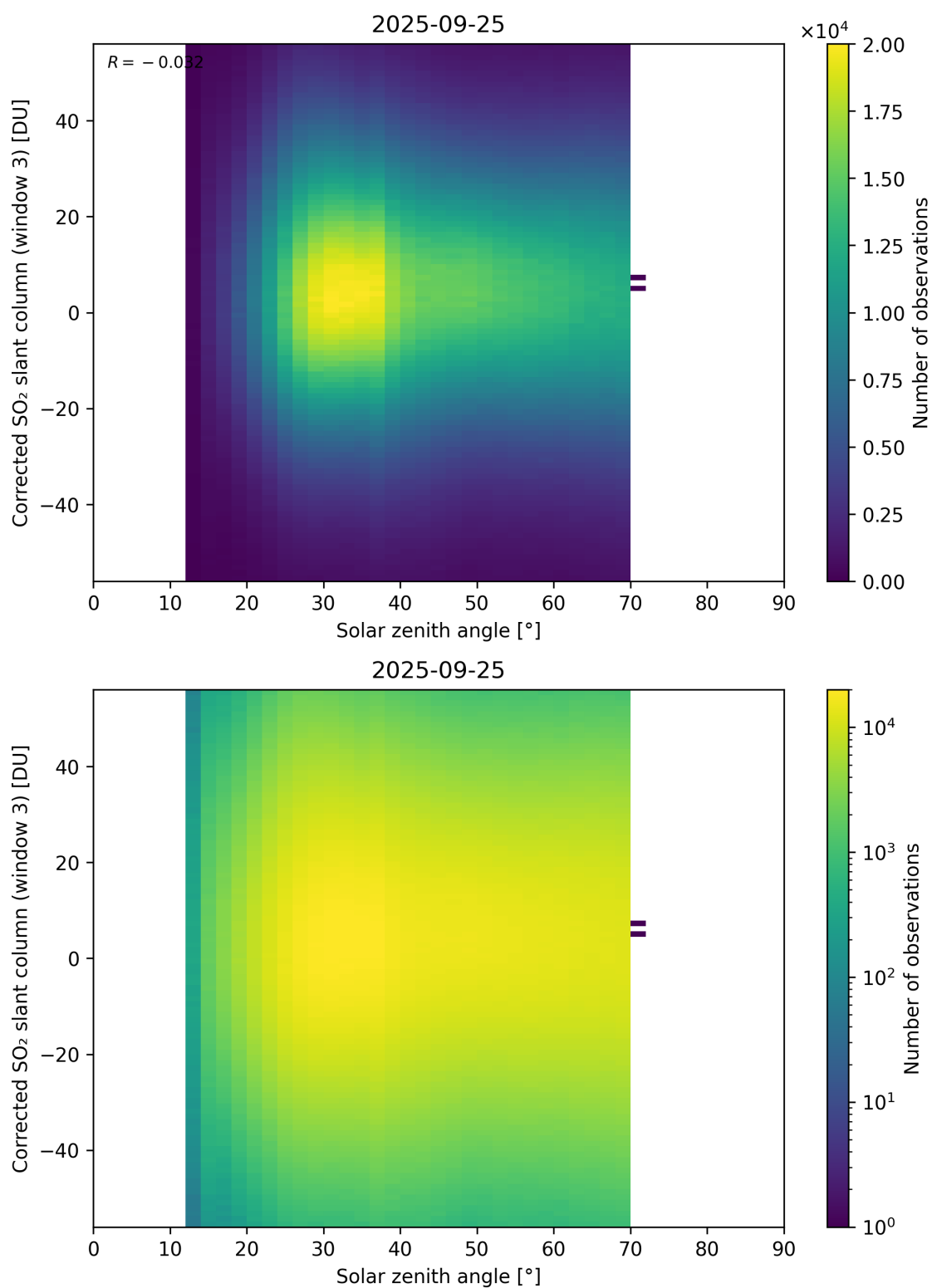
Figure 183: Scatter density plot of “Solar zenith angle” against “Corrected SO 2 slant column (window 3)” for 2025-09-25 to 2025-09-26.
