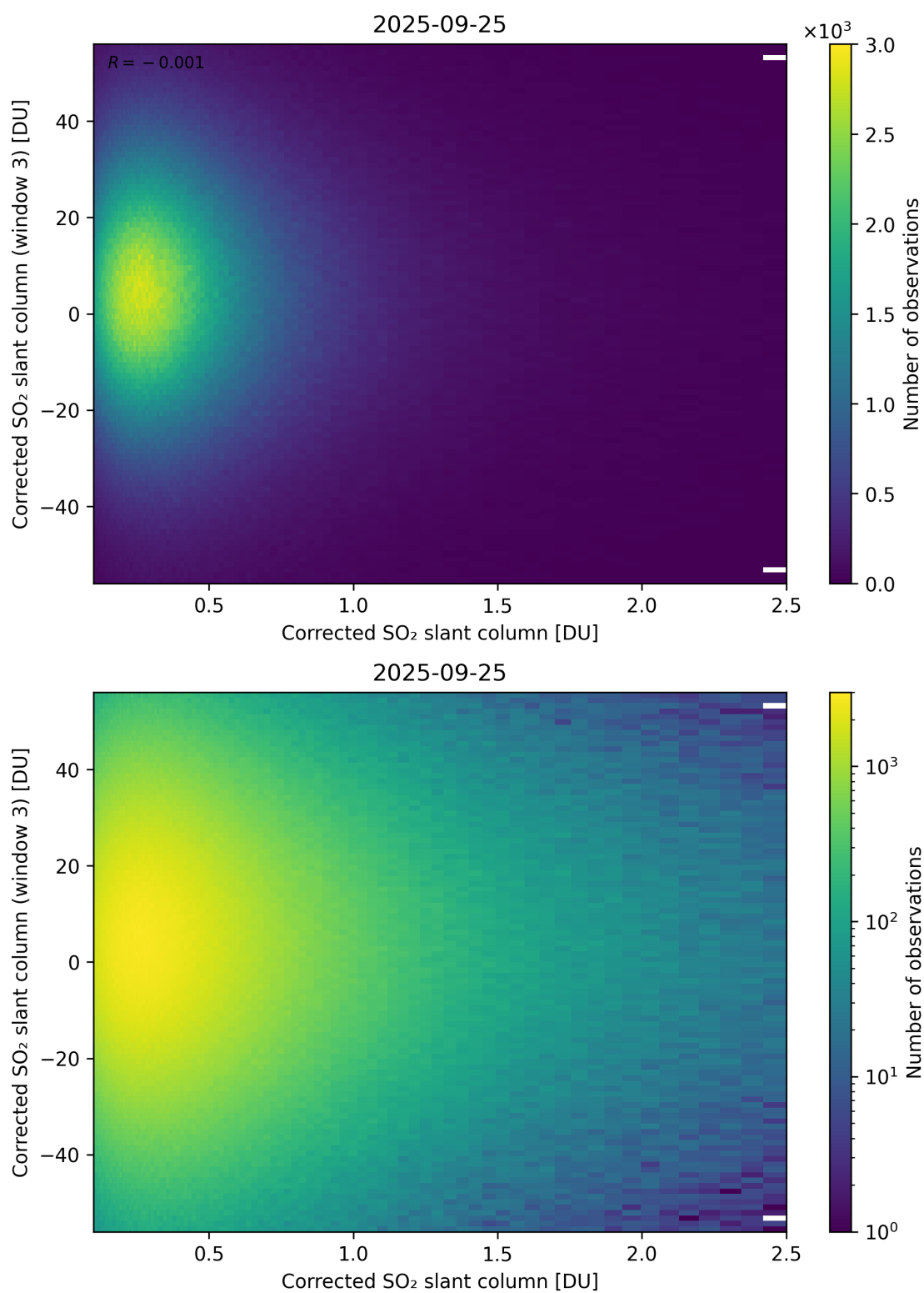
Figure 236: Scatter density plot of “Corrected SO 2 slant column” against “Corrected SO 2 slant column (window 3)” for 2025-09-25 to 2025-09-26.
