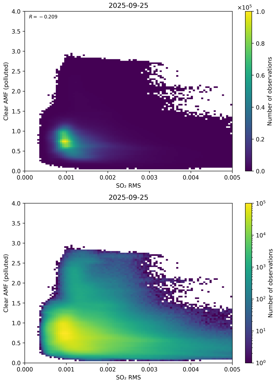
Figure 147: Scatter density plot of “SO 2 RMS” against “Clear AMF (polluted)” for 2025-09-25 to 2025-09-26.
