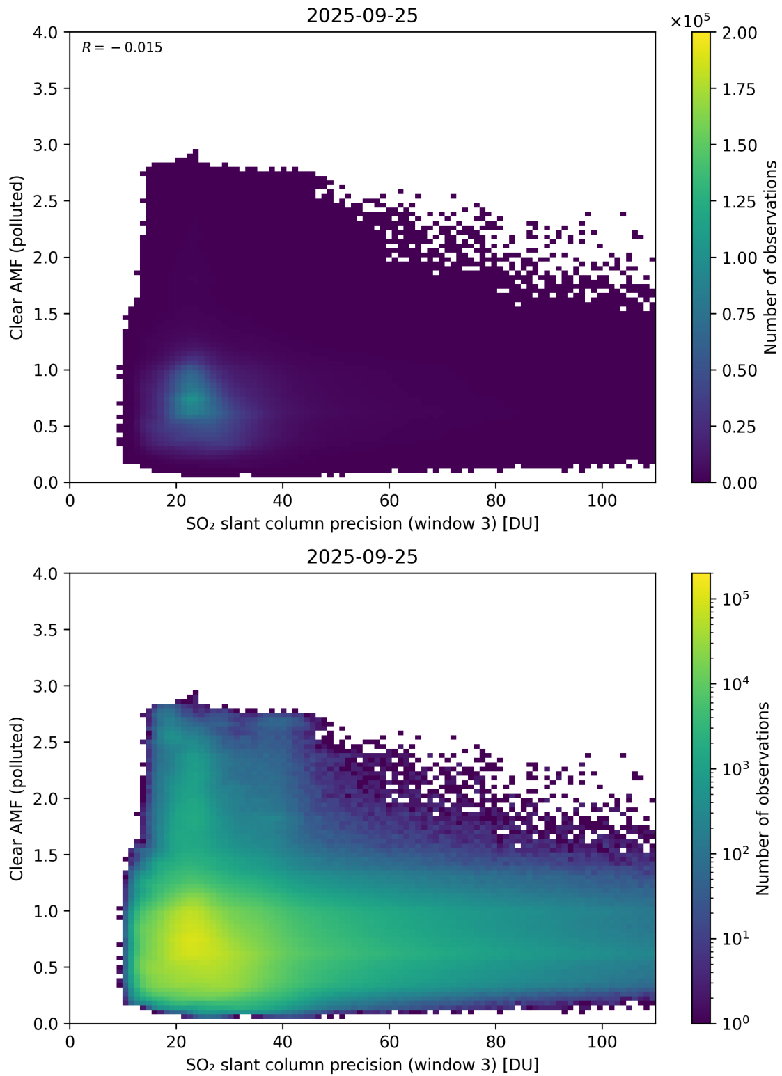
Figure 311: Scatter density plot of “SO 2 slant column precision (window 3)” against “Clear AMF (polluted)” for 2025-09-25 to 2025-09-26.
