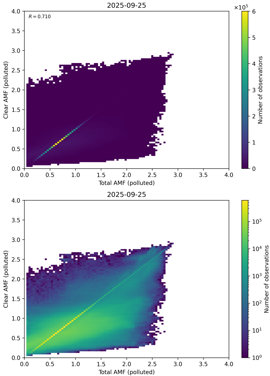
Figure 321: Scatter density plot of “Total AMF (polluted)” against “Clear AMF (polluted)” for 2025-09-25 to 2025-09-26.
