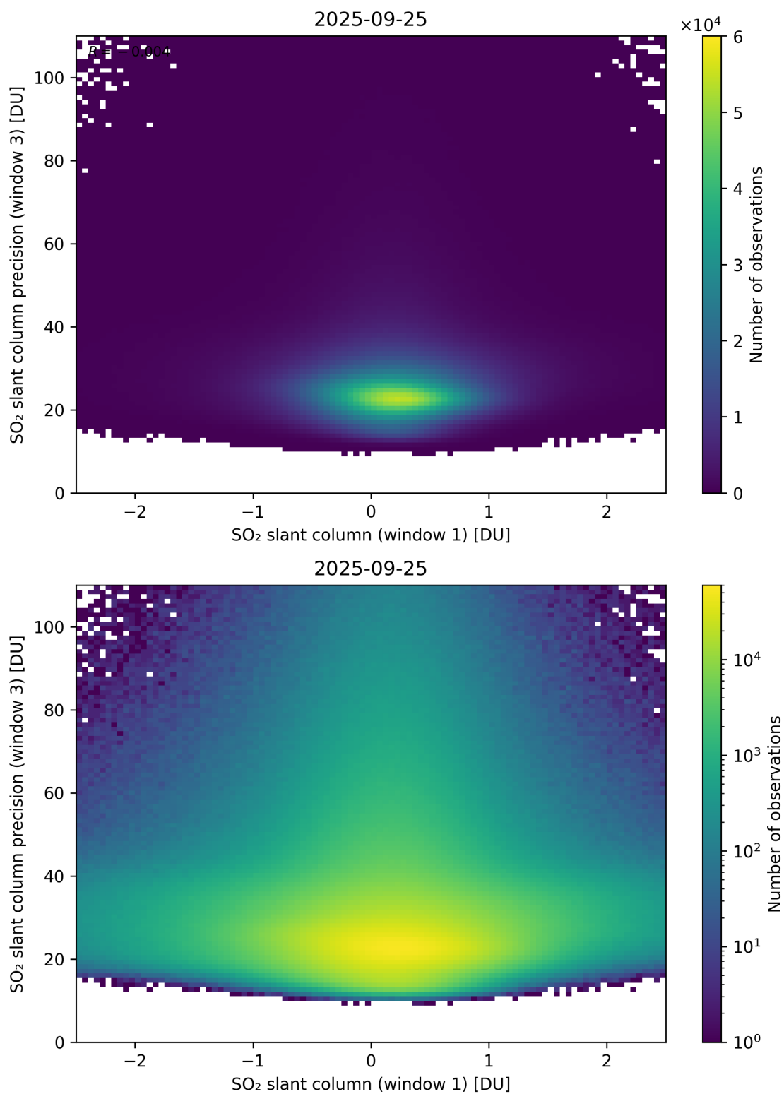
Figure 288: Scatter density plot of “SO 2 slant column (window 1)” against “SO 2 slant column precision (window 3)” for 2025-09-25 to 2025-09-26.
