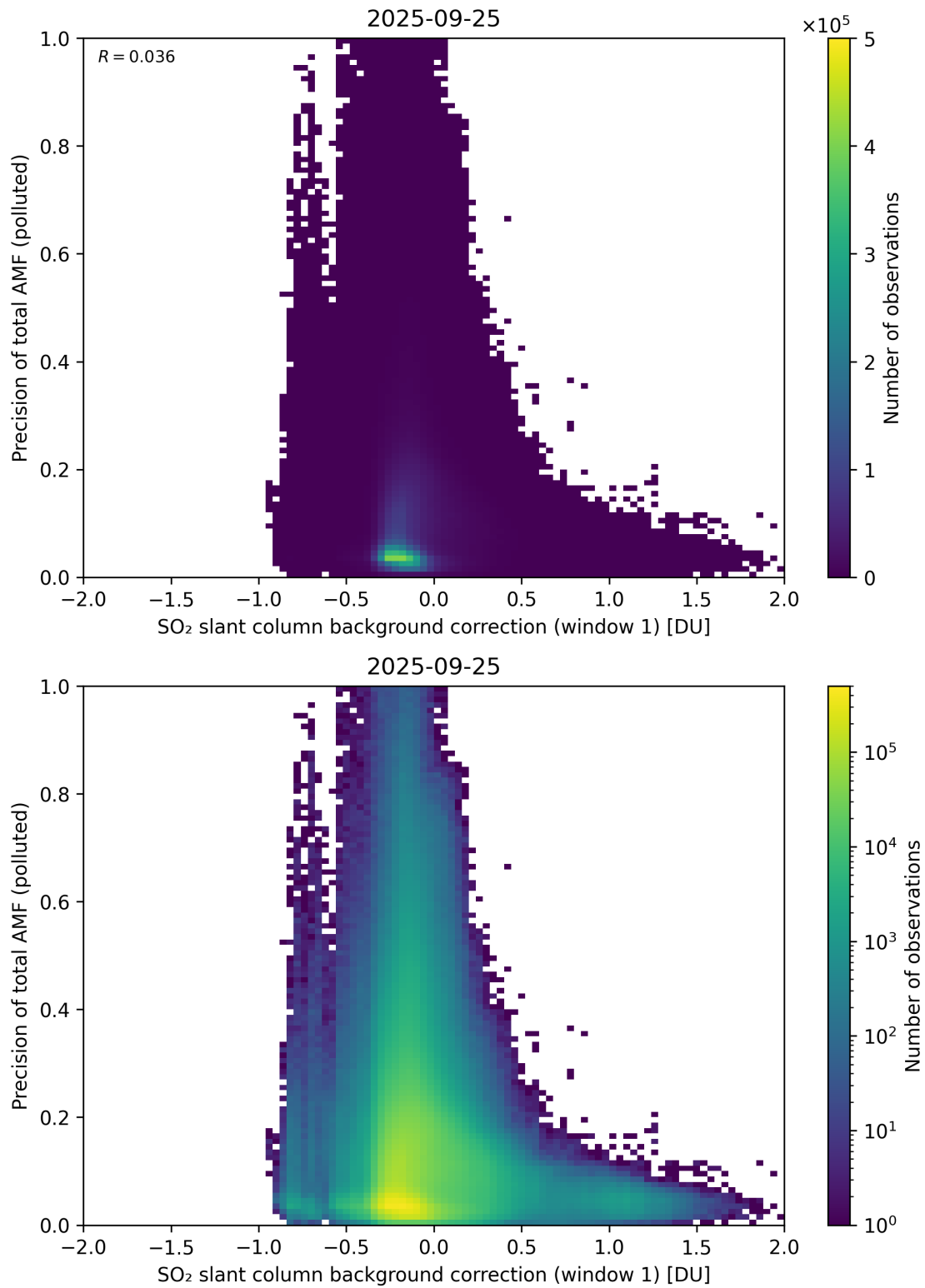
Figure 121: Scatter density plot of “SO 2 slant column background correction (window 1)” against “Precision of total AMF (polluted)” for 2025-09-25 to 2025-09-26.
