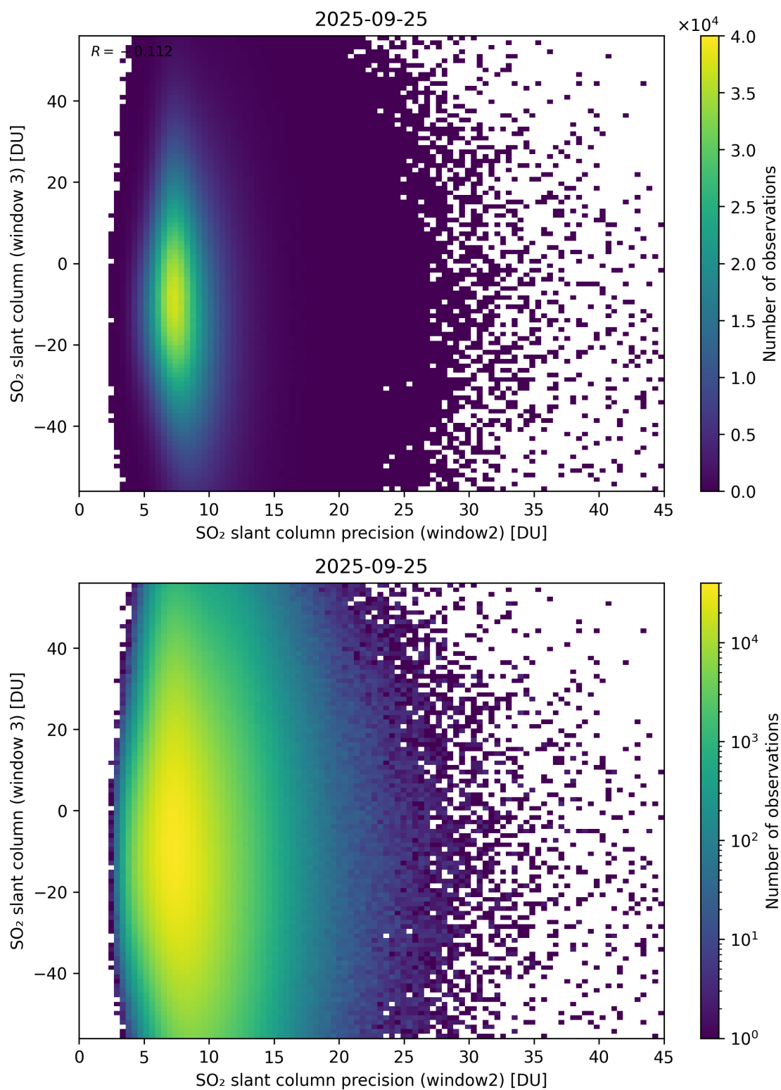
Figure 299: Scatter density plot of “SO 2 slant column precision (window2)” against “SO 2 slant column (window 3)” for 2025-09-25 to 2025-09-26.
