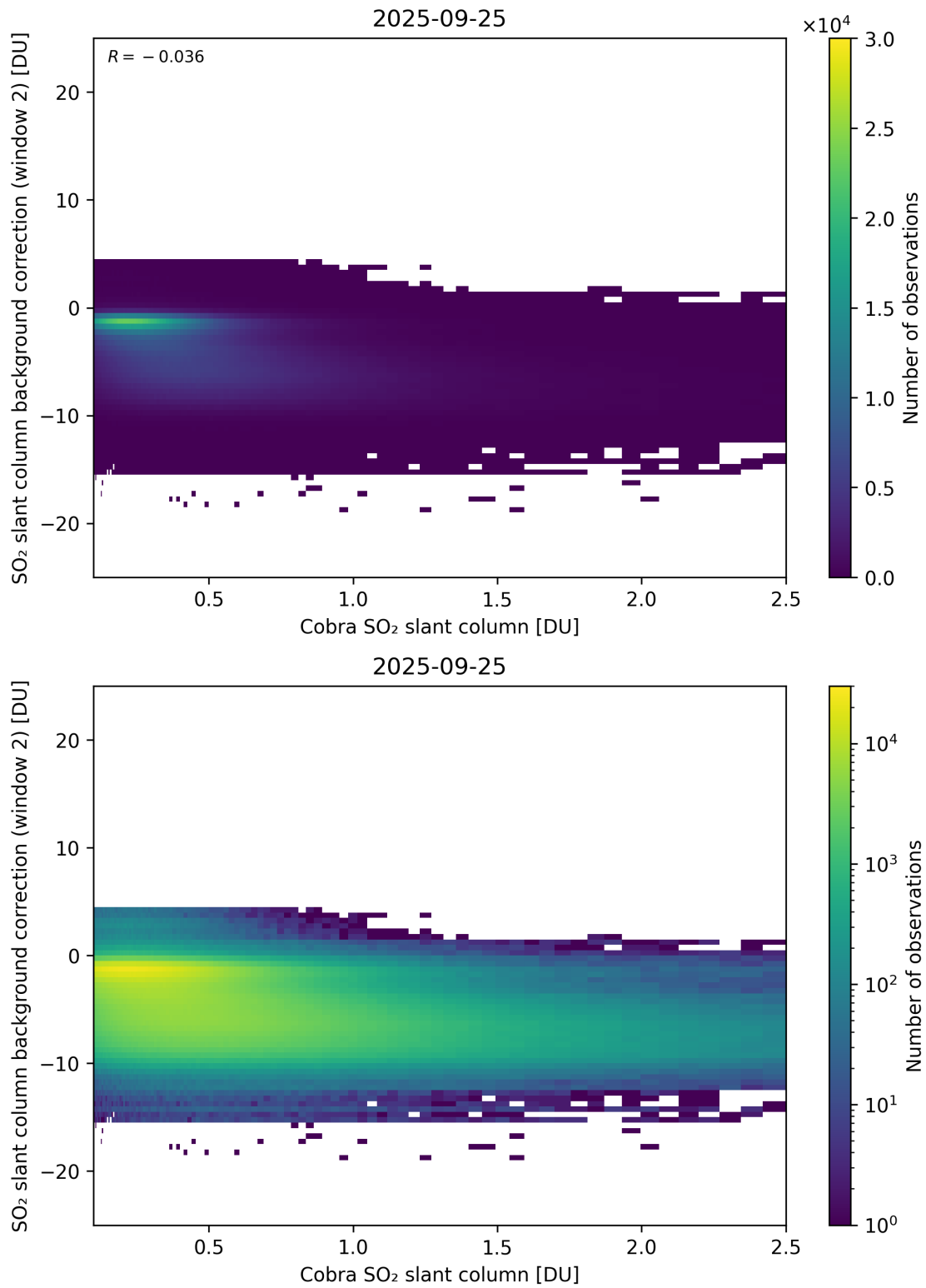
Figure 194: Scatter density plot of “Cobra SO 2 slant column” against “SO 2 slant column background correction (window 2)” for 2025-09-25 to 2025-09-26.
