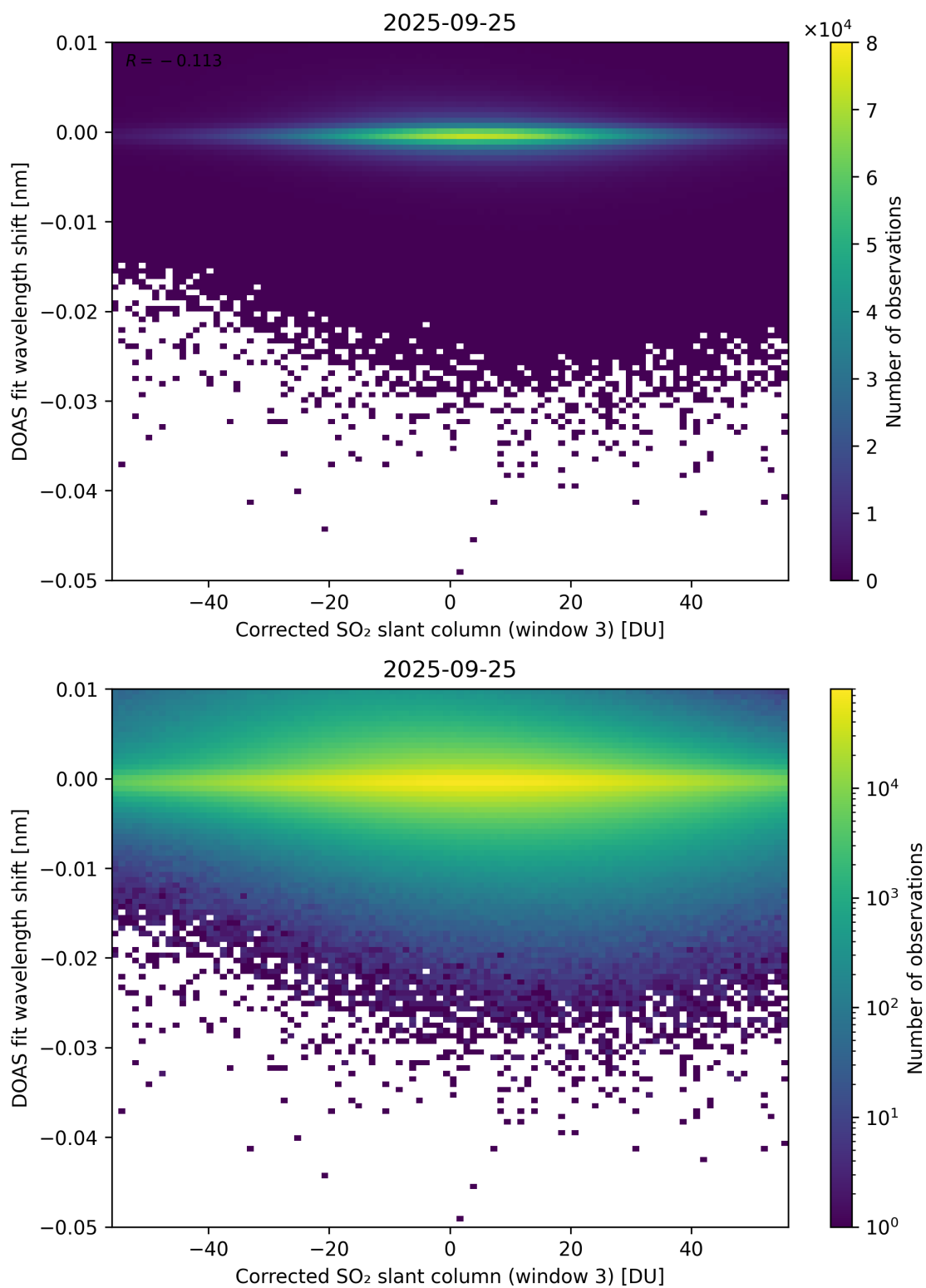
Figure 256: Scatter density plot of “Corrected SO 2 slant column (window 3)” against “DOAS fit wavelength shift” for 2025-09-25 to 2025-09-26.
