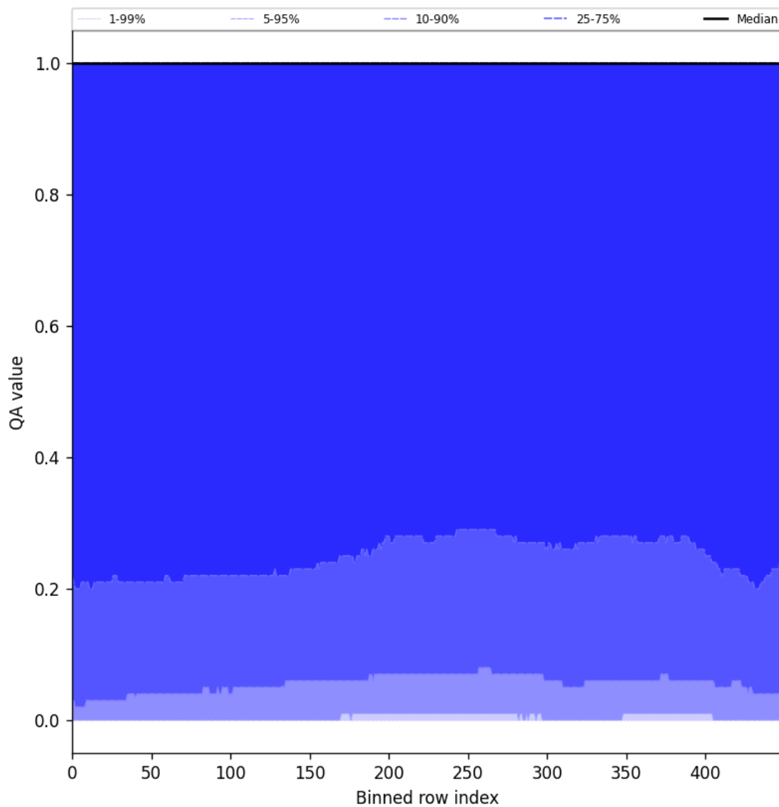
Figure 83: Along track statistics of “QA value” for 2025-09-25 to 2025-09-26
