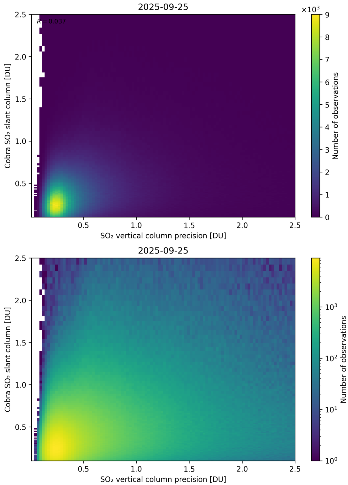
Figure 336: Scatter density plot of “SO 2 vertical column precision” against “Cobra SO 2 slant column” for 2025-09-25 to 2025-09-26.
