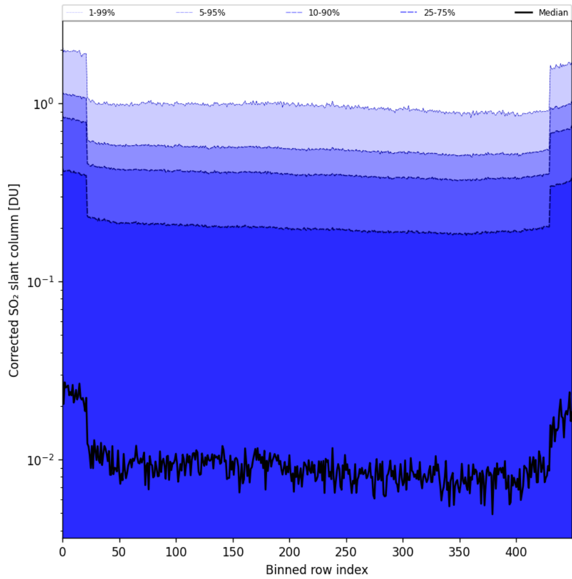
Figure 86: Along track statistics of "Corrected SO 2 slant column" for 2025-09-25 to 2025-09-26
