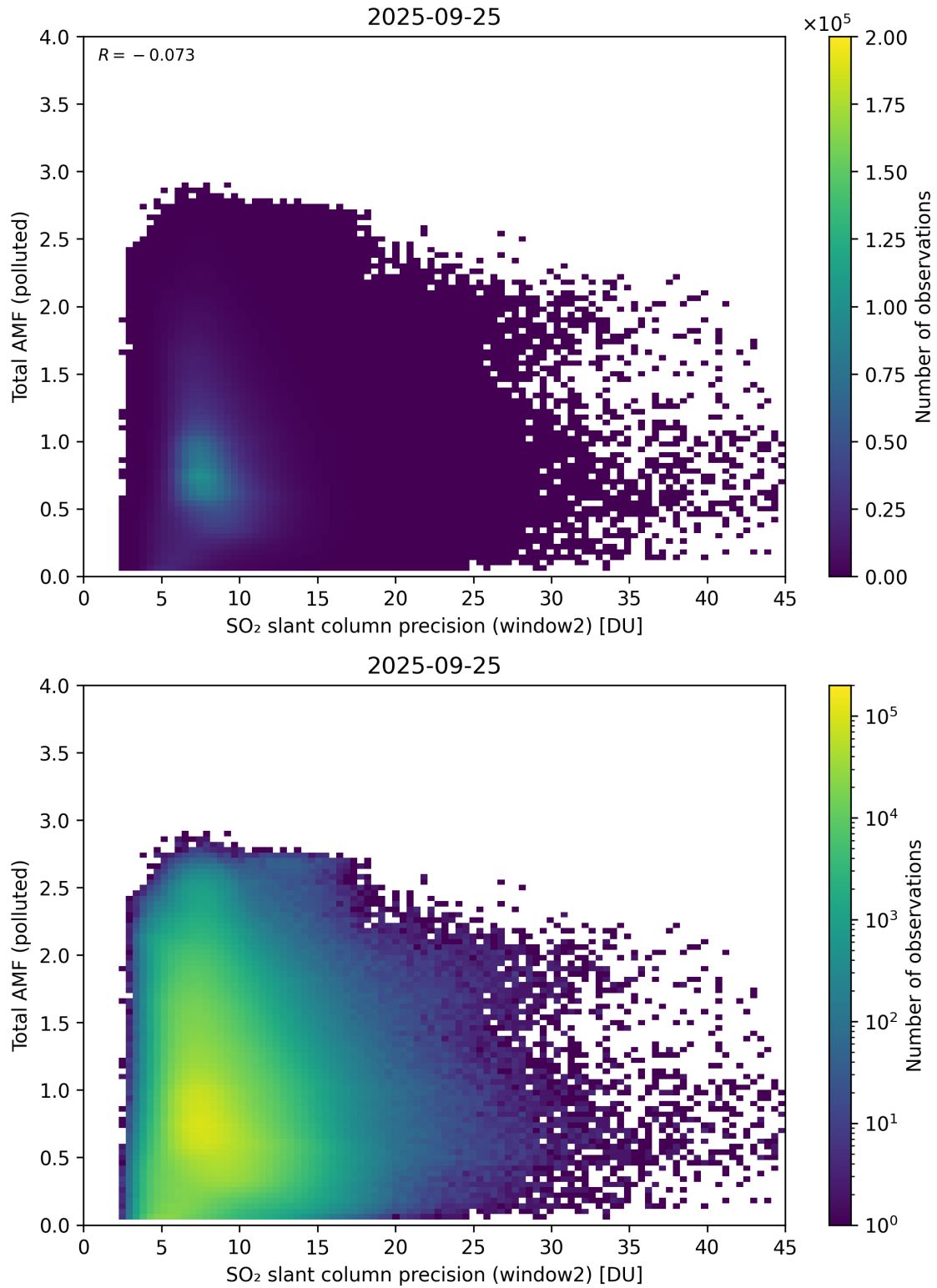
Figure 301: Scatter density plot of “SO 2 slant column precision (window2)” against “Total AMF (polluted)” for 2025-09-25 to 2025-09-26.
