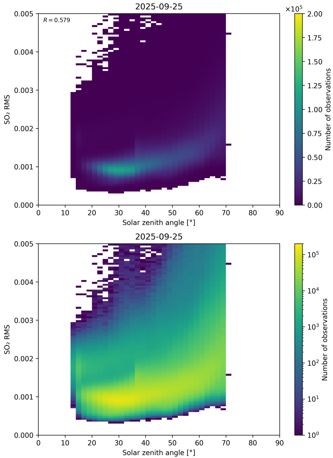
Figure 176: Scatter density plot of “Solar zenith angle” against “SO 2 RMS” for 2025-09-25 to 2025-09-26.
