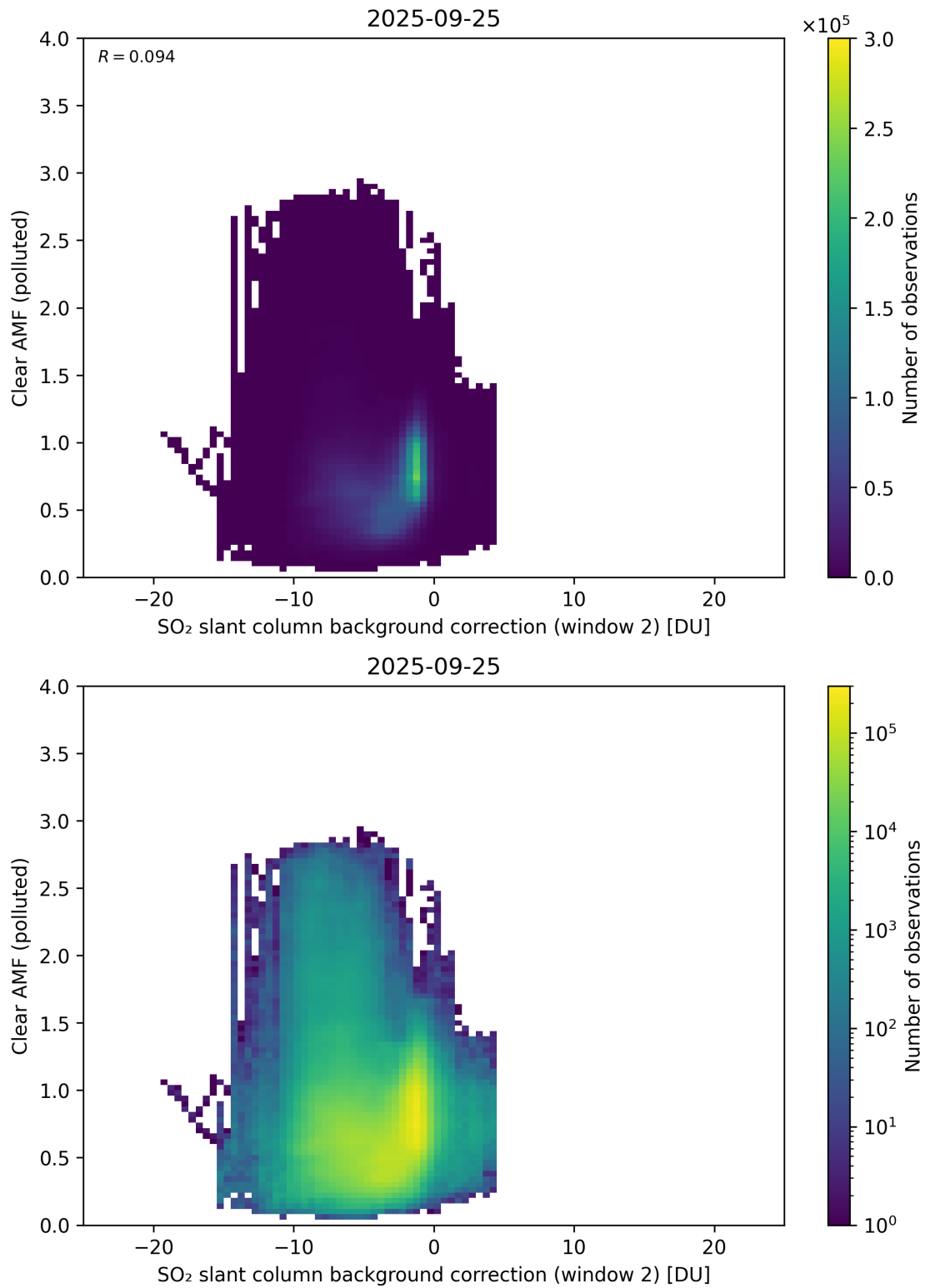
Figure 126: Scatter density plot of “SO 2 slant column background correction (window 2)” against “Clear AMF (polluted)” for 2025-09-25 to 2025-09-26.
