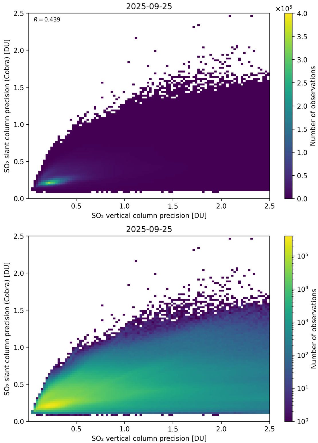
Figure 337: Scatter density plot of “SO 2 vertical column precision” against “SO 2 slant column precision (Cobra)” for 2025-09-25 to 2025-09-26.
