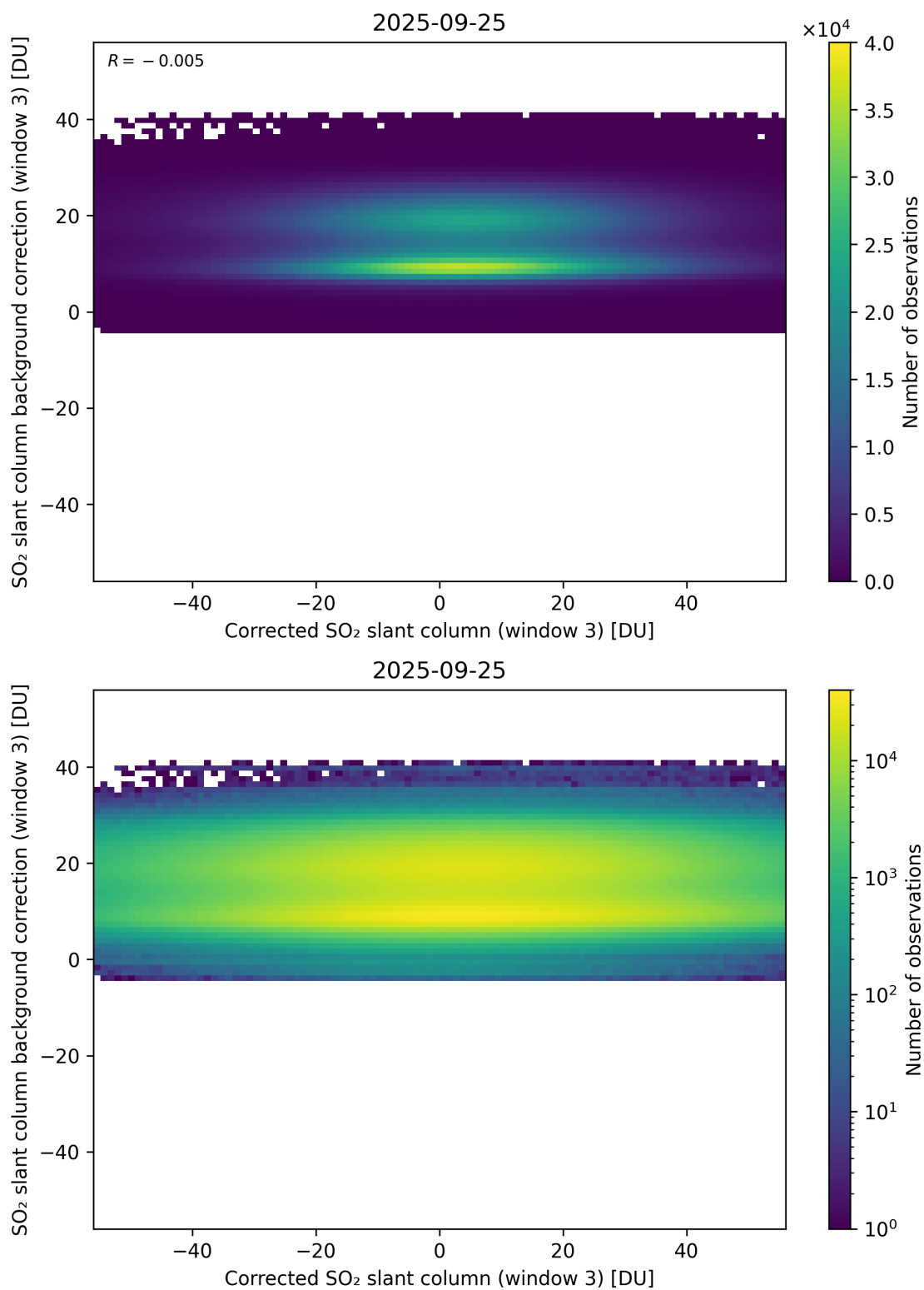
Figure 255: Scatter density plot of “Corrected SO 2 slant column (window 3)” against “SO 2 slant column background correction (window 3)” for 2025-09-25 to 2025-09-26.
