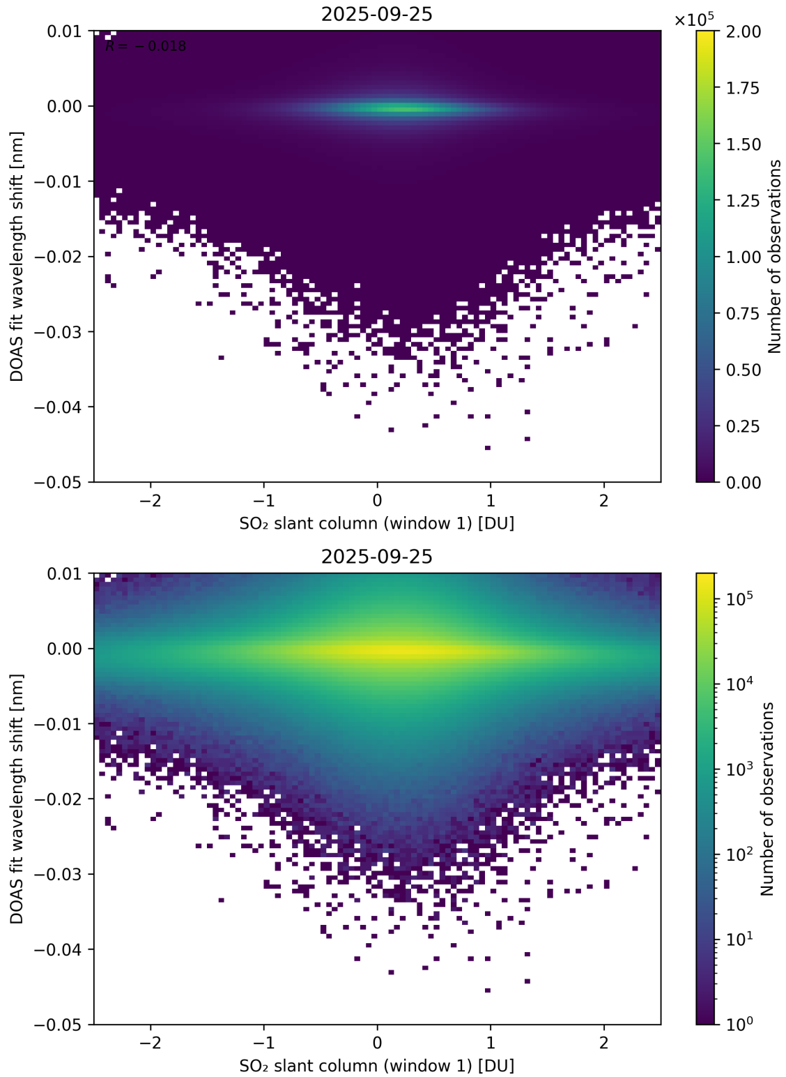
Figure 265: Scatter density plot of “SO 2 slant column (window 1)” against “DOAS fit wavelength shift” for 2025-09-25 to 2025-09-26.
