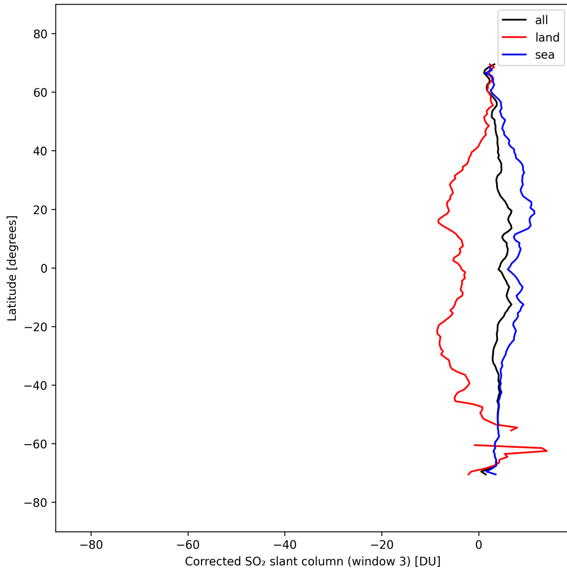
Figure 47: Zonal average of “Corrected SO 2 slant column (window 3)” for 2025-09-25 to 2025-09-26.
