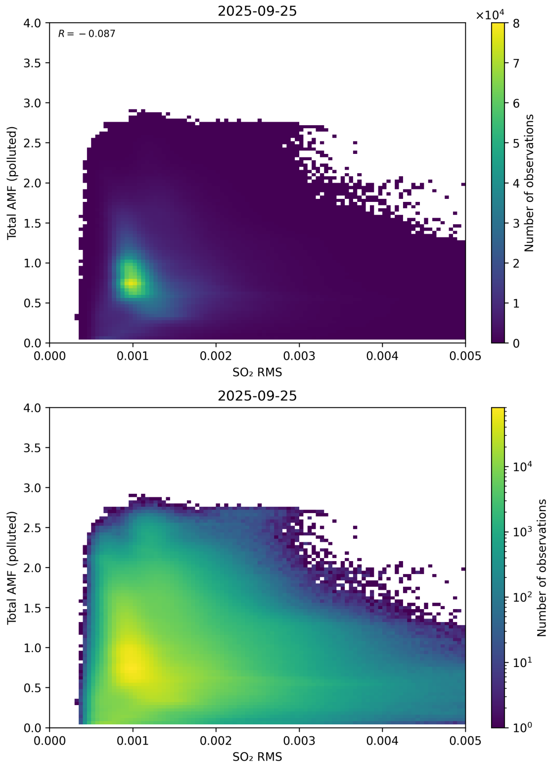
Figure 148: Scatter density plot of “SO 2 RMS” against “Total AMF (polluted)” for 2025-09-25 to 2025-09-26.
