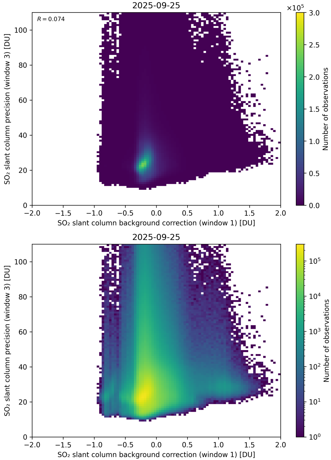
Figure 119: Scatter density plot of “SO 2 slant column background correction (window 1)” against “SO 2 slant column precision (window 3)” for 2025-09-25 to 2025-09-26.
