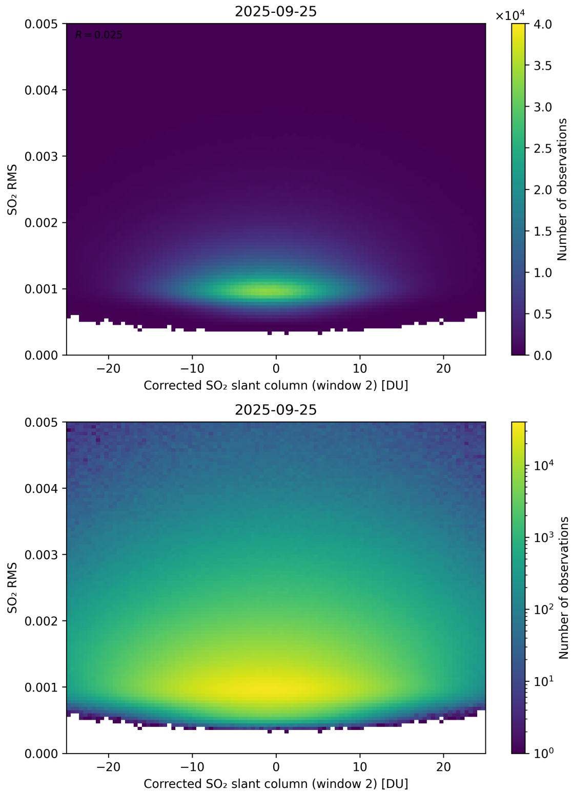
Figure 248: Scatter density plot of “Corrected SO 2 slant column (window 2)” against “SO 2 RMS” for 2025-09-25 to 2025-09-26.
