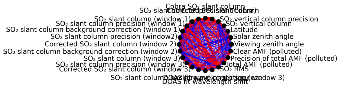
Figure 1: Map of correlation graph for 2025-09-25 to 2025-09-26.
