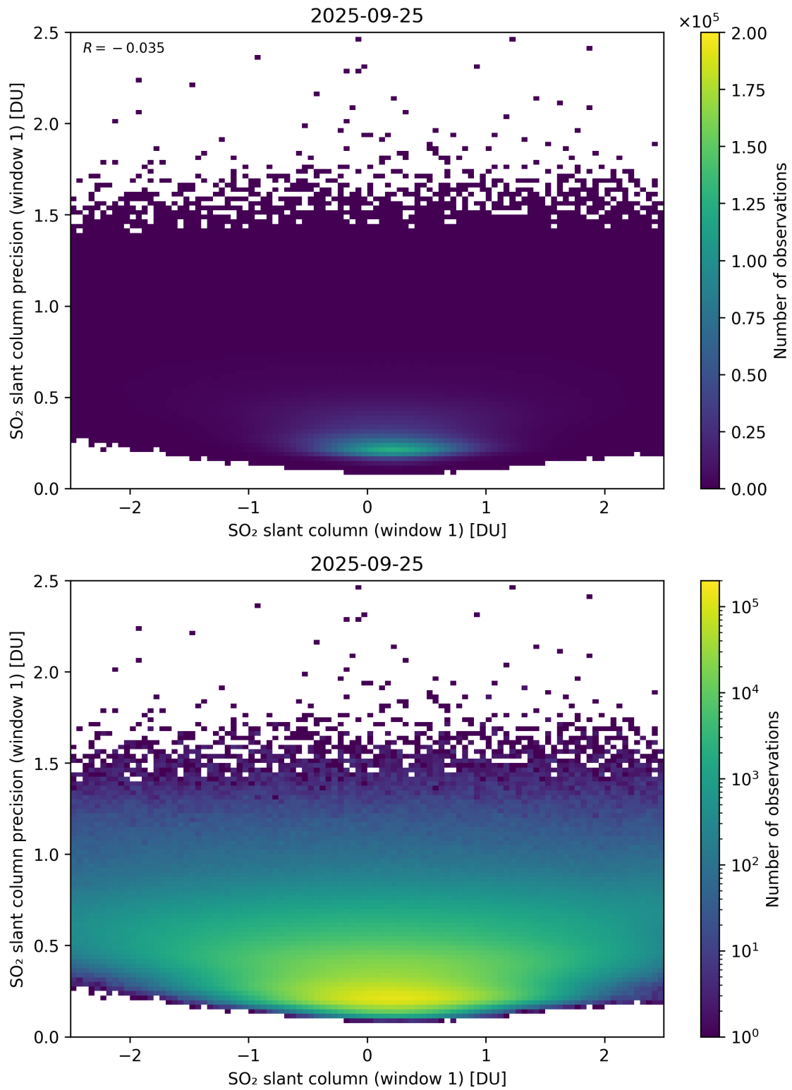
Figure 285: Scatter density plot of “SO 2 slant column (window 1)” against “SO 2 slant column precision (window 1)” for 2025-09-25 to 2025-09-26.
