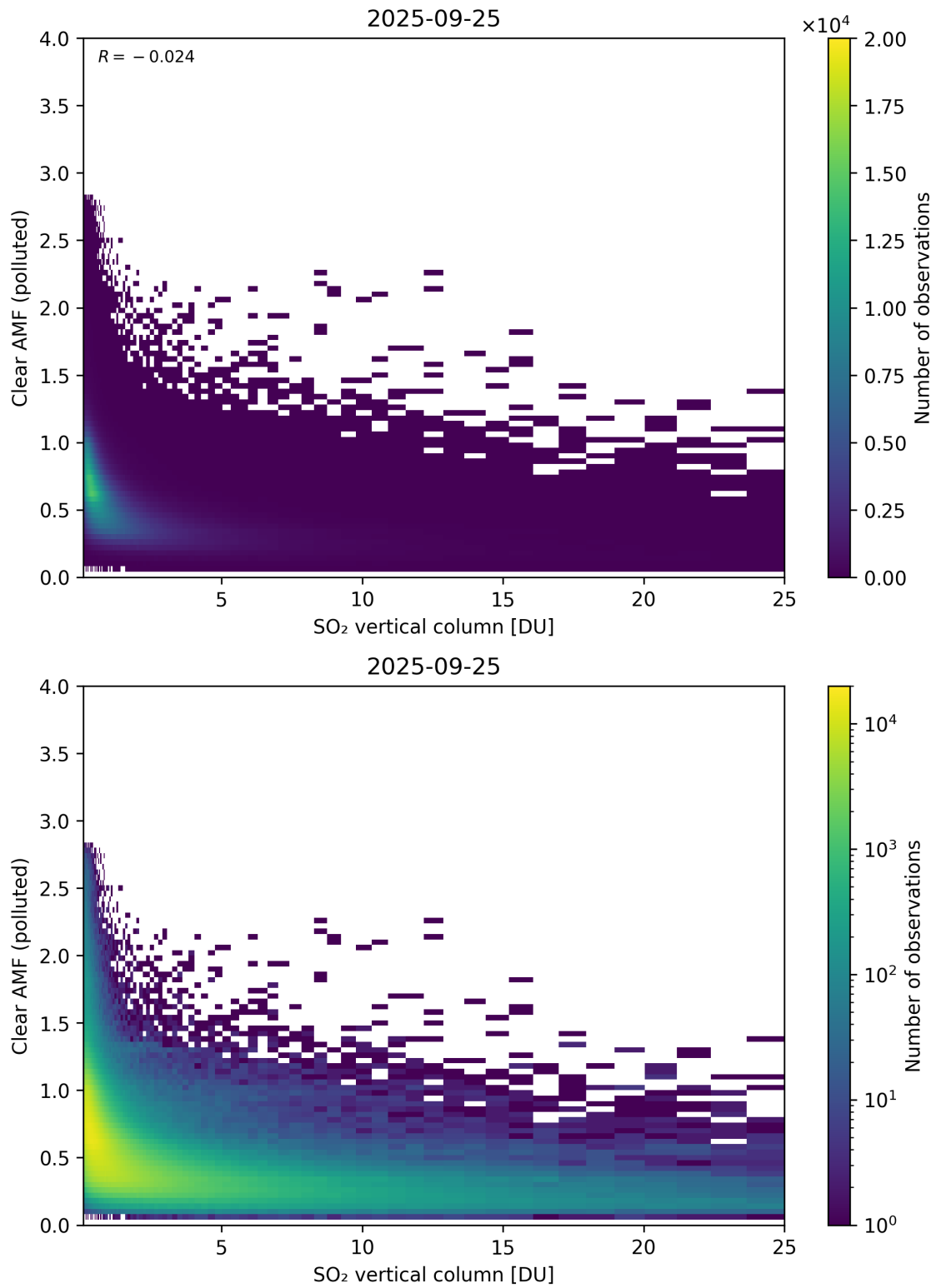
Figure 348: Scatter density plot of “SO 2 vertical column” against “Clear AMF (polluted)” for 2025-09-25 to 2025-09-26.
