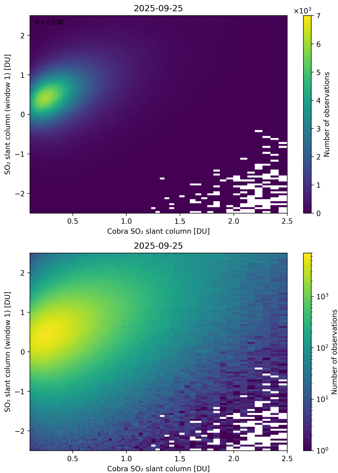
Figure 219: Scatter density plot of “Cobra SO 2 slant column” against “SO 2 slant column (window 1)” for 2025-09-25 to 2025-09-26.
