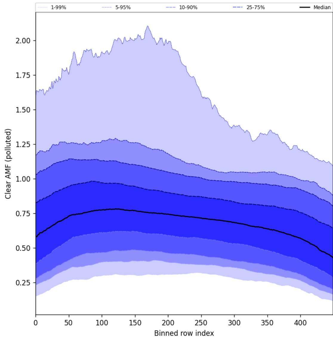
Figure 107: Along track statistics of “Clear AMF (polluted)” for 2025-09-25 to 2025-09-26
