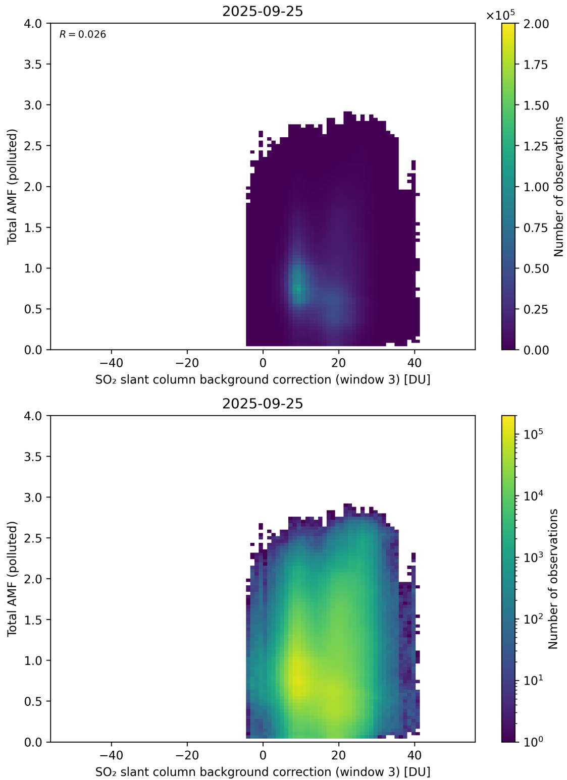
Figure 136: Scatter density plot of “SO 2 slant column background correction (window 3)” against “Total AMF (polluted)” for 2025-09-25 to 2025-09-26.
