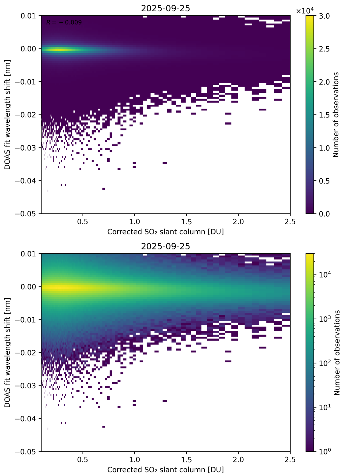
Figure 229: Scatter density plot of “Corrected SO 2 slant column” against “DOAS fit wavelength shift” for 2025-09-25 to 2025-09-26.
