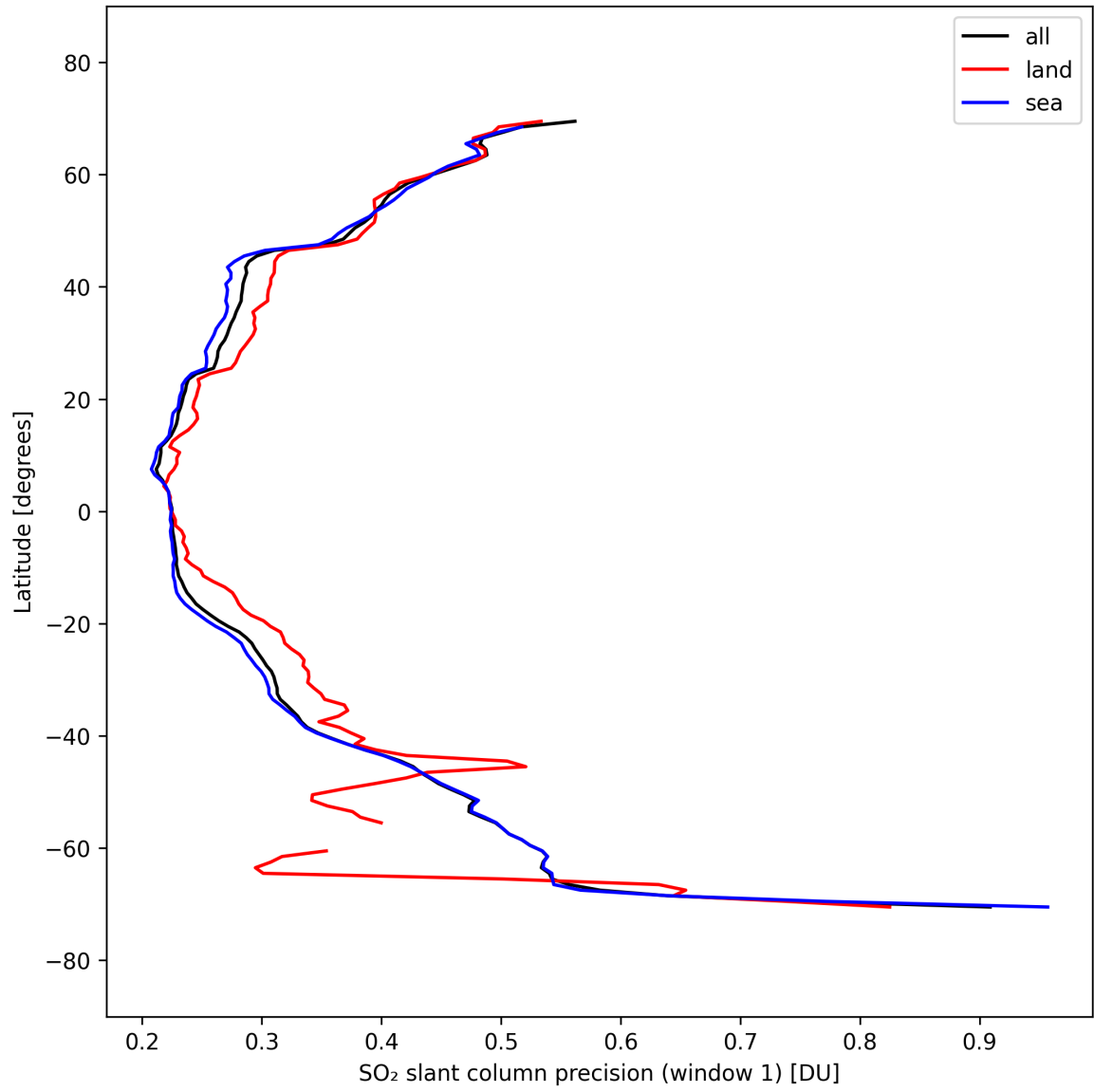
Figure 38: Zonal average of “SO 2 slant column precision (window 1)” for 2025-09-25 to 2025-09-26.
