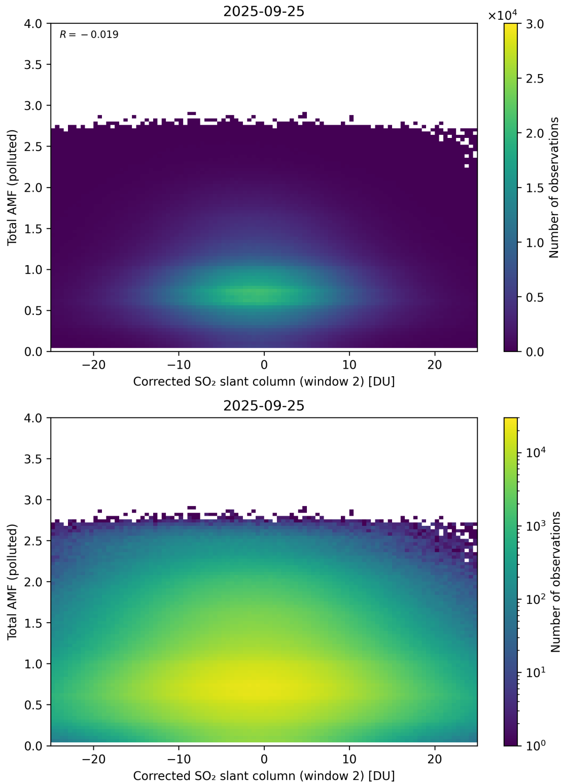
Figure 253: Scatter density plot of “Corrected SO 2 slant column (window 2)” against “Total AMF (polluted)” for 2025-09-25 to 2025-09-26.
