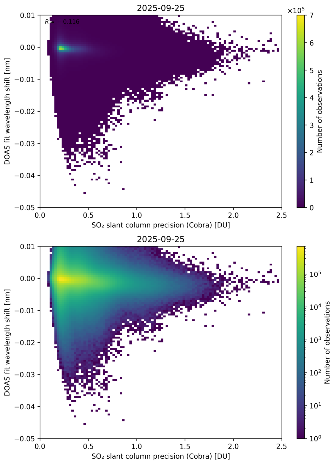
Figure 202: Scatter density plot of “SO 2 slant column precision (Cobra)” against “DOAS fit wavelength shift” for 2025-09-25 to 2025-09-26.
