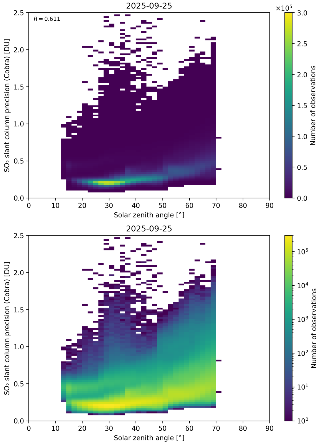
Figure 180: Scatter density plot of “Solar zenith angle” against “SO 2 slant column precision (Cobra)” for 2025-09-25 to 2025-09-26.
