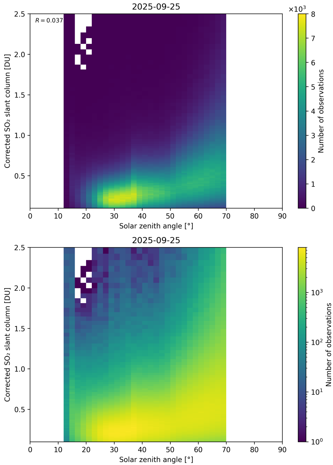
Figure 181: Scatter density plot of “Solar zenith angle” against “Corrected SO 2 slant column” for 2025-09-25 to 2025-09-26.
