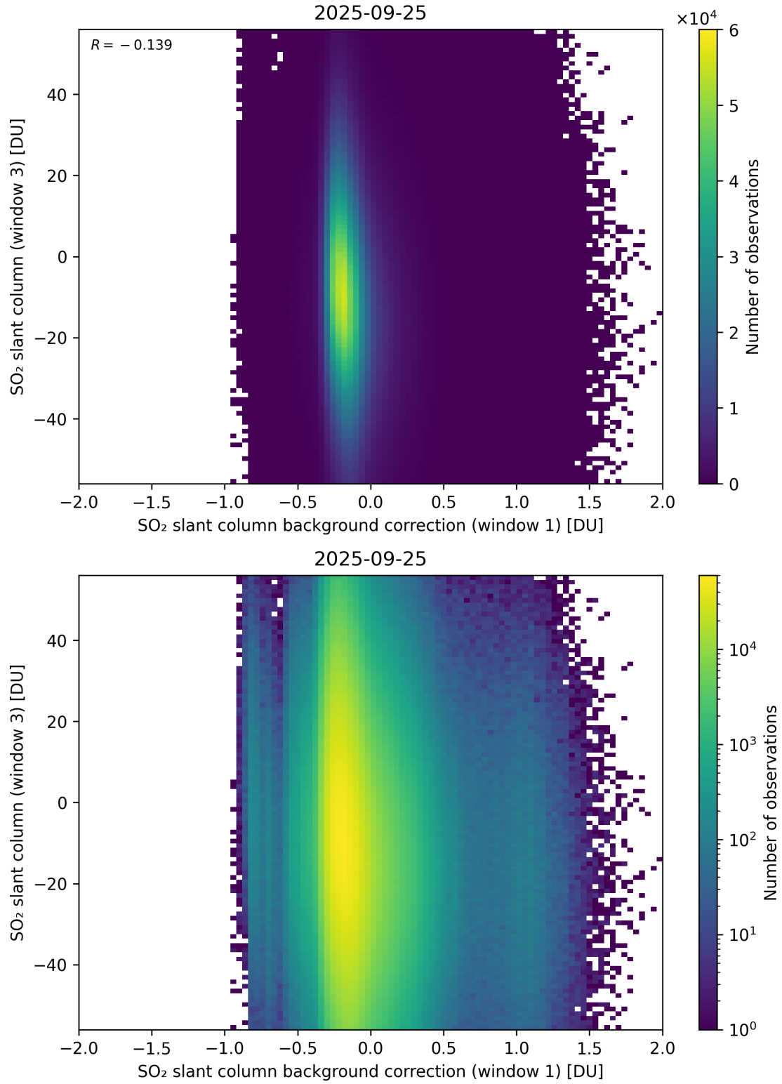
Figure 118: Scatter density plot of “SO 2 slant column background correction (window 1)” against “SO 2 slant column (window 3)” for 2025-09-25 to 2025-09-26.
