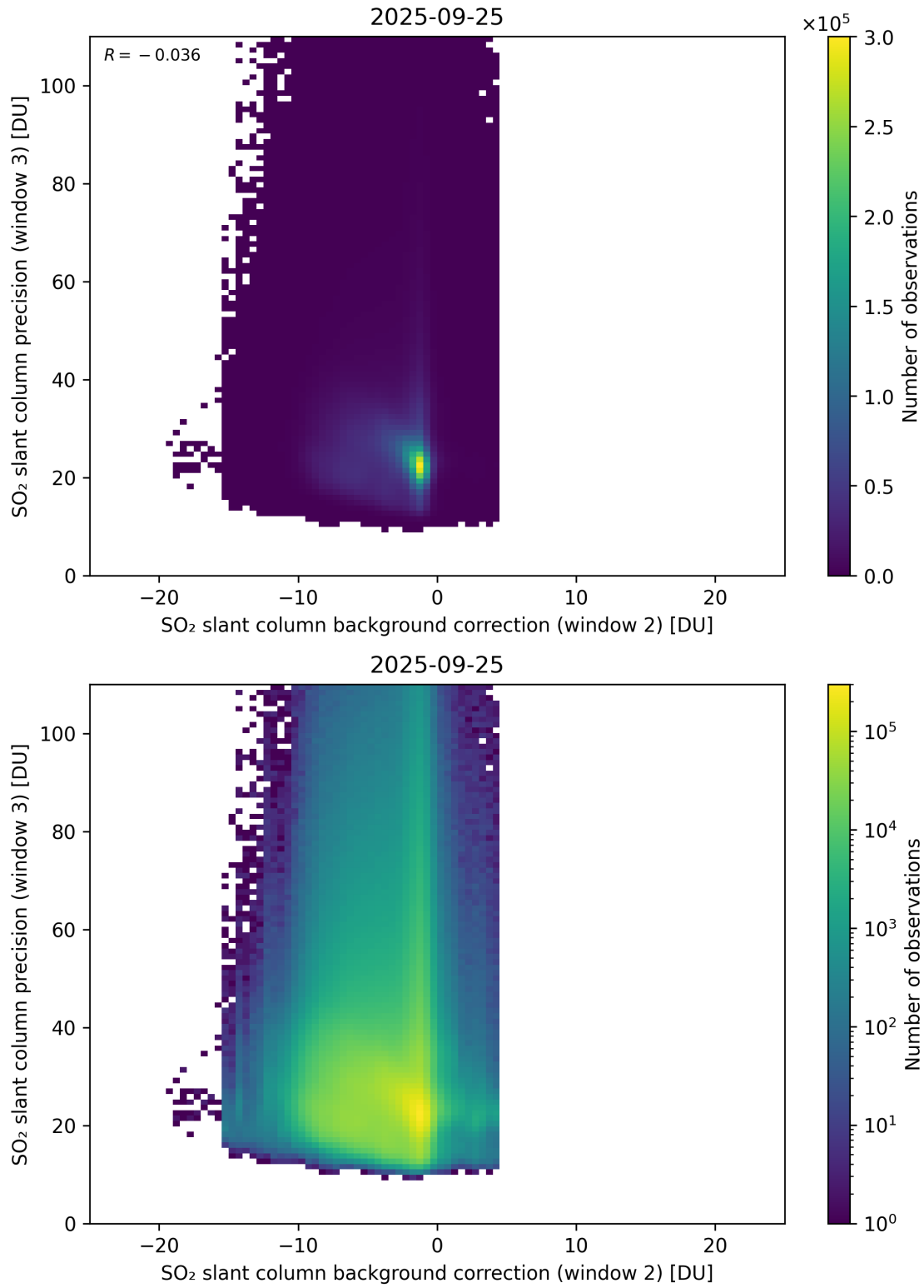
Figure 129: Scatter density plot of “SO 2 slant column background correction (window 2)” against “SO 2 slant column precision (window 3)” for 2025-09-25 to 2025-09-26.
