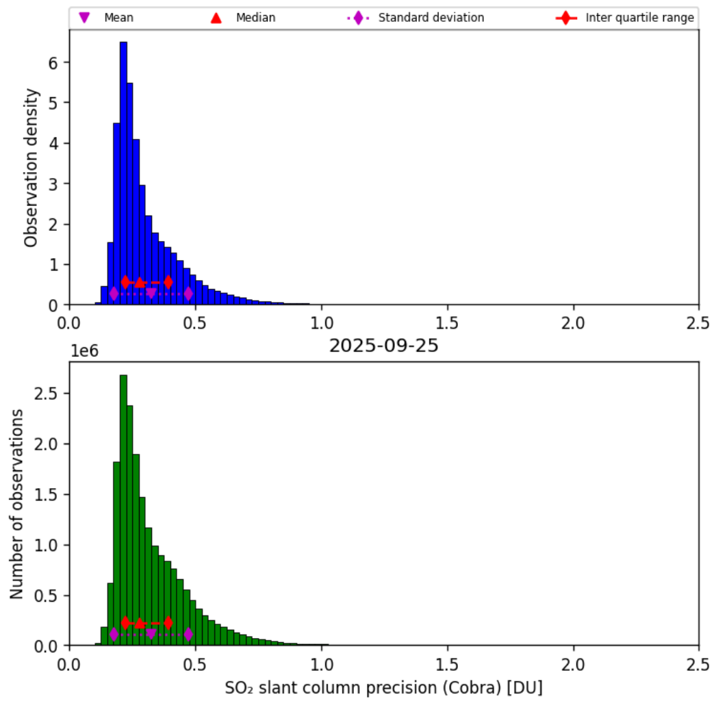
Figure 62: Histogram of “SO 2 slant column precision (Cobra)” for 2025-09-25 to 2025-09-26
