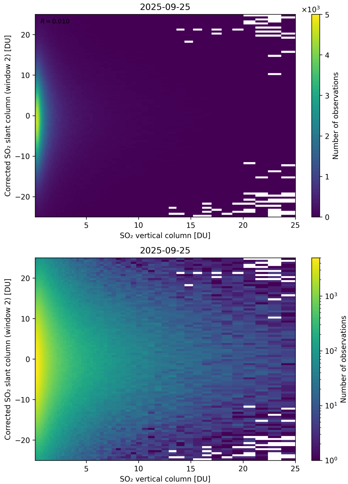
Figure 352: Scatter density plot of “SO 2 vertical column” against “Corrected SO 2 slant column (window 2)” for 2025-09-25 to 2025-09-26.
