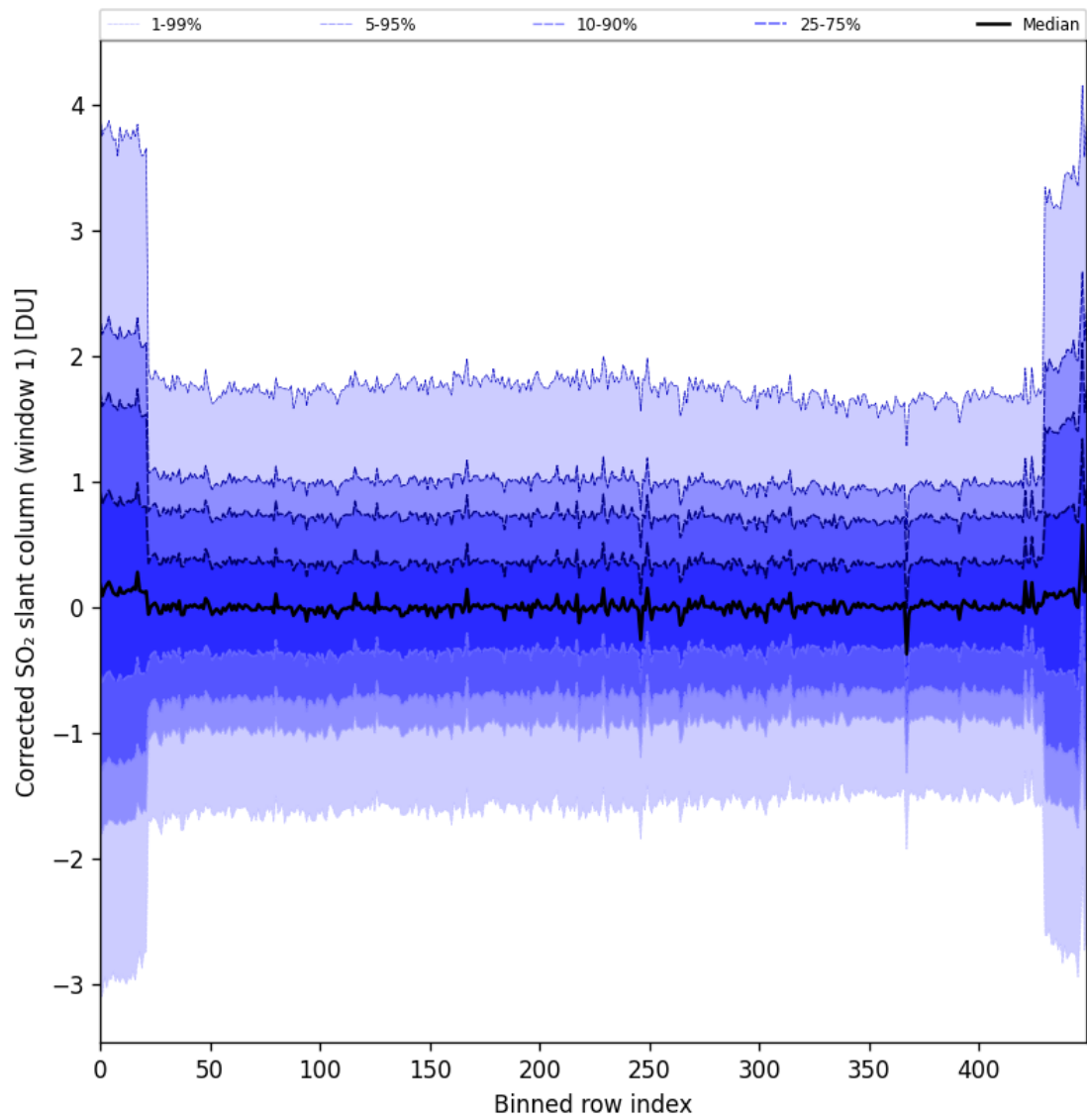
Figure 91: Along track statistics of “Corrected SO 2 slant column (window 1)” for 2025-09-26 to 2025-09-27
