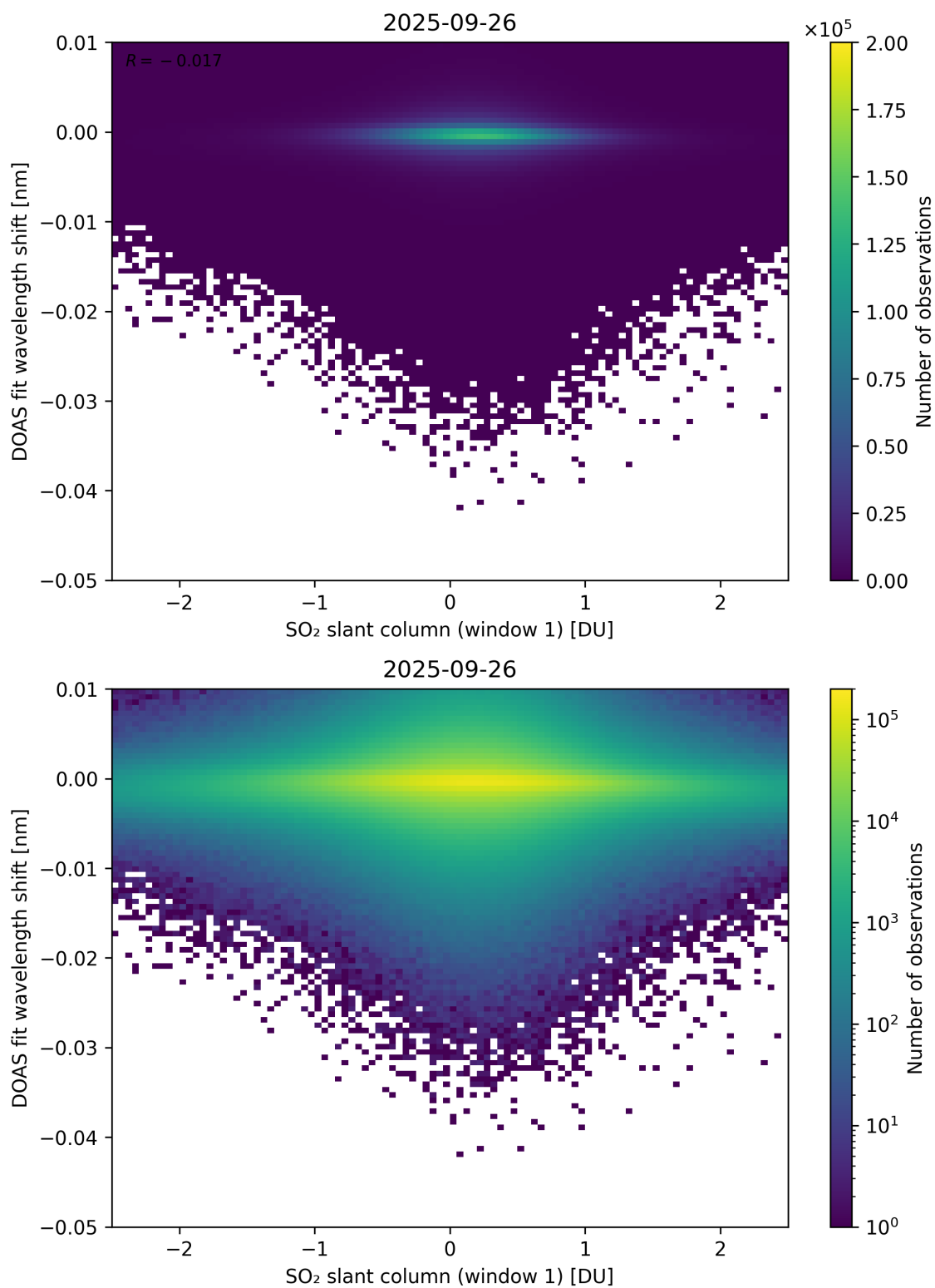
Figure 265: Scatter density plot of “SO 2 slant column (window 1)” against “DOAS fit wavelength shift” for 2025-09-26 to 2025-09-27.
