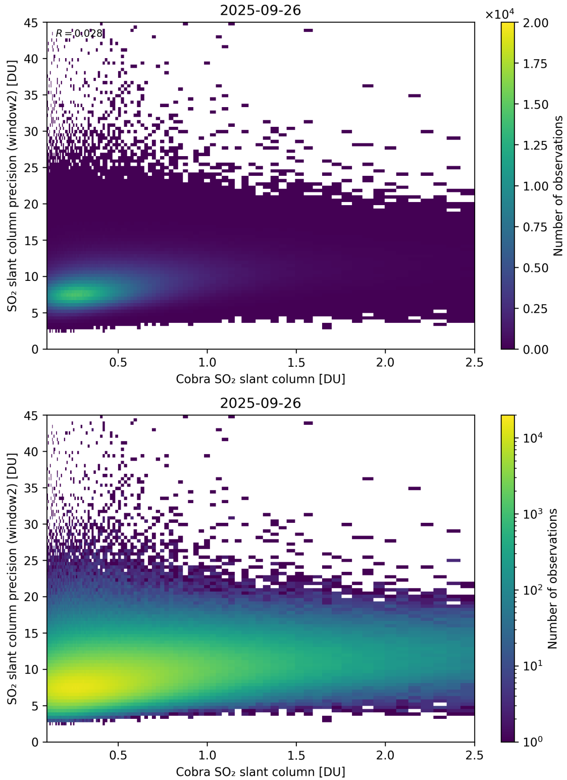
Figure 221: Scatter density plot of “Cobra SO 2 slant column” against “SO 2 slant column precision (window2)” for 2025-09-26 to 2025-09-27.
