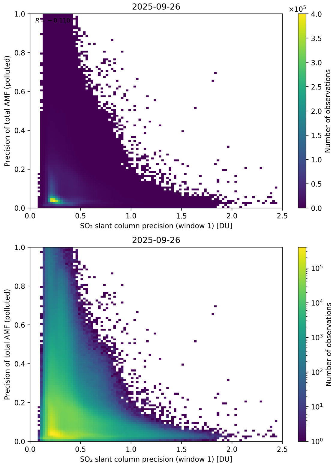
Figure 281: Scatter density plot of “SO 2 slant column precision (window 1)” against “Precision of total AMF (polluted)” for 2025-09-26 to 2025-09-27.
