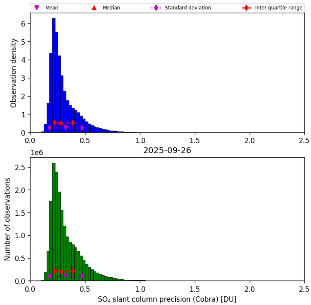
Figure 62: Histogram of “SO 2 slant column precision (Cobra)” for 2025-09-26 to 2025-09-27
