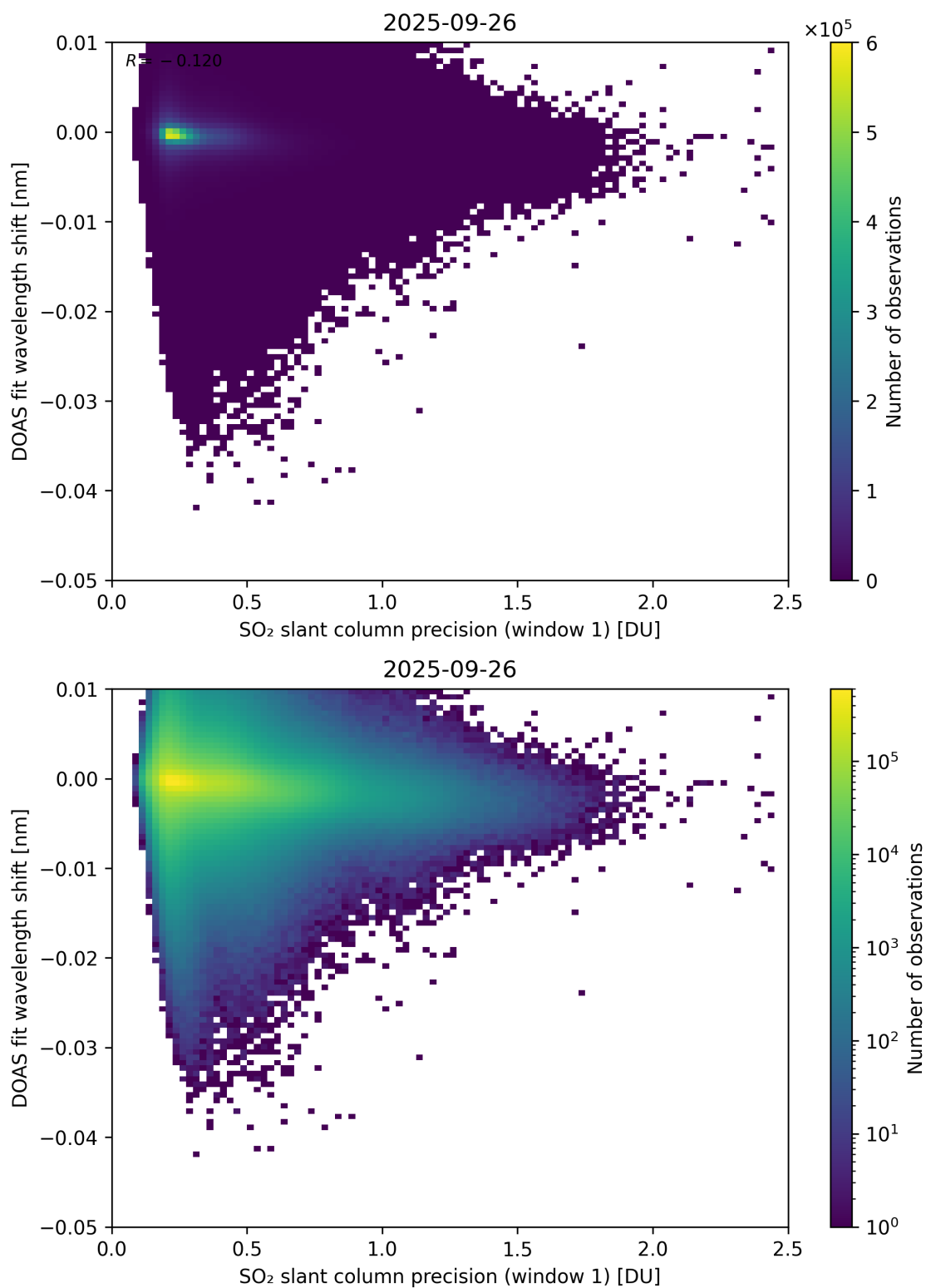
Figure 271: Scatter density plot of “SO 2 slant column precision (window 1)” against “DOAS fit wavelength shift” for 2025-09-26 to 2025-09-27.
