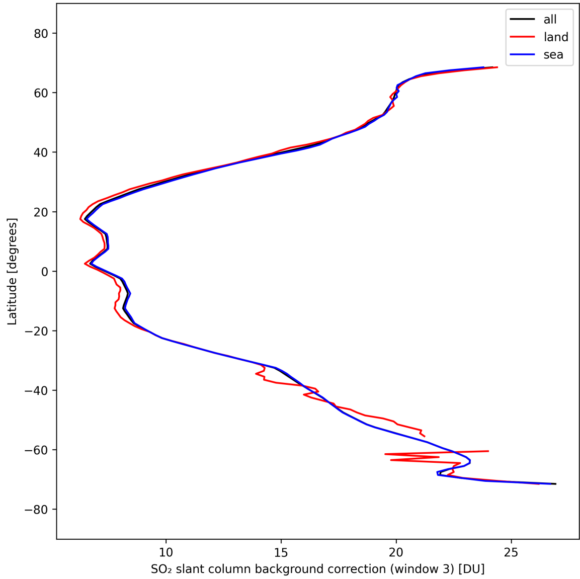
Figure 48: Zonal average of “SO 2 slant column background correction (window 3)” for 2025-09-26 to 2025-09-27.
