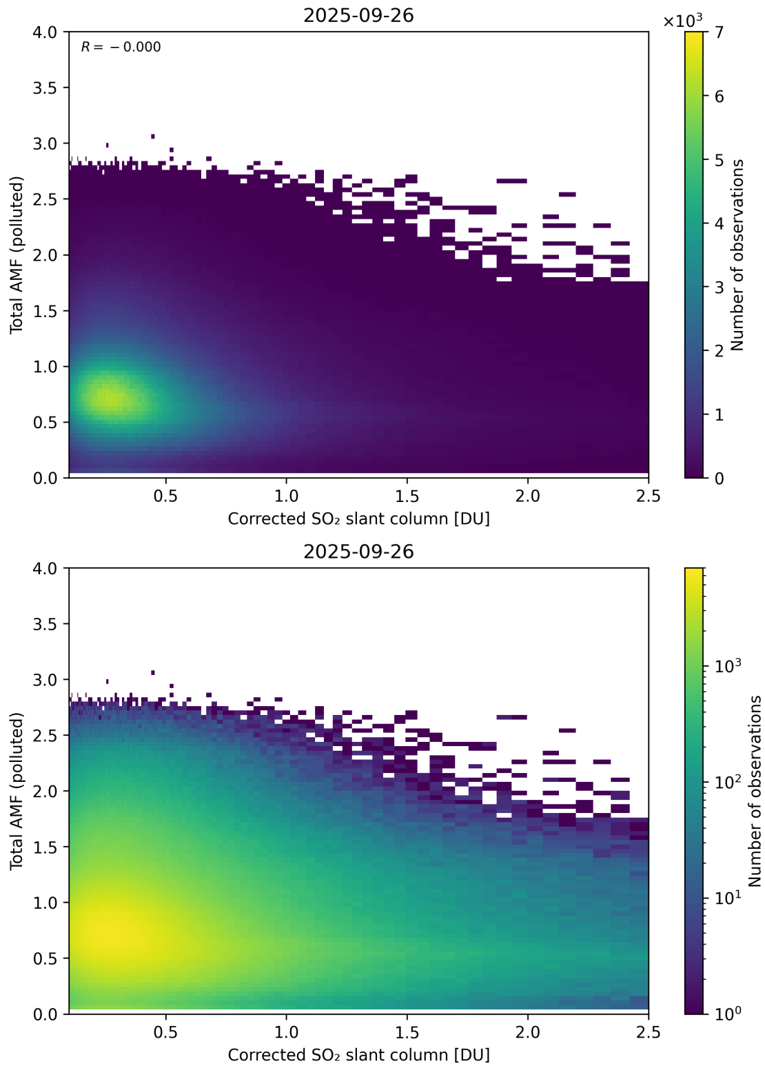
Figure 242: Scatter density plot of “Corrected SO 2 slant column” against “Total AMF (polluted)” for 2025-09-26 to 2025-09-27.
