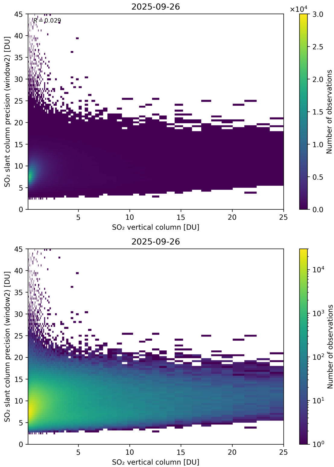
Figure 356: Scatter density plot of “SO 2 vertical column” against “SO 2 slant column precision (window2)” for 2025-09-26 to 2025-09-27.
