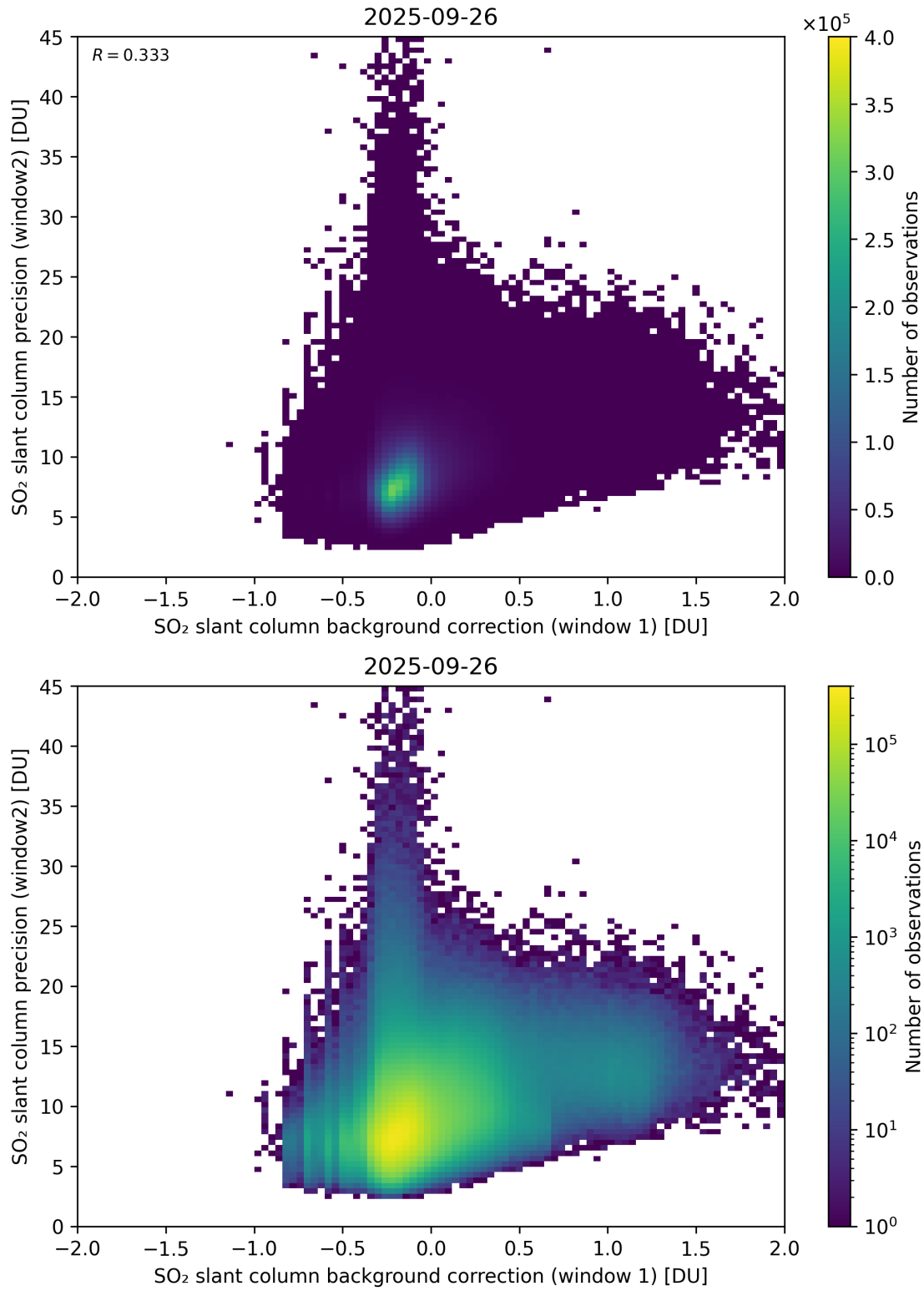
Figure 117: Scatter density plot of “SO 2 slant column background correction (window 1)” against “SO 2 slant column precision (window2)” for 2025-09-26 to 2025-09-27.
