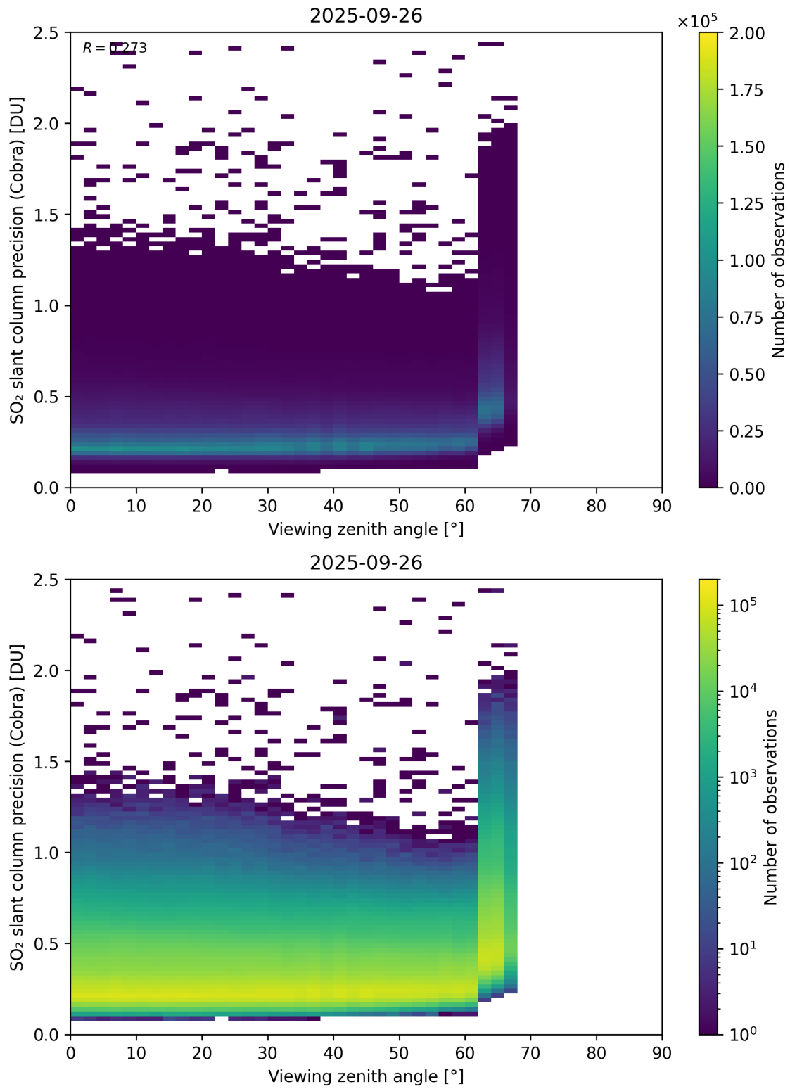
Figure 372: Scatter density plot of “Viewing zenith angle” against “SO 2 slant column precision (Cobra)” for 2025-09-26 to 2025-09-27.
