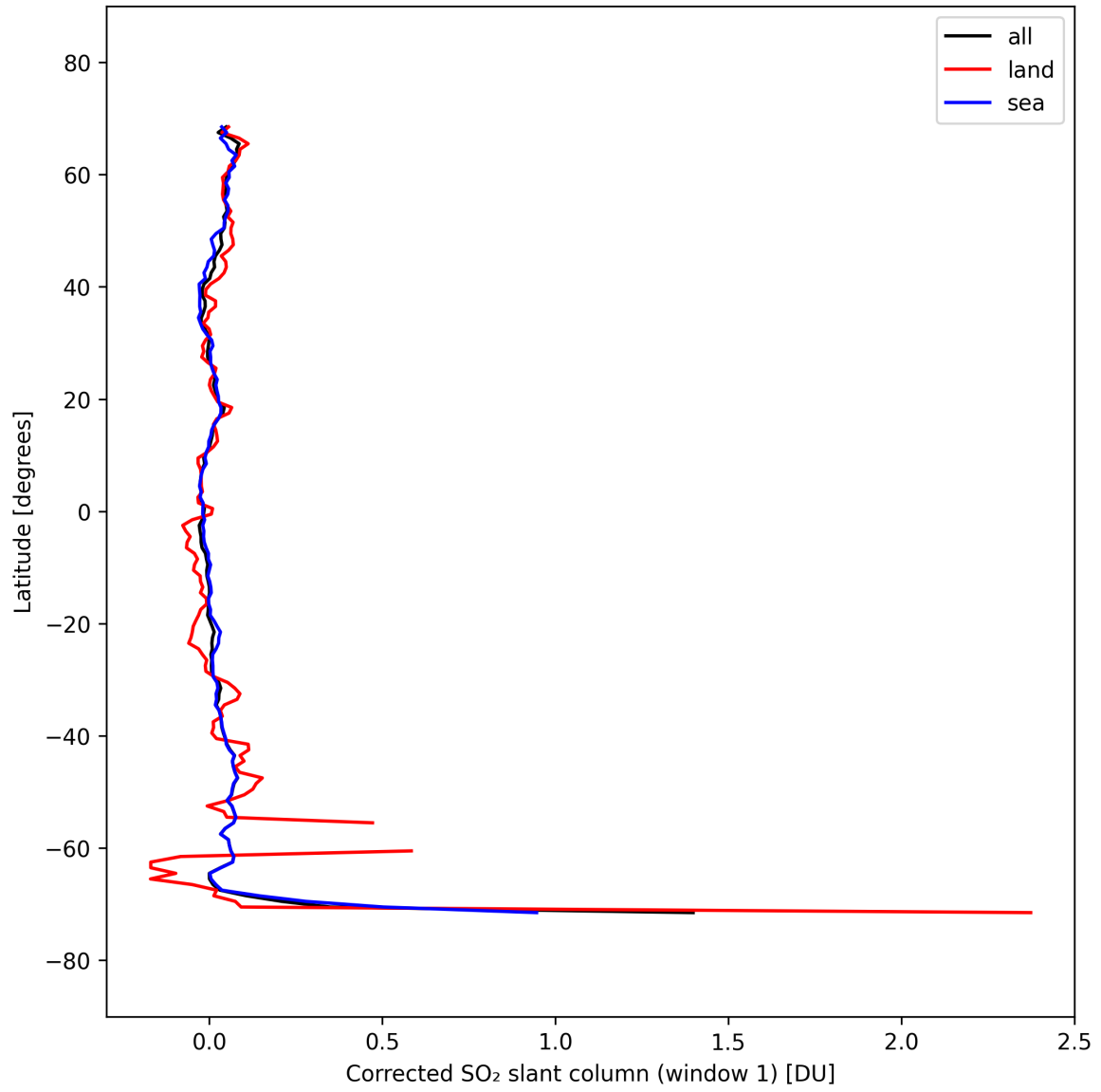
Figure 39: Zonal average of “Corrected SO 2 slant column (window 1)” for 2025-09-26 to 2025-09-27.
