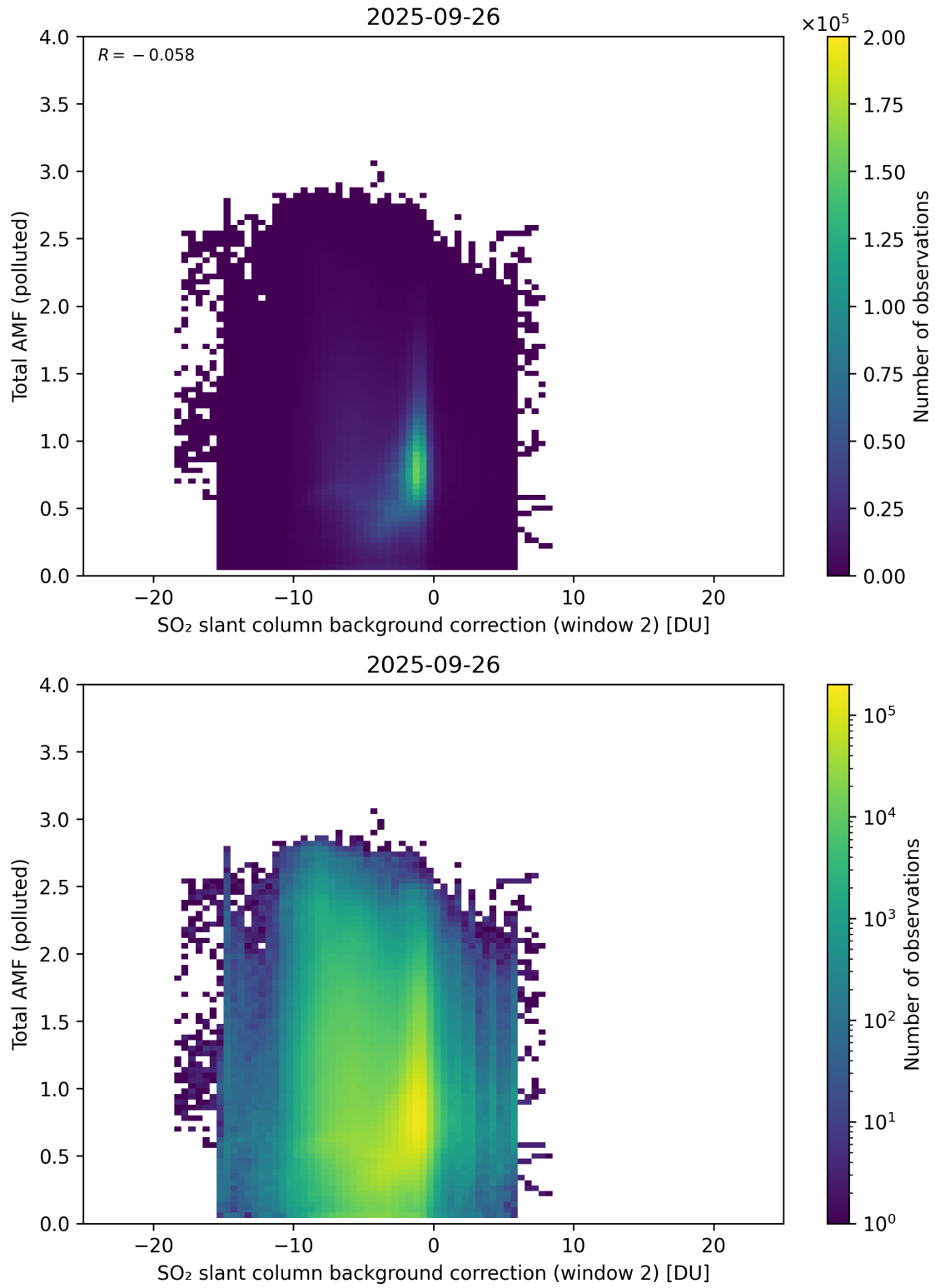
Figure 130: Scatter density plot of “SO 2 slant column background correction (window 2)” against “Total AMF (polluted)” for 2025-09-26 to 2025-09-27.
