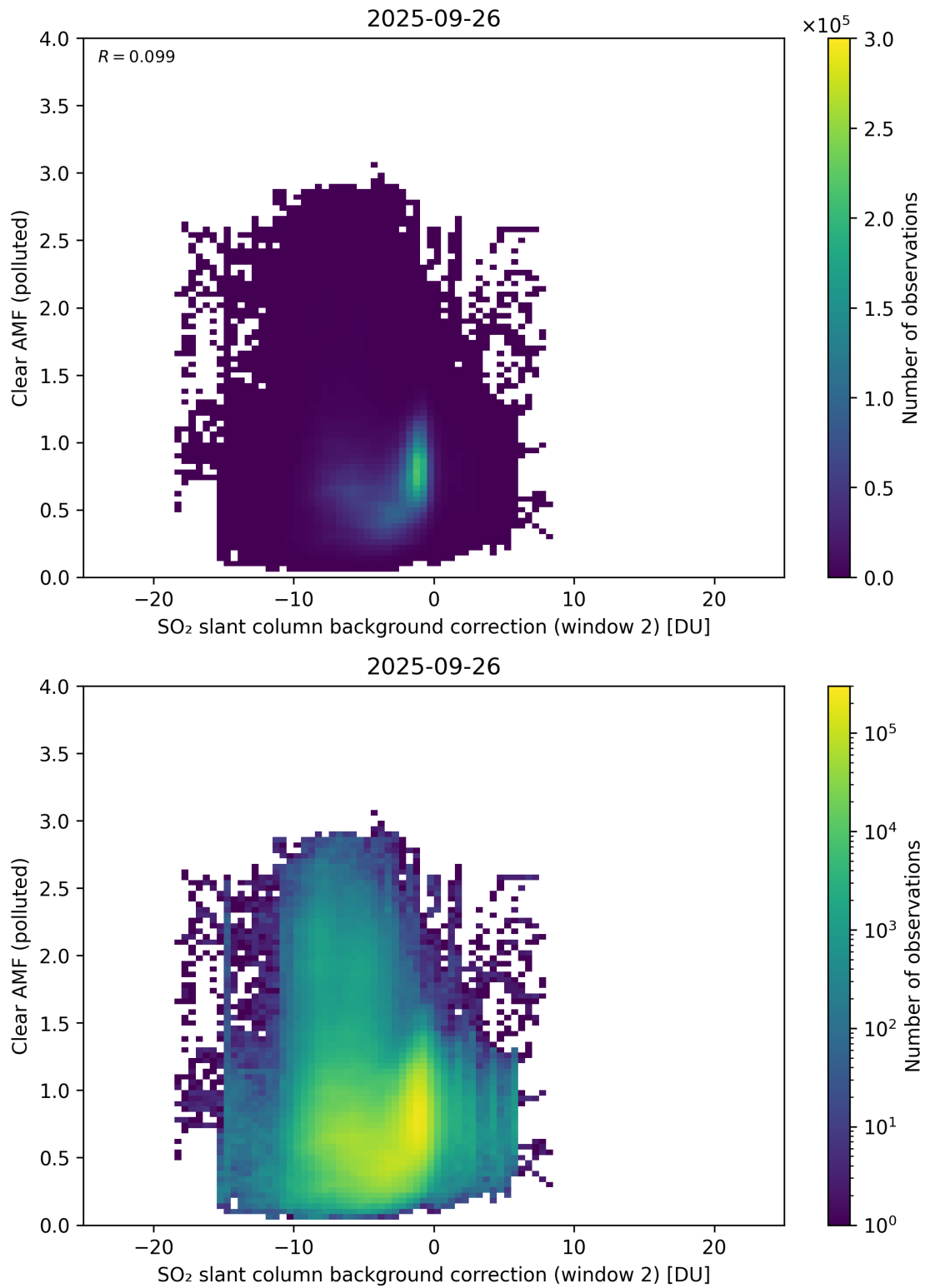
Figure 126: Scatter density plot of “SO 2 slant column background correction (window 2)” against “Clear AMF (polluted)” for 2025-09-26 to 2025-09-27.
