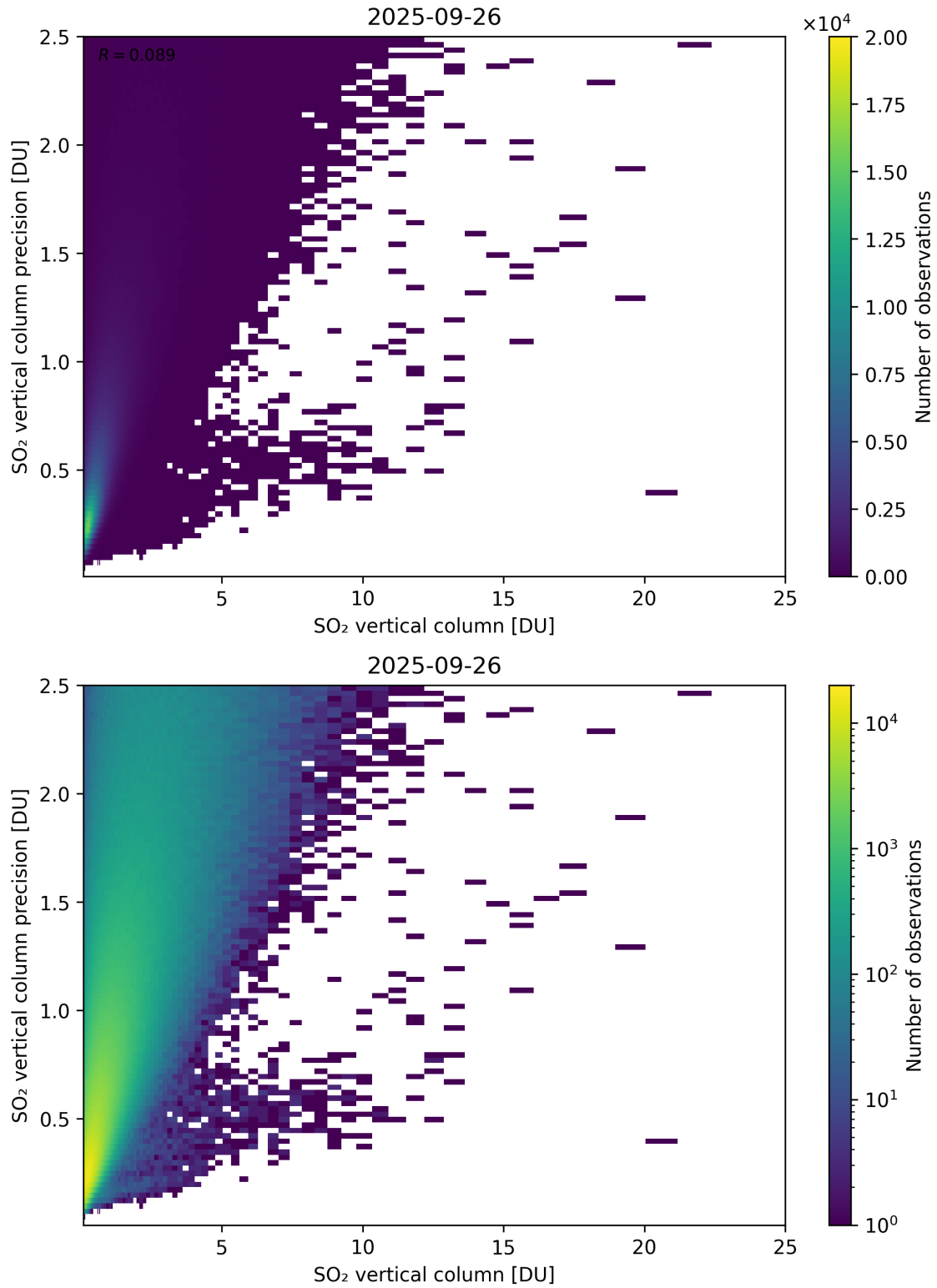
Figure 361: Scatter density plot of “SO 2 vertical column” against “SO 2 vertical column precision” for 2025-09-26 to 2025-09-27.
