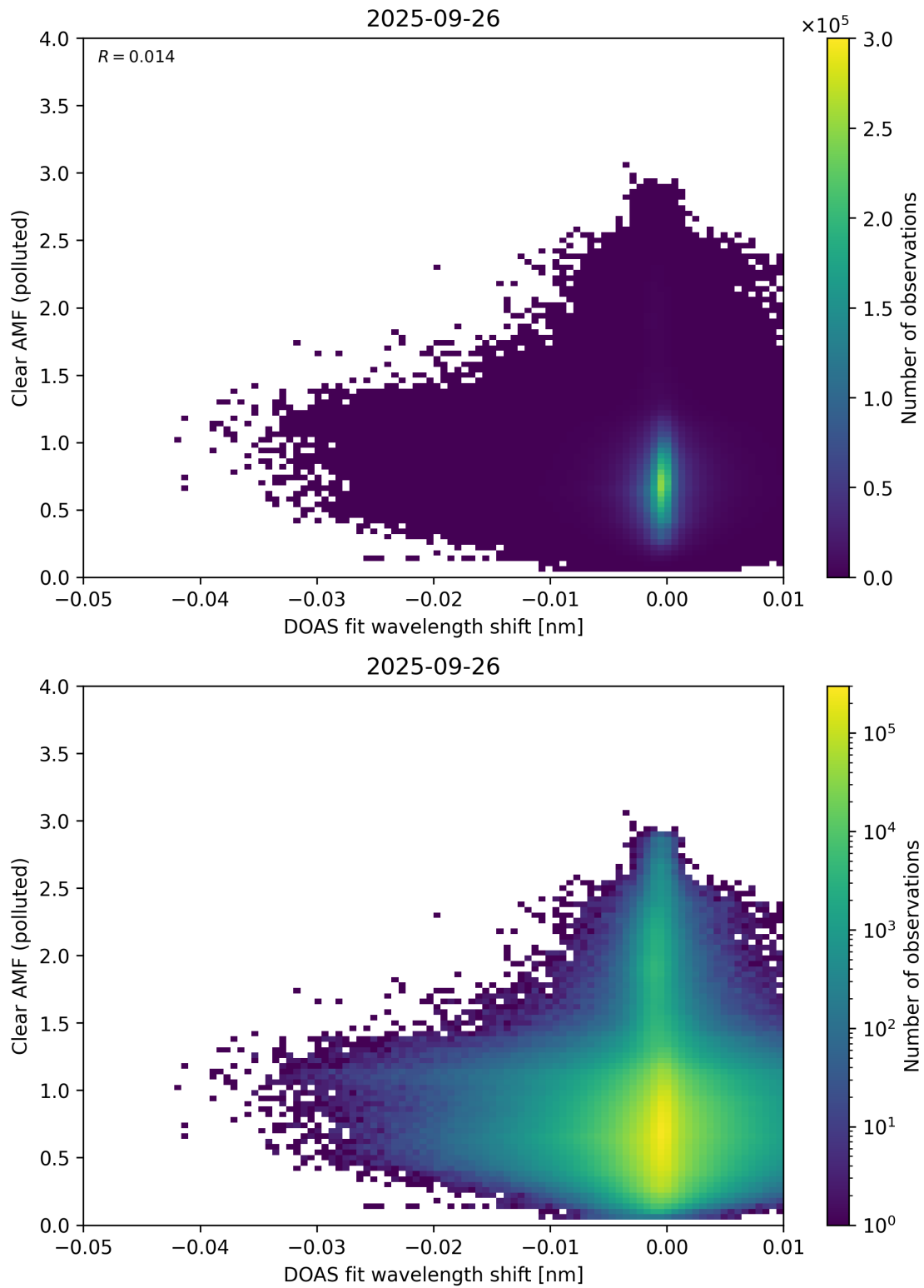
Figure 140: Scatter density plot of “DOAS fit wavelength shift” against “Clear AMF (polluted)” for 2025-09-26 to 2025-09-27.
