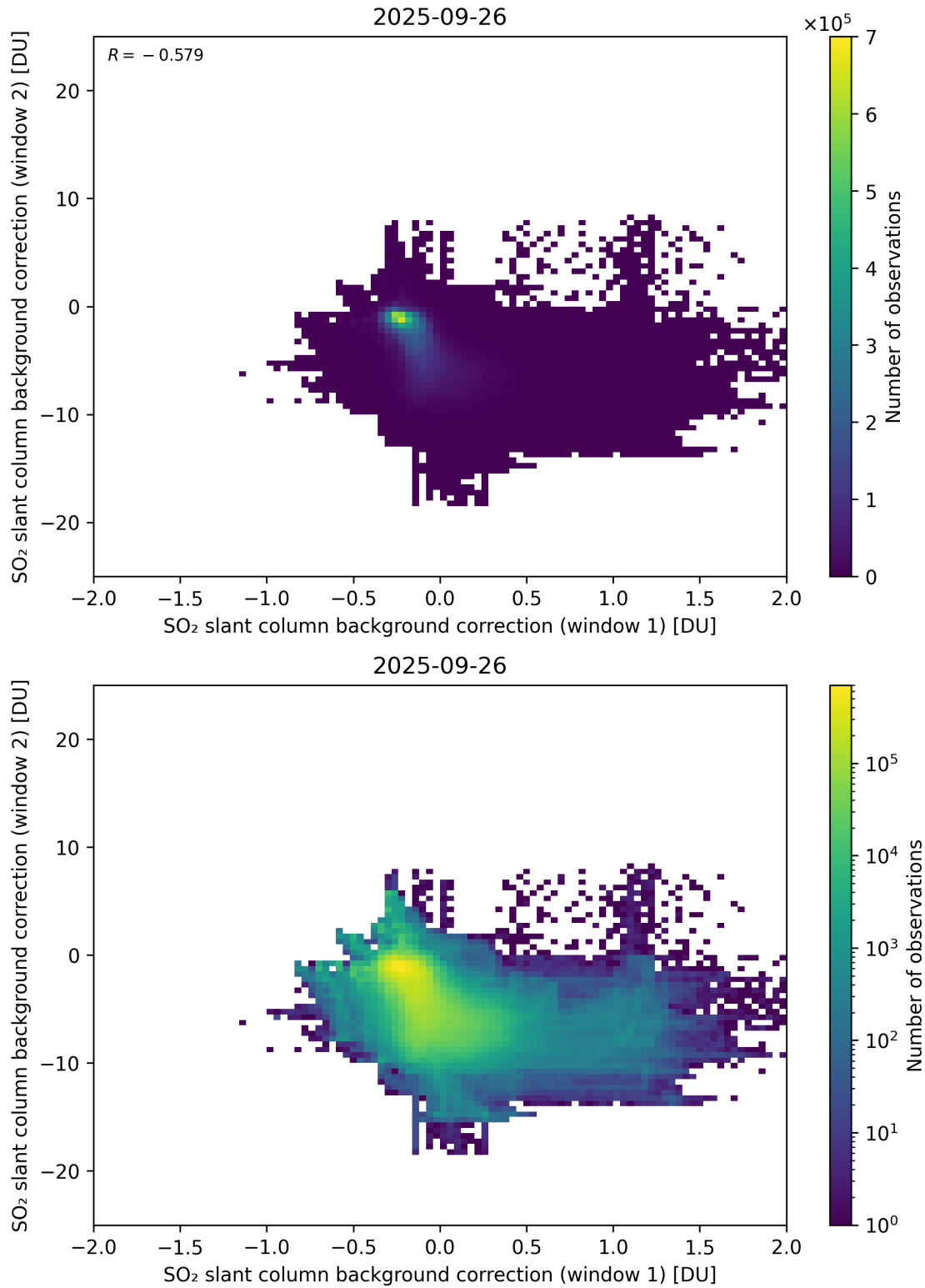
Figure 109: Scatter density plot of “SO 2 slant column background correction (window 1)” against “SO 2 slant column background correction (window 2)” for 2025-09-26 to 2025-09-27.
