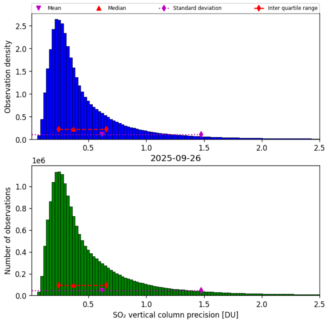
Figure 59: Histogram of “SO 2 vertical column precision” for 2025-09-26 to 2025-09-27
