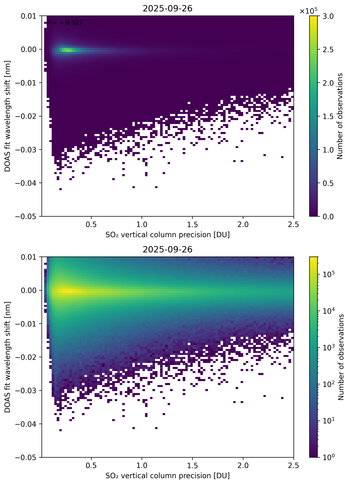
Figure 332: Scatter density plot of “SO 2 vertical column precision” against “DOAS fit wavelength shift” for 2025-09-26 to 2025-09-27.
