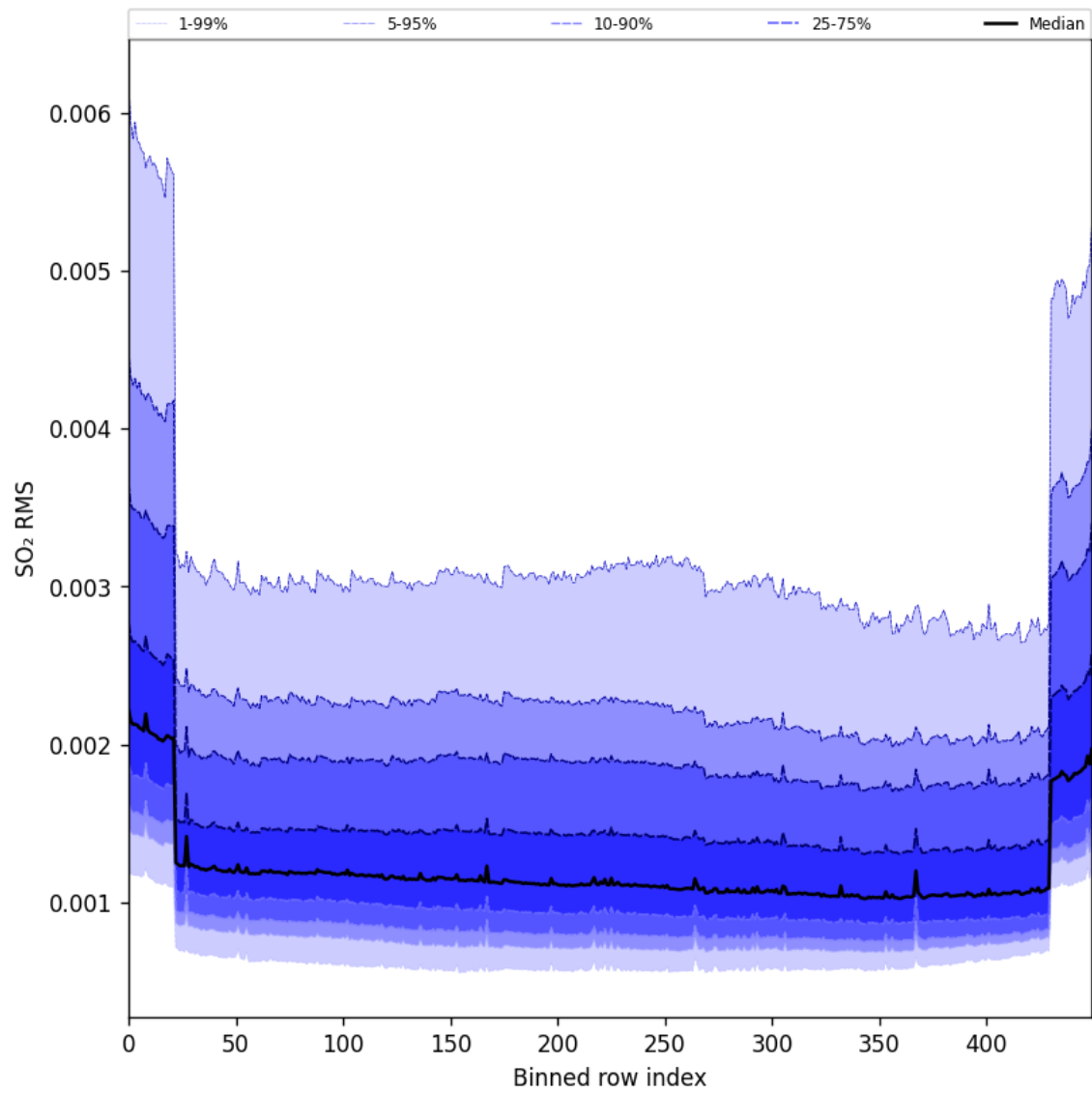
Figure 104: Along track statistics of “SO 2 RMS” for 2025-09-26 to 2025-09-27
