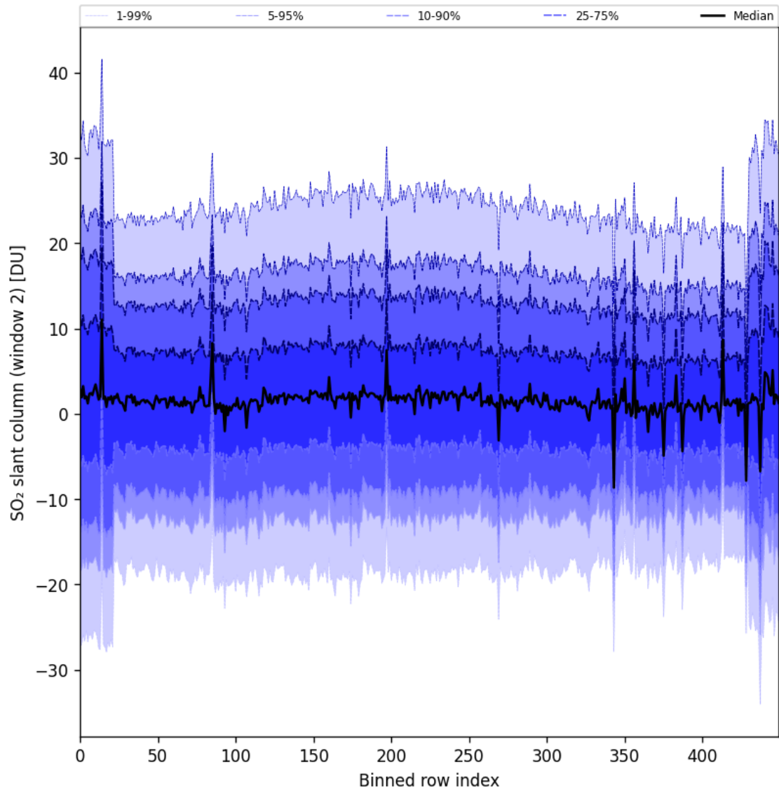
Figure 93: Along track statistics of “SO 2 slant column (window 2)” for 2025-09-26 to 2025-09-27
