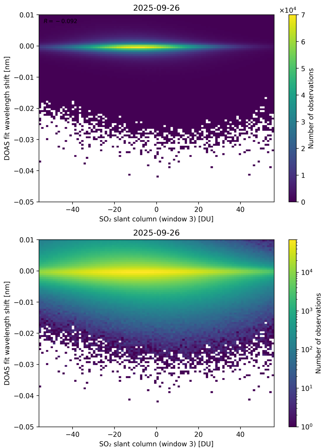
Figure 304: Scatter density plot of “SO 2 slant column (window 3)” against “DOAS fit wavelength shift” for 2025-09-26 to 2025-09-27.
