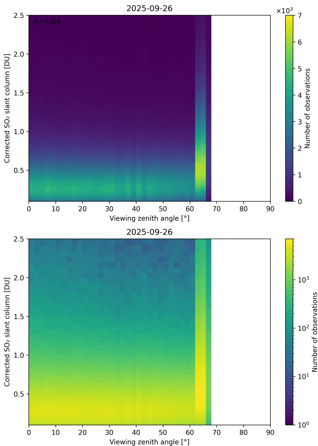
Figure 373: Scatter density plot of “Viewing zenith angle” against “Corrected SO 2 slant column” for 2025-09-26 to 2025-09-27.
