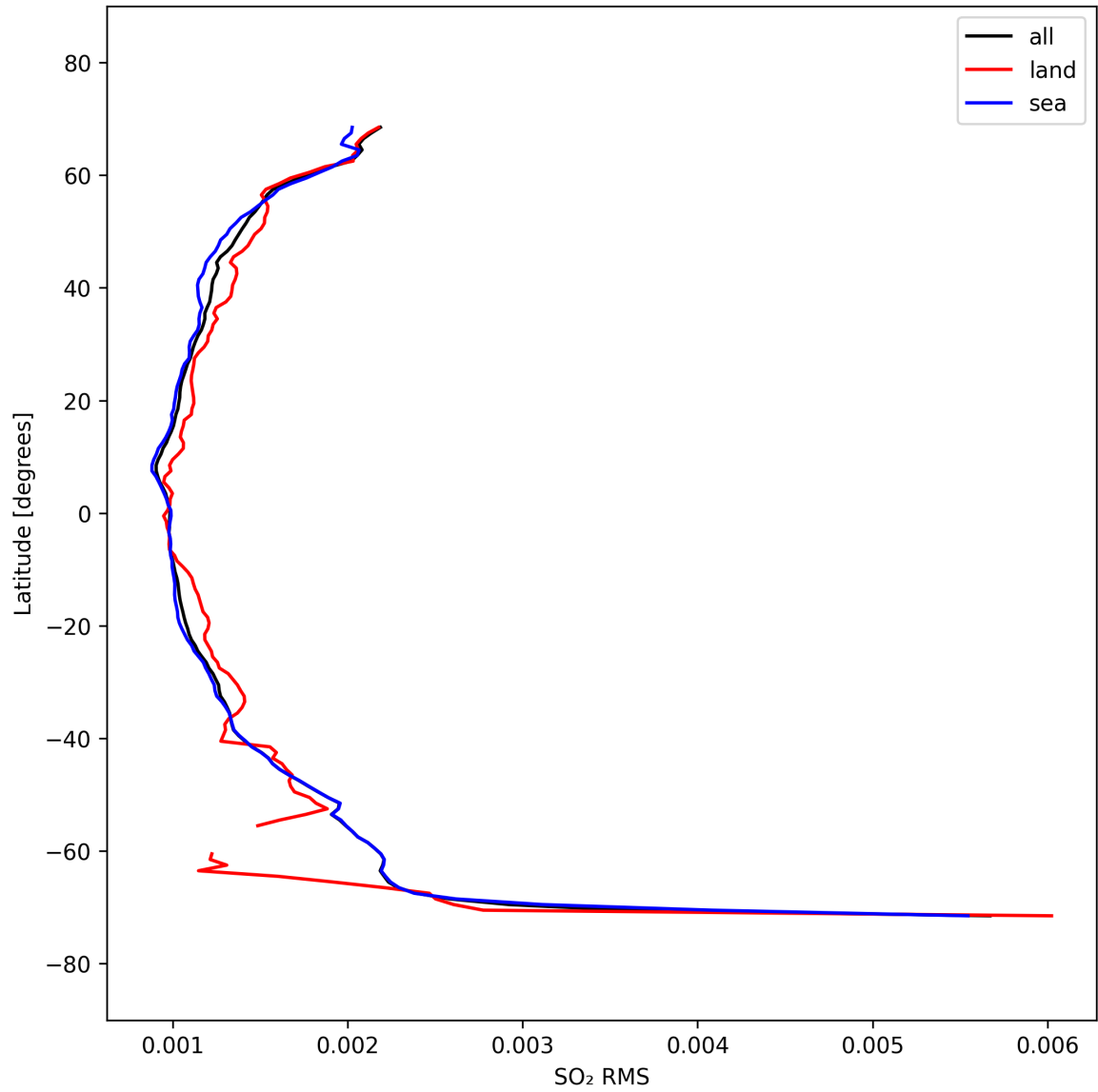
Figure 52: Zonal average of “SO 2 RMS” for 2025-09-26 to 2025-09-27.
