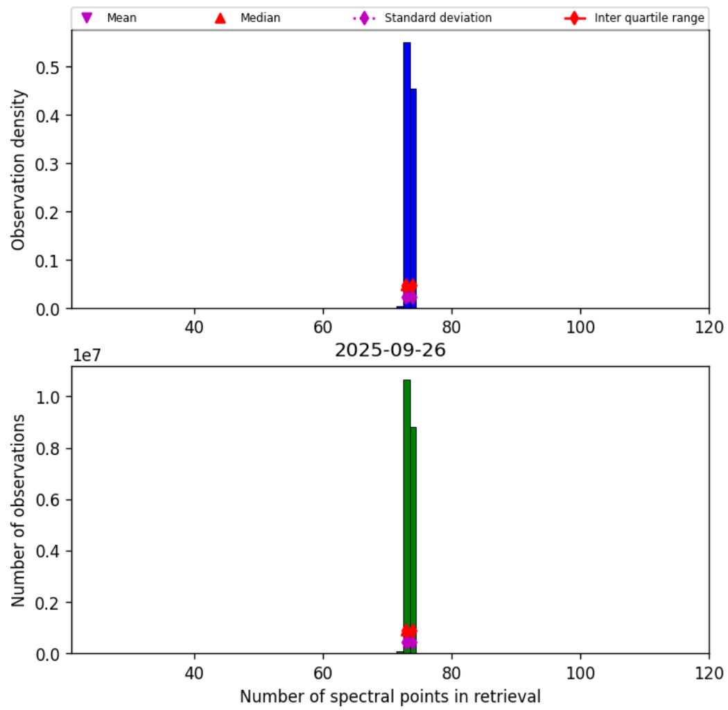
Figure 82: Histogram of “Number of spectral points in retrieval” for 2025-09-26 to 2025-09-27
