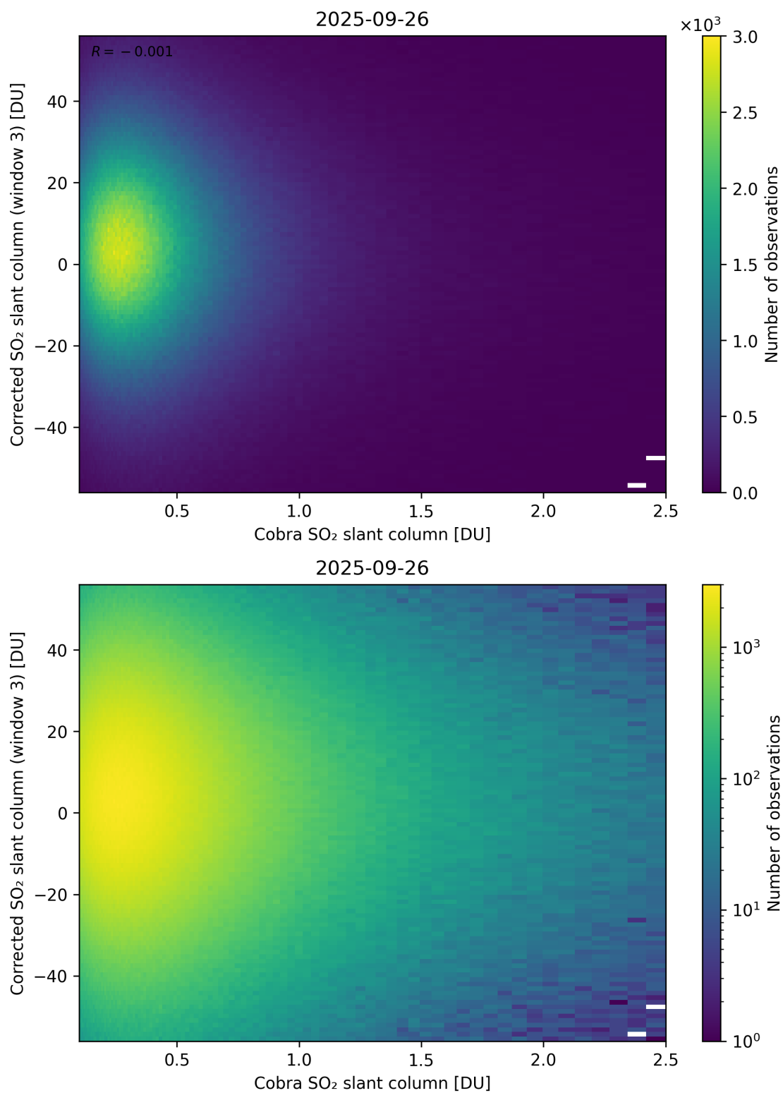
Figure 218: Scatter density plot of “Cobra SO 2 slant column” against “Corrected SO 2 slant column (window 3)” for 2025-09-26 to 2025-09-27.
