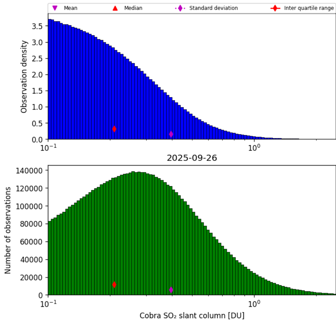
Figure 61: Histogram of “Cobra SO 2 slant column” for 2025-09-26 to 2025-09-27
