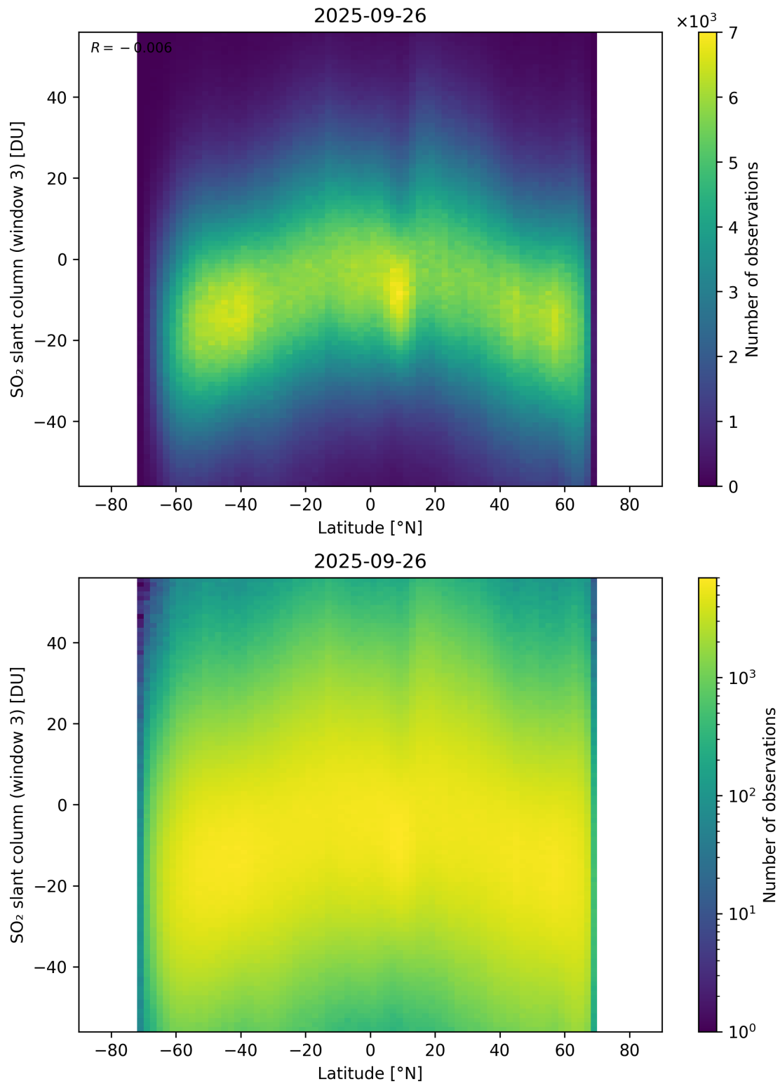
Figure 165: Scatter density plot of “Latitude” against “SO 2 slant column (window 3)” for 2025-09-26 to 2025-09-27.
