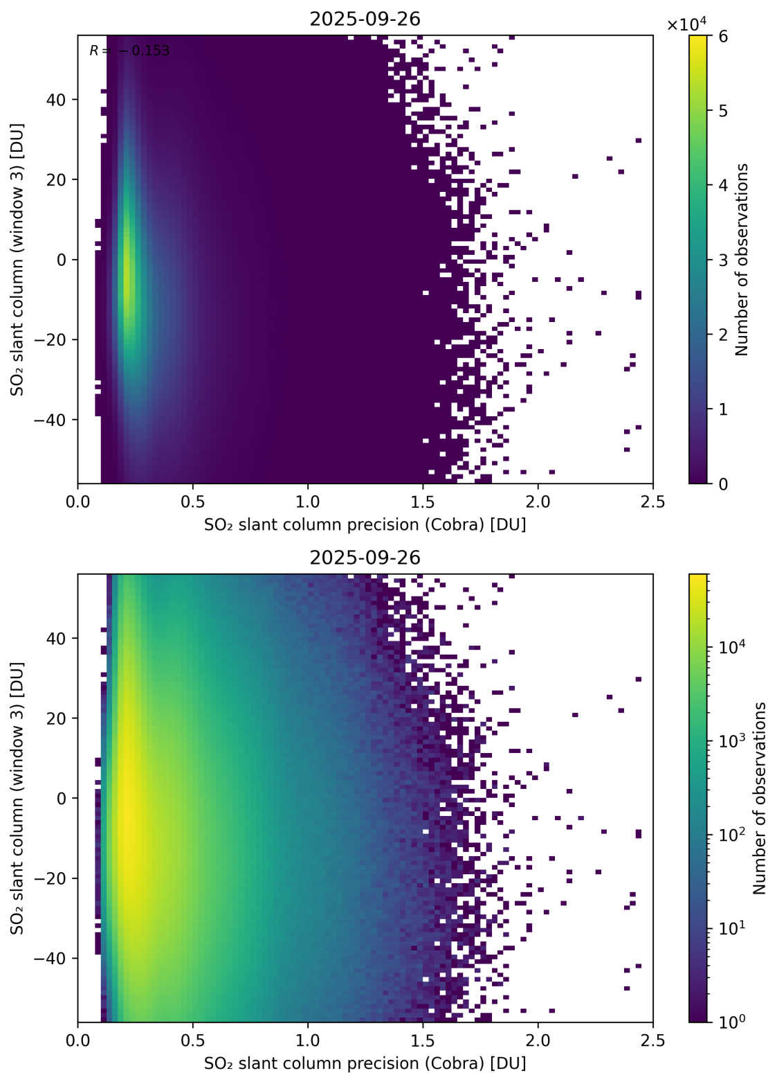
Figure 211: Scatter density plot of “SO 2 slant column precision (Cobra)” against “SO 2 slant column (window 3)” for 2025-09-26 to 2025-09-27.
