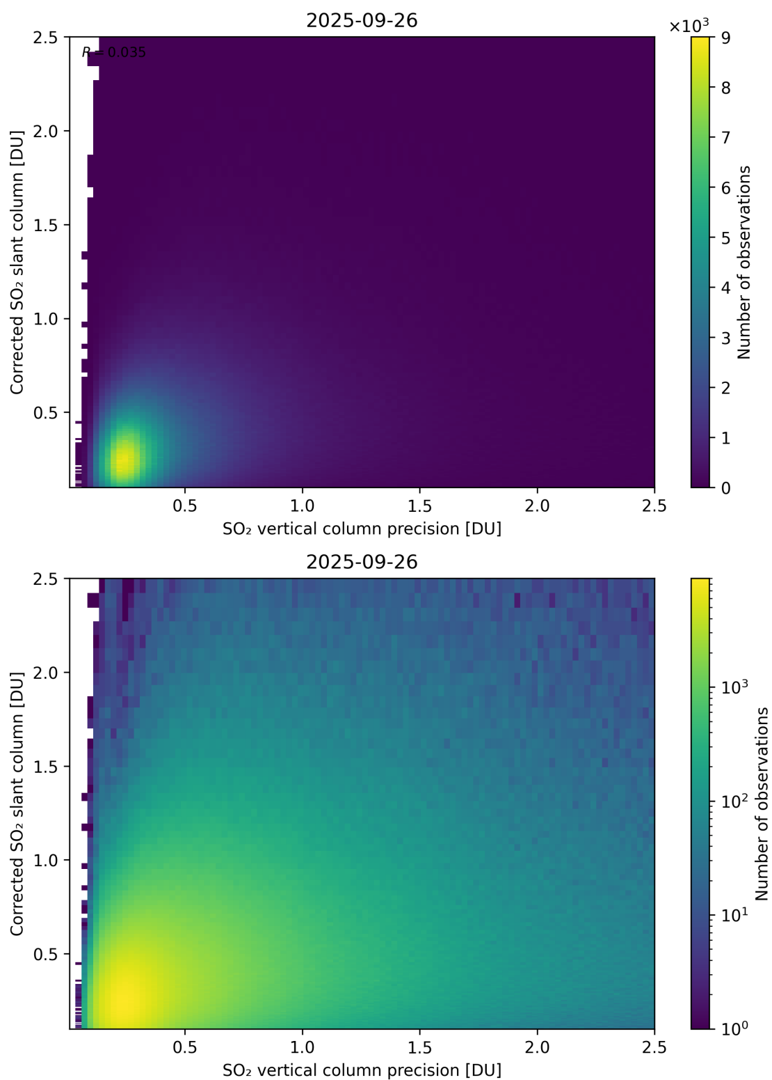
Figure 338: Scatter density plot of “SO 2 vertical column precision” against “Corrected SO 2 slant column” for 2025-09-26 to 2025-09-27.
