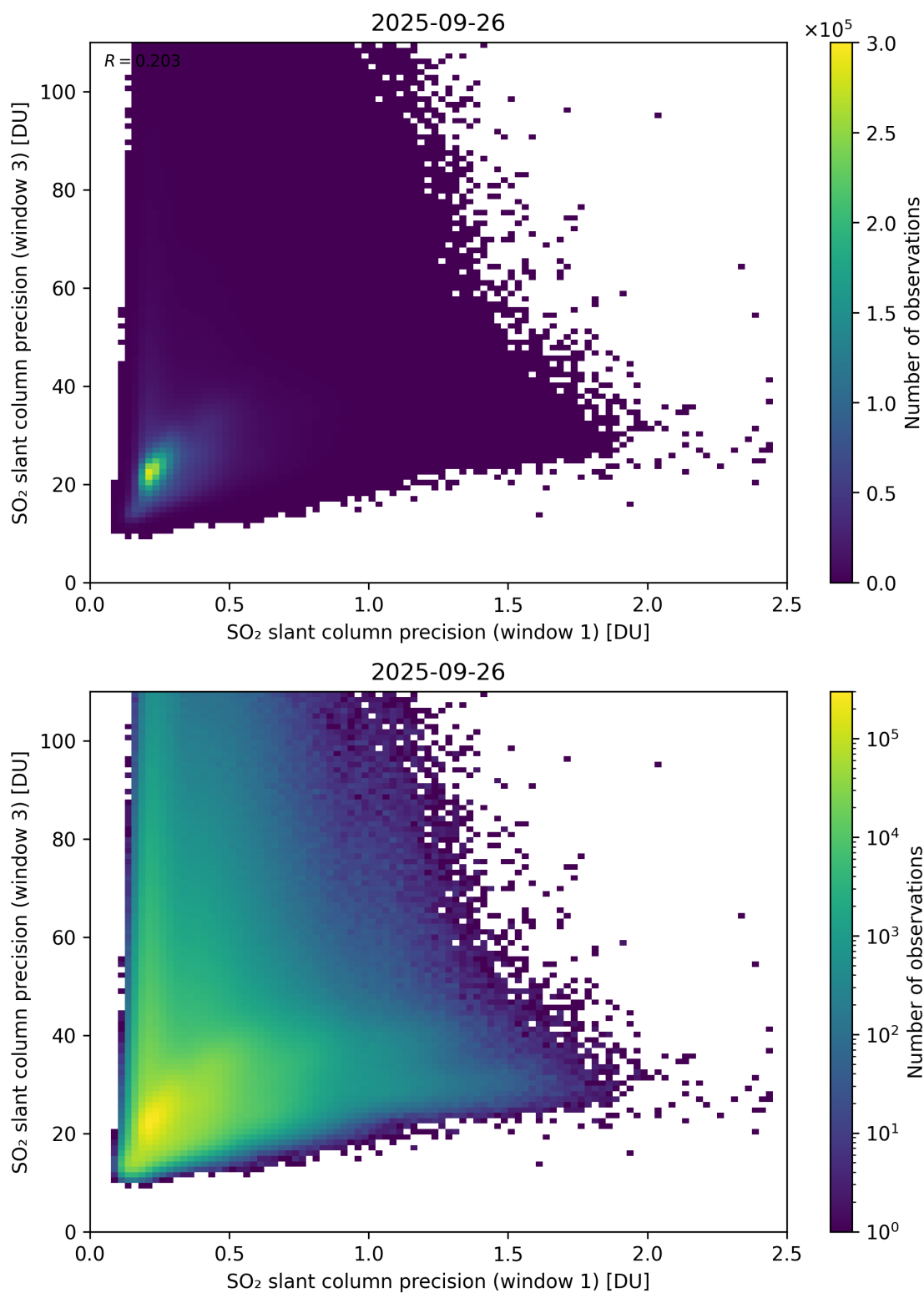
Figure 279: Scatter density plot of “SO 2 slant column precision (window 1)” against “SO 2 slant column precision (window 3)” for 2025-09-26 to 2025-09-27.
