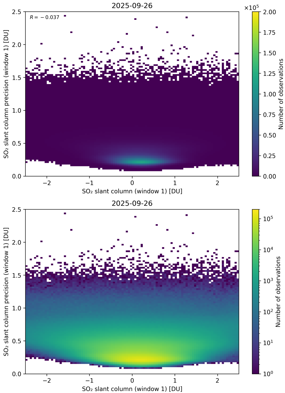
Figure 285: Scatter density plot of “SO 2 slant column (window 1)” against “SO 2 slant column precision (window 1)” for 2025-09-26 to 2025-09-27.
