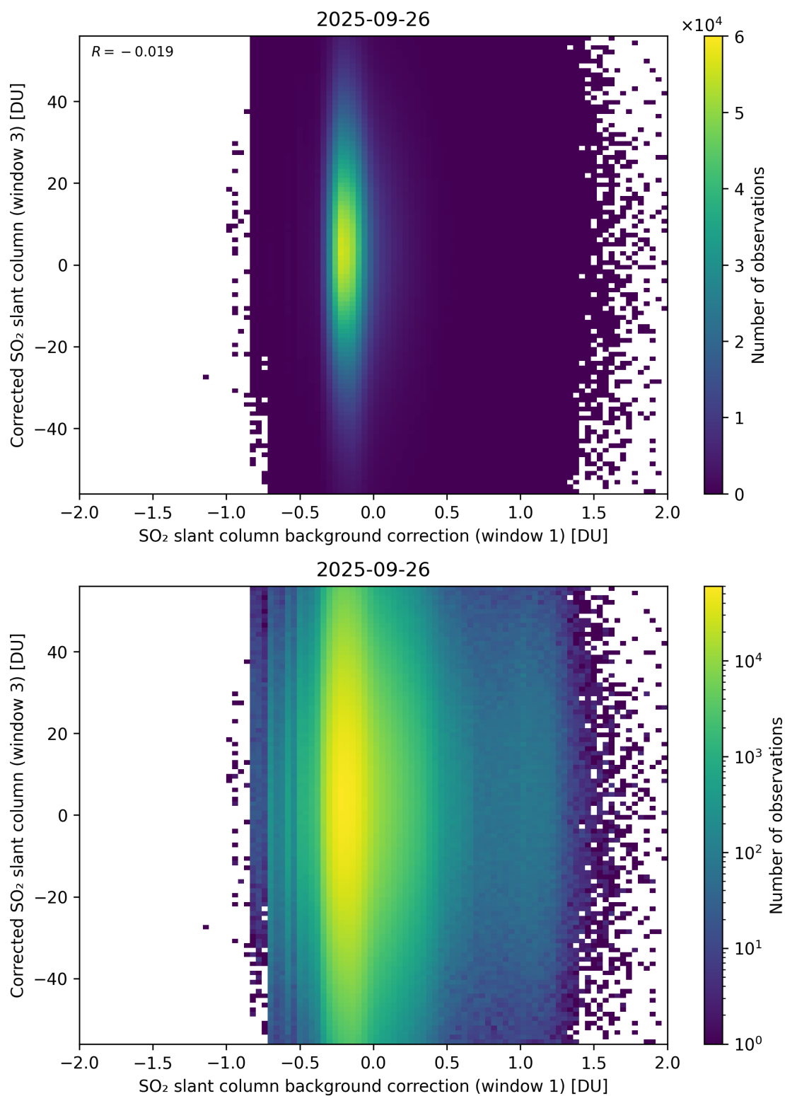
Figure 116: Scatter density plot of “SO 2 slant column background correction (window 1)” against “Corrected SO 2 slant column (window 3)” for 2025-09-26 to 2025-09-27.
