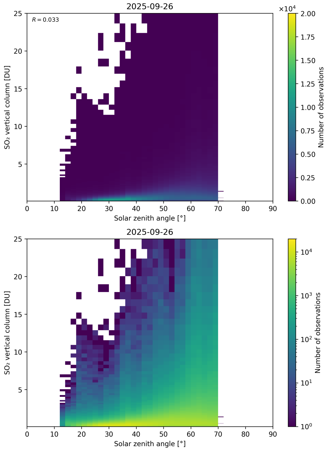
Figure 191: Scatter density plot of “Solar zenith angle” against “SO 2 vertical column” for 2025-09-26 to 2025-09-27.
