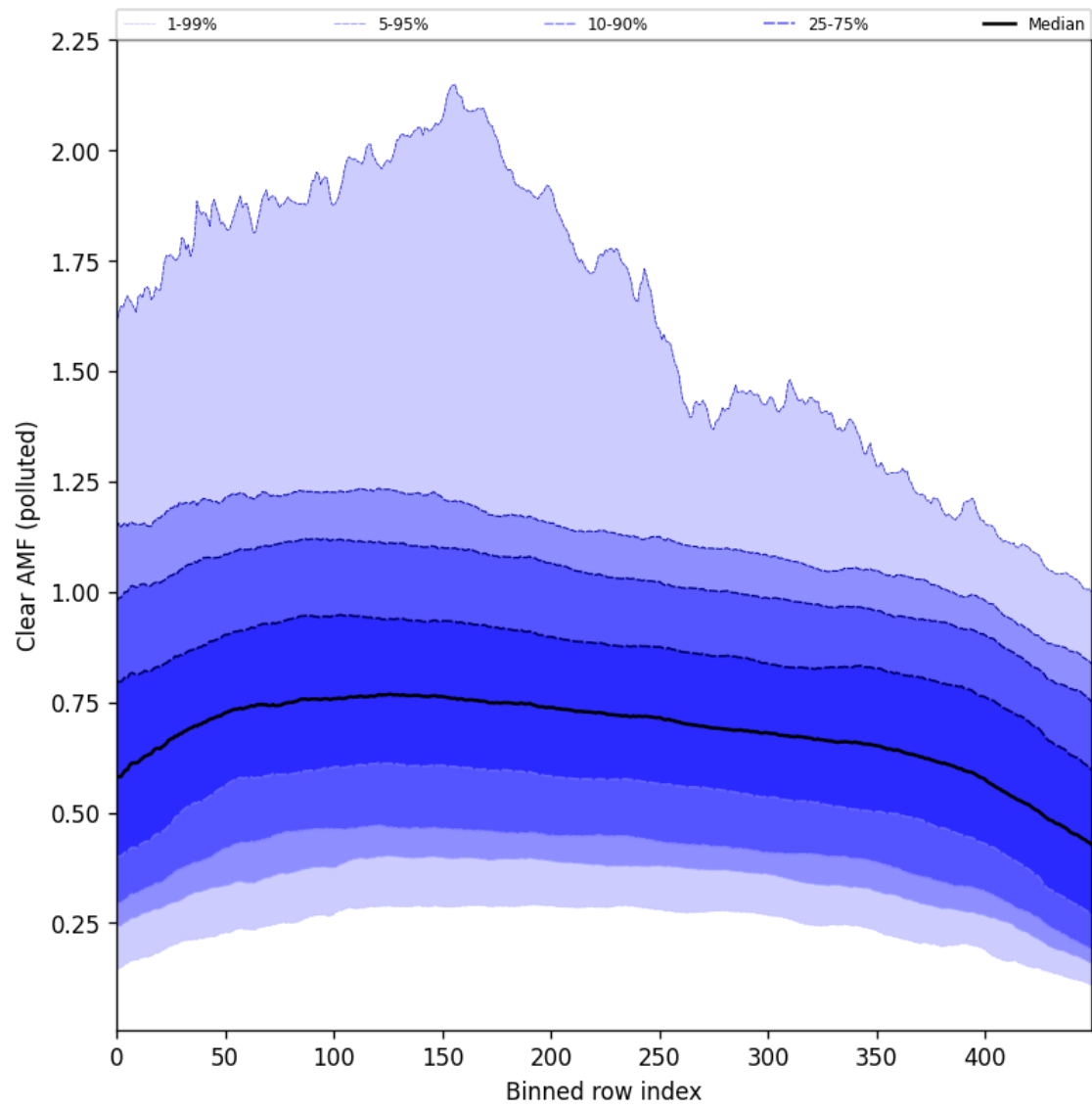
Figure 107: Along track statistics of “Clear AMF (polluted)” for 2025-09-26 to 2025-09-27
