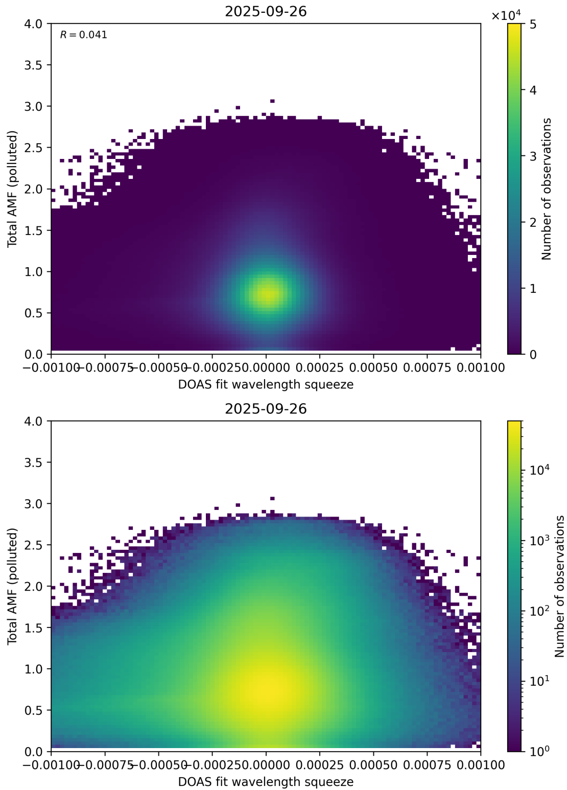
Figure 145: Scatter density plot of “DOAS fit wavelength squeeze” against “Total AMF (polluted)” for 2025-09-26 to 2025-09-27.
