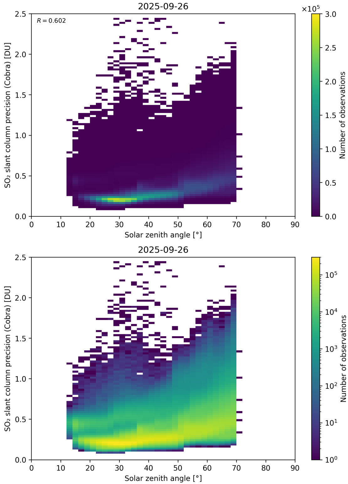
Figure 180: Scatter density plot of “Solar zenith angle” against “SO 2 slant column precision (Cobra)” for 2025-09-26 to 2025-09-27.
