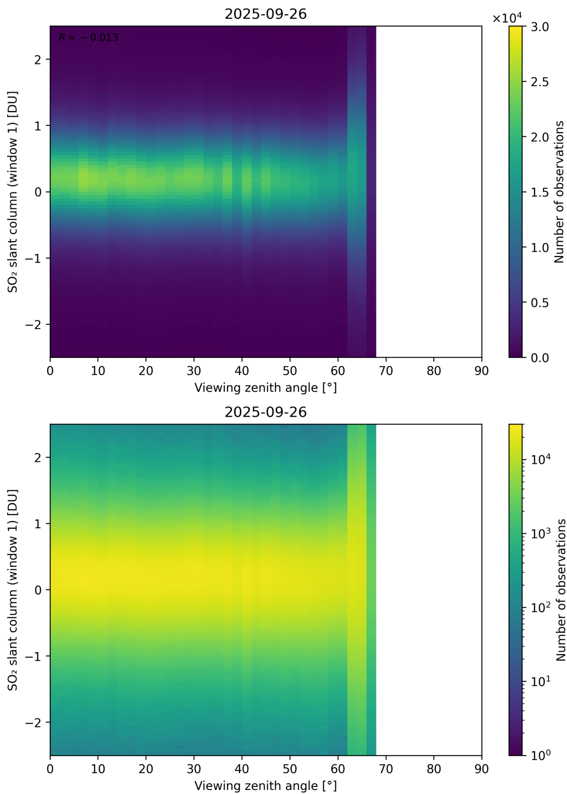
Figure 376: Scatter density plot of “Viewing zenith angle” against “SO 2 slant column (window 1)” for 2025-09-26 to 2025-09-27.
