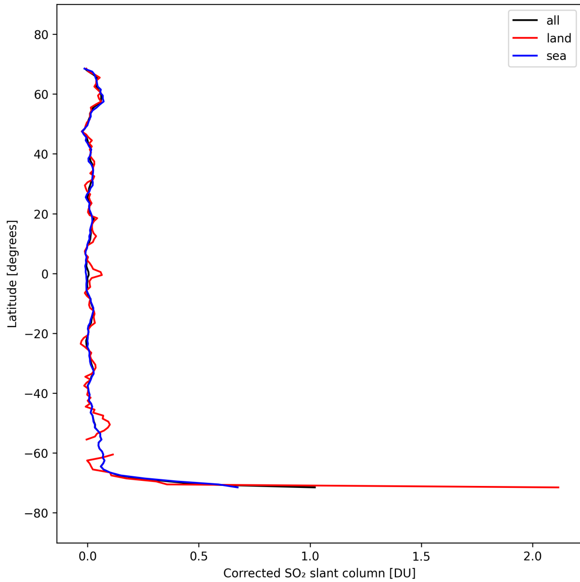
Figure 34: Zonal average of “Corrected SO 2 slant column” for 2025-09-26 to 2025-09-27.
