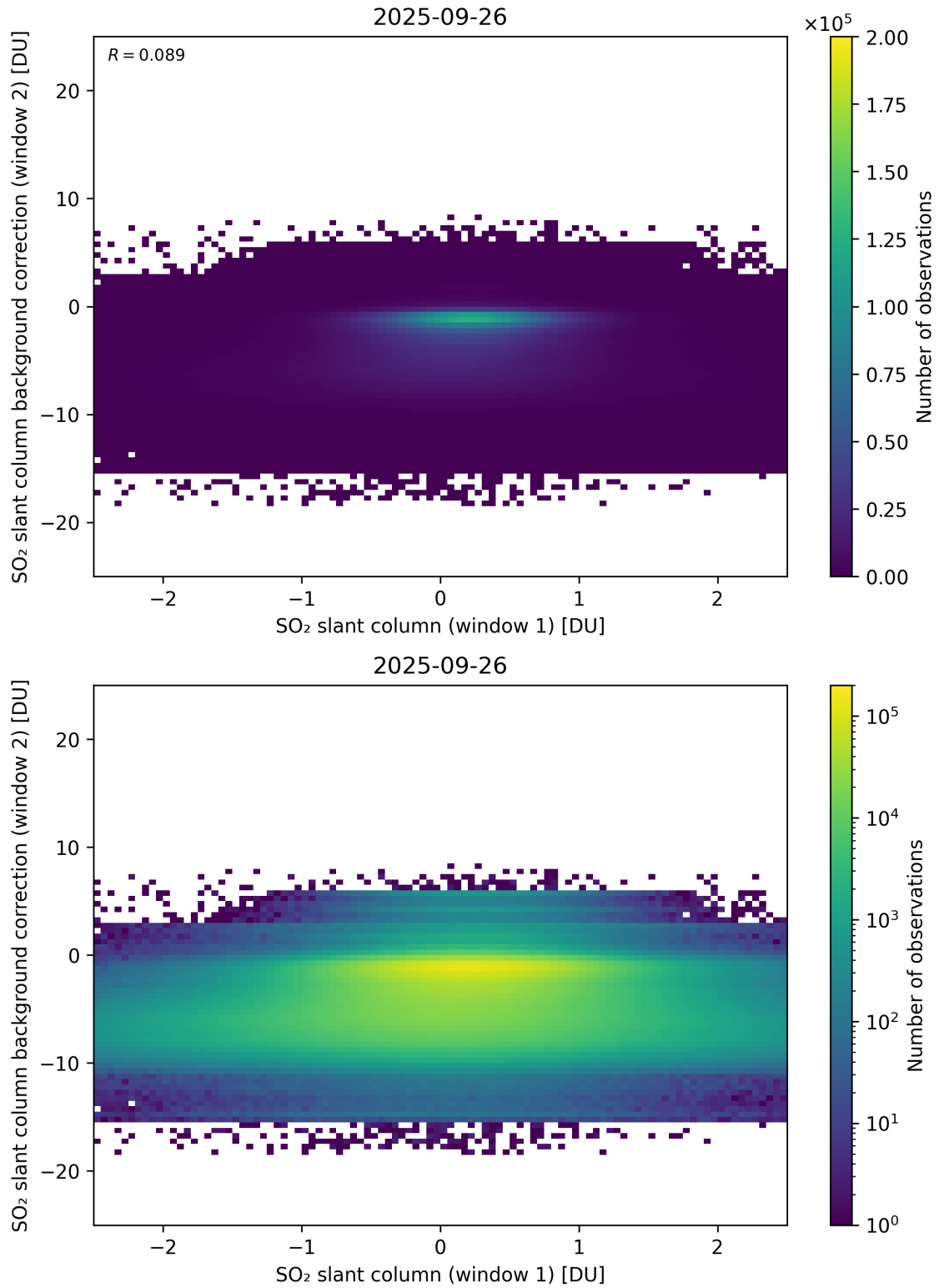
Figure 263: Scatter density plot of “SO 2 slant column (window 1)” against “SO 2 slant column background correction (window 2)” for 2025-09-26 to 2025-09-27.
