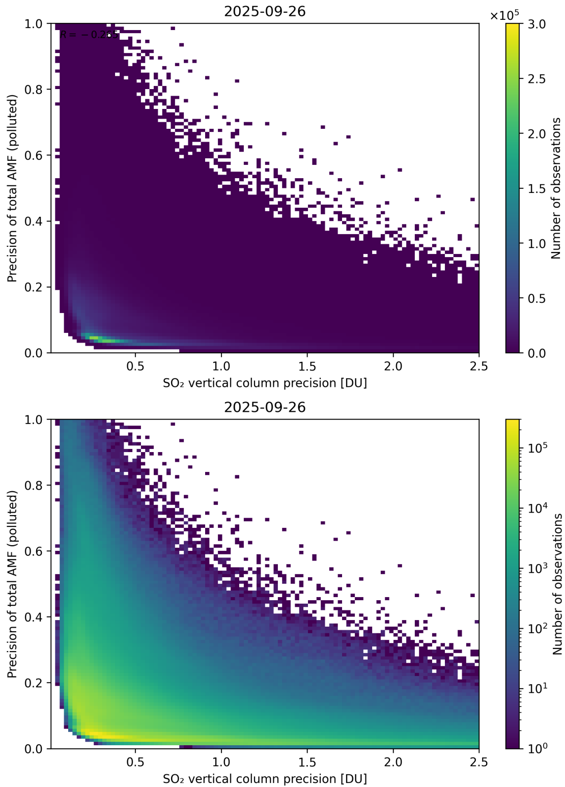
Figure 347: Scatter density plot of “SO 2 vertical column precision” against “Precision of total AMF (polluted)” for 2025-09-26 to 2025-09-27.
