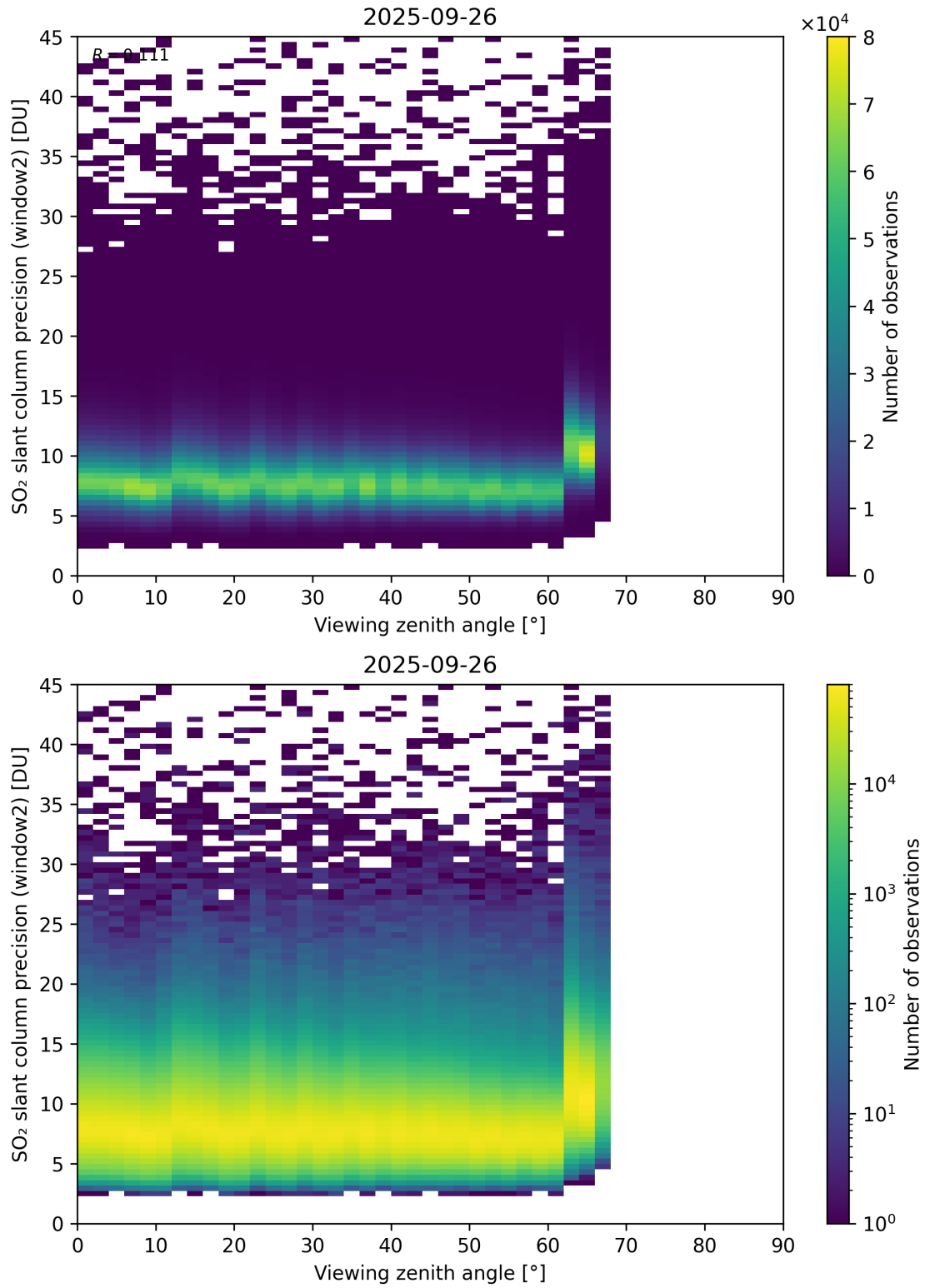
Figure 378: Scatter density plot of “Viewing zenith angle” against “SO 2 slant column precision (window2)” for 2025-09-26 to 2025-09-27.
