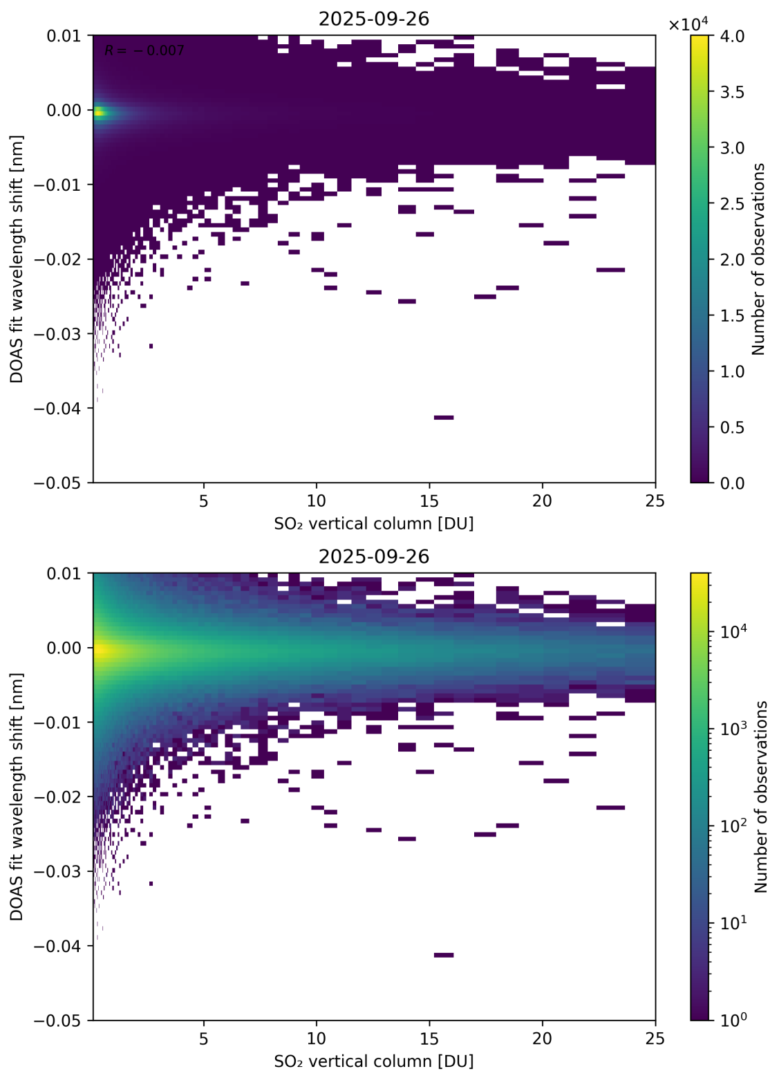
Figure 326: Scatter density plot of “SO 2 vertical column” against “DOAS fit wavelength shift” for 2025-09-26 to 2025-09-27.
