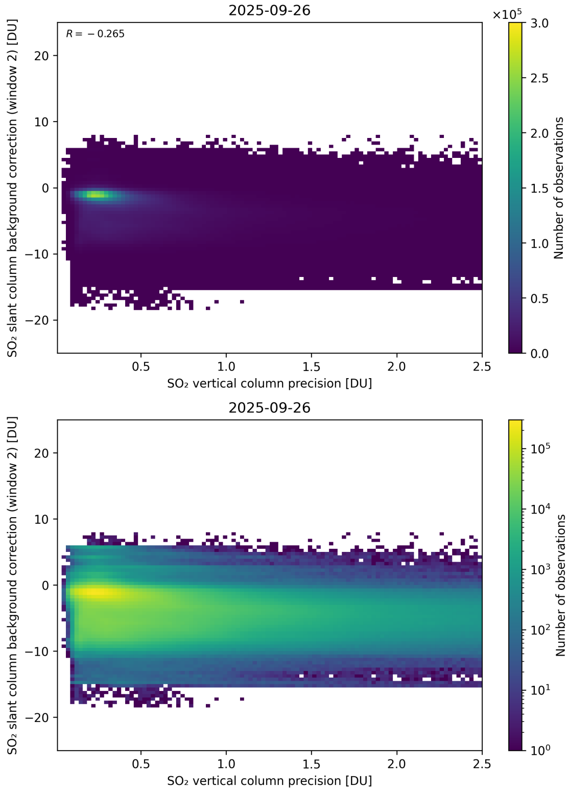
Figure 330: Scatter density plot of “SO 2 vertical column precision” against “SO 2 slant column background correction (window 2)” for 2025-09-26 to 2025-09-27.
