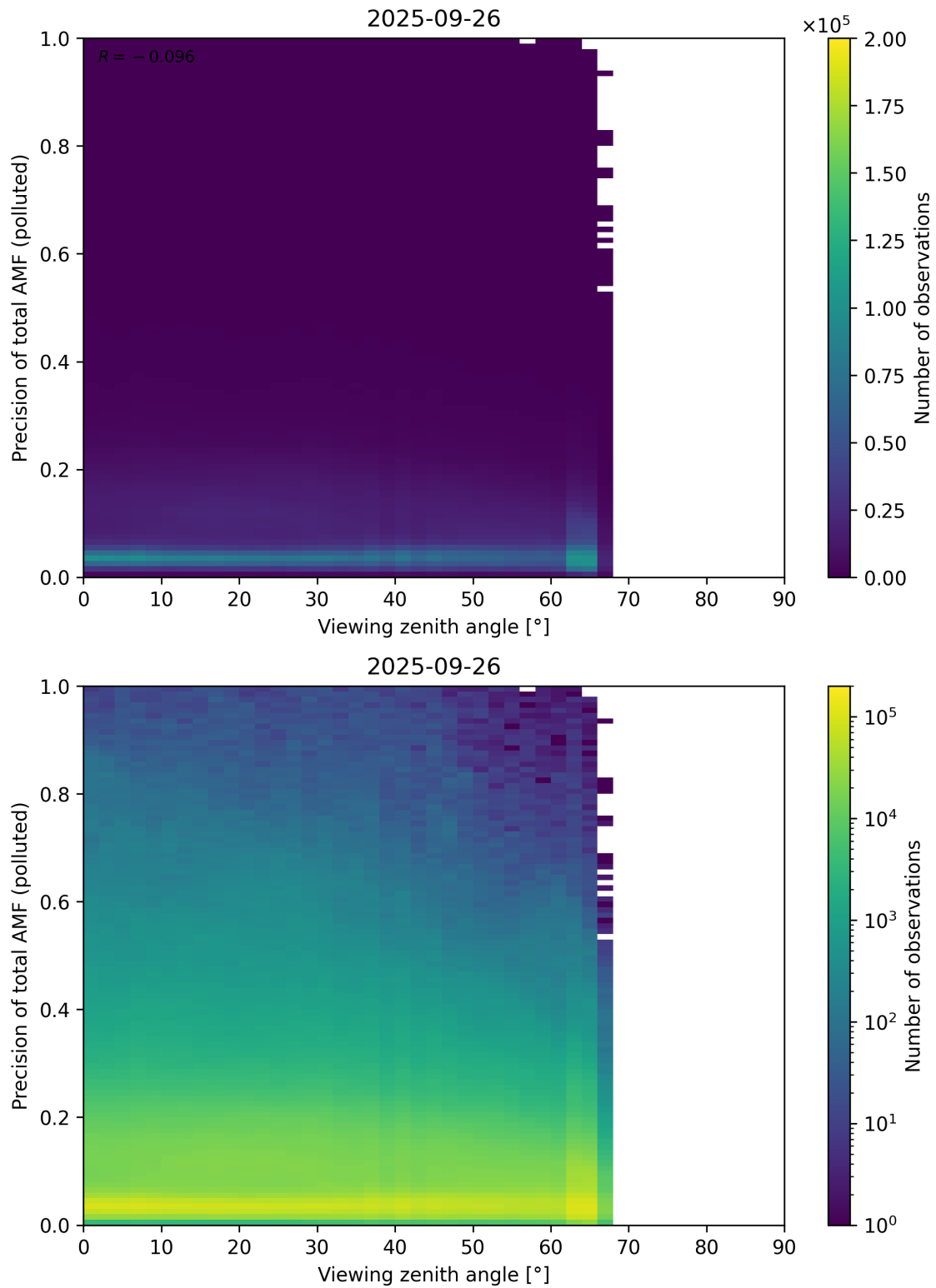
Figure 382: Scatter density plot of “Viewing zenith angle” against “Precision of total AMF (polluted)” for 2025-09-26 to 2025-09-27.
