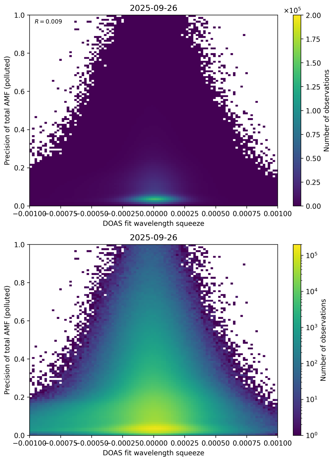
Figure 146: Scatter density plot of “DOAS fit wavelength squeeze” against “Precision of total AMF (polluted)” for 2025-09-26 to 2025-09-27.
