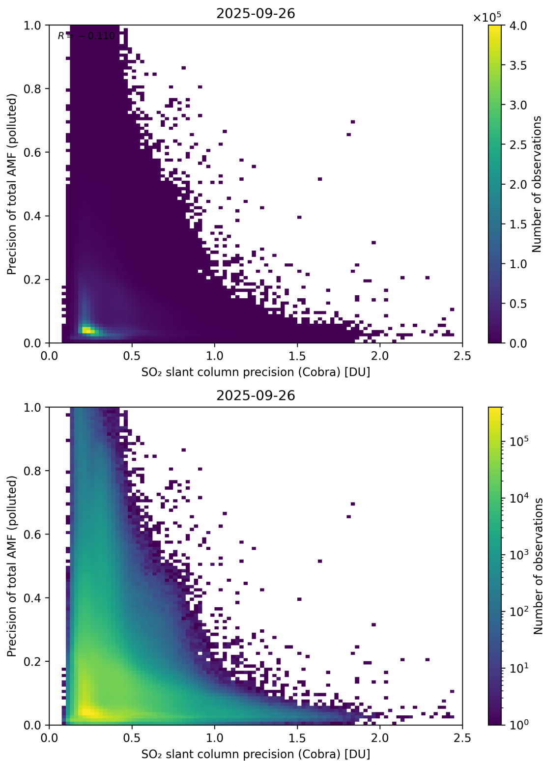
Figure 214: Scatter density plot of “SO 2 slant column precision (Cobra)” against “Precision of total AMF (polluted)” for 2025-09-26 to 2025-09-27.
