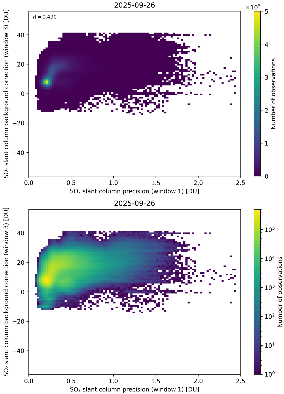
Figure 270: Scatter density plot of “SO 2 slant column precision (window 1)” against “SO 2 slant column background correction (window 3)” for 2025-09-26 to 2025-09-27.
