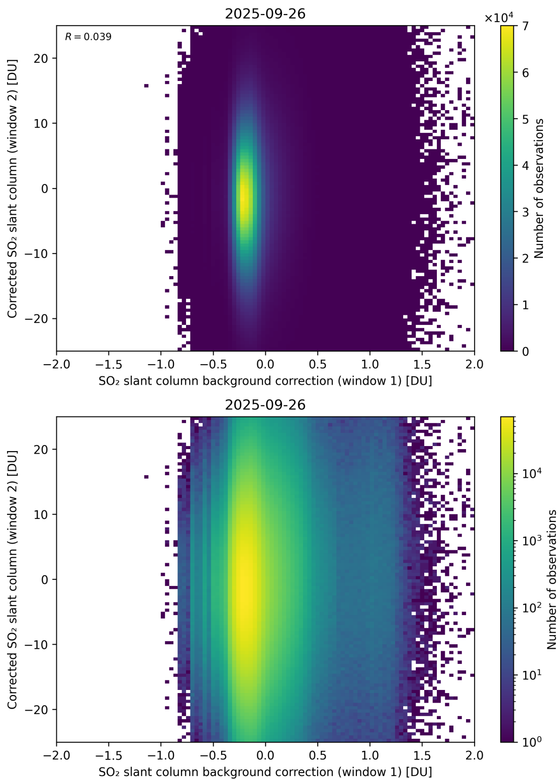
Figure 115: Scatter density plot of “SO 2 slant column background correction (window 1)” against “Corrected SO 2 slant column (window 2)” for 2025-09-26 to 2025-09-27.
