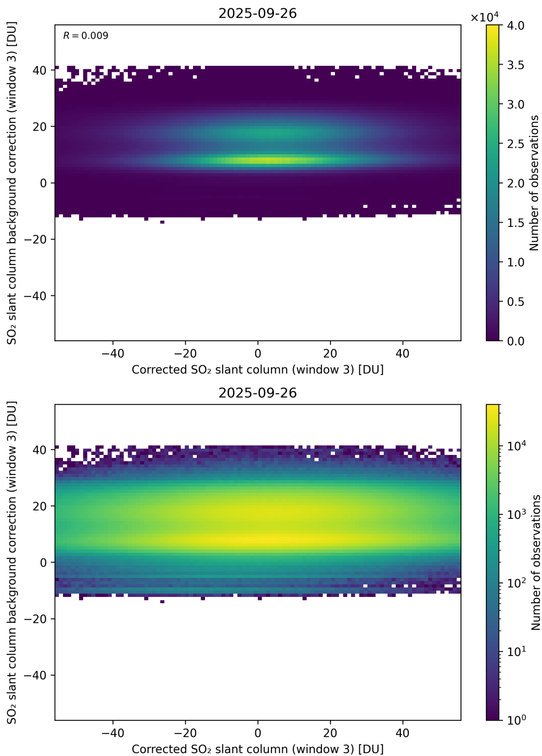
Figure 255: Scatter density plot of “Corrected SO 2 slant column (window 3)” against “SO 2 slant column background correction (window 3)” for 2025-09-26 to 2025-09-27.
