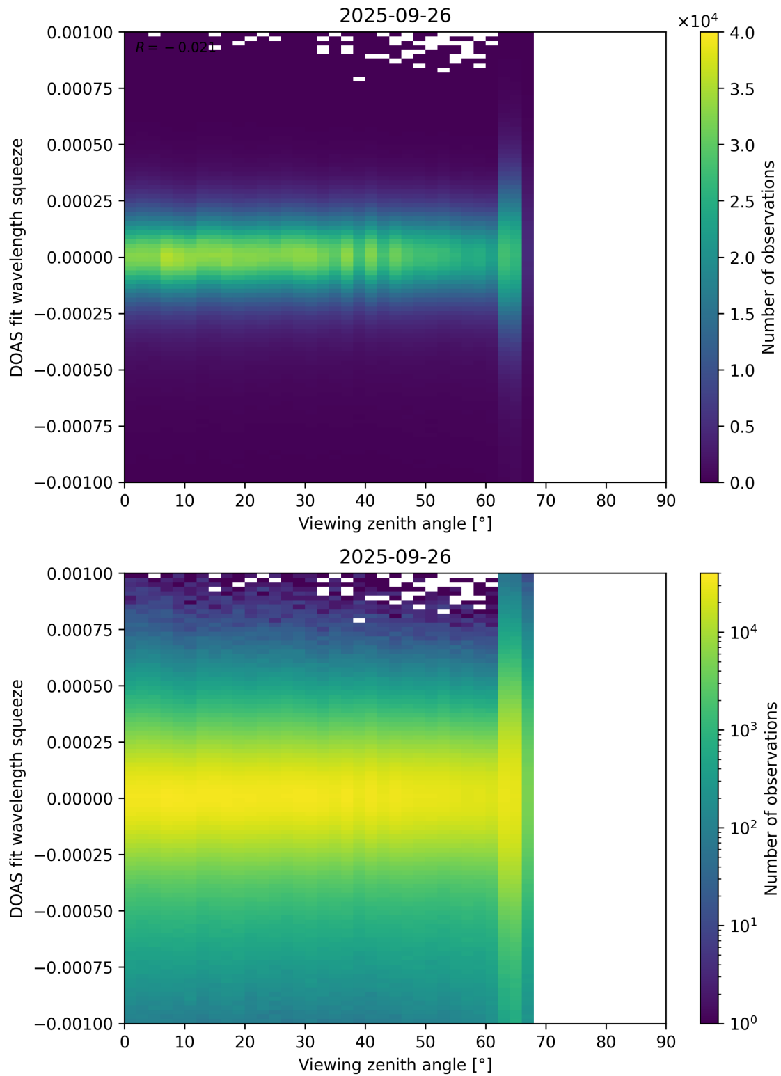
Figure 366: Scatter density plot of “Viewing zenith angle” against “DOAS fit wavelength squeeze” for 2025-09-26 to 2025-09-27.
