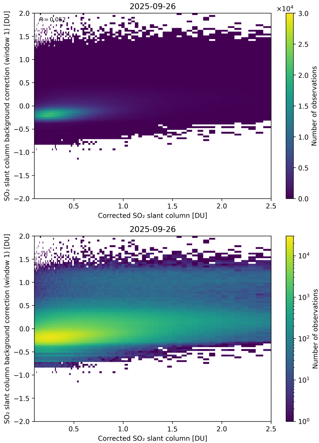
Figure 226: Scatter density plot of “Corrected SO 2 slant column” against “SO 2 slant column background correction (window 1)” for 2025-09-26 to 2025-09-27.
