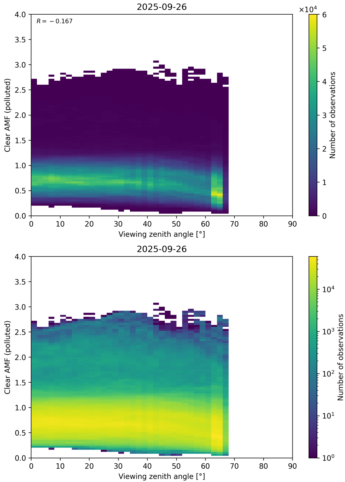
Figure 370: Scatter density plot of “Viewing zenith angle” against “Clear AMF (polluted)” for 2025-09-26 to 2025-09-27.
