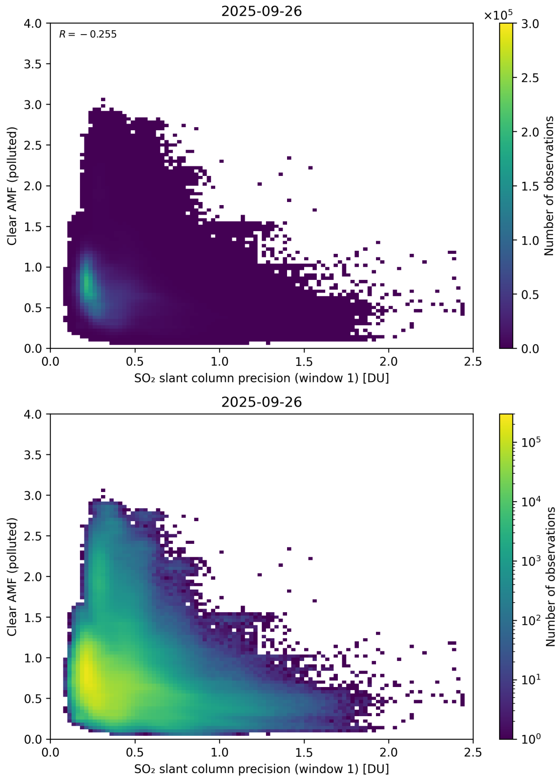
Figure 274: Scatter density plot of “SO 2 slant column precision (window 1)” against “Clear AMF (polluted)” for 2025-09-26 to 2025-09-27.
