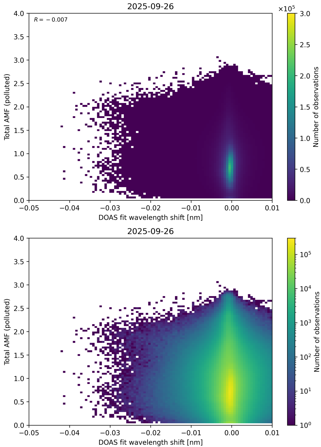
Figure 141: Scatter density plot of “DOAS fit wavelength shift” against “Total AMF (polluted)” for 2025-09-26 to 2025-09-27.
