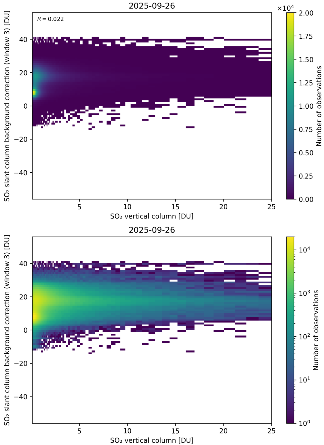
Figure 325: Scatter density plot of “SO 2 vertical column” against “SO 2 slant column background correction (window 3)” for 2025-09-26 to 2025-09-27.
