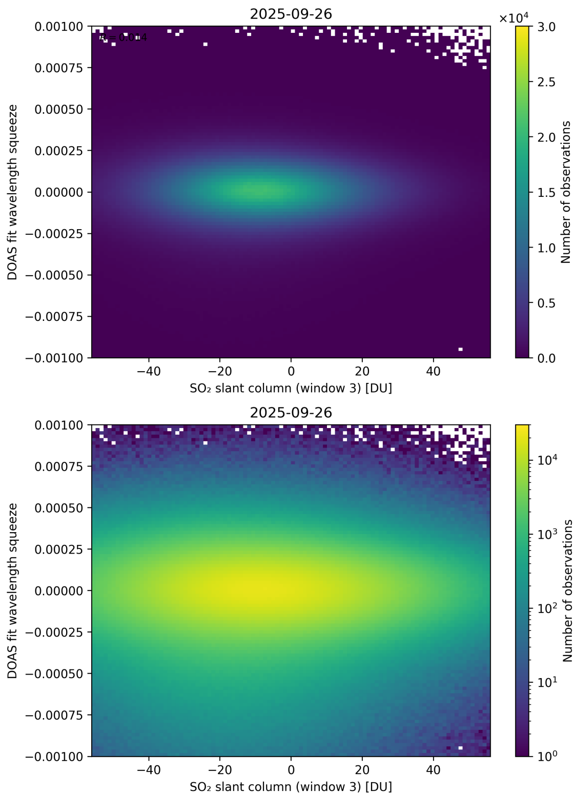
Figure 305: Scatter density plot of “SO 2 slant column (window 3)” against “DOAS fit wavelength squeeze” for 2025-09-26 to 2025-09-27.
