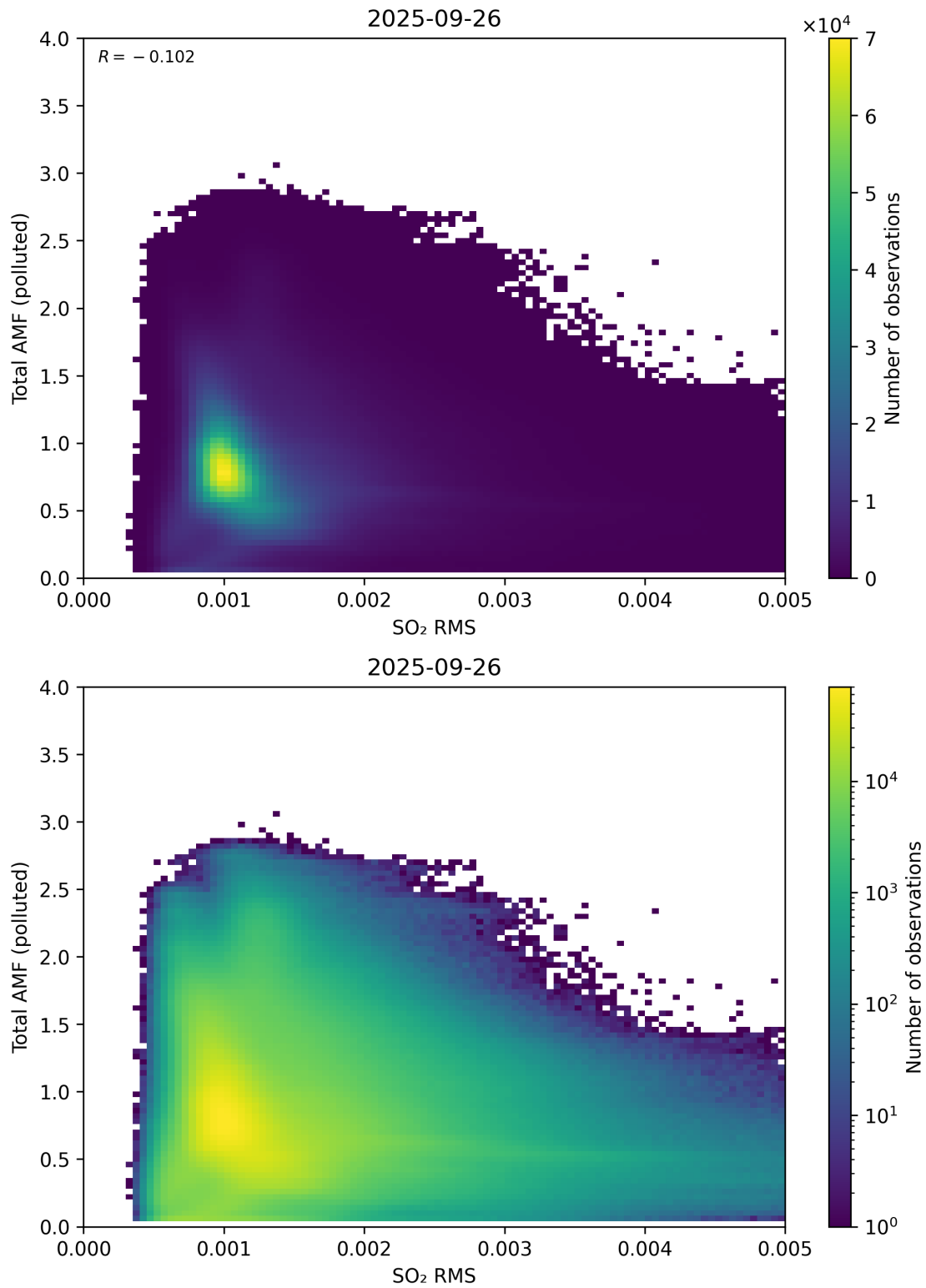
Figure 148: Scatter density plot of “SO 2 RMS” against “Total AMF (polluted)” for 2025-09-26 to 2025-09-27.
