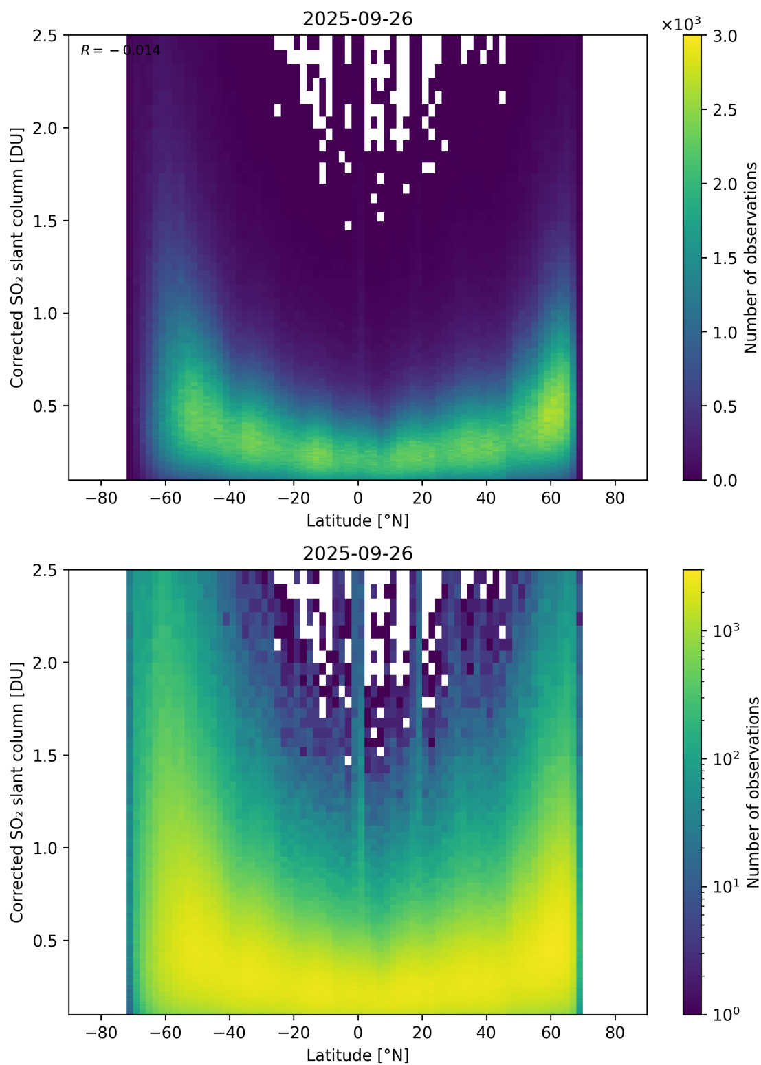
Figure 159: Scatter density plot of “Latitude” against “Corrected SO 2 slant column” for 2025-09-26 to 2025-09-27.
