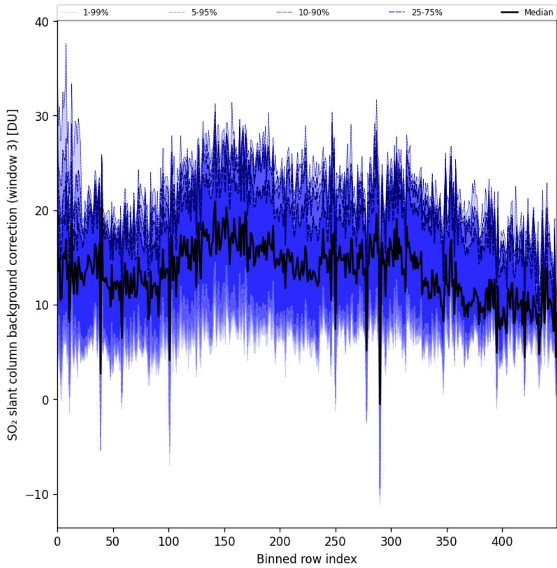
Figure 100: Along track statistics of “SO 2 slant column background correction (window 3)” for 2025-09-26 to 2025-09-27
