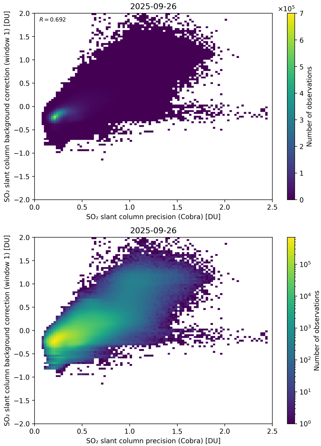
Figure 199: Scatter density plot of “SO 2 slant column precision (Cobra)” against “SO 2 slant column background correction (window 1)” for 2025-09-26 to 2025-09-27.
