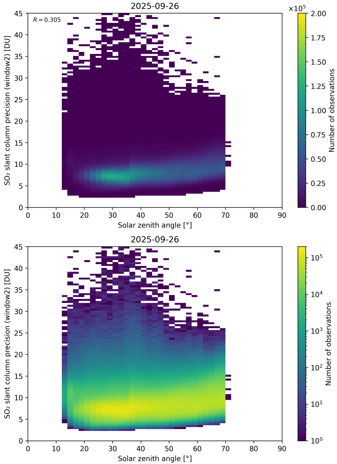
Figure 186: Scatter density plot of “Solar zenith angle” against “SO 2 slant column precision (window2)” for 2025-09-26 to 2025-09-27.
