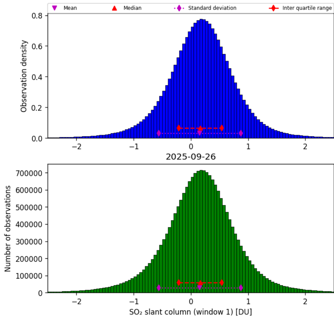
Figure 63: Histogram of “SO 2 slant column (window 1)” for 2025-09-26 to 2025-09-27
