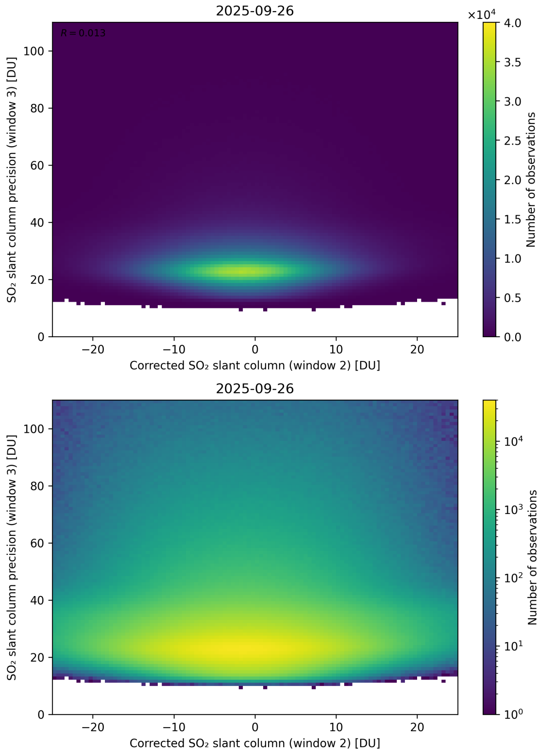
Figure 252: Scatter density plot of “Corrected SO 2 slant column (window 2)” against “SO 2 slant column precision (window 3)” for 2025-09-26 to 2025-09-27.
