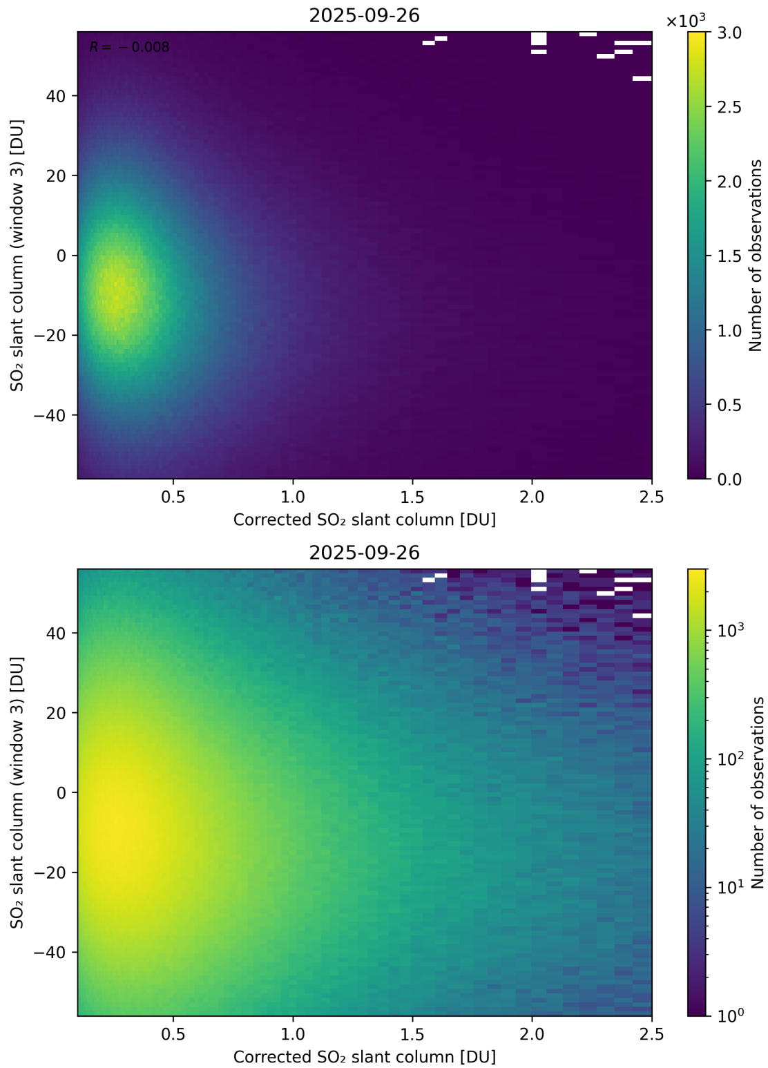
Figure 240: Scatter density plot of “Corrected SO 2 slant column” against “SO 2 slant column (window 3)” for 2025-09-26 to 2025-09-27.
