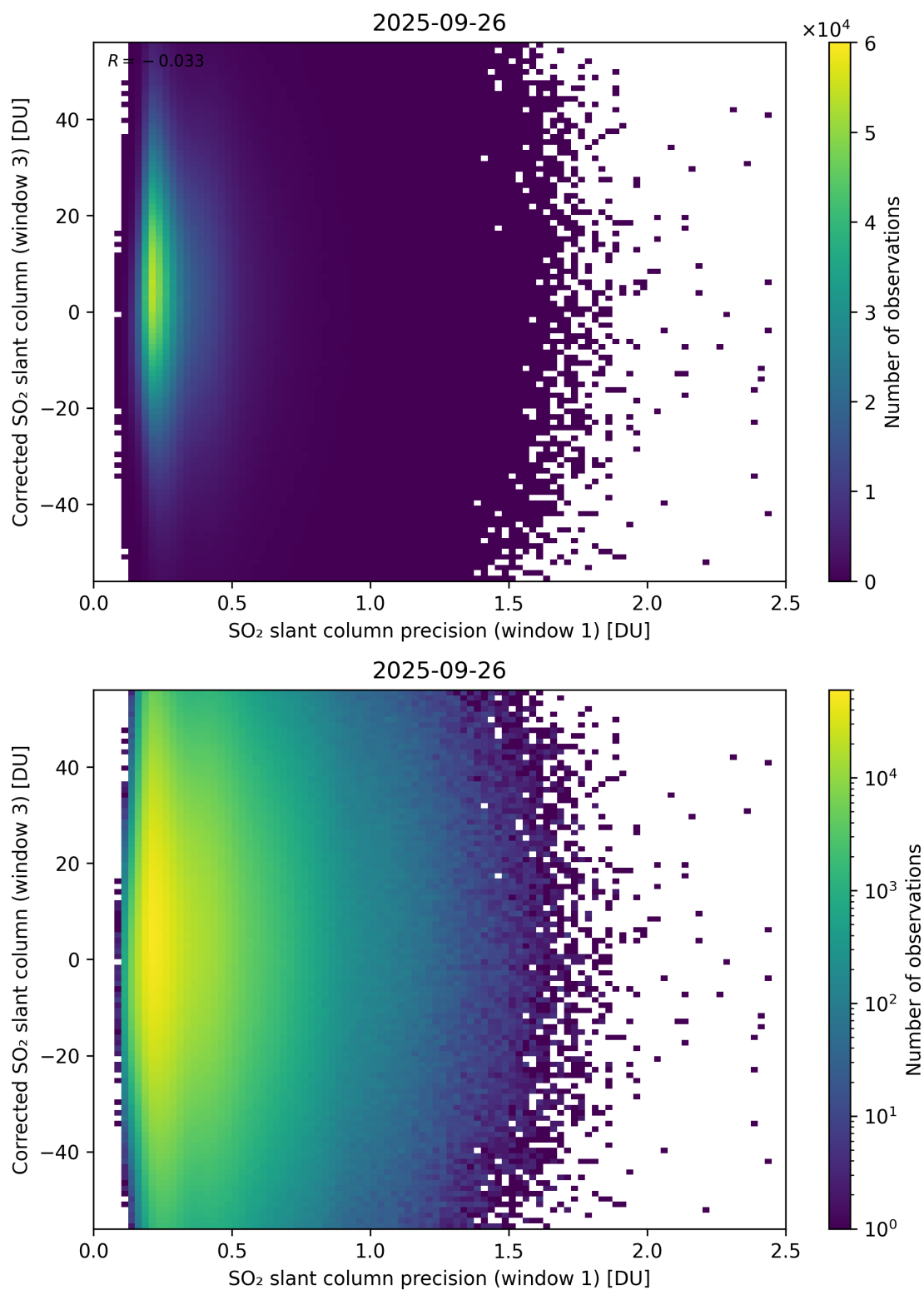
Figure 276: Scatter density plot of “SO 2 slant column precision (window 1)” against “Corrected SO 2 slant column (window 3)” for 2025-09-26 to 2025-09-27.
