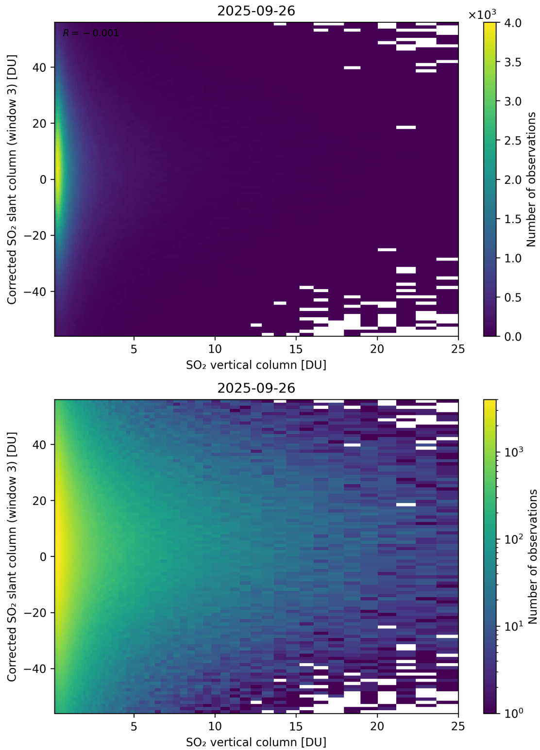
Figure 353: Scatter density plot of “SO 2 vertical column” against “Corrected SO 2 slant column (window 3)” for 2025-09-26 to 2025-09-27.
