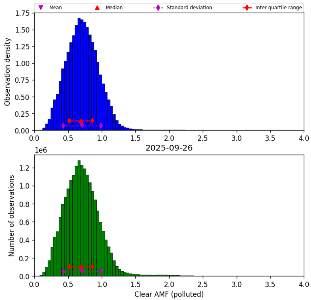
Figure 81: Histogram of “Clear AMF (polluted)” for 2025-09-26 to 2025-09-27
