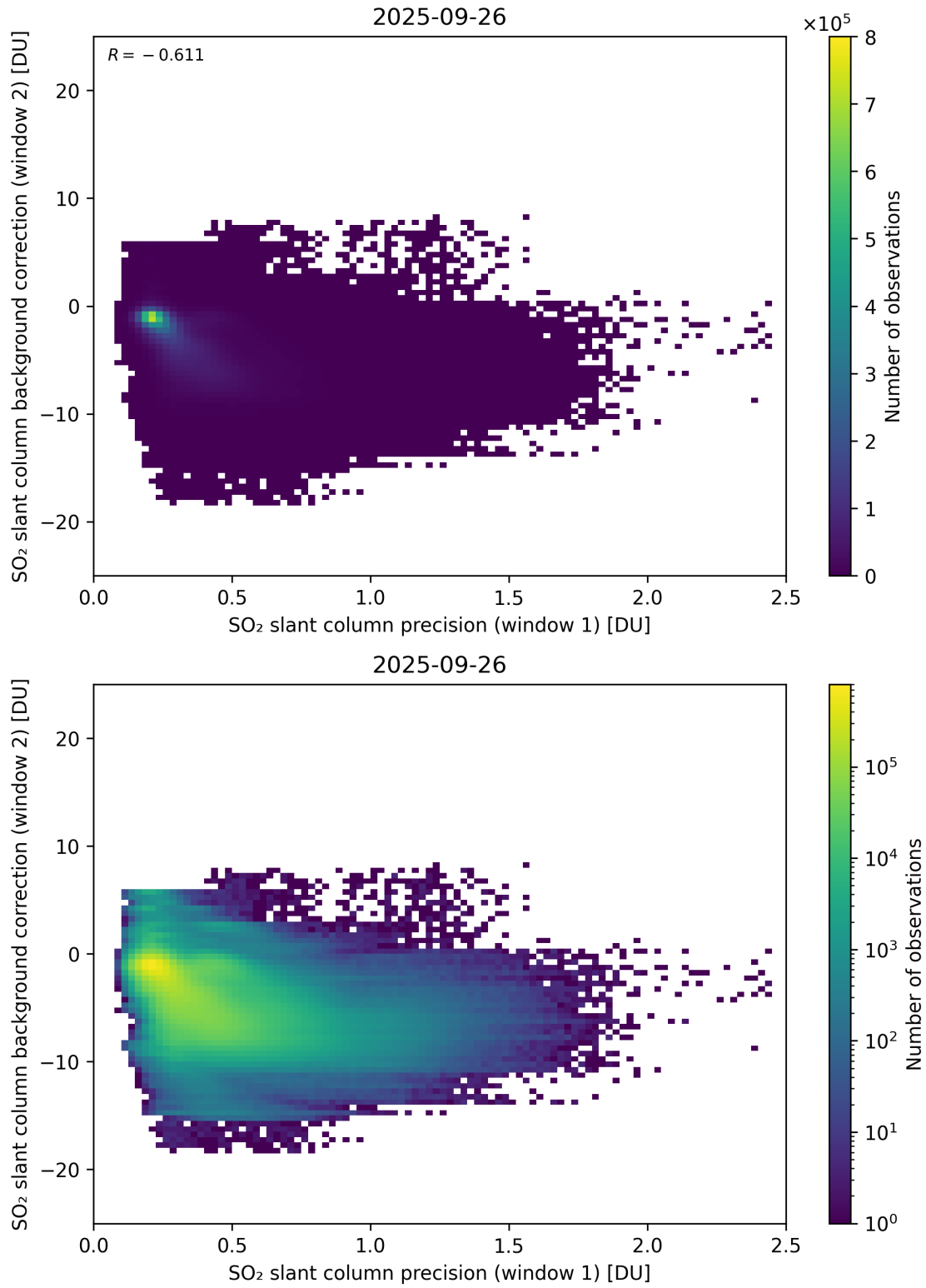
Figure 269: Scatter density plot of “SO 2 slant column precision (window 1)” against “SO 2 slant column background correction (window 2)” for 2025-09-26 to 2025-09-27.
