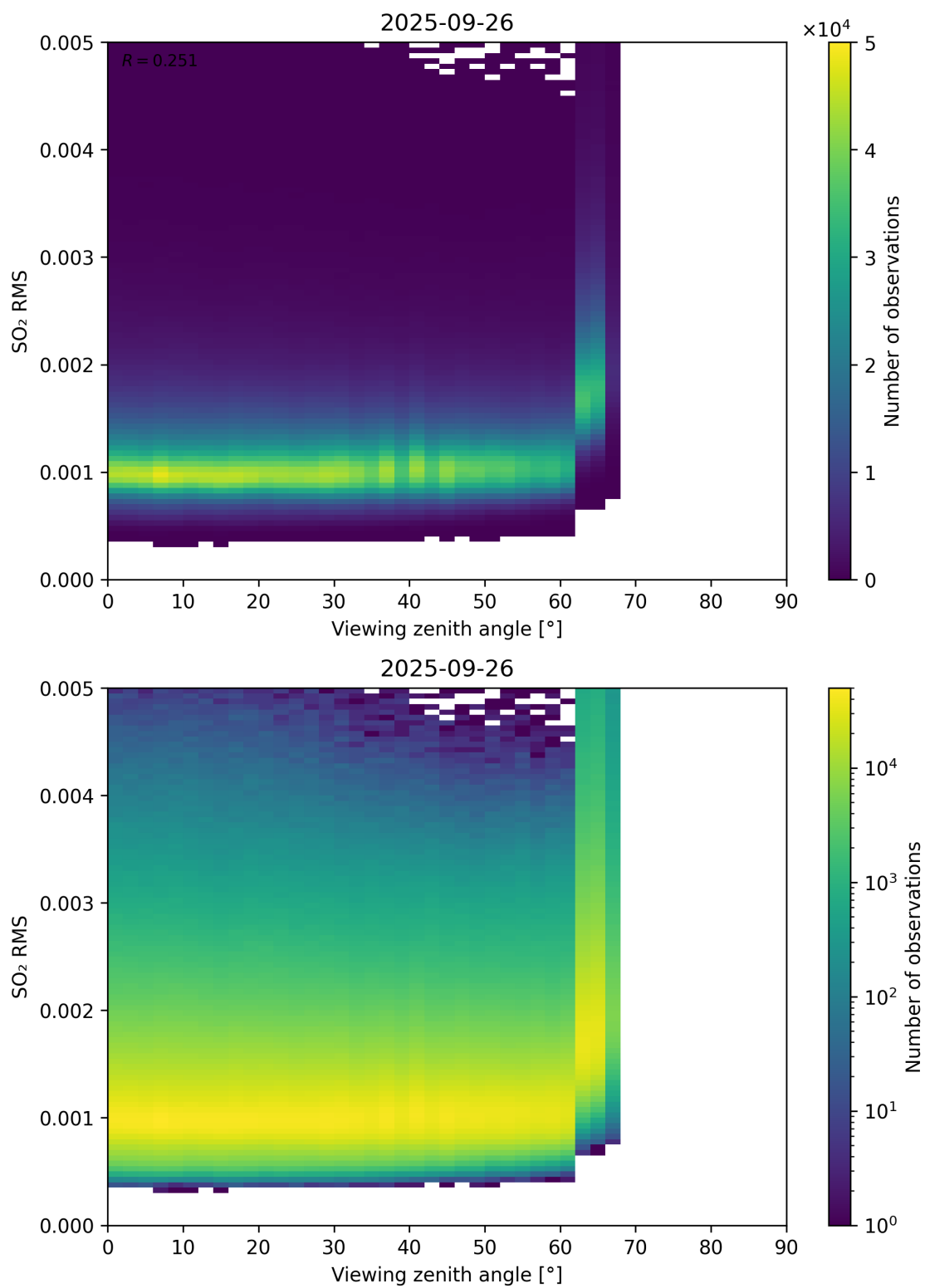
Figure 367: Scatter density plot of “Viewing zenith angle” against “SO 2 RMS” for 2025-09-26 to 2025-09-27.
