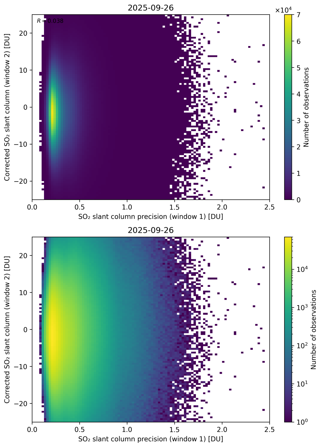
Figure 275: Scatter density plot of “SO 2 slant column precision (window 1)” against “Corrected SO 2 slant column (window 2)” for 2025-09-26 to 2025-09-27.
