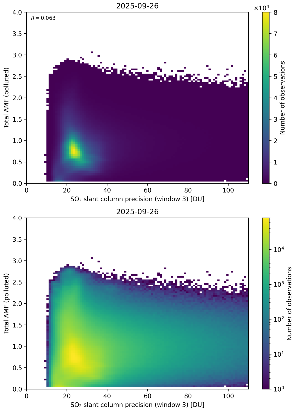
Figure 313: Scatter density plot of “SO 2 slant column precision (window 3)” against “Total AMF (polluted)” for 2025-09-26 to 2025-09-27.
