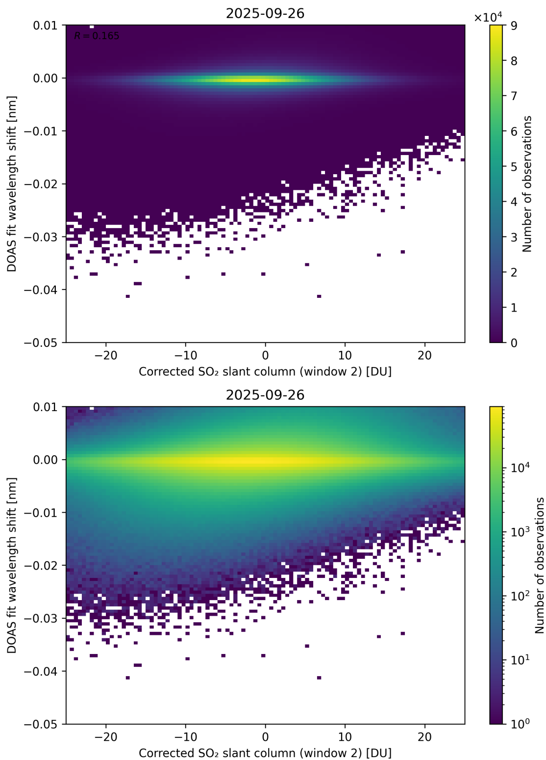
Figure 246: Scatter density plot of “Corrected SO 2 slant column (window 2)” against “DOAS fit wavelength shift” for 2025-09-26 to 2025-09-27.
