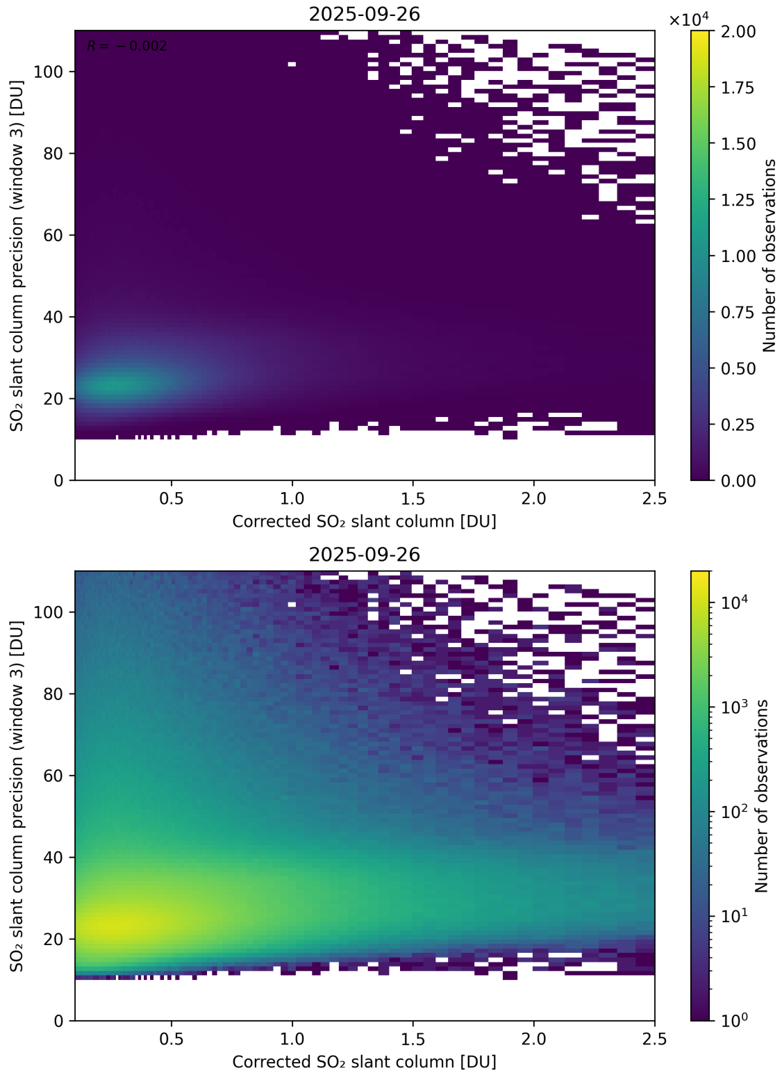
Figure 241: Scatter density plot of “Corrected SO 2 slant column” against “SO 2 slant column precision (window 3)” for 2025-09-26 to 2025-09-27.
