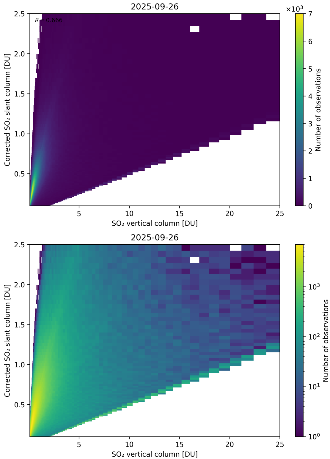
Figure 351: Scatter density plot of “SO 2 vertical column” against “Corrected SO 2 slant column” for 2025-09-26 to 2025-09-27.
