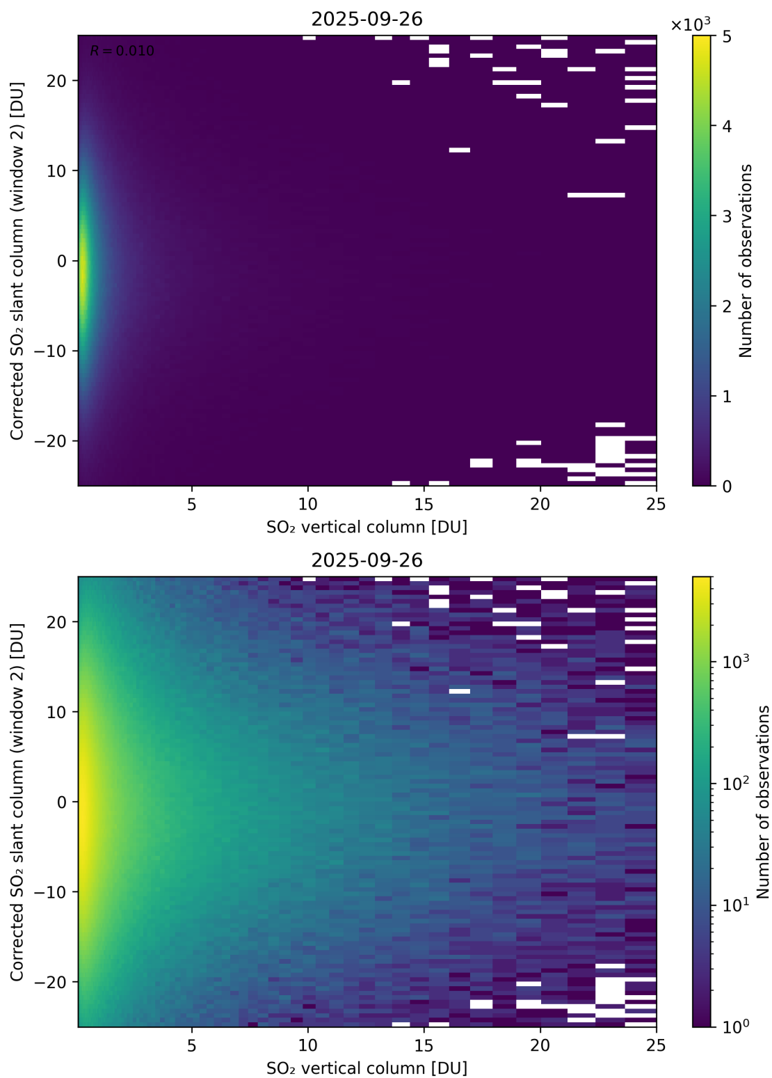
Figure 352: Scatter density plot of “SO 2 vertical column” against “Corrected SO 2 slant column (window 2)” for 2025-09-26 to 2025-09-27.
