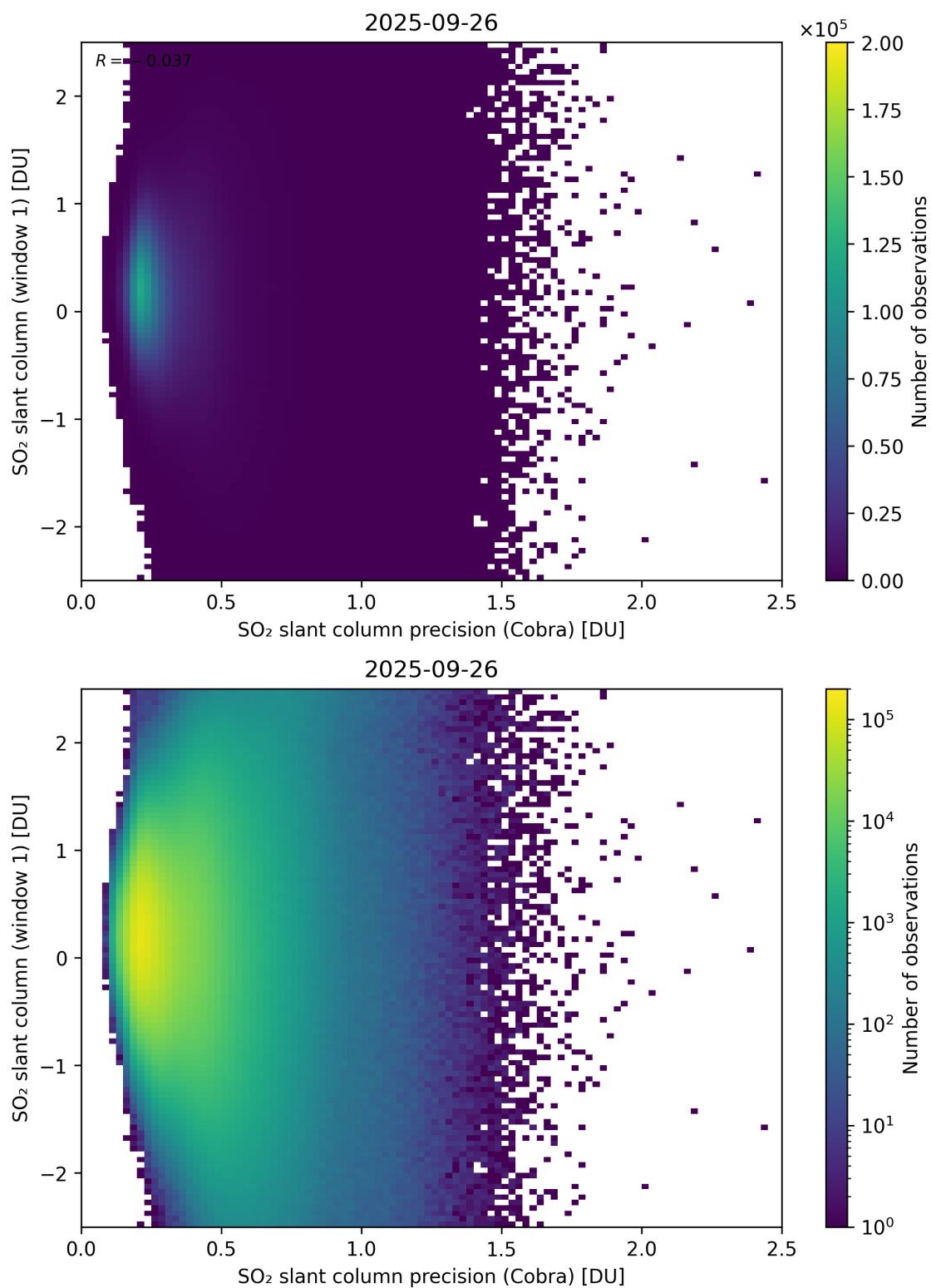
Figure 208: Scatter density plot of “SO 2 slant column precision (Cobra)” against “SO 2 slant column (window 1)” for 2025-09-26 to 2025-09-27.
