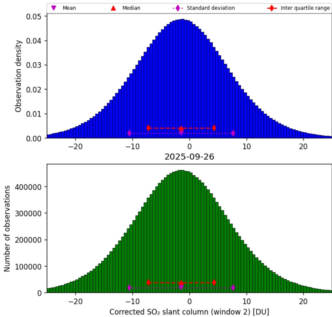
Figure 69: Histogram of “Corrected SO 2 slant column (window 2)” for 2025-09-26 to 2025-09-27
