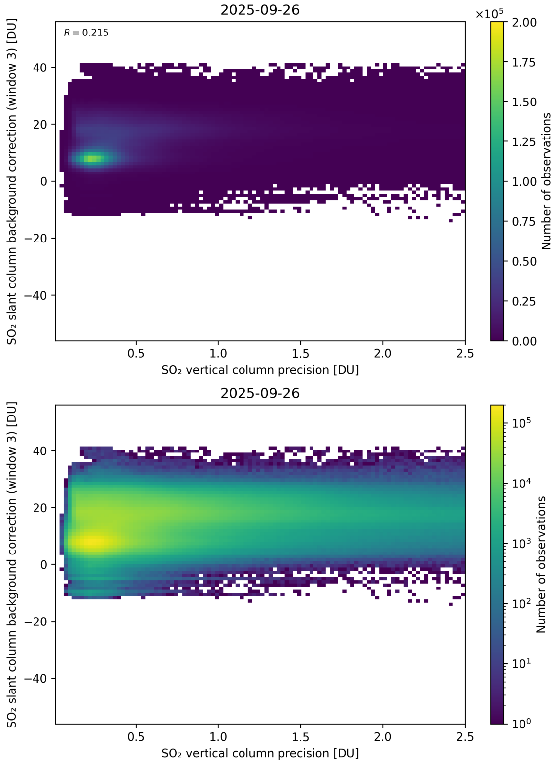
Figure 331: Scatter density plot of “SO 2 vertical column precision” against “SO 2 slant column background correction (window 3)” for 2025-09-26 to 2025-09-27.
