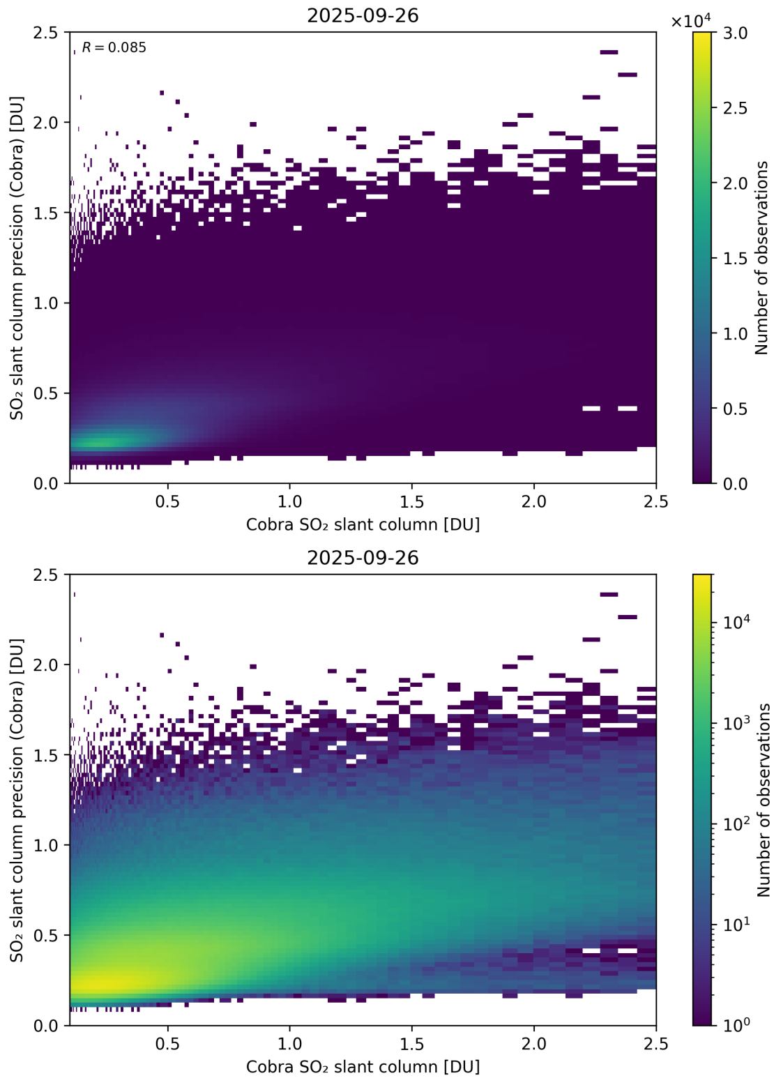
Figure 216: Scatter density plot of “Cobra SO 2 slant column” against “SO 2 slant column precision (Cobra)” for 2025-09-26 to 2025-09-27.
