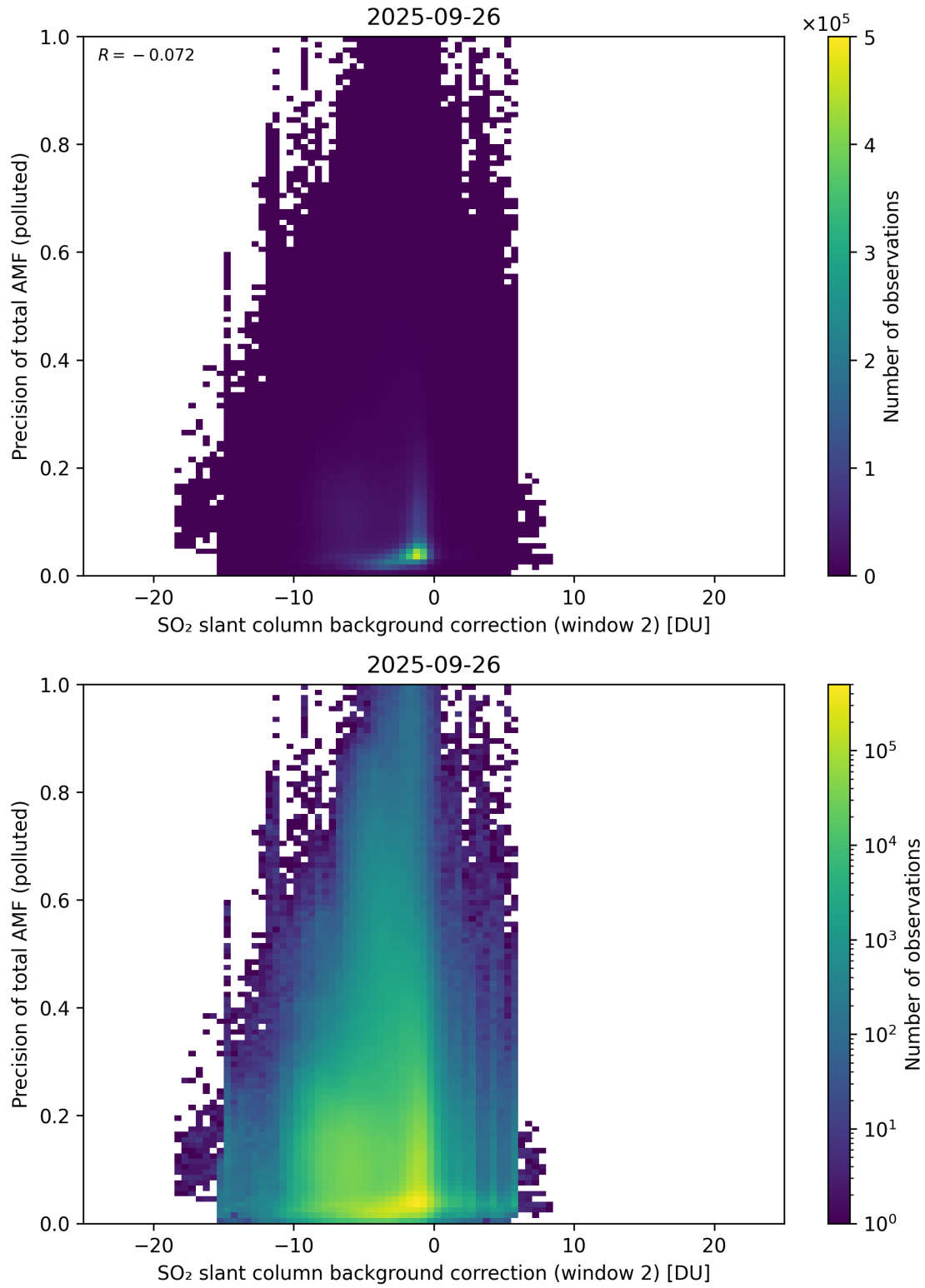
Figure 131: Scatter density plot of “SO 2 slant column background correction (window 2)” against “Precision of total AMF (polluted)” for 2025-09-26 to 2025-09-27.
