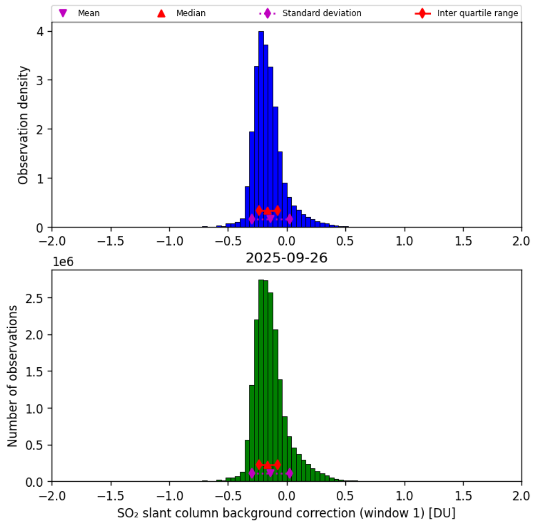
Figure 66: Histogram of “SO 2 slant column background correction (window 1)” for 2025-09-26 to 2025-09-27
