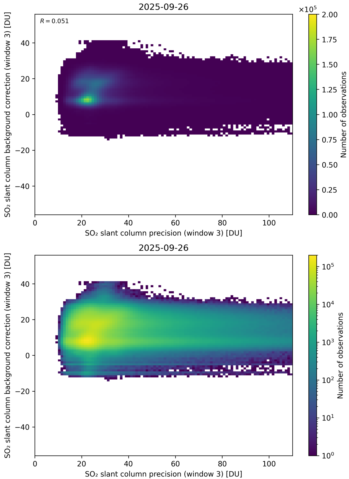
Figure 307: Scatter density plot of “SO 2 slant column precision (window 3)” against “SO 2 slant column background correction (window 3)” for 2025-09-26 to 2025-09-27.
