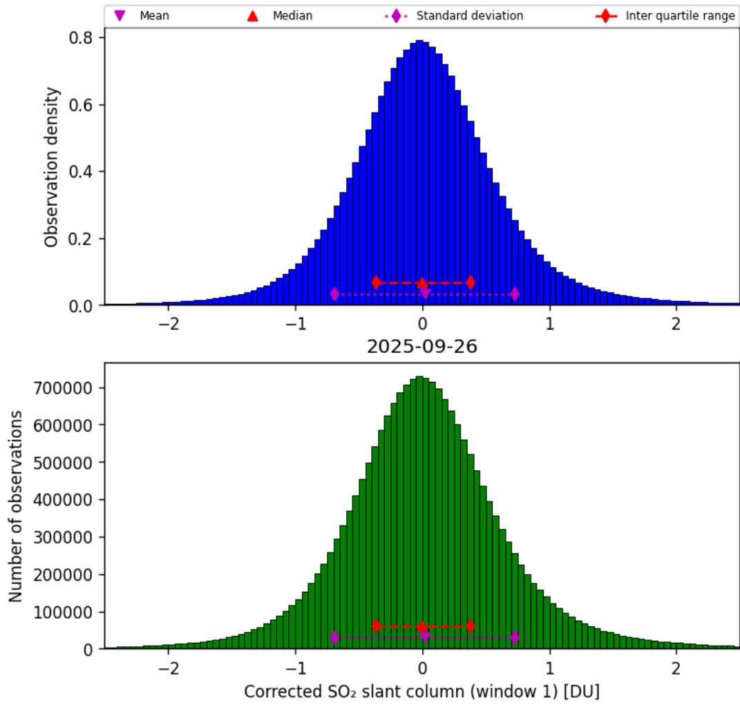
Figure 65: Histogram of “Corrected SO 2 slant column (window 1)” for 2025-09-26 to 2025-09-27
