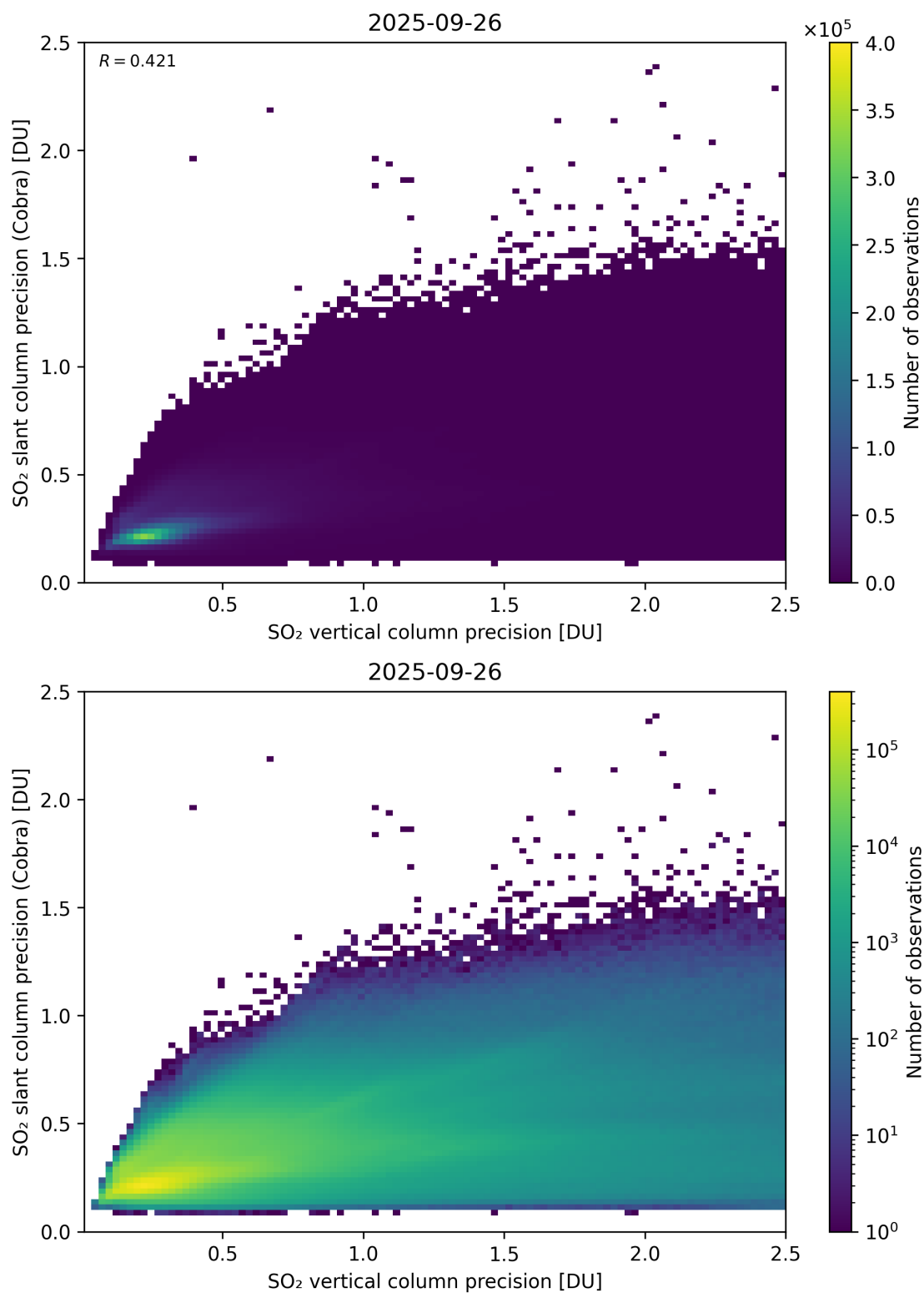
Figure 337: Scatter density plot of “SO 2 vertical column precision” against “SO 2 slant column precision (Cobra)” for 2025-09-26 to 2025-09-27.
