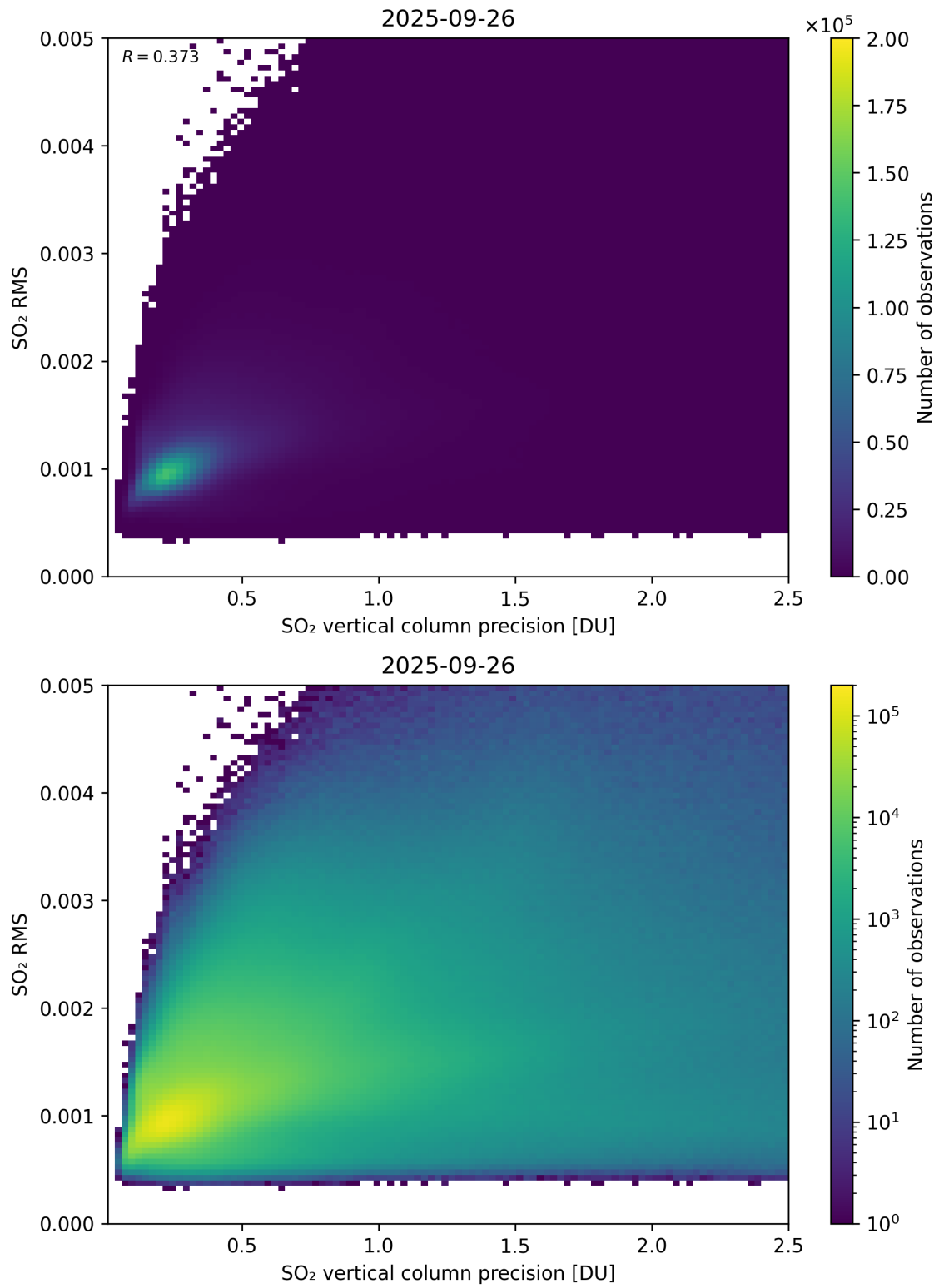
Figure 334: Scatter density plot of “SO 2 vertical column precision” against “SO 2 RMS” for 2025-09-26 to 2025-09-27.
