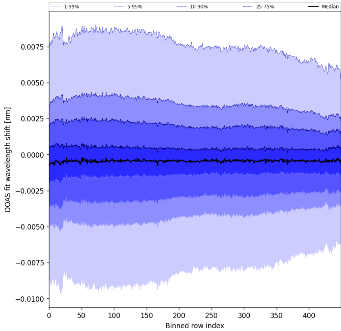
Figure 102: Along track statistics of “DOAS fit wavelength shift” for 2025-09-26 to 2025-09-27
