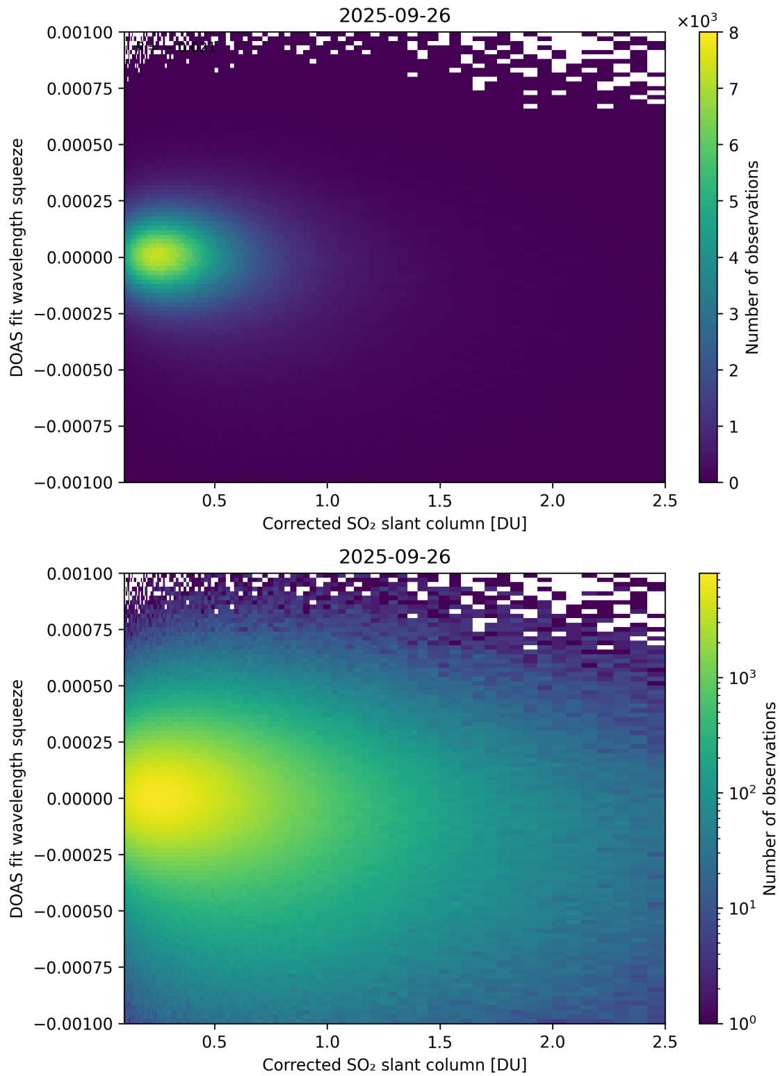
Figure 230: Scatter density plot of "Corrected SO 2 slant column" against "DOAS fit wavelength squeeze" for 2025-09-26 to 2025-09-27.
