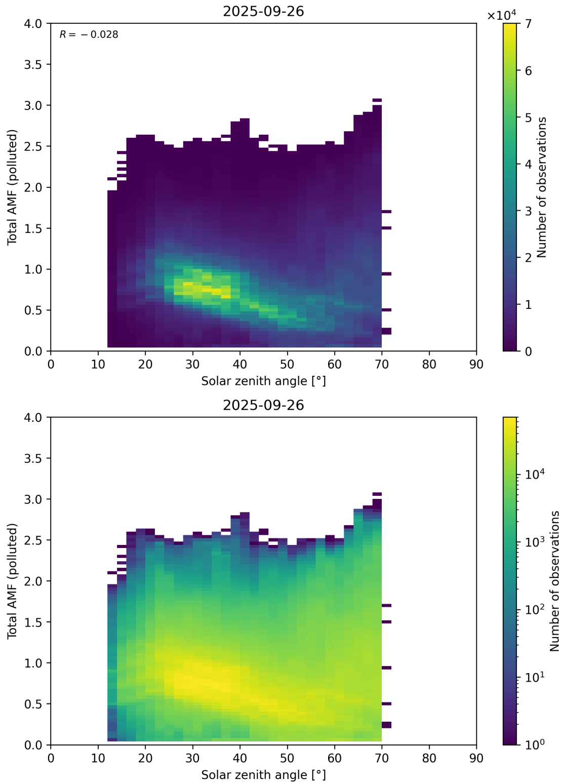
Figure 189: Scatter density plot of “Solar zenith angle” against “Total AMF (polluted)” for 2025-09-26 to 2025-09-27.
