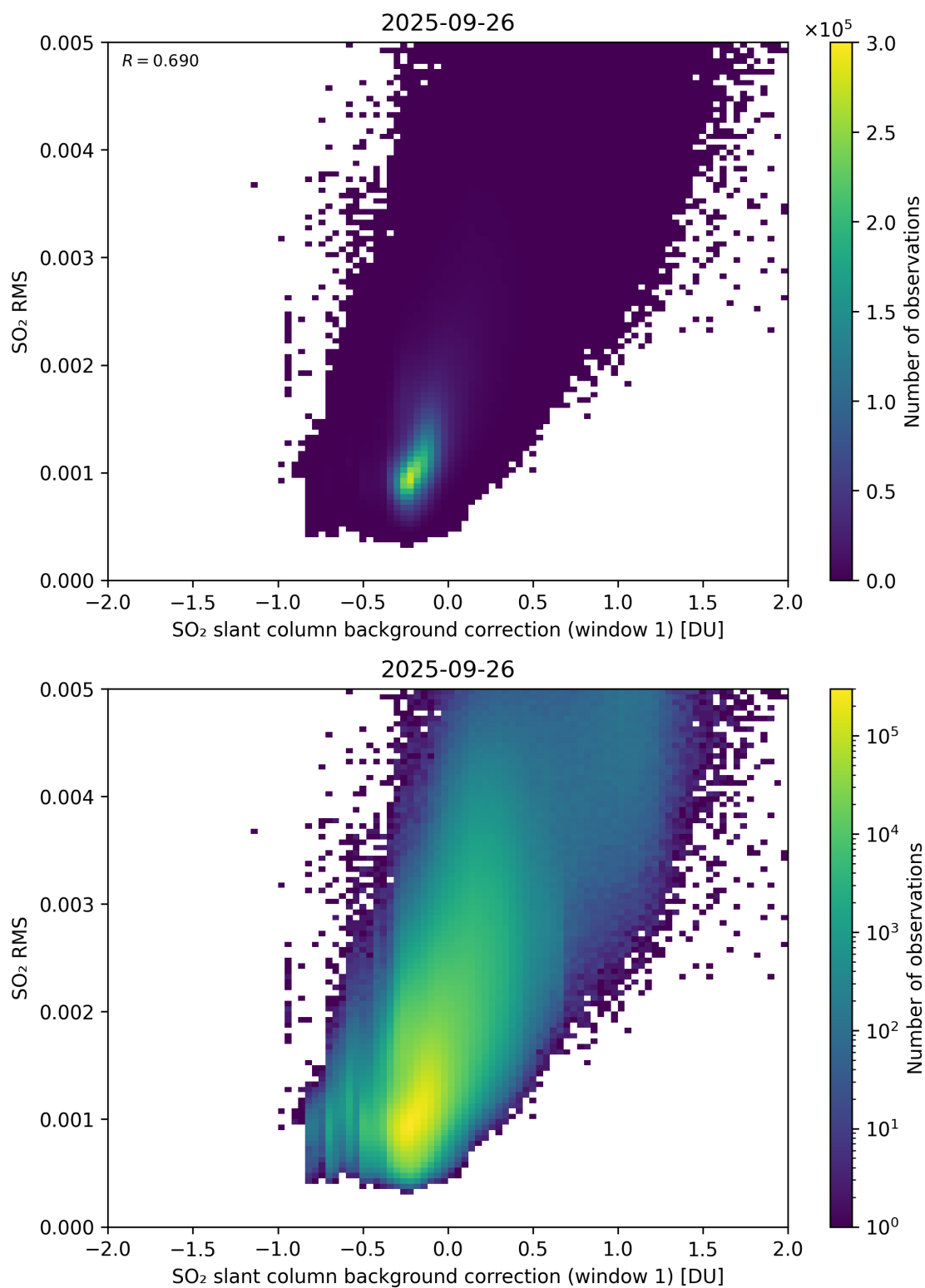
Figure 113: Scatter density plot of “SO 2 slant column background correction (window 1)” against “SO 2 RMS” for 2025-09-26 to 2025-09-27.
