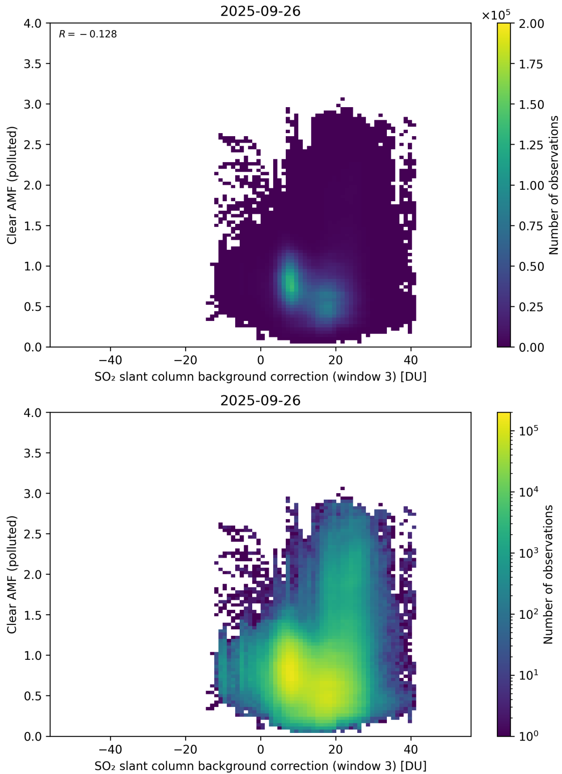
Figure 135: Scatter density plot of “SO 2 slant column background correction (window 3)” against “Clear AMF (polluted)” for 2025-09-26 to 2025-09-27.
