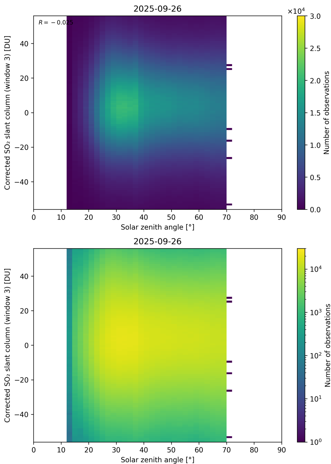
Figure 183: Scatter density plot of “Solar zenith angle” against “Corrected SO 2 slant column (window 3)” for 2025-09-26 to 2025-09-27.
