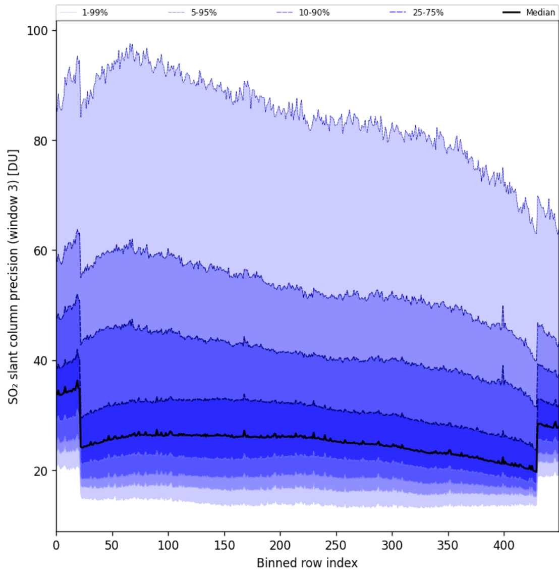
Figure 98: Along track statistics of “SO 2 slant column precision (window 3)” for 2025-09-26 to 2025-09-27
