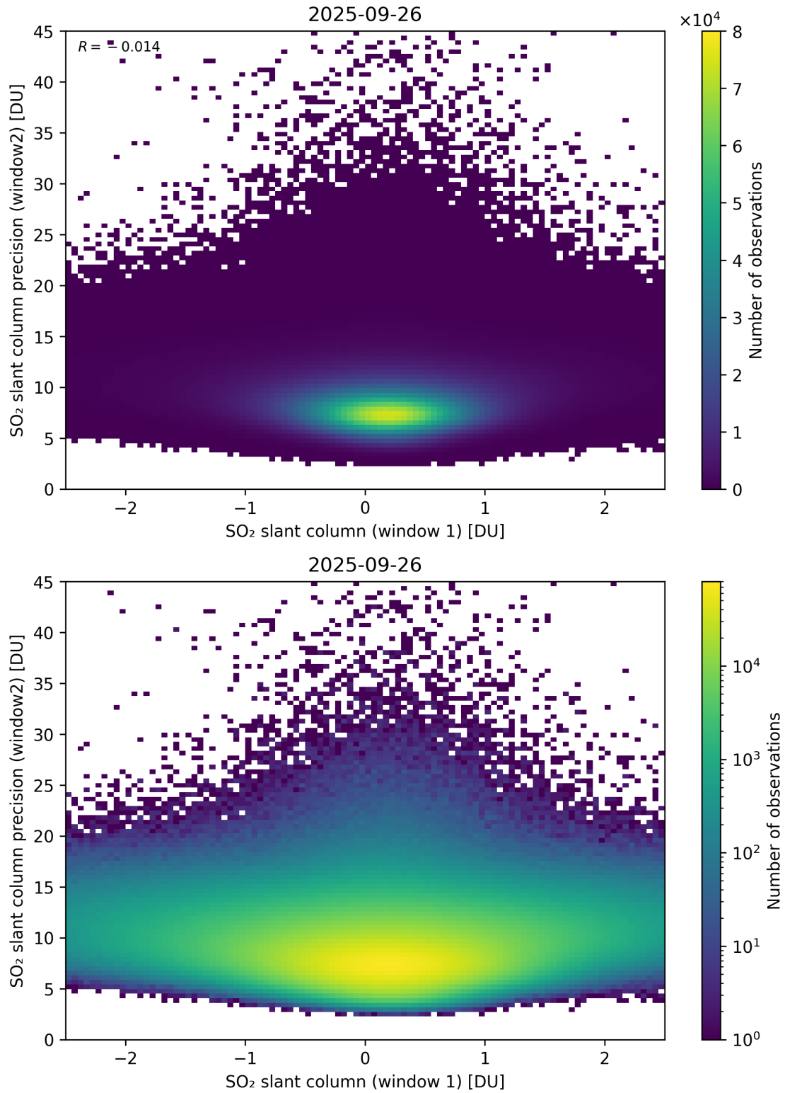
Figure 286: Scatter density plot of “SO 2 slant column (window 1)” against “SO 2 slant column precision (window2)” for 2025-09-26 to 2025-09-27.
