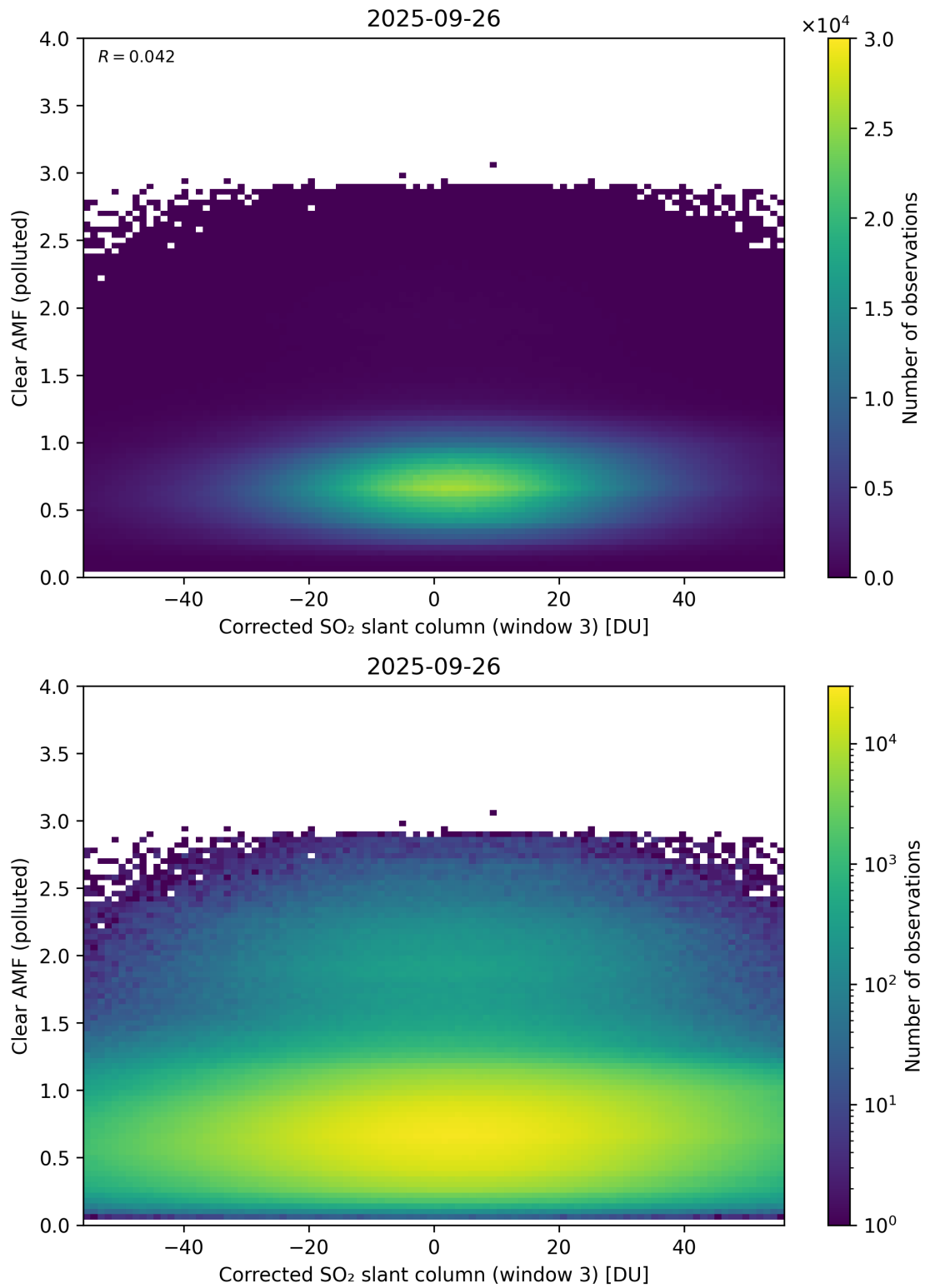
Figure 259: Scatter density plot of “Corrected SO 2 slant column (window 3)” against “Clear AMF (polluted)” for 2025-09-26 to 2025-09-27.
