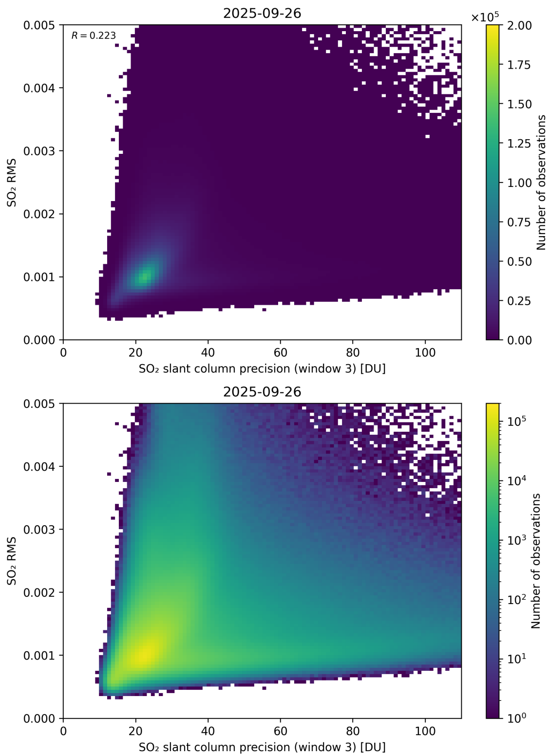
Figure 310: Scatter density plot of “SO 2 slant column precision (window 3)” against “SO 2 RMS” for 2025-09-26 to 2025-09-27.
