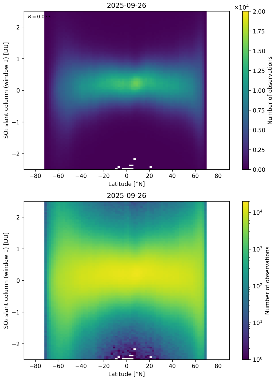
Figure 162: Scatter density plot of “Latitude” against “SO 2 slant column (window 1)” for 2025-09-26 to 2025-09-27.
