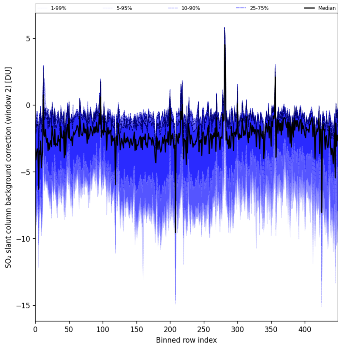
Figure 96: Along track statistics of “SO 2 slant column background correction (window 2)” for 2025-09-26 to 2025-09-27
