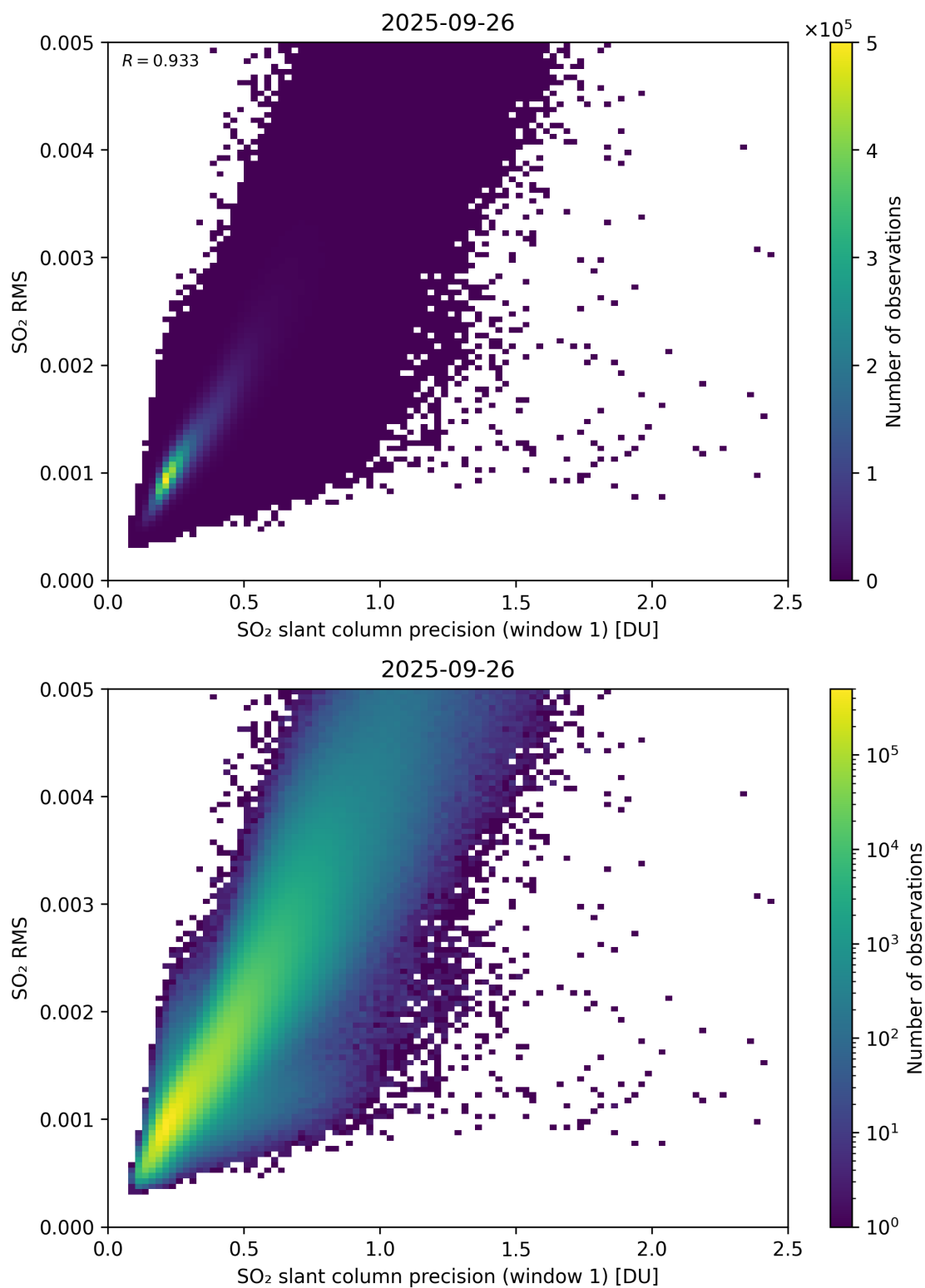
Figure 273: Scatter density plot of “SO 2 slant column precision (window 1)” against “SO 2 RMS” for 2025-09-26 to 2025-09-27.
