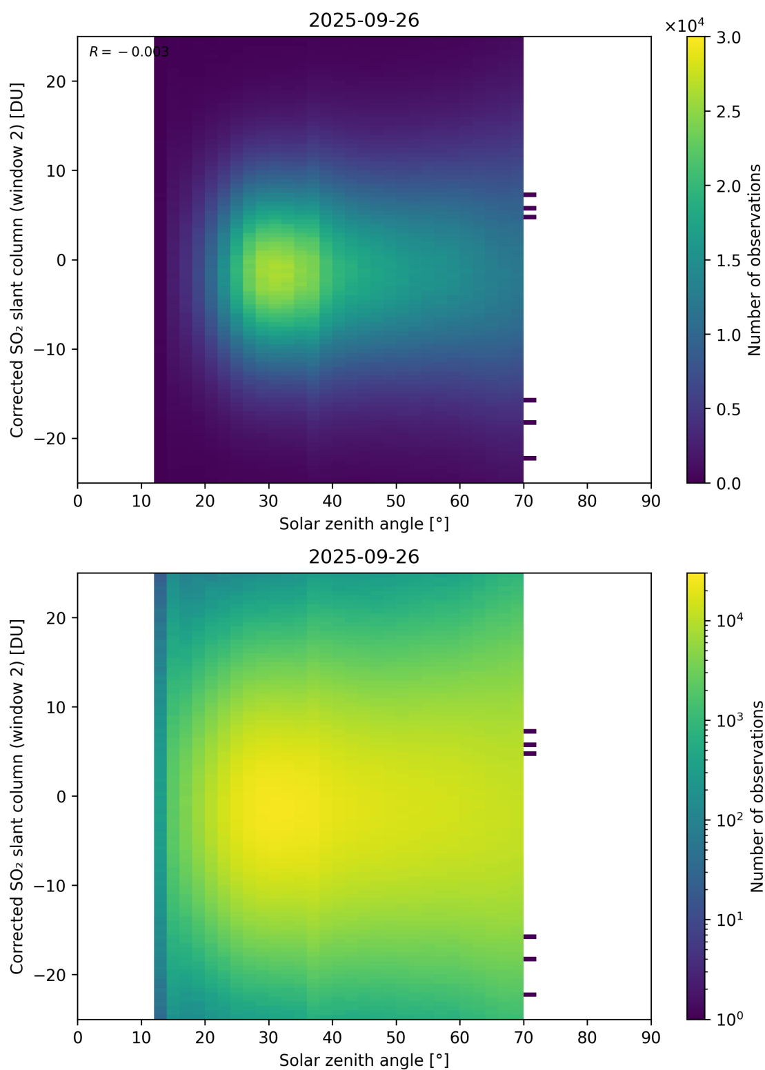
Figure 182: Scatter density plot of “Solar zenith angle” against “Corrected SO 2 slant column (window 2)” for 2025-09-26 to 2025-09-27.
