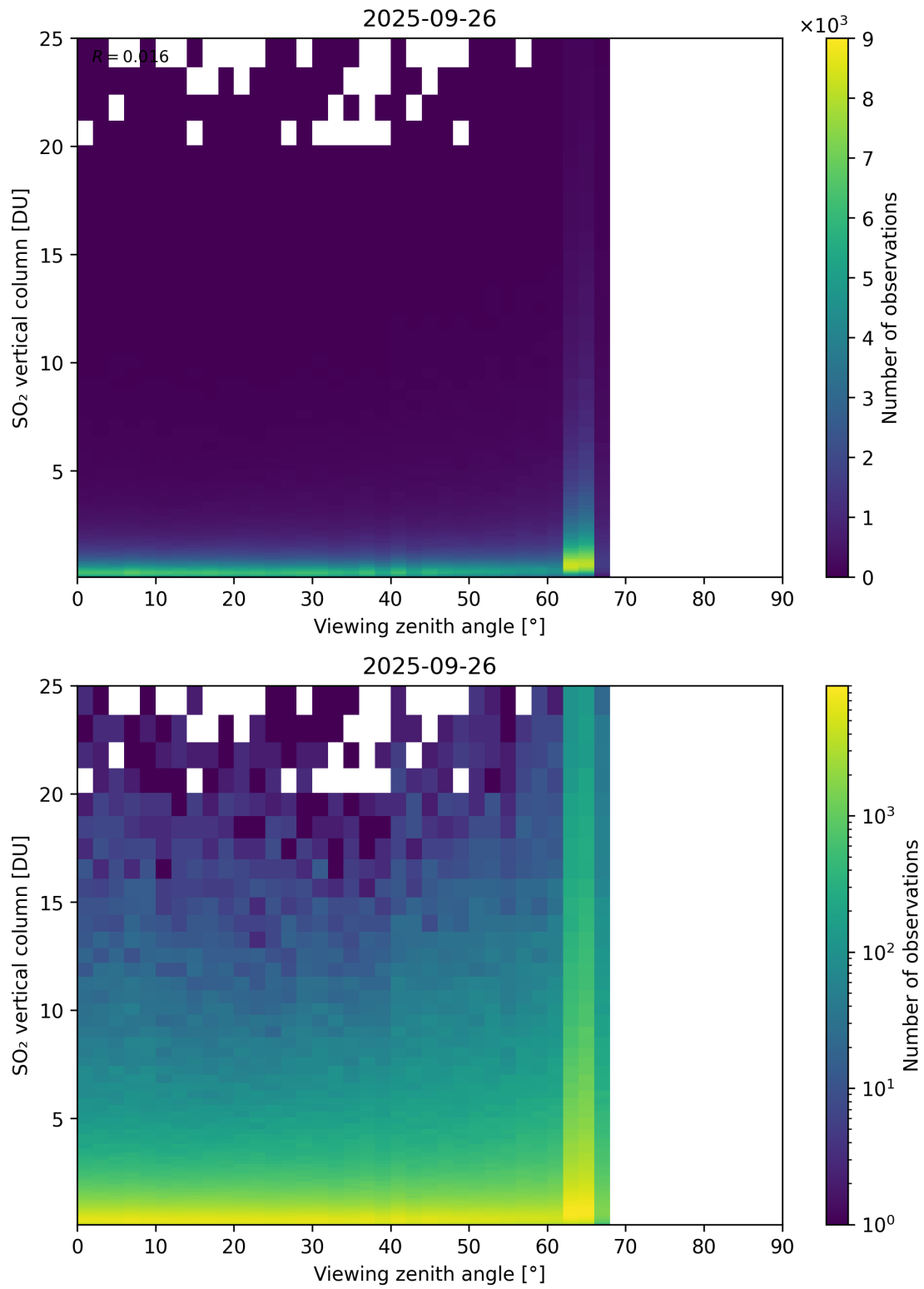
Figure 383: Scatter density plot of “Viewing zenith angle” against “SO 2 vertical column” for 2025-09-26 to 2025-09-27.
