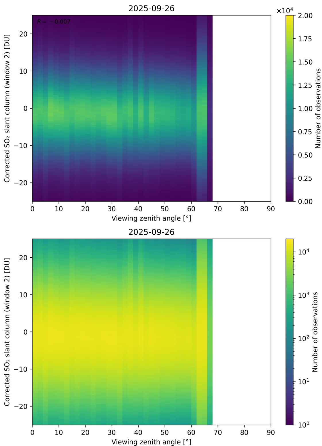
Figure 374: Scatter density plot of “Viewing zenith angle” against “Corrected SO 2 slant column (window 2)” for 2025-09-26 to 2025-09-27.
