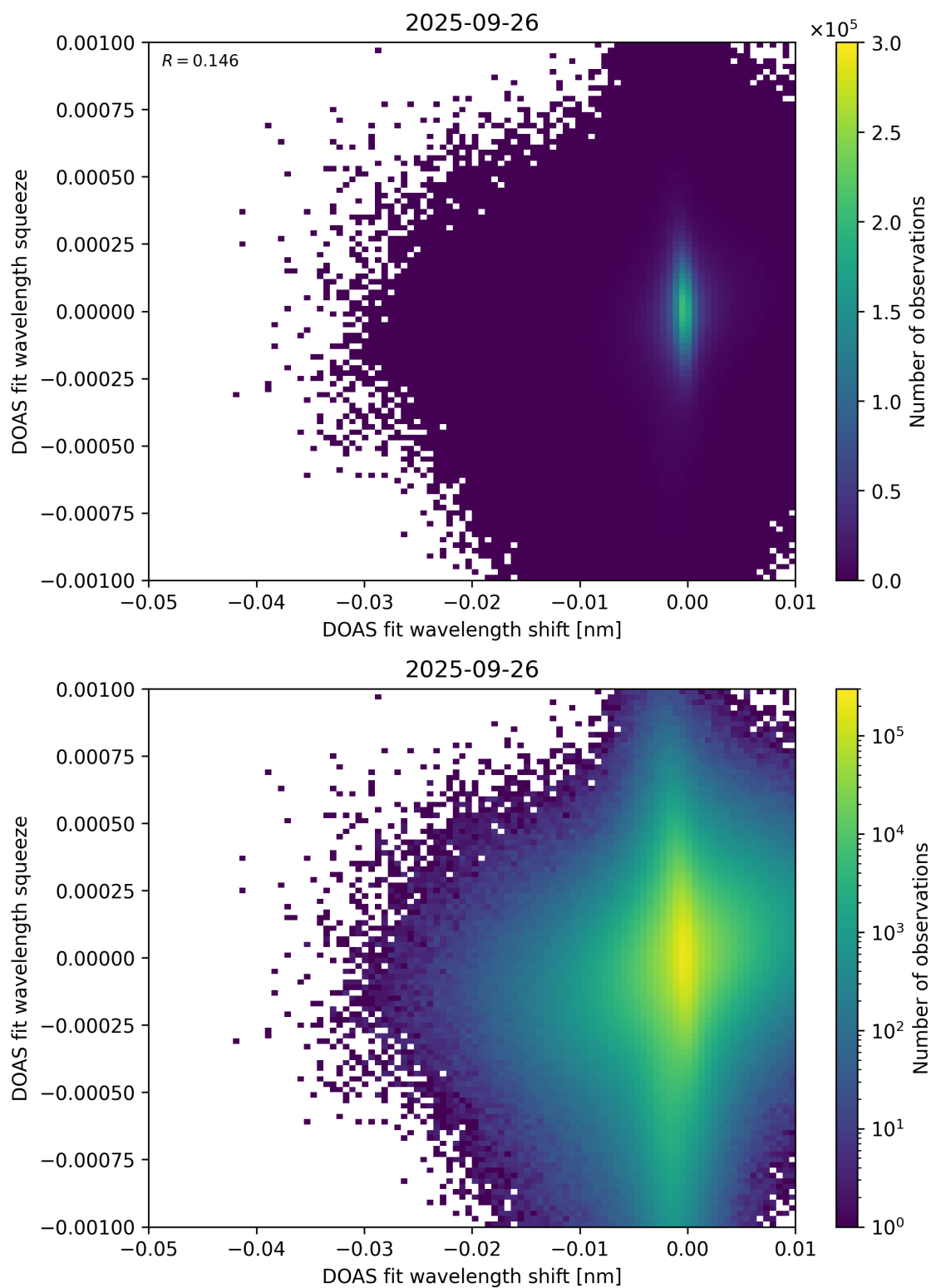
Figure 138: Scatter density plot of “DOAS fit wavelength shift” against “DOAS fit wavelength squeeze” for 2025-09-26 to 2025-09-27.
