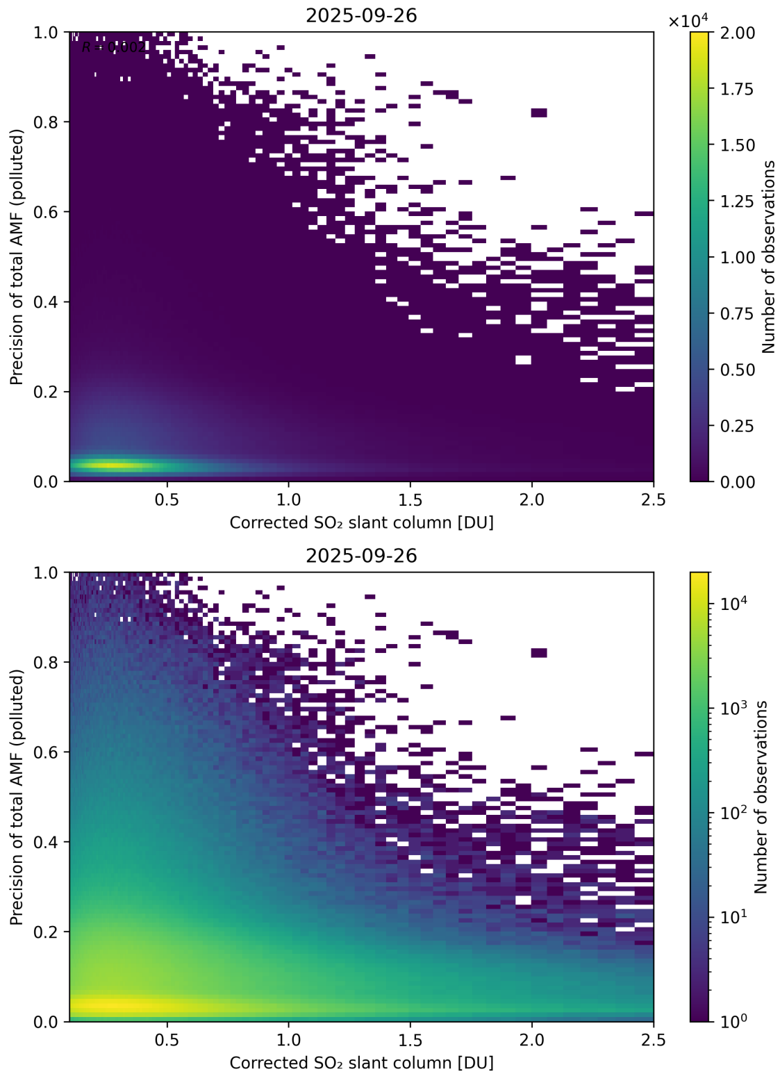
Figure 243: Scatter density plot of “Corrected SO 2 slant column” against “Precision of total AMF (polluted)” for 2025-09-26 to 2025-09-27.
