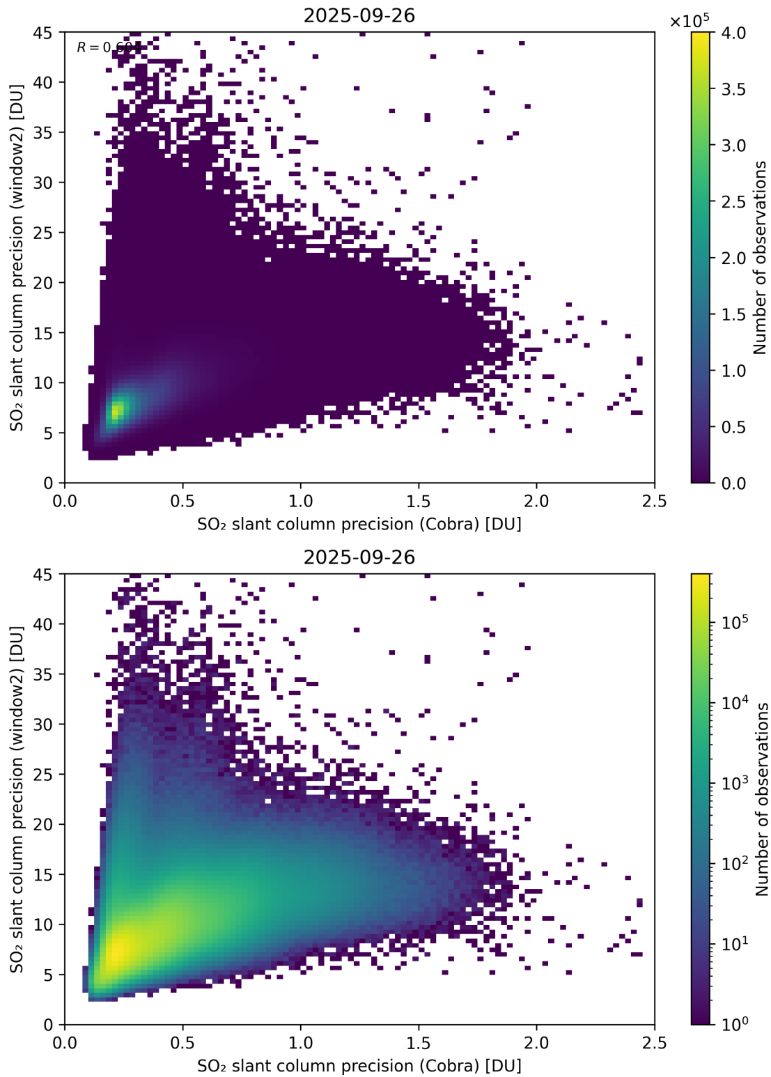
Figure 210: Scatter density plot of “SO 2 slant column precision (Cobra)” against “SO 2 slant column precision (window2)” for 2025-09-26 to 2025-09-27.
