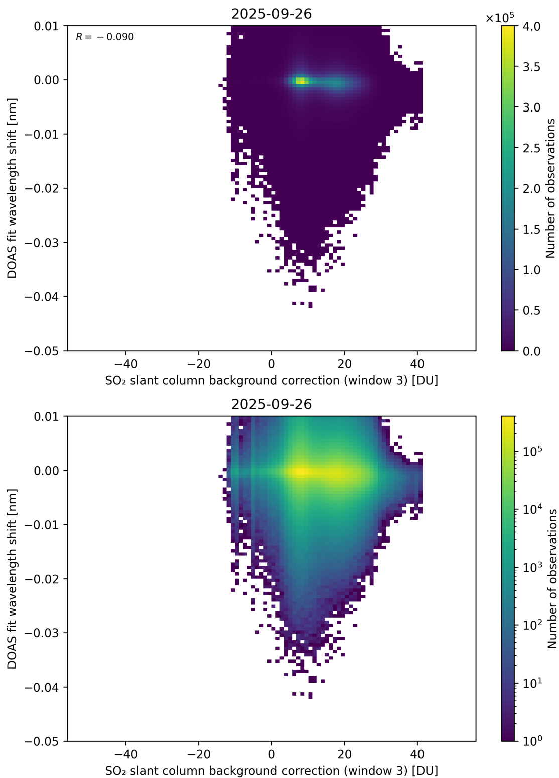
Figure 132: Scatter density plot of “SO 2 slant column background correction (window 3)” against “DOAS fit wavelength shift” for 2025-09-26 to 2025-09-27.
