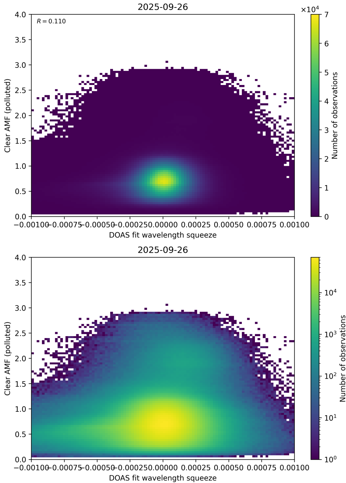
Figure 144: Scatter density plot of “DOAS fit wavelength squeeze” against “Clear AMF (polluted)” for 2025-09-26 to 2025-09-27.
