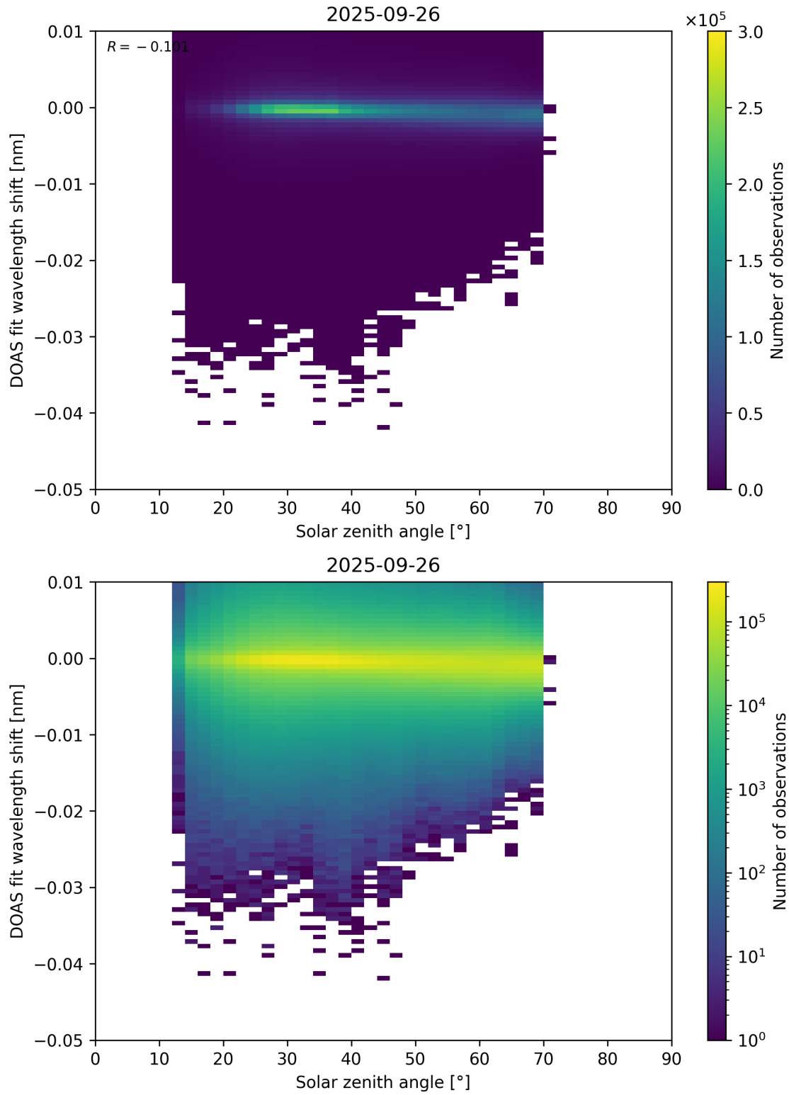
Figure 174: Scatter density plot of “Solar zenith angle” against “DOAS fit wavelength shift” for 2025-09-26 to 2025-09-27.
