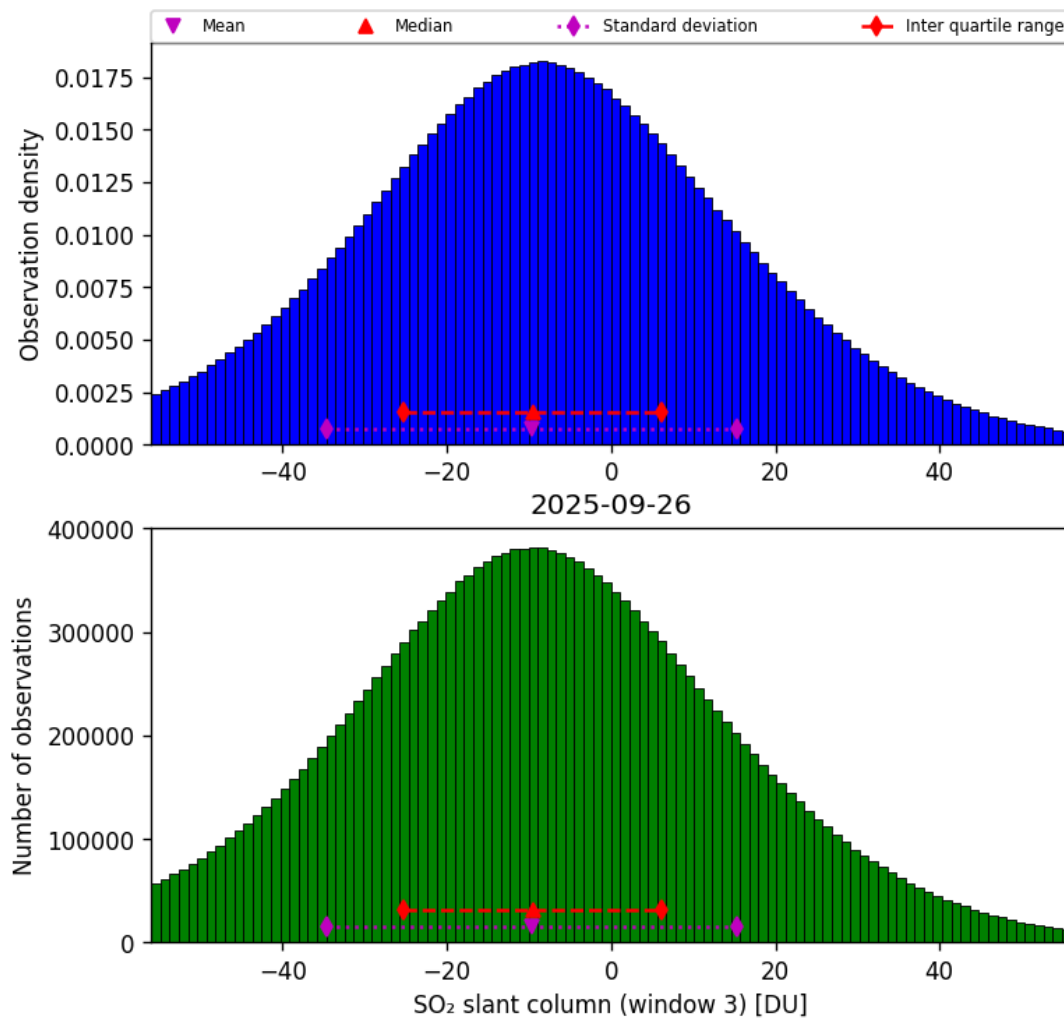
Figure 71: Histogram of “SO 2 slant column (window 3)” for 2025-09-26 to 2025-09-27
