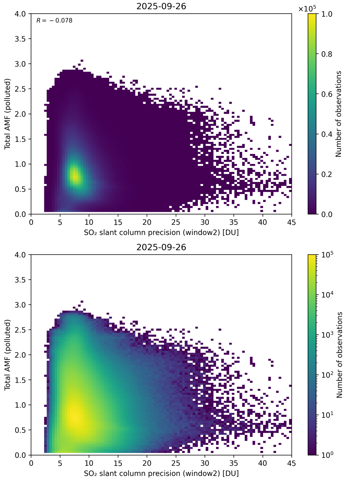
Figure 301: Scatter density plot of “SO 2 slant column precision (window2)” against “Total AMF (polluted)” for 2025-09-26 to 2025-09-27.
