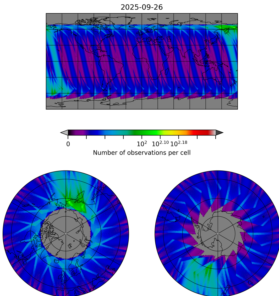
Figure 30: Map of the number of observations for 2025-09-26 to 2025-09-27
