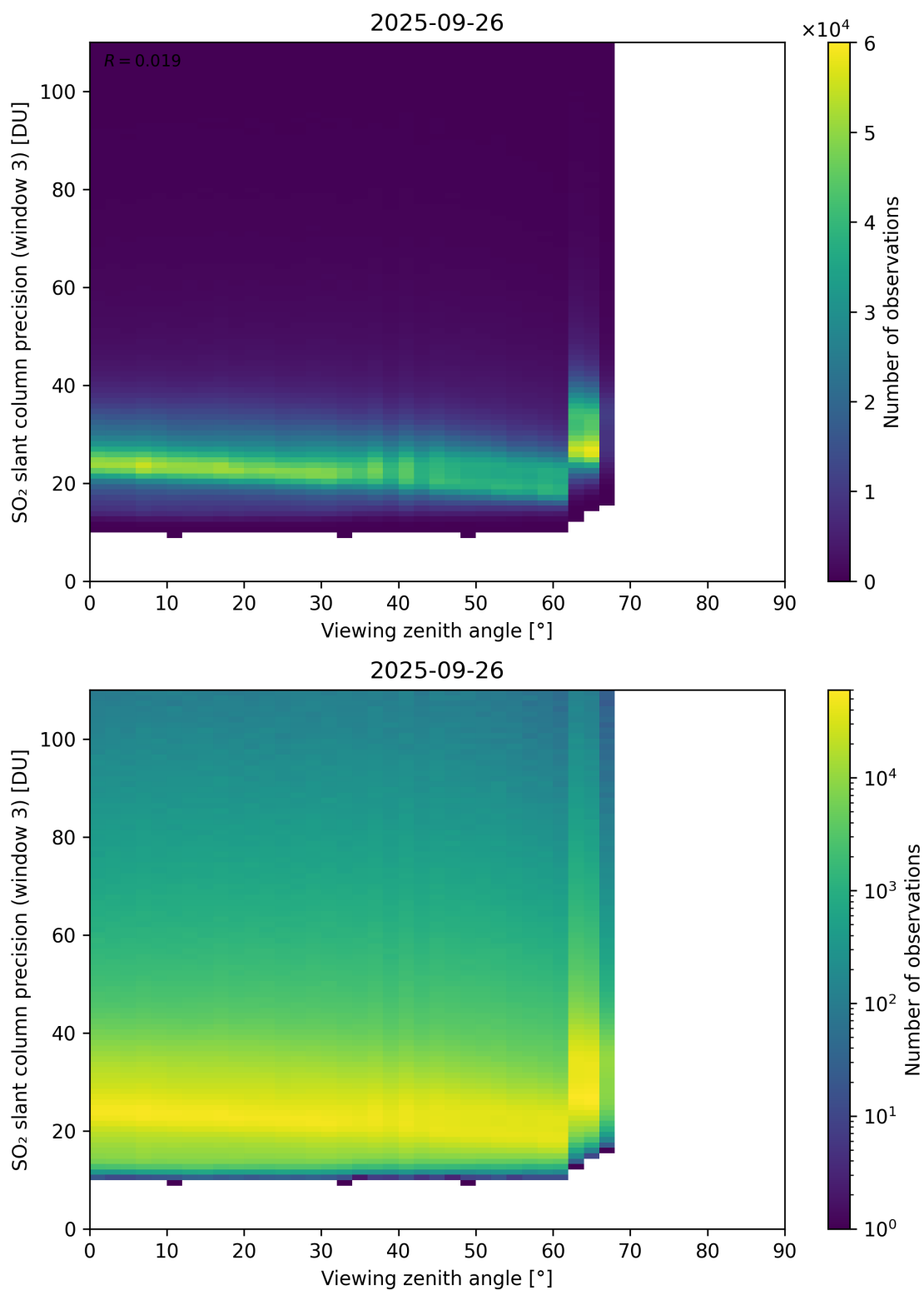
Figure 380: Scatter density plot of “Viewing zenith angle” against “SO 2 slant column precision (window 3)” for 2025-09-26 to 2025-09-27.
