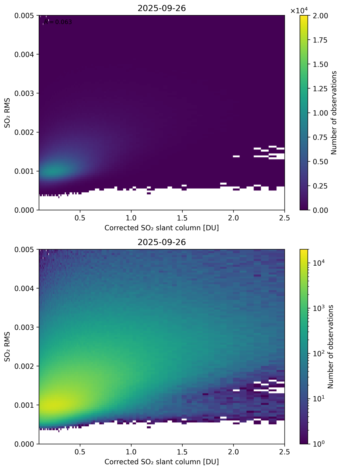
Figure 231: Scatter density plot of “Corrected SO 2 slant column” against “SO 2 RMS” for 2025-09-26 to 2025-09-27.
