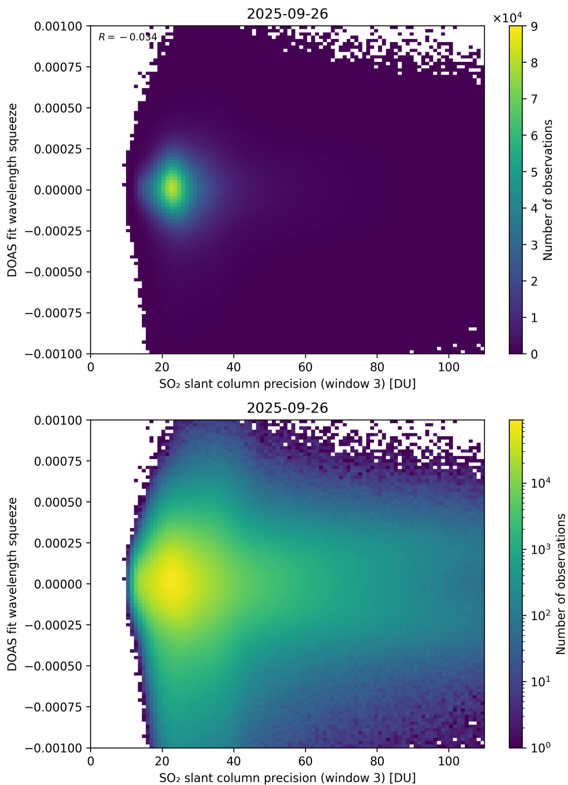
Figure 309: Scatter density plot of “SO 2 slant column precision (window 3)” against “DOAS fit wavelength squeeze” for 2025-09-26 to 2025-09-27.
