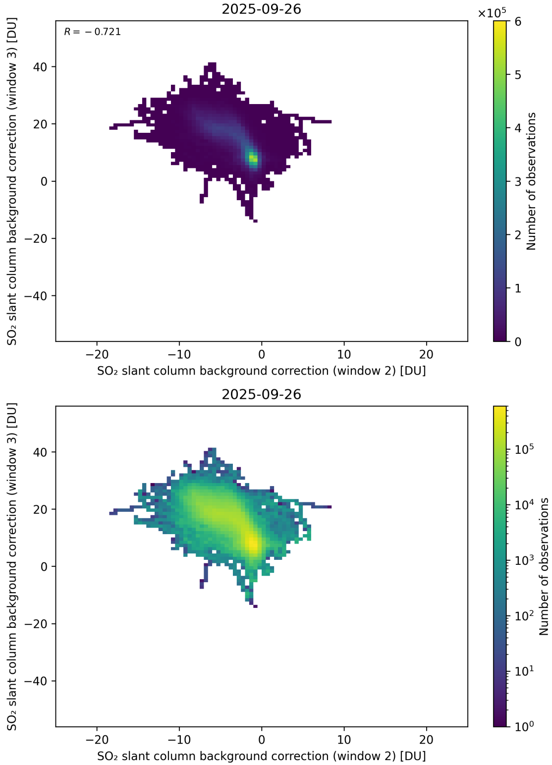
Figure 122: Scatter density plot of “SO 2 slant column background correction (window 2)” against “SO 2 slant column background correction (window 3)” for 2025-09-26 to 2025-09-27.
