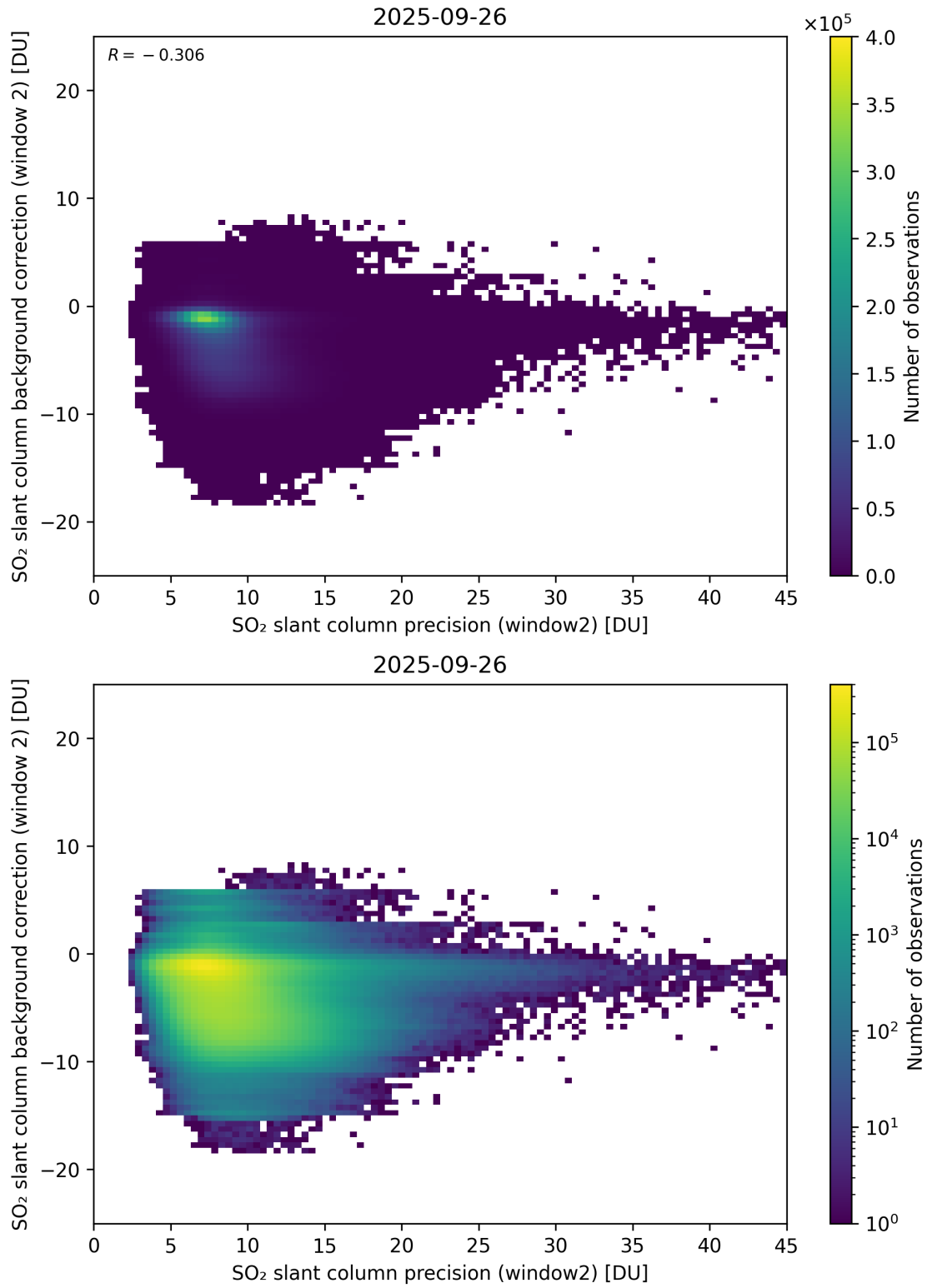
Figure 291: Scatter density plot of “SO 2 slant column precision (window2)” against “SO 2 slant column background correction (window 2)” for 2025-09-26 to 2025-09-27.
