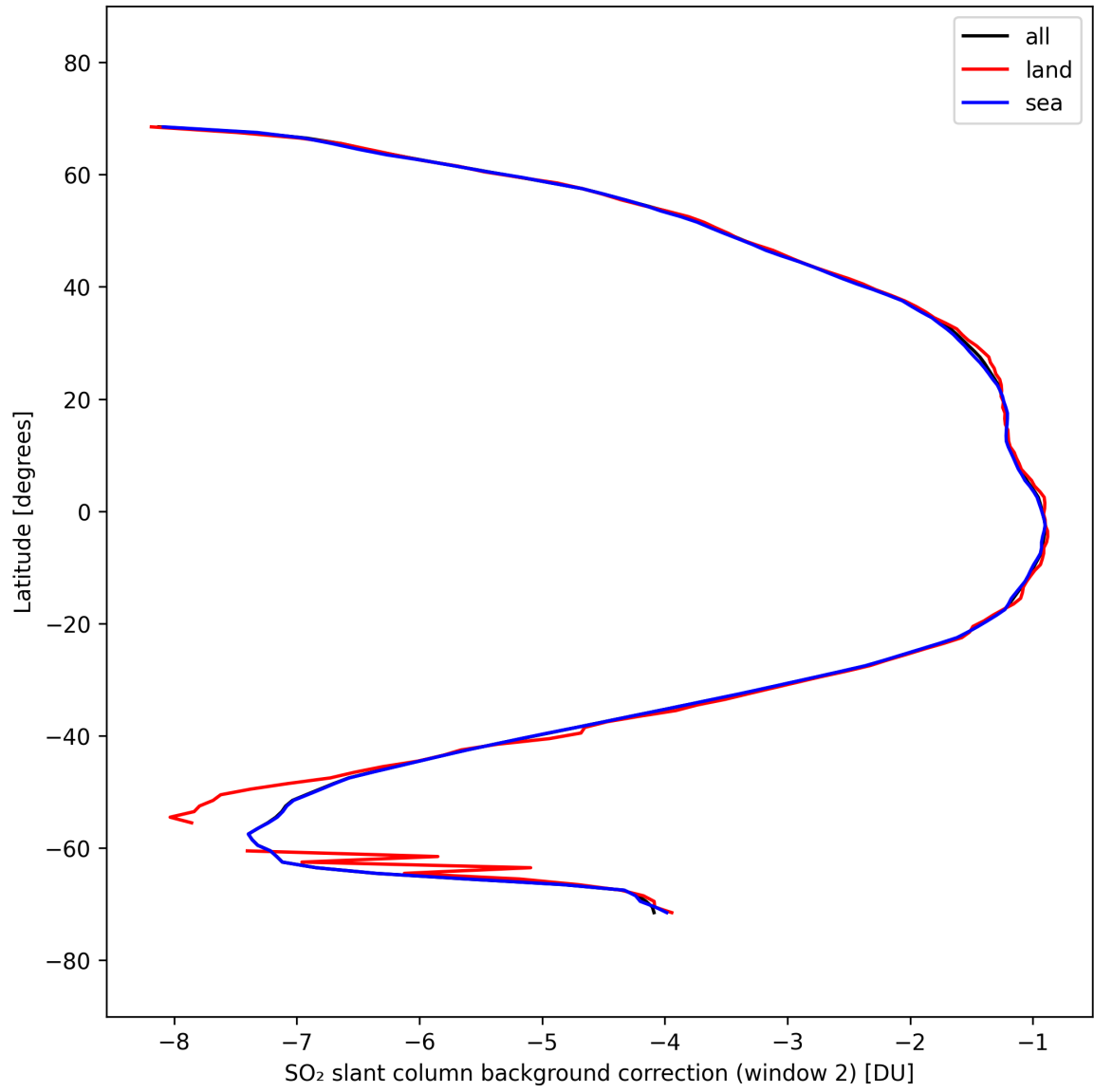
Figure 44: Zonal average of “SO 2 slant column background correction (window 2)” for 2025-09-26 to 2025-09-27.
