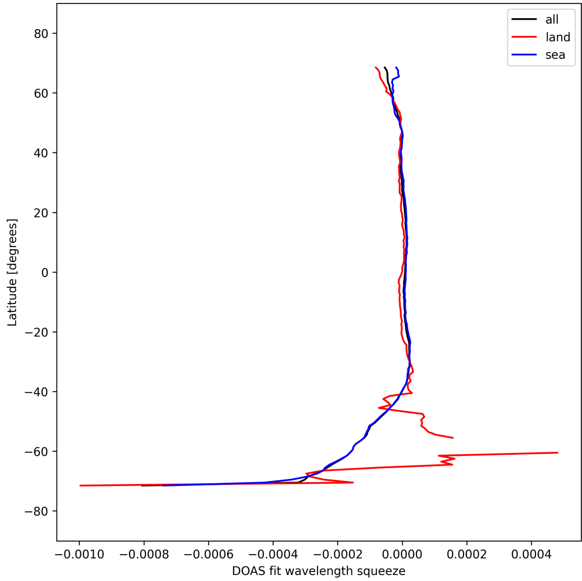
Figure 51: Zonal average of “DOAS fit wavelength squeeze” for 2025-09-26 to 2025-09-27.
