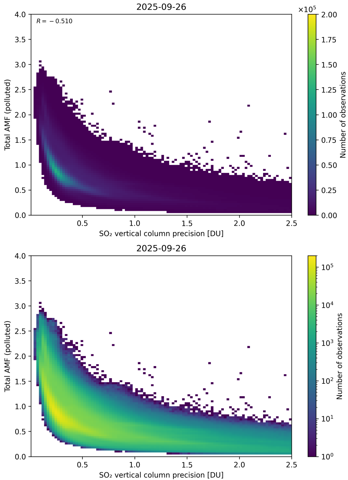
Figure 346: Scatter density plot of “SO 2 vertical column precision” against “Total AMF (polluted)” for 2025-09-26 to 2025-09-27.
