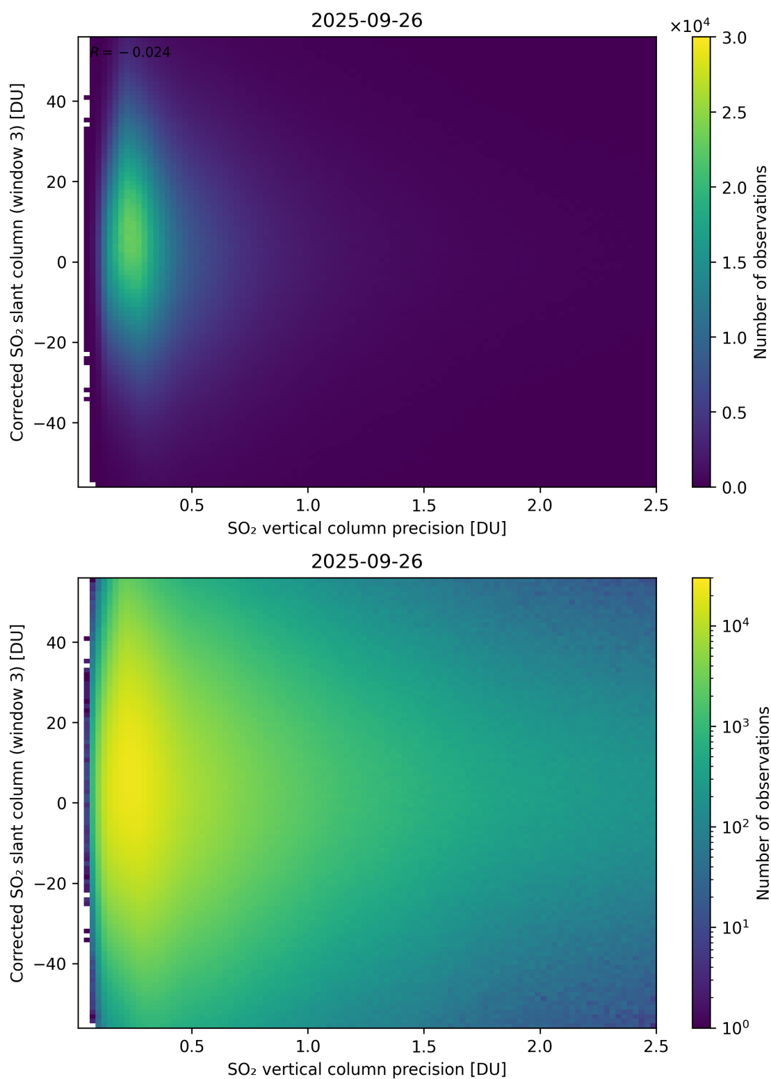
Figure 340: Scatter density plot of “SO 2 vertical column precision” against “Corrected SO 2 slant column (window 3)” for 2025-09-26 to 2025-09-27.
