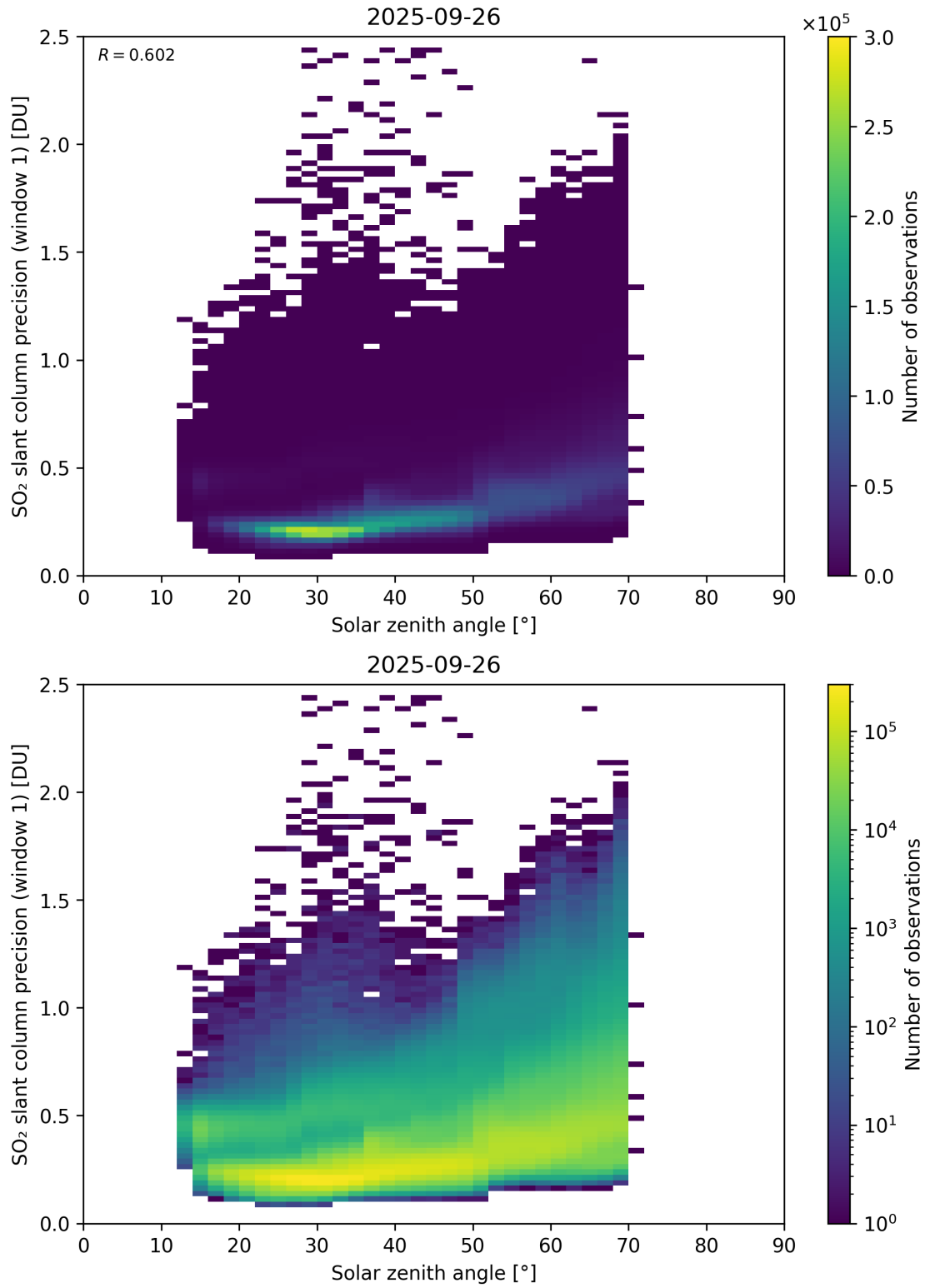
Figure 185: Scatter density plot of “Solar zenith angle” against “SO 2 slant column precision (window 1)” for 2025-09-26 to 2025-09-27.
