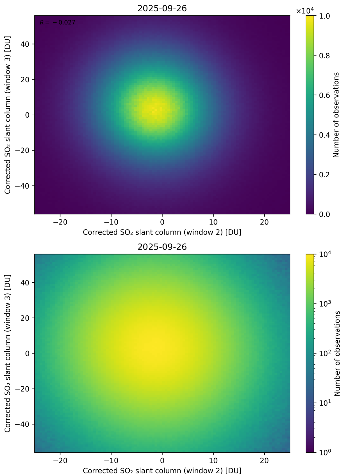
Figure 250: Scatter density plot of “Corrected SO 2 slant column (window 2)” against “Corrected SO 2 slant column (window 3)” for 2025-09-26 to 2025-09-27.
