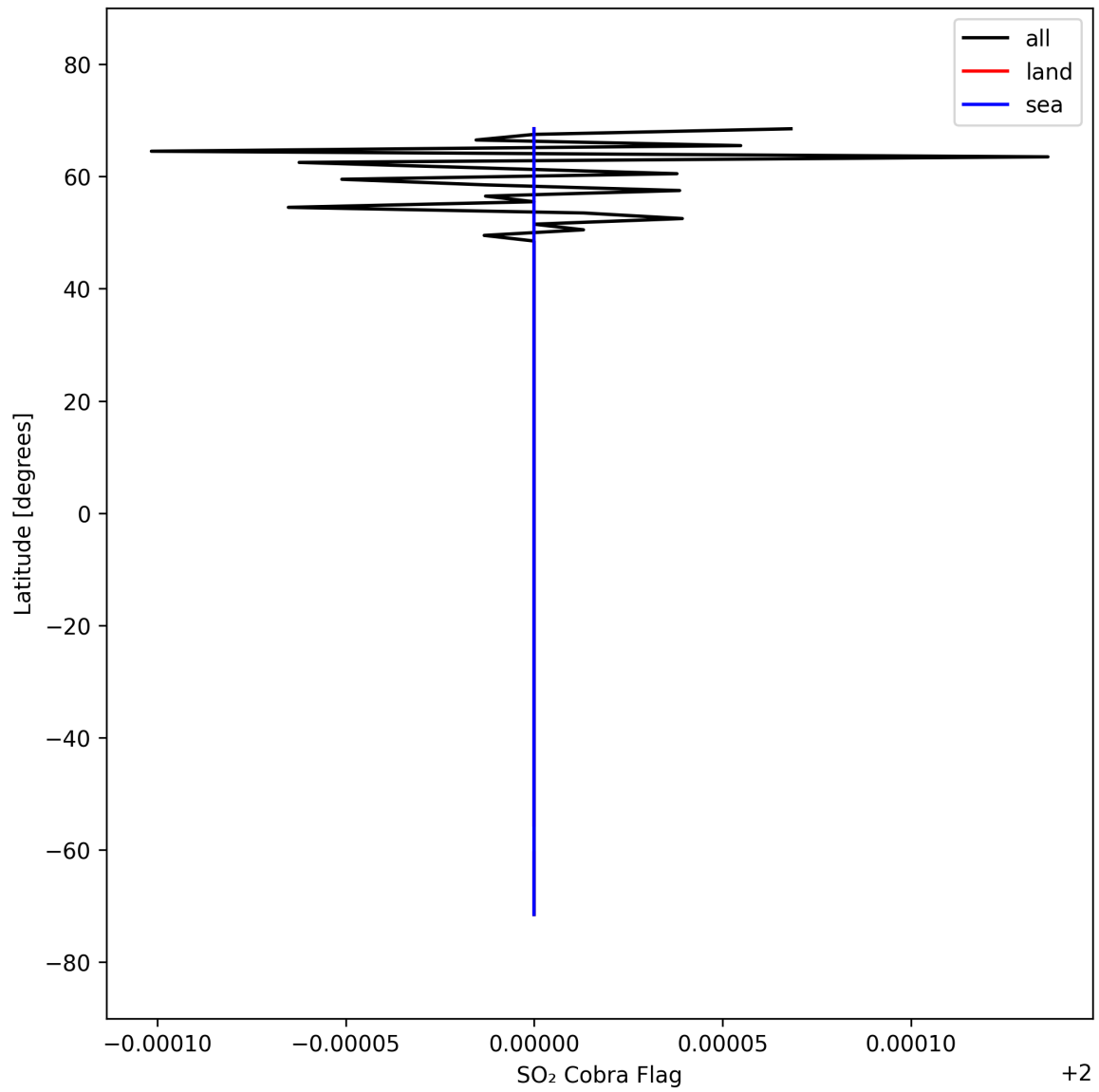
Figure 49: Zonal average of “SO 2 Cobra Flag” for 2025-09-26 to 2025-09-27.
