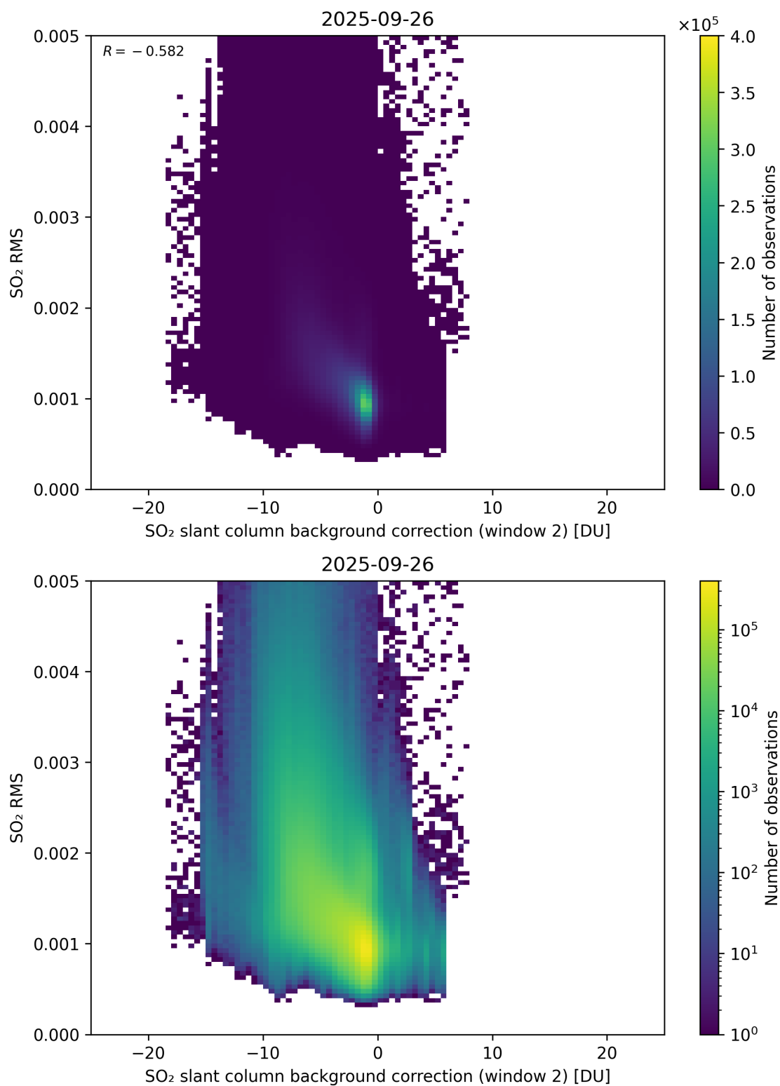
Figure 125: Scatter density plot of “SO 2 slant column background correction (window 2)” against “SO 2 RMS” for 2025-09-26 to 2025-09-27.
