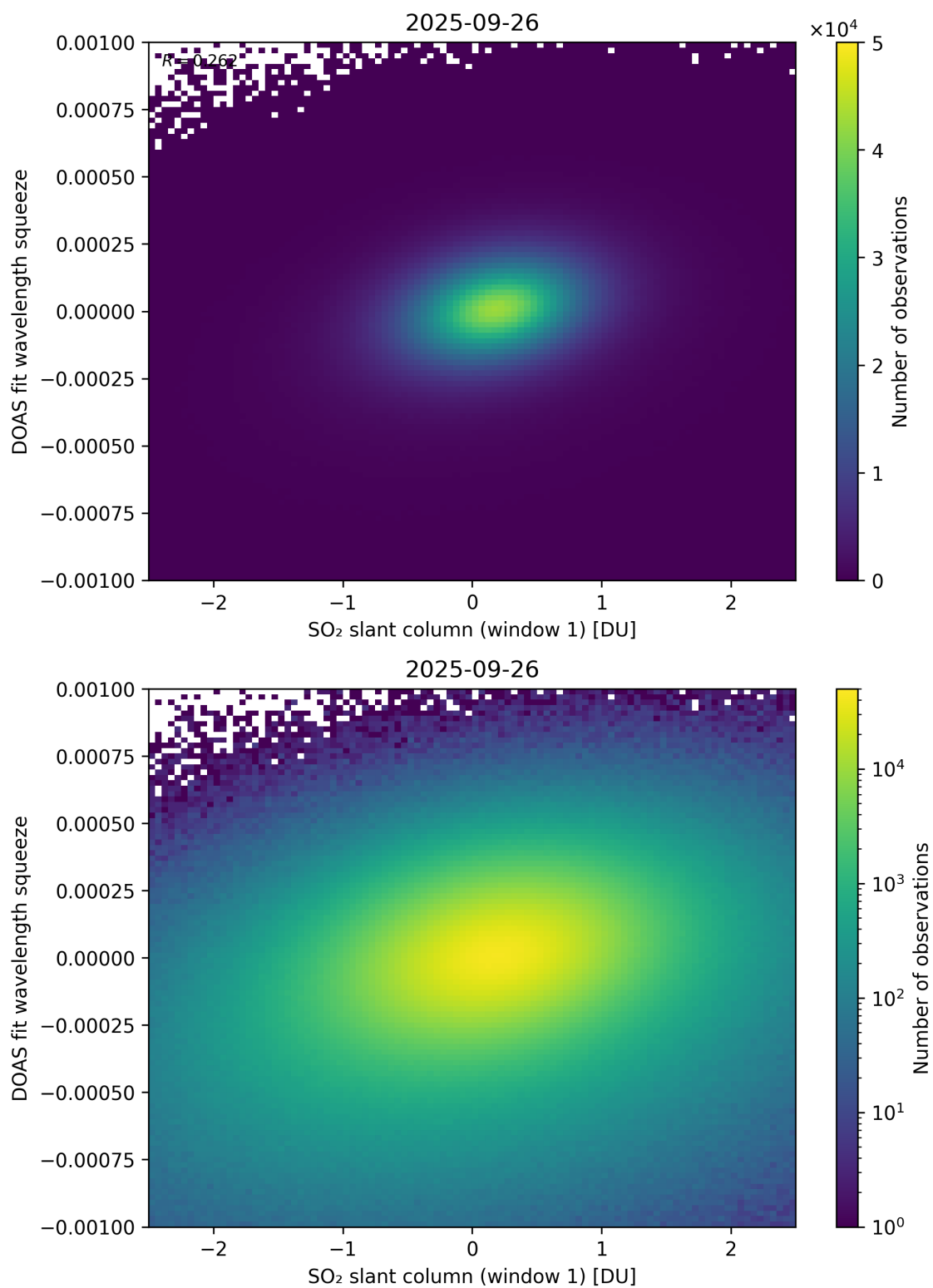
Figure 266: Scatter density plot of “SO 2 slant column (window 1)” against “DOAS fit wavelength squeeze” for 2025-09-26 to 2025-09-27.
