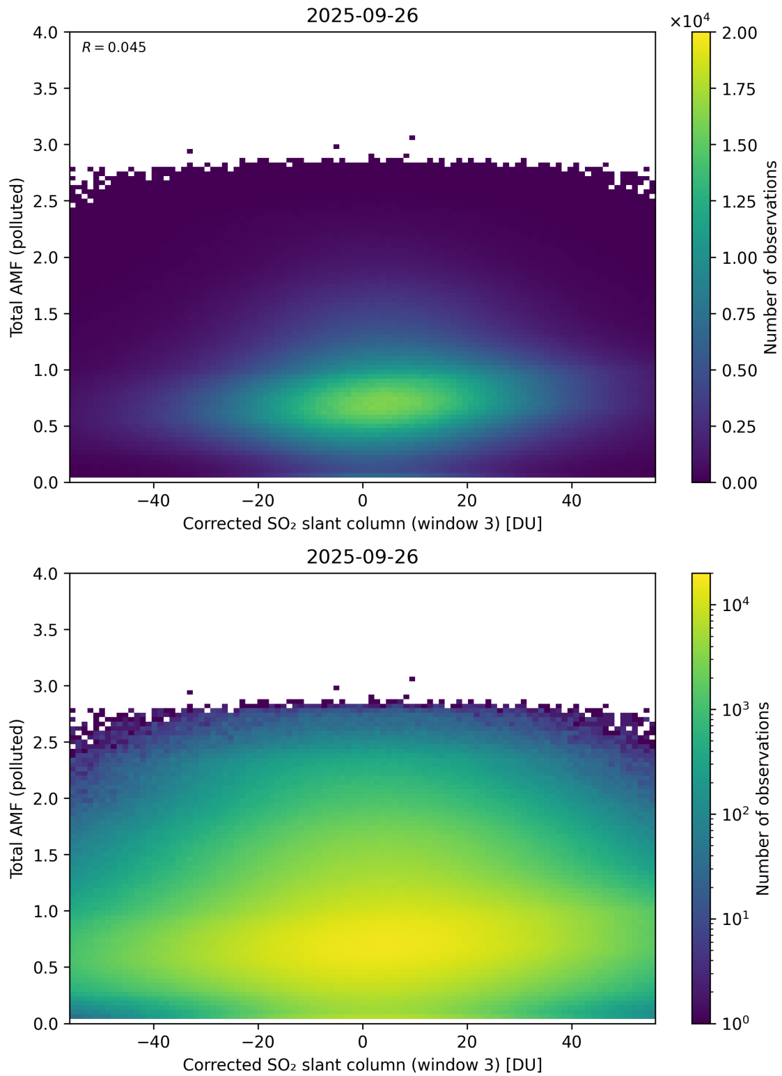
Figure 260: Scatter density plot of “Corrected SO 2 slant column (window 3)” against “Total AMF (polluted)” for 2025-09-26 to 2025-09-27.
