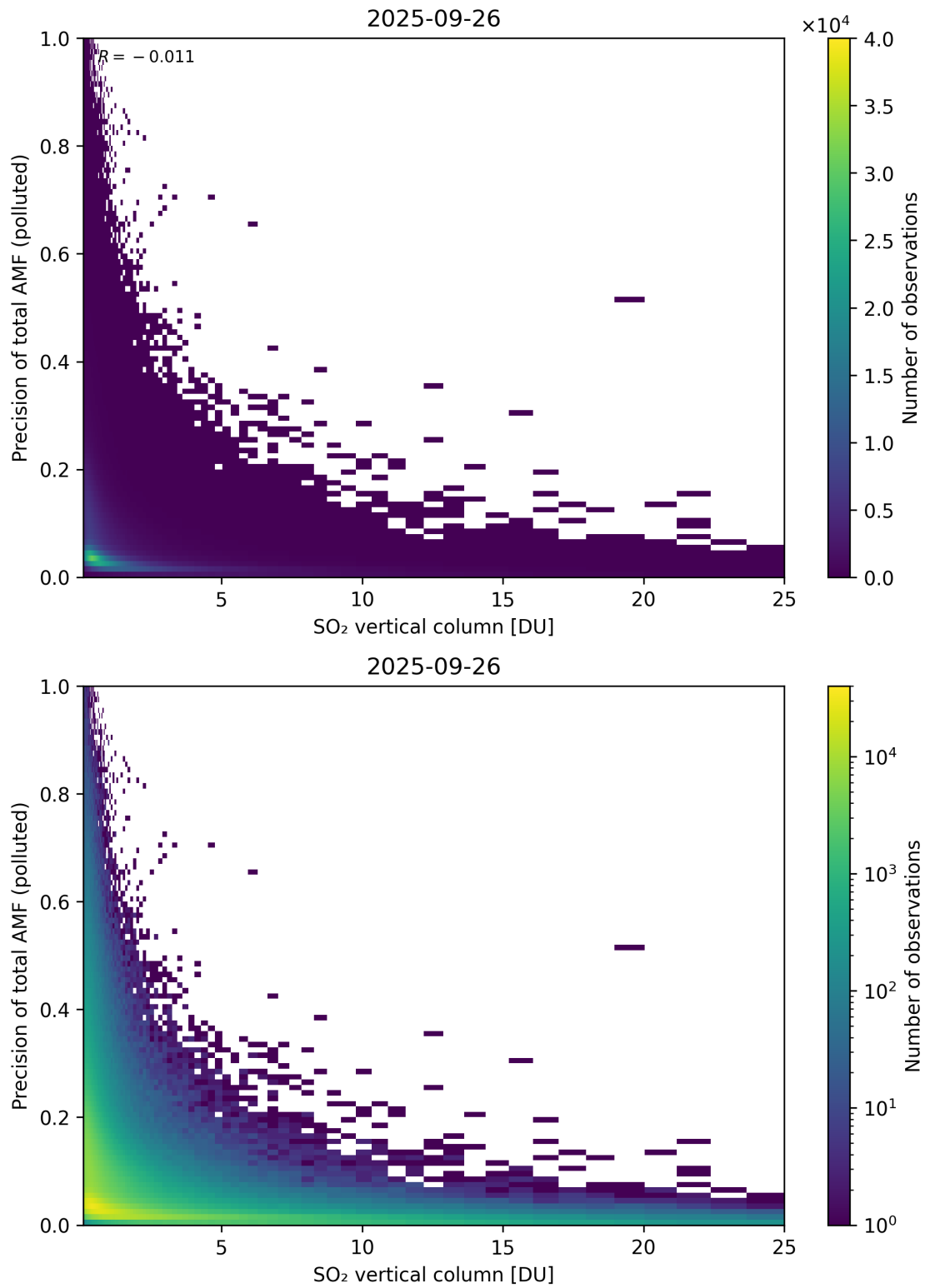
Figure 360: Scatter density plot of “SO 2 vertical column” against “Precision of total AMF (polluted)” for 2025-09-26 to 2025-09-27.
