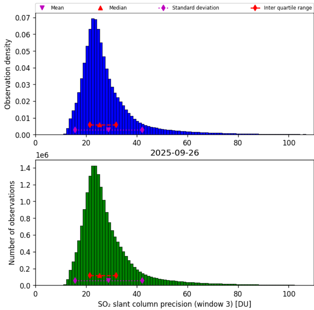
Figure 72: Histogram of “SO 2 slant column precision (window 3)” for 2025-09-26 to 2025-09-27
