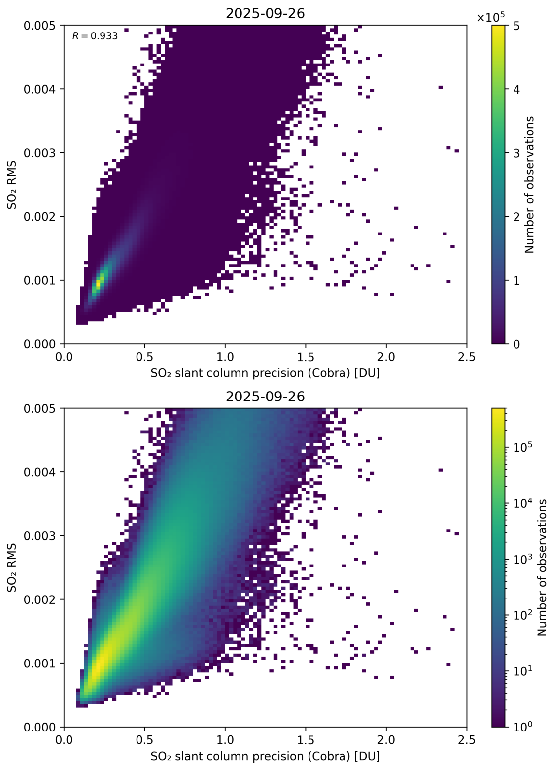
Figure 204: Scatter density plot of “SO 2 slant column precision (Cobra)” against “SO 2 RMS” for 2025-09-26 to 2025-09-27.
