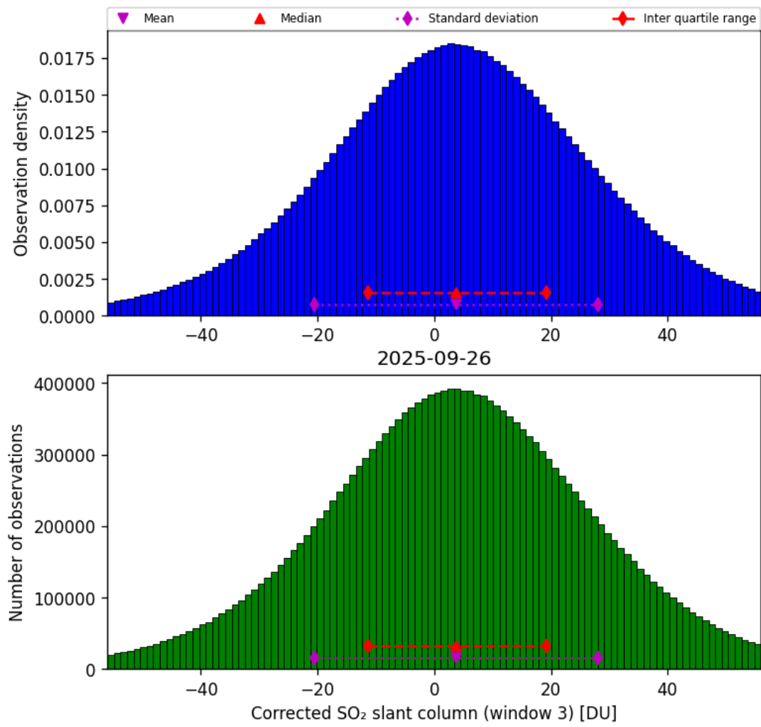
Figure 73: Histogram of “Corrected SO 2 slant column (window 3)” for 2025-09-26 to 2025-09-27
