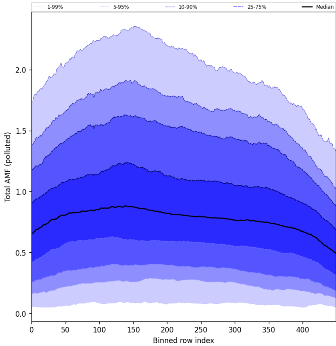
Figure 105: Along track statistics of “Total AMF (polluted)” for 2025-09-26 to 2025-09-27
