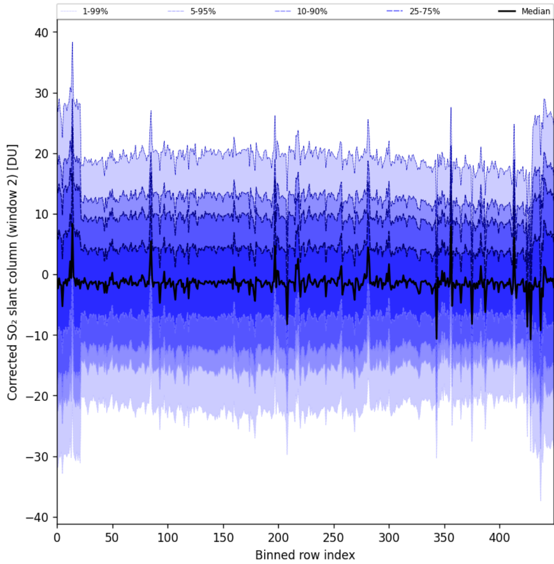
Figure 95: Along track statistics of “Corrected SO 2 slant column (window 2)” for 2025-09-26 to 2025-09-27
