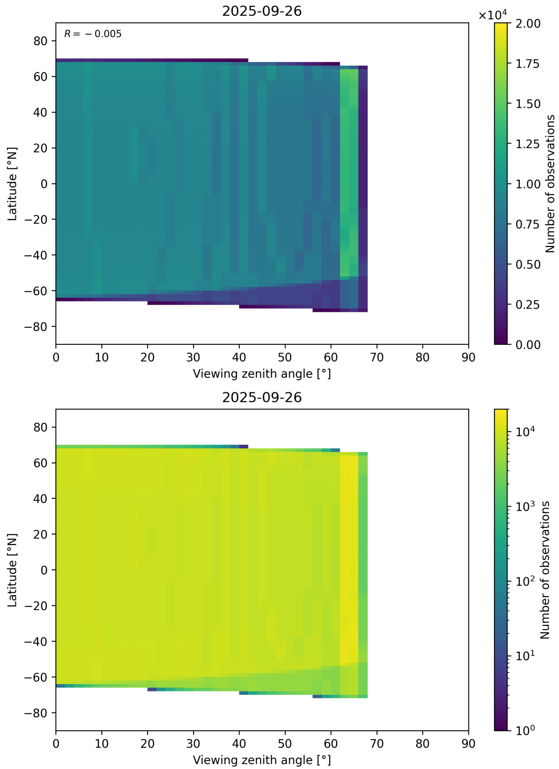
Figure 368: Scatter density plot of “Viewing zenith angle” against “Latitude” for 2025-09-26 to 2025-09-27.
