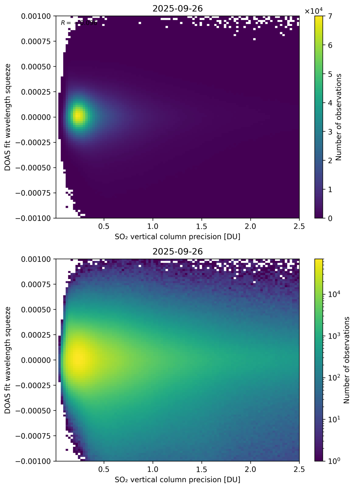
Figure 333: Scatter density plot of “SO 2 vertical column precision” against “DOAS fit wavelength squeeze” for 2025-09-26 to 2025-09-27.
