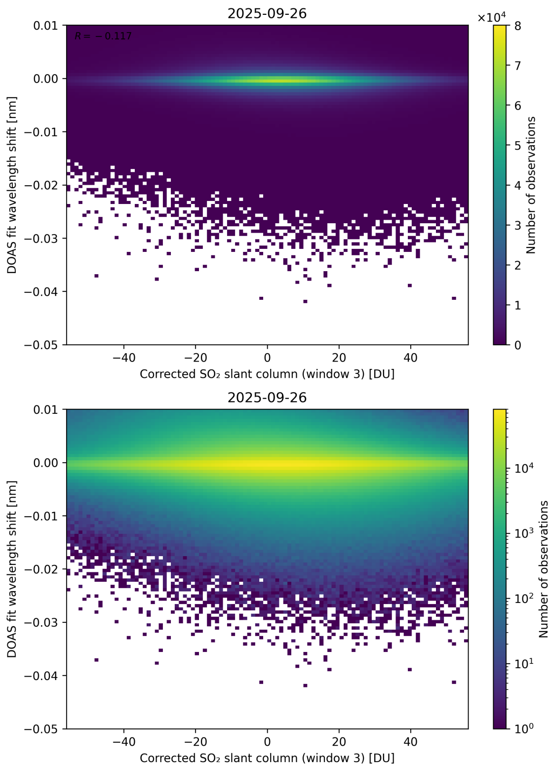
Figure 256: Scatter density plot of “Corrected SO 2 slant column (window 3)” against “DOAS fit wavelength shift” for 2025-09-26 to 2025-09-27.
