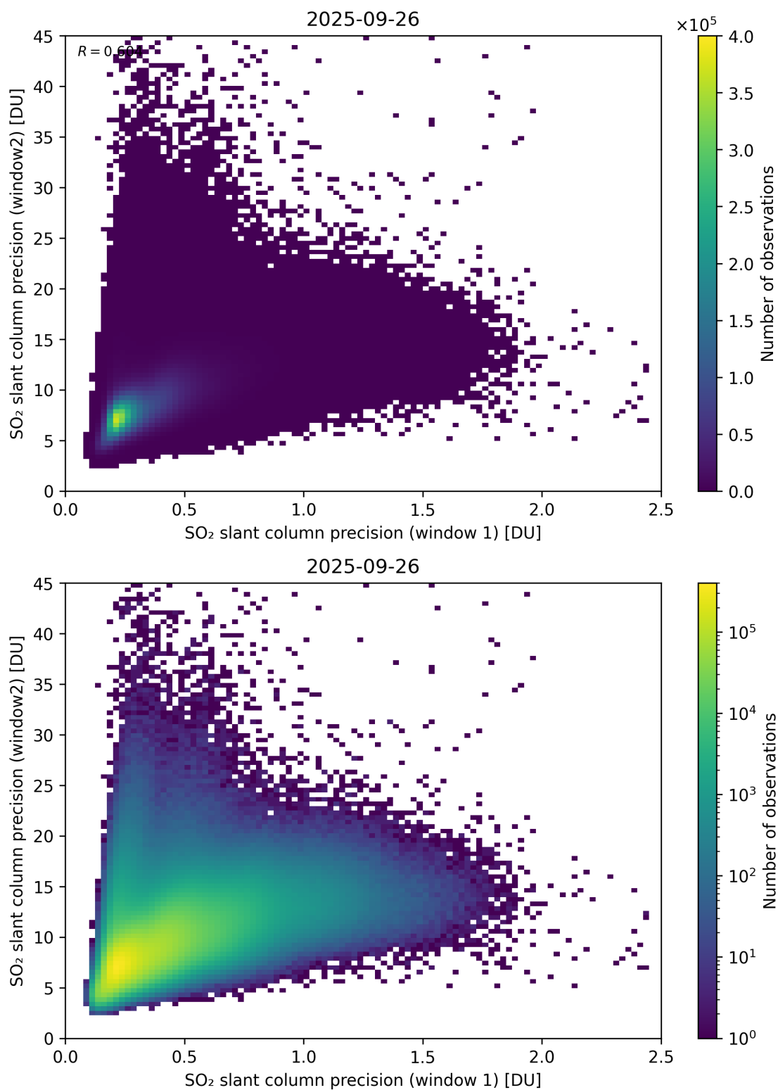
Figure 277: Scatter density plot of “SO 2 slant column precision (window 1)” against “SO 2 slant column precision (window2)” for 2025-09-26 to 2025-09-27.
