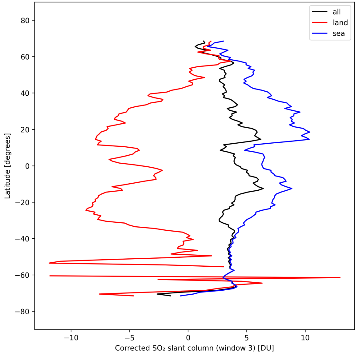
Figure 47: Zonal average of “Corrected SO 2 slant column (window 3)” for 2025-09-26 to 2025-09-27.
