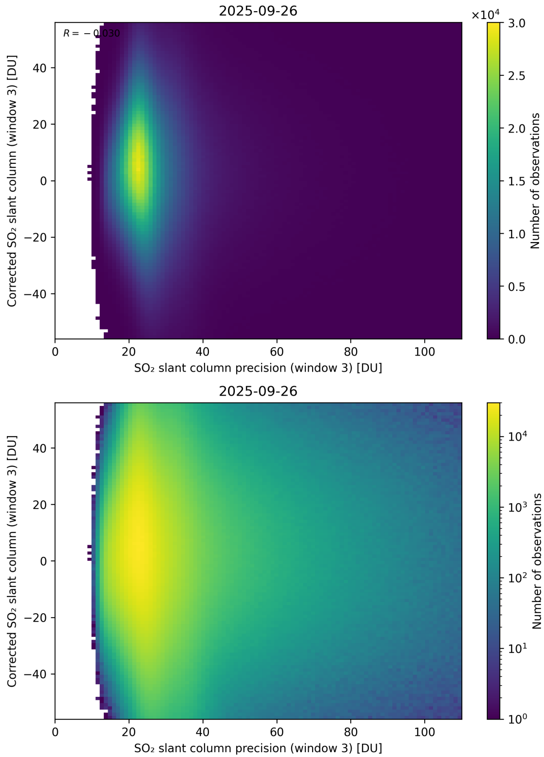
Figure 312: Scatter density plot of “SO 2 slant column precision (window 3)” against “Corrected SO 2 slant column (window 3)” for 2025-09-26 to 2025-09-27.
