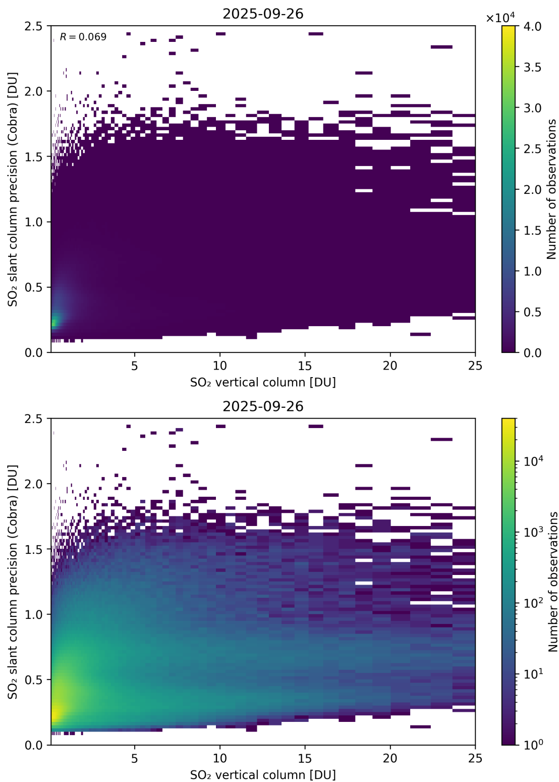
Figure 350: Scatter density plot of “SO 2 vertical column” against “SO 2 slant column precision (Cobra)” for 2025-09-26 to 2025-09-27.
