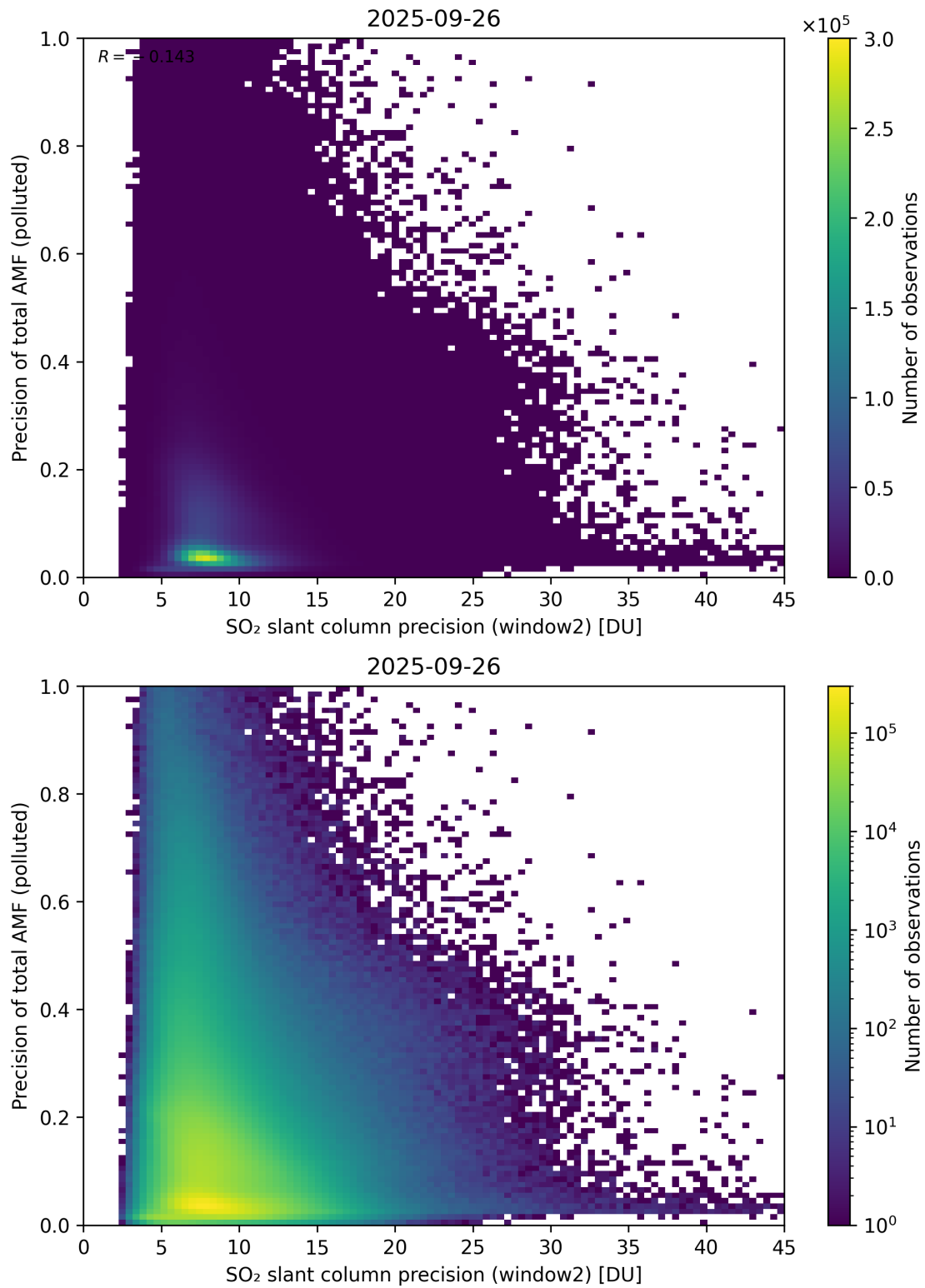
Figure 302: Scatter density plot of “SO 2 slant column precision (window2)” against “Precision of total AMF (polluted)” for 2025-09-26 to 2025-09-27.
