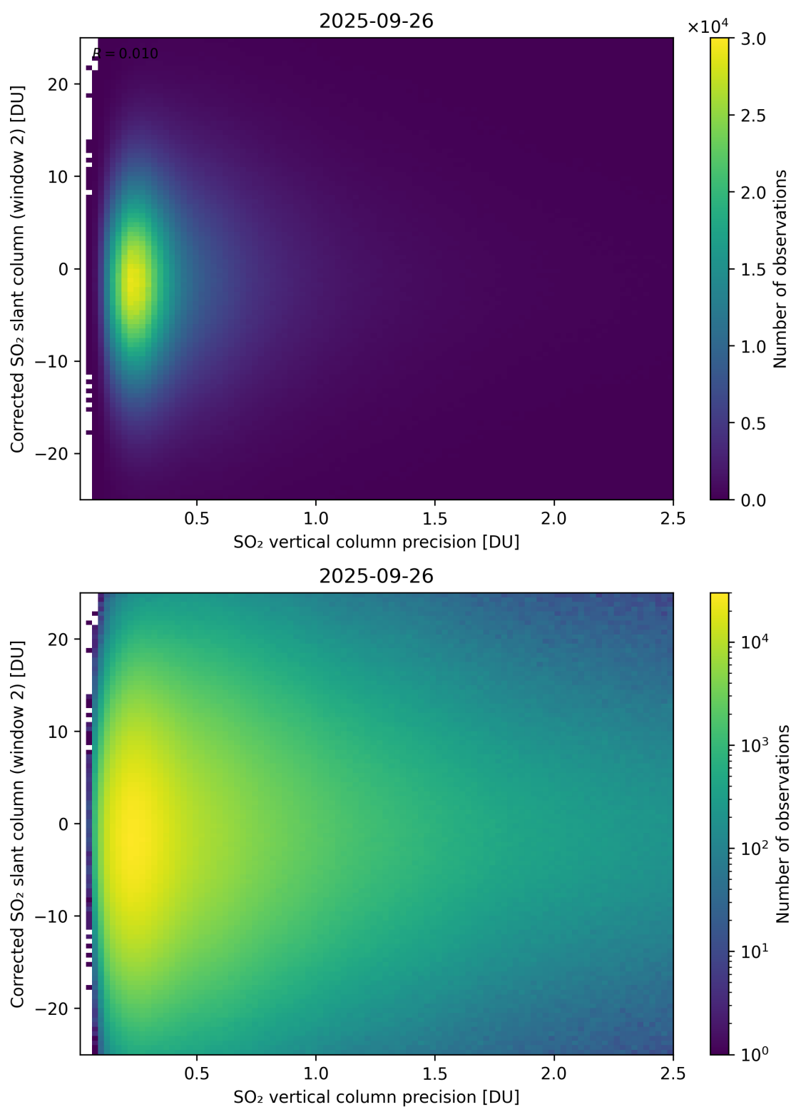
Figure 339: Scatter density plot of “SO 2 vertical column precision” against “Corrected SO 2 slant column (window 2)” for 2025-09-26 to 2025-09-27.
