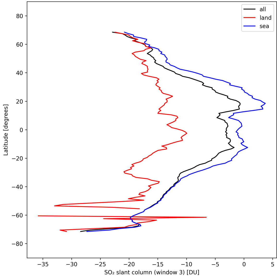
Figure 45: Zonal average of “SO 2 slant column (window 3)” for 2025-09-26 to 2025-09-27.
