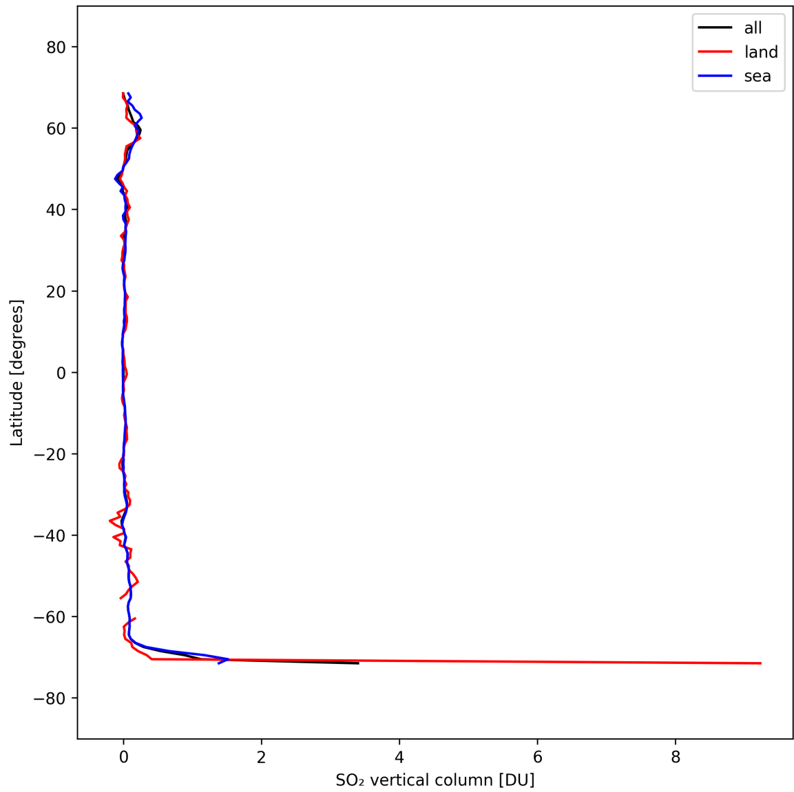
Figure 32: Zonal average of “SO 2 vertical column” for 2025-09-26 to 2025-09-27.
