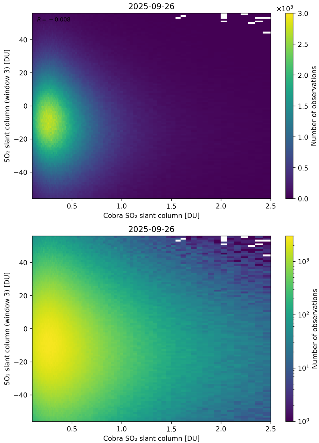
Figure 222: Scatter density plot of “Cobra SO 2 slant column” against “SO 2 slant column (window 3)” for 2025-09-26 to 2025-09-27.
