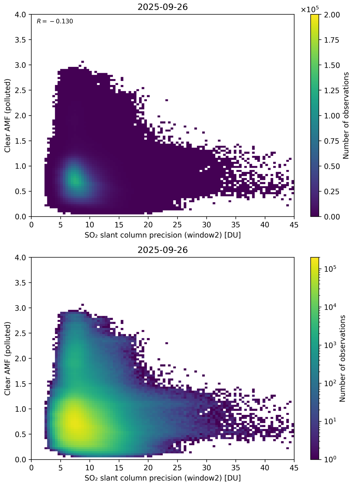
Figure 296: Scatter density plot of “SO 2 slant column precision (window2)” against “Clear AMF (polluted)” for 2025-09-26 to 2025-09-27.
