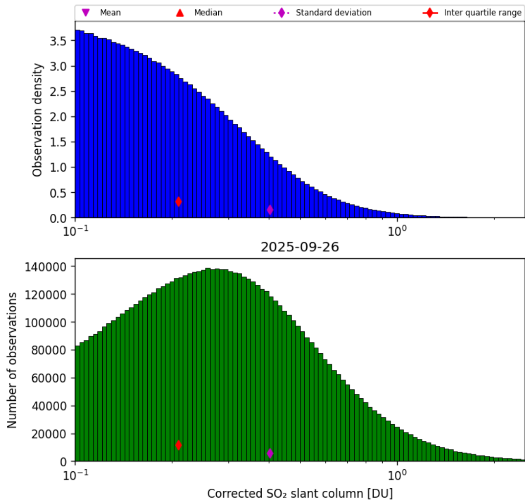
Figure 60: Histogram of “Corrected SO 2 slant column” for 2025-09-26 to 2025-09-27
