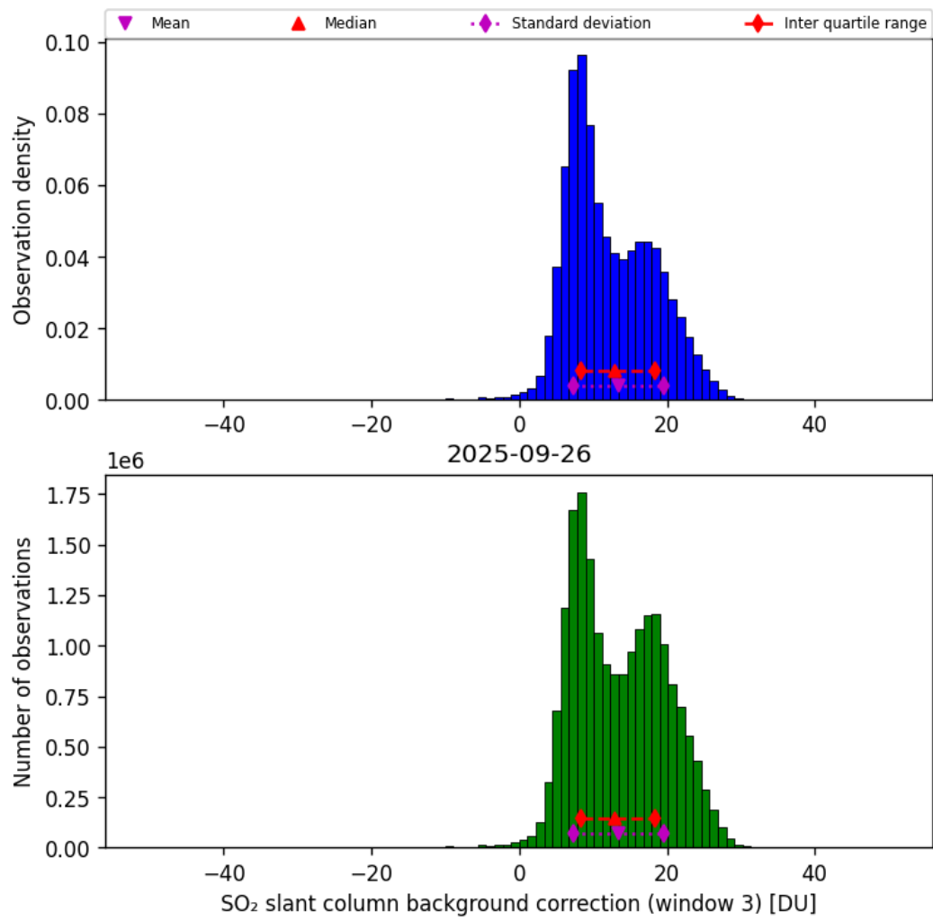
Figure 74: Histogram of “SO 2 slant column background correction (window 3)” for 2025-09-26 to 2025-09-27
