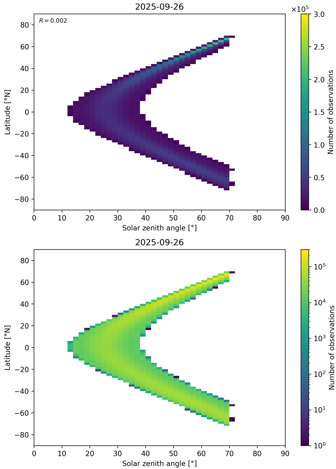
Figure 177: Scatter density plot of “Solar zenith angle” against “Latitude” for 2025-09-26 to 2025-09-27.
