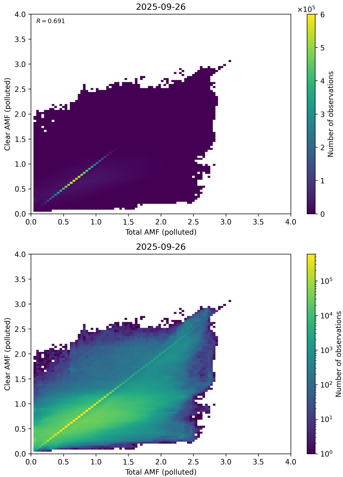
Figure 321: Scatter density plot of “Total AMF (polluted)” against “Clear AMF (polluted)” for 2025-09-26 to 2025-09-27.
