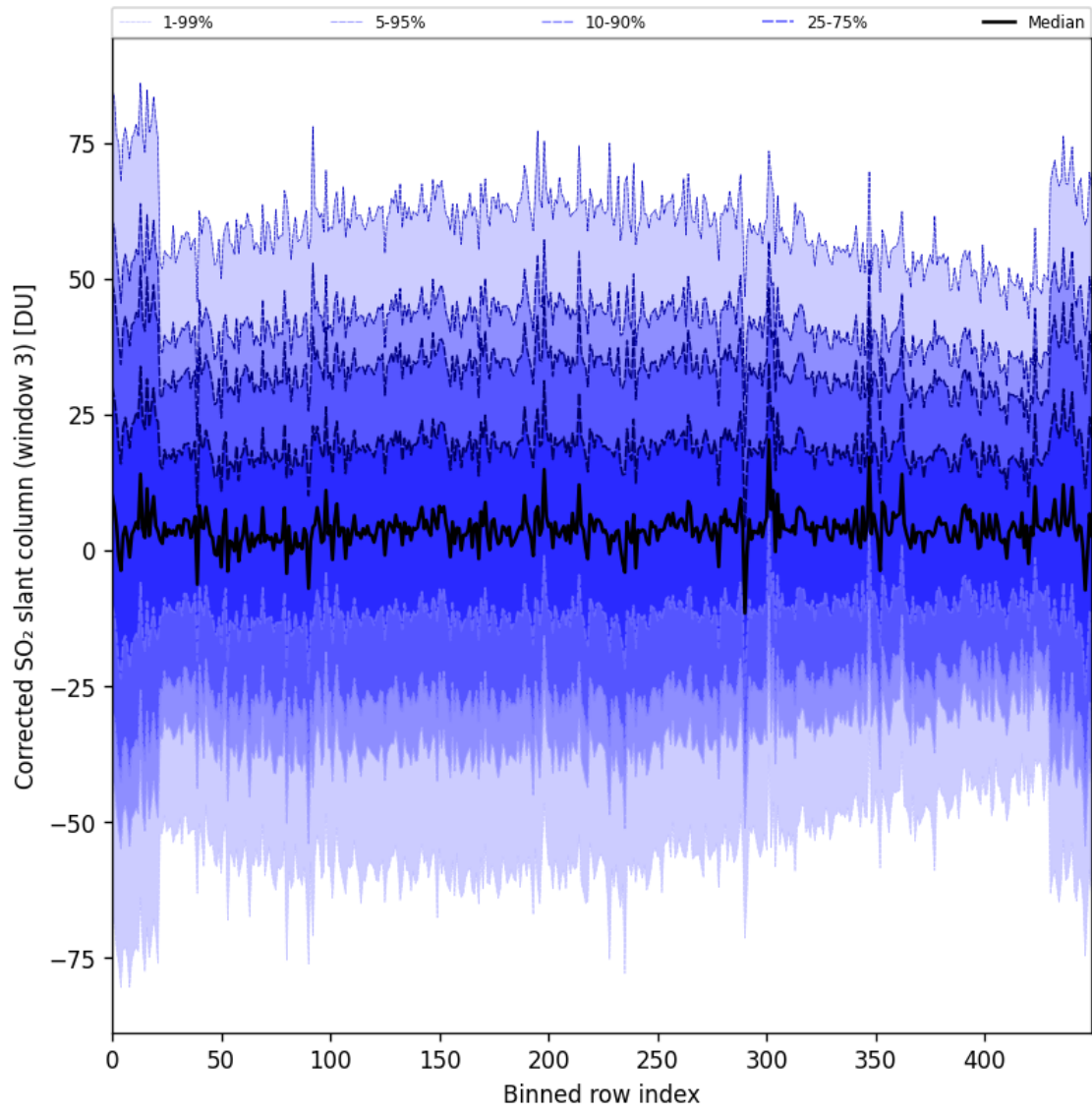
Figure 99: Along track statistics of “Corrected SO 2 slant column (window 3)” for 2025-09-26 to 2025-09-27
