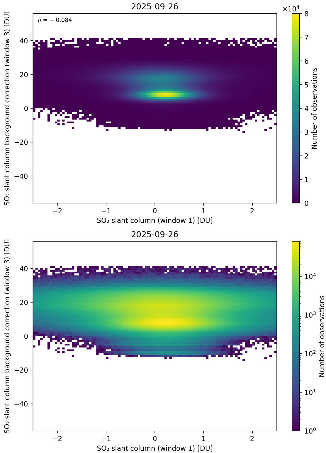
Figure 264: Scatter density plot of “SO 2 slant column (window 1)” against “SO 2 slant column background correction (window 3)” for 2025-09-26 to 2025-09-27.
