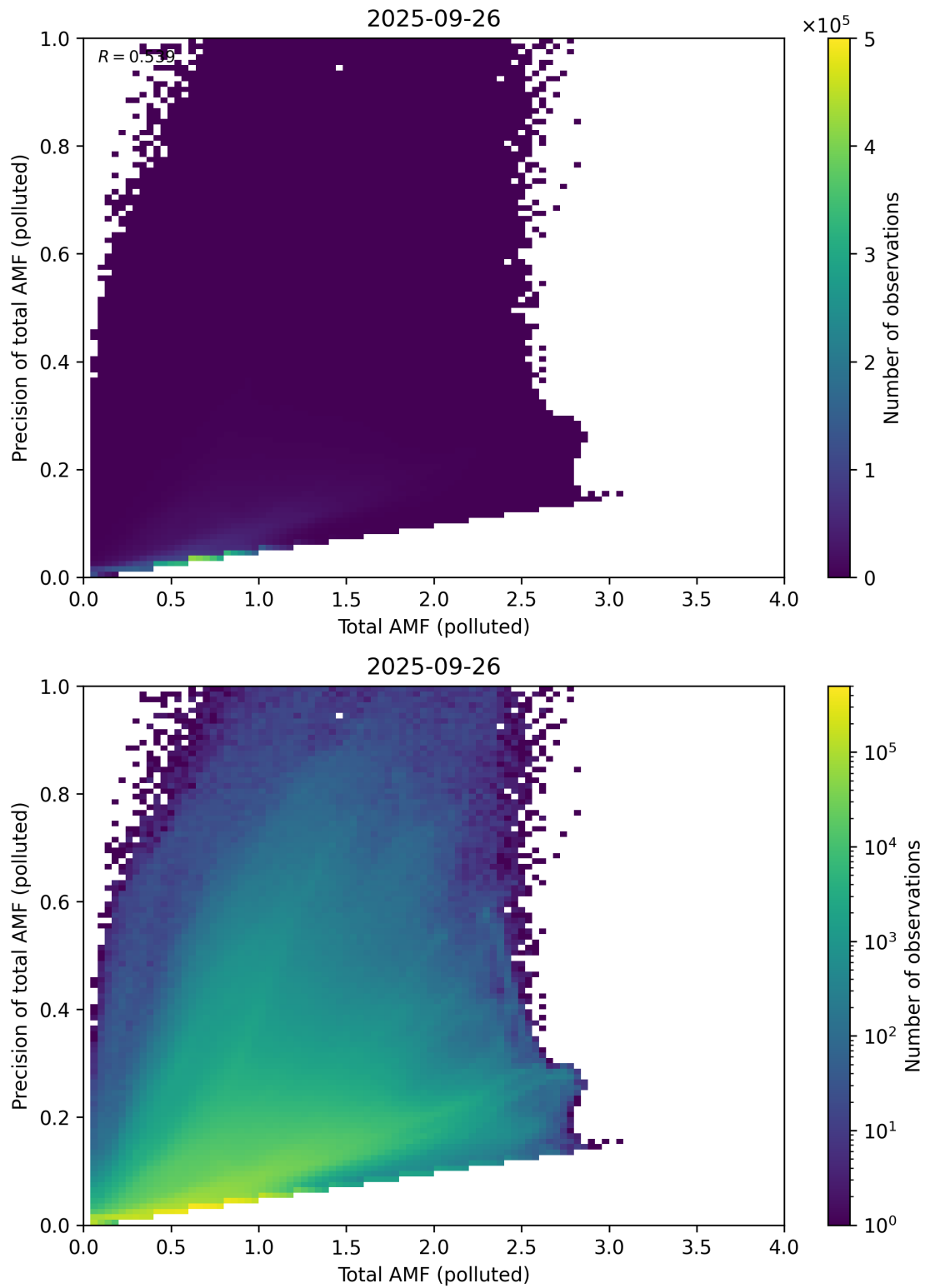
Figure 322: Scatter density plot of “Total AMF (polluted)” against “Precision of total AMF (polluted)” for 2025-09-26 to 2025-09-27.
