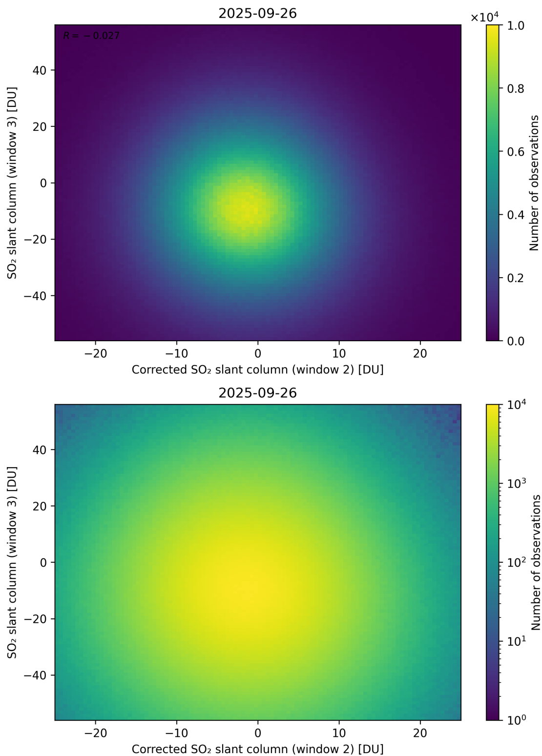
Figure 251: Scatter density plot of “Corrected SO 2 slant column (window 2)” against “SO 2 slant column (window 3)” for 2025-09-26 to 2025-09-27.
