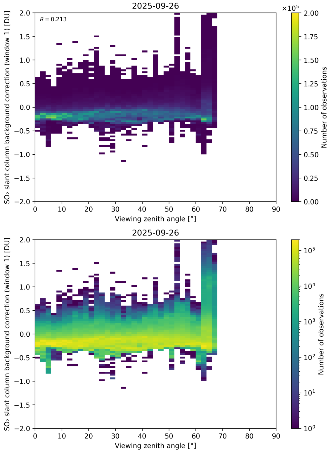
Figure 362: Scatter density plot of “Viewing zenith angle” against “SO 2 slant column background correction (window 1)” for 2025-09-26 to 2025-09-27.
