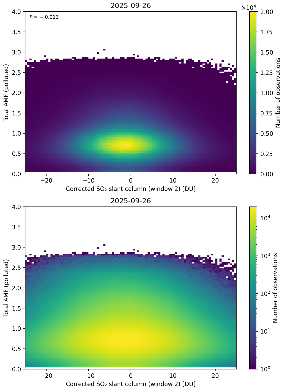
Figure 253: Scatter density plot of “Corrected SO 2 slant column (window 2)” against “Total AMF (polluted)” for 2025-09-26 to 2025-09-27.
