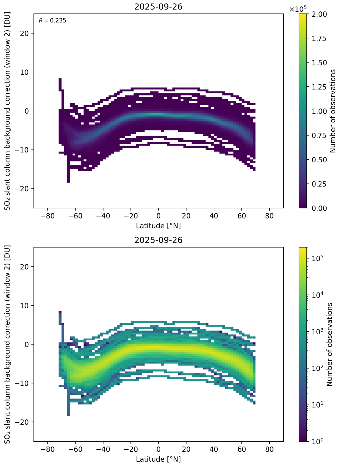
Figure 151: Scatter density plot of “Latitude” against “SO 2 slant column background correction (window 2)” for 2025-09-26 to 2025-09-27.
