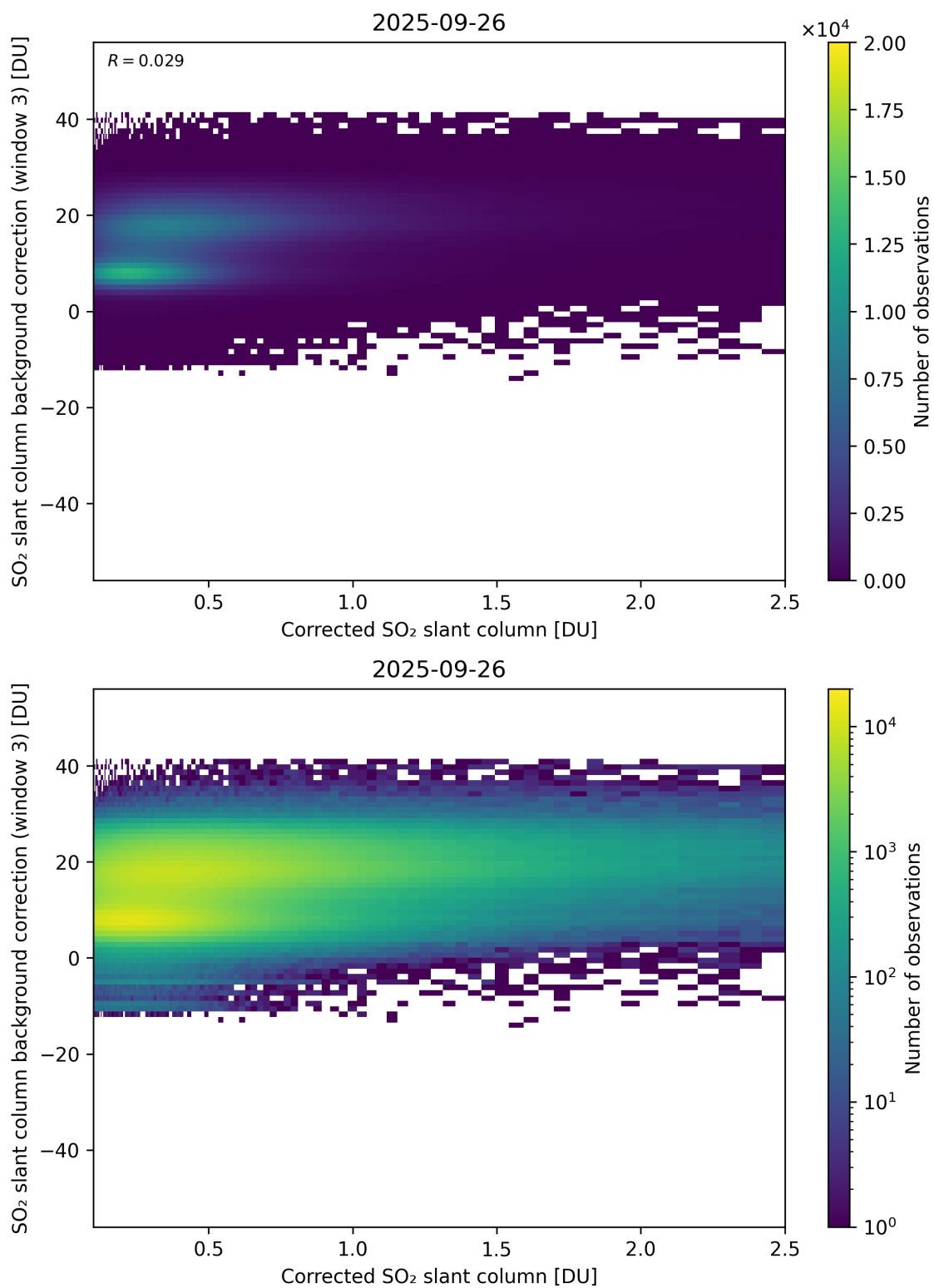
Figure 228: Scatter density plot of “Corrected SO 2 slant column” against “SO 2 slant column background correction (window 3)” for 2025-09-26 to 2025-09-27.
