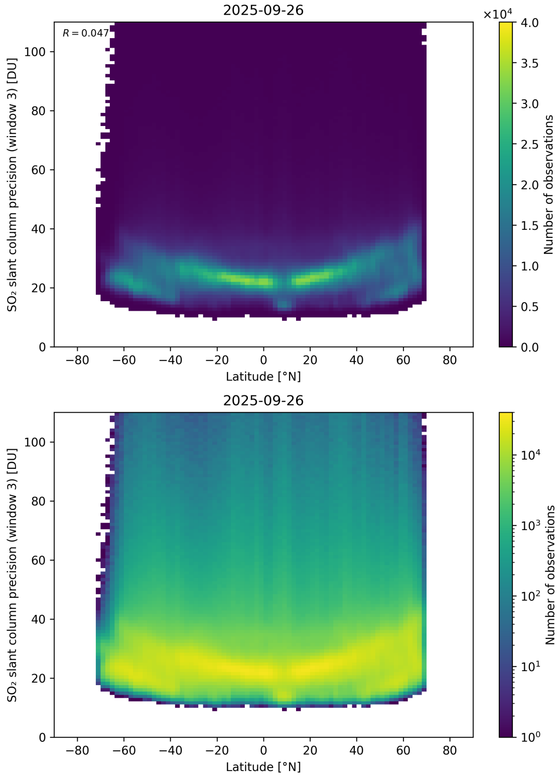
Figure 166: Scatter density plot of “Latitude” against “SO 2 slant column precision (window 3)” for 2025-09-26 to 2025-09-27.
