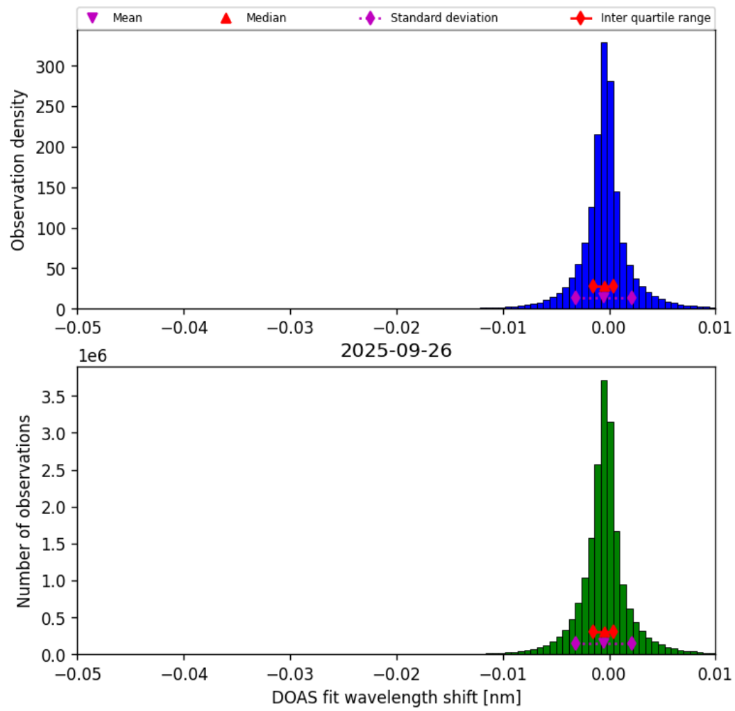
Figure 76: Histogram of “DOAS fit wavelength shift” for 2025-09-26 to 2025-09-27
