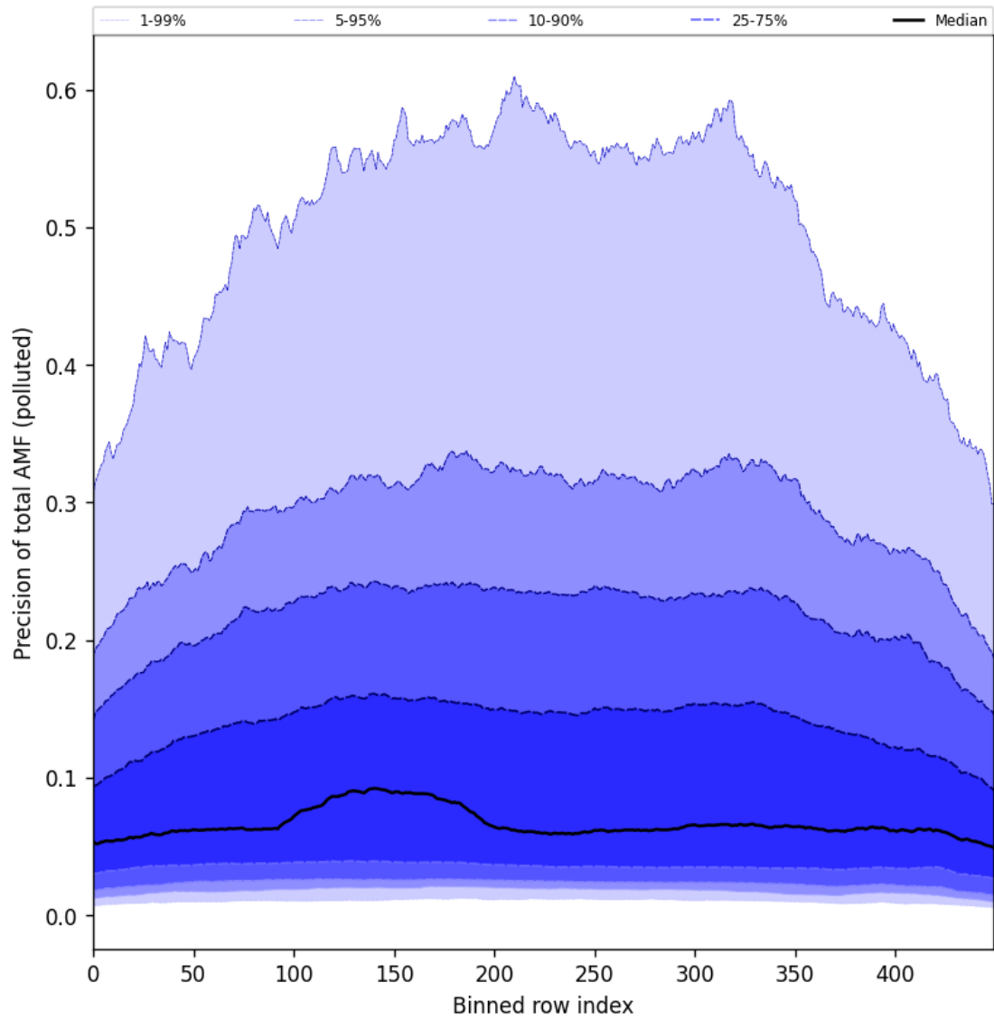
Figure 106: Along track statistics of “Precision of total AMF (polluted)” for 2025-09-26 to 2025-09-27
