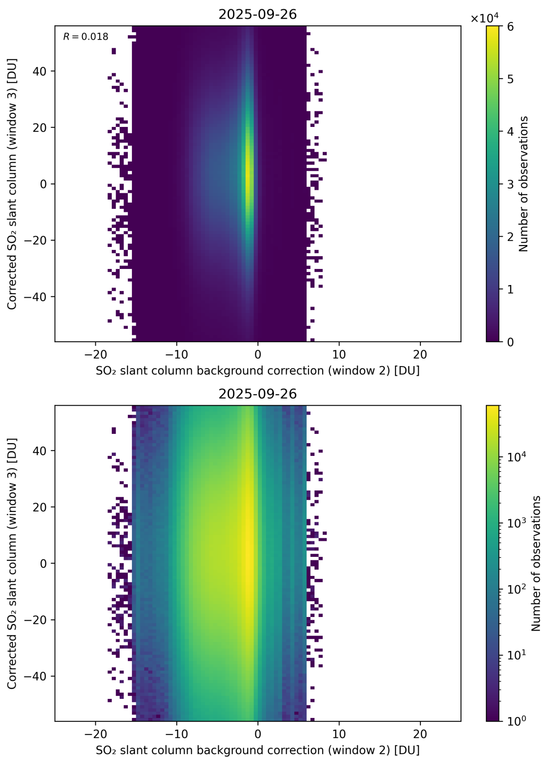
Figure 127: Scatter density plot of “SO 2 slant column background correction (window 2)” against “Corrected SO 2 slant column (window 3)” for 2025-09-26 to 2025-09-27.
