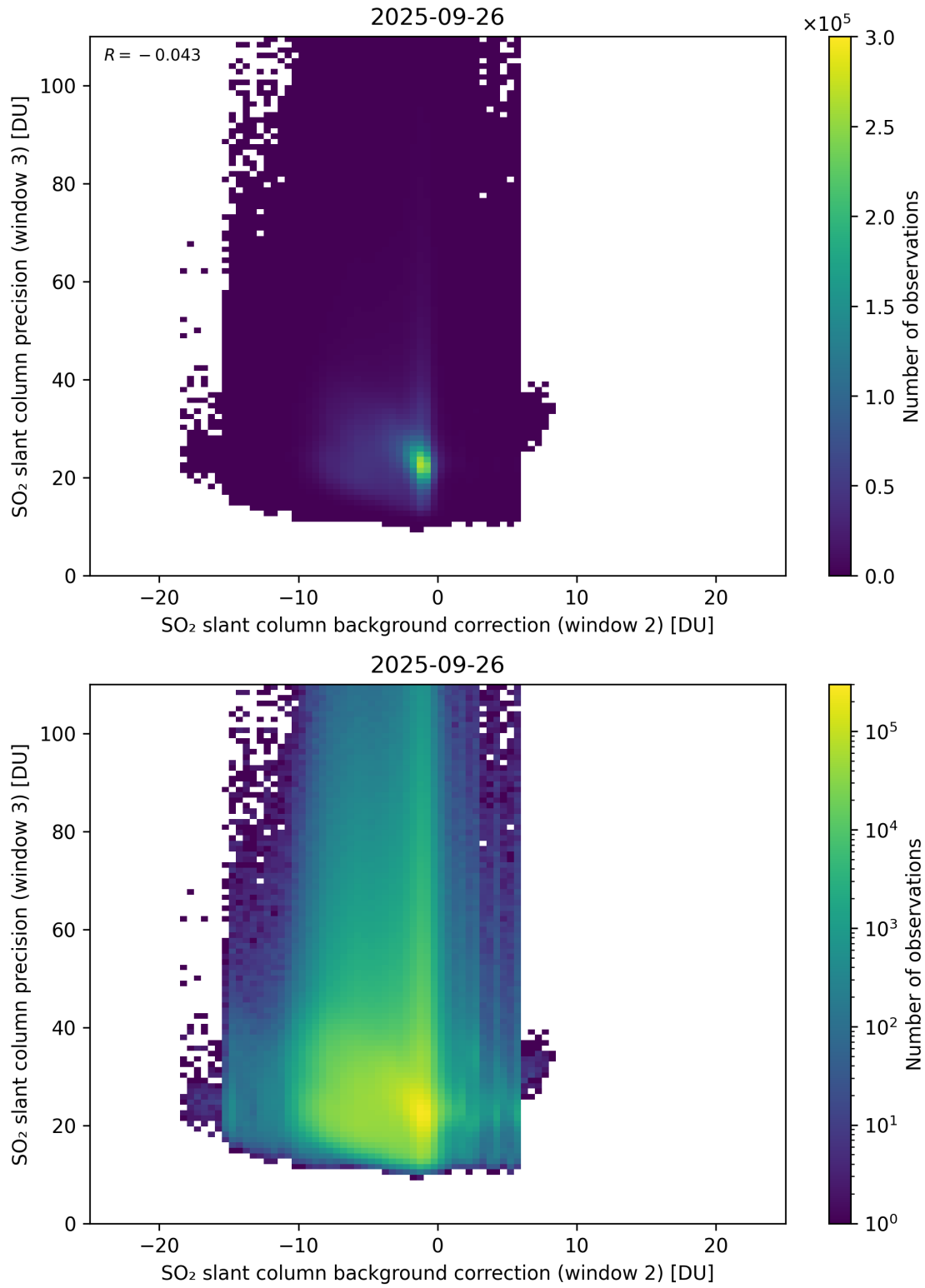
Figure 129: Scatter density plot of “SO 2 slant column background correction (window 2)” against “SO 2 slant column precision (window 3)” for 2025-09-26 to 2025-09-27.
