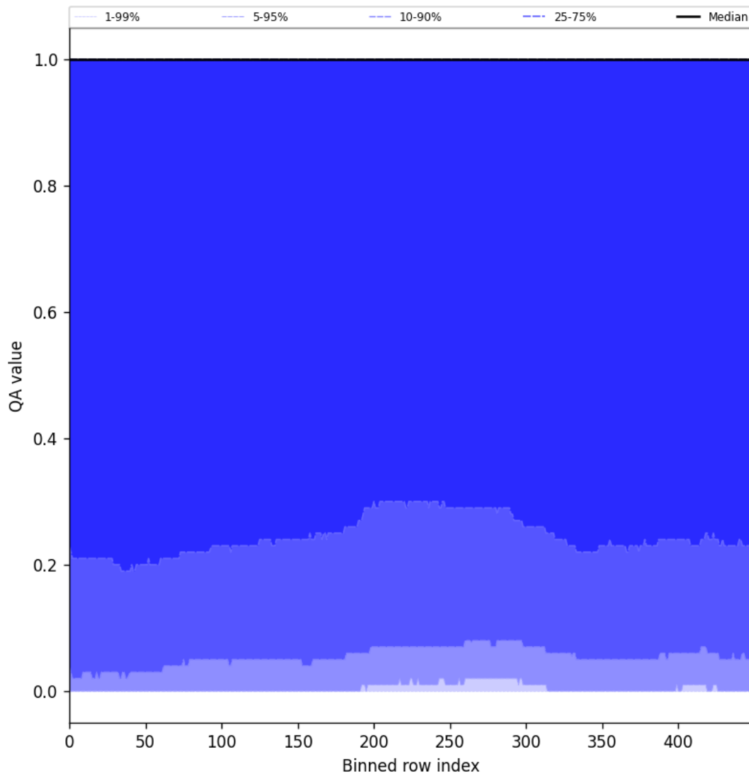
Figure 83: Along track statistics of “QA value” for 2025-09-26 to 2025-09-27
