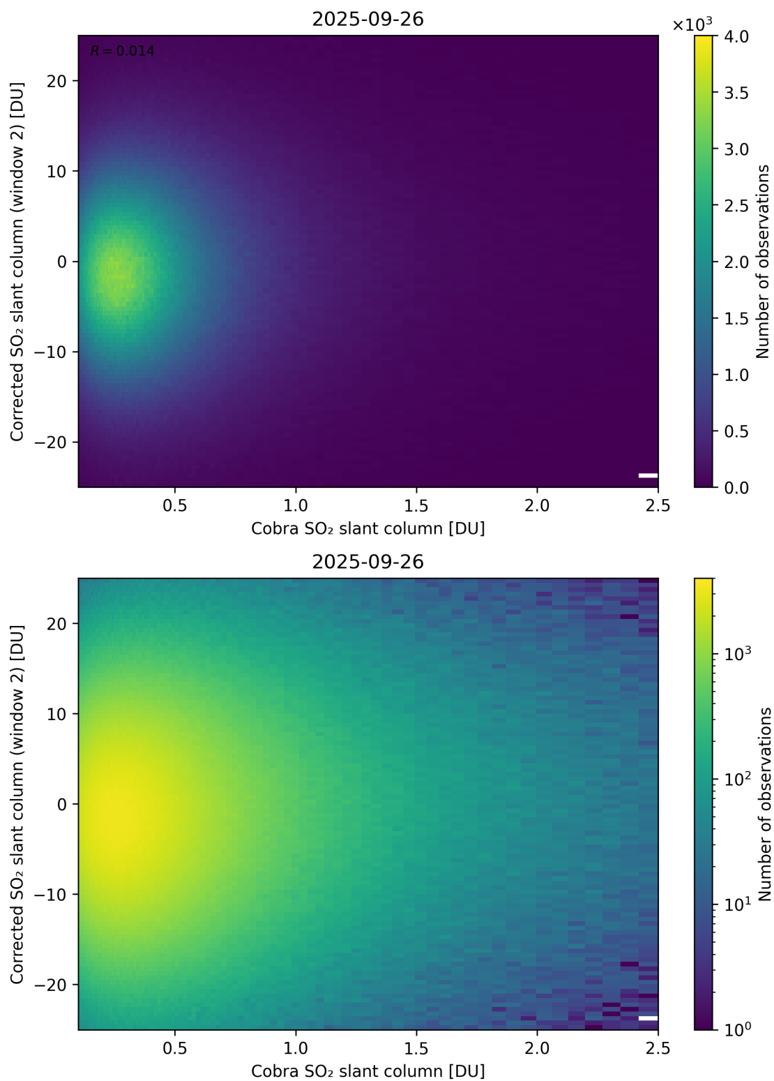
Figure 217: Scatter density plot of “Cobra SO 2 slant column” against “Corrected SO 2 slant column (window 2)” for 2025-09-26 to 2025-09-27.
