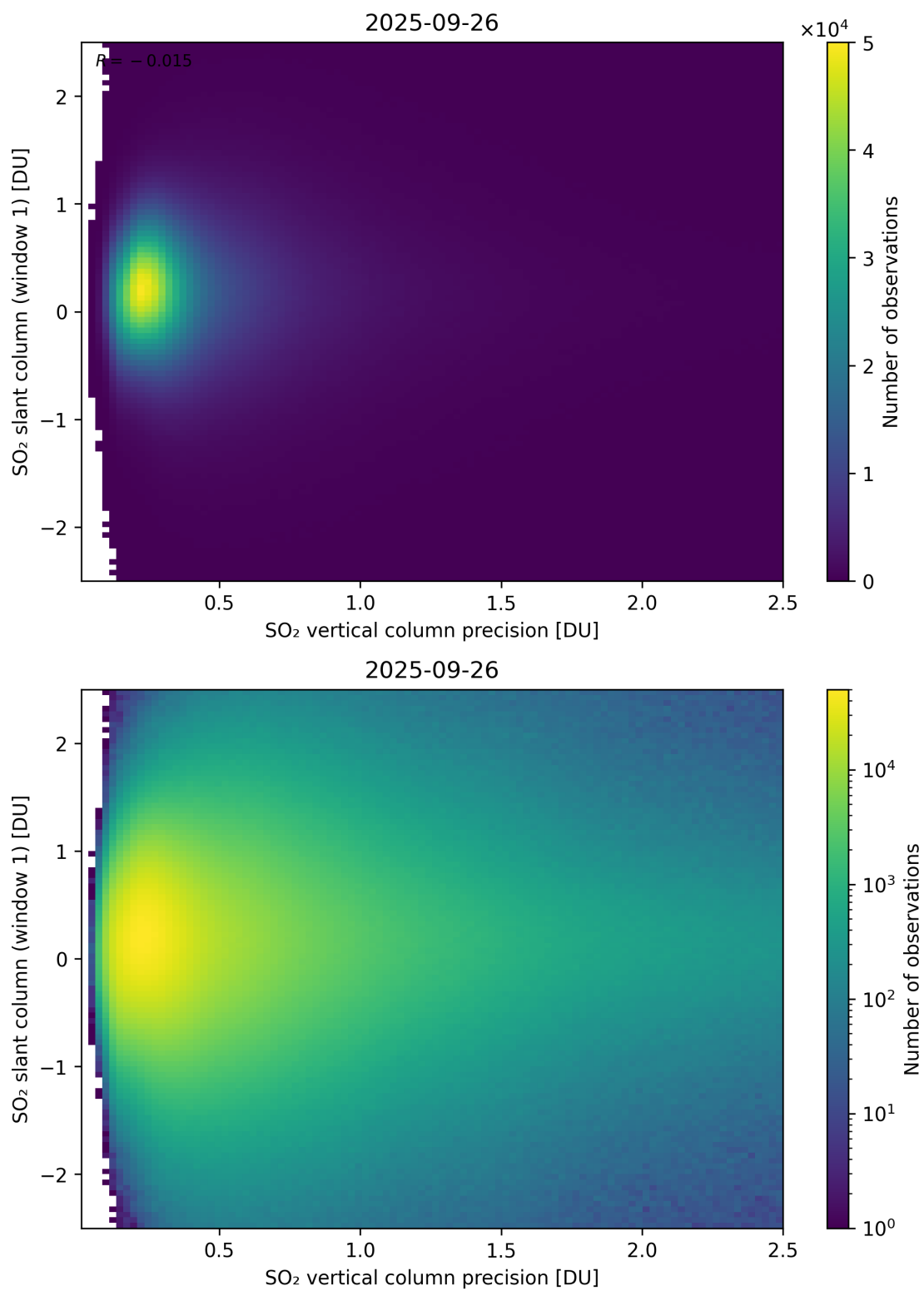
Figure 341: Scatter density plot of “SO 2 vertical column precision” against “SO 2 slant column (window 1)” for 2025-09-26 to 2025-09-27.
