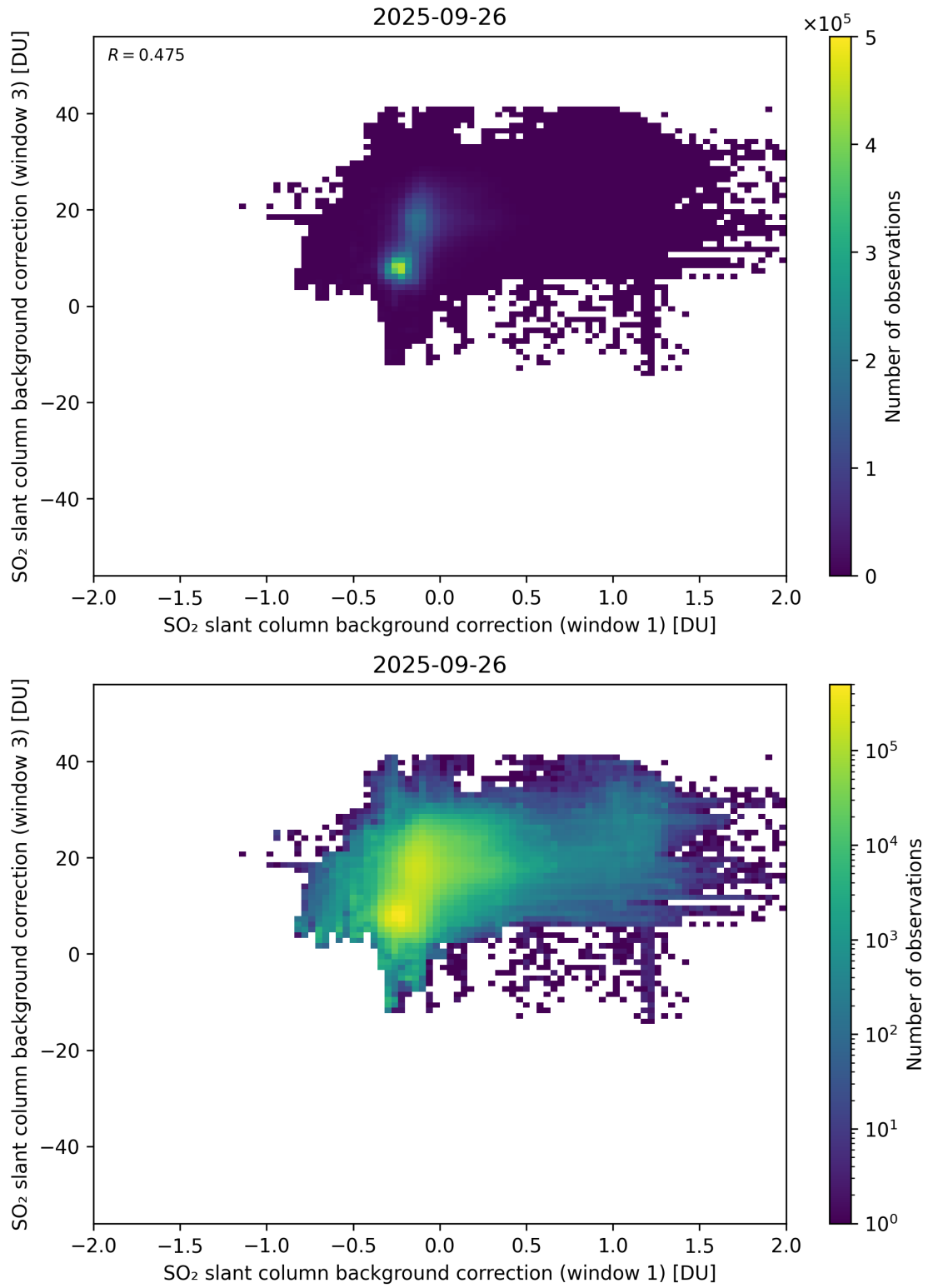
Figure 110: Scatter density plot of “SO 2 slant column background correction (window 1)” against “SO 2 slant column background correction (window 3)” for 2025-09-26 to 2025-09-27.
