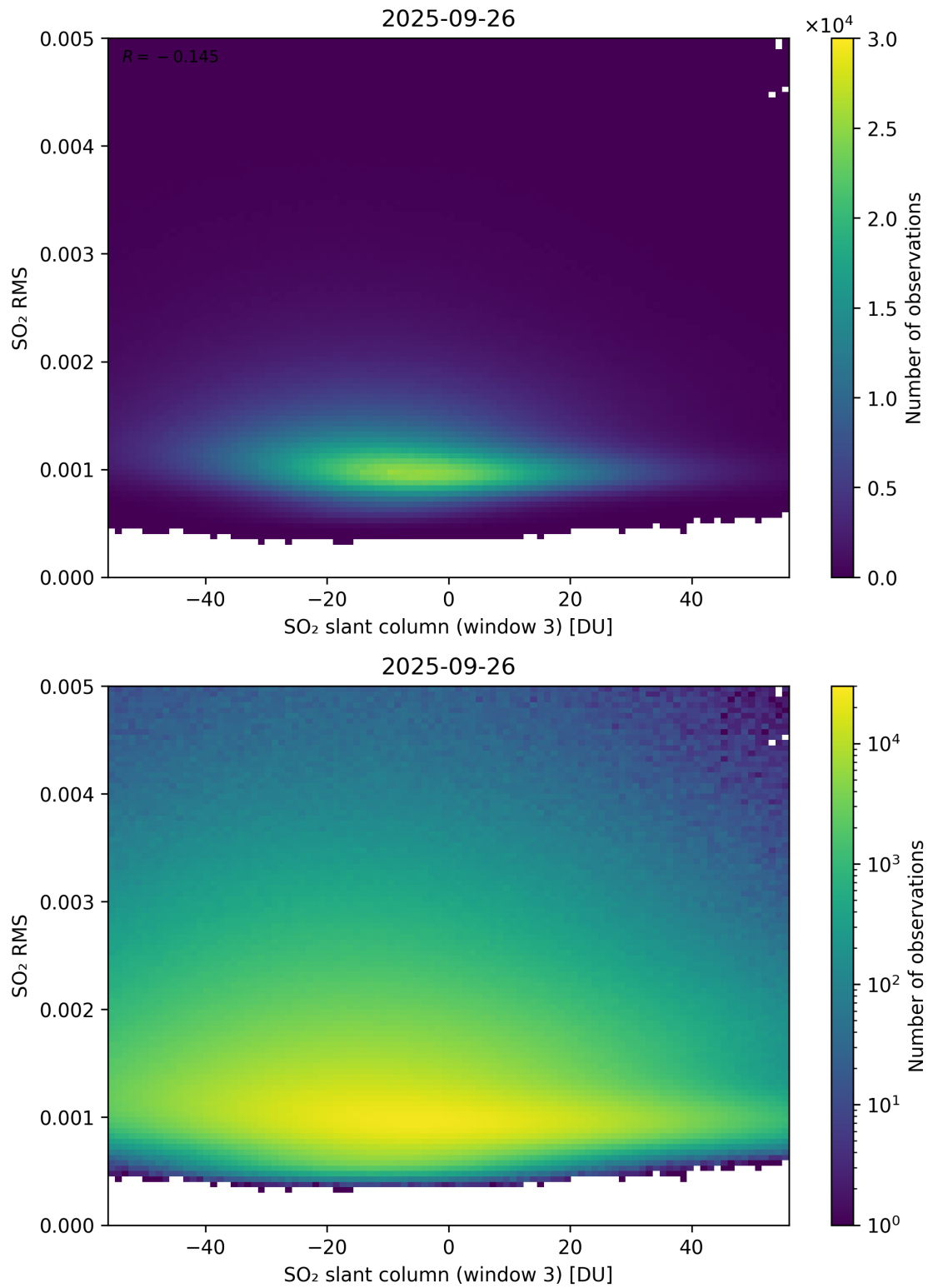
Figure 306: Scatter density plot of “SO 2 slant column (window 3)” against “SO 2 RMS” for 2025-09-26 to 2025-09-27.
