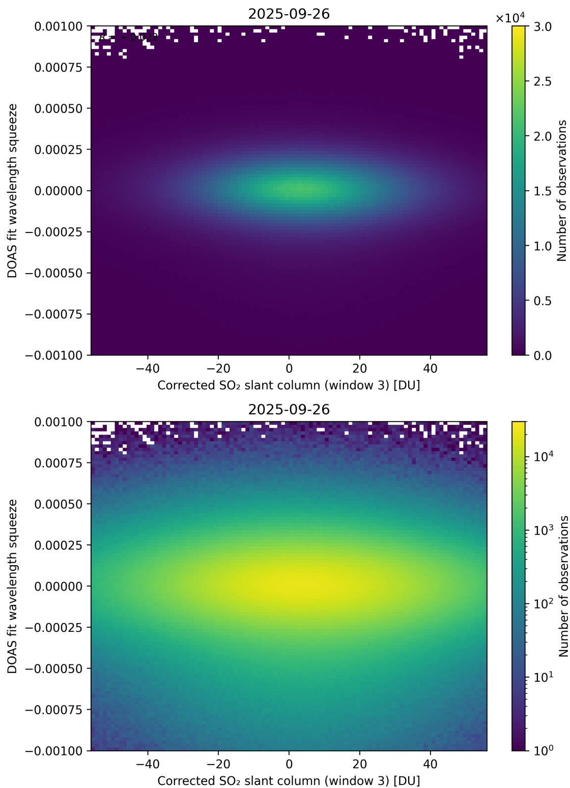
Figure 257: Scatter density plot of “Corrected SO 2 slant column (window 3)” against “DOAS fit wavelength squeeze” for 2025-09-26 to 2025-09-27.
