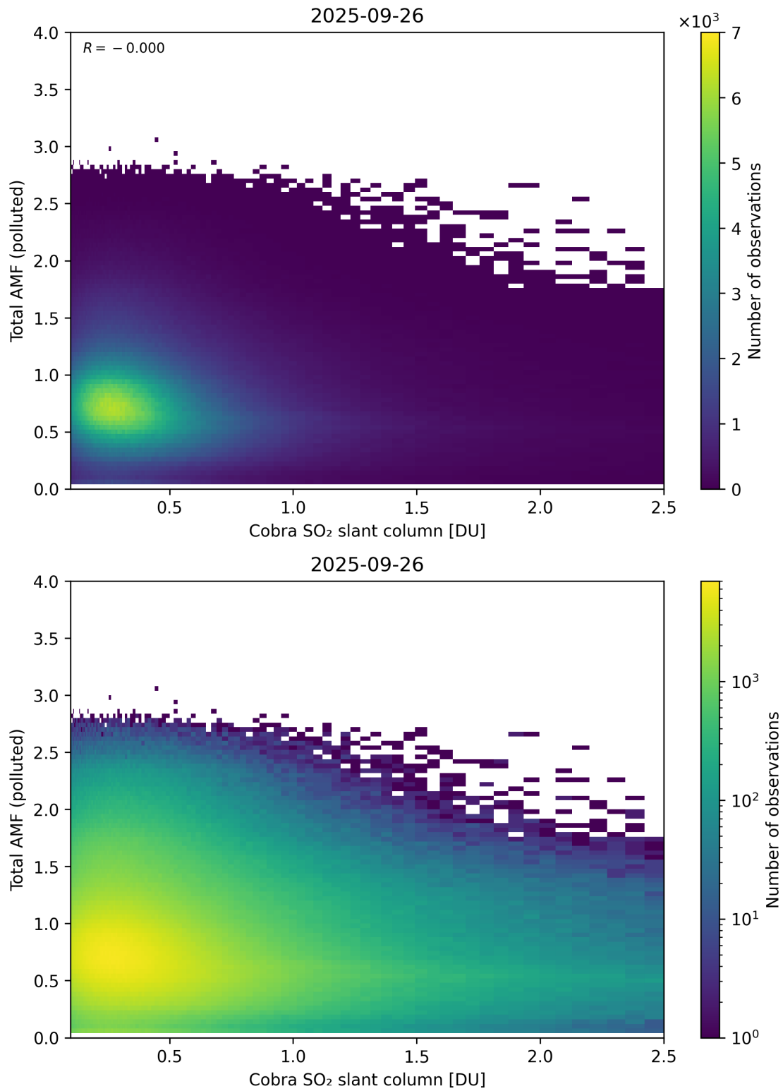
Figure 224: Scatter density plot of “Cobra SO 2 slant column” against “Total AMF (polluted)” for 2025-09-26 to 2025-09-27.
