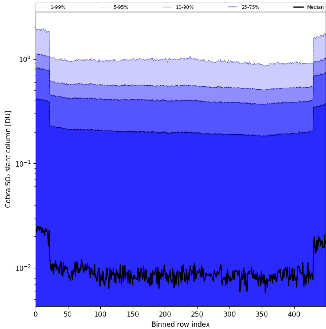
Figure 87: Along track statistics of “Cobra SO 2 slant column” for 2025-09-26 to 2025-09-27
