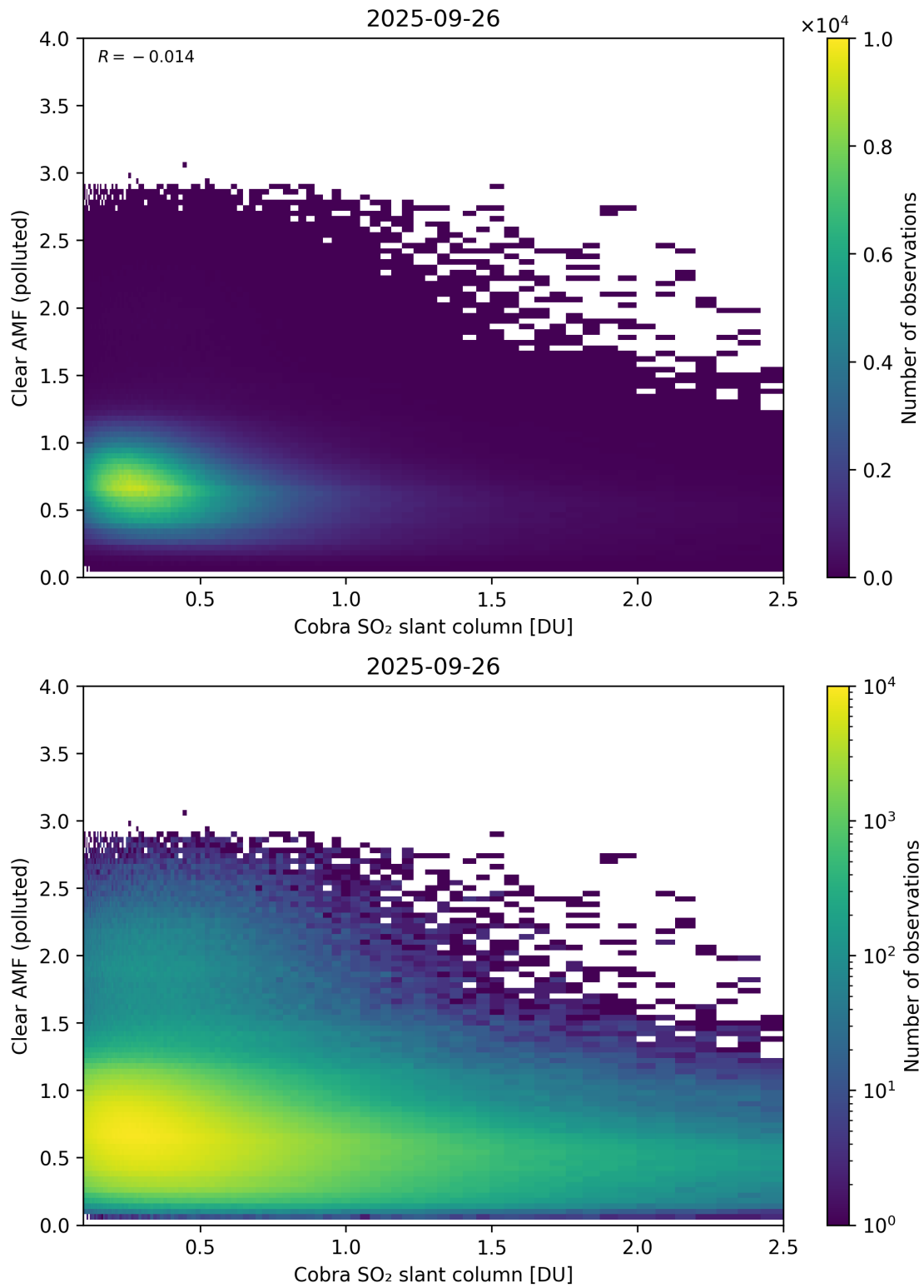
Figure 215: Scatter density plot of “Cobra SO 2 slant column” against “Clear AMF (polluted)” for 2025-09-26 to 2025-09-27.
