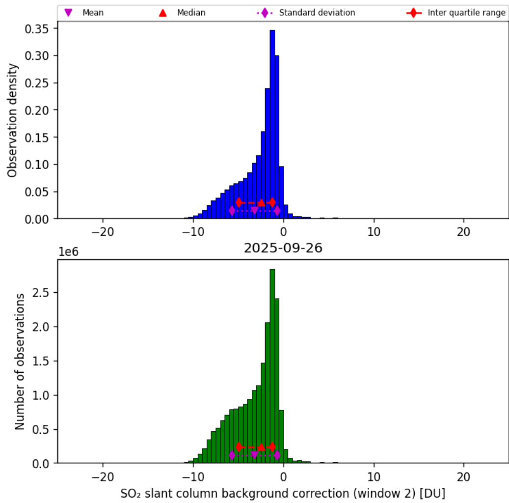
Figure 70: Histogram of “SO 2 slant column background correction (window 2)” for 2025-09-26 to 2025-09-27
