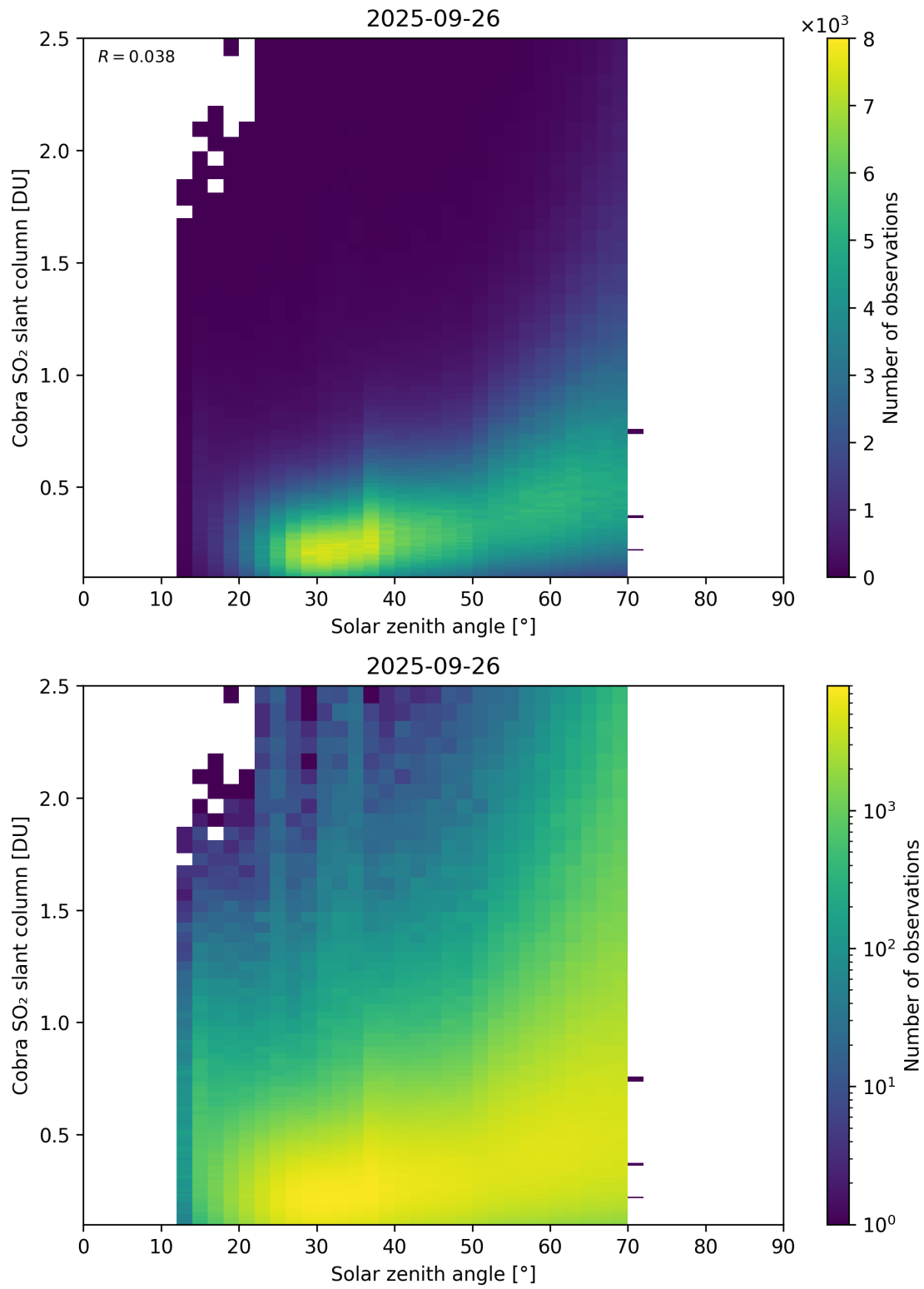
Figure 179: Scatter density plot of “Solar zenith angle” against “Cobra SO 2 slant column” for 2025-09-26 to 2025-09-27.
