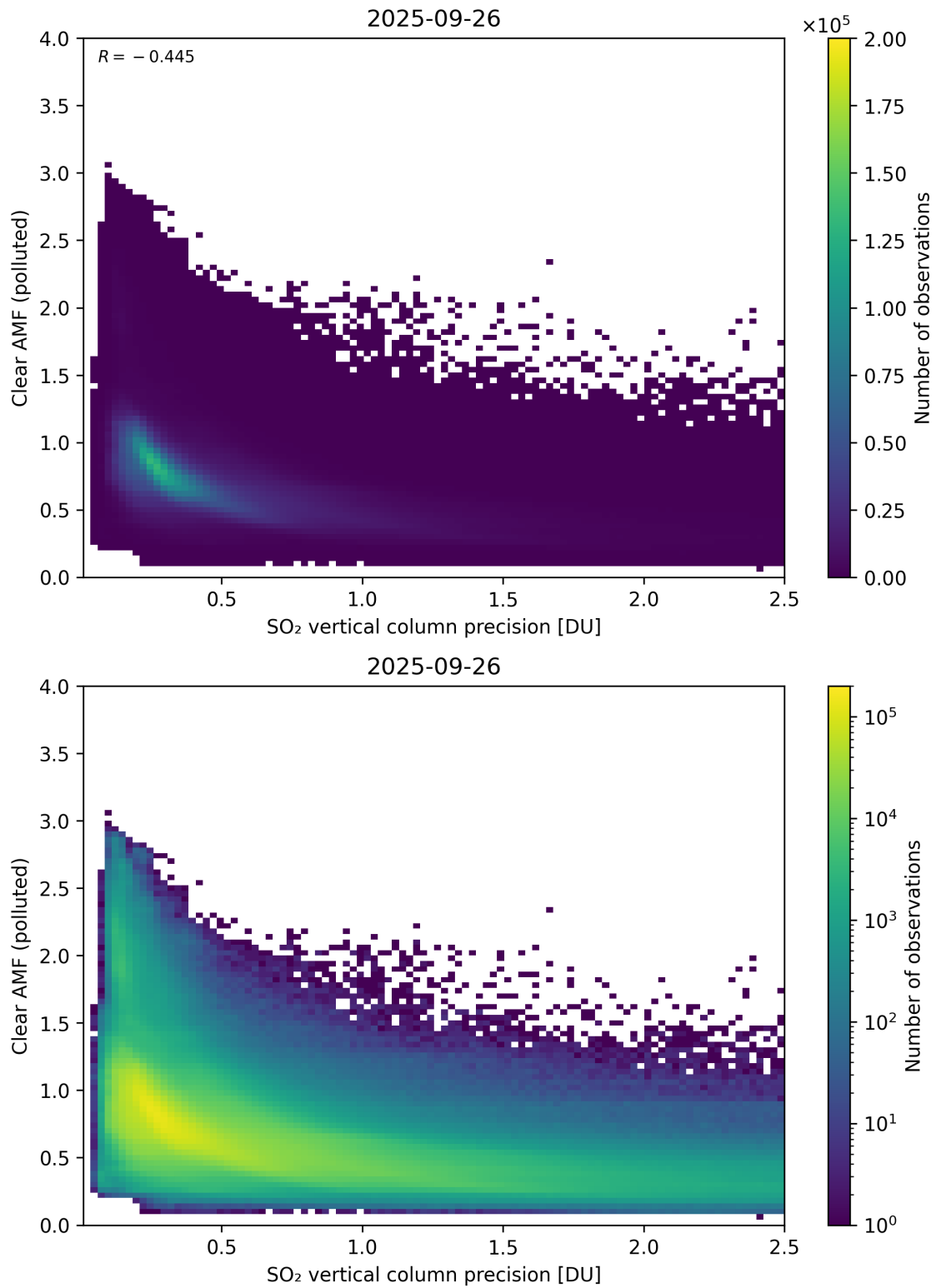
Figure 335: Scatter density plot of “SO 2 vertical column precision” against “Clear AMF (polluted)” for 2025-09-26 to 2025-09-27.
