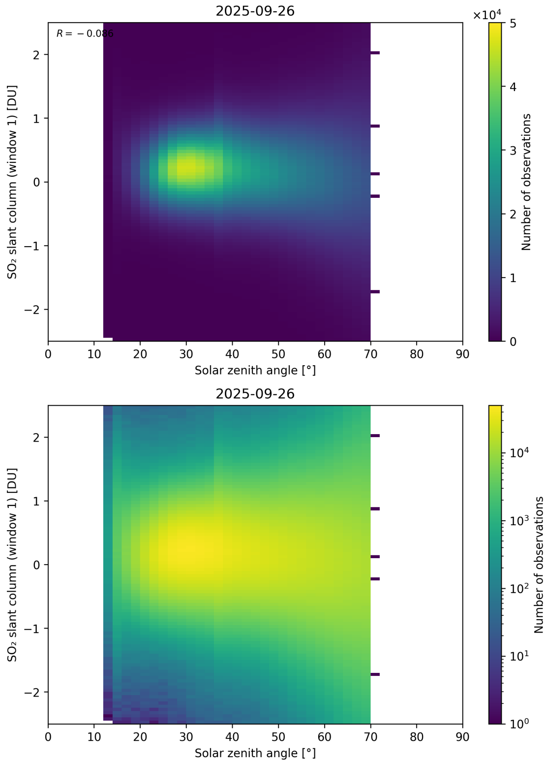
Figure 184: Scatter density plot of “Solar zenith angle” against “SO 2 slant column (window 1)” for 2025-09-26 to 2025-09-27.
