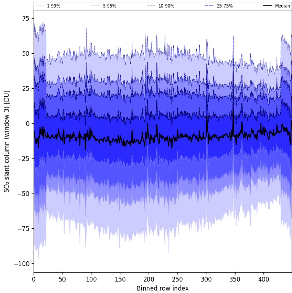
Figure 97: Along track statistics of “SO 2 slant column (window 3)” for 2025-09-26 to 2025-09-27
