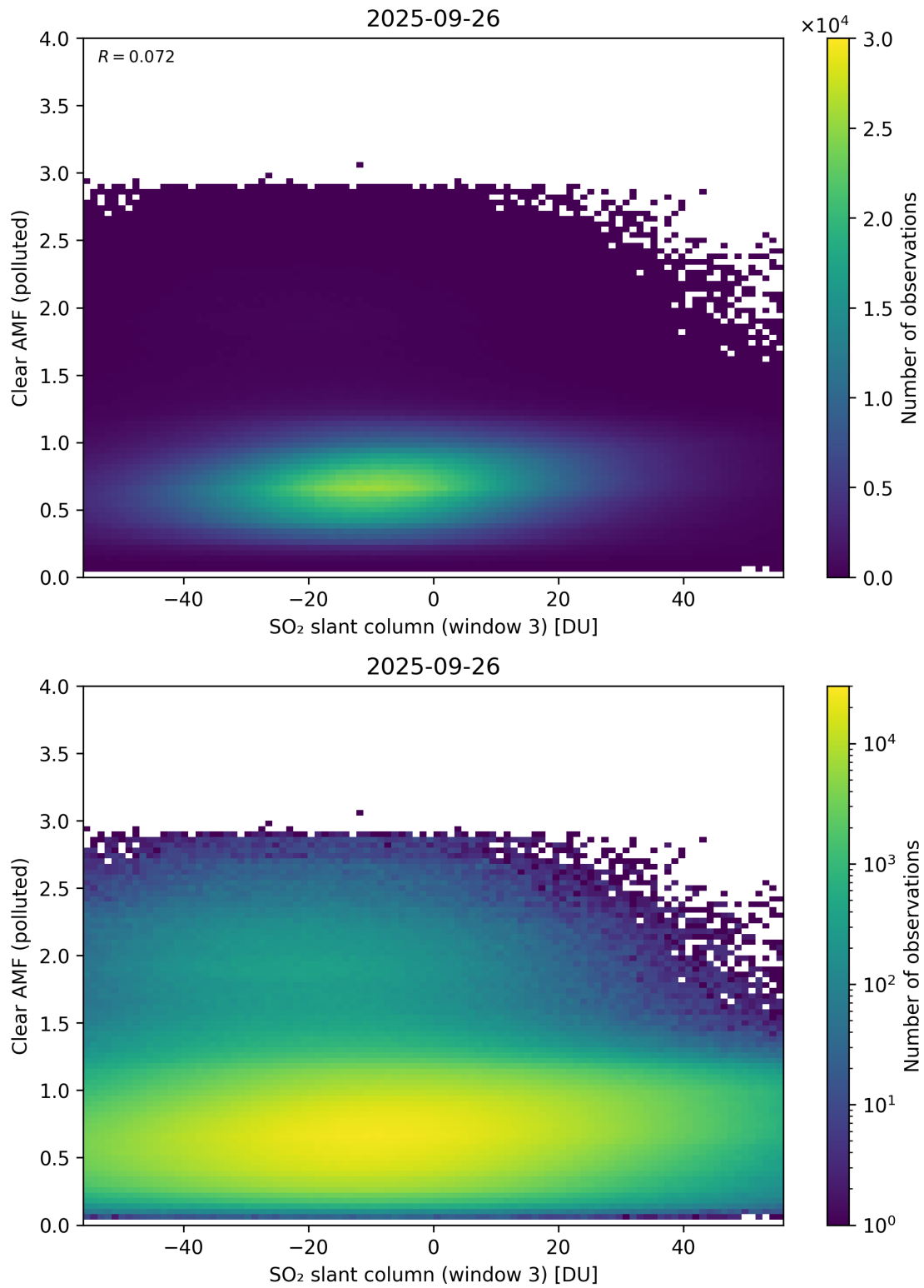
Figure 315: Scatter density plot of “SO 2 slant column (window 3)” against “Clear AMF (polluted)” for 2025-09-26 to 2025-09-27.
