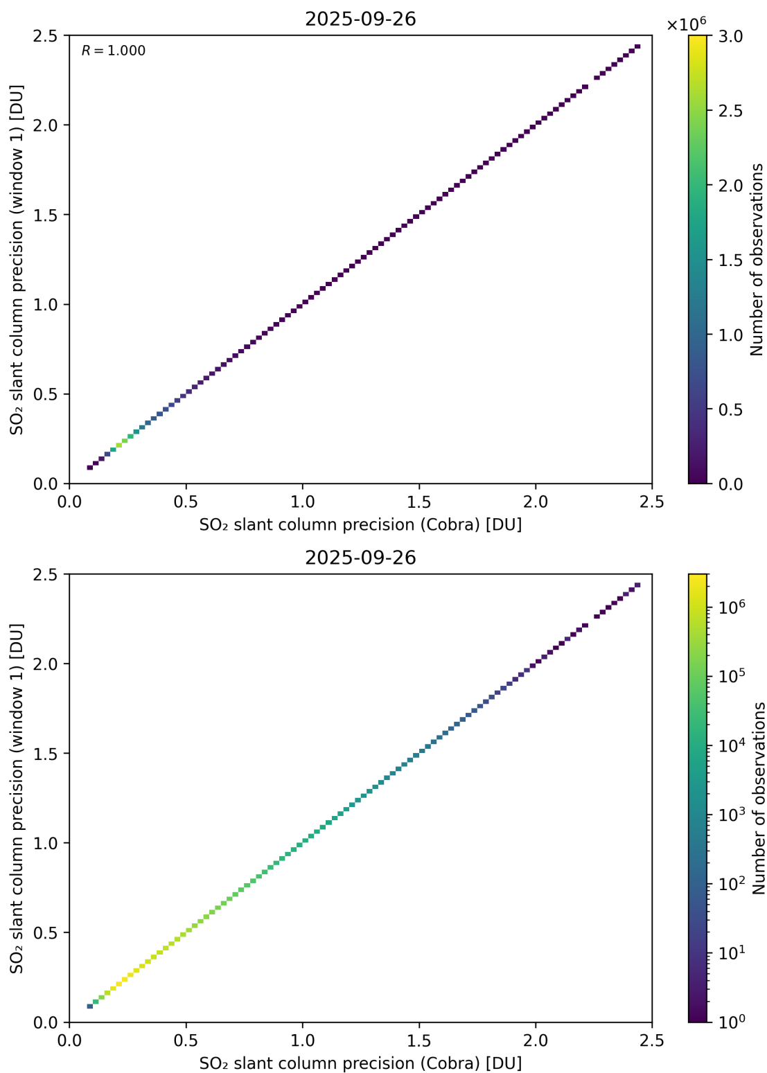
Figure 209: Scatter density plot of “SO 2 slant column precision (Cobra)” against “SO 2 slant column precision (window 1)” for 2025-09-26 to 2025-09-27.
