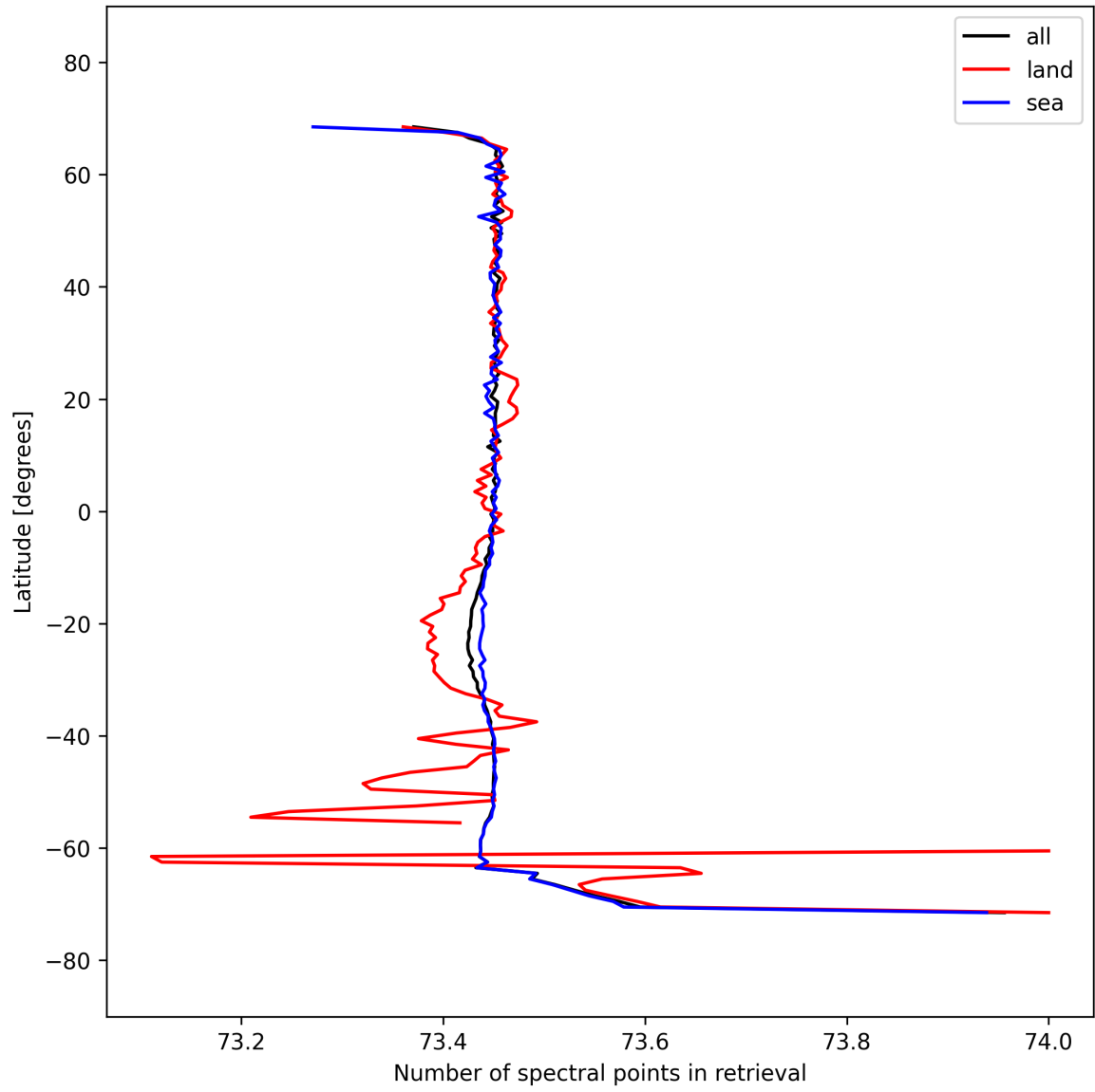
Figure 56: Zonal average of “Number of spectral points in retrieval” for 2025-09-26 to 2025-09-27.
