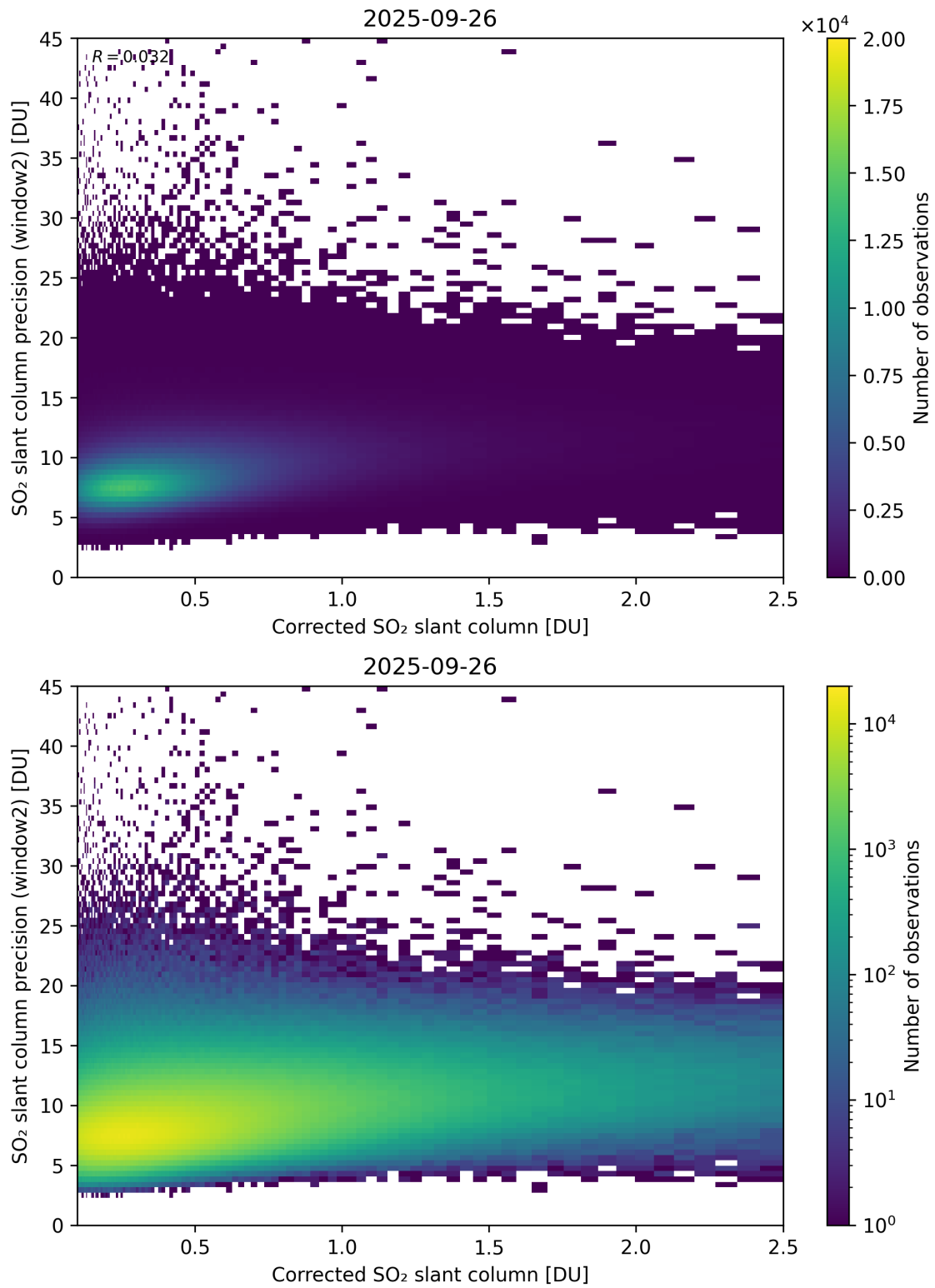
Figure 239: Scatter density plot of “Corrected SO 2 slant column” against “SO 2 slant column precision (window2)” for 2025-09-26 to 2025-09-27.
