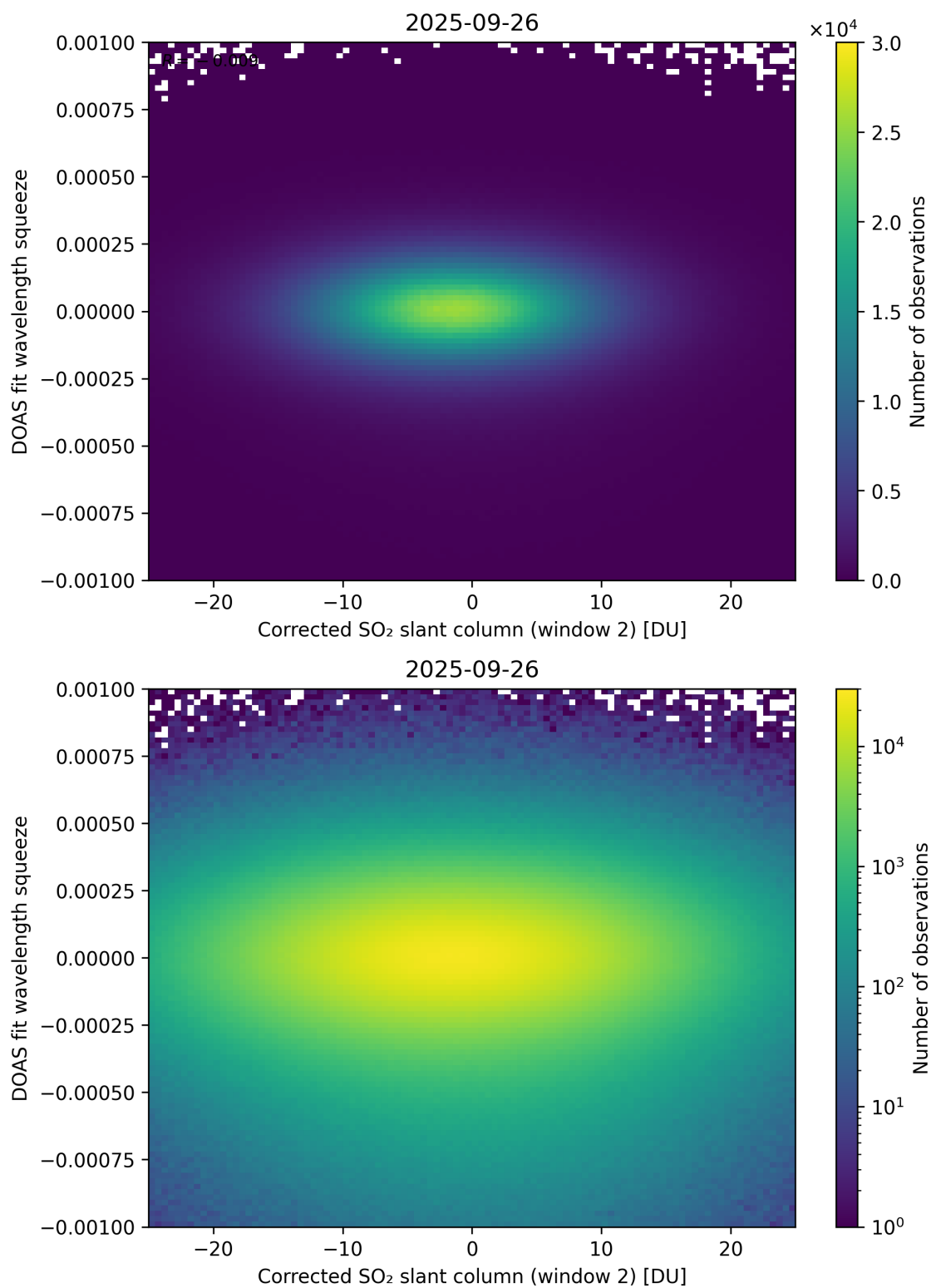
Figure 247: Scatter density plot of “Corrected SO 2 slant column (window 2)” against “DOAS fit wavelength squeeze” for 2025-09-26 to 2025-09-27.
