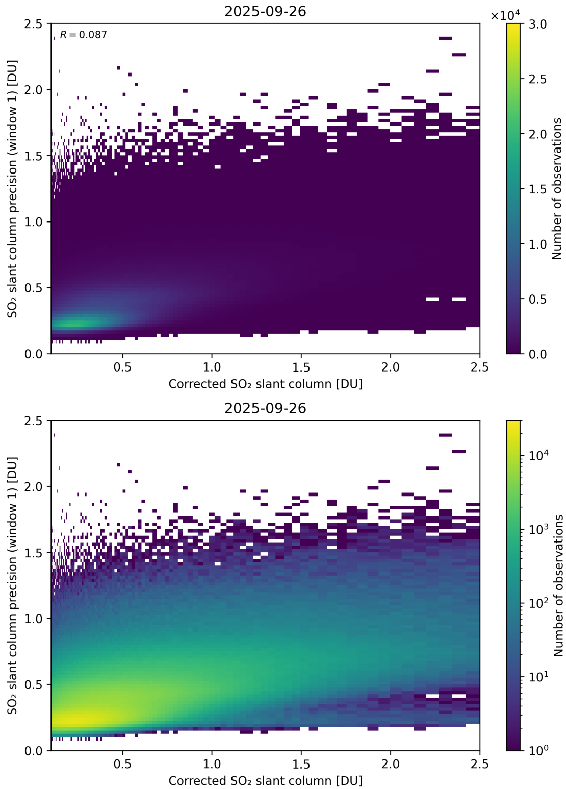
Figure 238: Scatter density plot of “Corrected SO 2 slant column” against “SO 2 slant column precision (window 1)” for 2025-09-26 to 2025-09-27.
