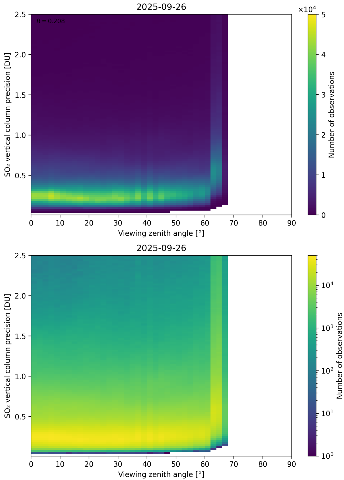
Figure 384: Scatter density plot of “Viewing zenith angle” against “SO 2 vertical column precision” for 2025-09-26 to 2025-09-27.
