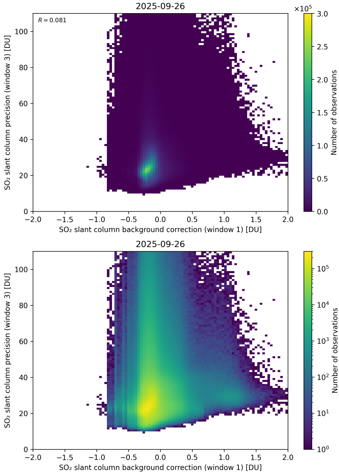
Figure 119: Scatter density plot of “SO 2 slant column background correction (window 1)” against “SO 2 slant column precision (window 3)” for 2025-09-26 to 2025-09-27.
