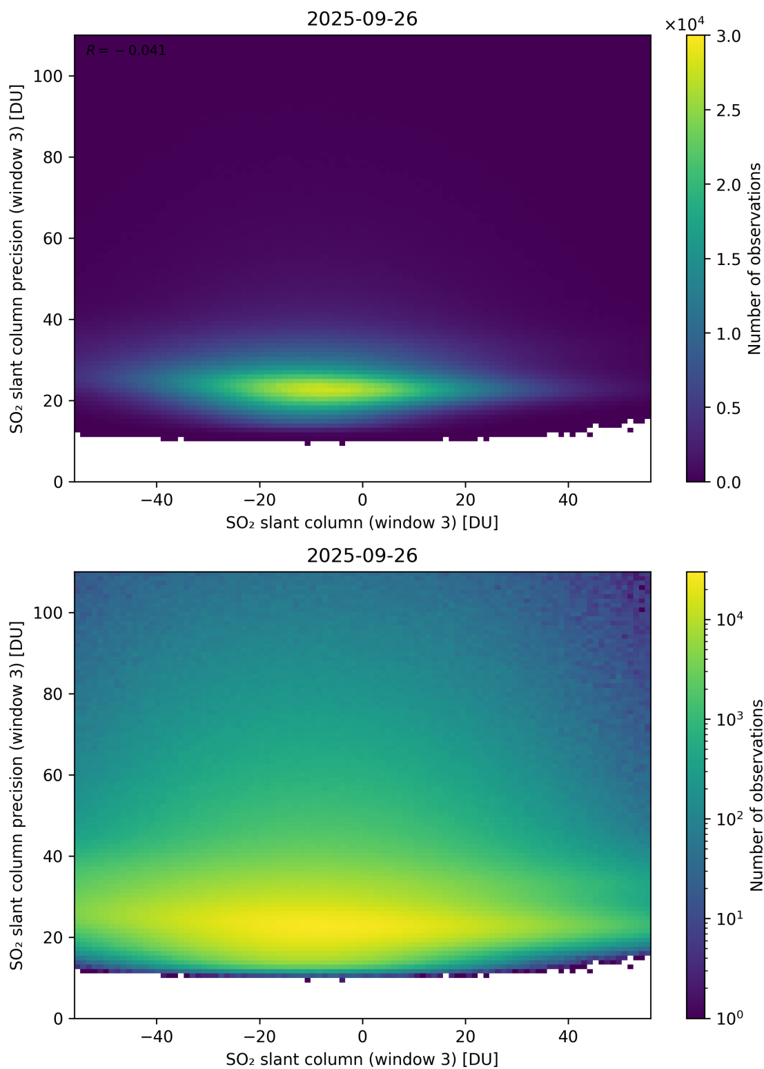
Figure 317: Scatter density plot of “SO 2 slant column (window 3)” against “SO 2 slant column precision (window 3)” for 2025-09-26 to 2025-09-27.
