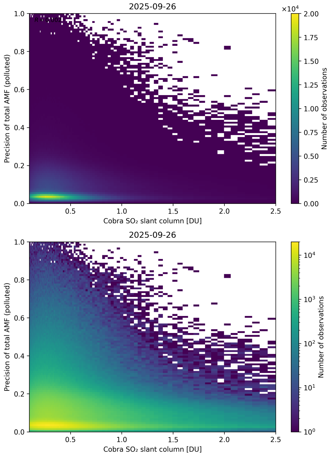
Figure 225: Scatter density plot of “Cobra SO 2 slant column” against “Precision of total AMF (polluted)” for 2025-09-26 to 2025-09-27.
