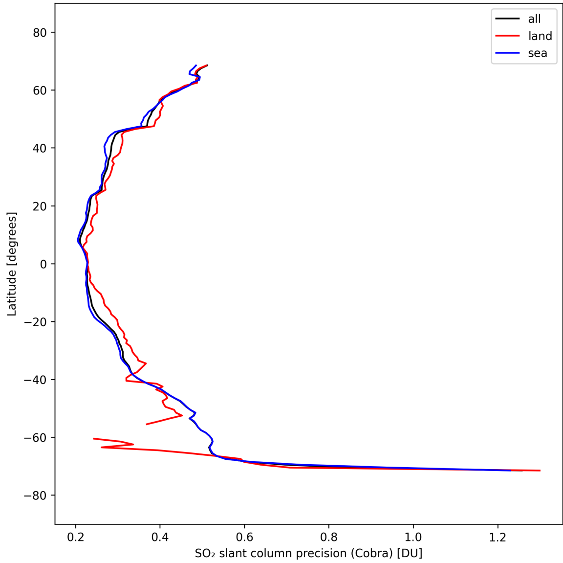
Figure 36: Zonal average of “SO 2 slant column precision (Cobra)” for 2025-09-26 to 2025-09-27.
