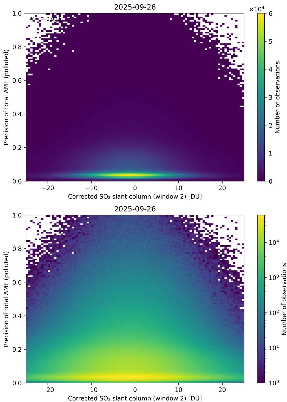
Figure 254: Scatter density plot of “Corrected SO 2 slant column (window 2)” against “Precision of total AMF (polluted)” for 2025-09-26 to 2025-09-27.
