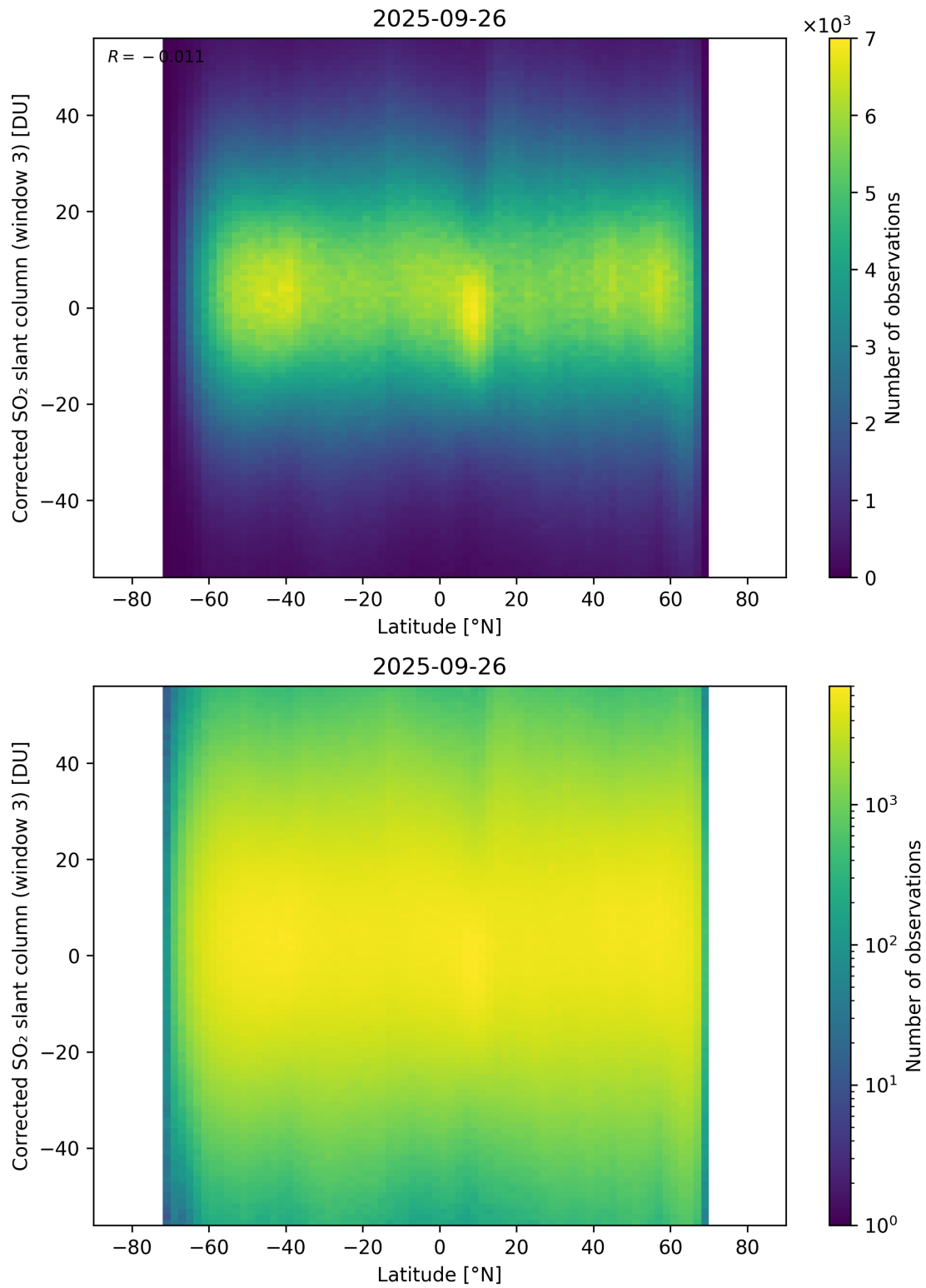
Figure 161: Scatter density plot of “Latitude” against “Corrected SO 2 slant column (window 3)” for 2025-09-26 to 2025-09-27.
