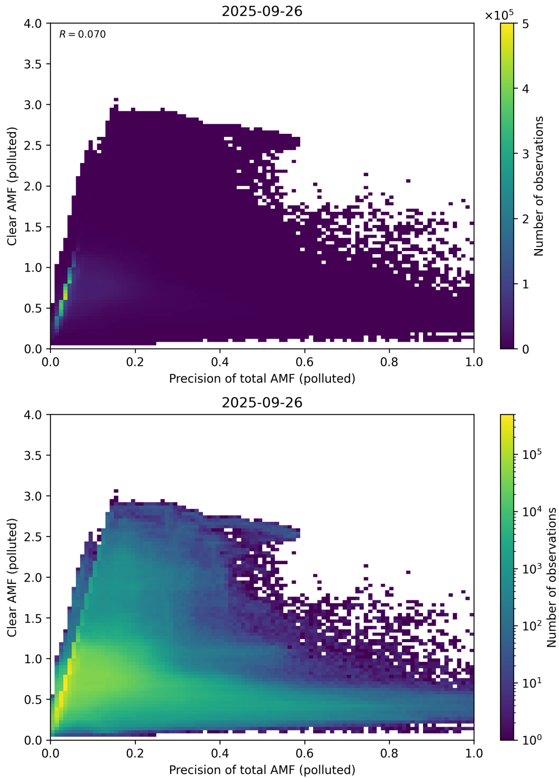
Figure 320: Scatter density plot of “Precision of total AMF (polluted)” against “Clear AMF (polluted)” for 2025-09-26 to 2025-09-27.
