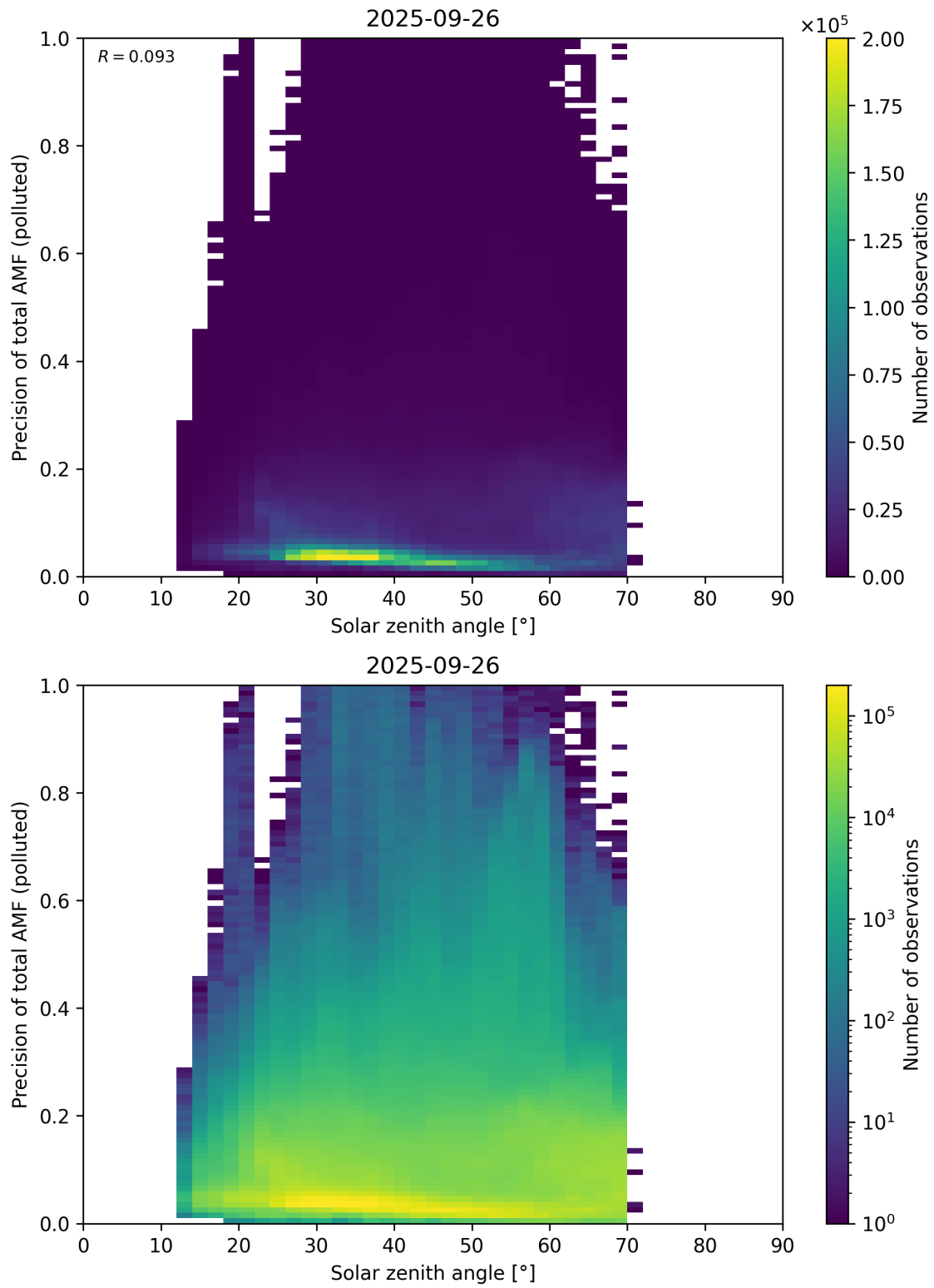
Figure 190: Scatter density plot of “Solar zenith angle” against “Precision of total AMF (polluted)” for 2025-09-26 to 2025-09-27.
