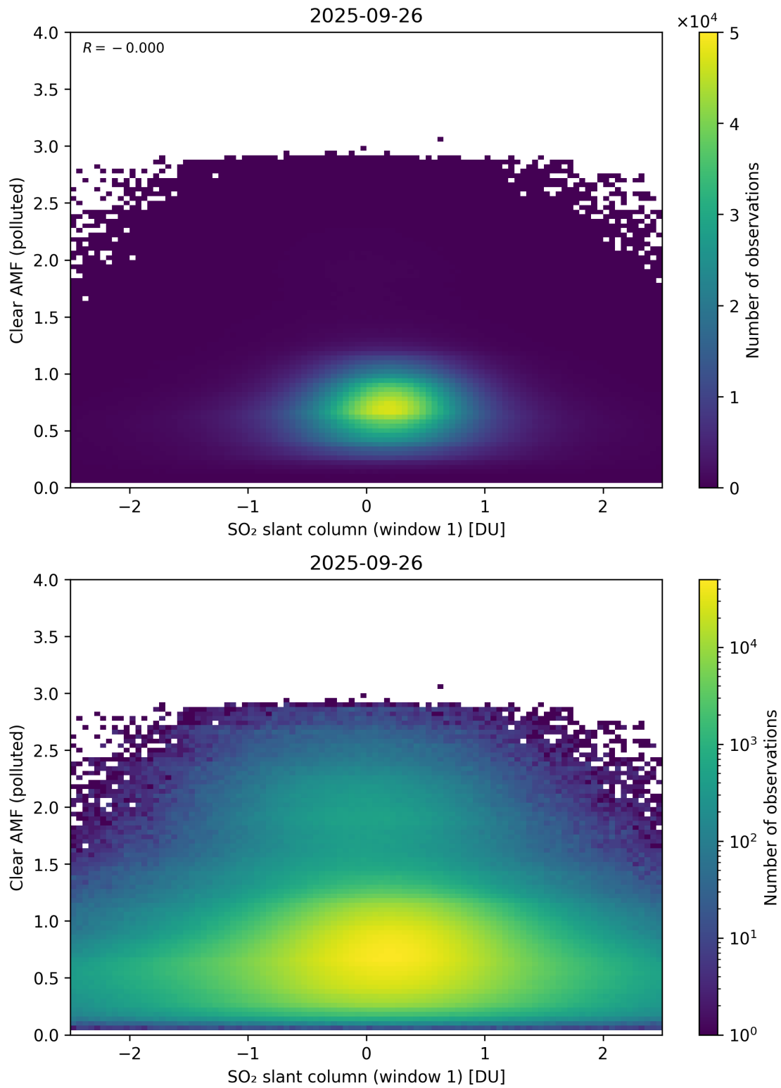
Figure 282: Scatter density plot of “SO 2 slant column (window 1)” against “Clear AMF (polluted)” for 2025-09-26 to 2025-09-27.
