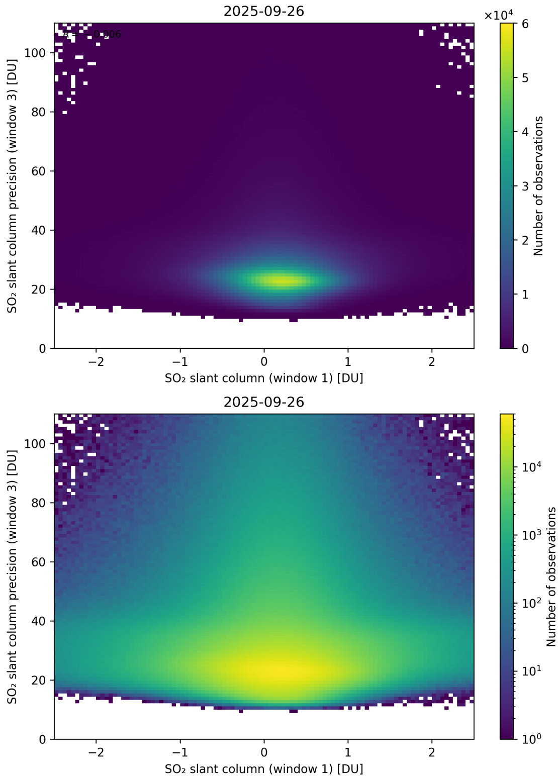
Figure 288: Scatter density plot of “SO 2 slant column (window 1)” against “SO 2 slant column precision (window 3)” for 2025-09-26 to 2025-09-27.
