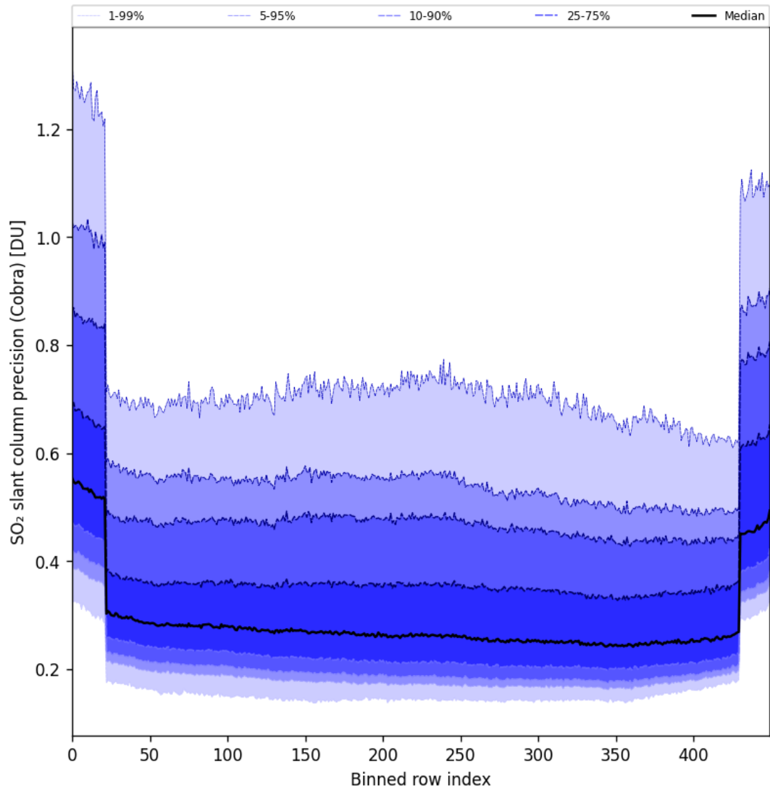
Figure 88: Along track statistics of “SO 2 slant column precision (Cobra)” for 2025-09-26 to 2025-09-27
