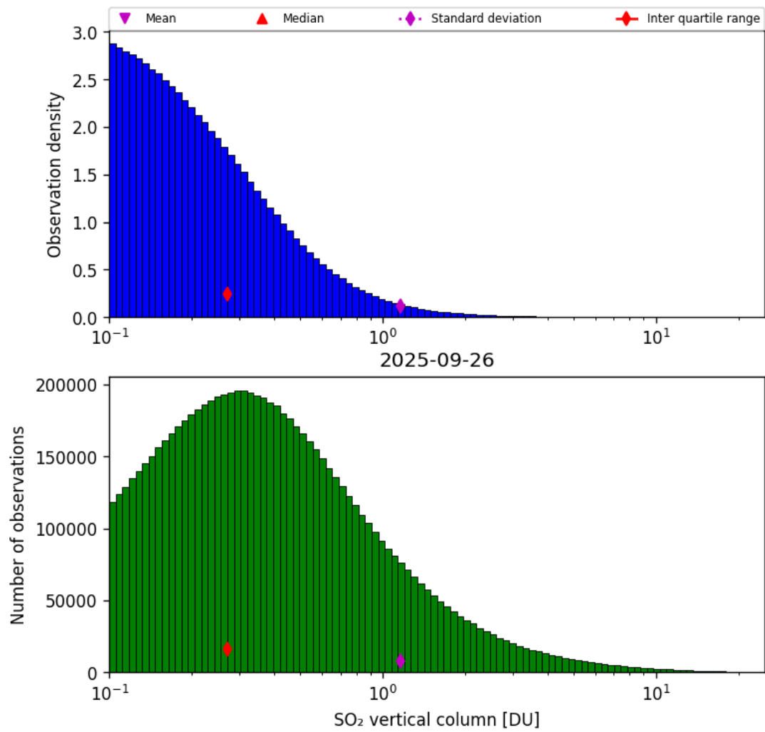
Figure 58: Histogram of “SO 2 vertical column” for 2025-09-26 to 2025-09-27
