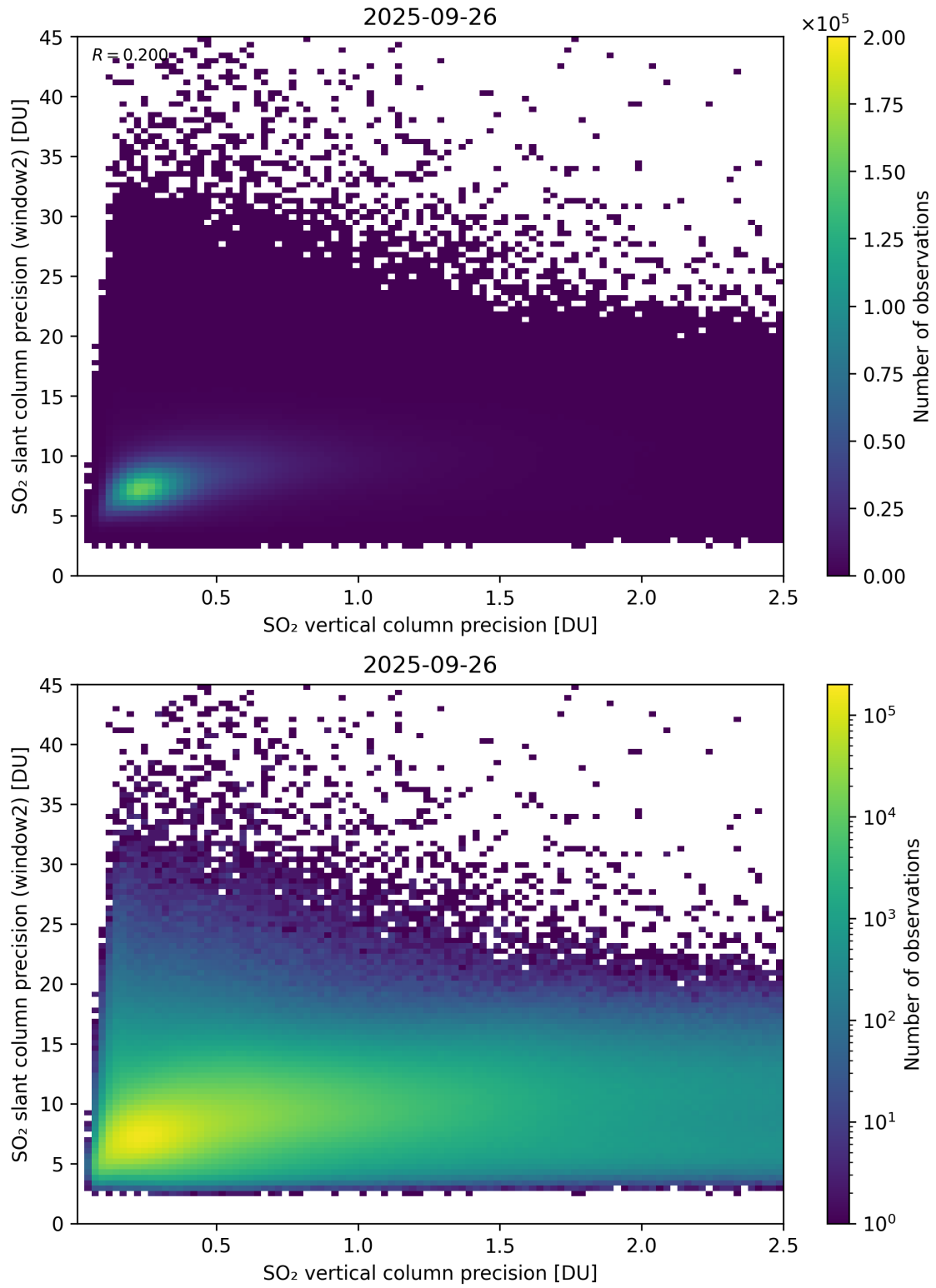
Figure 343: Scatter density plot of “SO 2 vertical column precision” against “SO 2 slant column precision (window2)” for 2025-09-26 to 2025-09-27.
