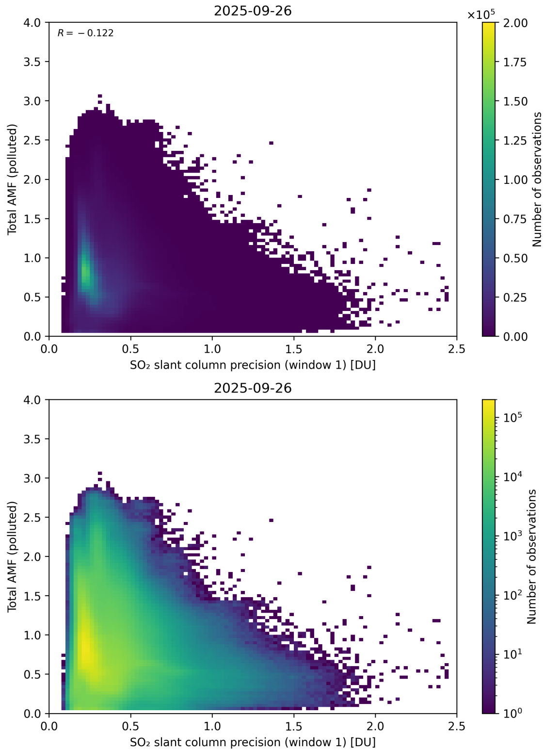
Figure 280: Scatter density plot of “SO 2 slant column precision (window 1)” against “Total AMF (polluted)” for 2025-09-26 to 2025-09-27.
