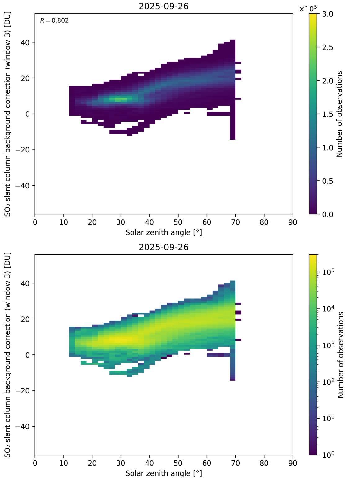
Figure 173: Scatter density plot of “Solar zenith angle” against “SO 2 slant column background correction (window 3)” for 2025-09-26 to 2025-09-27.
