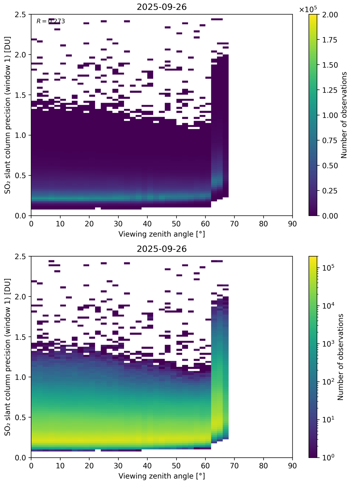
Figure 377: Scatter density plot of “Viewing zenith angle” against “SO 2 slant column precision (window 1)” for 2025-09-26 to 2025-09-27.
