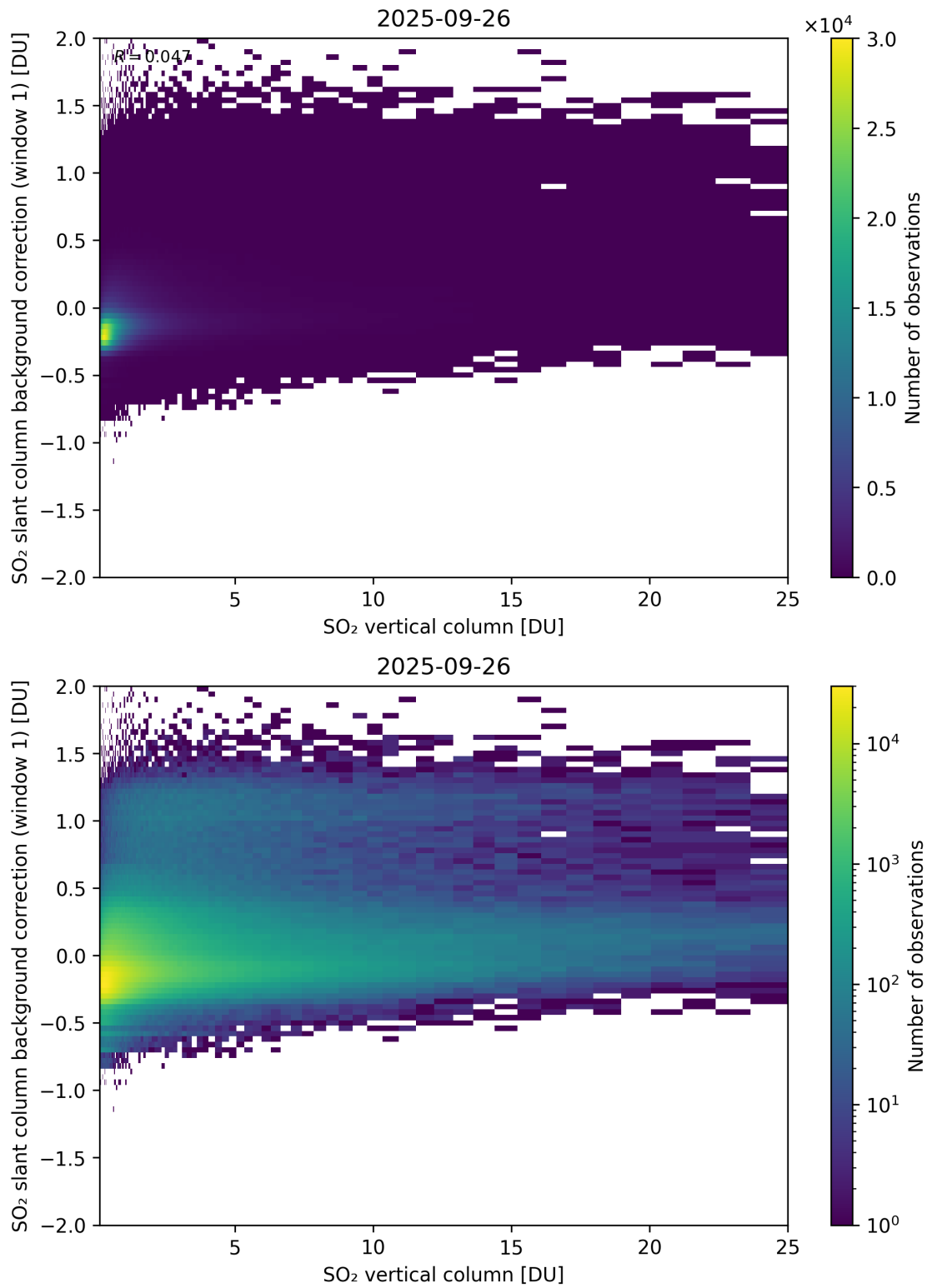
Figure 323: Scatter density plot of “SO 2 vertical column” against “SO 2 slant column background correction (window 1)” for 2025-09-26 to 2025-09-27.
