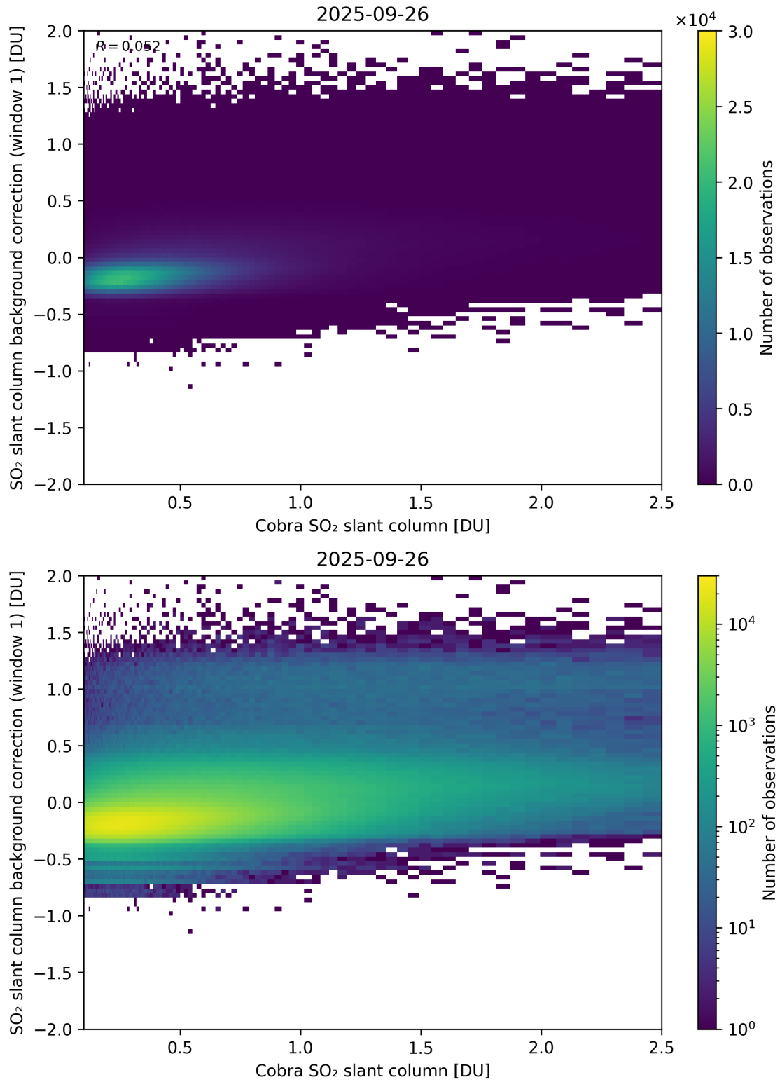
Figure 193: Scatter density plot of “Cobra SO 2 slant column” against “SO 2 slant column background correction (window 1)” for 2025-09-26 to 2025-09-27.
