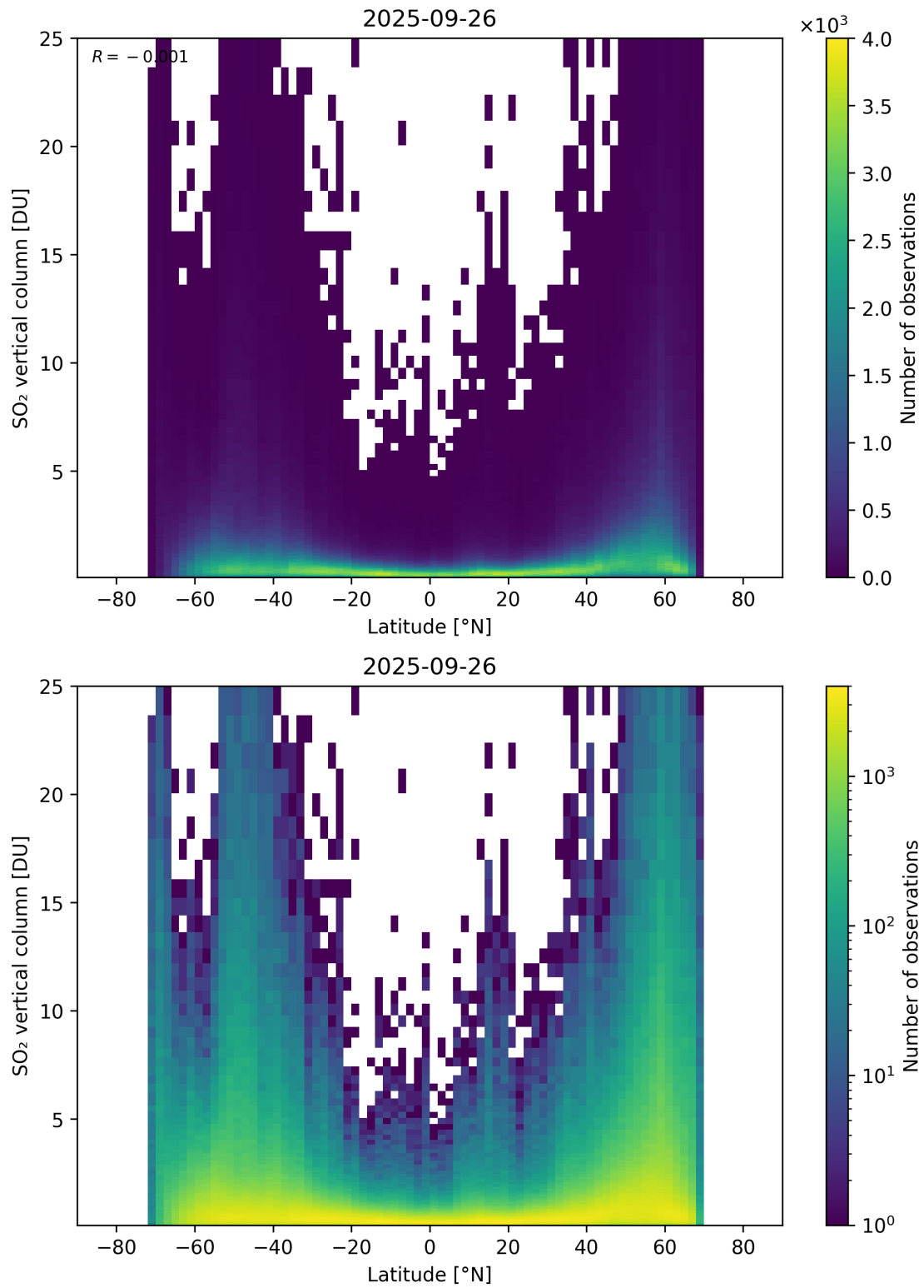
Figure 169: Scatter density plot of “Latitude” against “SO 2 vertical column” for 2025-09-26 to 2025-09-27.
