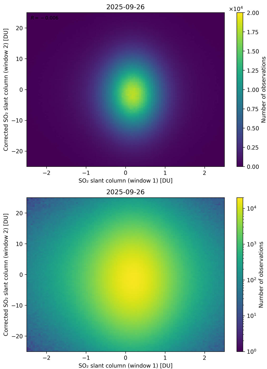
Figure 283: Scatter density plot of “SO 2 slant column (window 1)” against “Corrected SO 2 slant column (window 2)” for 2025-09-26 to 2025-09-27.
