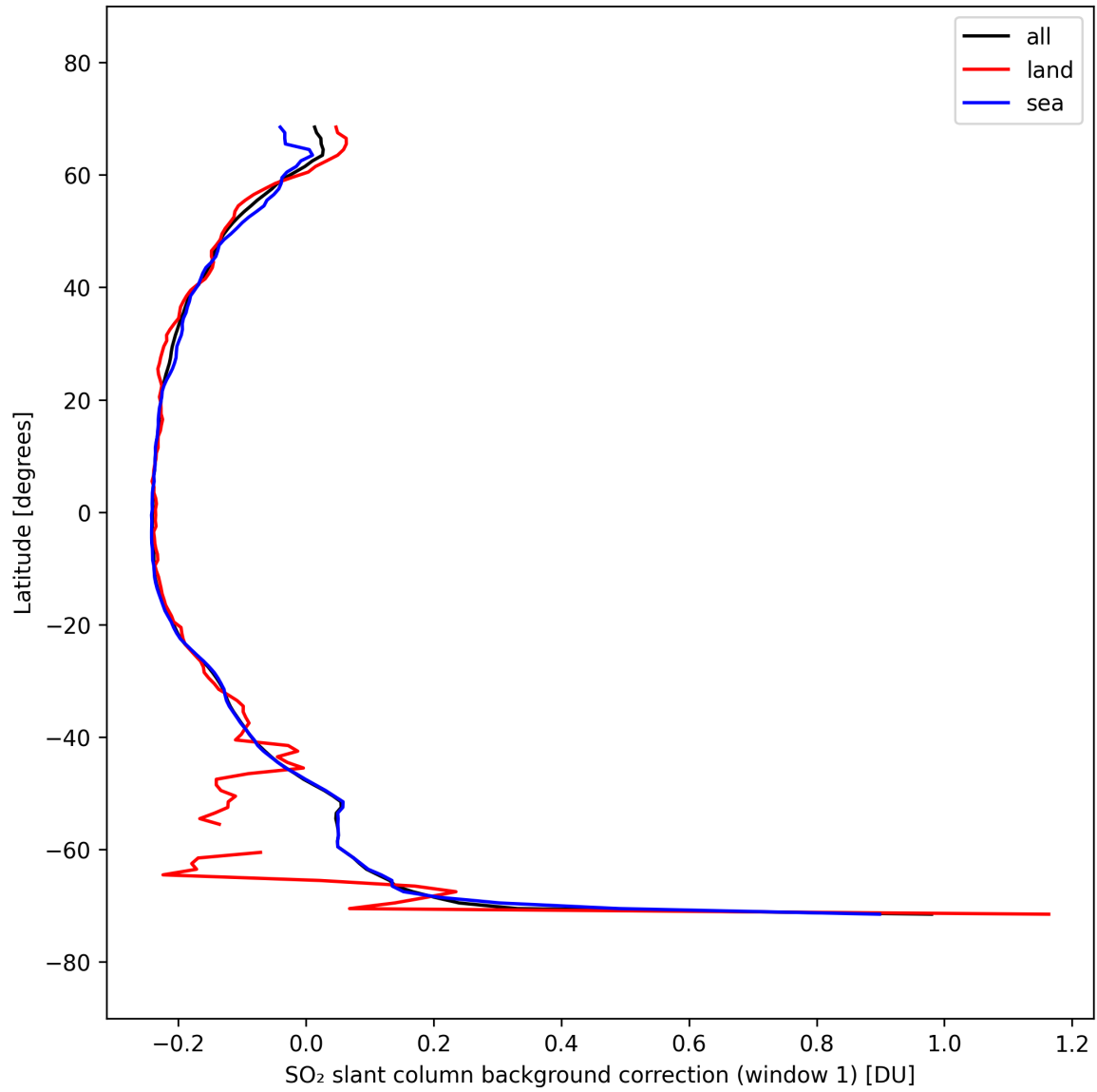
Figure 40: Zonal average of “SO 2 slant column background correction (window 1)” for 2025-09-26 to 2025-09-27.
