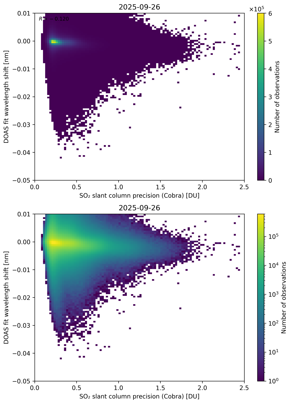
Figure 202: Scatter density plot of “SO 2 slant column precision (Cobra)” against “DOAS fit wavelength shift” for 2025-09-26 to 2025-09-27.
