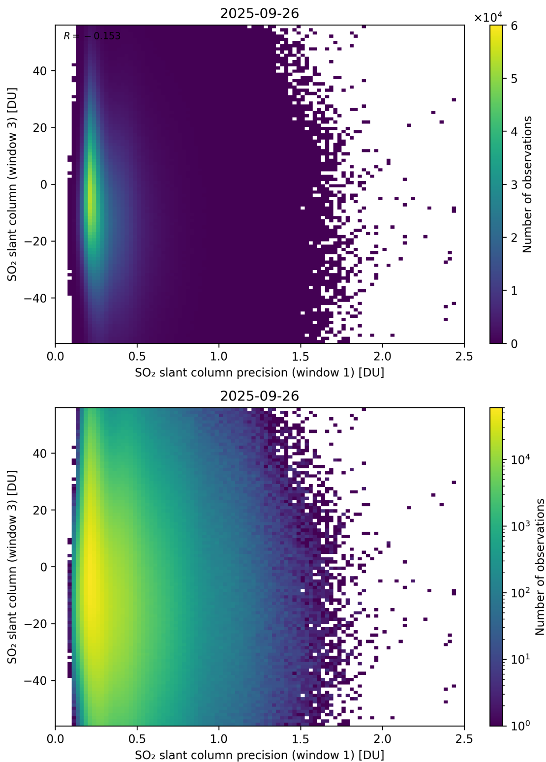
Figure 278: Scatter density plot of “SO 2 slant column precision (window 1)” against “SO 2 slant column (window 3)” for 2025-09-26 to 2025-09-27.
