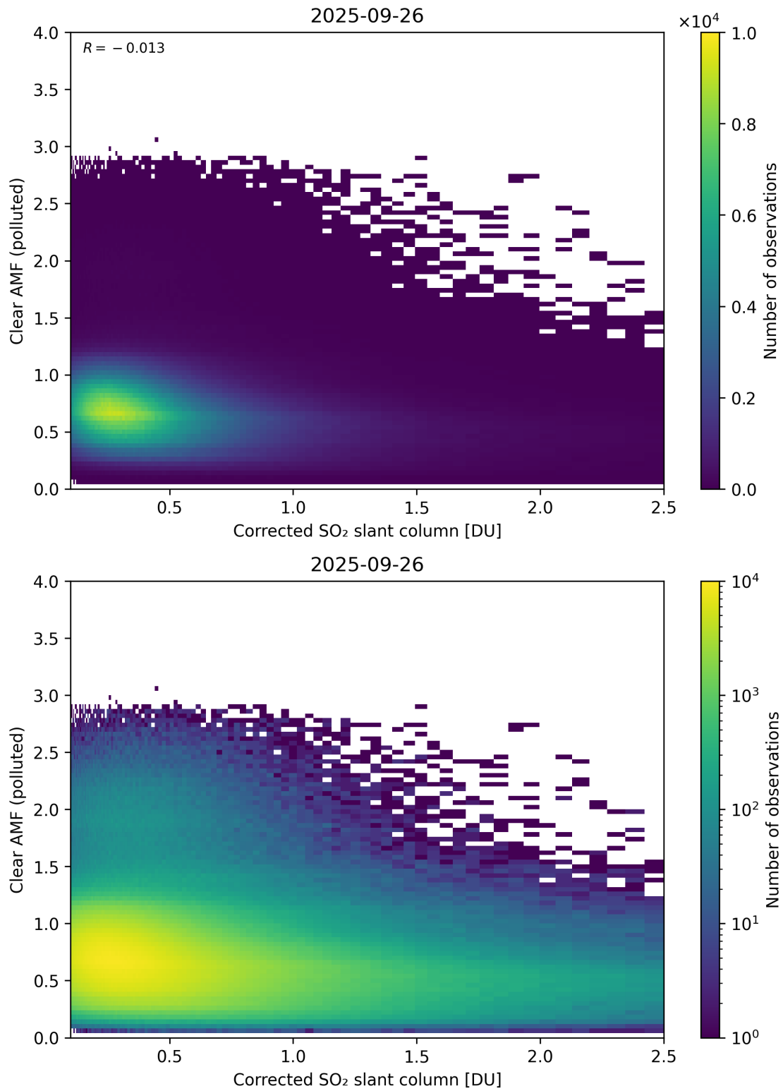
Figure 232: Scatter density plot of “Corrected SO 2 slant column” against “Clear AMF (polluted)” for 2025-09-26 to 2025-09-27.
