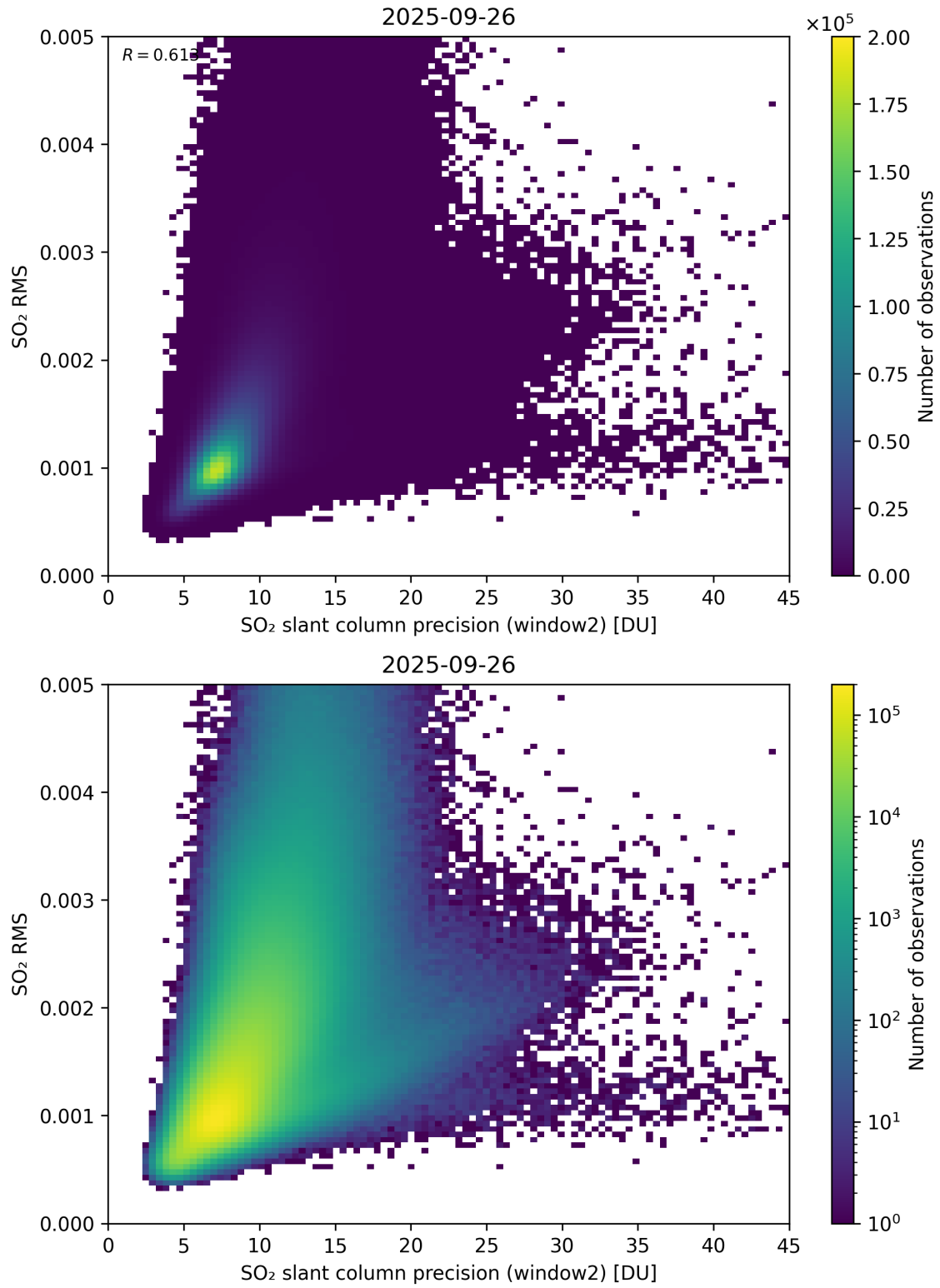
Figure 295: Scatter density plot of “SO 2 slant column precision (window2)” against “SO 2 RMS” for 2025-09-26 to 2025-09-27.
