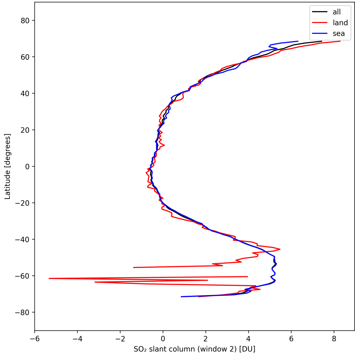
Figure 41: Zonal average of “SO 2 slant column (window 2)” for 2025-09-26 to 2025-09-27.
