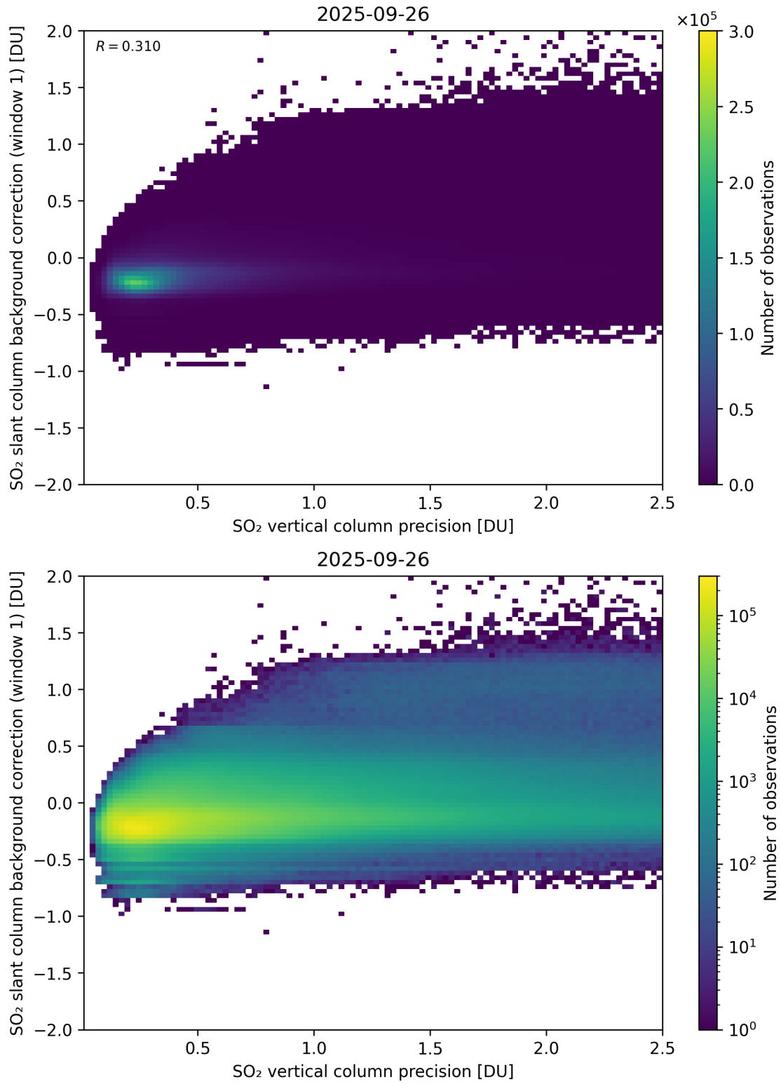
Figure 329: Scatter density plot of “SO 2 vertical column precision” against “SO 2 slant column background correction (window 1)” for 2025-09-26 to 2025-09-27.
