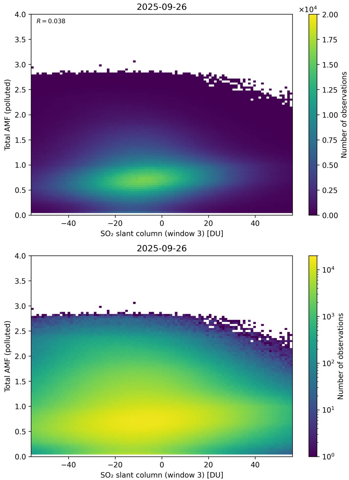
Figure 318: Scatter density plot of “SO 2 slant column (window 3)” against “Total AMF (polluted)” for 2025-09-26 to 2025-09-27.
