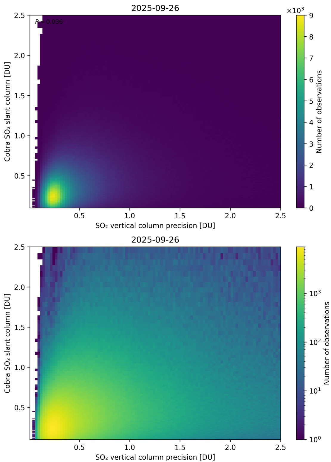
Figure 336: Scatter density plot of “SO 2 vertical column precision” against “Cobra SO 2 slant column” for 2025-09-26 to 2025-09-27.
