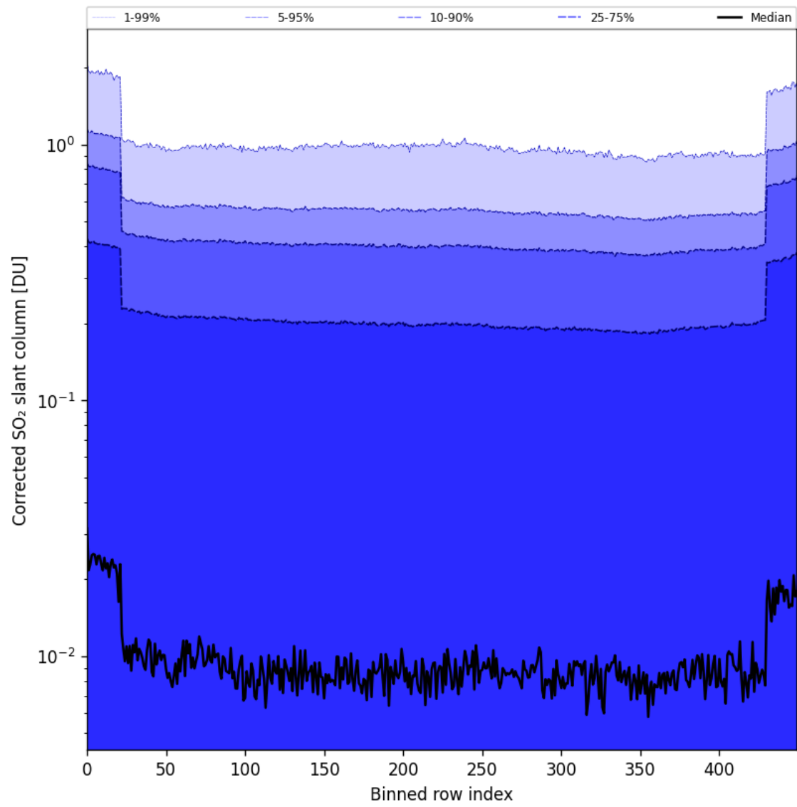
Figure 86: Along track statistics of “Corrected SO 2 slant column” for 2025-09-26 to 2025-09-27
