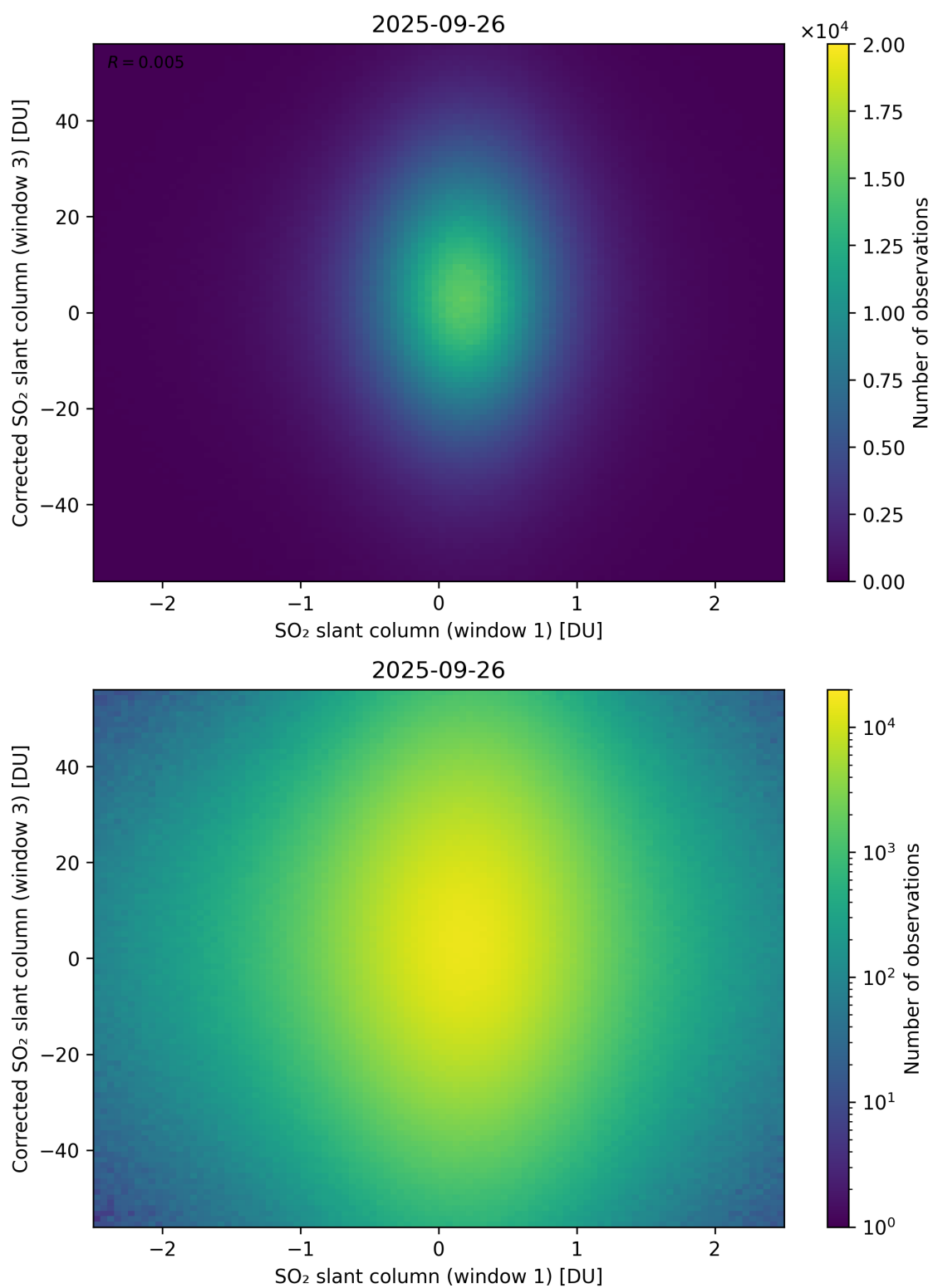
Figure 284: Scatter density plot of “SO 2 slant column (window 1)” against “Corrected SO 2 slant column (window 3)” for 2025-09-26 to 2025-09-27.
