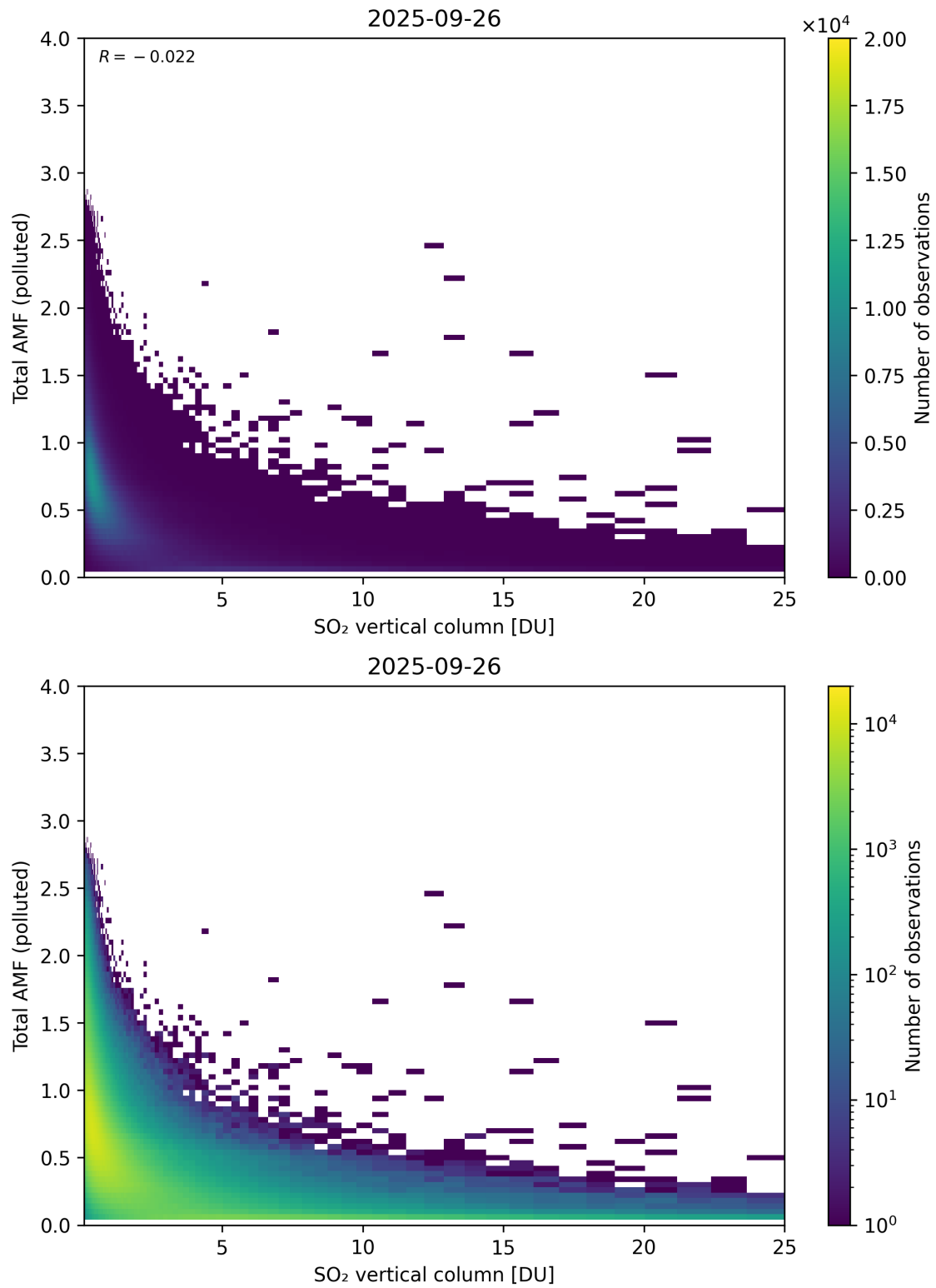
Figure 359: Scatter density plot of “SO 2 vertical column” against “Total AMF (polluted)” for 2025-09-26 to 2025-09-27.
