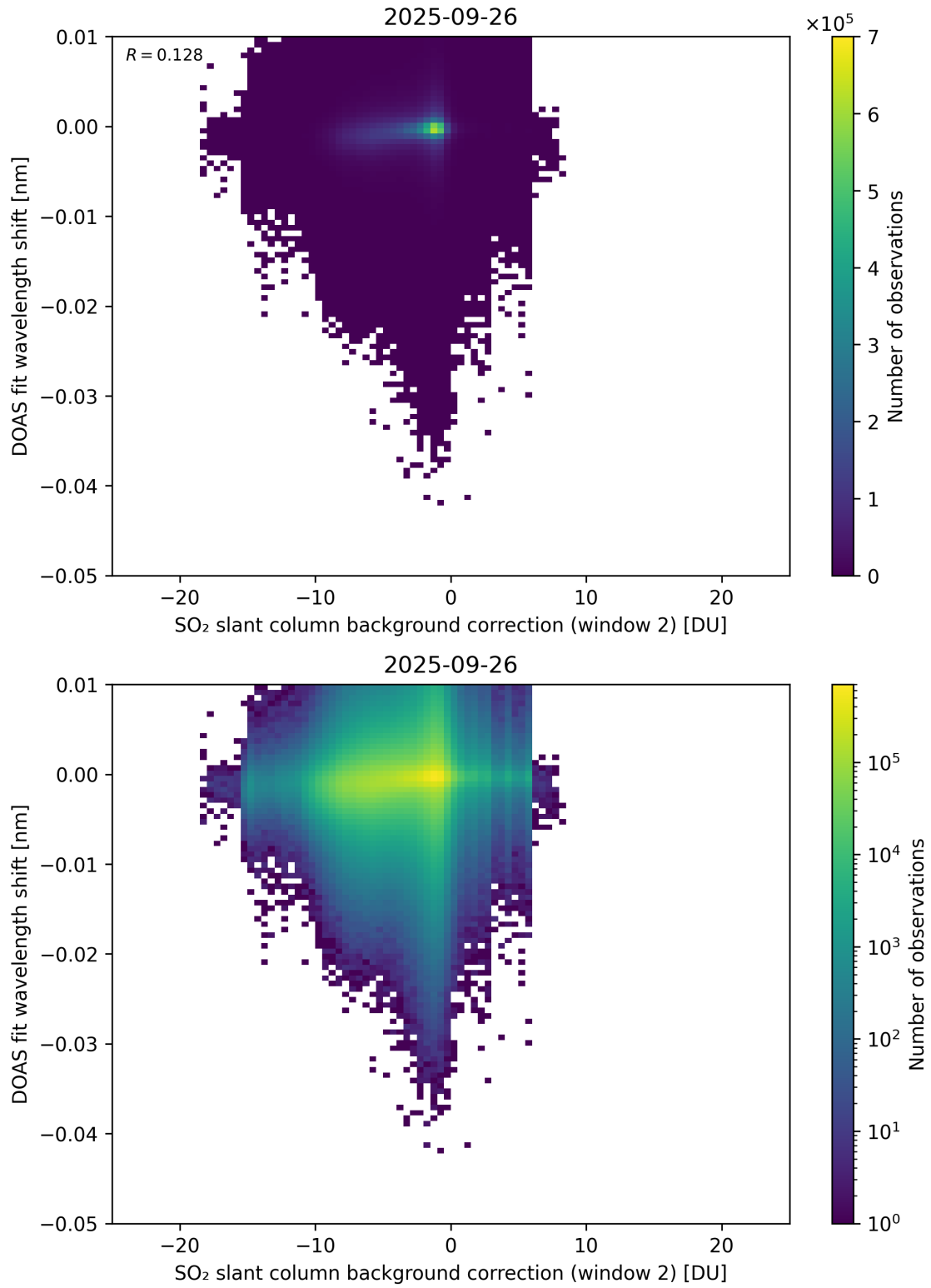
Figure 123: Scatter density plot of “SO 2 slant column background correction (window 2)” against “DOAS fit wavelength shift” for 2025-09-26 to 2025-09-27.
