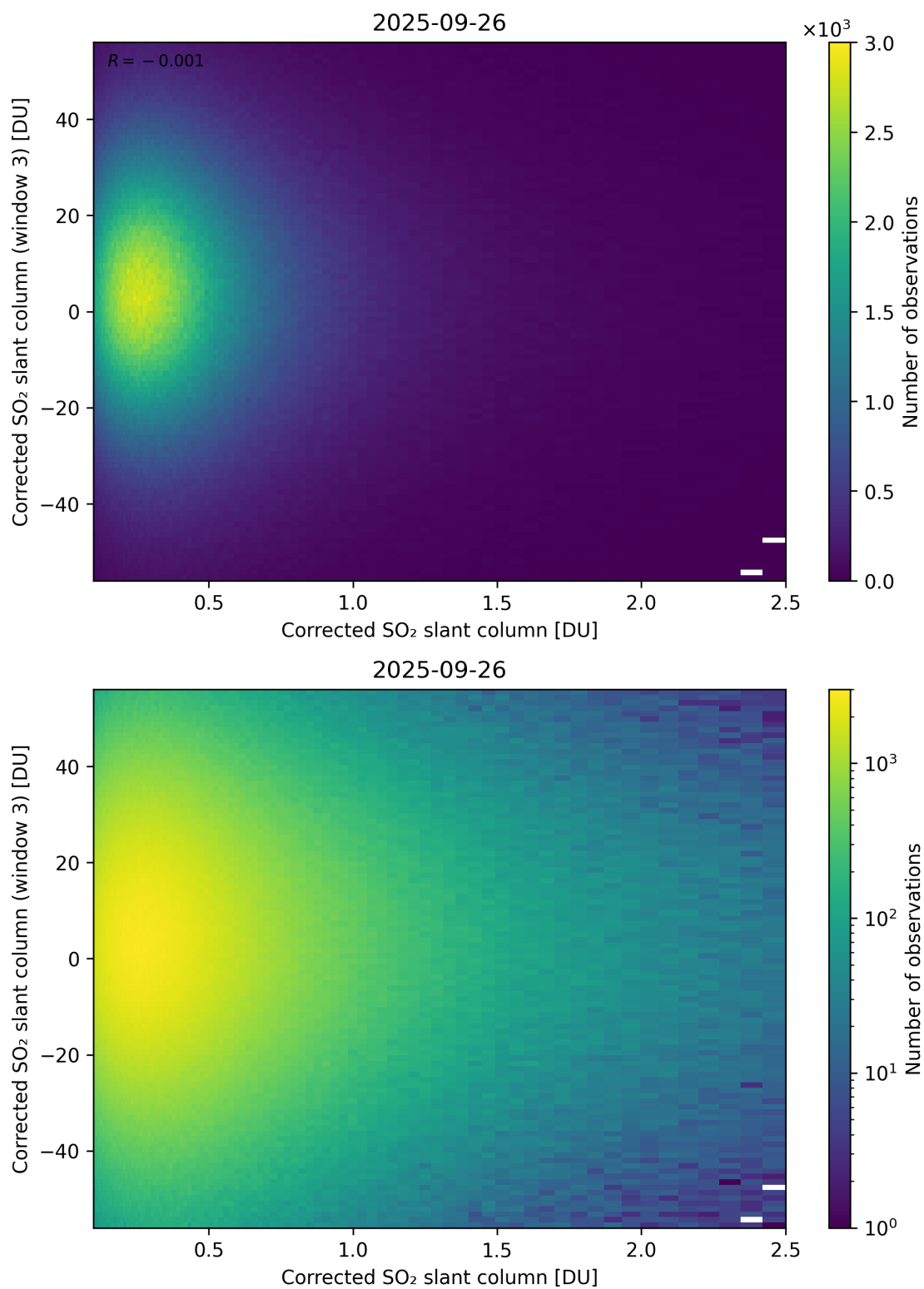
Figure 236: Scatter density plot of “Corrected SO 2 slant column” against “Corrected SO 2 slant column (window 3)” for 2025-09-26 to 2025-09-27.
