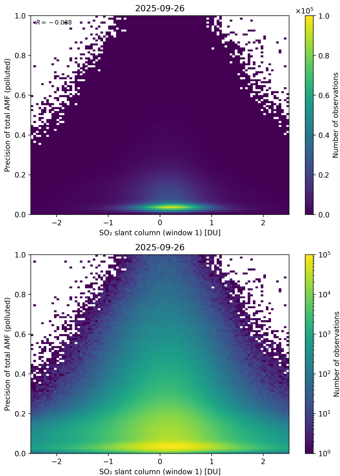
Figure 290: Scatter density plot of “SO 2 slant column (window 1)” against “Precision of total AMF (polluted)” for 2025-09-26 to 2025-09-27.
