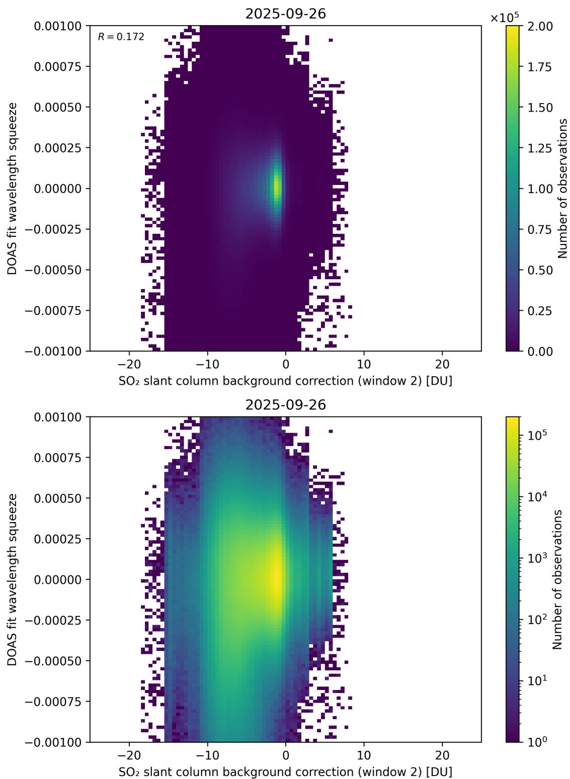
Figure 124: Scatter density plot of “SO 2 slant column background correction (window 2)” against “DOAS fit wavelength squeeze” for 2025-09-26 to 2025-09-27.
