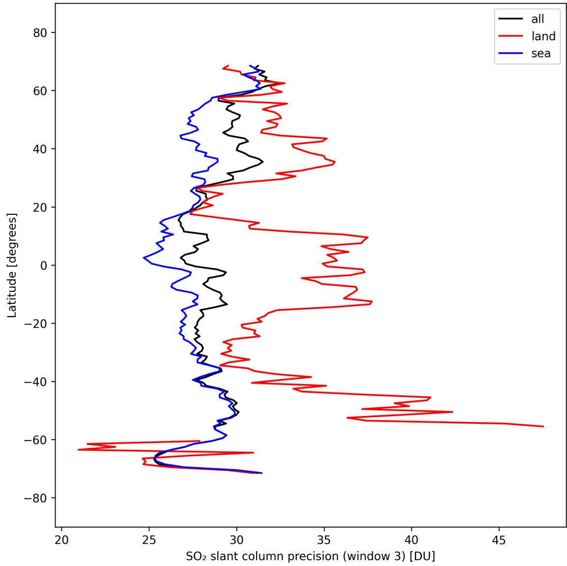
Figure 46: Zonal average of “SO 2 slant column precision (window 3)” for 2025-09-26 to 2025-09-27.
