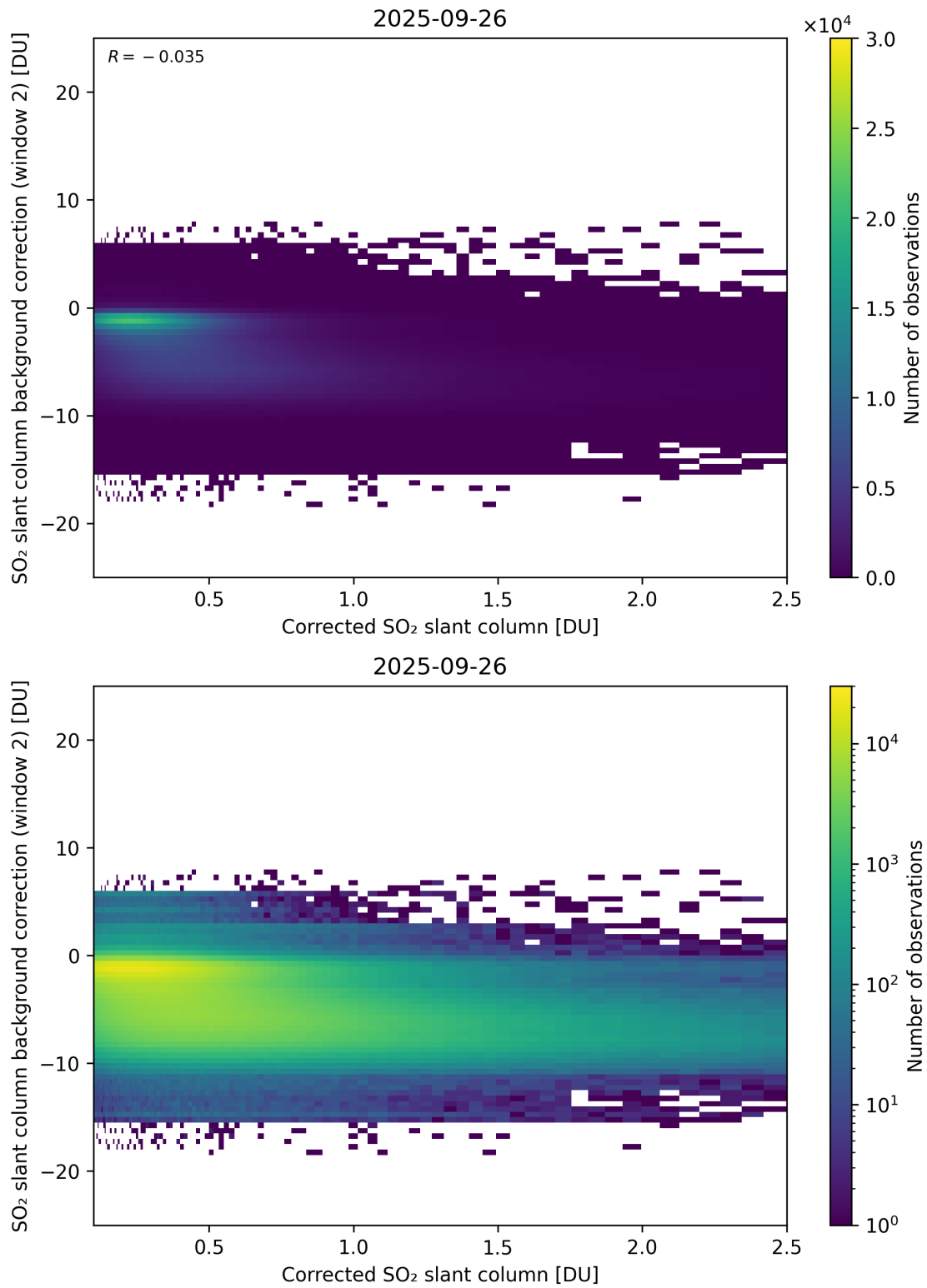
Figure 227: Scatter density plot of “Corrected SO 2 slant column” against “SO 2 slant column background correction (window 2)” for 2025-09-26 to 2025-09-27.
