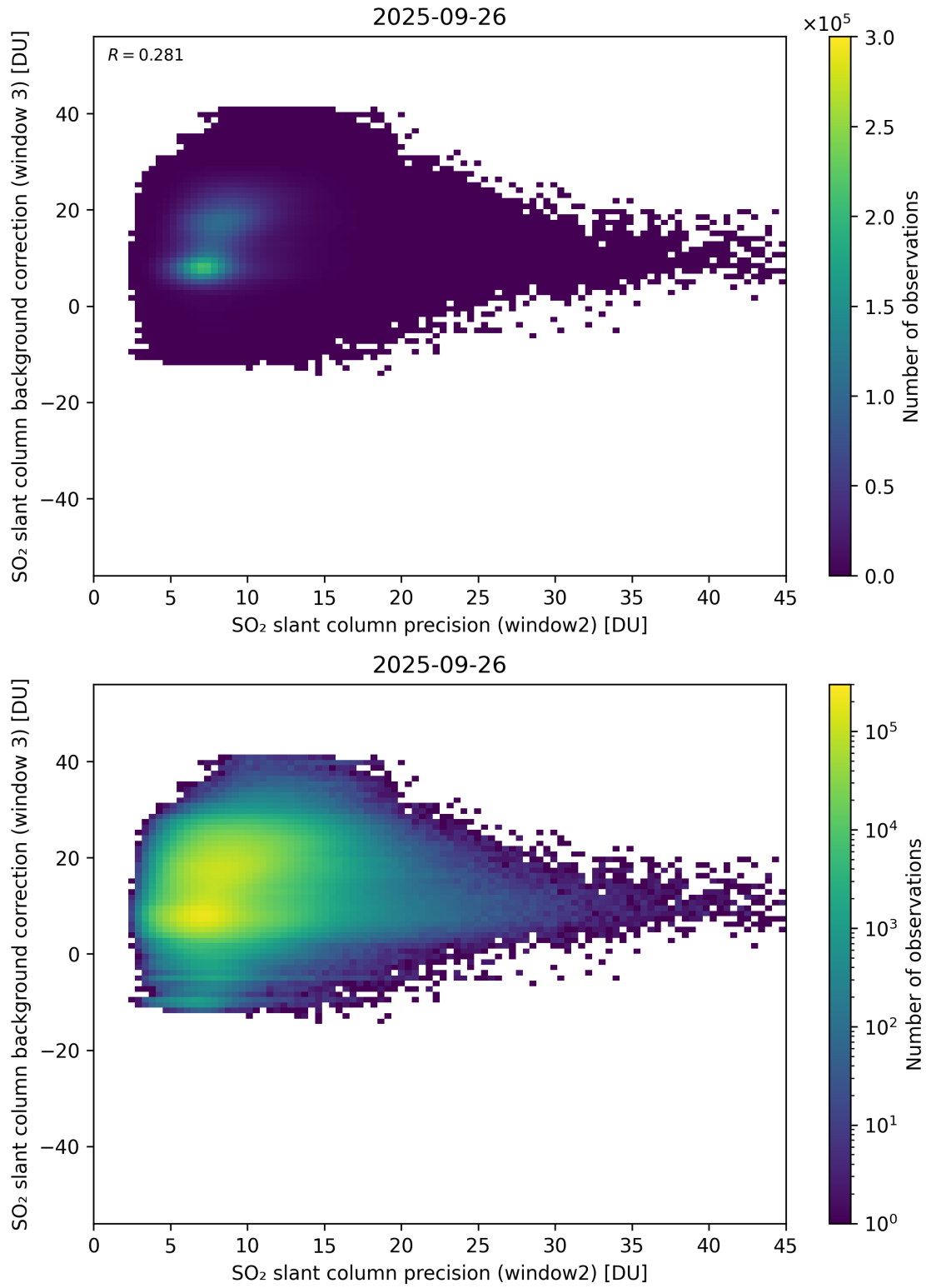
Figure 292: Scatter density plot of “SO 2 slant column precision (window2)” against “SO 2 slant column background correction (window 3)” for 2025-09-26 to 2025-09-27.
