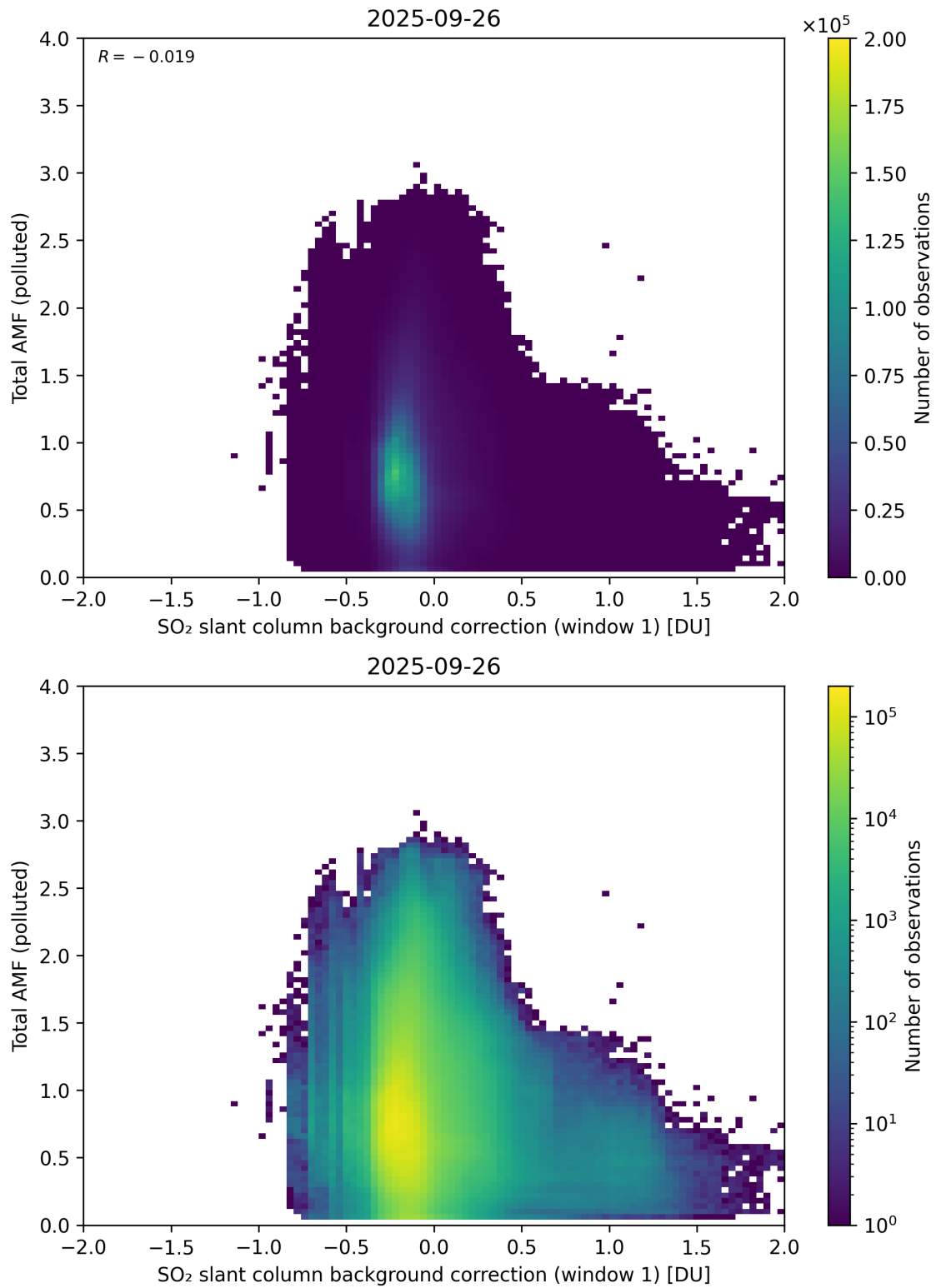
Figure 120: Scatter density plot of “SO 2 slant column background correction (window 1)” against “Total AMF (polluted)” for 2025-09-26 to 2025-09-27.
