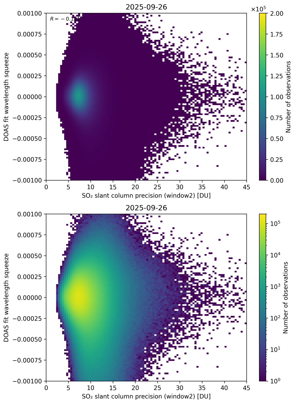
Figure 294: Scatter density plot of “SO 2 slant column precision (window2)” against “DOAS fit wavelength squeeze” for 2025-09-26 to 2025-09-27.
