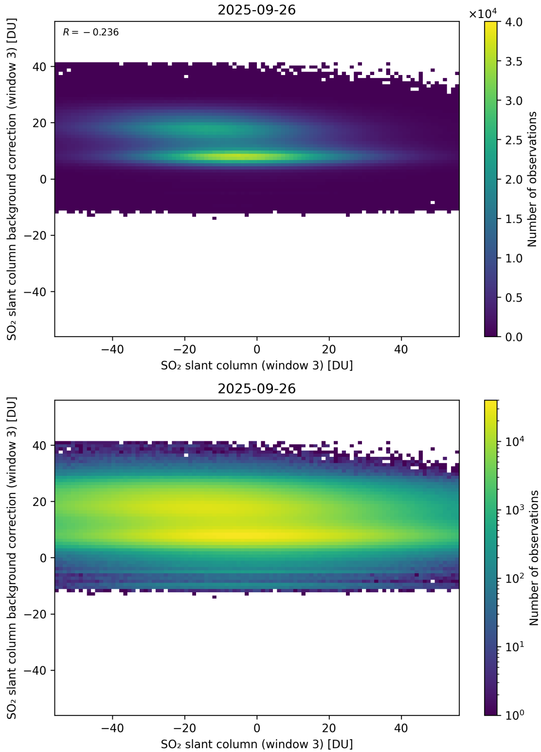
Figure 303: Scatter density plot of “SO 2 slant column (window 3)” against “SO 2 slant column background correction (window 3)” for 2025-09-26 to 2025-09-27.
