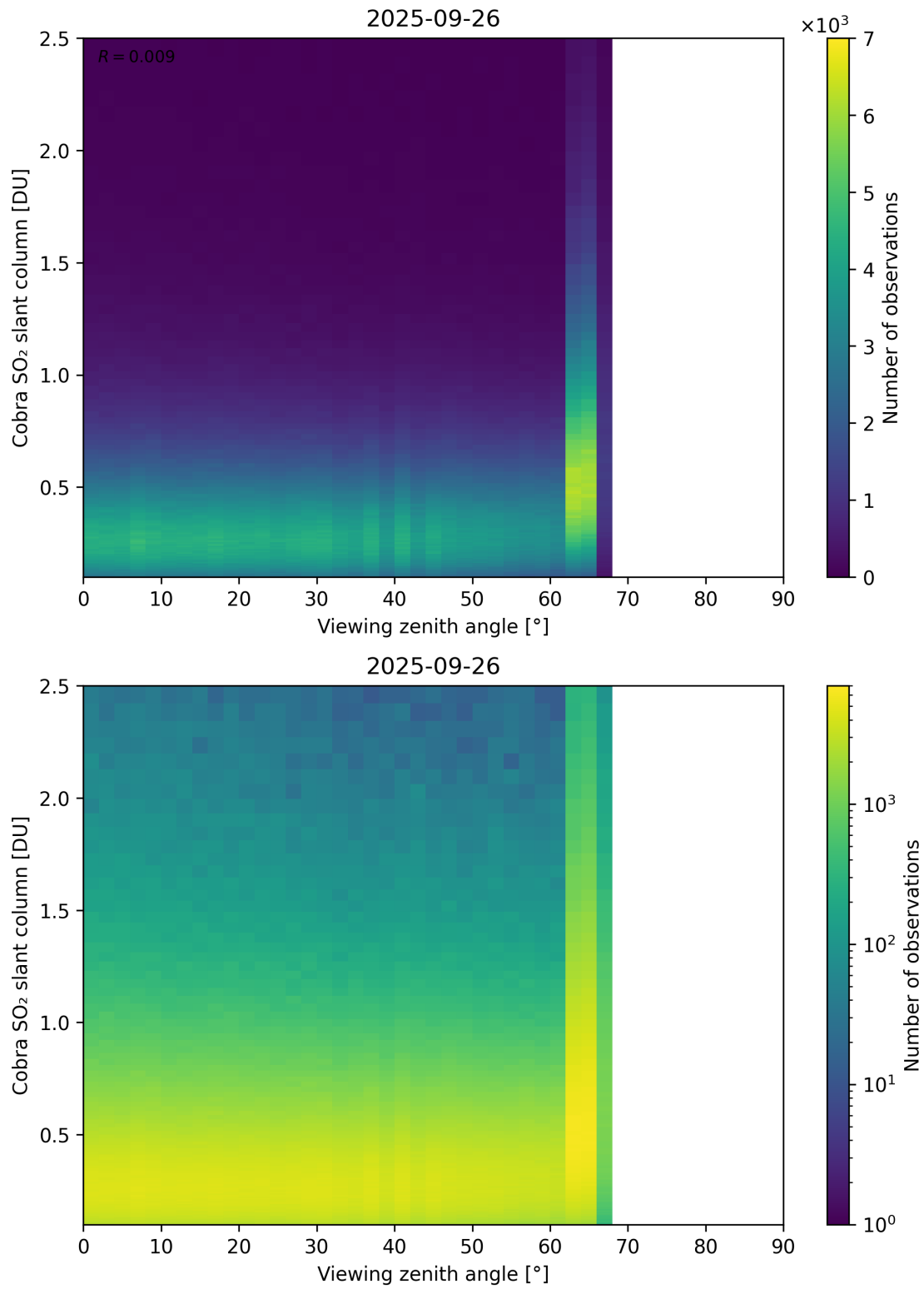
Figure 371: Scatter density plot of “Viewing zenith angle” against “Cobra SO 2 slant column” for 2025-09-26 to 2025-09-27.
