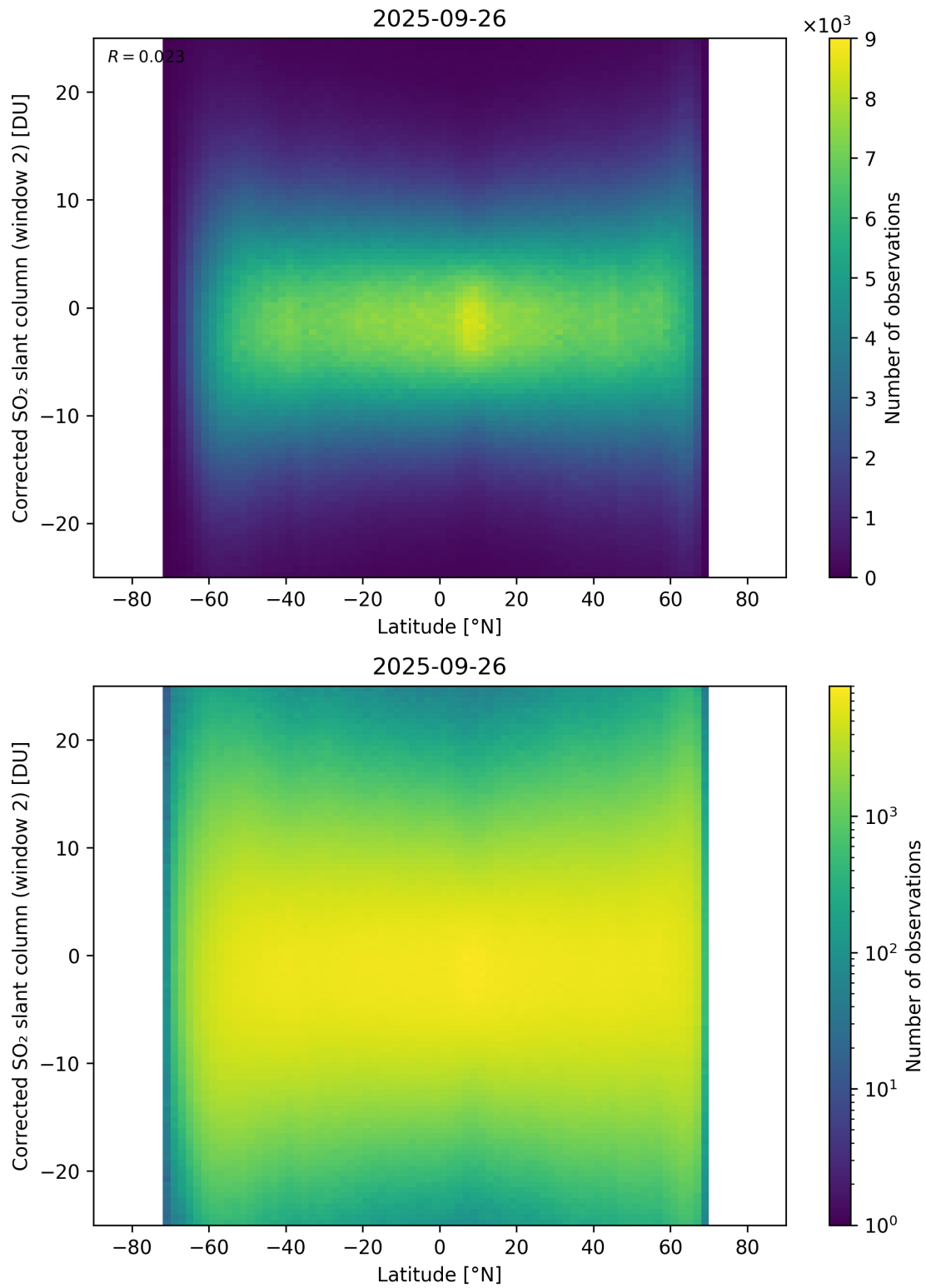
Figure 160: Scatter density plot of “Latitude” against “Corrected SO 2 slant column (window 2)” for 2025-09-26 to 2025-09-27.
