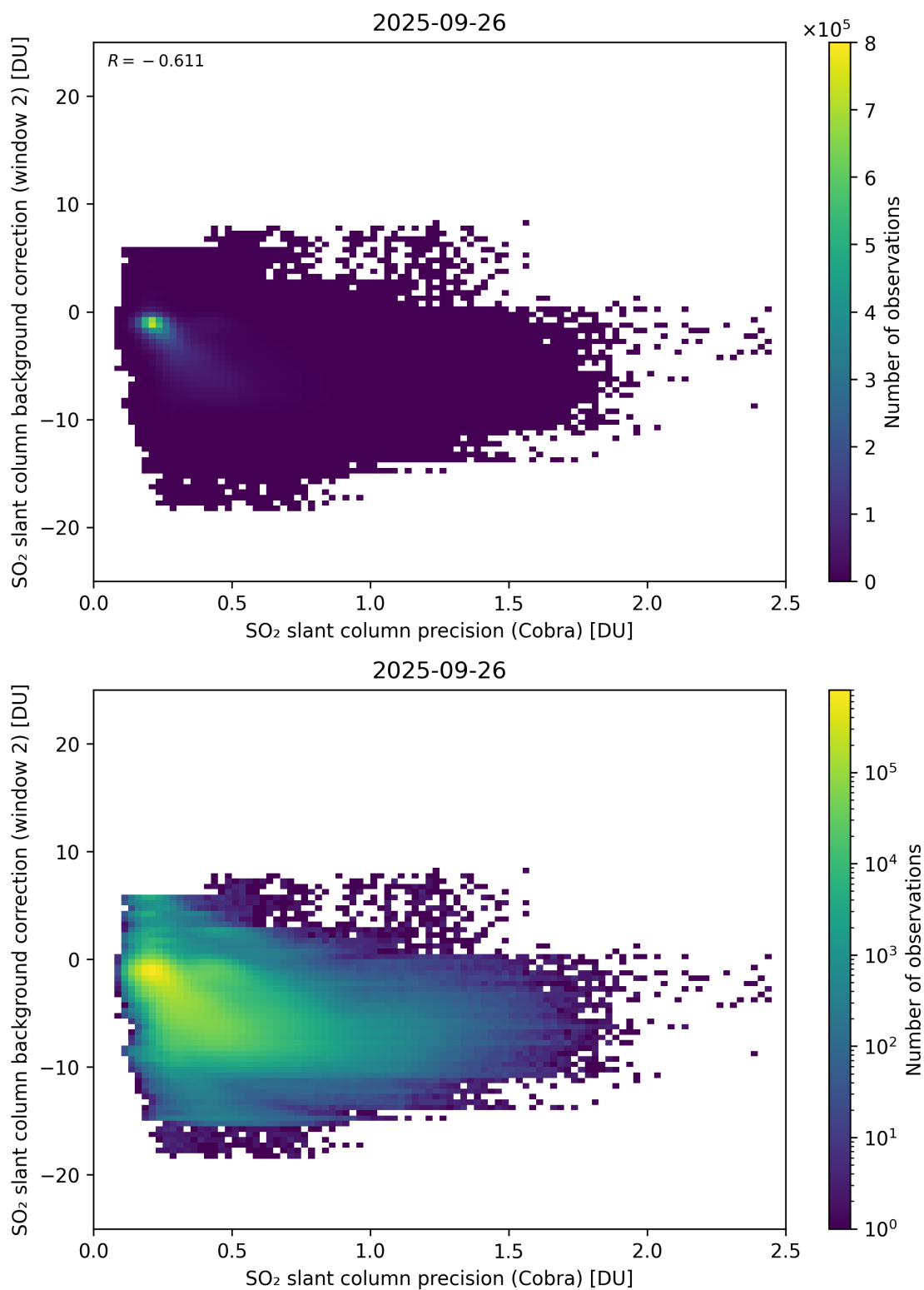
Figure 200: Scatter density plot of “SO 2 slant column precision (Cobra)” against “SO 2 slant column background correction (window 2)” for 2025-09-26 to 2025-09-27.
