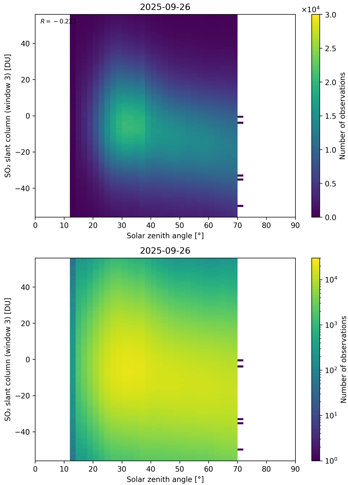
Figure 187: Scatter density plot of “Solar zenith angle” against “SO 2 slant column (window 3)” for 2025-09-26 to 2025-09-27.
