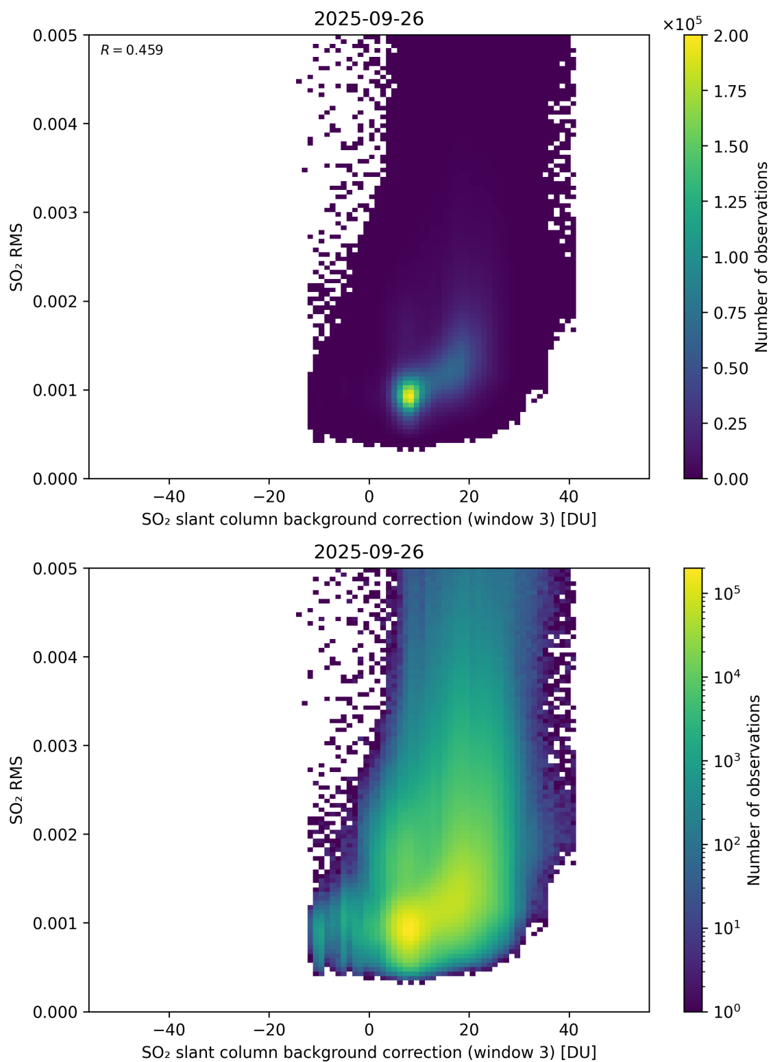
Figure 134: Scatter density plot of “SO 2 slant column background correction (window 3)” against “SO 2 RMS” for 2025-09-26 to 2025-09-27.
