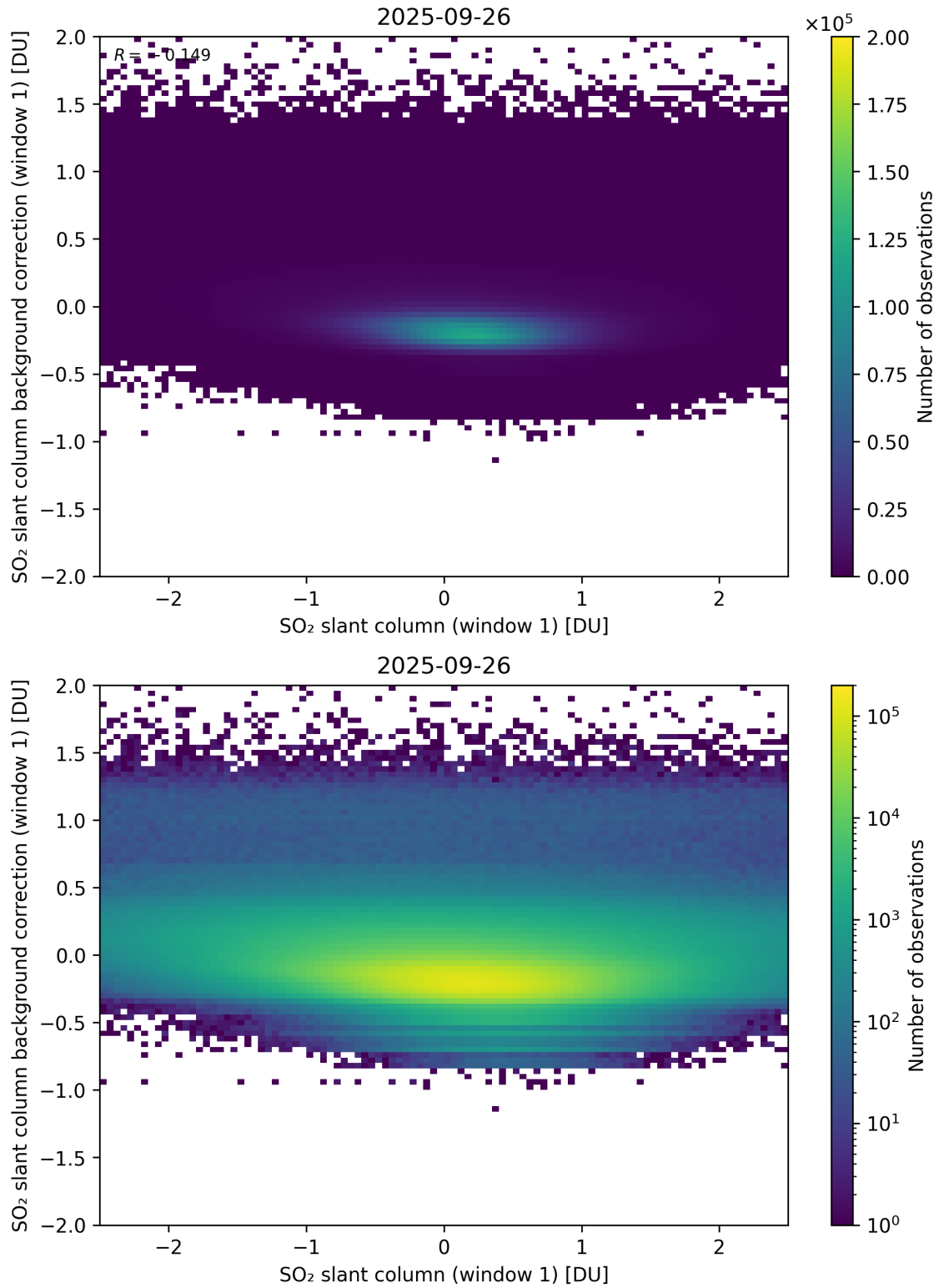
Figure 262: Scatter density plot of “SO 2 slant column (window 1)” against “SO 2 slant column background correction (window 1)” for 2025-09-26 to 2025-09-27.
