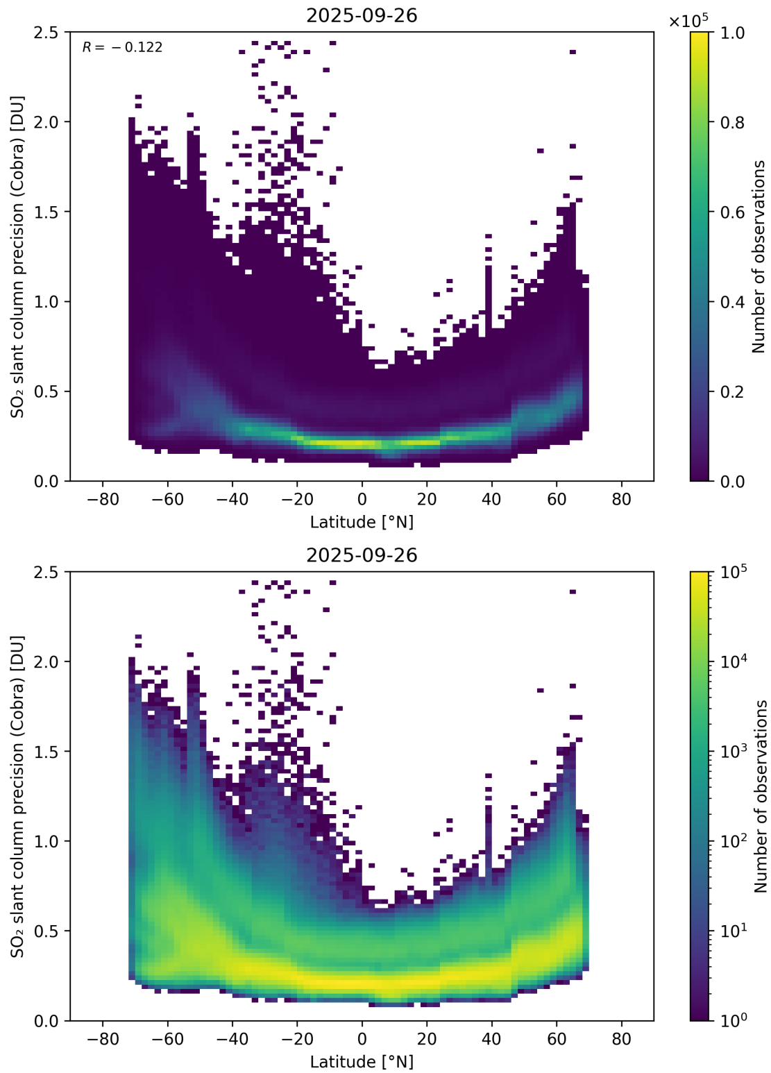
Figure 158: Scatter density plot of “Latitude” against “SO 2 slant column precision (Cobra)” for 2025-09-26 to 2025-09-27.
