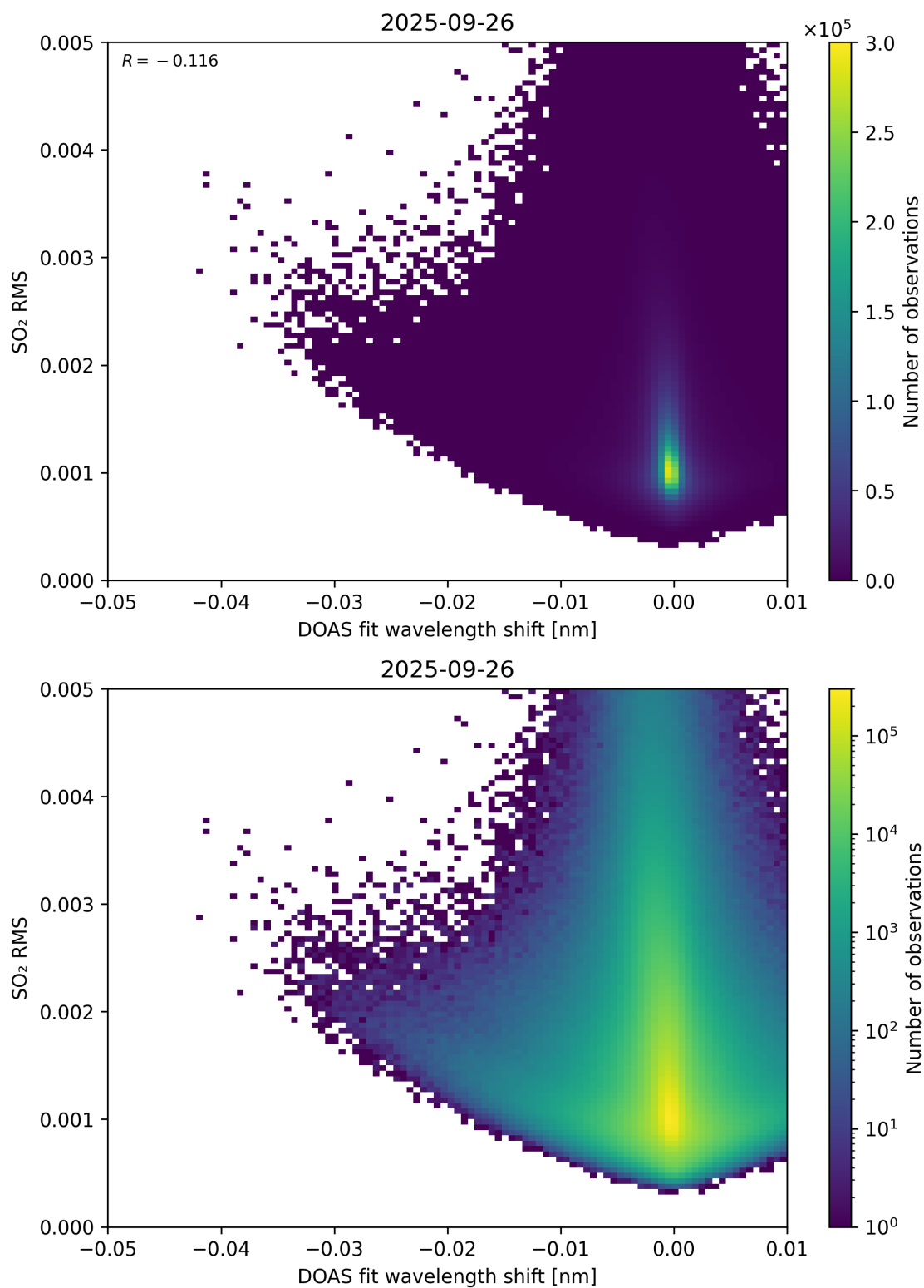
Figure 139: Scatter density plot of “DOAS fit wavelength shift” against “SO 2 RMS” for 2025-09-26 to 2025-09-27.
