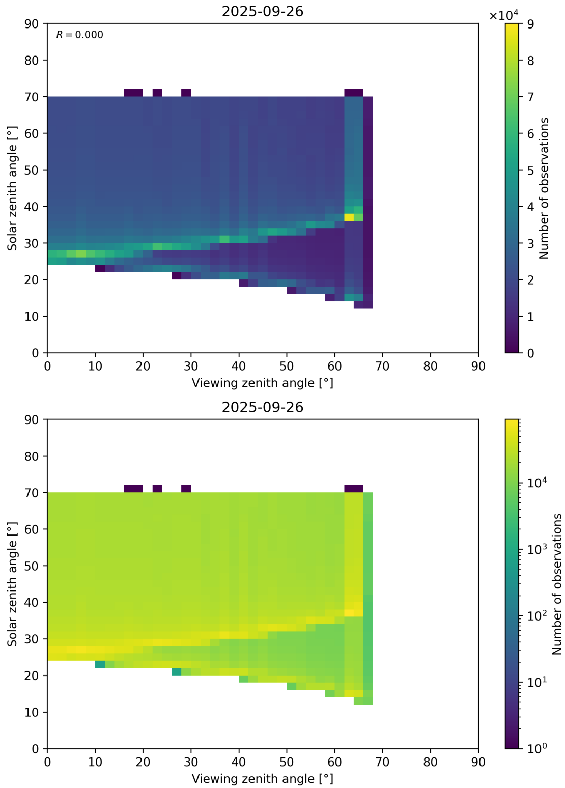
Figure 369: Scatter density plot of “Viewing zenith angle” against “Solar zenith angle” for 2025-09-26 to 2025-09-27.
