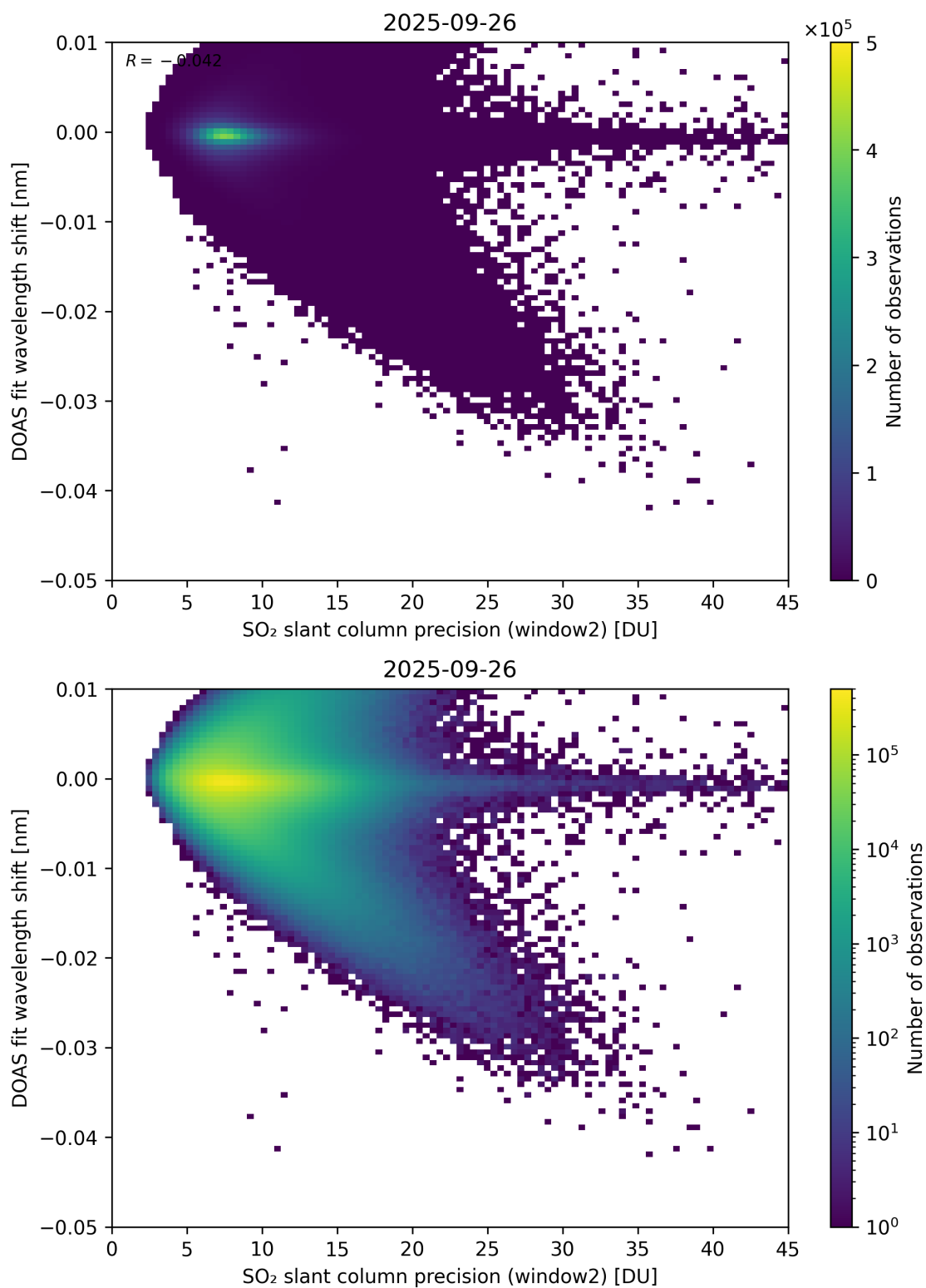
Figure 293: Scatter density plot of “SO 2 slant column precision (window2)” against “DOAS fit wavelength shift” for 2025-09-26 to 2025-09-27.
