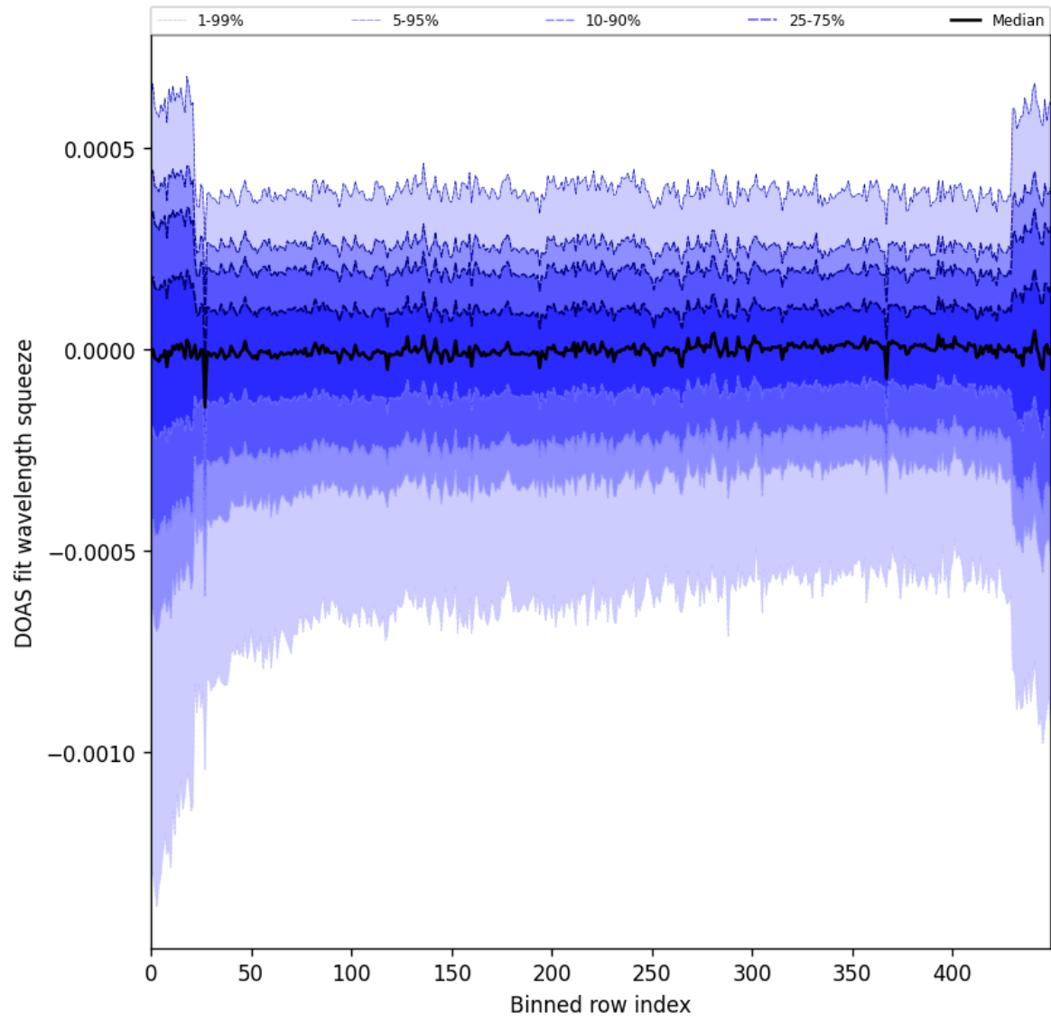
Figure 103: Along track statistics of “DOAS fit wavelength squeeze” for 2025-09-26 to 2025-09-27
