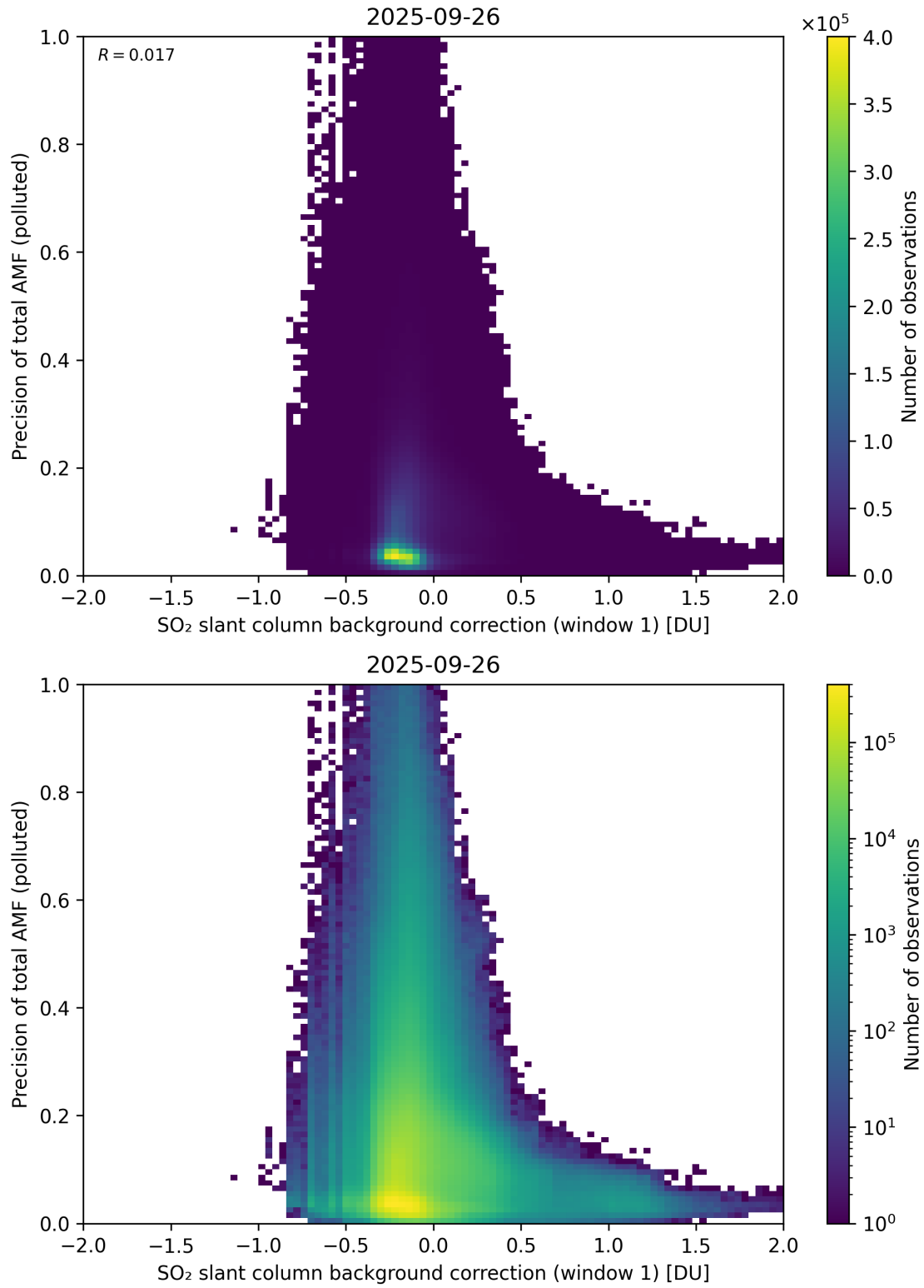
Figure 121: Scatter density plot of “SO 2 slant column background correction (window 1)” against “Precision of total AMF (polluted)” for 2025-09-26 to 2025-09-27.
