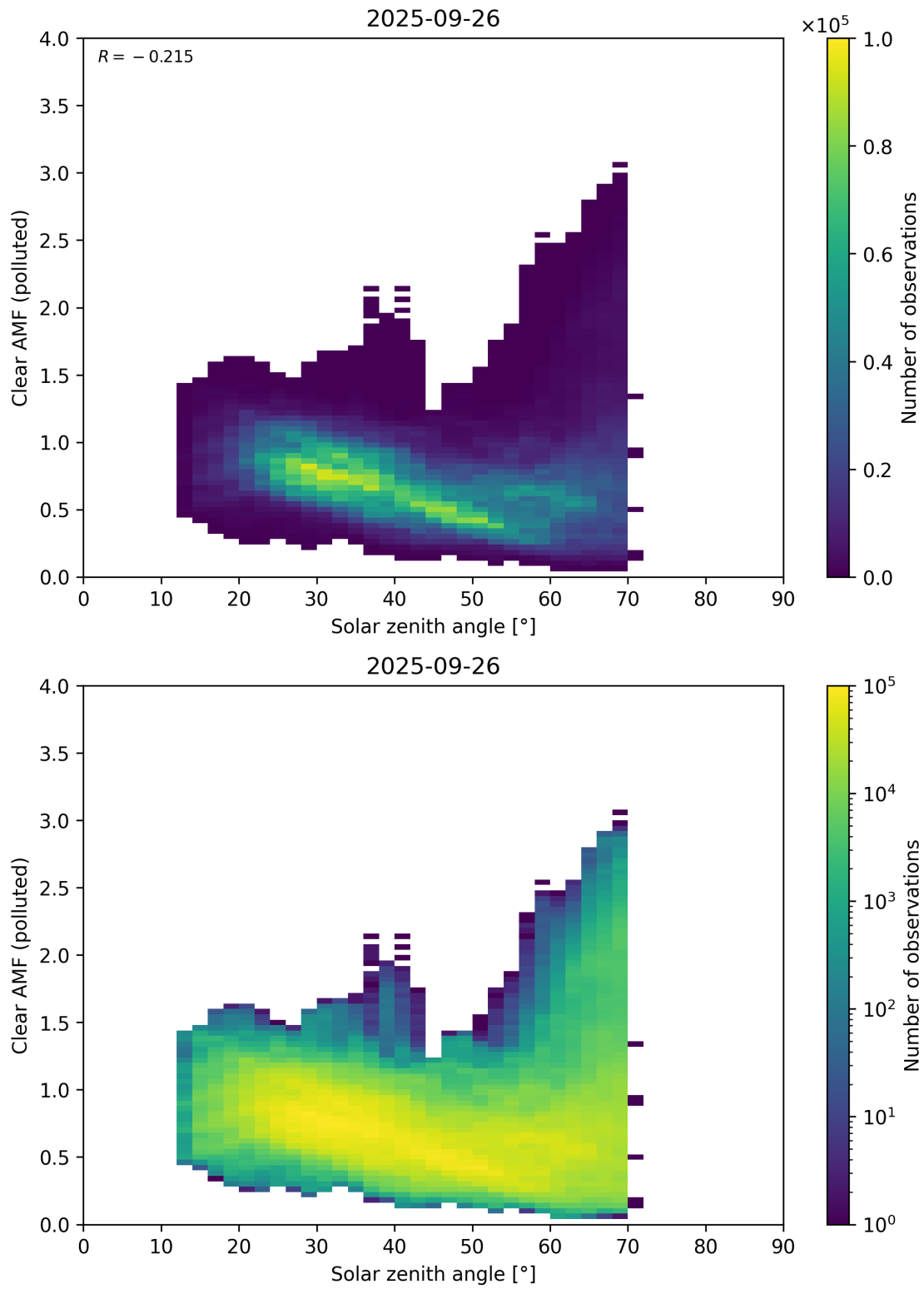
Figure 178: Scatter density plot of “Solar zenith angle” against “Clear AMF (polluted)” for 2025-09-26 to 2025-09-27.
