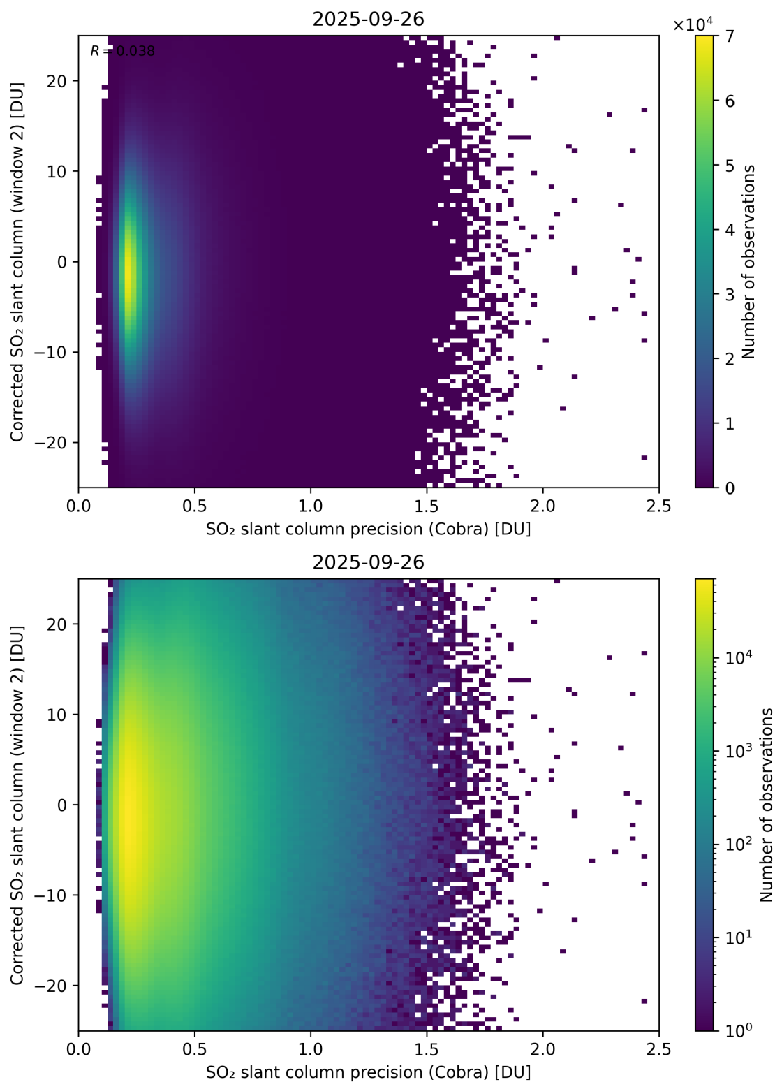
Figure 206: Scatter density plot of “SO 2 slant column precision (Cobra)” against “Corrected SO 2 slant column (window 2)” for 2025-09-26 to 2025-09-27.
