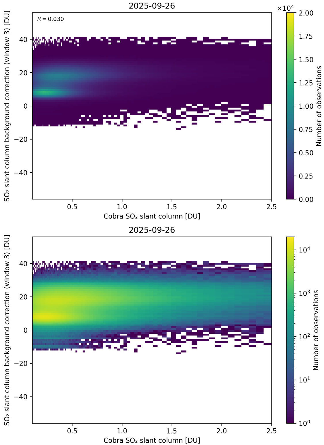
Figure 195: Scatter density plot of “Cobra SO 2 slant column” against “SO 2 slant column background correction (window 3)” for 2025-09-26 to 2025-09-27.
