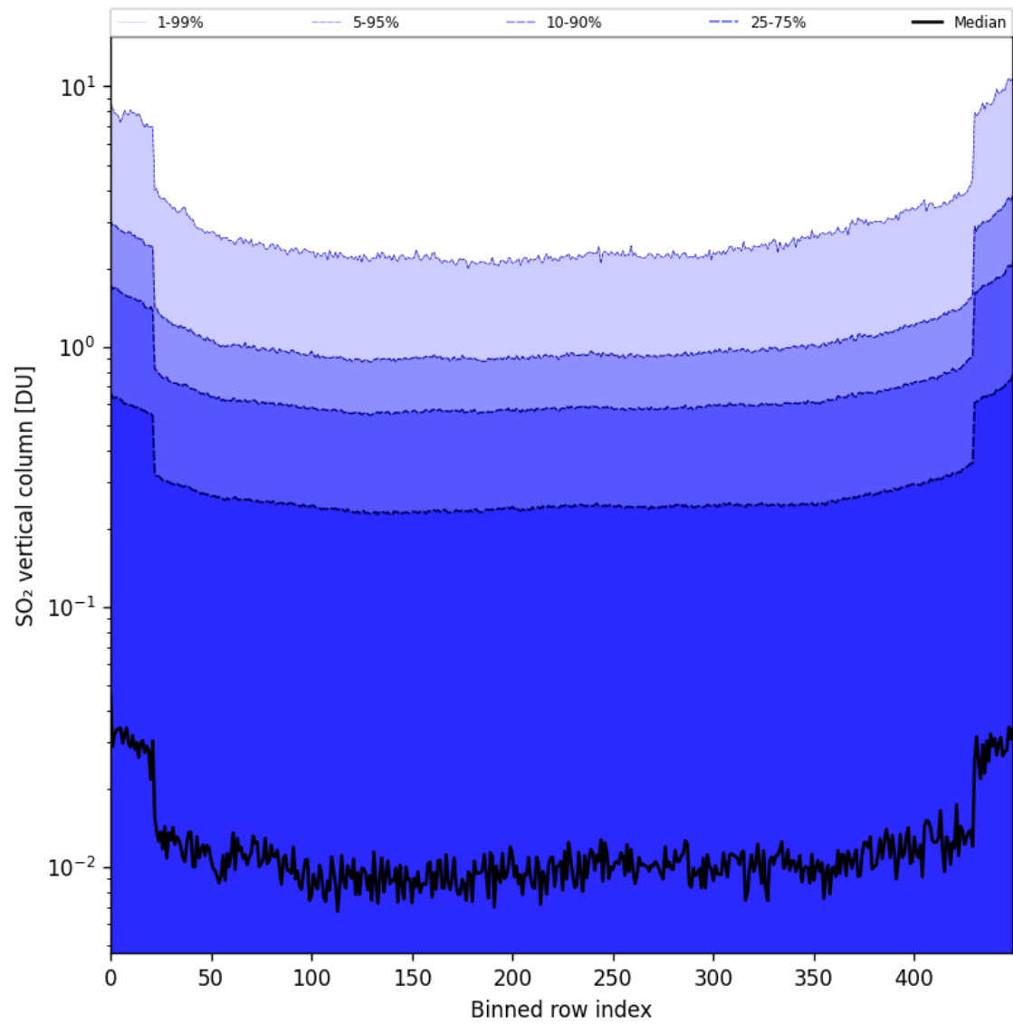
Figure 84: Along track statistics of “SO 2 vertical column” for 2025-09-26 to 2025-09-27
