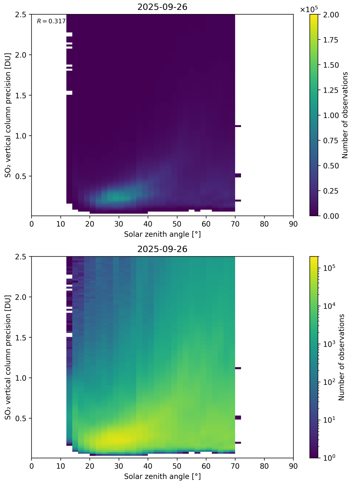
Figure 192: Scatter density plot of “Solar zenith angle” against “SO 2 vertical column precision” for 2025-09-26 to 2025-09-27.
