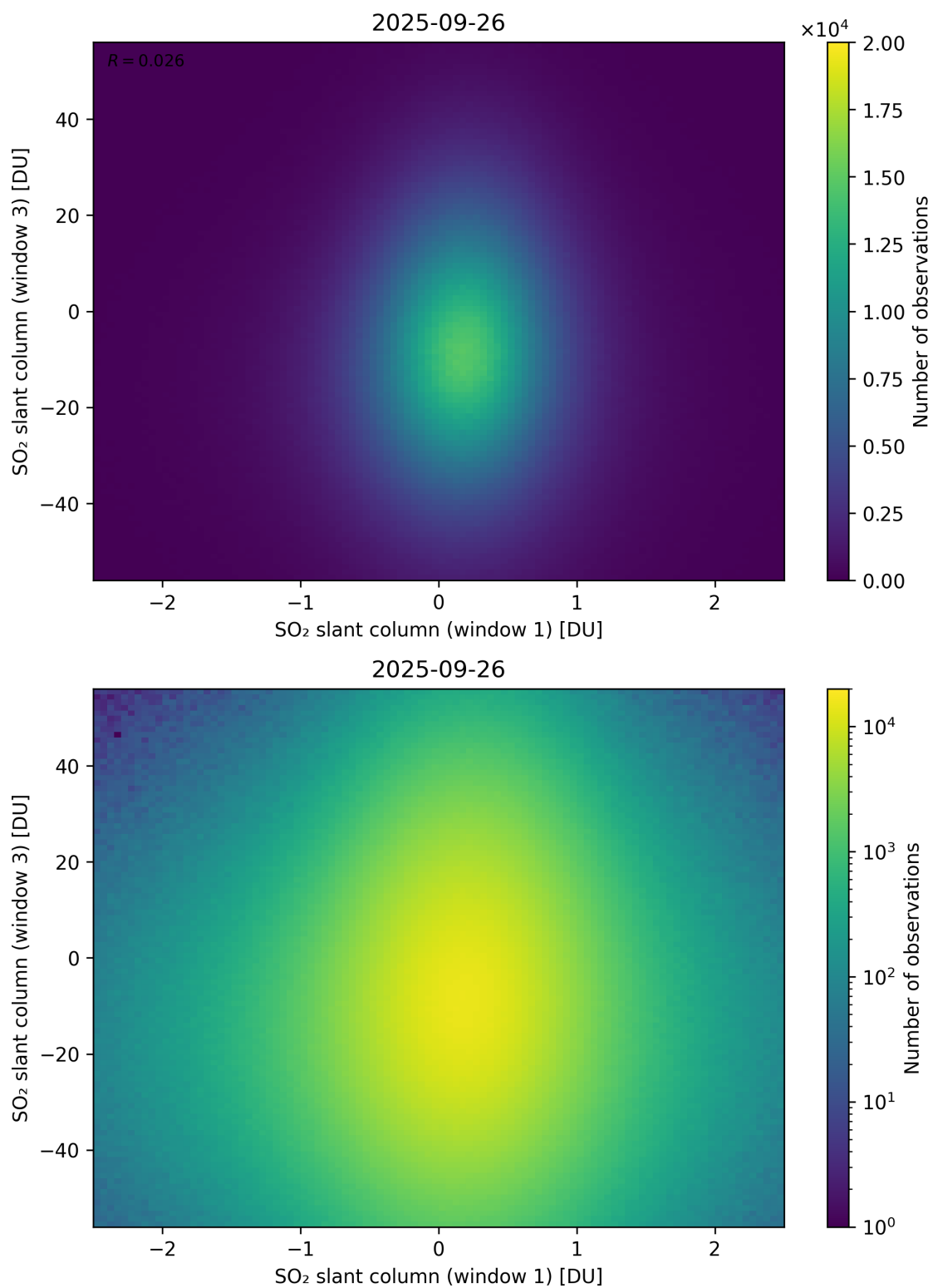
Figure 287: Scatter density plot of “SO 2 slant column (window 1)” against “SO 2 slant column (window 3)” for 2025-09-26 to 2025-09-27.
