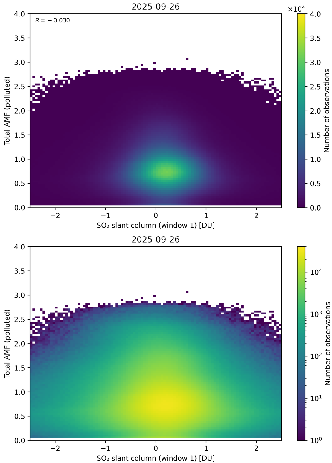
Figure 289: Scatter density plot of “SO 2 slant column (window 1)” against “Total AMF (polluted)” for 2025-09-26 to 2025-09-27.
