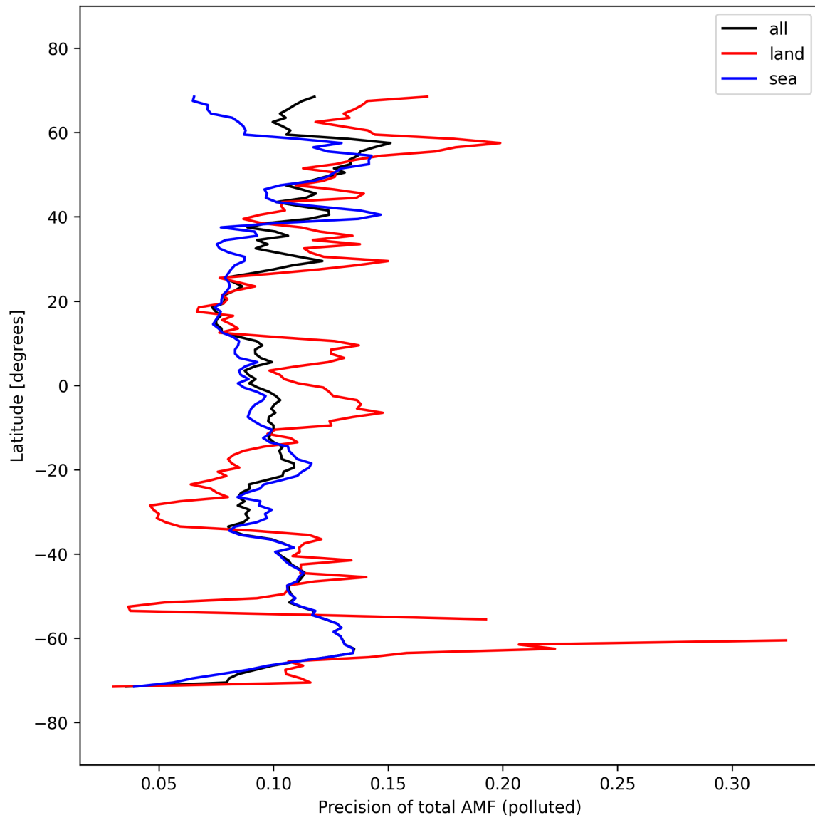
Figure 54: Zonal average of “Precision of total AMF (polluted)” for 2025-09-26 to 2025-09-27.
