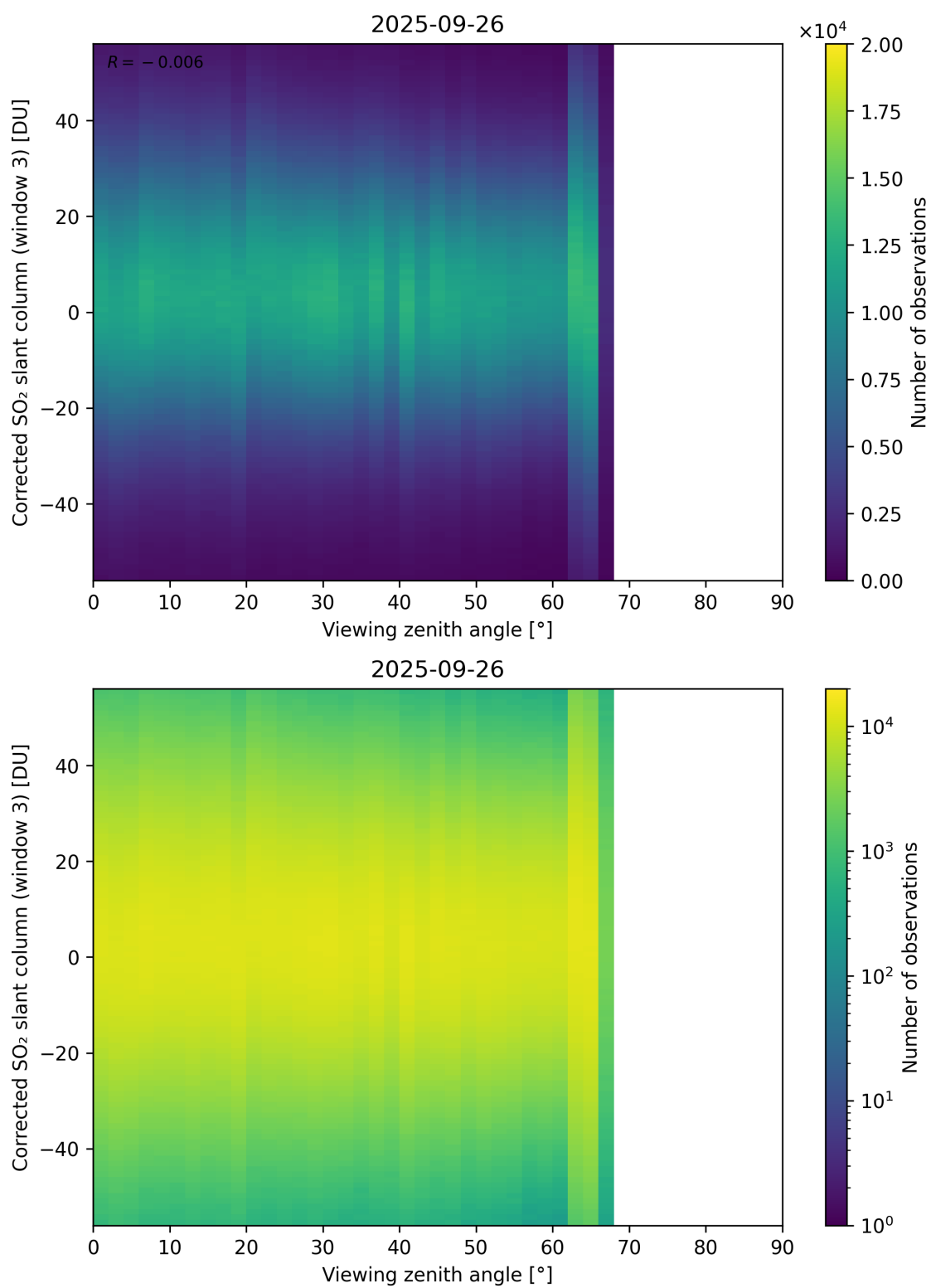
Figure 375: Scatter density plot of “Viewing zenith angle” against “Corrected SO 2 slant column (window 3)” for 2025-09-26 to 2025-09-27.
