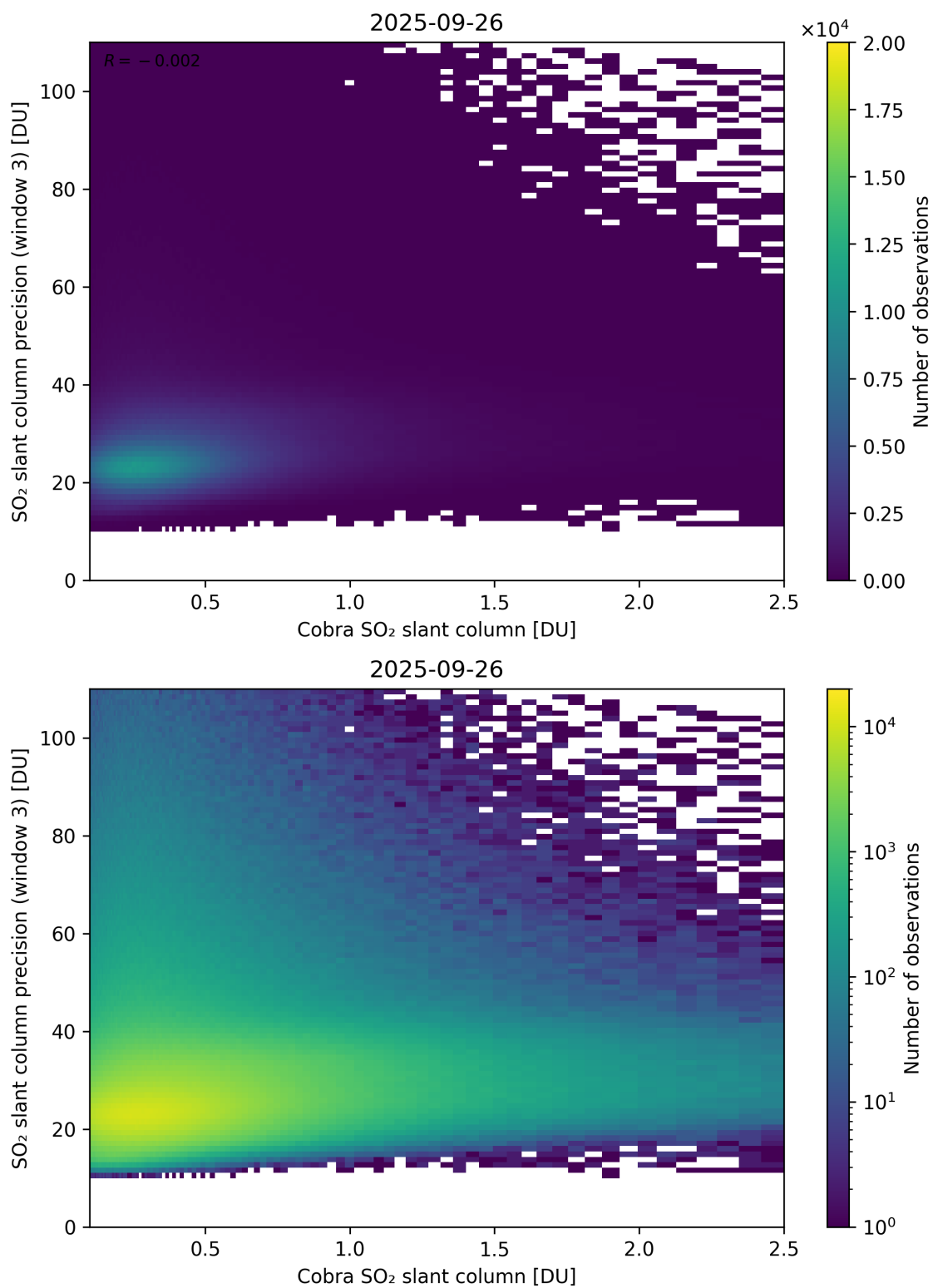
Figure 223: Scatter density plot of “Cobra SO 2 slant column” against “SO 2 slant column precision (window 3)” for 2025-09-26 to 2025-09-27.
