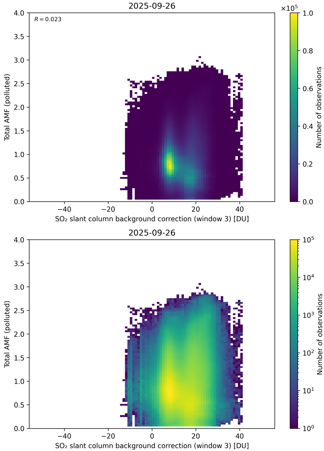
Figure 136: Scatter density plot of “SO 2 slant column background correction (window 3)” against “Total AMF (polluted)” for 2025-09-26 to 2025-09-27.
