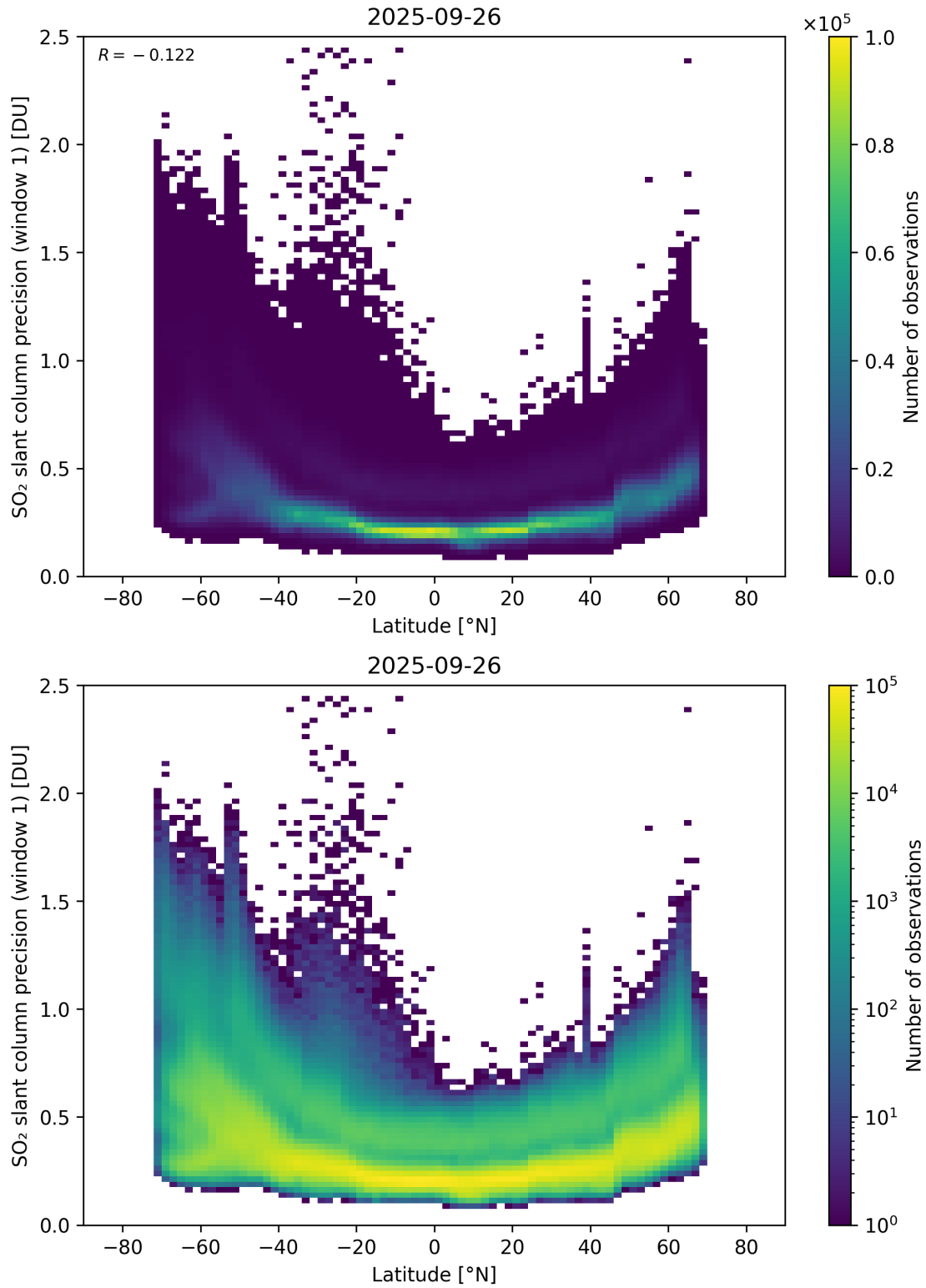
Figure 163: Scatter density plot of “Latitude” against “SO 2 slant column precision (window 1)” for 2025-09-26 to 2025-09-27.
