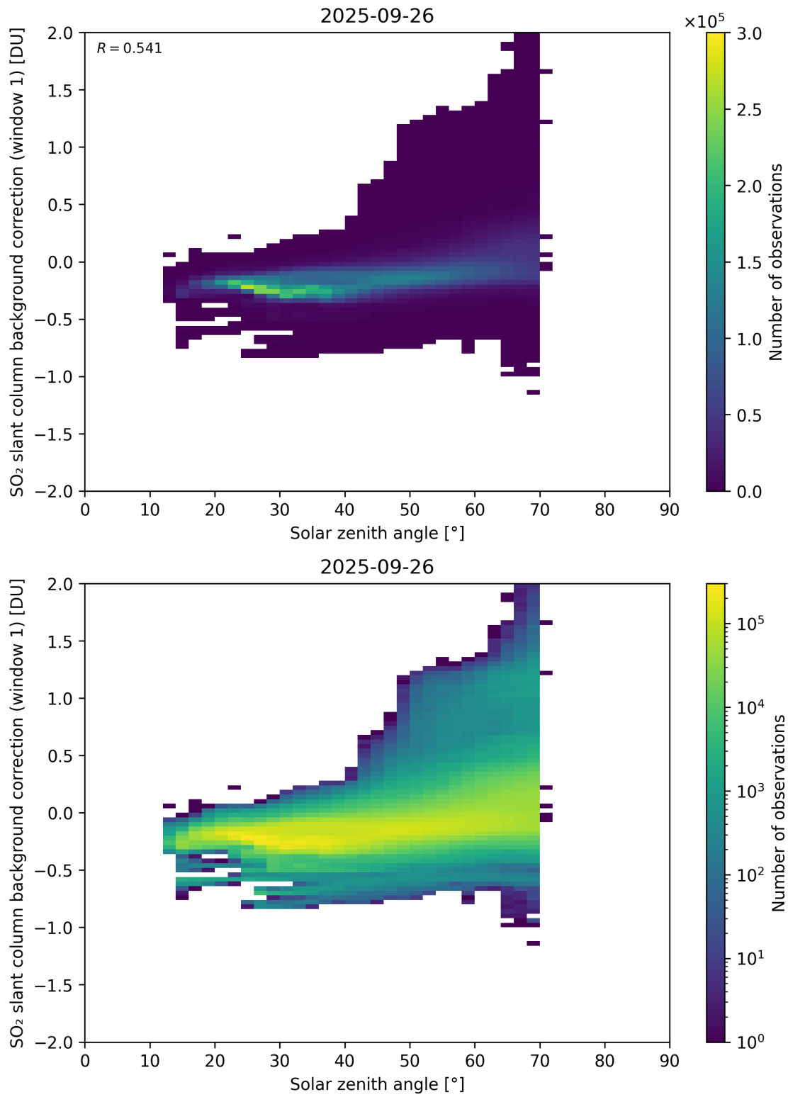
Figure 171: Scatter density plot of “Solar zenith angle” against “SO 2 slant column background correction (window 1)” for 2025-09-26 to 2025-09-27.
