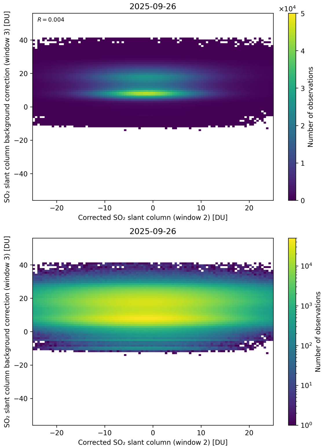
Figure 245: Scatter density plot of “Corrected SO 2 slant column (window 2)” against “SO 2 slant column background correction (window 3)” for 2025-09-26 to 2025-09-27.
