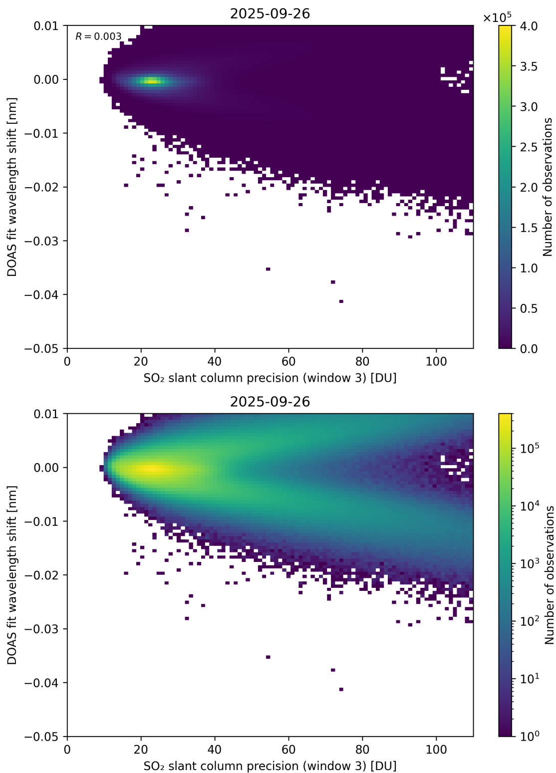
Figure 308: Scatter density plot of “SO 2 slant column precision (window 3)” against “DOAS fit wavelength shift” for 2025-09-26 to 2025-09-27.
