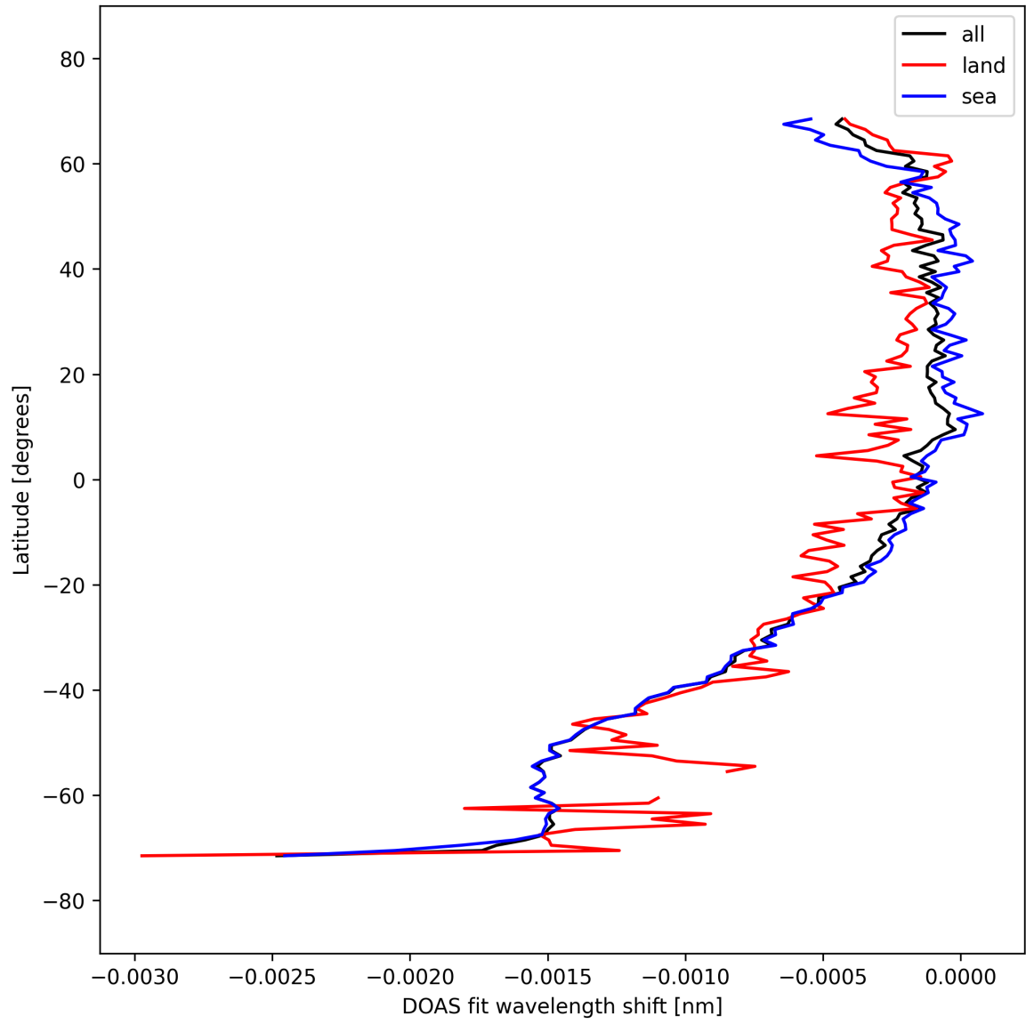
Figure 50: Zonal average of “DOAS fit wavelength shift” for 2025-09-26 to 2025-09-27.
