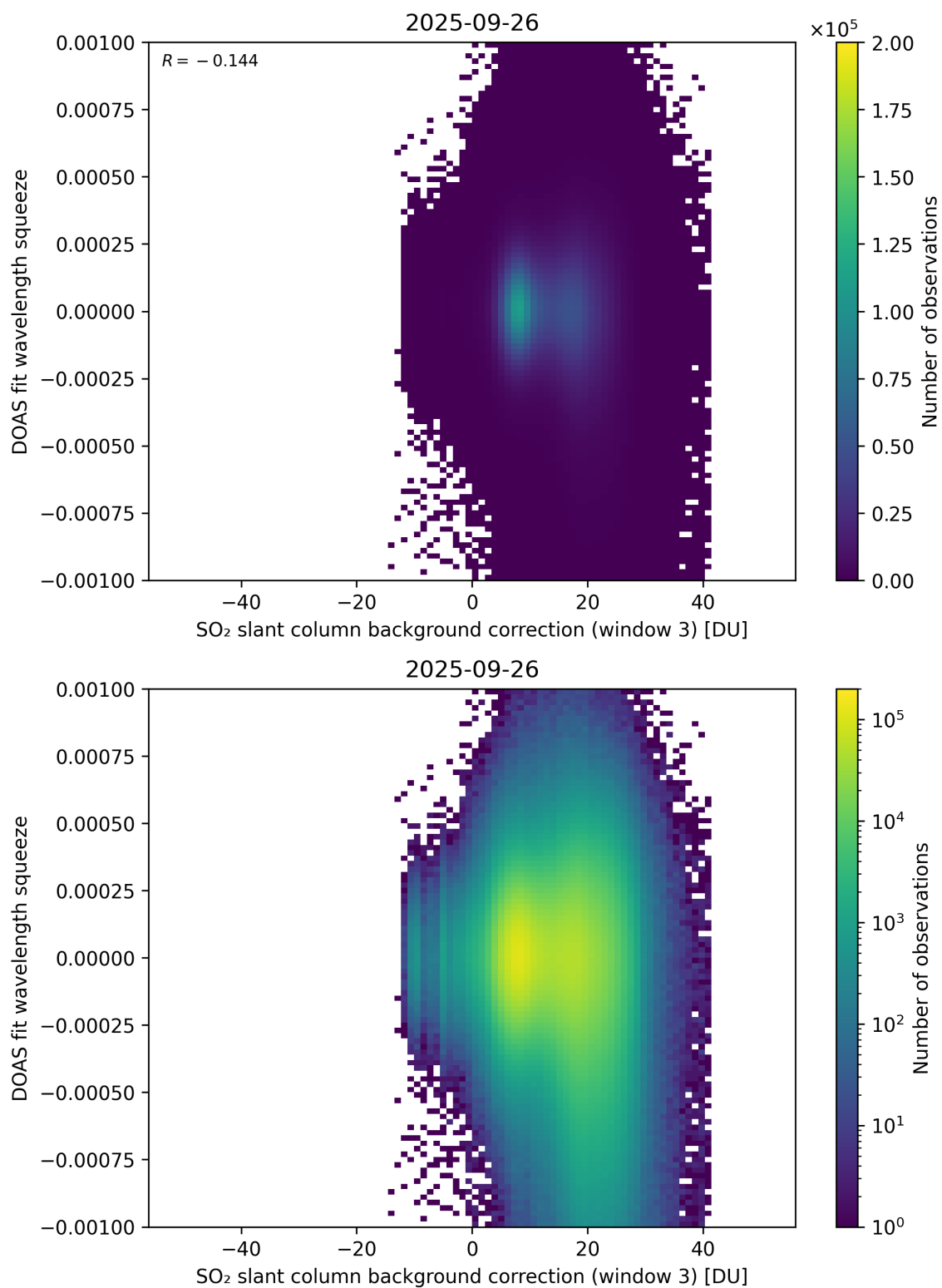
Figure 133: Scatter density plot of “SO 2 slant column background correction (window 3)” against “DOAS fit wavelength squeeze” for 2025-09-26 to 2025-09-27.
