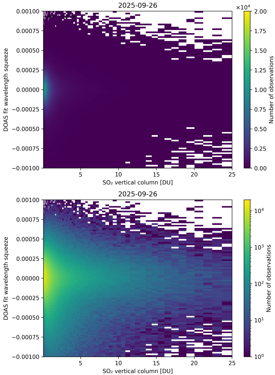
Figure 327: Scatter density plot of “SO 2 vertical column” against “DOAS fit wavelength squeeze” for 2025-09-26 to 2025-09-27.
