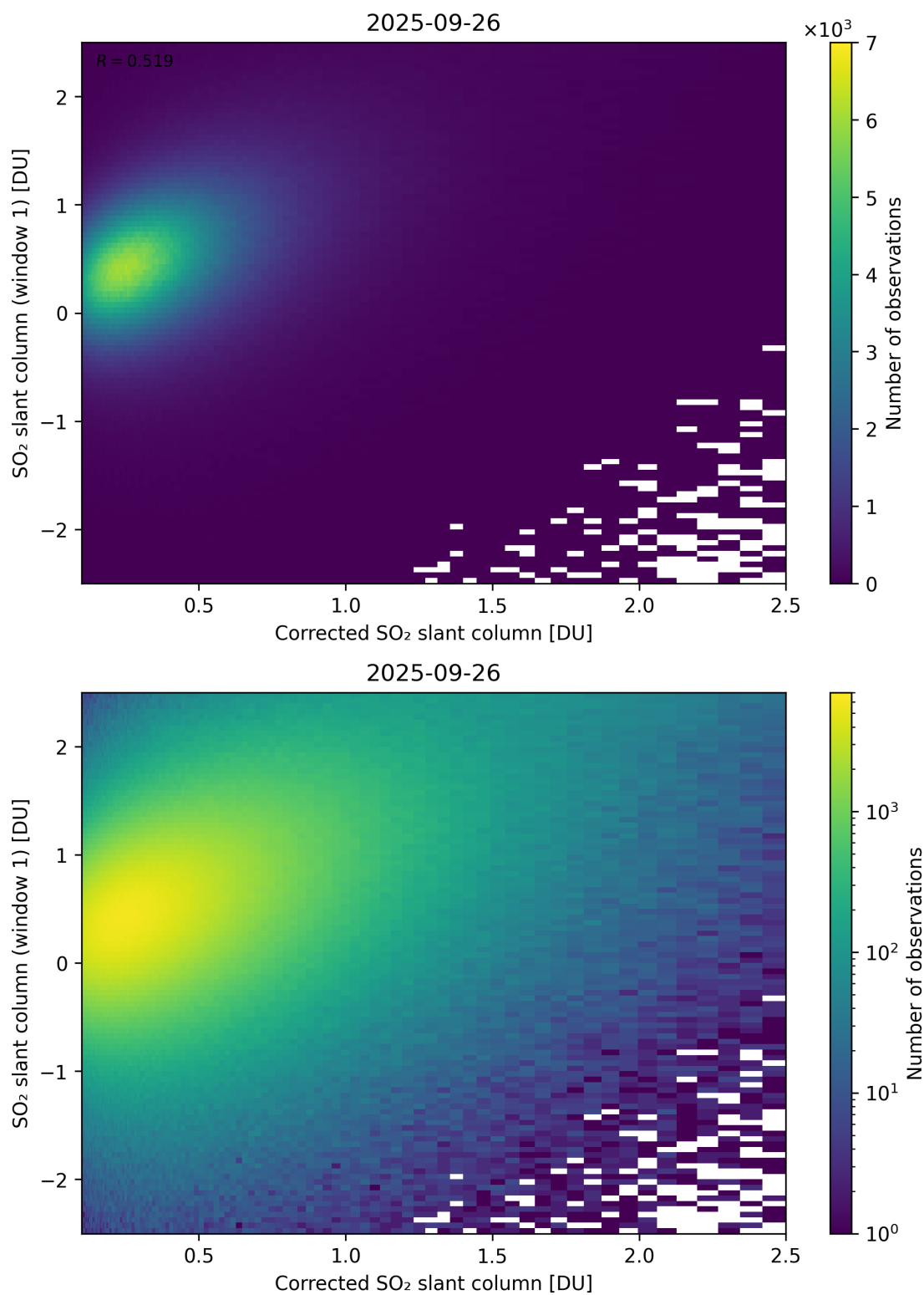
Figure 237: Scatter density plot of “Corrected SO 2 slant column” against “SO 2 slant column (window 1)” for 2025-09-26 to 2025-09-27.
