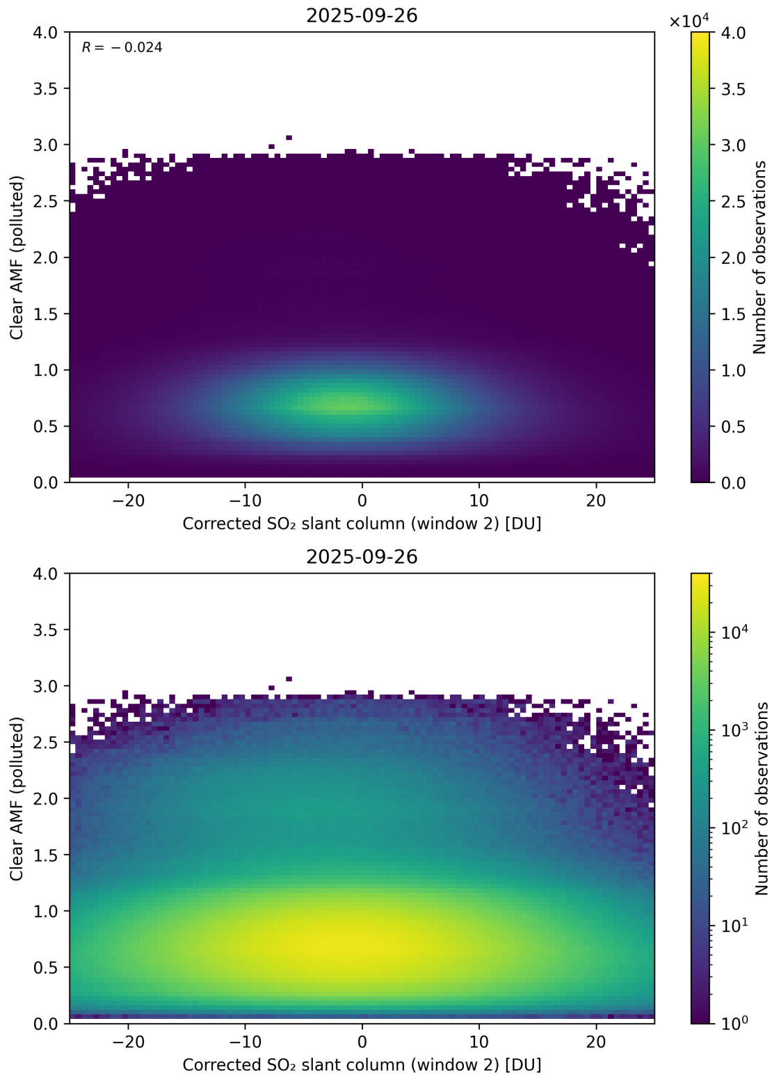
Figure 249: Scatter density plot of “Corrected SO 2 slant column (window 2)” against “Clear AMF (polluted)” for 2025-09-26 to 2025-09-27.
