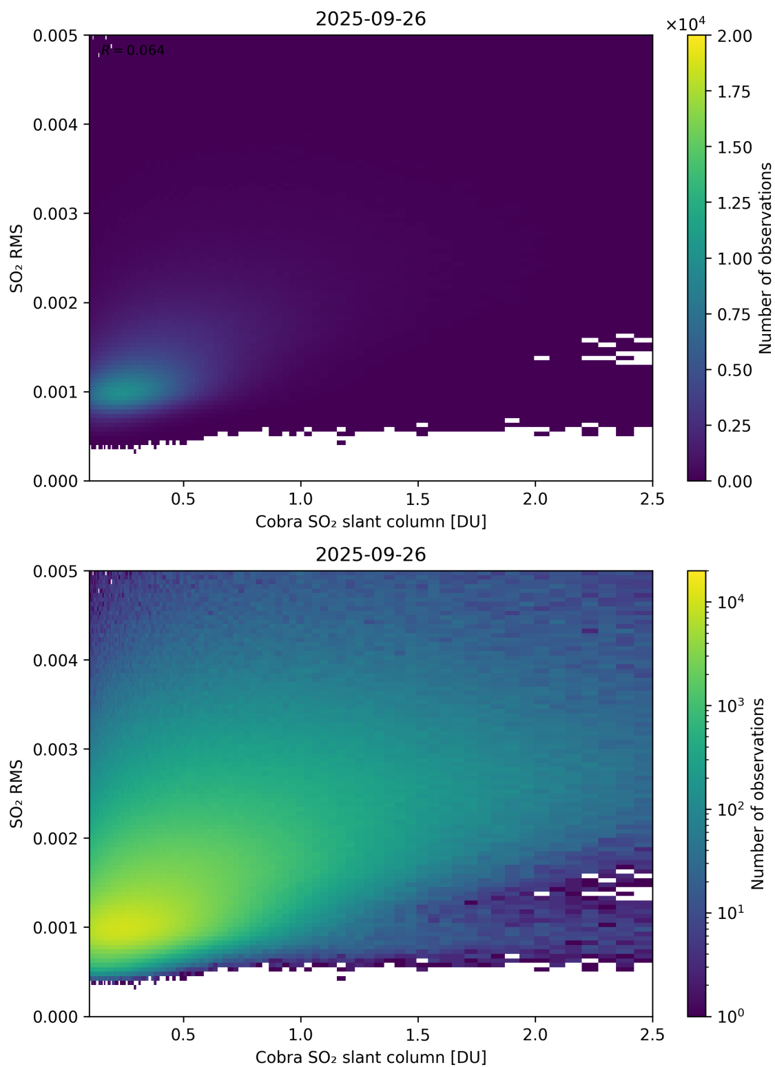
Figure 198: Scatter density plot of “Cobra SO 2 slant column” against “SO 2 RMS” for 2025-09-26 to 2025-09-27.
