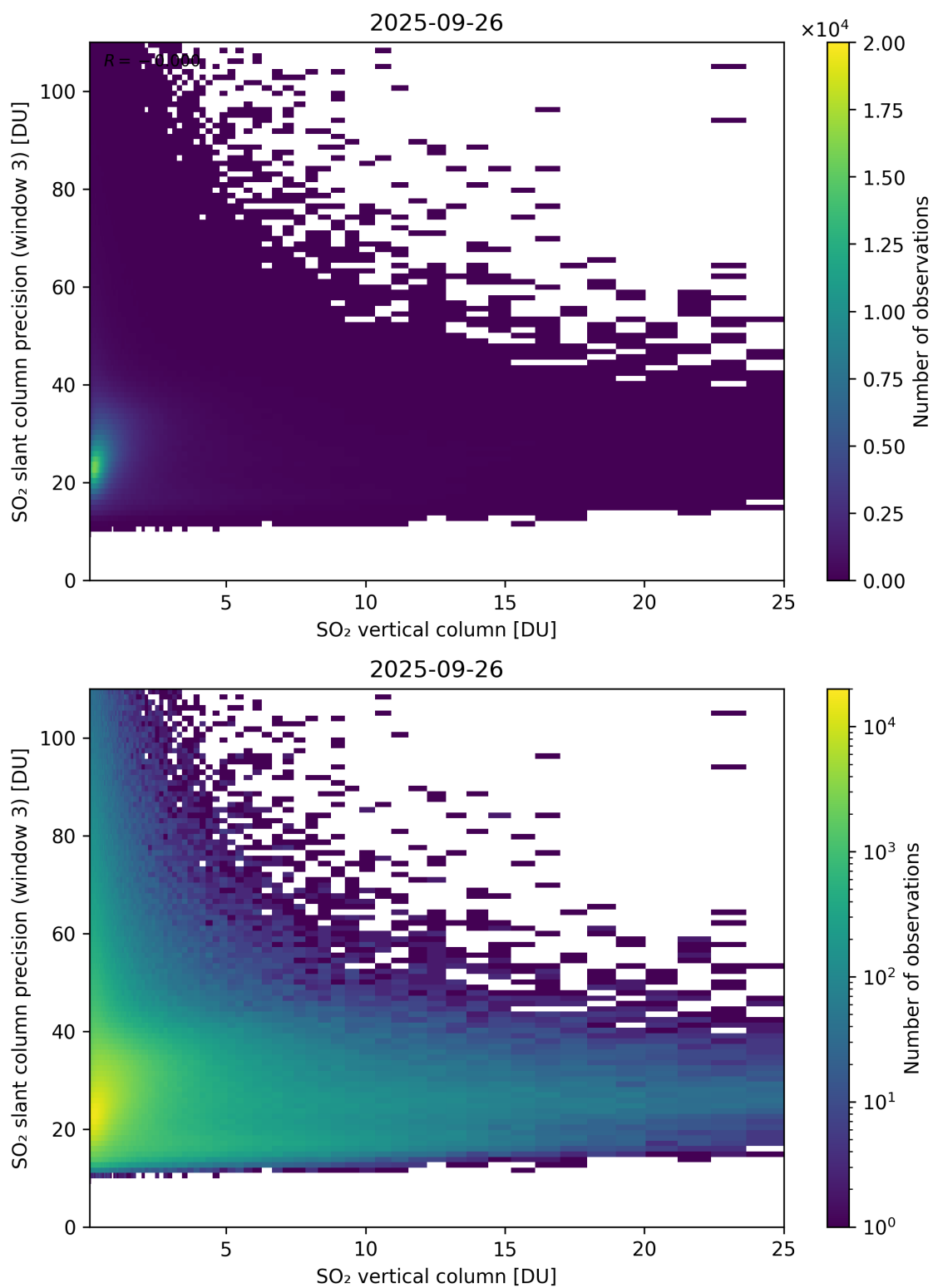
Figure 358: Scatter density plot of “SO 2 vertical column” against “SO 2 slant column precision (window 3)” for 2025-09-26 to 2025-09-27.
