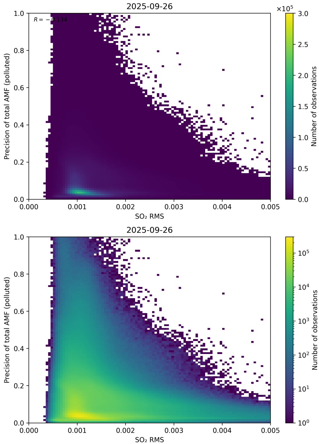
Figure 149: Scatter density plot of “SO 2 RMS” against “Precision of total AMF (polluted)” for 2025-09-26 to 2025-09-27.
