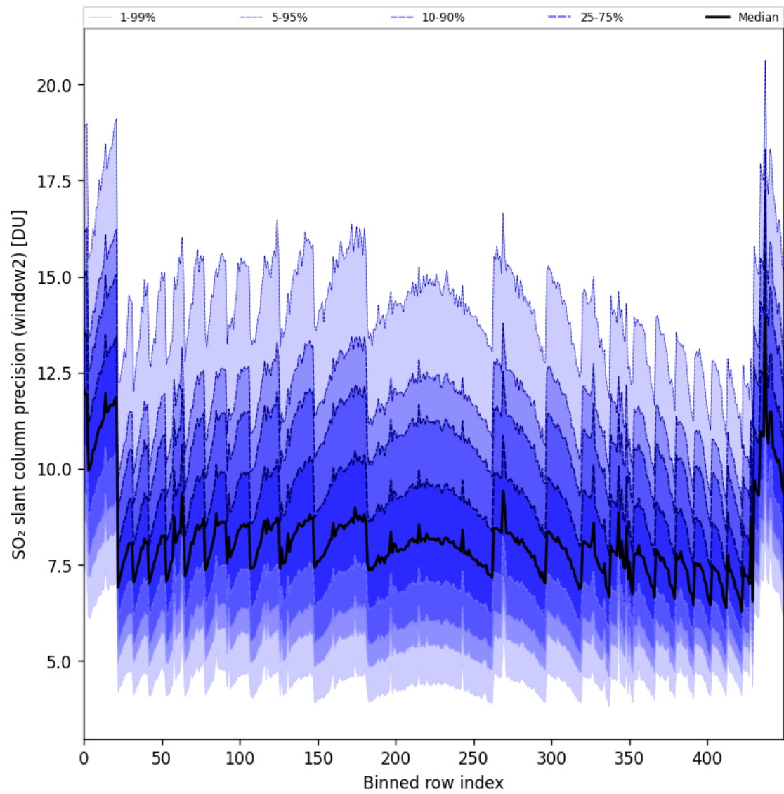
Figure 94: Along track statistics of “SO 2 slant column precision (window2)” for 2025-09-26 to 2025-09-27
