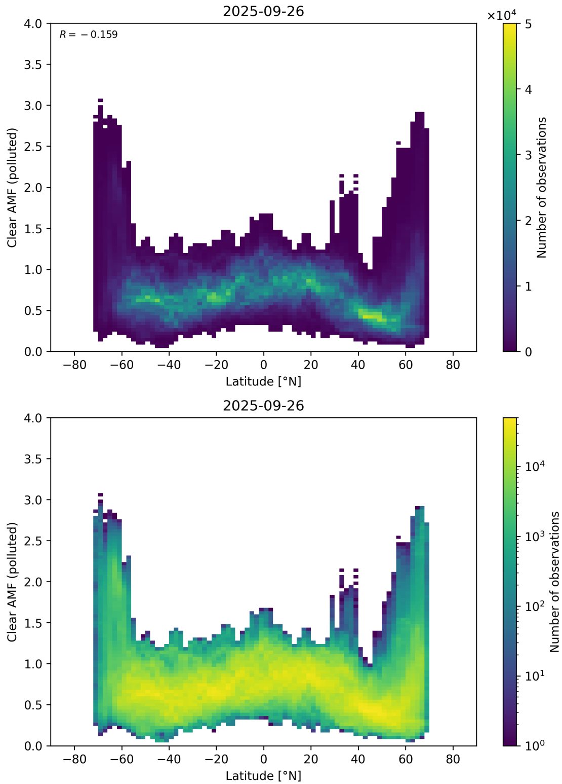
Figure 156: Scatter density plot of “Latitude” against “Clear AMF (polluted)” for 2025-09-26 to 2025-09-27.
