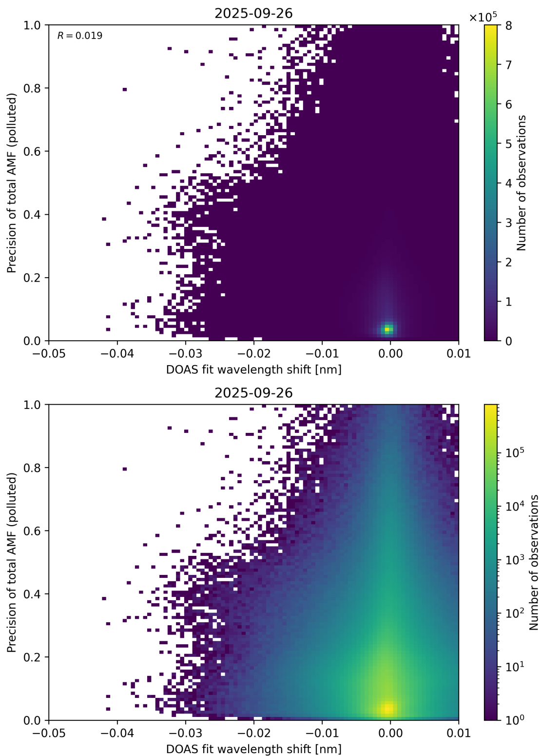
Figure 142: Scatter density plot of “DOAS fit wavelength shift” against “Precision of total AMF (polluted)” for 2025-09-26 to 2025-09-27.
