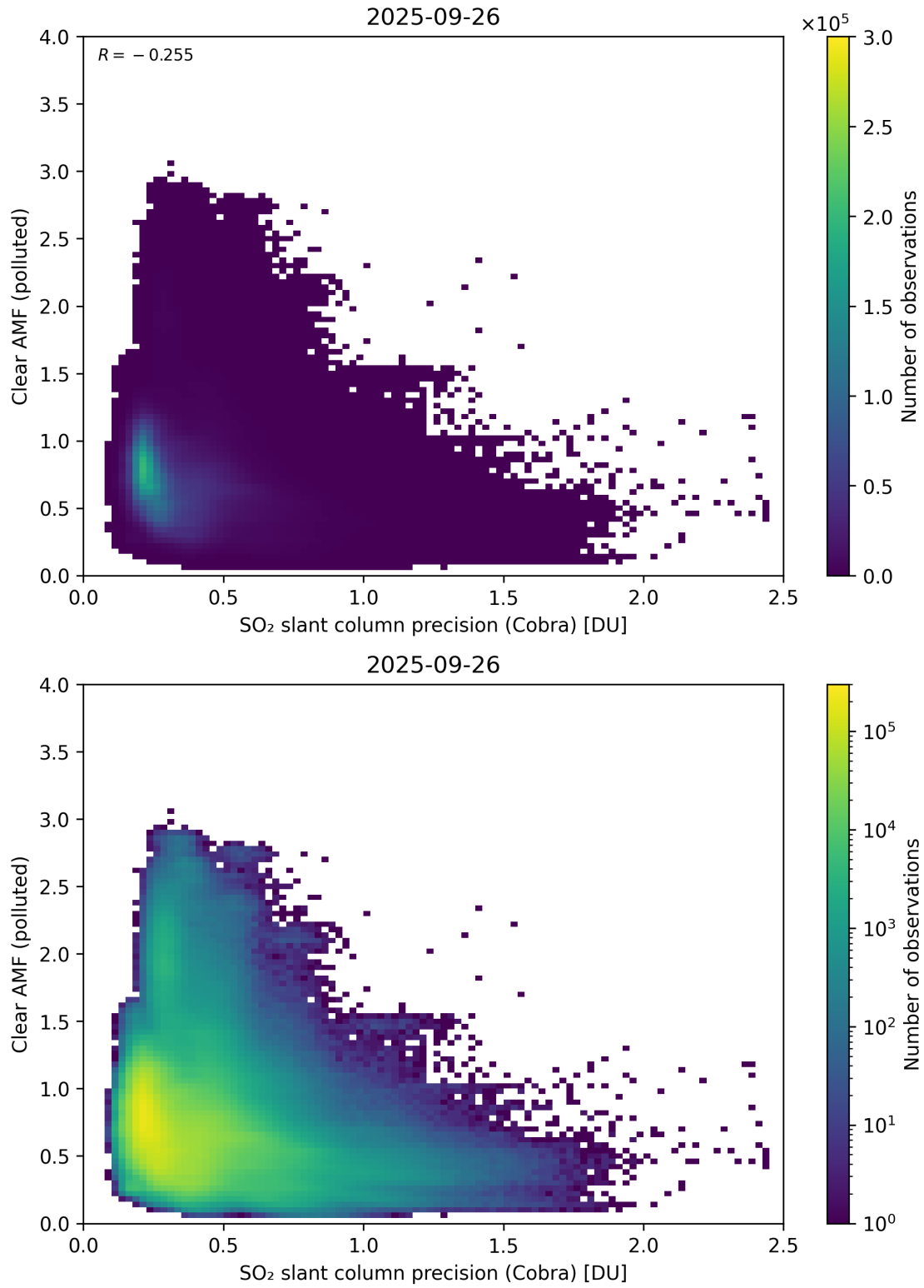
Figure 205: Scatter density plot of “SO 2 slant column precision (Cobra)” against “Clear AMF (polluted)” for 2025-09-26 to 2025-09-27.
