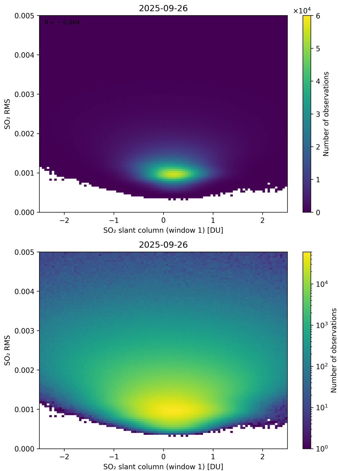
Figure 267: Scatter density plot of “SO 2 slant column (window 1)” against “SO 2 RMS” for 2025-09-26 to 2025-09-27.
