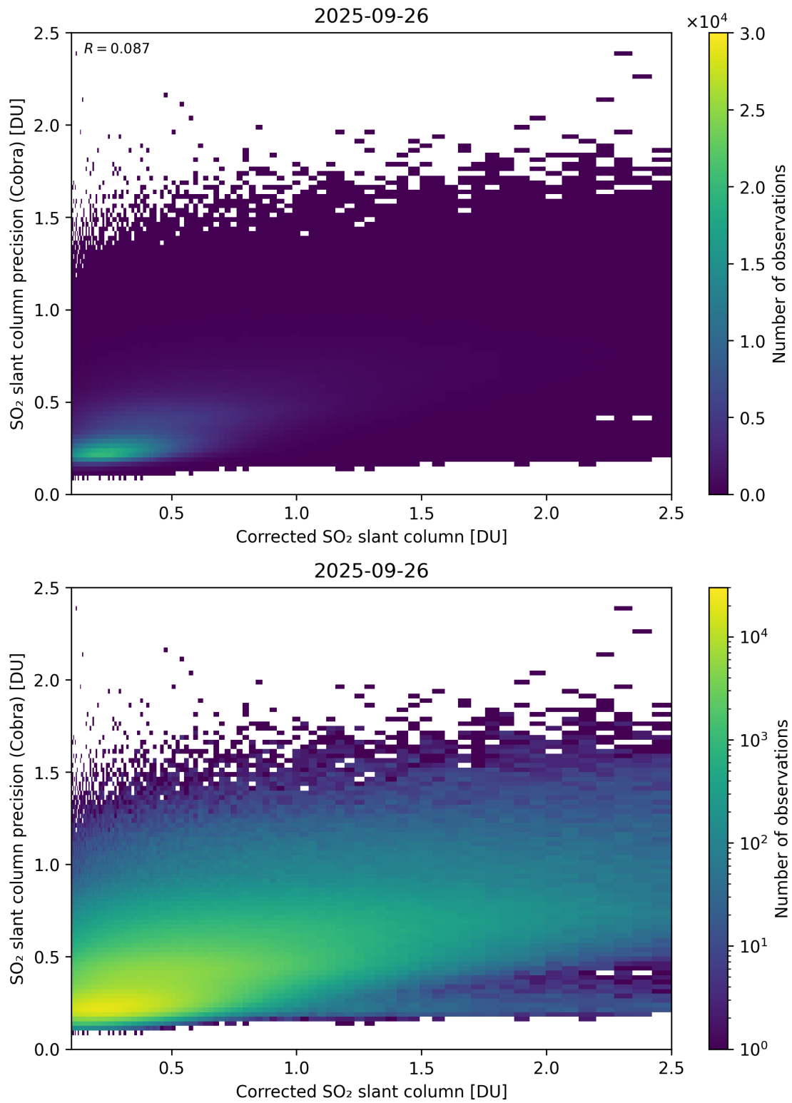
Figure 234: Scatter density plot of “Corrected SO 2 slant column” against “SO 2 slant column precision (Cobra)” for 2025-09-26 to 2025-09-27.
