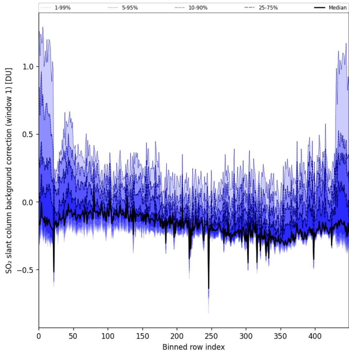
Figure 92: Along track statistics of “SO 2 slant column background correction (window 1)” for 2025-09-26 to 2025-09-27
