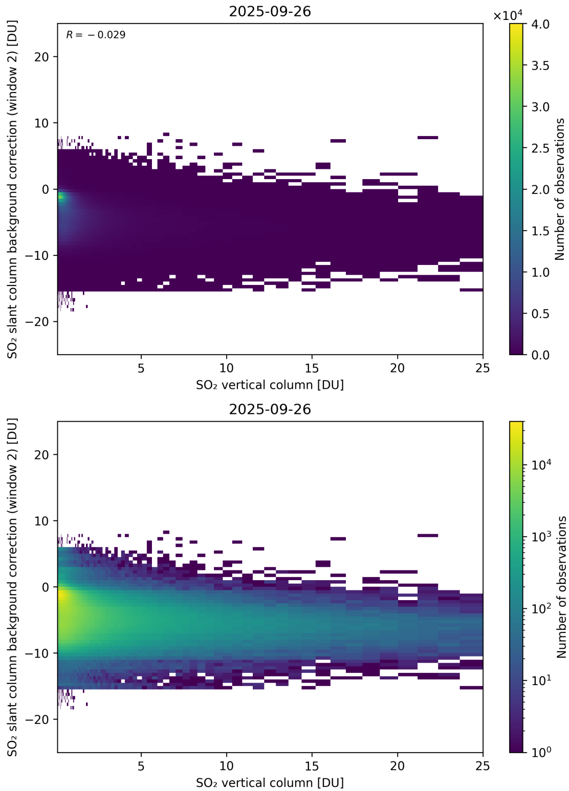
Figure 324: Scatter density plot of “SO 2 vertical column” against “SO 2 slant column background correction (window 2)” for 2025-09-26 to 2025-09-27.
