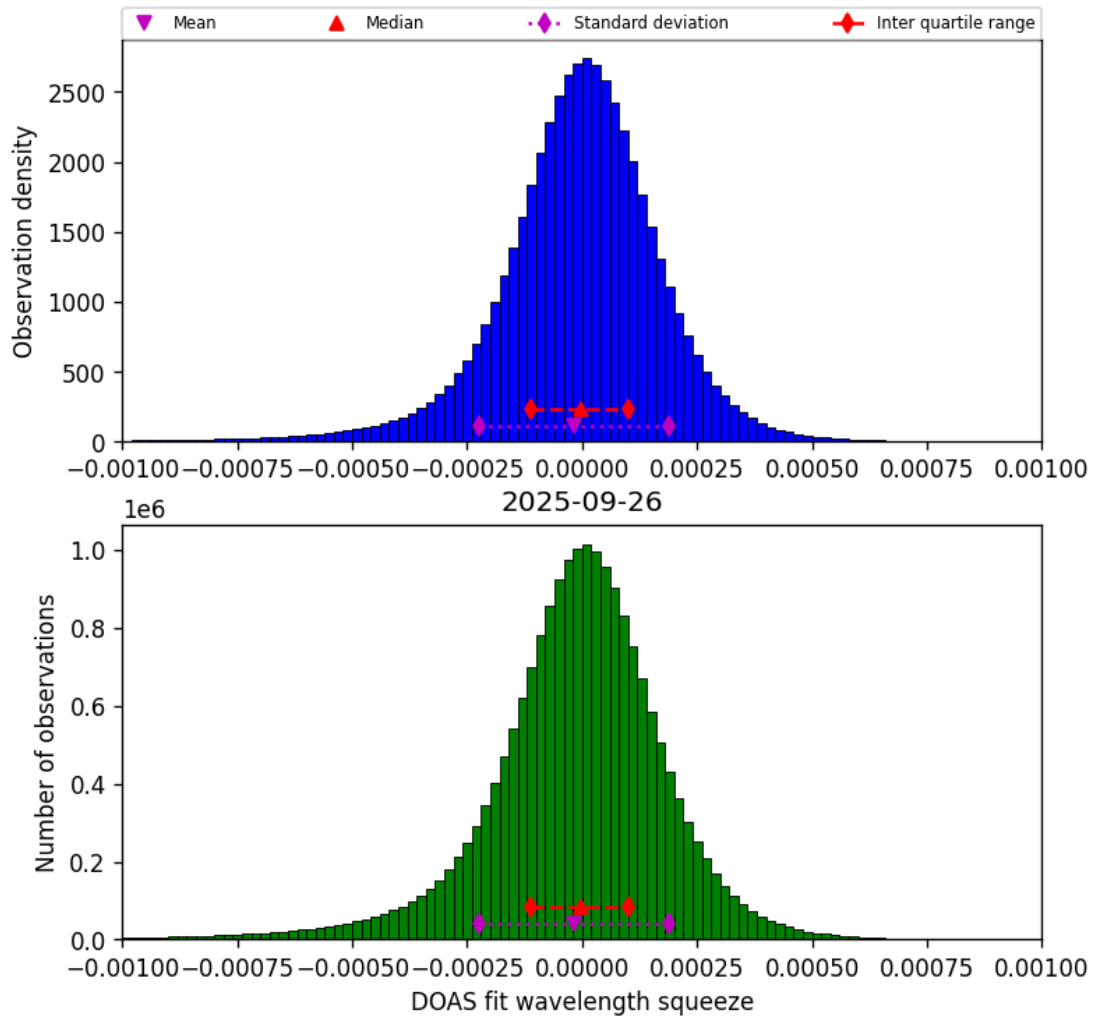
Figure 77: Histogram of “DOAS fit wavelength squeeze” for 2025-09-26 to 2025-09-27
