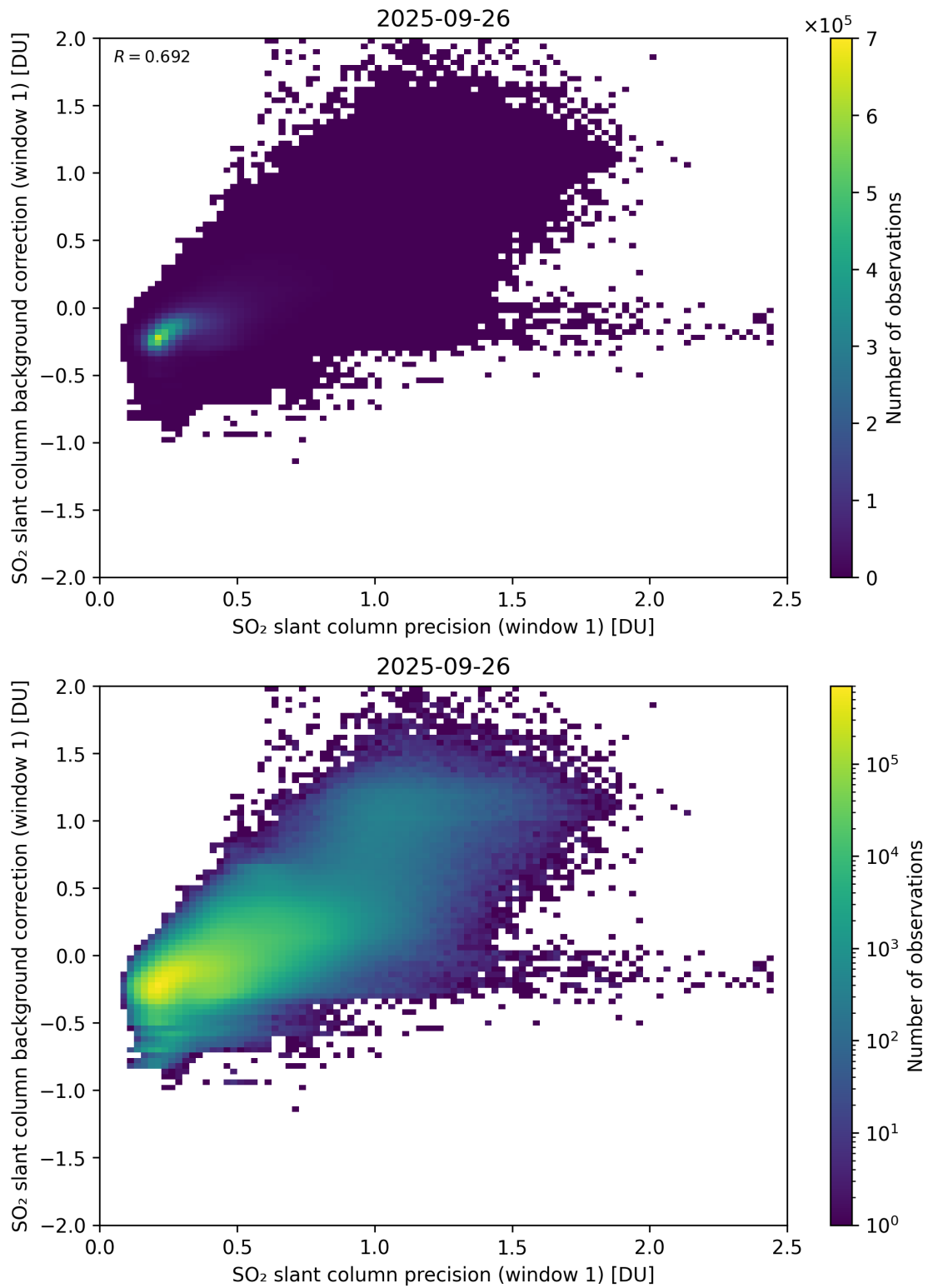
Figure 268: Scatter density plot of “SO 2 slant column precision (window 1)” against “SO 2 slant column background correction (window 1)” for 2025-09-26 to 2025-09-27.
