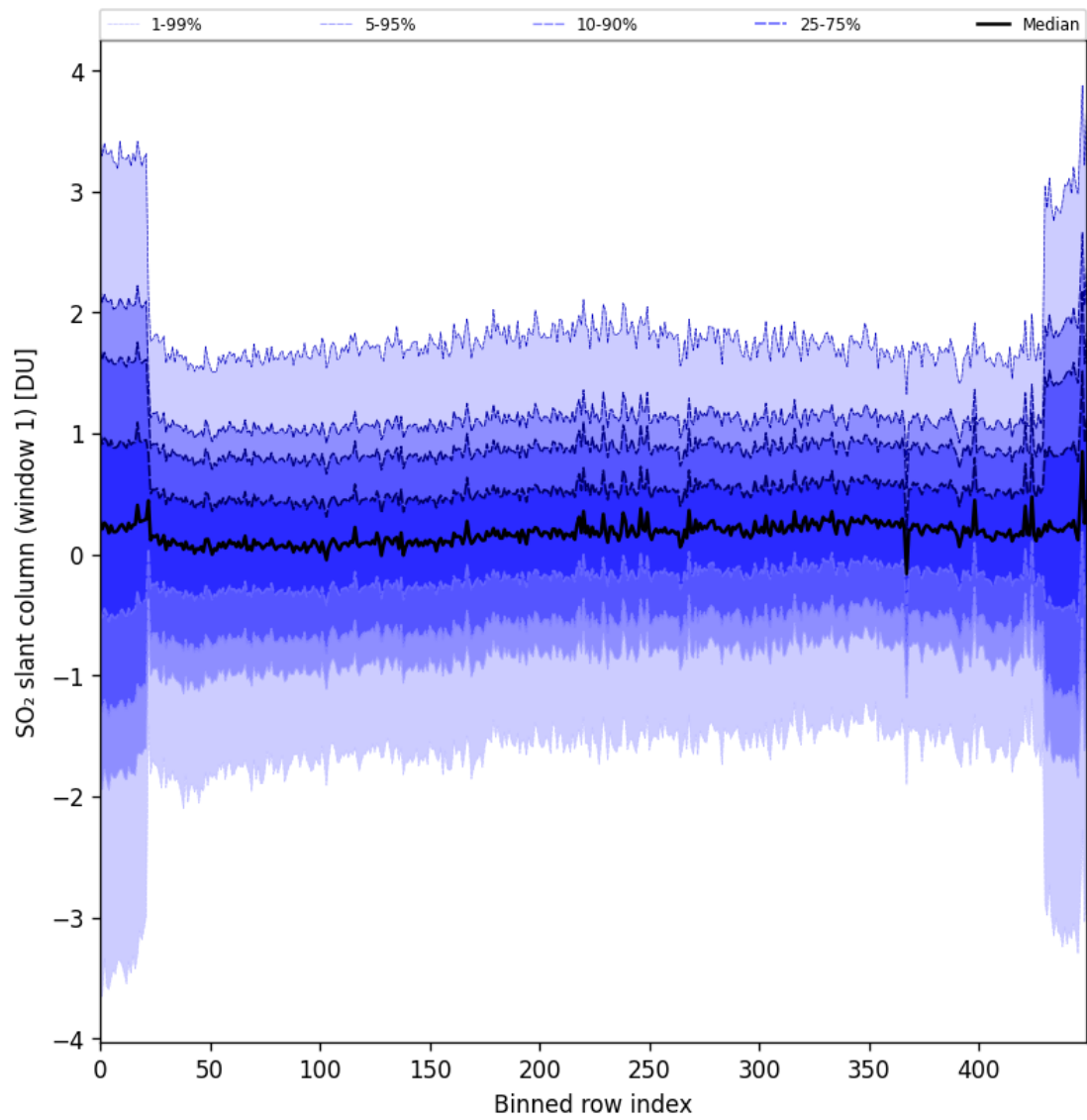
Figure 89: Along track statistics of “SO 2 slant column (window 1)” for 2025-09-26 to 2025-09-27
