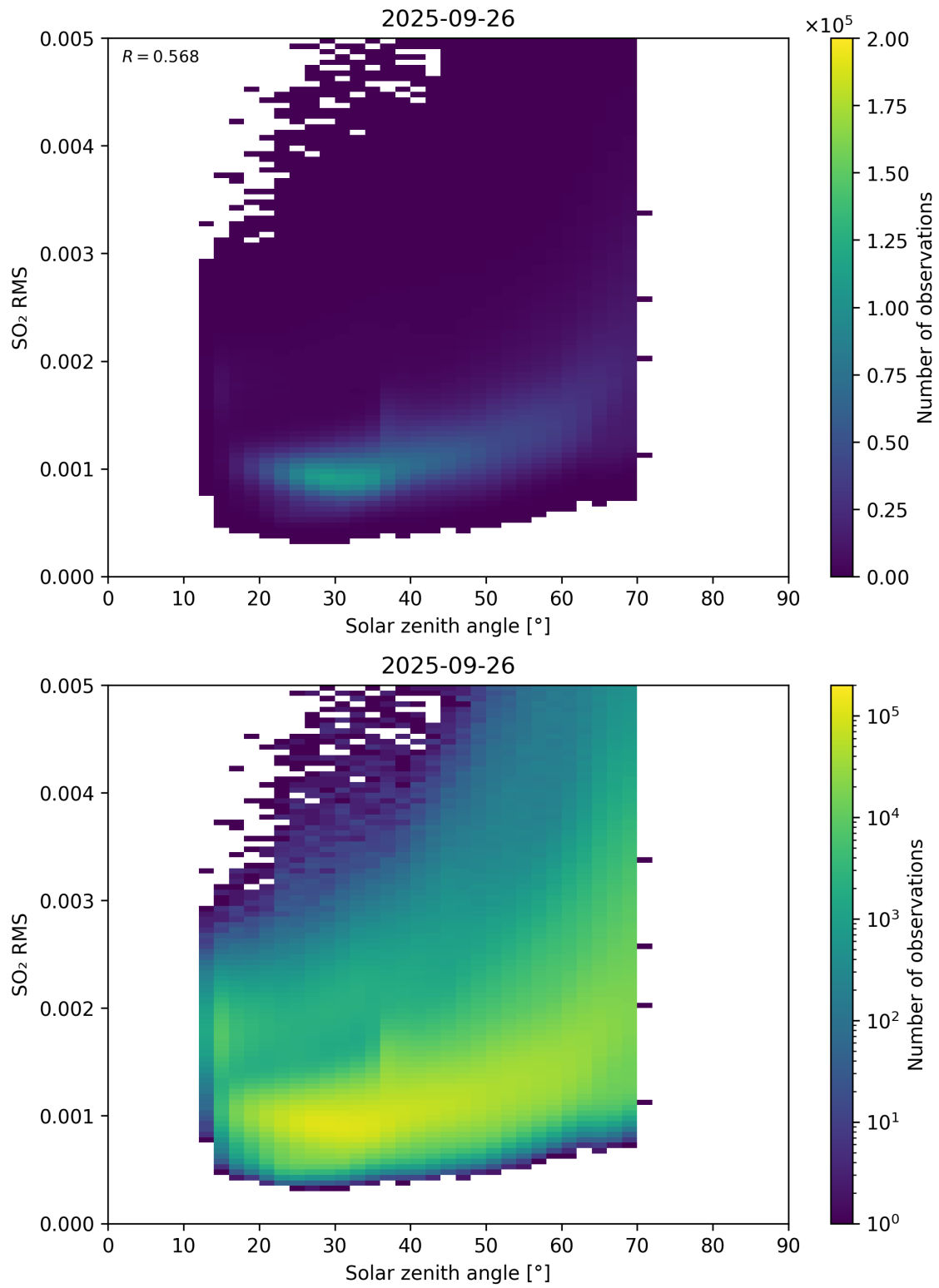
Figure 176: Scatter density plot of “Solar zenith angle” against “SO 2 RMS” for 2025-09-26 to 2025-09-27.
