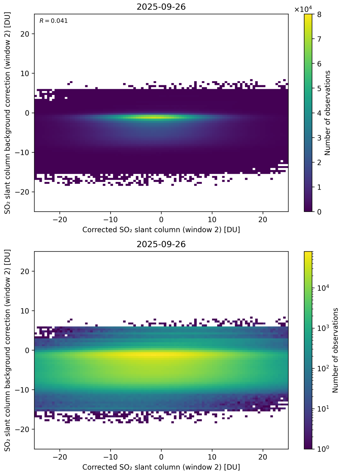
Figure 244: Scatter density plot of “Corrected SO 2 slant column (window 2)” against “SO 2 slant column background correction (window 2)” for 2025-09-26 to 2025-09-27.
