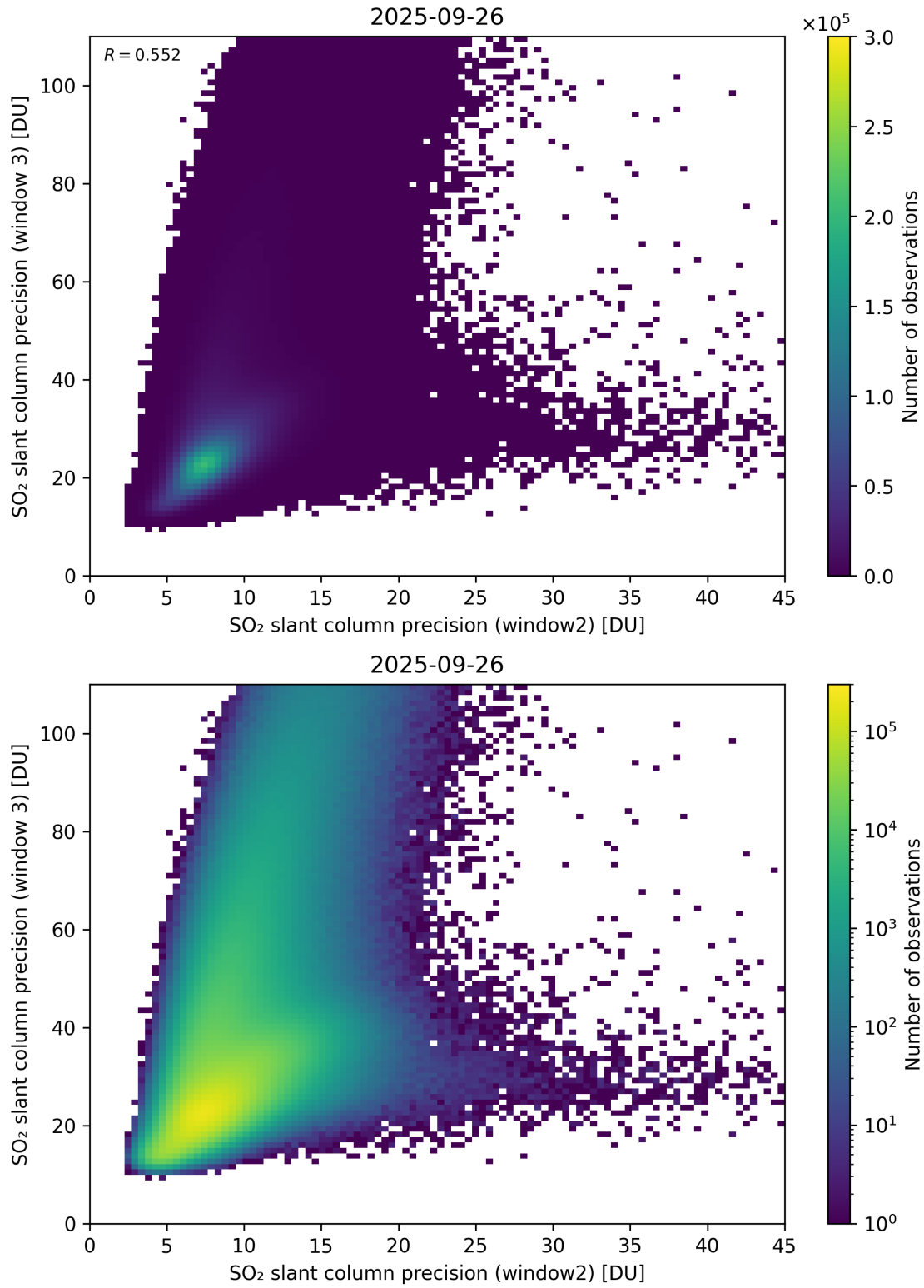
Figure 300: Scatter density plot of “SO 2 slant column precision (window2)” against “SO 2 slant column precision (window 3)” for 2025-09-26 to 2025-09-27.
