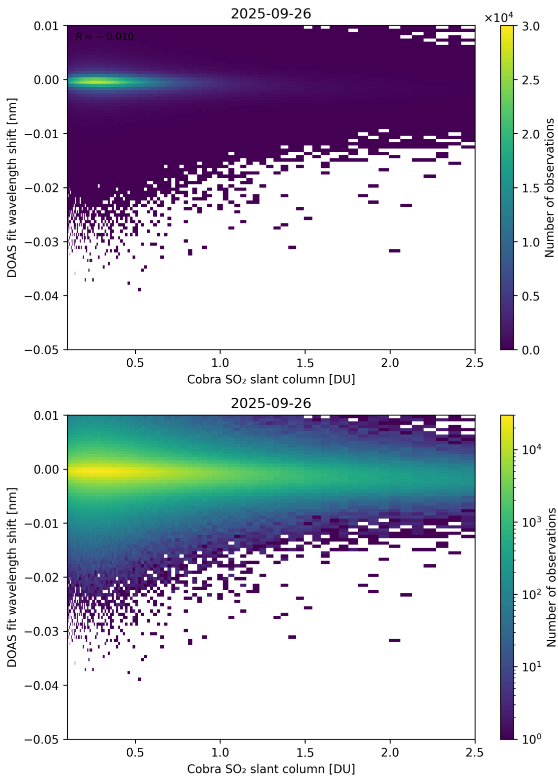
Figure 196: Scatter density plot of “Cobra SO 2 slant column” against “DOAS fit wavelength shift” for 2025-09-26 to 2025-09-27.
