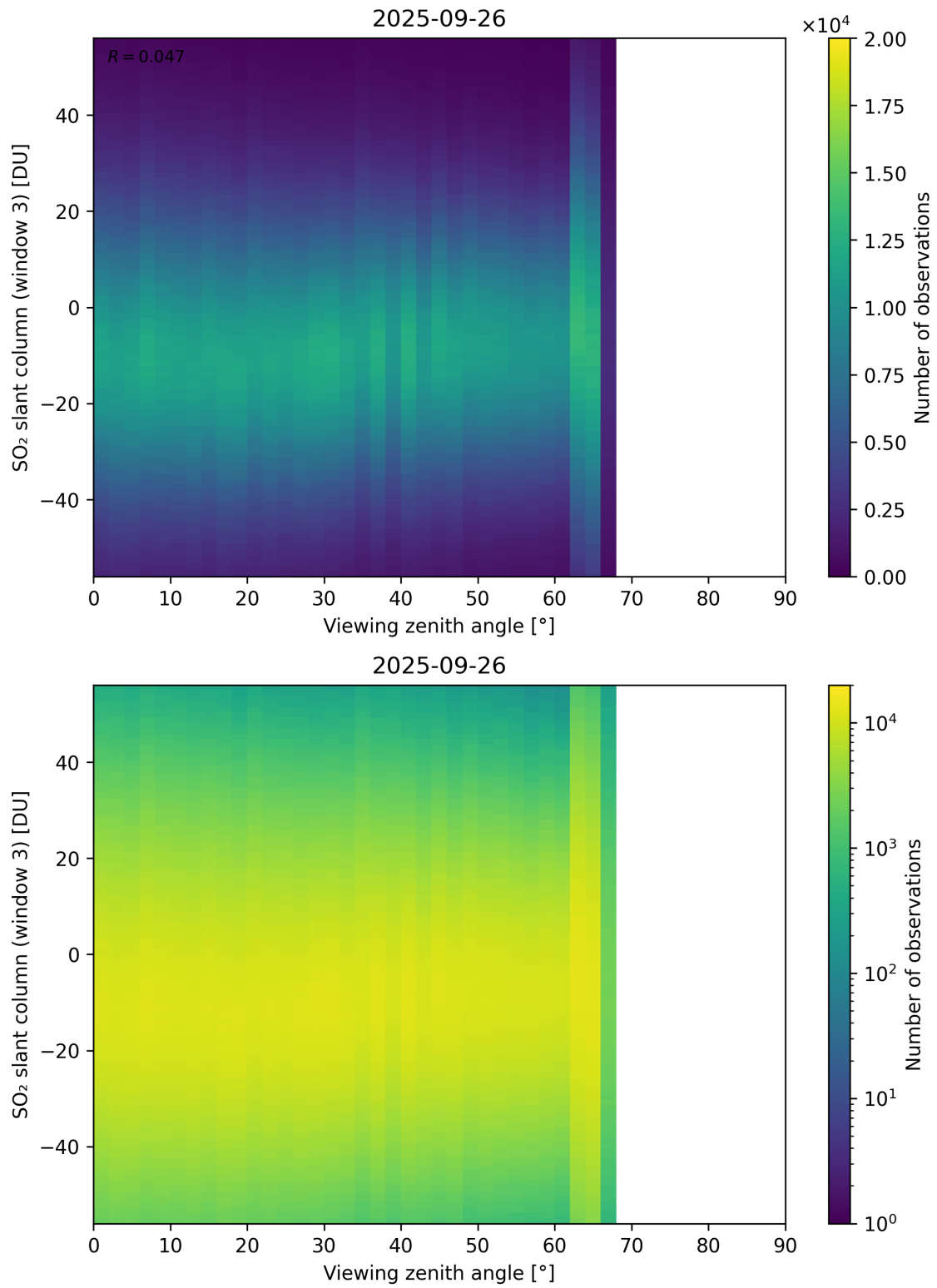
Figure 379: Scatter density plot of “Viewing zenith angle” against “SO 2 slant column (window 3)” for 2025-09-26 to 2025-09-27.
