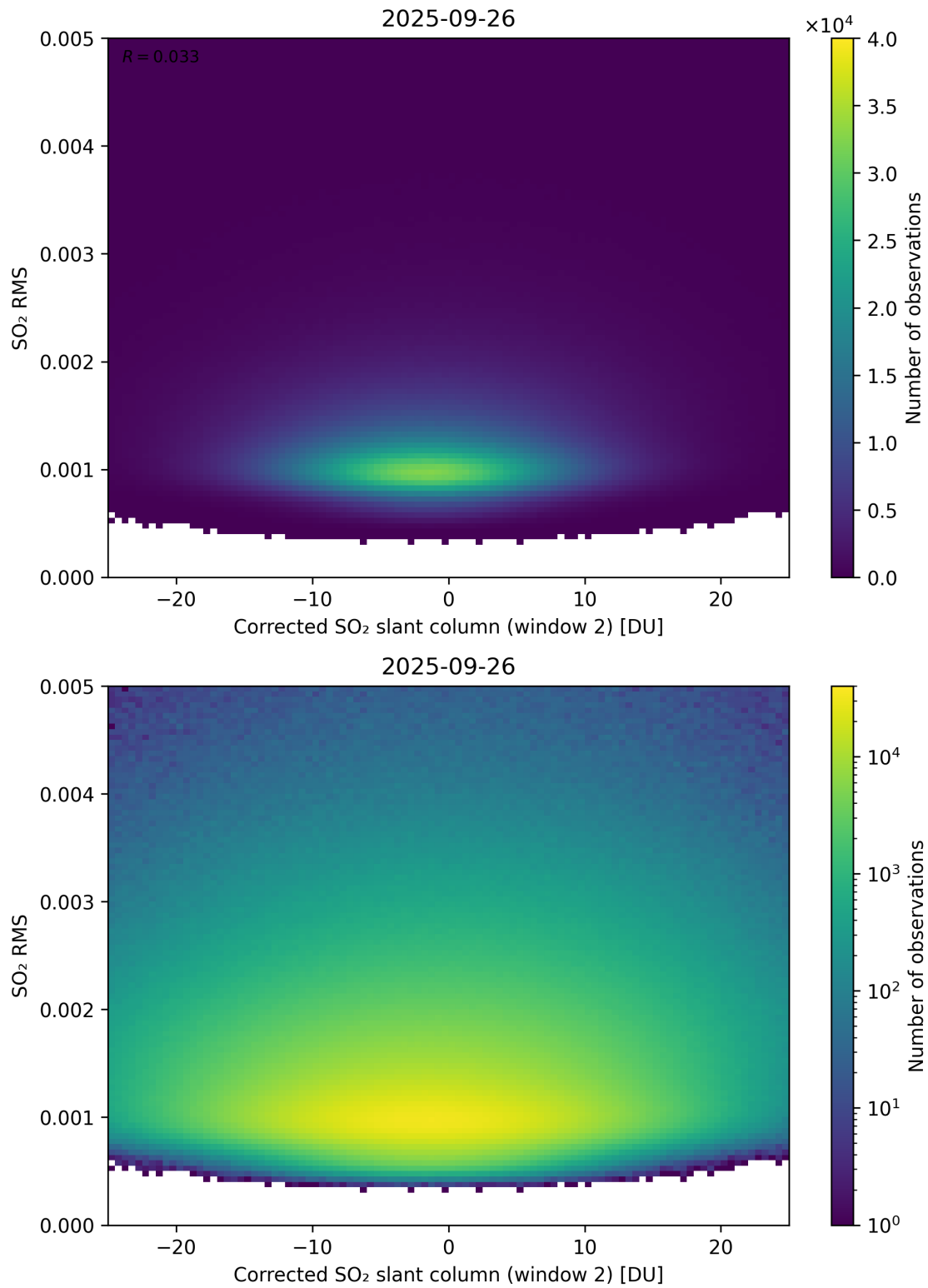
Figure 248: Scatter density plot of “Corrected SO 2 slant column (window 2)” against “SO 2 RMS” for 2025-09-26 to 2025-09-27.
