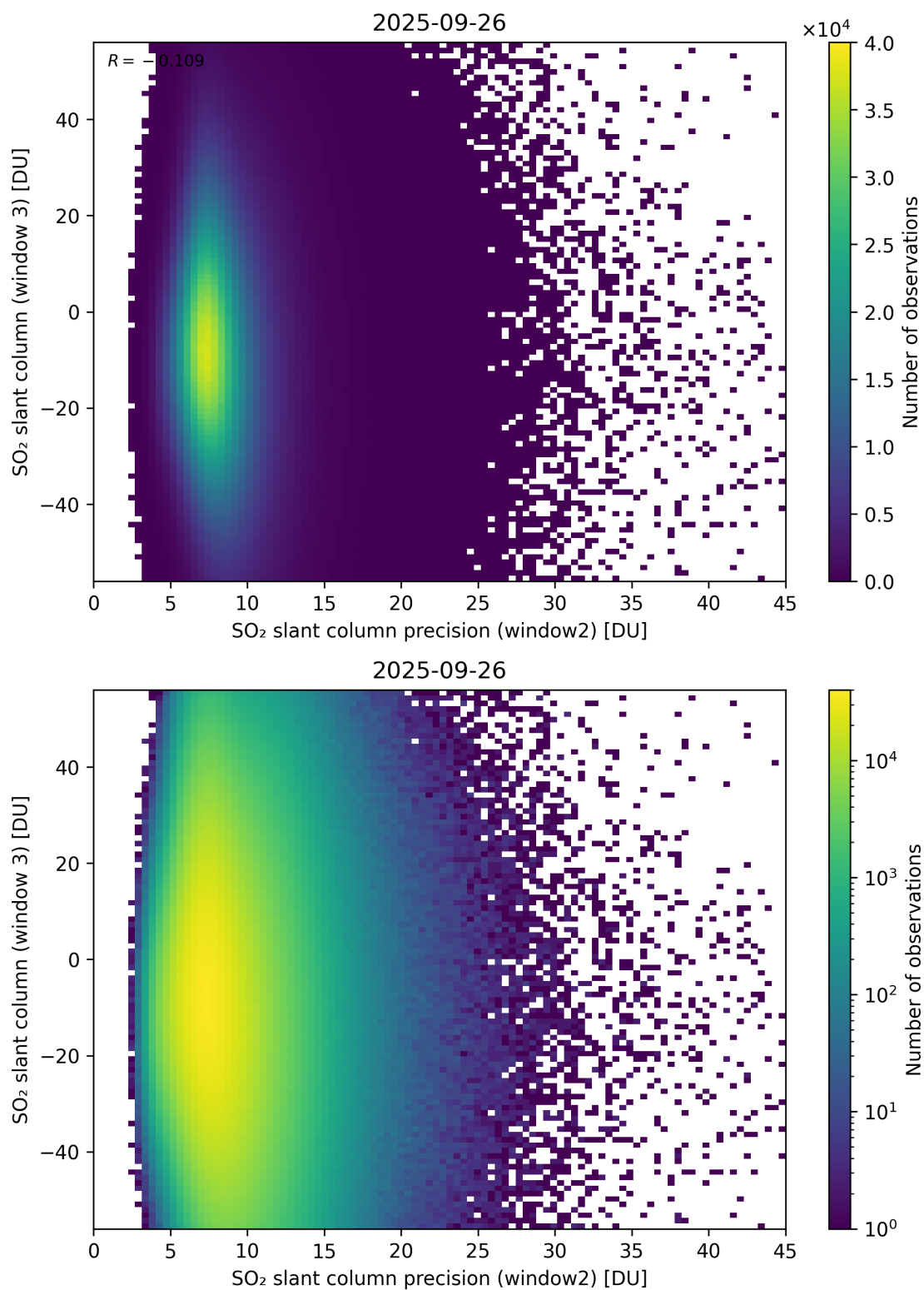
Figure 299: Scatter density plot of “SO 2 slant column precision (window2)” against “SO 2 slant column (window 3)” for 2025-09-26 to 2025-09-27.
