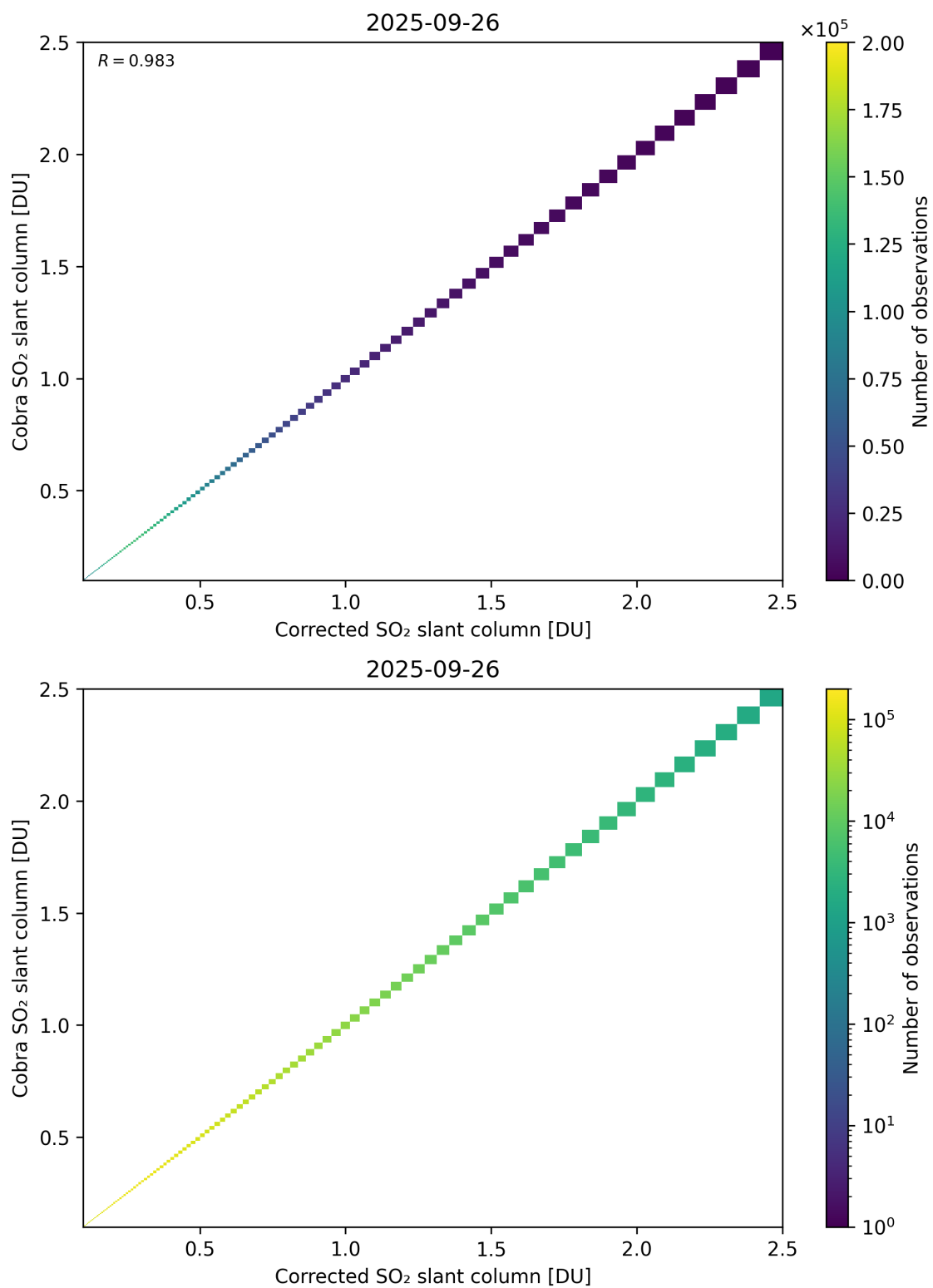
Figure 233: Scatter density plot of “Corrected SO 2 slant column” against “Cobra SO 2 slant column” for 2025-09-26 to 2025-09-27.
