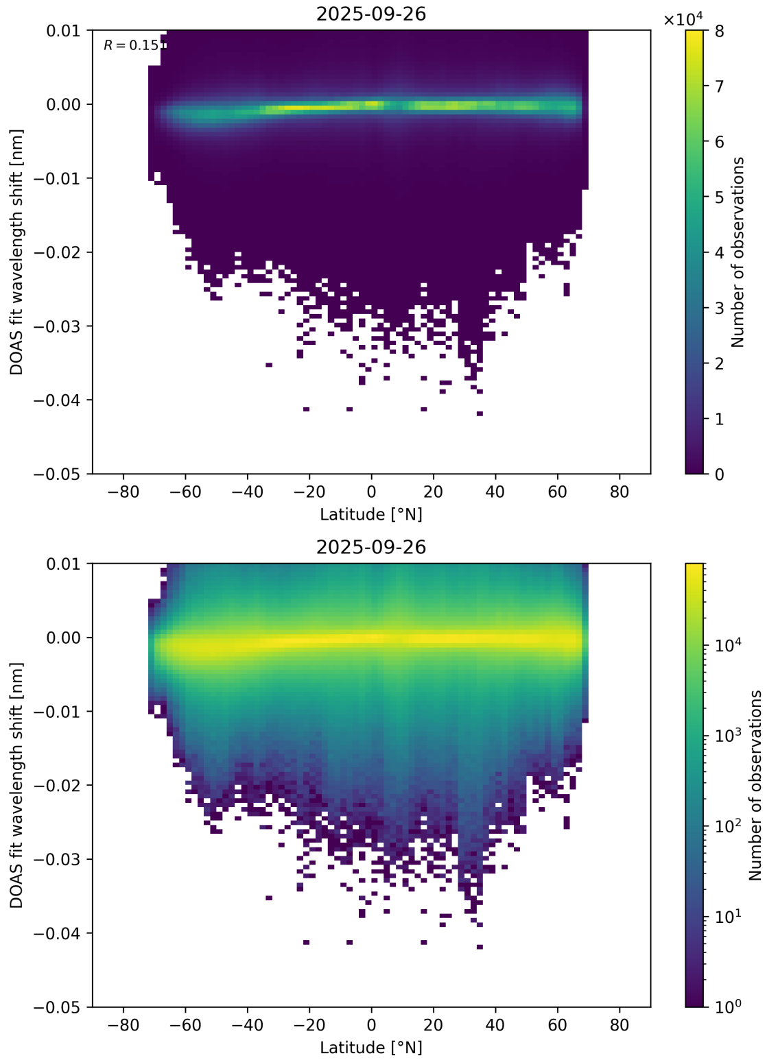
Figure 153: Scatter density plot of “Latitude” against “DOAS fit wavelength shift” for 2025-09-26 to 2025-09-27.
