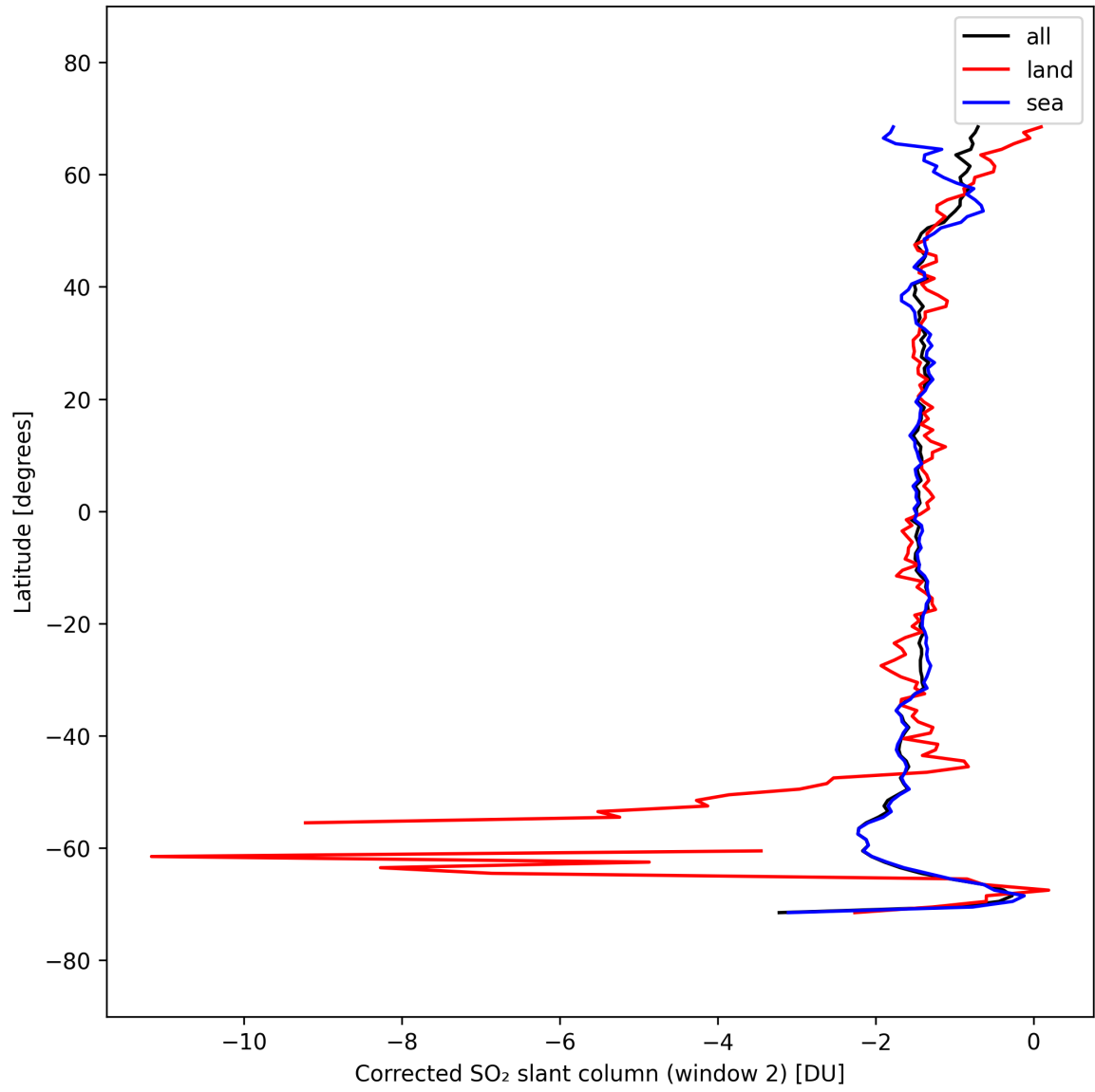
Figure 43: Zonal average of “Corrected SO 2 slant column (window 2)” for 2025-09-26 to 2025-09-27.
