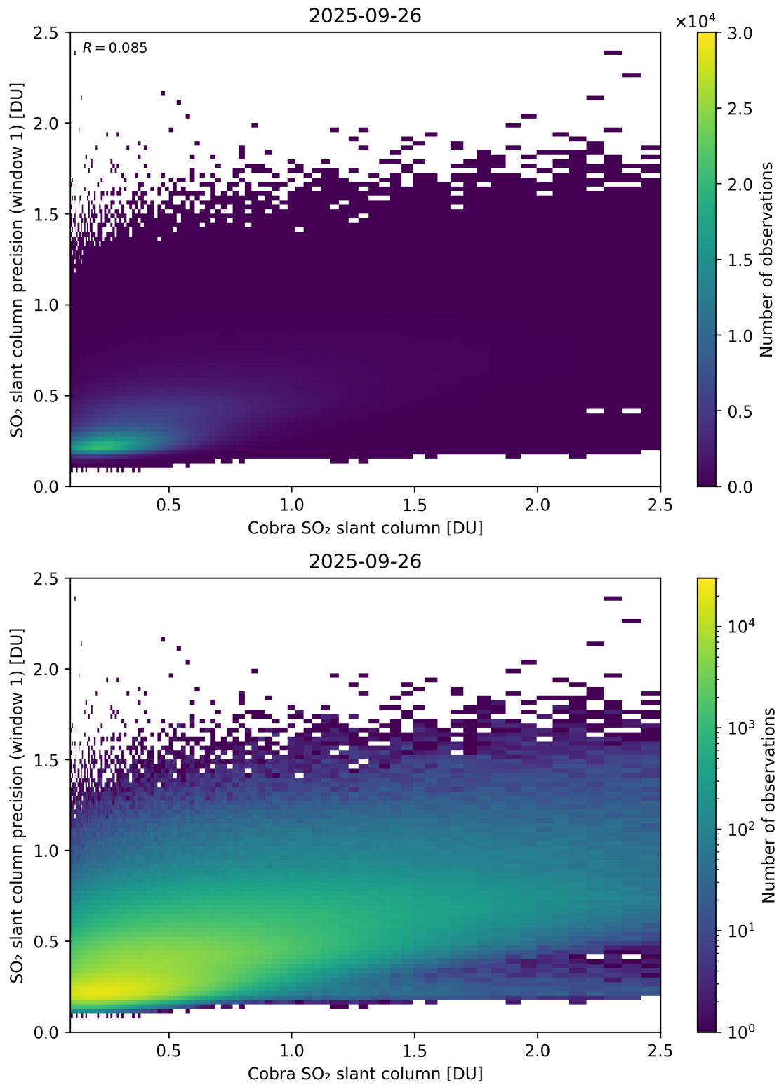
Figure 220: Scatter density plot of “Cobra SO 2 slant column” against “SO 2 slant column precision (window 1)” for 2025-09-26 to 2025-09-27.
