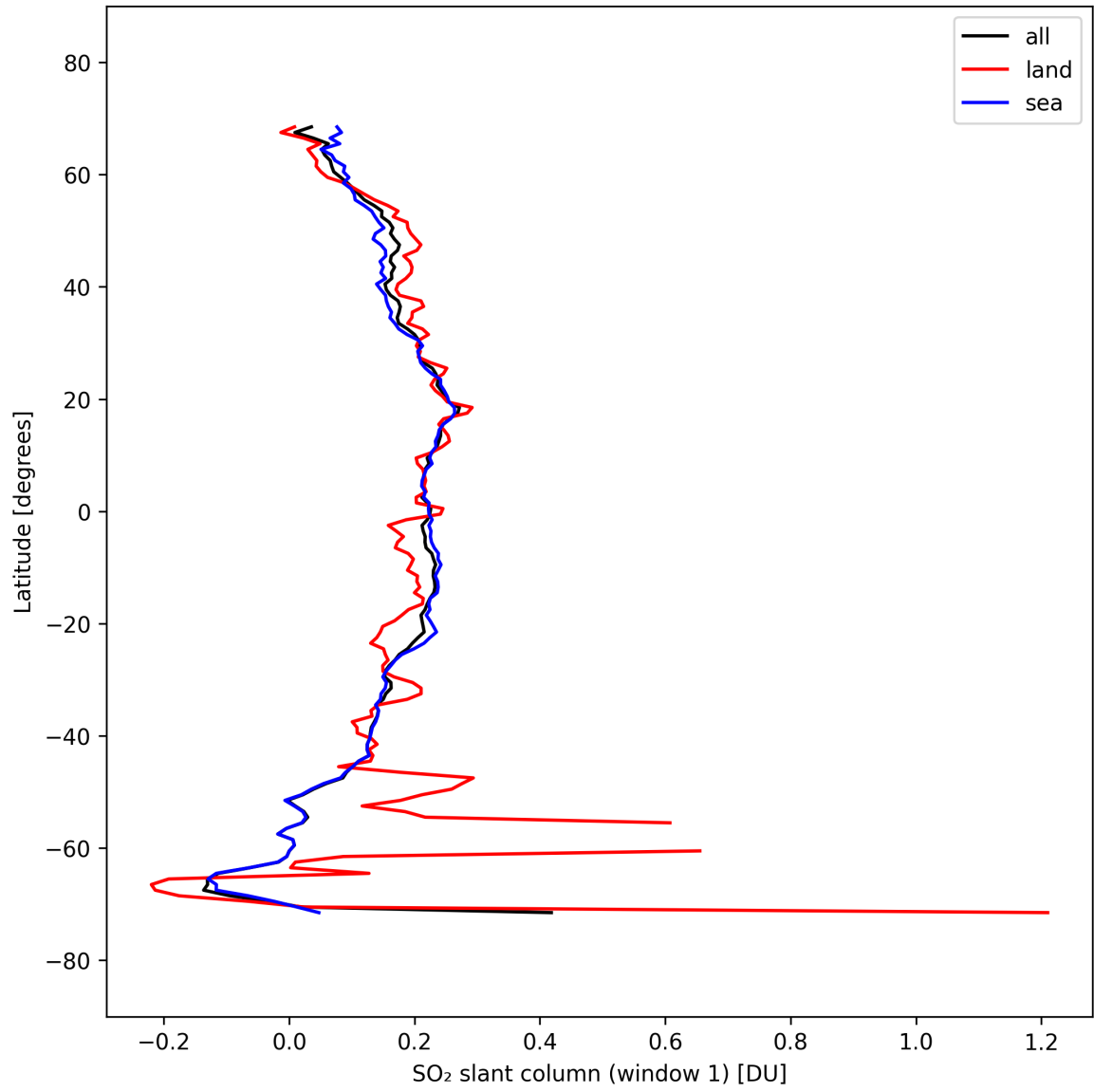
Figure 37: Zonal average of “SO 2 slant column (window 1)” for 2025-09-26 to 2025-09-27.
