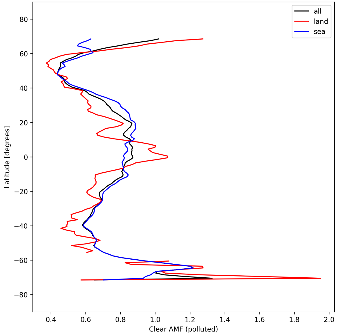
Figure 55: Zonal average of “Clear AMF (polluted)” for 2025-09-26 to 2025-09-27.
