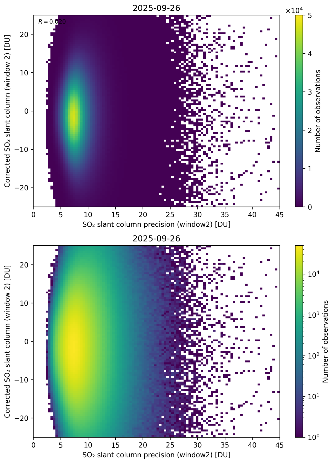
Figure 297: Scatter density plot of “SO 2 slant column precision (window2)” against “Corrected SO 2 slant column (window 2)” for 2025-09-26 to 2025-09-27.
