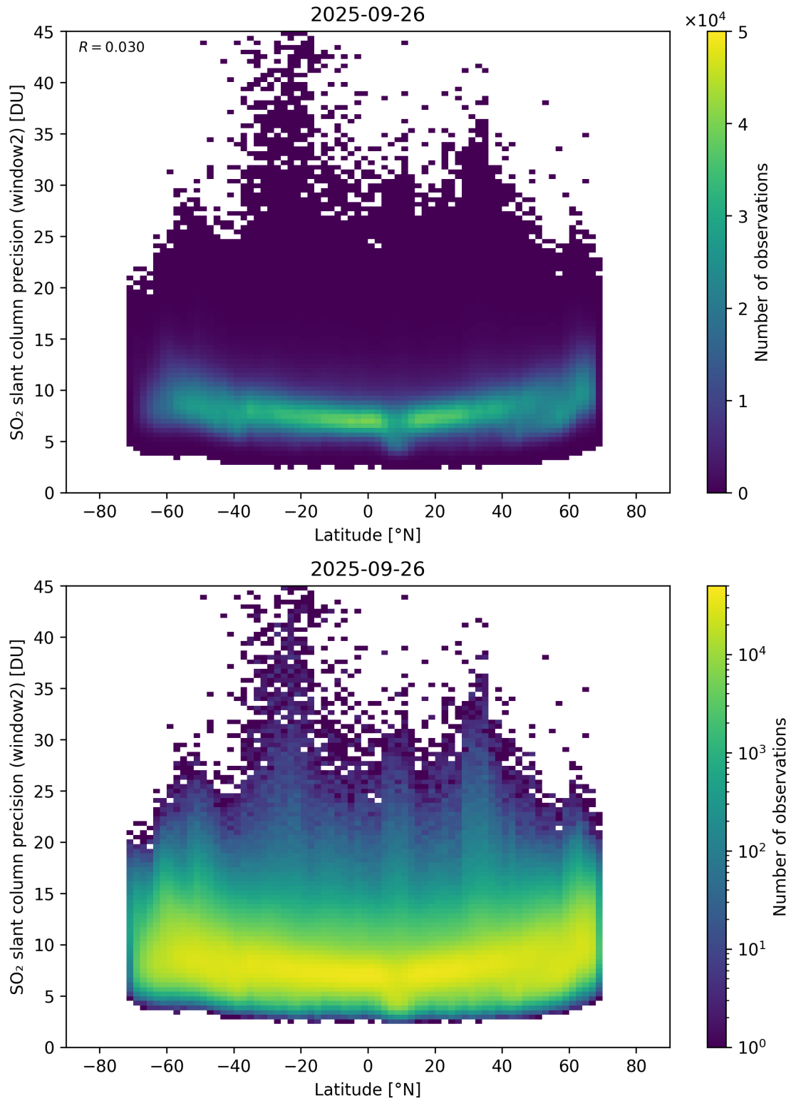
Figure 164: Scatter density plot of “Latitude” against “SO 2 slant column precision (window2)” for 2025-09-26 to 2025-09-27.
