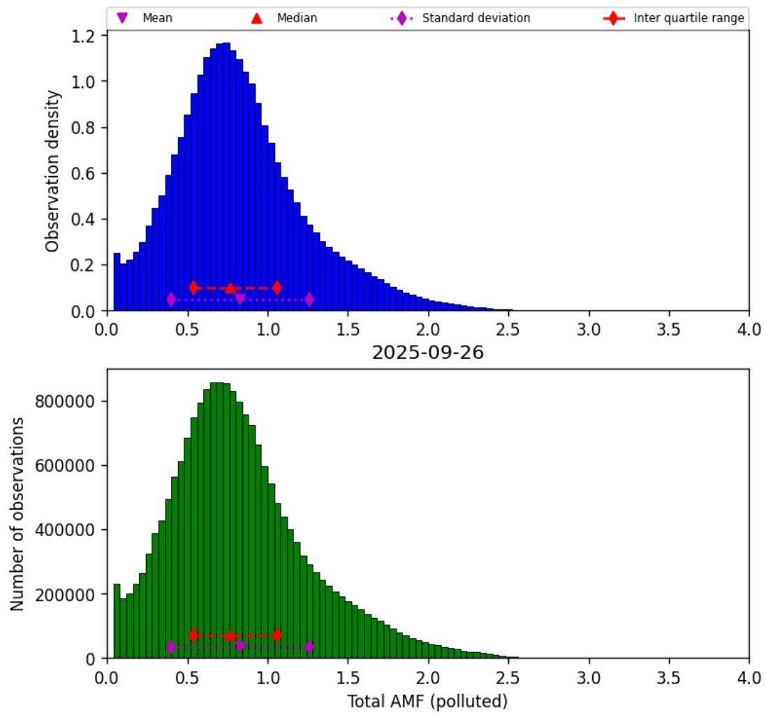
Figure 79: Histogram of “Total AMF (polluted)” for 2025-09-26 to 2025-09-27
