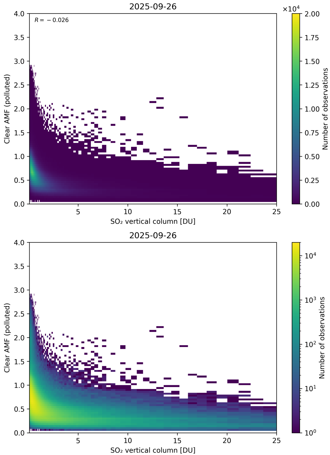
Figure 348: Scatter density plot of “SO 2 vertical column” against “Clear AMF (polluted)” for 2025-09-26 to 2025-09-27.
