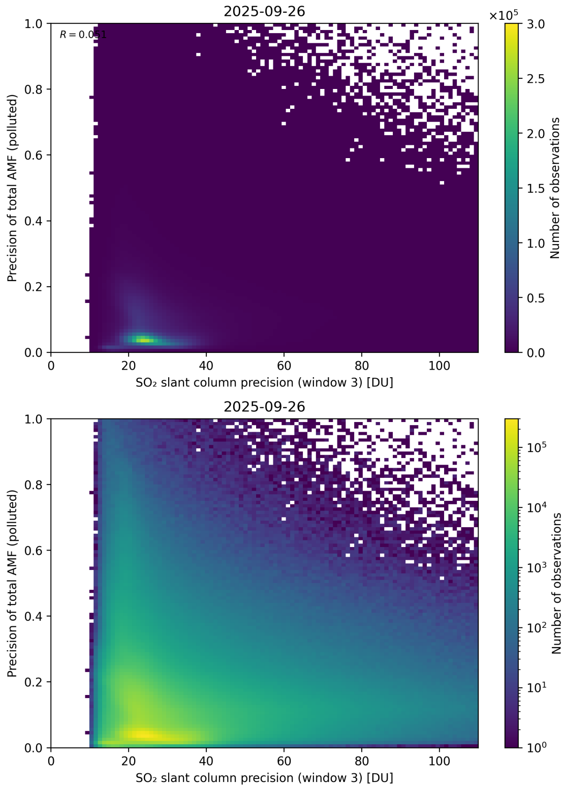
Figure 314: Scatter density plot of “SO 2 slant column precision (window 3)” against “Precision of total AMF (polluted)” for 2025-09-26 to 2025-09-27.
