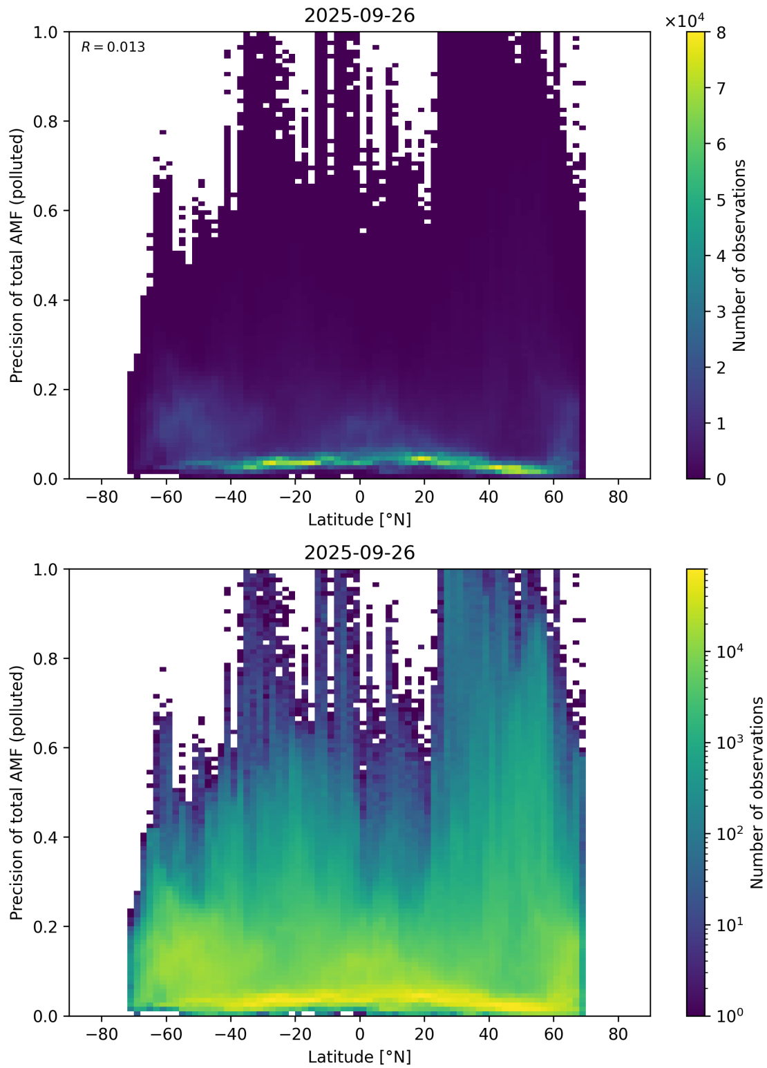
Figure 168: Scatter density plot of “Latitude” against “Precision of total AMF (polluted)” for 2025-09-26 to 2025-09-27.
