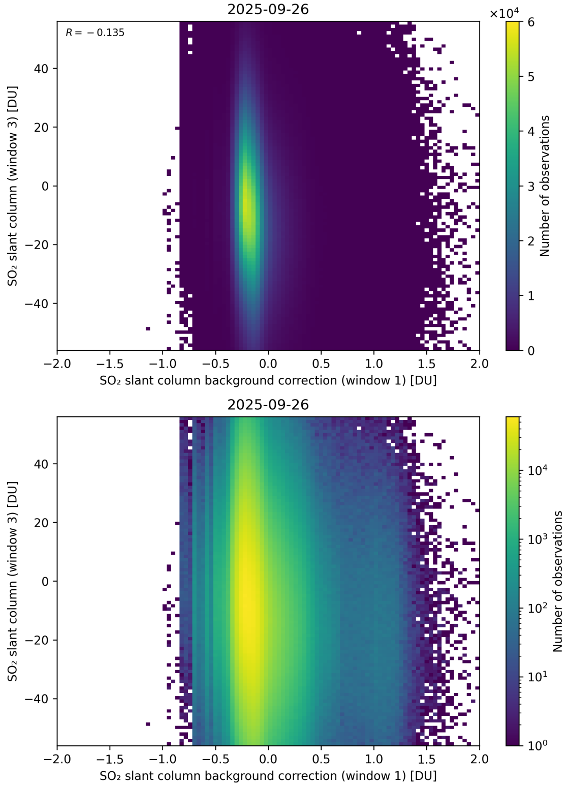
Figure 118: Scatter density plot of “SO 2 slant column background correction (window 1)” against “SO 2 slant column (window 3)” for 2025-09-26 to 2025-09-27.
