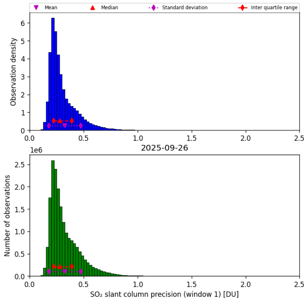
Figure 64: Histogram of “SO 2 slant column precision (window 1)” for 2025-09-26 to 2025-09-27
