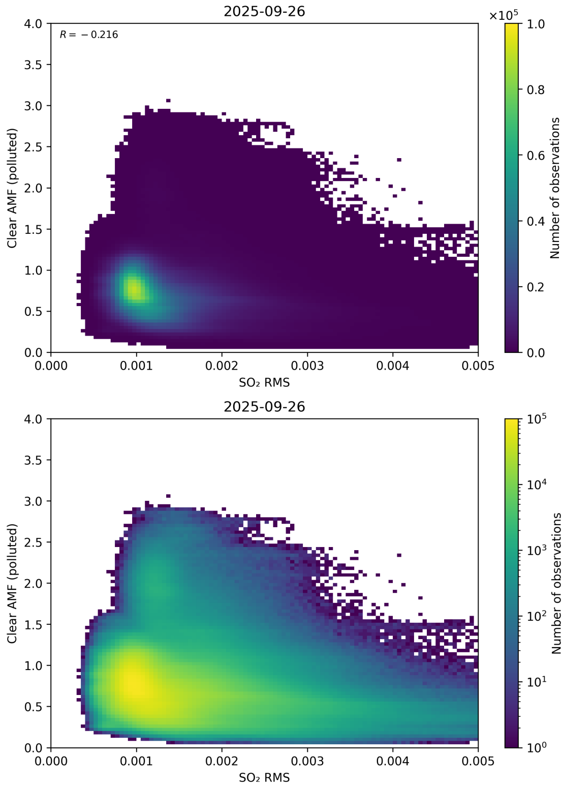
Figure 147: Scatter density plot of “SO 2 RMS” against “Clear AMF (polluted)” for 2025-09-26 to 2025-09-27.
