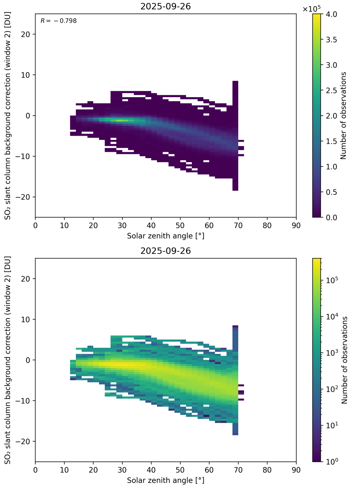
Figure 172: Scatter density plot of “Solar zenith angle” against “SO 2 slant column background correction (window 2)” for 2025-09-26 to 2025-09-27.
