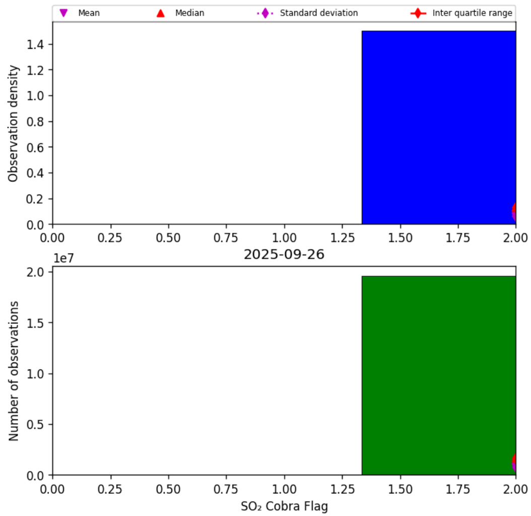
Figure 75: Histogram of “SO 2 Cobra Flag” for 2025-09-26 to 2025-09-27
