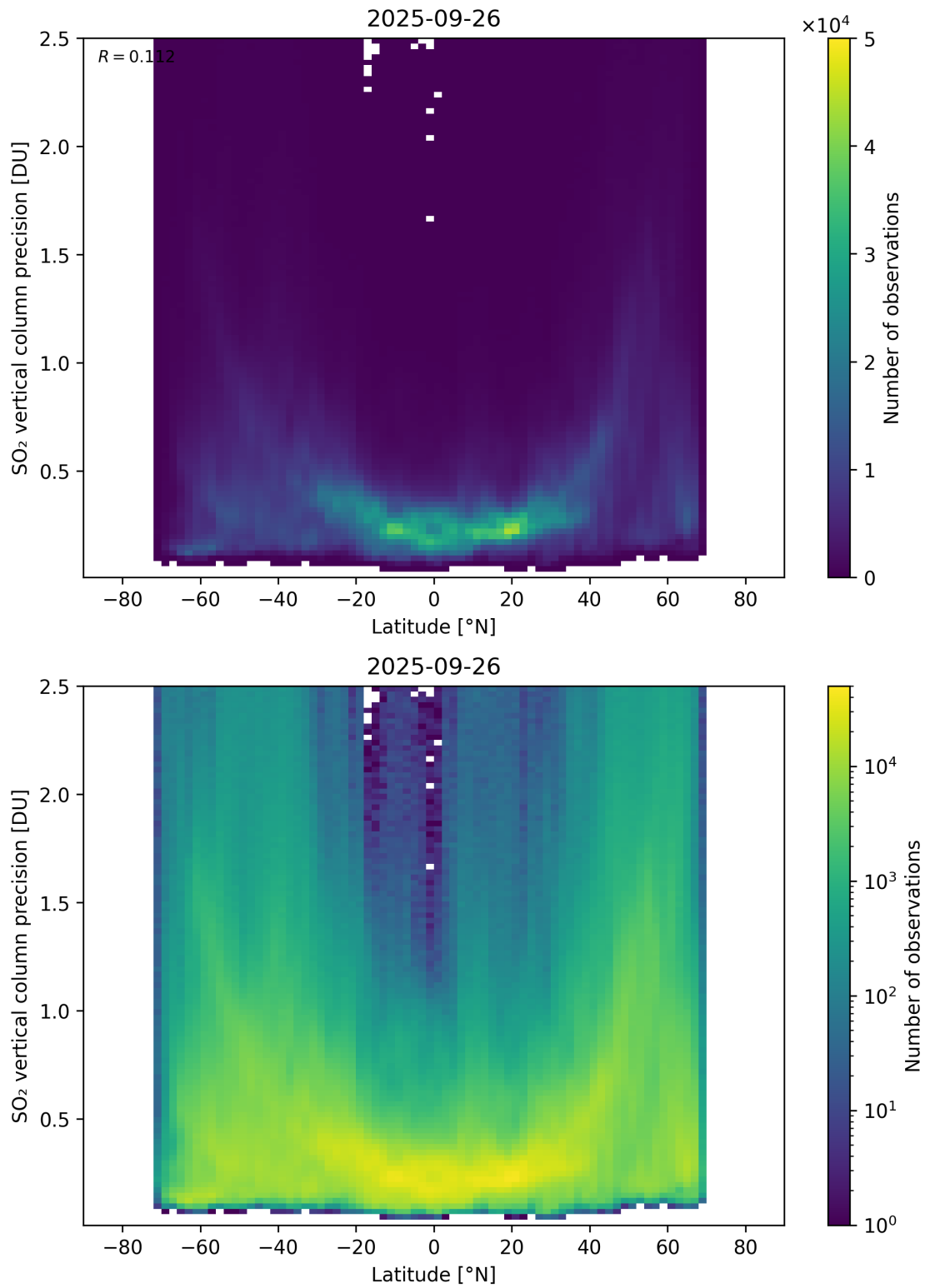
Figure 170: Scatter density plot of “Latitude” against “SO 2 vertical column precision” for 2025-09-26 to 2025-09-27.
