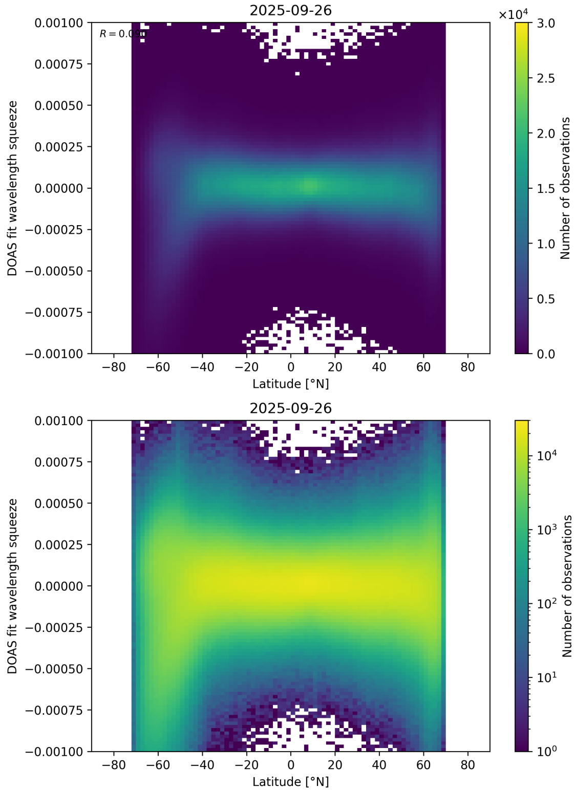
Figure 154: Scatter density plot of “Latitude” against “DOAS fit wavelength squeeze” for 2025-09-26 to 2025-09-27.
