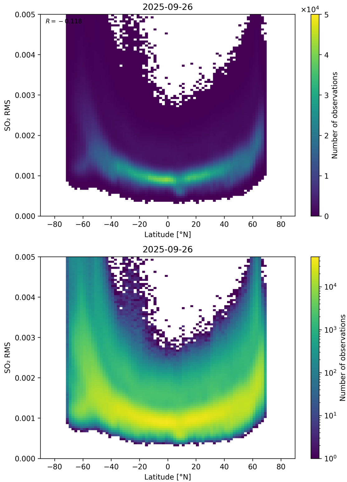
Figure 155: Scatter density plot of “Latitude” against “SO 2 RMS” for 2025-09-26 to 2025-09-27.
