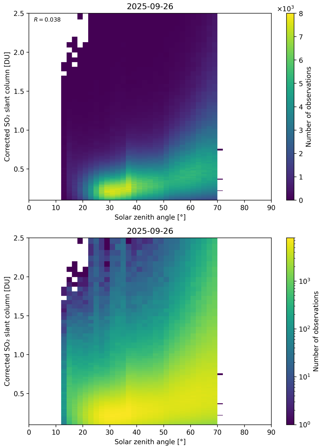
Figure 181: Scatter density plot of “Solar zenith angle” against “Corrected SO 2 slant column” for 2025-09-26 to 2025-09-27.
