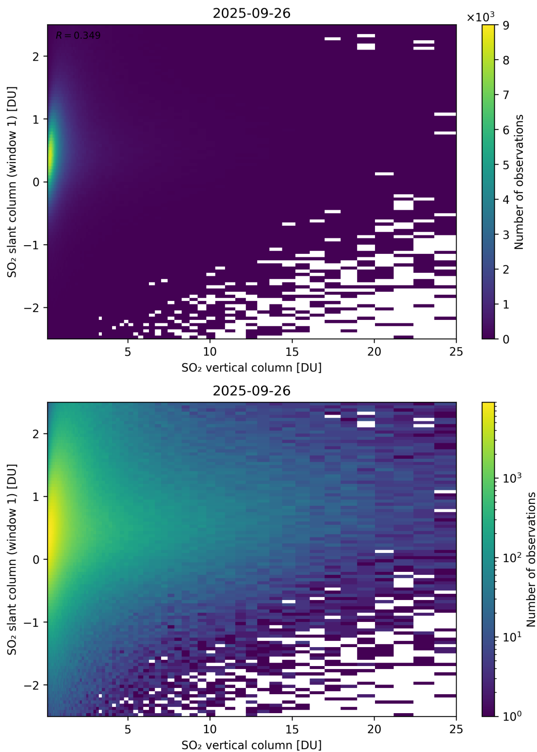
Figure 354: Scatter density plot of “SO 2 vertical column” against “SO 2 slant column (window 1)” for 2025-09-26 to 2025-09-27.
