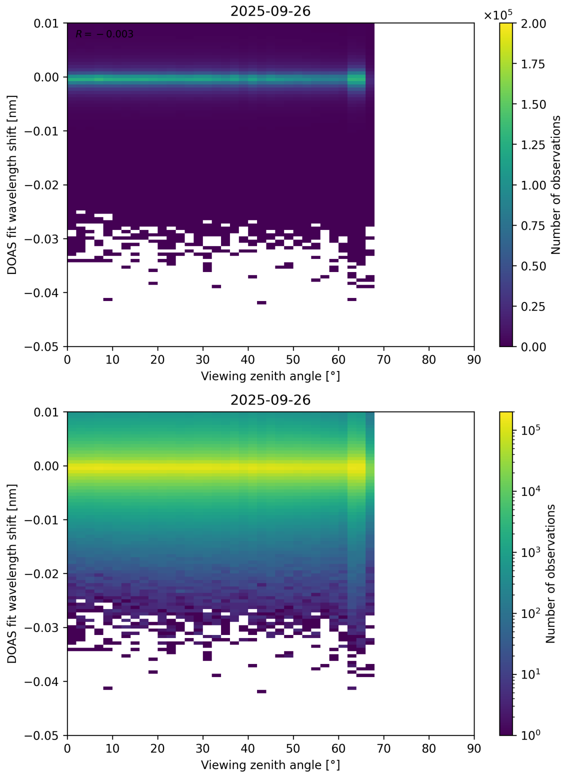
Figure 365: Scatter density plot of “Viewing zenith angle” against “DOAS fit wavelength shift” for 2025-09-26 to 2025-09-27.
