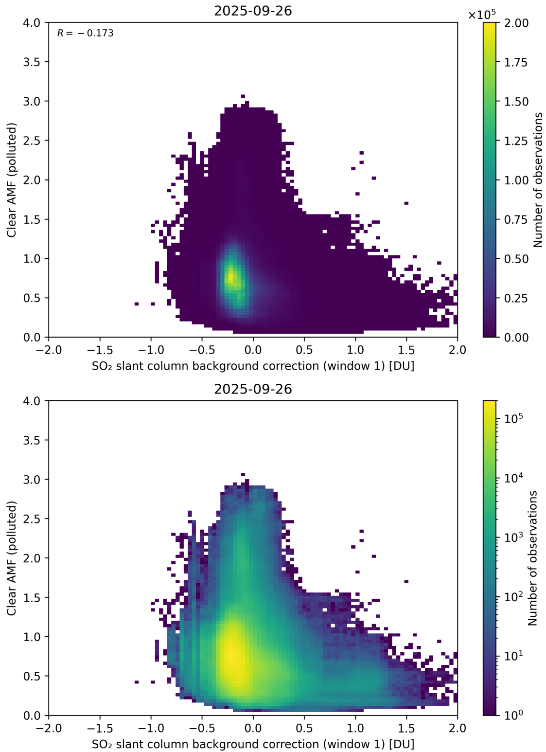
Figure 114: Scatter density plot of “SO 2 slant column background correction (window 1)” against “Clear AMF (polluted)” for 2025-09-26 to 2025-09-27.
