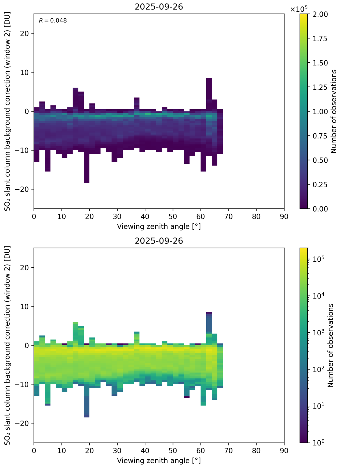
Figure 363: Scatter density plot of “Viewing zenith angle” against “SO 2 slant column background correction (window 2)” for 2025-09-26 to 2025-09-27.
