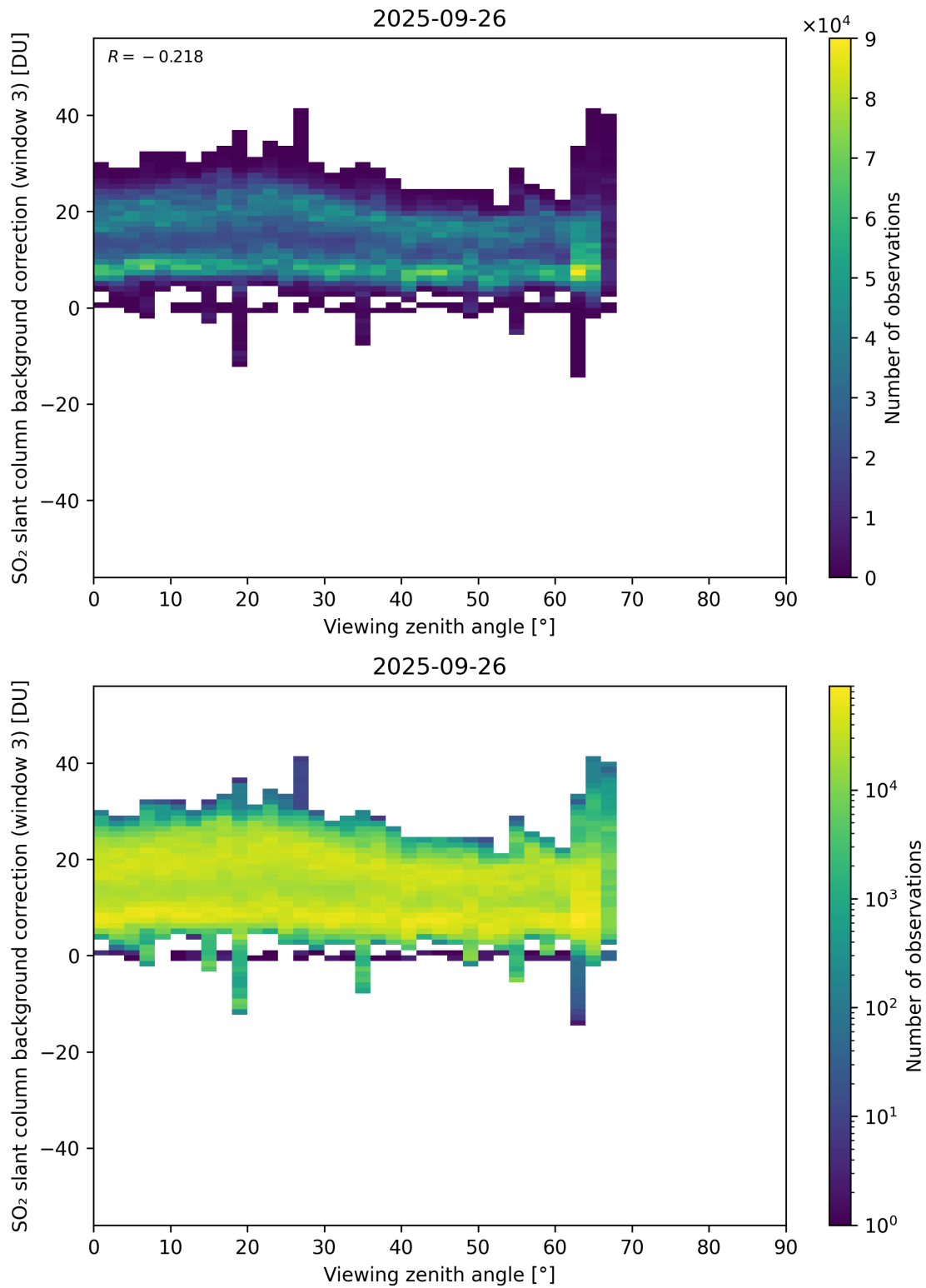
Figure 364: Scatter density plot of “Viewing zenith angle” against “SO 2 slant column background correction (window 3)” for 2025-09-26 to 2025-09-27.
