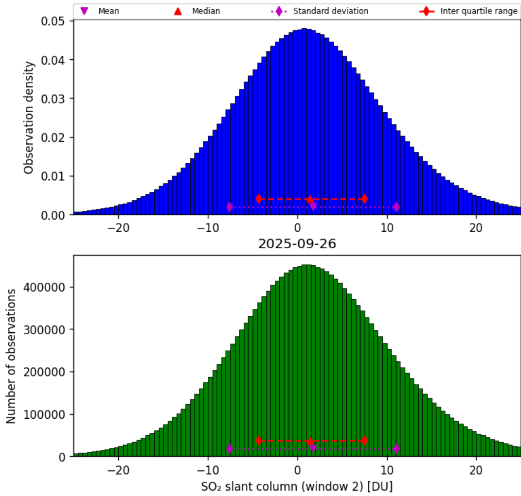
Figure 67: Histogram of “SO 2 slant column (window 2)” for 2025-09-26 to 2025-09-27
