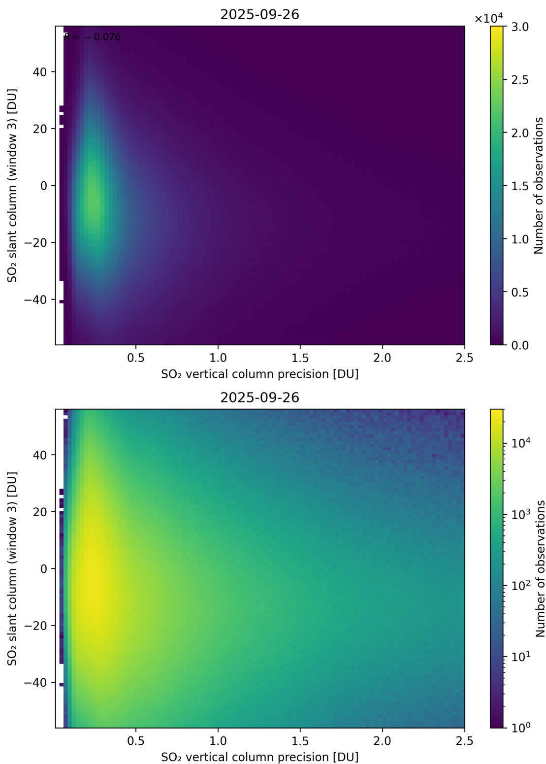
Figure 344: Scatter density plot of “SO 2 vertical column precision” against “SO 2 slant column (window 3)” for 2025-09-26 to 2025-09-27.
