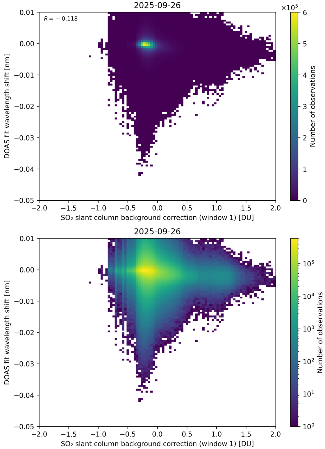
Figure 111: Scatter density plot of “SO 2 slant column background correction (window 1)” against “DOAS fit wavelength shift” for 2025-09-26 to 2025-09-27.
