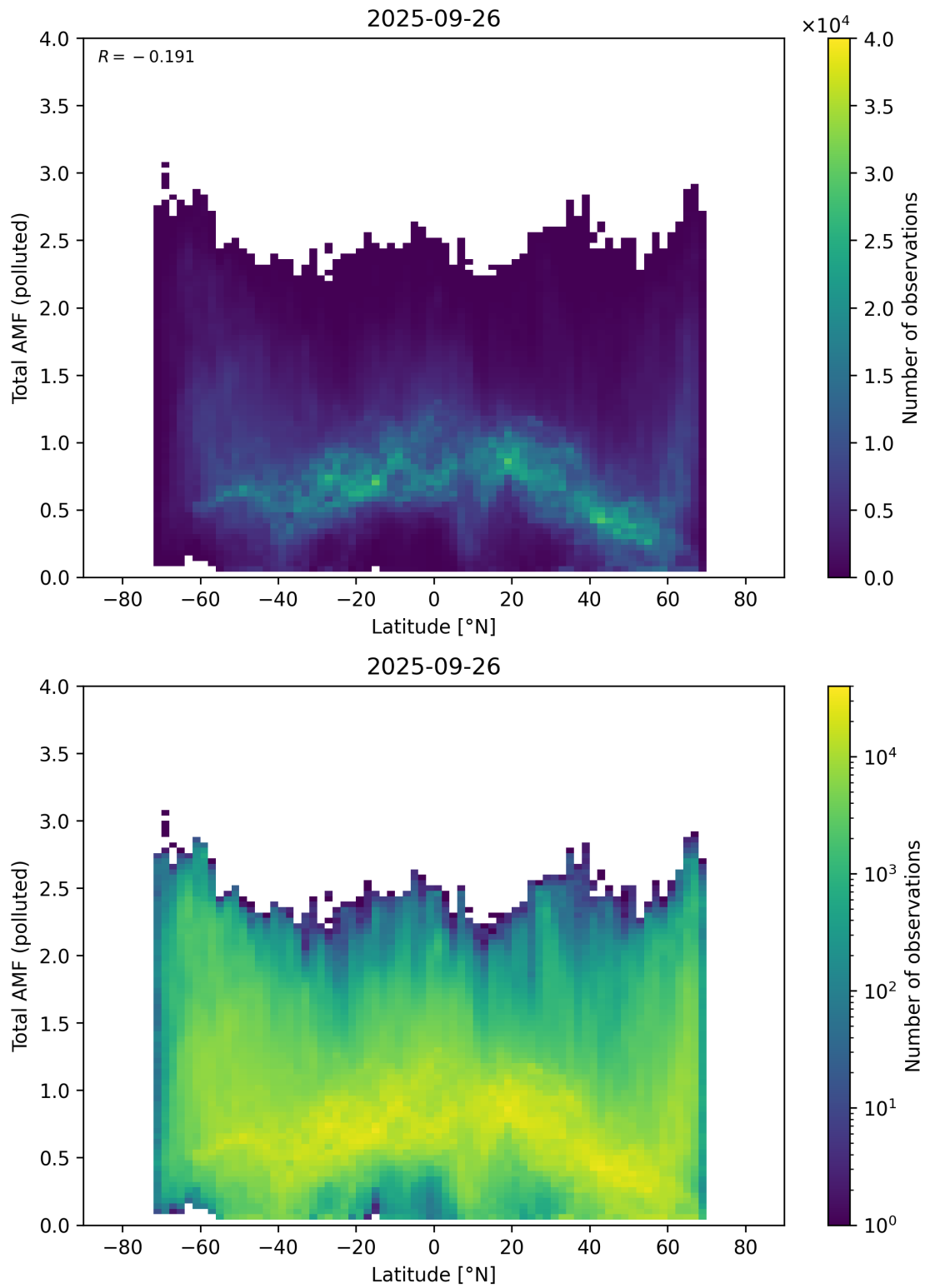
Figure 167: Scatter density plot of “Latitude” against “Total AMF (polluted)” for 2025-09-26 to 2025-09-27.
