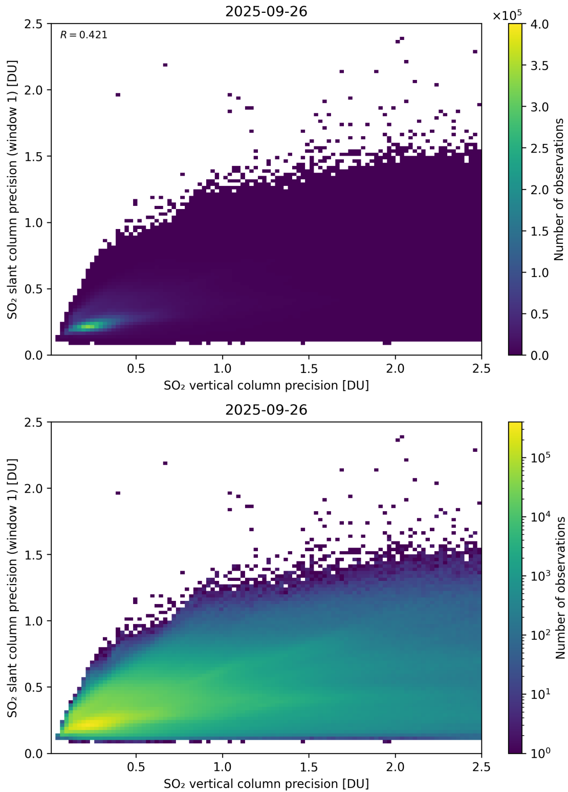
Figure 342: Scatter density plot of “SO 2 vertical column precision” against “SO 2 slant column precision (window 1)” for 2025-09-26 to 2025-09-27.
