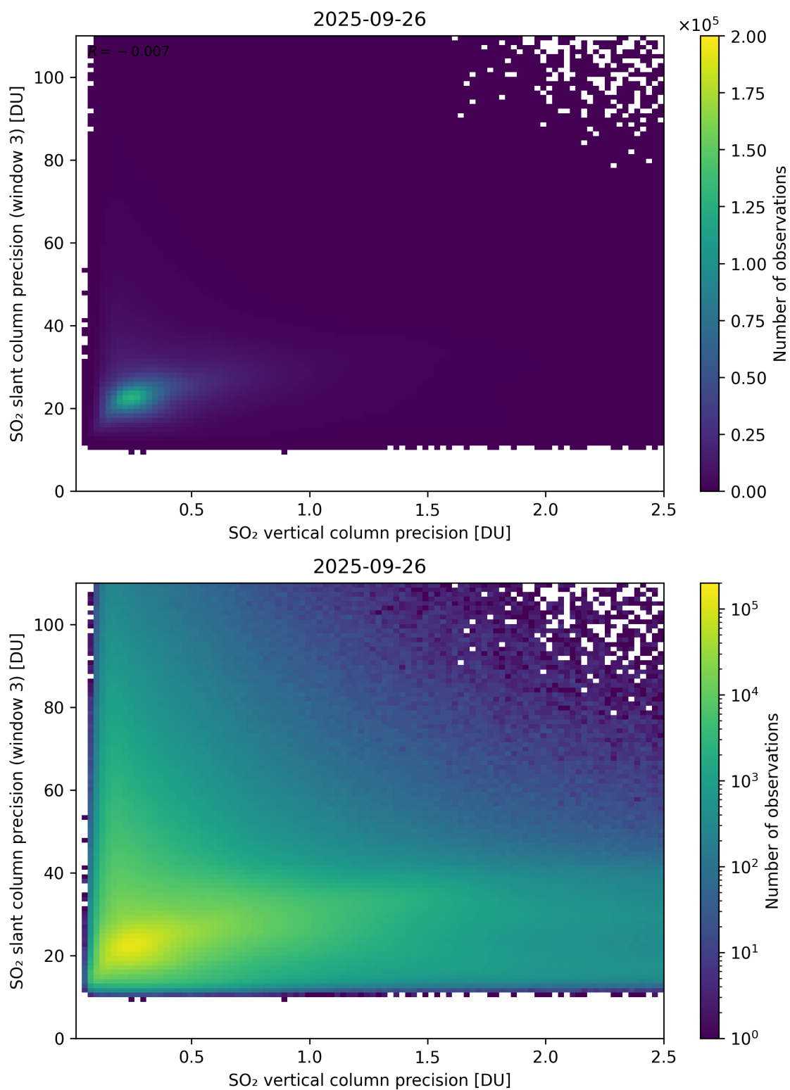
Figure 345: Scatter density plot of “SO 2 vertical column precision” against “SO 2 slant column precision (window 3)” for 2025-09-26 to 2025-09-27.
