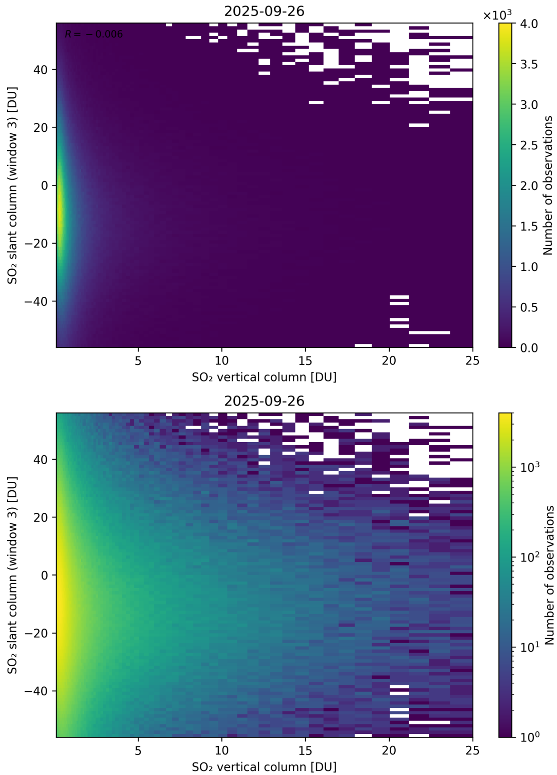
Figure 357: Scatter density plot of “SO 2 vertical column” against “SO 2 slant column (window 3)” for 2025-09-26 to 2025-09-27.
