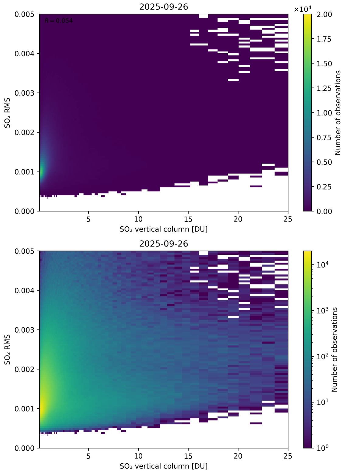
Figure 328: Scatter density plot of “SO 2 vertical column” against “SO 2 RMS” for 2025-09-26 to 2025-09-27.
