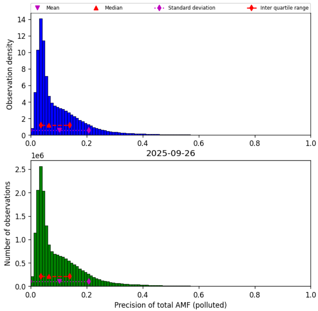
Figure 80: Histogram of “Precision of total AMF (polluted)” for 2025-09-26 to 2025-09-27
