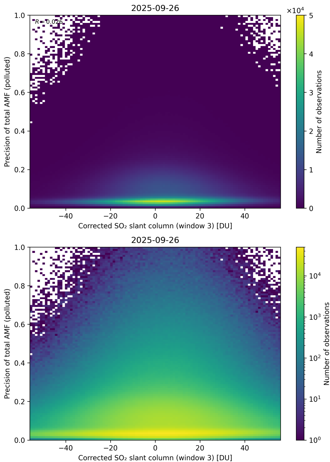
Figure 261: Scatter density plot of “Corrected SO 2 slant column (window 3)” against “Precision of total AMF (polluted)” for 2025-09-26 to 2025-09-27.
