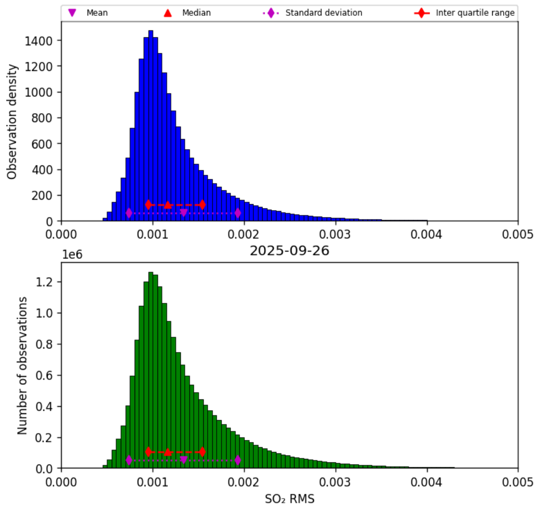
Figure 78: Histogram of “SO 2 RMS” for 2025-09-26 to 2025-09-27
