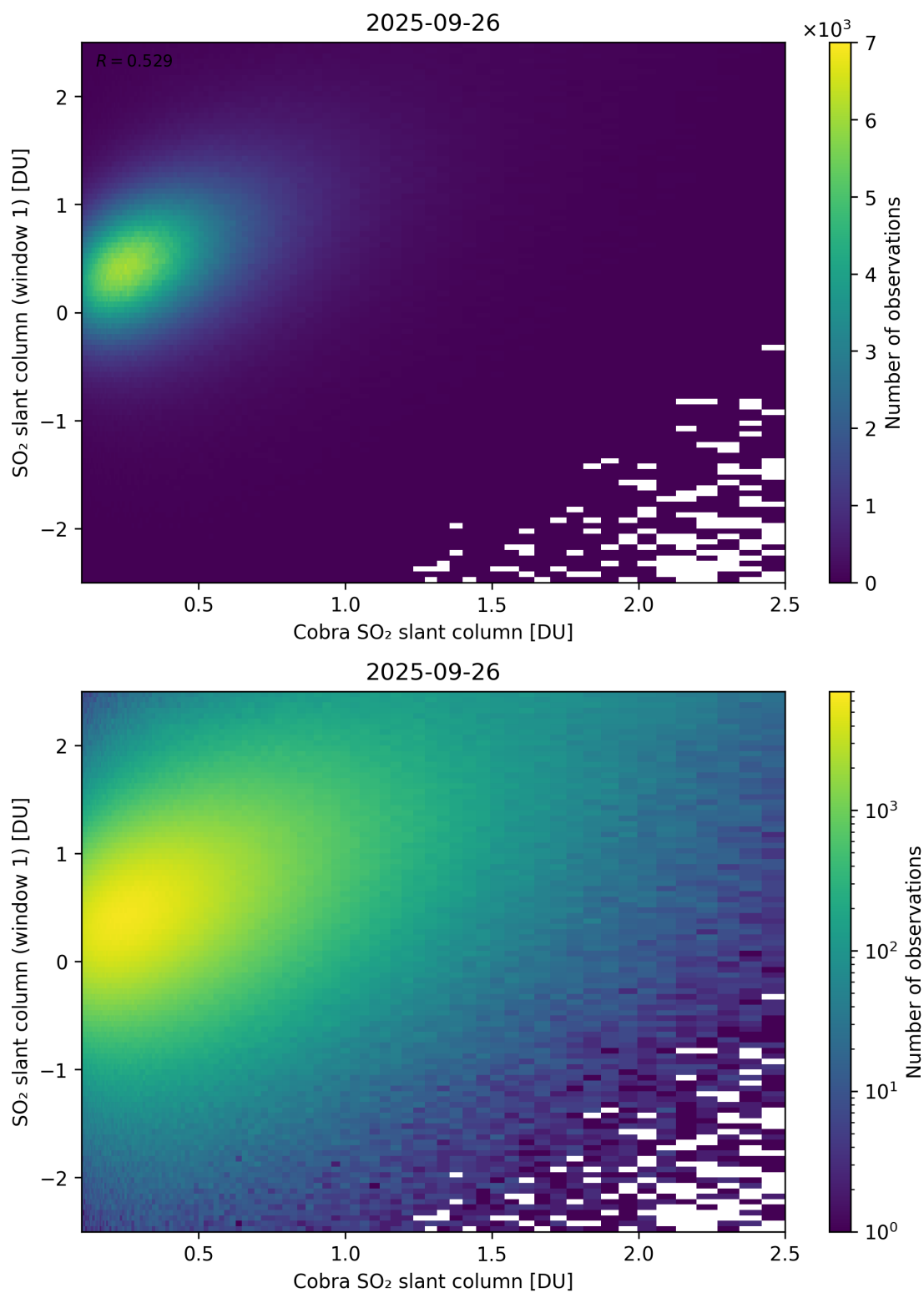
Figure 219: Scatter density plot of “Cobra SO 2 slant column” against “SO 2 slant column (window 1)” for 2025-09-26 to 2025-09-27.
