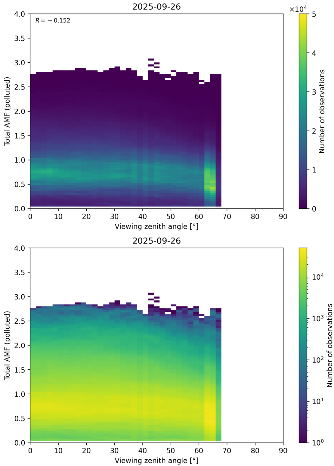
Figure 381: Scatter density plot of “Viewing zenith angle” against “Total AMF (polluted)” for 2025-09-26 to 2025-09-27.
