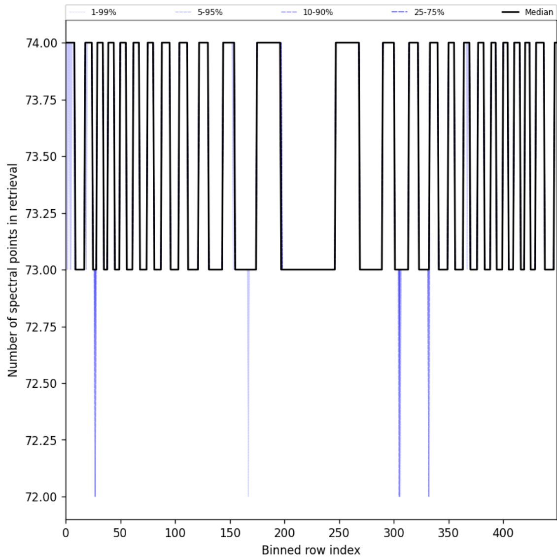
Figure 108: Along track statistics of “Number of spectral points in retrieval” for 2025-09-26 to 2025-09-27
