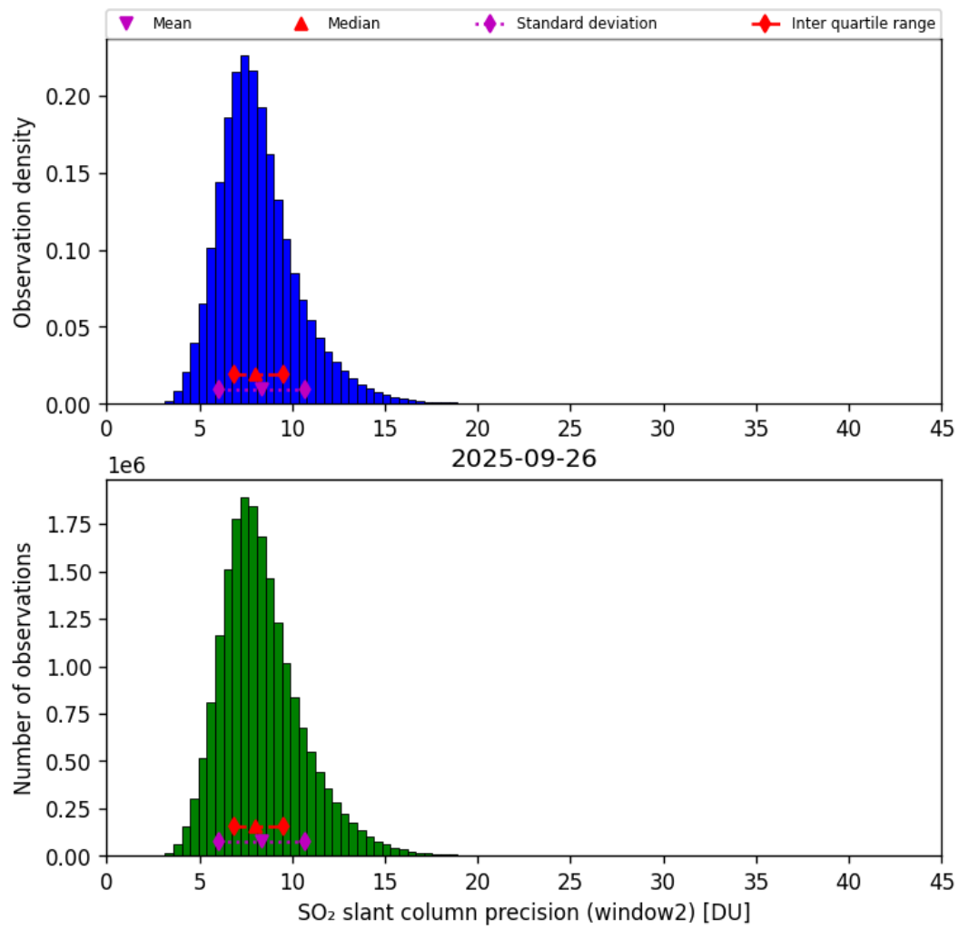
Figure 68: Histogram of “SO 2 slant column precision (window2)” for 2025-09-26 to 2025-09-27
