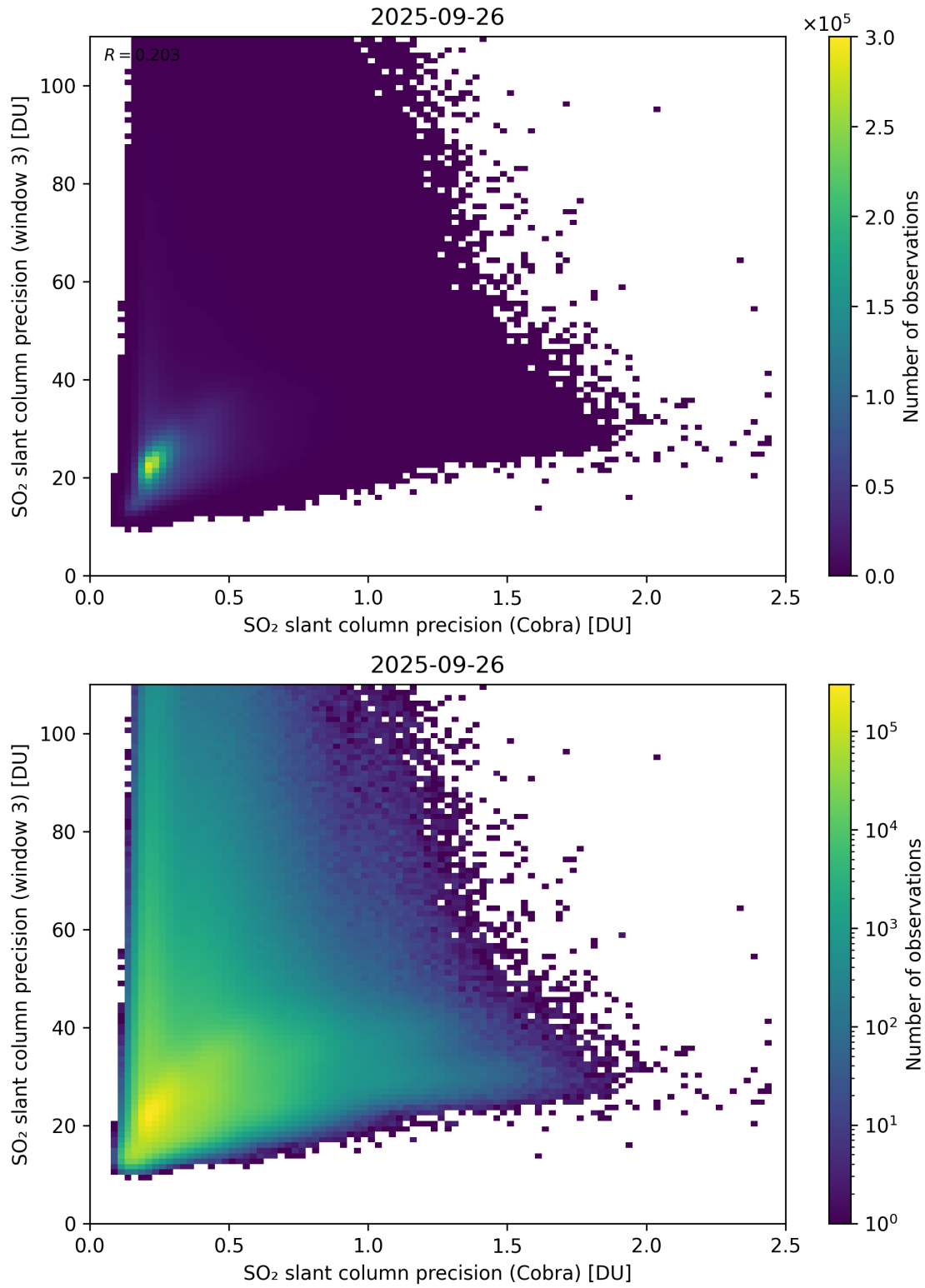
Figure 212: Scatter density plot of “SO 2 slant column precision (Cobra)” against “SO 2 slant column precision (window 3)” for 2025-09-26 to 2025-09-27.
