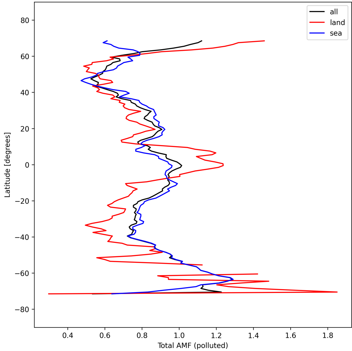
Figure 53: Zonal average of “Total AMF (polluted)” for 2025-09-26 to 2025-09-27.
