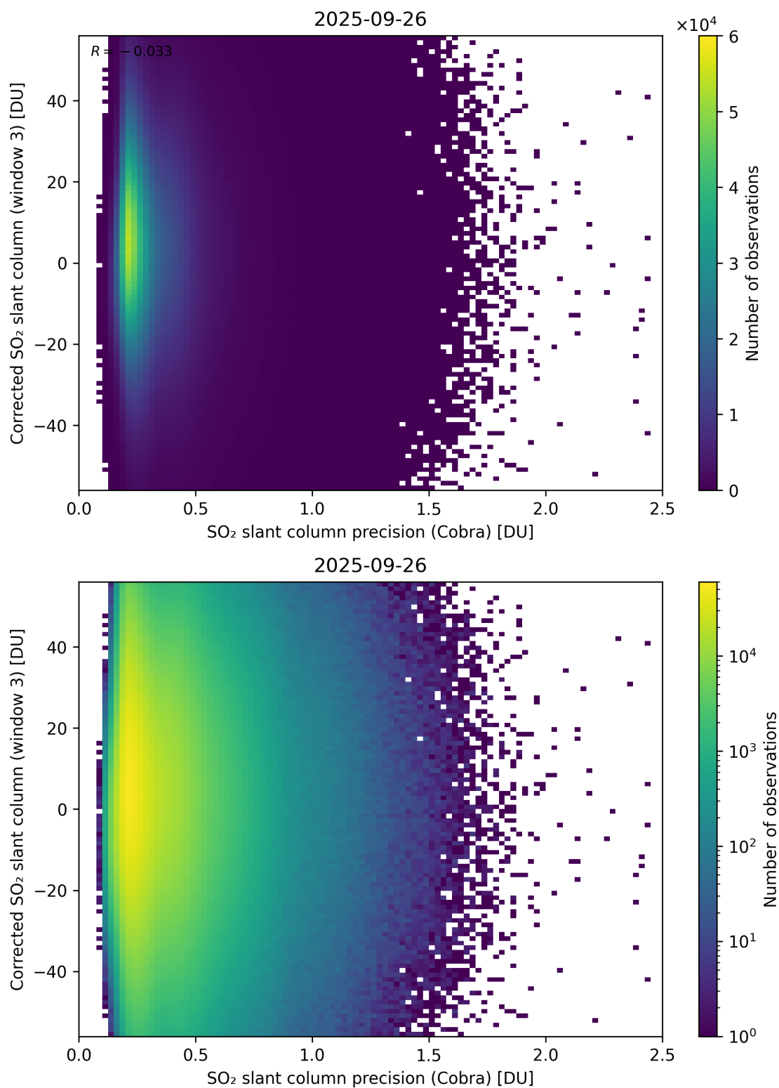
Figure 207: Scatter density plot of “SO 2 slant column precision (Cobra)” against “Corrected SO 2 slant column (window 3)” for 2025-09-26 to 2025-09-27.
