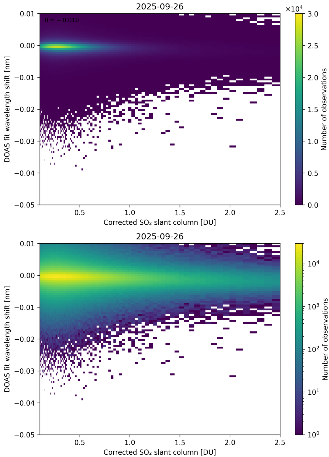
Figure 229: Scatter density plot of “Corrected SO 2 slant column” against “DOAS fit wavelength shift” for 2025-09-26 to 2025-09-27.
