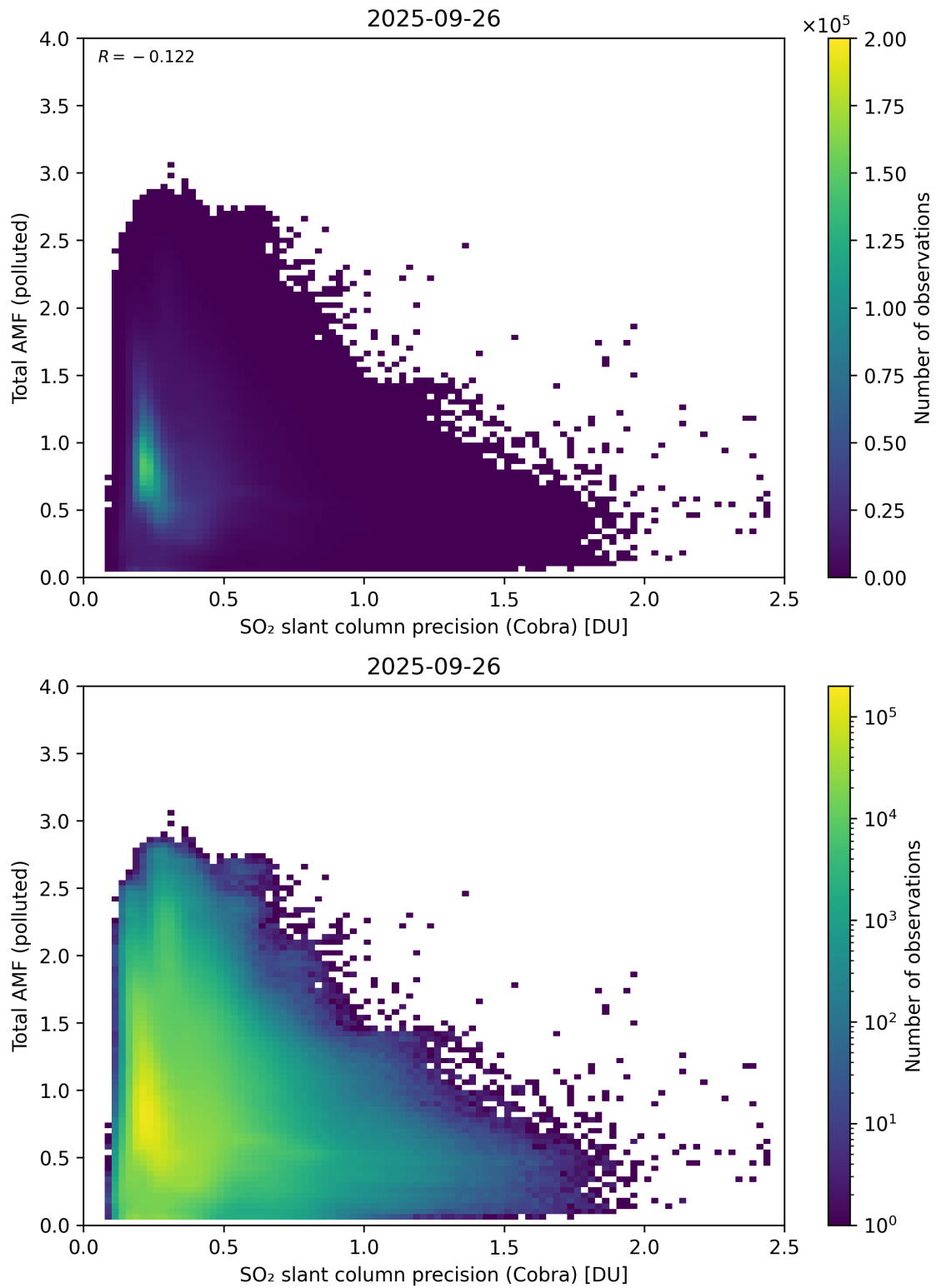
Figure 213: Scatter density plot of “SO 2 slant column precision (Cobra)” against “Total AMF (polluted)” for 2025-09-26 to 2025-09-27.
