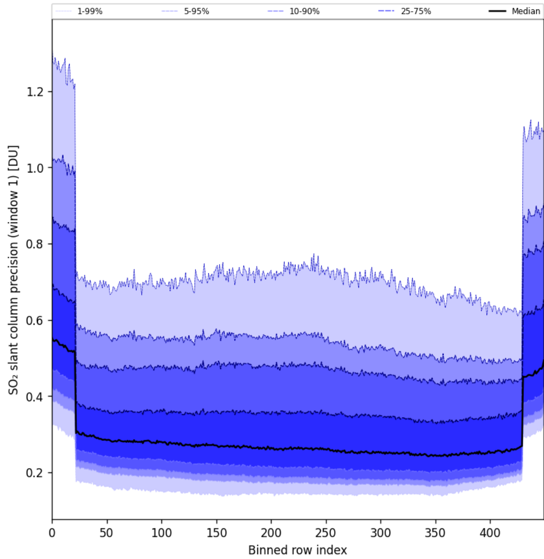
Figure 90: Along track statistics of “SO 2 slant column precision (window 1)” for 2025-09-26 to 2025-09-27
