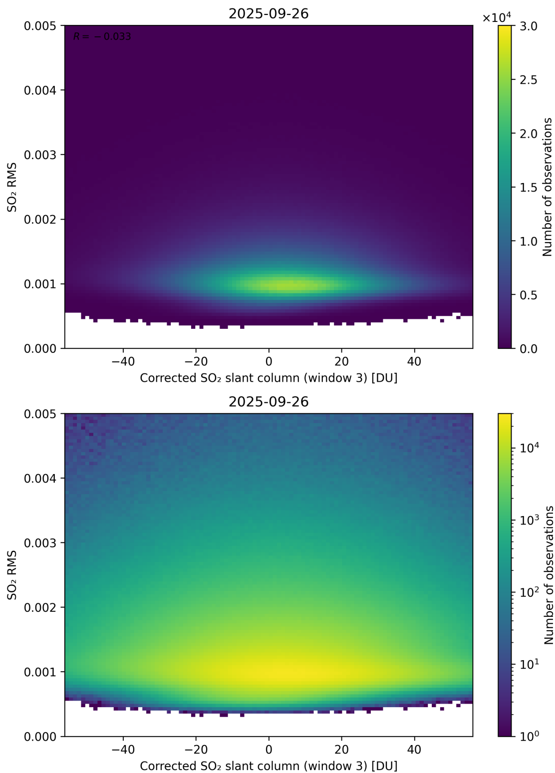
Figure 258: Scatter density plot of “Corrected SO 2 slant column (window 3)” against “SO 2 RMS” for 2025-09-26 to 2025-09-27.
