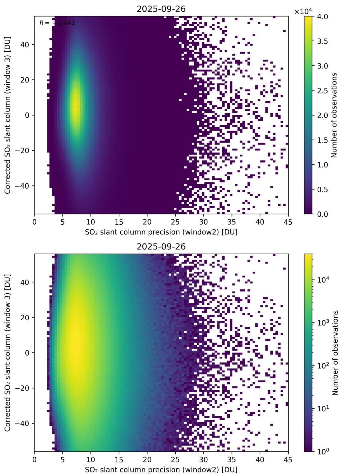
Figure 298: Scatter density plot of “SO 2 slant column precision (window2)” against “Corrected SO 2 slant column (window 3)” for 2025-09-26 to 2025-09-27.
