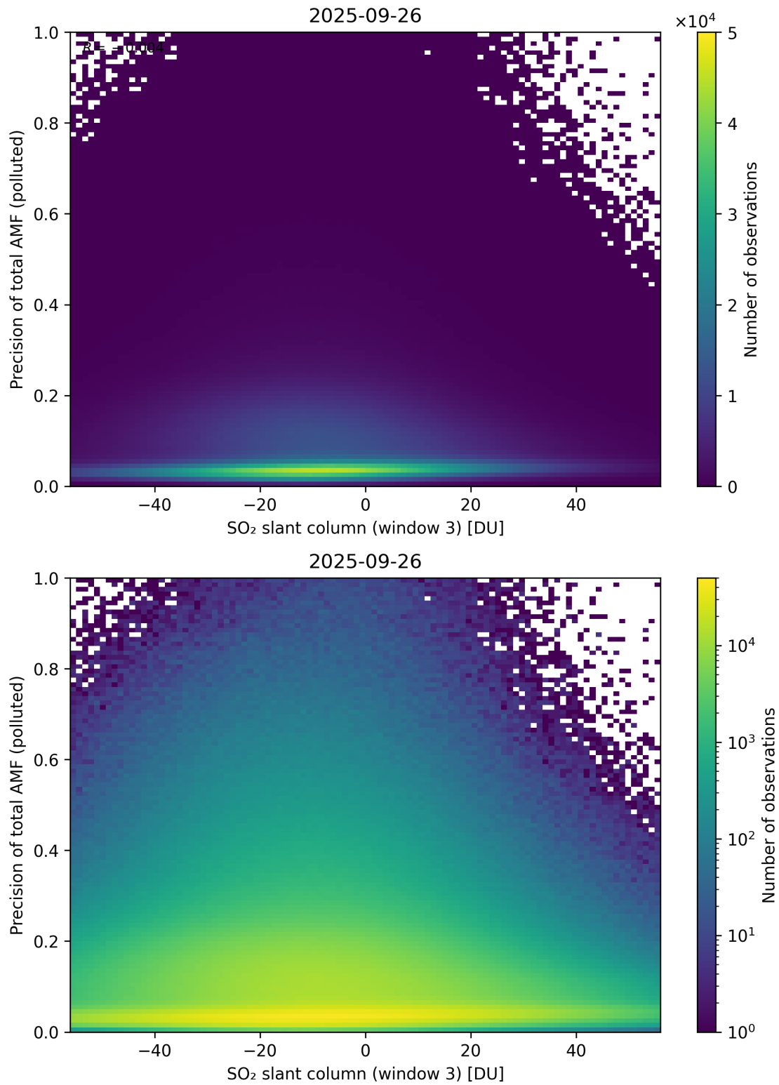
Figure 319: Scatter density plot of “SO 2 slant column (window 3)” against “Precision of total AMF (polluted)” for 2025-09-26 to 2025-09-27.
