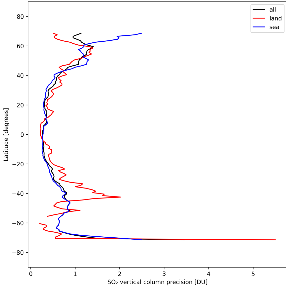
Figure 33: Zonal average of “SO 2 vertical column precision” for 2025-09-26 to 2025-09-27.
