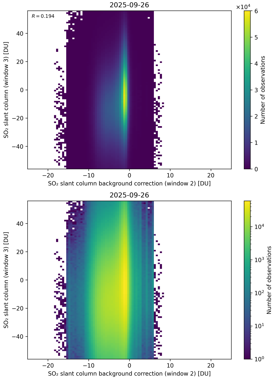
Figure 128: Scatter density plot of “SO 2 slant column background correction (window 2)” against “SO 2 slant column (window 3)” for 2025-09-26 to 2025-09-27.
