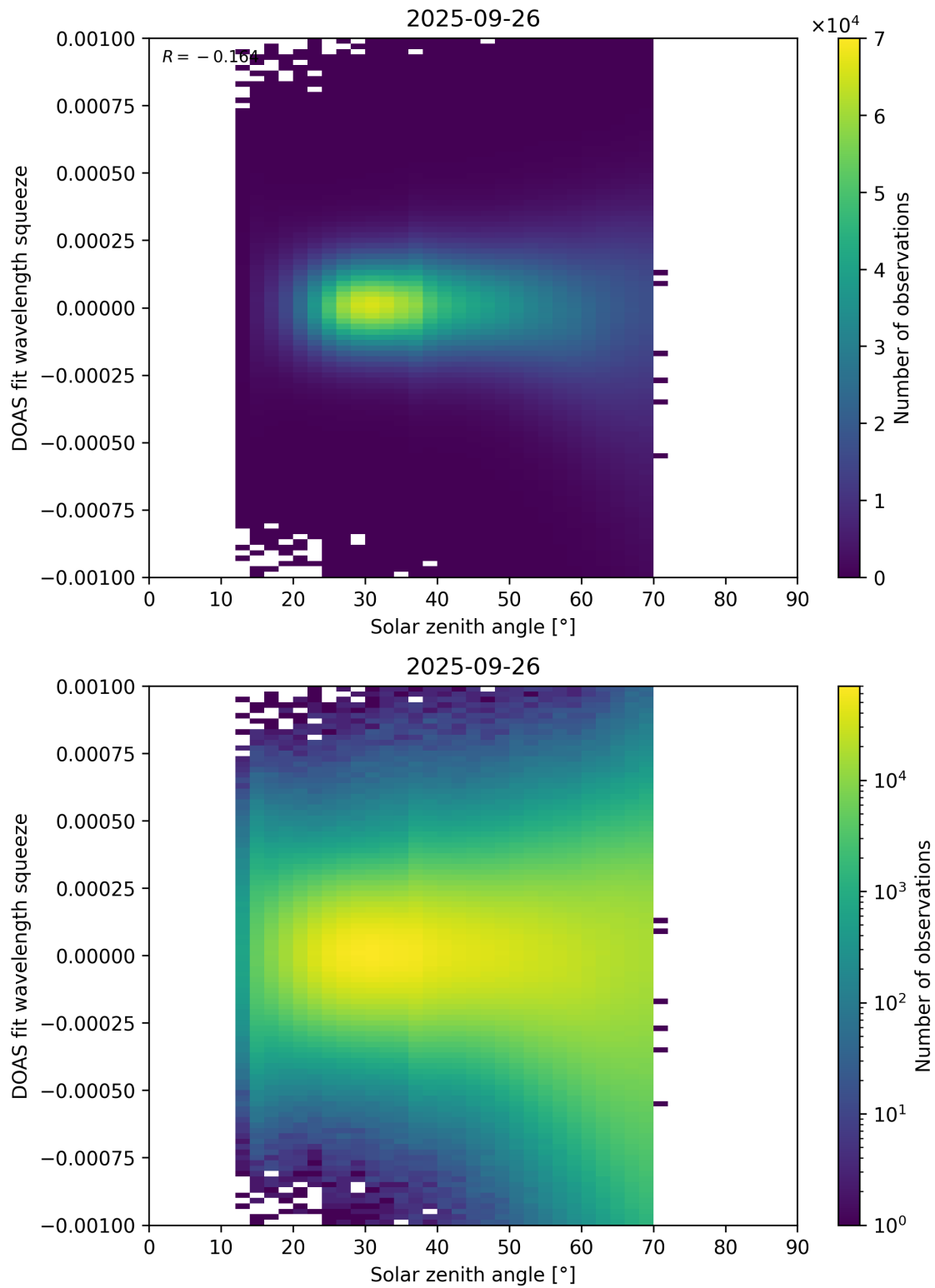
Figure 175: Scatter density plot of “Solar zenith angle” against “DOAS fit wavelength squeeze” for 2025-09-26 to 2025-09-27.
