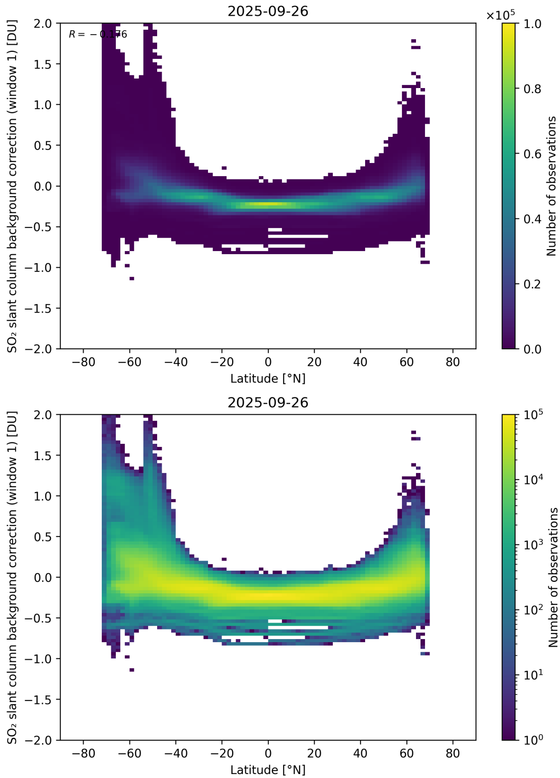
Figure 150: Scatter density plot of “Latitude” against “SO 2 slant column background correction (window 1)” for 2025-09-26 to 2025-09-27.
