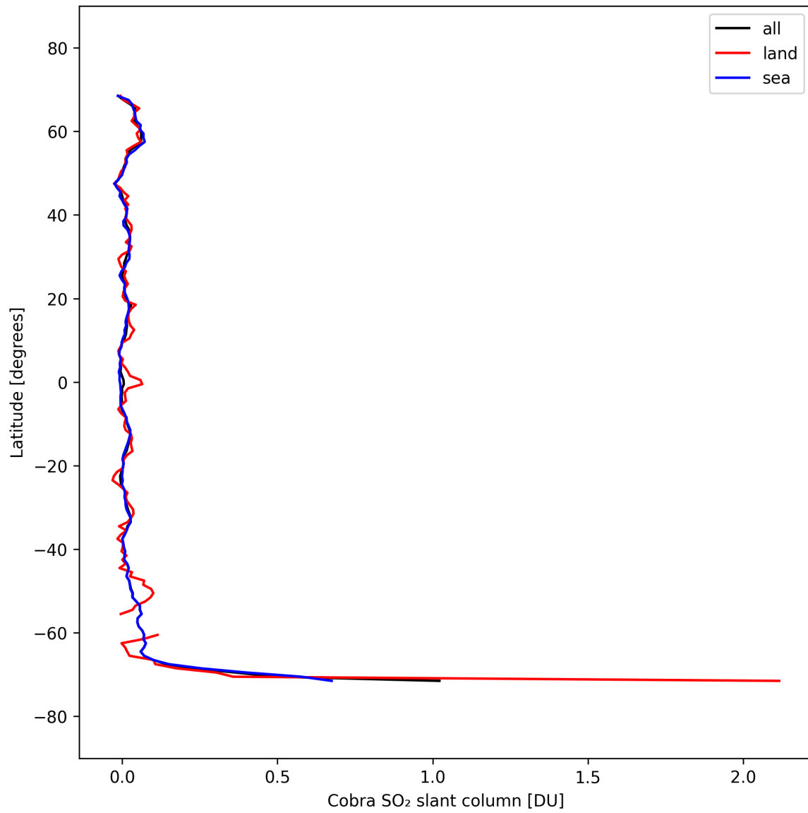
Figure 35: Zonal average of “Cobra SO 2 slant column” for 2025-09-26 to 2025-09-27.
