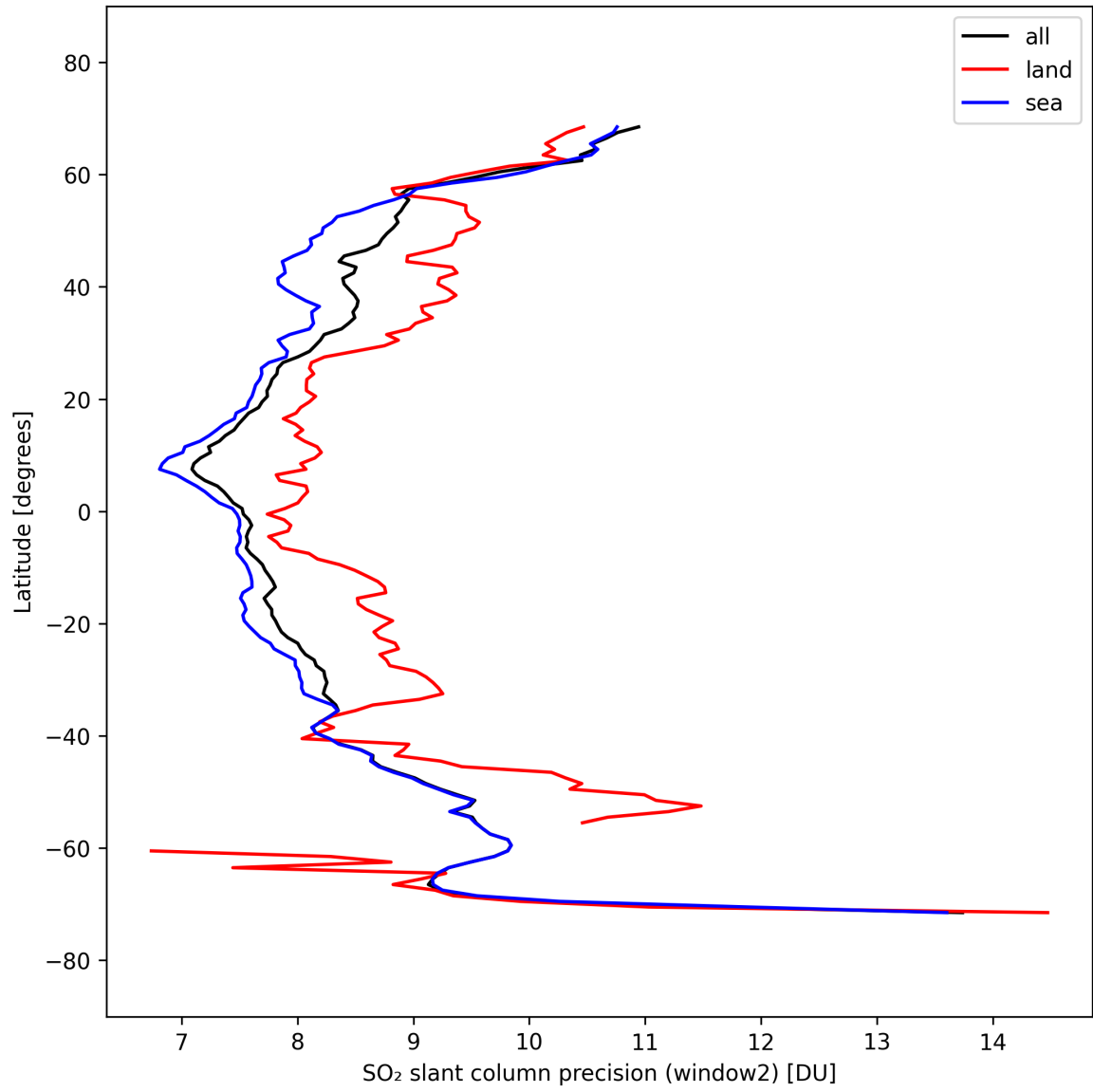
Figure 42: Zonal average of “SO 2 slant column precision (window2)” for 2025-09-26 to 2025-09-27.
