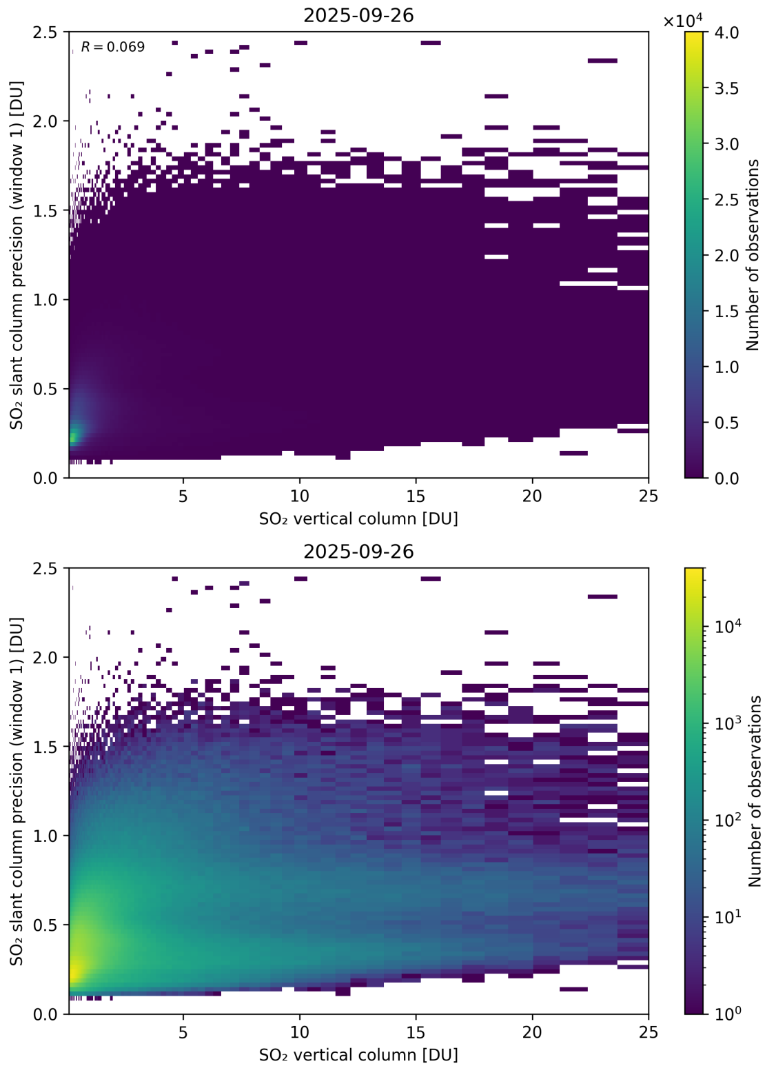
Figure 355: Scatter density plot of “SO 2 vertical column” against “SO 2 slant column precision (window 1)” for 2025-09-26 to 2025-09-27.
