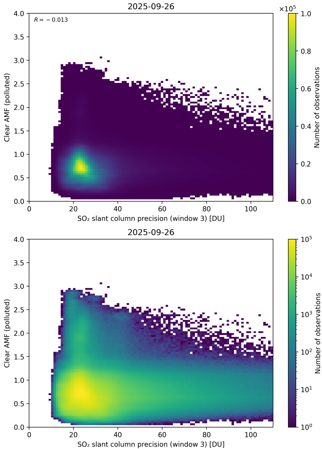
Figure 311: Scatter density plot of “SO 2 slant column precision (window 3)” against “Clear AMF (polluted)” for 2025-09-26 to 2025-09-27.
