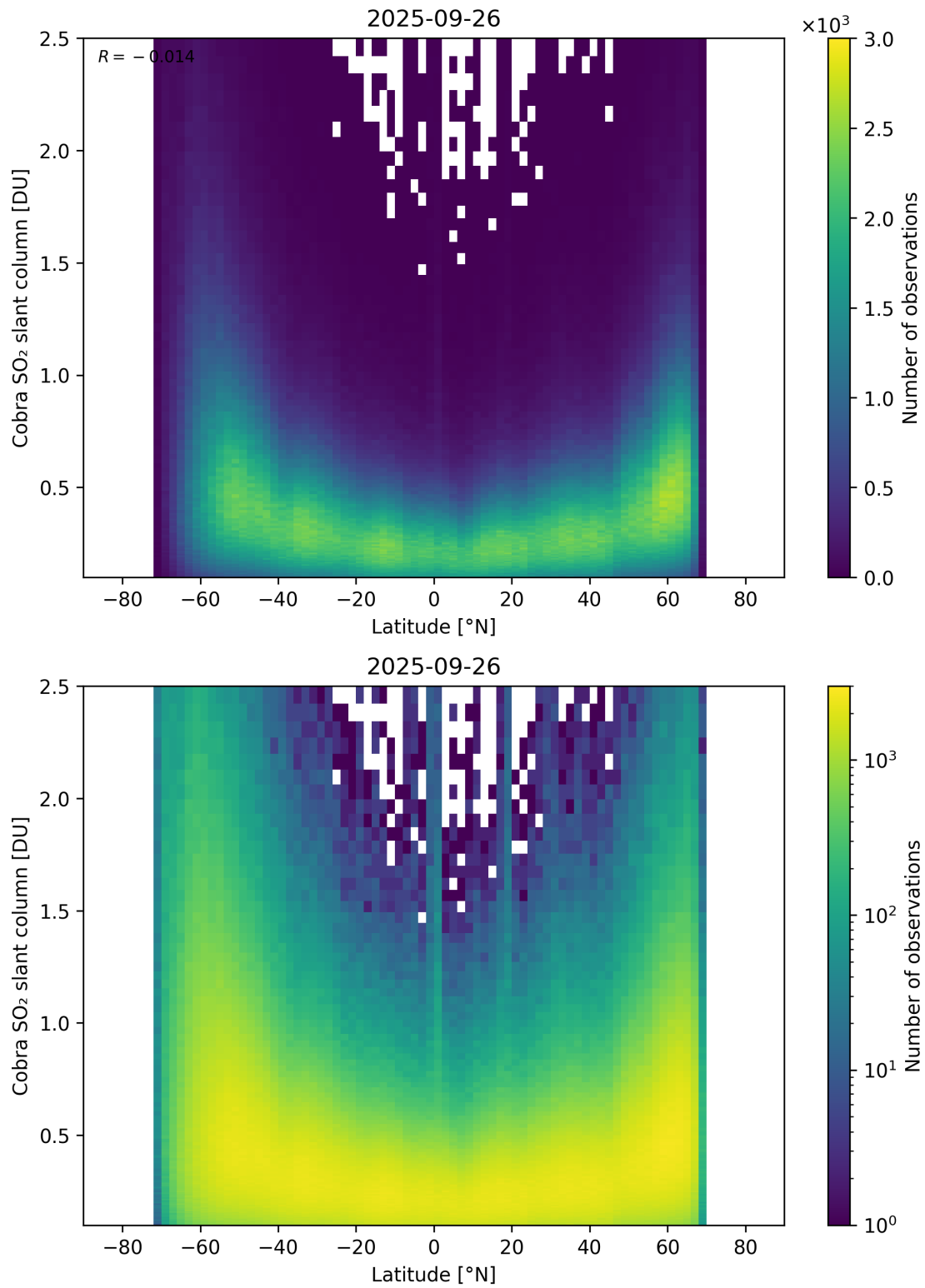
Figure 157: Scatter density plot of “Latitude” against “Cobra SO 2 slant column” for 2025-09-26 to 2025-09-27.
