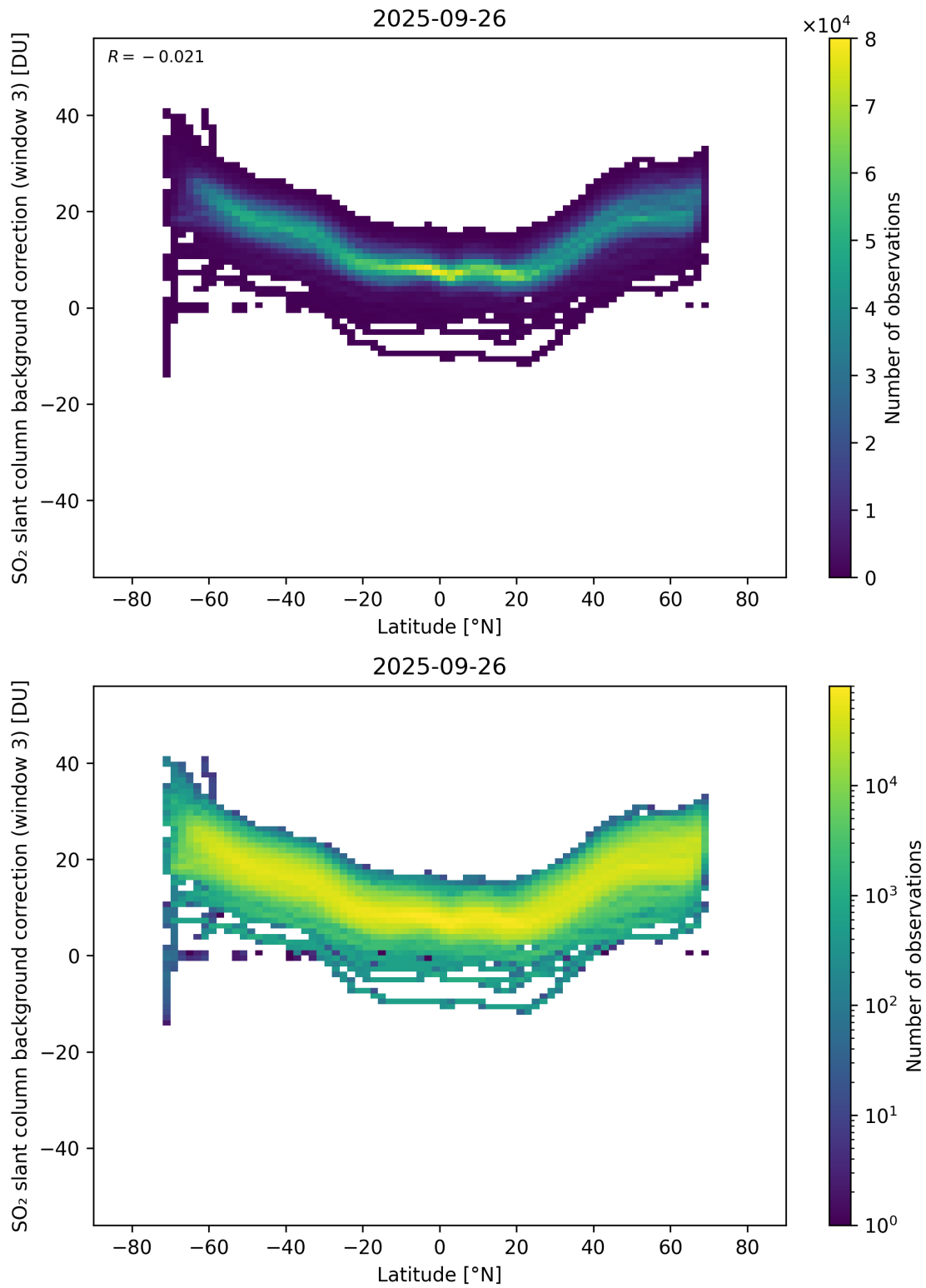
Figure 152: Scatter density plot of “Latitude” against “SO 2 slant column background correction (window 3)” for 2025-09-26 to 2025-09-27.
