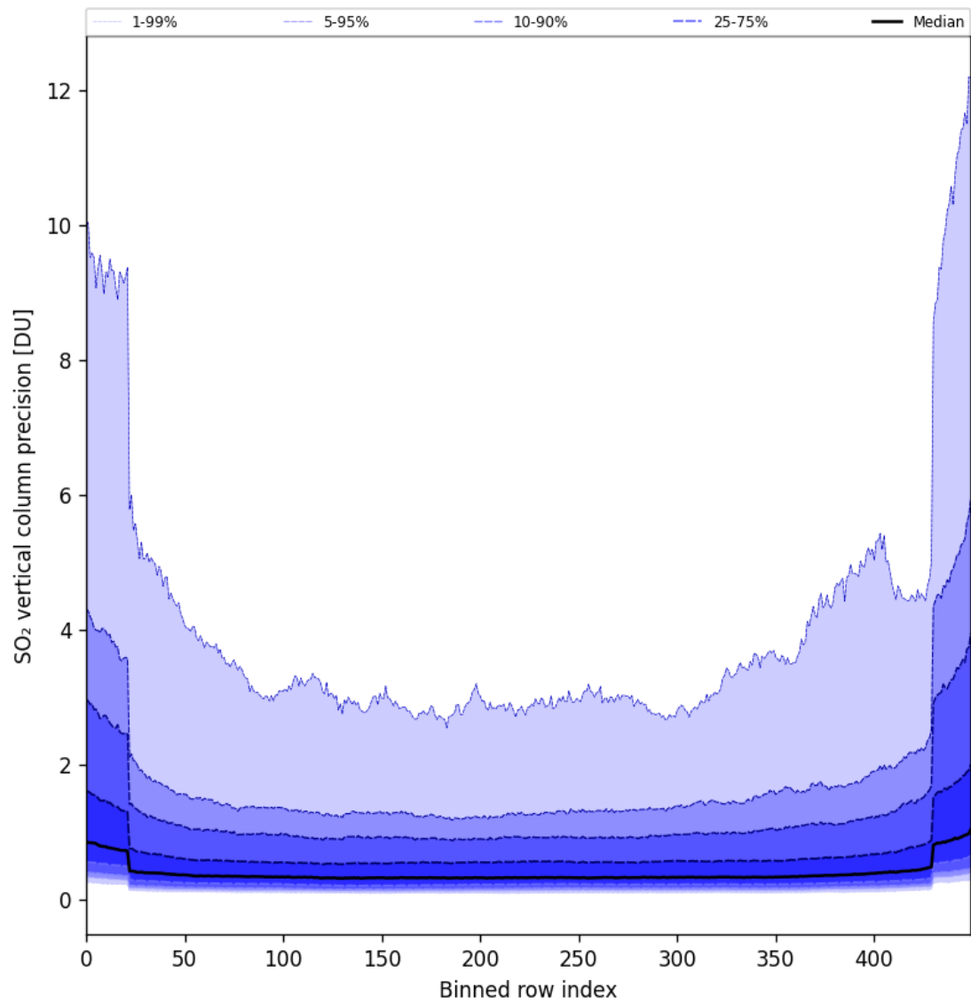
Figure 85: Along track statistics of “SO 2 vertical column precision” for 2025-09-26 to 2025-09-27
