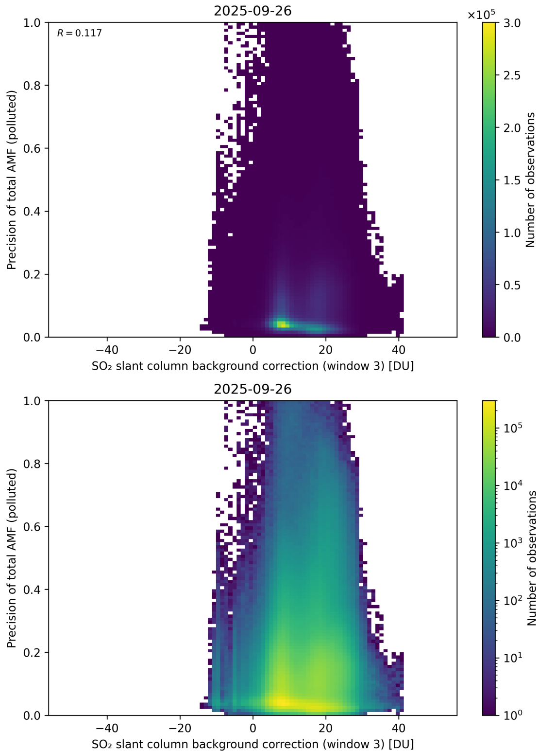
Figure 137: Scatter density plot of “SO 2 slant column background correction (window 3)” against “Precision of total AMF (polluted)” for 2025-09-26 to 2025-09-27.
