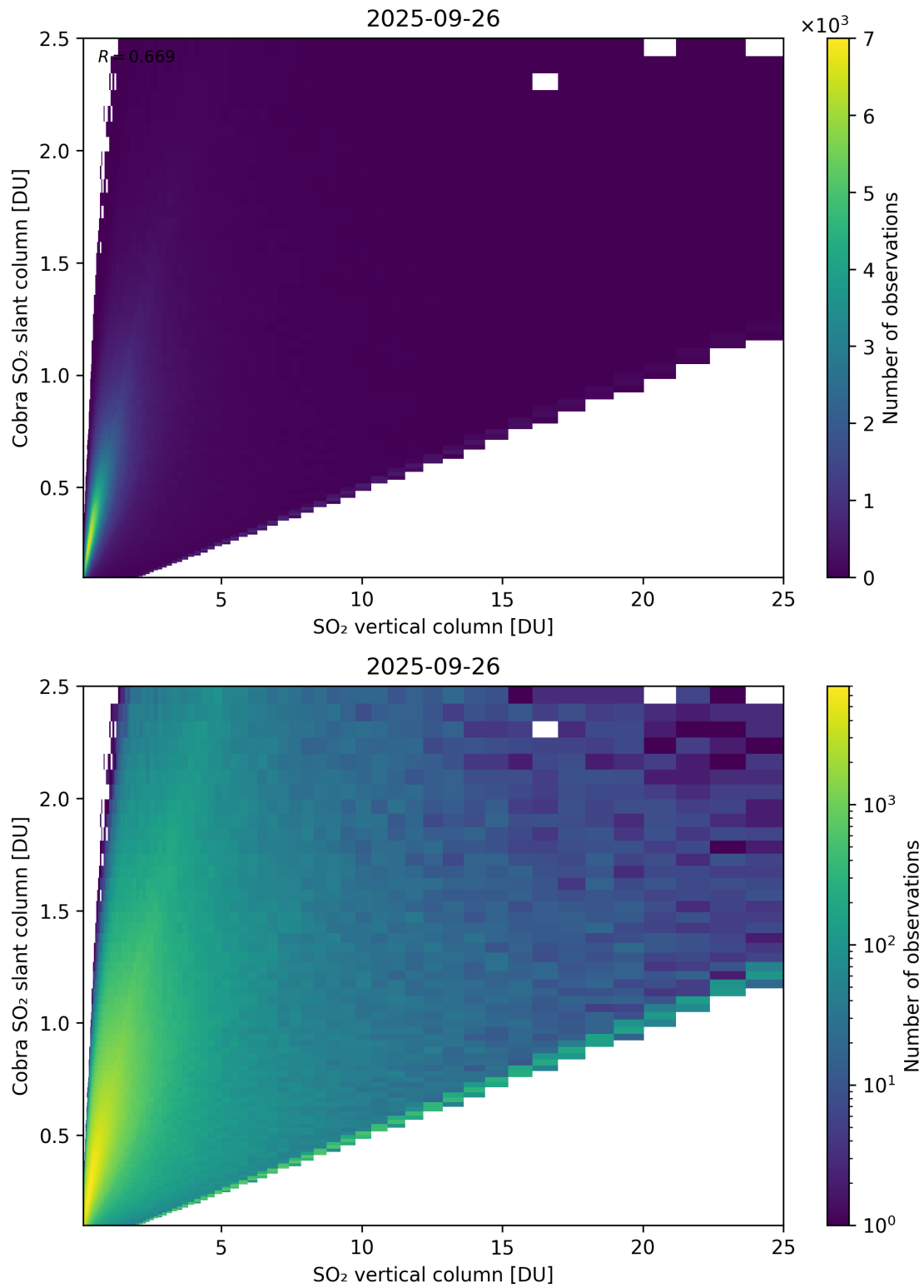
Figure 349: Scatter density plot of “SO 2 vertical column” against “Cobra SO 2 slant column” for 2025-09-26 to 2025-09-27.
