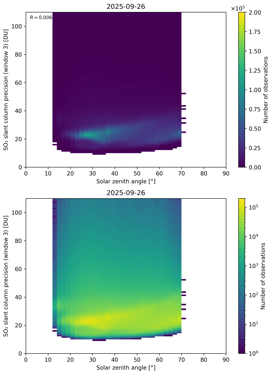
Figure 188: Scatter density plot of “Solar zenith angle” against “SO 2 slant column precision (window 3)” for 2025-09-26 to 2025-09-27.
