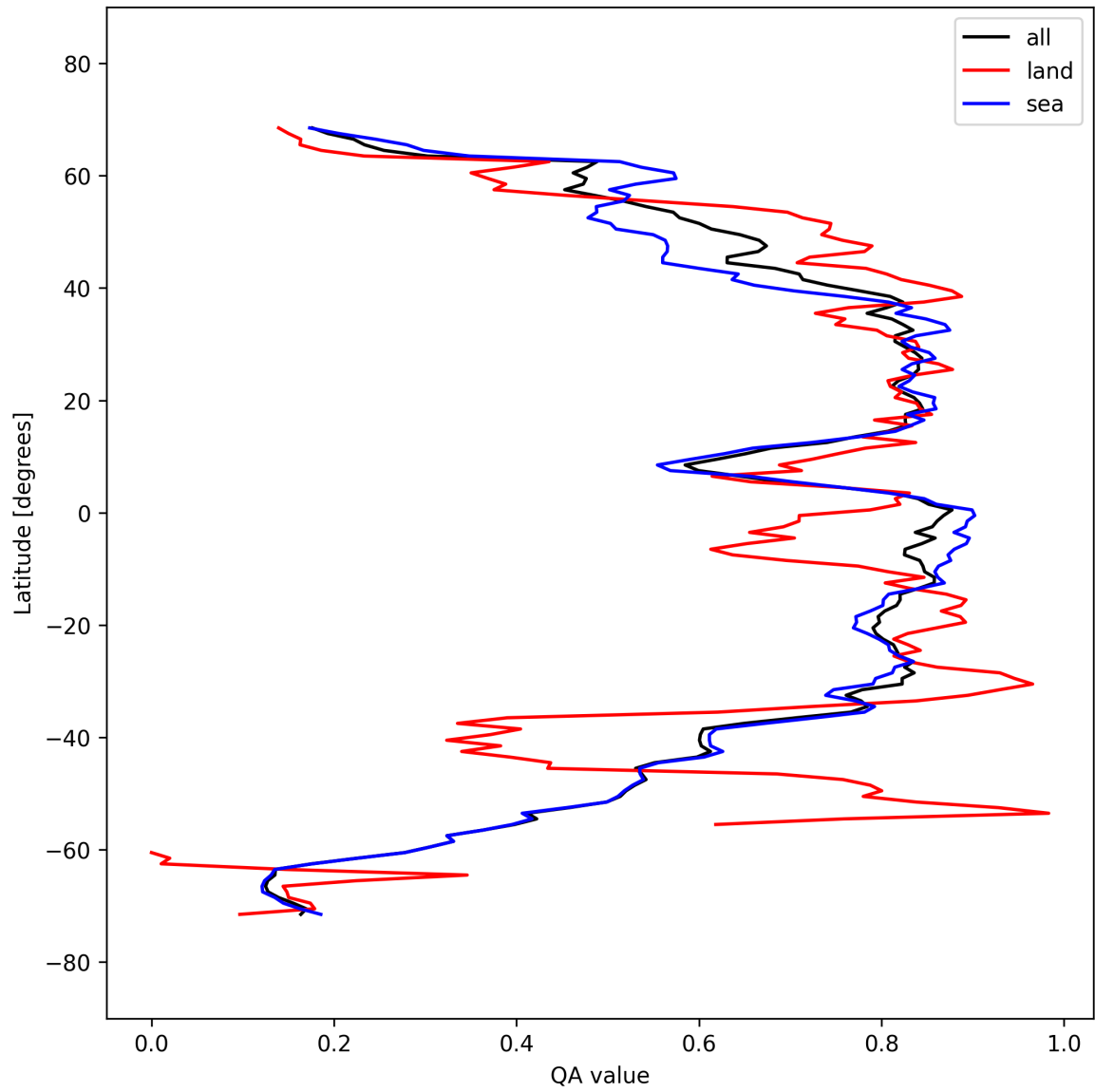
Figure 31: Zonal average of “QA value” for 2025-09-26 to 2025-09-27.
