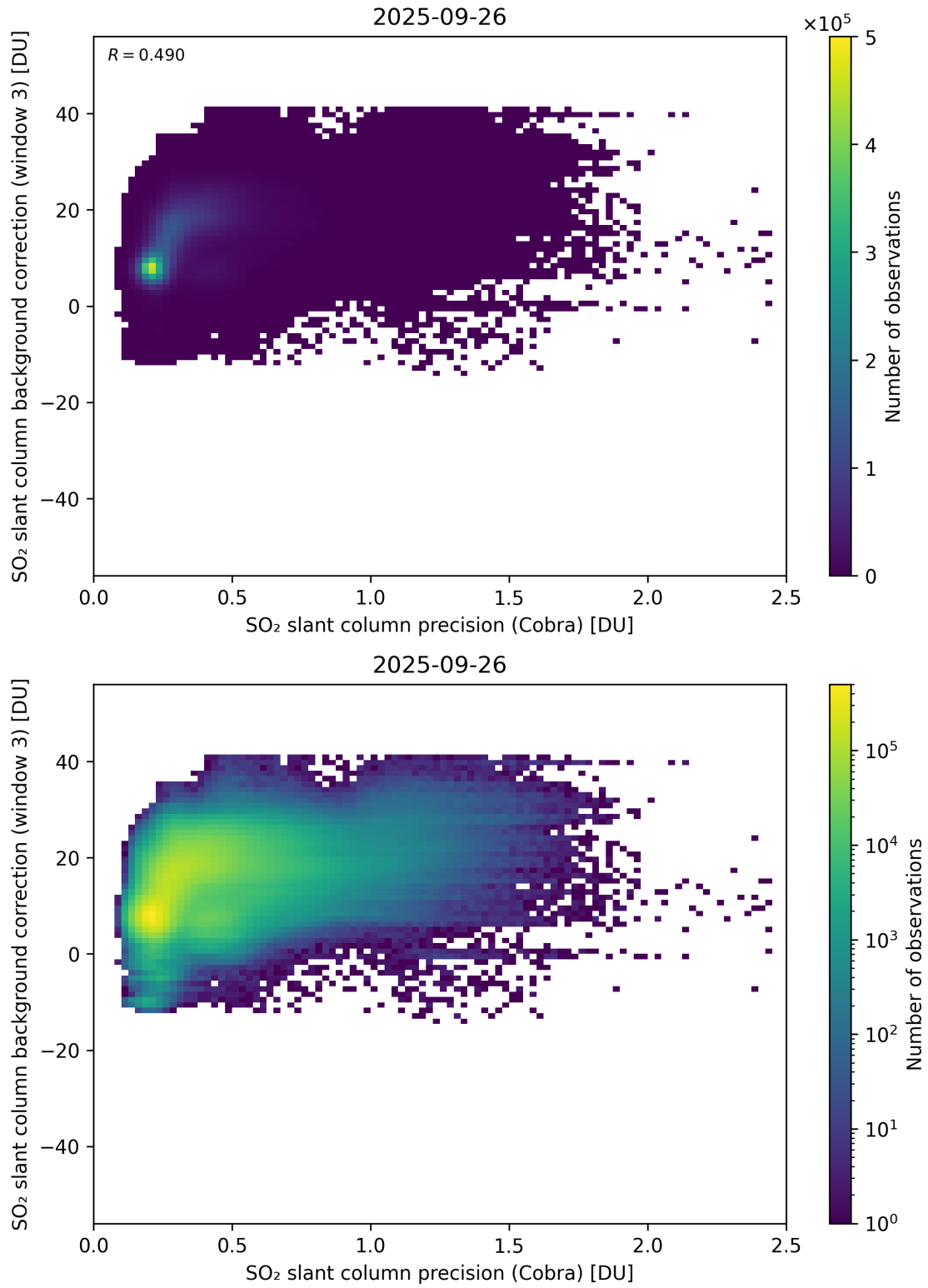
Figure 201: Scatter density plot of “SO 2 slant column precision (Cobra)” against “SO 2 slant column background correction (window 3)” for 2025-09-26 to 2025-09-27.
