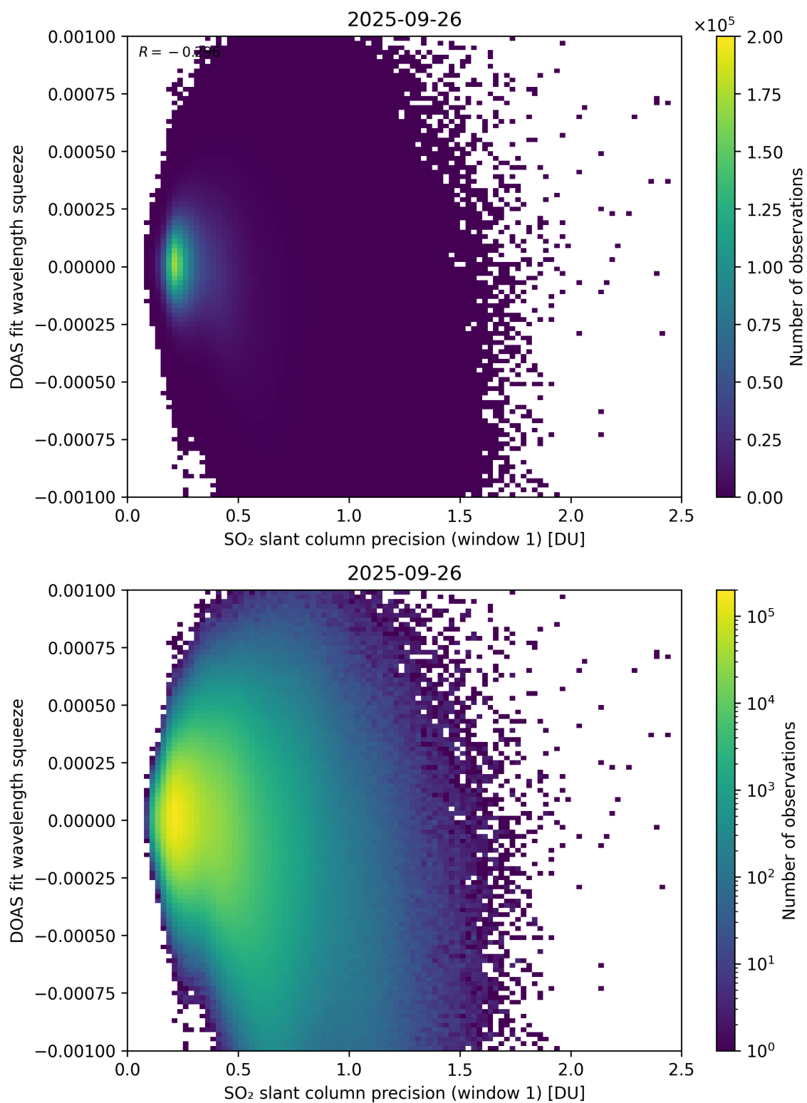
Figure 272: Scatter density plot of “SO 2 slant column precision (window 1)” against “DOAS fit wavelength squeeze” for 2025-09-26 to 2025-09-27.
