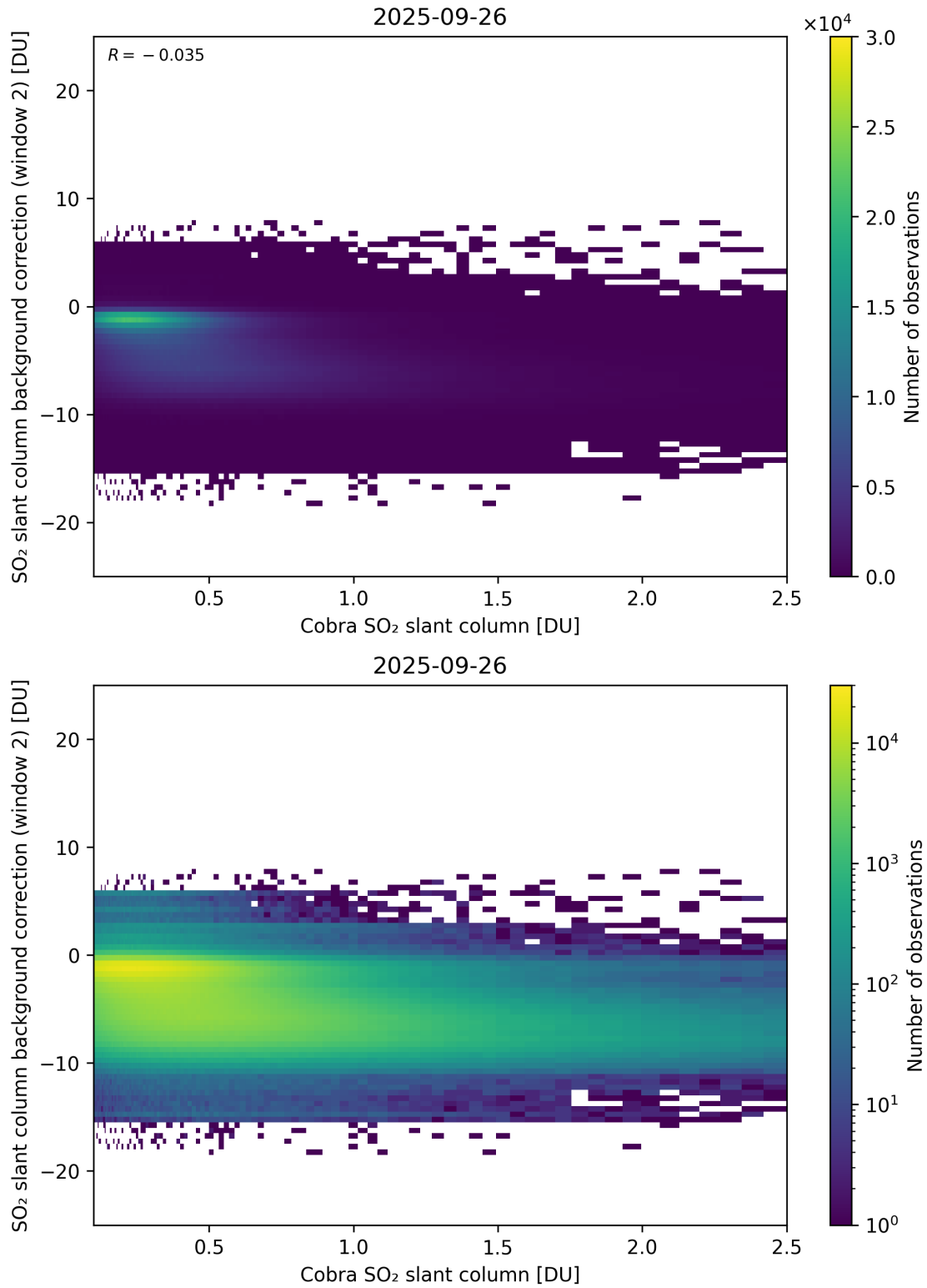
Figure 194: Scatter density plot of “Cobra SO 2 slant column” against “SO 2 slant column background correction (window 2)” for 2025-09-26 to 2025-09-27.
