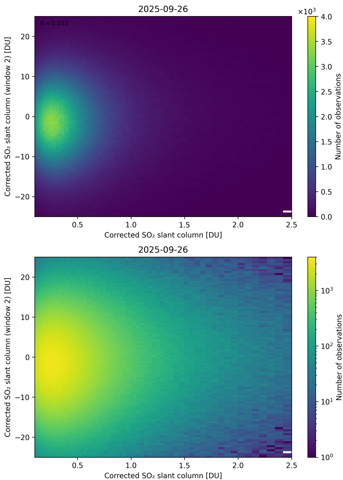
Figure 235: Scatter density plot of “Corrected SO 2 slant column” against “Corrected SO 2 slant column (window 2)” for 2025-09-26 to 2025-09-27.
