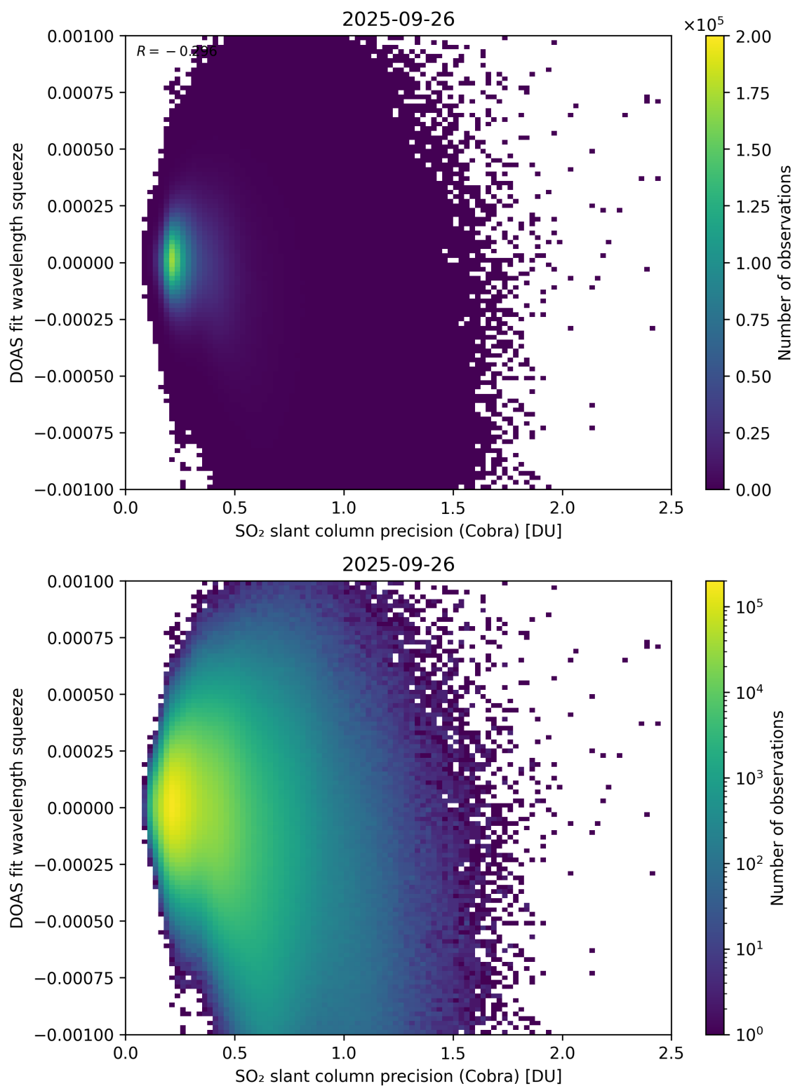
Figure 203: Scatter density plot of “SO 2 slant column precision (Cobra)” against “DOAS fit wavelength squeeze” for 2025-09-26 to 2025-09-27.
