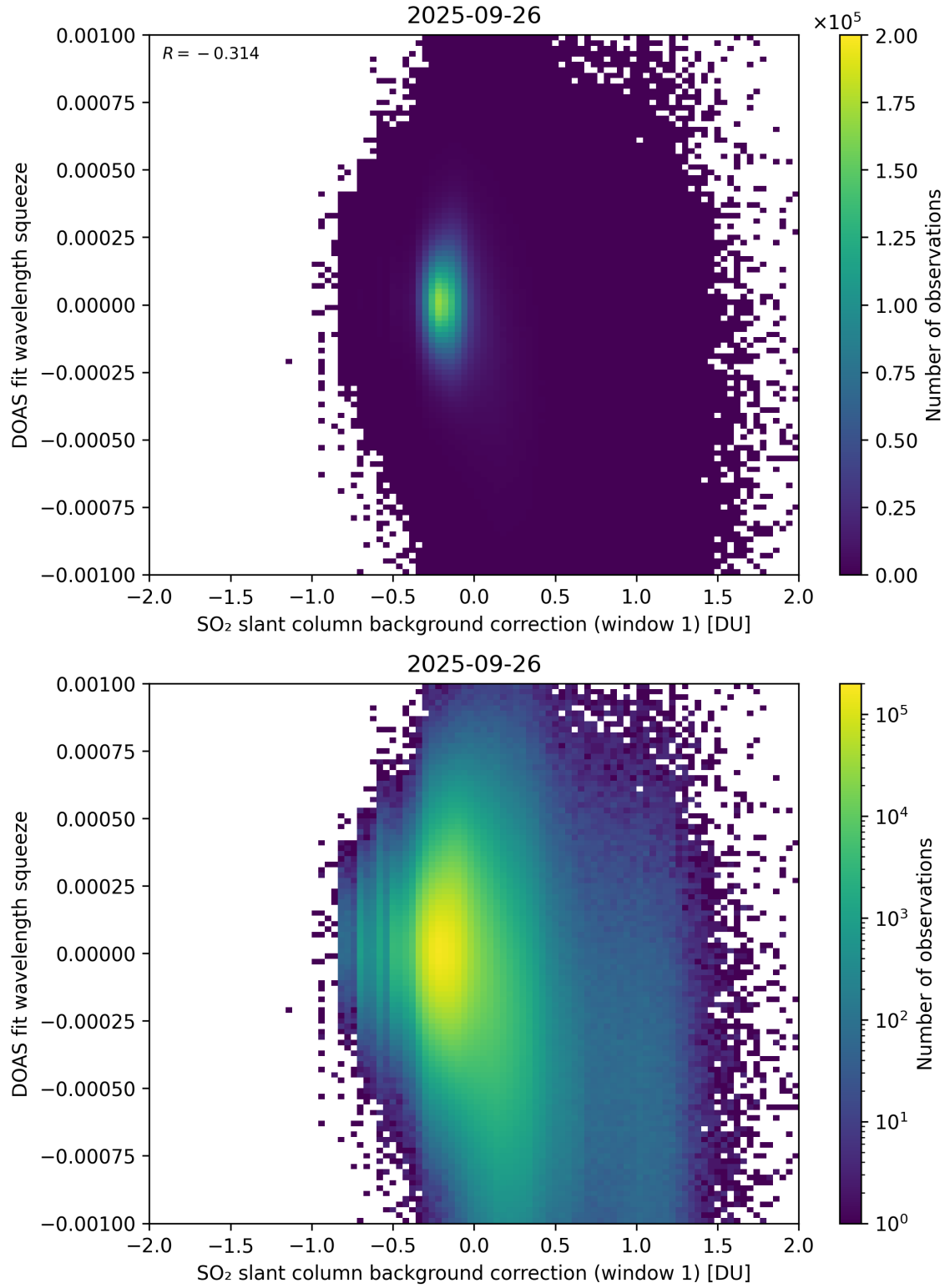
Figure 112: Scatter density plot of “SO 2 slant column background correction (window 1)” against “DOAS fit wavelength squeeze” for 2025-09-26 to 2025-09-27.
