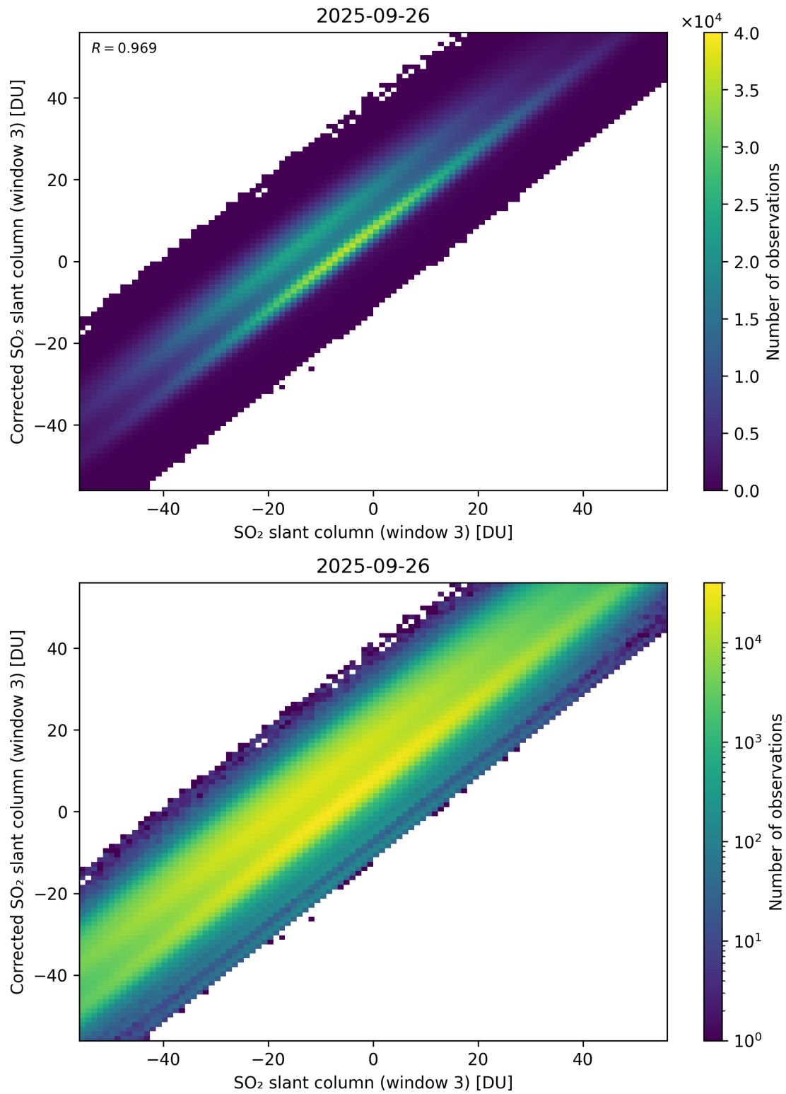
Figure 316: Scatter density plot of “SO 2 slant column (window 3)” against “Corrected SO 2 slant column (window 3)” for 2025-09-26 to 2025-09-27.
