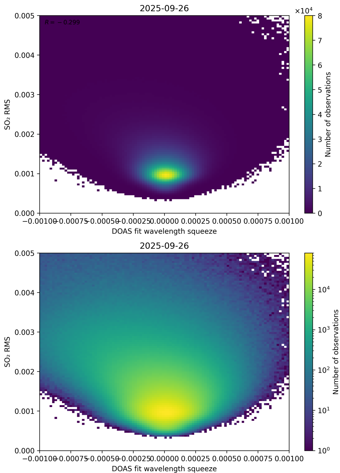
Figure 143: Scatter density plot of “DOAS fit wavelength squeeze” against “SO 2 RMS” for 2025-09-26 to 2025-09-27.
