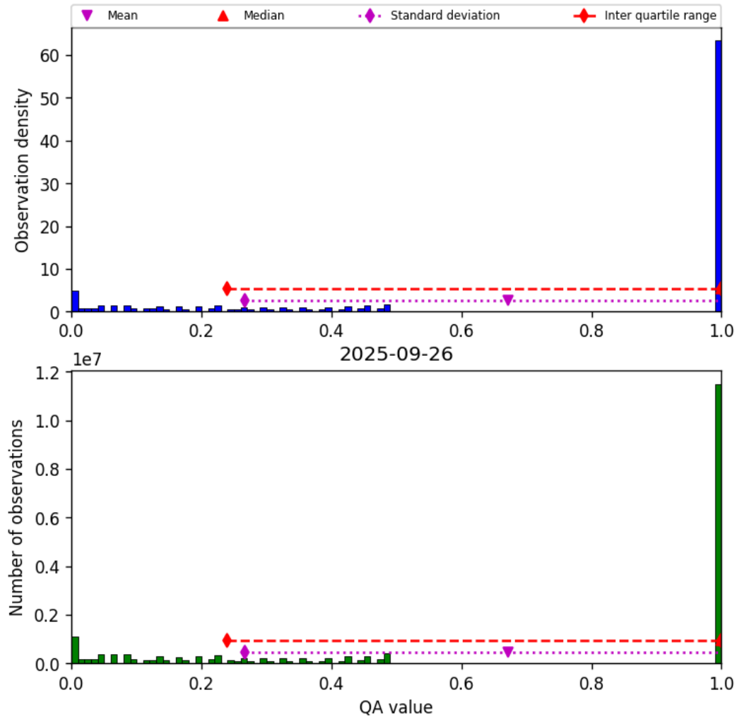
Figure 57: Histogram of “QA value” for 2025-09-26 to 2025-09-27
