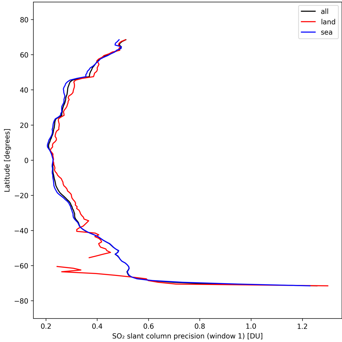
Figure 38: Zonal average of “SO 2 slant column precision (window 1)” for 2025-09-26 to 2025-09-27.
