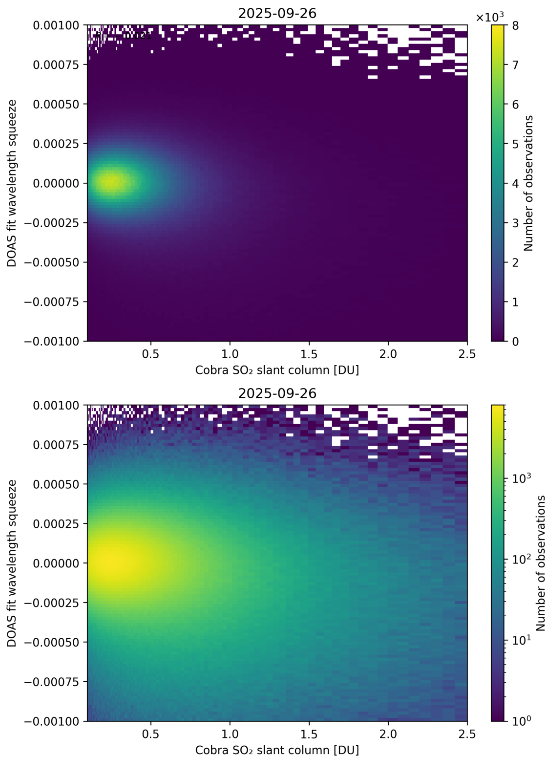
Figure 197: Scatter density plot of “Cobra SO 2 slant column” against “DOAS fit wavelength squeeze” for 2025-09-26 to 2025-09-27.
