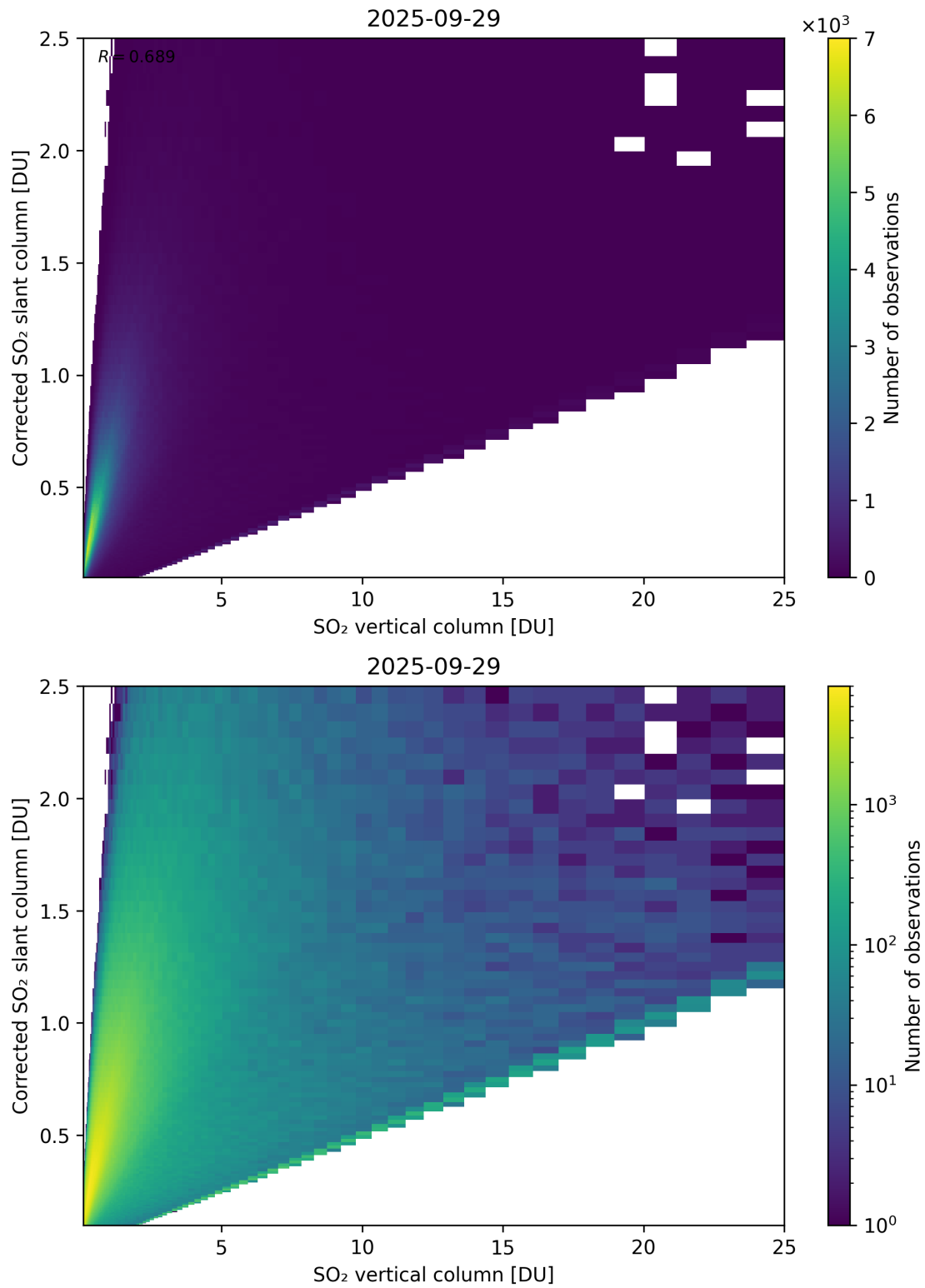
Figure 351: Scatter density plot of “SO 2 vertical column” against “Corrected SO 2 slant column” for 2025-09-28 to 2025-09-30.
