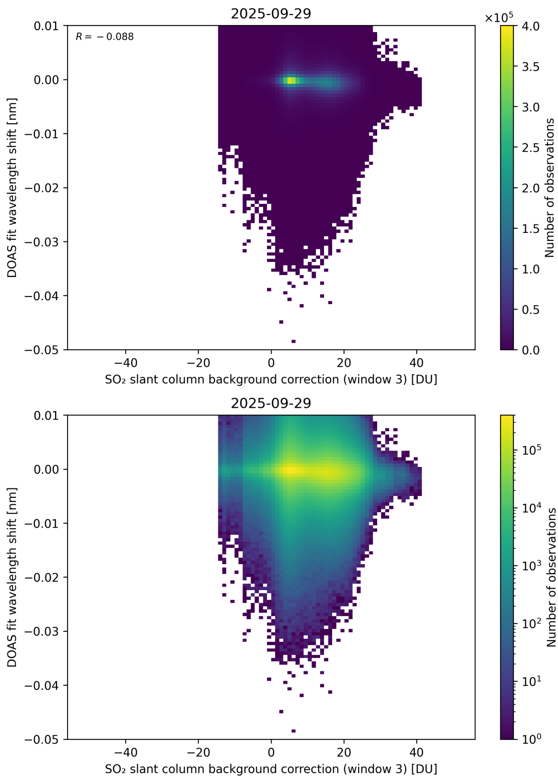
Figure 132: Scatter density plot of “SO 2 slant column background correction (window 3)” against “DOAS fit wavelength shift” for 2025-09-28 to 2025-09-30.
