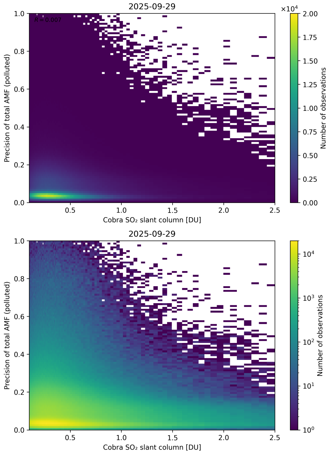
Figure 225: Scatter density plot of “Cobra SO 2 slant column” against “Precision of total AMF (polluted)” for 2025-09-28 to 2025-09-30.
