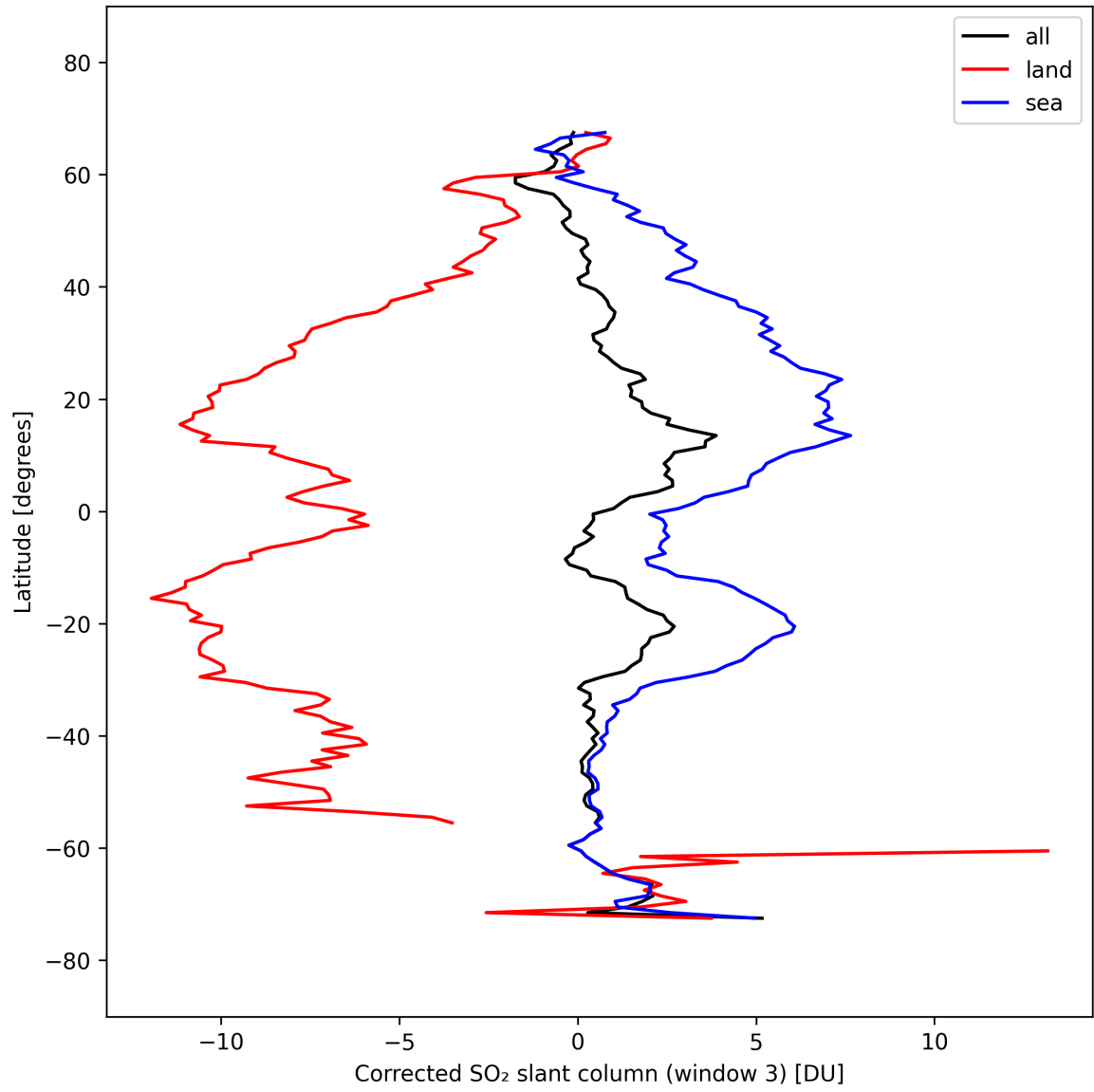
Figure 47: Zonal average of “Corrected SO 2 slant column (window 3)” for 2025-09-28 to 2025-09-30.
