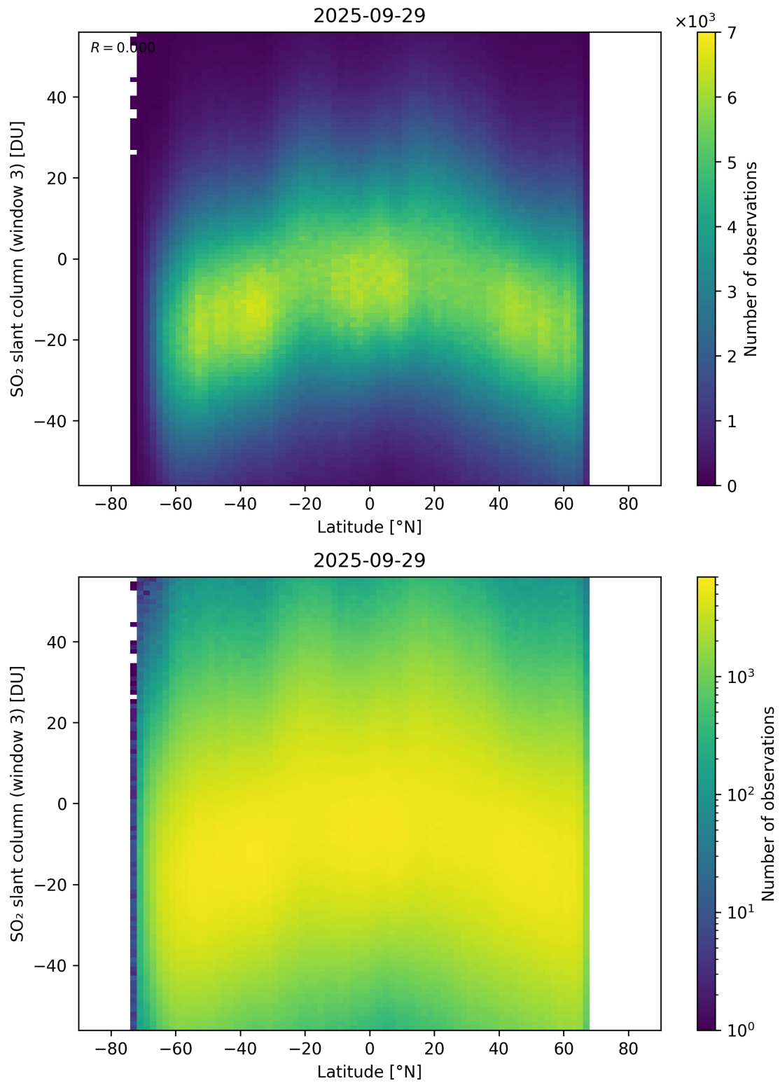
Figure 165: Scatter density plot of “Latitude” against “SO 2 slant column (window 3)” for 2025-09-28 to 2025-09-30.
