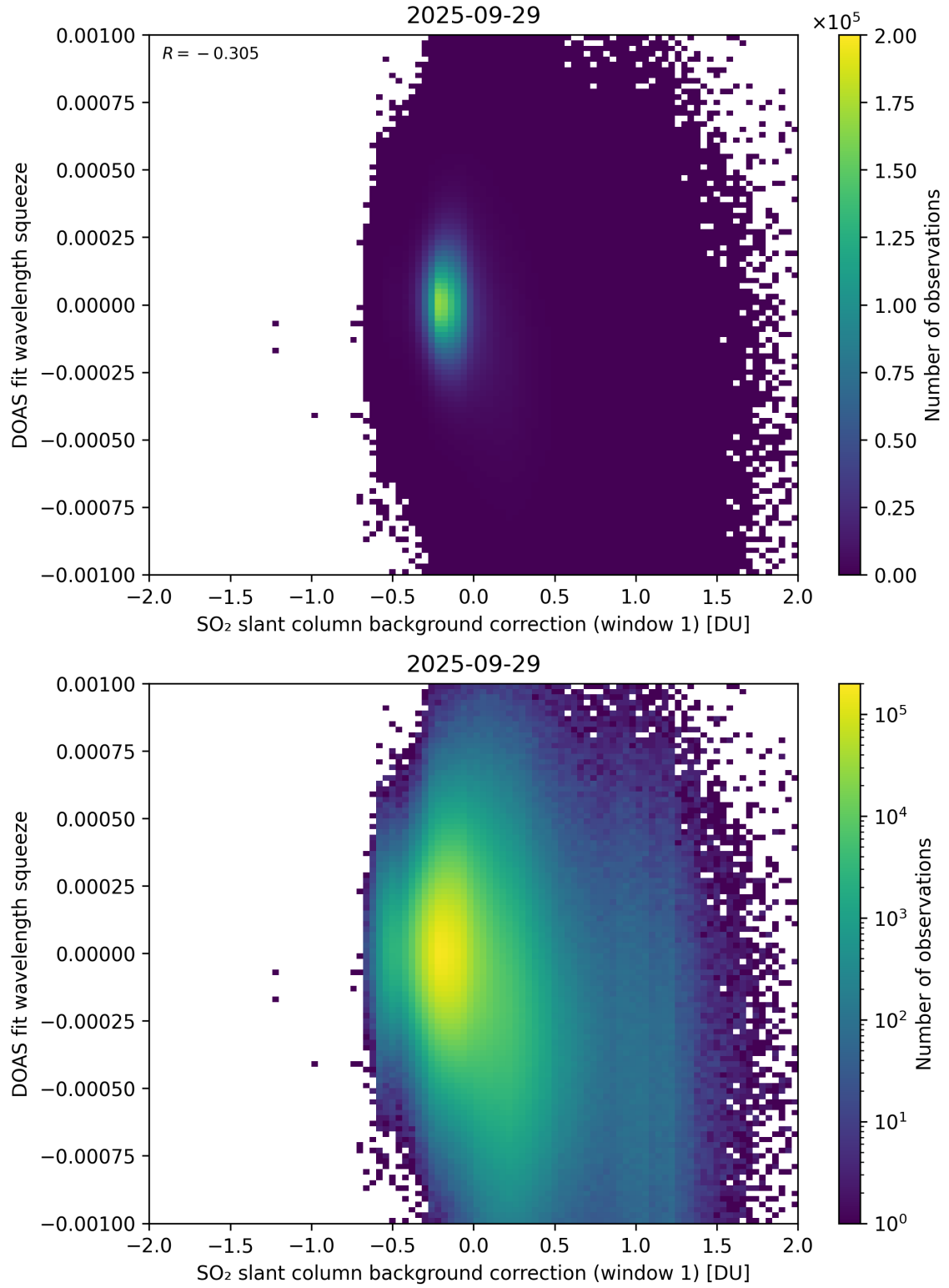
Figure 112: Scatter density plot of “SO 2 slant column background correction (window 1)” against “DOAS fit wavelength squeeze” for 2025-09-28 to 2025-09-30.
