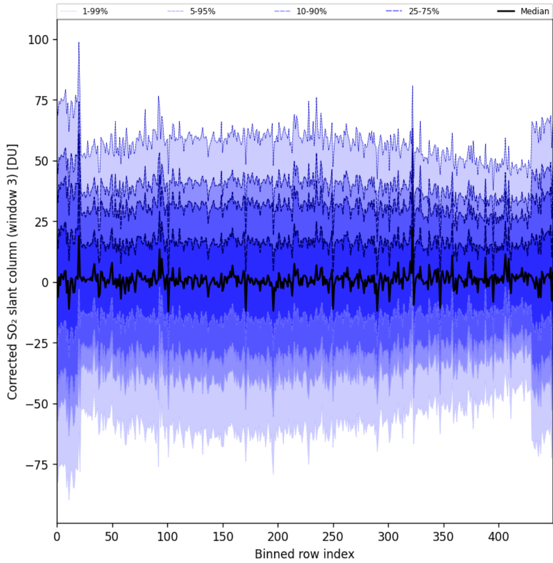
Figure 99: Along track statistics of “Corrected SO 2 slant column (window 3)” for 2025-09-28 to 2025-09-30
