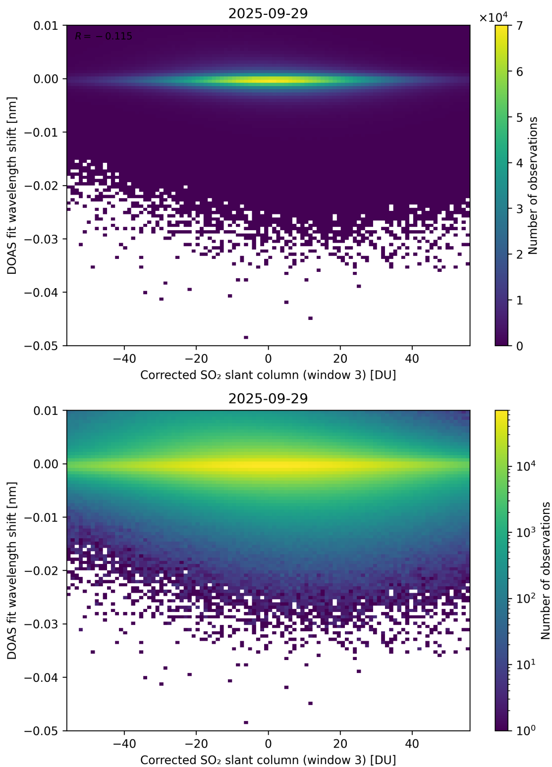
Figure 256: Scatter density plot of “Corrected SO 2 slant column (window 3)” against “DOAS fit wavelength shift” for 2025-09-28 to 2025-09-30.
