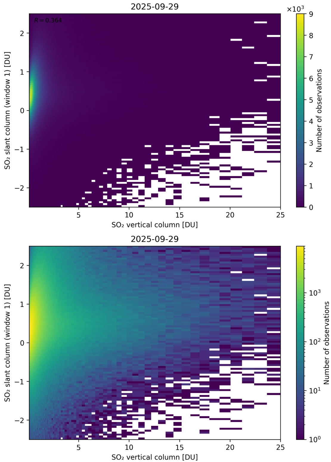
Figure 354: Scatter density plot of “SO 2 vertical column” against “SO 2 slant column (window 1)” for 2025-09-28 to 2025-09-30.
