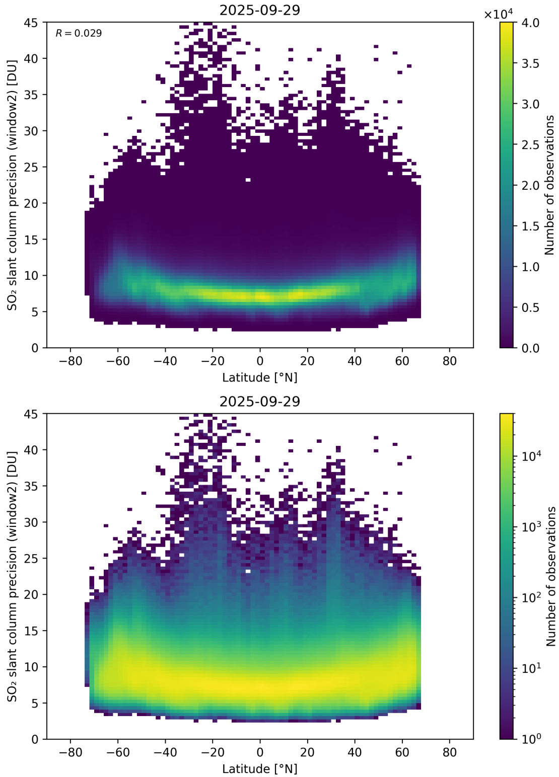
Figure 164: Scatter density plot of “Latitude” against “SO 2 slant column precision (window2)” for 2025-09-28 to 2025-09-30.
