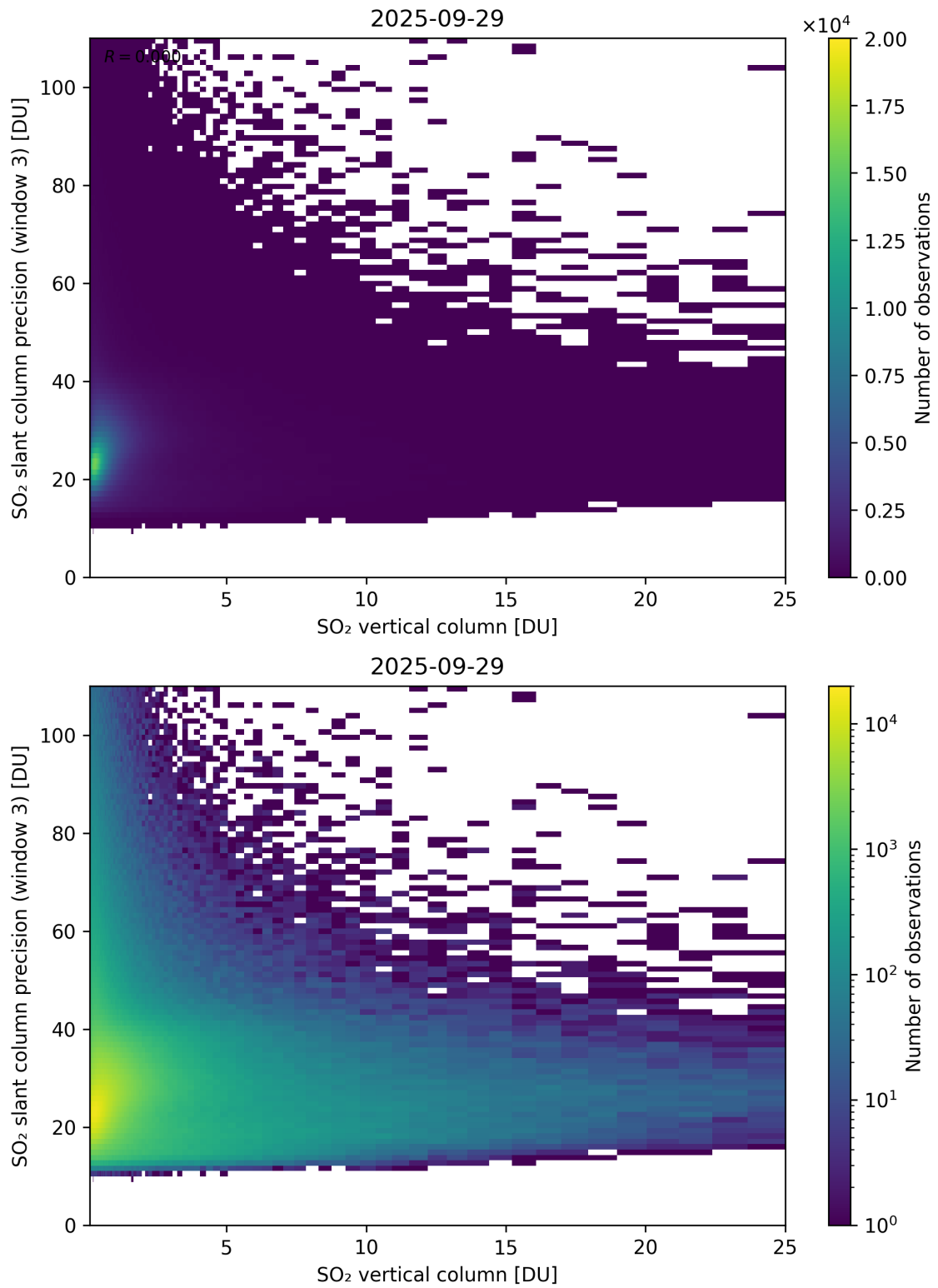
Figure 358: Scatter density plot of “SO 2 vertical column” against “SO 2 slant column precision (window 3)” for 2025-09-28 to 2025-09-30.
