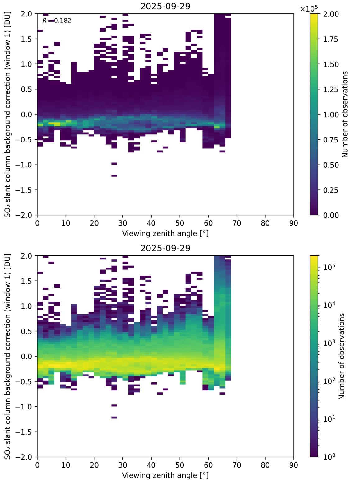
Figure 362: Scatter density plot of “Viewing zenith angle” against “SO 2 slant column background correction (window 1)” for 2025-09-28 to 2025-09-30.
