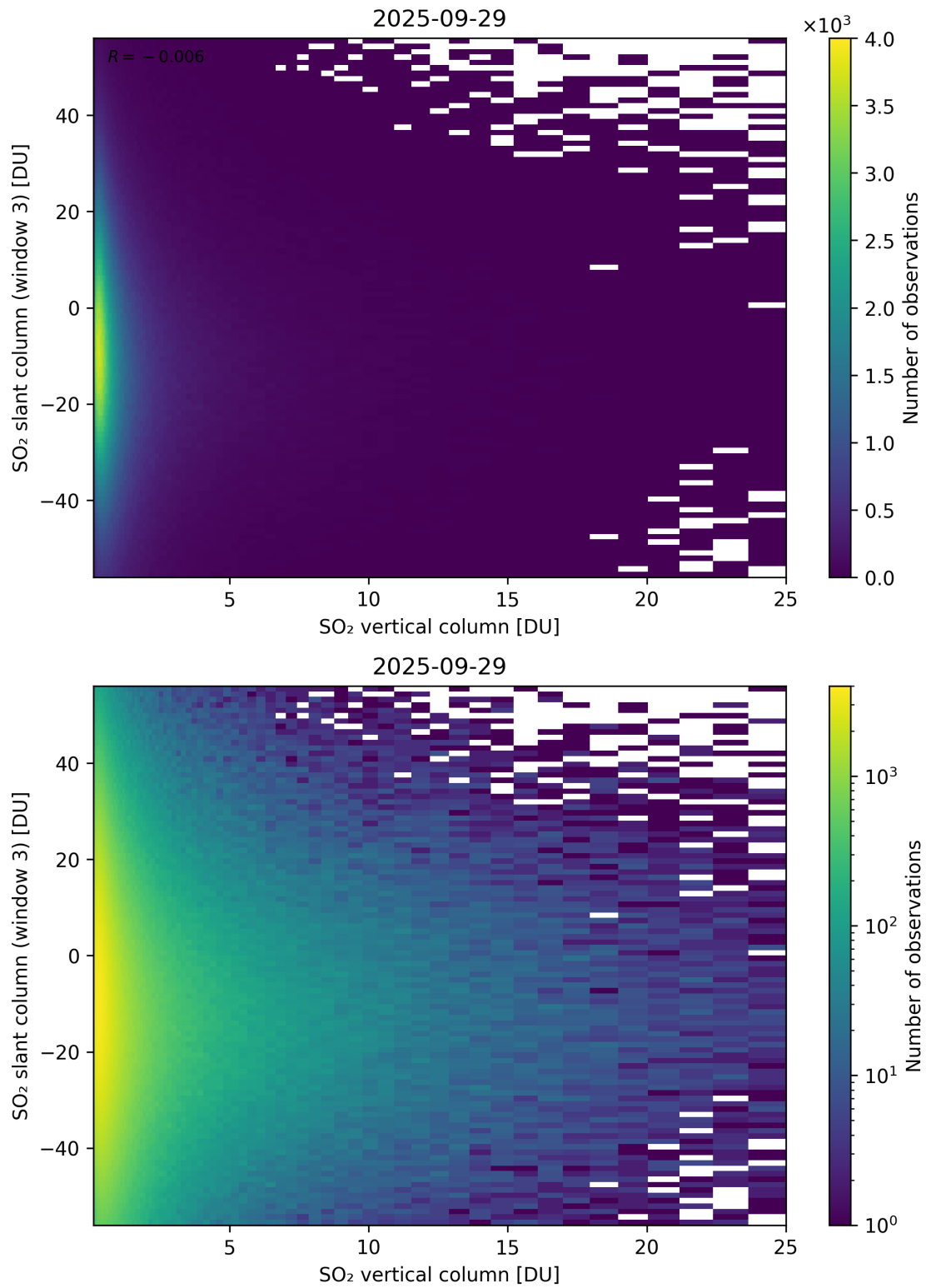
Figure 357: Scatter density plot of “SO 2 vertical column” against “SO 2 slant column (window 3)” for 2025-09-28 to 2025-09-30.
