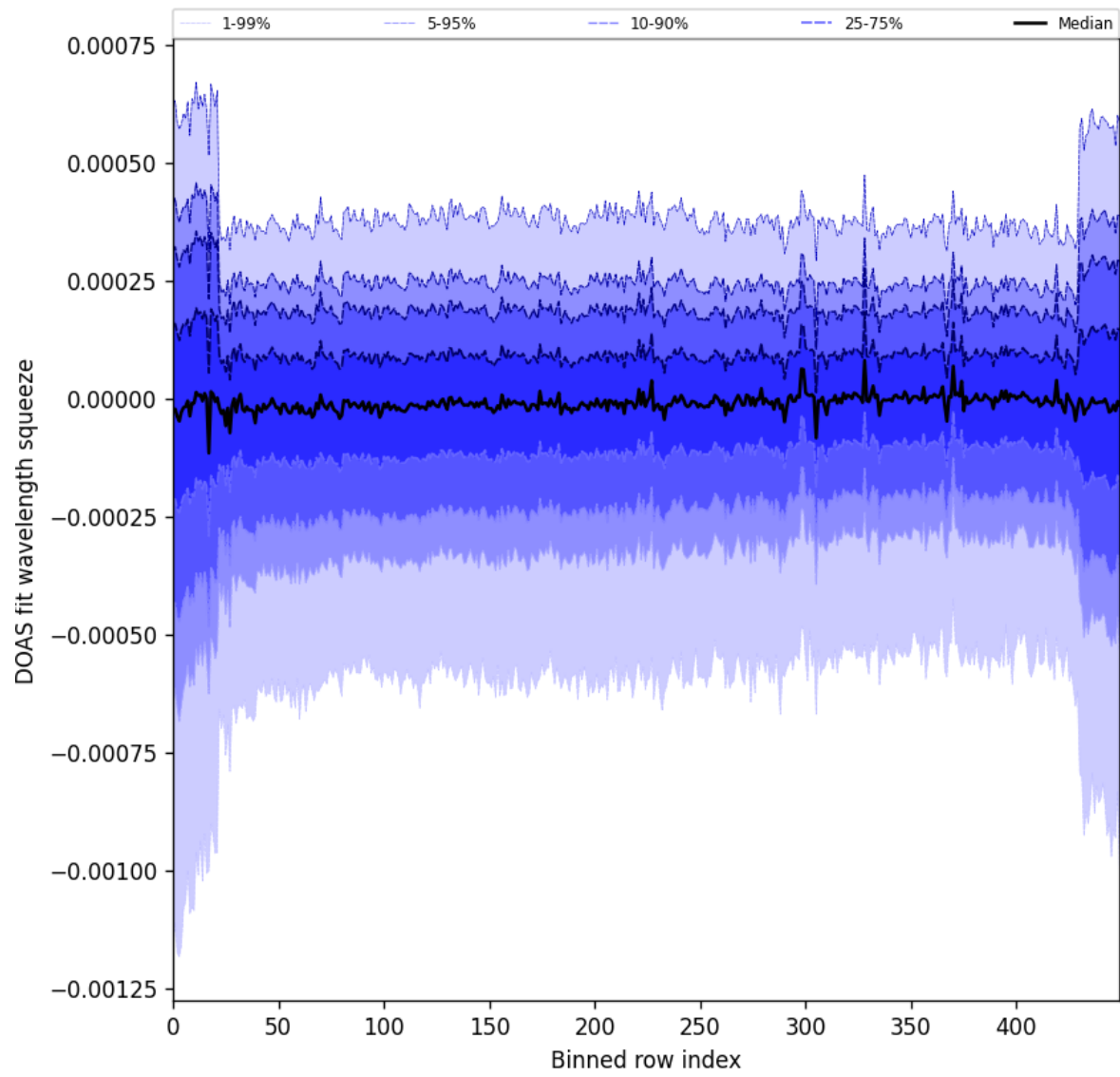
Figure 103: Along track statistics of “DOAS fit wavelength squeeze” for 2025-09-28 to 2025-09-30
