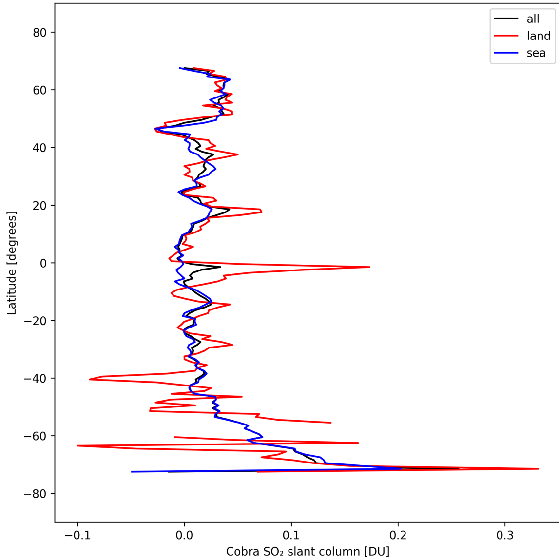
Figure 35: Zonal average of “Cobra SO 2 slant column” for 2025-09-28 to 2025-09-30.
