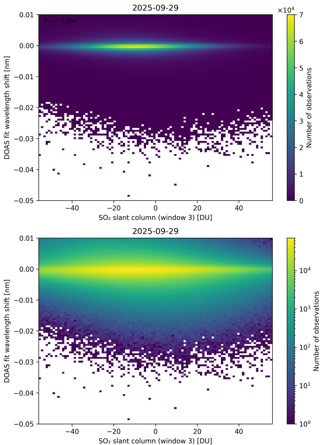
Figure 304: Scatter density plot of “SO 2 slant column (window 3)” against “DOAS fit wavelength shift” for 2025-09-28 to 2025-09-30.
