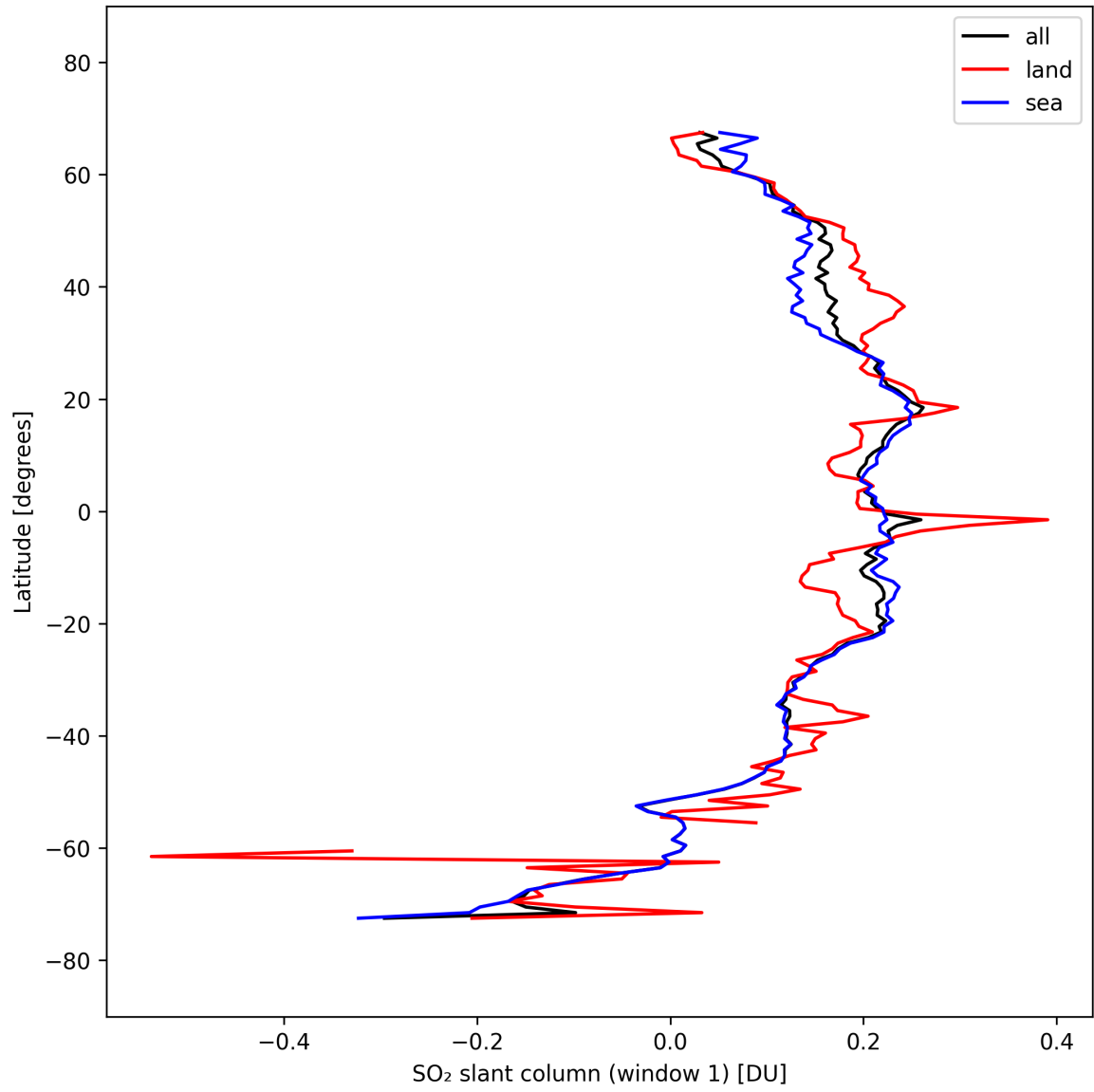
Figure 37: Zonal average of “SO 2 slant column (window 1)” for 2025-09-28 to 2025-09-30.
