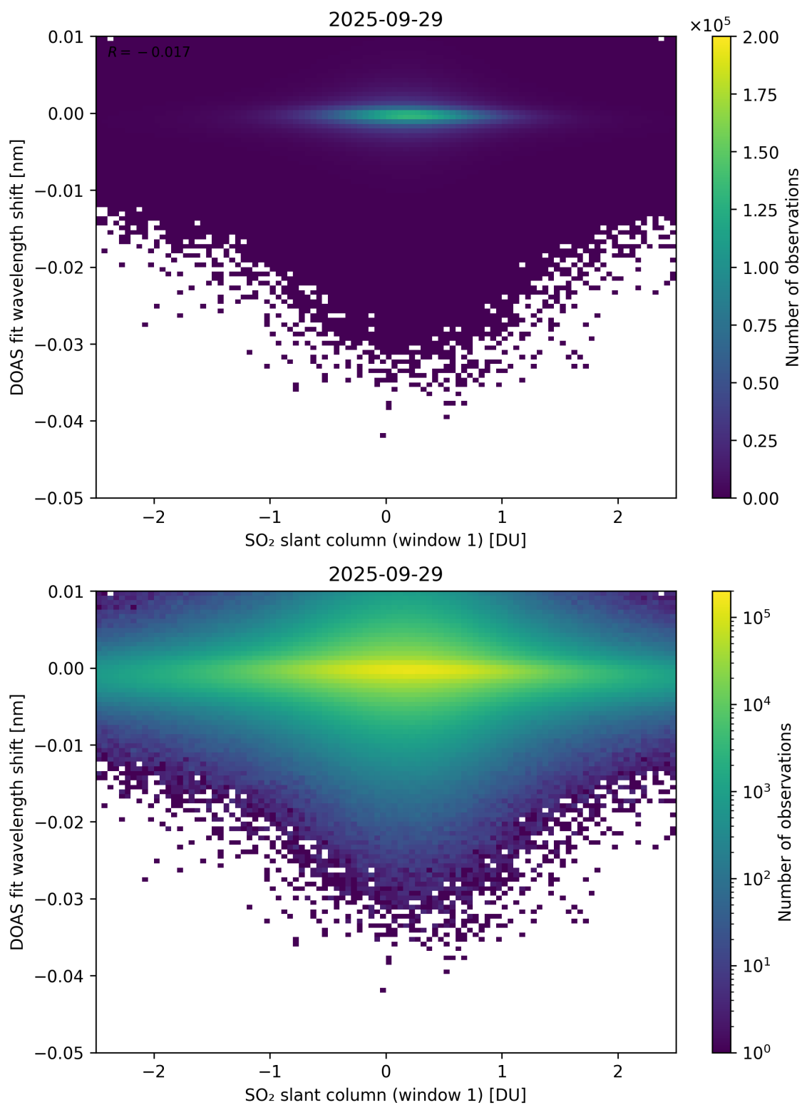
Figure 265: Scatter density plot of “SO 2 slant column (window 1)” against “DOAS fit wavelength shift” for 2025-09-28 to 2025-09-30.
