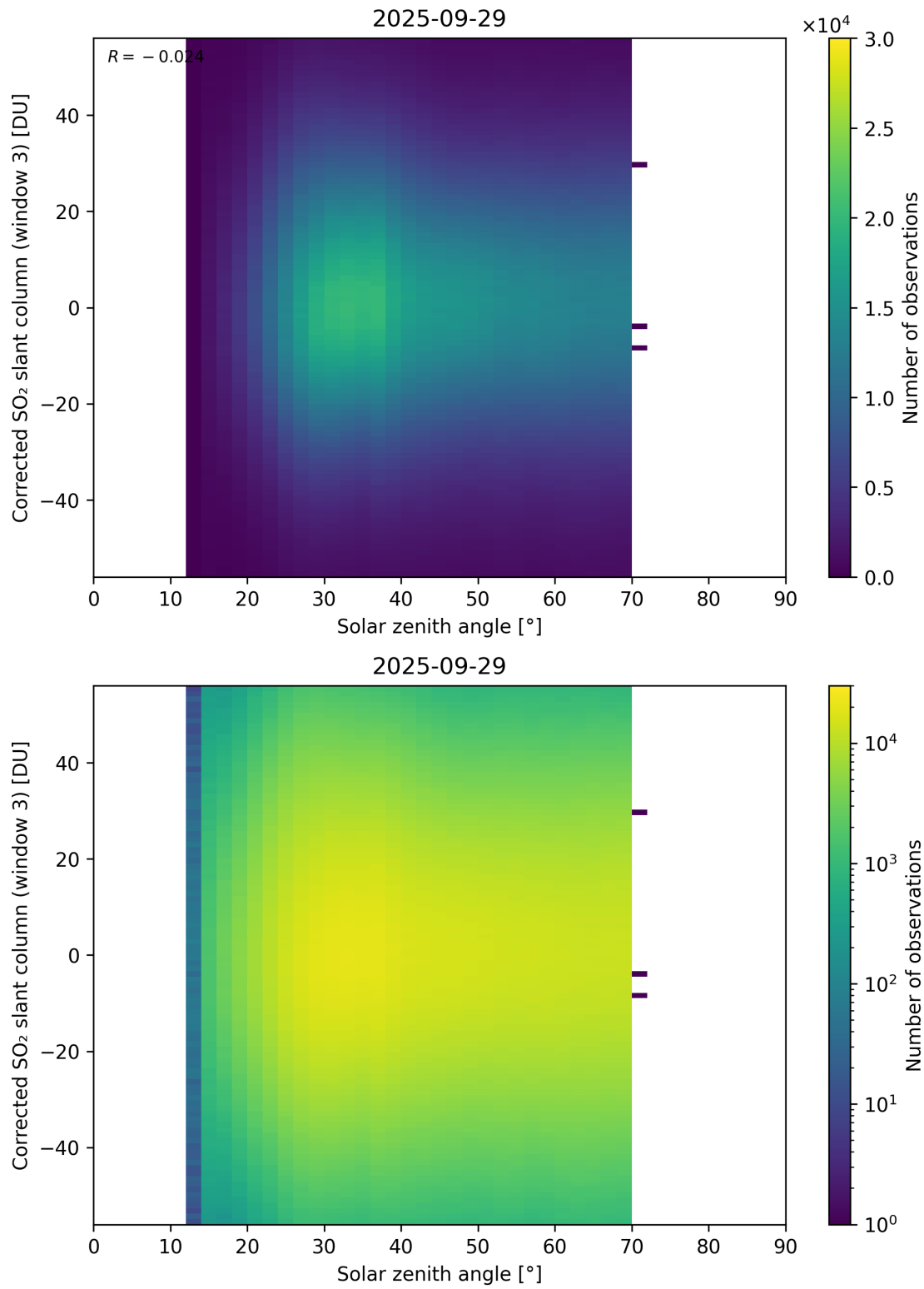
Figure 183: Scatter density plot of “Solar zenith angle” against “Corrected SO 2 slant column (window 3)” for 2025-09-28 to 2025-09-30.
