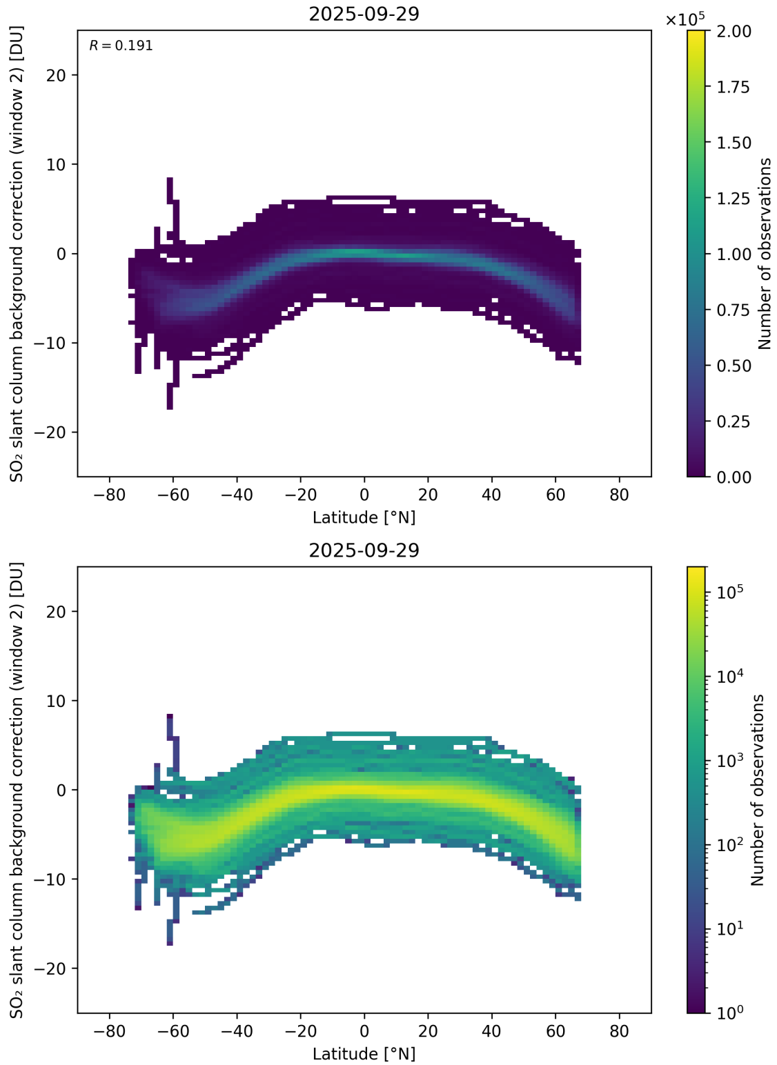
Figure 151: Scatter density plot of “Latitude” against “SO 2 slant column background correction (window 2)” for 2025-09-28 to 2025-09-30.
