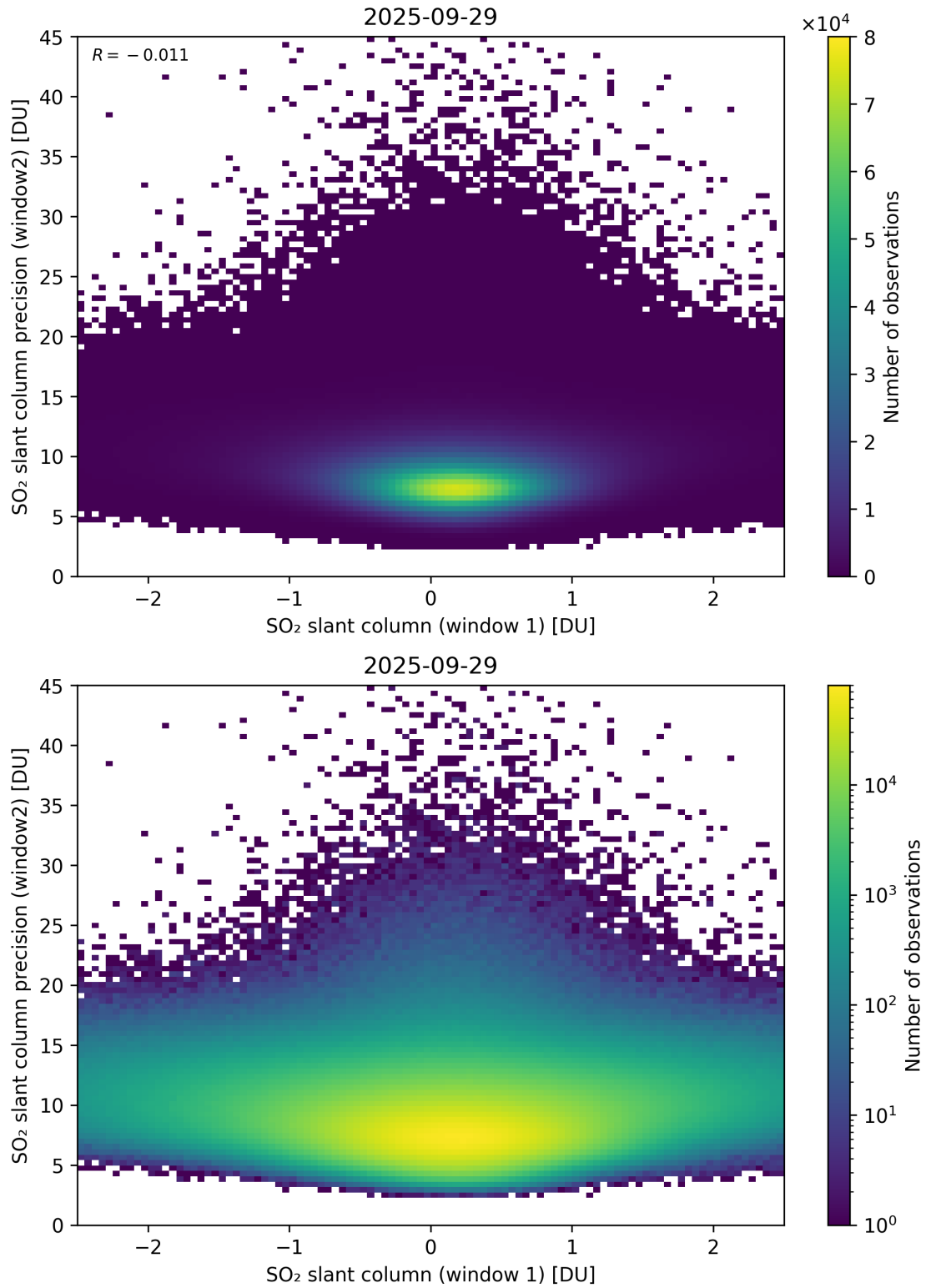
Figure 286: Scatter density plot of “SO 2 slant column (window 1)” against “SO 2 slant column precision (window2)” for 2025-09-28 to 2025-09-30.
