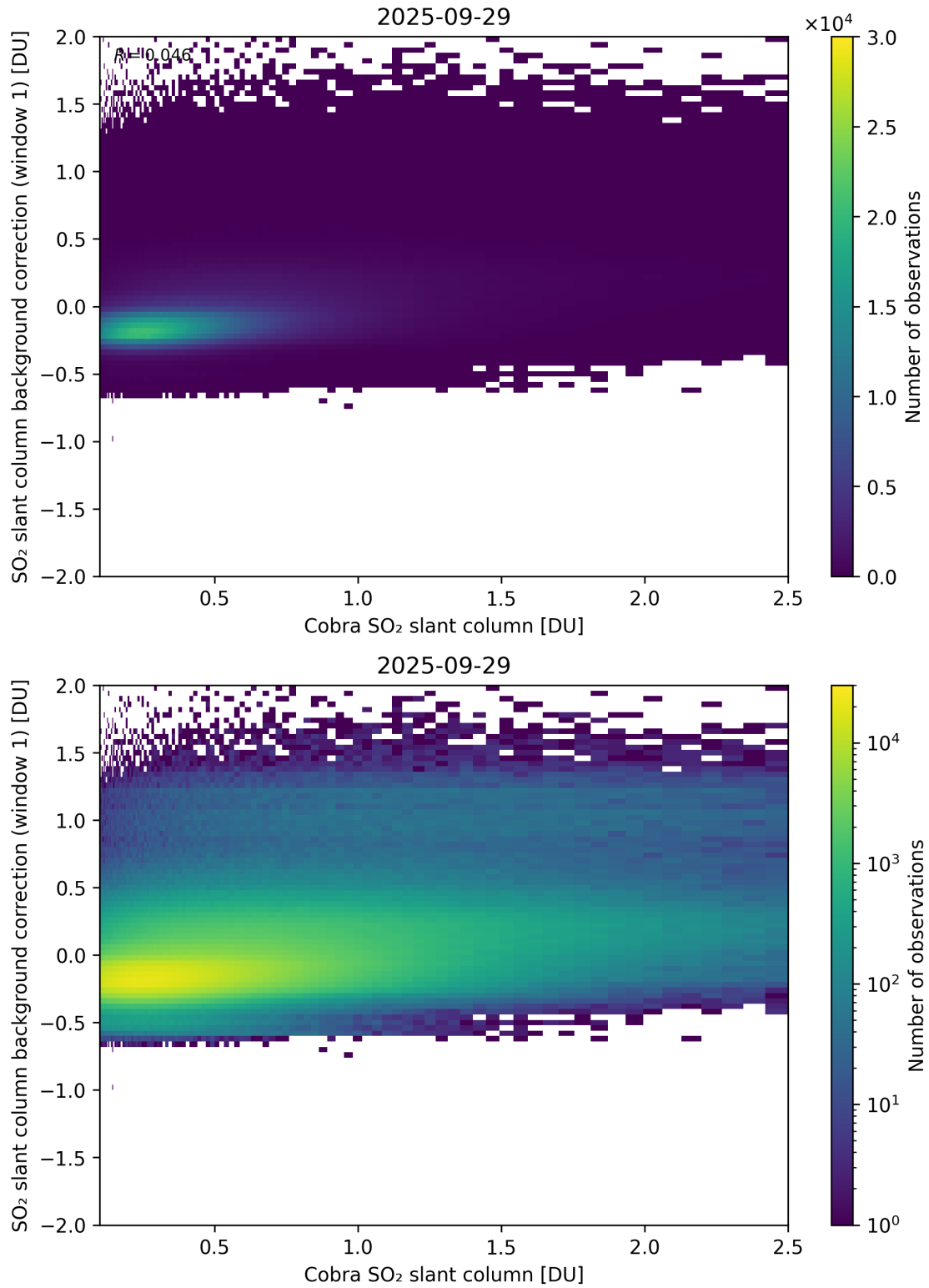
Figure 193: Scatter density plot of “Cobra SO 2 slant column” against “SO 2 slant column background correction (window 1)” for 2025-09-28 to 2025-09-30.
