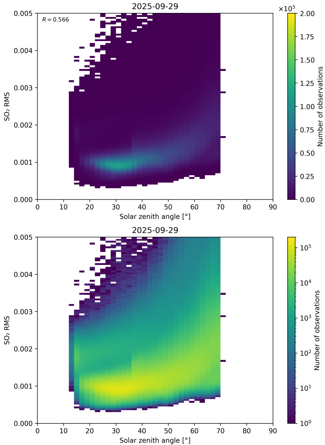
Figure 176: Scatter density plot of “Solar zenith angle” against “SO 2 RMS” for 2025-09-28 to 2025-09-30.
