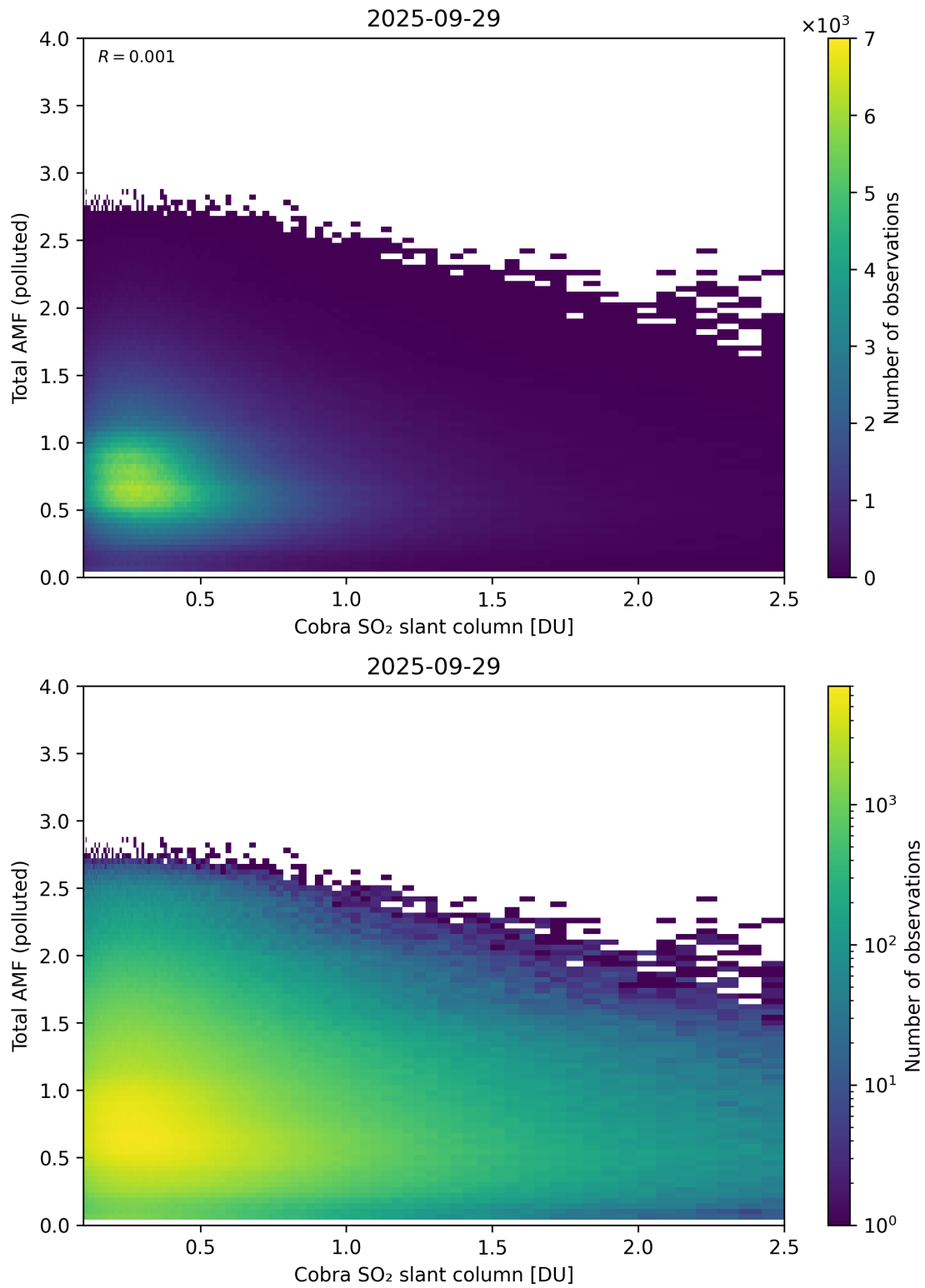
Figure 224: Scatter density plot of “Cobra SO 2 slant column” against “Total AMF (polluted)” for 2025-09-28 to 2025-09-30.
