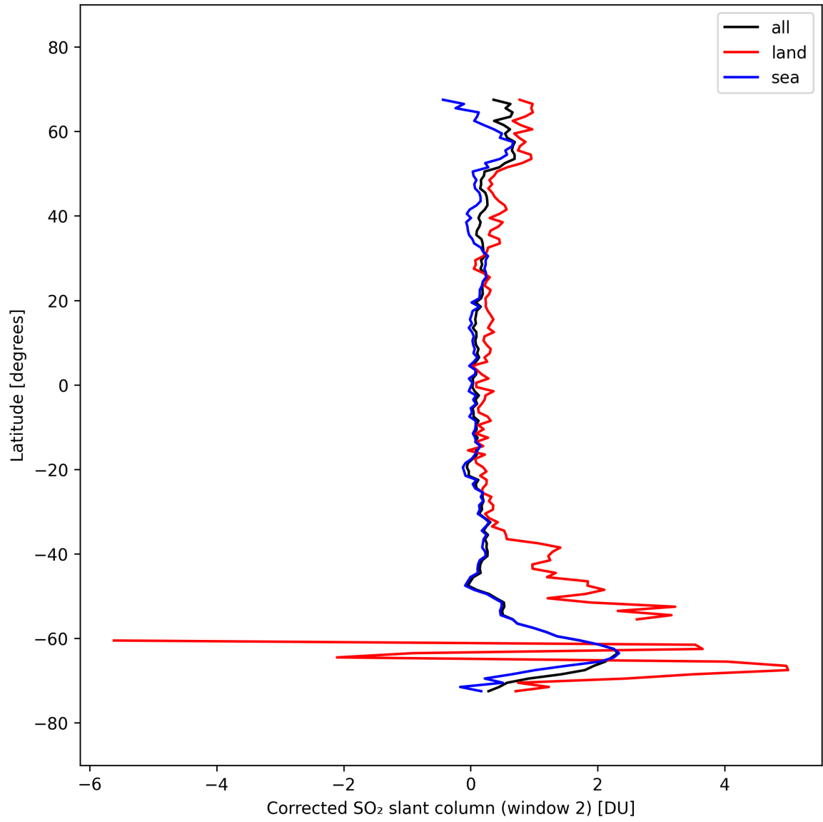
Figure 43: Zonal average of “Corrected SO 2 slant column (window 2)” for 2025-09-28 to 2025-09-30.
