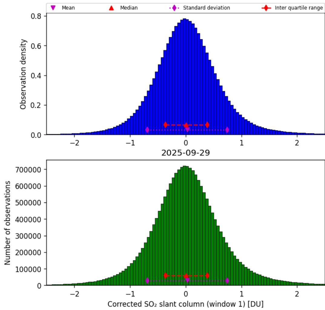
Figure 65: Histogram of “Corrected SO 2 slant column (window 1)” for 2025-09-28 to 2025-09-30
