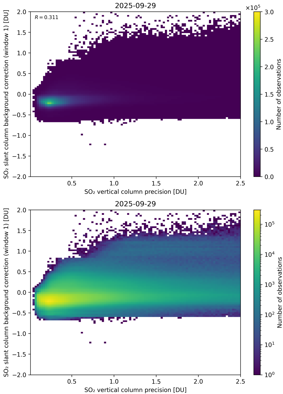
Figure 329: Scatter density plot of “SO 2 vertical column precision” against “SO 2 slant column background correction (window 1)” for 2025-09-28 to 2025-09-30.
