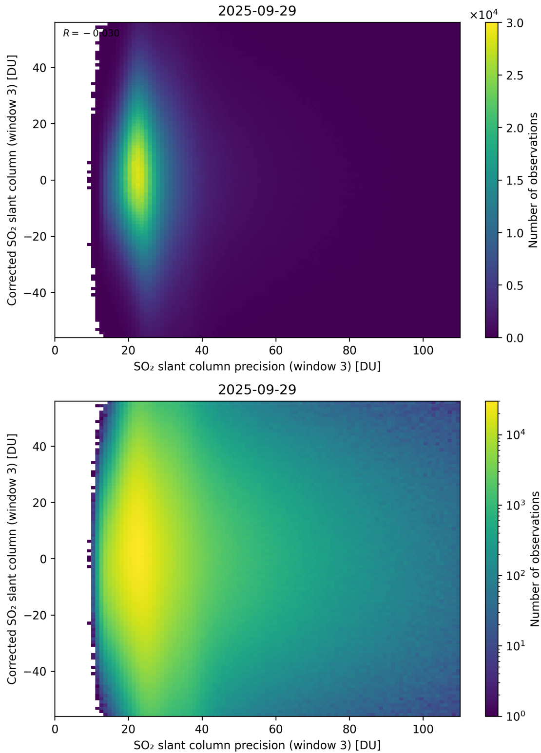
Figure 312: Scatter density plot of “SO 2 slant column precision (window 3)” against “Corrected SO 2 slant column (window 3)” for 2025-09-28 to 2025-09-30.
