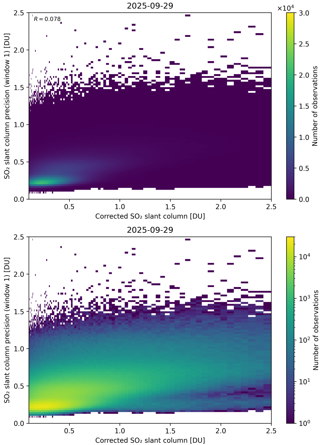
Figure 238: Scatter density plot of “Corrected SO 2 slant column” against “SO 2 slant column precision (window 1)” for 2025-09-28 to 2025-09-30.
