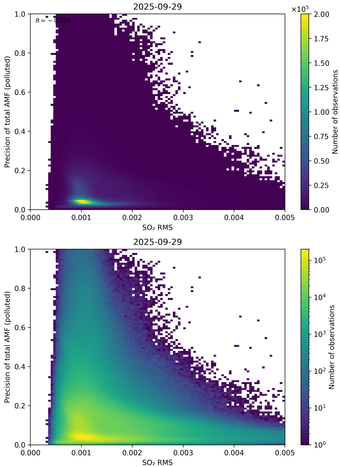
Figure 149: Scatter density plot of “SO 2 RMS” against “Precision of total AMF (polluted)” for 2025-09-28 to 2025-09-30.
