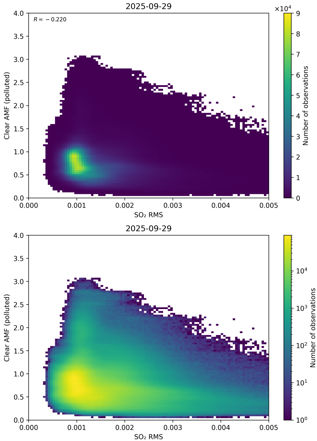
Figure 147: Scatter density plot of “SO 2 RMS” against “Clear AMF (polluted)” for 2025-09-28 to 2025-09-30.
