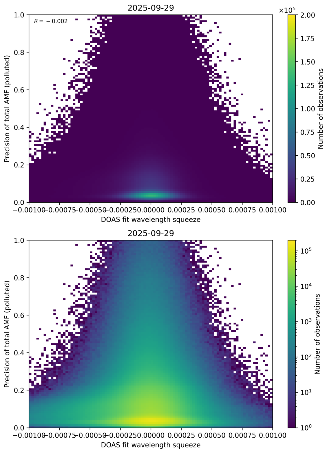
Figure 146: Scatter density plot of “DOAS fit wavelength squeeze” against “Precision of total AMF (polluted)” for 2025-09-28 to 2025-09-30.
