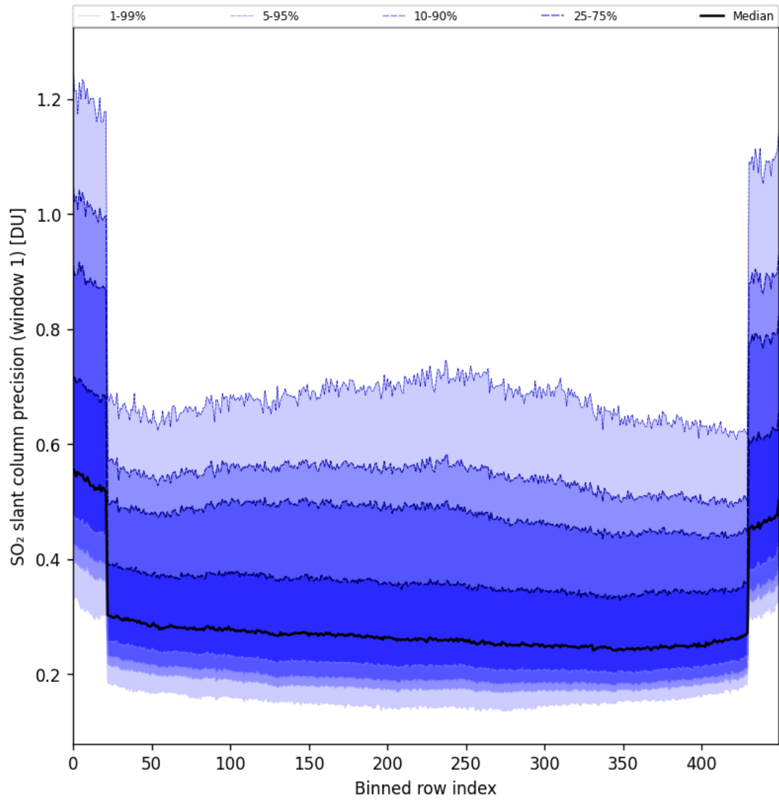
Figure 90: Along track statistics of “SO 2 slant column precision (window 1)” for 2025-09-28 to 2025-09-30
