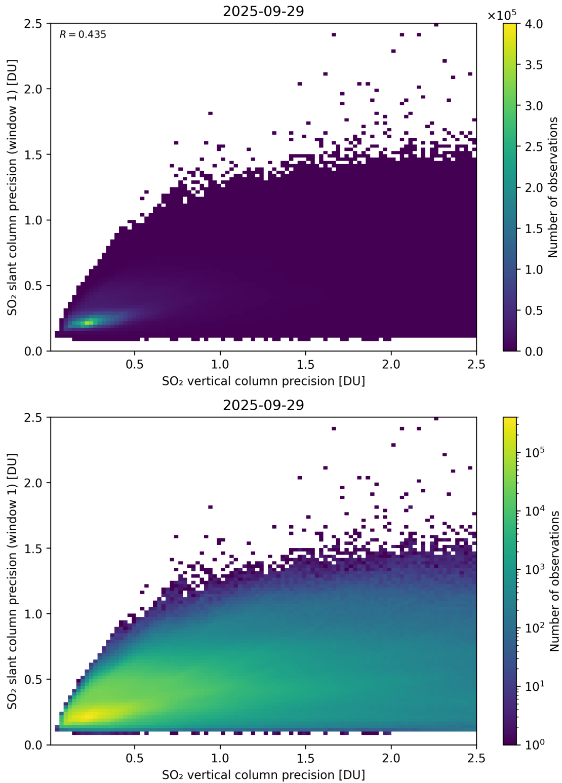
Figure 342: Scatter density plot of “SO 2 vertical column precision” against “SO 2 slant column precision (window 1)” for 2025-09-28 to 2025-09-30.
