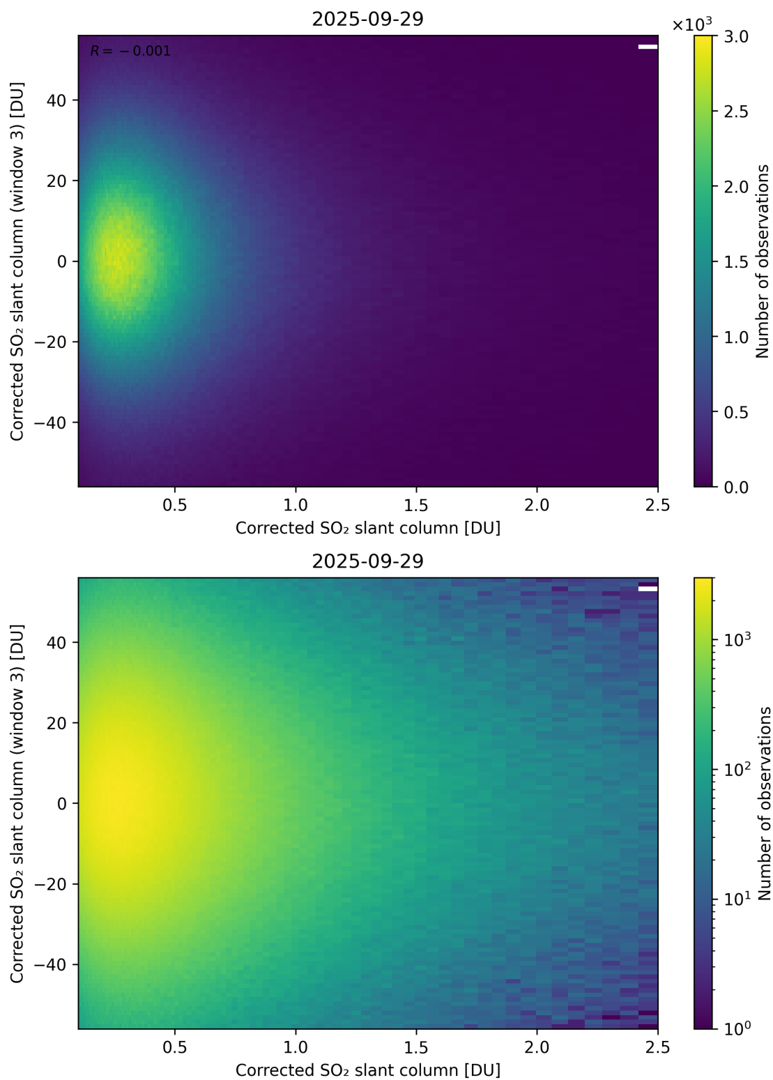
Figure 236: Scatter density plot of “Corrected SO 2 slant column” against “Corrected SO 2 slant column (window 3)” for 2025-09-28 to 2025-09-30.
