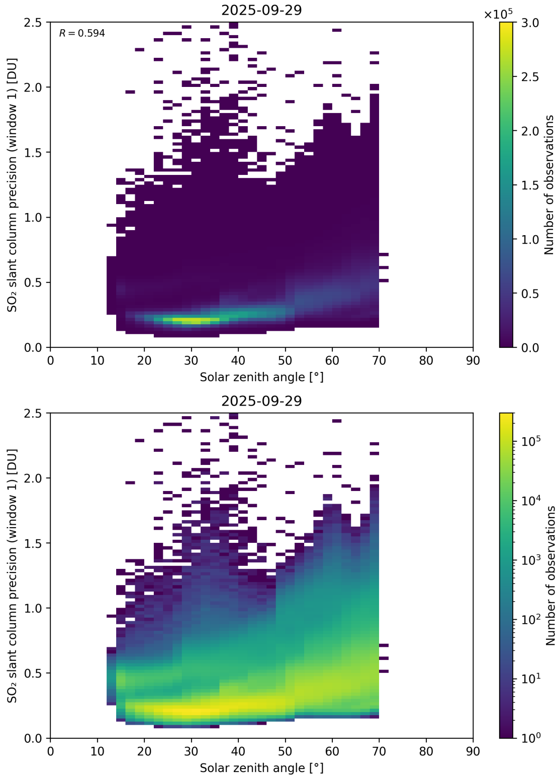
Figure 185: Scatter density plot of “Solar zenith angle” against “SO 2 slant column precision (window 1)” for 2025-09-28 to 2025-09-30.
