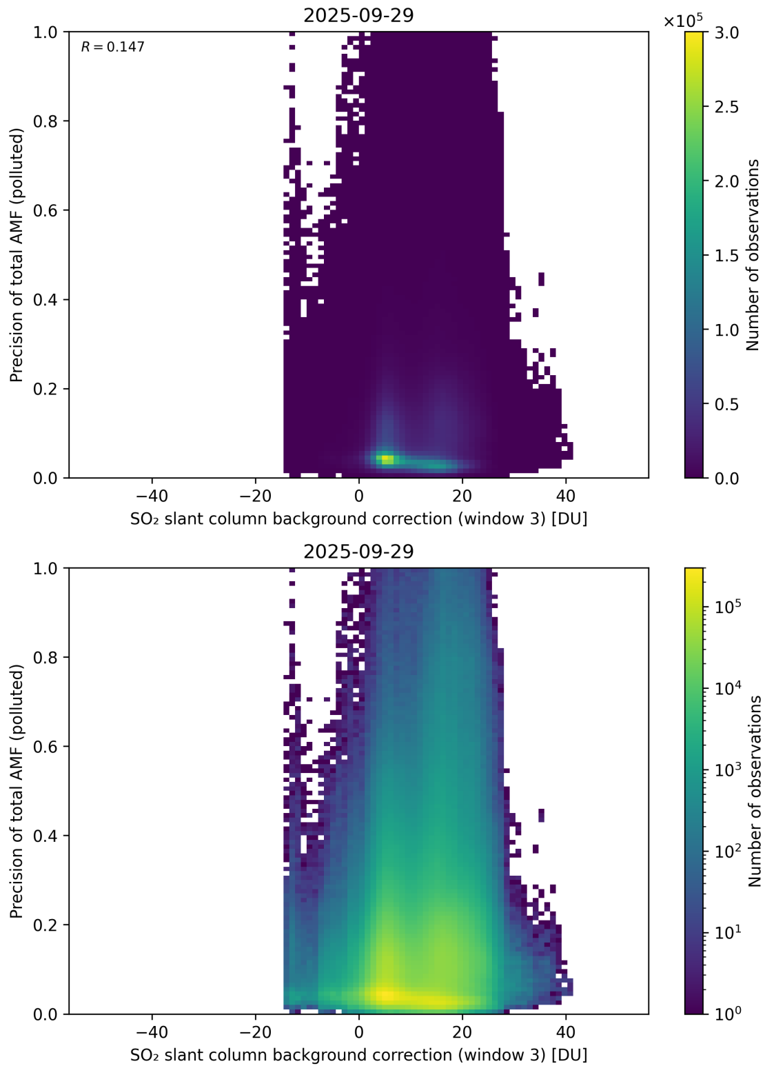
Figure 137: Scatter density plot of “SO 2 slant column background correction (window 3)” against “Precision of total AMF (polluted)” for 2025-09-28 to 2025-09-30.
