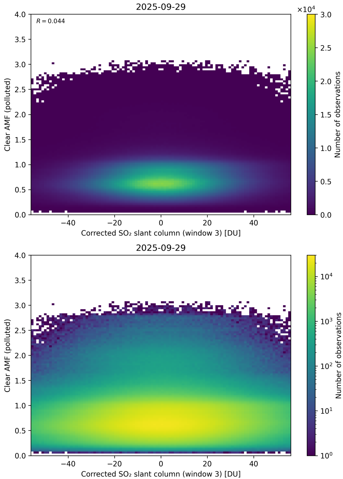
Figure 259: Scatter density plot of “Corrected SO 2 slant column (window 3)” against “Clear AMF (polluted)” for 2025-09-28 to 2025-09-30.
