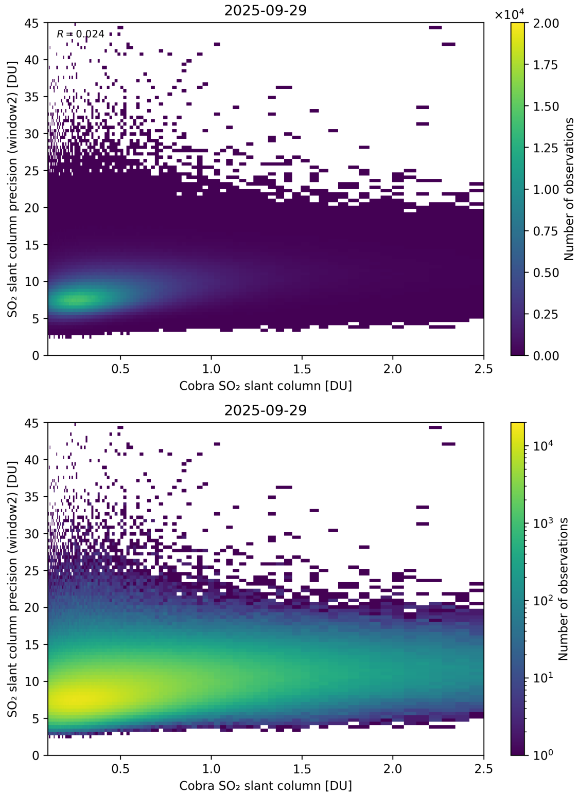
Figure 221: Scatter density plot of “Cobra SO 2 slant column” against “SO 2 slant column precision (window2)” for 2025-09-28 to 2025-09-30.
