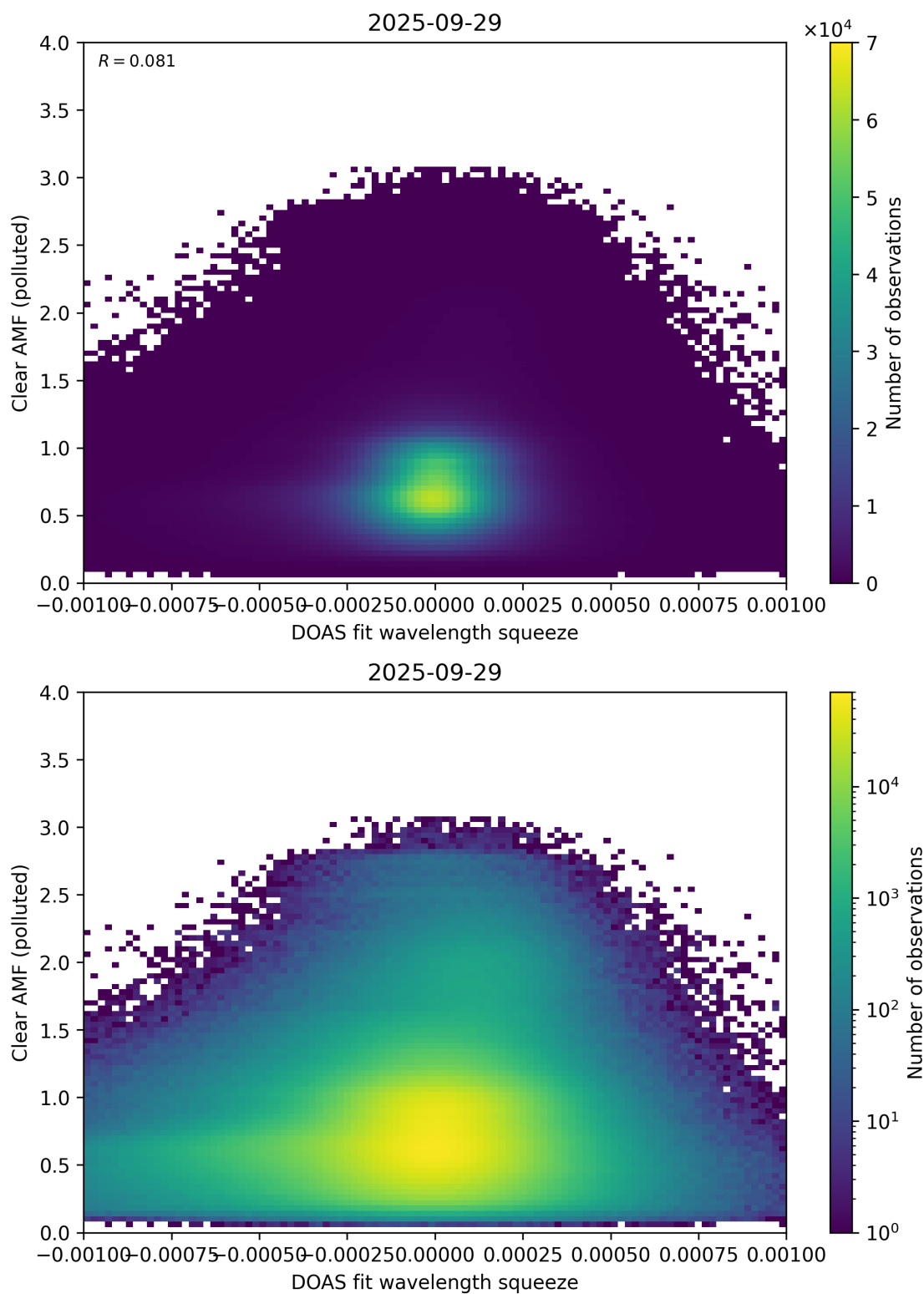
Figure 144: Scatter density plot of “DOAS fit wavelength squeeze” against “Clear AMF (polluted)” for 2025-09-28 to 2025-09-30.
