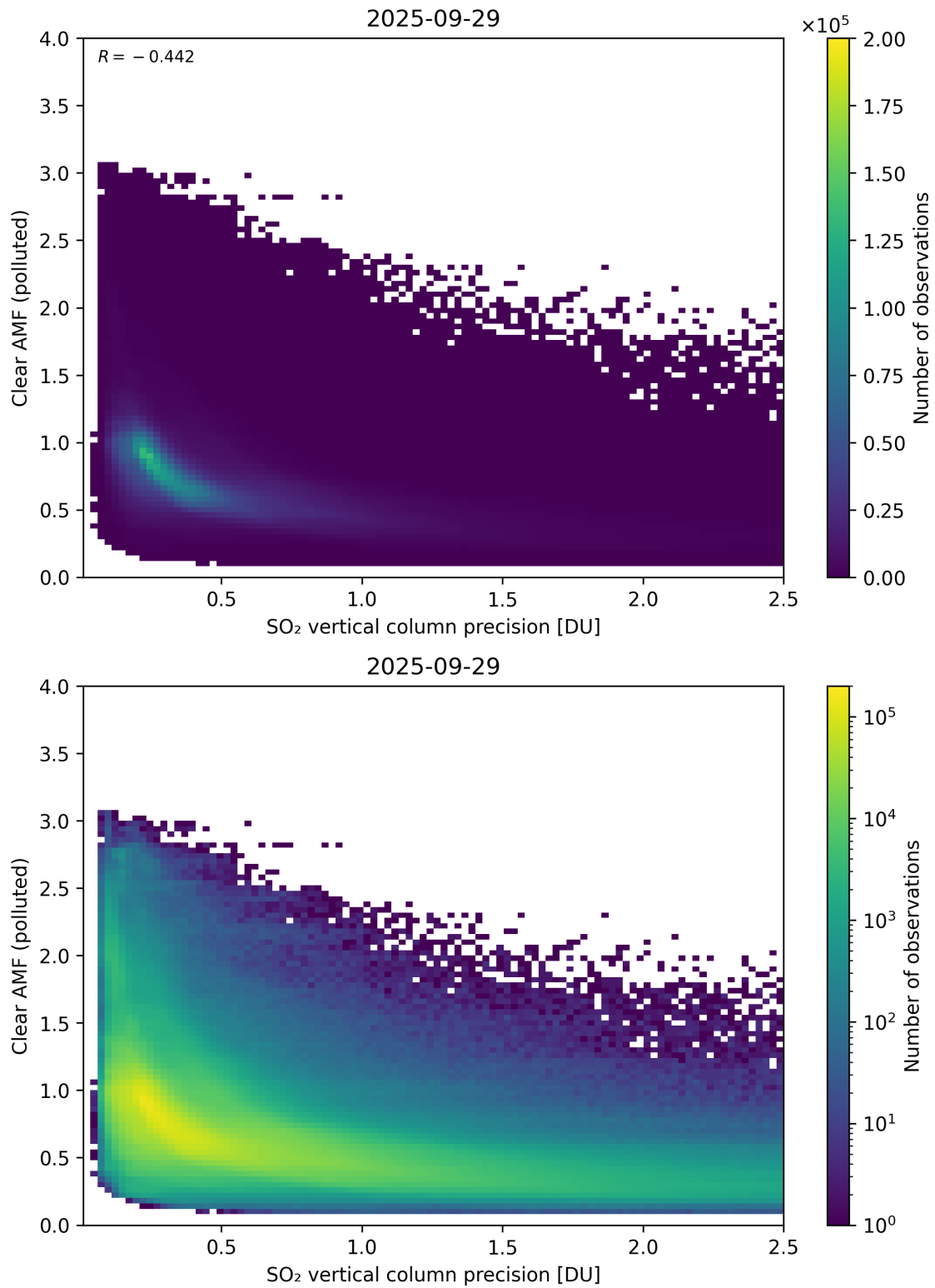
Figure 335: Scatter density plot of “SO 2 vertical column precision” against “Clear AMF (polluted)” for 2025-09-28 to 2025-09-30.
