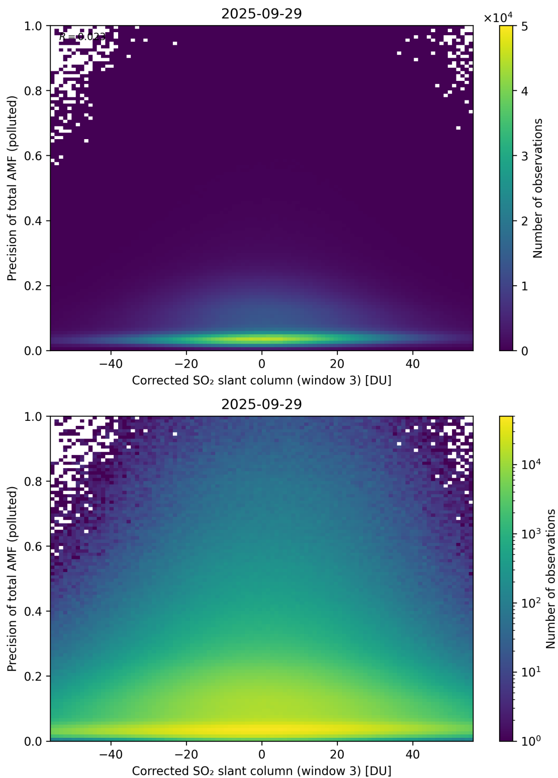
Figure 261: Scatter density plot of “Corrected SO 2 slant column (window 3)” against “Precision of total AMF (polluted)” for 2025-09-28 to 2025-09-30.
