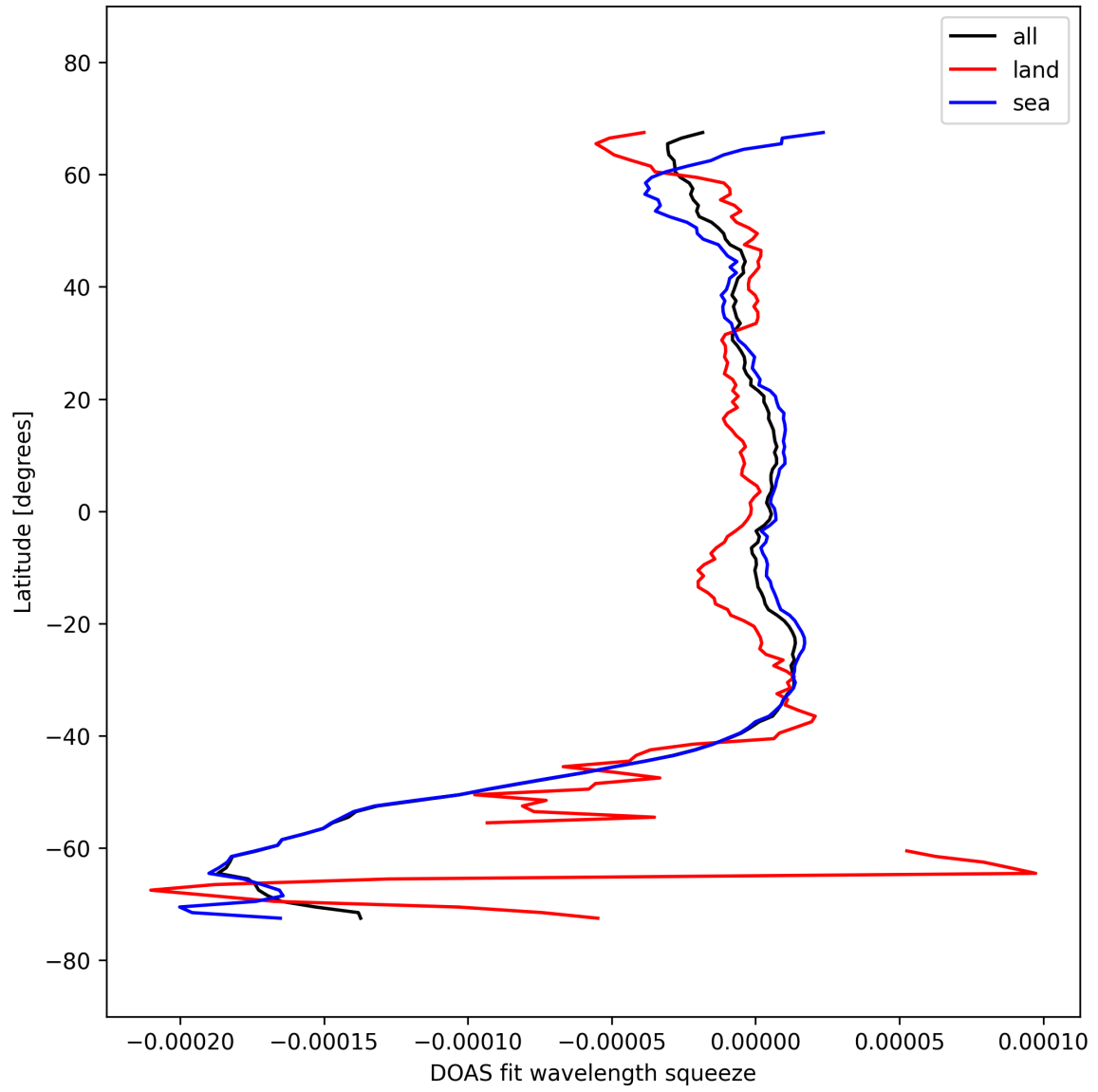
Figure 51: Zonal average of “DOAS fit wavelength squeeze” for 2025-09-28 to 2025-09-30.
