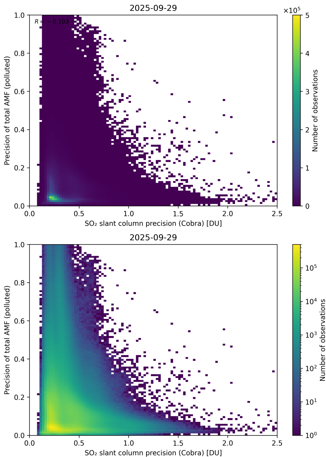
Figure 214: Scatter density plot of “SO 2 slant column precision (Cobra)” against “Precision of total AMF (polluted)” for 2025-09-28 to 2025-09-30.
