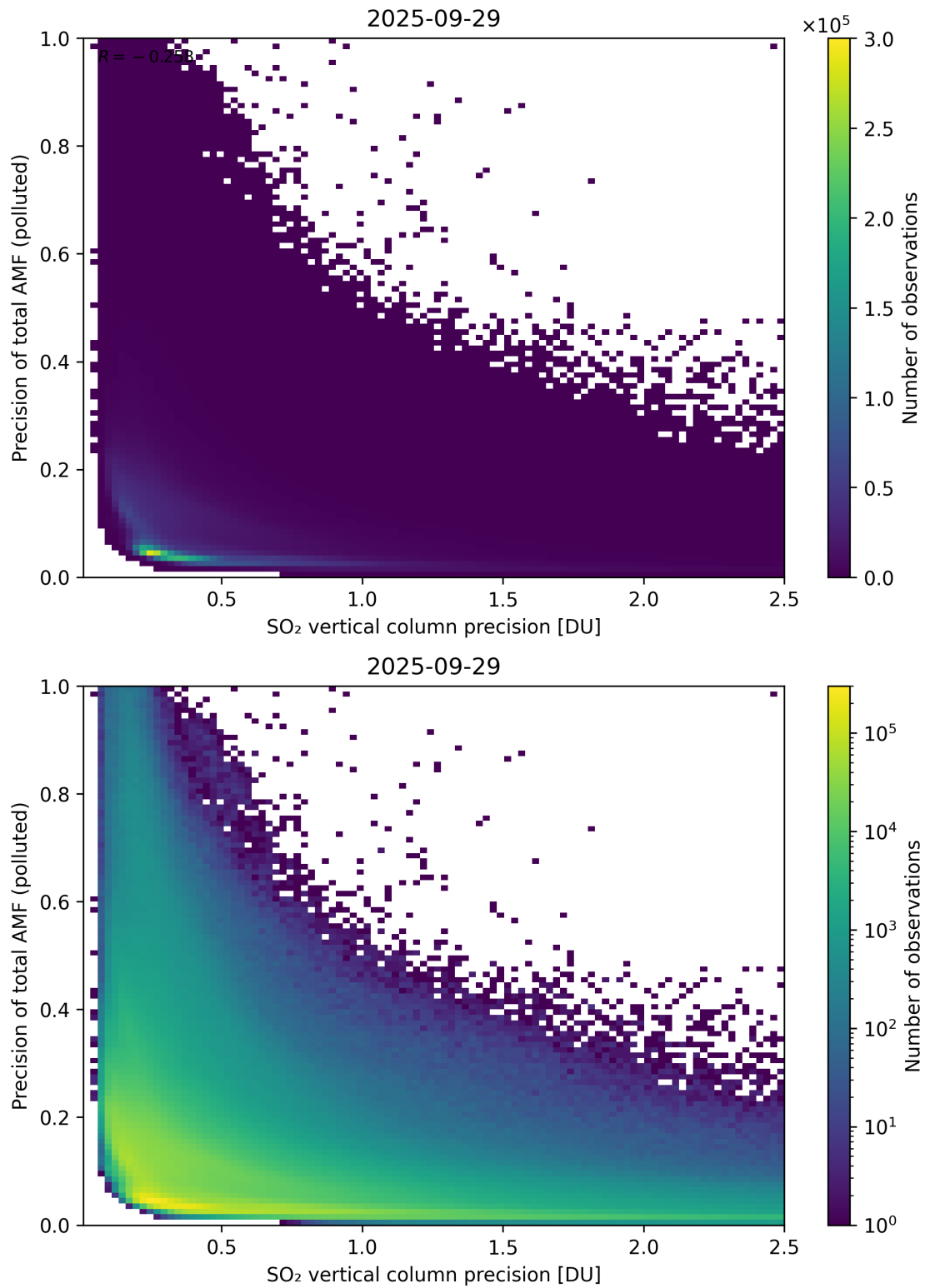
Figure 347: Scatter density plot of “SO 2 vertical column precision” against “Precision of total AMF (polluted)” for 2025-09-28 to 2025-09-30.
