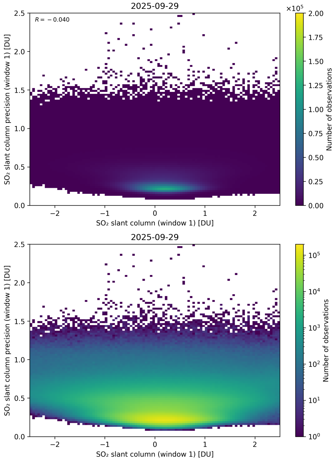
Figure 285: Scatter density plot of “SO 2 slant column (window 1)” against “SO 2 slant column precision (window 1)” for 2025-09-28 to 2025-09-30.
