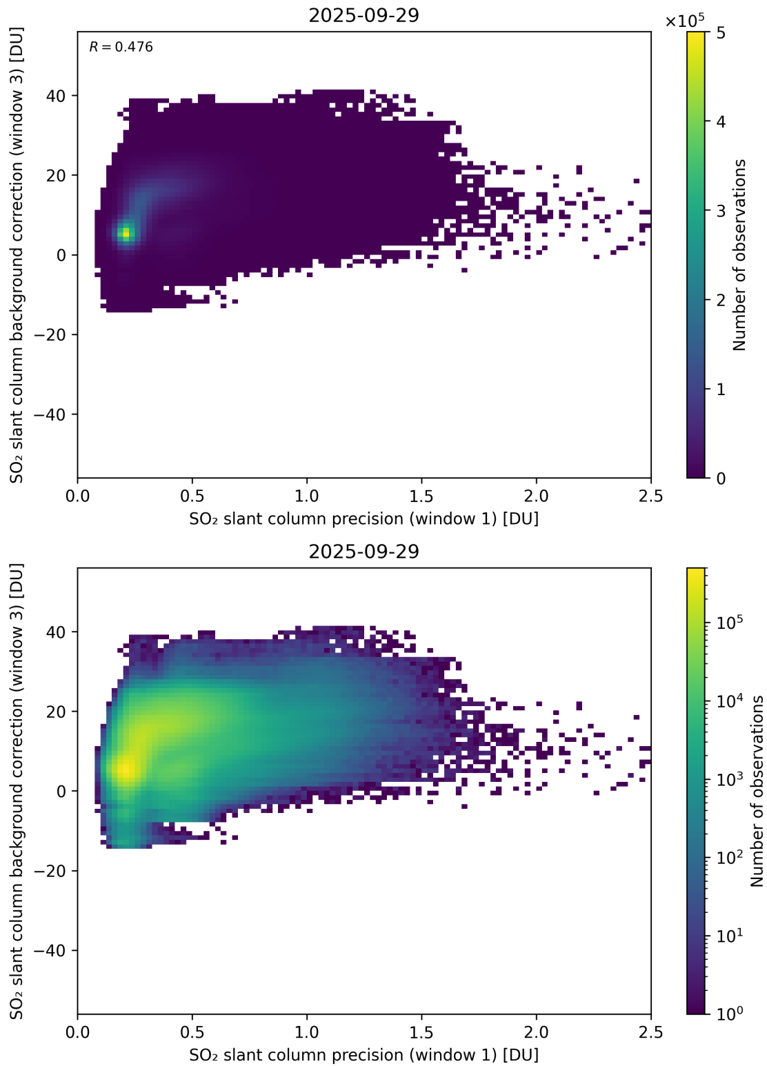
Figure 270: Scatter density plot of “SO 2 slant column precision (window 1)” against “SO 2 slant column background correction (window 3)” for 2025-09-28 to 2025-09-30.
