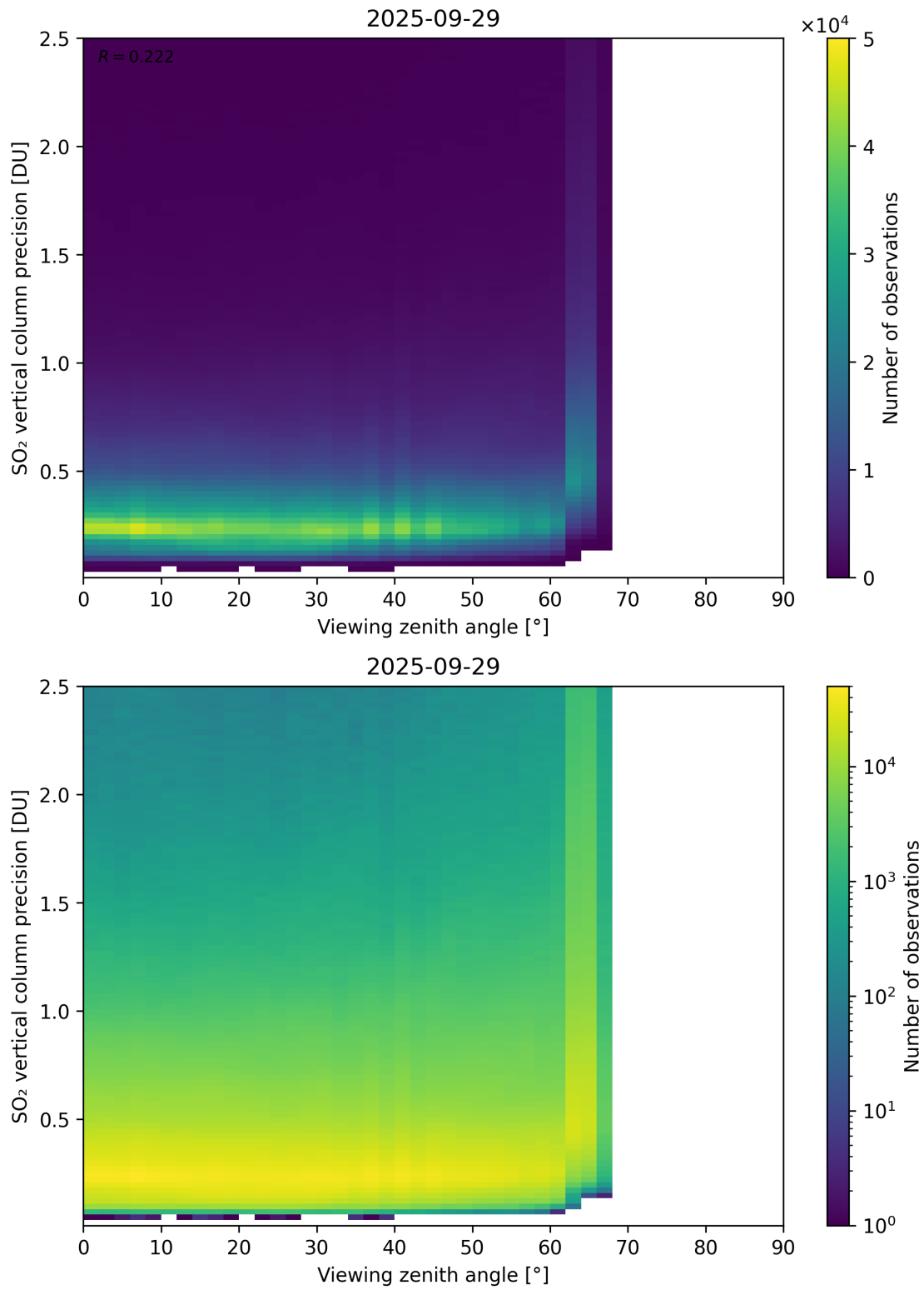
Figure 384: Scatter density plot of “Viewing zenith angle” against “SO 2 vertical column precision” for 2025-09-28 to 2025-09-30.
