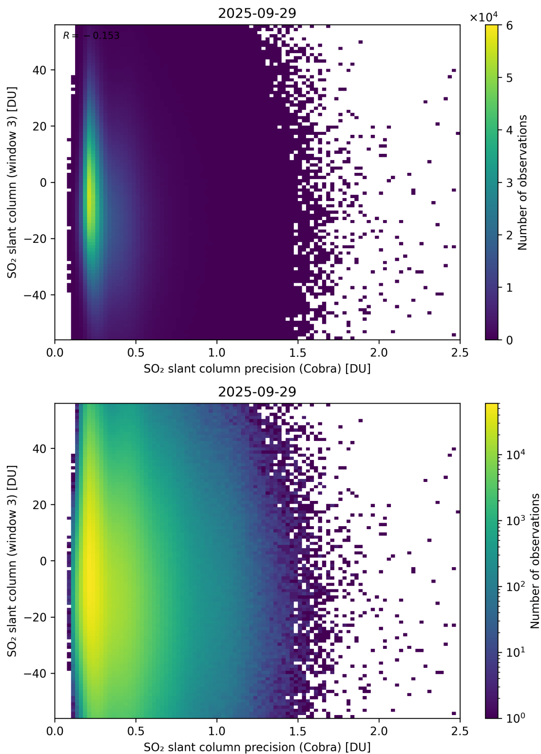
Figure 211: Scatter density plot of “SO 2 slant column precision (Cobra)” against “SO 2 slant column (window 3)” for 2025-09-28 to 2025-09-30.
