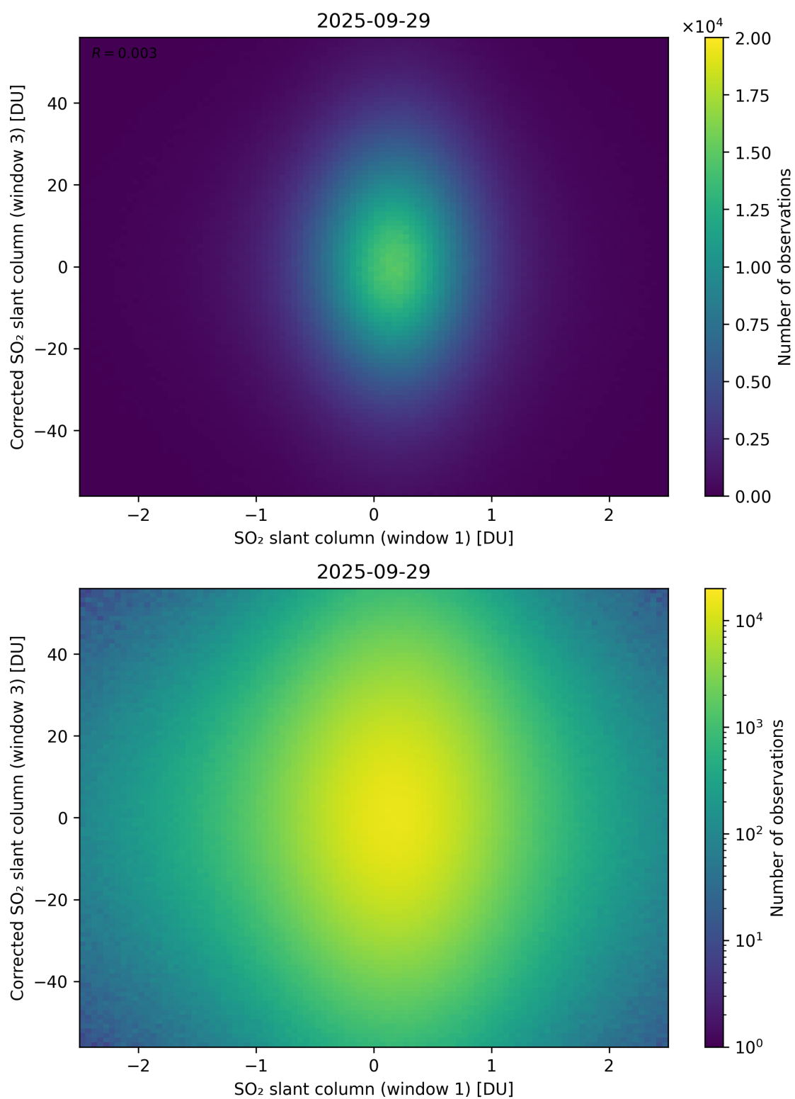
Figure 284: Scatter density plot of “SO 2 slant column (window 1)” against “Corrected SO 2 slant column (window 3)” for 2025-09-28 to 2025-09-30.
