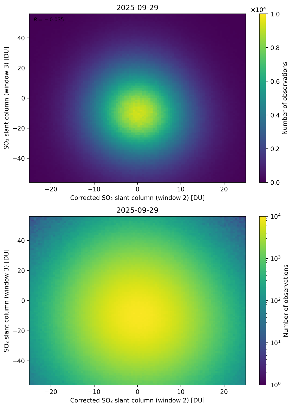
Figure 251: Scatter density plot of “Corrected SO 2 slant column (window 2)” against “SO 2 slant column (window 3)” for 2025-09-28 to 2025-09-30.
