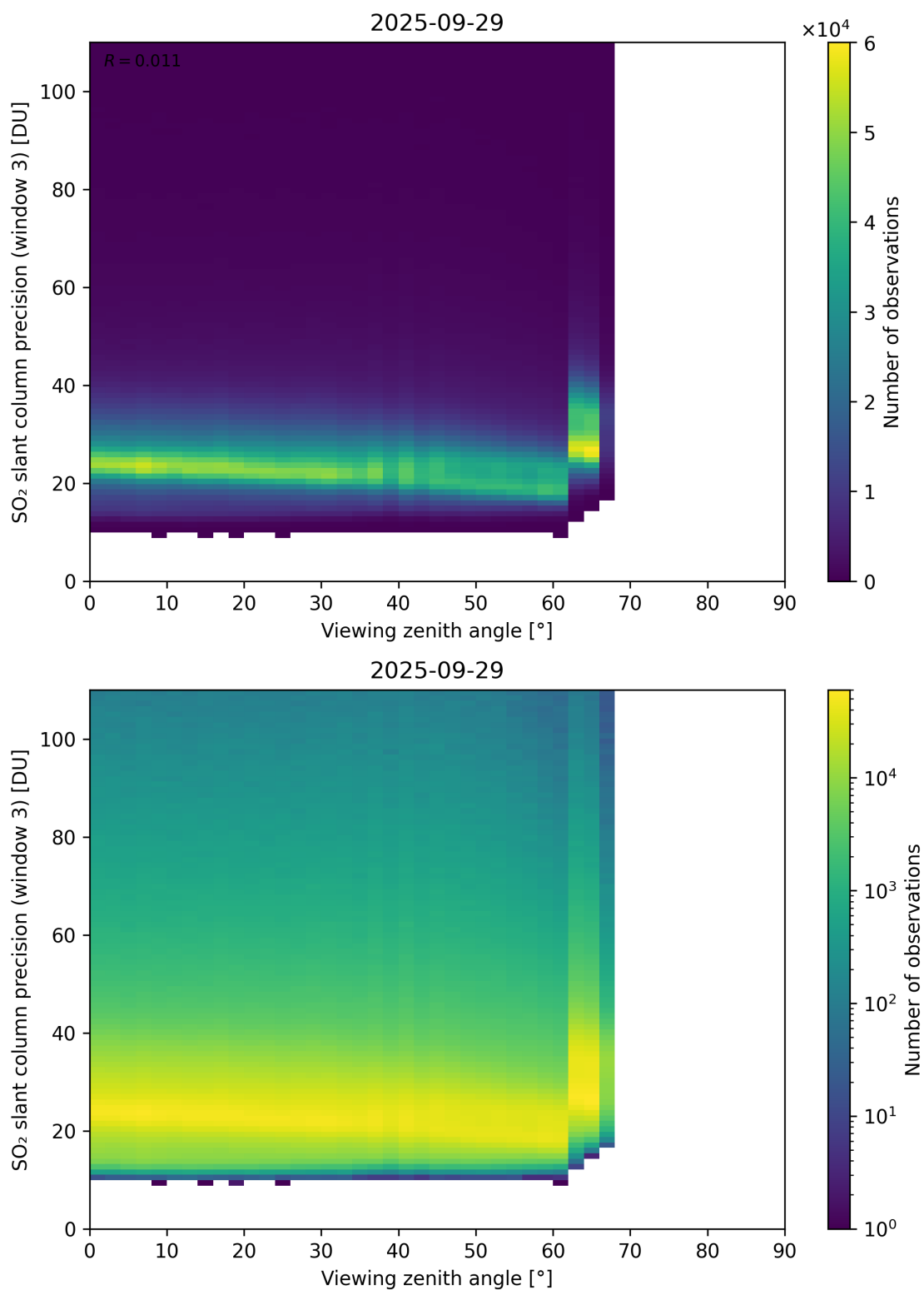
Figure 380: Scatter density plot of “Viewing zenith angle” against “SO 2 slant column precision (window 3)” for 2025-09-28 to 2025-09-30.
