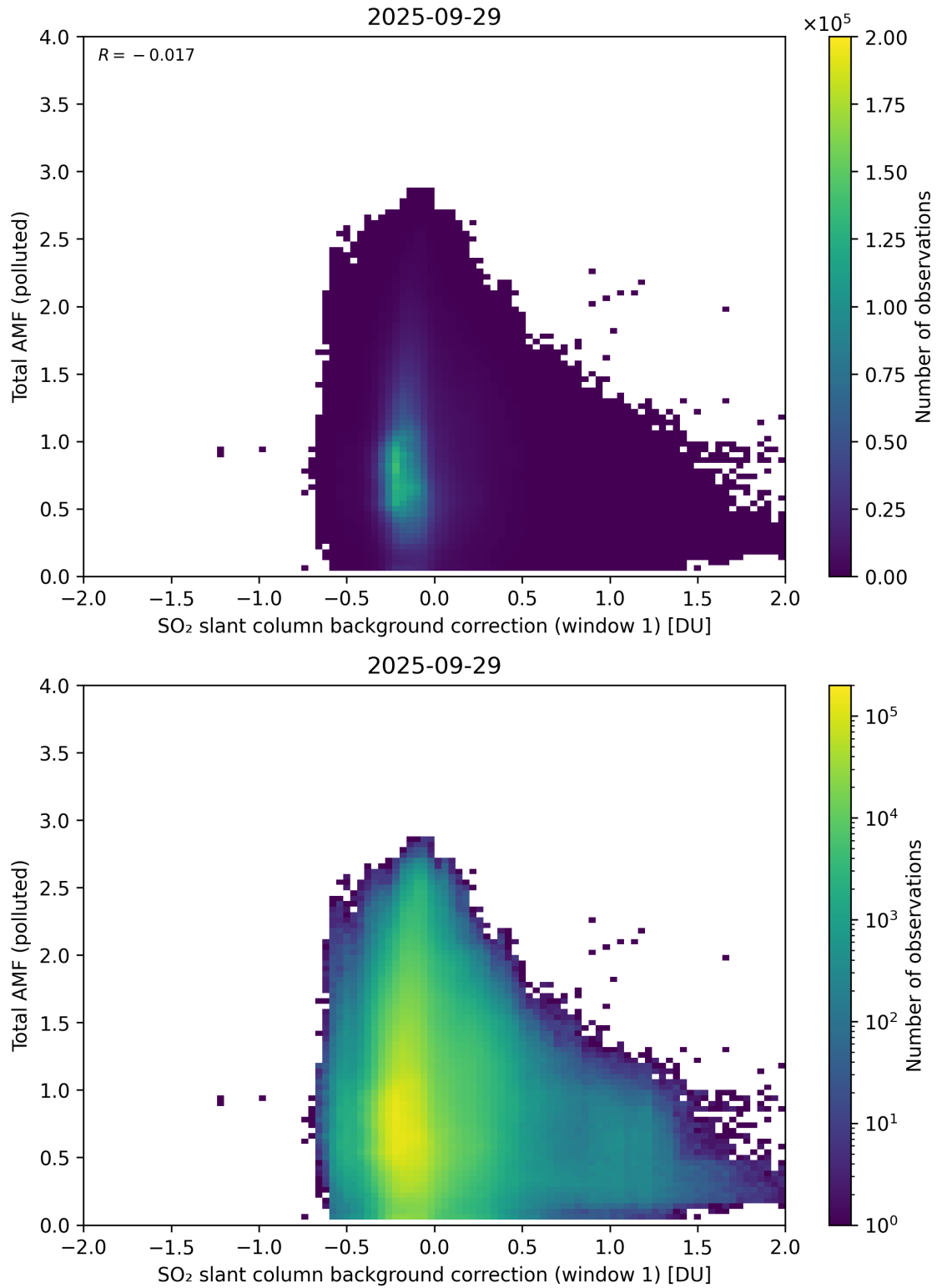
Figure 120: Scatter density plot of “SO 2 slant column background correction (window 1)” against “Total AMF (polluted)” for 2025-09-28 to 2025-09-30.
