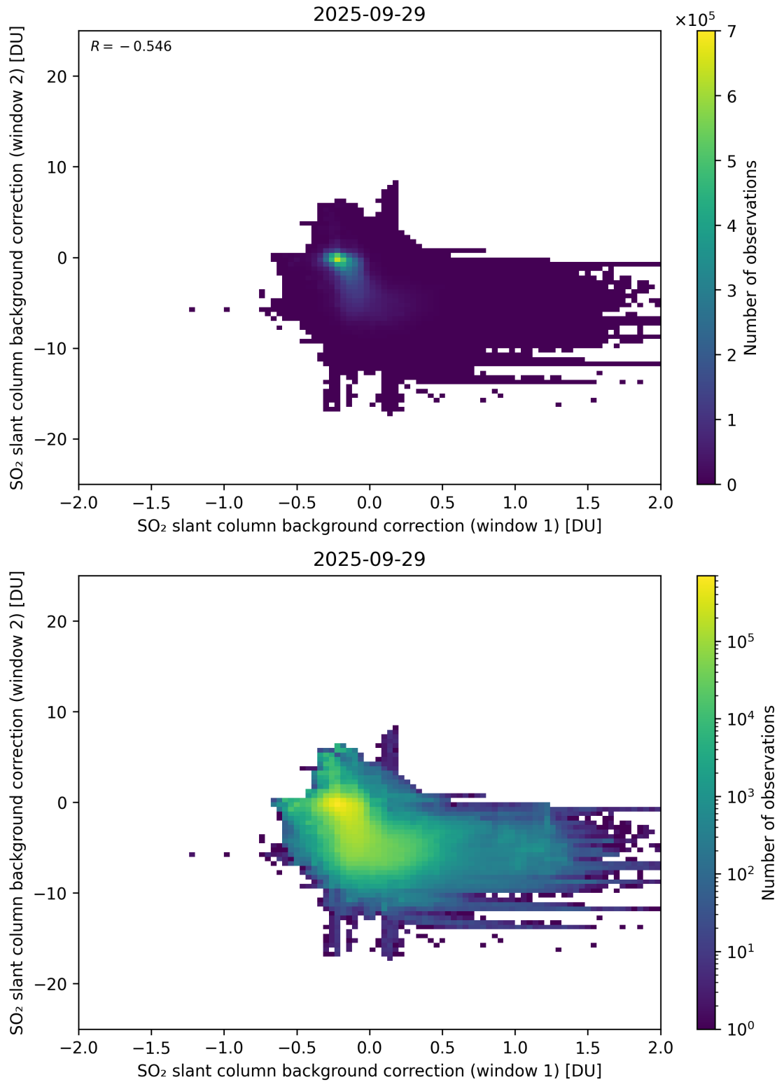
Figure 109: Scatter density plot of “SO 2 slant column background correction (window 1)” against “SO 2 slant column background correction (window 2)” for 2025-09-28 to 2025-09-30.
