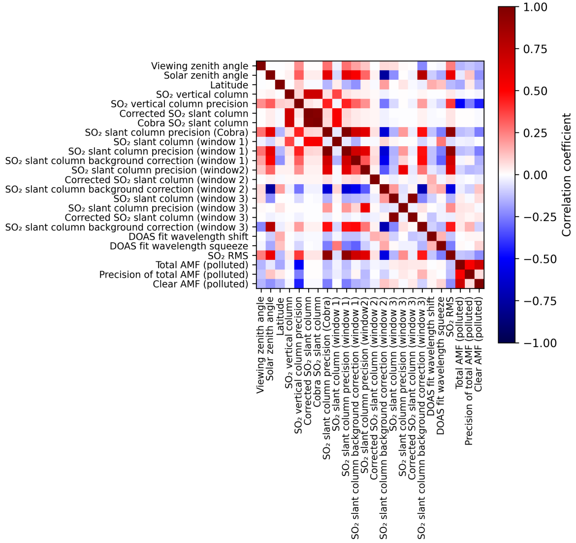
Figure 2: Map of correlation matrix for 2025-09-28 to 2025-09-30.
