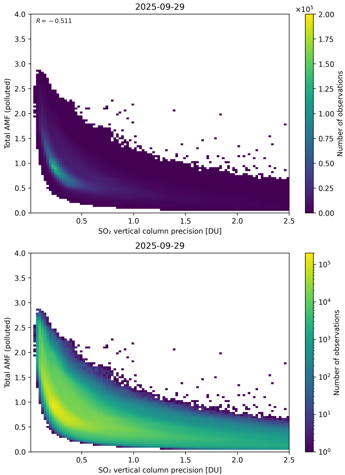
Figure 346: Scatter density plot of “SO 2 vertical column precision” against “Total AMF (polluted)” for 2025-09-28 to 2025-09-30.
