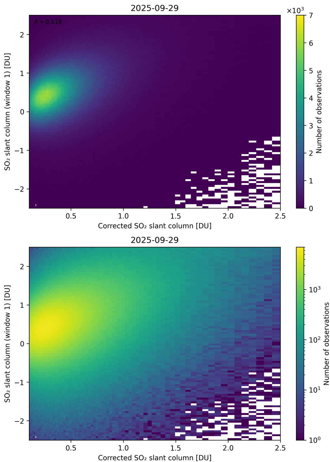
Figure 237: Scatter density plot of “Corrected SO 2 slant column” against “SO 2 slant column (window 1)” for 2025-09-28 to 2025-09-30.
