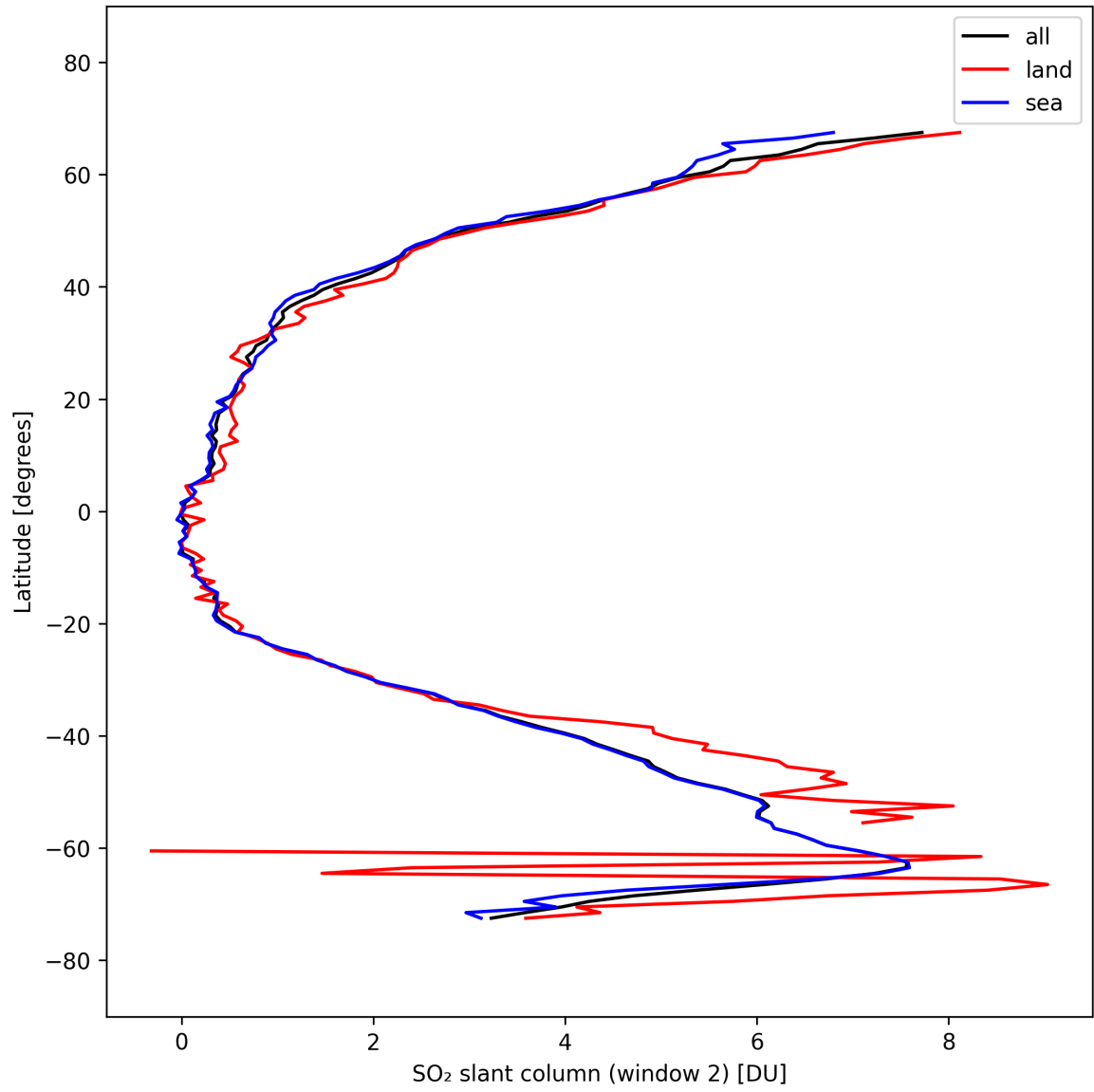
Figure 41: Zonal average of “SO 2 slant column (window 2)” for 2025-09-28 to 2025-09-30.
