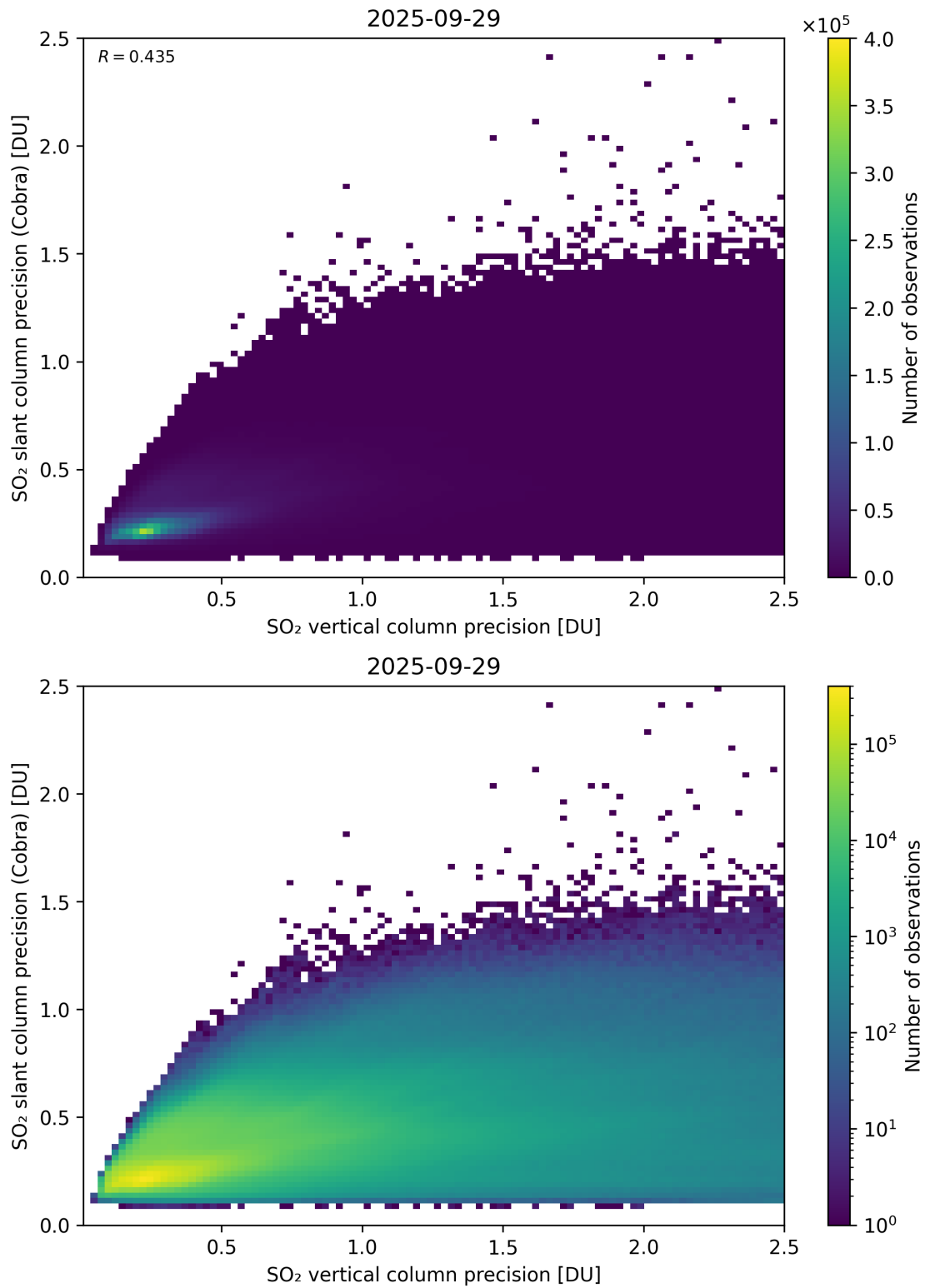
Figure 337: Scatter density plot of “SO 2 vertical column precision” against “SO 2 slant column precision (Cobra)” for 2025-09-28 to 2025-09-30.
