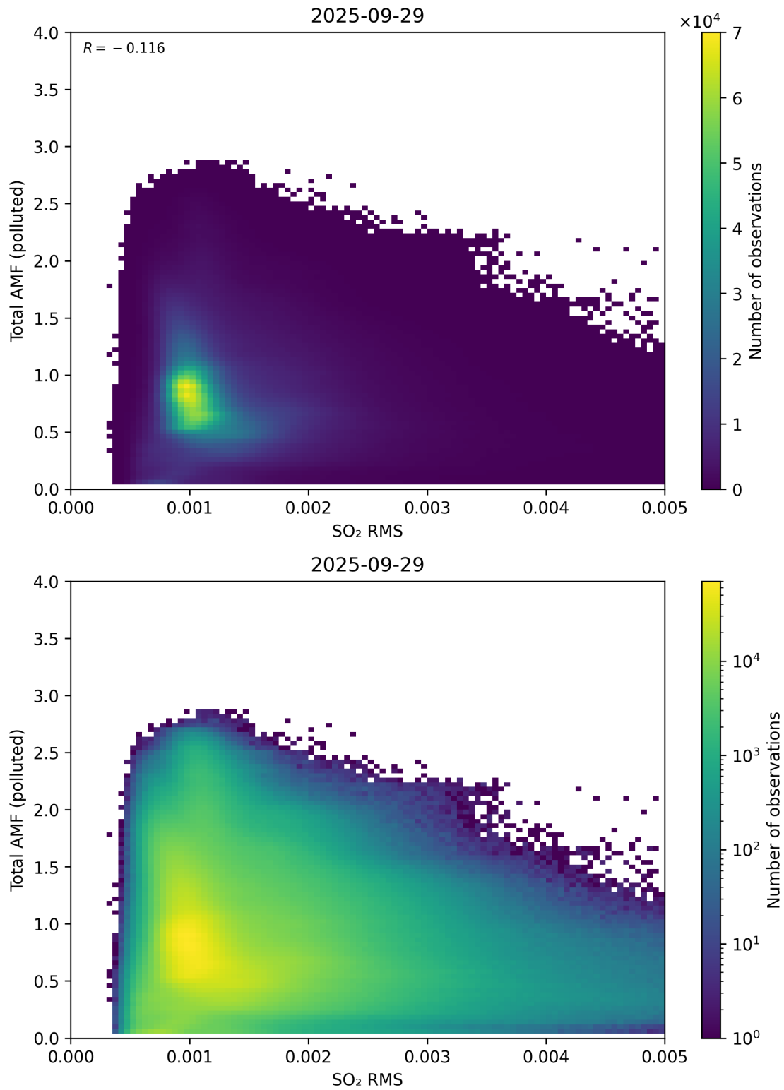
Figure 148: Scatter density plot of “SO 2 RMS” against “Total AMF (polluted)” for 2025-09-28 to 2025-09-30.
