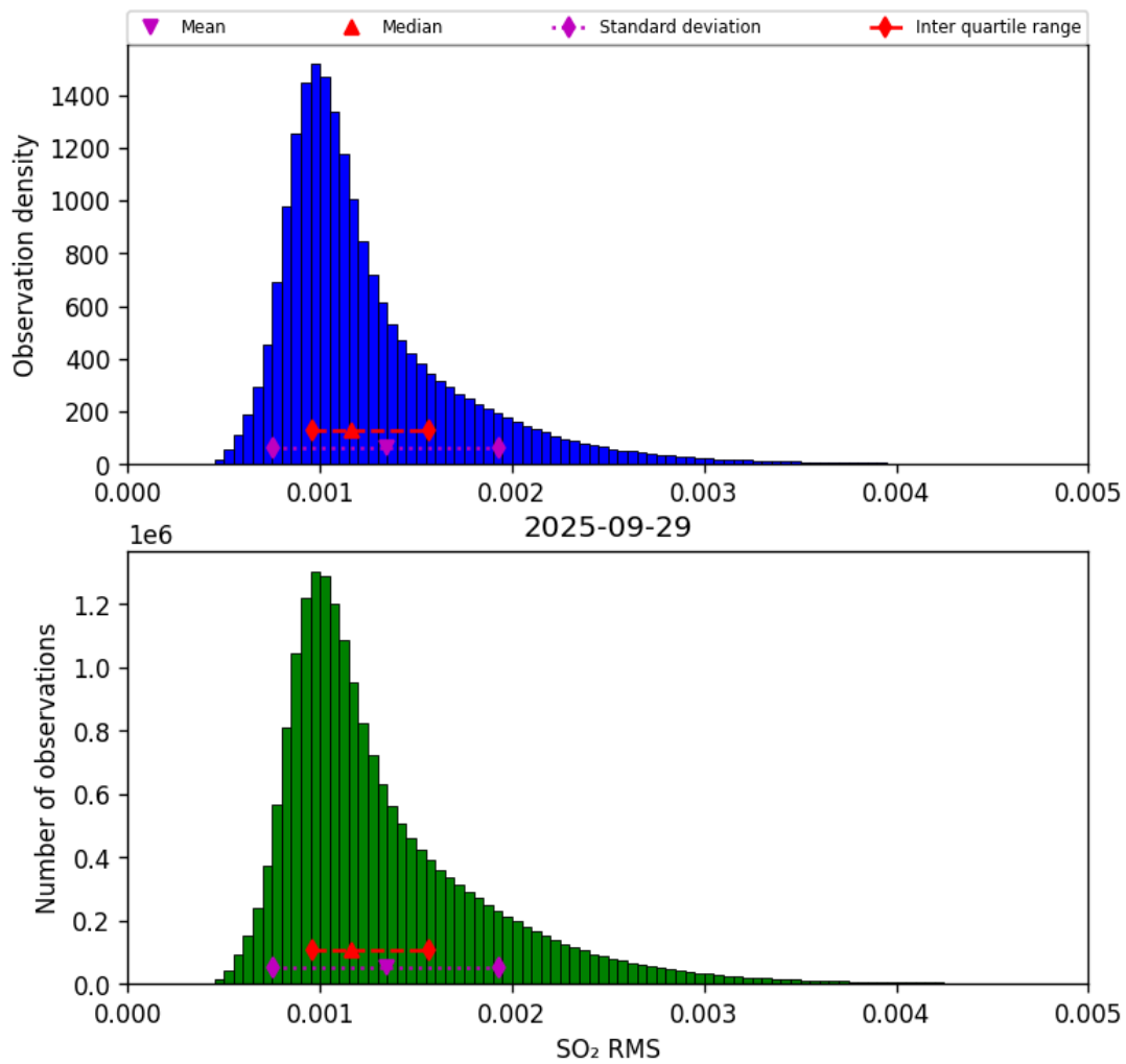
Figure 78: Histogram of “SO 2 RMS” for 2025-09-28 to 2025-09-30
