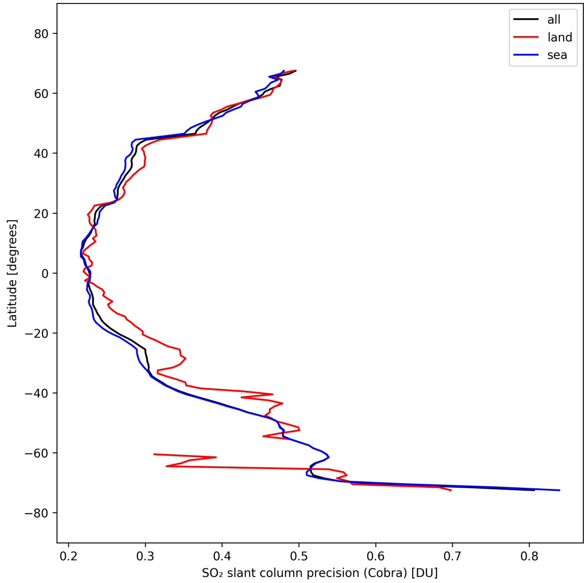
Figure 36: Zonal average of “SO 2 slant column precision (Cobra)” for 2025-09-28 to 2025-09-30.
