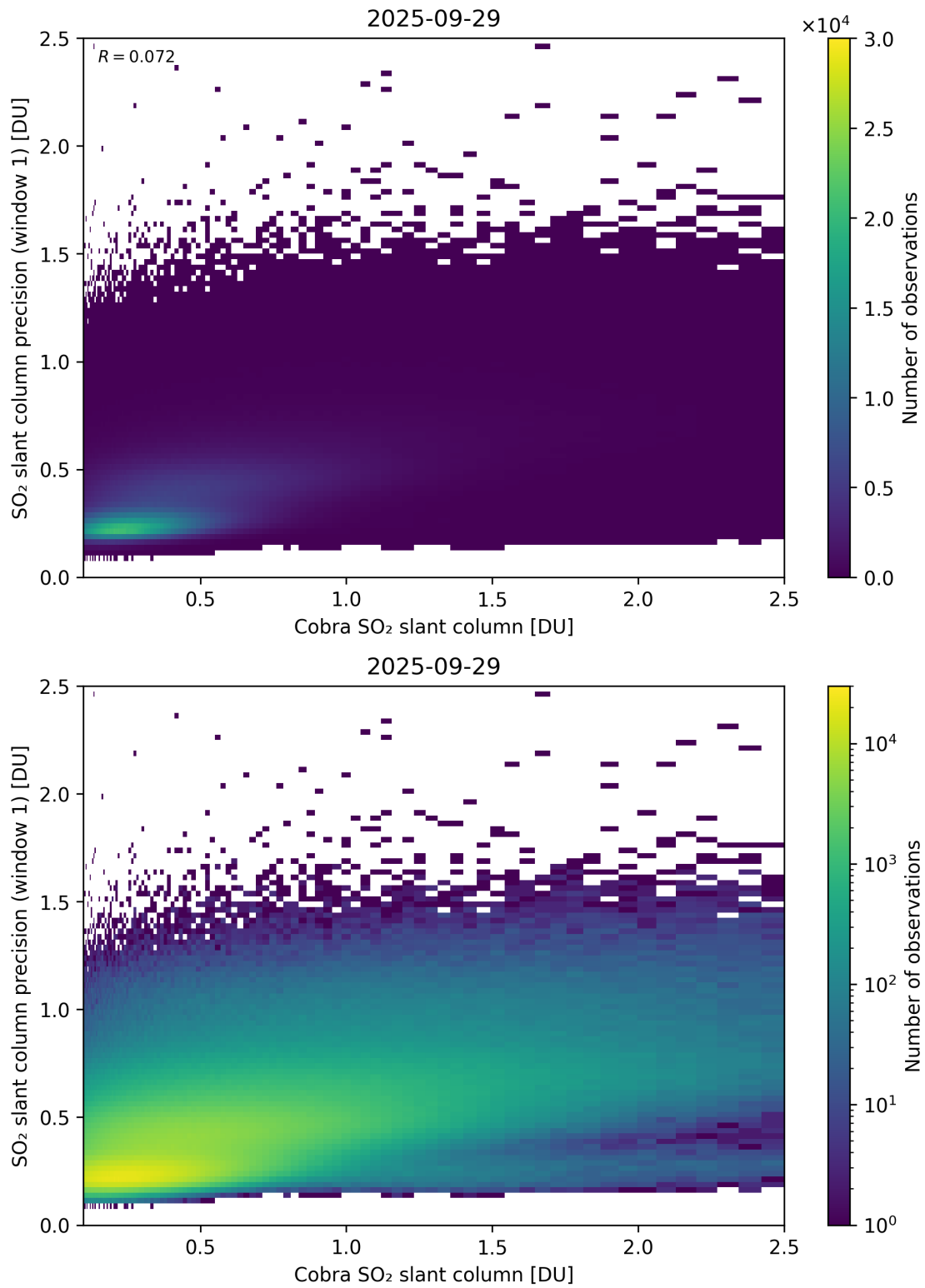
Figure 220: Scatter density plot of “Cobra SO 2 slant column” against “SO 2 slant column precision (window 1)” for 2025-09-28 to 2025-09-30.
