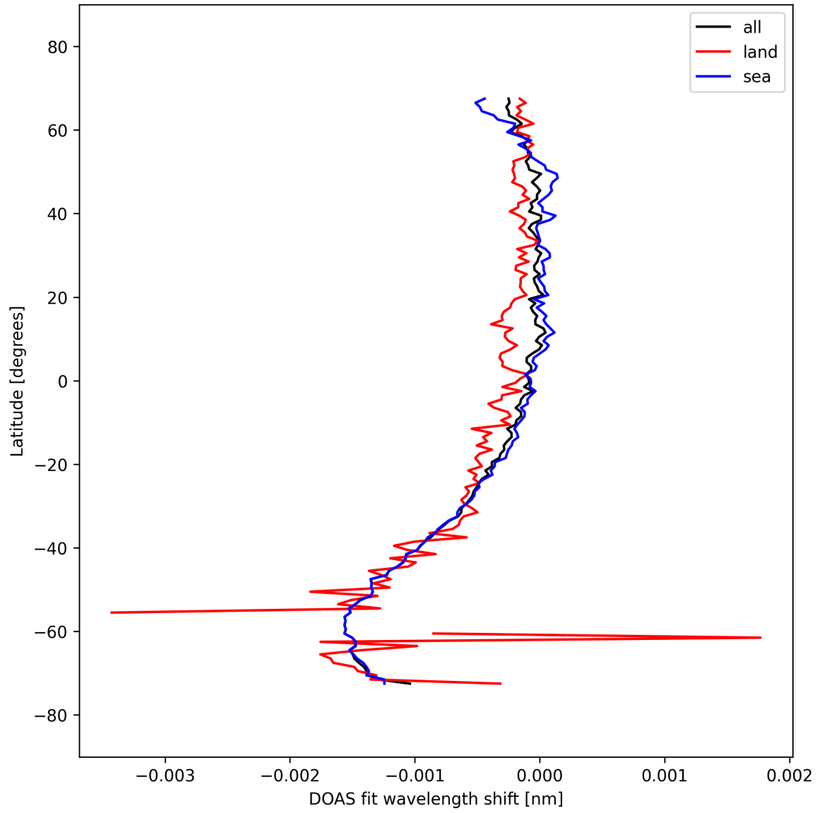
Figure 50: Zonal average of "DOAS fit wavelength shift" for 2025-09-28 to 2025-09-30.
