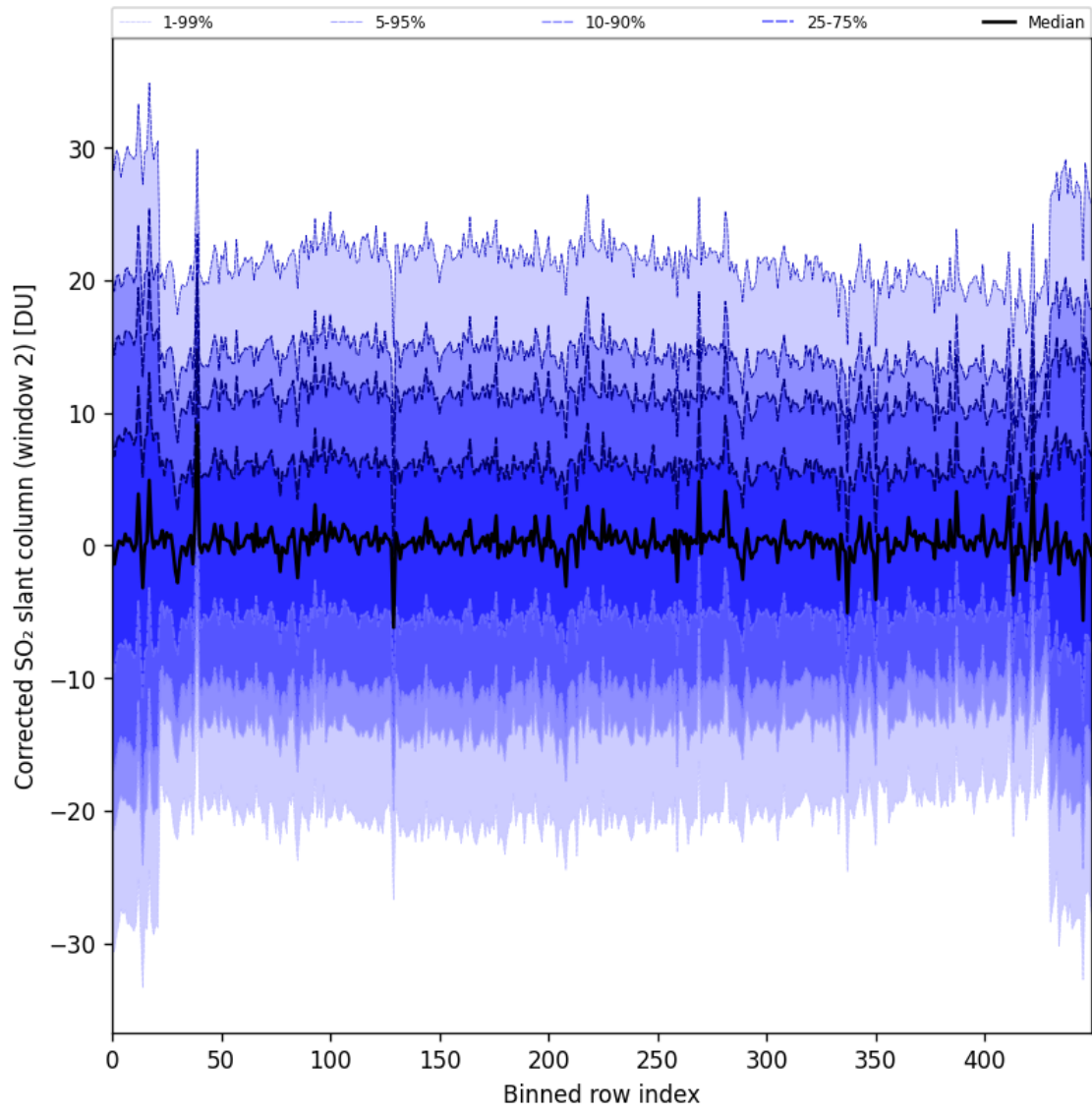
Figure 95: Along track statistics of “Corrected SO 2 slant column (window 2)” for 2025-09-28 to 2025-09-30
