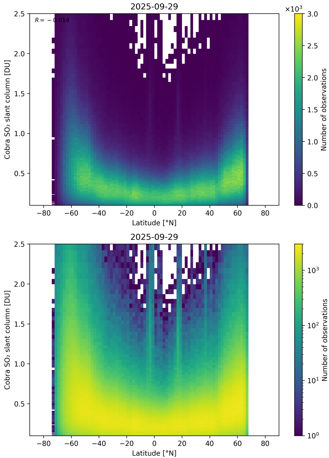
Figure 157: Scatter density plot of “Latitude” against “Cobra SO 2 slant column” for 2025-09-28 to 2025-09-30.
