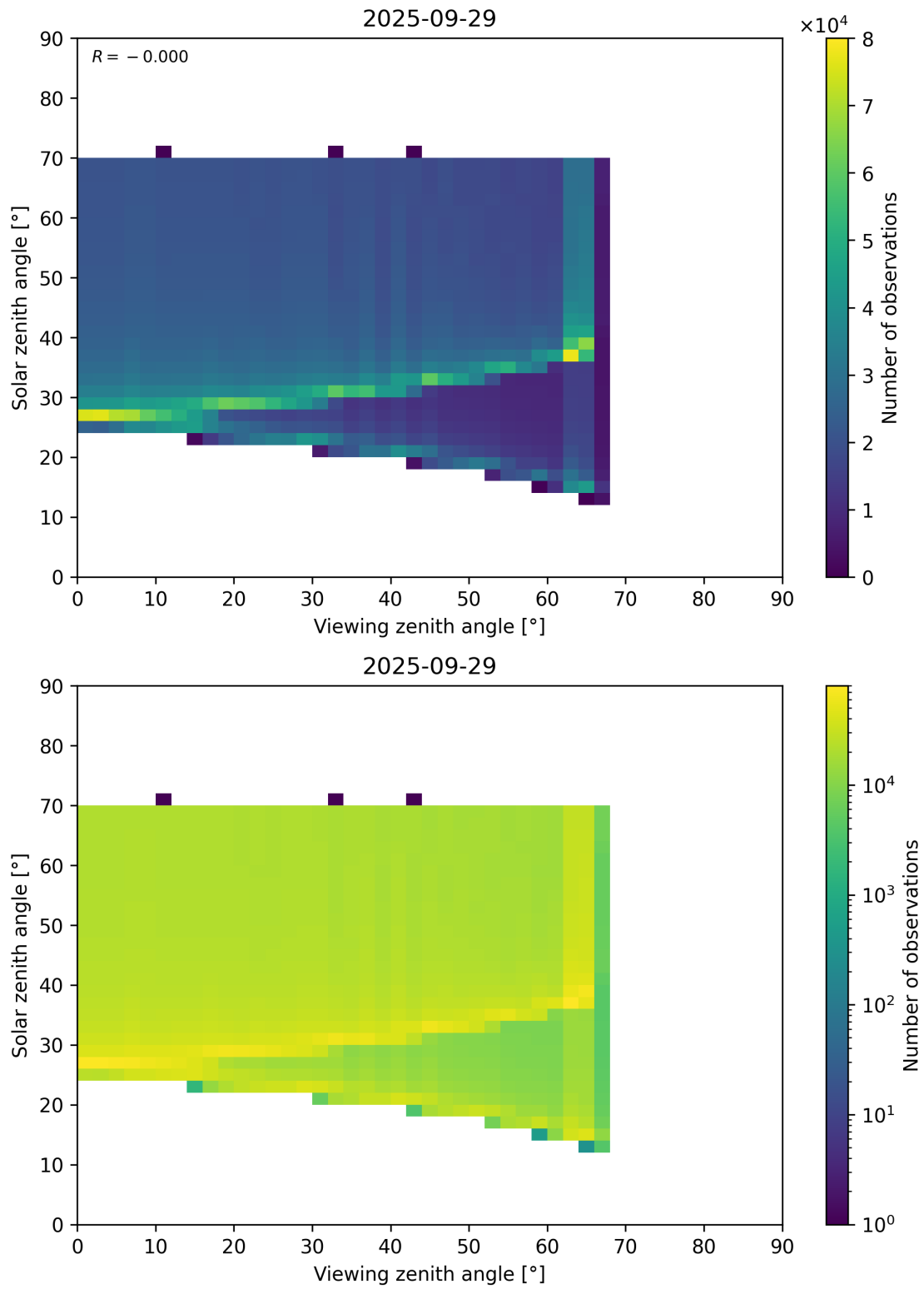
Figure 369: Scatter density plot of “Viewing zenith angle” against “Solar zenith angle” for 2025-09-28 to 2025-09-30.
