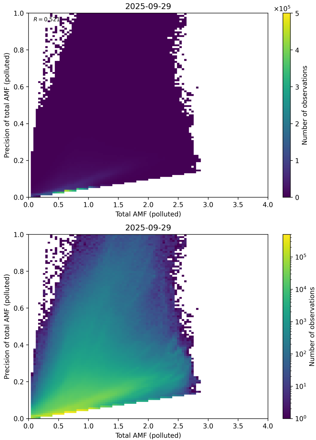
Figure 322: Scatter density plot of “Total AMF (polluted)” against “Precision of total AMF (polluted)” for 2025-09-28 to 2025-09-30.
