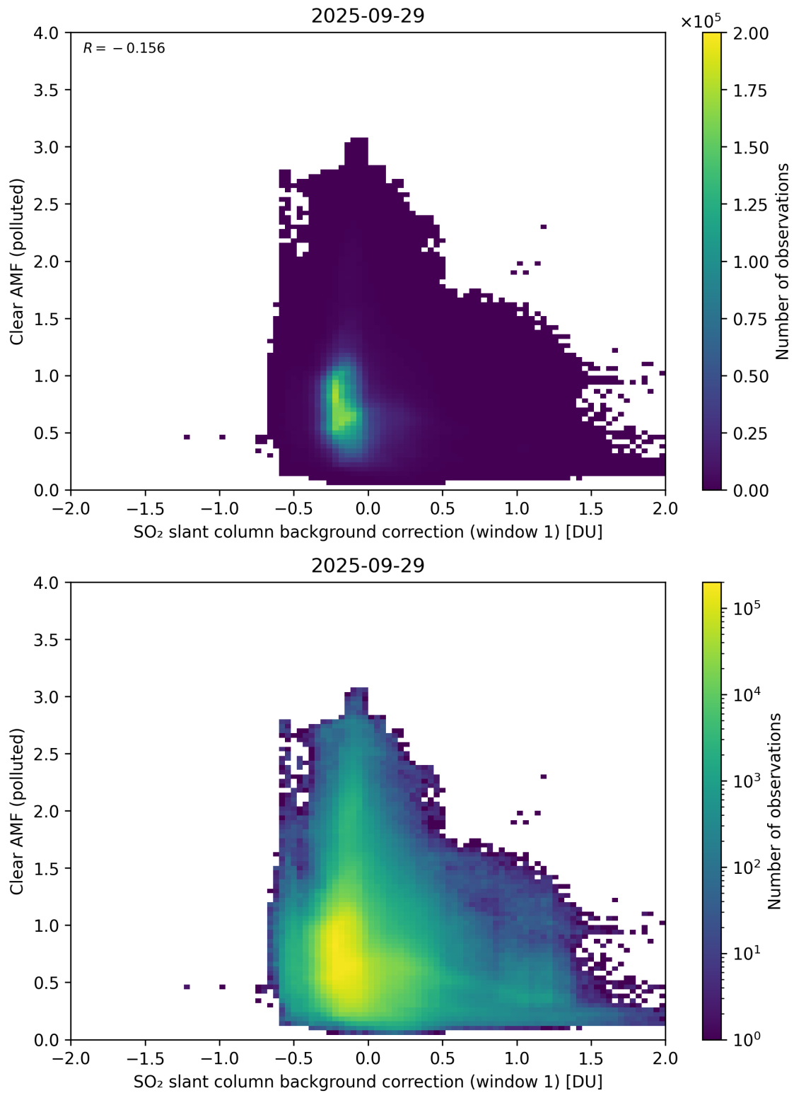
Figure 114: Scatter density plot of “SO 2 slant column background correction (window 1)” against “Clear AMF (polluted)” for 2025-09-28 to 2025-09-30.
