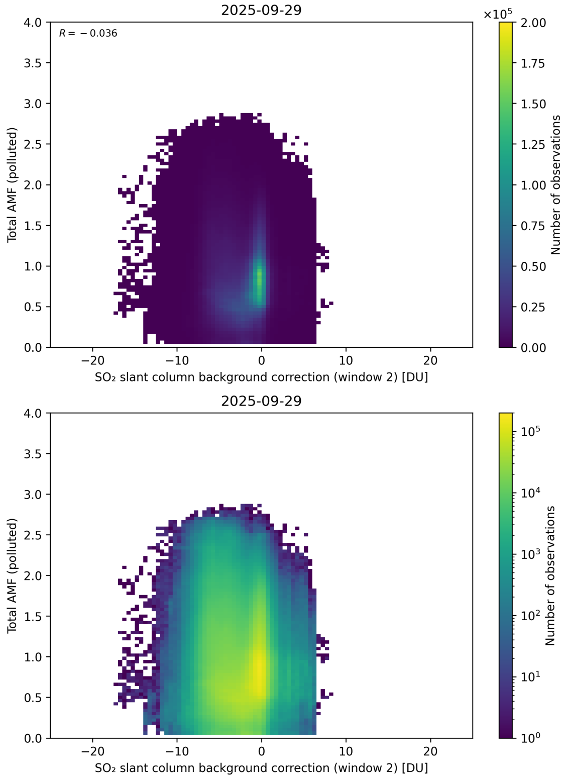
Figure 130: Scatter density plot of “SO 2 slant column background correction (window 2)” against “Total AMF (polluted)” for 2025-09-28 to 2025-09-30.
