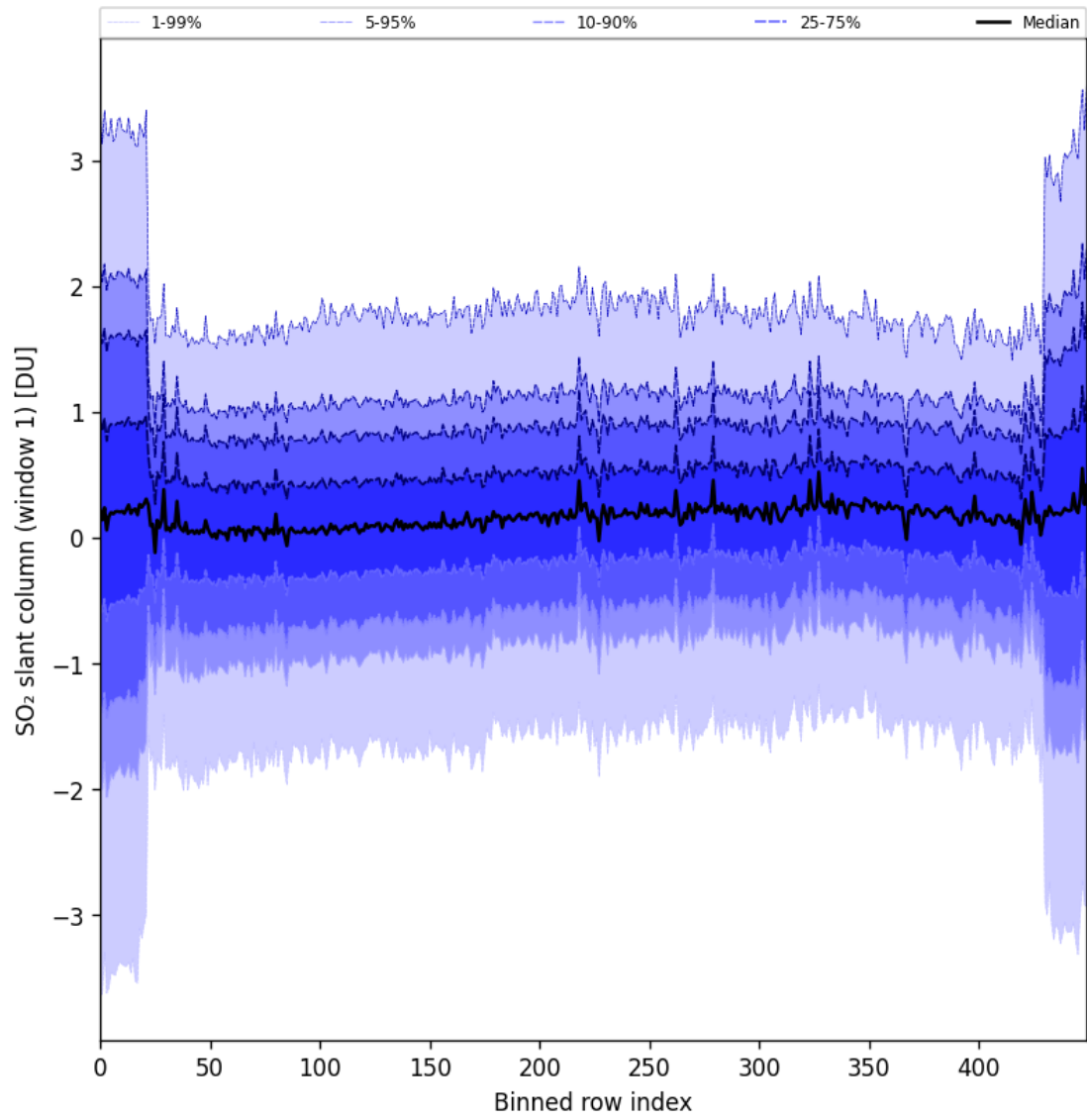
Figure 89: Along track statistics of “SO 2 slant column (window 1)” for 2025-09-28 to 2025-09-30
