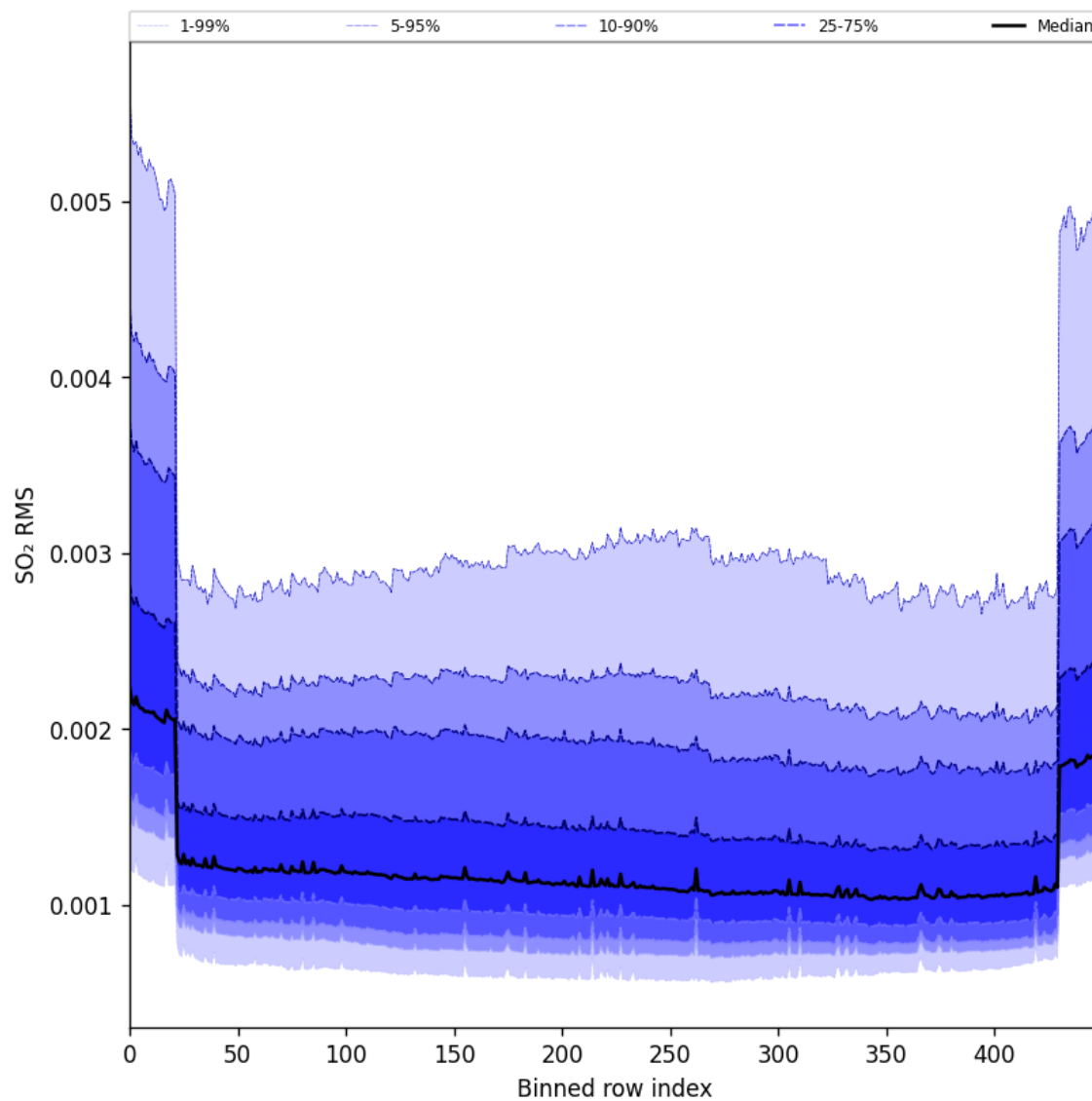
Figure 104: Along track statistics of “SO 2 RMS” for 2025-09-28 to 2025-09-30
