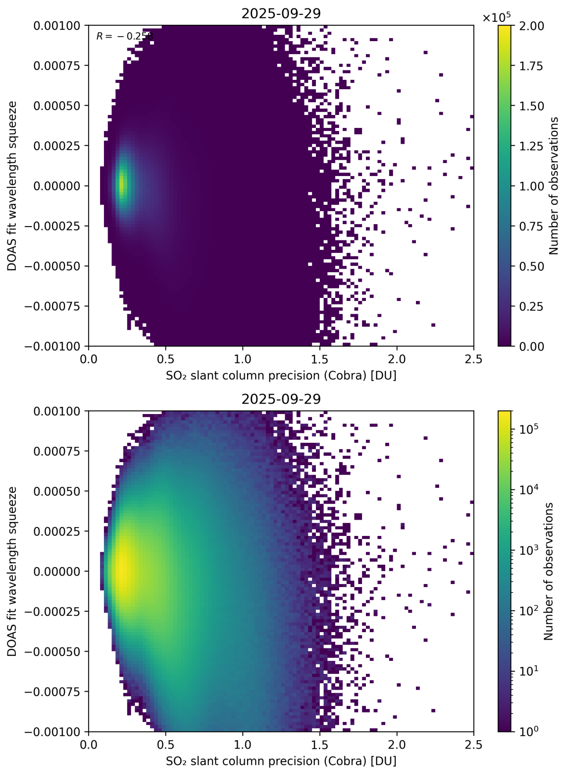
Figure 203: Scatter density plot of “SO 2 slant column precision (Cobra)” against “DOAS fit wavelength squeeze” for 2025-09-28 to 2025-09-30.
