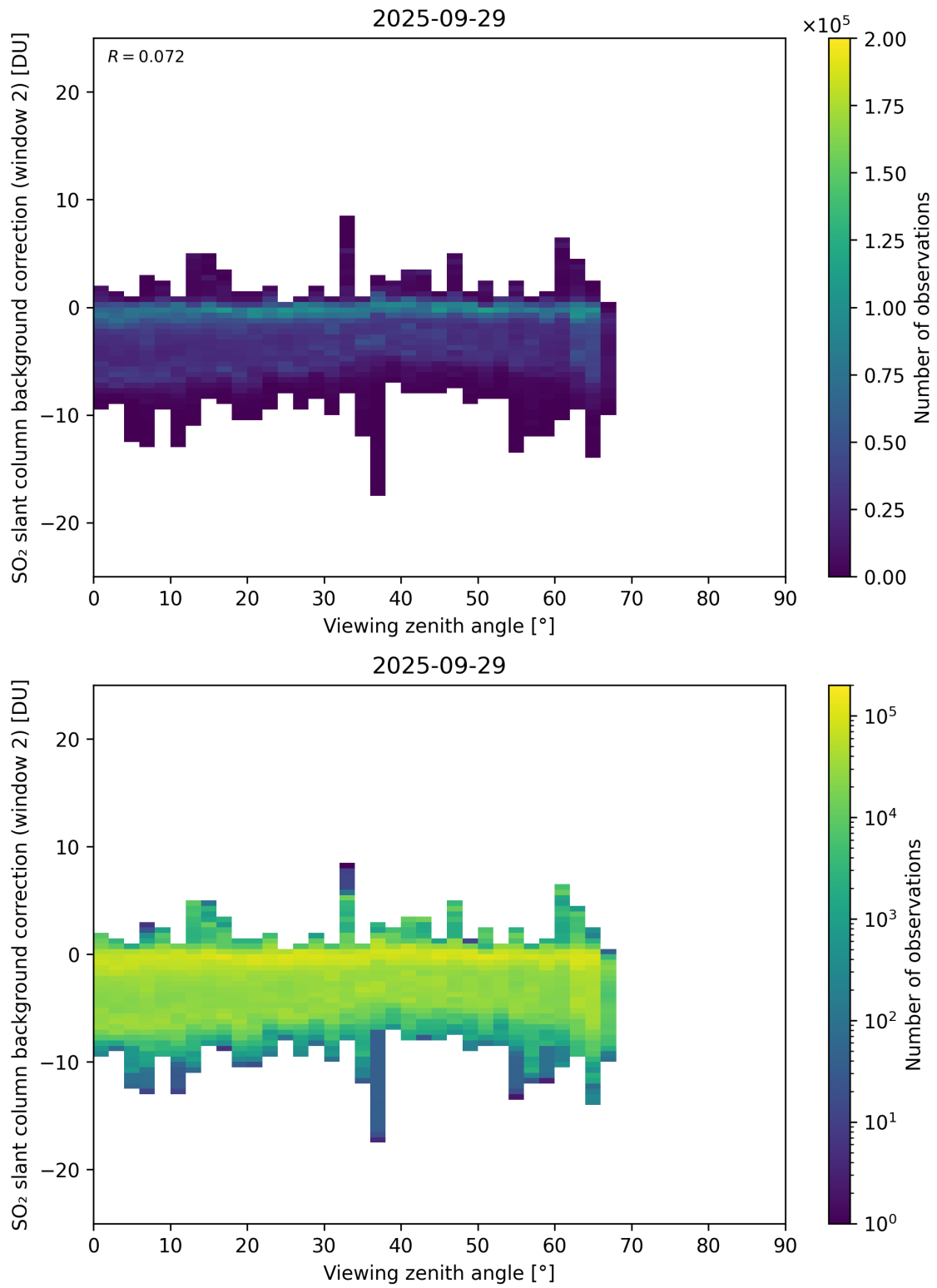
Figure 363: Scatter density plot of “Viewing zenith angle” against “SO 2 slant column background correction (window 2)” for 2025-09-28 to 2025-09-30.
