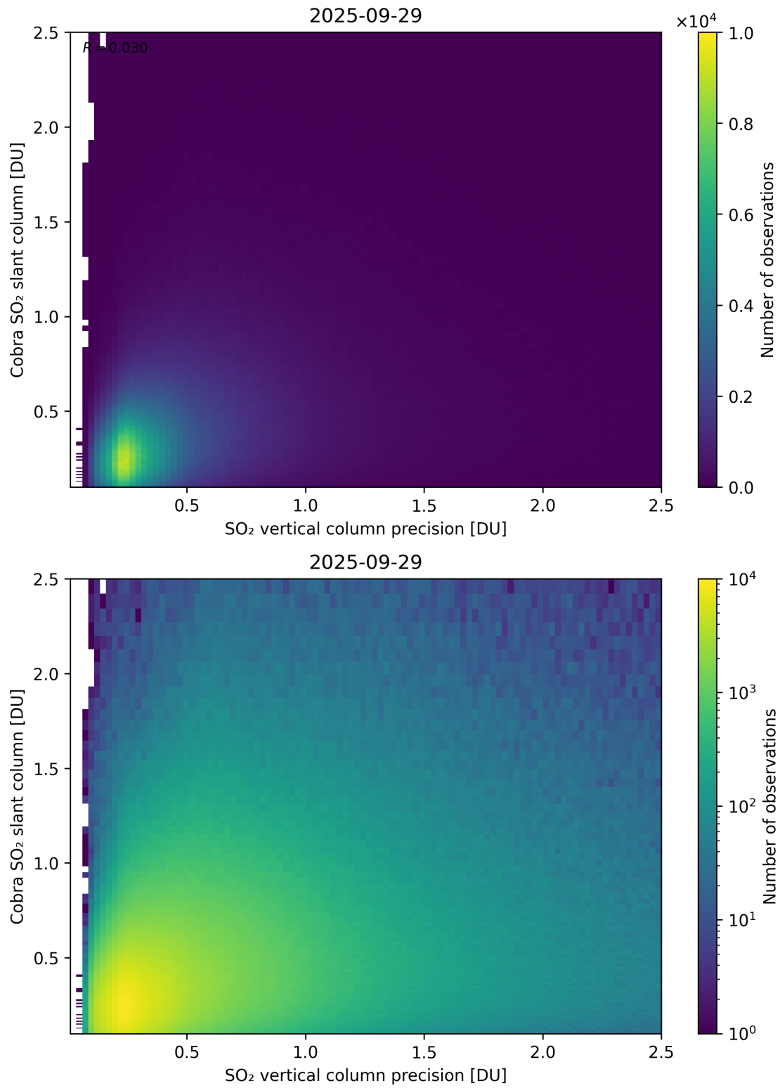
Figure 336: Scatter density plot of “SO 2 vertical column precision” against “Cobra SO 2 slant column” for 2025-09-28 to 2025-09-30.
