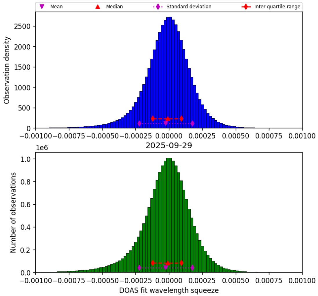
Figure 77: Histogram of “DOAS fit wavelength squeeze” for 2025-09-28 to 2025-09-30
