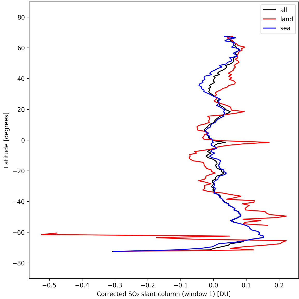
Figure 39: Zonal average of “Corrected SO 2 slant column (window 1)” for 2025-09-28 to 2025-09-30.
