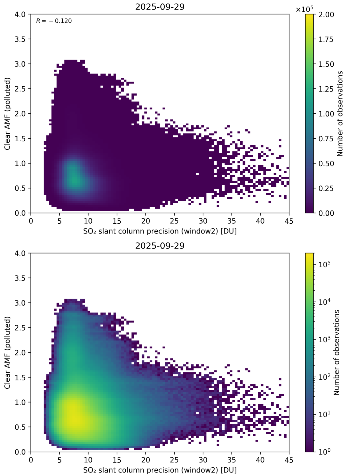
Figure 296: Scatter density plot of “SO 2 slant column precision (window2)” against “Clear AMF (polluted)” for 2025-09-28 to 2025-09-30.
