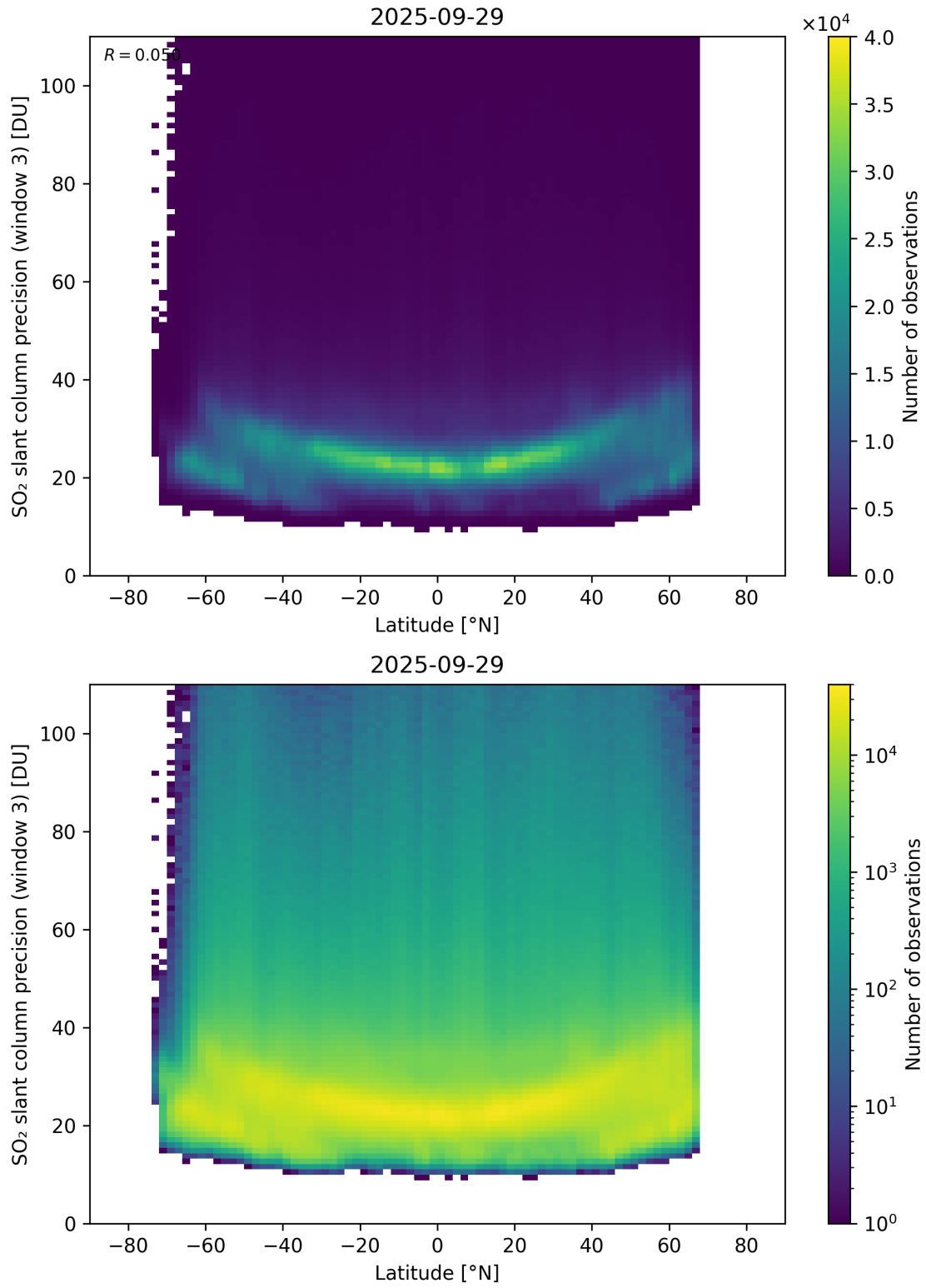
Figure 166: Scatter density plot of “Latitude” against “SO 2 slant column precision (window 3)” for 2025-09-28 to 2025-09-30.
