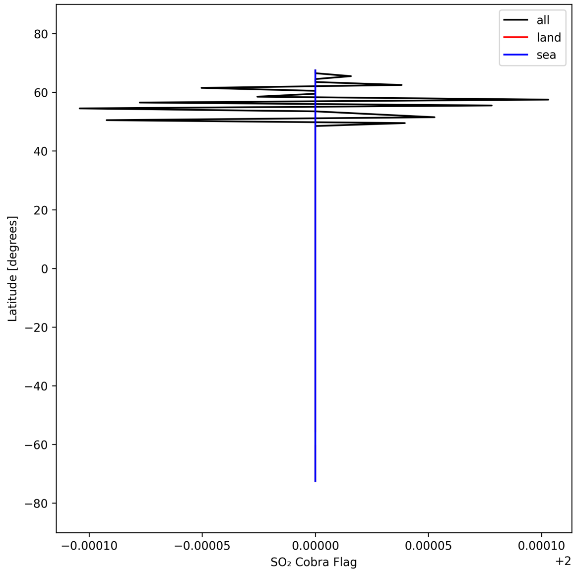
Figure 49: Zonal average of “SO 2 Cobra Flag” for 2025-09-28 to 2025-09-30.
