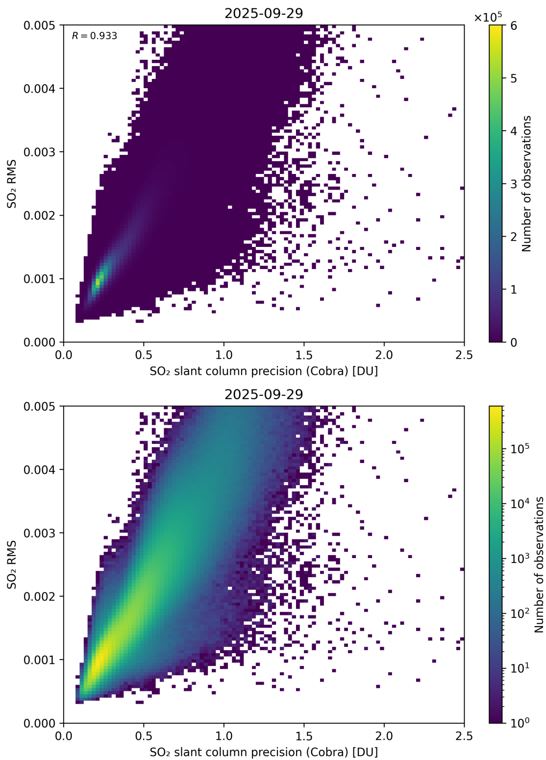
Figure 204: Scatter density plot of “SO 2 slant column precision (Cobra)” against “SO 2 RMS” for 2025-09-28 to 2025-09-30.
