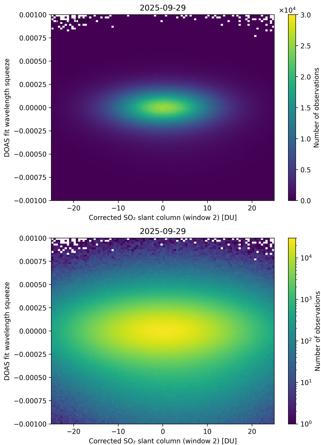
Figure 247: Scatter density plot of “Corrected SO 2 slant column (window 2)” against “DOAS fit wavelength squeeze” for 2025-09-28 to 2025-09-30.
