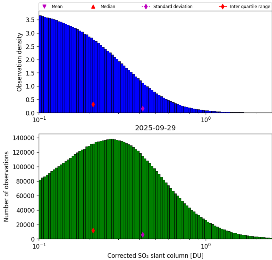
Figure 60: Histogram of "Corrected SO 2 slant column" for 2025-09-28 to 2025-09-30
