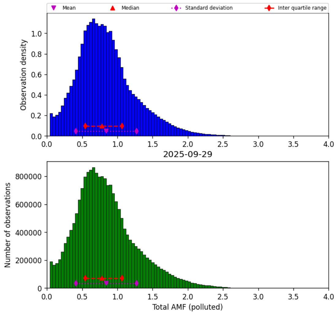
Figure 79: Histogram of “Total AMF (polluted)” for 2025-09-28 to 2025-09-30
