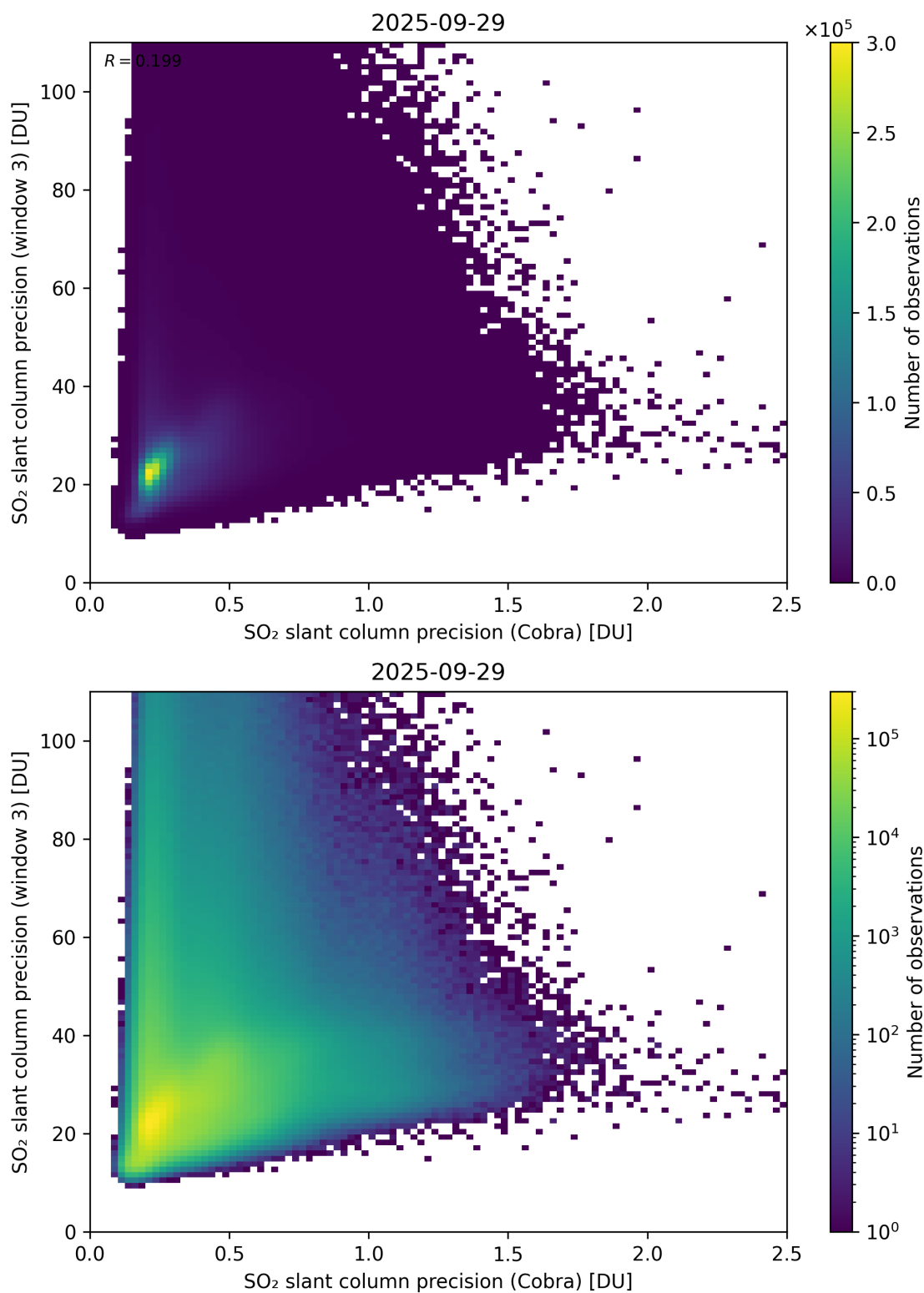
Figure 212: Scatter density plot of “SO 2 slant column precision (Cobra)” against “SO 2 slant column precision (window 3)” for 2025-09-28 to 2025-09-30.
