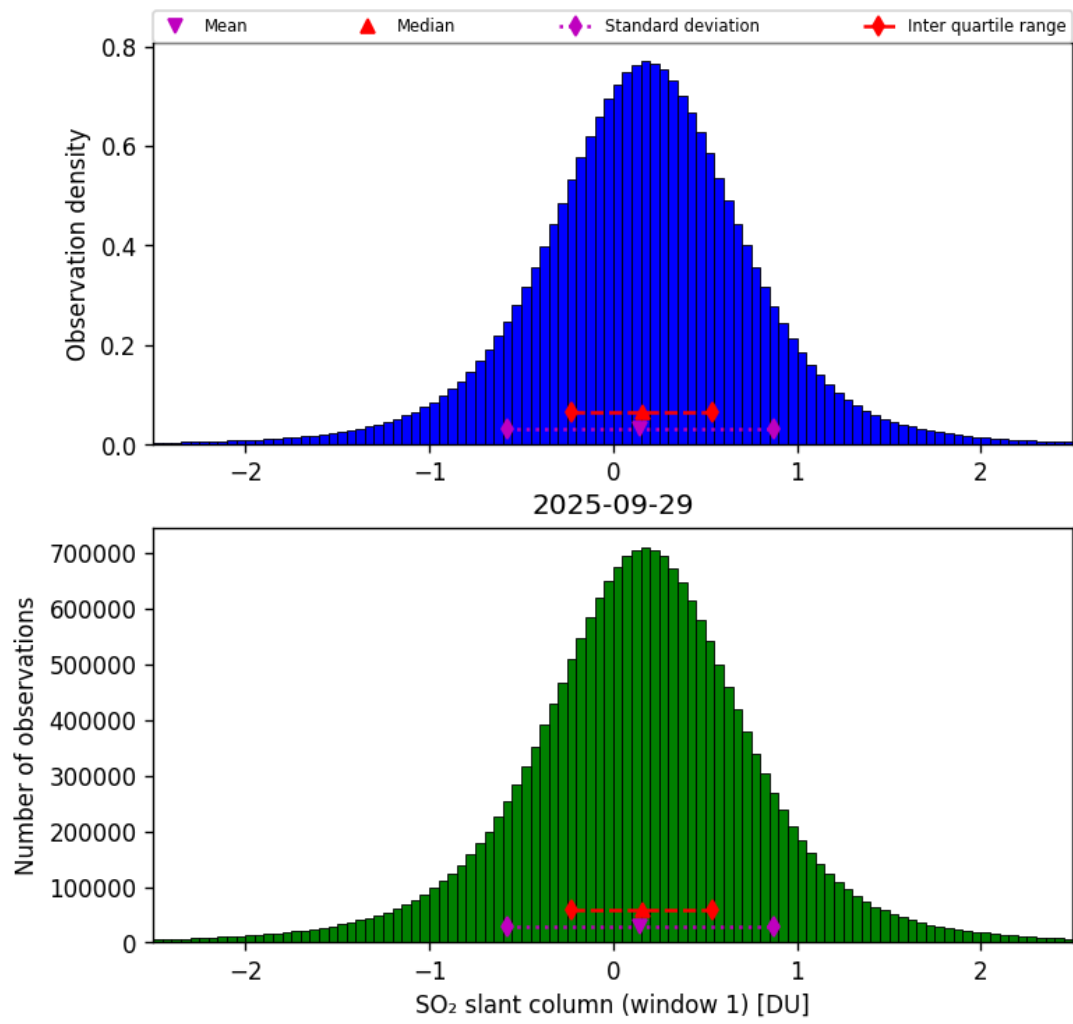
Figure 63: Histogram of “SO 2 slant column (window 1)” for 2025-09-28 to 2025-09-30
