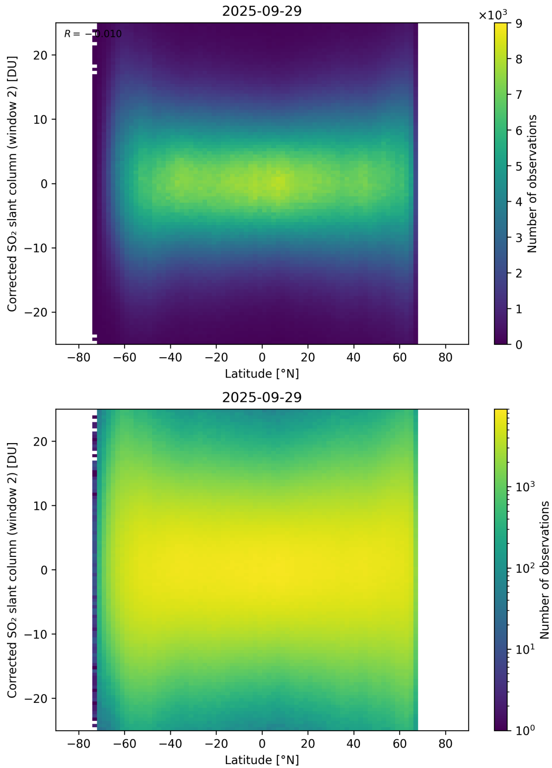
Figure 160: Scatter density plot of “Latitude” against “Corrected SO 2 slant column (window 2)” for 2025-09-28 to 2025-09-30.
