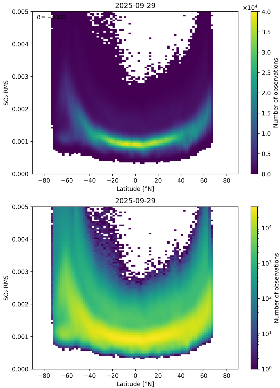
Figure 155: Scatter density plot of “Latitude” against “SO 2 RMS” for 2025-09-28 to 2025-09-30.
