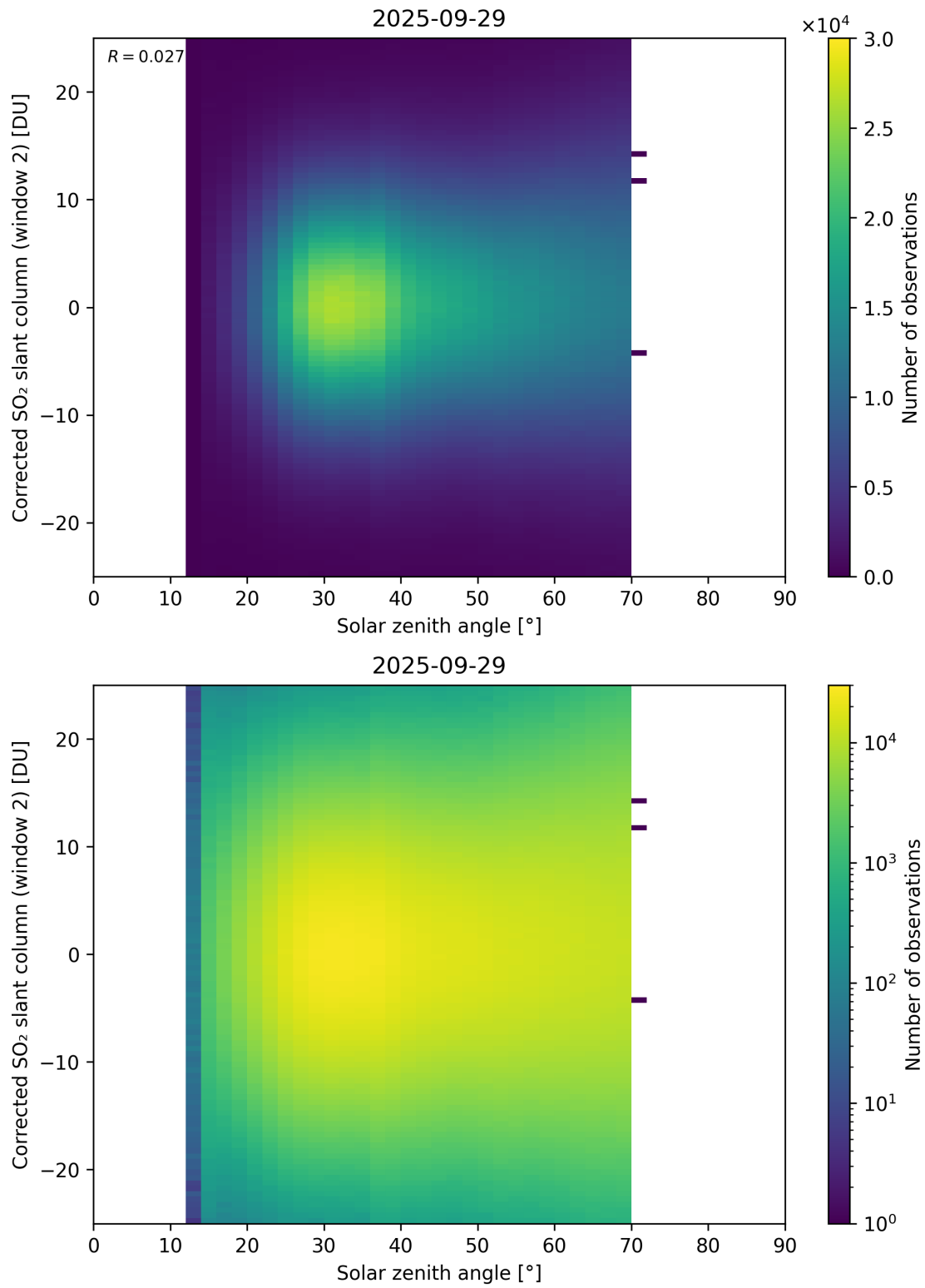
Figure 182: Scatter density plot of “Solar zenith angle” against “Corrected SO 2 slant column (window 2)” for 2025-09-28 to 2025-09-30.
