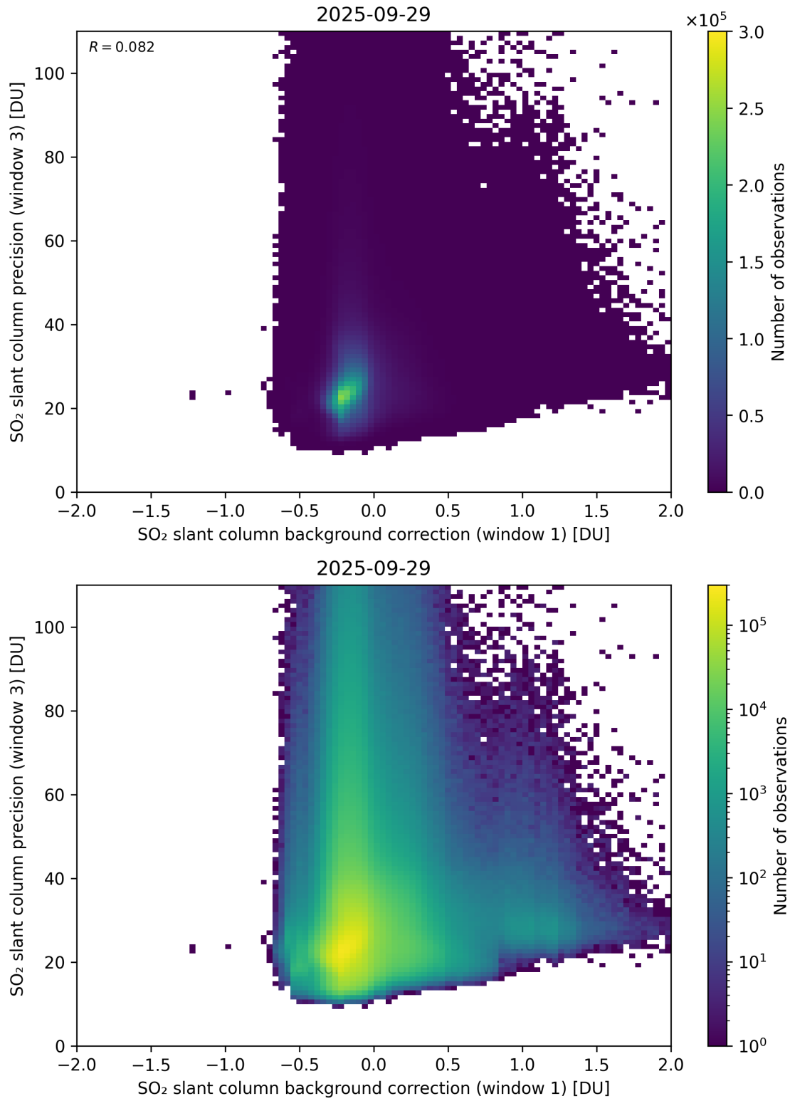
Figure 119: Scatter density plot of “SO 2 slant column background correction (window 1)” against “SO 2 slant column precision (window 3)” for 2025-09-28 to 2025-09-30.
