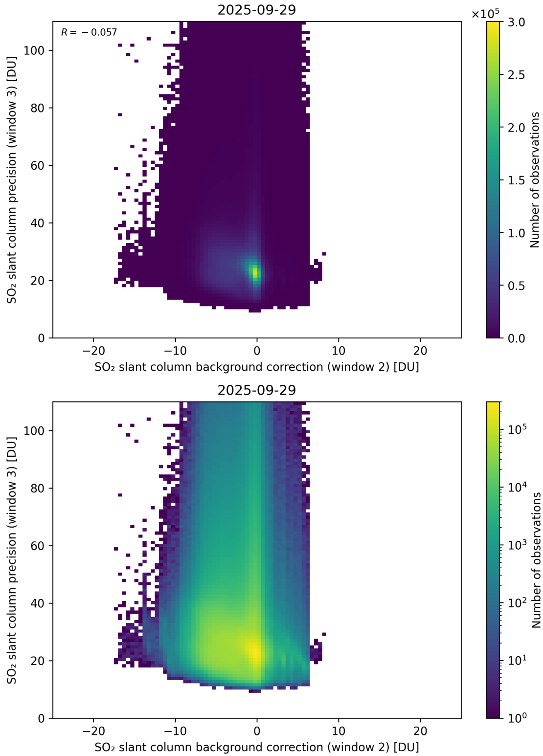
Figure 129: Scatter density plot of “SO 2 slant column background correction (window 2)” against “SO 2 slant column precision (window 3)” for 2025-09-28 to 2025-09-30.
