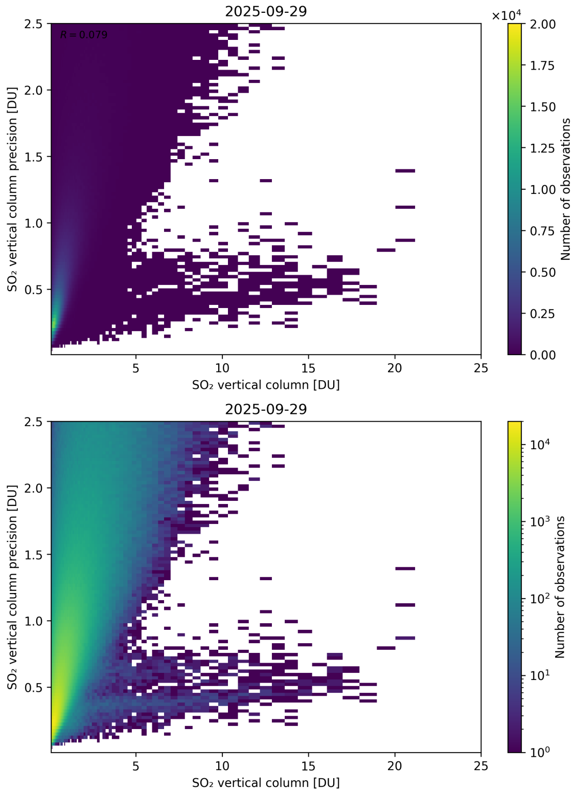
Figure 361: Scatter density plot of “SO 2 vertical column” against “SO 2 vertical column precision” for 2025-09-28 to 2025-09-30.
