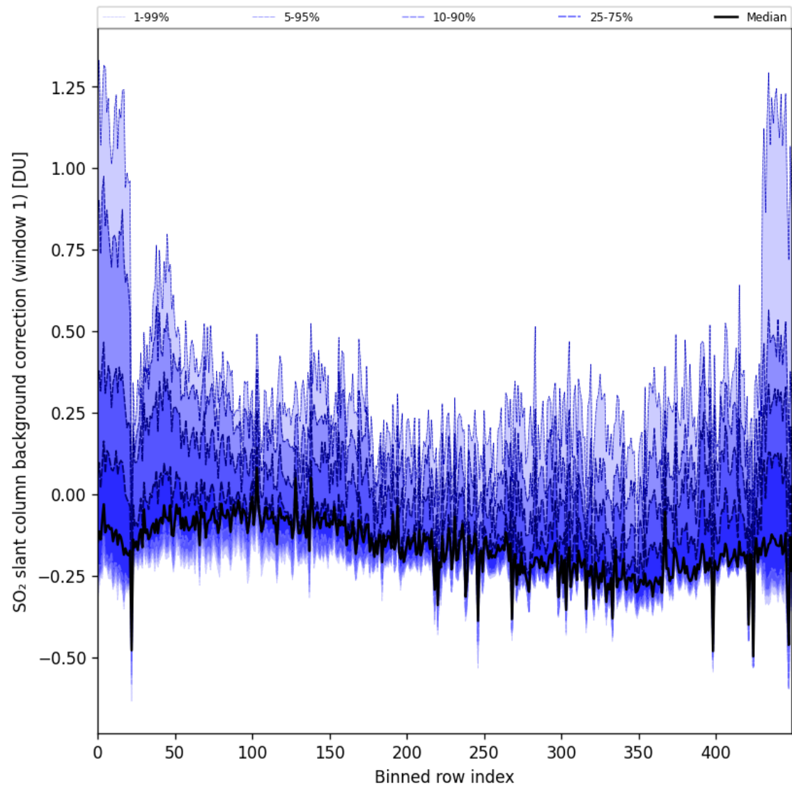
Figure 92: Along track statistics of “SO 2 slant column background correction (window 1)” for 2025-09-28 to 2025-09-30
