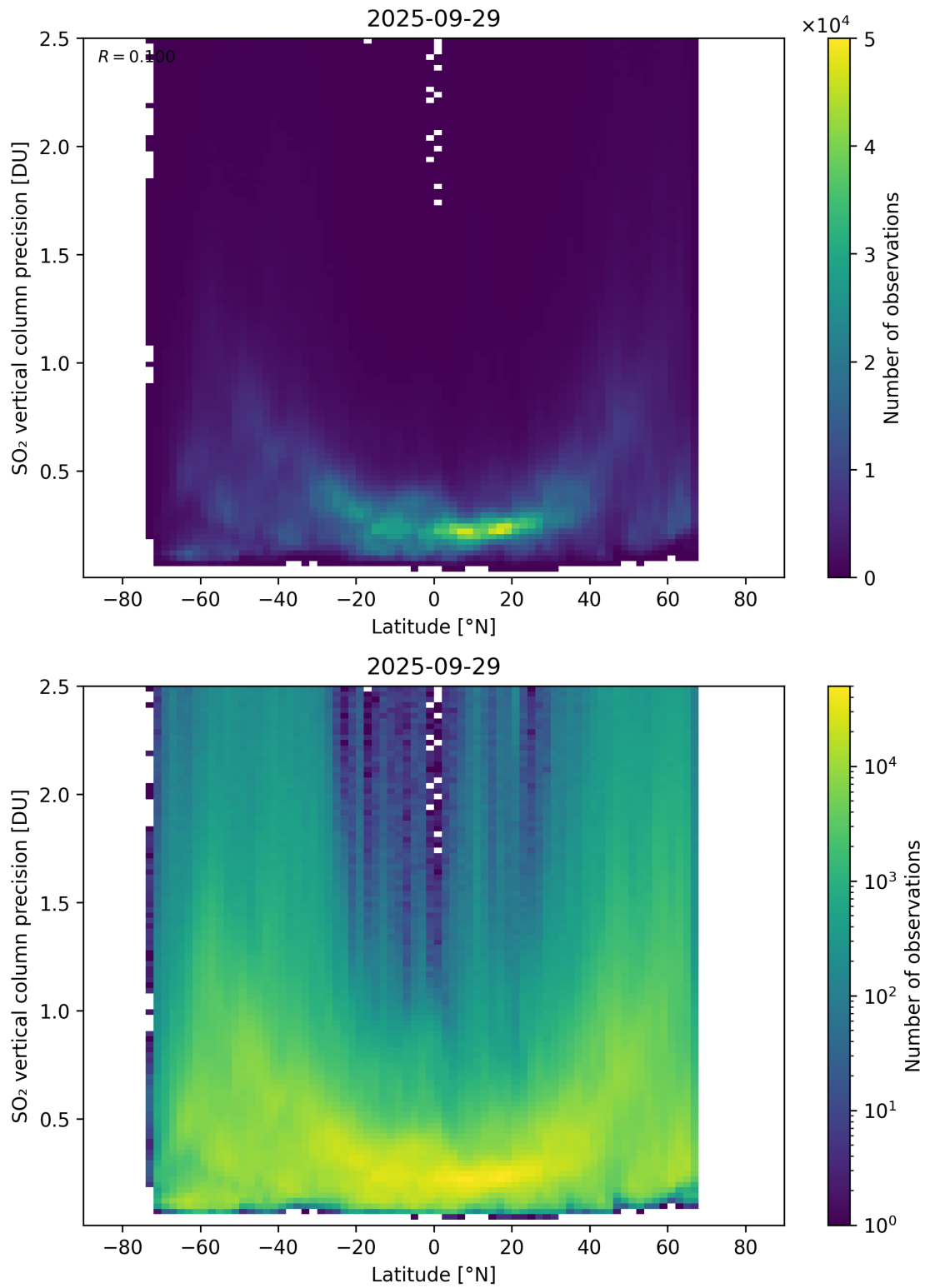
Figure 170: Scatter density plot of “Latitude” against “SO 2 vertical column precision” for 2025-09-28 to 2025-09-30.
