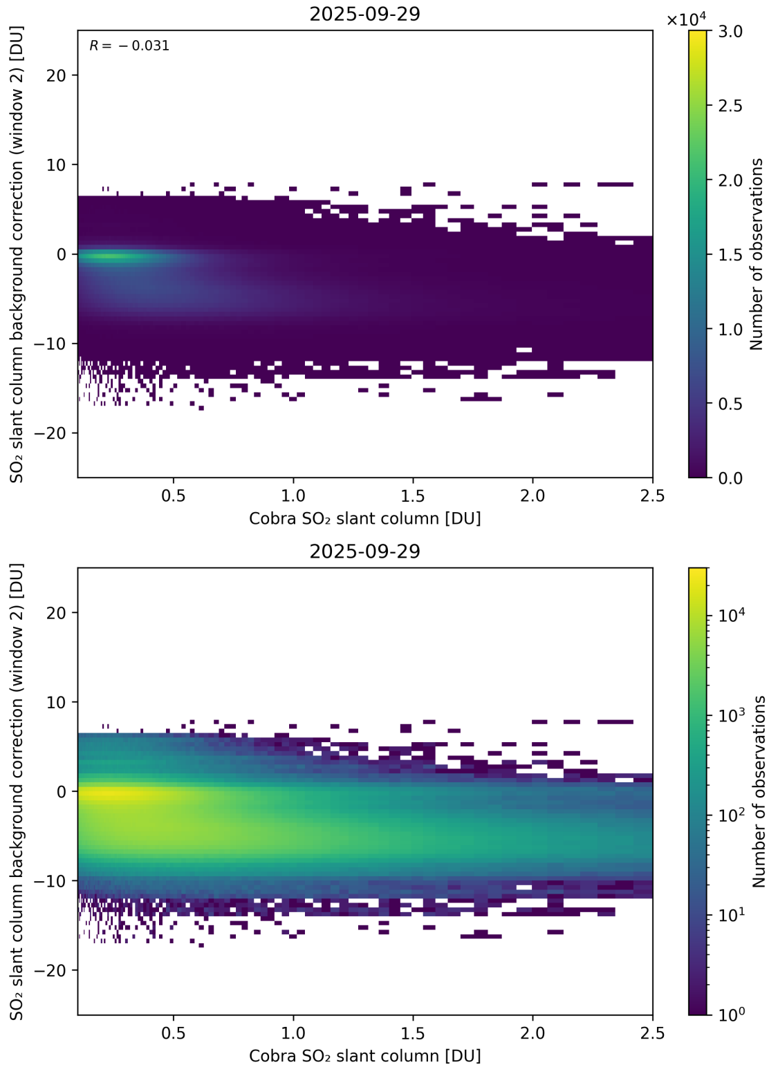
Figure 194: Scatter density plot of “Cobra SO 2 slant column” against “SO 2 slant column background correction (window 2)” for 2025-09-28 to 2025-09-30.
