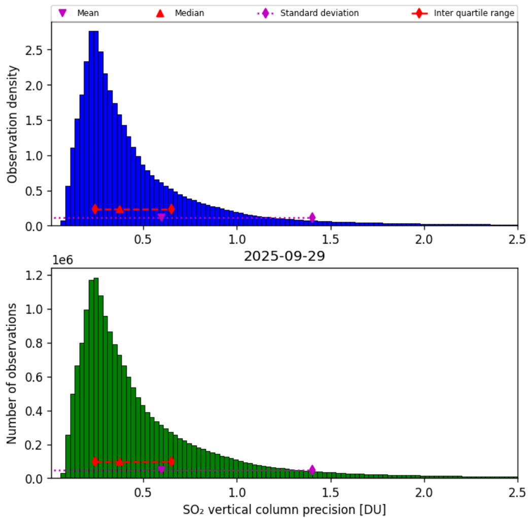
Figure 59: Histogram of “SO 2 vertical column precision” for 2025-09-28 to 2025-09-30
