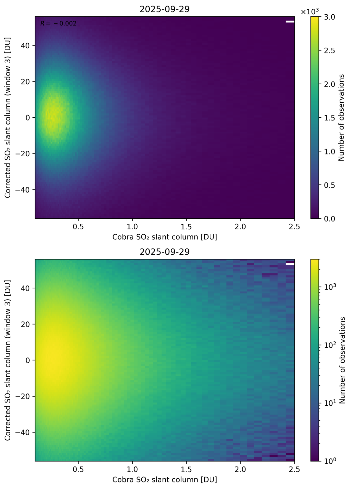
Figure 218: Scatter density plot of “Cobra SO 2 slant column” against “Corrected SO 2 slant column (window 3)” for 2025-09-28 to 2025-09-30.
