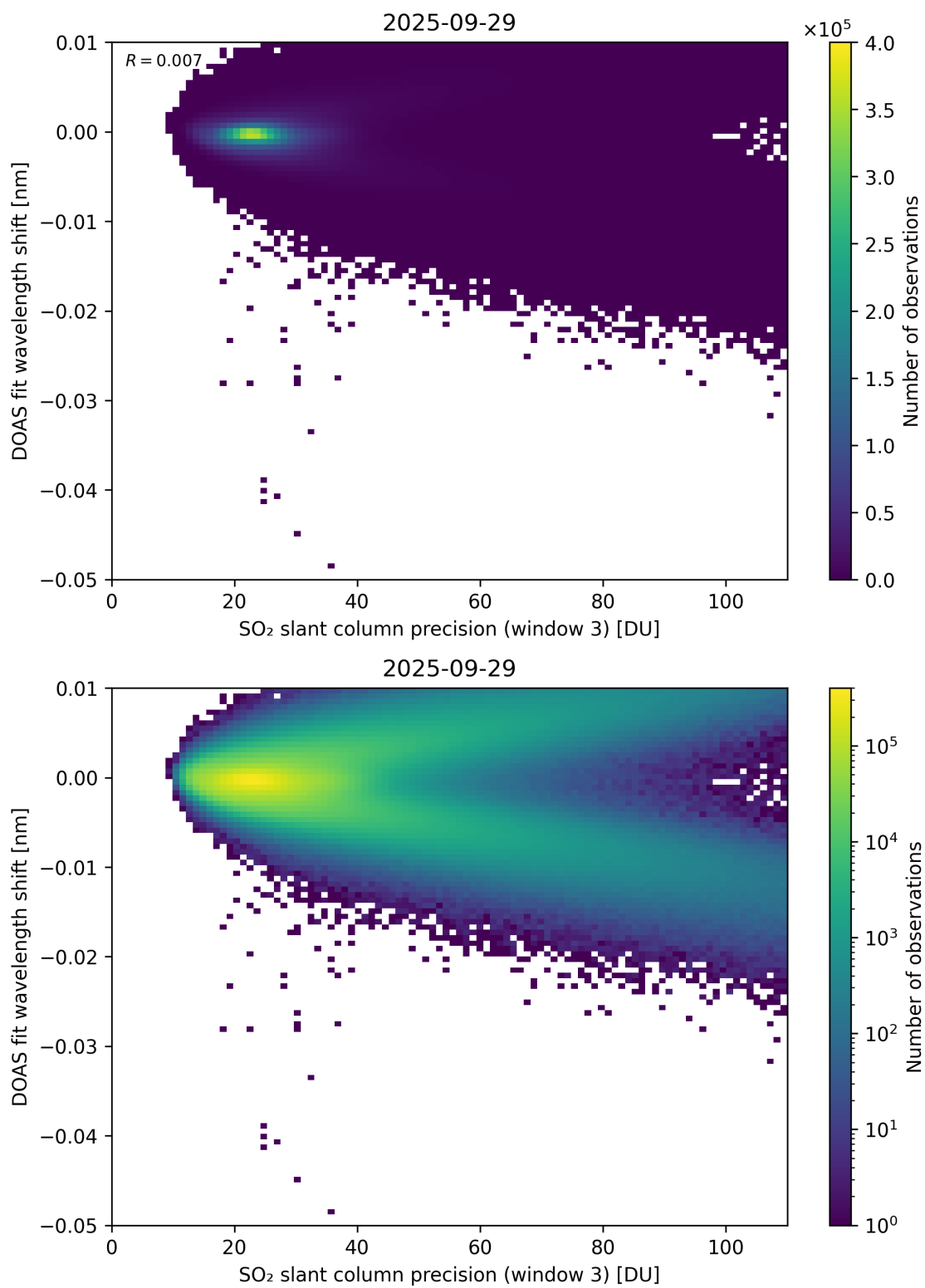
Figure 308: Scatter density plot of “SO 2 slant column precision (window 3)” against “DOAS fit wavelength shift” for 2025-09-28 to 2025-09-30.
