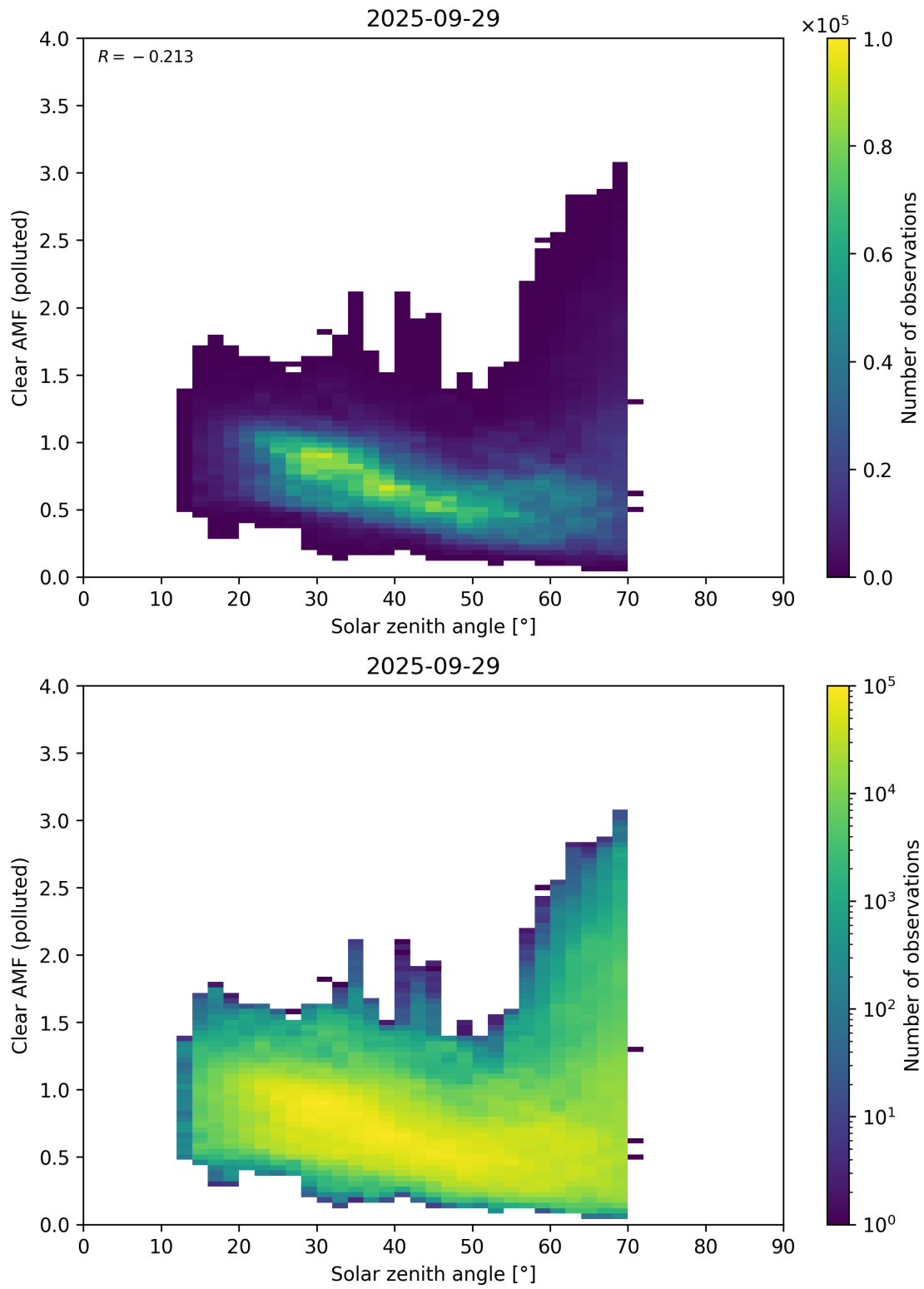
Figure 178: Scatter density plot of “Solar zenith angle” against “Clear AMF (polluted)” for 2025-09-28 to 2025-09-30.
