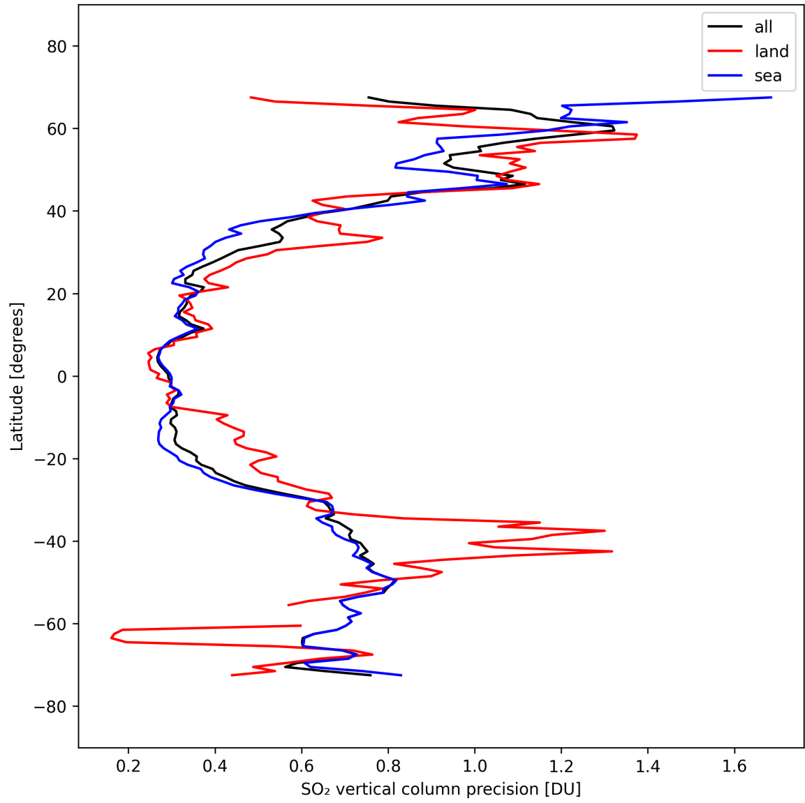
Figure 33: Zonal average of “SO 2 vertical column precision” for 2025-09-28 to 2025-09-30.
