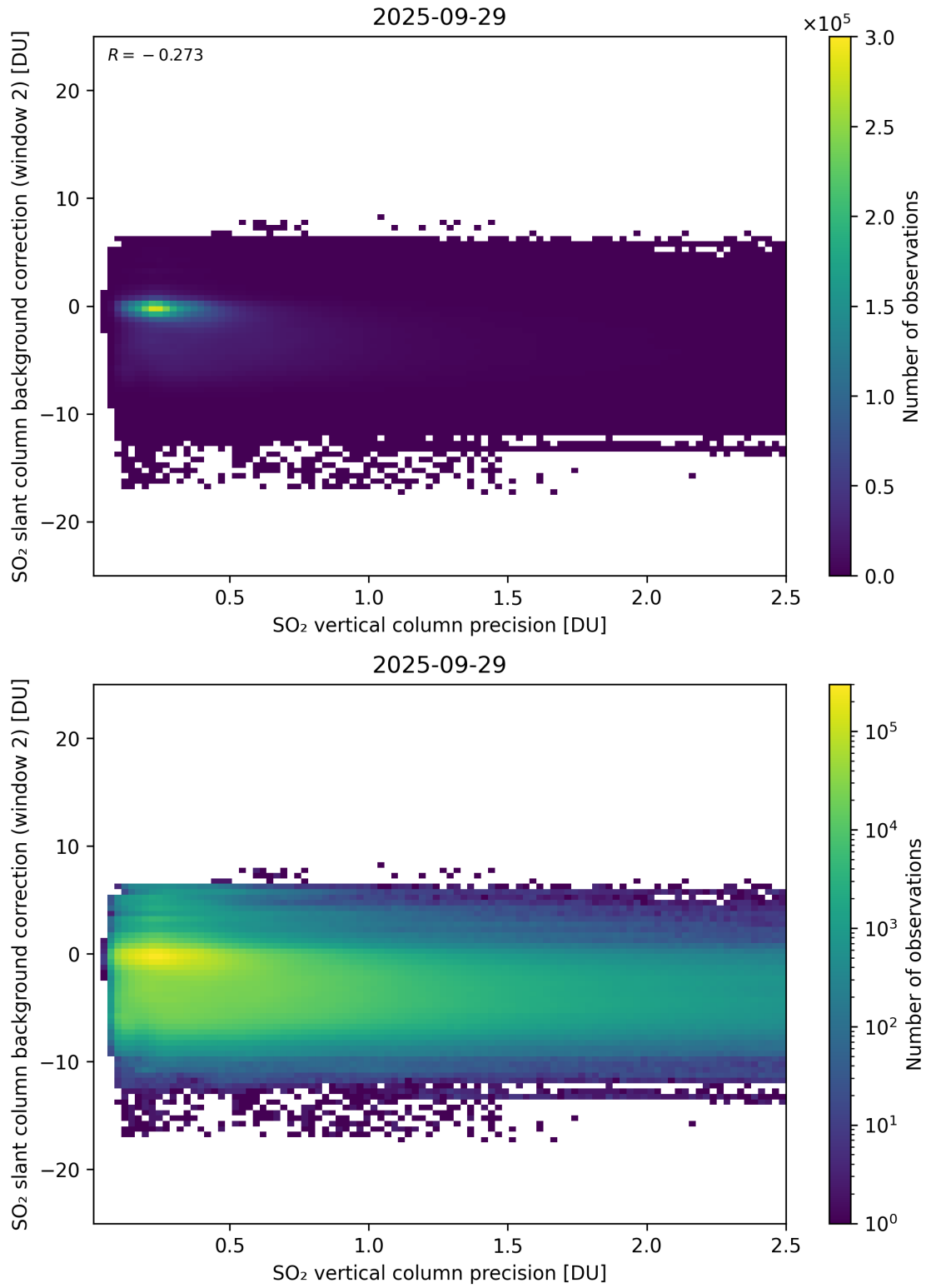
Figure 330: Scatter density plot of “SO 2 vertical column precision” against “SO 2 slant column background correction (window 2)” for 2025-09-28 to 2025-09-30.
