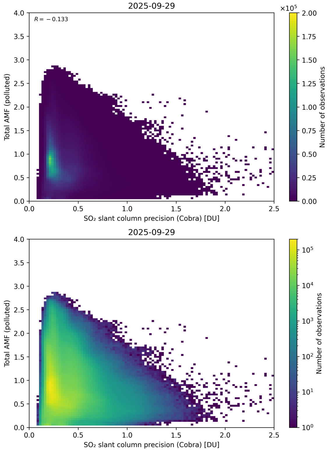
Figure 213: Scatter density plot of “SO 2 slant column precision (Cobra)” against “Total AMF (polluted)” for 2025-09-28 to 2025-09-30.
