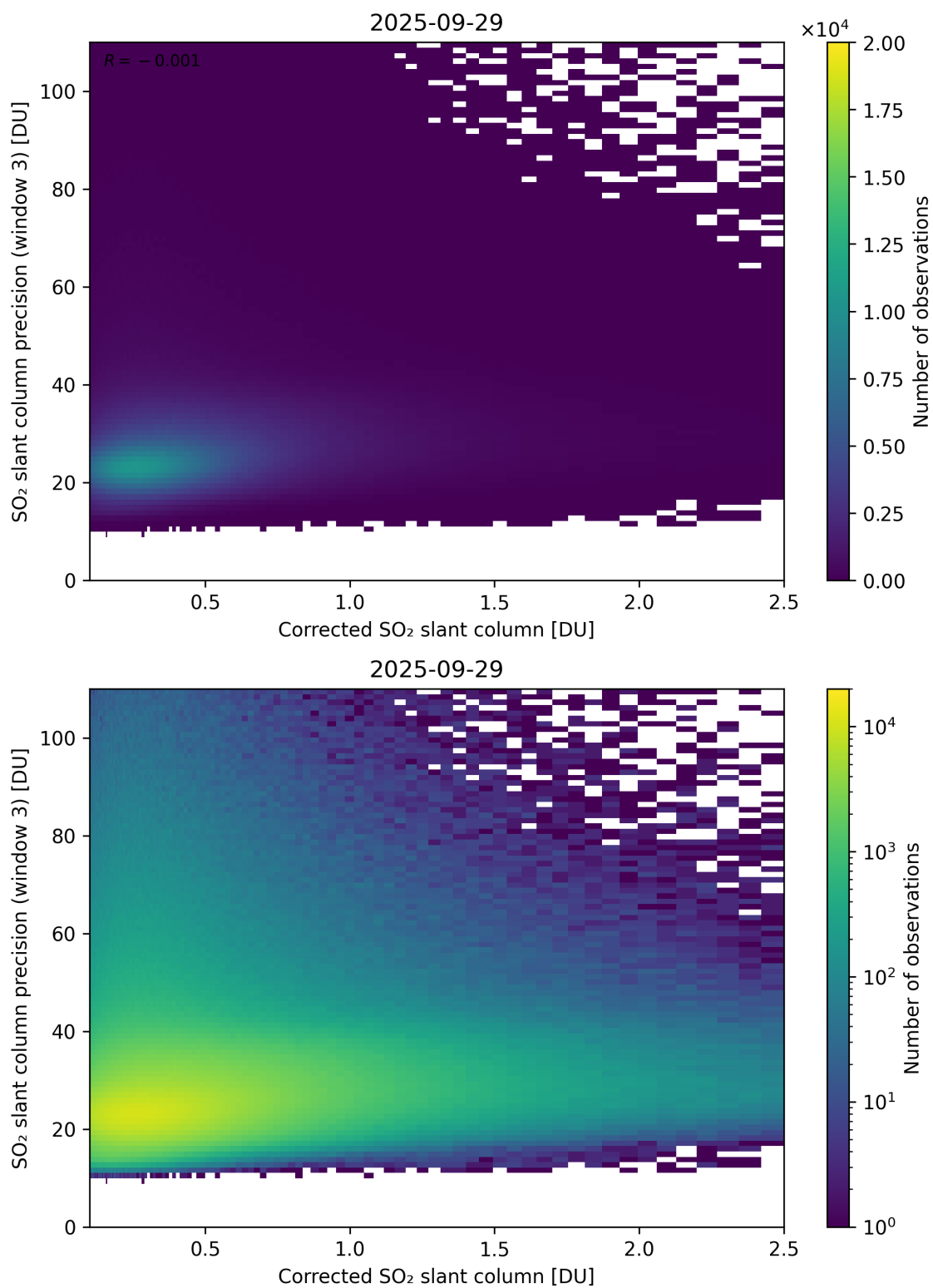
Figure 241: Scatter density plot of “Corrected SO 2 slant column” against “SO 2 slant column precision (window 3)” for 2025-09-28 to 2025-09-30.
