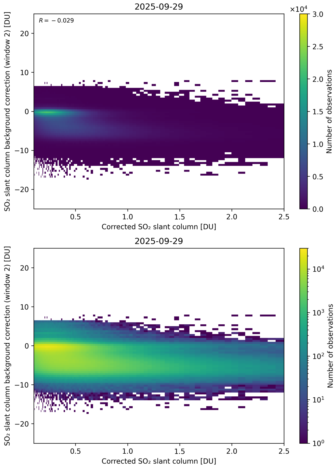
Figure 227: Scatter density plot of “Corrected SO 2 slant column” against “SO 2 slant column background correction (window 2)” for 2025-09-28 to 2025-09-30.
