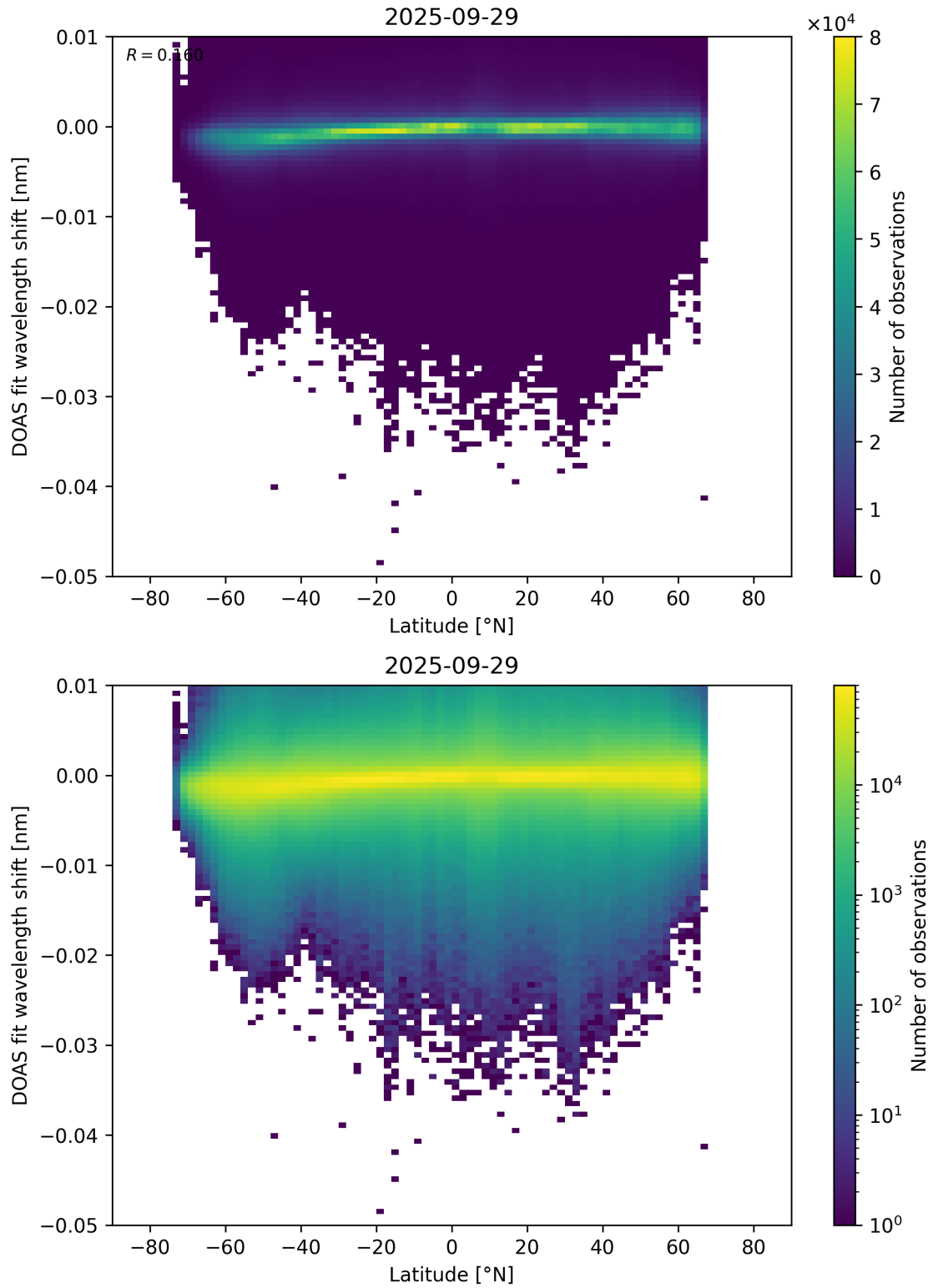
Figure 153: Scatter density plot of “Latitude” against “DOAS fit wavelength shift” for 2025-09-28 to 2025-09-30.
