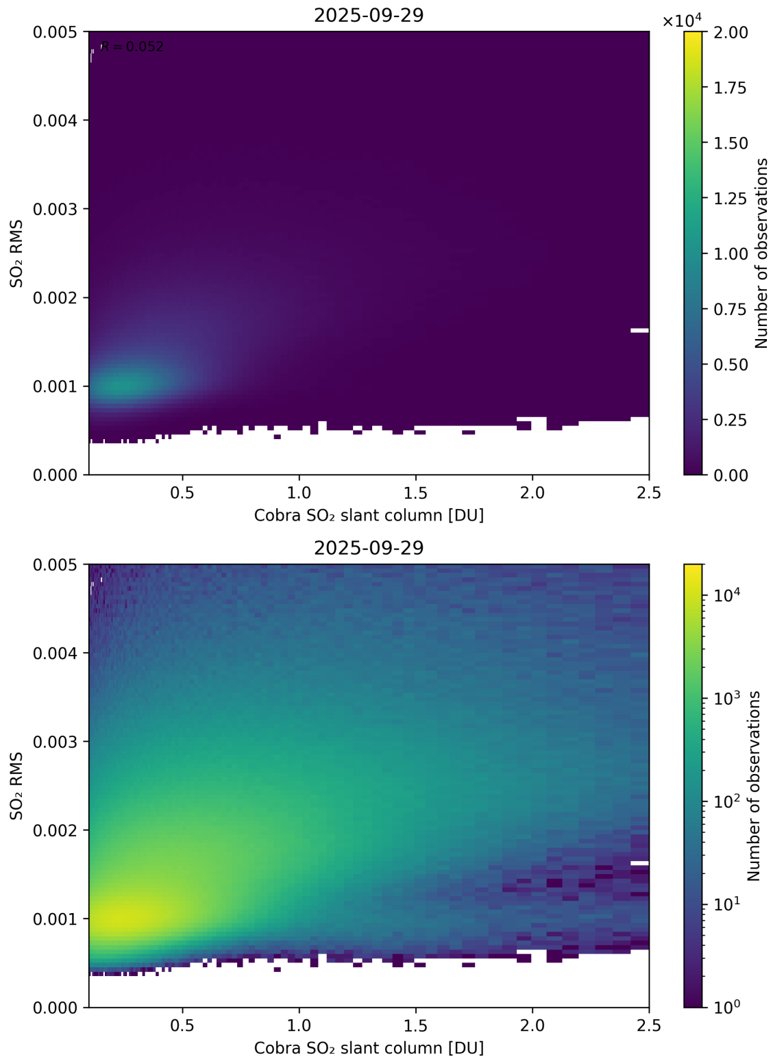
Figure 198: Scatter density plot of “Cobra SO 2 slant column” against “SO 2 RMS” for 2025-09-28 to 2025-09-30.
