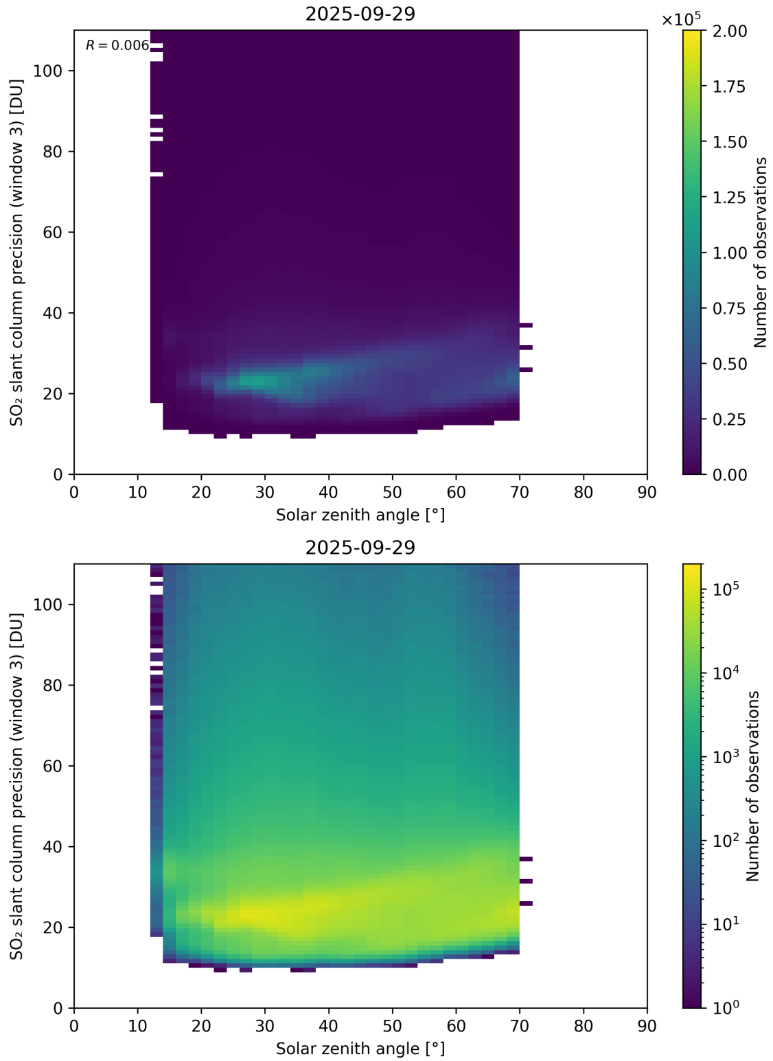
Figure 188: Scatter density plot of “Solar zenith angle” against “SO 2 slant column precision (window 3)” for 2025-09-28 to 2025-09-30.
