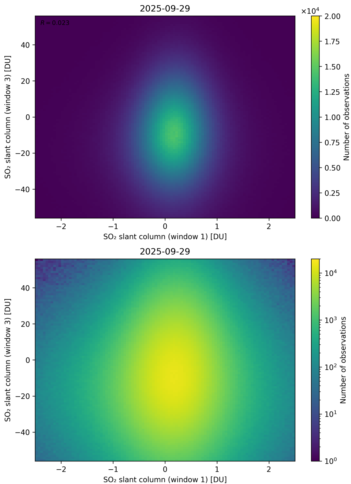
Figure 287: Scatter density plot of “SO 2 slant column (window 1)” against “SO 2 slant column (window 3)” for 2025-09-28 to 2025-09-30.
