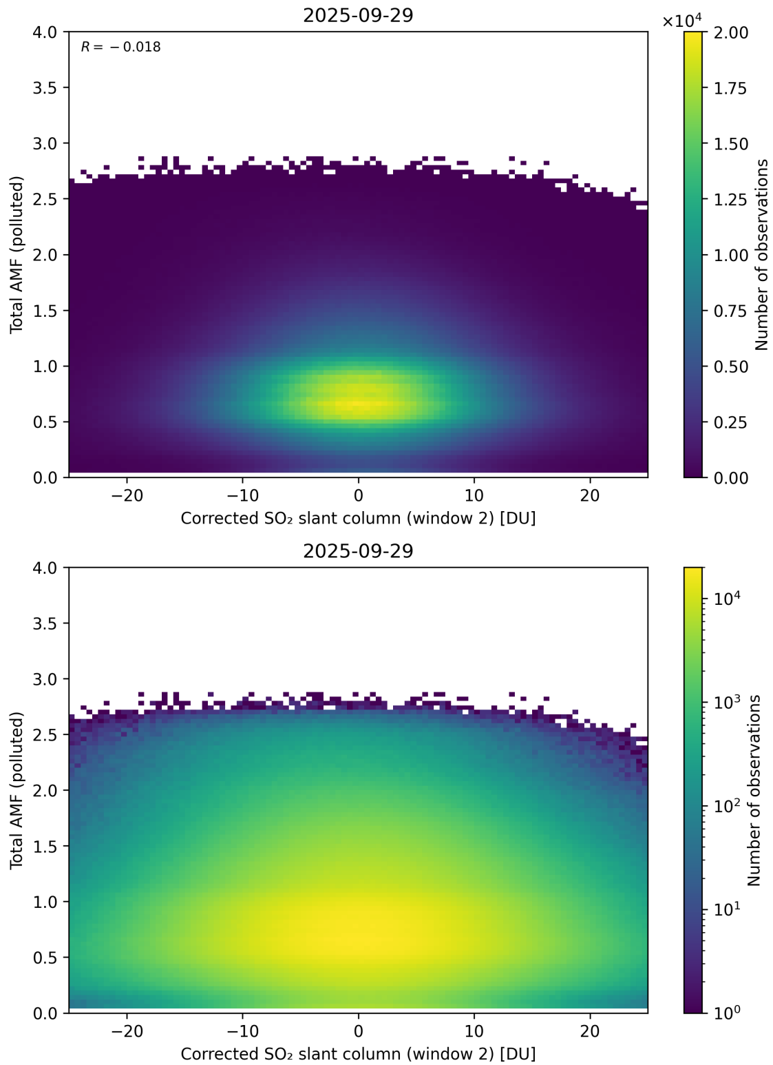
Figure 253: Scatter density plot of “Corrected SO 2 slant column (window 2)” against “Total AMF (polluted)” for 2025-09-28 to 2025-09-30.
