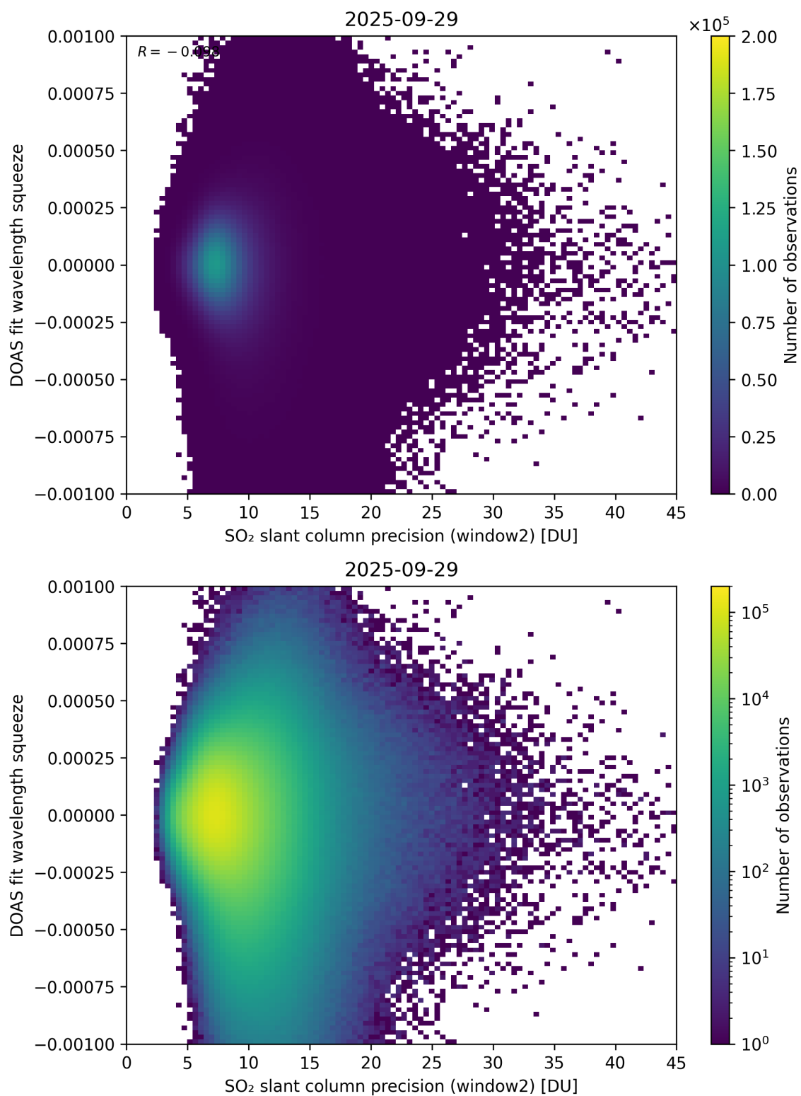
Figure 294: Scatter density plot of “SO 2 slant column precision (window2)” against “DOAS fit wavelength squeeze” for 2025-09-28 to 2025-09-30.
