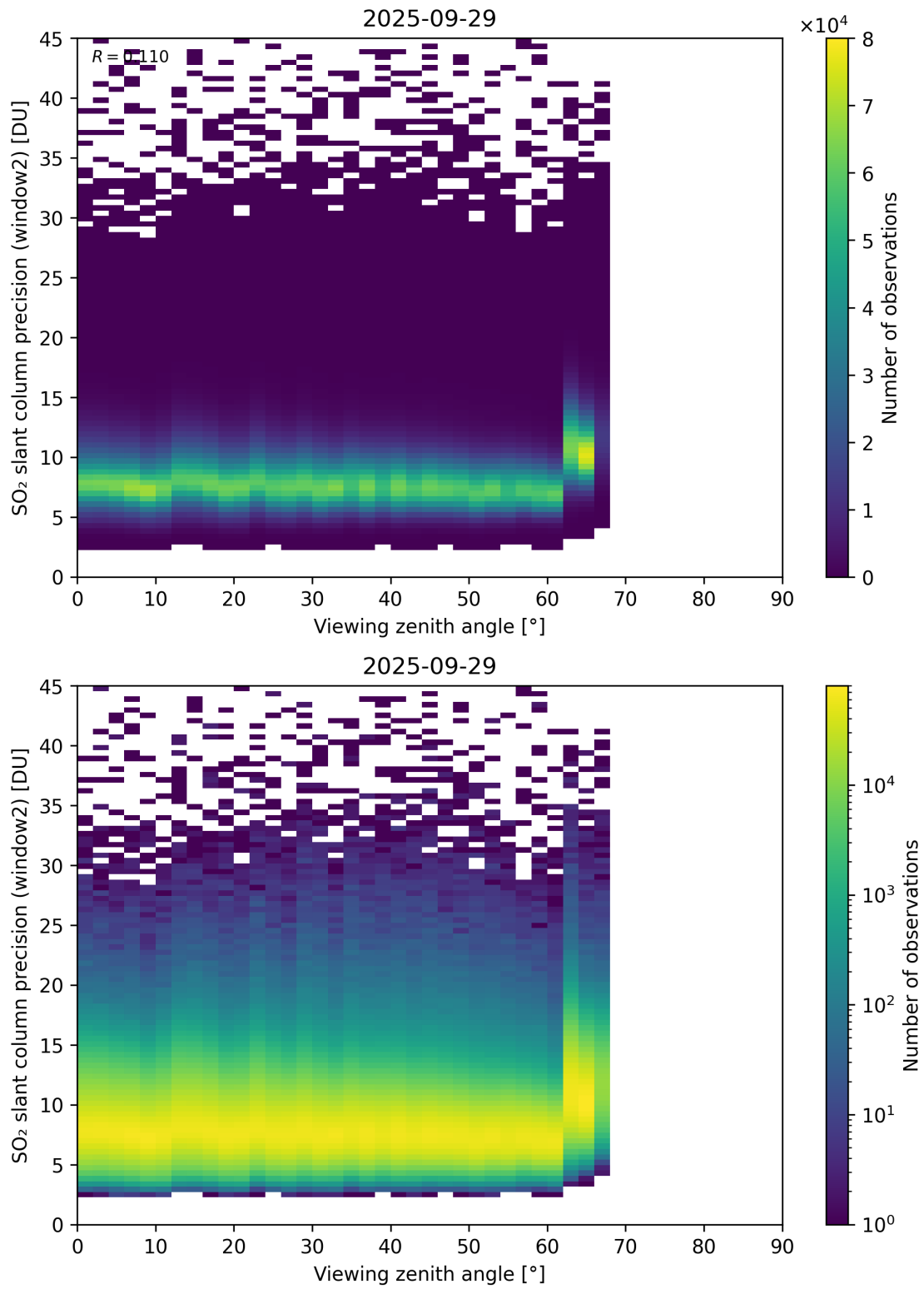
Figure 378: Scatter density plot of “Viewing zenith angle” against “SO 2 slant column precision (window2)” for 2025-09-28 to 2025-09-30.
