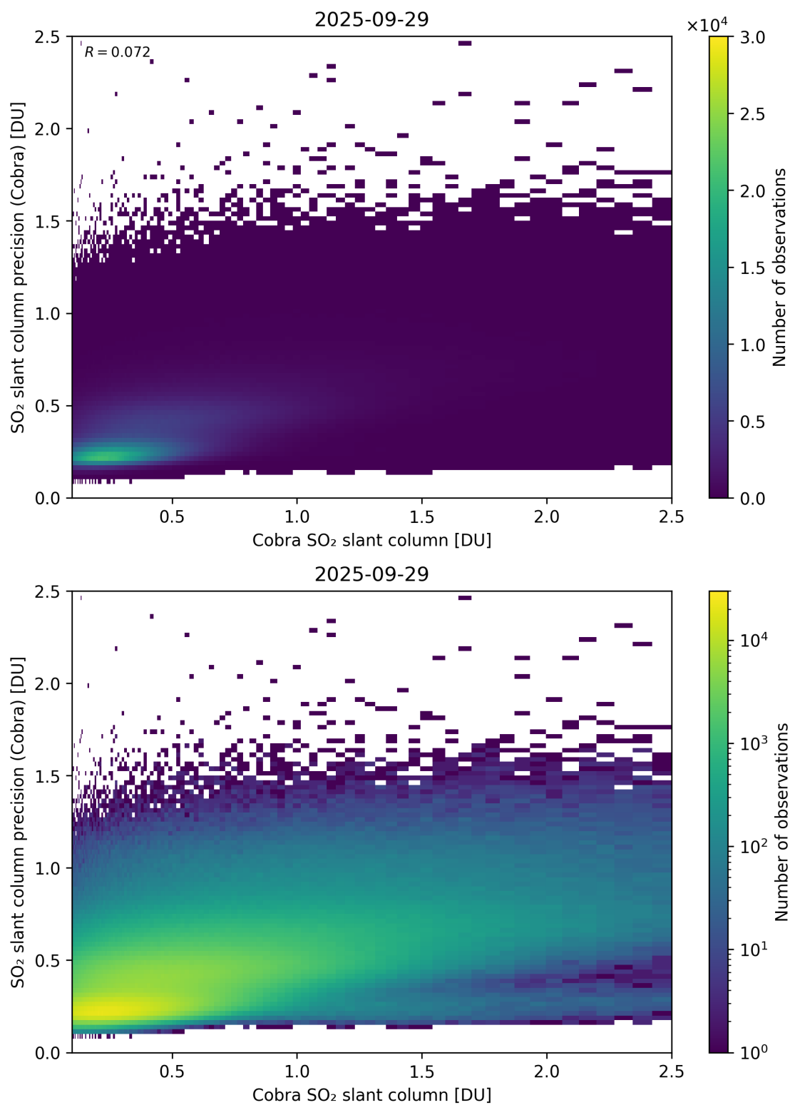
Figure 216: Scatter density plot of “Cobra SO 2 slant column” against “SO 2 slant column precision (Cobra)” for 2025-09-28 to 2025-09-30.
