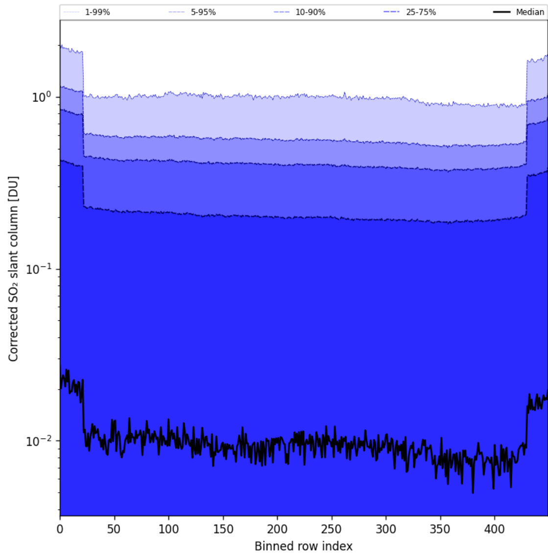
Figure 86: Along track statistics of “Corrected SO 2 slant column” for 2025-09-28 to 2025-09-30
