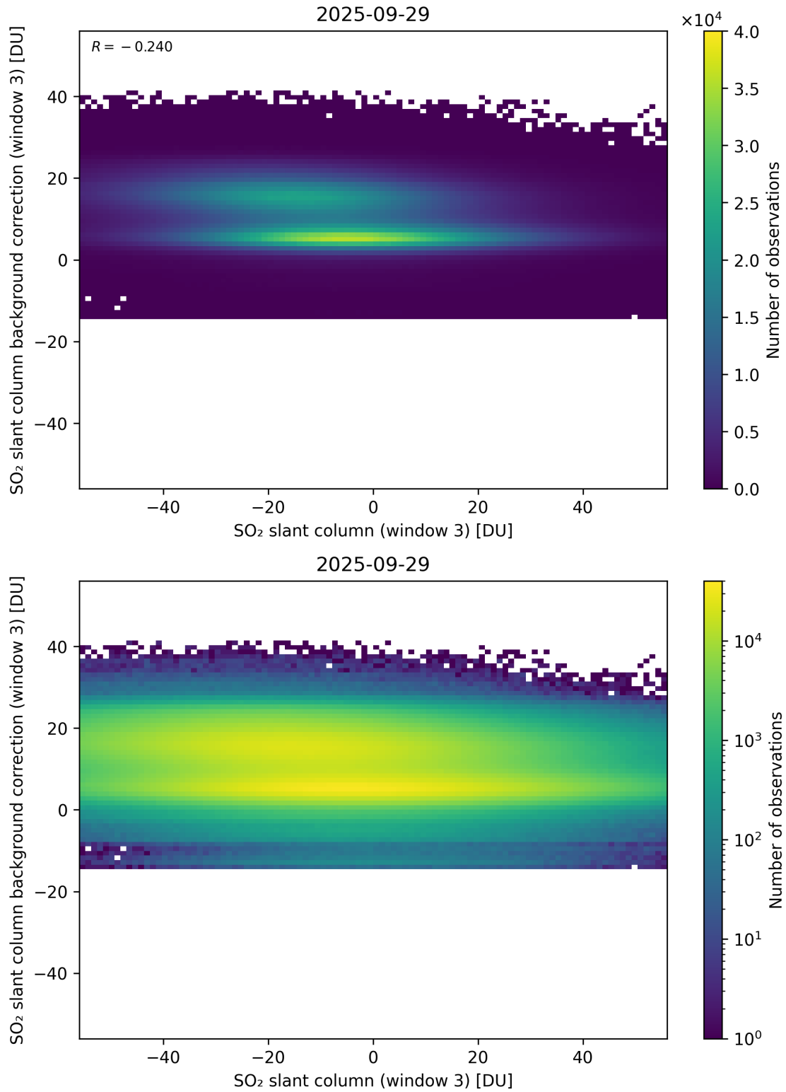
Figure 303: Scatter density plot of “SO 2 slant column (window 3)” against “SO 2 slant column background correction (window 3)” for 2025-09-28 to 2025-09-30.
