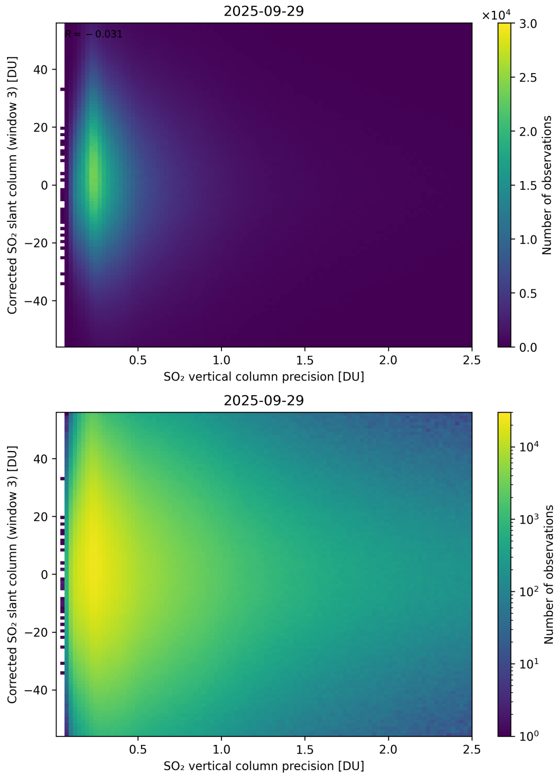
Figure 340: Scatter density plot of “SO 2 vertical column precision” against “Corrected SO 2 slant column (window 3)” for 2025-09-28 to 2025-09-30.
