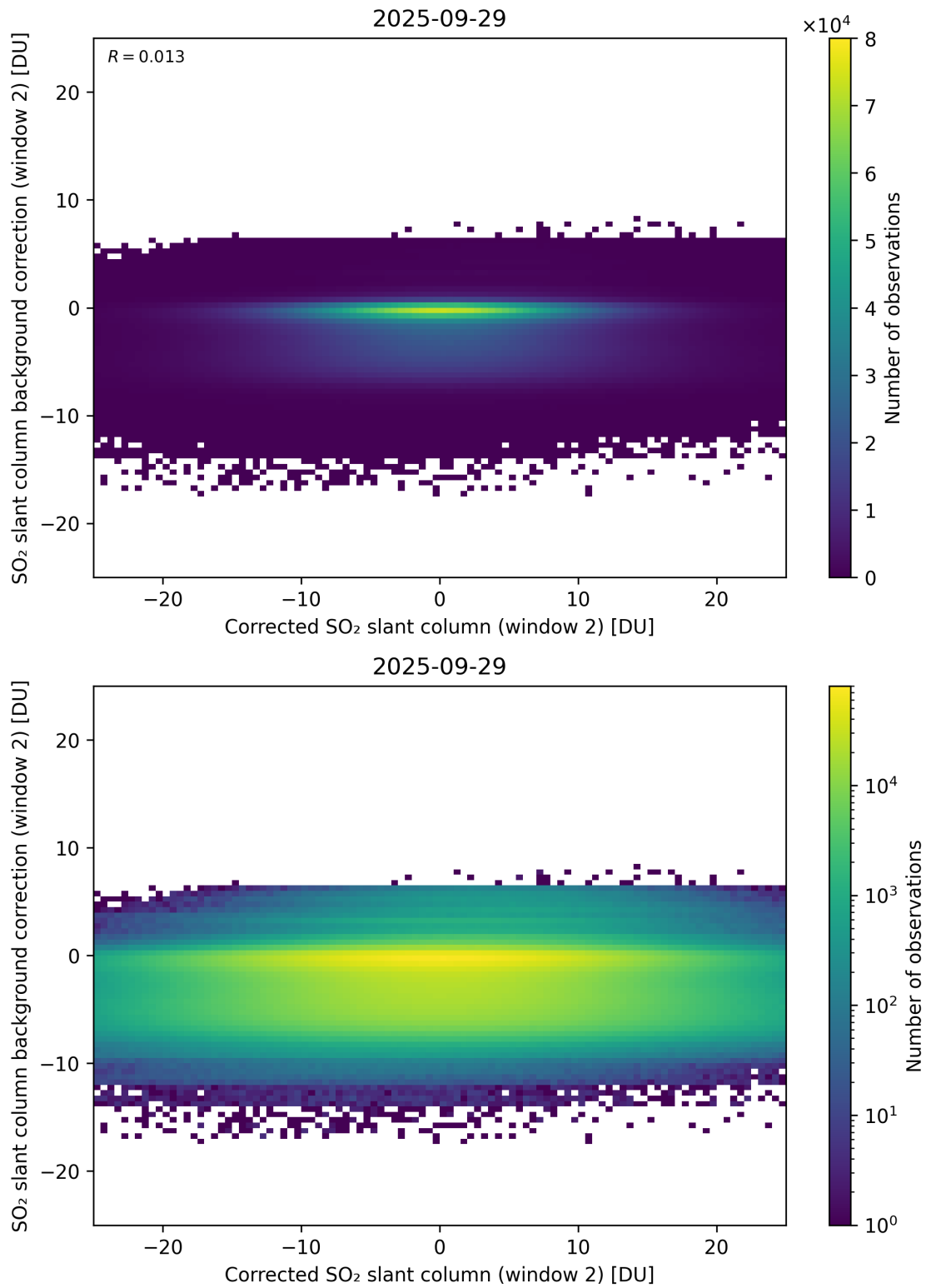
Figure 244: Scatter density plot of “Corrected SO 2 slant column (window 2)” against “SO 2 slant column background correction (window 2)” for 2025-09-28 to 2025-09-30.
