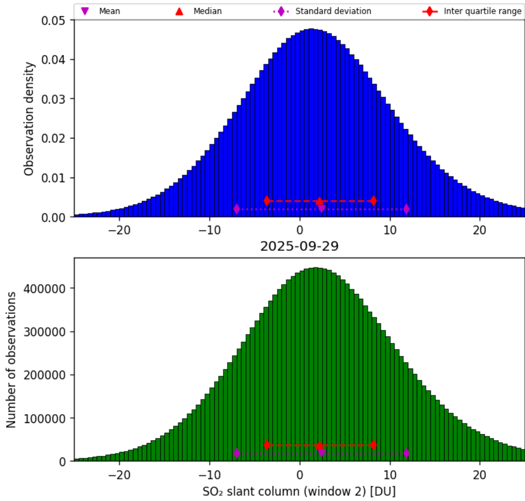
Figure 67: Histogram of “SO 2 slant column (window 2)” for 2025-09-28 to 2025-09-30
