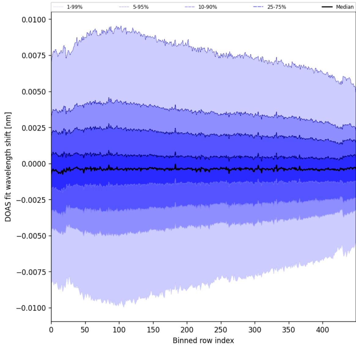
Figure 102: Along track statistics of “DOAS fit wavelength shift” for 2025-09-28 to 2025-09-30
