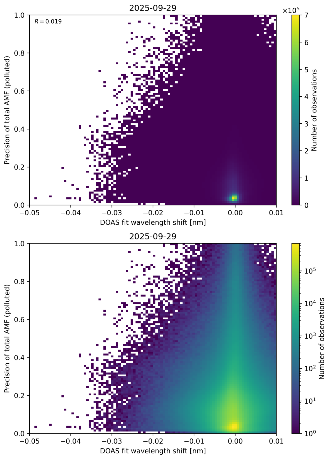
Figure 142: Scatter density plot of “DOAS fit wavelength shift” against “Precision of total AMF (polluted)” for 2025-09-28 to 2025-09-30.
