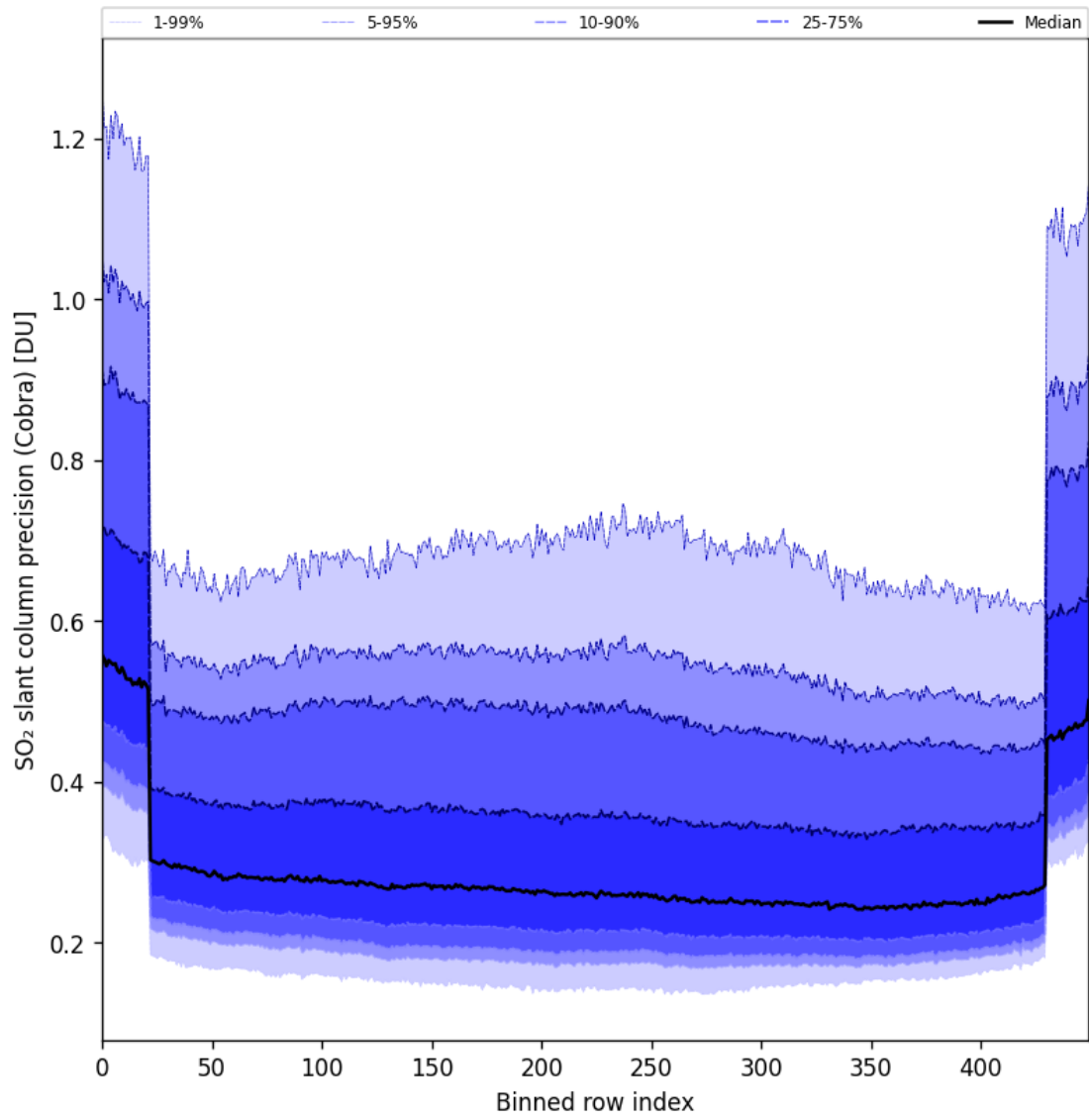
Figure 88: Along track statistics of “SO 2 slant column precision (Cobra)” for 2025-09-28 to 2025-09-30
