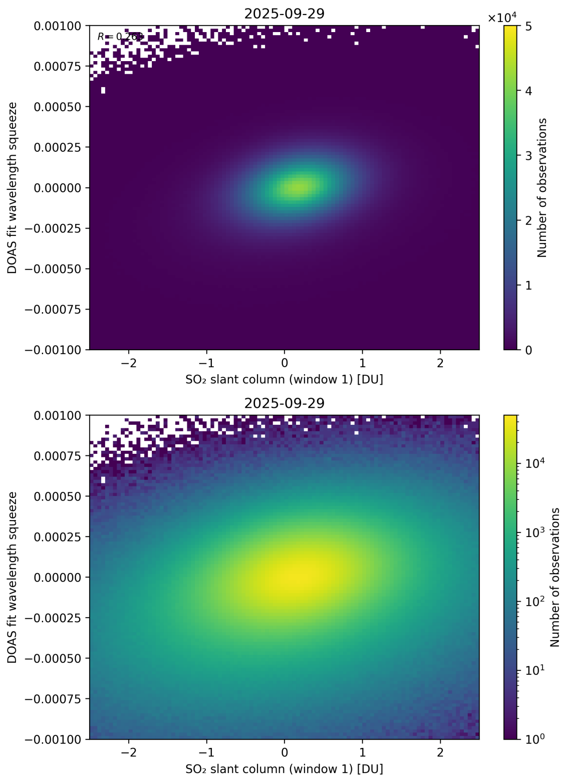
Figure 266: Scatter density plot of “SO 2 slant column (window 1)” against “DOAS fit wavelength squeeze” for 2025-09-28 to 2025-09-30.
