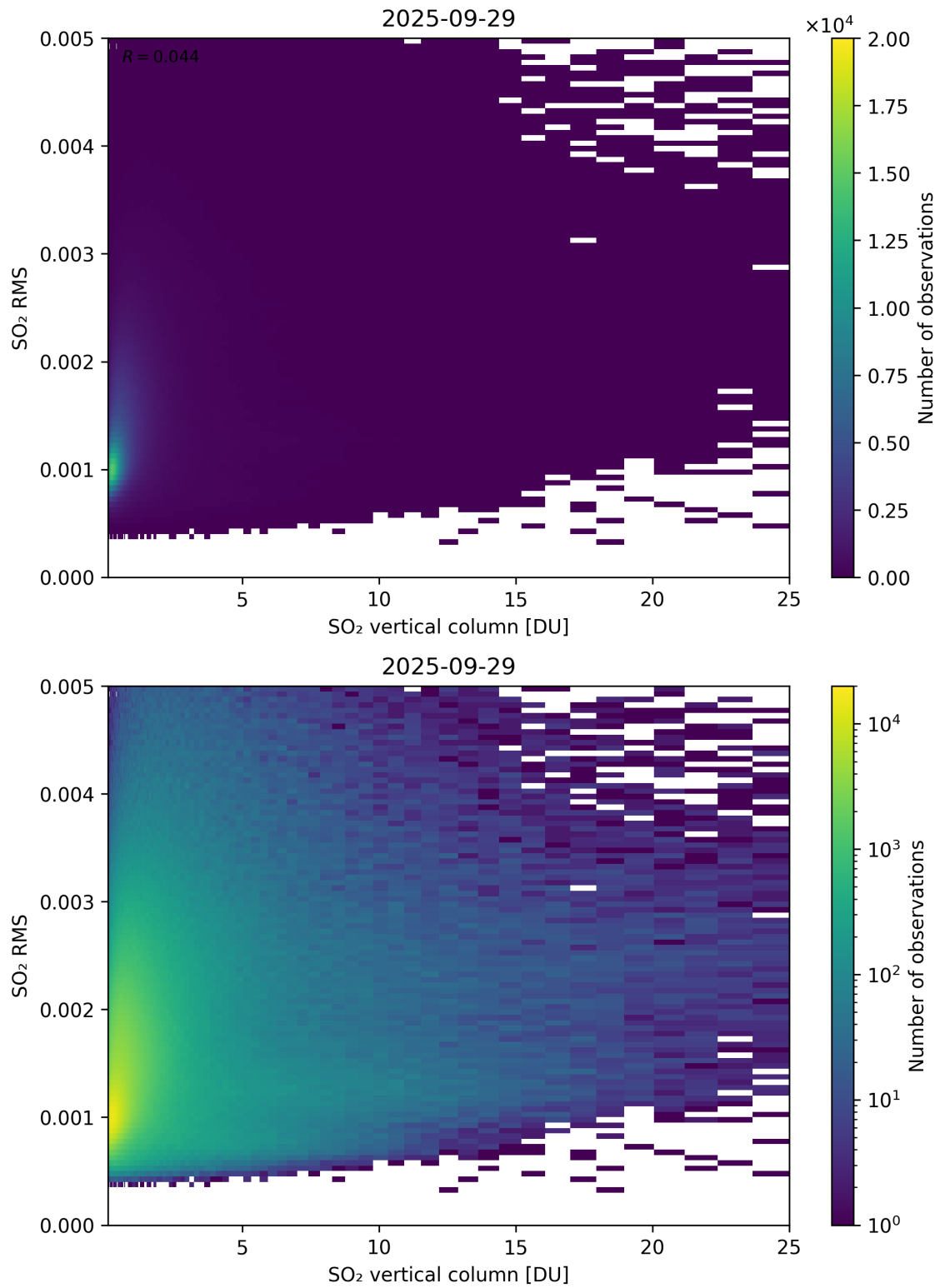
Figure 328: Scatter density plot of “SO 2 vertical column” against “SO 2 RMS” for 2025-09-28 to 2025-09-30.
