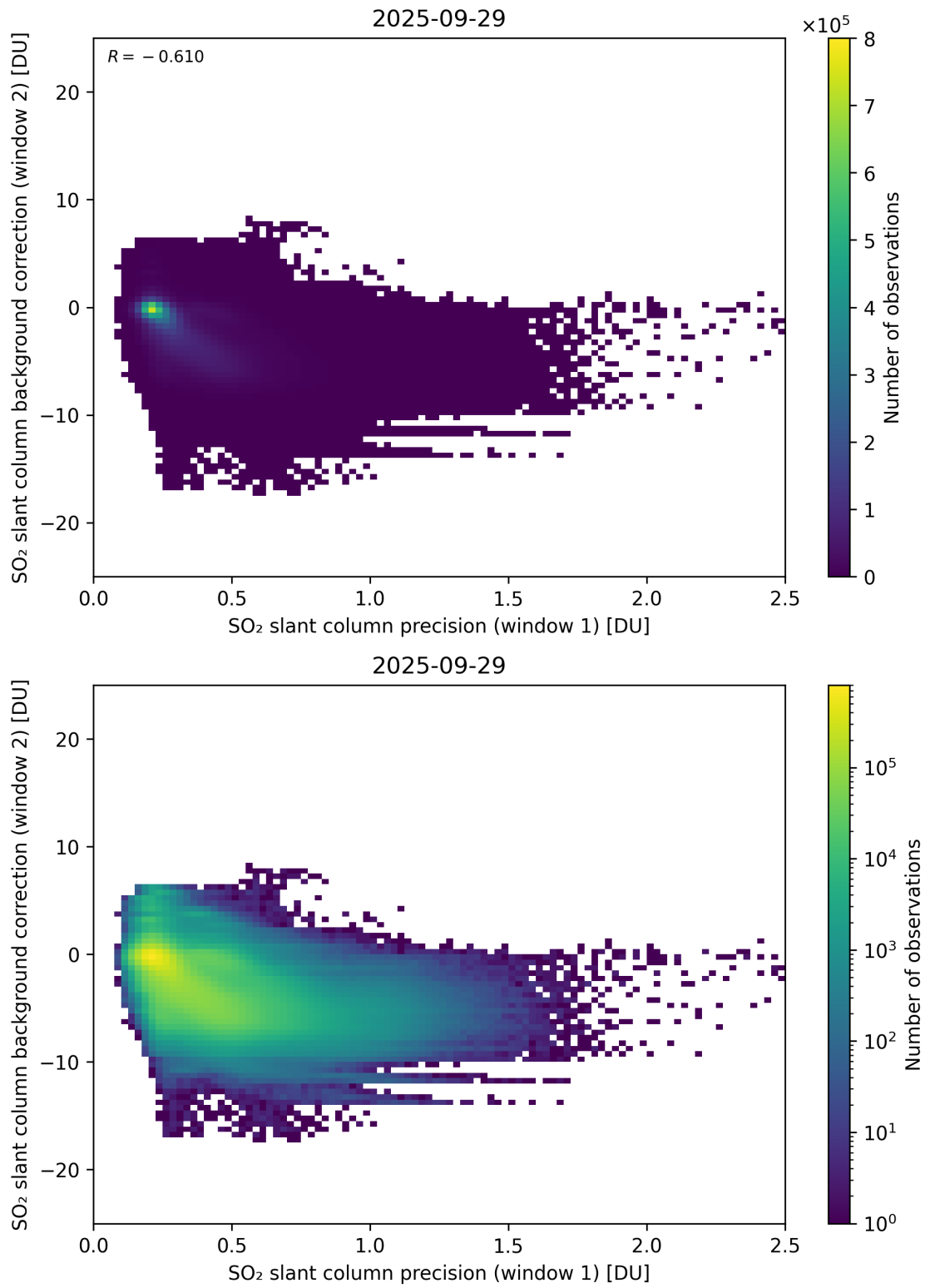
Figure 269: Scatter density plot of “SO 2 slant column precision (window 1)” against “SO 2 slant column background correction (window 2)” for 2025-09-28 to 2025-09-30.
