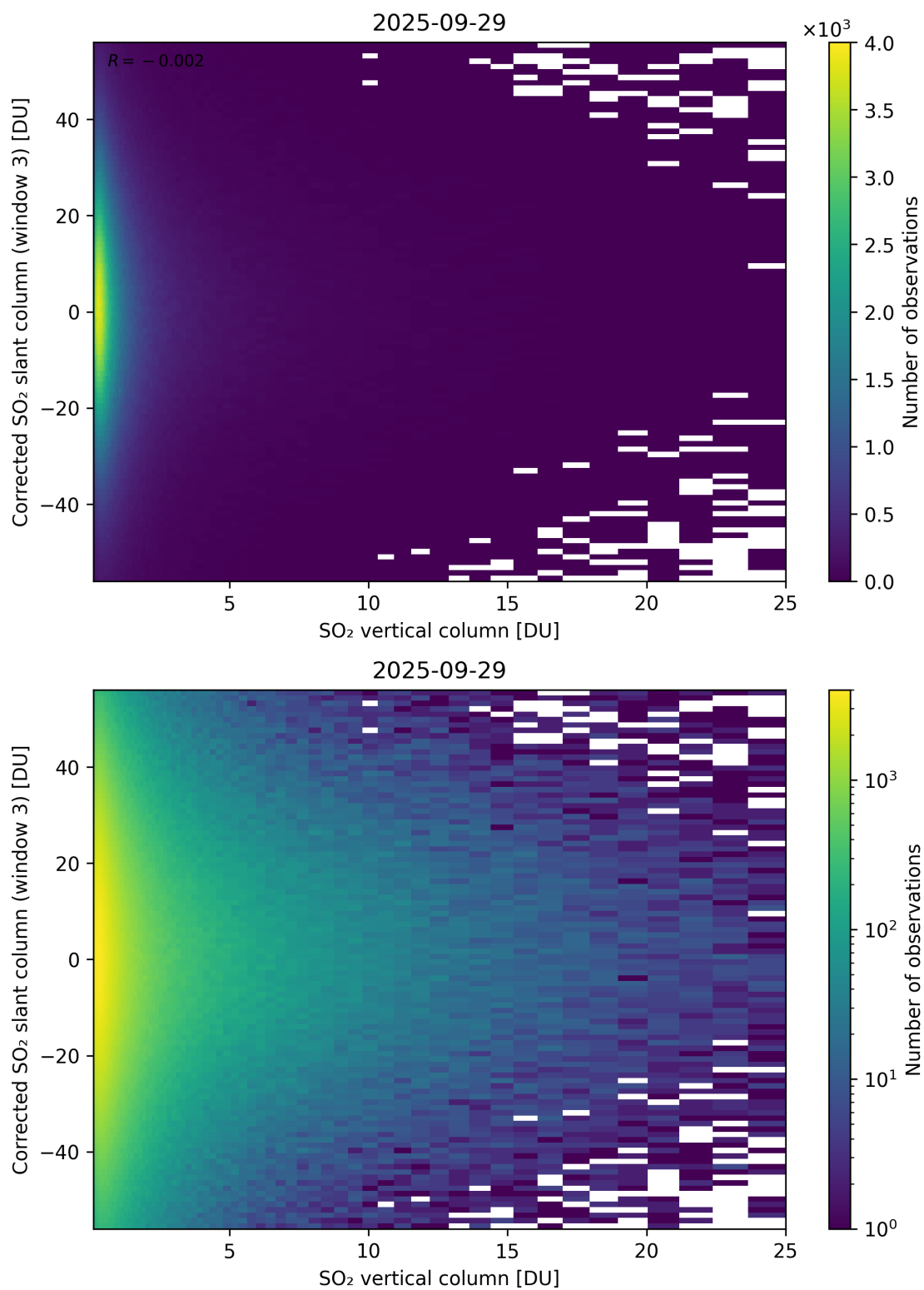
Figure 353: Scatter density plot of “SO 2 vertical column” against “Corrected SO 2 slant column (window 3)” for 2025-09-28 to 2025-09-30.
