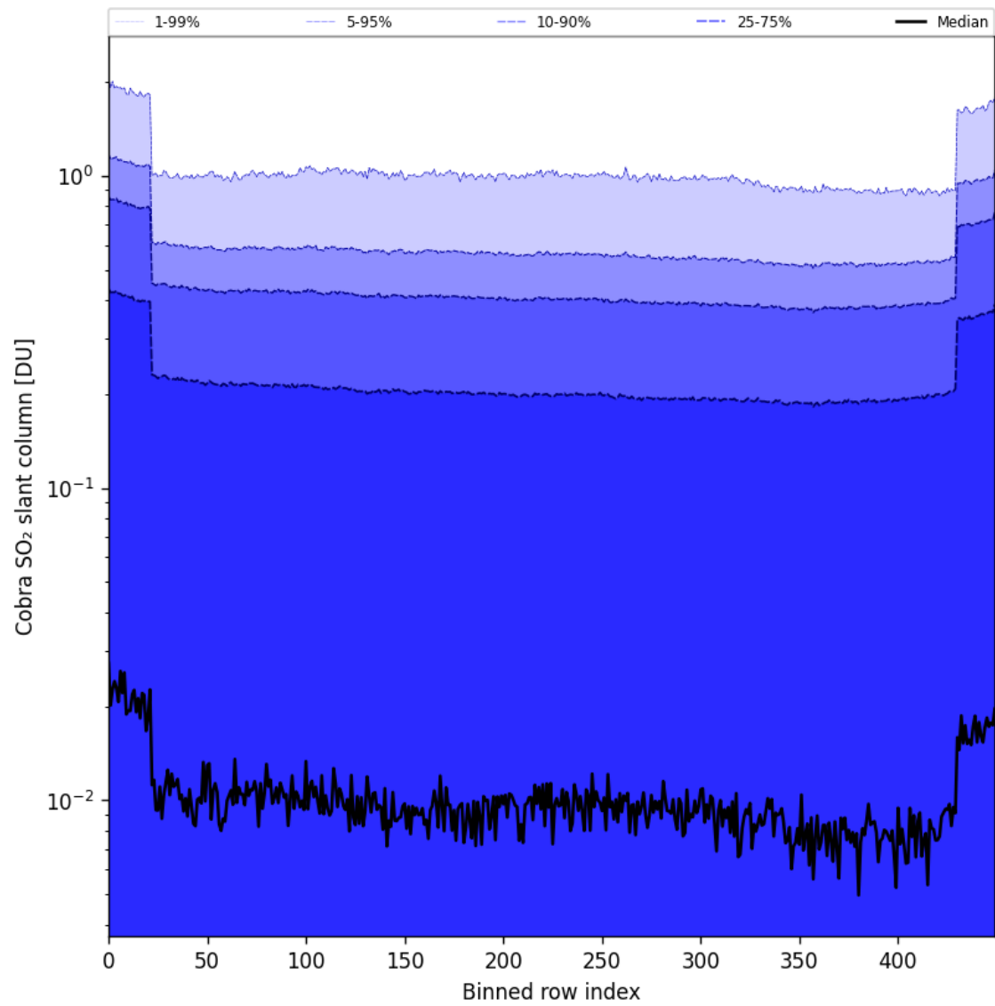
Figure 87: Along track statistics of “Cobra SO 2 slant column” for 2025-09-28 to 2025-09-30
