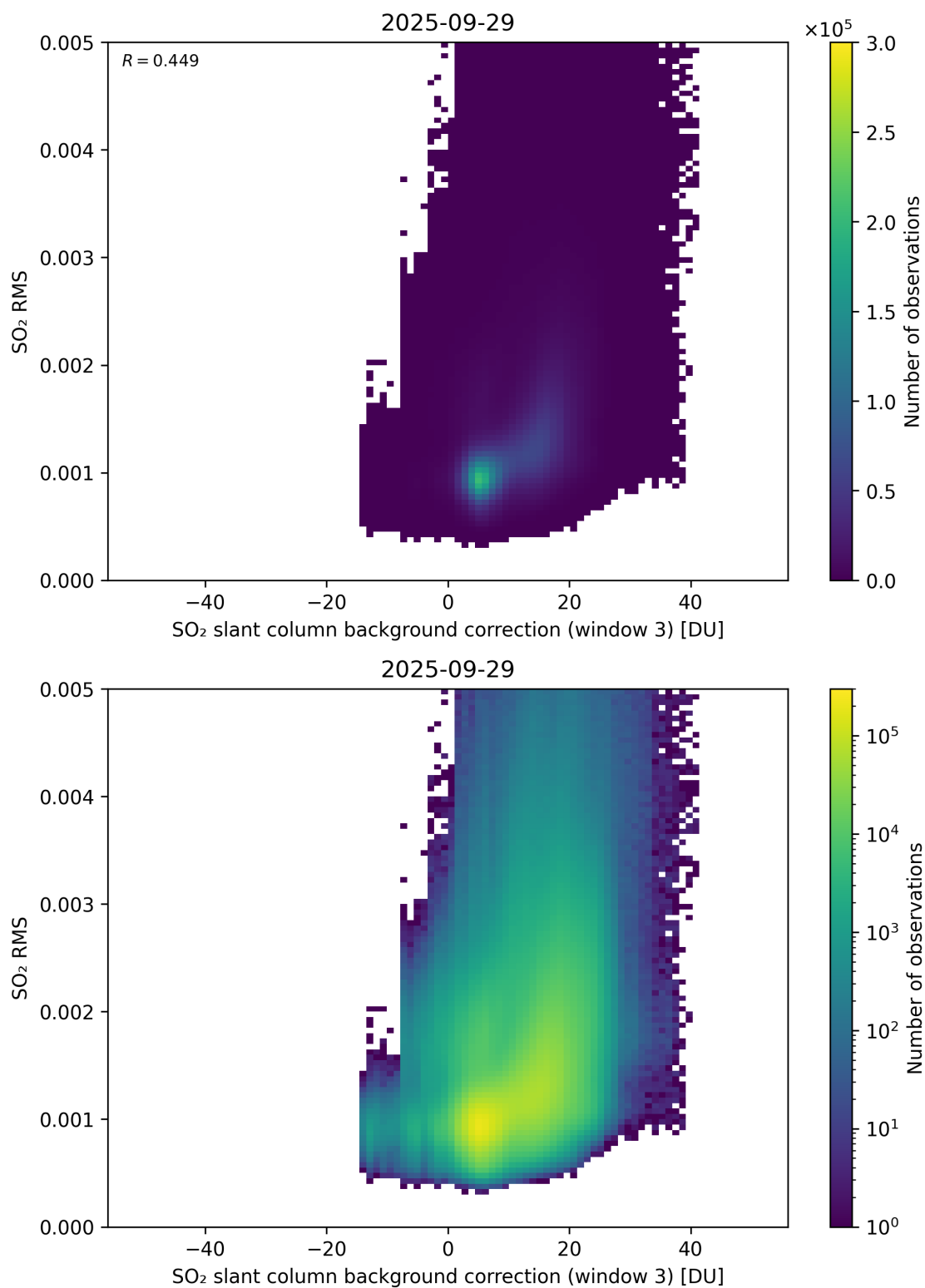
Figure 134: Scatter density plot of “SO 2 slant column background correction (window 3)” against “SO 2 RMS” for 2025-09-28 to 2025-09-30.
