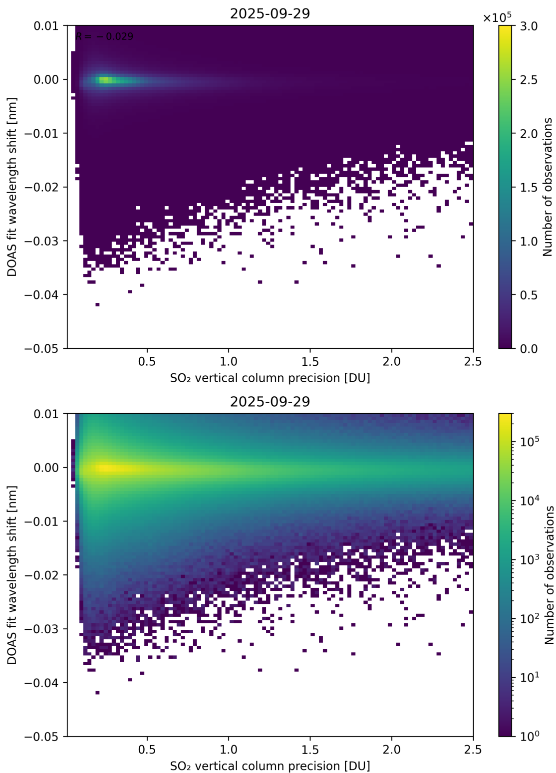
Figure 332: Scatter density plot of “SO 2 vertical column precision” against “DOAS fit wavelength shift” for 2025-09-28 to 2025-09-30.
