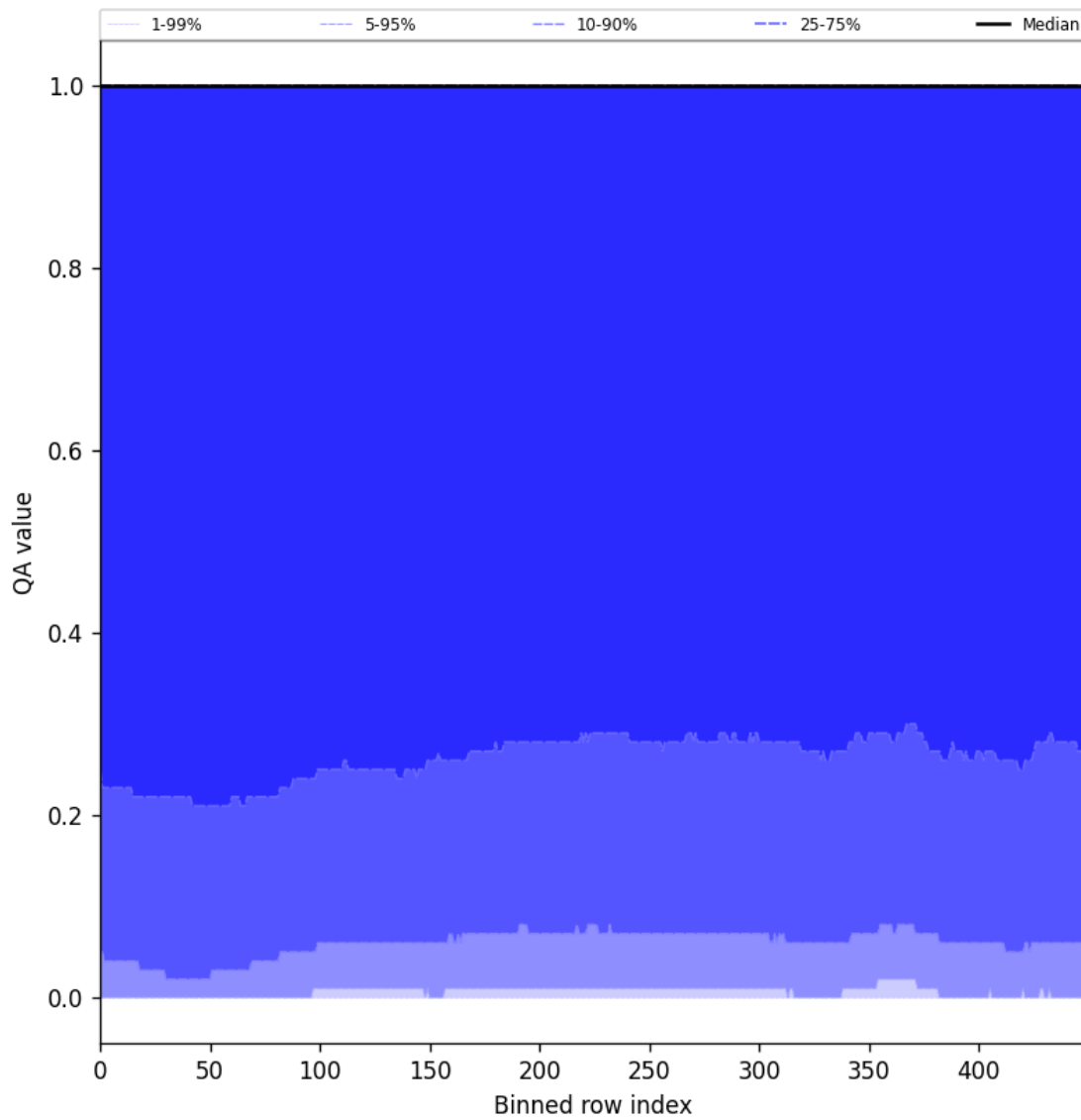
Figure 83: Along track statistics of “QA value” for 2025-09-28 to 2025-09-30
