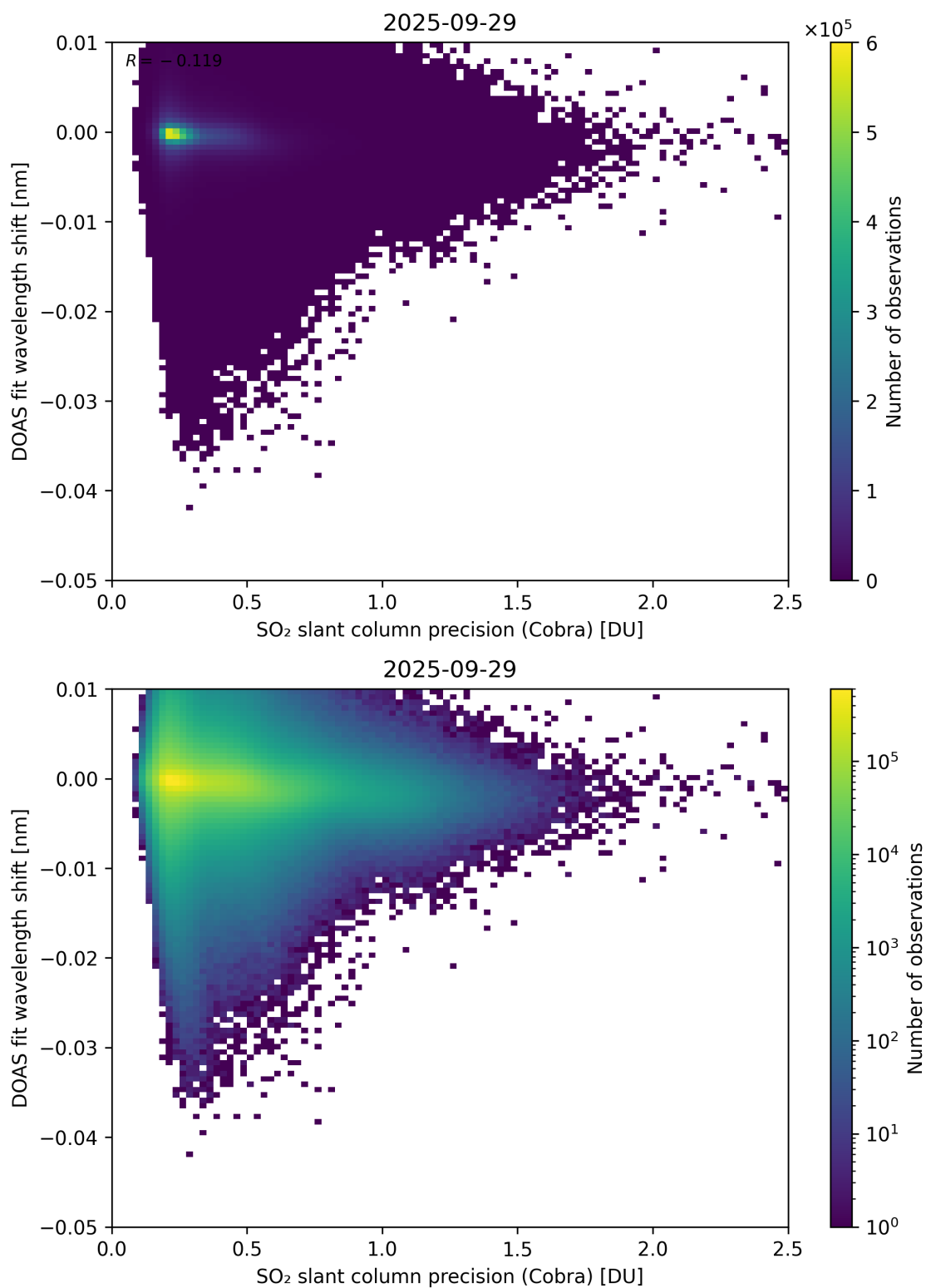
Figure 202: Scatter density plot of “SO 2 slant column precision (Cobra)” against “DOAS fit wavelength shift” for 2025-09-28 to 2025-09-30.
