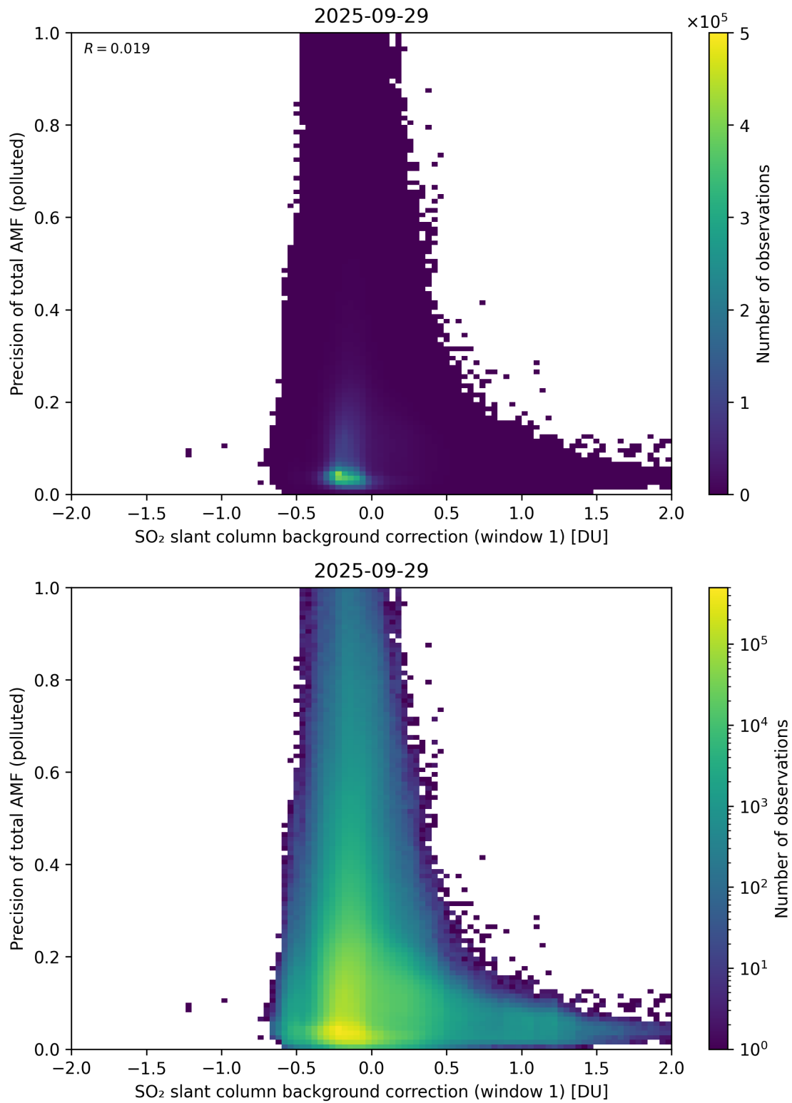
Figure 121: Scatter density plot of “SO 2 slant column background correction (window 1)” against “Precision of total AMF (polluted)” for 2025-09-28 to 2025-09-30.
