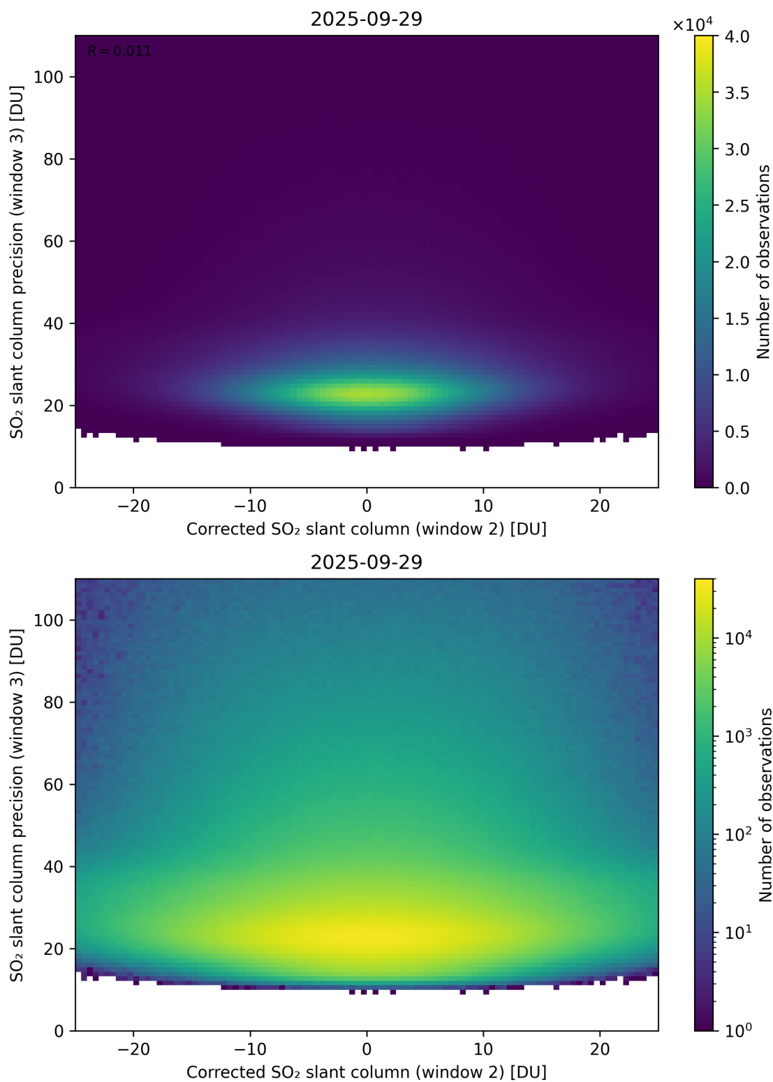
Figure 252: Scatter density plot of “Corrected SO 2 slant column (window 2)” against “SO 2 slant column precision (window 3)” for 2025-09-28 to 2025-09-30.
