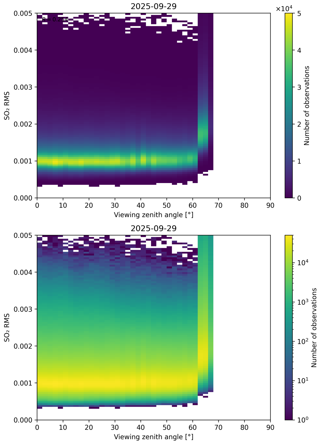
Figure 367: Scatter density plot of “Viewing zenith angle” against “SO 2 RMS” for 2025-09-28 to 2025-09-30.
