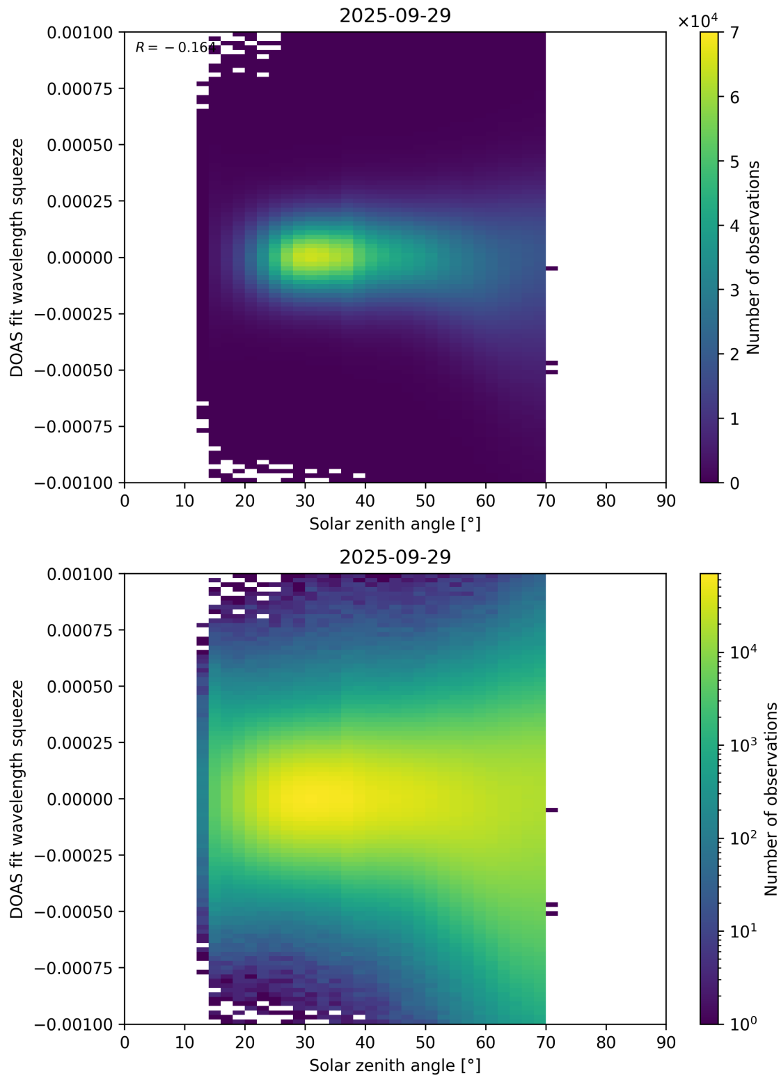
Figure 175: Scatter density plot of “Solar zenith angle” against “DOAS fit wavelength squeeze” for 2025-09-28 to 2025-09-30.
