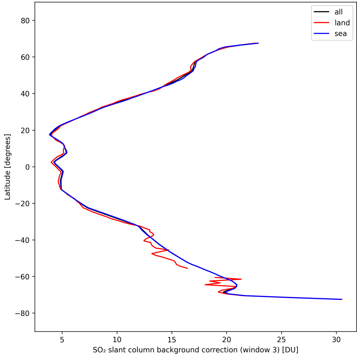
Figure 48: Zonal average of “SO 2 slant column background correction (window 3)” for 2025-09-28 to 2025-09-30.
