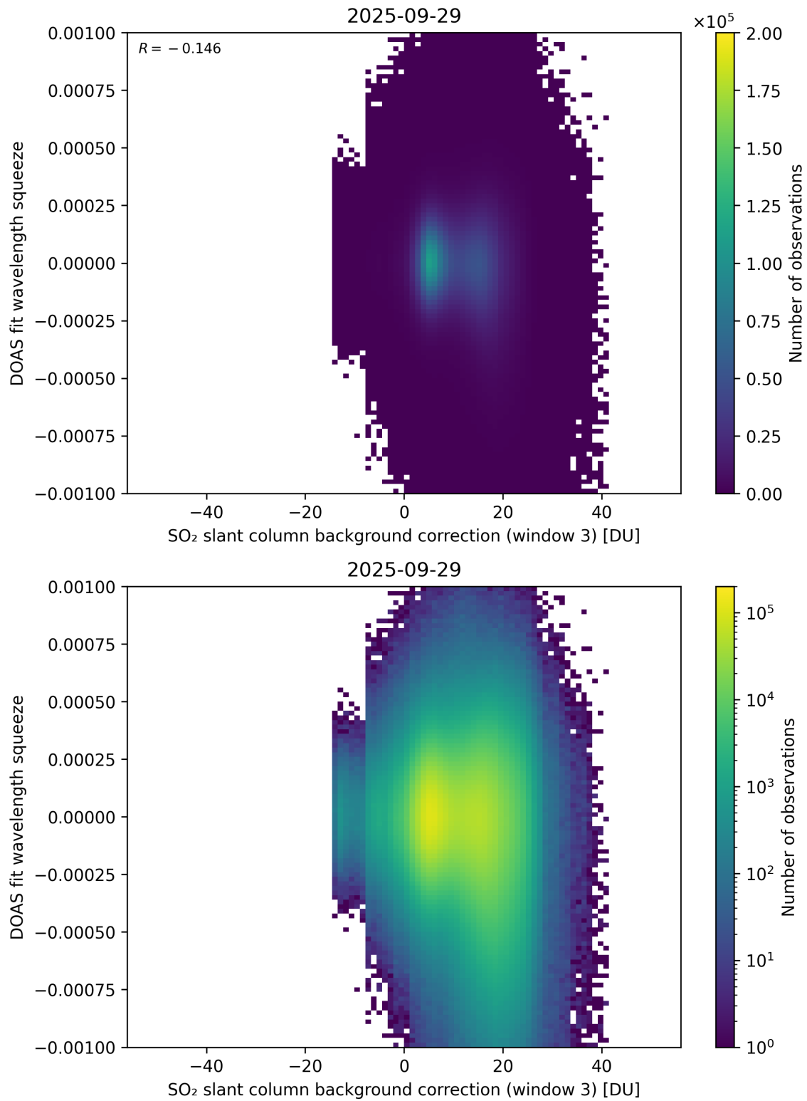
Figure 133: Scatter density plot of “SO 2 slant column background correction (window 3)” against “DOAS fit wavelength squeeze” for 2025-09-28 to 2025-09-30.
