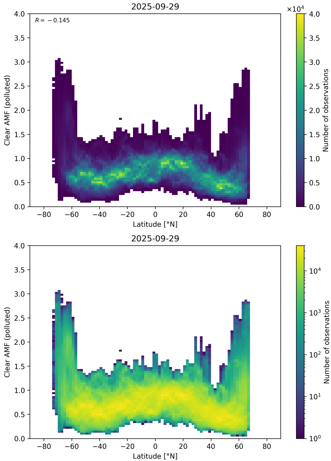
Figure 156: Scatter density plot of “Latitude” against “Clear AMF (polluted)” for 2025-09-28 to 2025-09-30.
