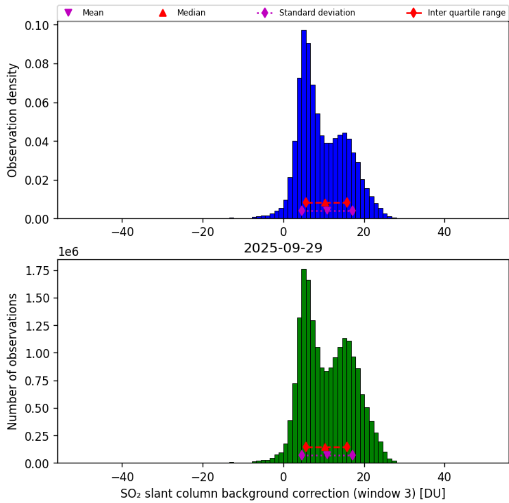
Figure 74: Histogram of “SO 2 slant column background correction (window 3)” for 2025-09-28 to 2025-09-30
