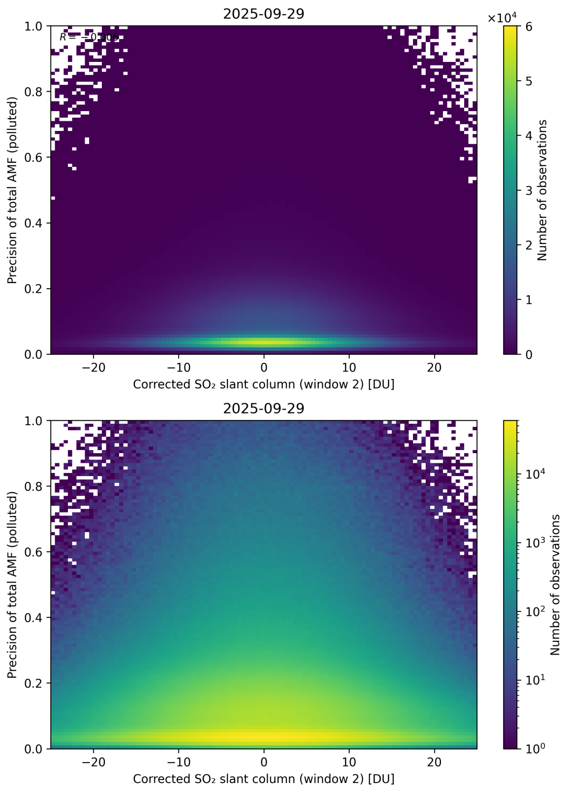
Figure 254: Scatter density plot of “Corrected SO 2 slant column (window 2)” against “Precision of total AMF (polluted)” for 2025-09-28 to 2025-09-30.
