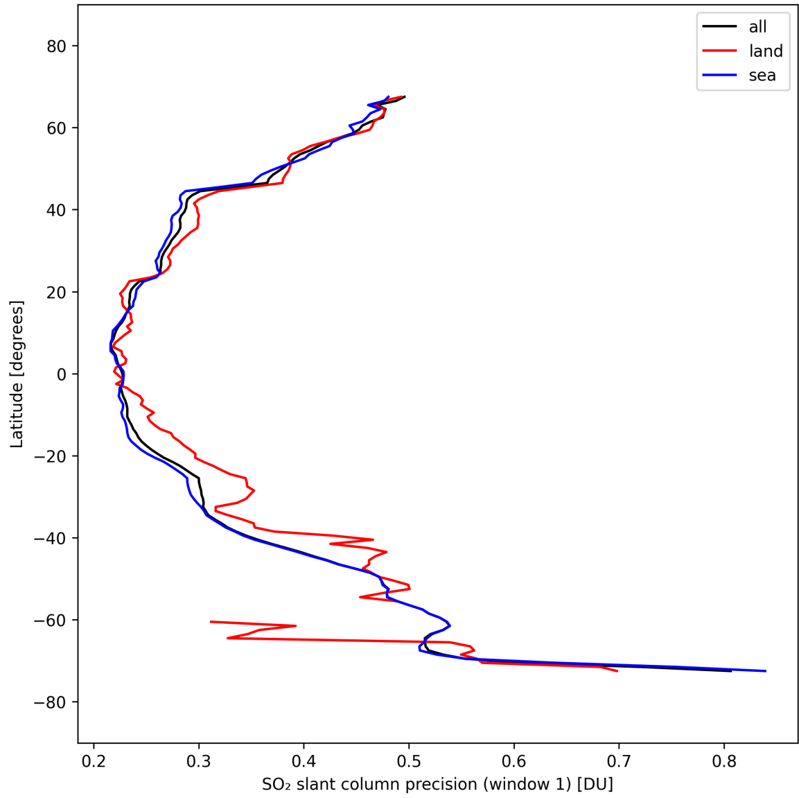
Figure 38: Zonal average of “SO 2 slant column precision (window 1)” for 2025-09-28 to 2025-09-30.
