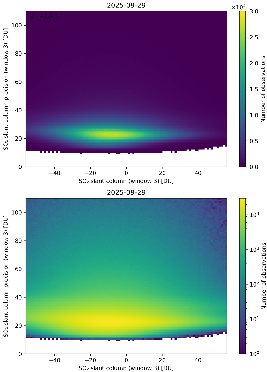
Figure 317: Scatter density plot of “SO 2 slant column (window 3)” against “SO 2 slant column precision (window 3)” for 2025-09-28 to 2025-09-30.
