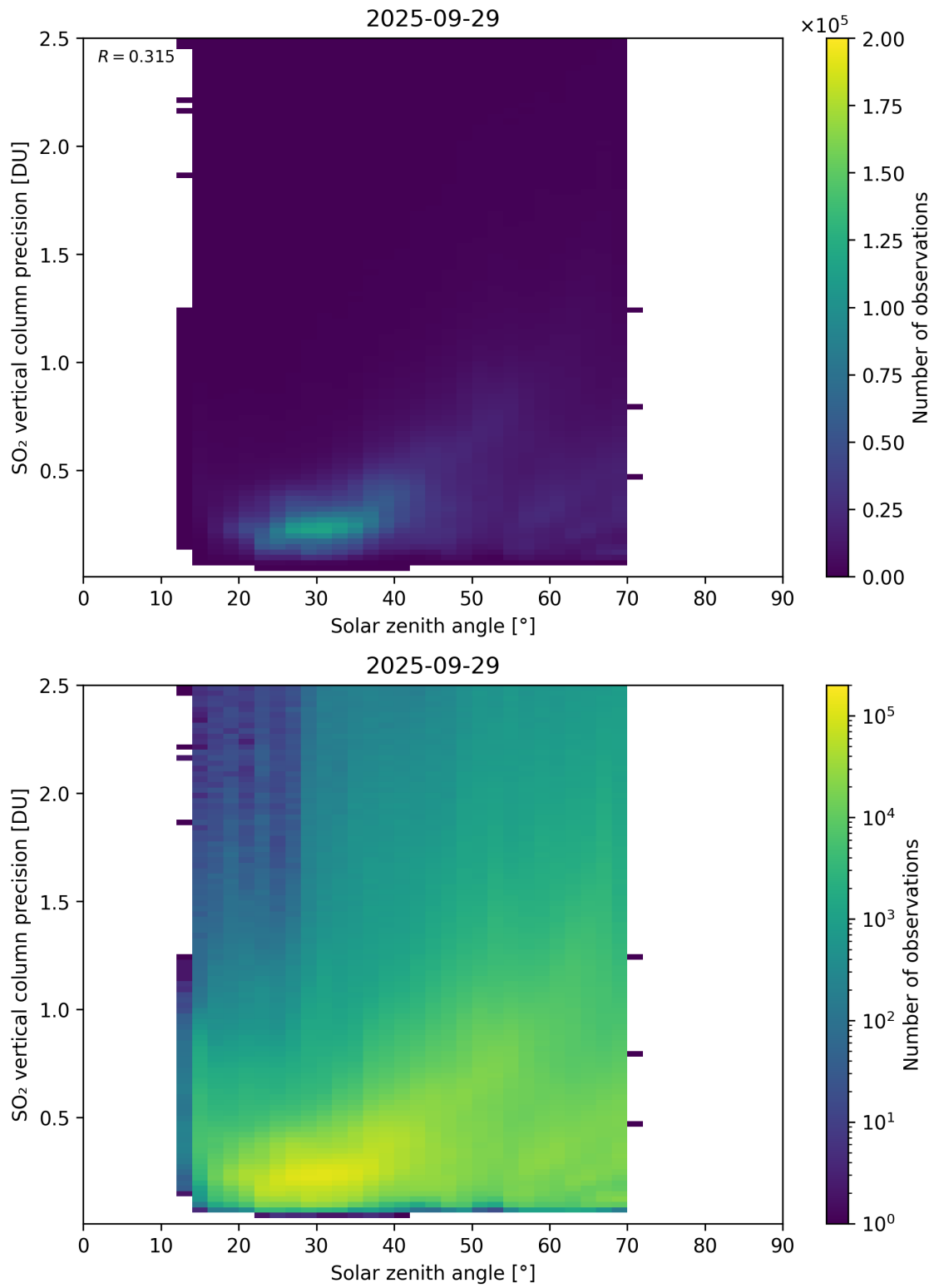
Figure 192: Scatter density plot of “Solar zenith angle” against “SO 2 vertical column precision” for 2025-09-28 to 2025-09-30.
