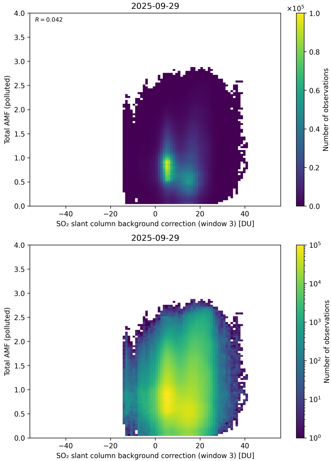
Figure 136: Scatter density plot of “SO 2 slant column background correction (window 3)” against “Total AMF (polluted)” for 2025-09-28 to 2025-09-30.
