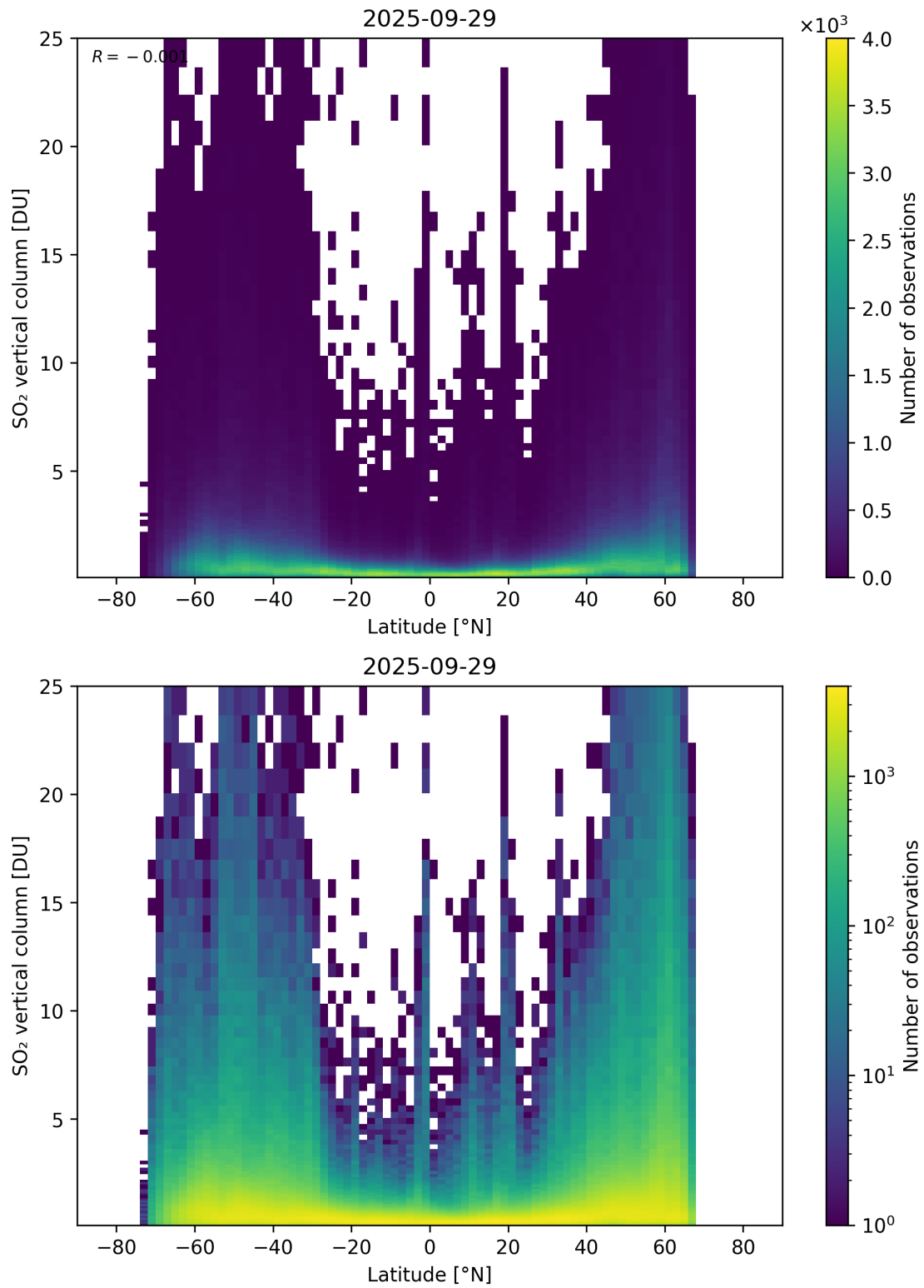
Figure 169: Scatter density plot of “Latitude” against “SO 2 vertical column” for 2025-09-28 to 2025-09-30.
