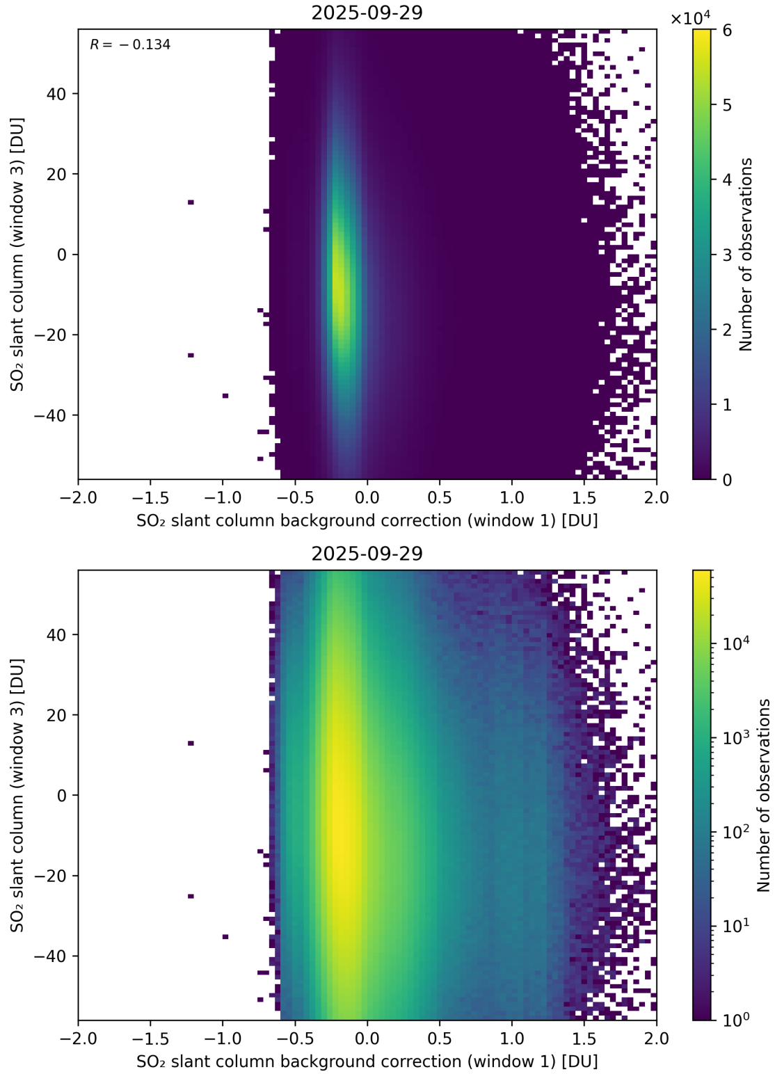
Figure 118: Scatter density plot of “SO 2 slant column background correction (window 1)” against “SO 2 slant column (window 3)” for 2025-09-28 to 2025-09-30.
