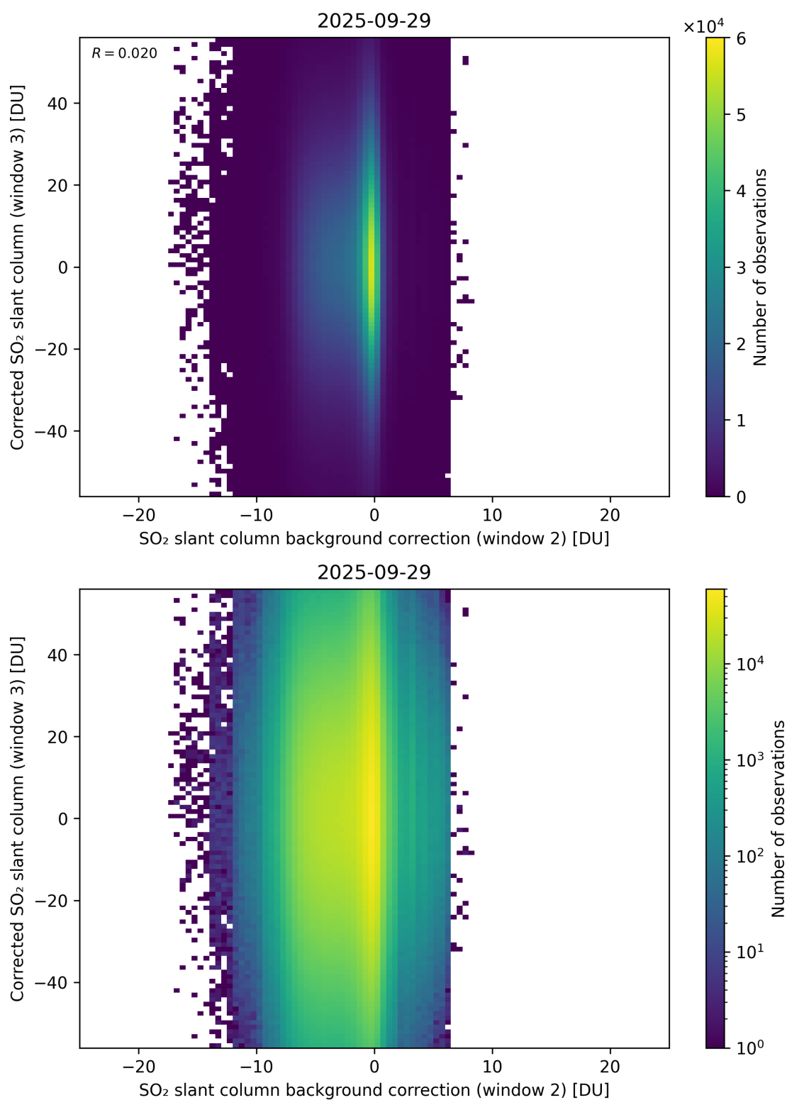
Figure 127: Scatter density plot of “SO 2 slant column background correction (window 2)” against “Corrected SO 2 slant column (window 3)” for 2025-09-28 to 2025-09-30.
