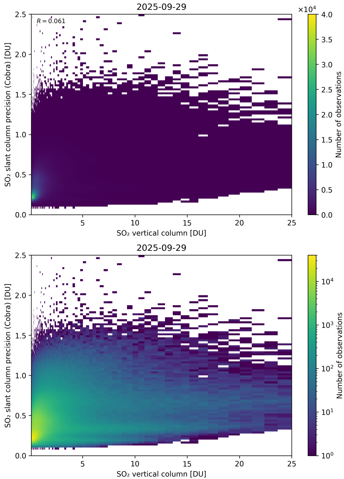
Figure 350: Scatter density plot of “SO 2 vertical column” against “SO 2 slant column precision (Cobra)” for 2025-09-28 to 2025-09-30.
