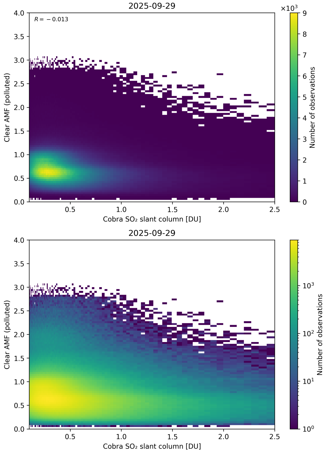
Figure 215: Scatter density plot of “Cobra SO 2 slant column” against “Clear AMF (polluted)” for 2025-09-28 to 2025-09-30.
