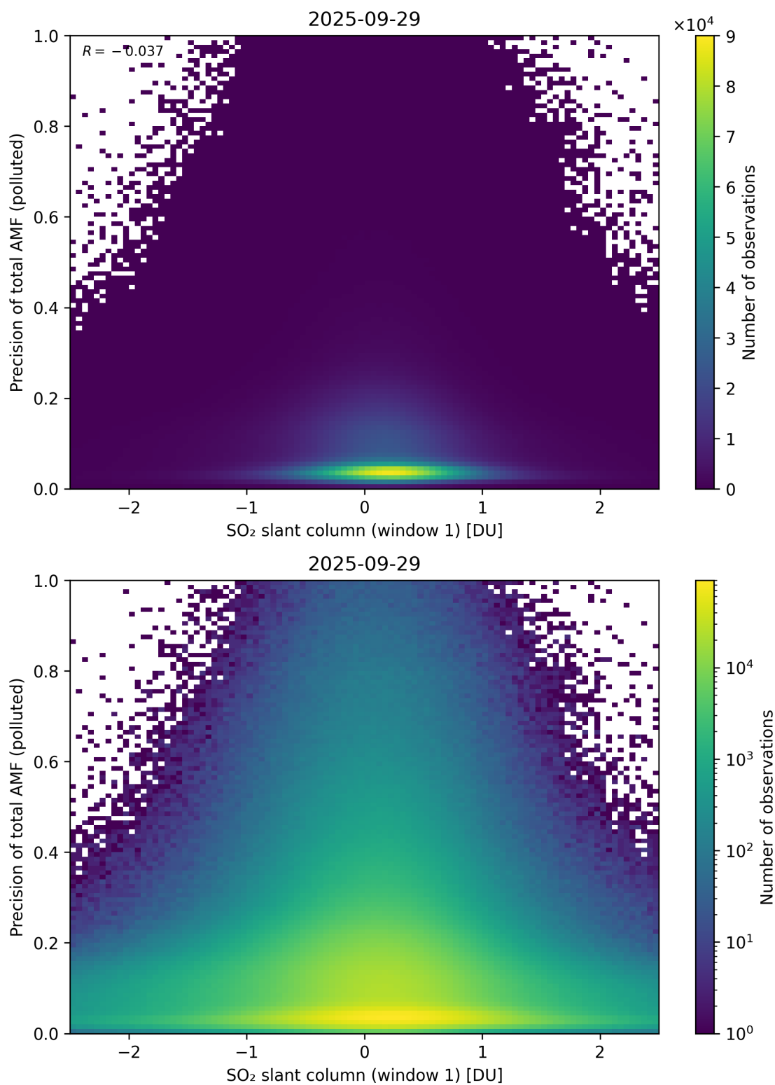
Figure 290: Scatter density plot of “SO 2 slant column (window 1)” against “Precision of total AMF (polluted)” for 2025-09-28 to 2025-09-30.
