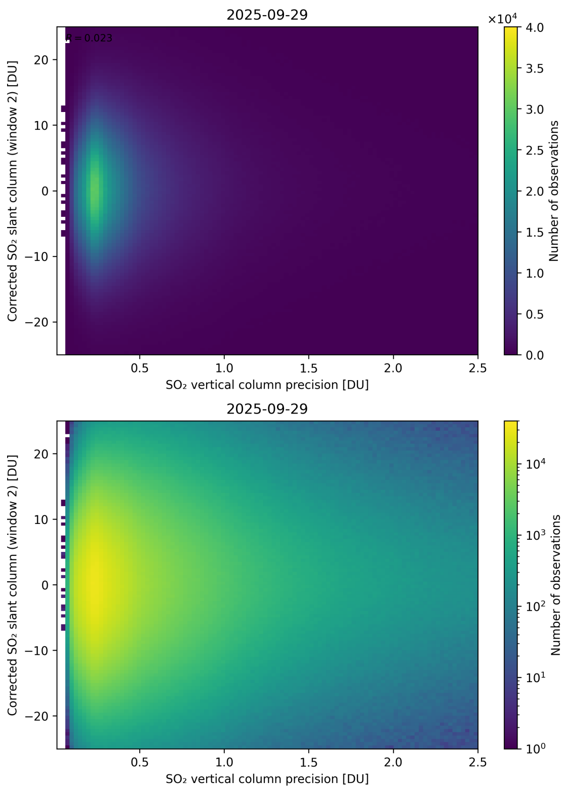
Figure 339: Scatter density plot of “SO 2 vertical column precision” against “Corrected SO 2 slant column (window 2)” for 2025-09-28 to 2025-09-30.
