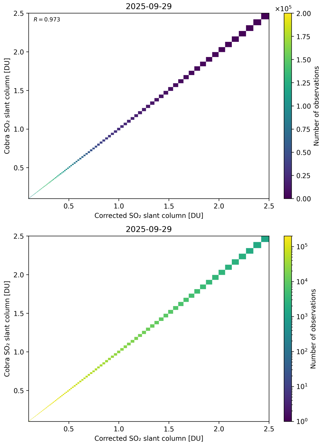
Figure 233: Scatter density plot of “Corrected SO 2 slant column” against “Cobra SO 2 slant column” for 2025-09-28 to 2025-09-30.
