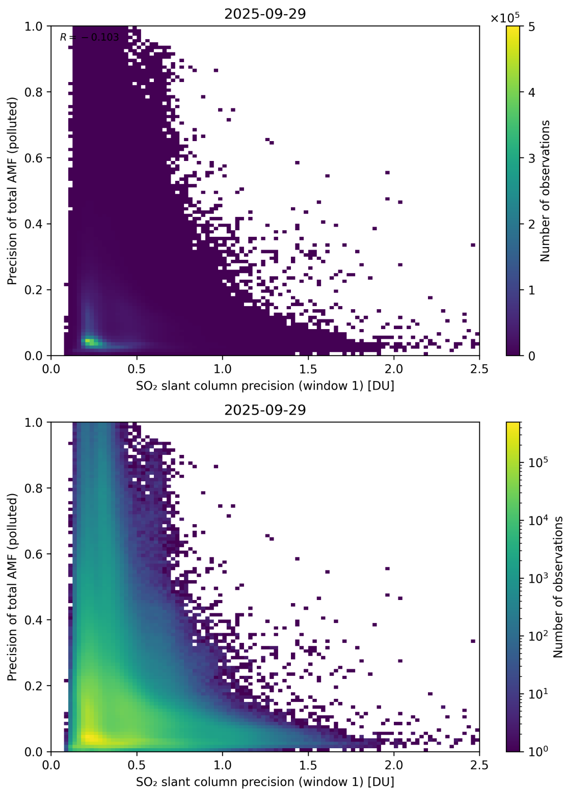
Figure 281: Scatter density plot of “SO 2 slant column precision (window 1)” against “Precision of total AMF (polluted)” for 2025-09-28 to 2025-09-30.
