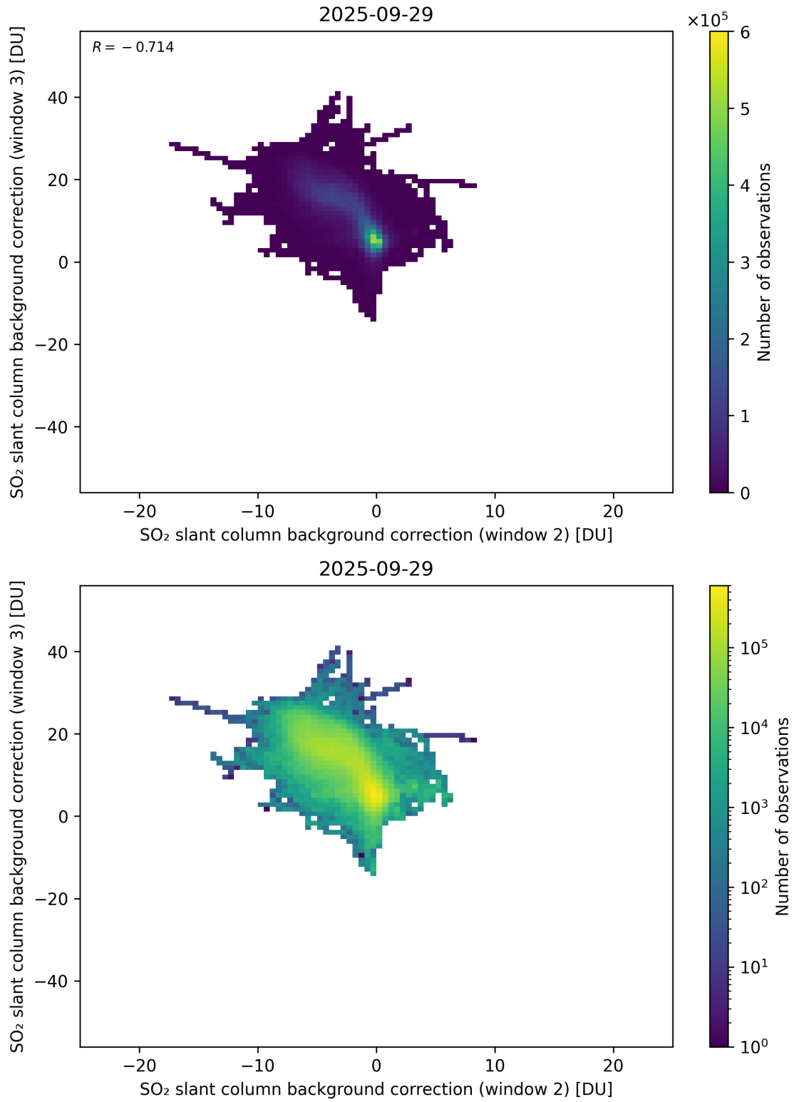
Figure 122: Scatter density plot of “SO 2 slant column background correction (window 2)” against “SO 2 slant column background correction (window 3)” for 2025-09-28 to 2025-09-30.
