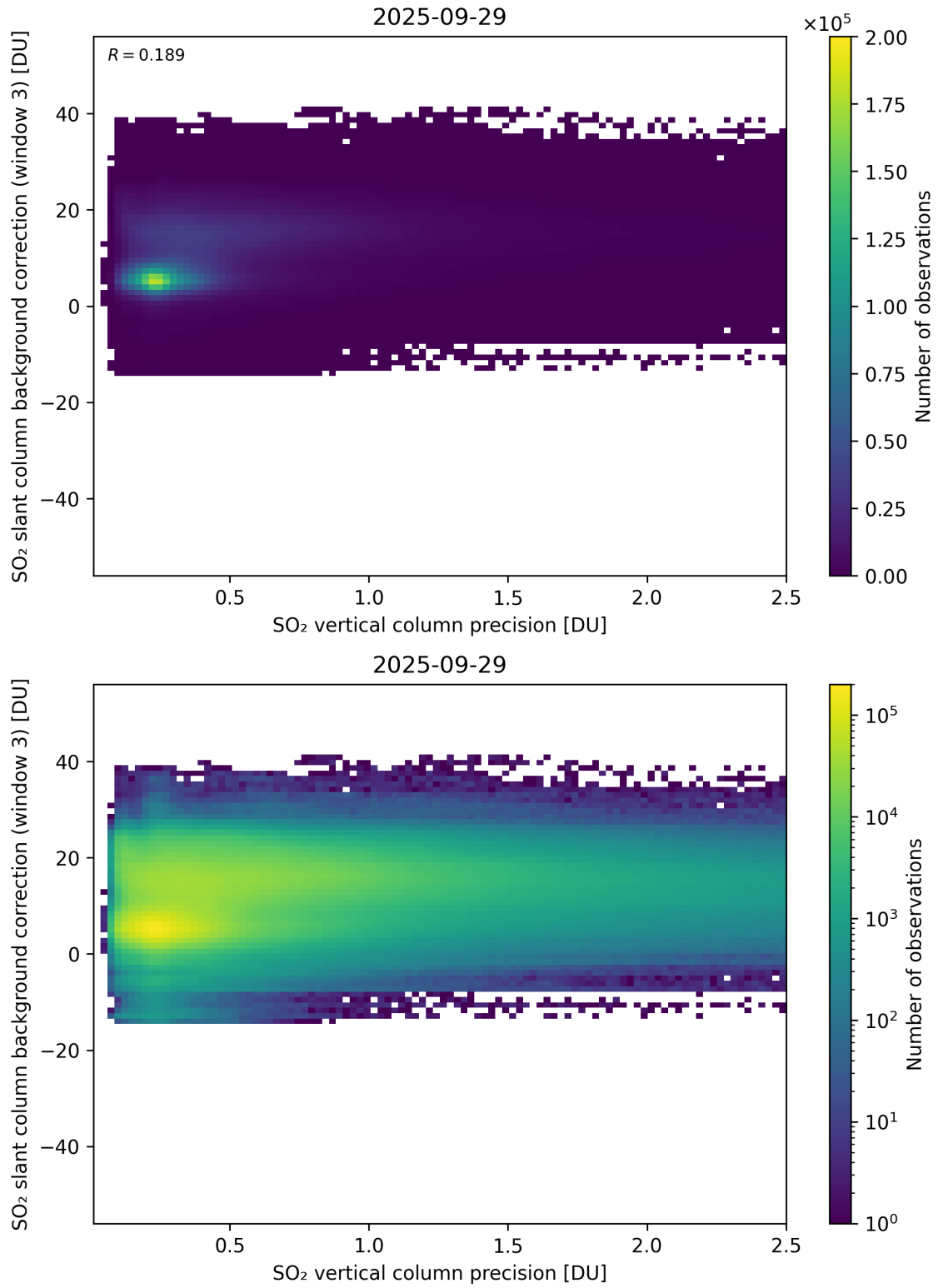
Figure 331: Scatter density plot of “SO 2 vertical column precision” against “SO 2 slant column background correction (window 3)” for 2025-09-28 to 2025-09-30.
