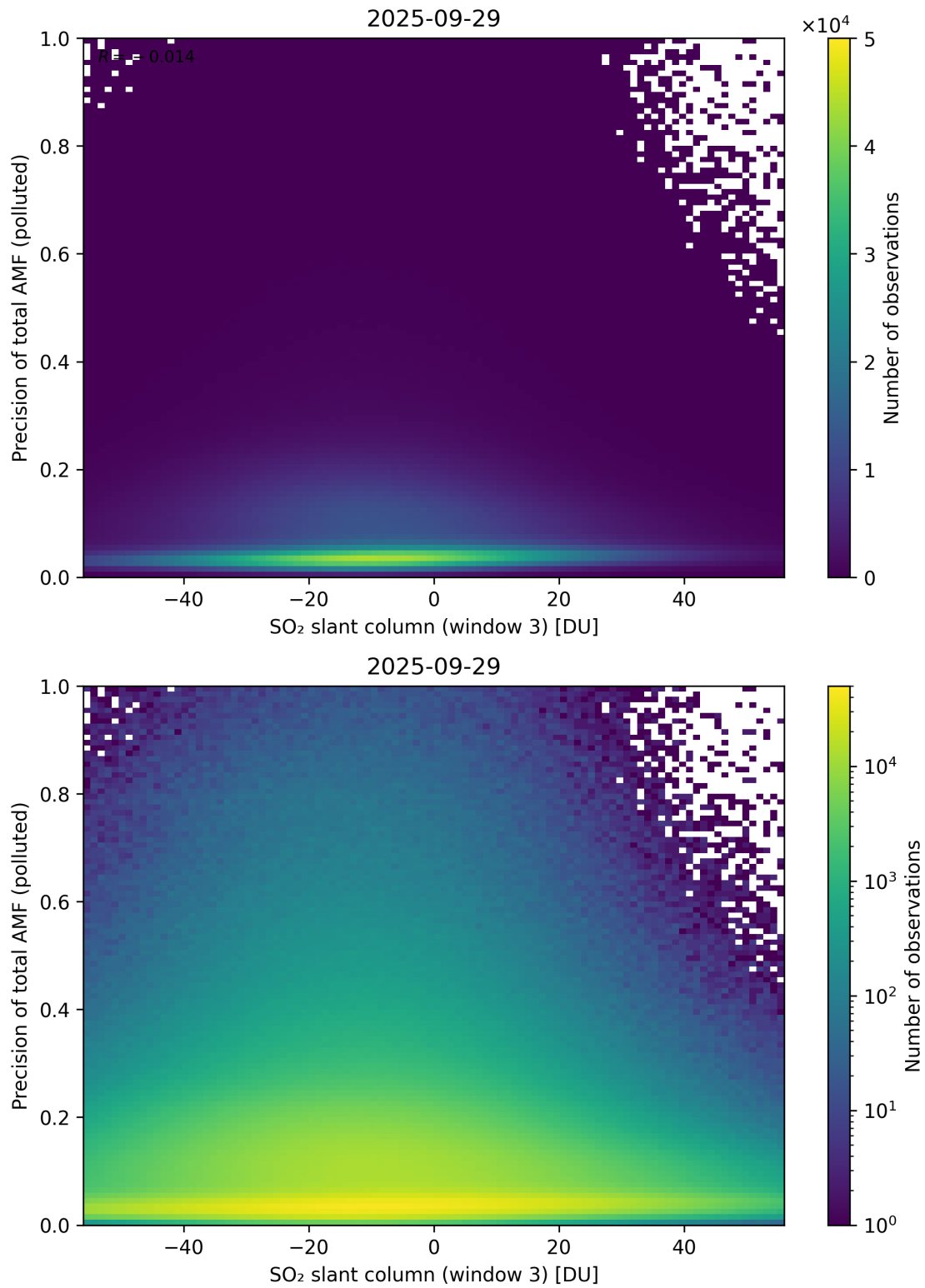
Figure 319: Scatter density plot of “SO 2 slant column (window 3)” against “Precision of total AMF (polluted)” for 2025-09-28 to 2025-09-30.
