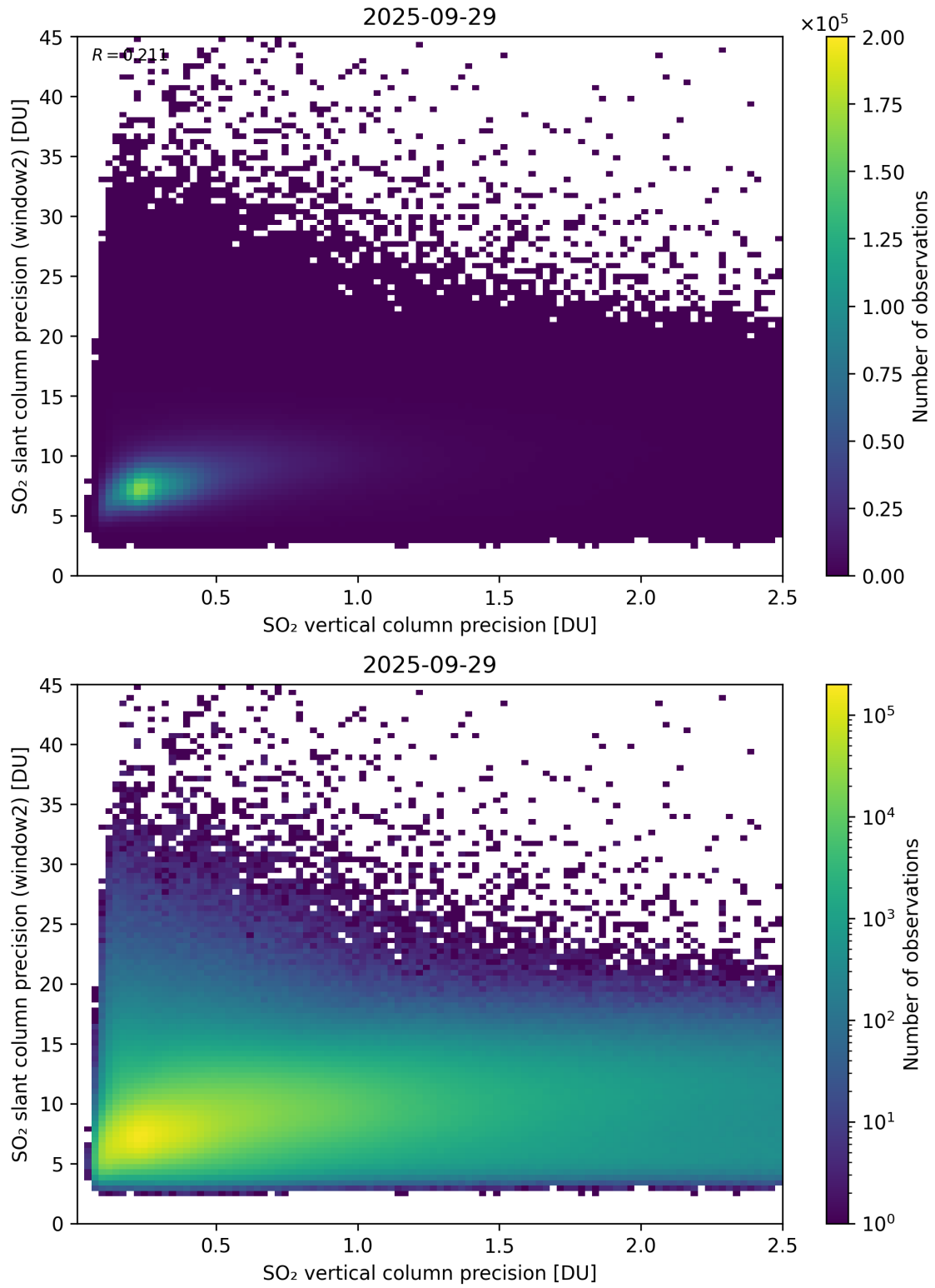
Figure 343: Scatter density plot of “SO 2 vertical column precision” against “SO 2 slant column precision (window2)” for 2025-09-28 to 2025-09-30.
