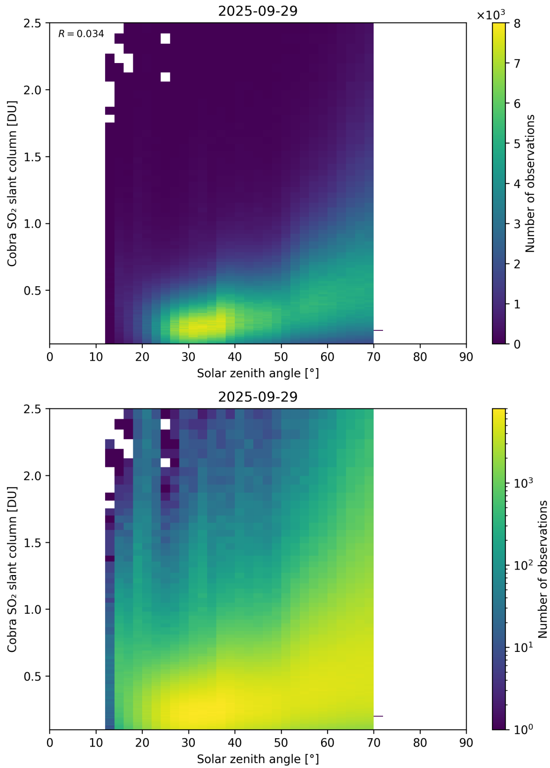
Figure 179: Scatter density plot of “Solar zenith angle” against “Cobra SO 2 slant column” for 2025-09-28 to 2025-09-30.
