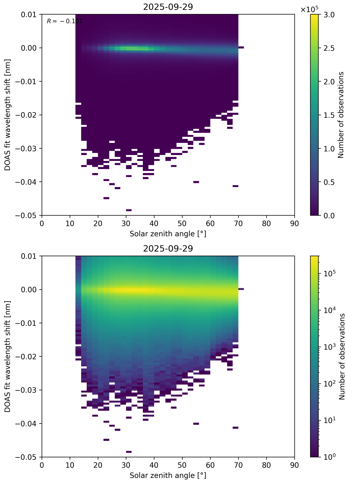
Figure 174: Scatter density plot of “Solar zenith angle” against “DOAS fit wavelength shift” for 2025-09-28 to 2025-09-30.
