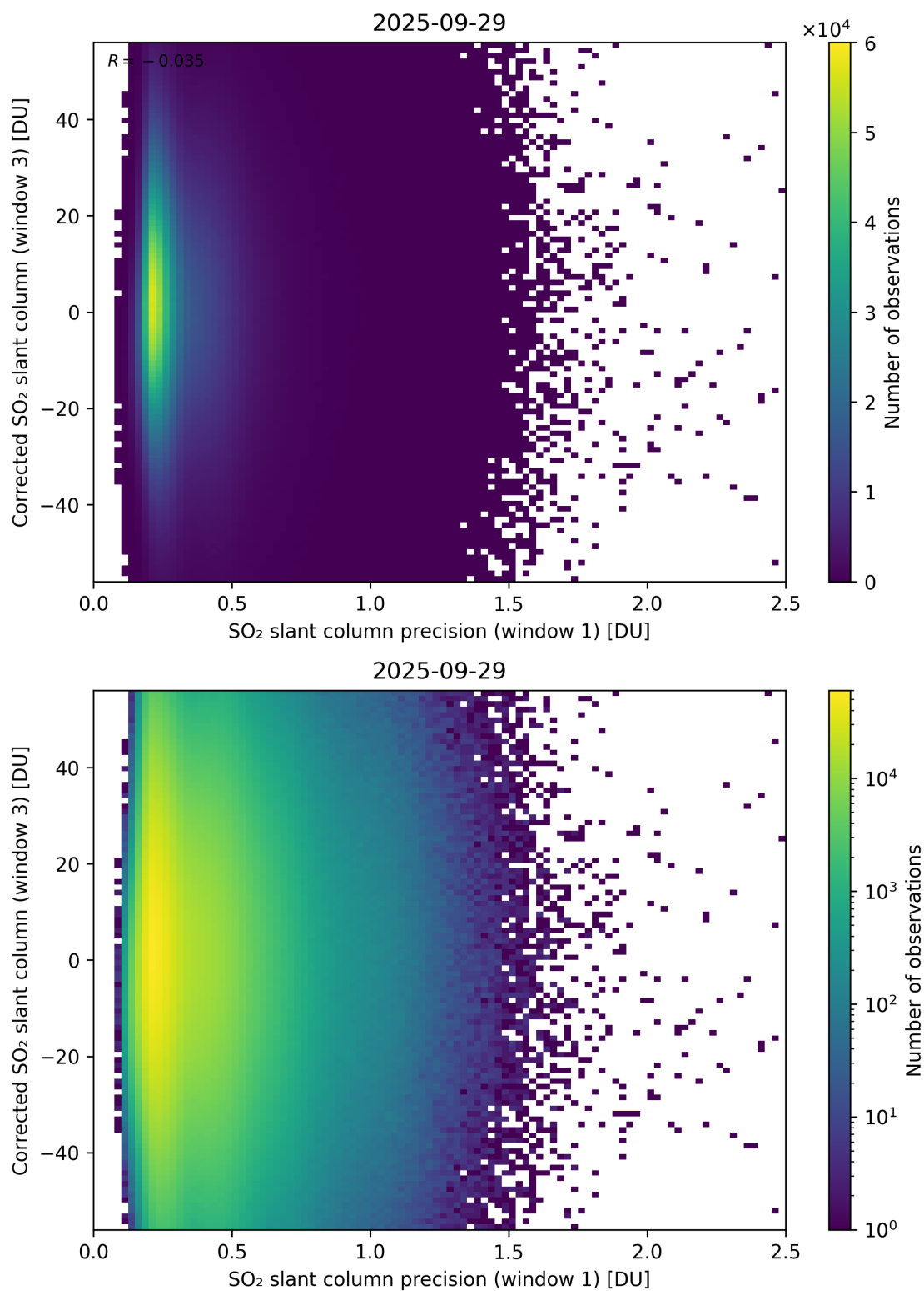
Figure 276: Scatter density plot of “SO 2 slant column precision (window 1)” against “Corrected SO 2 slant column (window 3)” for 2025-09-28 to 2025-09-30.
