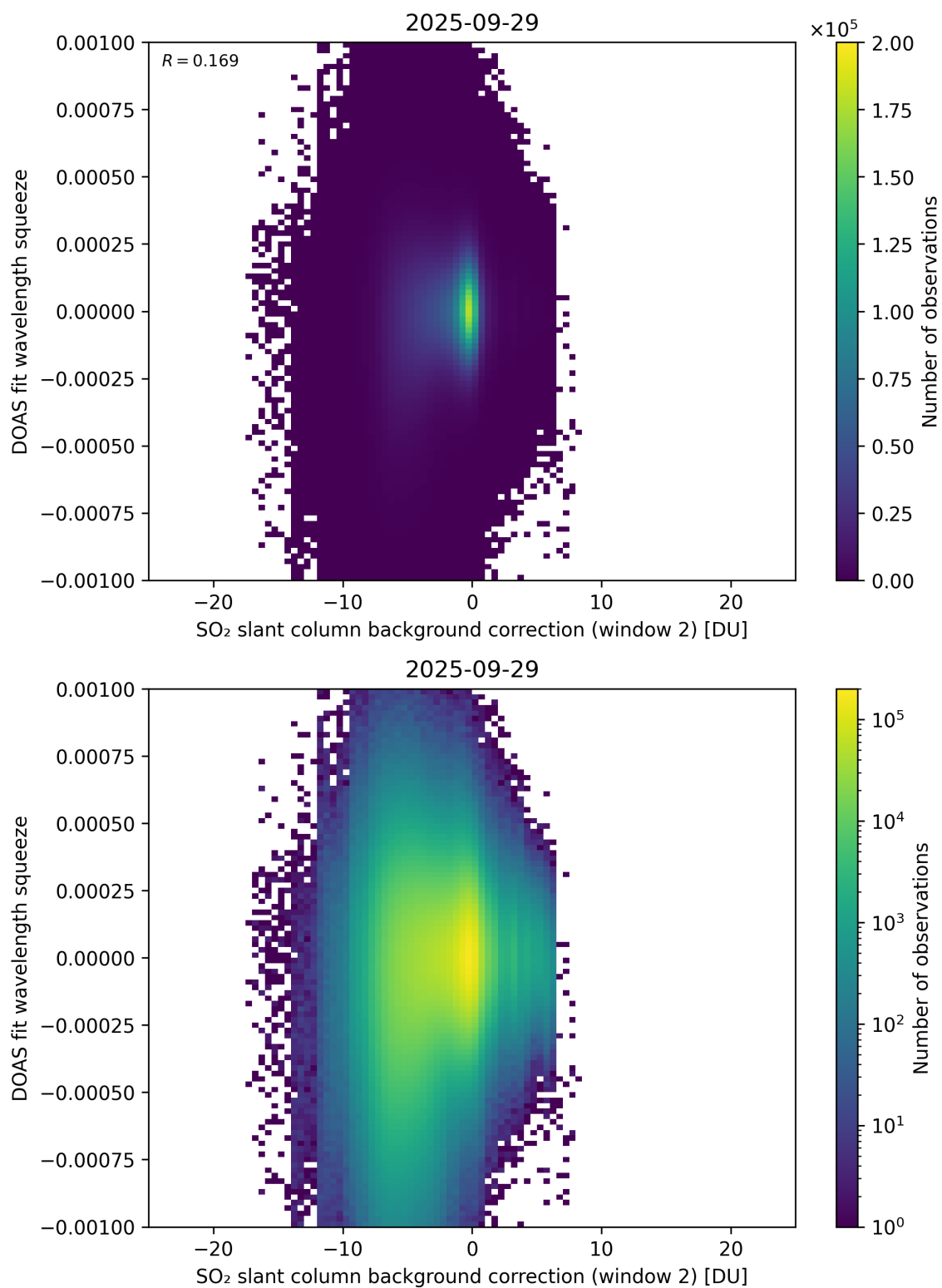
Figure 124: Scatter density plot of “SO 2 slant column background correction (window 2)” against “DOAS fit wavelength squeeze” for 2025-09-28 to 2025-09-30.
