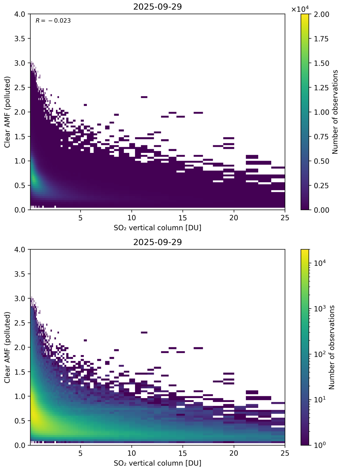
Figure 348: Scatter density plot of “SO 2 vertical column” against “Clear AMF (polluted)” for 2025-09-28 to 2025-09-30.
