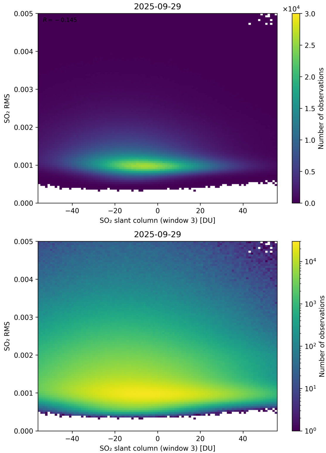
Figure 306: Scatter density plot of “SO 2 slant column (window 3)” against “SO 2 RMS” for 2025-09-28 to 2025-09-30.
