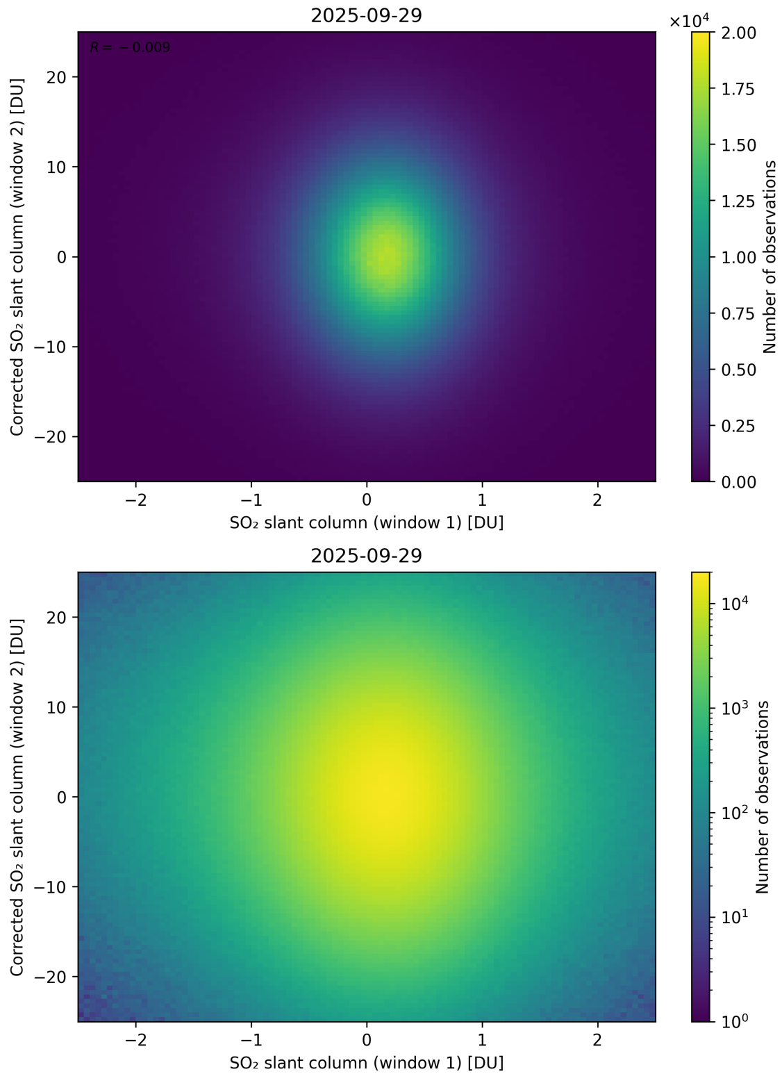
Figure 283: Scatter density plot of “SO 2 slant column (window 1)” against “Corrected SO 2 slant column (window 2)” for 2025-09-28 to 2025-09-30.
