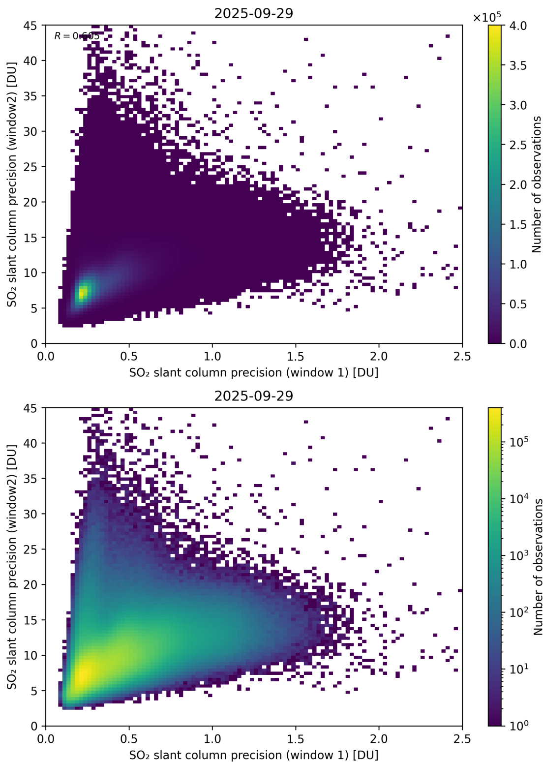
Figure 277: Scatter density plot of “SO 2 slant column precision (window 1)” against “SO 2 slant column precision (window2)” for 2025-09-28 to 2025-09-30.
