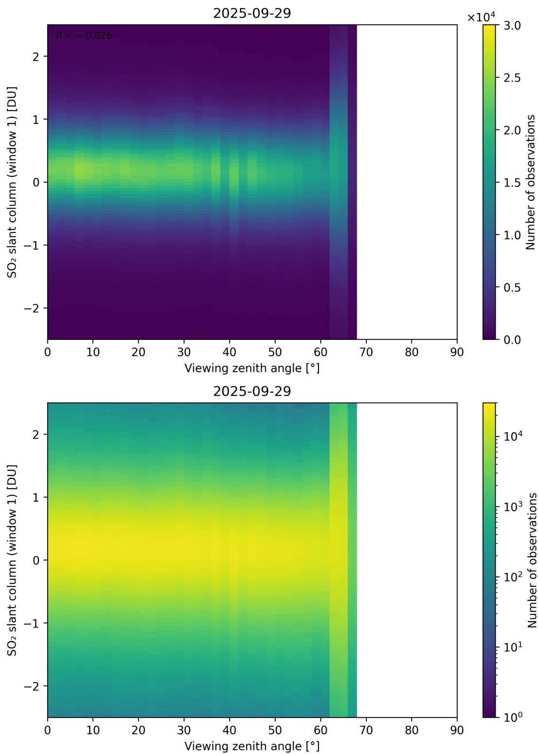
Figure 376: Scatter density plot of “Viewing zenith angle” against “SO 2 slant column (window 1)” for 2025-09-28 to 2025-09-30.
