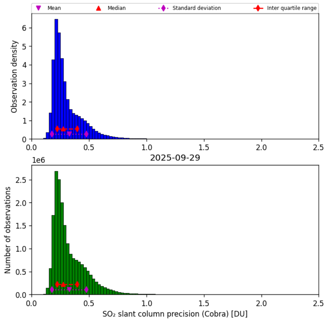
Figure 62: Histogram of “SO 2 slant column precision (Cobra)” for 2025-09-28 to 2025-09-30
