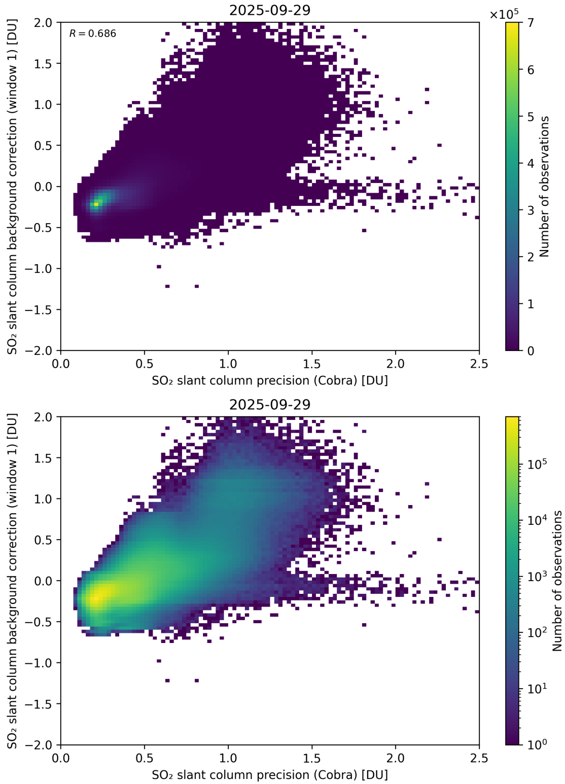
Figure 199: Scatter density plot of “SO 2 slant column precision (Cobra)” against “SO 2 slant column background correction (window 1)” for 2025-09-28 to 2025-09-30.
