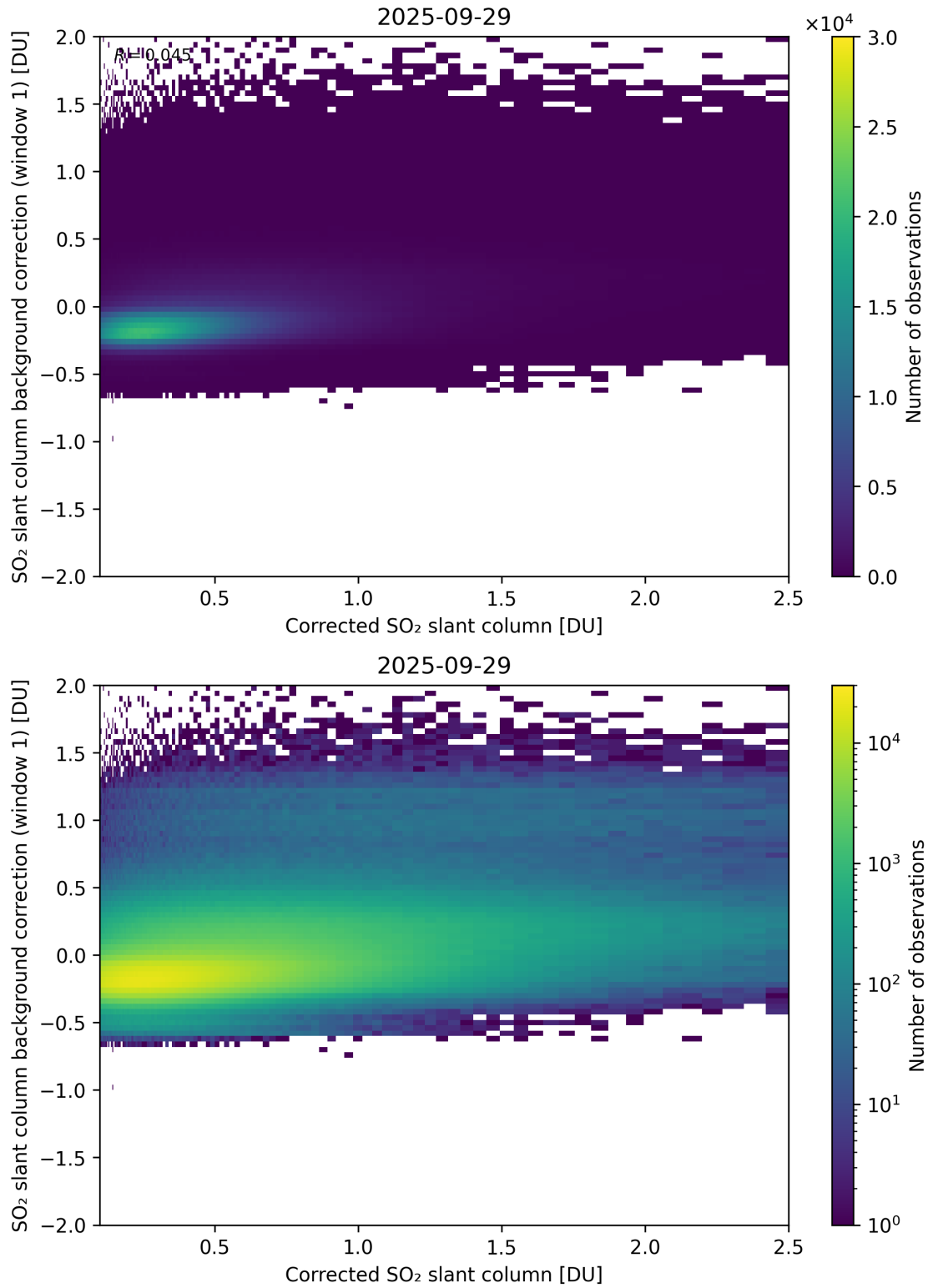
Figure 226: Scatter density plot of “Corrected SO 2 slant column” against “SO 2 slant column background correction (window 1)” for 2025-09-28 to 2025-09-30.
