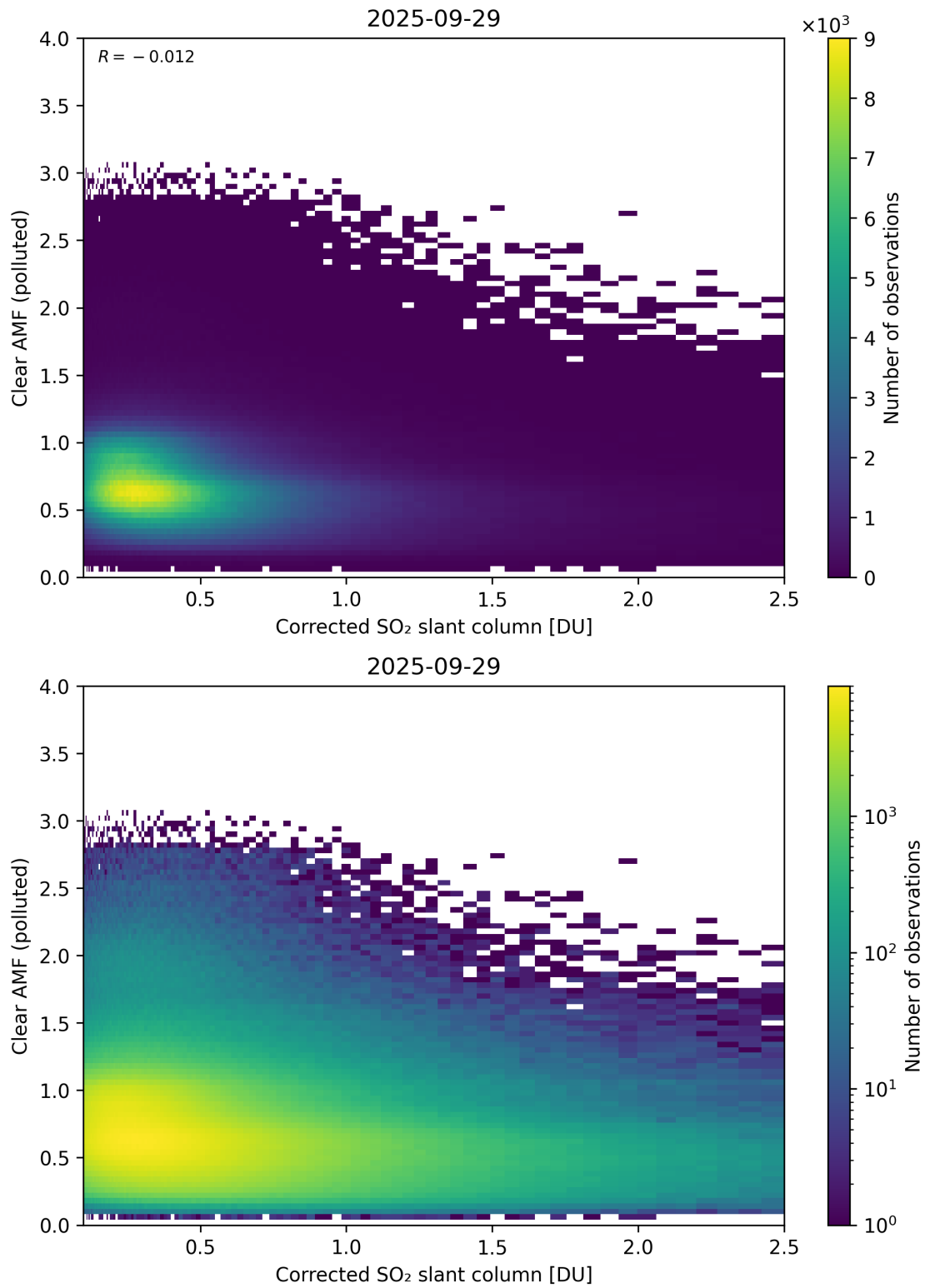
Figure 232: Scatter density plot of “Corrected SO 2 slant column” against “Clear AMF (polluted)” for 2025-09-28 to 2025-09-30.
