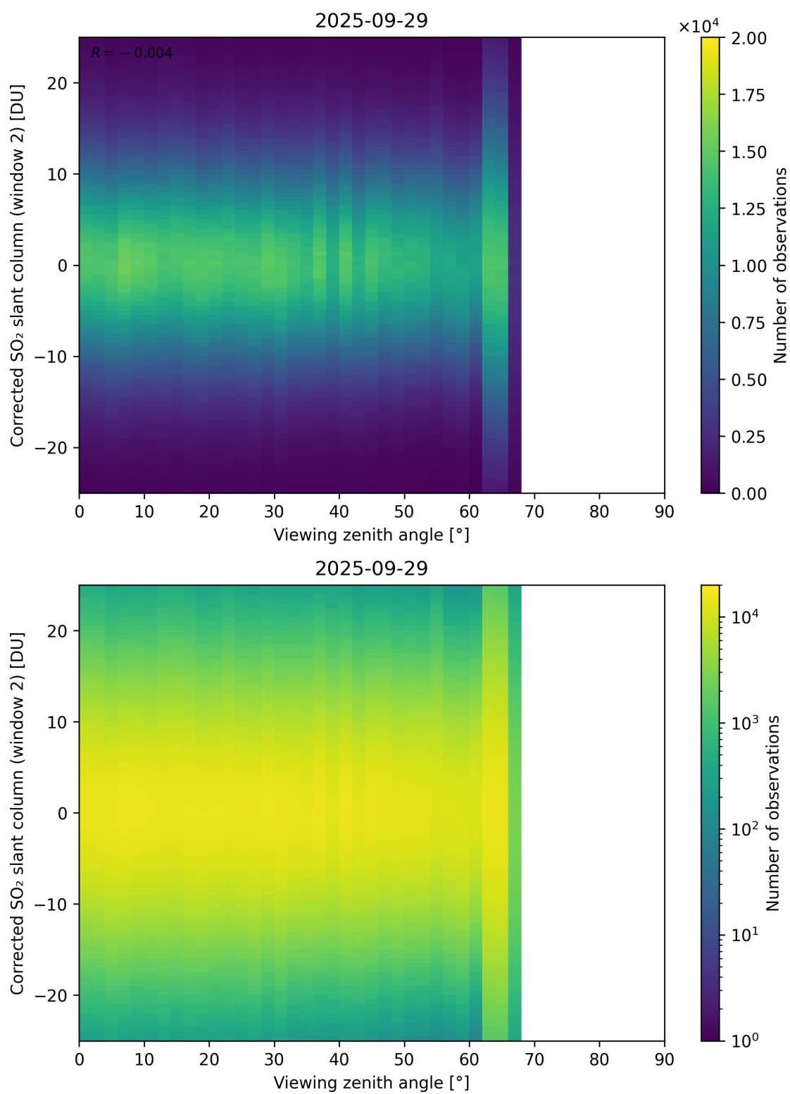
Figure 374: Scatter density plot of “Viewing zenith angle” against “Corrected SO 2 slant column (window 2)” for 2025-09-28 to 2025-09-30.
