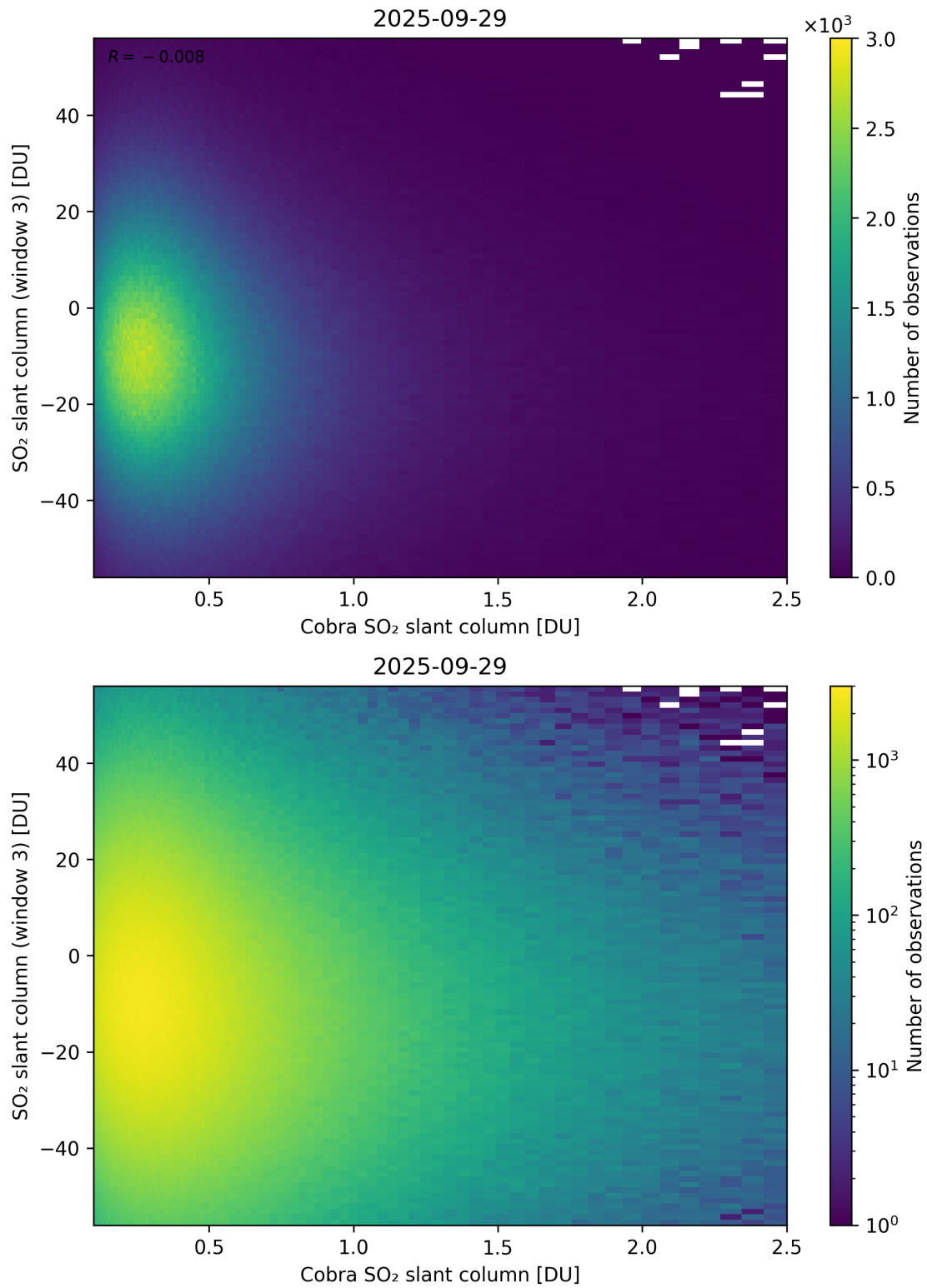
Figure 222: Scatter density plot of “Cobra SO 2 slant column” against “SO 2 slant column (window 3)” for 2025-09-28 to 2025-09-30.
