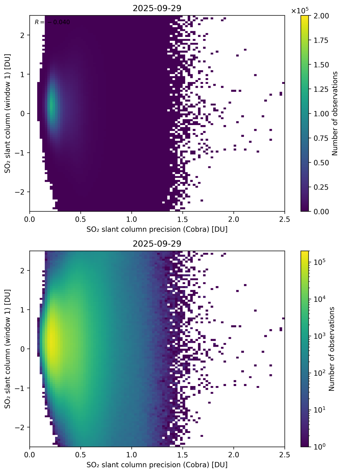
Figure 208: Scatter density plot of “SO 2 slant column precision (Cobra)” against “SO 2 slant column (window 1)” for 2025-09-28 to 2025-09-30.
