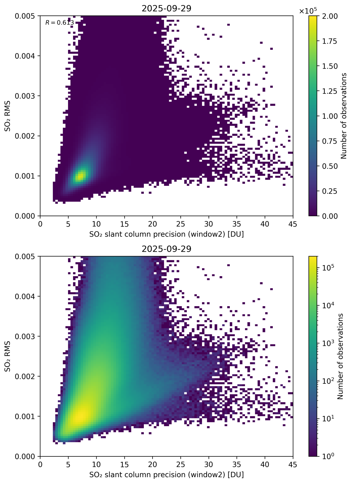
Figure 295: Scatter density plot of “SO 2 slant column precision (window2)” against “SO 2 RMS” for 2025-09-28 to 2025-09-30.
