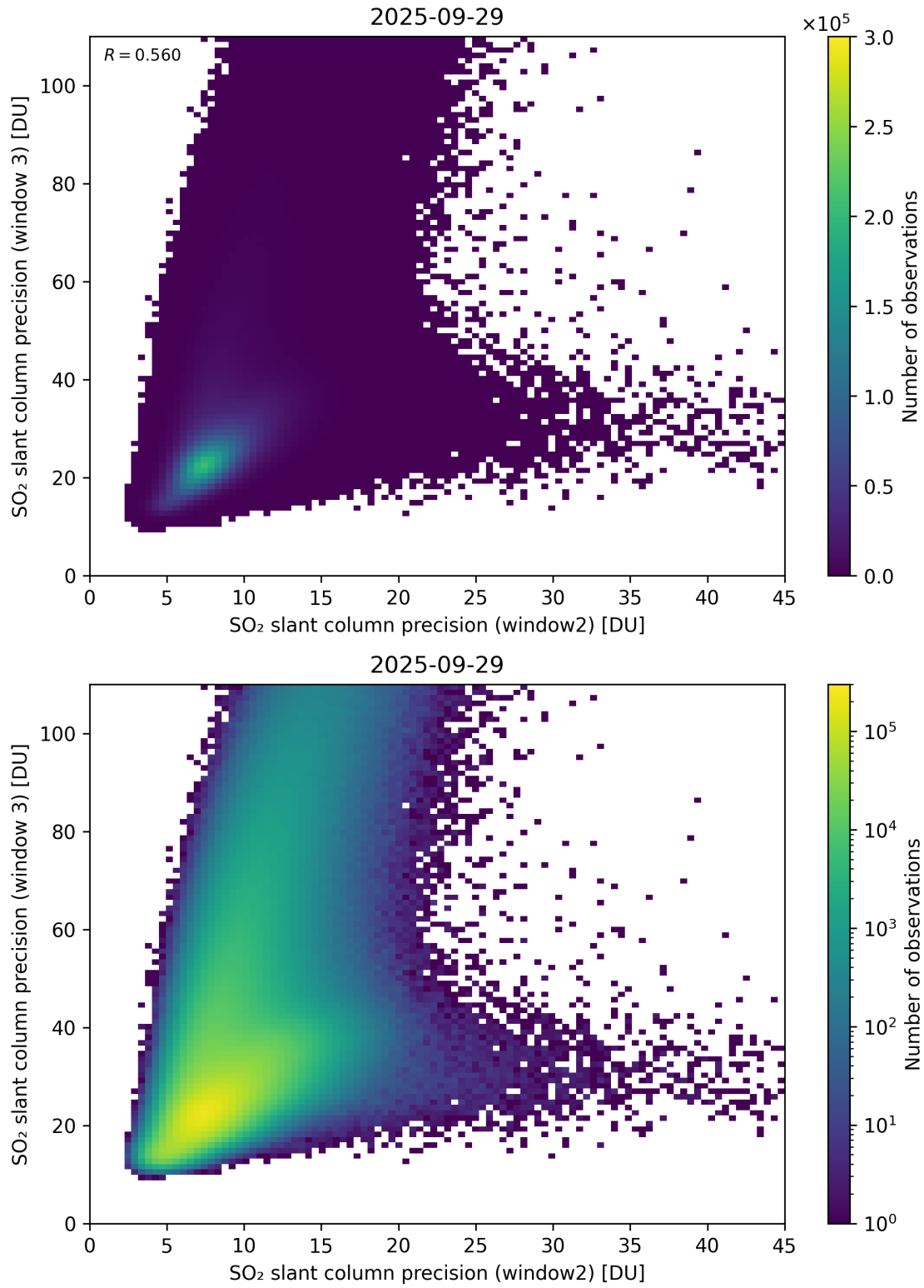
Figure 300: Scatter density plot of “SO 2 slant column precision (window2)” against “SO 2 slant column precision (window 3)” for 2025-09-28 to 2025-09-30.
