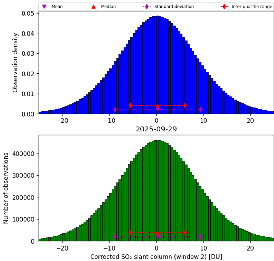
Figure 69: Histogram of “Corrected SO 2 slant column (window 2)” for 2025-09-28 to 2025-09-30
