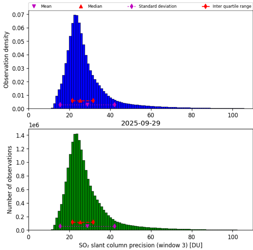
Figure 72: Histogram of “SO 2 slant column precision (window 3)” for 2025-09-28 to 2025-09-30
