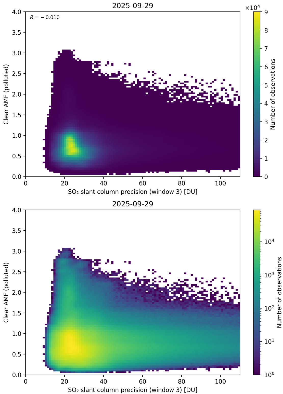
Figure 311: Scatter density plot of “SO 2 slant column precision (window 3)” against “Clear AMF (polluted)” for 2025-09-28 to 2025-09-30.
