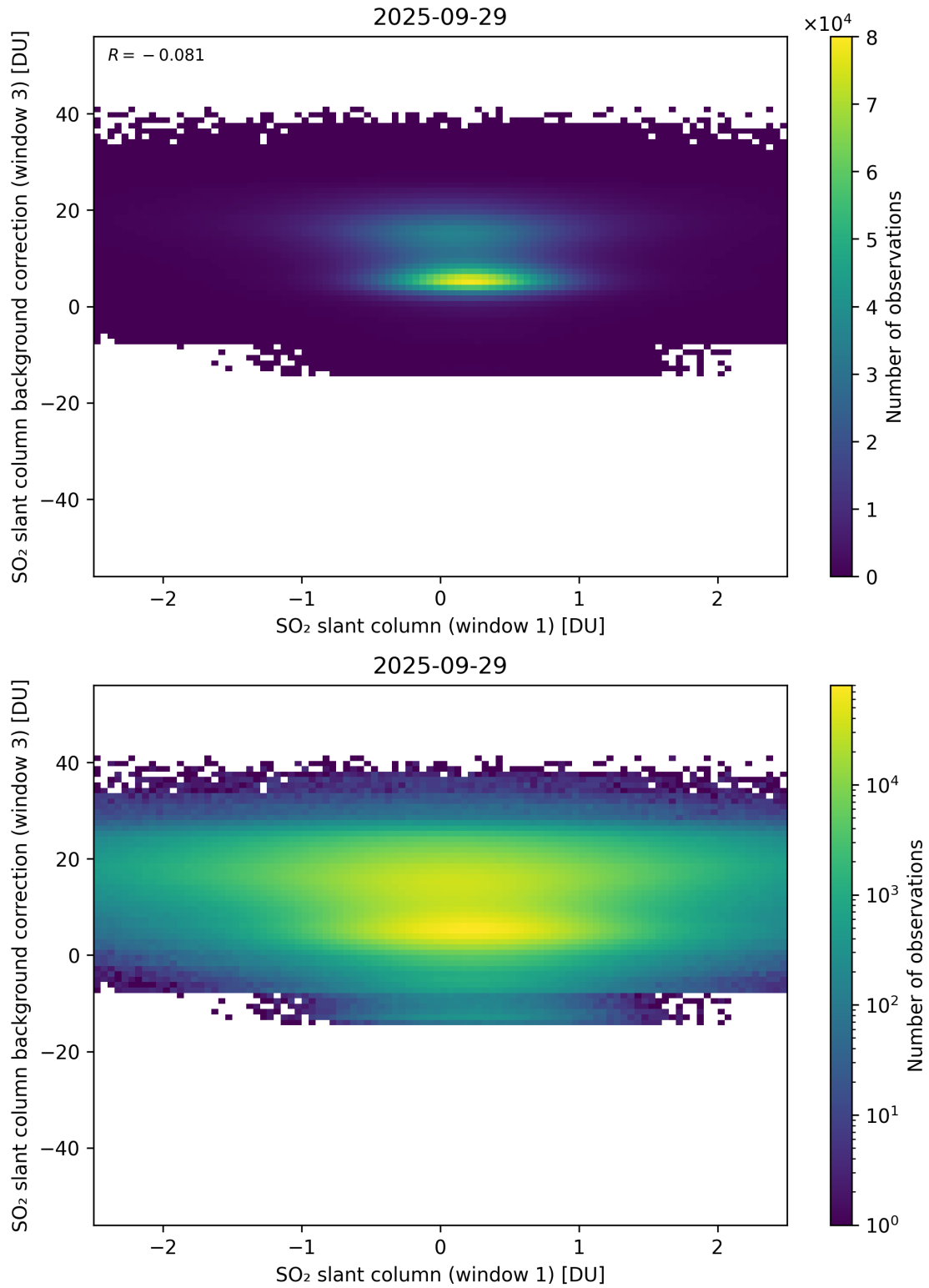
Figure 264: Scatter density plot of “SO 2 slant column (window 1)” against “SO 2 slant column background correction (window 3)” for 2025-09-28 to 2025-09-30.
