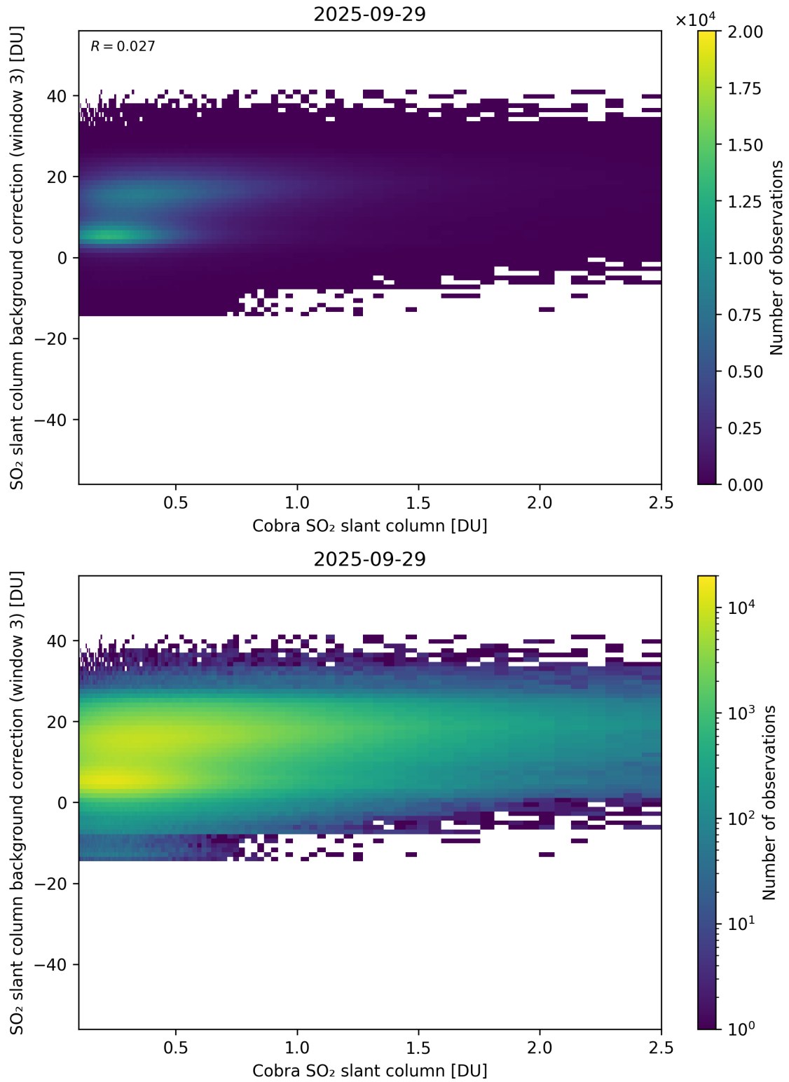
Figure 195: Scatter density plot of “Cobra SO 2 slant column” against “SO 2 slant column background correction (window 3)” for 2025-09-28 to 2025-09-30.
