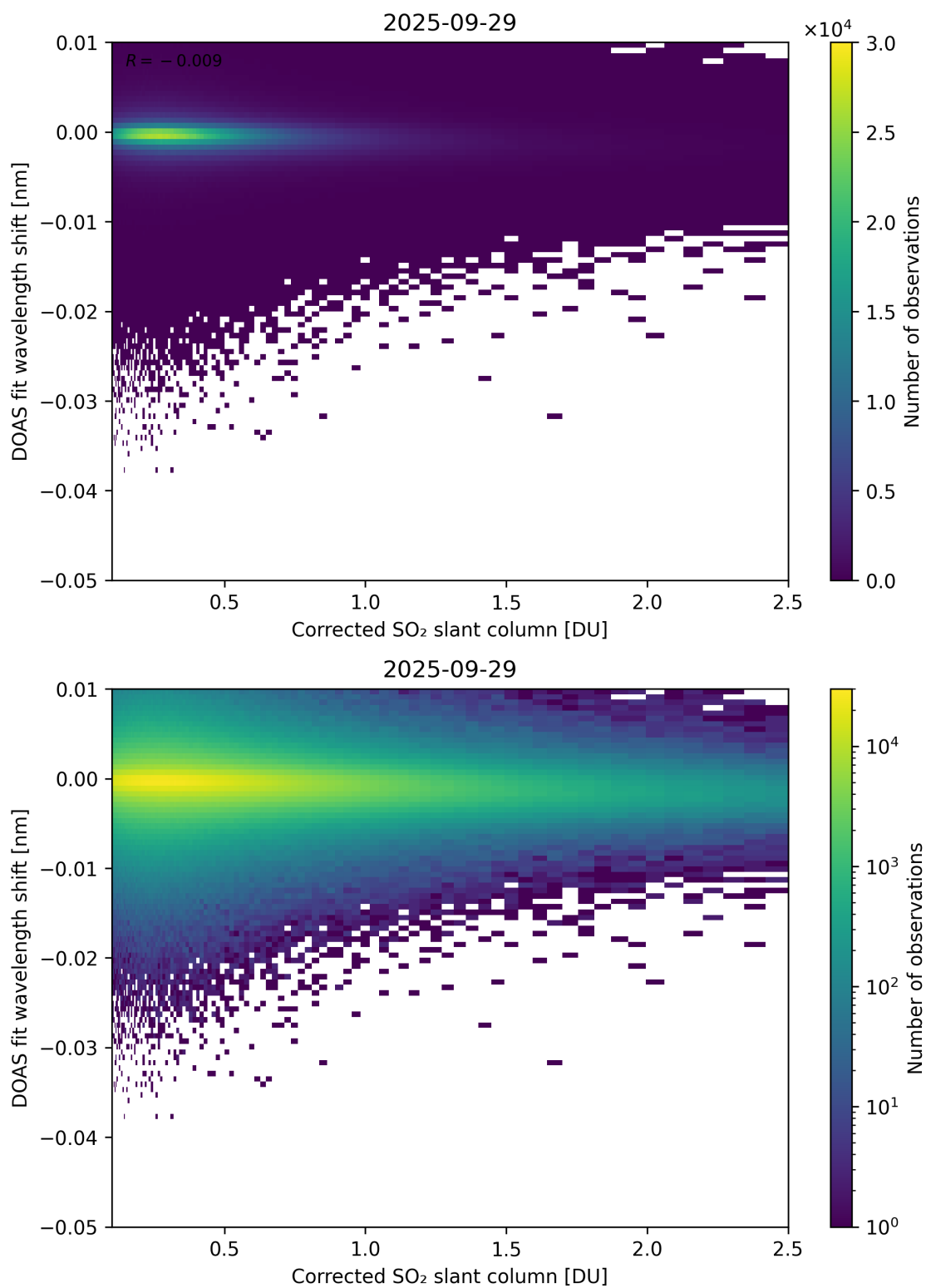
Figure 229: Scatter density plot of “Corrected SO 2 slant column” against “DOAS fit wavelength shift” for 2025-09-28 to 2025-09-30.
