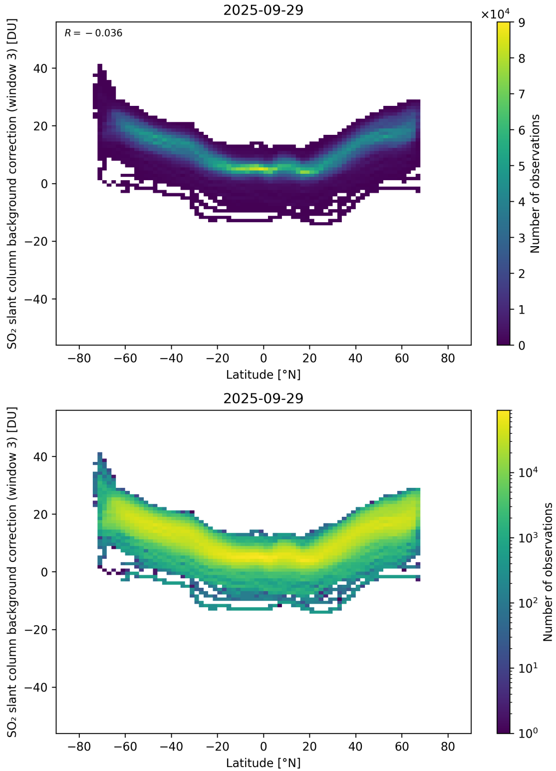
Figure 152: Scatter density plot of “Latitude” against “SO 2 slant column background correction (window 3)” for 2025-09-28 to 2025-09-30.
