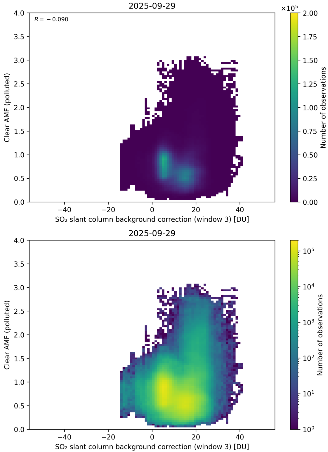
Figure 135: Scatter density plot of “SO 2 slant column background correction (window 3)” against “Clear AMF (polluted)” for 2025-09-28 to 2025-09-30.
