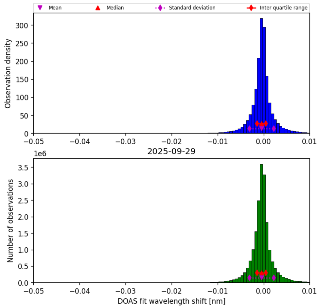
Figure 76: Histogram of “DOAS fit wavelength shift” for 2025-09-28 to 2025-09-30
