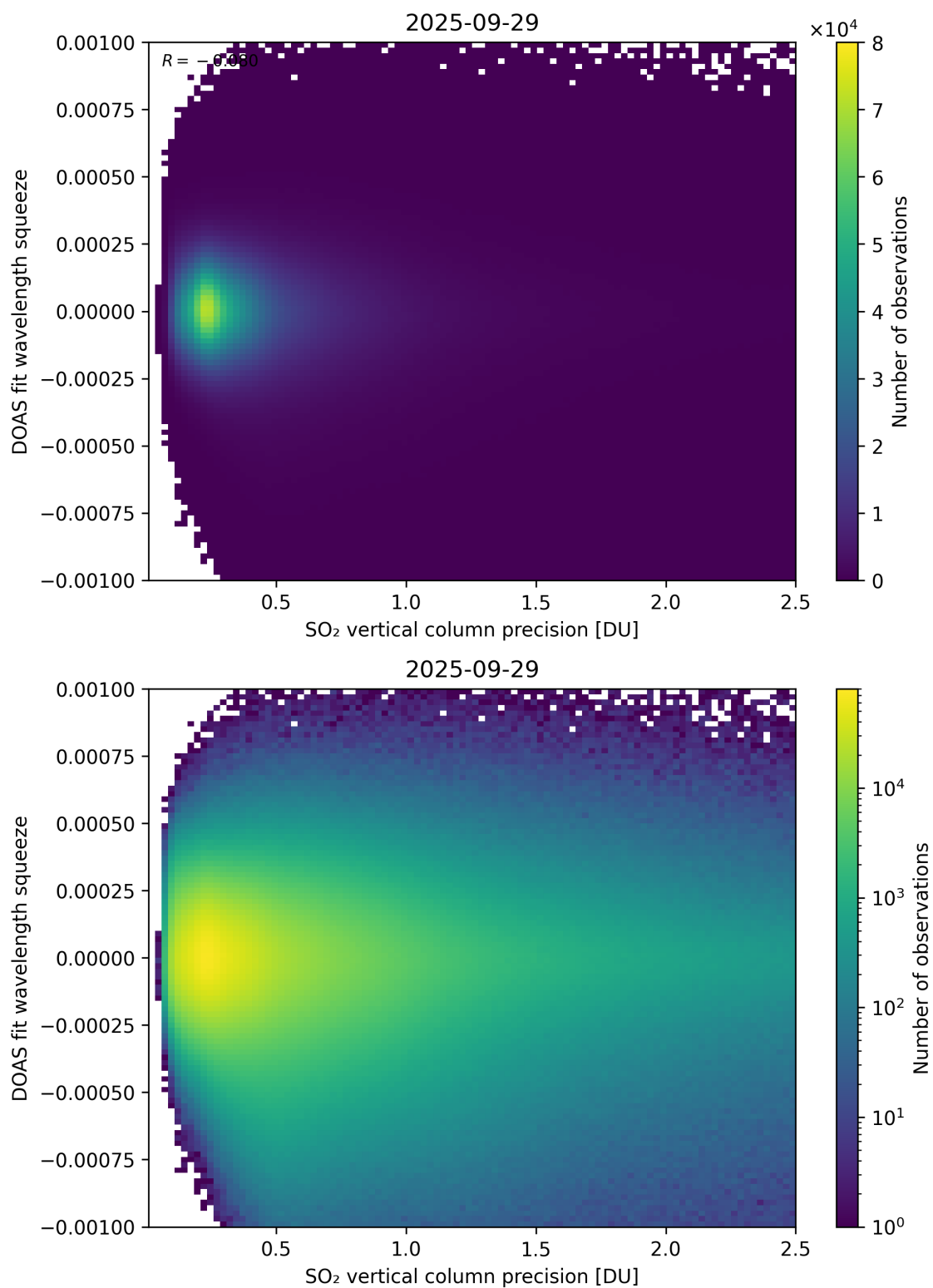
Figure 333: Scatter density plot of “SO 2 vertical column precision” against “DOAS fit wavelength squeeze” for 2025-09-28 to 2025-09-30.
