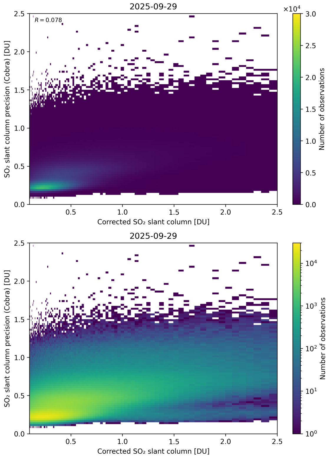
Figure 234: Scatter density plot of “Corrected SO 2 slant column” against “SO 2 slant column precision (Cobra)” for 2025-09-28 to 2025-09-30.
