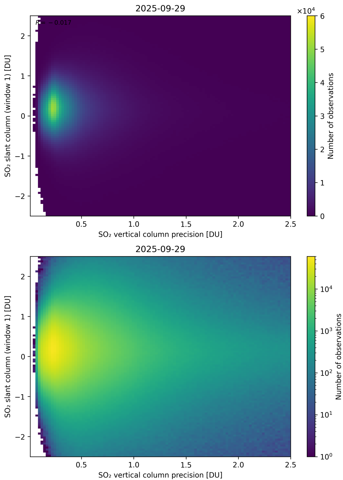
Figure 341: Scatter density plot of “SO 2 vertical column precision” against “SO 2 slant column (window 1)” for 2025-09-28 to 2025-09-30.
