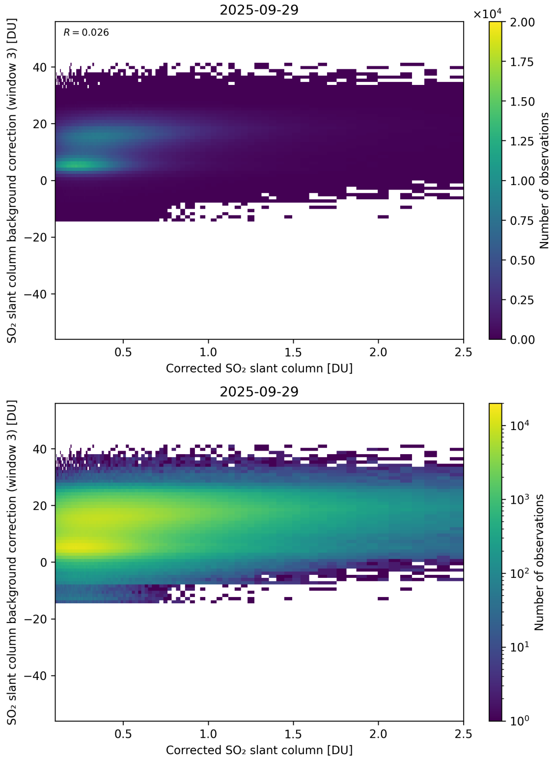
Figure 228: Scatter density plot of “Corrected SO 2 slant column” against “SO 2 slant column background correction (window 3)” for 2025-09-28 to 2025-09-30.
