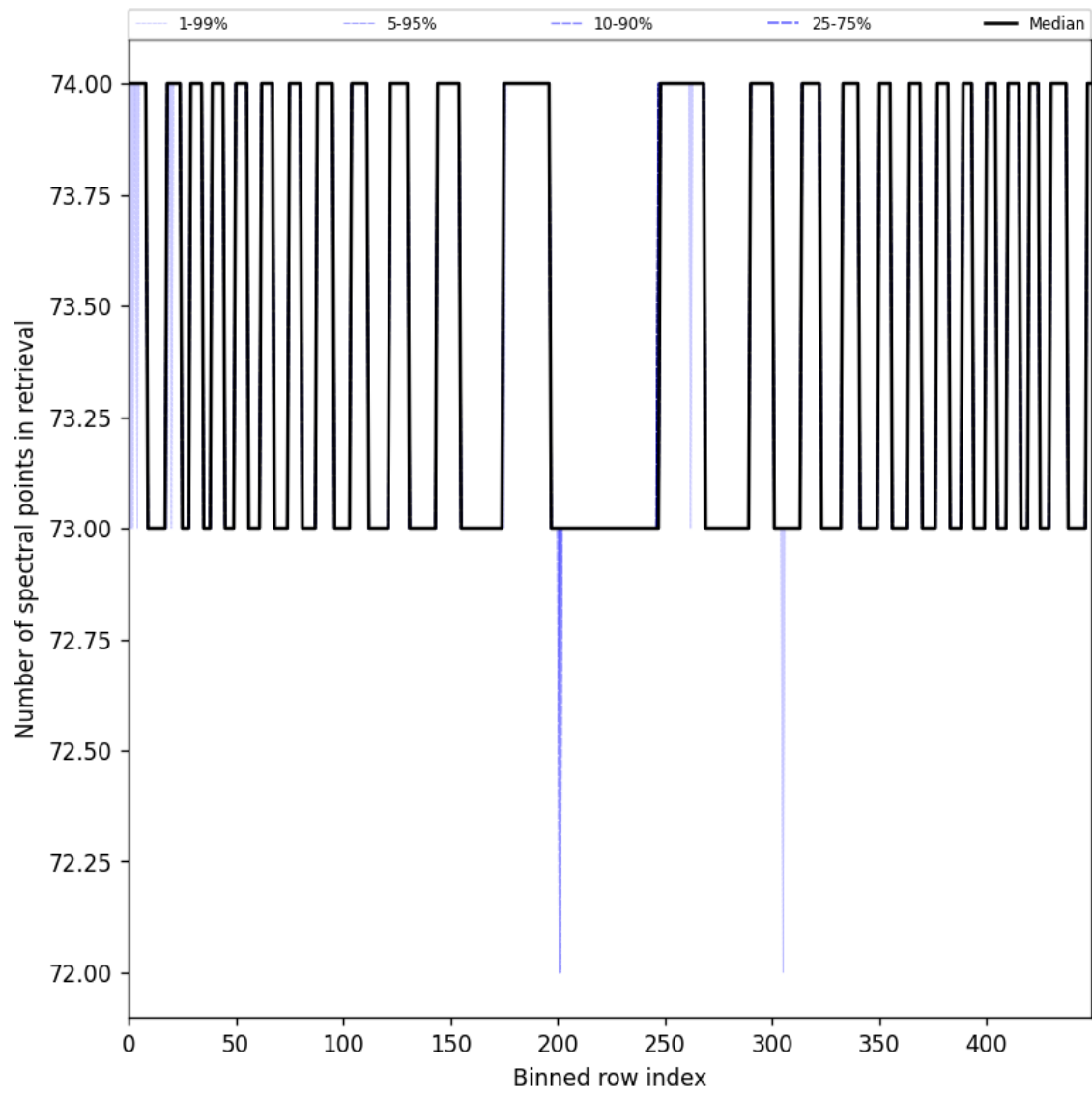
Figure 108: Along track statistics of “Number of spectral points in retrieval” for 2025-09-28 to 2025-09-30
