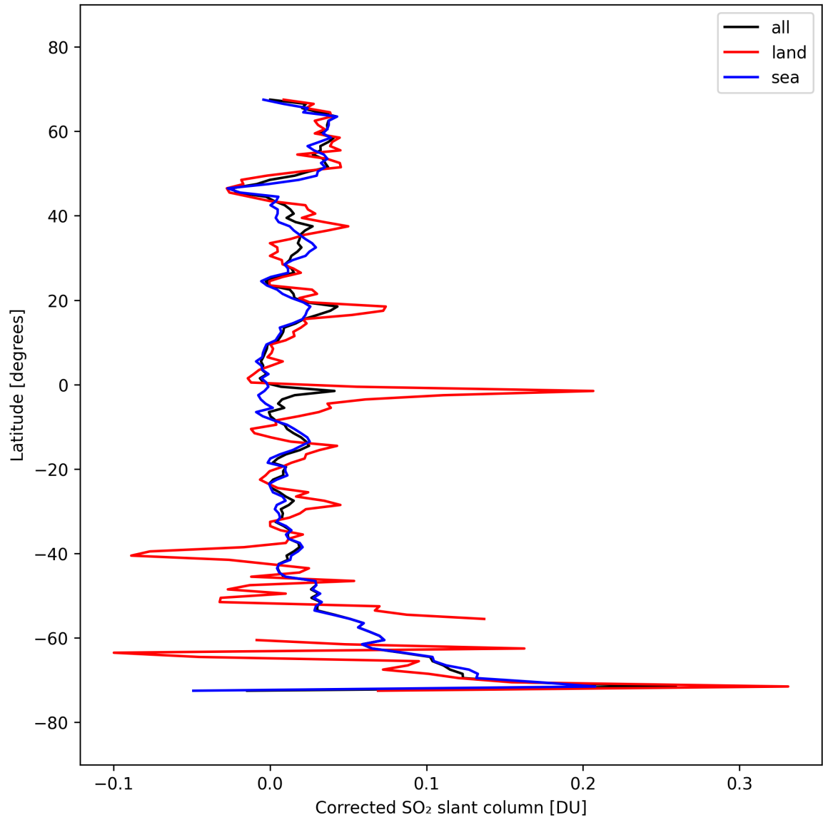
Figure 34: Zonal average of “Corrected SO 2 slant column” for 2025-09-28 to 2025-09-30.
