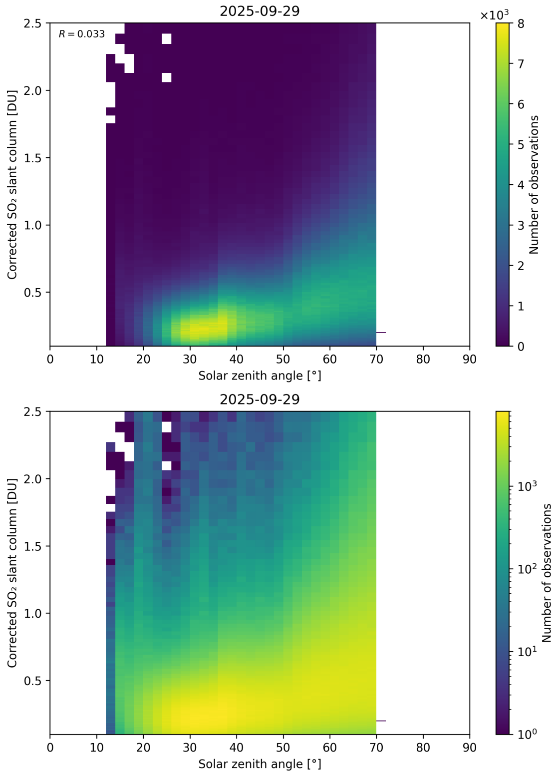
Figure 181: Scatter density plot of “Solar zenith angle” against “Corrected SO 2 slant column” for 2025-09-28 to 2025-09-30.
