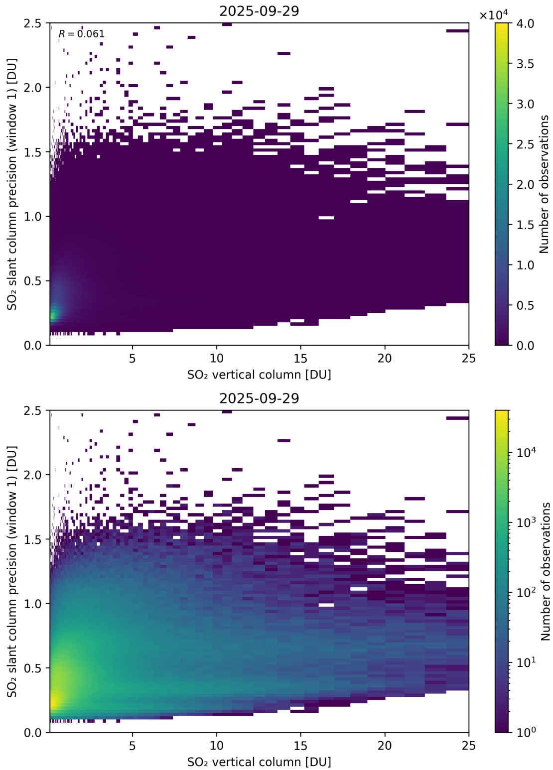
Figure 355: Scatter density plot of “SO 2 vertical column” against “SO 2 slant column precision (window 1)” for 2025-09-28 to 2025-09-30.
