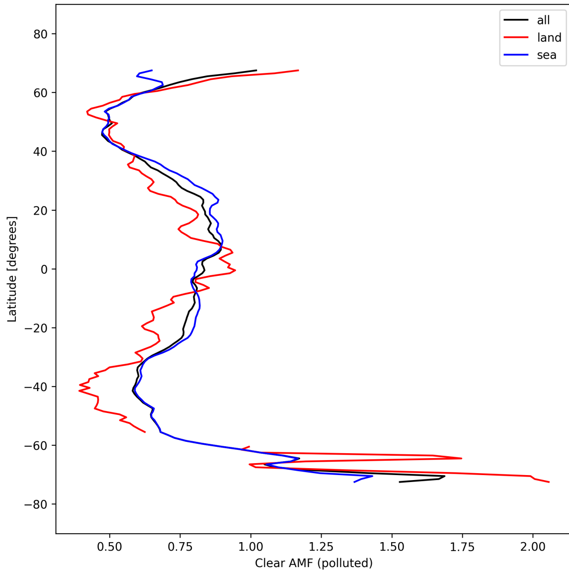
Figure 55: Zonal average of “Clear AMF (polluted)” for 2025-09-28 to 2025-09-30.
