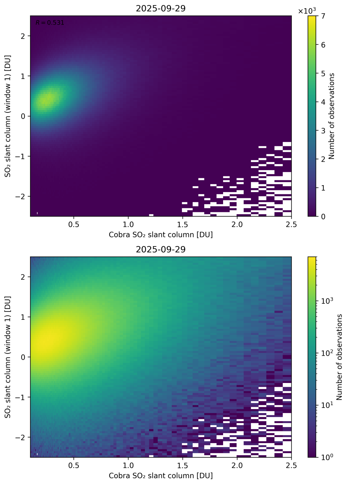
Figure 219: Scatter density plot of “Cobra SO 2 slant column” against “SO 2 slant column (window 1)” for 2025-09-28 to 2025-09-30.
