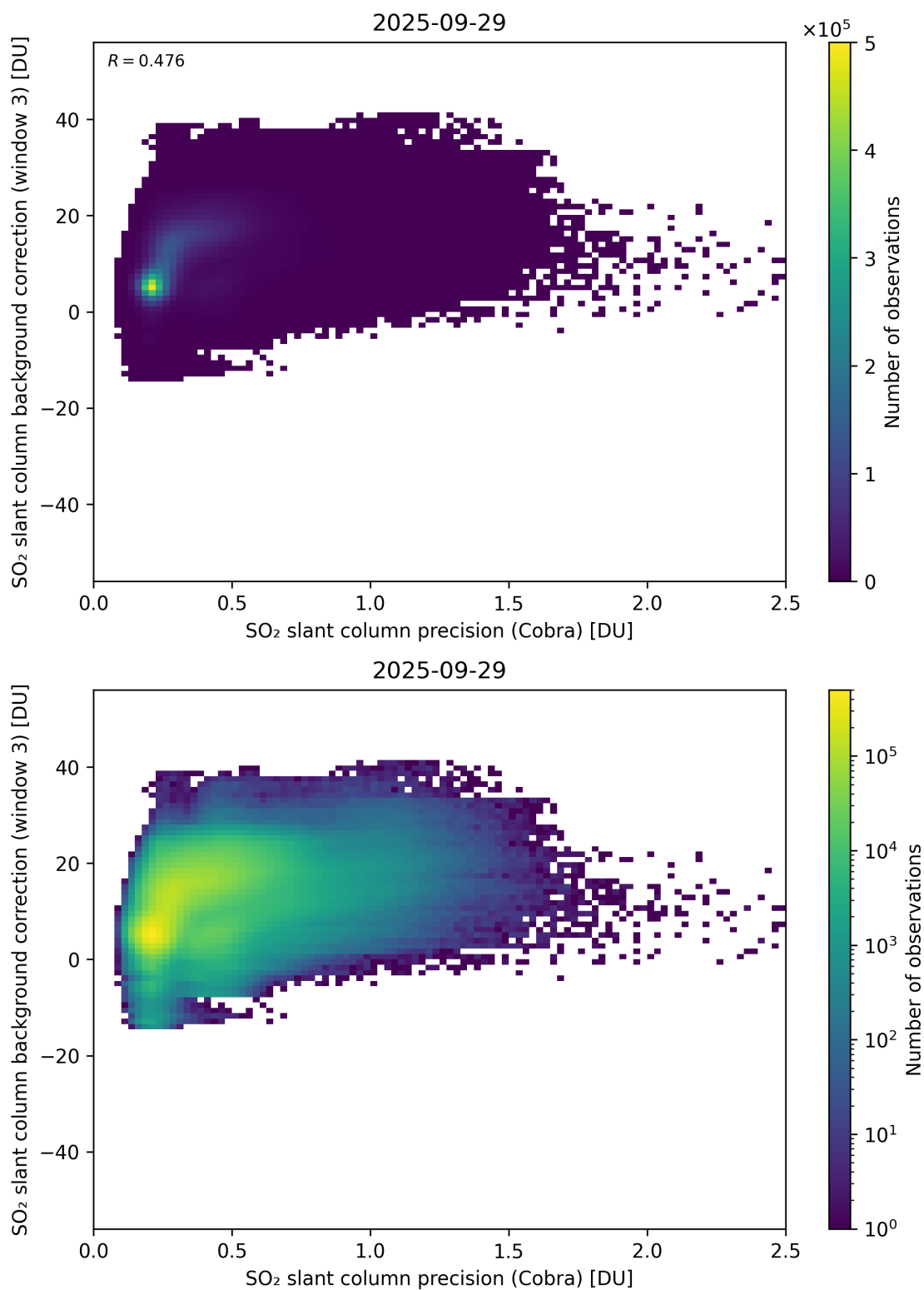
Figure 201: Scatter density plot of “SO 2 slant column precision (Cobra)” against “SO 2 slant column background correction (window 3)” for 2025-09-28 to 2025-09-30.
