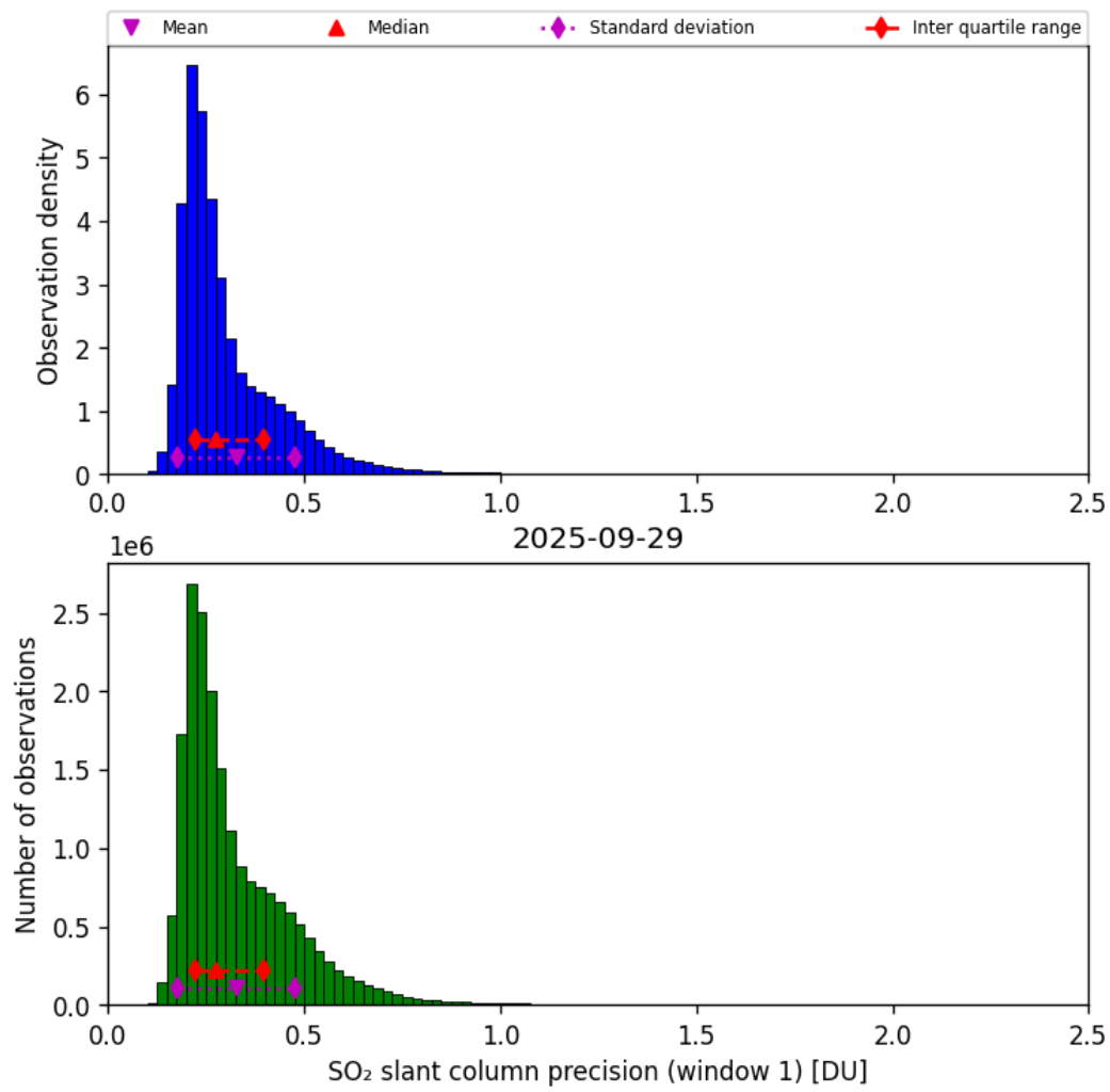
Figure 64: Histogram of “SO 2 slant column precision (window 1)” for 2025-09-28 to 2025-09-30
