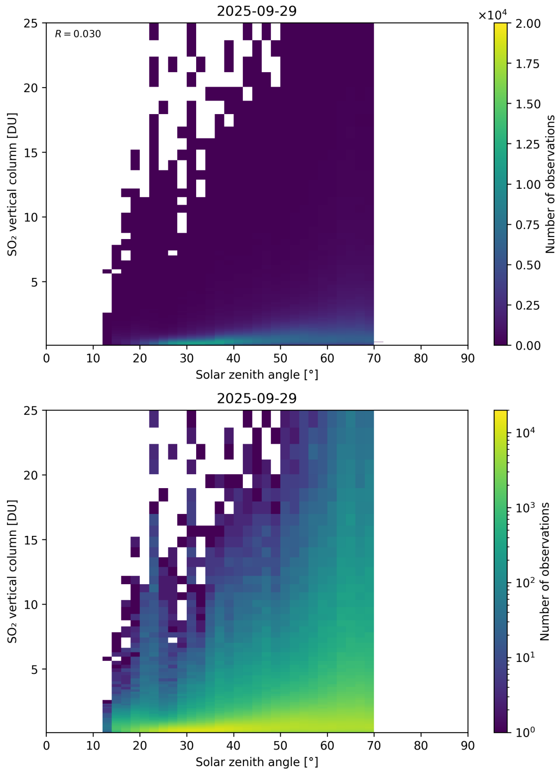
Figure 191: Scatter density plot of “Solar zenith angle” against “SO 2 vertical column” for 2025-09-28 to 2025-09-30.
