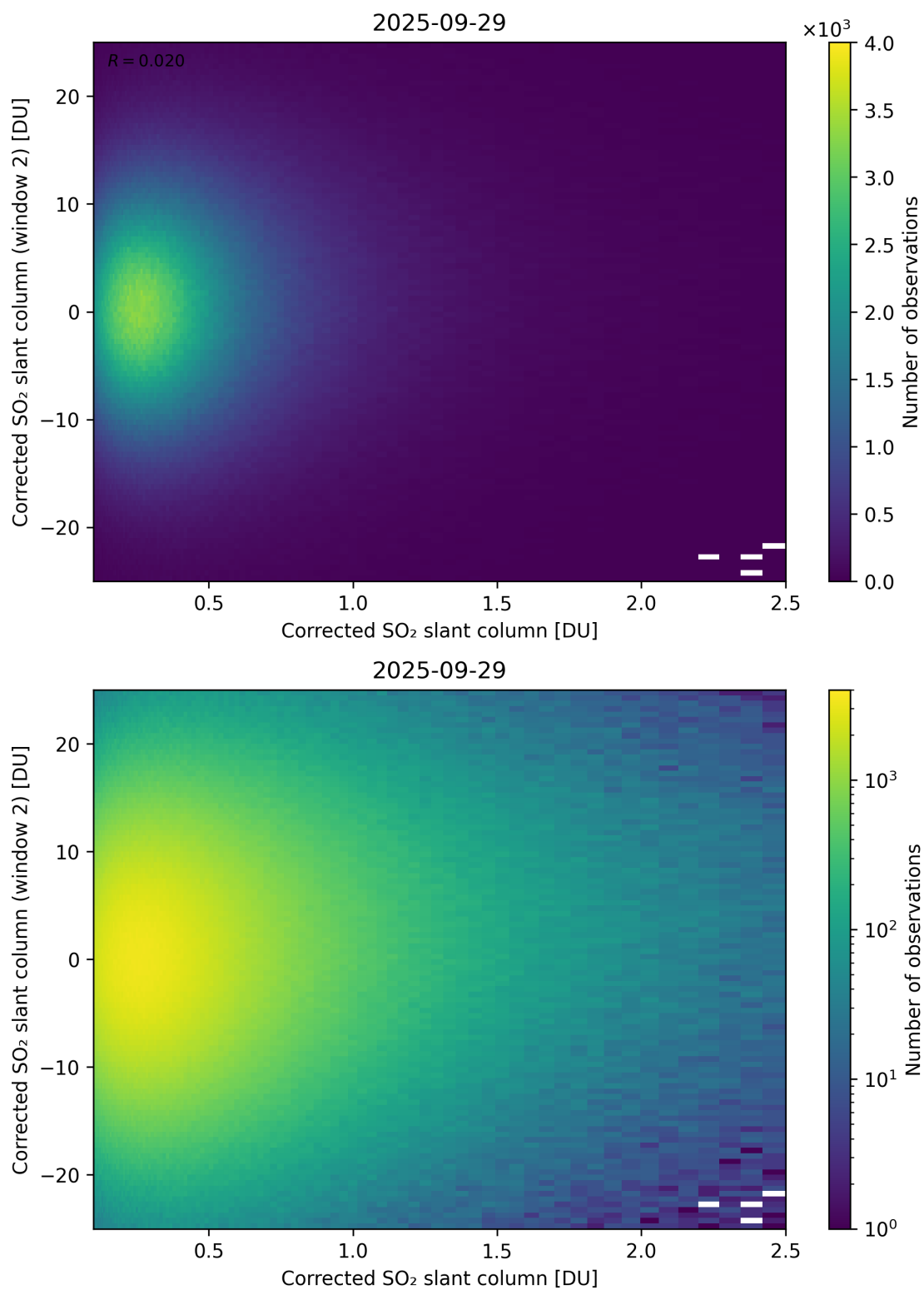
Figure 235: Scatter density plot of “Corrected SO 2 slant column” against “Corrected SO 2 slant column (window 2)” for 2025-09-28 to 2025-09-30.
