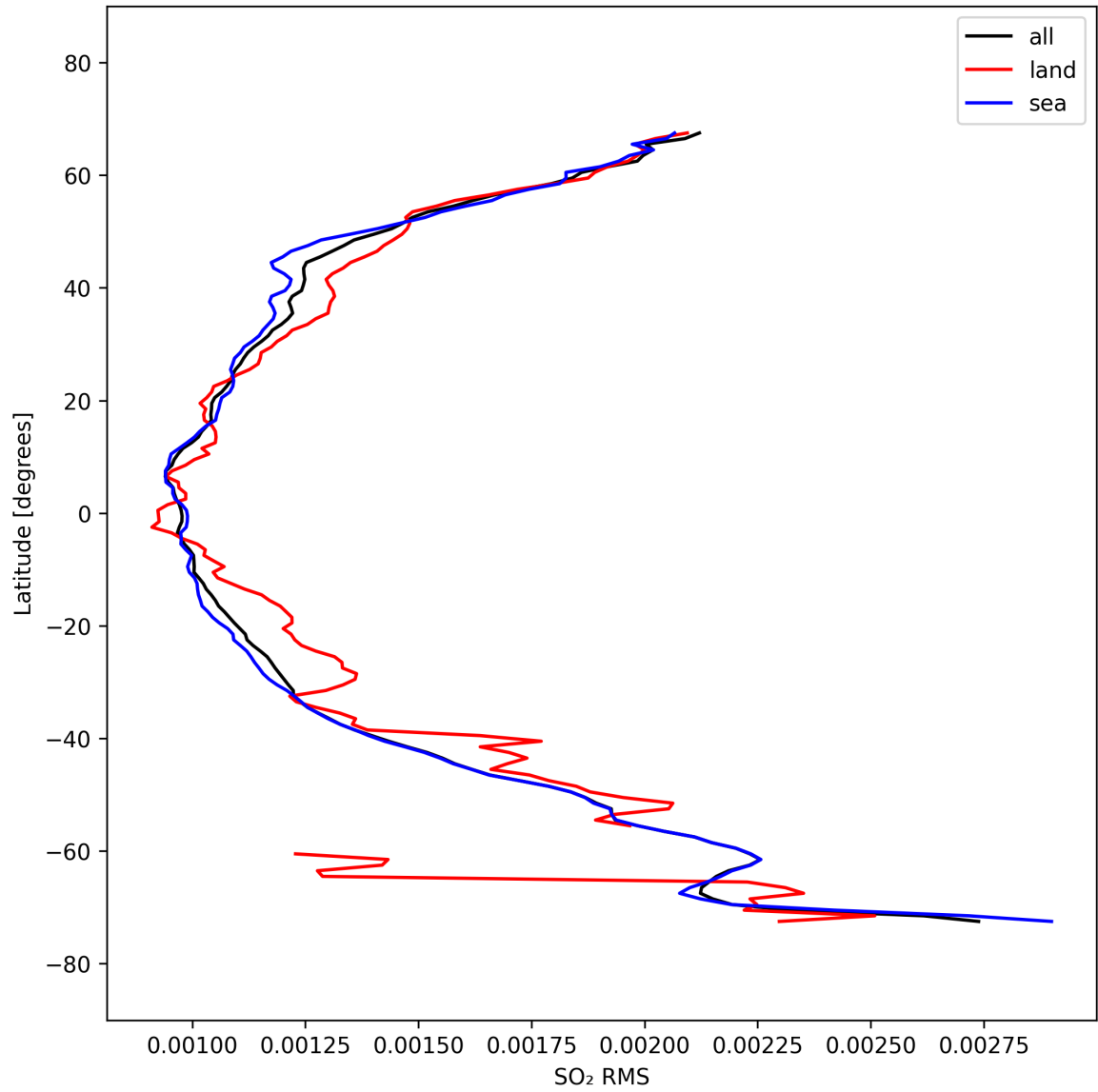
Figure 52: Zonal average of “SO 2 RMS” for 2025-09-28 to 2025-09-30.
