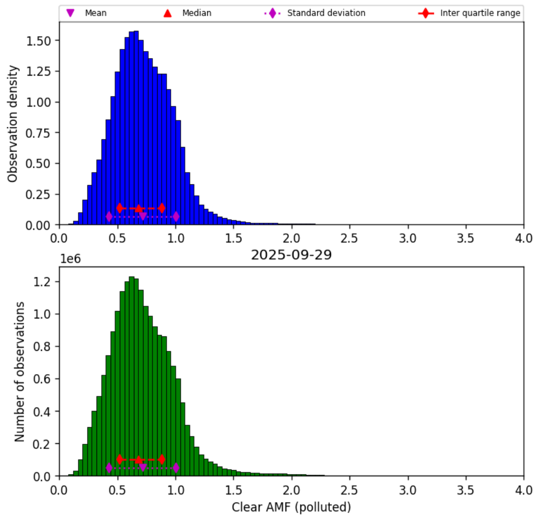
Figure 81: Histogram of "Clear AMF (polluted)" for 2025-09-28 to 2025-09-30
