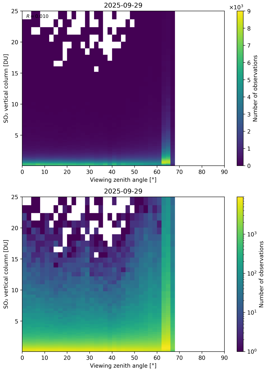
Figure 383: Scatter density plot of “Viewing zenith angle” against “SO 2 vertical column” for 2025-09-28 to 2025-09-30.
