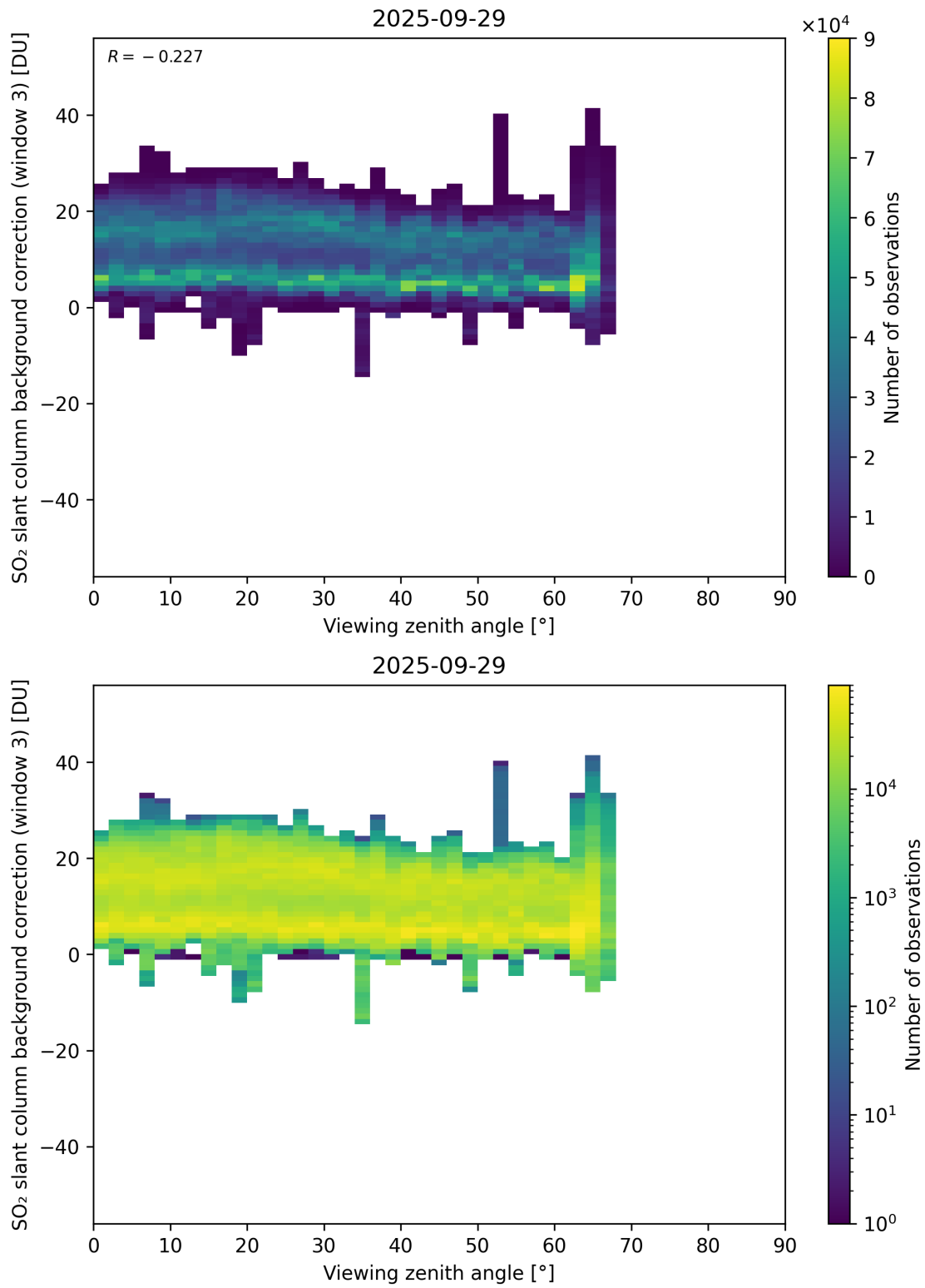
Figure 364: Scatter density plot of “Viewing zenith angle” against “SO 2 slant column background correction (window 3)” for 2025-09-28 to 2025-09-30.
