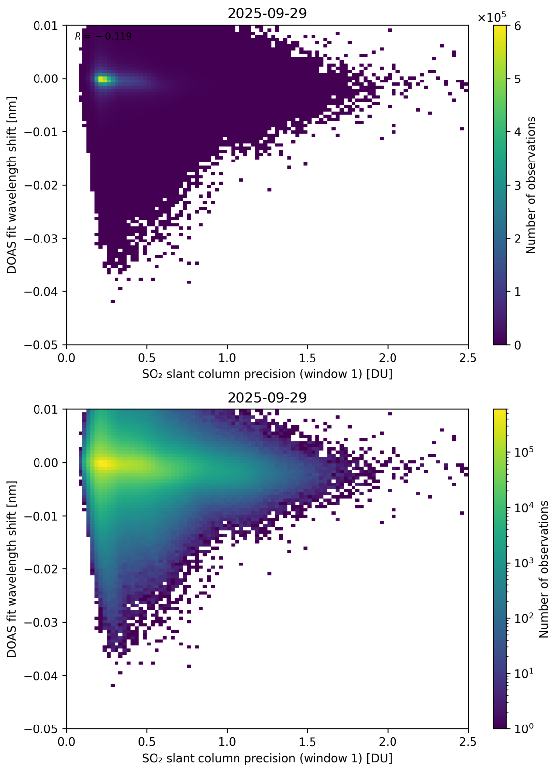
Figure 271: Scatter density plot of “SO 2 slant column precision (window 1)” against “DOAS fit wavelength shift” for 2025-09-28 to 2025-09-30.
