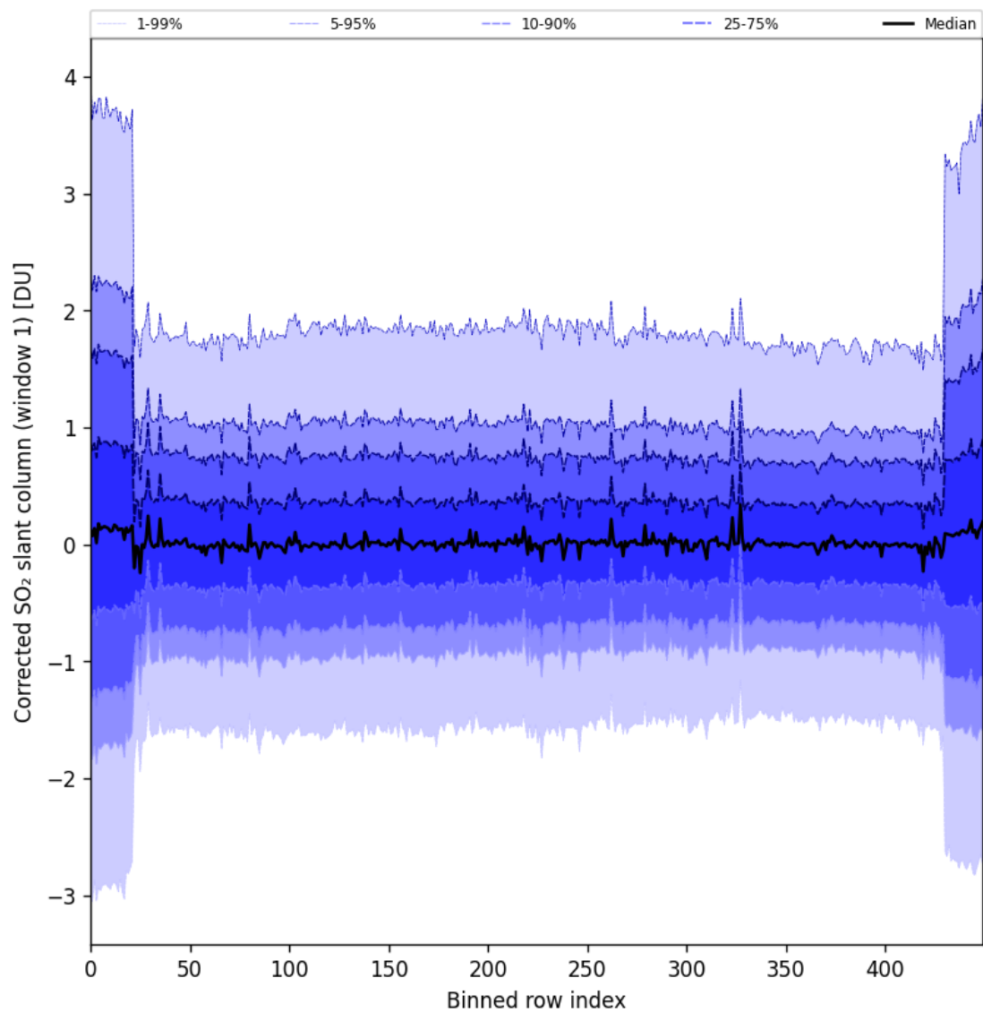
Figure 91: Along track statistics of “Corrected SO 2 slant column (window 1)” for 2025-09-28 to 2025-09-30
