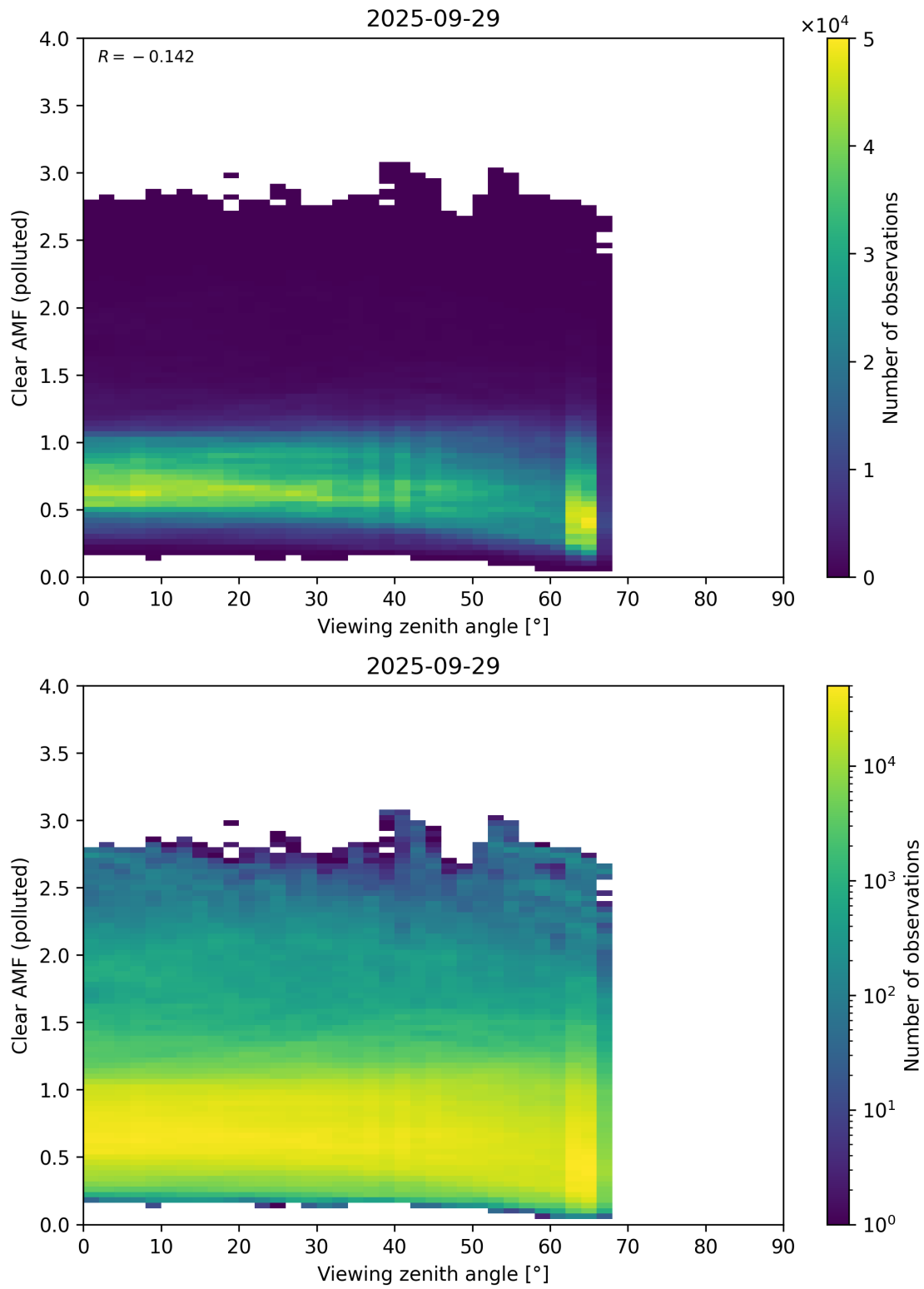
Figure 370: Scatter density plot of “Viewing zenith angle” against “Clear AMF (polluted)” for 2025-09-28 to 2025-09-30.
