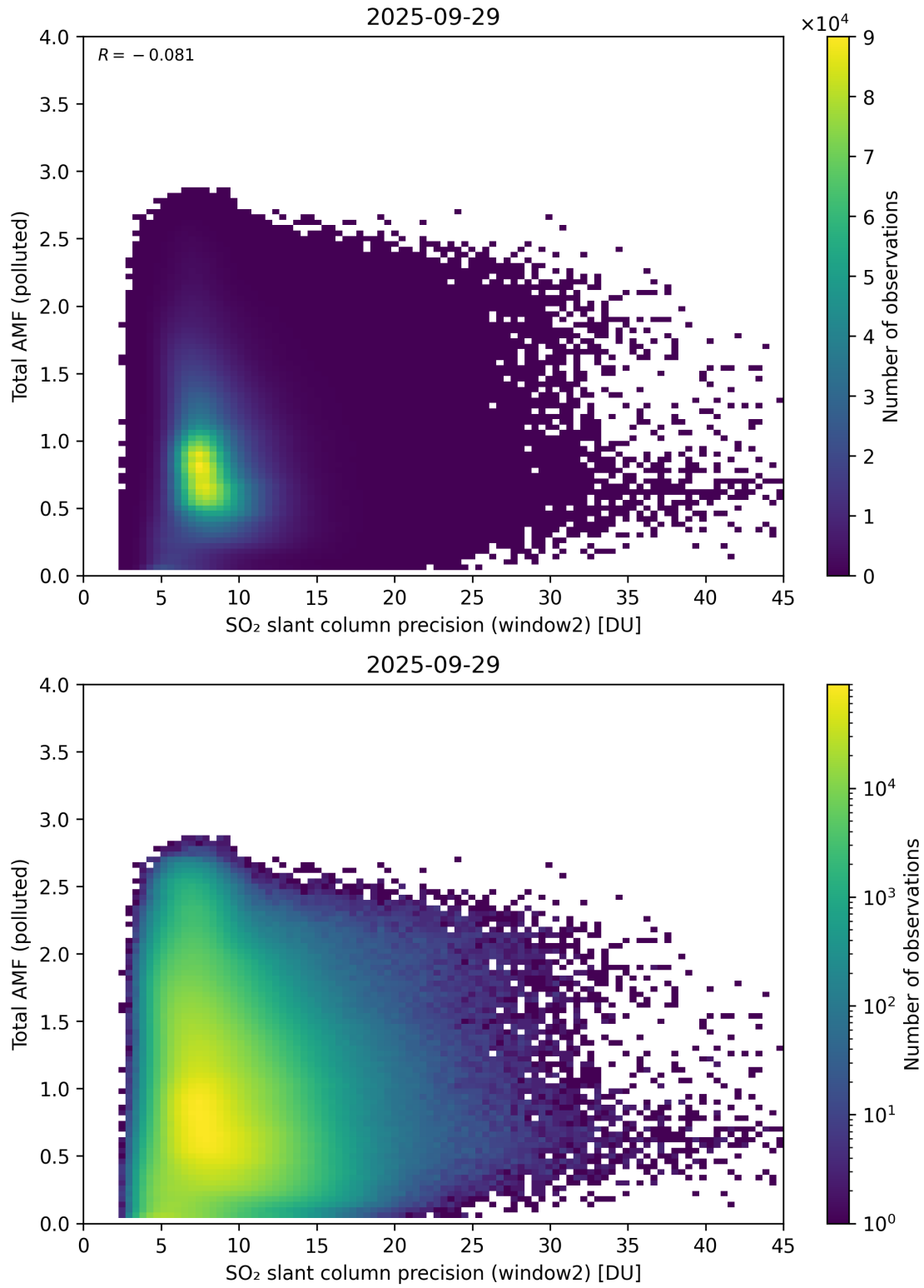
Figure 301: Scatter density plot of “SO 2 slant column precision (window2)” against “Total AMF (polluted)” for 2025-09-28 to 2025-09-30.
