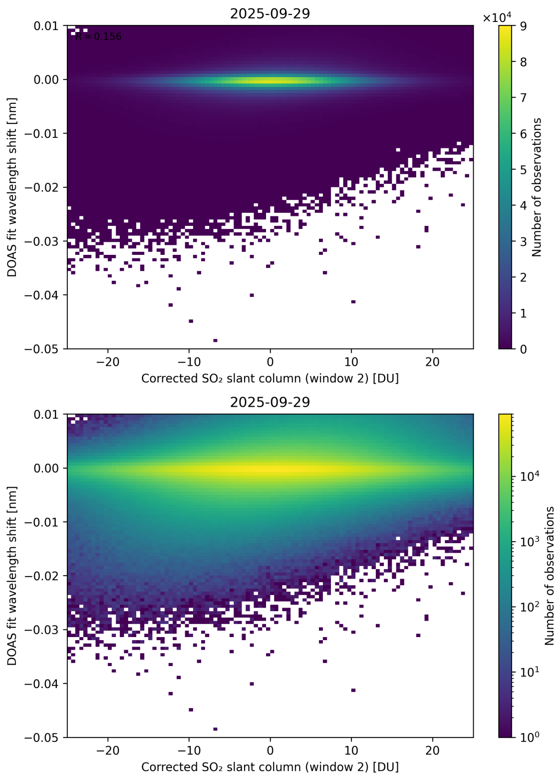
Figure 246: Scatter density plot of “Corrected SO 2 slant column (window 2)” against “DOAS fit wavelength shift” for 2025-09-28 to 2025-09-30.
