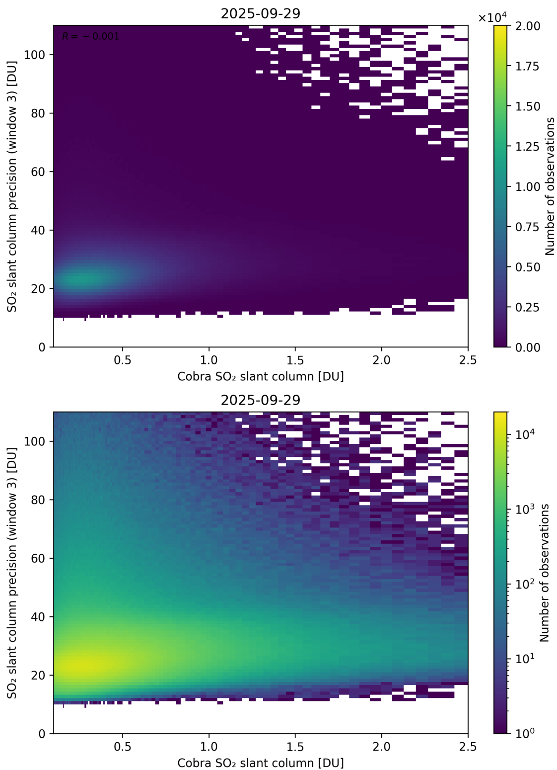
Figure 223: Scatter density plot of “Cobra SO 2 slant column” against “SO 2 slant column precision (window 3)” for 2025-09-28 to 2025-09-30.
