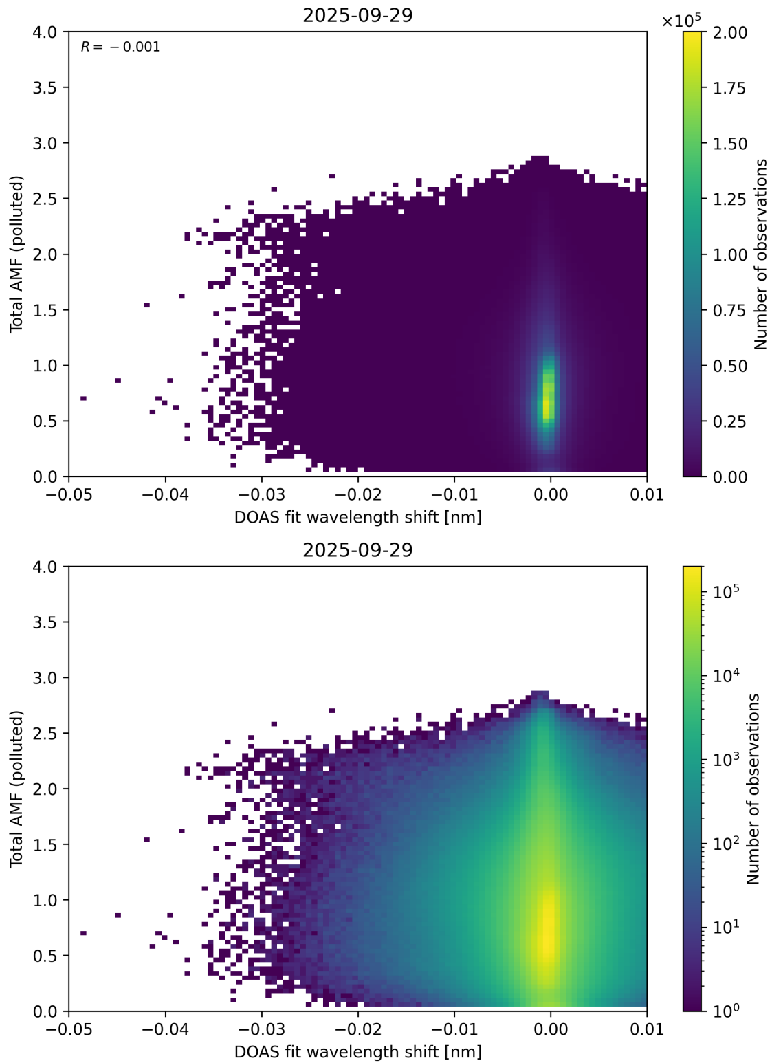
Figure 141: Scatter density plot of “DOAS fit wavelength shift” against “Total AMF (polluted)” for 2025-09-28 to 2025-09-30.
