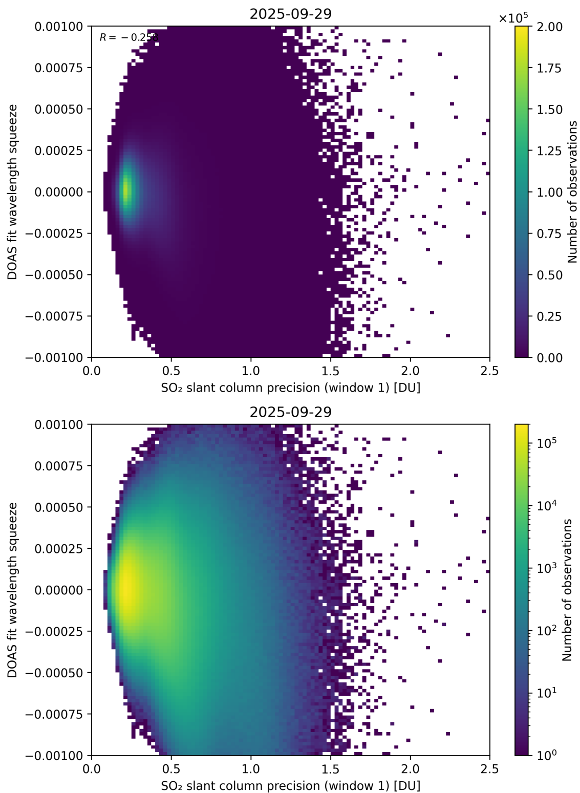
Figure 272: Scatter density plot of “SO 2 slant column precision (window 1)” against “DOAS fit wavelength squeeze” for 2025-09-28 to 2025-09-30.
