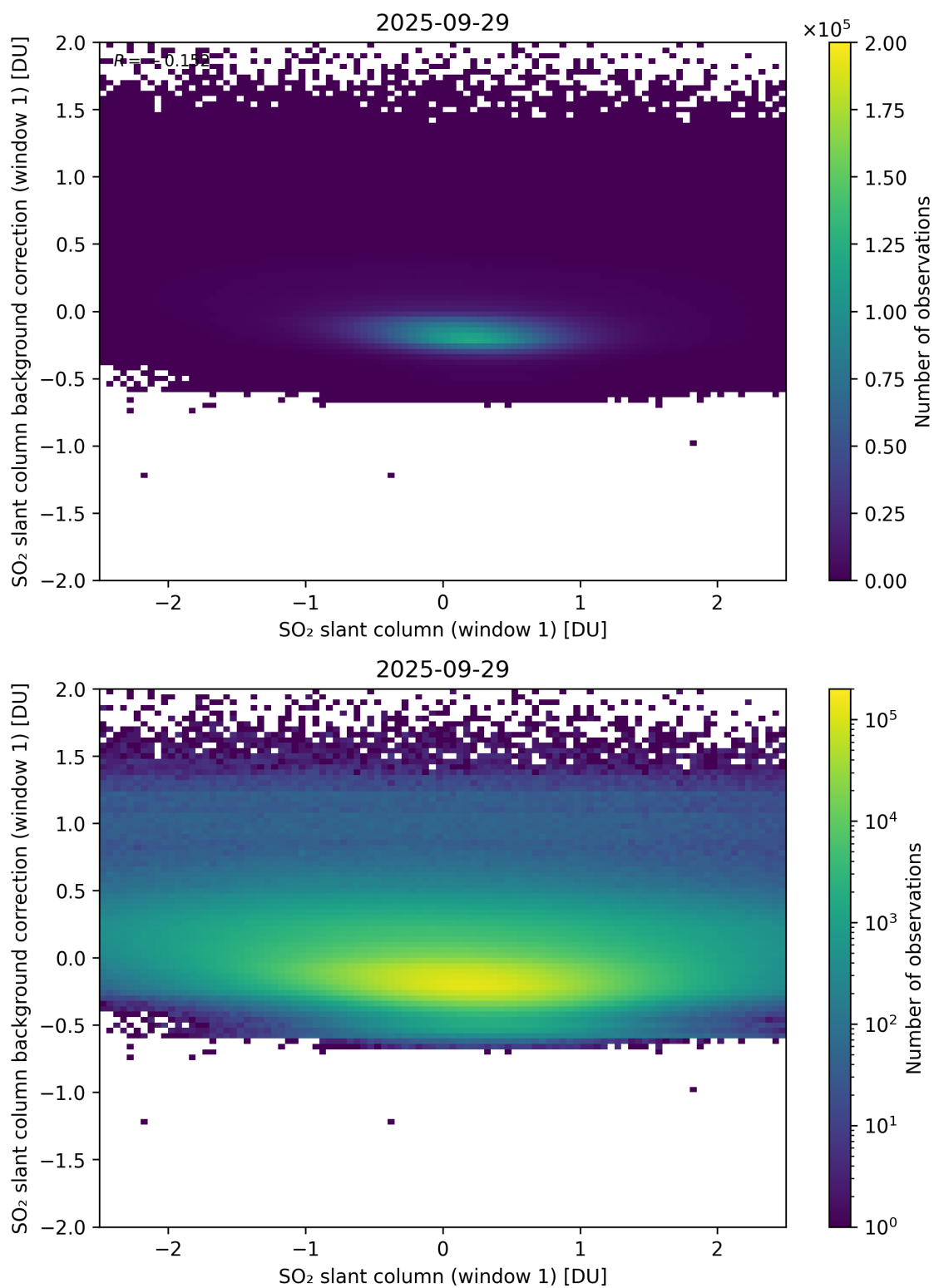
Figure 262: Scatter density plot of “SO 2 slant column (window 1)” against “SO 2 slant column background correction (window 1)” for 2025-09-28 to 2025-09-30.
