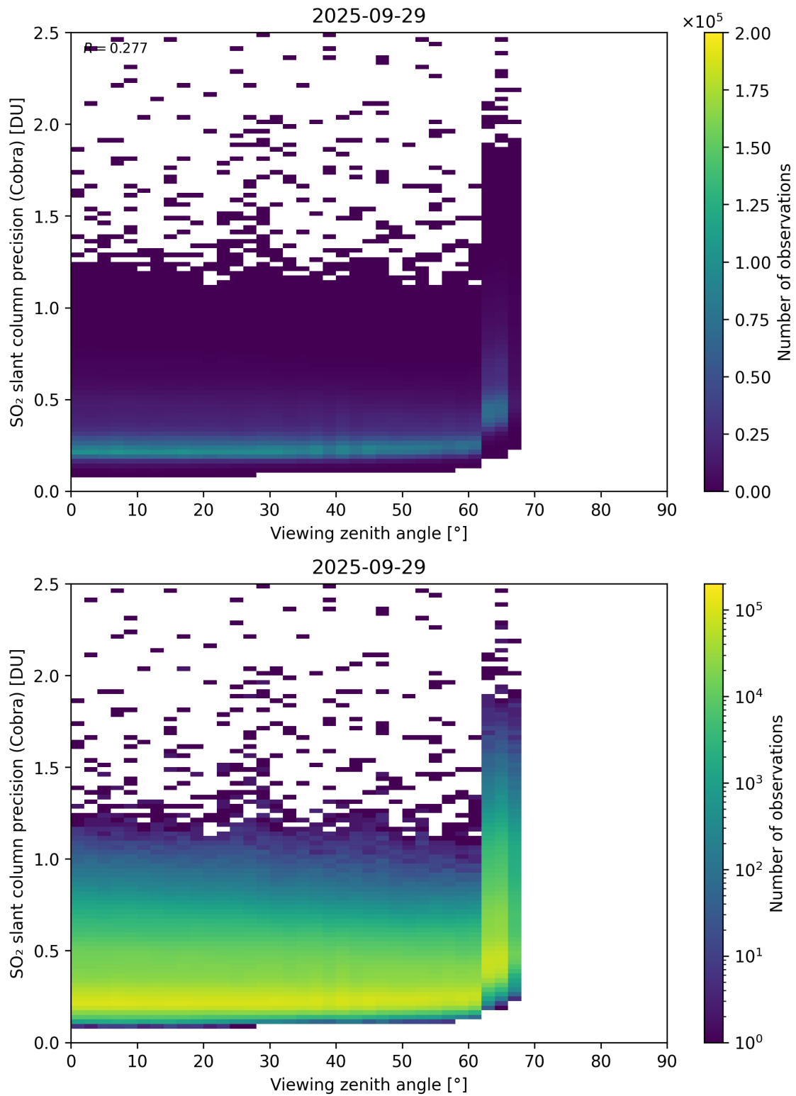
Figure 372: Scatter density plot of “Viewing zenith angle” against “SO 2 slant column precision (Cobra)” for 2025-09-28 to 2025-09-30.
