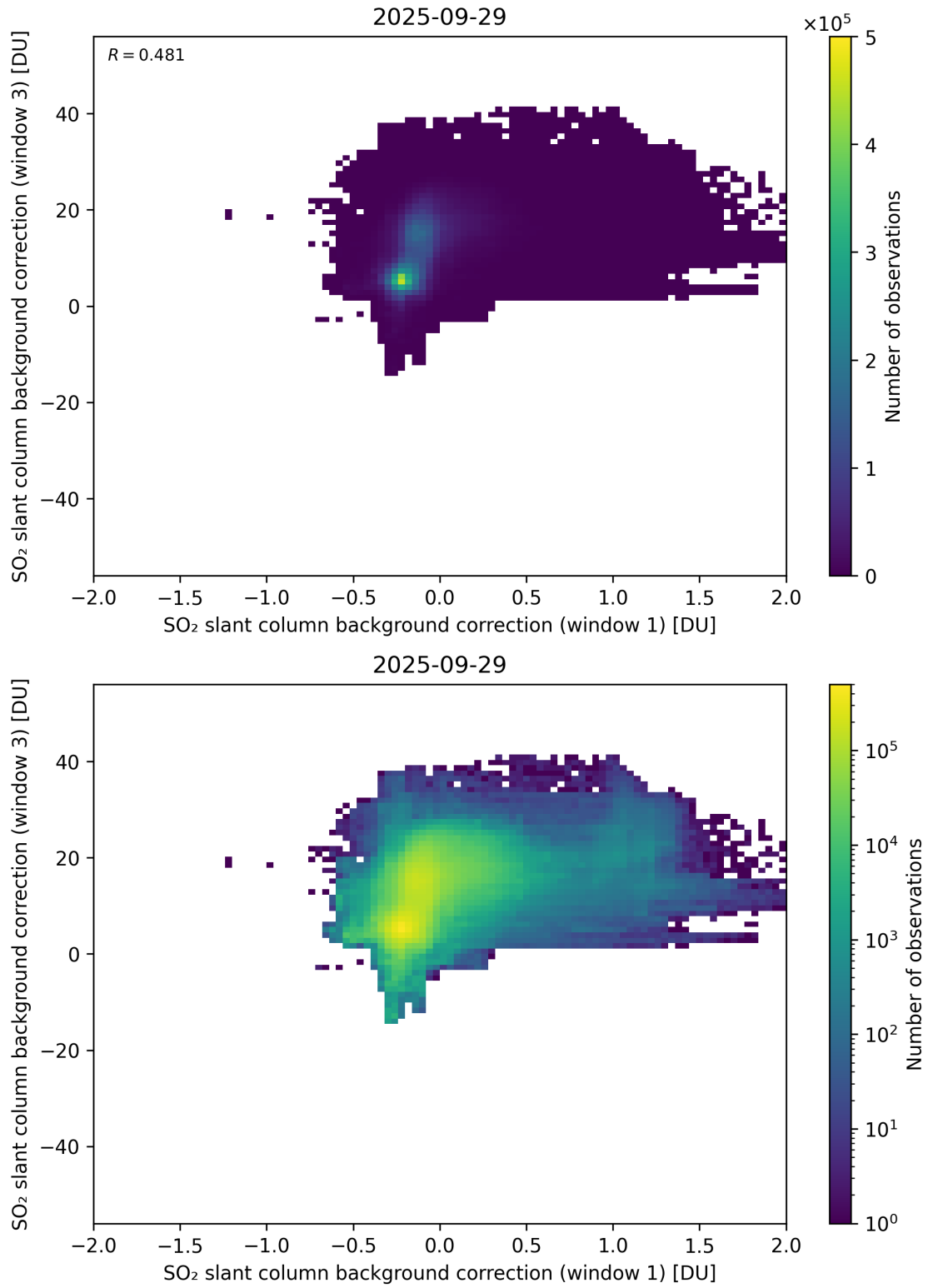
Figure 110: Scatter density plot of “SO 2 slant column background correction (window 1)” against “SO 2 slant column background correction (window 3)” for 2025-09-28 to 2025-09-30.
