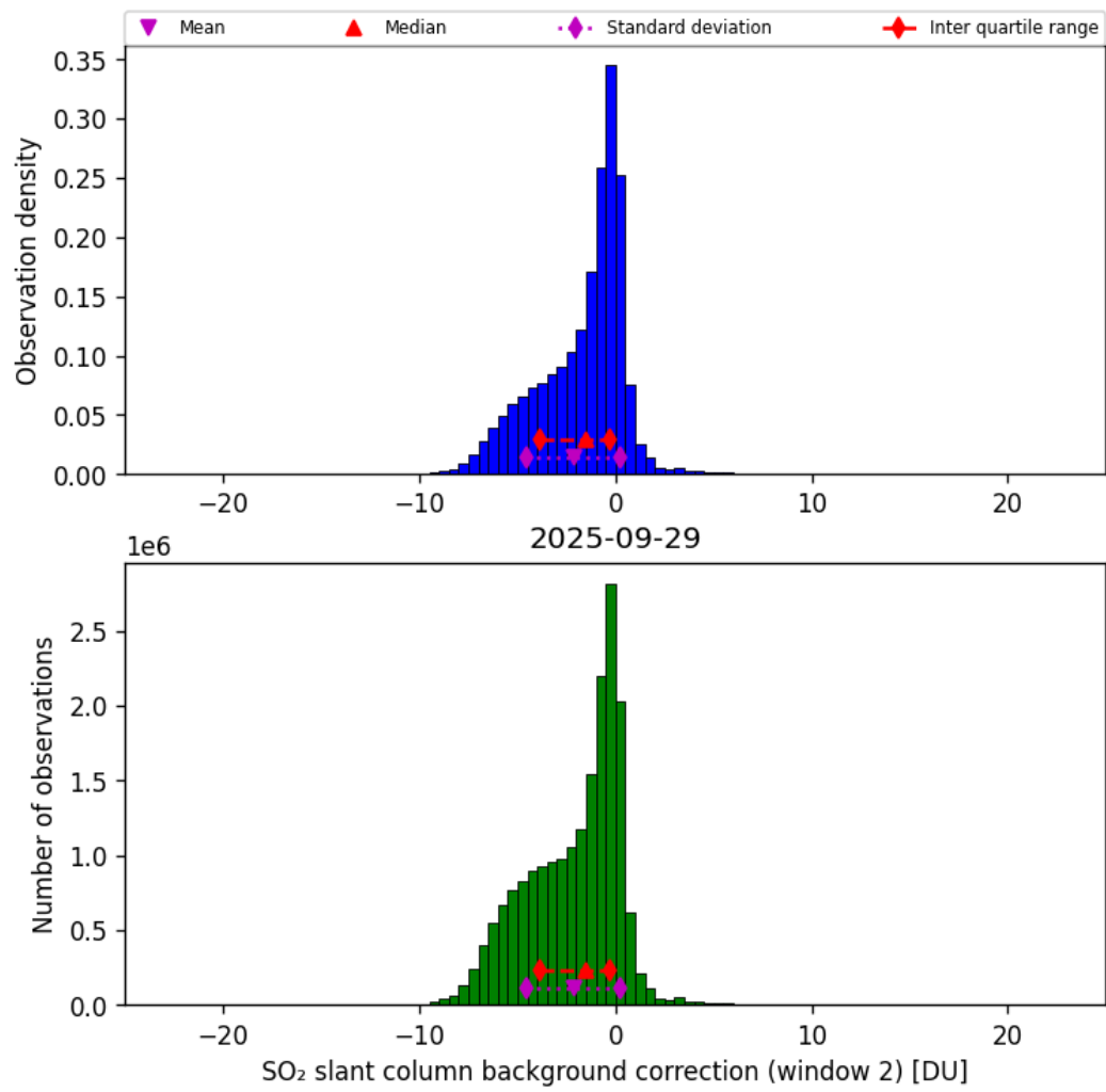
Figure 70: Histogram of “SO 2 slant column background correction (window 2)” for 2025-09-28 to 2025-09-30
