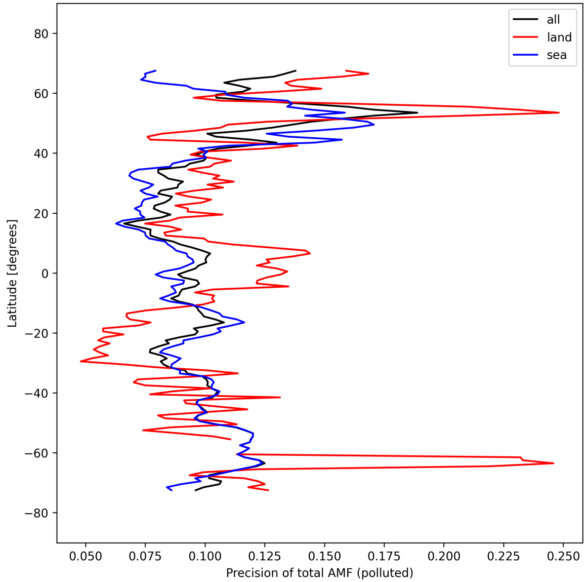
Figure 54: Zonal average of “Precision of total AMF (polluted)” for 2025-09-28 to 2025-09-30.
