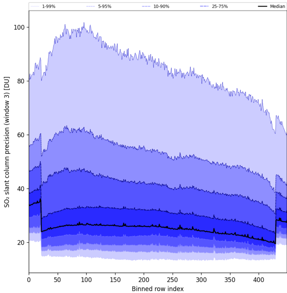
Figure 98: Along track statistics of “SO 2 slant column precision (window 3)” for 2025-09-28 to 2025-09-30
