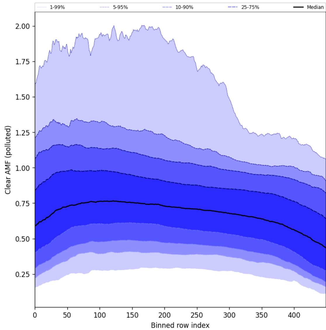
Figure 107: Along track statistics of “Clear AMF (polluted)” for 2025-09-28 to 2025-09-30
