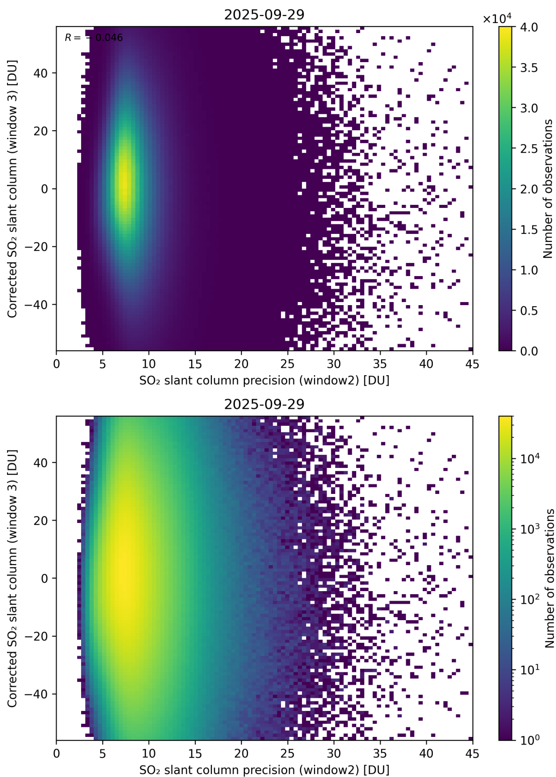
Figure 298: Scatter density plot of “SO 2 slant column precision (window2)” against “Corrected SO 2 slant column (window 3)” for 2025-09-28 to 2025-09-30.
