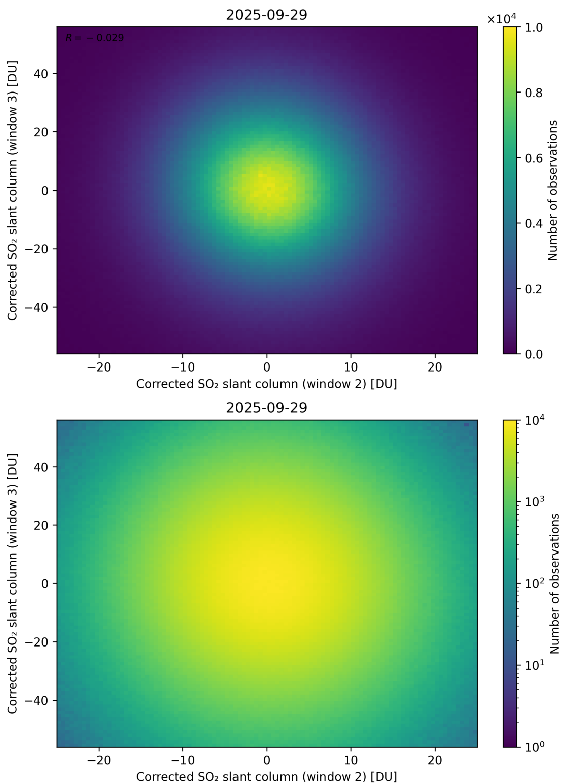
Figure 250: Scatter density plot of “Corrected SO 2 slant column (window 2)” against “Corrected SO 2 slant column (window 3)” for 2025-09-28 to 2025-09-30.
