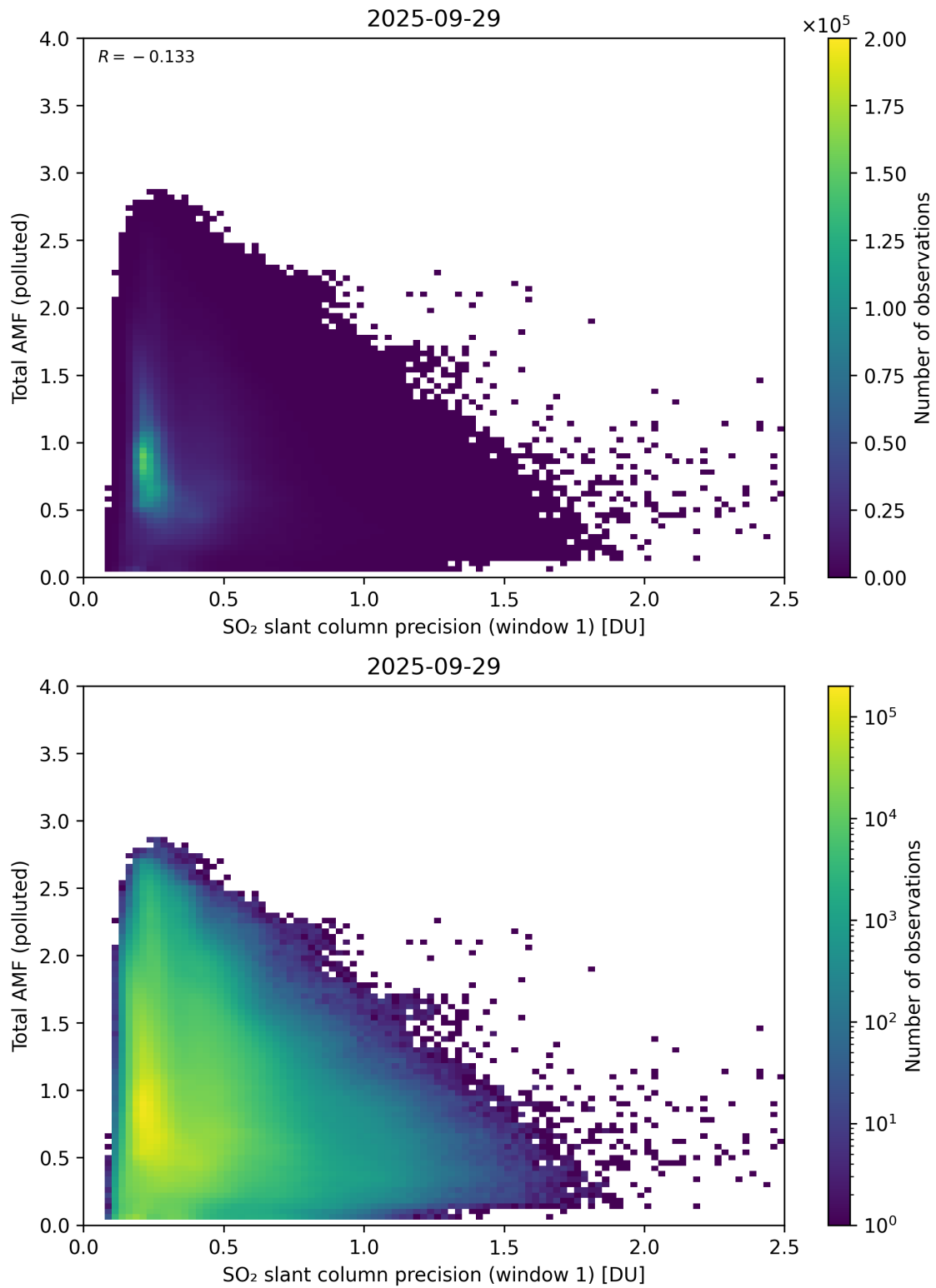
Figure 280: Scatter density plot of “SO 2 slant column precision (window 1)” against “Total AMF (polluted)” for 2025-09-28 to 2025-09-30.
