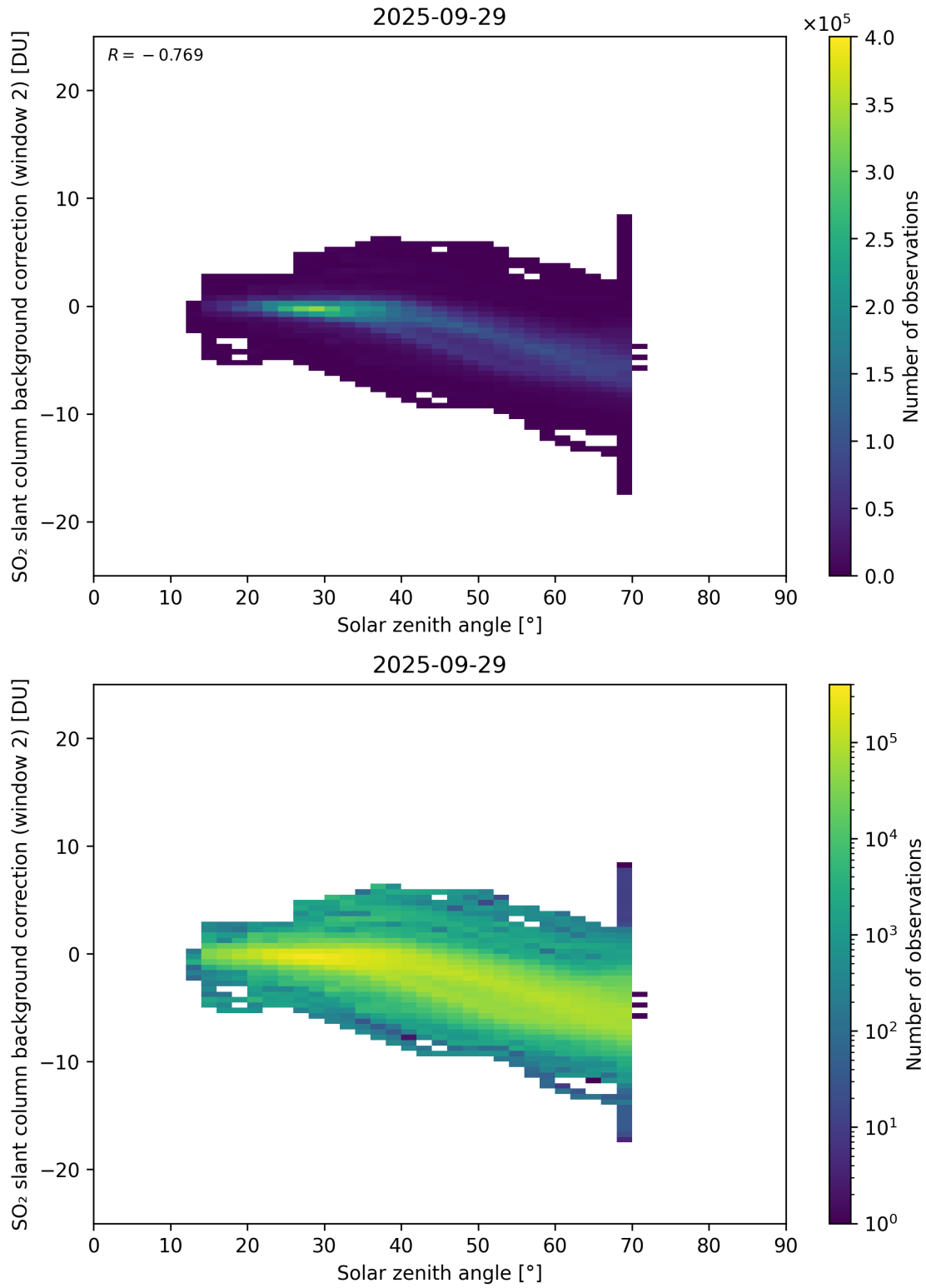
Figure 172: Scatter density plot of “Solar zenith angle” against “SO 2 slant column background correction (window 2)” for 2025-09-28 to 2025-09-30.
