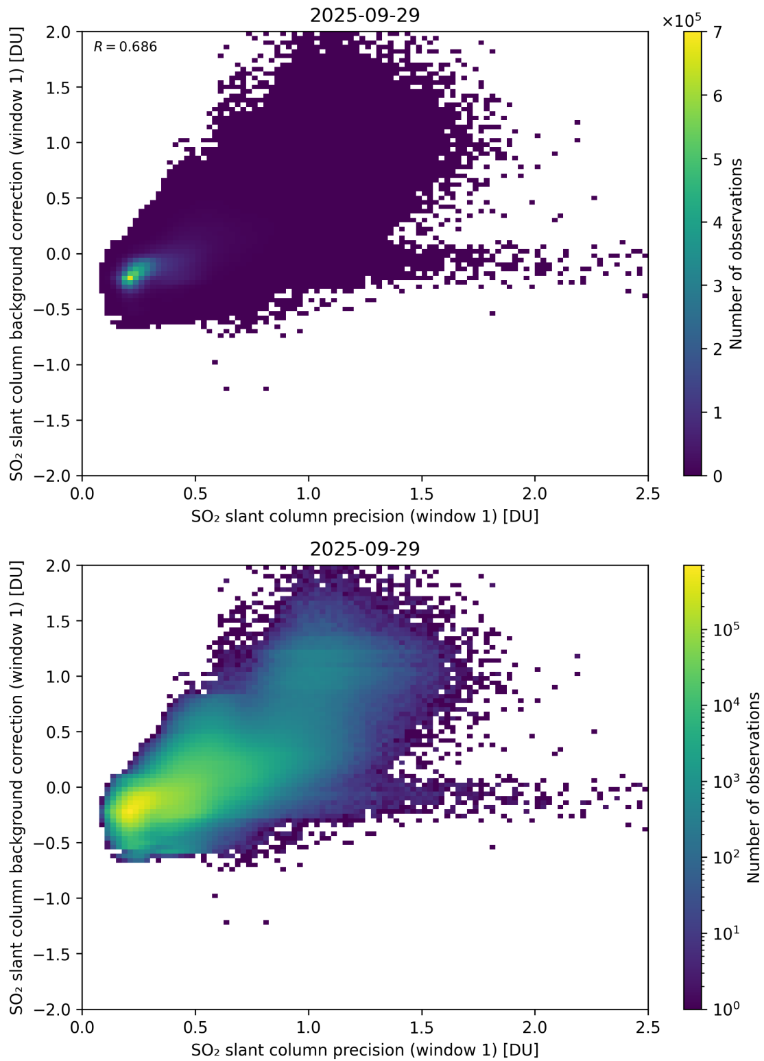
Figure 268: Scatter density plot of “SO 2 slant column precision (window 1)” against “SO 2 slant column background correction (window 1)” for 2025-09-28 to 2025-09-30.
