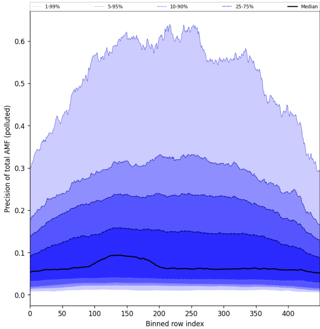
Figure 106: Along track statistics of “Precision of total AMF (polluted)” for 2025-09-28 to 2025-09-30
