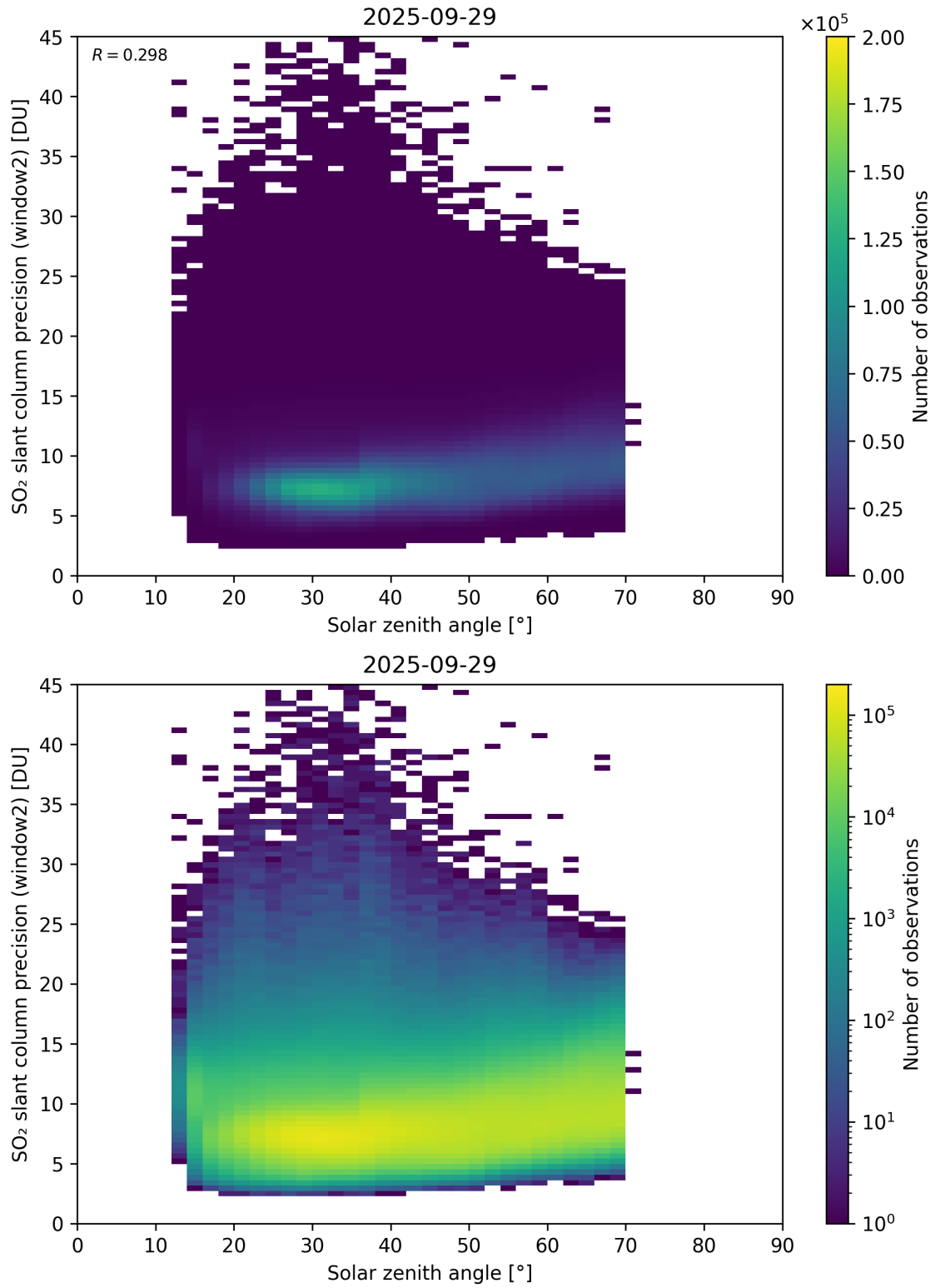
Figure 186: Scatter density plot of “Solar zenith angle” against “SO 2 slant column precision (window2)” for 2025-09-28 to 2025-09-30.
