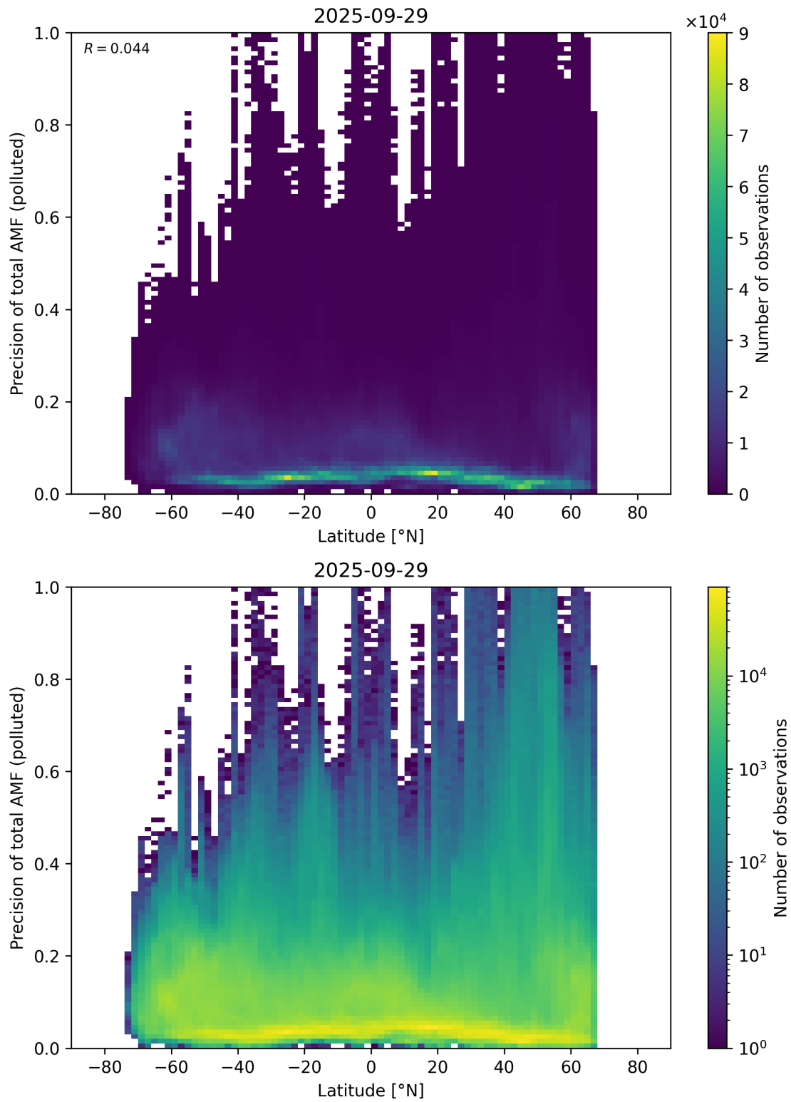
Figure 168: Scatter density plot of “Latitude” against “Precision of total AMF (polluted)” for 2025-09-28 to 2025-09-30.
