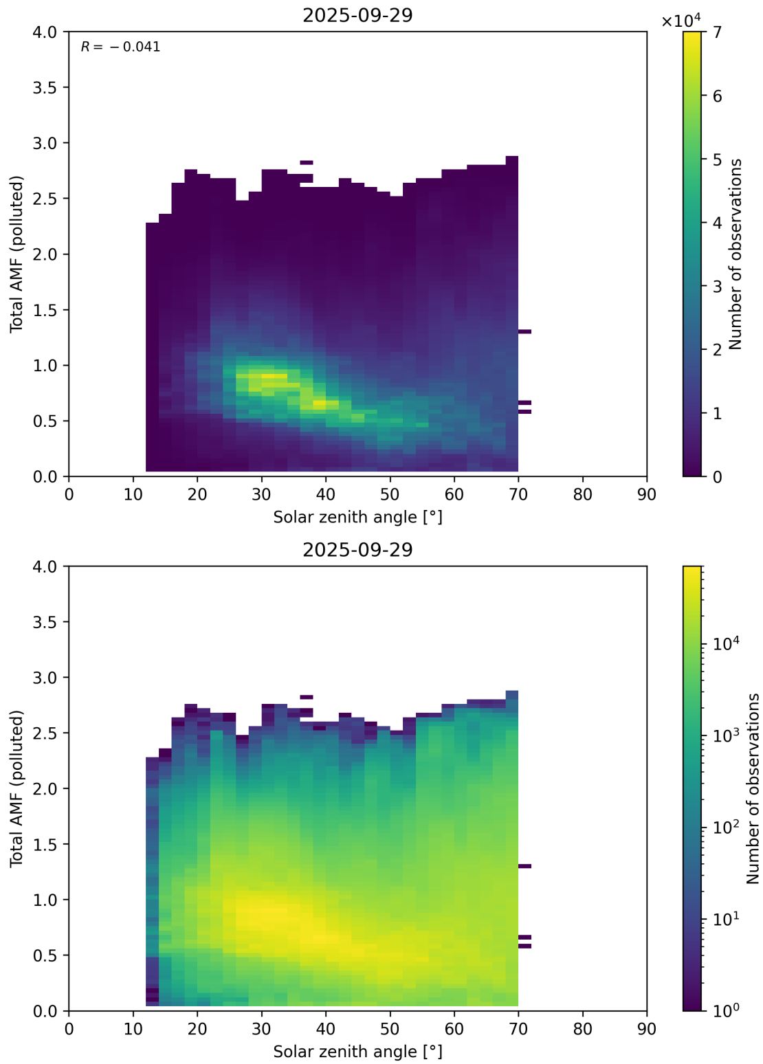
Figure 189: Scatter density plot of “Solar zenith angle” against “Total AMF (polluted)” for 2025-09-28 to 2025-09-30.
