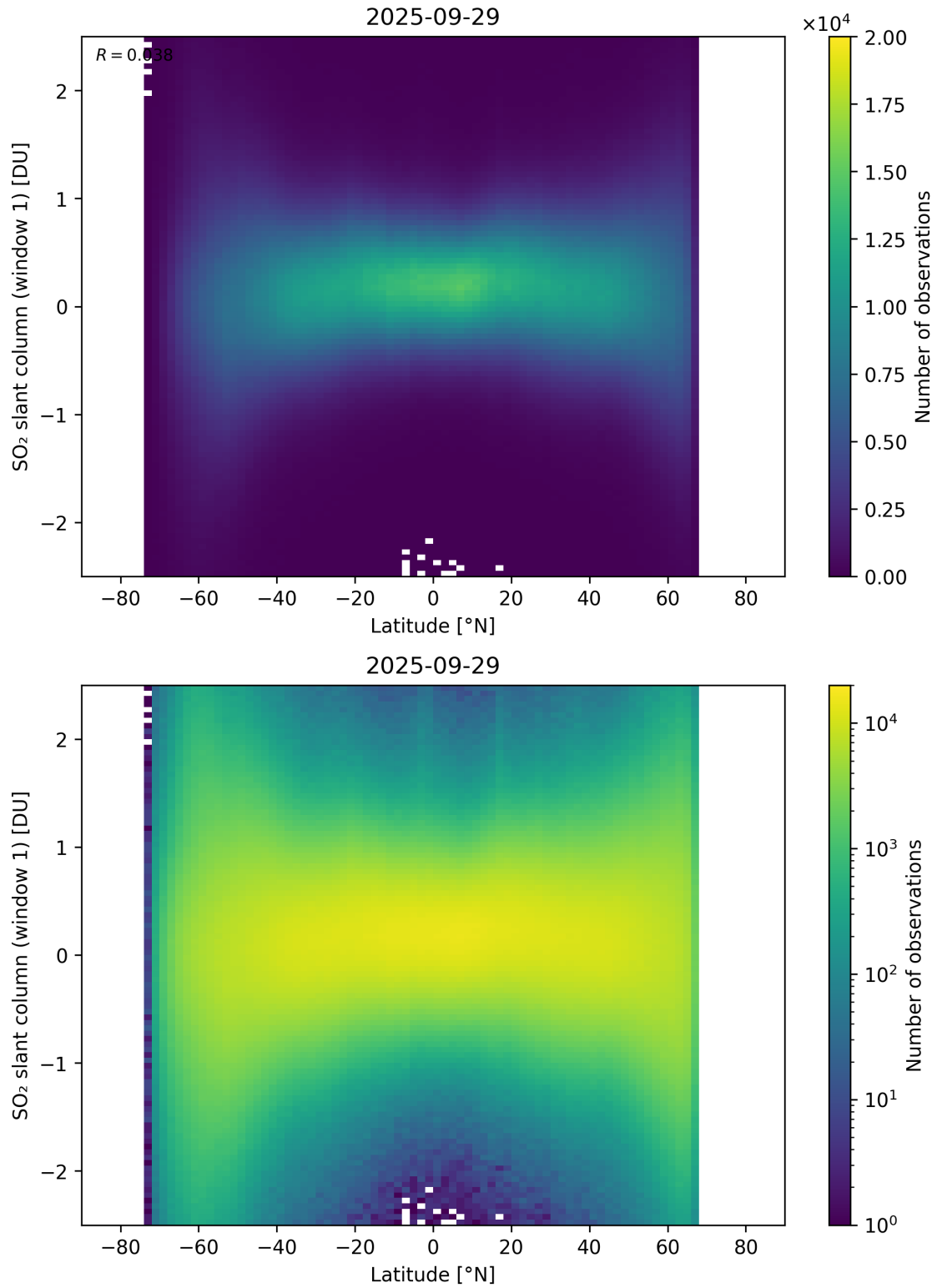
Figure 162: Scatter density plot of “Latitude” against “SO 2 slant column (window 1)” for 2025-09-28 to 2025-09-30.
