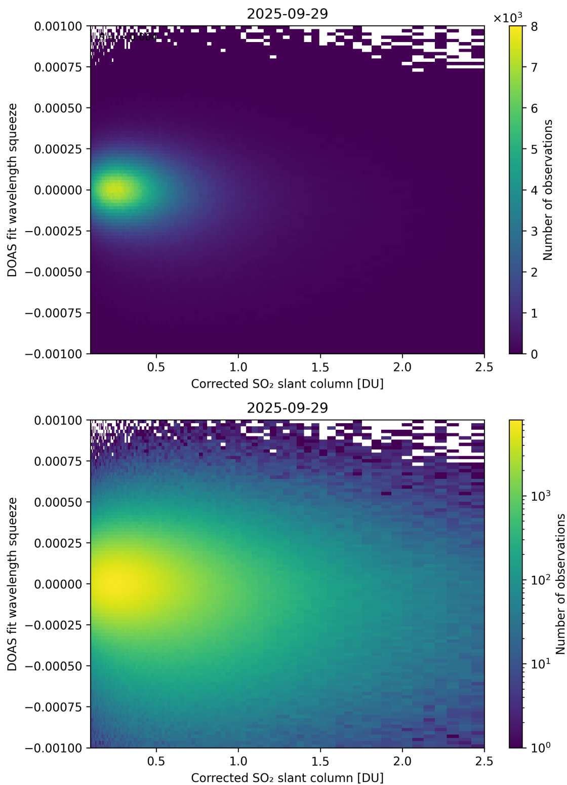
Figure 230: Scatter density plot of “Corrected SO 2 slant column” against “DOAS fit wavelength squeeze” for 2025-09-28 to 2025-09-30.
