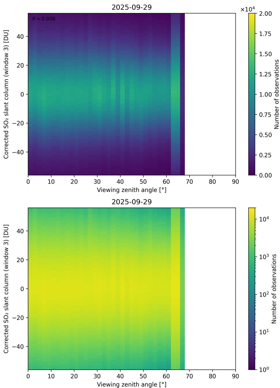
Figure 375: Scatter density plot of “Viewing zenith angle” against “Corrected SO 2 slant column (window 3)” for 2025-09-28 to 2025-09-30.
