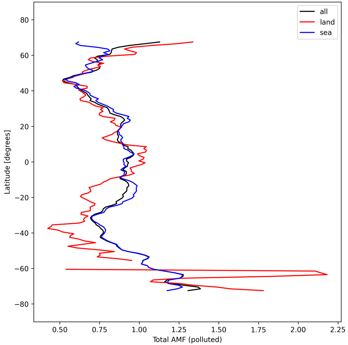
Figure 53: Zonal average of “Total AMF (polluted)” for 2025-09-28 to 2025-09-30.
