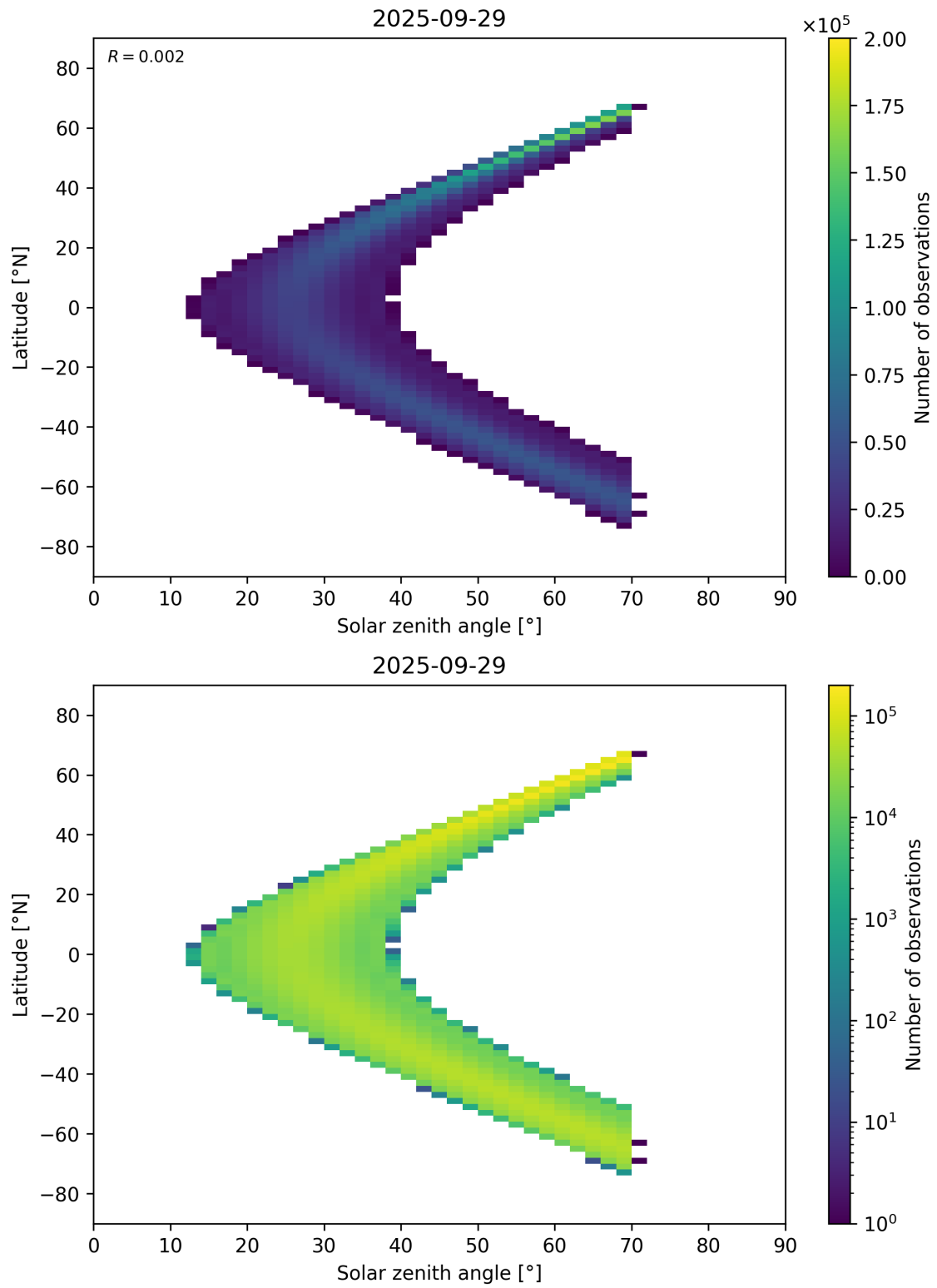
Figure 177: Scatter density plot of “Solar zenith angle” against “Latitude” for 2025-09-28 to 2025-09-30.
