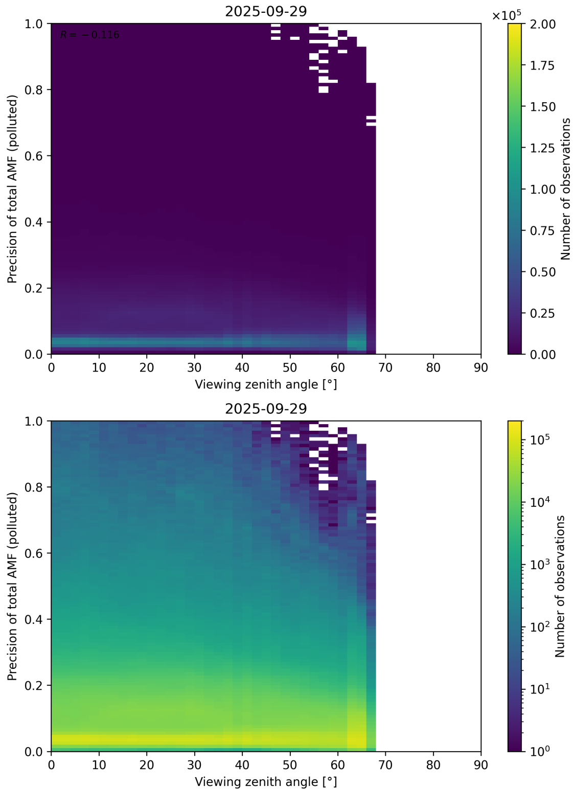
Figure 382: Scatter density plot of “Viewing zenith angle” against “Precision of total AMF (polluted)” for 2025-09-28 to 2025-09-30.
