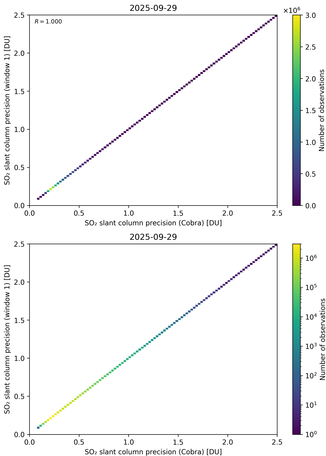
Figure 209: Scatter density plot of “SO 2 slant column precision (Cobra)” against “SO 2 slant column precision (window 1)” for 2025-09-28 to 2025-09-30.
