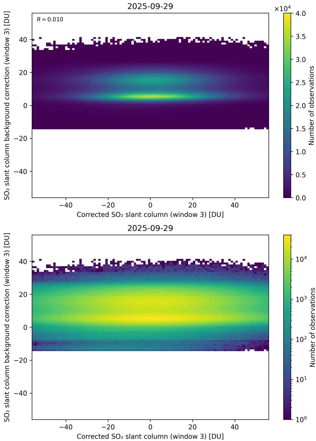
Figure 255: Scatter density plot of “Corrected SO 2 slant column (window 3)” against “SO 2 slant column background correction (window 3)” for 2025-09-28 to 2025-09-30.
