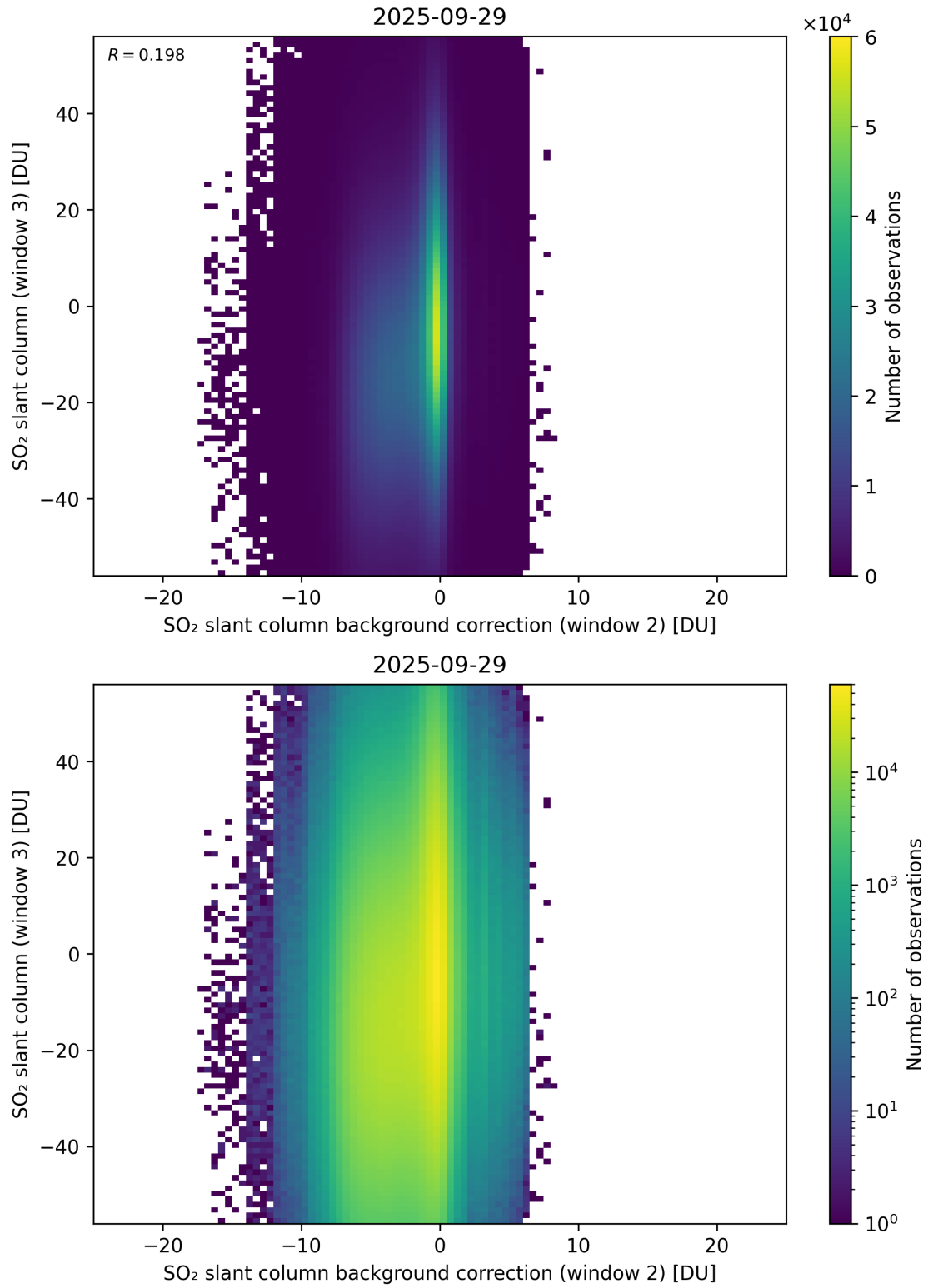
Figure 128: Scatter density plot of “SO 2 slant column background correction (window 2)” against “SO 2 slant column (window 3)” for 2025-09-28 to 2025-09-30.
