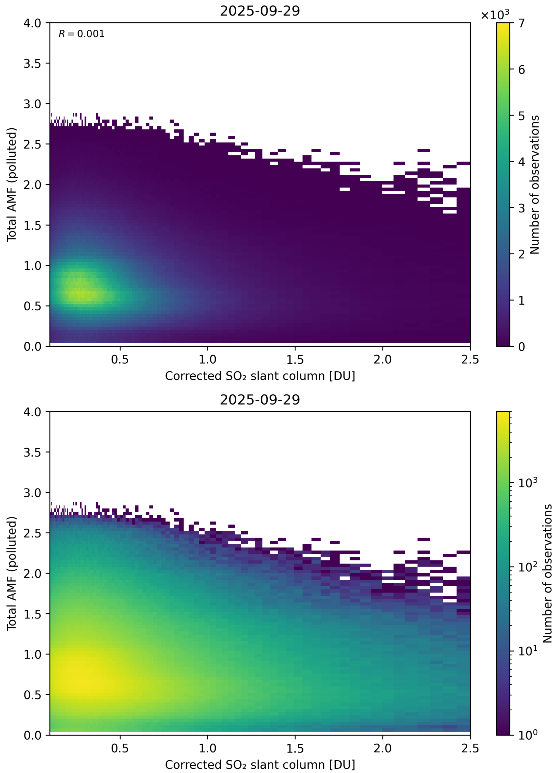
Figure 242: Scatter density plot of “Corrected SO 2 slant column” against “Total AMF (polluted)” for 2025-09-28 to 2025-09-30.
