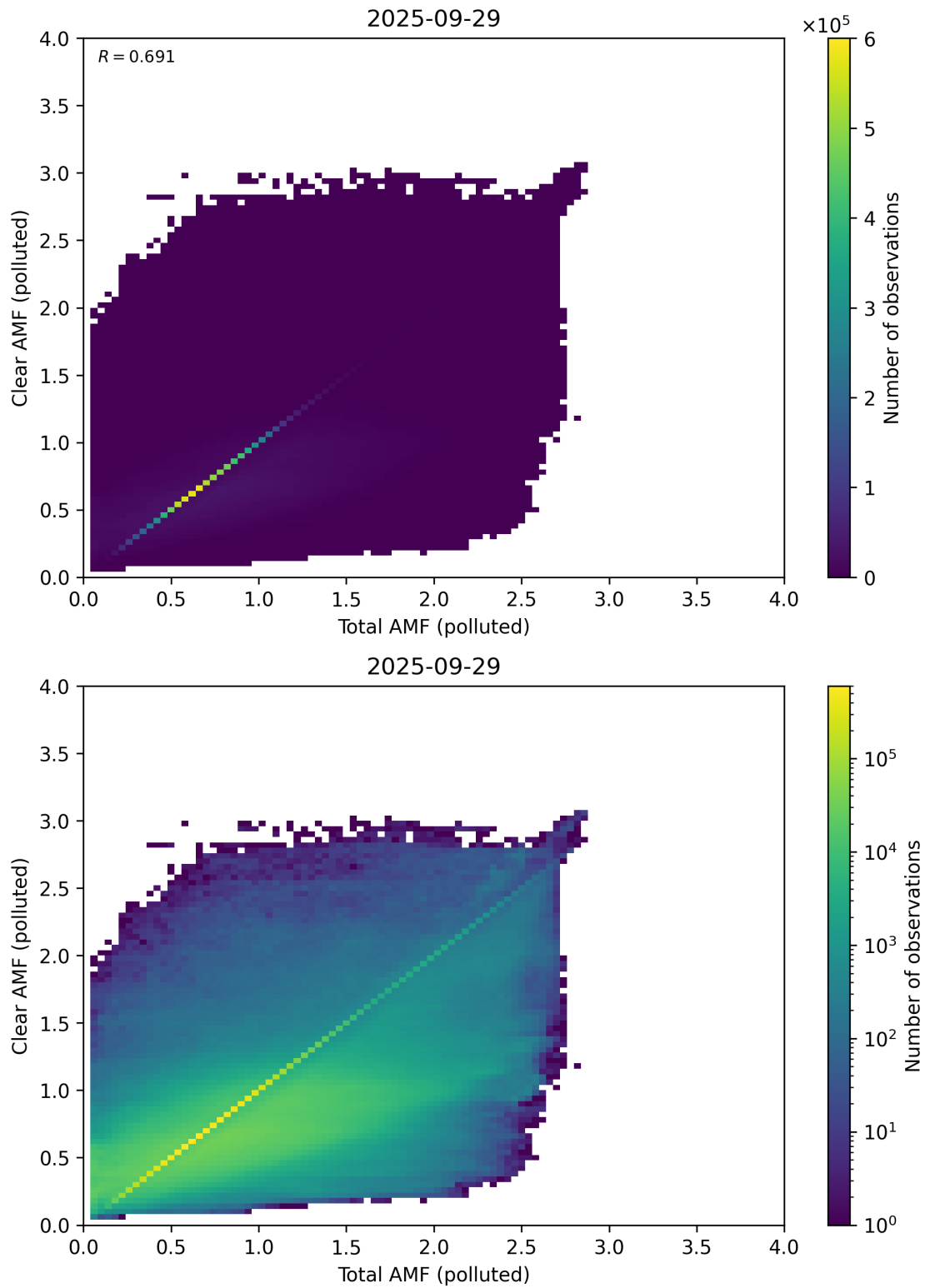
Figure 321: Scatter density plot of “Total AMF (polluted)” against “Clear AMF (polluted)” for 2025-09-28 to 2025-09-30.
