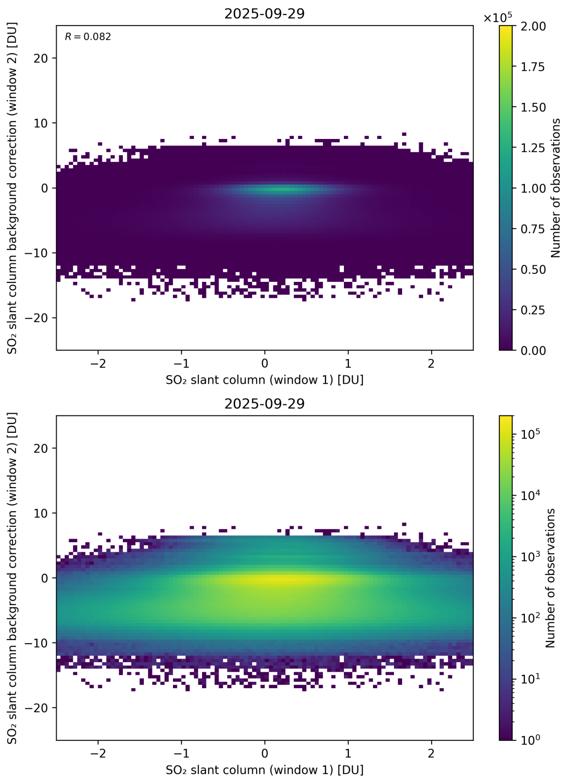
Figure 263: Scatter density plot of “SO 2 slant column (window 1)” against “SO 2 slant column background correction (window 2)” for 2025-09-28 to 2025-09-30.
