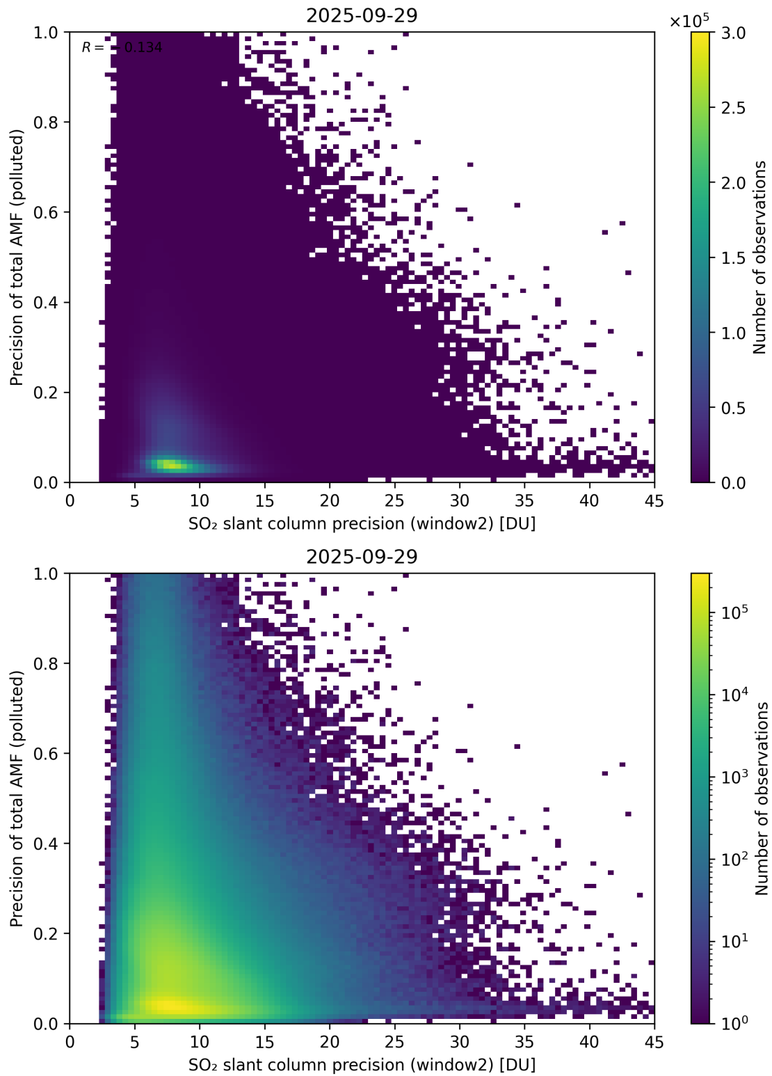
Figure 302: Scatter density plot of “SO 2 slant column precision (window2)” against “Precision of total AMF (polluted)” for 2025-09-28 to 2025-09-30.
