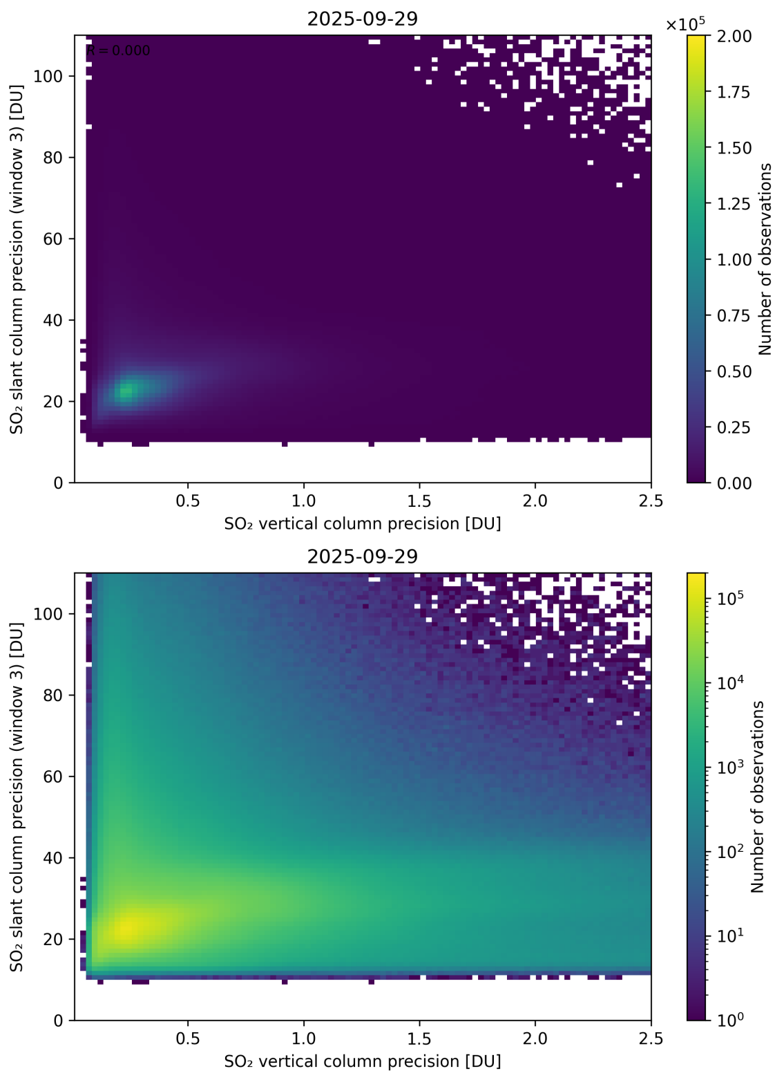
Figure 345: Scatter density plot of “SO 2 vertical column precision” against “SO 2 slant column precision (window 3)” for 2025-09-28 to 2025-09-30.
