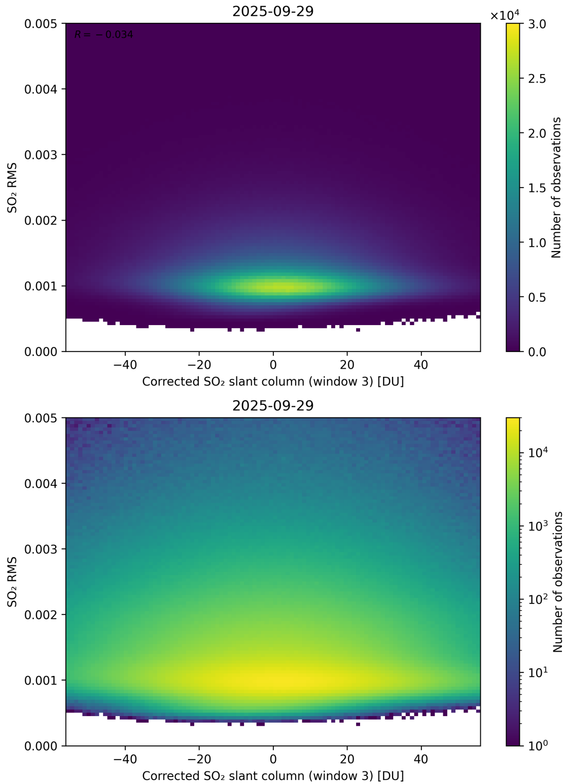
Figure 258: Scatter density plot of “Corrected SO 2 slant column (window 3)” against “SO 2 RMS” for 2025-09-28 to 2025-09-30.
