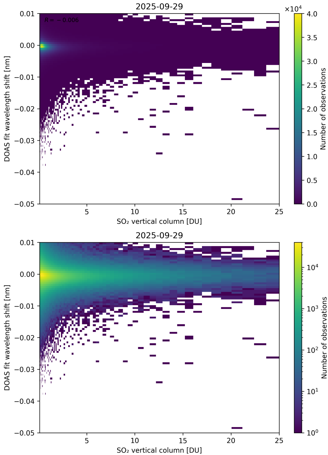
Figure 326: Scatter density plot of “SO 2 vertical column” against “DOAS fit wavelength shift” for 2025-09-28 to 2025-09-30.
