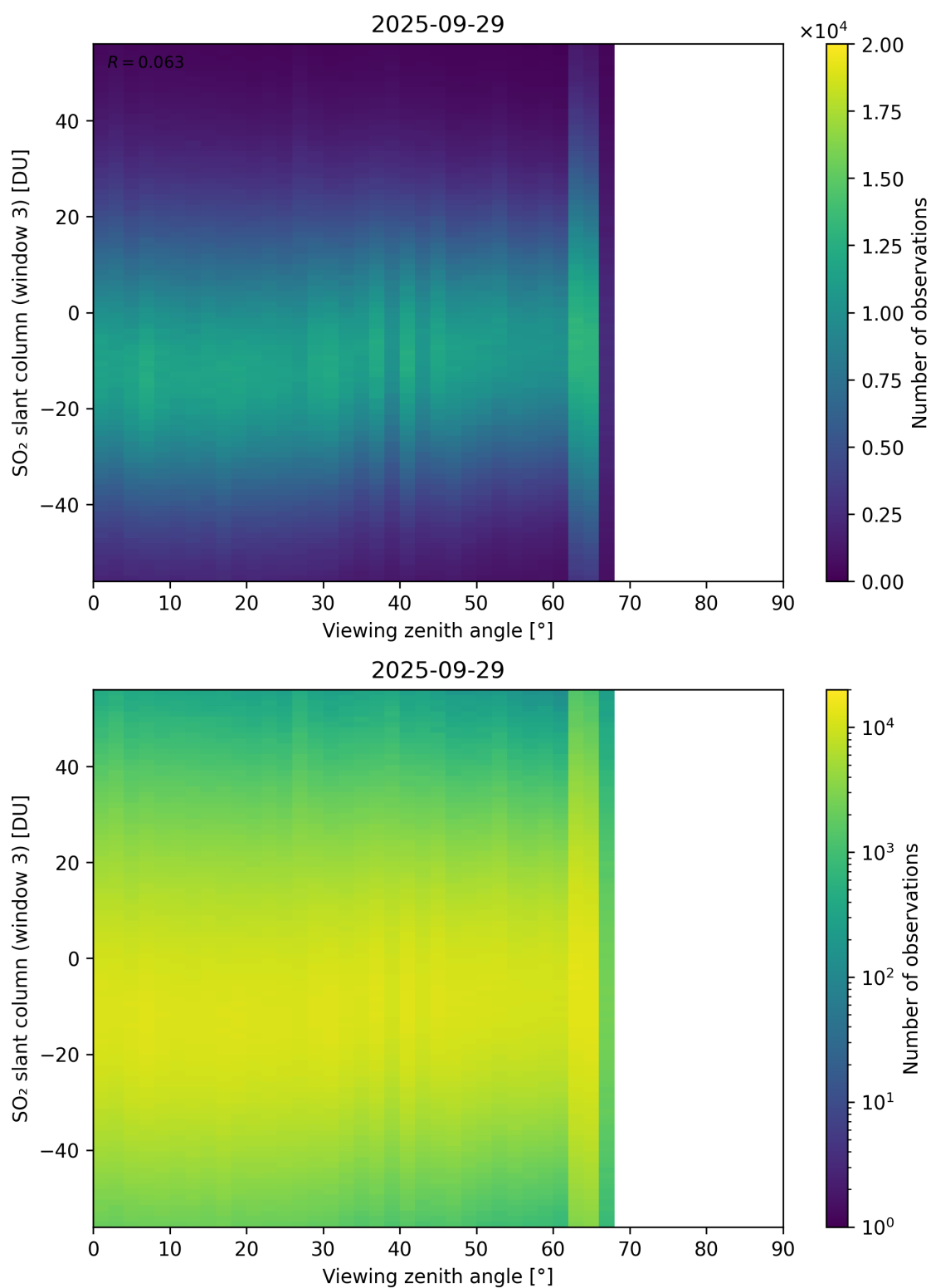
Figure 379: Scatter density plot of “Viewing zenith angle” against “SO 2 slant column (window 3)” for 2025-09-28 to 2025-09-30.
