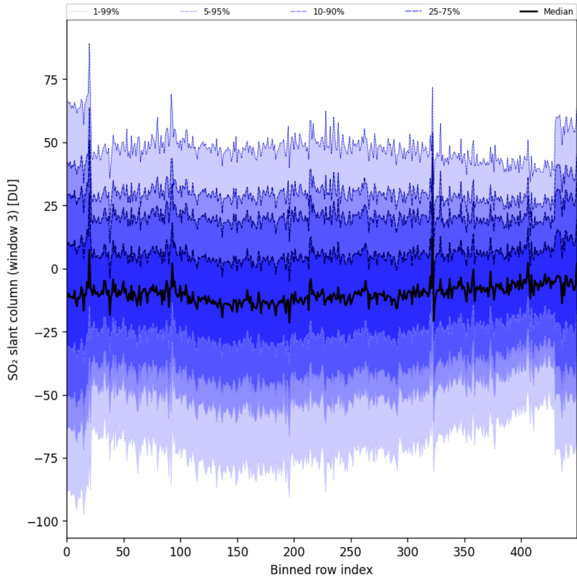
Figure 97: Along track statistics of “SO 2 slant column (window 3)” for 2025-09-28 to 2025-09-30
