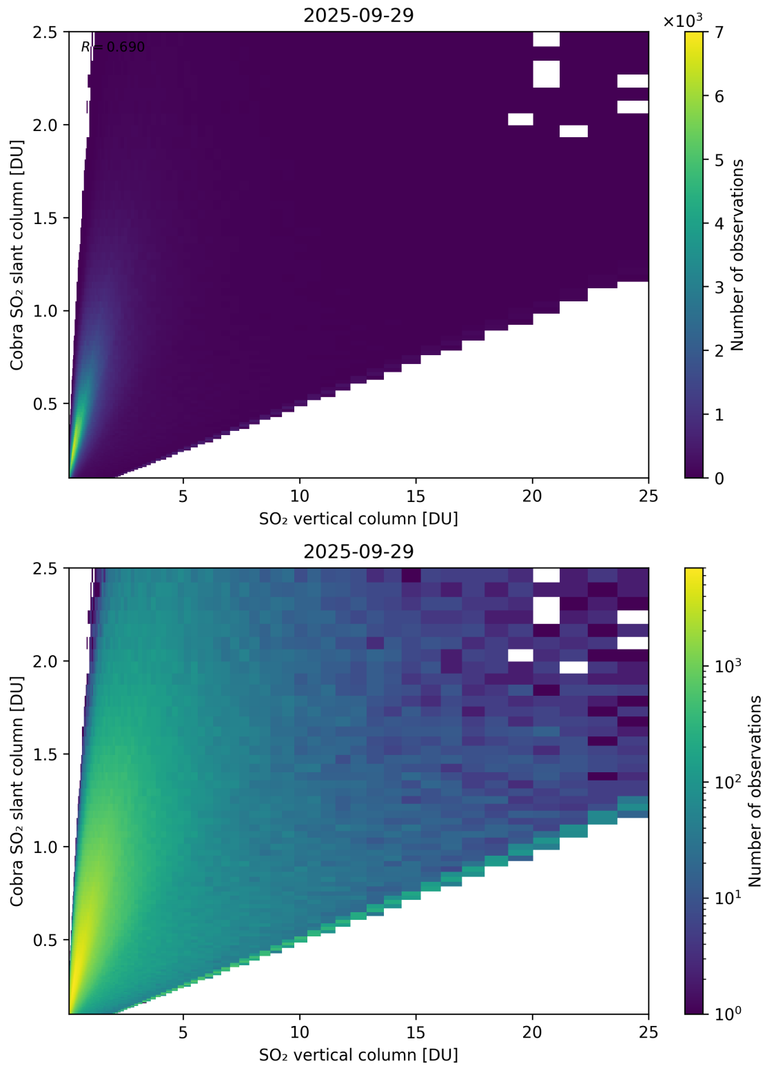
Figure 349: Scatter density plot of “SO 2 vertical column” against “Cobra SO 2 slant column” for 2025-09-28 to 2025-09-30.
