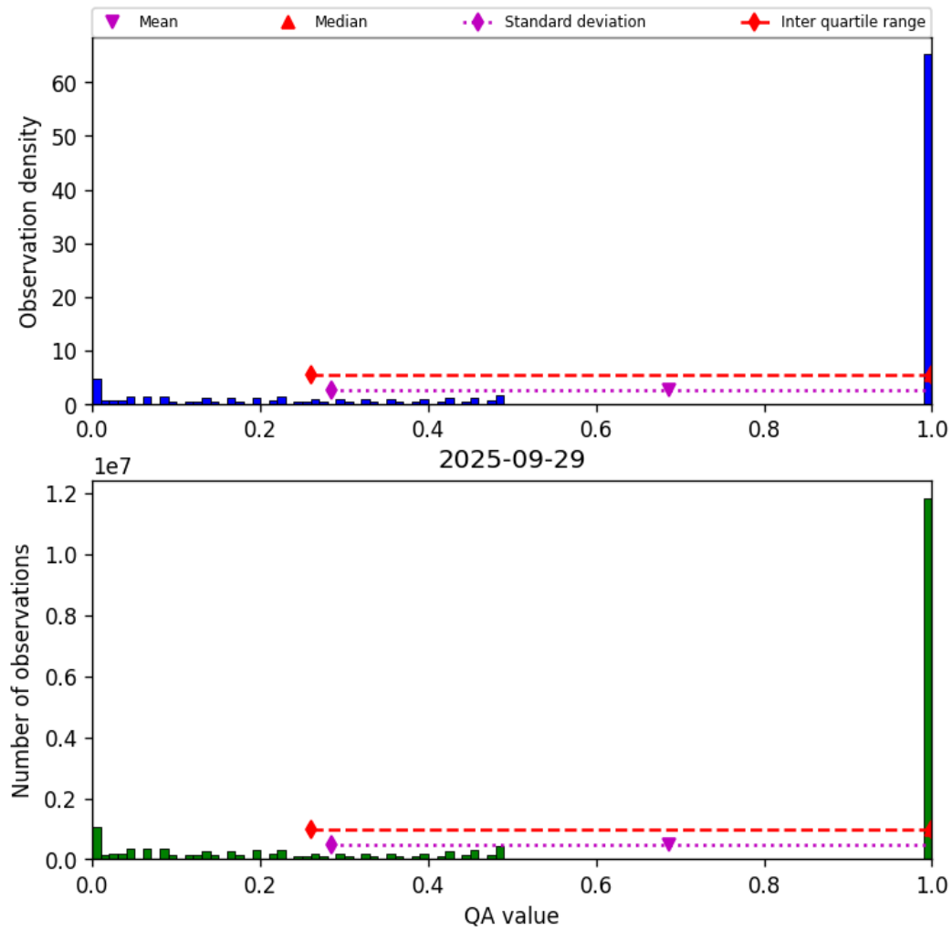
Figure 57: Histogram of “QA value” for 2025-09-28 to 2025-09-30
