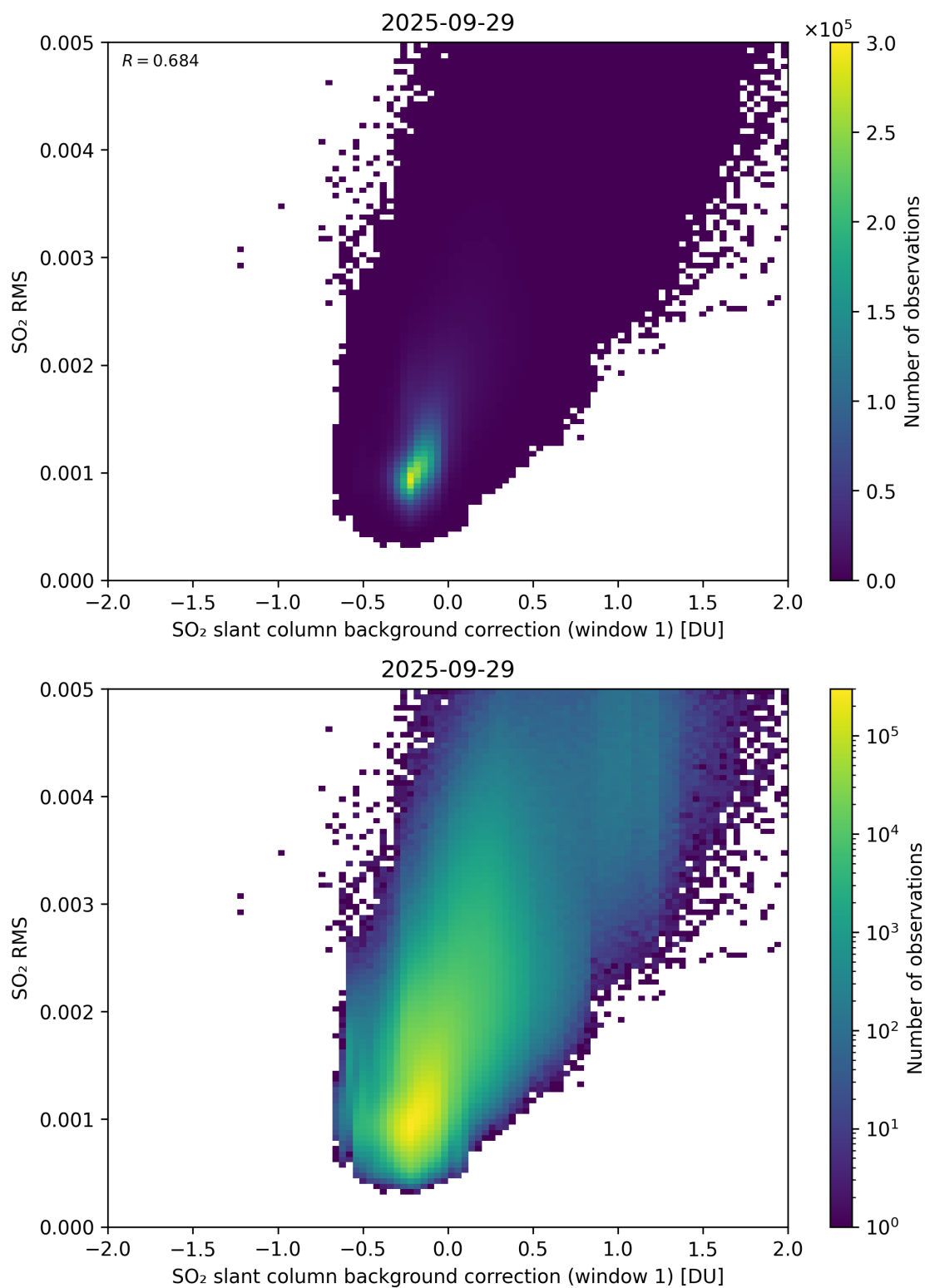
Figure 113: Scatter density plot of “SO 2 slant column background correction (window 1)” against “SO 2 RMS” for 2025-09-28 to 2025-09-30.
