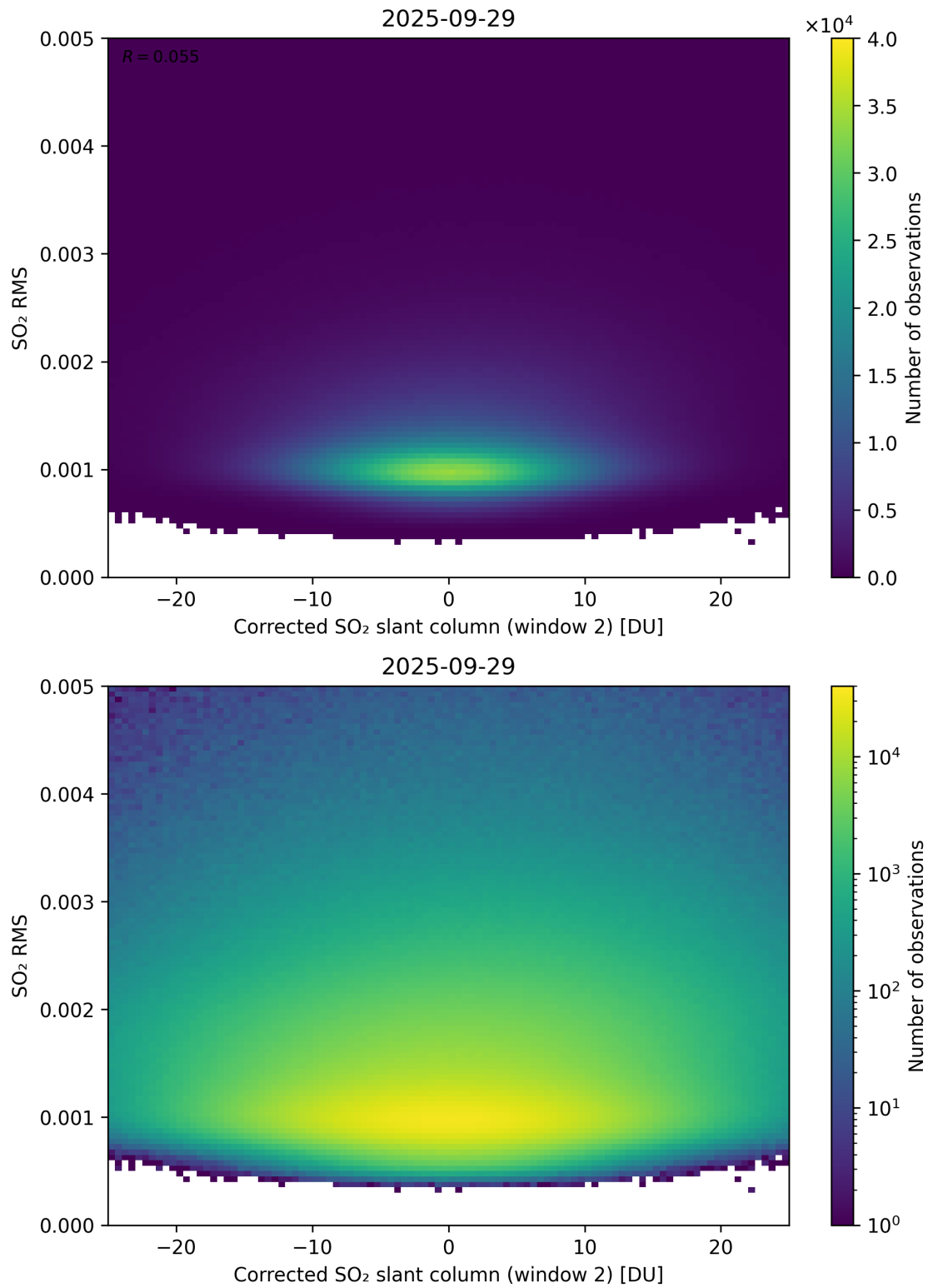
Figure 248: Scatter density plot of “Corrected SO 2 slant column (window 2)” against “SO 2 RMS” for 2025-09-28 to 2025-09-30.
