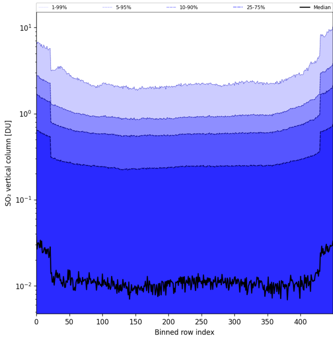
Figure 84: Along track statistics of “SO 2 vertical column” for 2025-09-28 to 2025-09-30
