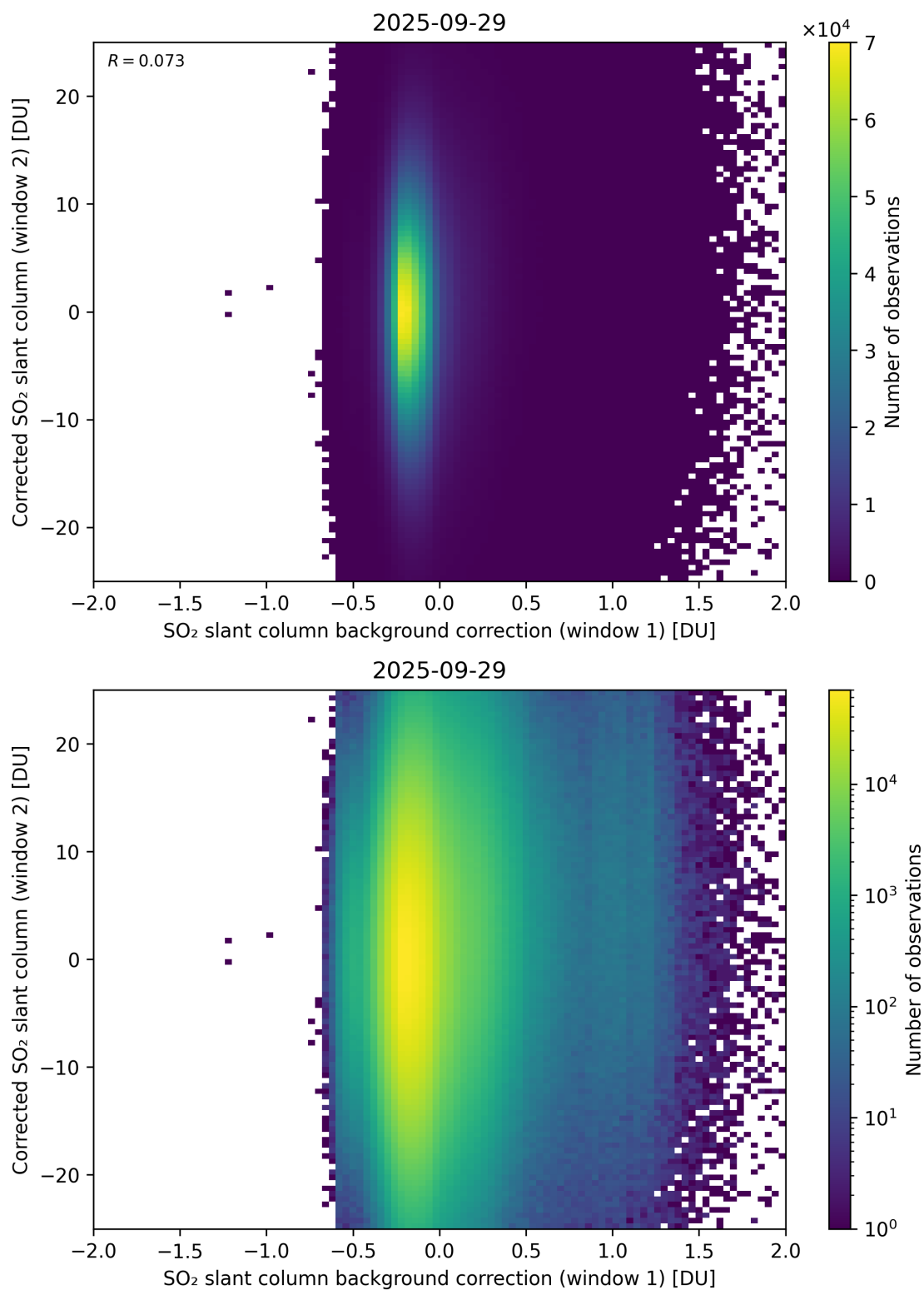
Figure 115: Scatter density plot of “SO 2 slant column background correction (window 1)” against “Corrected SO 2 slant column (window 2)” for 2025-09-28 to 2025-09-30.
