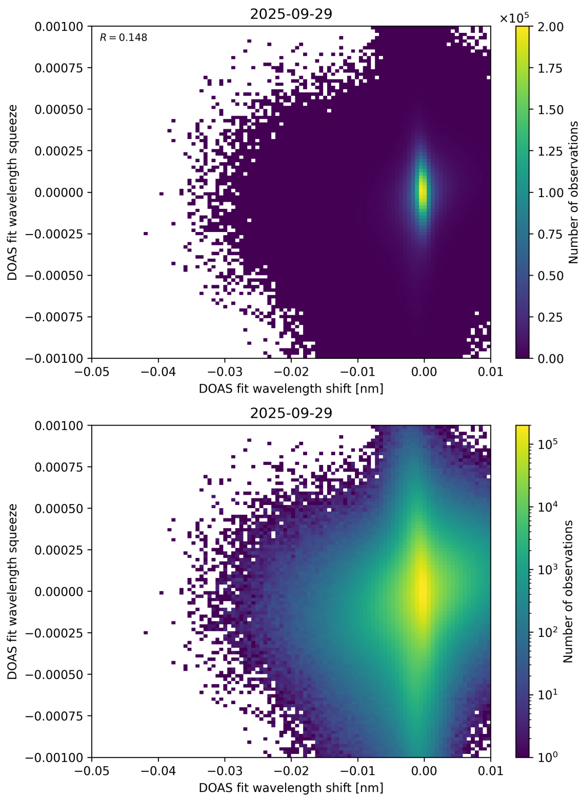
Figure 138: Scatter density plot of “DOAS fit wavelength shift” against “DOAS fit wavelength squeeze” for 2025-09-28 to 2025-09-30.
