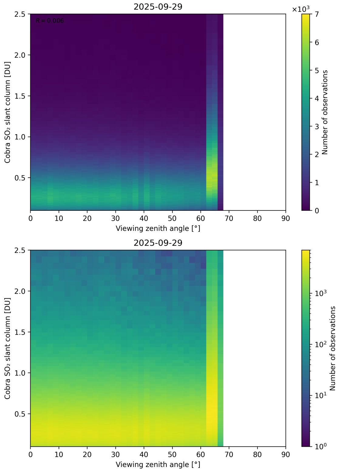
Figure 371: Scatter density plot of “Viewing zenith angle” against “Cobra SO 2 slant column” for 2025-09-28 to 2025-09-30.
