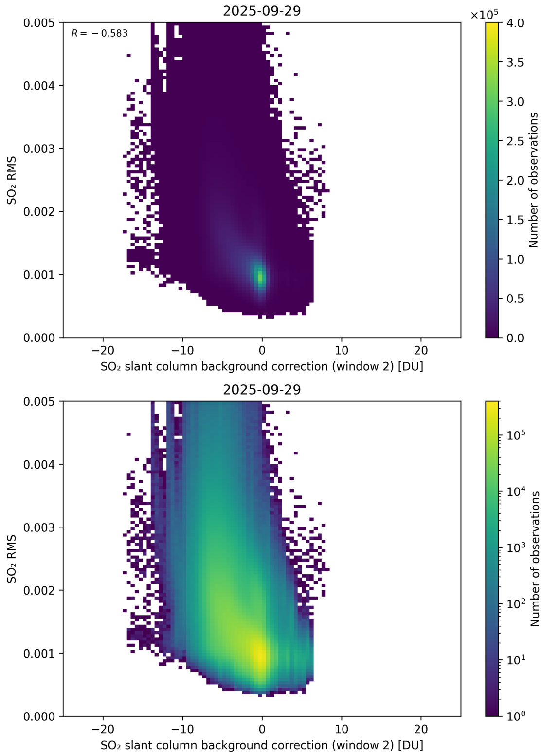
Figure 125: Scatter density plot of “SO 2 slant column background correction (window 2)” against “SO 2 RMS” for 2025-09-28 to 2025-09-30.
