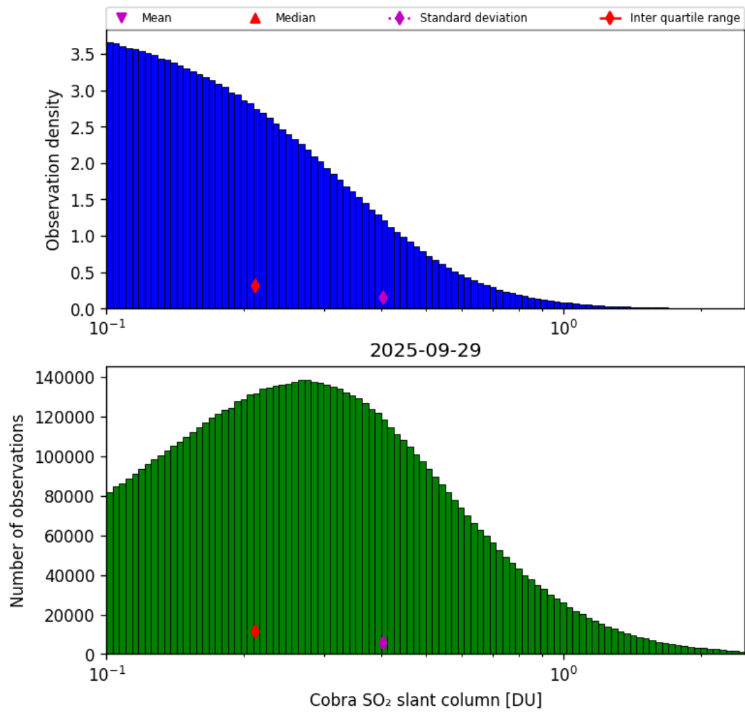
Figure 61: Histogram of “Cobra SO 2 slant column” for 2025-09-28 to 2025-09-30
