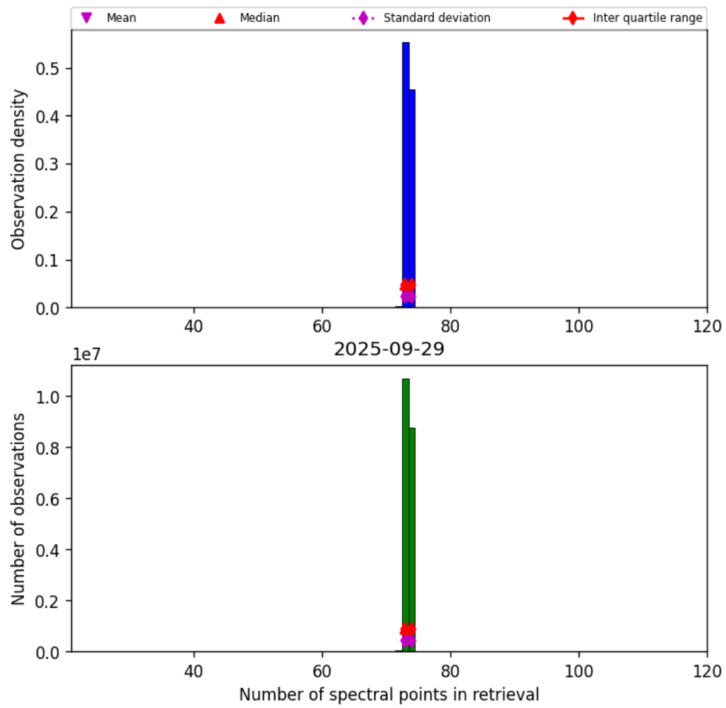
Figure 82: Histogram of “Number of spectral points in retrieval” for 2025-09-28 to 2025-09-30
