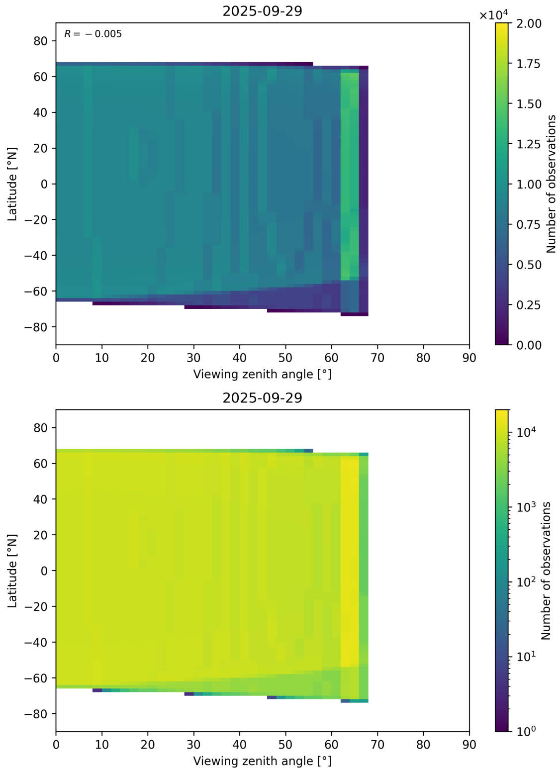
Figure 368: Scatter density plot of “Viewing zenith angle” against “Latitude” for 2025-09-28 to 2025-09-30.
