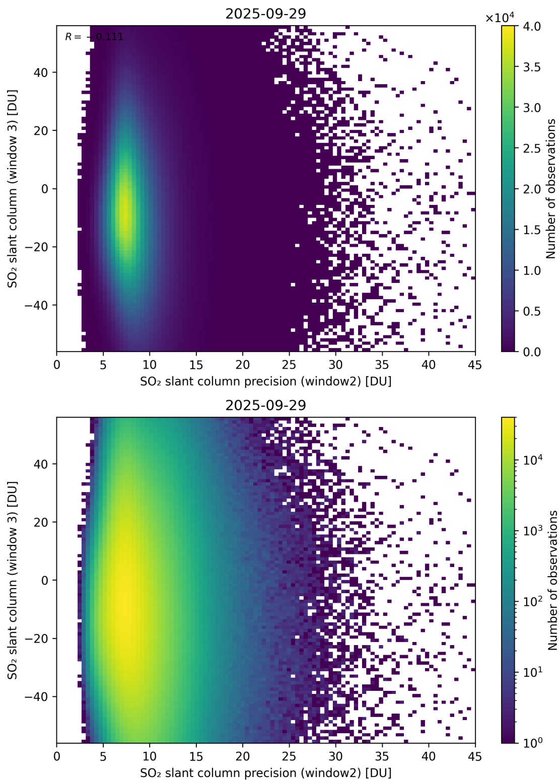
Figure 299: Scatter density plot of “SO 2 slant column precision (window2)” against “SO 2 slant column (window 3)” for 2025-09-28 to 2025-09-30.
