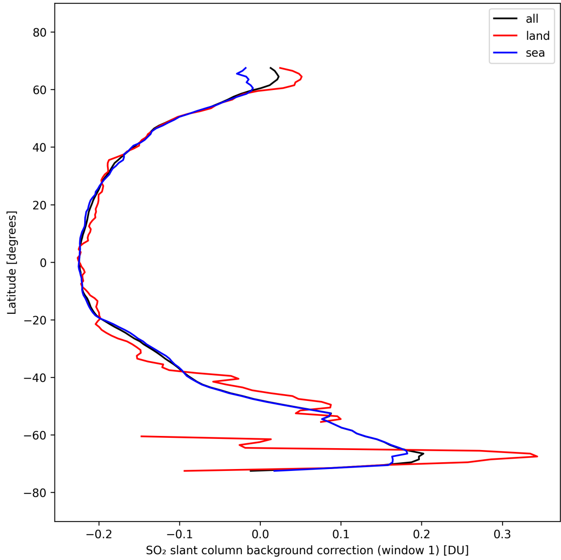
Figure 40: Zonal average of “SO 2 slant column background correction (window 1)” for 2025-09-28 to 2025-09-30.
