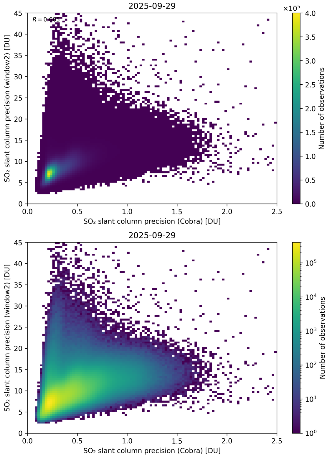
Figure 210: Scatter density plot of “SO 2 slant column precision (Cobra)” against “SO 2 slant column precision (window2)” for 2025-09-28 to 2025-09-30.
