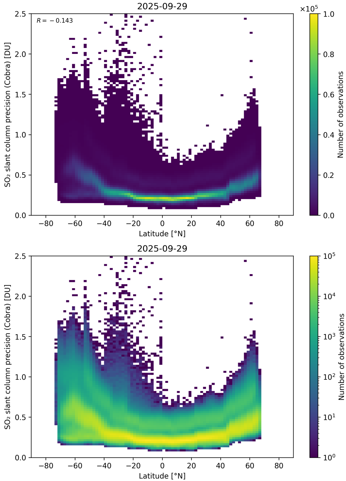
Figure 158: Scatter density plot of “Latitude” against “SO 2 slant column precision (Cobra)” for 2025-09-28 to 2025-09-30.
