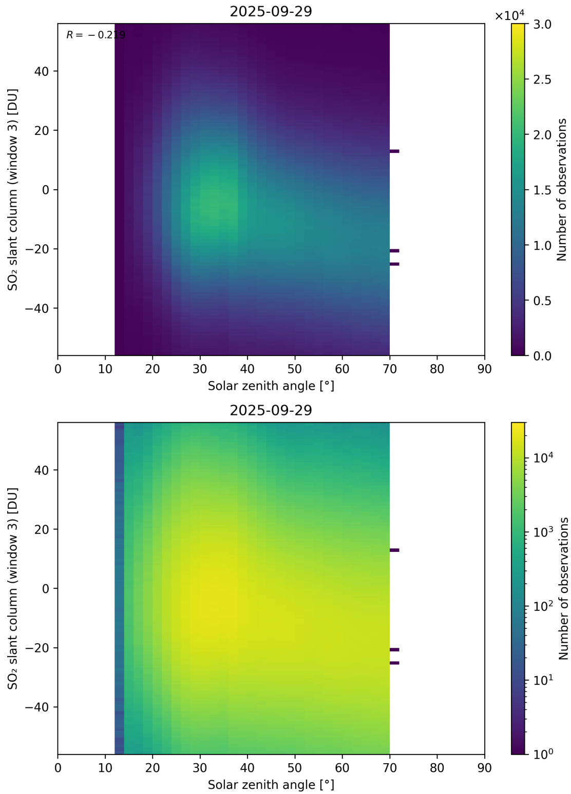
Figure 187: Scatter density plot of “Solar zenith angle” against “SO 2 slant column (window 3)” for 2025-09-28 to 2025-09-30.
