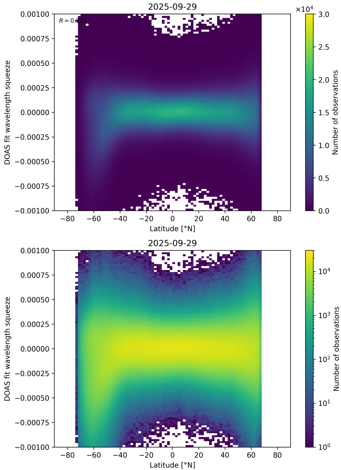
Figure 154: Scatter density plot of “Latitude” against “DOAS fit wavelength squeeze” for 2025-09-28 to 2025-09-30.
