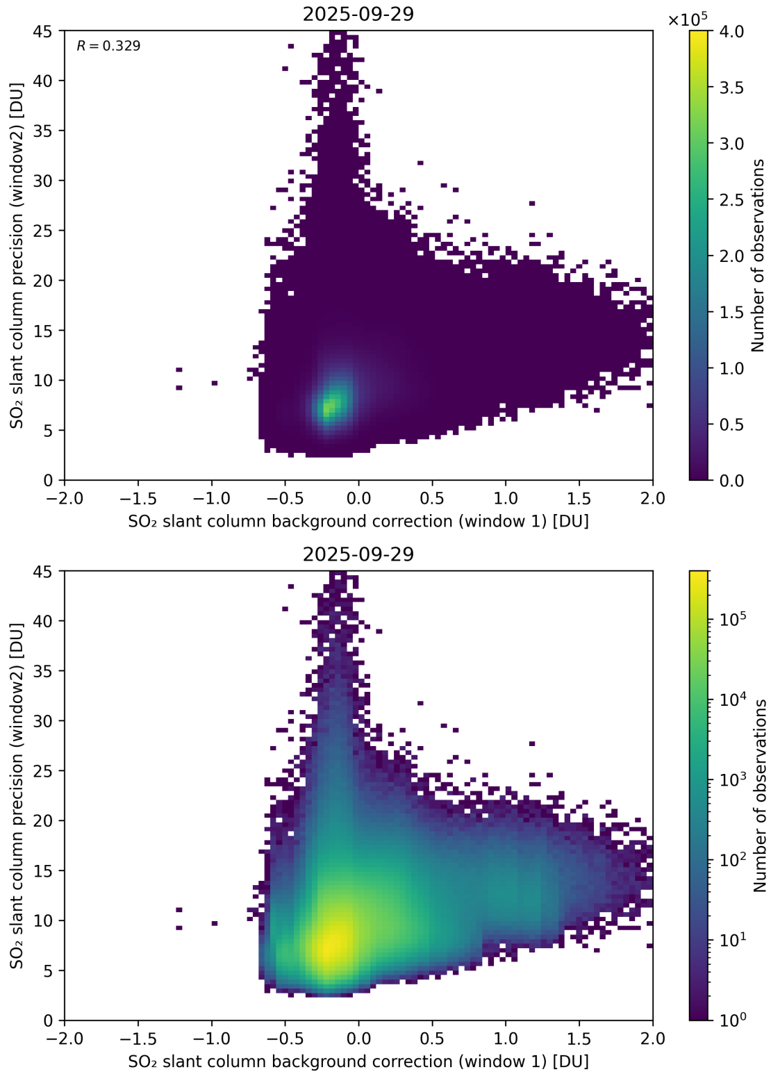
Figure 117: Scatter density plot of “SO 2 slant column background correction (window 1)” against “SO 2 slant column precision (window2)” for 2025-09-28 to 2025-09-30.
