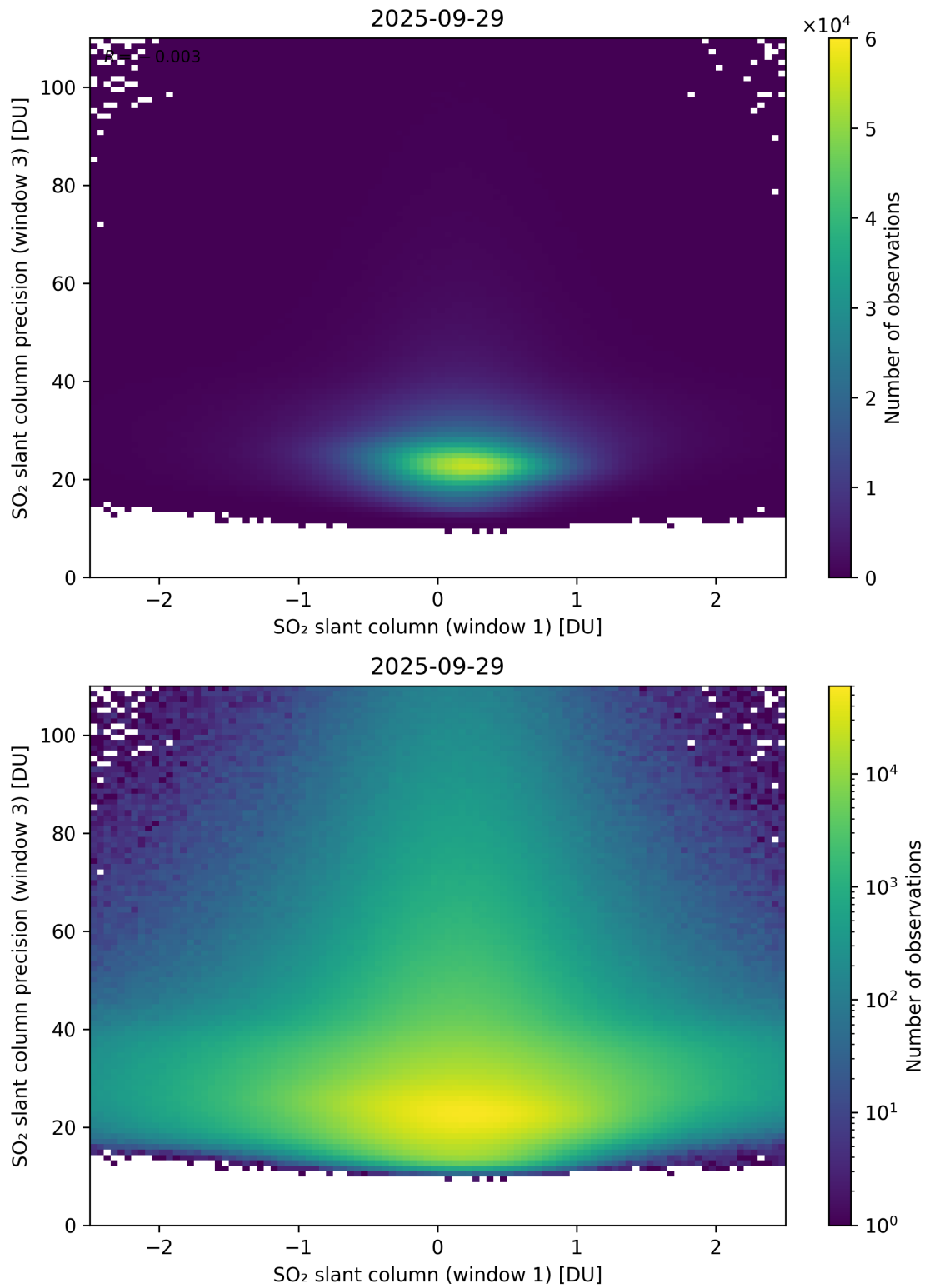
Figure 288: Scatter density plot of “SO 2 slant column (window 1)” against “SO 2 slant column precision (window 3)” for 2025-09-28 to 2025-09-30.
