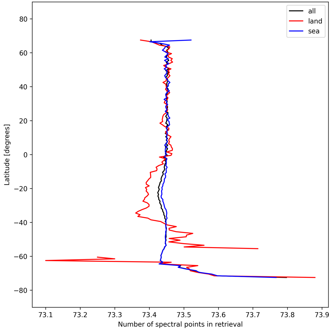
Figure 56: Zonal average of “Number of spectral points in retrieval” for 2025-09-28 to 2025-09-30.
