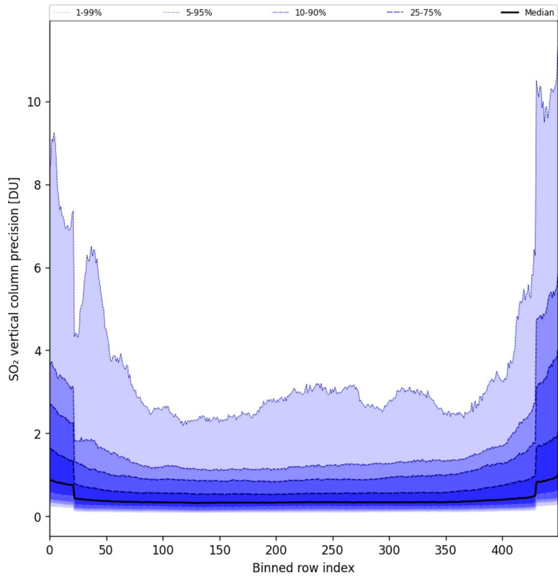
Figure 85: Along track statistics of “SO 2 vertical column precision” for 2025-09-28 to 2025-09-30
