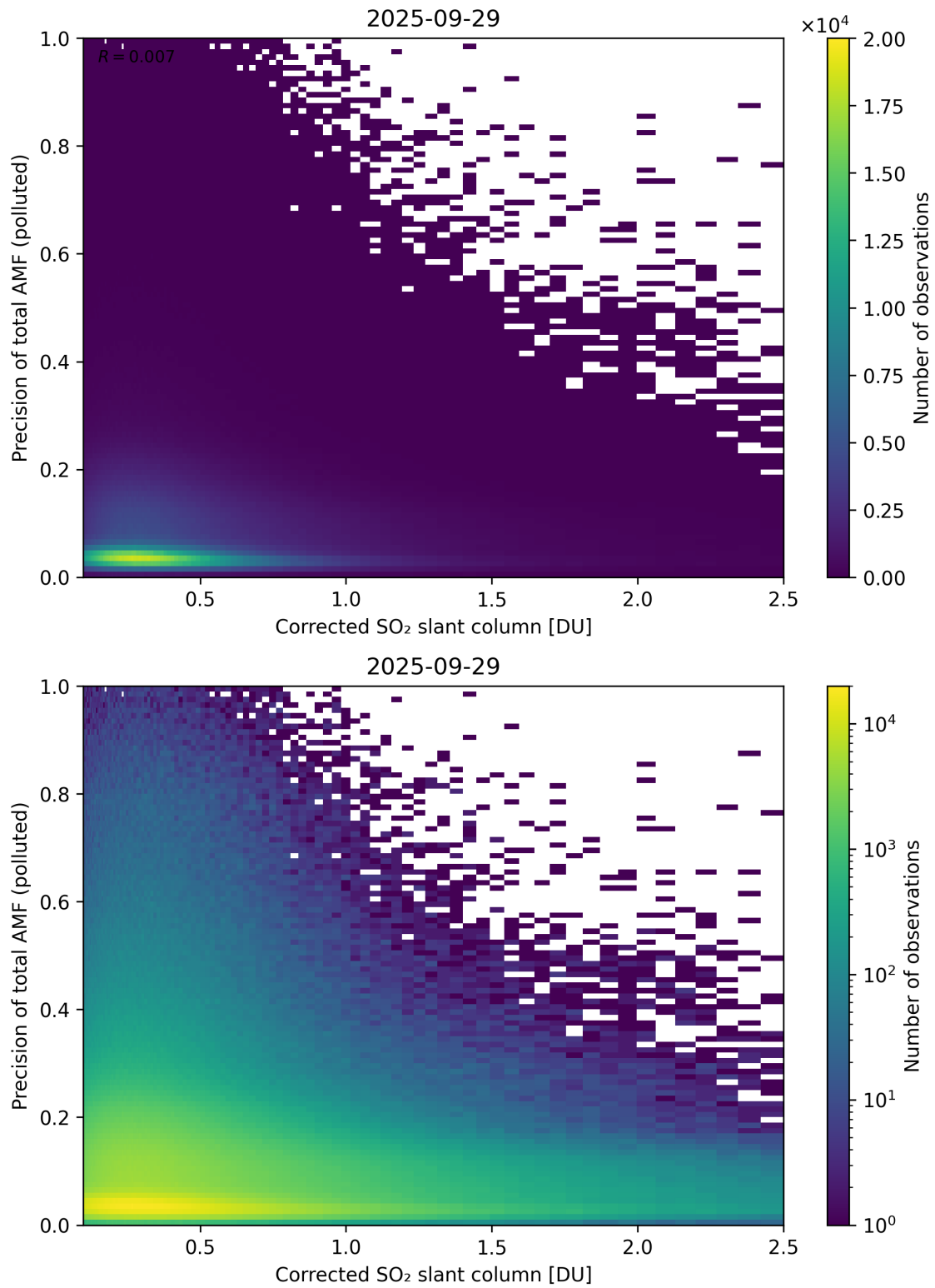
Figure 243: Scatter density plot of “Corrected SO 2 slant column” against “Precision of total AMF (polluted)” for 2025-09-28 to 2025-09-30.
