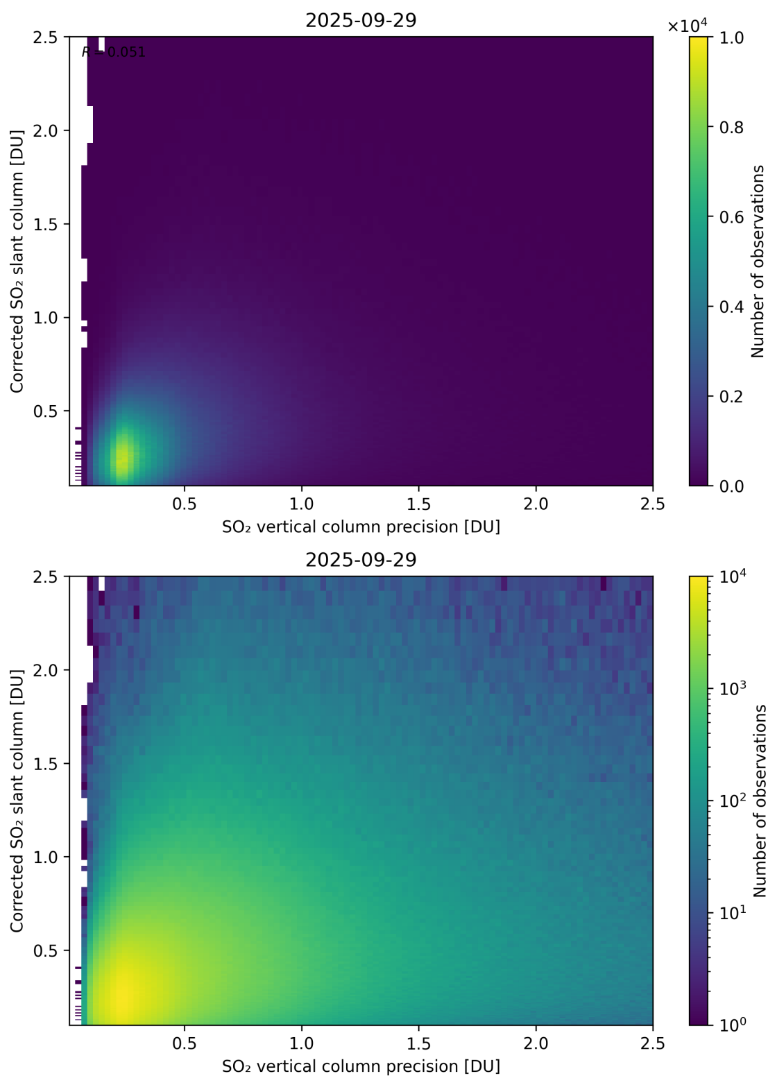
Figure 338: Scatter density plot of “SO 2 vertical column precision” against “Corrected SO 2 slant column” for 2025-09-28 to 2025-09-30.
