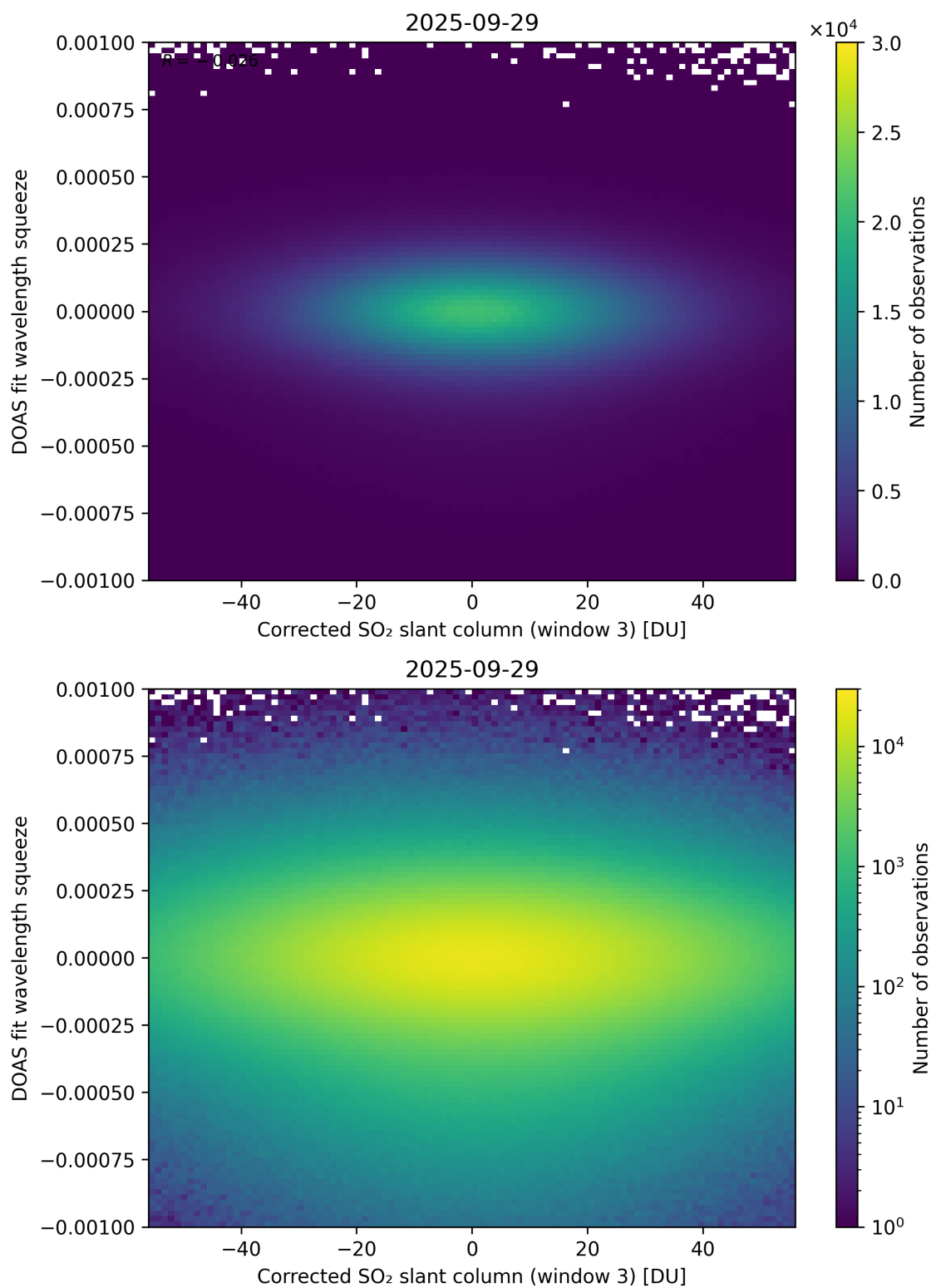
Figure 257: Scatter density plot of “Corrected SO 2 slant column (window 3)” against “DOAS fit wavelength squeeze” for 2025-09-28 to 2025-09-30.
