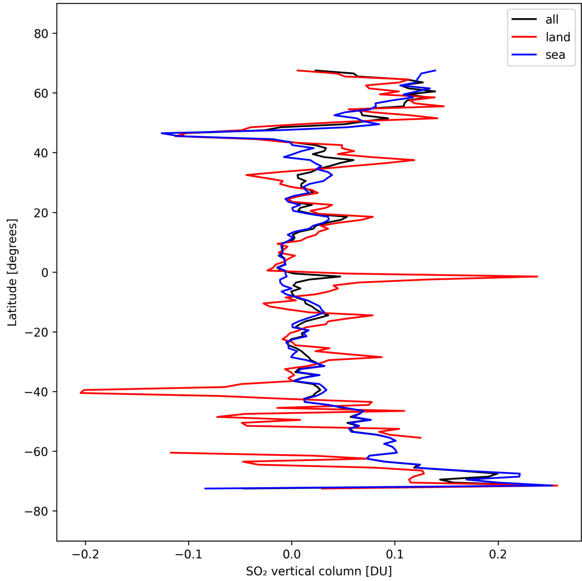
Figure 32: Zonal average of “SO 2 vertical column” for 2025-09-28 to 2025-09-30.
