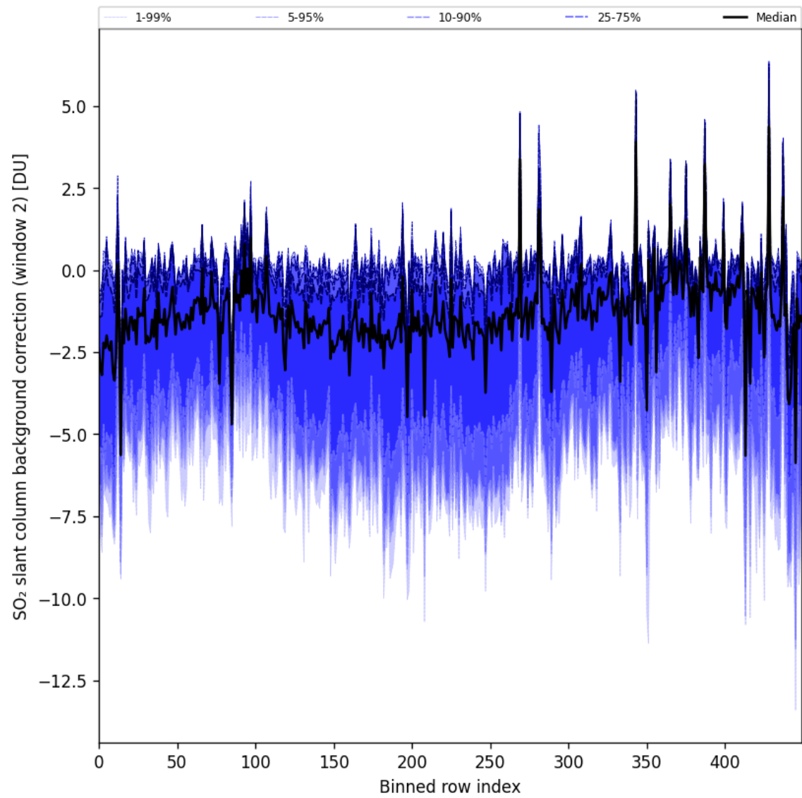
Figure 96: Along track statistics of “SO 2 slant column background correction (window 2)” for 2025-09-28 to 2025-09-30
