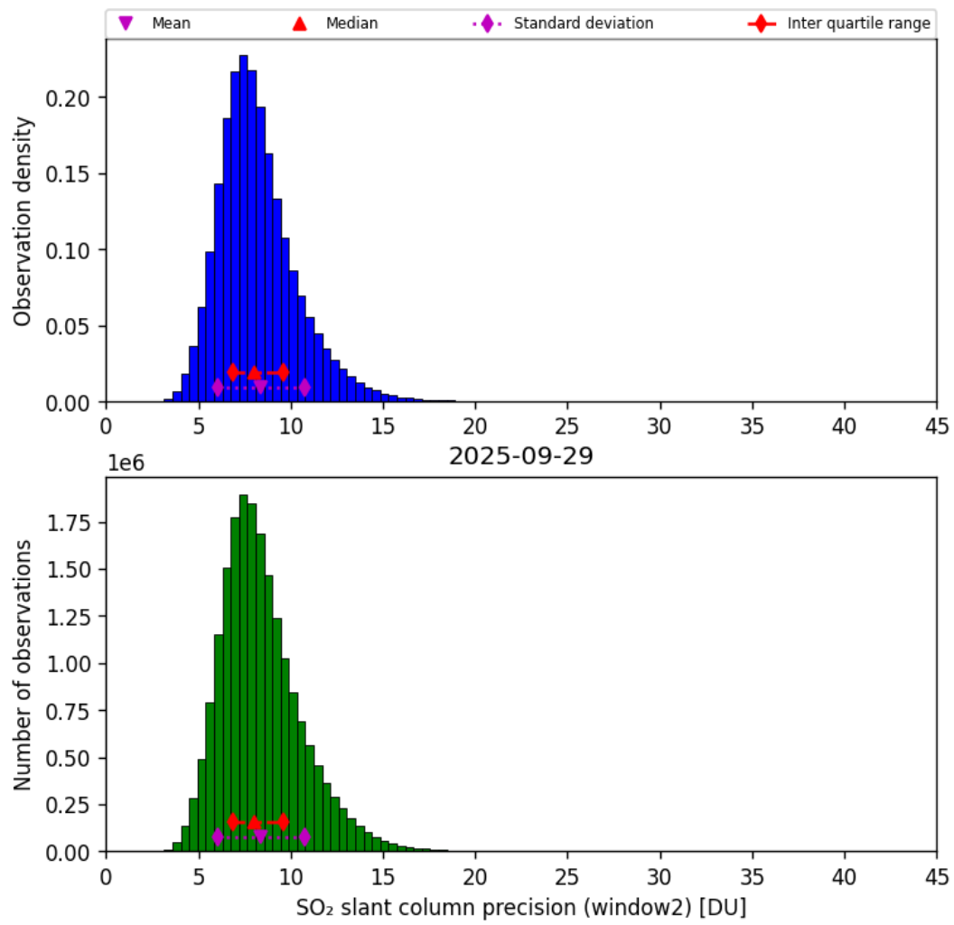
Figure 68: Histogram of “SO 2 slant column precision (window2)” for 2025-09-28 to 2025-09-30
