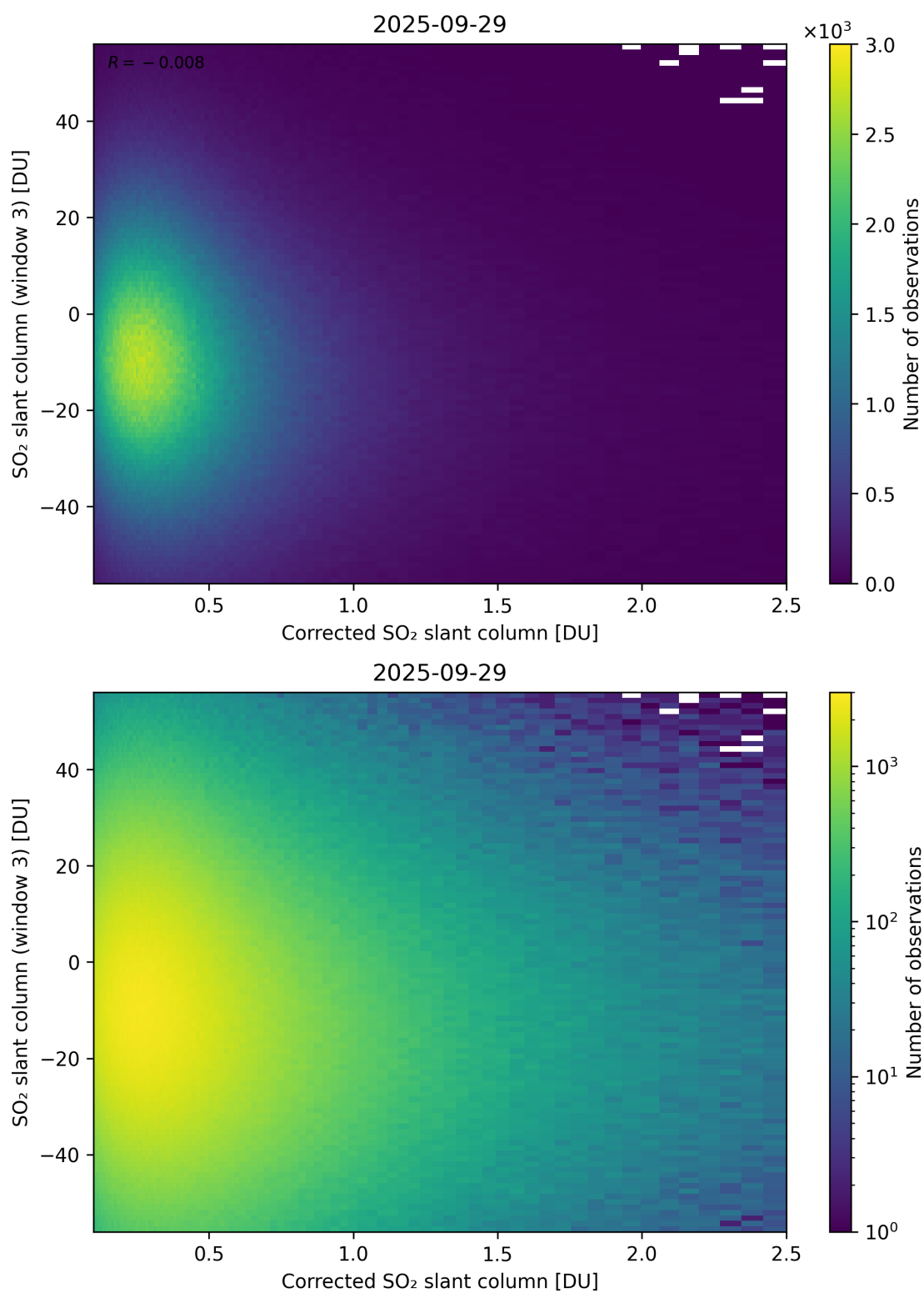
Figure 240: Scatter density plot of “Corrected SO 2 slant column” against “SO 2 slant column (window 3)” for 2025-09-28 to 2025-09-30.
