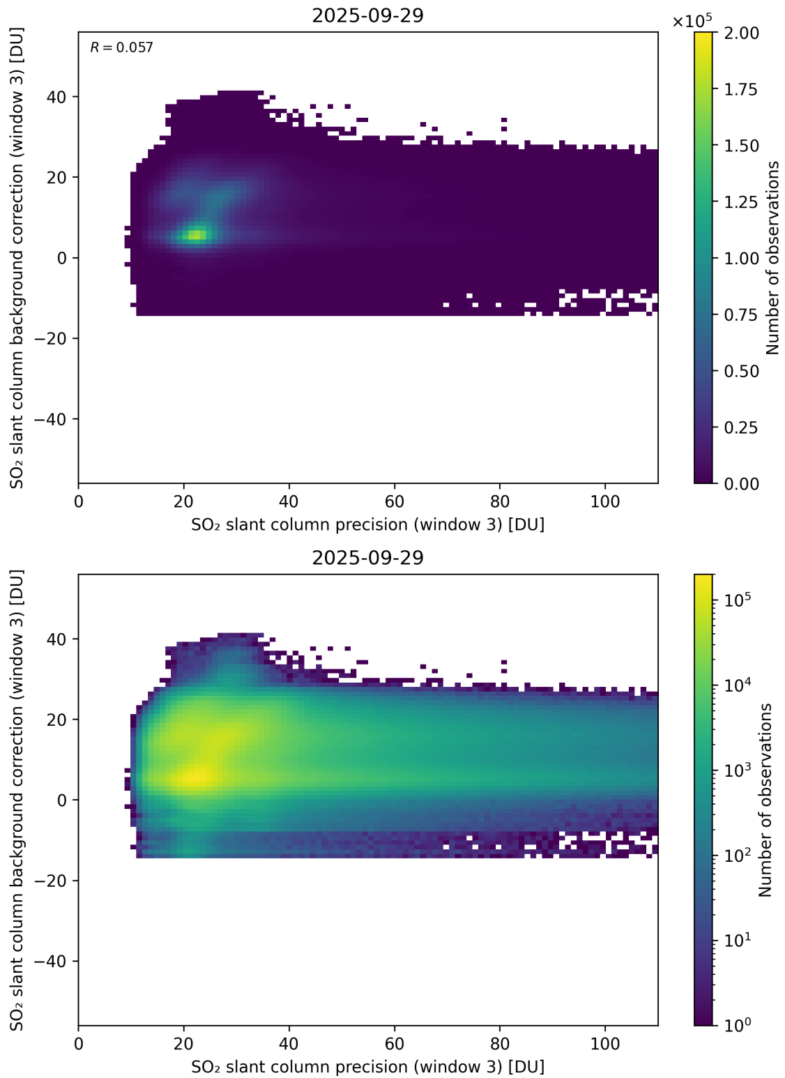
Figure 307: Scatter density plot of “SO 2 slant column precision (window 3)” against “SO 2 slant column background correction (window 3)” for 2025-09-28 to 2025-09-30.
