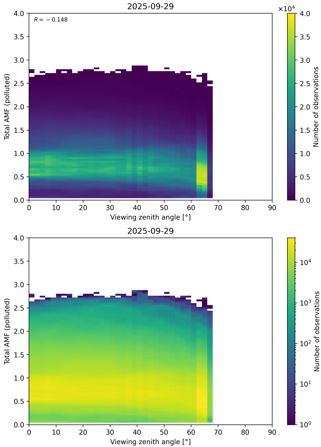
Figure 381: Scatter density plot of “Viewing zenith angle” against “Total AMF (polluted)” for 2025-09-28 to 2025-09-30.
