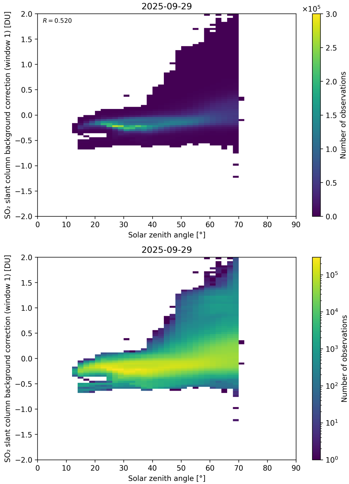
Figure 171: Scatter density plot of “Solar zenith angle” against “SO 2 slant column background correction (window 1)” for 2025-09-28 to 2025-09-30.
