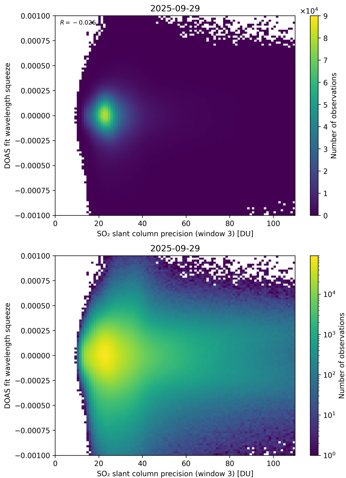
Figure 309: Scatter density plot of “SO 2 slant column precision (window 3)” against “DOAS fit wavelength squeeze” for 2025-09-28 to 2025-09-30.
