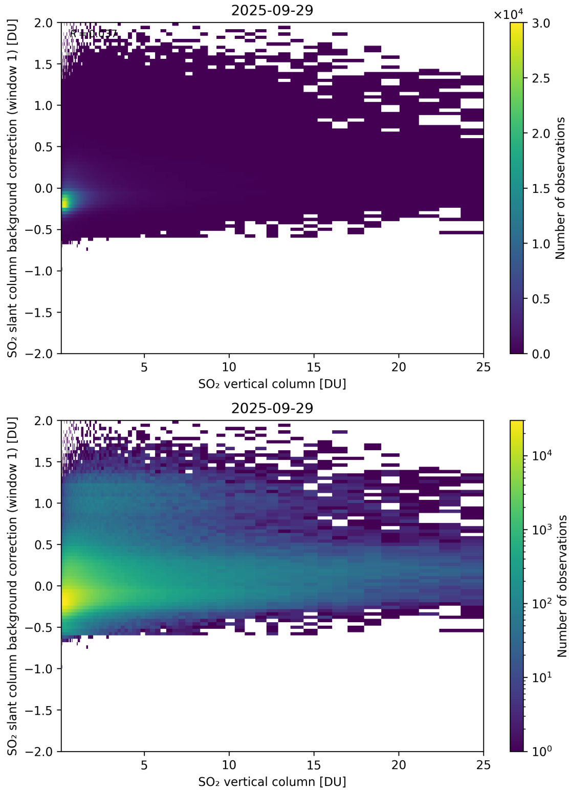
Figure 323: Scatter density plot of “SO 2 vertical column” against “SO 2 slant column background correction (window 1)” for 2025-09-28 to 2025-09-30.
