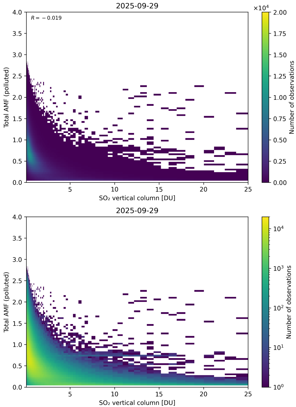
Figure 359: Scatter density plot of “SO 2 vertical column” against “Total AMF (polluted)” for 2025-09-28 to 2025-09-30.
