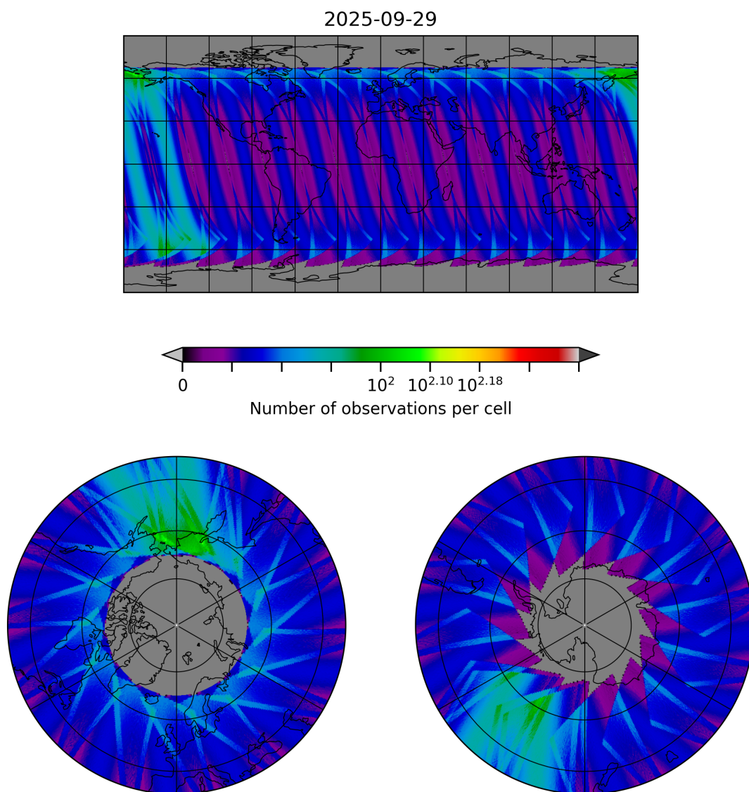
Figure 30: Map of the number of observations for 2025-09-28 to 2025-09-30
