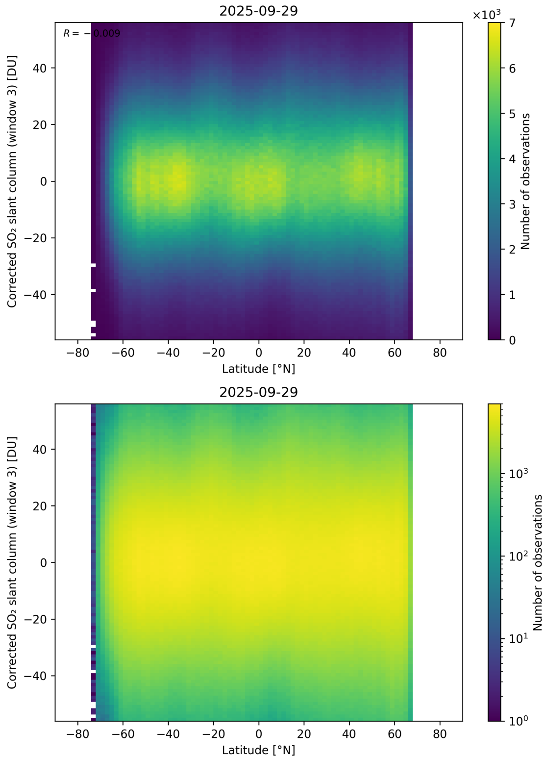
Figure 161: Scatter density plot of “Latitude” against “Corrected SO 2 slant column (window 3)” for 2025-09-28 to 2025-09-30.
