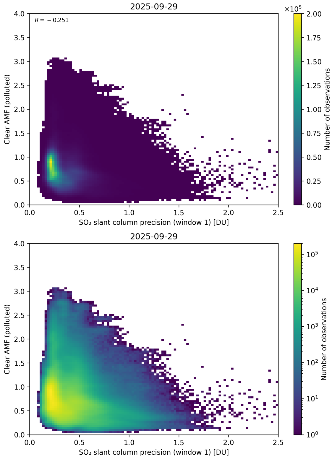
Figure 274: Scatter density plot of “SO 2 slant column precision (window 1)” against “Clear AMF (polluted)” for 2025-09-28 to 2025-09-30.
