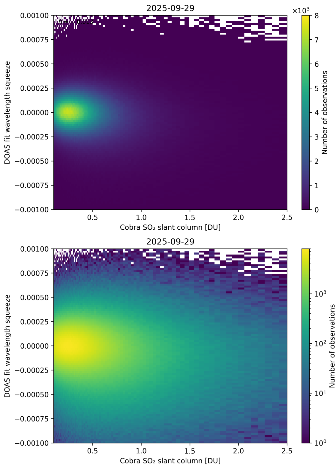
Figure 197: Scatter density plot of “Cobra SO 2 slant column” against “DOAS fit wavelength squeeze” for 2025-09-28 to 2025-09-30.
