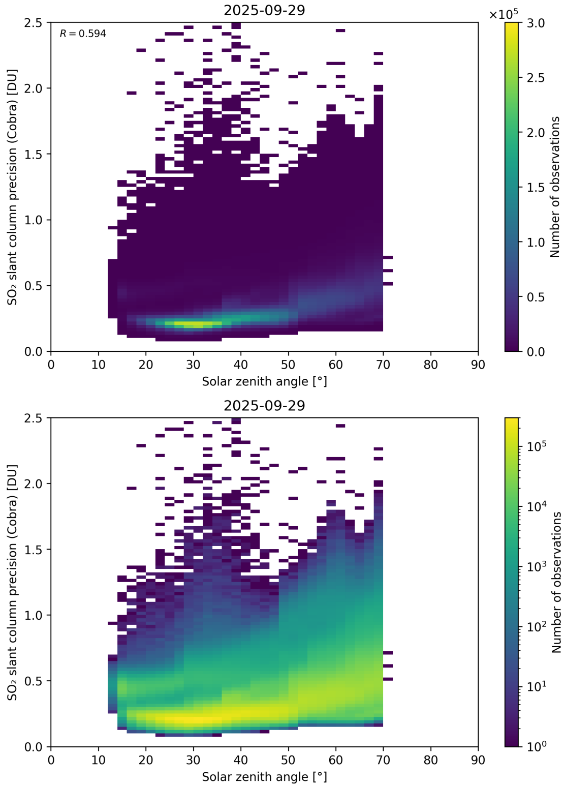
Figure 180: Scatter density plot of “Solar zenith angle” against “SO 2 slant column precision (Cobra)” for 2025-09-28 to 2025-09-30.
