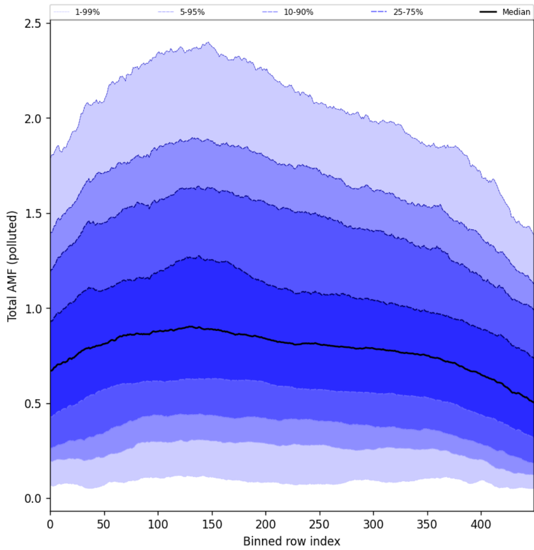
Figure 105: Along track statistics of “Total AMF (polluted)” for 2025-09-28 to 2025-09-30
