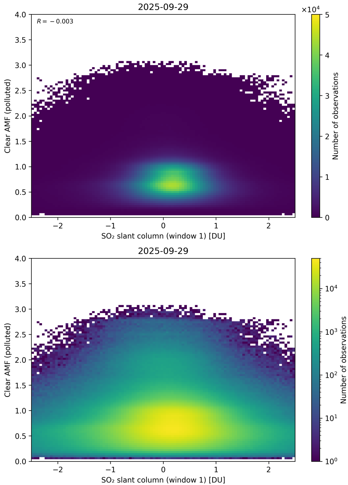
Figure 282: Scatter density plot of “SO 2 slant column (window 1)” against “Clear AMF (polluted)” for 2025-09-28 to 2025-09-30.
