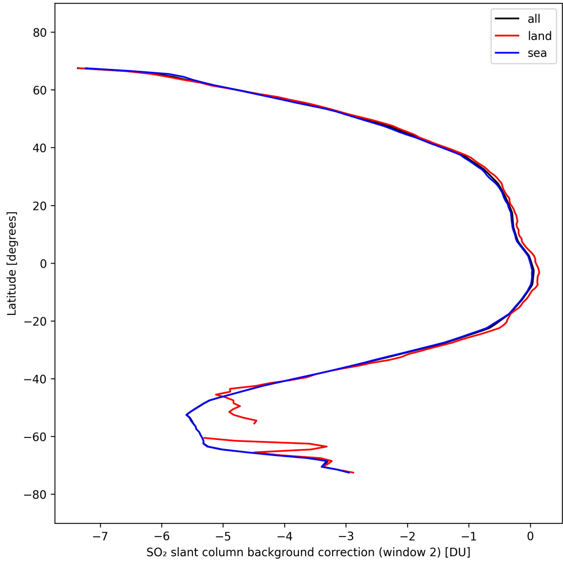
Figure 44: Zonal average of “SO 2 slant column background correction (window 2)” for 2025-09-28 to 2025-09-30.
