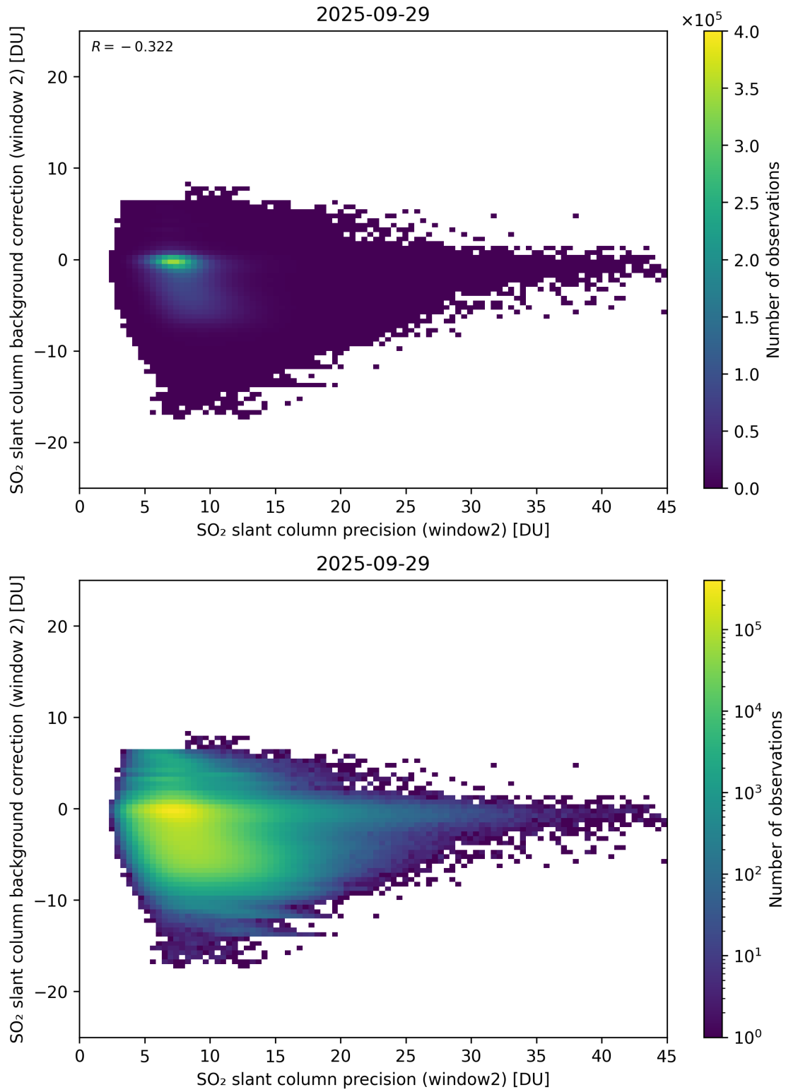
Figure 291: Scatter density plot of “SO 2 slant column precision (window2)” against “SO 2 slant column background correction (window 2)” for 2025-09-28 to 2025-09-30.
