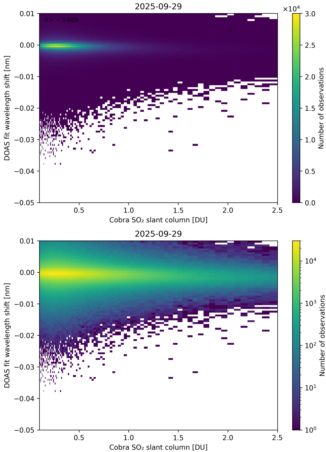
Figure 196: Scatter density plot of “Cobra SO 2 slant column” against “DOAS fit wavelength shift” for 2025-09-28 to 2025-09-30.
