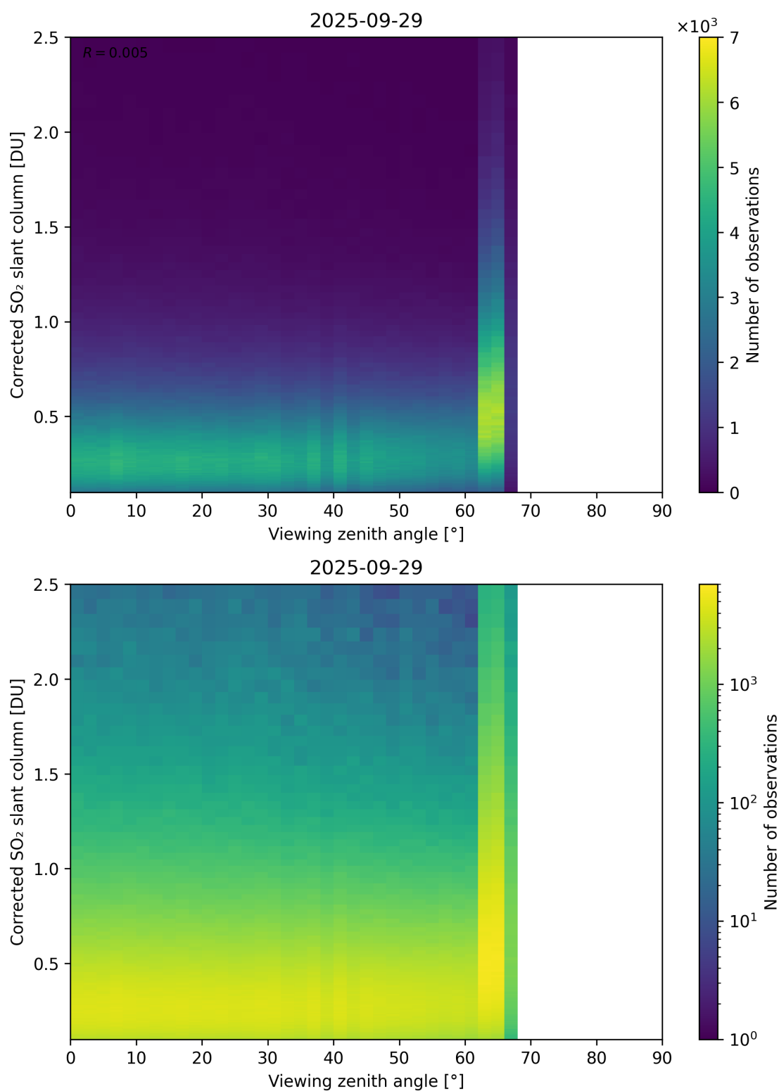
Figure 373: Scatter density plot of “Viewing zenith angle” against “Corrected SO 2 slant column” for 2025-09-28 to 2025-09-30.
