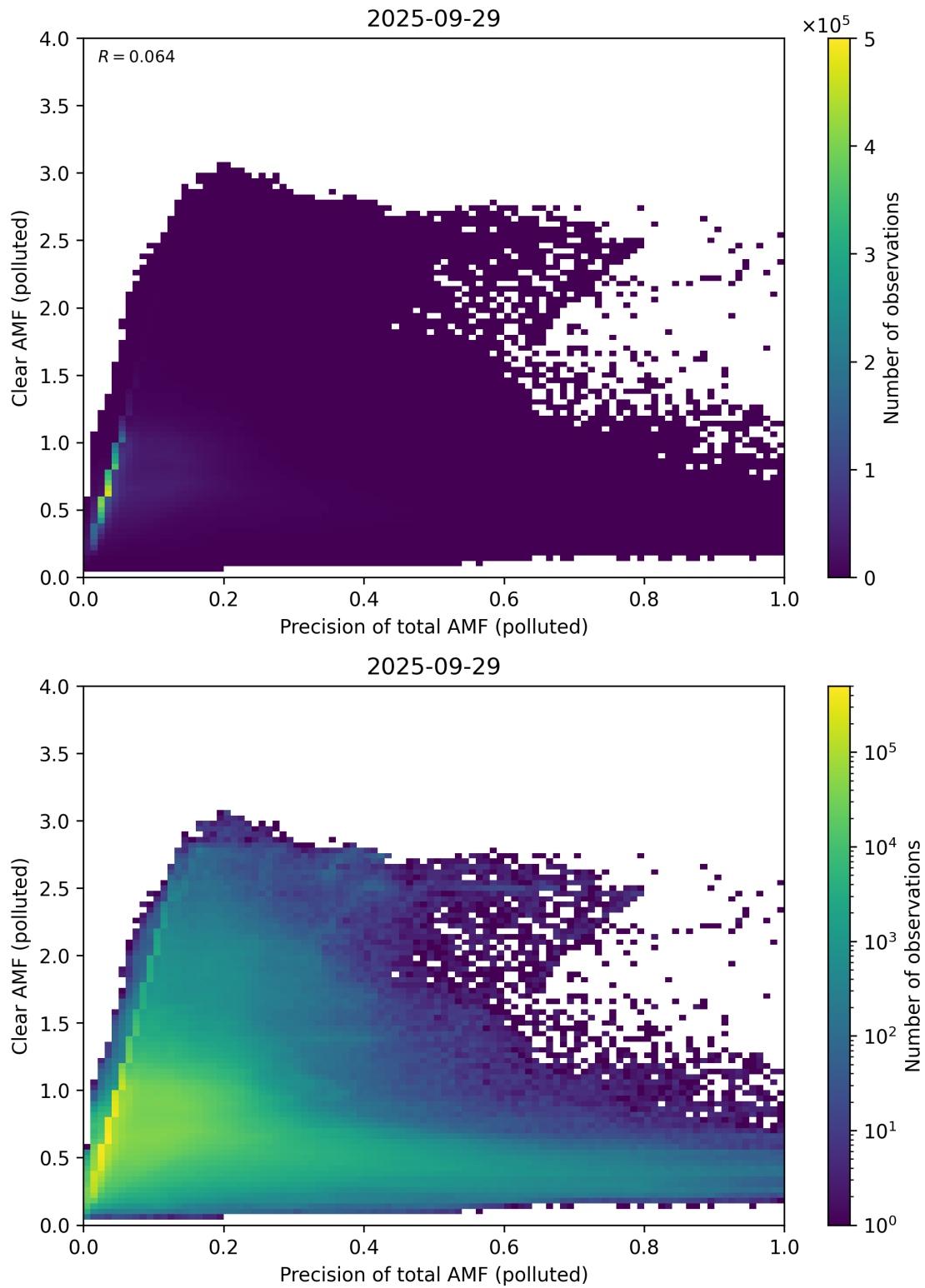
Figure 320: Scatter density plot of “Precision of total AMF (polluted)” against “Clear AMF (polluted)” for 2025-09-28 to 2025-09-30.
