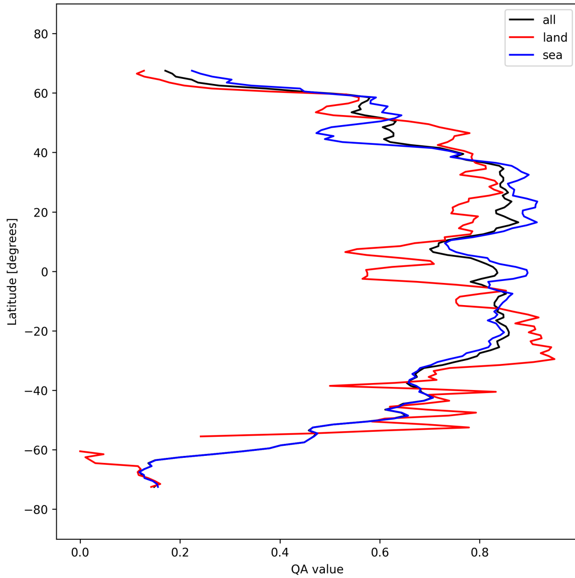
Figure 31: Zonal average of “QA value” for 2025-09-28 to 2025-09-30.
