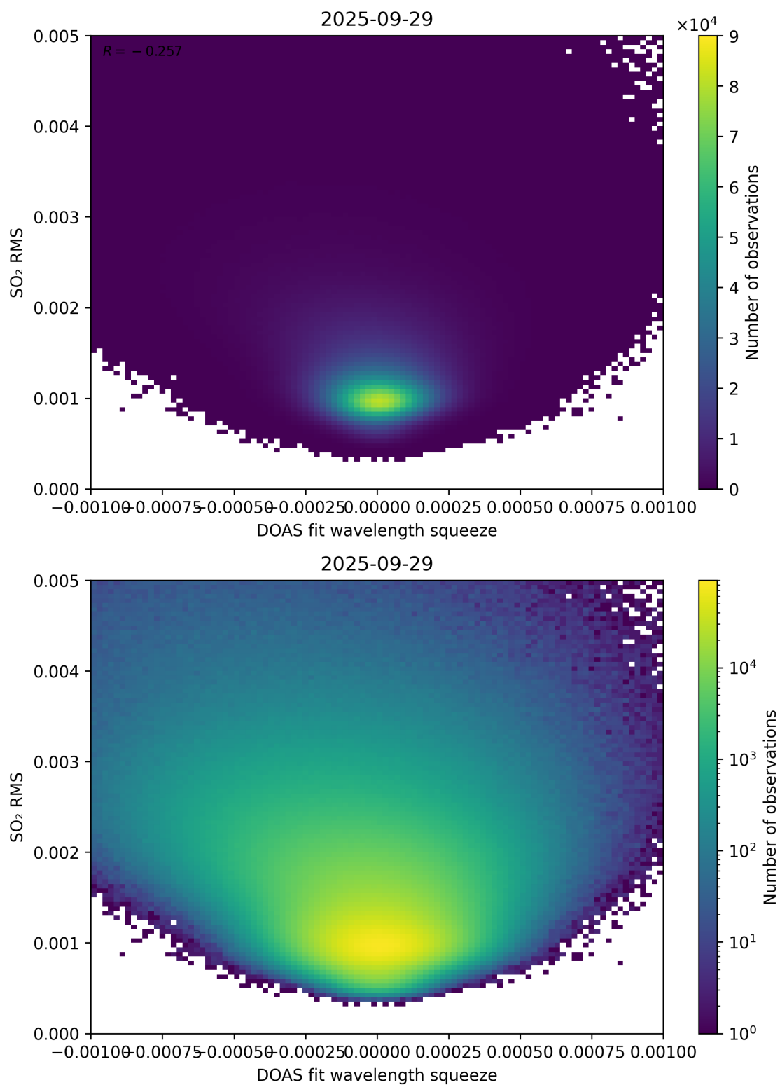
Figure 143: Scatter density plot of “DOAS fit wavelength squeeze” against “SO 2 RMS” for 2025-09-28 to 2025-09-30.
