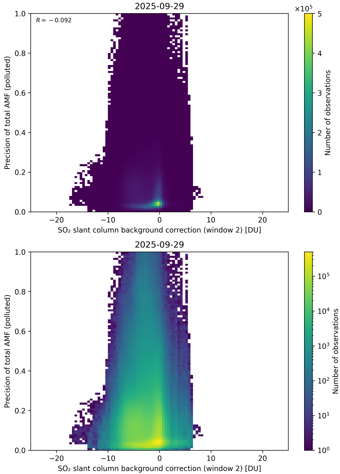
Figure 131: Scatter density plot of “SO 2 slant column background correction (window 2)” against “Precision of total AMF (polluted)” for 2025-09-28 to 2025-09-30.
