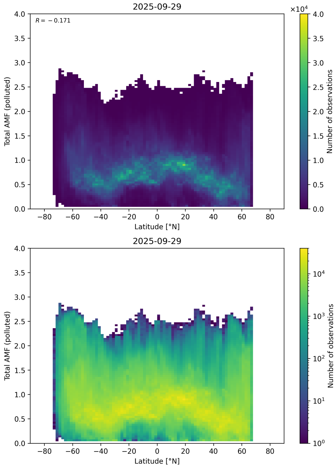
Figure 167: Scatter density plot of “Latitude” against “Total AMF (polluted)” for 2025-09-28 to 2025-09-30.
