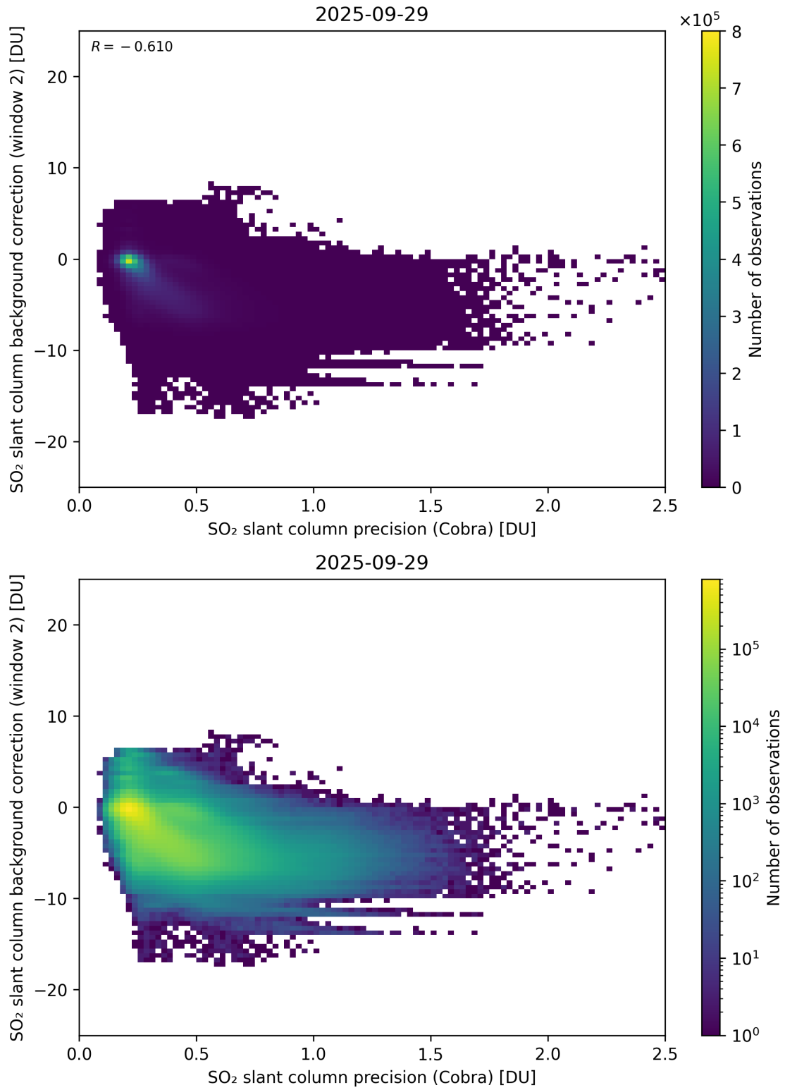
Figure 200: Scatter density plot of “SO 2 slant column precision (Cobra)” against “SO 2 slant column background correction (window 2)” for 2025-09-28 to 2025-09-30.
