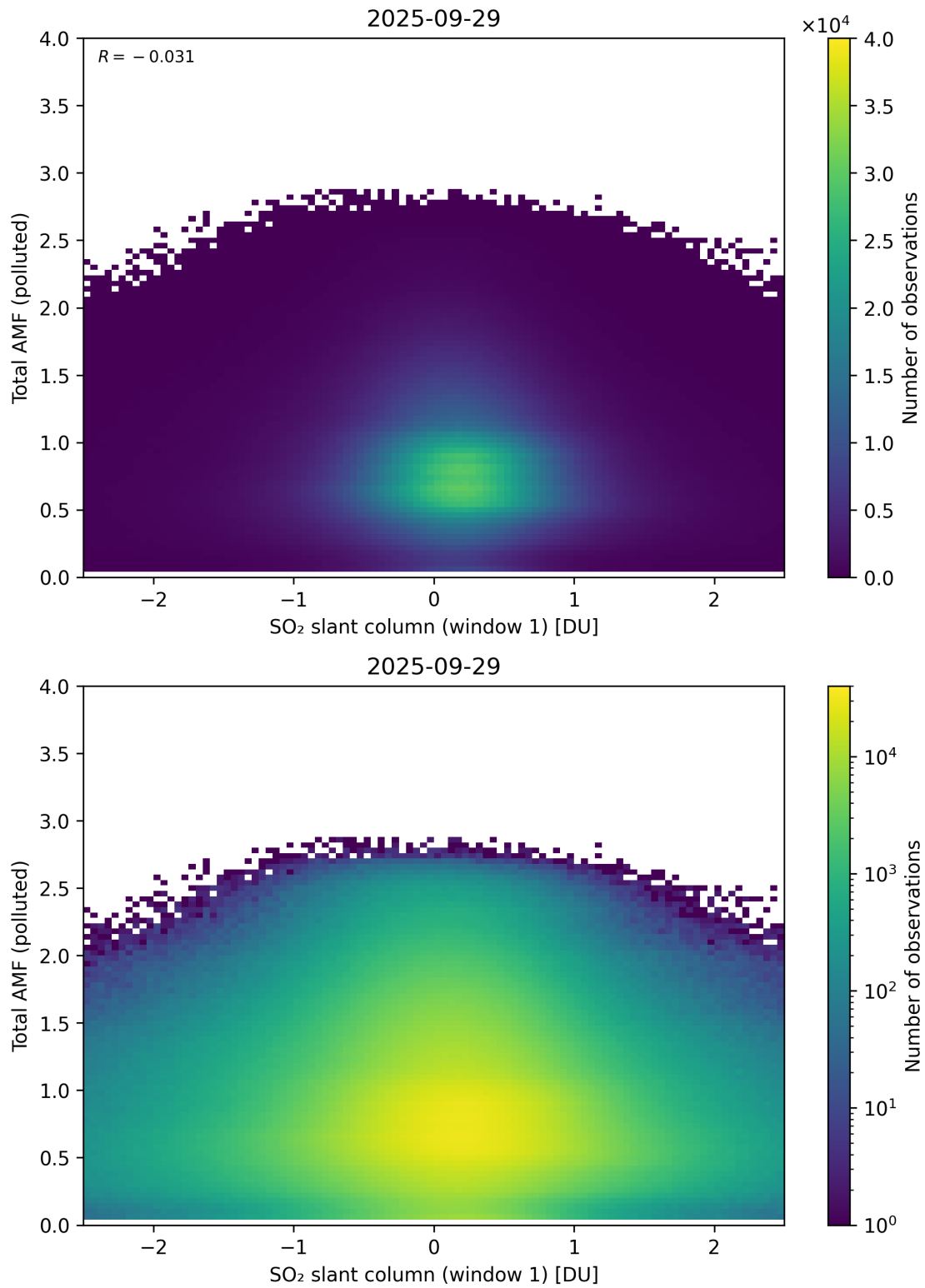
Figure 289: Scatter density plot of “SO 2 slant column (window 1)” against “Total AMF (polluted)” for 2025-09-28 to 2025-09-30.
