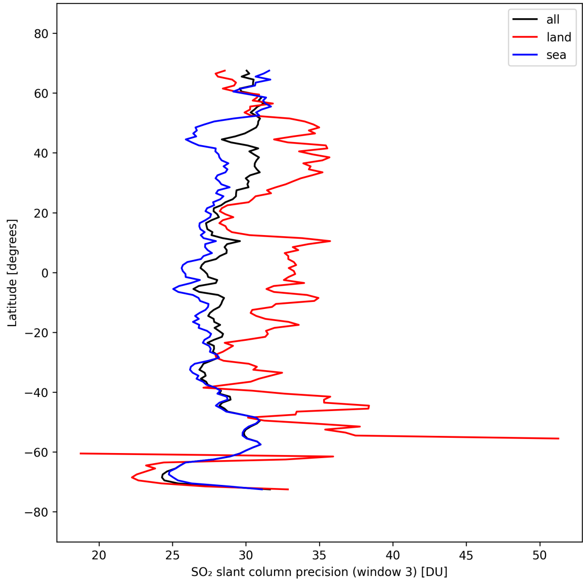
Figure 46: Zonal average of “SO 2 slant column precision (window 3)” for 2025-09-28 to 2025-09-30.
