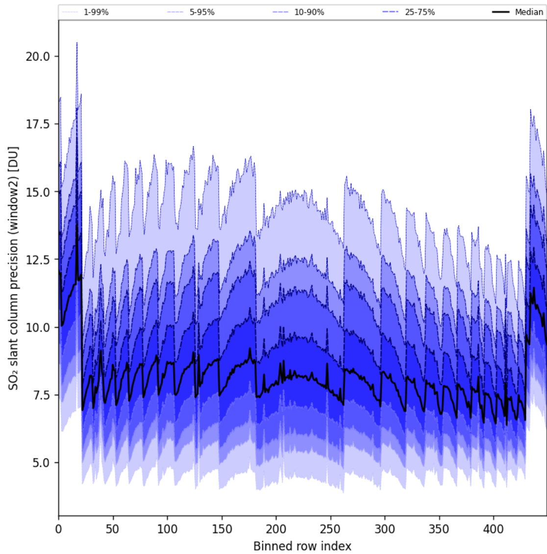
Figure 94: Along track statistics of “SO 2 slant column precision (window2)” for 2025-09-28 to 2025-09-30
