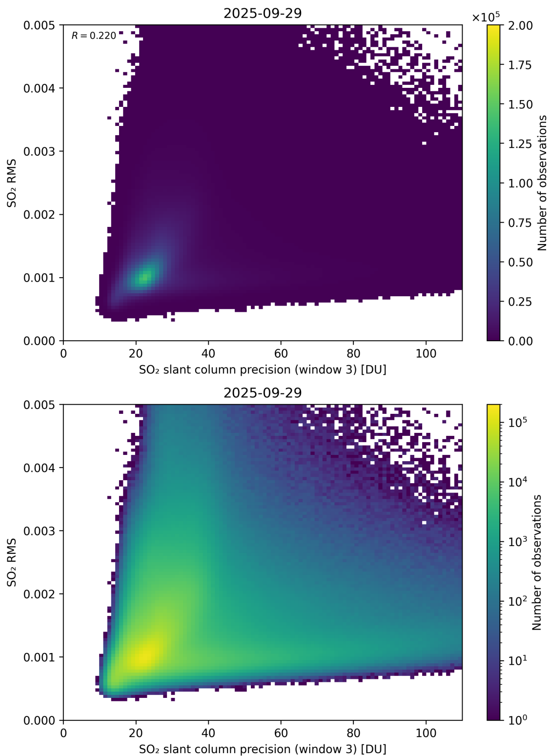
Figure 310: Scatter density plot of “SO 2 slant column precision (window 3)” against “SO 2 RMS” for 2025-09-28 to 2025-09-30.
