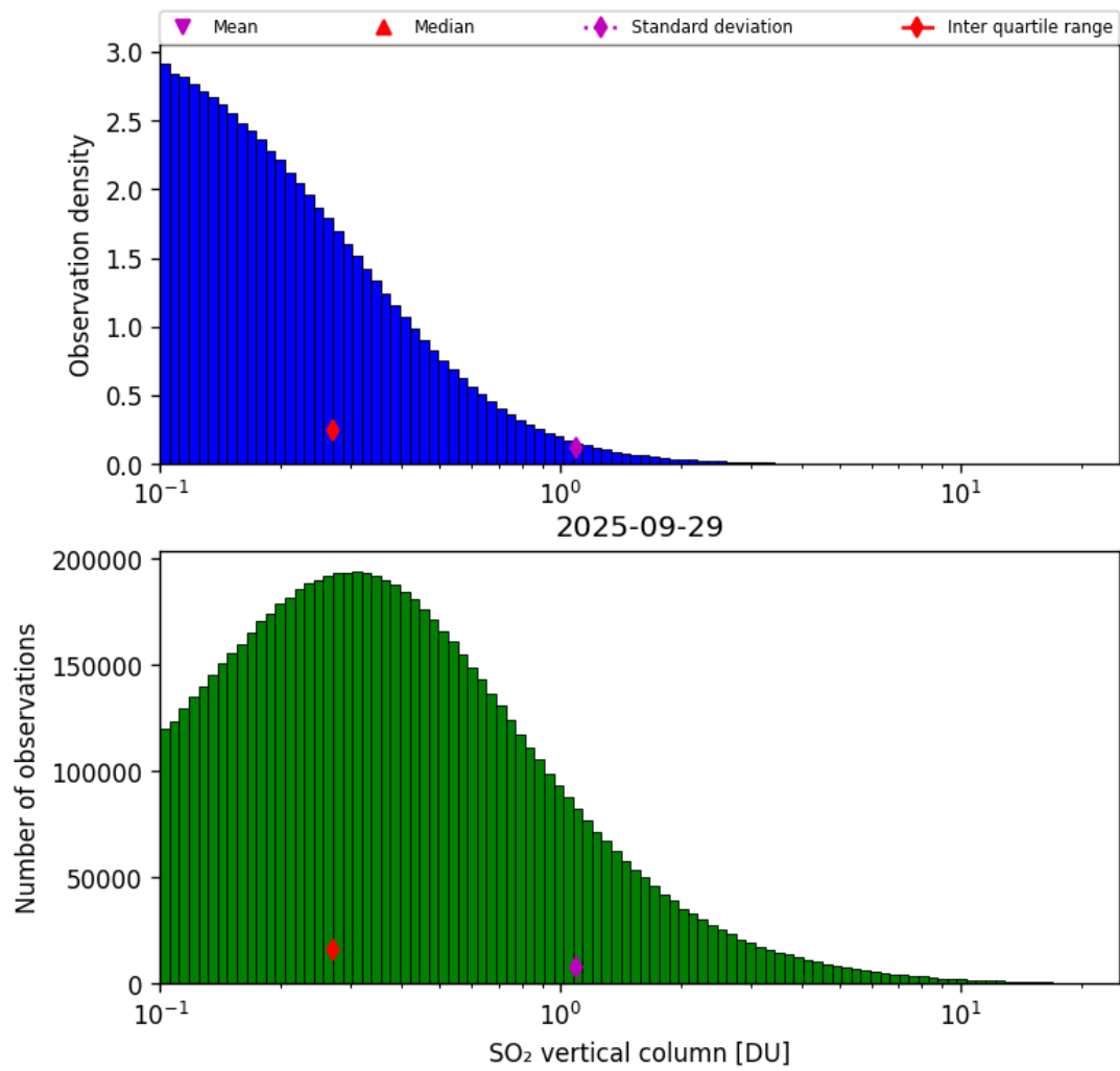
Figure 58: Histogram of “SO 2 vertical column” for 2025-09-28 to 2025-09-30
