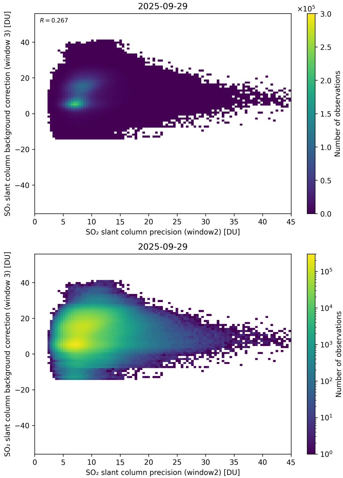
Figure 292: Scatter density plot of “SO 2 slant column precision (window2)” against “SO 2 slant column background correction (window 3)” for 2025-09-28 to 2025-09-30.
