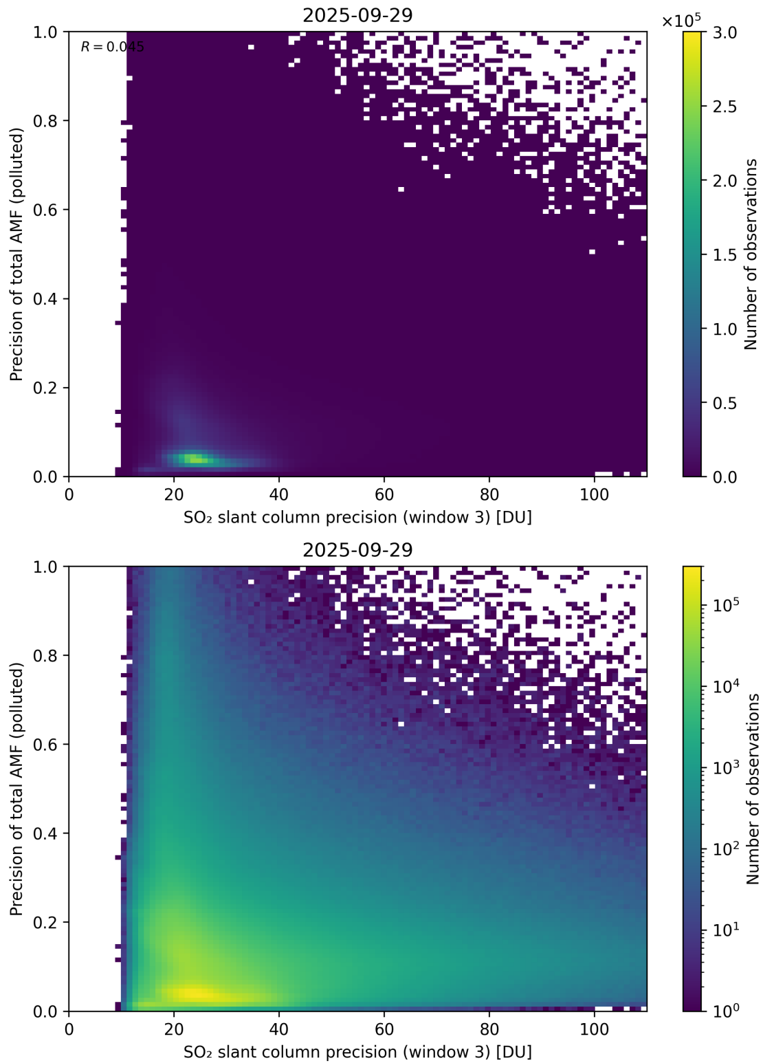
Figure 314: Scatter density plot of “SO 2 slant column precision (window 3)” against “Precision of total AMF (polluted)” for 2025-09-28 to 2025-09-30.
