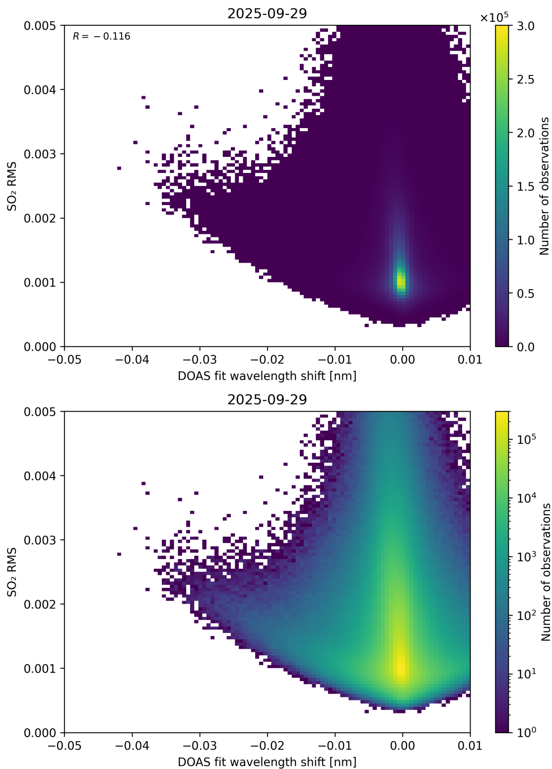
Figure 139: Scatter density plot of “DOAS fit wavelength shift” against “SO 2 RMS” for 2025-09-28 to 2025-09-30.
