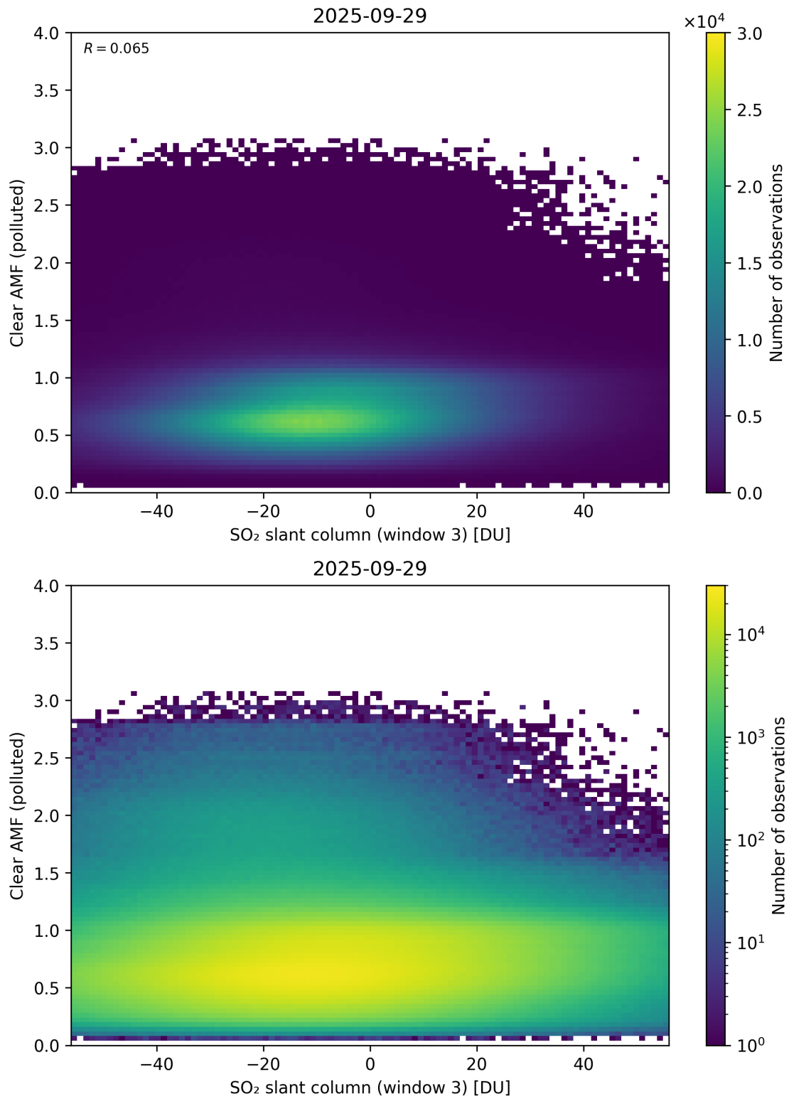
Figure 315: Scatter density plot of “SO 2 slant column (window 3)” against “Clear AMF (polluted)” for 2025-09-28 to 2025-09-30.
