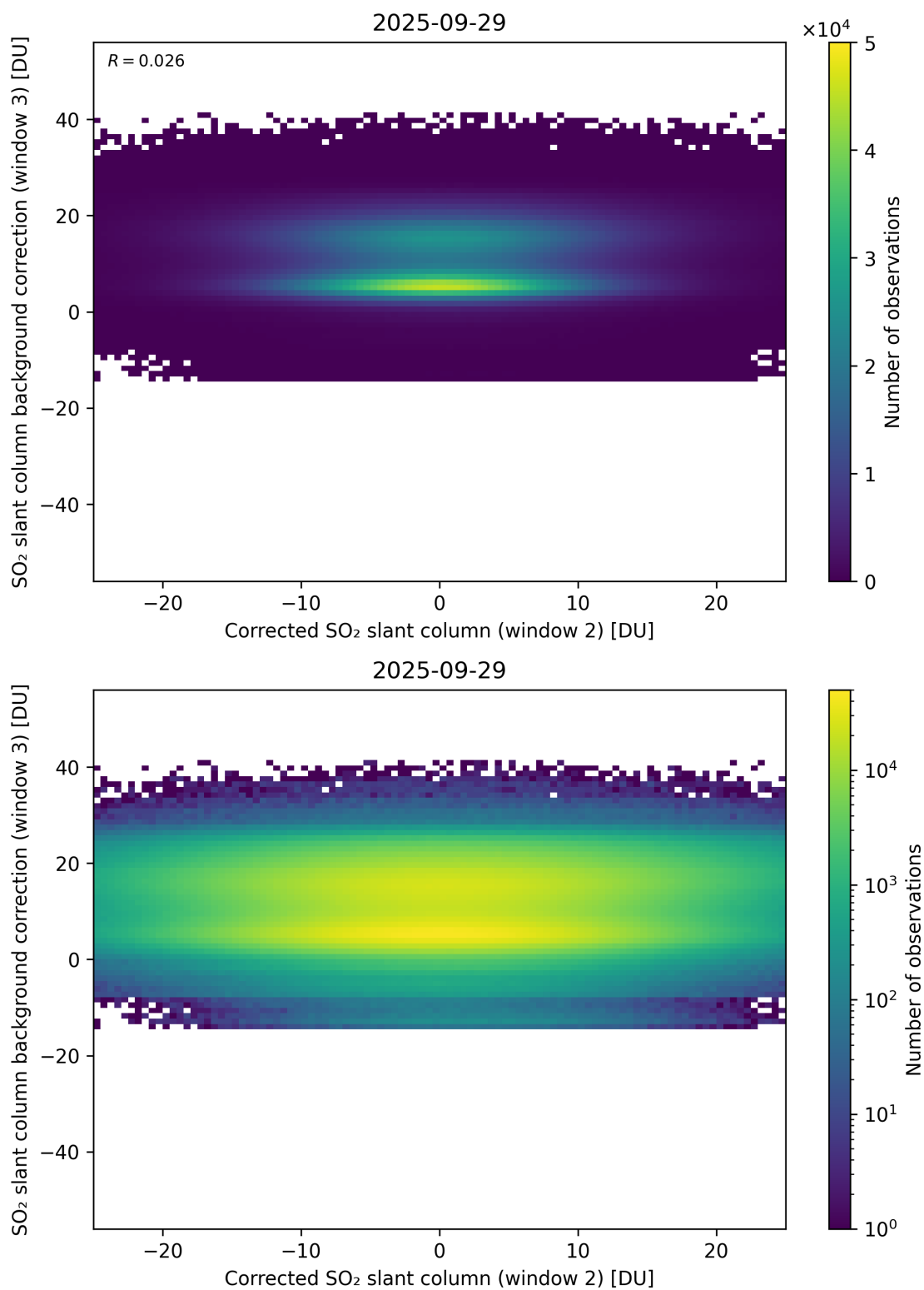
Figure 245: Scatter density plot of “Corrected SO 2 slant column (window 2)” against “SO 2 slant column background correction (window 3)” for 2025-09-28 to 2025-09-30.
