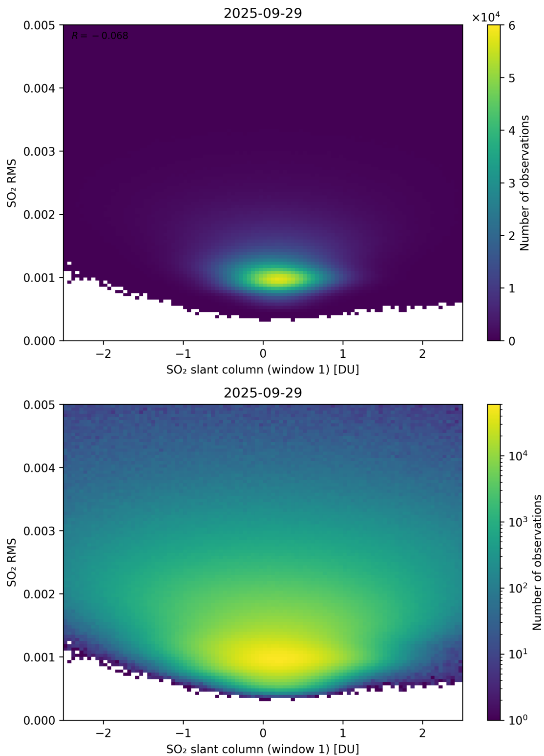
Figure 267: Scatter density plot of “SO 2 slant column (window 1)” against “SO 2 RMS” for 2025-09-28 to 2025-09-30.
