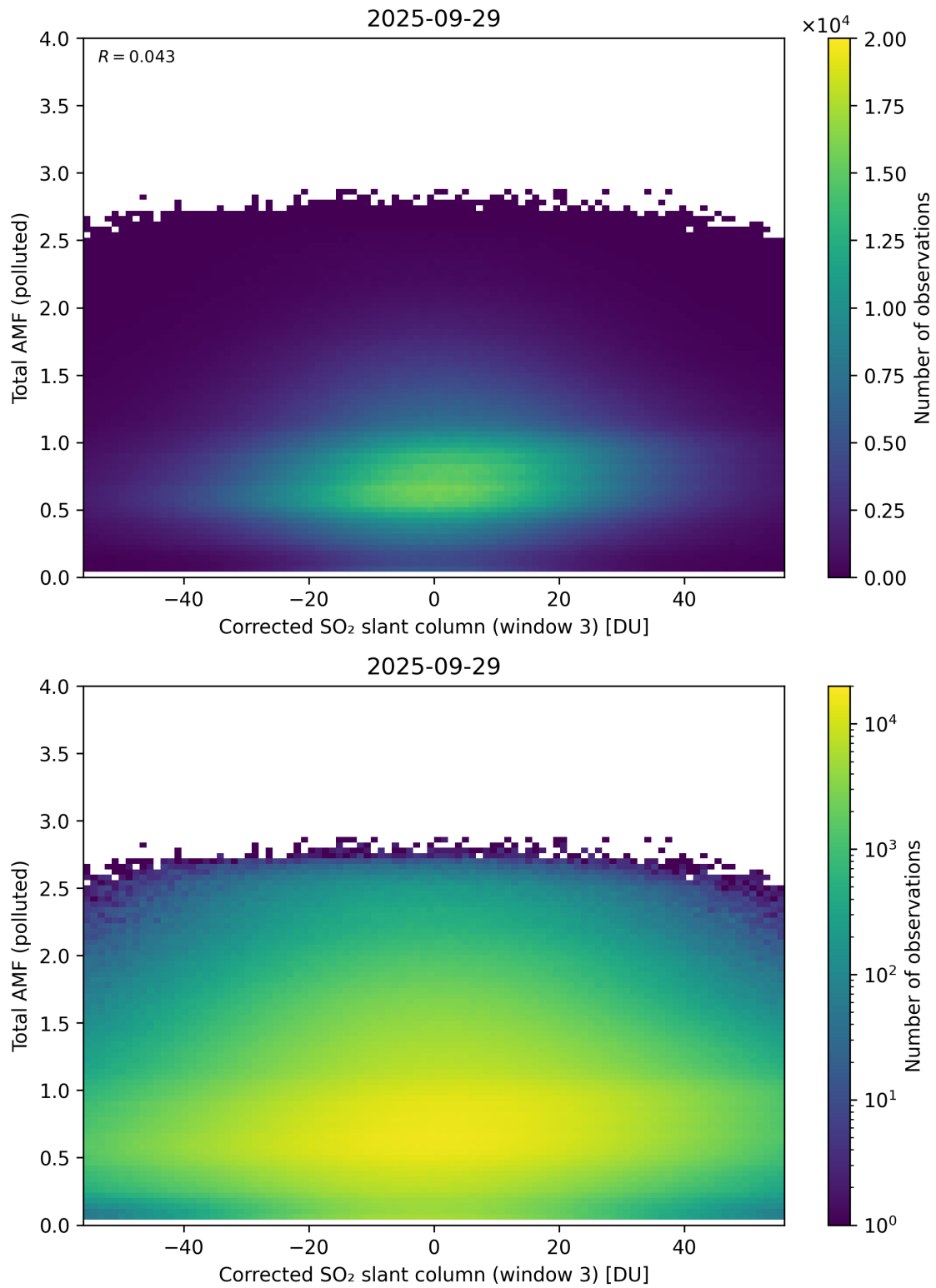
Figure 260: Scatter density plot of “Corrected SO 2 slant column (window 3)” against “Total AMF (polluted)” for 2025-09-28 to 2025-09-30.
