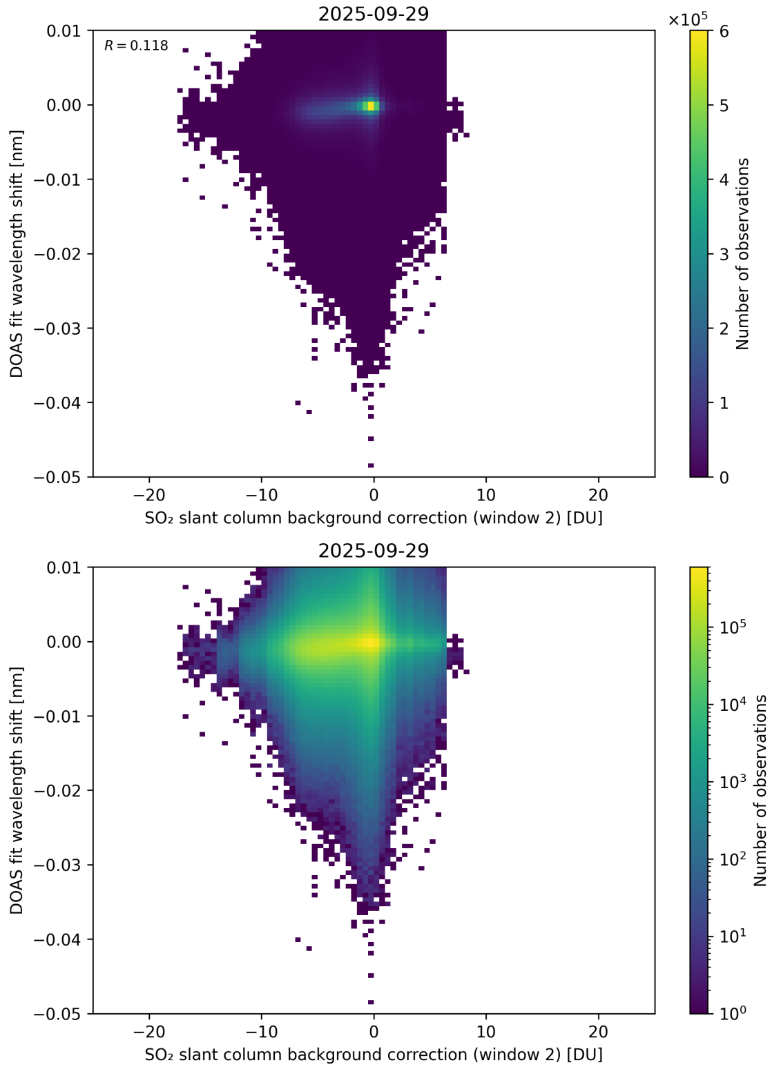
Figure 123: Scatter density plot of “SO 2 slant column background correction (window 2)” against “DOAS fit wavelength shift” for 2025-09-28 to 2025-09-30.
