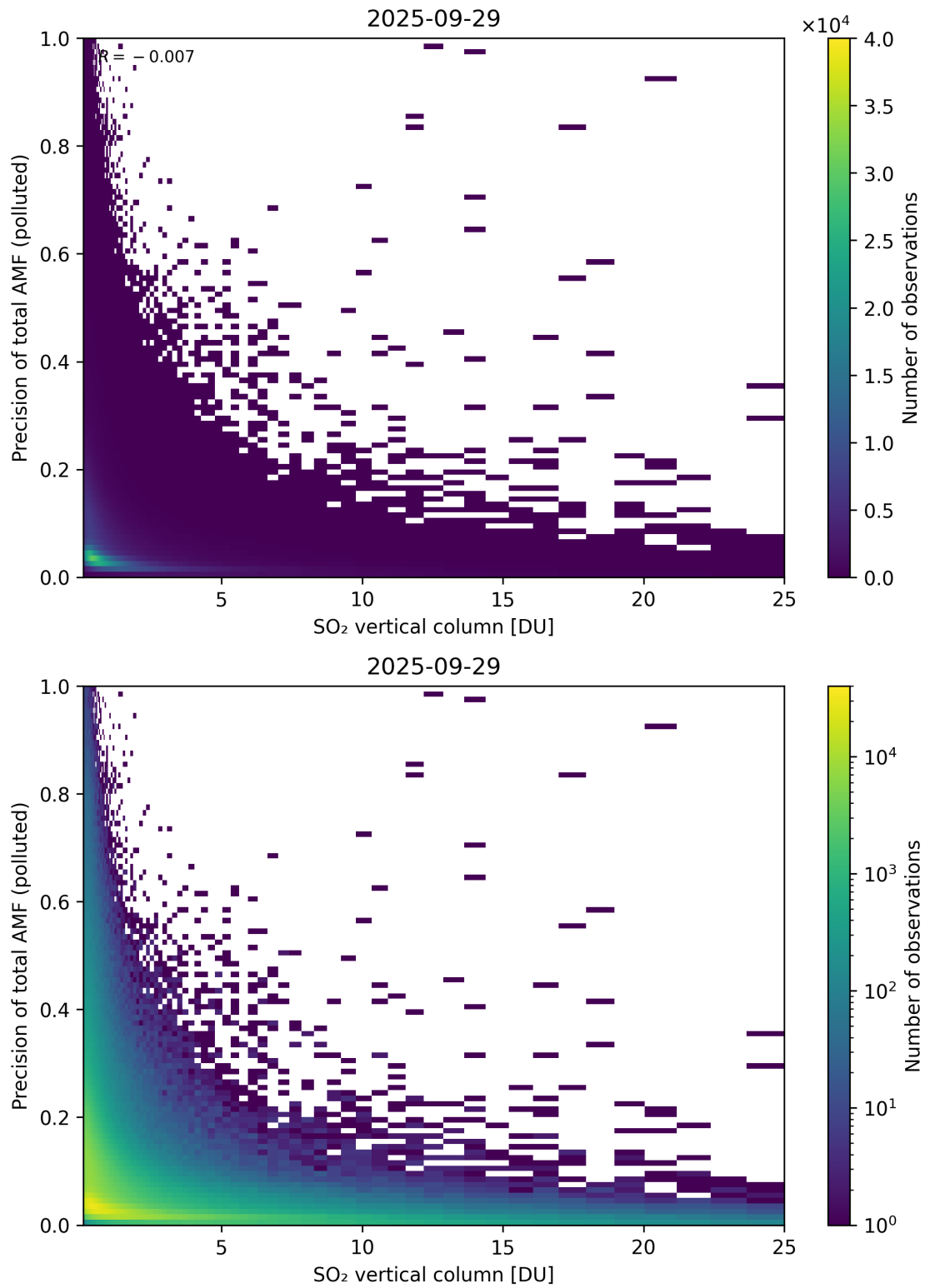
Figure 360: Scatter density plot of “SO 2 vertical column” against “Precision of total AMF (polluted)” for 2025-09-28 to 2025-09-30.
