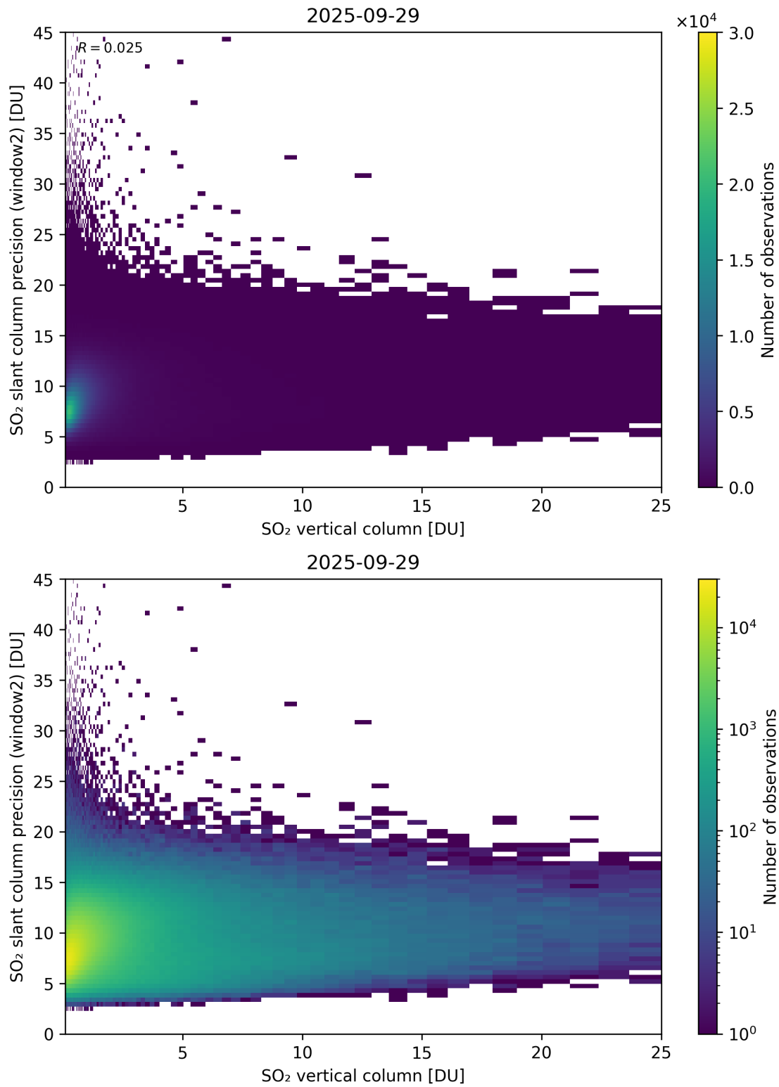
Figure 356: Scatter density plot of “SO 2 vertical column” against “SO 2 slant column precision (window2)” for 2025-09-28 to 2025-09-30.
