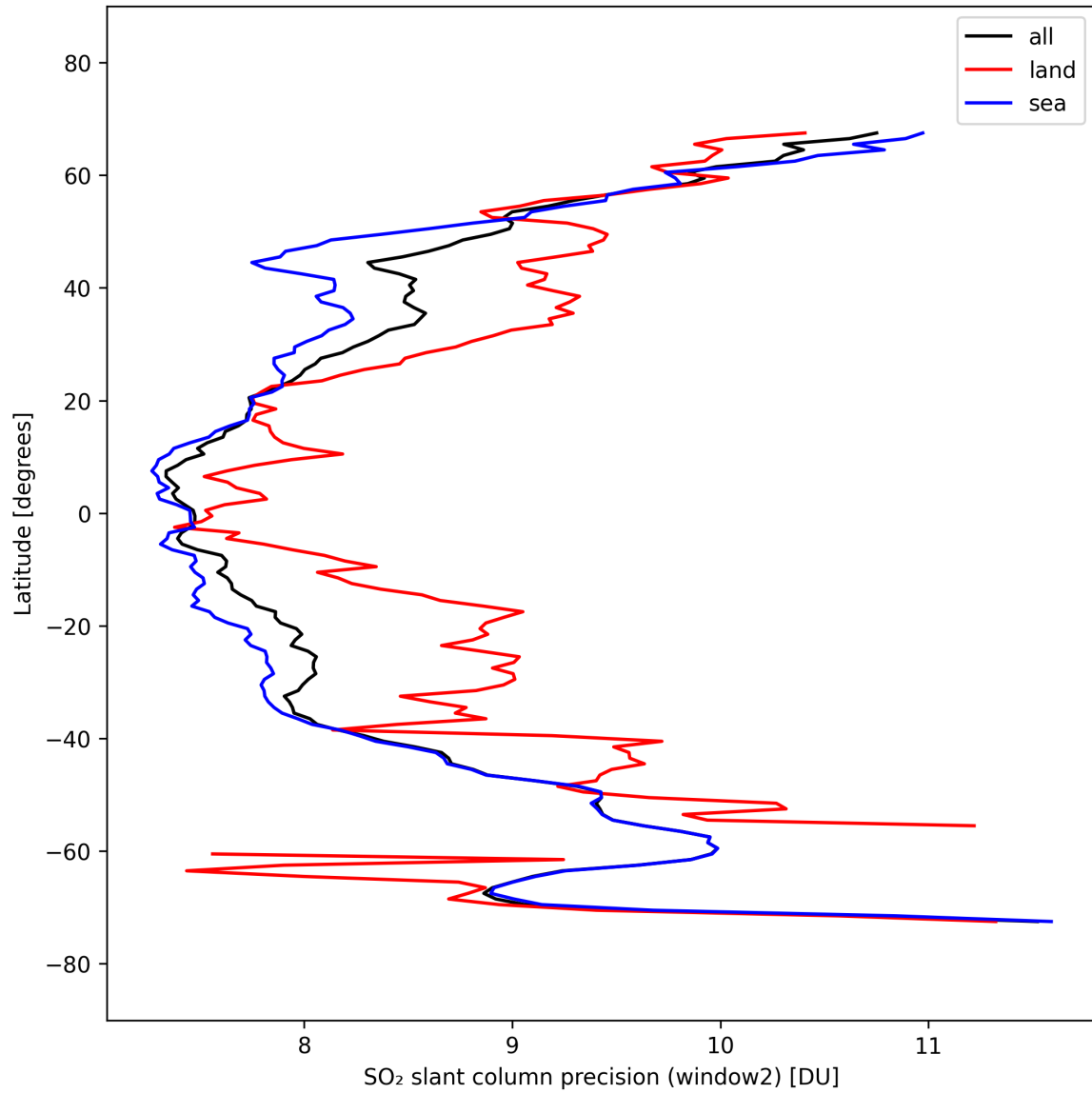
Figure 42: Zonal average of “SO 2 slant column precision (window2)” for 2025-09-28 to 2025-09-30.
