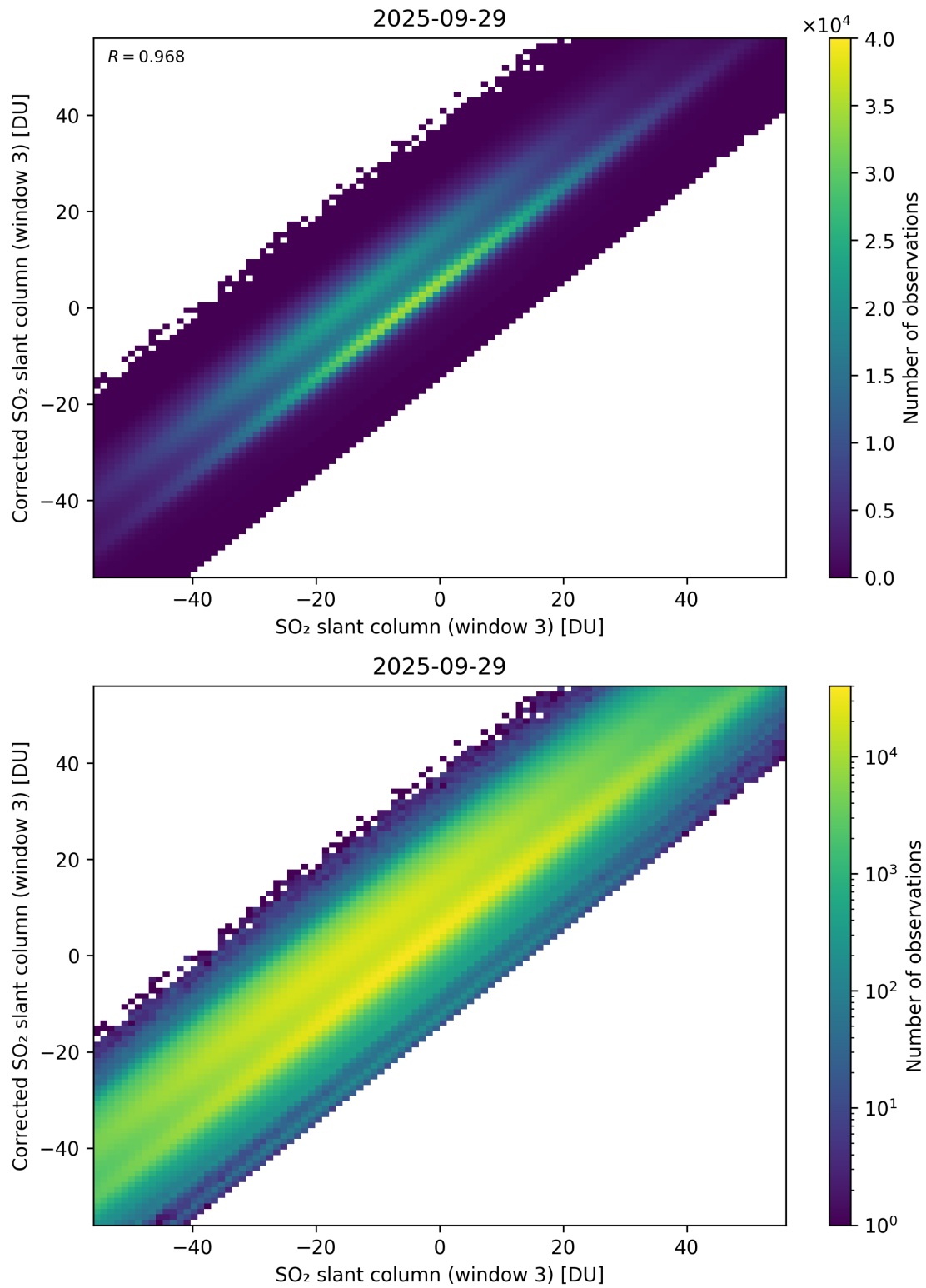
Figure 316: Scatter density plot of “SO 2 slant column (window 3)” against “Corrected SO 2 slant column (window 3)” for 2025-09-28 to 2025-09-30.
