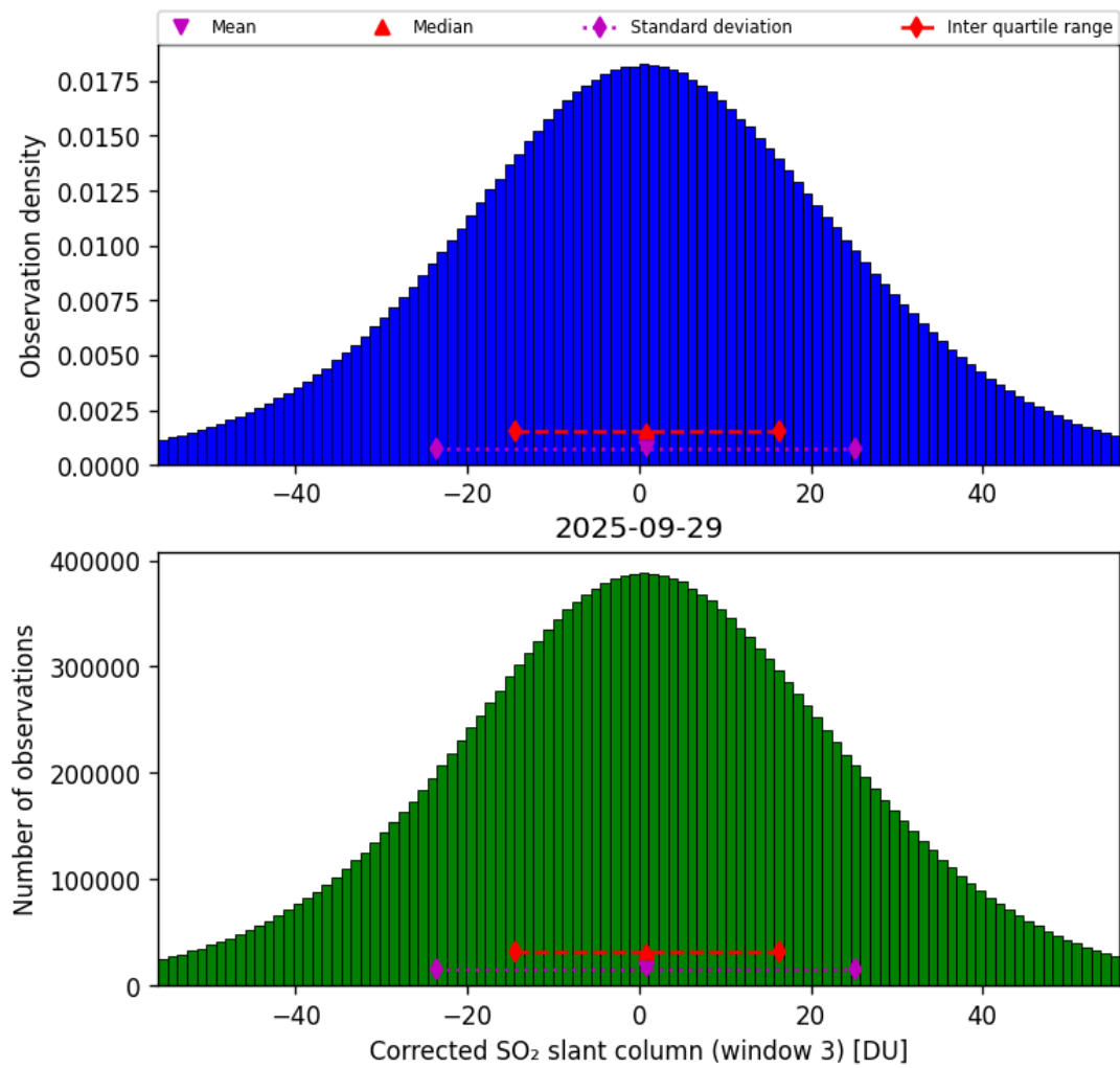
Figure 73: Histogram of “Corrected SO 2 slant column (window 3)” for 2025-09-28 to 2025-09-30
