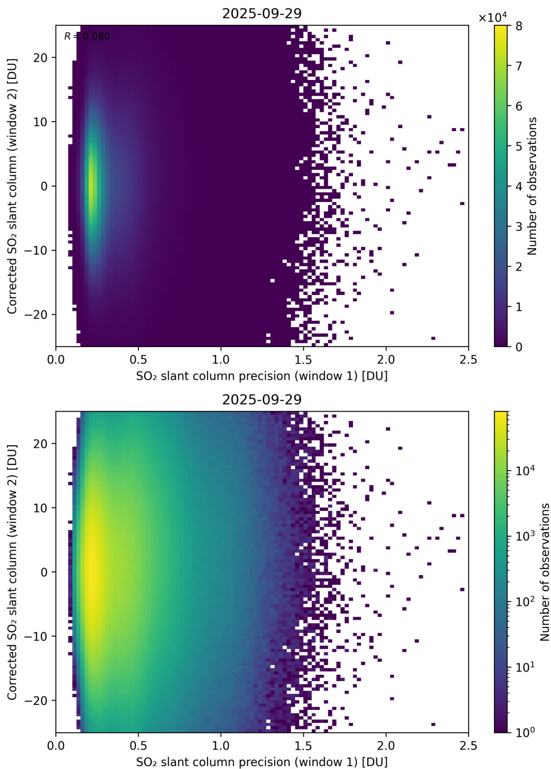
Figure 275: Scatter density plot of “SO 2 slant column precision (window 1)” against “Corrected SO 2 slant column (window 2)” for 2025-09-28 to 2025-09-30.
