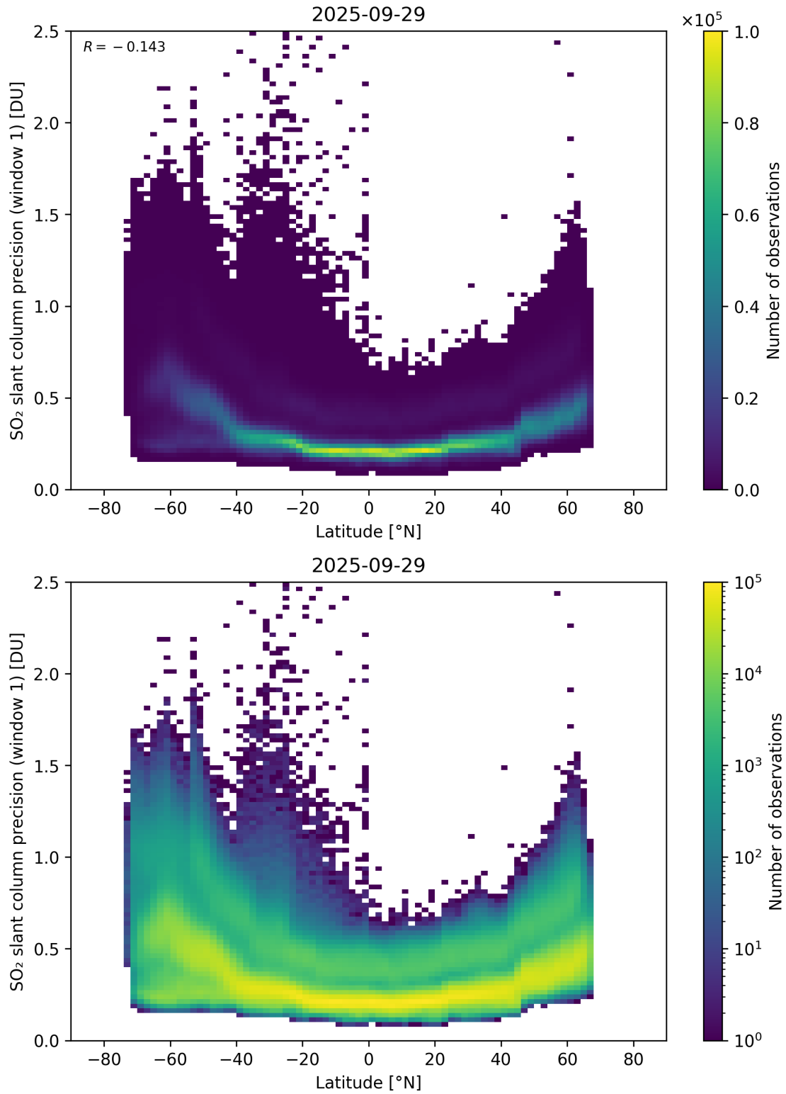
Figure 163: Scatter density plot of “Latitude” against “SO 2 slant column precision (window 1)” for 2025-09-28 to 2025-09-30.
