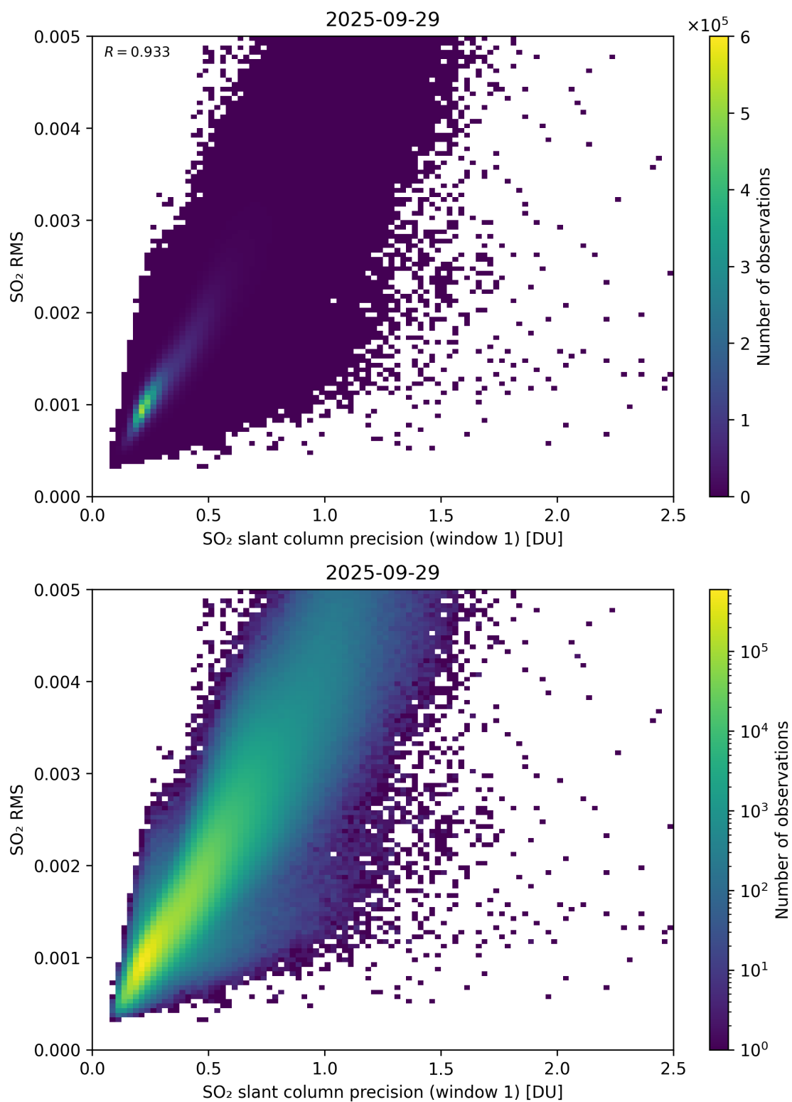
Figure 273: Scatter density plot of “SO 2 slant column precision (window 1)” against “SO 2 RMS” for 2025-09-28 to 2025-09-30.
