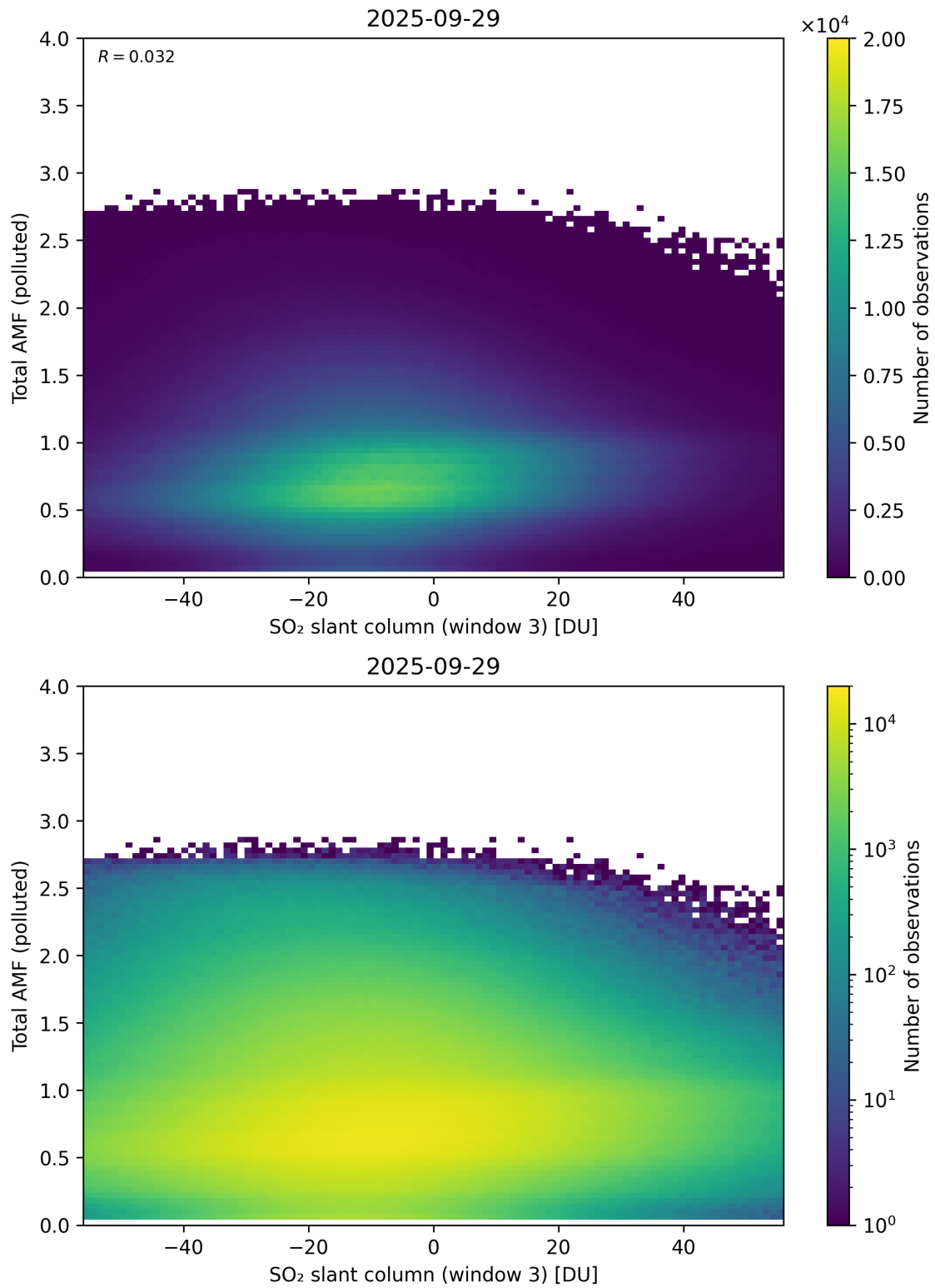
Figure 318: Scatter density plot of “SO 2 slant column (window 3)” against “Total AMF (polluted)” for 2025-09-28 to 2025-09-30.
