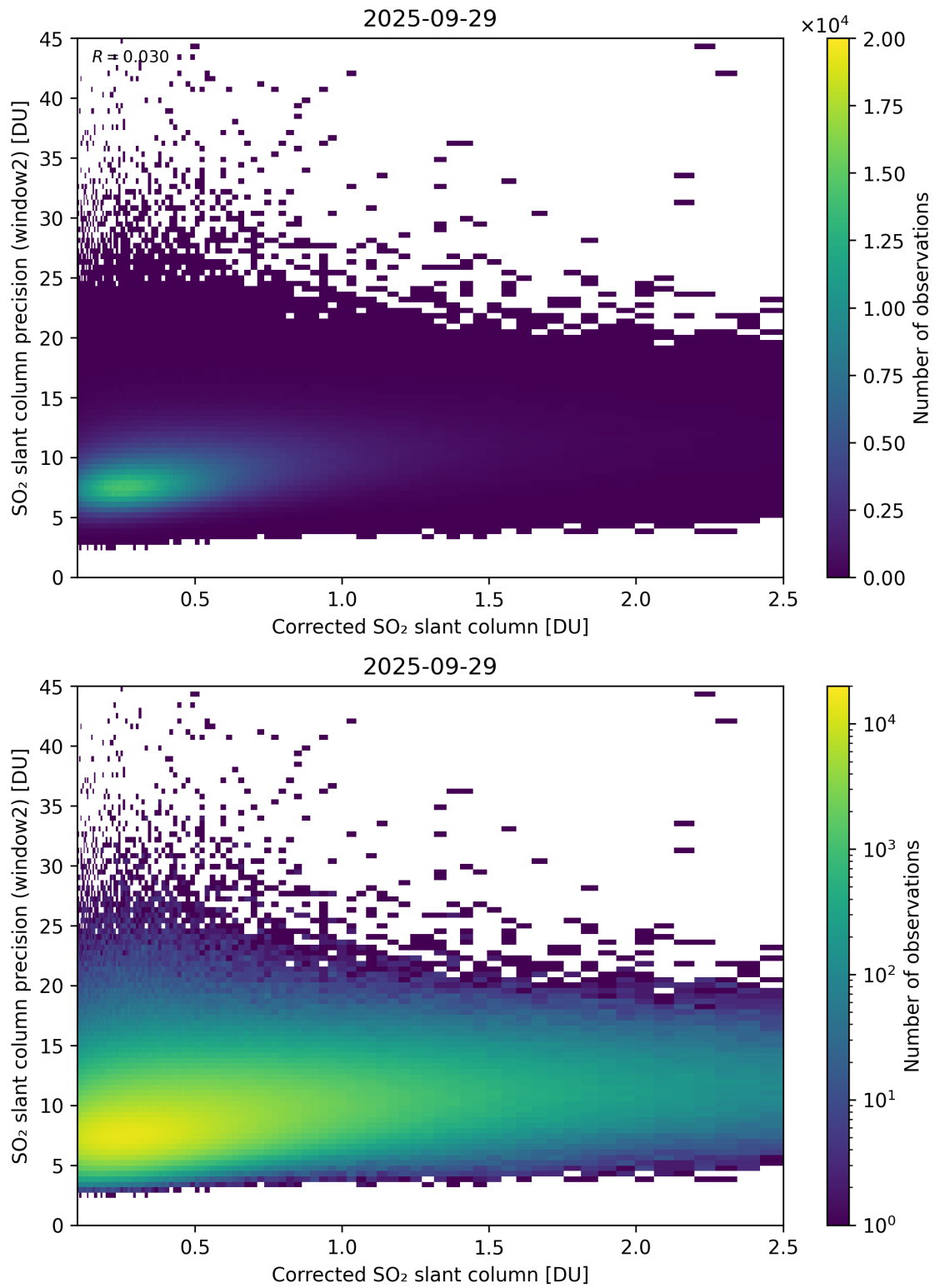
Figure 239: Scatter density plot of “Corrected SO 2 slant column” against “SO 2 slant column precision (window2)” for 2025-09-28 to 2025-09-30.
