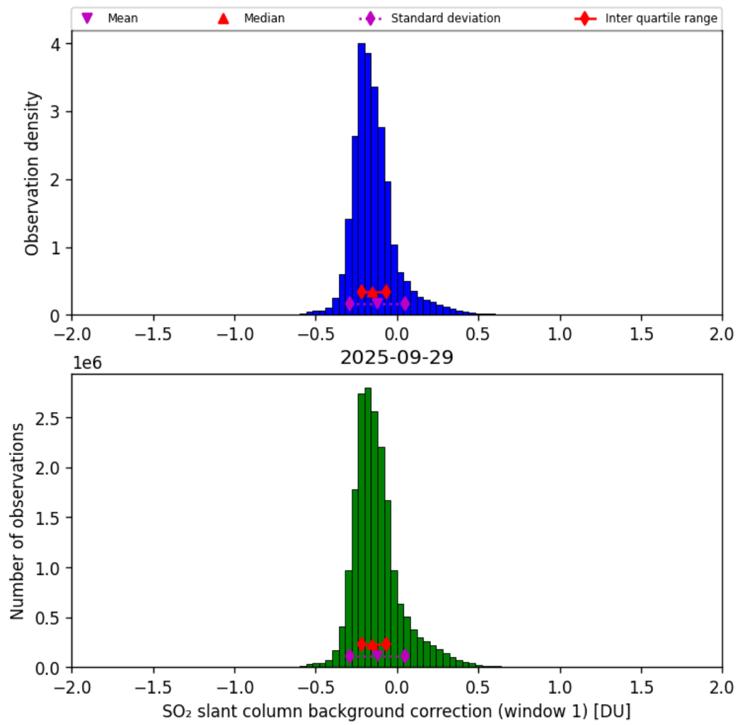
Figure 66: Histogram of “SO 2 slant column background correction (window 1)” for 2025-09-28 to 2025-09-30
