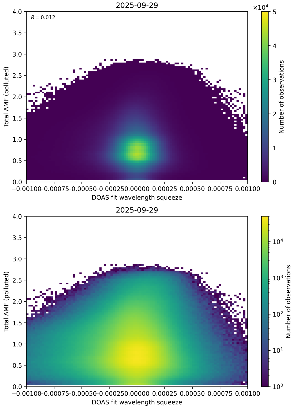
Figure 145: Scatter density plot of “DOAS fit wavelength squeeze” against “Total AMF (polluted)” for 2025-09-28 to 2025-09-30.
