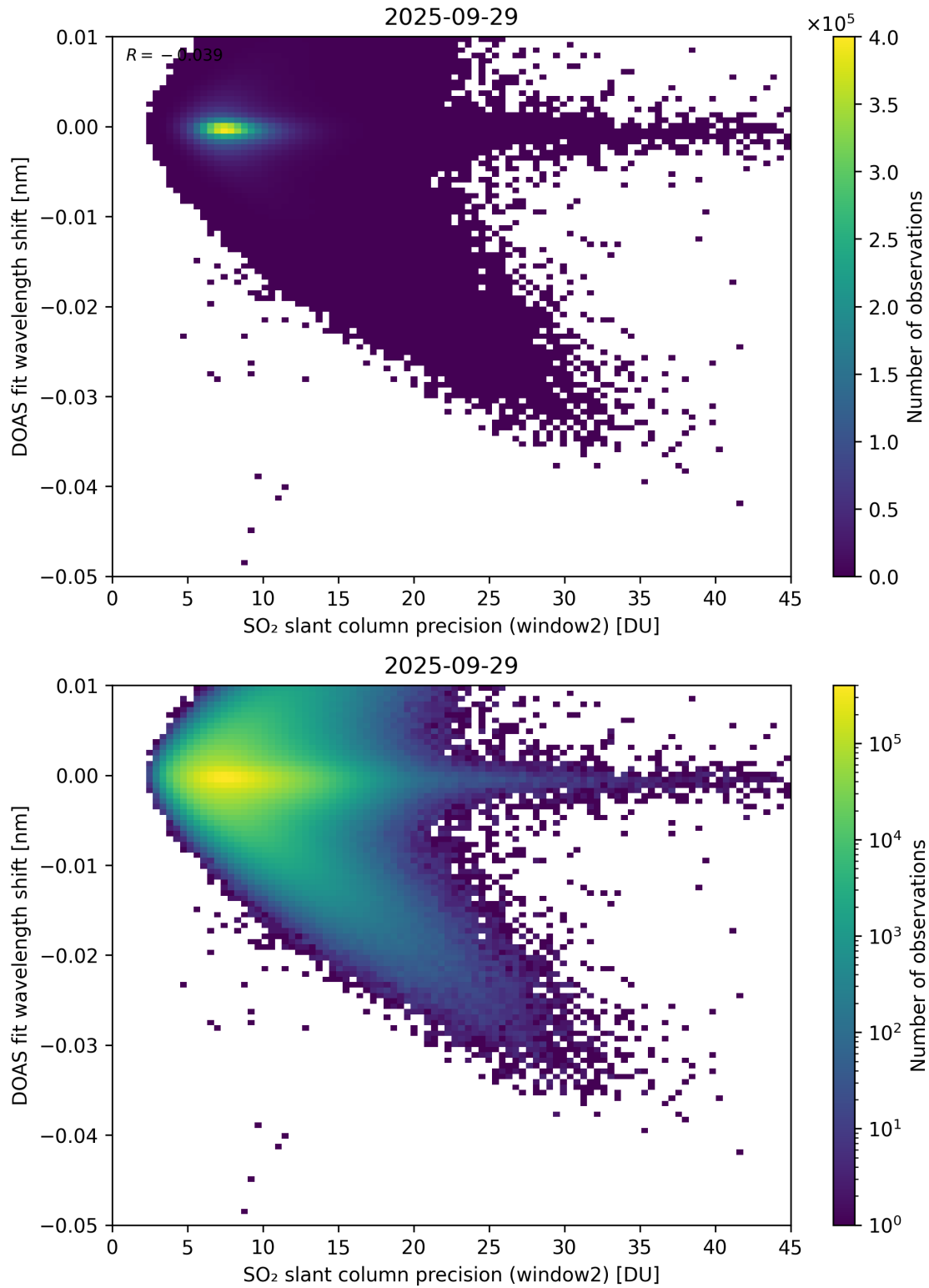
Figure 293: Scatter density plot of “SO 2 slant column precision (window2)” against “DOAS fit wavelength shift” for 2025-09-28 to 2025-09-30.
