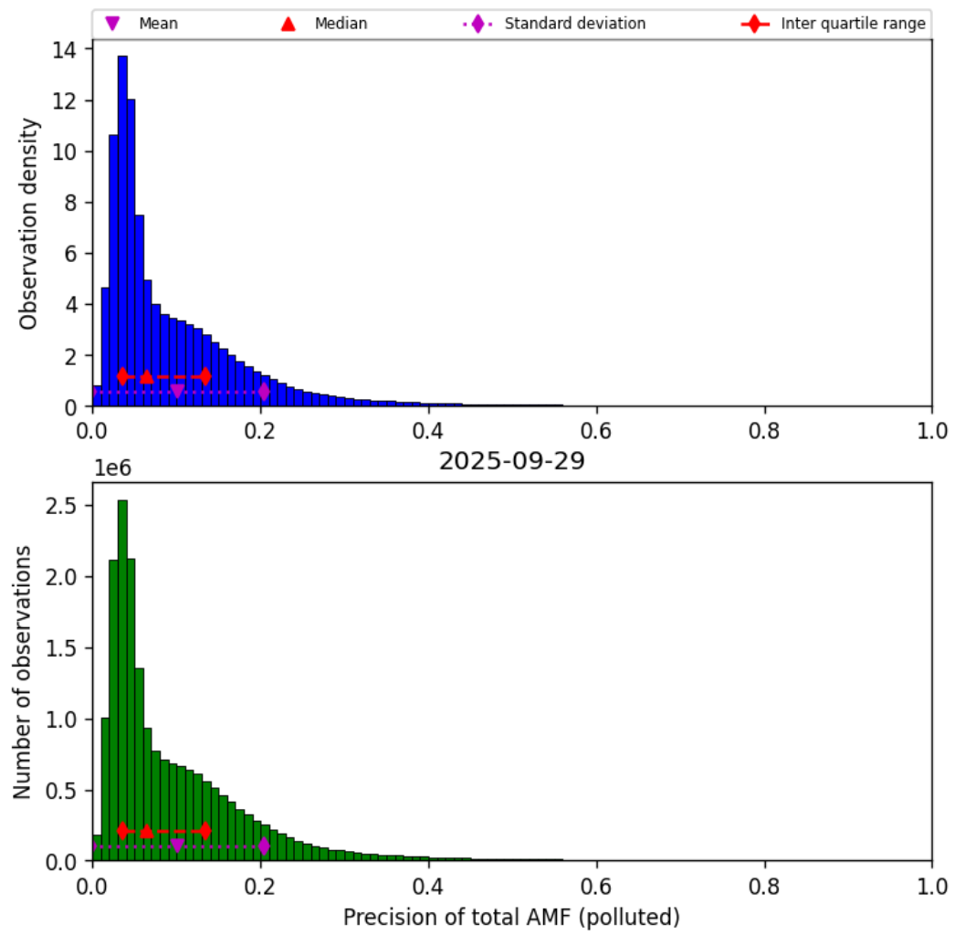
Figure 80: Histogram of “Precision of total AMF (polluted)” for 2025-09-28 to 2025-09-30
