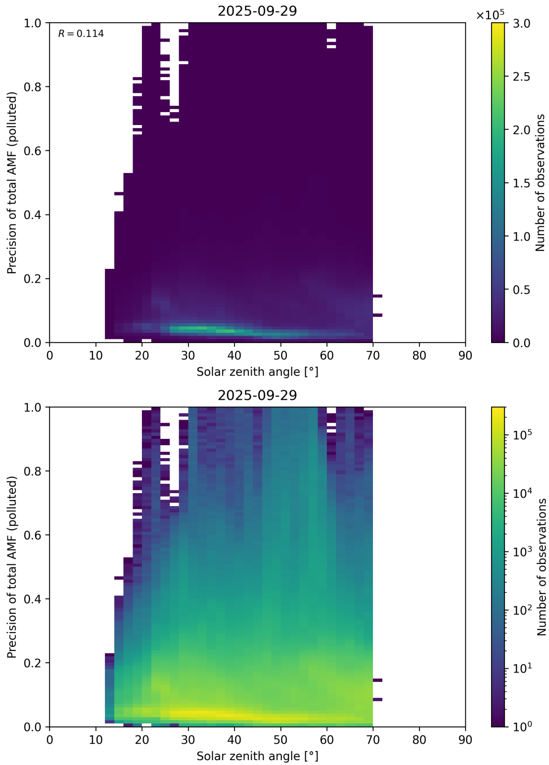
Figure 190: Scatter density plot of “Solar zenith angle” against “Precision of total AMF (polluted)” for 2025-09-28 to 2025-09-30.
