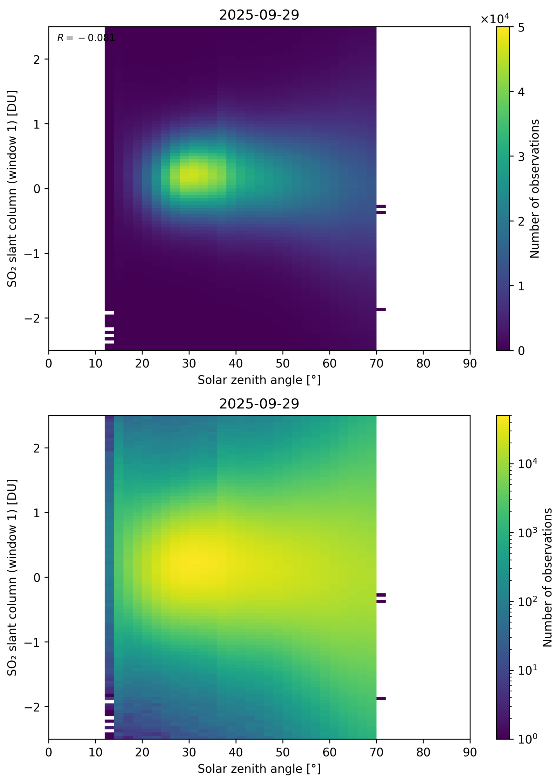
Figure 184: Scatter density plot of “Solar zenith angle” against “SO 2 slant column (window 1)” for 2025-09-28 to 2025-09-30.
