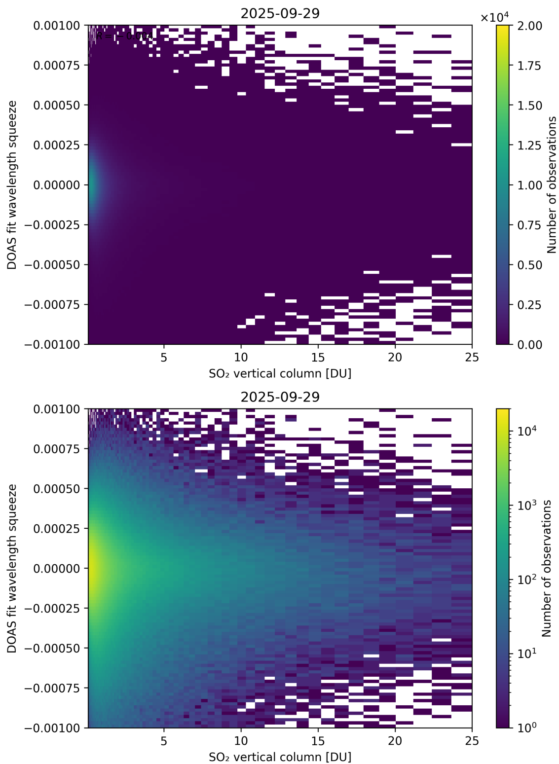
Figure 327: Scatter density plot of “SO 2 vertical column” against “DOAS fit wavelength squeeze” for 2025-09-28 to 2025-09-30.
