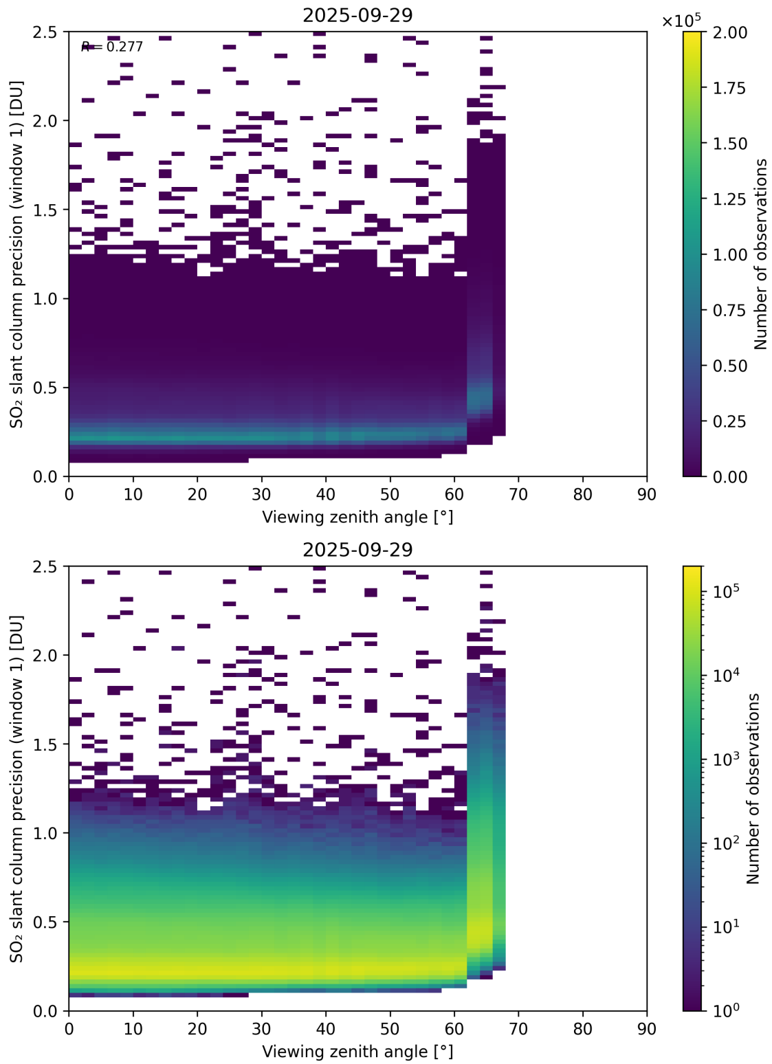
Figure 377: Scatter density plot of “Viewing zenith angle” against “SO 2 slant column precision (window 1)” for 2025-09-28 to 2025-09-30.
