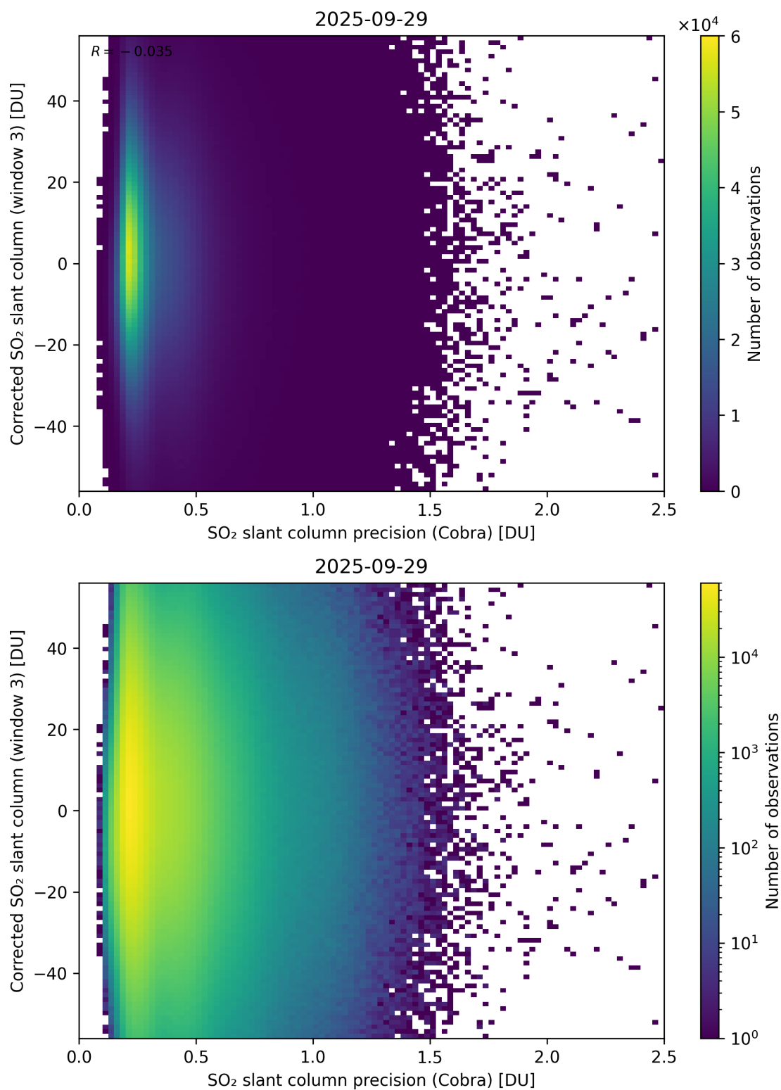
Figure 207: Scatter density plot of “SO 2 slant column precision (Cobra)” against “Corrected SO 2 slant column (window 3)” for 2025-09-28 to 2025-09-30.
