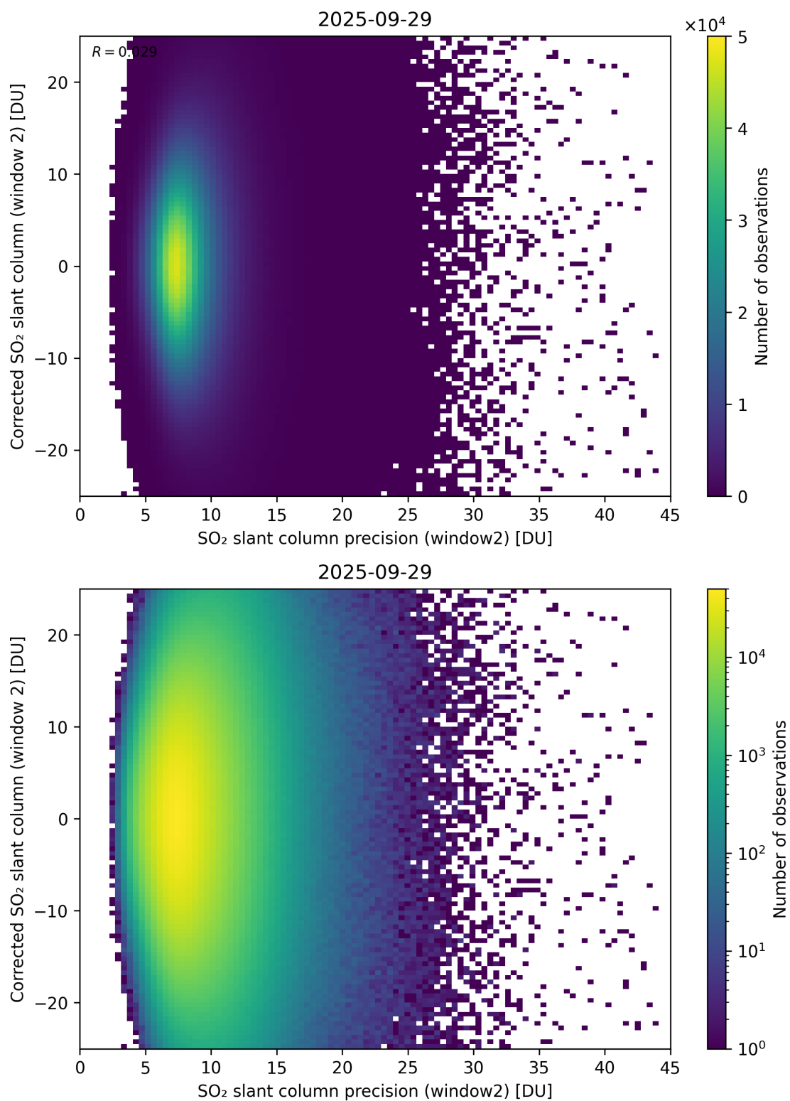
Figure 297: Scatter density plot of “SO 2 slant column precision (window2)” against “Corrected SO 2 slant column (window 2)” for 2025-09-28 to 2025-09-30.
