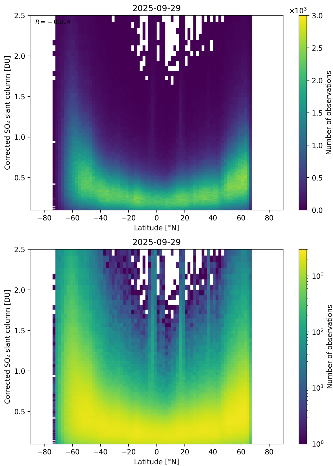
Figure 159: Scatter density plot of “Latitude” against “Corrected SO 2 slant column” for 2025-09-28 to 2025-09-30.
