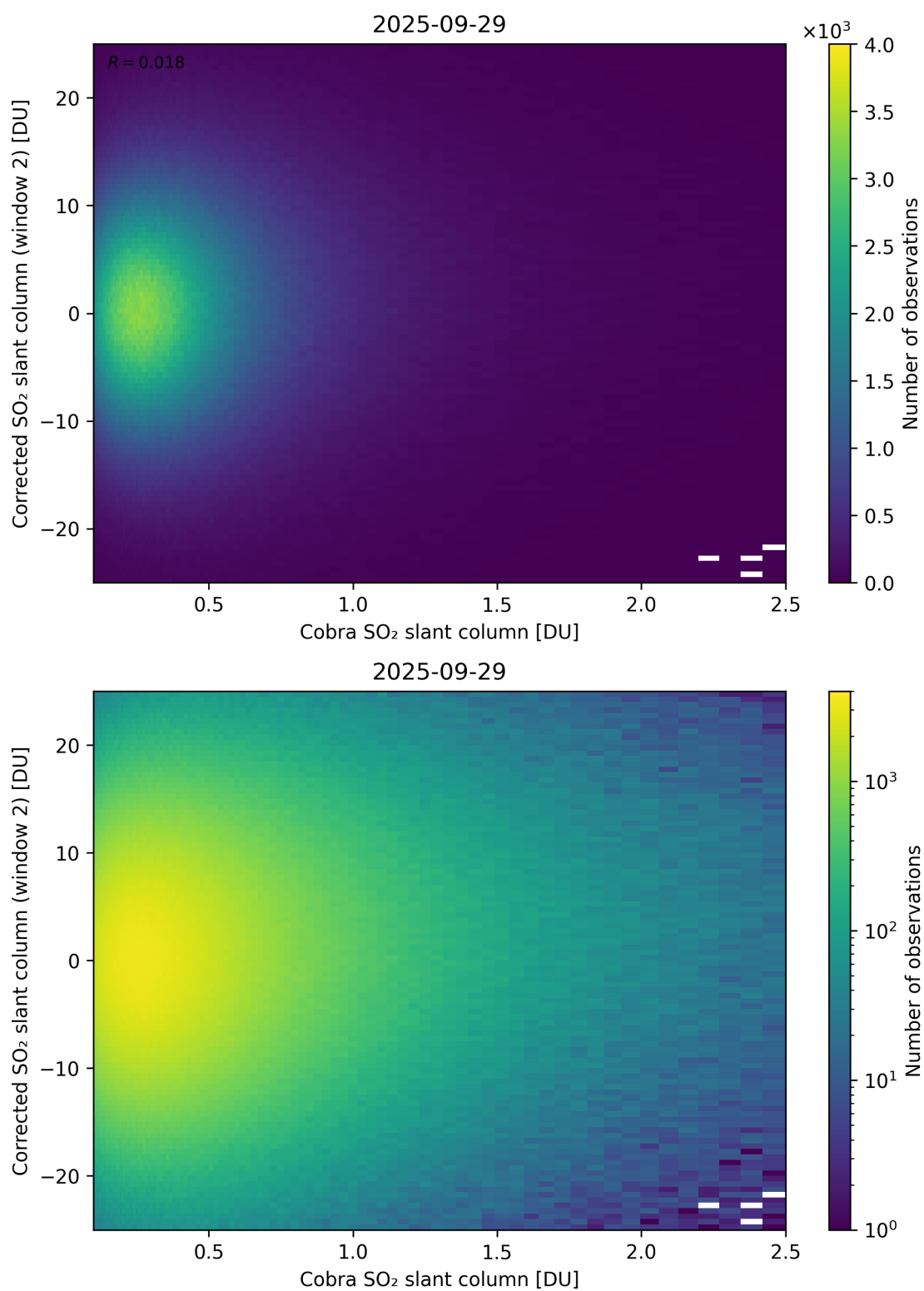
Figure 217: Scatter density plot of “Cobra SO 2 slant column” against “Corrected SO 2 slant column (window 2)” for 2025-09-28 to 2025-09-30.
