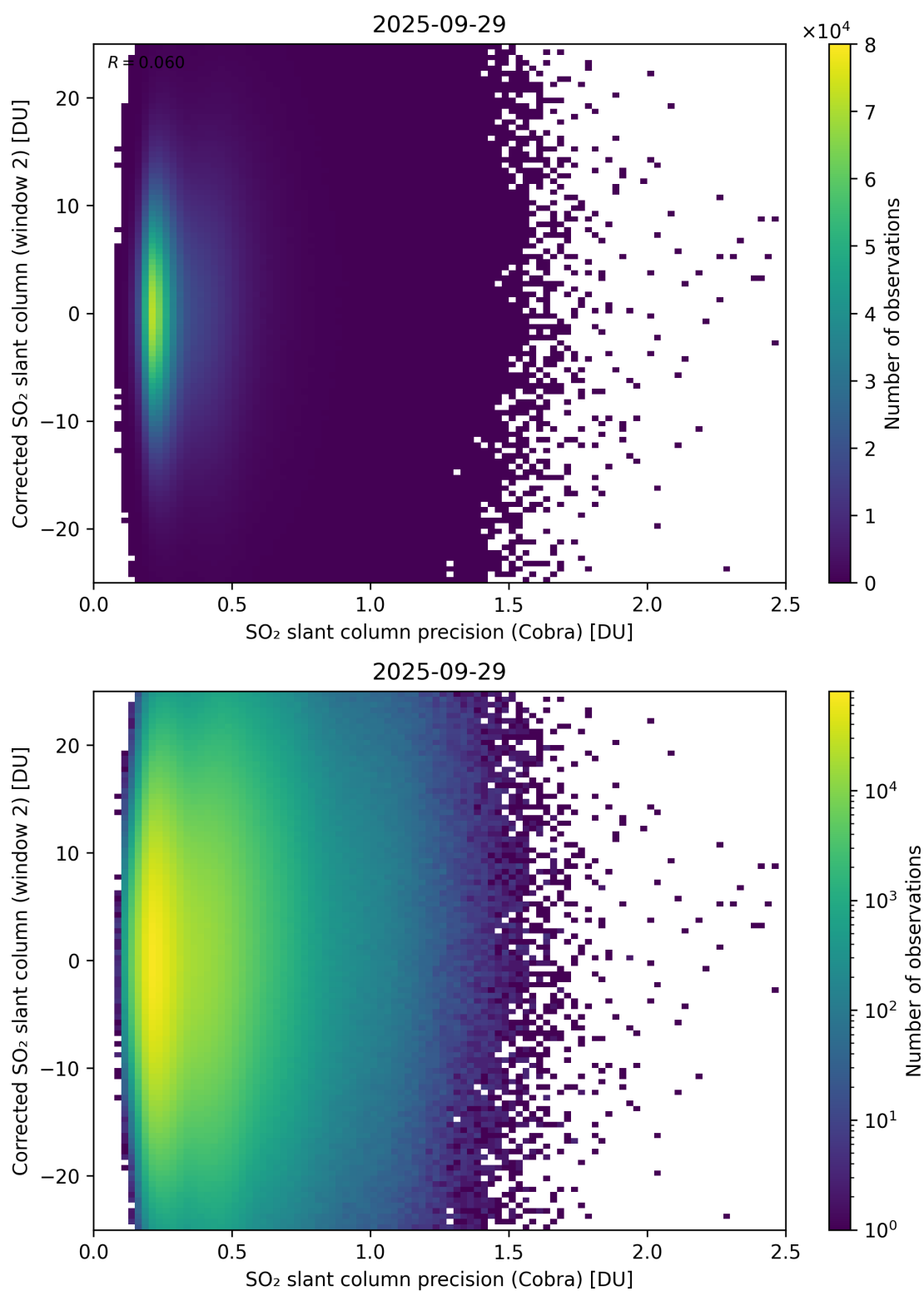
Figure 206: Scatter density plot of “SO 2 slant column precision (Cobra)” against “Corrected SO 2 slant column (window 2)” for 2025-09-28 to 2025-09-30.
