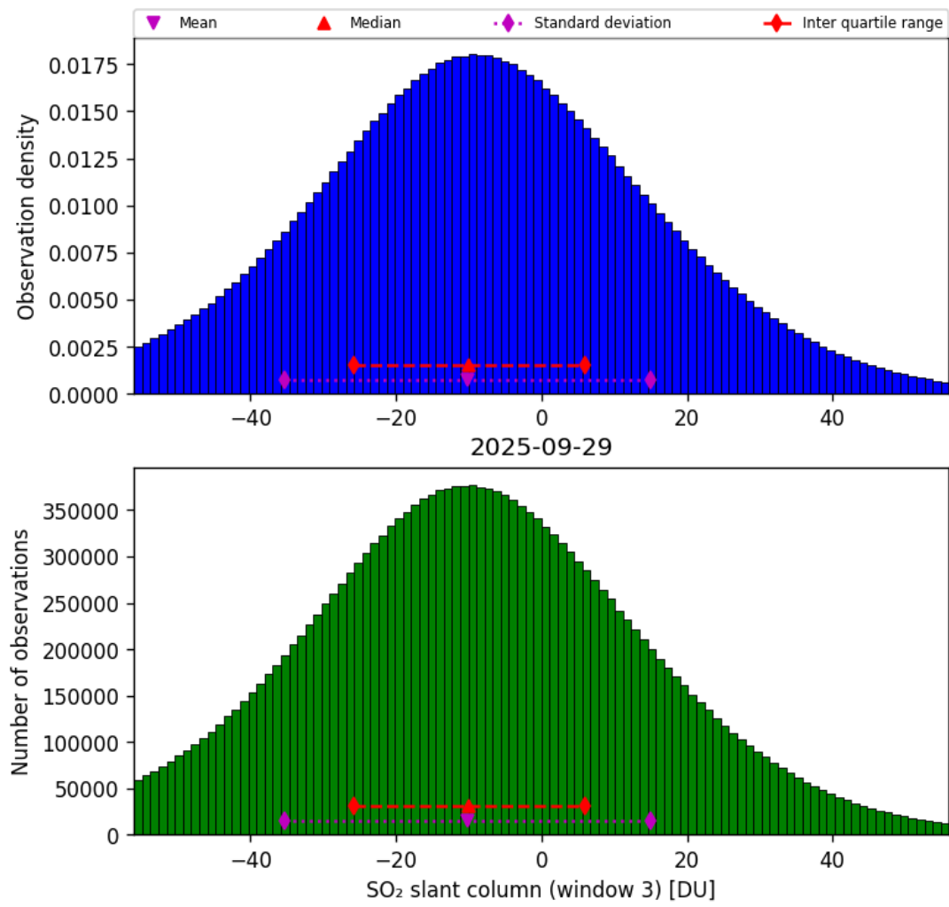
Figure 71: Histogram of “SO 2 slant column (window 3)” for 2025-09-28 to 2025-09-30
