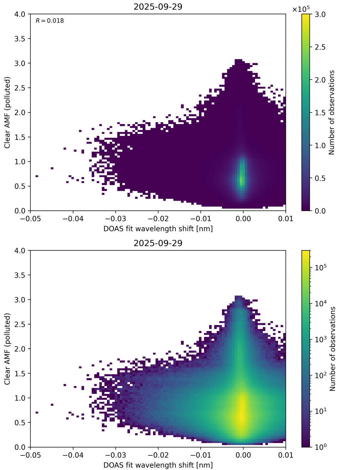
Figure 140: Scatter density plot of “DOAS fit wavelength shift” against “Clear AMF (polluted)” for 2025-09-28 to 2025-09-30.
