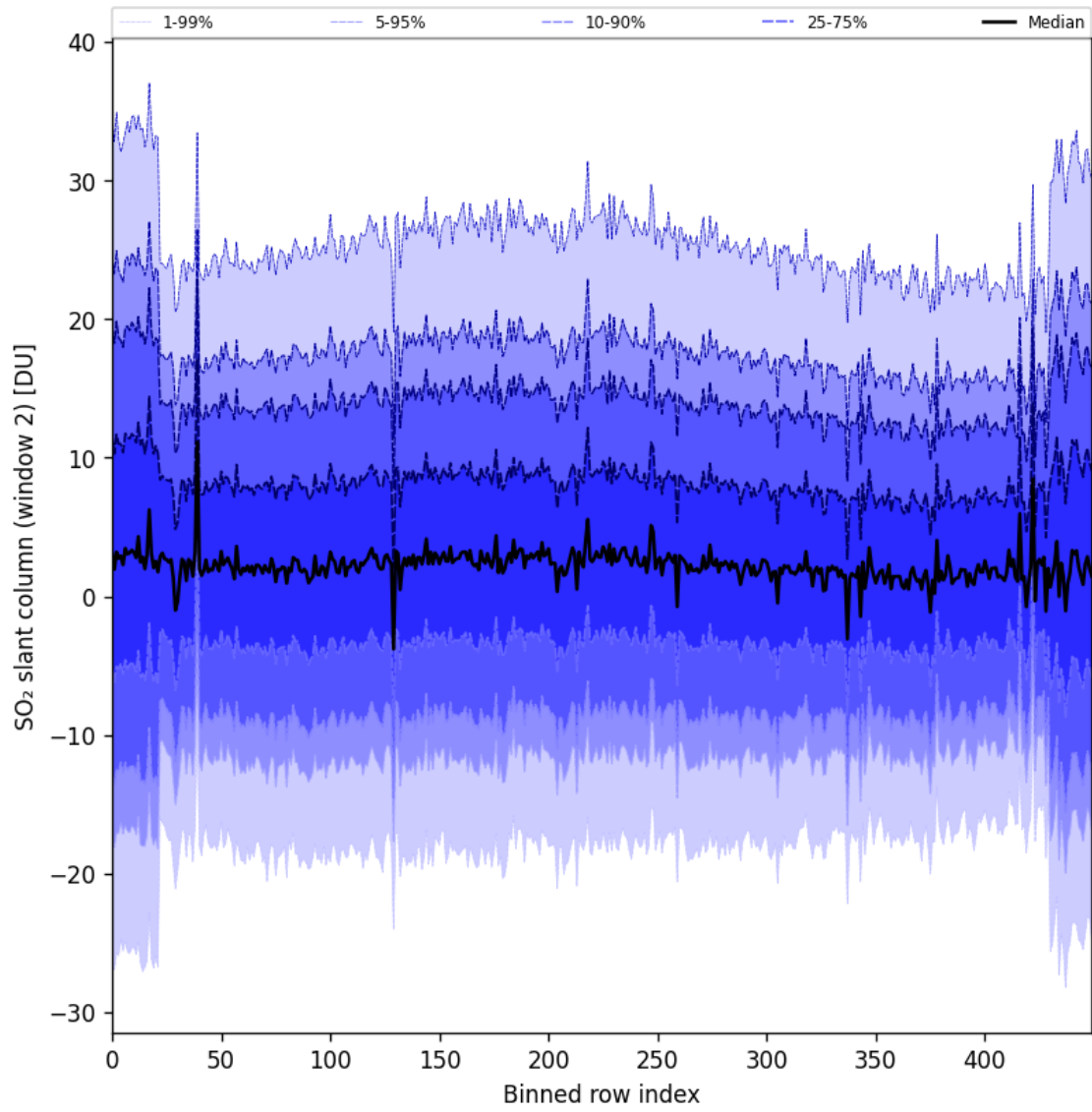
Figure 93: Along track statistics of “SO 2 slant column (window 2)” for 2025-09-28 to 2025-09-30
