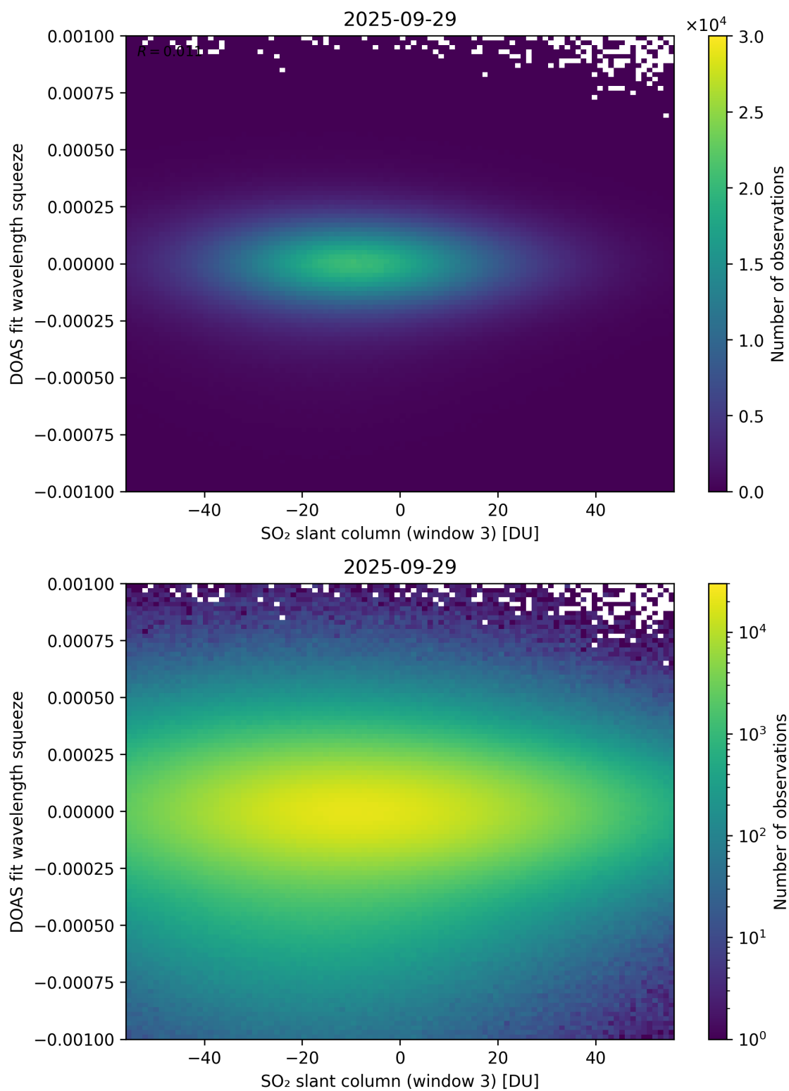
Figure 305: Scatter density plot of “SO 2 slant column (window 3)” against “DOAS fit wavelength squeeze” for 2025-09-28 to 2025-09-30.
