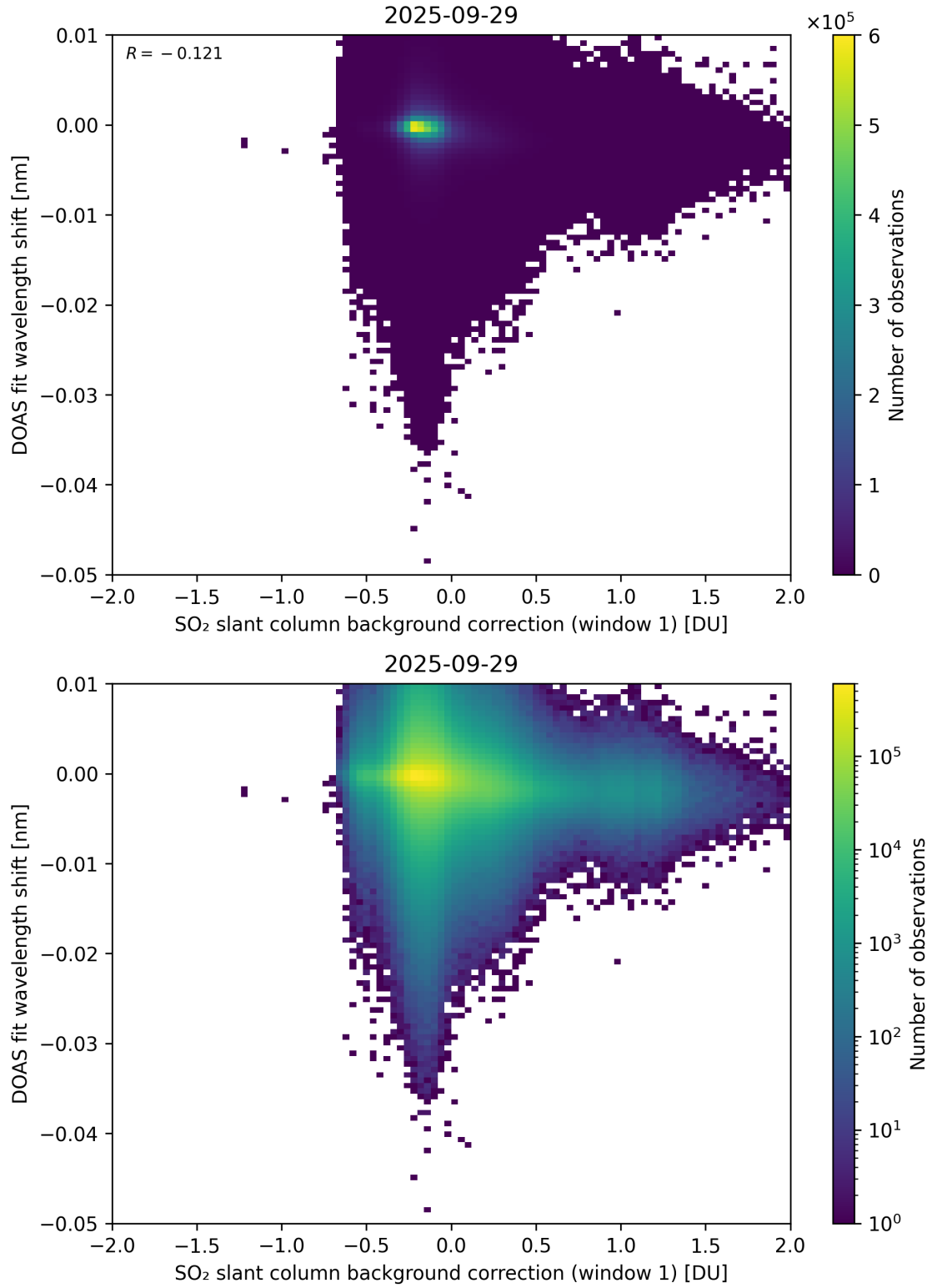
Figure 111: Scatter density plot of “SO 2 slant column background correction (window 1)” against “DOAS fit wavelength shift” for 2025-09-28 to 2025-09-30.
