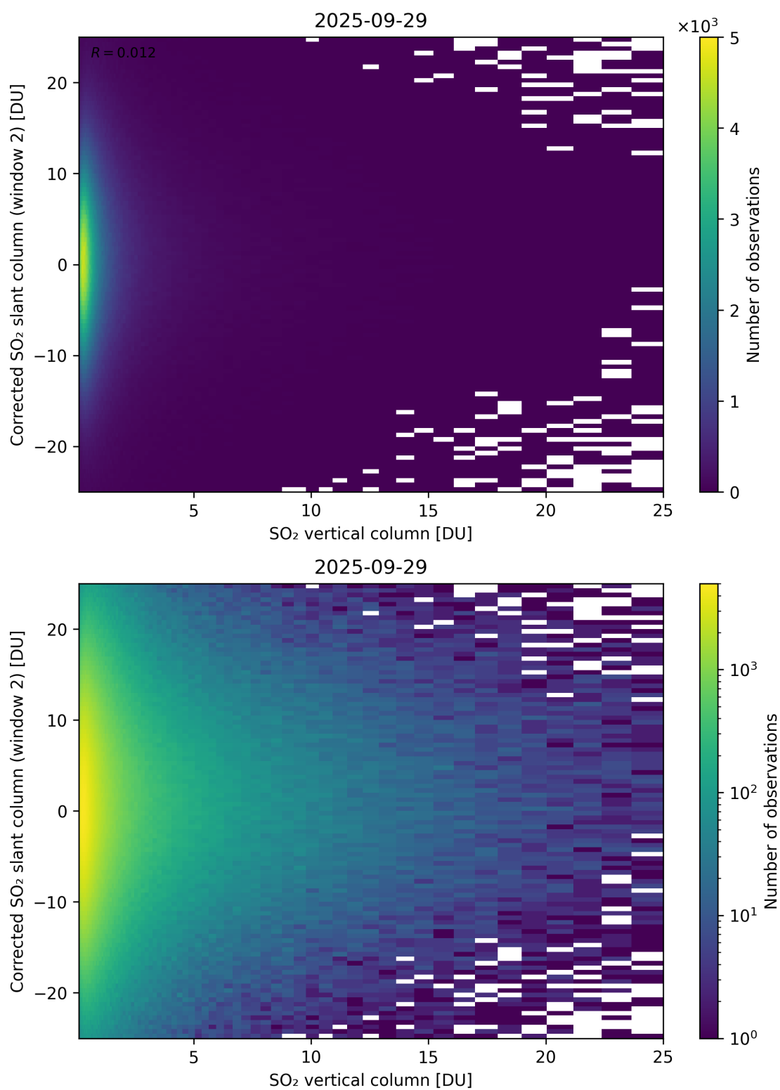
Figure 352: Scatter density plot of “SO 2 vertical column” against “Corrected SO 2 slant column (window 2)” for 2025-09-28 to 2025-09-30.
