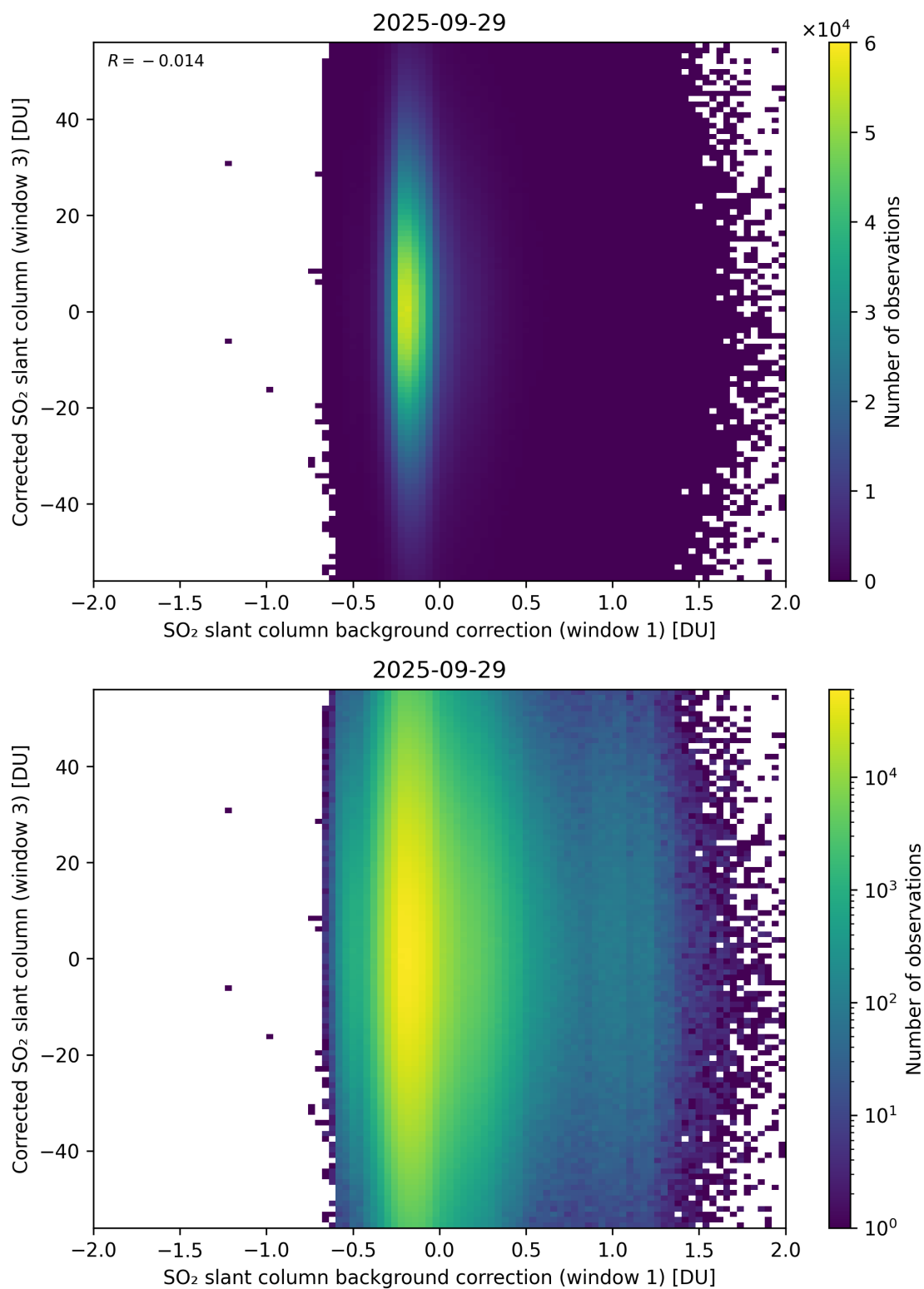
Figure 116: Scatter density plot of “SO 2 slant column background correction (window 1)” against “Corrected SO 2 slant column (window 3)” for 2025-09-28 to 2025-09-30.
