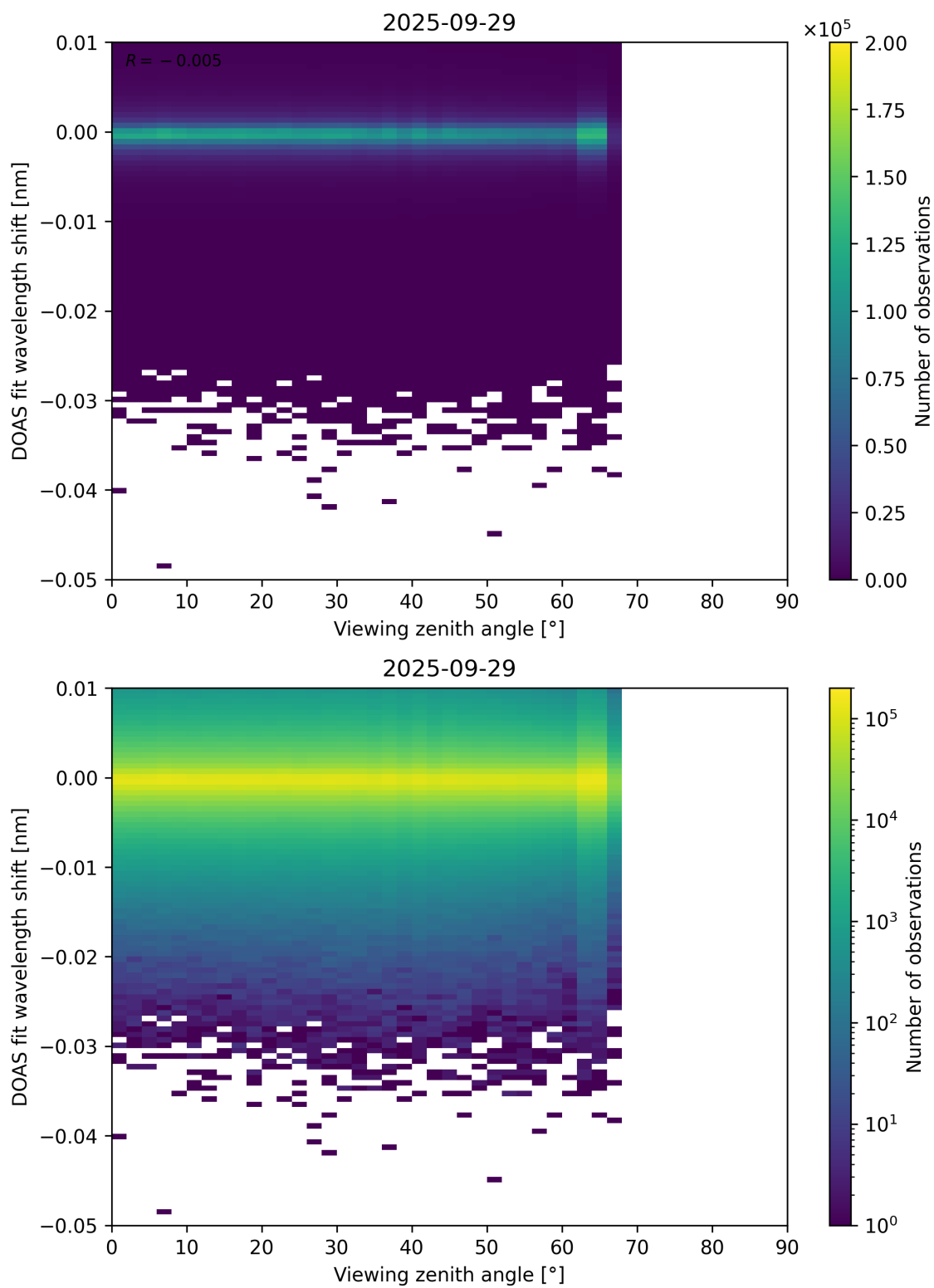
Figure 365: Scatter density plot of “Viewing zenith angle” against “DOAS fit wavelength shift” for 2025-09-28 to 2025-09-30.
