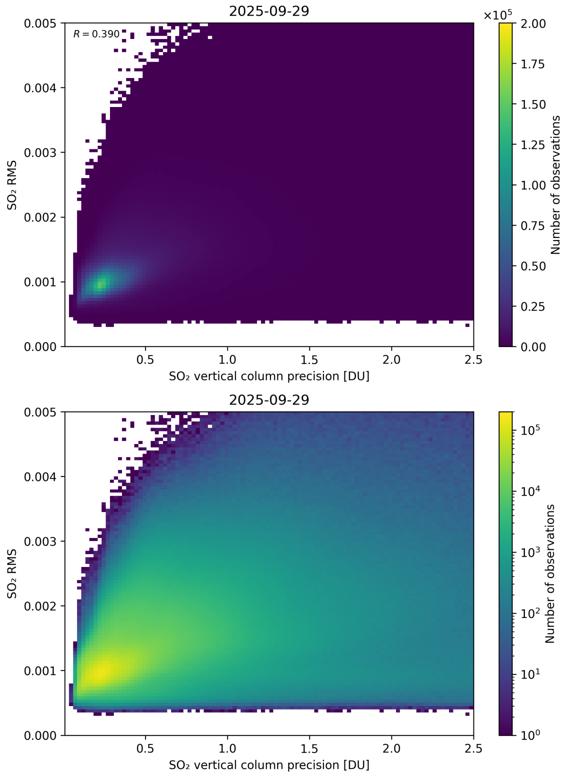
Figure 334: Scatter density plot of “SO 2 vertical column precision” against “SO 2 RMS” for 2025-09-28 to 2025-09-30.
