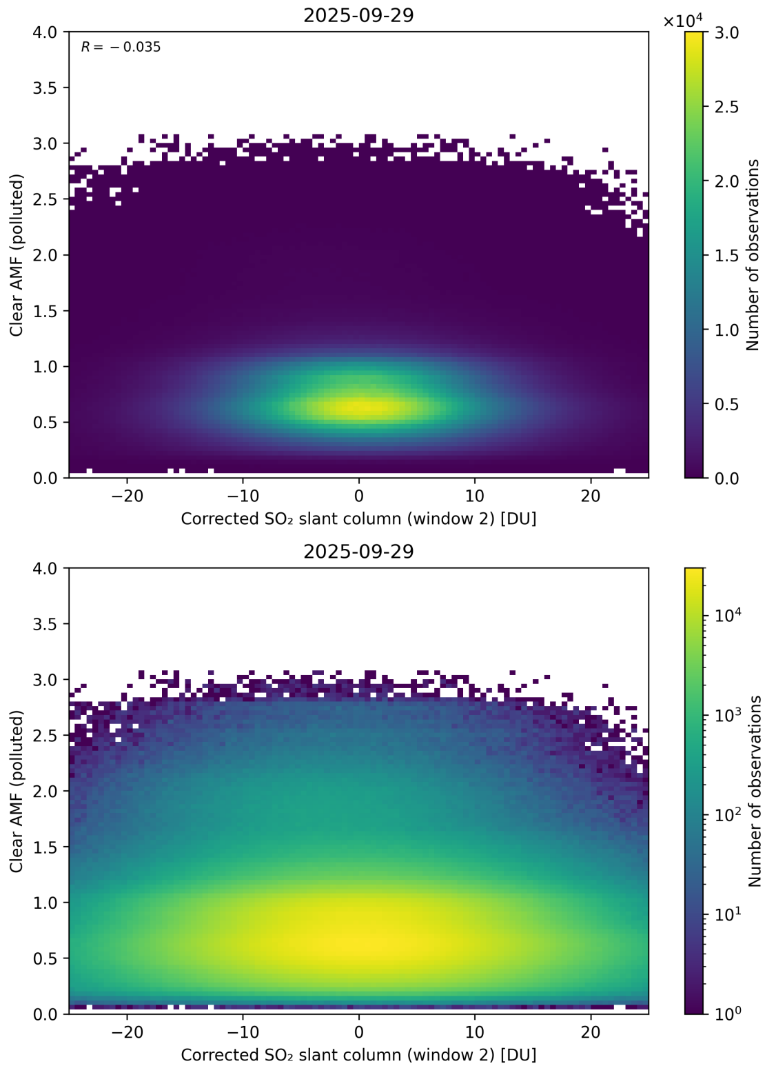
Figure 249: Scatter density plot of “Corrected SO 2 slant column (window 2)” against “Clear AMF (polluted)” for 2025-09-28 to 2025-09-30.
