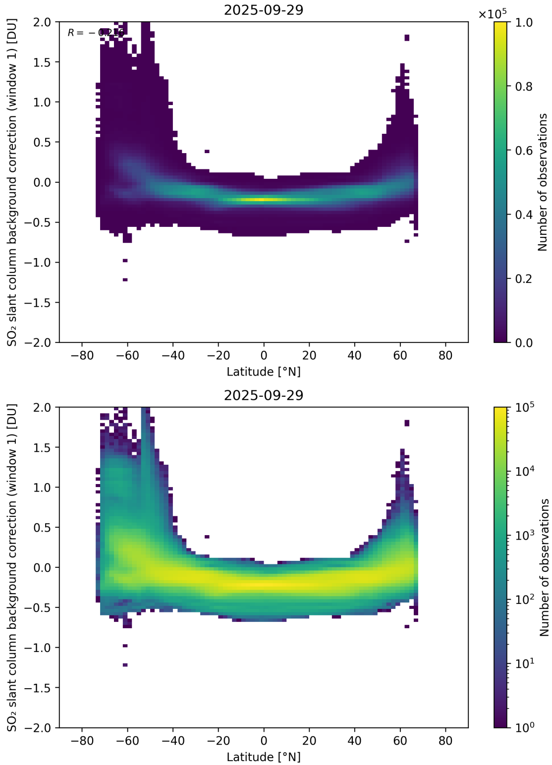
Figure 150: Scatter density plot of “Latitude” against “SO 2 slant column background correction (window 1)” for 2025-09-28 to 2025-09-30.
