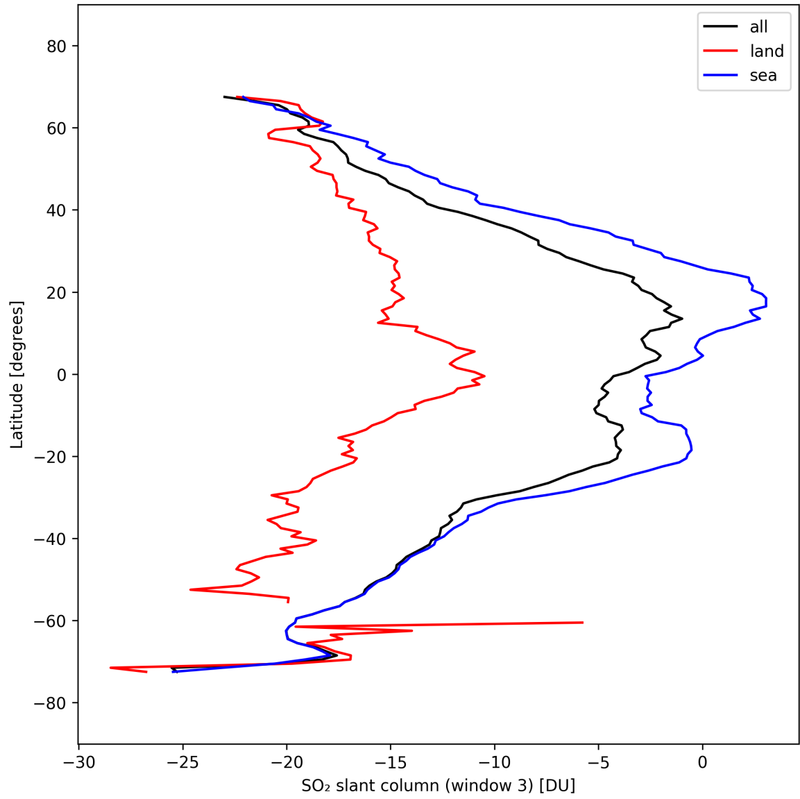
Figure 45: Zonal average of “SO 2 slant column (window 3)” for 2025-09-28 to 2025-09-30.
