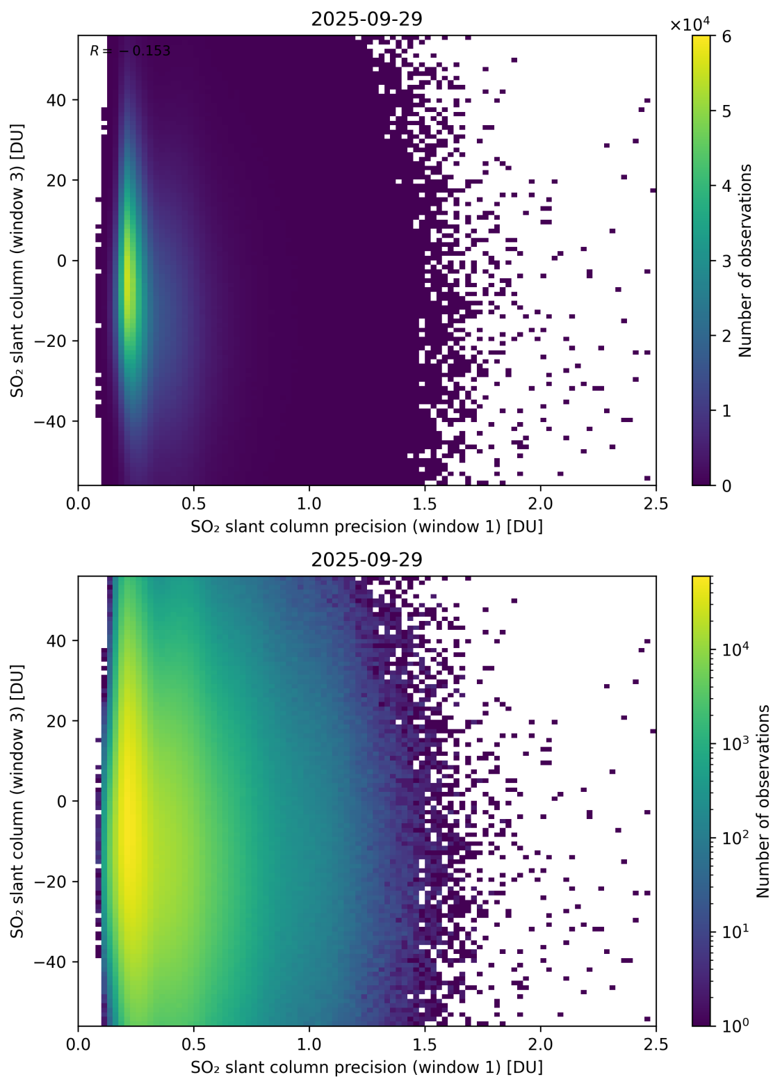
Figure 278: Scatter density plot of “SO 2 slant column precision (window 1)” against “SO 2 slant column (window 3)” for 2025-09-28 to 2025-09-30.
