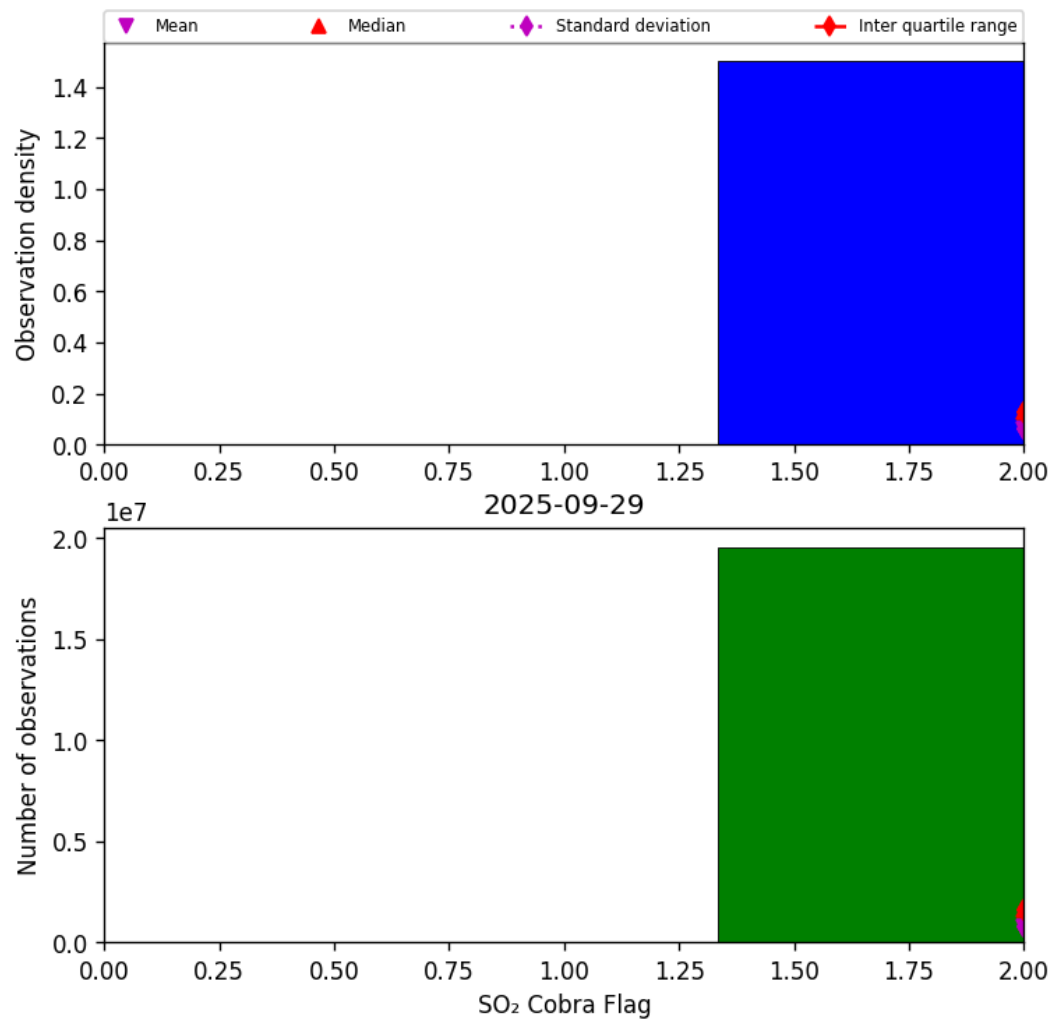
Figure 75: Histogram of “SO 2 Cobra Flag” for 2025-09-28 to 2025-09-30
