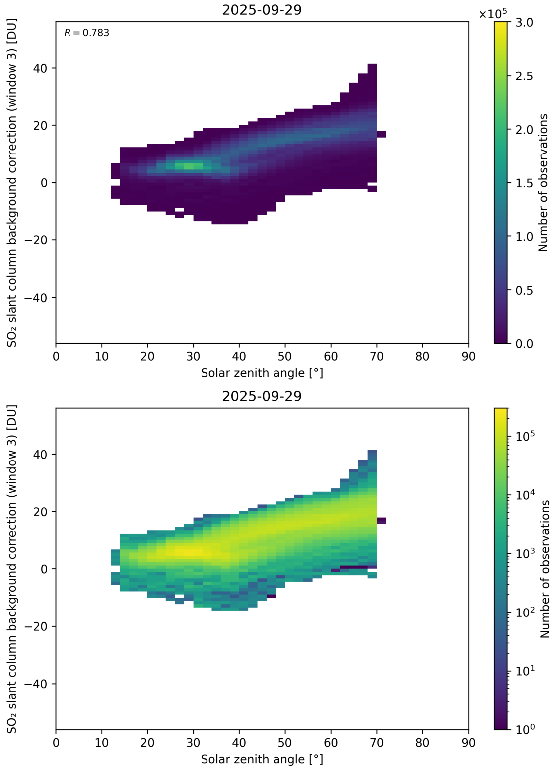
Figure 173: Scatter density plot of “Solar zenith angle” against “SO 2 slant column background correction (window 3)” for 2025-09-28 to 2025-09-30.
