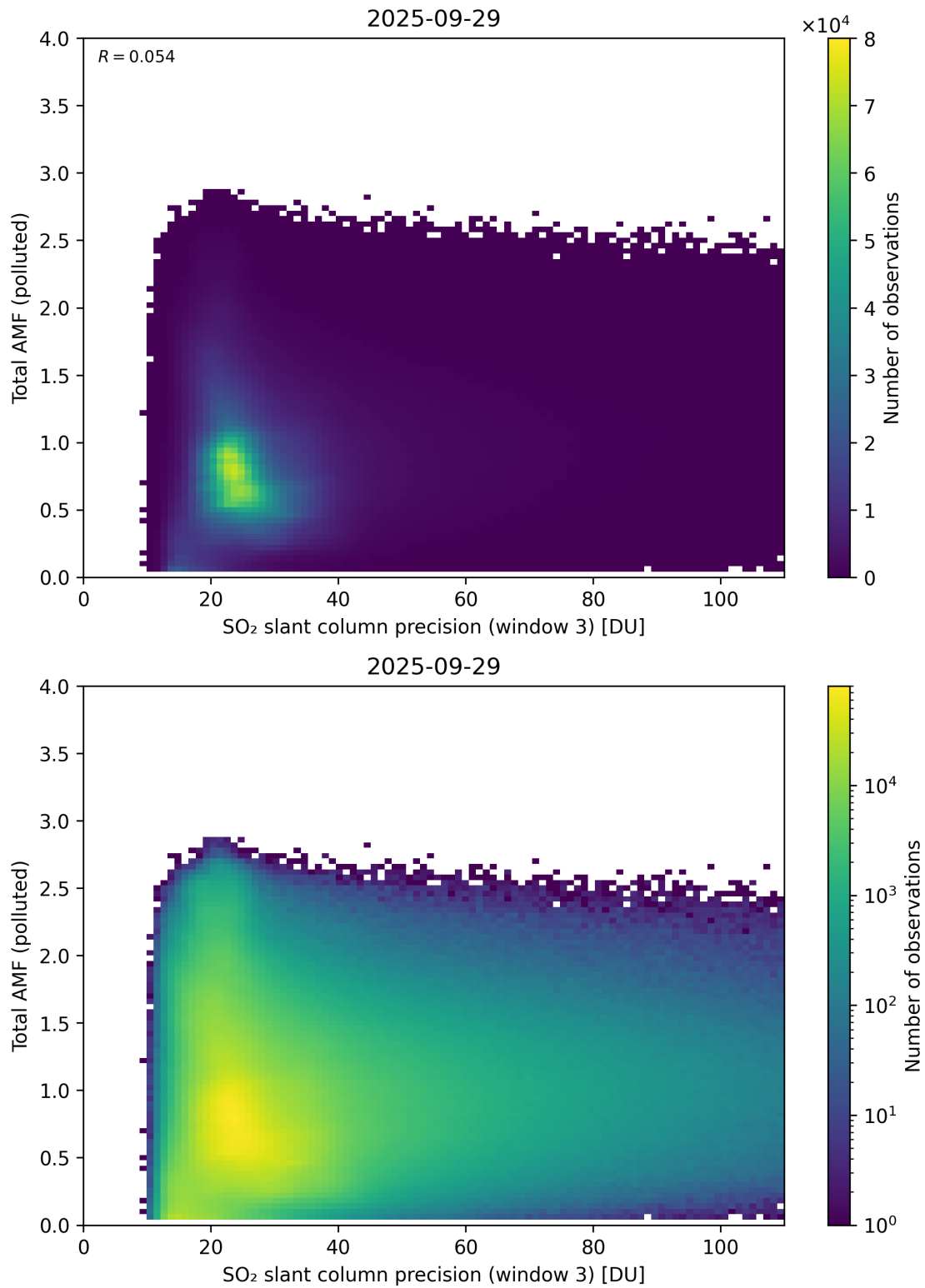
Figure 313: Scatter density plot of “SO 2 slant column precision (window 3)” against “Total AMF (polluted)” for 2025-09-28 to 2025-09-30.
