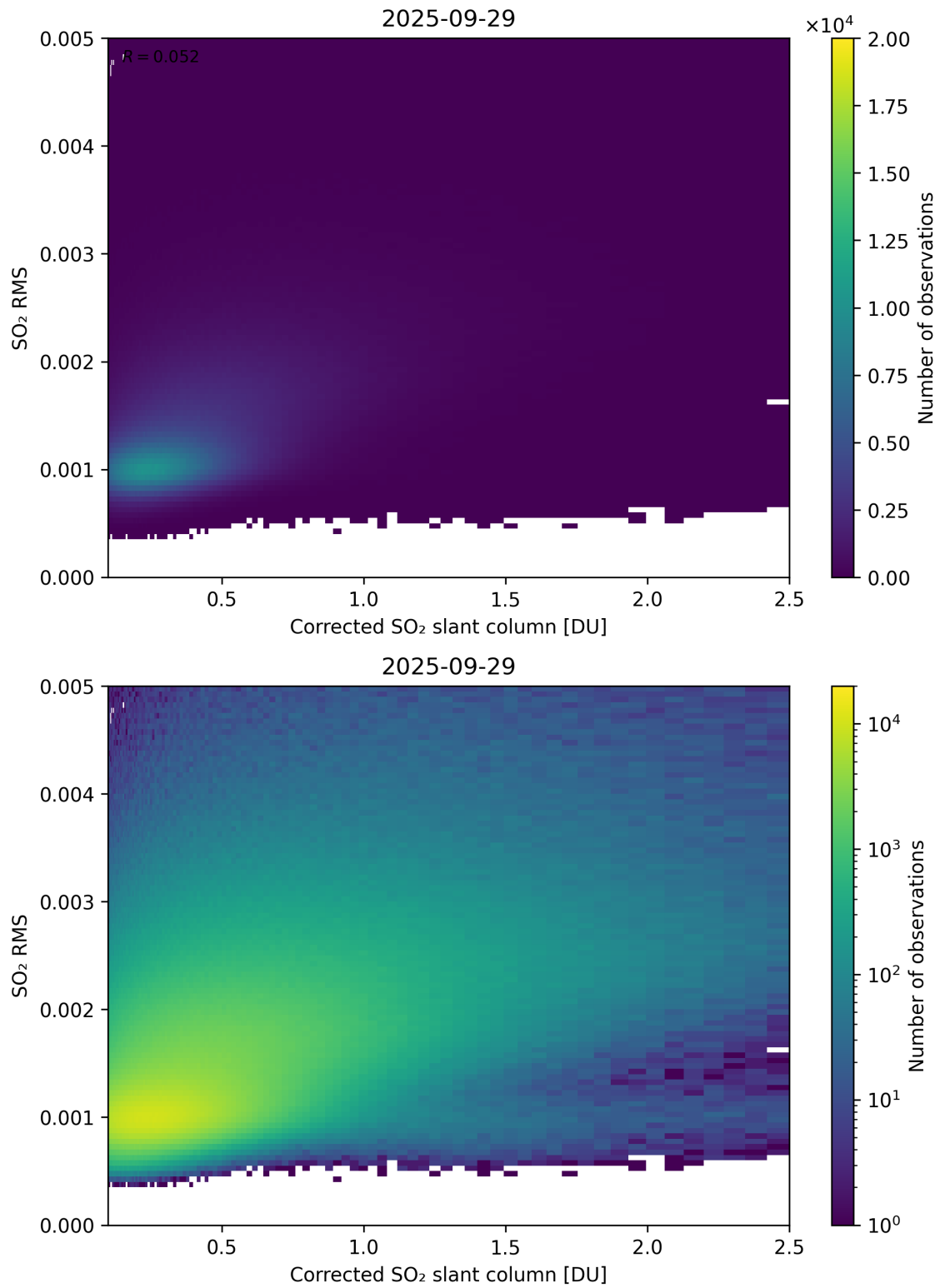
Figure 231: Scatter density plot of “Corrected SO 2 slant column” against “SO 2 RMS” for 2025-09-28 to 2025-09-30.
