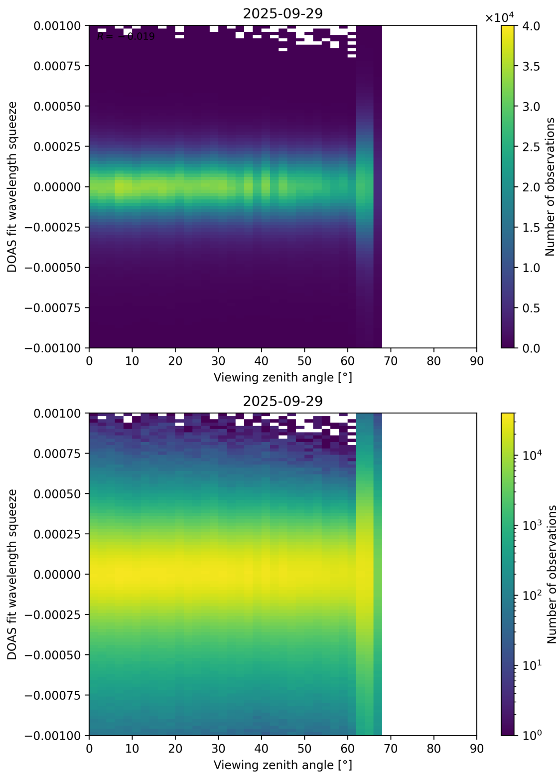
Figure 366: Scatter density plot of “Viewing zenith angle” against “DOAS fit wavelength squeeze” for 2025-09-28 to 2025-09-30.
