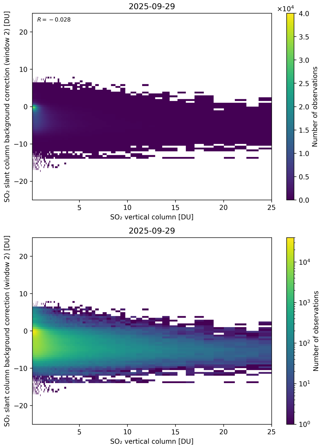
Figure 324: Scatter density plot of “SO 2 vertical column” against “SO 2 slant column background correction (window 2)” for 2025-09-28 to 2025-09-30.
