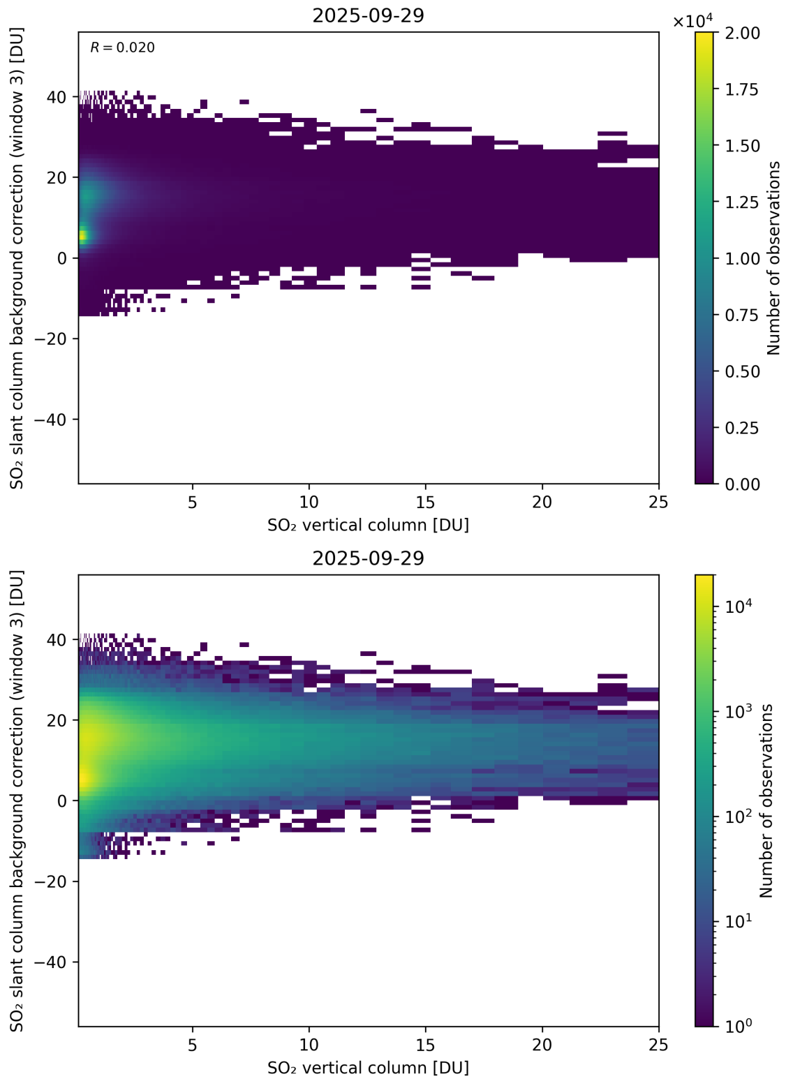
Figure 325: Scatter density plot of “SO 2 vertical column” against “SO 2 slant column background correction (window 3)” for 2025-09-28 to 2025-09-30.
