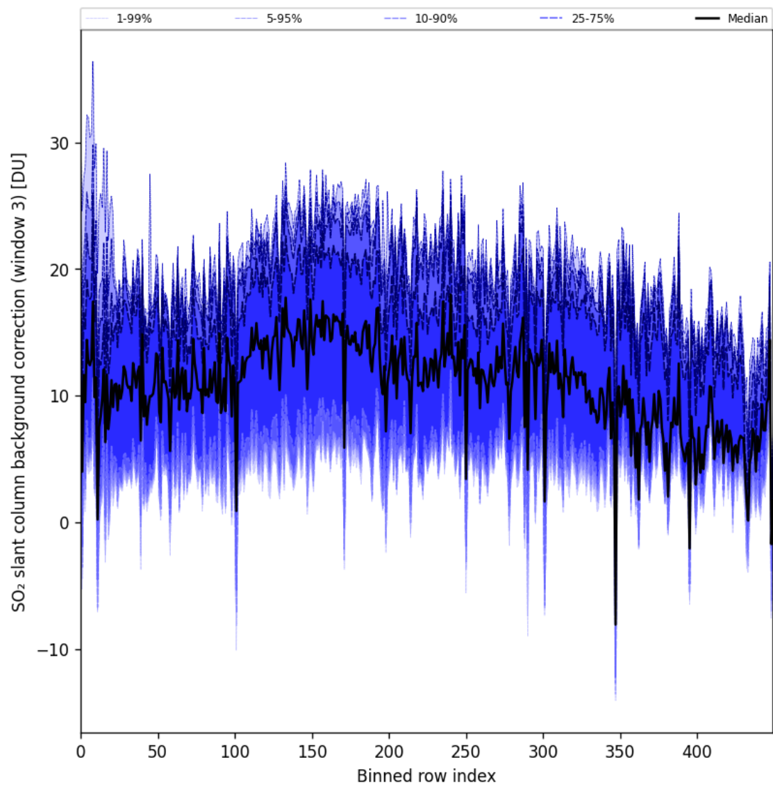
Figure 100: Along track statistics of “SO 2 slant column background correction (window 3)” for 2025-09-28 to 2025-09-30
