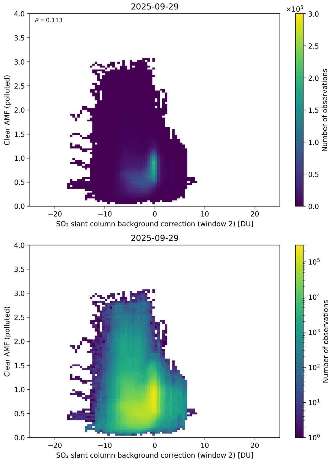
Figure 126: Scatter density plot of “SO 2 slant column background correction (window 2)” against “Clear AMF (polluted)” for 2025-09-28 to 2025-09-30.
