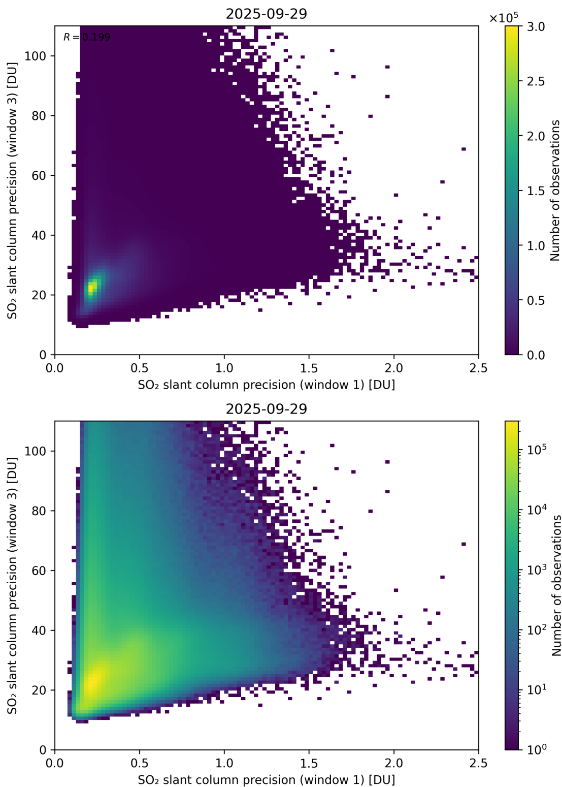
Figure 279: Scatter density plot of “SO 2 slant column precision (window 1)” against “SO 2 slant column precision (window 3)” for 2025-09-28 to 2025-09-30.
