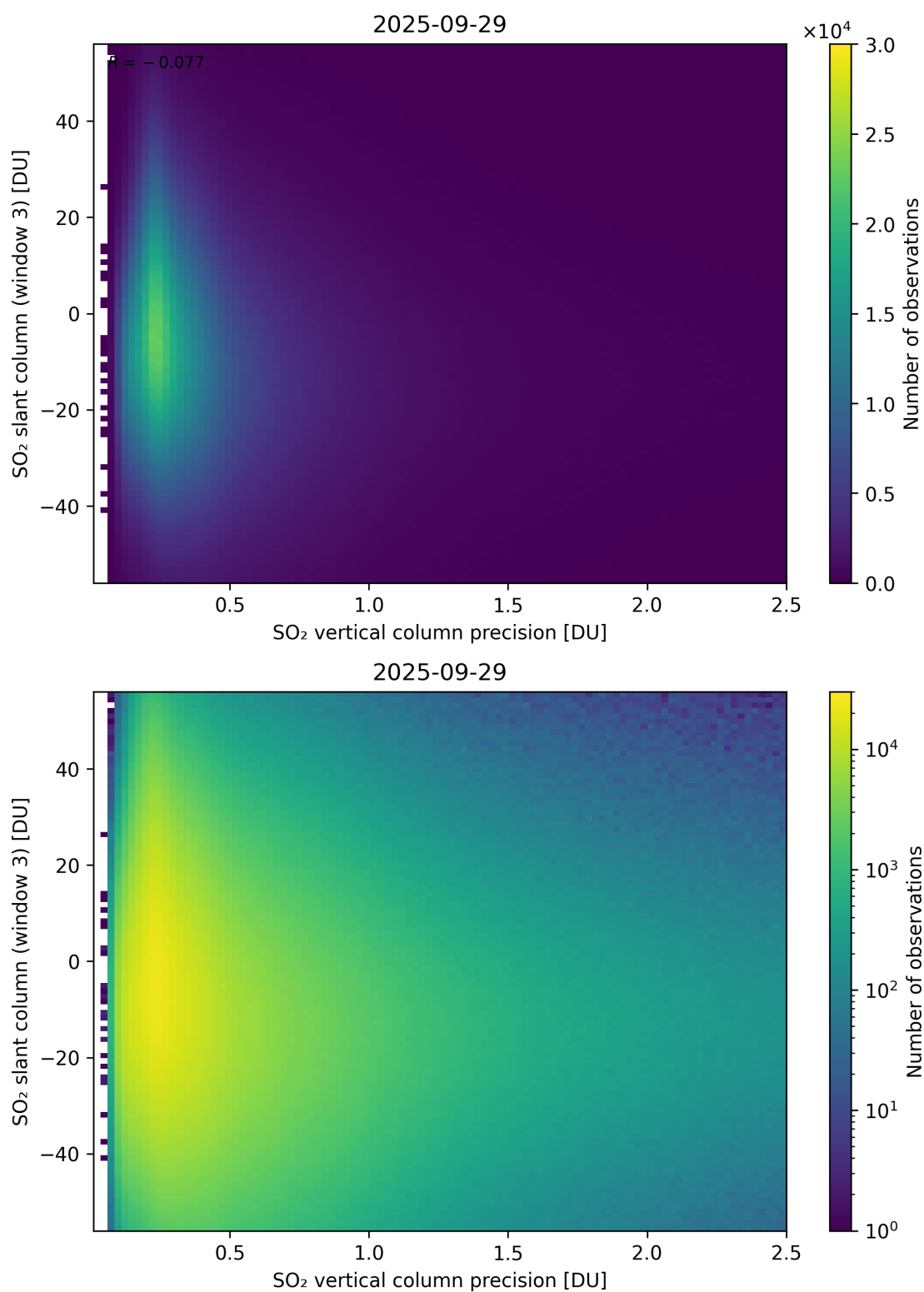
Figure 344: Scatter density plot of “SO 2 vertical column precision” against “SO 2 slant column (window 3)” for 2025-09-28 to 2025-09-30.
