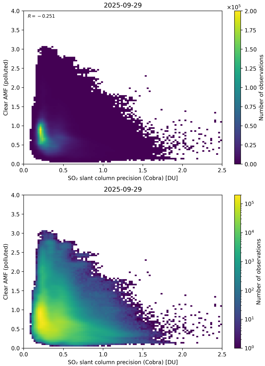
Figure 205: Scatter density plot of “SO 2 slant column precision (Cobra)” against “Clear AMF (polluted)” for 2025-09-28 to 2025-09-30.
