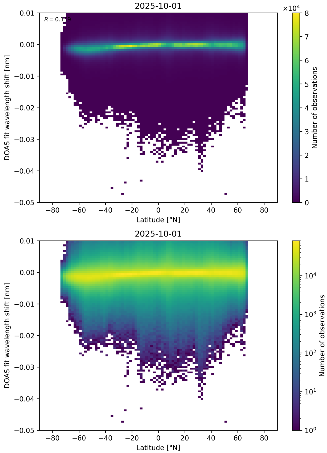
Figure 153: Scatter density plot of “Latitude” against “DOAS fit wavelength shift” for 2025-10-01 to 2025-10-02.
