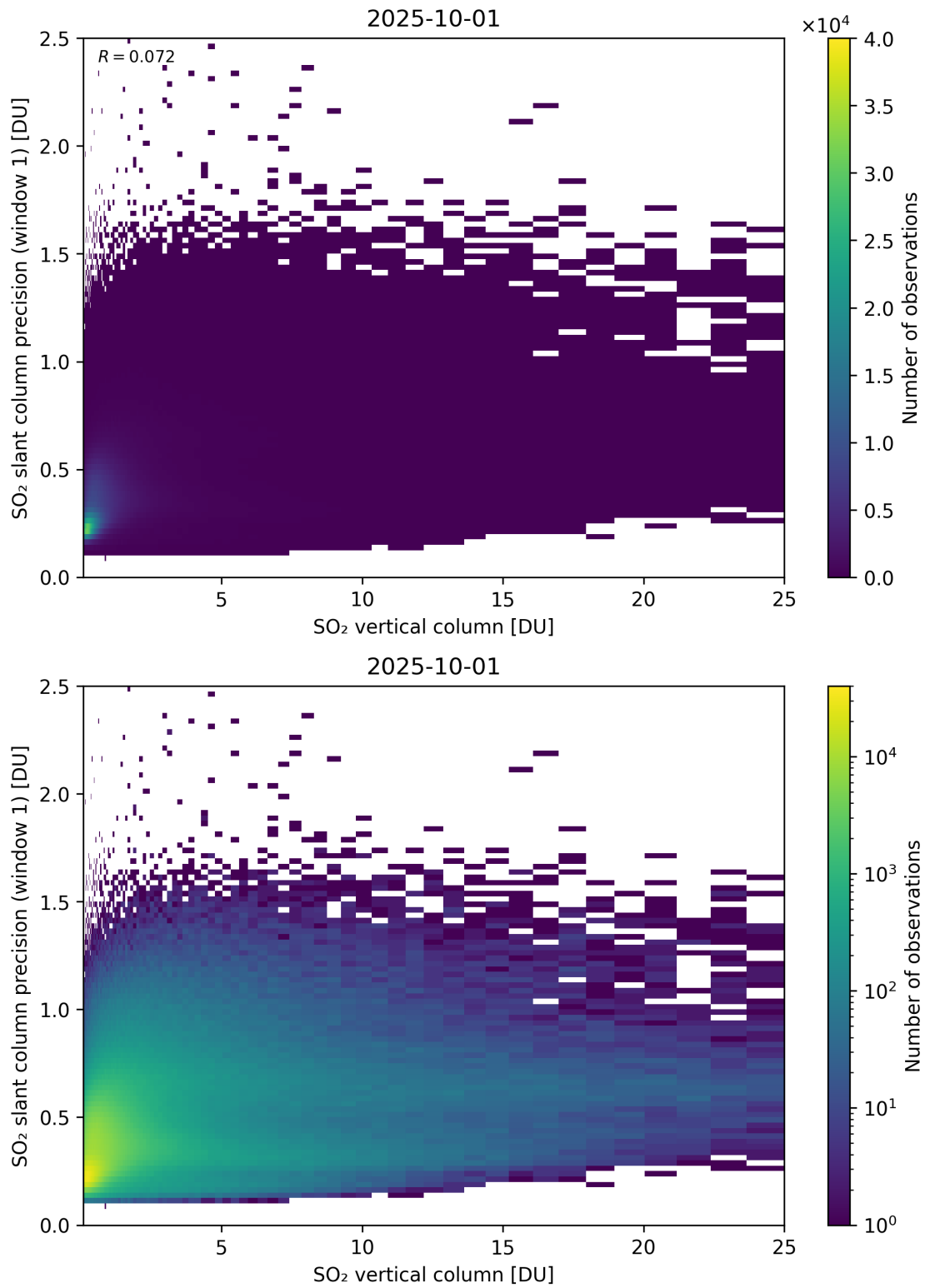
Figure 355: Scatter density plot of “SO 2 vertical column” against “SO 2 slant column precision (window 1)” for 2025-10-01 to 2025-10-02.
