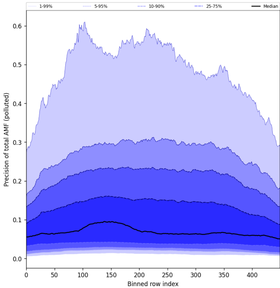
Figure 106: Along track statistics of “Precision of total AMF (polluted)” for 2025-10-01 to 2025-10-02
