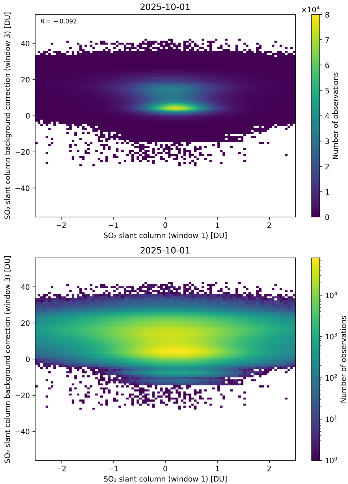
Figure 264: Scatter density plot of “SO 2 slant column (window 1)” against “SO 2 slant column background correction (window 3)” for 2025-10-01 to 2025-10-02.
