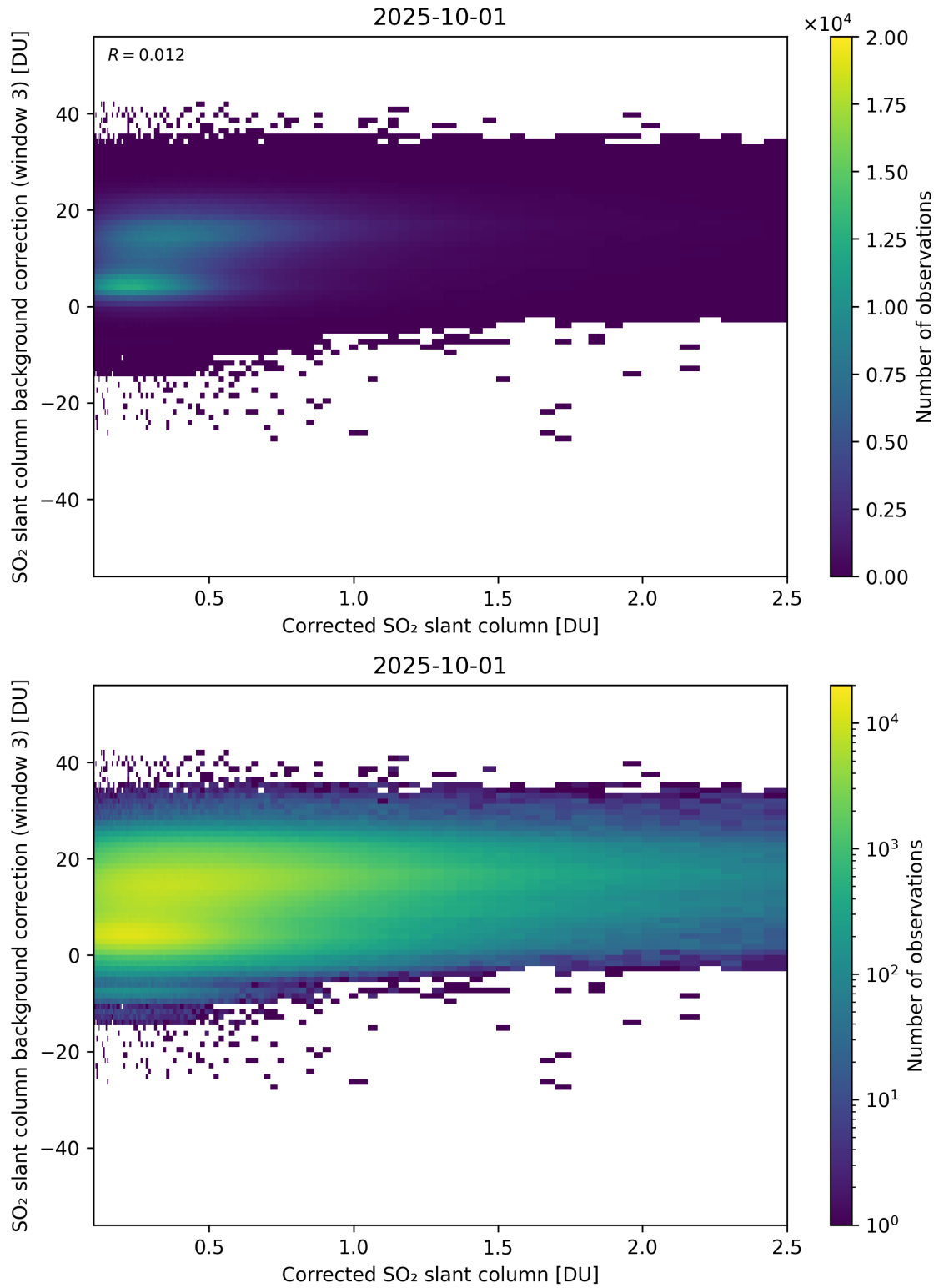
Figure 228: Scatter density plot of “Corrected SO 2 slant column” against “SO 2 slant column background correction (window 3)” for 2025-10-01 to 2025-10-02.
