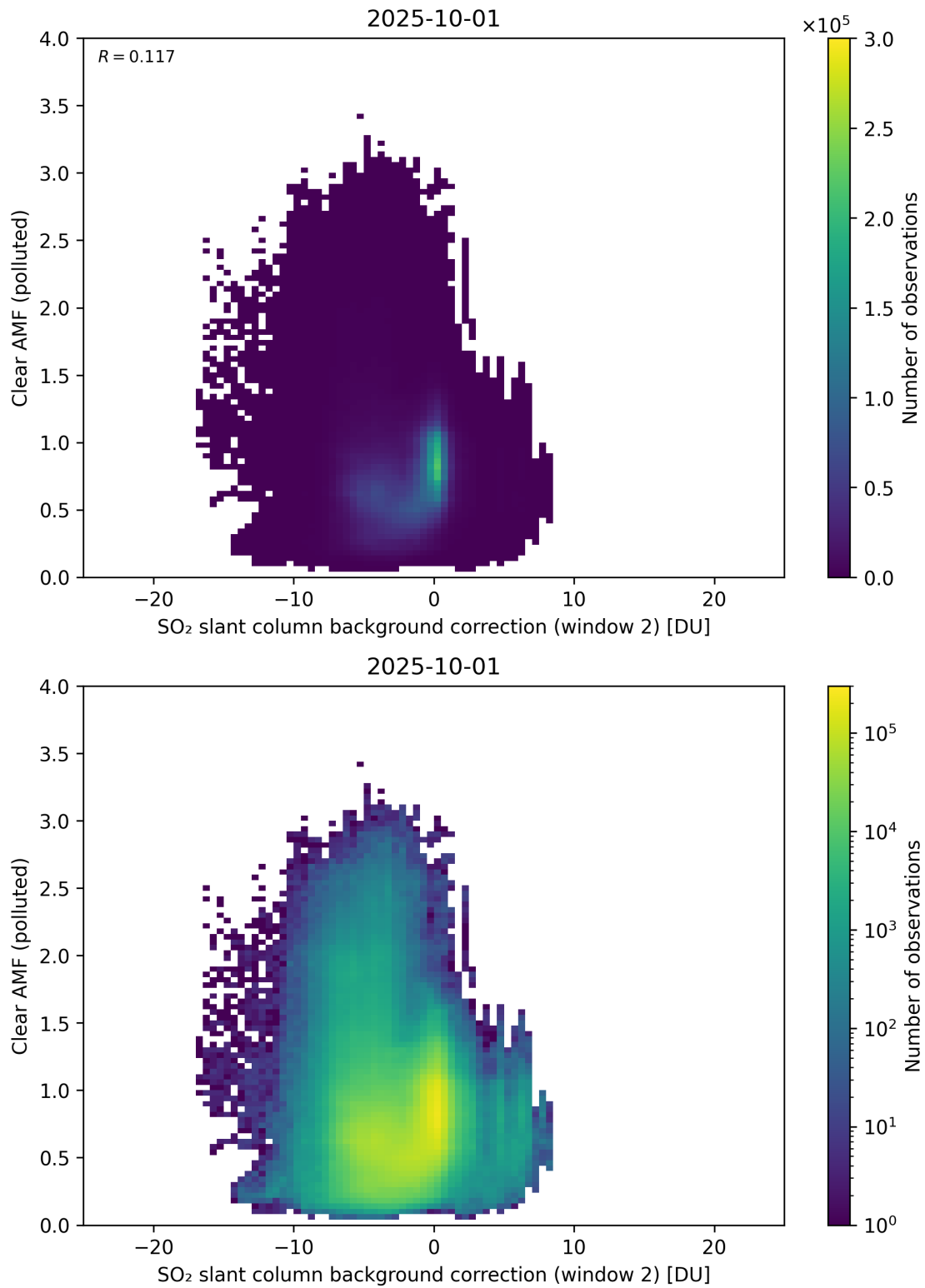
Figure 126: Scatter density plot of “SO 2 slant column background correction (window 2)” against “Clear AMF (polluted)” for 2025-10-01 to 2025-10-02.
