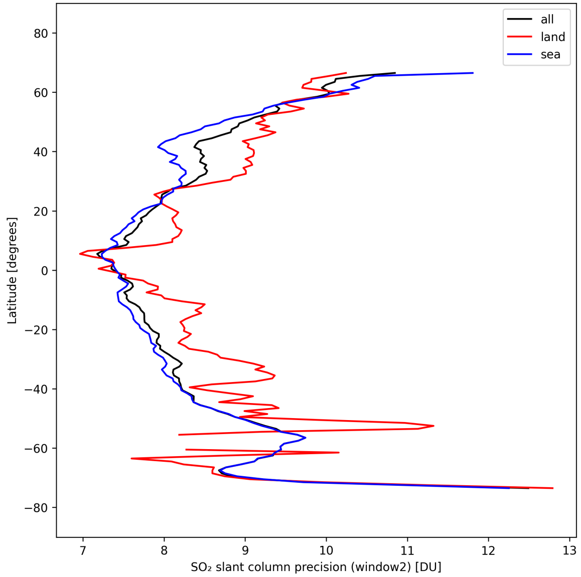
Figure 42: Zonal average of “SO 2 slant column precision (window2)” for 2025-10-01 to 2025-10-02.
