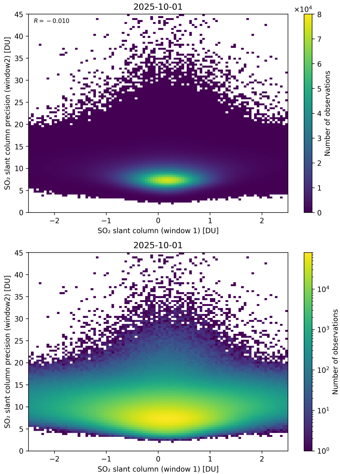
Figure 286: Scatter density plot of “SO 2 slant column (window 1)” against “SO 2 slant column precision (window2)” for 2025-10-01 to 2025-10-02.
