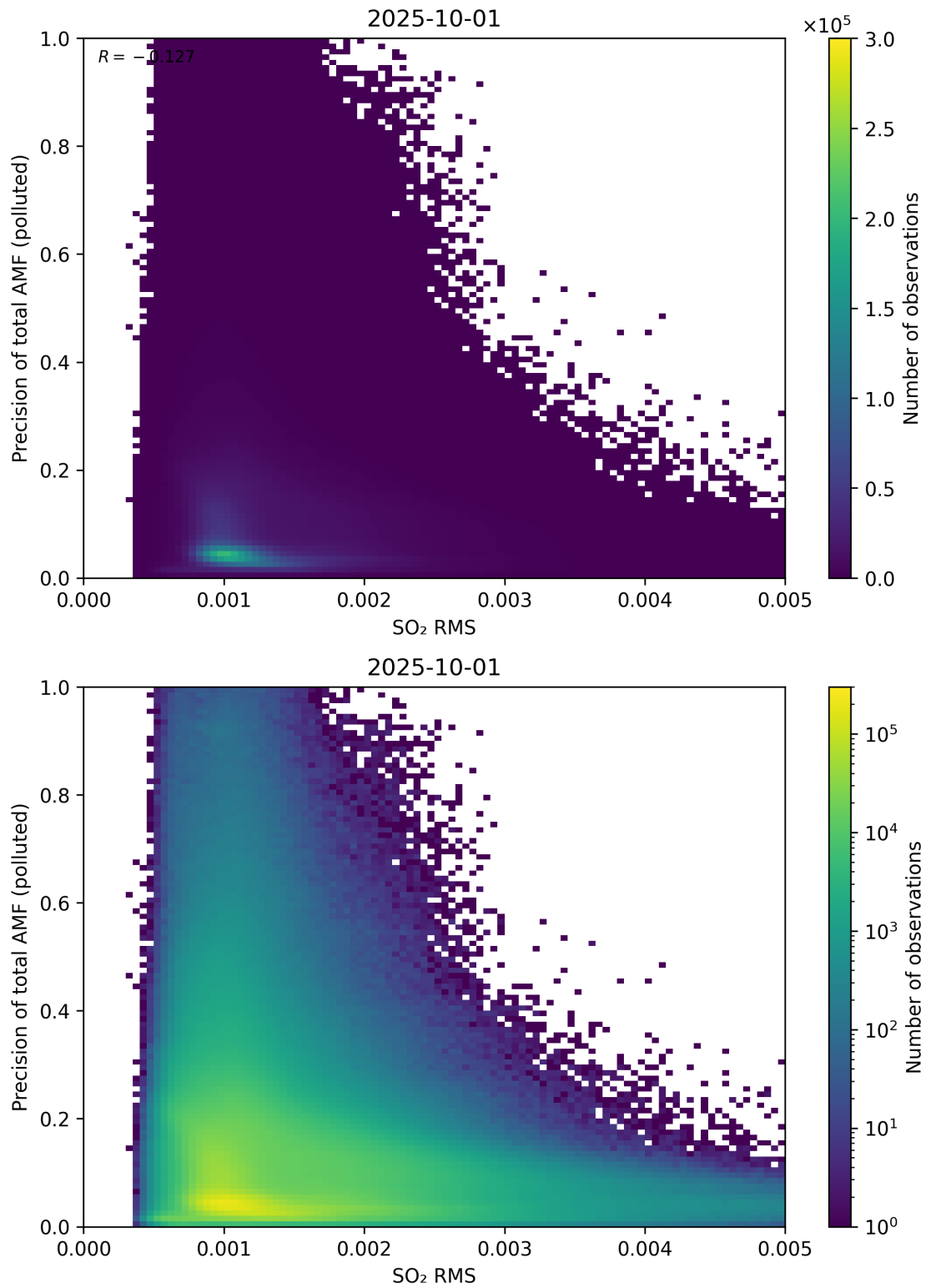
Figure 149: Scatter density plot of “SO 2 RMS” against “Precision of total AMF (polluted)” for 2025-10-01 to 2025-10-02.
