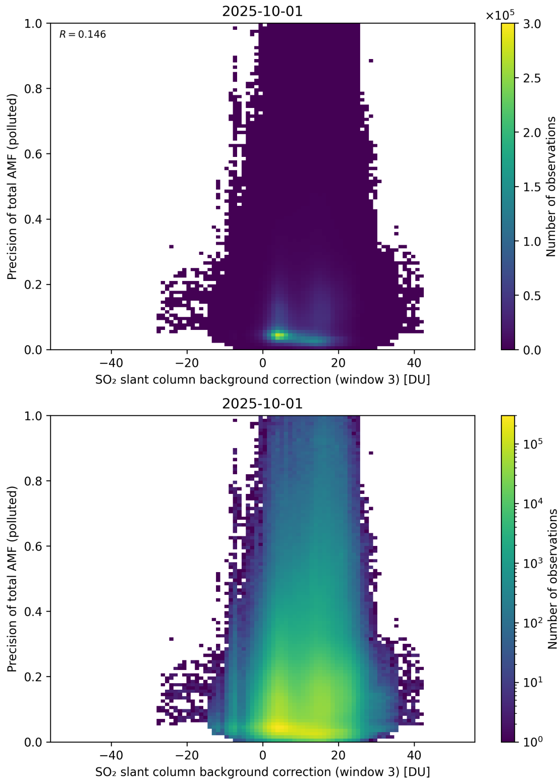
Figure 137: Scatter density plot of “SO 2 slant column background correction (window 3)” against “Precision of total AMF (polluted)” for 2025-10-01 to 2025-10-02.
