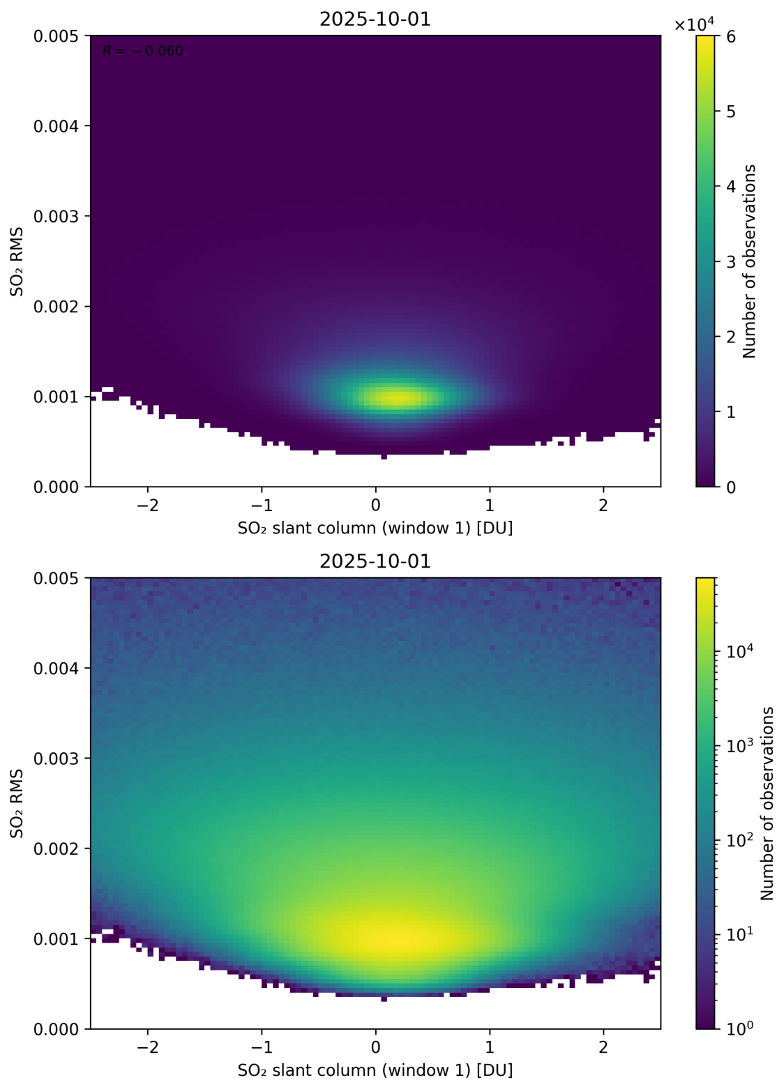
Figure 267: Scatter density plot of “SO 2 slant column (window 1)” against “SO 2 RMS” for 2025-10-01 to 2025-10-02.
