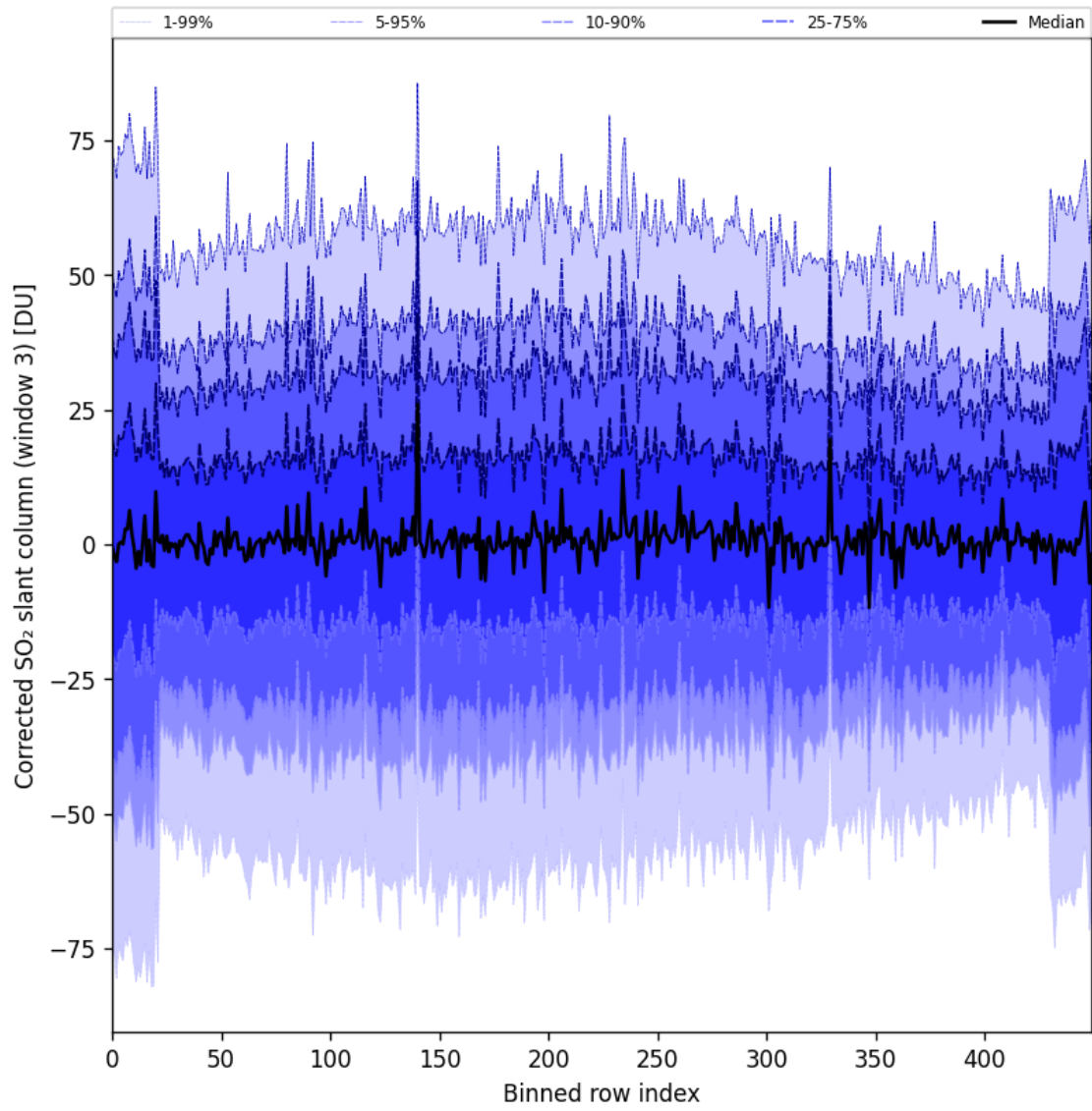
Figure 99: Along track statistics of “Corrected SO 2 slant column (window 3)” for 2025-10-01 to 2025-10-02
