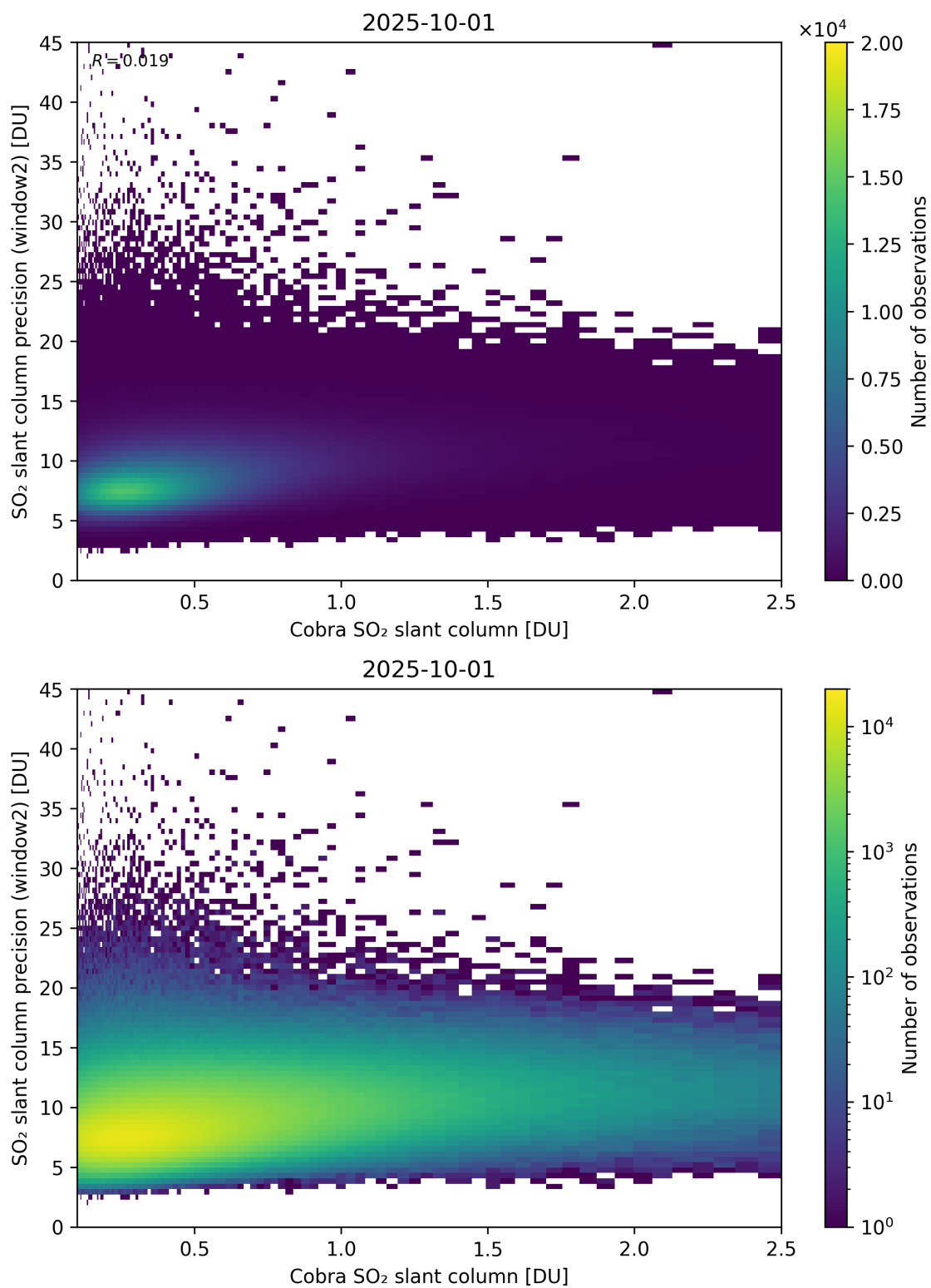
Figure 221: Scatter density plot of “Cobra SO 2 slant column” against “SO 2 slant column precision (window2)” for 2025-10-01 to 2025-10-02.
