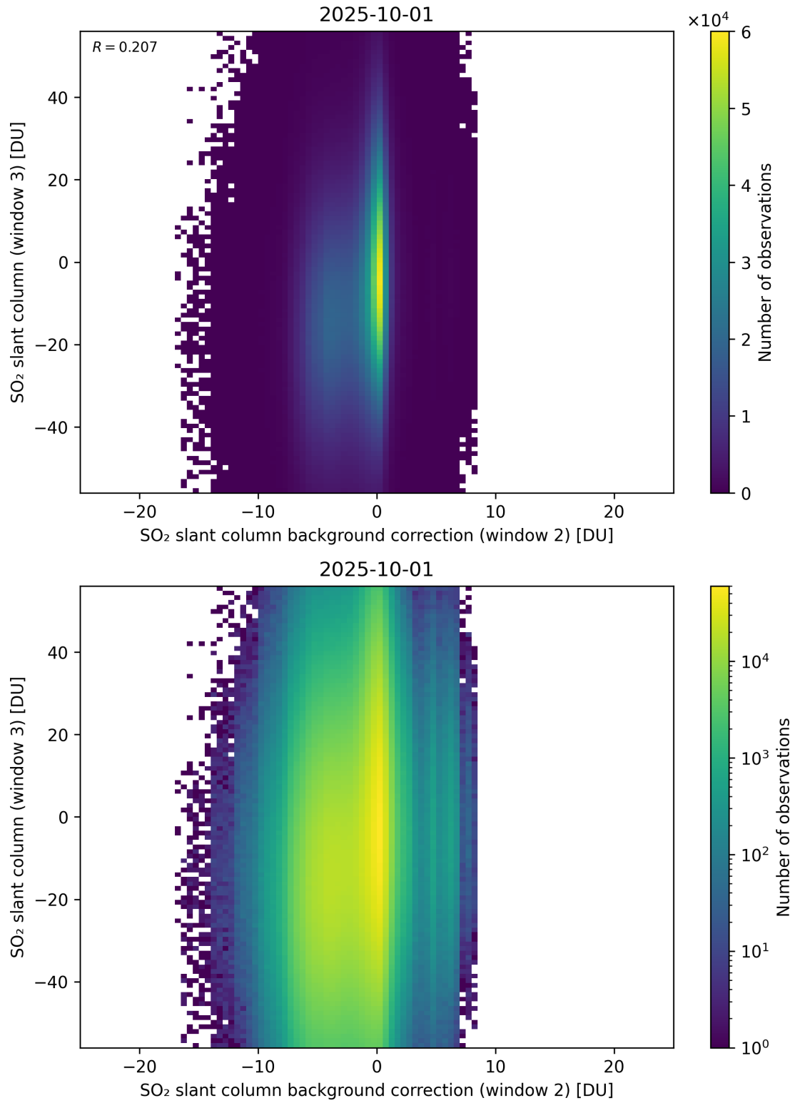
Figure 128: Scatter density plot of “SO 2 slant column background correction (window 2)” against “SO 2 slant column (window 3)” for 2025-10-01 to 2025-10-02.
