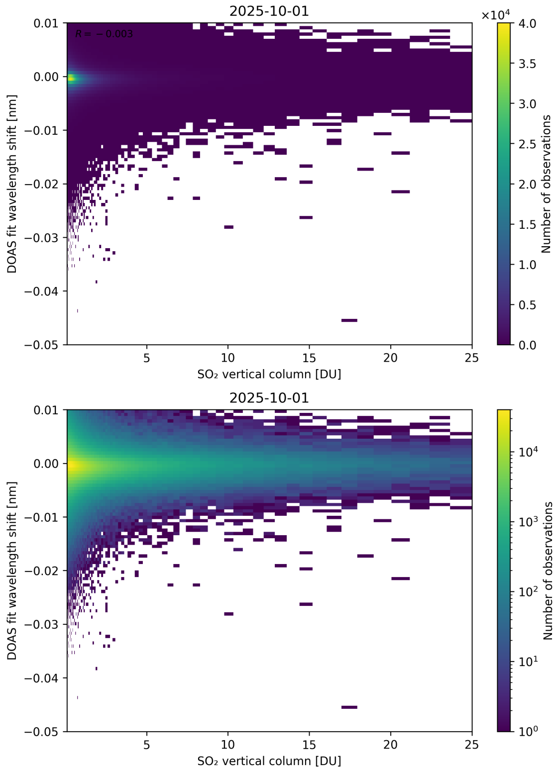
Figure 326: Scatter density plot of “SO 2 vertical column” against “DOAS fit wavelength shift” for 2025-10-01 to 2025-10-02.
