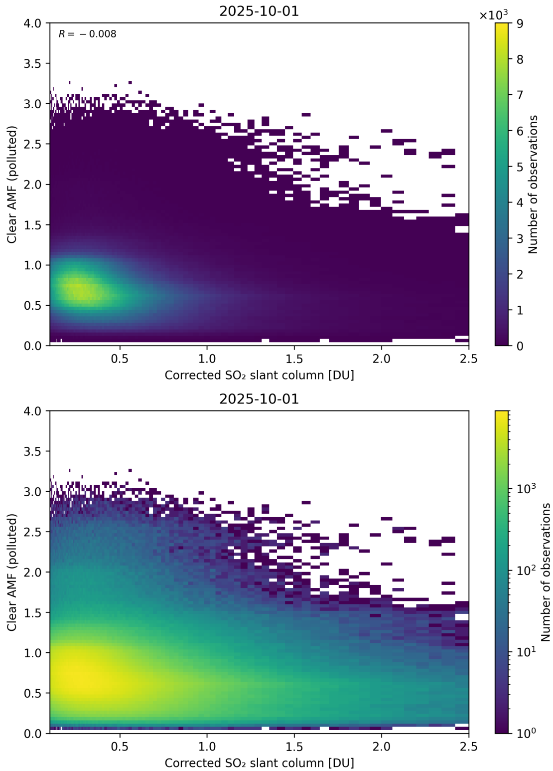
Figure 232: Scatter density plot of “Corrected SO 2 slant column” against “Clear AMF (polluted)” for 2025-10-01 to 2025-10-02.
