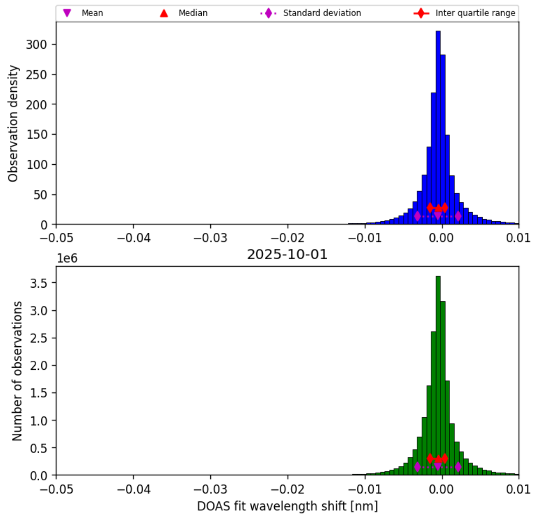
Figure 76: Histogram of “DOAS fit wavelength shift” for 2025-10-01 to 2025-10-02
