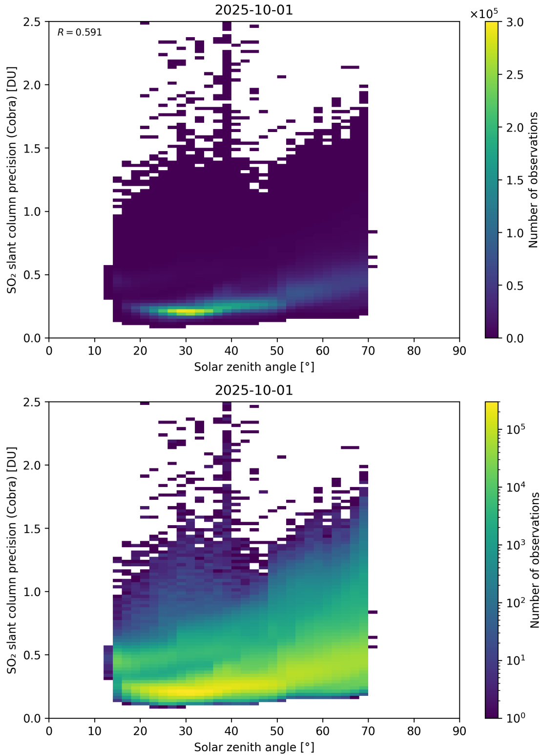
Figure 180: Scatter density plot of “Solar zenith angle” against “SO 2 slant column precision (Cobra)” for 2025-10-01 to 2025-10-02.
