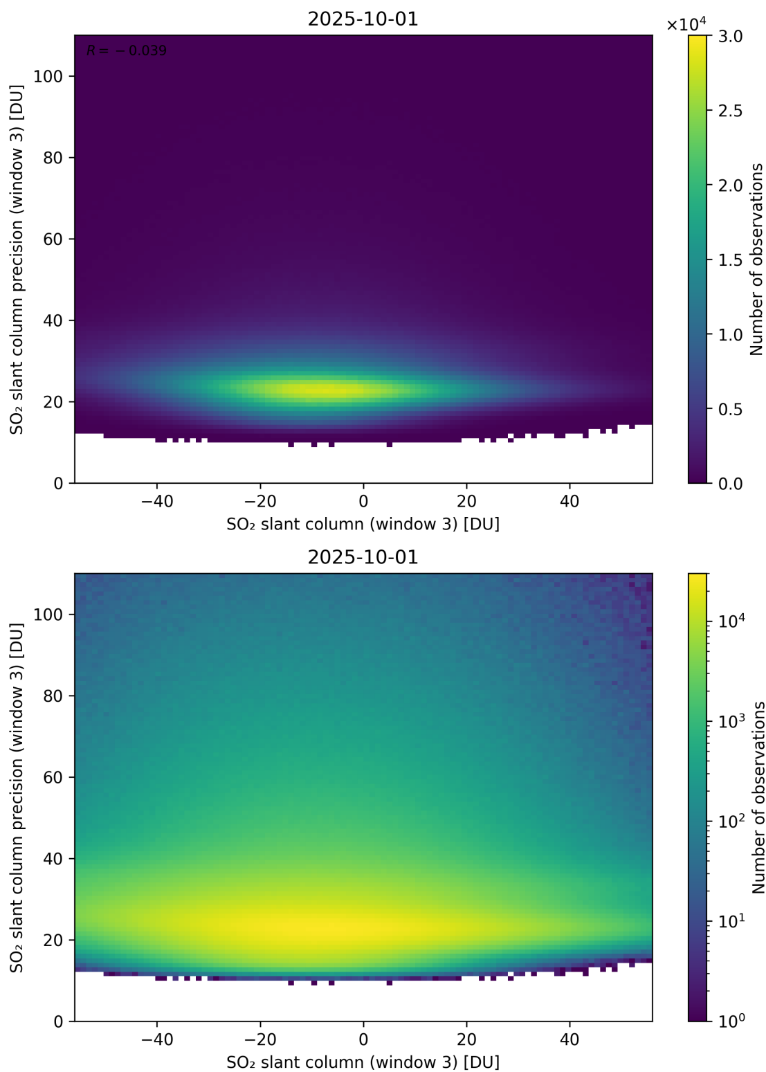
Figure 317: Scatter density plot of “SO 2 slant column (window 3)” against “SO 2 slant column precision (window 3)” for 2025-10-01 to 2025-10-02.
