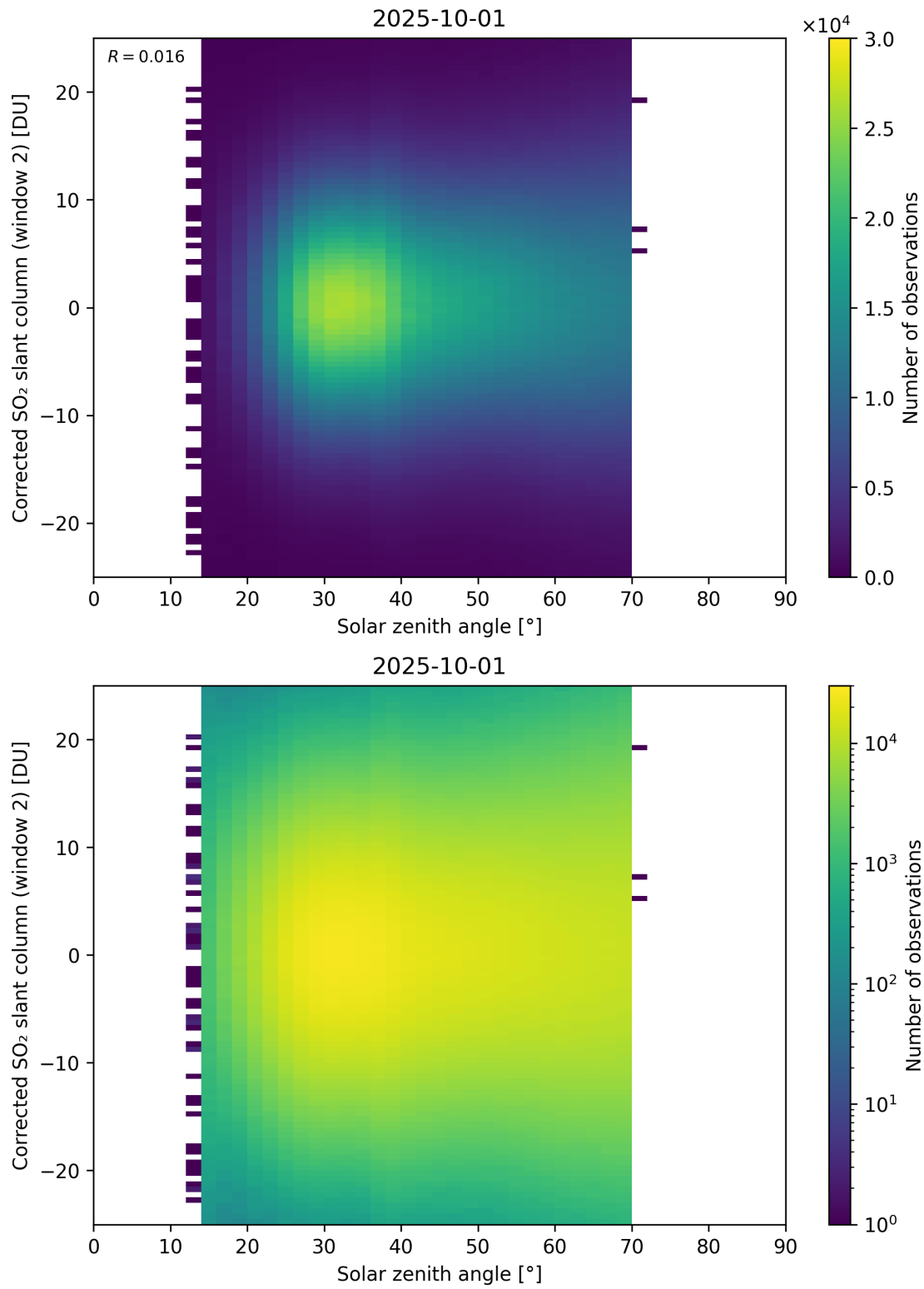
Figure 182: Scatter density plot of “Solar zenith angle” against “Corrected SO 2 slant column (window 2)” for 2025-10-01 to 2025-10-02.
