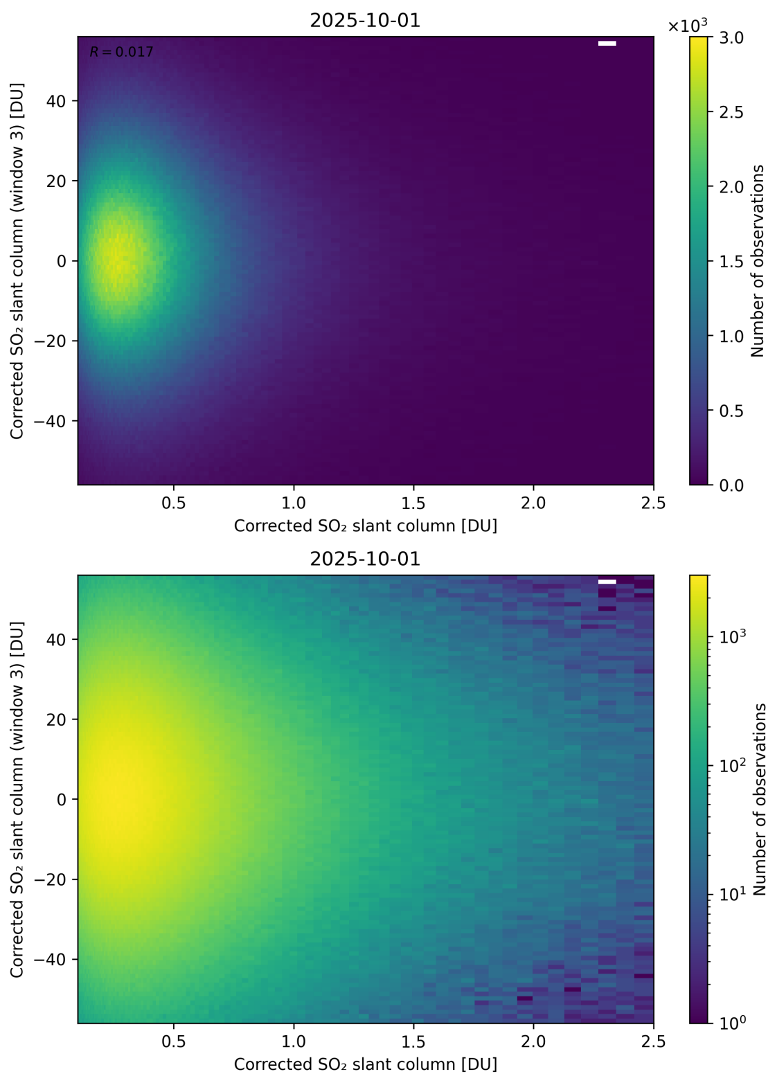
Figure 236: Scatter density plot of “Corrected SO 2 slant column” against “Corrected SO 2 slant column (window 3)” for 2025-10-01 to 2025-10-02.
