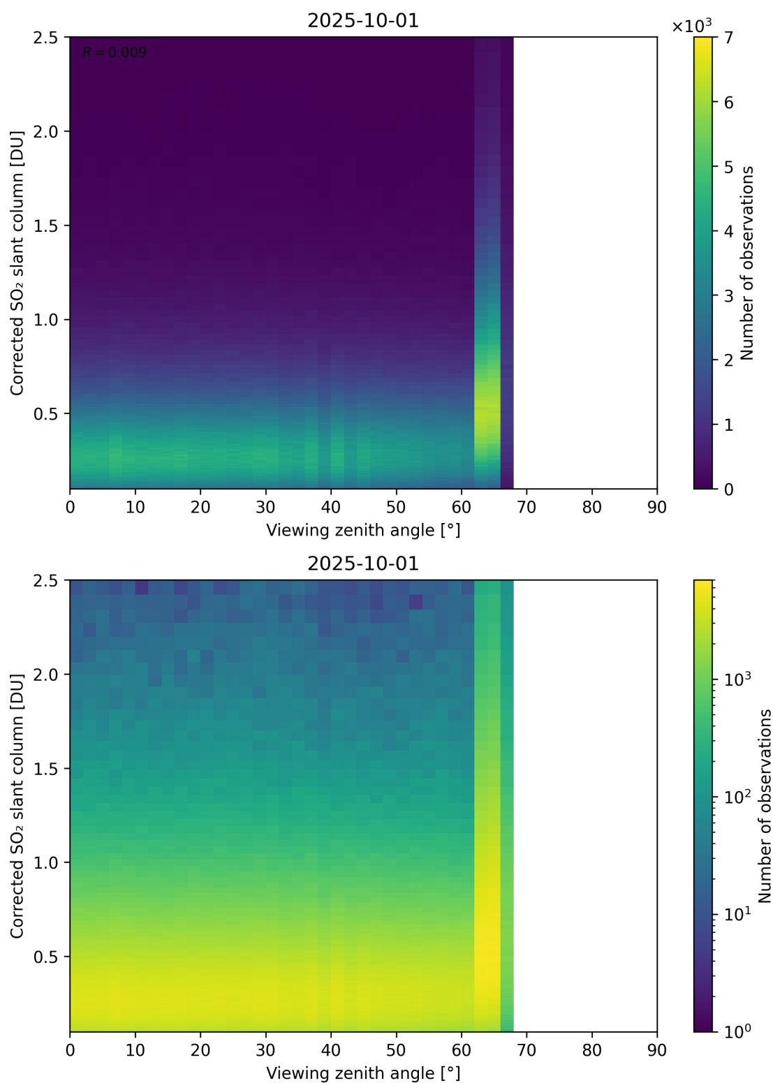
Figure 373: Scatter density plot of “Viewing zenith angle” against “Corrected SO 2 slant column” for 2025-10-01 to 2025-10-02.
