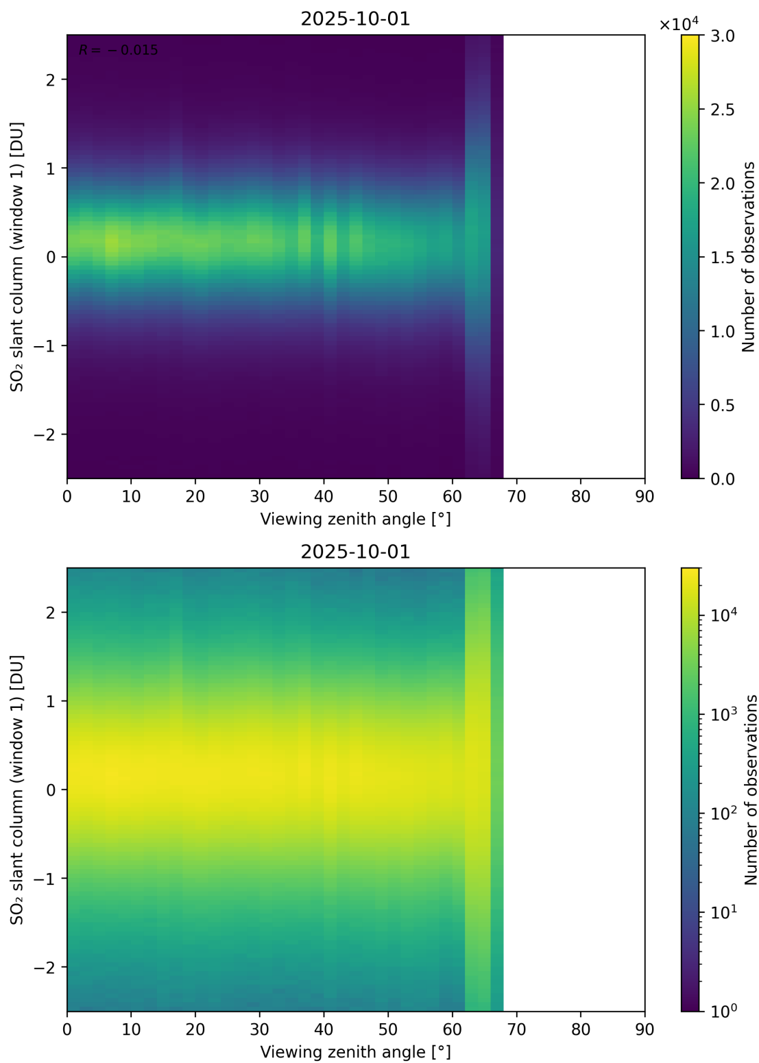
Figure 376: Scatter density plot of “Viewing zenith angle” against “SO 2 slant column (window 1)” for 2025-10-01 to 2025-10-02.
