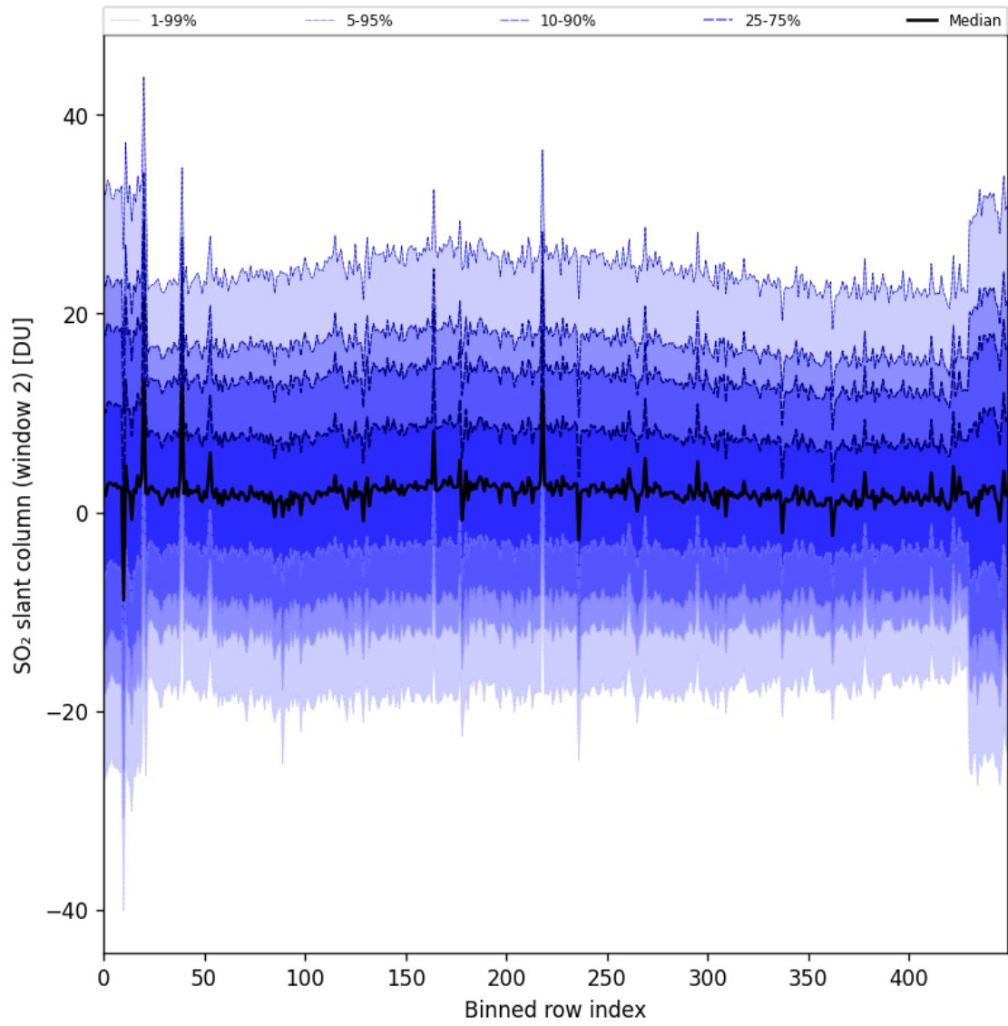
Figure 93: Along track statistics of “SO 2 slant column (window 2)” for 2025-10-01 to 2025-10-02
