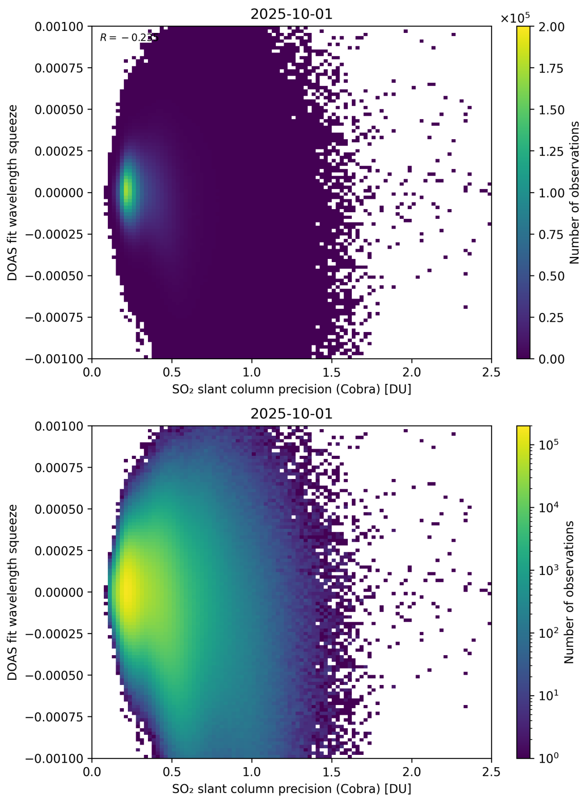
Figure 203: Scatter density plot of “SO 2 slant column precision (Cobra)” against “DOAS fit wavelength squeeze” for 2025-10-01 to 2025-10-02.
