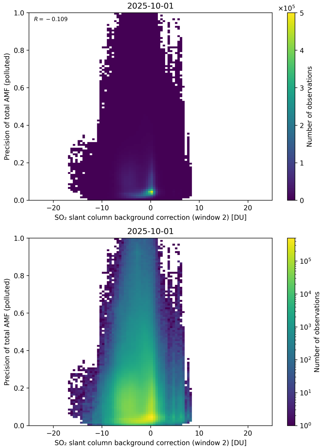
Figure 131: Scatter density plot of “SO 2 slant column background correction (window 2)” against “Precision of total AMF (polluted)” for 2025-10-01 to 2025-10-02.
