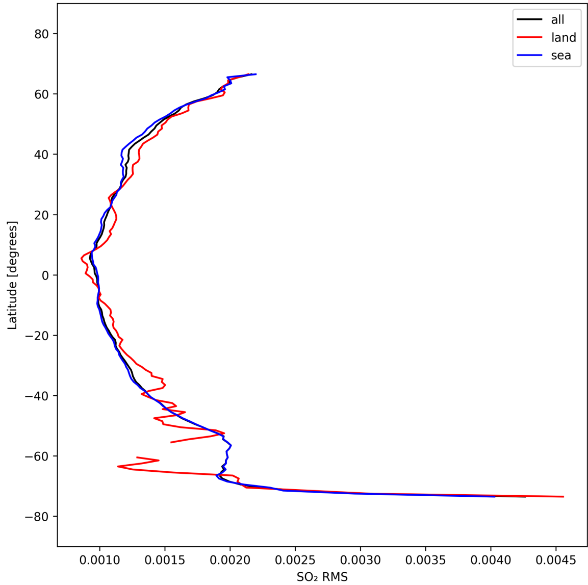
Figure 52: Zonal average of “SO 2 RMS” for 2025-10-01 to 2025-10-02.
