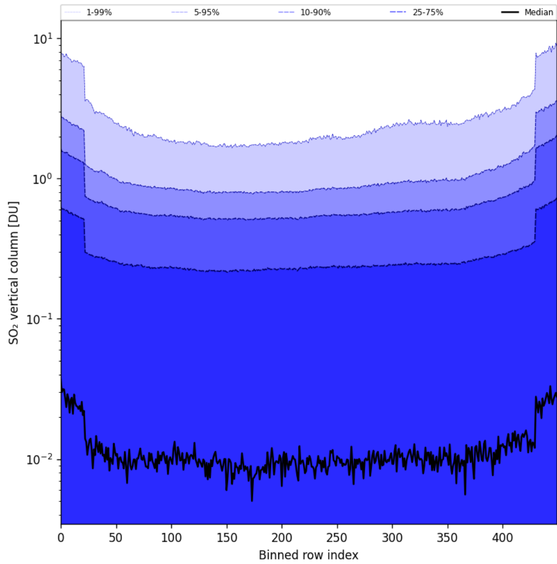
Figure 84: Along track statistics of “SO 2 vertical column” for 2025-10-01 to 2025-10-02
