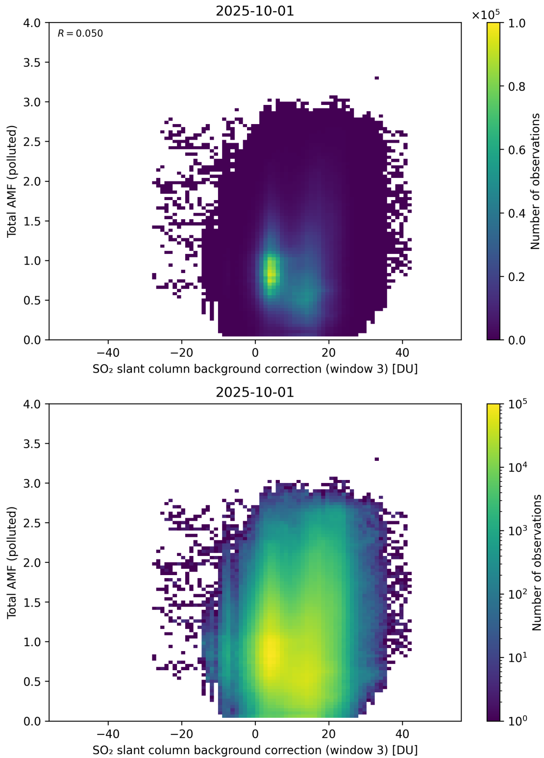
Figure 136: Scatter density plot of “SO 2 slant column background correction (window 3)” against “Total AMF (polluted)” for 2025-10-01 to 2025-10-02.
