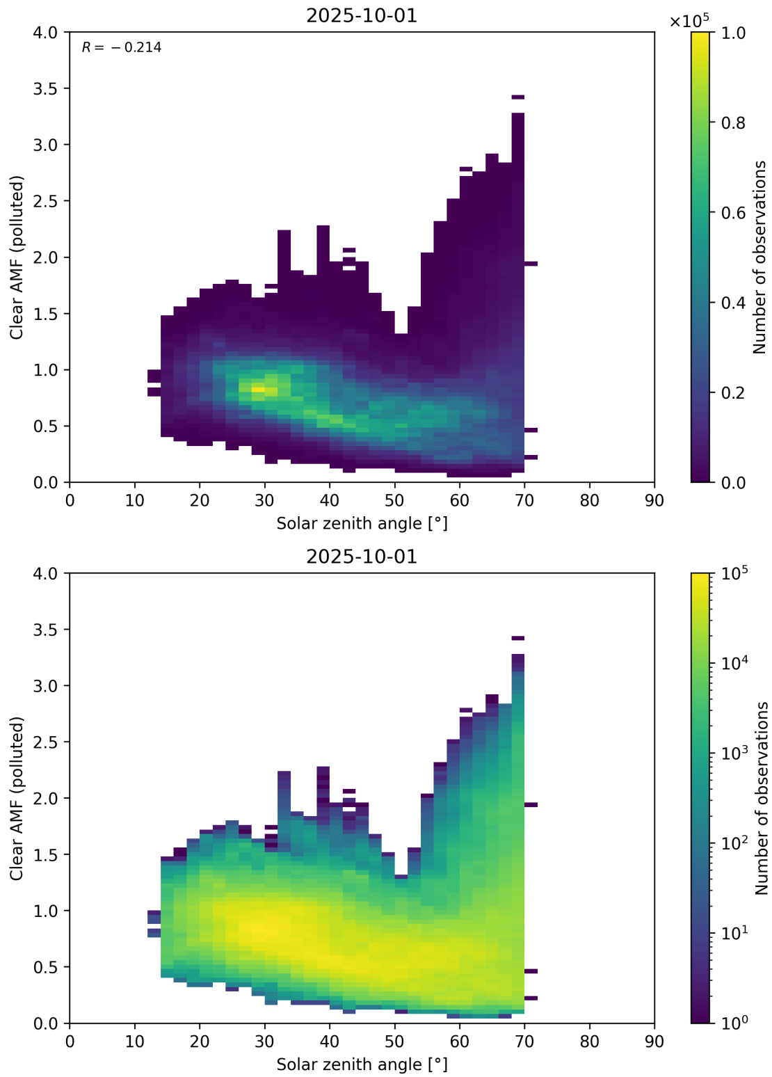
Figure 178: Scatter density plot of “Solar zenith angle” against “Clear AMF (polluted)” for 2025-10-01 to 2025-10-02.
