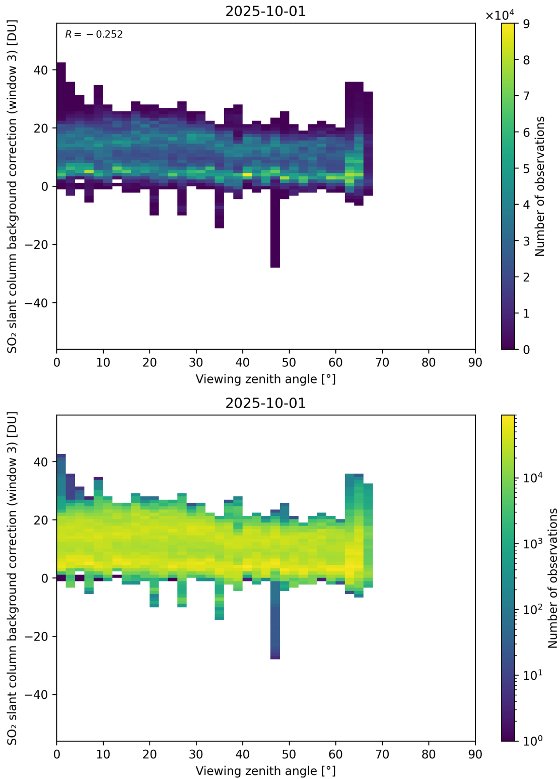
Figure 364: Scatter density plot of “Viewing zenith angle” against “SO 2 slant column background correction (window 3)” for 2025-10-01 to 2025-10-02.
