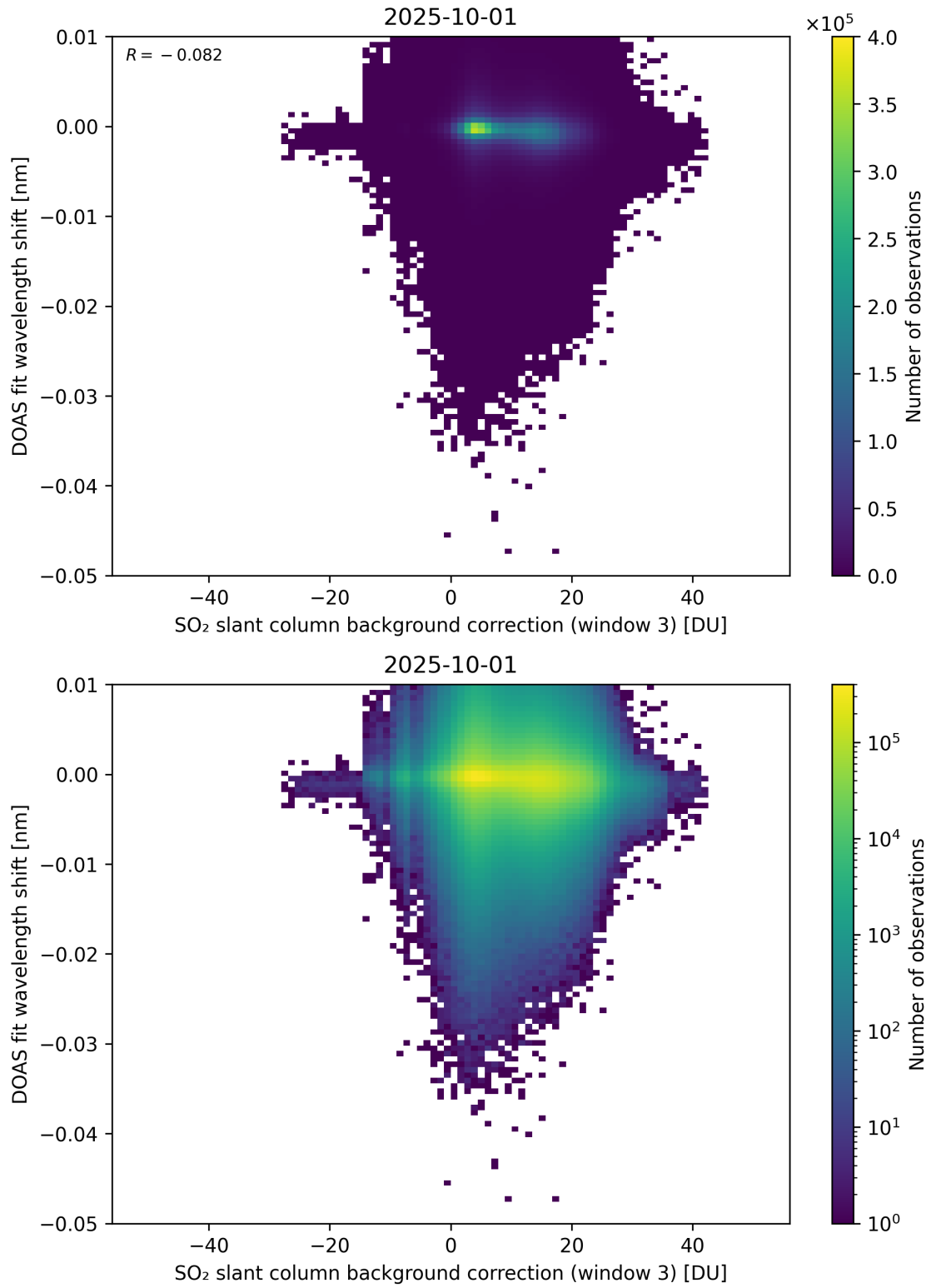
Figure 132: Scatter density plot of “SO 2 slant column background correction (window 3)” against “DOAS fit wavelength shift” for 2025-10-01 to 2025-10-02.
