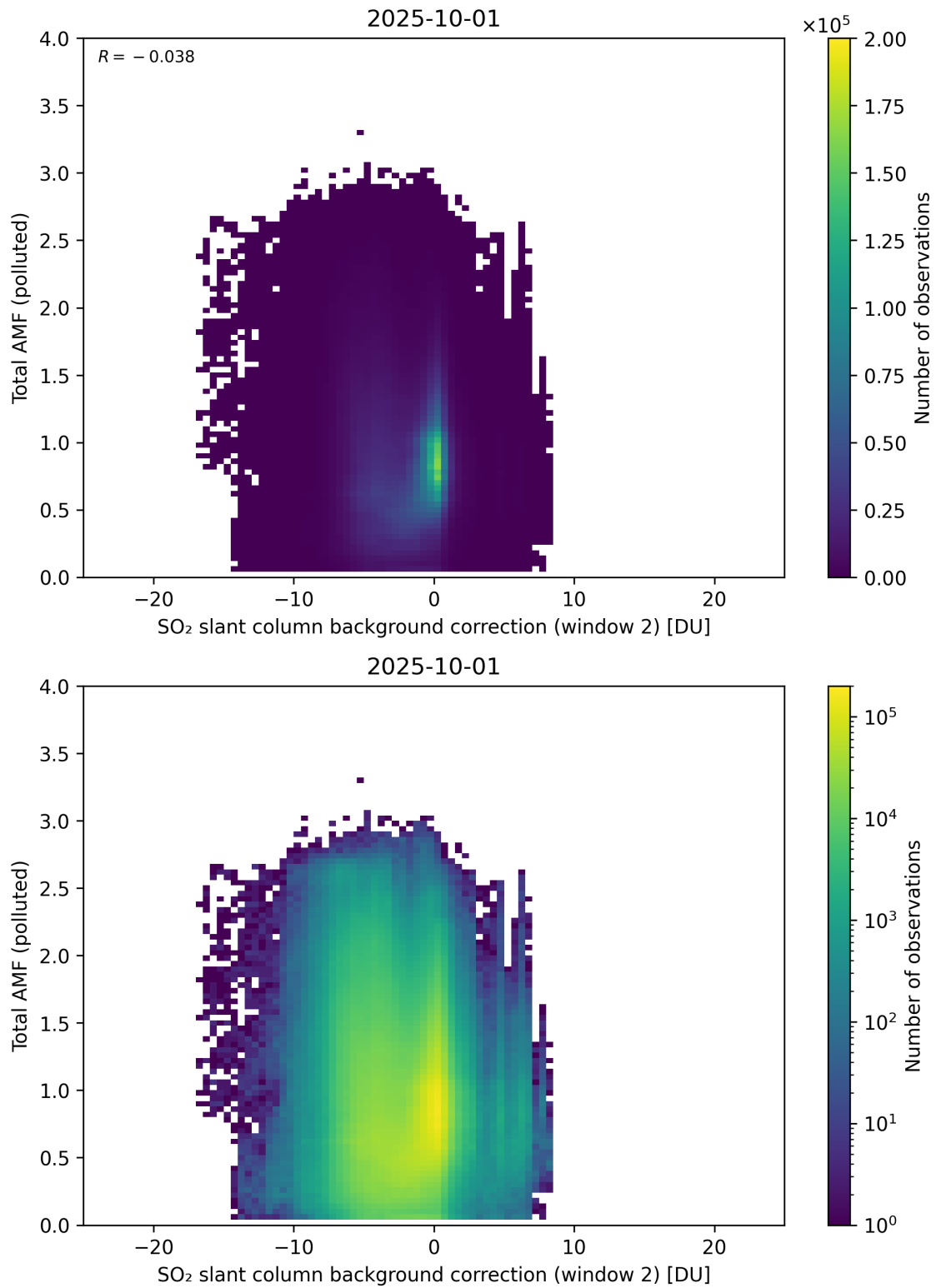
Figure 130: Scatter density plot of “SO 2 slant column background correction (window 2)” against “Total AMF (polluted)” for 2025-10-01 to 2025-10-02.
