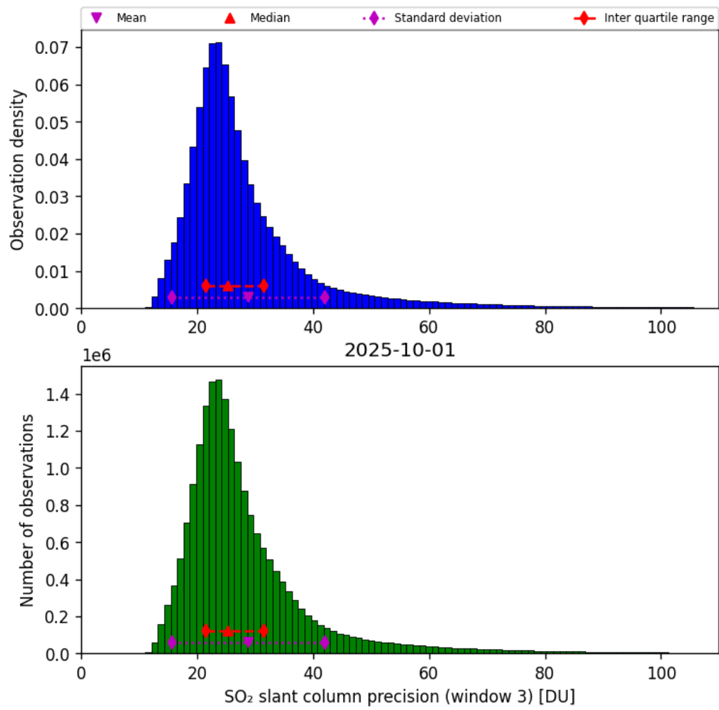
Figure 72: Histogram of “SO 2 slant column precision (window 3)” for 2025-10-01 to 2025-10-02
