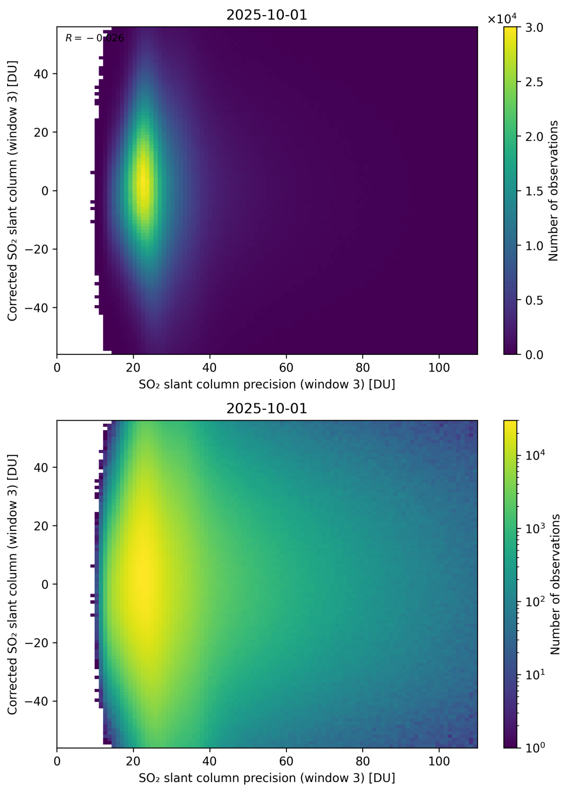
Figure 312: Scatter density plot of “SO 2 slant column precision (window 3)” against “Corrected SO 2 slant column (window 3)” for 2025-10-01 to 2025-10-02.
