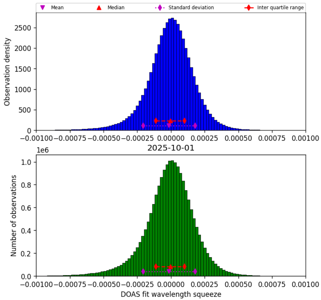
Figure 77: Histogram of “DOAS fit wavelength squeeze” for 2025-10-01 to 2025-10-02
