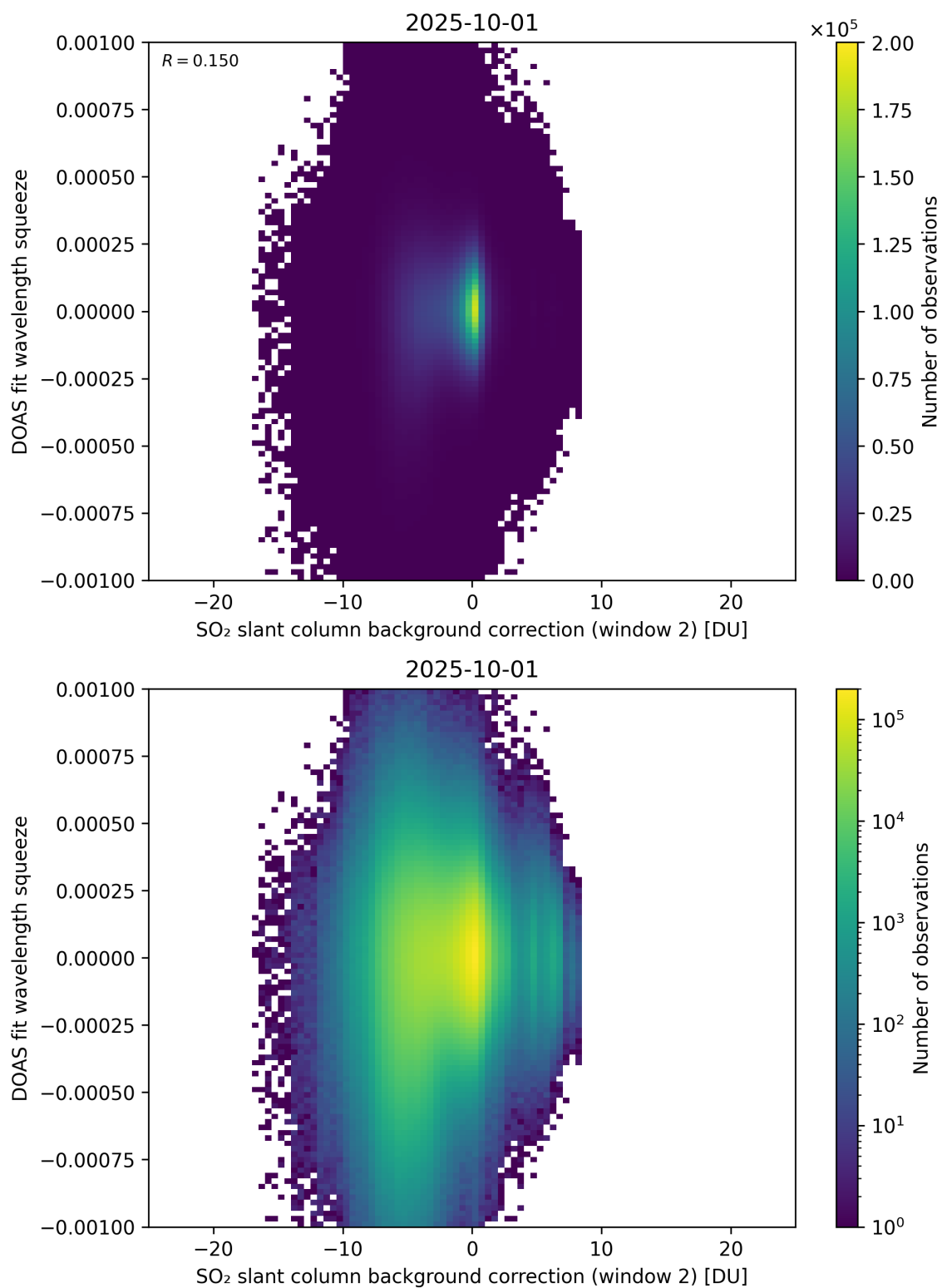
Figure 124: Scatter density plot of “SO 2 slant column background correction (window 2)” against “DOAS fit wavelength squeeze” for 2025-10-01 to 2025-10-02.
