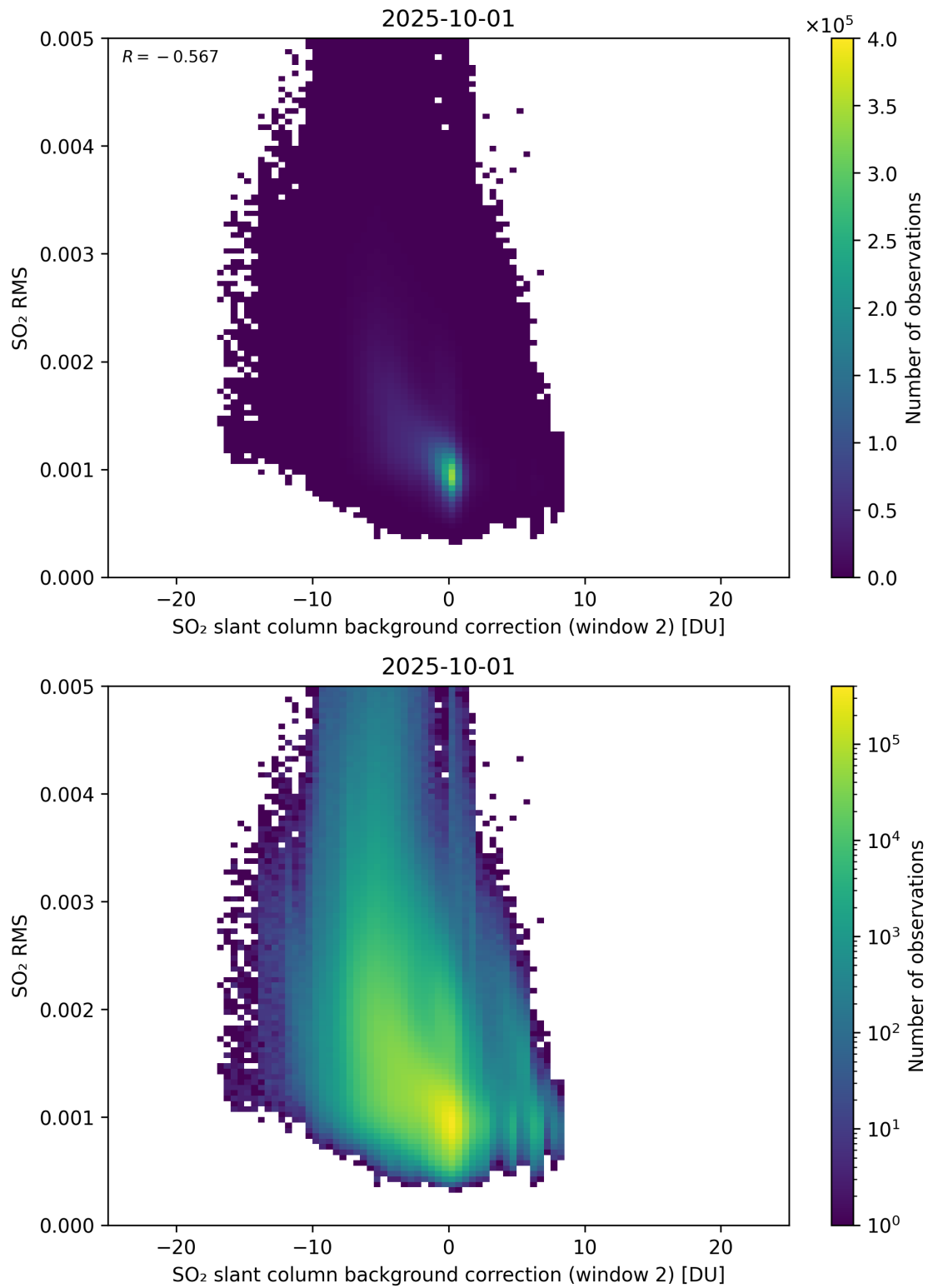
Figure 125: Scatter density plot of “SO 2 slant column background correction (window 2)” against “SO 2 RMS” for 2025-10-01 to 2025-10-02.
