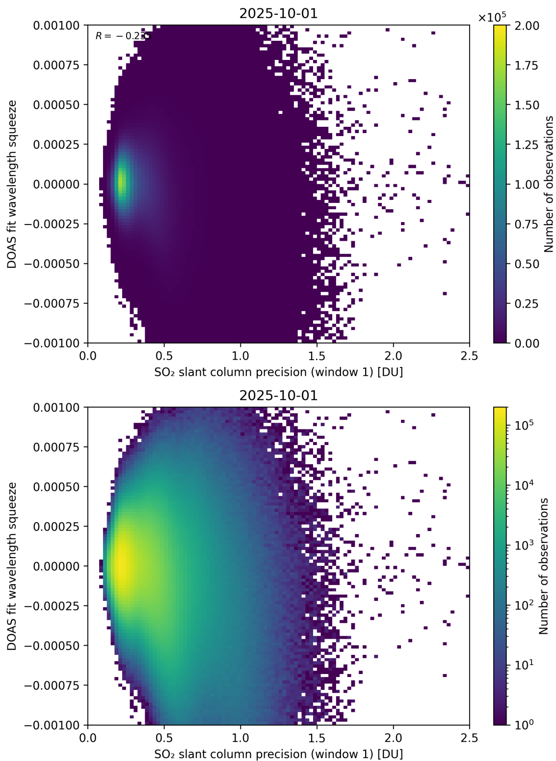
Figure 272: Scatter density plot of “SO 2 slant column precision (window 1)” against “DOAS fit wavelength squeeze” for 2025-10-01 to 2025-10-02.
