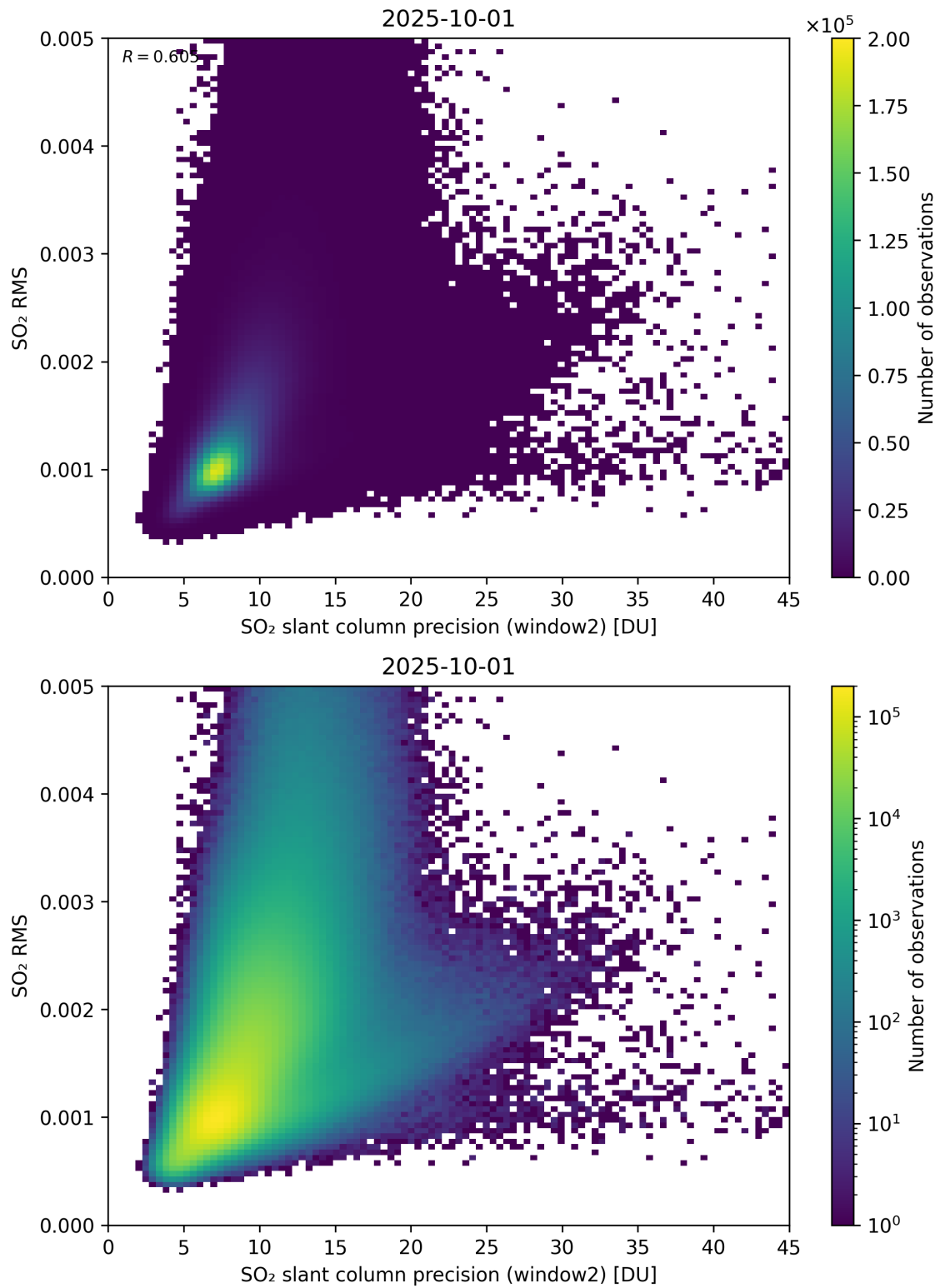
Figure 295: Scatter density plot of “SO 2 slant column precision (window2)” against “SO 2 RMS” for 2025-10-01 to 2025-10-02.
