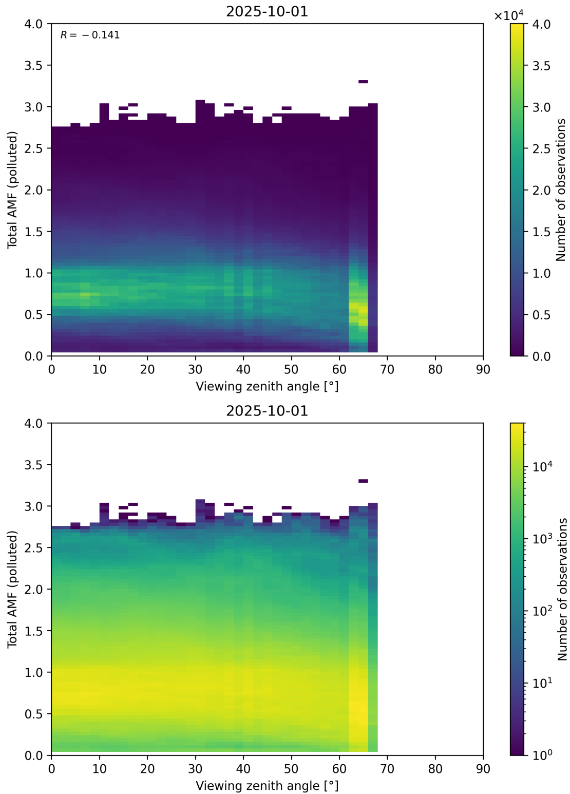
Figure 381: Scatter density plot of “Viewing zenith angle” against “Total AMF (polluted)” for 2025-10-01 to 2025-10-02.
