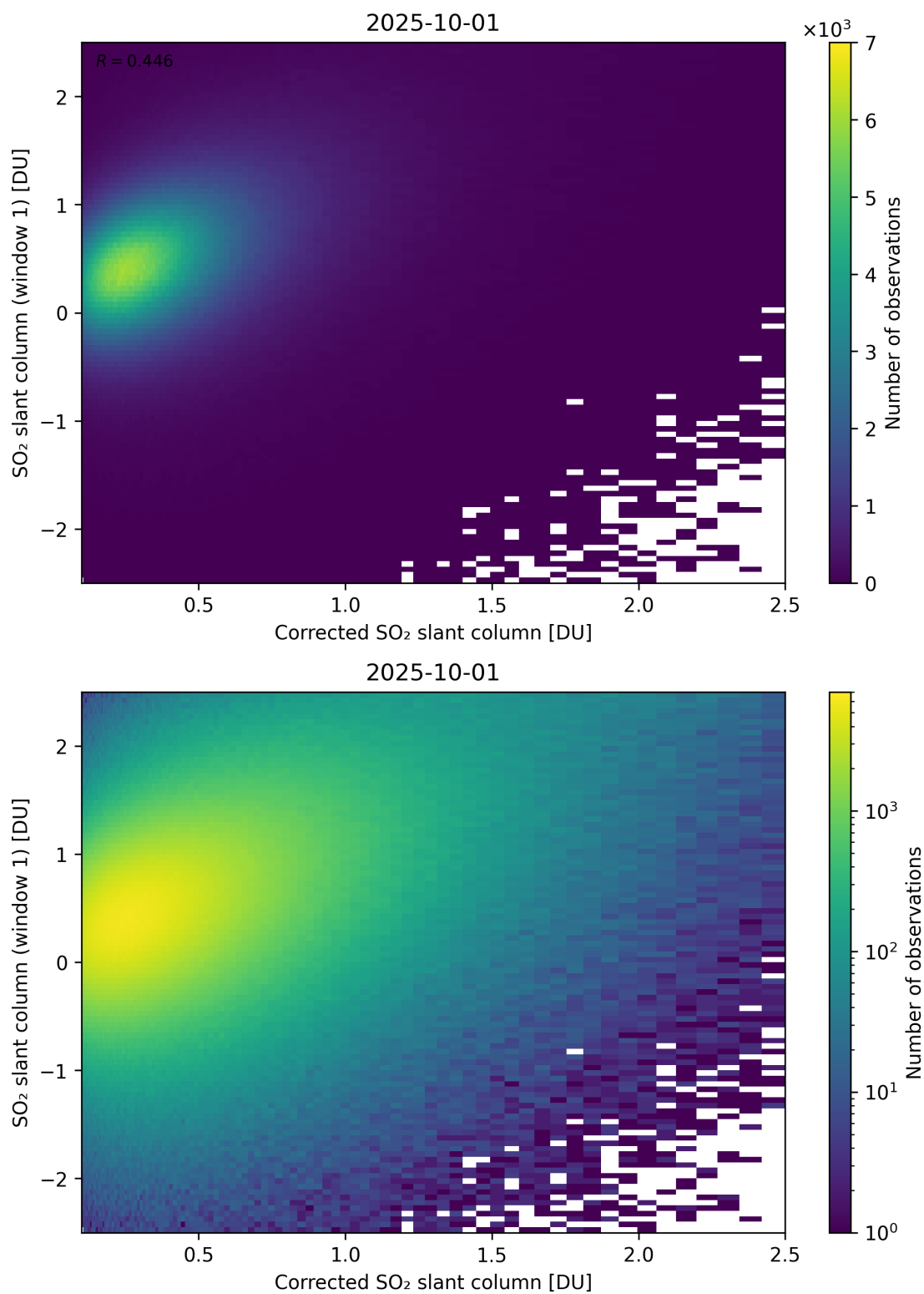
Figure 237: Scatter density plot of “Corrected SO 2 slant column” against “SO 2 slant column (window 1)” for 2025-10-01 to 2025-10-02.
