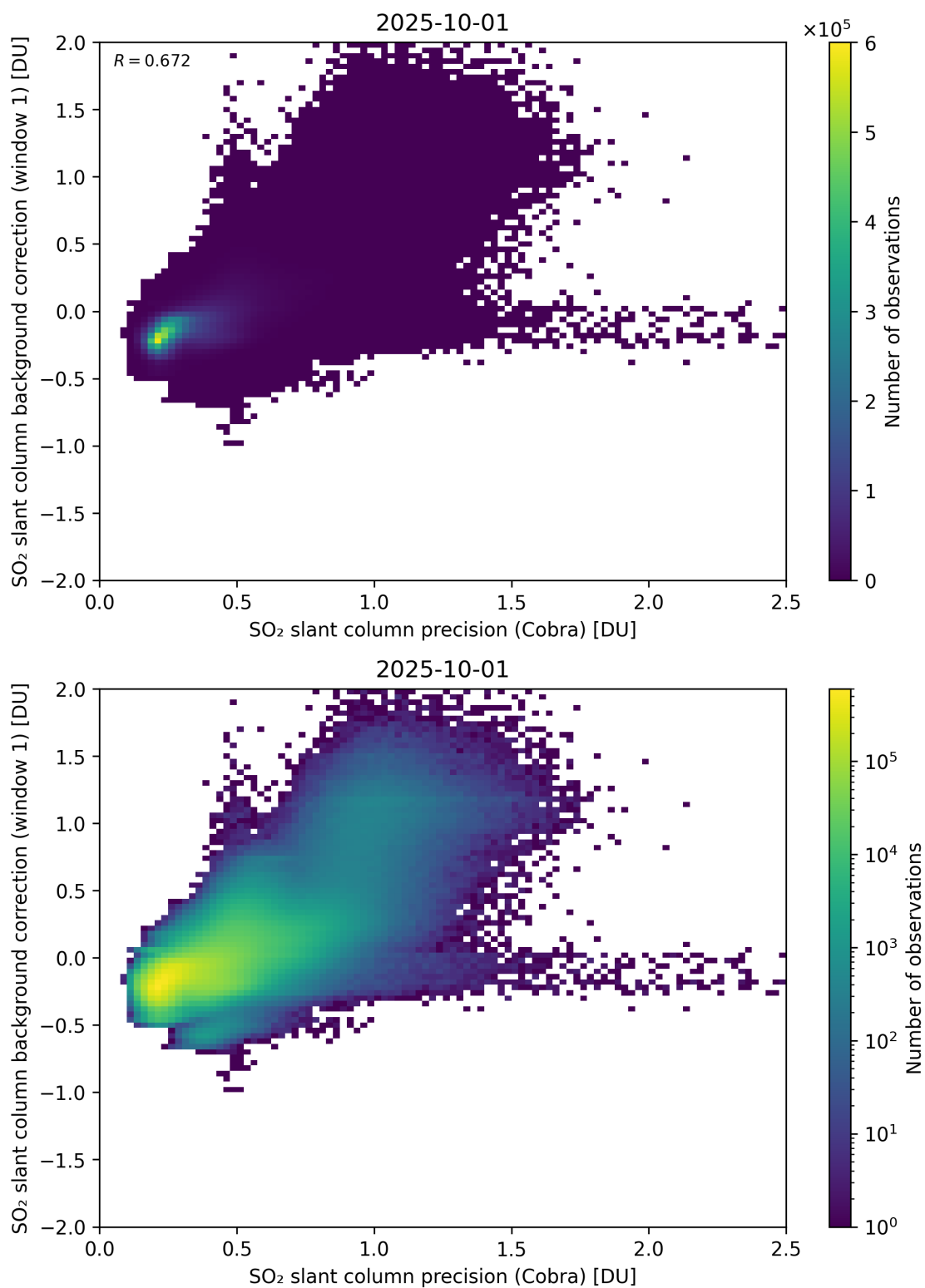
Figure 199: Scatter density plot of “SO 2 slant column precision (Cobra)” against “SO 2 slant column background correction (window 1)” for 2025-10-01 to 2025-10-02.
