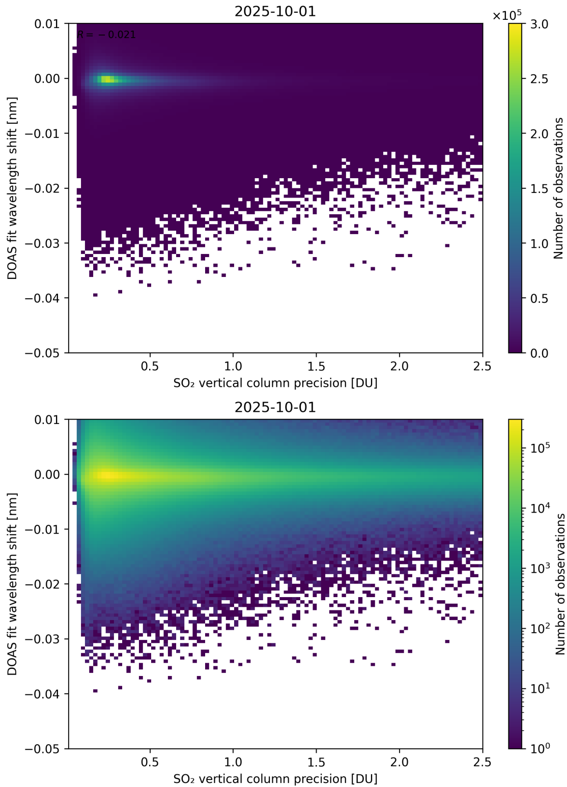
Figure 332: Scatter density plot of “SO 2 vertical column precision” against “DOAS fit wavelength shift” for 2025-10-01 to 2025-10-02.
