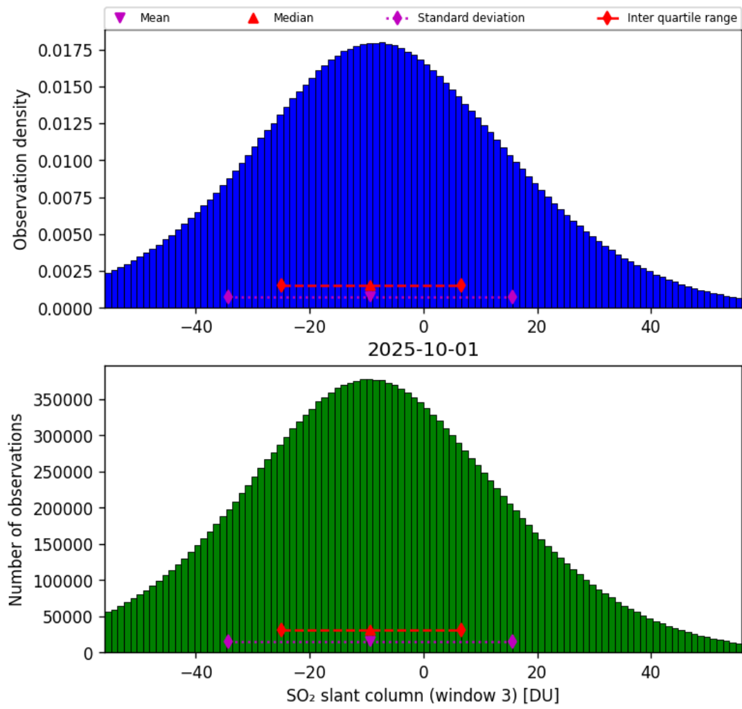
Figure 71: Histogram of “SO 2 slant column (window 3)” for 2025-10-01 to 2025-10-02
