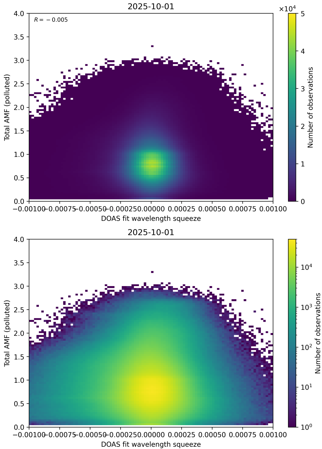
Figure 145: Scatter density plot of “DOAS fit wavelength squeeze” against “Total AMF (polluted)” for 2025-10-01 to 2025-10-02.
