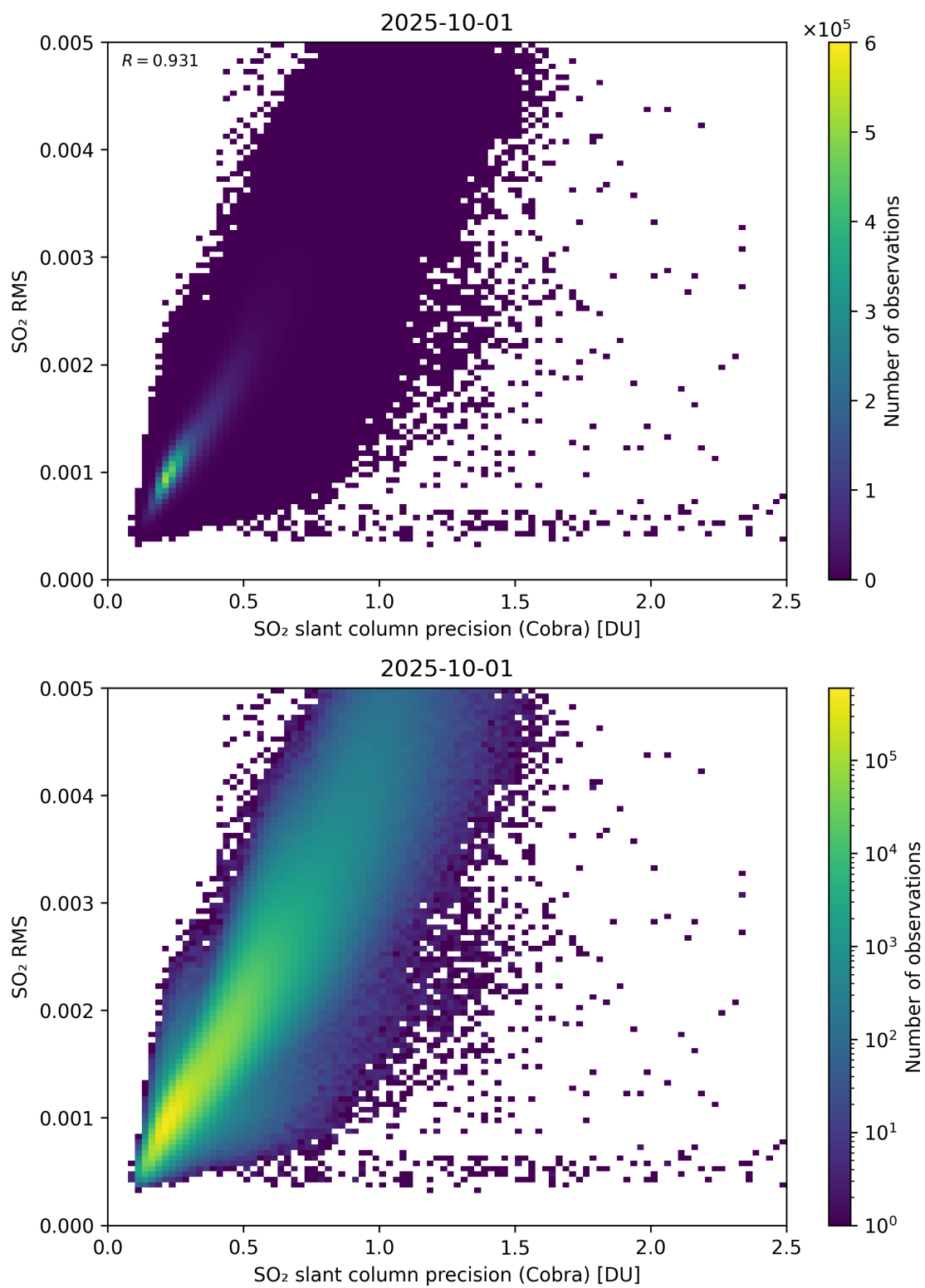
Figure 204: Scatter density plot of “SO 2 slant column precision (Cobra)” against “SO 2 RMS” for 2025-10-01 to 2025-10-02.
