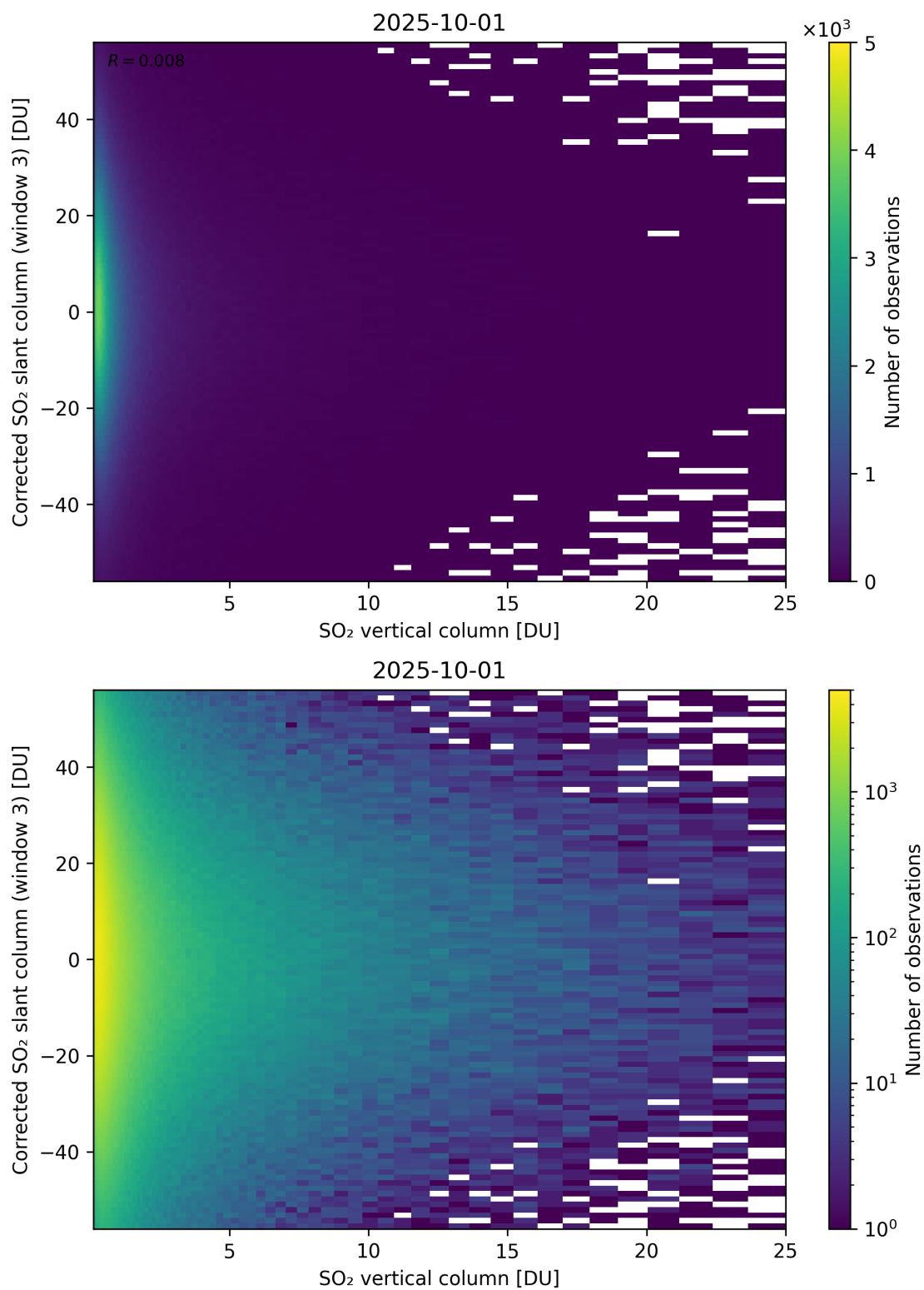
Figure 353: Scatter density plot of “SO 2 vertical column” against “Corrected SO 2 slant column (window 3)” for 2025-10-01 to 2025-10-02.
