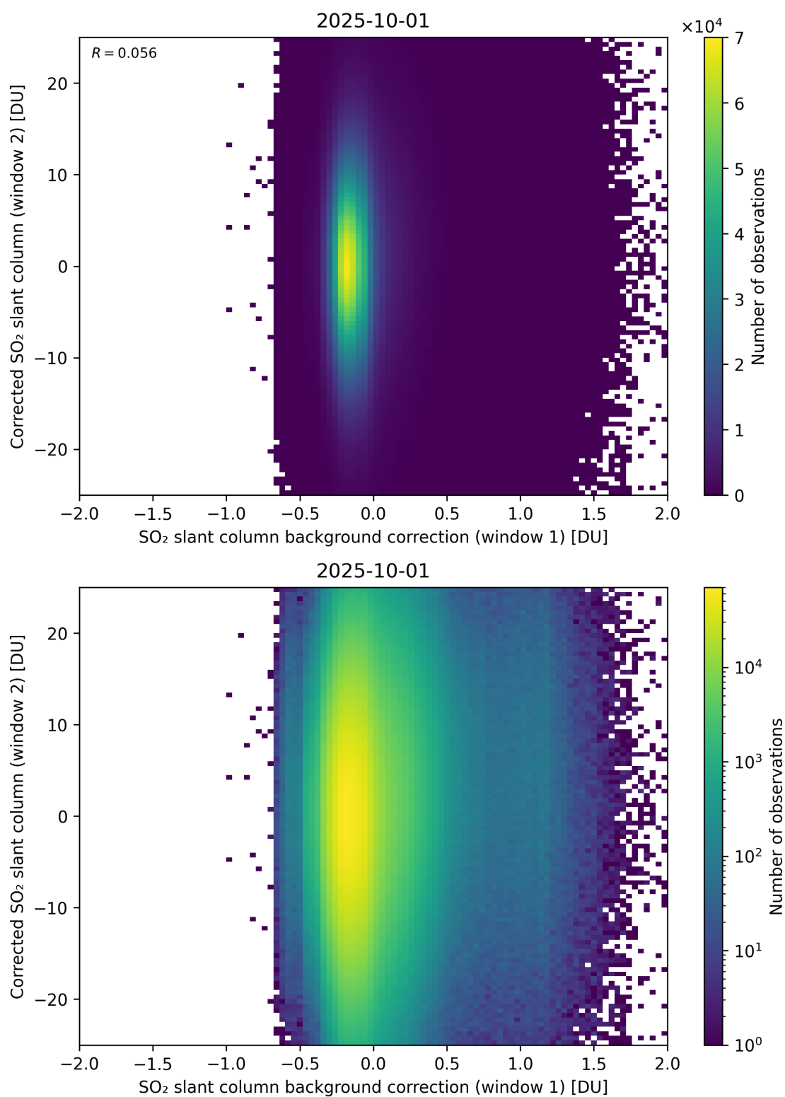
Figure 115: Scatter density plot of “SO 2 slant column background correction (window 1)” against “Corrected SO 2 slant column (window 2)” for 2025-10-01 to 2025-10-02.
