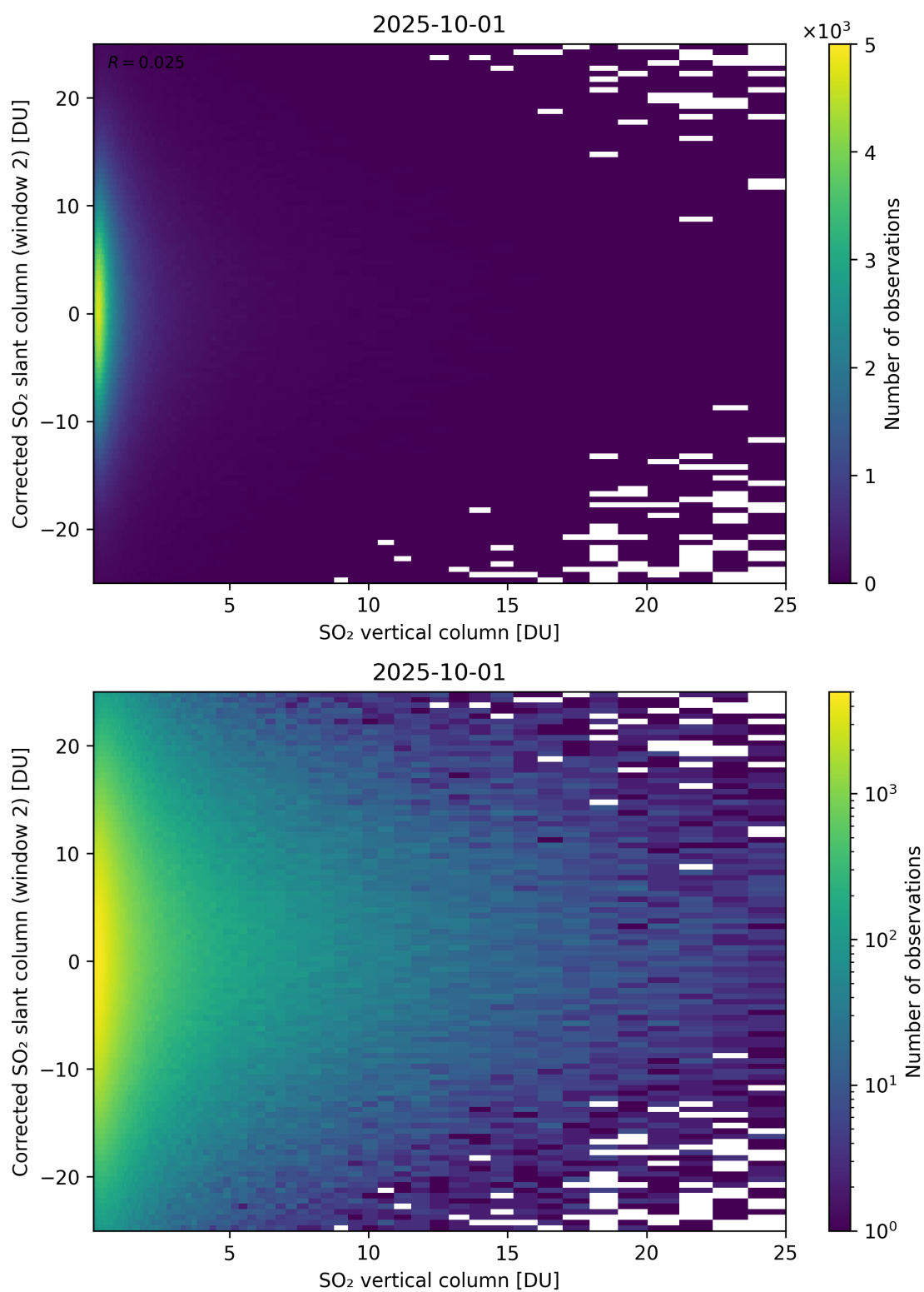
Figure 352: Scatter density plot of “SO 2 vertical column” against “Corrected SO 2 slant column (window 2)” for 2025-10-01 to 2025-10-02.
