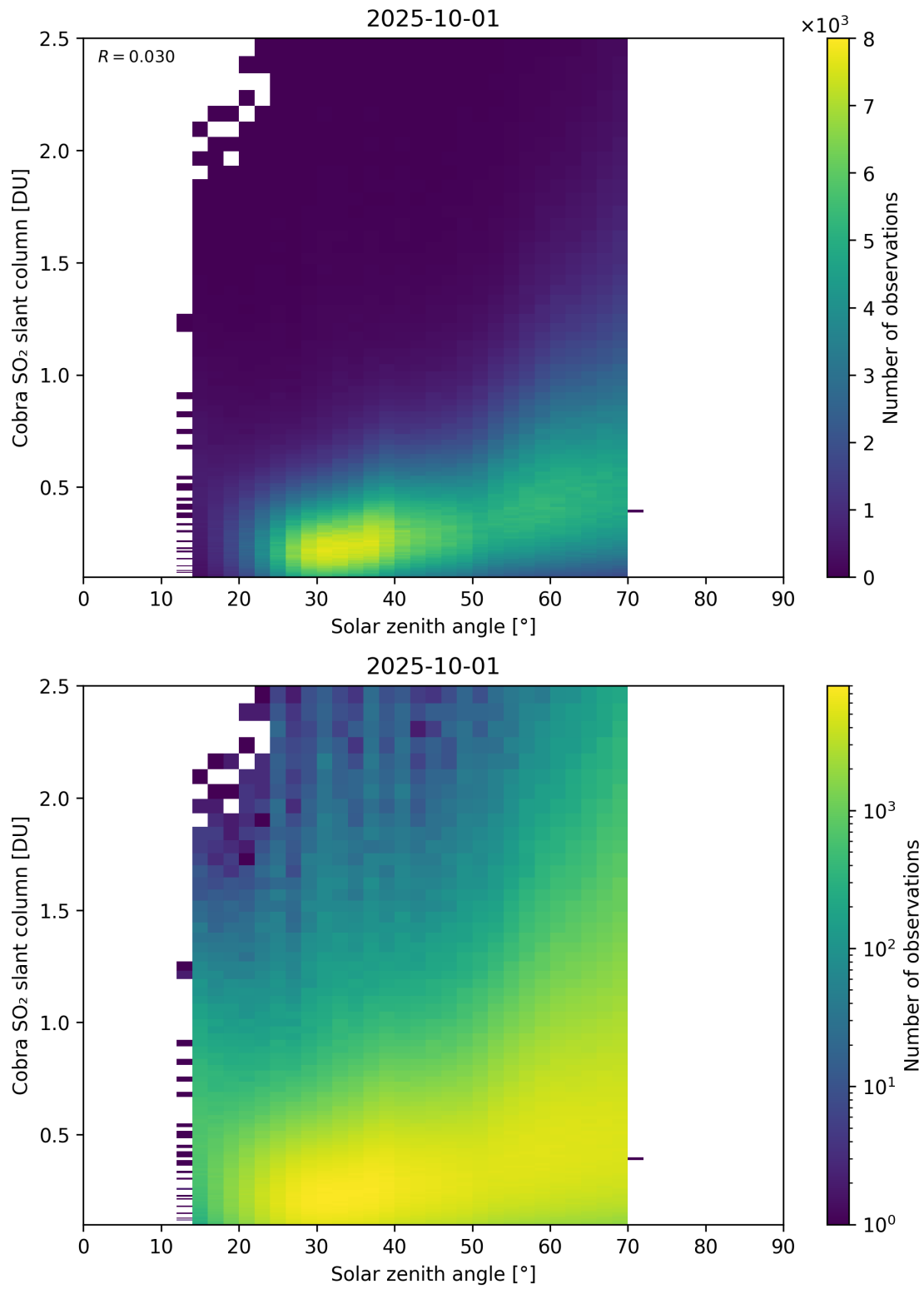
Figure 179: Scatter density plot of “Solar zenith angle” against “Cobra SO 2 slant column” for 2025-10-01 to 2025-10-02.
