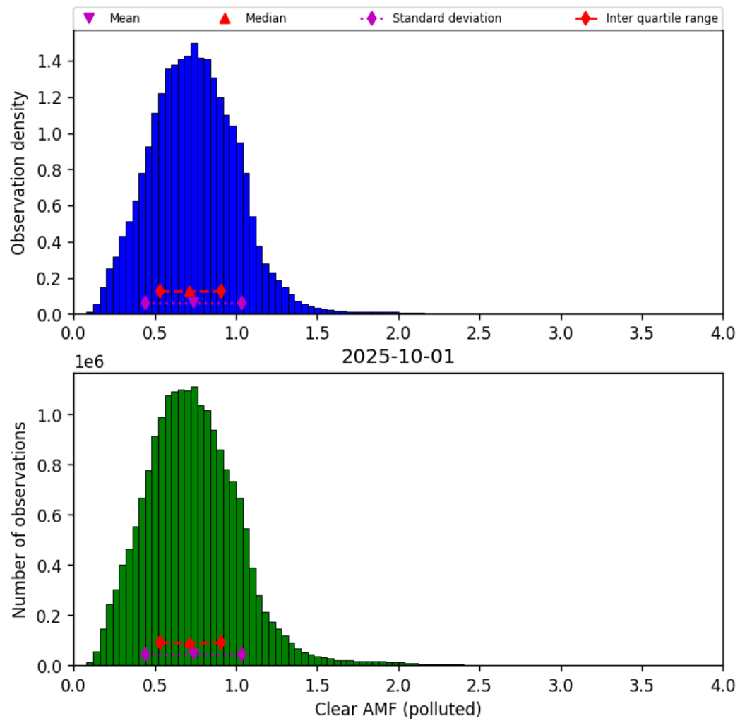
Figure 81: Histogram of “Clear AMF (polluted)” for 2025-10-01 to 2025-10-02
