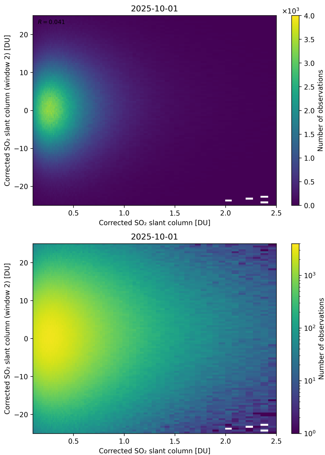
Figure 235: Scatter density plot of “Corrected SO 2 slant column” against “Corrected SO 2 slant column (window 2)” for 2025-10-01 to 2025-10-02.
