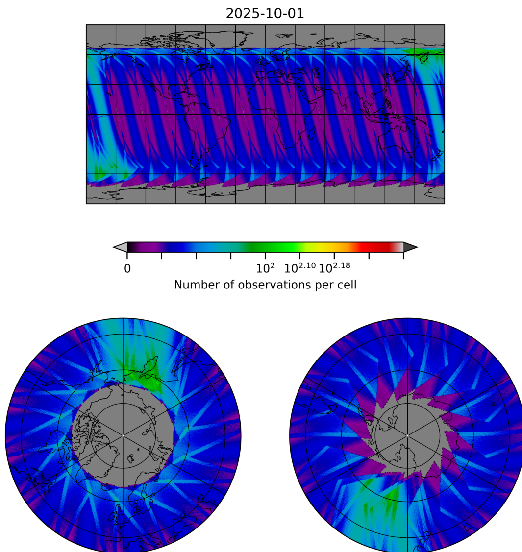
Figure 30: Map of the number of observations for 2025-10-01 to 2025-10-02
