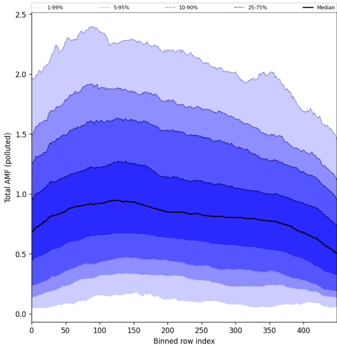
Figure 105: Along track statistics of “Total AMF (polluted)” for 2025-10-01 to 2025-10-02
