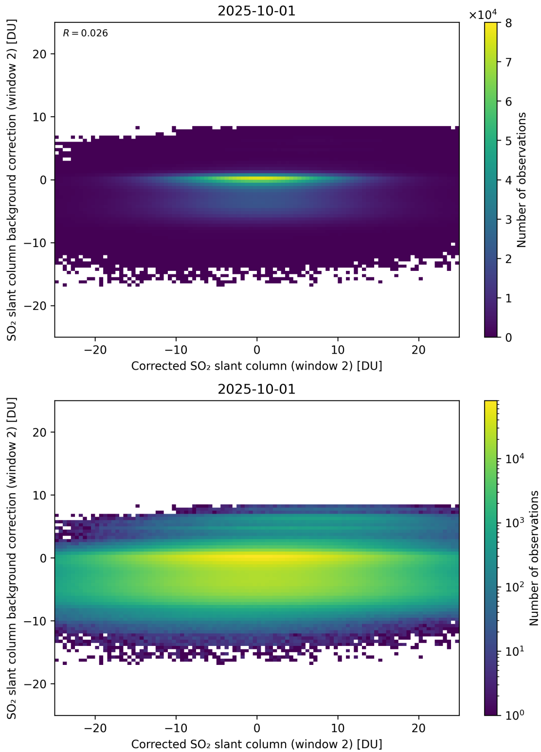
Figure 244: Scatter density plot of “Corrected SO 2 slant column (window 2)” against “SO 2 slant column background correction (window 2)” for 2025-10-01 to 2025-10-02.
