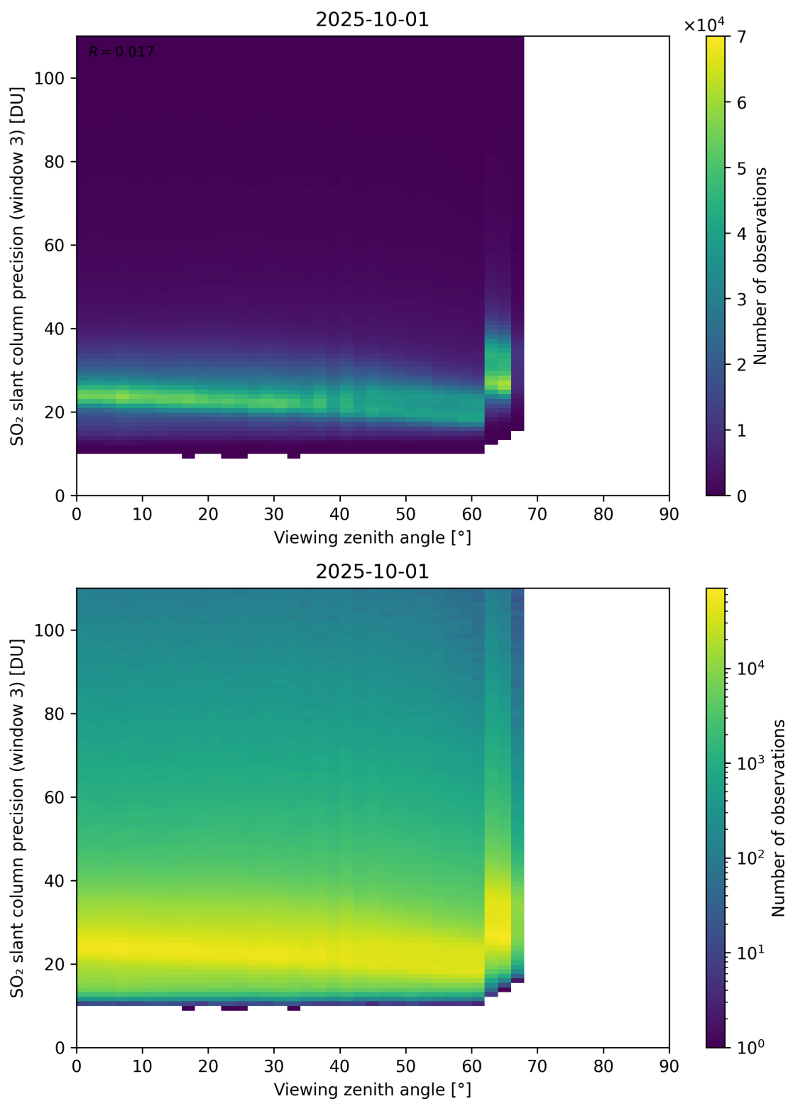
Figure 380: Scatter density plot of “Viewing zenith angle” against “SO 2 slant column precision (window 3)” for 2025-10-01 to 2025-10-02.
