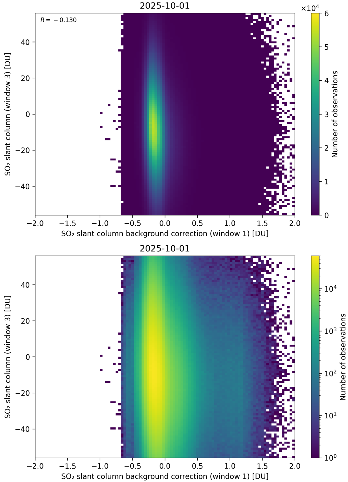
Figure 118: Scatter density plot of “SO 2 slant column background correction (window 1)” against “SO 2 slant column (window 3)” for 2025-10-01 to 2025-10-02.
