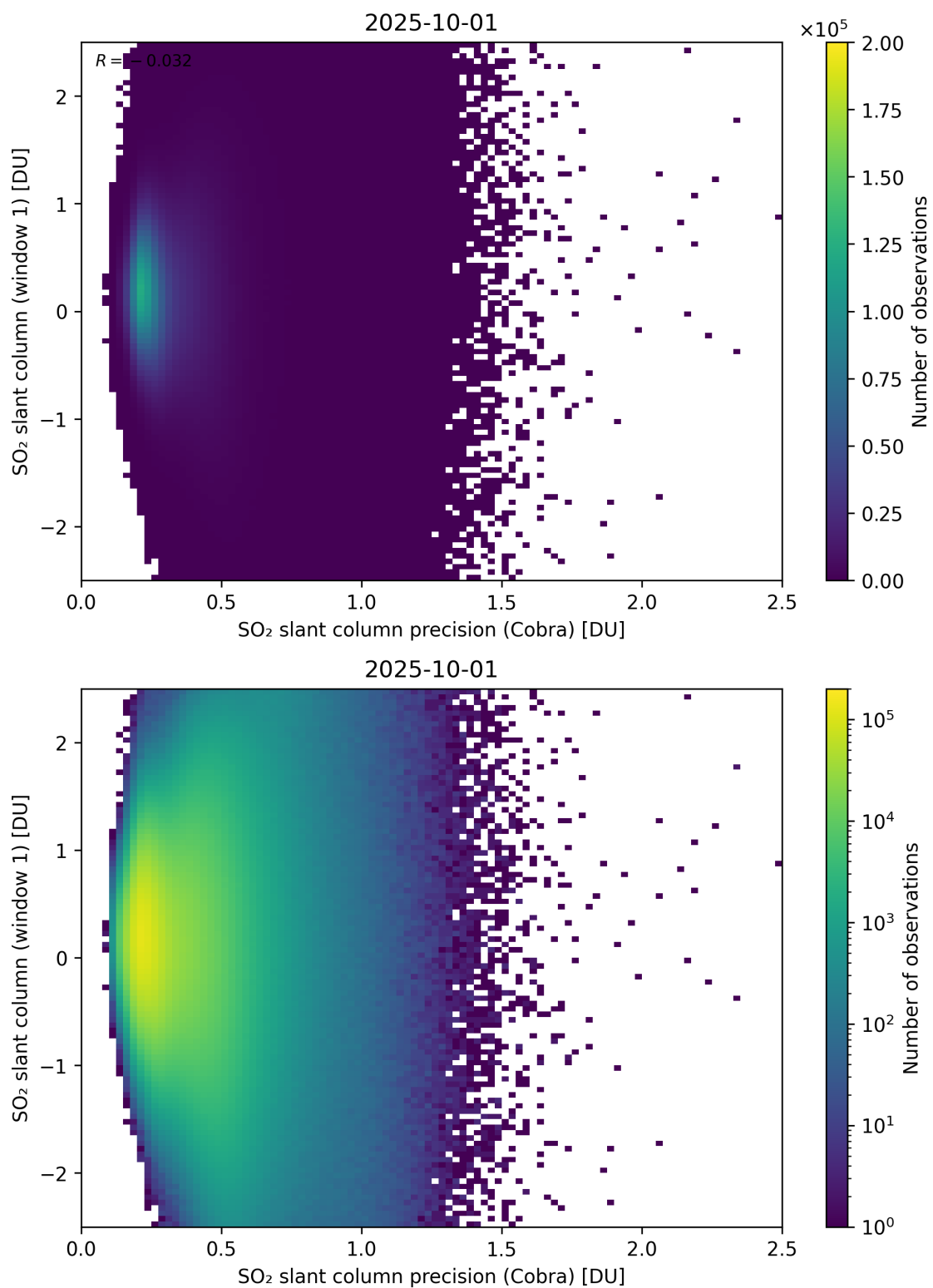
Figure 208: Scatter density plot of “SO 2 slant column precision (Cobra)” against “SO 2 slant column (window 1)” for 2025-10-01 to 2025-10-02.
