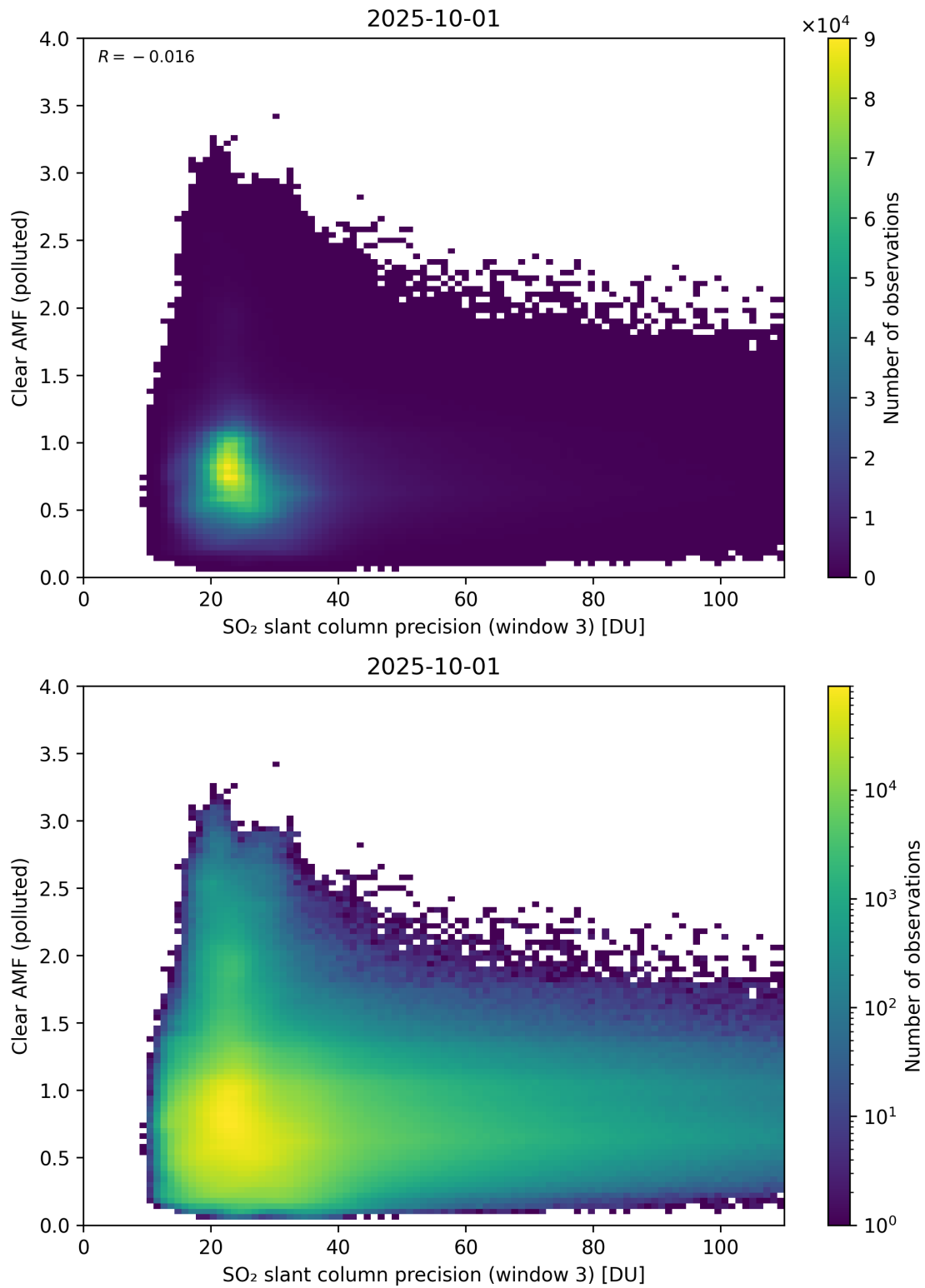
Figure 311: Scatter density plot of “SO 2 slant column precision (window 3)” against “Clear AMF (polluted)” for 2025-10-01 to 2025-10-02.
