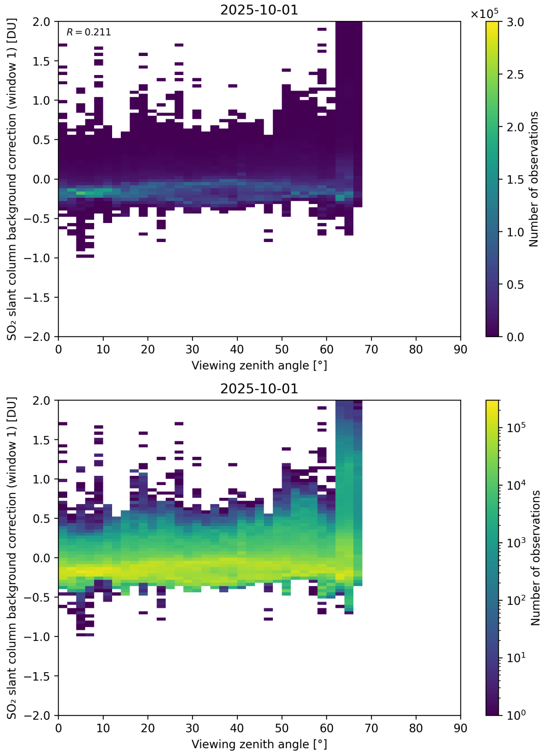
Figure 362: Scatter density plot of “Viewing zenith angle” against “SO 2 slant column background correction (window 1)” for 2025-10-01 to 2025-10-02.
