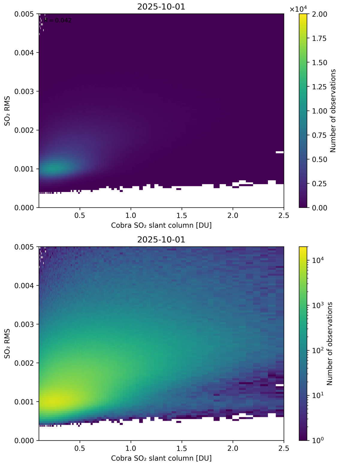
Figure 198: Scatter density plot of “Cobra SO 2 slant column” against “SO 2 RMS” for 2025-10-01 to 2025-10-02.
