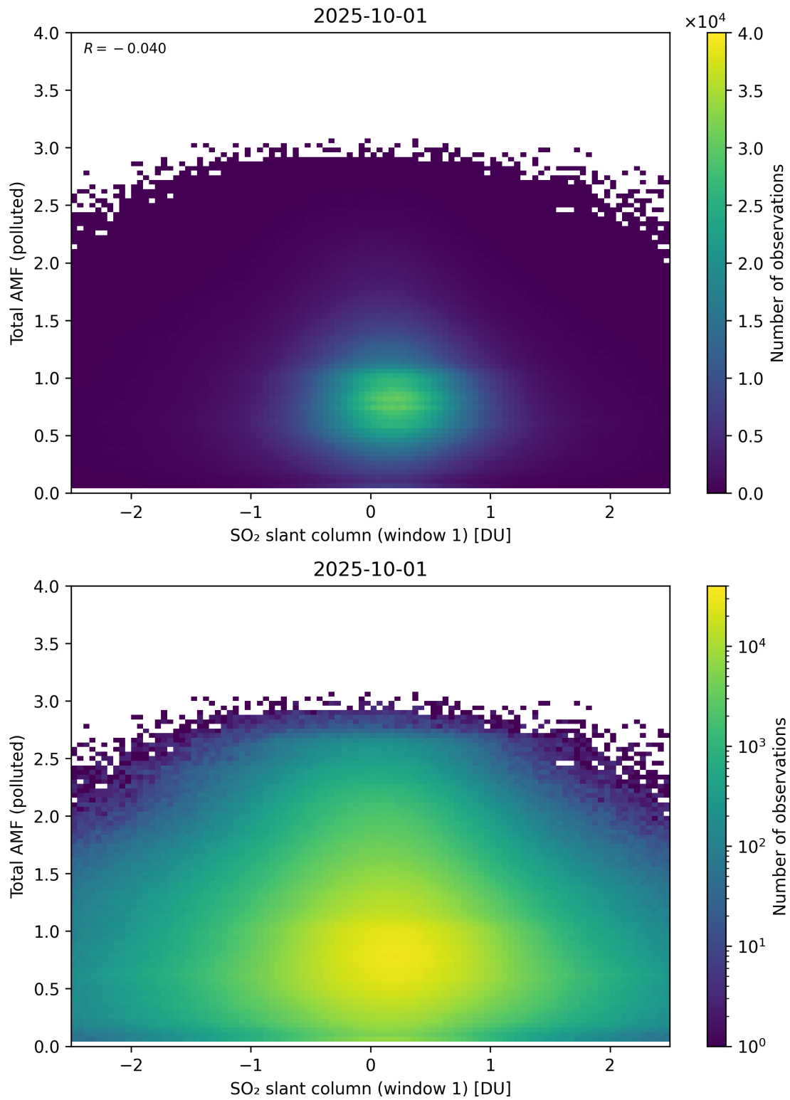
Figure 289: Scatter density plot of “SO 2 slant column (window 1)” against “Total AMF (polluted)” for 2025-10-01 to 2025-10-02.
