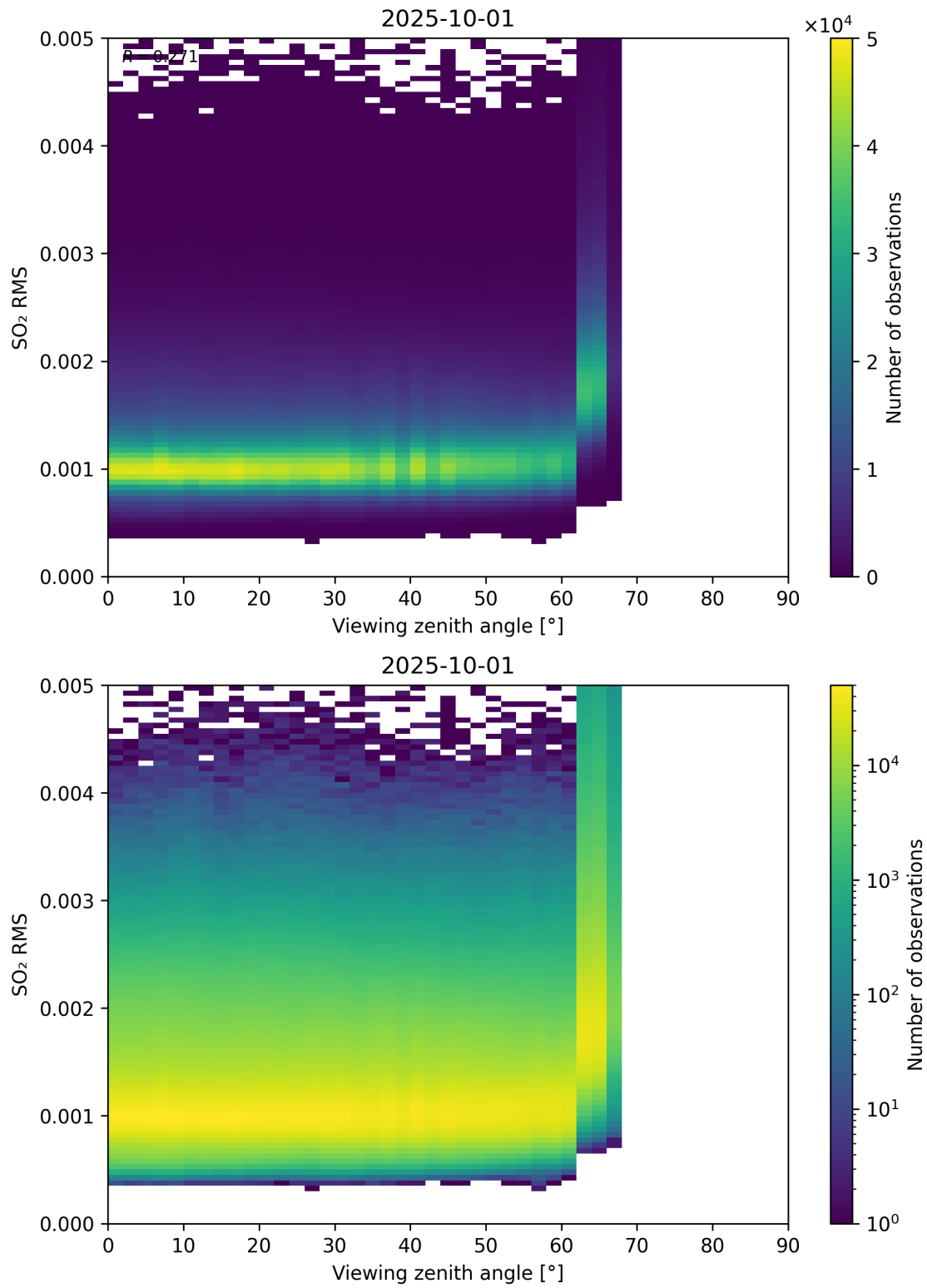
Figure 367: Scatter density plot of “Viewing zenith angle” against “SO 2 RMS” for 2025-10-01 to 2025-10-02.
