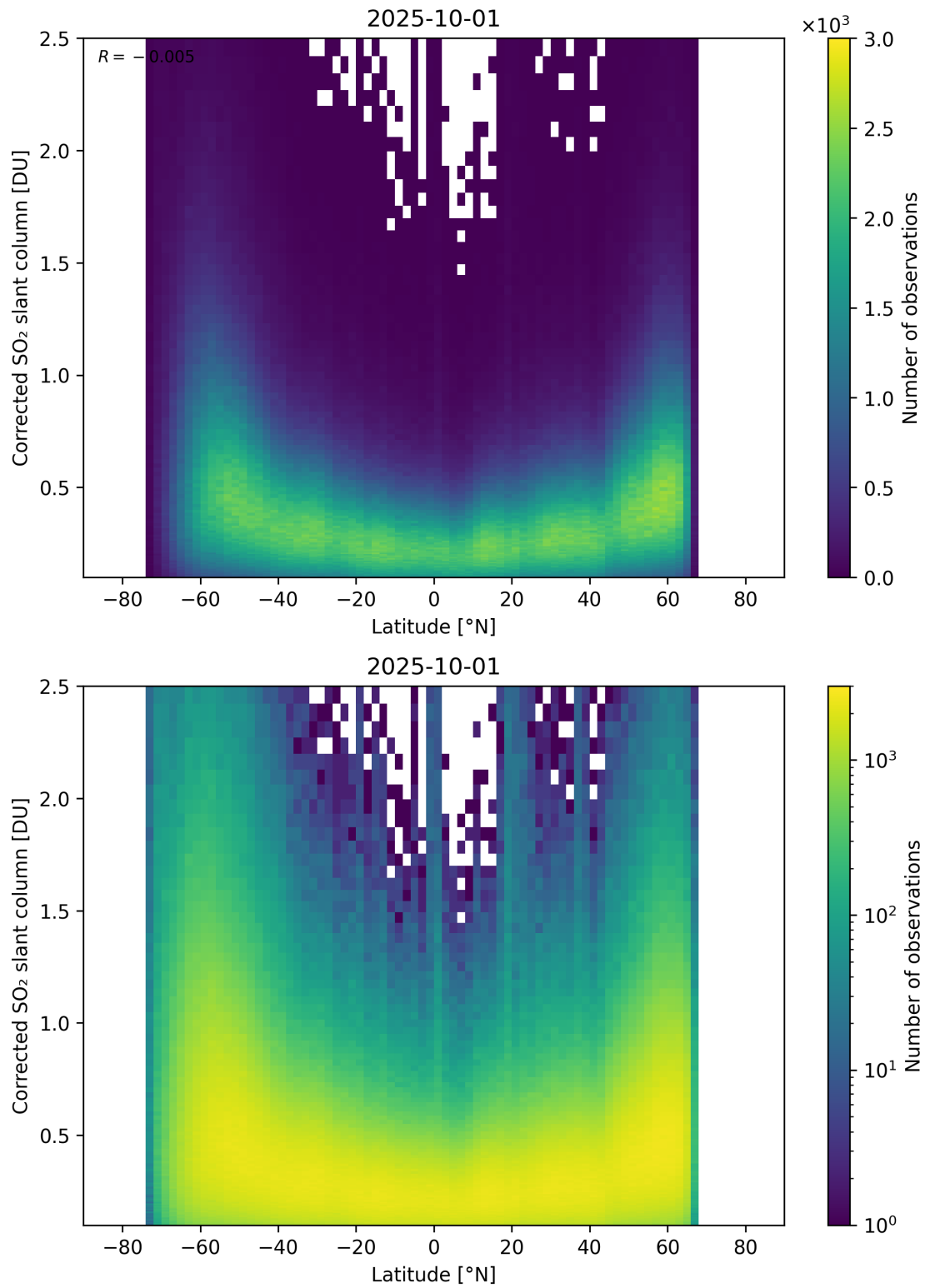
Figure 159: Scatter density plot of “Latitude” against “Corrected SO 2 slant column” for 2025-10-01 to 2025-10-02.
