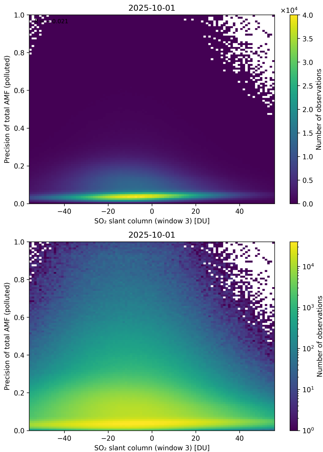
Figure 319: Scatter density plot of “SO 2 slant column (window 3)” against “Precision of total AMF (polluted)” for 2025-10-01 to 2025-10-02.
