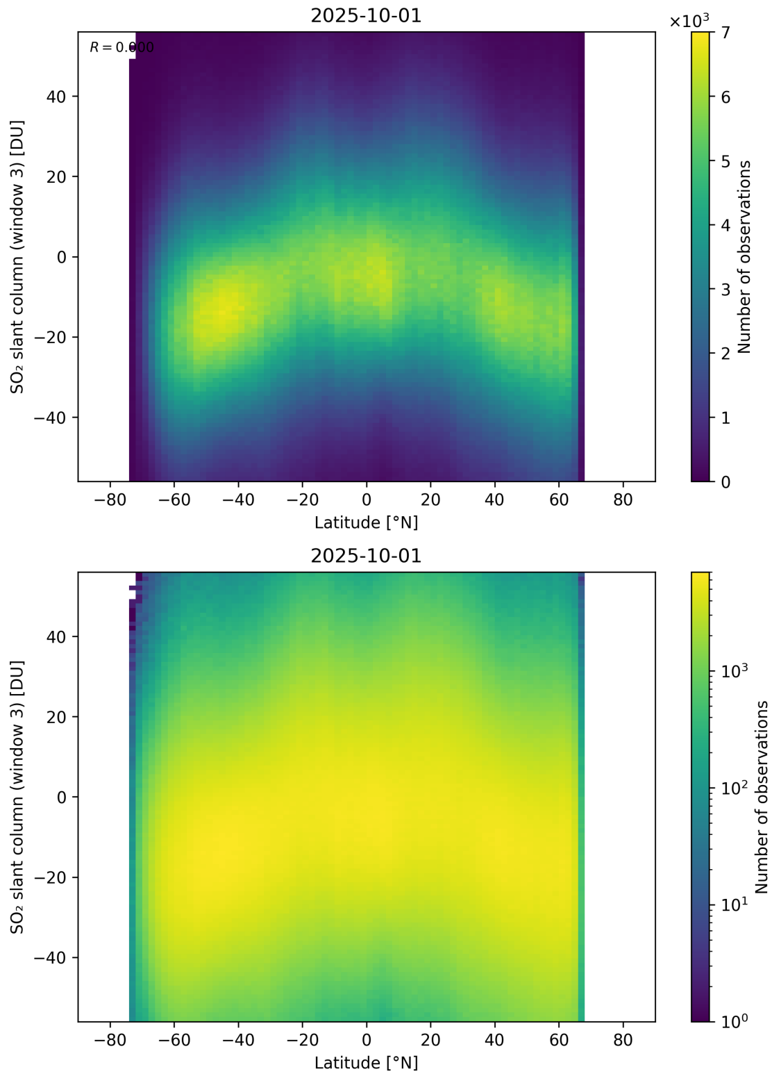
Figure 165: Scatter density plot of “Latitude” against “SO 2 slant column (window 3)” for 2025-10-01 to 2025-10-02.
