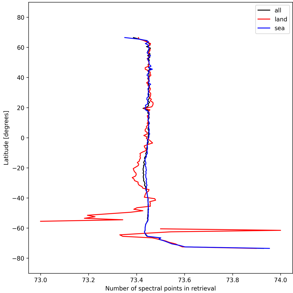
Figure 56: Zonal average of “Number of spectral points in retrieval” for 2025-10-01 to 2025-10-02.
