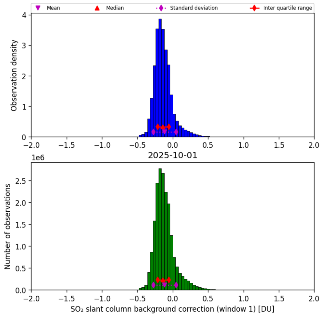
Figure 66: Histogram of “SO 2 slant column background correction (window 1)” for 2025-10-01 to 2025-10-02
