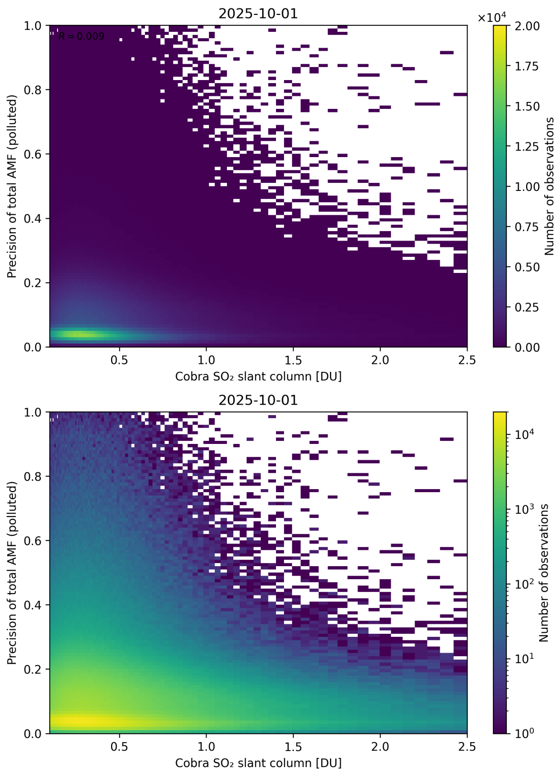
Figure 225: Scatter density plot of “Cobra SO 2 slant column” against “Precision of total AMF (polluted)” for 2025-10-01 to 2025-10-02.
