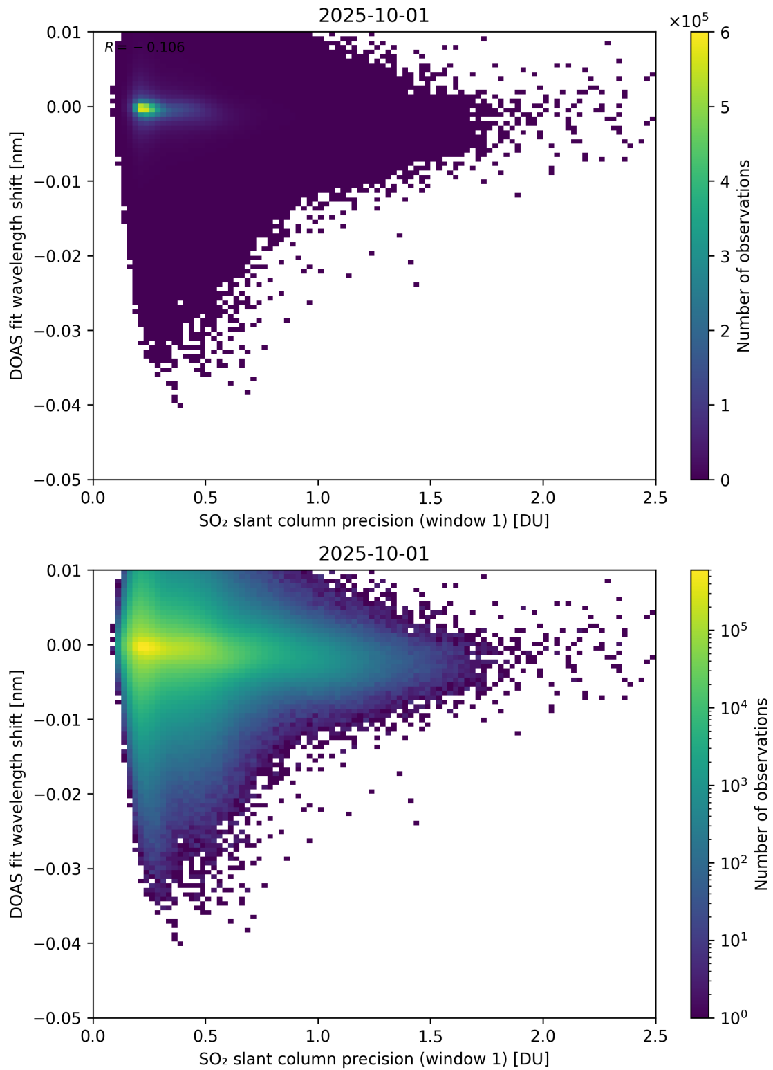
Figure 271: Scatter density plot of “SO 2 slant column precision (window 1)” against “DOAS fit wavelength shift” for 2025-10-01 to 2025-10-02.
