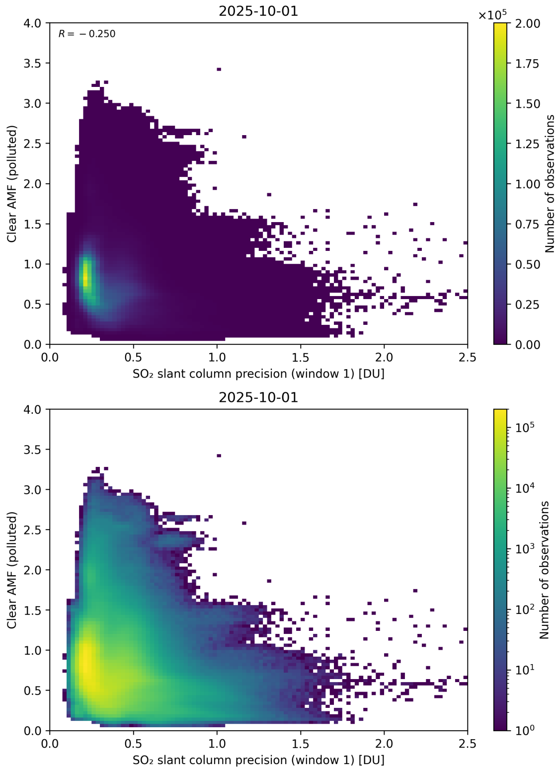
Figure 274: Scatter density plot of “SO 2 slant column precision (window 1)” against “Clear AMF (polluted)” for 2025-10-01 to 2025-10-02.
