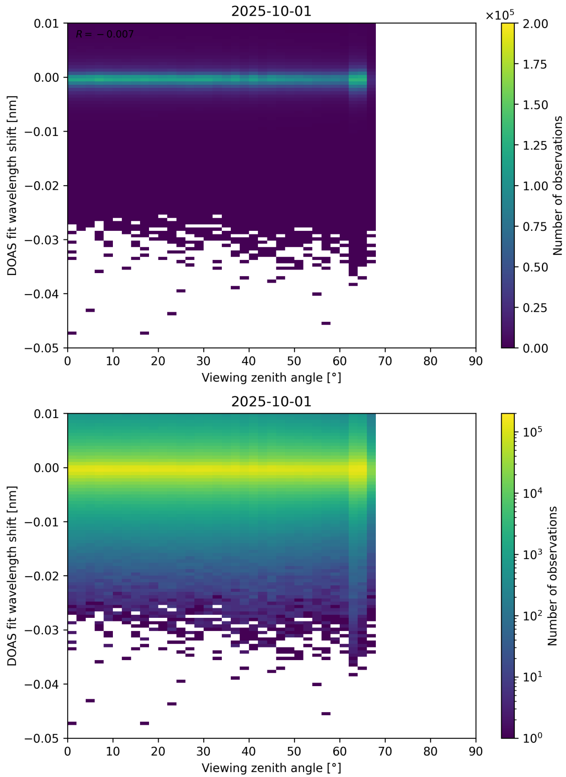
Figure 365: Scatter density plot of “Viewing zenith angle” against “DOAS fit wavelength shift” for 2025-10-01 to 2025-10-02.
