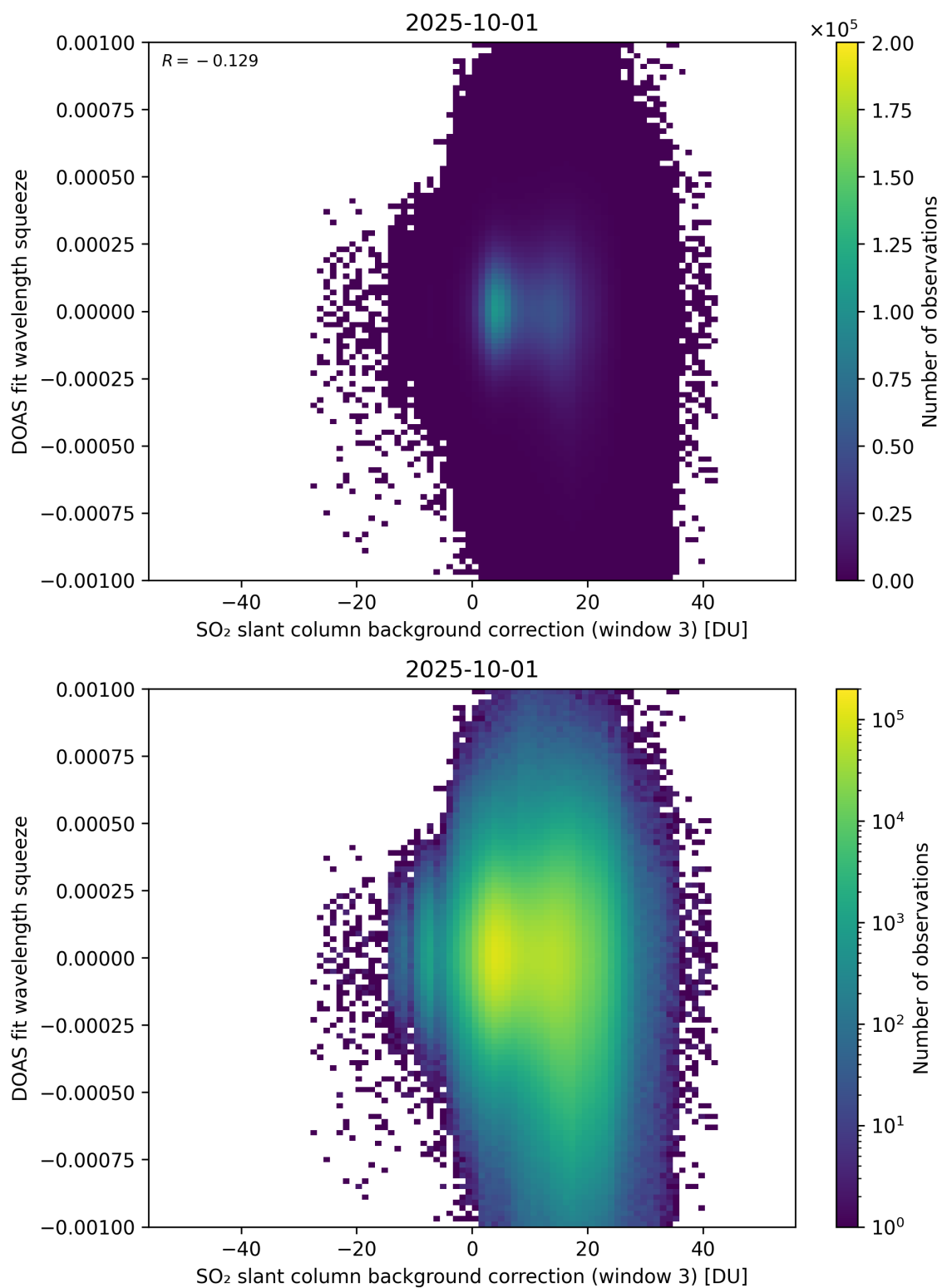
Figure 133: Scatter density plot of “SO 2 slant column background correction (window 3)” against “DOAS fit wavelength squeeze” for 2025-10-01 to 2025-10-02.
