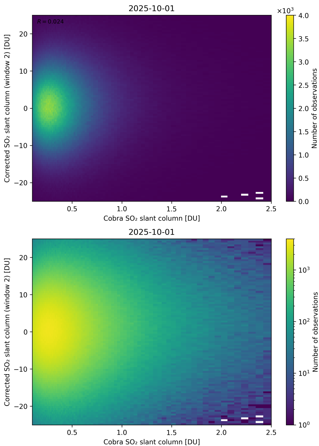
Figure 217: Scatter density plot of “Cobra SO 2 slant column” against “Corrected SO 2 slant column (window 2)” for 2025-10-01 to 2025-10-02.
