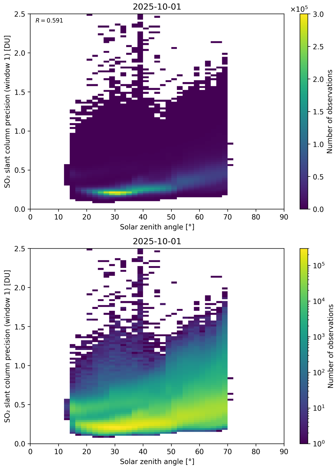
Figure 185: Scatter density plot of “Solar zenith angle” against “SO 2 slant column precision (window 1)” for 2025-10-01 to 2025-10-02.
