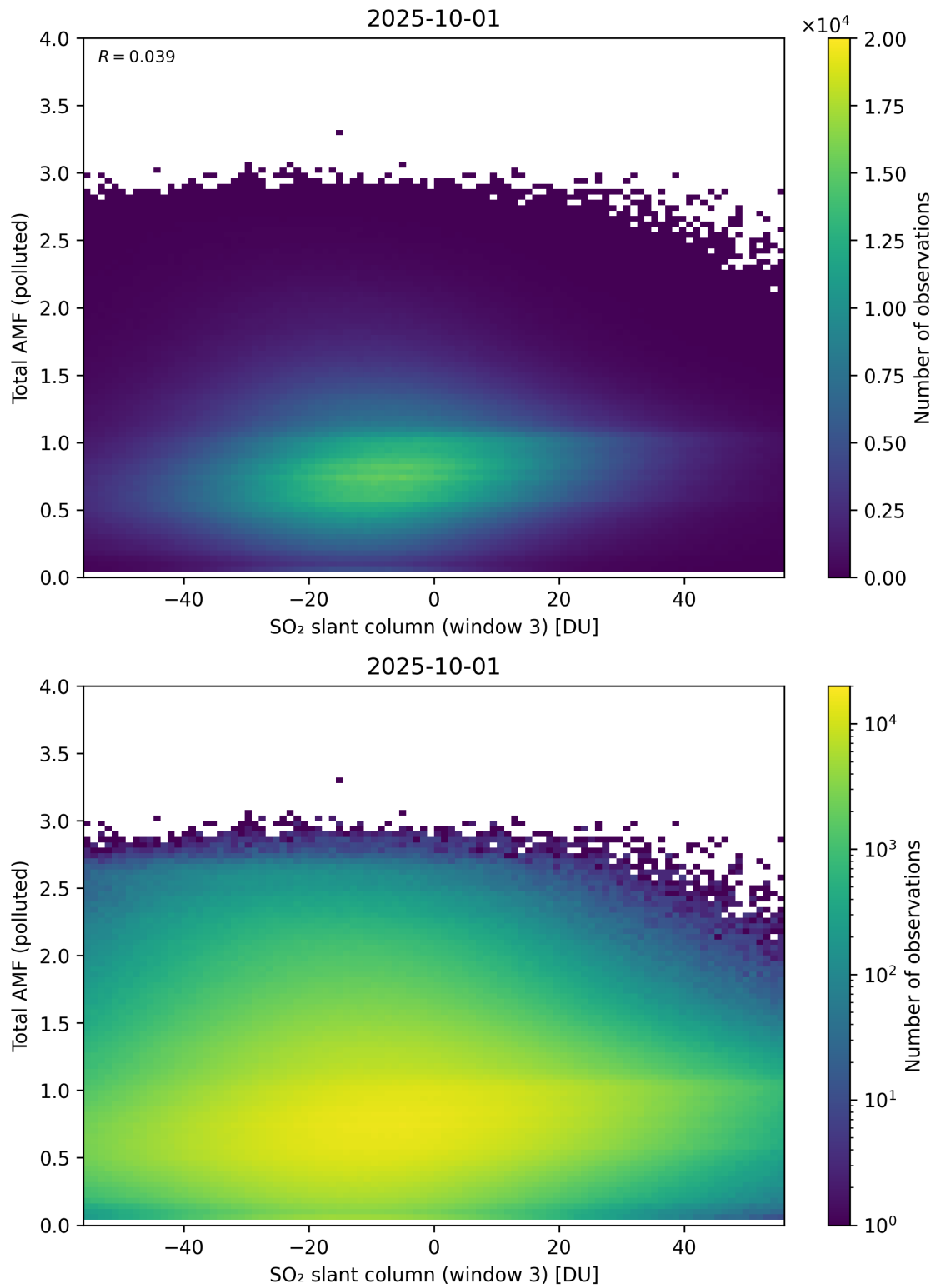
Figure 318: Scatter density plot of “SO 2 slant column (window 3)” against “Total AMF (polluted)” for 2025-10-01 to 2025-10-02.
