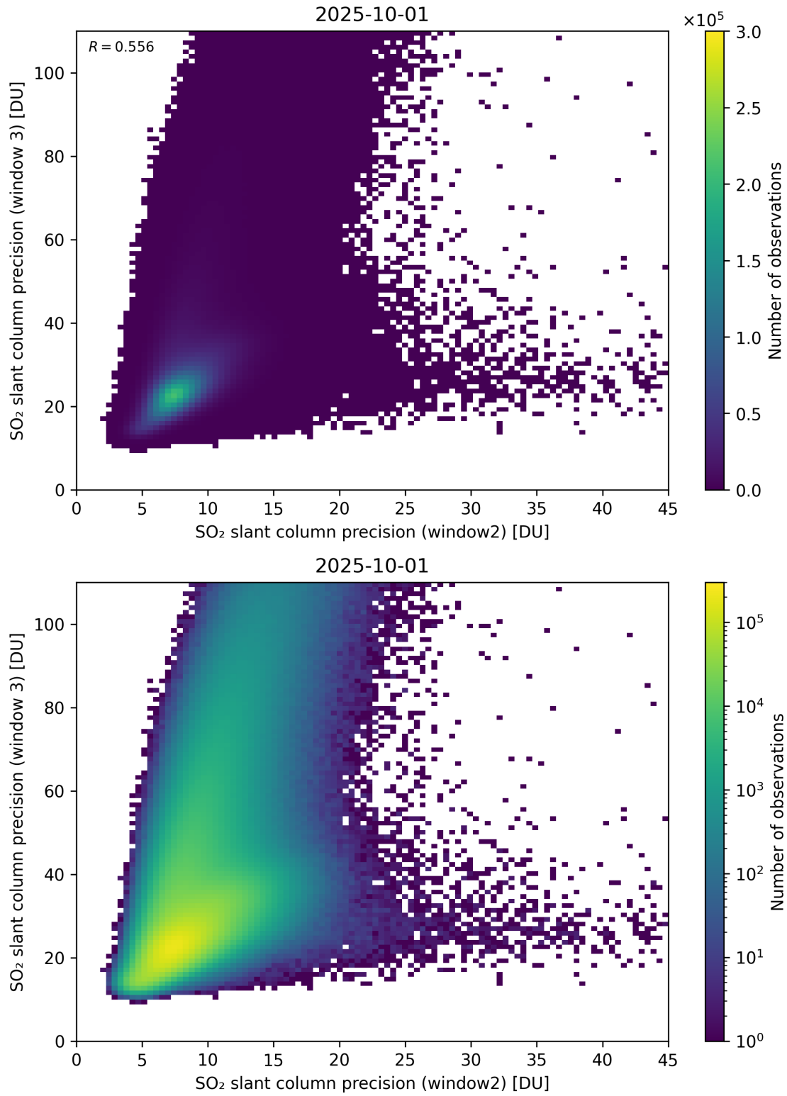
Figure 300: Scatter density plot of “SO 2 slant column precision (window2)” against “SO 2 slant column precision (window 3)” for 2025-10-01 to 2025-10-02.
