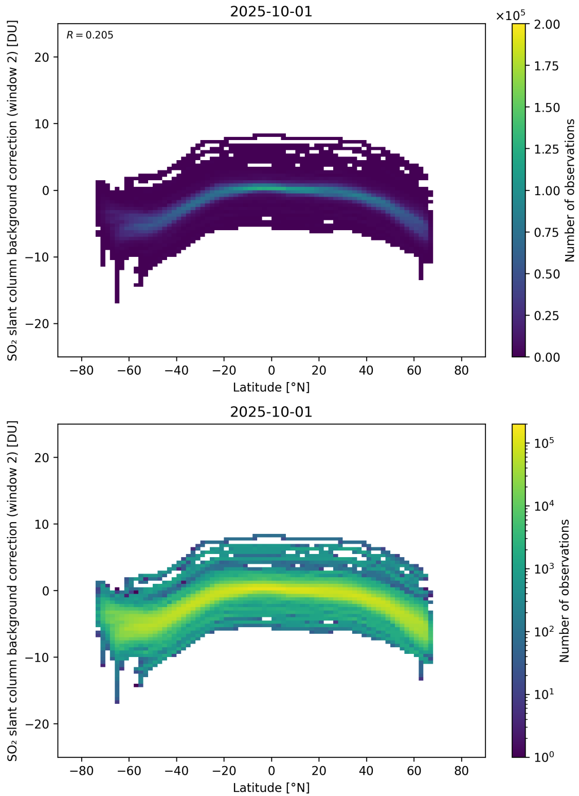
Figure 151: Scatter density plot of “Latitude” against “SO 2 slant column background correction (window 2)” for 2025-10-01 to 2025-10-02.
