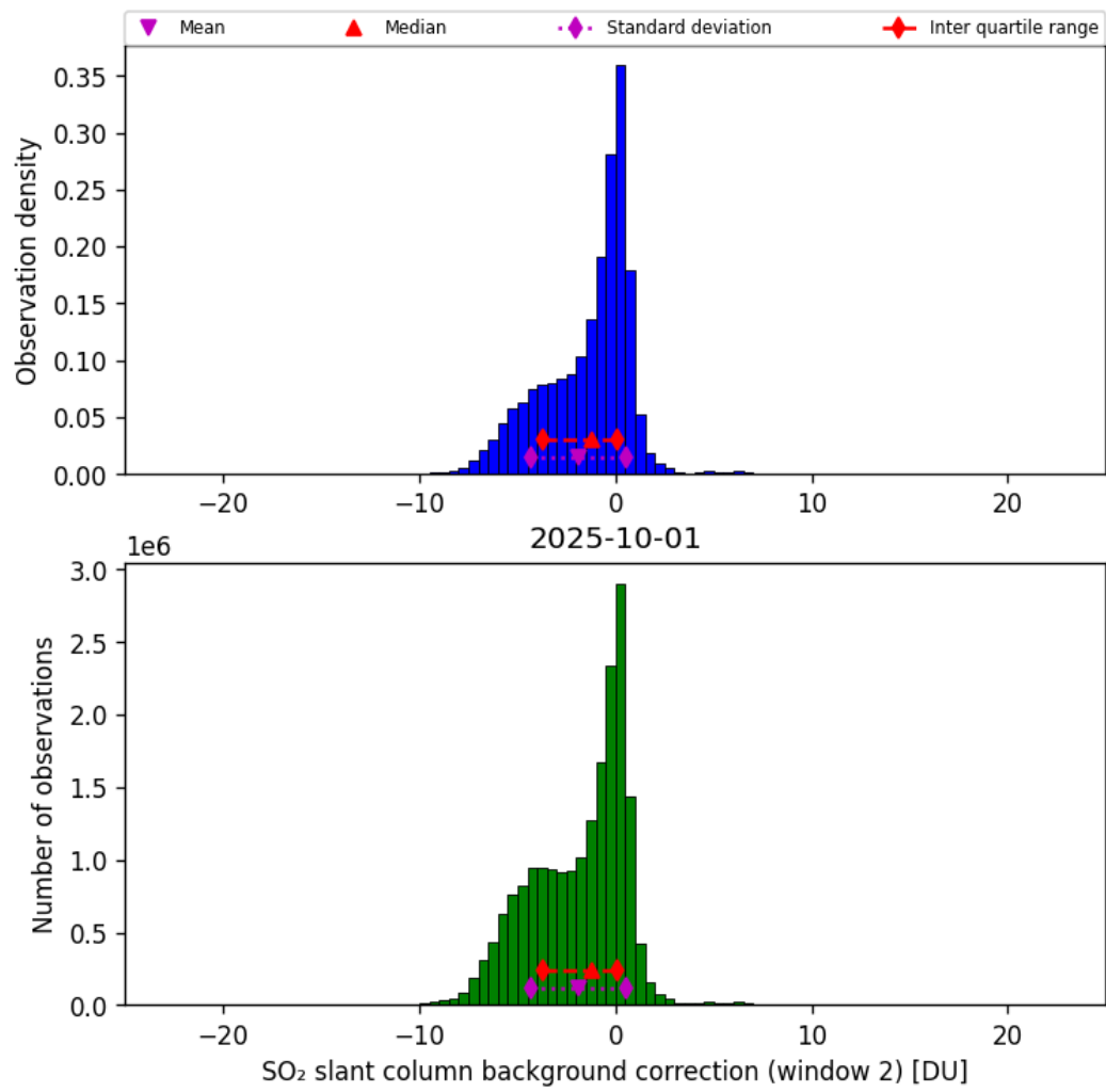
Figure 70: Histogram of “SO 2 slant column background correction (window 2)” for 2025-10-01 to 2025-10-02
