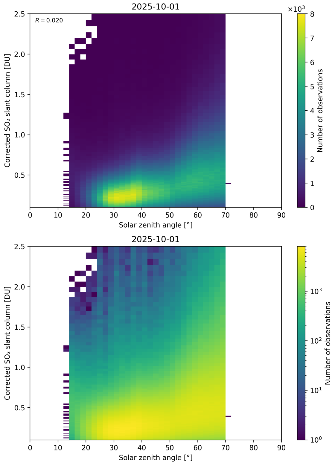
Figure 181: Scatter density plot of “Solar zenith angle” against “Corrected SO 2 slant column” for 2025-10-01 to 2025-10-02.
