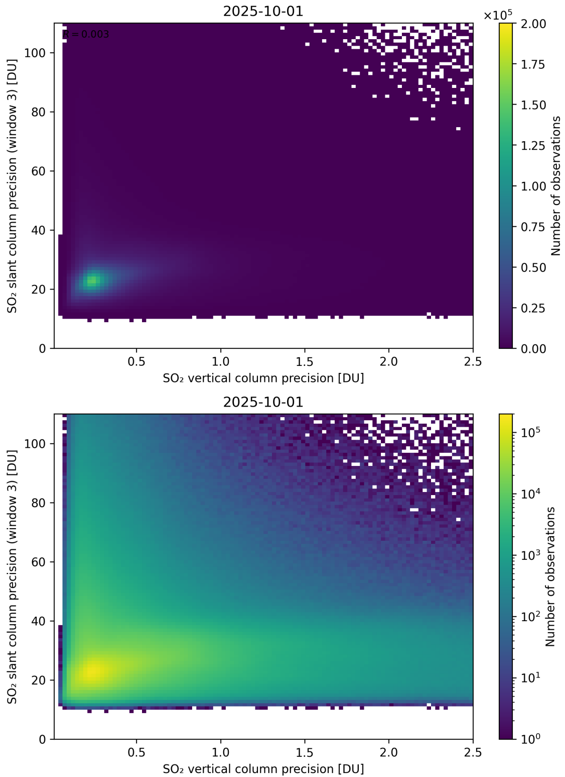
Figure 345: Scatter density plot of “SO 2 vertical column precision” against “SO 2 slant column precision (window 3)” for 2025-10-01 to 2025-10-02.
