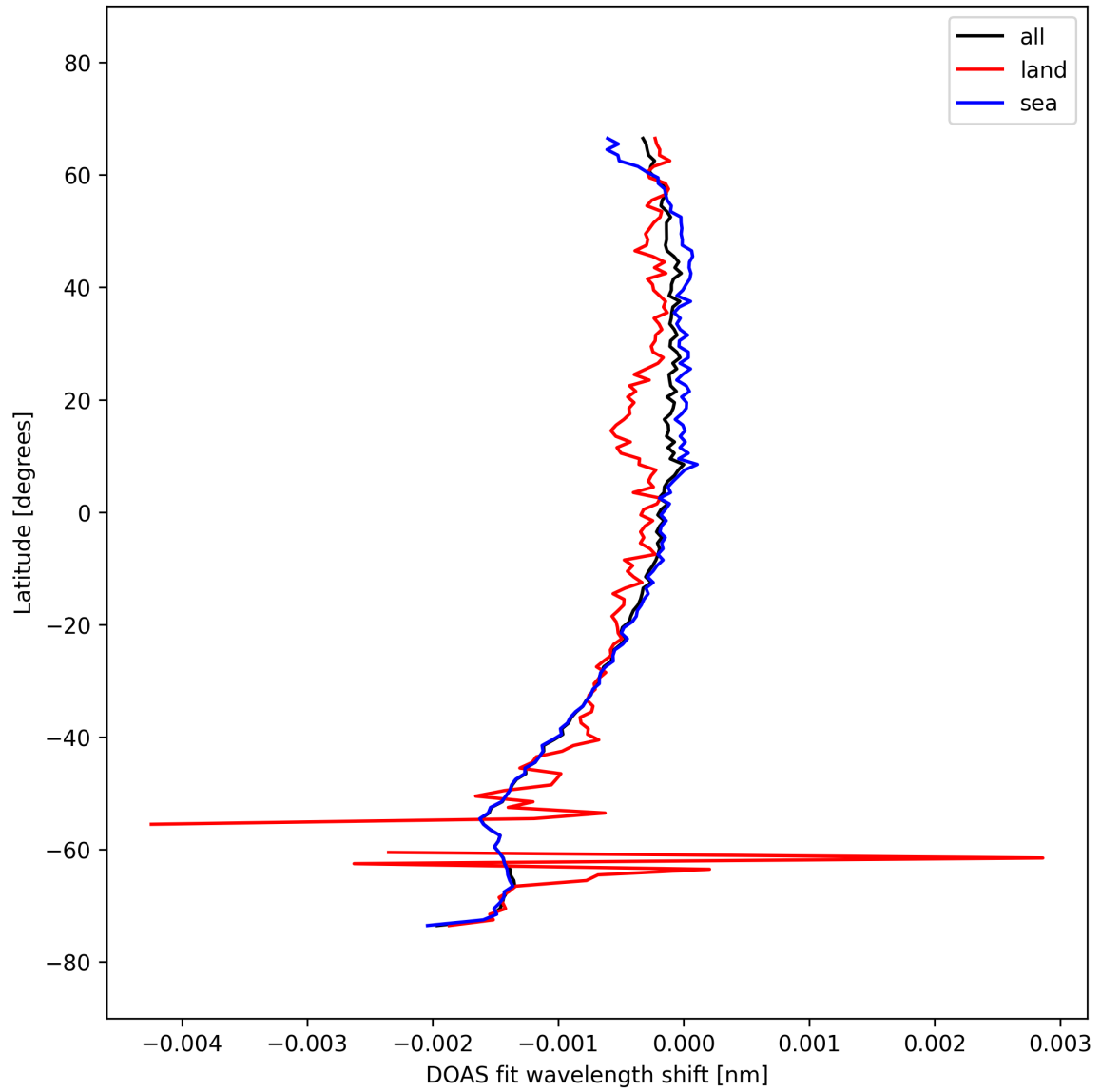
Figure 50: Zonal average of "DOAS fit wavelength shift" for 2025-10-01 to 2025-10-02.
