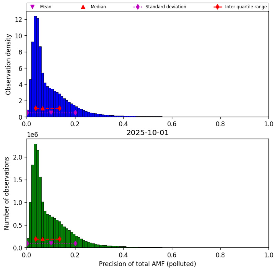
Figure 80: Histogram of “Precision of total AMF (polluted)” for 2025-10-01 to 2025-10-02
