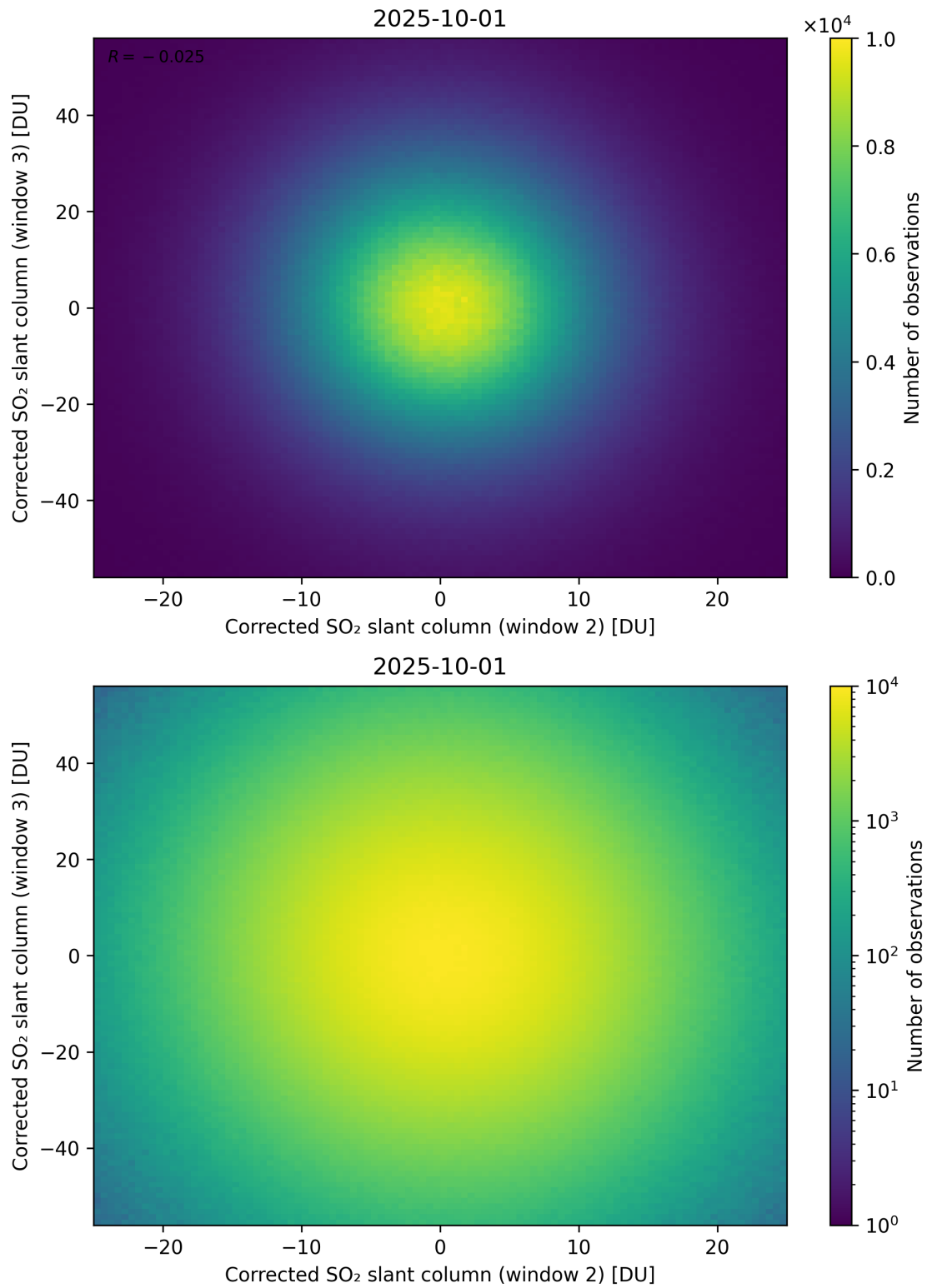
Figure 250: Scatter density plot of “Corrected SO 2 slant column (window 2)” against “Corrected SO 2 slant column (window 3)” for 2025-10-01 to 2025-10-02.
