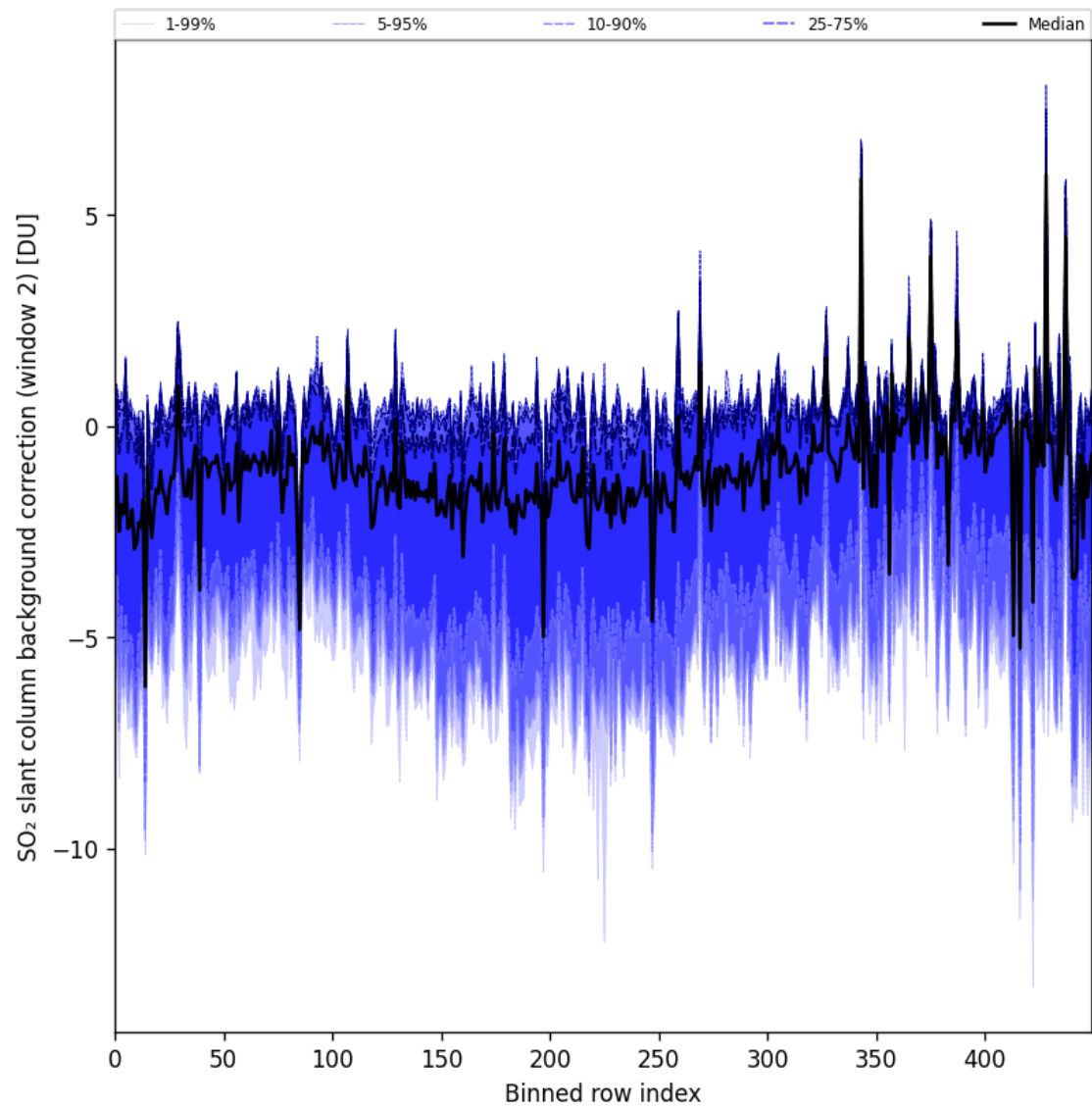
Figure 96: Along track statistics of “SO 2 slant column background correction (window 2)” for 2025-10-01 to 2025-10-02
