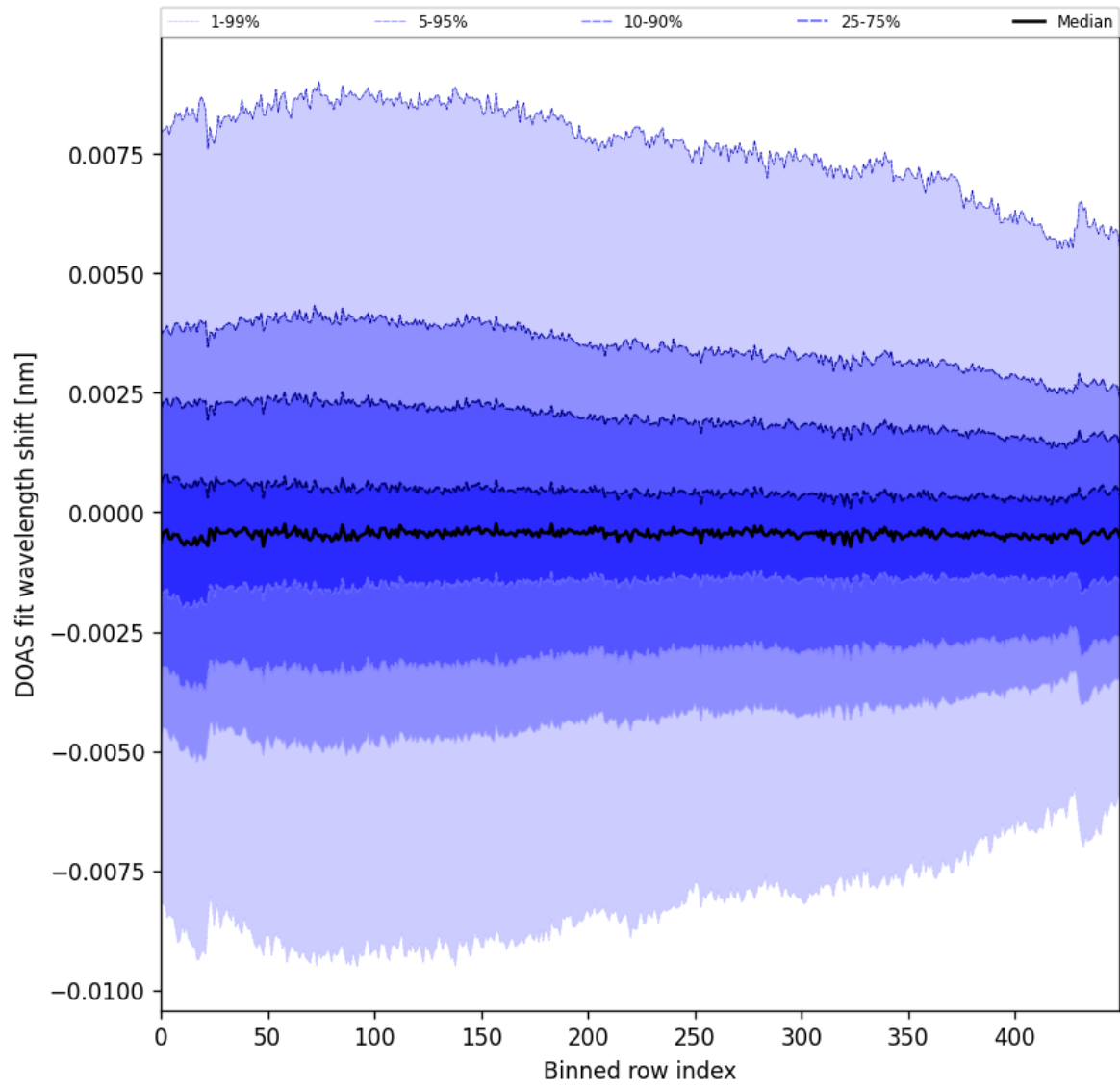
Figure 102: Along track statistics of “DOAS fit wavelength shift” for 2025-10-01 to 2025-10-02
