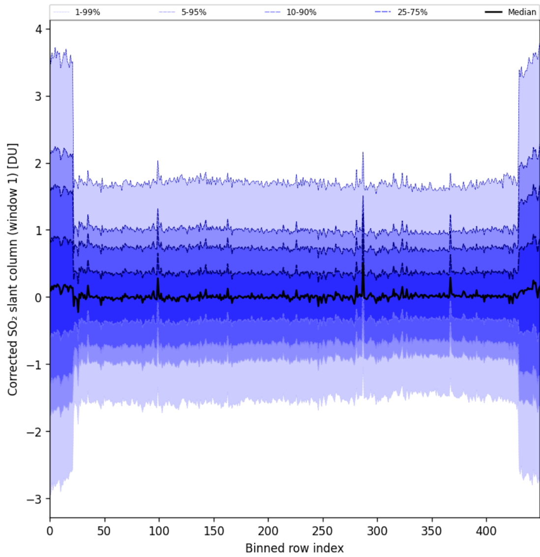
Figure 91: Along track statistics of “Corrected SO 2 slant column (window 1)” for 2025-10-01 to 2025-10-02
