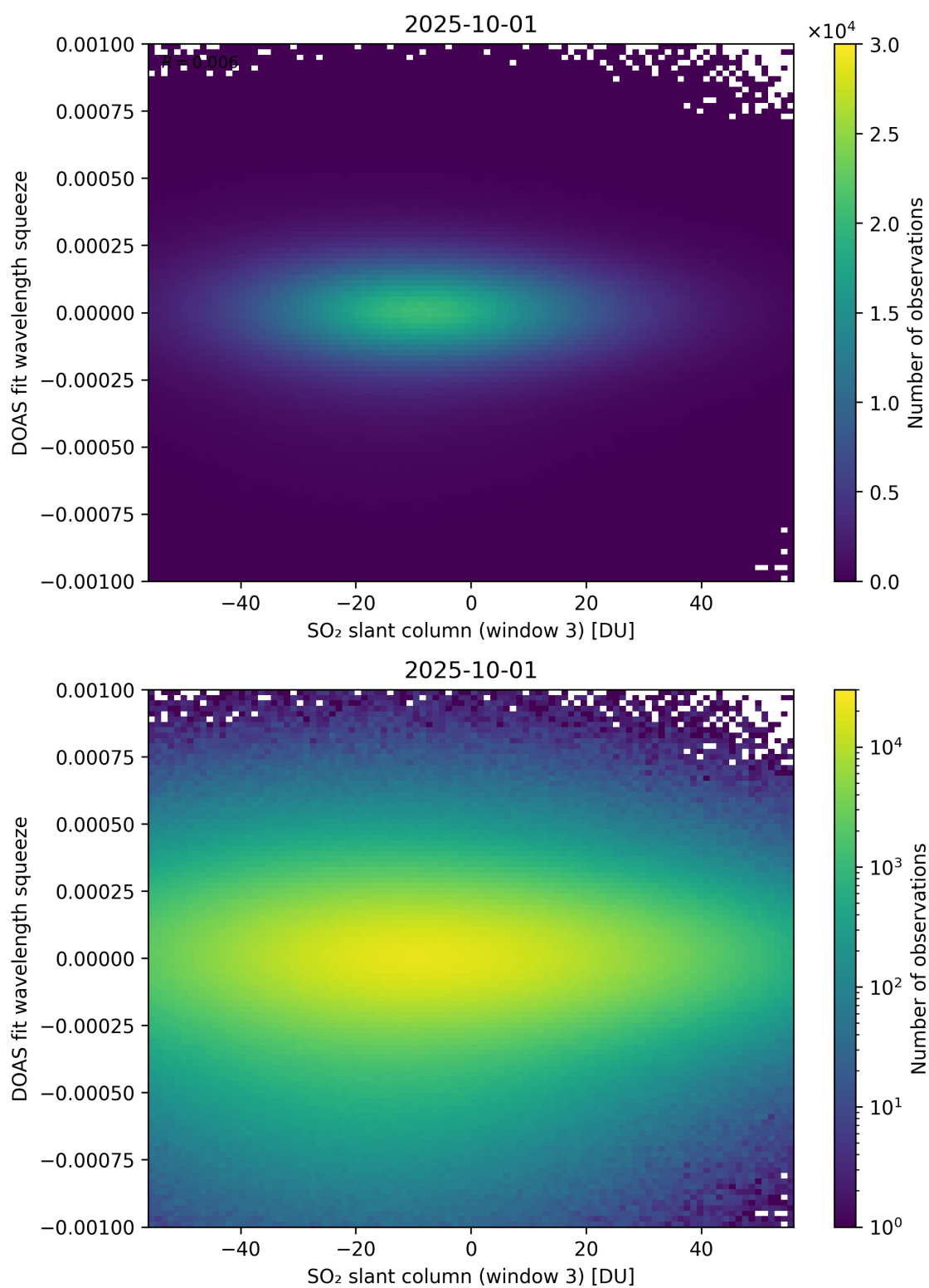
Figure 305: Scatter density plot of “SO 2 slant column (window 3)” against “DOAS fit wavelength squeeze” for 2025-10-01 to 2025-10-02.
