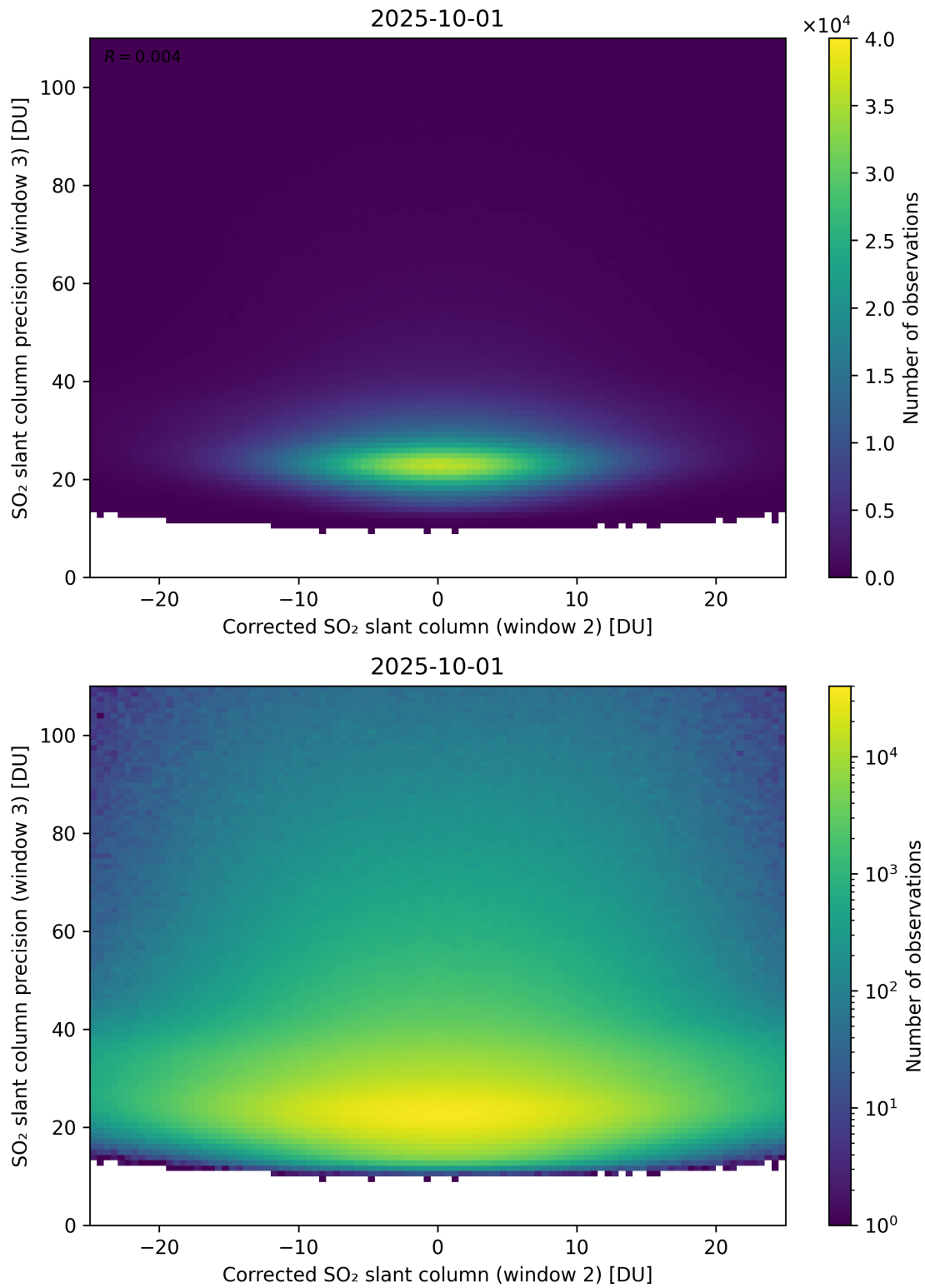
Figure 252: Scatter density plot of “Corrected SO 2 slant column (window 2)” against “SO 2 slant column precision (window 3)” for 2025-10-01 to 2025-10-02.
