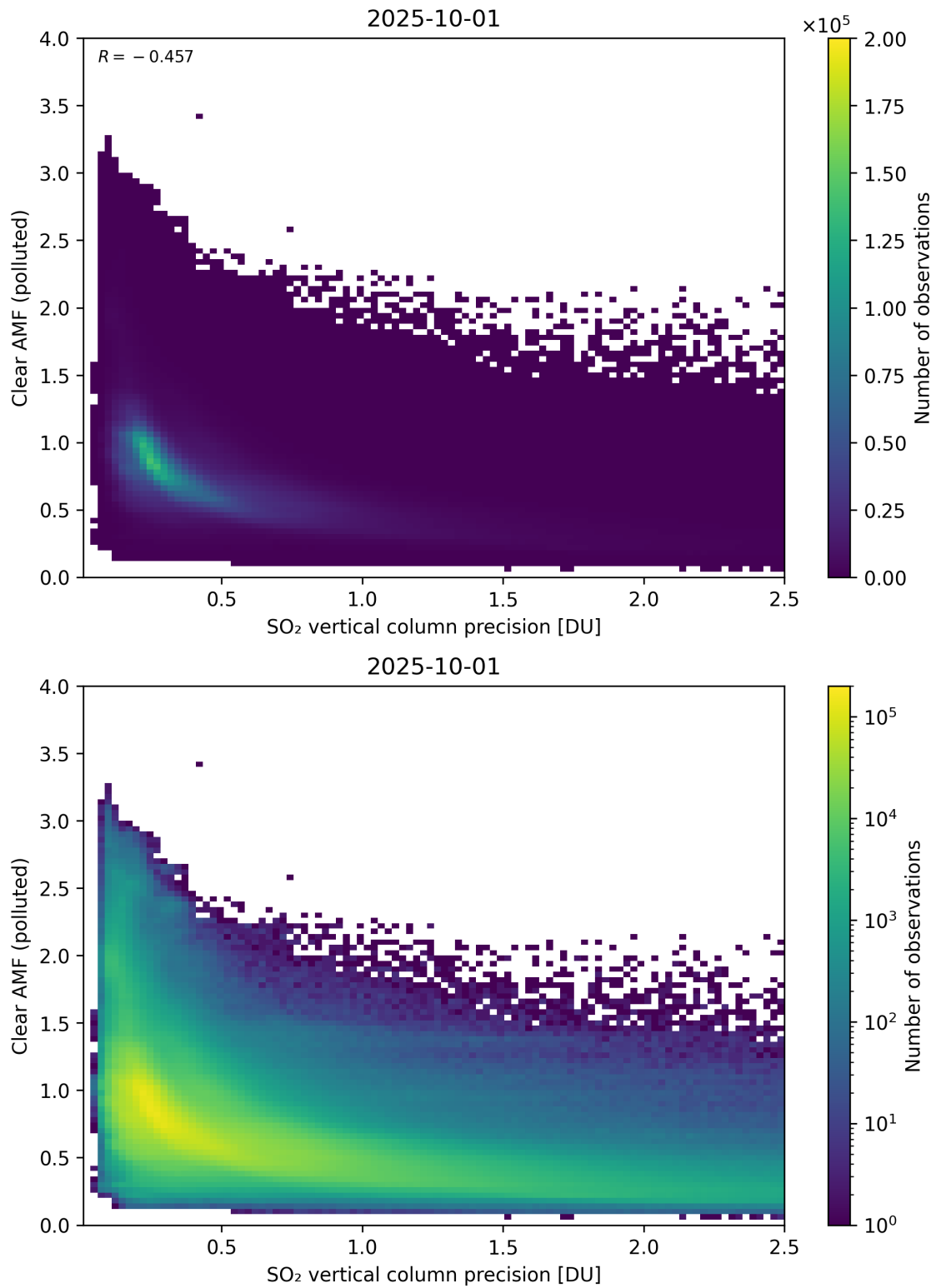
Figure 335: Scatter density plot of “SO 2 vertical column precision” against “Clear AMF (polluted)” for 2025-10-01 to 2025-10-02.
