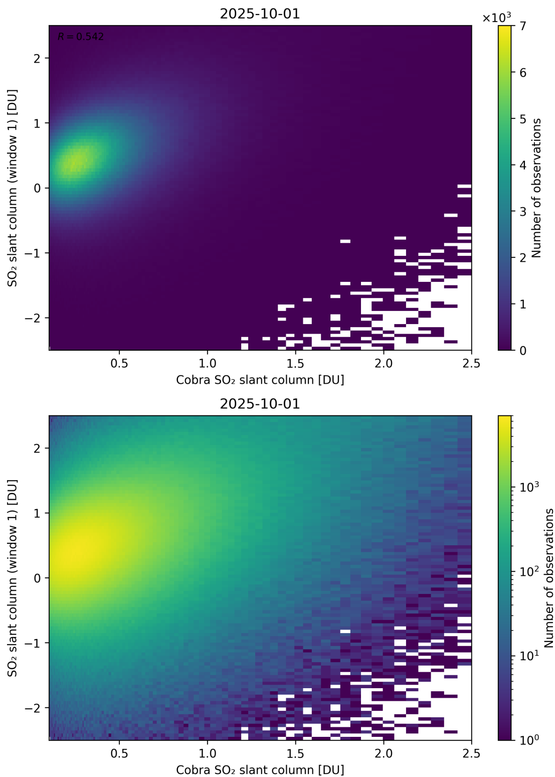
Figure 219: Scatter density plot of “Cobra SO 2 slant column” against “SO 2 slant column (window 1)” for 2025-10-01 to 2025-10-02.
