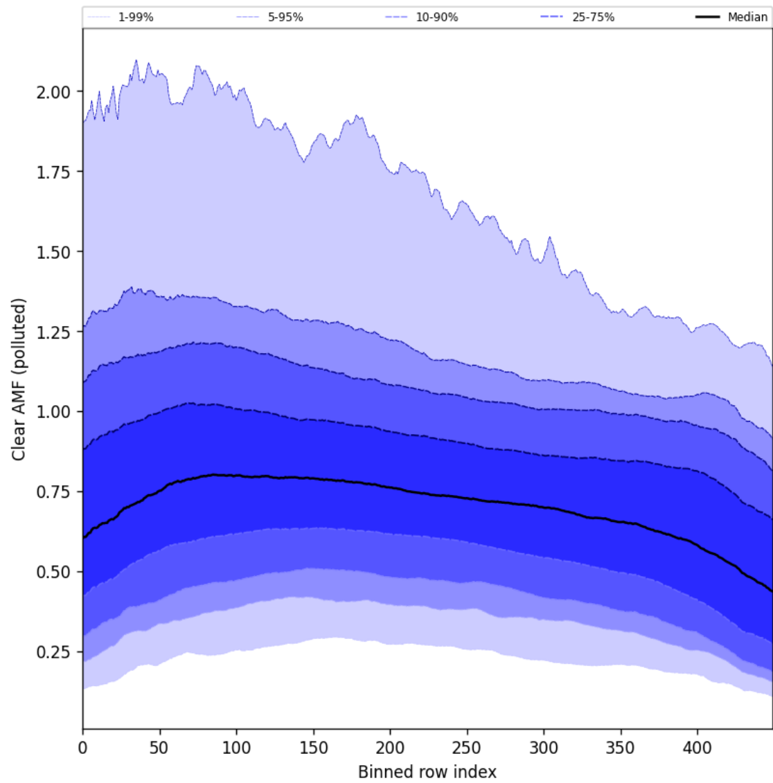
Figure 107: Along track statistics of “Clear AMF (polluted)” for 2025-10-01 to 2025-10-02
