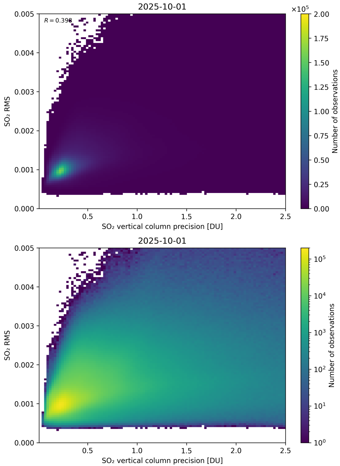
Figure 334: Scatter density plot of “SO 2 vertical column precision” against “SO 2 RMS” for 2025-10-01 to 2025-10-02.
