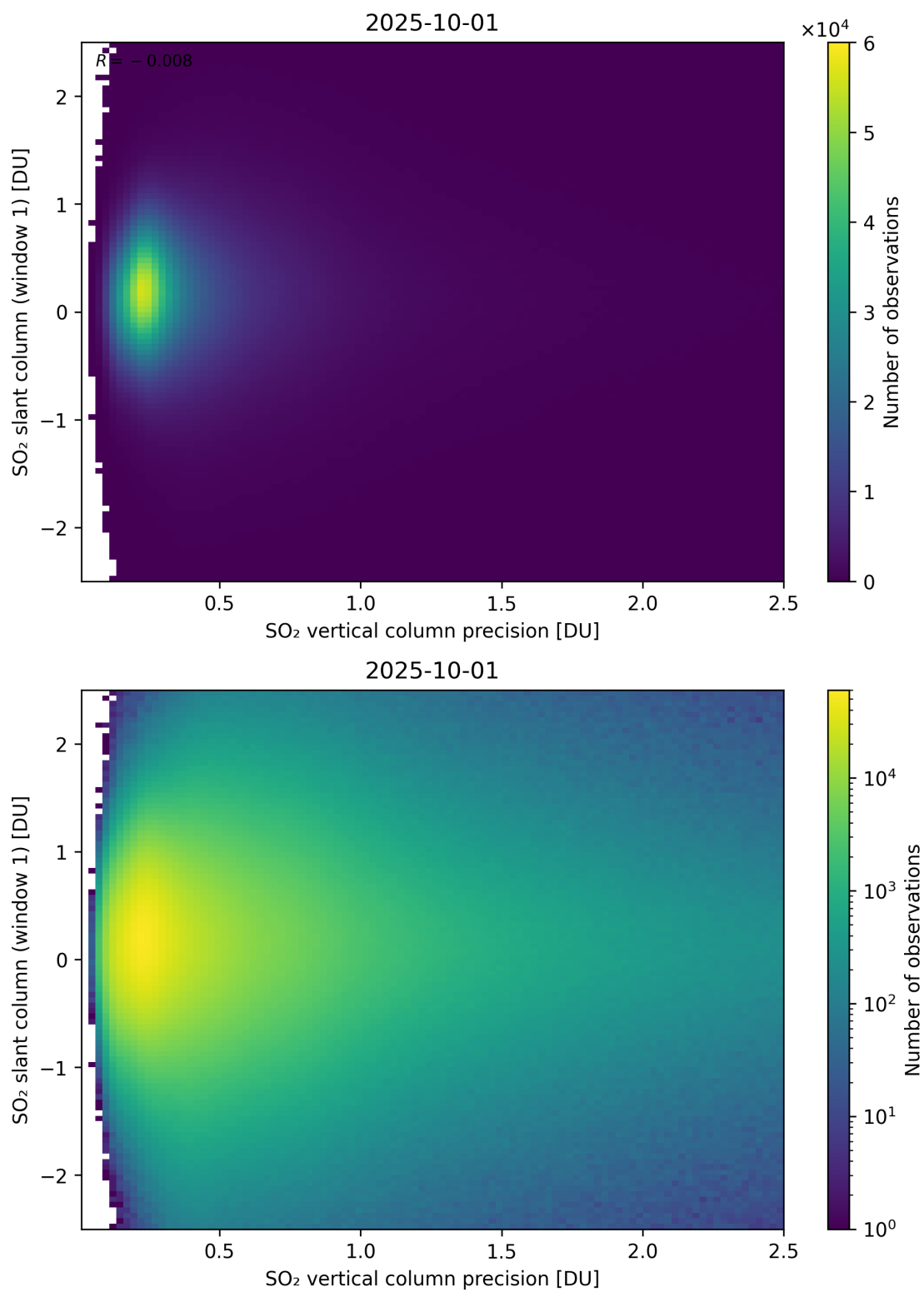
Figure 341: Scatter density plot of “SO 2 vertical column precision” against “SO 2 slant column (window 1)” for 2025-10-01 to 2025-10-02.
