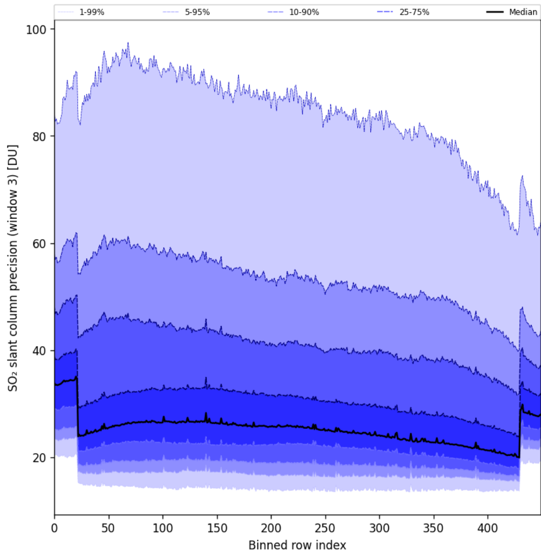
Figure 98: Along track statistics of “SO 2 slant column precision (window 3)” for 2025-10-01 to 2025-10-02
