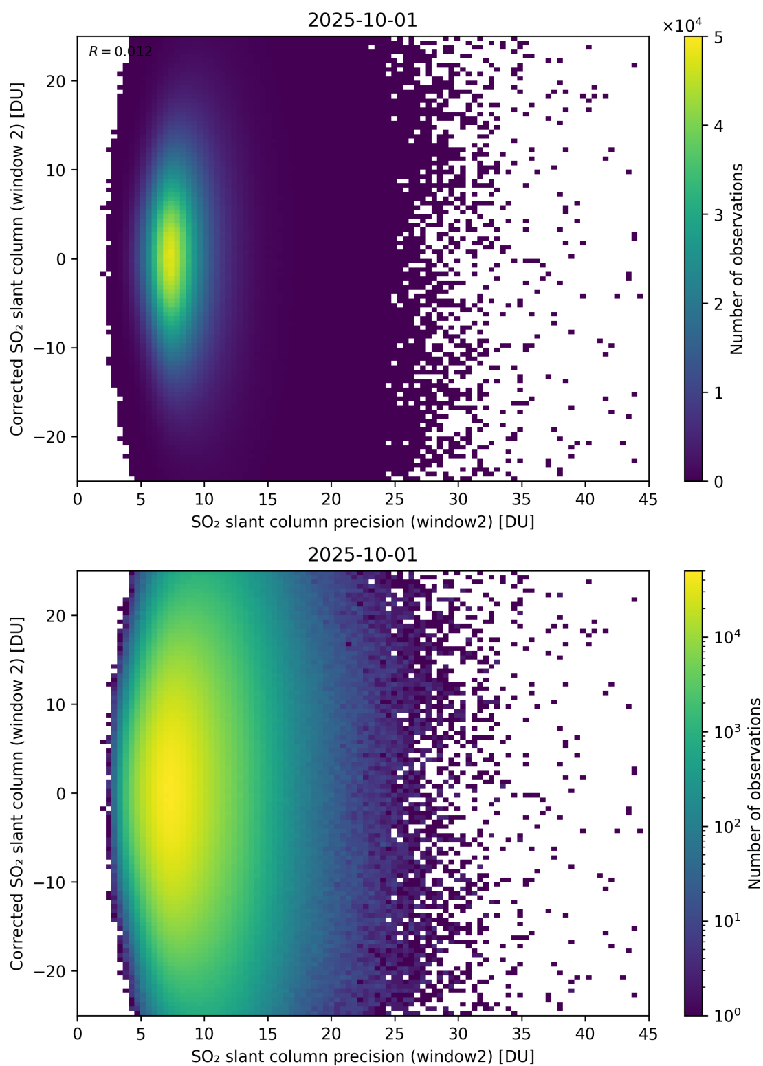
Figure 297: Scatter density plot of “SO 2 slant column precision (window2)” against “Corrected SO 2 slant column (window 2)” for 2025-10-01 to 2025-10-02.
