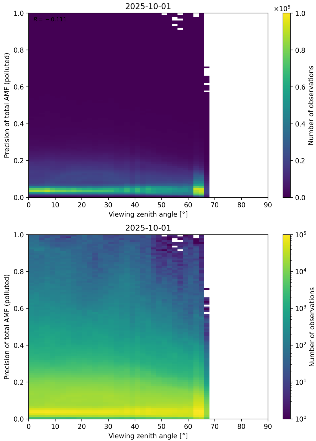
Figure 382: Scatter density plot of “Viewing zenith angle” against “Precision of total AMF (polluted)” for 2025-10-01 to 2025-10-02.
