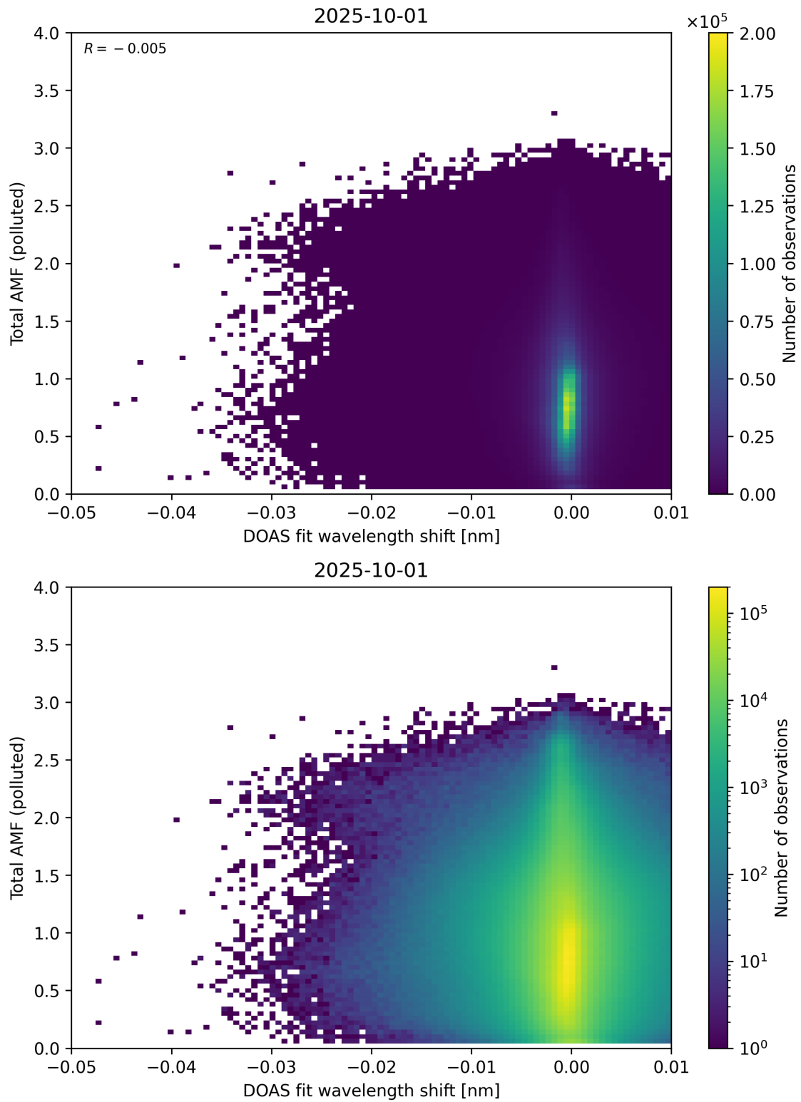
Figure 141: Scatter density plot of “DOAS fit wavelength shift” against “Total AMF (polluted)” for 2025-10-01 to 2025-10-02.
