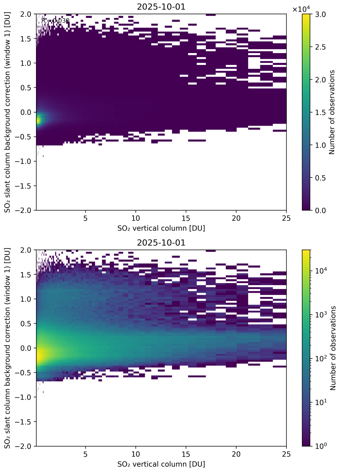
Figure 323: Scatter density plot of “SO 2 vertical column” against “SO 2 slant column background correction (window 1)” for 2025-10-01 to 2025-10-02.
