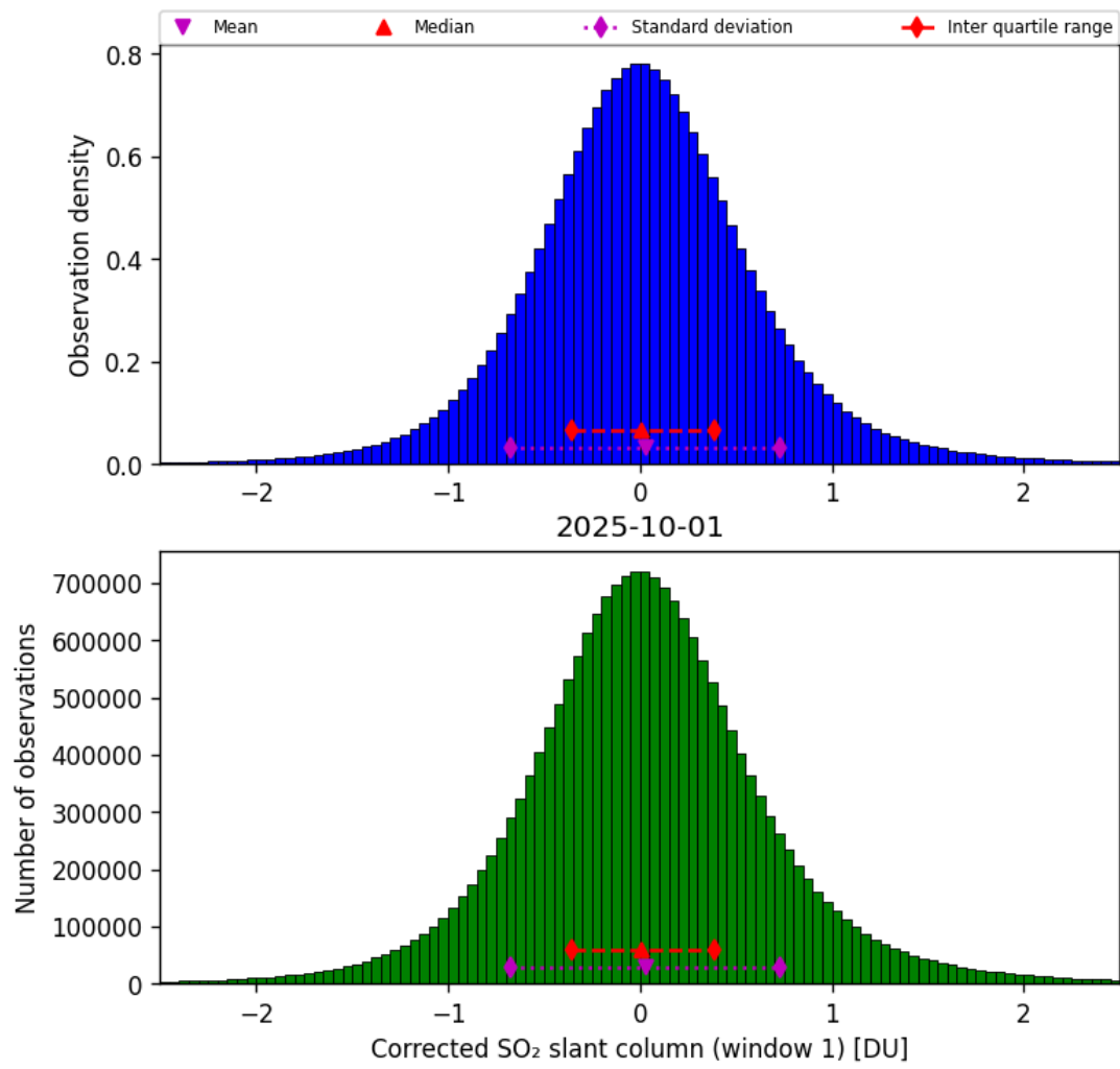
Figure 65: Histogram of “Corrected SO 2 slant column (window 1)” for 2025-10-01 to 2025-10-02
