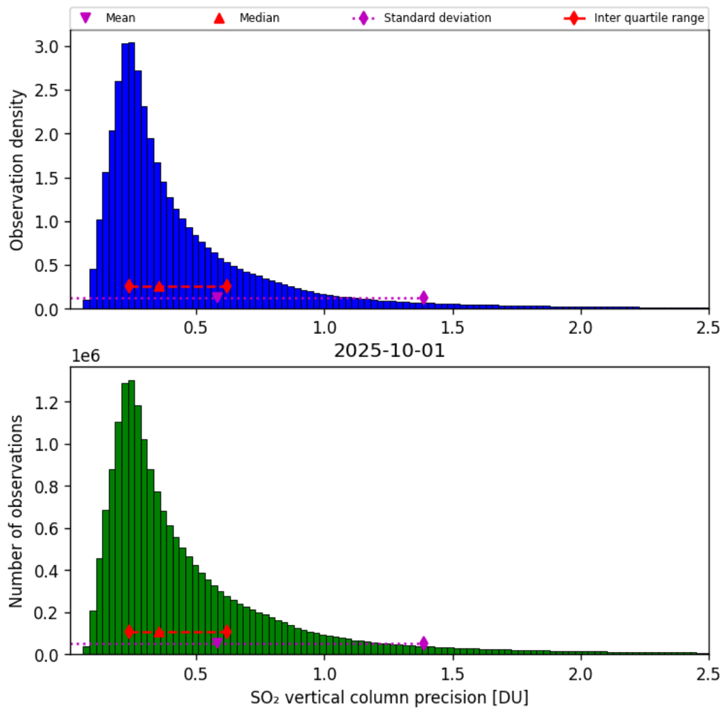
Figure 59: Histogram of “SO 2 vertical column precision” for 2025-10-01 to 2025-10-02
