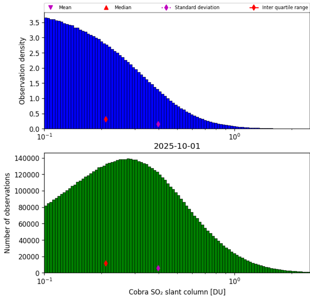
Figure 61: Histogram of “Cobra SO 2 slant column” for 2025-10-01 to 2025-10-02
