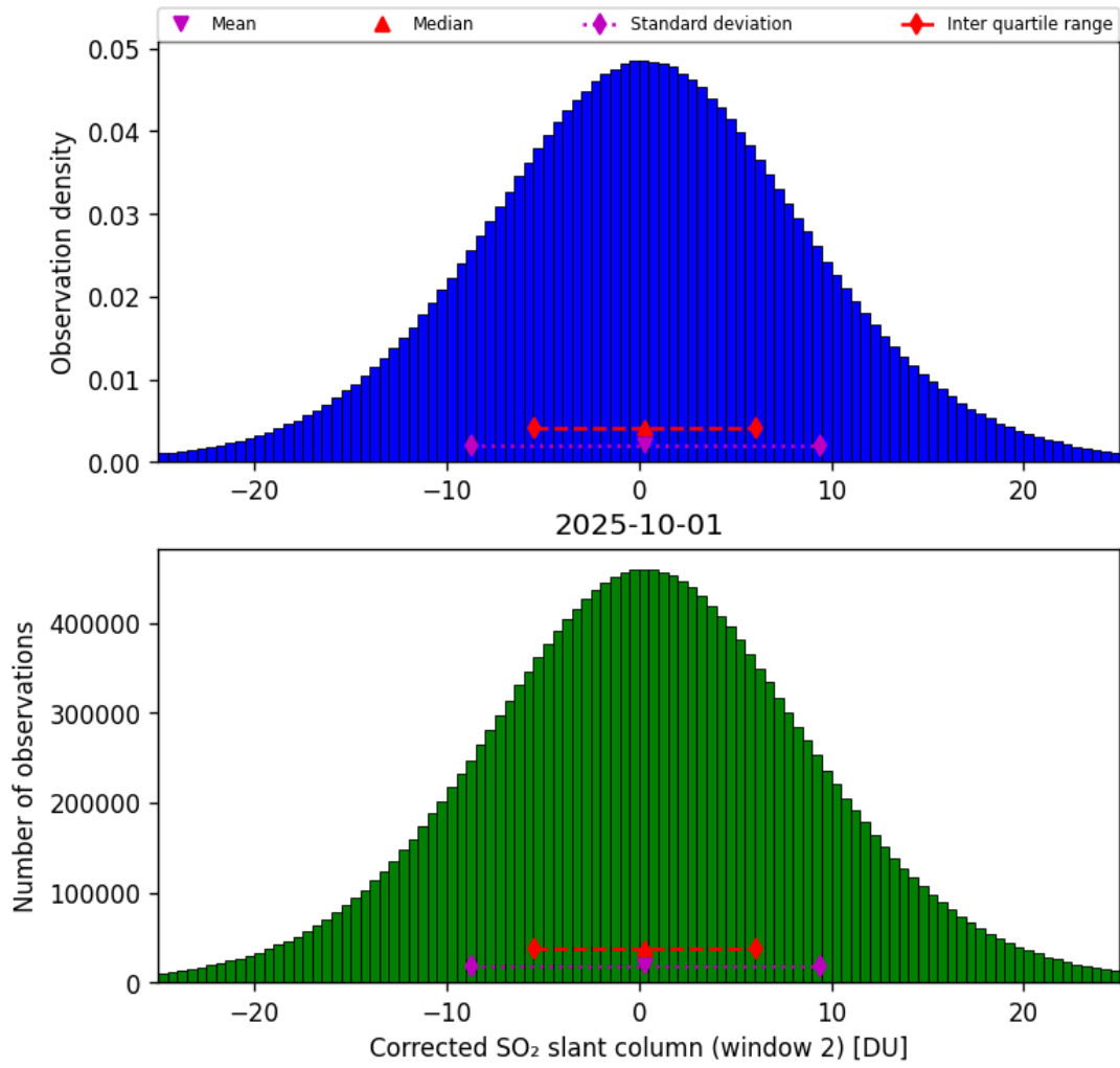
Figure 69: Histogram of “Corrected SO 2 slant column (window 2)” for 2025-10-01 to 2025-10-02
