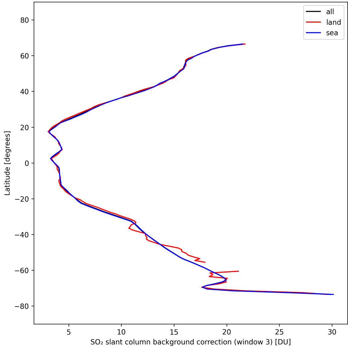
Figure 48: Zonal average of “SO 2 slant column background correction (window 3)” for 2025-10-01 to 2025-10-02.
