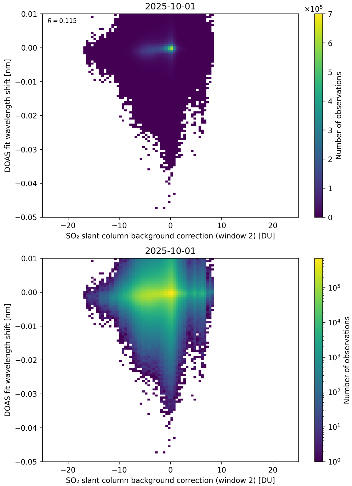
Figure 123: Scatter density plot of “SO 2 slant column background correction (window 2)” against “DOAS fit wavelength shift” for 2025-10-01 to 2025-10-02.
