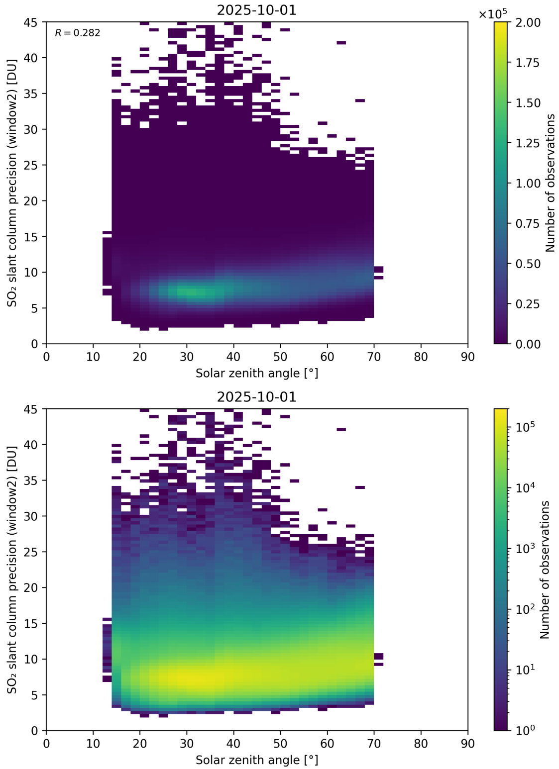
Figure 186: Scatter density plot of “Solar zenith angle” against “SO 2 slant column precision (window2)” for 2025-10-01 to 2025-10-02.
