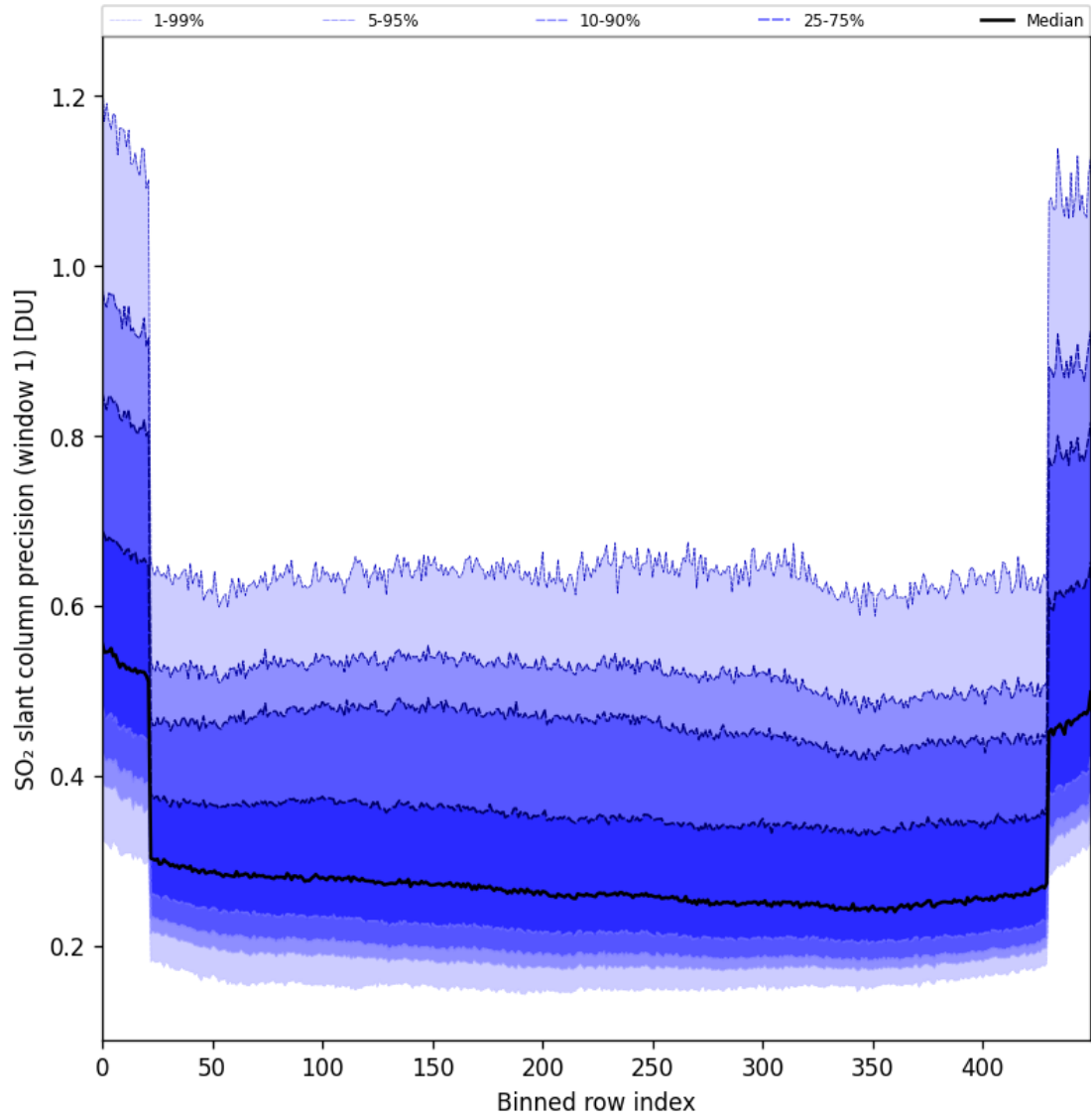
Figure 90: Along track statistics of “SO 2 slant column precision (window 1)” for 2025-10-01 to 2025-10-02
