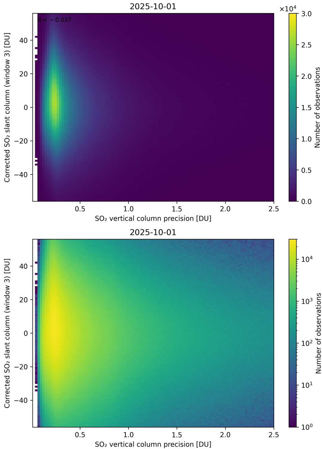
Figure 340: Scatter density plot of “SO 2 vertical column precision” against “Corrected SO 2 slant column (window 3)” for 2025-10-01 to 2025-10-02.
