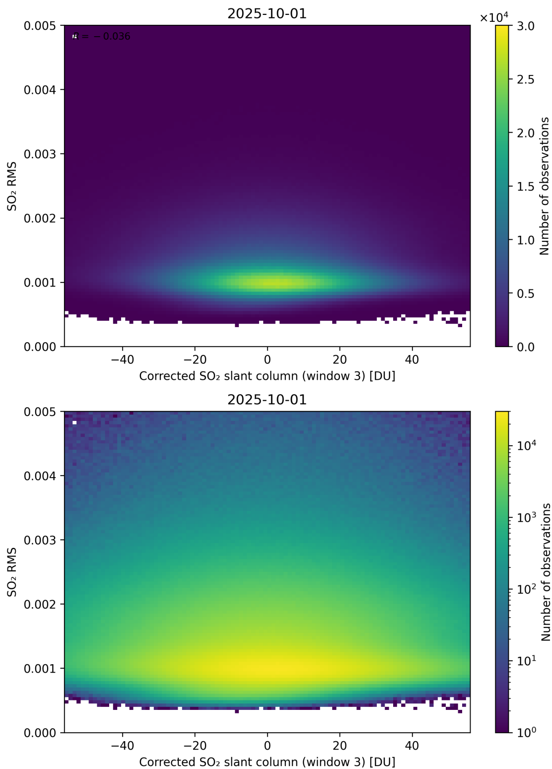
Figure 258: Scatter density plot of “Corrected SO 2 slant column (window 3)” against “SO 2 RMS” for 2025-10-01 to 2025-10-02.
