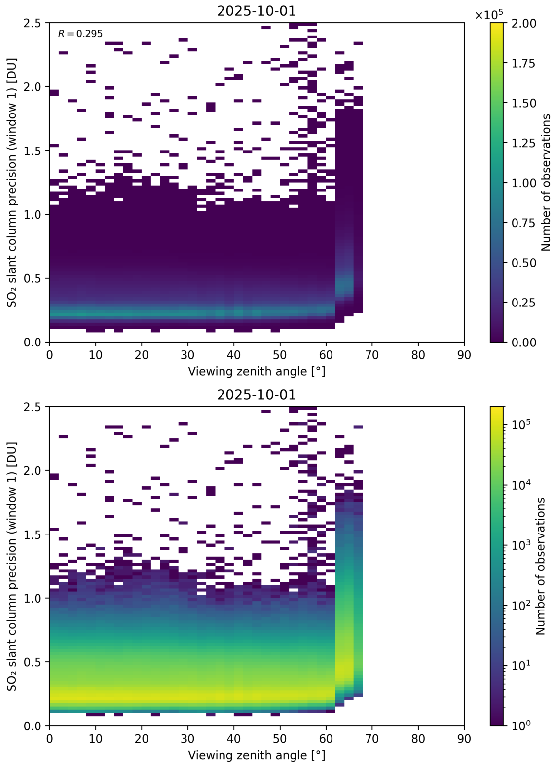
Figure 377: Scatter density plot of “Viewing zenith angle” against “SO 2 slant column precision (window 1)” for 2025-10-01 to 2025-10-02.
