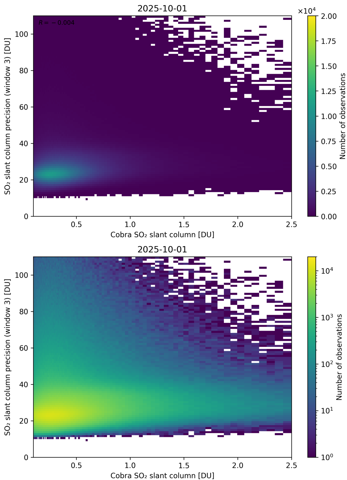
Figure 223: Scatter density plot of “Cobra SO 2 slant column” against “SO 2 slant column precision (window 3)” for 2025-10-01 to 2025-10-02.
