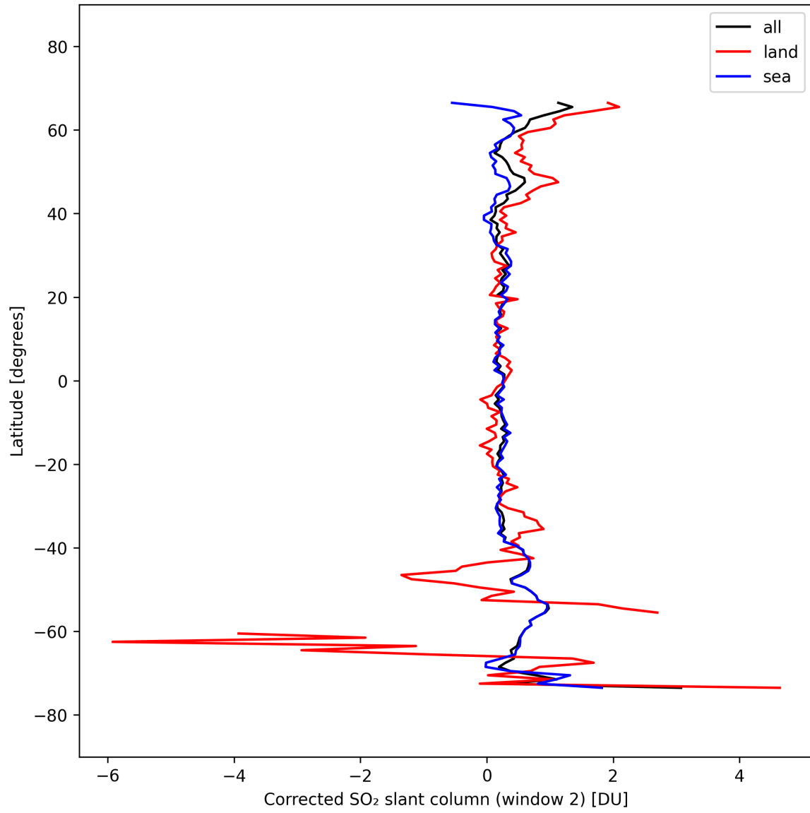
Figure 43: Zonal average of “Corrected SO 2 slant column (window 2)” for 2025-10-01 to 2025-10-02.
