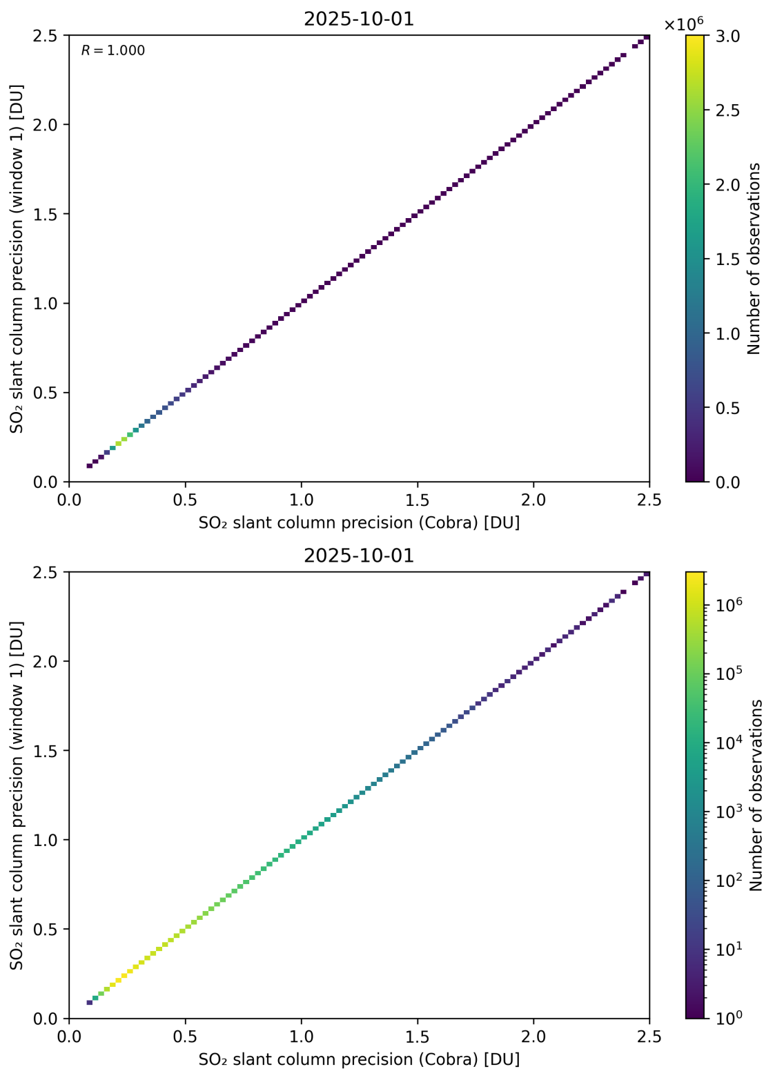
Figure 209: Scatter density plot of “SO 2 slant column precision (Cobra)” against “SO 2 slant column precision (window 1)” for 2025-10-01 to 2025-10-02.
