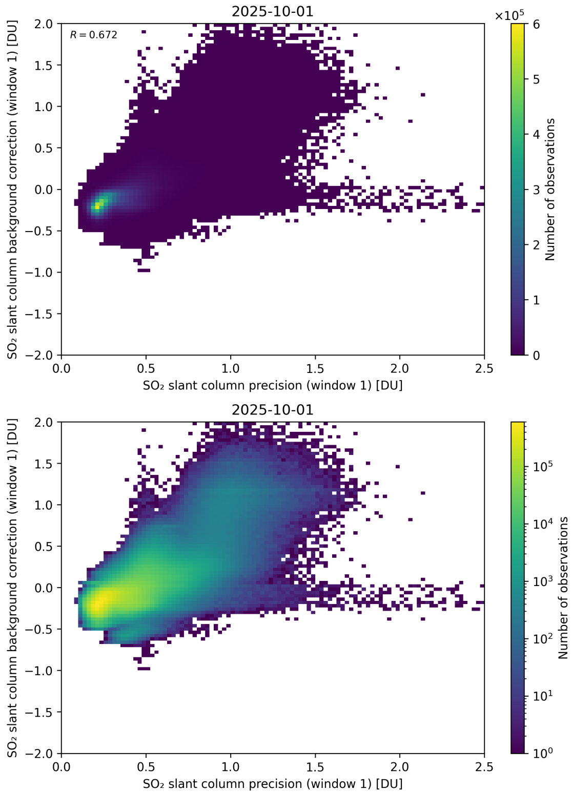
Figure 268: Scatter density plot of “SO 2 slant column precision (window 1)” against “SO 2 slant column background correction (window 1)” for 2025-10-01 to 2025-10-02.
