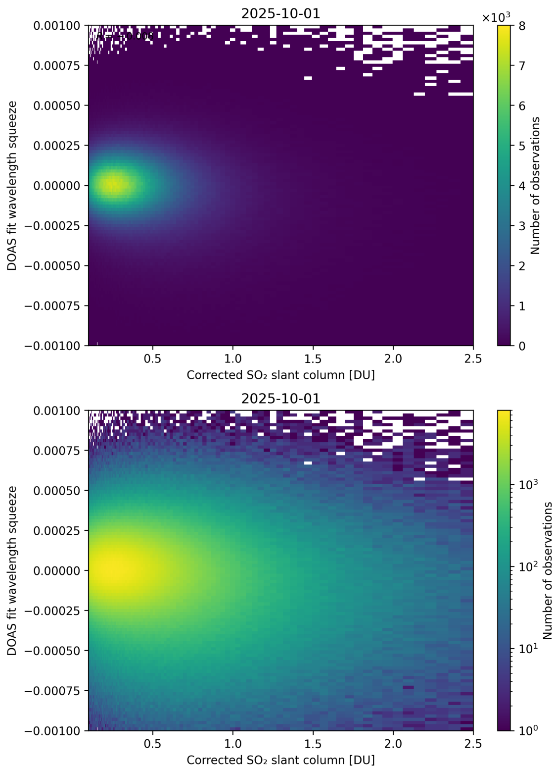
Figure 230: Scatter density plot of “Corrected SO 2 slant column” against “DOAS fit wavelength squeeze” for 2025-10-01 to 2025-10-02.
