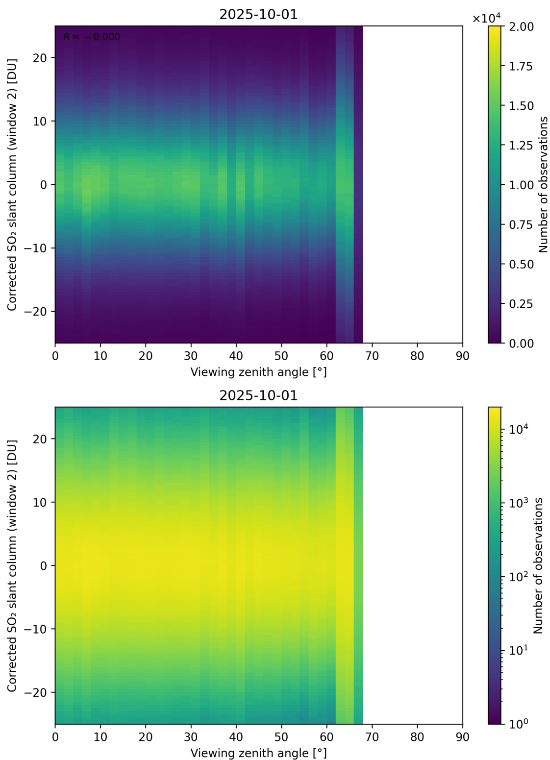
Figure 374: Scatter density plot of “Viewing zenith angle” against “Corrected SO 2 slant column (window 2)” for 2025-10-01 to 2025-10-02.
