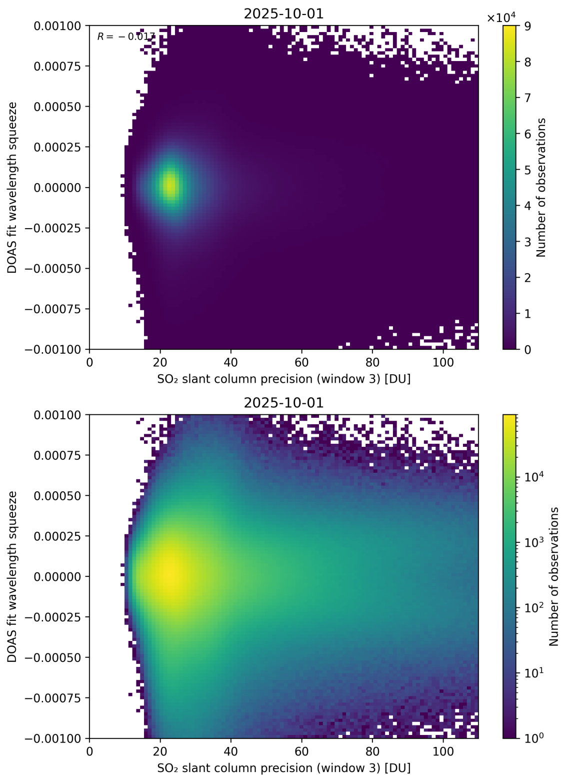
Figure 309: Scatter density plot of “SO 2 slant column precision (window 3)” against “DOAS fit wavelength squeeze” for 2025-10-01 to 2025-10-02.
