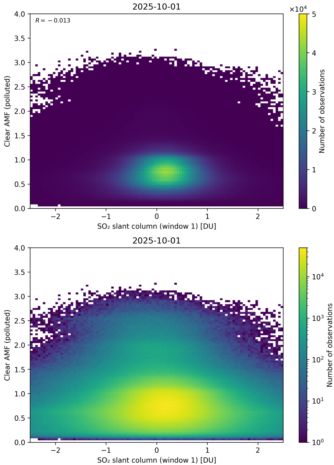
Figure 282: Scatter density plot of “SO 2 slant column (window 1)” against “Clear AMF (polluted)” for 2025-10-01 to 2025-10-02.
