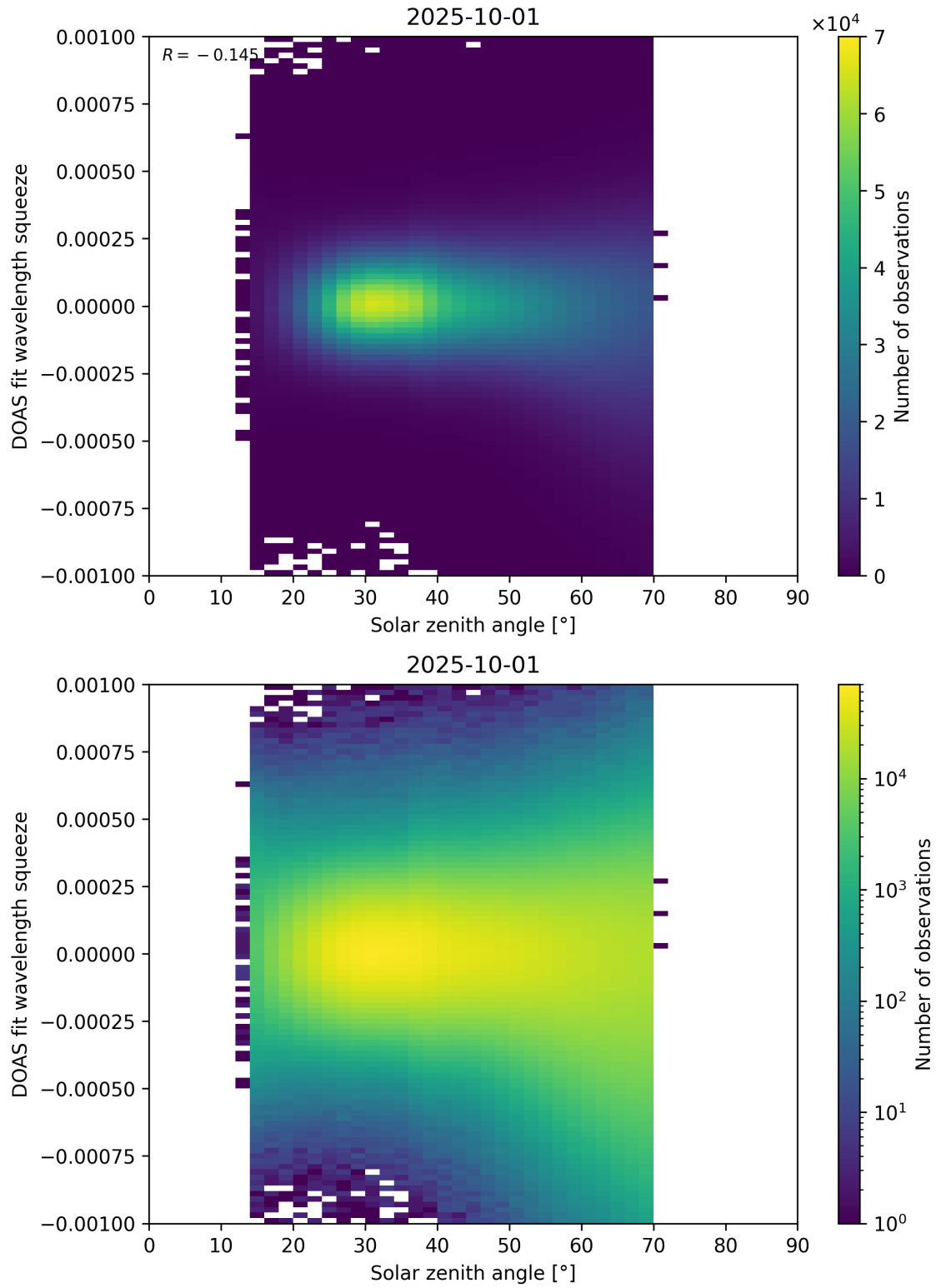
Figure 175: Scatter density plot of “Solar zenith angle” against “DOAS fit wavelength squeeze” for 2025-10-01 to 2025-10-02.
