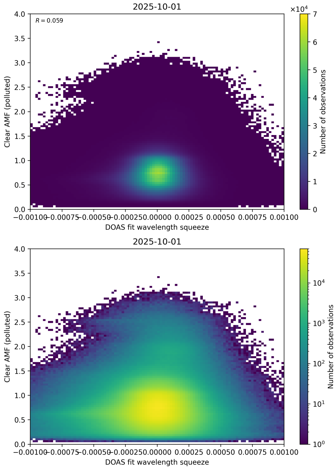
Figure 144: Scatter density plot of “DOAS fit wavelength squeeze” against “Clear AMF (polluted)” for 2025-10-01 to 2025-10-02.
