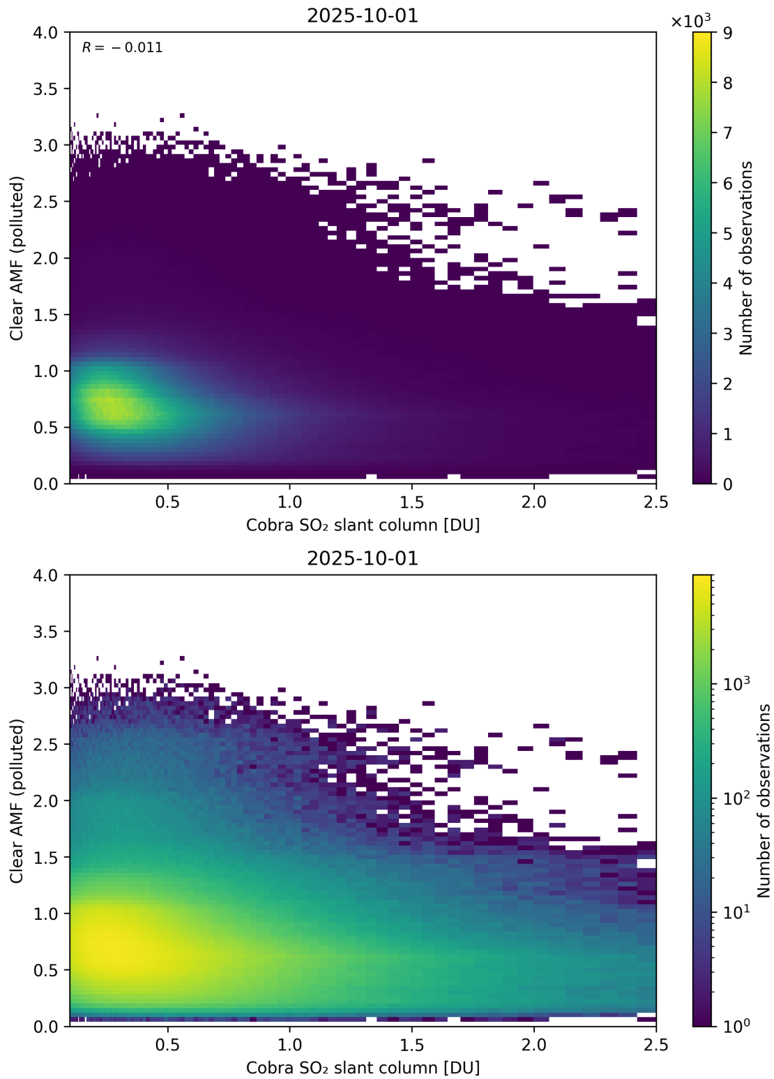
Figure 215: Scatter density plot of “Cobra SO 2 slant column” against “Clear AMF (polluted)” for 2025-10-01 to 2025-10-02.
