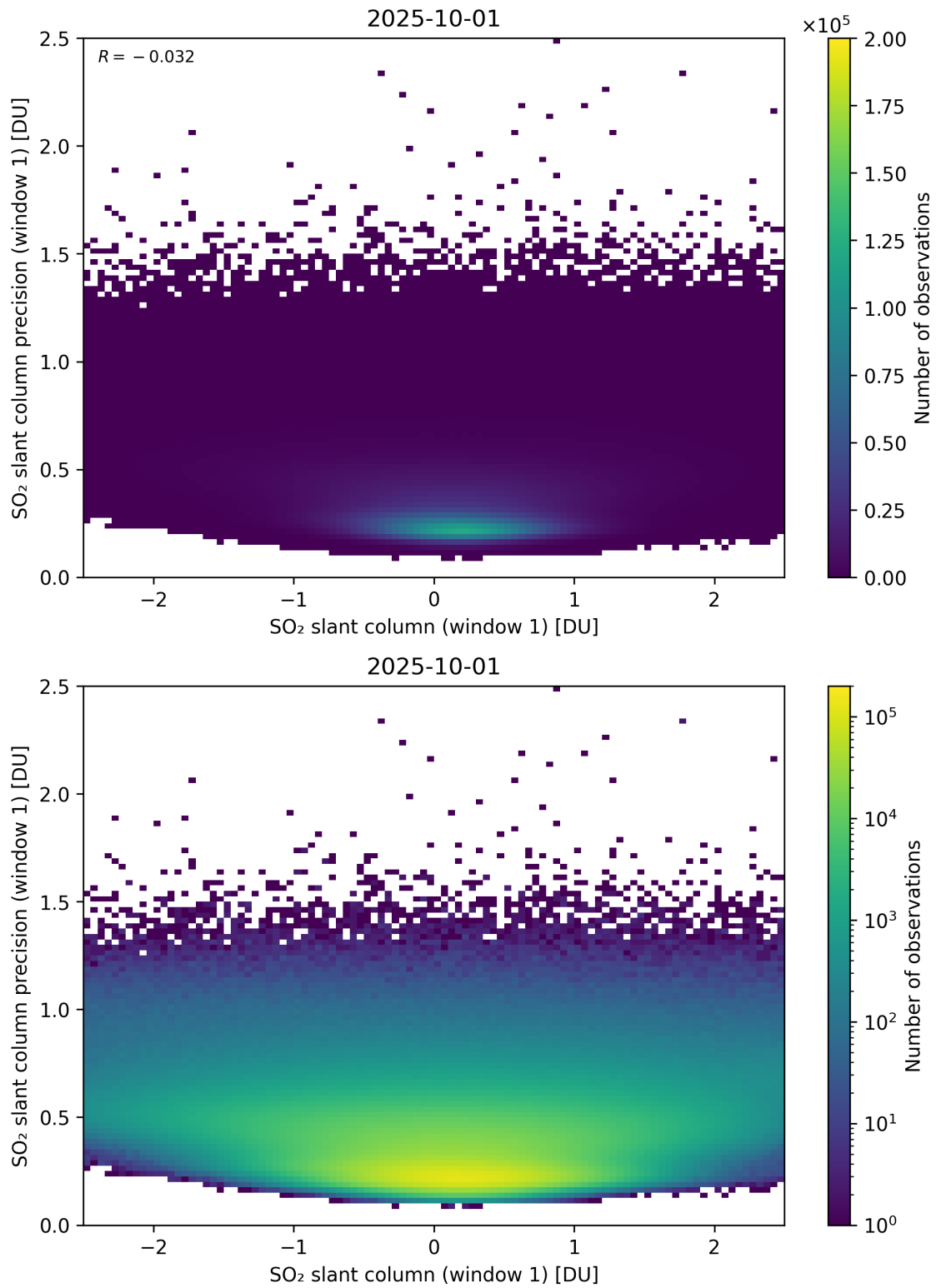
Figure 285: Scatter density plot of “SO 2 slant column (window 1)” against “SO 2 slant column precision (window 1)” for 2025-10-01 to 2025-10-02.
