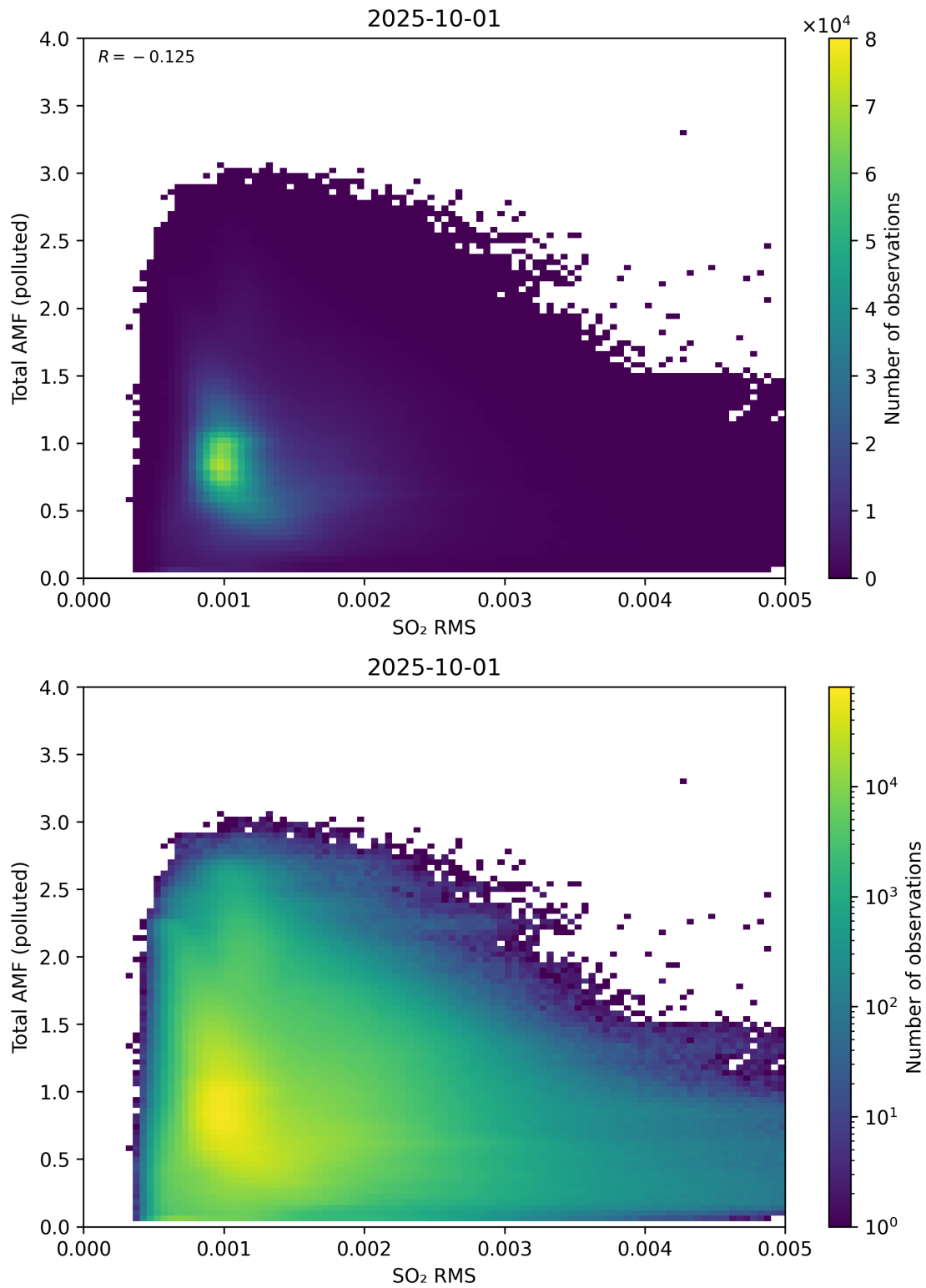
Figure 148: Scatter density plot of “SO 2 RMS” against “Total AMF (polluted)” for 2025-10-01 to 2025-10-02.
