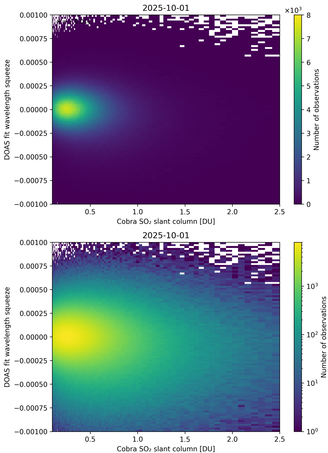
Figure 197: Scatter density plot of “Cobra SO 2 slant column” against “DOAS fit wavelength squeeze” for 2025-10-01 to 2025-10-02.
