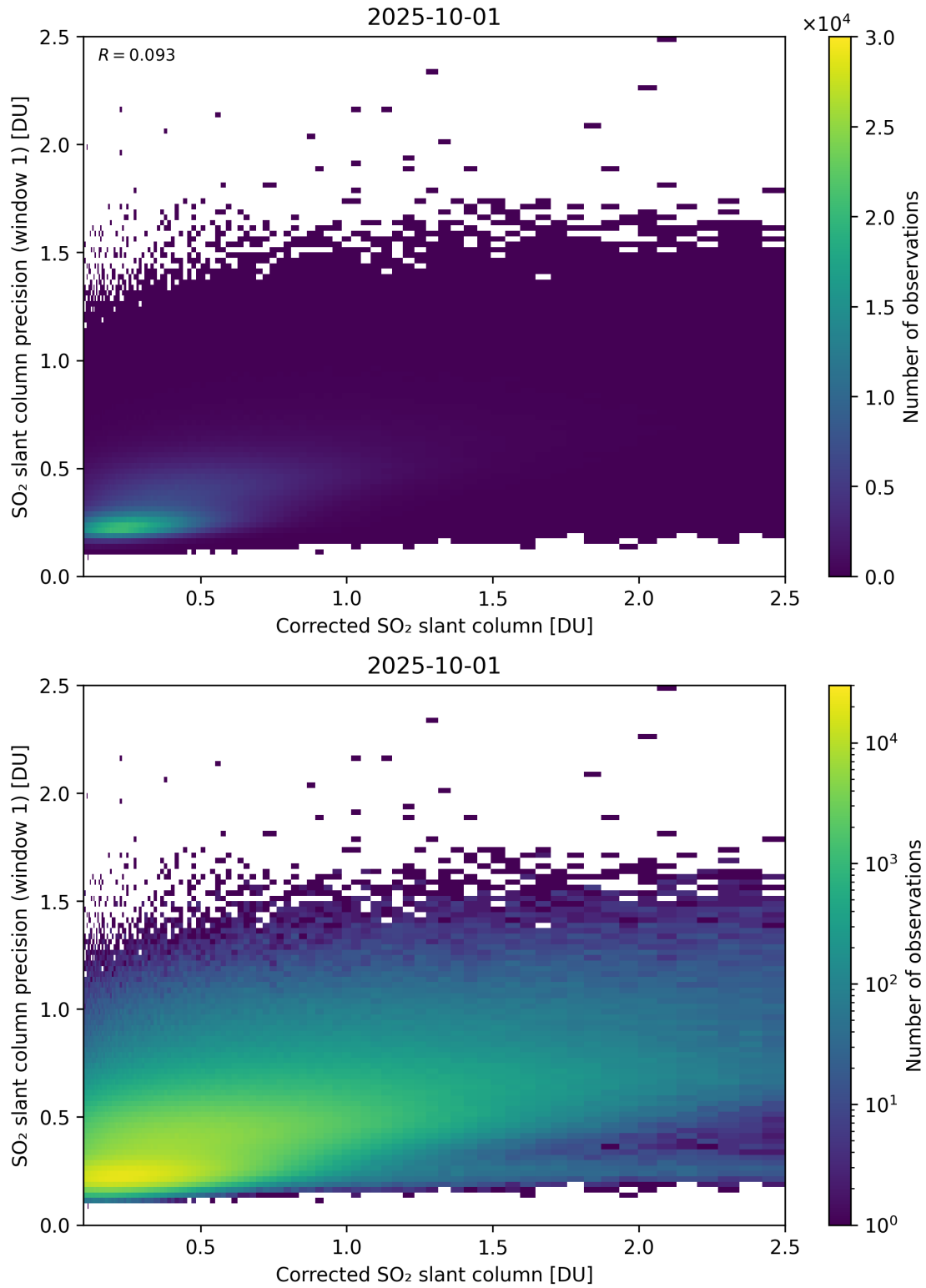
Figure 238: Scatter density plot of “Corrected SO 2 slant column” against “SO 2 slant column precision (window 1)” for 2025-10-01 to 2025-10-02.
