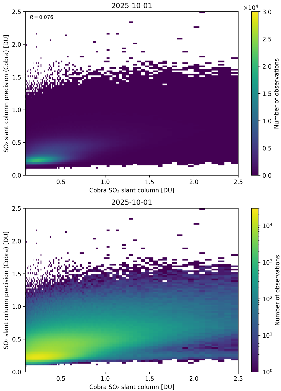
Figure 216: Scatter density plot of “Cobra SO 2 slant column” against “SO 2 slant column precision (Cobra)” for 2025-10-01 to 2025-10-02.
