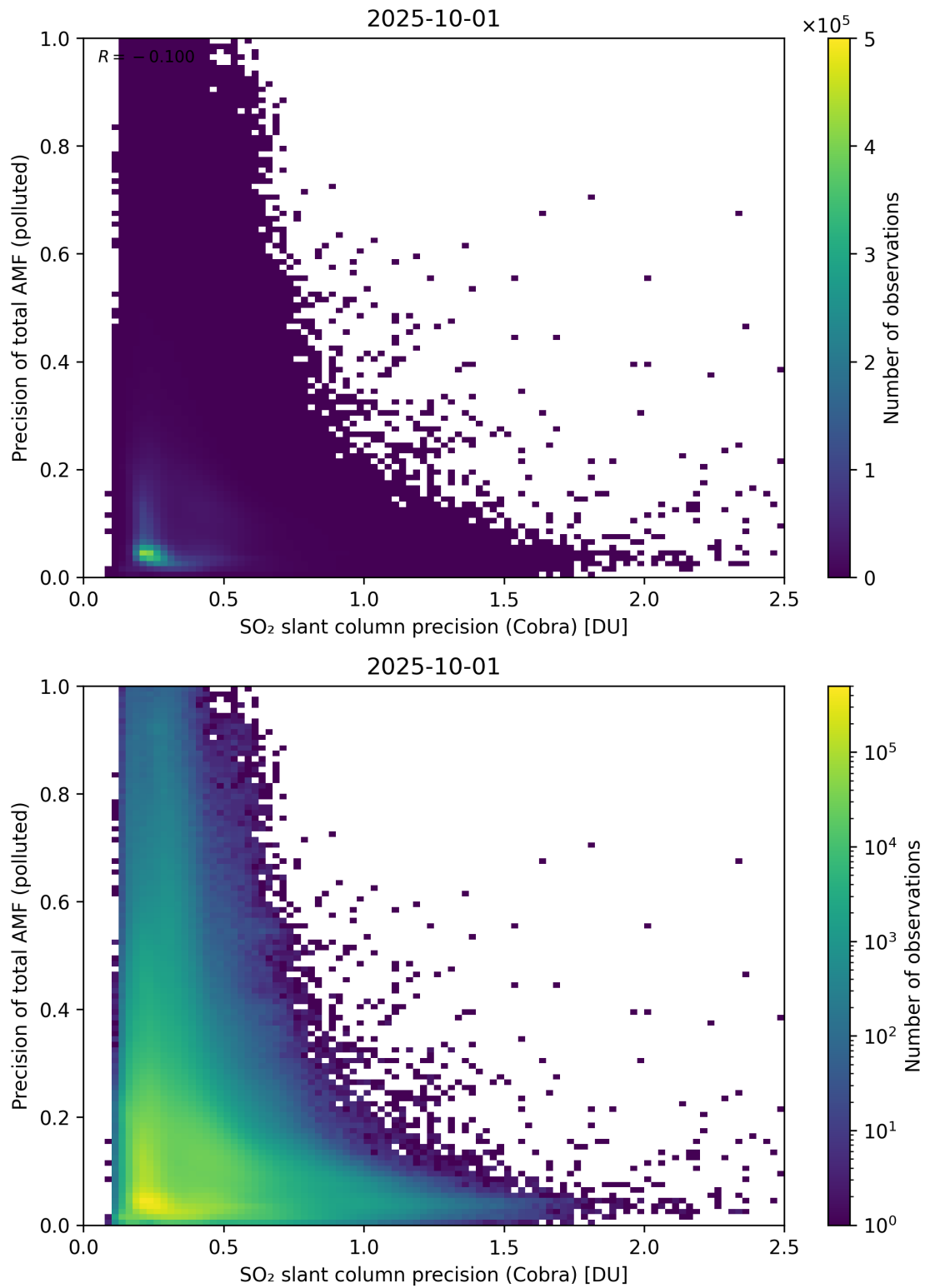
Figure 214: Scatter density plot of “SO 2 slant column precision (Cobra)” against “Precision of total AMF (polluted)” for 2025-10-01 to 2025-10-02.
