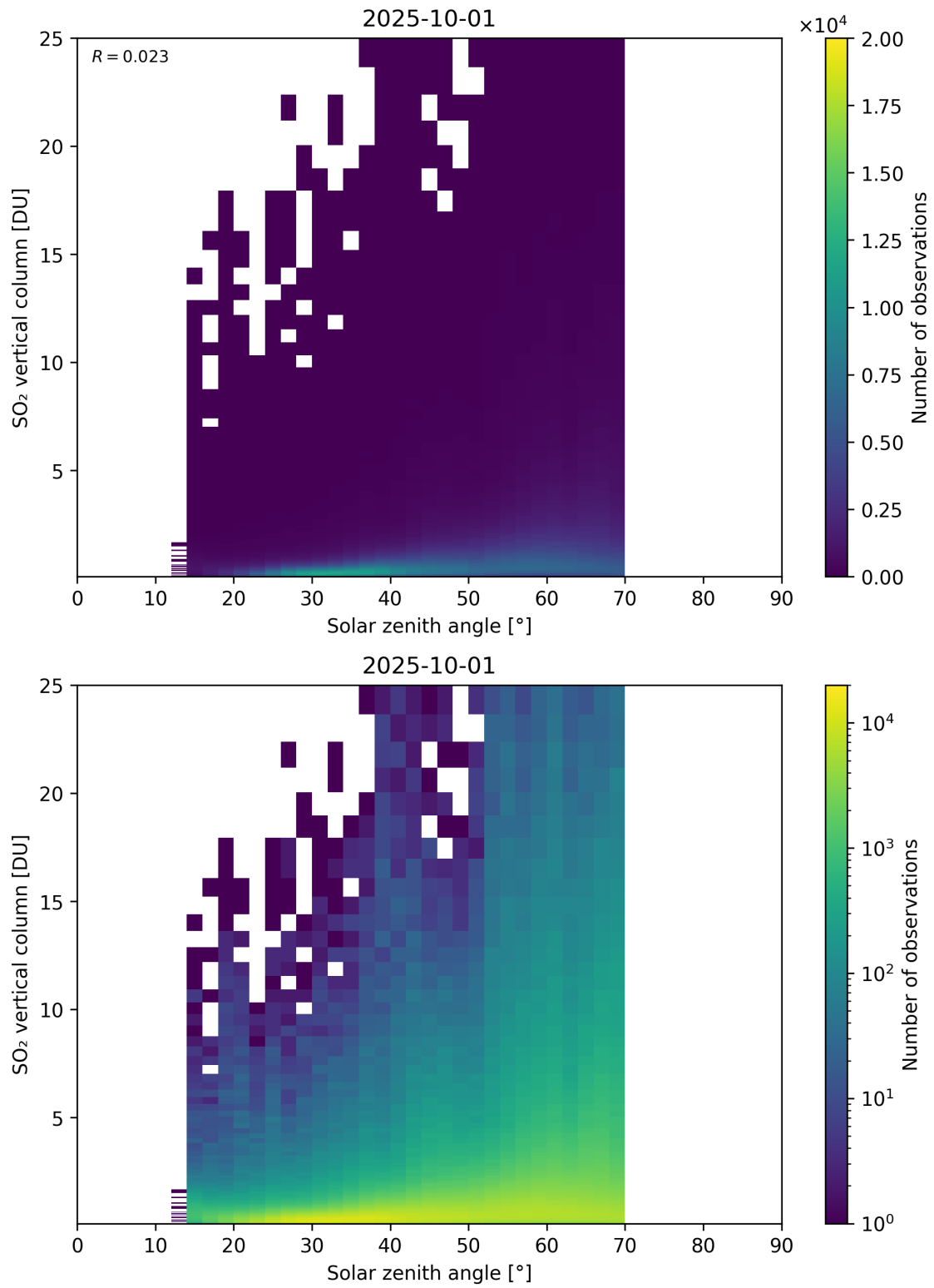
Figure 191: Scatter density plot of “Solar zenith angle” against “SO 2 vertical column” for 2025-10-01 to 2025-10-02.
