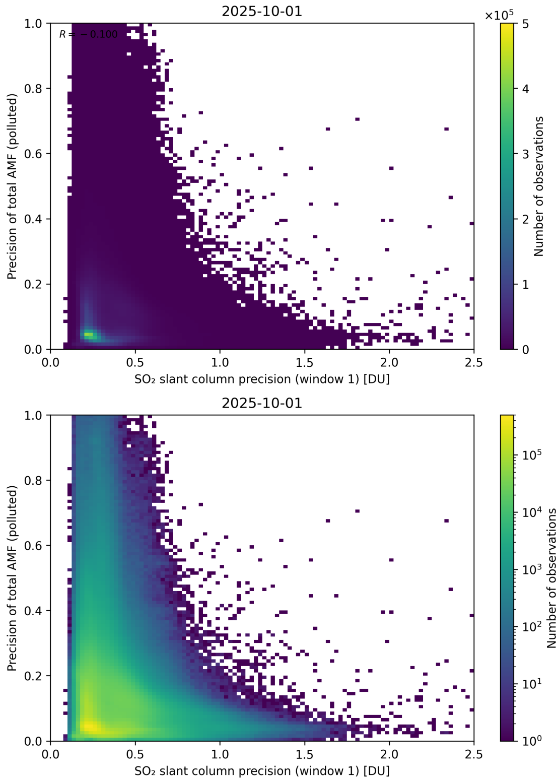
Figure 281: Scatter density plot of “SO 2 slant column precision (window 1)” against “Precision of total AMF (polluted)” for 2025-10-01 to 2025-10-02.
