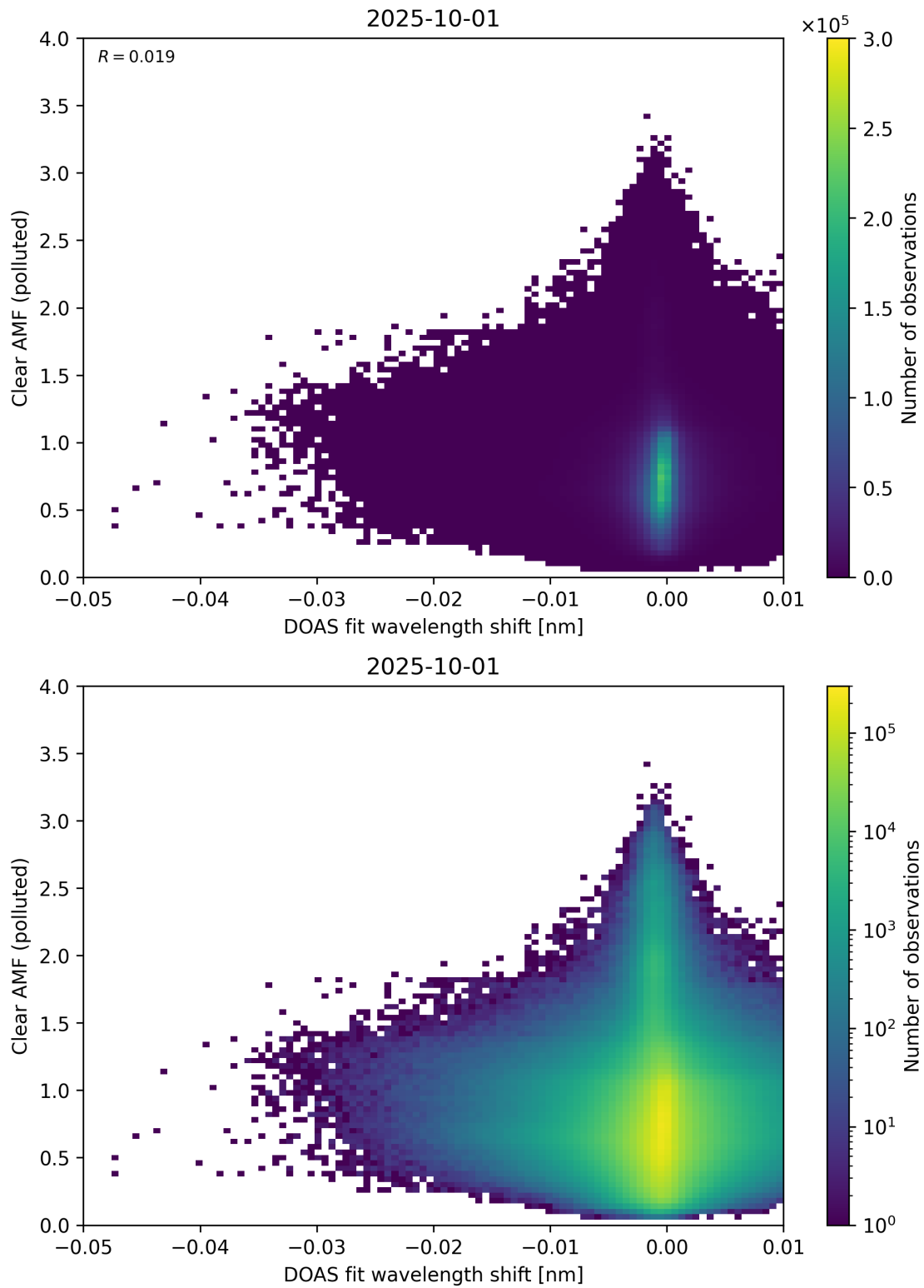
Figure 140: Scatter density plot of “DOAS fit wavelength shift” against “Clear AMF (polluted)” for 2025-10-01 to 2025-10-02.
