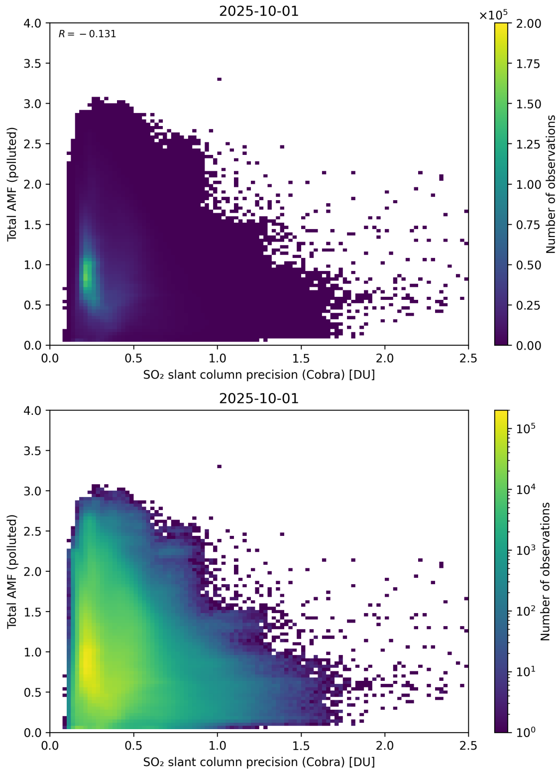
Figure 213: Scatter density plot of “SO 2 slant column precision (Cobra)” against “Total AMF (polluted)” for 2025-10-01 to 2025-10-02.
