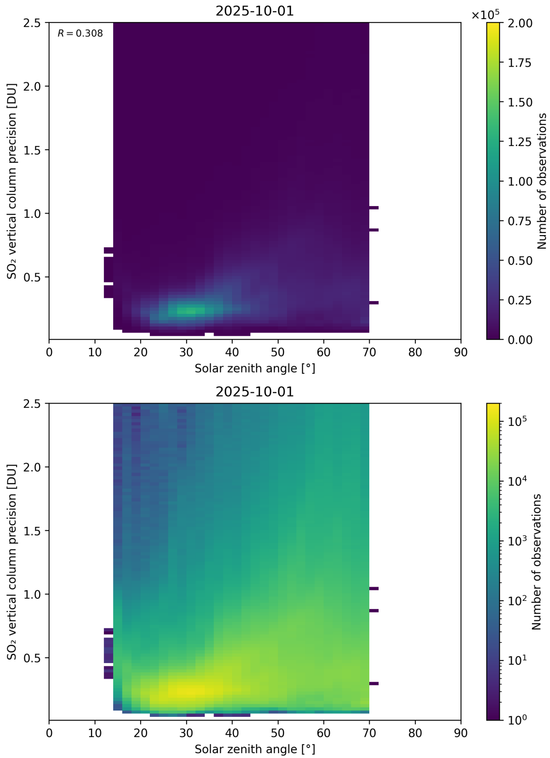
Figure 192: Scatter density plot of “Solar zenith angle” against “SO 2 vertical column precision” for 2025-10-01 to 2025-10-02.
