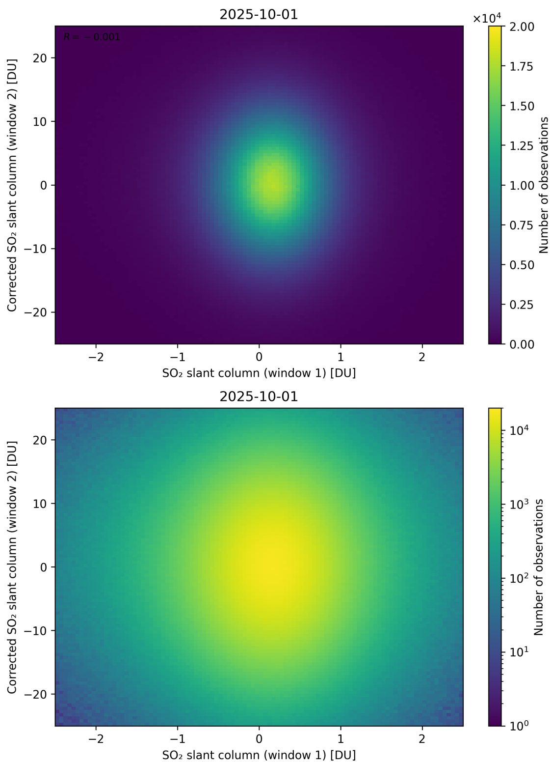
Figure 283: Scatter density plot of “SO 2 slant column (window 1)” against “Corrected SO 2 slant column (window 2)” for 2025-10-01 to 2025-10-02.
