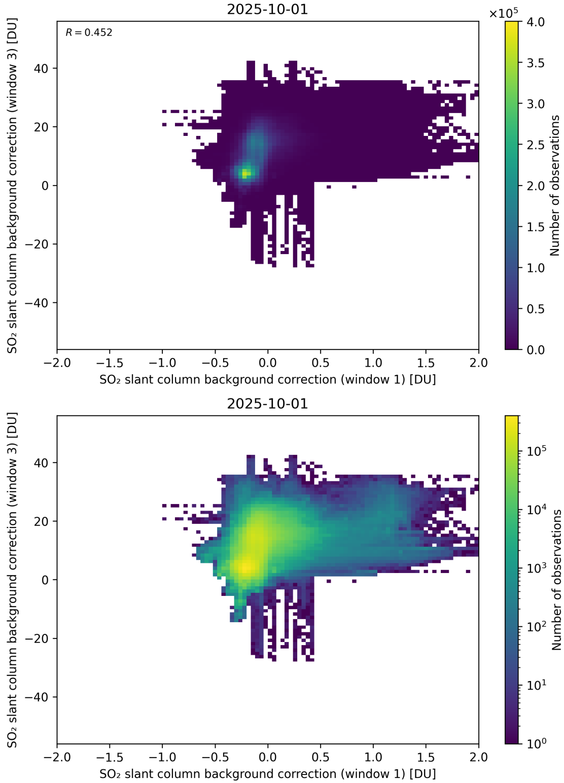
Figure 110: Scatter density plot of “SO 2 slant column background correction (window 1)” against “SO 2 slant column background correction (window 3)” for 2025-10-01 to 2025-10-02.
