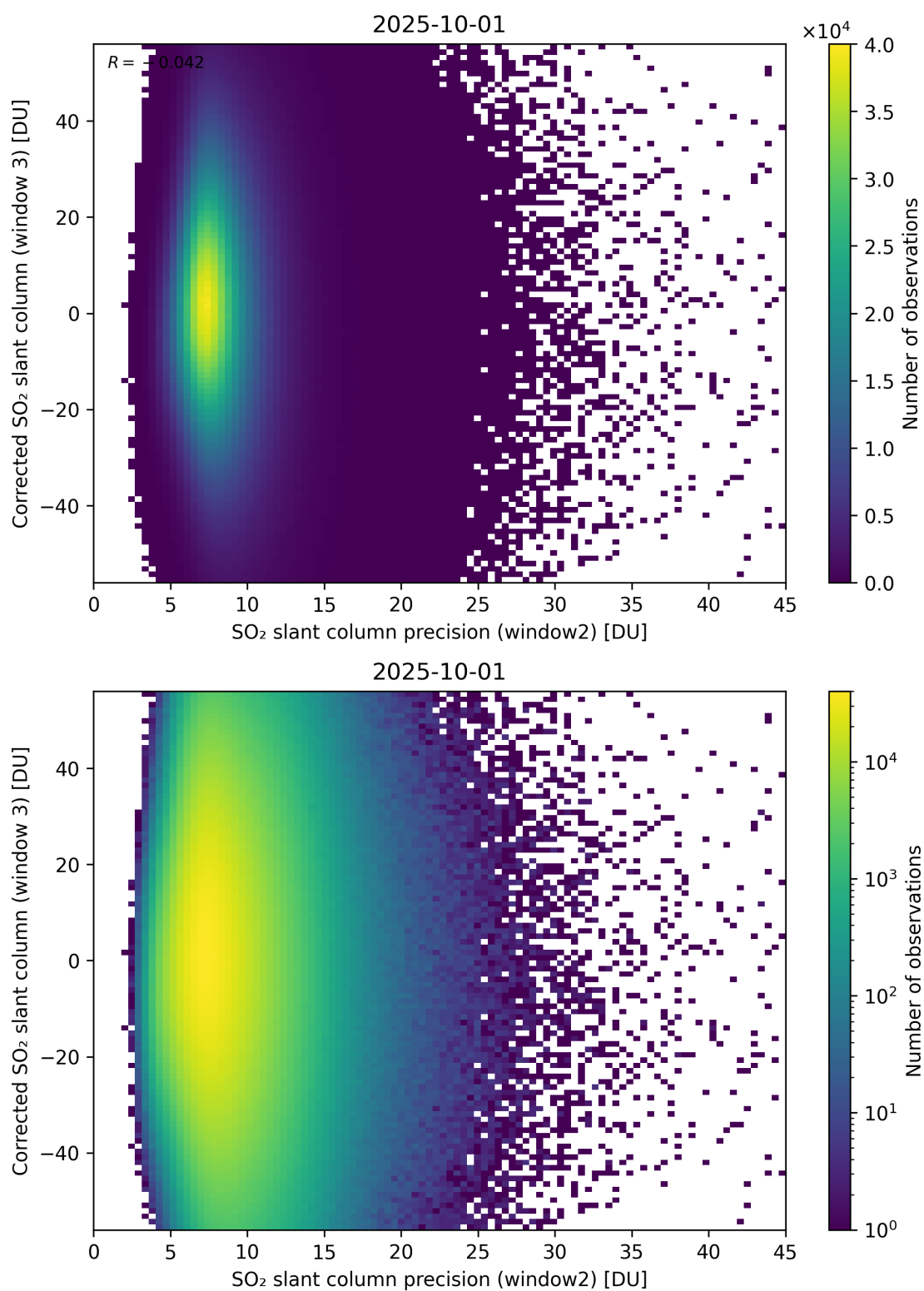
Figure 298: Scatter density plot of “SO 2 slant column precision (window2)” against “Corrected SO 2 slant column (window 3)” for 2025-10-01 to 2025-10-02.
