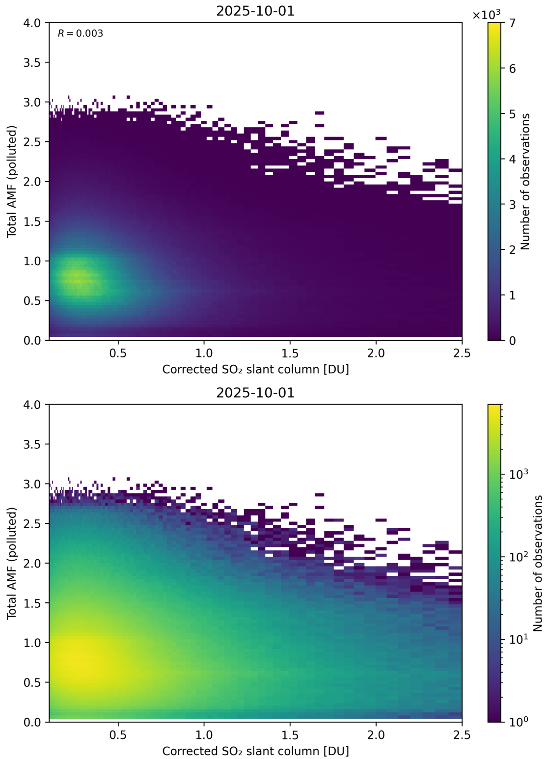
Figure 242: Scatter density plot of “Corrected SO 2 slant column” against “Total AMF (polluted)” for 2025-10-01 to 2025-10-02.
