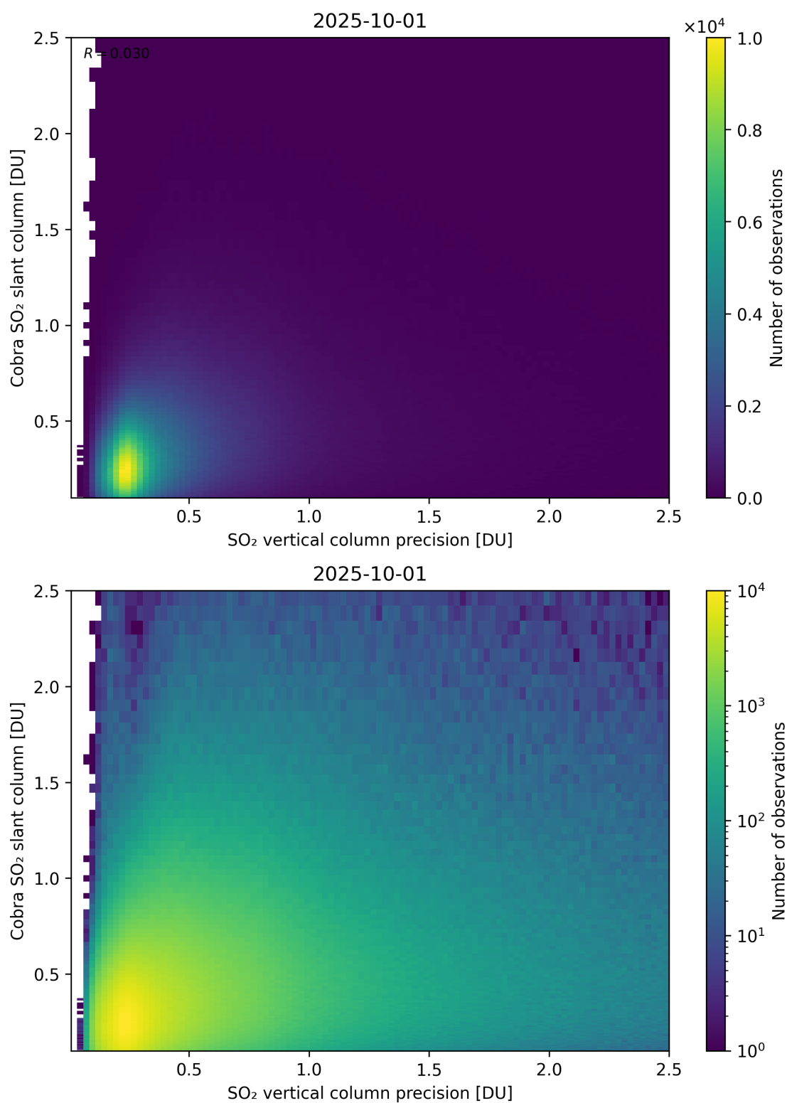
Figure 336: Scatter density plot of “SO 2 vertical column precision” against “Cobra SO 2 slant column” for 2025-10-01 to 2025-10-02.
