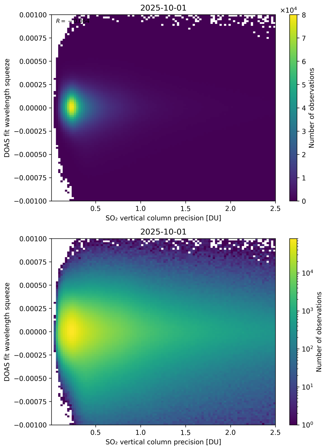
Figure 333: Scatter density plot of “SO 2 vertical column precision” against “DOAS fit wavelength squeeze” for 2025-10-01 to 2025-10-02.
