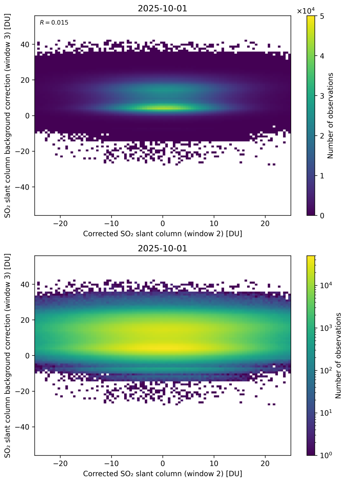
Figure 245: Scatter density plot of “Corrected SO 2 slant column (window 2)” against “SO 2 slant column background correction (window 3)” for 2025-10-01 to 2025-10-02.
