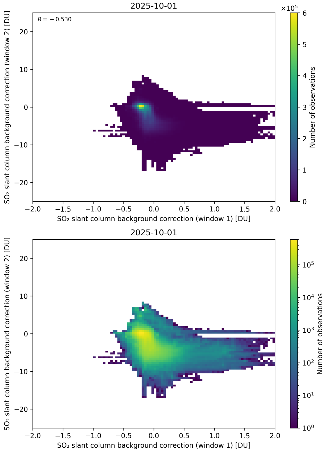
Figure 109: Scatter density plot of “SO 2 slant column background correction (window 1)” against “SO 2 slant column background correction (window 2)” for 2025-10-01 to 2025-10-02.
