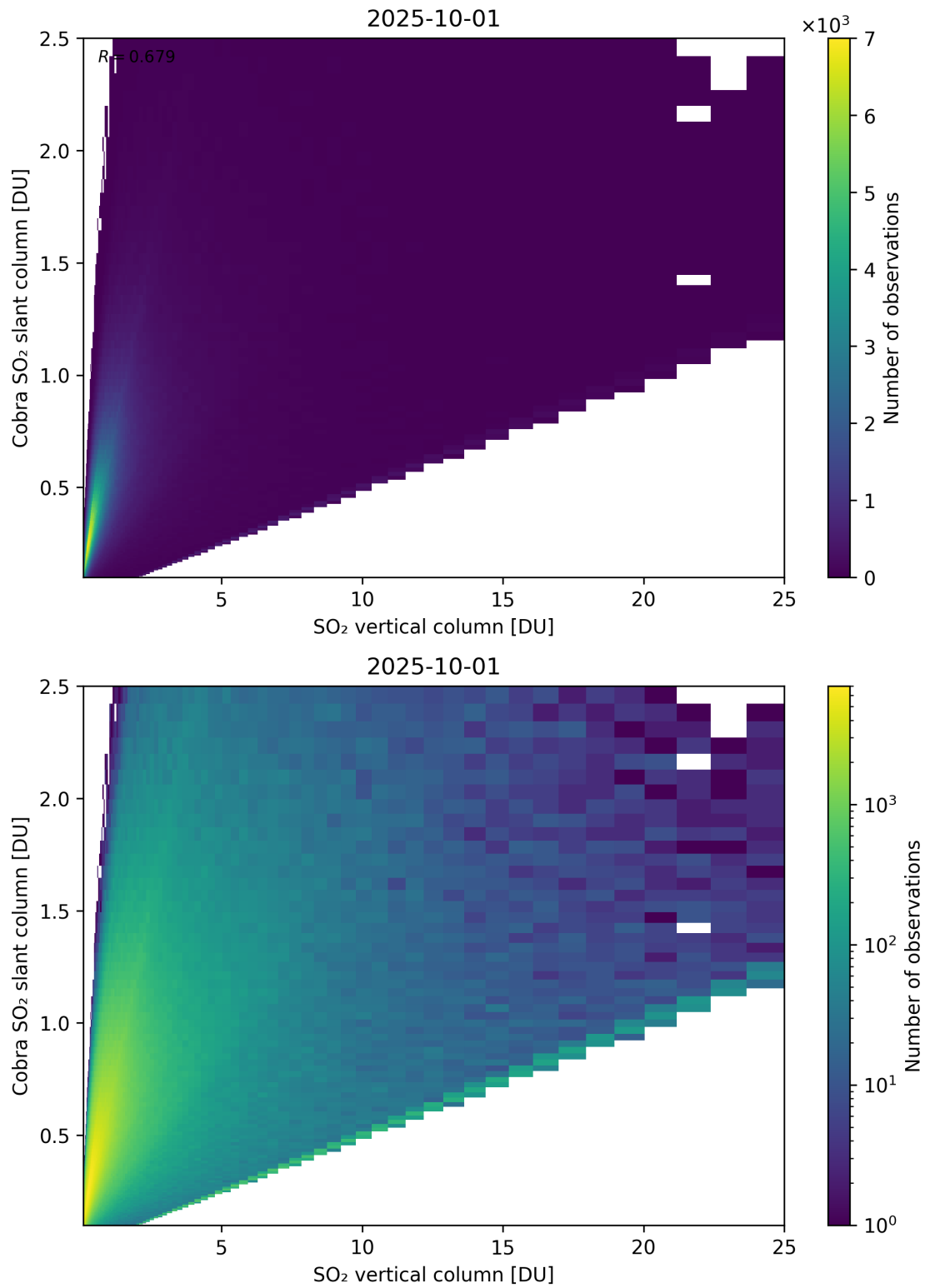
Figure 349: Scatter density plot of “SO 2 vertical column” against “Cobra SO 2 slant column” for 2025-10-01 to 2025-10-02.
