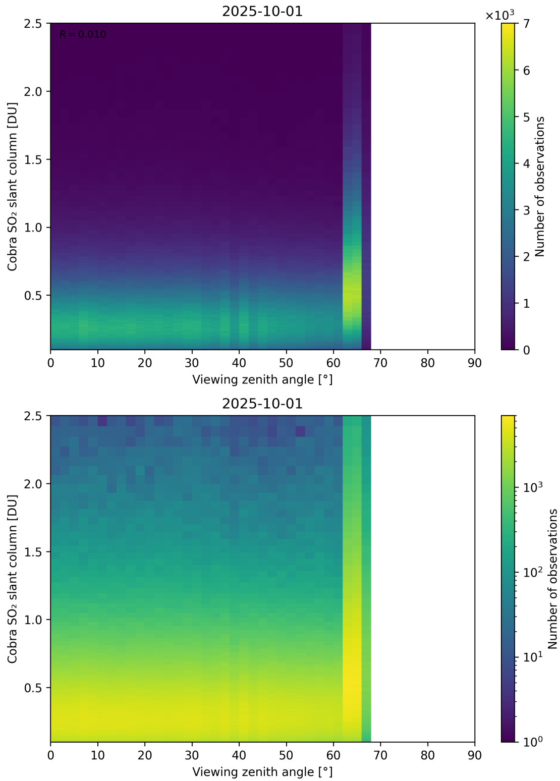
Figure 371: Scatter density plot of “Viewing zenith angle” against “Cobra SO 2 slant column” for 2025-10-01 to 2025-10-02.
