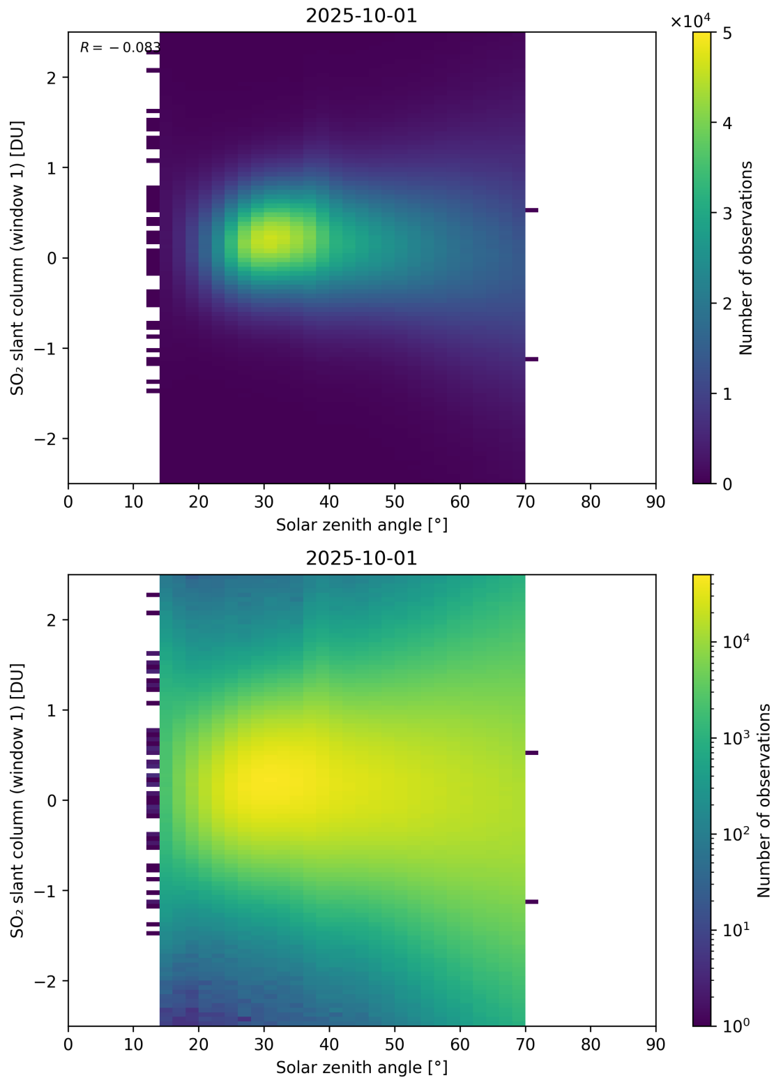
Figure 184: Scatter density plot of “Solar zenith angle” against “SO 2 slant column (window 1)” for 2025-10-01 to 2025-10-02.
