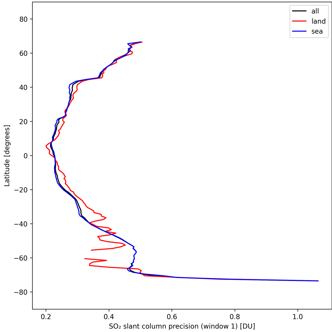
Figure 38: Zonal average of “SO 2 slant column precision (window 1)” for 2025-10-01 to 2025-10-02.
