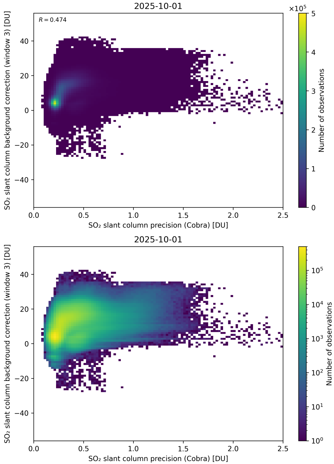
Figure 201: Scatter density plot of “SO 2 slant column precision (Cobra)” against “SO 2 slant column background correction (window 3)” for 2025-10-01 to 2025-10-02.
