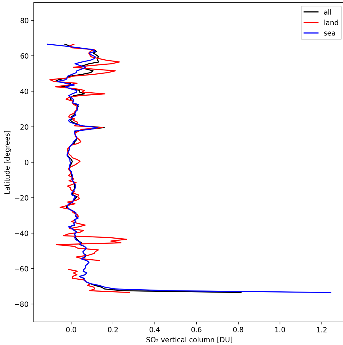
Figure 32: Zonal average of “SO 2 vertical column” for 2025-10-01 to 2025-10-02.
