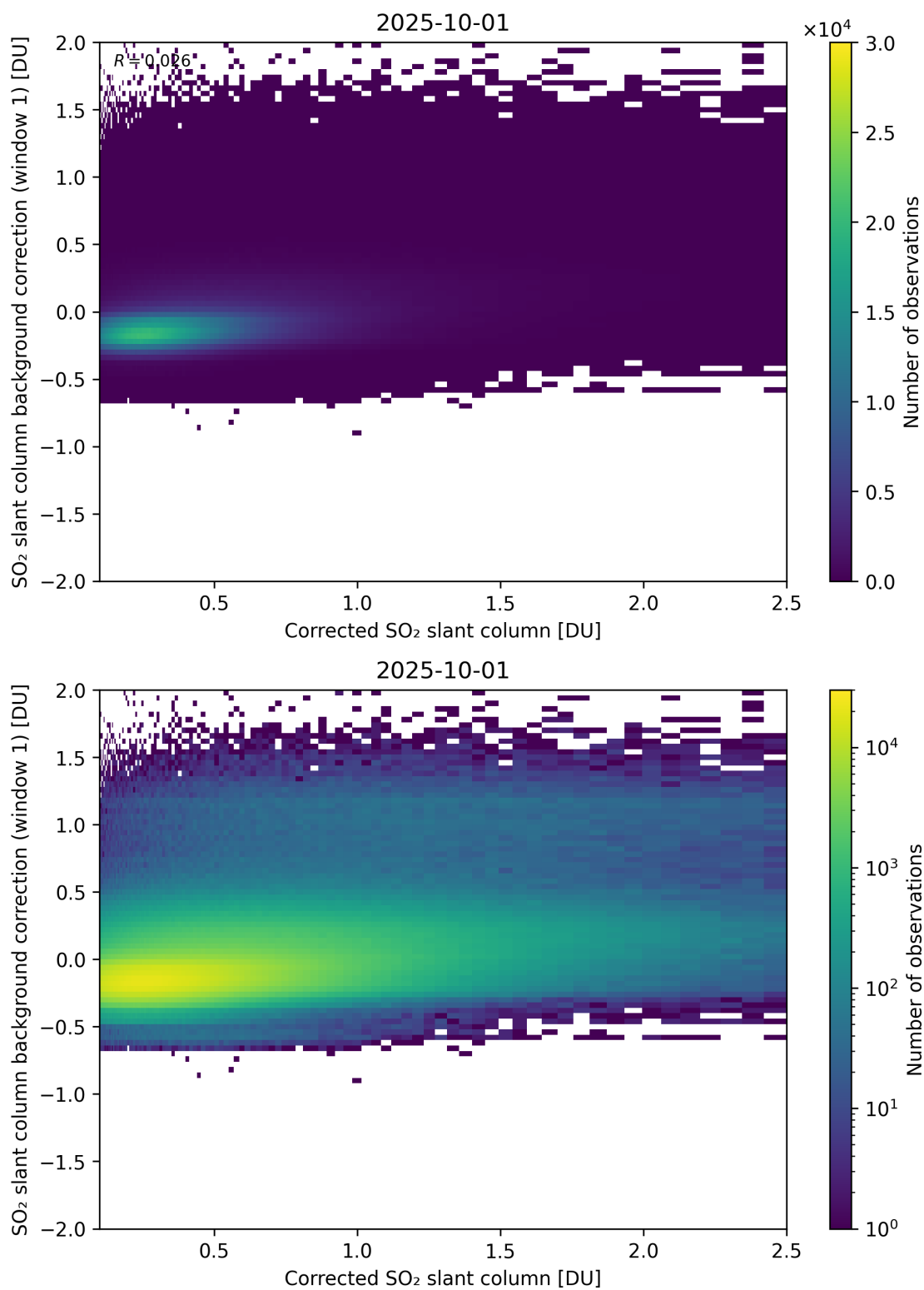
Figure 226: Scatter density plot of “Corrected SO 2 slant column” against “SO 2 slant column background correction (window 1)” for 2025-10-01 to 2025-10-02.
