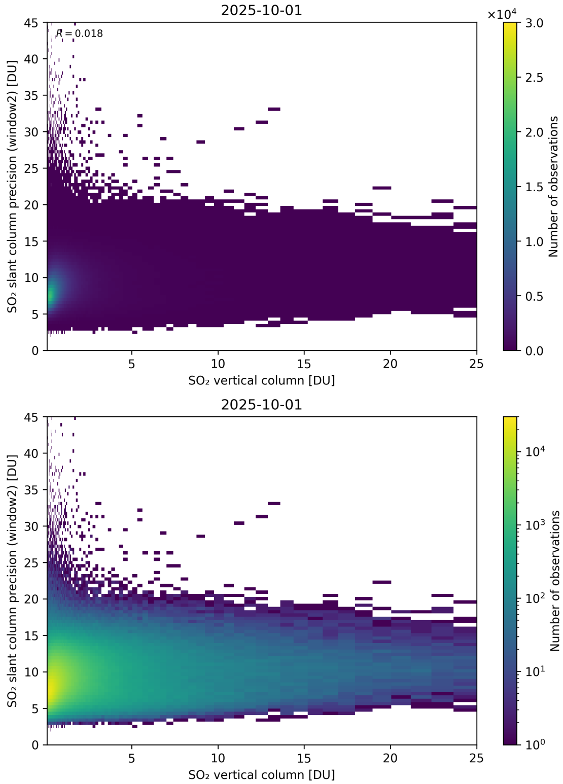
Figure 356: Scatter density plot of “SO 2 vertical column” against “SO 2 slant column precision (window2)” for 2025-10-01 to 2025-10-02.
