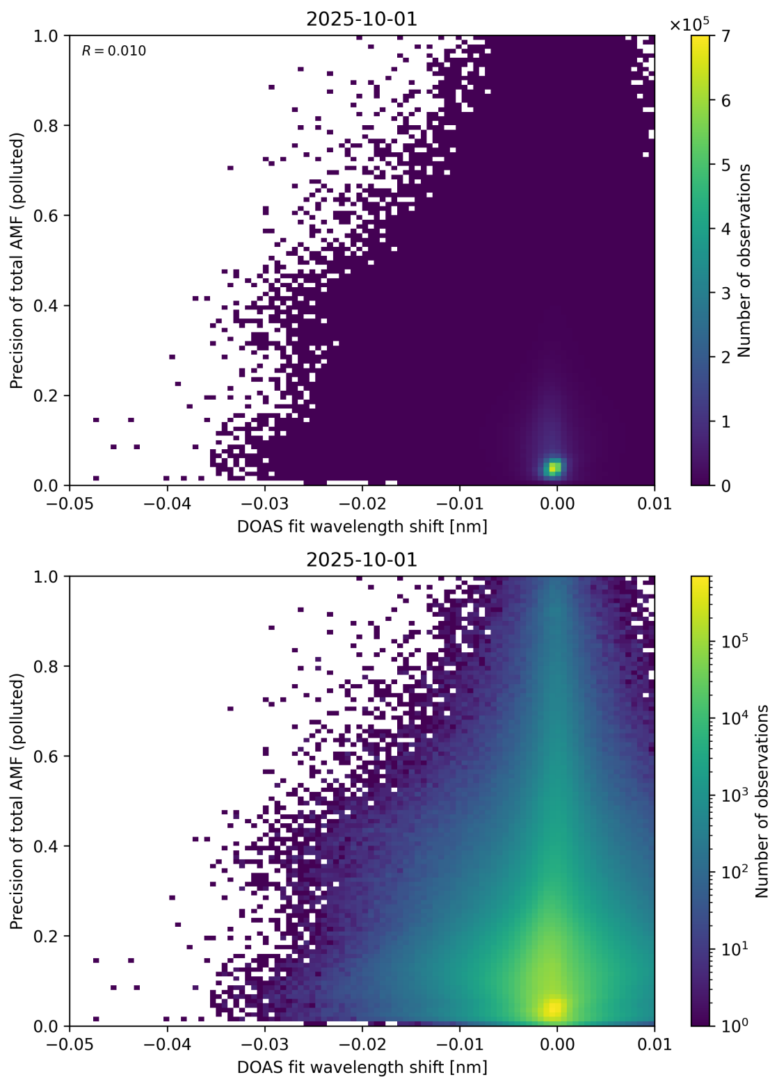
Figure 142: Scatter density plot of “DOAS fit wavelength shift” against “Precision of total AMF (polluted)” for 2025-10-01 to 2025-10-02.
