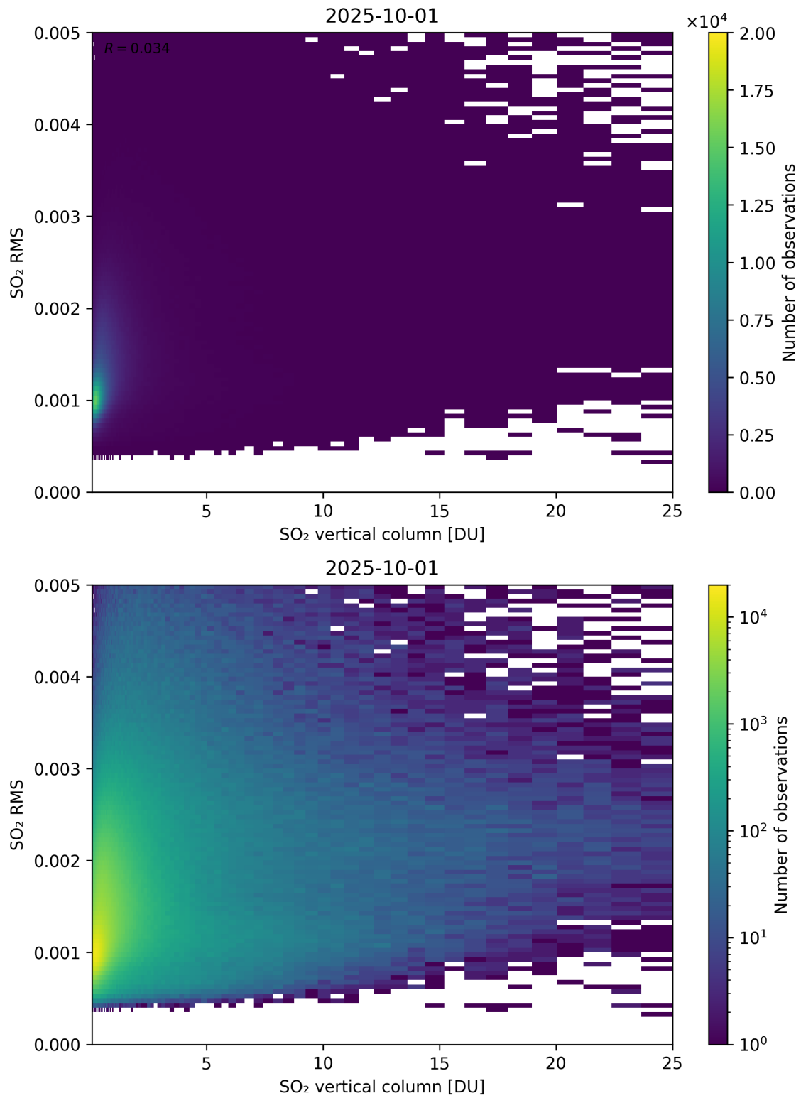
Figure 328: Scatter density plot of “SO 2 vertical column” against “SO 2 RMS” for 2025-10-01 to 2025-10-02.
