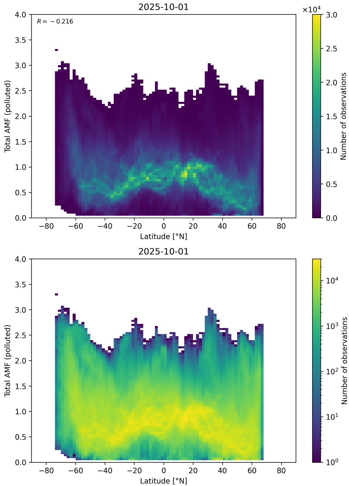
Figure 167: Scatter density plot of “Latitude” against “Total AMF (polluted)” for 2025-10-01 to 2025-10-02.
