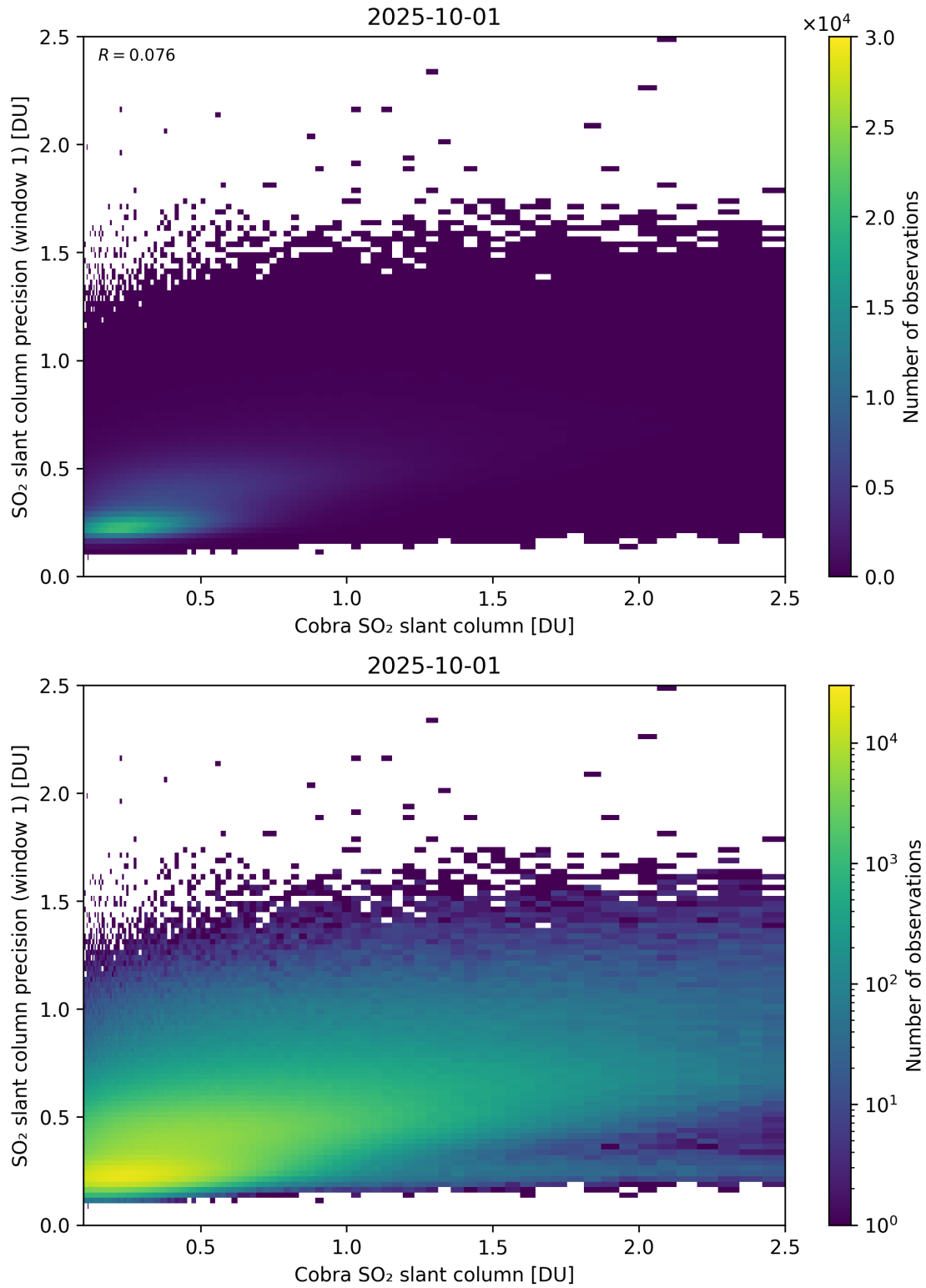
Figure 220: Scatter density plot of “Cobra SO 2 slant column” against “SO 2 slant column precision (window 1)” for 2025-10-01 to 2025-10-02.
