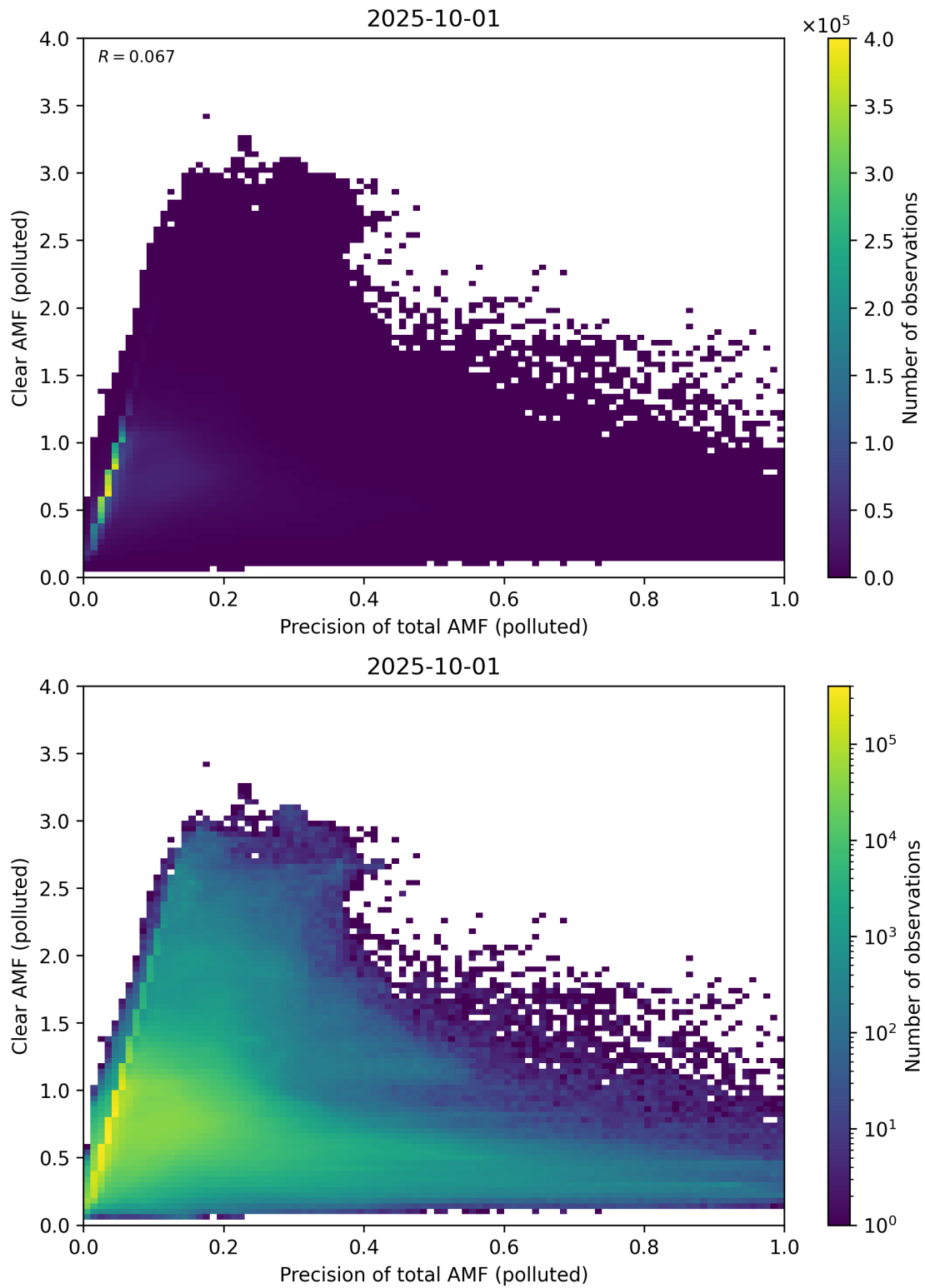
Figure 320: Scatter density plot of “Precision of total AMF (polluted)” against “Clear AMF (polluted)” for 2025-10-01 to 2025-10-02.
