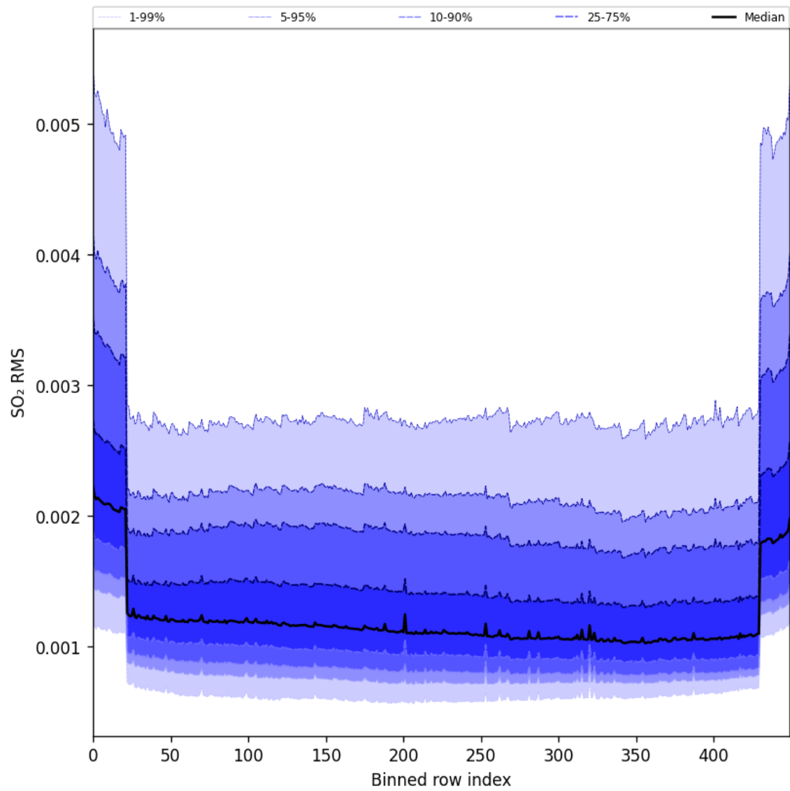
Figure 104: Along track statistics of “SO 2 RMS” for 2025-10-01 to 2025-10-02
