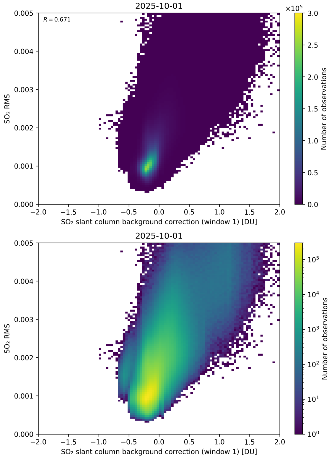
Figure 113: Scatter density plot of “SO 2 slant column background correction (window 1)” against “SO 2 RMS” for 2025-10-01 to 2025-10-02.
