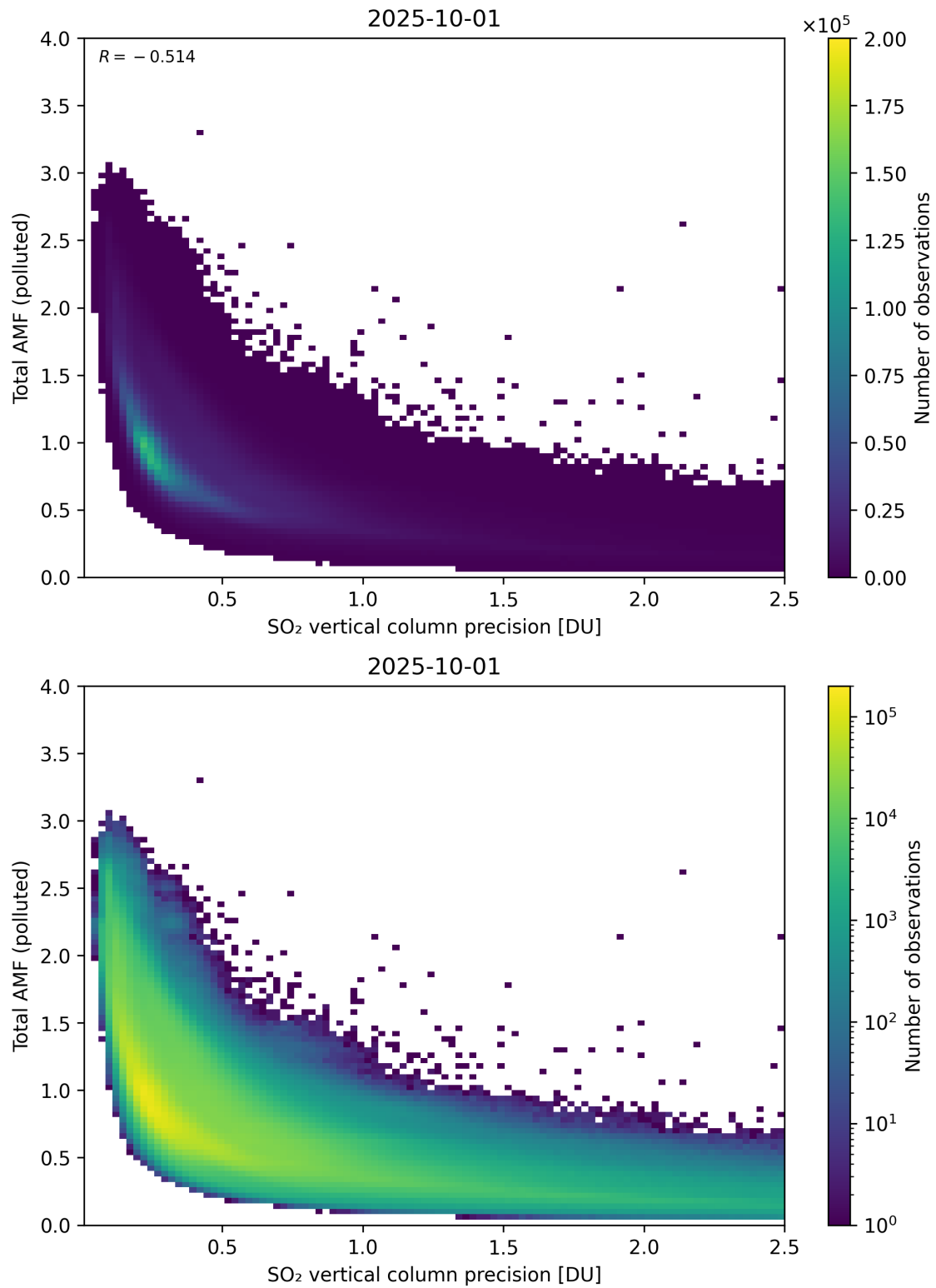
Figure 346: Scatter density plot of “SO 2 vertical column precision” against “Total AMF (polluted)” for 2025-10-01 to 2025-10-02.
