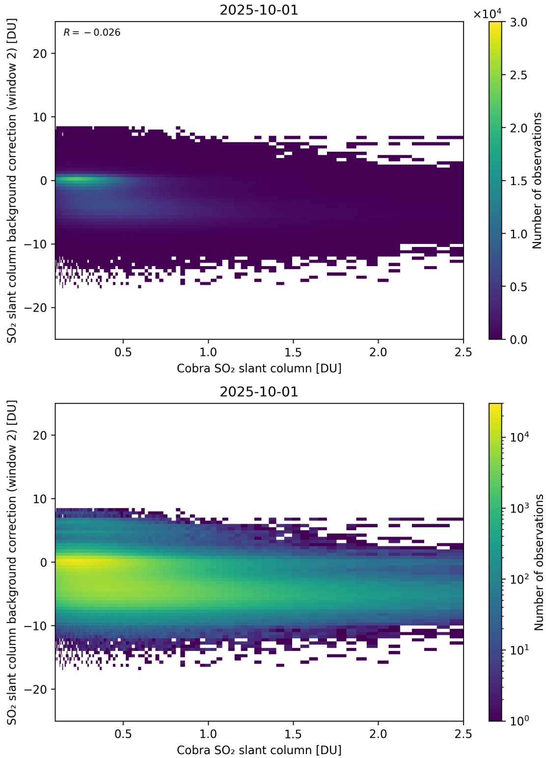
Figure 194: Scatter density plot of “Cobra SO 2 slant column” against “SO 2 slant column background correction (window 2)” for 2025-10-01 to 2025-10-02.
