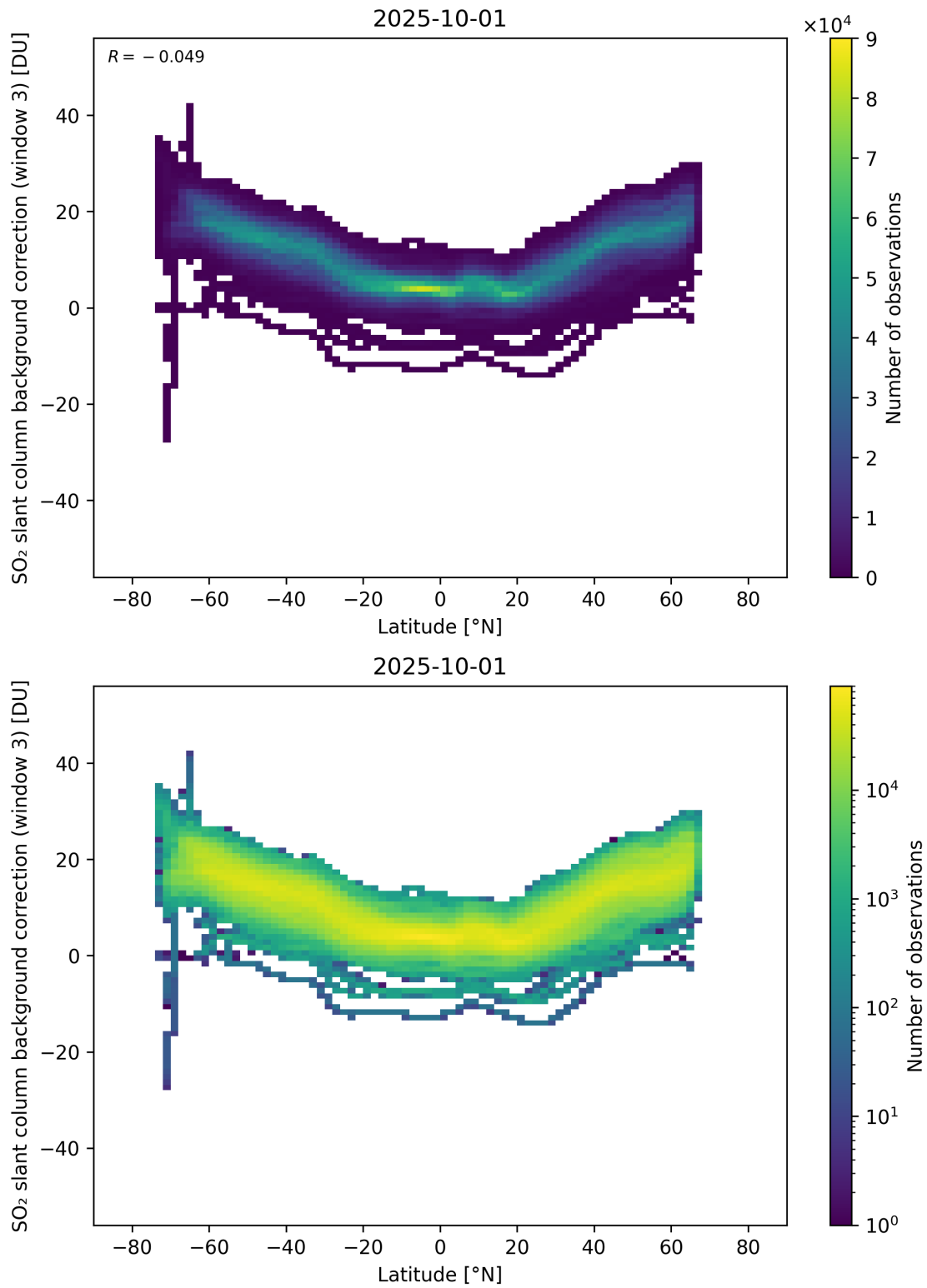
Figure 152: Scatter density plot of “Latitude” against “SO 2 slant column background correction (window 3)” for 2025-10-01 to 2025-10-02.
