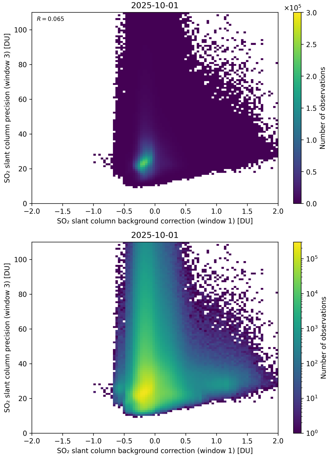
Figure 119: Scatter density plot of “SO 2 slant column background correction (window 1)” against “SO 2 slant column precision (window 3)” for 2025-10-01 to 2025-10-02.
