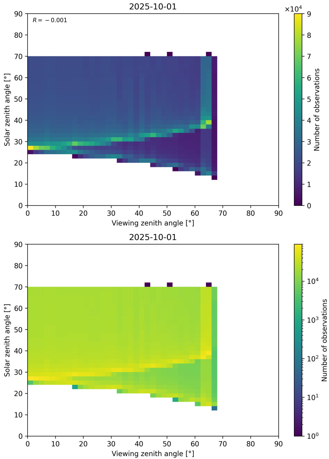
Figure 369: Scatter density plot of “Viewing zenith angle” against “Solar zenith angle” for 2025-10-01 to 2025-10-02.
