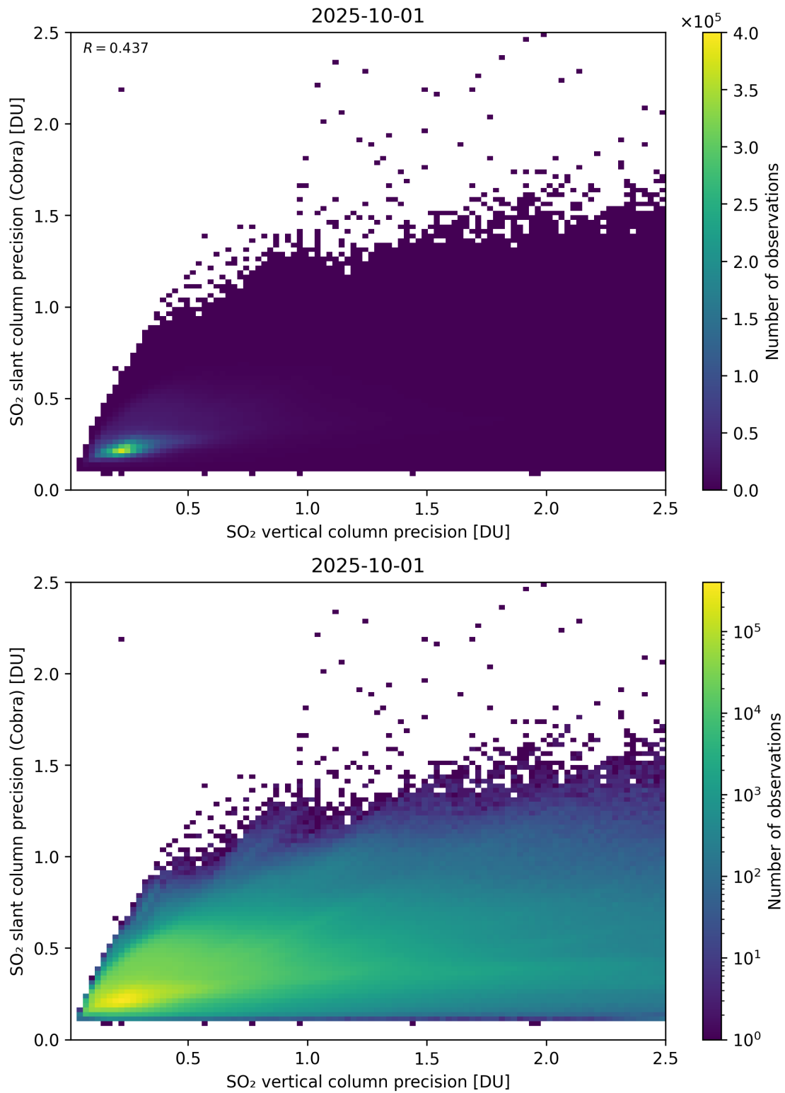
Figure 337: Scatter density plot of “SO 2 vertical column precision” against “SO 2 slant column precision (Cobra)” for 2025-10-01 to 2025-10-02.
