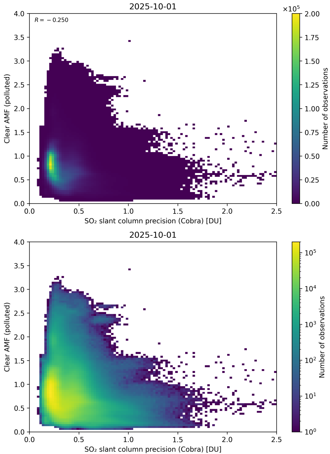
Figure 205: Scatter density plot of “SO 2 slant column precision (Cobra)” against “Clear AMF (polluted)” for 2025-10-01 to 2025-10-02.
