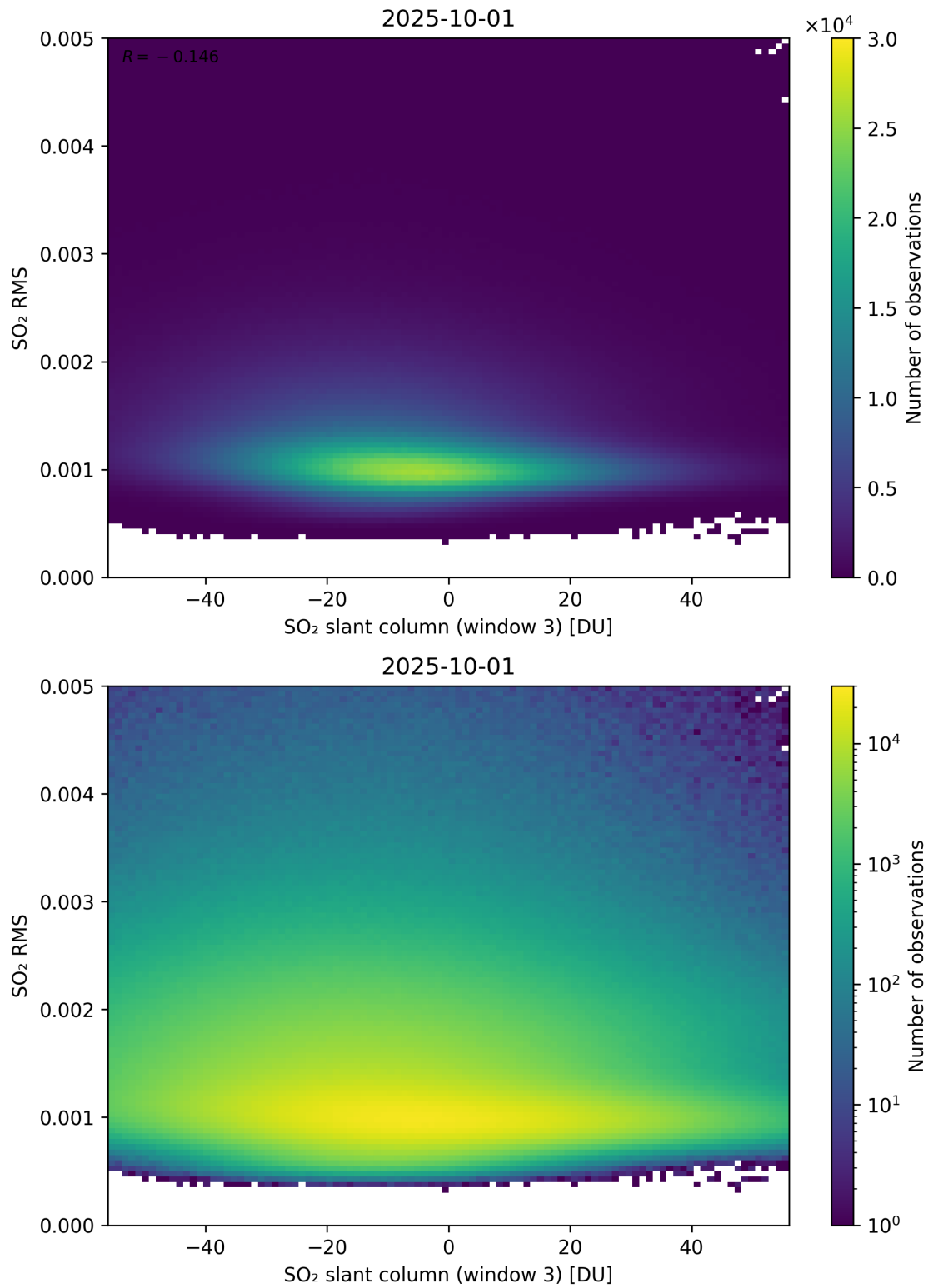
Figure 306: Scatter density plot of “SO 2 slant column (window 3)” against “SO 2 RMS” for 2025-10-01 to 2025-10-02.
