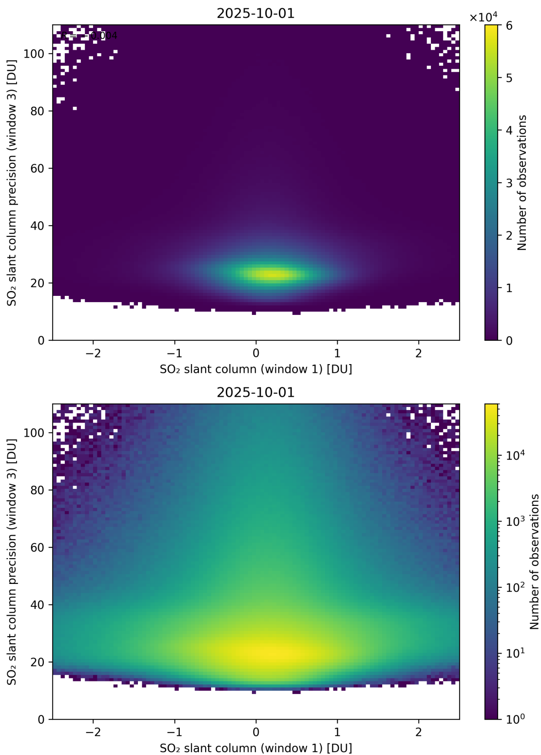
Figure 288: Scatter density plot of “SO 2 slant column (window 1)” against “SO 2 slant column precision (window 3)” for 2025-10-01 to 2025-10-02.
