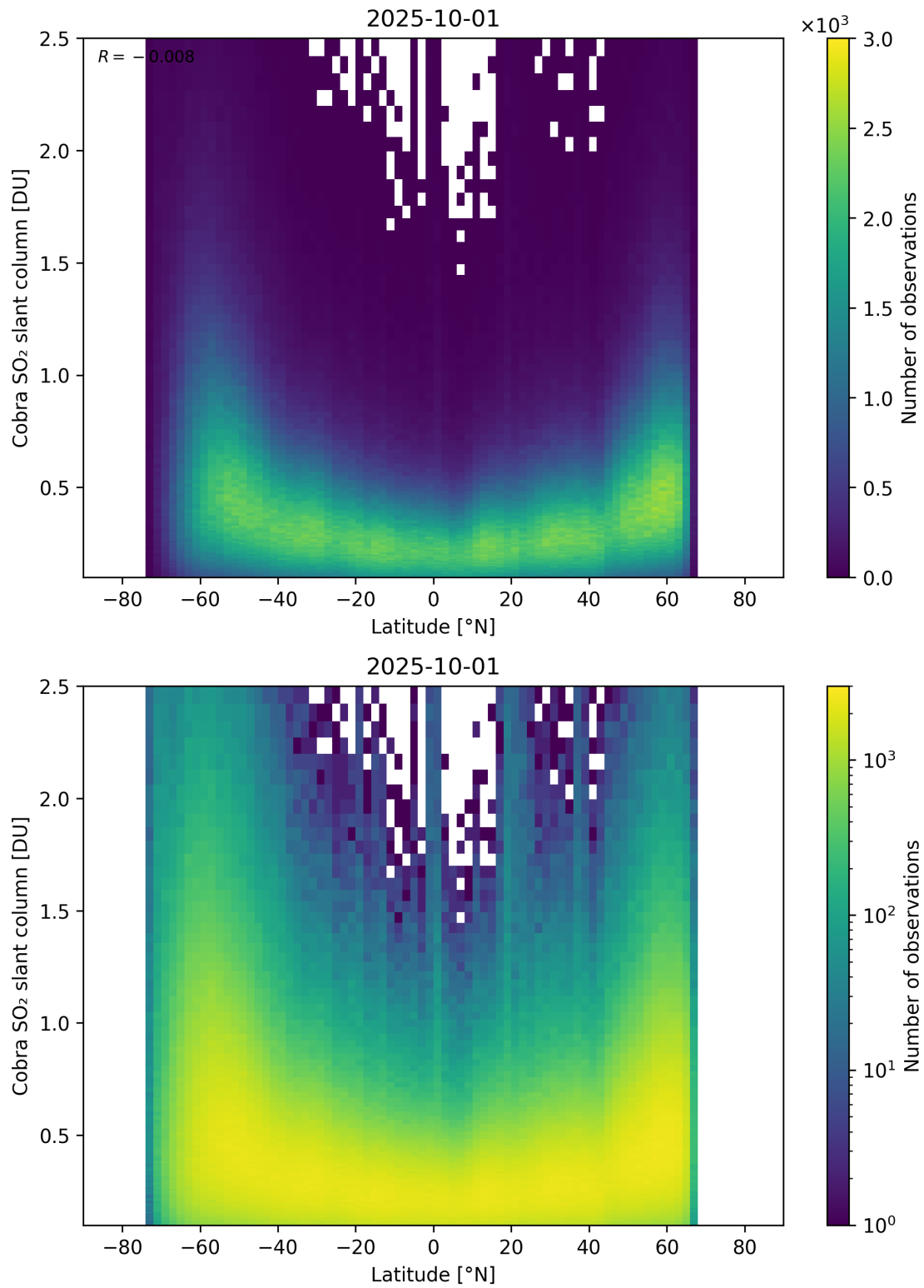
Figure 157: Scatter density plot of “Latitude” against “Cobra SO 2 slant column” for 2025-10-01 to 2025-10-02.
