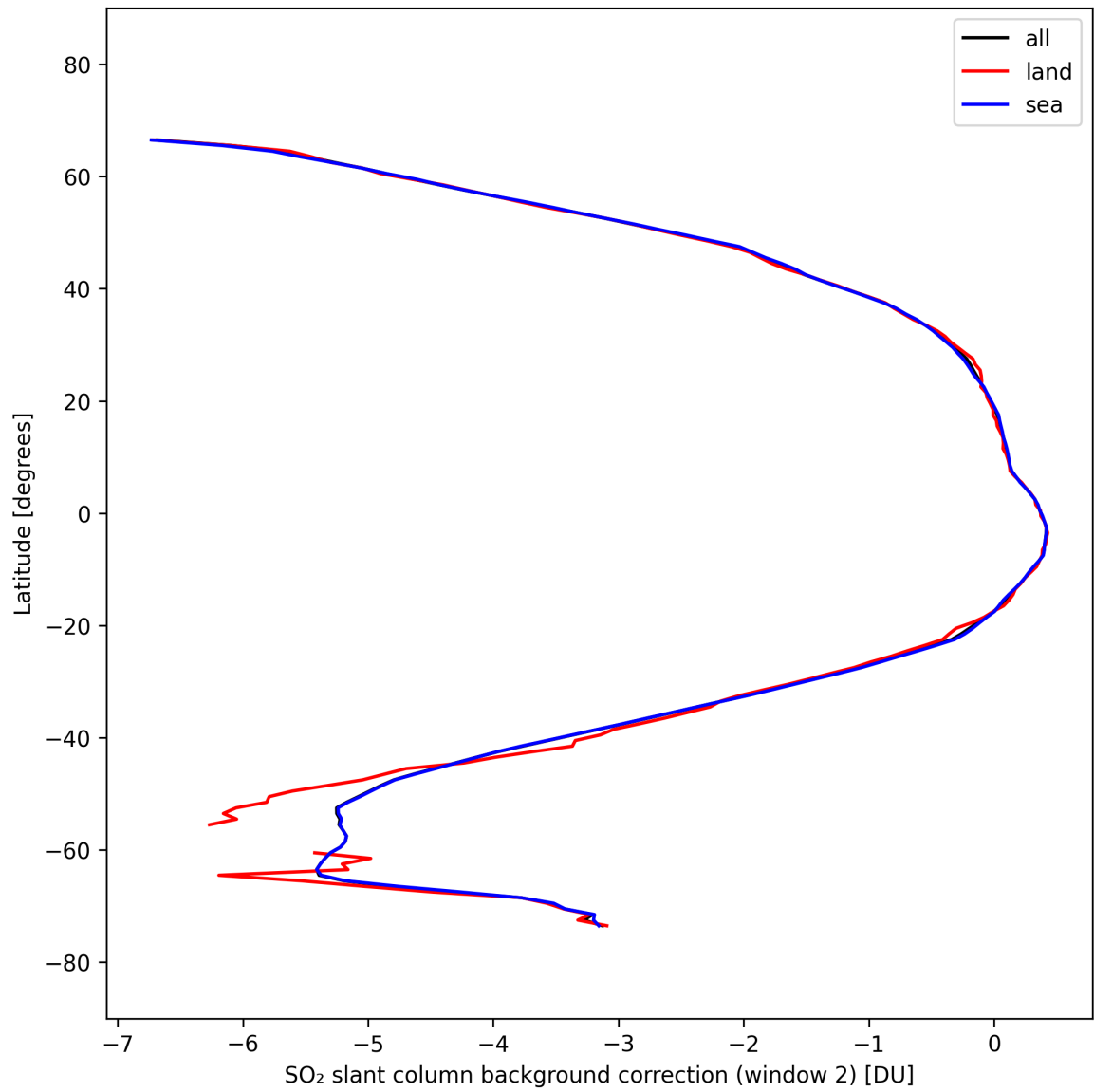
Figure 44: Zonal average of “SO 2 slant column background correction (window 2)” for 2025-10-01 to 2025-10-02.
