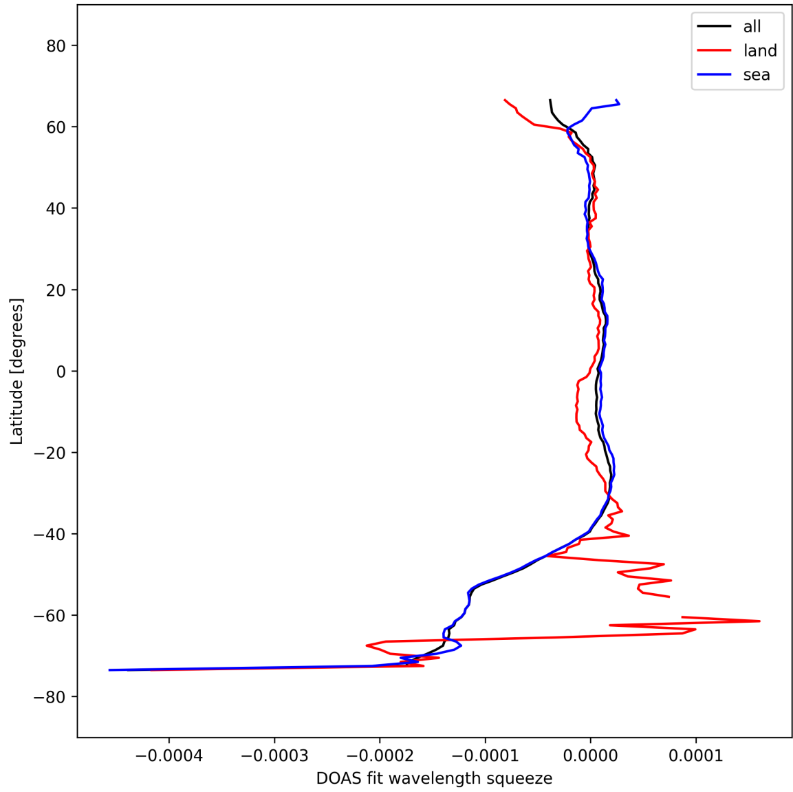
Figure 51: Zonal average of “DOAS fit wavelength squeeze” for 2025-10-01 to 2025-10-02.
