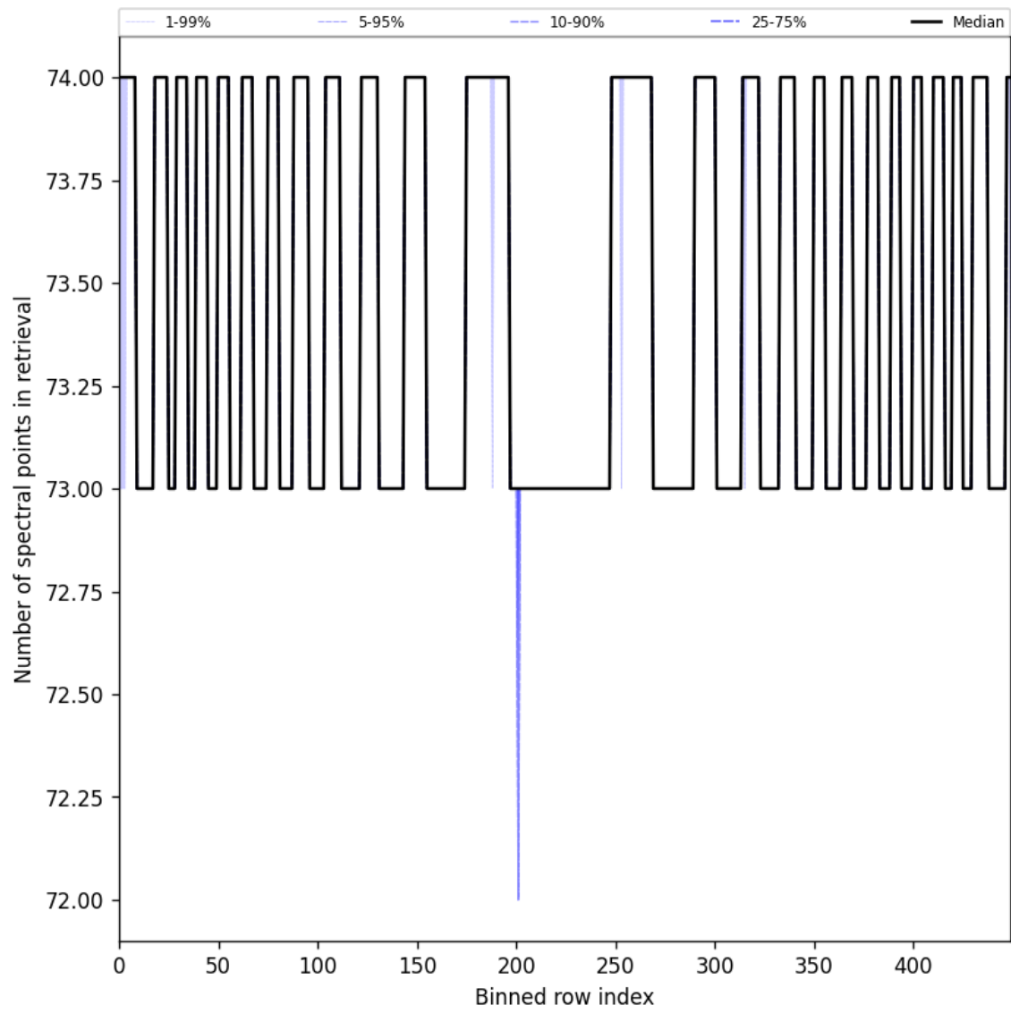
Figure 108: Along track statistics of “Number of spectral points in retrieval” for 2025-10-01 to 2025-10-02
