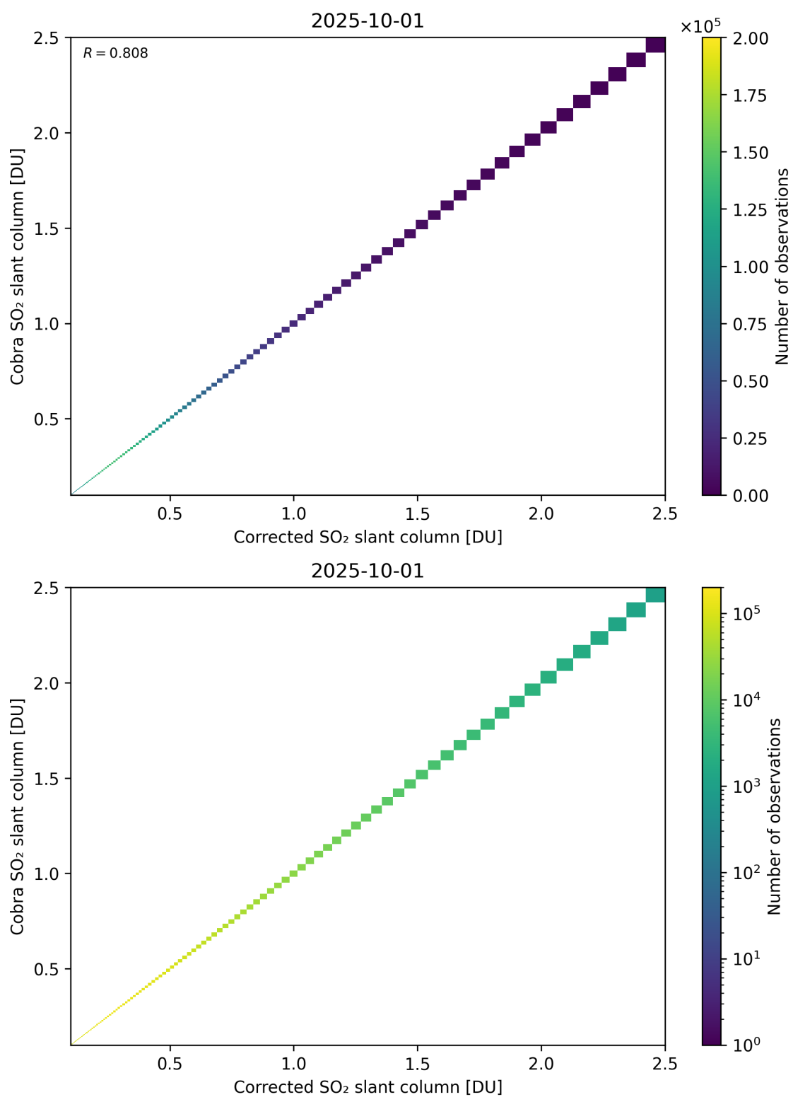
Figure 233: Scatter density plot of “Corrected SO 2 slant column” against “Cobra SO 2 slant column” for 2025-10-01 to 2025-10-02.
