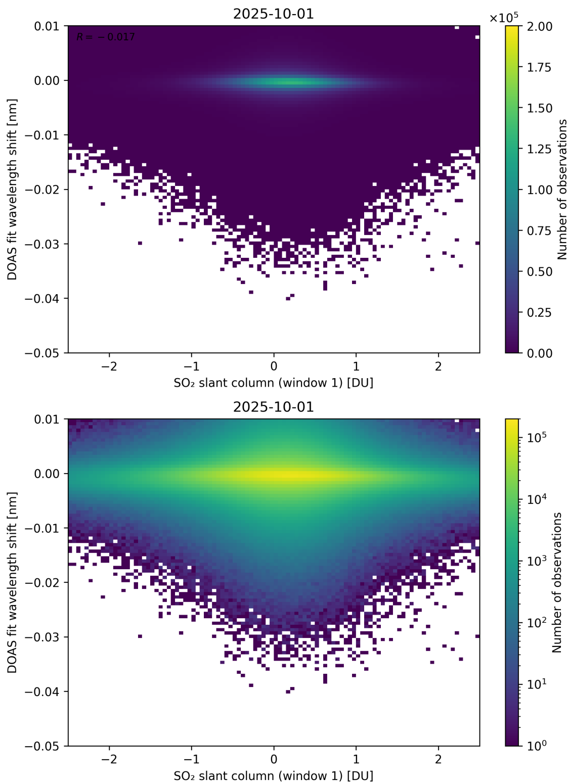
Figure 265: Scatter density plot of “SO 2 slant column (window 1)” against “DOAS fit wavelength shift” for 2025-10-01 to 2025-10-02.
