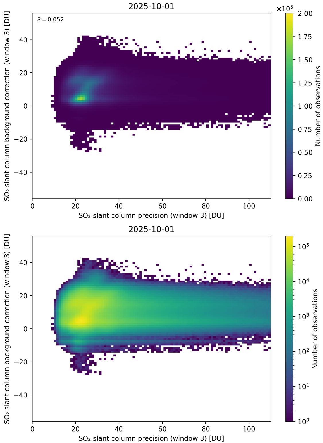
Figure 307: Scatter density plot of “SO 2 slant column precision (window 3)” against “SO 2 slant column background correction (window 3)” for 2025-10-01 to 2025-10-02.
