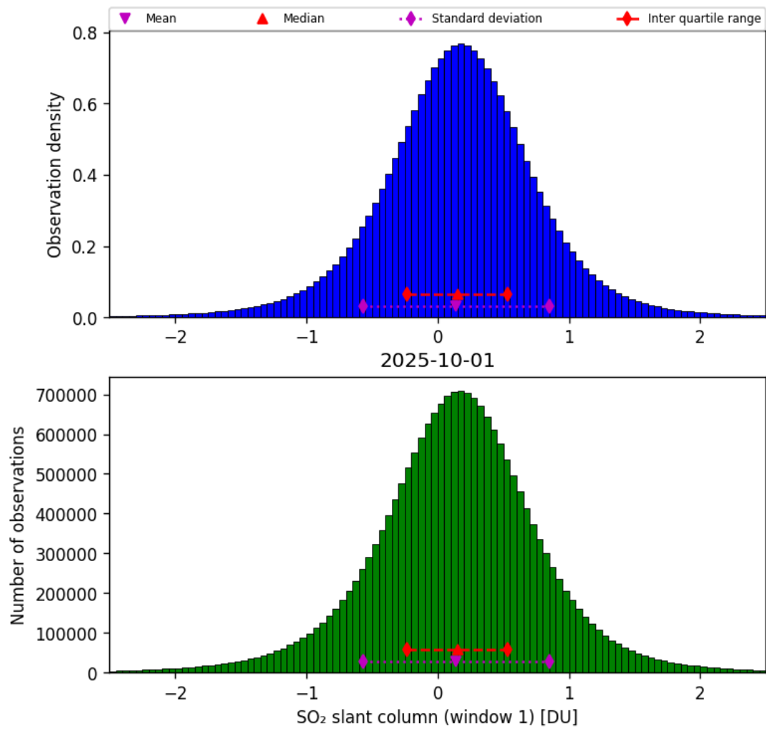
Figure 63: Histogram of “SO 2 slant column (window 1)” for 2025-10-01 to 2025-10-02
