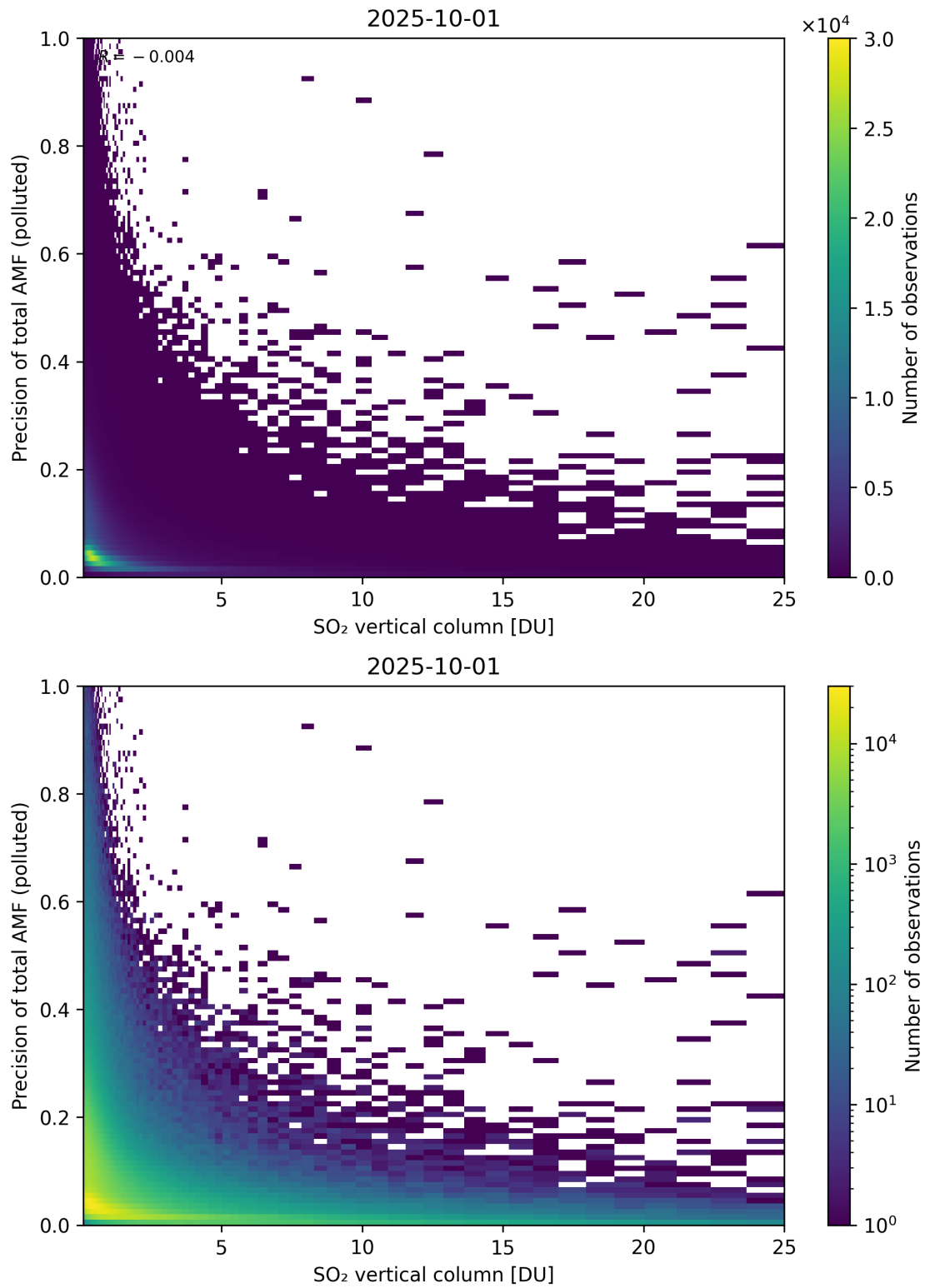
Figure 360: Scatter density plot of “SO 2 vertical column” against “Precision of total AMF (polluted)” for 2025-10-01 to 2025-10-02.
