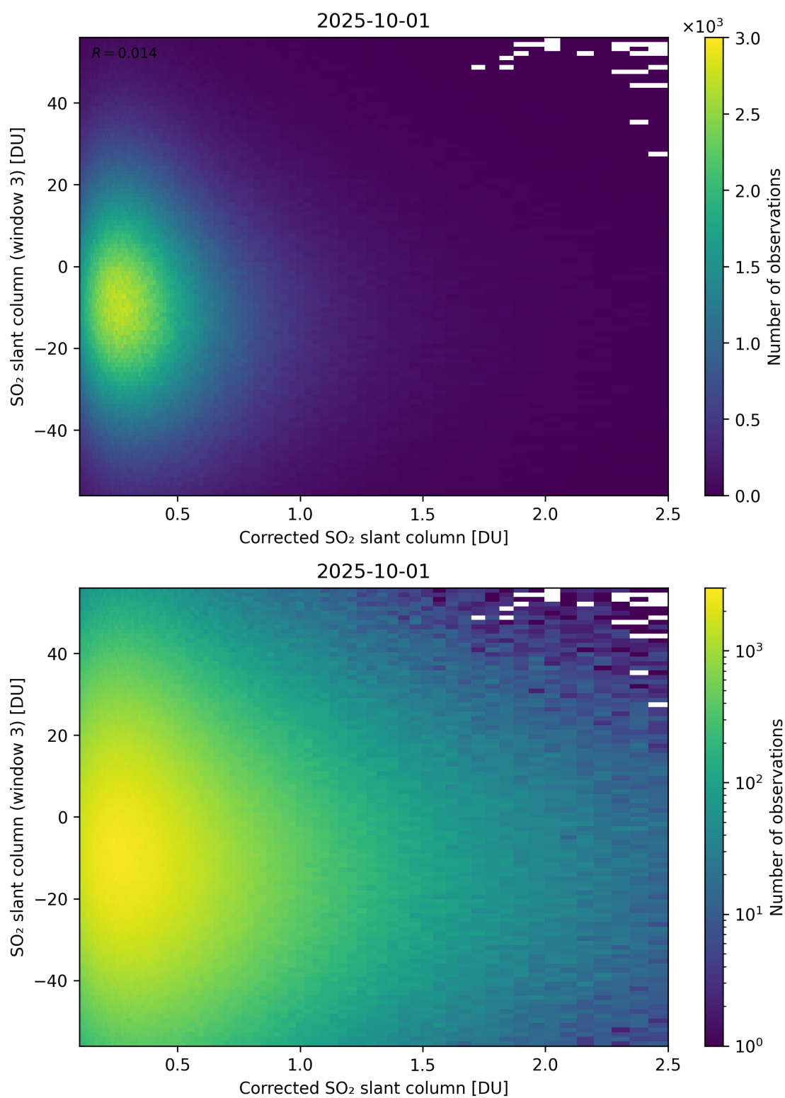
Figure 240: Scatter density plot of “Corrected SO 2 slant column” against “SO 2 slant column (window 3)” for 2025-10-01 to 2025-10-02.
