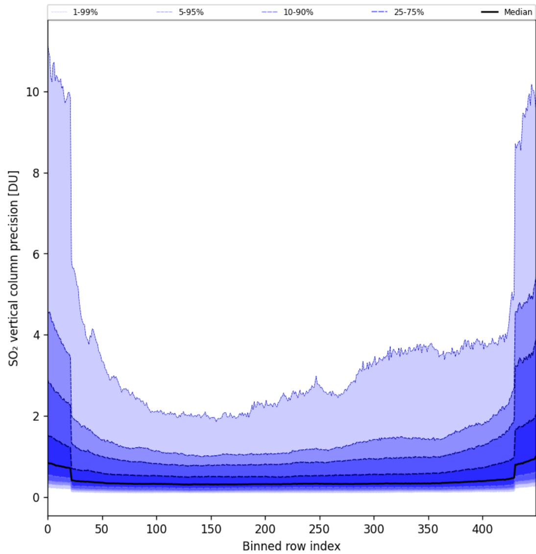
Figure 85: Along track statistics of “SO 2 vertical column precision” for 2025-10-01 to 2025-10-02
