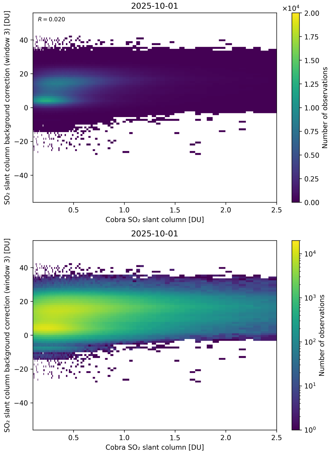
Figure 195: Scatter density plot of “Cobra SO 2 slant column” against “SO 2 slant column background correction (window 3)” for 2025-10-01 to 2025-10-02.
