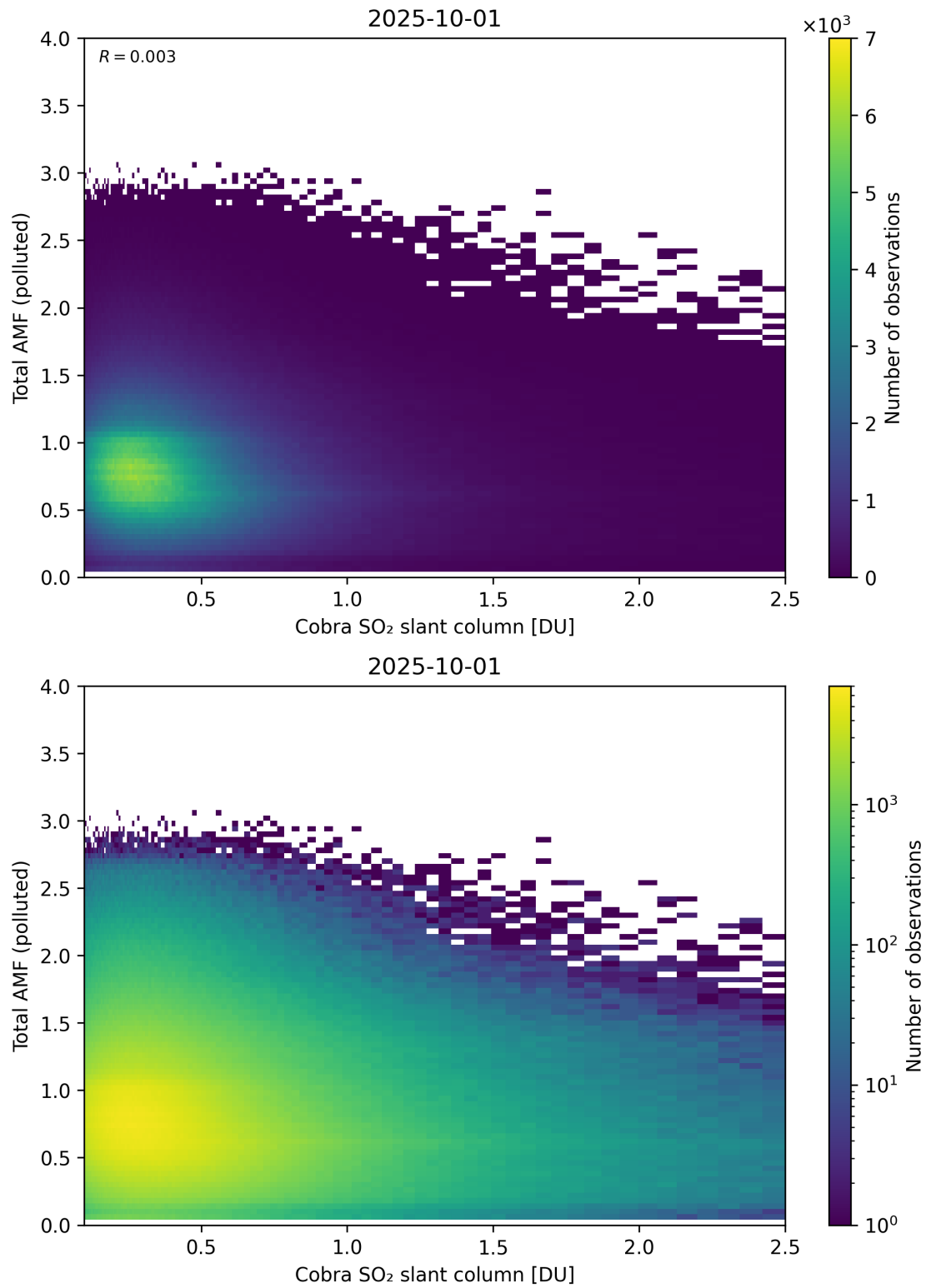
Figure 224: Scatter density plot of “Cobra SO 2 slant column” against “Total AMF (polluted)” for 2025-10-01 to 2025-10-02.
