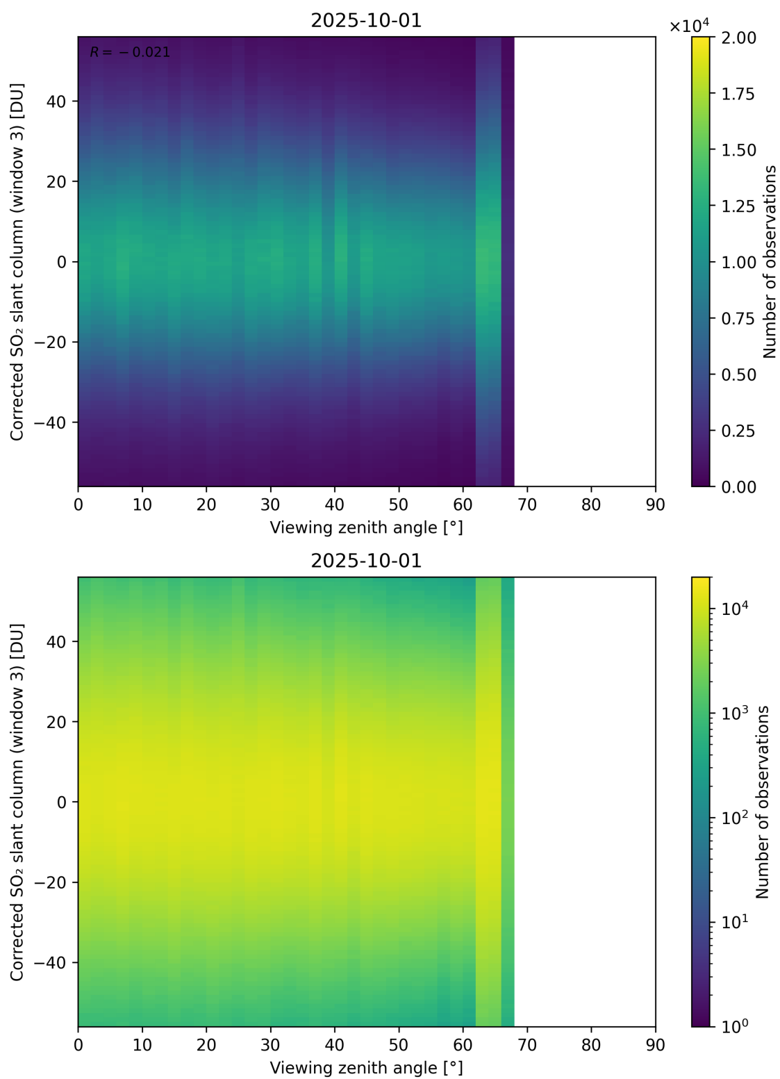
Figure 375: Scatter density plot of “Viewing zenith angle” against “Corrected SO 2 slant column (window 3)” for 2025-10-01 to 2025-10-02.
