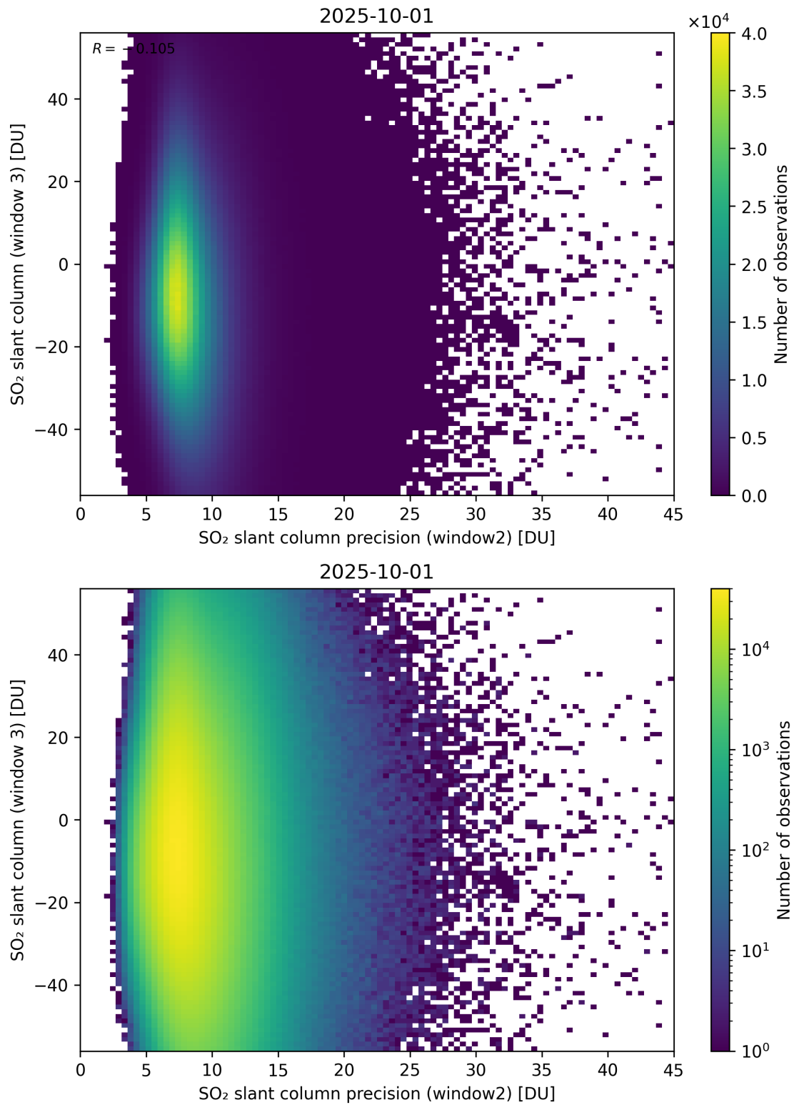
Figure 299: Scatter density plot of “SO 2 slant column precision (window2)” against “SO 2 slant column (window 3)” for 2025-10-01 to 2025-10-02.
