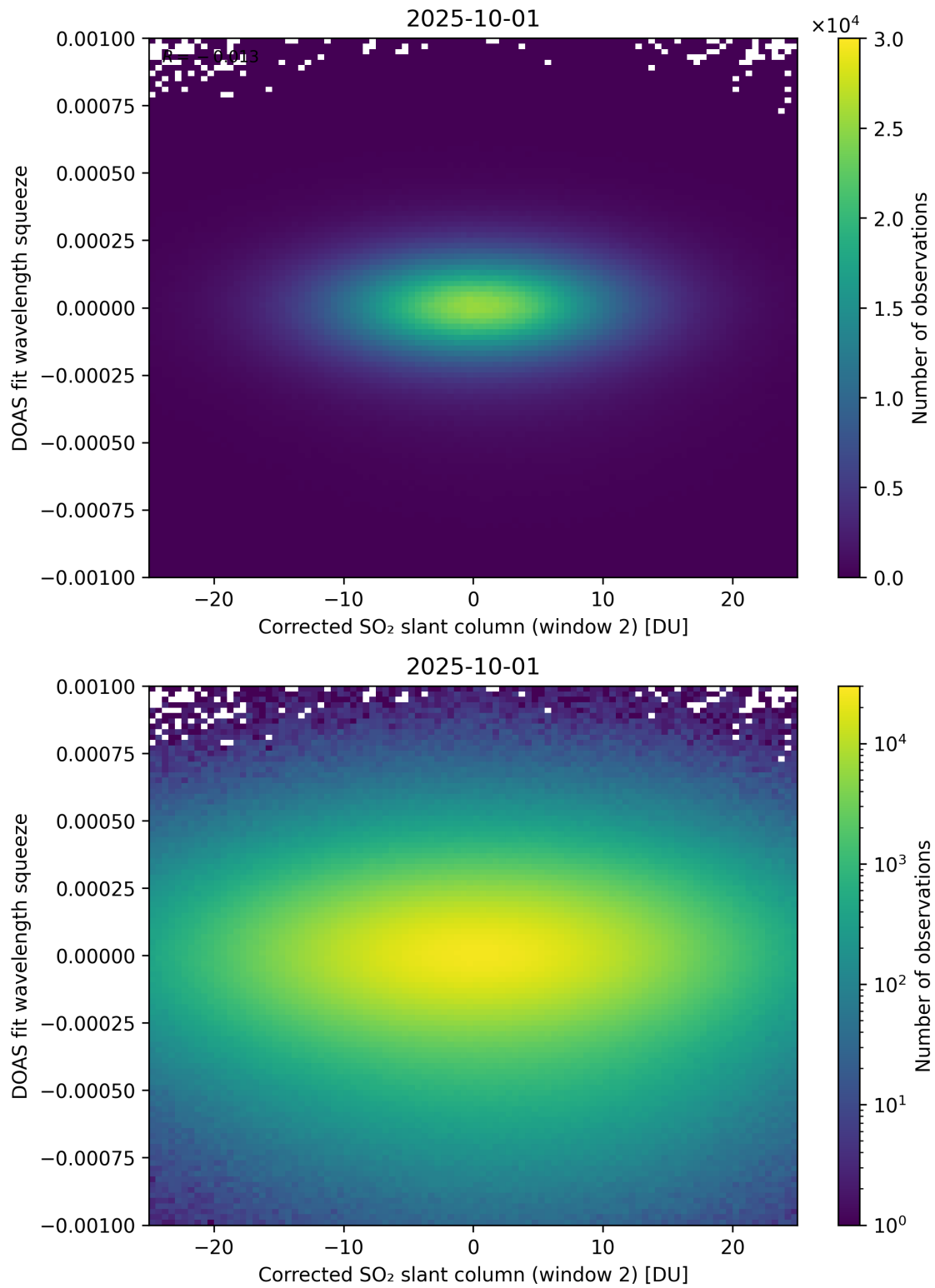
Figure 247: Scatter density plot of “Corrected SO 2 slant column (window 2)” against “DOAS fit wavelength squeeze” for 2025-10-01 to 2025-10-02.
