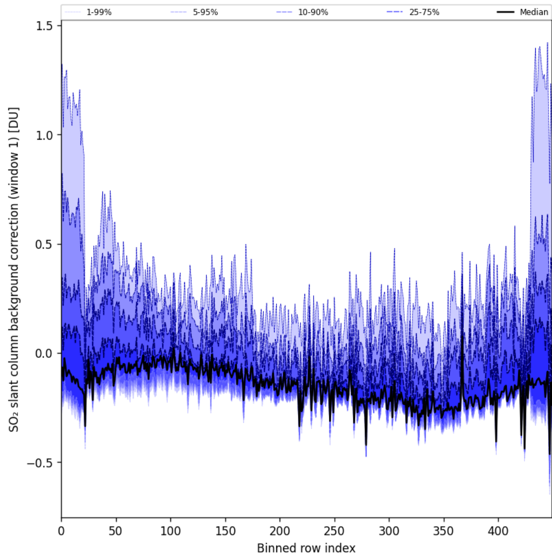
Figure 92: Along track statistics of “SO 2 slant column background correction (window 1)” for 2025-10-01 to 2025-10-02
