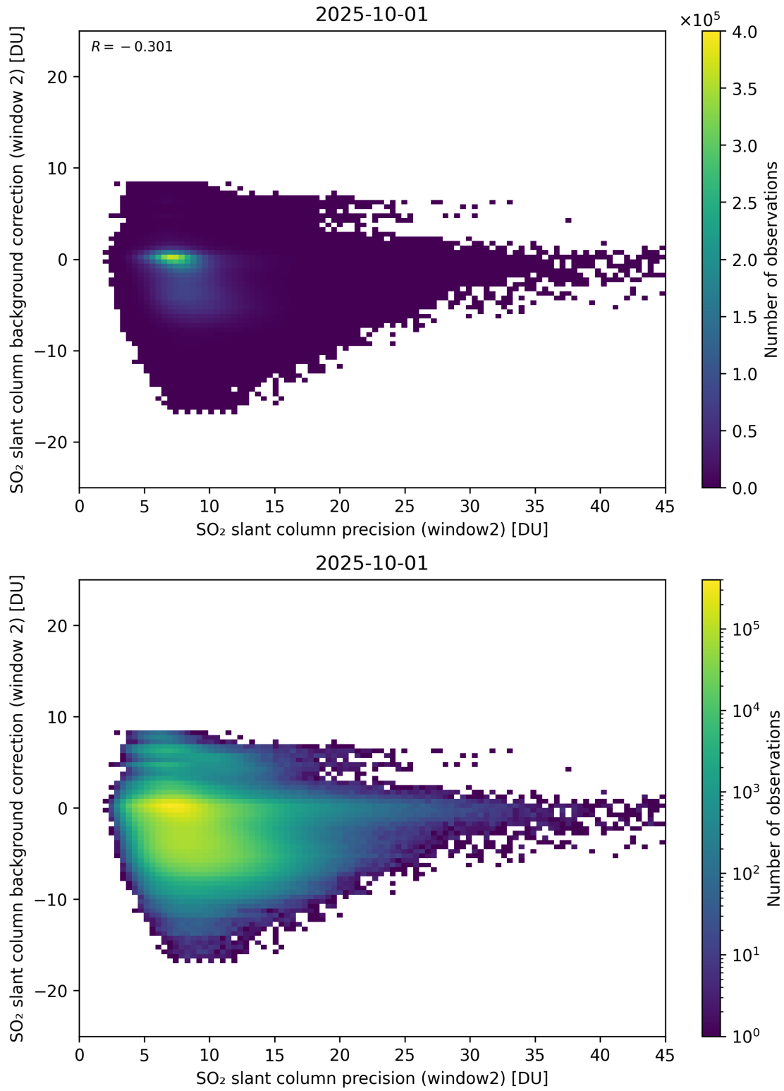
Figure 291: Scatter density plot of “SO 2 slant column precision (window2)” against “SO 2 slant column background correction (window 2)” for 2025-10-01 to 2025-10-02.
