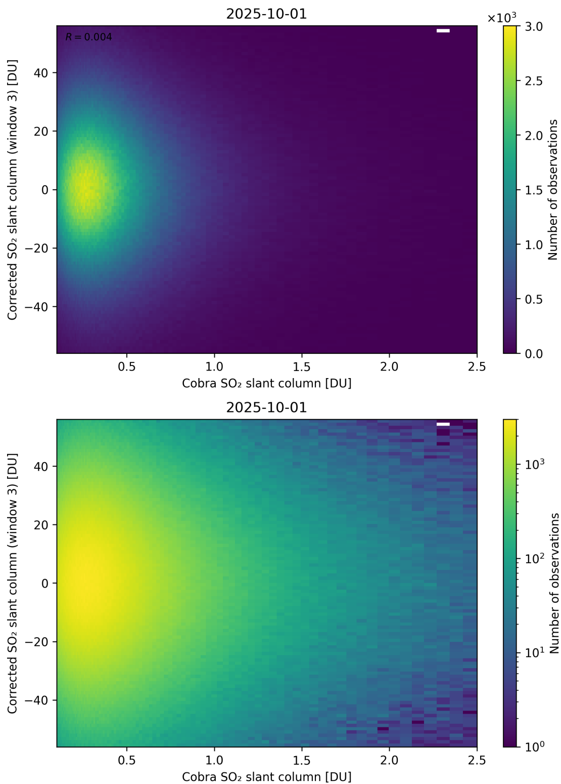
Figure 218: Scatter density plot of “Cobra SO 2 slant column” against “Corrected SO 2 slant column (window 3)” for 2025-10-01 to 2025-10-02.
