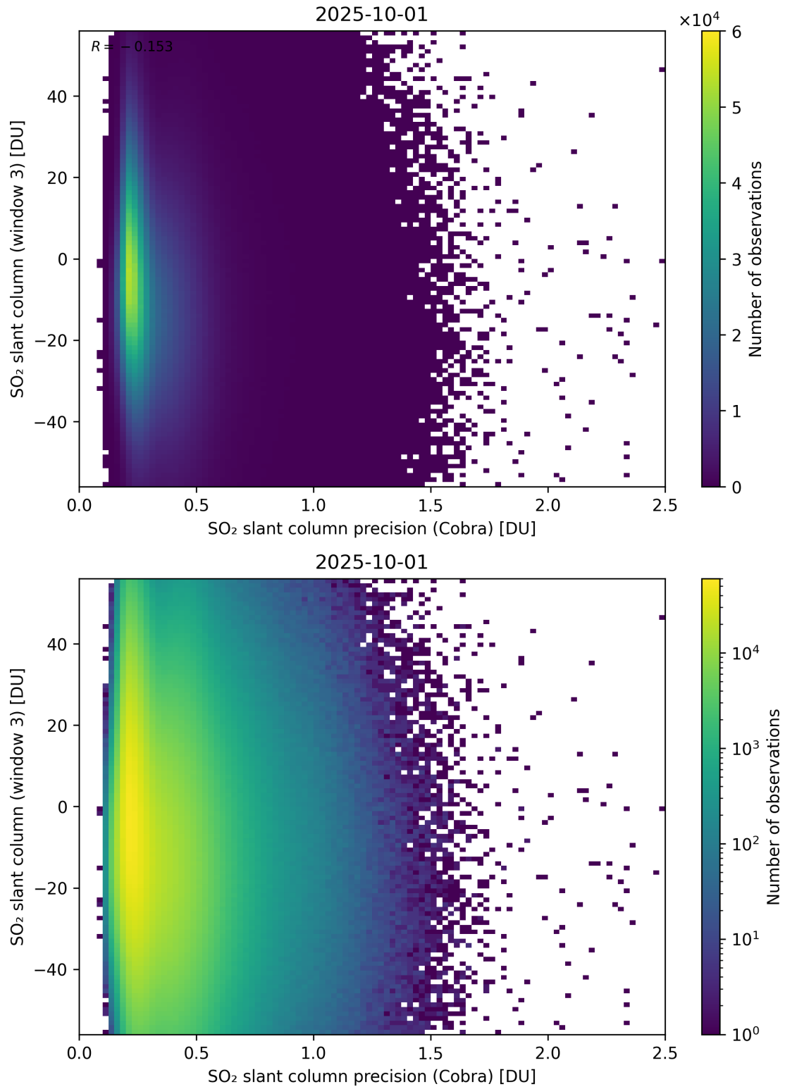
Figure 211: Scatter density plot of “SO 2 slant column precision (Cobra)” against “SO 2 slant column (window 3)” for 2025-10-01 to 2025-10-02.
