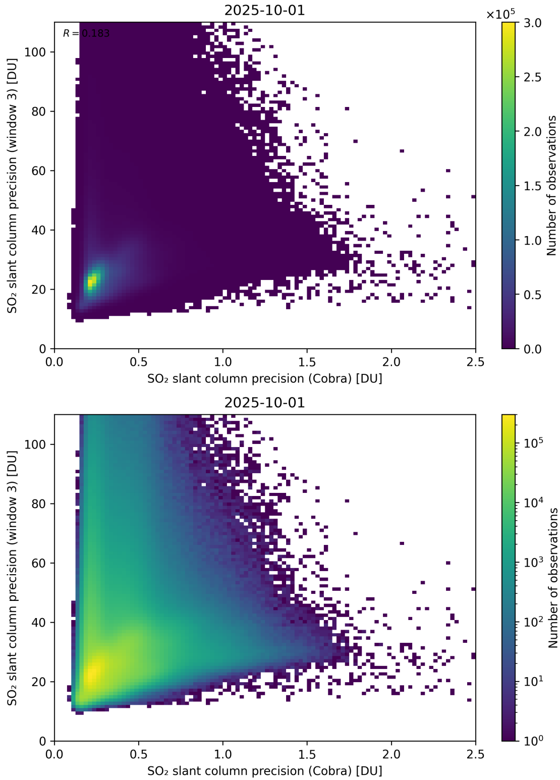
Figure 212: Scatter density plot of “SO 2 slant column precision (Cobra)” against “SO 2 slant column precision (window 3)” for 2025-10-01 to 2025-10-02.
