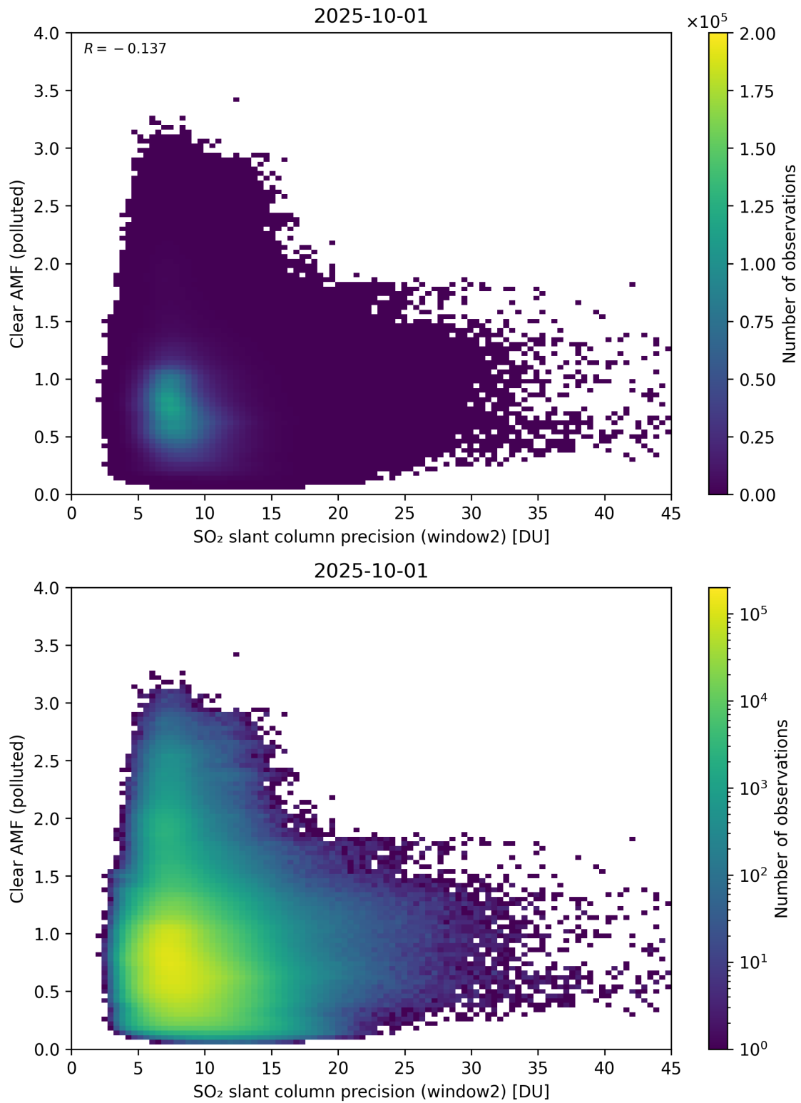
Figure 296: Scatter density plot of “SO 2 slant column precision (window2)” against “Clear AMF (polluted)” for 2025-10-01 to 2025-10-02.
