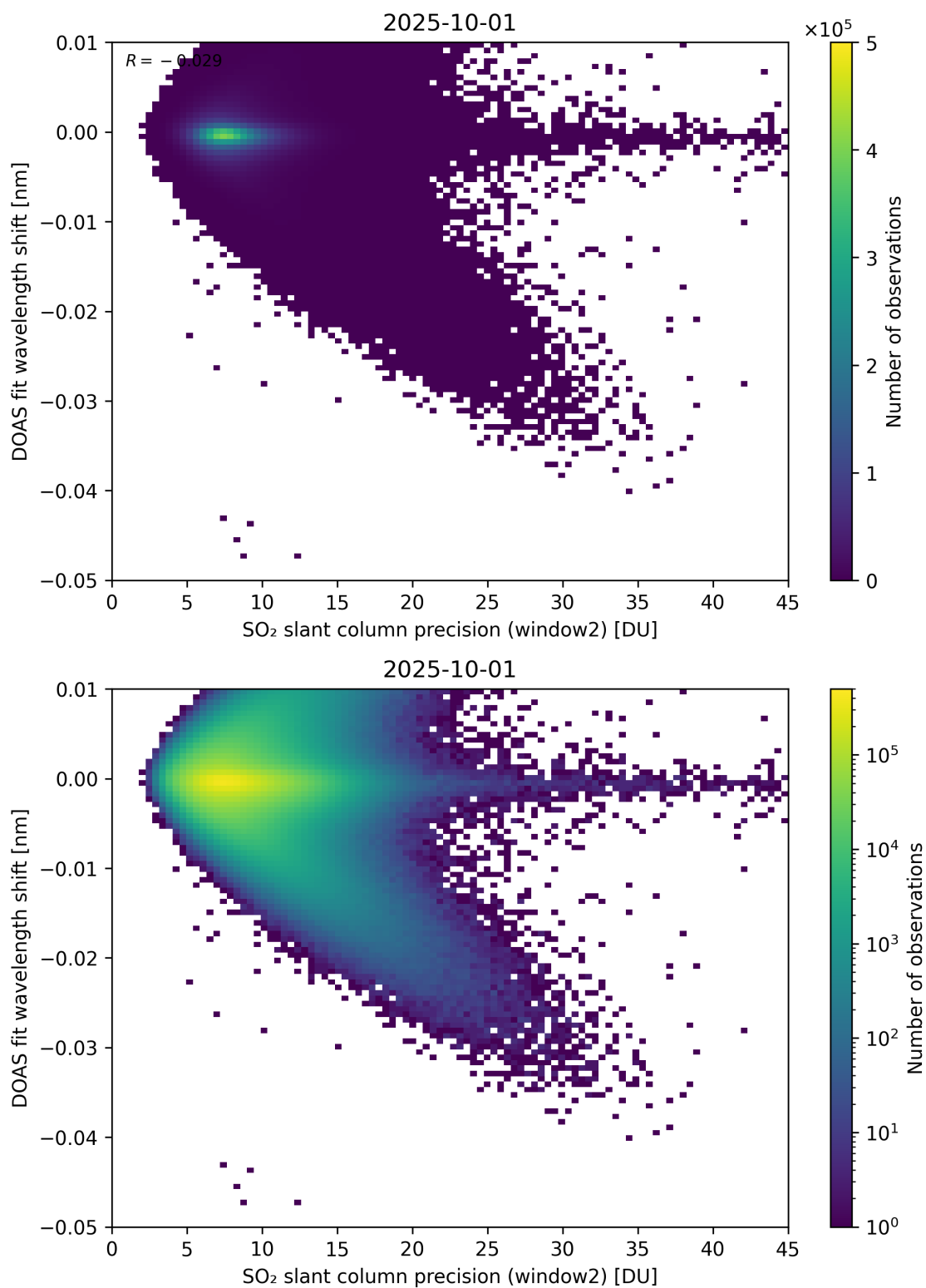
Figure 293: Scatter density plot of “SO 2 slant column precision (window2)” against “DOAS fit wavelength shift” for 2025-10-01 to 2025-10-02.
