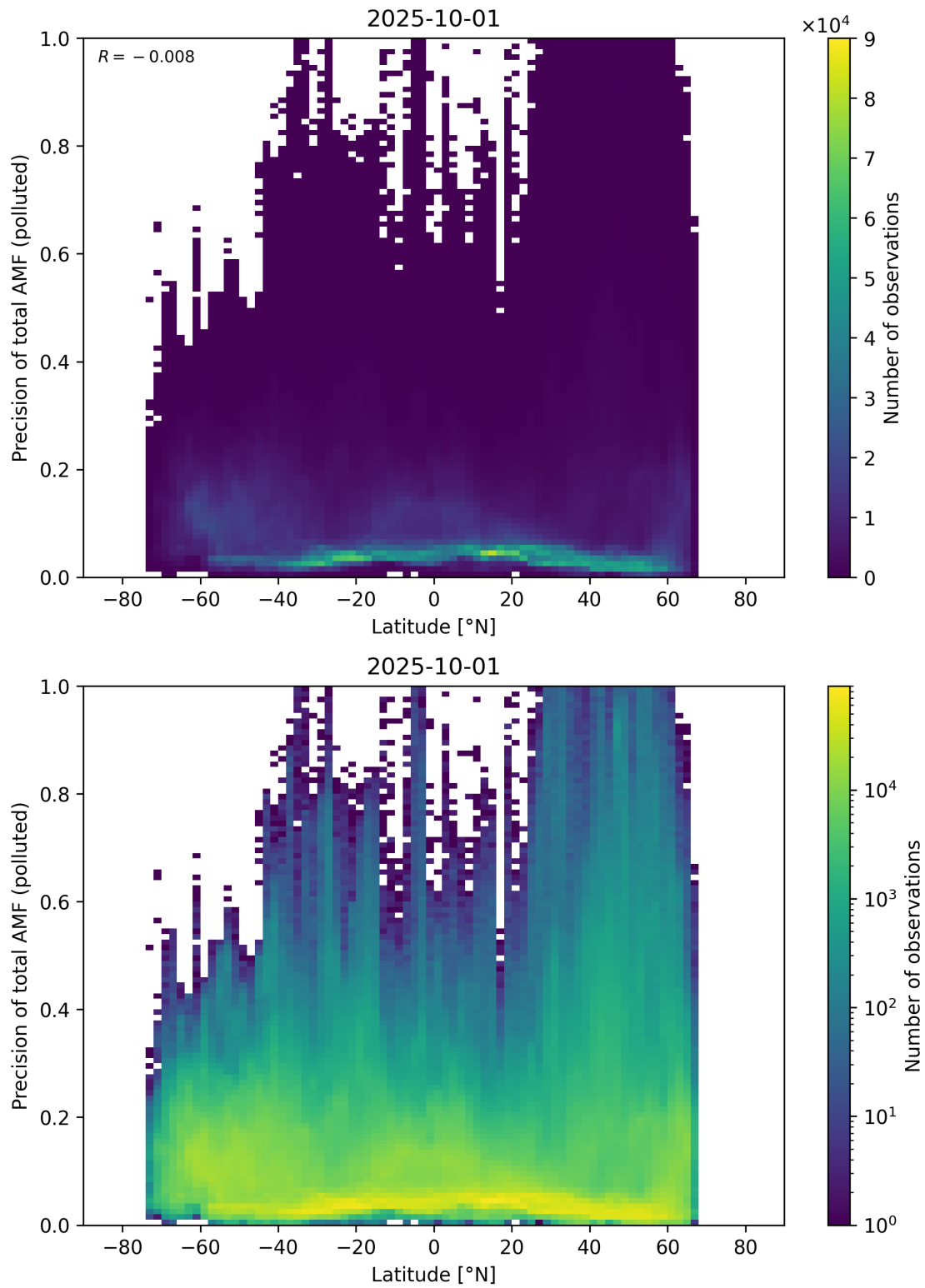
Figure 168: Scatter density plot of “Latitude” against “Precision of total AMF (polluted)” for 2025-10-01 to 2025-10-02.
