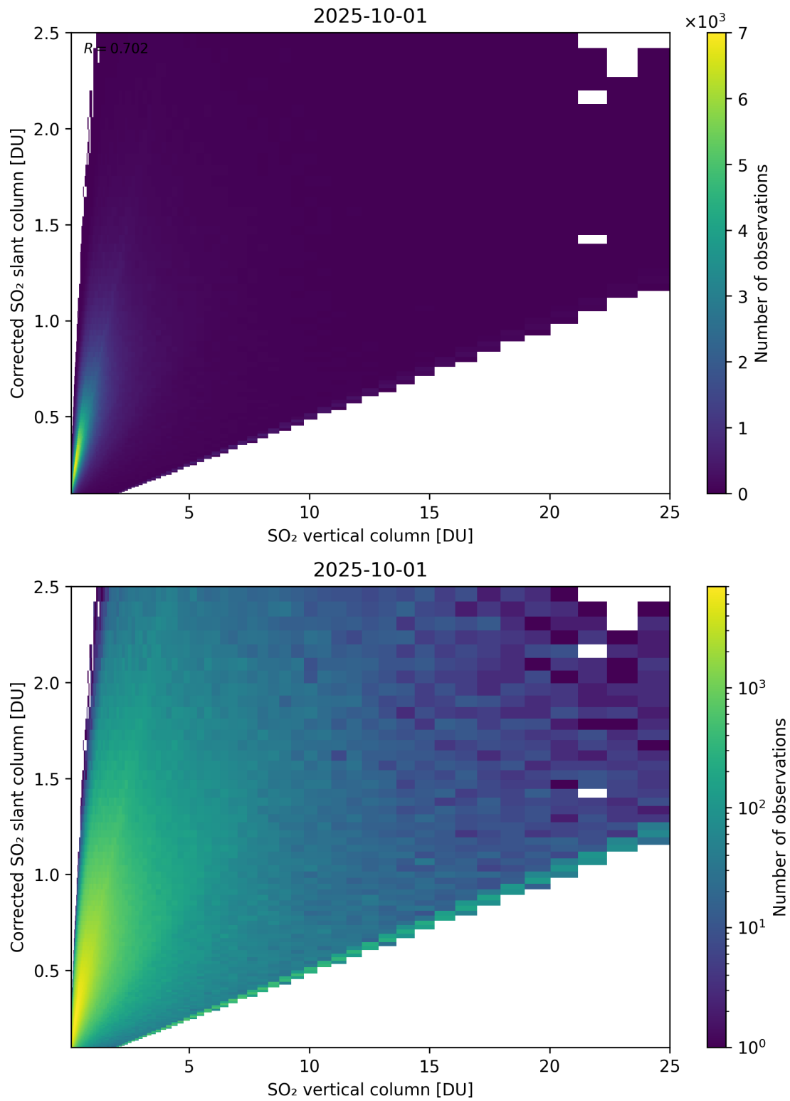
Figure 351: Scatter density plot of “SO 2 vertical column” against “Corrected SO 2 slant column” for 2025-10-01 to 2025-10-02.
