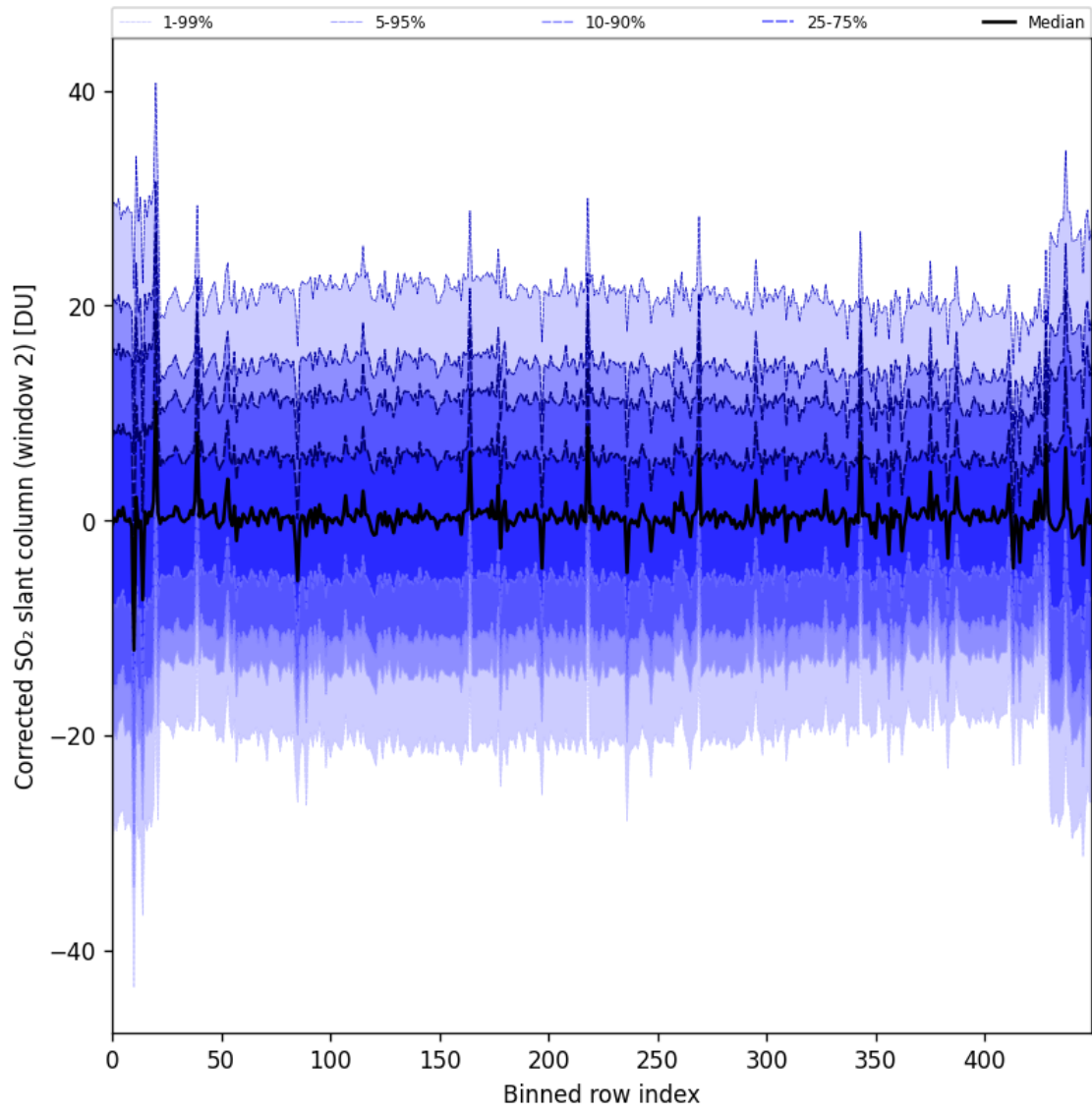
Figure 95: Along track statistics of “Corrected SO 2 slant column (window 2)” for 2025-10-01 to 2025-10-02
