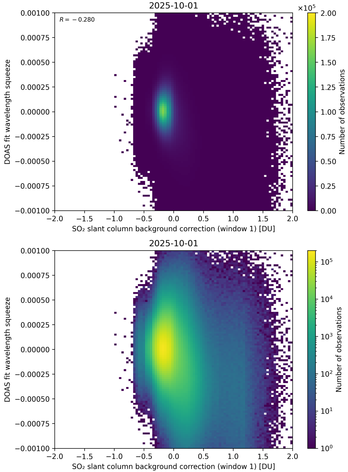
Figure 112: Scatter density plot of “SO 2 slant column background correction (window 1)” against “DOAS fit wavelength squeeze” for 2025-10-01 to 2025-10-02.
