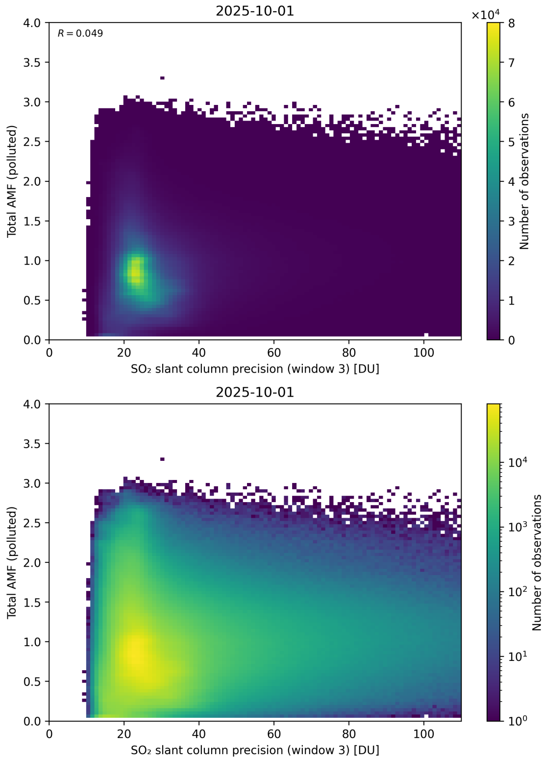
Figure 313: Scatter density plot of “SO 2 slant column precision (window 3)” against “Total AMF (polluted)” for 2025-10-01 to 2025-10-02.
