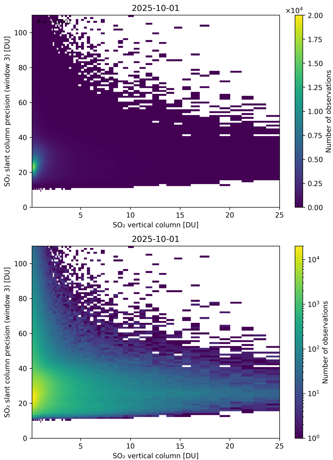
Figure 358: Scatter density plot of “SO 2 vertical column” against “SO 2 slant column precision (window 3)” for 2025-10-01 to 2025-10-02.
