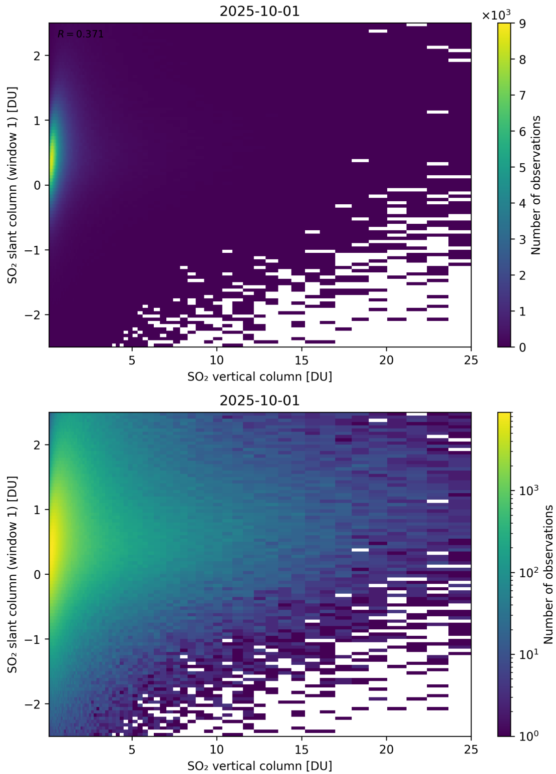
Figure 354: Scatter density plot of “SO 2 vertical column” against “SO 2 slant column (window 1)” for 2025-10-01 to 2025-10-02.
