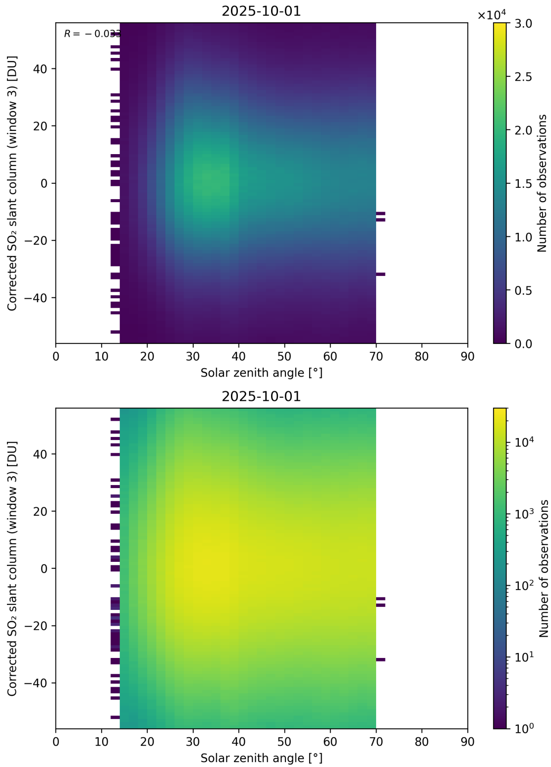
Figure 183: Scatter density plot of “Solar zenith angle” against “Corrected SO 2 slant column (window 3)” for 2025-10-01 to 2025-10-02.
