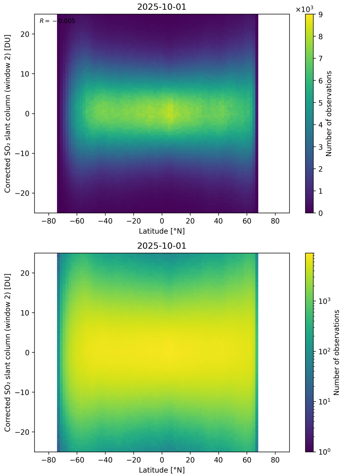
Figure 160: Scatter density plot of “Latitude” against “Corrected SO 2 slant column (window 2)” for 2025-10-01 to 2025-10-02.
