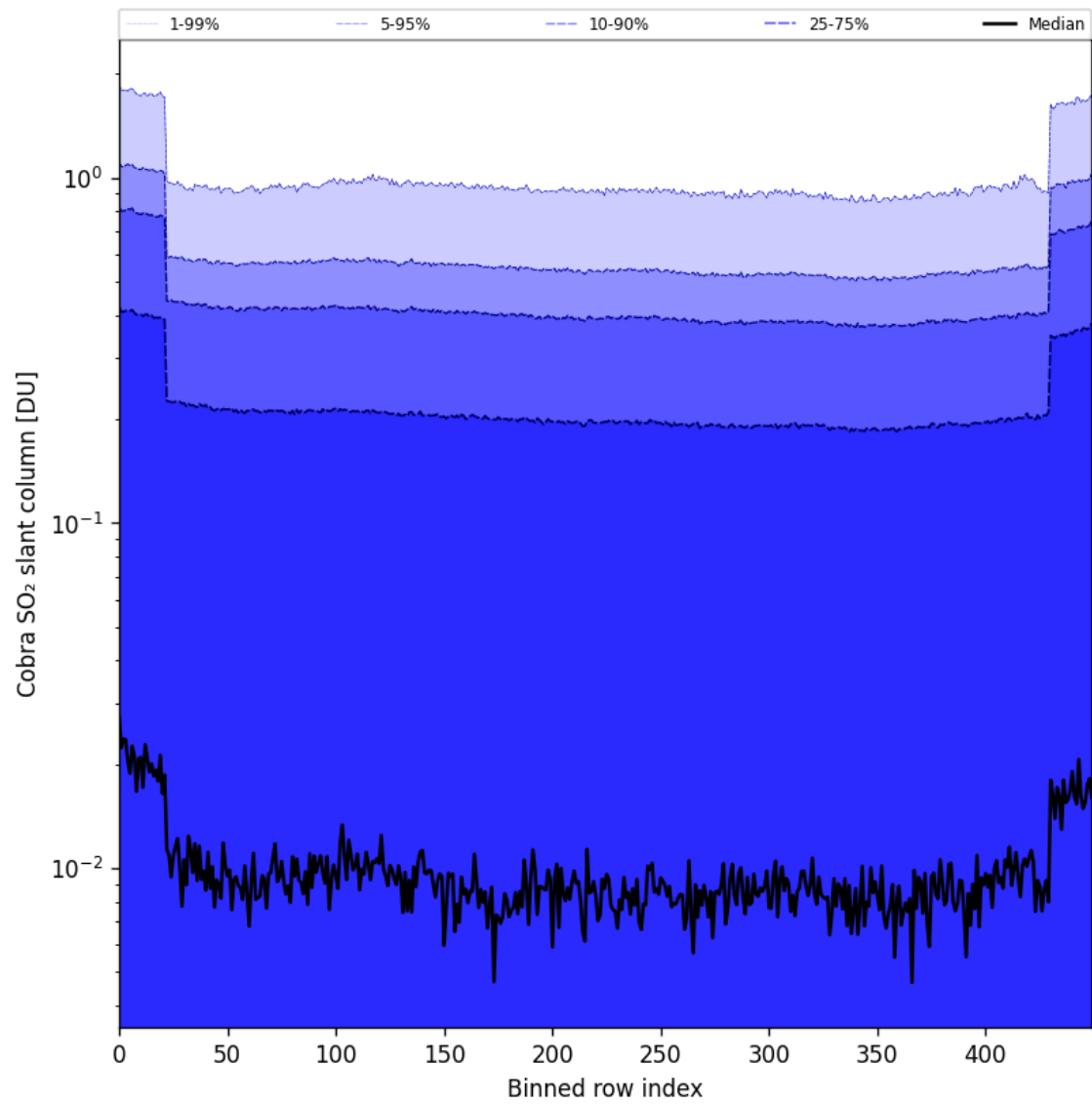
Figure 87: Along track statistics of "Cobra SO 2 slant column" for 2025-10-01 to 2025-10-02
