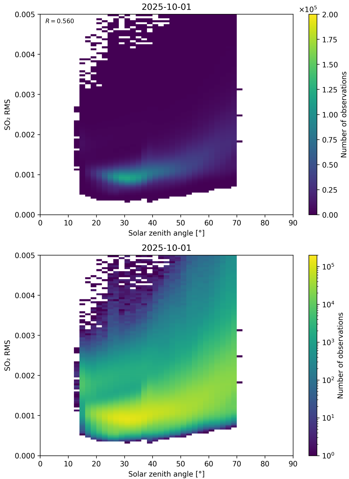
Figure 176: Scatter density plot of “Solar zenith angle” against “SO 2 RMS” for 2025-10-01 to 2025-10-02.
