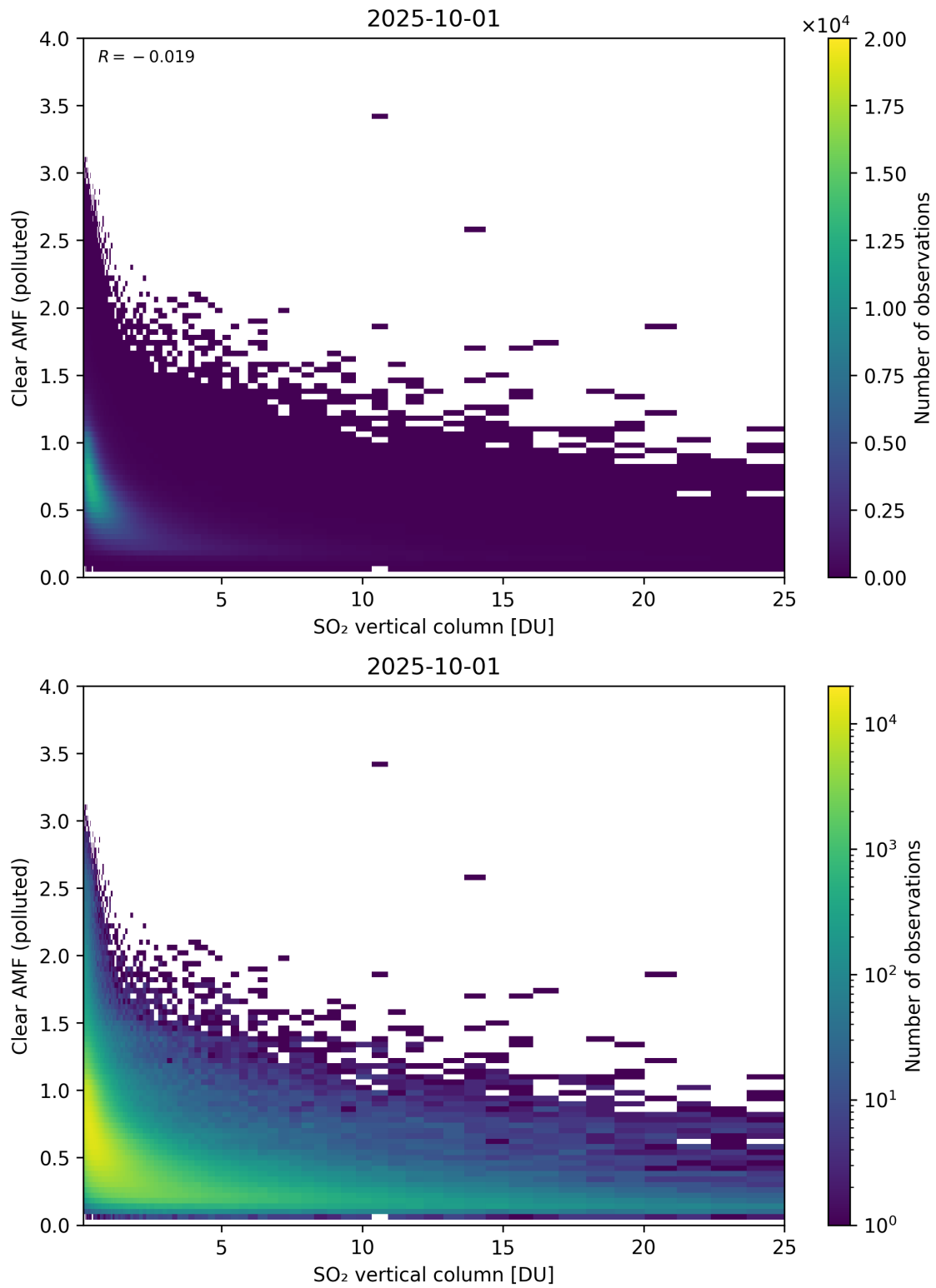
Figure 348: Scatter density plot of “SO 2 vertical column” against “Clear AMF (polluted)” for 2025-10-01 to 2025-10-02.
