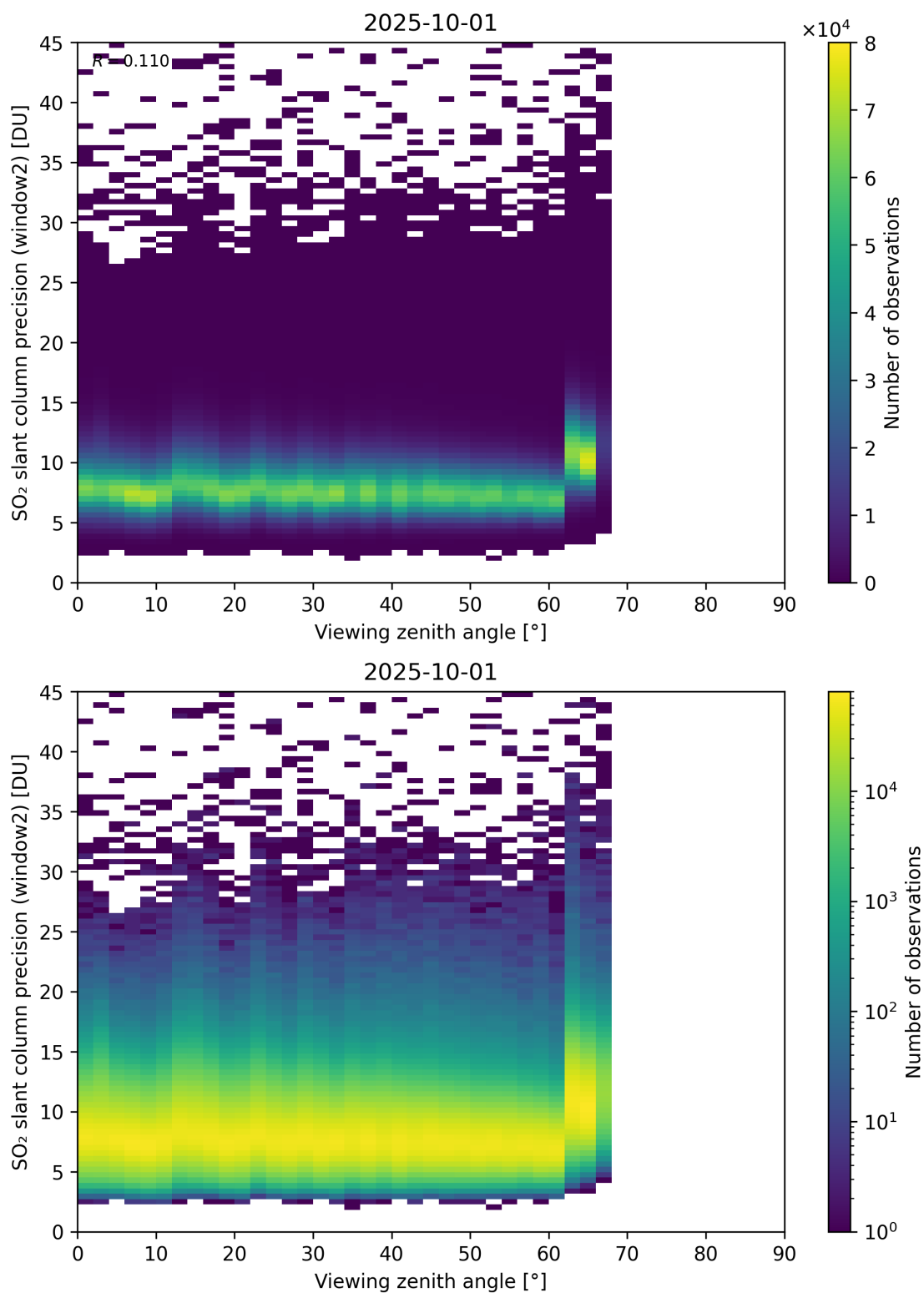
Figure 378: Scatter density plot of “Viewing zenith angle” against “SO 2 slant column precision (window2)” for 2025-10-01 to 2025-10-02.
