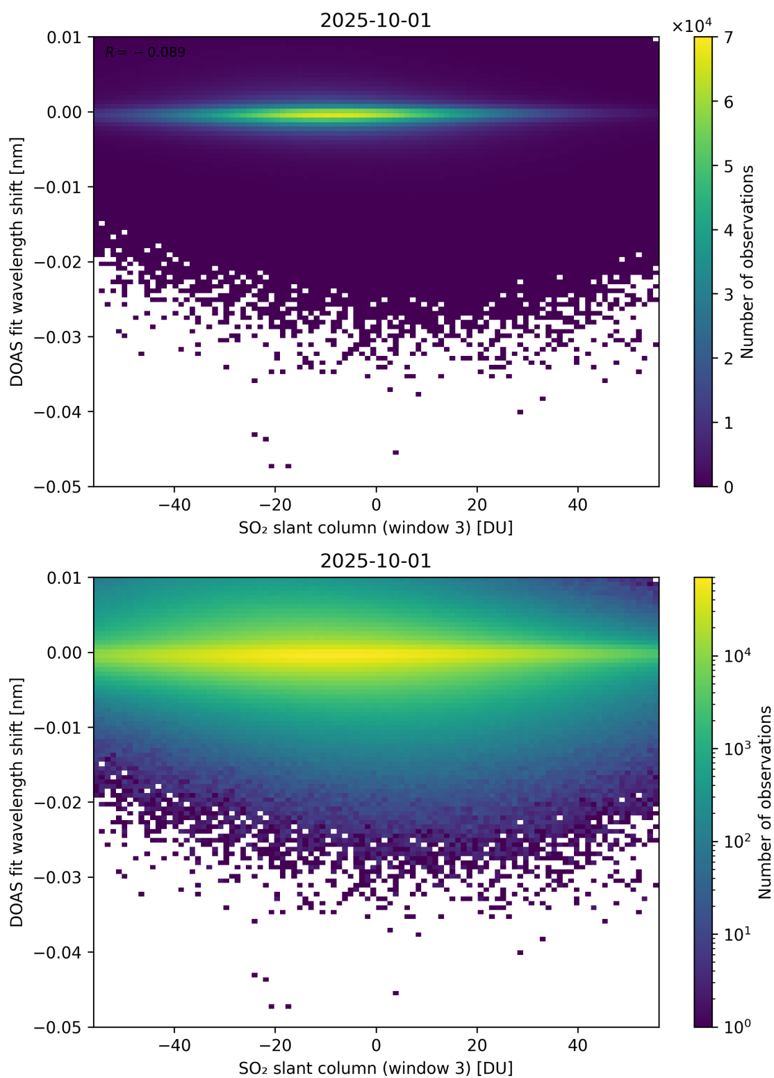
Figure 304: Scatter density plot of “SO 2 slant column (window 3)” against “DOAS fit wavelength shift” for 2025-10-01 to 2025-10-02.
