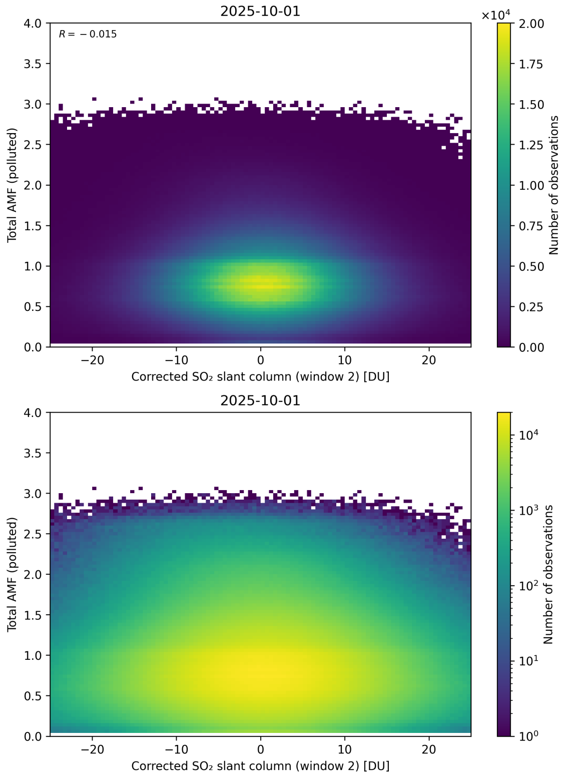
Figure 253: Scatter density plot of “Corrected SO 2 slant column (window 2)” against “Total AMF (polluted)” for 2025-10-01 to 2025-10-02.
