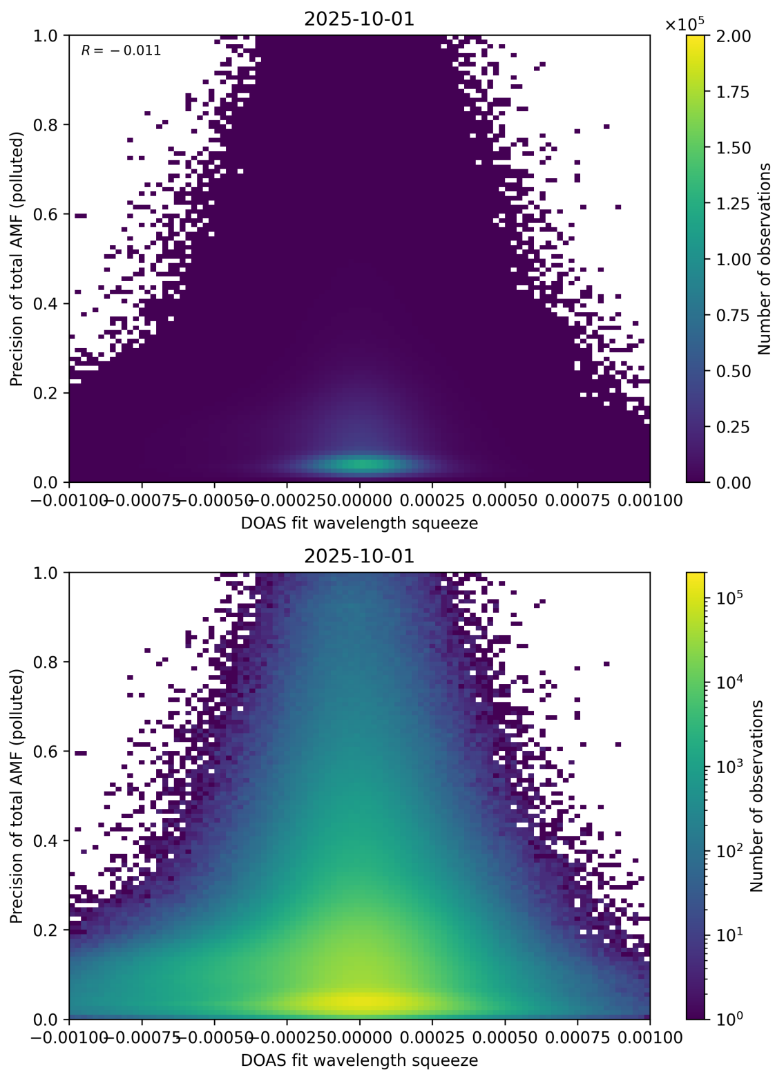
Figure 146: Scatter density plot of “DOAS fit wavelength squeeze” against “Precision of total AMF (polluted)” for 2025-10-01 to 2025-10-02.
