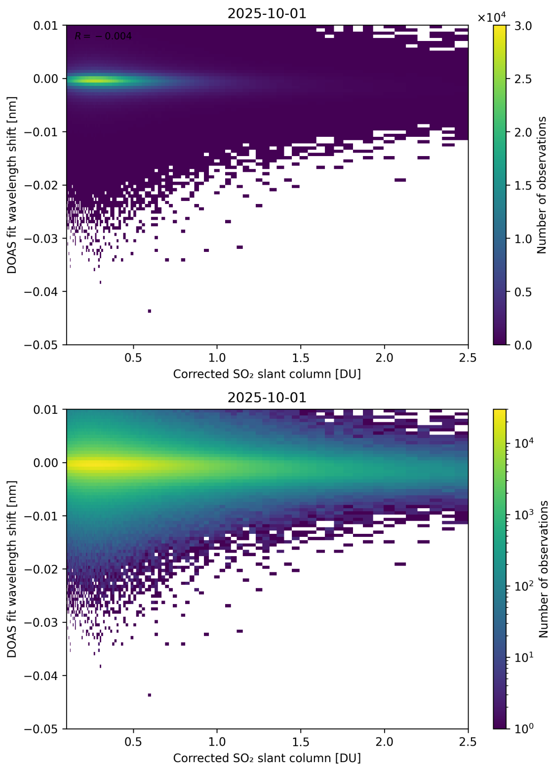
Figure 229: Scatter density plot of “Corrected SO 2 slant column” against “DOAS fit wavelength shift” for 2025-10-01 to 2025-10-02.
