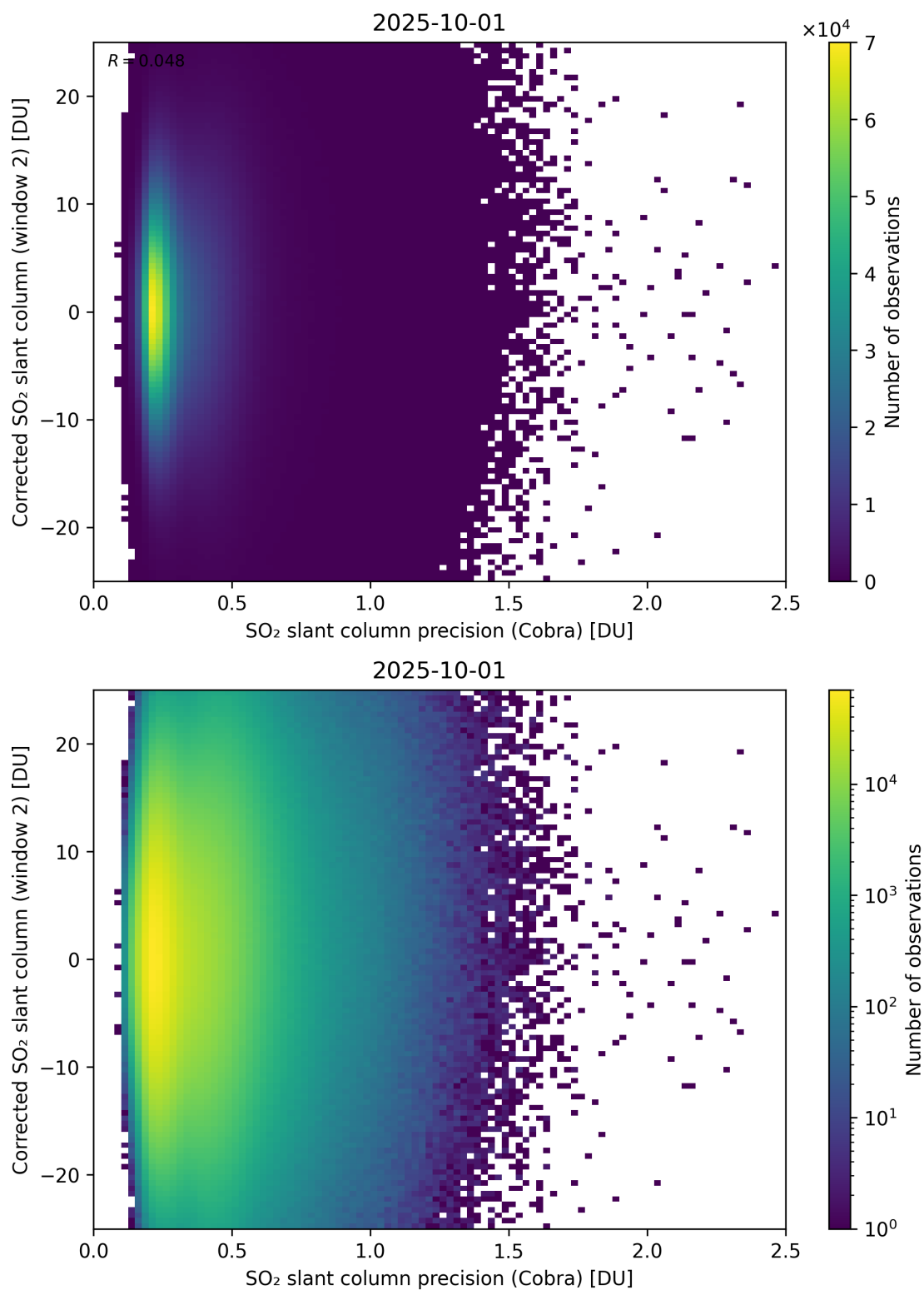
Figure 206: Scatter density plot of “SO 2 slant column precision (Cobra)” against “Corrected SO 2 slant column (window 2)” for 2025-10-01 to 2025-10-02.
