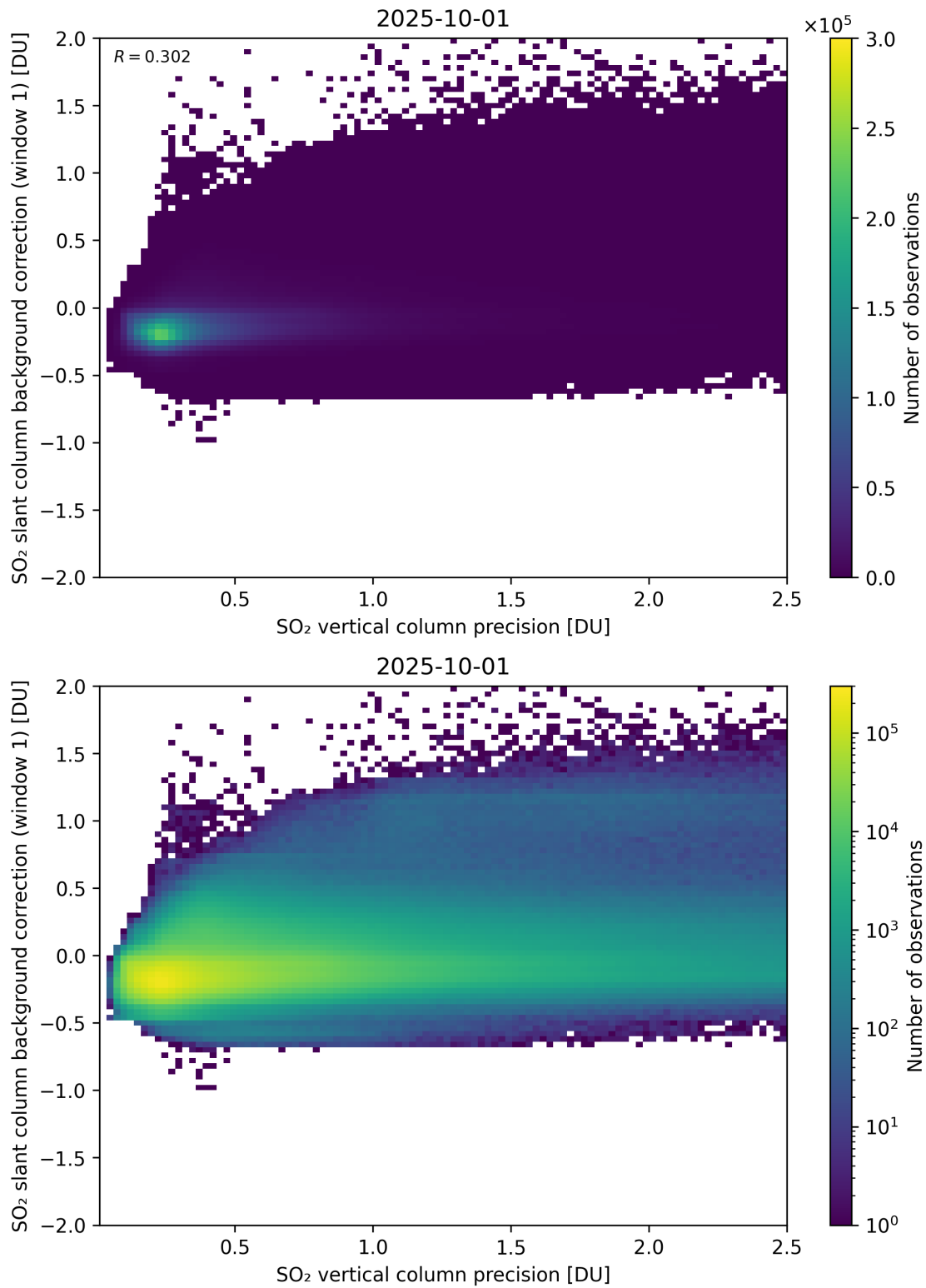
Figure 329: Scatter density plot of “SO 2 vertical column precision” against “SO 2 slant column background correction (window 1)” for 2025-10-01 to 2025-10-02.
