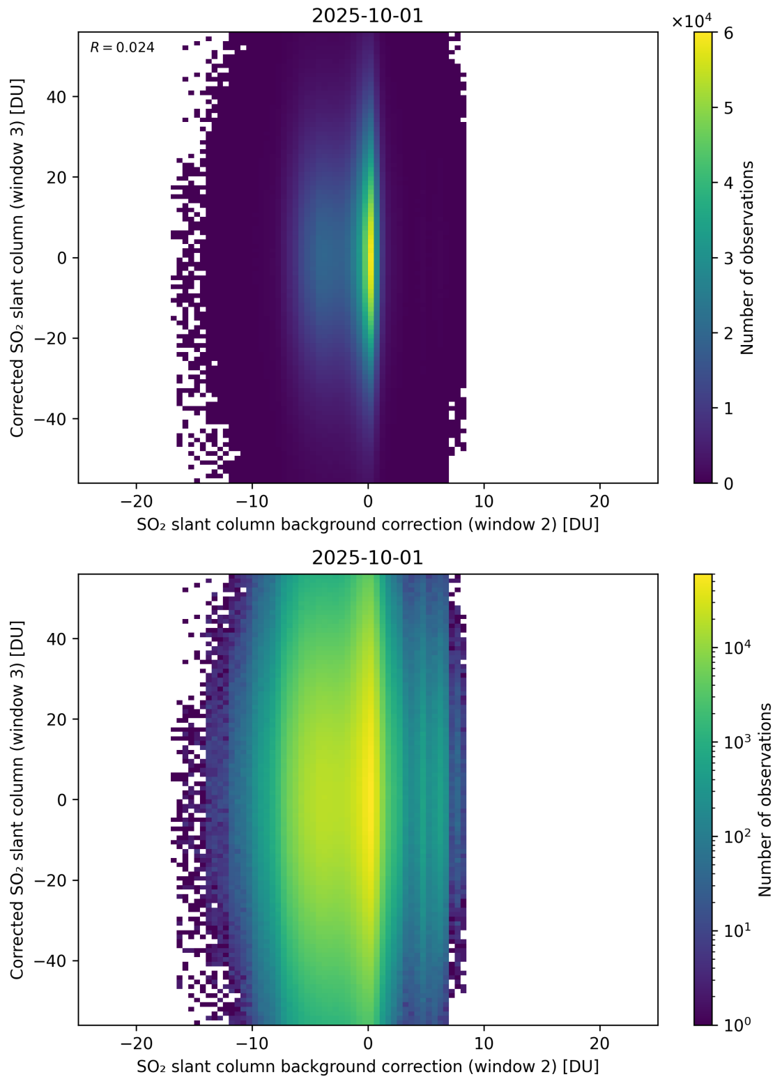
Figure 127: Scatter density plot of “SO 2 slant column background correction (window 2)” against “Corrected SO 2 slant column (window 3)” for 2025-10-01 to 2025-10-02.
