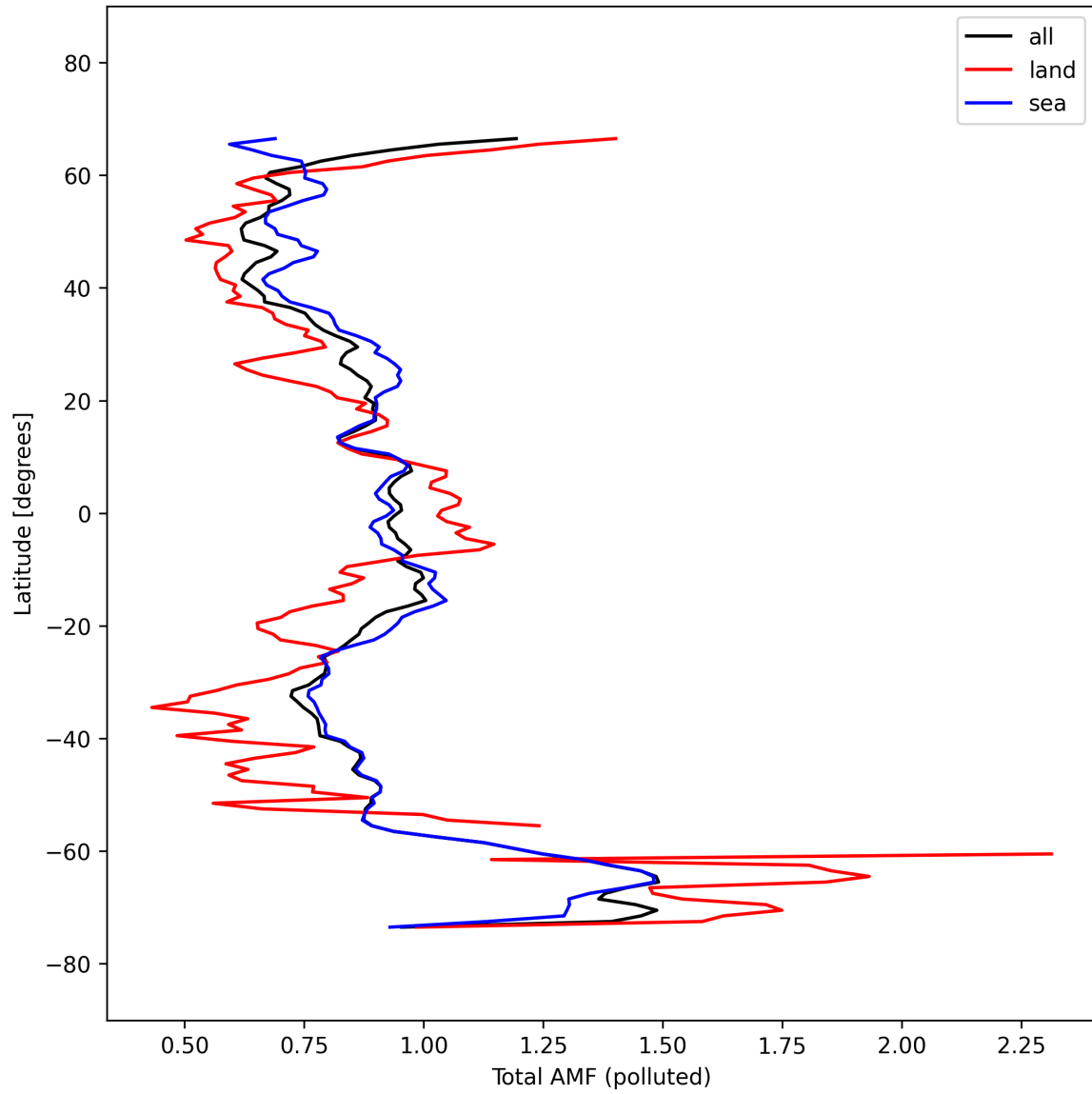
Figure 53: Zonal average of “Total AMF (polluted)” for 2025-10-01 to 2025-10-02.
