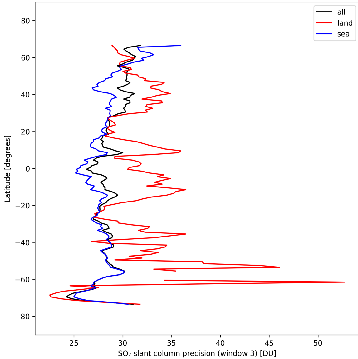
Figure 46: Zonal average of “SO 2 slant column precision (window 3)” for 2025-10-01 to 2025-10-02.
