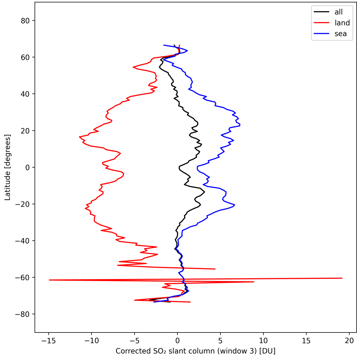
Figure 47: Zonal average of "Corrected SO 2 slant column (window 3)" for 2025-10-01 to 2025-10-02.
