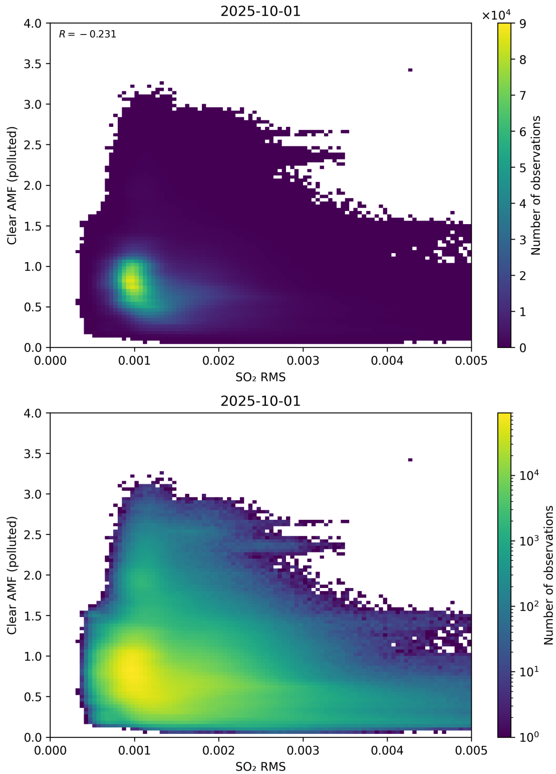
Figure 147: Scatter density plot of “SO 2 RMS” against “Clear AMF (polluted)” for 2025-10-01 to 2025-10-02.
