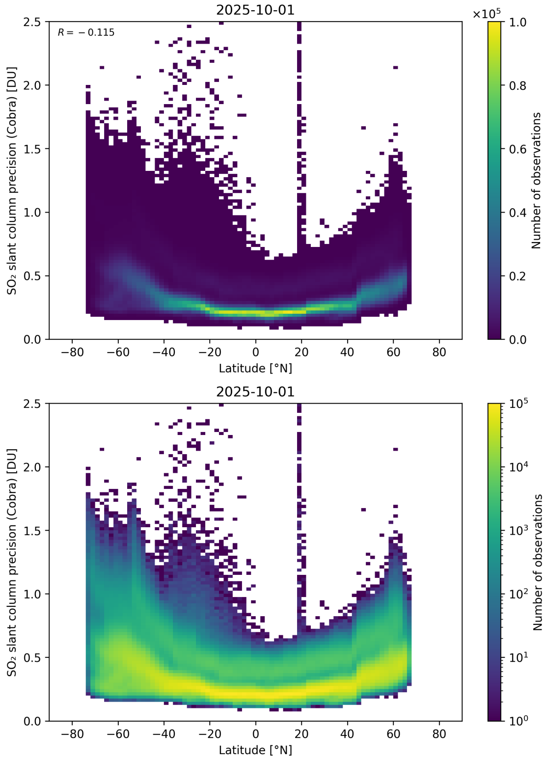
Figure 158: Scatter density plot of “Latitude” against “SO 2 slant column precision (Cobra)” for 2025-10-01 to 2025-10-02.
