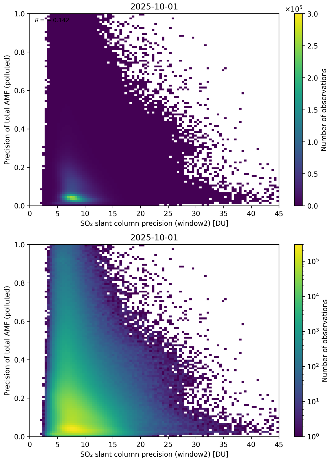
Figure 302: Scatter density plot of “SO 2 slant column precision (window2)” against “Precision of total AMF (polluted)” for 2025-10-01 to 2025-10-02.
