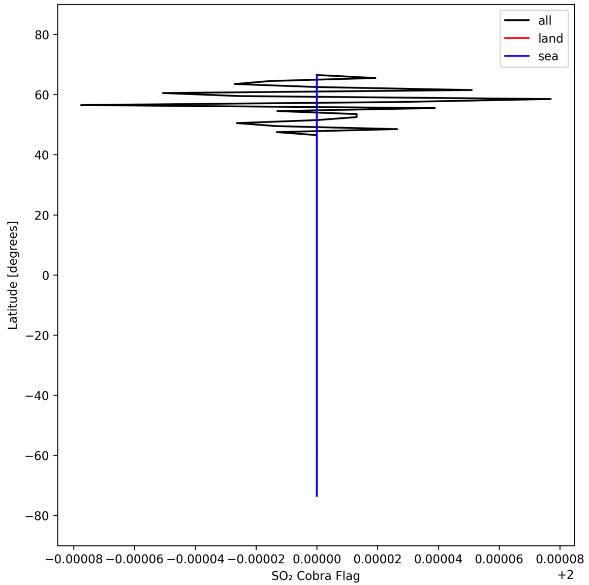
Figure 49: Zonal average of “SO 2 Cobra Flag” for 2025-10-01 to 2025-10-02.
