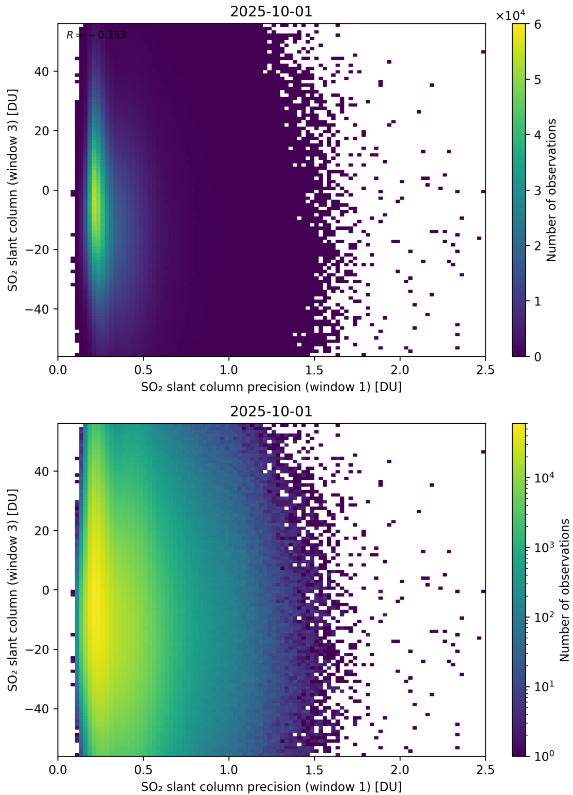
Figure 278: Scatter density plot of “SO 2 slant column precision (window 1)” against “SO 2 slant column (window 3)” for 2025-10-01 to 2025-10-02.
