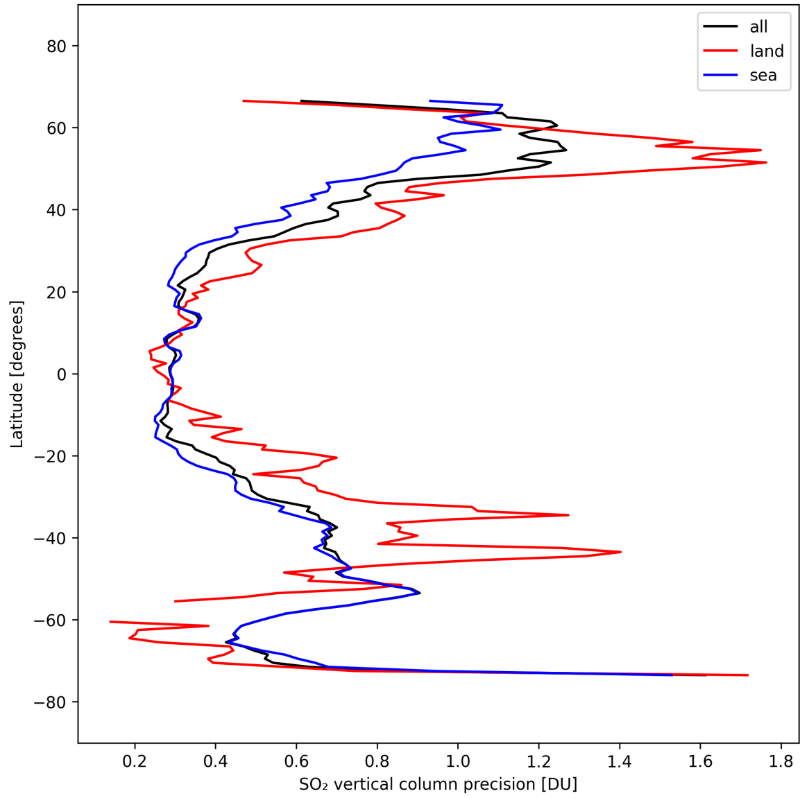
Figure 33: Zonal average of “SO 2 vertical column precision” for 2025-10-01 to 2025-10-02.
