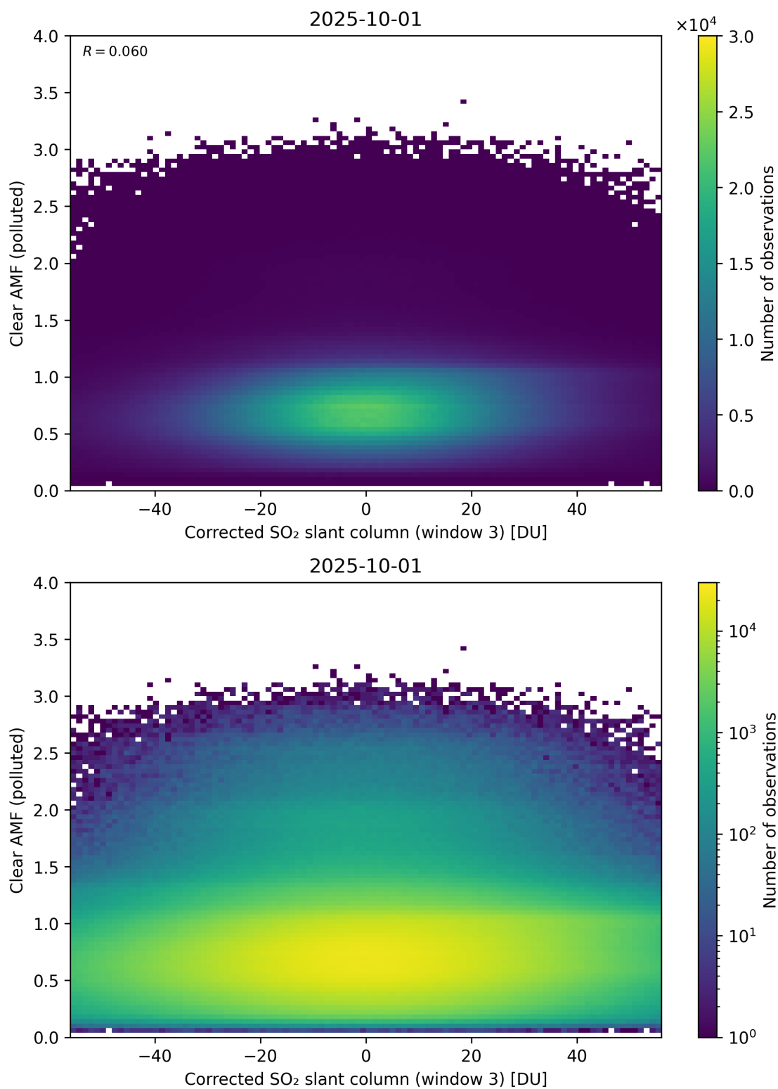
Figure 259: Scatter density plot of “Corrected SO 2 slant column (window 3)” against “Clear AMF (polluted)” for 2025-10-01 to 2025-10-02.
