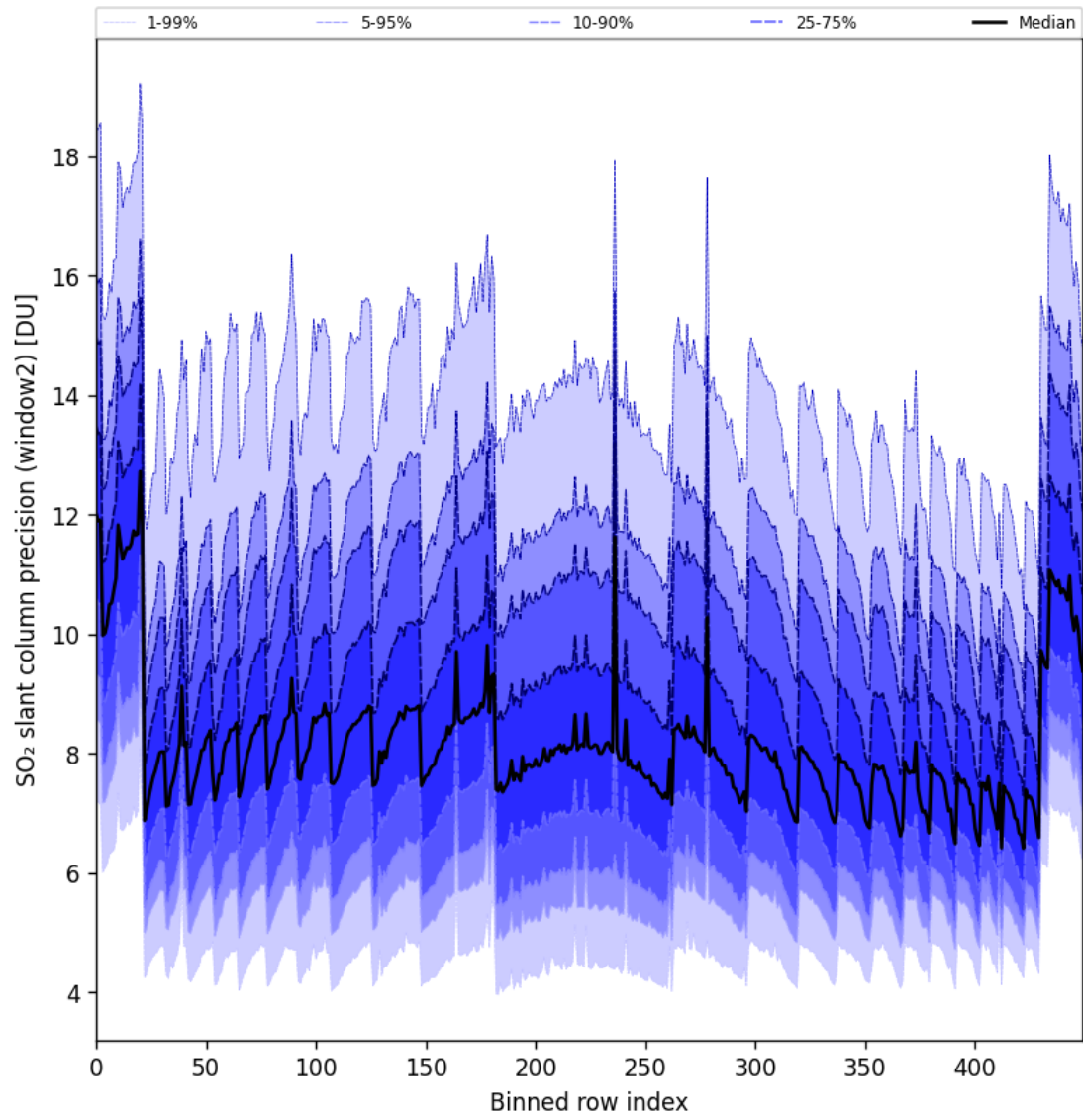
Figure 94: Along track statistics of “SO 2 slant column precision (window2)” for 2025-10-01 to 2025-10-02
