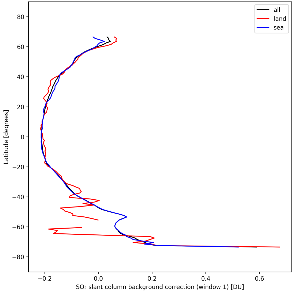
Figure 40: Zonal average of “SO 2 slant column background correction (window 1)” for 2025-10-01 to 2025-10-02.
