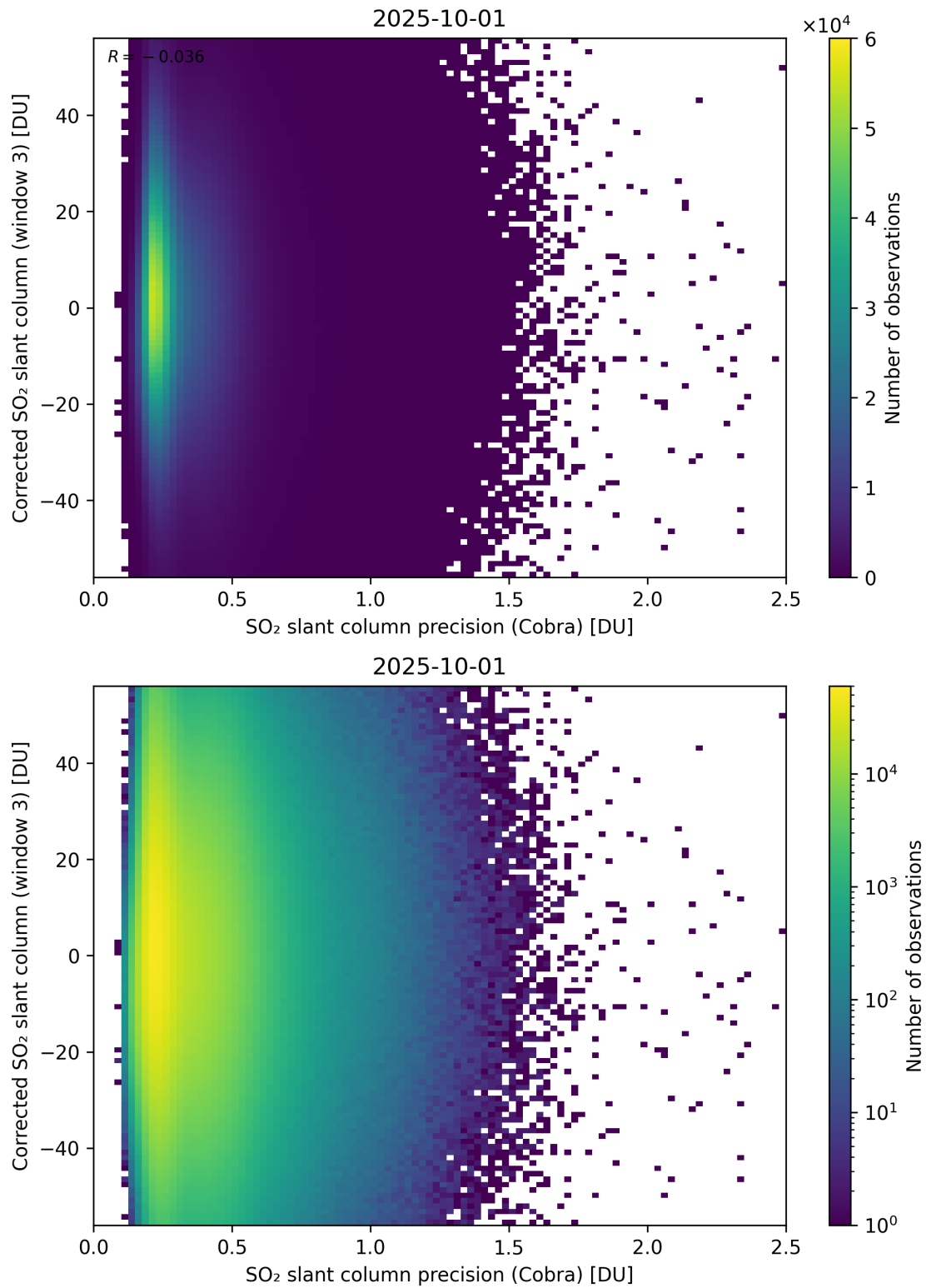
Figure 207: Scatter density plot of “SO 2 slant column precision (Cobra)” against “Corrected SO 2 slant column (window 3)” for 2025-10-01 to 2025-10-02.
