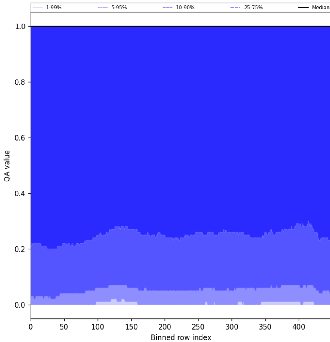
Figure 83: Along track statistics of “QA value” for 2025-10-01 to 2025-10-02
