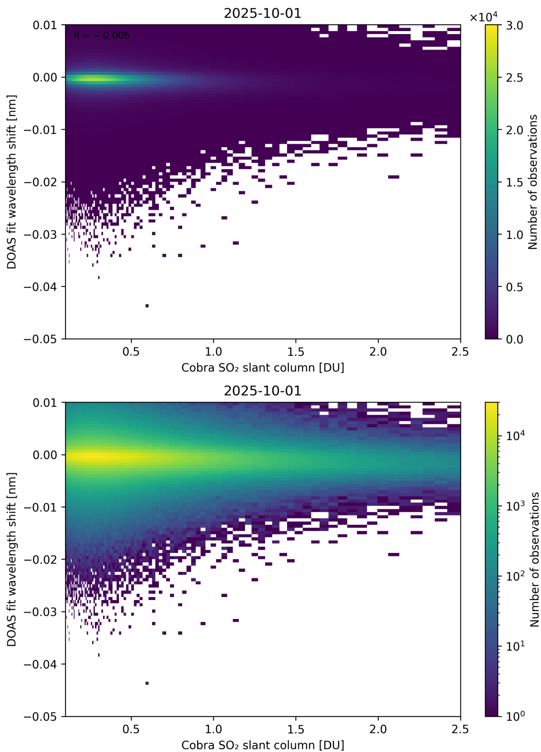
Figure 196: Scatter density plot of “Cobra SO 2 slant column” against “DOAS fit wavelength shift” for 2025-10-01 to 2025-10-02.
