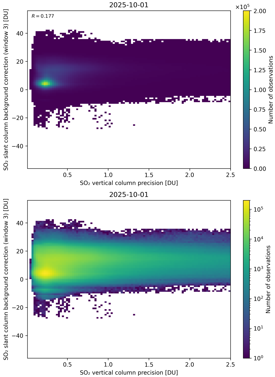
Figure 331: Scatter density plot of “SO 2 vertical column precision” against “SO 2 slant column background correction (window 3)” for 2025-10-01 to 2025-10-02.
