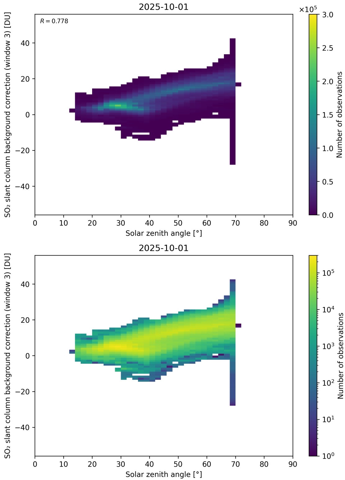
Figure 173: Scatter density plot of “Solar zenith angle” against “SO 2 slant column background correction (window 3)” for 2025-10-01 to 2025-10-02.
