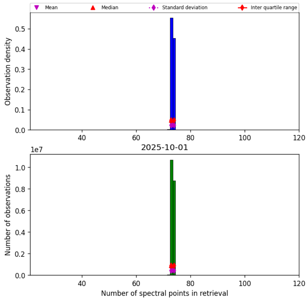
Figure 82: Histogram of “Number of spectral points in retrieval” for 2025-10-01 to 2025-10-02
