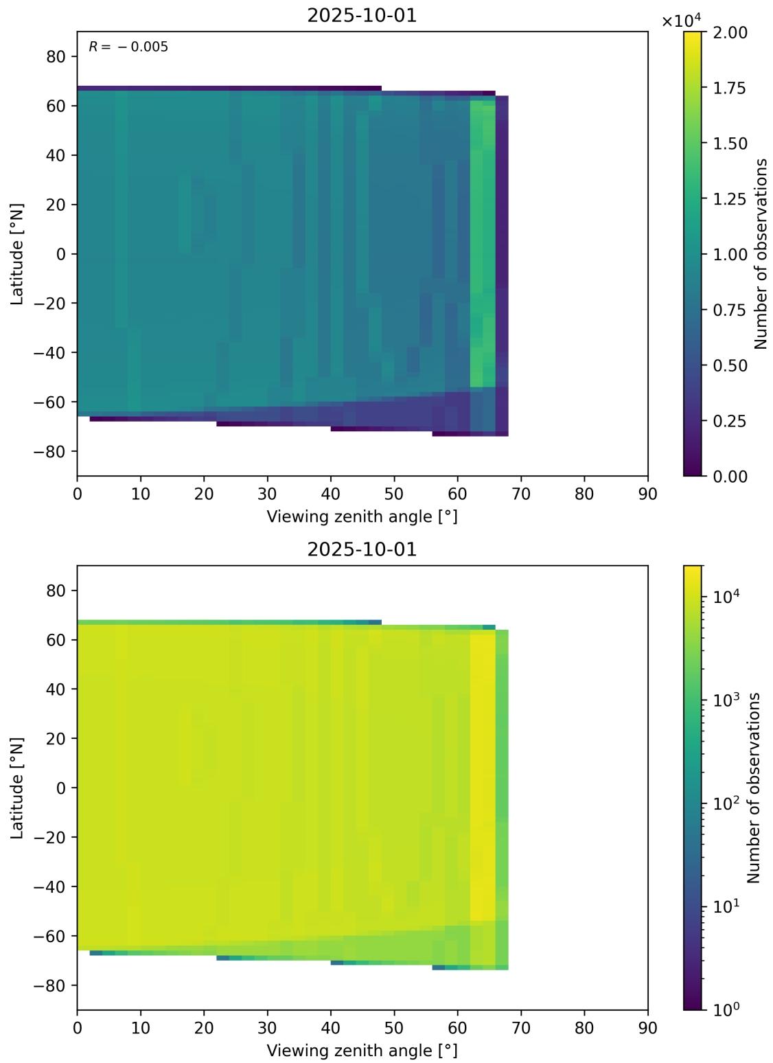
Figure 368: Scatter density plot of “Viewing zenith angle” against “Latitude” for 2025-10-01 to 2025-10-02.
