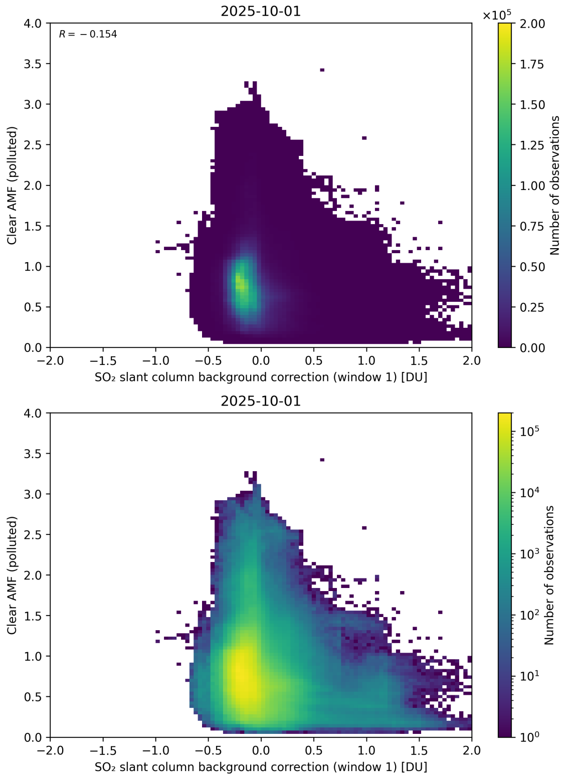
Figure 114: Scatter density plot of “SO 2 slant column background correction (window 1)” against “Clear AMF (polluted)” for 2025-10-01 to 2025-10-02.
