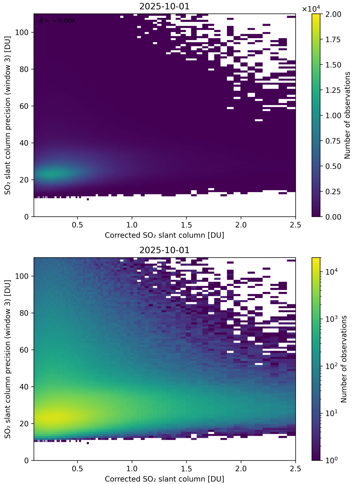
Figure 241: Scatter density plot of “Corrected SO 2 slant column” against “SO 2 slant column precision (window 3)” for 2025-10-01 to 2025-10-02.
