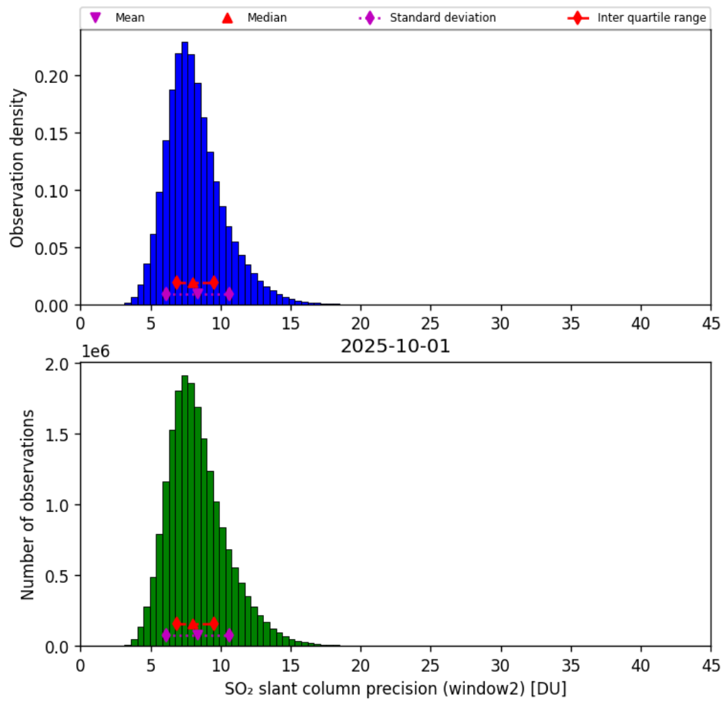
Figure 68: Histogram of “SO 2 slant column precision (window2)” for 2025-10-01 to 2025-10-02
