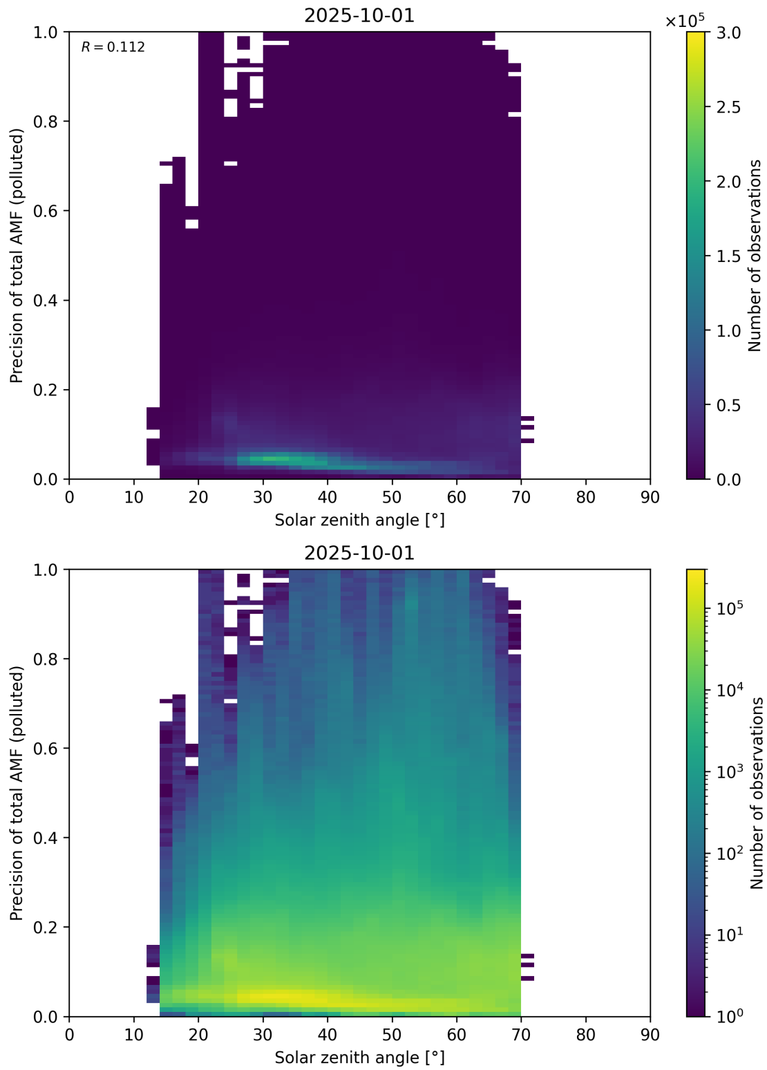
Figure 190: Scatter density plot of “Solar zenith angle” against “Precision of total AMF (polluted)” for 2025-10-01 to 2025-10-02.
