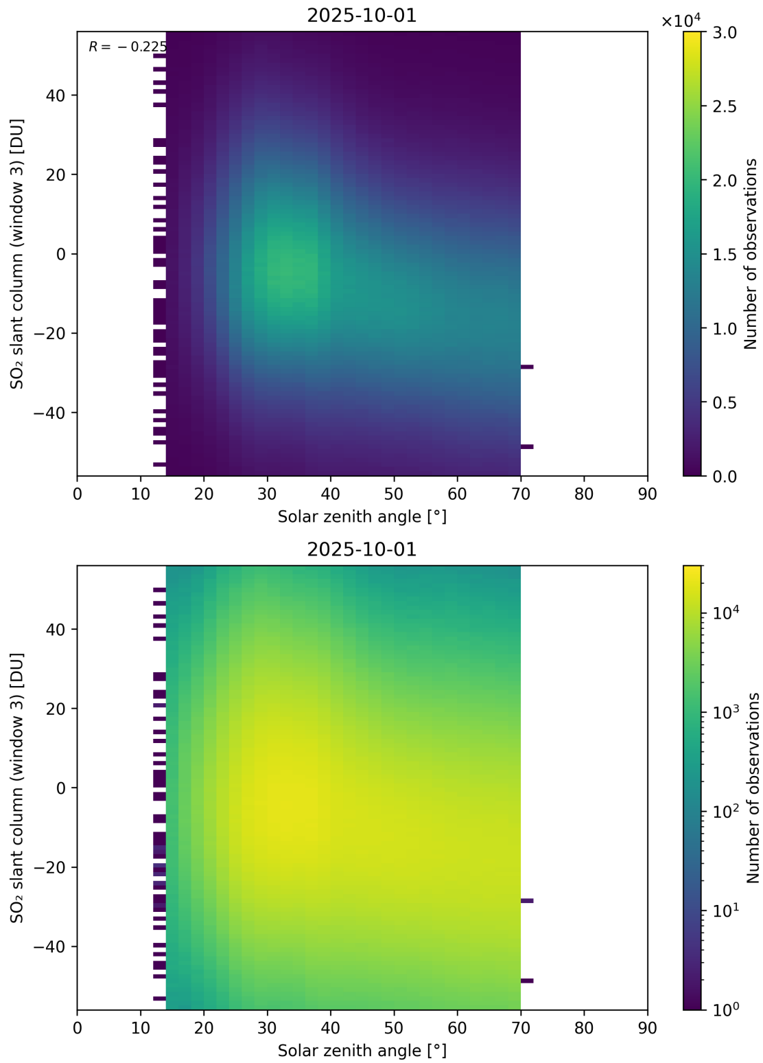
Figure 187: Scatter density plot of “Solar zenith angle” against “SO 2 slant column (window 3)” for 2025-10-01 to 2025-10-02.
