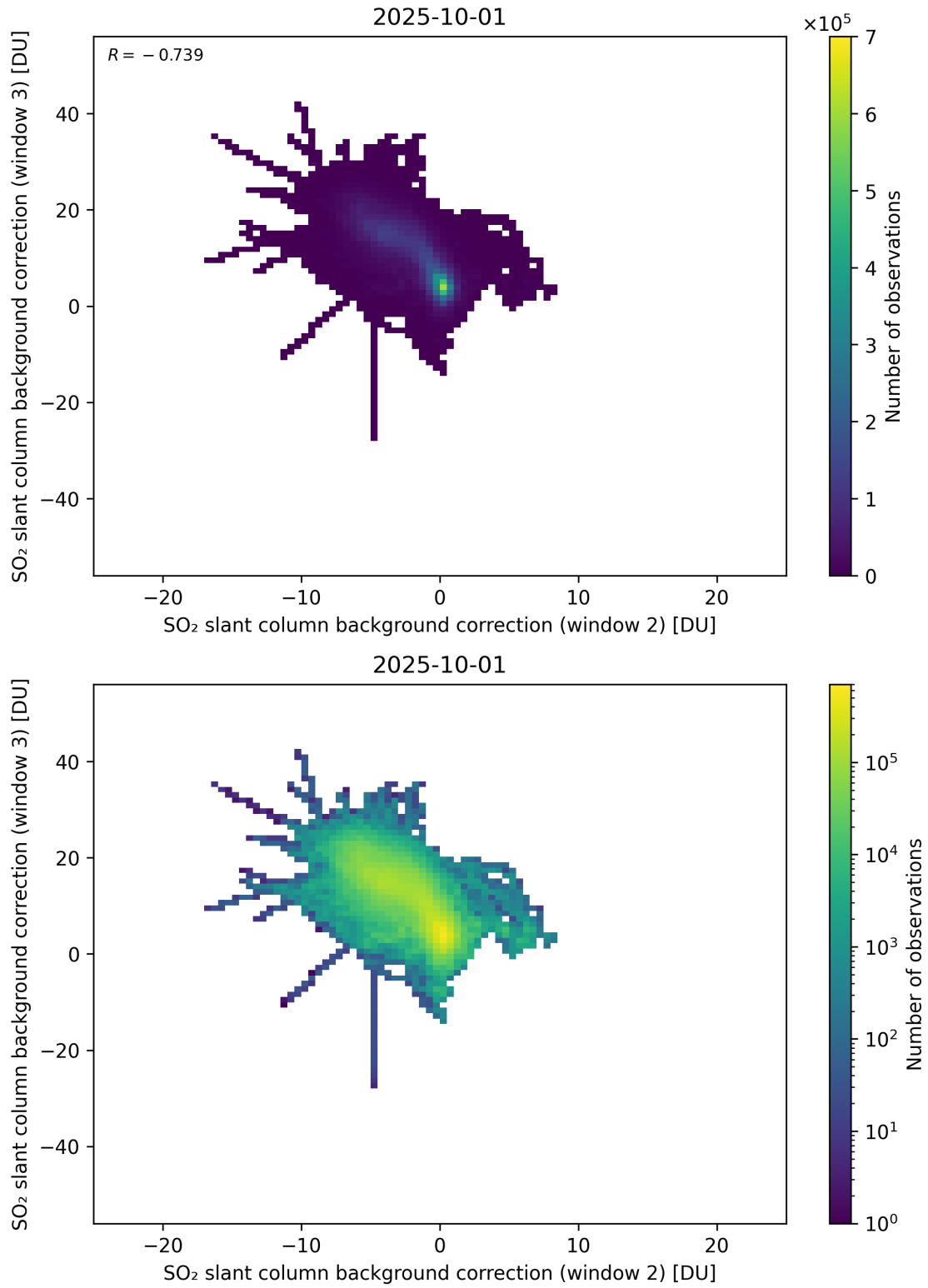
Figure 122: Scatter density plot of “SO 2 slant column background correction (window 2)” against “SO 2 slant column background correction (window 3)” for 2025-10-01 to 2025-10-02.
