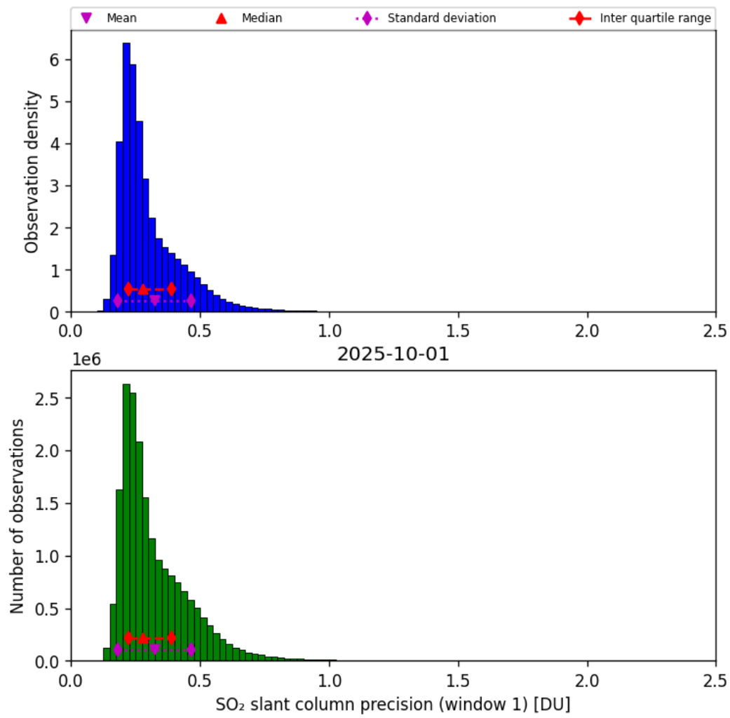
Figure 64: Histogram of “SO 2 slant column precision (window 1)” for 2025-10-01 to 2025-10-02
