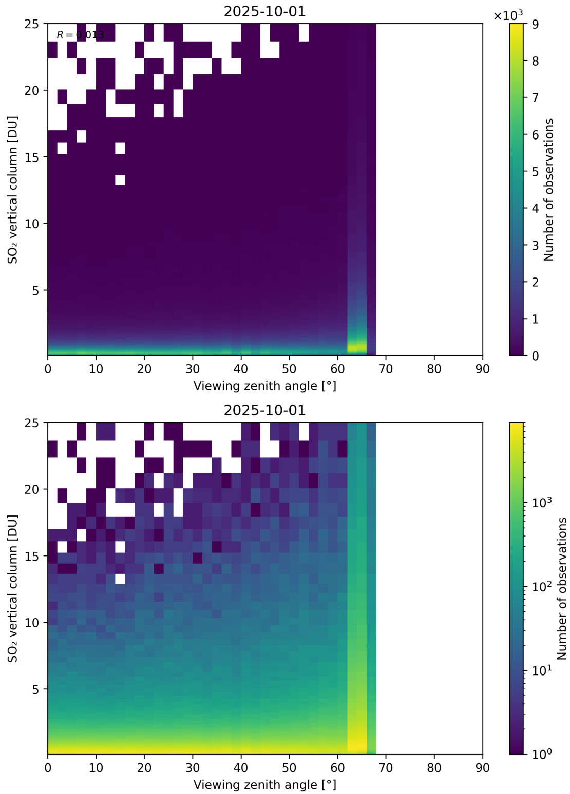
Figure 383: Scatter density plot of “Viewing zenith angle” against “SO 2 vertical column” for 2025-10-01 to 2025-10-02.
