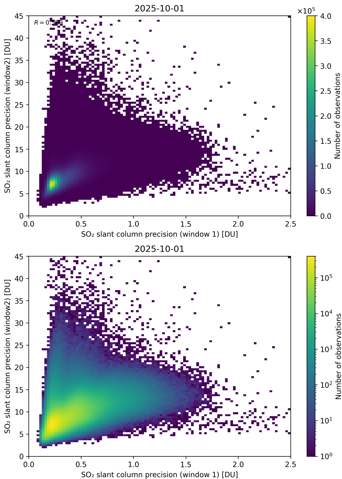
Figure 277: Scatter density plot of “SO 2 slant column precision (window 1)” against “SO 2 slant column precision (window2)” for 2025-10-01 to 2025-10-02.
