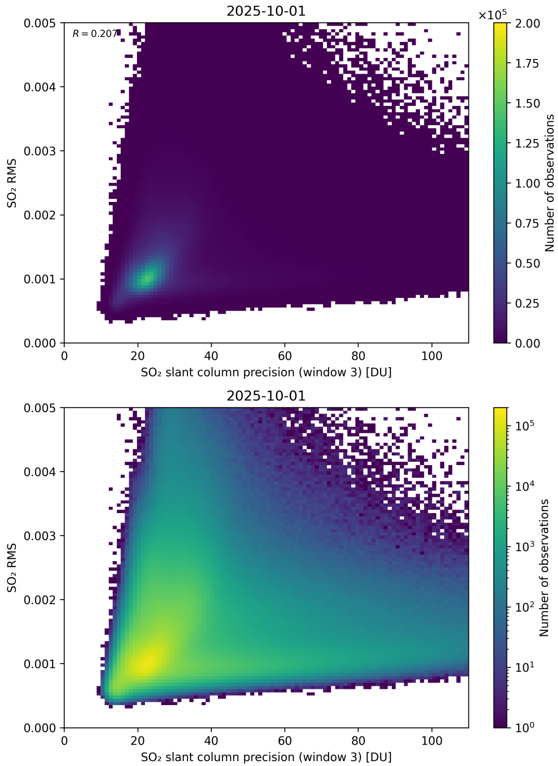
Figure 310: Scatter density plot of “SO 2 slant column precision (window 3)” against “SO 2 RMS” for 2025-10-01 to 2025-10-02.
