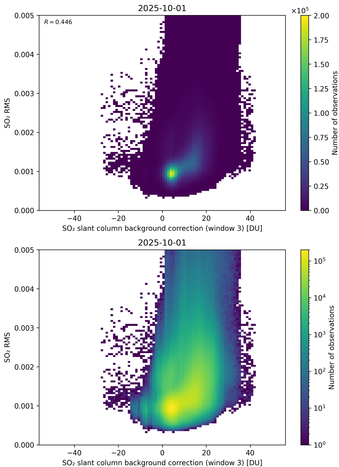
Figure 134: Scatter density plot of “SO 2 slant column background correction (window 3)” against “SO 2 RMS” for 2025-10-01 to 2025-10-02.
