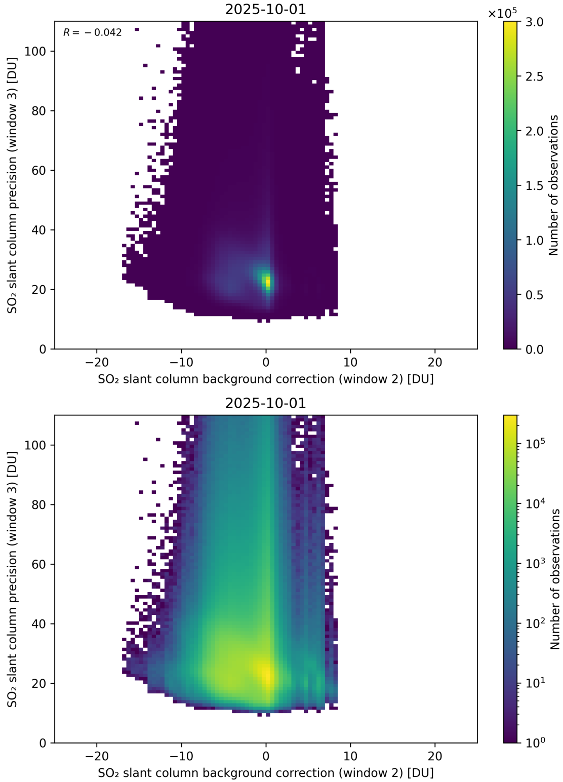
Figure 129: Scatter density plot of “SO 2 slant column background correction (window 2)” against “SO 2 slant column precision (window 3)” for 2025-10-01 to 2025-10-02.
