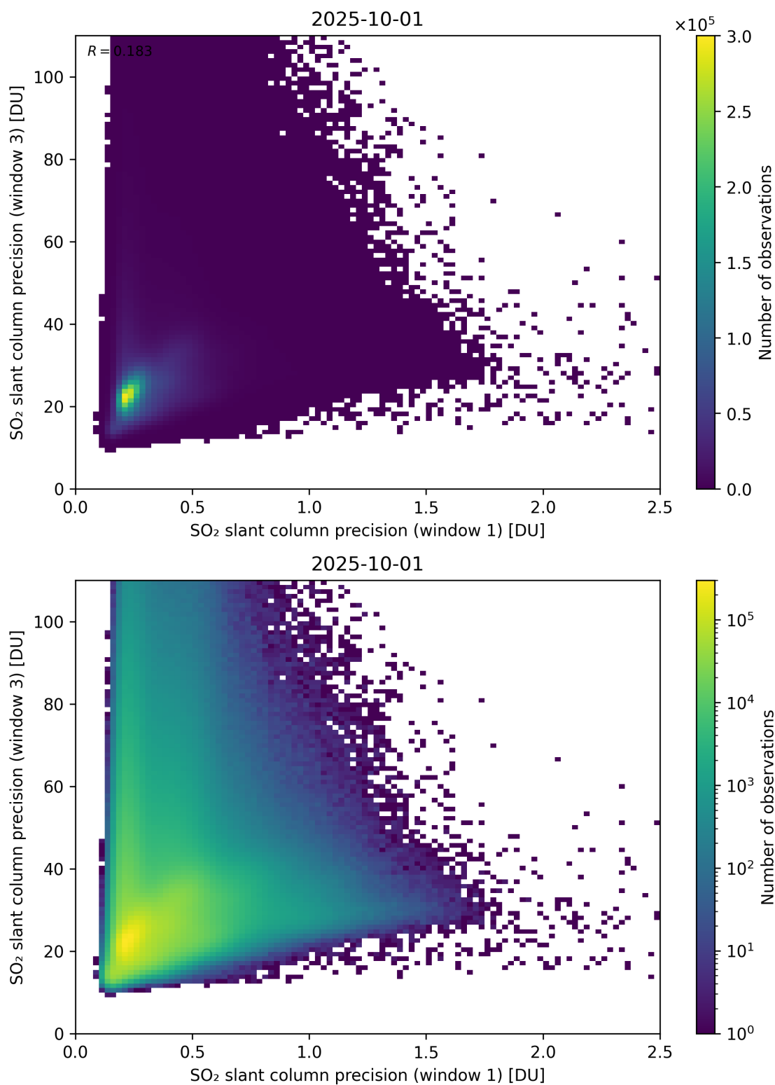
Figure 279: Scatter density plot of “SO 2 slant column precision (window 1)” against “SO 2 slant column precision (window 3)” for 2025-10-01 to 2025-10-02.
