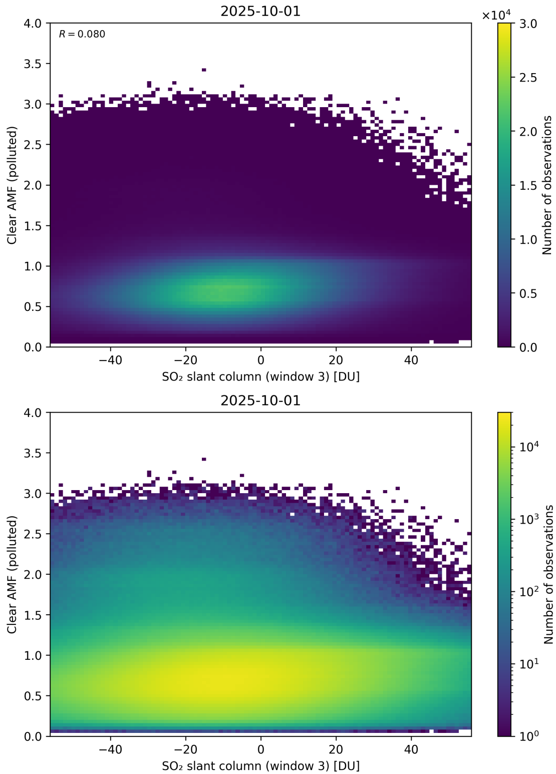
Figure 315: Scatter density plot of “SO 2 slant column (window 3)” against “Clear AMF (polluted)” for 2025-10-01 to 2025-10-02.
