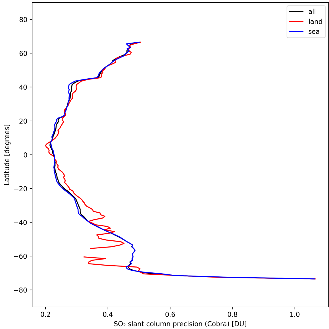
Figure 36: Zonal average of “SO 2 slant column precision (Cobra)” for 2025-10-01 to 2025-10-02.
