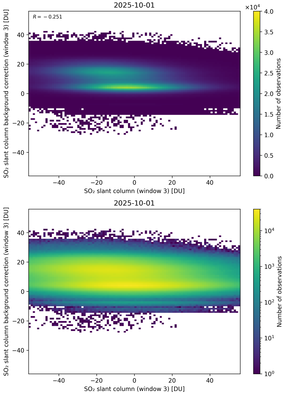
Figure 303: Scatter density plot of “SO 2 slant column (window 3)” against “SO 2 slant column background correction (window 3)” for 2025-10-01 to 2025-10-02.
