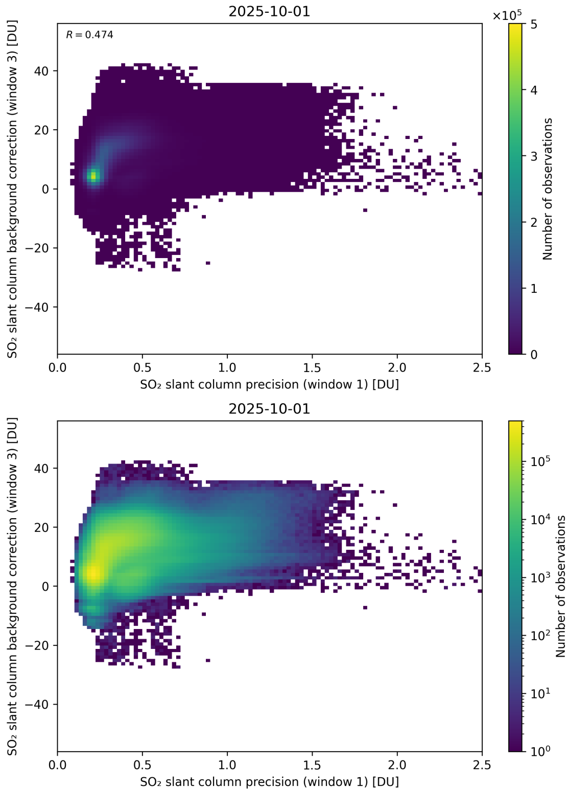
Figure 270: Scatter density plot of “SO 2 slant column precision (window 1)” against “SO 2 slant column background correction (window 3)” for 2025-10-01 to 2025-10-02.
