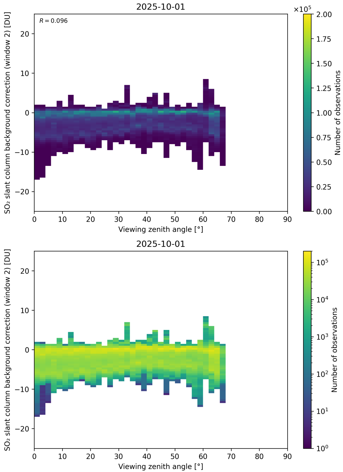
Figure 363: Scatter density plot of “Viewing zenith angle” against “SO 2 slant column background correction (window 2)” for 2025-10-01 to 2025-10-02.
