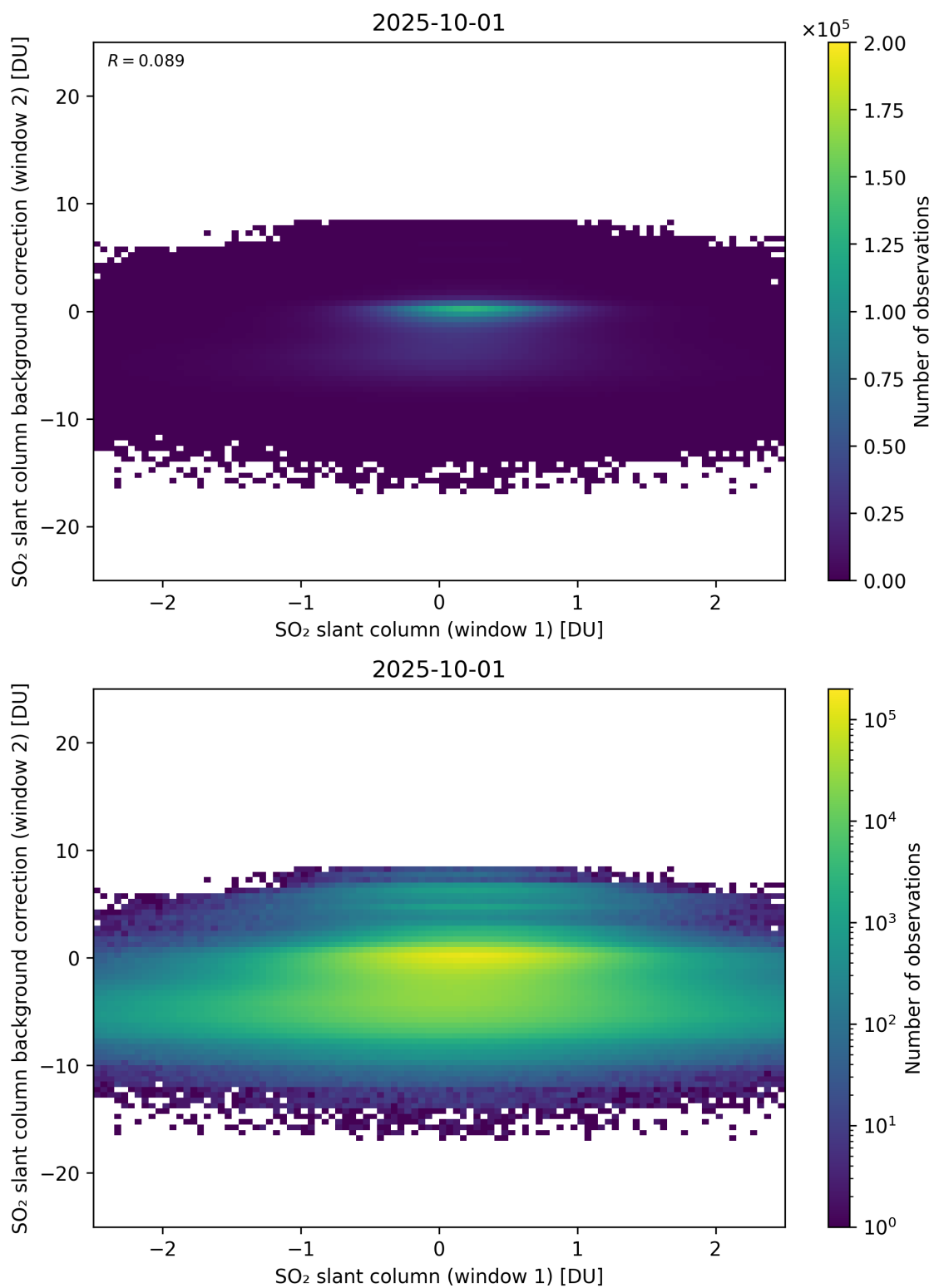
Figure 263: Scatter density plot of “SO 2 slant column (window 1)” against “SO 2 slant column background correction (window 2)” for 2025-10-01 to 2025-10-02.
