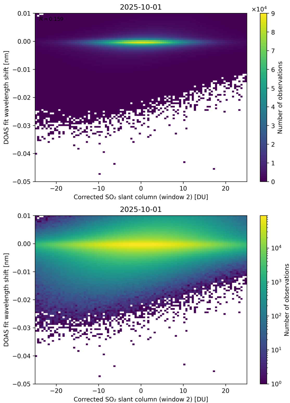
Figure 246: Scatter density plot of “Corrected SO 2 slant column (window 2)” against “DOAS fit wavelength shift” for 2025-10-01 to 2025-10-02.
