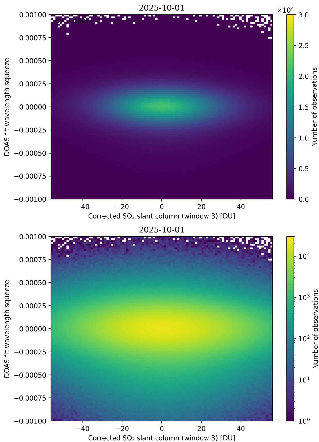
Figure 257: Scatter density plot of “Corrected SO 2 slant column (window 3)” against “DOAS fit wavelength squeeze” for 2025-10-01 to 2025-10-02.
