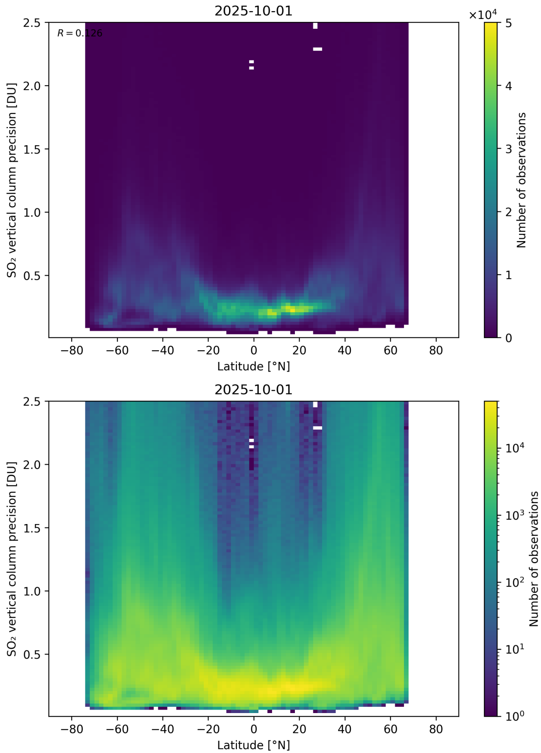
Figure 170: Scatter density plot of “Latitude” against “SO 2 vertical column precision” for 2025-10-01 to 2025-10-02.
