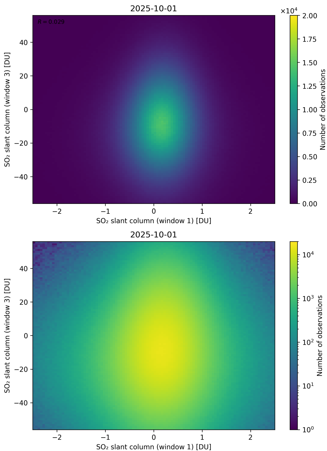
Figure 287: Scatter density plot of “SO 2 slant column (window 1)” against “SO 2 slant column (window 3)” for 2025-10-01 to 2025-10-02.
