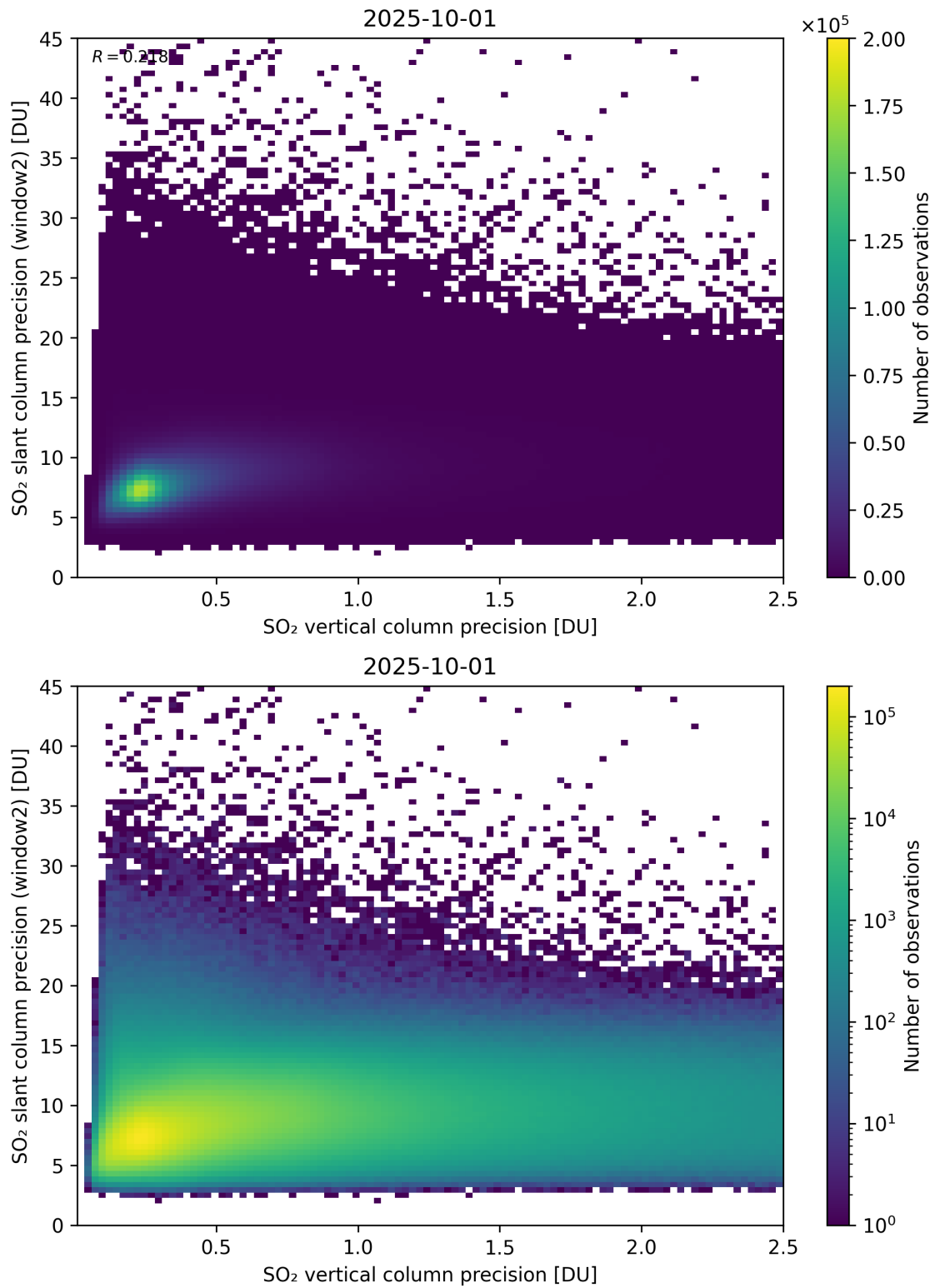
Figure 343: Scatter density plot of “SO 2 vertical column precision” against “SO 2 slant column precision (window2)” for 2025-10-01 to 2025-10-02.
