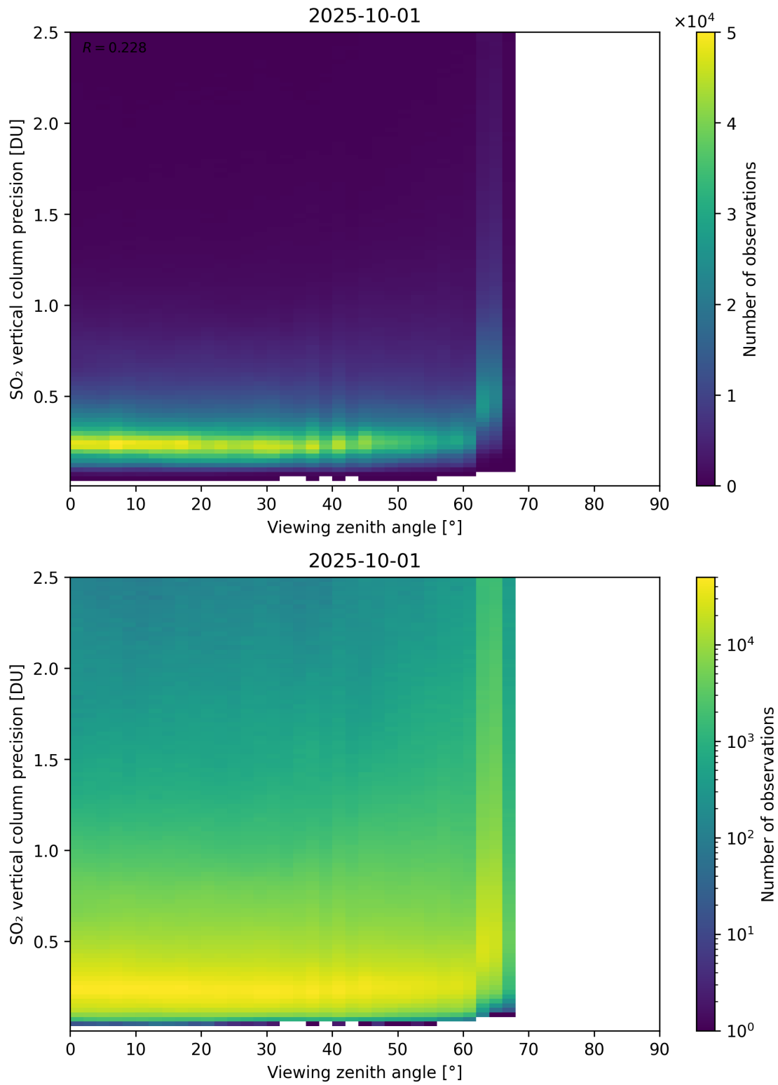
Figure 384: Scatter density plot of “Viewing zenith angle” against “SO 2 vertical column precision” for 2025-10-01 to 2025-10-02.
