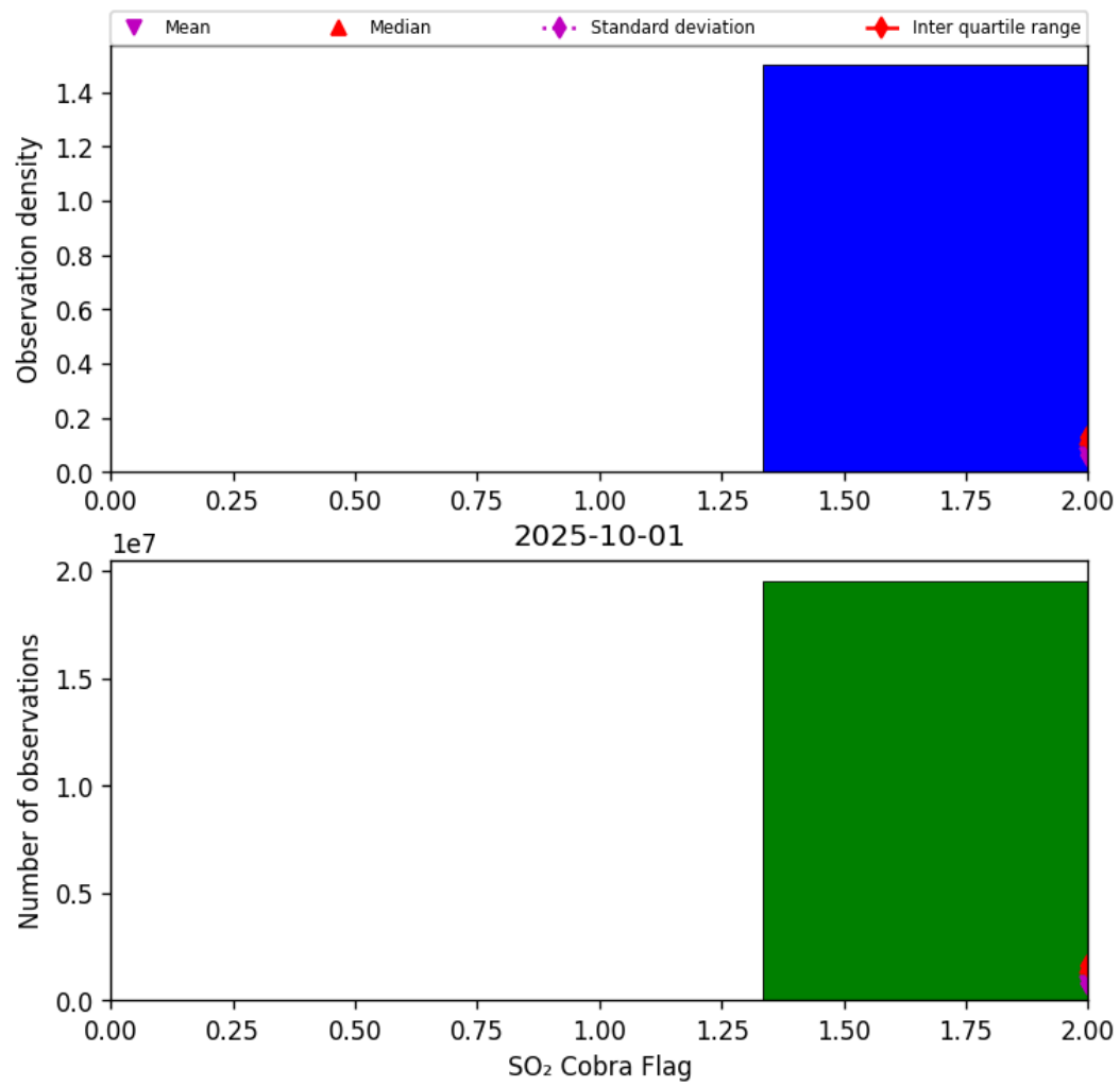
Figure 75: Histogram of "SO 2 Cobra Flag" for 2025-10-01 to 2025-10-02
