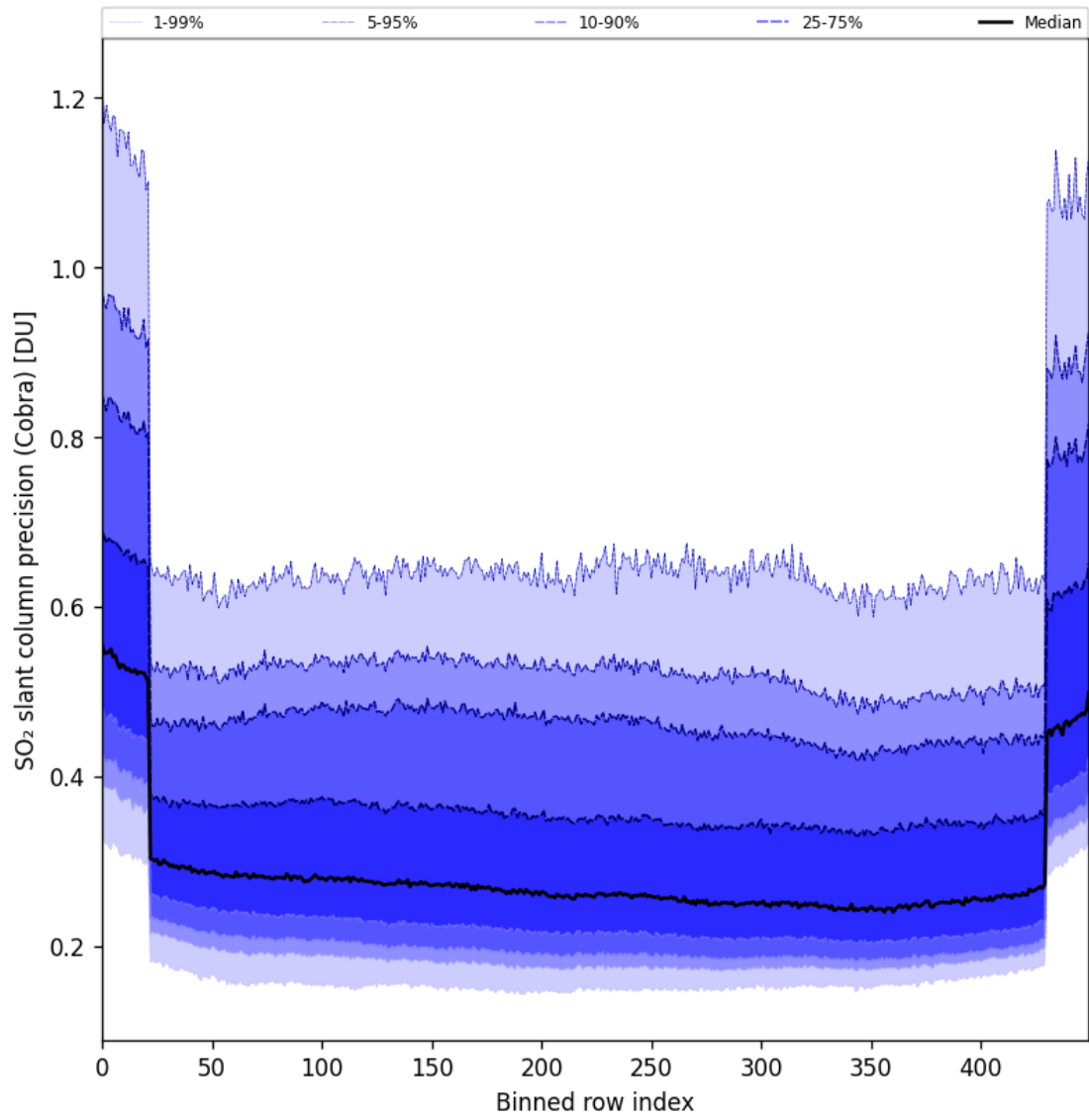
Figure 88: Along track statistics of “SO 2 slant column precision (Cobra)” for 2025-10-01 to 2025-10-02
