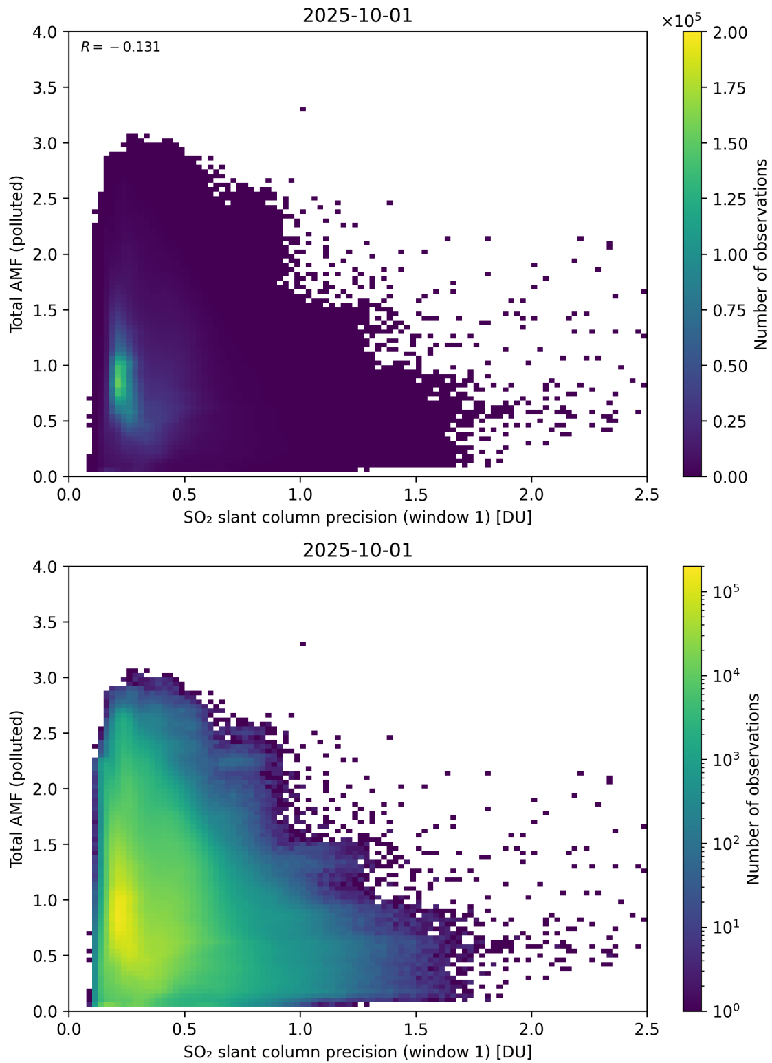
Figure 280: Scatter density plot of “SO 2 slant column precision (window 1)” against “Total AMF (polluted)” for 2025-10-01 to 2025-10-02.
