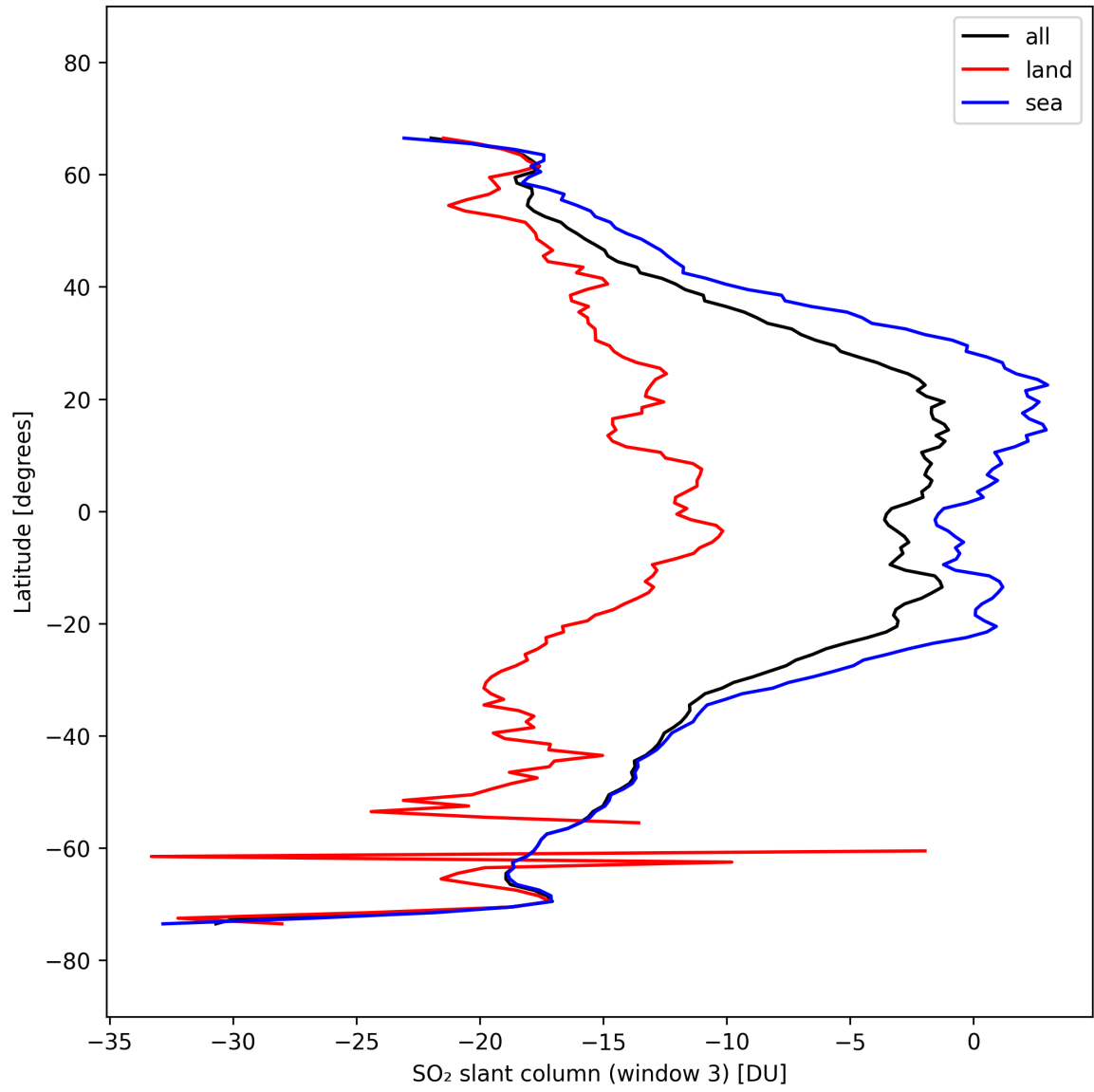
Figure 45: Zonal average of “SO 2 slant column (window 3)” for 2025-10-01 to 2025-10-02.
