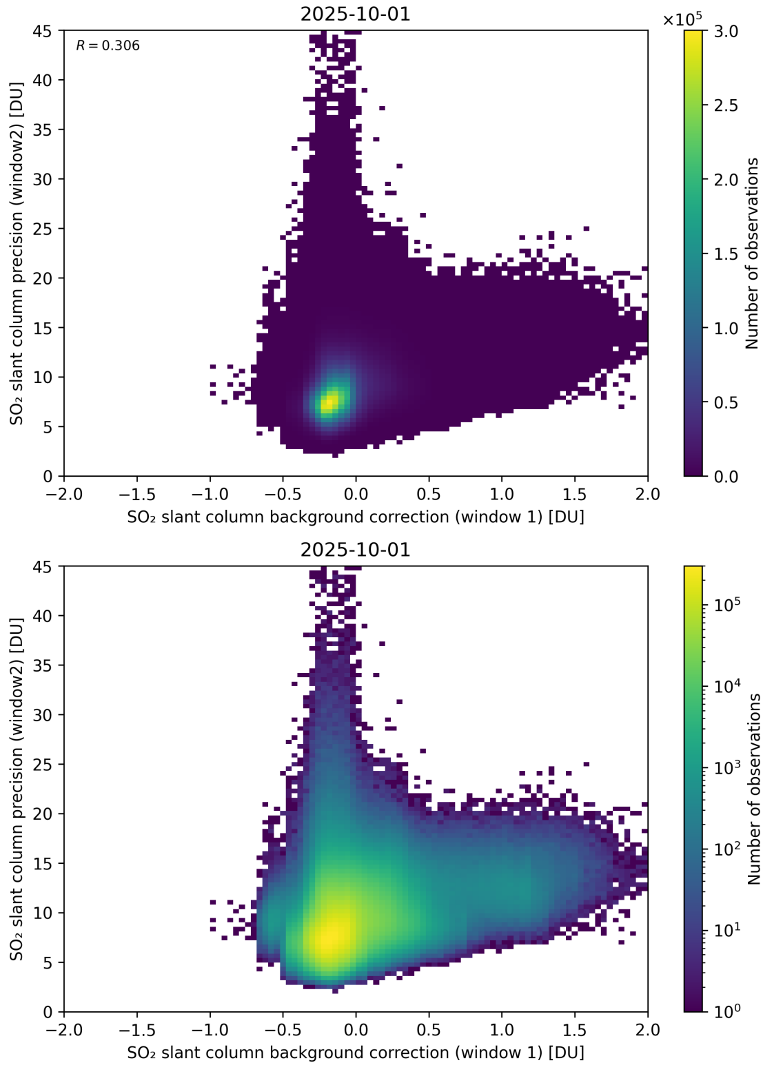
Figure 117: Scatter density plot of “SO 2 slant column background correction (window 1)” against “SO 2 slant column precision (window2)” for 2025-10-01 to 2025-10-02.
