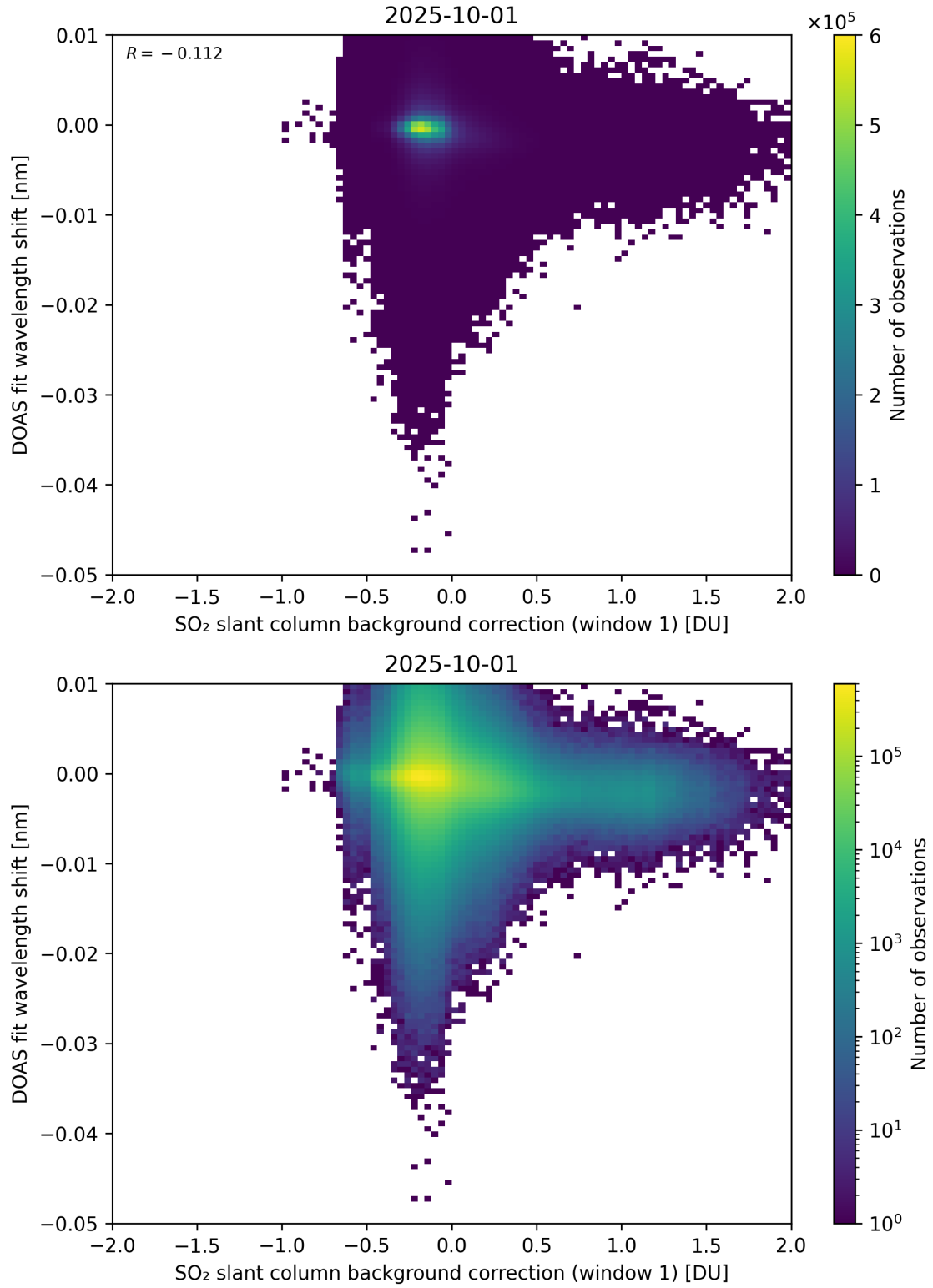
Figure 111: Scatter density plot of “SO 2 slant column background correction (window 1)” against “DOAS fit wavelength shift” for 2025-10-01 to 2025-10-02.
