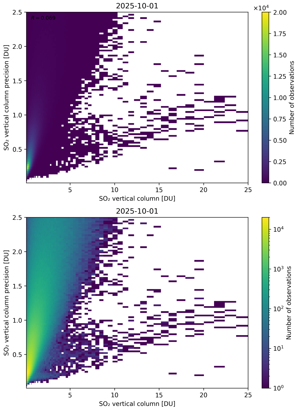
Figure 361: Scatter density plot of “SO 2 vertical column” against “SO 2 vertical column precision” for 2025-10-01 to 2025-10-02.
