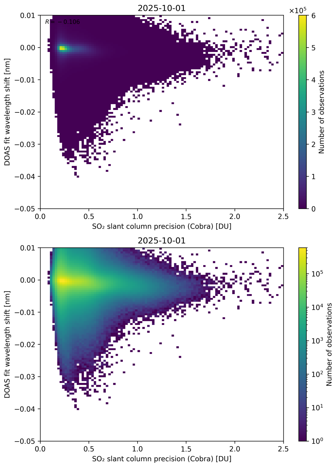
Figure 202: Scatter density plot of “SO 2 slant column precision (Cobra)” against “DOAS fit wavelength shift” for 2025-10-01 to 2025-10-02.
