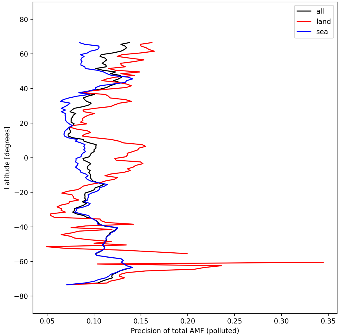
Figure 54: Zonal average of “Precision of total AMF (polluted)” for 2025-10-01 to 2025-10-02.
