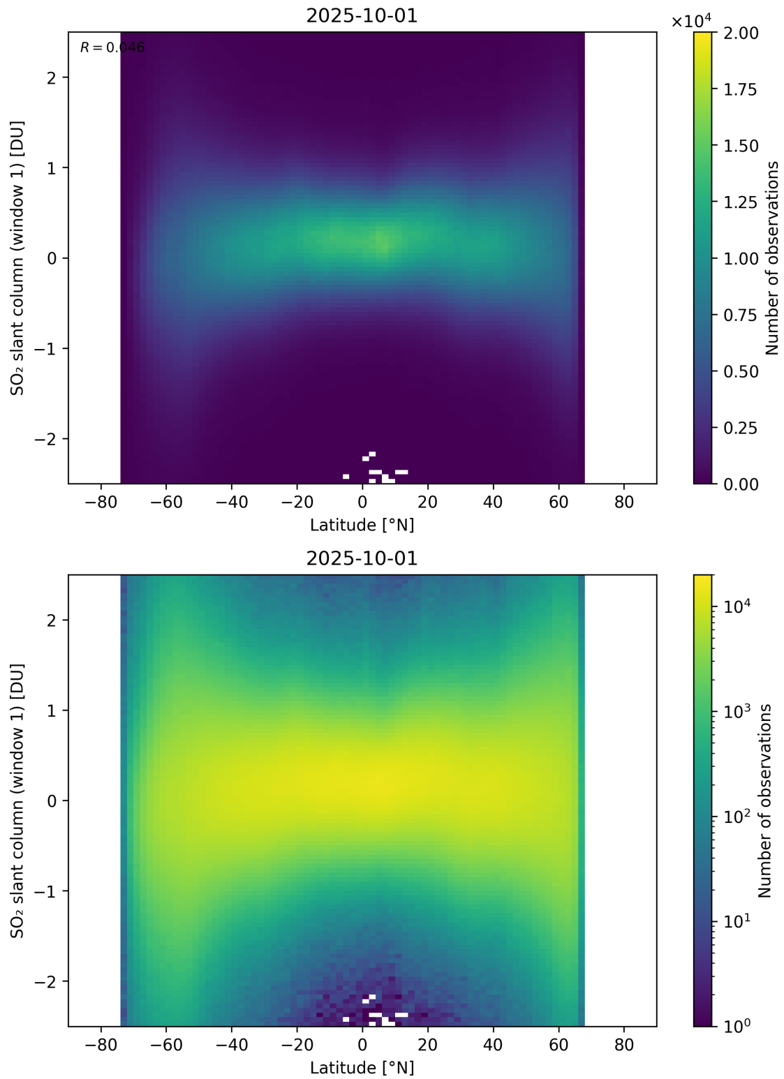
Figure 162: Scatter density plot of “Latitude” against “SO 2 slant column (window 1)” for 2025-10-01 to 2025-10-02.
