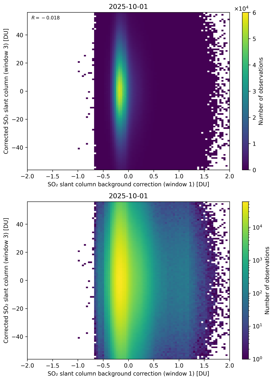
Figure 116: Scatter density plot of “SO 2 slant column background correction (window 1)” against “Corrected SO 2 slant column (window 3)” for 2025-10-01 to 2025-10-02.
