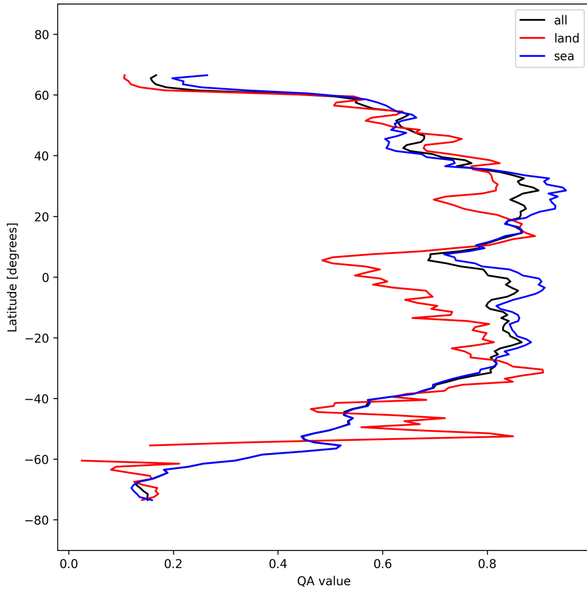
Figure 31: Zonal average of “QA value” for 2025-10-01 to 2025-10-02.
