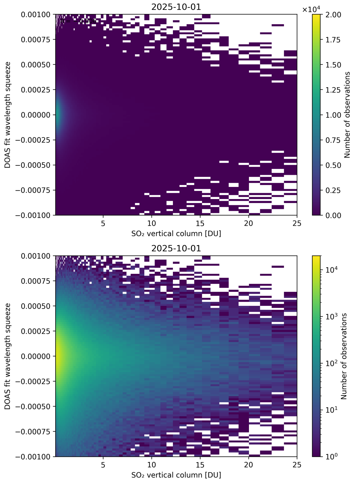
Figure 327: Scatter density plot of “SO 2 vertical column” against “DOAS fit wavelength squeeze” for 2025-10-01 to 2025-10-02.
