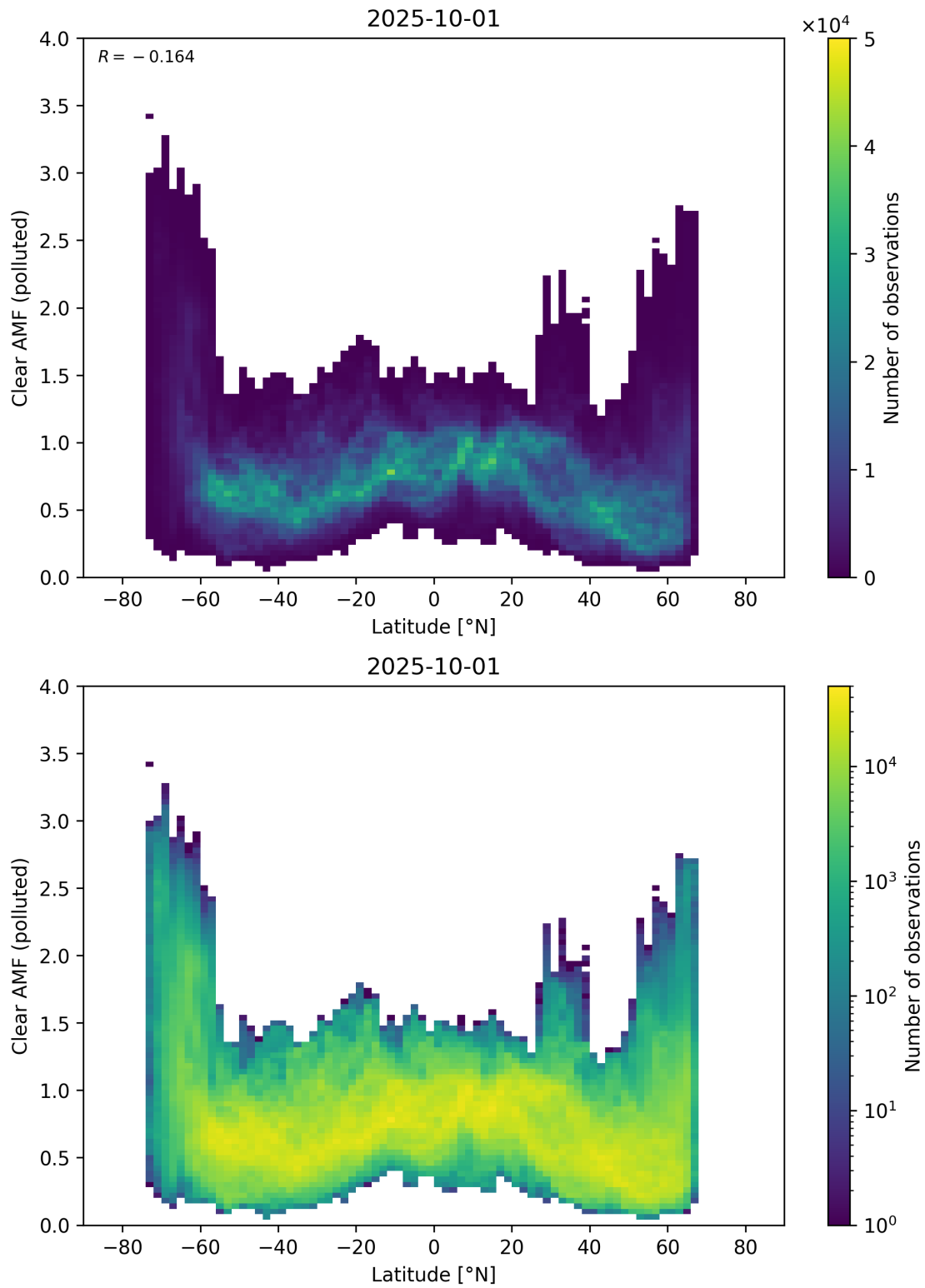
Figure 156: Scatter density plot of “Latitude” against “Clear AMF (polluted)” for 2025-10-01 to 2025-10-02.
