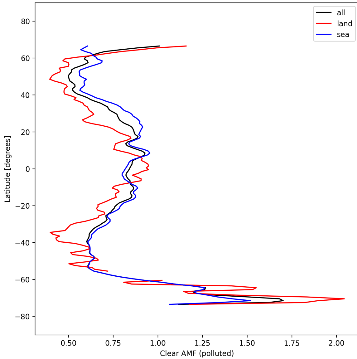
Figure 55: Zonal average of “Clear AMF (polluted)” for 2025-10-01 to 2025-10-02.
