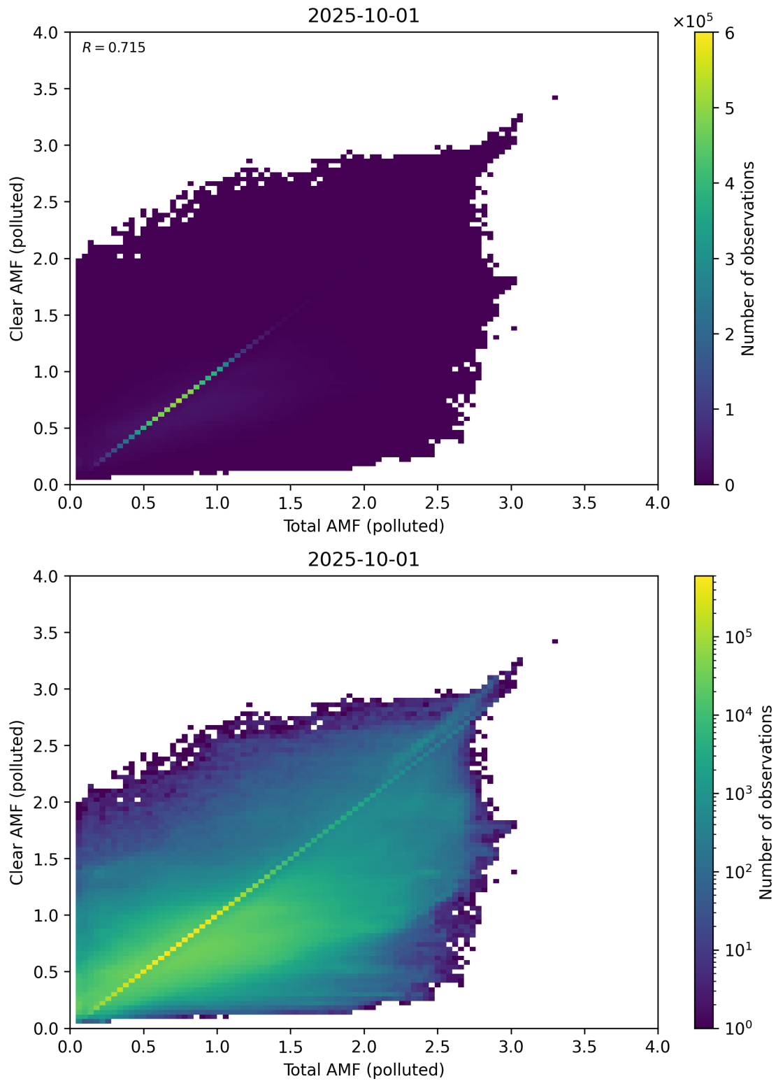
Figure 321: Scatter density plot of “Total AMF (polluted)” against “Clear AMF (polluted)” for 2025-10-01 to 2025-10-02.
