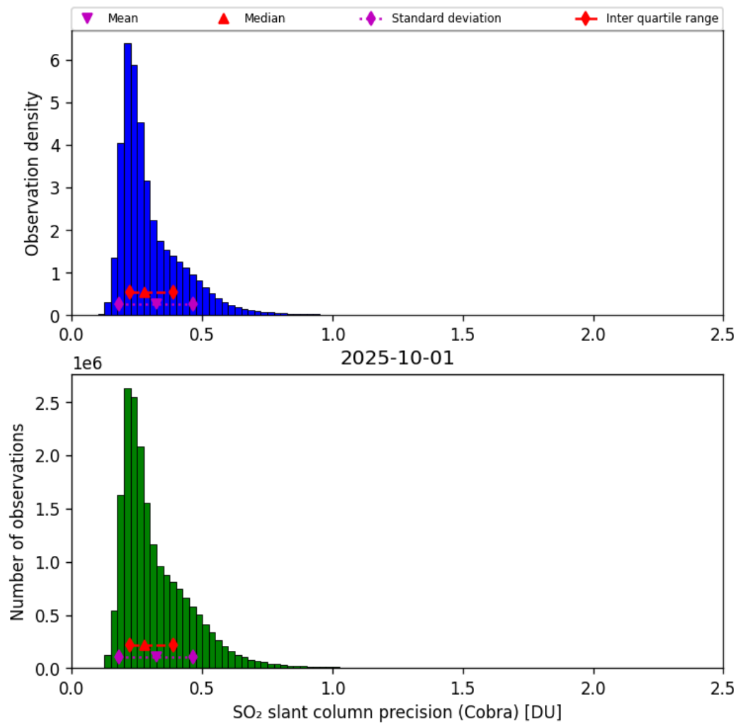
Figure 62: Histogram of “SO 2 slant column precision (Cobra)” for 2025-10-01 to 2025-10-02
