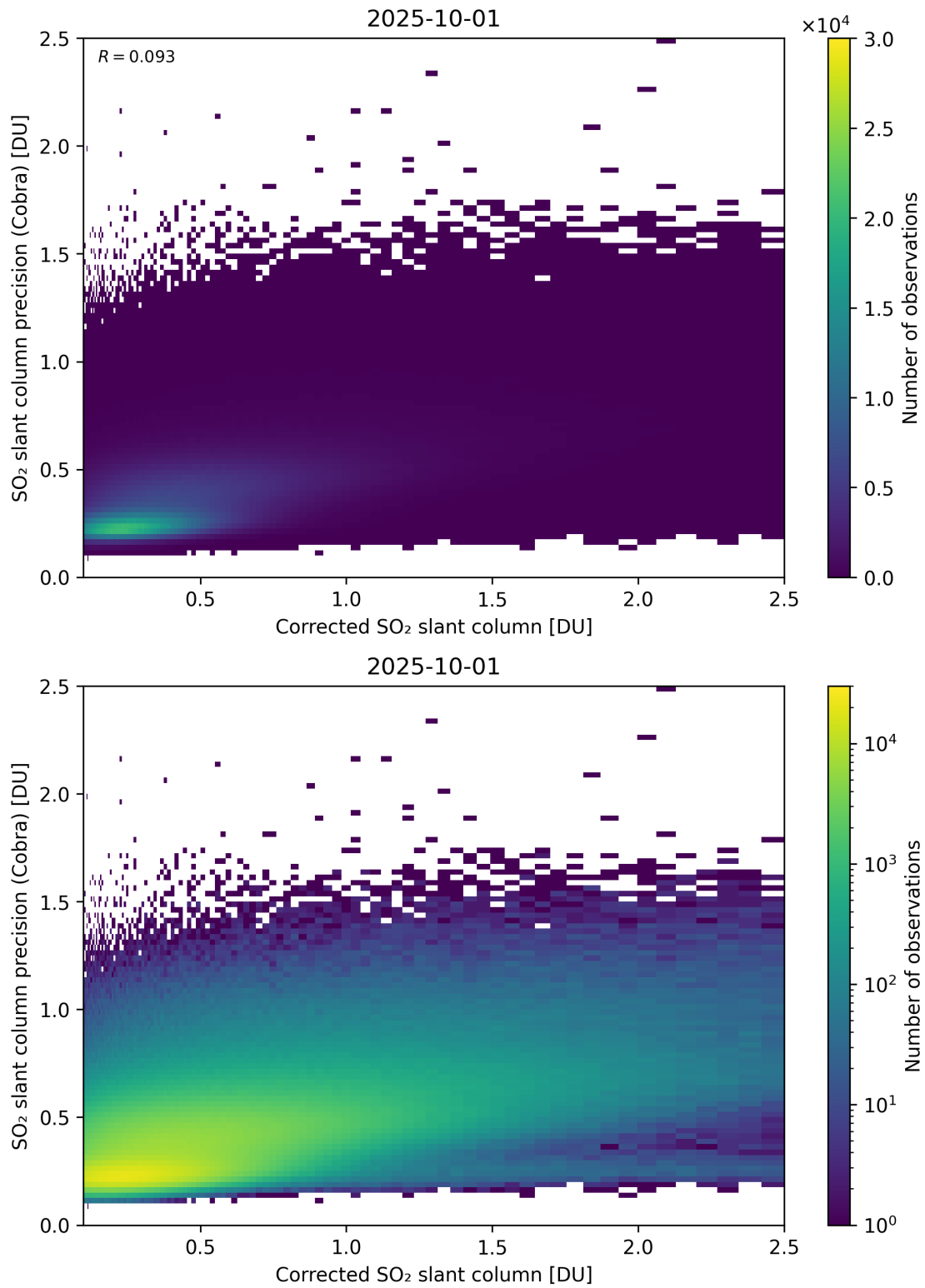
Figure 234: Scatter density plot of “Corrected SO 2 slant column” against “SO 2 slant column precision (Cobra)” for 2025-10-01 to 2025-10-02.
