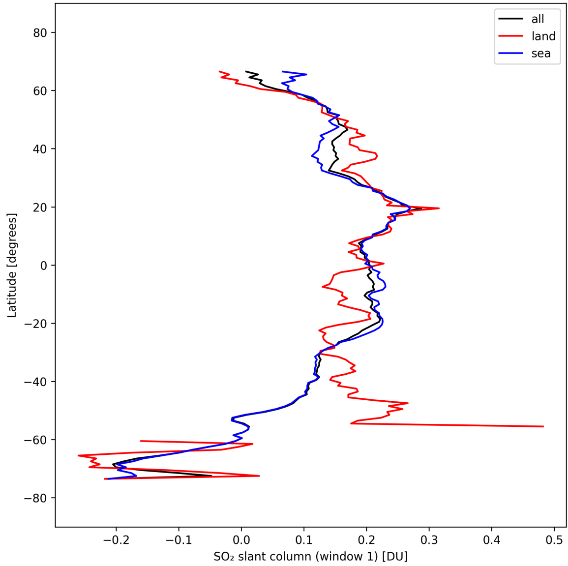
Figure 37: Zonal average of “SO 2 slant column (window 1)” for 2025-10-01 to 2025-10-02.
