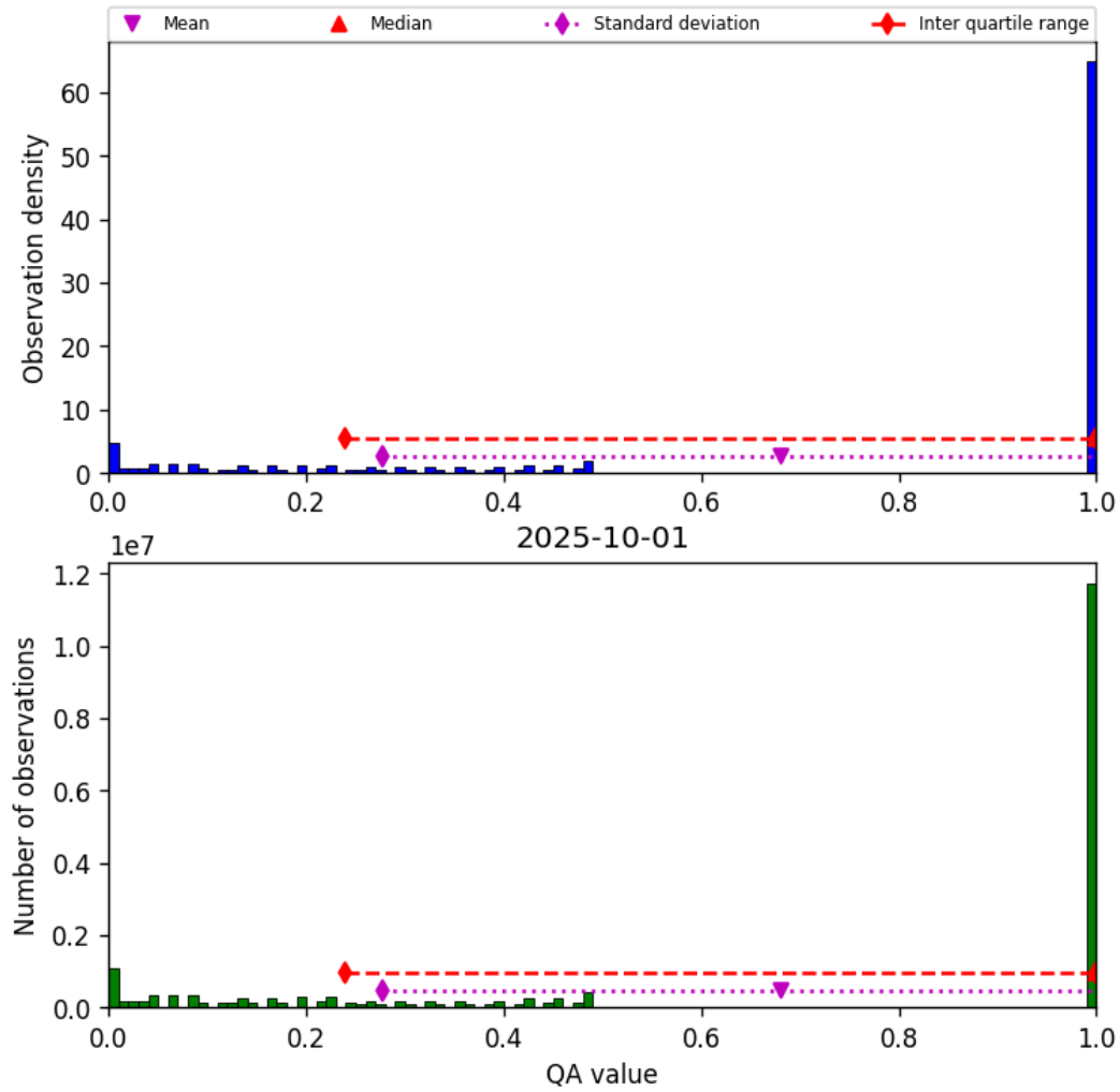
Figure 57: Histogram of “QA value” for 2025-10-01 to 2025-10-02
