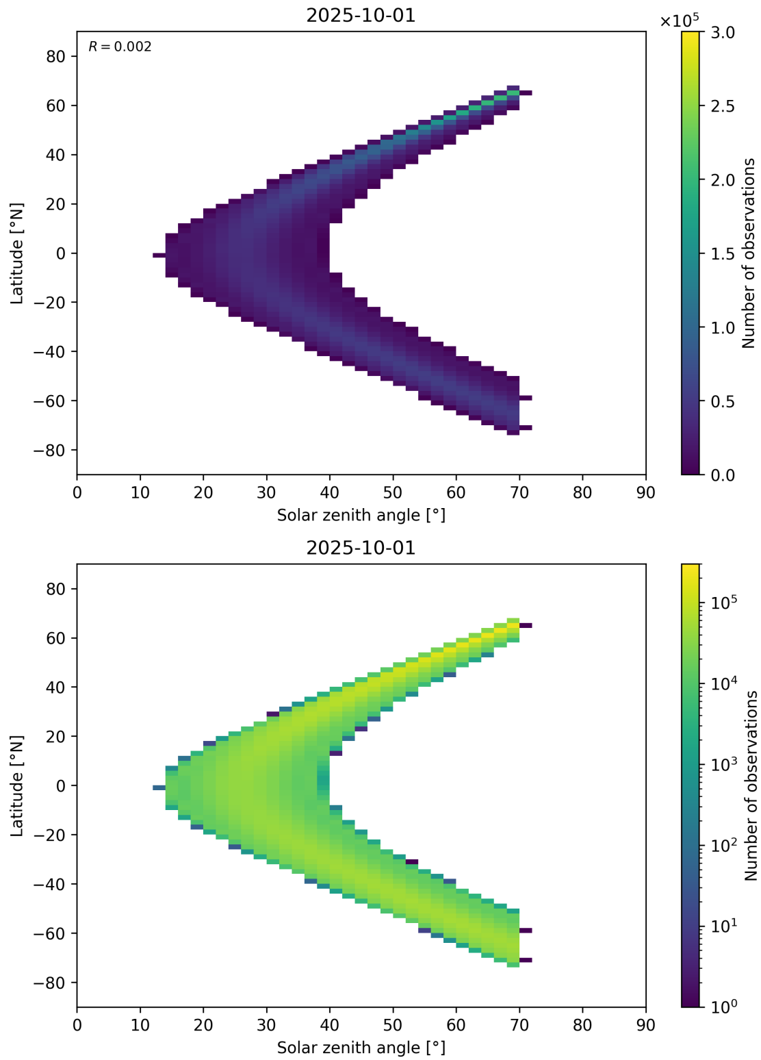
Figure 177: Scatter density plot of “Solar zenith angle” against “Latitude” for 2025-10-01 to 2025-10-02.
