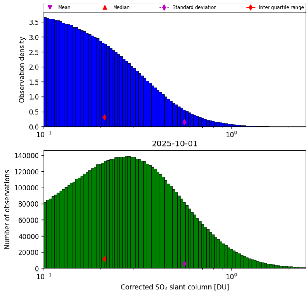
Figure 60: Histogram of “Corrected SO 2 slant column” for 2025-10-01 to 2025-10-02
