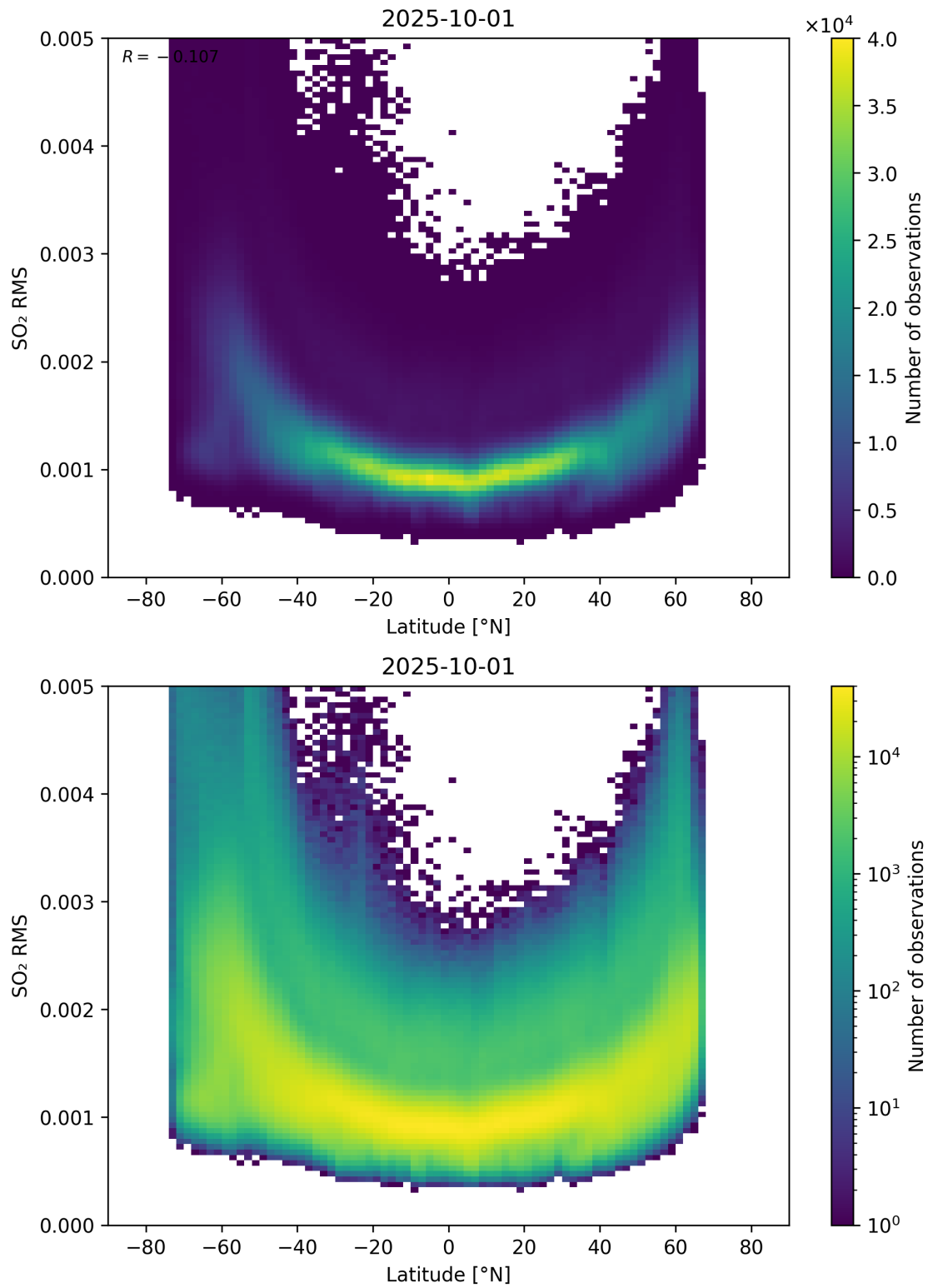
Figure 155: Scatter density plot of “Latitude” against “SO 2 RMS” for 2025-10-01 to 2025-10-02.
