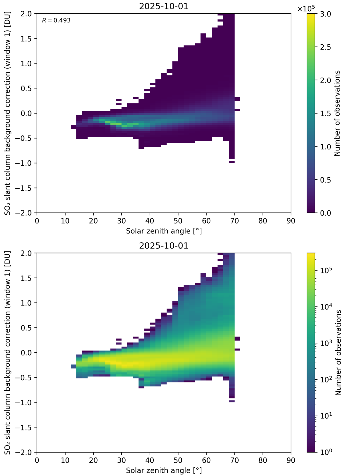
Figure 171: Scatter density plot of “Solar zenith angle” against “SO 2 slant column background correction (window 1)” for 2025-10-01 to 2025-10-02.
