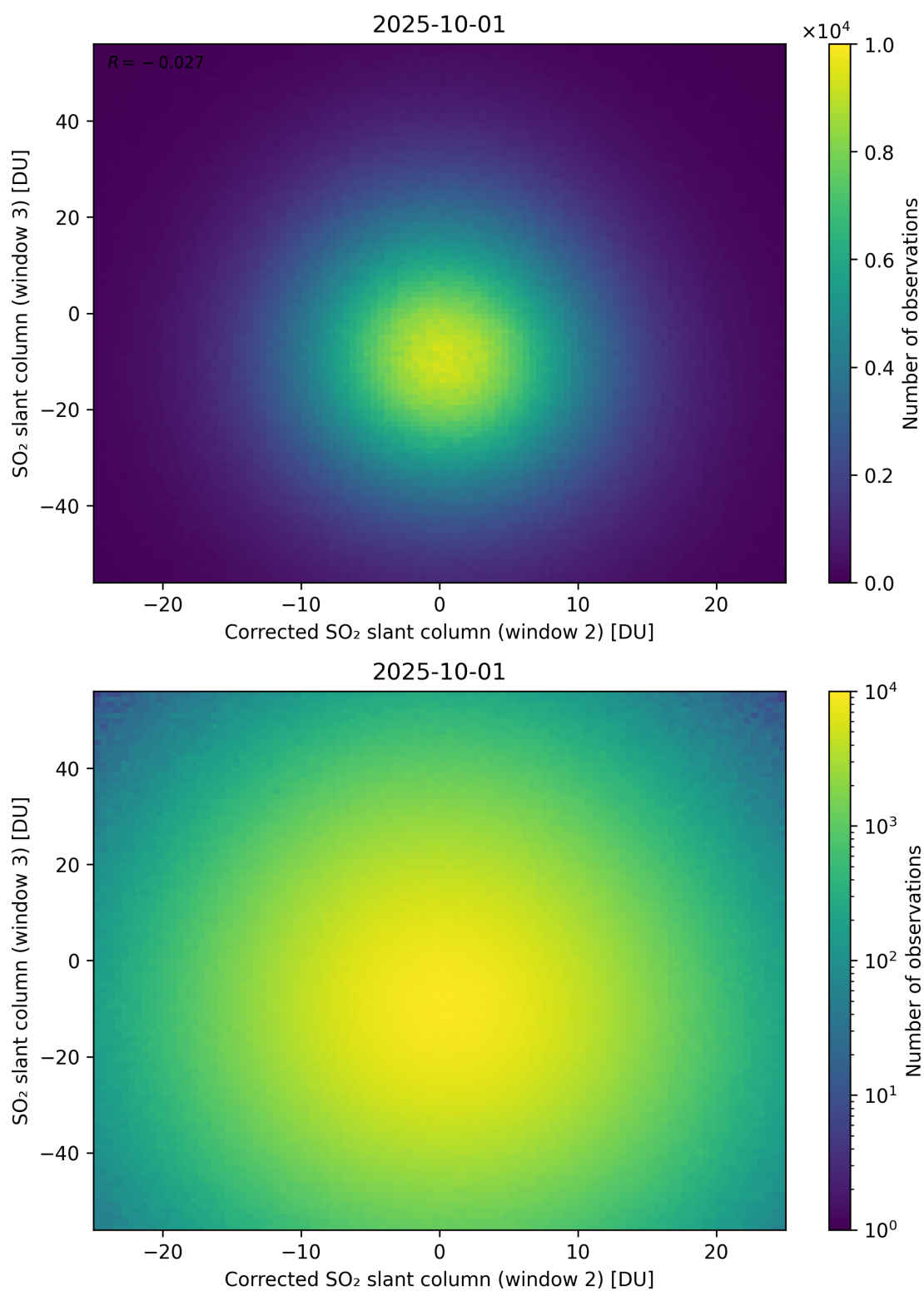
Figure 251: Scatter density plot of “Corrected SO 2 slant column (window 2)” against “SO 2 slant column (window 3)” for 2025-10-01 to 2025-10-02.
