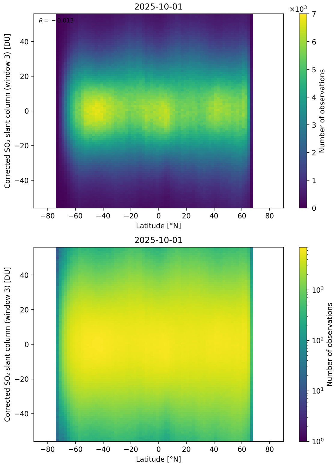
Figure 161: Scatter density plot of “Latitude” against “Corrected SO 2 slant column (window 3)” for 2025-10-01 to 2025-10-02.
