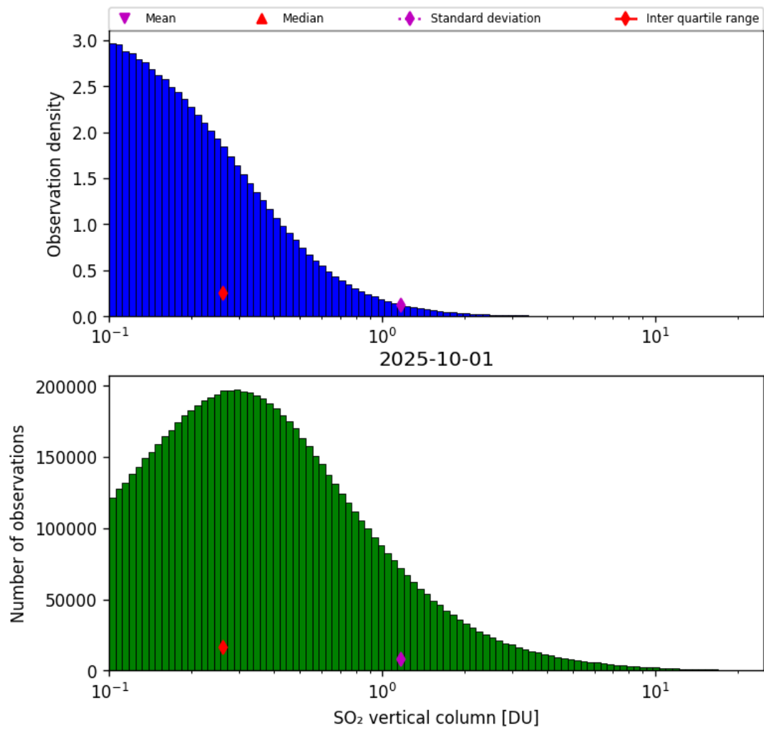
Figure 58: Histogram of “SO 2 vertical column” for 2025-10-01 to 2025-10-02
