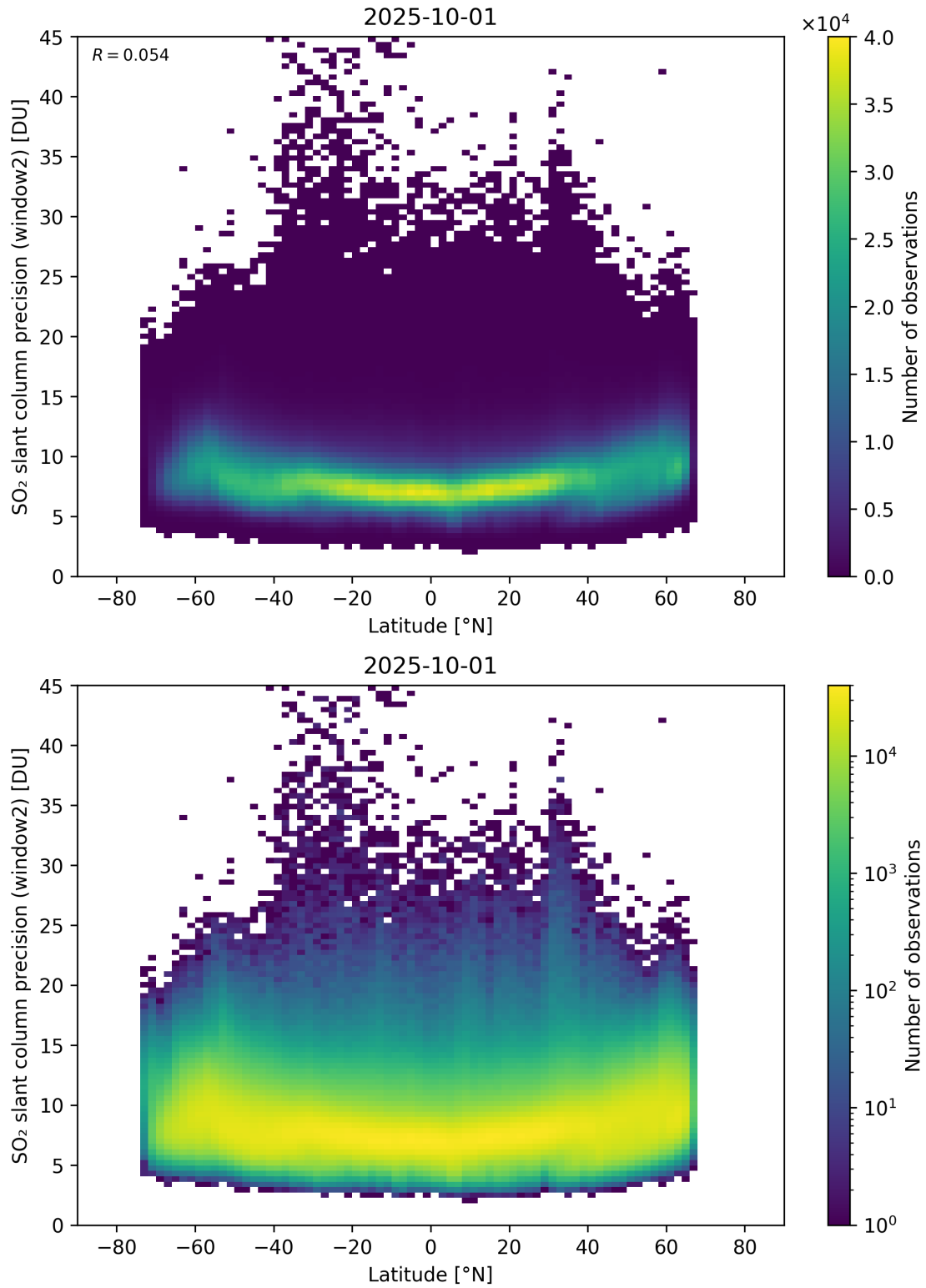
Figure 164: Scatter density plot of “Latitude” against “SO 2 slant column precision (window2)” for 2025-10-01 to 2025-10-02.
