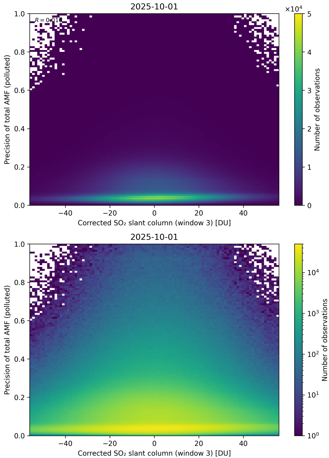
Figure 261: Scatter density plot of “Corrected SO 2 slant column (window 3)” against “Precision of total AMF (polluted)” for 2025-10-01 to 2025-10-02.
