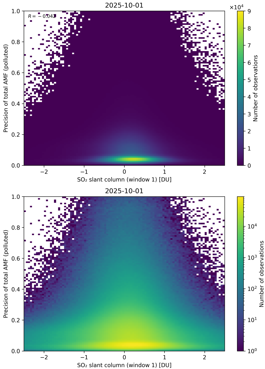
Figure 290: Scatter density plot of “SO 2 slant column (window 1)” against “Precision of total AMF (polluted)” for 2025-10-01 to 2025-10-02.
