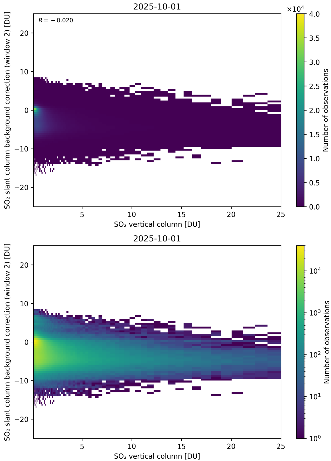
Figure 324: Scatter density plot of “SO 2 vertical column” against “SO 2 slant column background correction (window 2)” for 2025-10-01 to 2025-10-02.
