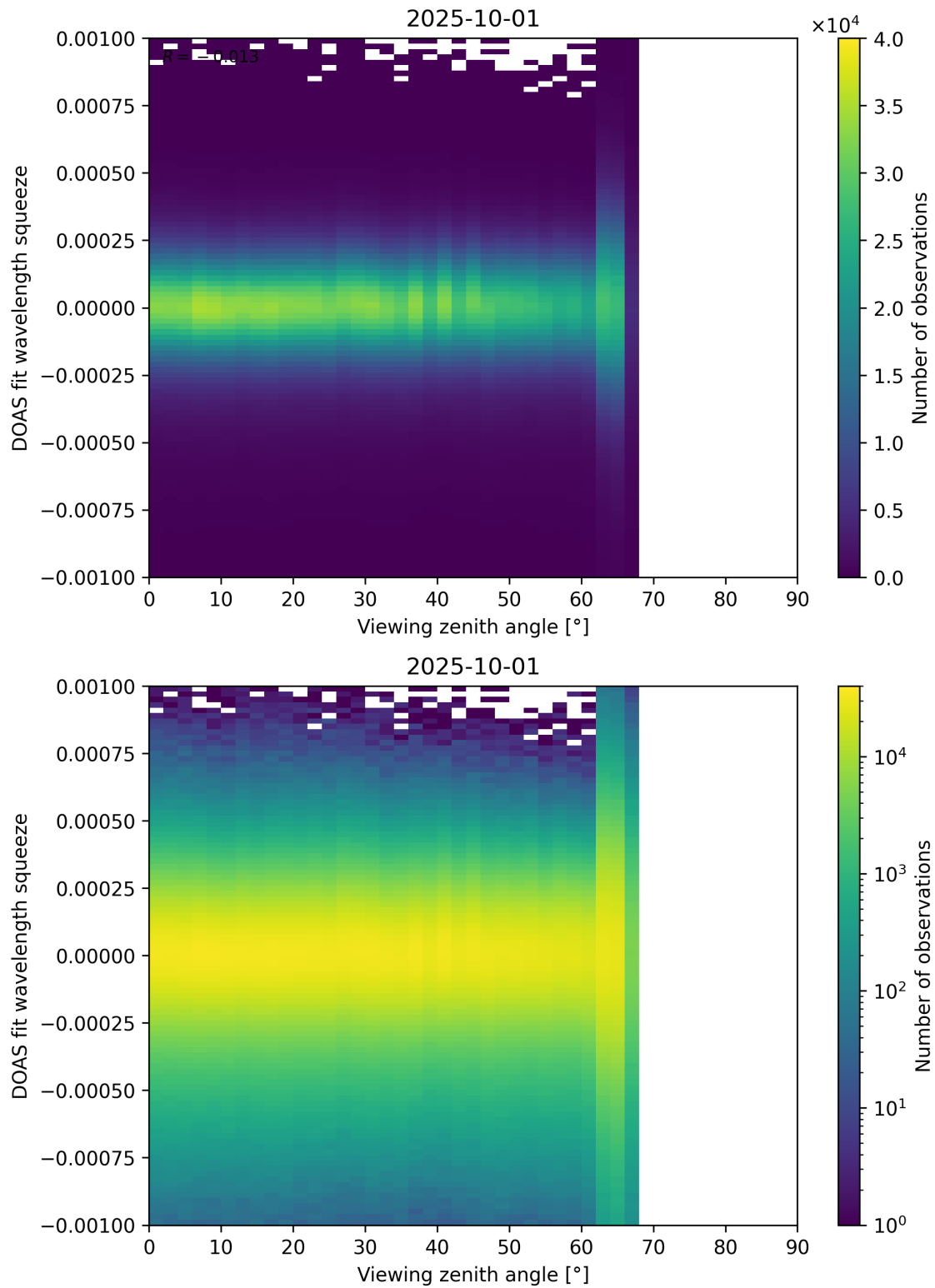
Figure 366: Scatter density plot of “Viewing zenith angle” against “DOAS fit wavelength squeeze” for 2025-10-01 to 2025-10-02.
