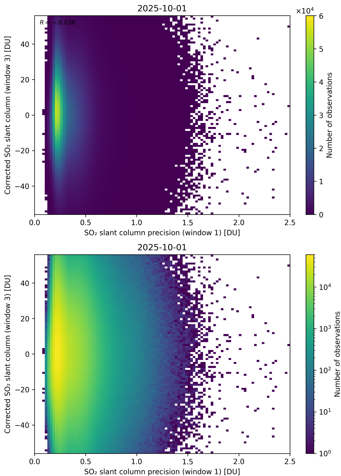
Figure 276: Scatter density plot of “SO 2 slant column precision (window 1)” against “Corrected SO 2 slant column (window 3)” for 2025-10-01 to 2025-10-02.
