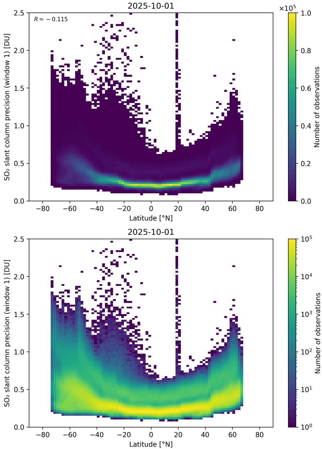
Figure 163: Scatter density plot of “Latitude” against “SO 2 slant column precision (window 1)” for 2025-10-01 to 2025-10-02.
