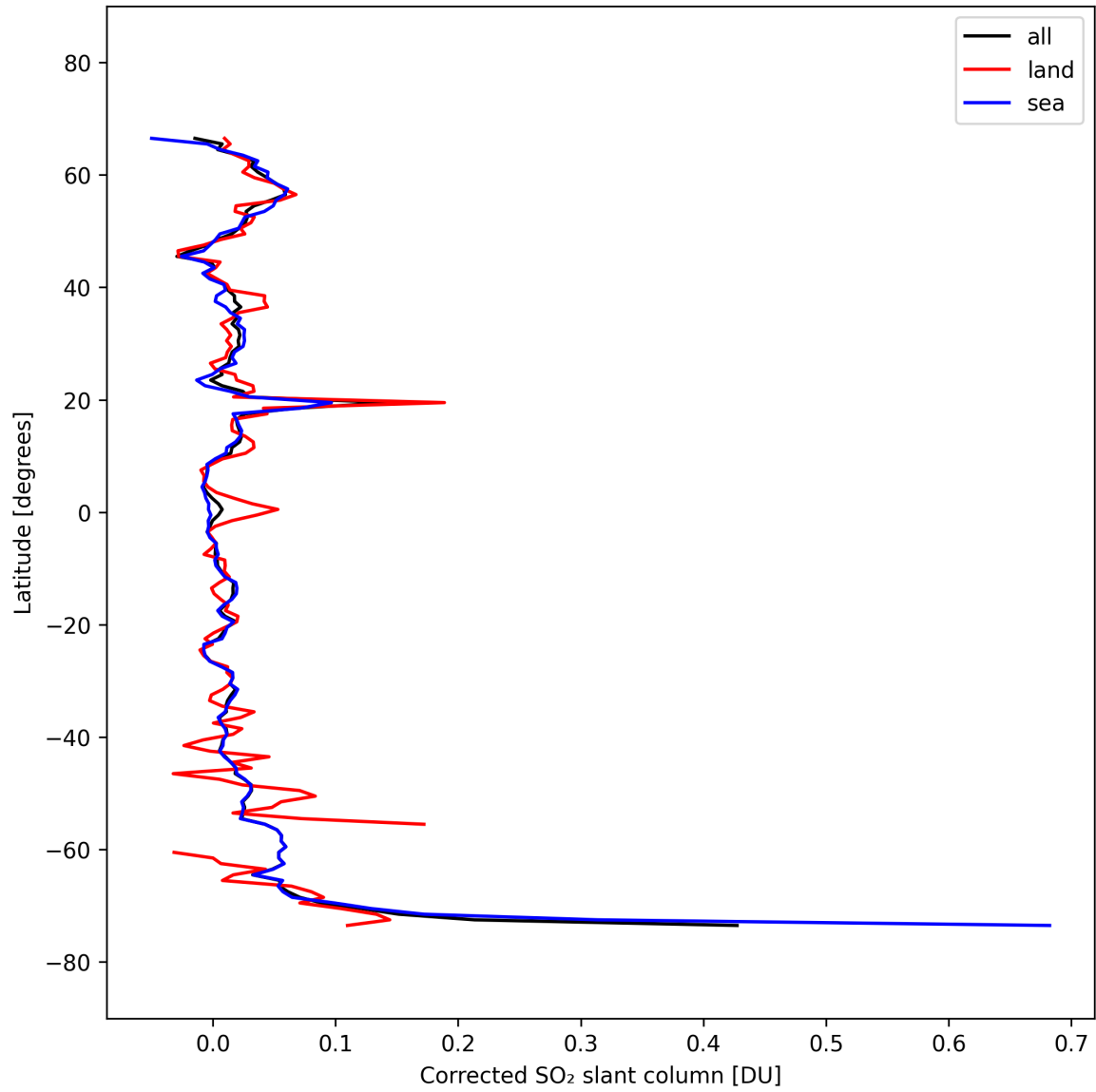
Figure 34: Zonal average of “Corrected SO 2 slant column” for 2025-10-01 to 2025-10-02.
