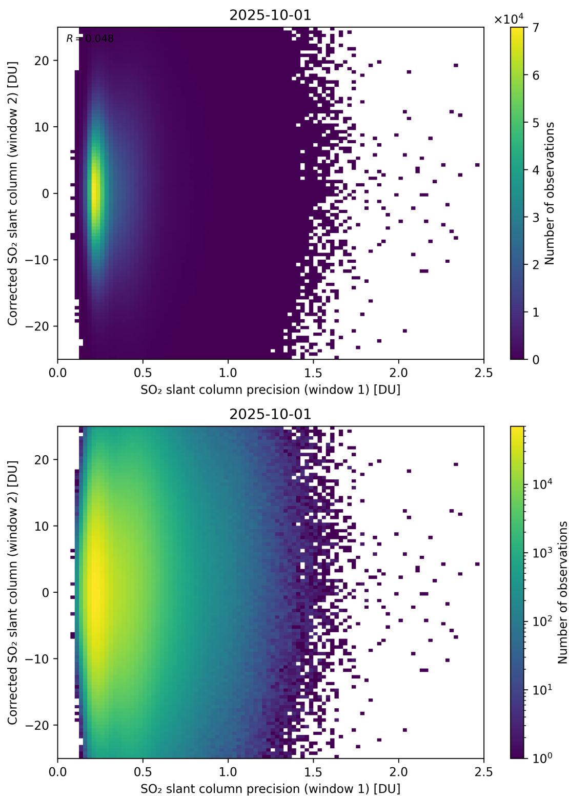
Figure 275: Scatter density plot of “SO 2 slant column precision (window 1)” against “Corrected SO 2 slant column (window 2)” for 2025-10-01 to 2025-10-02.
