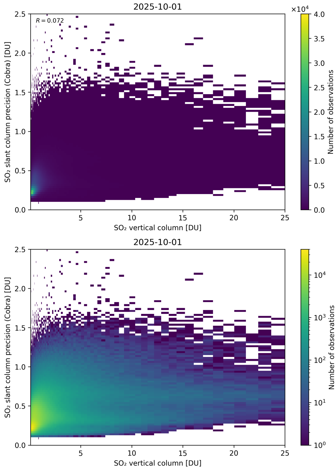
Figure 350: Scatter density plot of “SO 2 vertical column” against “SO 2 slant column precision (Cobra)” for 2025-10-01 to 2025-10-02.
