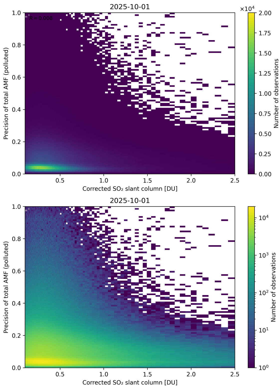
Figure 243: Scatter density plot of “Corrected SO 2 slant column” against “Precision of total AMF (polluted)” for 2025-10-01 to 2025-10-02.
