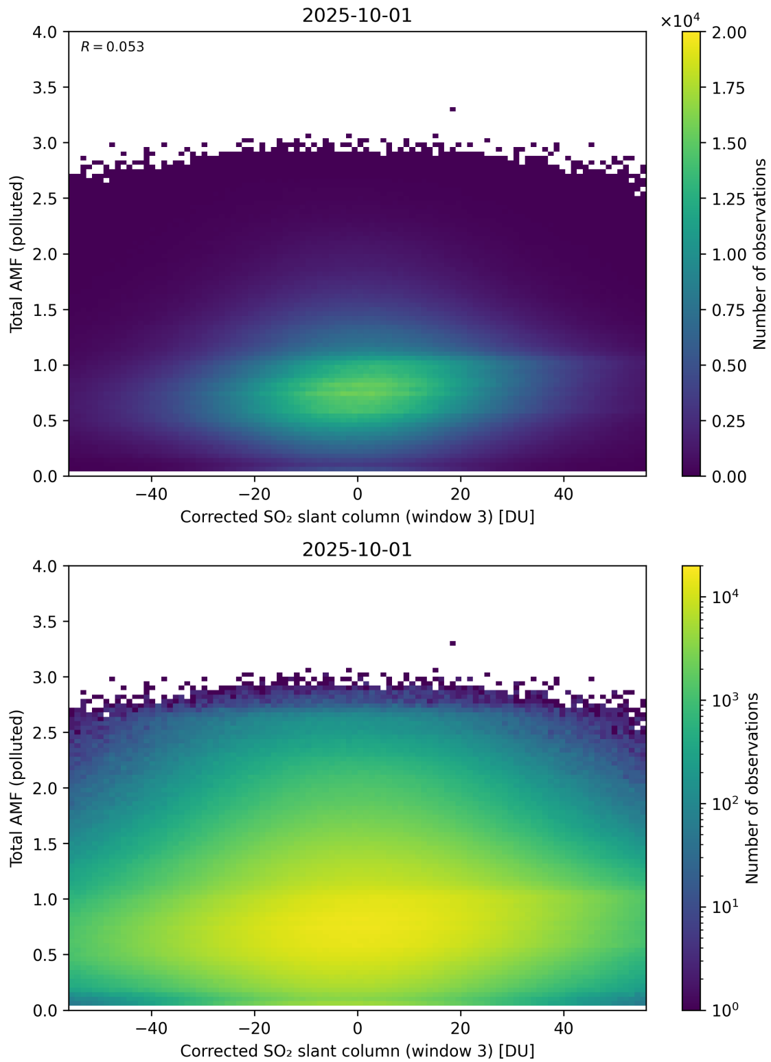
Figure 260: Scatter density plot of “Corrected SO 2 slant column (window 3)” against “Total AMF (polluted)” for 2025-10-01 to 2025-10-02.
