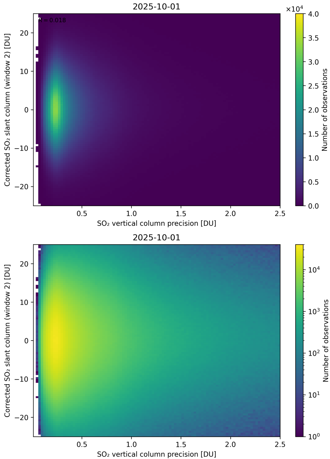
Figure 339: Scatter density plot of “SO 2 vertical column precision” against “Corrected SO 2 slant column (window 2)” for 2025-10-01 to 2025-10-02.
