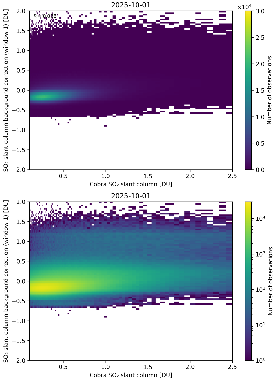
Figure 193: Scatter density plot of “Cobra SO 2 slant column” against “SO 2 slant column background correction (window 1)” for 2025-10-01 to 2025-10-02.
