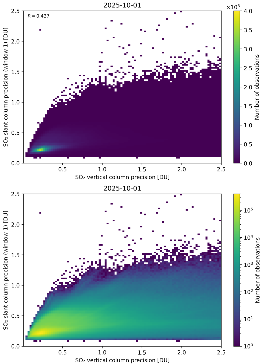
Figure 342: Scatter density plot of “SO 2 vertical column precision” against “SO 2 slant column precision (window 1)” for 2025-10-01 to 2025-10-02.
