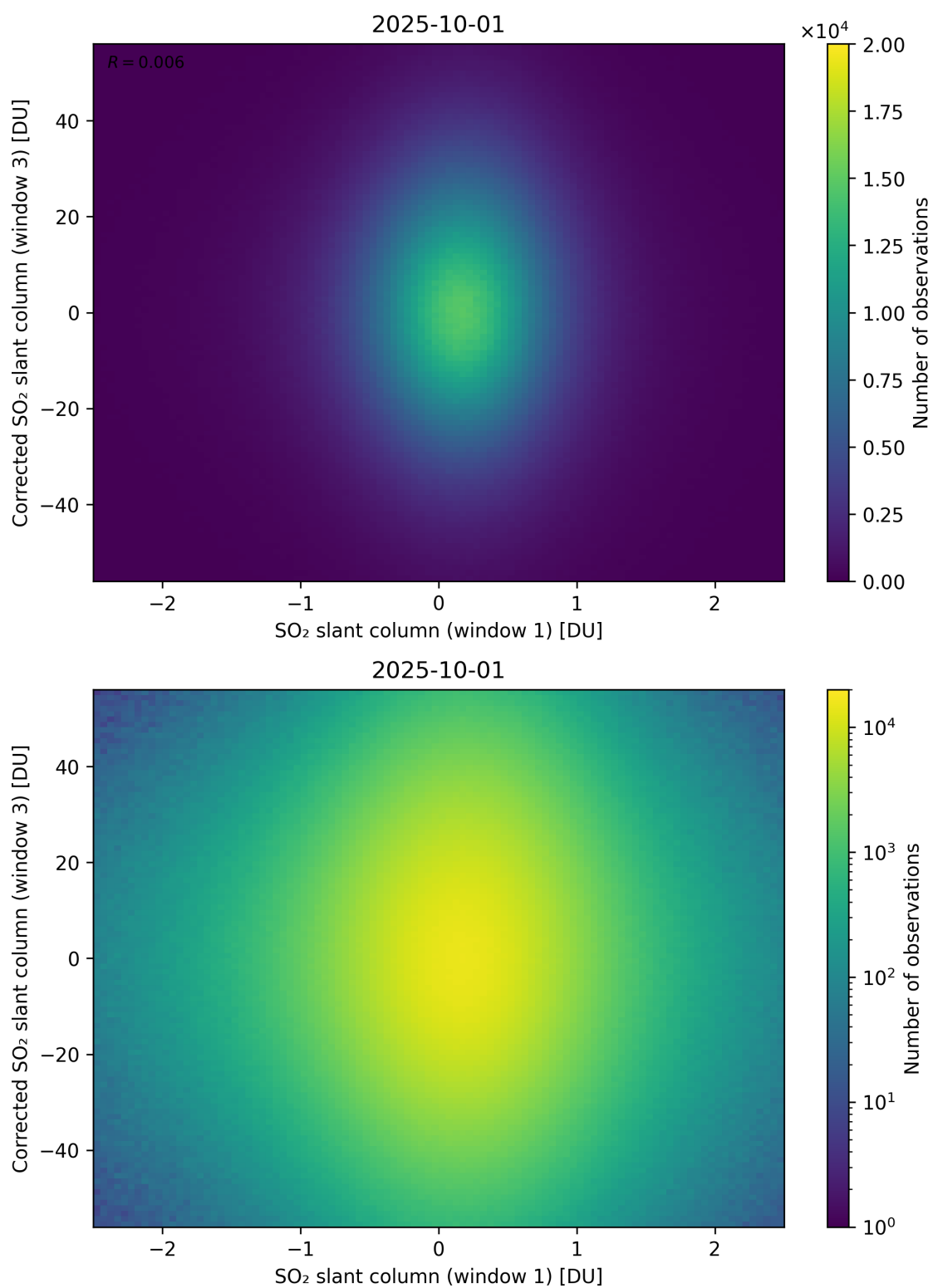
Figure 284: Scatter density plot of “SO 2 slant column (window 1)” against “Corrected SO 2 slant column (window 3)” for 2025-10-01 to 2025-10-02.
