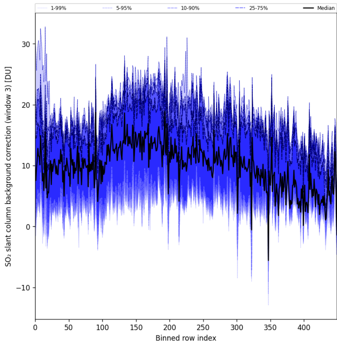
Figure 100: Along track statistics of “SO 2 slant column background correction (window 3)” for 2025-10-01 to 2025-10-02
