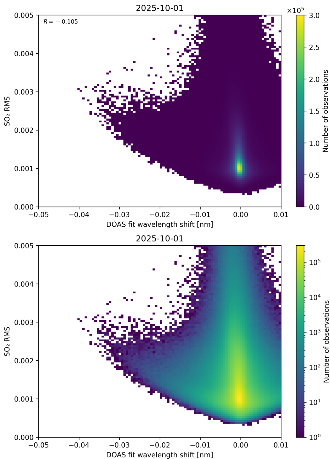
Figure 139: Scatter density plot of “DOAS fit wavelength shift” against “SO 2 RMS” for 2025-10-01 to 2025-10-02.
