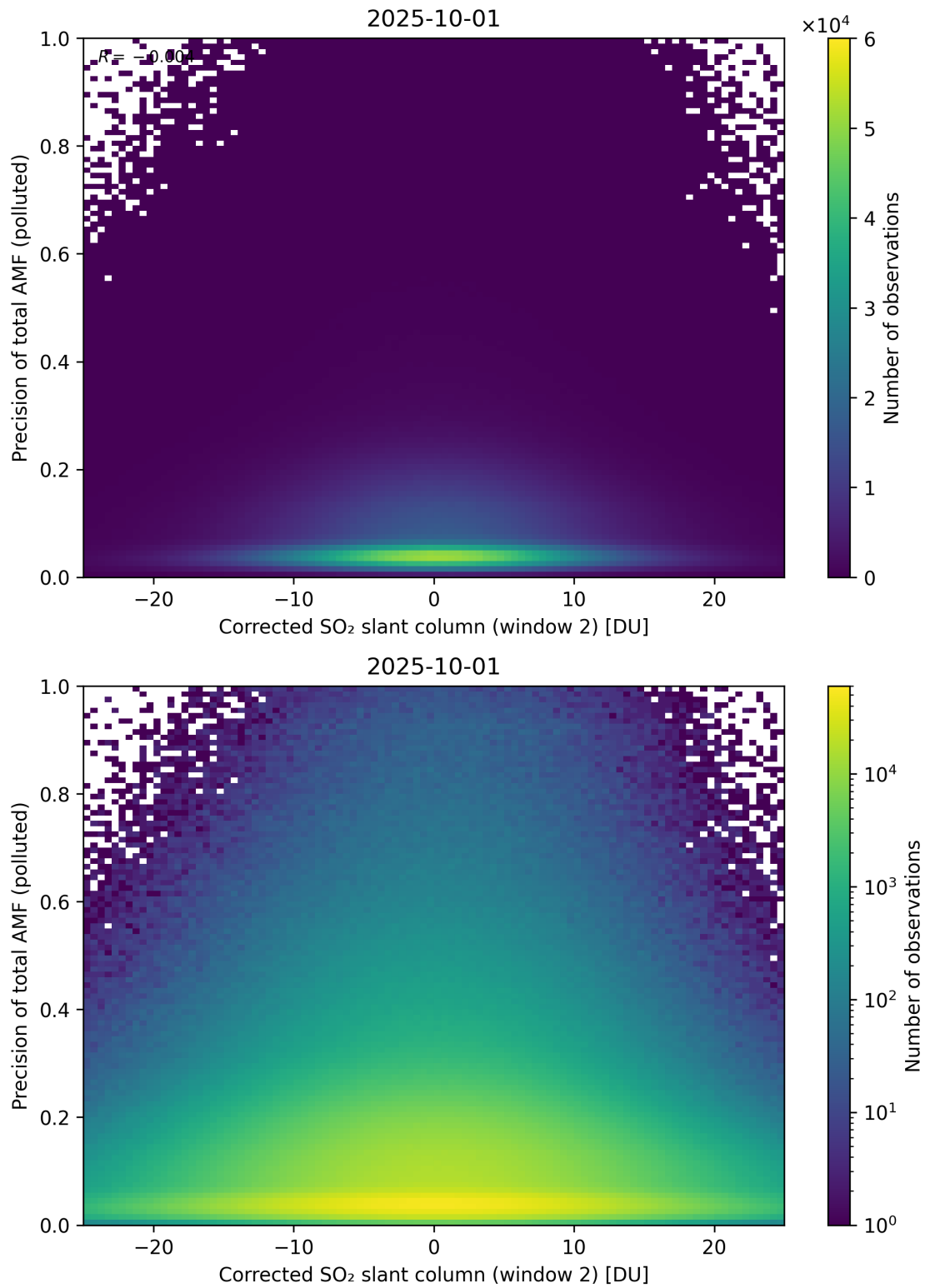
Figure 254: Scatter density plot of “Corrected SO 2 slant column (window 2)” against “Precision of total AMF (polluted)” for 2025-10-01 to 2025-10-02.
