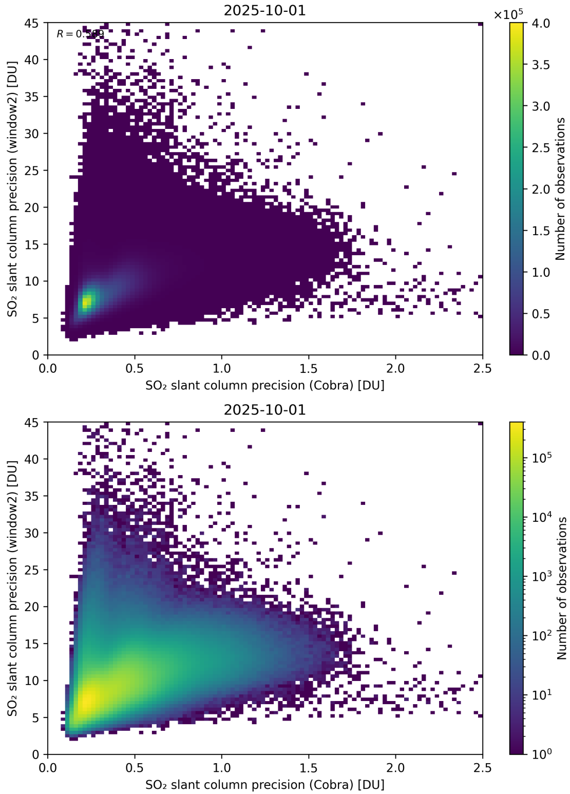
Figure 210: Scatter density plot of “SO 2 slant column precision (Cobra)” against “SO 2 slant column precision (window2)” for 2025-10-01 to 2025-10-02.
