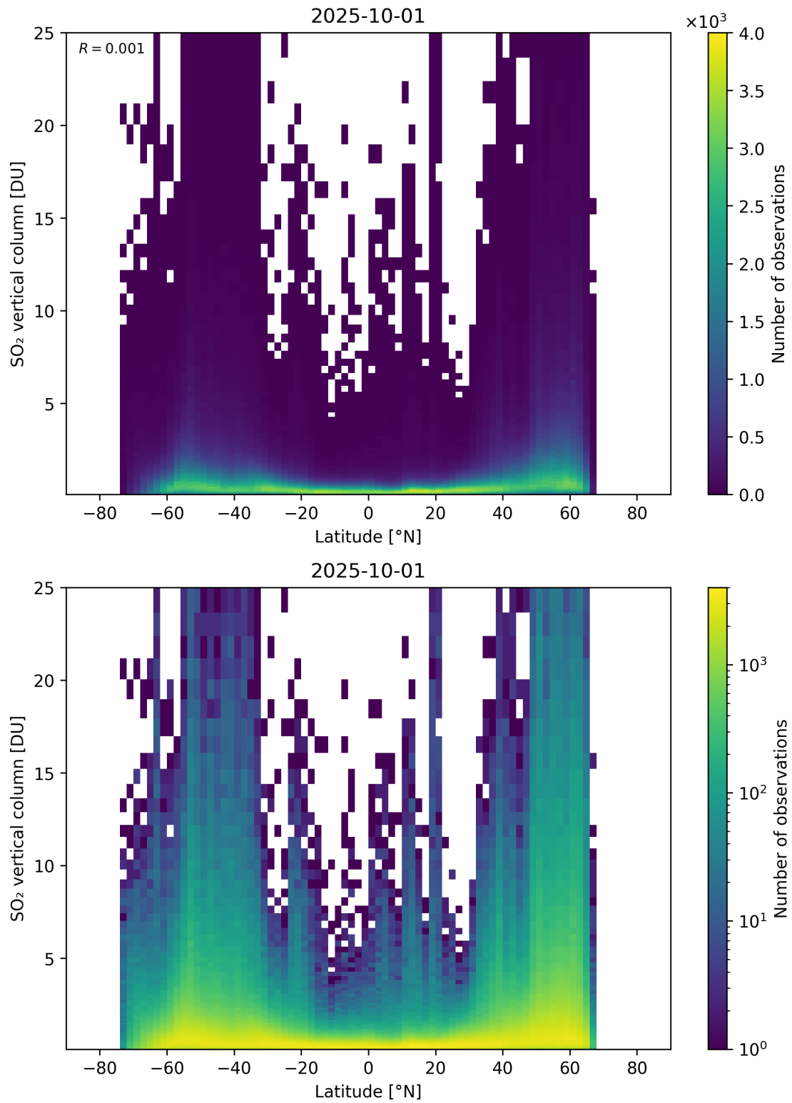
Figure 169: Scatter density plot of “Latitude” against “SO 2 vertical column” for 2025-10-01 to 2025-10-02.
