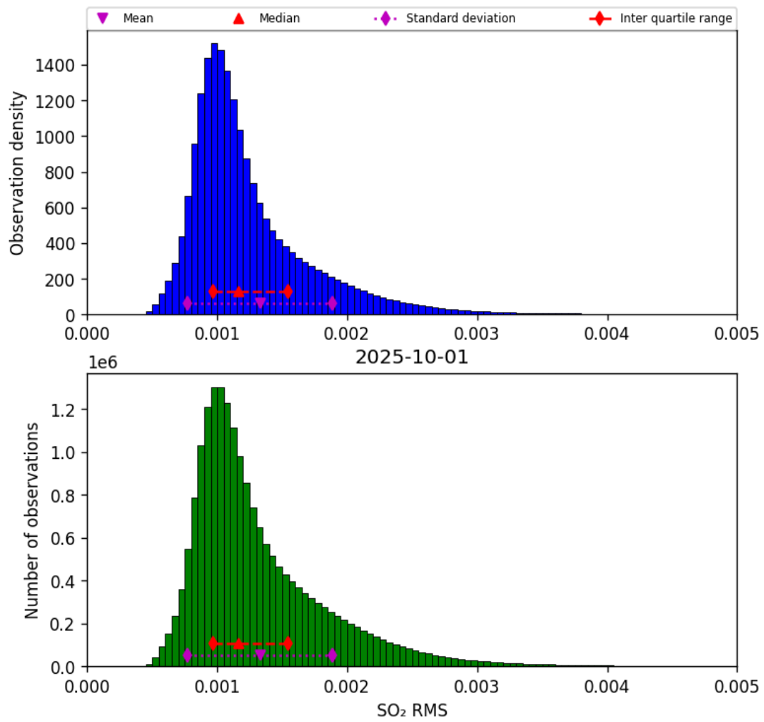
Figure 78: Histogram of “SO 2 RMS” for 2025-10-01 to 2025-10-02
