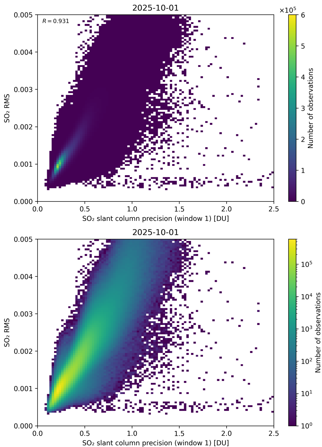
Figure 273: Scatter density plot of “SO 2 slant column precision (window 1)” against “SO 2 RMS” for 2025-10-01 to 2025-10-02.
