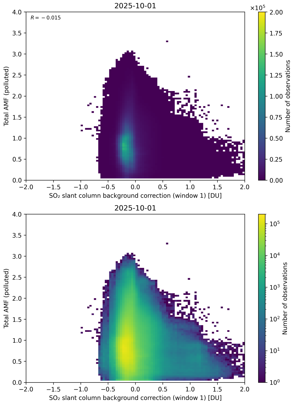
Figure 120: Scatter density plot of “SO 2 slant column background correction (window 1)” against “Total AMF (polluted)” for 2025-10-01 to 2025-10-02.
