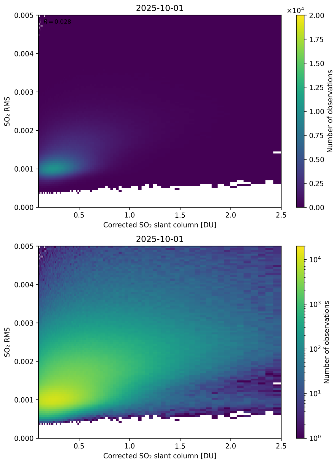
Figure 231: Scatter density plot of “Corrected SO 2 slant column” against “SO 2 RMS” for 2025-10-01 to 2025-10-02.
