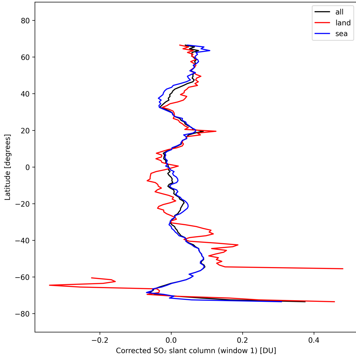
Figure 39: Zonal average of “Corrected SO 2 slant column (window 1)” for 2025-10-01 to 2025-10-02.
