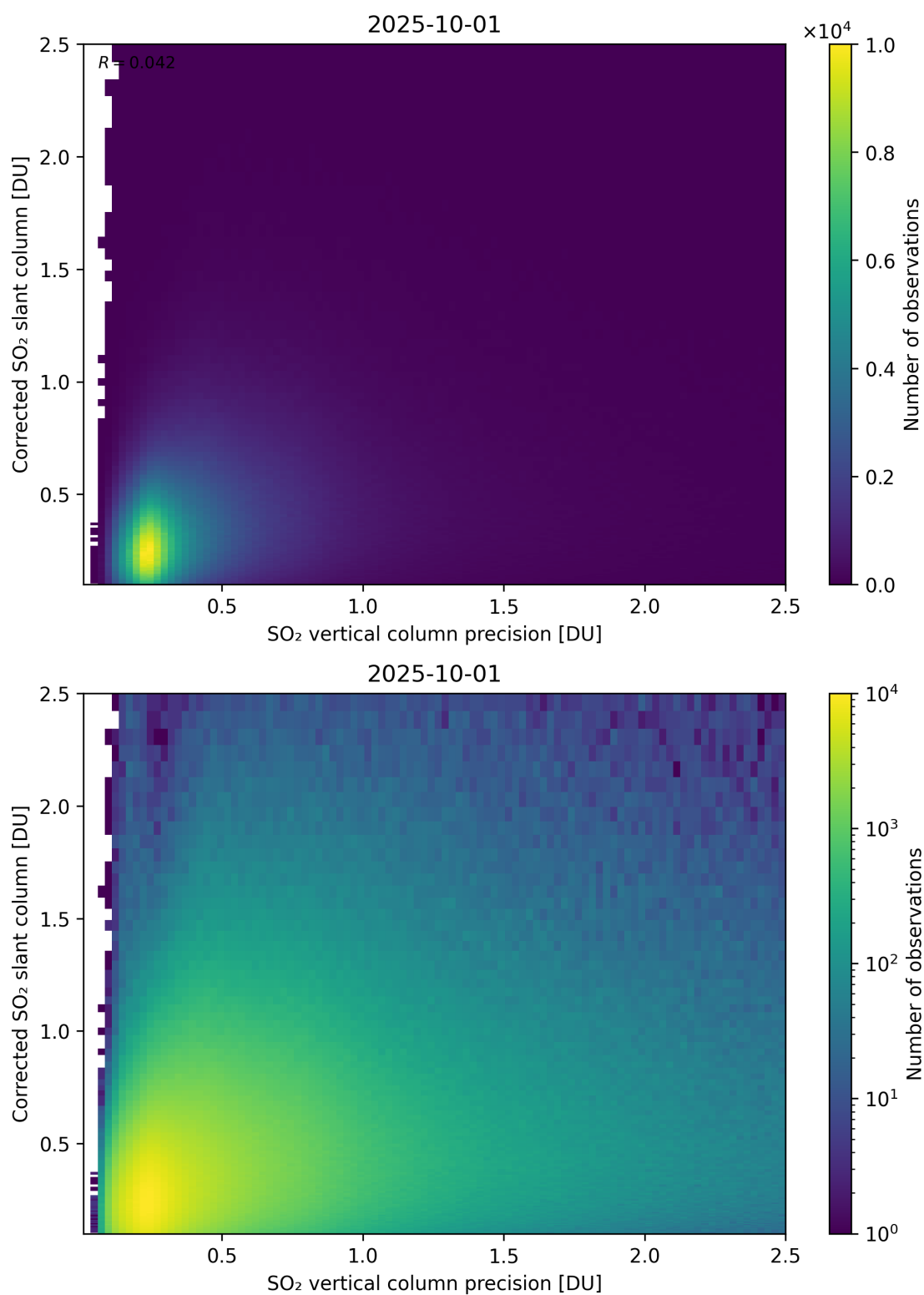
Figure 338: Scatter density plot of “SO 2 vertical column precision” against “Corrected SO 2 slant column” for 2025-10-01 to 2025-10-02.
