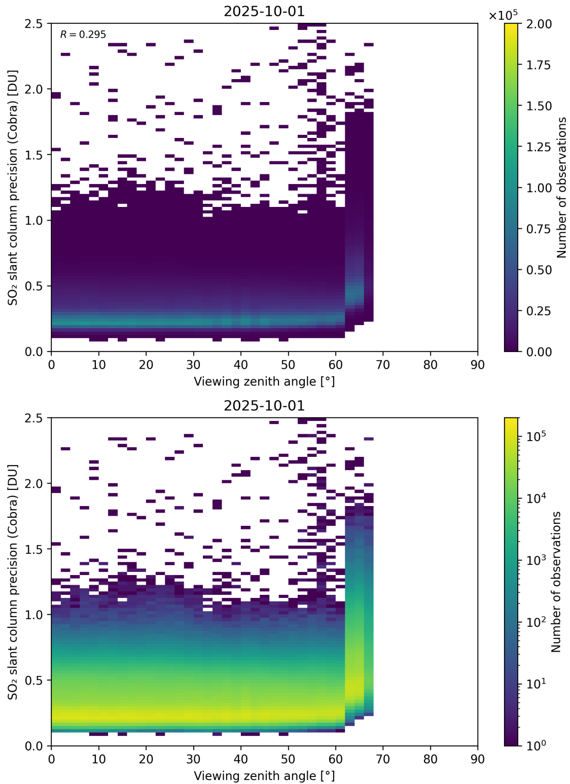
Figure 372: Scatter density plot of “Viewing zenith angle” against “SO 2 slant column precision (Cobra)” for 2025-10-01 to 2025-10-02.
