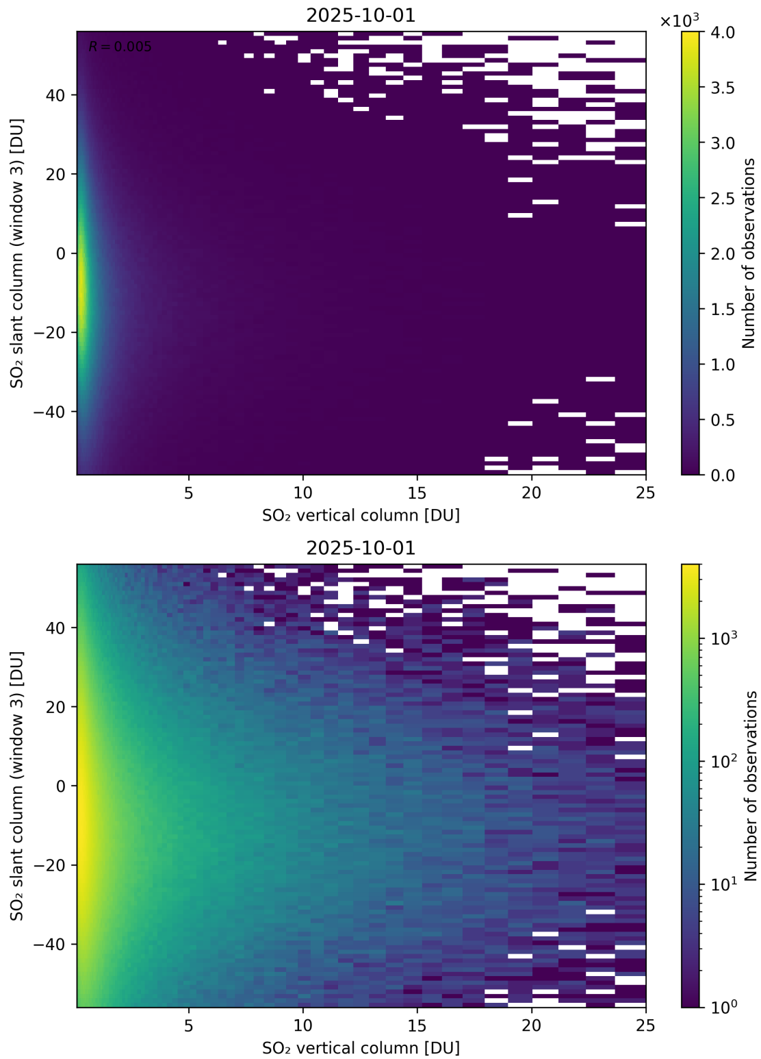
Figure 357: Scatter density plot of “SO 2 vertical column” against “SO 2 slant column (window 3)” for 2025-10-01 to 2025-10-02.
