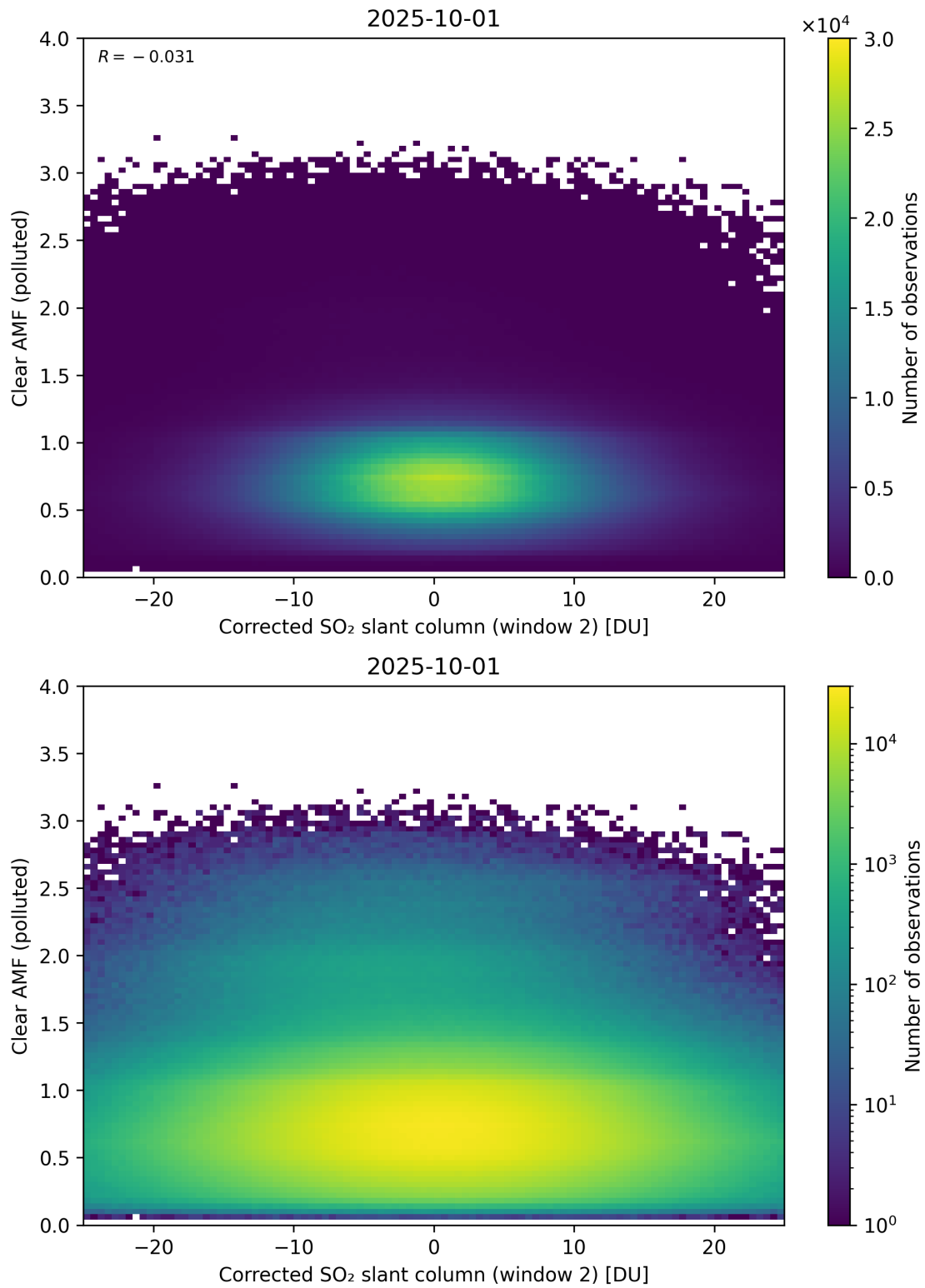
Figure 249: Scatter density plot of “Corrected SO 2 slant column (window 2)” against “Clear AMF (polluted)” for 2025-10-01 to 2025-10-02.
