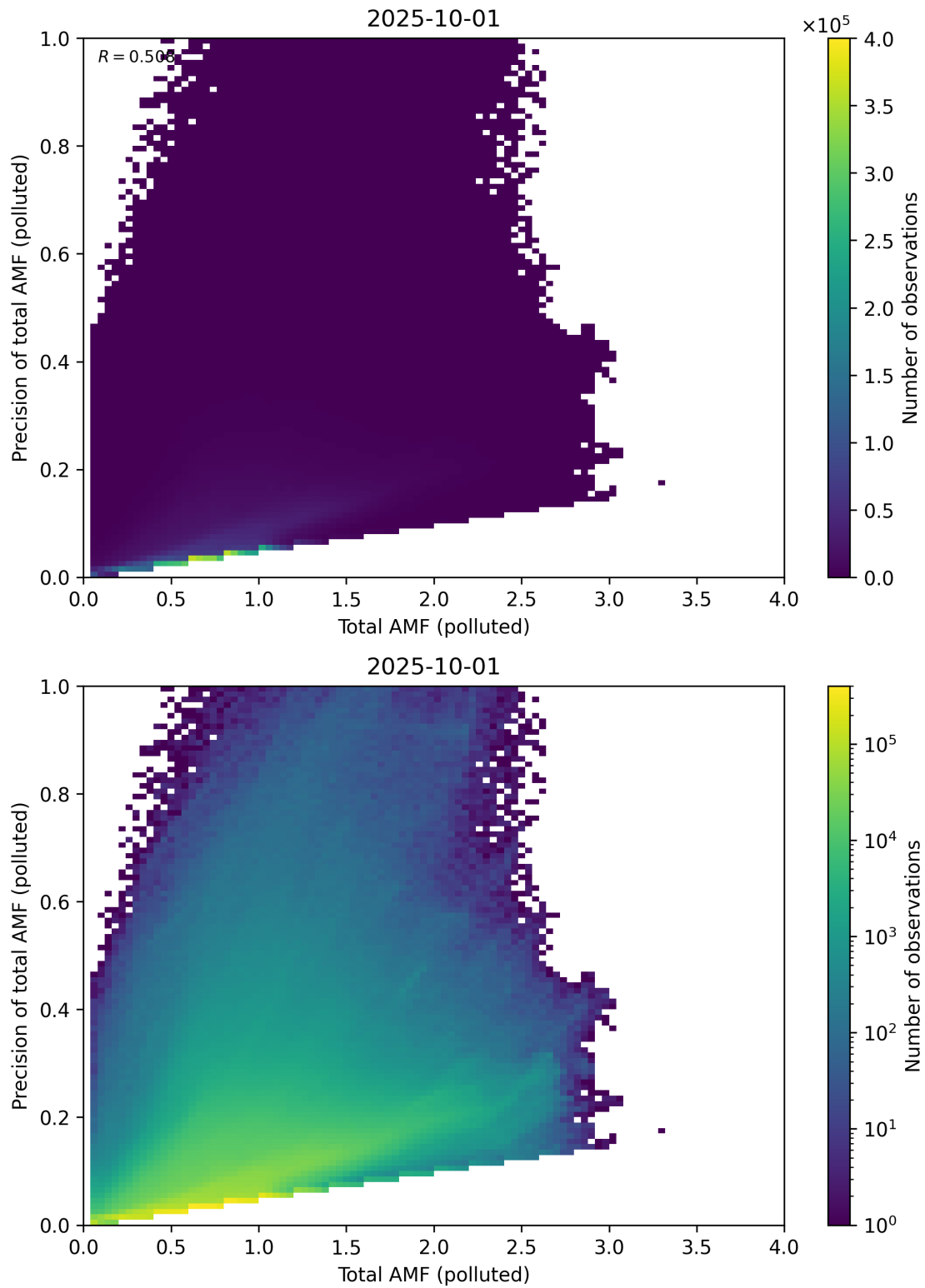
Figure 322: Scatter density plot of “Total AMF (polluted)” against “Precision of total AMF (polluted)” for 2025-10-01 to 2025-10-02.
