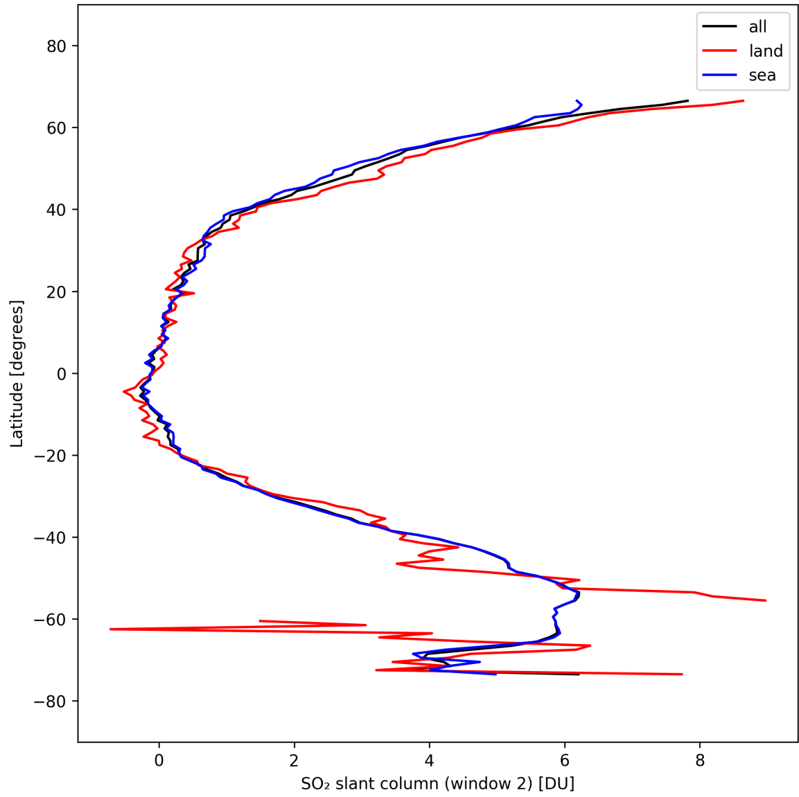
Figure 41: Zonal average of “SO 2 slant column (window 2)” for 2025-10-01 to 2025-10-02.
