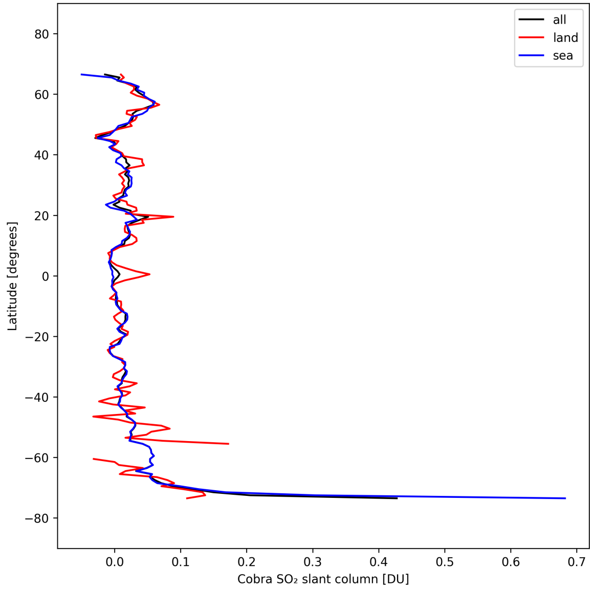
Figure 35: Zonal average of “Cobra SO 2 slant column” for 2025-10-01 to 2025-10-02.
