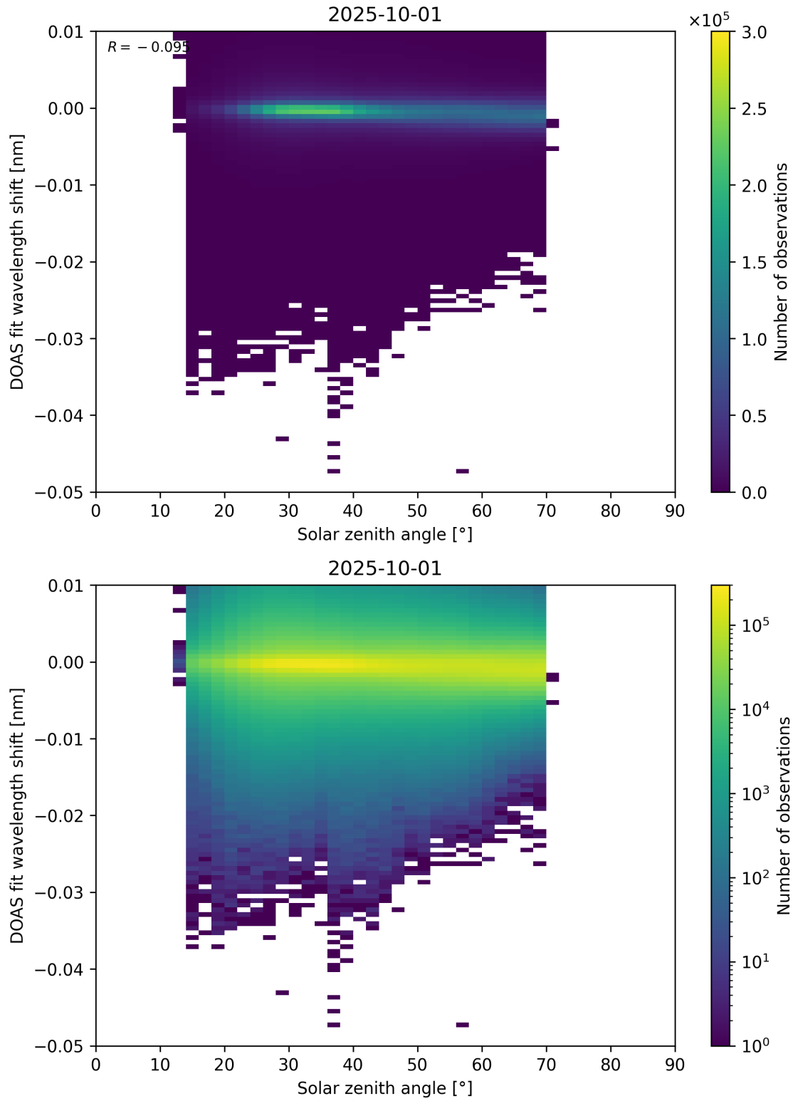
Figure 174: Scatter density plot of “Solar zenith angle” against “DOAS fit wavelength shift” for 2025-10-01 to 2025-10-02.
