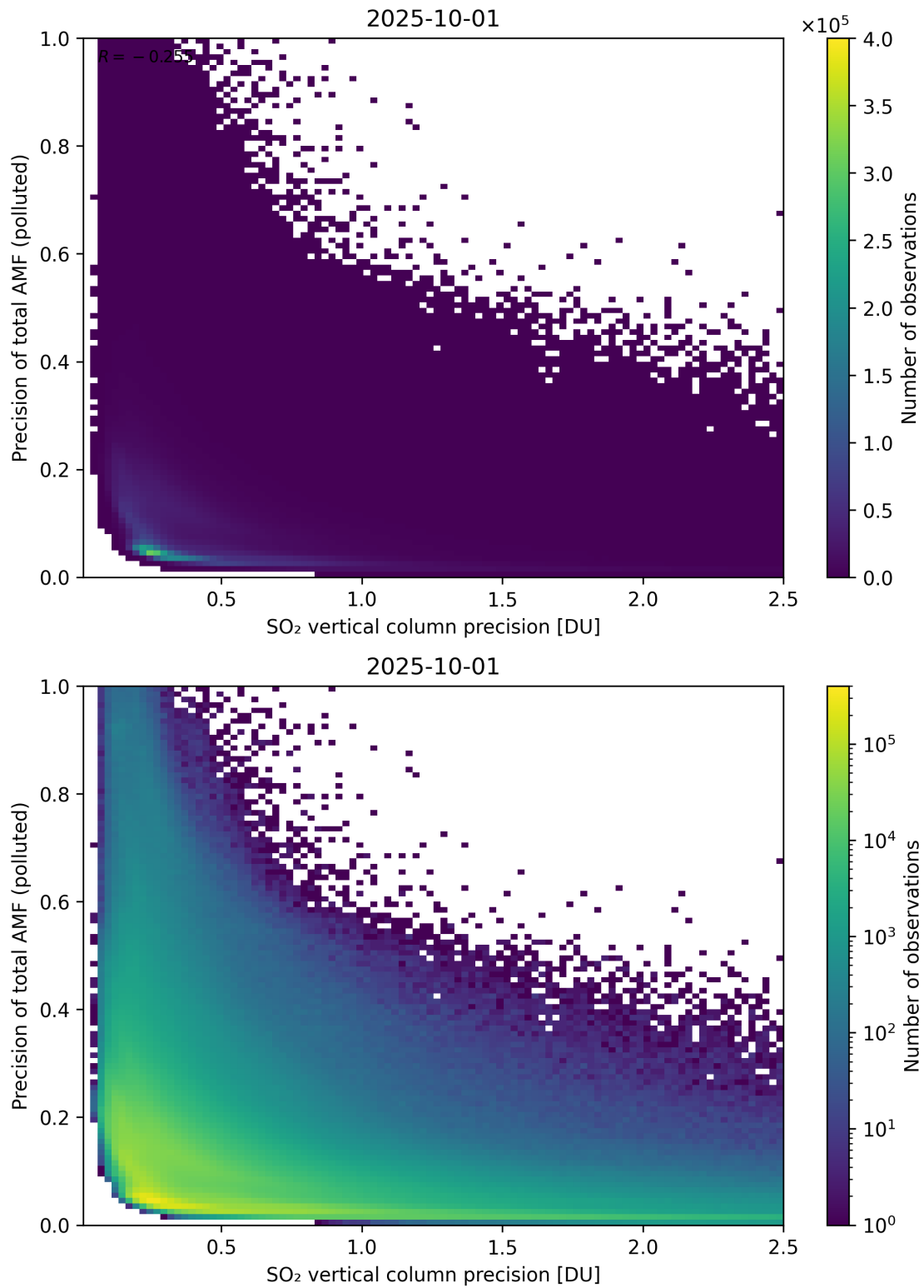
Figure 347: Scatter density plot of “SO 2 vertical column precision” against “Precision of total AMF (polluted)” for 2025-10-01 to 2025-10-02.
