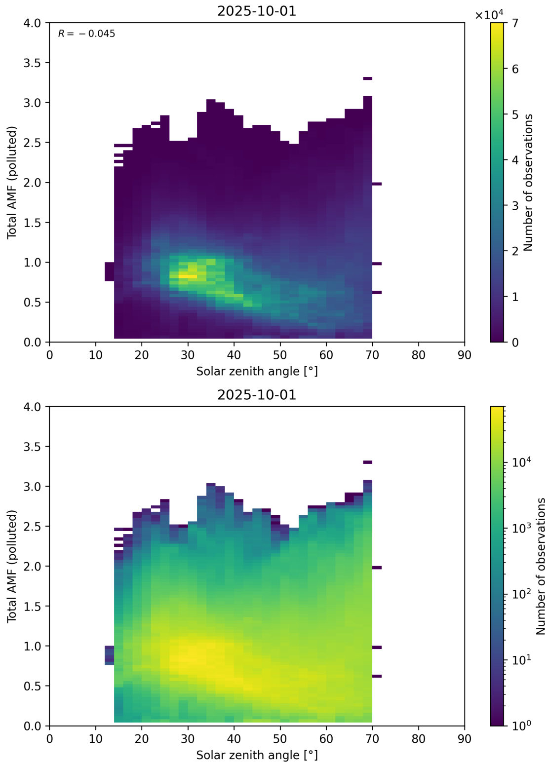
Figure 189: Scatter density plot of “Solar zenith angle” against “Total AMF (polluted)” for 2025-10-01 to 2025-10-02.
