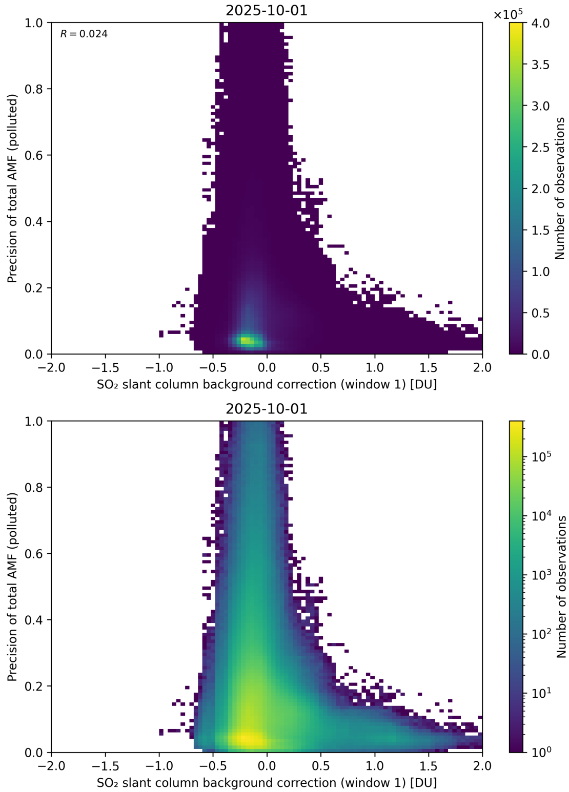
Figure 121: Scatter density plot of “SO 2 slant column background correction (window 1)” against “Precision of total AMF (polluted)” for 2025-10-01 to 2025-10-02.
