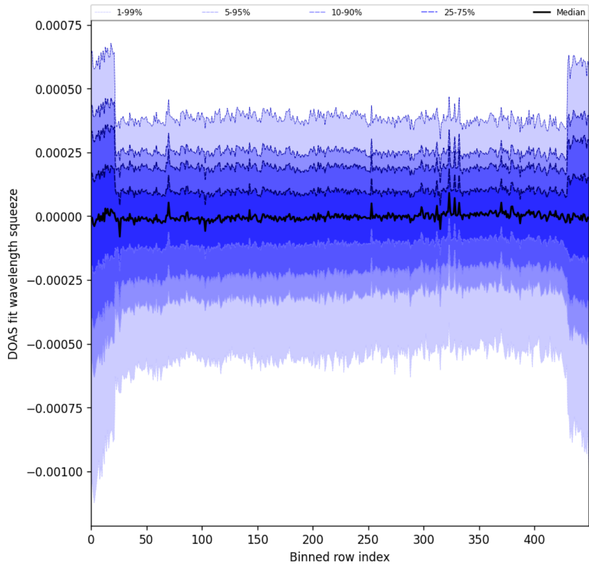
Figure 103: Along track statistics of “DOAS fit wavelength squeeze” for 2025-10-01 to 2025-10-02
