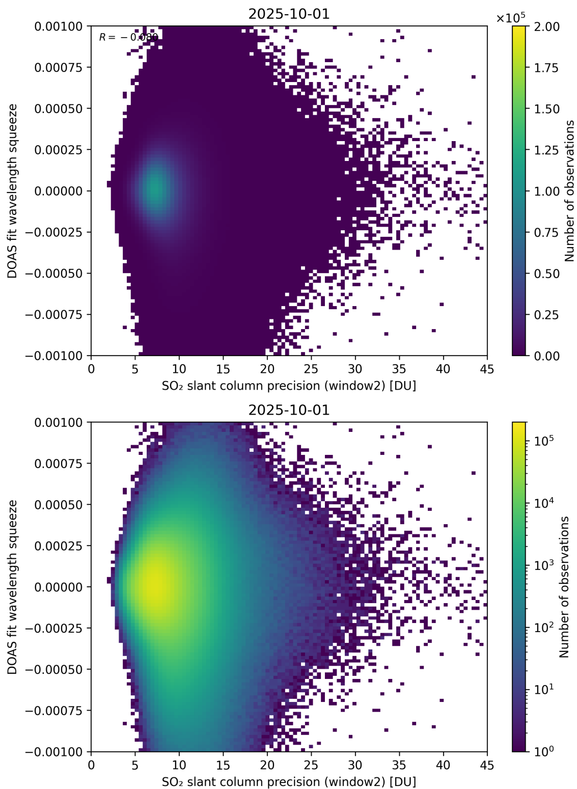
Figure 294: Scatter density plot of “SO 2 slant column precision (window2)” against “DOAS fit wavelength squeeze” for 2025-10-01 to 2025-10-02.
