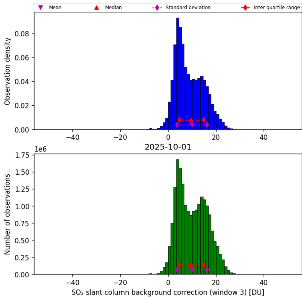
Figure 74: Histogram of “SO 2 slant column background correction (window 3)” for 2025-10-01 to 2025-10-02
