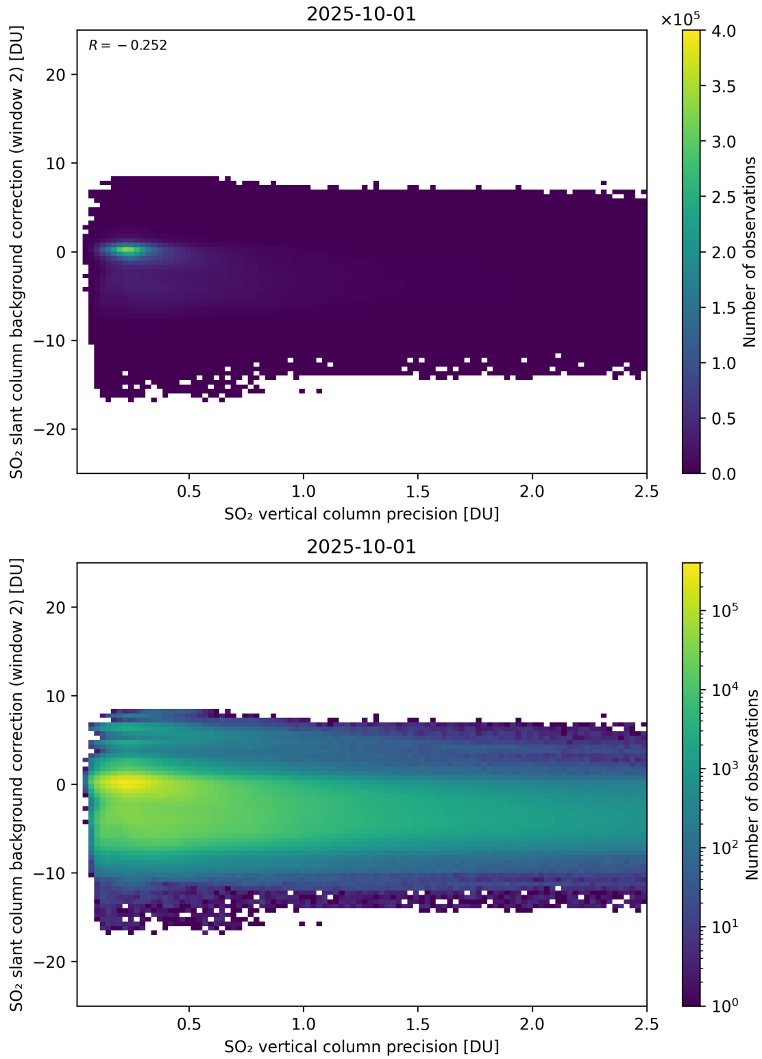
Figure 330: Scatter density plot of “SO 2 vertical column precision” against “SO 2 slant column background correction (window 2)” for 2025-10-01 to 2025-10-02.
