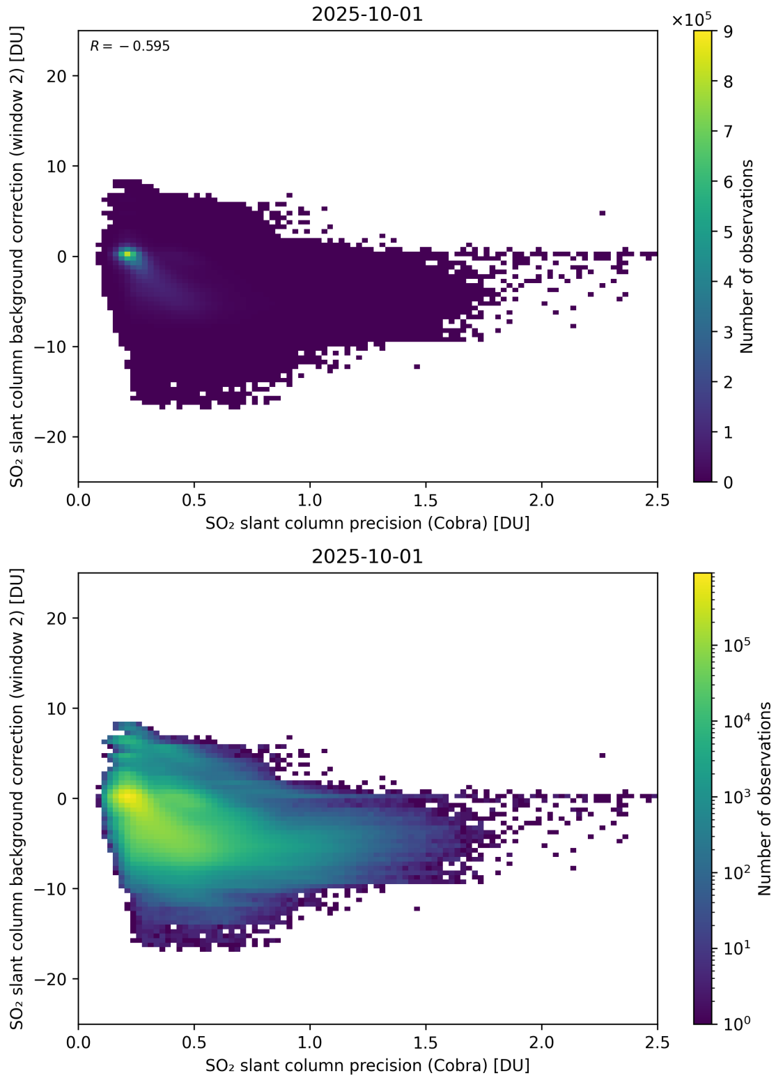
Figure 200: Scatter density plot of “SO 2 slant column precision (Cobra)” against “SO 2 slant column background correction (window 2)” for 2025-10-01 to 2025-10-02.
