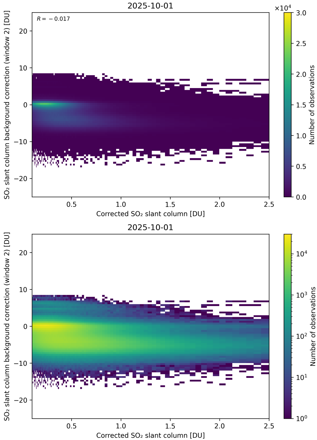
Figure 227: Scatter density plot of “Corrected SO 2 slant column” against “SO 2 slant column background correction (window 2)” for 2025-10-01 to 2025-10-02.
