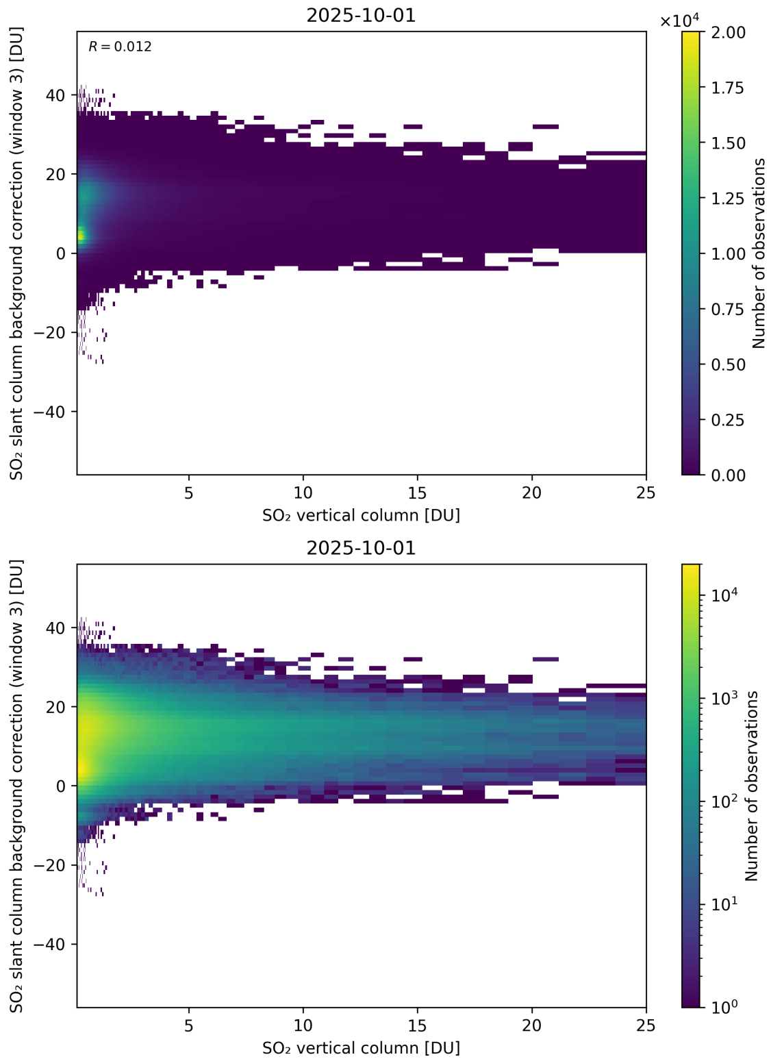
Figure 325: Scatter density plot of “SO 2 vertical column” against “SO 2 slant column background correction (window 3)” for 2025-10-01 to 2025-10-02.
