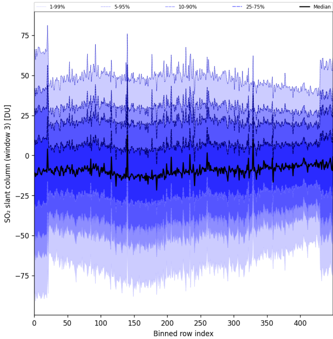
Figure 97: Along track statistics of “SO 2 slant column (window 3)” for 2025-10-01 to 2025-10-02
