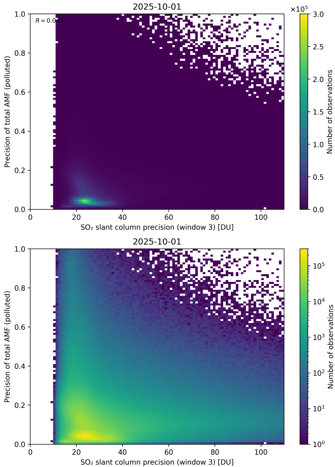
Figure 314: Scatter density plot of “SO 2 slant column precision (window 3)” against “Precision of total AMF (polluted)” for 2025-10-01 to 2025-10-02.
