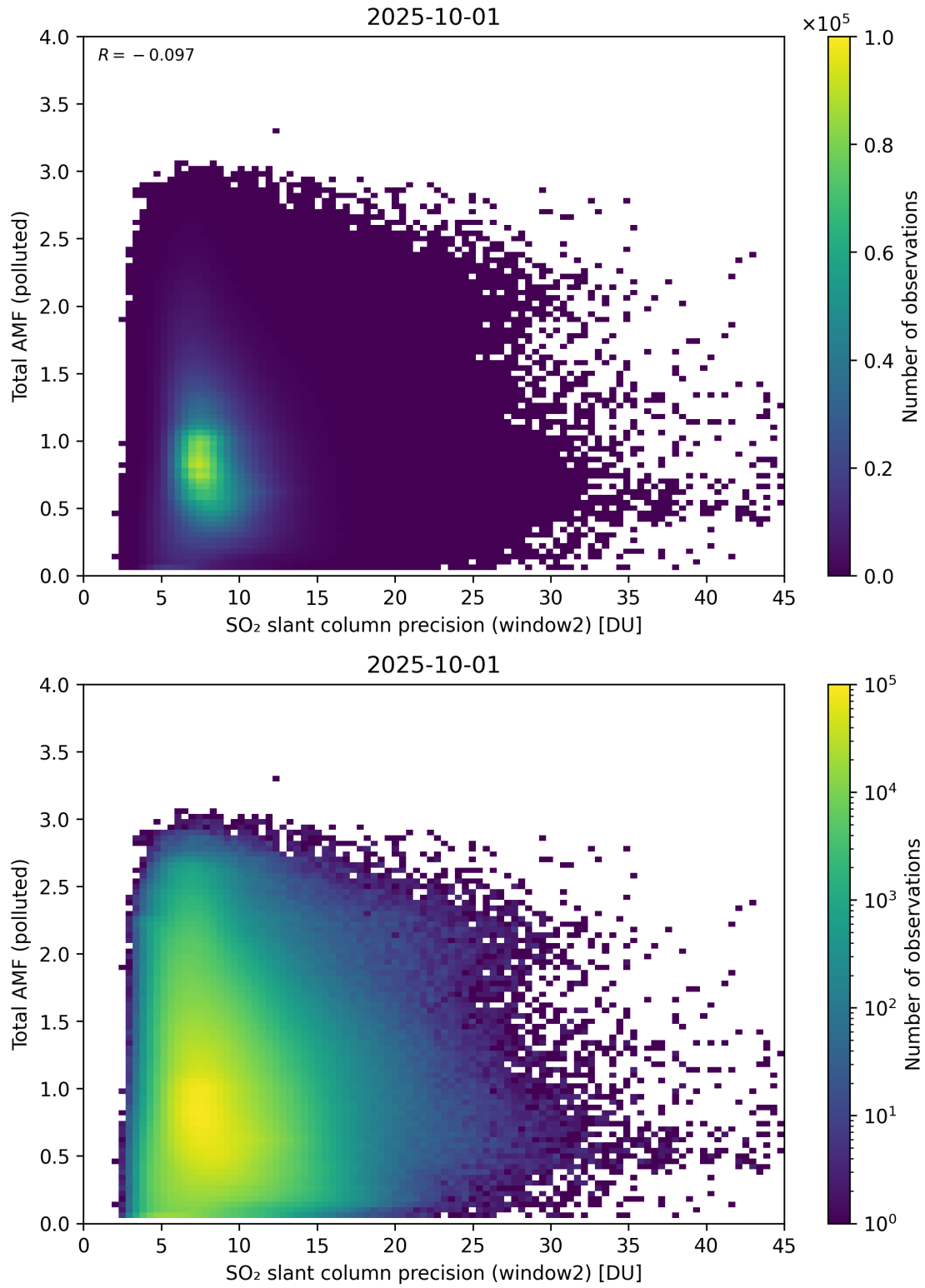
Figure 301: Scatter density plot of “SO 2 slant column precision (window2)” against “Total AMF (polluted)” for 2025-10-01 to 2025-10-02.
