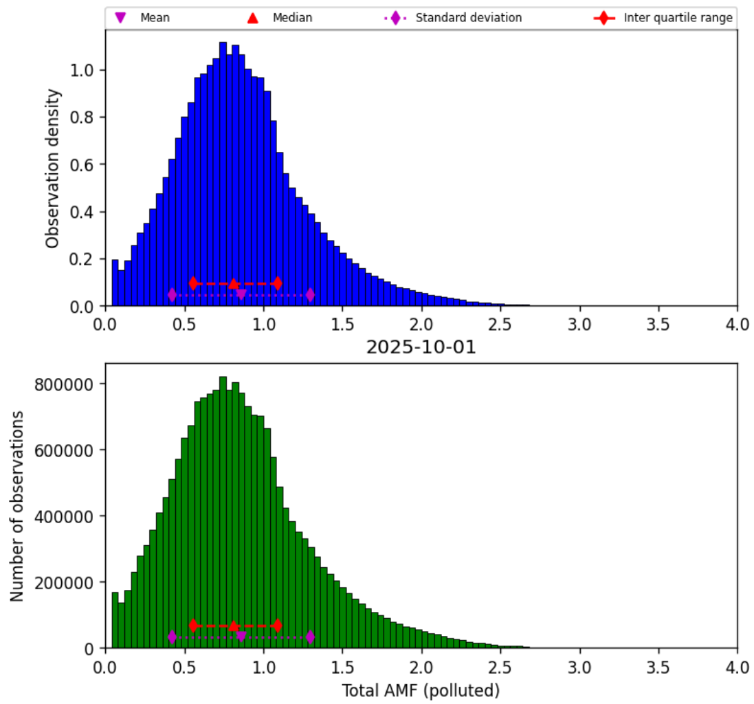
Figure 79: Histogram of “Total AMF (polluted)” for 2025-10-01 to 2025-10-02
