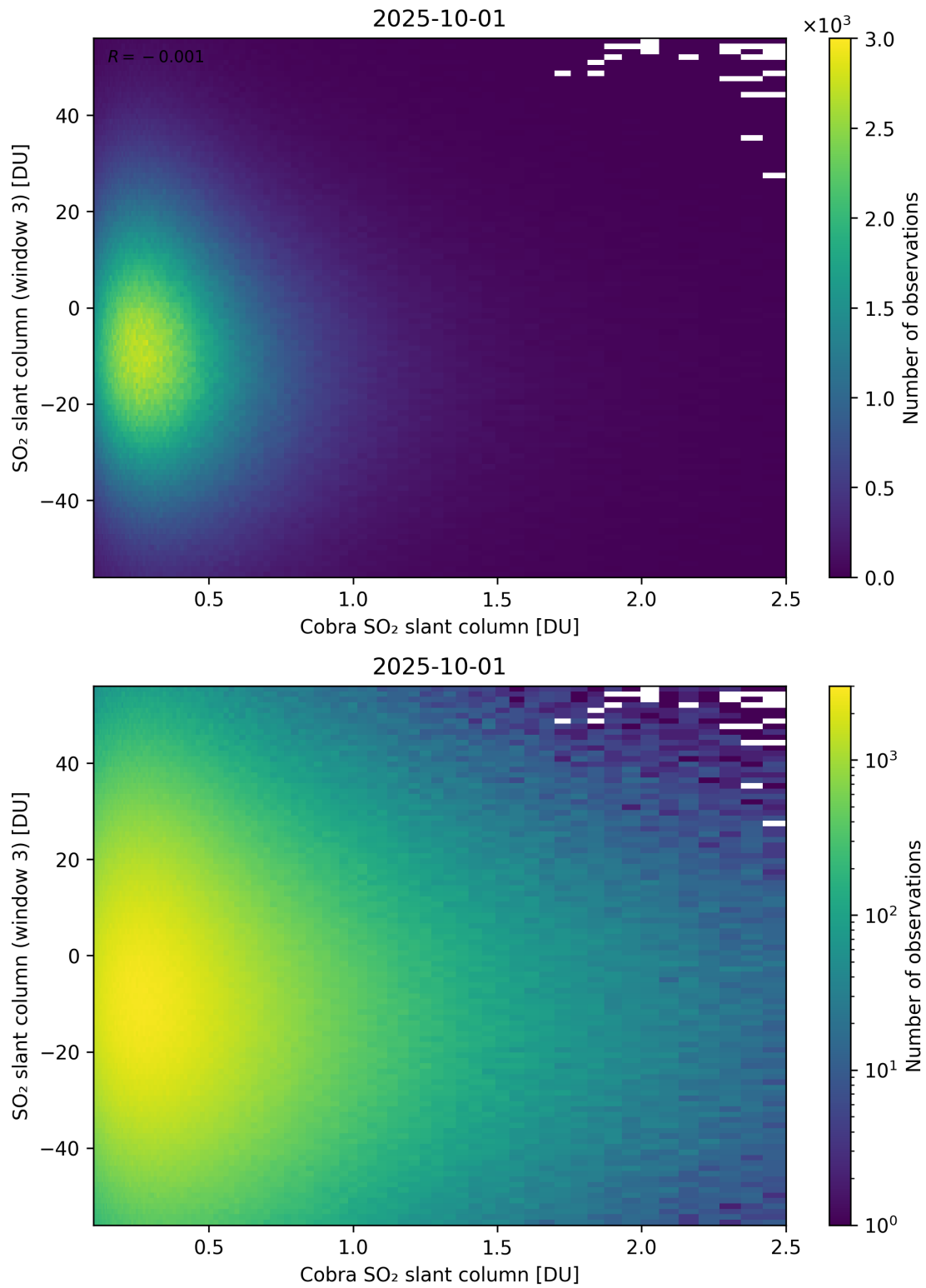
Figure 222: Scatter density plot of “Cobra SO 2 slant column” against “SO 2 slant column (window 3)” for 2025-10-01 to 2025-10-02.
