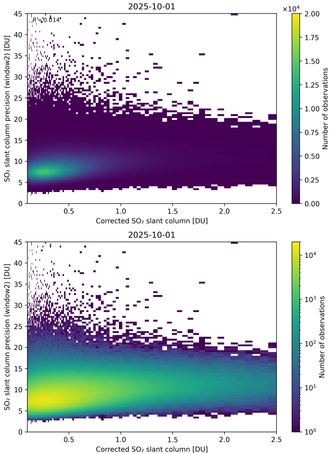
Figure 239: Scatter density plot of “Corrected SO 2 slant column” against “SO 2 slant column precision (window2)” for 2025-10-01 to 2025-10-02.
