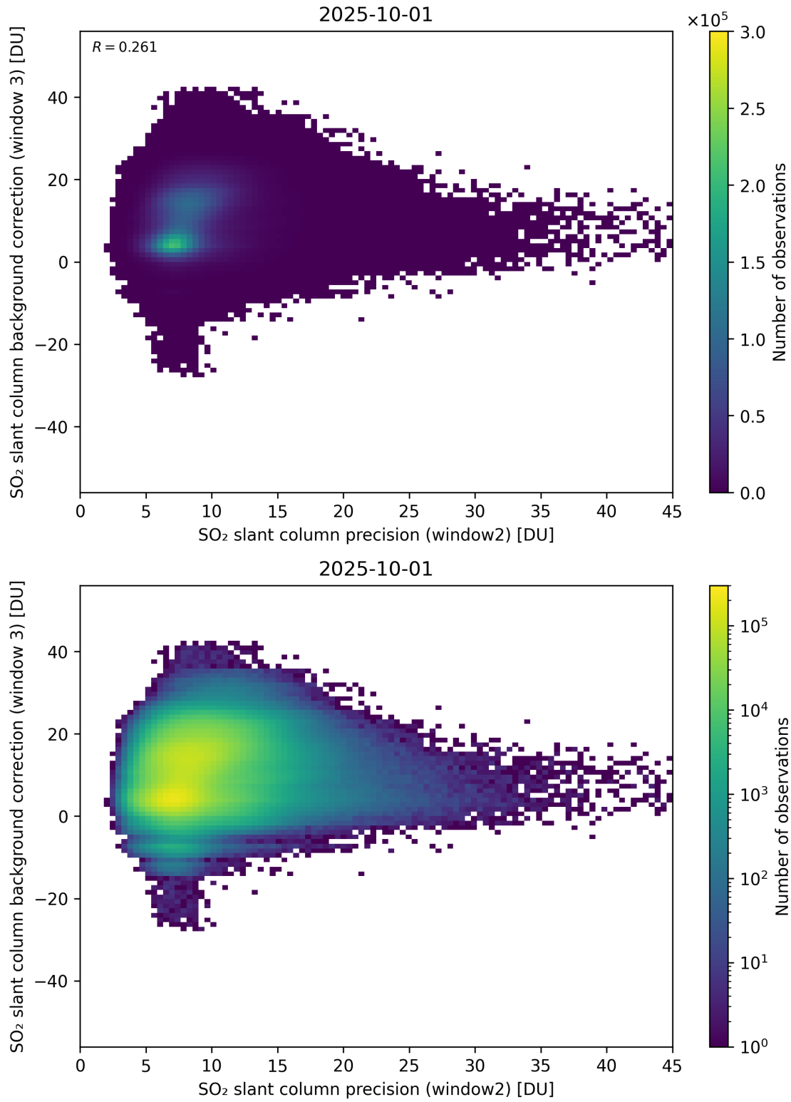
Figure 292: Scatter density plot of “SO 2 slant column precision (window2)” against “SO 2 slant column background correction (window 3)” for 2025-10-01 to 2025-10-02.
