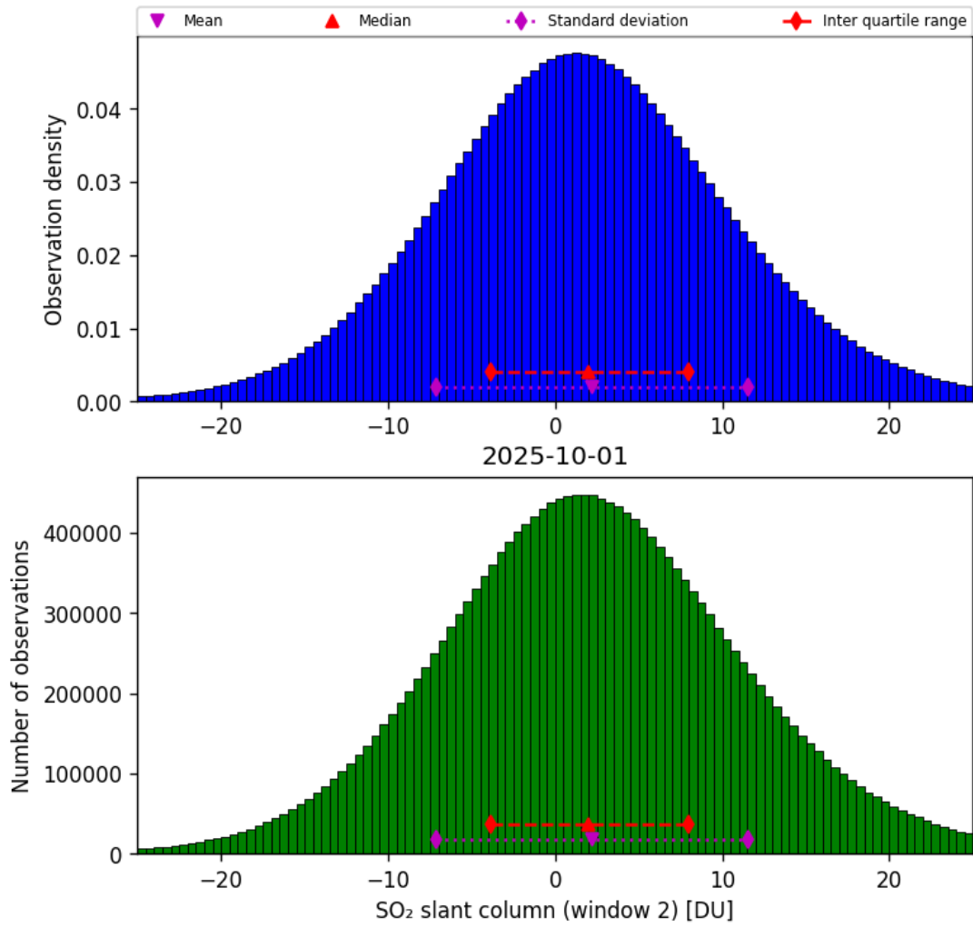
Figure 67: Histogram of “SO 2 slant column (window 2)” for 2025-10-01 to 2025-10-02
