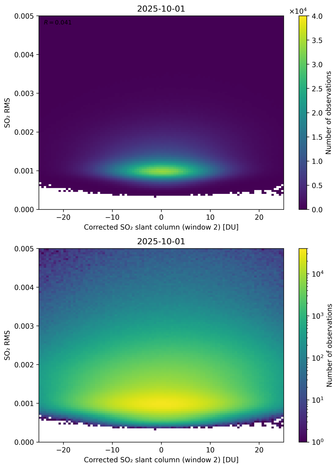
Figure 248: Scatter density plot of “Corrected SO 2 slant column (window 2)” against “SO 2 RMS” for 2025-10-01 to 2025-10-02.
