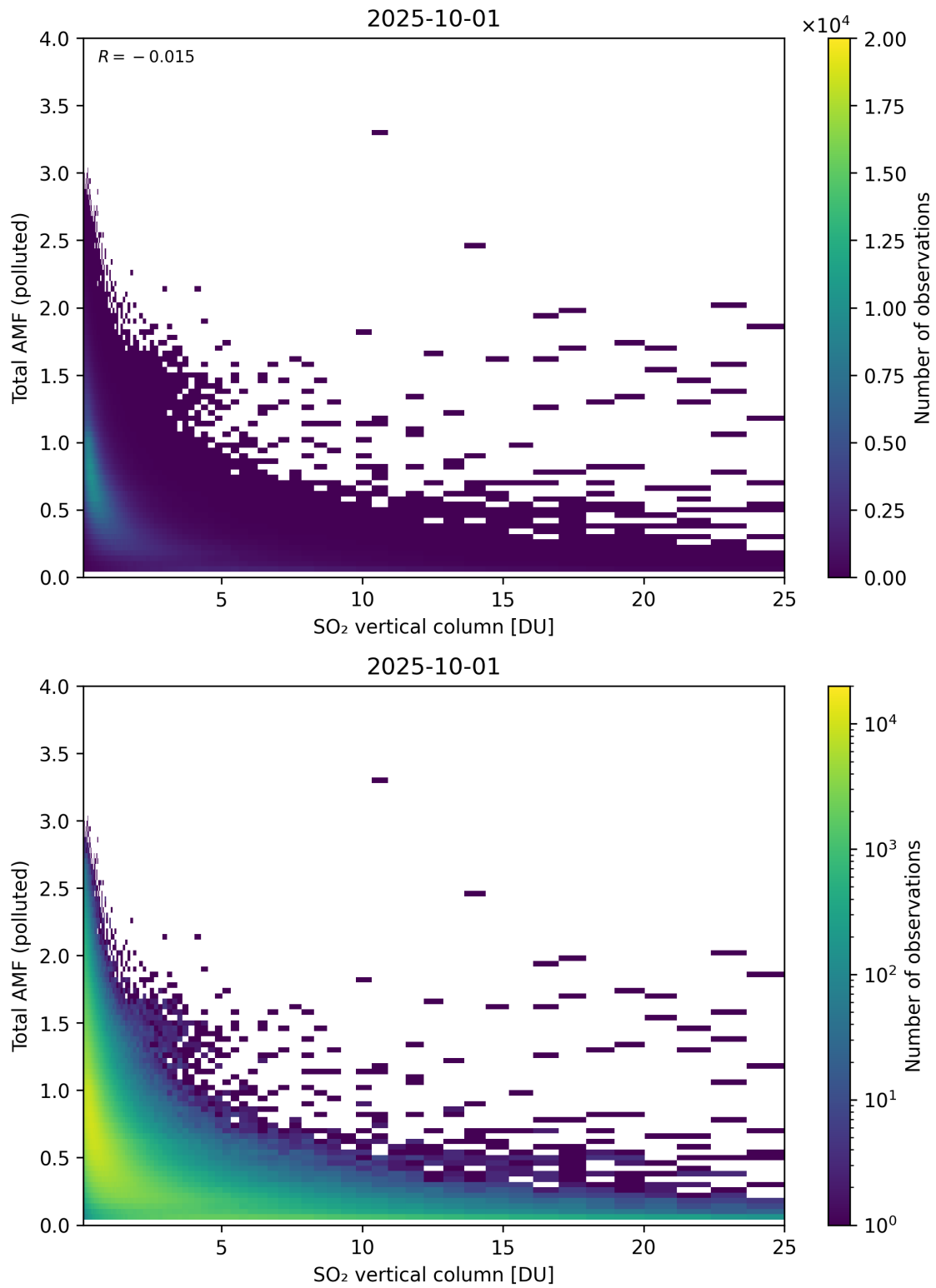
Figure 359: Scatter density plot of “SO 2 vertical column” against “Total AMF (polluted)” for 2025-10-01 to 2025-10-02.
