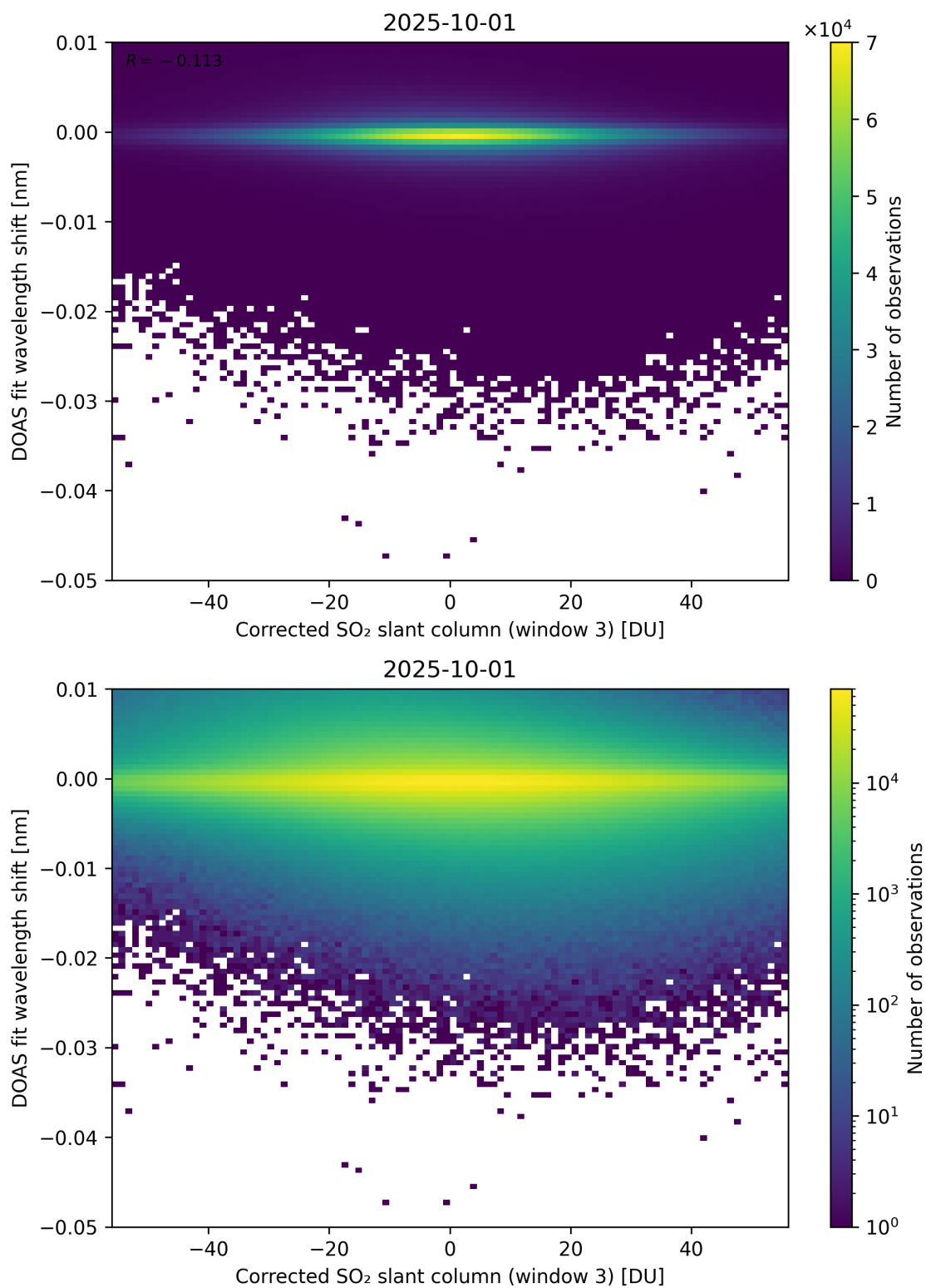
Figure 256: Scatter density plot of “Corrected SO 2 slant column (window 3)” against “DOAS fit wavelength shift” for 2025-10-01 to 2025-10-02.
