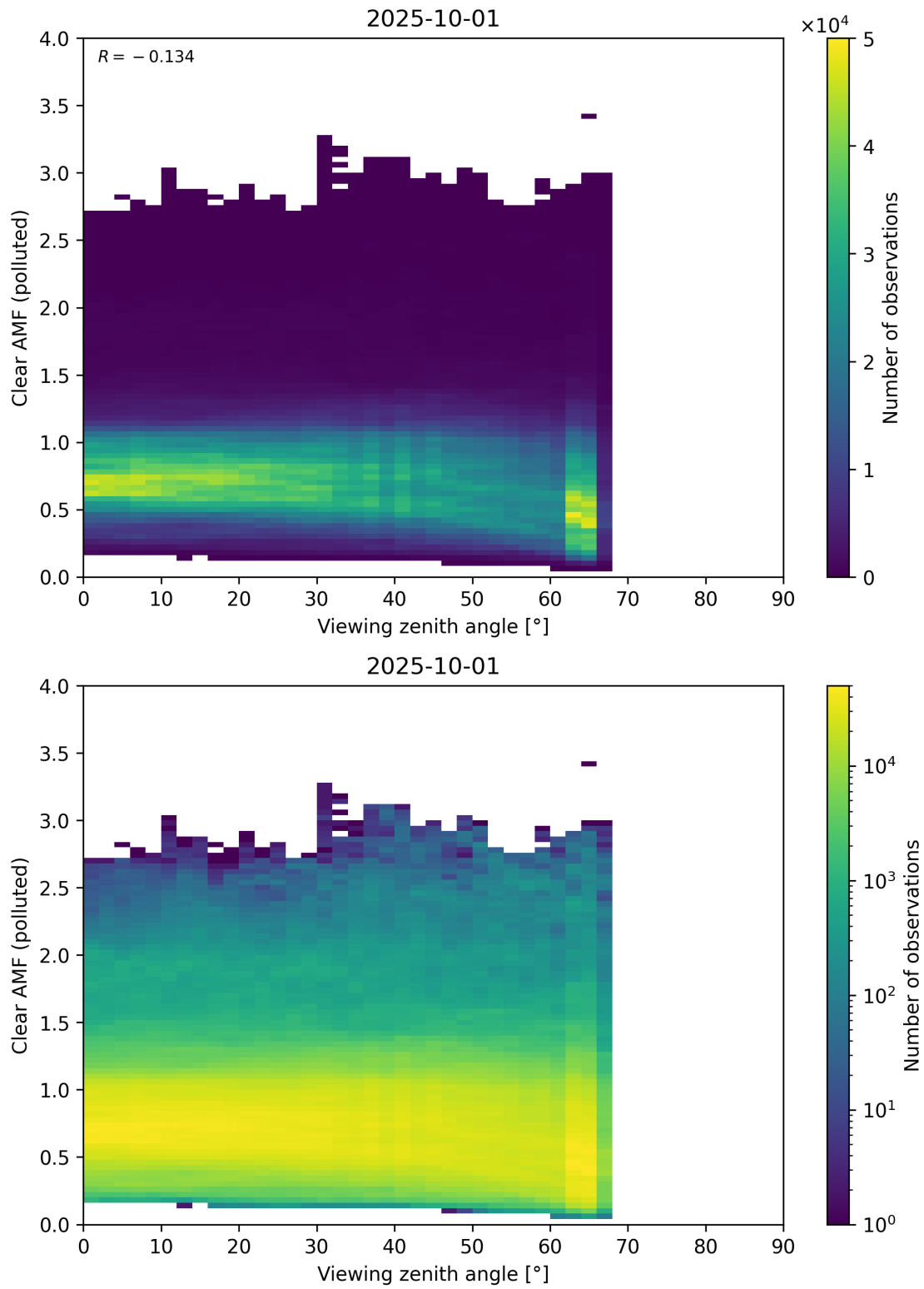
Figure 370: Scatter density plot of “Viewing zenith angle” against “Clear AMF (polluted)” for 2025-10-01 to 2025-10-02.
