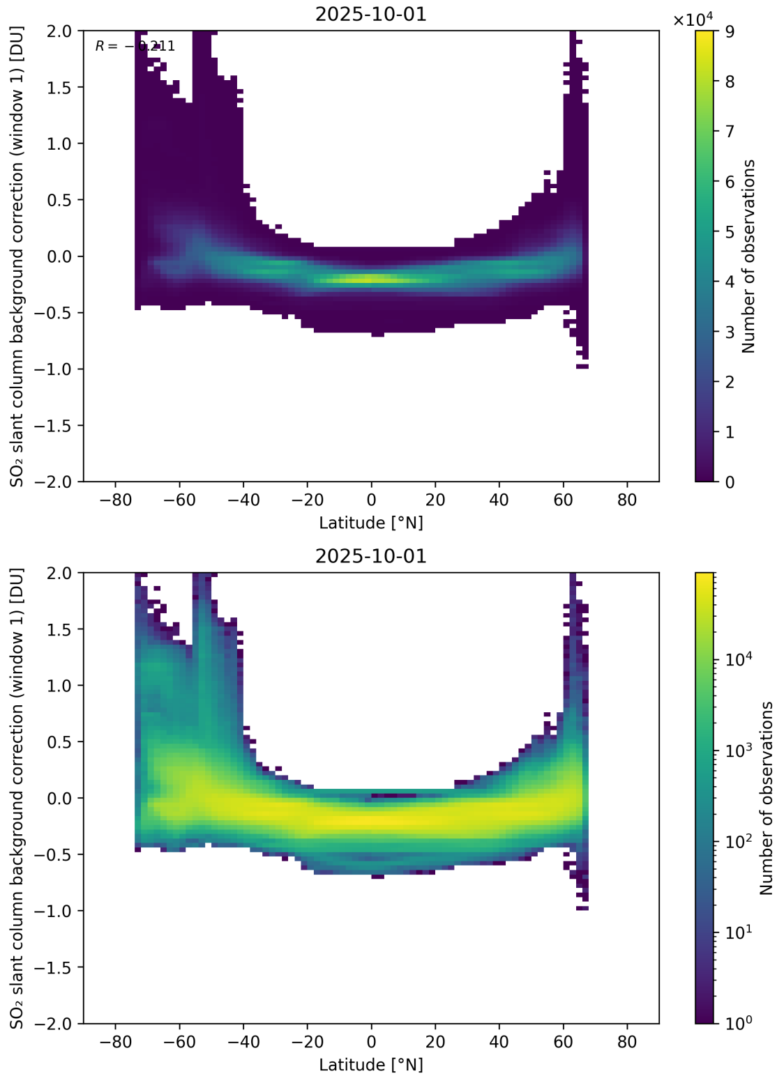
Figure 150: Scatter density plot of “Latitude” against “SO 2 slant column background correction (window 1)” for 2025-10-01 to 2025-10-02.
