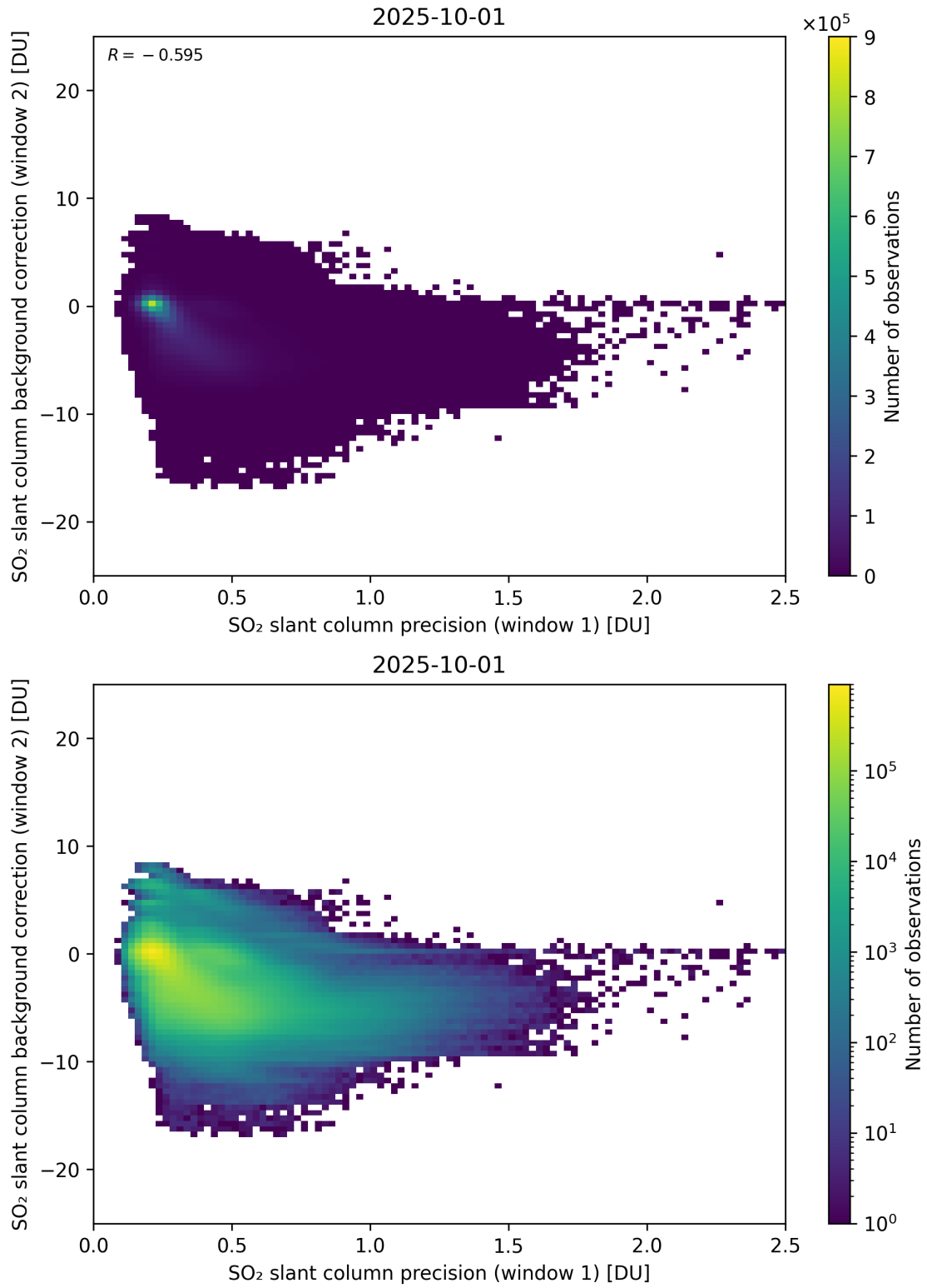
Figure 269: Scatter density plot of “SO 2 slant column precision (window 1)” against “SO 2 slant column background correction (window 2)” for 2025-10-01 to 2025-10-02.
