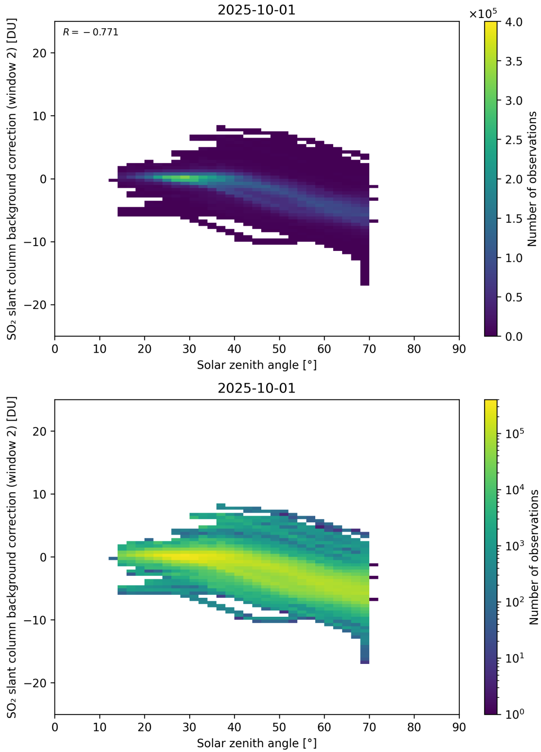
Figure 172: Scatter density plot of “Solar zenith angle” against “SO 2 slant column background correction (window 2)” for 2025-10-01 to 2025-10-02.
