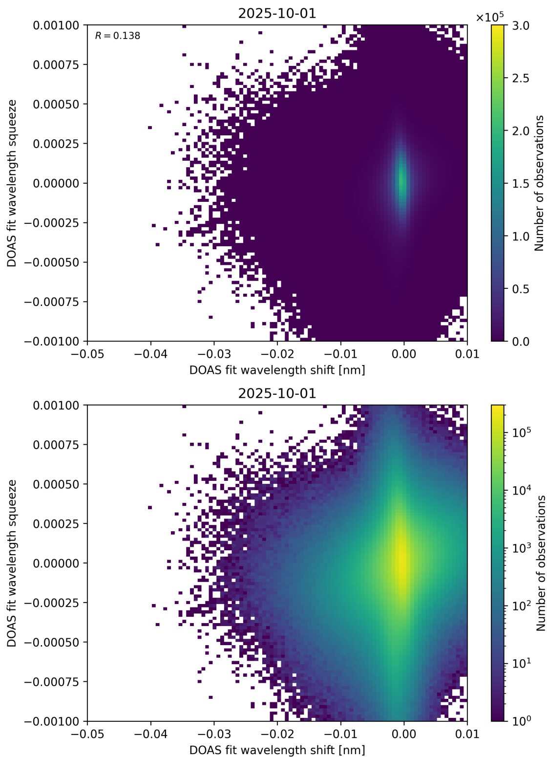
Figure 138: Scatter density plot of “DOAS fit wavelength shift” against “DOAS fit wavelength squeeze” for 2025-10-01 to 2025-10-02.
