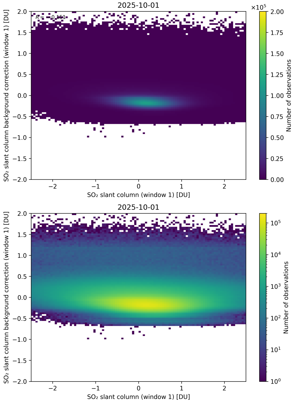
Figure 262: Scatter density plot of “SO 2 slant column (window 1)” against “SO 2 slant column background correction (window 1)” for 2025-10-01 to 2025-10-02.
