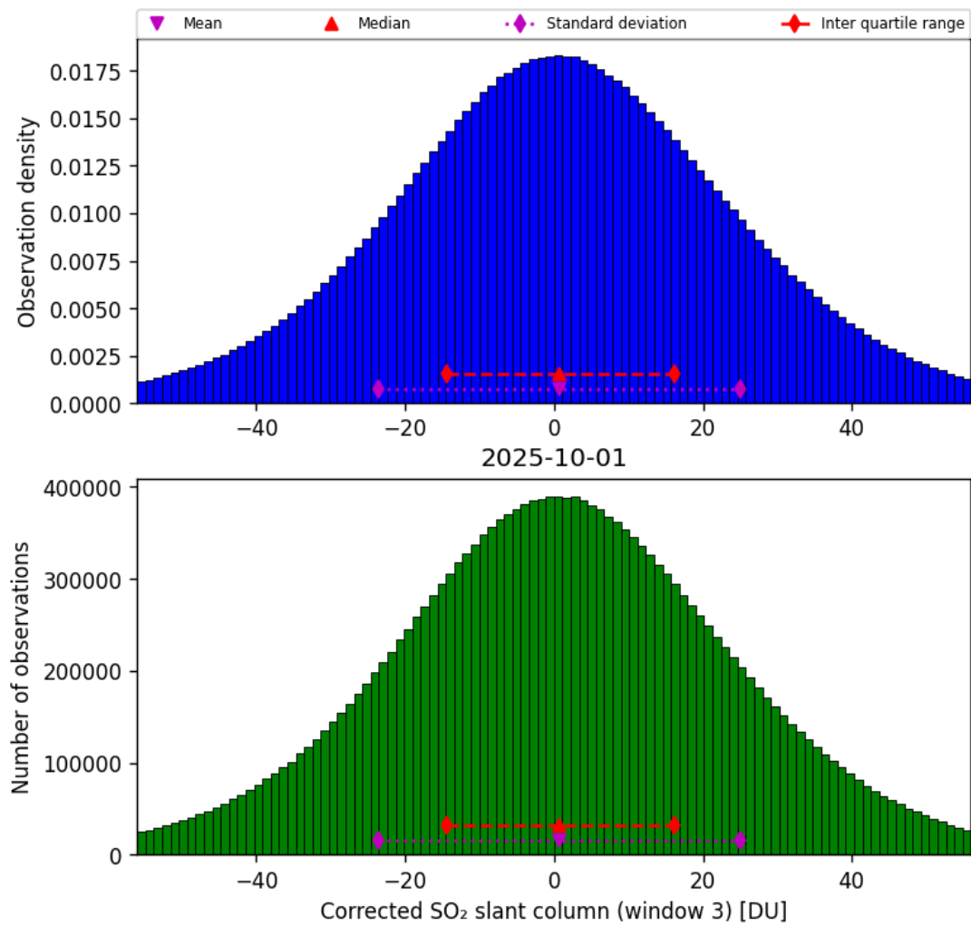
Figure 73: Histogram of “Corrected SO 2 slant column (window 3)” for 2025-10-01 to 2025-10-02
