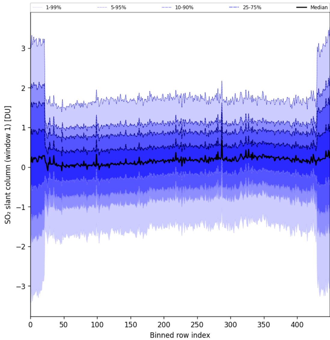
Figure 89: Along track statistics of “SO 2 slant column (window 1)” for 2025-10-01 to 2025-10-02
