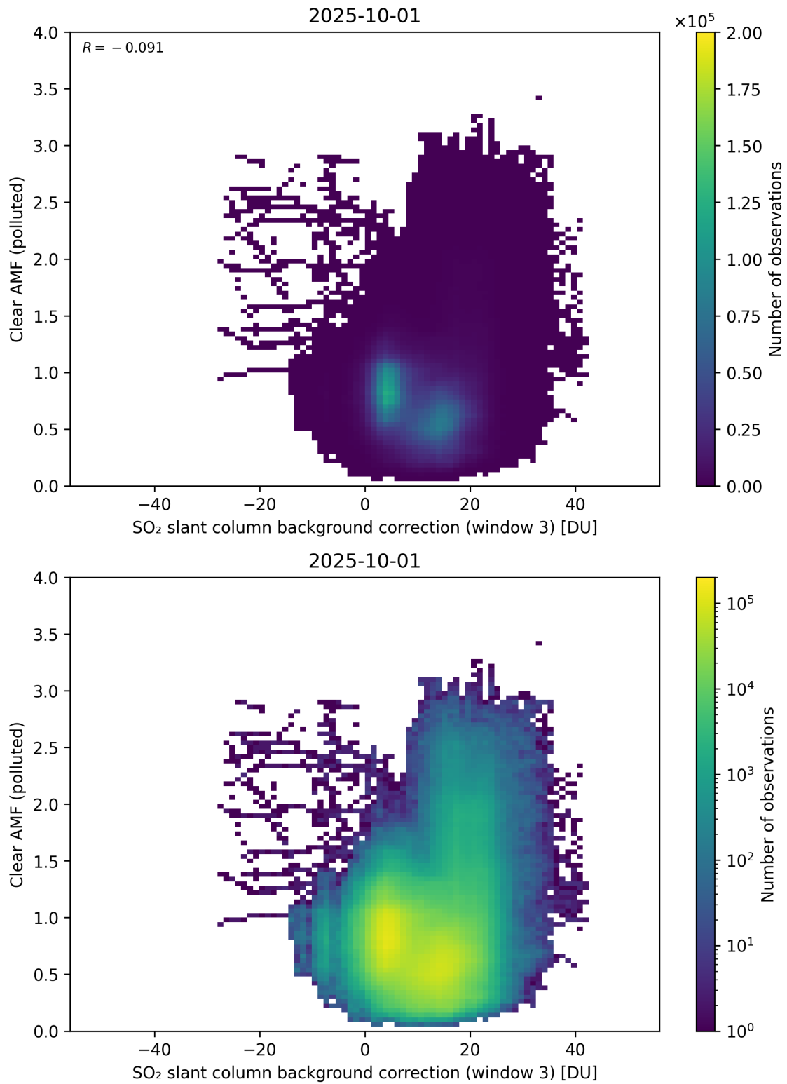
Figure 135: Scatter density plot of “SO 2 slant column background correction (window 3)” against “Clear AMF (polluted)” for 2025-10-01 to 2025-10-02.
