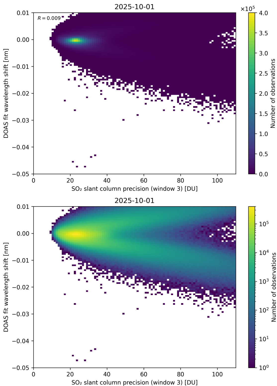
Figure 308: Scatter density plot of “SO 2 slant column precision (window 3)” against “DOAS fit wavelength shift” for 2025-10-01 to 2025-10-02.
