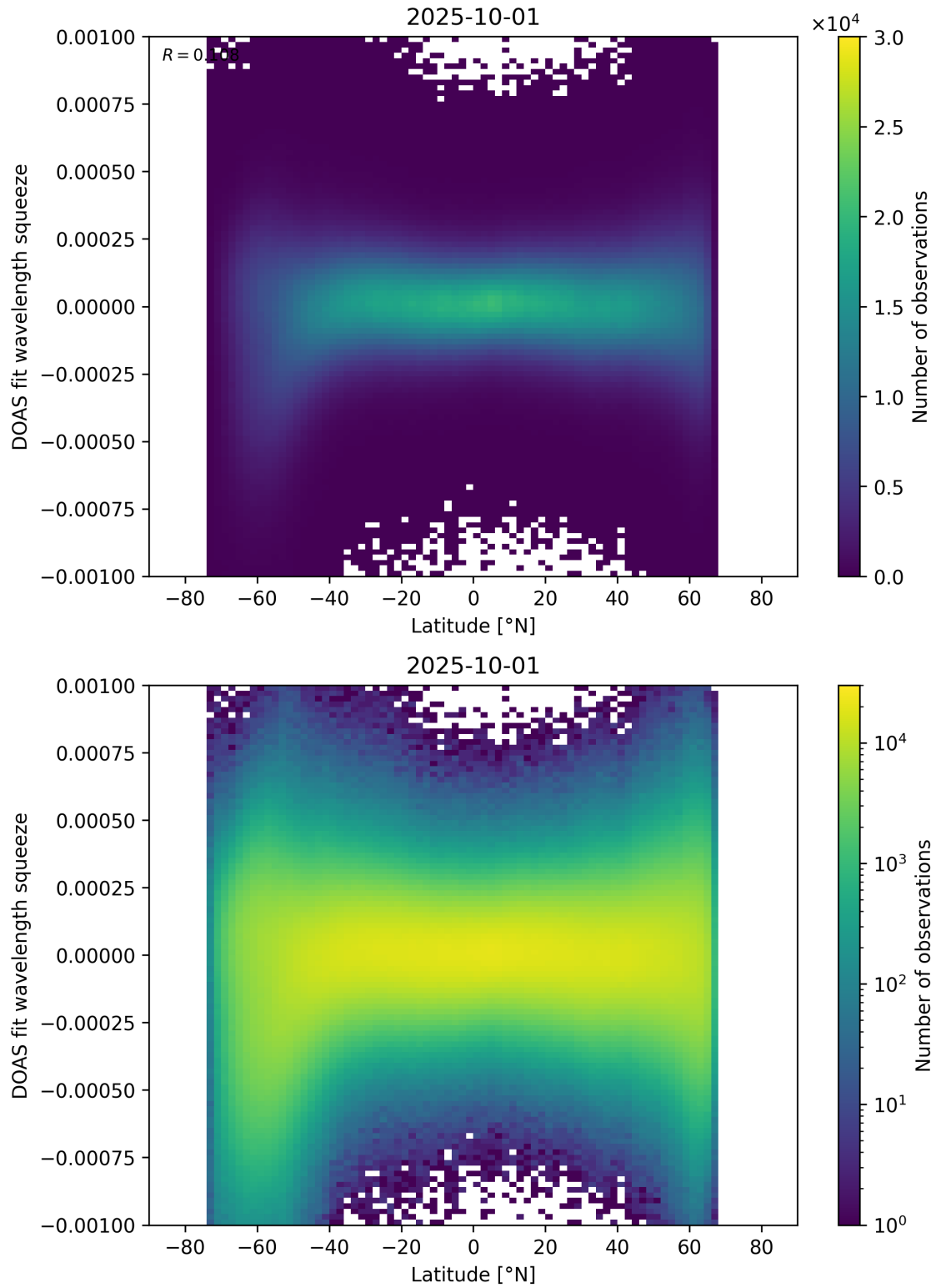
Figure 154: Scatter density plot of “Latitude” against “DOAS fit wavelength squeeze” for 2025-10-01 to 2025-10-02.
