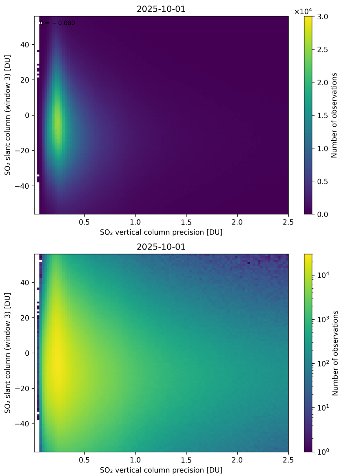
Figure 344: Scatter density plot of “SO 2 vertical column precision” against “SO 2 slant column (window 3)” for 2025-10-01 to 2025-10-02.
