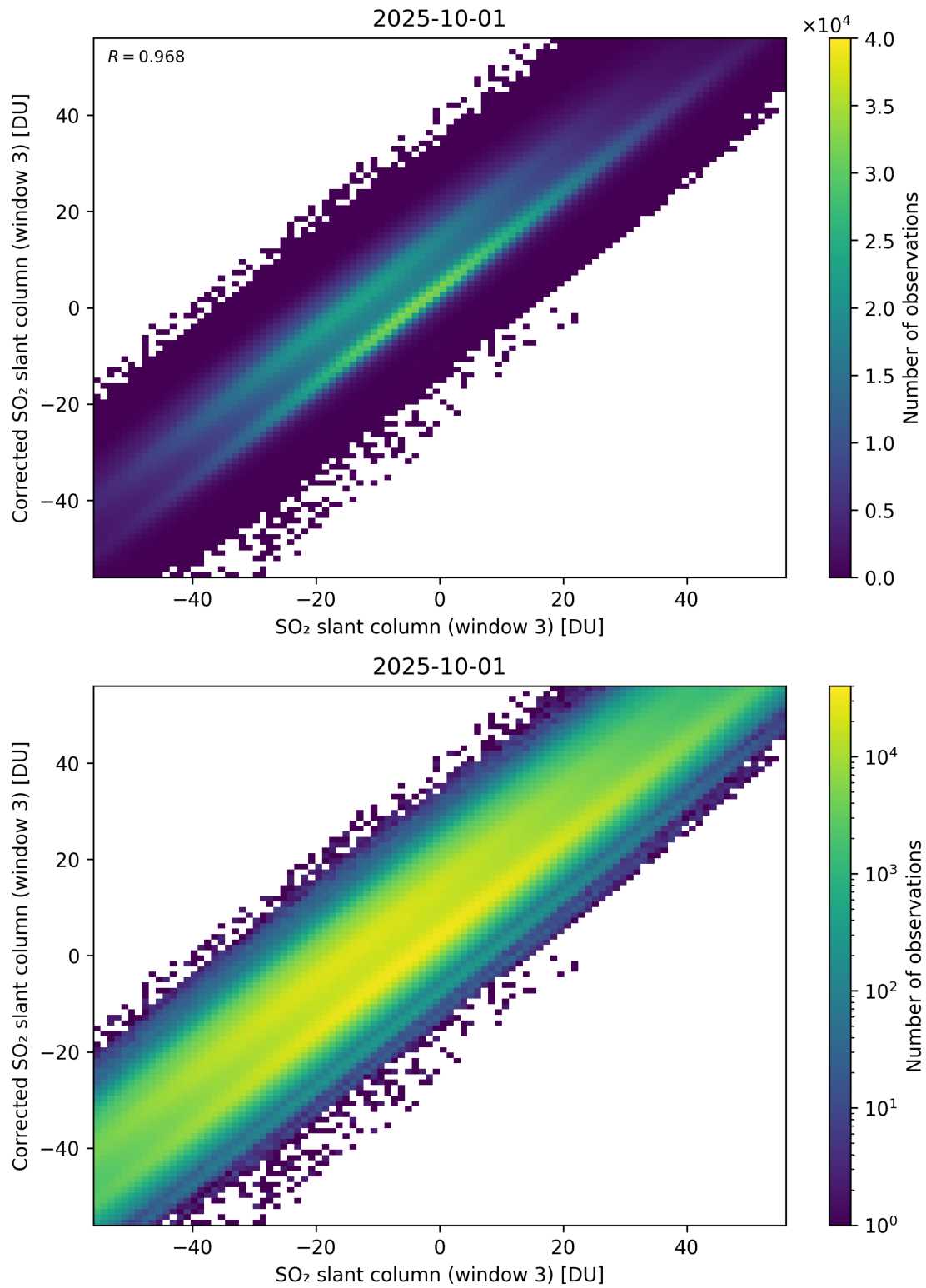
Figure 316: Scatter density plot of “SO 2 slant column (window 3)” against “Corrected SO 2 slant column (window 3)” for 2025-10-01 to 2025-10-02.
