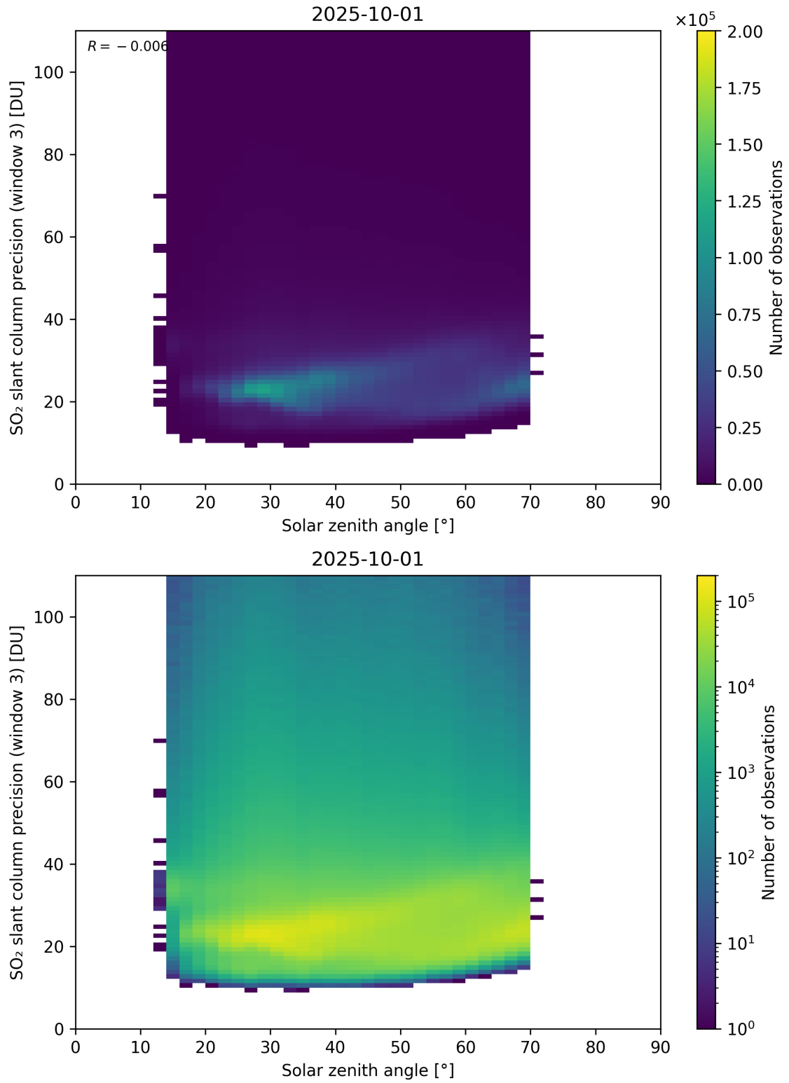
Figure 188: Scatter density plot of “Solar zenith angle” against “SO 2 slant column precision (window 3)” for 2025-10-01 to 2025-10-02.
