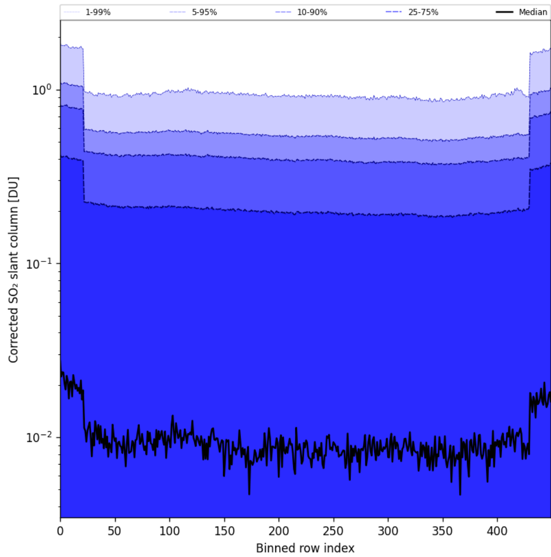
Figure 86: Along track statistics of “Corrected SO 2 slant column” for 2025-10-01 to 2025-10-02
