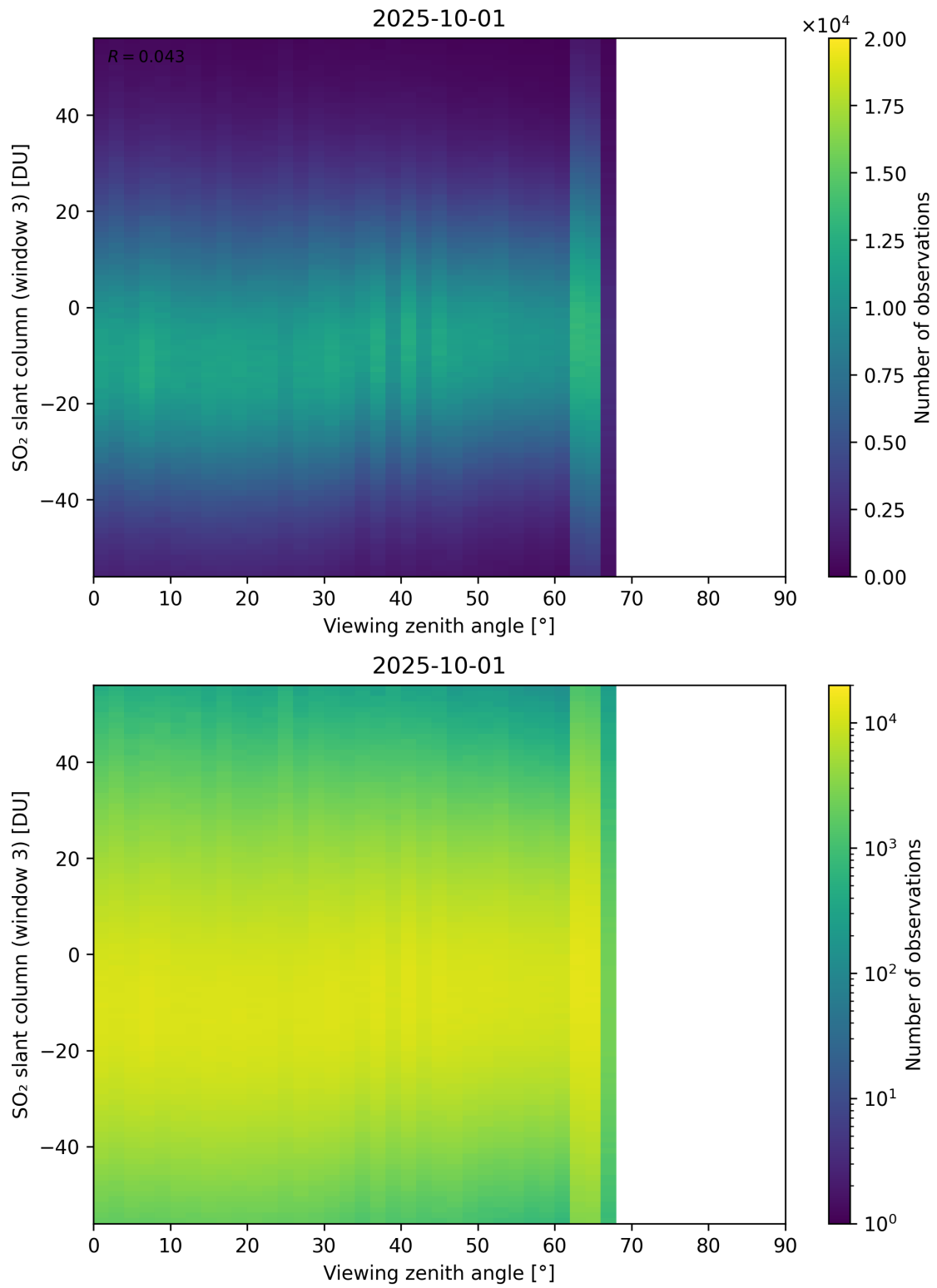
Figure 379: Scatter density plot of “Viewing zenith angle” against “SO 2 slant column (window 3)” for 2025-10-01 to 2025-10-02.
