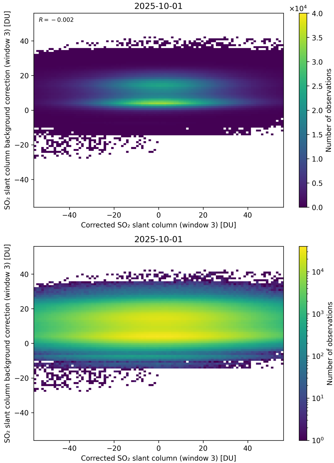
Figure 255: Scatter density plot of “Corrected SO 2 slant column (window 3)” against “SO 2 slant column background correction (window 3)” for 2025-10-01 to 2025-10-02.
