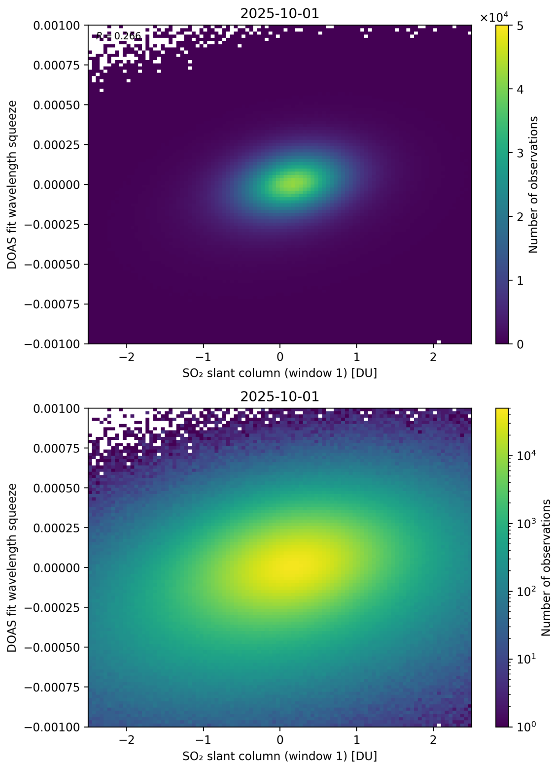
Figure 266: Scatter density plot of “SO 2 slant column (window 1)” against “DOAS fit wavelength squeeze” for 2025-10-01 to 2025-10-02.
