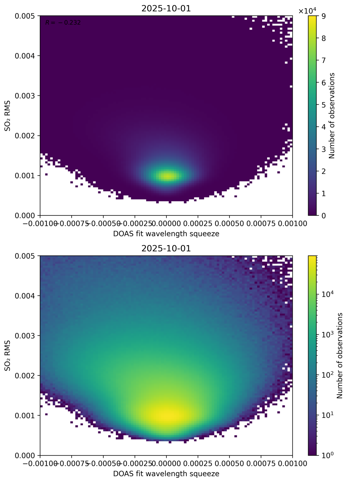
Figure 143: Scatter density plot of “DOAS fit wavelength squeeze” against “SO 2 RMS” for 2025-10-01 to 2025-10-02.
