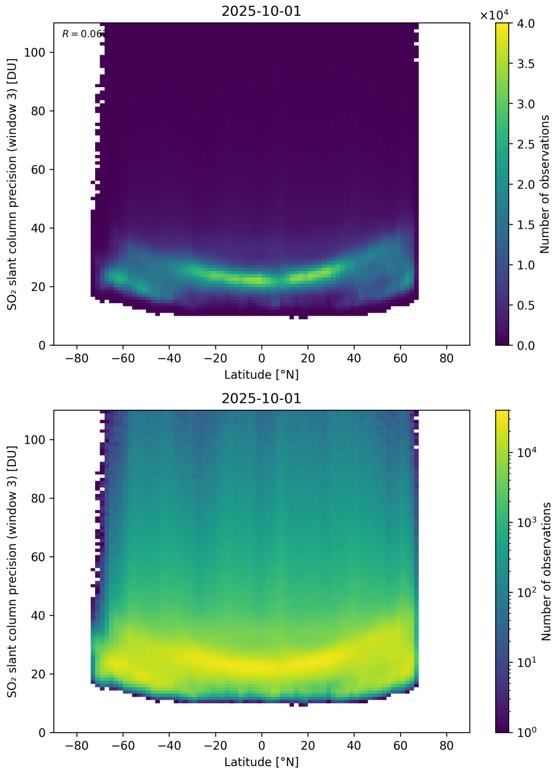
Figure 166: Scatter density plot of “Latitude” against “SO 2 slant column precision (window 3)” for 2025-10-01 to 2025-10-02.
