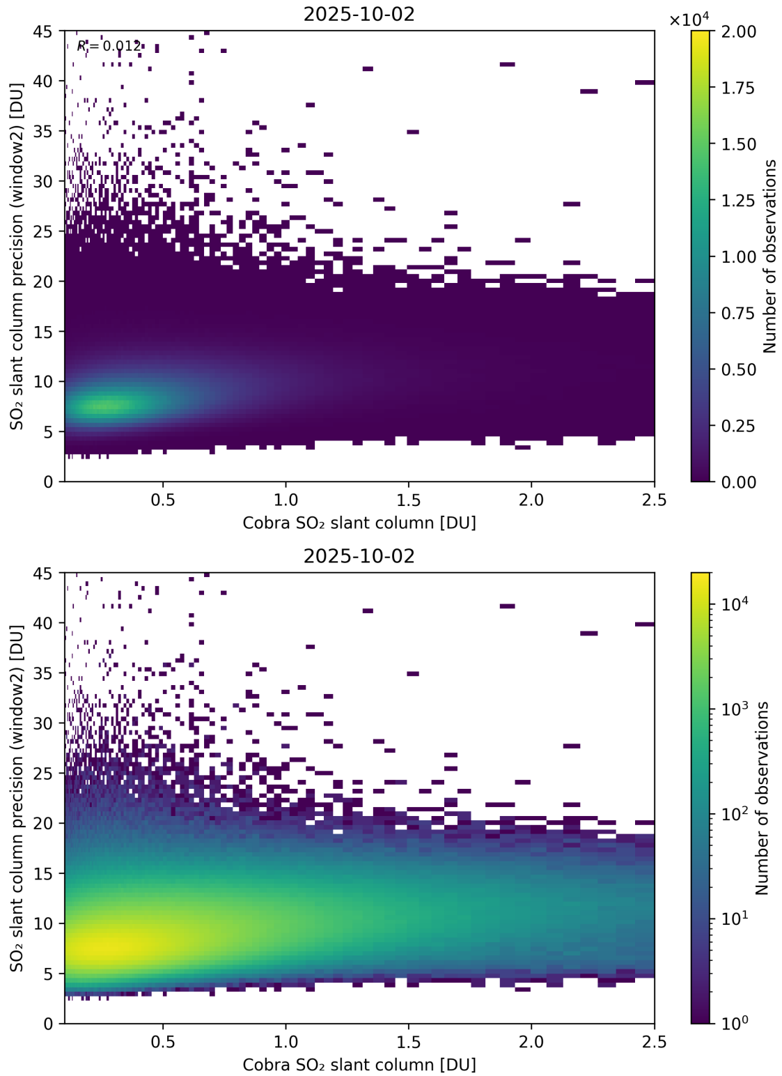
Figure 221: Scatter density plot of “Cobra SO 2 slant column” against “SO 2 slant column precision (window2)” for 2025-10-01 to 2025-10-03.
