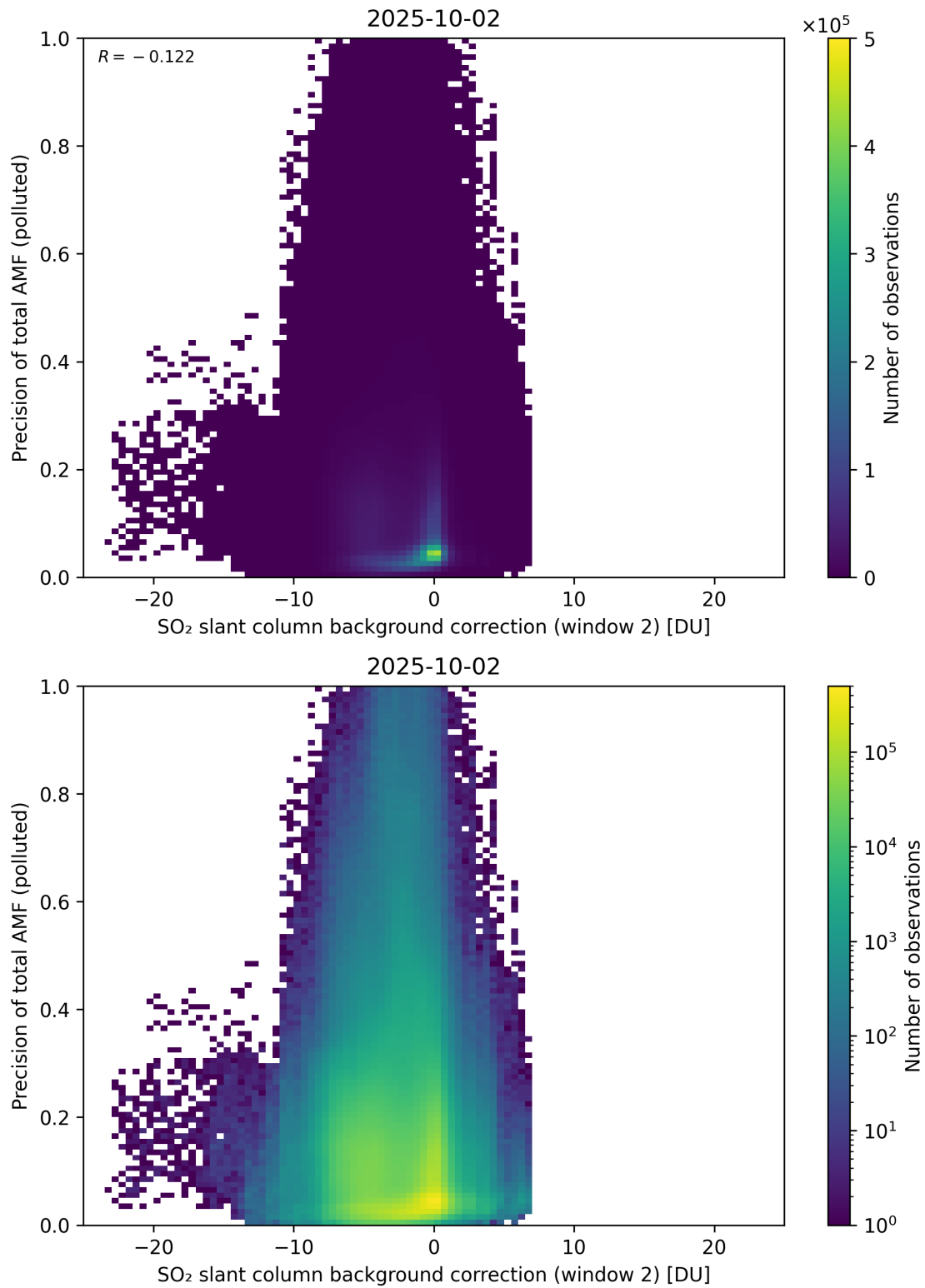
Figure 131: Scatter density plot of “SO 2 slant column background correction (window 2)” against “Precision of total AMF (polluted)” for 2025-10-01 to 2025-10-03.
