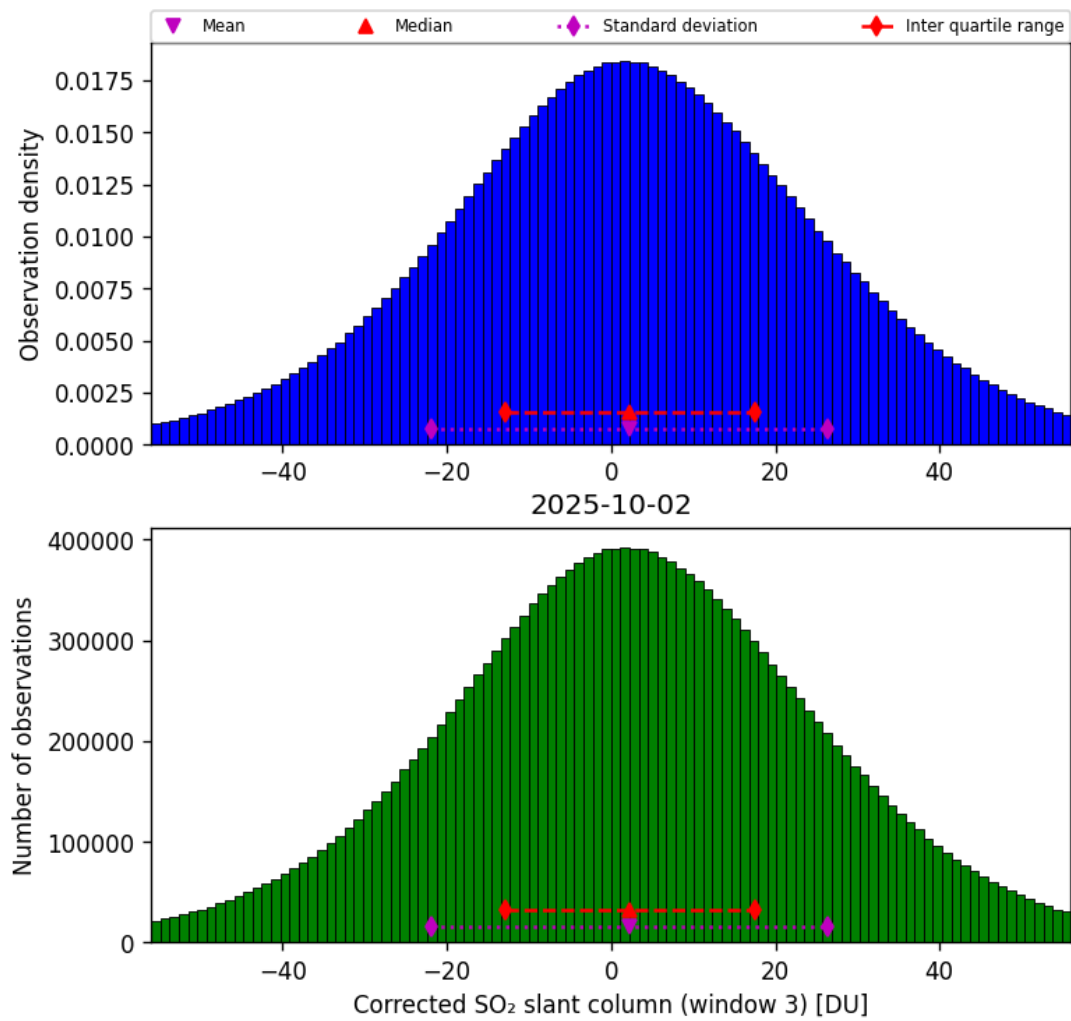
Figure 73: Histogram of “Corrected SO 2 slant column (window 3)” for 2025-10-01 to 2025-10-03
