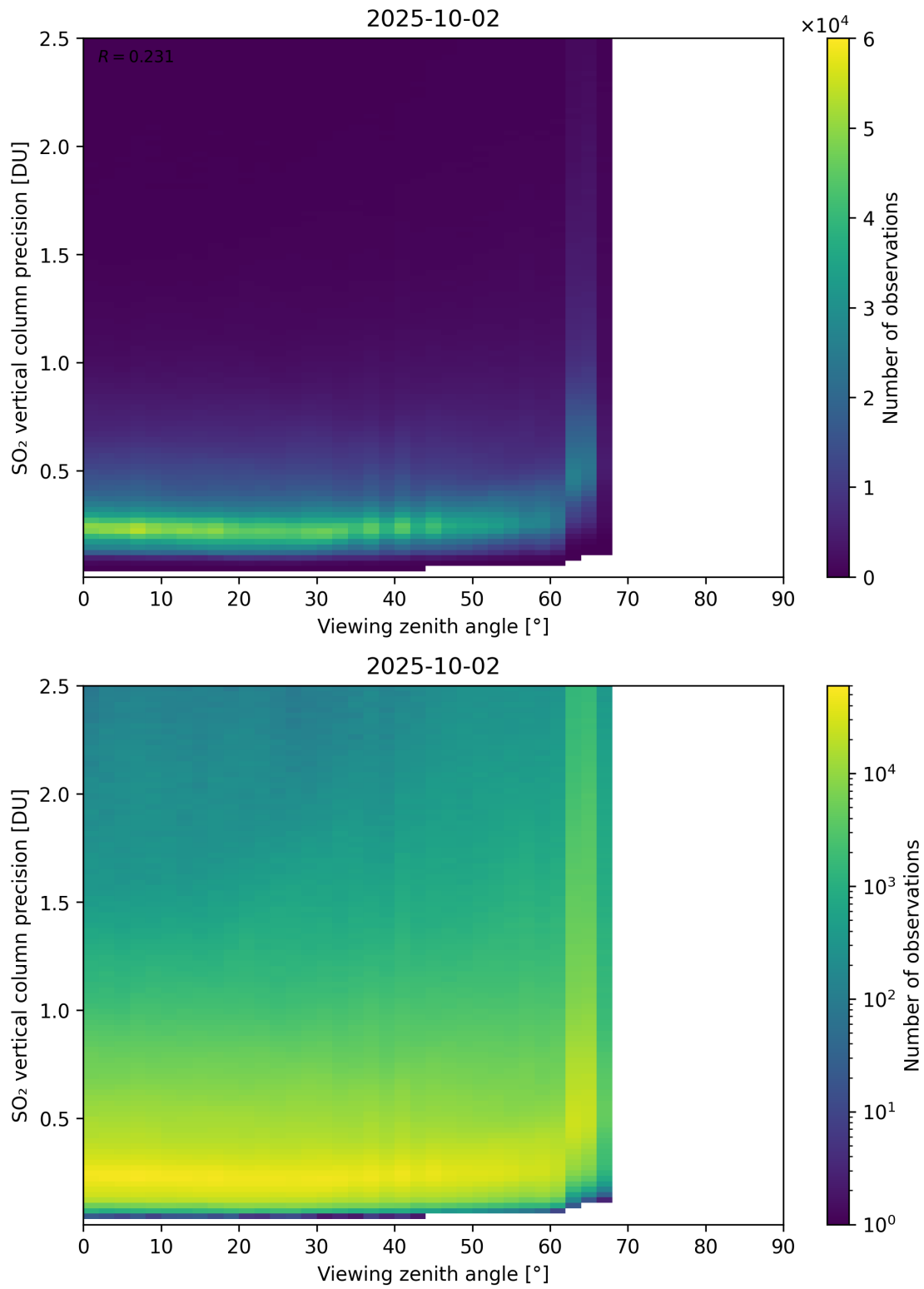
Figure 384: Scatter density plot of “Viewing zenith angle” against “SO 2 vertical column precision” for 2025-10-01 to 2025-10-03.
