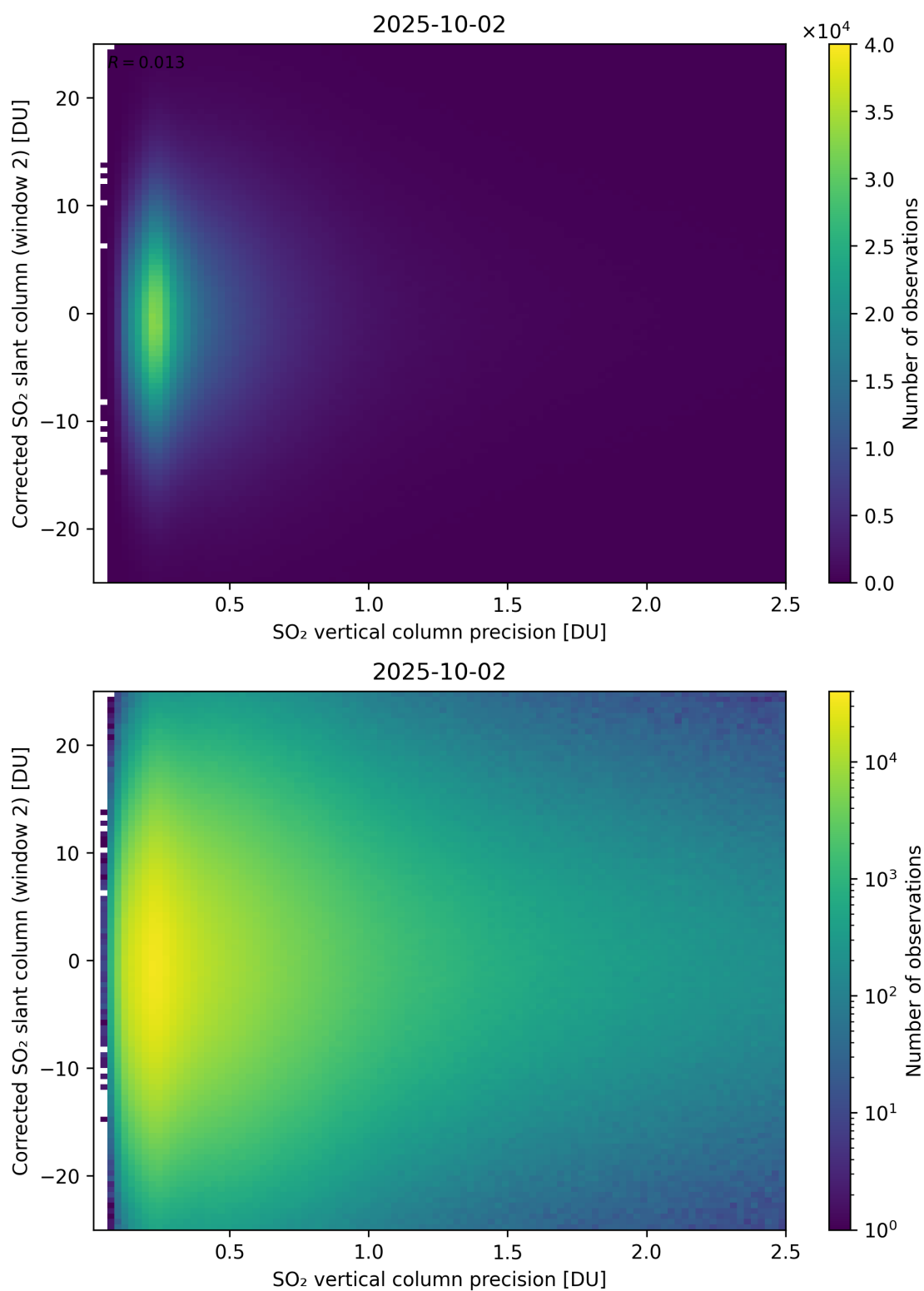
Figure 339: Scatter density plot of “SO 2 vertical column precision” against “Corrected SO 2 slant column (window 2)” for 2025-10-01 to 2025-10-03.
