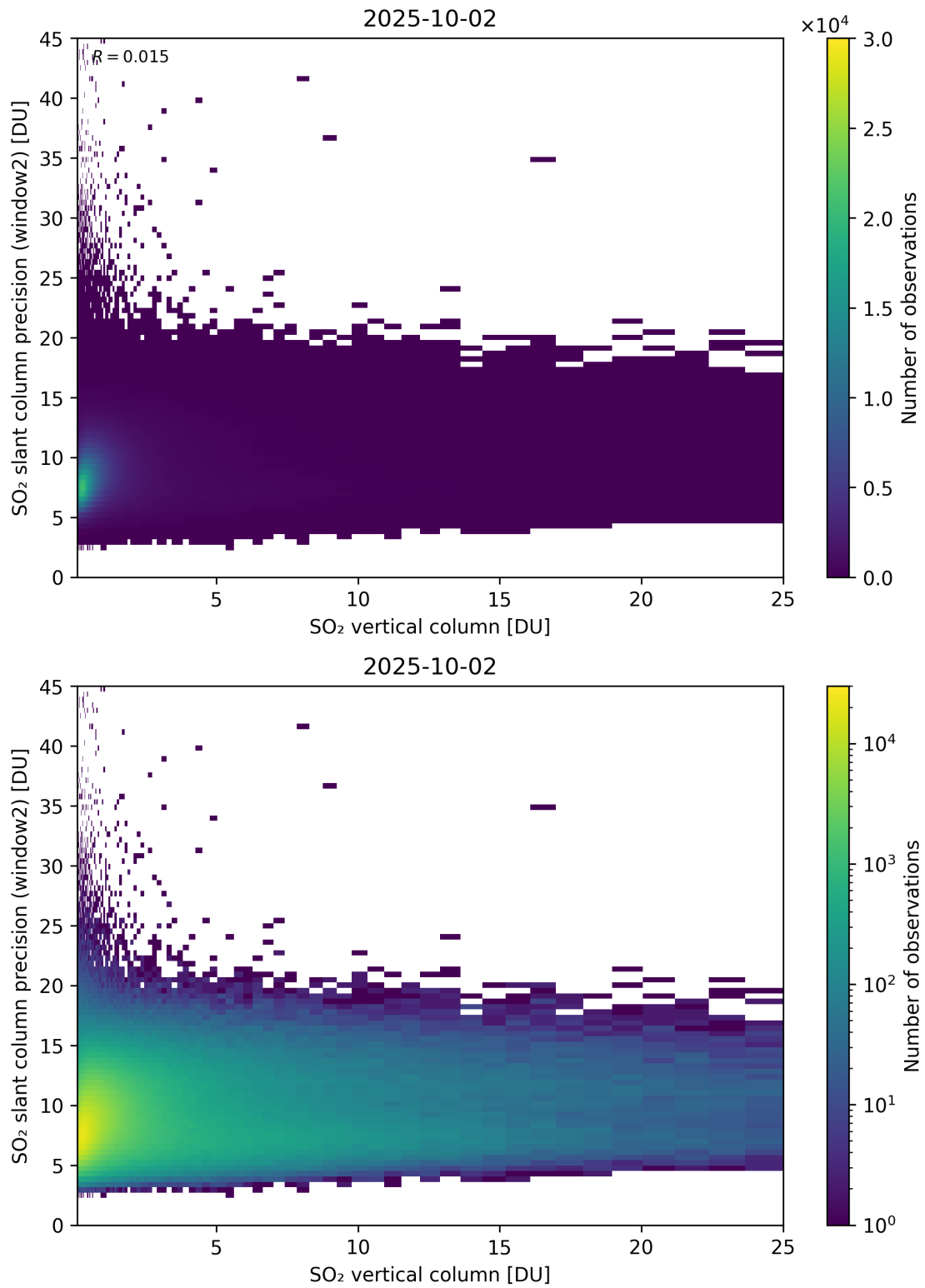
Figure 356: Scatter density plot of “SO 2 vertical column” against “SO 2 slant column precision (window2)” for 2025-10-01 to 2025-10-03.
