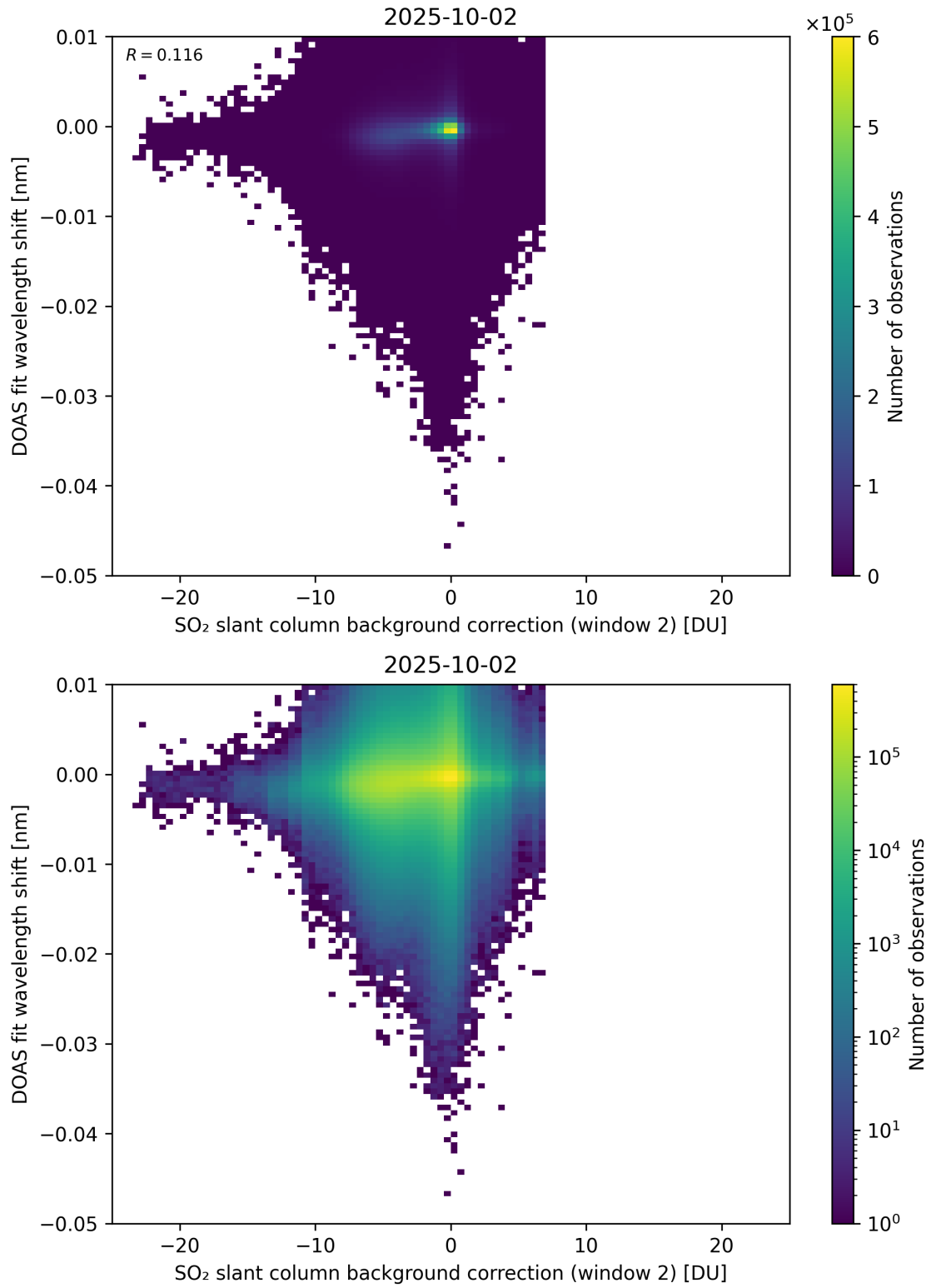
Figure 123: Scatter density plot of “SO 2 slant column background correction (window 2)” against “DOAS fit wavelength shift” for 2025-10-01 to 2025-10-03.
