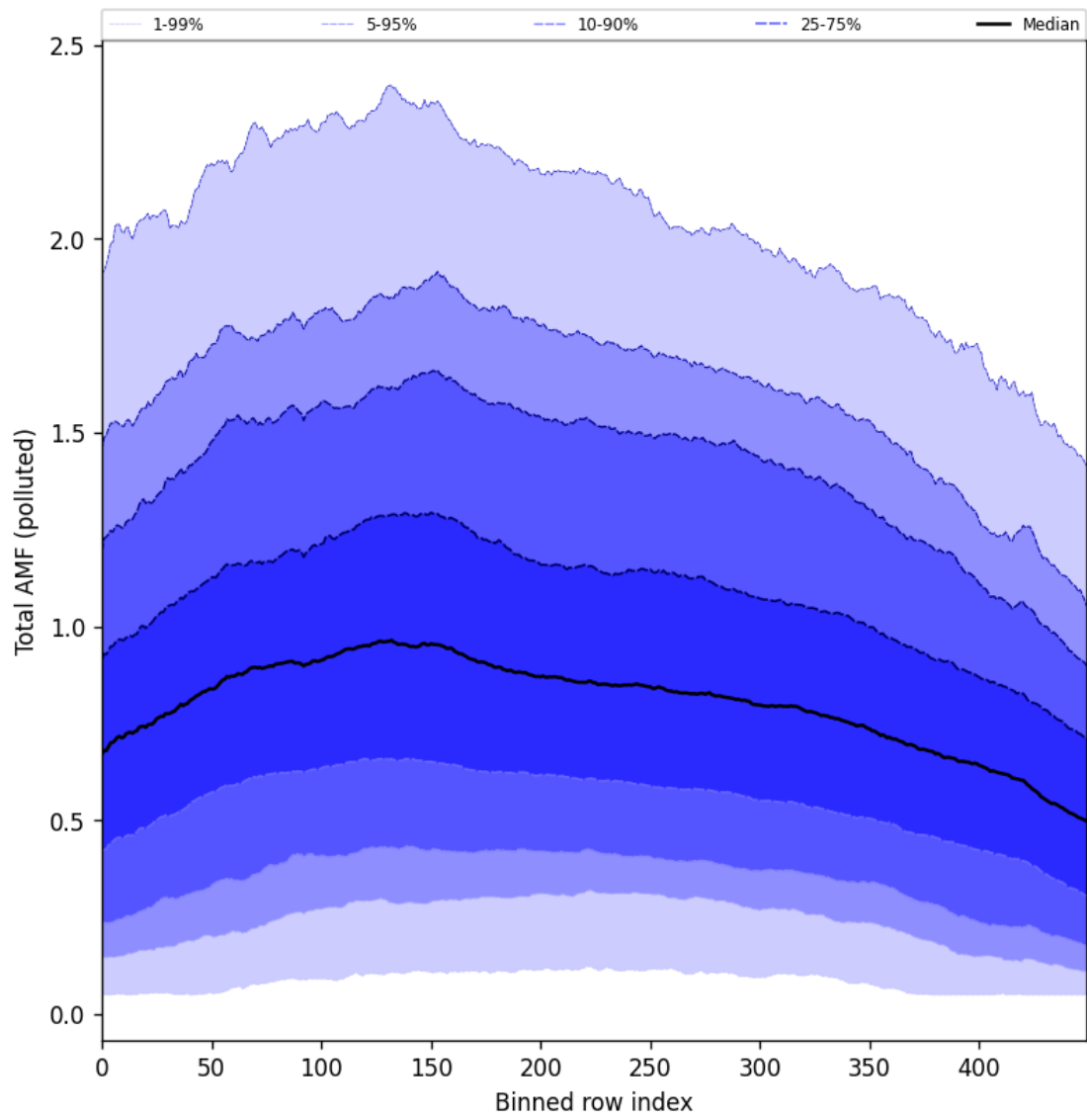
Figure 105: Along track statistics of “Total AMF (polluted)” for 2025-10-01 to 2025-10-03
