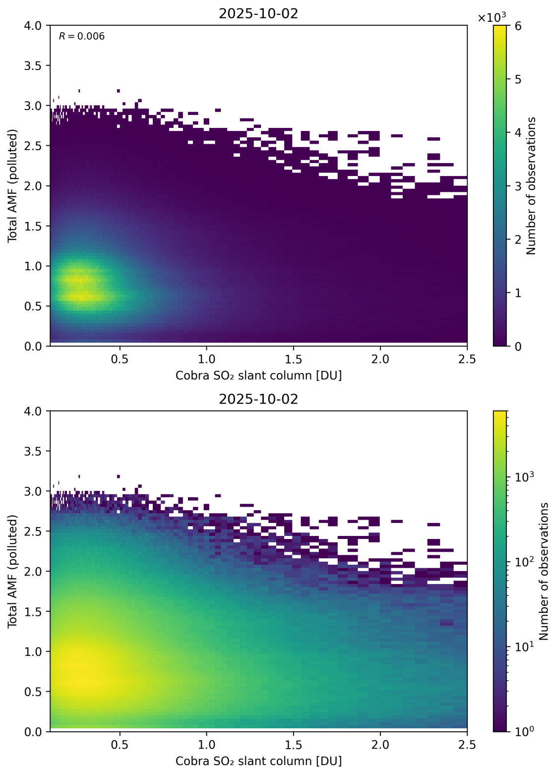
Figure 224: Scatter density plot of “Cobra SO 2 slant column” against “Total AMF (polluted)” for 2025-10-01 to 2025-10-03.
