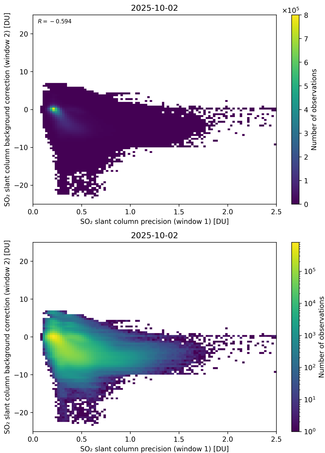
Figure 269: Scatter density plot of “SO 2 slant column precision (window 1)” against “SO 2 slant column background correction (window 2)” for 2025-10-01 to 2025-10-03.
