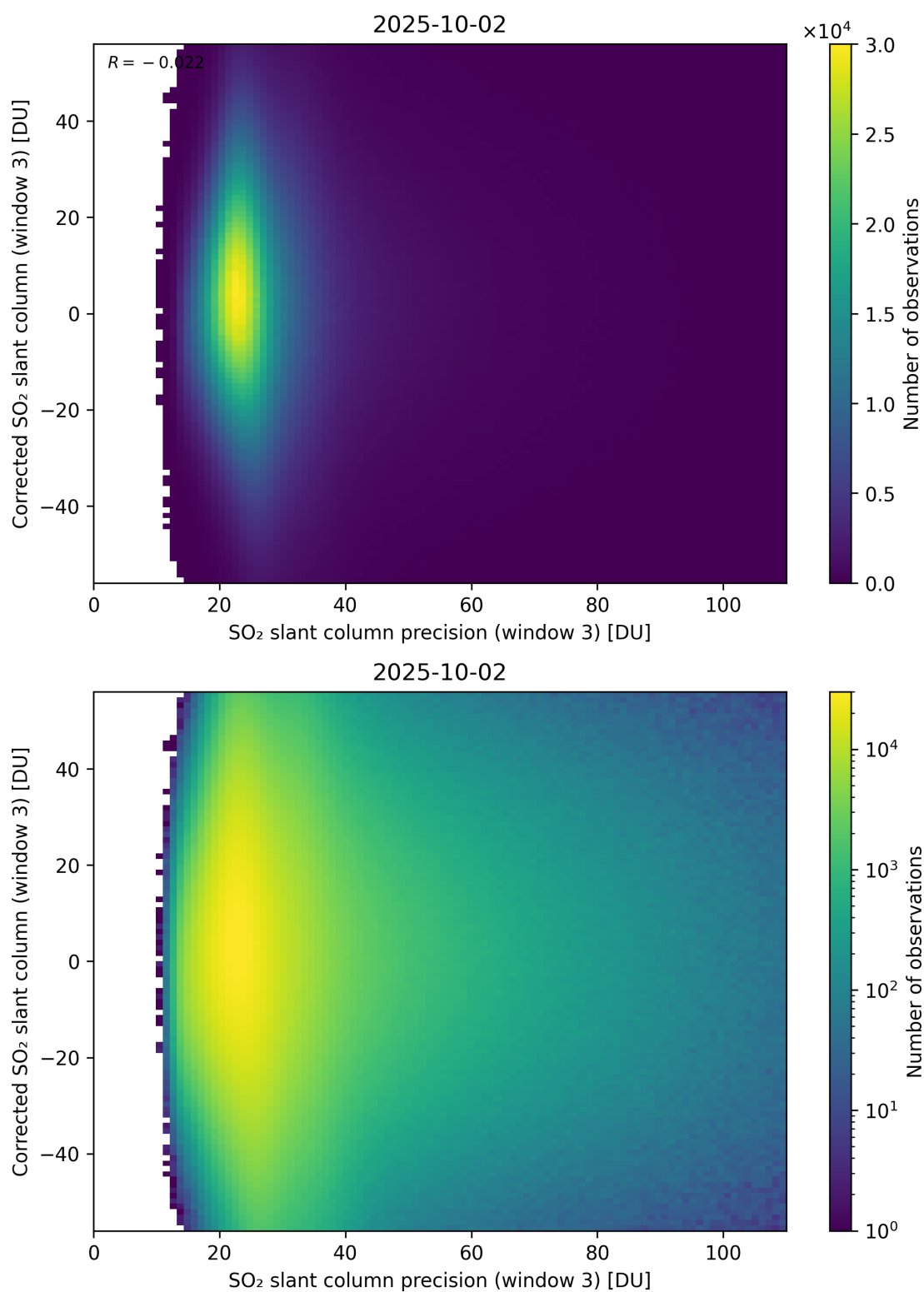
Figure 312: Scatter density plot of “SO 2 slant column precision (window 3)” against “Corrected SO 2 slant column (window 3)” for 2025-10-01 to 2025-10-03.
