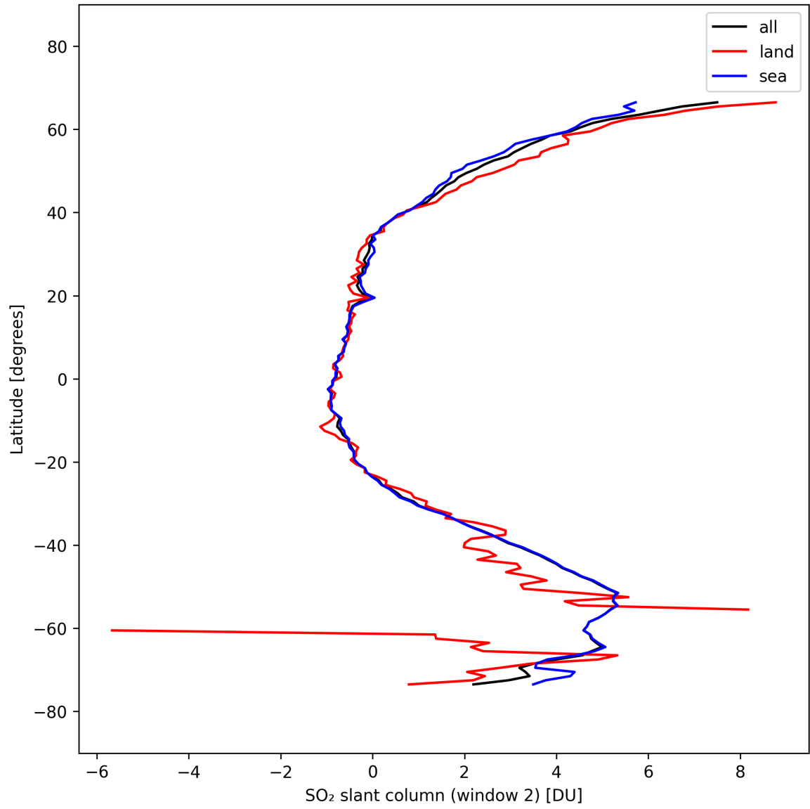
Figure 41: Zonal average of “SO 2 slant column (window 2)” for 2025-10-01 to 2025-10-03.
