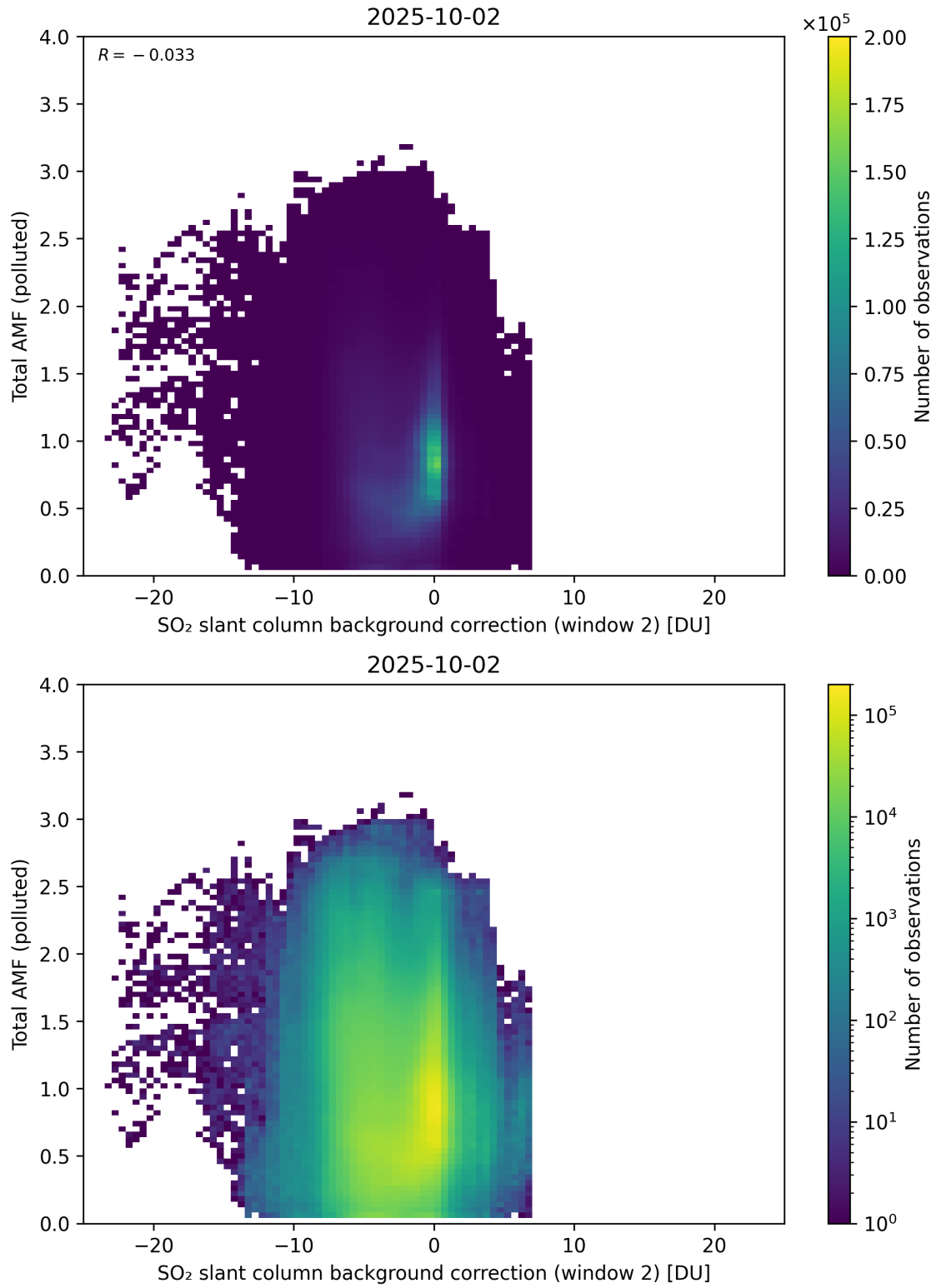
Figure 130: Scatter density plot of “SO 2 slant column background correction (window 2)” against “Total AMF (polluted)” for 2025-10-01 to 2025-10-03.
