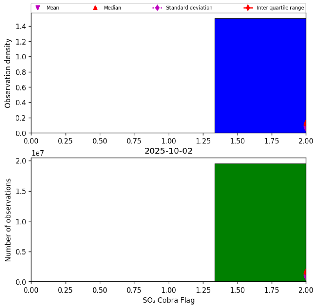
Figure 75: Histogram of “SO 2 Cobra Flag” for 2025-10-01 to 2025-10-03
