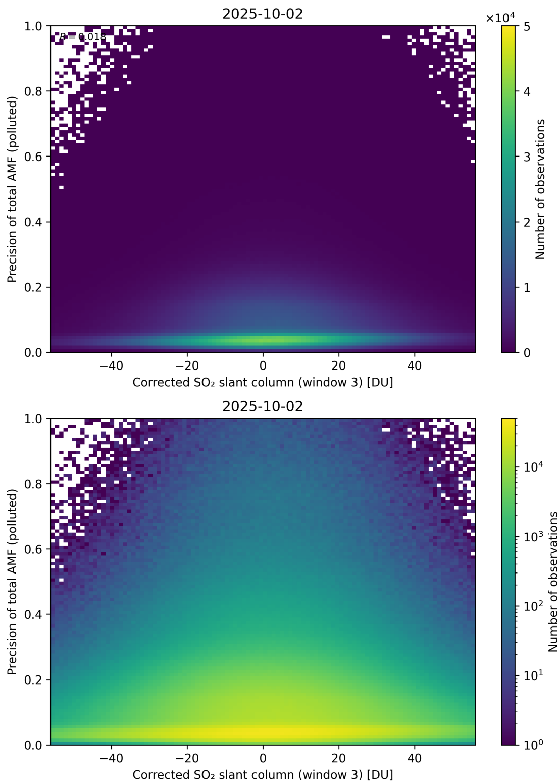
Figure 261: Scatter density plot of “Corrected SO 2 slant column (window 3)” against “Precision of total AMF (polluted)” for 2025-10-01 to 2025-10-03.
