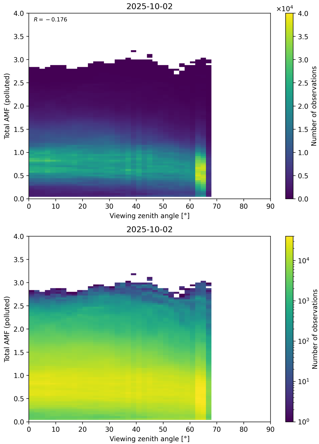
Figure 381: Scatter density plot of “Viewing zenith angle” against “Total AMF (polluted)” for 2025-10-01 to 2025-10-03.
