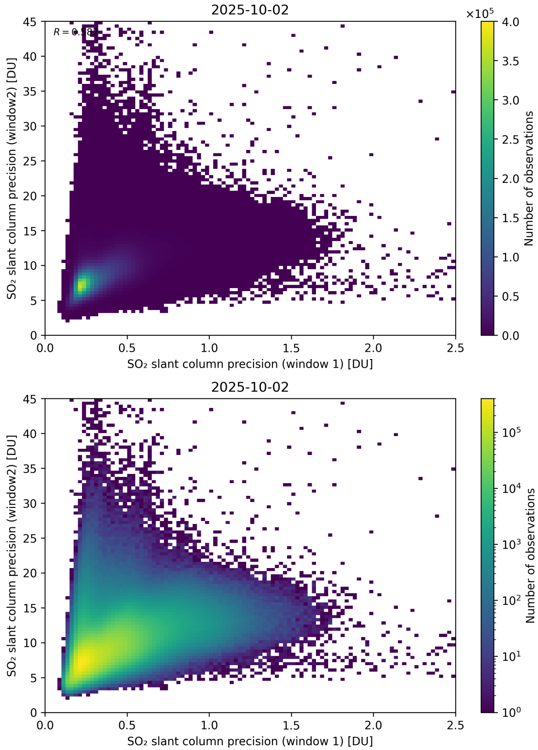
Figure 277: Scatter density plot of “SO 2 slant column precision (window 1)” against “SO 2 slant column precision (window2)” for 2025-10-01 to 2025-10-03.
