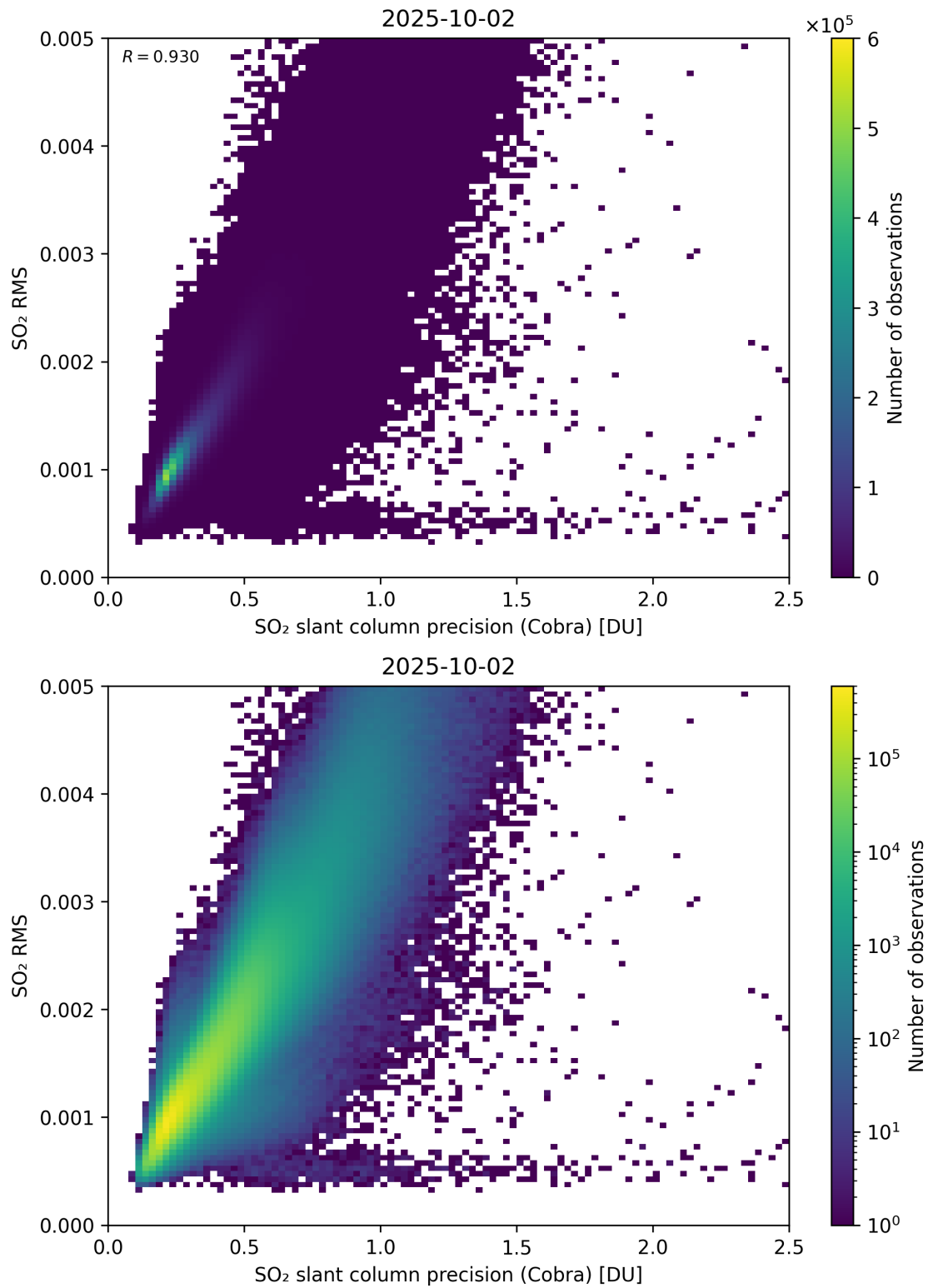
Figure 204: Scatter density plot of “SO 2 slant column precision (Cobra)” against “SO 2 RMS” for 2025-10-01 to 2025-10-03.
