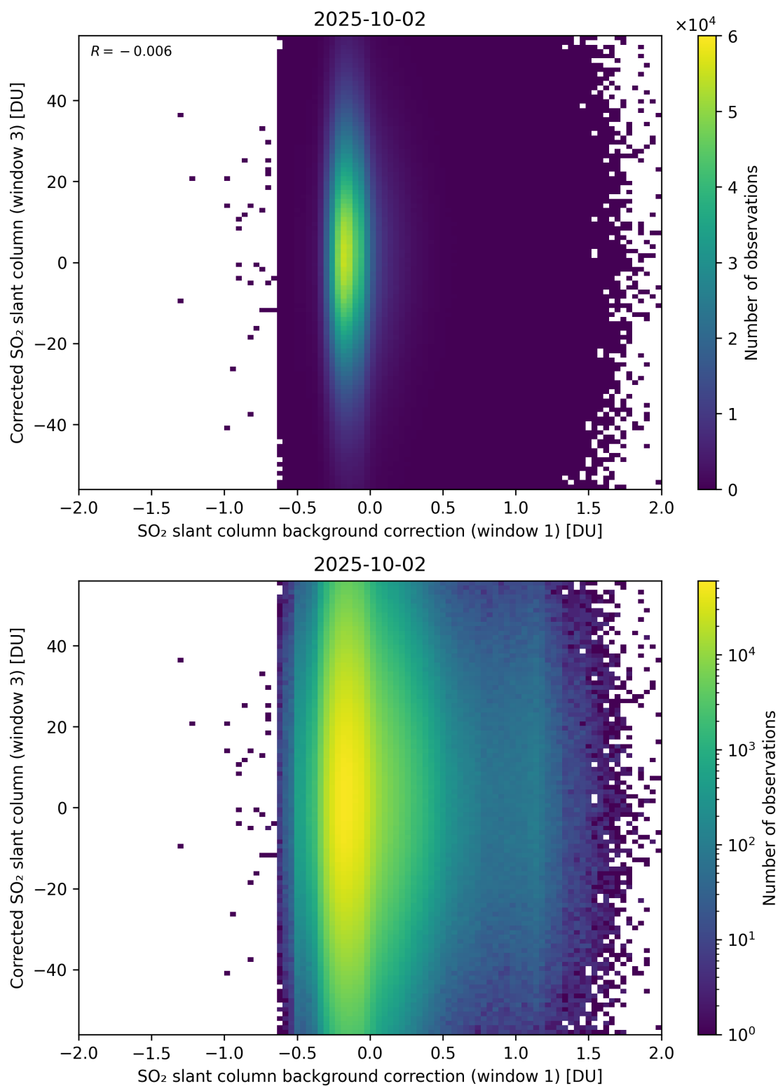
Figure 116: Scatter density plot of “SO 2 slant column background correction (window 1)” against “Corrected SO 2 slant column (window 3)” for 2025-10-01 to 2025-10-03.
