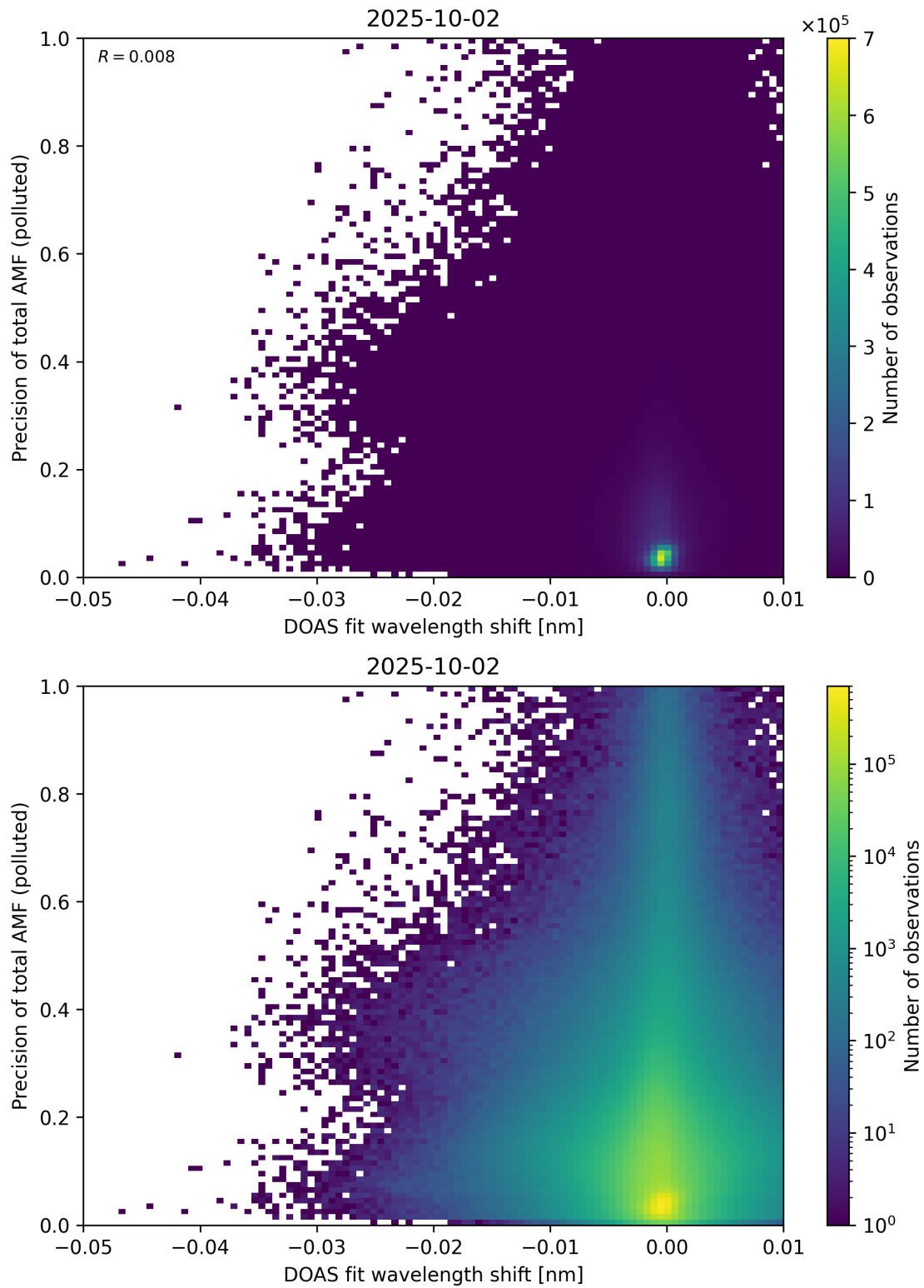
Figure 142: Scatter density plot of “DOAS fit wavelength shift” against “Precision of total AMF (polluted)” for 2025-10-01 to 2025-10-03.
