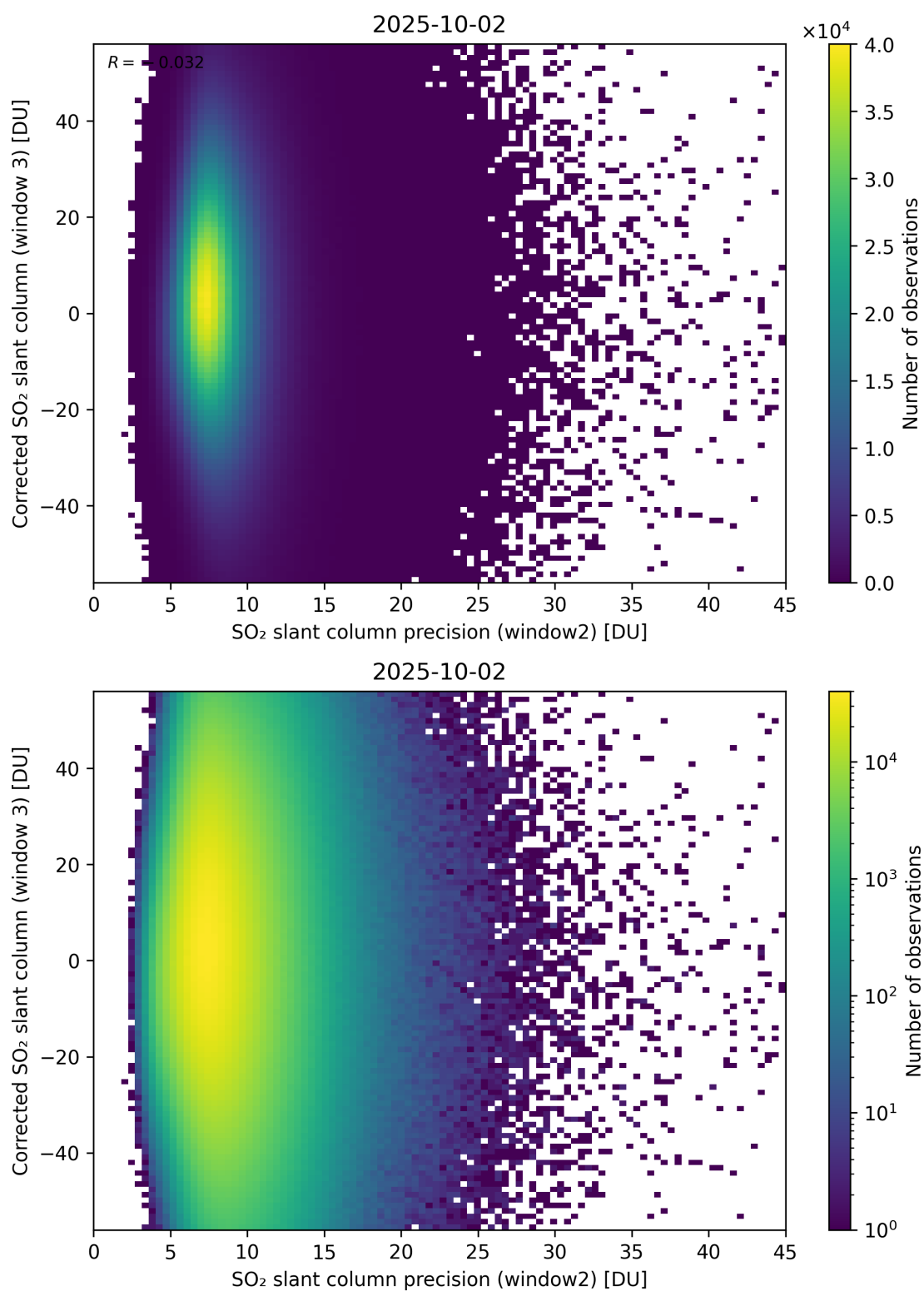
Figure 298: Scatter density plot of “SO 2 slant column precision (window2)” against “Corrected SO 2 slant column (window 3)” for 2025-10-01 to 2025-10-03.
