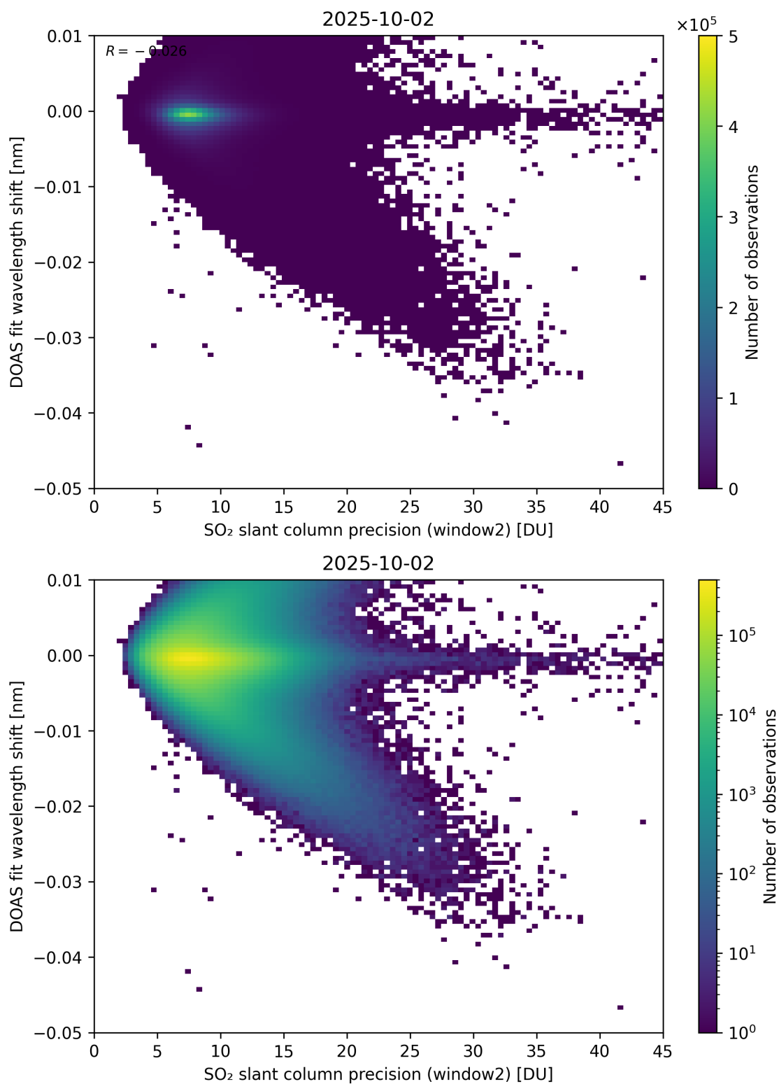
Figure 293: Scatter density plot of “SO 2 slant column precision (window2)” against “DOAS fit wavelength shift” for 2025-10-01 to 2025-10-03.
