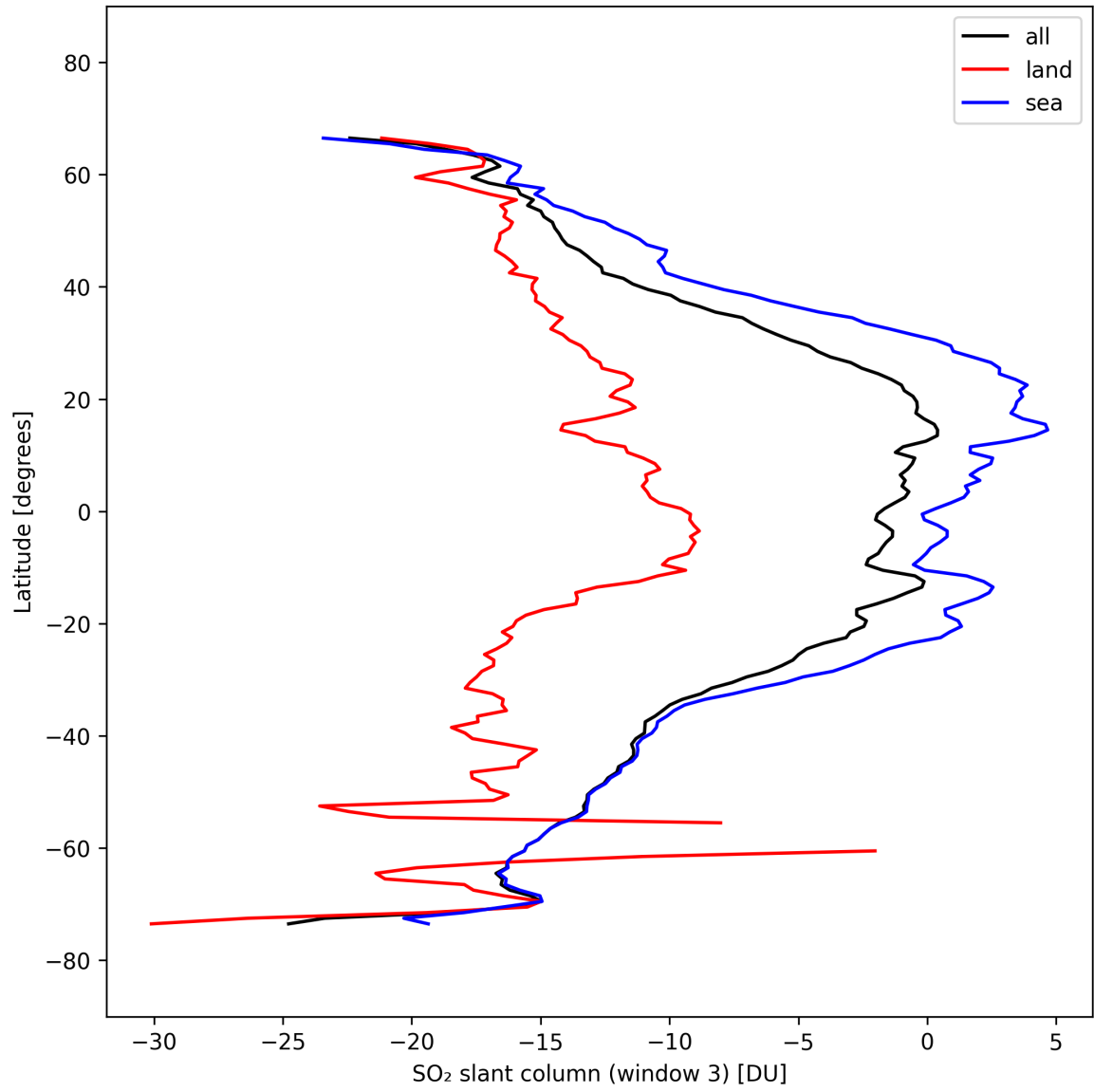
Figure 45: Zonal average of “SO 2 slant column (window 3)” for 2025-10-01 to 2025-10-03.
