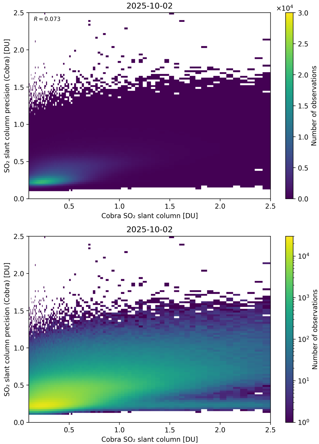
Figure 216: Scatter density plot of “Cobra SO 2 slant column” against “SO 2 slant column precision (Cobra)” for 2025-10-01 to 2025-10-03.
