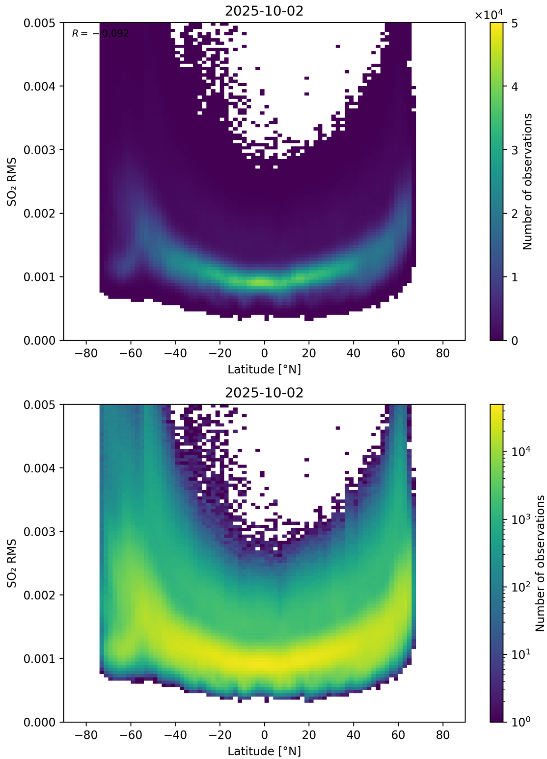
Figure 155: Scatter density plot of “Latitude” against “SO 2 RMS” for 2025-10-01 to 2025-10-03.
