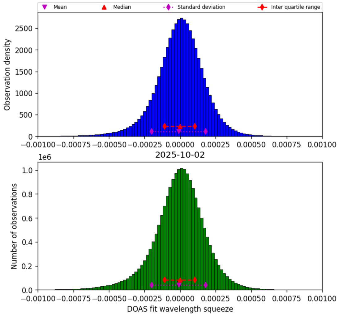
Figure 77: Histogram of “DOAS fit wavelength squeeze” for 2025-10-01 to 2025-10-03
