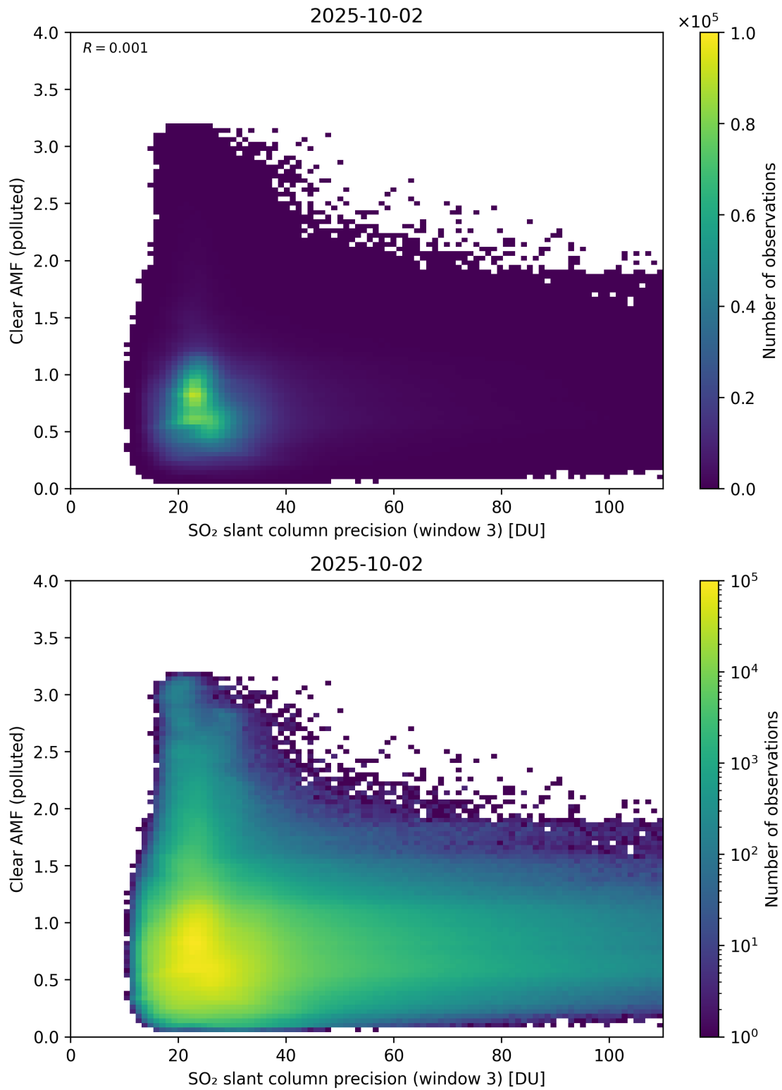
Figure 311: Scatter density plot of “SO 2 slant column precision (window 3)” against “Clear AMF (polluted)” for 2025-10-01 to 2025-10-03.
