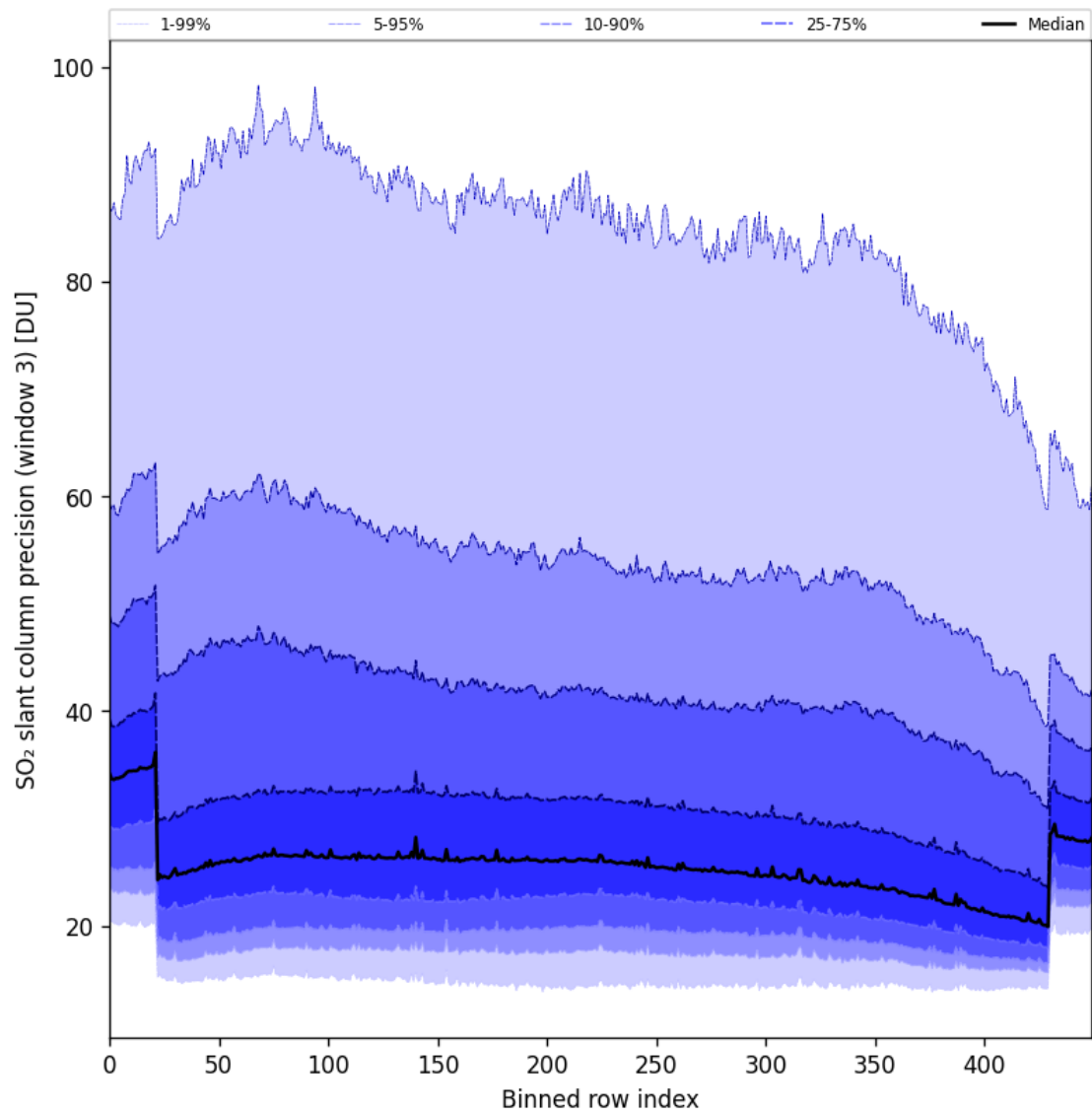
Figure 98: Along track statistics of “SO 2 slant column precision (window 3)” for 2025-10-01 to 2025-10-03
