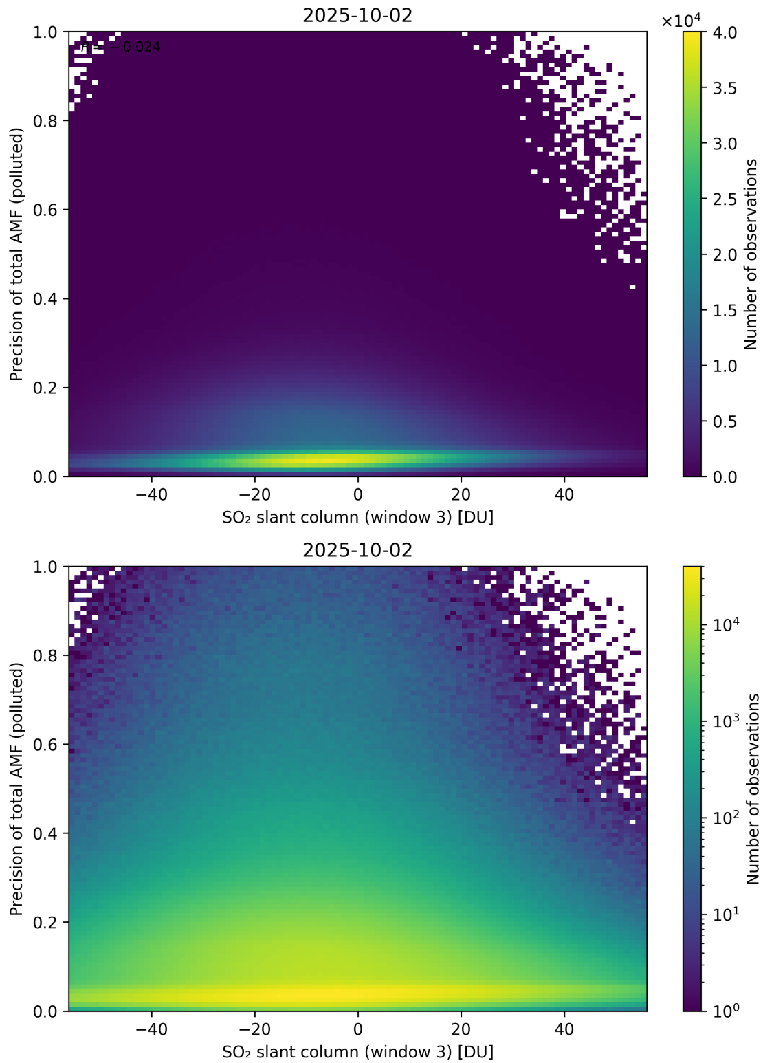
Figure 319: Scatter density plot of “SO 2 slant column (window 3)” against “Precision of total AMF (polluted)” for 2025-10-01 to 2025-10-03.
