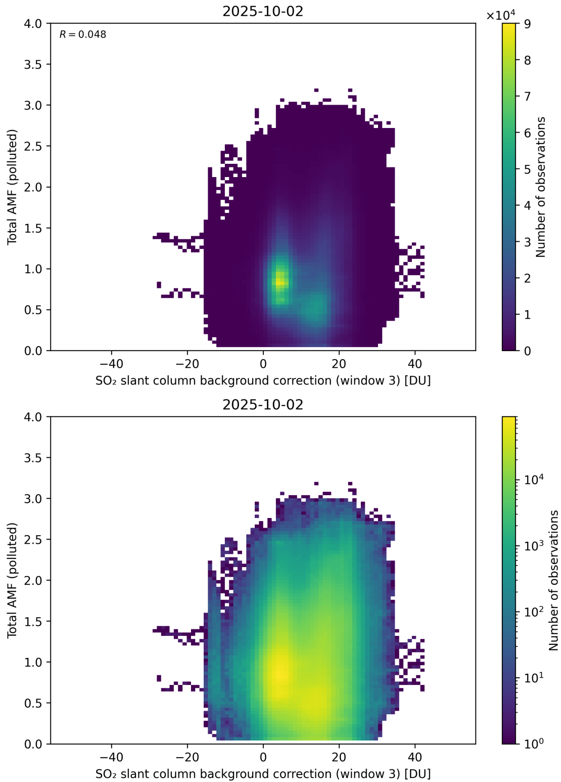
Figure 136: Scatter density plot of “SO 2 slant column background correction (window 3)” against “Total AMF (polluted)” for 2025-10-01 to 2025-10-03.
