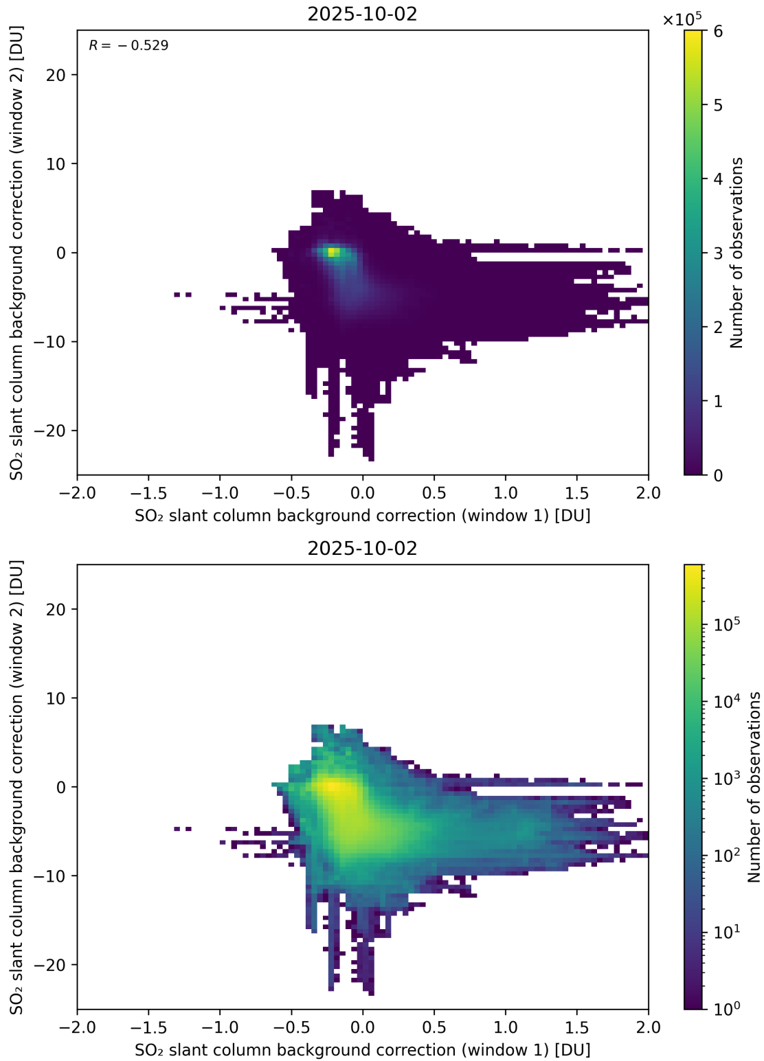
Figure 109: Scatter density plot of “SO 2 slant column background correction (window 1)” against “SO 2 slant column background correction (window 2)” for 2025-10-01 to 2025-10-03.
