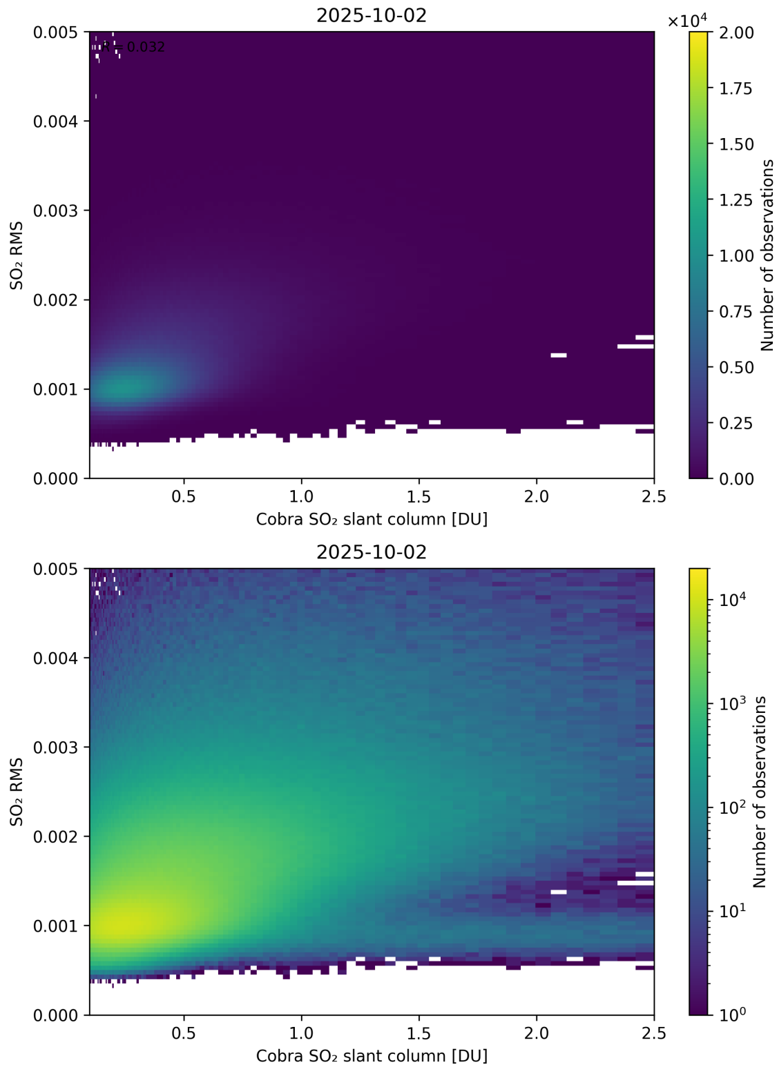
Figure 198: Scatter density plot of “Cobra SO 2 slant column” against “SO 2 RMS” for 2025-10-01 to 2025-10-03.
