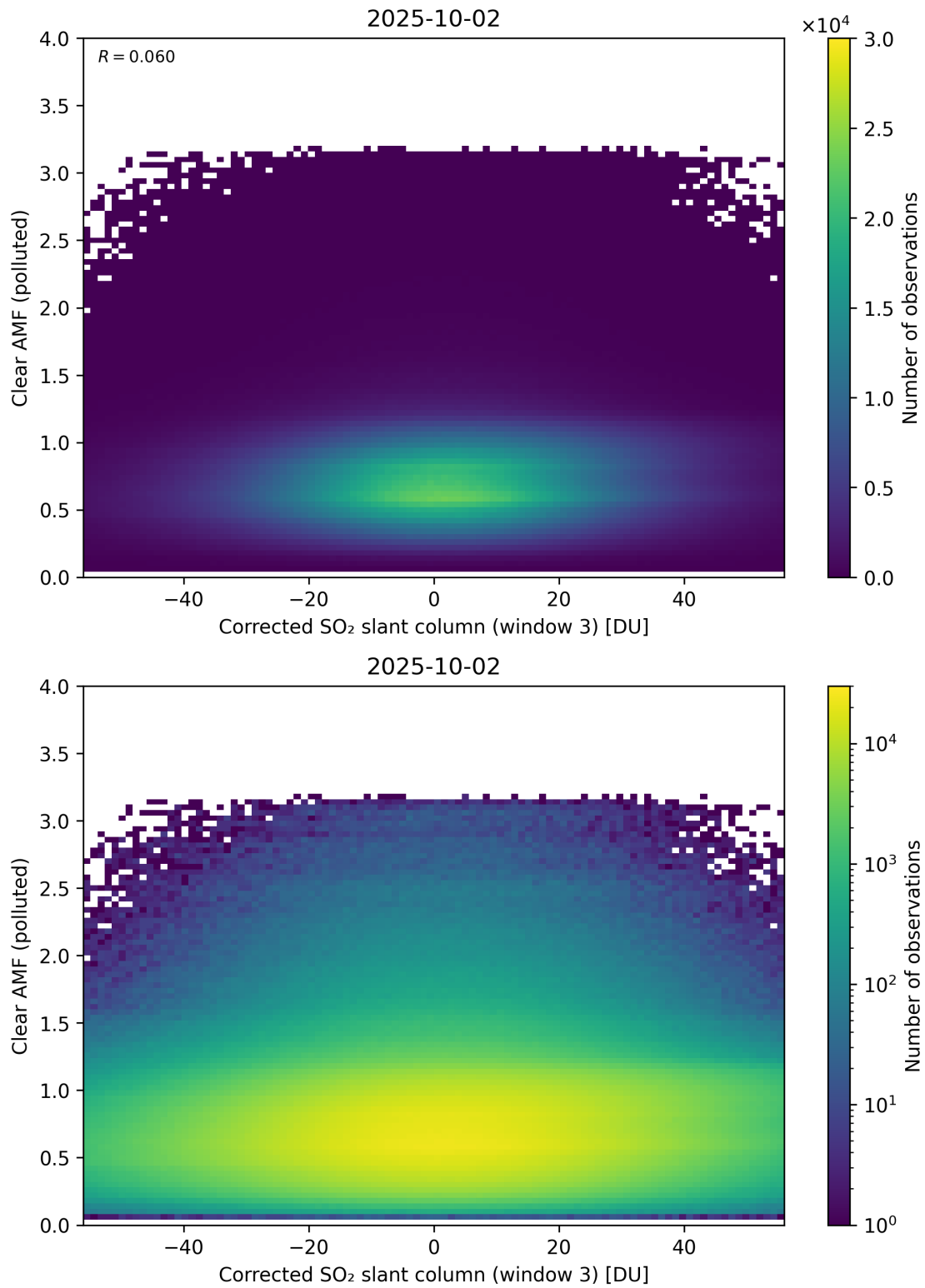
Figure 259: Scatter density plot of “Corrected SO 2 slant column (window 3)” against “Clear AMF (polluted)” for 2025-10-01 to 2025-10-03.
