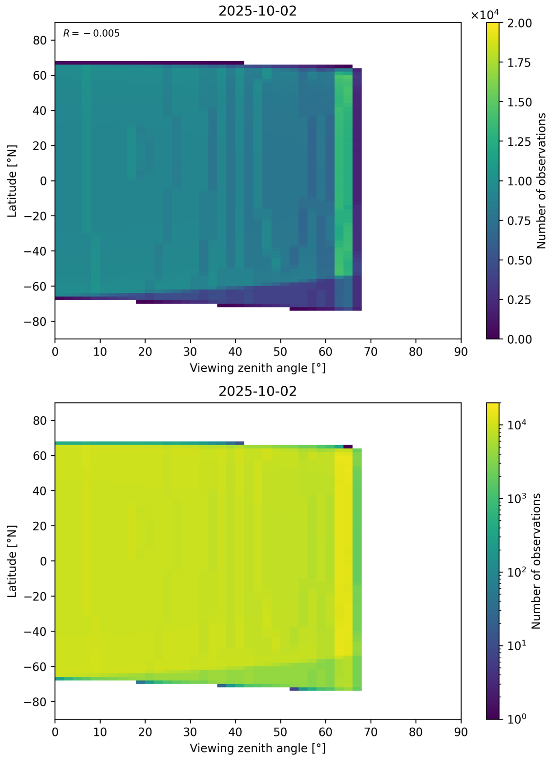
Figure 368: Scatter density plot of “Viewing zenith angle” against “Latitude” for 2025-10-01 to 2025-10-03.
