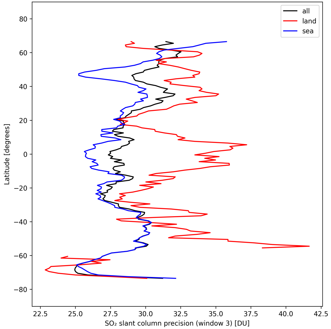
Figure 46: Zonal average of “SO 2 slant column precision (window 3)” for 2025-10-01 to 2025-10-03.
