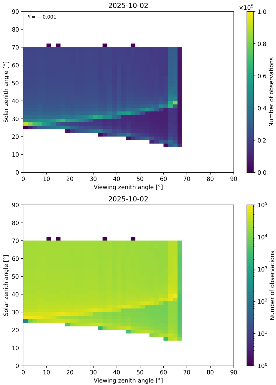
Figure 369: Scatter density plot of “Viewing zenith angle” against “Solar zenith angle” for 2025-10-01 to 2025-10-03.
