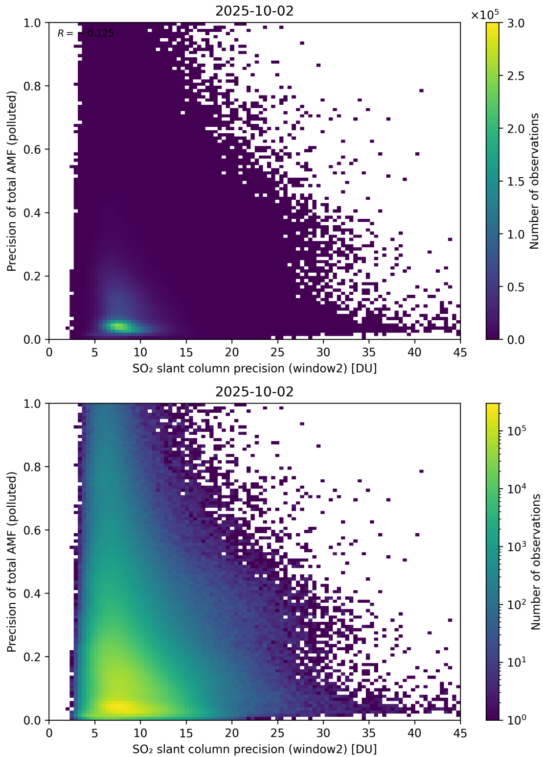
Figure 302: Scatter density plot of “SO 2 slant column precision (window2)” against “Precision of total AMF (polluted)” for 2025-10-01 to 2025-10-03.
