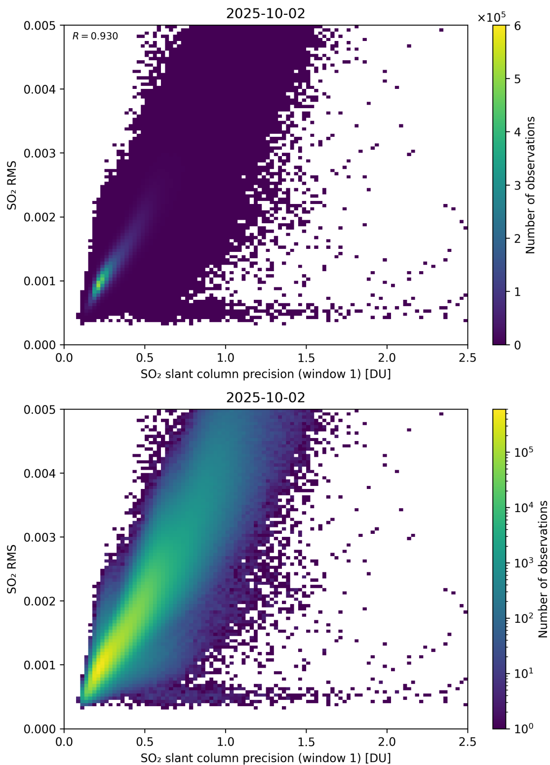
Figure 273: Scatter density plot of “SO 2 slant column precision (window 1)” against “SO 2 RMS” for 2025-10-01 to 2025-10-03.
