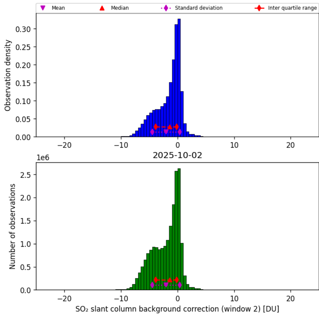
Figure 70: Histogram of “SO 2 slant column background correction (window 2)” for 2025-10-01 to 2025-10-03
