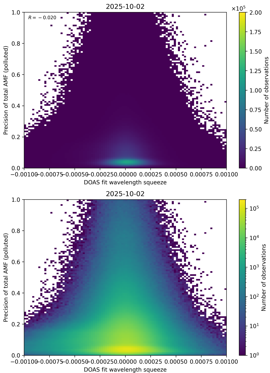
Figure 146: Scatter density plot of “DOAS fit wavelength squeeze” against “Precision of total AMF (polluted)” for 2025-10-01 to 2025-10-03.
