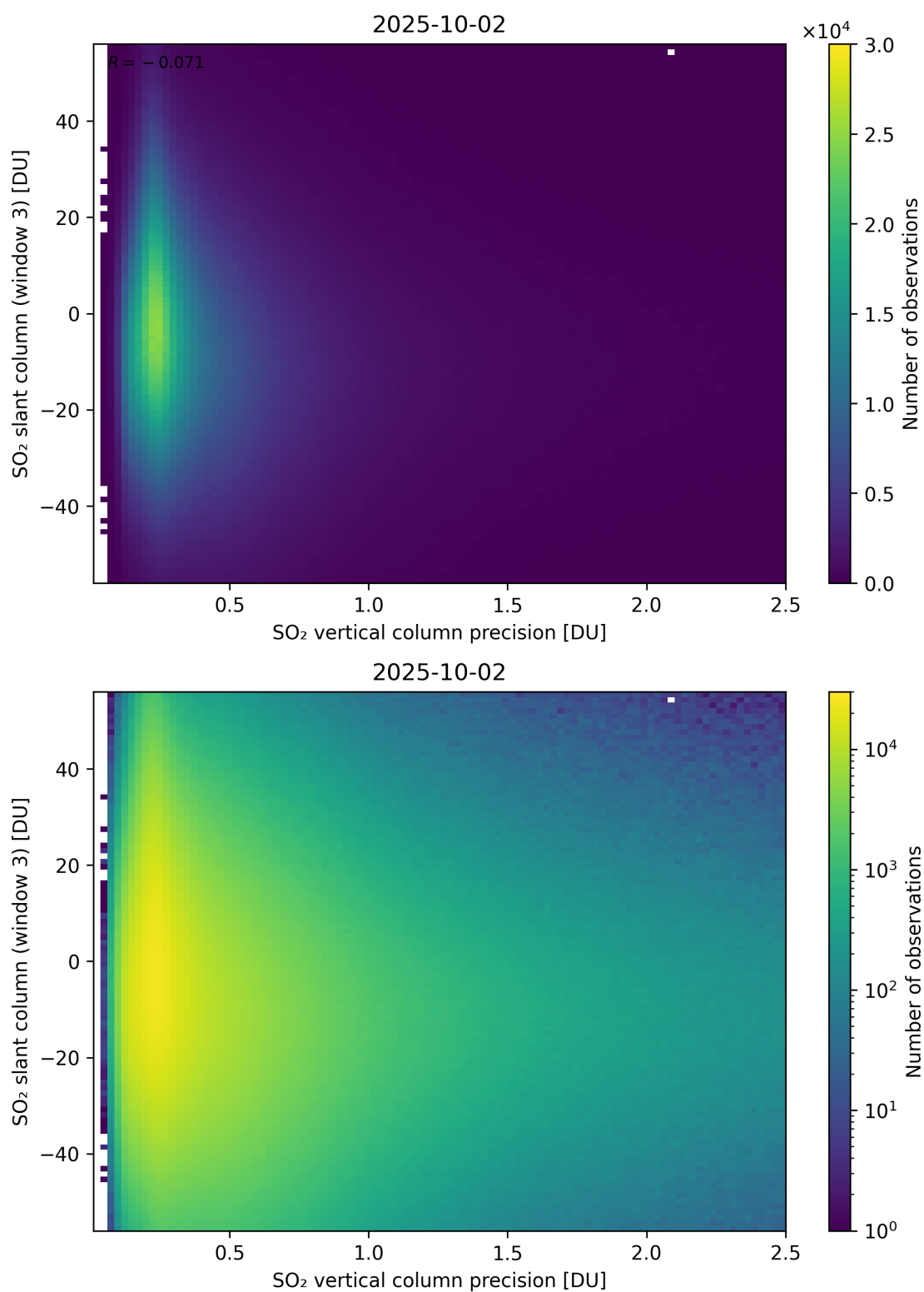
Figure 344: Scatter density plot of “SO 2 vertical column precision” against “SO 2 slant column (window 3)” for 2025-10-01 to 2025-10-03.
