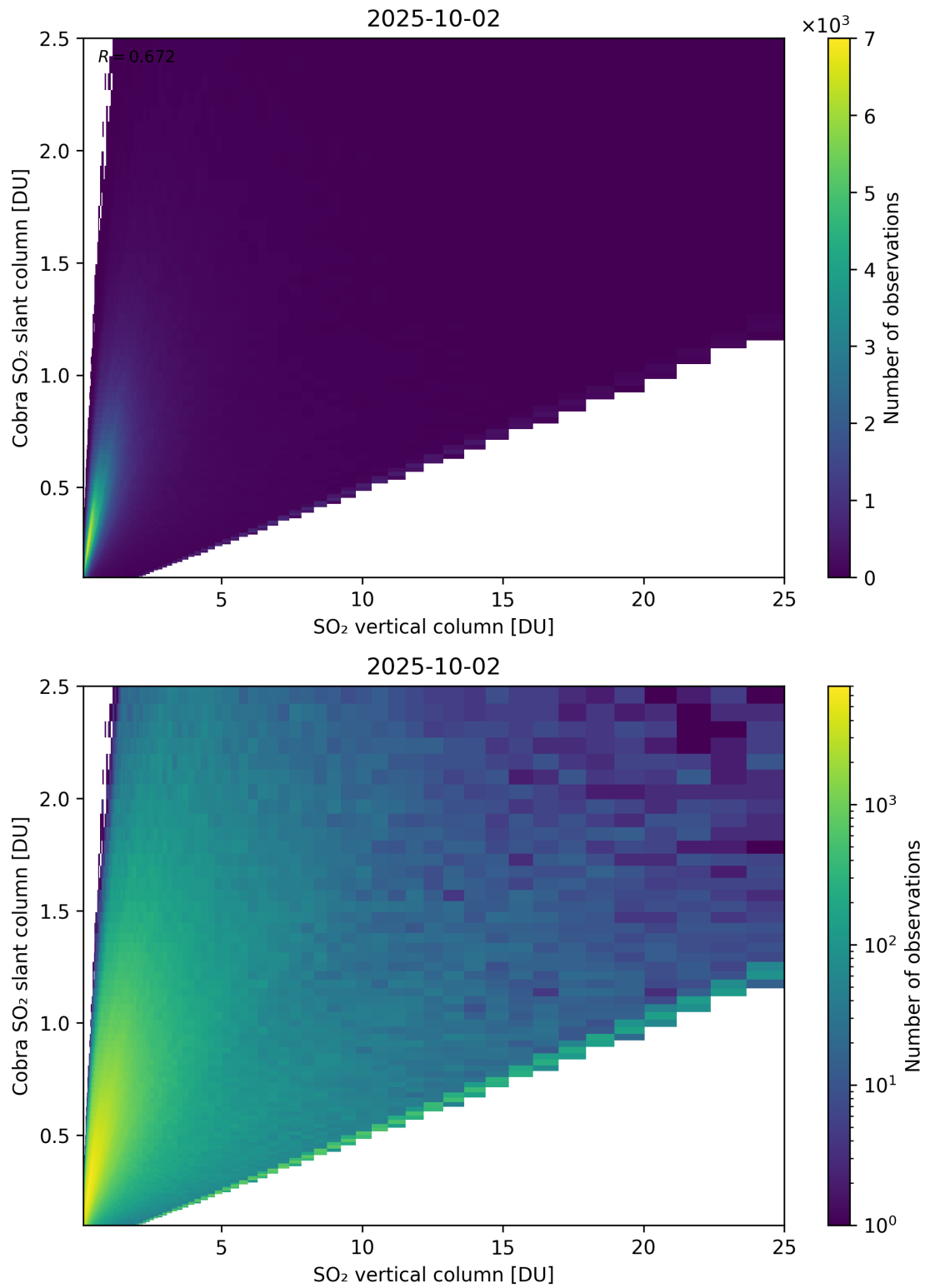
Figure 349: Scatter density plot of “SO 2 vertical column” against “Cobra SO 2 slant column” for 2025-10-01 to 2025-10-03.
