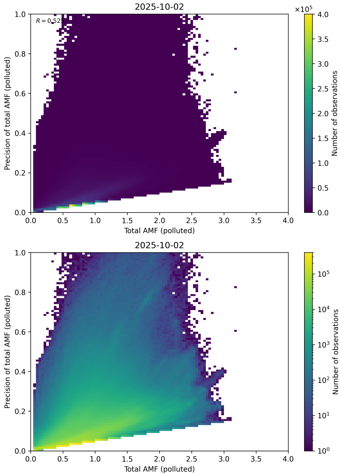
Figure 322: Scatter density plot of “Total AMF (polluted)” against “Precision of total AMF (polluted)” for 2025-10-01 to 2025-10-03.
