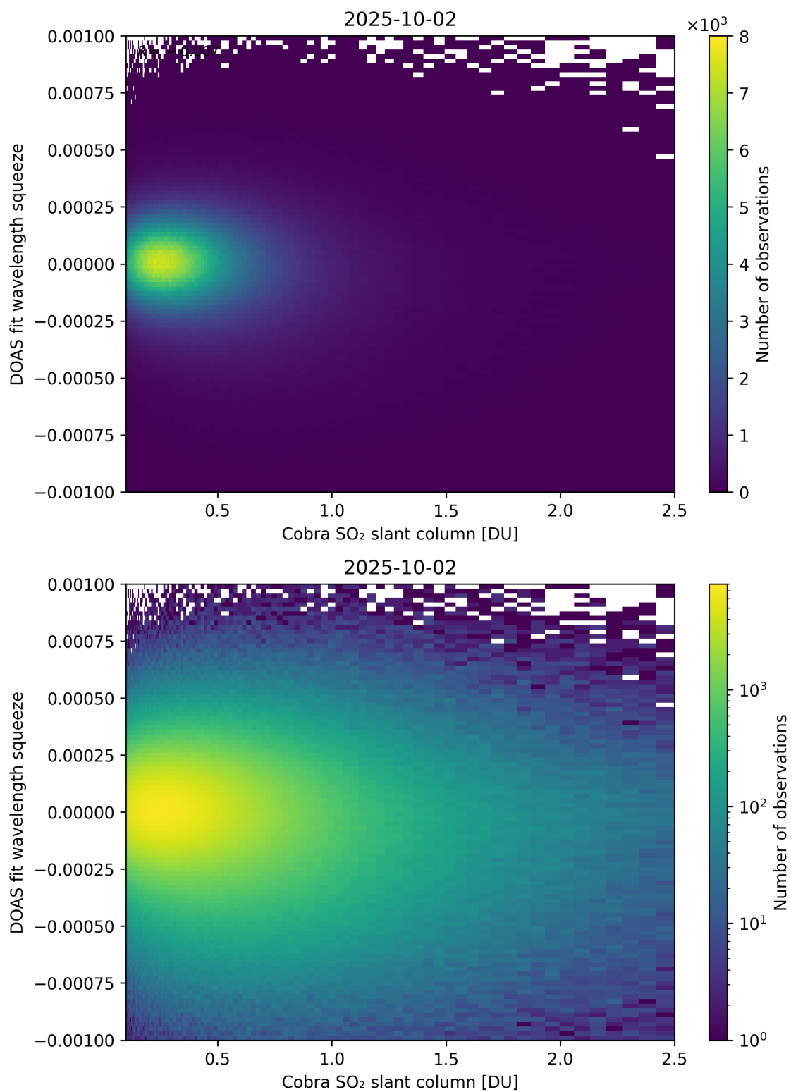
Figure 197: Scatter density plot of “Cobra SO 2 slant column” against “DOAS fit wavelength squeeze” for 2025-10-01 to 2025-10-03.
