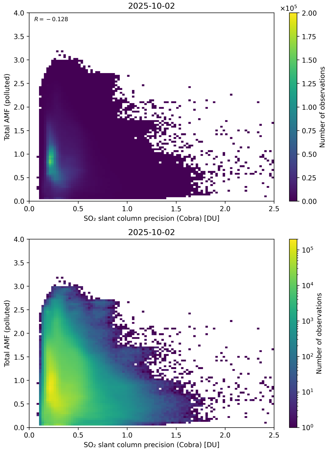
Figure 213: Scatter density plot of “SO 2 slant column precision (Cobra)” against “Total AMF (polluted)” for 2025-10-01 to 2025-10-03.
