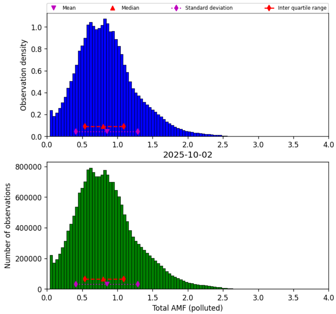
Figure 79: Histogram of “Total AMF (polluted)” for 2025-10-01 to 2025-10-03
