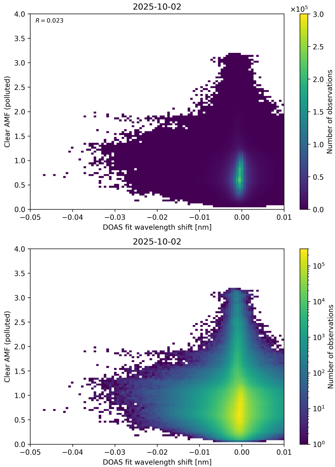
Figure 140: Scatter density plot of “DOAS fit wavelength shift” against “Clear AMF (polluted)” for 2025-10-01 to 2025-10-03.
