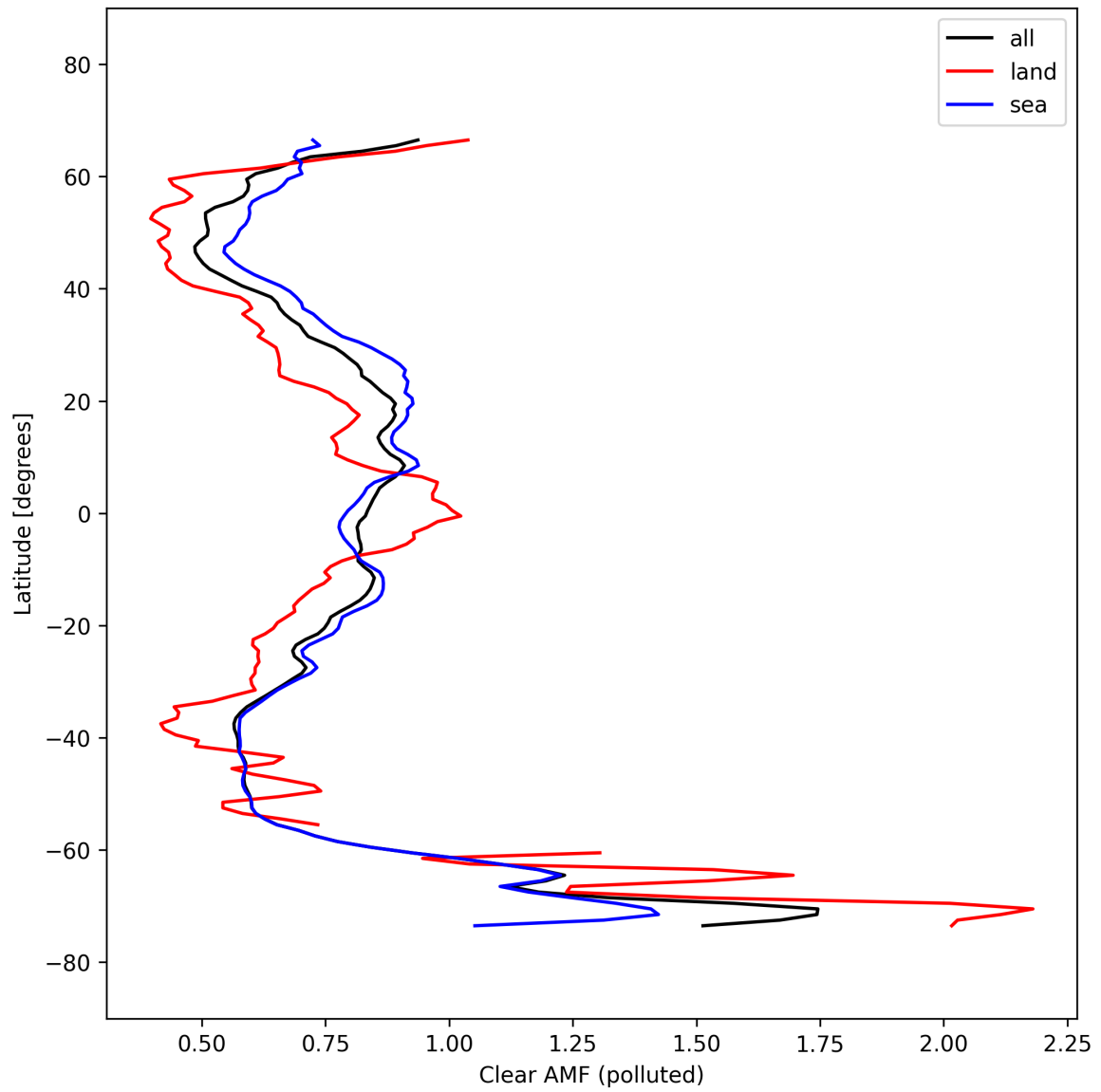
Figure 55: Zonal average of “Clear AMF (polluted)” for 2025-10-01 to 2025-10-03.
