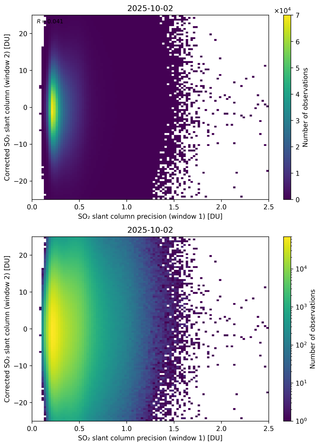
Figure 275: Scatter density plot of “SO 2 slant column precision (window 1)” against “Corrected SO 2 slant column (window 2)” for 2025-10-01 to 2025-10-03.
