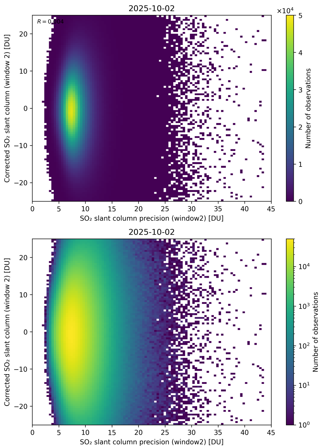
Figure 297: Scatter density plot of “SO 2 slant column precision (window2)” against “Corrected SO 2 slant column (window 2)” for 2025-10-01 to 2025-10-03.
