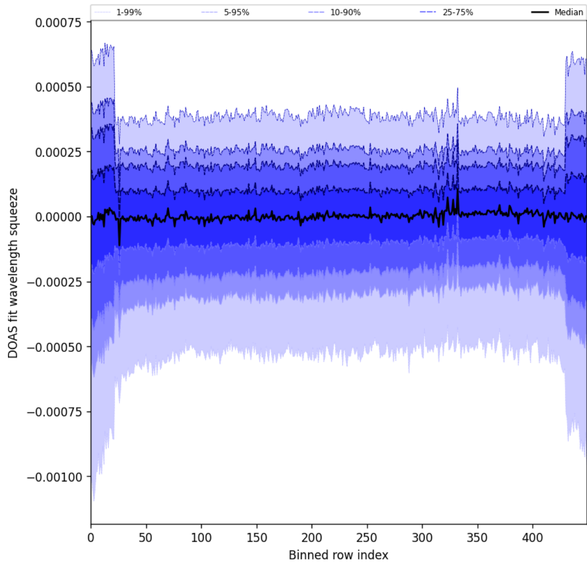
Figure 103: Along track statistics of “DOAS fit wavelength squeeze” for 2025-10-01 to 2025-10-03
