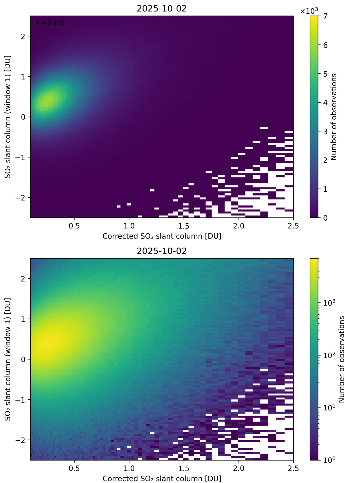
Figure 237: Scatter density plot of “Corrected SO 2 slant column” against “SO 2 slant column (window 1)” for 2025-10-01 to 2025-10-03.
