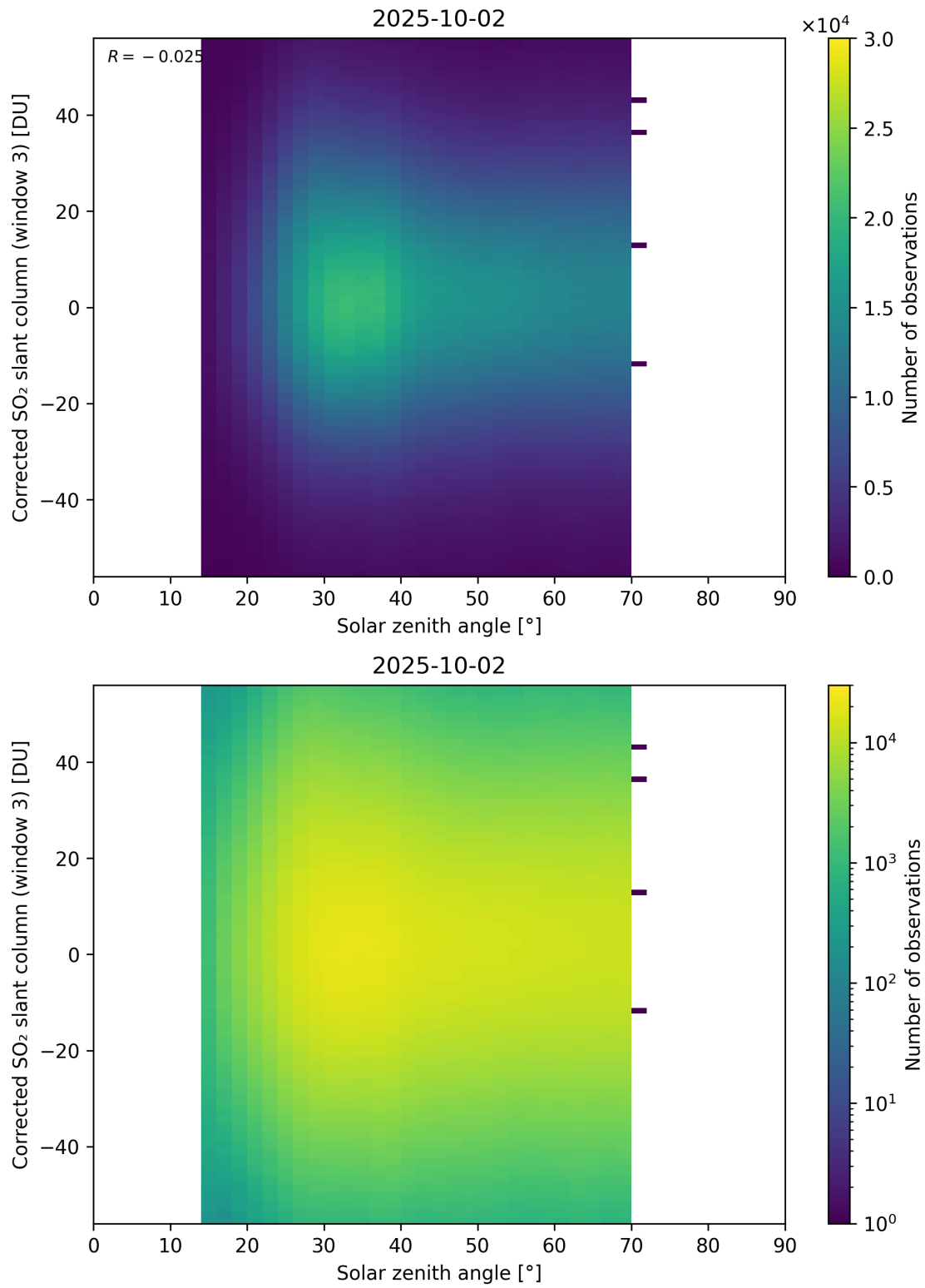
Figure 183: Scatter density plot of “Solar zenith angle” against “Corrected SO 2 slant column (window 3)” for 2025-10-01 to 2025-10-03.
