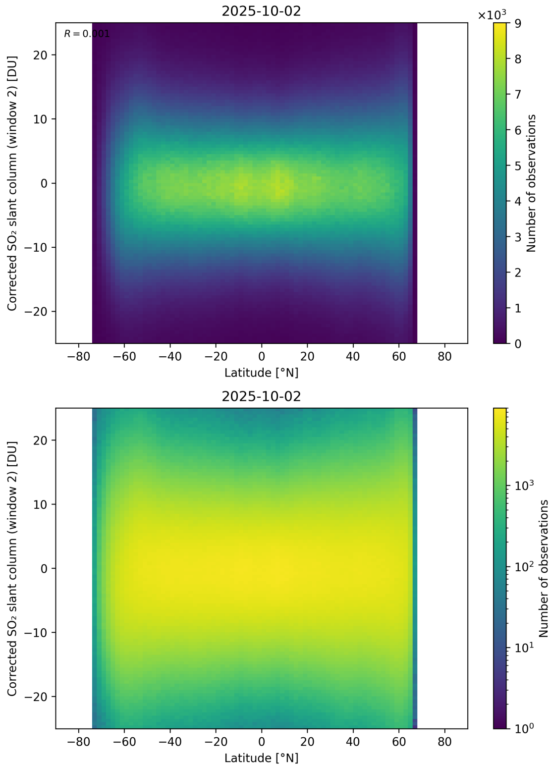
Figure 160: Scatter density plot of “Latitude” against “Corrected SO 2 slant column (window 2)” for 2025-10-01 to 2025-10-03.
