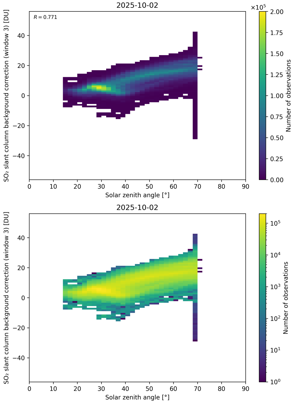
Figure 173: Scatter density plot of “Solar zenith angle” against “SO 2 slant column background correction (window 3)” for 2025-10-01 to 2025-10-03.
