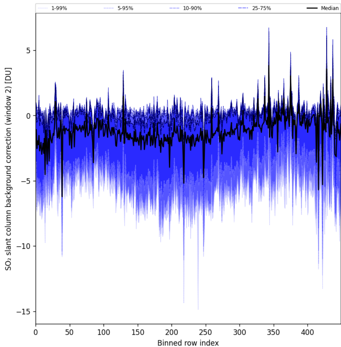
Figure 96: Along track statistics of “SO 2 slant column background correction (window 2)” for 2025-10-01 to 2025-10-03
