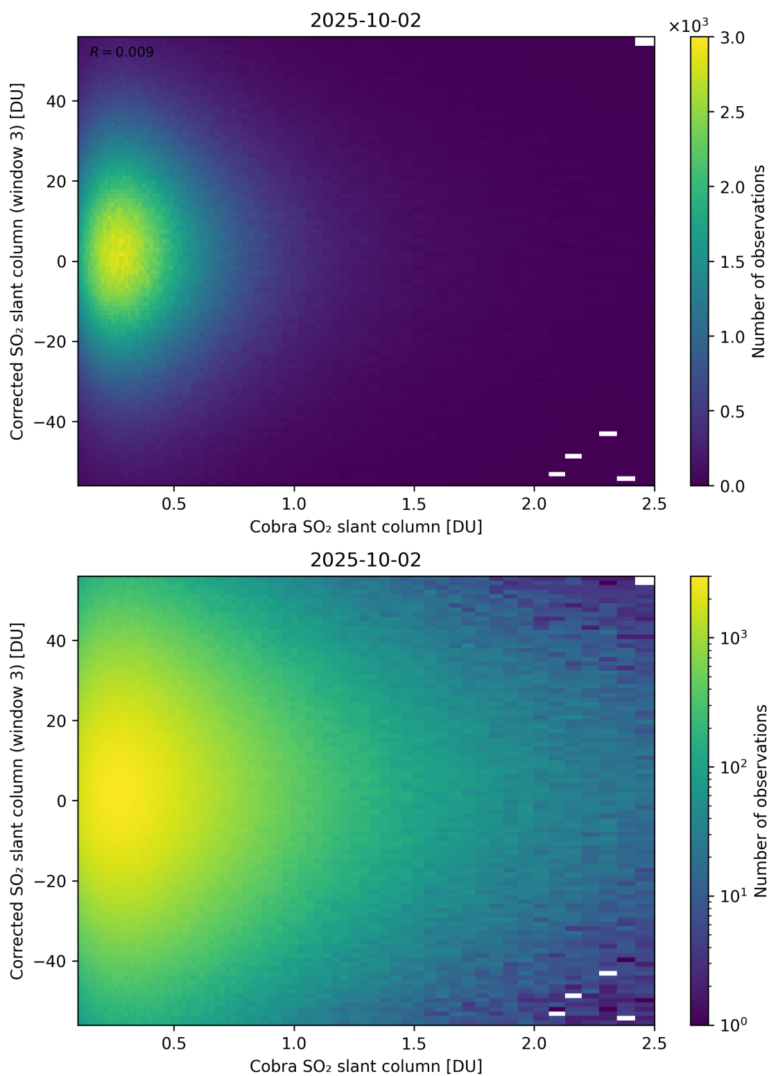
Figure 218: Scatter density plot of “Cobra SO 2 slant column” against “Corrected SO 2 slant column (window 3)” for 2025-10-01 to 2025-10-03.
