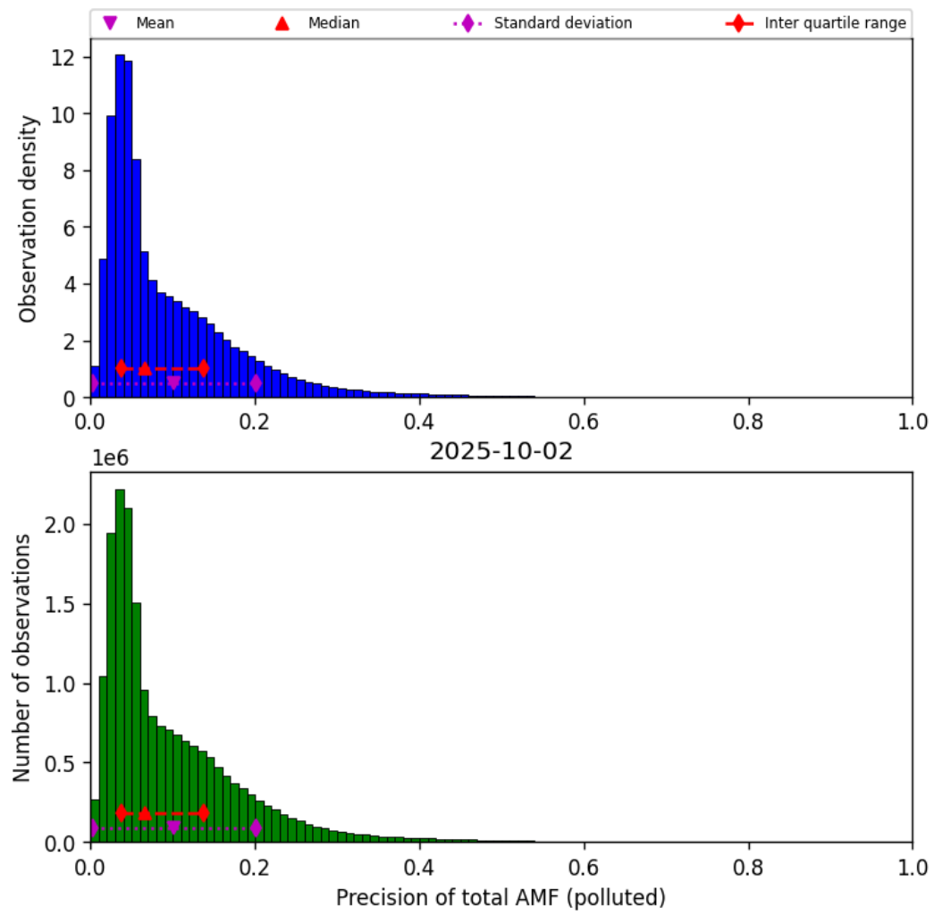
Figure 80: Histogram of “Precision of total AMF (polluted)” for 2025-10-01 to 2025-10-03
