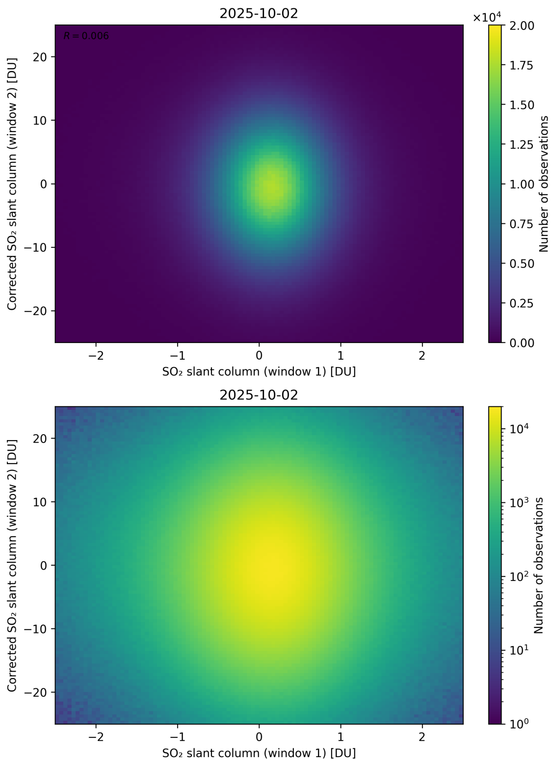
Figure 283: Scatter density plot of “SO 2 slant column (window 1)” against “Corrected SO 2 slant column (window 2)” for 2025-10-01 to 2025-10-03.
