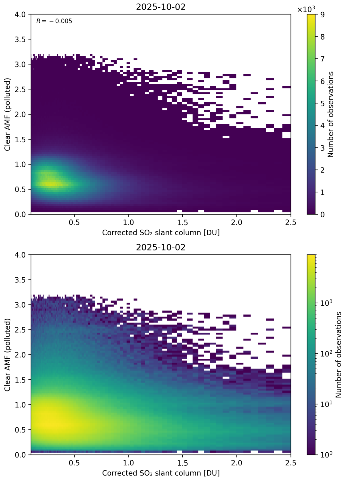
Figure 232: Scatter density plot of “Corrected SO 2 slant column” against “Clear AMF (polluted)” for 2025-10-01 to 2025-10-03.
