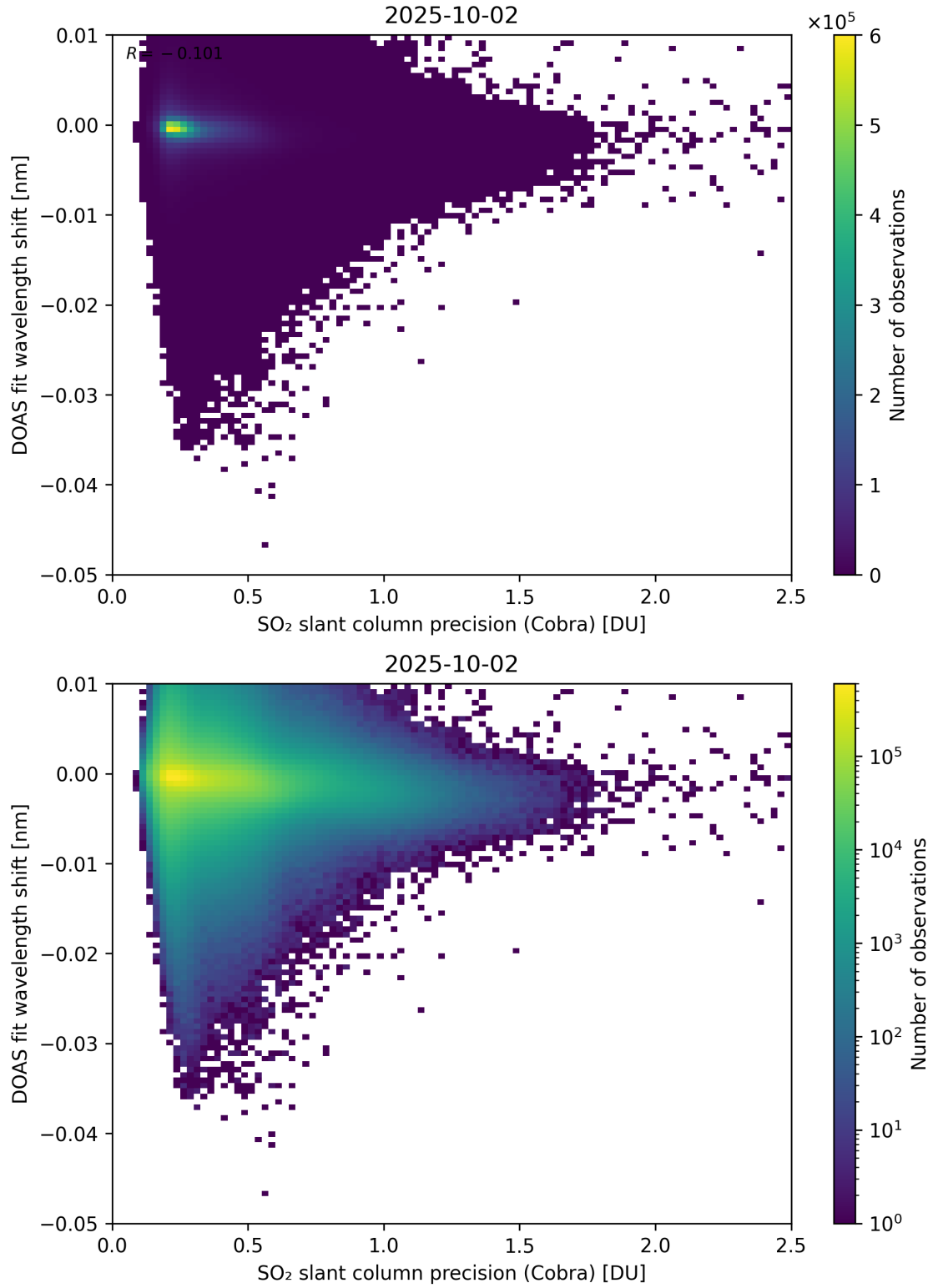
Figure 202: Scatter density plot of “SO 2 slant column precision (Cobra)” against “DOAS fit wavelength shift” for 2025-10-01 to 2025-10-03.
