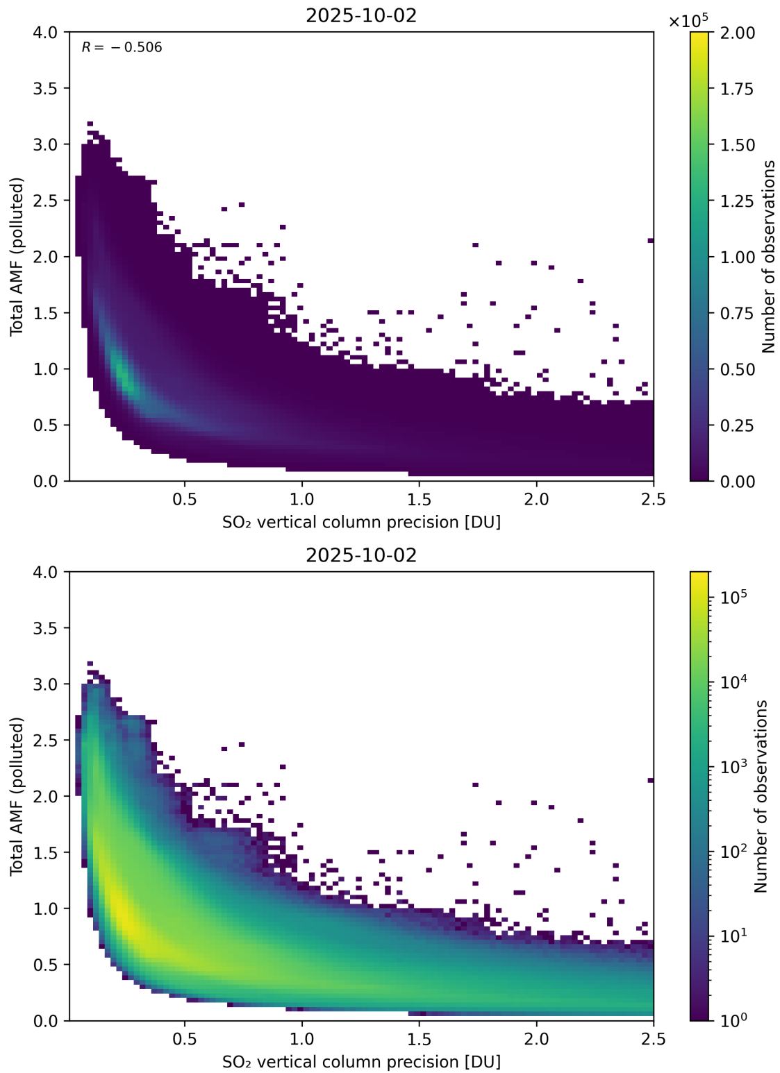
Figure 346: Scatter density plot of “SO 2 vertical column precision” against “Total AMF (polluted)” for 2025-10-01 to 2025-10-03.
