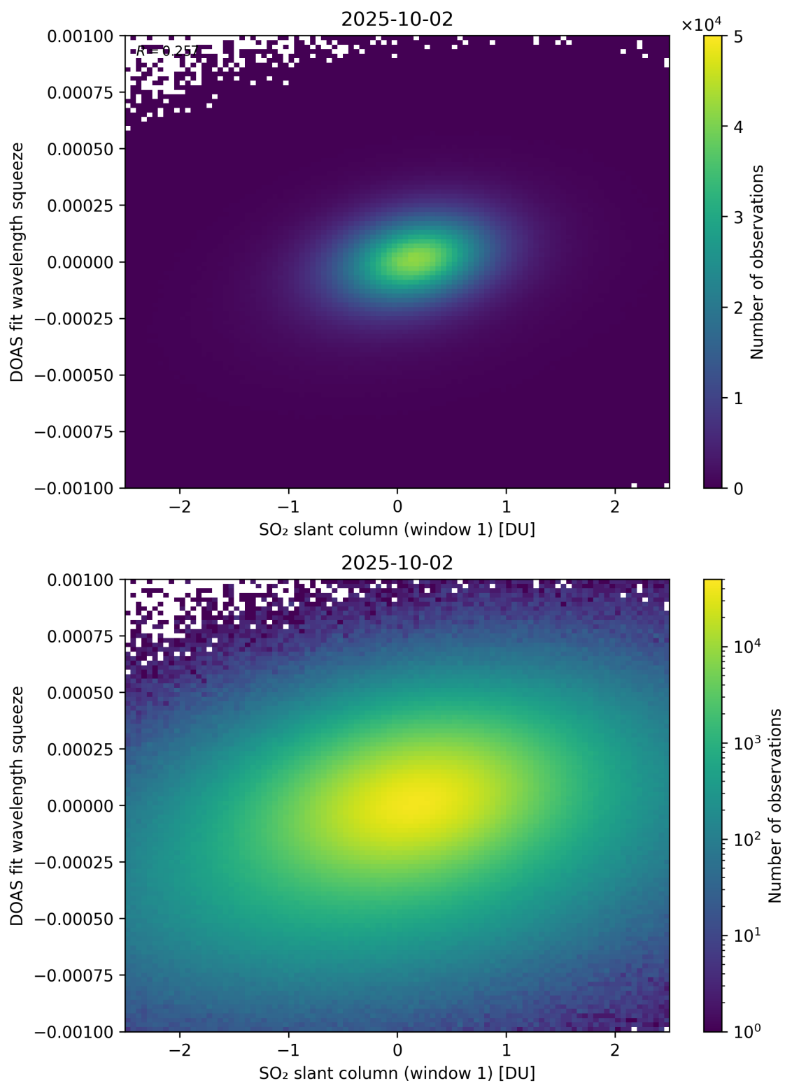
Figure 266: Scatter density plot of “SO 2 slant column (window 1)” against “DOAS fit wavelength squeeze” for 2025-10-01 to 2025-10-03.
