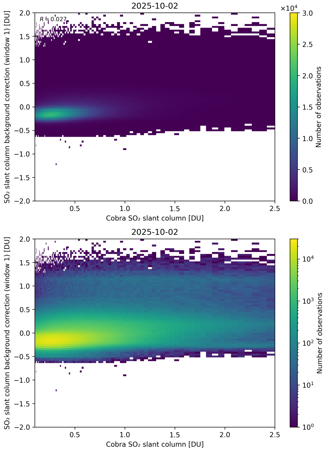
Figure 193: Scatter density plot of “Cobra SO 2 slant column” against “SO 2 slant column background correction (window 1)” for 2025-10-01 to 2025-10-03.
