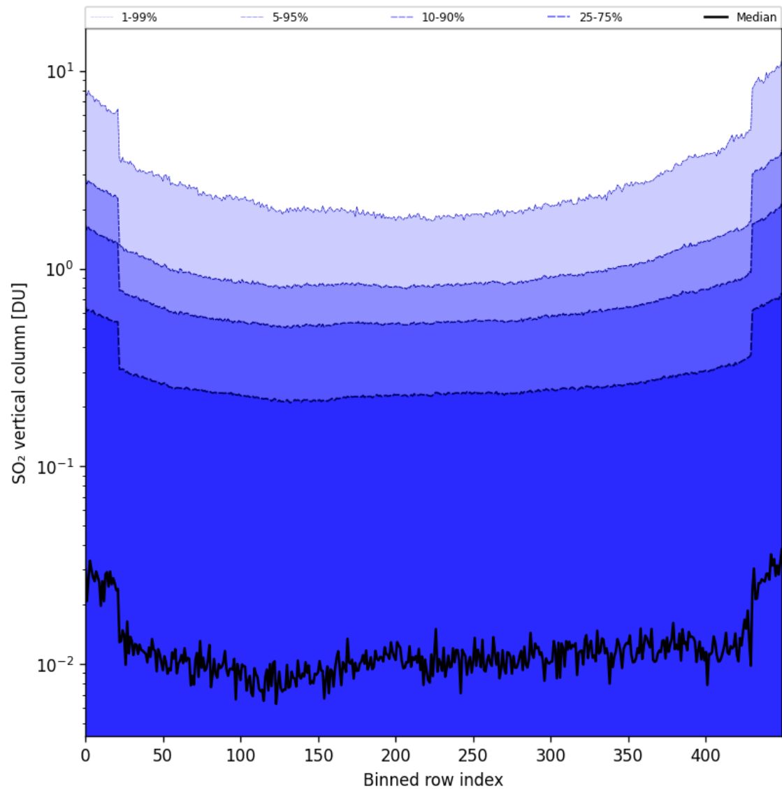
Figure 84: Along track statistics of “SO 2 vertical column” for 2025-10-01 to 2025-10-03
