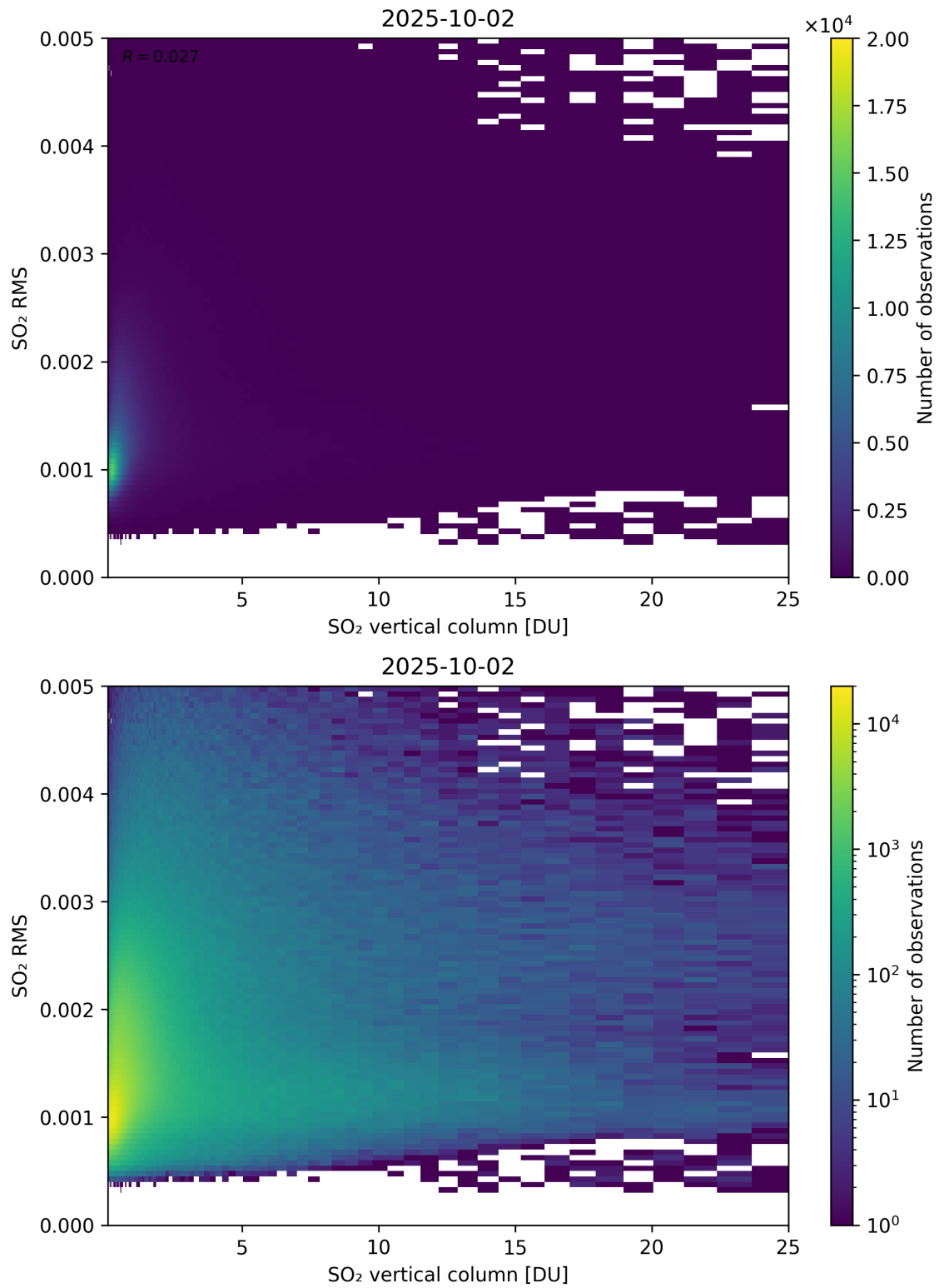
Figure 328: Scatter density plot of “SO 2 vertical column” against “SO 2 RMS” for 2025-10-01 to 2025-10-03.
