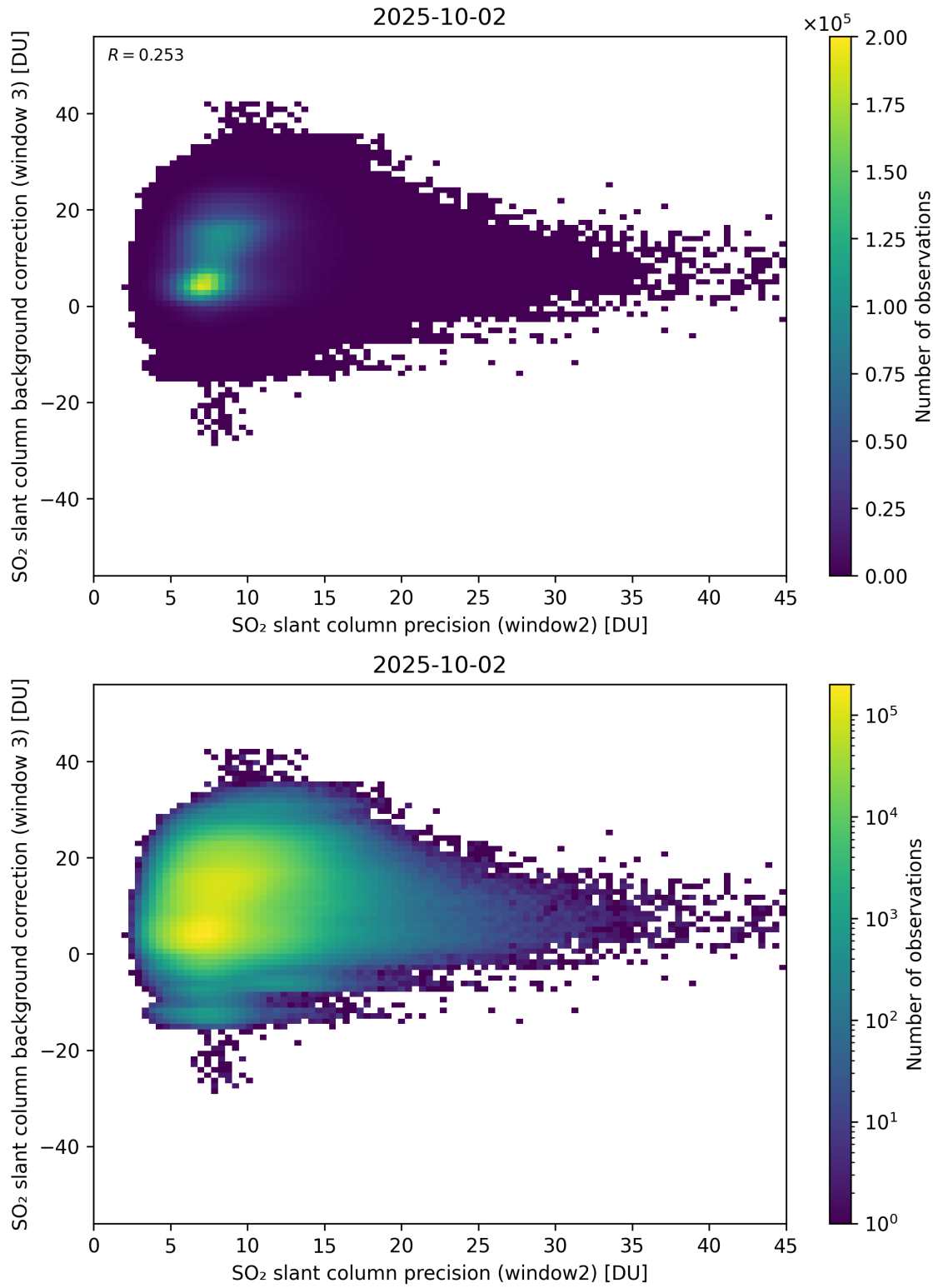
Figure 292: Scatter density plot of “SO 2 slant column precision (window2)” against “SO 2 slant column background correction (window 3)” for 2025-10-01 to 2025-10-03.
