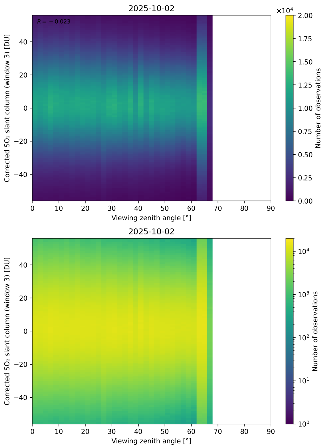
Figure 375: Scatter density plot of “Viewing zenith angle” against “Corrected SO 2 slant column (window 3)” for 2025-10-01 to 2025-10-03.
