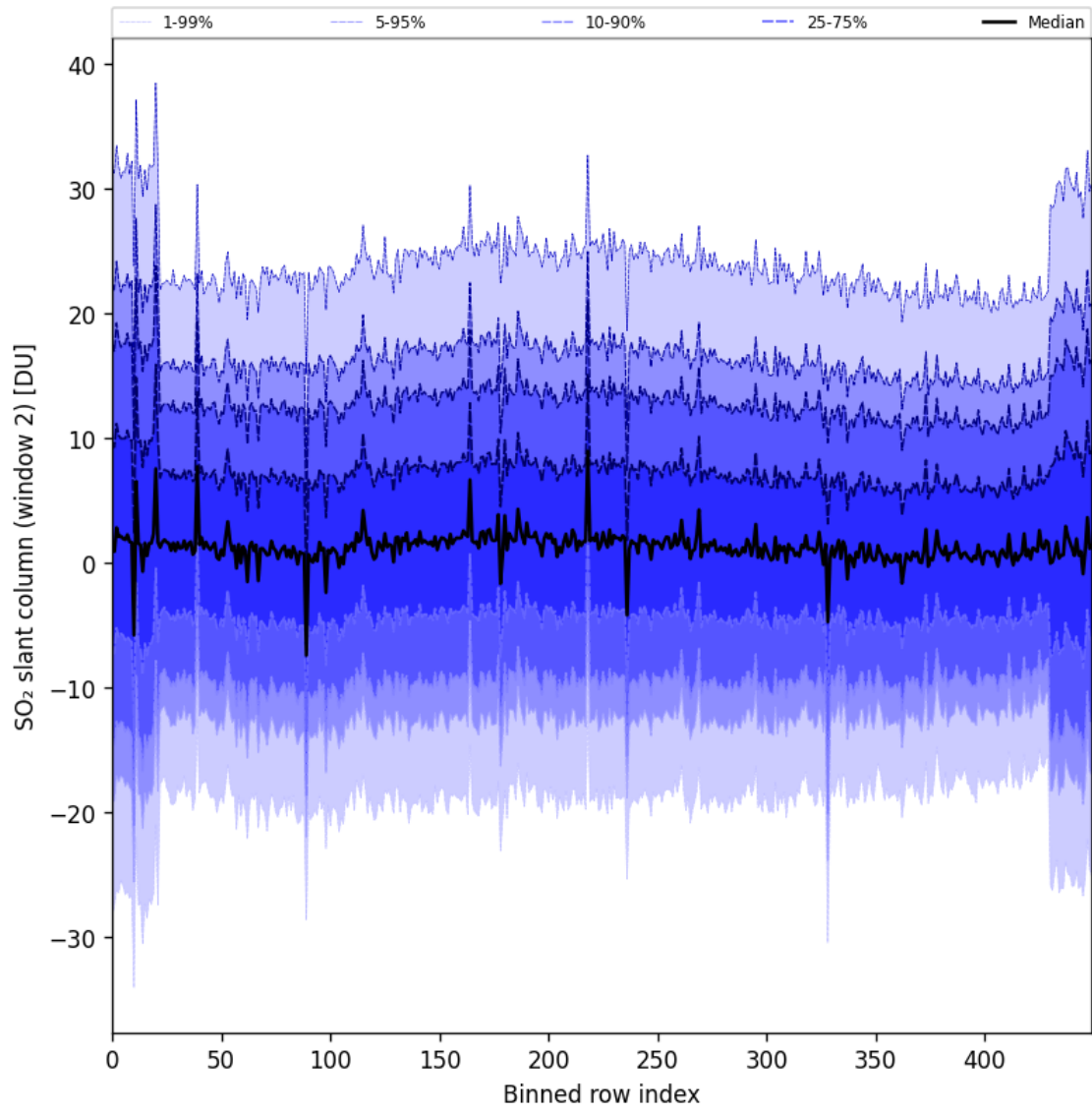
Figure 93: Along track statistics of “SO 2 slant column (window 2)” for 2025-10-01 to 2025-10-03
