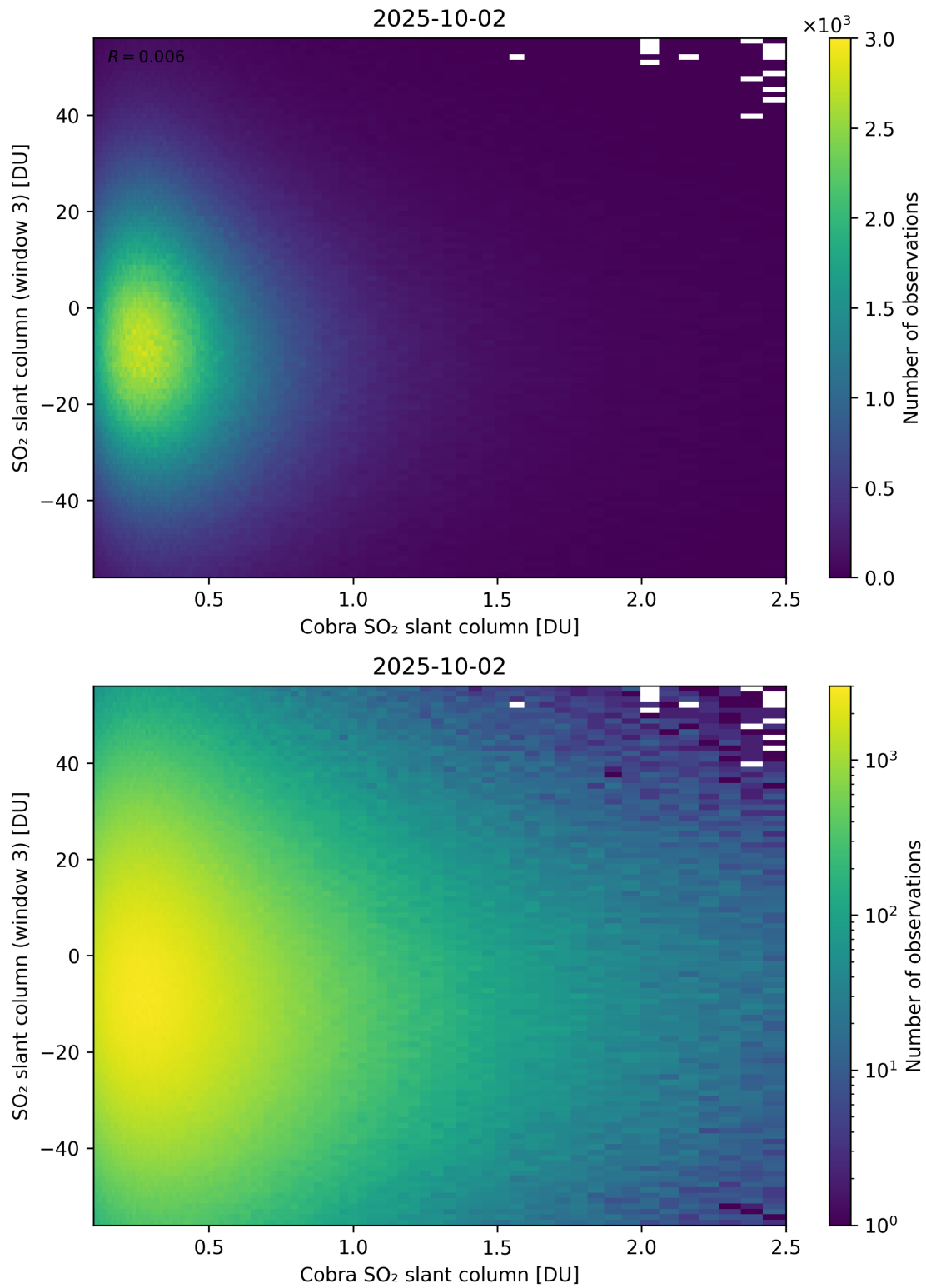
Figure 222: Scatter density plot of “Cobra SO 2 slant column” against “SO 2 slant column (window 3)” for 2025-10-01 to 2025-10-03.
