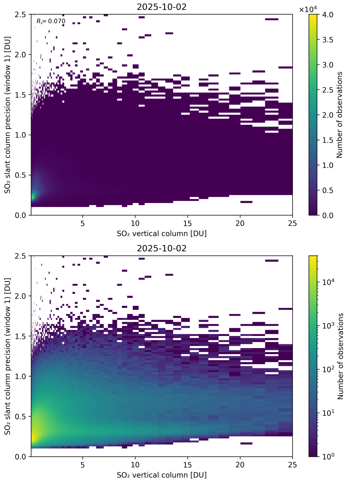
Figure 355: Scatter density plot of “SO 2 vertical column” against “SO 2 slant column precision (window 1)” for 2025-10-01 to 2025-10-03.
