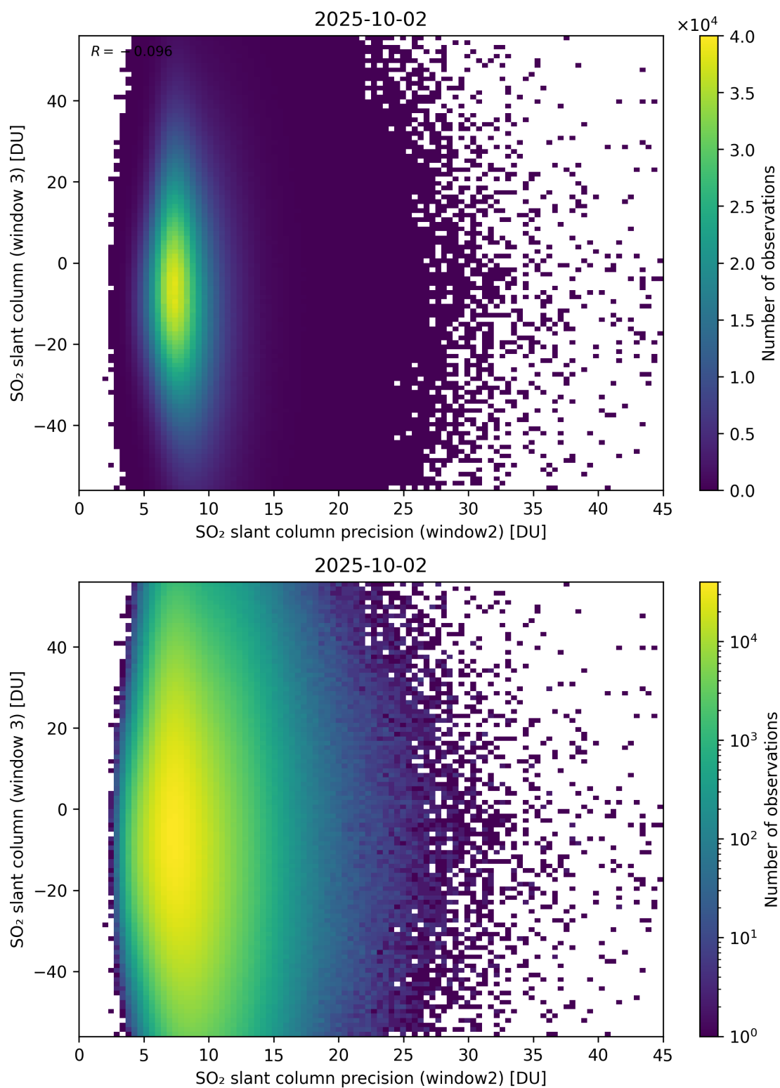
Figure 299: Scatter density plot of “SO 2 slant column precision (window2)” against “SO 2 slant column (window 3)” for 2025-10-01 to 2025-10-03.
