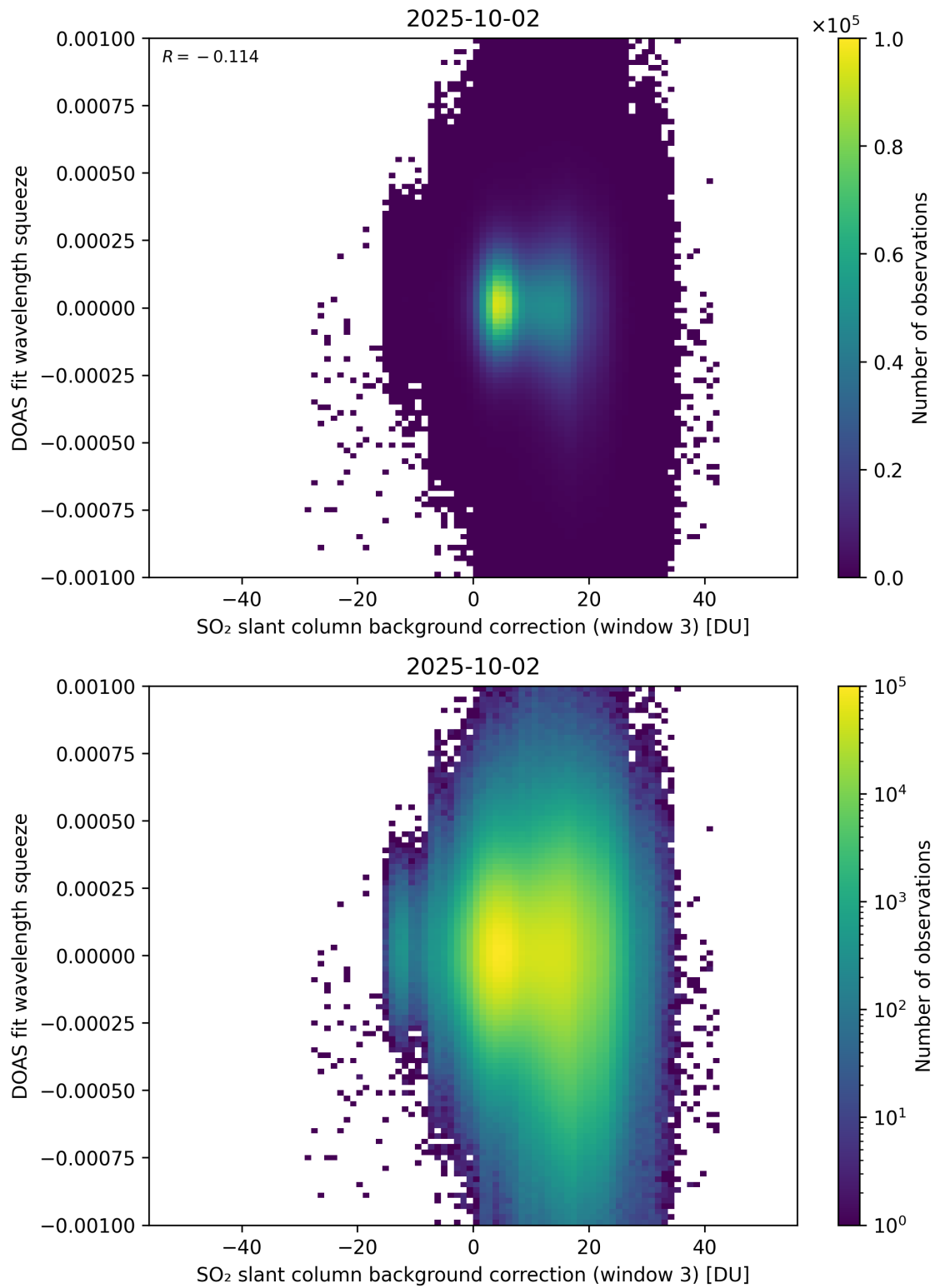
Figure 133: Scatter density plot of “SO 2 slant column background correction (window 3)” against “DOAS fit wavelength squeeze” for 2025-10-01 to 2025-10-03.
