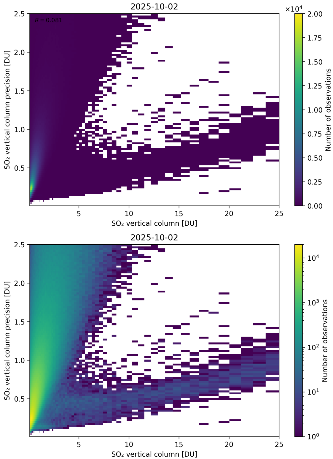
Figure 361: Scatter density plot of “SO 2 vertical column” against “SO 2 vertical column precision” for 2025-10-01 to 2025-10-03.
