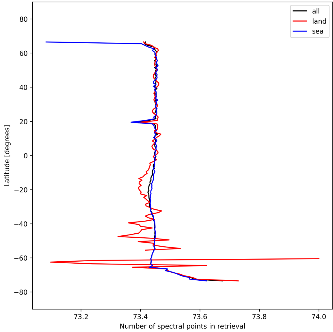
Figure 56: Zonal average of “Number of spectral points in retrieval” for 2025-10-01 to 2025-10-03.
