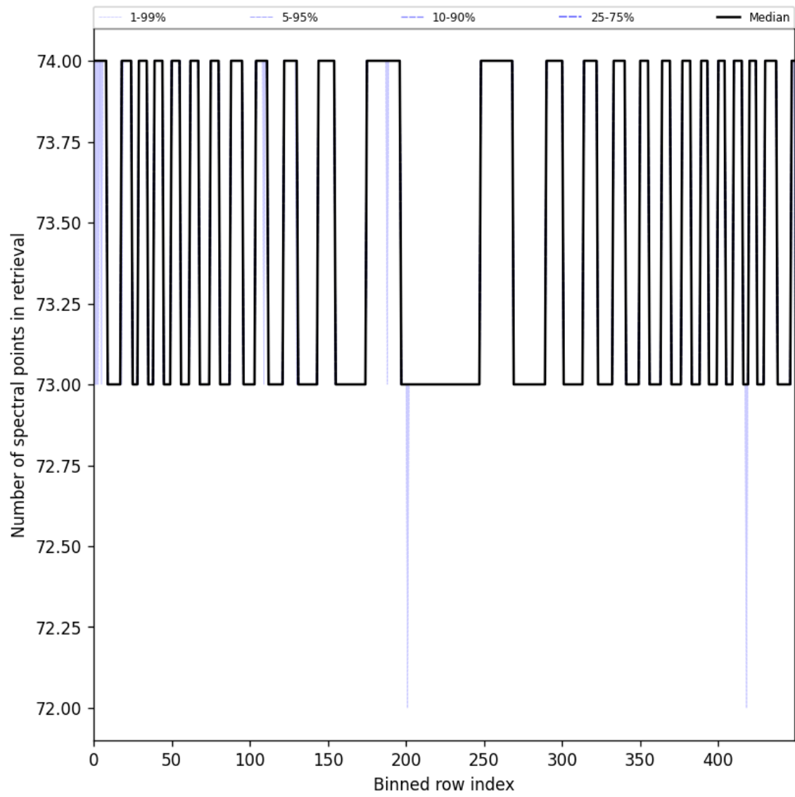
Figure 108: Along track statistics of “Number of spectral points in retrieval” for 2025-10-01 to 2025-10-03
