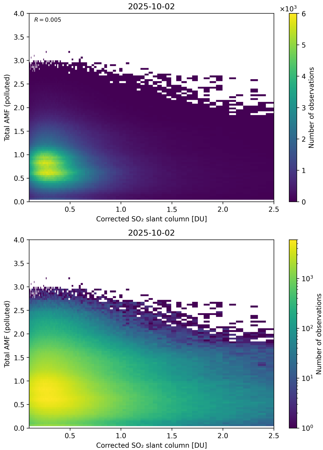
Figure 242: Scatter density plot of “Corrected SO 2 slant column” against “Total AMF (polluted)” for 2025-10-01 to 2025-10-03.
