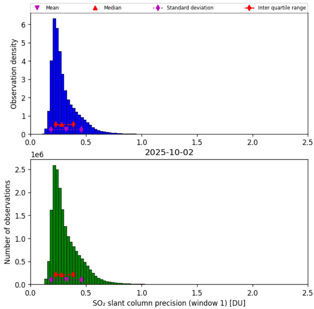
Figure 64: Histogram of “SO 2 slant column precision (window 1)” for 2025-10-01 to 2025-10-03
