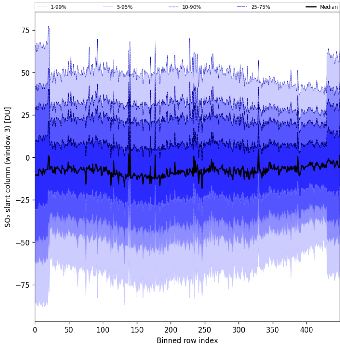
Figure 97: Along track statistics of “SO 2 slant column (window 3)” for 2025-10-01 to 2025-10-03
