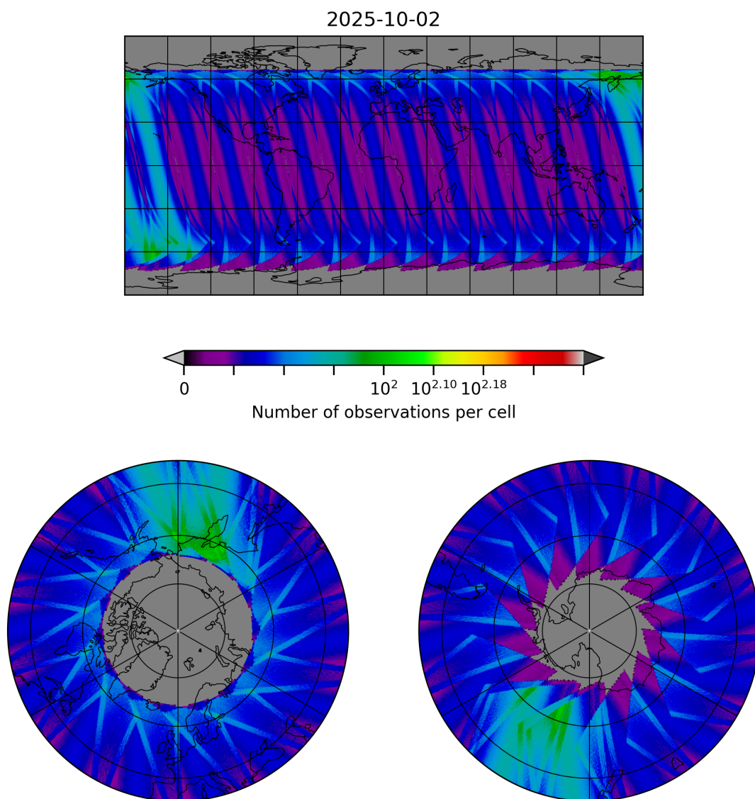
Figure 30: Map of the number of observations for 2025-10-01 to 2025-10-03
