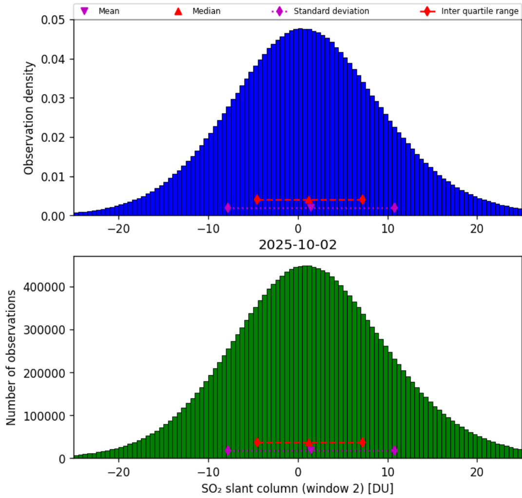
Figure 67: Histogram of “SO 2 slant column (window 2)” for 2025-10-01 to 2025-10-03
