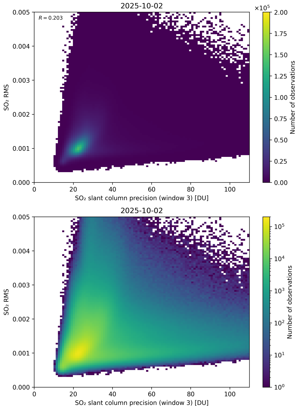
Figure 310: Scatter density plot of “SO 2 slant column precision (window 3)” against “SO 2 RMS” for 2025-10-01 to 2025-10-03.
