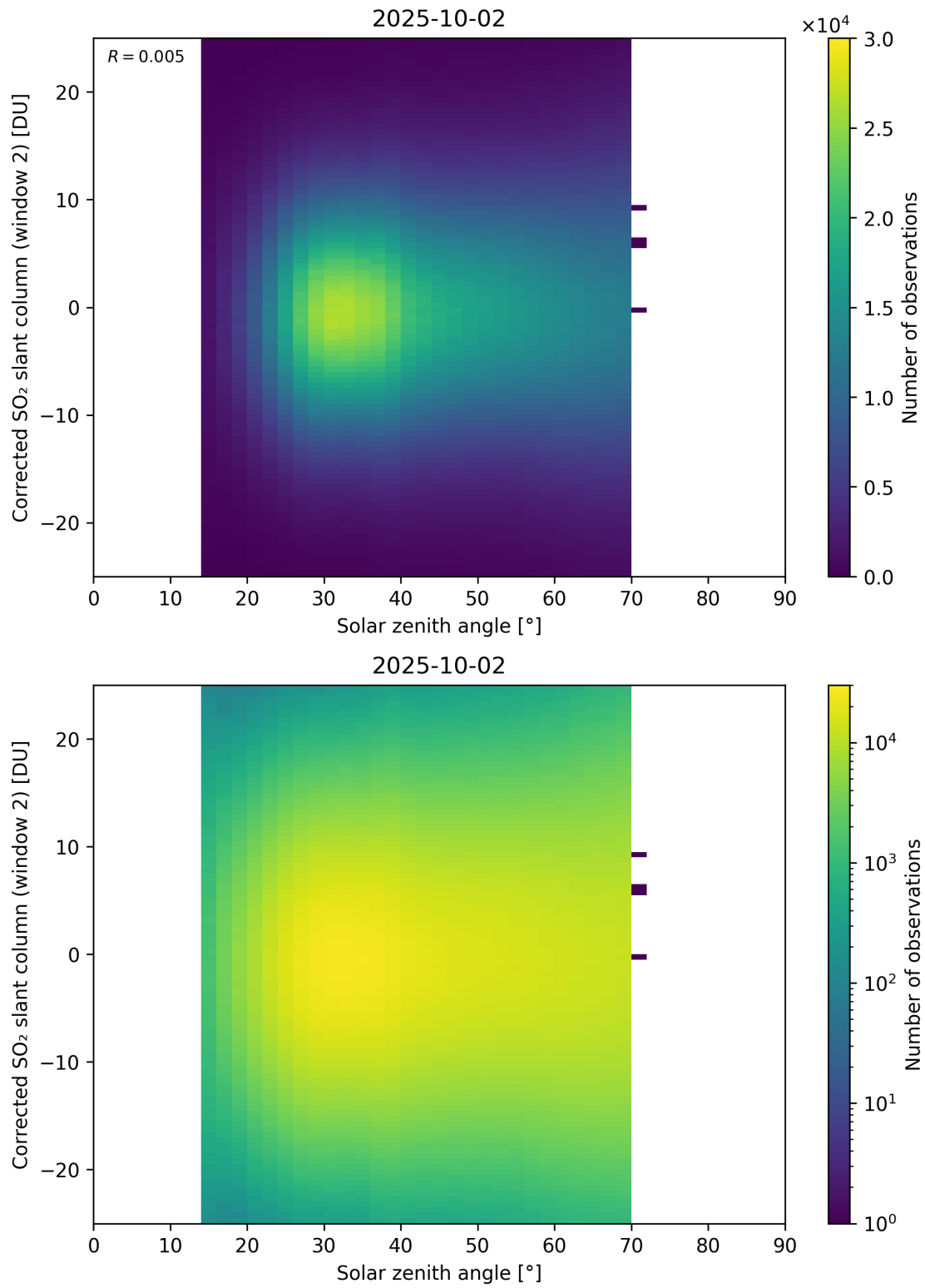
Figure 182: Scatter density plot of “Solar zenith angle” against “Corrected SO 2 slant column (window 2)” for 2025-10-01 to 2025-10-03.
