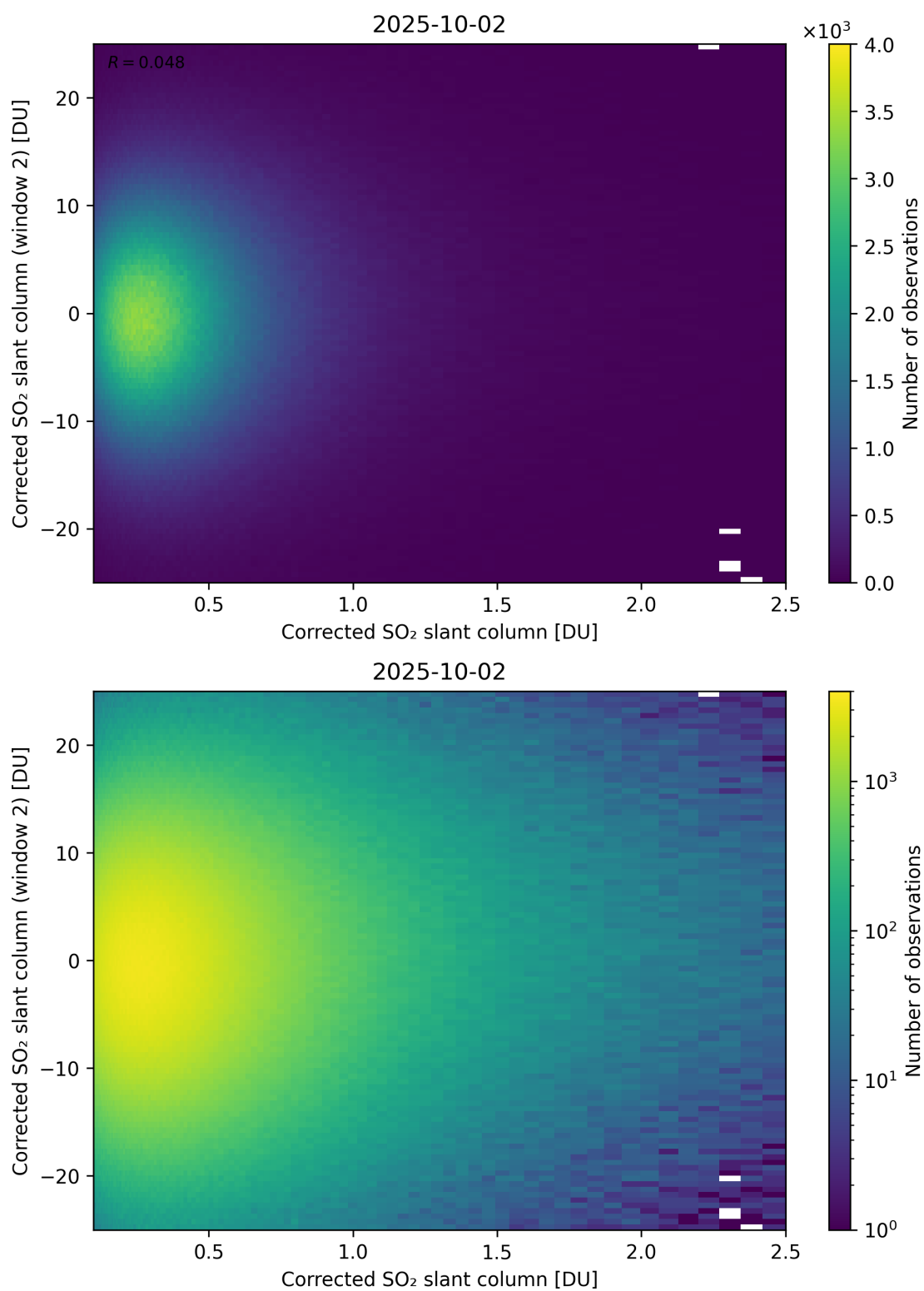
Figure 235: Scatter density plot of “Corrected SO 2 slant column” against “Corrected SO 2 slant column (window 2)” for 2025-10-01 to 2025-10-03.
