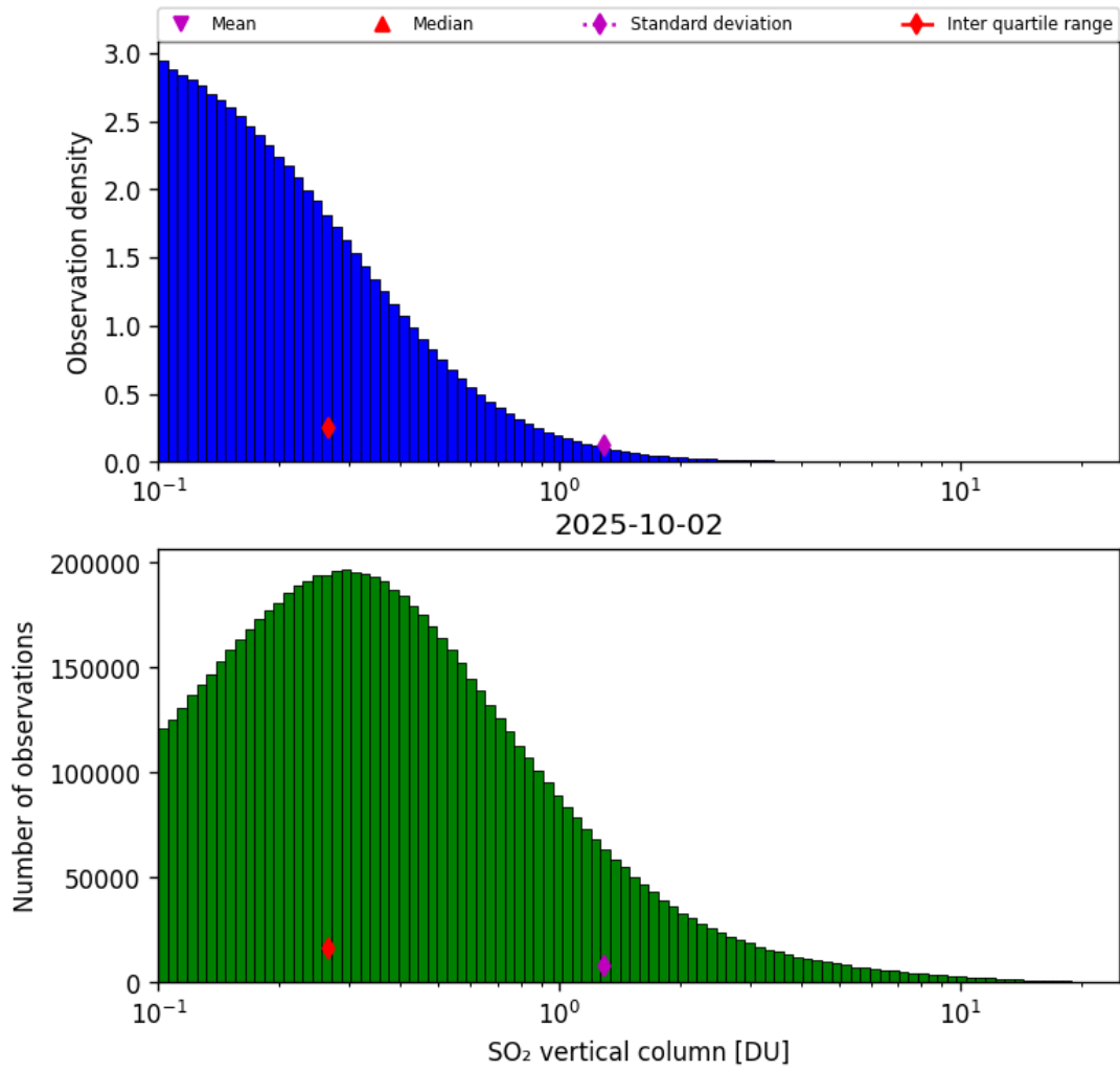
Figure 58: Histogram of “SO 2 vertical column” for 2025-10-01 to 2025-10-03
