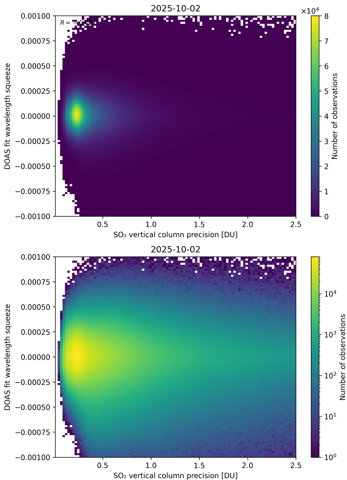
Figure 333: Scatter density plot of “SO 2 vertical column precision” against “DOAS fit wavelength squeeze” for 2025-10-01 to 2025-10-03.
