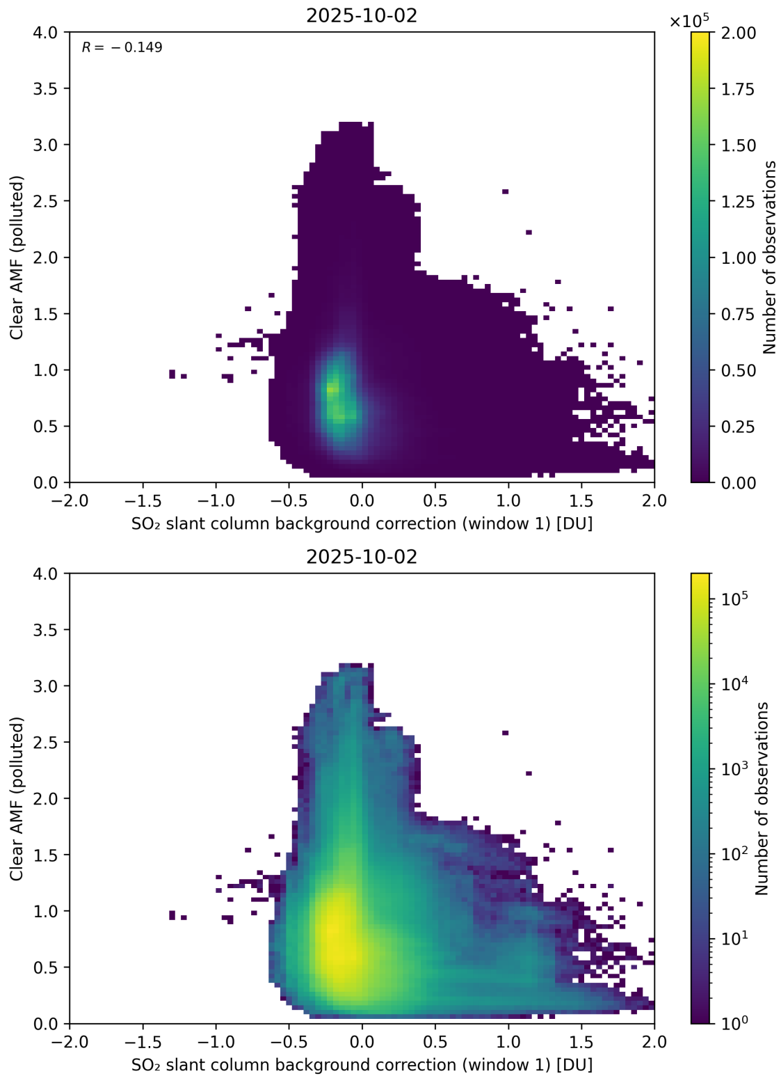
Figure 114: Scatter density plot of “SO 2 slant column background correction (window 1)” against “Clear AMF (polluted)” for 2025-10-01 to 2025-10-03.
