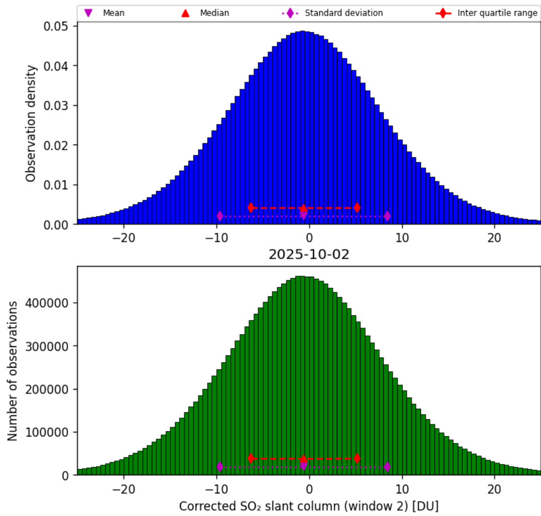
Figure 69: Histogram of “Corrected SO 2 slant column (window 2)” for 2025-10-01 to 2025-10-03
