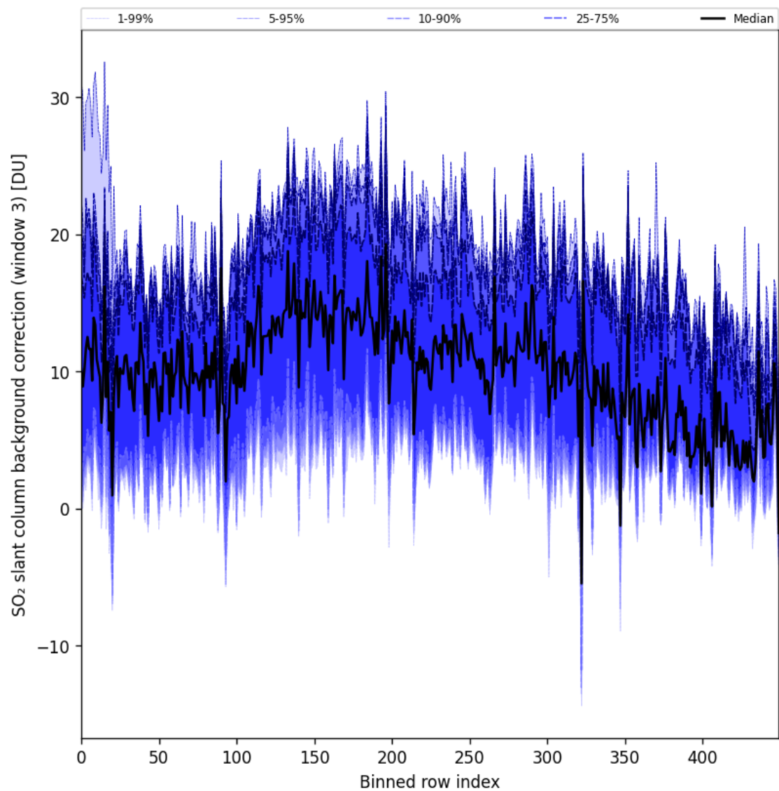
Figure 100: Along track statistics of “SO 2 slant column background correction (window 3)” for 2025-10-01 to 2025-10-03
