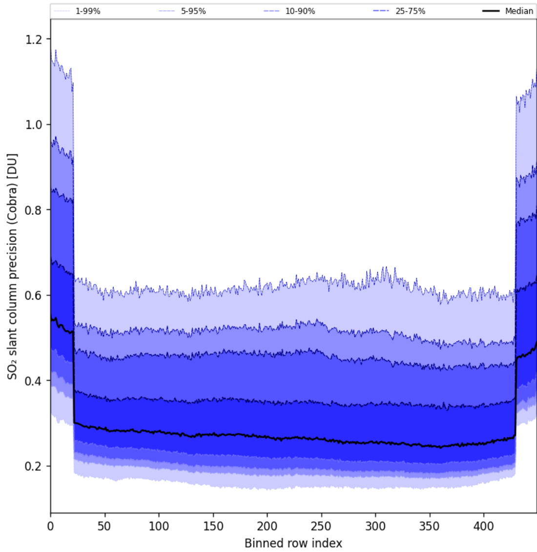
Figure 88: Along track statistics of “SO 2 slant column precision (Cobra)” for 2025-10-01 to 2025-10-03
