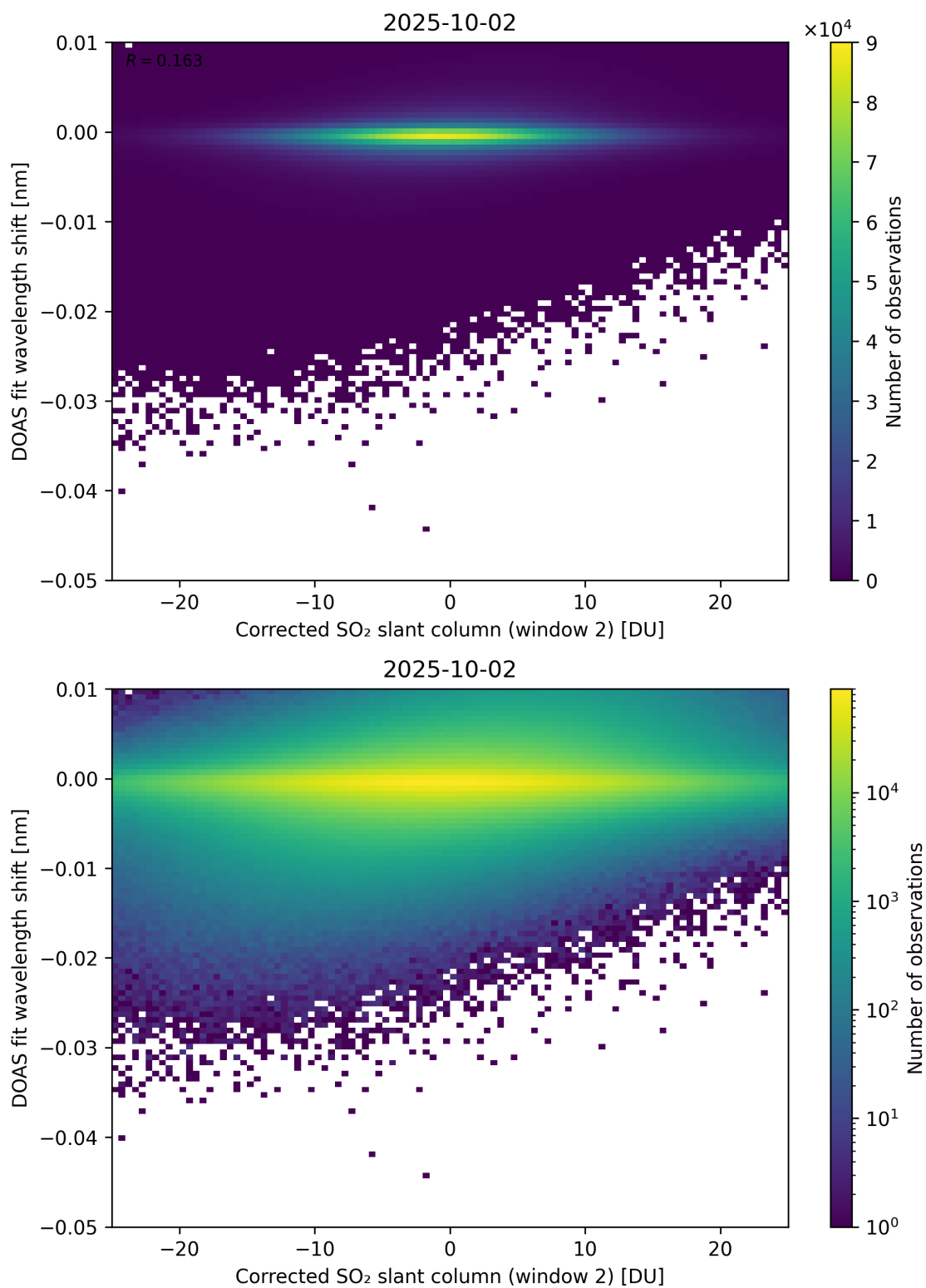
Figure 246: Scatter density plot of “Corrected SO 2 slant column (window 2)” against “DOAS fit wavelength shift” for 2025-10-01 to 2025-10-03.
