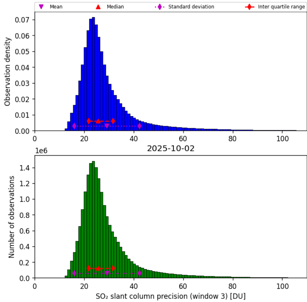
Figure 72: Histogram of “SO 2 slant column precision (window 3)” for 2025-10-01 to 2025-10-03
