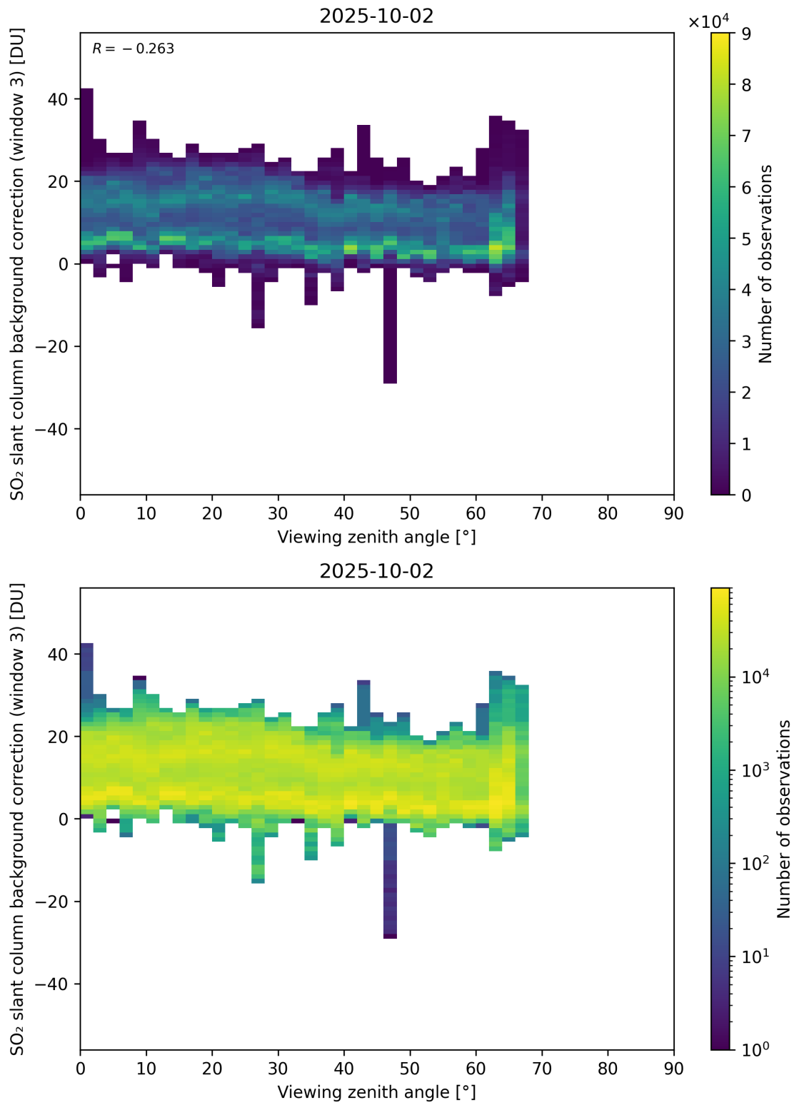
Figure 364: Scatter density plot of “Viewing zenith angle” against “SO 2 slant column background correction (window 3)” for 2025-10-01 to 2025-10-03.
