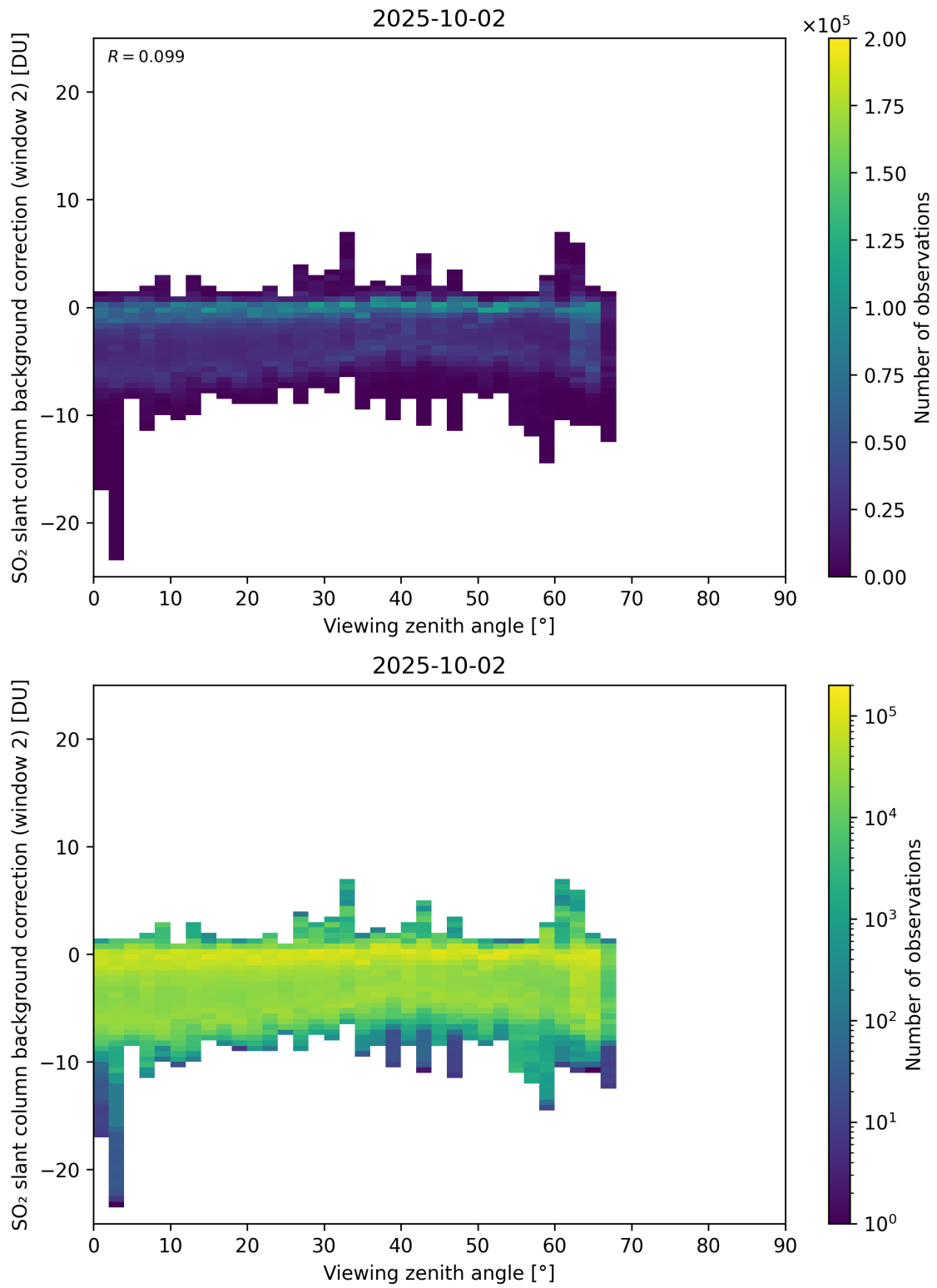
Figure 363: Scatter density plot of “Viewing zenith angle” against “SO 2 slant column background correction (window 2)” for 2025-10-01 to 2025-10-03.
