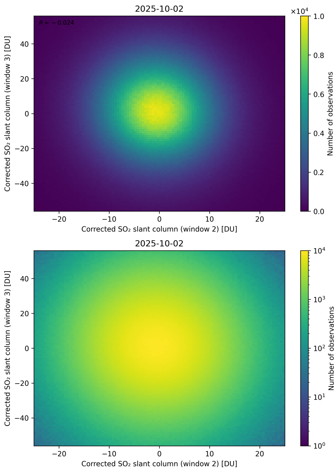
Figure 250: Scatter density plot of “Corrected SO 2 slant column (window 2)” against “Corrected SO 2 slant column (window 3)” for 2025-10-01 to 2025-10-03.
