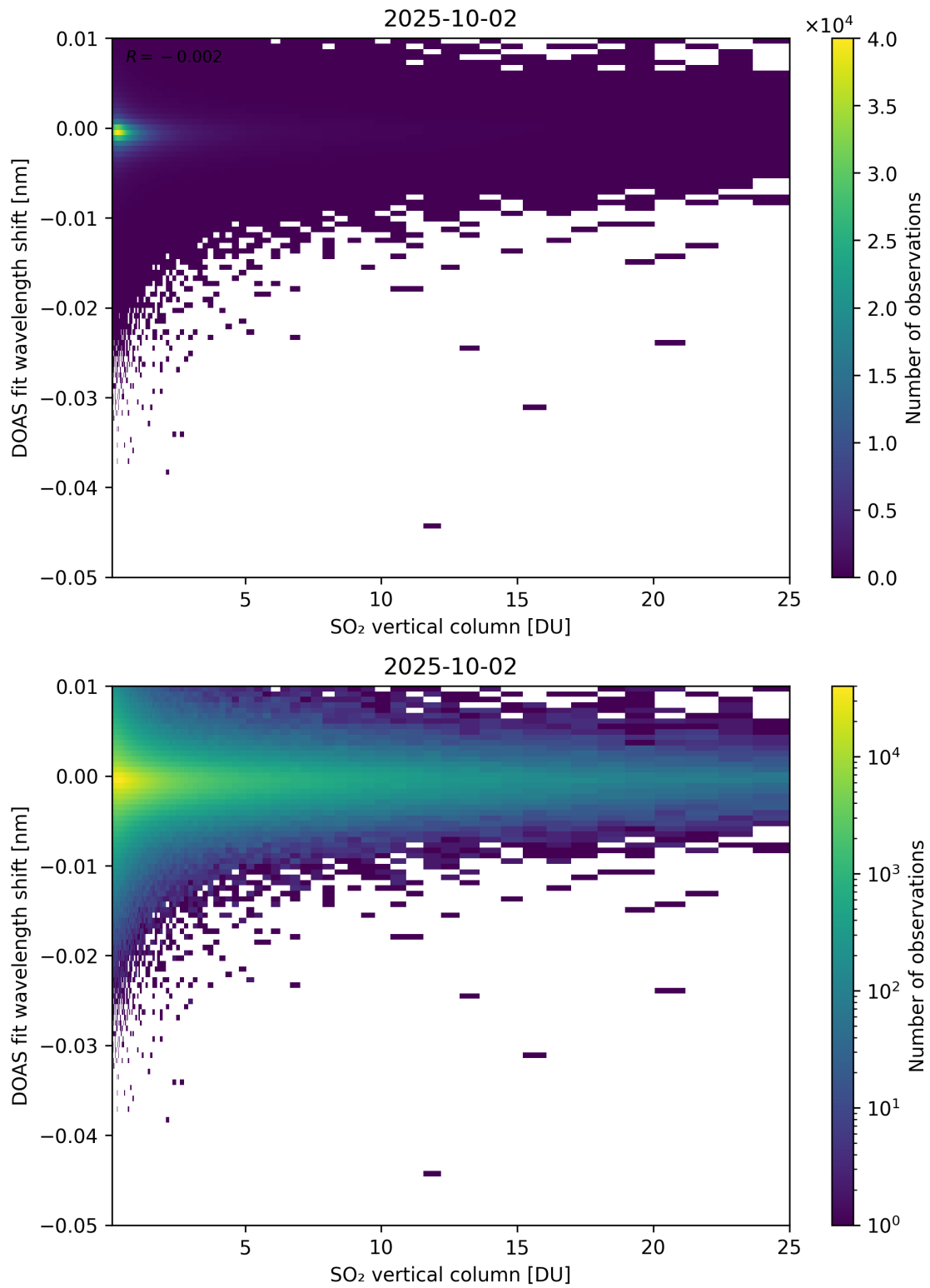
Figure 326: Scatter density plot of “SO 2 vertical column” against “DOAS fit wavelength shift” for 2025-10-01 to 2025-10-03.
