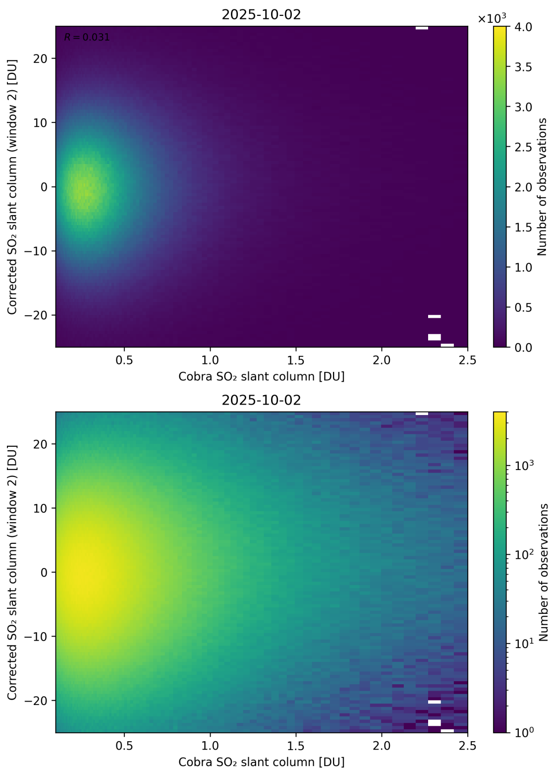
Figure 217: Scatter density plot of “Cobra SO 2 slant column” against “Corrected SO 2 slant column (window 2)” for 2025-10-01 to 2025-10-03.
