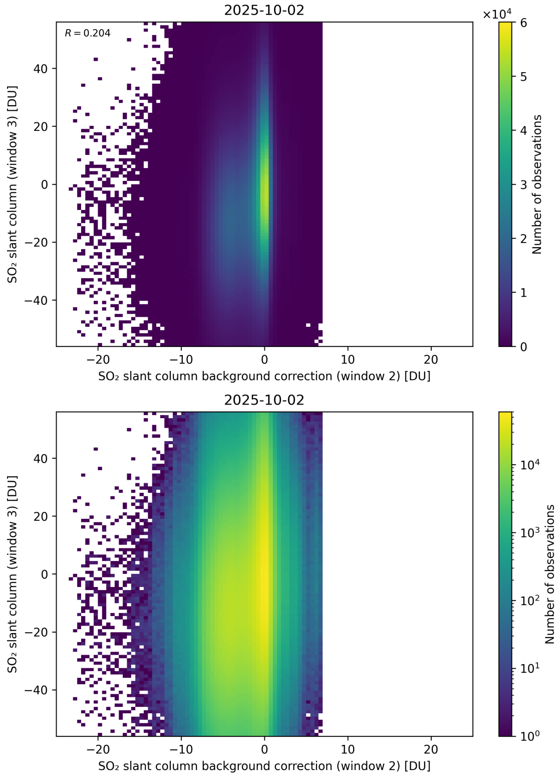
Figure 128: Scatter density plot of “SO 2 slant column background correction (window 2)” against “SO 2 slant column (window 3)” for 2025-10-01 to 2025-10-03.
