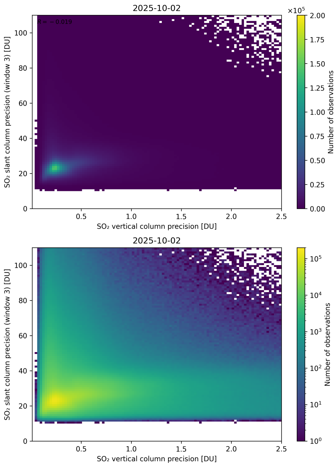
Figure 345: Scatter density plot of “SO 2 vertical column precision” against “SO 2 slant column precision (window 3)” for 2025-10-01 to 2025-10-03.
