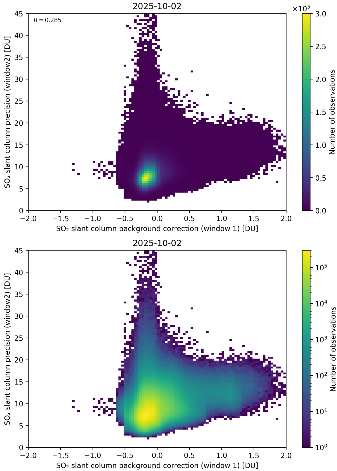
Figure 117: Scatter density plot of “SO 2 slant column background correction (window 1)” against “SO 2 slant column precision (window2)” for 2025-10-01 to 2025-10-03.
