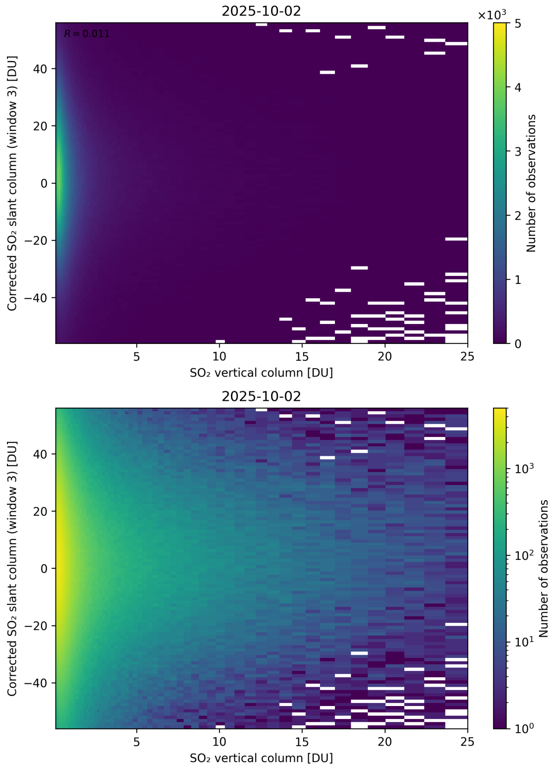
Figure 353: Scatter density plot of “SO 2 vertical column” against “Corrected SO 2 slant column (window 3)” for 2025-10-01 to 2025-10-03.
