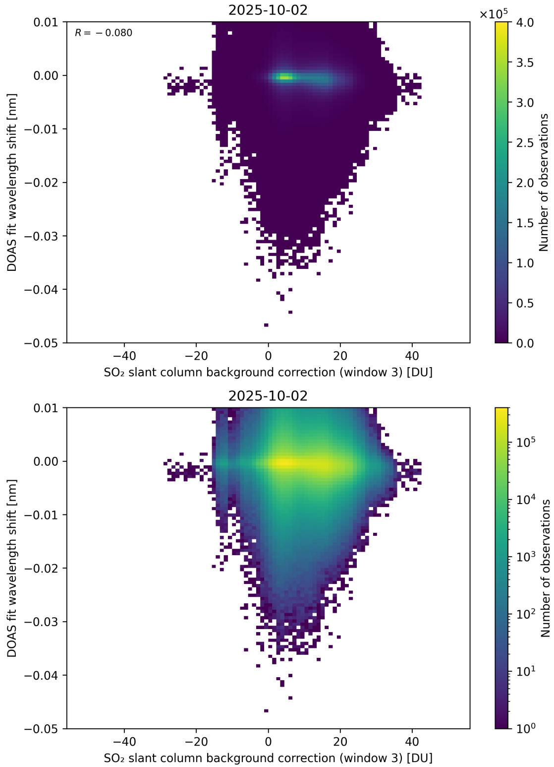
Figure 132: Scatter density plot of “SO 2 slant column background correction (window 3)” against “DOAS fit wavelength shift” for 2025-10-01 to 2025-10-03.
