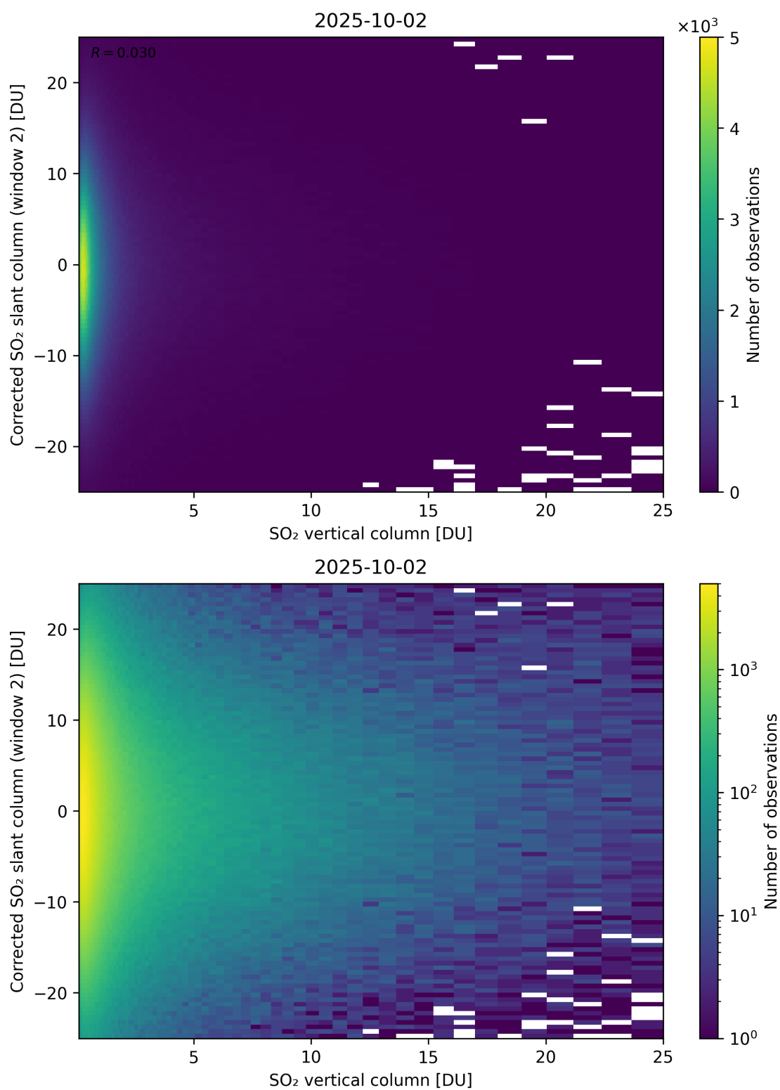
Figure 352: Scatter density plot of “SO 2 vertical column” against “Corrected SO 2 slant column (window 2)” for 2025-10-01 to 2025-10-03.
