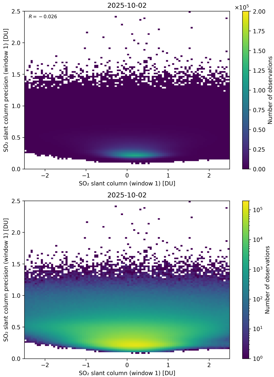
Figure 285: Scatter density plot of “SO 2 slant column (window 1)” against “SO 2 slant column precision (window 1)” for 2025-10-01 to 2025-10-03.
