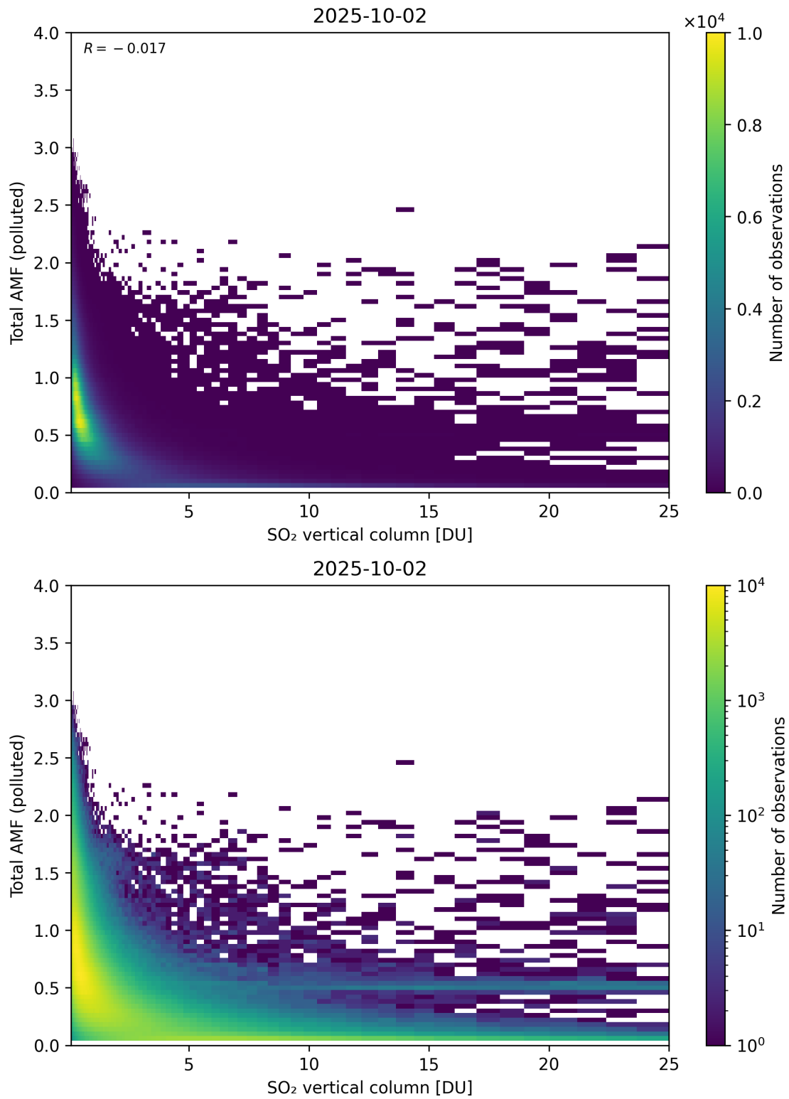
Figure 359: Scatter density plot of “SO 2 vertical column” against “Total AMF (polluted)” for 2025-10-01 to 2025-10-03.
