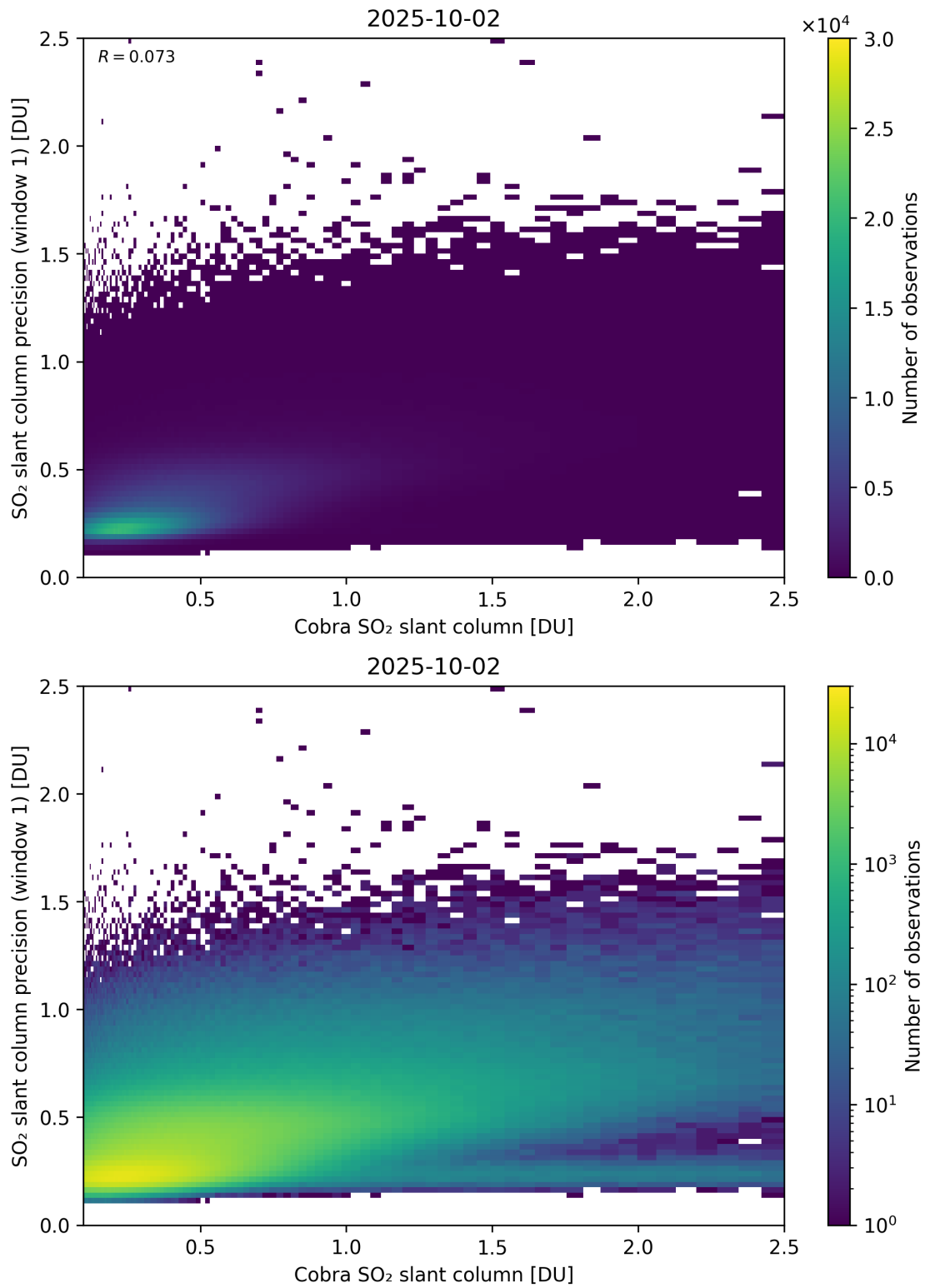
Figure 220: Scatter density plot of “Cobra SO 2 slant column” against “SO 2 slant column precision (window 1)” for 2025-10-01 to 2025-10-03.
