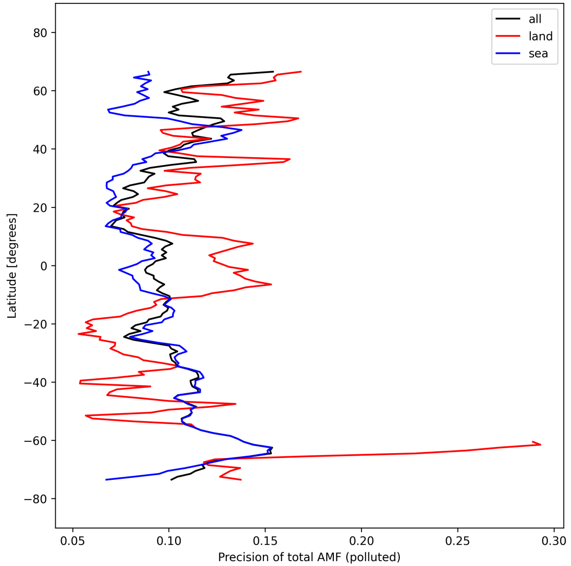
Figure 54: Zonal average of “Precision of total AMF (polluted)” for 2025-10-01 to 2025-10-03.
