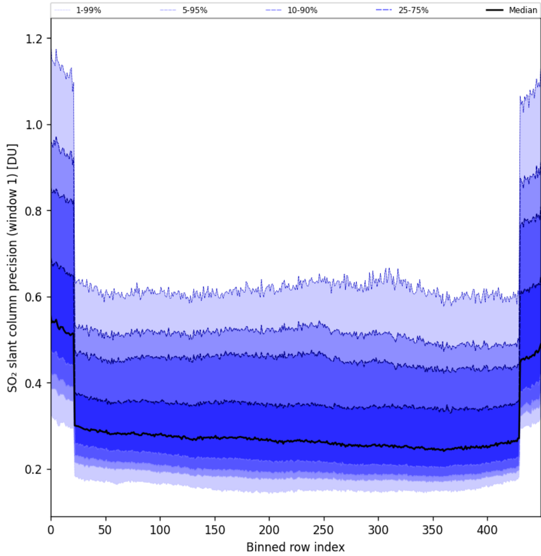
Figure 90: Along track statistics of “SO 2 slant column precision (window 1)” for 2025-10-01 to 2025-10-03
