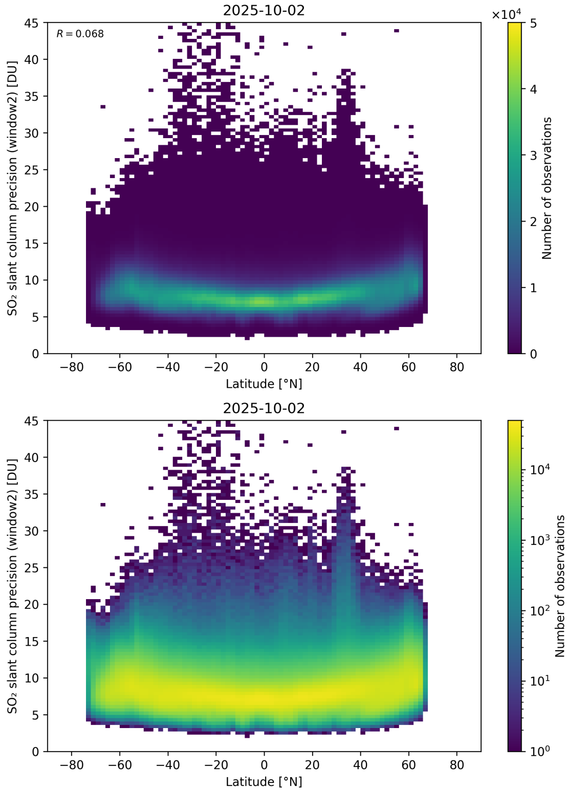
Figure 164: Scatter density plot of “Latitude” against “SO 2 slant column precision (window2)” for 2025-10-01 to 2025-10-03.
