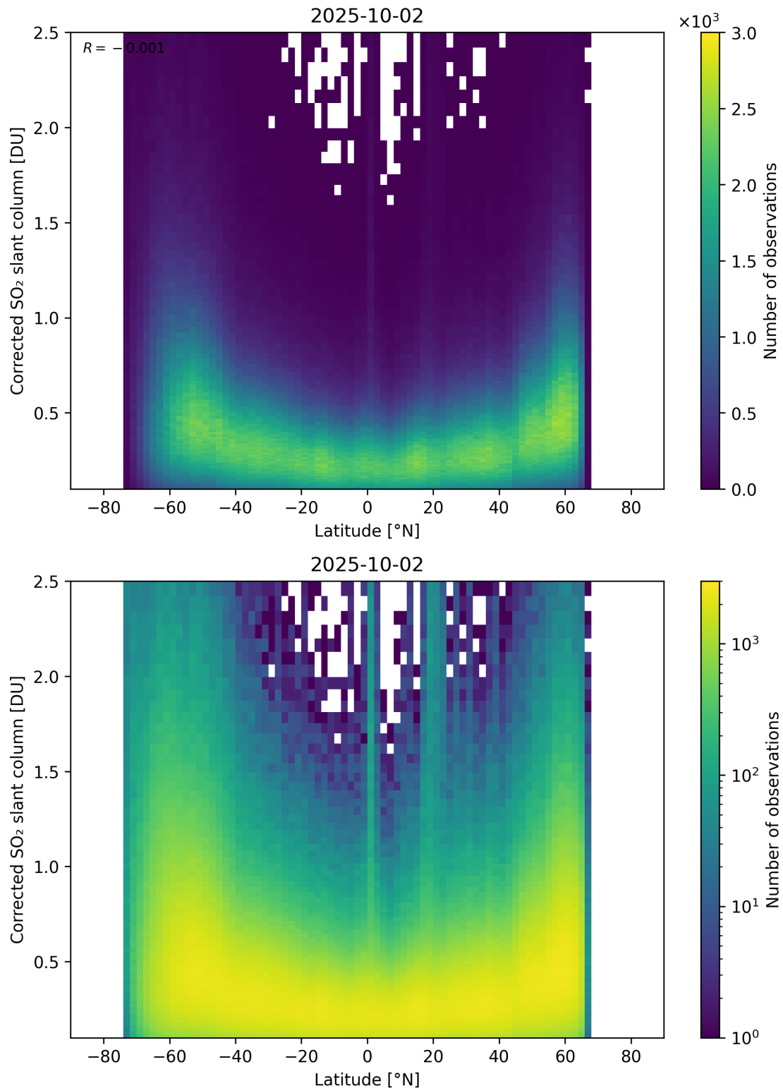
Figure 159: Scatter density plot of “Latitude” against “Corrected SO 2 slant column” for 2025-10-01 to 2025-10-03.
