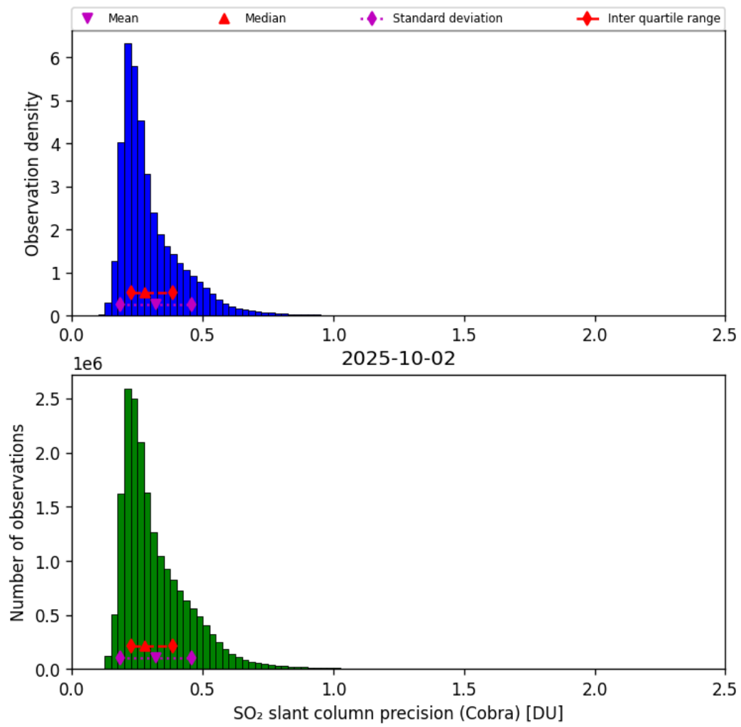
Figure 62: Histogram of “SO 2 slant column precision (Cobra)” for 2025-10-01 to 2025-10-03
