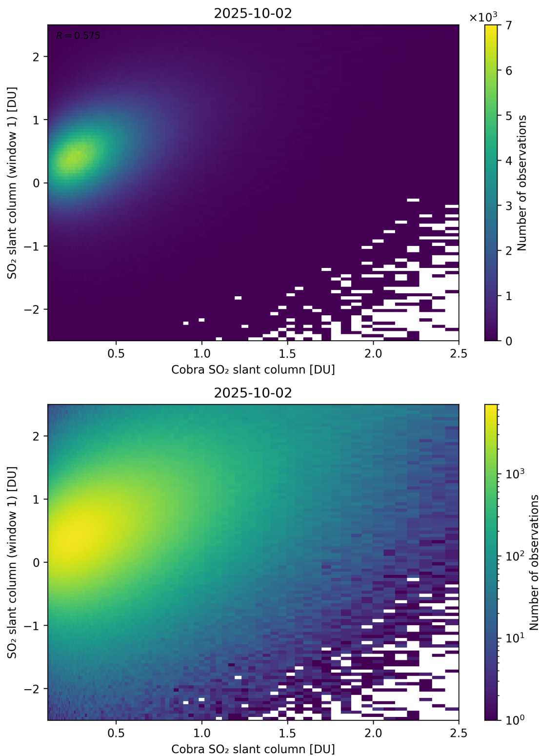
Figure 219: Scatter density plot of “Cobra SO 2 slant column” against “SO 2 slant column (window 1)” for 2025-10-01 to 2025-10-03.
