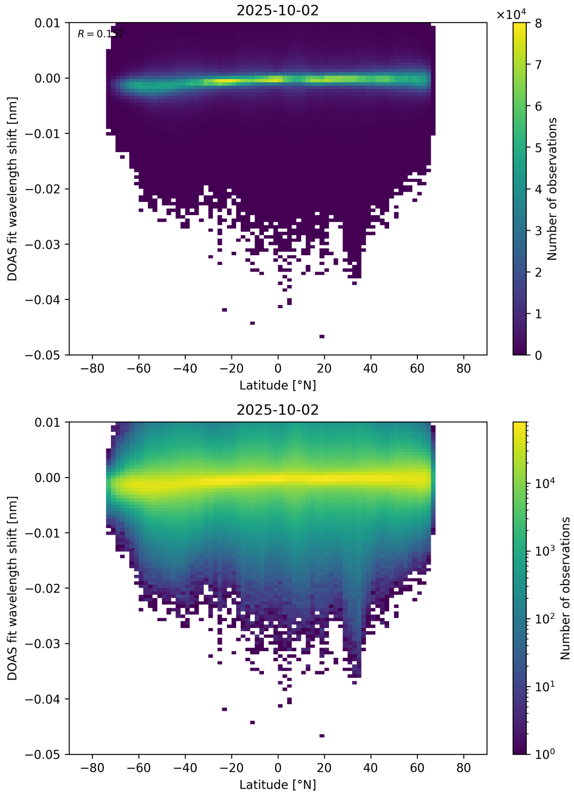
Figure 153: Scatter density plot of “Latitude” against “DOAS fit wavelength shift” for 2025-10-01 to 2025-10-03.
