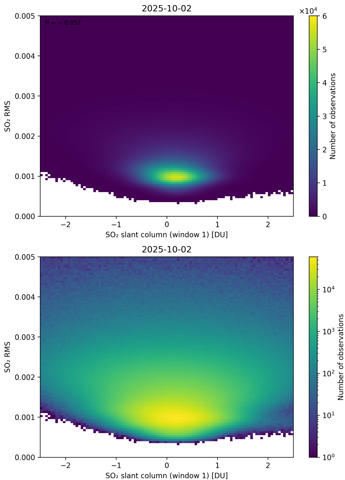
Figure 267: Scatter density plot of “SO 2 slant column (window 1)” against “SO 2 RMS” for 2025-10-01 to 2025-10-03.
