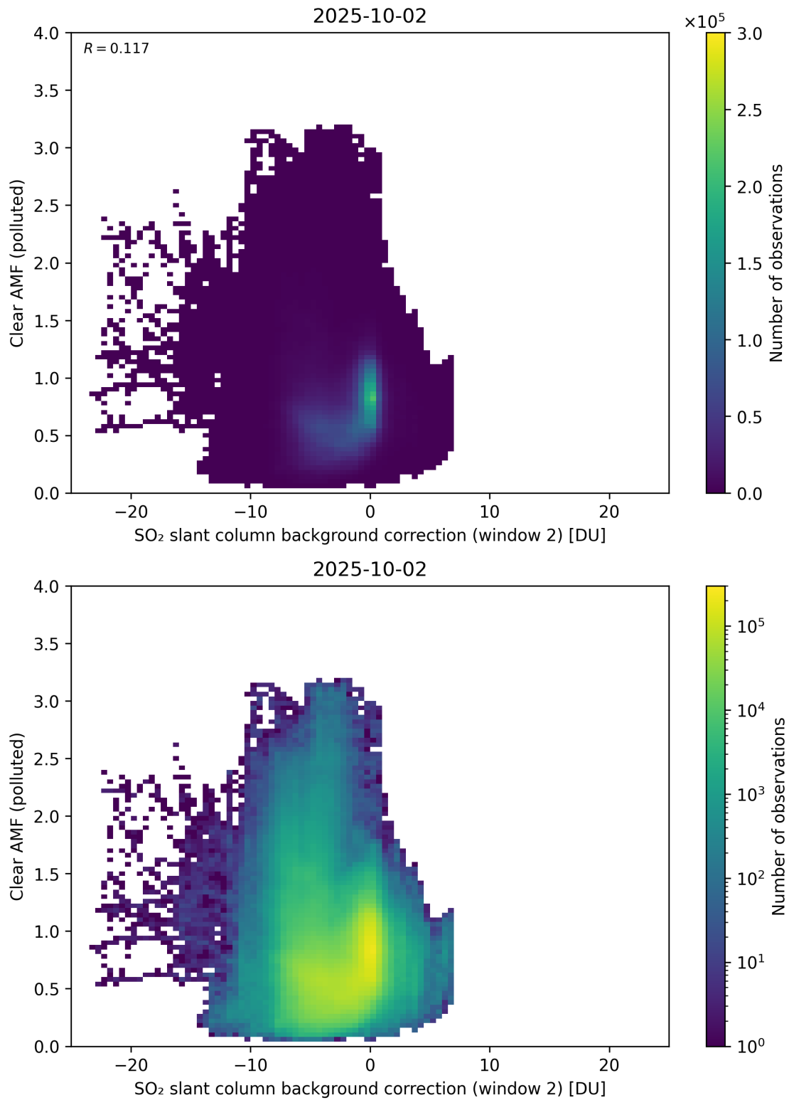
Figure 126: Scatter density plot of “SO 2 slant column background correction (window 2)” against “Clear AMF (polluted)” for 2025-10-01 to 2025-10-03.
