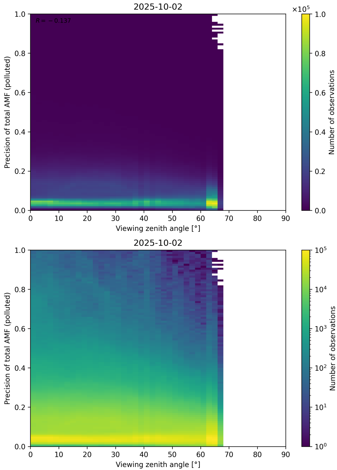
Figure 382: Scatter density plot of “Viewing zenith angle” against “Precision of total AMF (polluted)” for 2025-10-01 to 2025-10-03.
