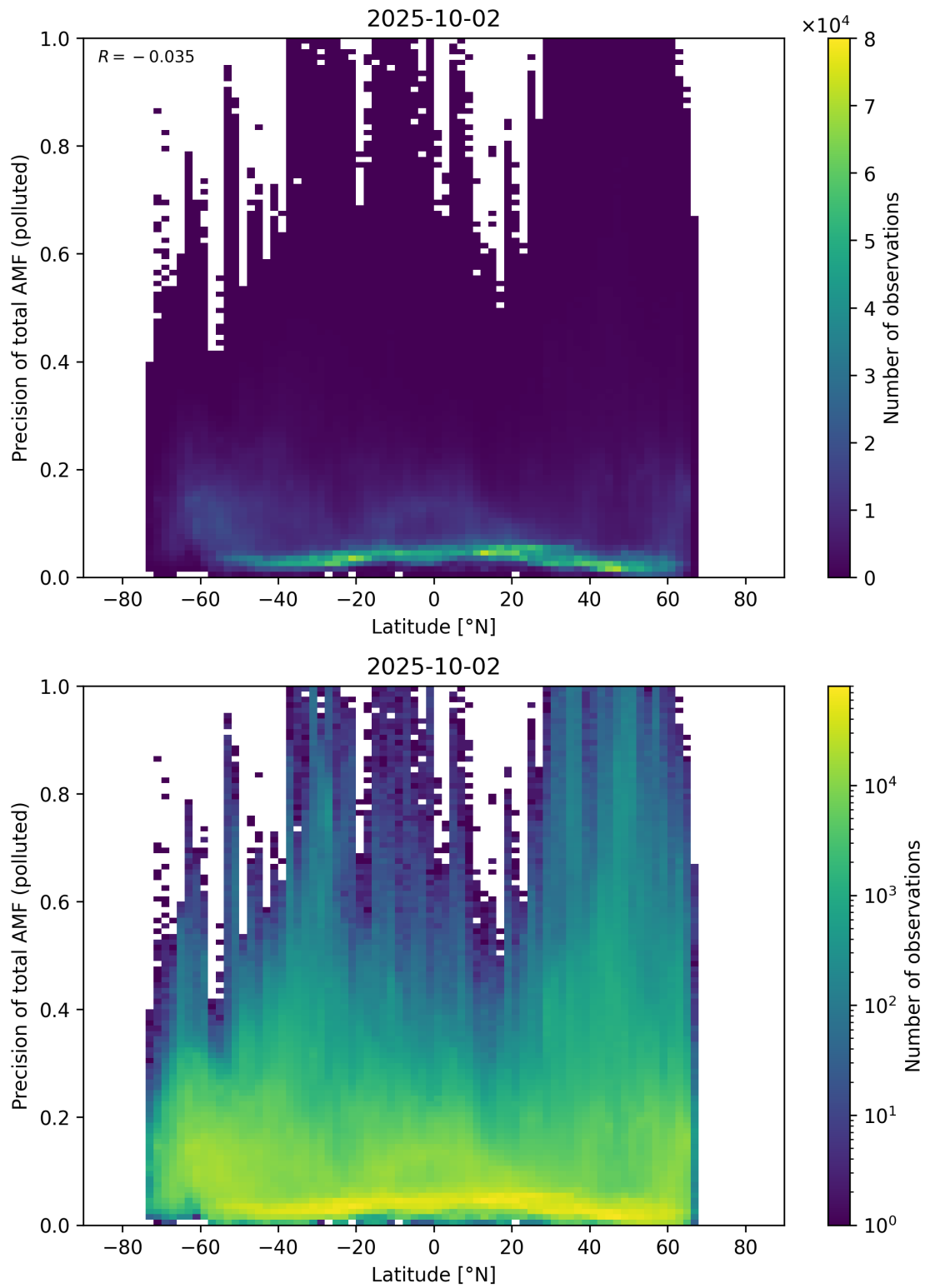
Figure 168: Scatter density plot of “Latitude” against “Precision of total AMF (polluted)” for 2025-10-01 to 2025-10-03.
