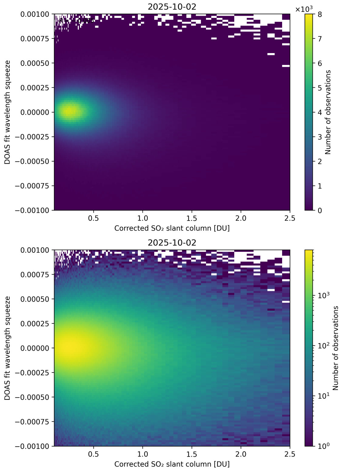
Figure 230: Scatter density plot of "Corrected SO 2 slant column" against "DOAS fit wavelength squeeze" for 2025-10-01 to 2025-10-03.
