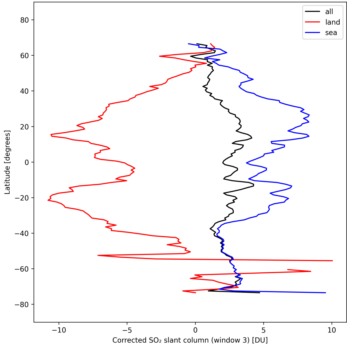
Figure 47: Zonal average of “Corrected SO 2 slant column (window 3)” for 2025-10-01 to 2025-10-03.
