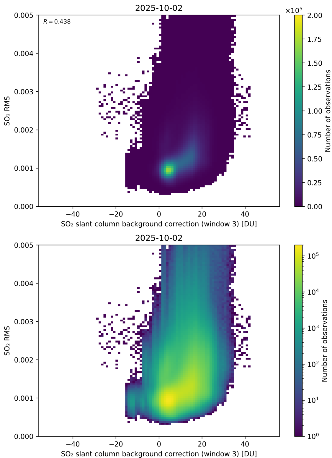
Figure 134: Scatter density plot of “SO 2 slant column background correction (window 3)” against “SO 2 RMS” for 2025-10-01 to 2025-10-03.
