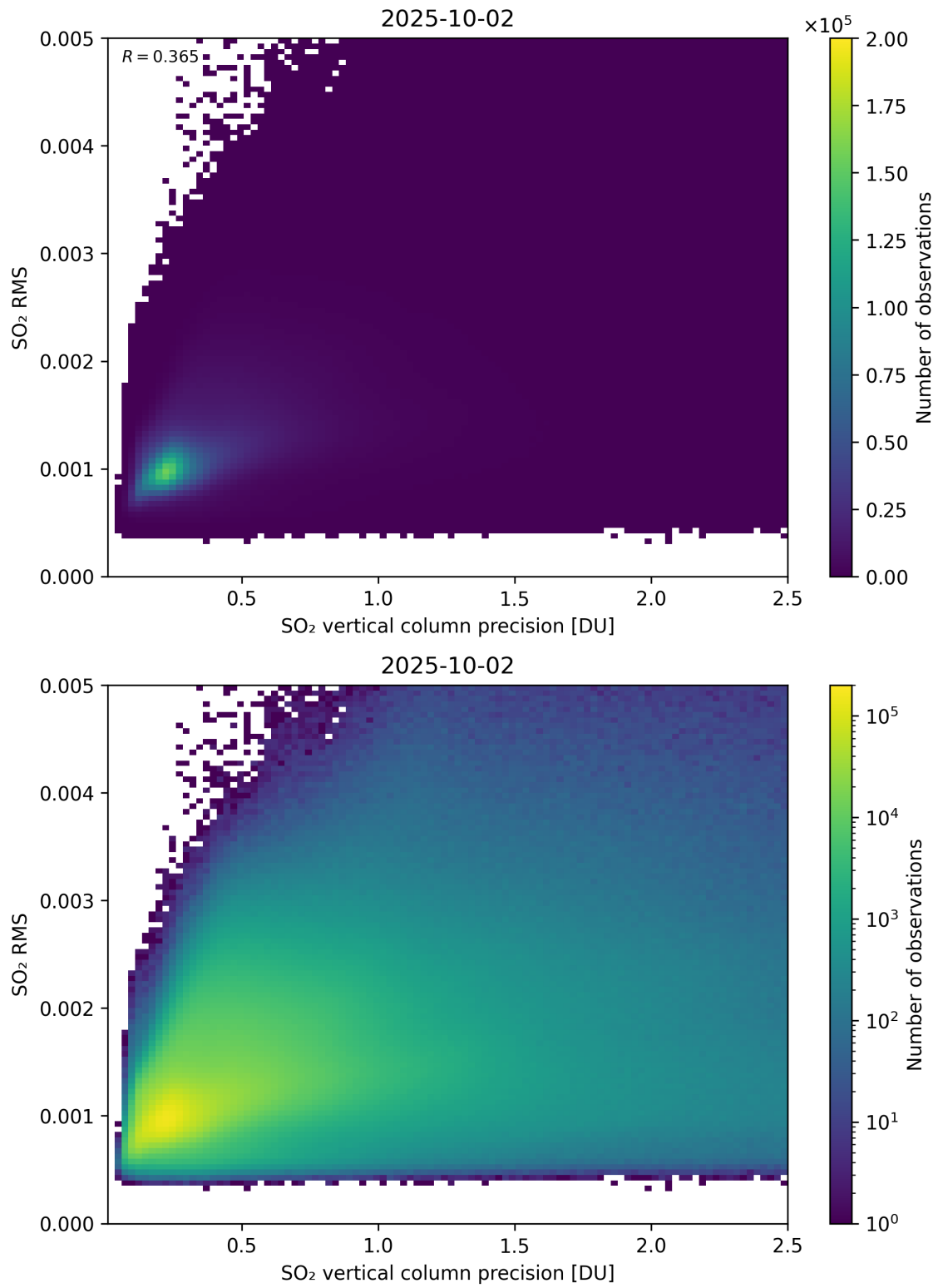
Figure 334: Scatter density plot of “SO 2 vertical column precision” against “SO 2 RMS” for 2025-10-01 to 2025-10-03.
