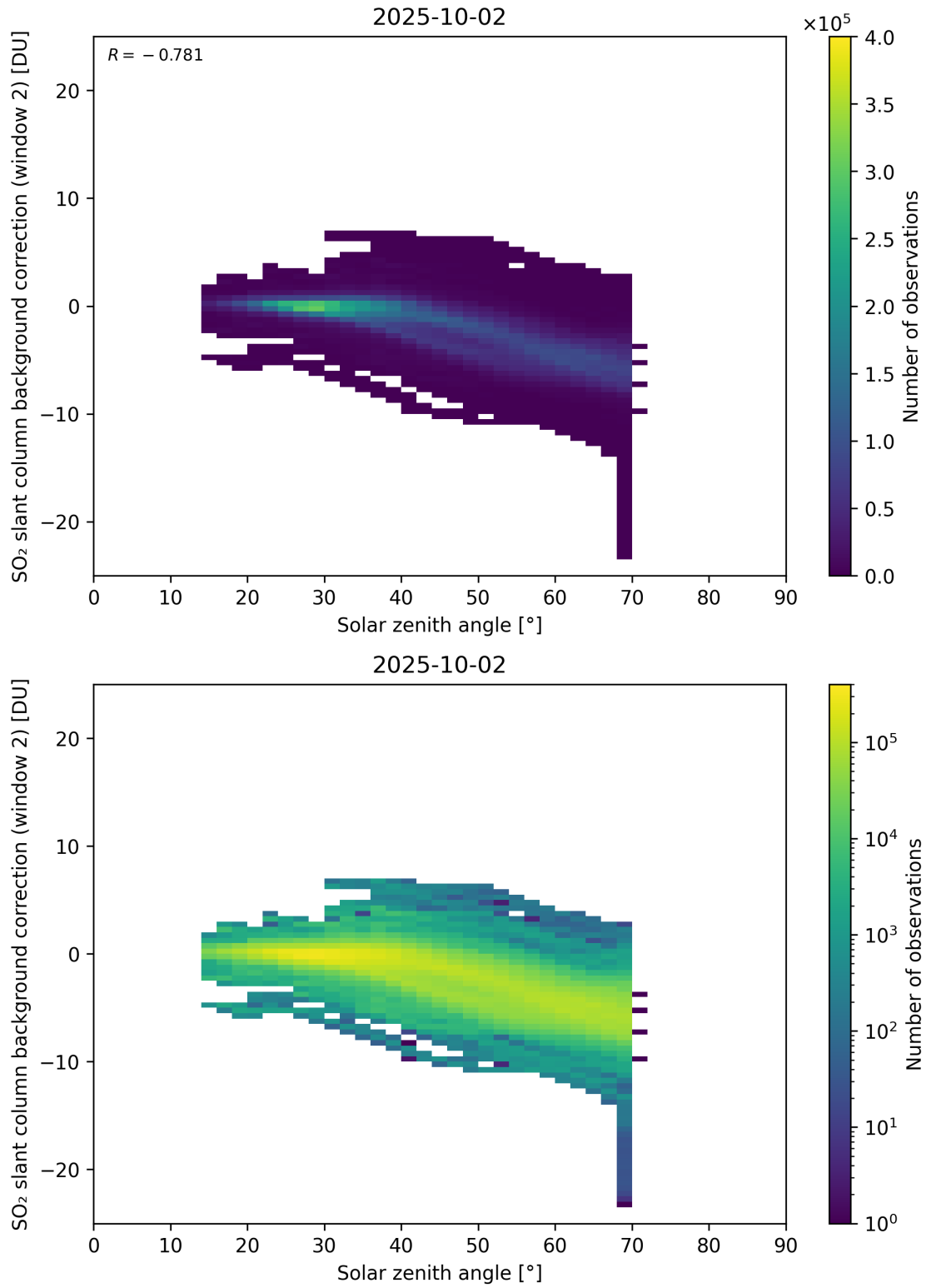
Figure 172: Scatter density plot of “Solar zenith angle” against “SO 2 slant column background correction (window 2)” for 2025-10-01 to 2025-10-03.
