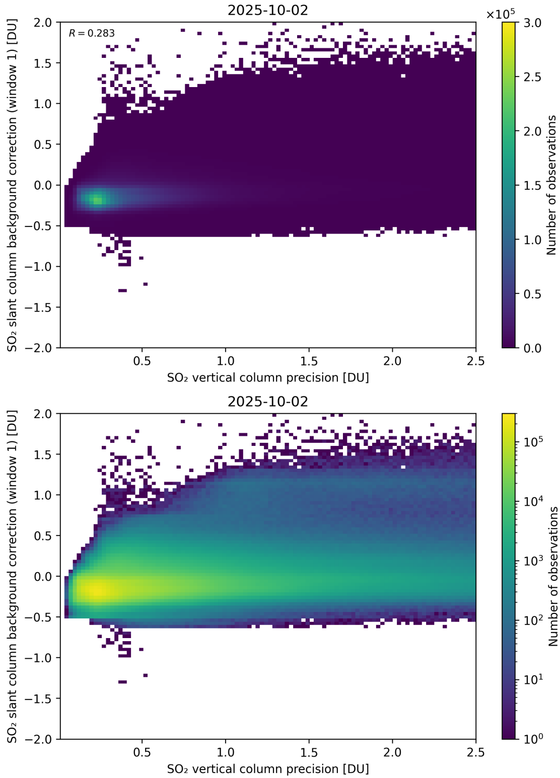
Figure 329: Scatter density plot of “SO 2 vertical column precision” against “SO 2 slant column background correction (window 1)” for 2025-10-01 to 2025-10-03.
