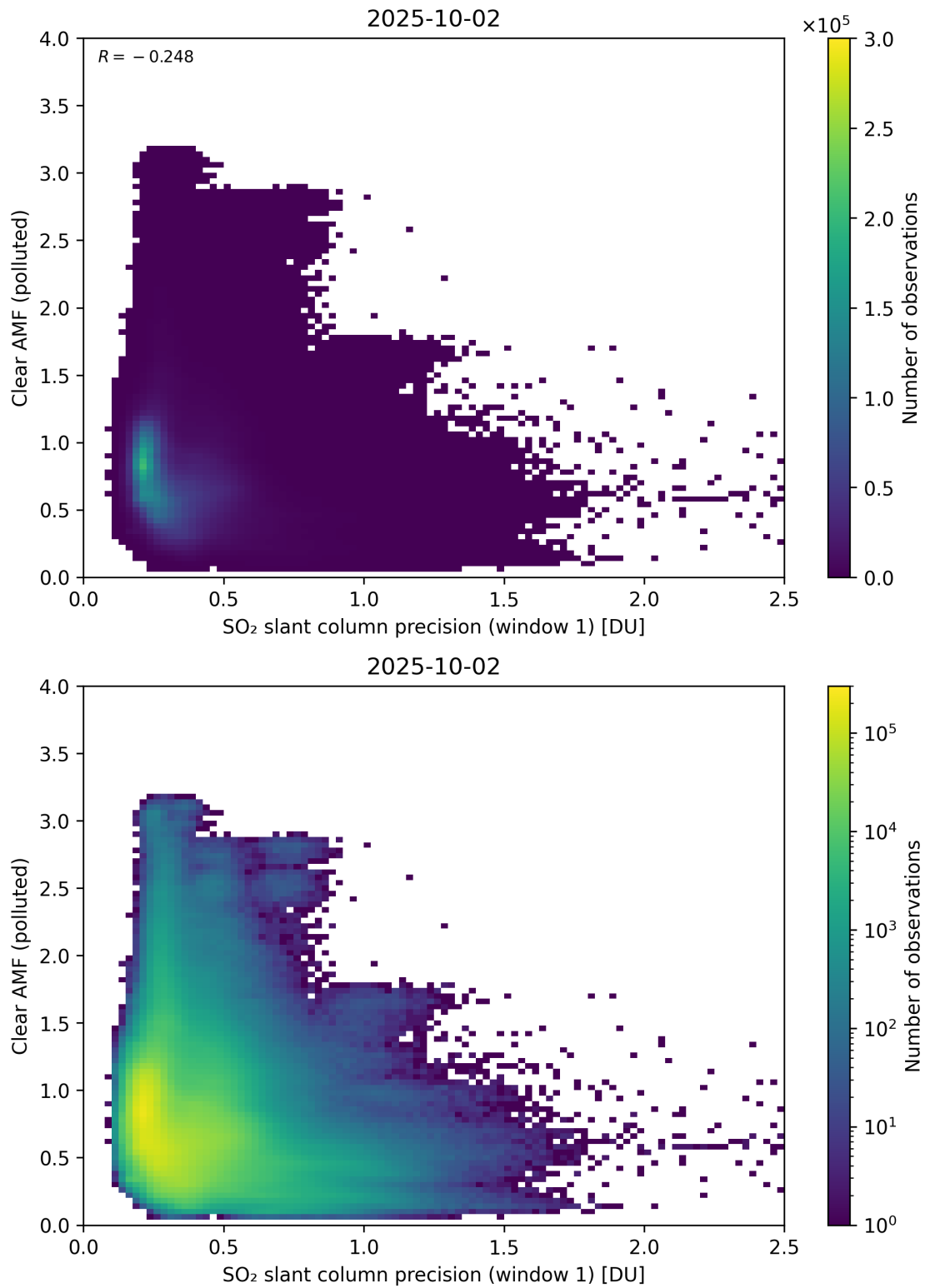
Figure 274: Scatter density plot of “SO 2 slant column precision (window 1)” against “Clear AMF (polluted)” for 2025-10-01 to 2025-10-03.
