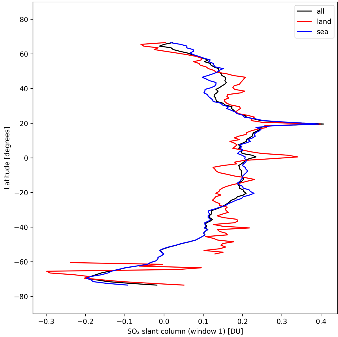
Figure 37: Zonal average of “SO 2 slant column (window 1)” for 2025-10-01 to 2025-10-03.
