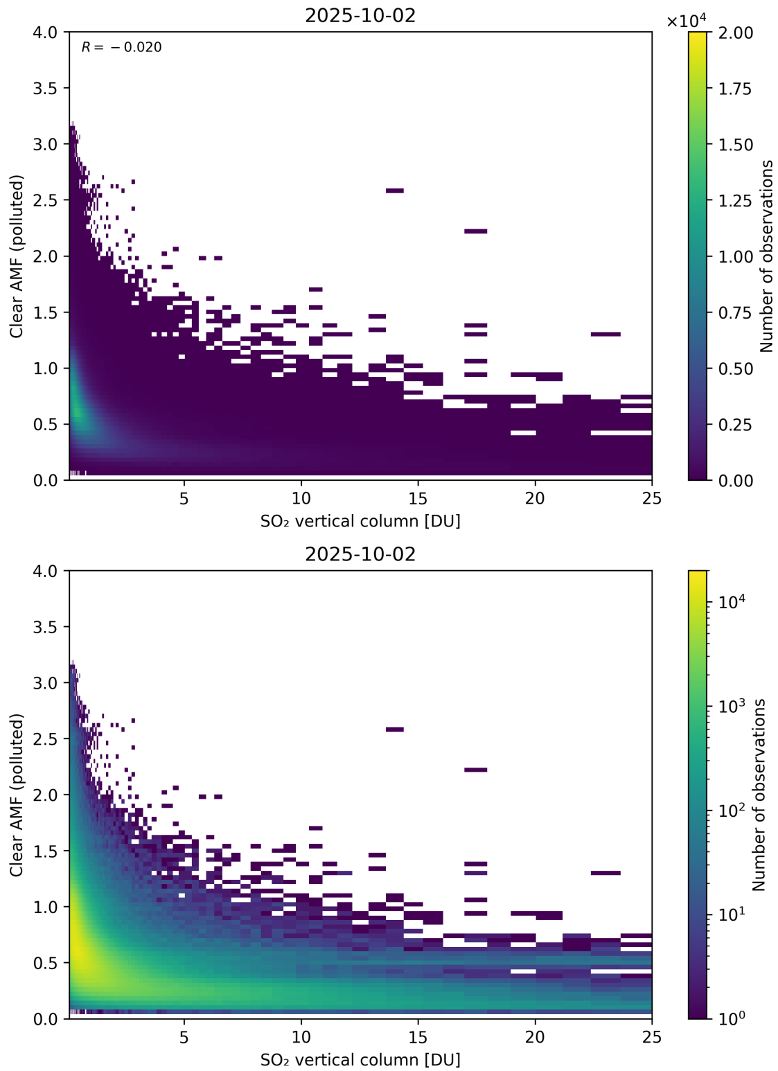
Figure 348: Scatter density plot of “SO 2 vertical column” against “Clear AMF (polluted)” for 2025-10-01 to 2025-10-03.
