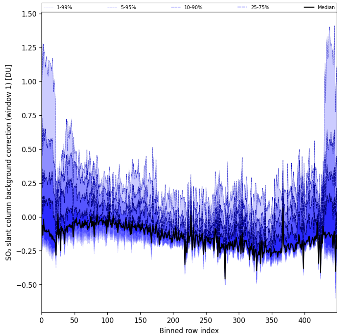
Figure 92: Along track statistics of “SO 2 slant column background correction (window 1)” for 2025-10-01 to 2025-10-03
