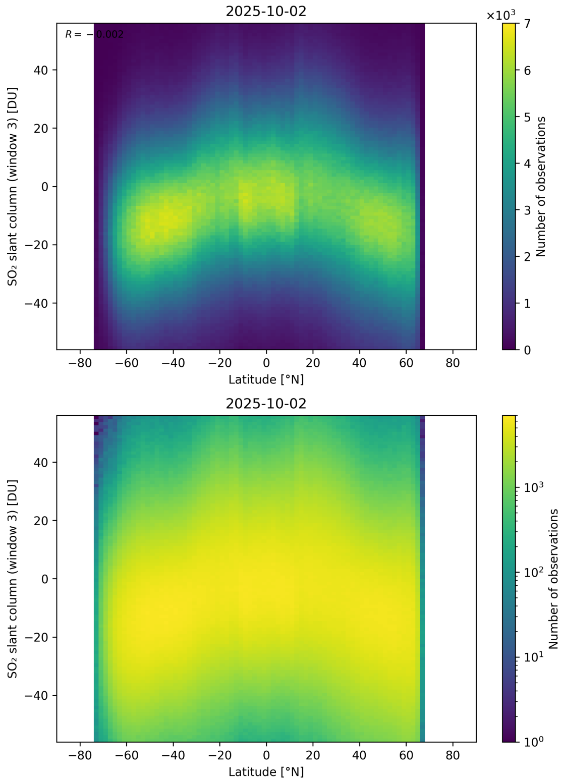
Figure 165: Scatter density plot of “Latitude” against “SO 2 slant column (window 3)” for 2025-10-01 to 2025-10-03.
