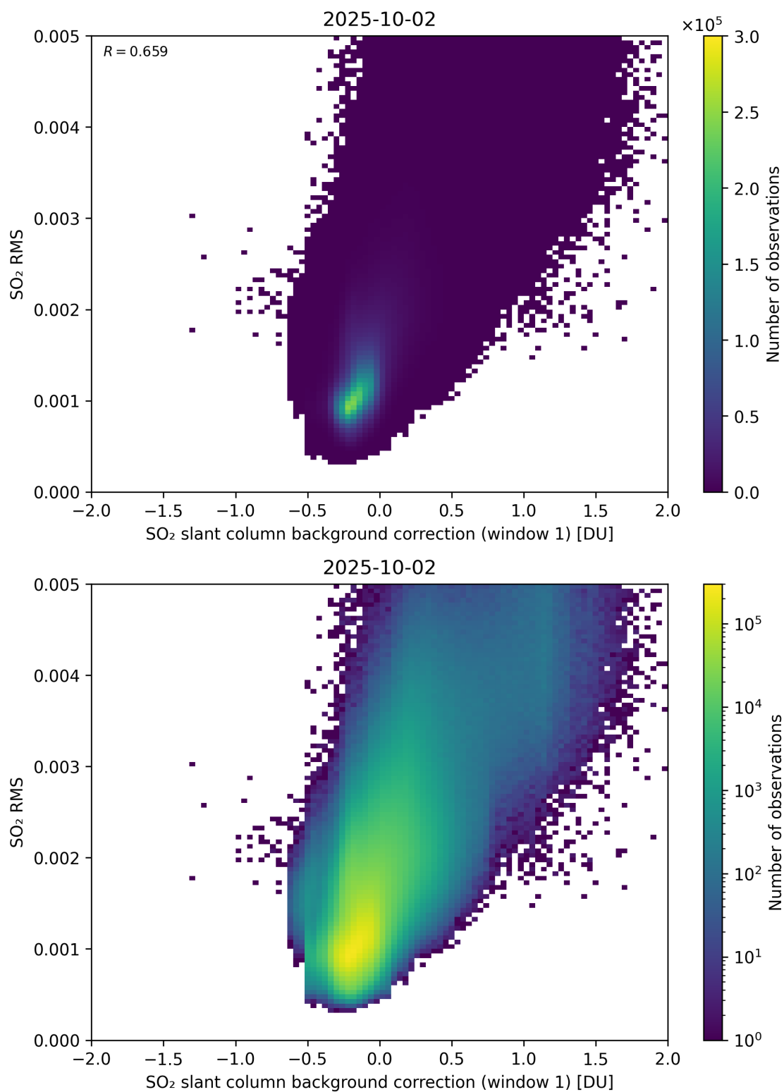
Figure 113: Scatter density plot of “SO 2 slant column background correction (window 1)” against “SO 2 RMS” for 2025-10-01 to 2025-10-03.
