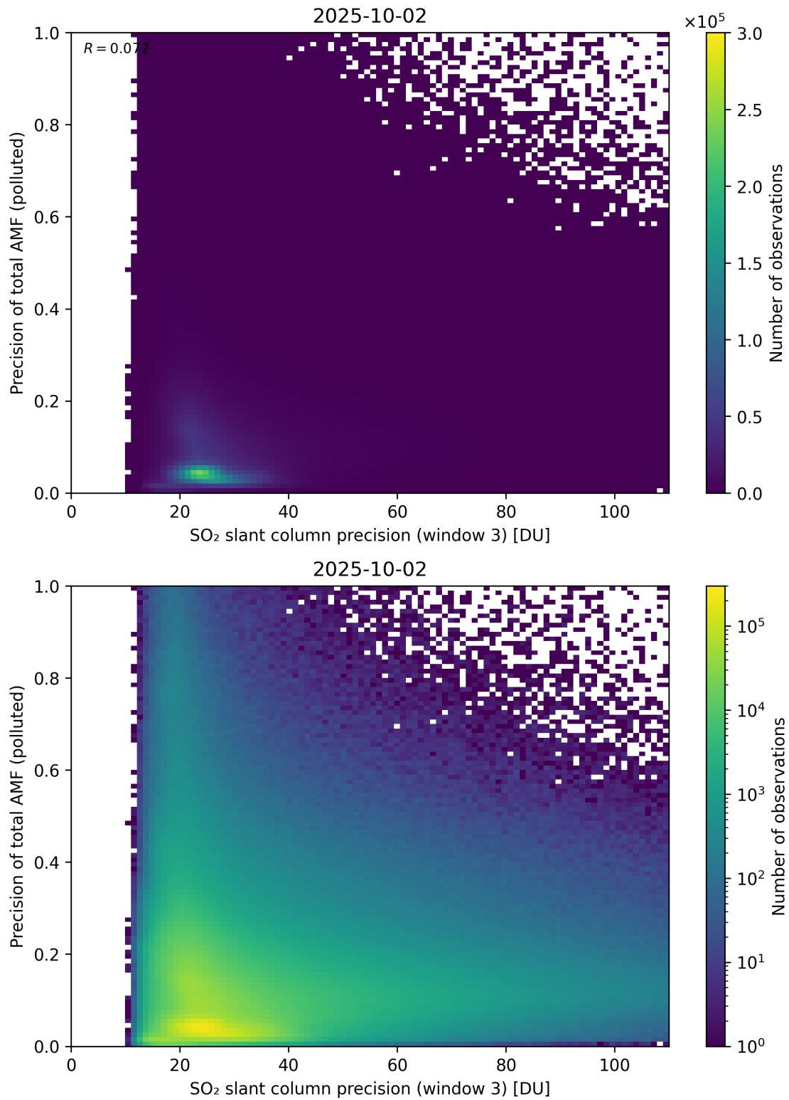
Figure 314: Scatter density plot of “SO 2 slant column precision (window 3)” against “Precision of total AMF (polluted)” for 2025-10-01 to 2025-10-03.
