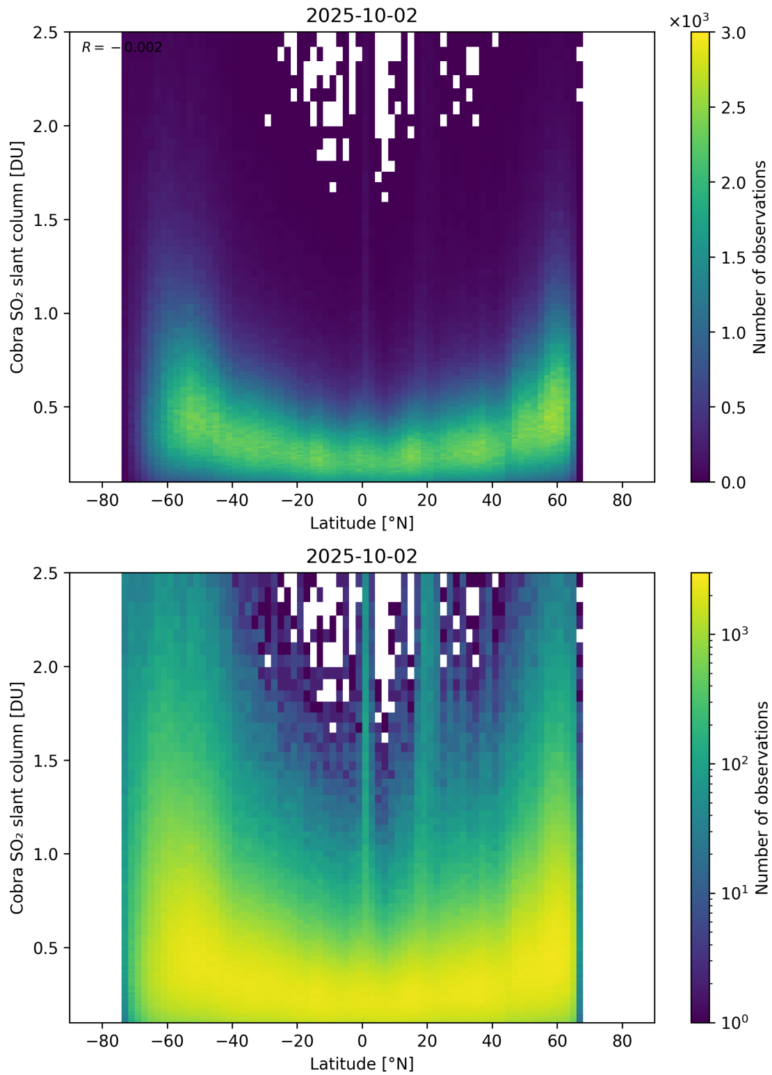
Figure 157: Scatter density plot of “Latitude” against “Cobra SO 2 slant column” for 2025-10-01 to 2025-10-03.
