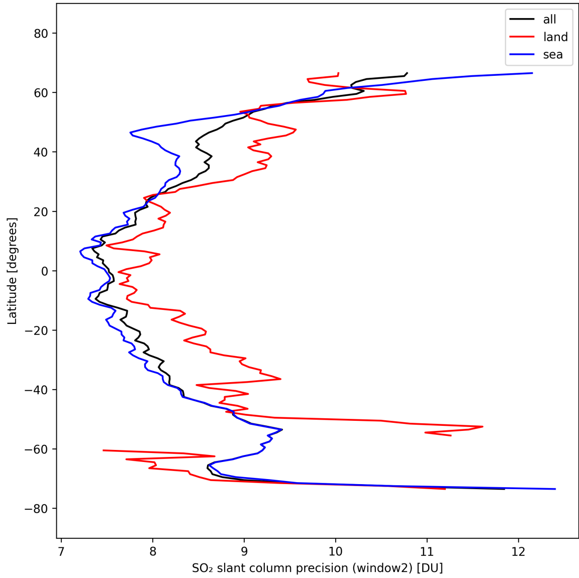
Figure 42: Zonal average of “SO 2 slant column precision (window2)” for 2025-10-01 to 2025-10-03.
