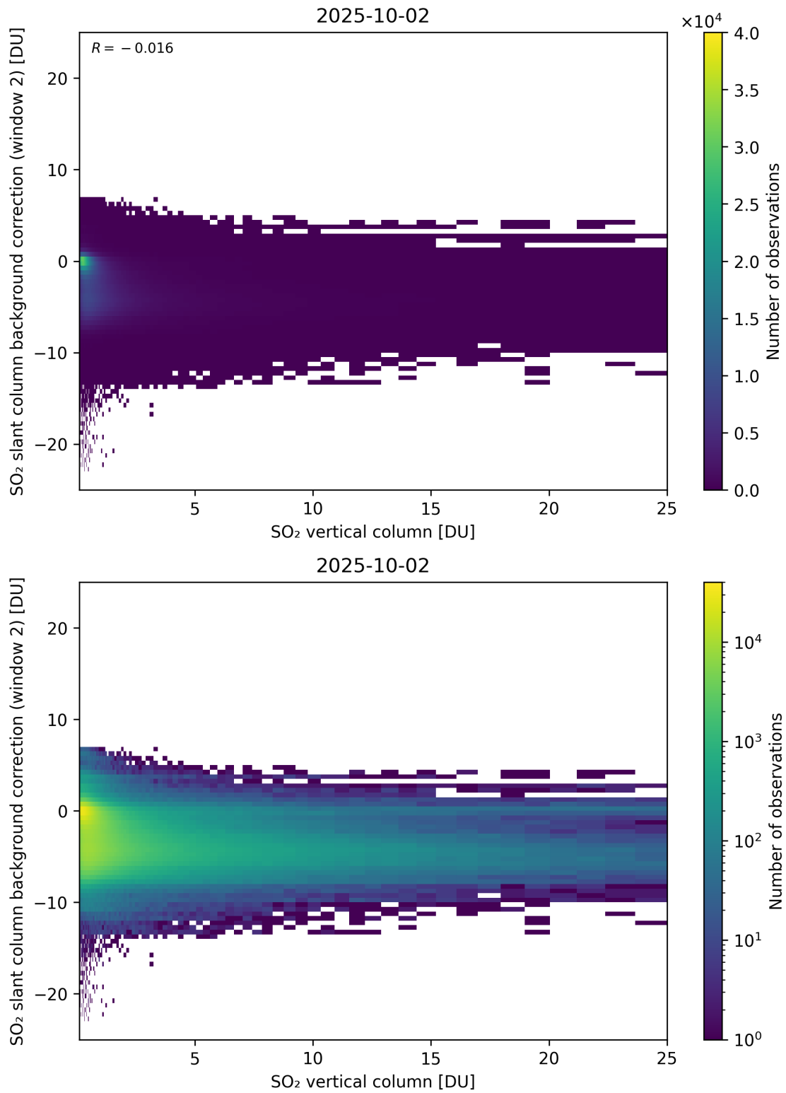
Figure 324: Scatter density plot of “SO 2 vertical column” against “SO 2 slant column background correction (window 2)” for 2025-10-01 to 2025-10-03.
