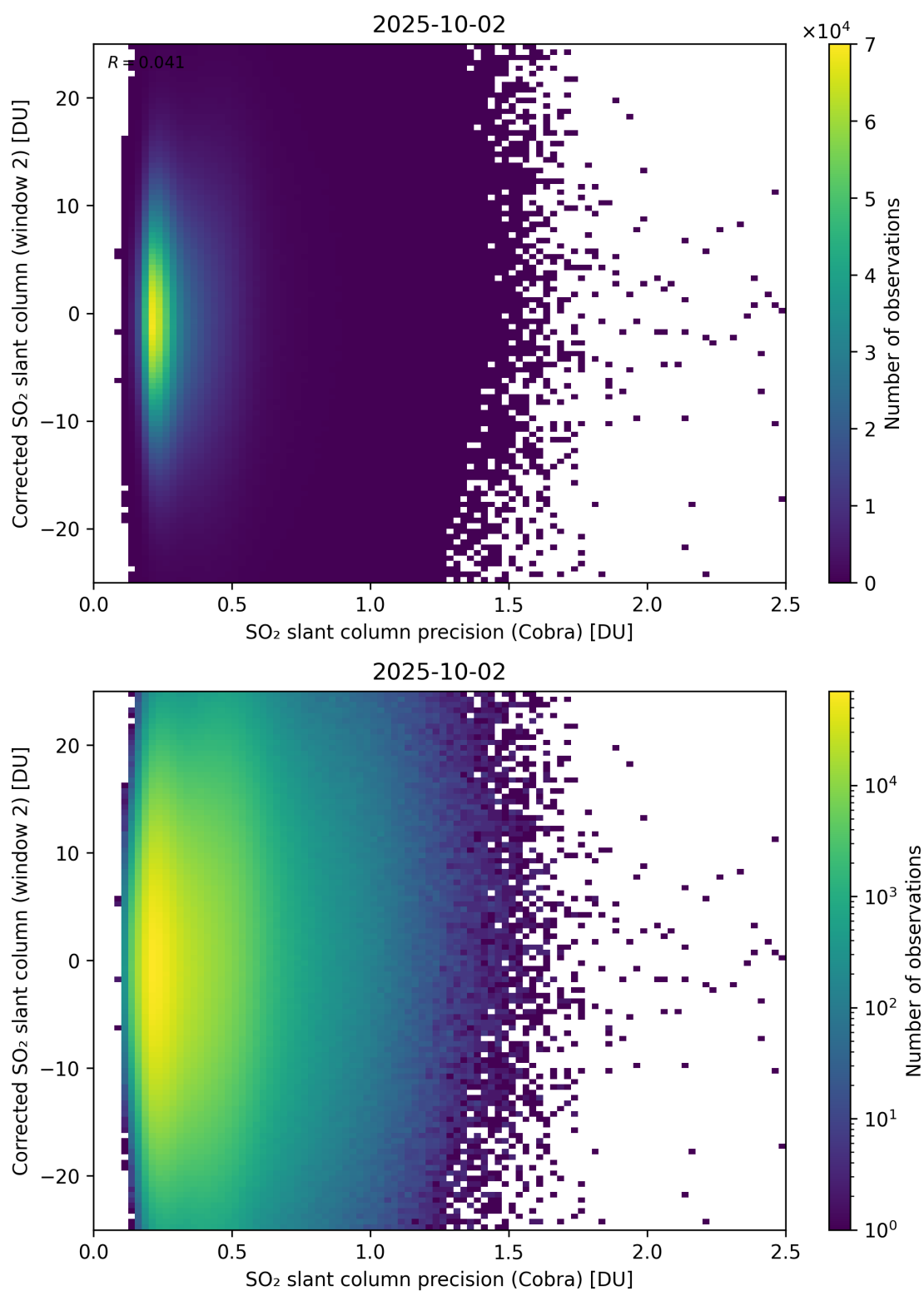
Figure 206: Scatter density plot of “SO 2 slant column precision (Cobra)” against “Corrected SO 2 slant column (window 2)” for 2025-10-01 to 2025-10-03.
