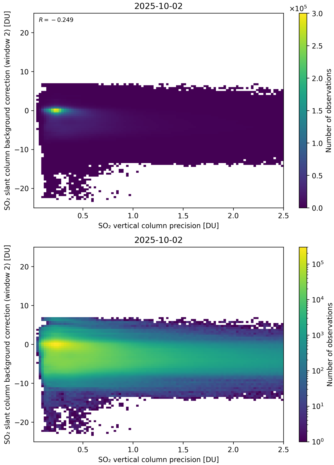
Figure 330: Scatter density plot of “SO 2 vertical column precision” against “SO 2 slant column background correction (window 2)” for 2025-10-01 to 2025-10-03.
