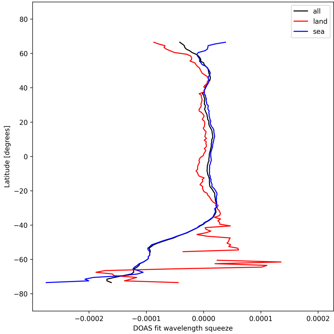
Figure 51: Zonal average of “DOAS fit wavelength squeeze” for 2025-10-01 to 2025-10-03.
