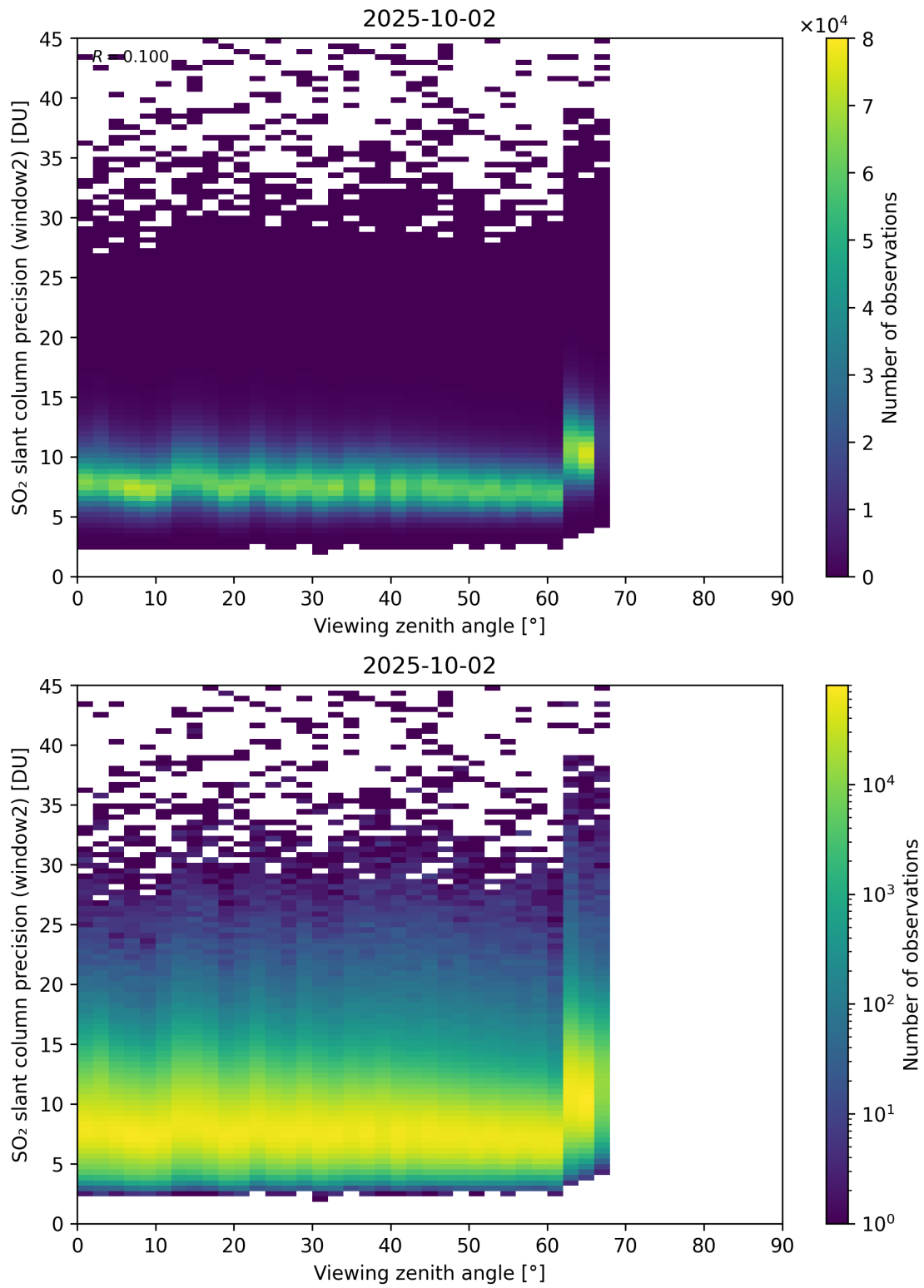
Figure 378: Scatter density plot of “Viewing zenith angle” against “SO 2 slant column precision (window2)” for 2025-10-01 to 2025-10-03.
