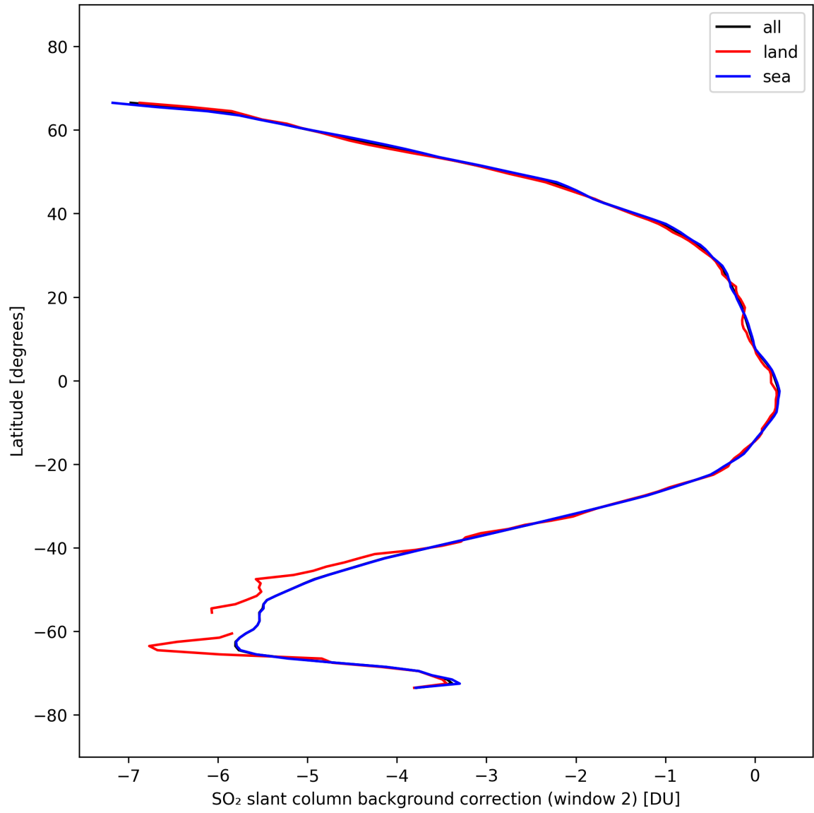
Figure 44: Zonal average of “SO 2 slant column background correction (window 2)” for 2025-10-01 to 2025-10-03.
