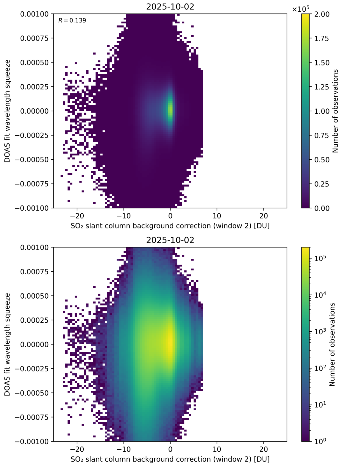
Figure 124: Scatter density plot of “SO 2 slant column background correction (window 2)” against “DOAS fit wavelength squeeze” for 2025-10-01 to 2025-10-03.
