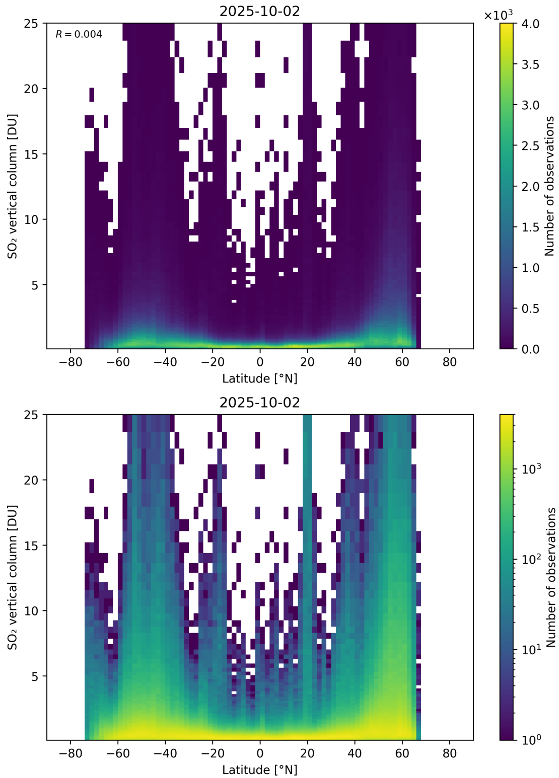
Figure 169: Scatter density plot of “Latitude” against “SO 2 vertical column” for 2025-10-01 to 2025-10-03.
