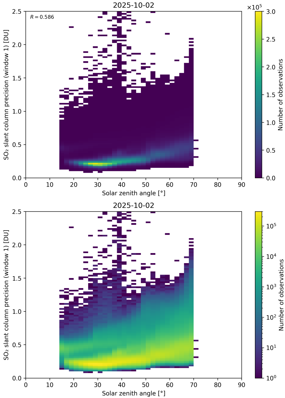
Figure 185: Scatter density plot of “Solar zenith angle” against “SO 2 slant column precision (window 1)” for 2025-10-01 to 2025-10-03.
