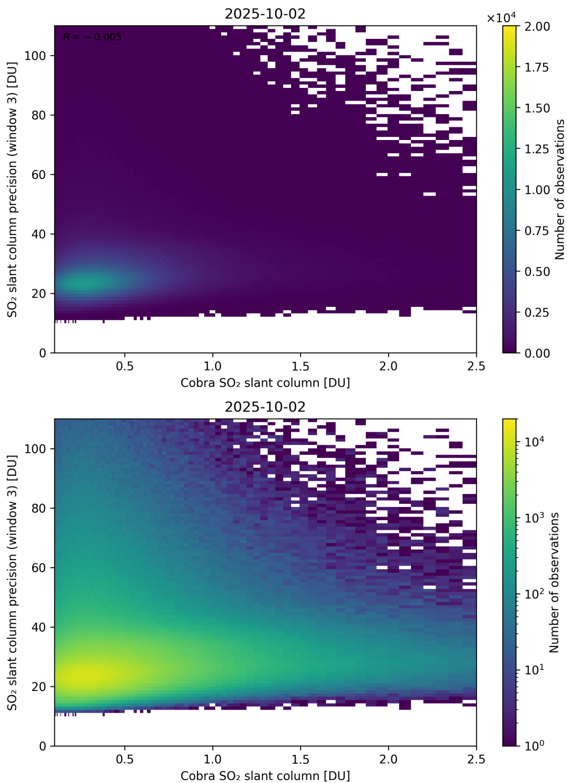
Figure 223: Scatter density plot of “Cobra SO 2 slant column” against “SO 2 slant column precision (window 3)” for 2025-10-01 to 2025-10-03.
