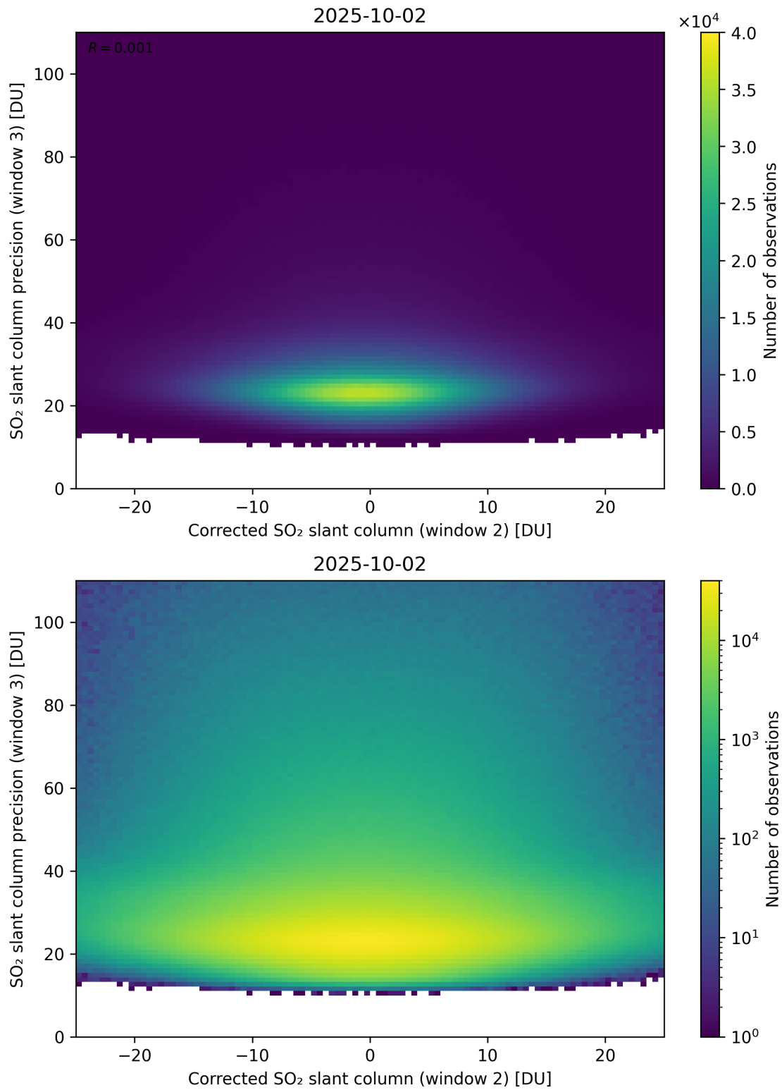
Figure 252: Scatter density plot of “Corrected SO 2 slant column (window 2)” against “SO 2 slant column precision (window 3)” for 2025-10-01 to 2025-10-03.
