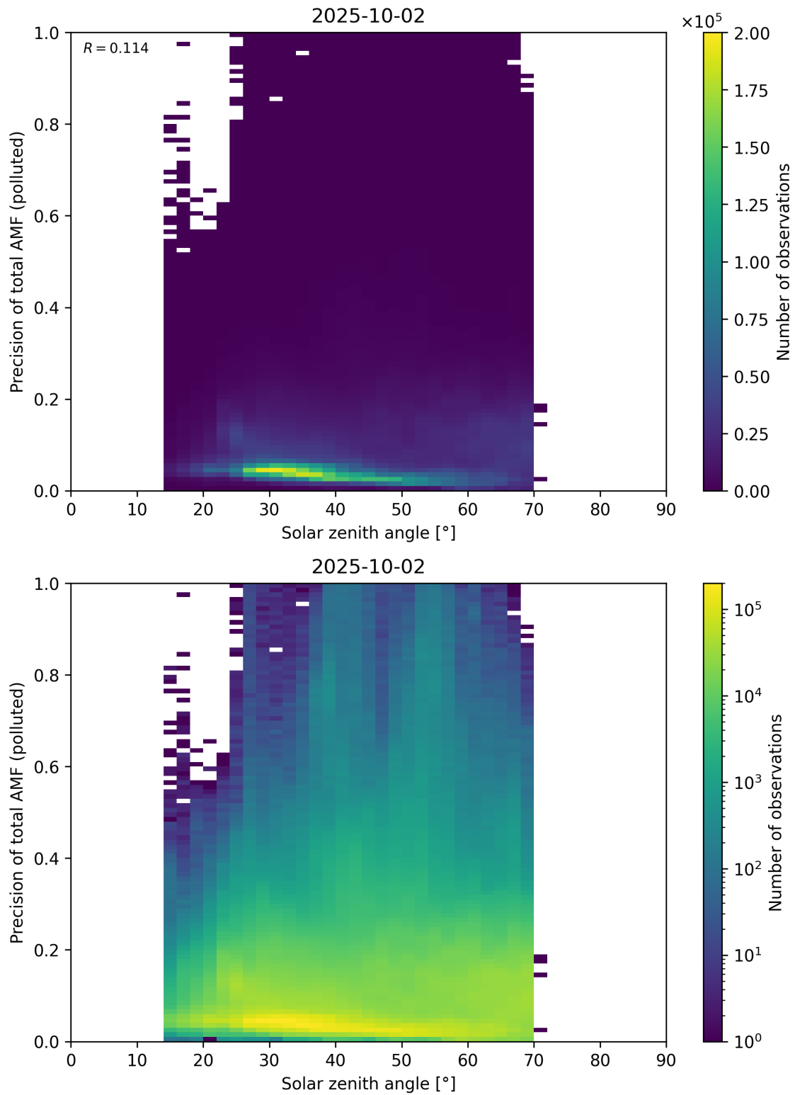
Figure 190: Scatter density plot of “Solar zenith angle” against “Precision of total AMF (polluted)” for 2025-10-01 to 2025-10-03.
