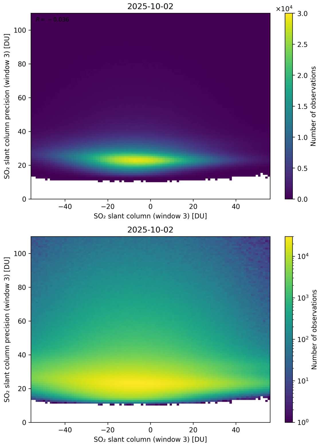
Figure 317: Scatter density plot of “SO 2 slant column (window 3)” against “SO 2 slant column precision (window 3)” for 2025-10-01 to 2025-10-03.
