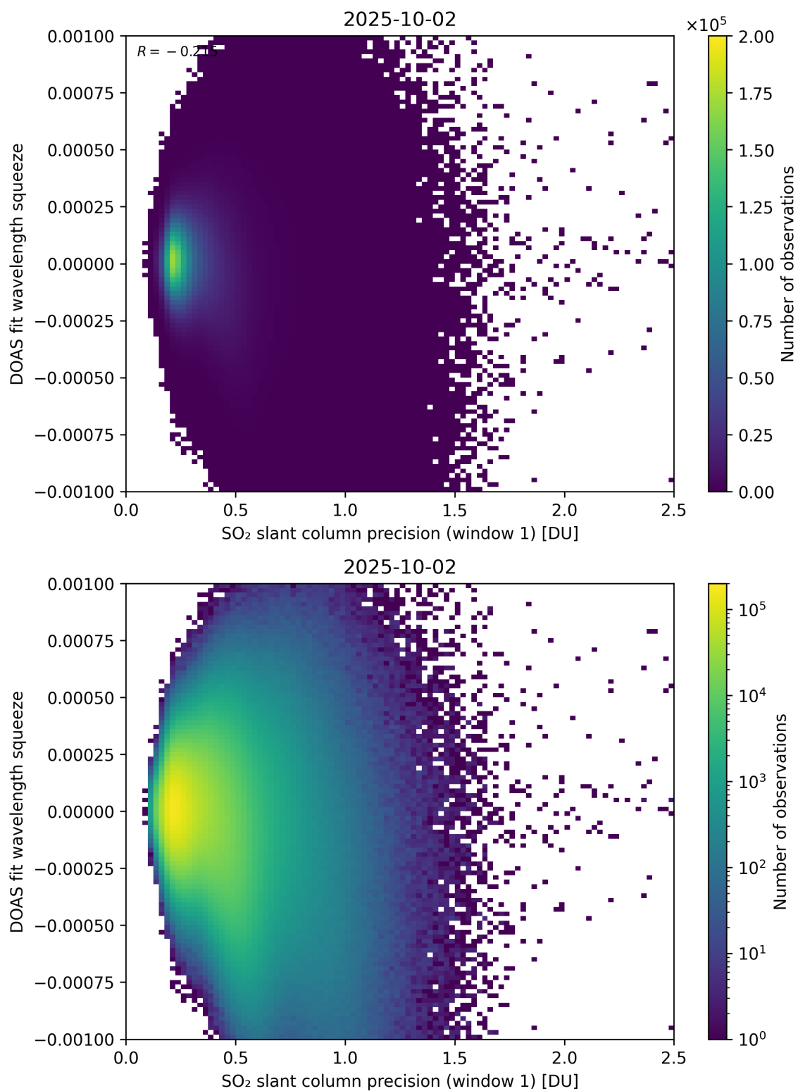
Figure 272: Scatter density plot of “SO 2 slant column precision (window 1)” against “DOAS fit wavelength squeeze” for 2025-10-01 to 2025-10-03.
