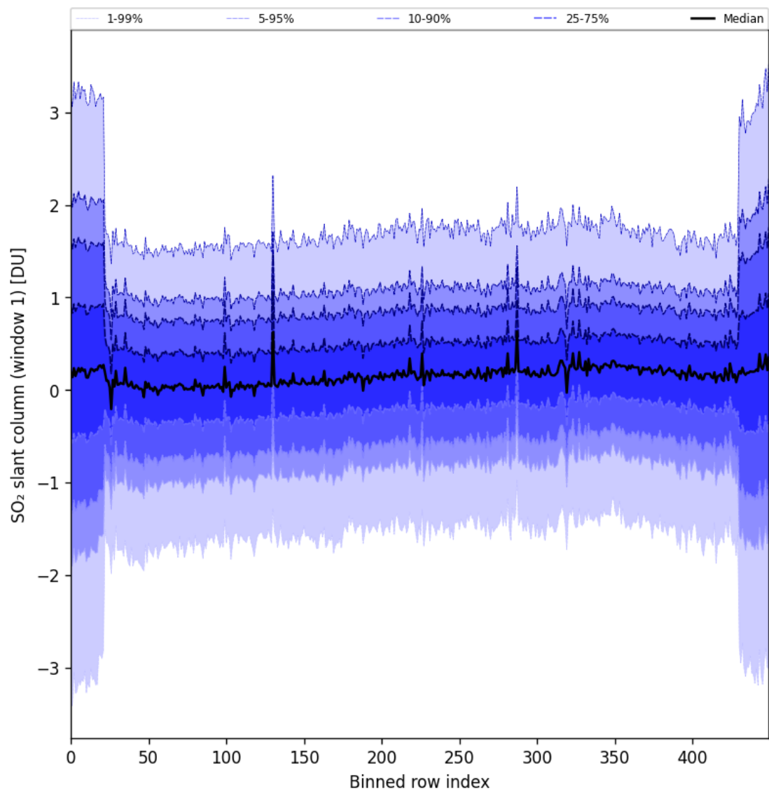
Figure 89: Along track statistics of “SO 2 slant column (window 1)” for 2025-10-01 to 2025-10-03
