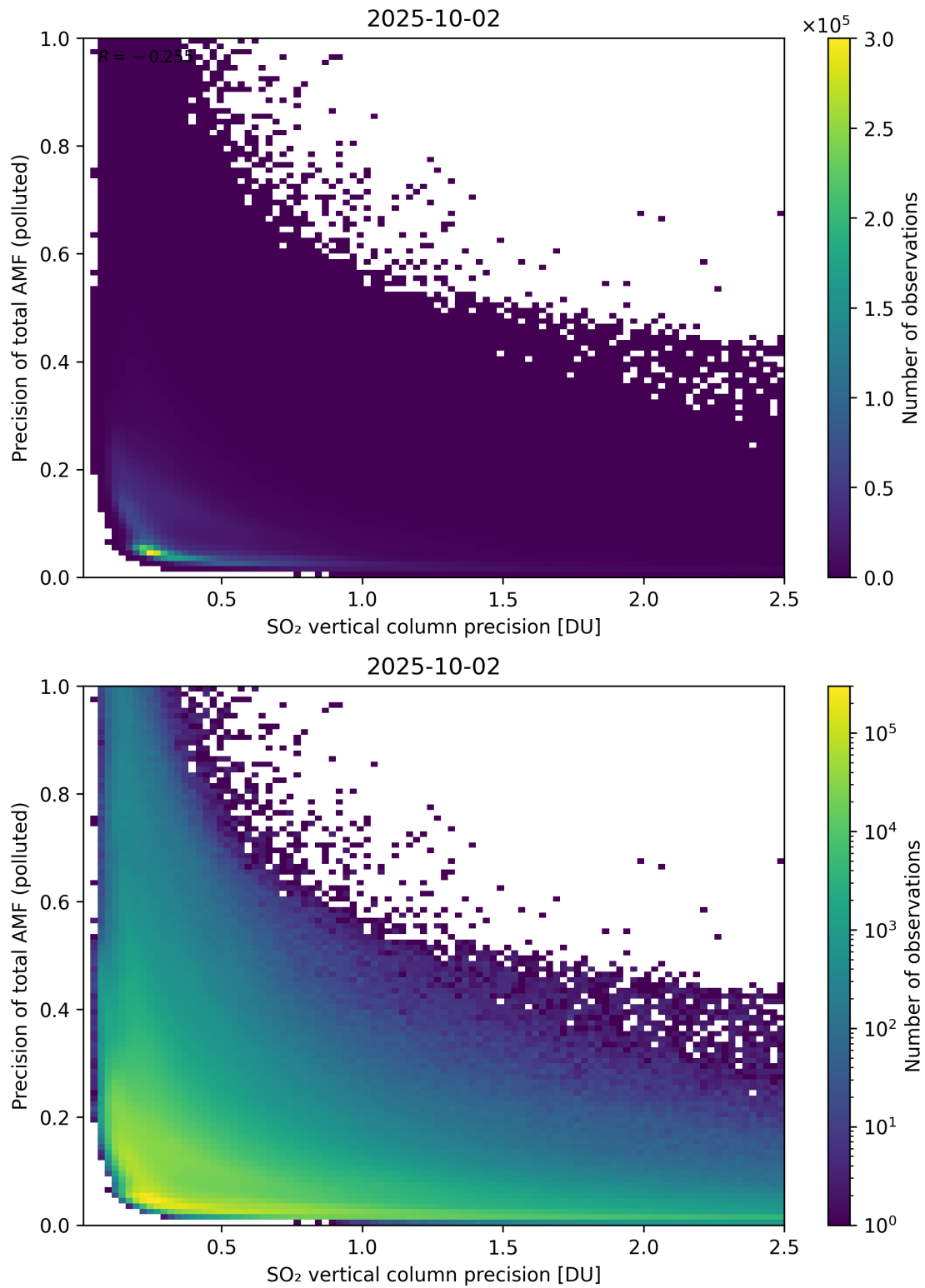
Figure 347: Scatter density plot of “SO 2 vertical column precision” against “Precision of total AMF (polluted)” for 2025-10-01 to 2025-10-03.
