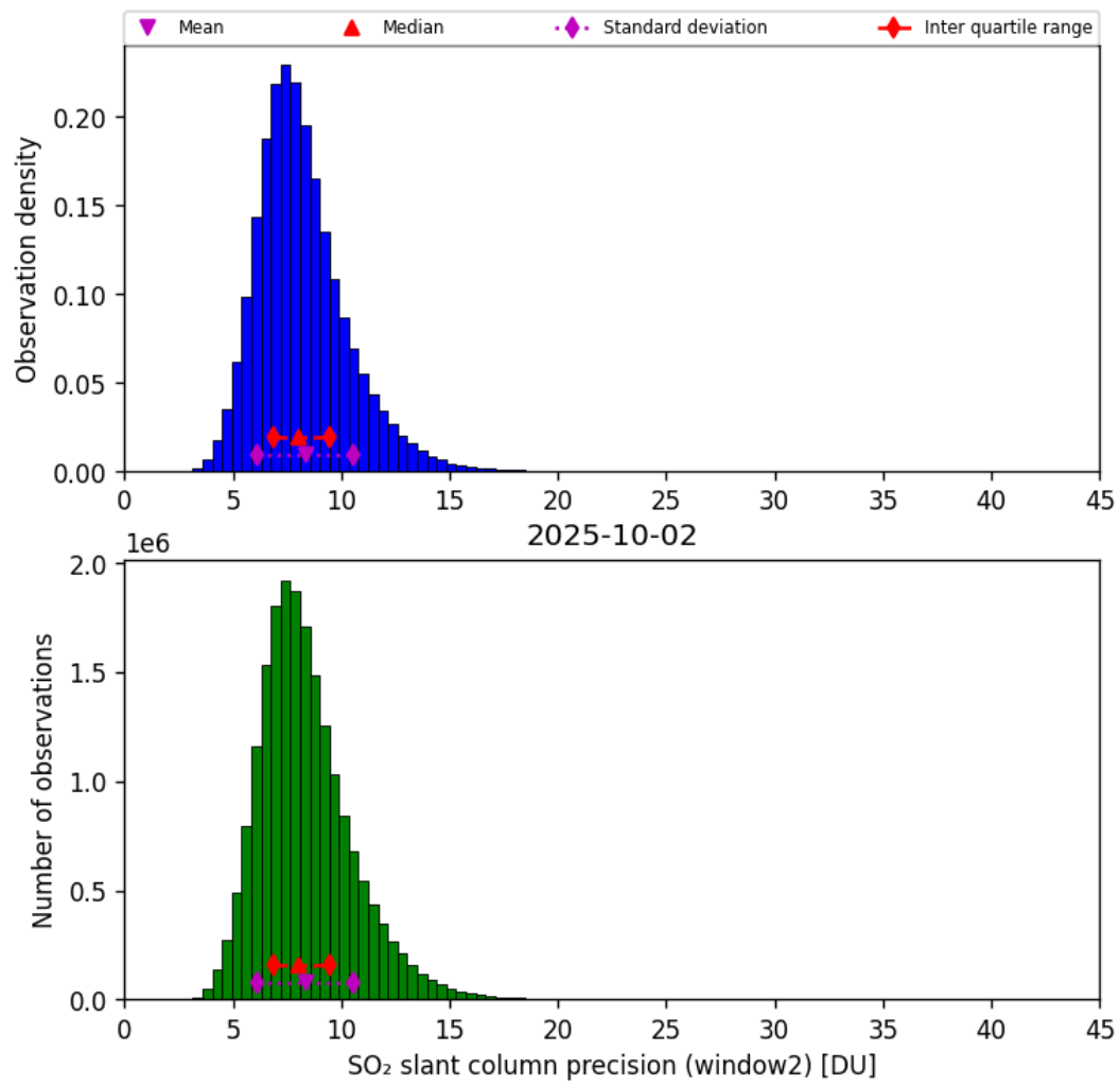
Figure 68: Histogram of “SO 2 slant column precision (window2)” for 2025-10-01 to 2025-10-03
