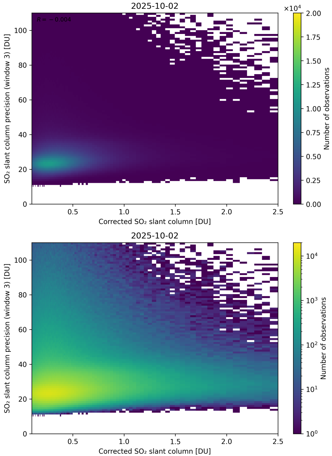
Figure 241: Scatter density plot of “Corrected SO 2 slant column” against “SO 2 slant column precision (window 3)” for 2025-10-01 to 2025-10-03.
