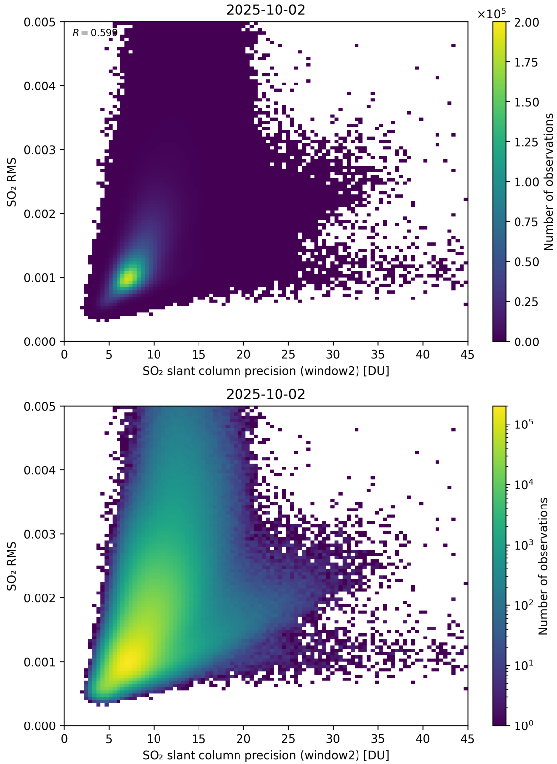
Figure 295: Scatter density plot of “SO 2 slant column precision (window2)” against “SO 2 RMS” for 2025-10-01 to 2025-10-03.
