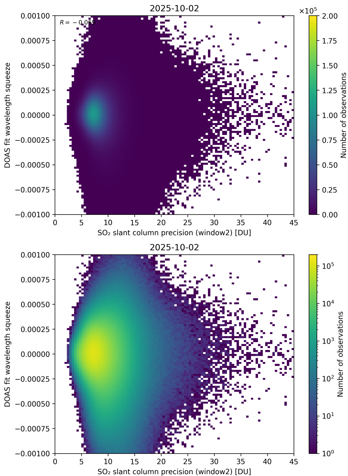
Figure 294: Scatter density plot of “SO 2 slant column precision (window2)” against “DOAS fit wavelength squeeze” for 2025-10-01 to 2025-10-03.
