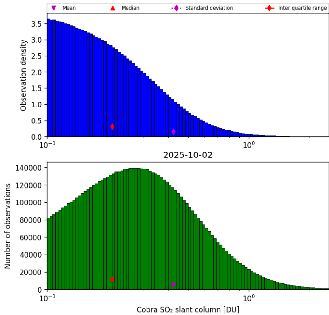
Figure 61: Histogram of “Cobra SO 2 slant column” for 2025-10-01 to 2025-10-03
