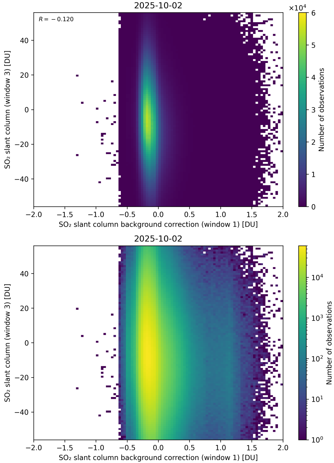
Figure 118: Scatter density plot of “SO 2 slant column background correction (window 1)” against “SO 2 slant column (window 3)” for 2025-10-01 to 2025-10-03.
