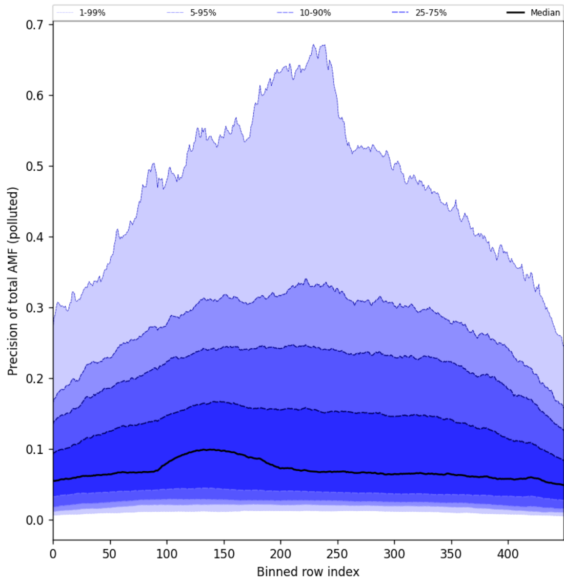
Figure 106: Along track statistics of “Precision of total AMF (polluted)” for 2025-10-01 to 2025-10-03
