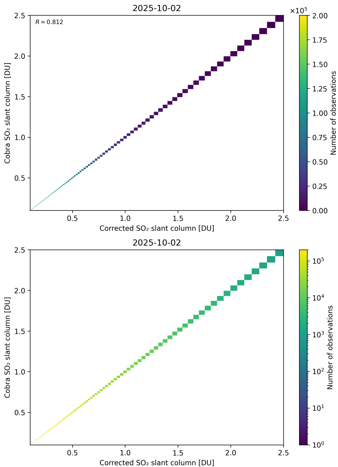
Figure 233: Scatter density plot of “Corrected SO 2 slant column” against “Cobra SO 2 slant column” for 2025-10-01 to 2025-10-03.
