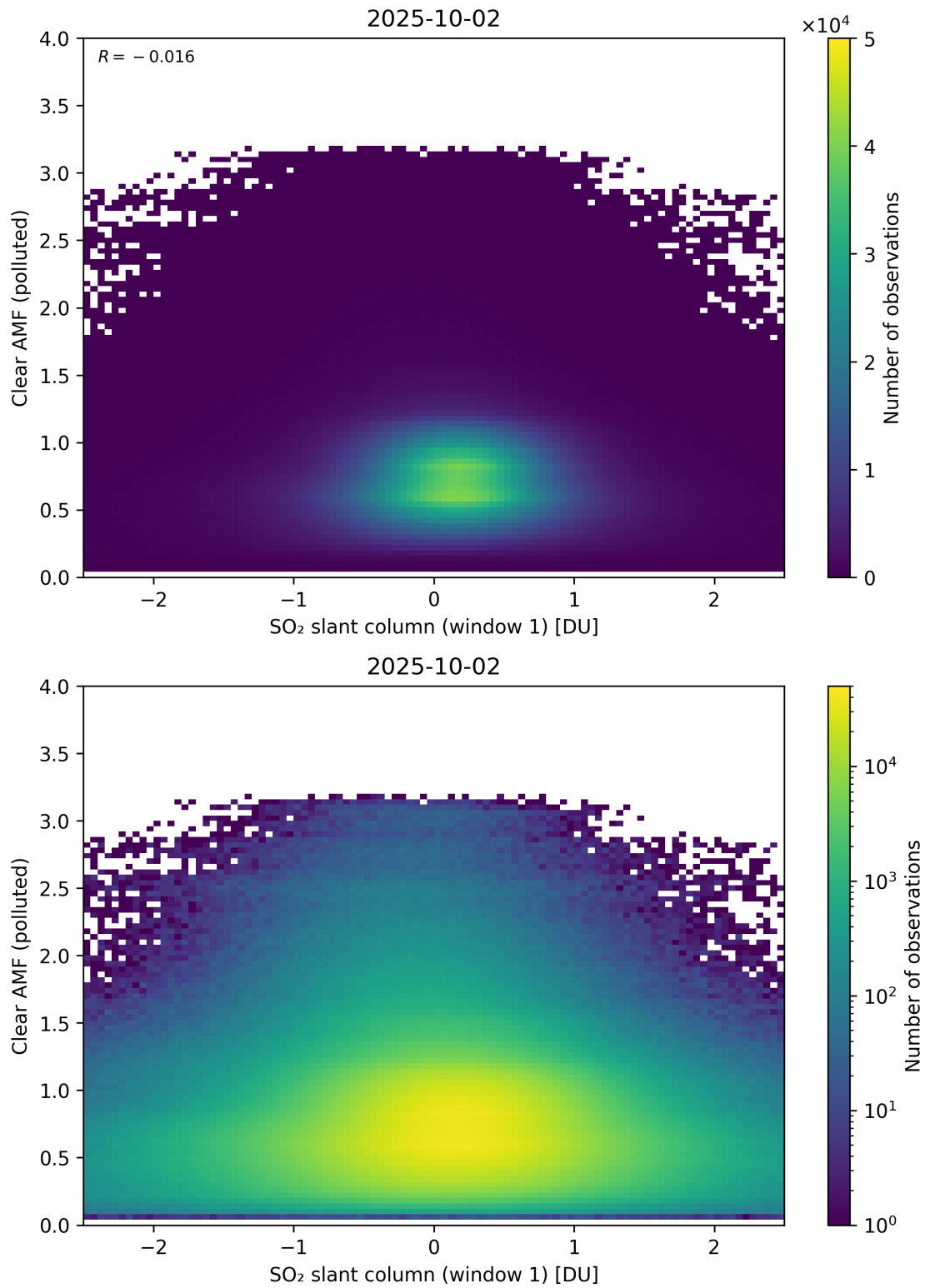
Figure 282: Scatter density plot of “SO 2 slant column (window 1)” against “Clear AMF (polluted)” for 2025-10-01 to 2025-10-03.
