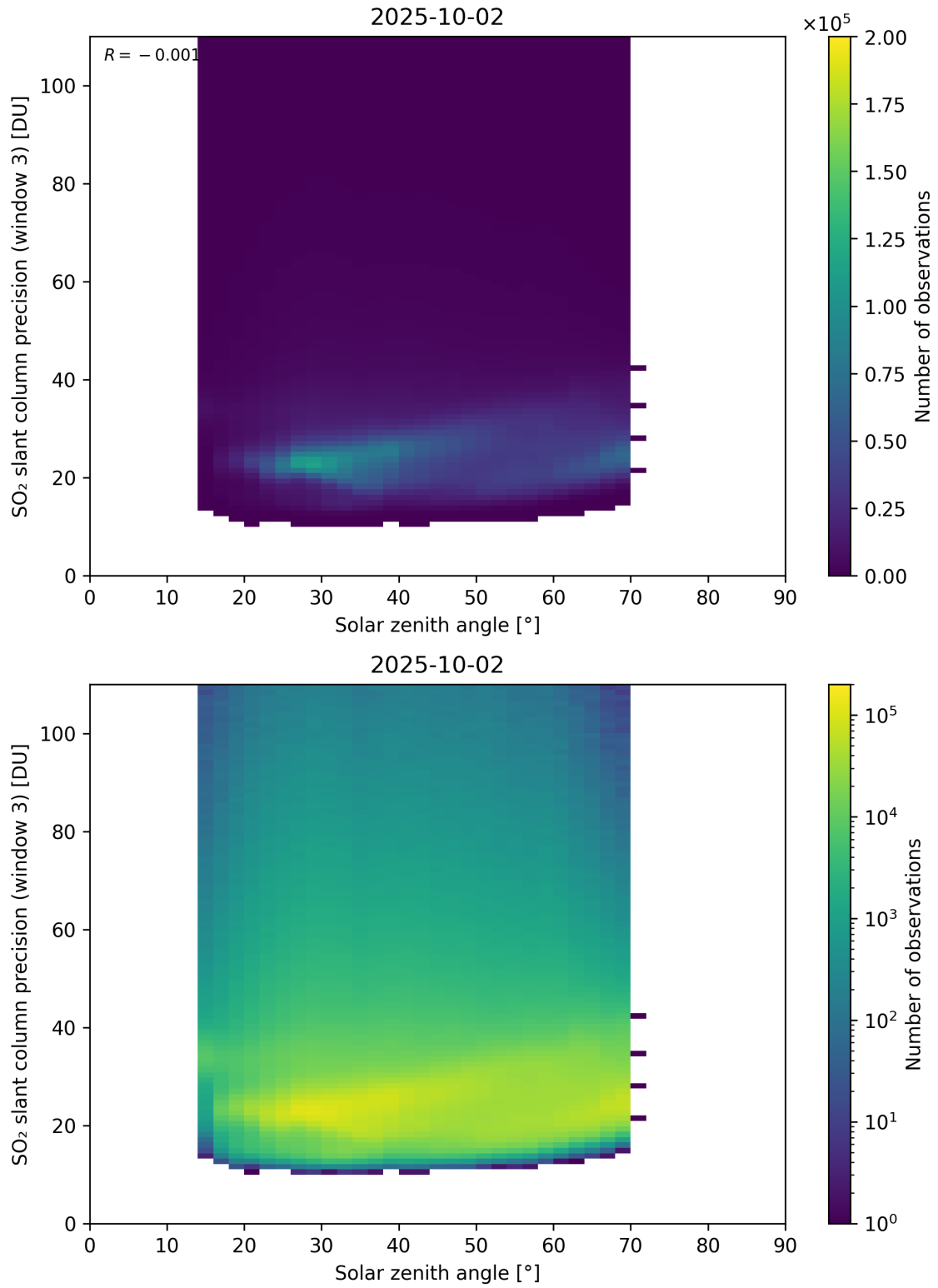
Figure 188: Scatter density plot of “Solar zenith angle” against “SO 2 slant column precision (window 3)” for 2025-10-01 to 2025-10-03.
