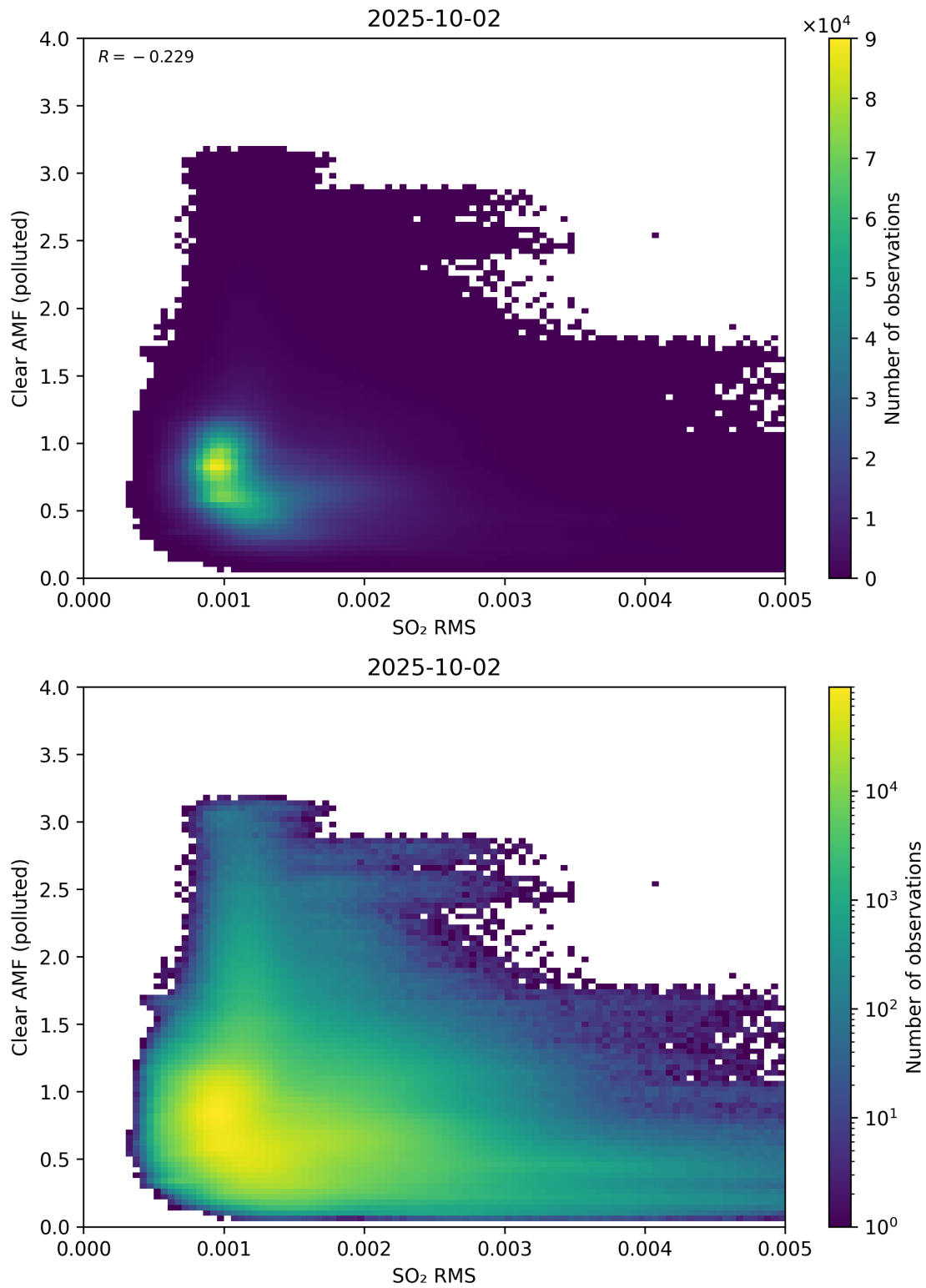
Figure 147: Scatter density plot of “SO 2 RMS” against “Clear AMF (polluted)” for 2025-10-01 to 2025-10-03.
