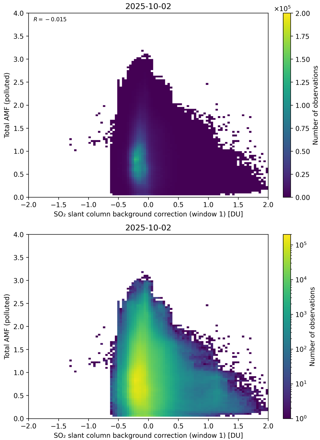
Figure 120: Scatter density plot of “SO 2 slant column background correction (window 1)” against “Total AMF (polluted)” for 2025-10-01 to 2025-10-03.
