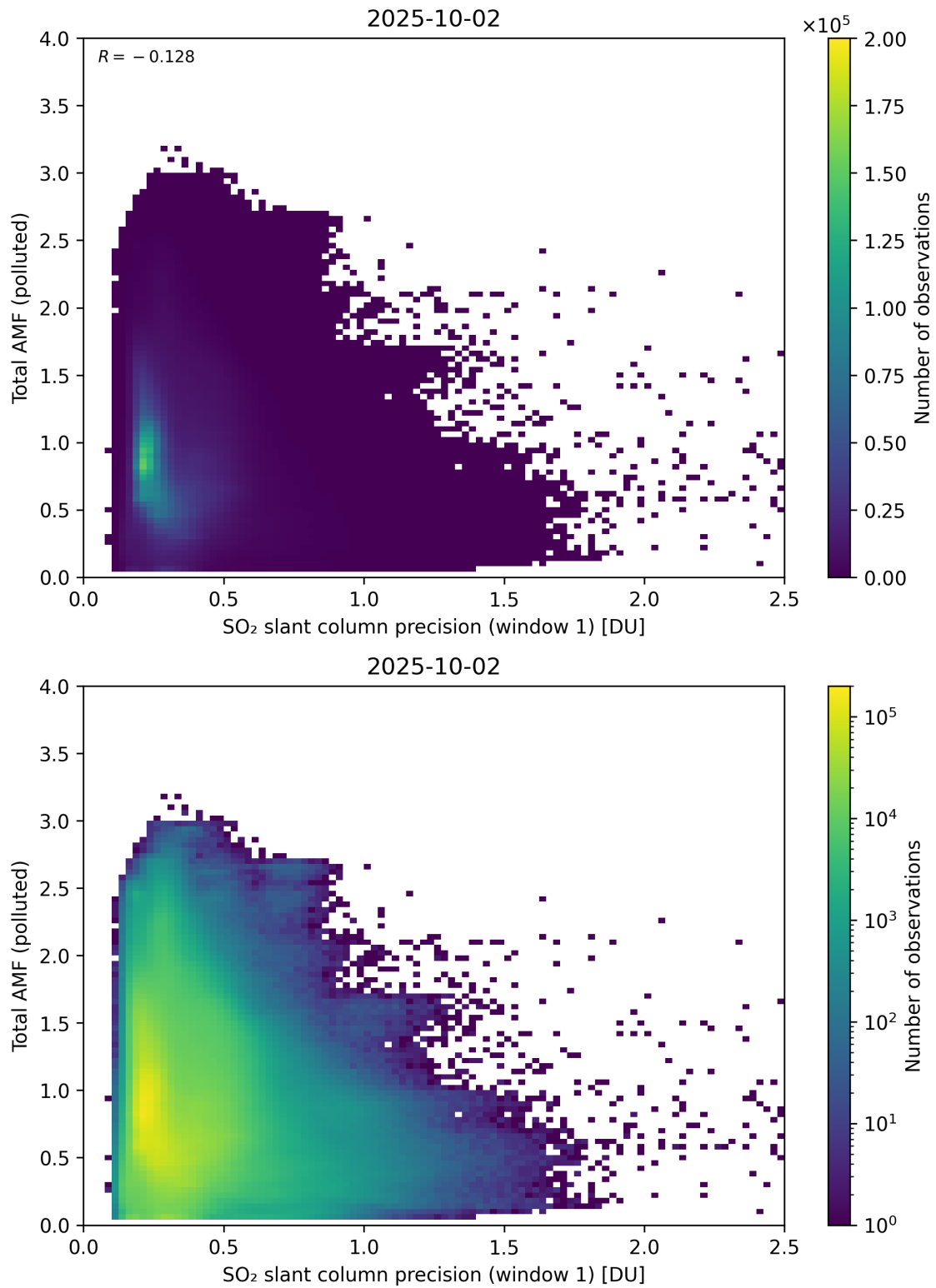
Figure 280: Scatter density plot of “SO 2 slant column precision (window 1)” against “Total AMF (polluted)” for 2025-10-01 to 2025-10-03.
