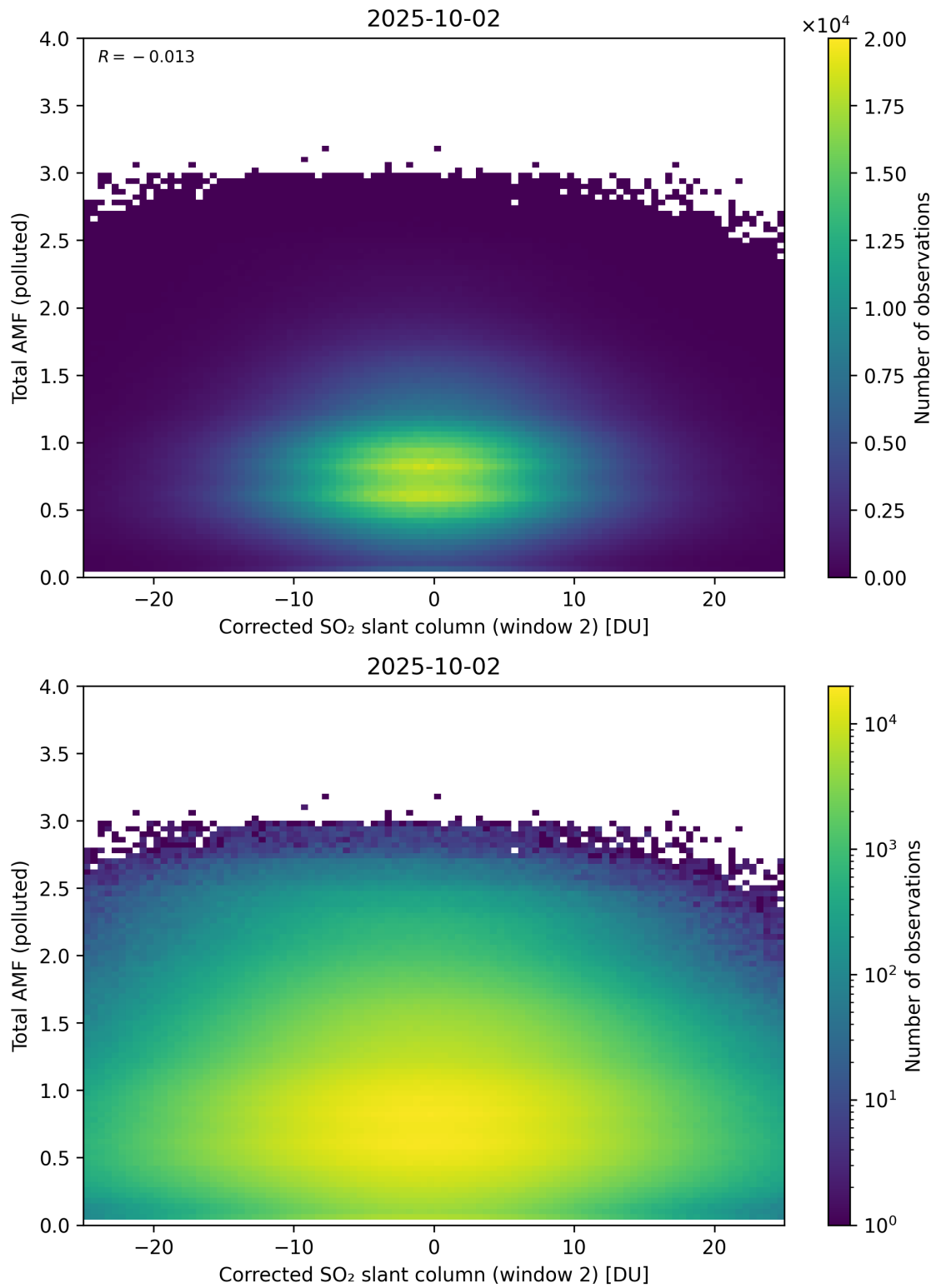
Figure 253: Scatter density plot of “Corrected SO 2 slant column (window 2)” against “Total AMF (polluted)” for 2025-10-01 to 2025-10-03.
