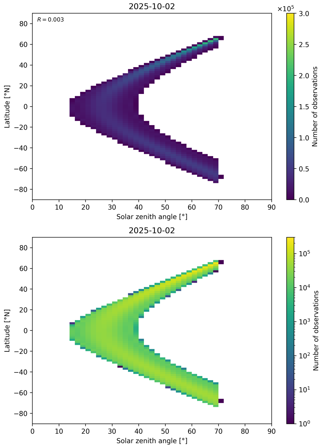
Figure 177: Scatter density plot of “Solar zenith angle” against “Latitude” for 2025-10-01 to 2025-10-03.
