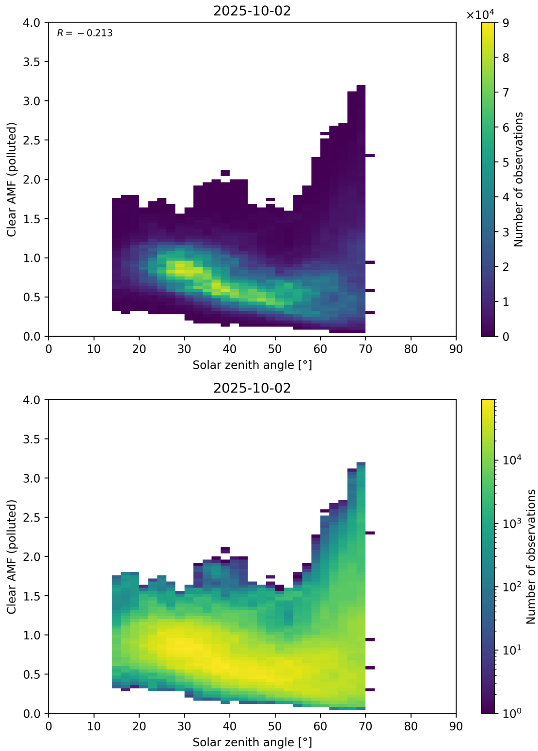
Figure 178: Scatter density plot of “Solar zenith angle” against “Clear AMF (polluted)” for 2025-10-01 to 2025-10-03.
