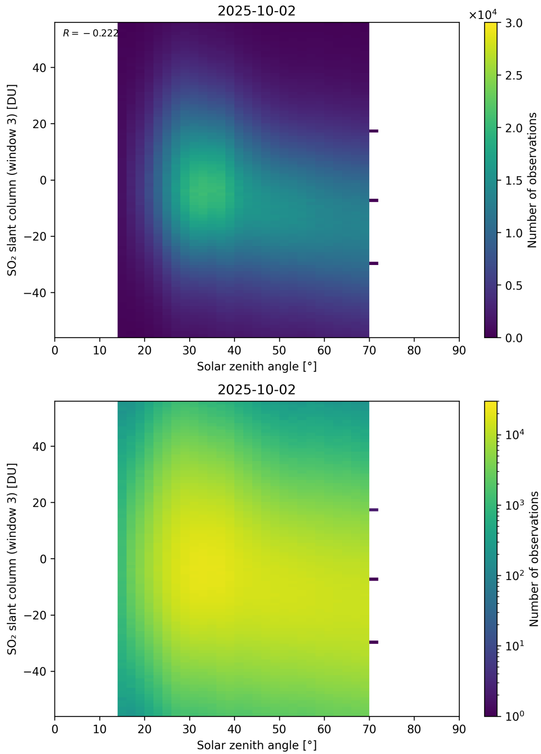
Figure 187: Scatter density plot of “Solar zenith angle” against “SO 2 slant column (window 3)” for 2025-10-01 to 2025-10-03.
