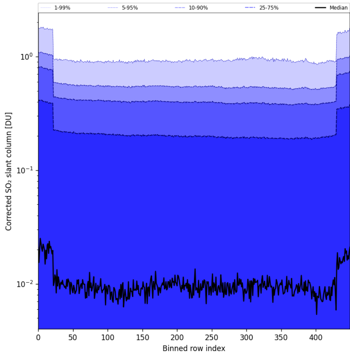
Figure 86: Along track statistics of “Corrected SO 2 slant column” for 2025-10-01 to 2025-10-03
