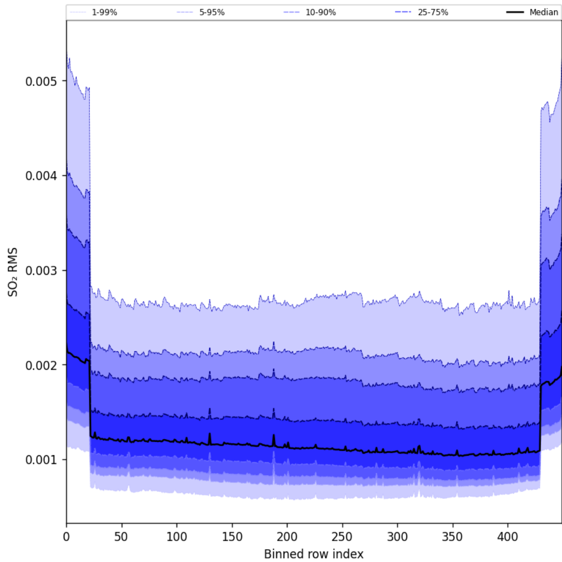
Figure 104: Along track statistics of “SO 2 RMS” for 2025-10-01 to 2025-10-03
