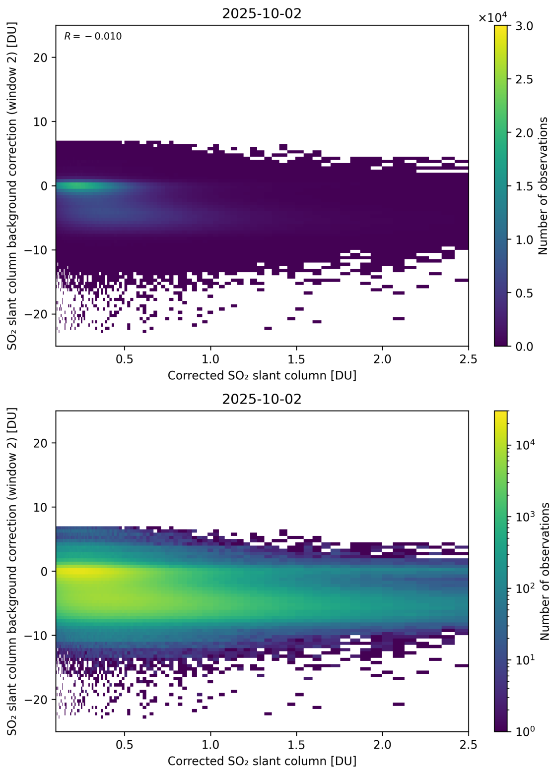
Figure 227: Scatter density plot of “Corrected SO 2 slant column” against “SO 2 slant column background correction (window 2)” for 2025-10-01 to 2025-10-03.
