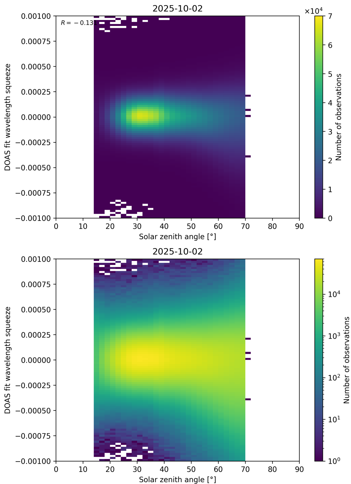
Figure 175: Scatter density plot of “Solar zenith angle” against “DOAS fit wavelength squeeze” for 2025-10-01 to 2025-10-03.
