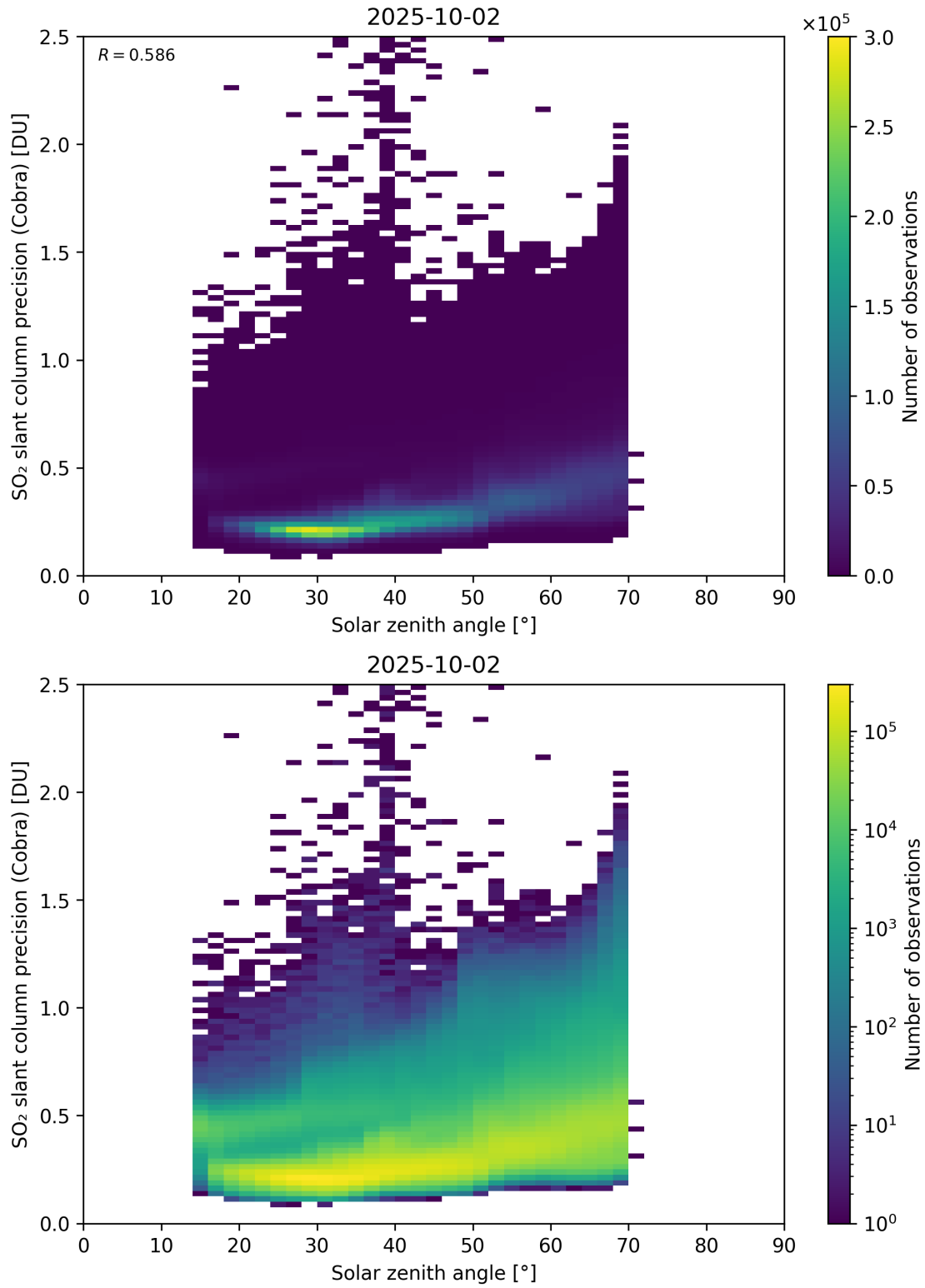
Figure 180: Scatter density plot of “Solar zenith angle” against “SO 2 slant column precision (Cobra)” for 2025-10-01 to 2025-10-03.
