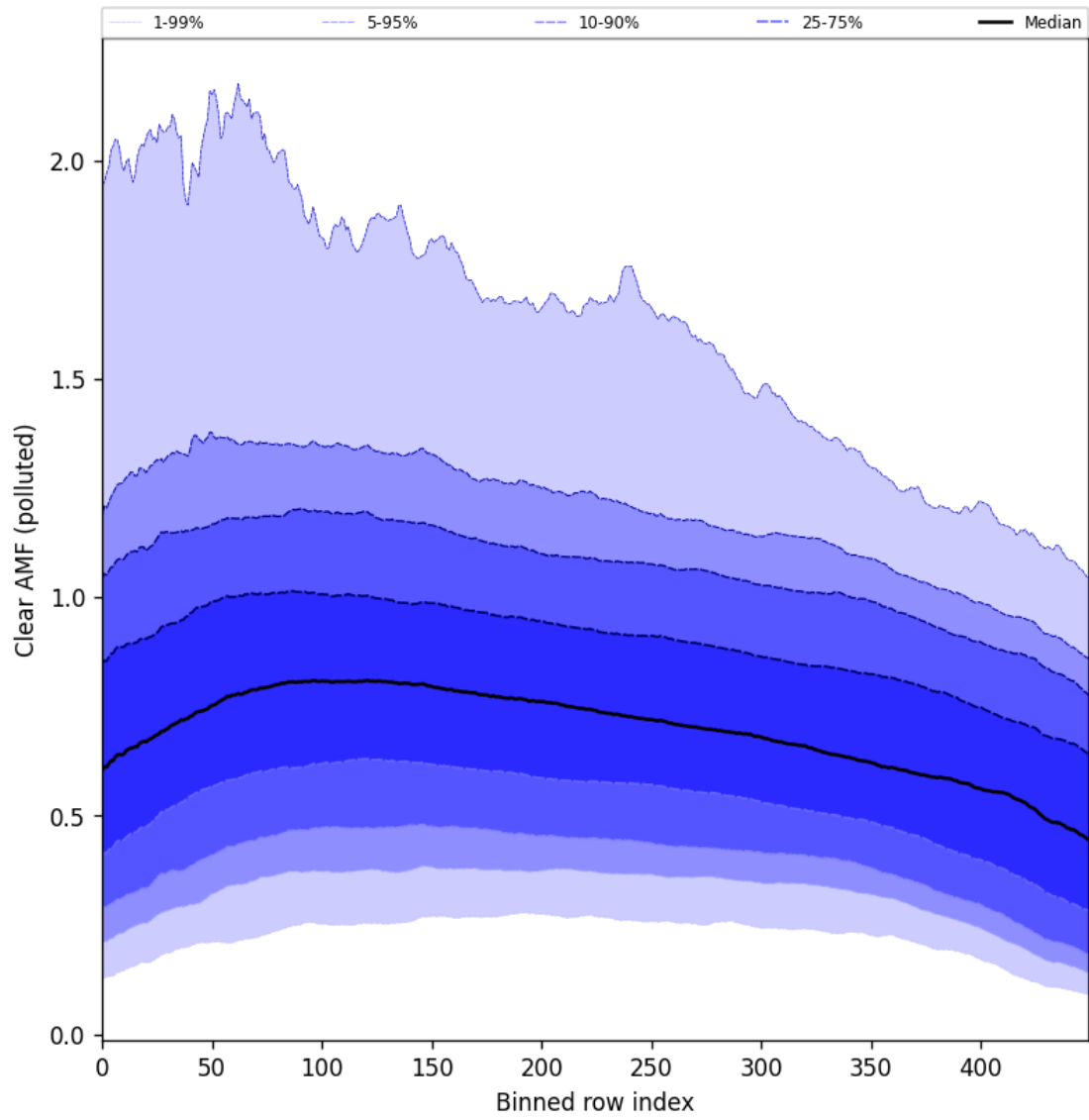
Figure 107: Along track statistics of “Clear AMF (polluted)” for 2025-10-01 to 2025-10-03
