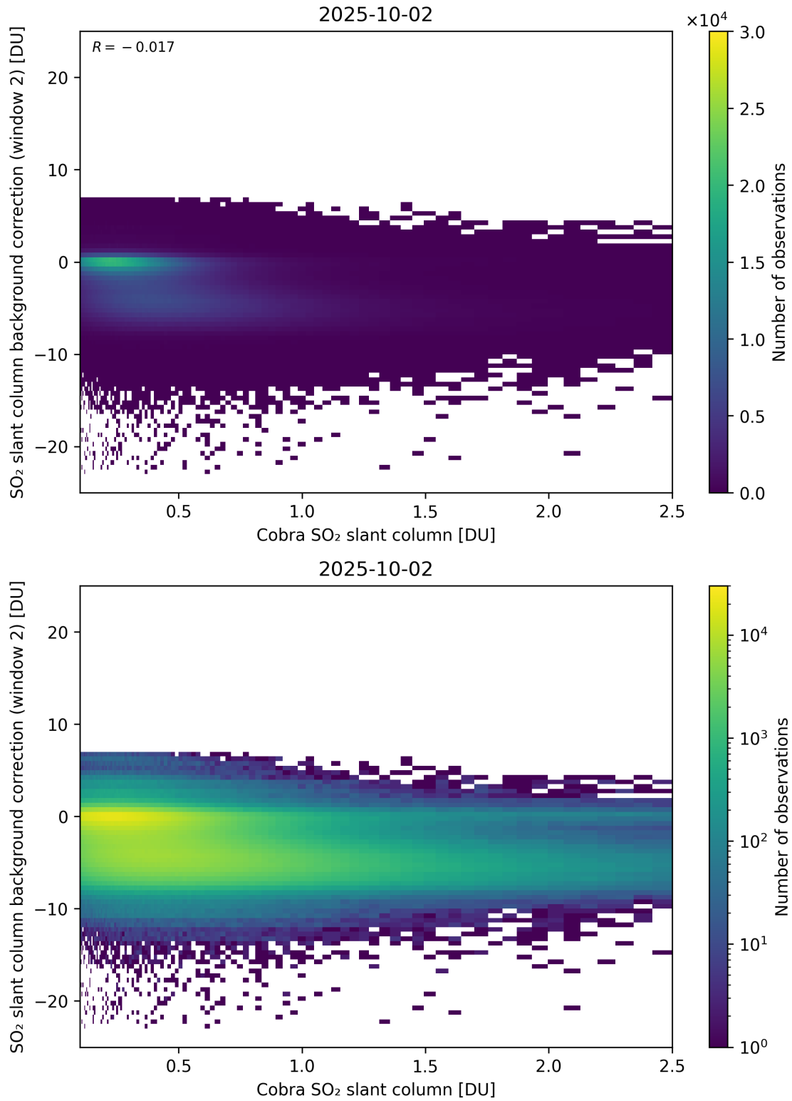
Figure 194: Scatter density plot of “Cobra SO 2 slant column” against “SO 2 slant column background correction (window 2)” for 2025-10-01 to 2025-10-03.
