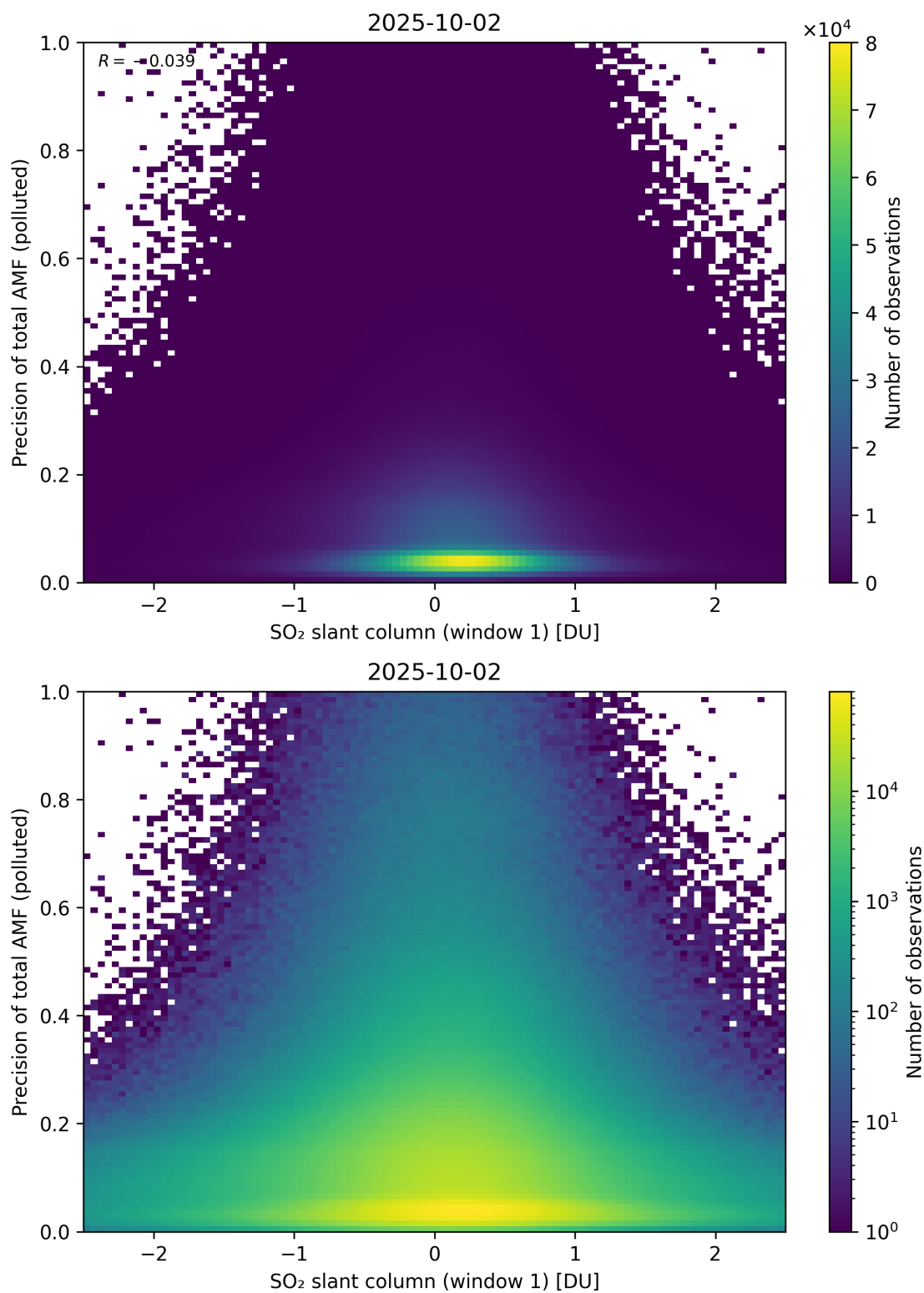
Figure 290: Scatter density plot of “SO 2 slant column (window 1)” against “Precision of total AMF (polluted)” for 2025-10-01 to 2025-10-03.
