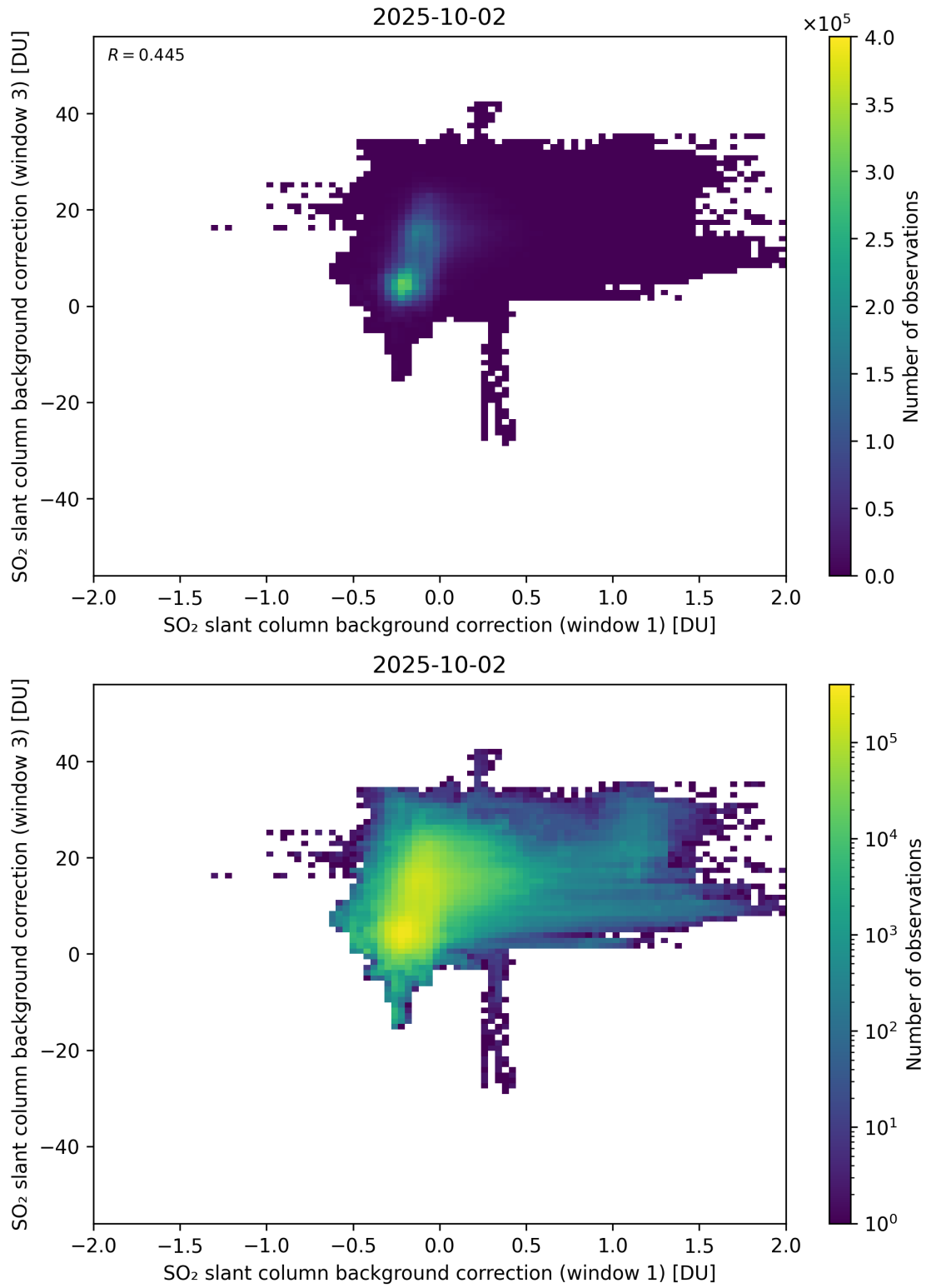
Figure 110: Scatter density plot of “SO 2 slant column background correction (window 1)” against “SO 2 slant column background correction (window 3)” for 2025-10-01 to 2025-10-03.
