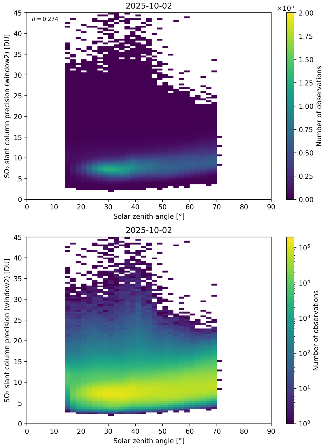
Figure 186: Scatter density plot of “Solar zenith angle” against “SO 2 slant column precision (window2)” for 2025-10-01 to 2025-10-03.
