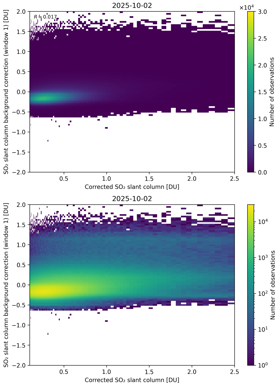
Figure 226: Scatter density plot of “Corrected SO 2 slant column” against “SO 2 slant column background correction (window 1)” for 2025-10-01 to 2025-10-03.
