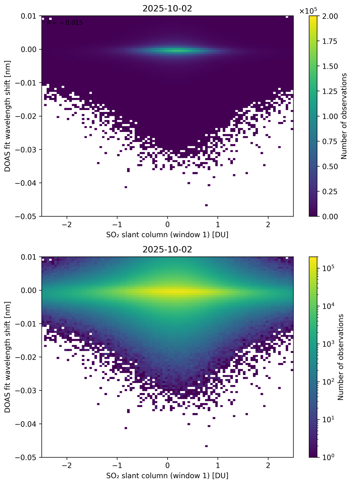
Figure 265: Scatter density plot of “SO 2 slant column (window 1)” against “DOAS fit wavelength shift” for 2025-10-01 to 2025-10-03.
