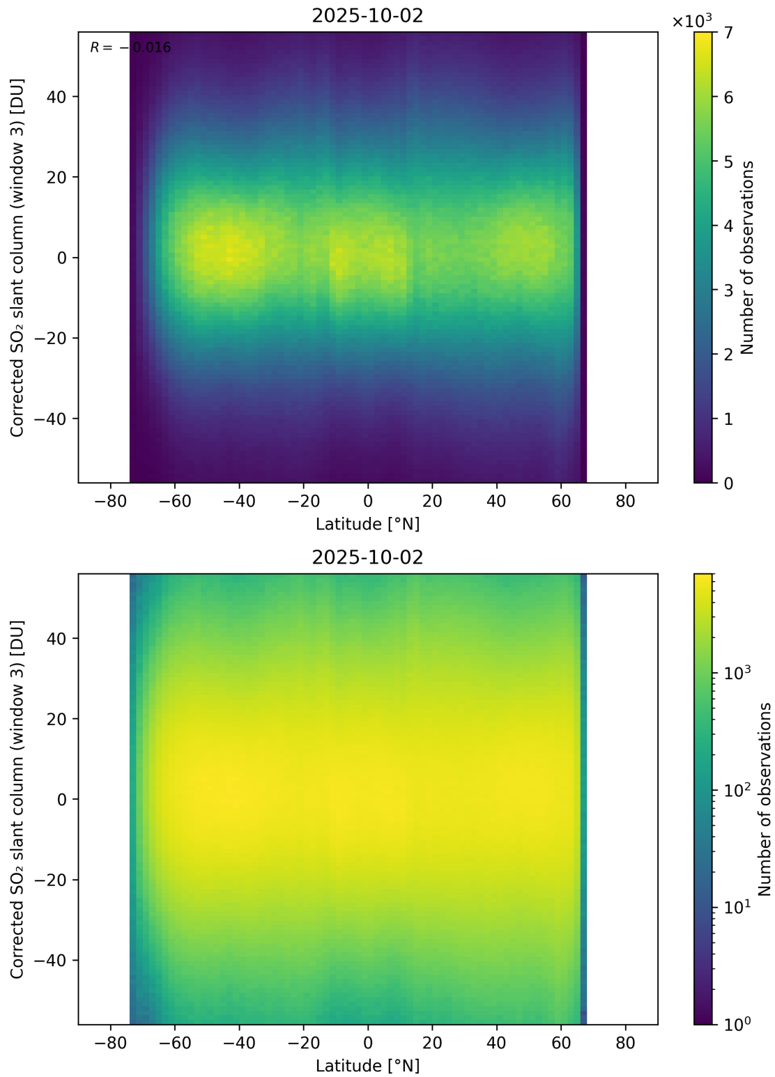
Figure 161: Scatter density plot of “Latitude” against “Corrected SO 2 slant column (window 3)” for 2025-10-01 to 2025-10-03.
