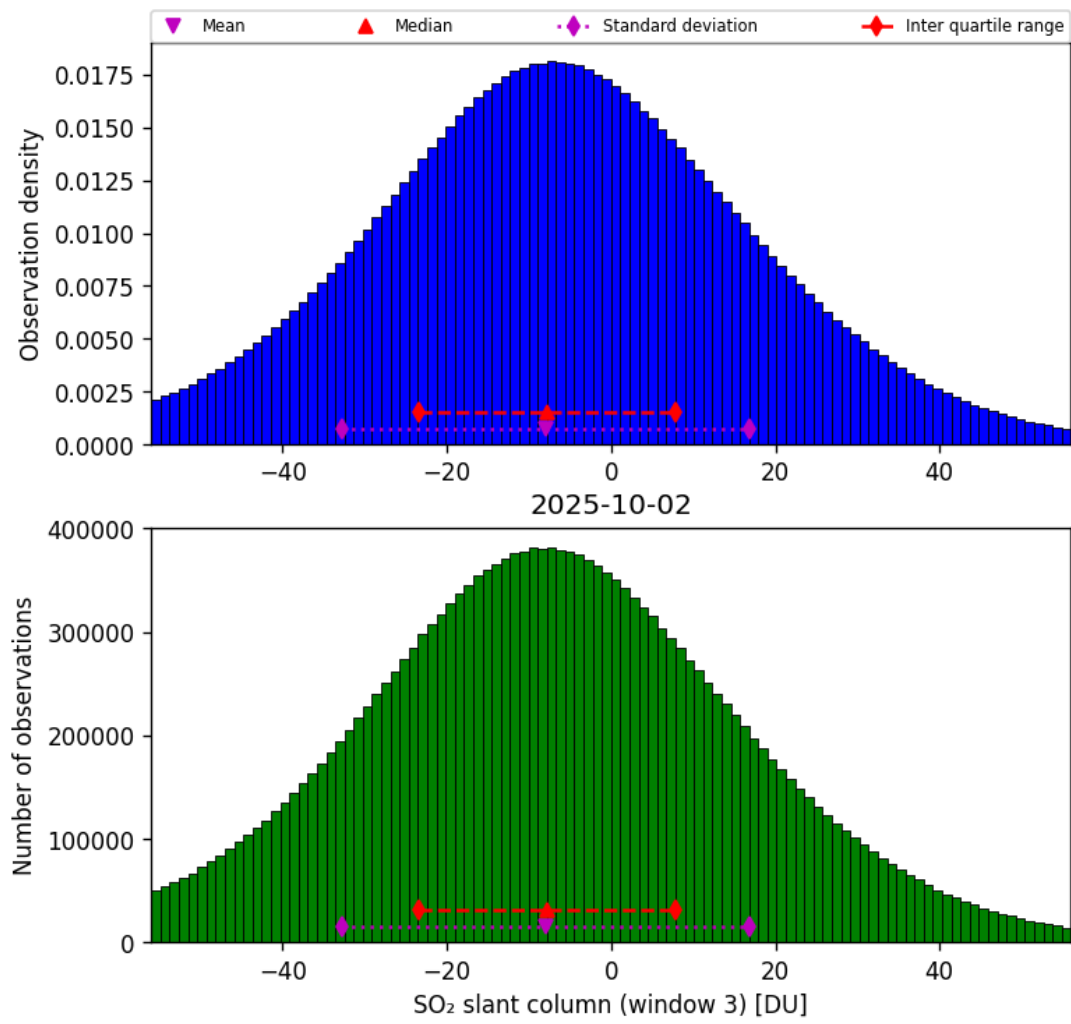
Figure 71: Histogram of “SO 2 slant column (window 3)” for 2025-10-01 to 2025-10-03
