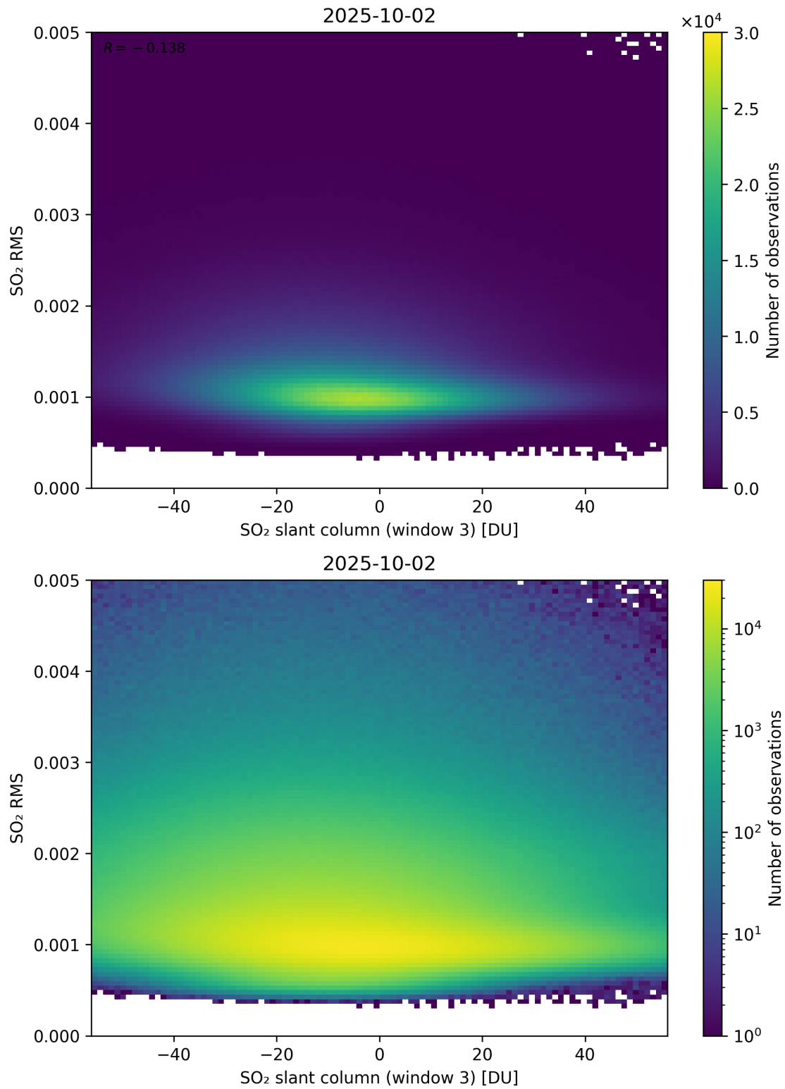
Figure 306: Scatter density plot of “SO 2 slant column (window 3)” against “SO 2 RMS” for 2025-10-01 to 2025-10-03.
