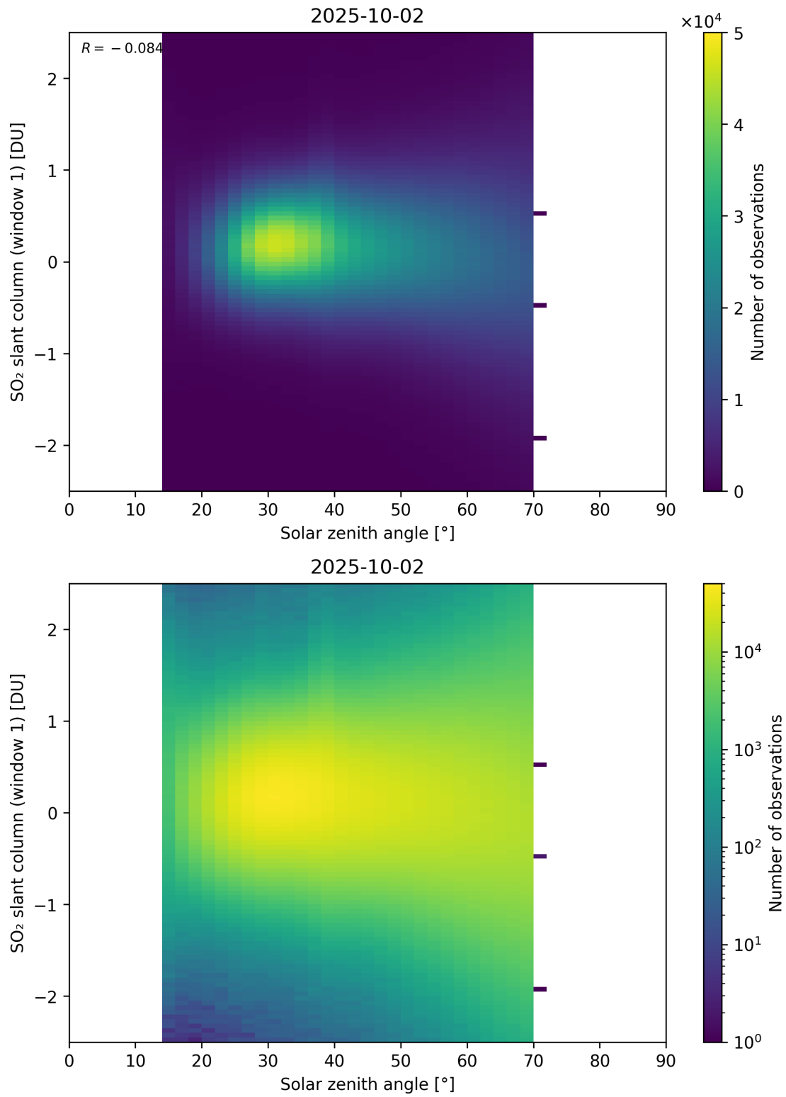
Figure 184: Scatter density plot of “Solar zenith angle” against “SO 2 slant column (window 1)” for 2025-10-01 to 2025-10-03.
