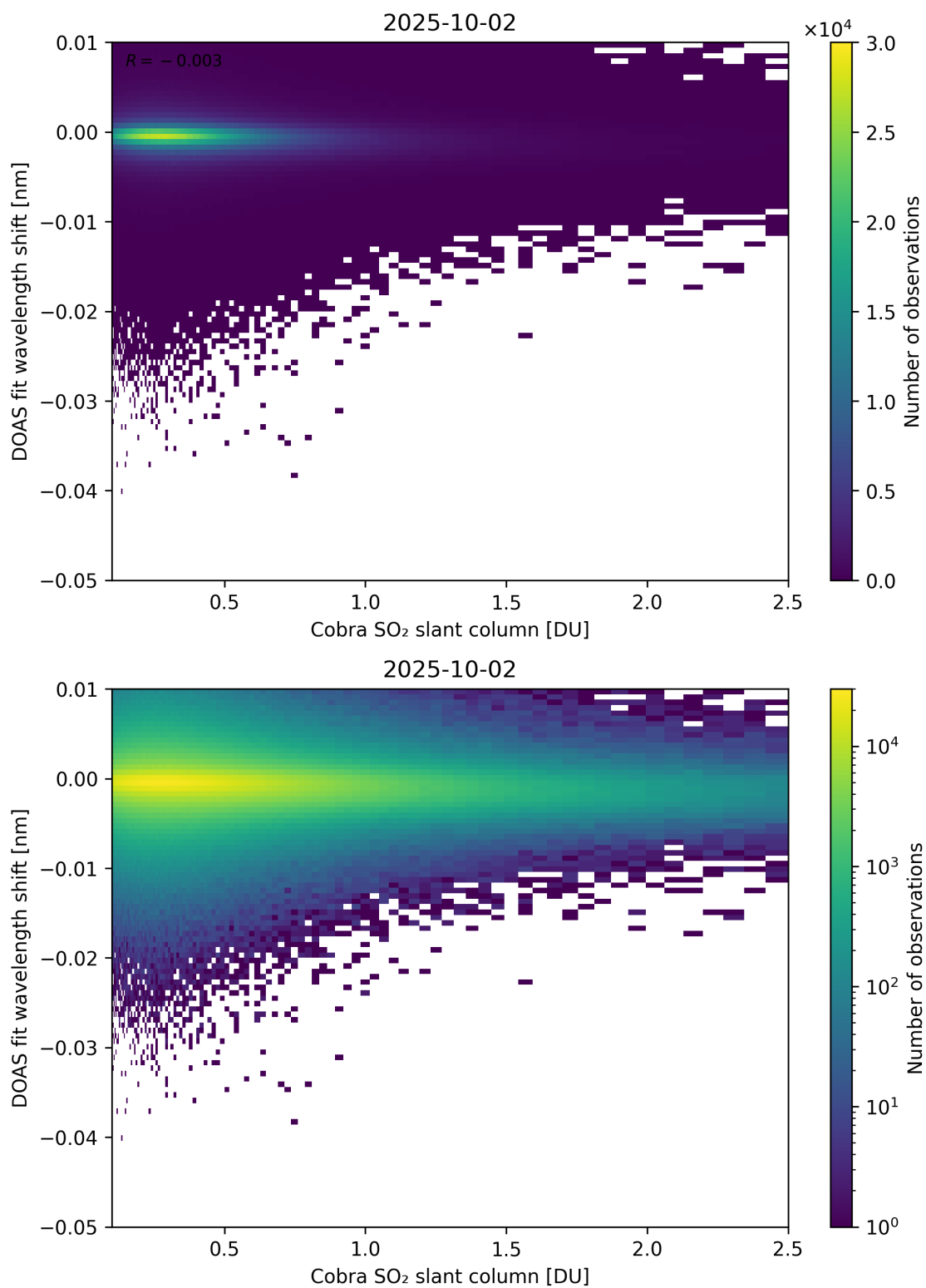
Figure 196: Scatter density plot of “Cobra SO 2 slant column” against “DOAS fit wavelength shift” for 2025-10-01 to 2025-10-03.
