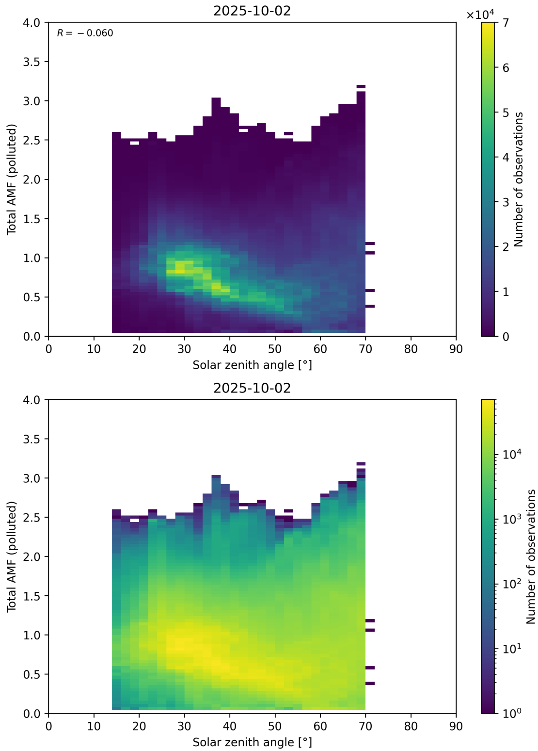
Figure 189: Scatter density plot of “Solar zenith angle” against “Total AMF (polluted)” for 2025-10-01 to 2025-10-03.
