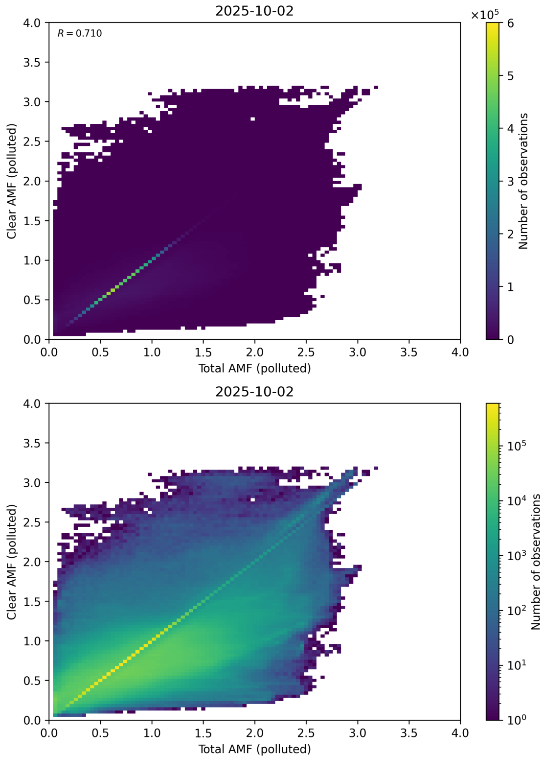
Figure 321: Scatter density plot of “Total AMF (polluted)” against “Clear AMF (polluted)” for 2025-10-01 to 2025-10-03.
