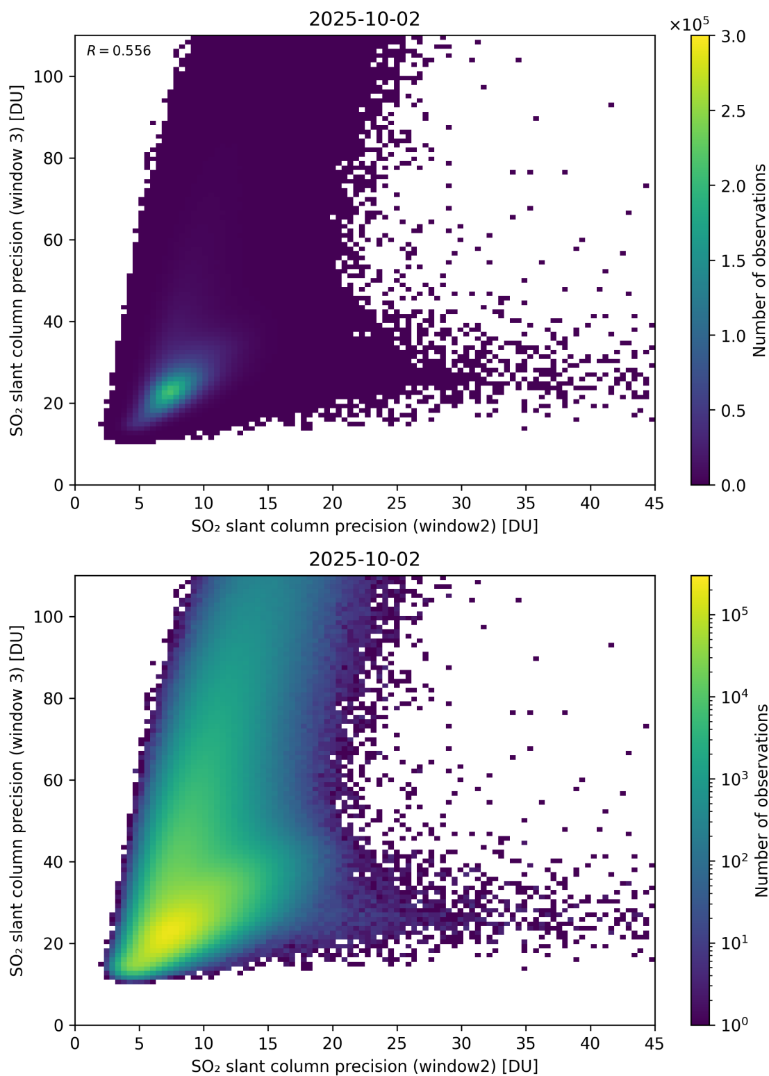
Figure 300: Scatter density plot of “SO 2 slant column precision (window2)” against “SO 2 slant column precision (window 3)” for 2025-10-01 to 2025-10-03.
