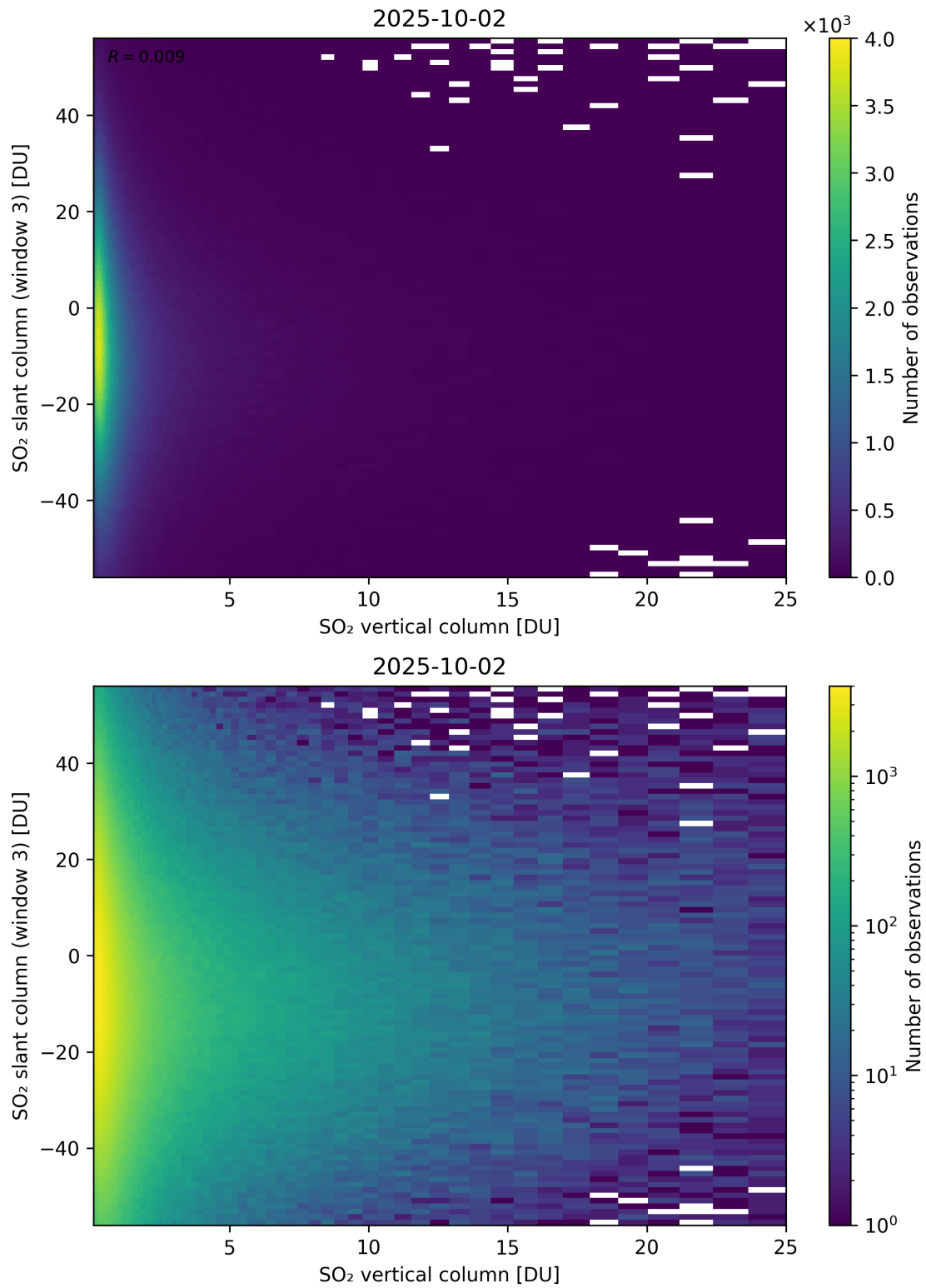
Figure 357: Scatter density plot of “SO 2 vertical column” against “SO 2 slant column (window 3)” for 2025-10-01 to 2025-10-03.
