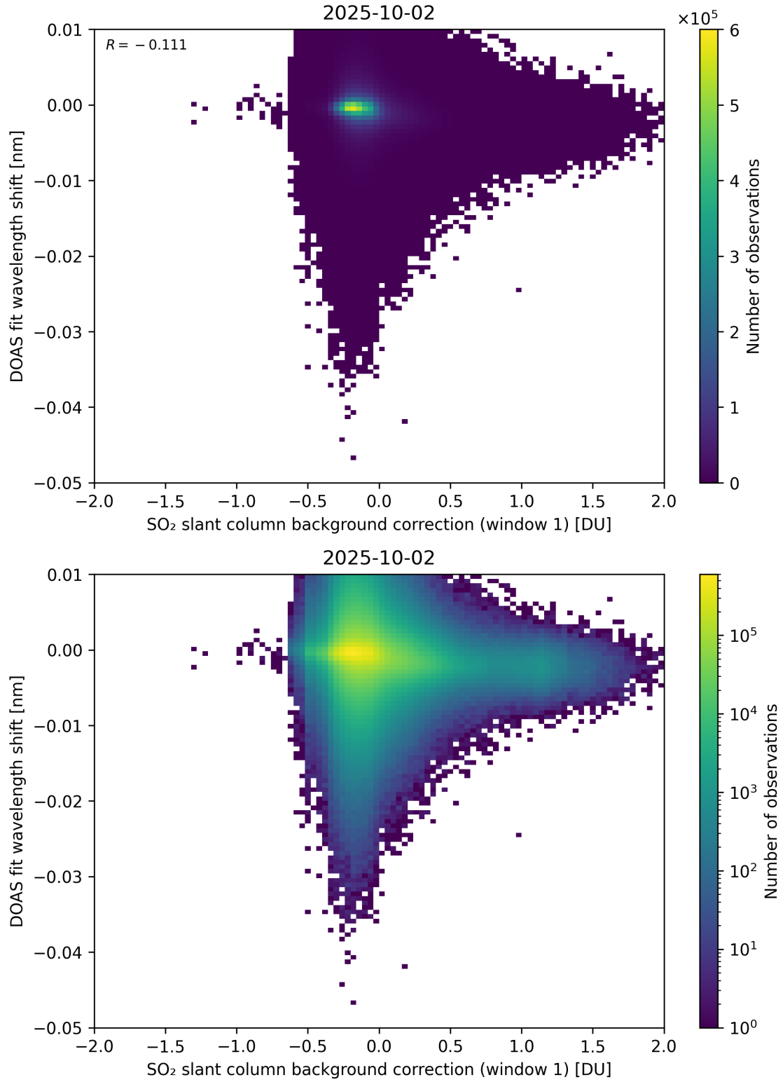
Figure 111: Scatter density plot of “SO 2 slant column background correction (window 1)” against “DOAS fit wavelength shift” for 2025-10-01 to 2025-10-03.
