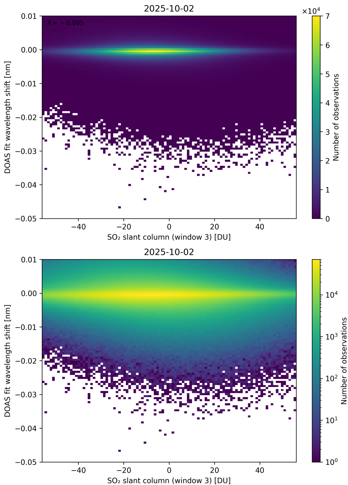
Figure 304: Scatter density plot of “SO 2 slant column (window 3)” against “DOAS fit wavelength shift” for 2025-10-01 to 2025-10-03.
