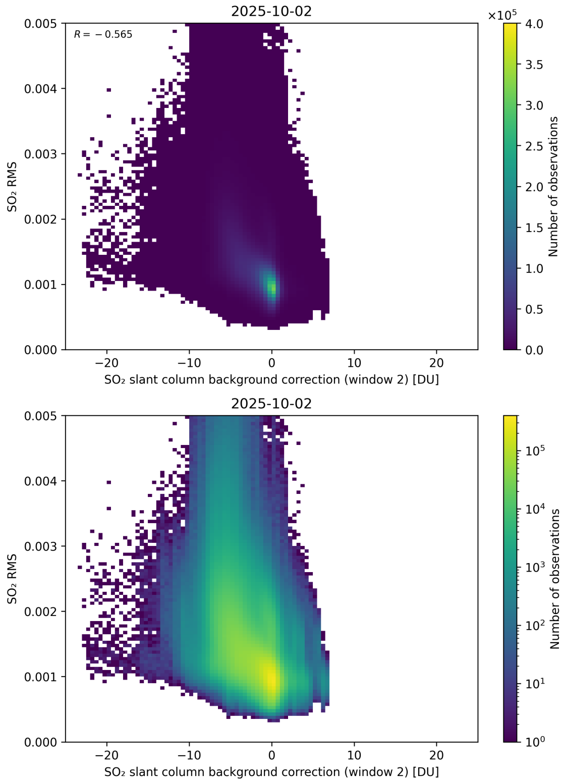
Figure 125: Scatter density plot of “SO 2 slant column background correction (window 2)” against “SO 2 RMS” for 2025-10-01 to 2025-10-03.
