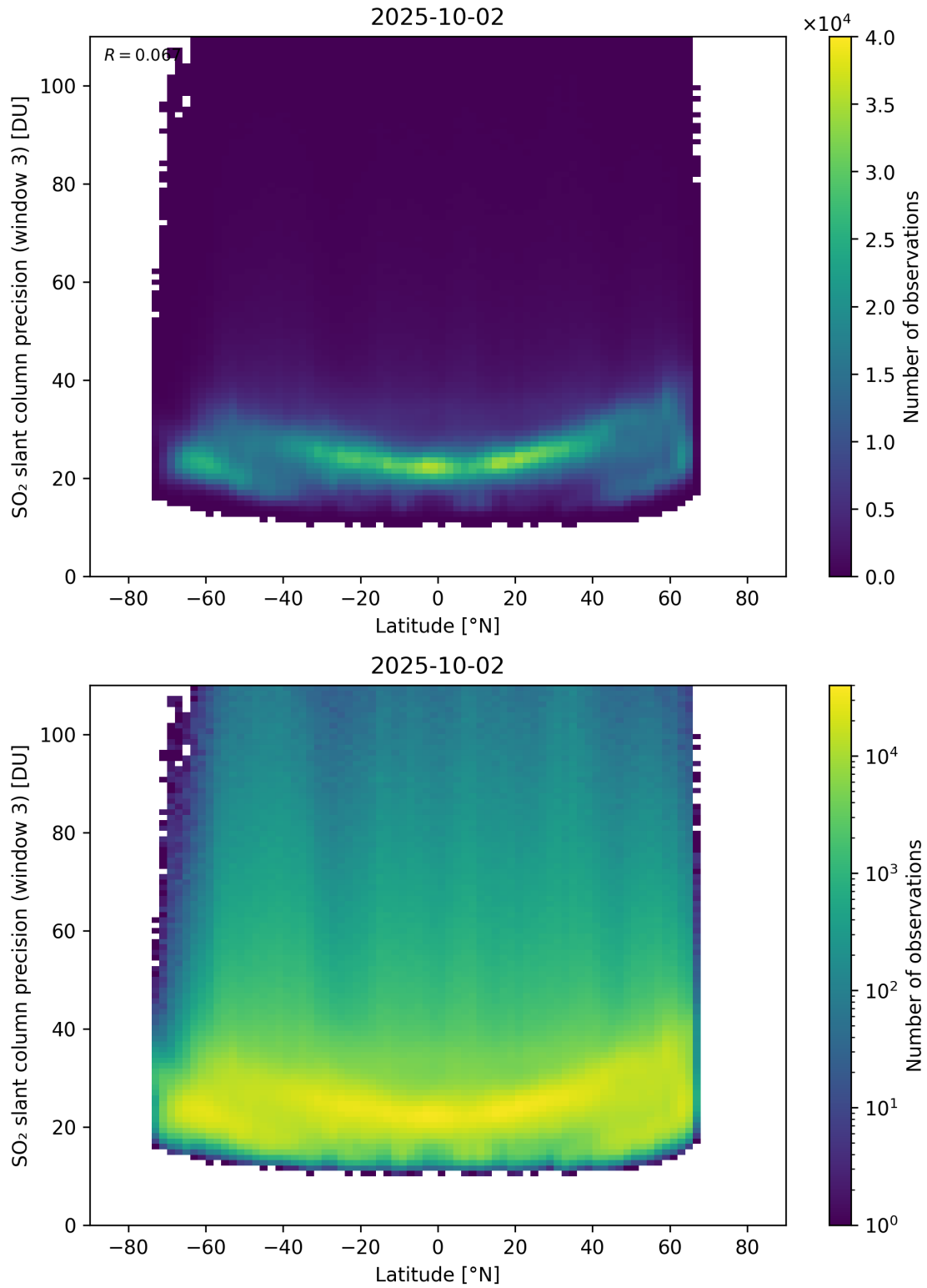
Figure 166: Scatter density plot of “Latitude” against “SO 2 slant column precision (window 3)” for 2025-10-01 to 2025-10-03.
