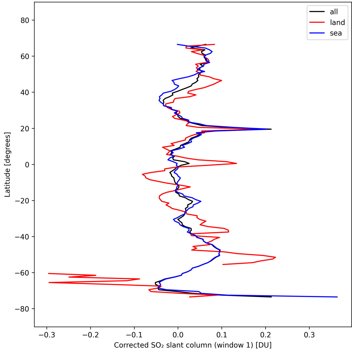
Figure 39: Zonal average of “Corrected SO 2 slant column (window 1)” for 2025-10-01 to 2025-10-03.
