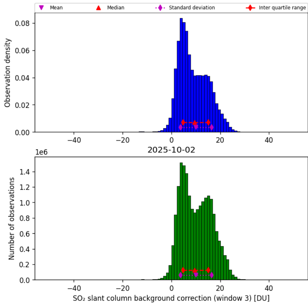
Figure 74: Histogram of “SO 2 slant column background correction (window 3)” for 2025-10-01 to 2025-10-03
