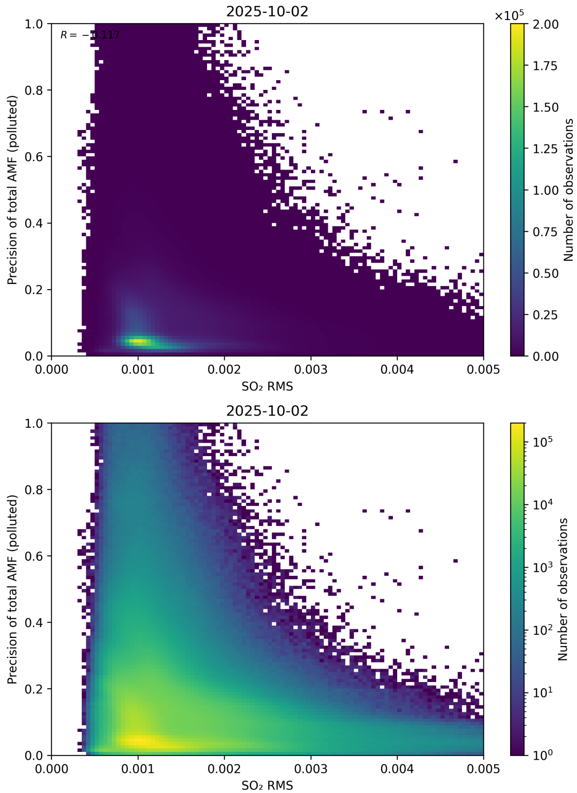
Figure 149: Scatter density plot of “SO 2 RMS” against “Precision of total AMF (polluted)” for 2025-10-01 to 2025-10-03.
