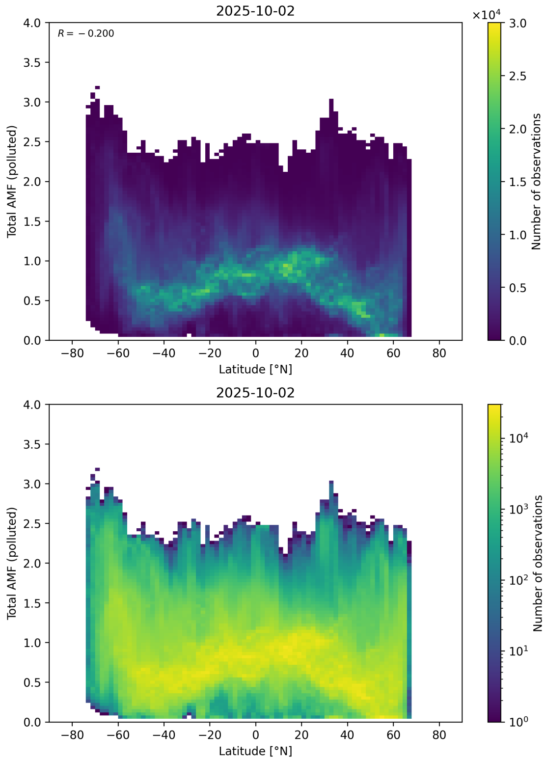
Figure 167: Scatter density plot of “Latitude” against “Total AMF (polluted)” for 2025-10-01 to 2025-10-03.
