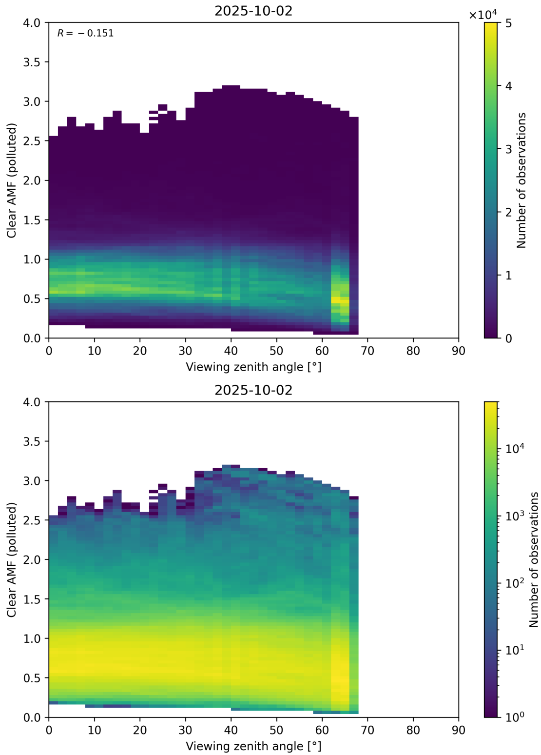
Figure 370: Scatter density plot of “Viewing zenith angle” against “Clear AMF (polluted)” for 2025-10-01 to 2025-10-03.
