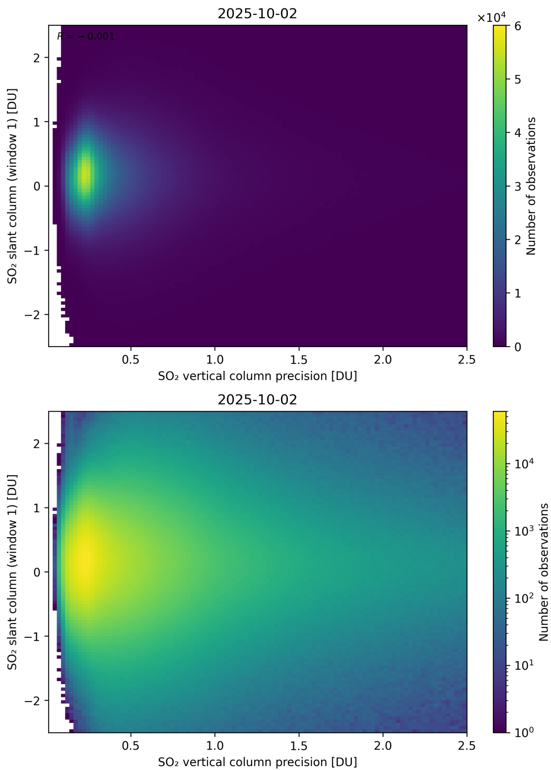
Figure 341: Scatter density plot of “SO 2 vertical column precision” against “SO 2 slant column (window 1)” for 2025-10-01 to 2025-10-03.
