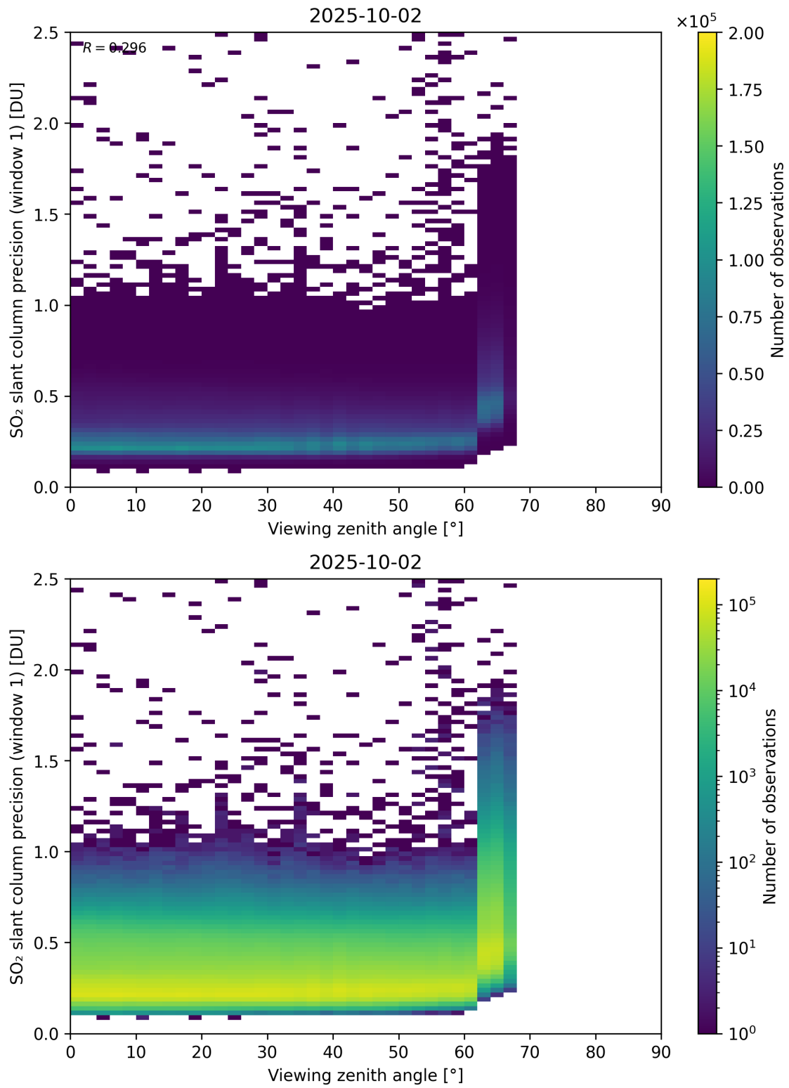
Figure 377: Scatter density plot of “Viewing zenith angle” against “SO 2 slant column precision (window 1)” for 2025-10-01 to 2025-10-03.
