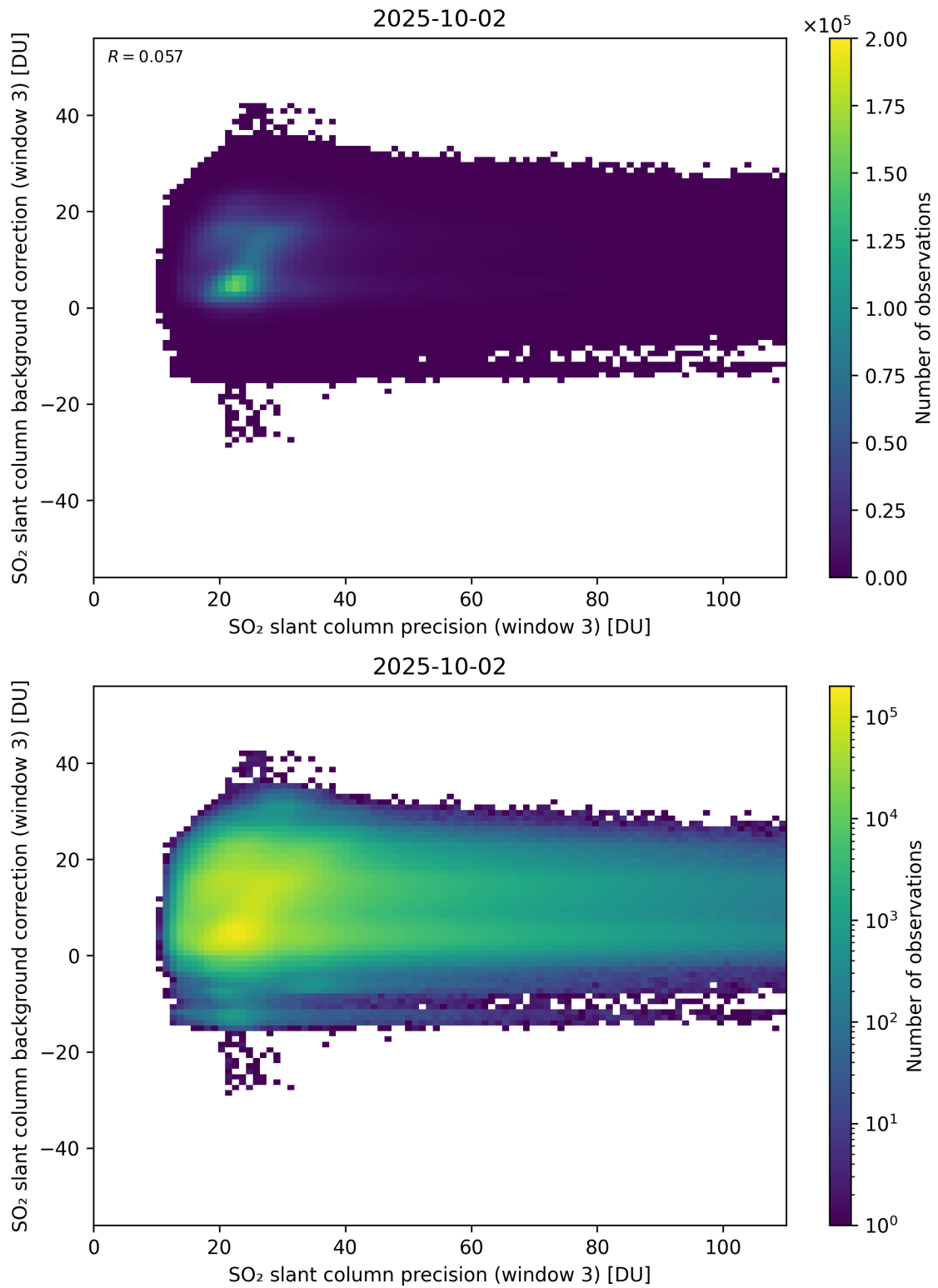
Figure 307: Scatter density plot of “SO 2 slant column precision (window 3)” against “SO 2 slant column background correction (window 3)” for 2025-10-01 to 2025-10-03.
