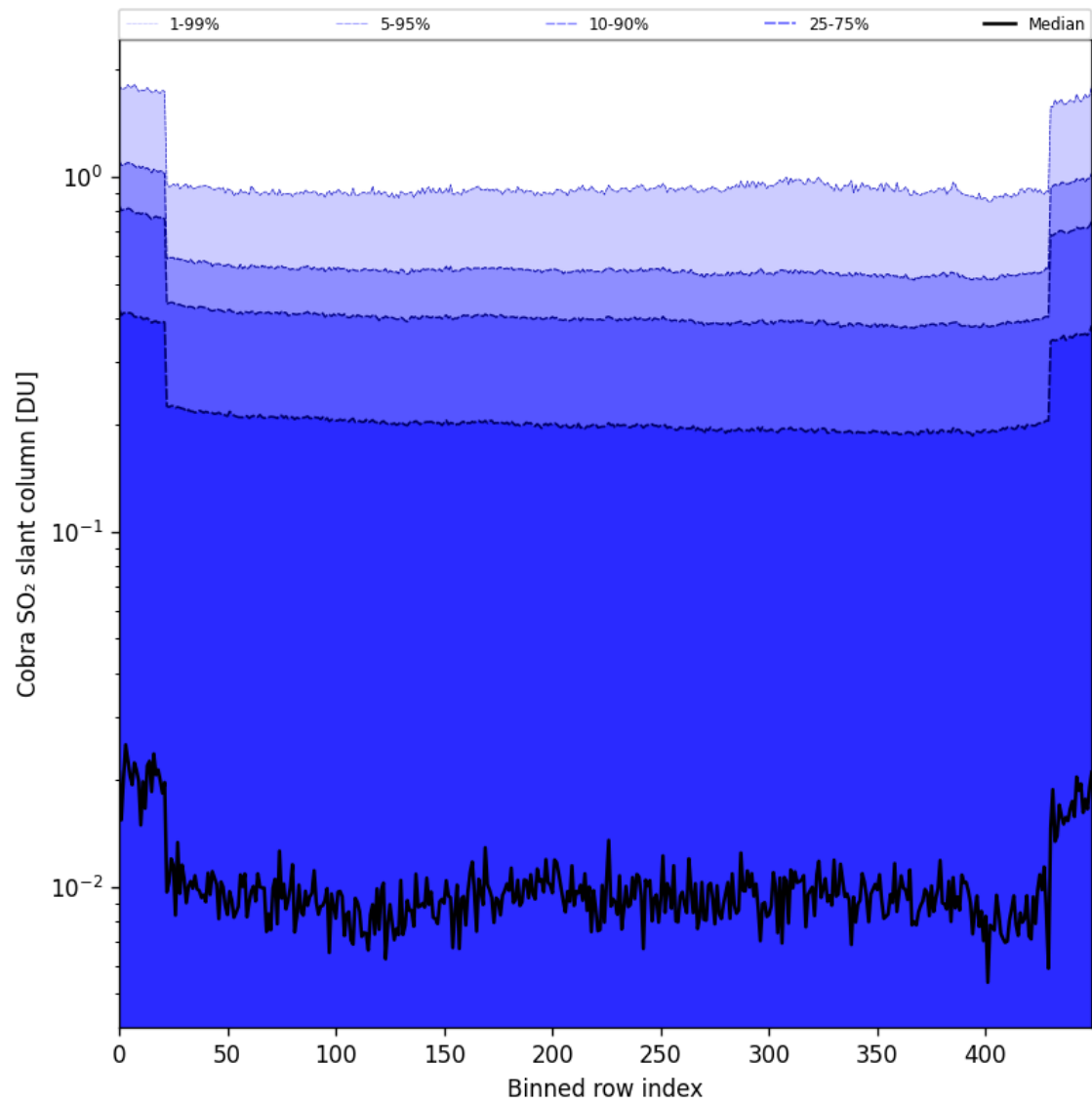
Figure 87: Along track statistics of “Cobra SO 2 slant column” for 2025-10-01 to 2025-10-03
