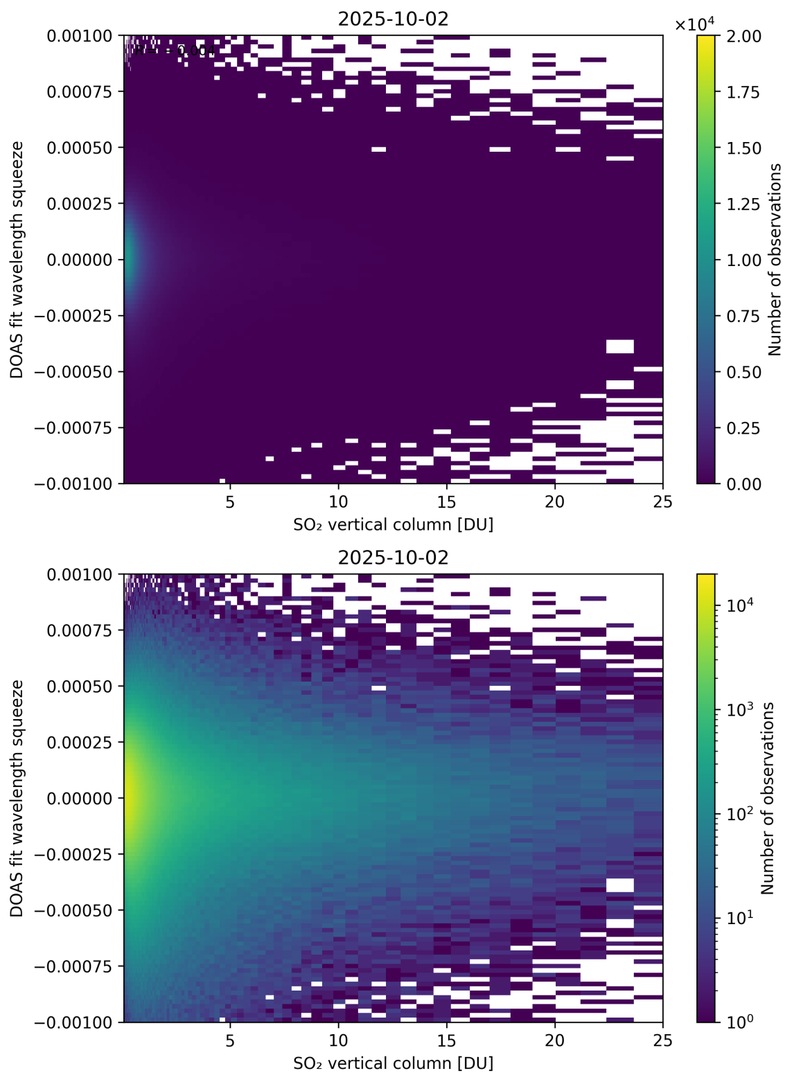
Figure 327: Scatter density plot of “SO 2 vertical column” against “DOAS fit wavelength squeeze” for 2025-10-01 to 2025-10-03.
