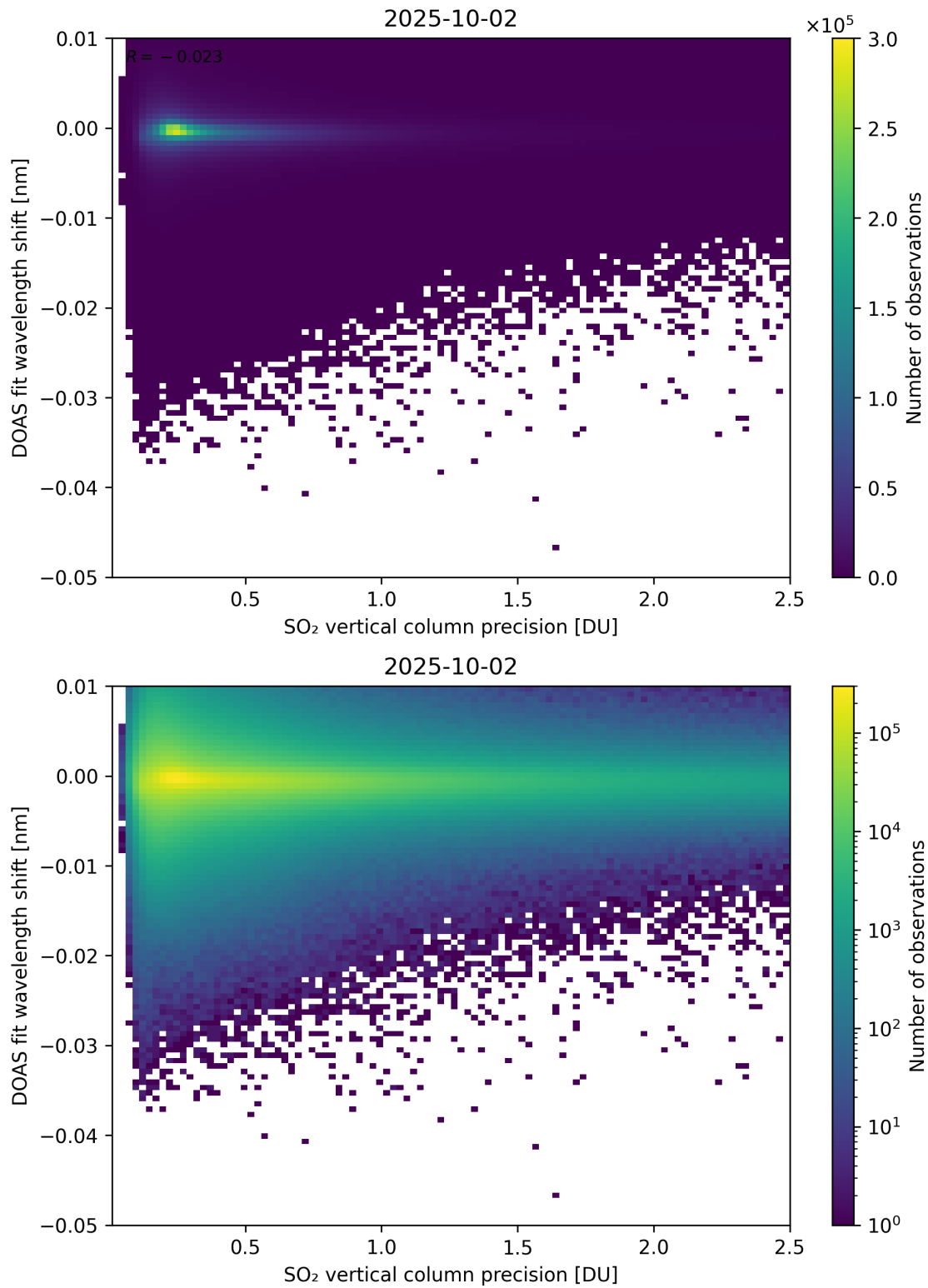
Figure 332: Scatter density plot of “SO 2 vertical column precision” against “DOAS fit wavelength shift” for 2025-10-01 to 2025-10-03.
