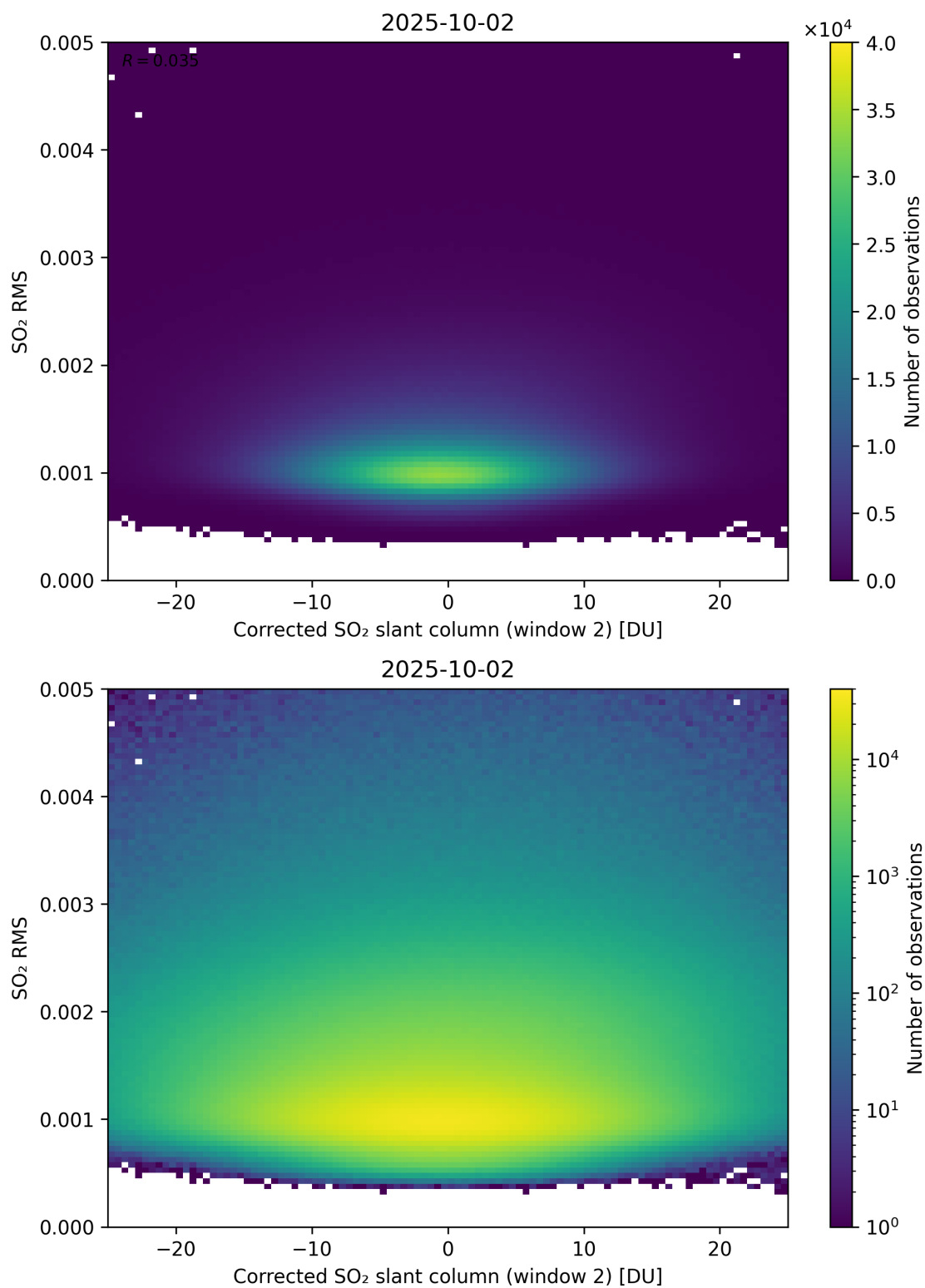
Figure 248: Scatter density plot of “Corrected SO 2 slant column (window 2)” against “SO 2 RMS” for 2025-10-01 to 2025-10-03.
