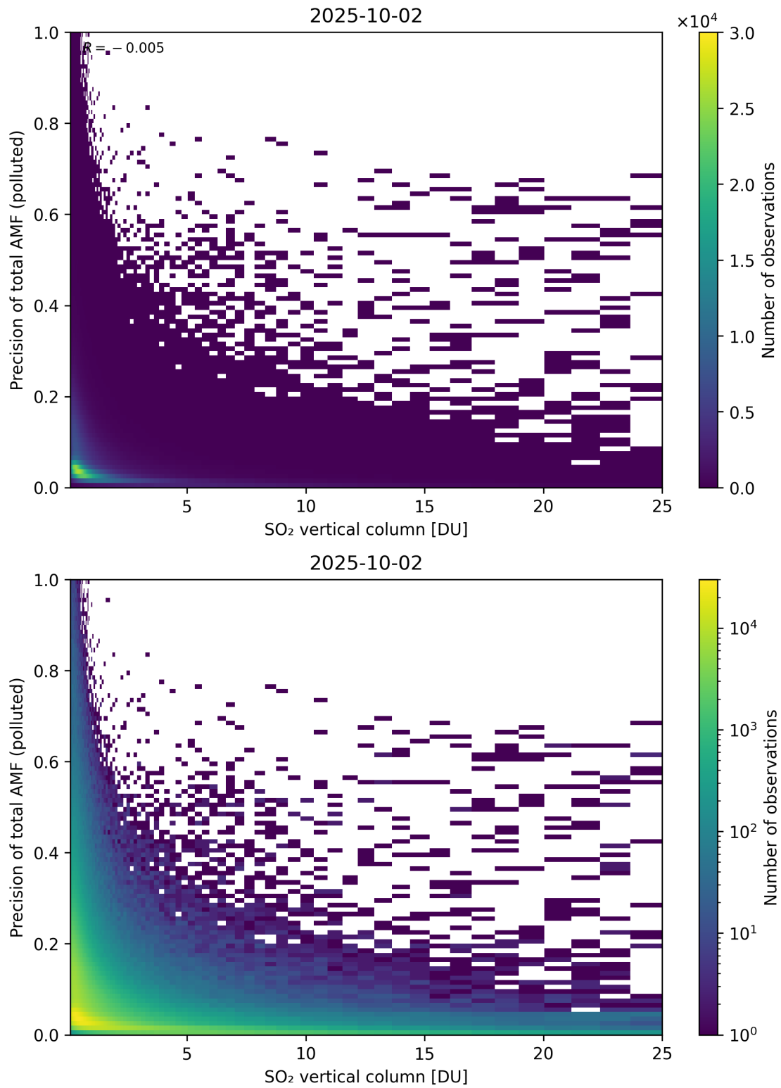
Figure 360: Scatter density plot of “SO 2 vertical column” against “Precision of total AMF (polluted)” for 2025-10-01 to 2025-10-03.
