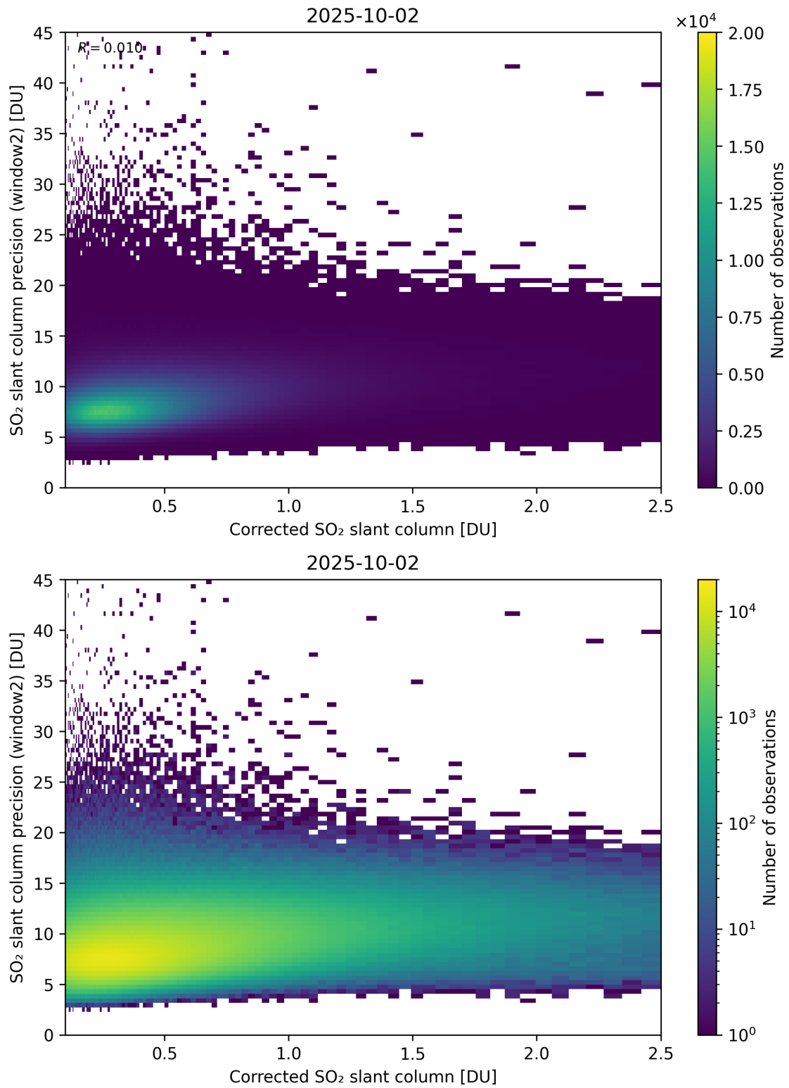
Figure 239: Scatter density plot of “Corrected SO 2 slant column” against “SO 2 slant column precision (window2)” for 2025-10-01 to 2025-10-03.
