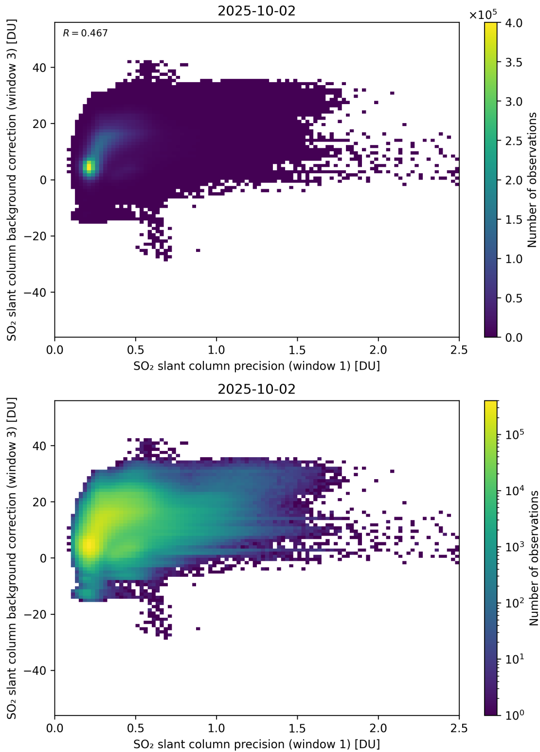
Figure 270: Scatter density plot of “SO 2 slant column precision (window 1)” against “SO 2 slant column background correction (window 3)” for 2025-10-01 to 2025-10-03.
