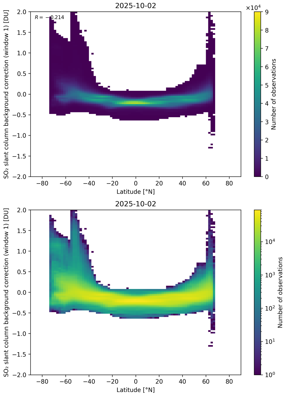
Figure 150: Scatter density plot of “Latitude” against “SO 2 slant column background correction (window 1)” for 2025-10-01 to 2025-10-03.
