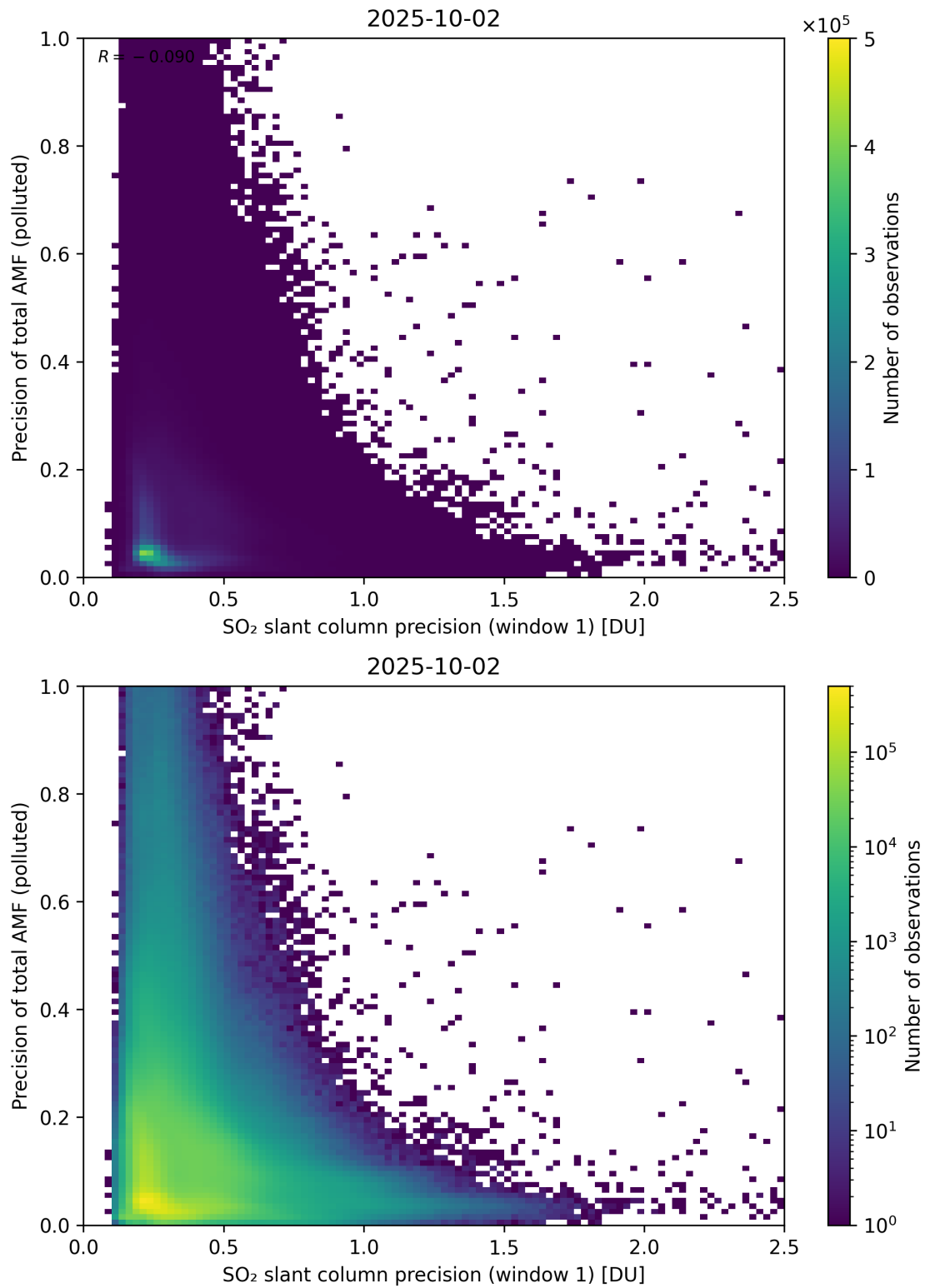
Figure 281: Scatter density plot of “SO 2 slant column precision (window 1)” against “Precision of total AMF (polluted)” for 2025-10-01 to 2025-10-03.
