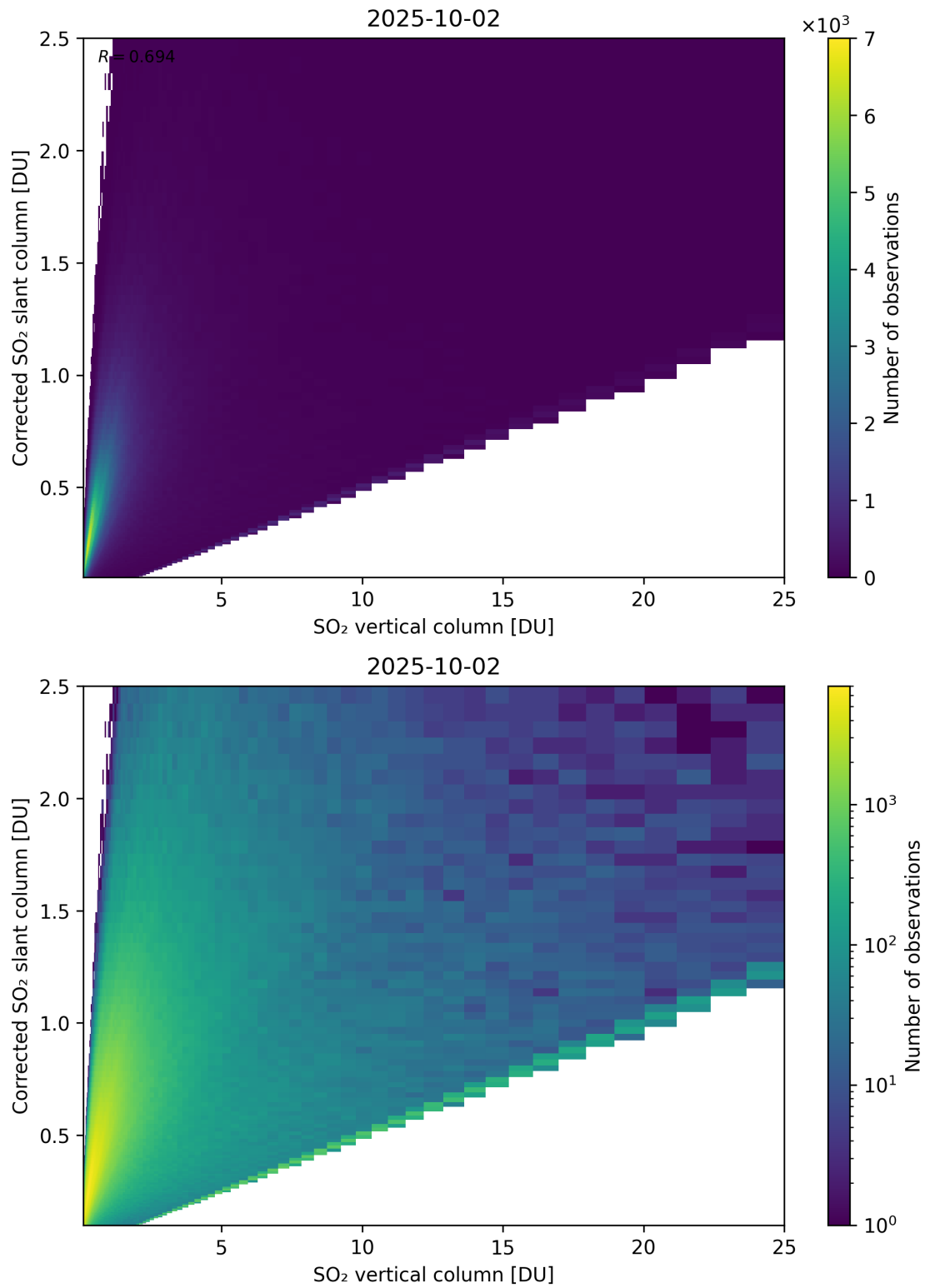
Figure 351: Scatter density plot of “SO 2 vertical column” against “Corrected SO 2 slant column” for 2025-10-01 to 2025-10-03.
