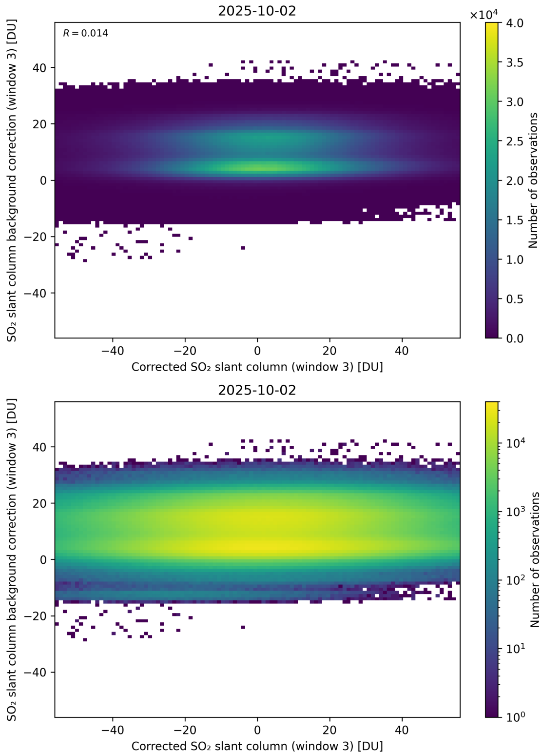
Figure 255: Scatter density plot of “Corrected SO 2 slant column (window 3)” against “SO 2 slant column background correction (window 3)” for 2025-10-01 to 2025-10-03.
