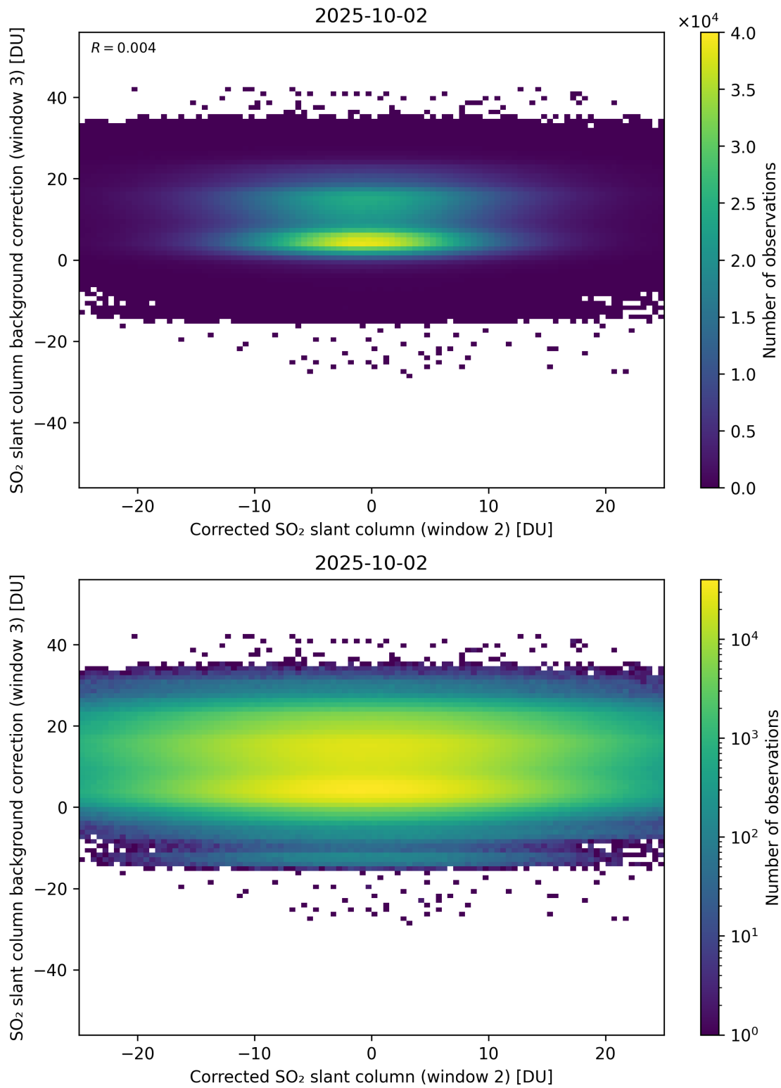
Figure 245: Scatter density plot of “Corrected SO 2 slant column (window 2)” against “SO 2 slant column background correction (window 3)” for 2025-10-01 to 2025-10-03.
