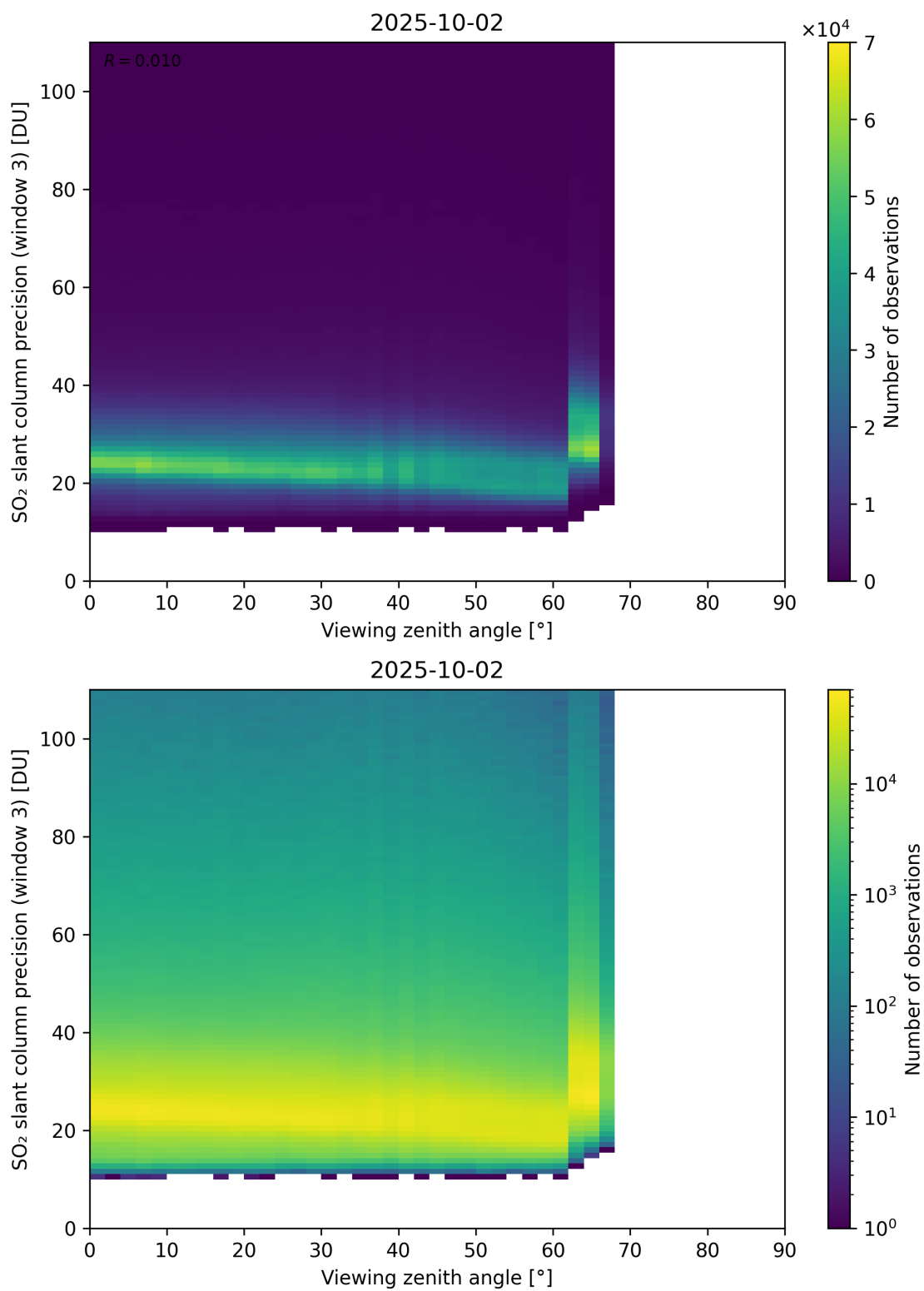
Figure 380: Scatter density plot of “Viewing zenith angle” against “SO 2 slant column precision (window 3)” for 2025-10-01 to 2025-10-03.
