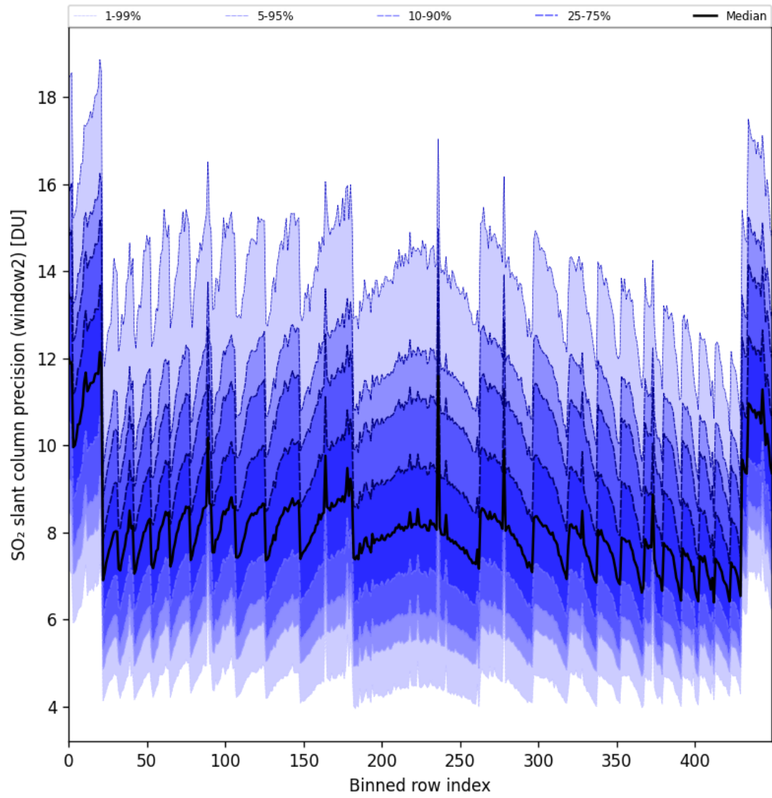
Figure 94: Along track statistics of “SO 2 slant column precision (window2)” for 2025-10-01 to 2025-10-03
