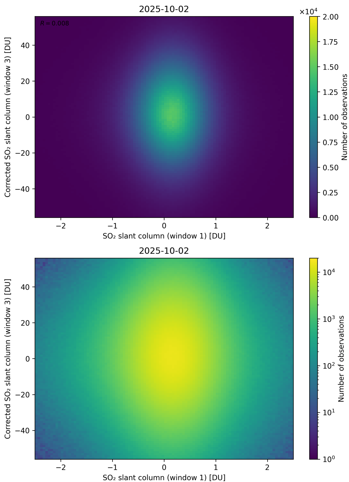
Figure 284: Scatter density plot of “SO 2 slant column (window 1)” against “Corrected SO 2 slant column (window 3)” for 2025-10-01 to 2025-10-03.
