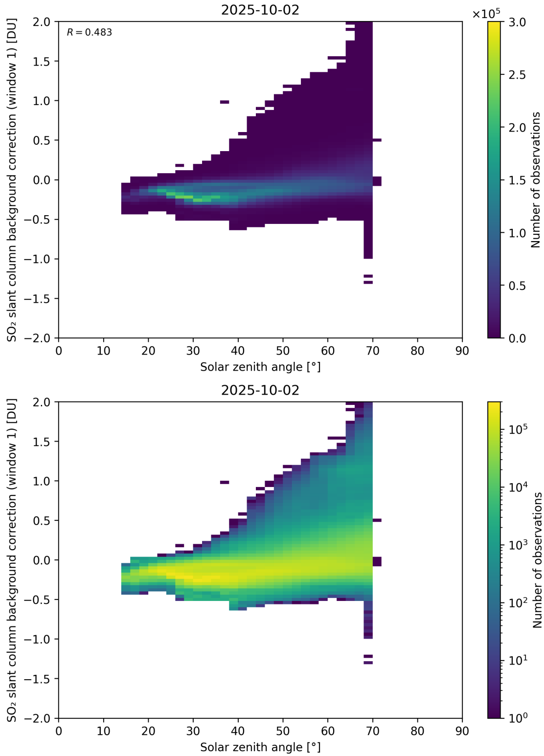
Figure 171: Scatter density plot of “Solar zenith angle” against “SO 2 slant column background correction (window 1)” for 2025-10-01 to 2025-10-03.
