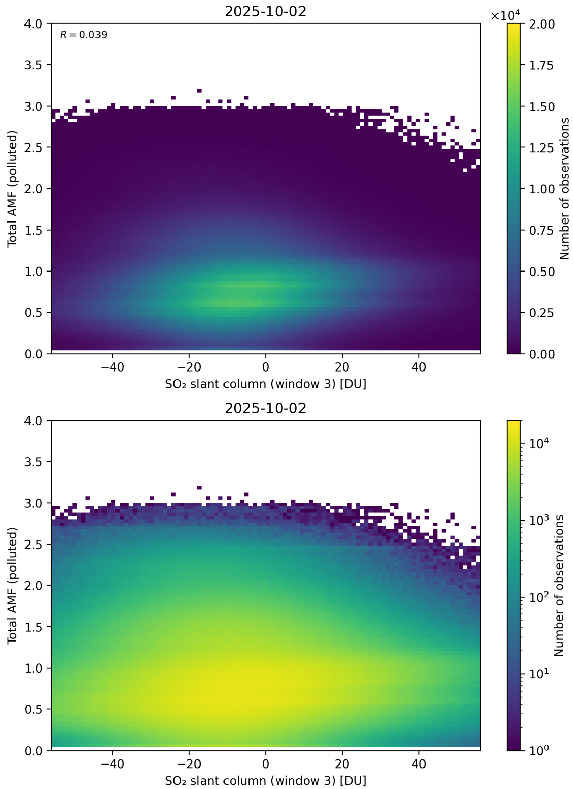
Figure 318: Scatter density plot of “SO 2 slant column (window 3)” against “Total AMF (polluted)” for 2025-10-01 to 2025-10-03.
