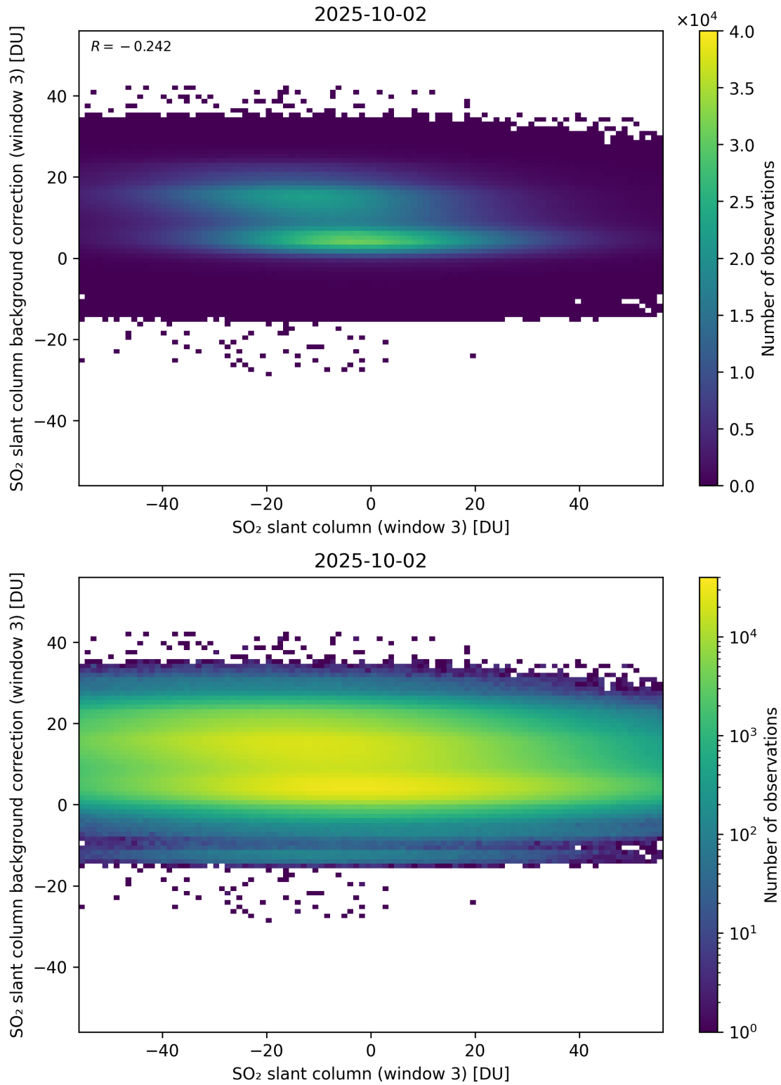
Figure 303: Scatter density plot of “SO 2 slant column (window 3)” against “SO 2 slant column background correction (window 3)” for 2025-10-01 to 2025-10-03.
