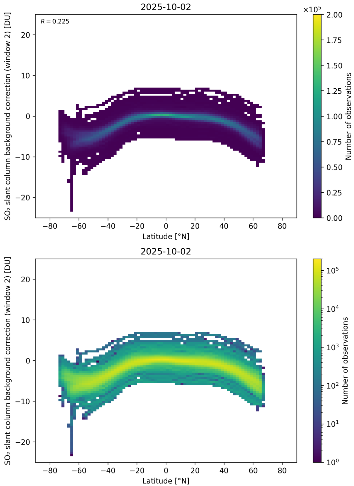
Figure 151: Scatter density plot of “Latitude” against “SO 2 slant column background correction (window 2)” for 2025-10-01 to 2025-10-03.
