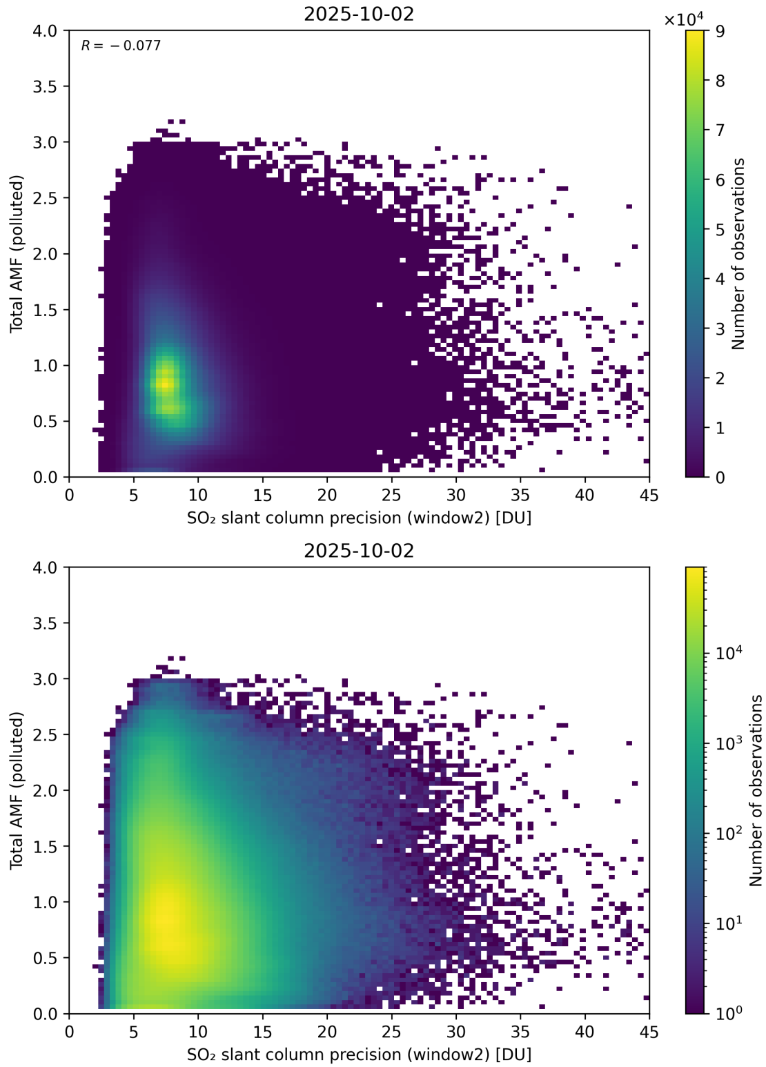
Figure 301: Scatter density plot of “SO 2 slant column precision (window2)” against “Total AMF (polluted)” for 2025-10-01 to 2025-10-03.
