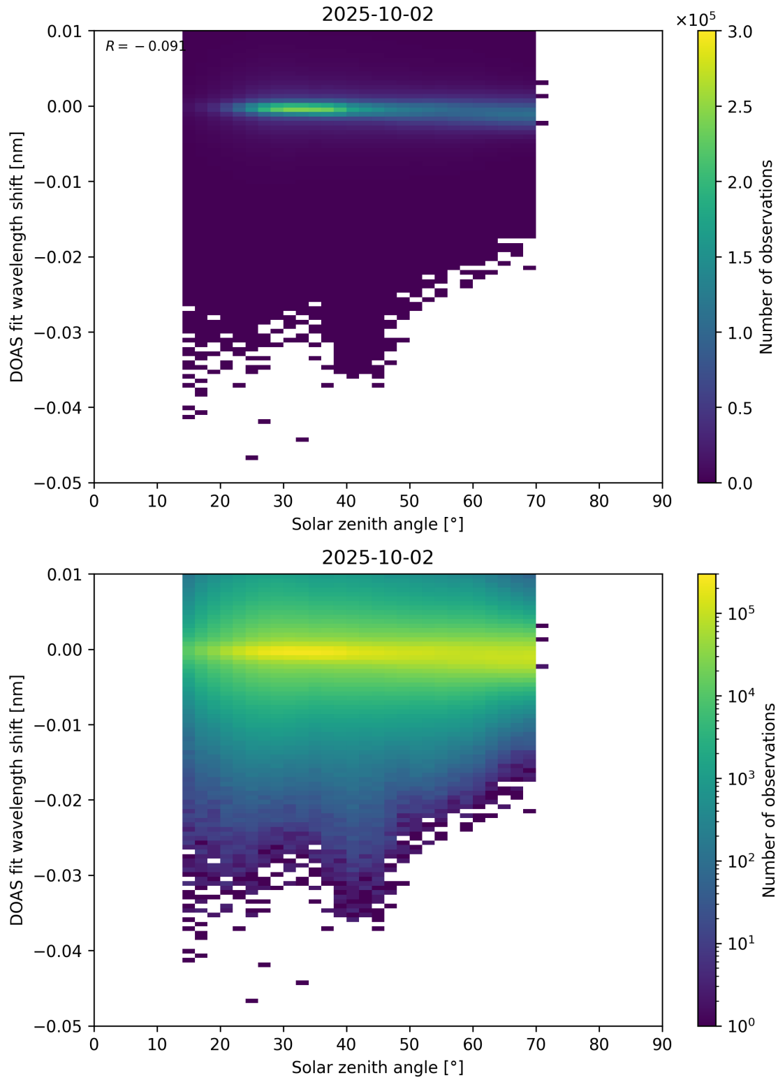
Figure 174: Scatter density plot of “Solar zenith angle” against “DOAS fit wavelength shift” for 2025-10-01 to 2025-10-03.
