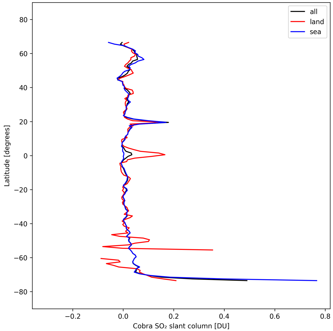
Figure 35: Zonal average of “Cobra SO 2 slant column” for 2025-10-01 to 2025-10-03.
