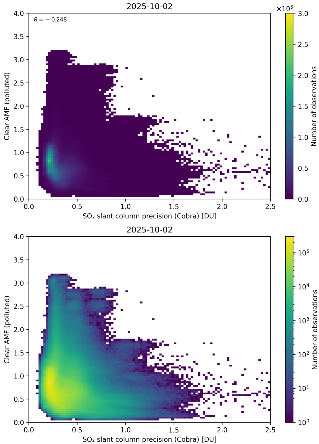
Figure 205: Scatter density plot of “SO 2 slant column precision (Cobra)” against “Clear AMF (polluted)” for 2025-10-01 to 2025-10-03.
