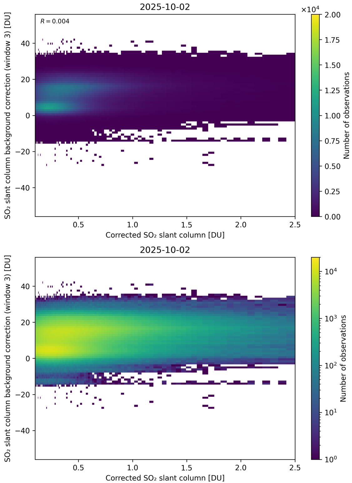
Figure 228: Scatter density plot of “Corrected SO 2 slant column” against “SO 2 slant column background correction (window 3)” for 2025-10-01 to 2025-10-03.
