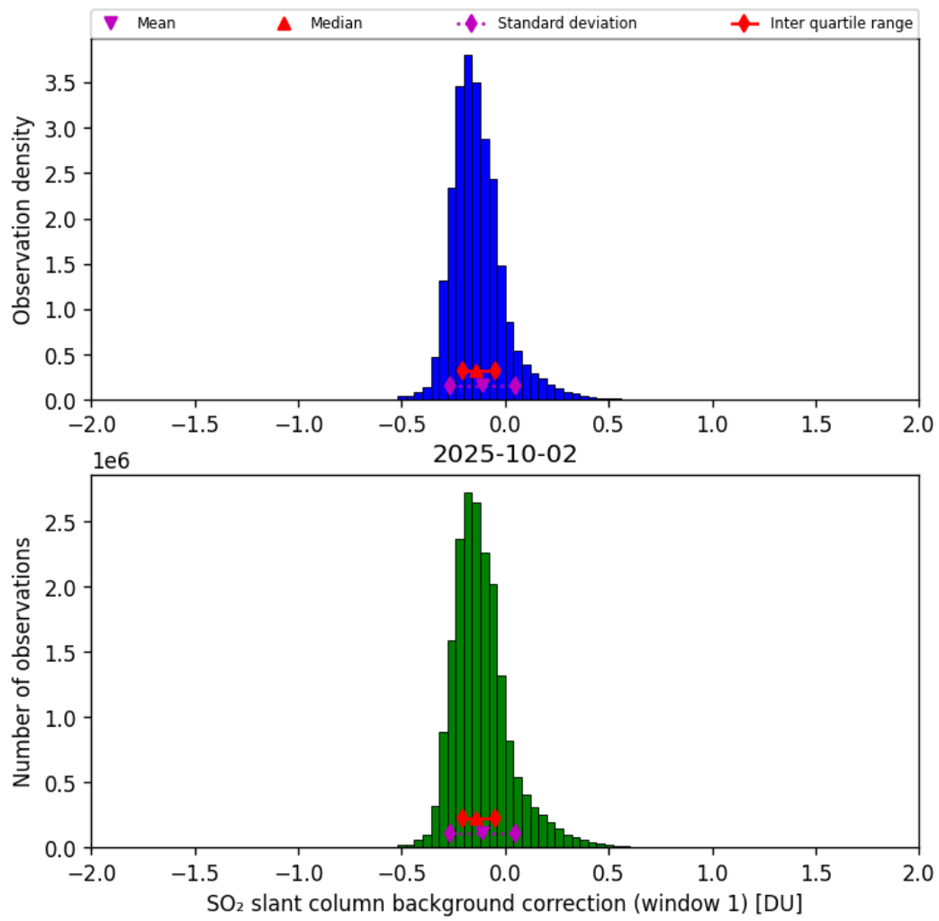
Figure 66: Histogram of “SO 2 slant column background correction (window 1)” for 2025-10-01 to 2025-10-03
