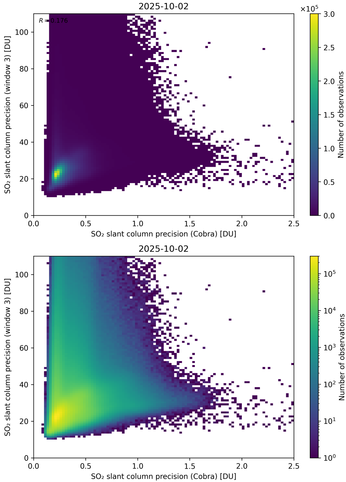
Figure 212: Scatter density plot of “SO 2 slant column precision (Cobra)” against “SO 2 slant column precision (window 3)” for 2025-10-01 to 2025-10-03.
