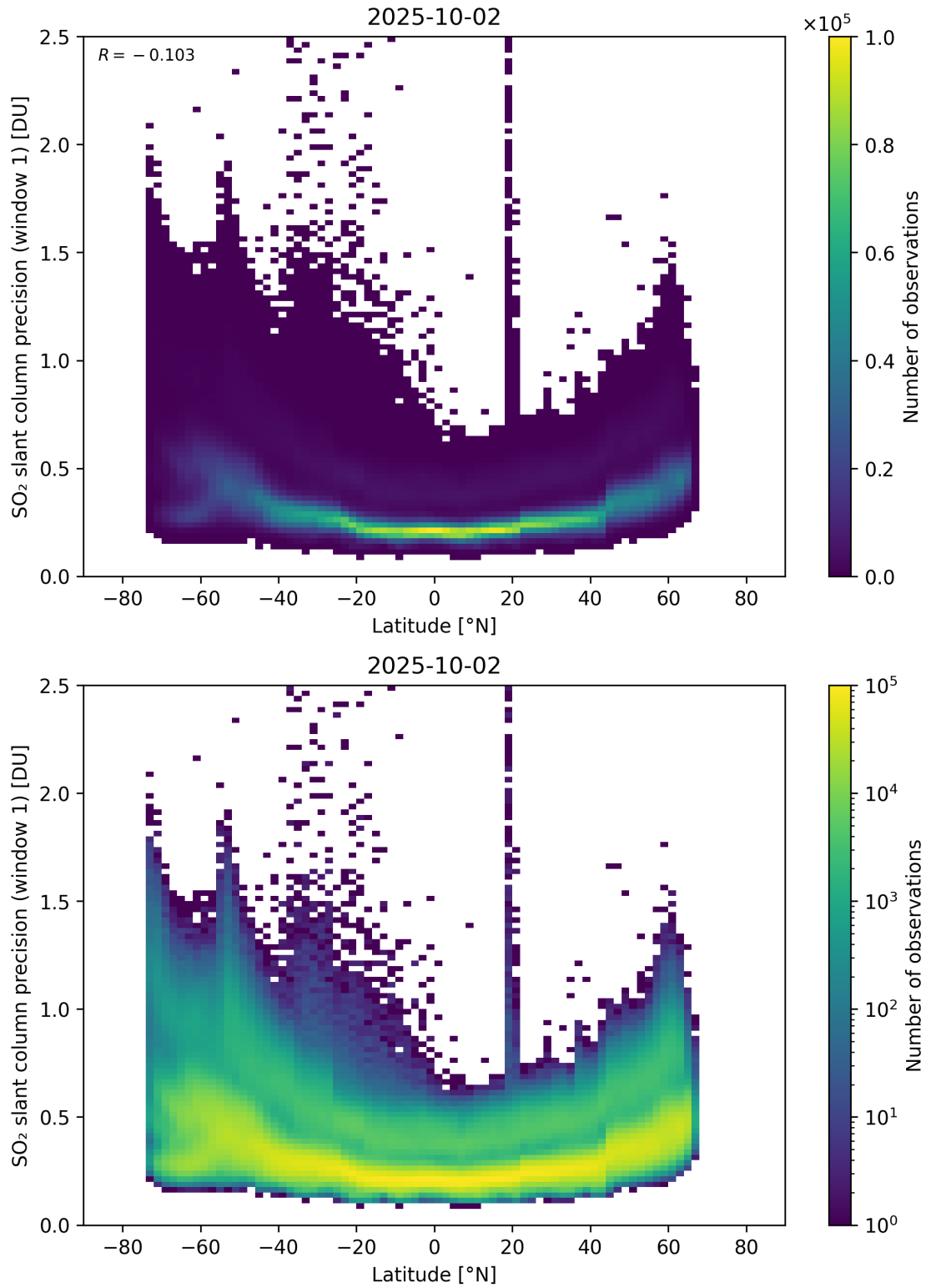
Figure 163: Scatter density plot of “Latitude” against “SO 2 slant column precision (window 1)” for 2025-10-01 to 2025-10-03.
