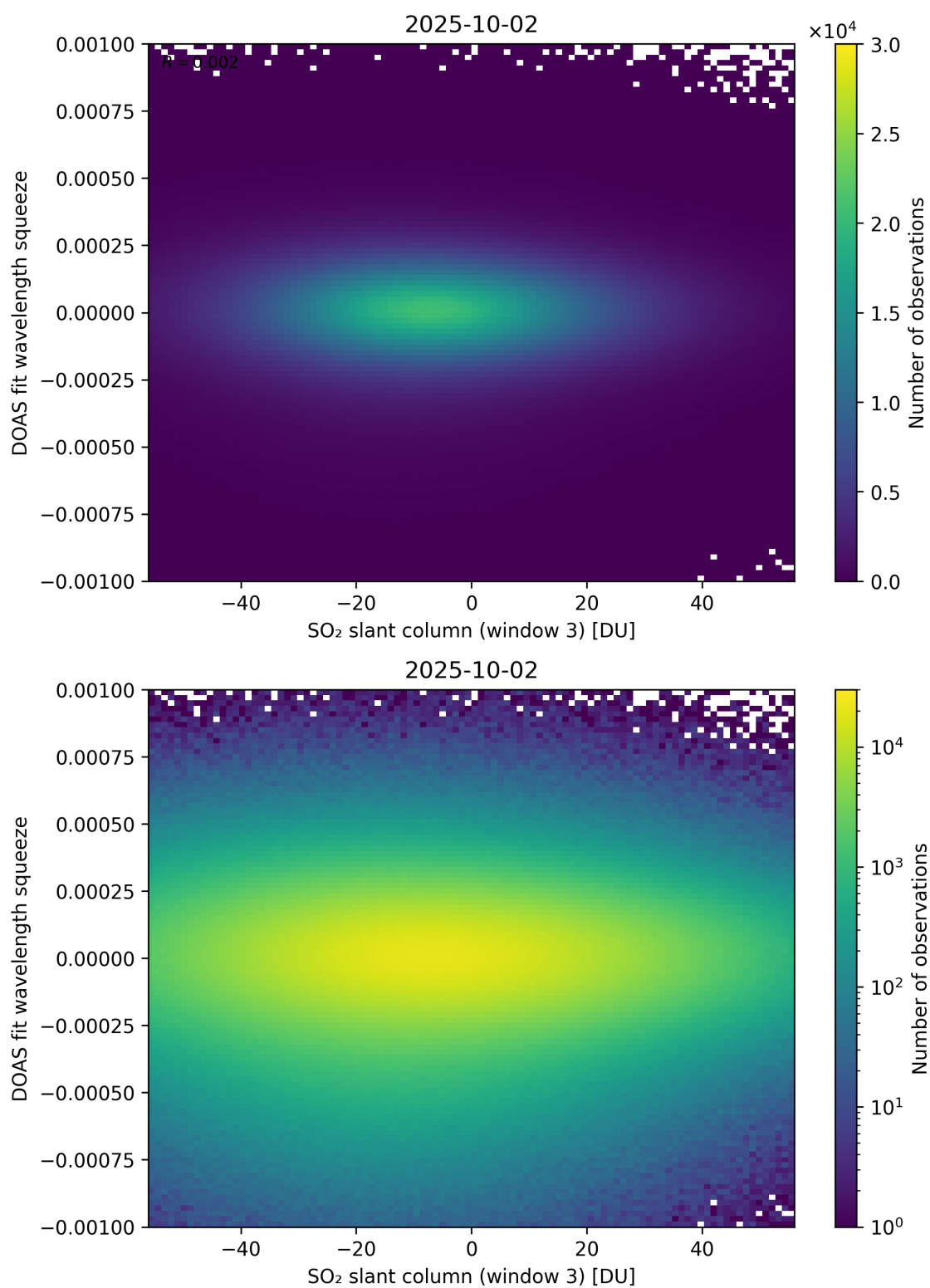
Figure 305: Scatter density plot of “SO 2 slant column (window 3)” against “DOAS fit wavelength squeeze” for 2025-10-01 to 2025-10-03.
