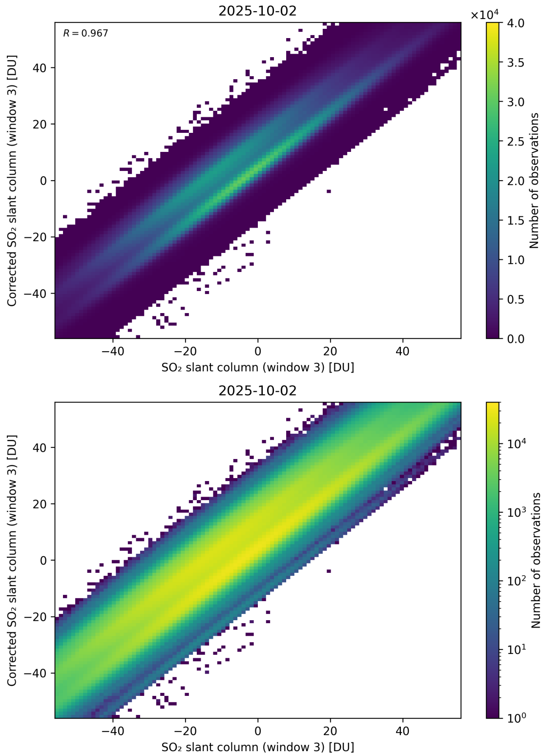
Figure 316: Scatter density plot of “SO 2 slant column (window 3)” against “Corrected SO 2 slant column (window 3)” for 2025-10-01 to 2025-10-03.
