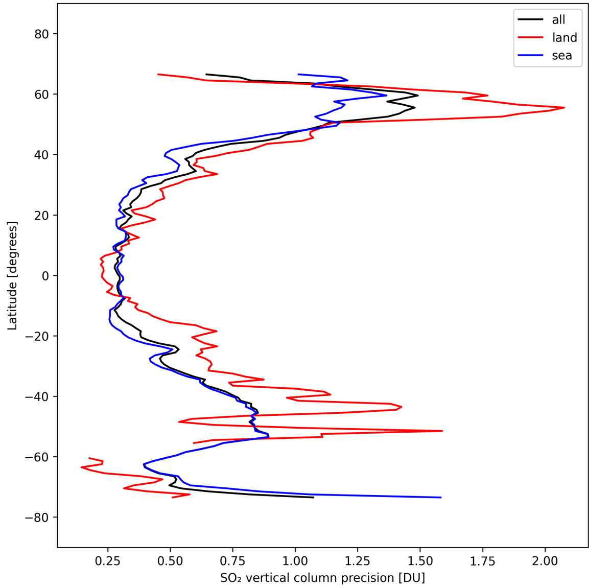
Figure 33: Zonal average of “SO 2 vertical column precision” for 2025-10-01 to 2025-10-03.
