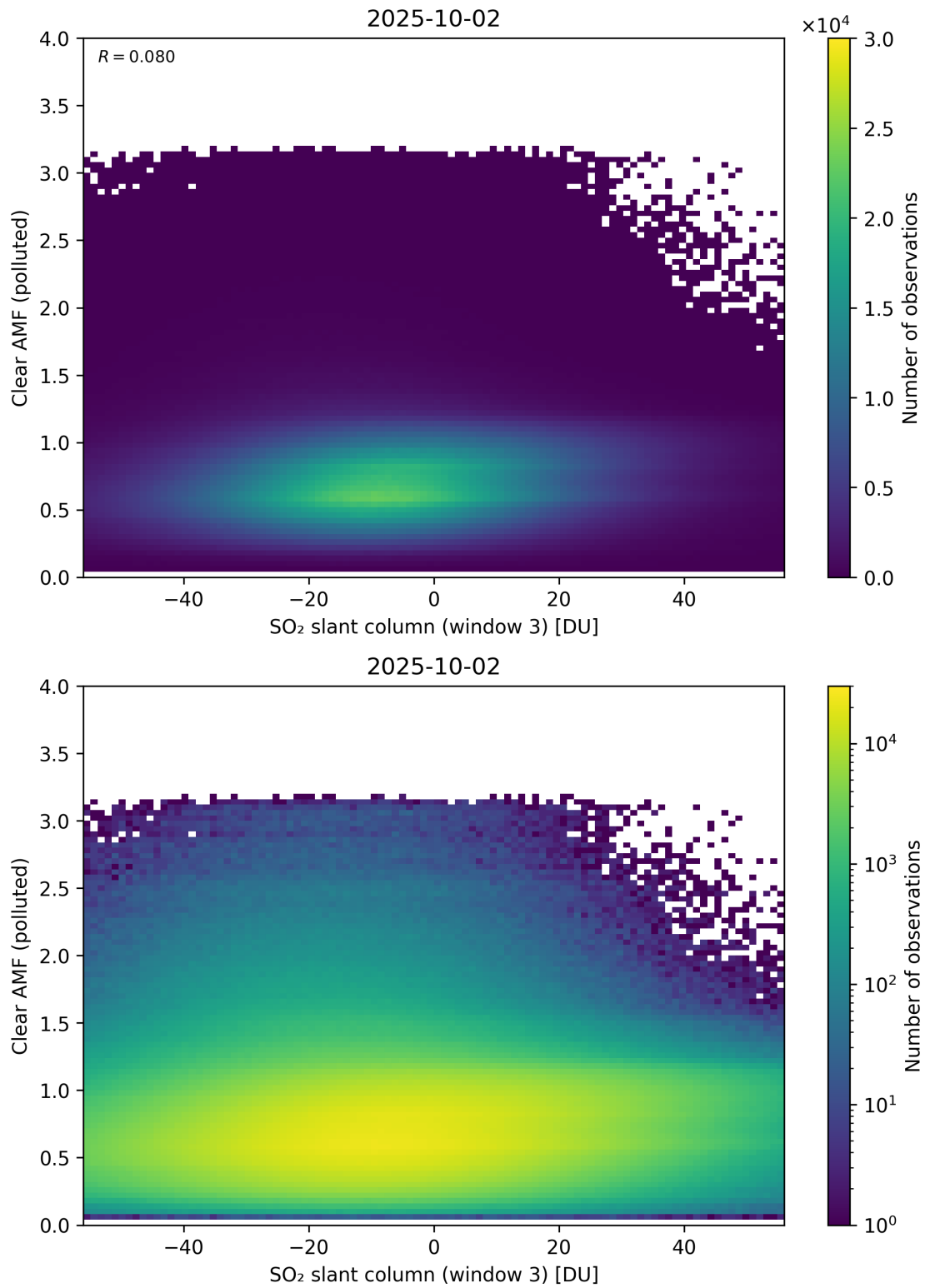
Figure 315: Scatter density plot of “SO 2 slant column (window 3)” against “Clear AMF (polluted)” for 2025-10-01 to 2025-10-03.
