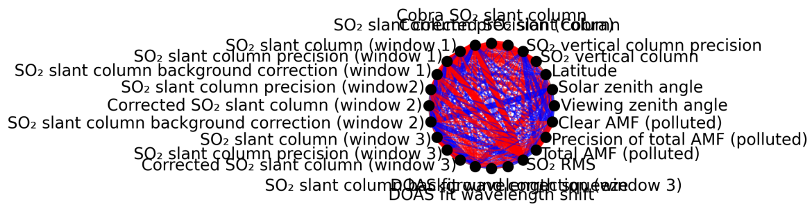
Figure 1: Map of correlation graph for 2025-10-01 to 2025-10-03.
