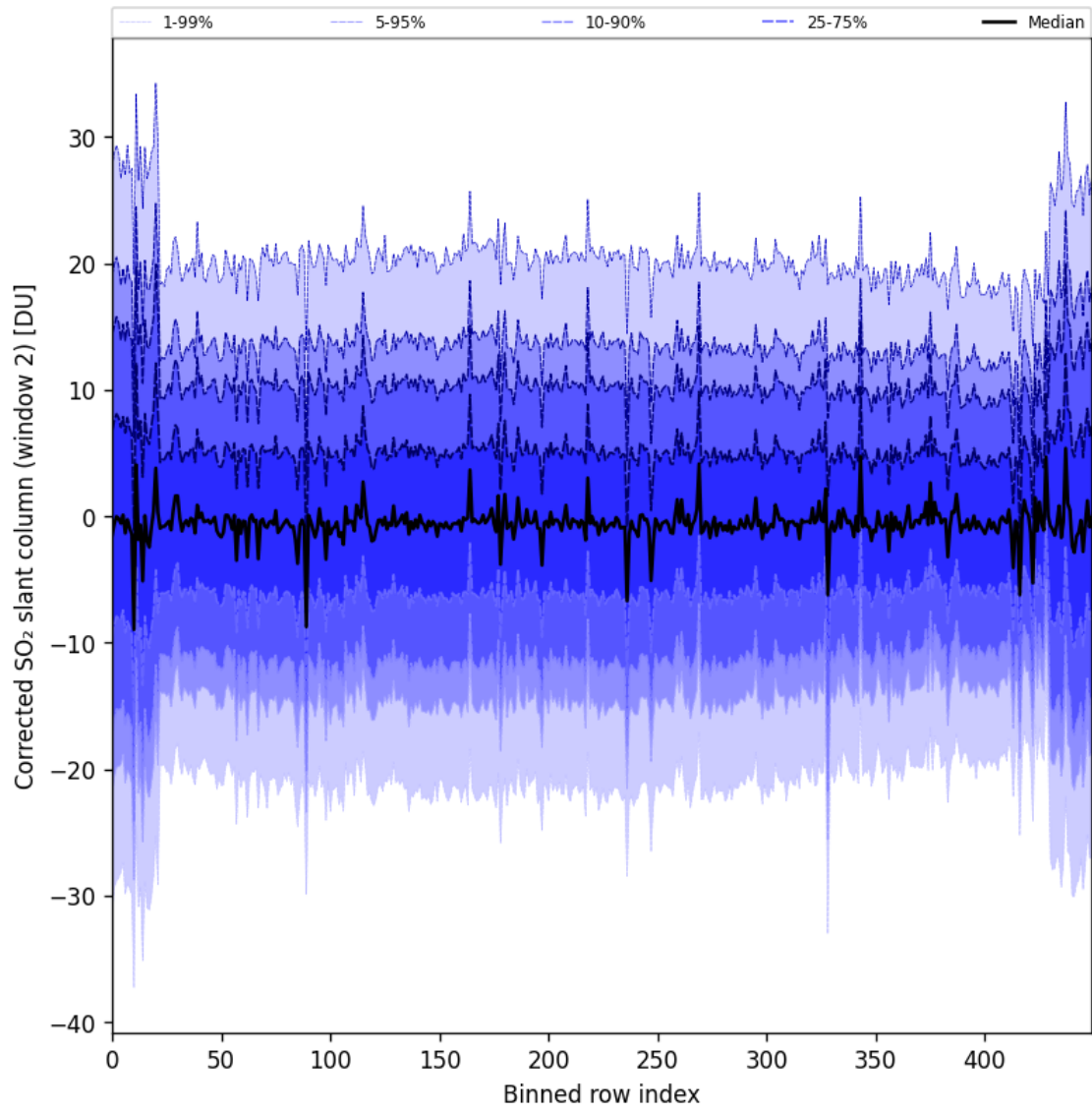
Figure 95: Along track statistics of “Corrected SO 2 slant column (window 2)” for 2025-10-01 to 2025-10-03
