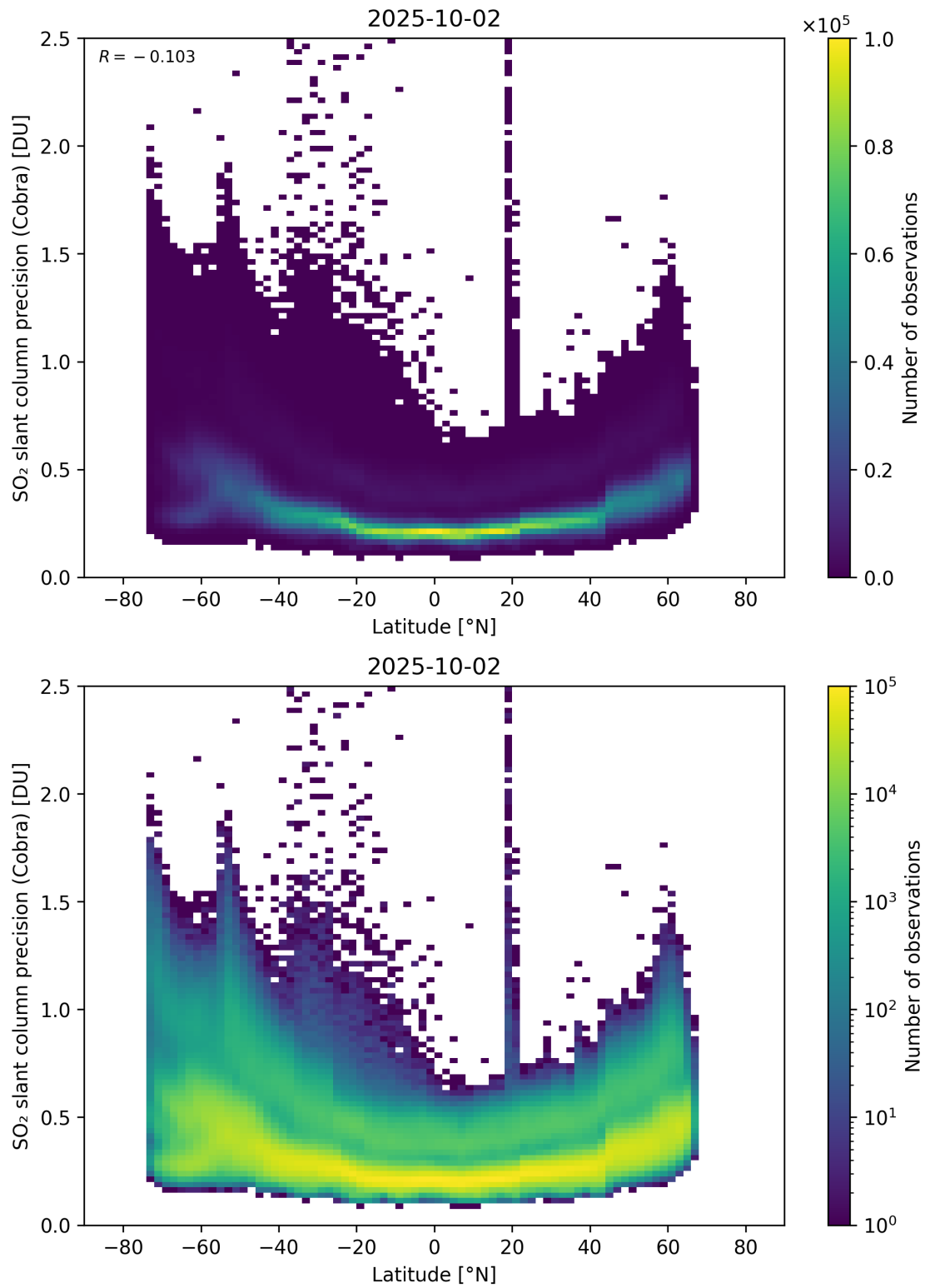
Figure 158: Scatter density plot of “Latitude” against “SO 2 slant column precision (Cobra)” for 2025-10-01 to 2025-10-03.
