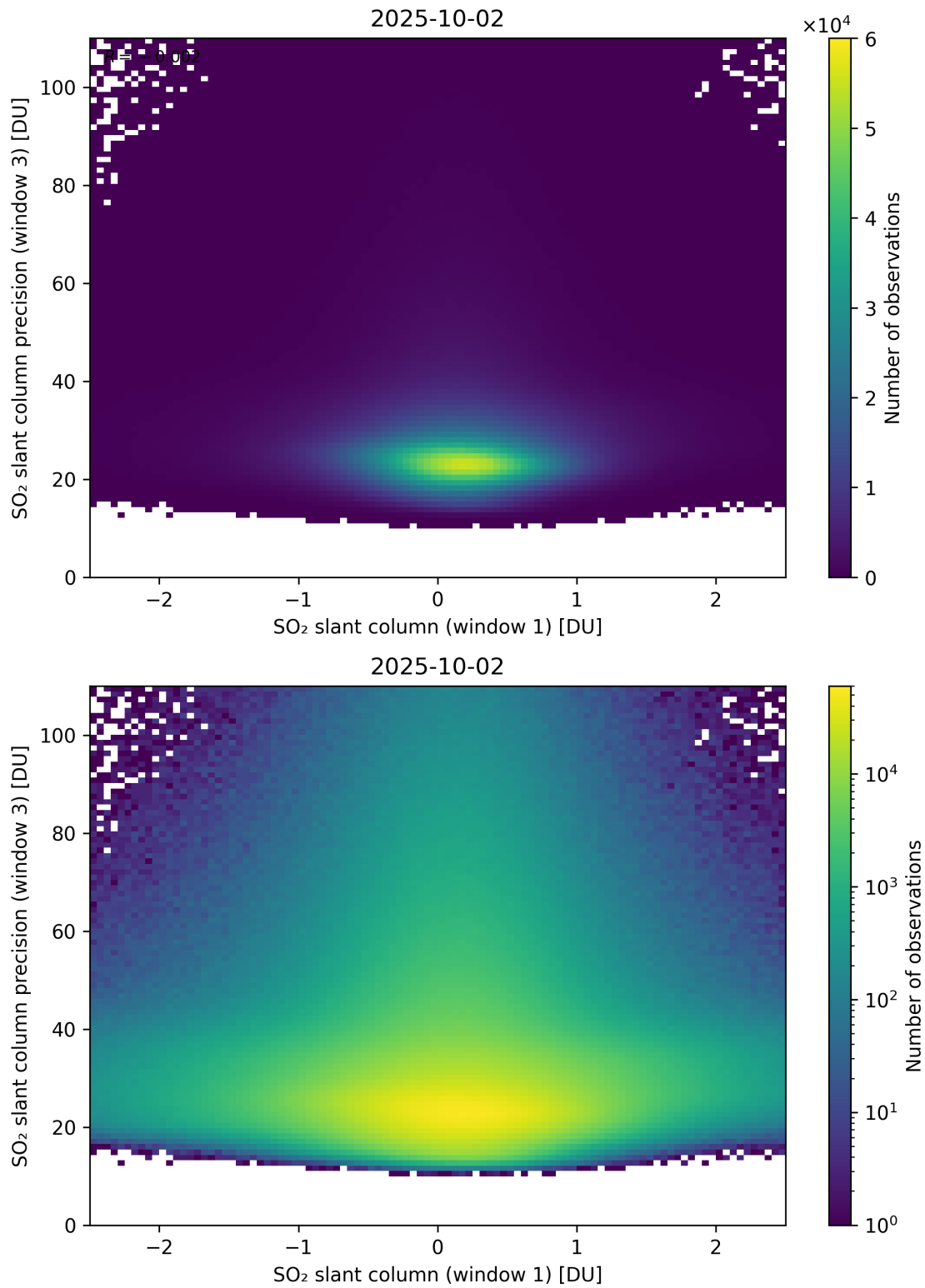
Figure 288: Scatter density plot of “SO 2 slant column (window 1)” against “SO 2 slant column precision (window 3)” for 2025-10-01 to 2025-10-03.
