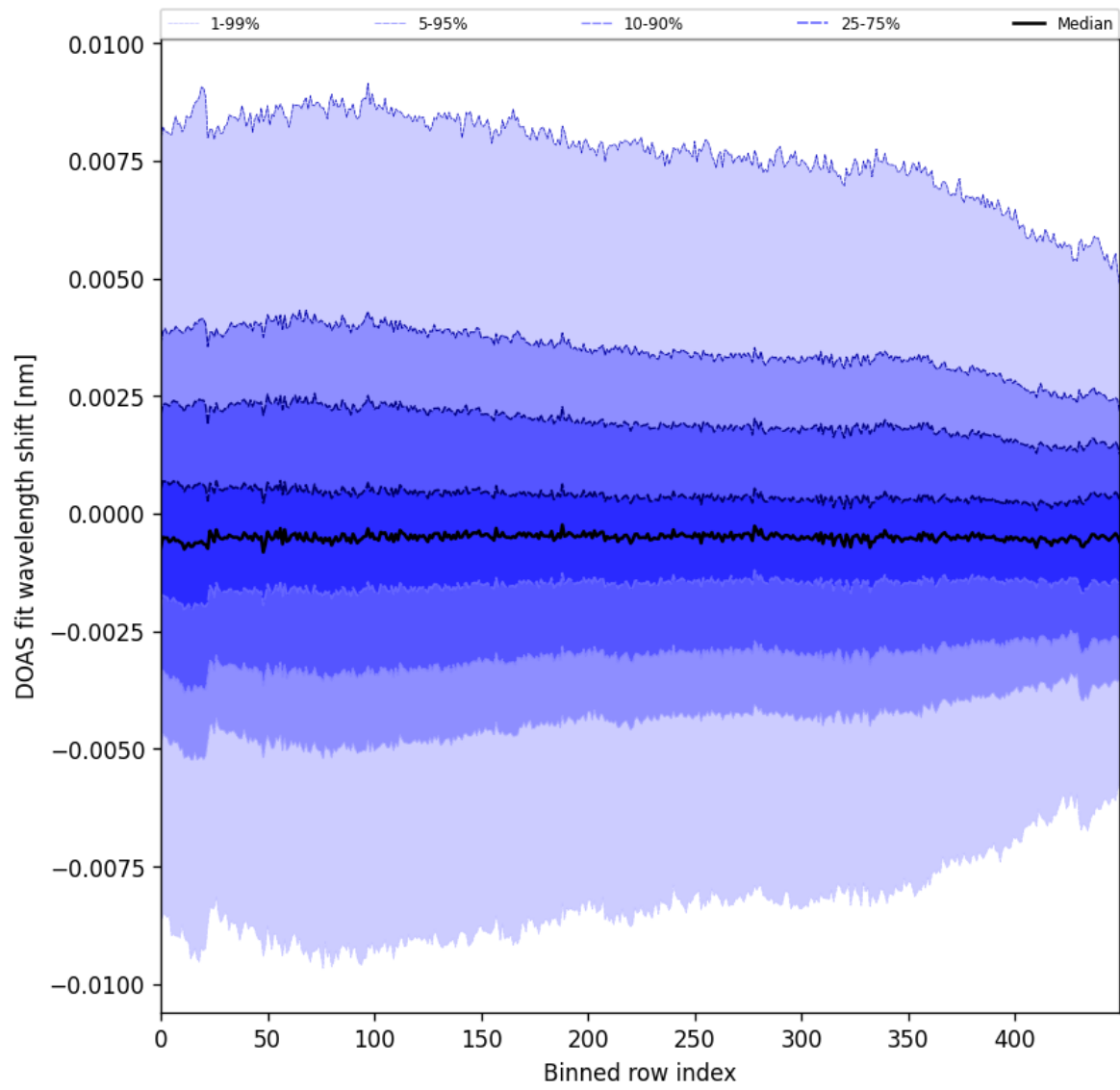
Figure 102: Along track statistics of “DOAS fit wavelength shift” for 2025-10-01 to 2025-10-03
