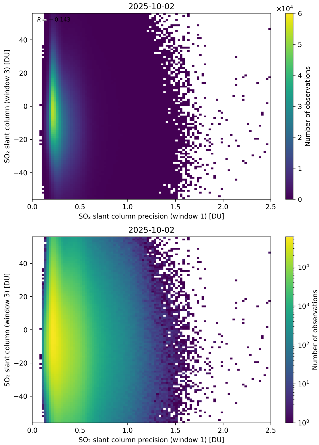
Figure 278: Scatter density plot of “SO 2 slant column precision (window 1)” against “SO 2 slant column (window 3)” for 2025-10-01 to 2025-10-03.
