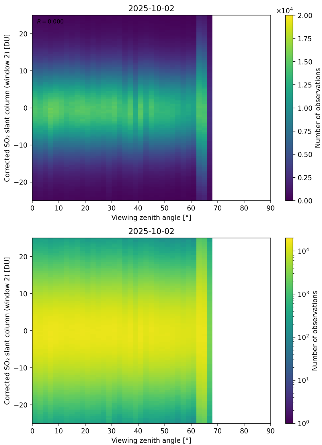
Figure 374: Scatter density plot of “Viewing zenith angle” against “Corrected SO 2 slant column (window 2)” for 2025-10-01 to 2025-10-03.
