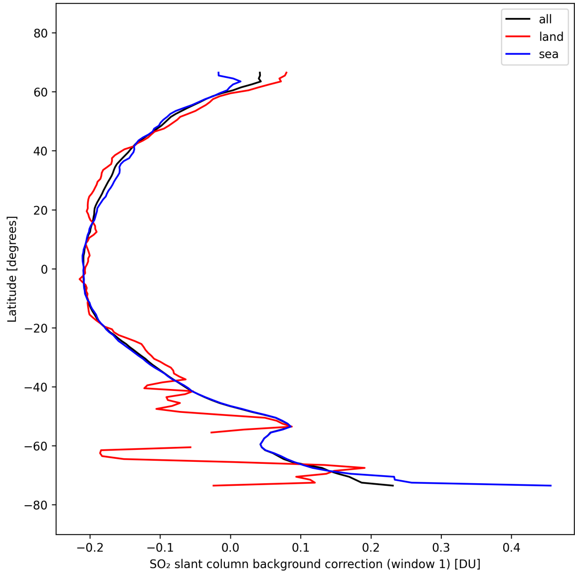
Figure 40: Zonal average of “SO 2 slant column background correction (window 1)” for 2025-10-01 to 2025-10-03.
