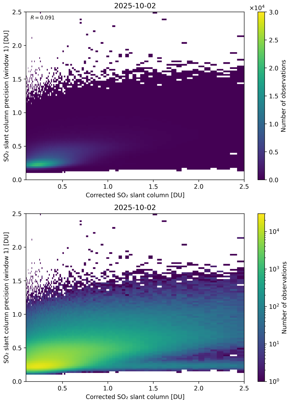
Figure 238: Scatter density plot of “Corrected SO 2 slant column” against “SO 2 slant column precision (window 1)” for 2025-10-01 to 2025-10-03.
