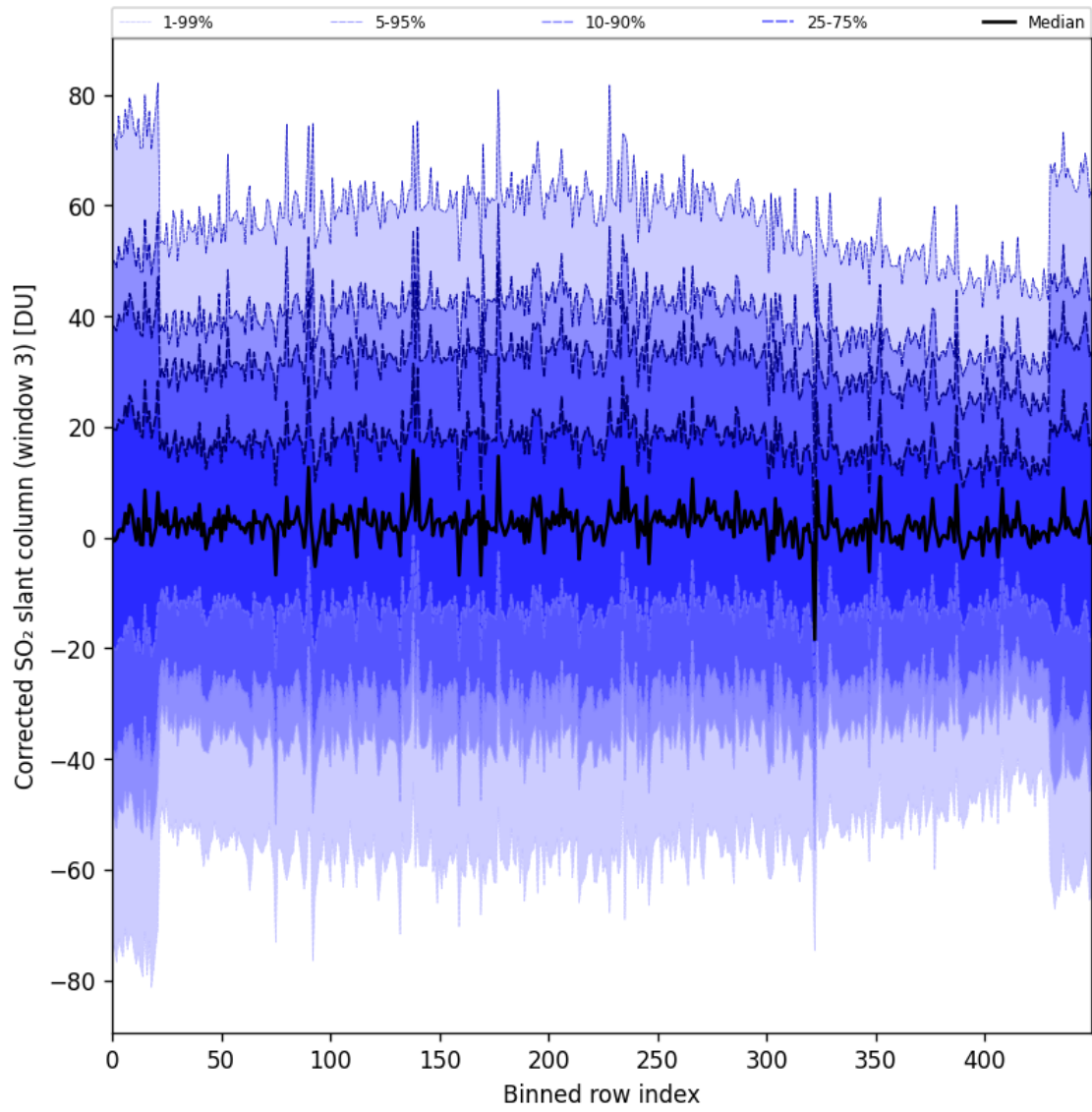
Figure 99: Along track statistics of “Corrected SO 2 slant column (window 3)” for 2025-10-01 to 2025-10-03
