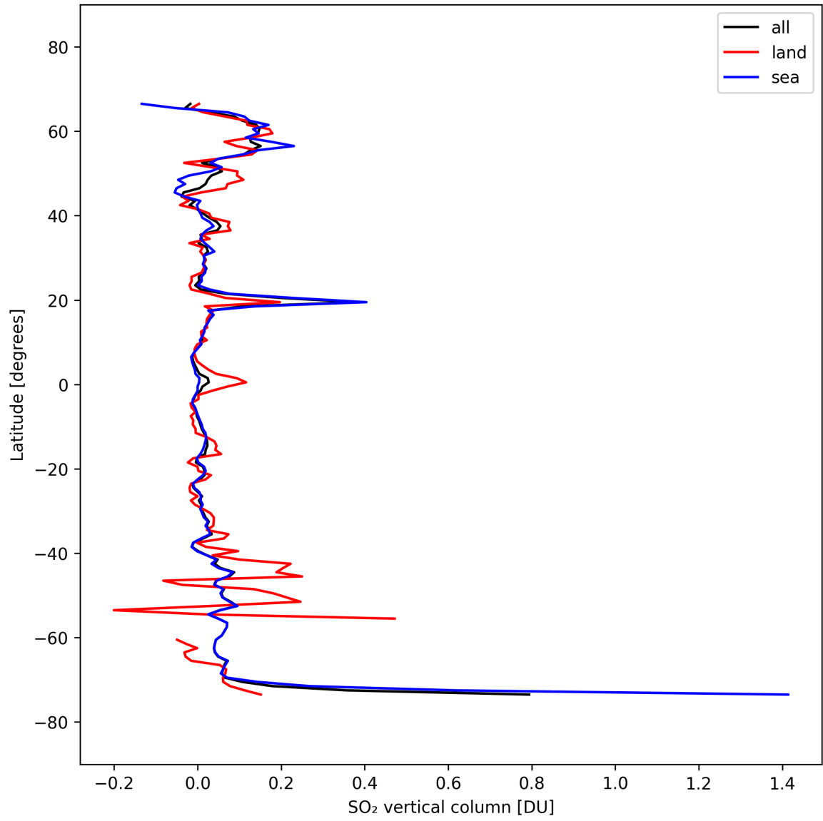
Figure 32: Zonal average of “SO 2 vertical column” for 2025-10-01 to 2025-10-03.
