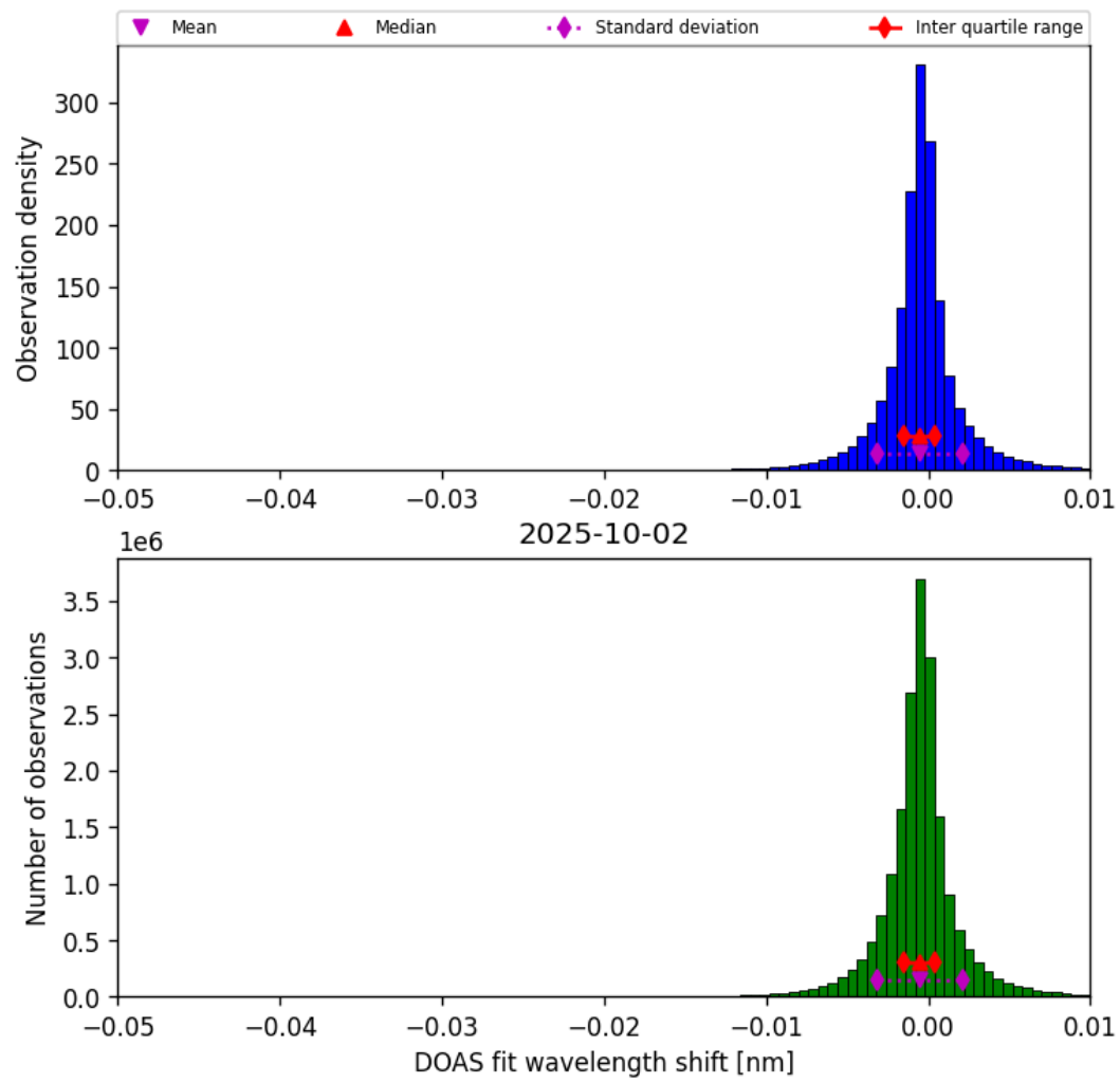
Figure 76: Histogram of “DOAS fit wavelength shift” for 2025-10-01 to 2025-10-03
