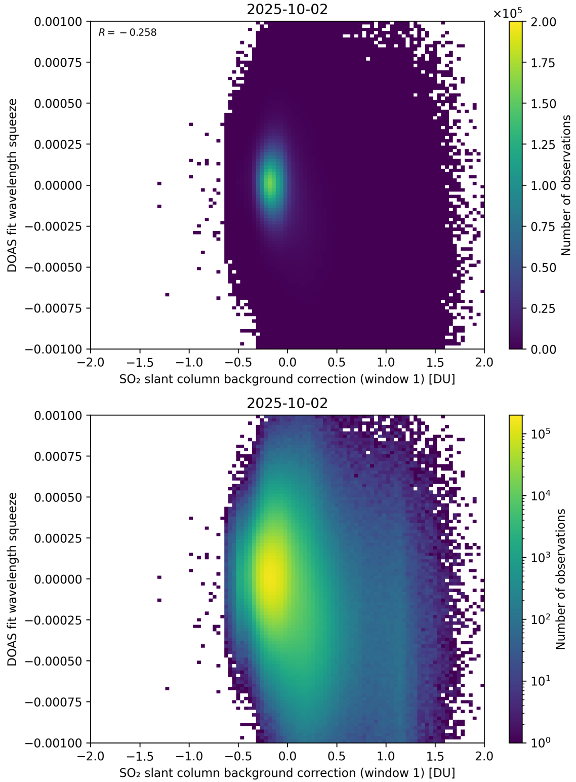
Figure 112: Scatter density plot of “SO 2 slant column background correction (window 1)” against “DOAS fit wavelength squeeze” for 2025-10-01 to 2025-10-03.
