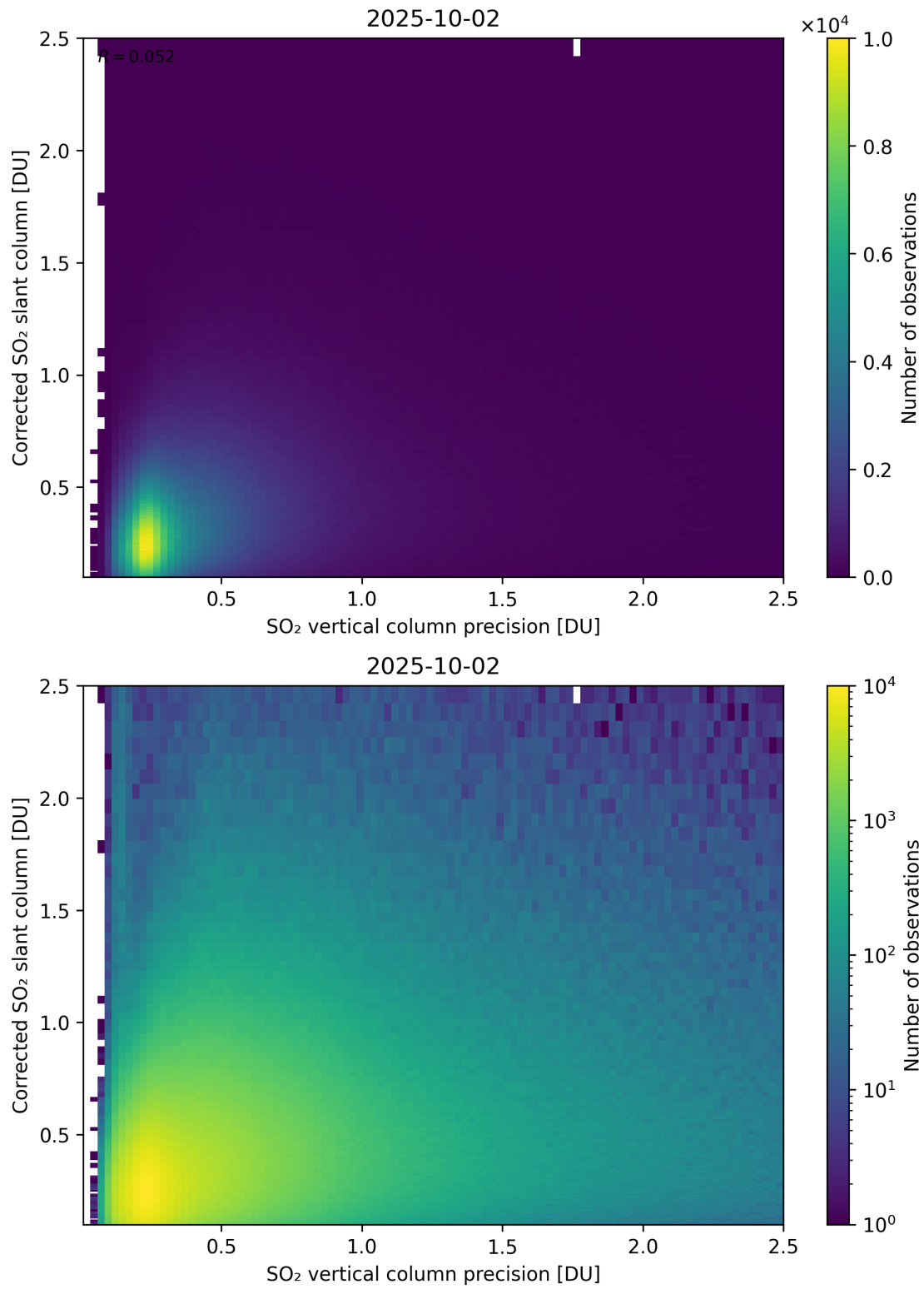
Figure 338: Scatter density plot of “SO 2 vertical column precision” against “Corrected SO 2 slant column” for 2025-10-01 to 2025-10-03.
