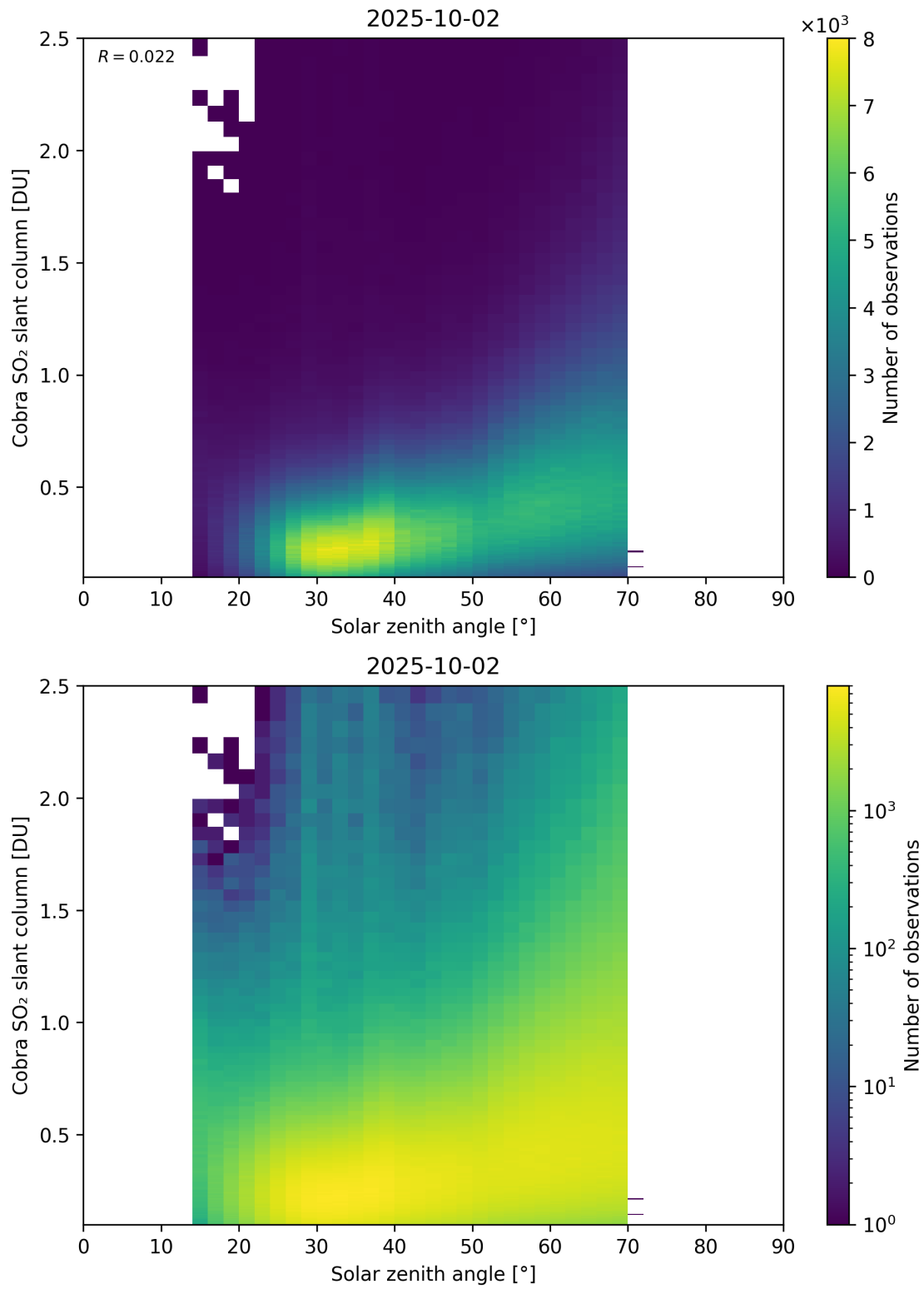
Figure 179: Scatter density plot of “Solar zenith angle” against “Cobra SO 2 slant column” for 2025-10-01 to 2025-10-03.
