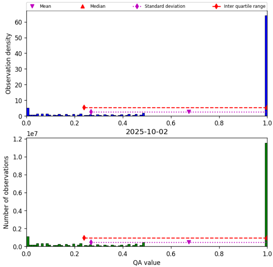
Figure 57: Histogram of “QA value” for 2025-10-01 to 2025-10-03
