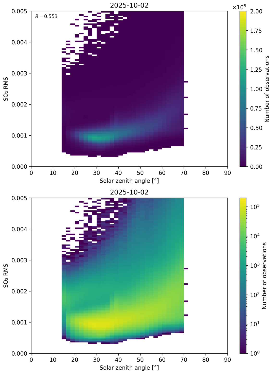
Figure 176: Scatter density plot of “Solar zenith angle” against “SO 2 RMS” for 2025-10-01 to 2025-10-03.
