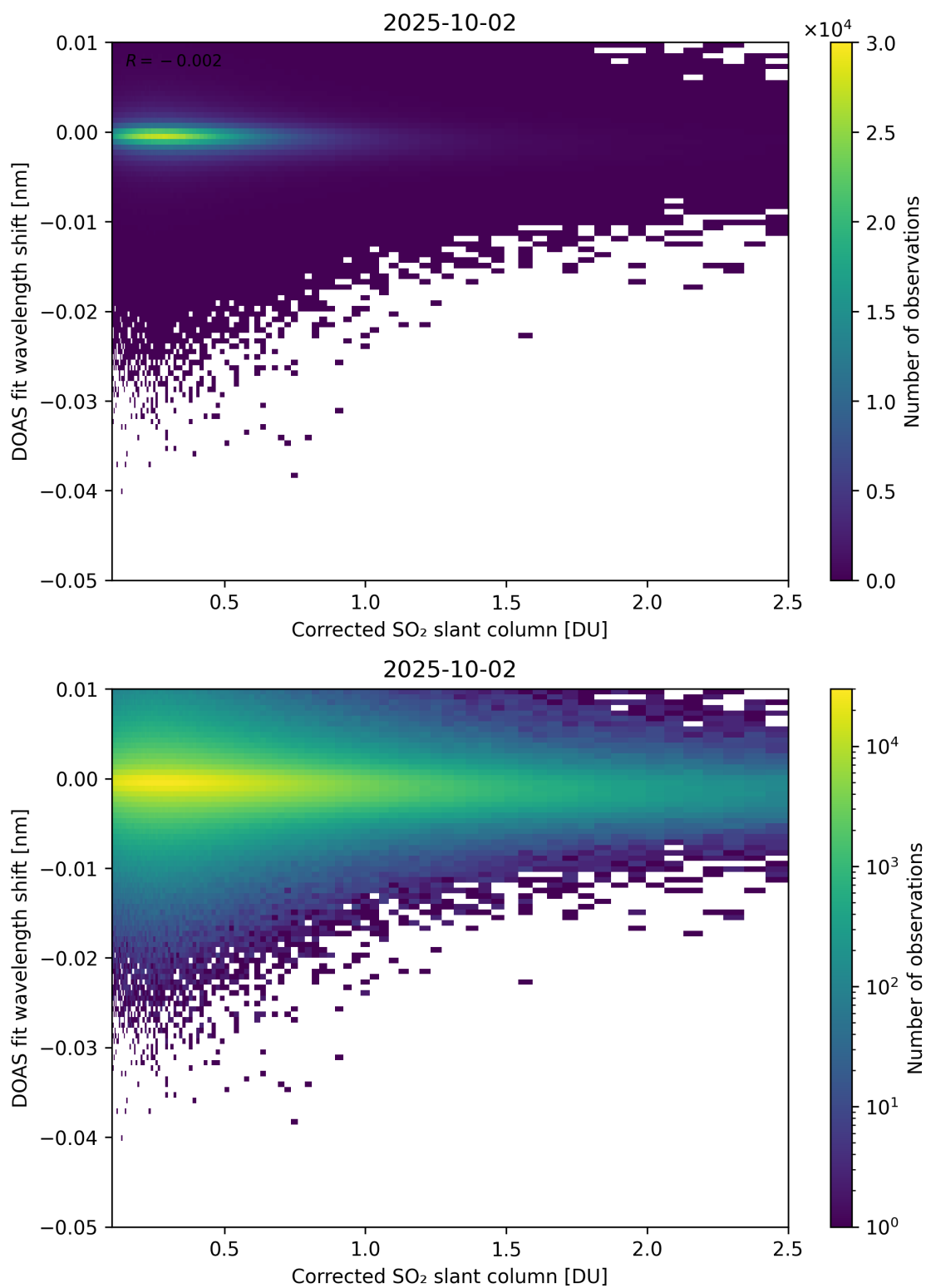
Figure 229: Scatter density plot of “Corrected SO 2 slant column” against “DOAS fit wavelength shift” for 2025-10-01 to 2025-10-03.
