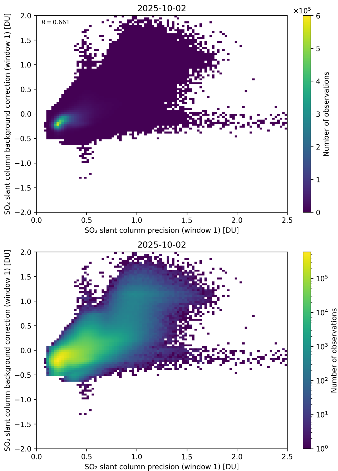
Figure 268: Scatter density plot of “SO 2 slant column precision (window 1)” against “SO 2 slant column background correction (window 1)” for 2025-10-01 to 2025-10-03.
