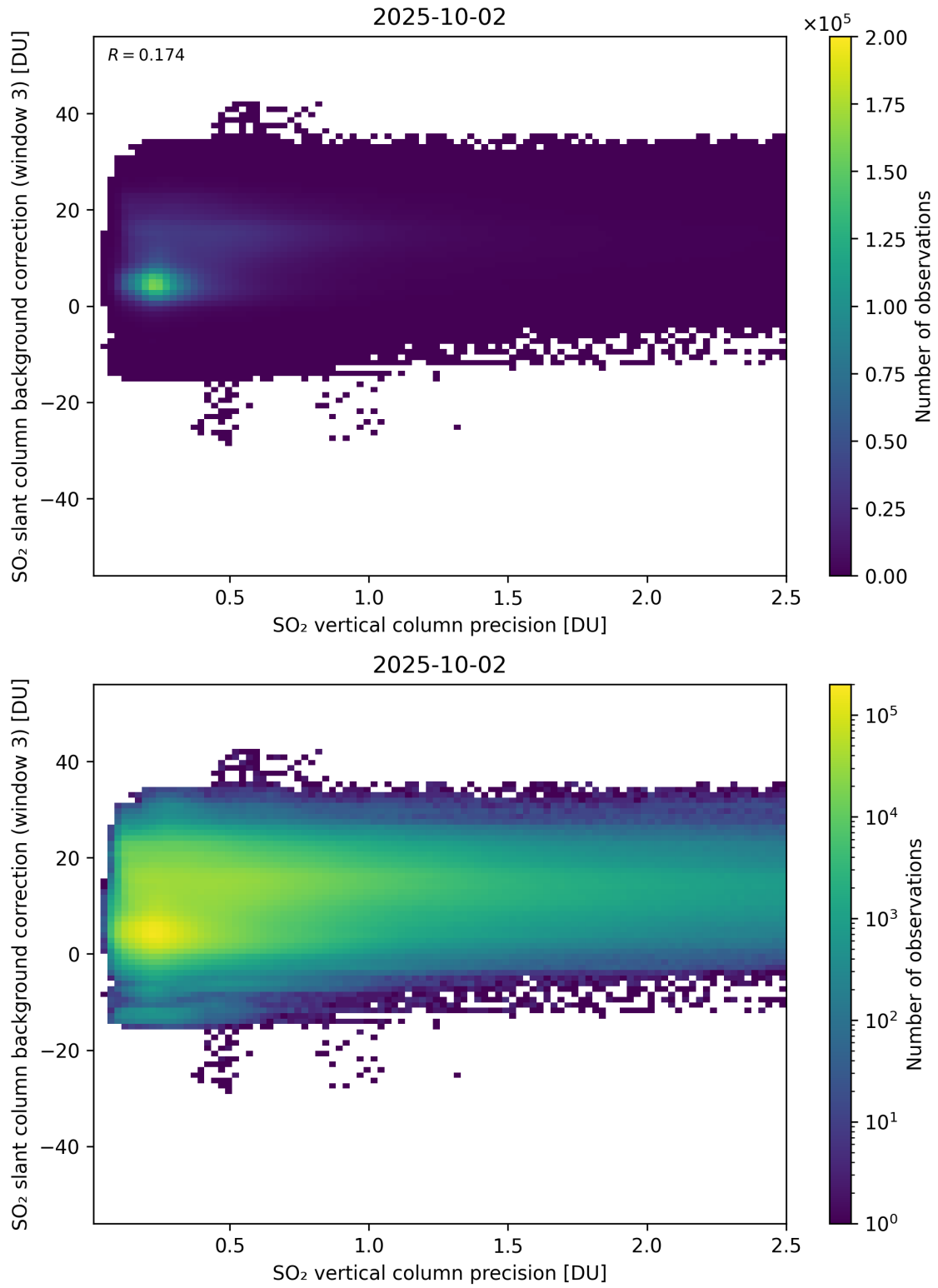
Figure 331: Scatter density plot of “SO 2 vertical column precision” against “SO 2 slant column background correction (window 3)” for 2025-10-01 to 2025-10-03.
