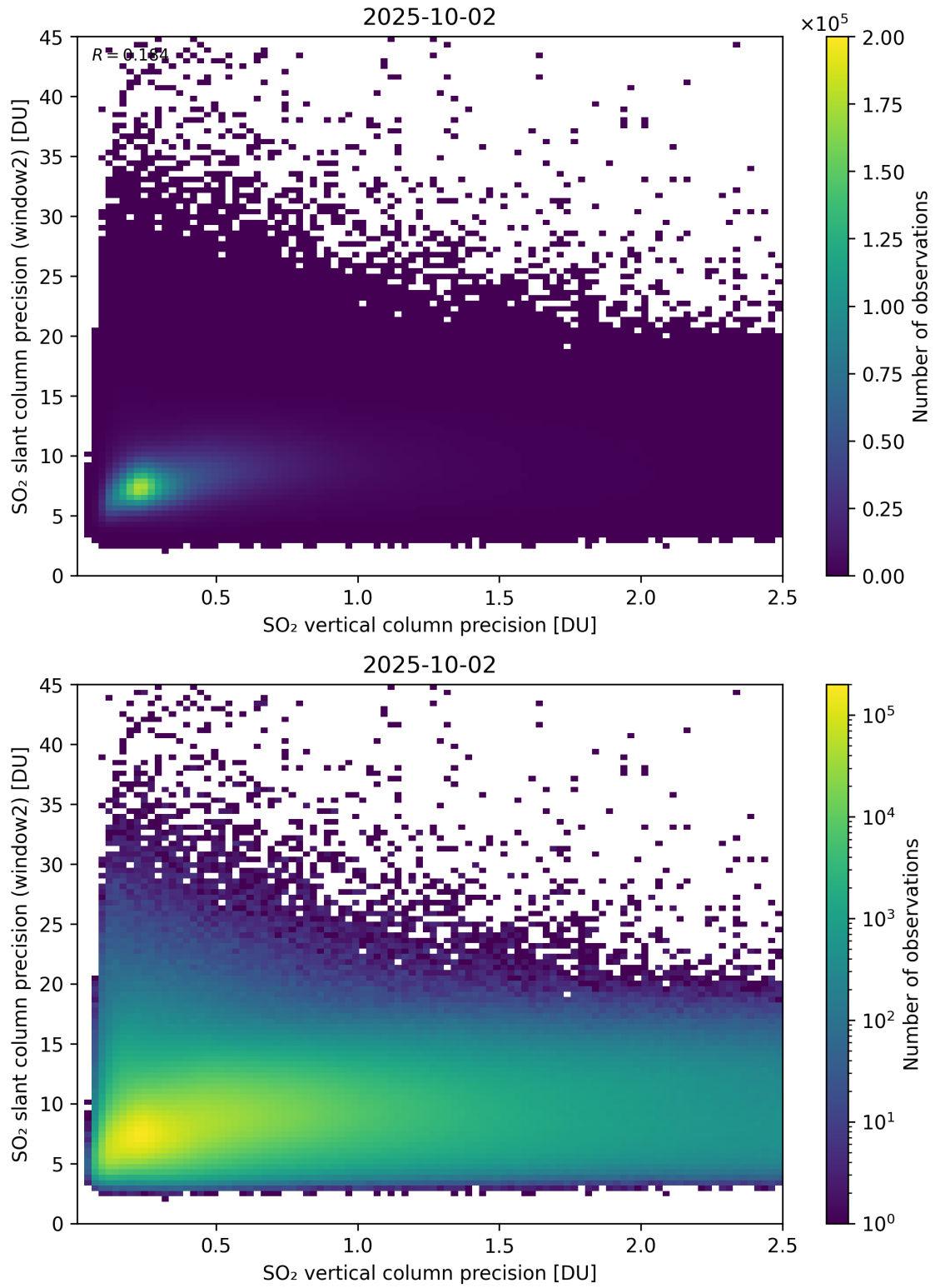
Figure 343: Scatter density plot of “SO 2 vertical column precision” against “SO 2 slant column precision (window2)” for 2025-10-01 to 2025-10-03.
