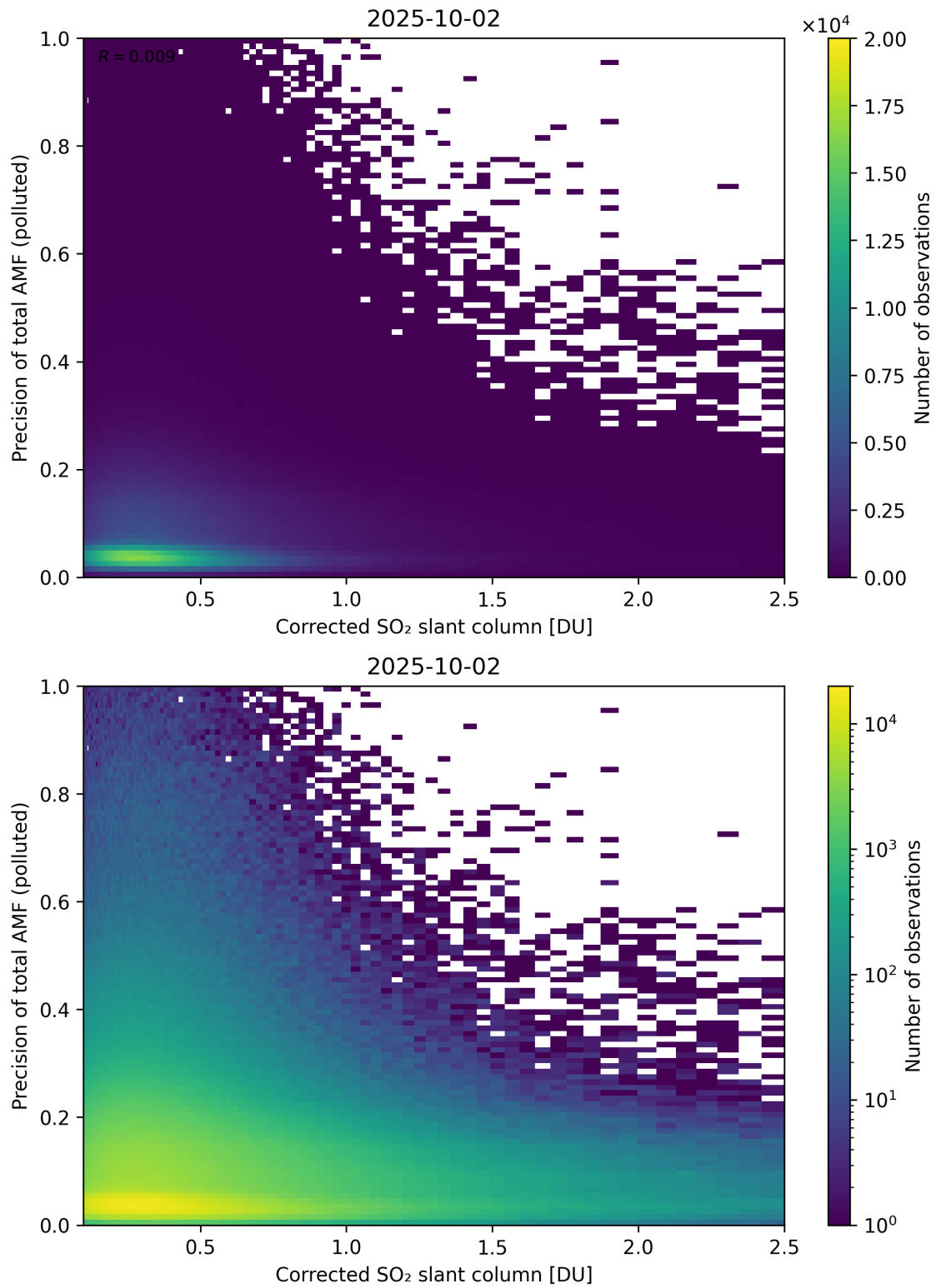
Figure 243: Scatter density plot of “Corrected SO 2 slant column” against “Precision of total AMF (polluted)” for 2025-10-01 to 2025-10-03.
