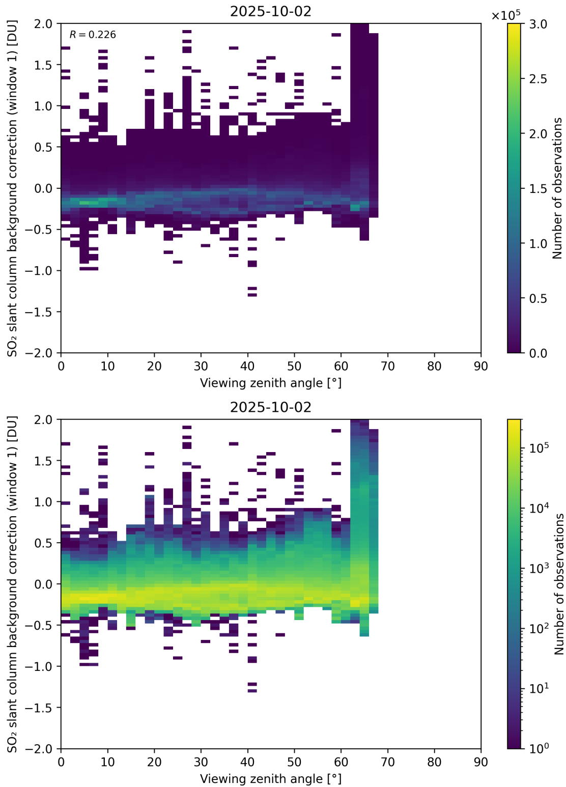
Figure 362: Scatter density plot of “Viewing zenith angle” against “SO 2 slant column background correction (window 1)” for 2025-10-01 to 2025-10-03.
