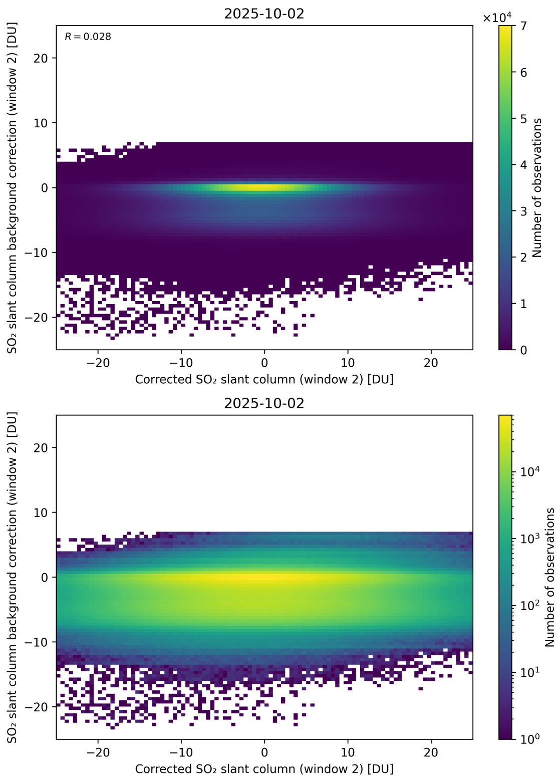
Figure 244: Scatter density plot of “Corrected SO 2 slant column (window 2)” against “SO 2 slant column background correction (window 2)” for 2025-10-01 to 2025-10-03.
