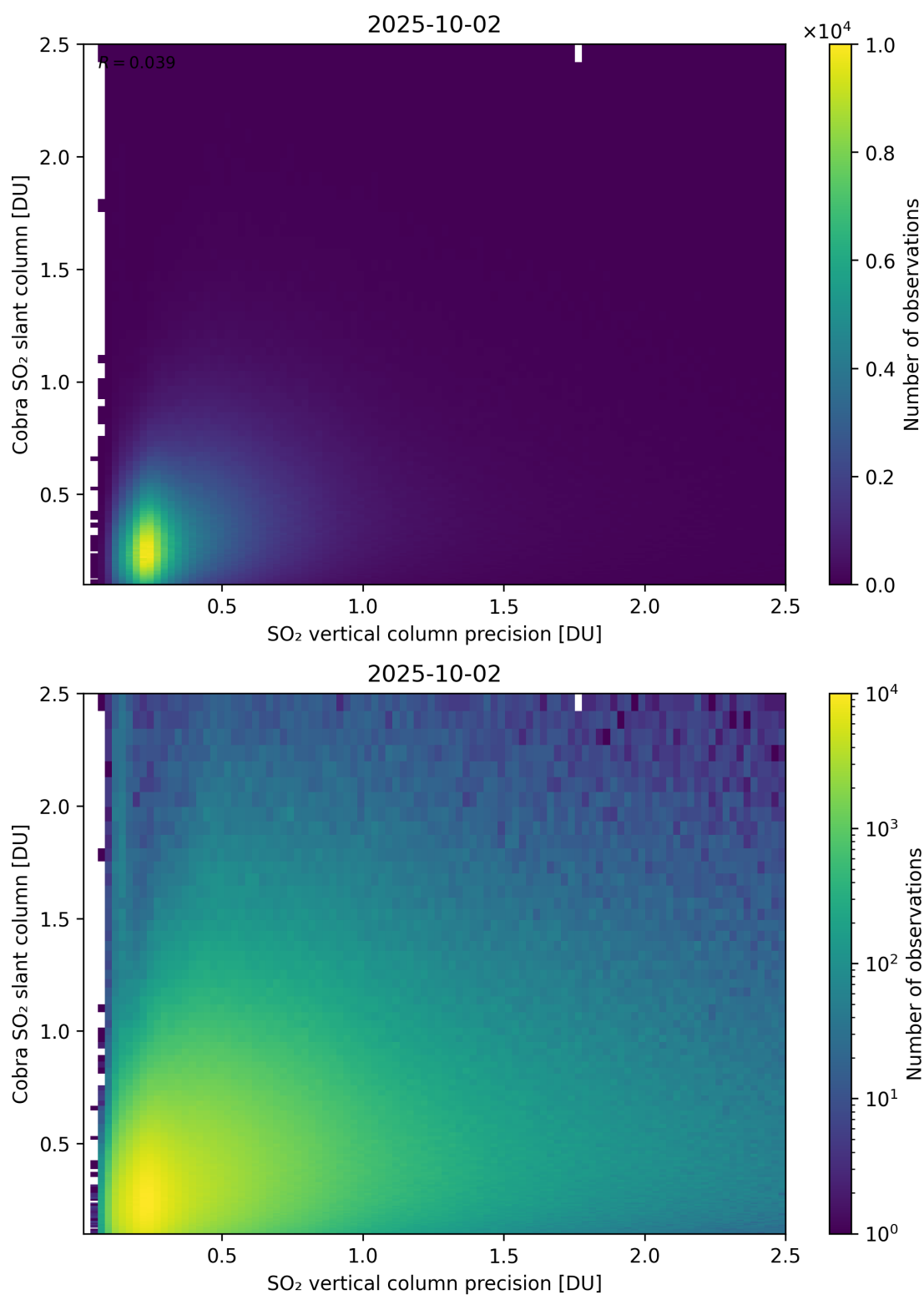
Figure 336: Scatter density plot of “SO 2 vertical column precision” against “Cobra SO 2 slant column” for 2025-10-01 to 2025-10-03.
