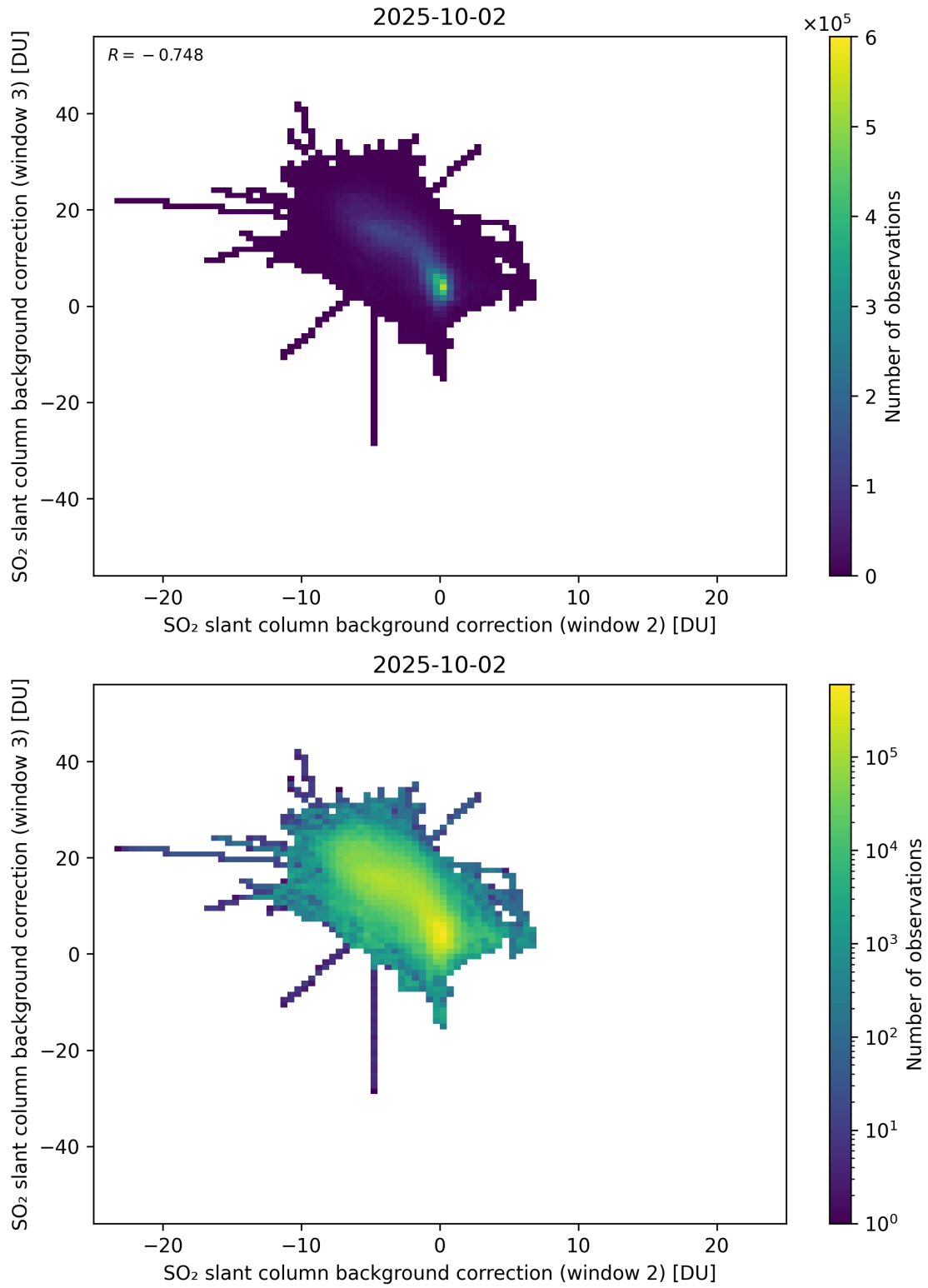
Figure 122: Scatter density plot of “SO 2 slant column background correction (window 2)” against “SO 2 slant column background correction (window 3)” for 2025-10-01 to 2025-10-03.
