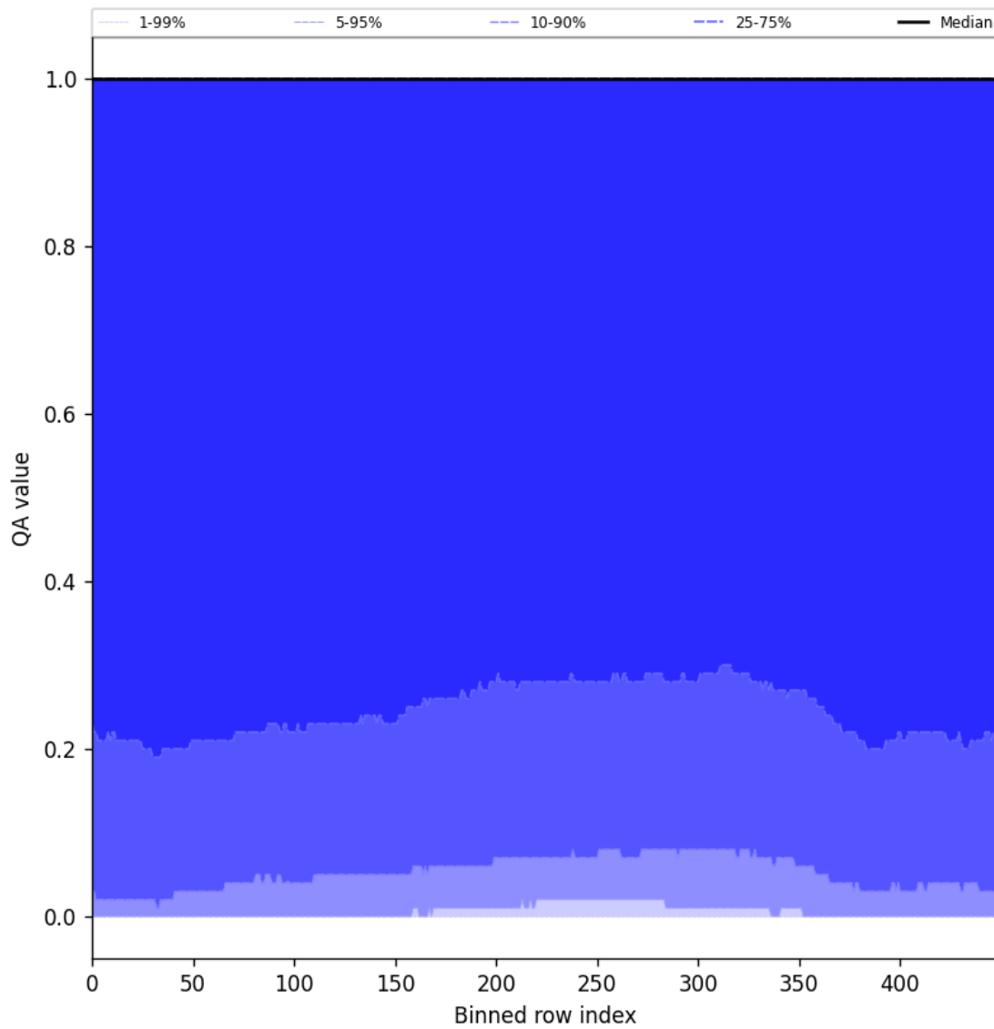
Figure 83: Along track statistics of “QA value” for 2025-10-01 to 2025-10-03
