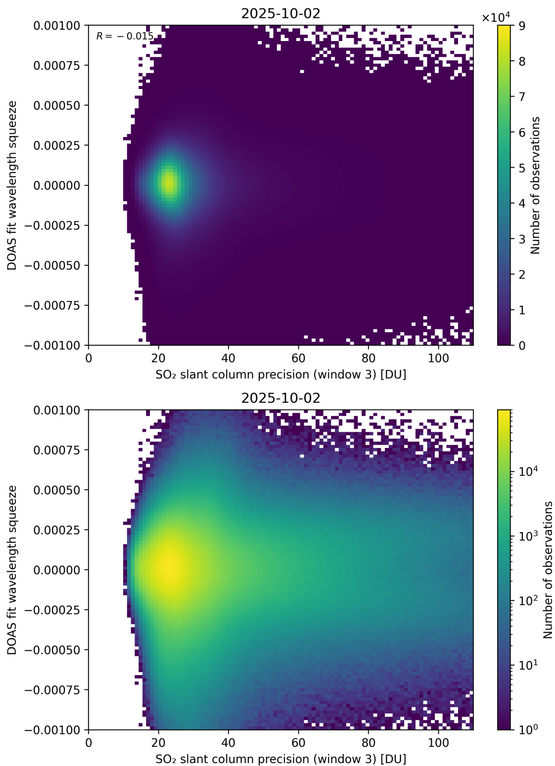
Figure 309: Scatter density plot of “SO 2 slant column precision (window 3)” against “DOAS fit wavelength squeeze” for 2025-10-01 to 2025-10-03.
