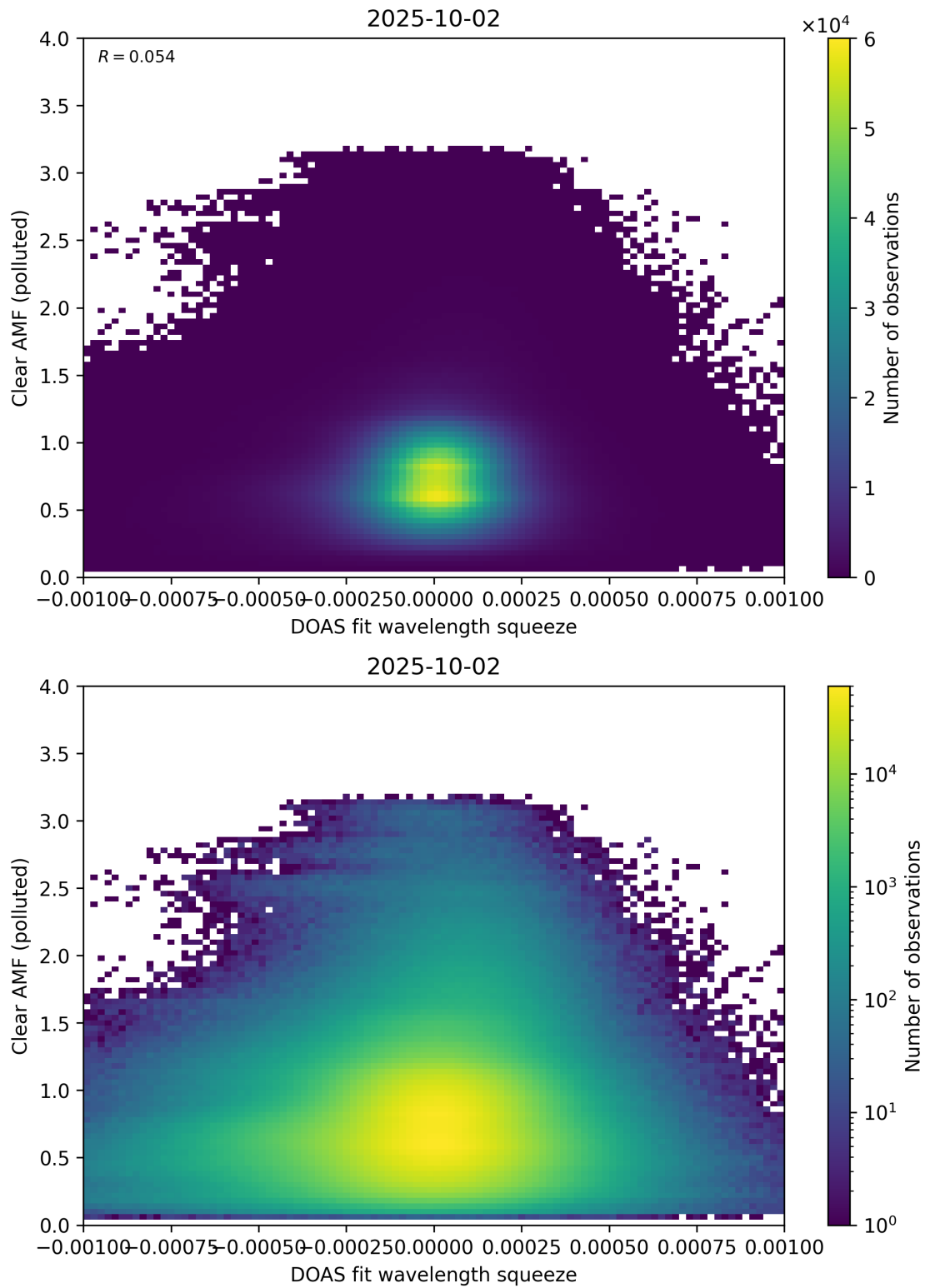
Figure 144: Scatter density plot of “DOAS fit wavelength squeeze” against “Clear AMF (polluted)” for 2025-10-01 to 2025-10-03.
