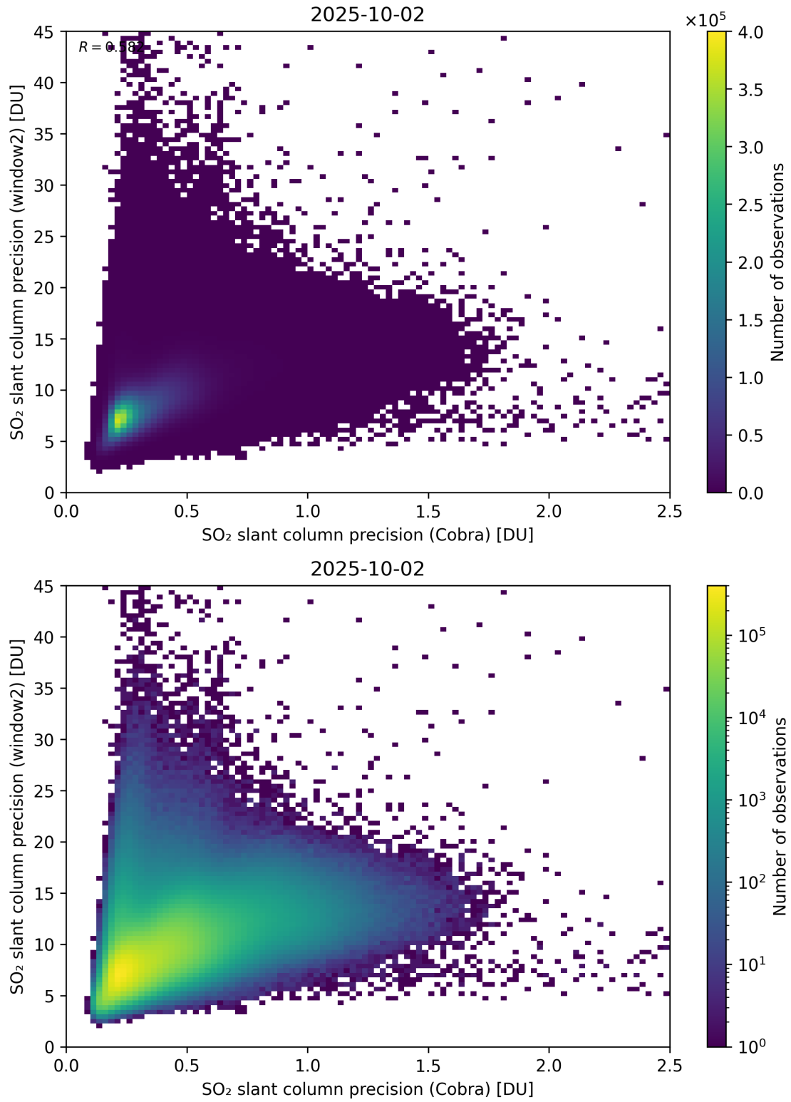
Figure 210: Scatter density plot of “SO 2 slant column precision (Cobra)” against “SO 2 slant column precision (window2)” for 2025-10-01 to 2025-10-03.
