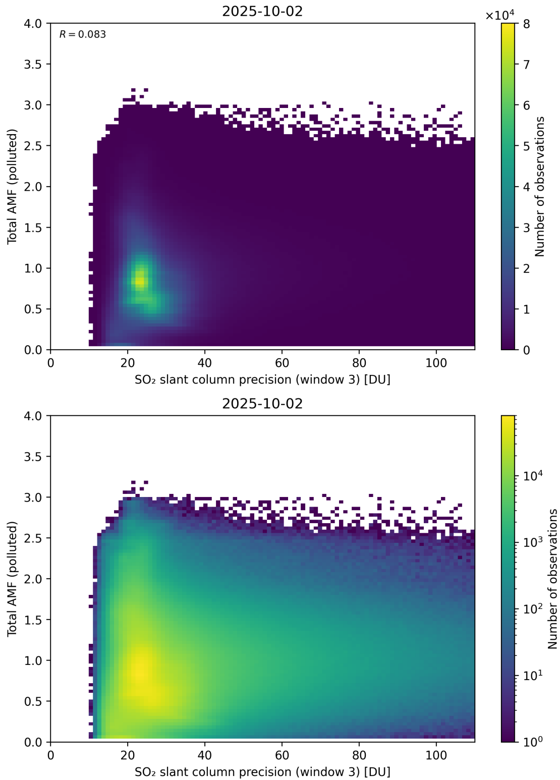
Figure 313: Scatter density plot of “SO 2 slant column precision (window 3)” against “Total AMF (polluted)” for 2025-10-01 to 2025-10-03.
