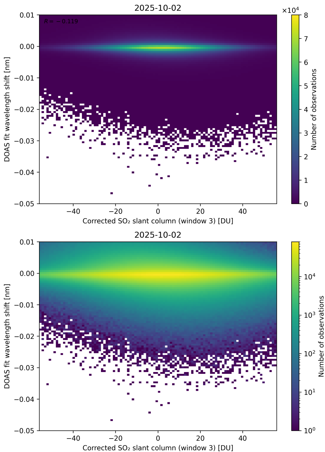
Figure 256: Scatter density plot of “Corrected SO 2 slant column (window 3)” against “DOAS fit wavelength shift” for 2025-10-01 to 2025-10-03.
