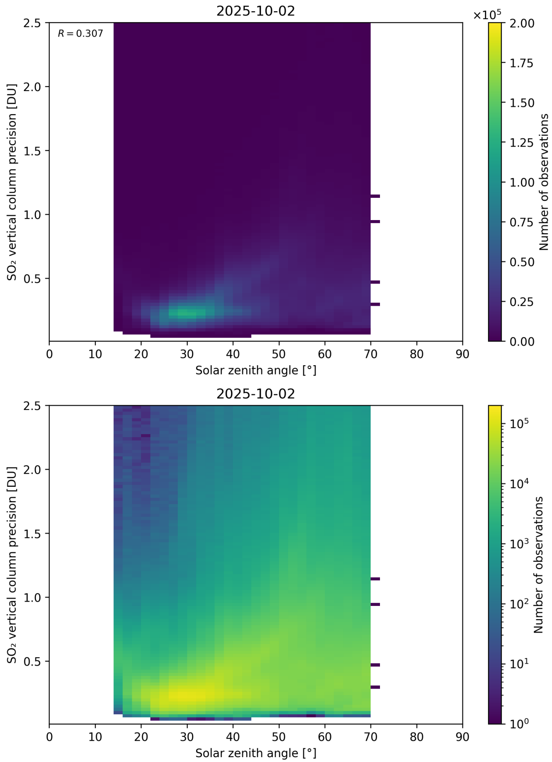
Figure 192: Scatter density plot of “Solar zenith angle” against “SO 2 vertical column precision” for 2025-10-01 to 2025-10-03.
