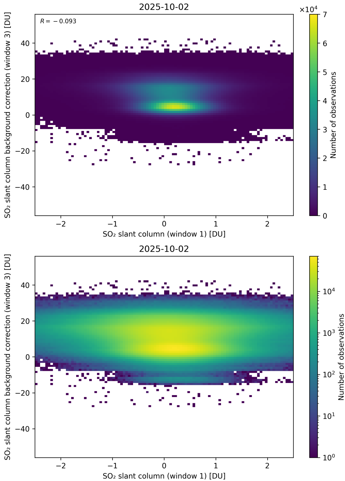
Figure 264: Scatter density plot of “SO 2 slant column (window 1)” against “SO 2 slant column background correction (window 3)” for 2025-10-01 to 2025-10-03.
