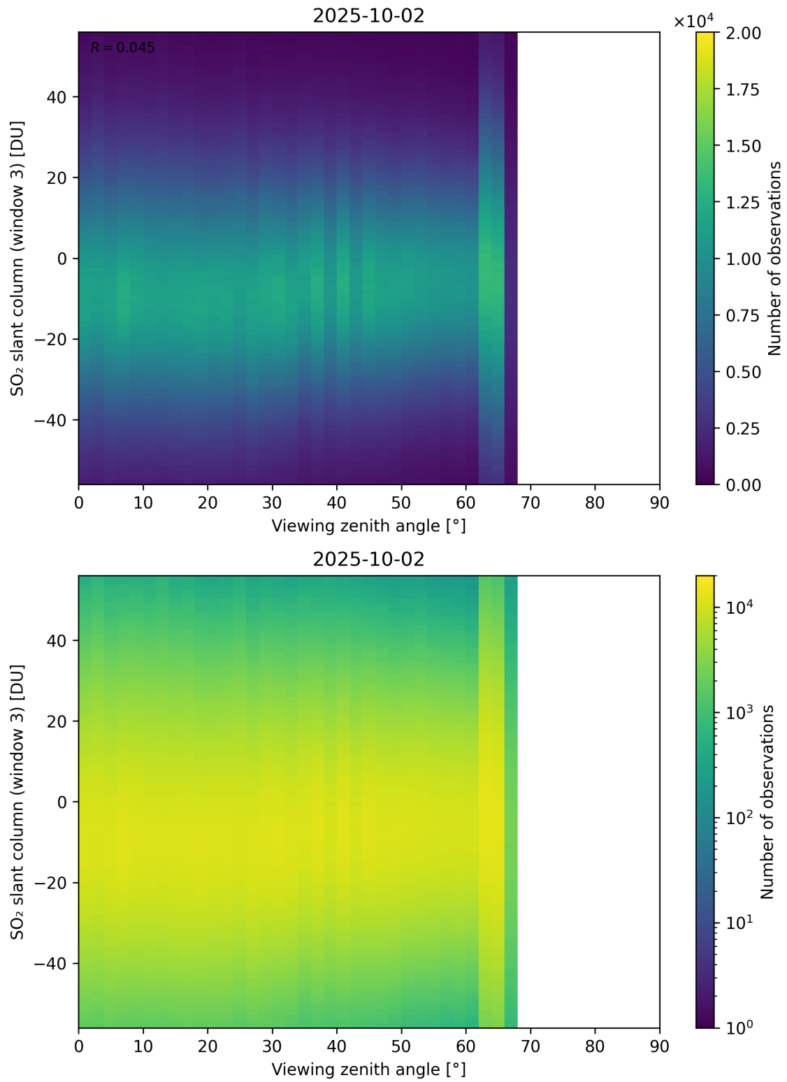
Figure 379: Scatter density plot of “Viewing zenith angle” against “SO 2 slant column (window 3)” for 2025-10-01 to 2025-10-03.
