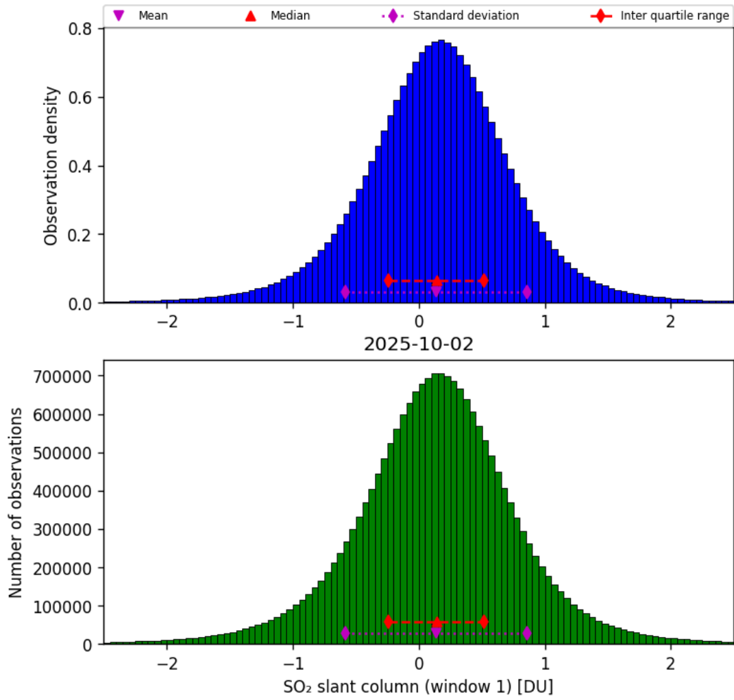
Figure 63: Histogram of “SO 2 slant column (window 1)” for 2025-10-01 to 2025-10-03
