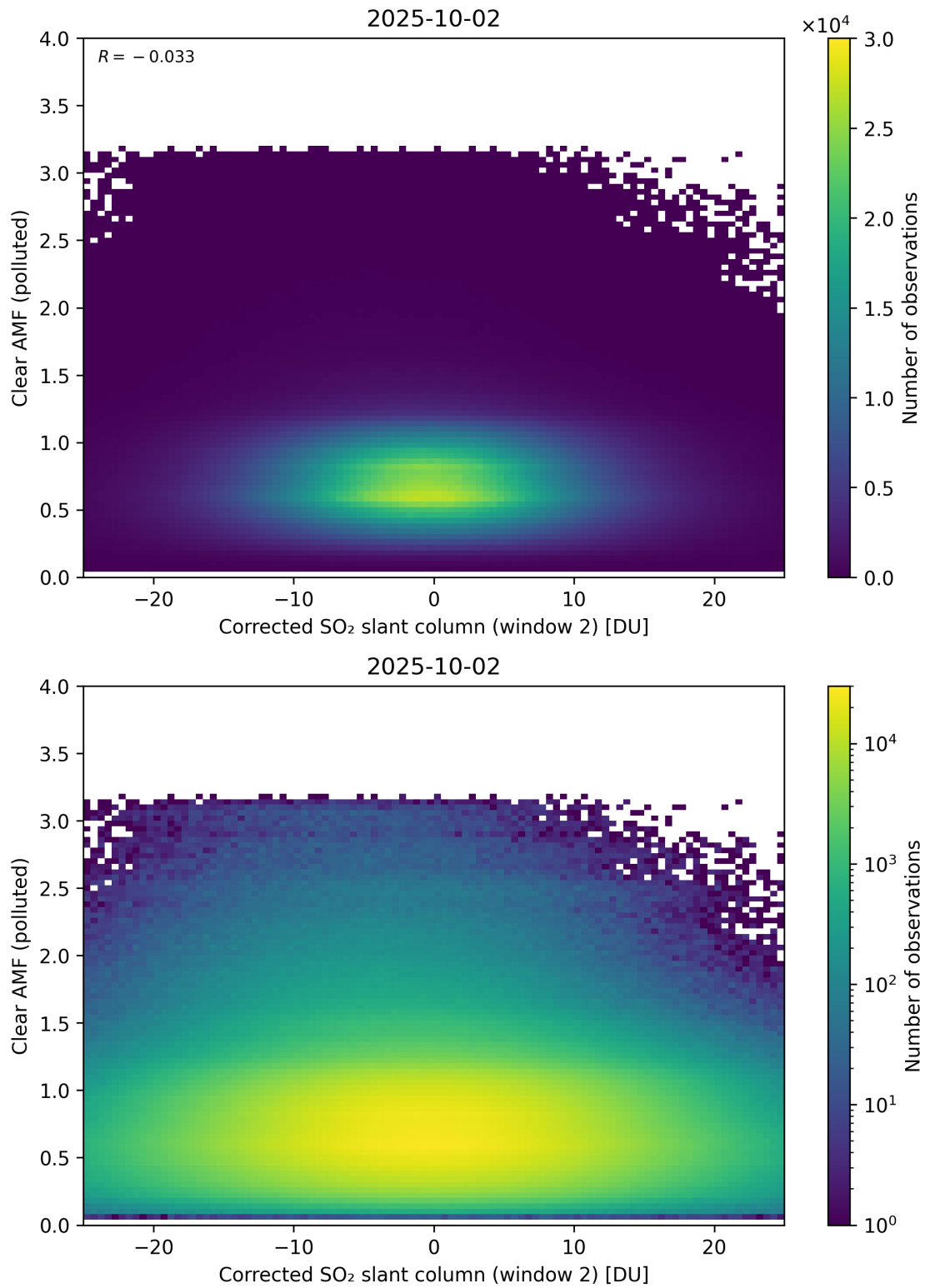
Figure 249: Scatter density plot of “Corrected SO 2 slant column (window 2)” against “Clear AMF (polluted)” for 2025-10-01 to 2025-10-03.
