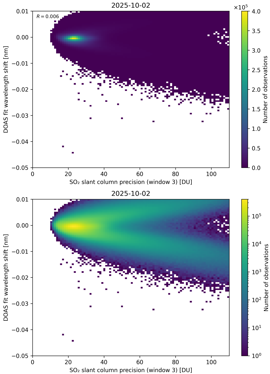
Figure 308: Scatter density plot of “SO 2 slant column precision (window 3)” against “DOAS fit wavelength shift” for 2025-10-01 to 2025-10-03.
