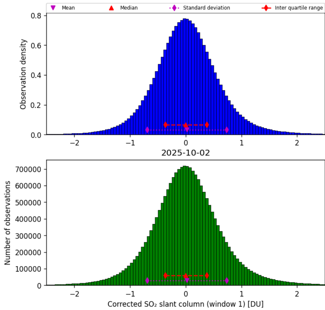
Figure 65: Histogram of “Corrected SO 2 slant column (window 1)” for 2025-10-01 to 2025-10-03
