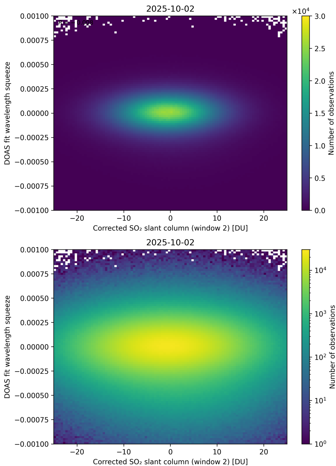
Figure 247: Scatter density plot of “Corrected SO 2 slant column (window 2)” against “DOAS fit wavelength squeeze” for 2025-10-01 to 2025-10-03.
