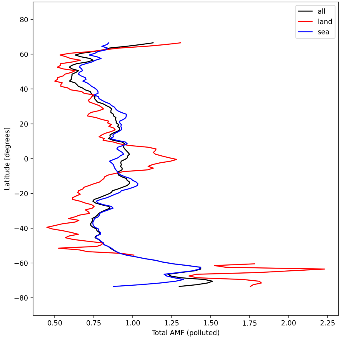
Figure 53: Zonal average of “Total AMF (polluted)” for 2025-10-01 to 2025-10-03.
