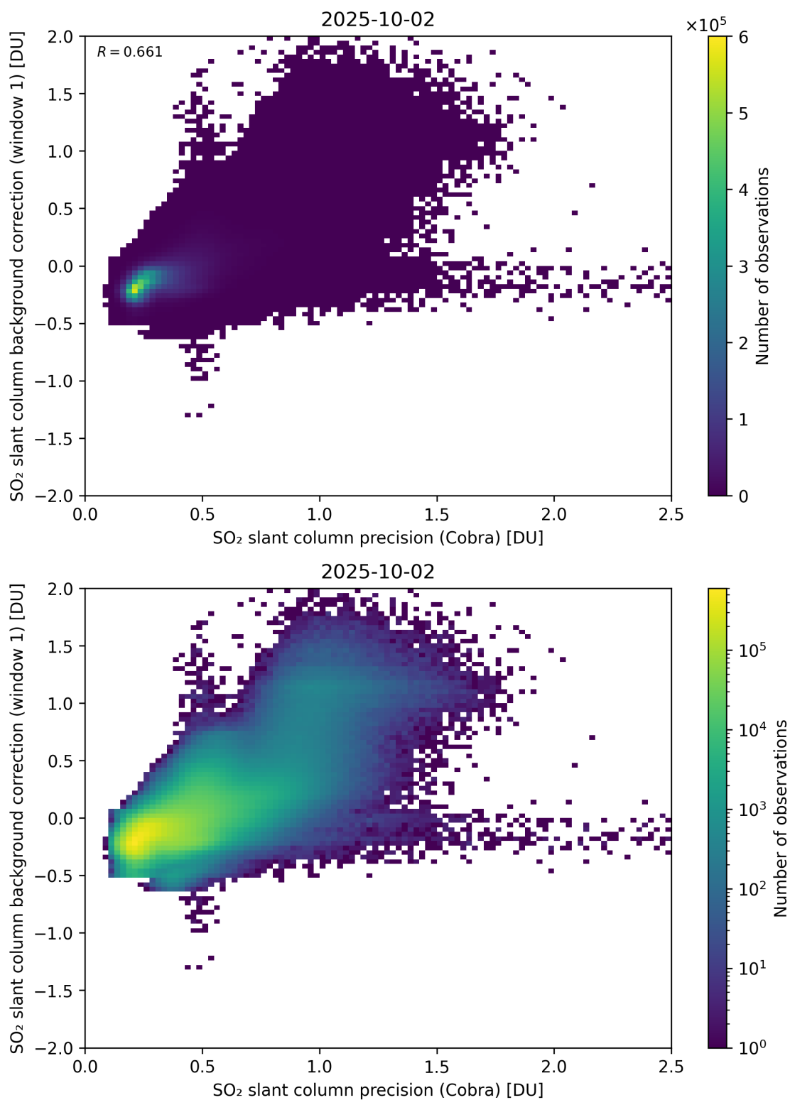
Figure 199: Scatter density plot of “SO 2 slant column precision (Cobra)” against “SO 2 slant column background correction (window 1)” for 2025-10-01 to 2025-10-03.
