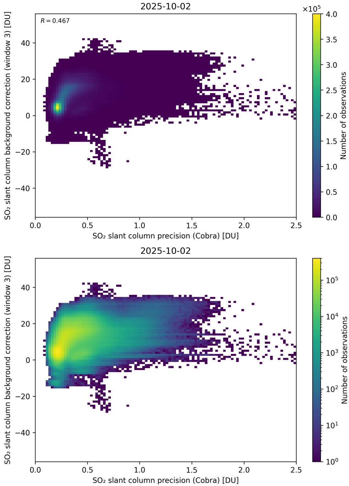
Figure 201: Scatter density plot of “SO 2 slant column precision (Cobra)” against “SO 2 slant column background correction (window 3)” for 2025-10-01 to 2025-10-03.
