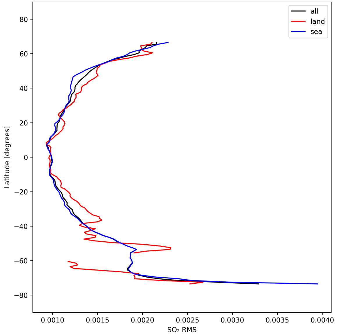
Figure 52: Zonal average of “ \text{SO}_2 RMS” for 2025-10-01 to 2025-10-03.
