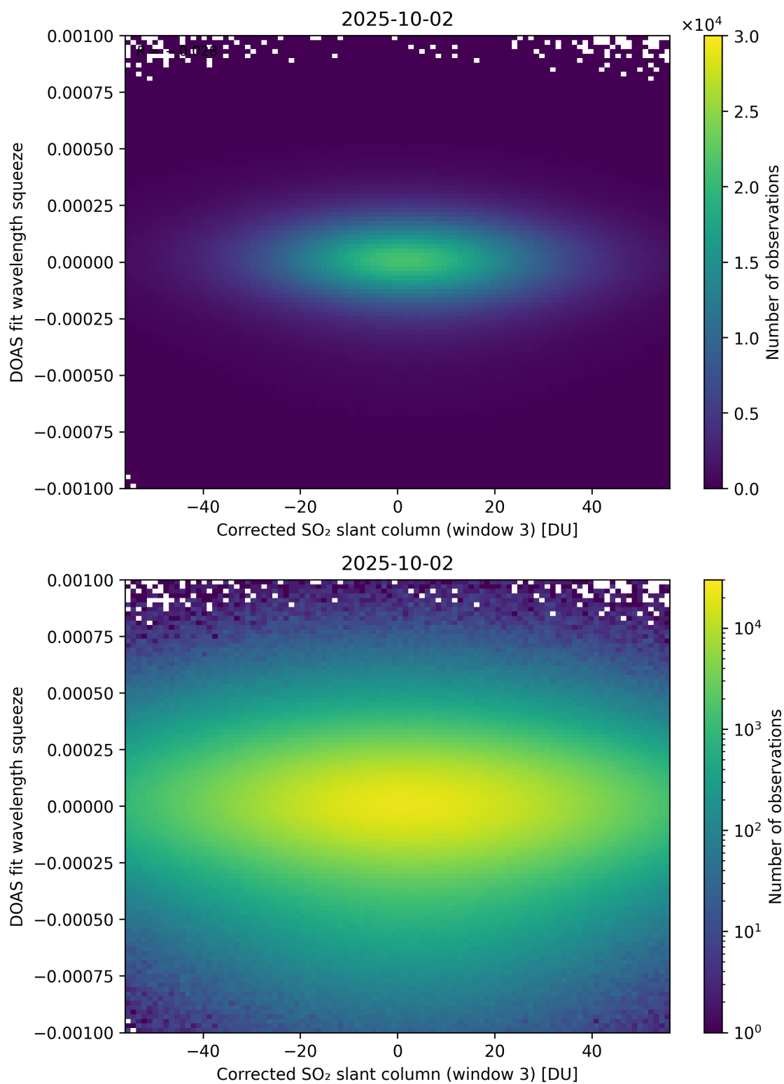
Figure 257: Scatter density plot of “Corrected SO 2 slant column (window 3)” against “DOAS fit wavelength squeeze” for 2025-10-01 to 2025-10-03.
