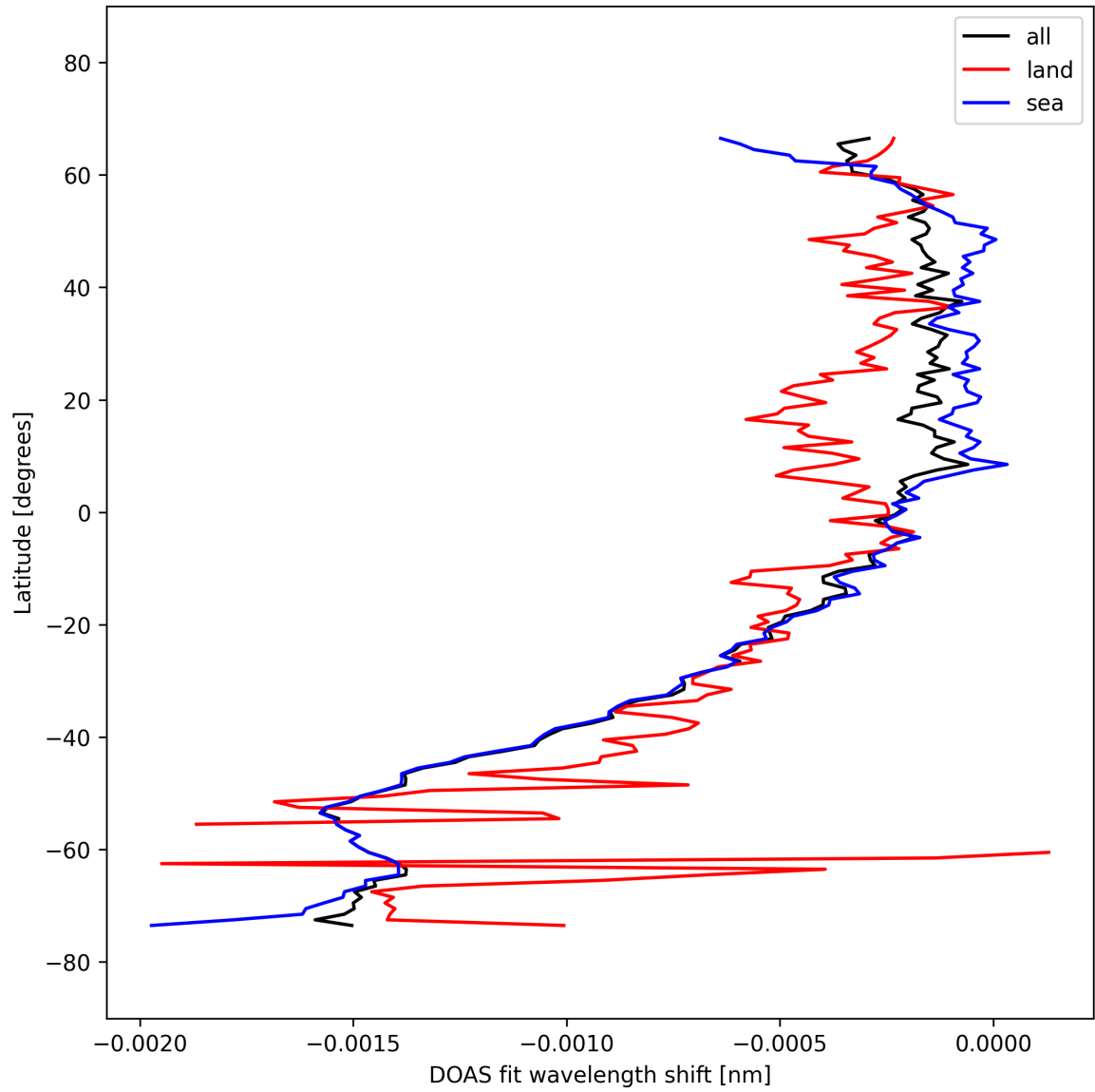
Figure 50: Zonal average of “DOAS fit wavelength shift” for 2025-10-01 to 2025-10-03.
