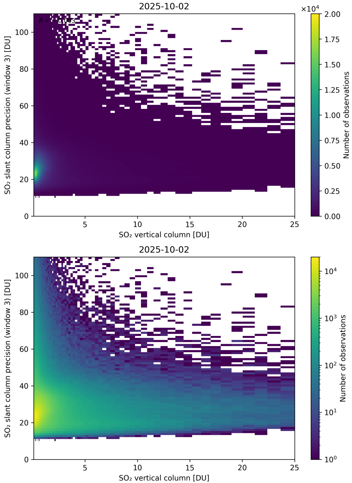
Figure 358: Scatter density plot of “SO 2 vertical column” against “SO 2 slant column precision (window 3)” for 2025-10-01 to 2025-10-03.
