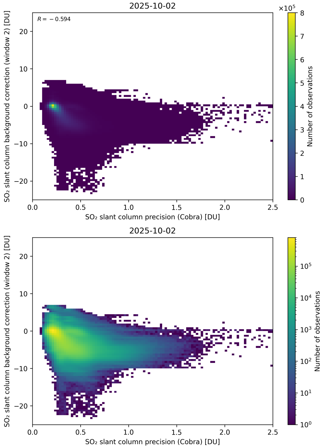
Figure 200: Scatter density plot of “SO 2 slant column precision (Cobra)” against “SO 2 slant column background correction (window 2)” for 2025-10-01 to 2025-10-03.
