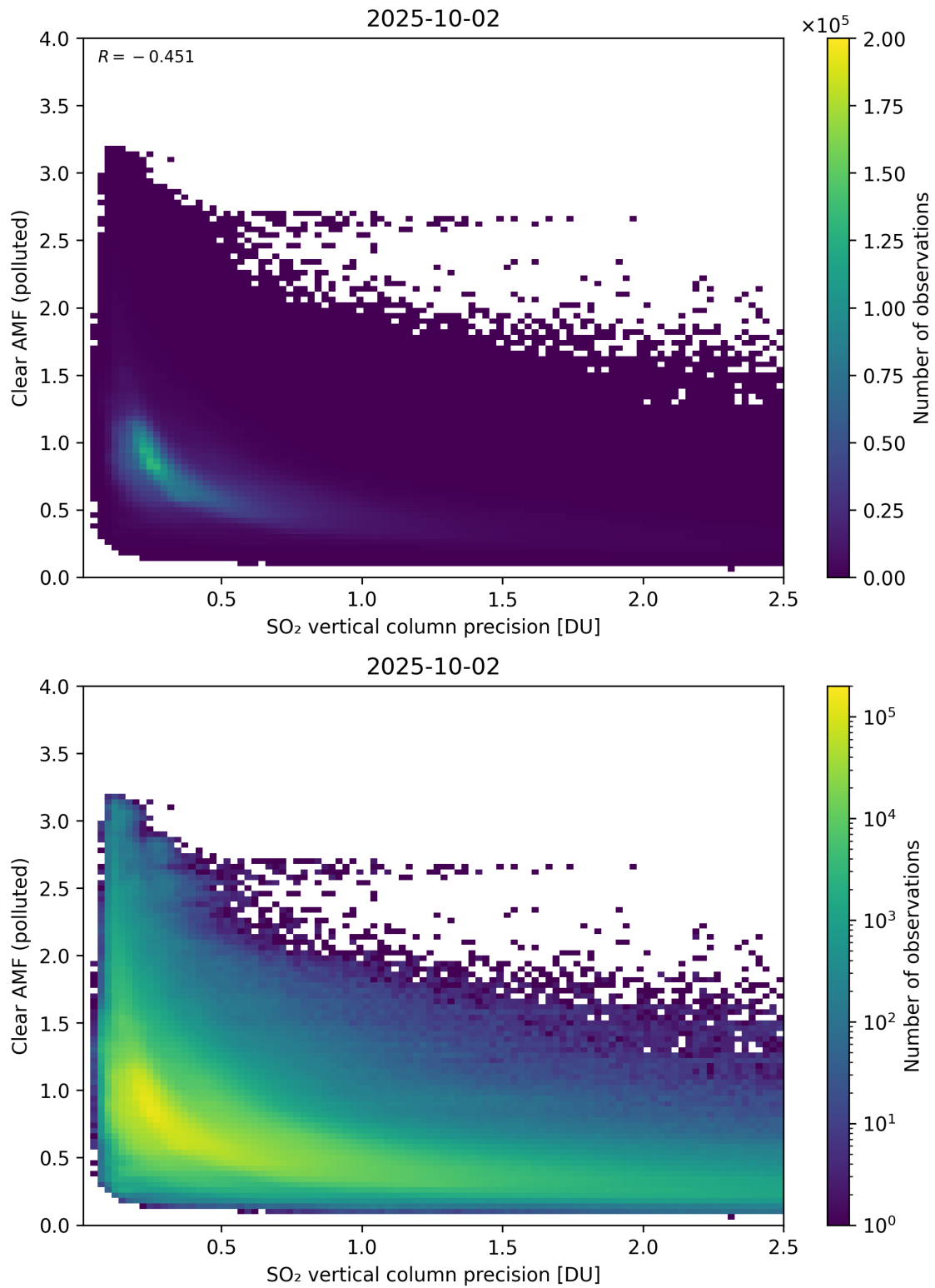
Figure 335: Scatter density plot of “SO 2 vertical column precision” against “Clear AMF (polluted)” for 2025-10-01 to 2025-10-03.
