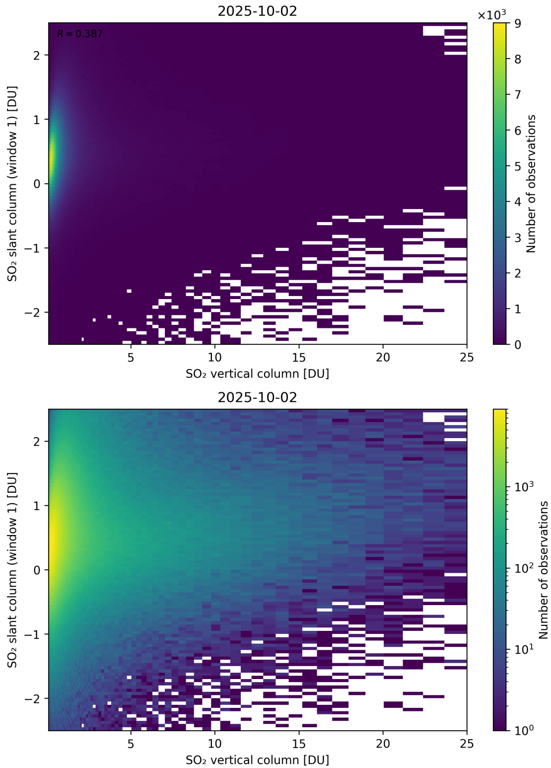
Figure 354: Scatter density plot of “SO 2 vertical column” against “SO 2 slant column (window 1)” for 2025-10-01 to 2025-10-03.
