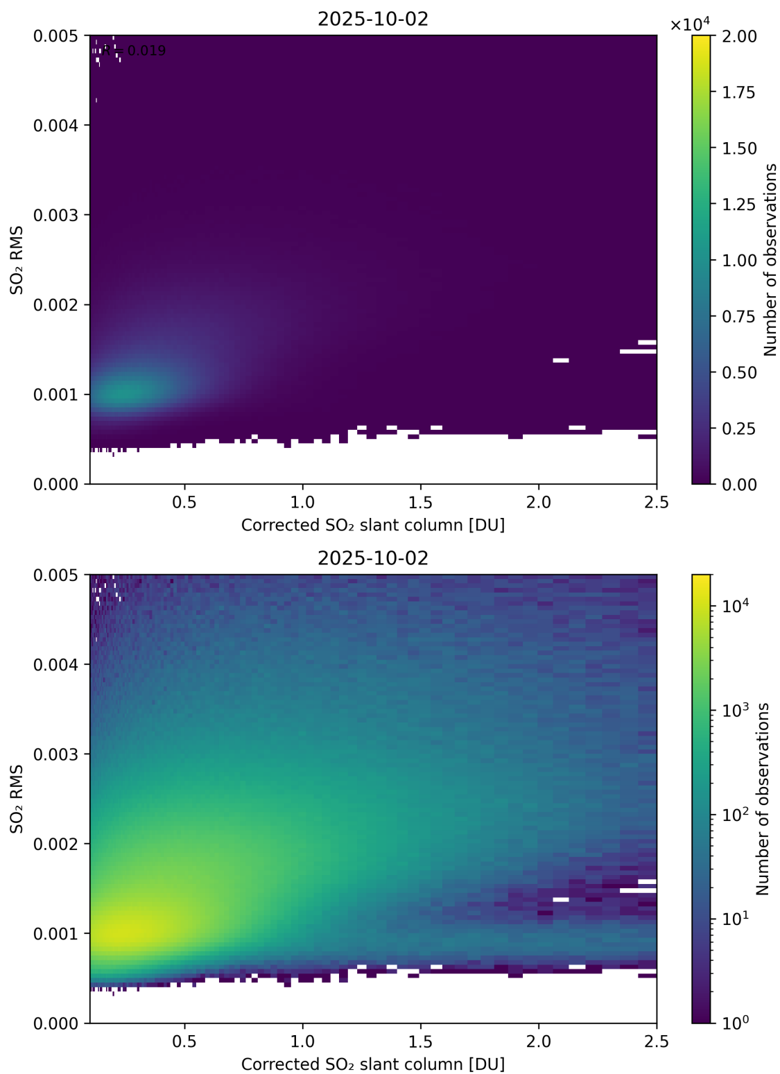
Figure 231: Scatter density plot of “Corrected SO 2 slant column” against “SO 2 RMS” for 2025-10-01 to 2025-10-03.
