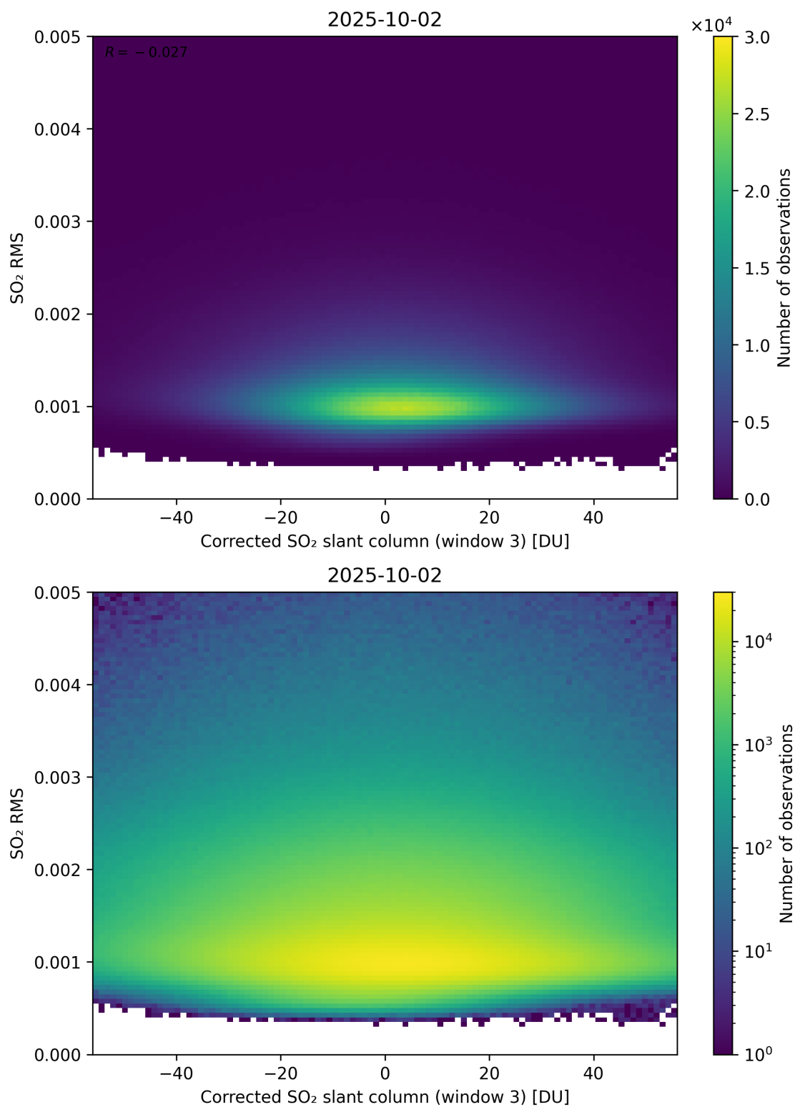
Figure 258: Scatter density plot of “Corrected SO 2 slant column (window 3)” against “SO 2 RMS” for 2025-10-01 to 2025-10-03.
