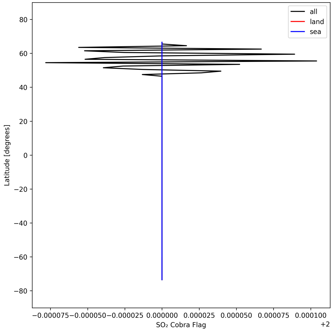
Figure 49: Zonal average of “SO 2 Cobra Flag” for 2025-10-01 to 2025-10-03.
