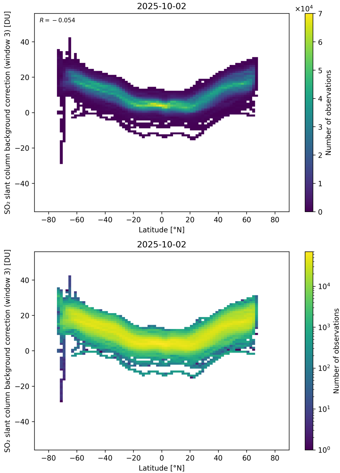
Figure 152: Scatter density plot of “Latitude” against “SO 2 slant column background correction (window 3)” for 2025-10-01 to 2025-10-03.
