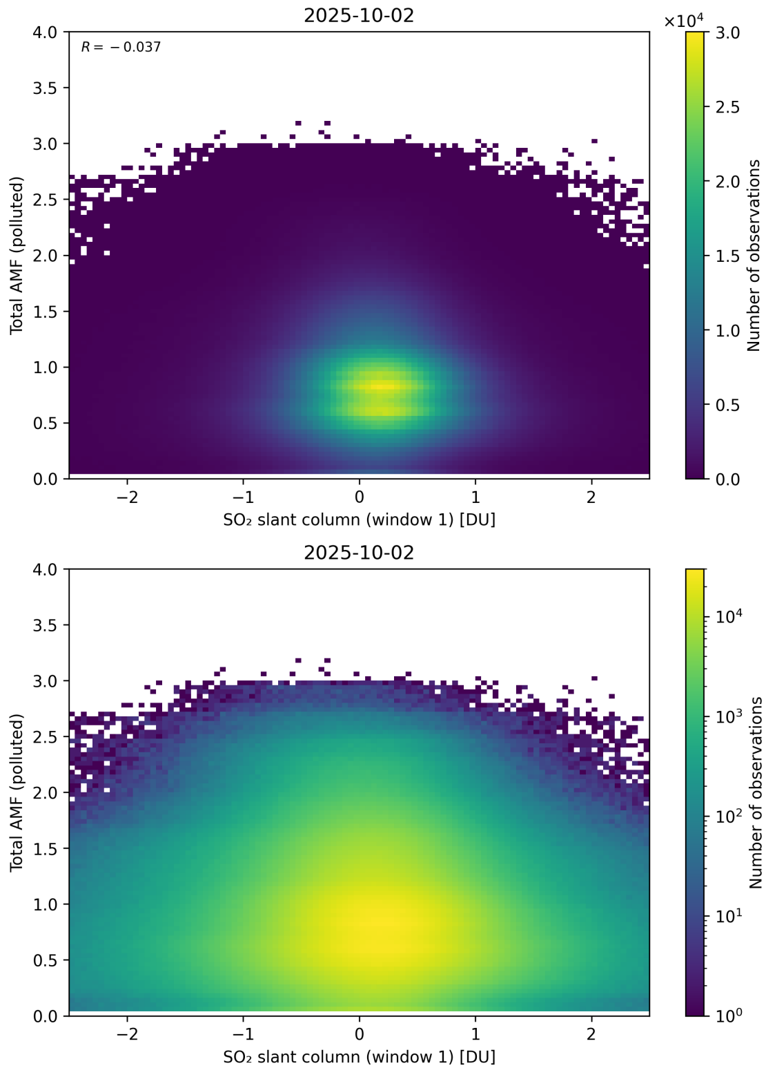
Figure 289: Scatter density plot of “SO 2 slant column (window 1)” against “Total AMF (polluted)” for 2025-10-01 to 2025-10-03.
