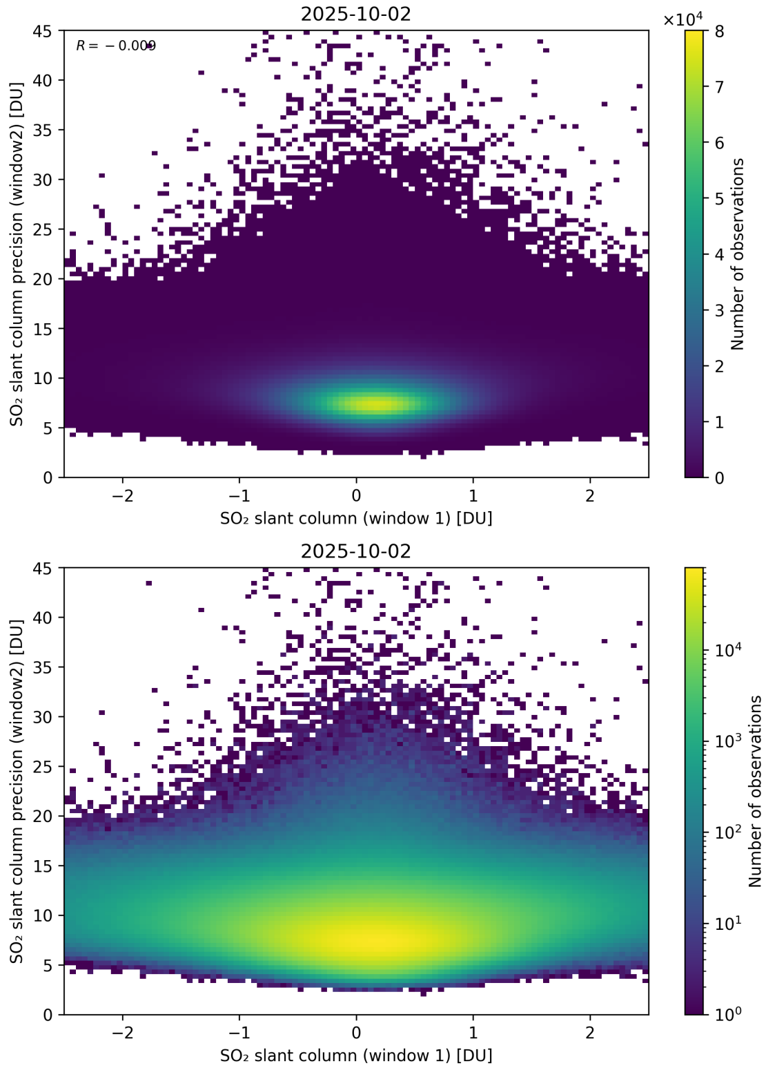
Figure 286: Scatter density plot of “SO 2 slant column (window 1)” against “SO 2 slant column precision (window2)” for 2025-10-01 to 2025-10-03.
