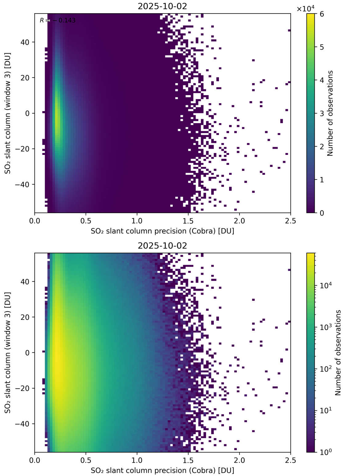
Figure 211: Scatter density plot of “SO 2 slant column precision (Cobra)” against “SO 2 slant column (window 3)” for 2025-10-01 to 2025-10-03.
