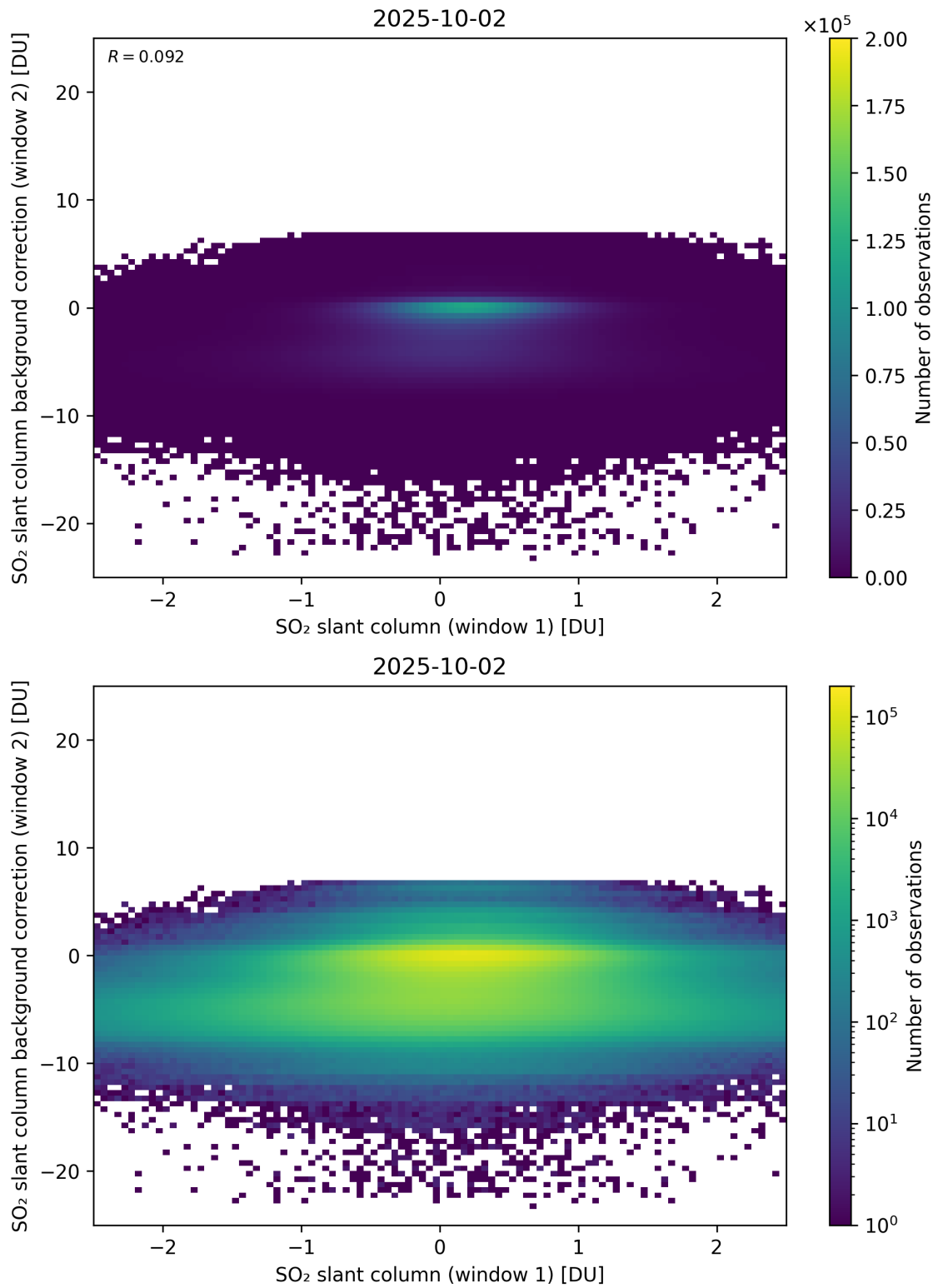
Figure 263: Scatter density plot of “SO 2 slant column (window 1)” against “SO 2 slant column background correction (window 2)” for 2025-10-01 to 2025-10-03.
