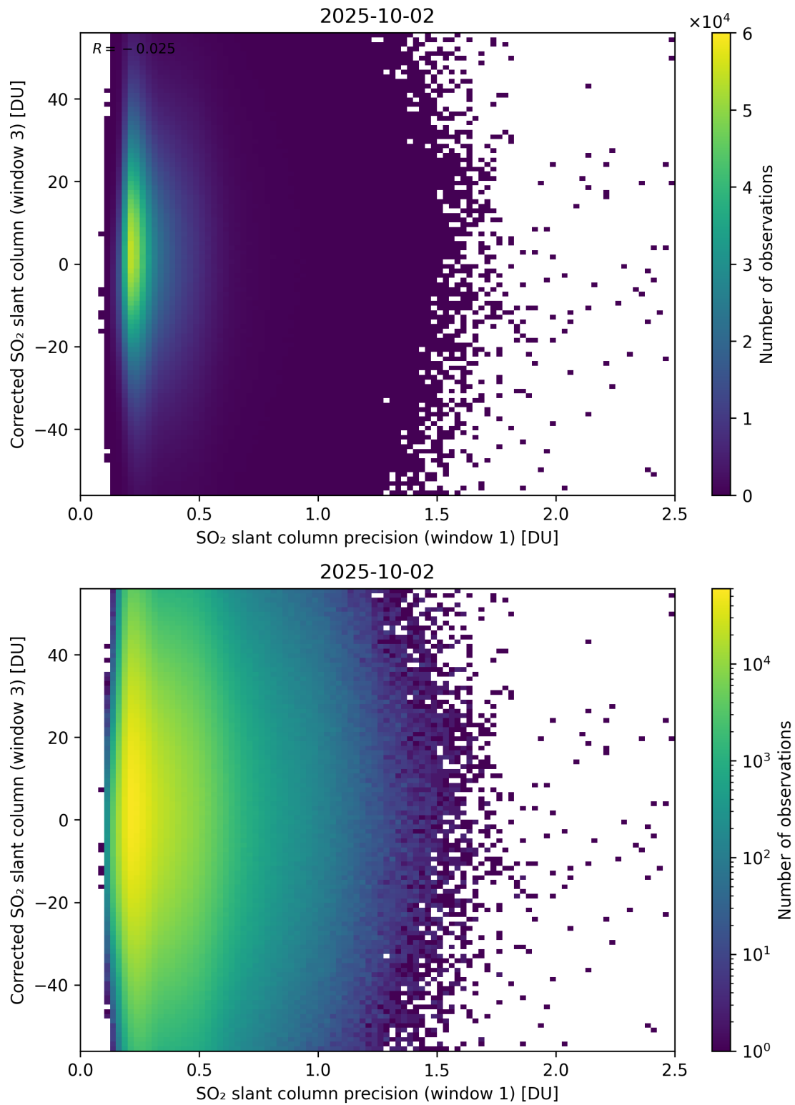
Figure 276: Scatter density plot of “SO 2 slant column precision (window 1)” against “Corrected SO 2 slant column (window 3)” for 2025-10-01 to 2025-10-03.
