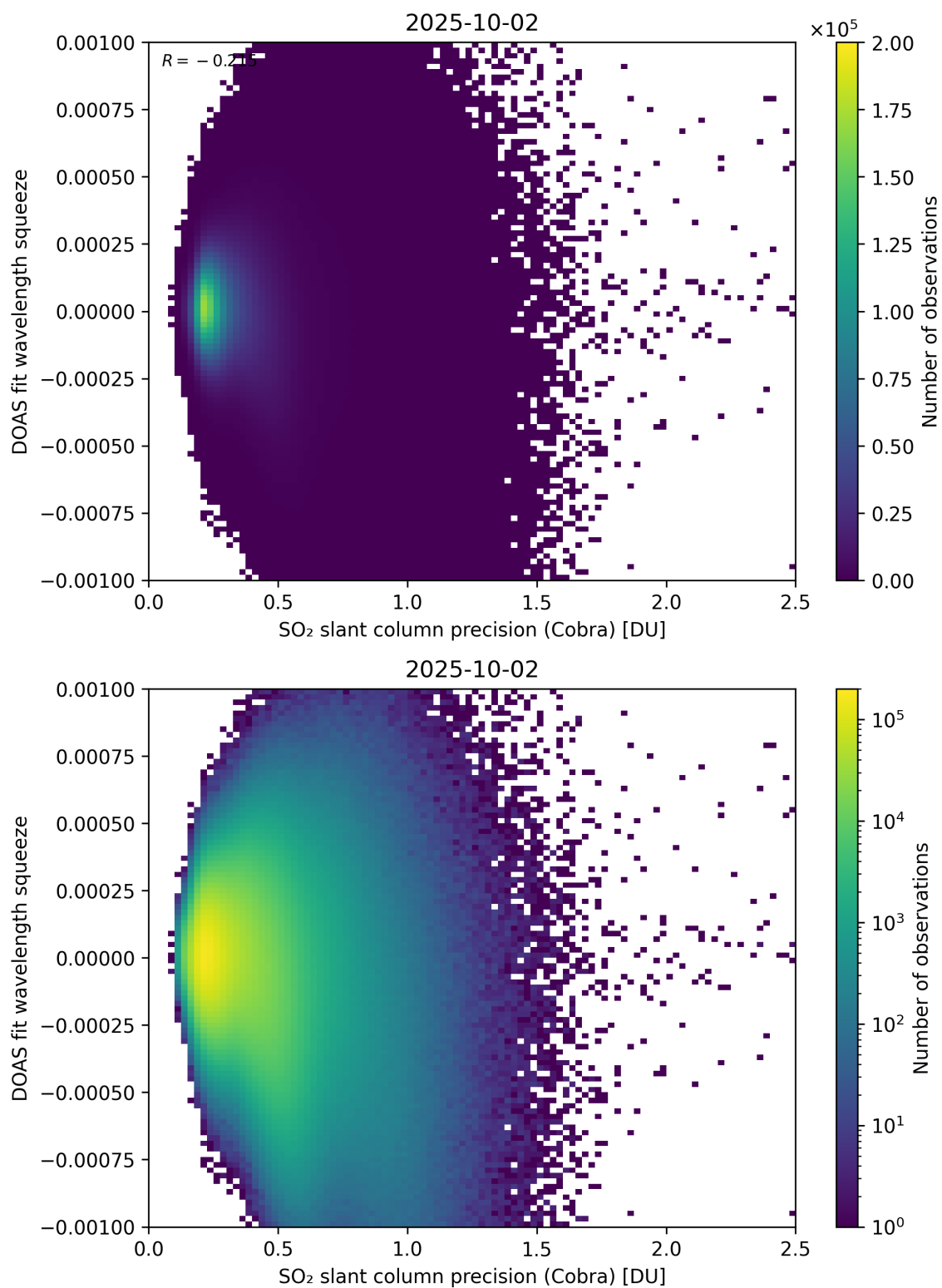
Figure 203: Scatter density plot of “SO 2 slant column precision (Cobra)” against “DOAS fit wavelength squeeze” for 2025-10-01 to 2025-10-03.
