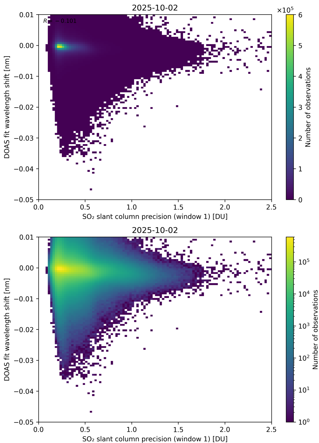
Figure 271: Scatter density plot of “SO 2 slant column precision (window 1)” against “DOAS fit wavelength shift” for 2025-10-01 to 2025-10-03.
