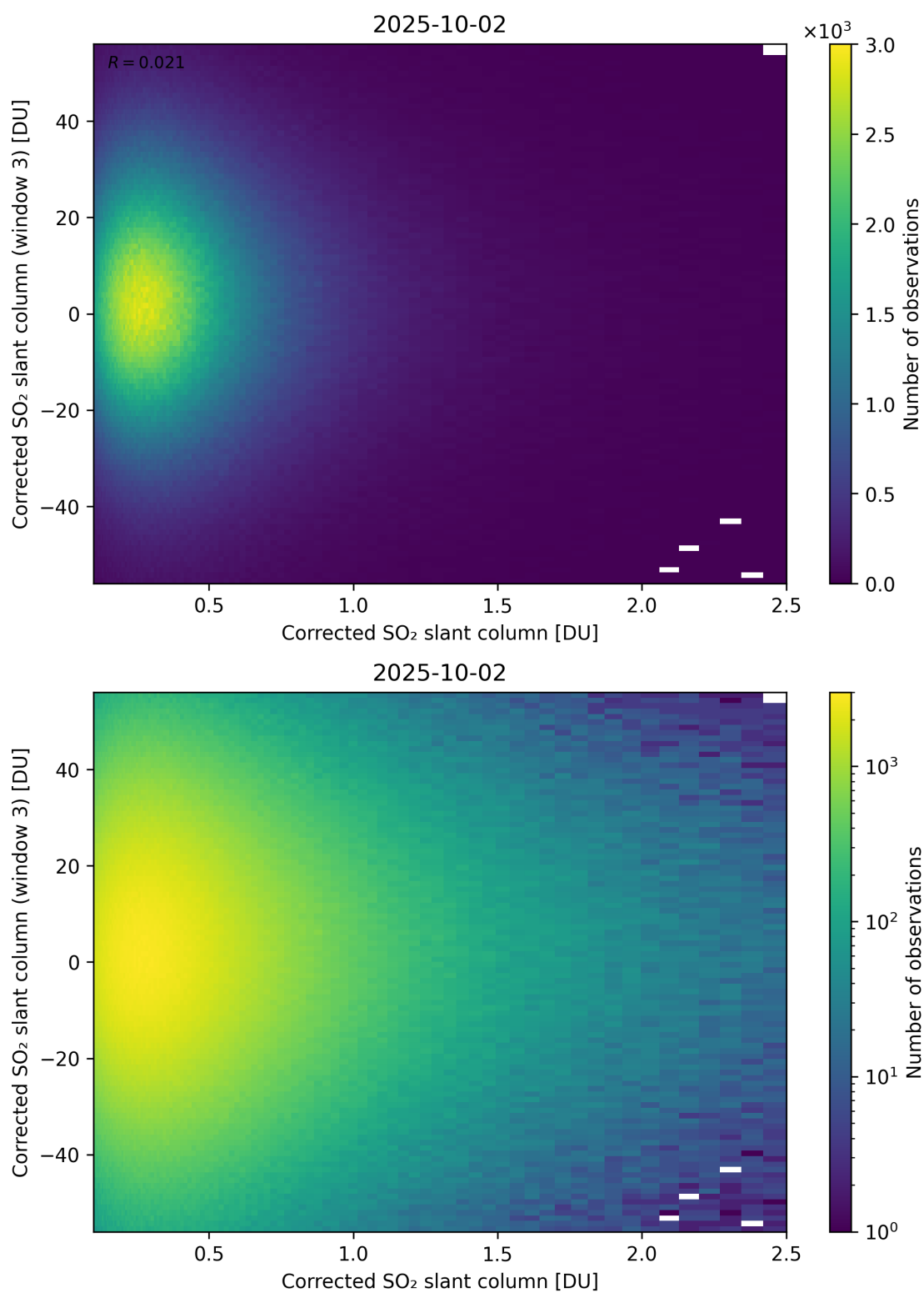
Figure 236: Scatter density plot of “Corrected SO 2 slant column” against “Corrected SO 2 slant column (window 3)” for 2025-10-01 to 2025-10-03.
