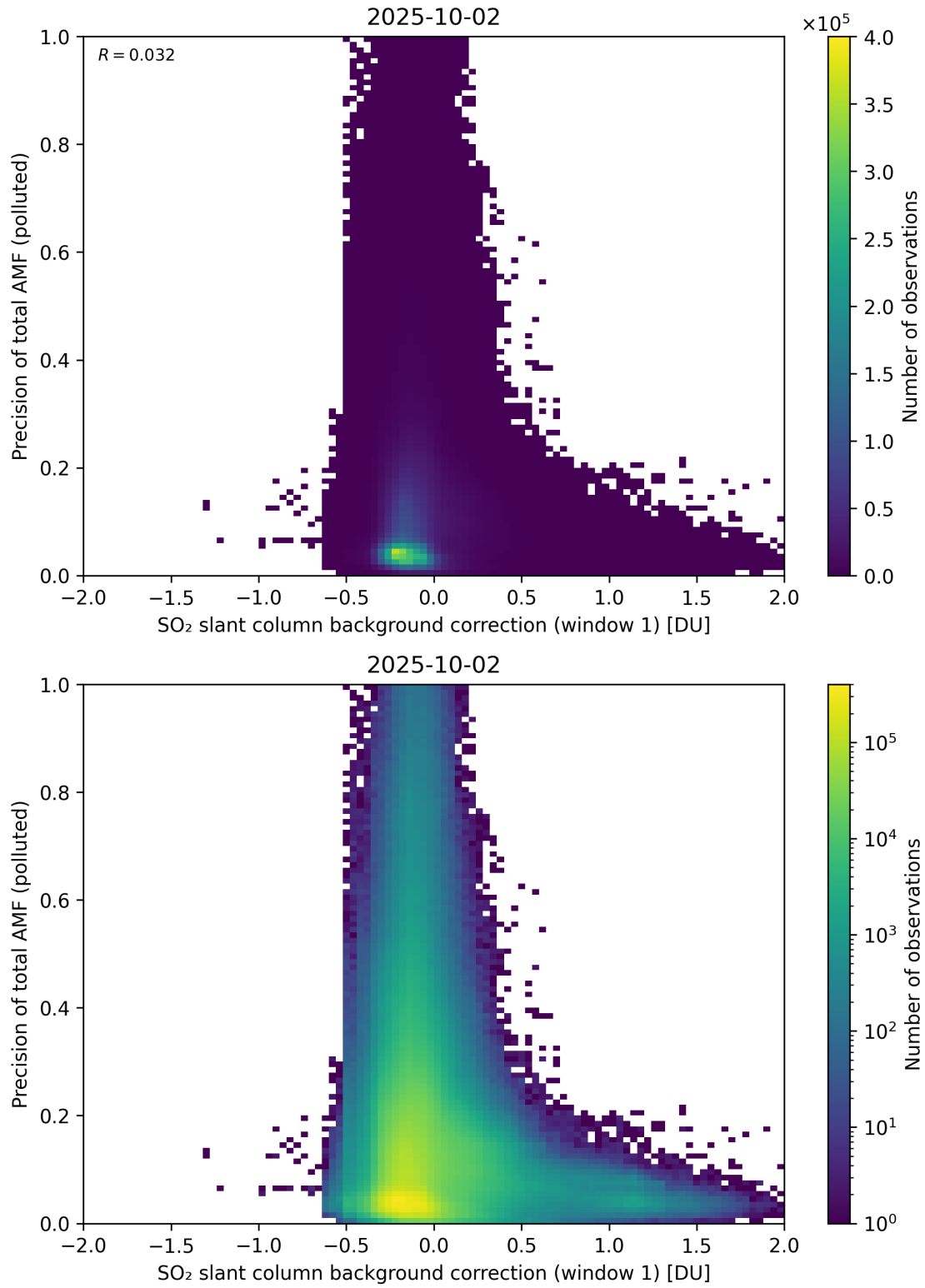
Figure 121: Scatter density plot of “SO 2 slant column background correction (window 1)” against “Precision of total AMF (polluted)” for 2025-10-01 to 2025-10-03.
