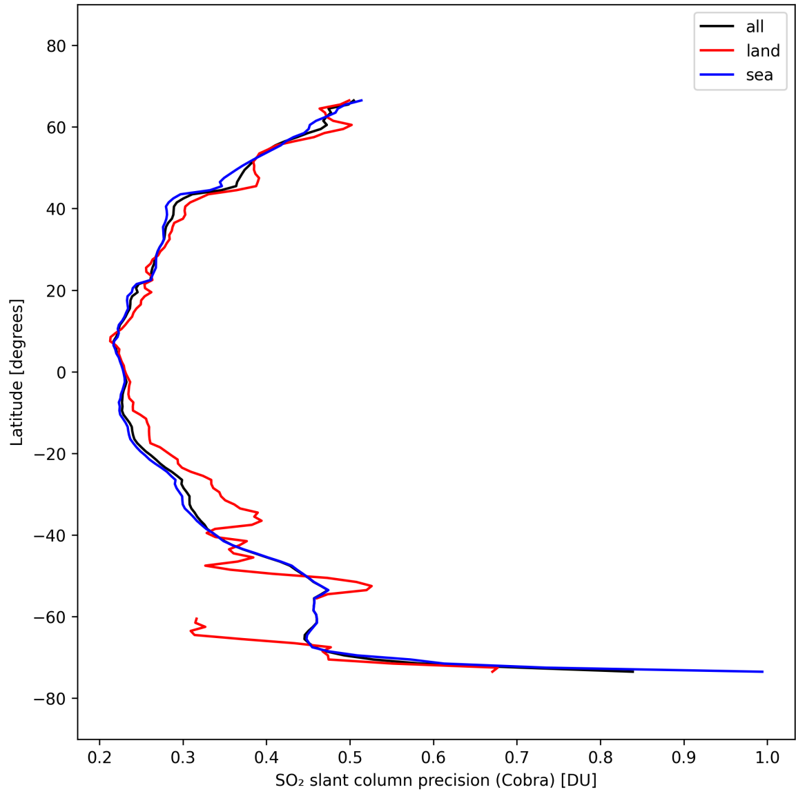
Figure 36: Zonal average of “SO 2 slant column precision (Cobra)” for 2025-10-01 to 2025-10-03.
