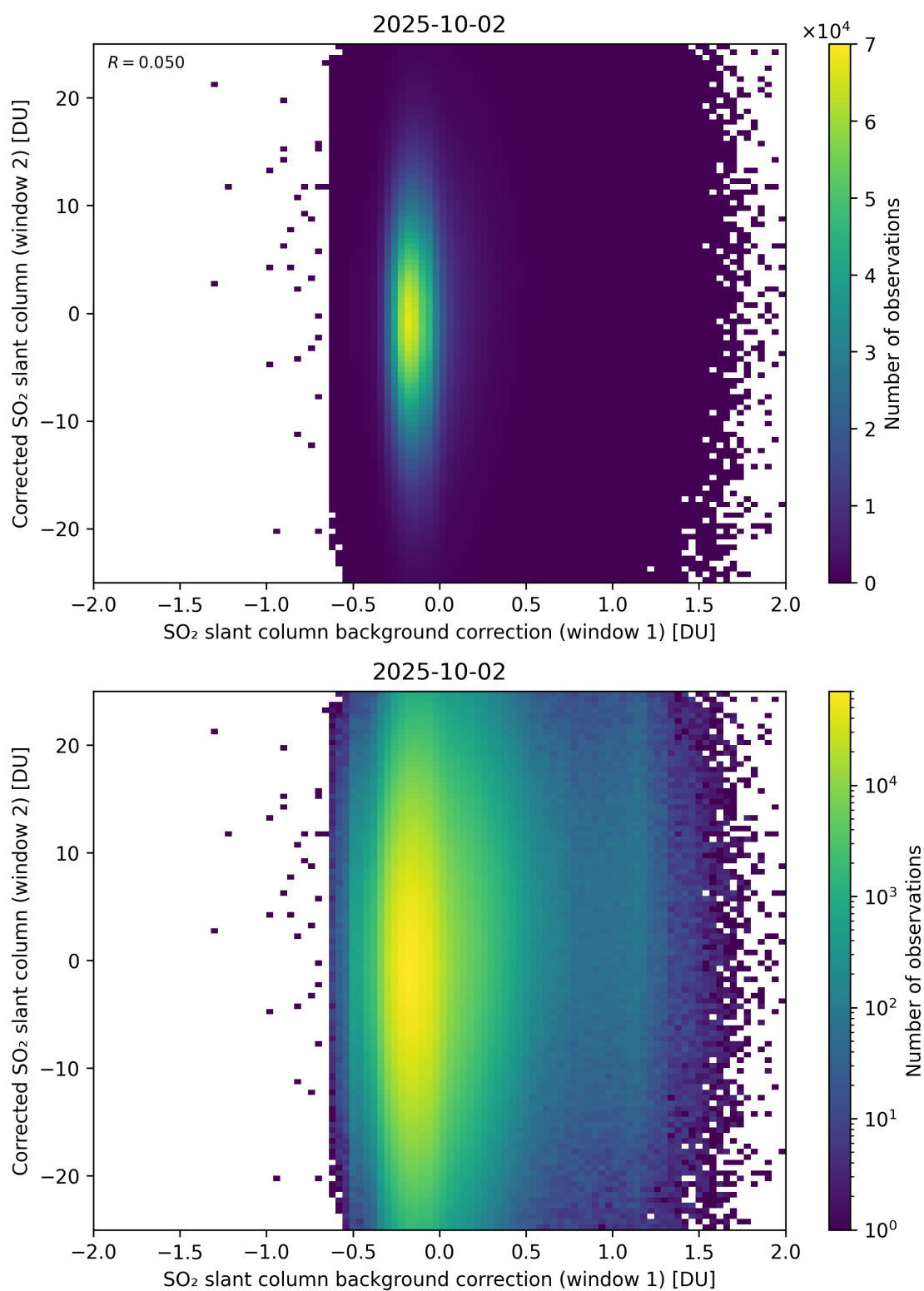
Figure 115: Scatter density plot of “SO 2 slant column background correction (window 1)” against “Corrected SO 2 slant column (window 2)” for 2025-10-01 to 2025-10-03.
