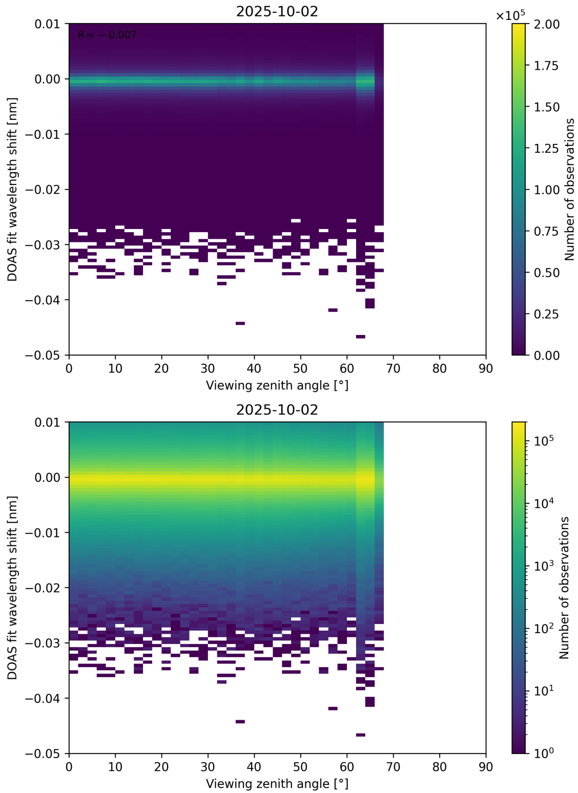
Figure 365: Scatter density plot of “Viewing zenith angle” against “DOAS fit wavelength shift” for 2025-10-01 to 2025-10-03.
