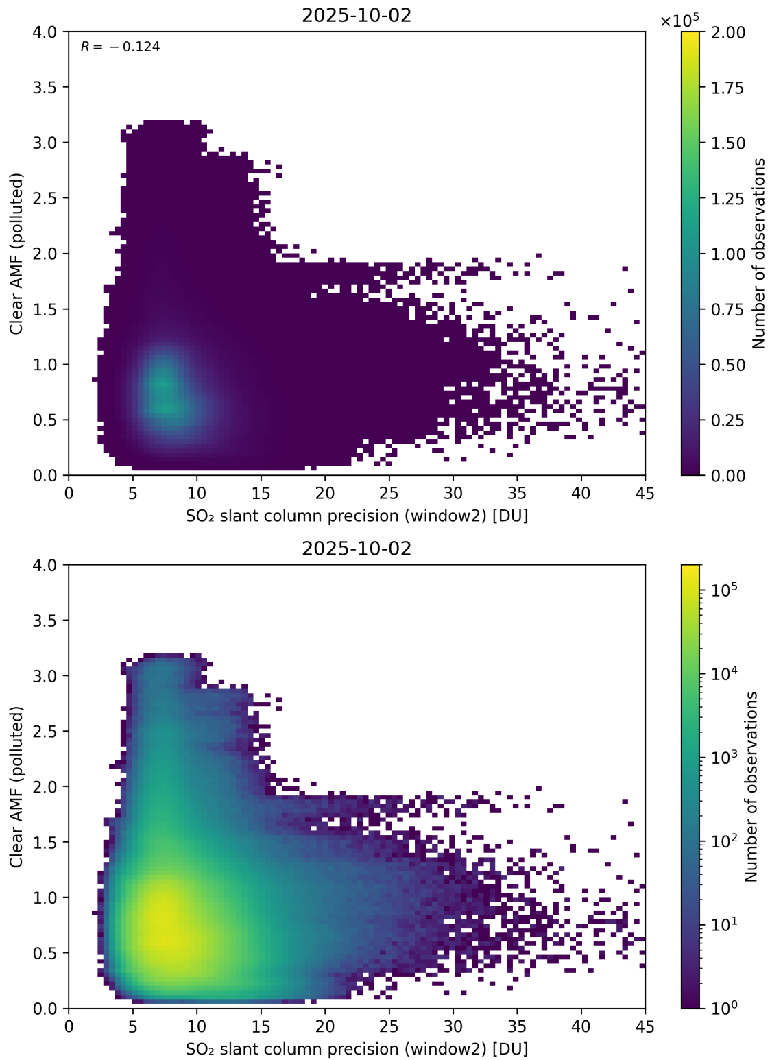
Figure 296: Scatter density plot of “SO 2 slant column precision (window2)” against “Clear AMF (polluted)” for 2025-10-01 to 2025-10-03.
