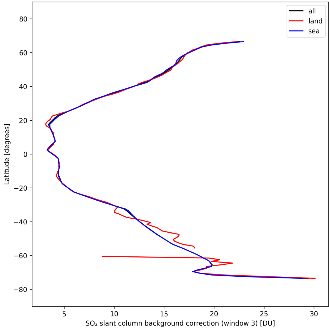
Figure 48: Zonal average of “SO 2 slant column background correction (window 3)” for 2025-10-01 to 2025-10-03.
