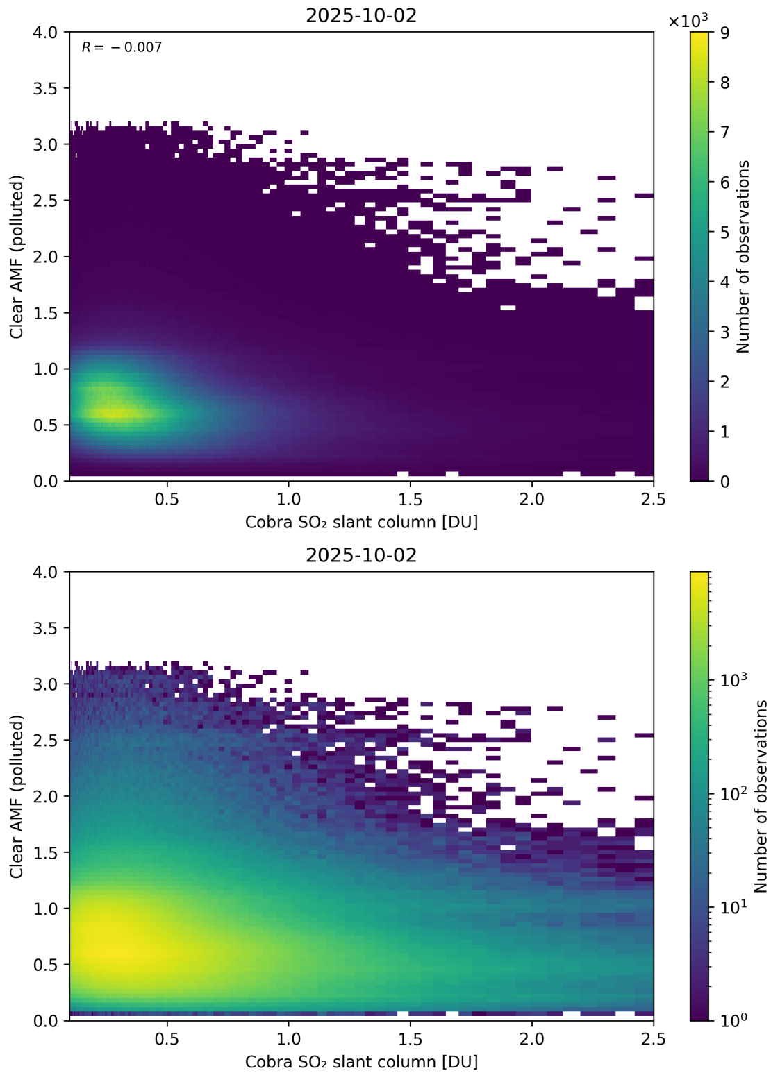
Figure 215: Scatter density plot of “Cobra SO 2 slant column” against “Clear AMF (polluted)” for 2025-10-01 to 2025-10-03.
