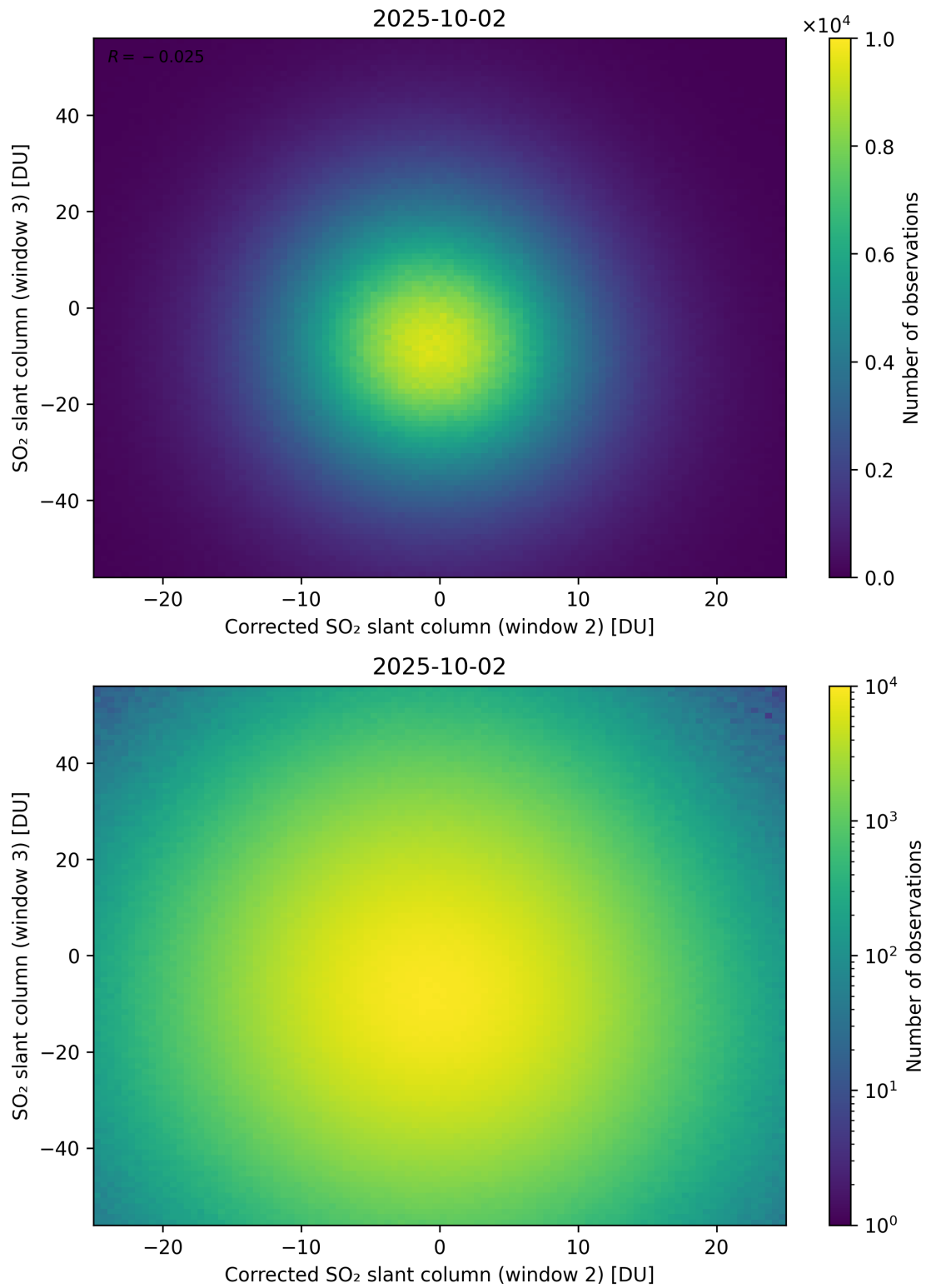
Figure 251: Scatter density plot of “Corrected SO 2 slant column (window 2)” against “SO 2 slant column (window 3)” for 2025-10-01 to 2025-10-03.
