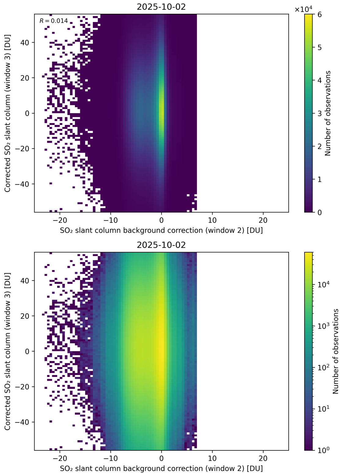
Figure 127: Scatter density plot of “SO 2 slant column background correction (window 2)” against “Corrected SO 2 slant column (window 3)” for 2025-10-01 to 2025-10-03.
