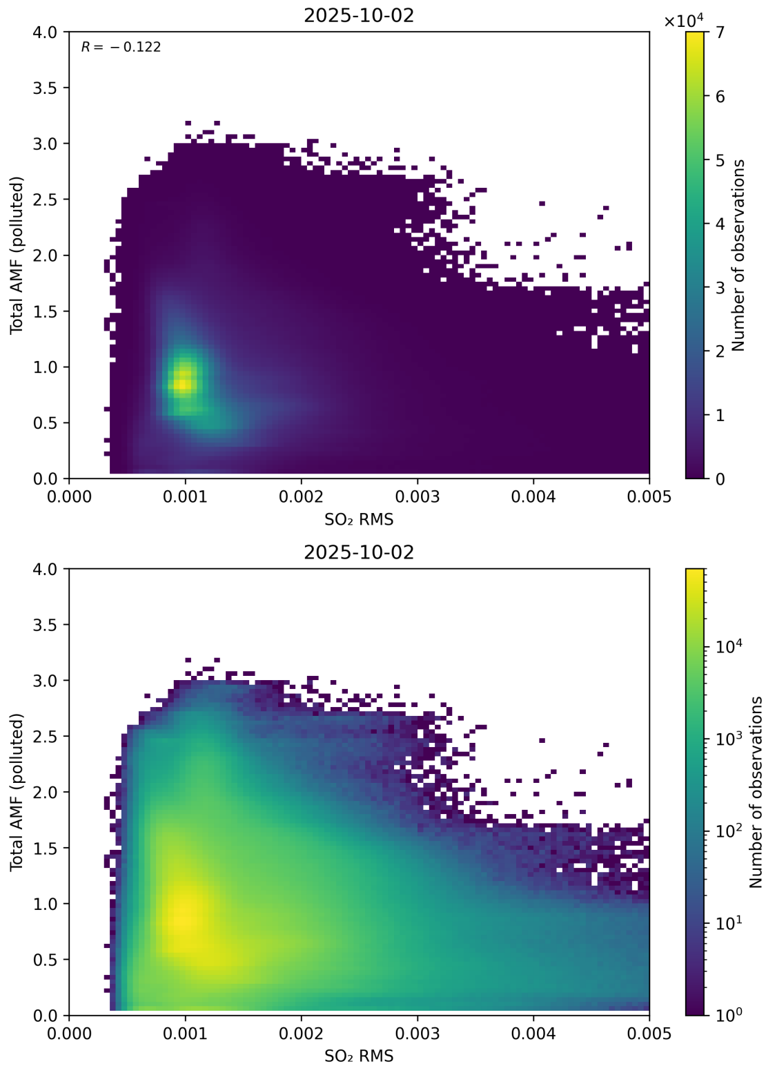
Figure 148: Scatter density plot of “SO 2 RMS” against “Total AMF (polluted)” for 2025-10-01 to 2025-10-03.
