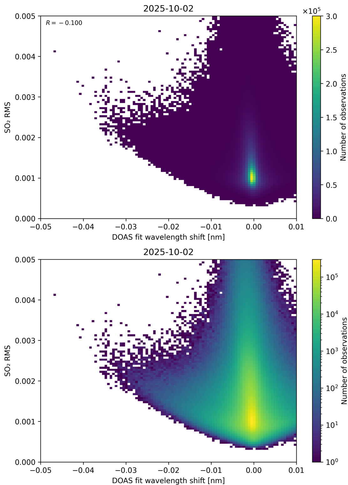
Figure 139: Scatter density plot of “DOAS fit wavelength shift” against “SO 2 RMS” for 2025-10-01 to 2025-10-03.
