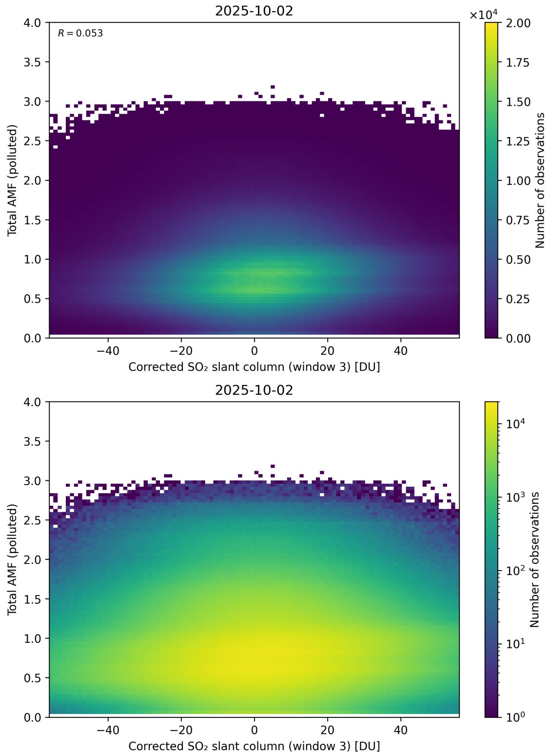
Figure 260: Scatter density plot of “Corrected SO 2 slant column (window 3)” against “Total AMF (polluted)” for 2025-10-01 to 2025-10-03.
