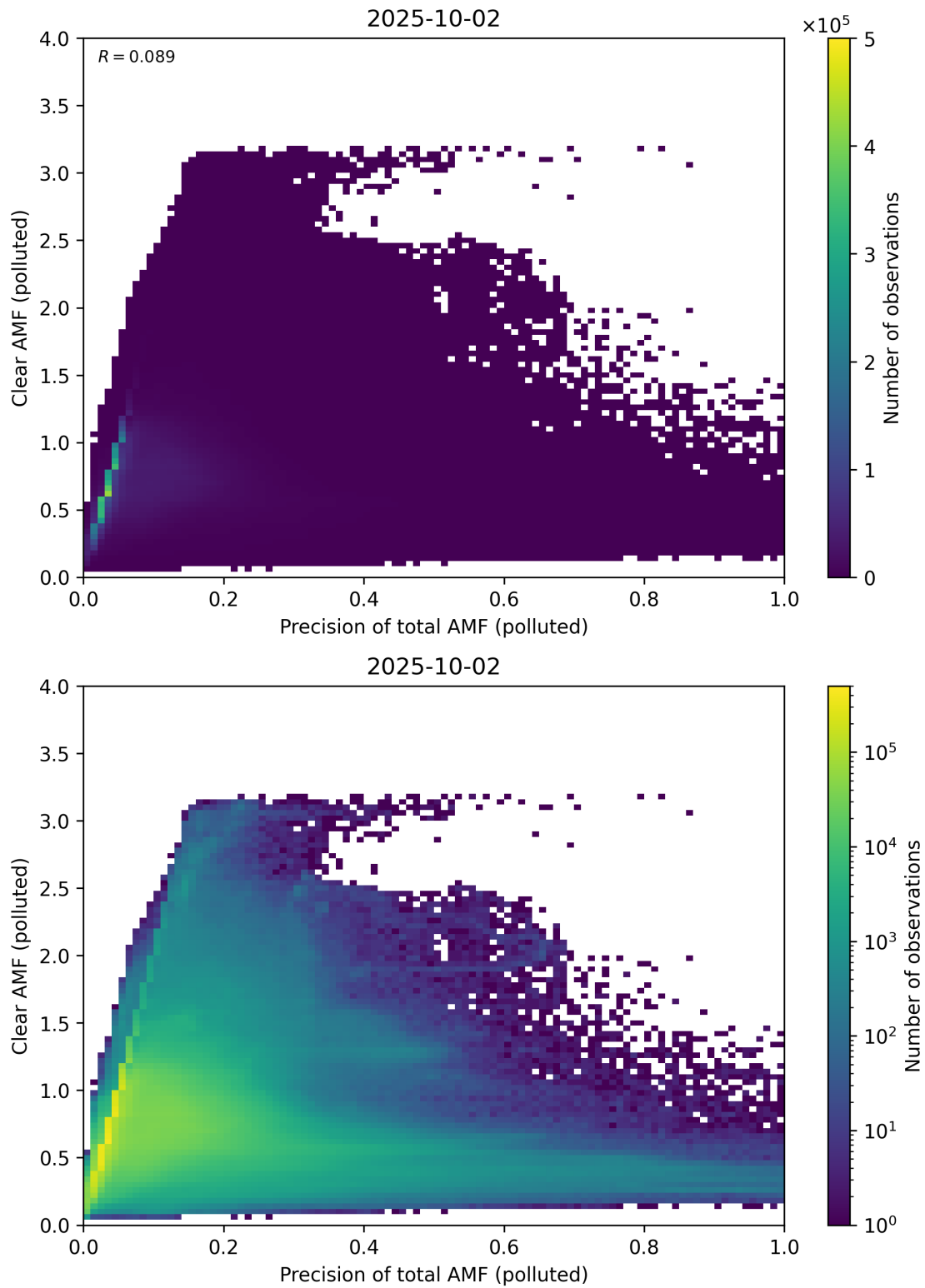
Figure 320: Scatter density plot of “Precision of total AMF (polluted)” against “Clear AMF (polluted)” for 2025-10-01 to 2025-10-03.
