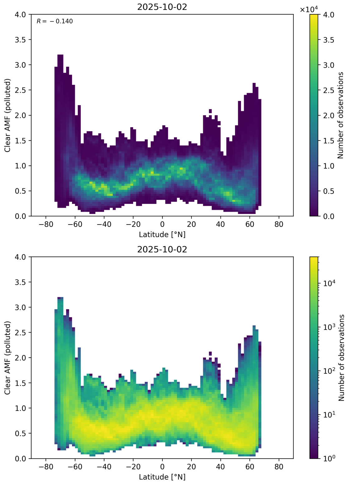
Figure 156: Scatter density plot of “Latitude” against “Clear AMF (polluted)” for 2025-10-01 to 2025-10-03.
