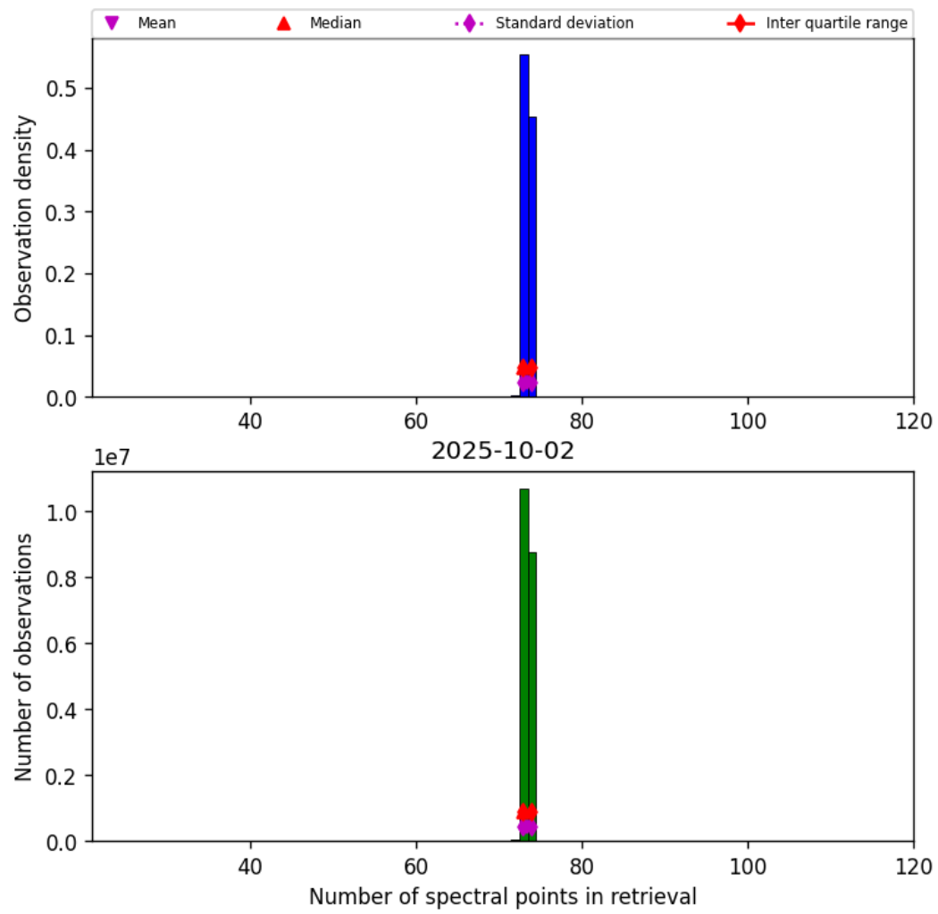
Figure 82: Histogram of “Number of spectral points in retrieval” for 2025-10-01 to 2025-10-03
