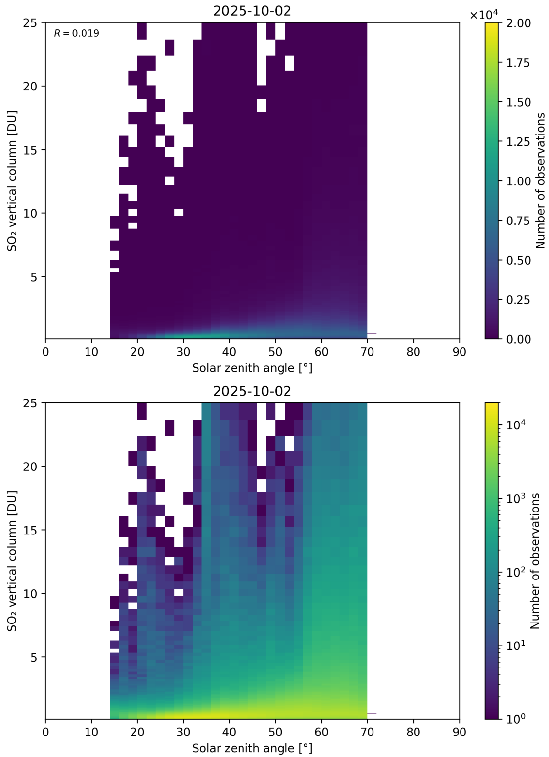
Figure 191: Scatter density plot of “Solar zenith angle” against “SO 2 vertical column” for 2025-10-01 to 2025-10-03.
