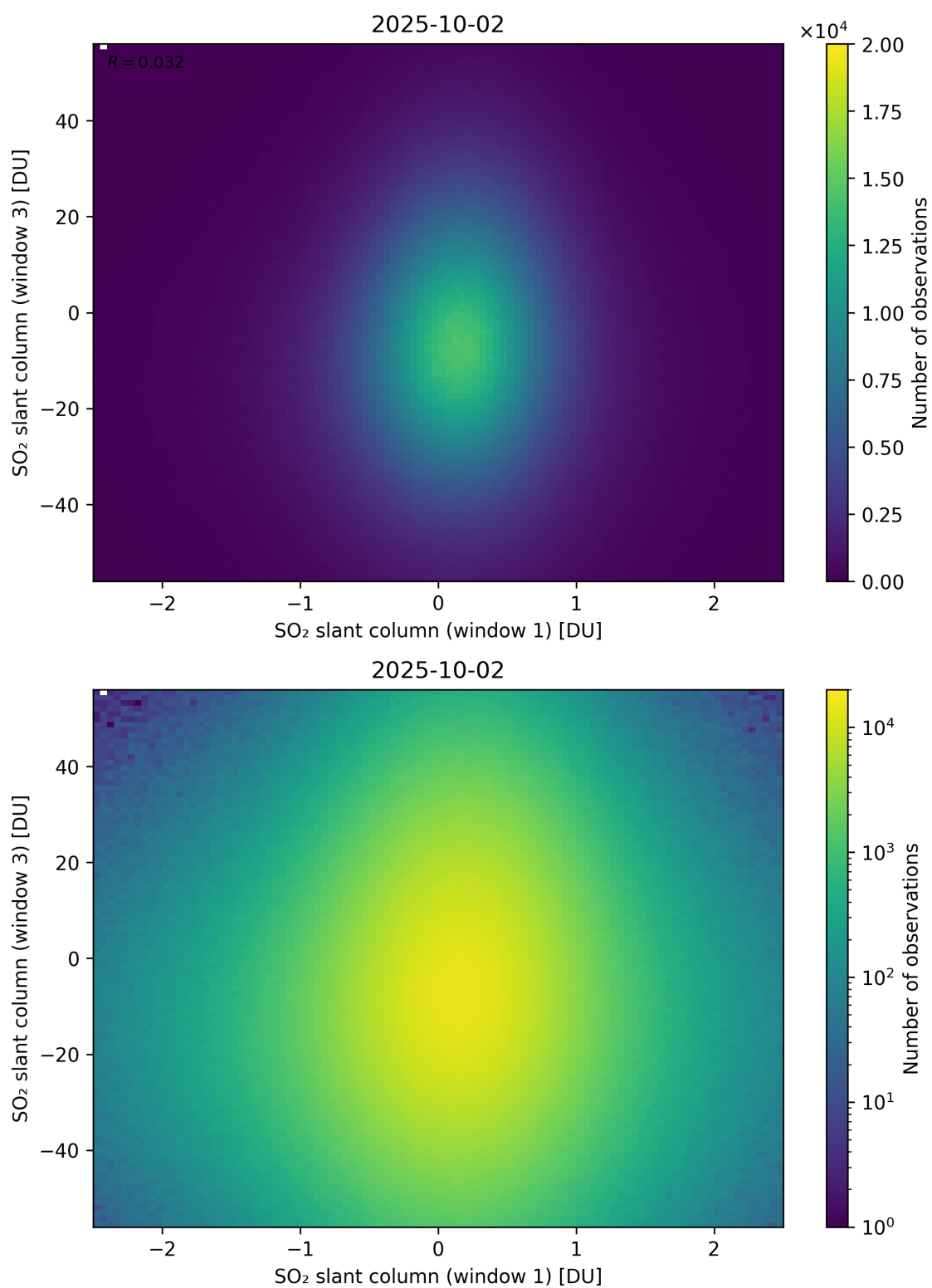
Figure 287: Scatter density plot of “SO 2 slant column (window 1)” against “SO 2 slant column (window 3)” for 2025-10-01 to 2025-10-03.
