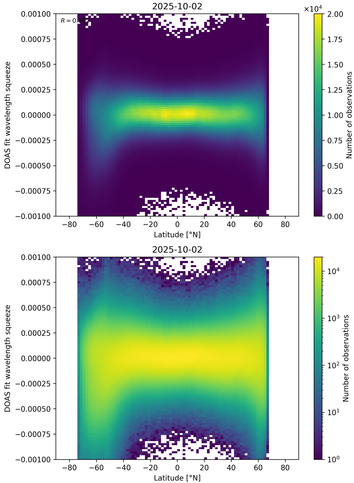
Figure 154: Scatter density plot of “Latitude” against “DOAS fit wavelength squeeze” for 2025-10-01 to 2025-10-03.
