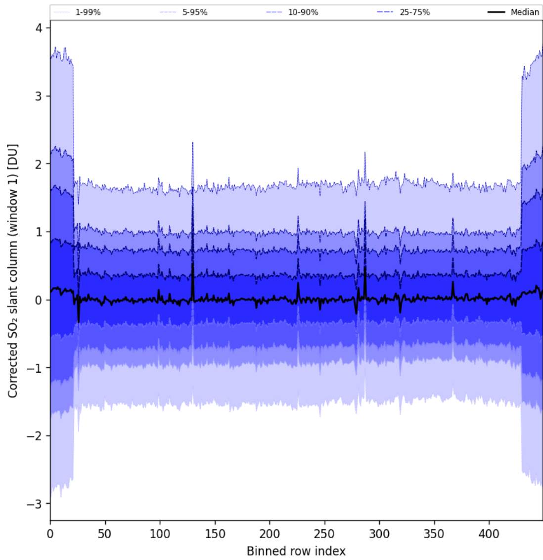
Figure 91: Along track statistics of “Corrected SO 2 slant column (window 1)” for 2025-10-01 to 2025-10-03
