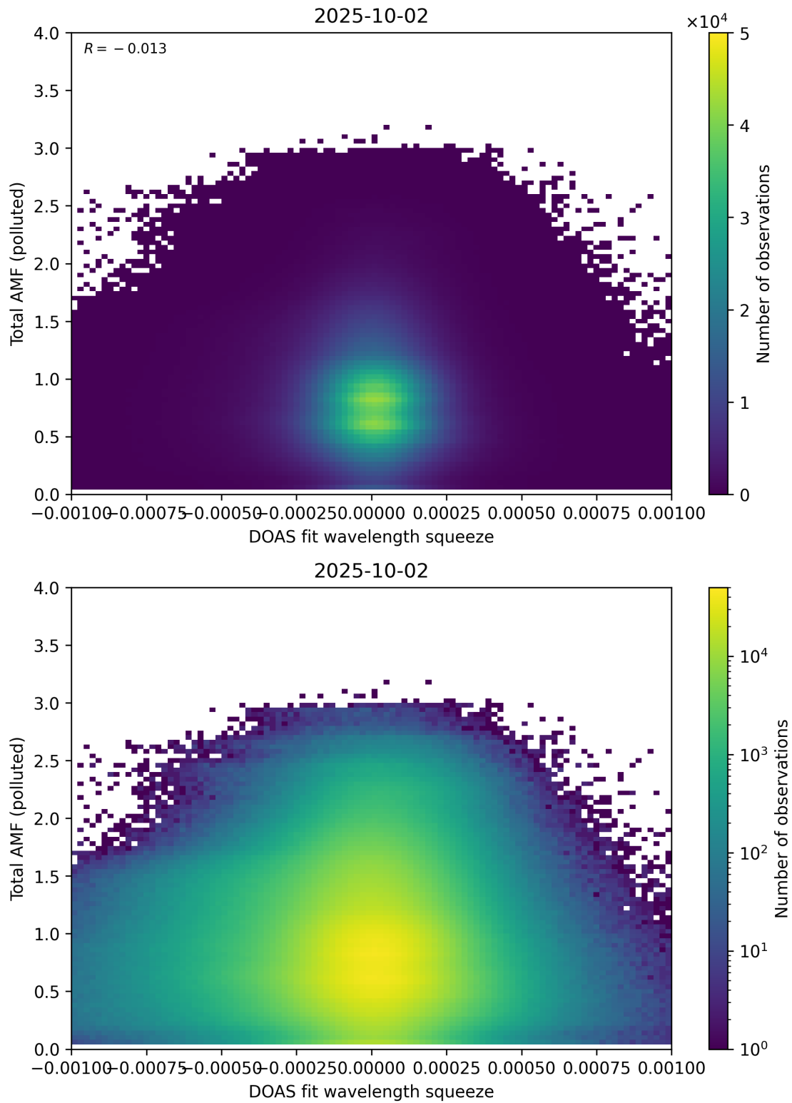
Figure 145: Scatter density plot of “DOAS fit wavelength squeeze” against “Total AMF (polluted)” for 2025-10-01 to 2025-10-03.
