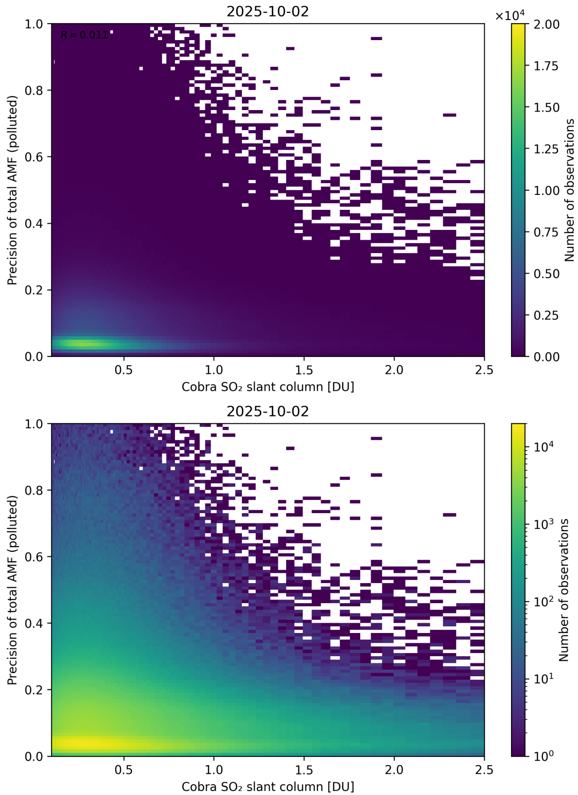
Figure 225: Scatter density plot of “Cobra SO 2 slant column” against “Precision of total AMF (polluted)” for 2025-10-01 to 2025-10-03.
