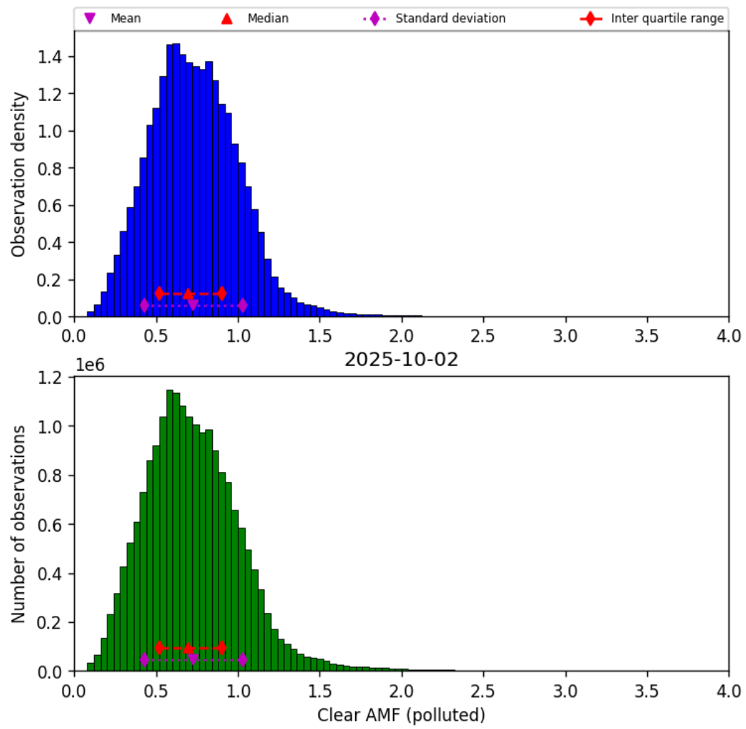
Figure 81: Histogram of “Clear AMF (polluted)” for 2025-10-01 to 2025-10-03
