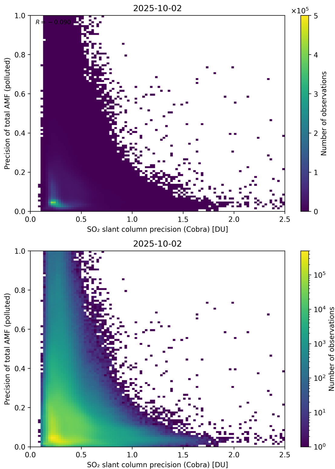
Figure 214: Scatter density plot of “SO 2 slant column precision (Cobra)” against “Precision of total AMF (polluted)” for 2025-10-01 to 2025-10-03.
