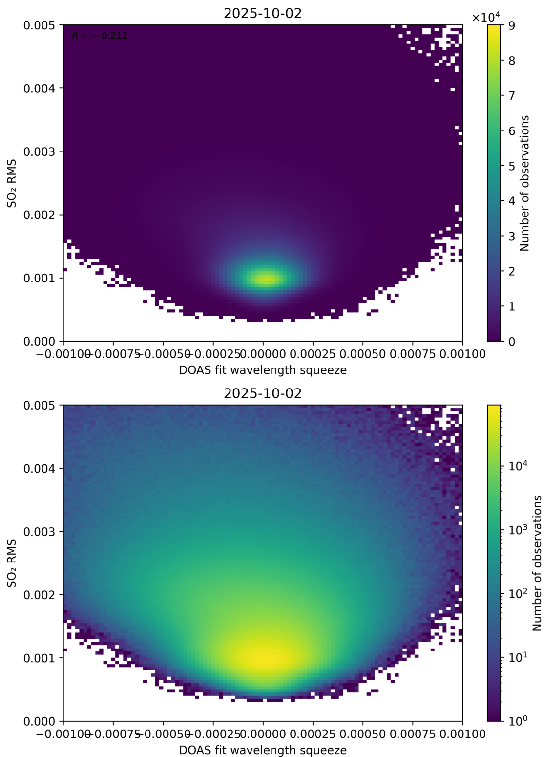
Figure 143: Scatter density plot of “DOAS fit wavelength squeeze” against “SO 2 RMS” for 2025-10-01 to 2025-10-03.
