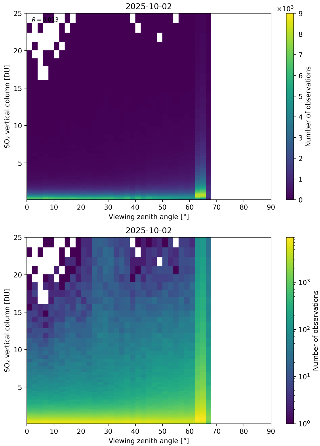
Figure 383: Scatter density plot of “Viewing zenith angle” against “SO 2 vertical column” for 2025-10-01 to 2025-10-03.
