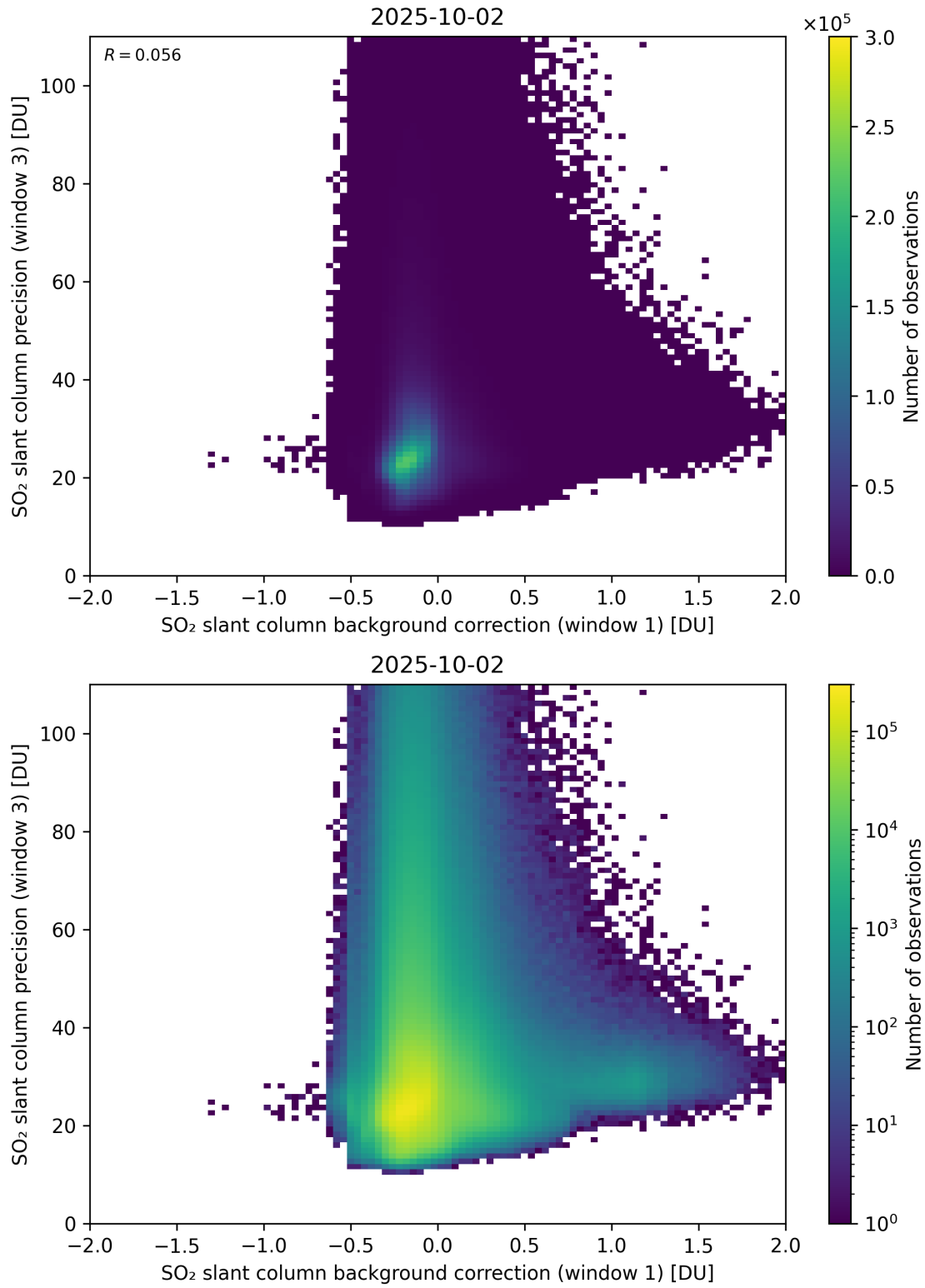
Figure 119: Scatter density plot of “SO 2 slant column background correction (window 1)” against “SO 2 slant column precision (window 3)” for 2025-10-01 to 2025-10-03.
