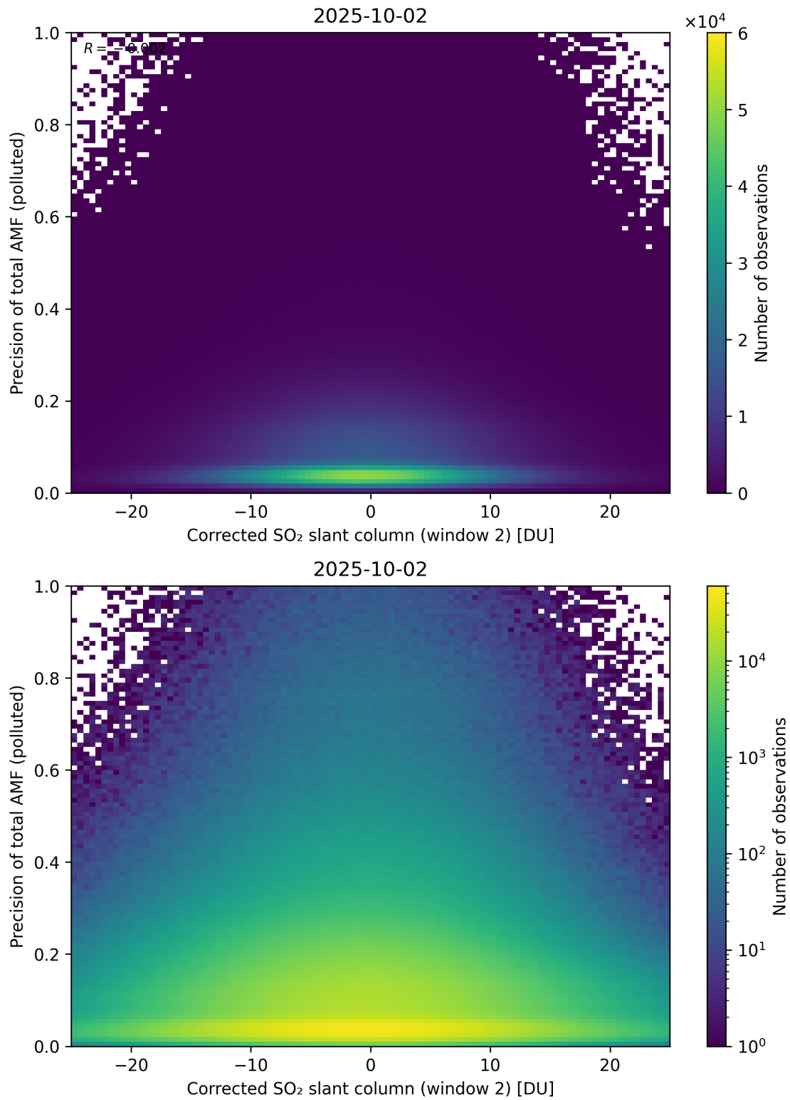
Figure 254: Scatter density plot of “Corrected SO 2 slant column (window 2)” against “Precision of total AMF (polluted)” for 2025-10-01 to 2025-10-03.
