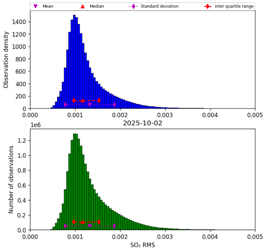
Figure 78: Histogram of “SO 2 RMS” for 2025-10-01 to 2025-10-03
