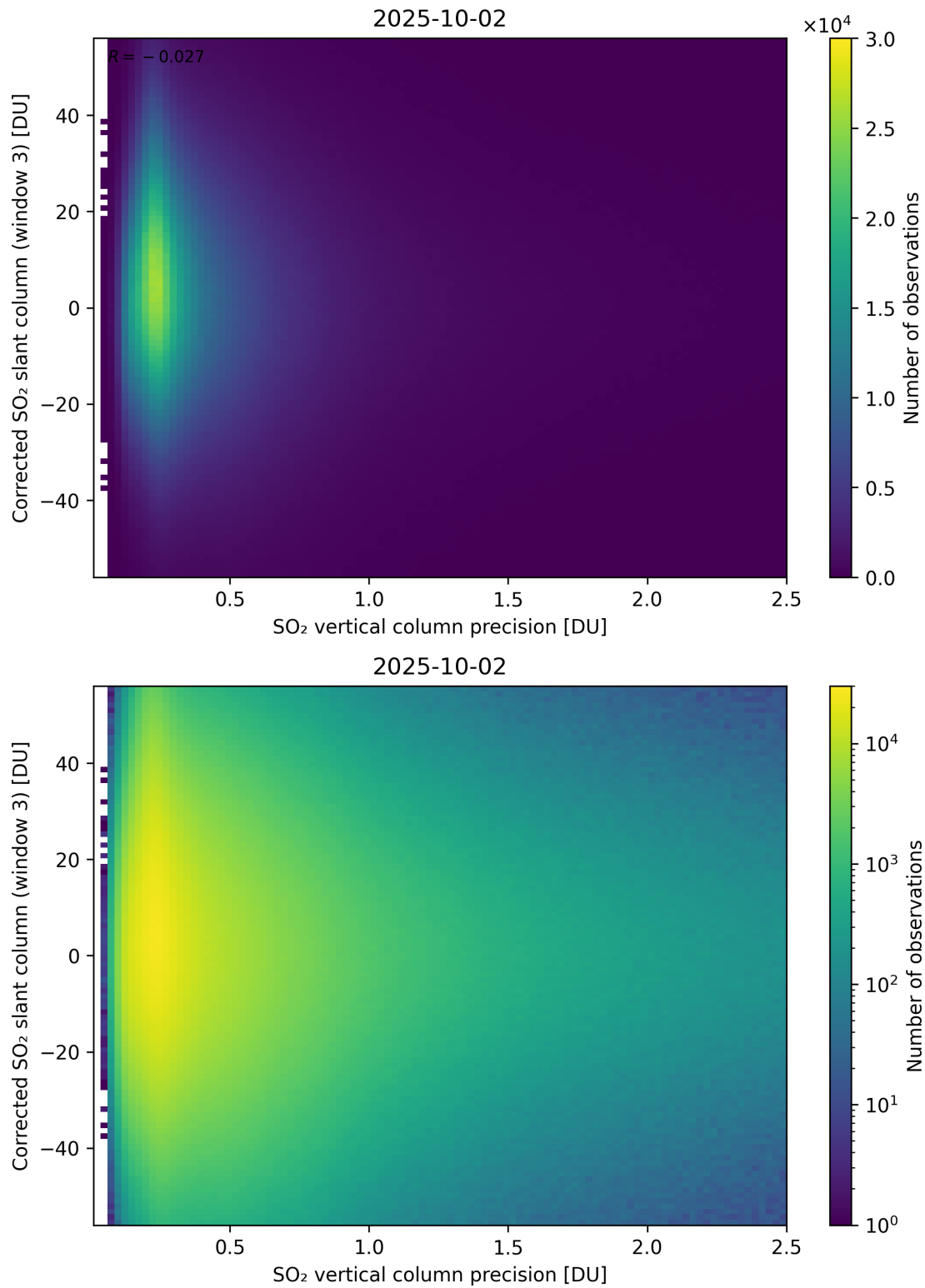
Figure 340: Scatter density plot of “SO 2 vertical column precision” against “Corrected SO 2 slant column (window 3)” for 2025-10-01 to 2025-10-03.
