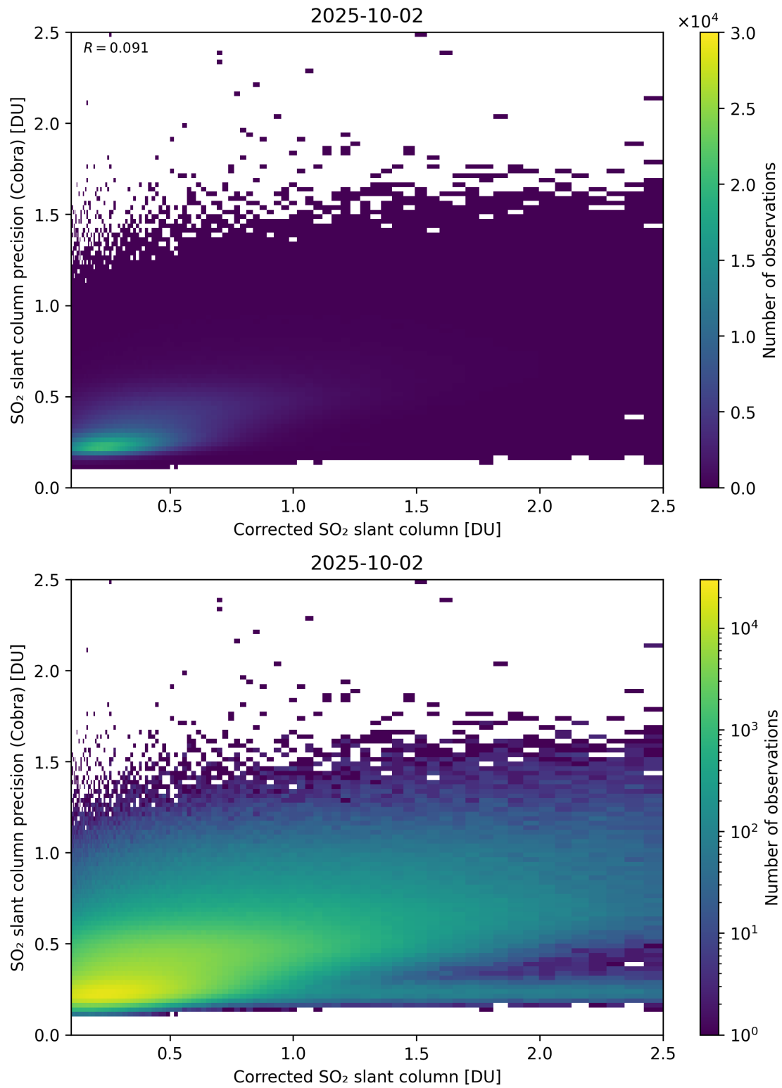
Figure 234: Scatter density plot of “Corrected SO 2 slant column” against “SO 2 slant column precision (Cobra)” for 2025-10-01 to 2025-10-03.
