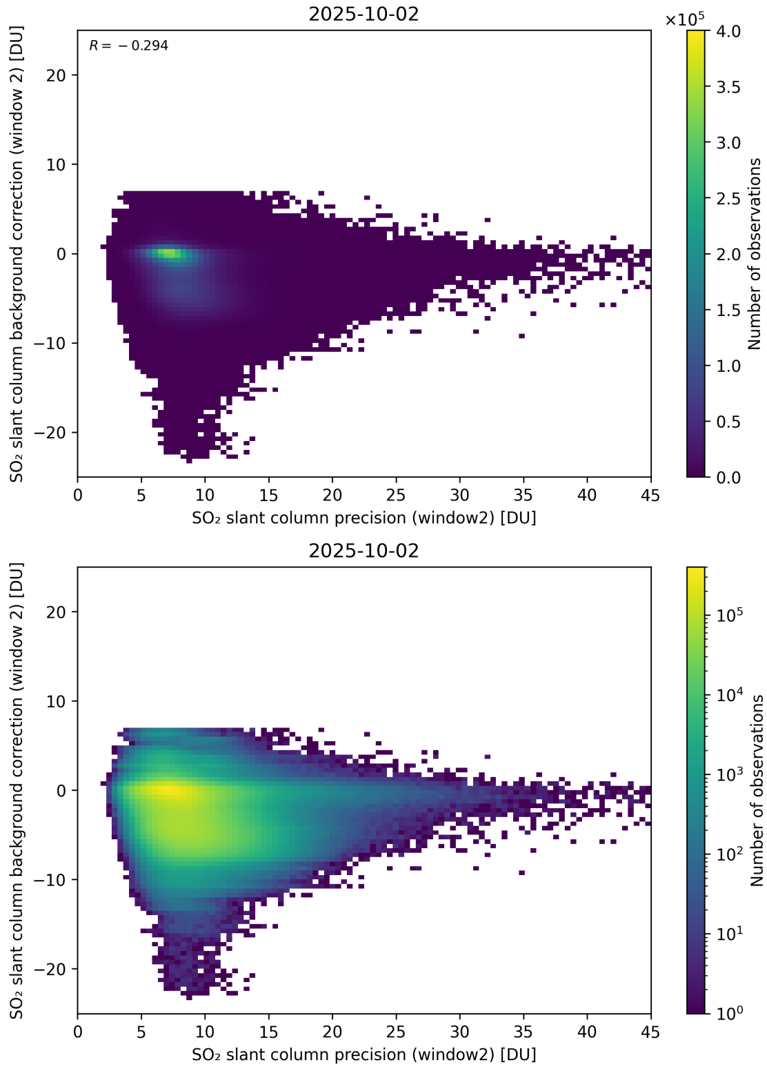
Figure 291: Scatter density plot of “SO 2 slant column precision (window2)” against “SO 2 slant column background correction (window 2)” for 2025-10-01 to 2025-10-03.
