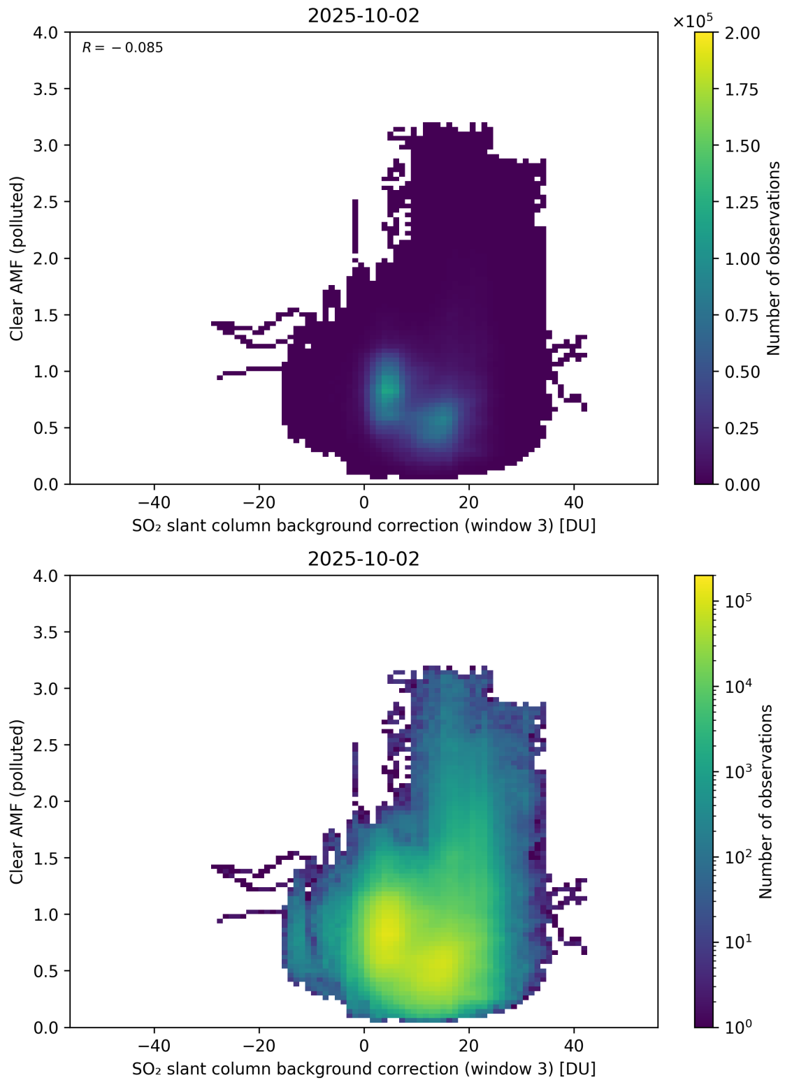
Figure 135: Scatter density plot of “SO 2 slant column background correction (window 3)” against “Clear AMF (polluted)” for 2025-10-01 to 2025-10-03.
