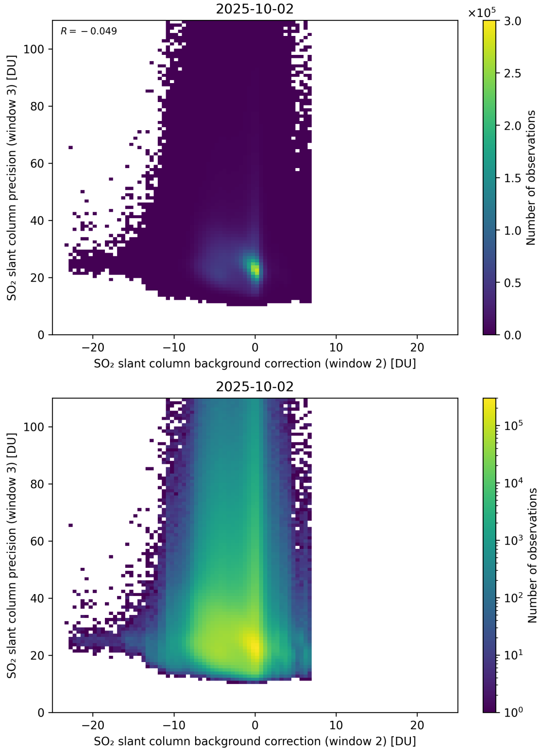
Figure 129: Scatter density plot of “SO 2 slant column background correction (window 2)” against “SO 2 slant column precision (window 3)” for 2025-10-01 to 2025-10-03.
