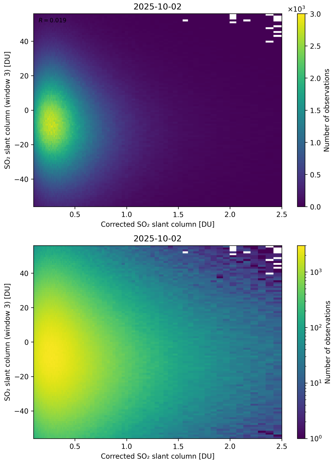
Figure 240: Scatter density plot of “Corrected SO 2 slant column” against “SO 2 slant column (window 3)” for 2025-10-01 to 2025-10-03.
