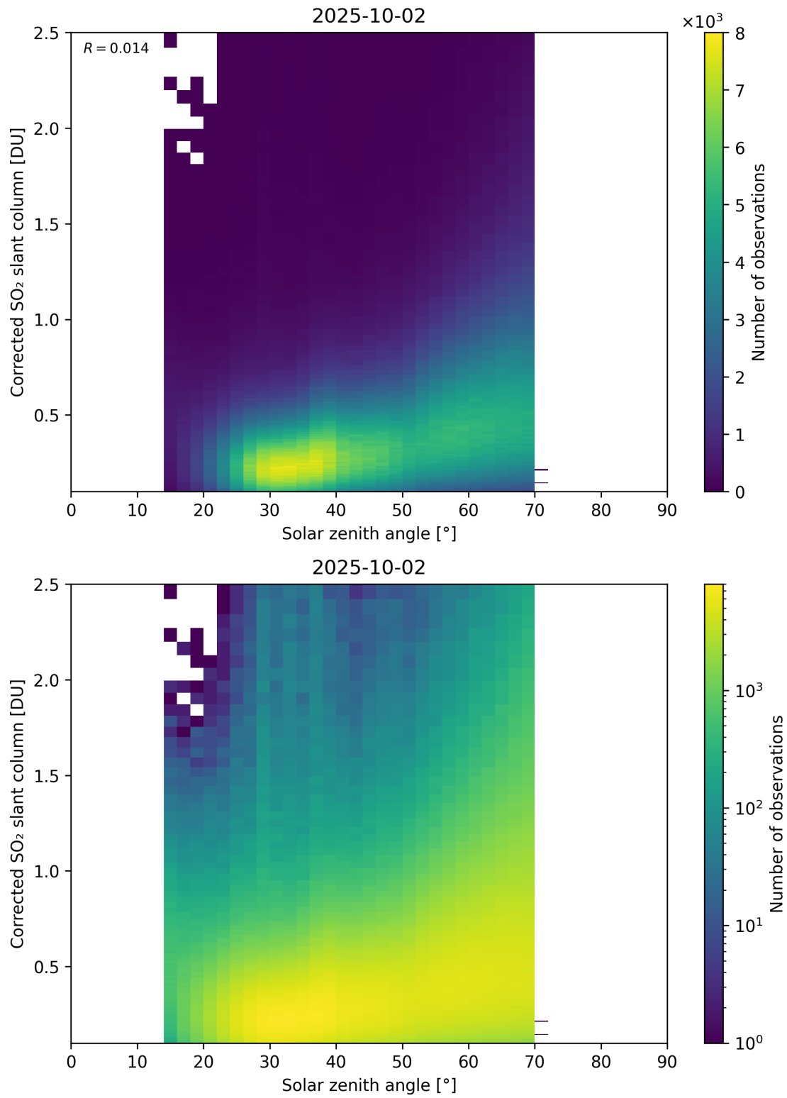
Figure 181: Scatter density plot of “Solar zenith angle” against “Corrected SO 2 slant column” for 2025-10-01 to 2025-10-03.
