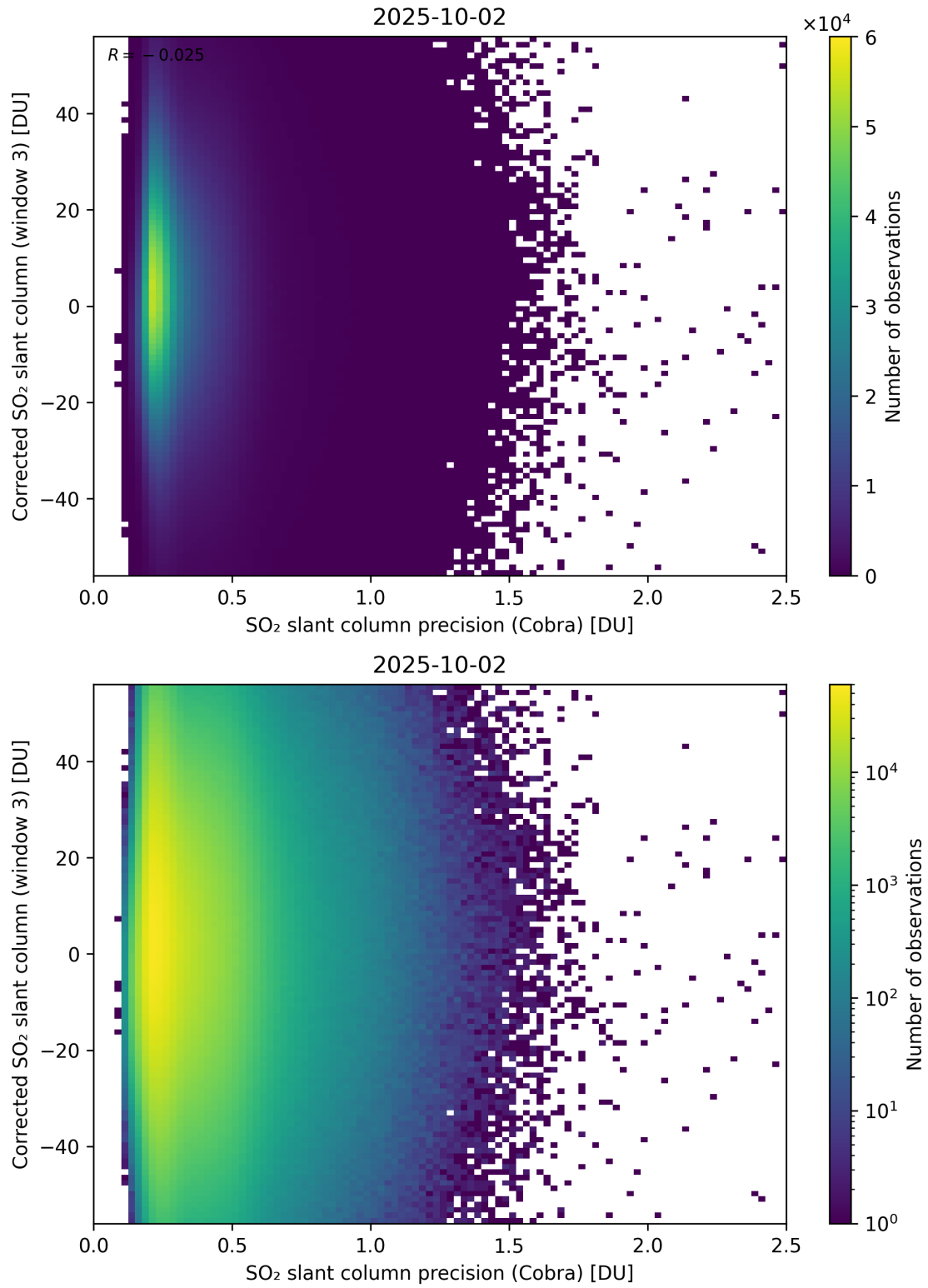
Figure 207: Scatter density plot of “SO 2 slant column precision (Cobra)” against “Corrected SO 2 slant column (window 3)” for 2025-10-01 to 2025-10-03.
