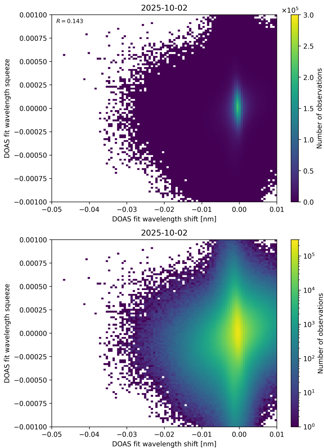
Figure 138: Scatter density plot of “DOAS fit wavelength shift” against “DOAS fit wavelength squeeze” for 2025-10-01 to 2025-10-03.
