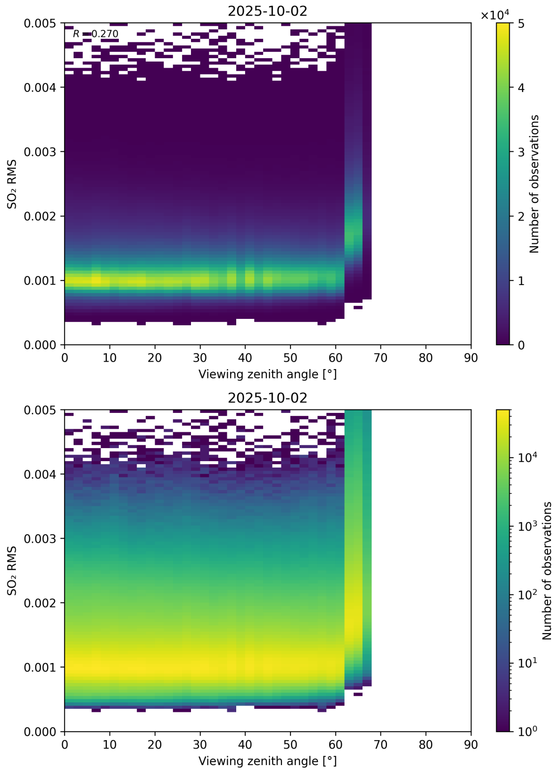
Figure 367: Scatter density plot of “Viewing zenith angle” against “SO 2 RMS” for 2025-10-01 to 2025-10-03.
