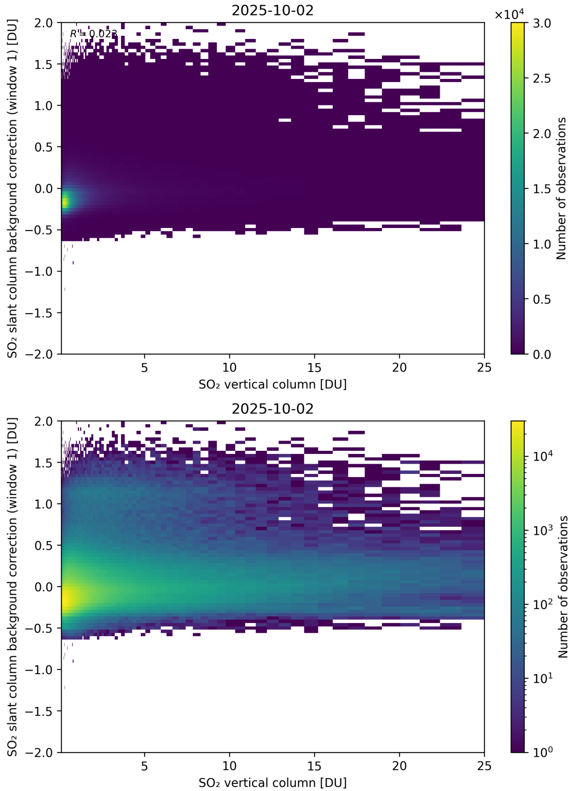
Figure 323: Scatter density plot of “SO 2 vertical column” against “SO 2 slant column background correction (window 1)” for 2025-10-01 to 2025-10-03.
