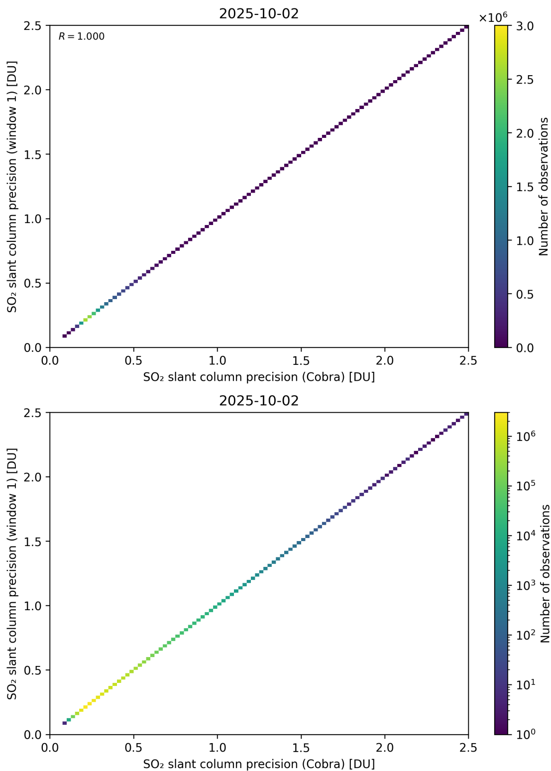
Figure 209: Scatter density plot of “SO 2 slant column precision (Cobra)” against “SO 2 slant column precision (window 1)” for 2025-10-01 to 2025-10-03.
