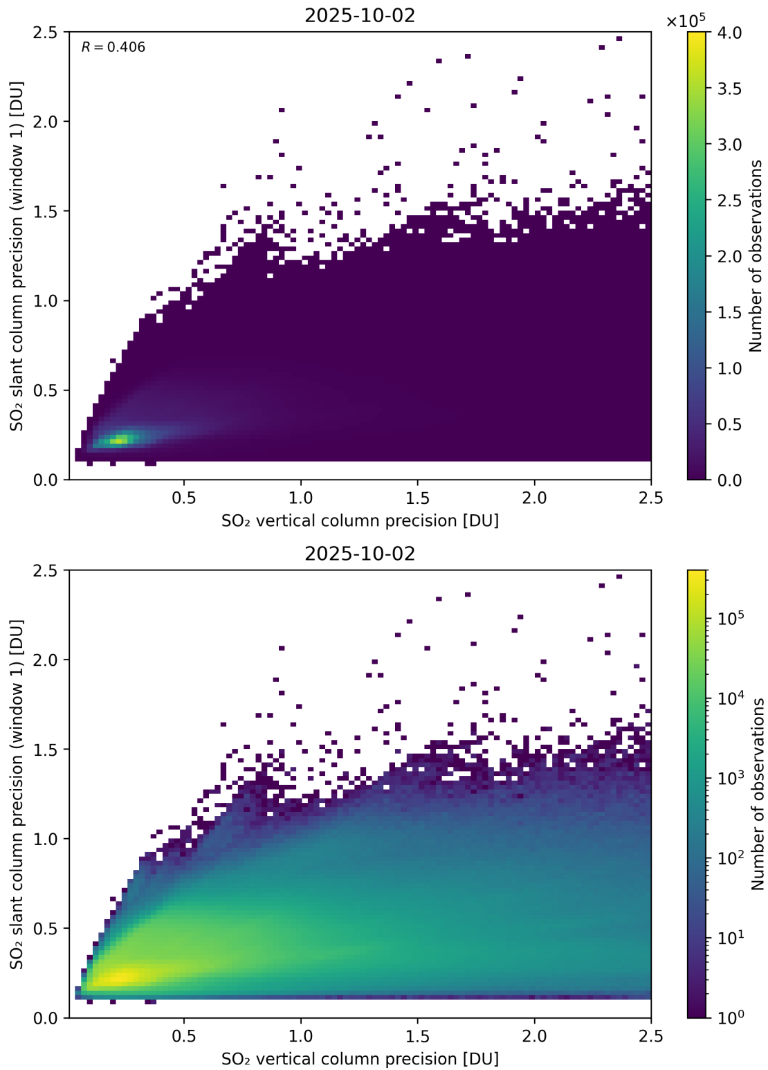
Figure 342: Scatter density plot of “SO 2 vertical column precision” against “SO 2 slant column precision (window 1)” for 2025-10-01 to 2025-10-03.
