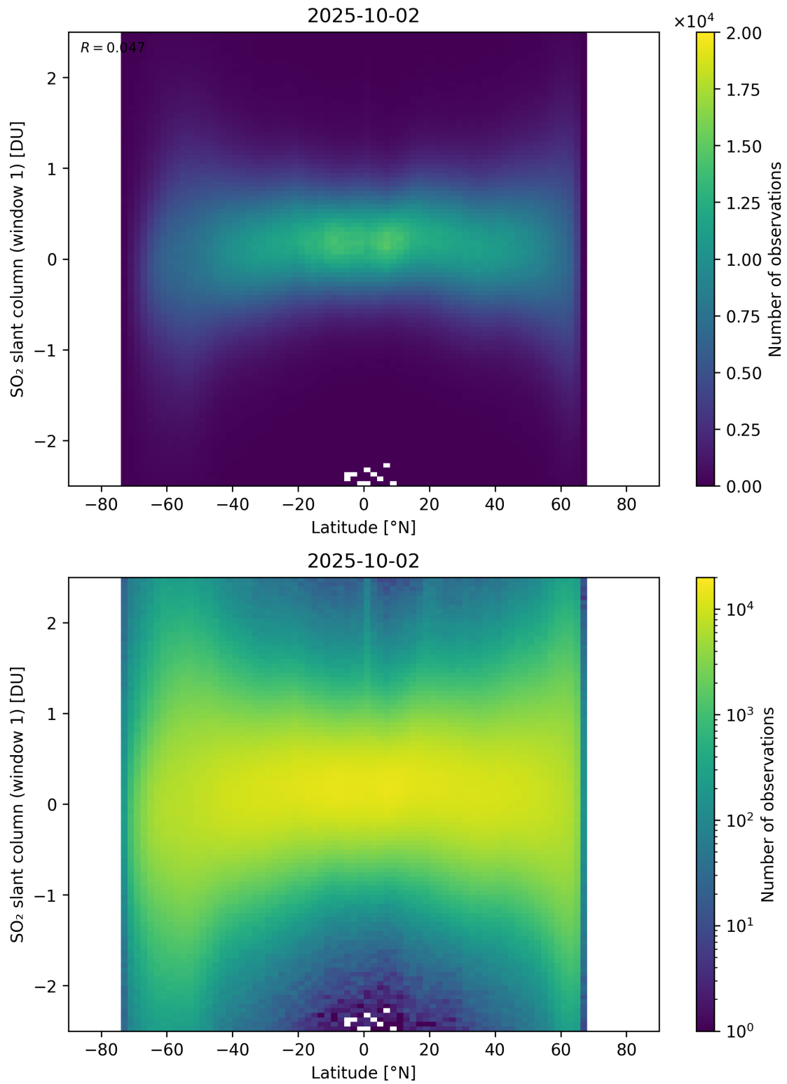
Figure 162: Scatter density plot of “Latitude” against “SO 2 slant column (window 1)” for 2025-10-01 to 2025-10-03.
