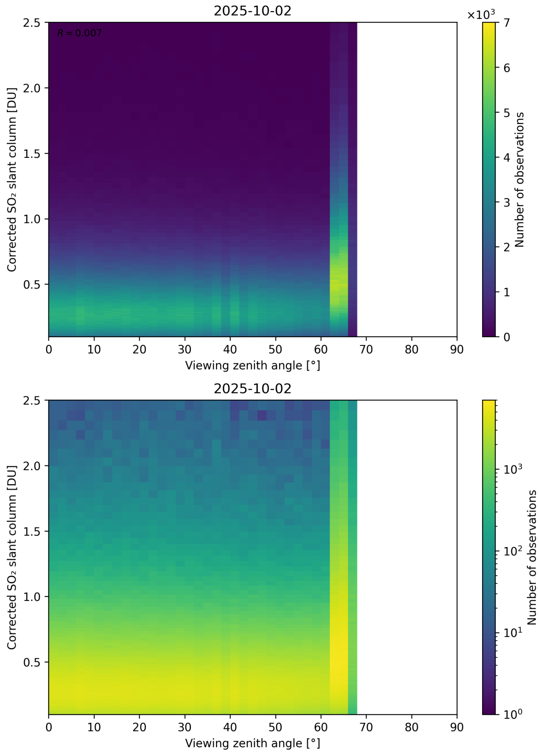
Figure 373: Scatter density plot of “Viewing zenith angle” against “Corrected SO 2 slant column” for 2025-10-01 to 2025-10-03.
