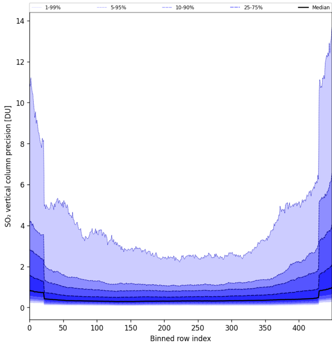
Figure 85: Along track statistics of “SO 2 vertical column precision” for 2025-10-01 to 2025-10-03
