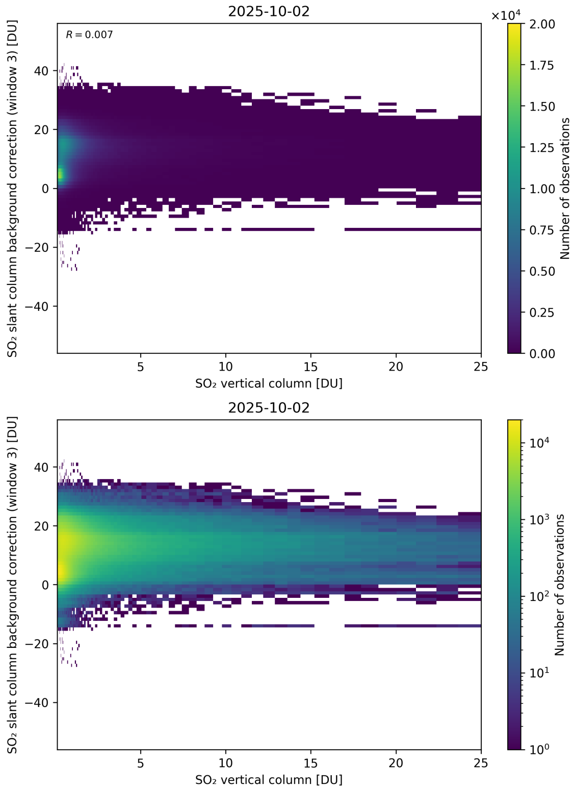
Figure 325: Scatter density plot of “SO 2 vertical column” against “SO 2 slant column background correction (window 3)” for 2025-10-01 to 2025-10-03.
