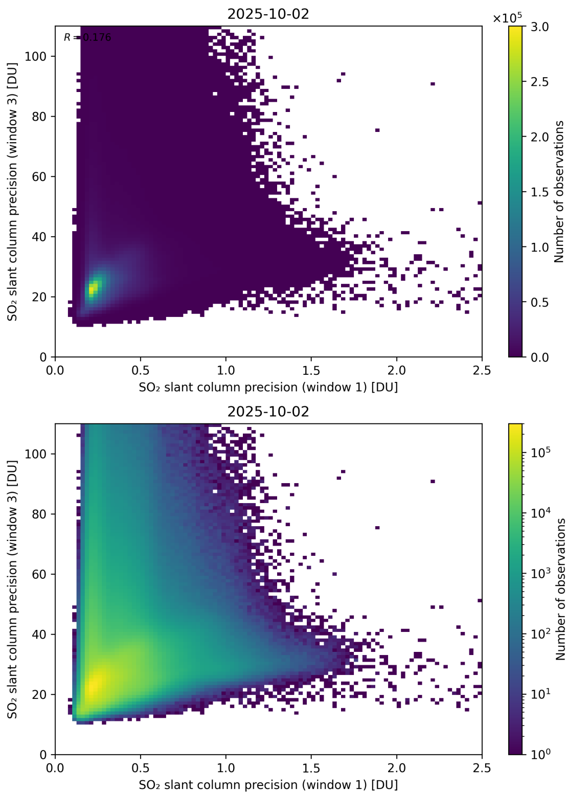
Figure 279: Scatter density plot of “SO 2 slant column precision (window 1)” against “SO 2 slant column precision (window 3)” for 2025-10-01 to 2025-10-03.
