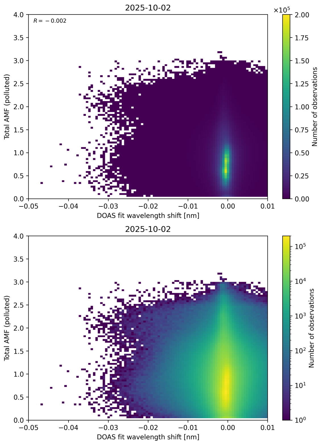
Figure 141: Scatter density plot of “DOAS fit wavelength shift” against “Total AMF (polluted)” for 2025-10-01 to 2025-10-03.
