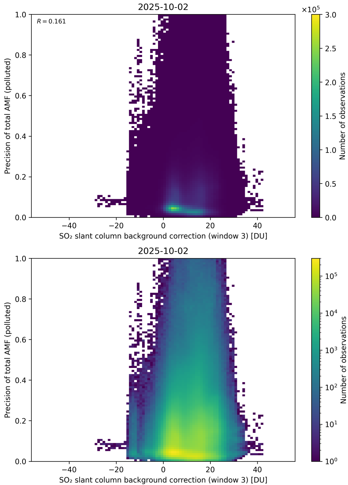
Figure 137: Scatter density plot of “SO 2 slant column background correction (window 3)” against “Precision of total AMF (polluted)” for 2025-10-01 to 2025-10-03.
