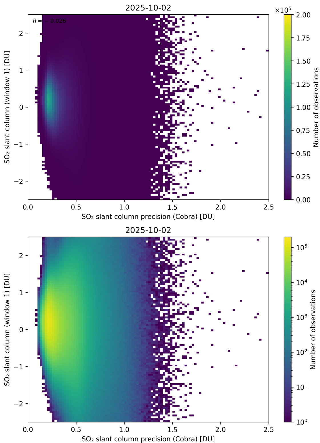
Figure 208: Scatter density plot of “SO 2 slant column precision (Cobra)” against “SO 2 slant column (window 1)” for 2025-10-01 to 2025-10-03.
