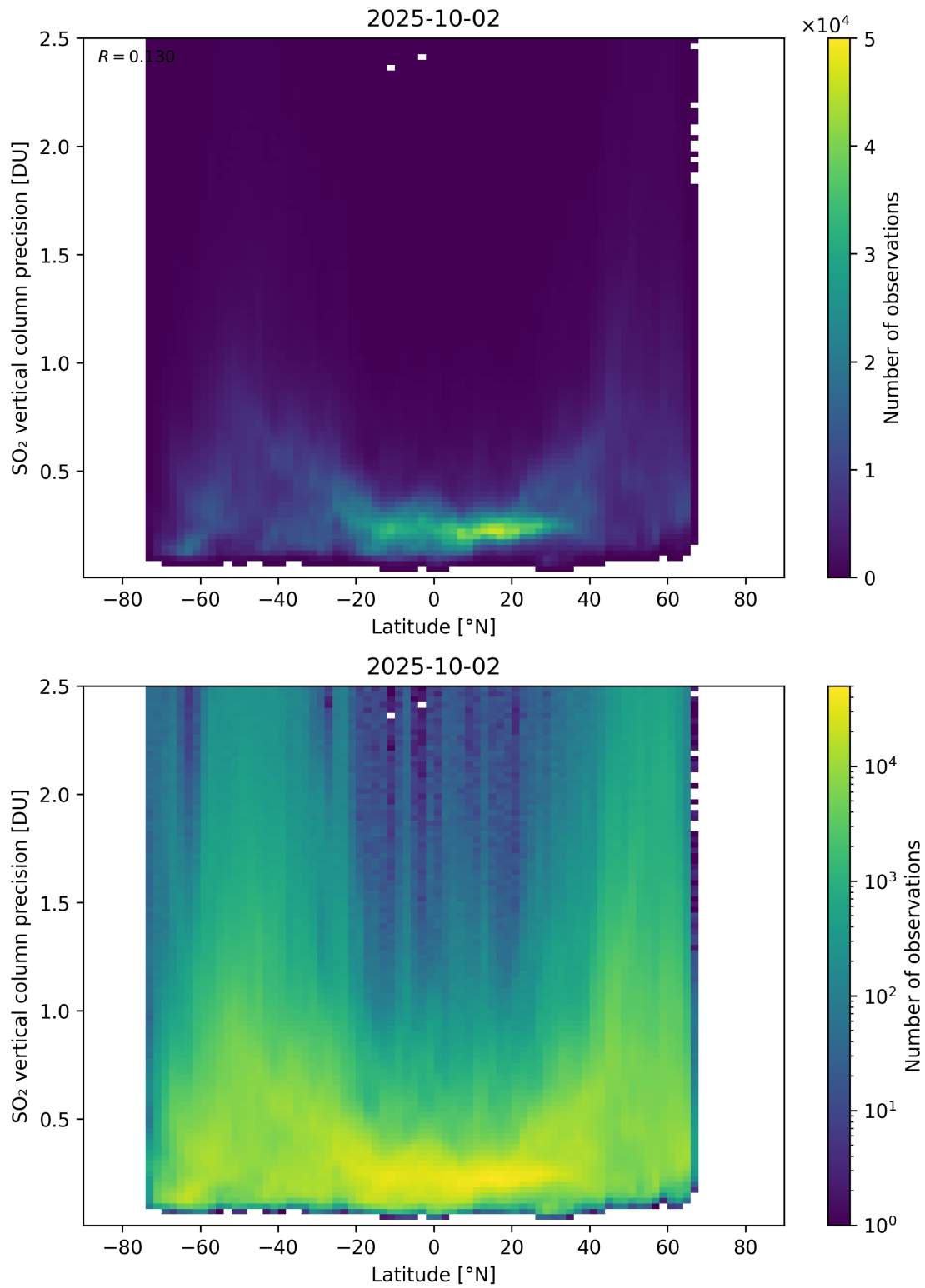
Figure 170: Scatter density plot of “Latitude” against “SO 2 vertical column precision” for 2025-10-01 to 2025-10-03.
