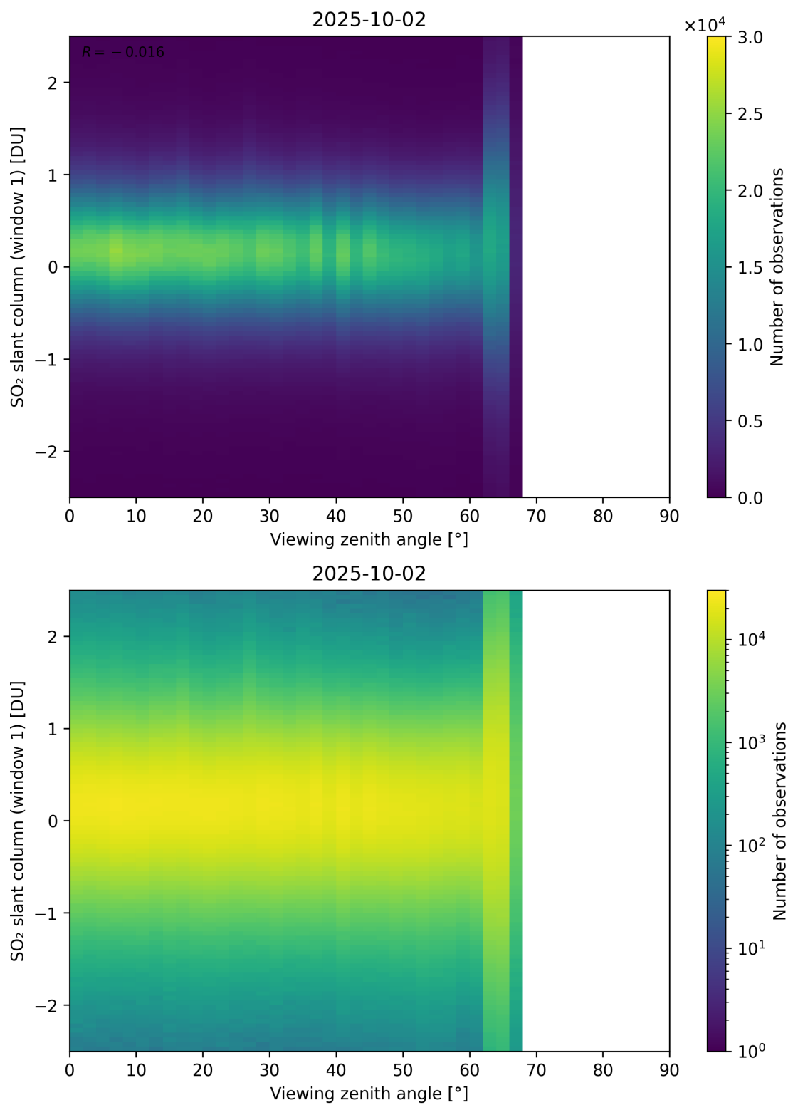
Figure 376: Scatter density plot of “Viewing zenith angle” against “SO 2 slant column (window 1)” for 2025-10-01 to 2025-10-03.
