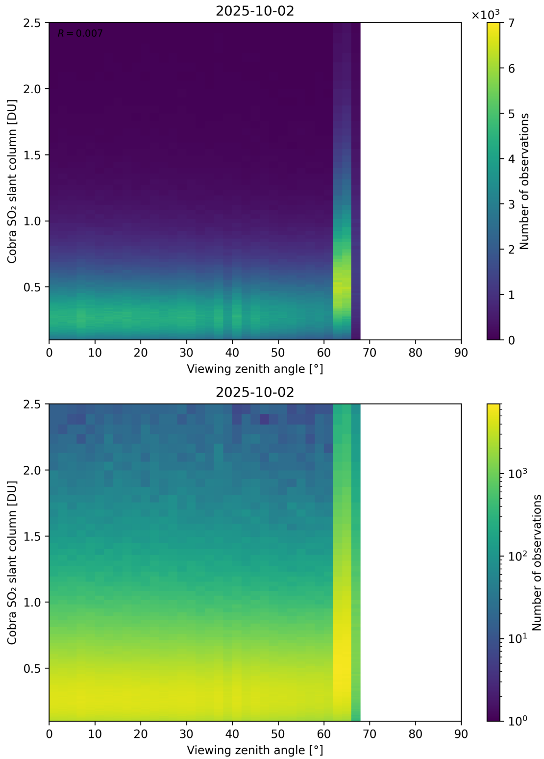
Figure 371: Scatter density plot of “Viewing zenith angle” against “Cobra SO 2 slant column” for 2025-10-01 to 2025-10-03.
