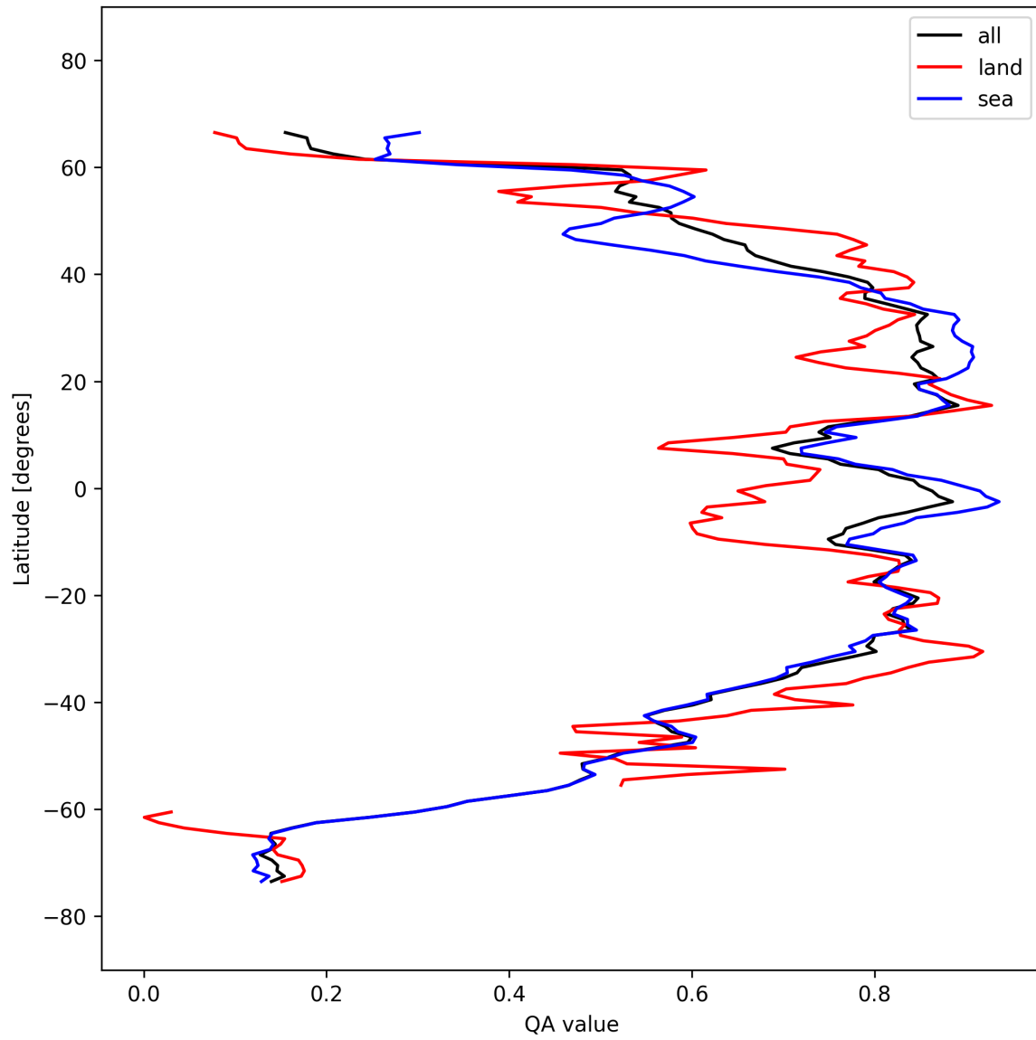
Figure 31: Zonal average of “QA value” for 2025-10-01 to 2025-10-03.
