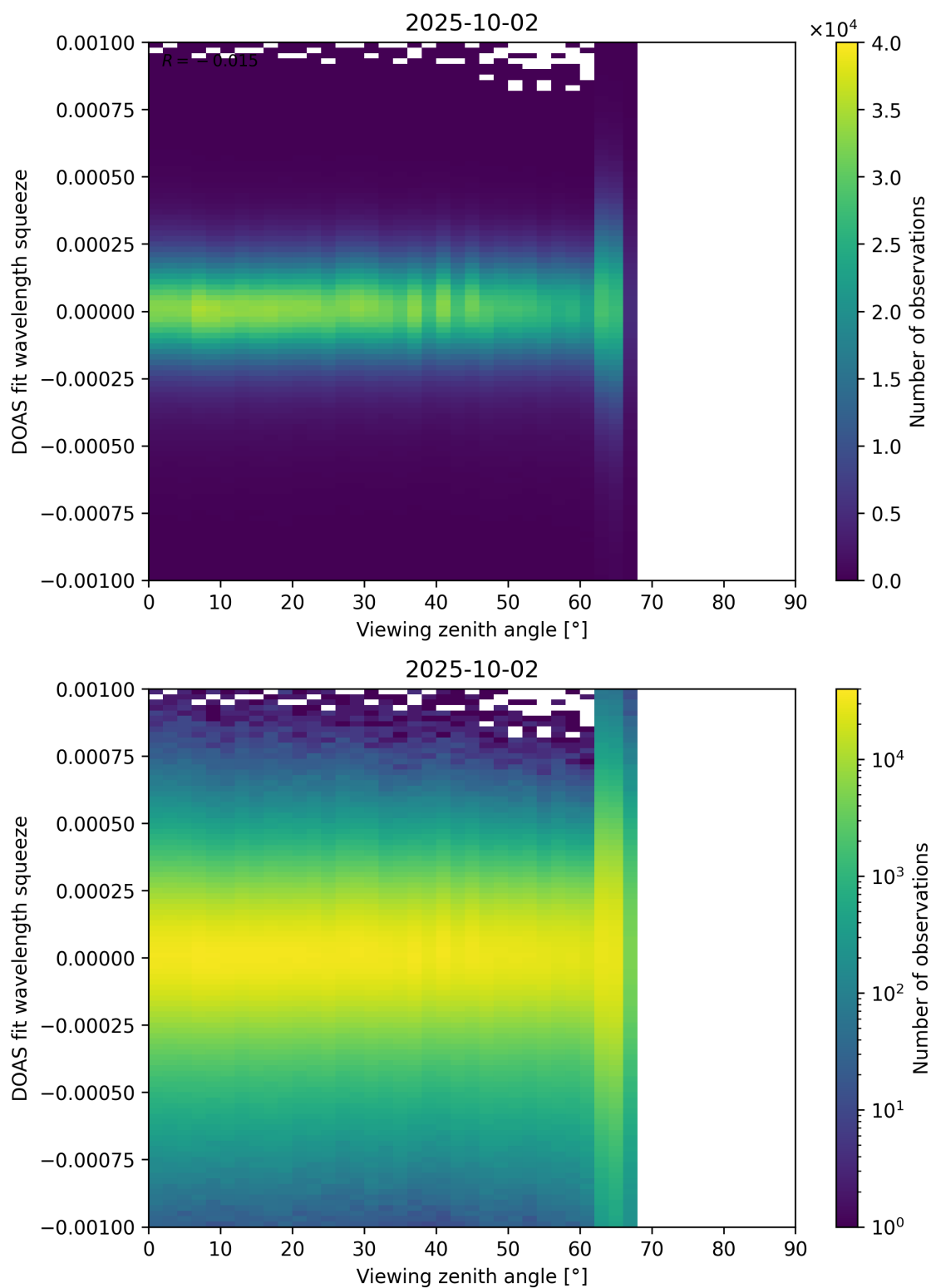
Figure 366: Scatter density plot of “Viewing zenith angle” against “DOAS fit wavelength squeeze” for 2025-10-01 to 2025-10-03.
