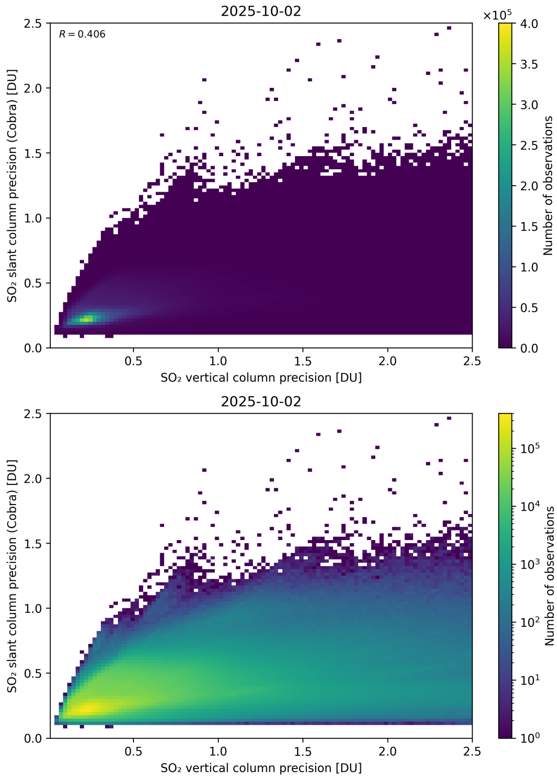
Figure 337: Scatter density plot of “SO 2 vertical column precision” against “SO 2 slant column precision (Cobra)” for 2025-10-01 to 2025-10-03.
