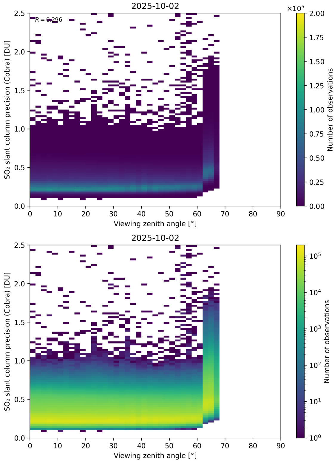
Figure 372: Scatter density plot of “Viewing zenith angle” against “SO 2 slant column precision (Cobra)” for 2025-10-01 to 2025-10-03.
