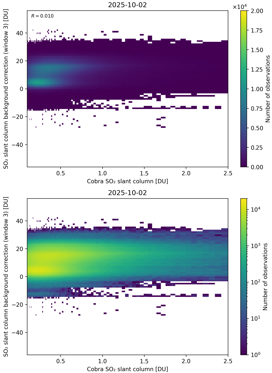
Figure 195: Scatter density plot of “Cobra SO 2 slant column” against “SO 2 slant column background correction (window 3)” for 2025-10-01 to 2025-10-03.
