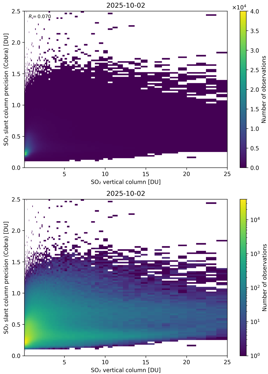
Figure 350: Scatter density plot of “SO 2 vertical column” against “SO 2 slant column precision (Cobra)” for 2025-10-01 to 2025-10-03.
