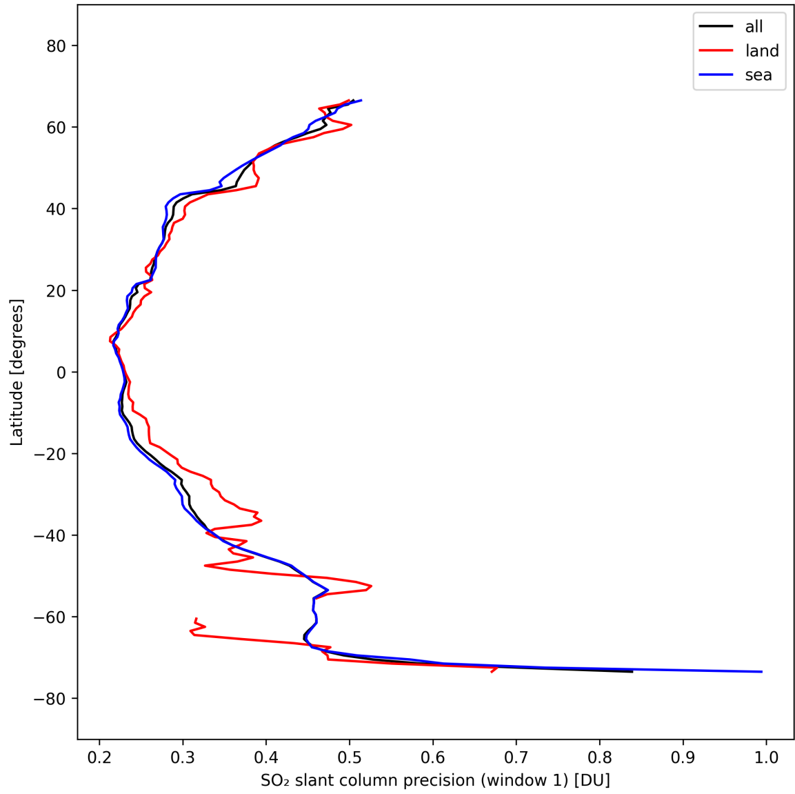
Figure 38: Zonal average of “SO 2 slant column precision (window 1)” for 2025-10-01 to 2025-10-03.
