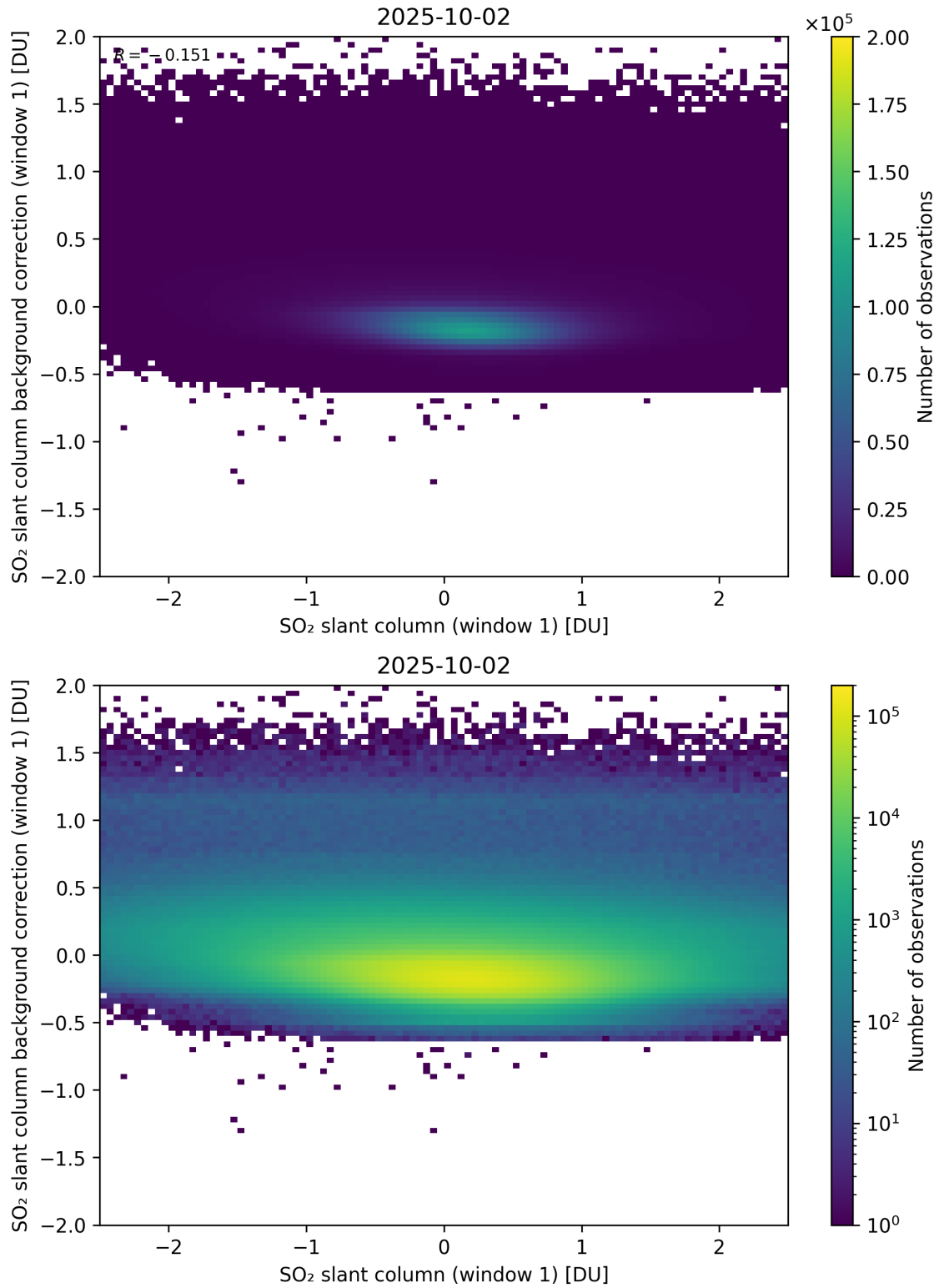
Figure 262: Scatter density plot of “SO 2 slant column (window 1)” against “SO 2 slant column background correction (window 1)” for 2025-10-01 to 2025-10-03.
