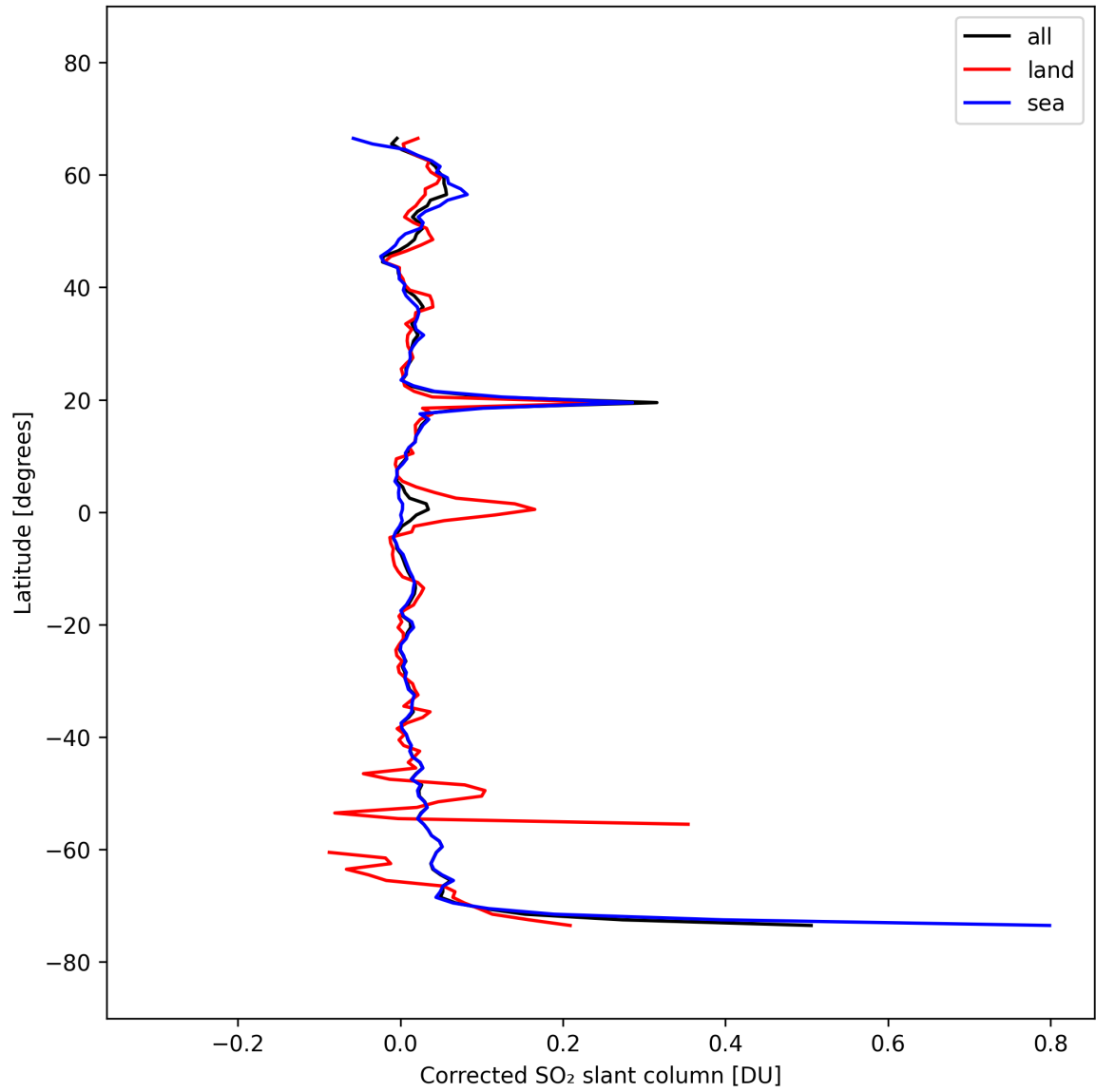
Figure 34: Zonal average of “Corrected SO 2 slant column” for 2025-10-01 to 2025-10-03.
