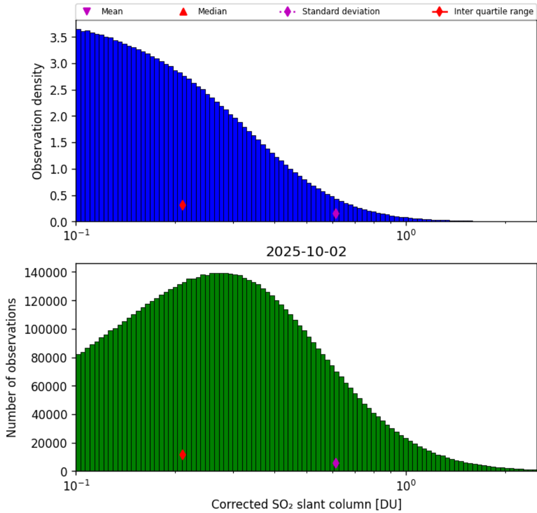
Figure 60: Histogram of "Corrected SO 2 slant column" for 2025-10-01 to 2025-10-03
