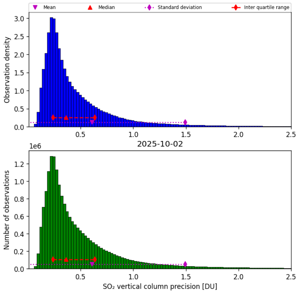
Figure 59: Histogram of "SO 2 vertical column precision" for 2025-10-01 to 2025-10-03
