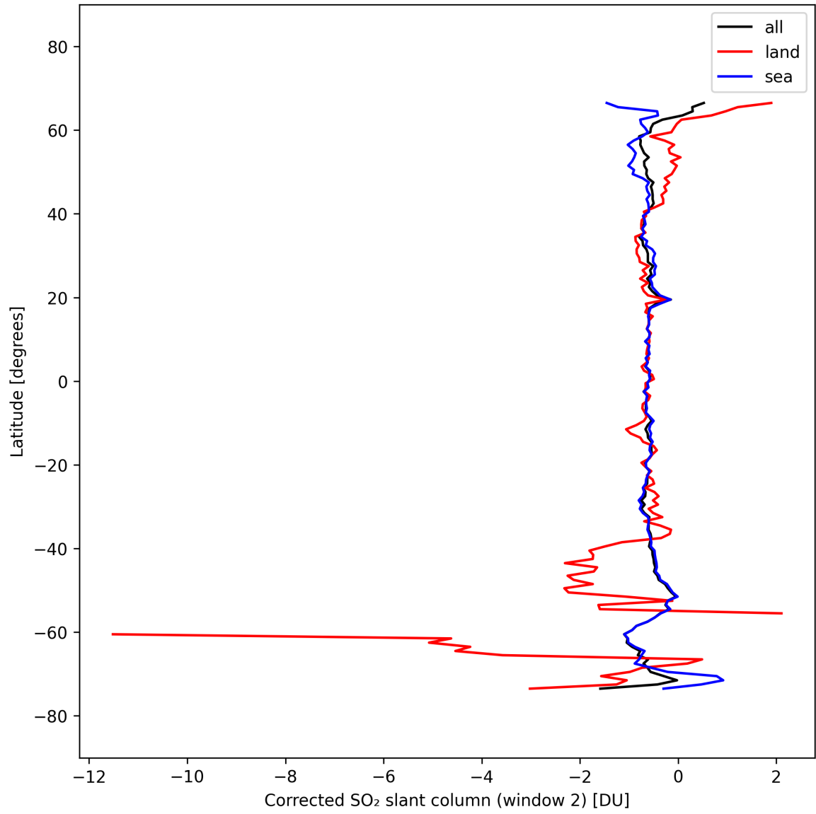
Figure 43: Zonal average of “Corrected SO 2 slant column (window 2)” for 2025-10-01 to 2025-10-03.
