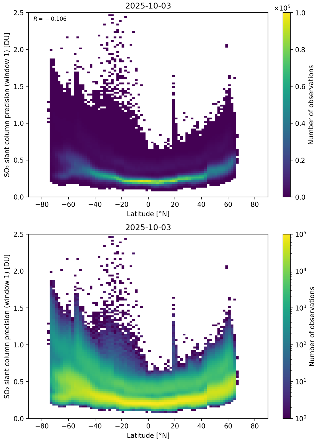
Figure 163: Scatter density plot of “Latitude” against “SO 2 slant column precision (window 1)” for 2025-10-02 to 2025-10-04.
