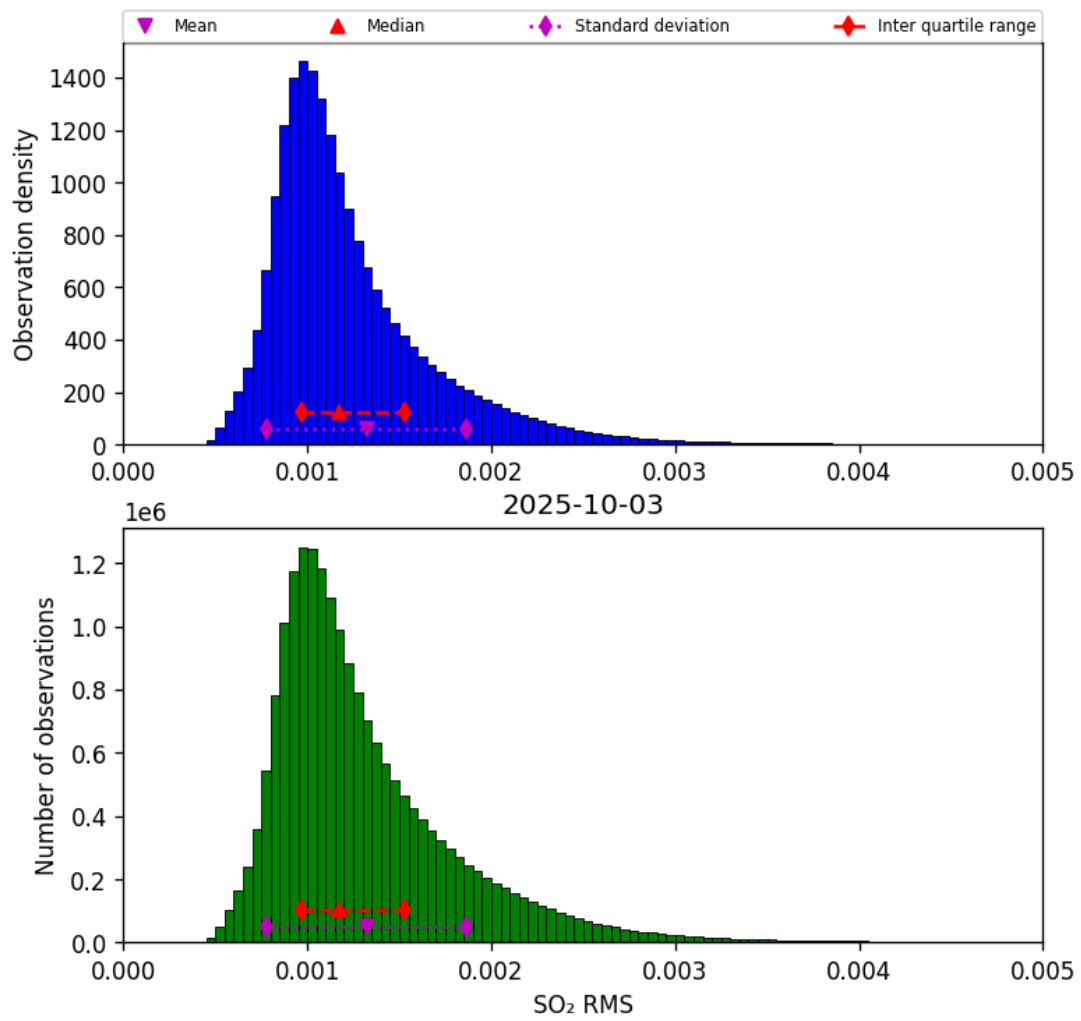
Figure 78: Histogram of “SO 2 RMS” for 2025-10-02 to 2025-10-04
