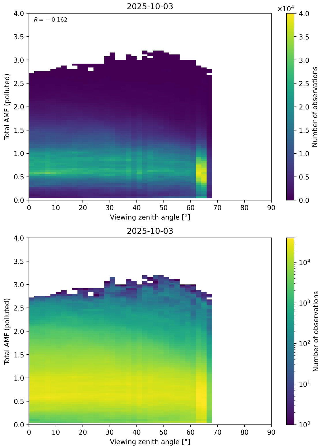
Figure 381: Scatter density plot of “Viewing zenith angle” against “Total AMF (polluted)” for 2025-10-02 to 2025-10-04.
