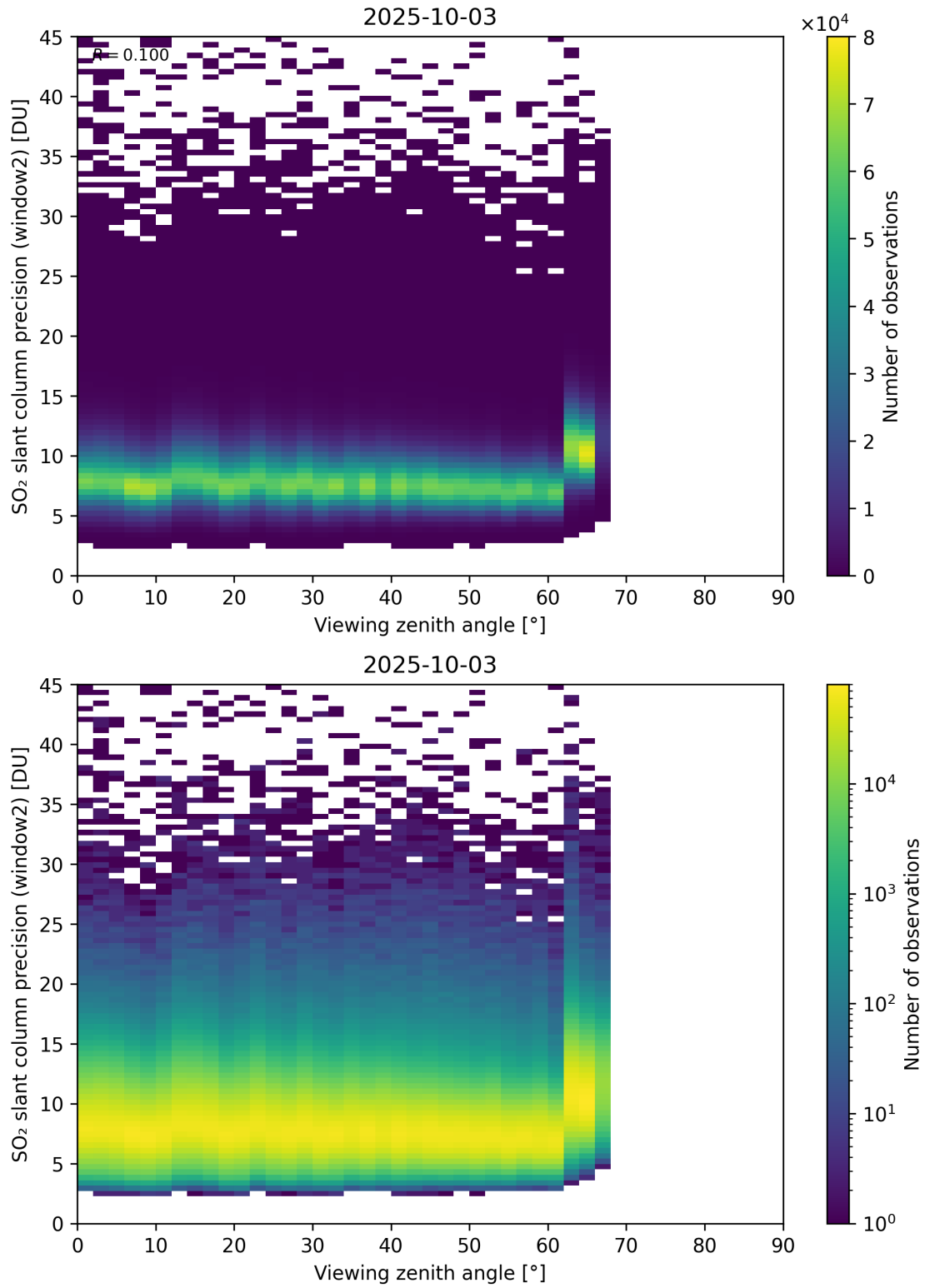
Figure 378: Scatter density plot of “Viewing zenith angle” against “SO 2 slant column precision (window2)” for 2025-10-02 to 2025-10-04.
