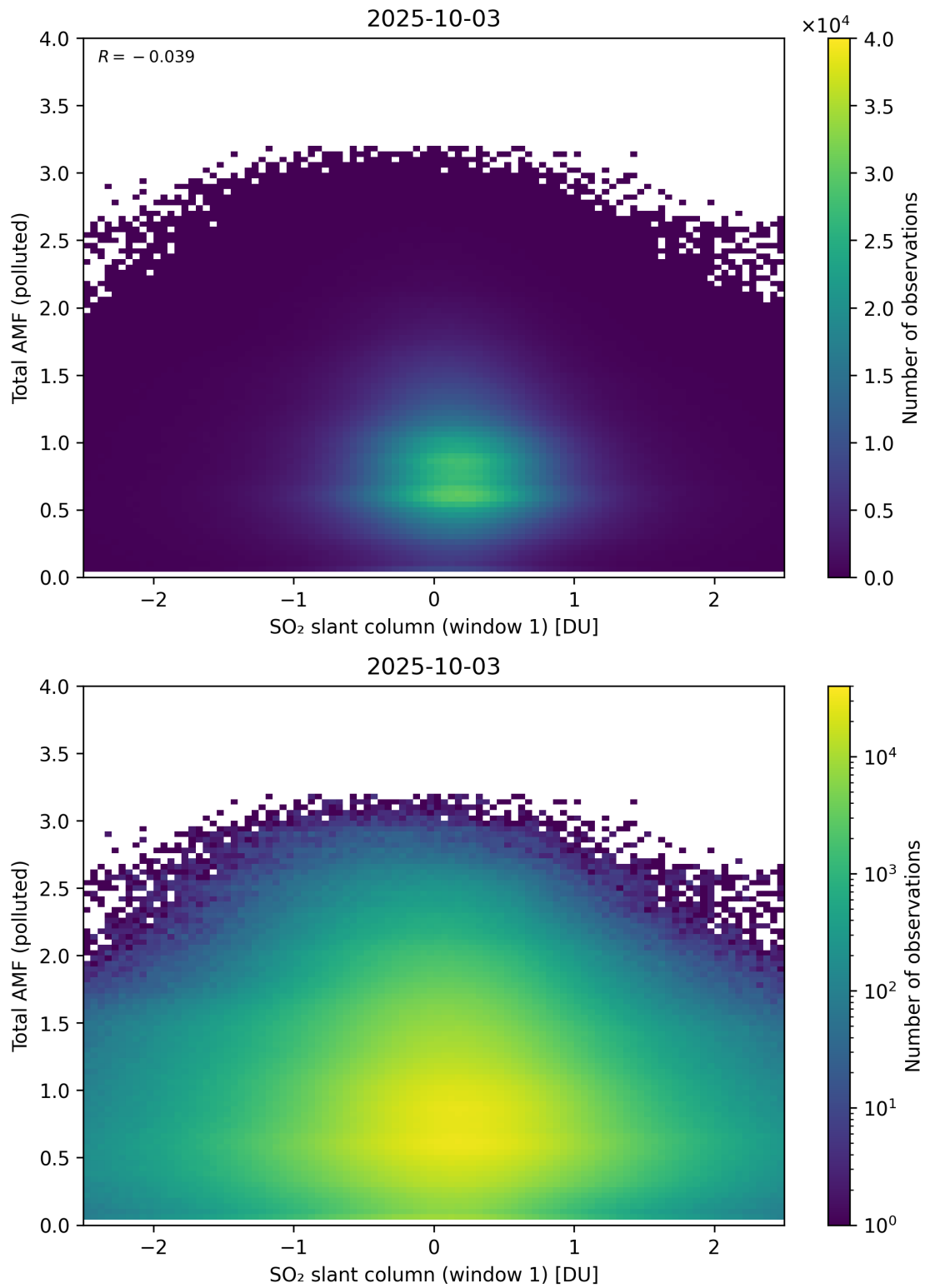
Figure 289: Scatter density plot of “SO 2 slant column (window 1)” against “Total AMF (polluted)” for 2025-10-02 to 2025-10-04.
