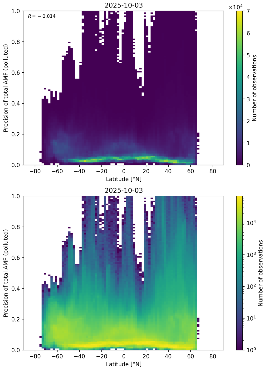
Figure 168: Scatter density plot of “Latitude” against “Precision of total AMF (polluted)” for 2025-10-02 to 2025-10-04.
