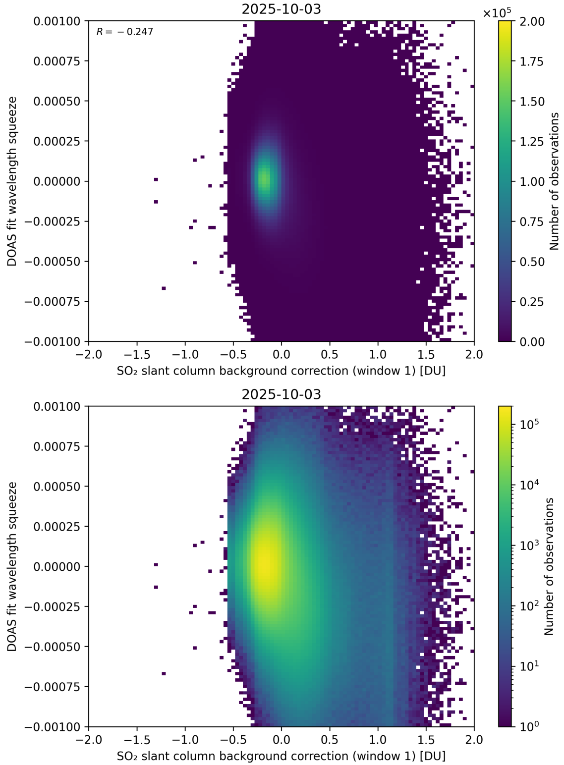
Figure 112: Scatter density plot of “SO 2 slant column background correction (window 1)” against “DOAS fit wavelength squeeze” for 2025-10-02 to 2025-10-04.
