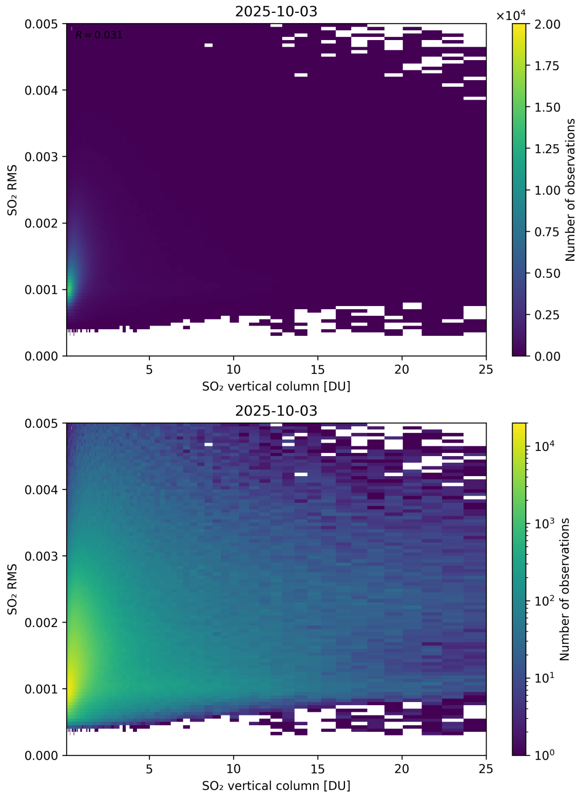
Figure 328: Scatter density plot of “SO 2 vertical column” against “SO 2 RMS” for 2025-10-02 to 2025-10-04.
