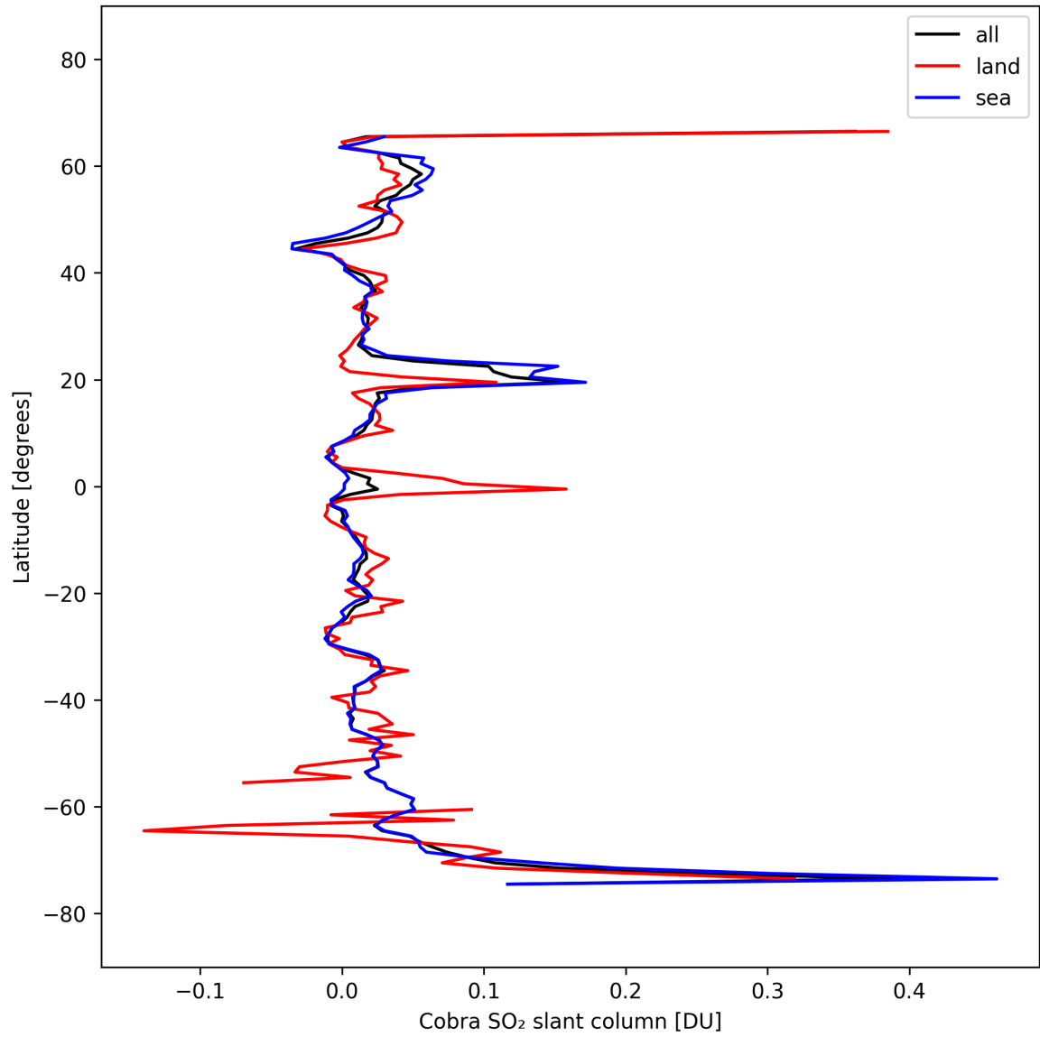
Figure 35: Zonal average of “Cobra SO 2 slant column” for 2025-10-02 to 2025-10-04.
