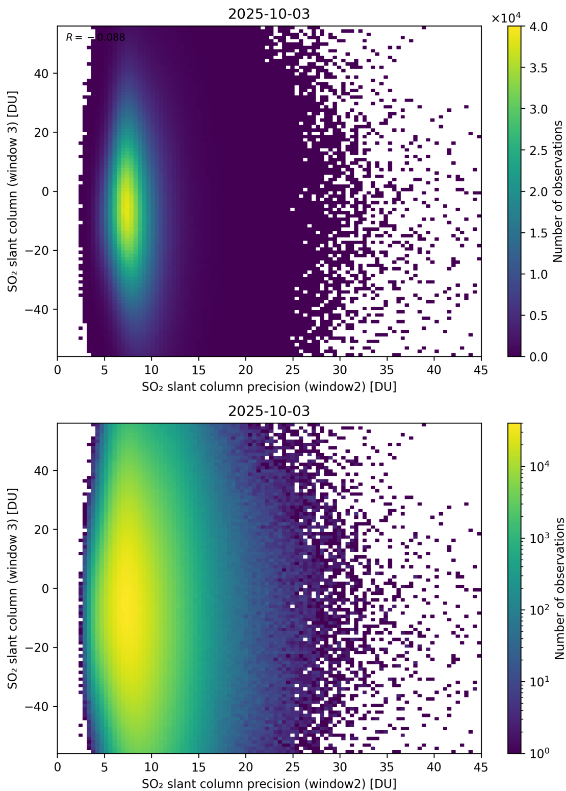
Figure 299: Scatter density plot of “SO 2 slant column precision (window2)” against “SO 2 slant column (window 3)” for 2025-10-02 to 2025-10-04.
