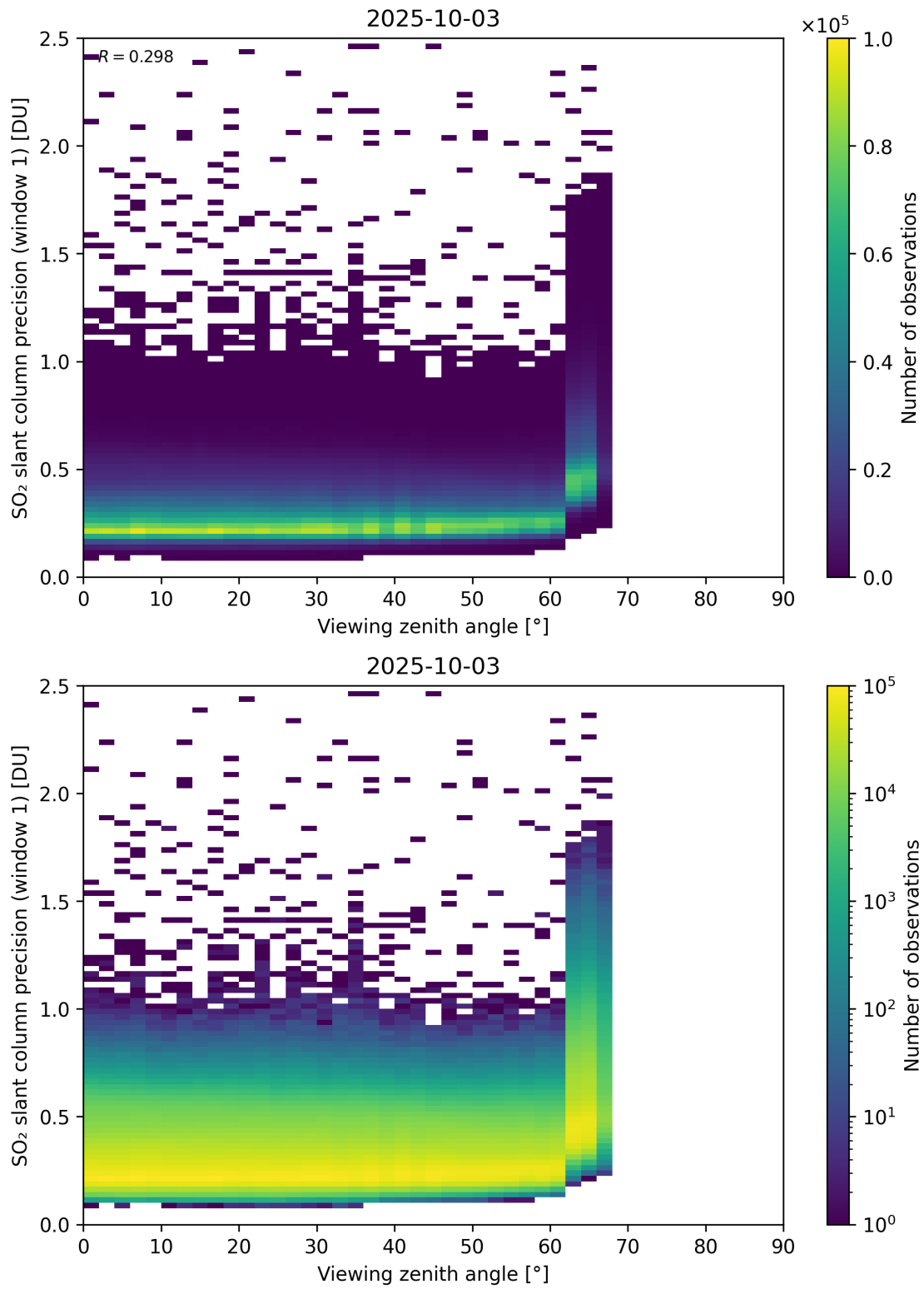
Figure 377: Scatter density plot of “Viewing zenith angle” against “SO 2 slant column precision (window 1)” for 2025-10-02 to 2025-10-04.
