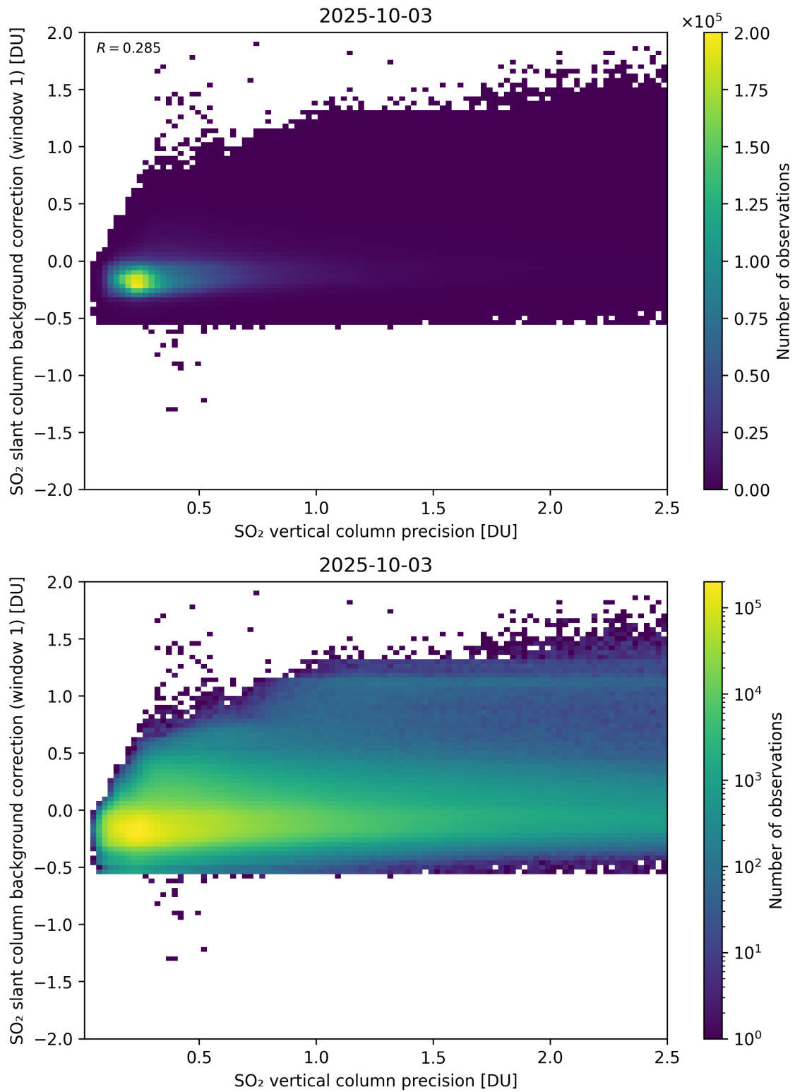
Figure 329: Scatter density plot of “SO 2 vertical column precision” against “SO 2 slant column background correction (window 1)” for 2025-10-02 to 2025-10-04.
