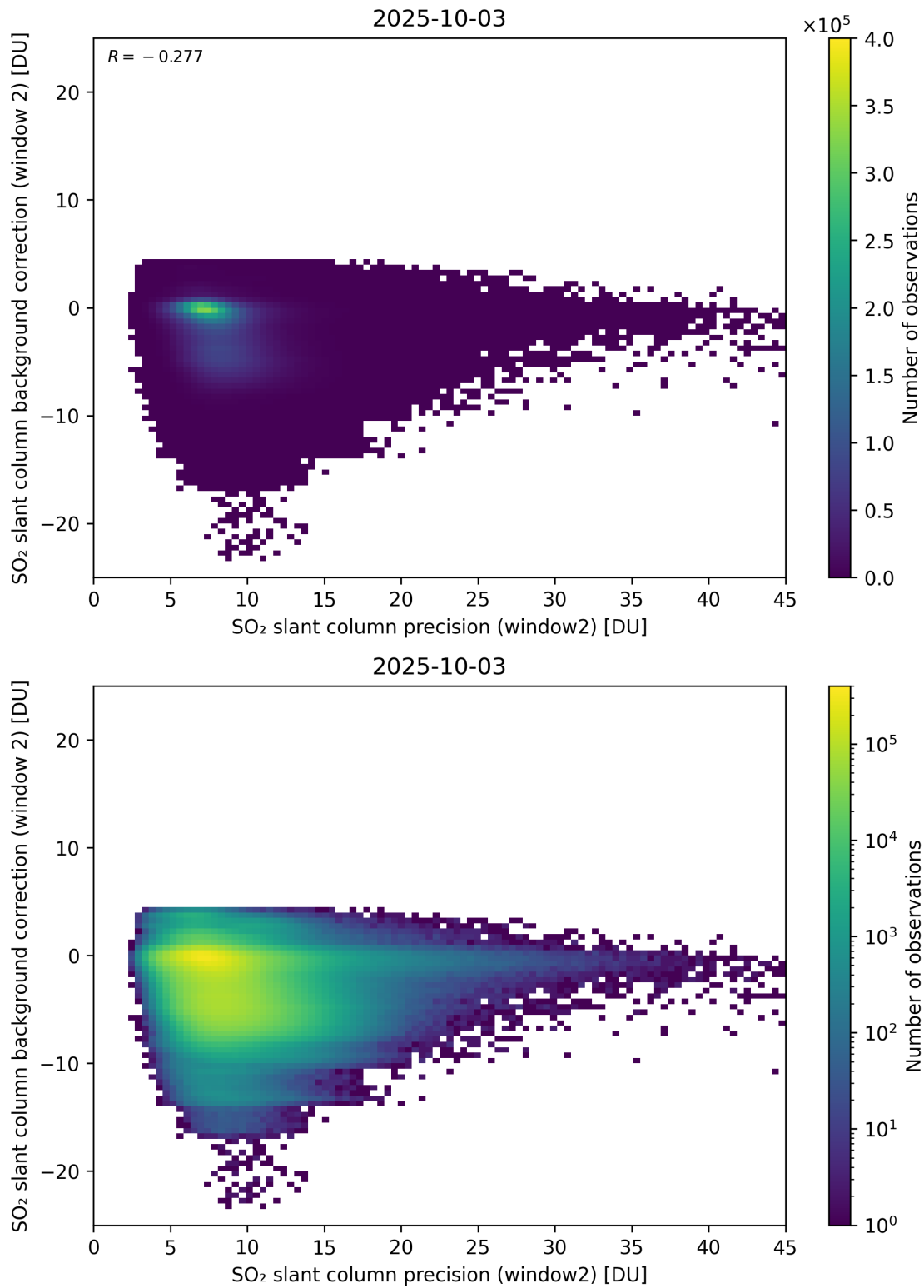
Figure 291: Scatter density plot of “SO 2 slant column precision (window2)” against “SO 2 slant column background correction (window 2)” for 2025-10-02 to 2025-10-04.
