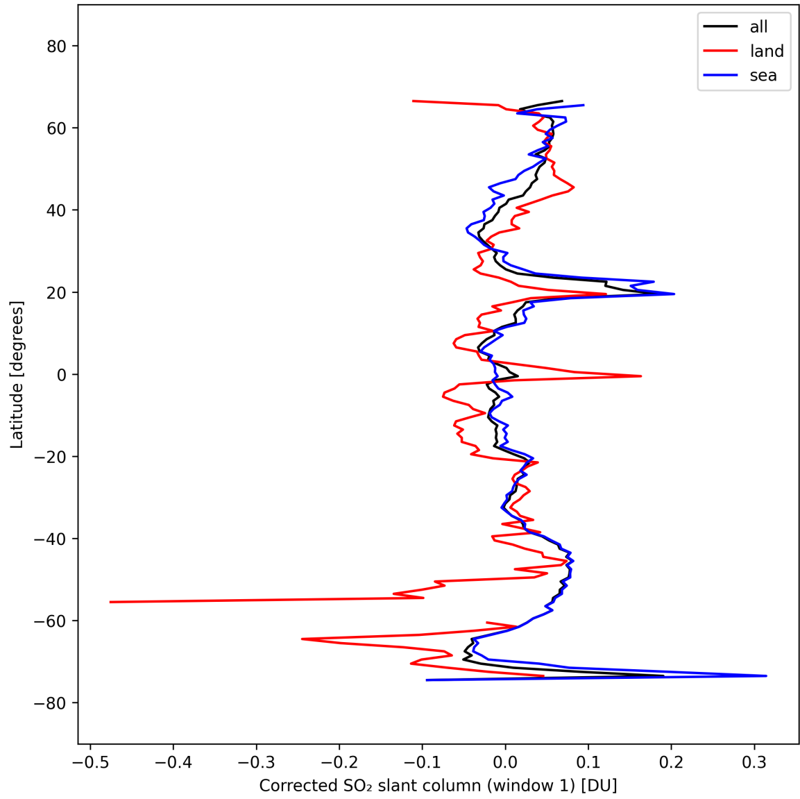
Figure 39: Zonal average of “Corrected SO 2 slant column (window 1)” for 2025-10-02 to 2025-10-04.
