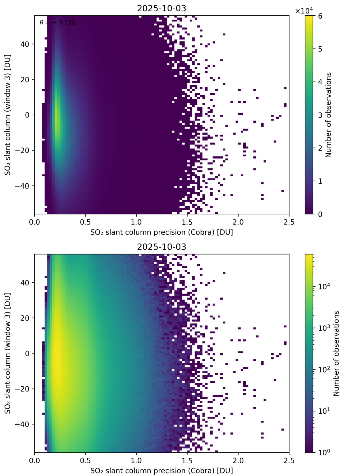
Figure 211: Scatter density plot of “SO 2 slant column precision (Cobra)” against “SO 2 slant column (window 3)” for 2025-10-02 to 2025-10-04.
