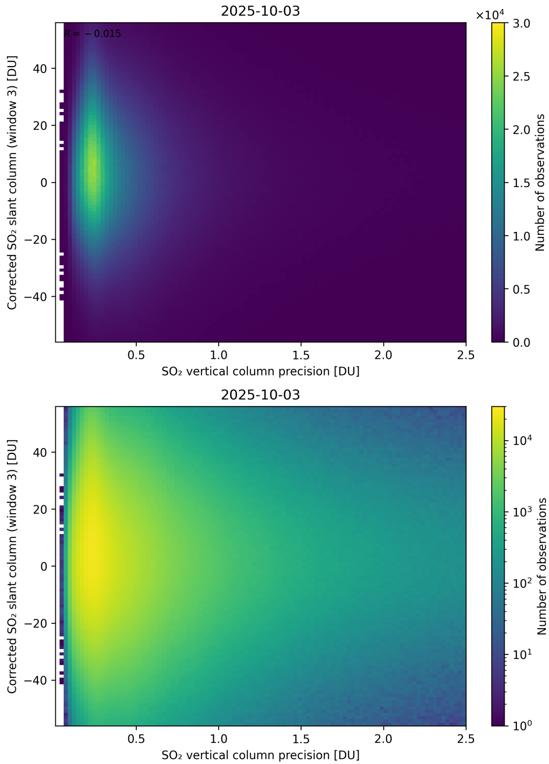
Figure 340: Scatter density plot of “SO 2 vertical column precision” against “Corrected SO 2 slant column (window 3)” for 2025-10-02 to 2025-10-04.
