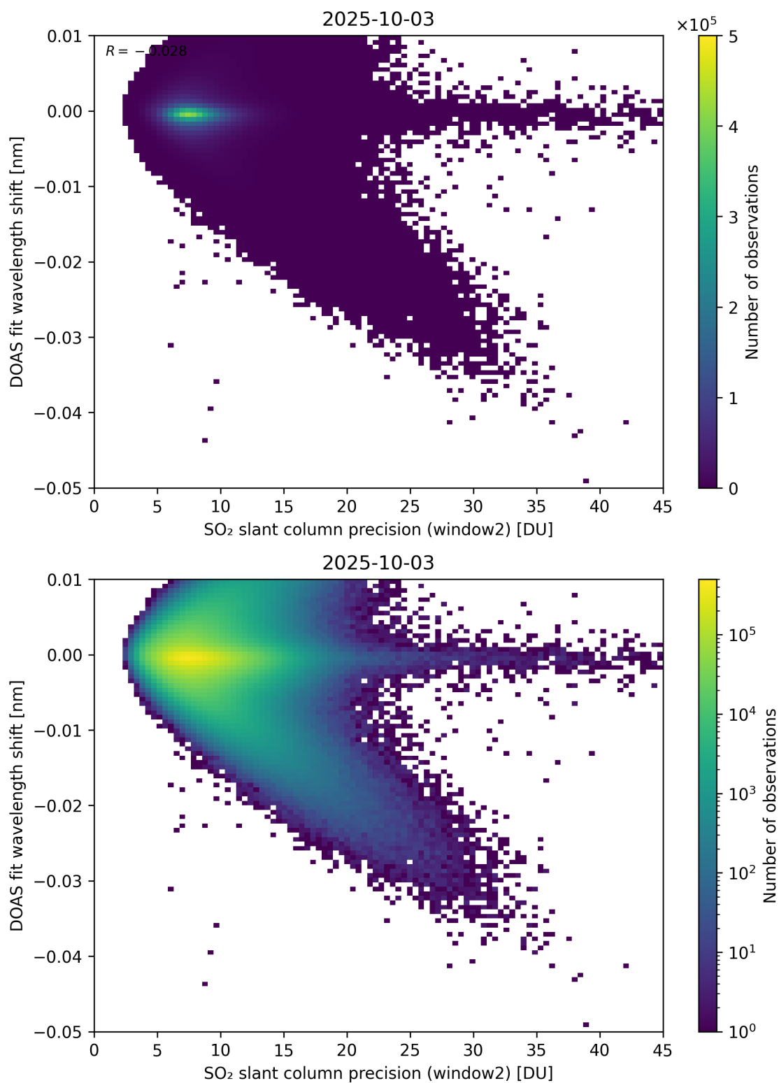
Figure 293: Scatter density plot of “SO 2 slant column precision (window2)” against “DOAS fit wavelength shift” for 2025-10-02 to 2025-10-04.
