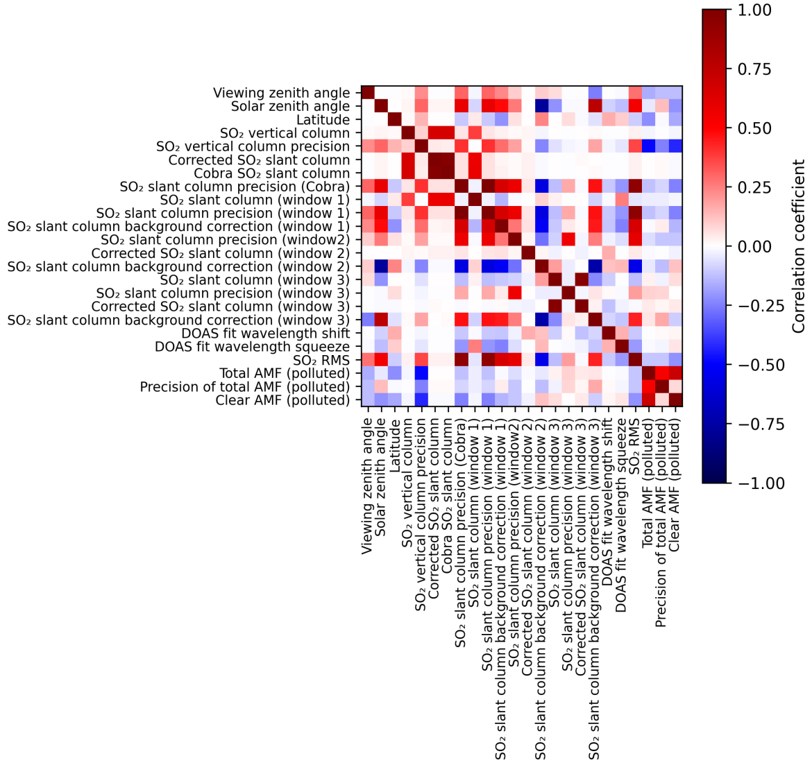
Figure 2: Map of correlation matrix for 2025-10-02 to 2025-10-04.
