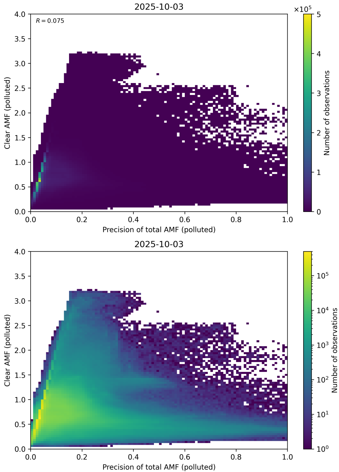
Figure 320: Scatter density plot of “Precision of total AMF (polluted)” against “Clear AMF (polluted)” for 2025-10-02 to 2025-10-04.
