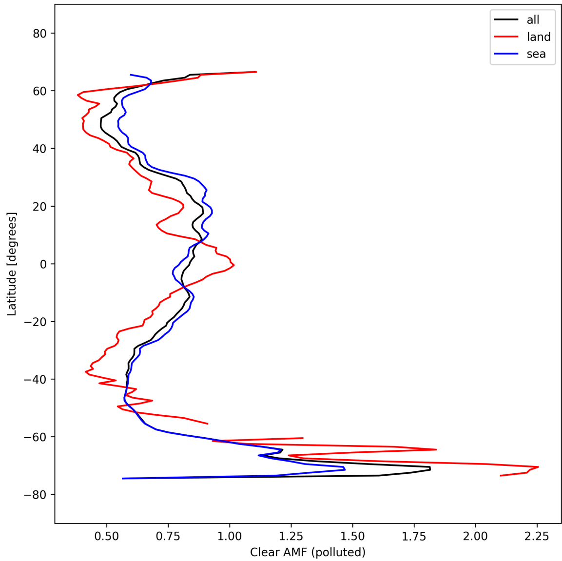
Figure 55: Zonal average of “Clear AMF (polluted)” for 2025-10-02 to 2025-10-04.
