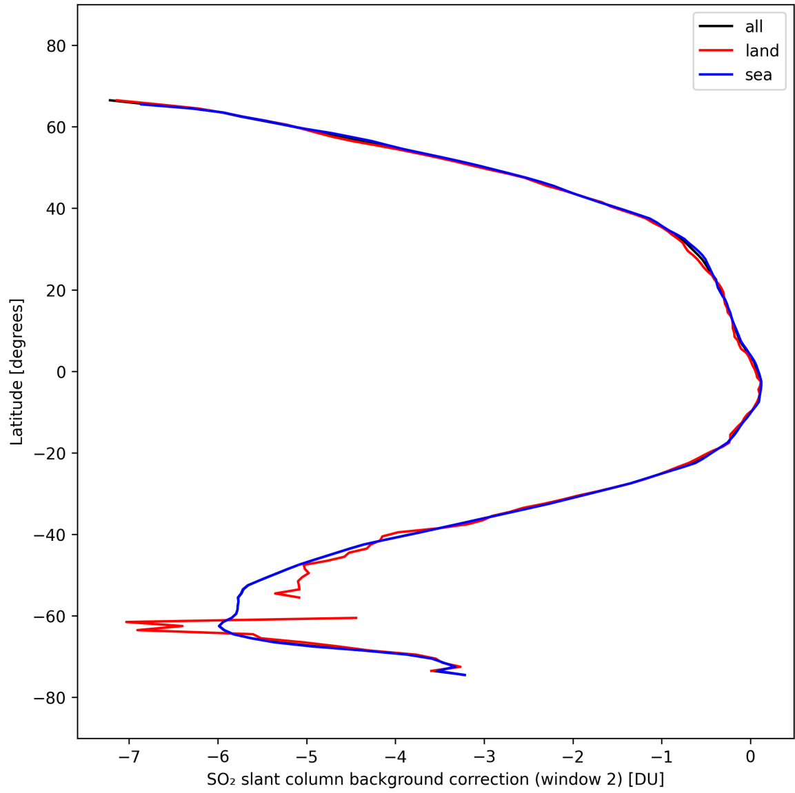
Figure 44: Zonal average of “SO 2 slant column background correction (window 2)” for 2025-10-02 to 2025-10-04.
