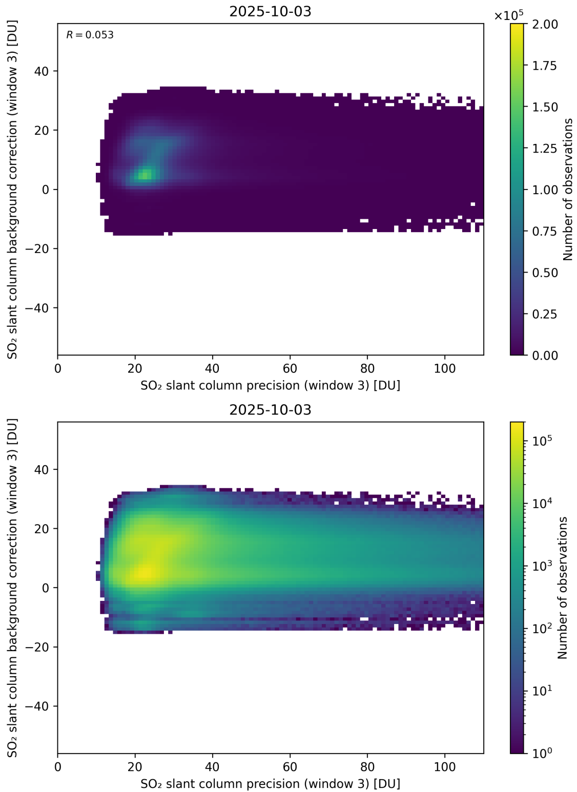
Figure 307: Scatter density plot of “SO 2 slant column precision (window 3)” against “SO 2 slant column background correction (window 3)” for 2025-10-02 to 2025-10-04.
