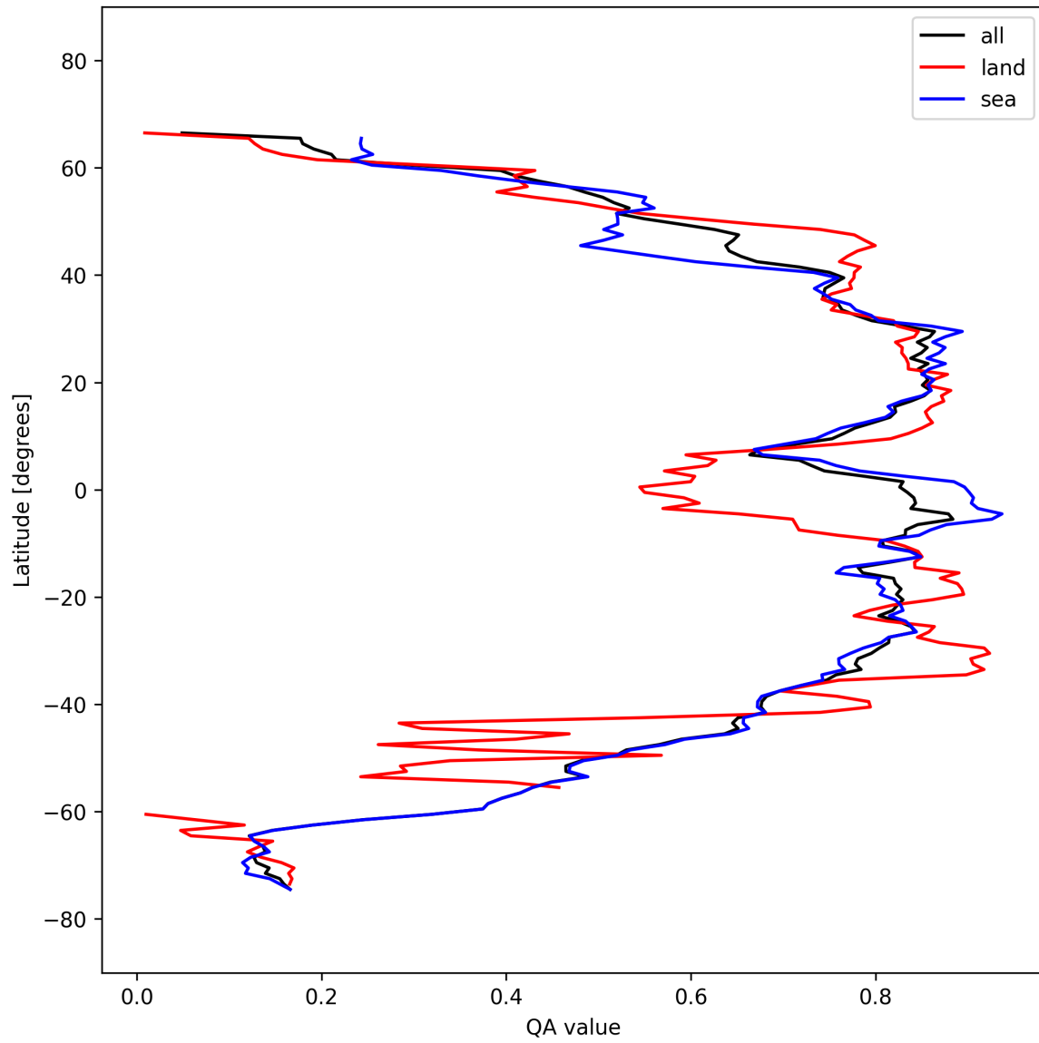
Figure 31: Zonal average of “QA value” for 2025-10-02 to 2025-10-04.
