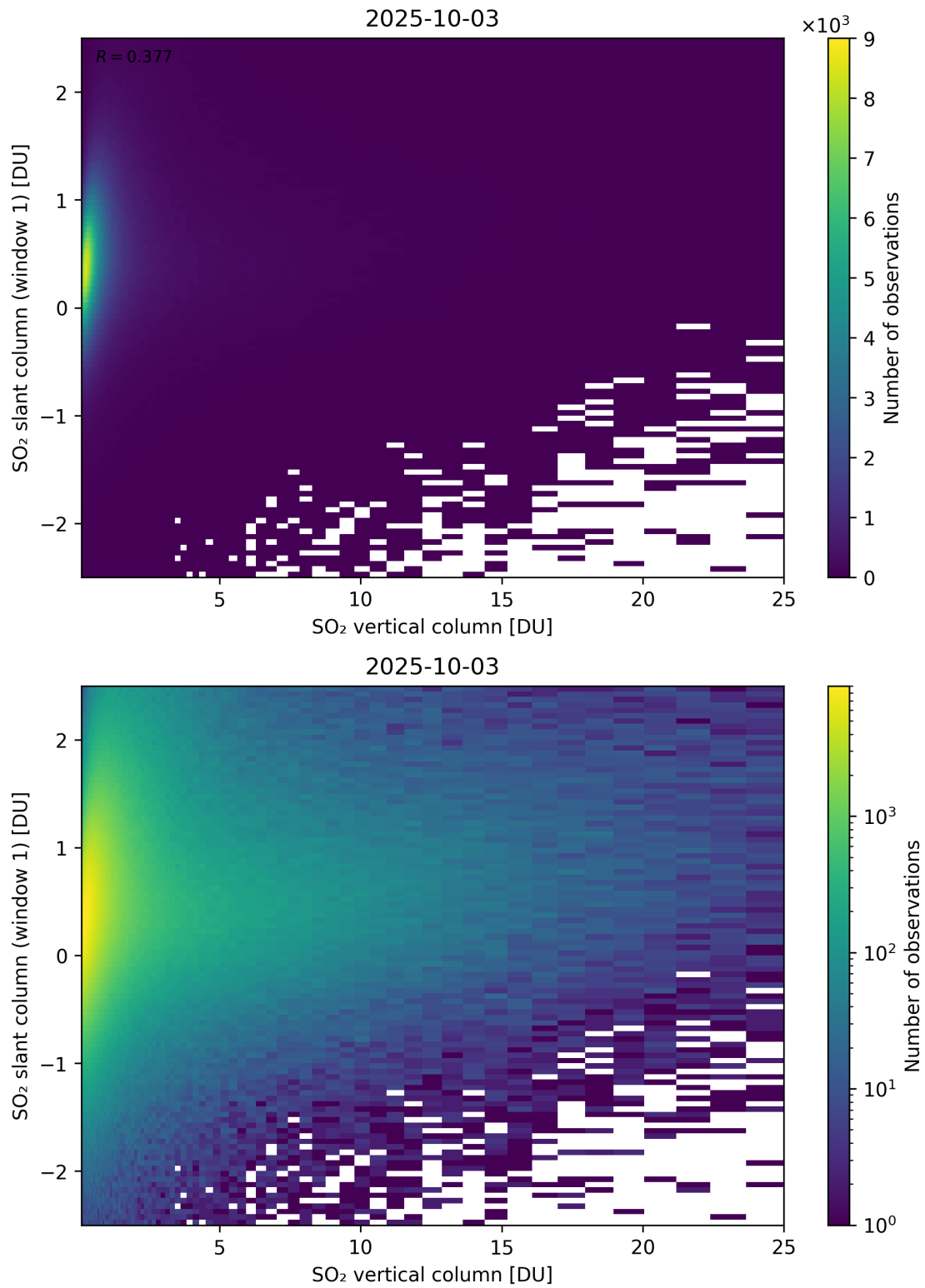
Figure 354: Scatter density plot of “SO 2 vertical column” against “SO 2 slant column (window 1)” for 2025-10-02 to 2025-10-04.
