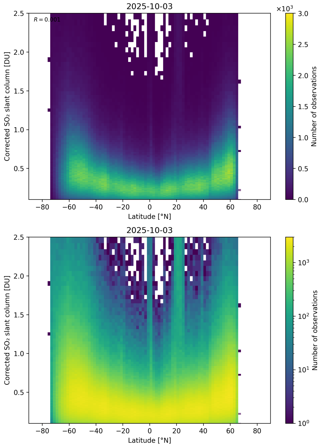
Figure 159: Scatter density plot of “Latitude” against “Corrected SO 2 slant column” for 2025-10-02 to 2025-10-04.
