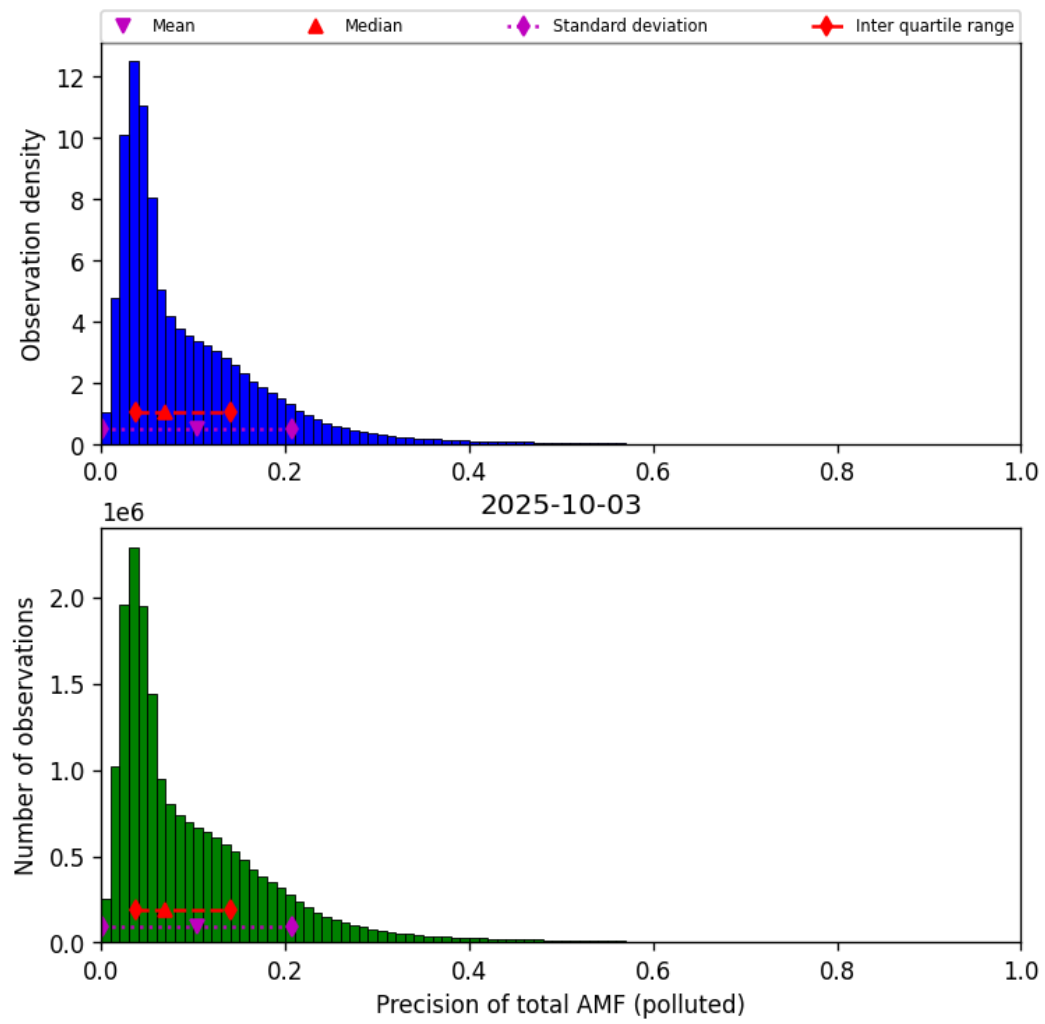
Figure 80: Histogram of “Precision of total AMF (polluted)” for 2025-10-02 to 2025-10-04
