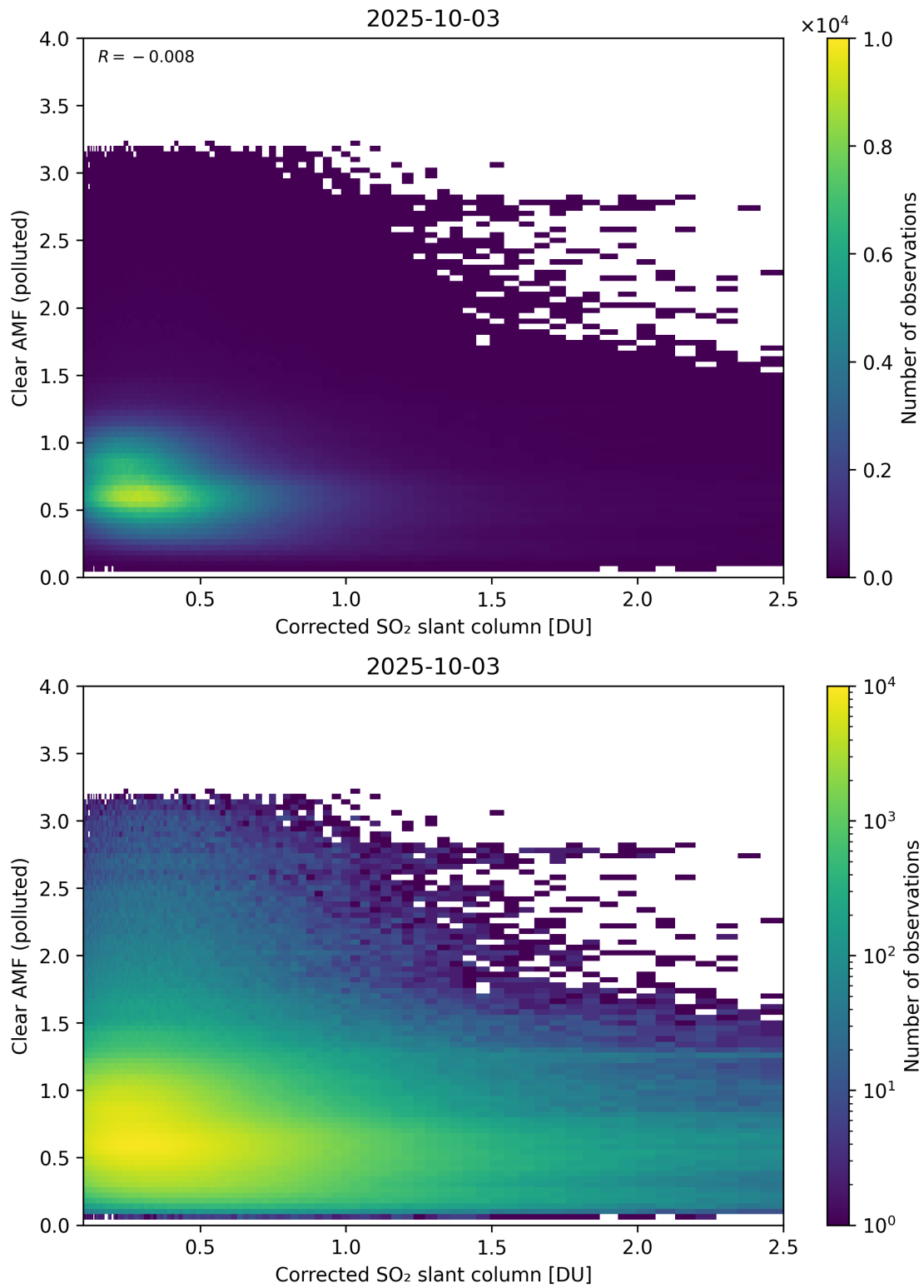
Figure 232: Scatter density plot of “Corrected SO 2 slant column” against “Clear AMF (polluted)” for 2025-10-02 to 2025-10-04.
