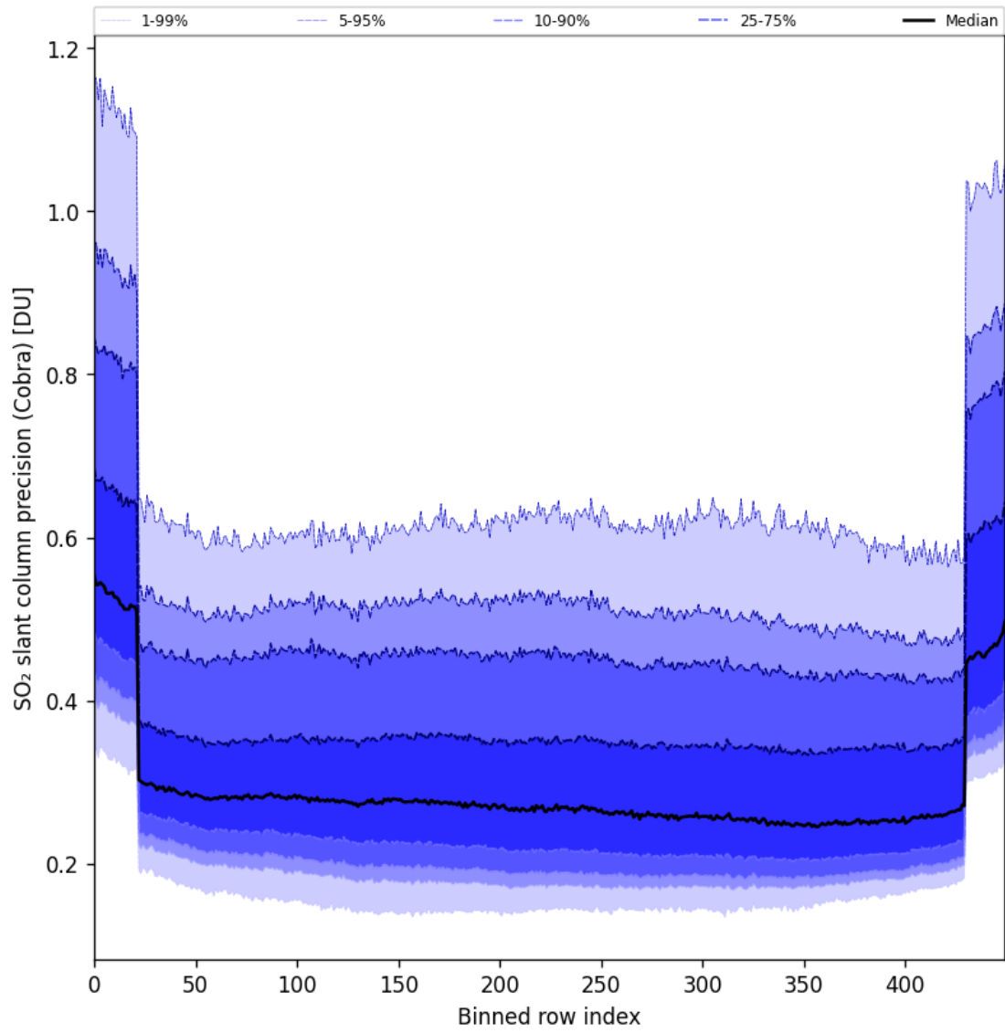
Figure 88: Along track statistics of “SO 2 slant column precision (Cobra)” for 2025-10-02 to 2025-10-04
