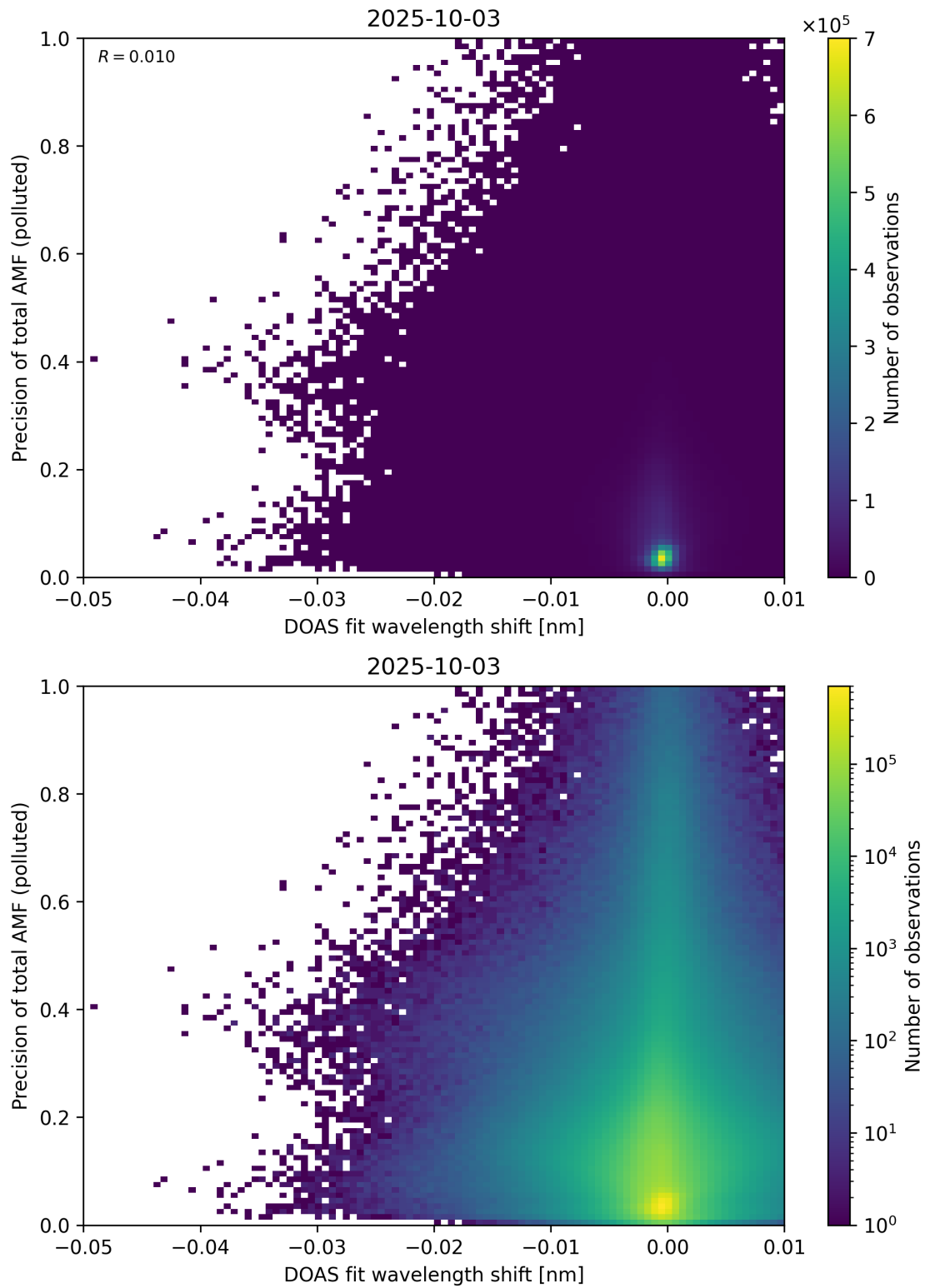
Figure 142: Scatter density plot of “DOAS fit wavelength shift” against “Precision of total AMF (polluted)” for 2025-10-02 to 2025-10-04.
