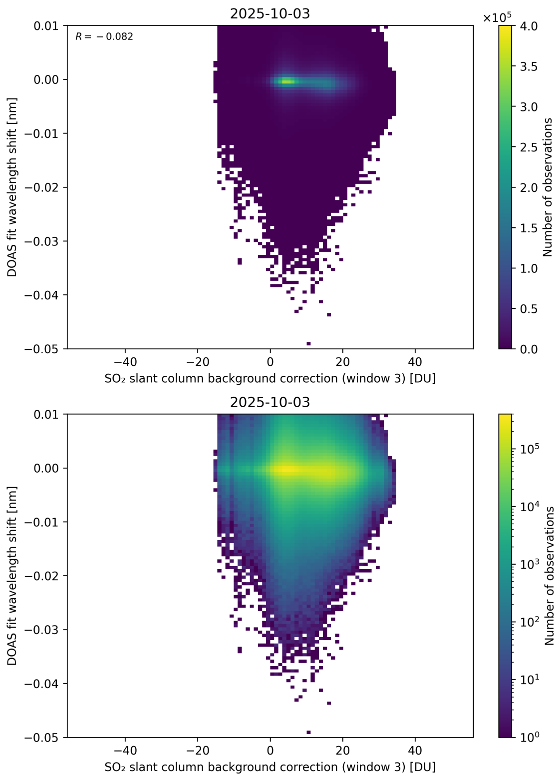
Figure 132: Scatter density plot of “SO 2 slant column background correction (window 3)” against “DOAS fit wavelength shift” for 2025-10-02 to 2025-10-04.
