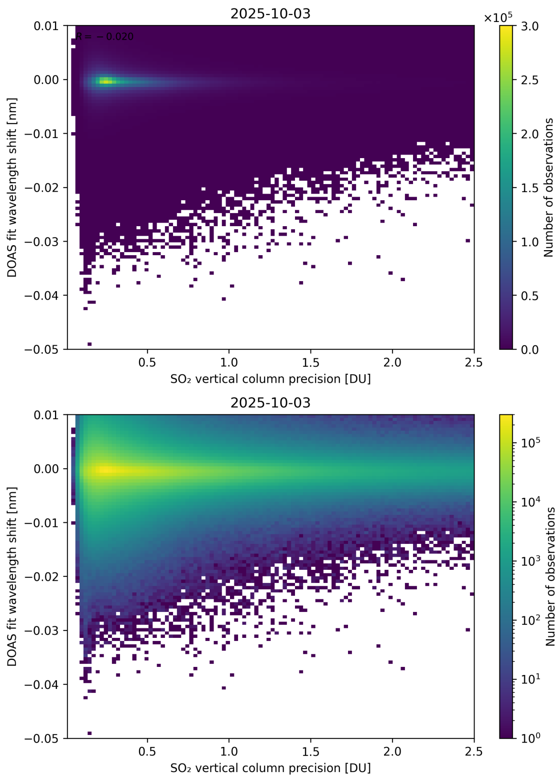
Figure 332: Scatter density plot of “SO 2 vertical column precision” against “DOAS fit wavelength shift” for 2025-10-02 to 2025-10-04.
