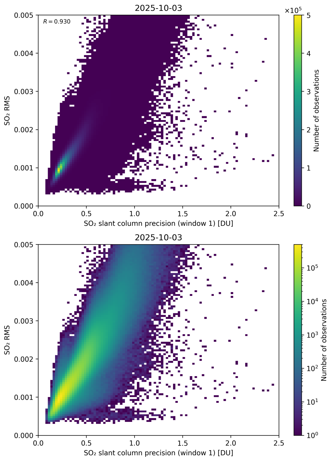
Figure 273: Scatter density plot of “SO 2 slant column precision (window 1)” against “SO 2 RMS” for 2025-10-02 to 2025-10-04.
