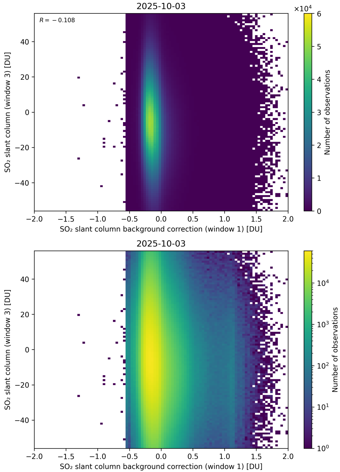
Figure 118: Scatter density plot of “SO 2 slant column background correction (window 1)” against “SO 2 slant column (window 3)” for 2025-10-02 to 2025-10-04.
