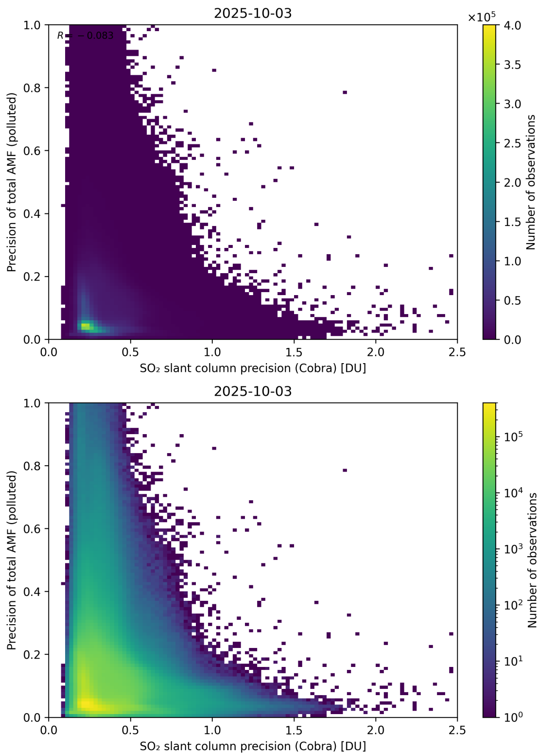
Figure 214: Scatter density plot of “SO 2 slant column precision (Cobra)” against “Precision of total AMF (polluted)” for 2025-10-02 to 2025-10-04.
