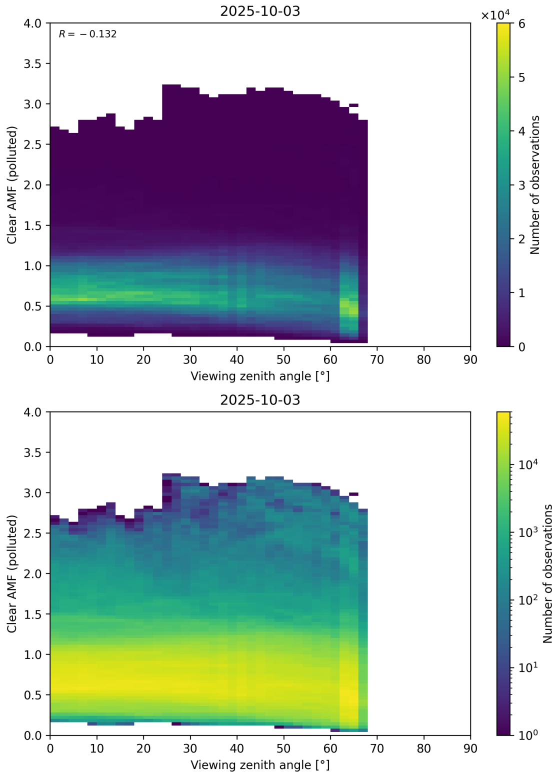
Figure 370: Scatter density plot of “Viewing zenith angle” against “Clear AMF (polluted)” for 2025-10-02 to 2025-10-04.
