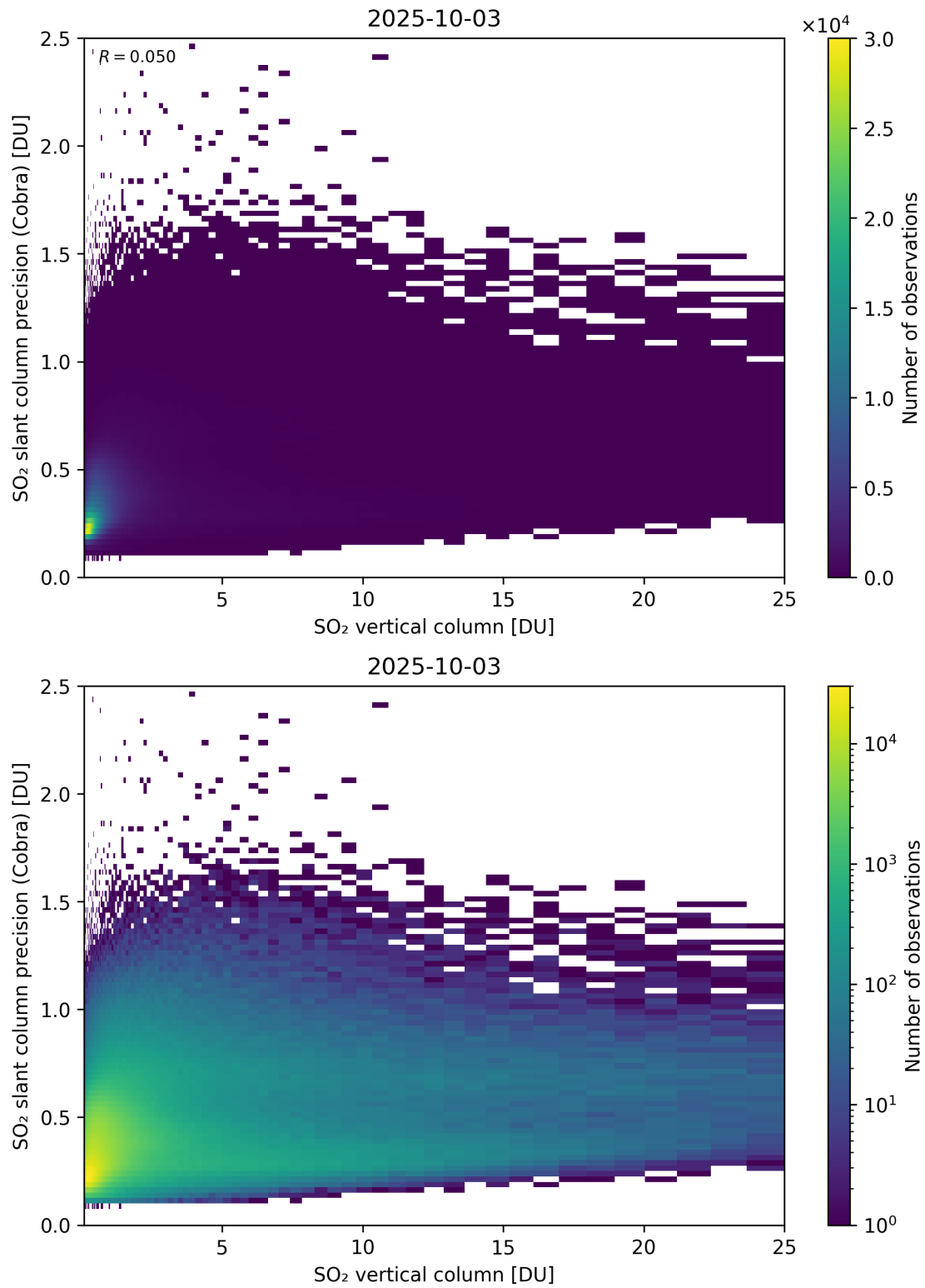
Figure 350: Scatter density plot of “SO 2 vertical column” against “SO 2 slant column precision (Cobra)” for 2025-10-02 to 2025-10-04.
