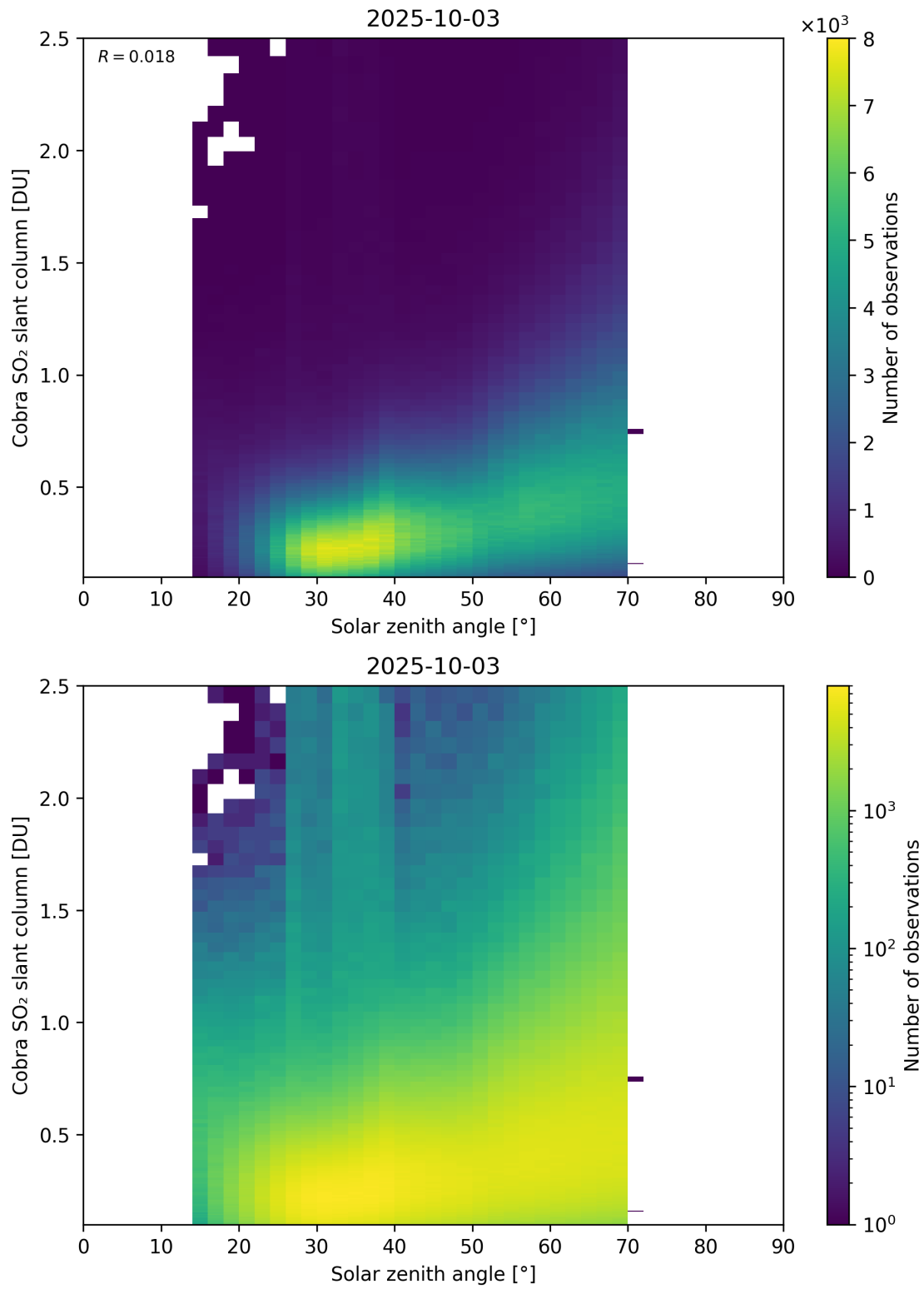
Figure 179: Scatter density plot of “Solar zenith angle” against “Cobra SO 2 slant column” for 2025-10-02 to 2025-10-04.
