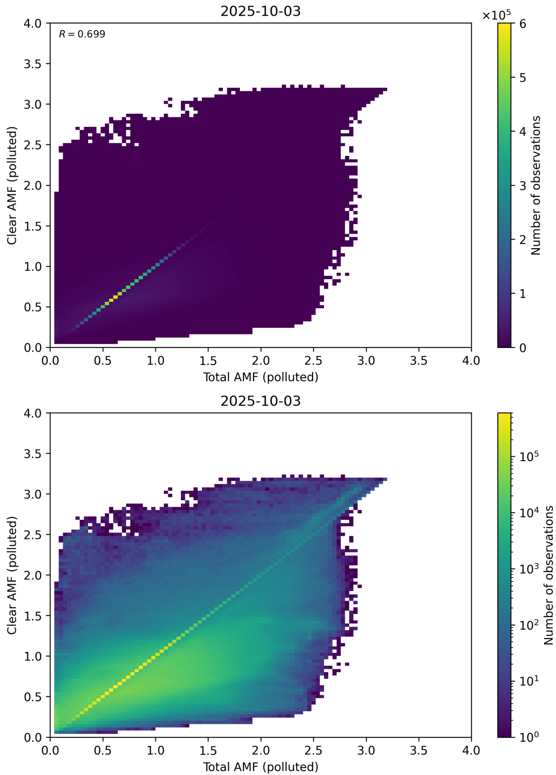
Figure 321: Scatter density plot of “Total AMF (polluted)” against “Clear AMF (polluted)” for 2025-10-02 to 2025-10-04.
