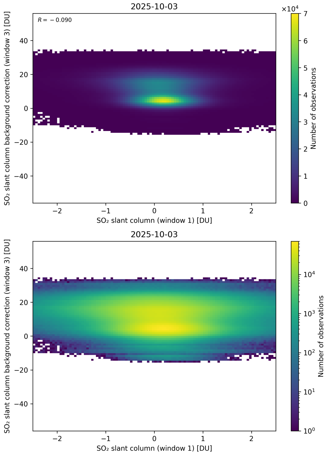
Figure 264: Scatter density plot of “SO 2 slant column (window 1)” against “SO 2 slant column background correction (window 3)” for 2025-10-02 to 2025-10-04.
