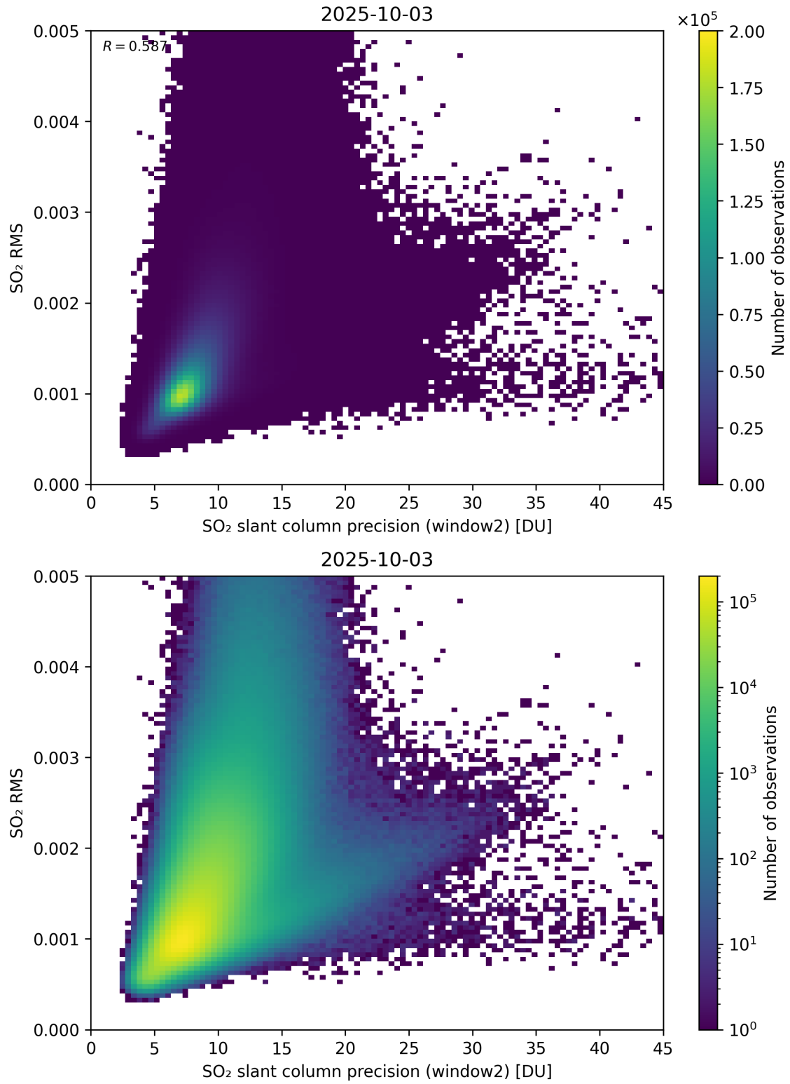
Figure 295: Scatter density plot of “SO 2 slant column precision (window2)” against “SO 2 RMS” for 2025-10-02 to 2025-10-04.
