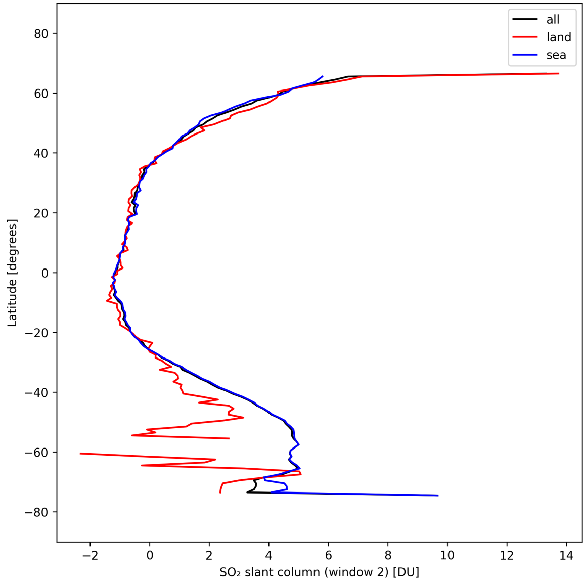
Figure 41: Zonal average of “SO 2 slant column (window 2)” for 2025-10-02 to 2025-10-04.
