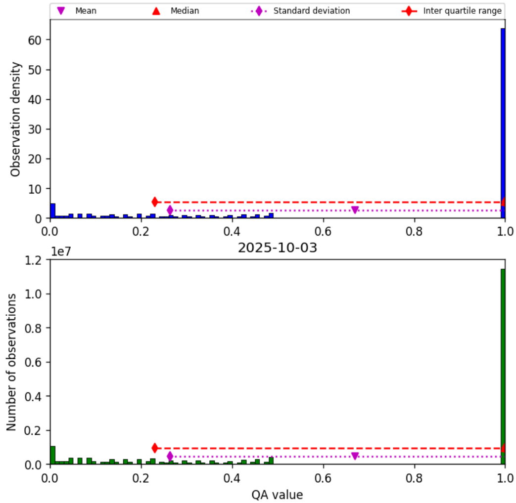
Figure 57: Histogram of “QA value” for 2025-10-02 to 2025-10-04
