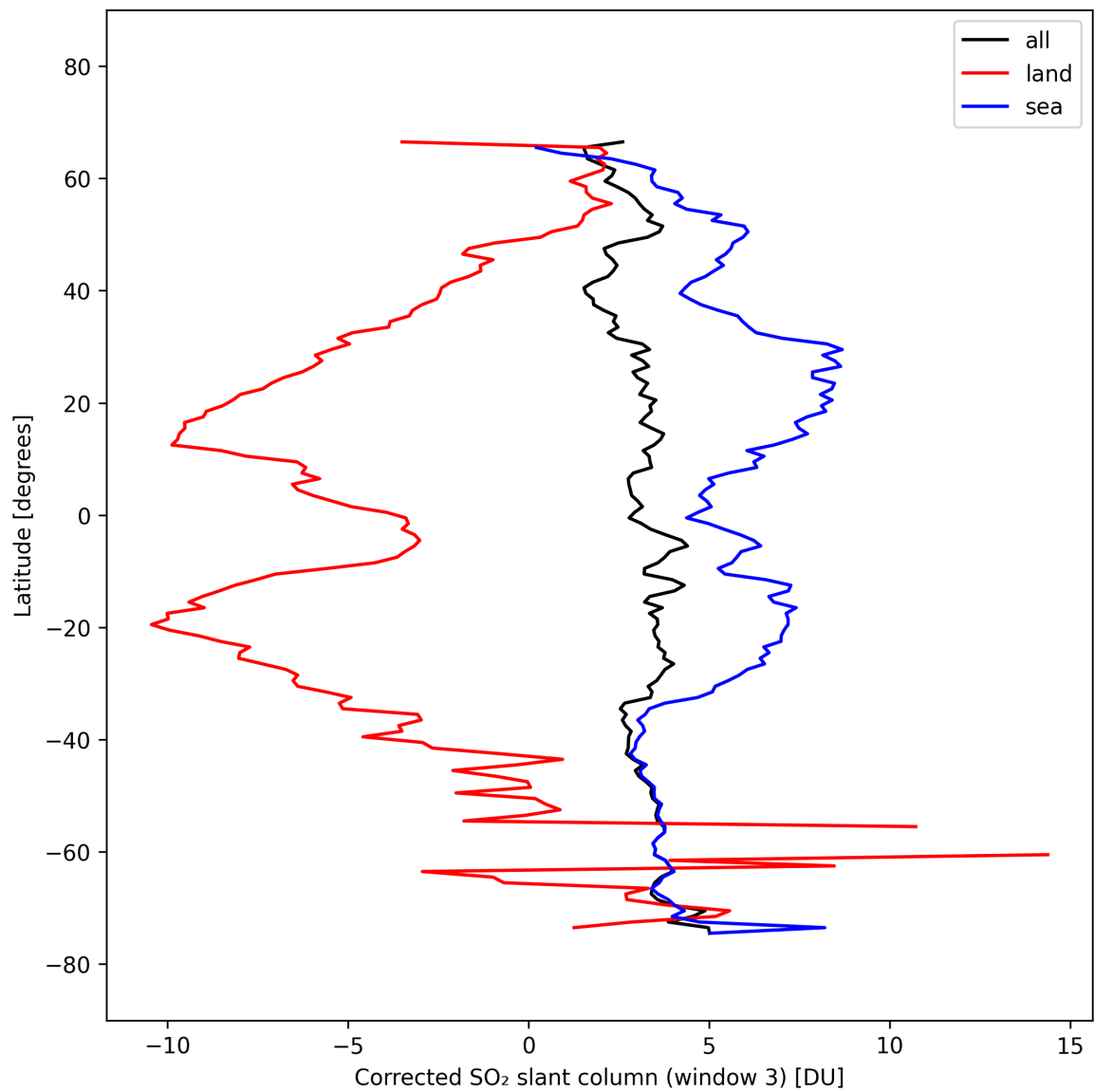
Figure 47: Zonal average of “Corrected SO 2 slant column (window 3)” for 2025-10-02 to 2025-10-04.
