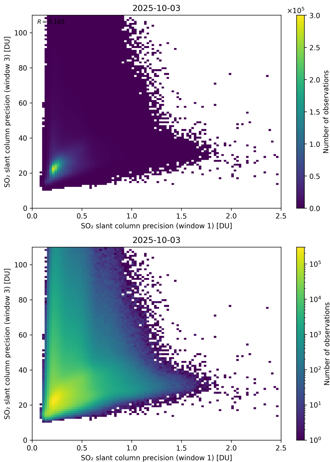
Figure 279: Scatter density plot of “SO 2 slant column precision (window 1)” against “SO 2 slant column precision (window 3)” for 2025-10-02 to 2025-10-04.
