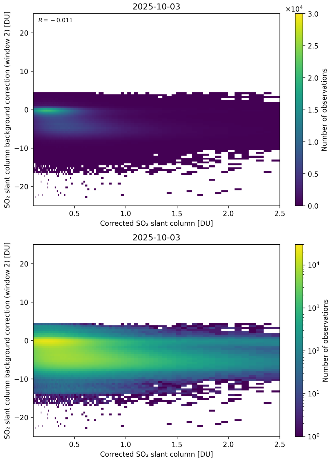
Figure 227: Scatter density plot of “Corrected SO 2 slant column” against “SO 2 slant column background correction (window 2)” for 2025-10-02 to 2025-10-04.
