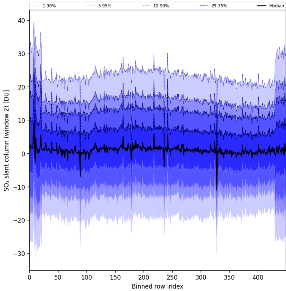
Figure 93: Along track statistics of “SO 2 slant column (window 2)” for 2025-10-02 to 2025-10-04
