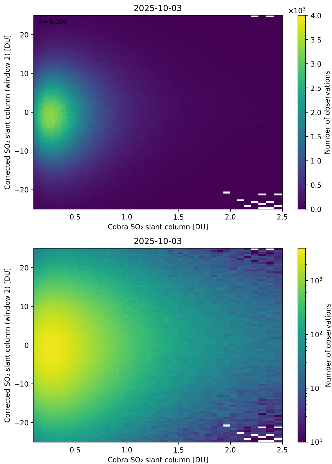
Figure 217: Scatter density plot of “Cobra SO 2 slant column” against “Corrected SO 2 slant column (window 2)” for 2025-10-02 to 2025-10-04.
