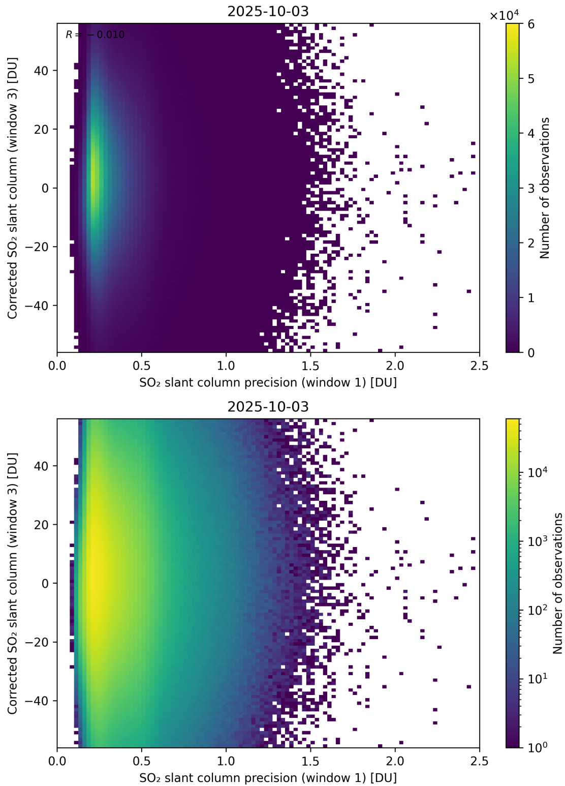
Figure 276: Scatter density plot of “SO 2 slant column precision (window 1)” against “Corrected SO 2 slant column (window 3)” for 2025-10-02 to 2025-10-04.
