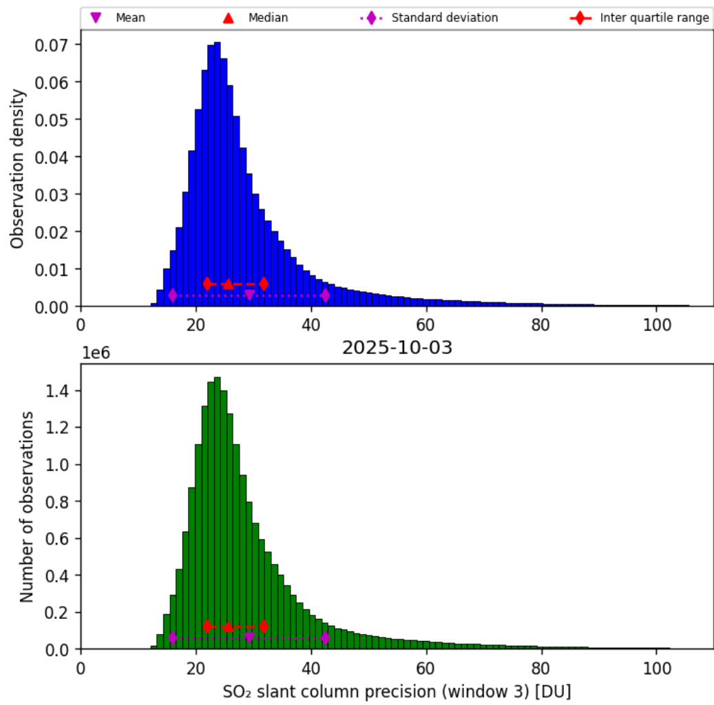
Figure 72: Histogram of “SO 2 slant column precision (window 3)” for 2025-10-02 to 2025-10-04
