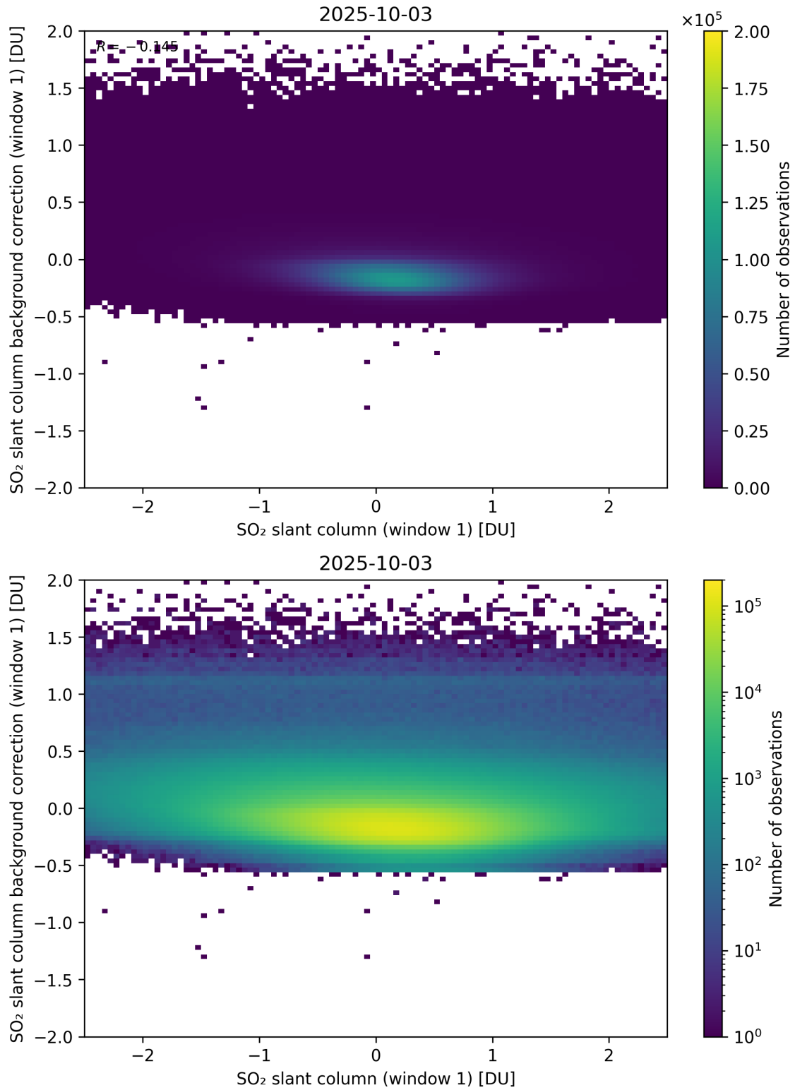
Figure 262: Scatter density plot of “SO 2 slant column (window 1)” against “SO 2 slant column background correction (window 1)” for 2025-10-02 to 2025-10-04.
