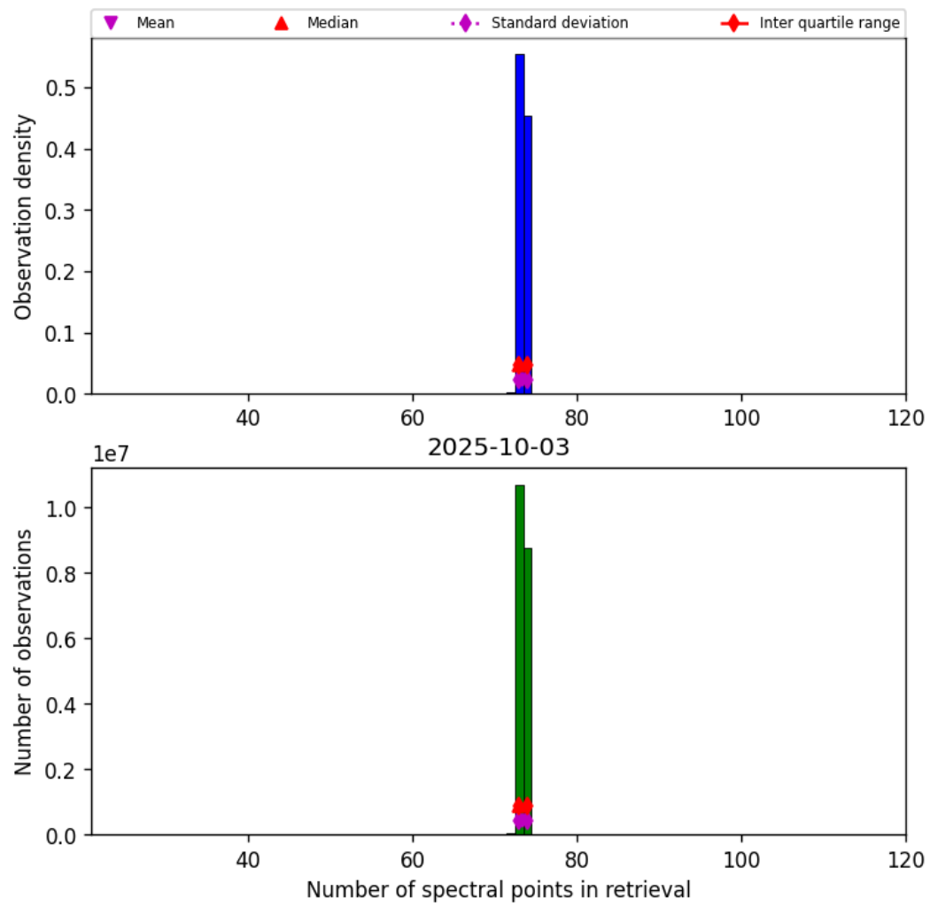
Figure 82: Histogram of “Number of spectral points in retrieval” for 2025-10-02 to 2025-10-04
