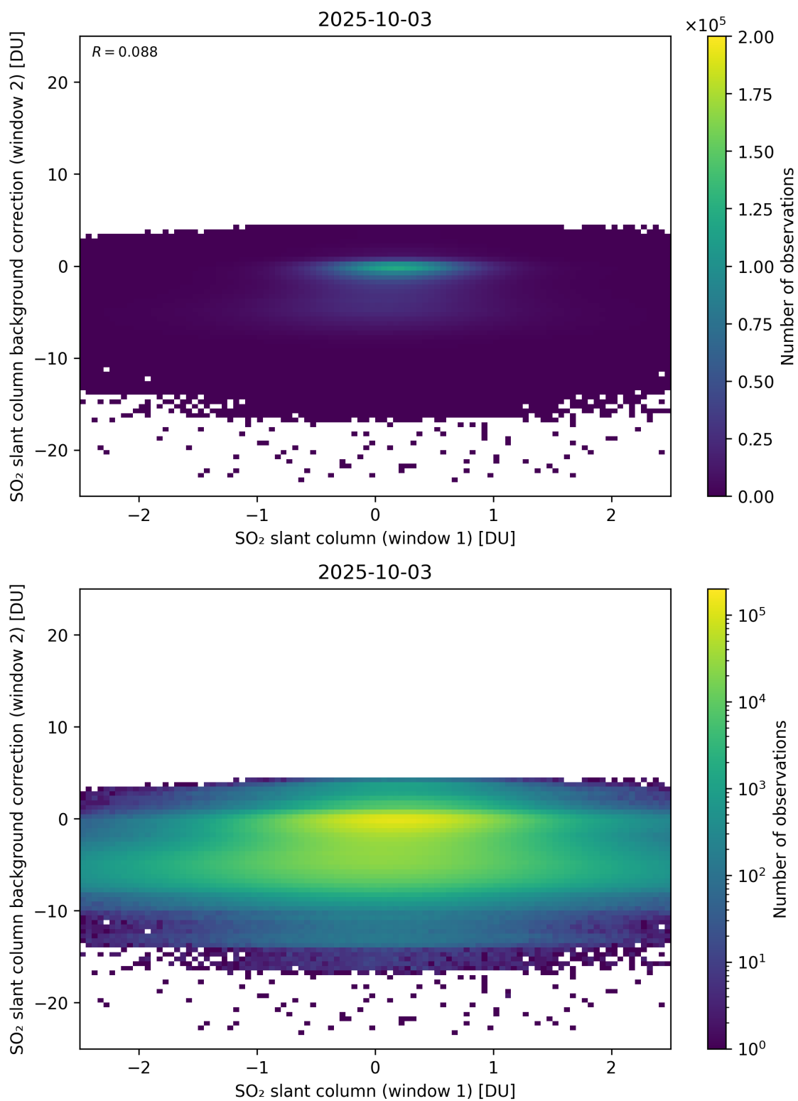
Figure 263: Scatter density plot of “SO 2 slant column (window 1)” against “SO 2 slant column background correction (window 2)” for 2025-10-02 to 2025-10-04.
