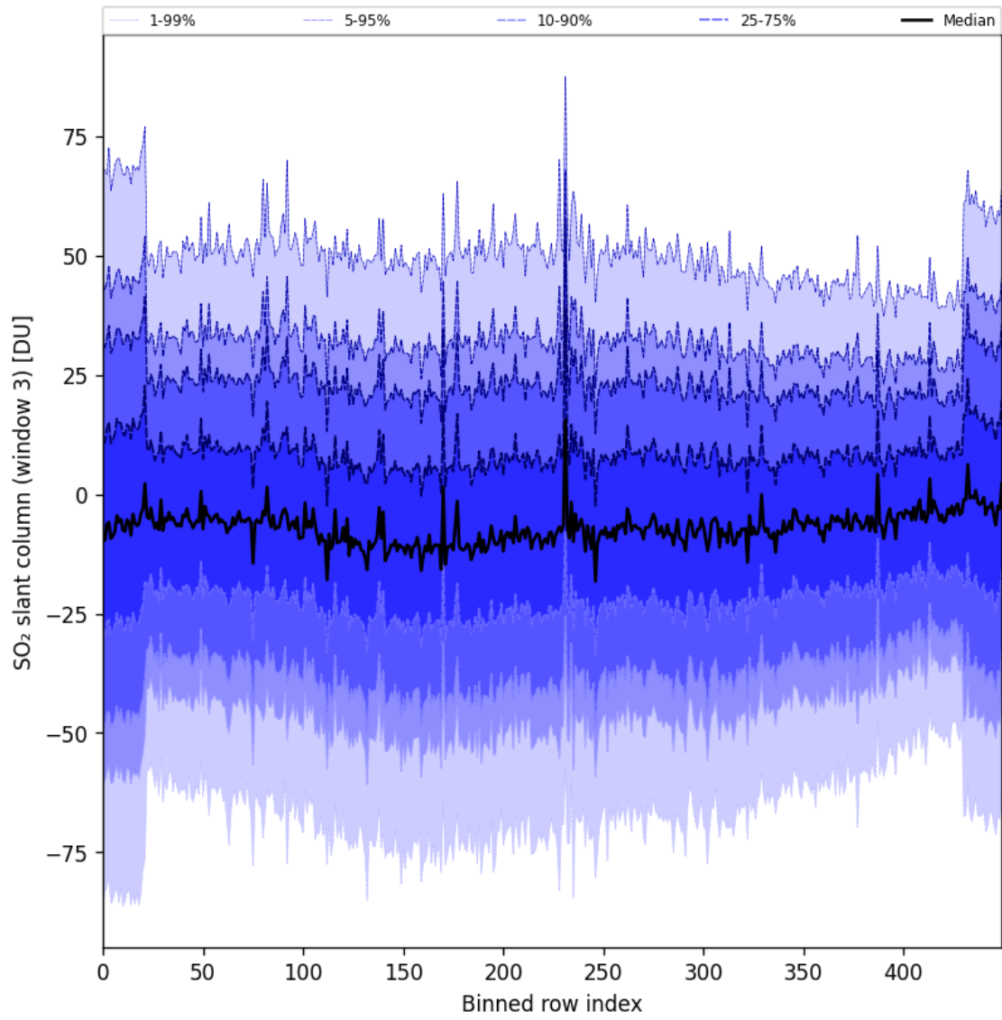
Figure 97: Along track statistics of “SO 2 slant column (window 3)” for 2025-10-02 to 2025-10-04
