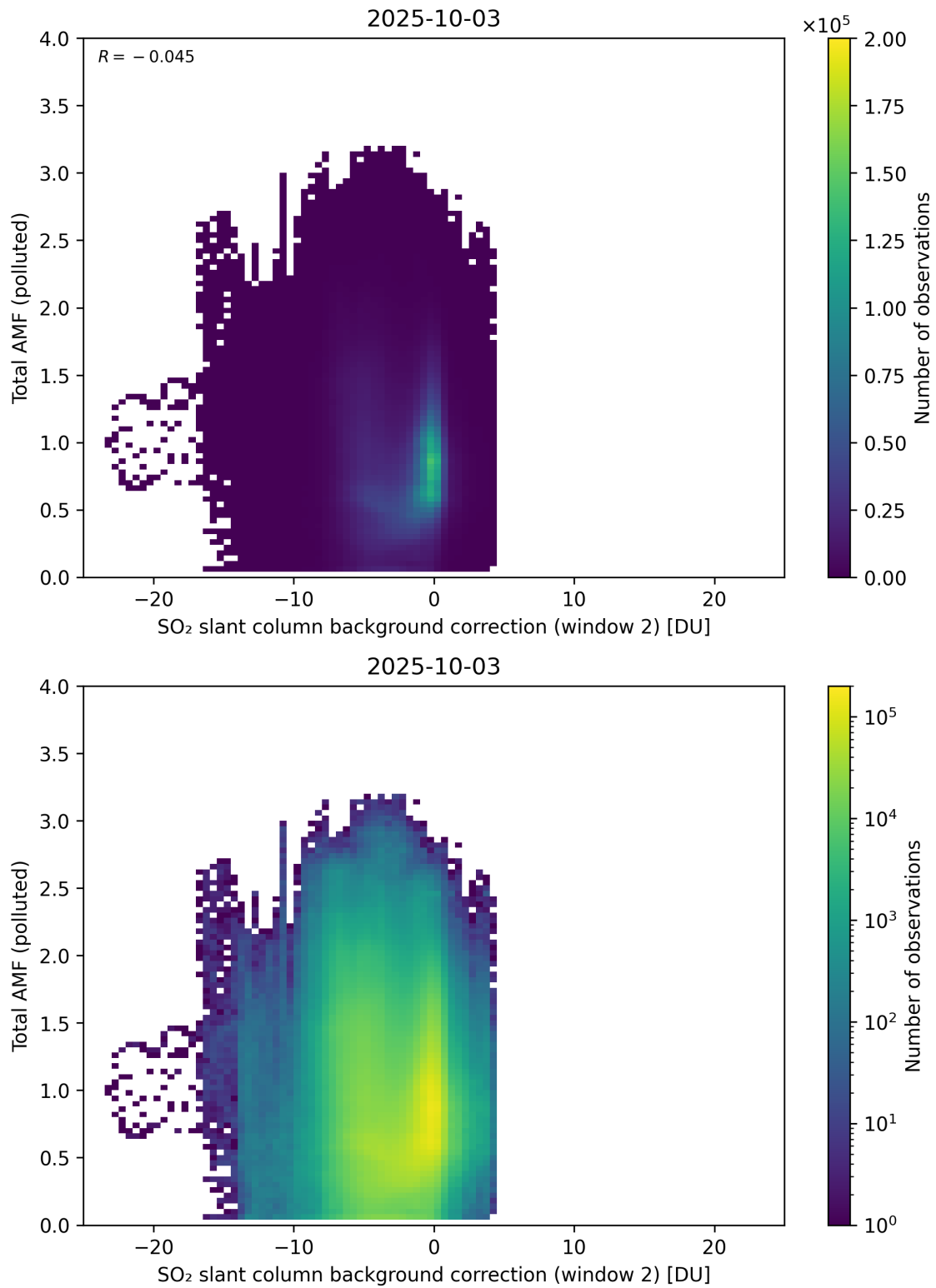
Figure 130: Scatter density plot of “SO 2 slant column background correction (window 2)” against “Total AMF (polluted)” for 2025-10-02 to 2025-10-04.
