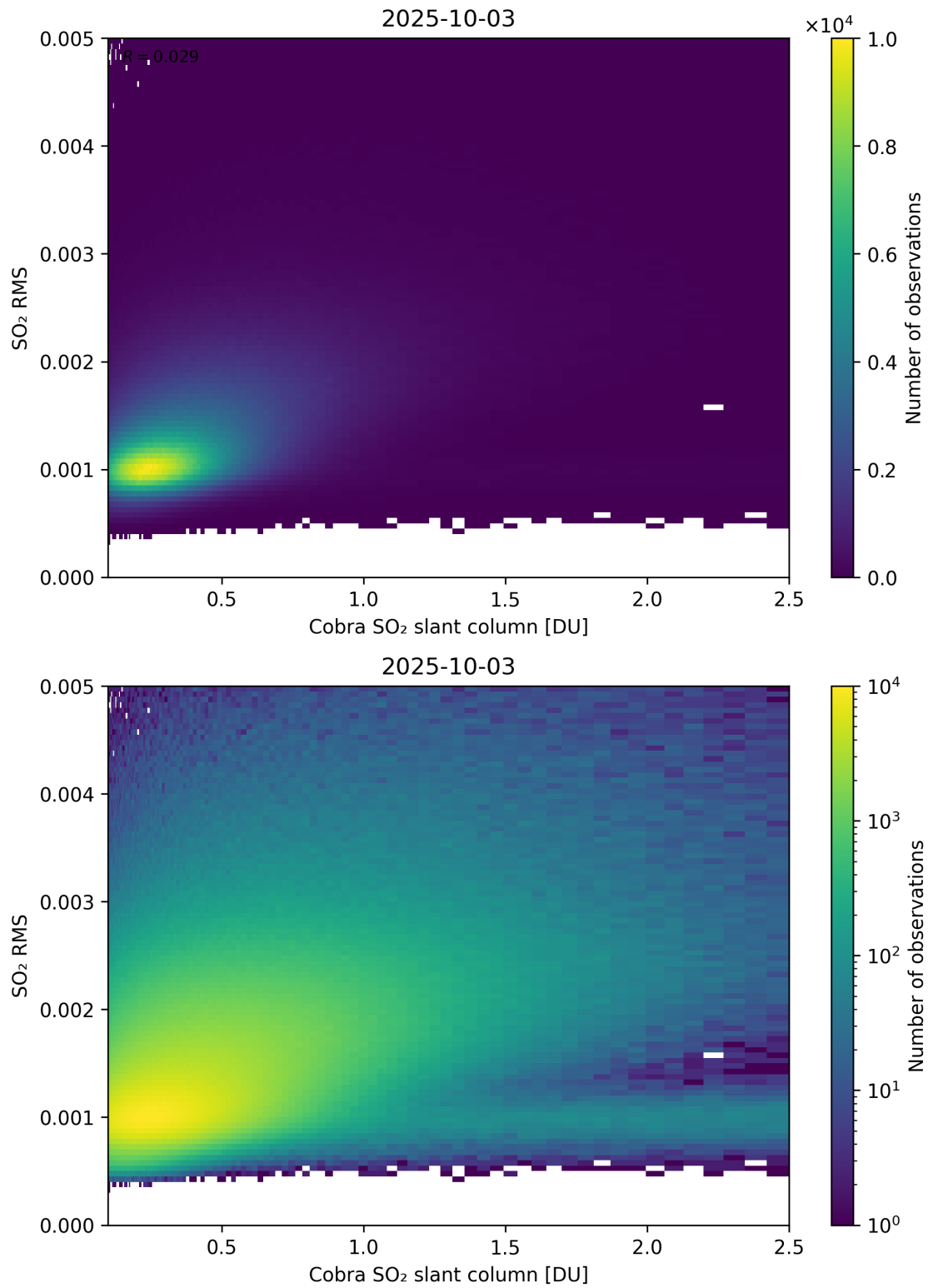
Figure 198: Scatter density plot of “Cobra SO 2 slant column” against “SO 2 RMS” for 2025-10-02 to 2025-10-04.
