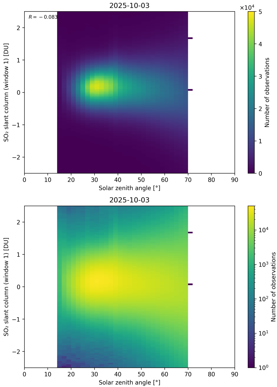
Figure 184: Scatter density plot of “Solar zenith angle” against “SO 2 slant column (window 1)” for 2025-10-02 to 2025-10-04.
