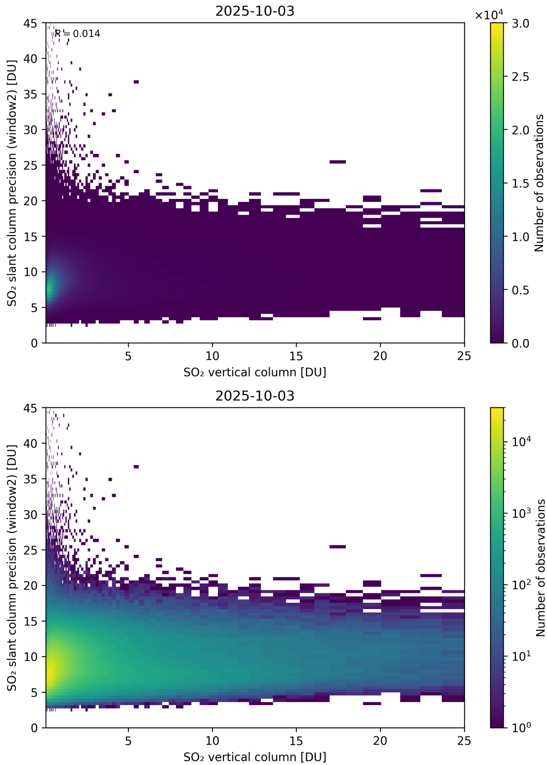
Figure 356: Scatter density plot of “SO 2 vertical column” against “SO 2 slant column precision (window2)” for 2025-10-02 to 2025-10-04.
