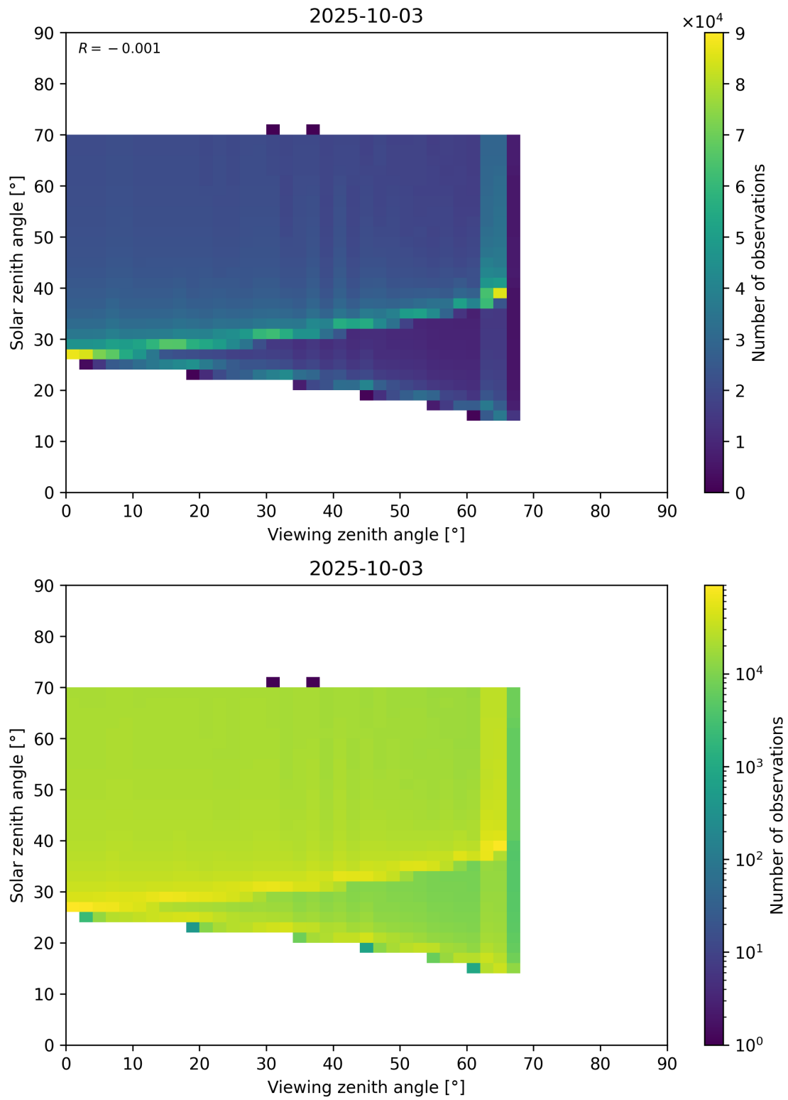
Figure 369: Scatter density plot of “Viewing zenith angle” against “Solar zenith angle” for 2025-10-02 to 2025-10-04.
