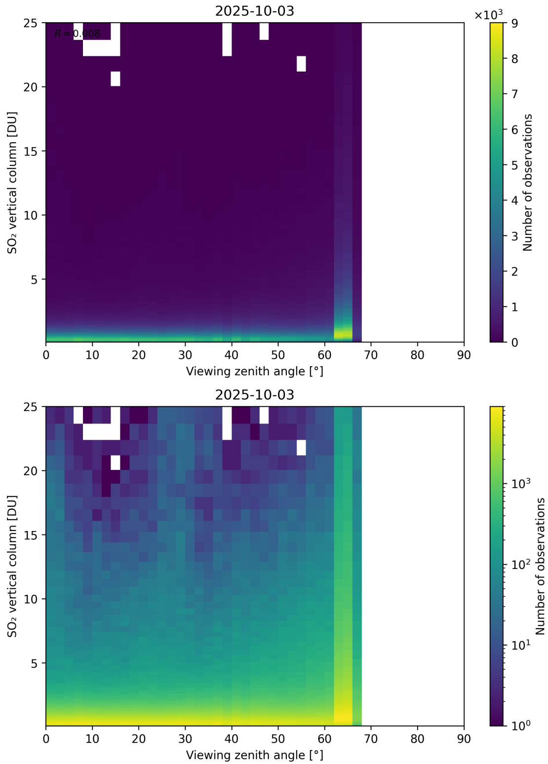
Figure 383: Scatter density plot of “Viewing zenith angle” against “SO 2 vertical column” for 2025-10-02 to 2025-10-04.
