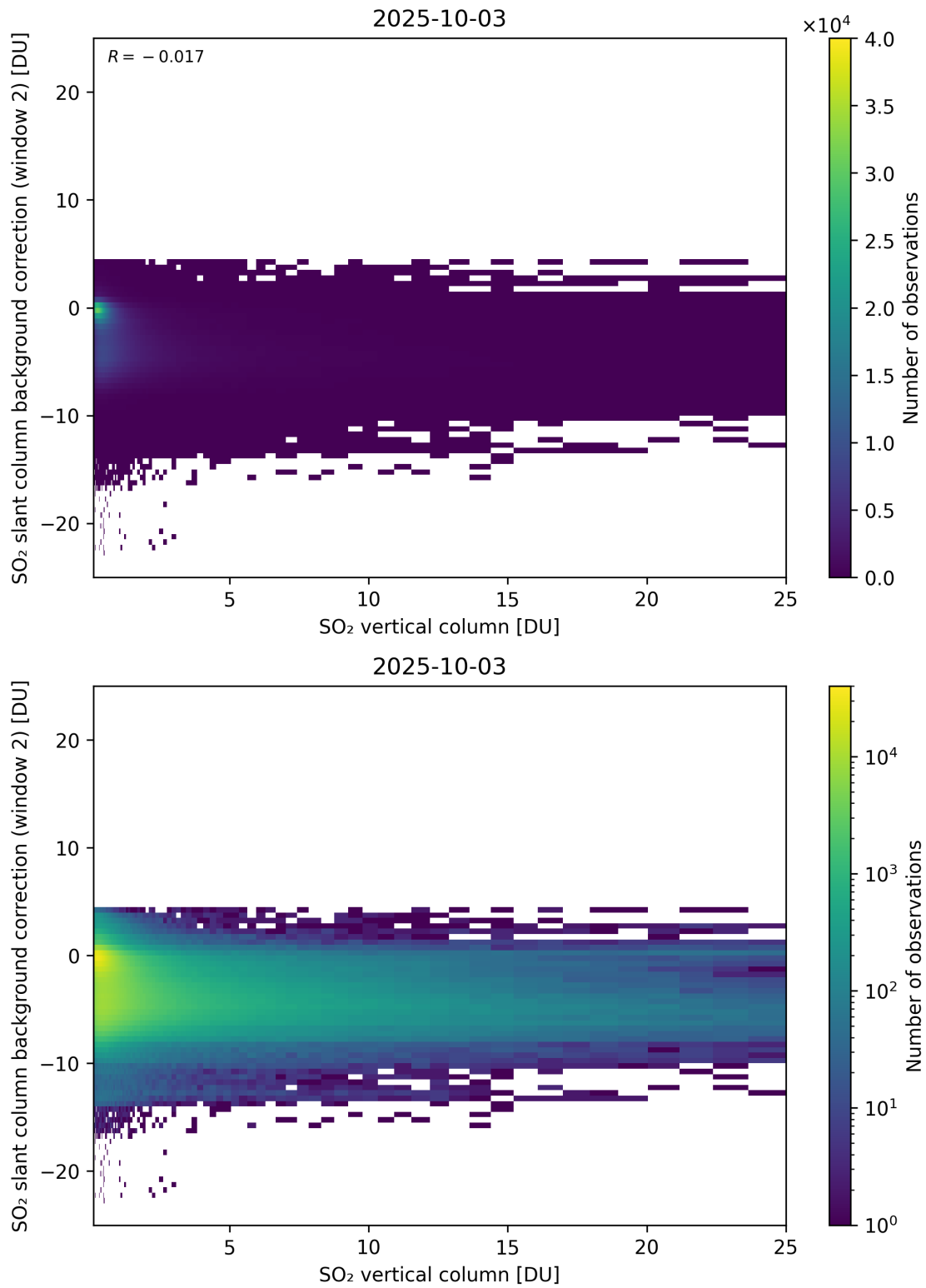
Figure 324: Scatter density plot of “SO 2 vertical column” against “SO 2 slant column background correction (window 2)” for 2025-10-02 to 2025-10-04.
