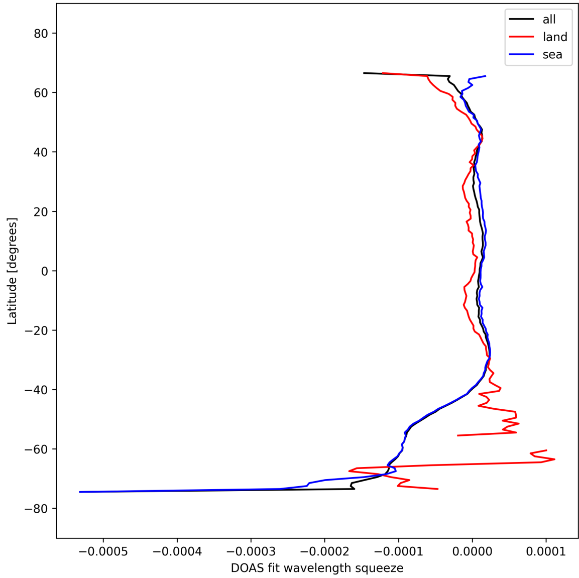
Figure 51: Zonal average of “DOAS fit wavelength squeeze” for 2025-10-02 to 2025-10-04.
