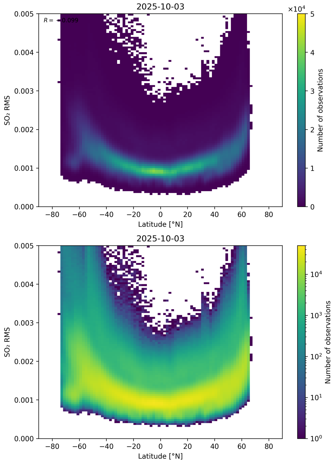
Figure 155: Scatter density plot of “Latitude” against “SO 2 RMS” for 2025-10-02 to 2025-10-04.
