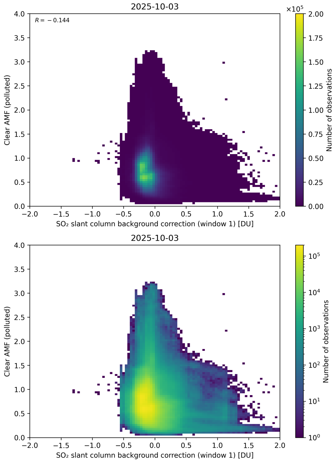
Figure 114: Scatter density plot of “SO 2 slant column background correction (window 1)” against “Clear AMF (polluted)” for 2025-10-02 to 2025-10-04.
