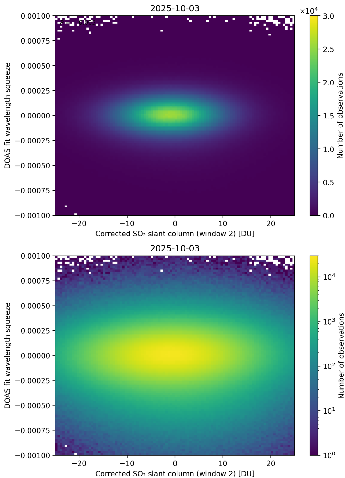
Figure 247: Scatter density plot of “Corrected SO 2 slant column (window 2)” against “DOAS fit wavelength squeeze” for 2025-10-02 to 2025-10-04.
