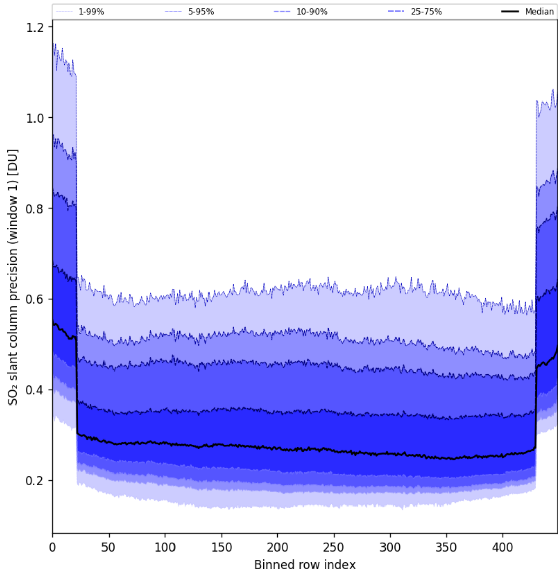
Figure 90: Along track statistics of “SO 2 slant column precision (window 1)” for 2025-10-02 to 2025-10-04
