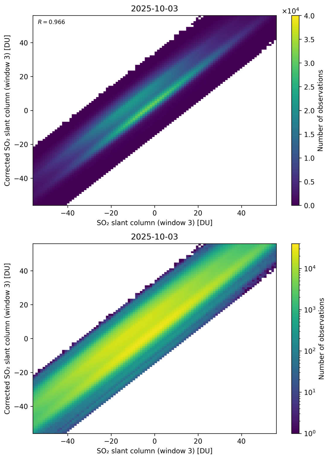
Figure 316: Scatter density plot of “SO 2 slant column (window 3)” against “Corrected SO 2 slant column (window 3)” for 2025-10-02 to 2025-10-04.
