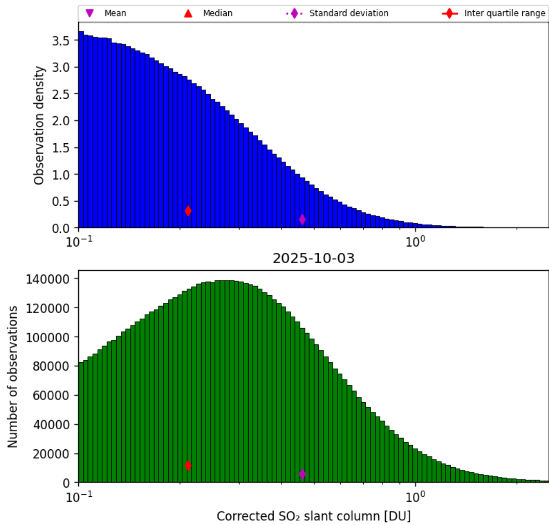
Figure 60: Histogram of "Corrected SO 2 slant column" for 2025-10-02 to 2025-10-04
