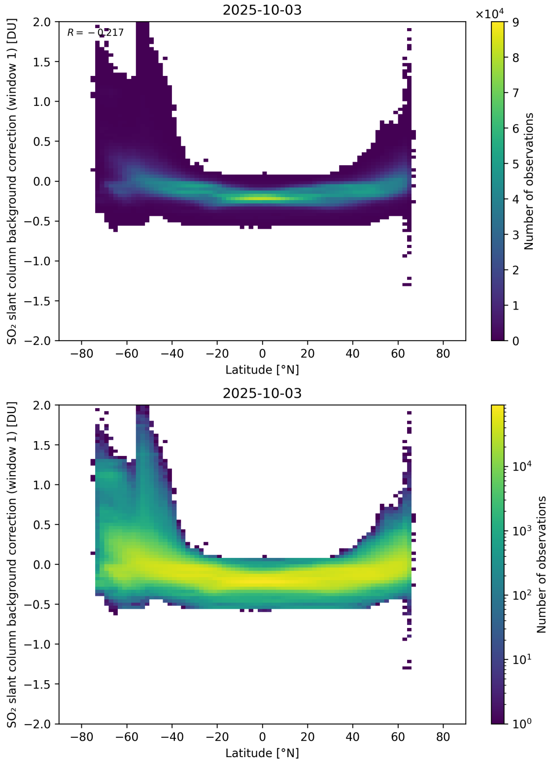
Figure 150: Scatter density plot of “Latitude” against “SO 2 slant column background correction (window 1)” for 2025-10-02 to 2025-10-04.
