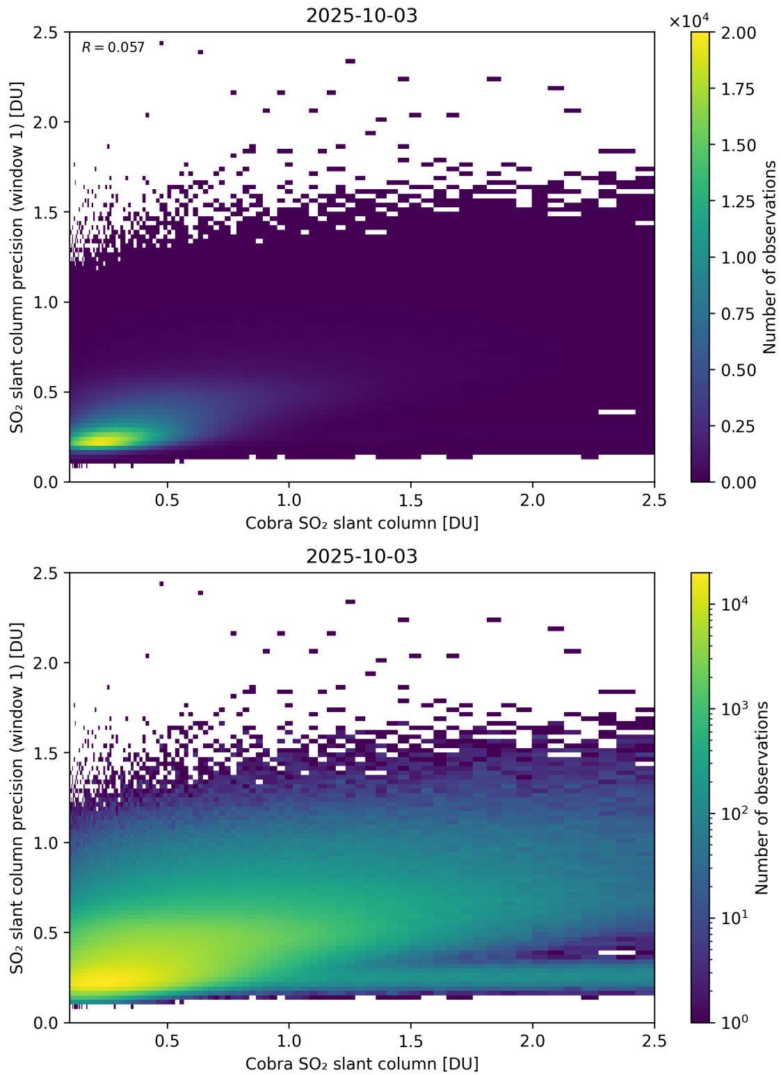
Figure 220: Scatter density plot of “Cobra SO 2 slant column” against “SO 2 slant column precision (window 1)” for 2025-10-02 to 2025-10-04.
