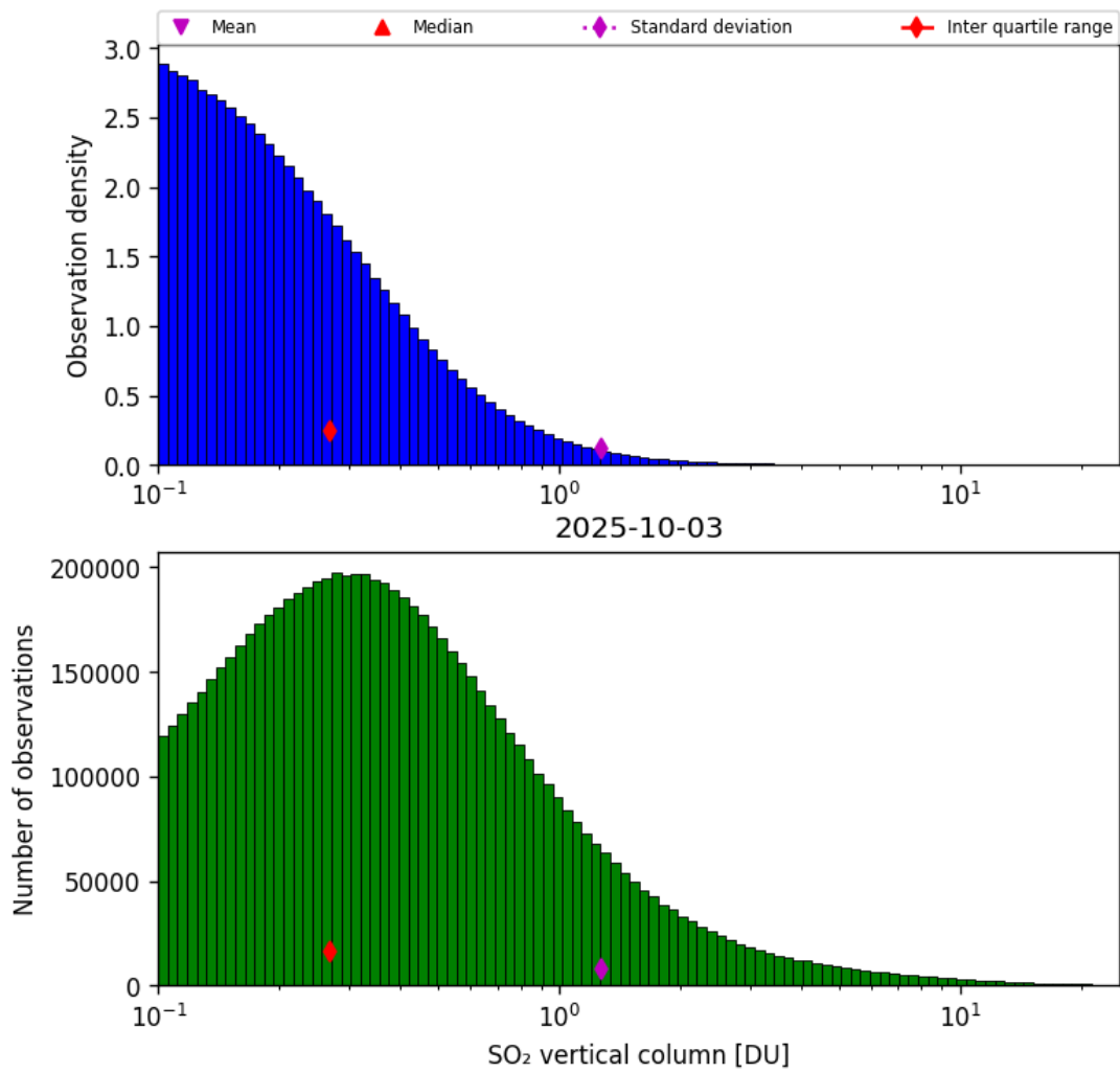
Figure 58: Histogram of “SO 2 vertical column” for 2025-10-02 to 2025-10-04
