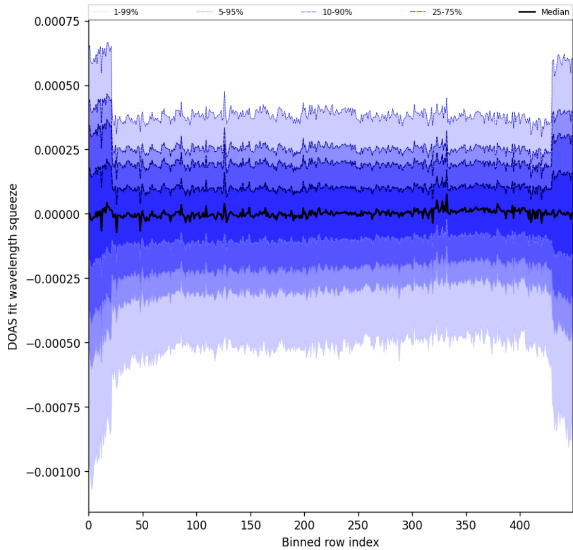
Figure 103: Along track statistics of “DOAS fit wavelength squeeze” for 2025-10-02 to 2025-10-04
