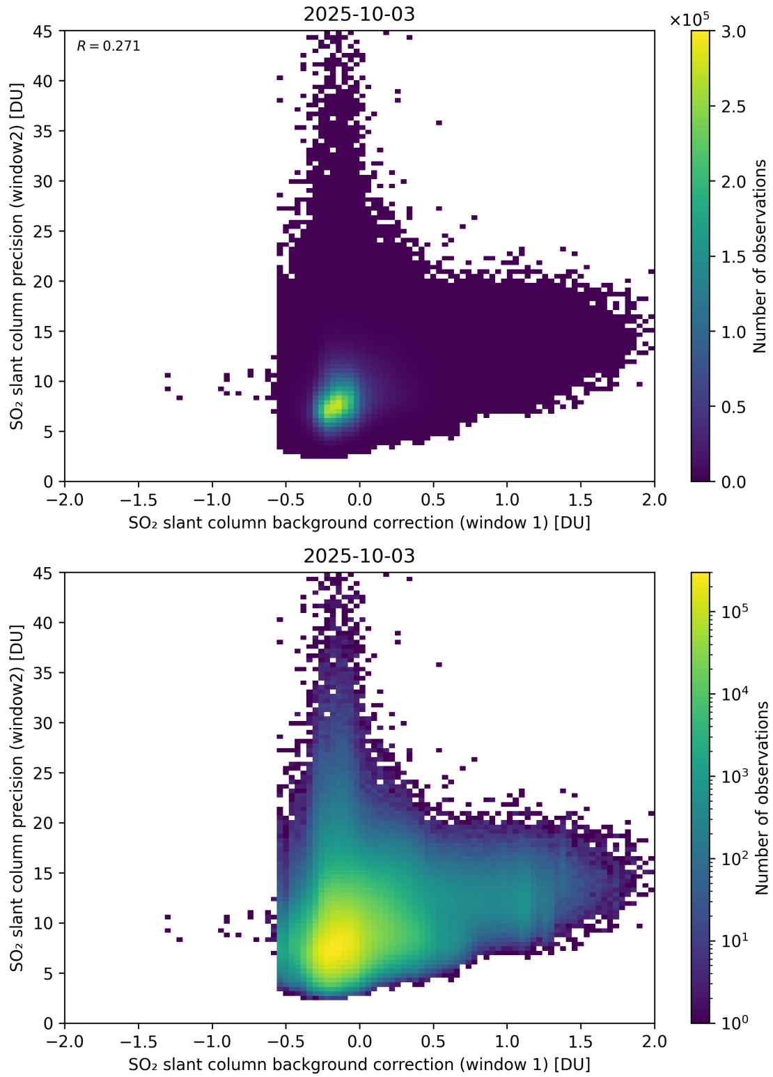
Figure 117: Scatter density plot of “SO 2 slant column background correction (window 1)” against “SO 2 slant column precision (window2)” for 2025-10-02 to 2025-10-04.
