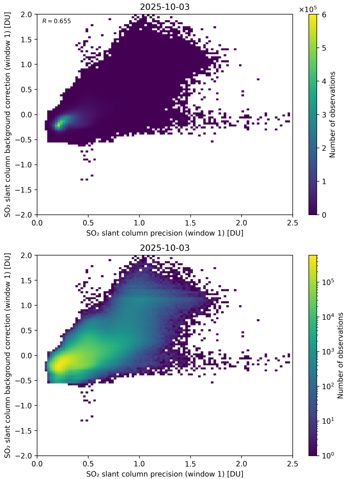
Figure 268: Scatter density plot of “SO 2 slant column precision (window 1)” against “SO 2 slant column background correction (window 1)” for 2025-10-02 to 2025-10-04.
