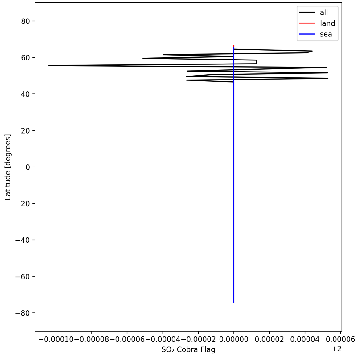
Figure 49: Zonal average of “SO 2 Cobra Flag” for 2025-10-02 to 2025-10-04.
