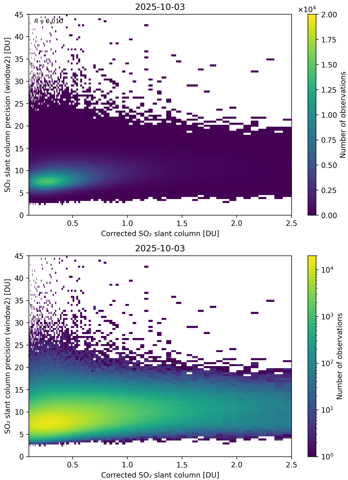
Figure 239: Scatter density plot of “Corrected SO 2 slant column” against “SO 2 slant column precision (window2)” for 2025-10-02 to 2025-10-04.
