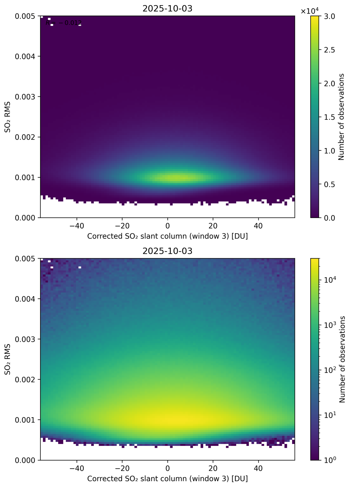
Figure 258: Scatter density plot of “Corrected SO 2 slant column (window 3)” against “SO 2 RMS” for 2025-10-02 to 2025-10-04.
