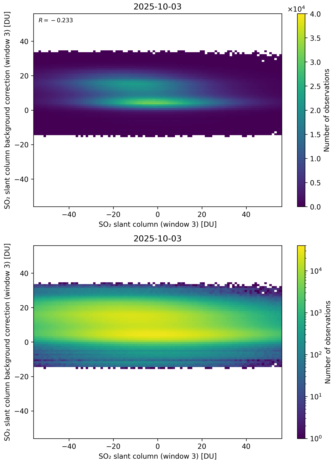
Figure 303: Scatter density plot of “SO 2 slant column (window 3)” against “SO 2 slant column background correction (window 3)” for 2025-10-02 to 2025-10-04.
