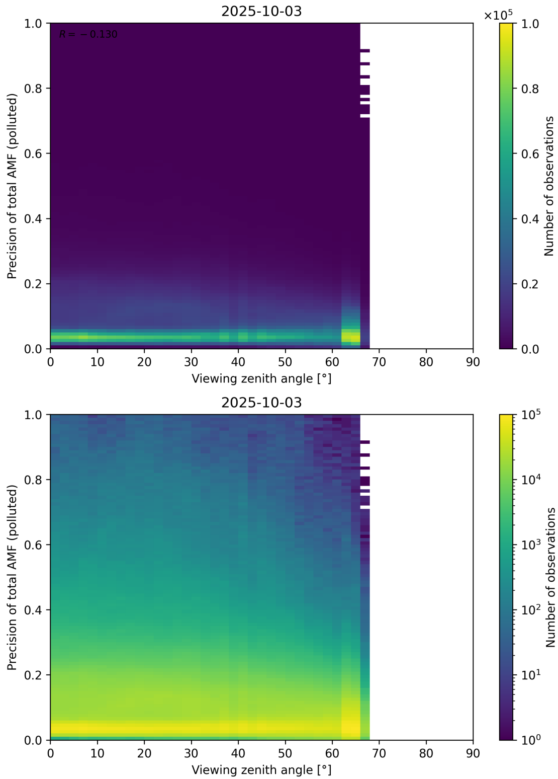
Figure 382: Scatter density plot of “Viewing zenith angle” against “Precision of total AMF (polluted)” for 2025-10-02 to 2025-10-04.
