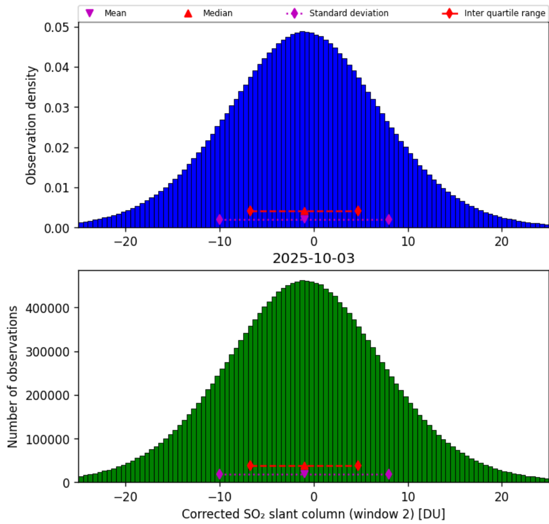
Figure 69: Histogram of “Corrected SO 2 slant column (window 2)” for 2025-10-02 to 2025-10-04
