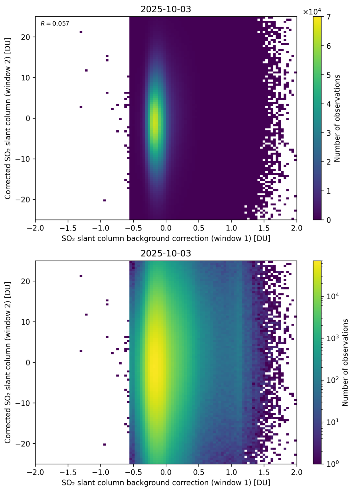
Figure 115: Scatter density plot of “SO 2 slant column background correction (window 1)” against “Corrected SO 2 slant column (window 2)” for 2025-10-02 to 2025-10-04.
