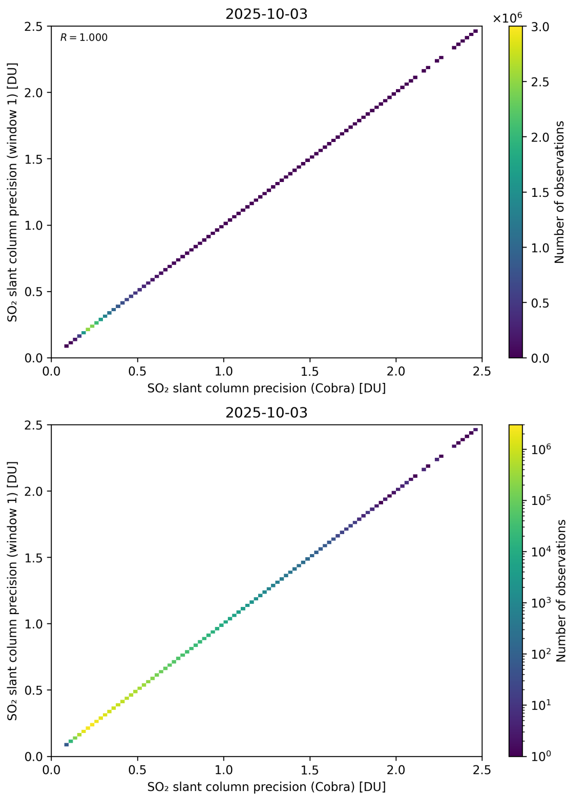
Figure 209: Scatter density plot of “SO 2 slant column precision (Cobra)” against “SO 2 slant column precision (window 1)” for 2025-10-02 to 2025-10-04.
