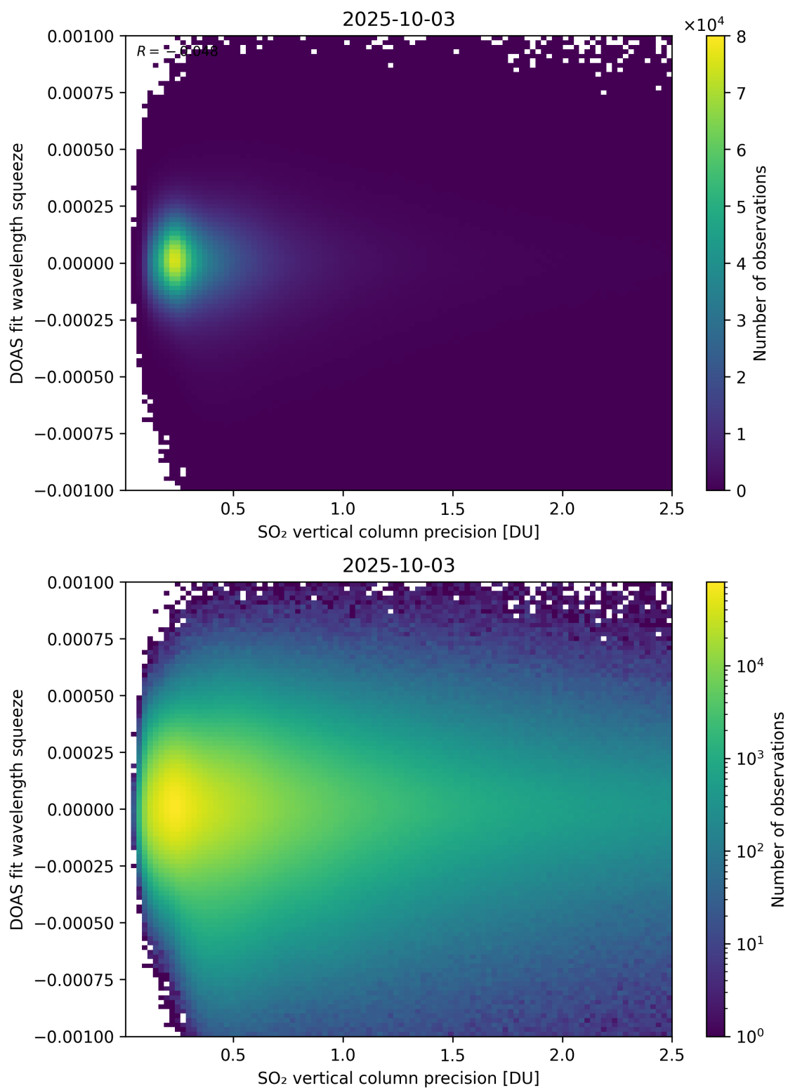
Figure 333: Scatter density plot of “SO 2 vertical column precision” against “DOAS fit wavelength squeeze” for 2025-10-02 to 2025-10-04.
