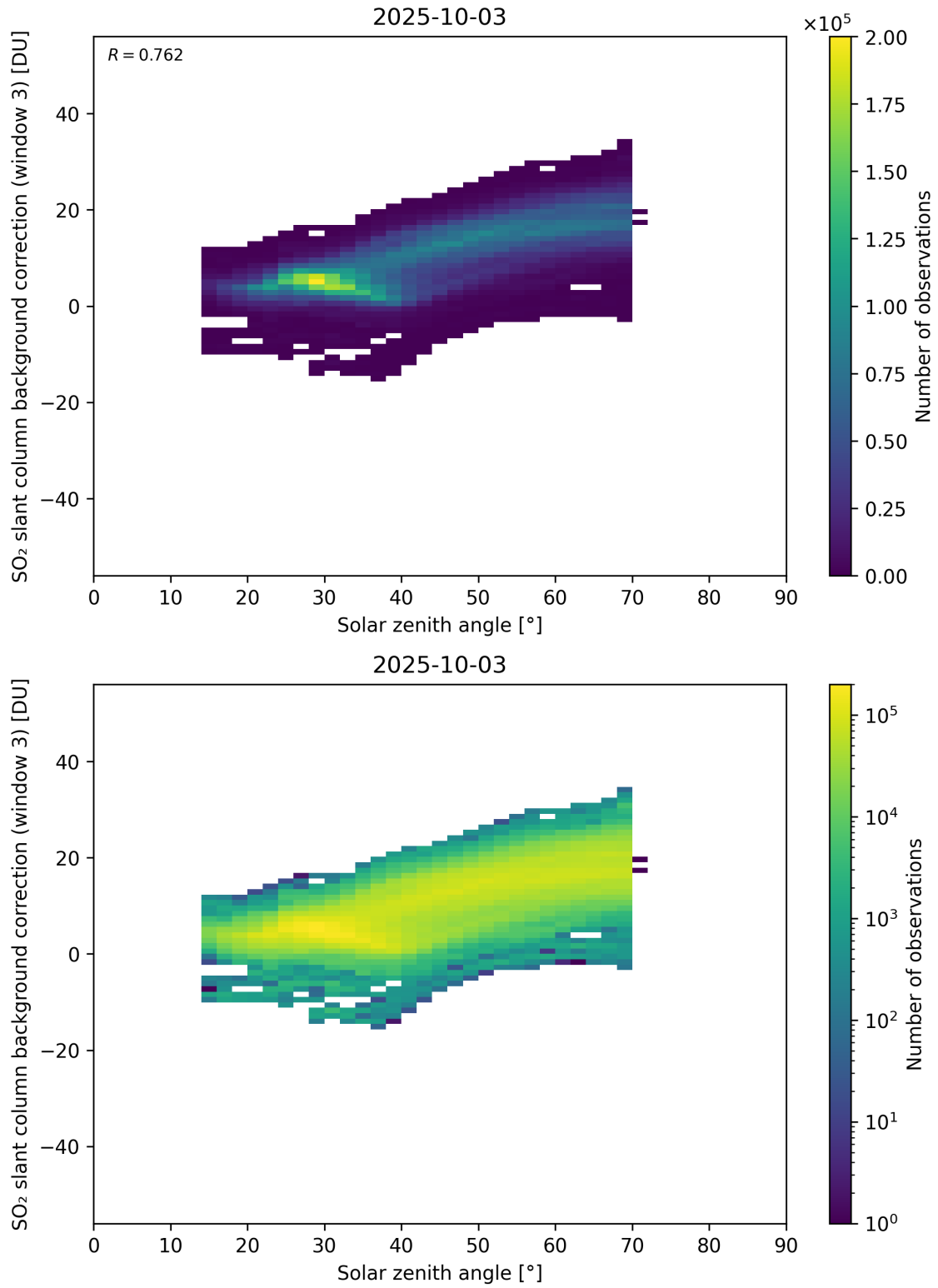
Figure 173: Scatter density plot of “Solar zenith angle” against “SO 2 slant column background correction (window 3)” for 2025-10-02 to 2025-10-04.
