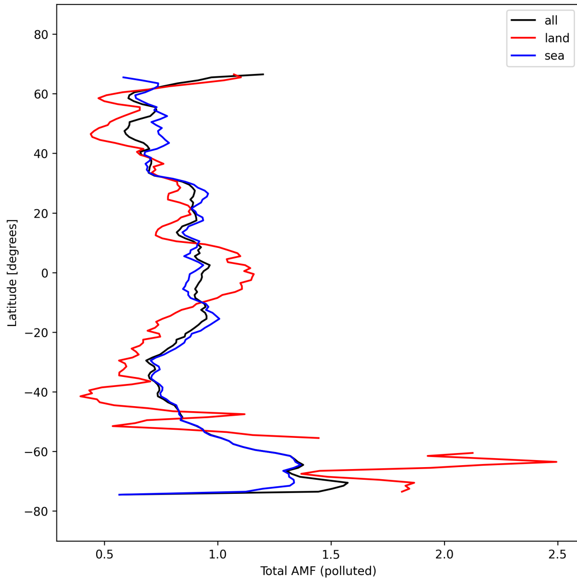
Figure 53: Zonal average of “Total AMF (polluted)” for 2025-10-02 to 2025-10-04.
