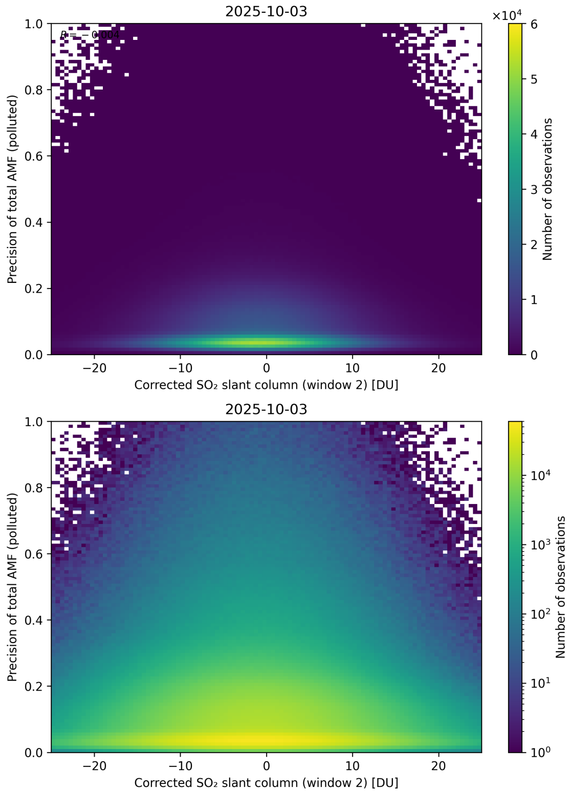
Figure 254: Scatter density plot of “Corrected SO 2 slant column (window 2)” against “Precision of total AMF (polluted)” for 2025-10-02 to 2025-10-04.
