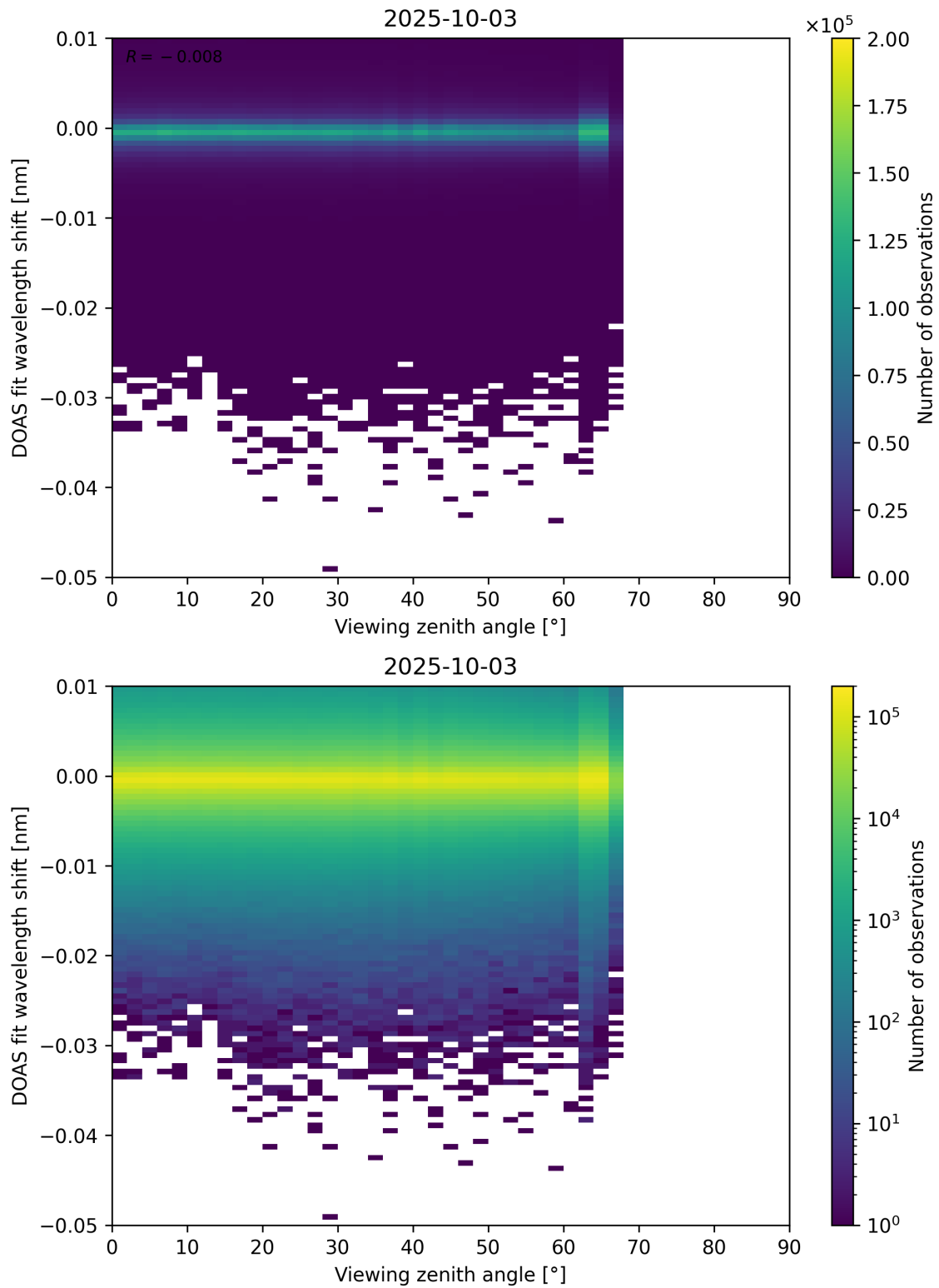
Figure 365: Scatter density plot of “Viewing zenith angle” against “DOAS fit wavelength shift” for 2025-10-02 to 2025-10-04.
