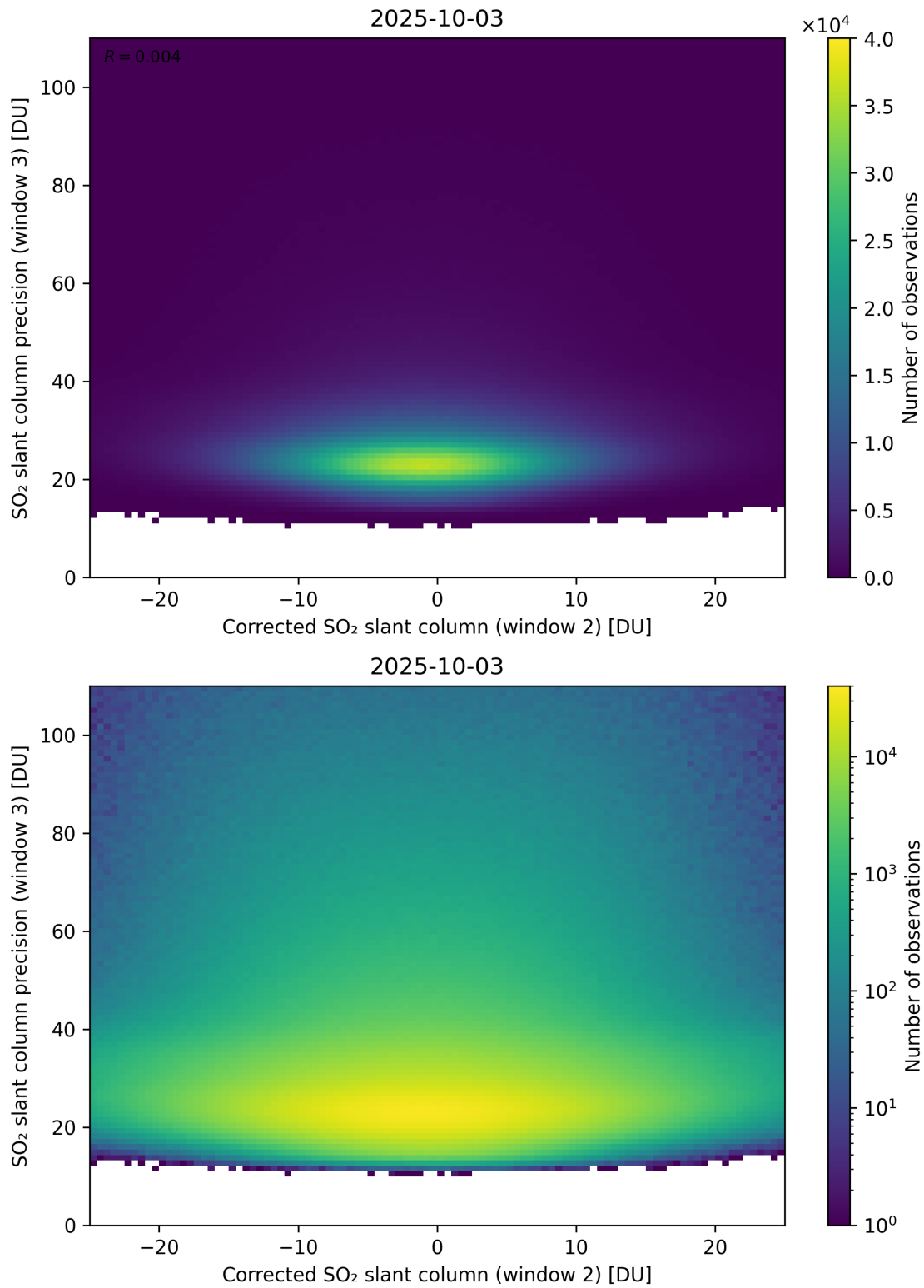
Figure 252: Scatter density plot of “Corrected SO 2 slant column (window 2)” against “SO 2 slant column precision (window 3)” for 2025-10-02 to 2025-10-04.
