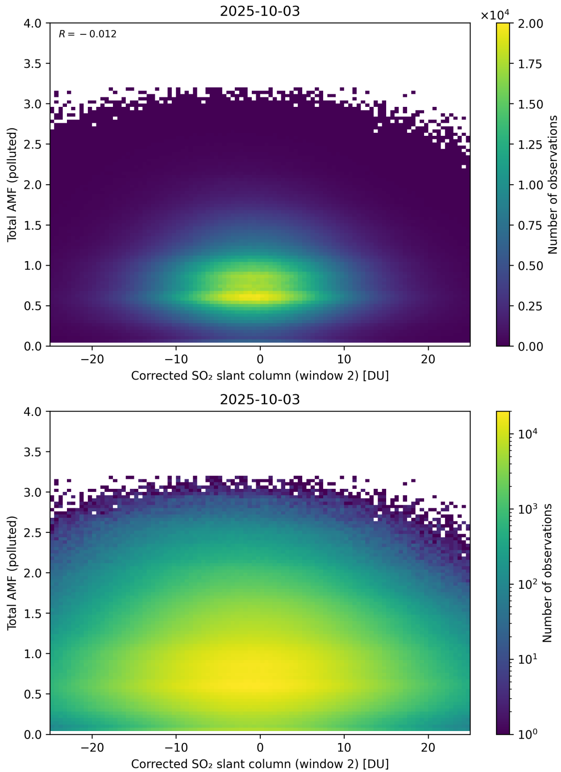
Figure 253: Scatter density plot of “Corrected SO 2 slant column (window 2)” against “Total AMF (polluted)” for 2025-10-02 to 2025-10-04.
