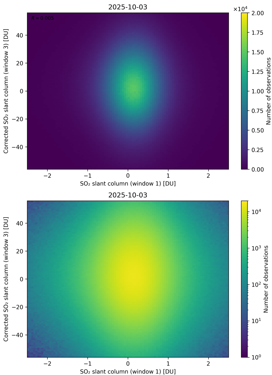
Figure 284: Scatter density plot of “SO 2 slant column (window 1)” against “Corrected SO 2 slant column (window 3)” for 2025-10-02 to 2025-10-04.
