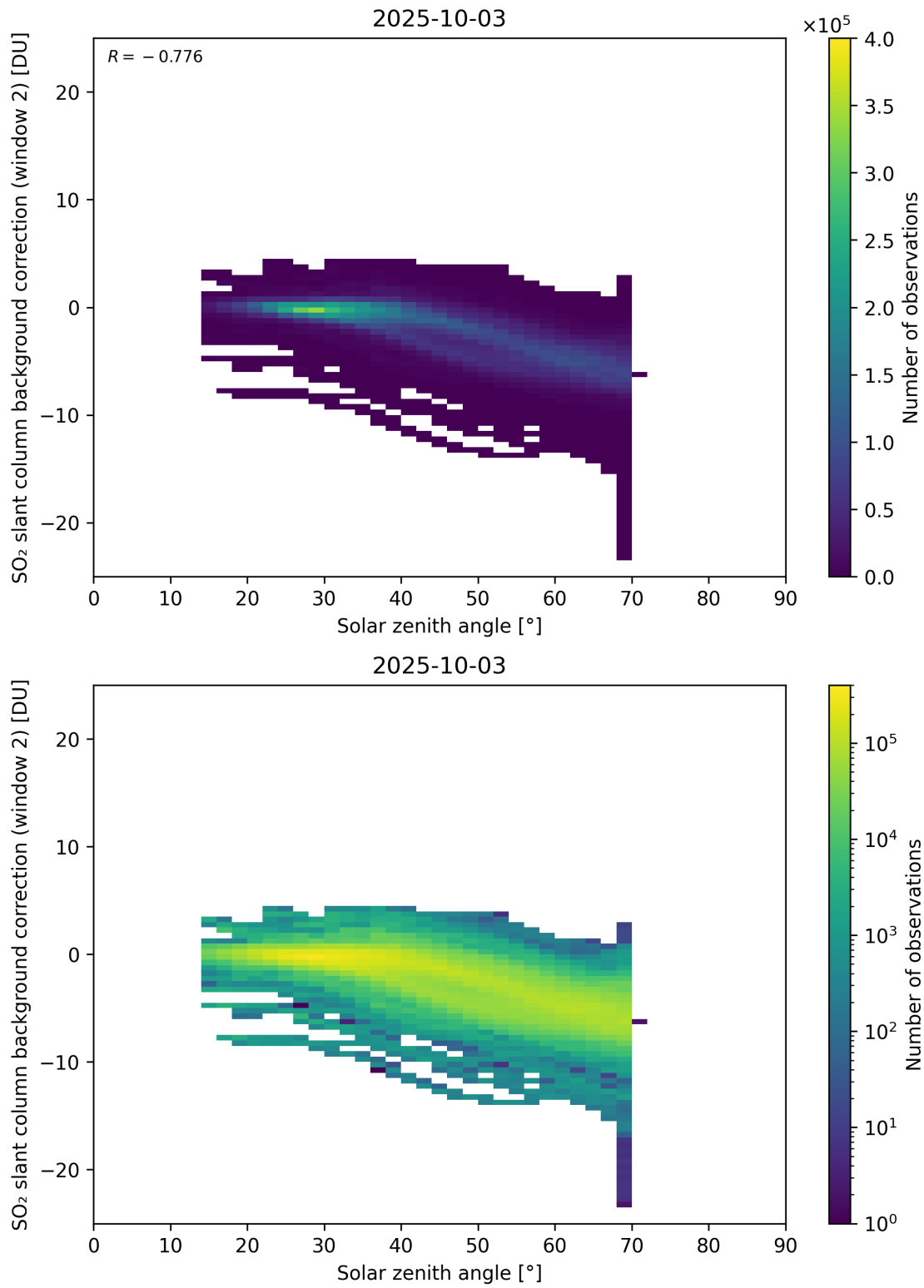
Figure 172: Scatter density plot of “Solar zenith angle” against “SO 2 slant column background correction (window 2)” for 2025-10-02 to 2025-10-04.
