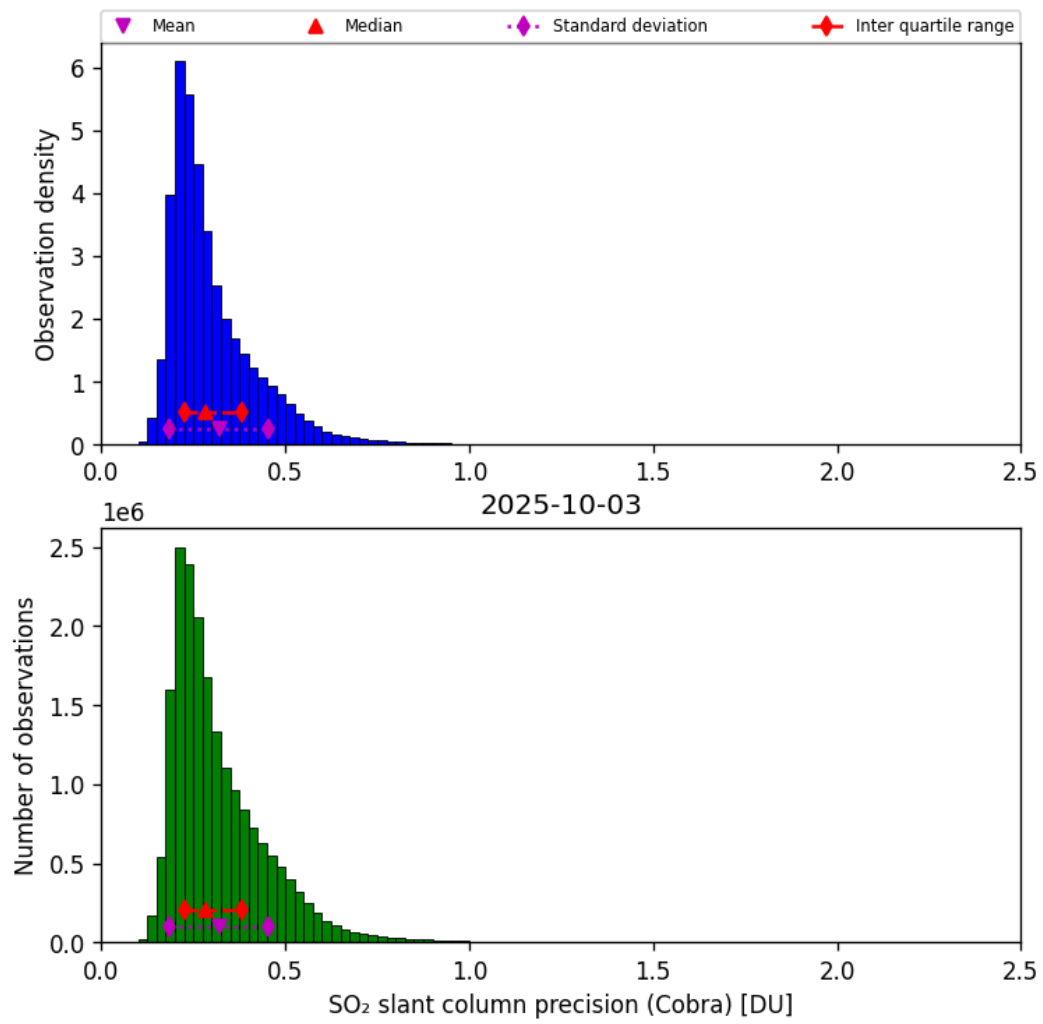
Figure 62: Histogram of “SO 2 slant column precision (Cobra)” for 2025-10-02 to 2025-10-04
