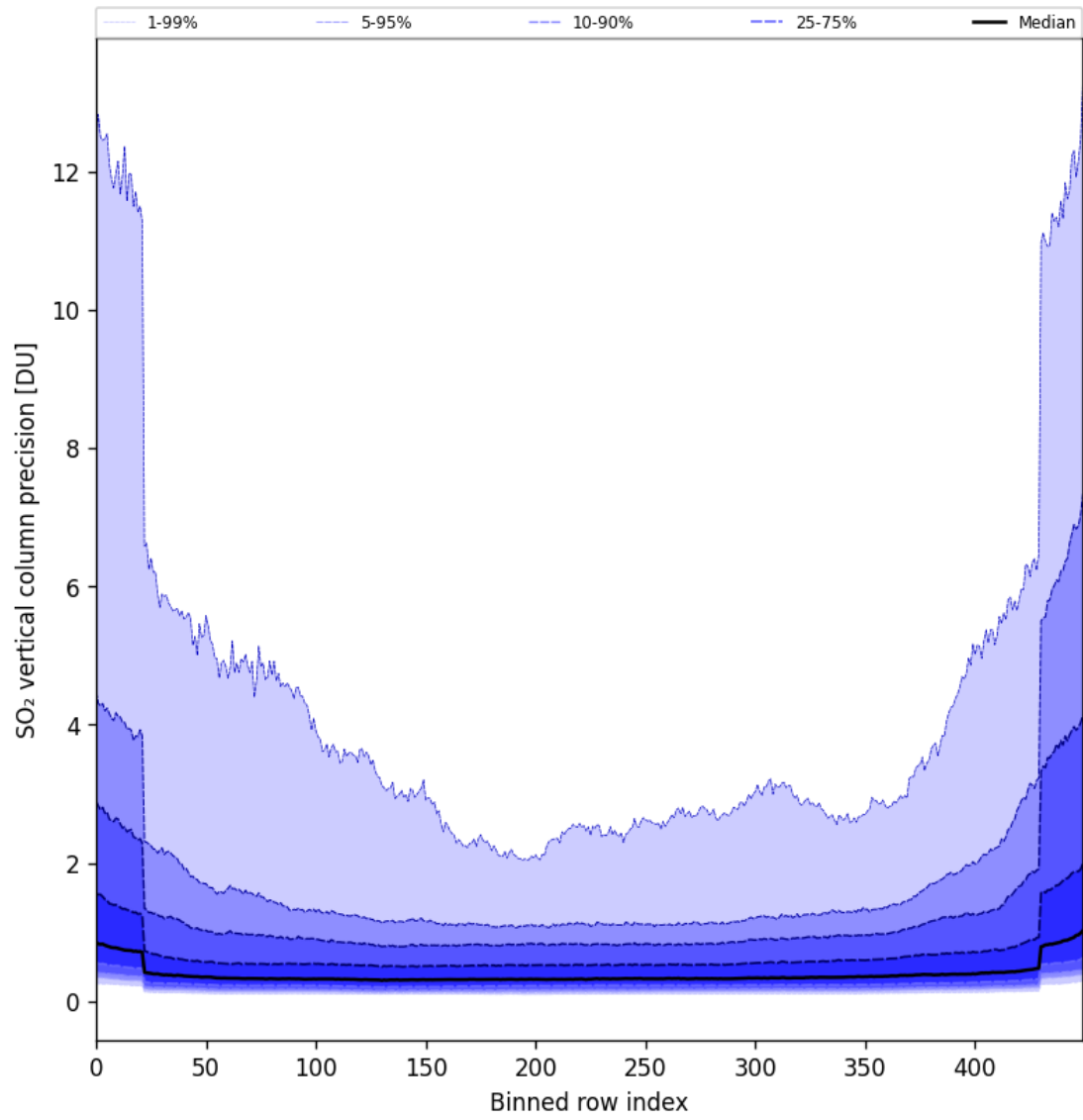
Figure 85: Along track statistics of “SO 2 vertical column precision” for 2025-10-02 to 2025-10-04
