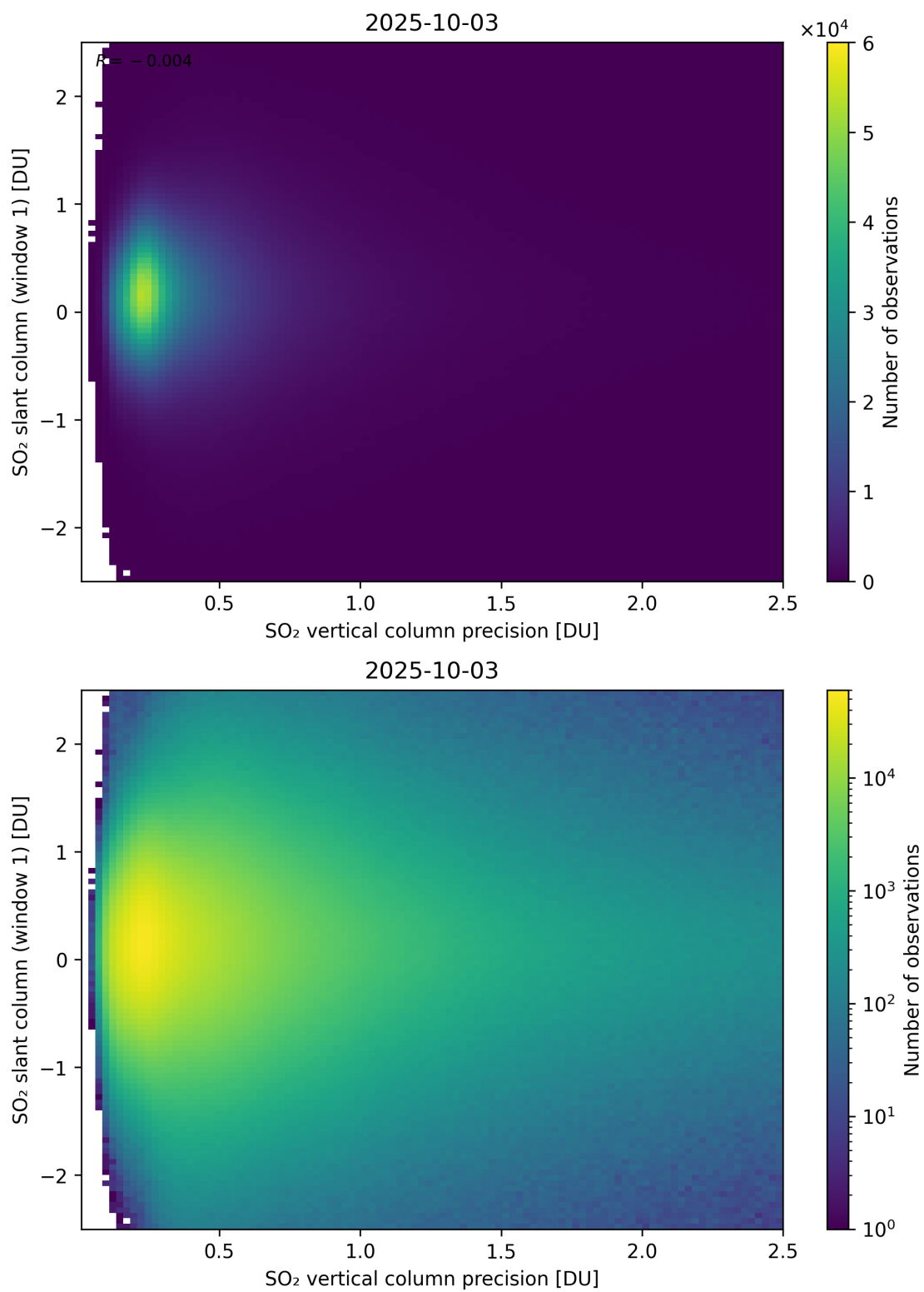
Figure 341: Scatter density plot of “SO 2 vertical column precision” against “SO 2 slant column (window 1)” for 2025-10-02 to 2025-10-04.
