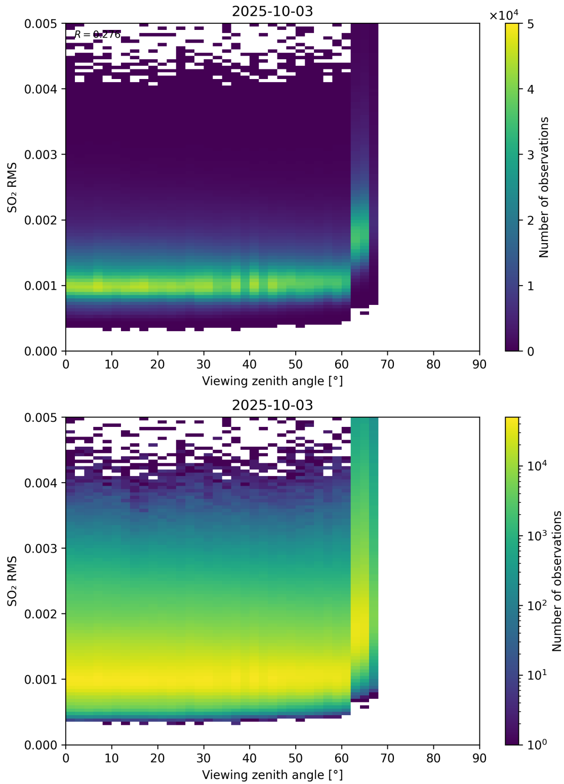
Figure 367: Scatter density plot of “Viewing zenith angle” against “SO 2 RMS” for 2025-10-02 to 2025-10-04.
