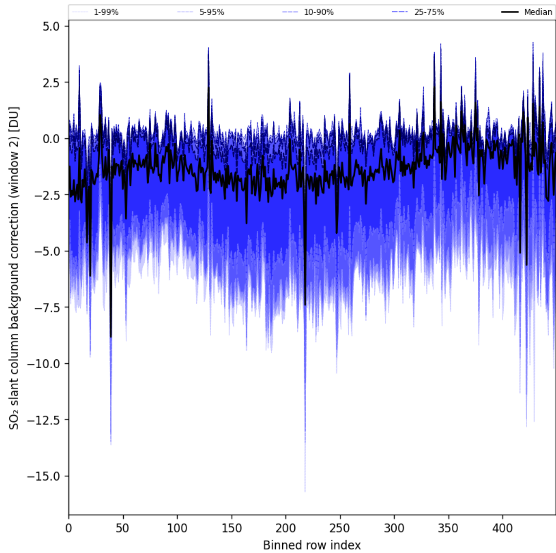
Figure 96: Along track statistics of “SO 2 slant column background correction (window 2)” for 2025-10-02 to 2025-10-04
