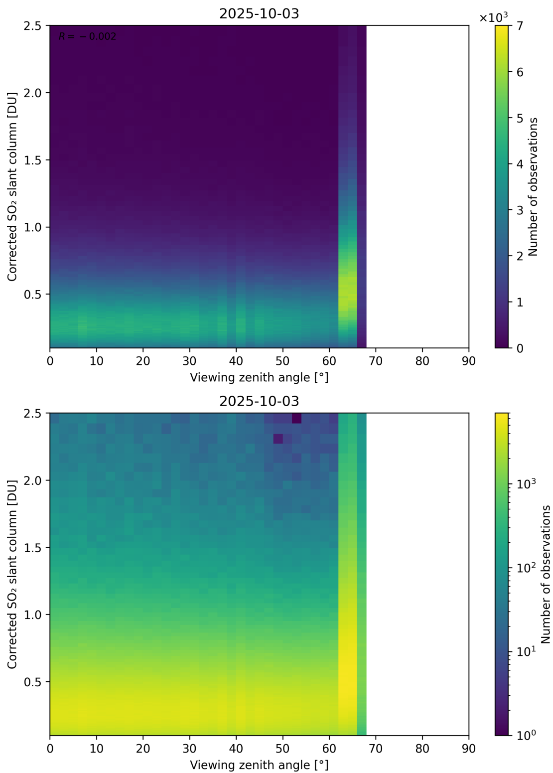
Figure 373: Scatter density plot of “Viewing zenith angle” against “Corrected SO 2 slant column” for 2025-10-02 to 2025-10-04.
