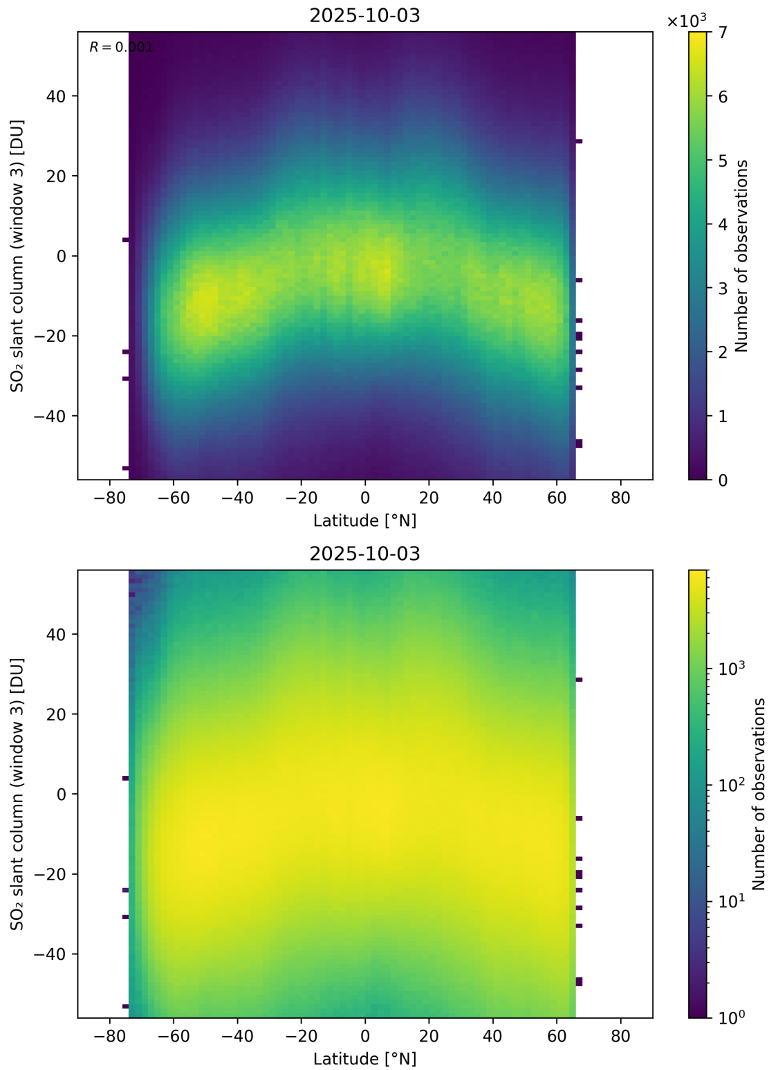
Figure 165: Scatter density plot of “Latitude” against “SO 2 slant column (window 3)” for 2025-10-02 to 2025-10-04.
