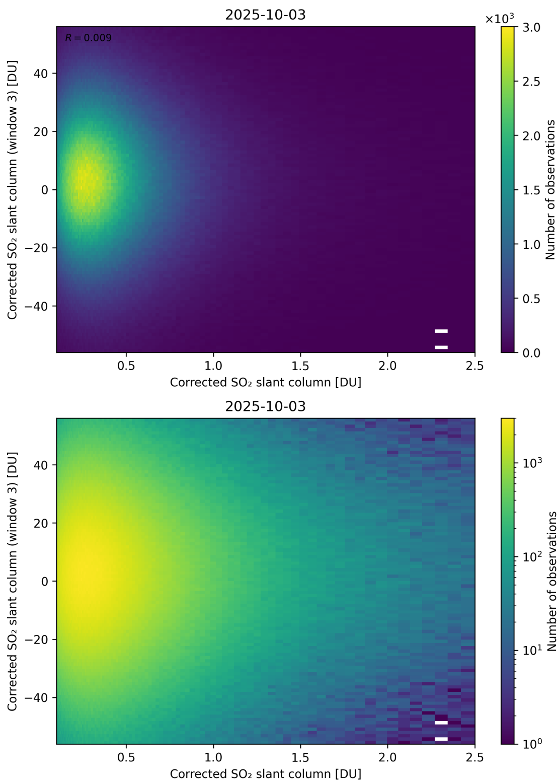
Figure 236: Scatter density plot of “Corrected SO 2 slant column” against “Corrected SO 2 slant column (window 3)” for 2025-10-02 to 2025-10-04.
