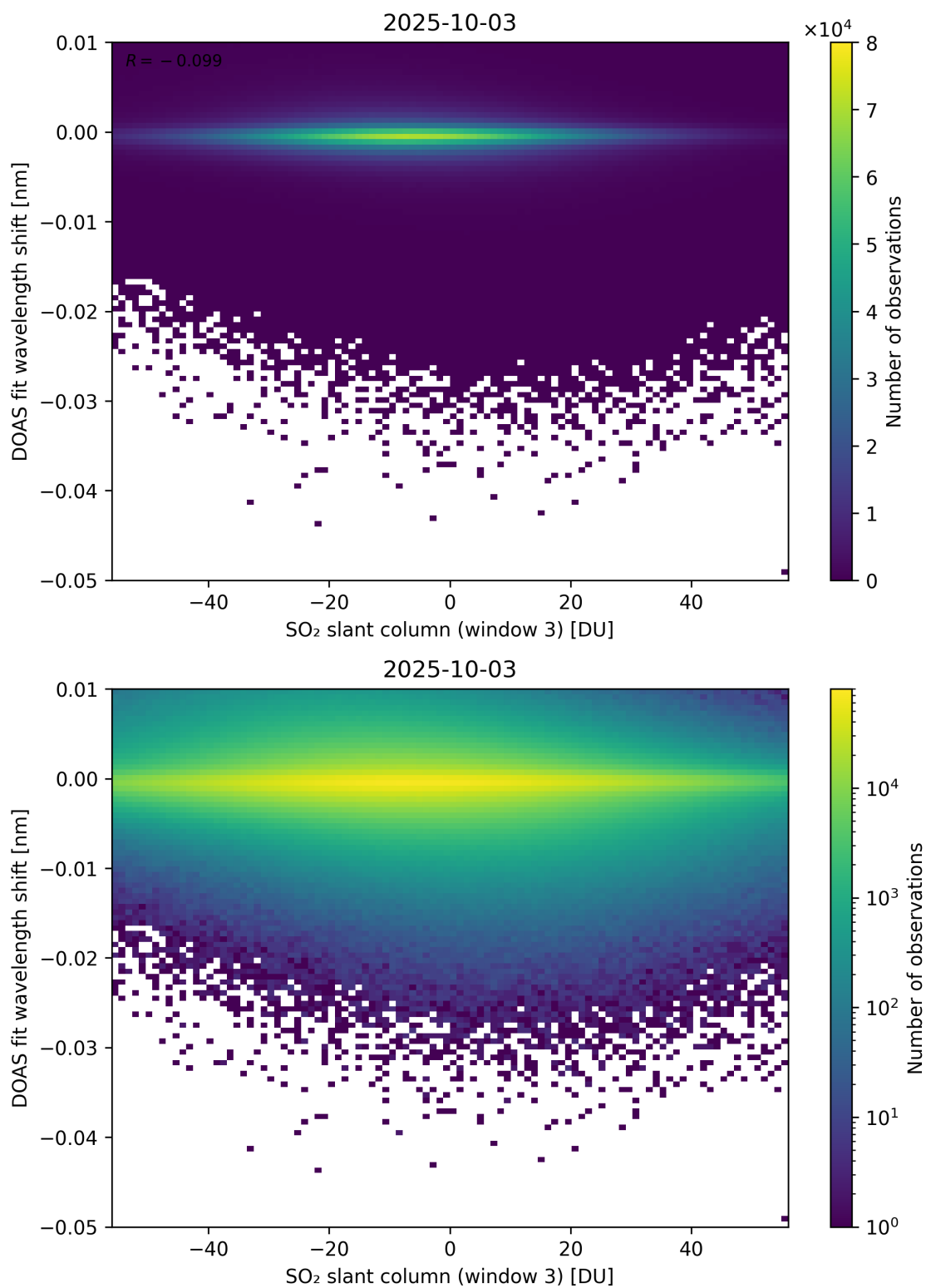
Figure 304: Scatter density plot of “SO 2 slant column (window 3)” against “DOAS fit wavelength shift” for 2025-10-02 to 2025-10-04.
