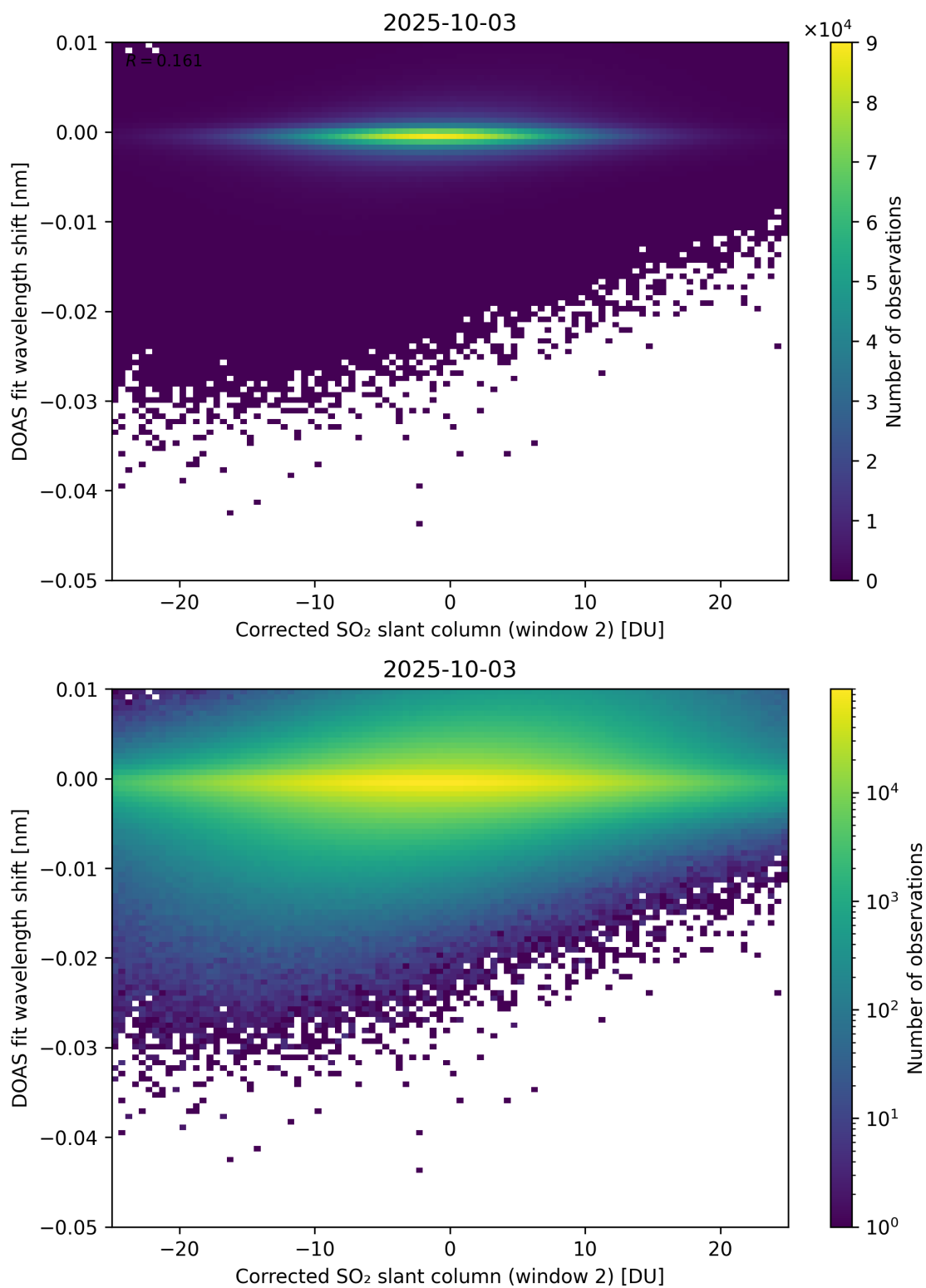
Figure 246: Scatter density plot of “Corrected SO 2 slant column (window 2)” against “DOAS fit wavelength shift” for 2025-10-02 to 2025-10-04.
