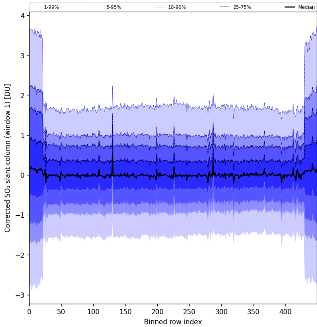
Figure 91: Along track statistics of “Corrected SO 2 slant column (window 1)” for 2025-10-02 to 2025-10-04
