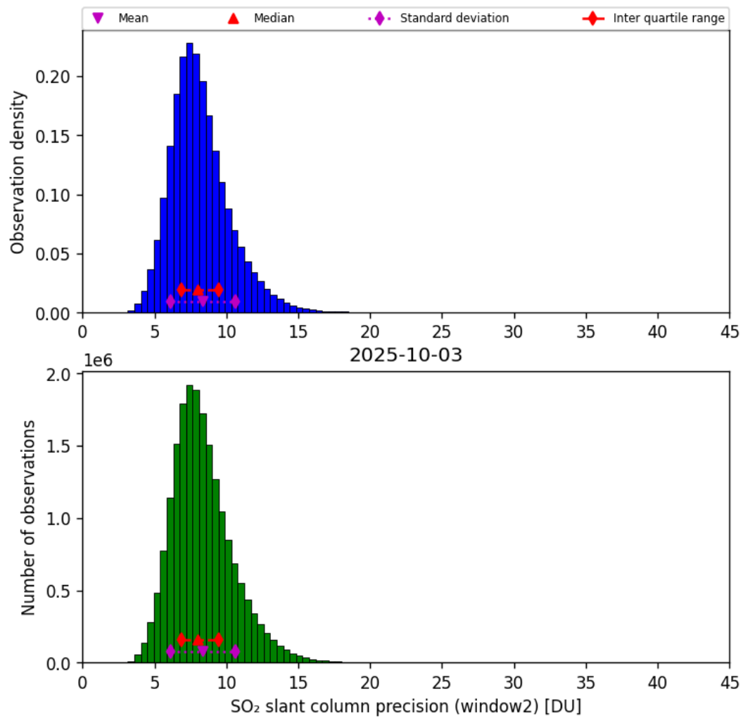
Figure 68: Histogram of “SO 2 slant column precision (window2)” for 2025-10-02 to 2025-10-04
