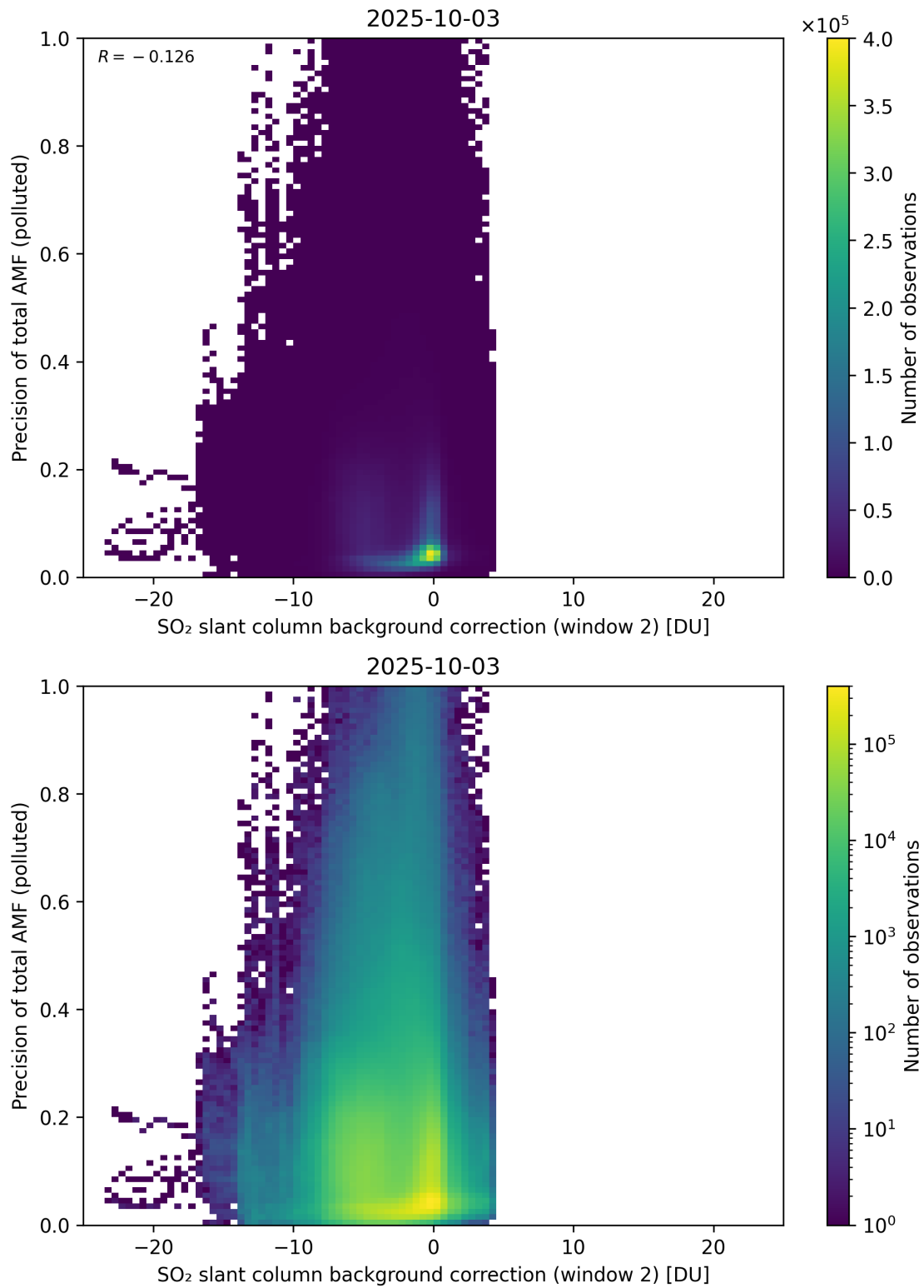
Figure 131: Scatter density plot of “SO 2 slant column background correction (window 2)” against “Precision of total AMF (polluted)” for 2025-10-02 to 2025-10-04.
