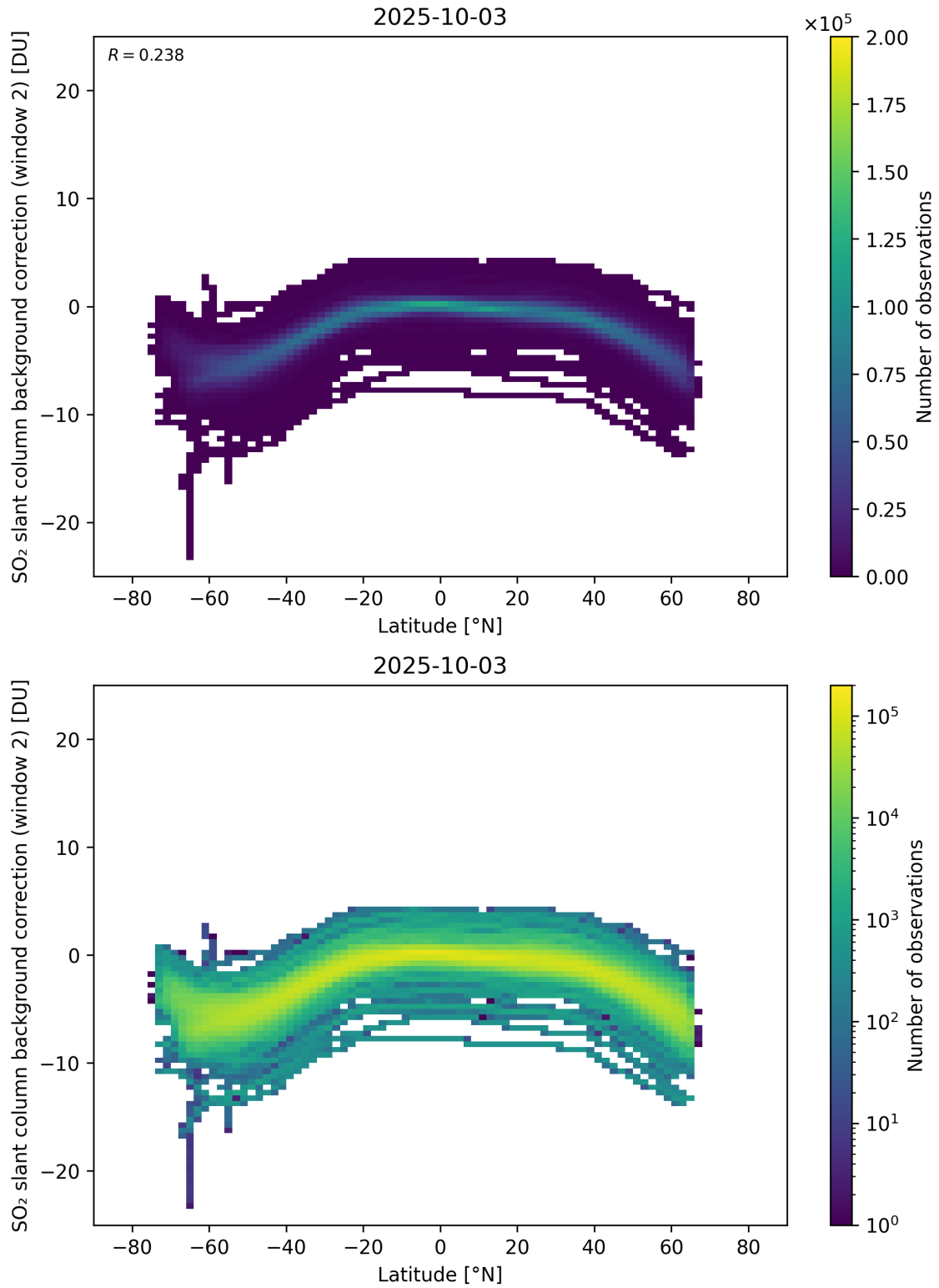
Figure 151: Scatter density plot of “Latitude” against “SO 2 slant column background correction (window 2)” for 2025-10-02 to 2025-10-04.
