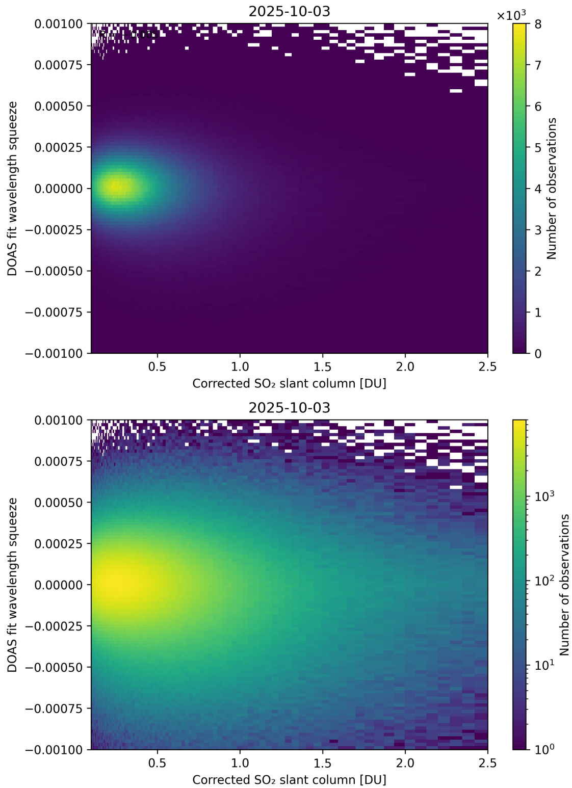
Figure 230: Scatter density plot of "Corrected SO 2 slant column" against "DOAS fit wavelength squeeze" for 2025-10-02 to 2025-10-04.
