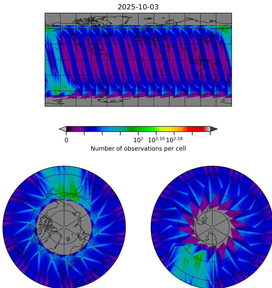
Figure 30: Map of the number of observations for 2025-10-02 to 2025-10-04
