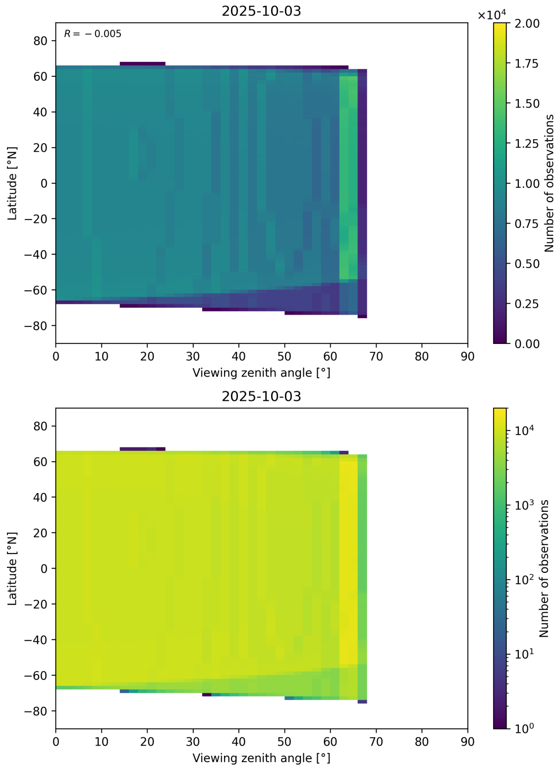
Figure 368: Scatter density plot of “Viewing zenith angle” against “Latitude” for 2025-10-02 to 2025-10-04.
