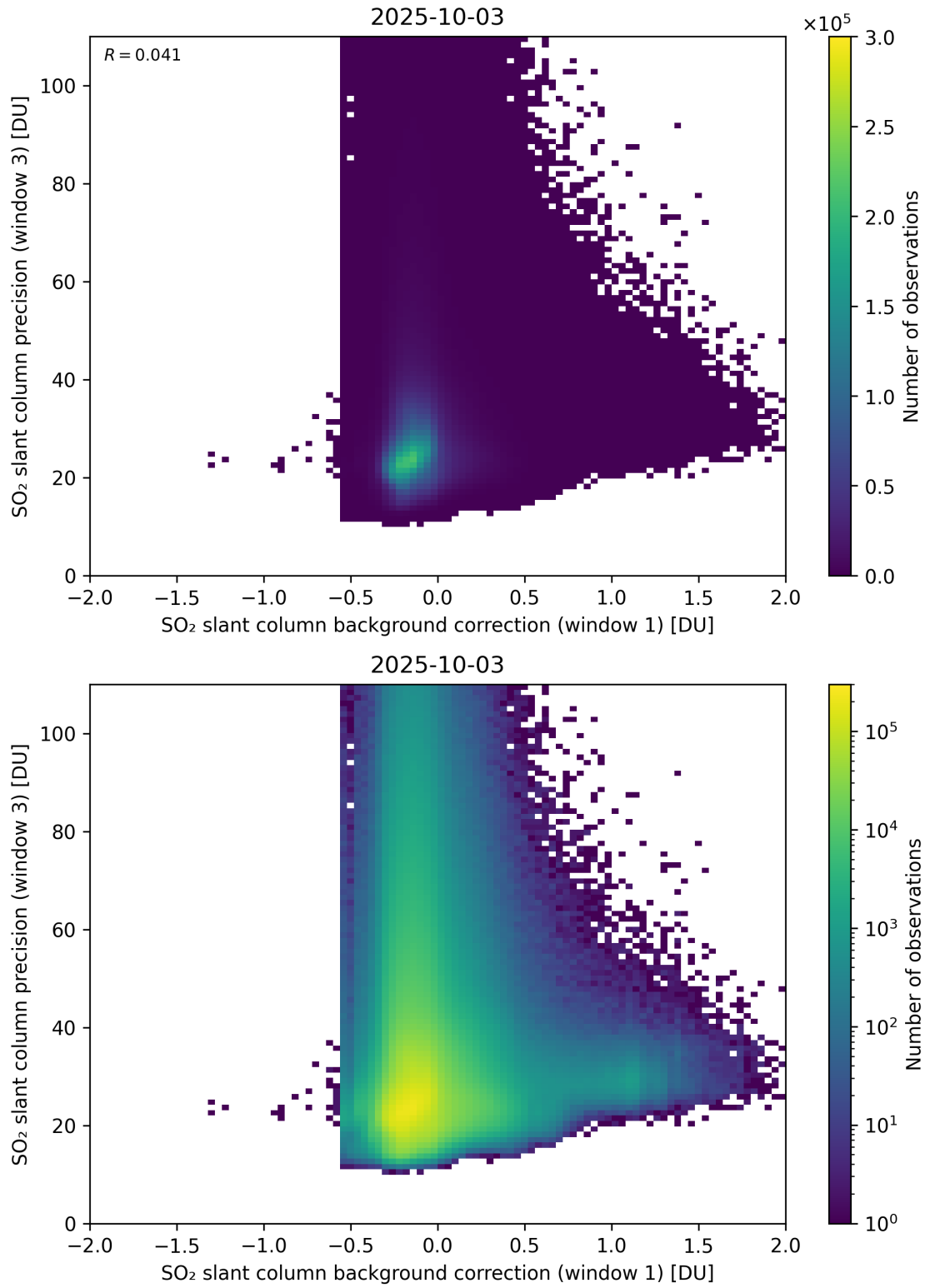
Figure 119: Scatter density plot of “SO 2 slant column background correction (window 1)” against “SO 2 slant column precision (window 3)” for 2025-10-02 to 2025-10-04.
