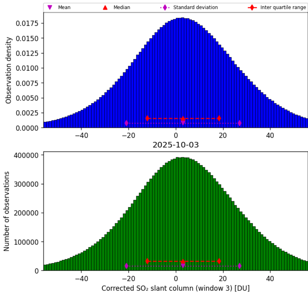
Figure 73: Histogram of “Corrected SO 2 slant column (window 3)” for 2025-10-02 to 2025-10-04
