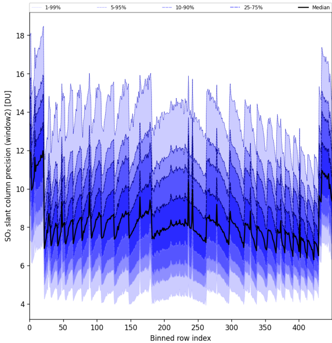
Figure 94: Along track statistics of “SO 2 slant column precision (window2)” for 2025-10-02 to 2025-10-04
