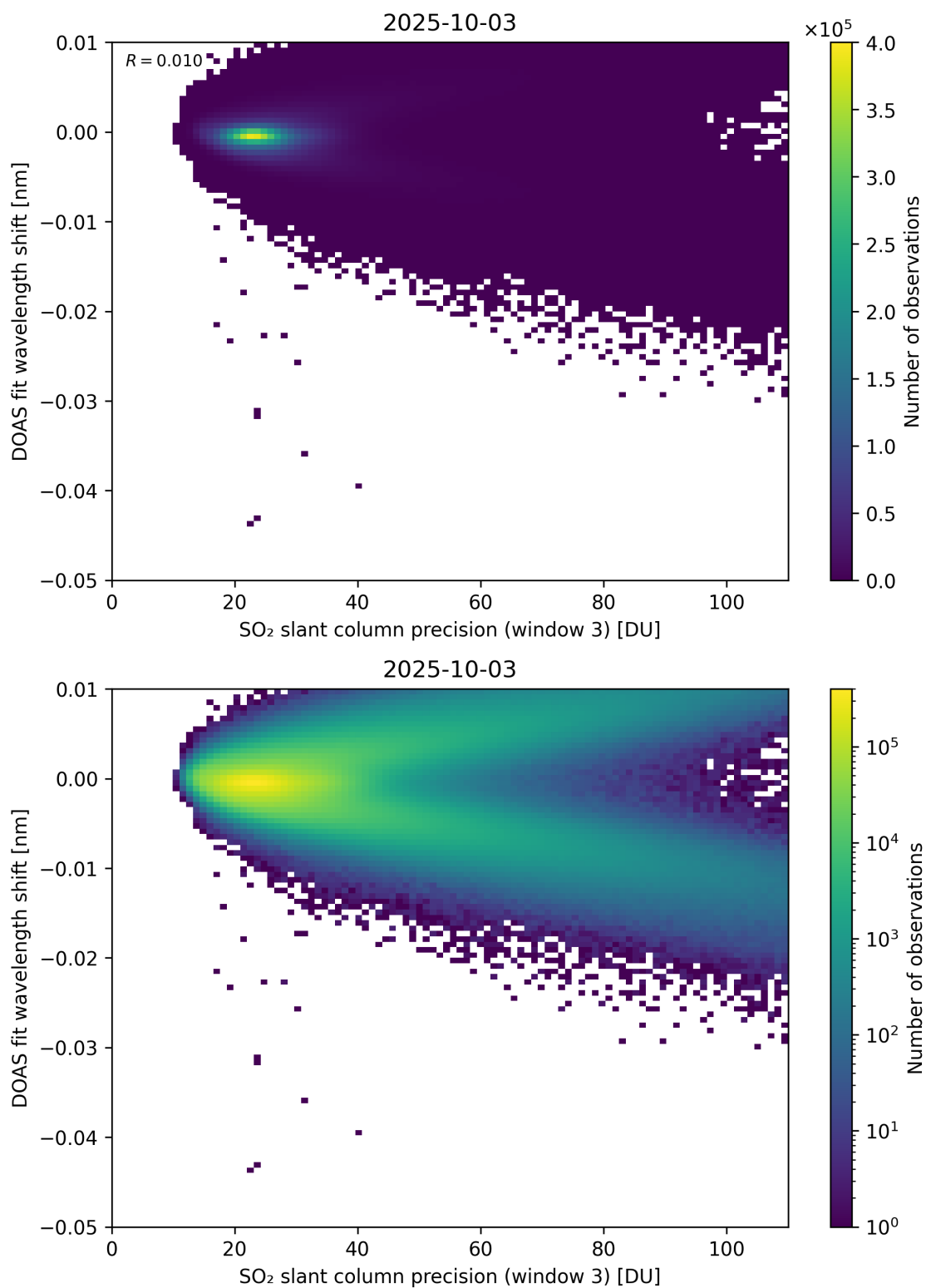
Figure 308: Scatter density plot of “SO 2 slant column precision (window 3)” against “DOAS fit wavelength shift” for 2025-10-02 to 2025-10-04.
