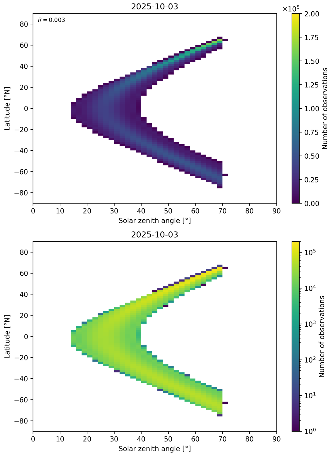
Figure 177: Scatter density plot of “Solar zenith angle” against “Latitude” for 2025-10-02 to 2025-10-04.
