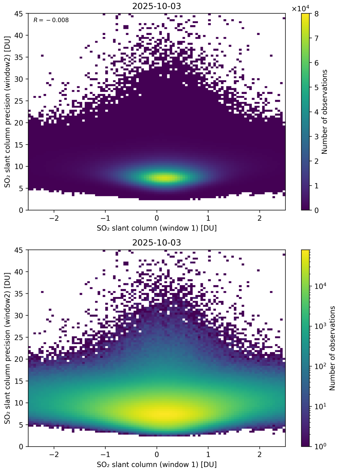
Figure 286: Scatter density plot of “SO 2 slant column (window 1)” against “SO 2 slant column precision (window2)” for 2025-10-02 to 2025-10-04.
