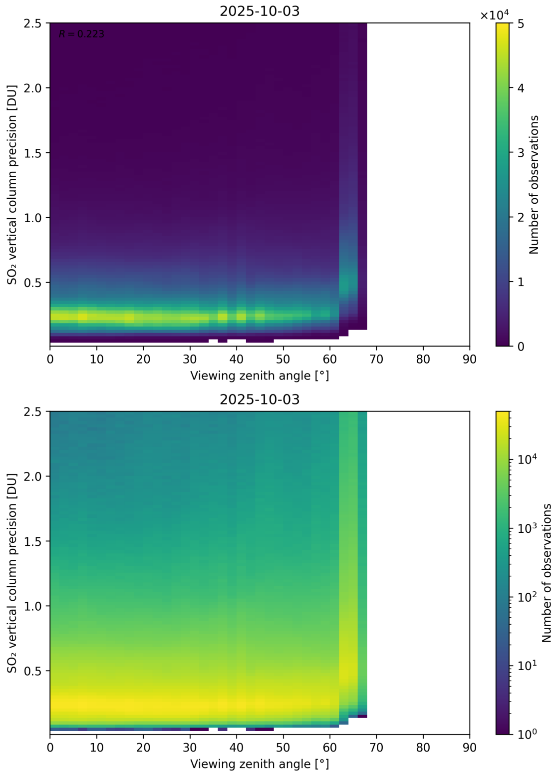
Figure 384: Scatter density plot of “Viewing zenith angle” against “SO 2 vertical column precision” for 2025-10-02 to 2025-10-04.
