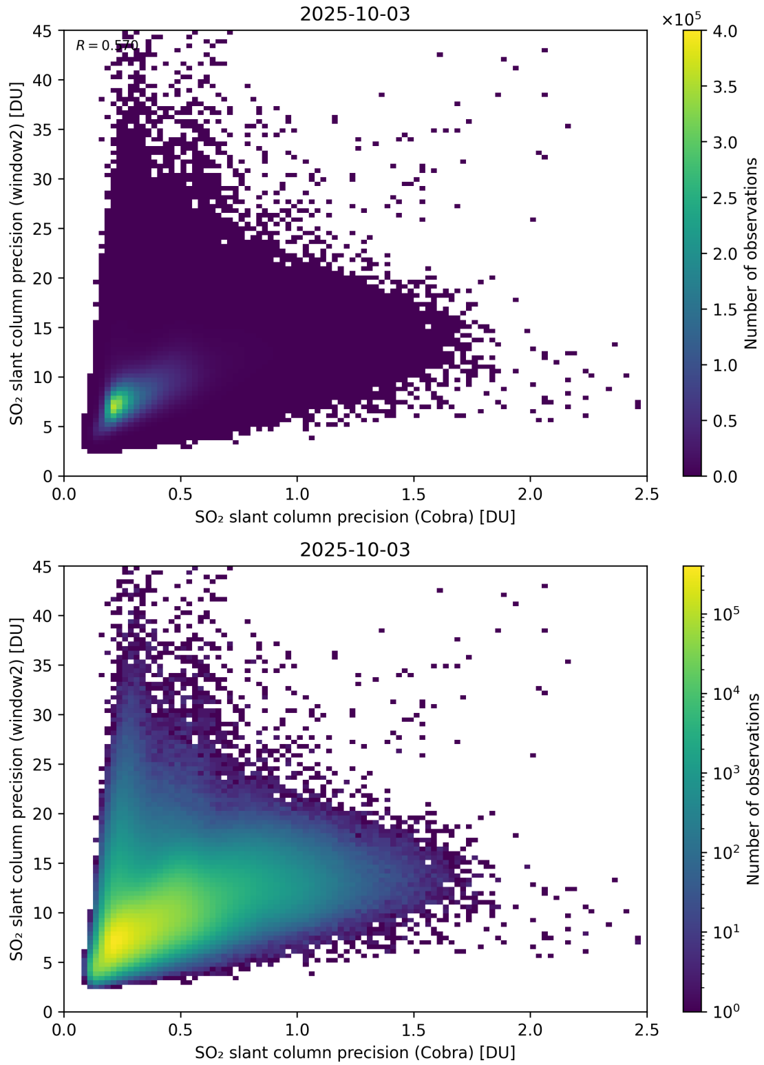
Figure 210: Scatter density plot of “SO 2 slant column precision (Cobra)” against “SO 2 slant column precision (window2)” for 2025-10-02 to 2025-10-04.
