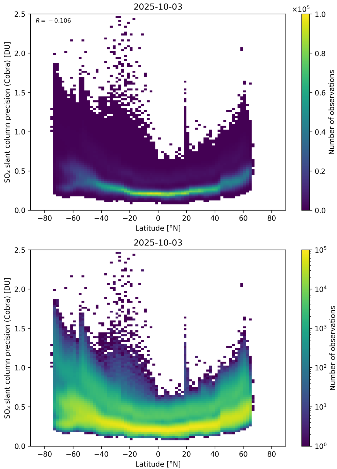
Figure 158: Scatter density plot of “Latitude” against “SO 2 slant column precision (Cobra)” for 2025-10-02 to 2025-10-04.
