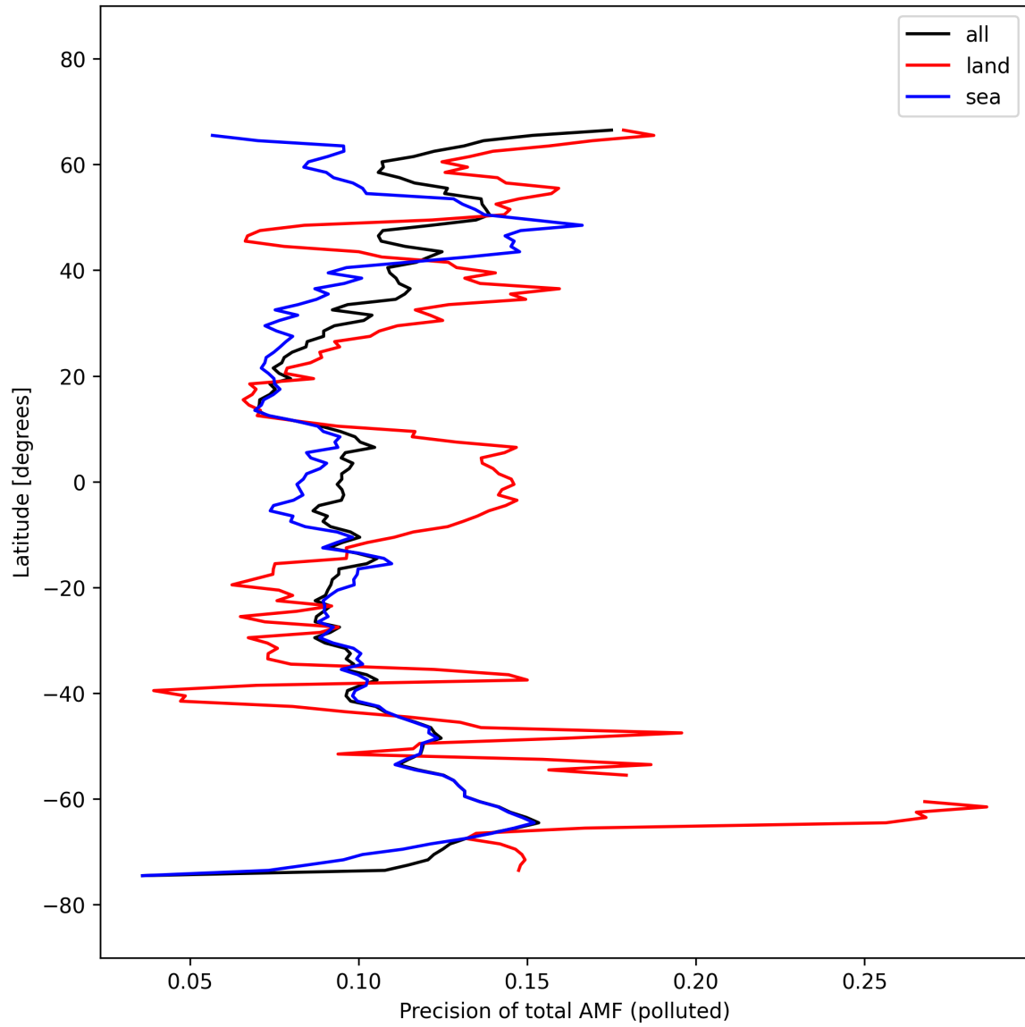
Figure 54: Zonal average of “Precision of total AMF (polluted)” for 2025-10-02 to 2025-10-04.
