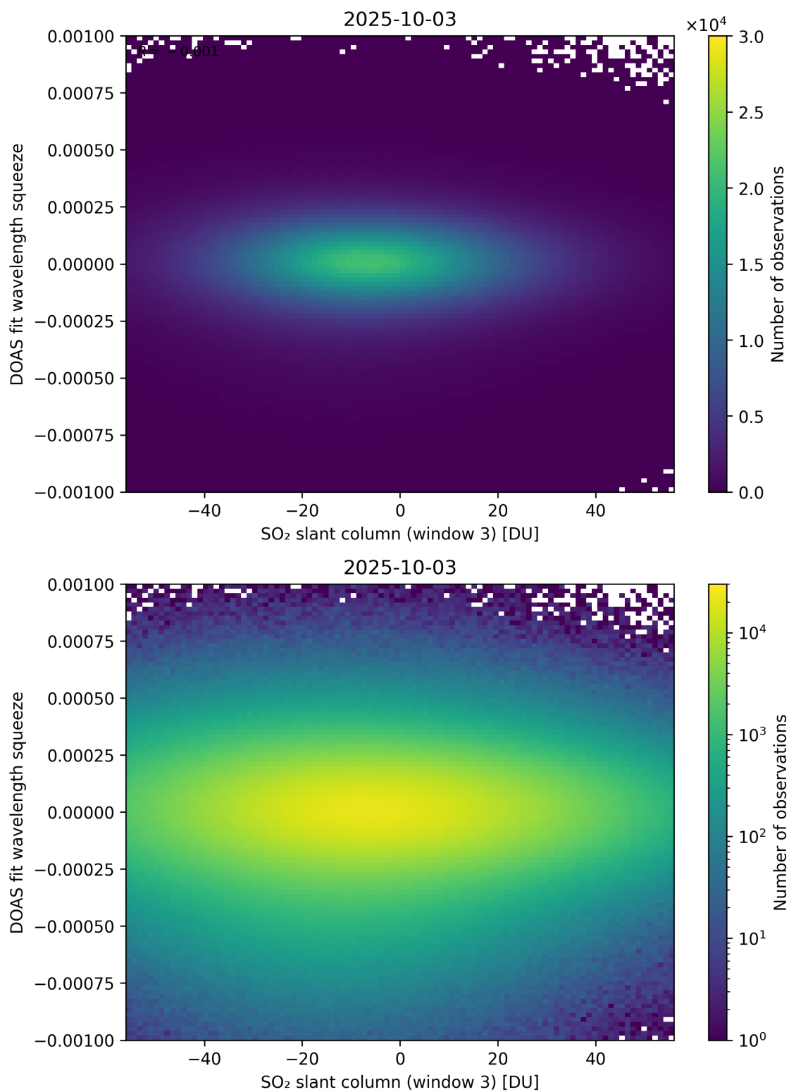
Figure 305: Scatter density plot of “SO 2 slant column (window 3)” against “DOAS fit wavelength squeeze” for 2025-10-02 to 2025-10-04.
