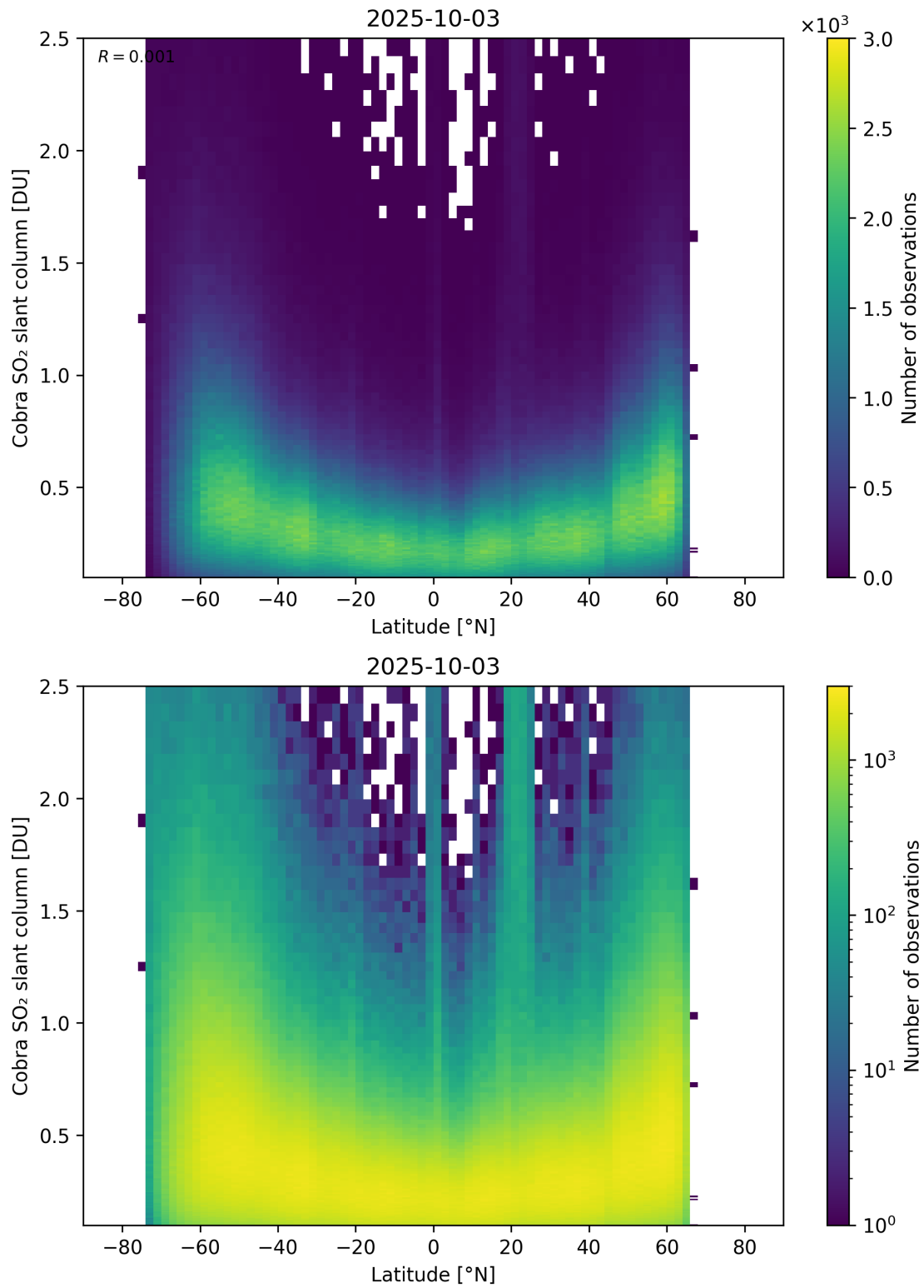
Figure 157: Scatter density plot of “Latitude” against “Cobra SO 2 slant column” for 2025-10-02 to 2025-10-04.
