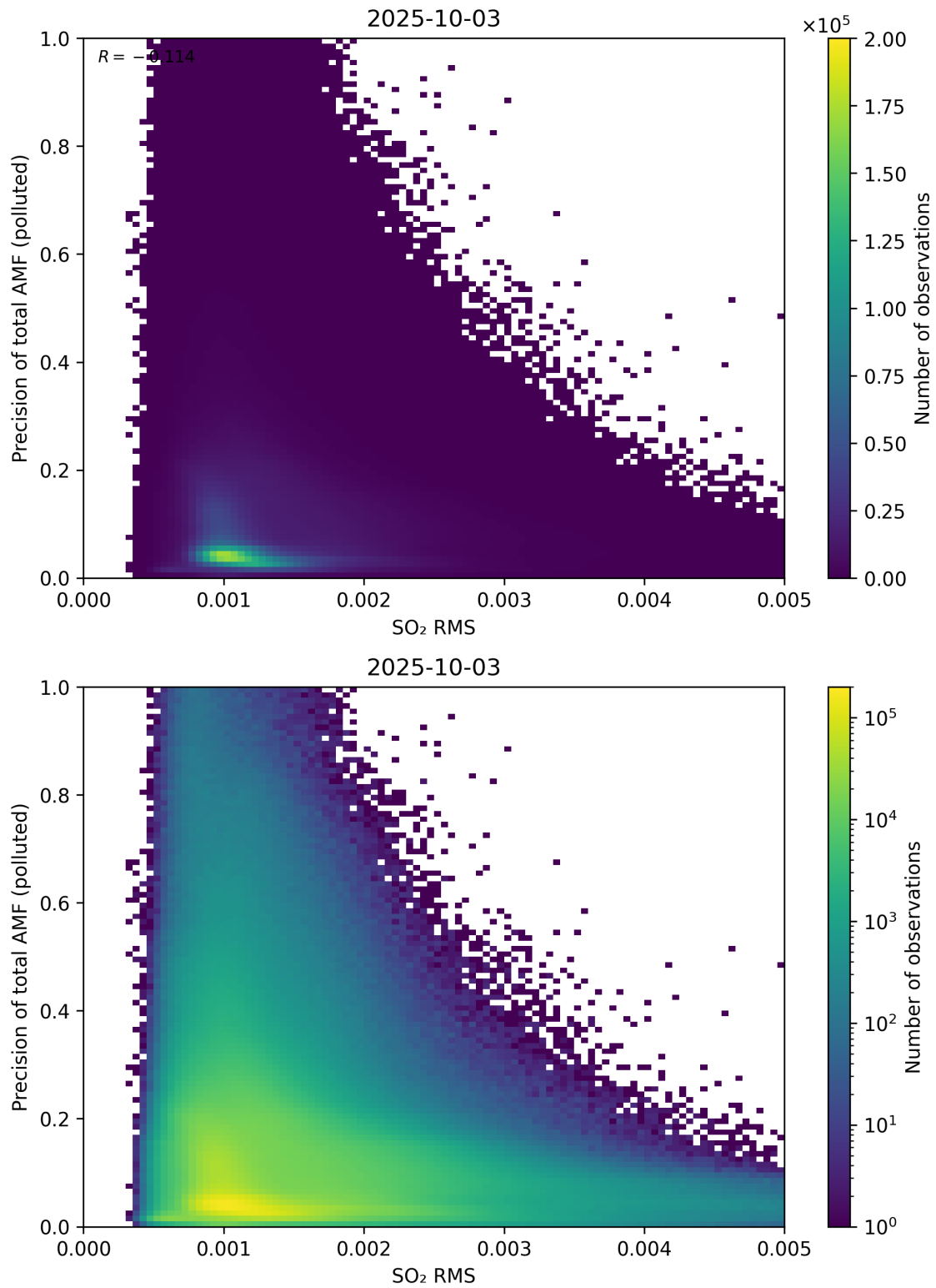
Figure 149: Scatter density plot of “SO 2 RMS” against “Precision of total AMF (polluted)” for 2025-10-02 to 2025-10-04.
