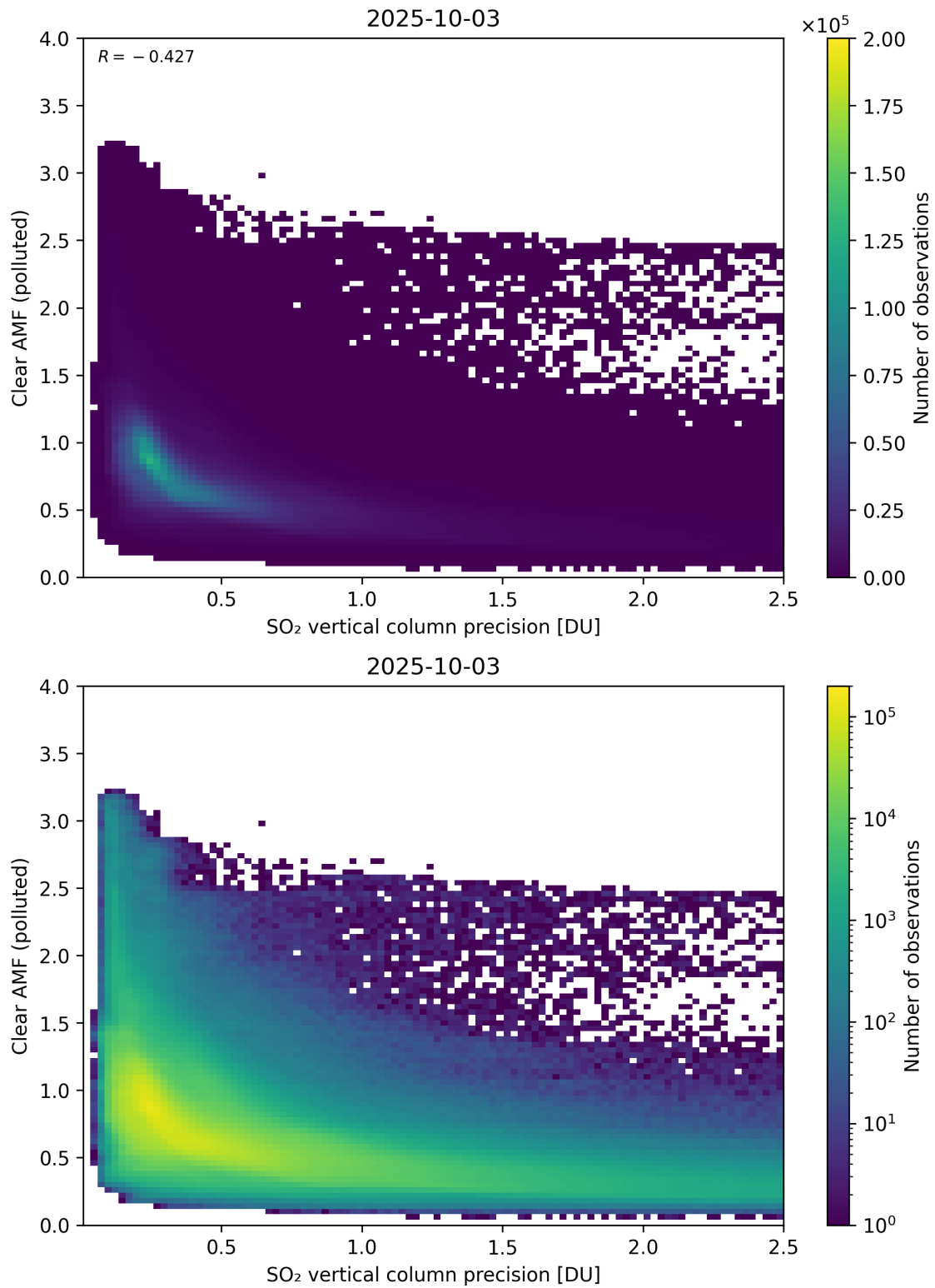
Figure 335: Scatter density plot of “SO 2 vertical column precision” against “Clear AMF (polluted)” for 2025-10-02 to 2025-10-04.
