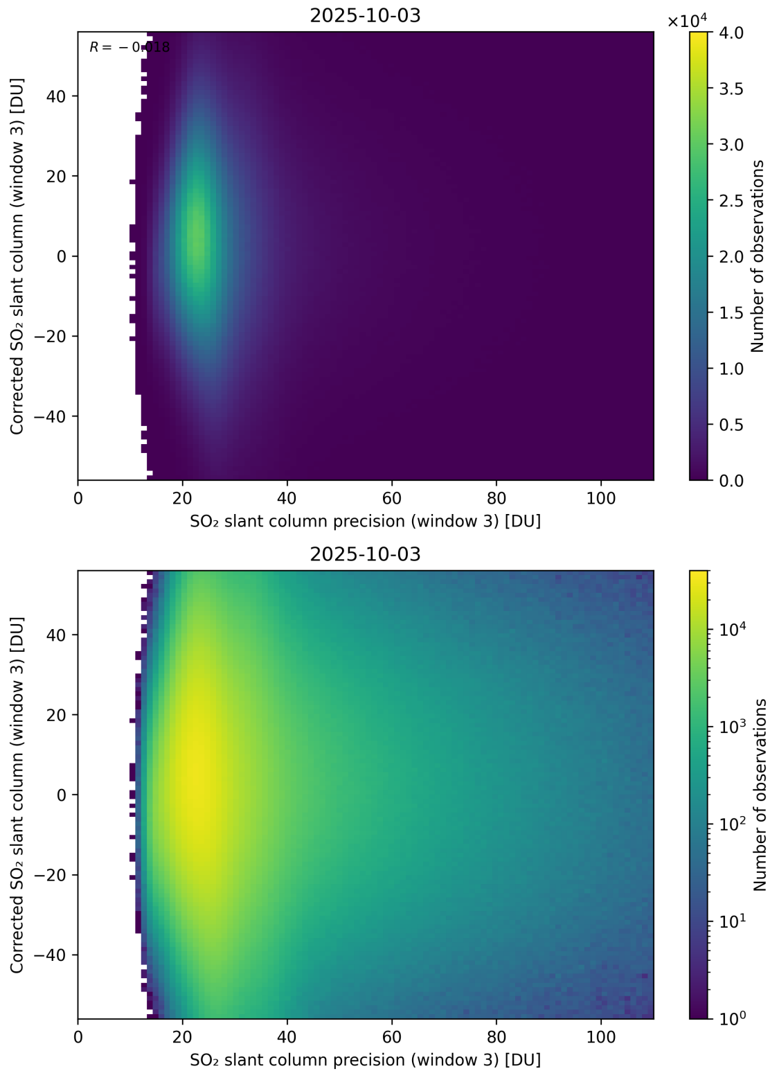
Figure 312: Scatter density plot of “SO 2 slant column precision (window 3)” against “Corrected SO 2 slant column (window 3)” for 2025-10-02 to 2025-10-04.
