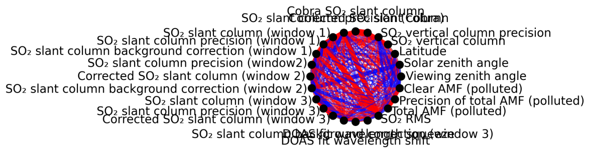
Figure 1: Map of correlation graph for 2025-10-02 to 2025-10-04.
