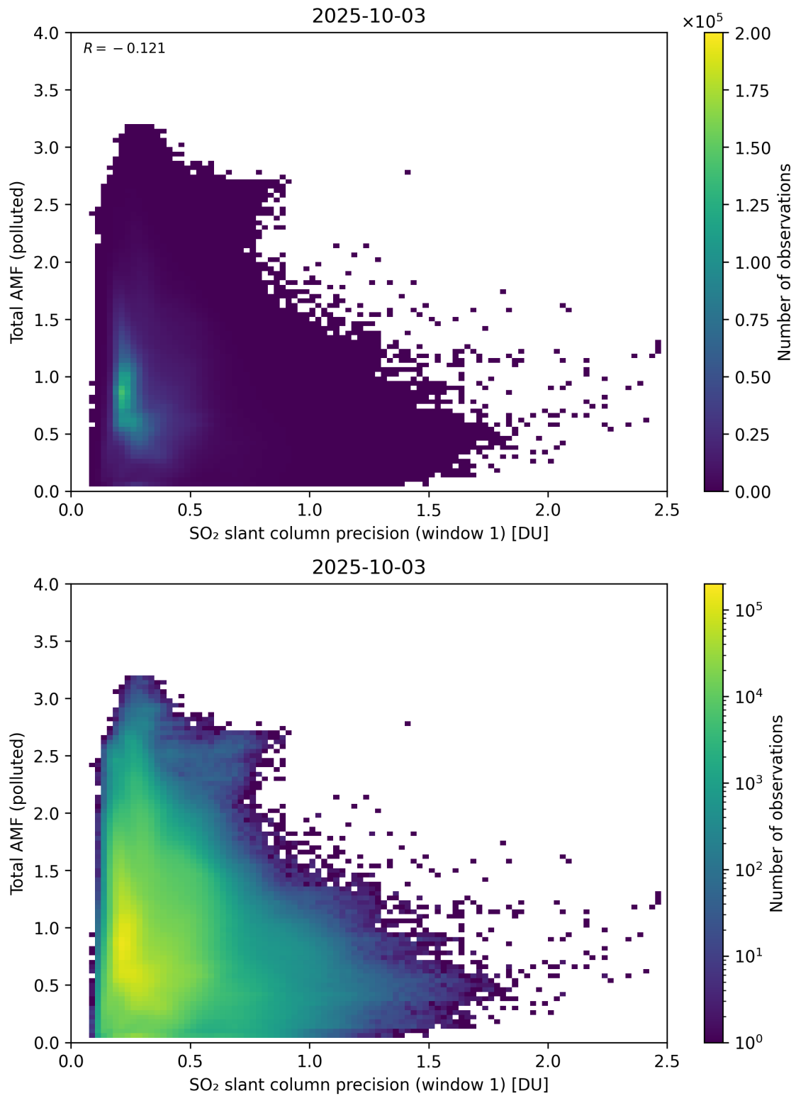
Figure 280: Scatter density plot of “SO 2 slant column precision (window 1)” against “Total AMF (polluted)” for 2025-10-02 to 2025-10-04.
