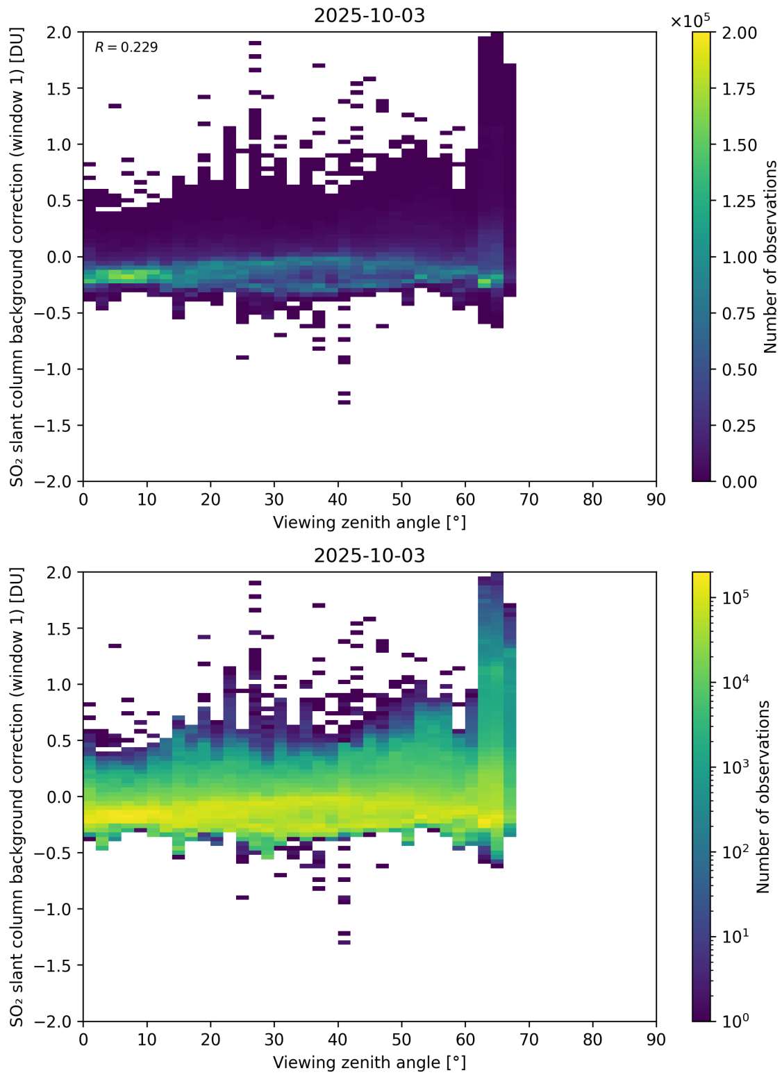
Figure 362: Scatter density plot of “Viewing zenith angle” against “SO 2 slant column background correction (window 1)” for 2025-10-02 to 2025-10-04.
