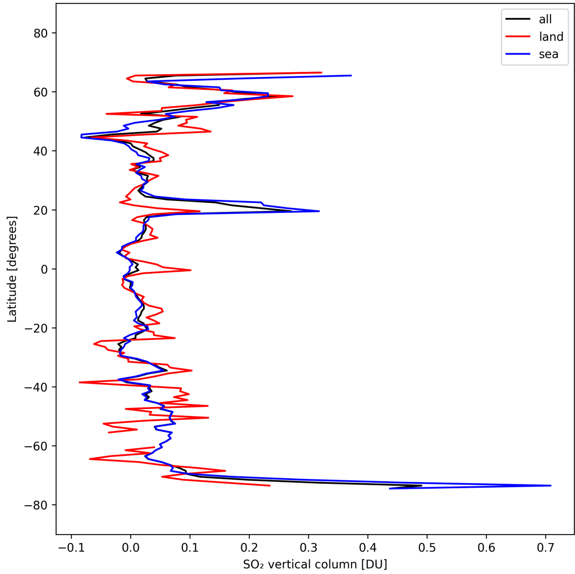
Figure 32: Zonal average of “SO 2 vertical column” for 2025-10-02 to 2025-10-04.
