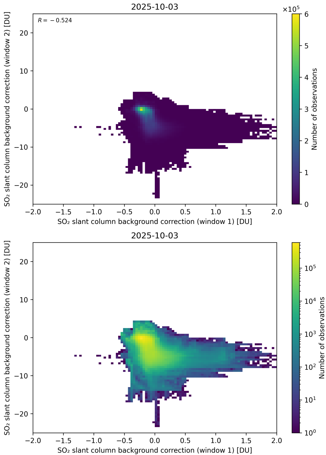
Figure 109: Scatter density plot of “SO 2 slant column background correction (window 1)” against “SO 2 slant column background correction (window 2)” for 2025-10-02 to 2025-10-04.
