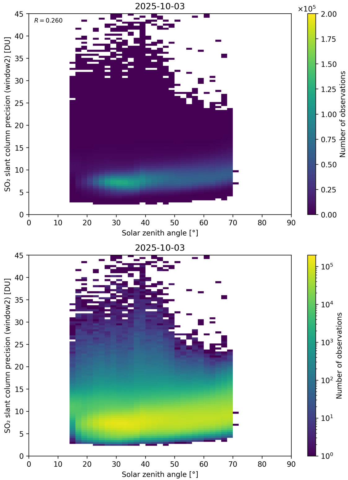
Figure 186: Scatter density plot of “Solar zenith angle” against “SO 2 slant column precision (window2)” for 2025-10-02 to 2025-10-04.
