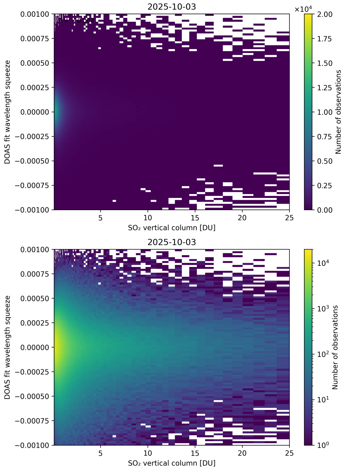
Figure 327: Scatter density plot of “SO 2 vertical column” against “DOAS fit wavelength squeeze” for 2025-10-02 to 2025-10-04.
