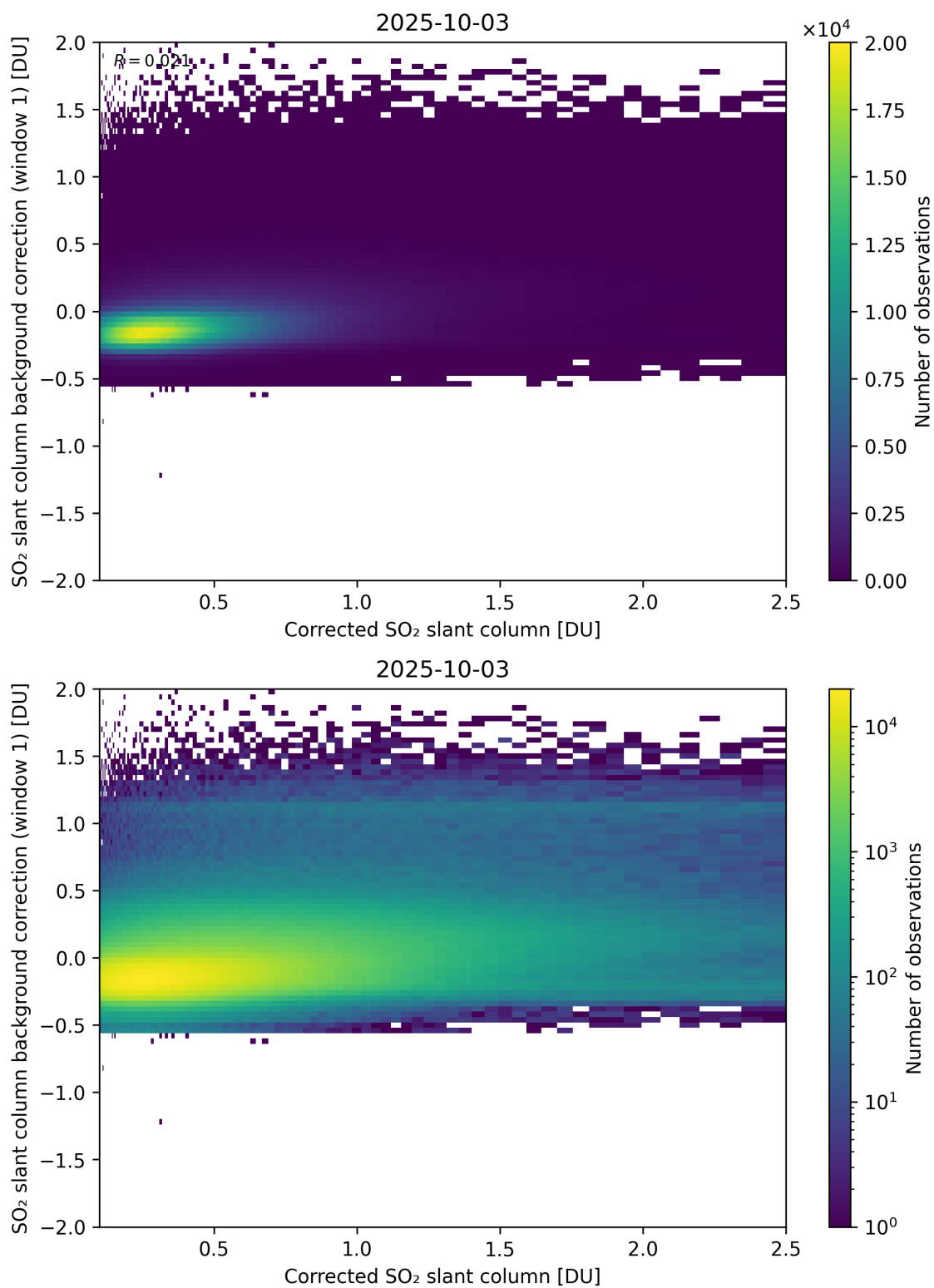
Figure 226: Scatter density plot of “Corrected SO 2 slant column” against “SO 2 slant column background correction (window 1)” for 2025-10-02 to 2025-10-04.
