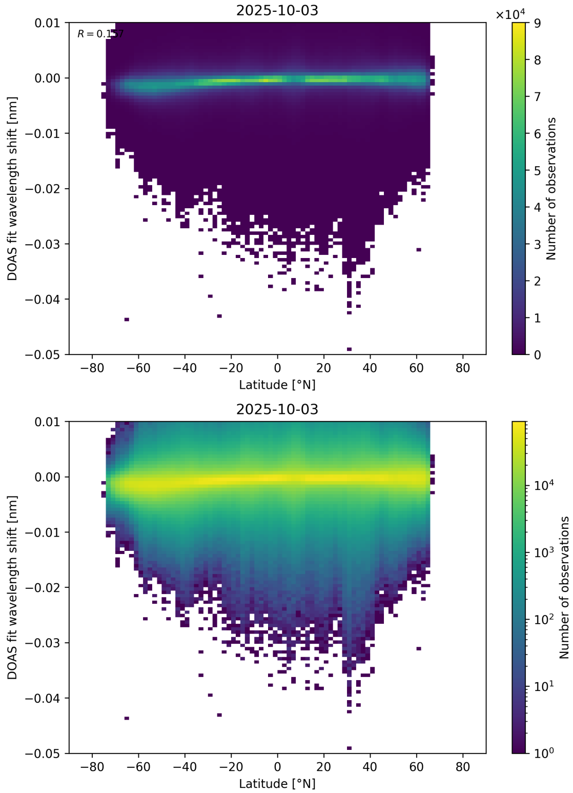
Figure 153: Scatter density plot of “Latitude” against “DOAS fit wavelength shift” for 2025-10-02 to 2025-10-04.
