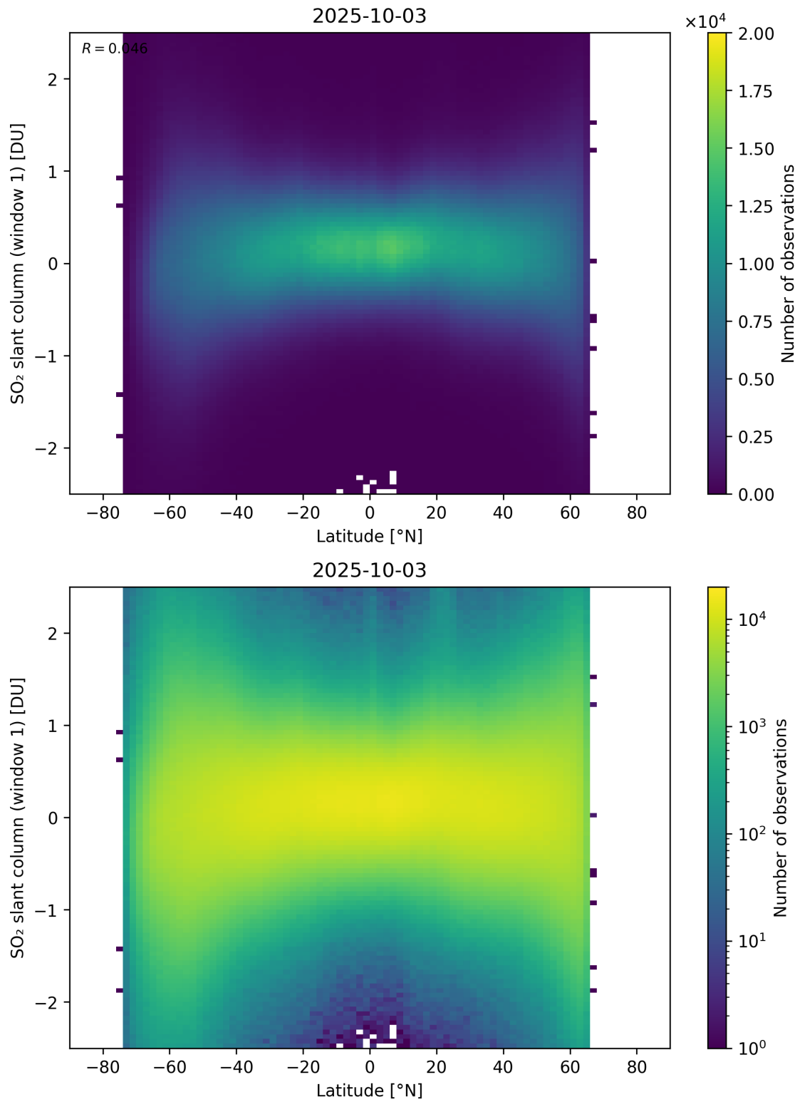
Figure 162: Scatter density plot of “Latitude” against “SO 2 slant column (window 1)” for 2025-10-02 to 2025-10-04.
