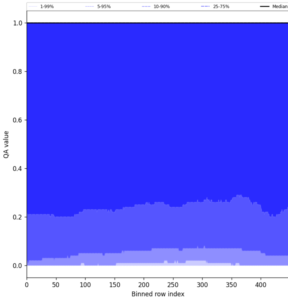
Figure 83: Along track statistics of “QA value” for 2025-10-02 to 2025-10-04
