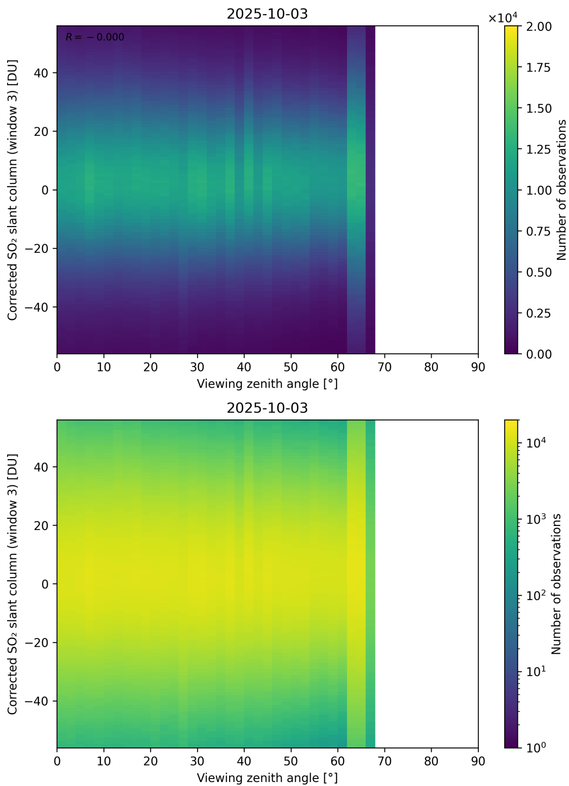
Figure 375: Scatter density plot of “Viewing zenith angle” against “Corrected SO 2 slant column (window 3)” for 2025-10-02 to 2025-10-04.
