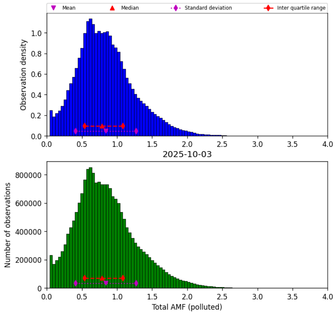
Figure 79: Histogram of “Total AMF (polluted)” for 2025-10-02 to 2025-10-04
