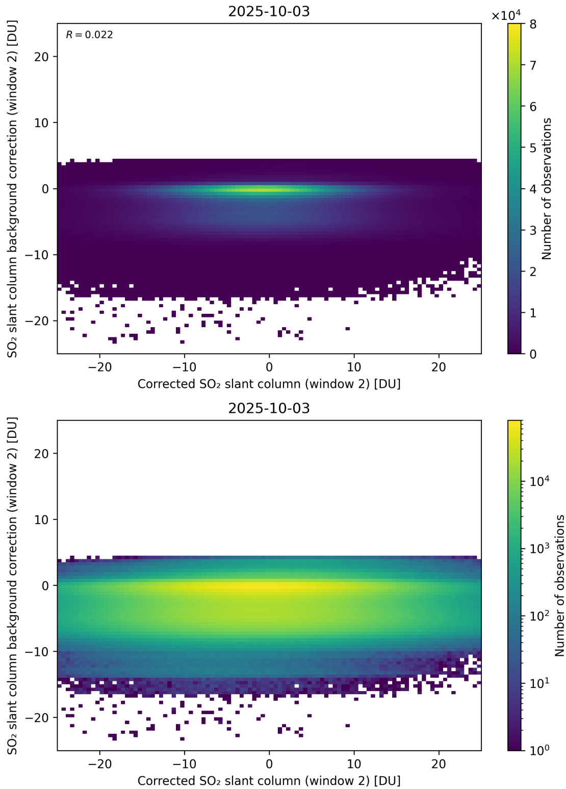
Figure 244: Scatter density plot of “Corrected SO 2 slant column (window 2)” against “SO 2 slant column background correction (window 2)” for 2025-10-02 to 2025-10-04.
