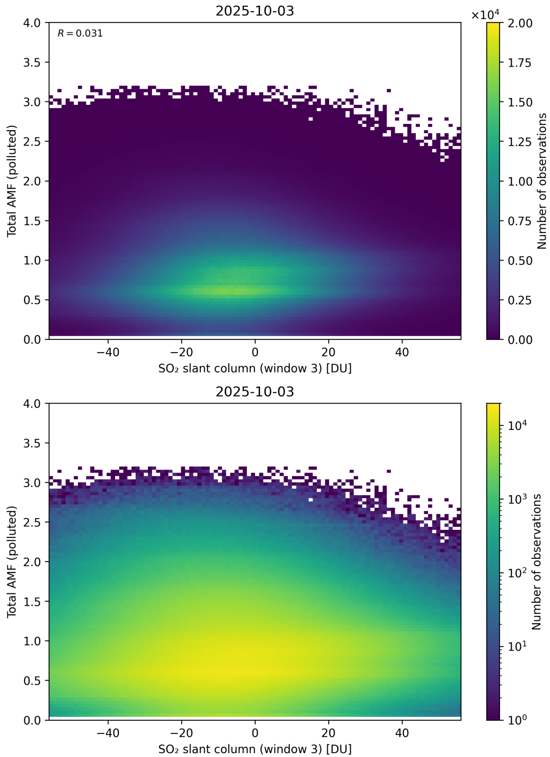
Figure 318: Scatter density plot of “SO 2 slant column (window 3)” against “Total AMF (polluted)” for 2025-10-02 to 2025-10-04.
