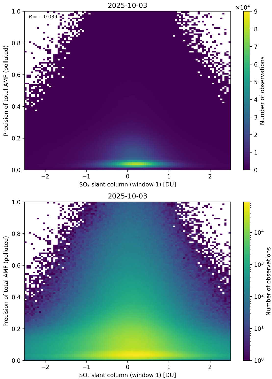
Figure 290: Scatter density plot of “SO 2 slant column (window 1)” against “Precision of total AMF (polluted)” for 2025-10-02 to 2025-10-04.
