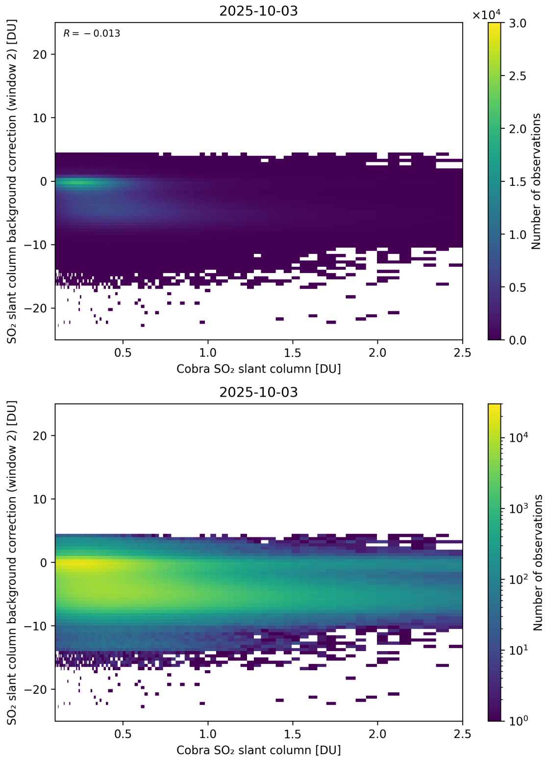
Figure 194: Scatter density plot of “Cobra SO 2 slant column” against “SO 2 slant column background correction (window 2)” for 2025-10-02 to 2025-10-04.
