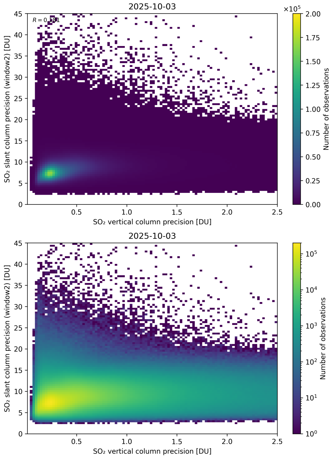
Figure 343: Scatter density plot of “SO 2 vertical column precision” against “SO 2 slant column precision (window2)” for 2025-10-02 to 2025-10-04.
