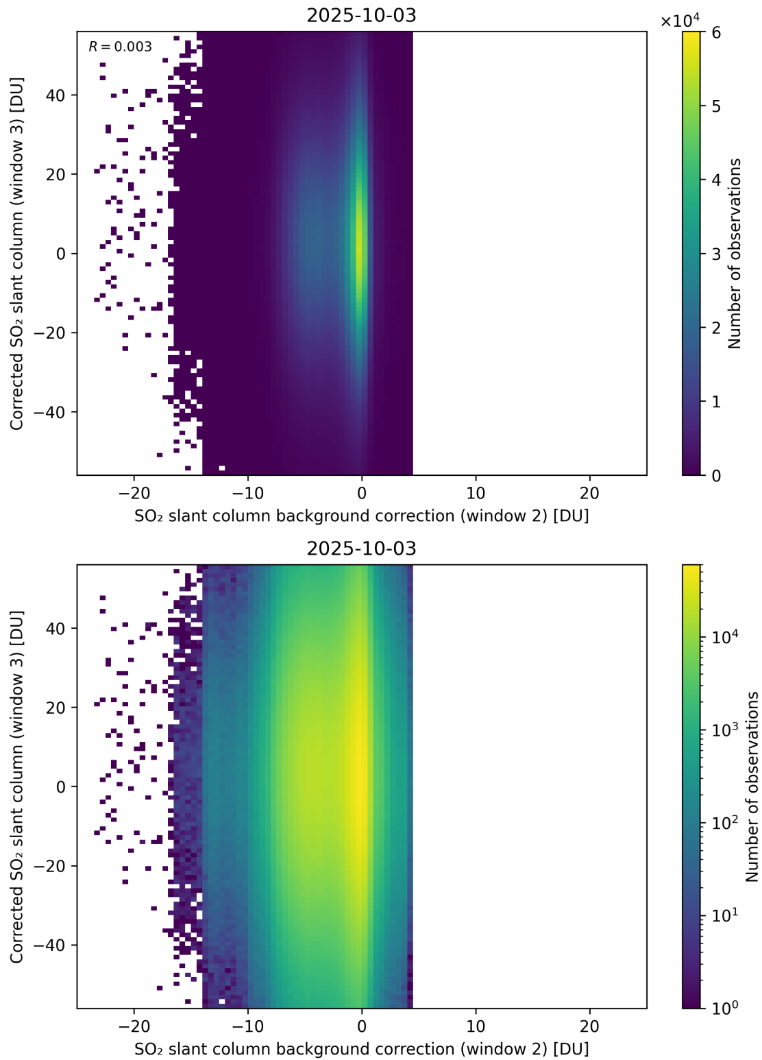
Figure 127: Scatter density plot of “SO 2 slant column background correction (window 2)” against “Corrected SO 2 slant column (window 3)” for 2025-10-02 to 2025-10-04.
