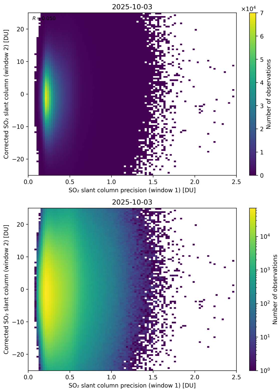
Figure 275: Scatter density plot of “SO 2 slant column precision (window 1)” against “Corrected SO 2 slant column (window 2)” for 2025-10-02 to 2025-10-04.
