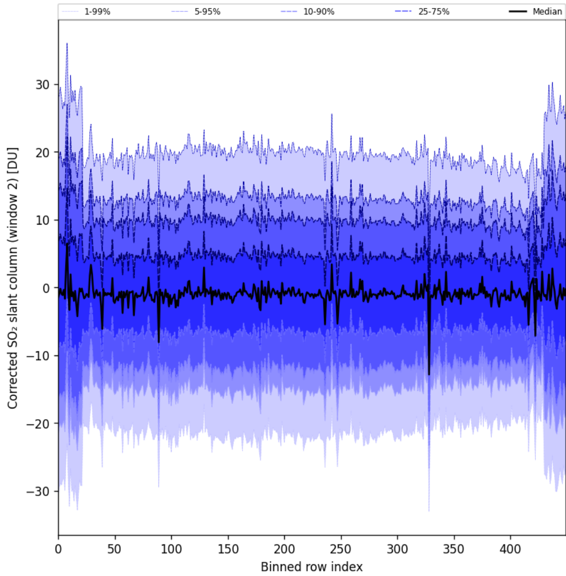
Figure 95: Along track statistics of “Corrected SO 2 slant column (window 2)” for 2025-10-02 to 2025-10-04
