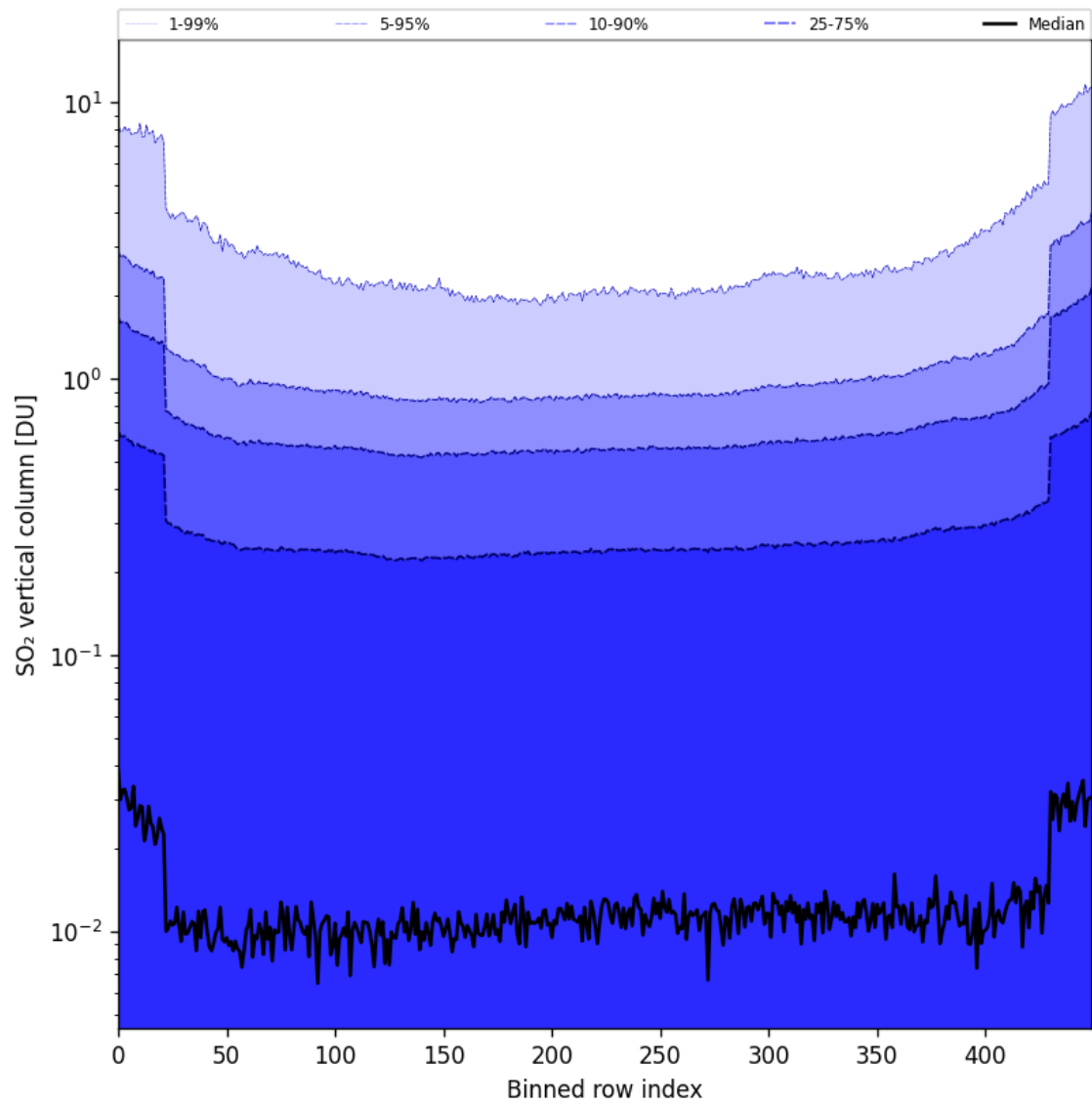
Figure 84: Along track statistics of “SO 2 vertical column” for 2025-10-02 to 2025-10-04
