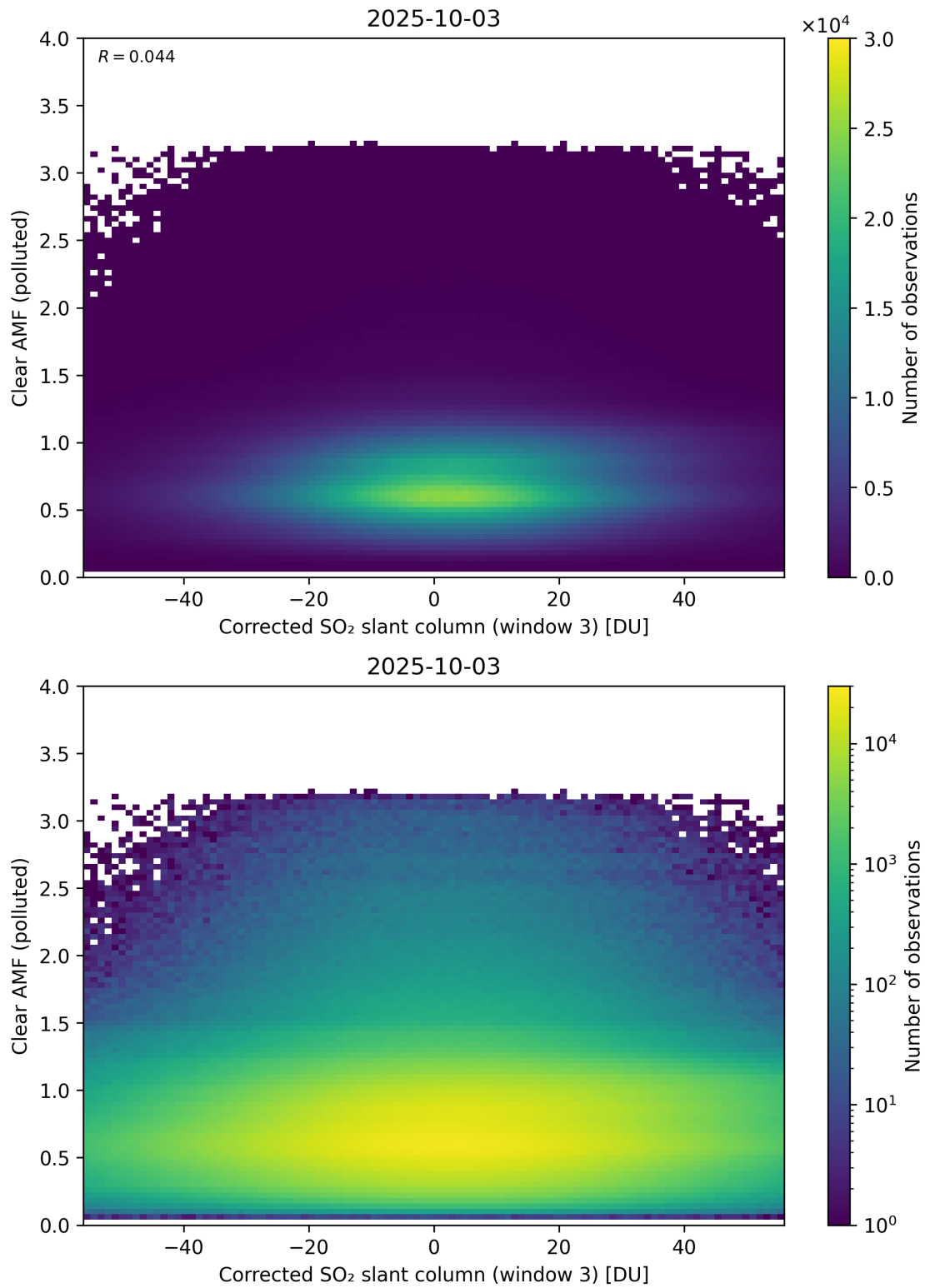
Figure 259: Scatter density plot of “Corrected SO 2 slant column (window 3)” against “Clear AMF (polluted)” for 2025-10-02 to 2025-10-04.
