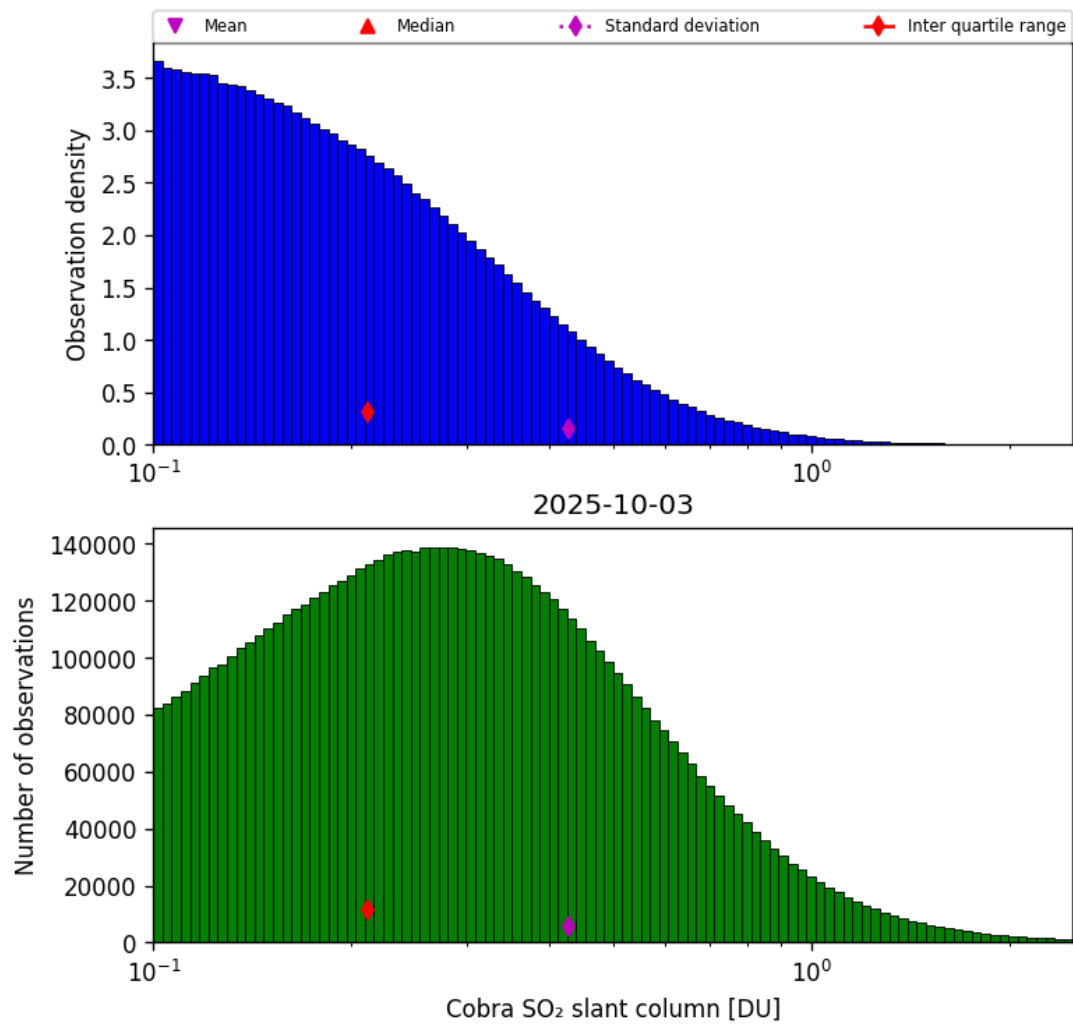
Figure 61: Histogram of “Cobra SO 2 slant column” for 2025-10-02 to 2025-10-04
