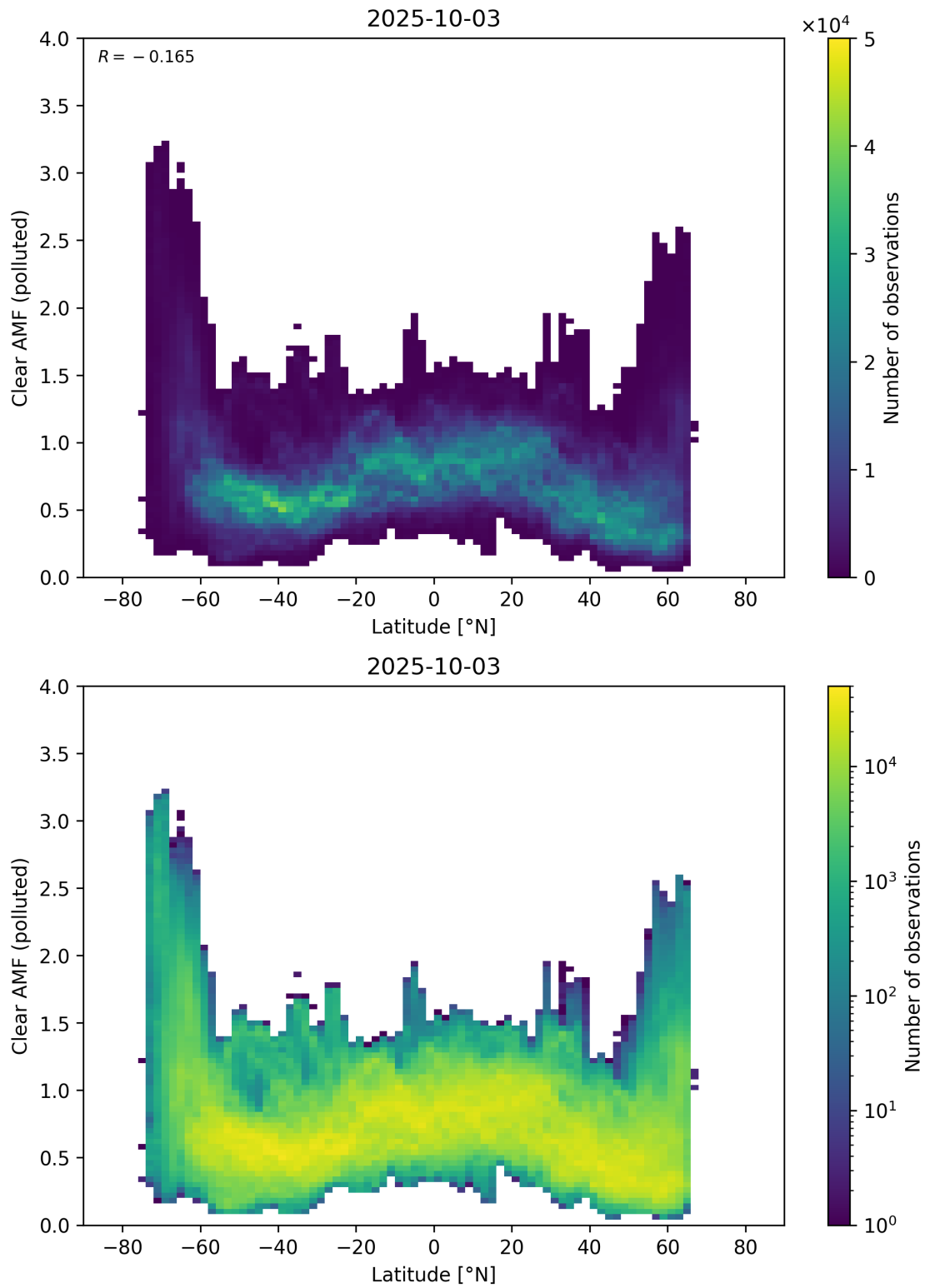
Figure 156: Scatter density plot of “Latitude” against “Clear AMF (polluted)” for 2025-10-02 to 2025-10-04.
