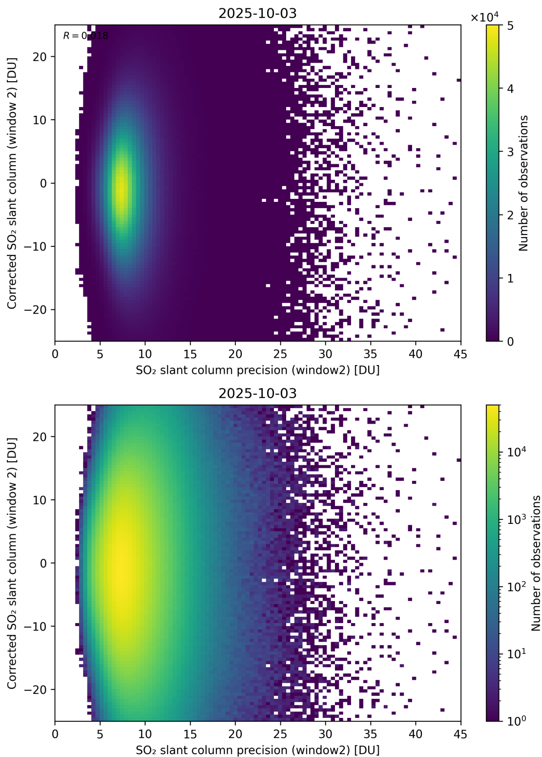
Figure 297: Scatter density plot of “SO 2 slant column precision (window2)” against “Corrected SO 2 slant column (window 2)” for 2025-10-02 to 2025-10-04.
