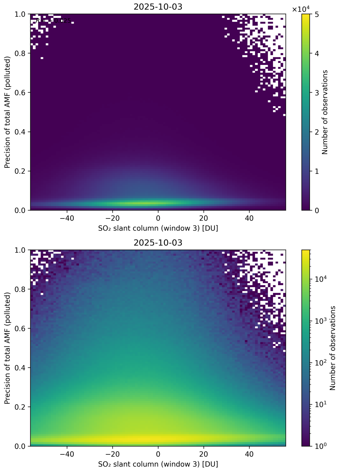
Figure 319: Scatter density plot of “SO 2 slant column (window 3)” against “Precision of total AMF (polluted)” for 2025-10-02 to 2025-10-04.
