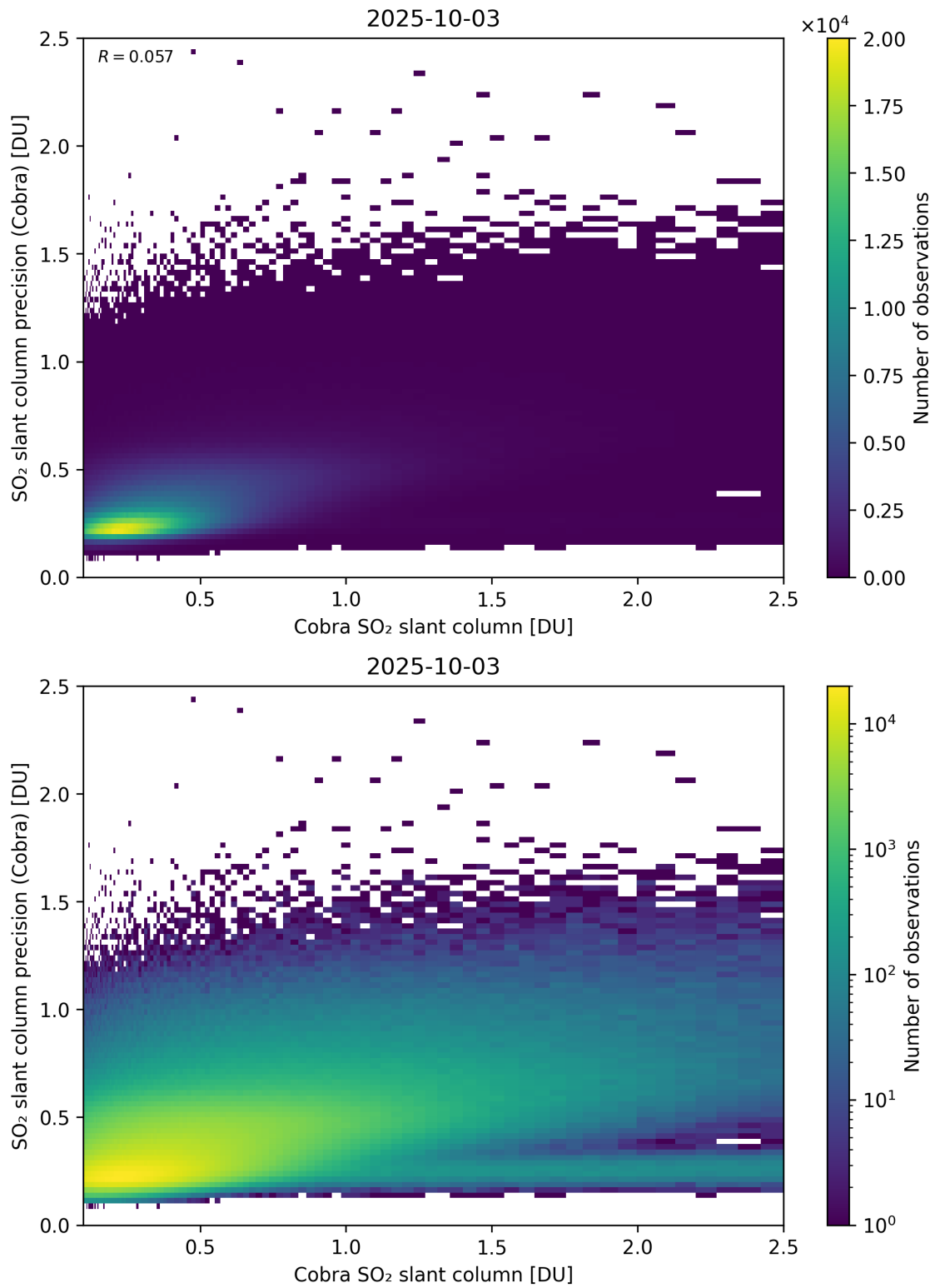
Figure 216: Scatter density plot of “Cobra SO 2 slant column” against “SO 2 slant column precision (Cobra)” for 2025-10-02 to 2025-10-04.
