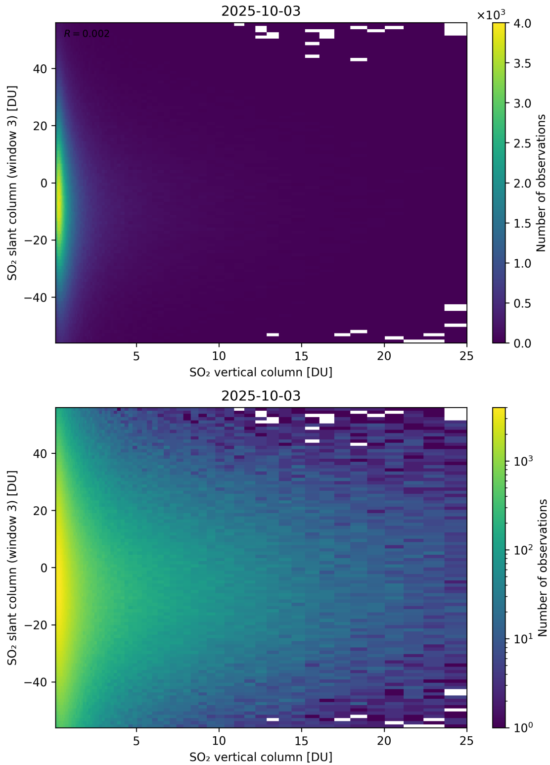
Figure 357: Scatter density plot of “SO 2 vertical column” against “SO 2 slant column (window 3)” for 2025-10-02 to 2025-10-04.
