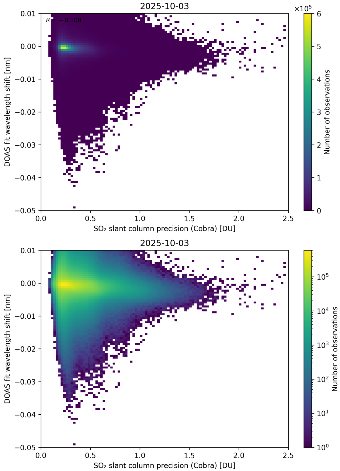
Figure 202: Scatter density plot of “SO 2 slant column precision (Cobra)” against “DOAS fit wavelength shift” for 2025-10-02 to 2025-10-04.
