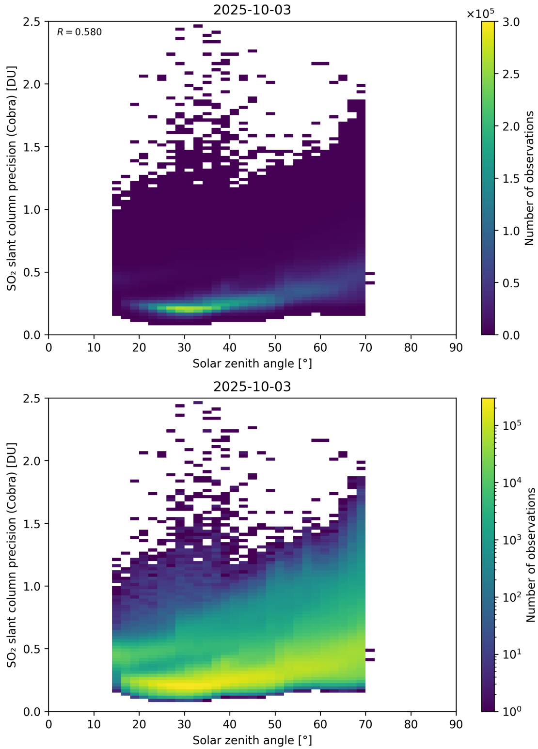
Figure 180: Scatter density plot of “Solar zenith angle” against “SO 2 slant column precision (Cobra)” for 2025-10-02 to 2025-10-04.
