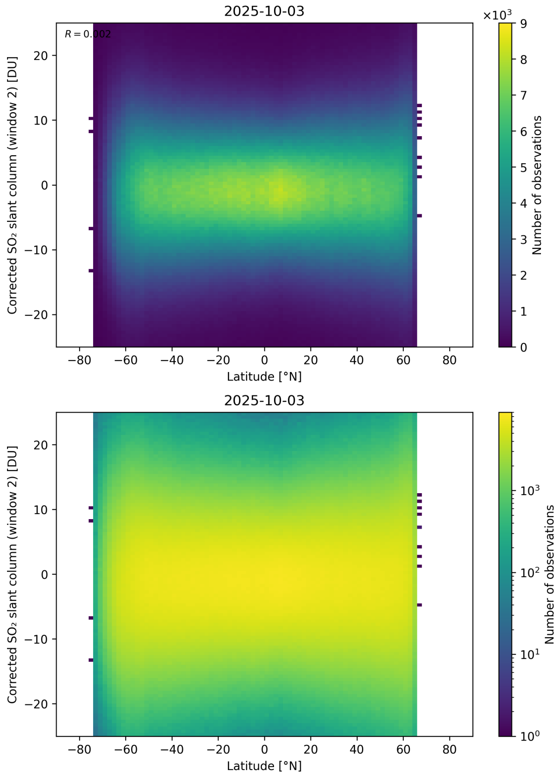
Figure 160: Scatter density plot of “Latitude” against “Corrected SO 2 slant column (window 2)” for 2025-10-02 to 2025-10-04.
