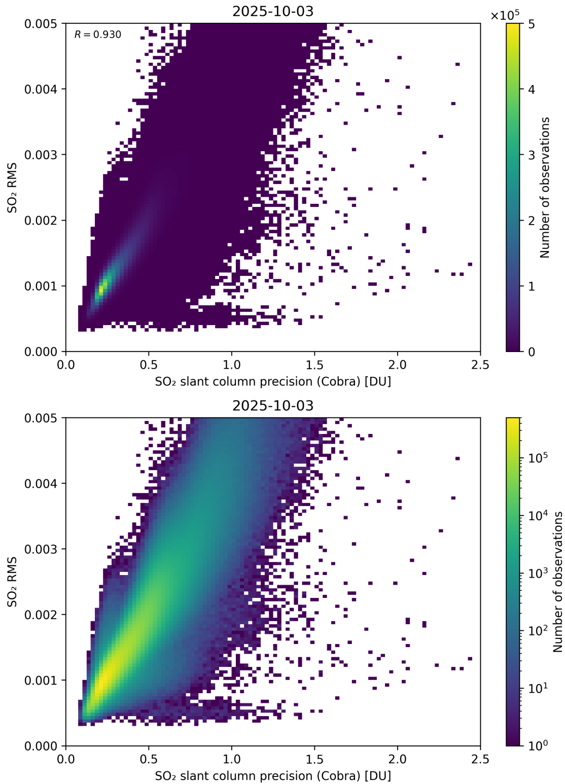
Figure 204: Scatter density plot of “SO 2 slant column precision (Cobra)” against “SO 2 RMS” for 2025-10-02 to 2025-10-04.
