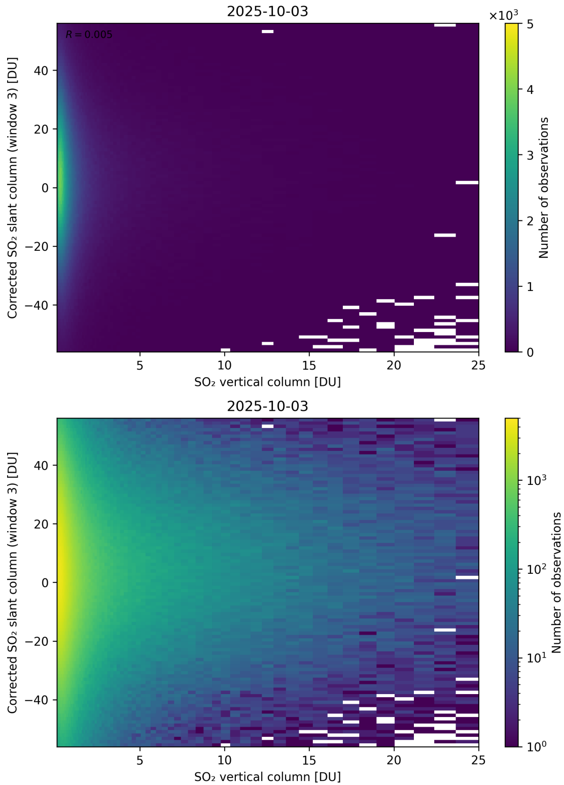
Figure 353: Scatter density plot of “SO 2 vertical column” against “Corrected SO 2 slant column (window 3)” for 2025-10-02 to 2025-10-04.
