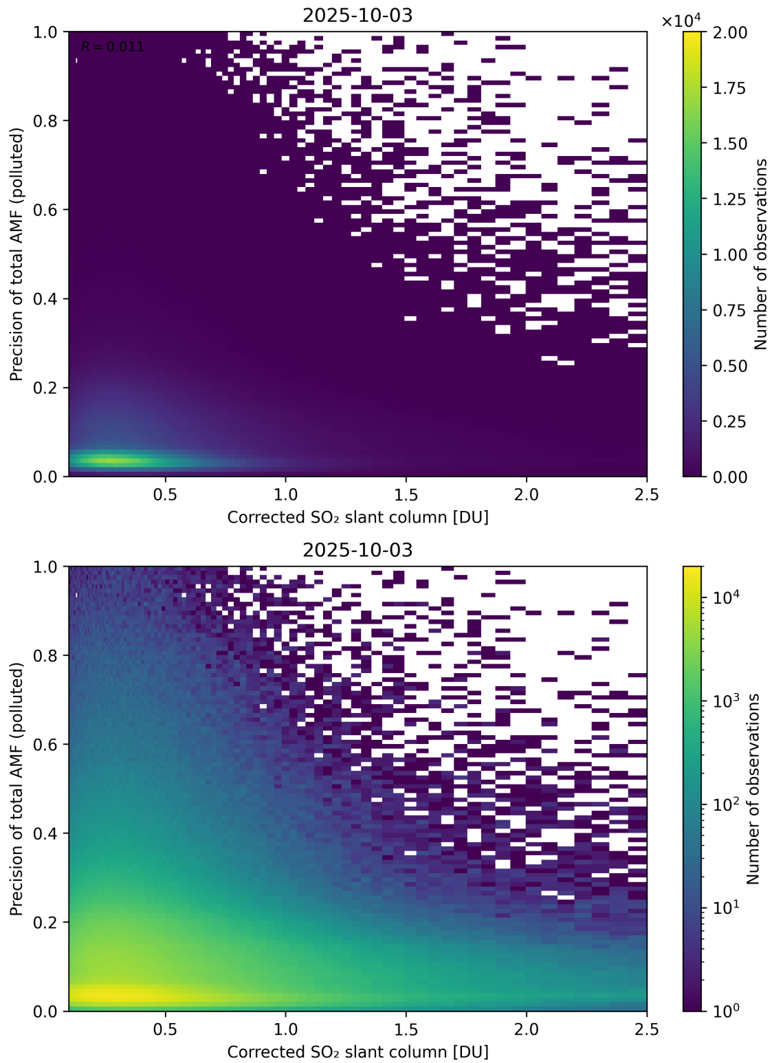
Figure 243: Scatter density plot of “Corrected SO 2 slant column” against “Precision of total AMF (polluted)” for 2025-10-02 to 2025-10-04.
