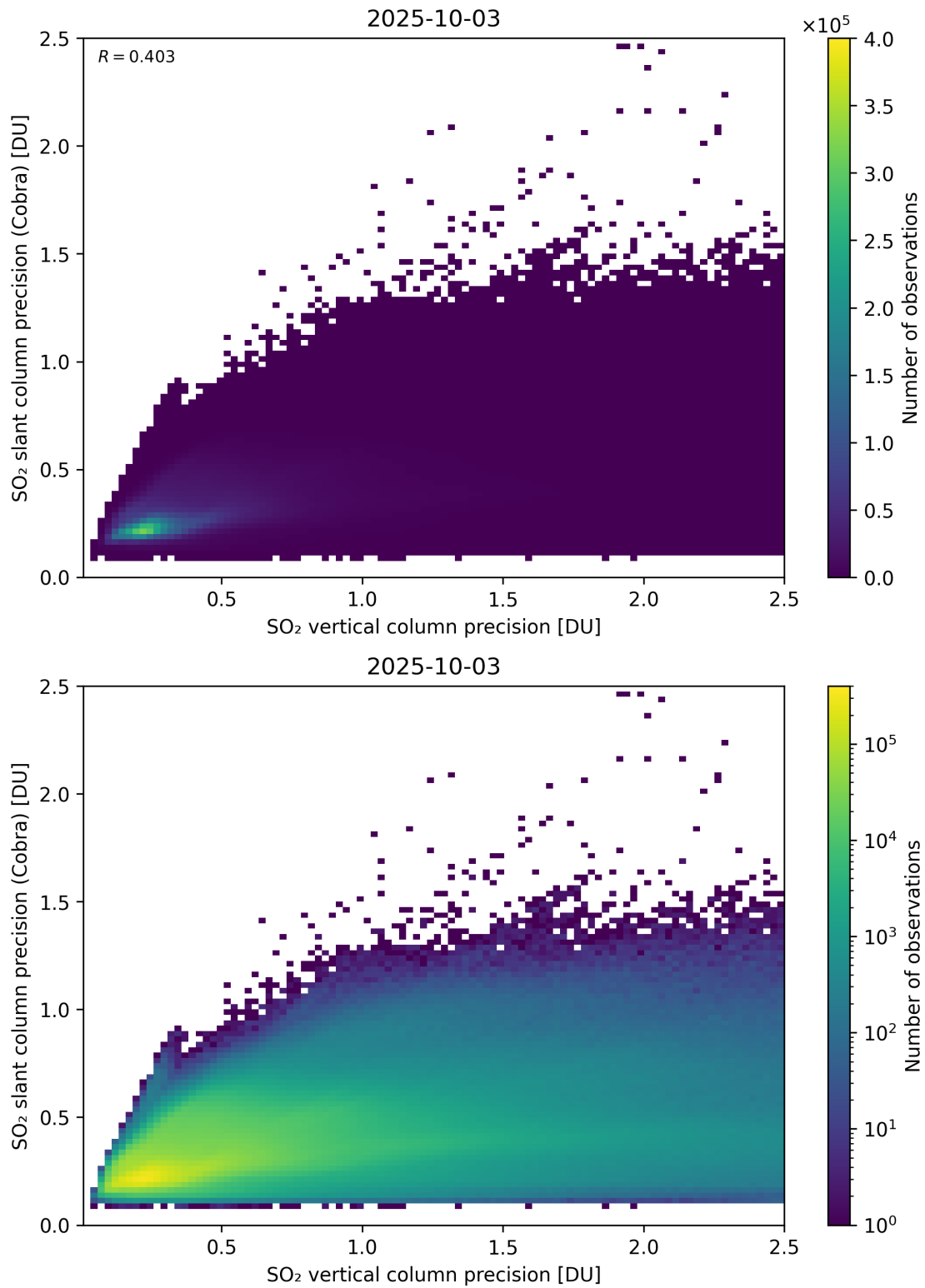
Figure 337: Scatter density plot of “SO 2 vertical column precision” against “SO 2 slant column precision (Cobra)” for 2025-10-02 to 2025-10-04.
