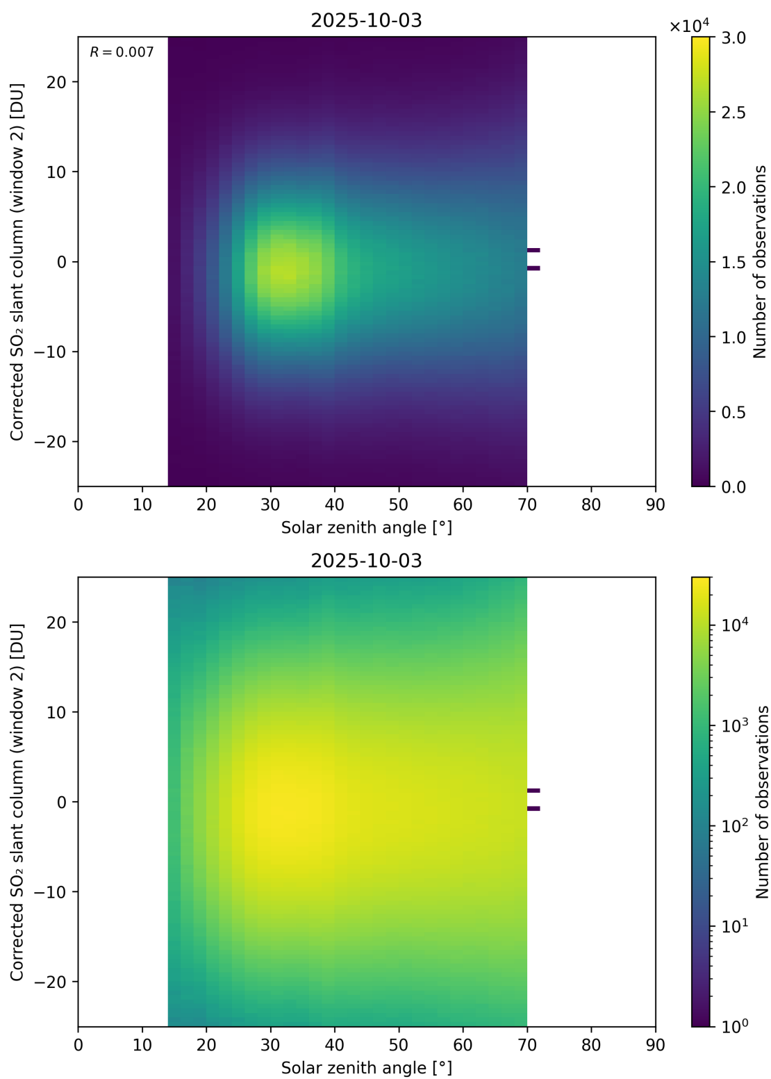
Figure 182: Scatter density plot of “Solar zenith angle” against “Corrected SO 2 slant column (window 2)” for 2025-10-02 to 2025-10-04.
