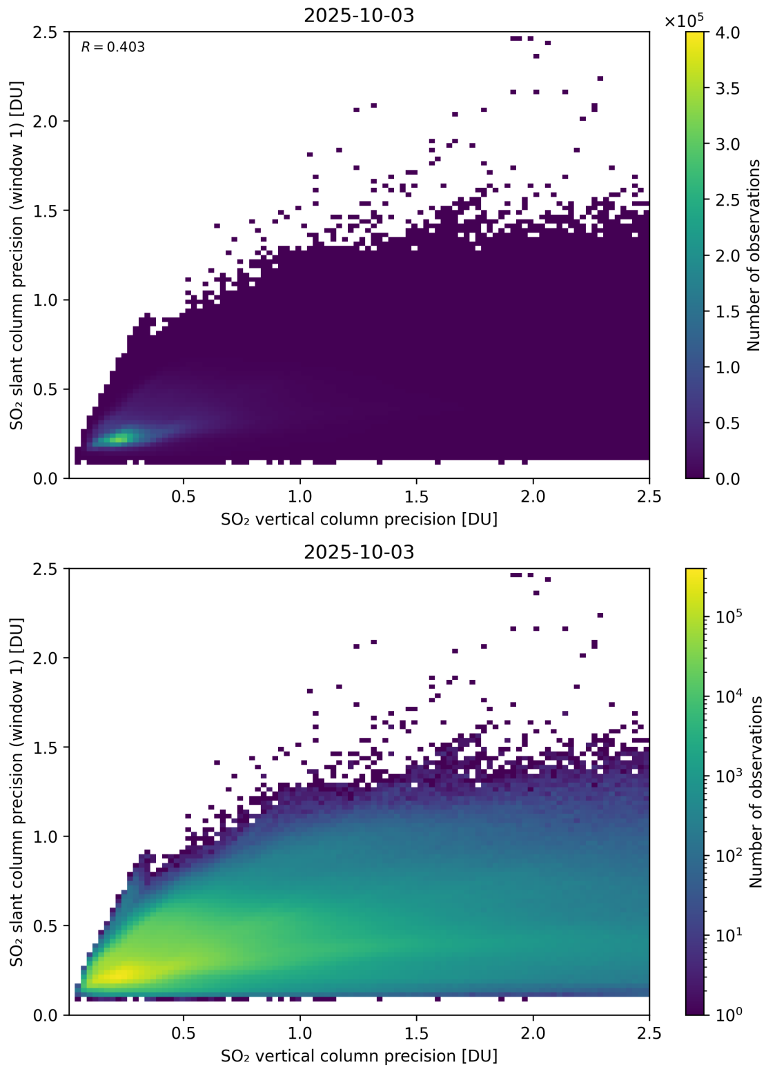
Figure 342: Scatter density plot of “SO 2 vertical column precision” against “SO 2 slant column precision (window 1)” for 2025-10-02 to 2025-10-04.
