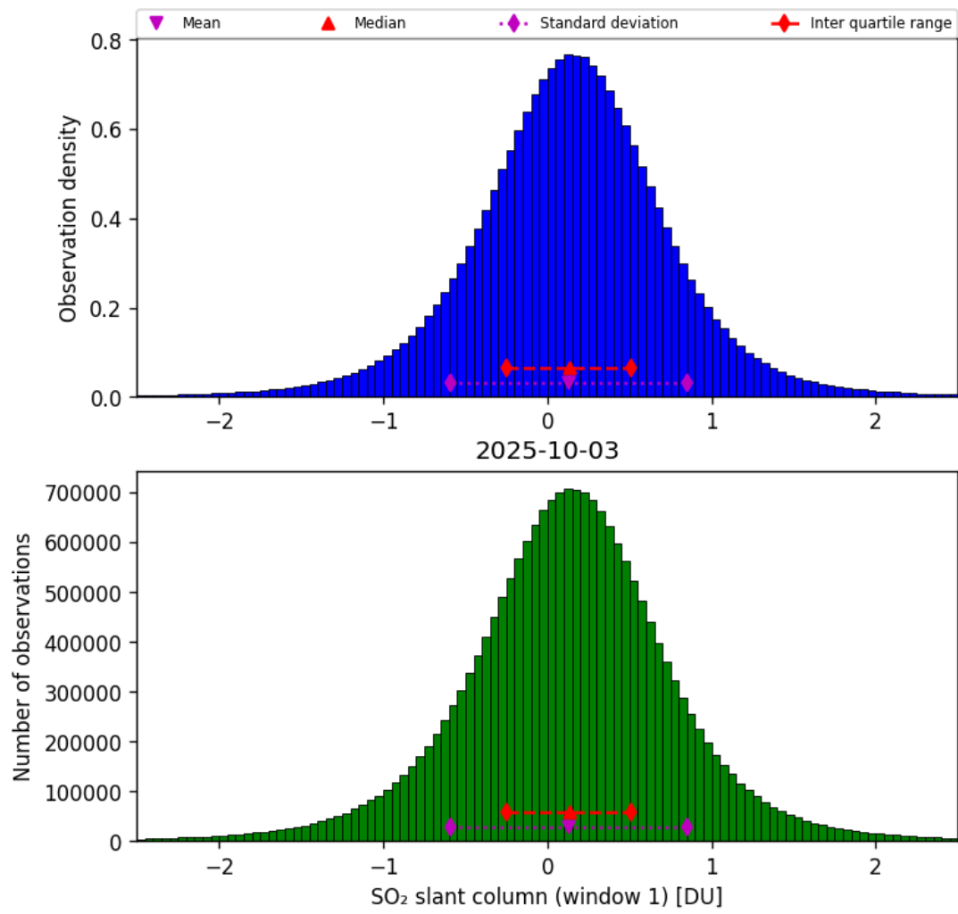
Figure 63: Histogram of “SO 2 slant column (window 1)” for 2025-10-02 to 2025-10-04
