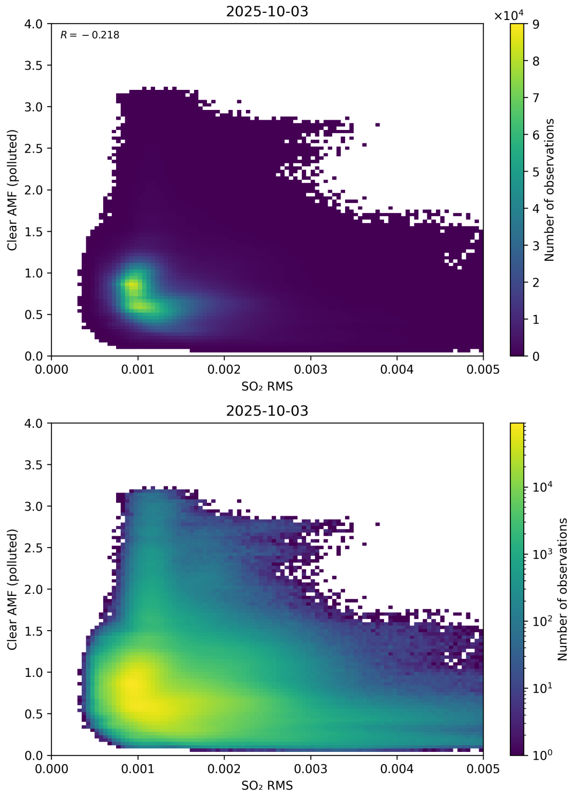
Figure 147: Scatter density plot of “SO 2 RMS” against “Clear AMF (polluted)” for 2025-10-02 to 2025-10-04.
