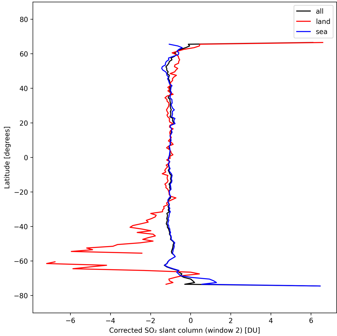
Figure 43: Zonal average of “Corrected SO 2 slant column (window 2)” for 2025-10-02 to 2025-10-04.
