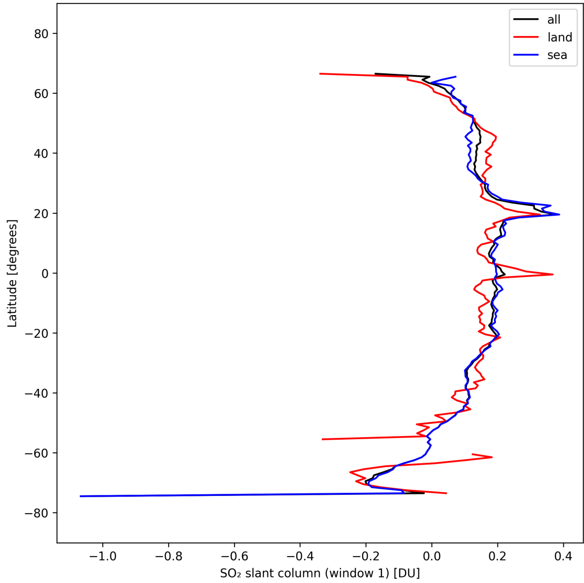
Figure 37: Zonal average of “SO 2 slant column (window 1)” for 2025-10-02 to 2025-10-04.
