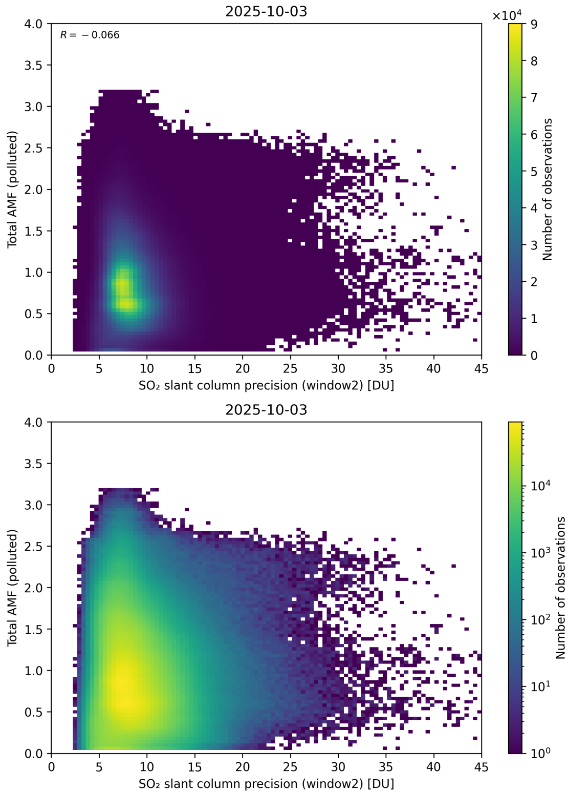
Figure 301: Scatter density plot of “SO 2 slant column precision (window2)” against “Total AMF (polluted)” for 2025-10-02 to 2025-10-04.
