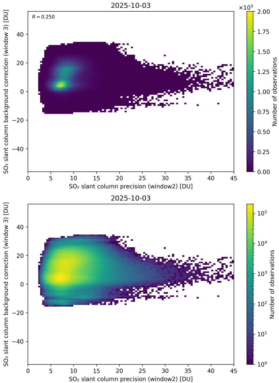
Figure 292: Scatter density plot of “SO 2 slant column precision (window2)” against “SO 2 slant column background correction (window 3)” for 2025-10-02 to 2025-10-04.
