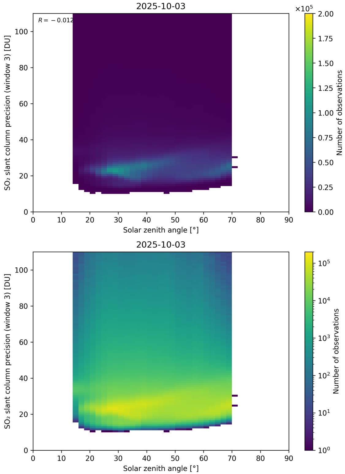
Figure 188: Scatter density plot of “Solar zenith angle” against “SO 2 slant column precision (window 3)” for 2025-10-02 to 2025-10-04.
