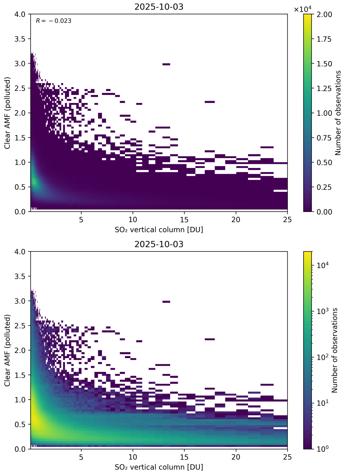
Figure 348: Scatter density plot of “SO 2 vertical column” against “Clear AMF (polluted)” for 2025-10-02 to 2025-10-04.
