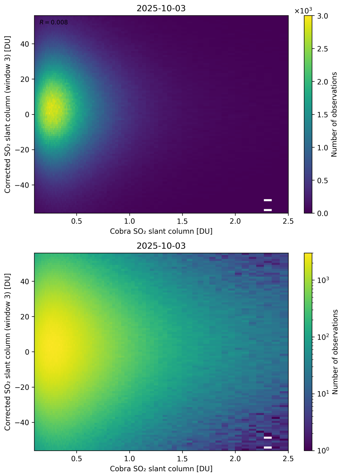
Figure 218: Scatter density plot of “Cobra SO 2 slant column” against “Corrected SO 2 slant column (window 3)” for 2025-10-02 to 2025-10-04.
