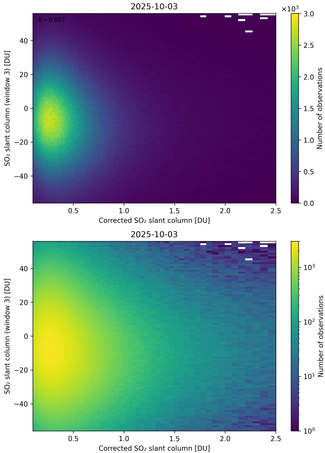
Figure 240: Scatter density plot of “Corrected SO 2 slant column” against “SO 2 slant column (window 3)” for 2025-10-02 to 2025-10-04.
