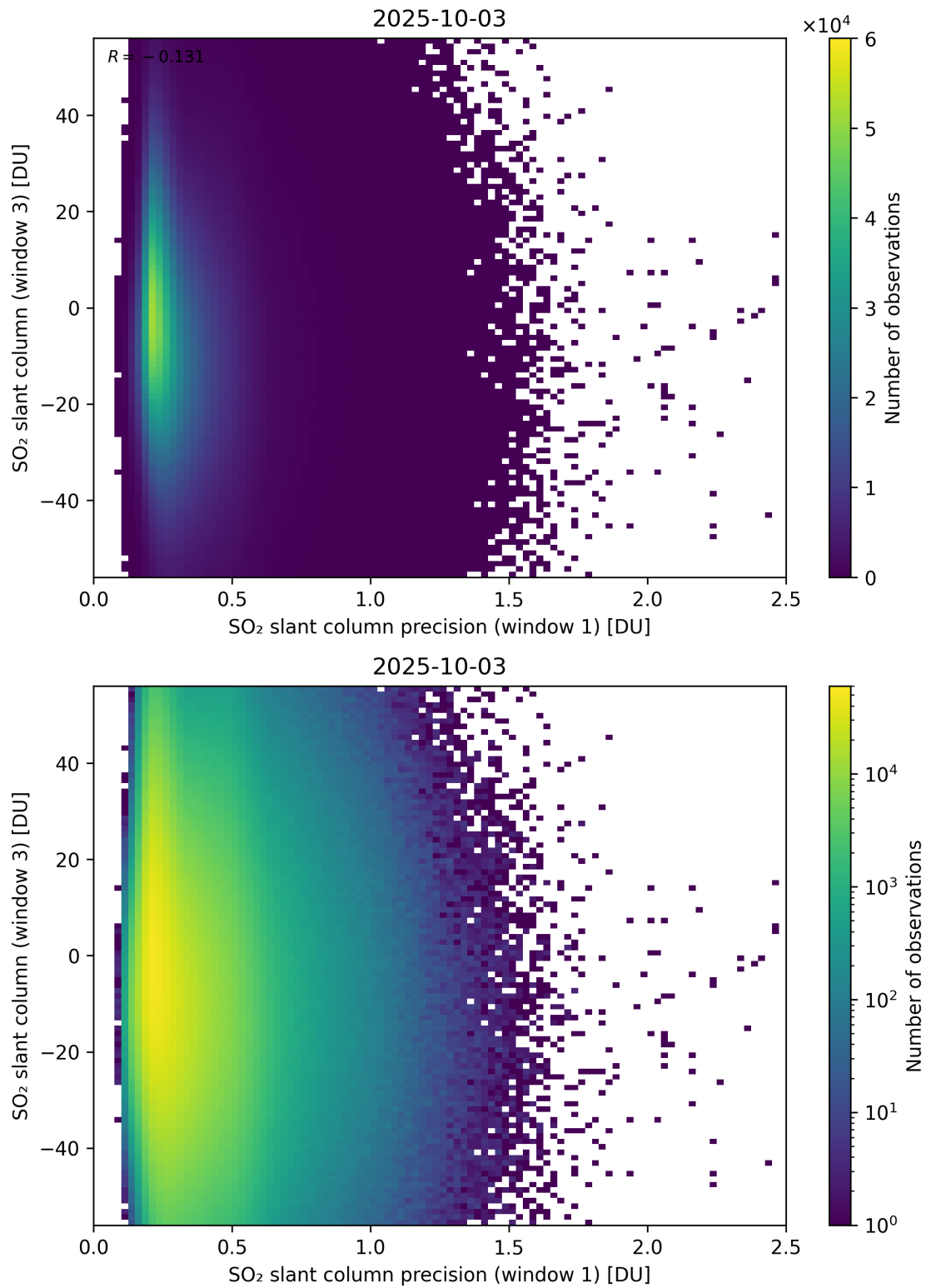
Figure 278: Scatter density plot of “SO 2 slant column precision (window 1)” against “SO 2 slant column (window 3)” for 2025-10-02 to 2025-10-04.
