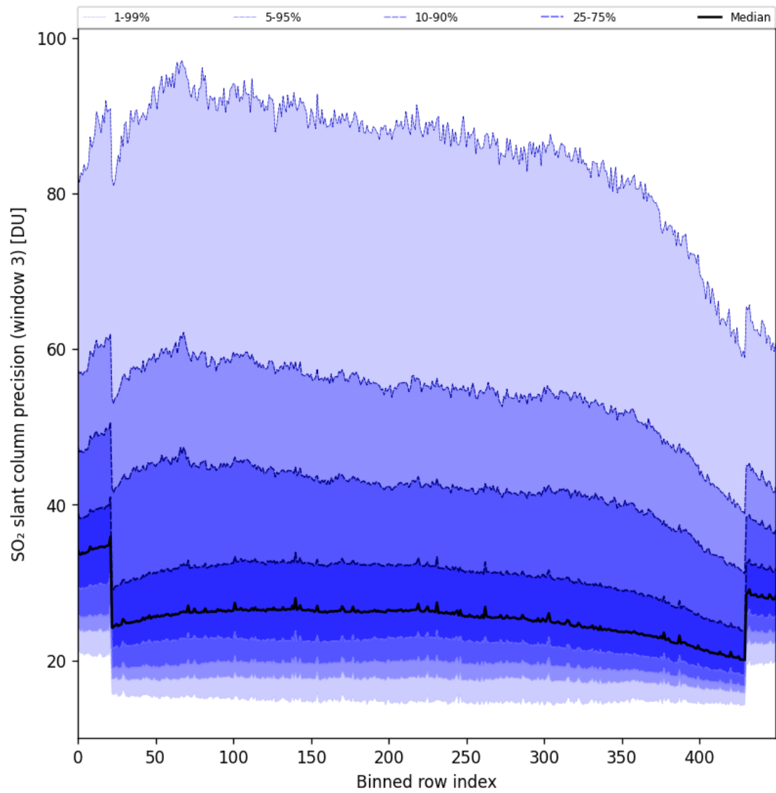
Figure 98: Along track statistics of “SO 2 slant column precision (window 3)” for 2025-10-02 to 2025-10-04
