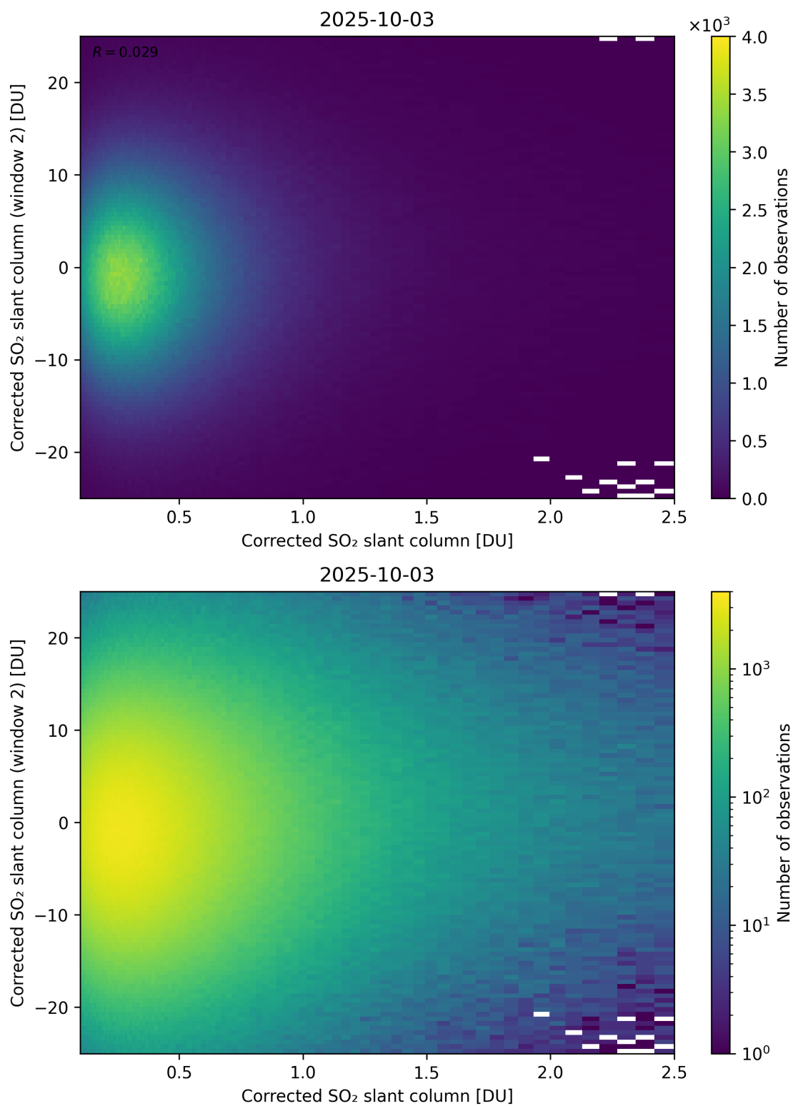
Figure 235: Scatter density plot of “Corrected SO 2 slant column” against “Corrected SO 2 slant column (window 2)” for 2025-10-02 to 2025-10-04.
