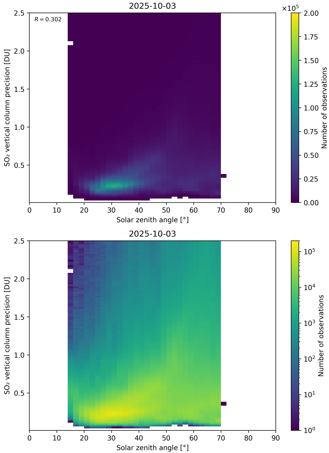
Figure 192: Scatter density plot of “Solar zenith angle” against “SO 2 vertical column precision” for 2025-10-02 to 2025-10-04.
