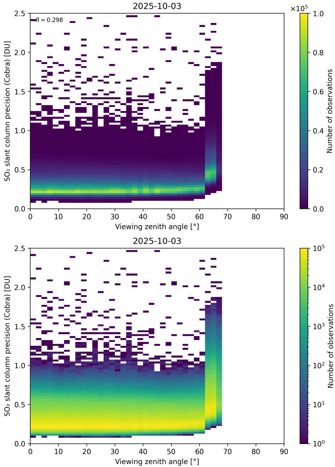
Figure 372: Scatter density plot of “Viewing zenith angle” against “SO 2 slant column precision (Cobra)” for 2025-10-02 to 2025-10-04.
