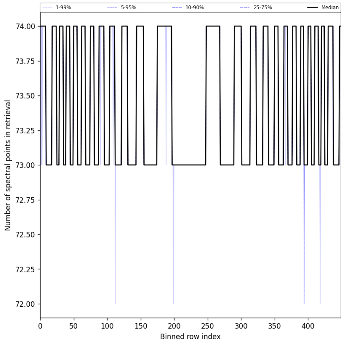
Figure 108: Along track statistics of “Number of spectral points in retrieval” for 2025-10-02 to 2025-10-04
