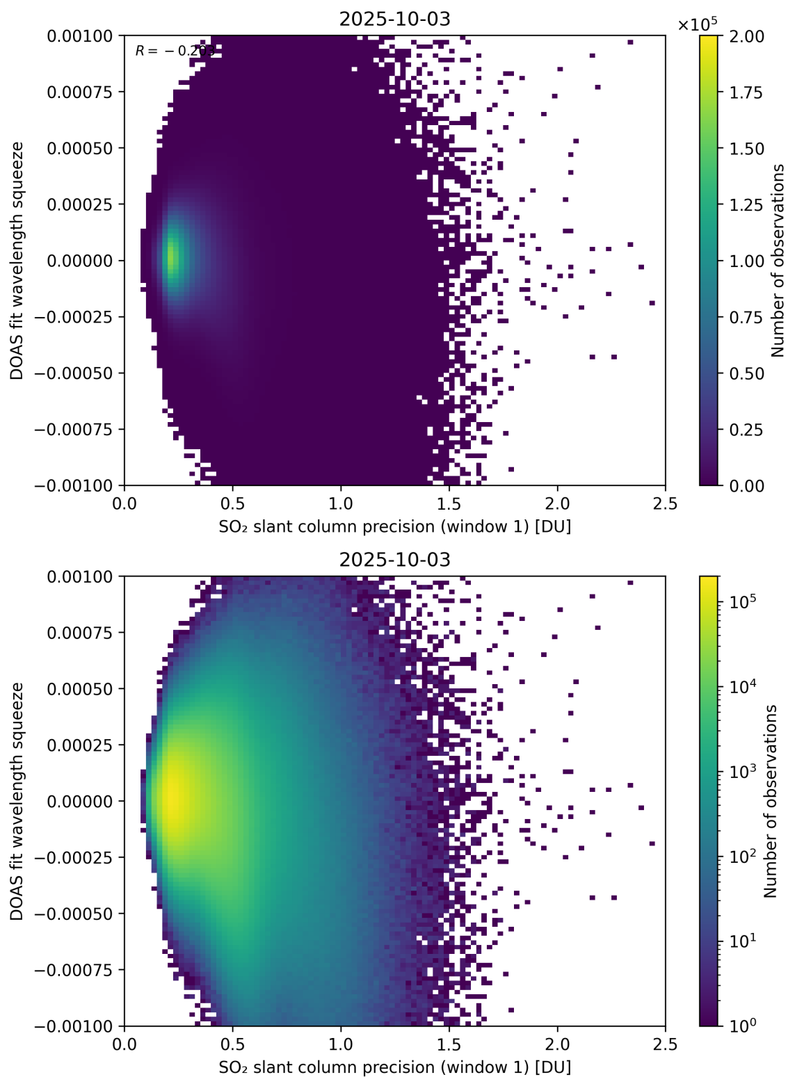
Figure 272: Scatter density plot of “SO 2 slant column precision (window 1)” against “DOAS fit wavelength squeeze” for 2025-10-02 to 2025-10-04.
