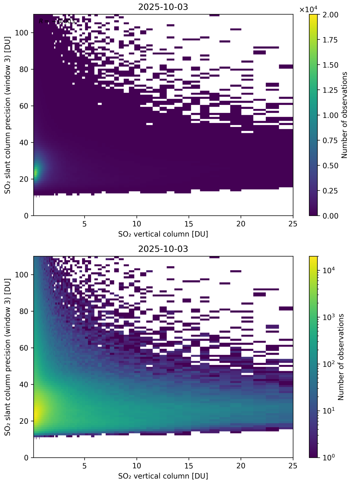
Figure 358: Scatter density plot of “SO 2 vertical column” against “SO 2 slant column precision (window 3)” for 2025-10-02 to 2025-10-04.
