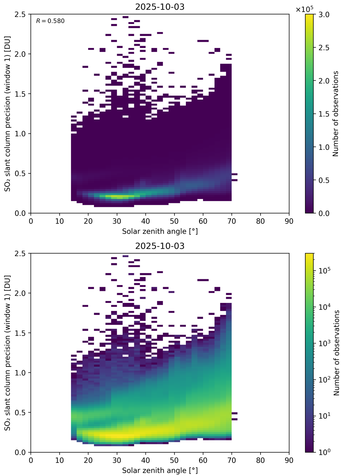
Figure 185: Scatter density plot of “Solar zenith angle” against “SO 2 slant column precision (window 1)” for 2025-10-02 to 2025-10-04.
