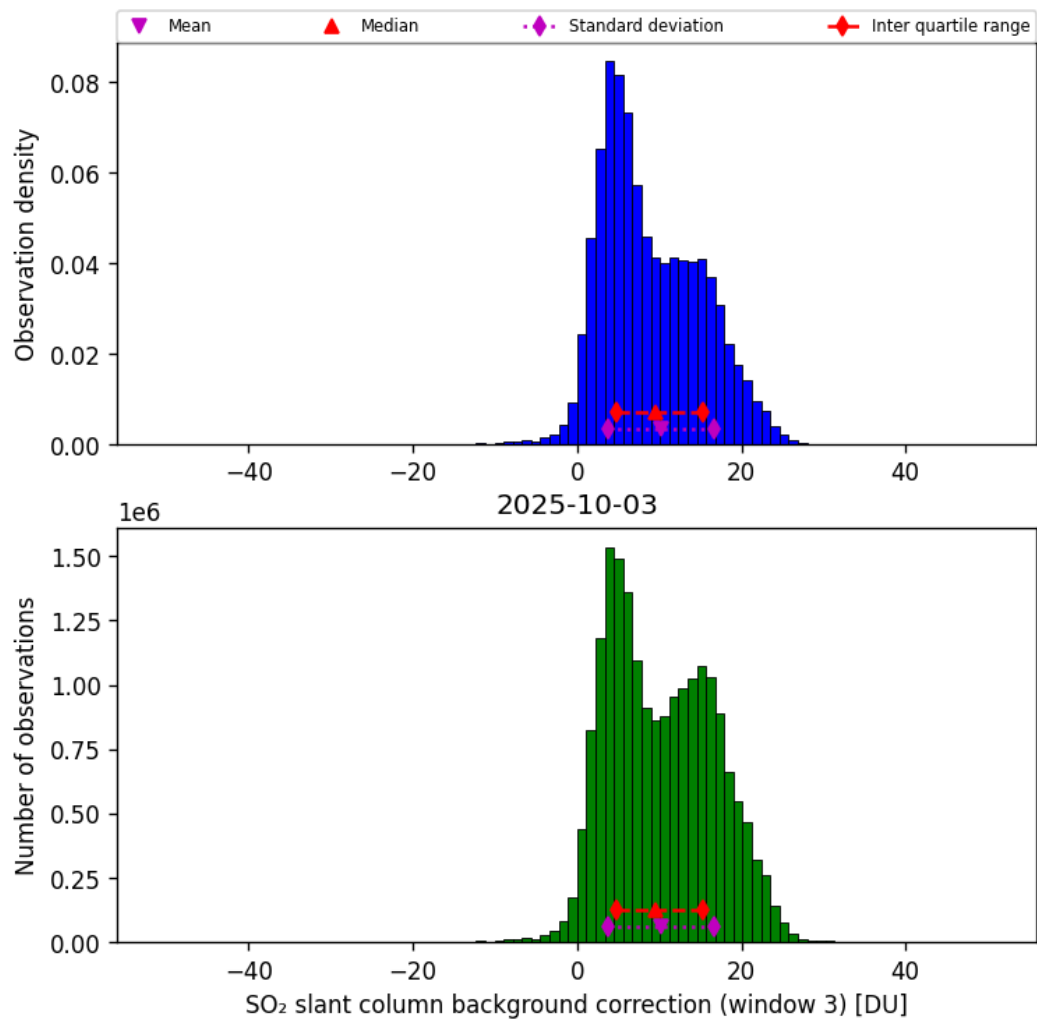
Figure 74: Histogram of “SO 2 slant column background correction (window 3)” for 2025-10-02 to 2025-10-04
