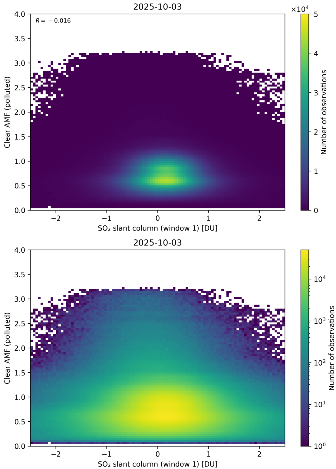
Figure 282: Scatter density plot of “SO 2 slant column (window 1)” against “Clear AMF (polluted)” for 2025-10-02 to 2025-10-04.
