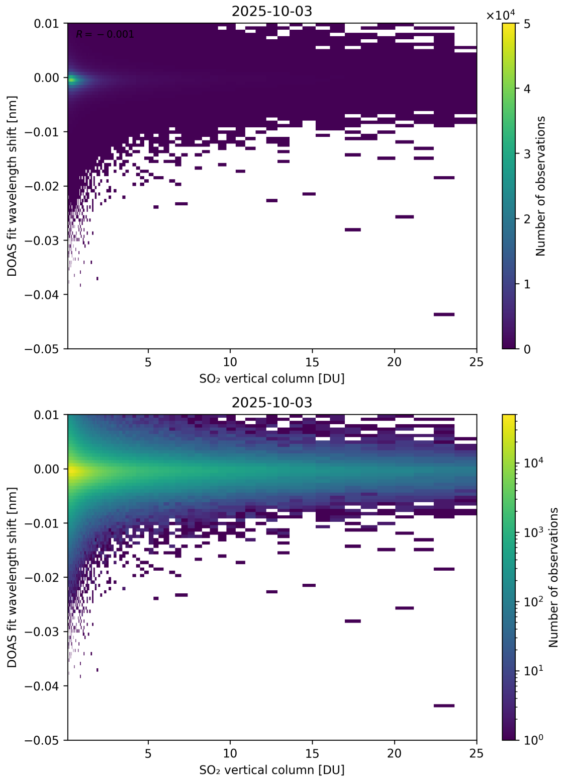
Figure 326: Scatter density plot of “SO 2 vertical column” against “DOAS fit wavelength shift” for 2025-10-02 to 2025-10-04.
