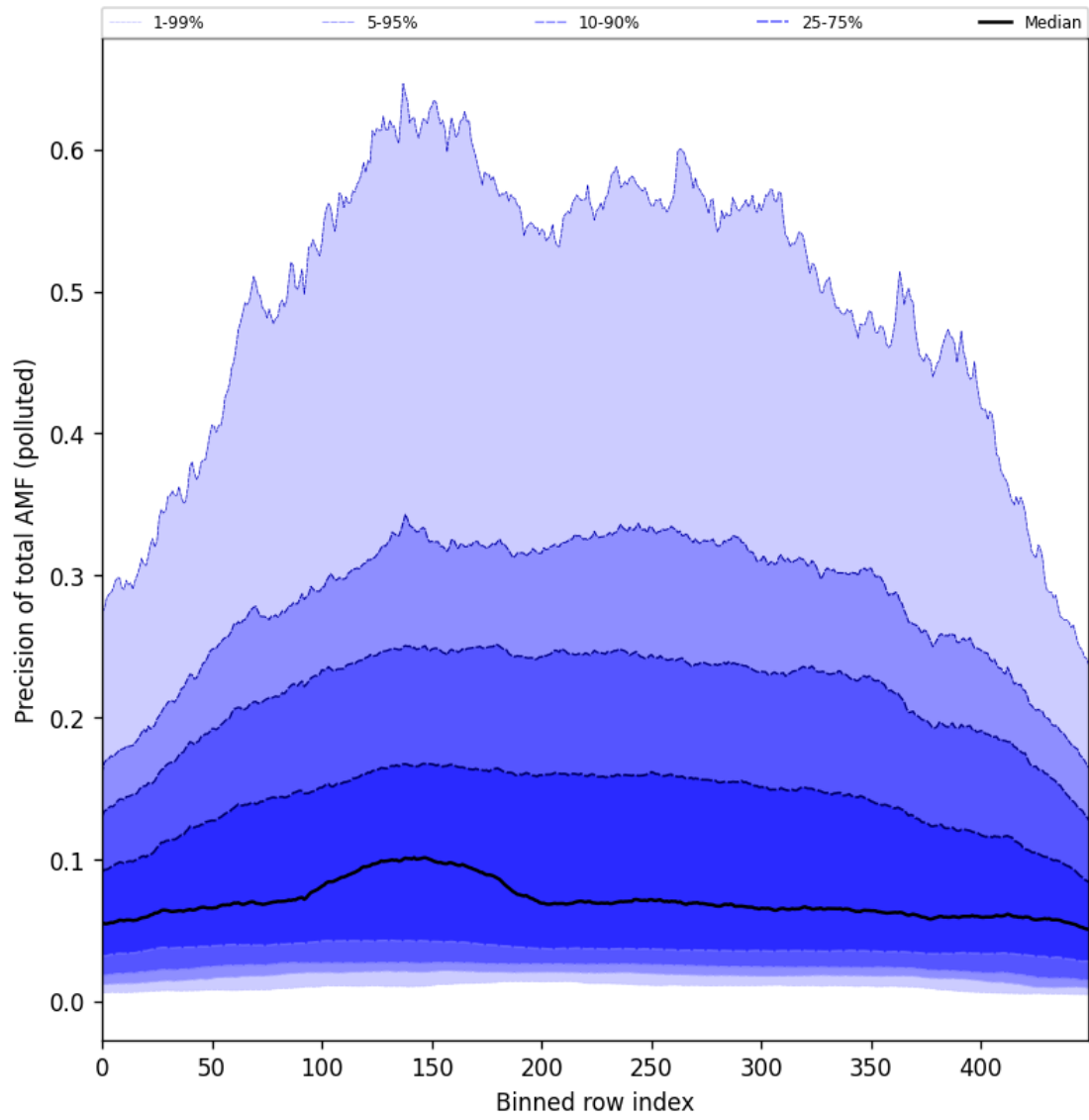
Figure 106: Along track statistics of “Precision of total AMF (polluted)” for 2025-10-02 to 2025-10-04
