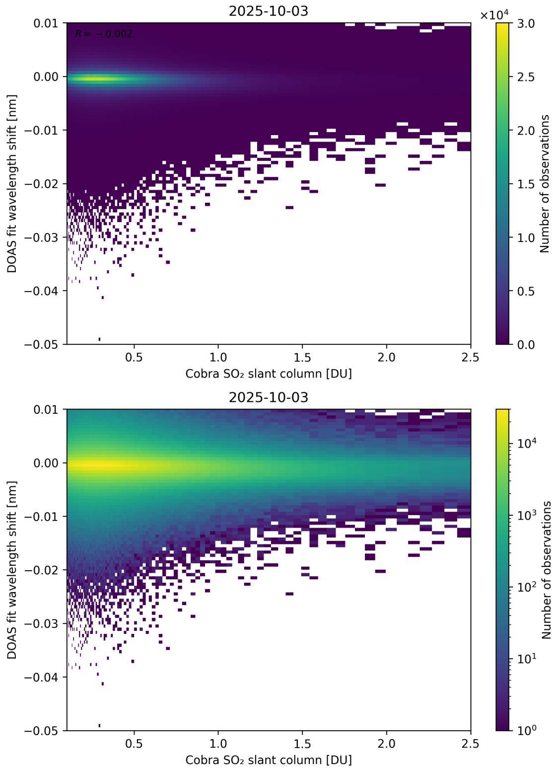
Figure 196: Scatter density plot of “Cobra SO 2 slant column” against “DOAS fit wavelength shift” for 2025-10-02 to 2025-10-04.
