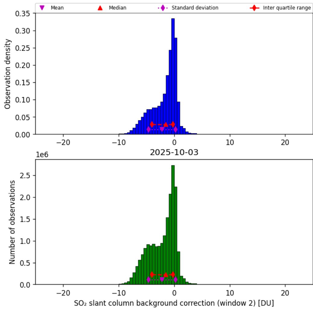
Figure 70: Histogram of “SO 2 slant column background correction (window 2)” for 2025-10-02 to 2025-10-04
