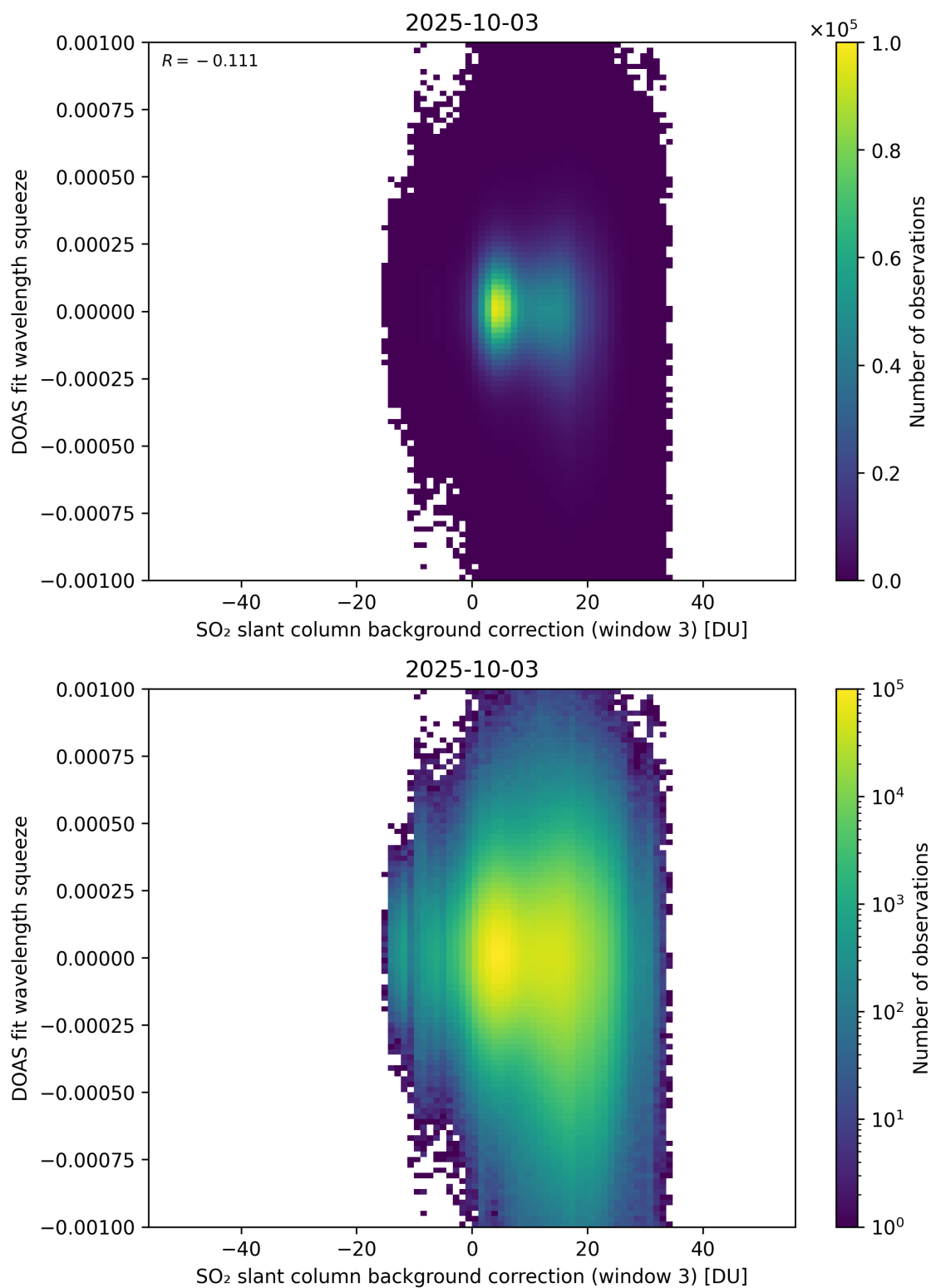
Figure 133: Scatter density plot of “SO 2 slant column background correction (window 3)” against “DOAS fit wavelength squeeze” for 2025-10-02 to 2025-10-04.
