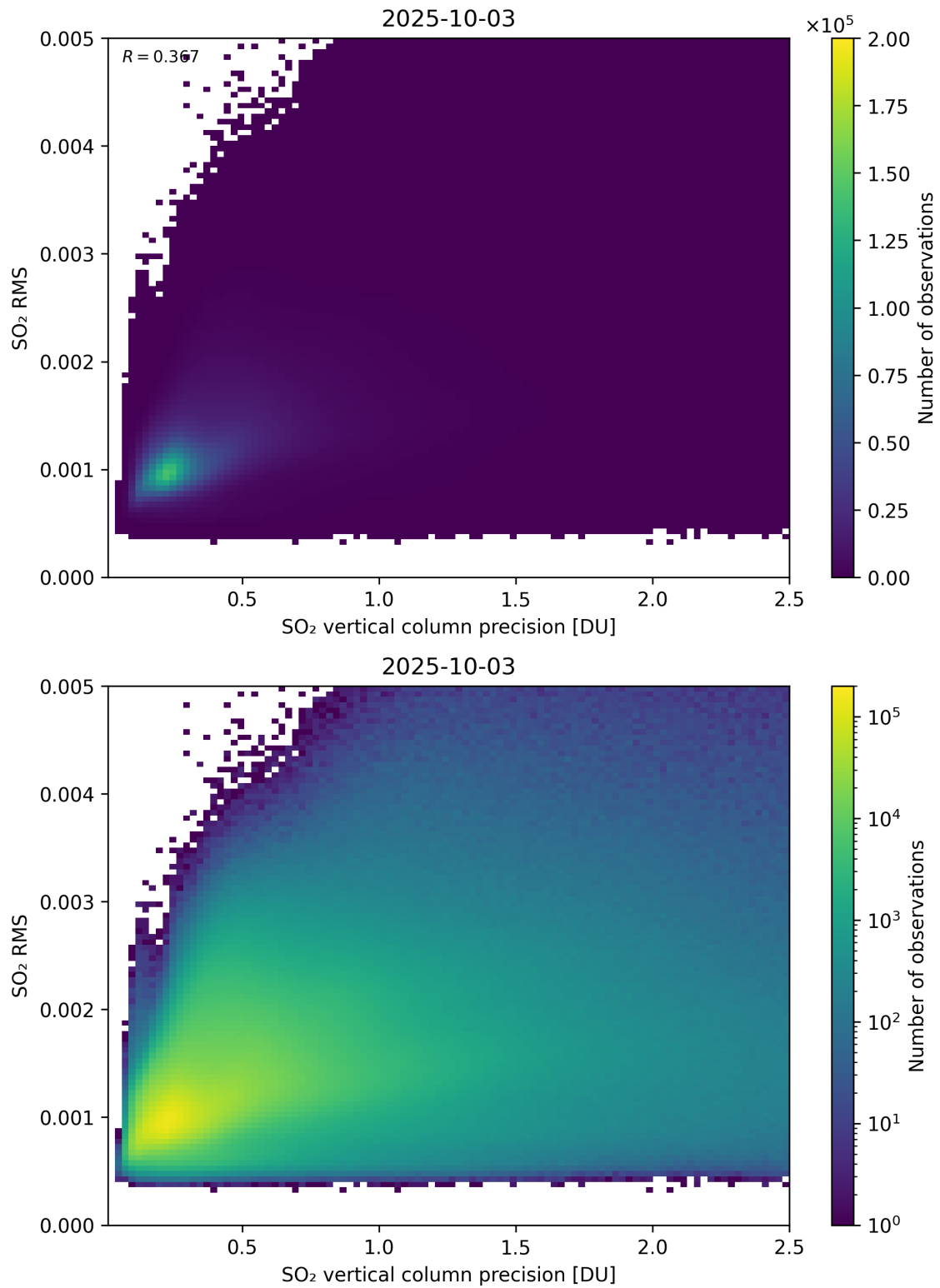
Figure 334: Scatter density plot of “SO 2 vertical column precision” against “SO 2 RMS” for 2025-10-02 to 2025-10-04.
