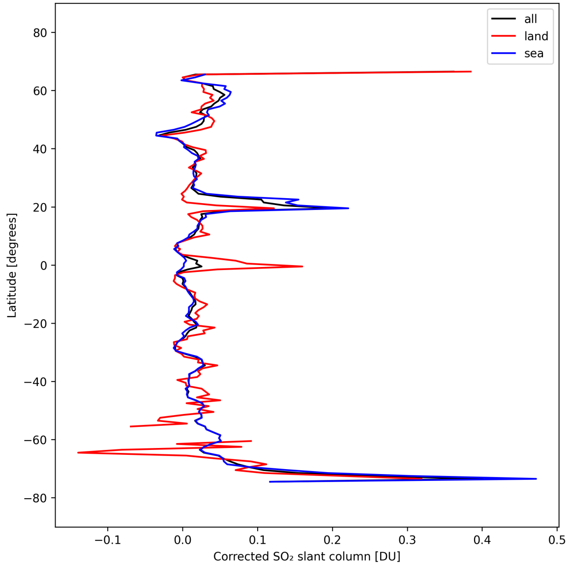
Figure 34: Zonal average of “Corrected SO 2 slant column” for 2025-10-02 to 2025-10-04.
