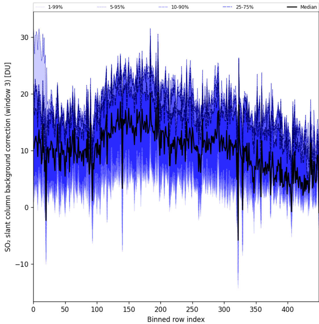
Figure 100: Along track statistics of “SO 2 slant column background correction (window 3)” for 2025-10-02 to 2025-10-04
