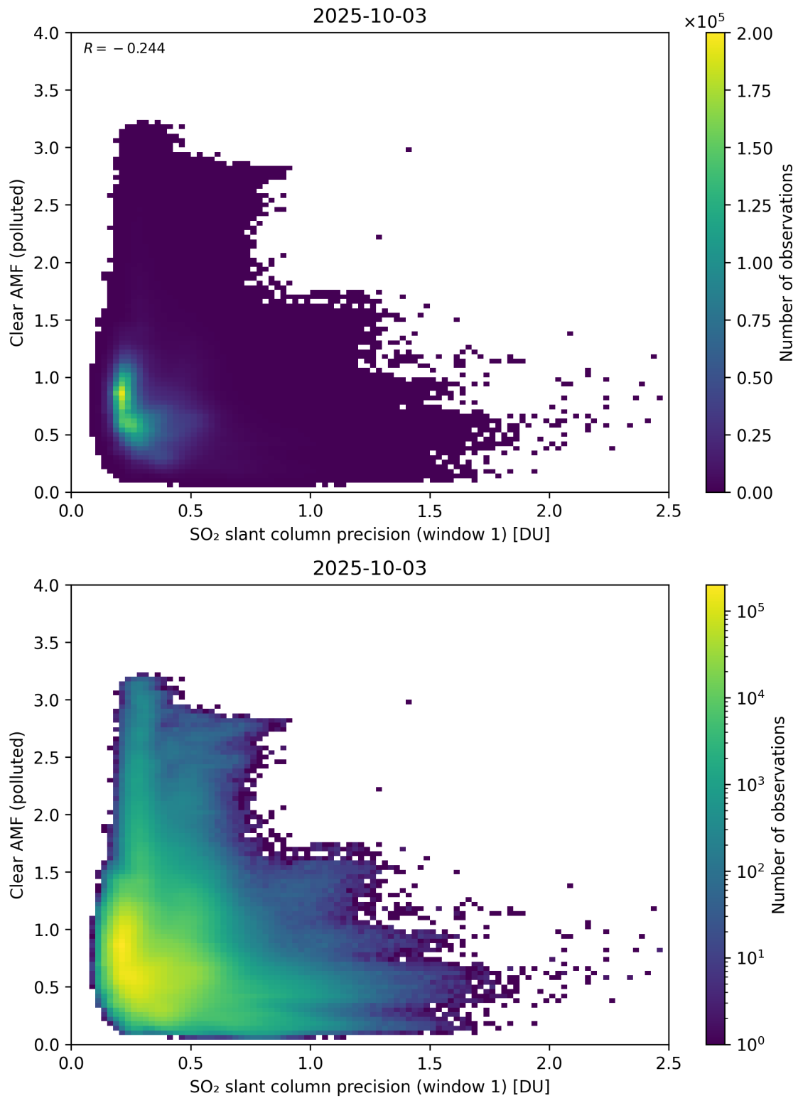
Figure 274: Scatter density plot of “SO 2 slant column precision (window 1)” against “Clear AMF (polluted)” for 2025-10-02 to 2025-10-04.
