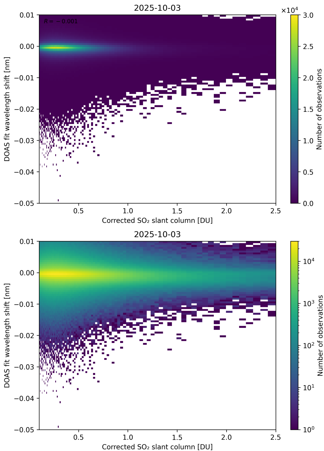
Figure 229: Scatter density plot of “Corrected SO 2 slant column” against “DOAS fit wavelength shift” for 2025-10-02 to 2025-10-04.
