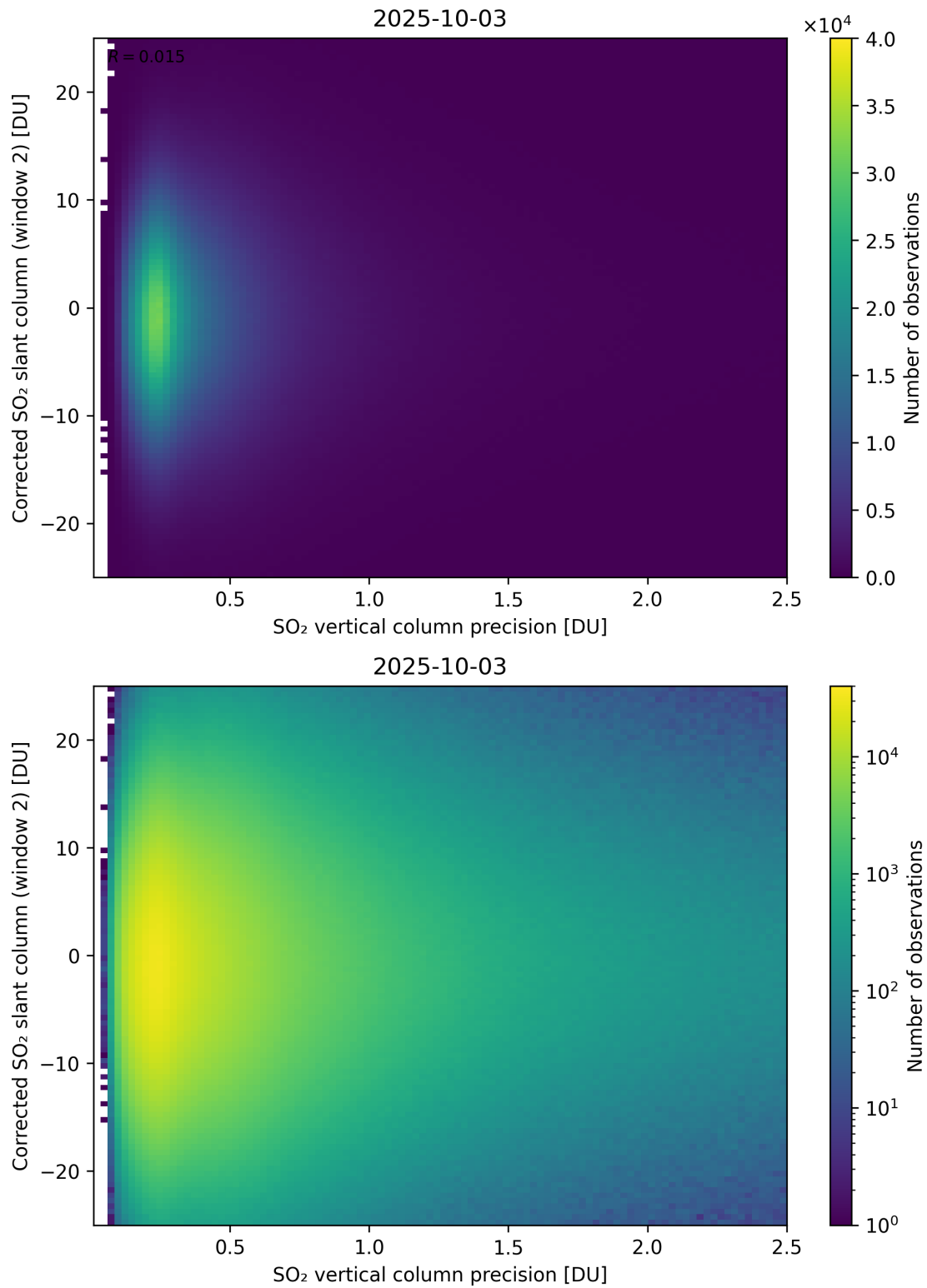
Figure 339: Scatter density plot of “SO 2 vertical column precision” against “Corrected SO 2 slant column (window 2)” for 2025-10-02 to 2025-10-04.
