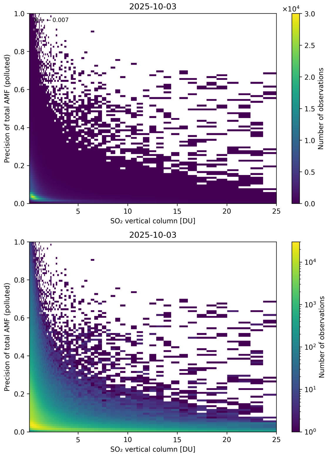
Figure 360: Scatter density plot of “SO 2 vertical column” against “Precision of total AMF (polluted)” for 2025-10-02 to 2025-10-04.
