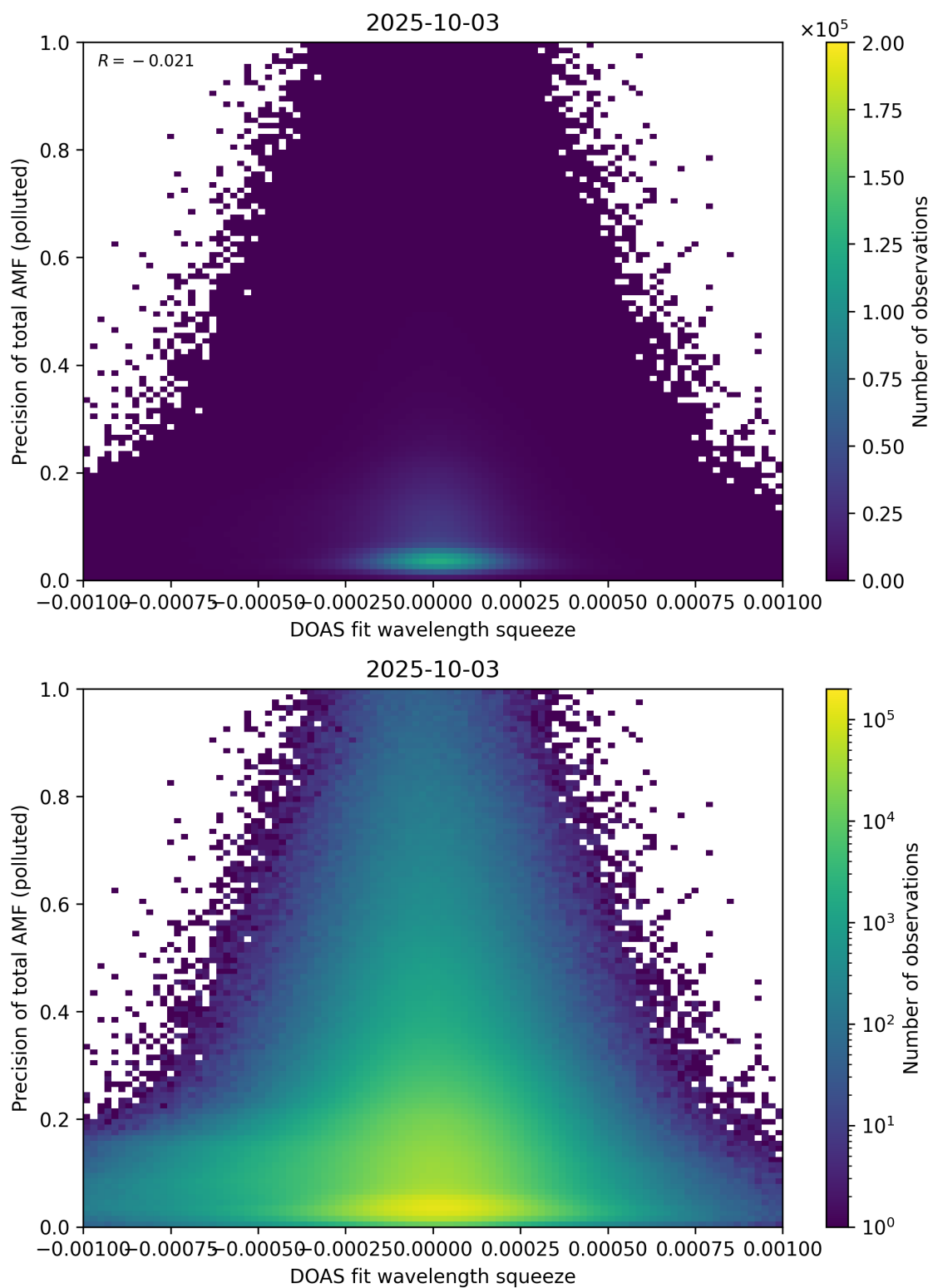
Figure 146: Scatter density plot of “DOAS fit wavelength squeeze” against “Precision of total AMF (polluted)” for 2025-10-02 to 2025-10-04.
