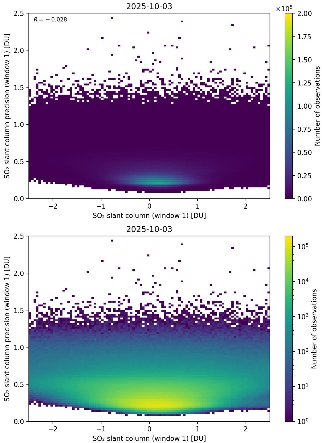
Figure 285: Scatter density plot of “SO 2 slant column (window 1)” against “SO 2 slant column precision (window 1)” for 2025-10-02 to 2025-10-04.
