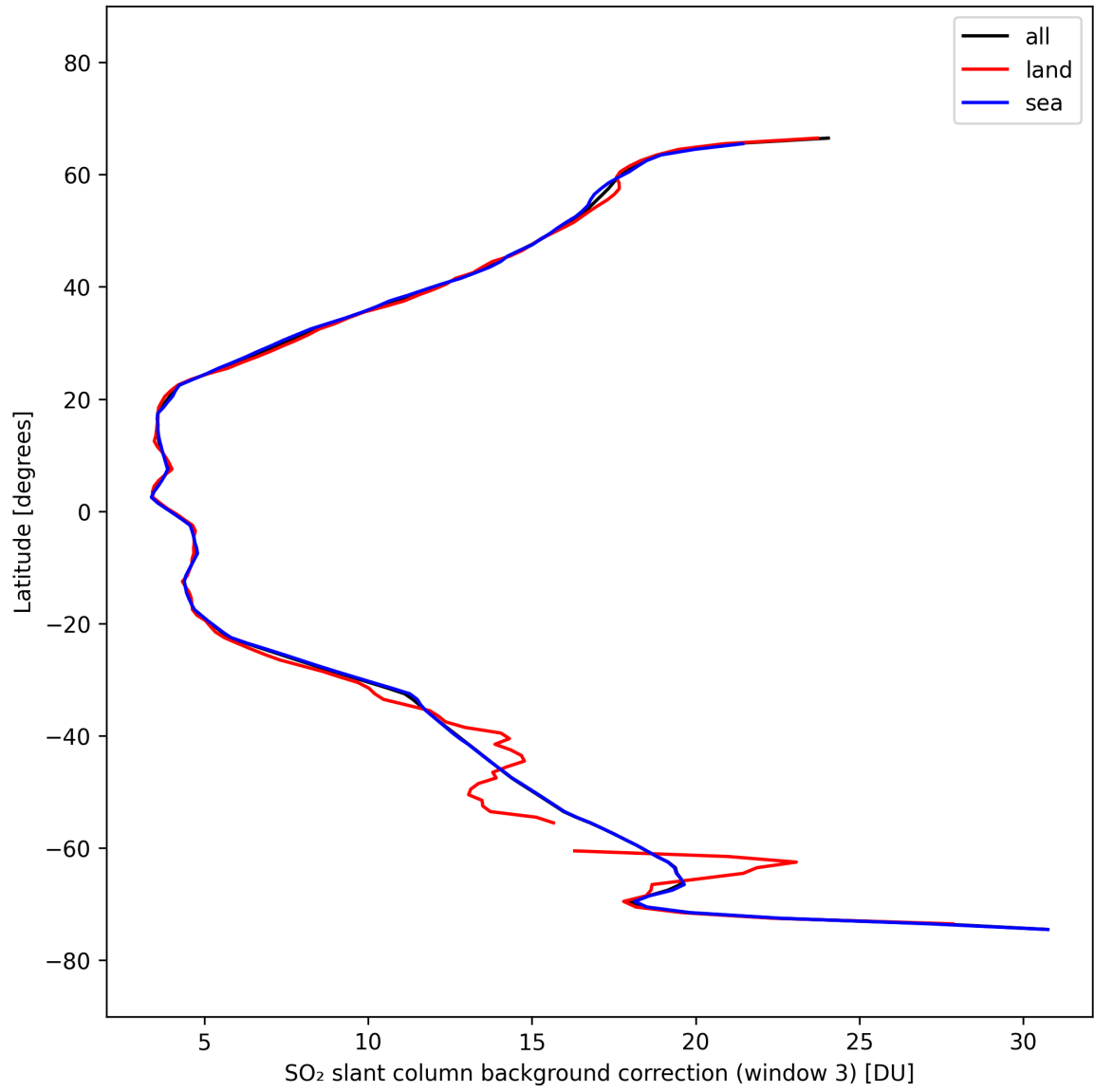
Figure 48: Zonal average of “SO 2 slant column background correction (window 3)” for 2025-10-02 to 2025-10-04.
