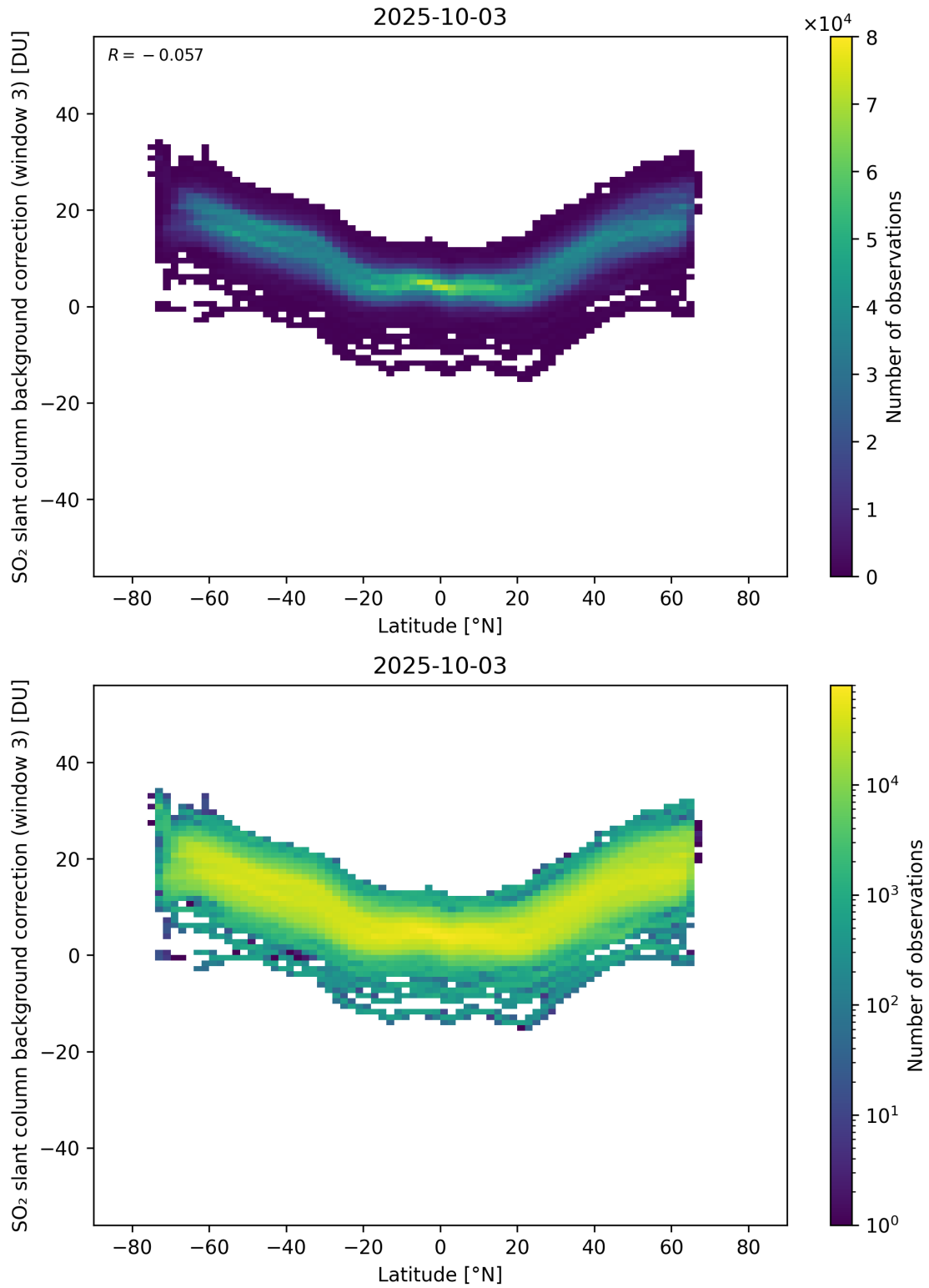
Figure 152: Scatter density plot of “Latitude” against “SO 2 slant column background correction (window 3)” for 2025-10-02 to 2025-10-04.
