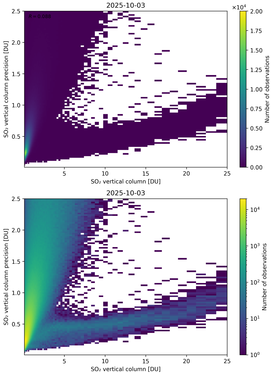
Figure 361: Scatter density plot of “SO 2 vertical column” against “SO 2 vertical column precision” for 2025-10-02 to 2025-10-04.
