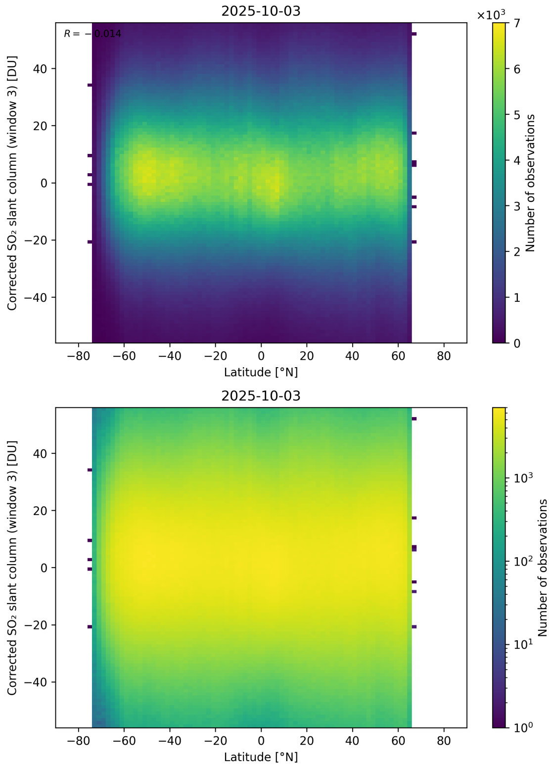
Figure 161: Scatter density plot of “Latitude” against “Corrected SO 2 slant column (window 3)” for 2025-10-02 to 2025-10-04.
