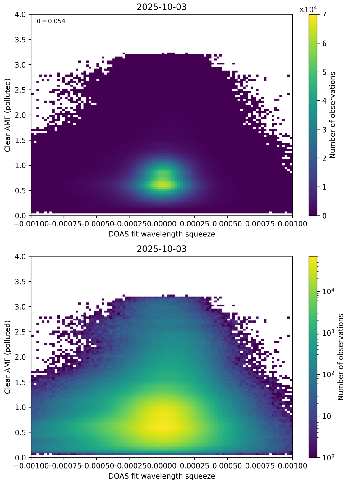
Figure 144: Scatter density plot of “DOAS fit wavelength squeeze” against “Clear AMF (polluted)” for 2025-10-02 to 2025-10-04.
