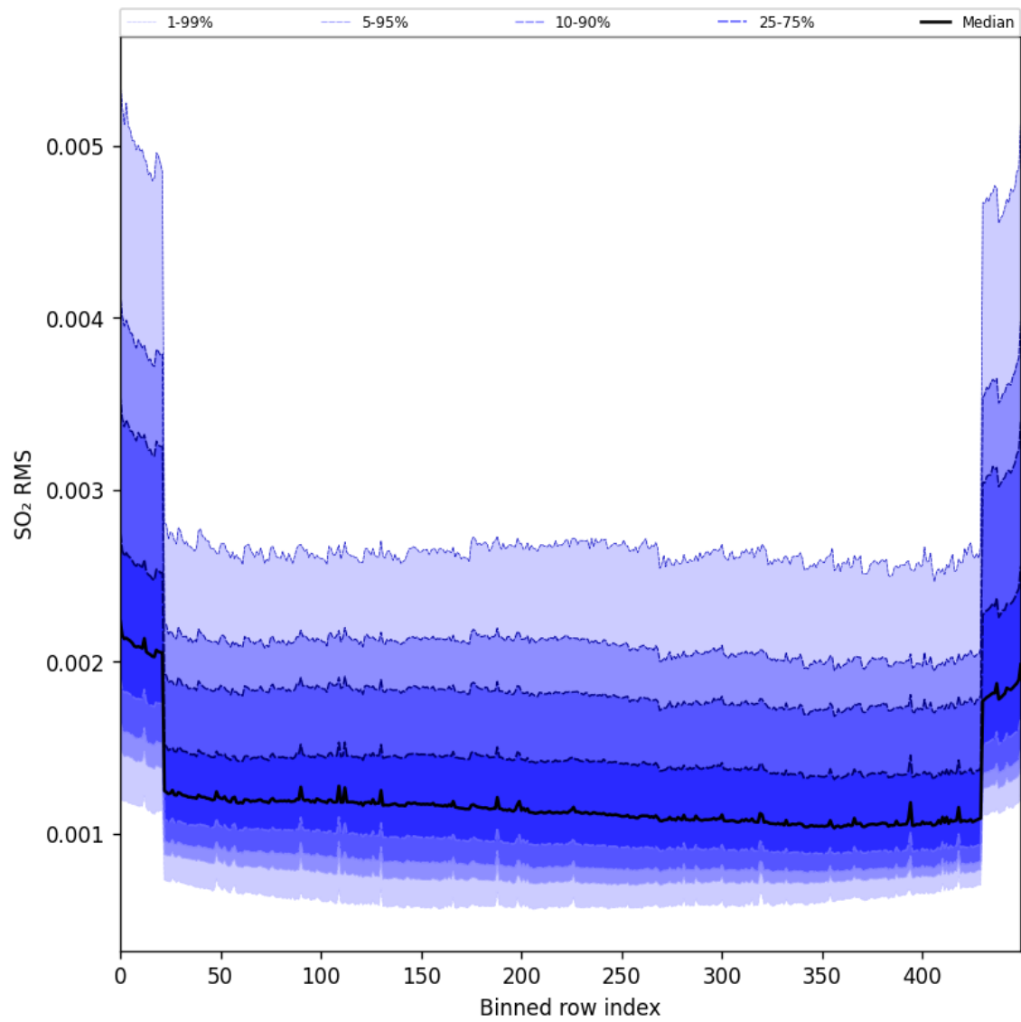
Figure 104: Along track statistics of “SO 2 RMS” for 2025-10-02 to 2025-10-04
