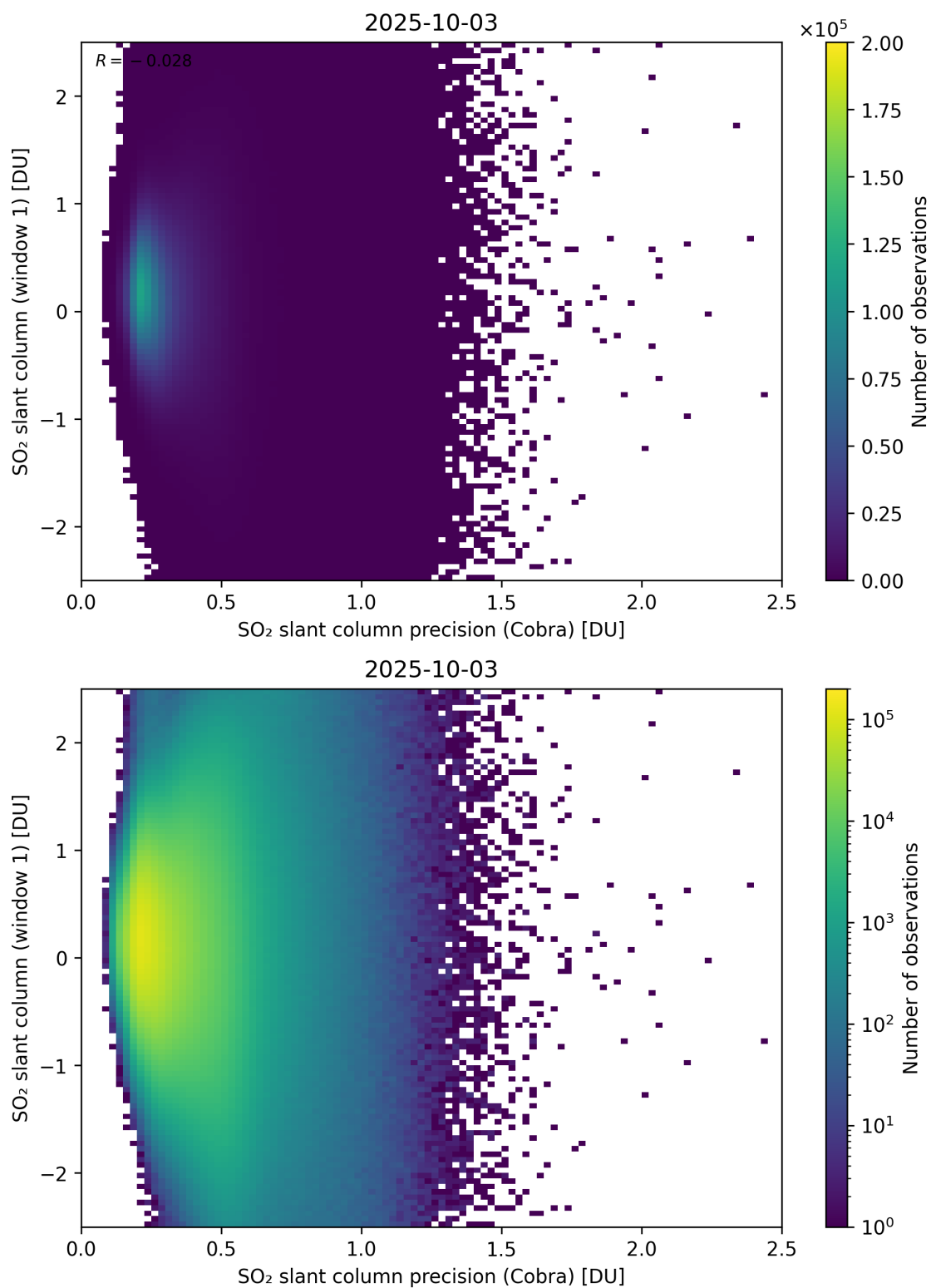
Figure 208: Scatter density plot of “SO 2 slant column precision (Cobra)” against “SO 2 slant column (window 1)” for 2025-10-02 to 2025-10-04.
