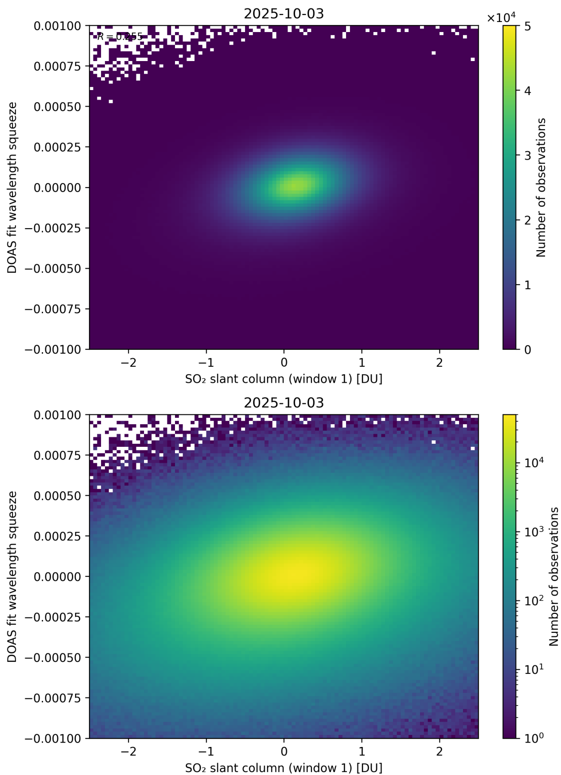
Figure 266: Scatter density plot of “SO 2 slant column (window 1)” against “DOAS fit wavelength squeeze” for 2025-10-02 to 2025-10-04.
