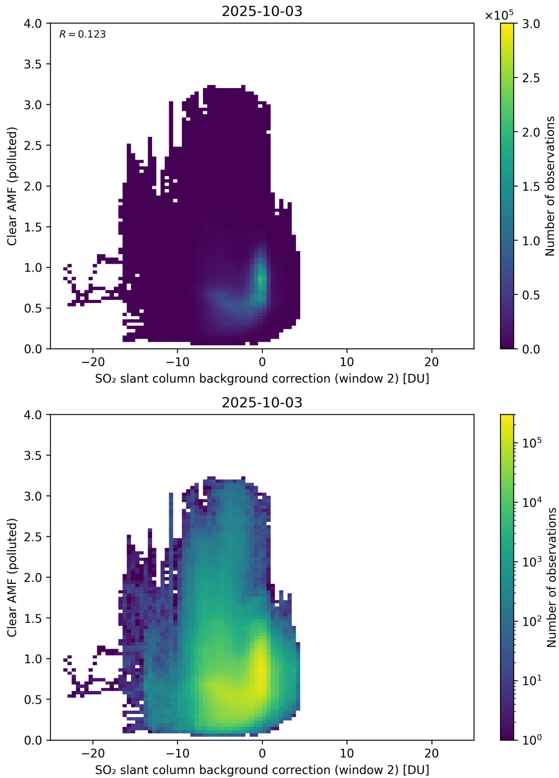
Figure 126: Scatter density plot of “SO 2 slant column background correction (window 2)” against “Clear AMF (polluted)” for 2025-10-02 to 2025-10-04.
