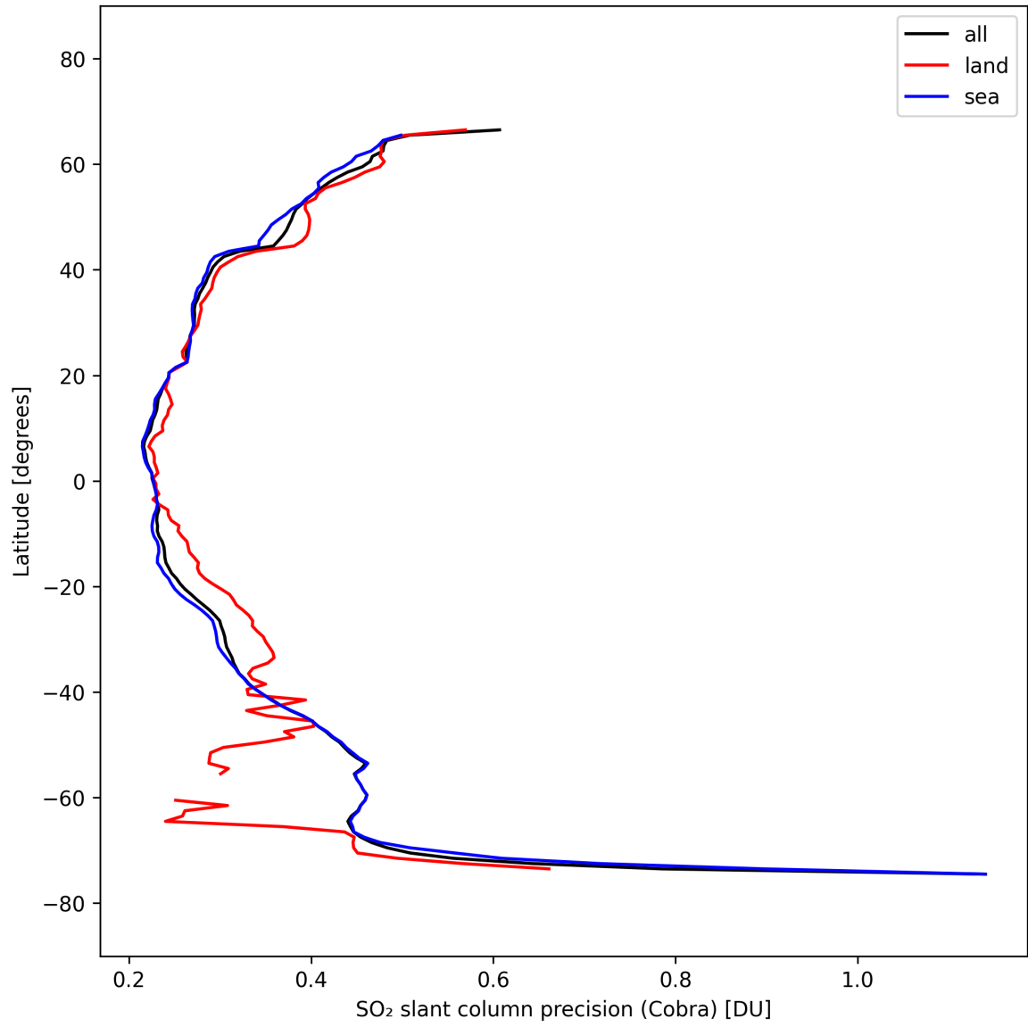
Figure 36: Zonal average of “SO 2 slant column precision (Cobra)” for 2025-10-02 to 2025-10-04.
