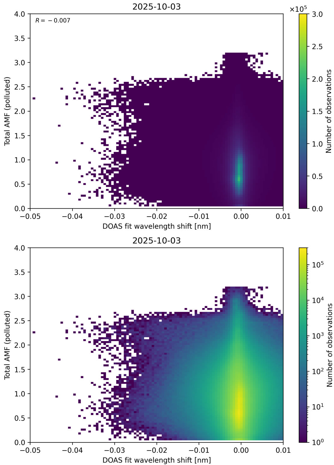
Figure 141: Scatter density plot of “DOAS fit wavelength shift” against “Total AMF (polluted)” for 2025-10-02 to 2025-10-04.
