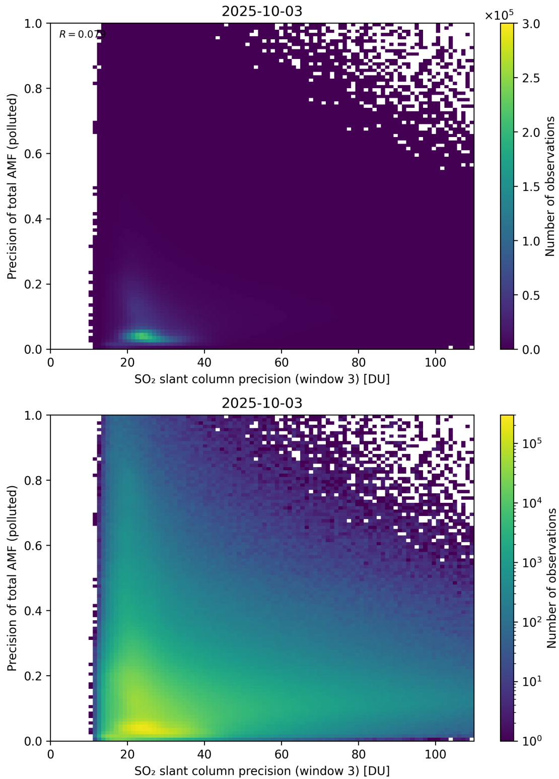
Figure 314: Scatter density plot of “SO 2 slant column precision (window 3)” against “Precision of total AMF (polluted)” for 2025-10-02 to 2025-10-04.
