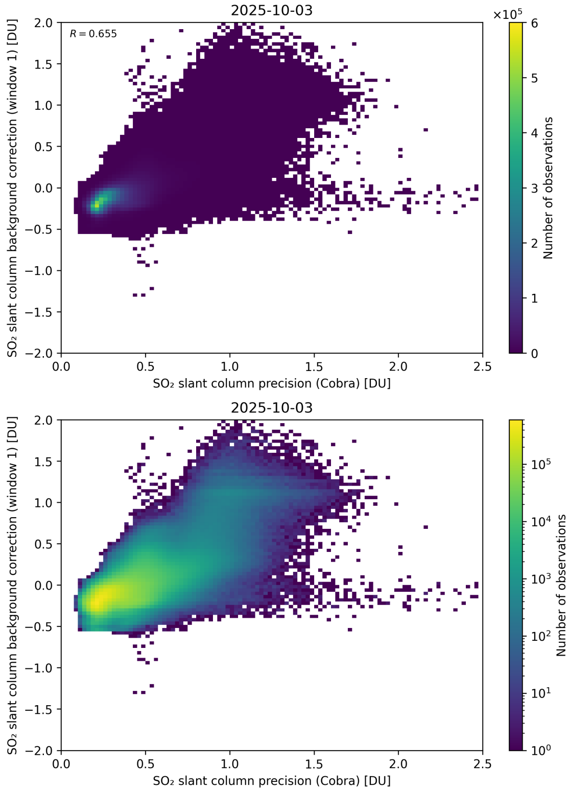
Figure 199: Scatter density plot of “SO 2 slant column precision (Cobra)” against “SO 2 slant column background correction (window 1)” for 2025-10-02 to 2025-10-04.
