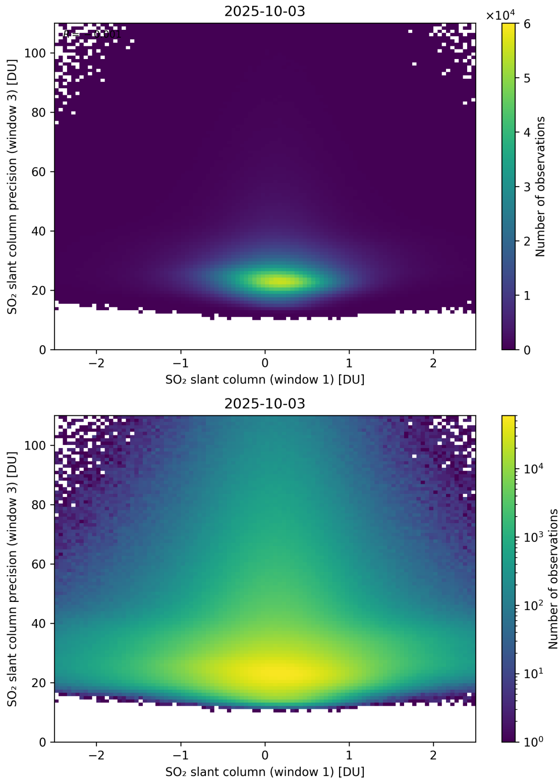
Figure 288: Scatter density plot of “SO 2 slant column (window 1)” against “SO 2 slant column precision (window 3)” for 2025-10-02 to 2025-10-04.
