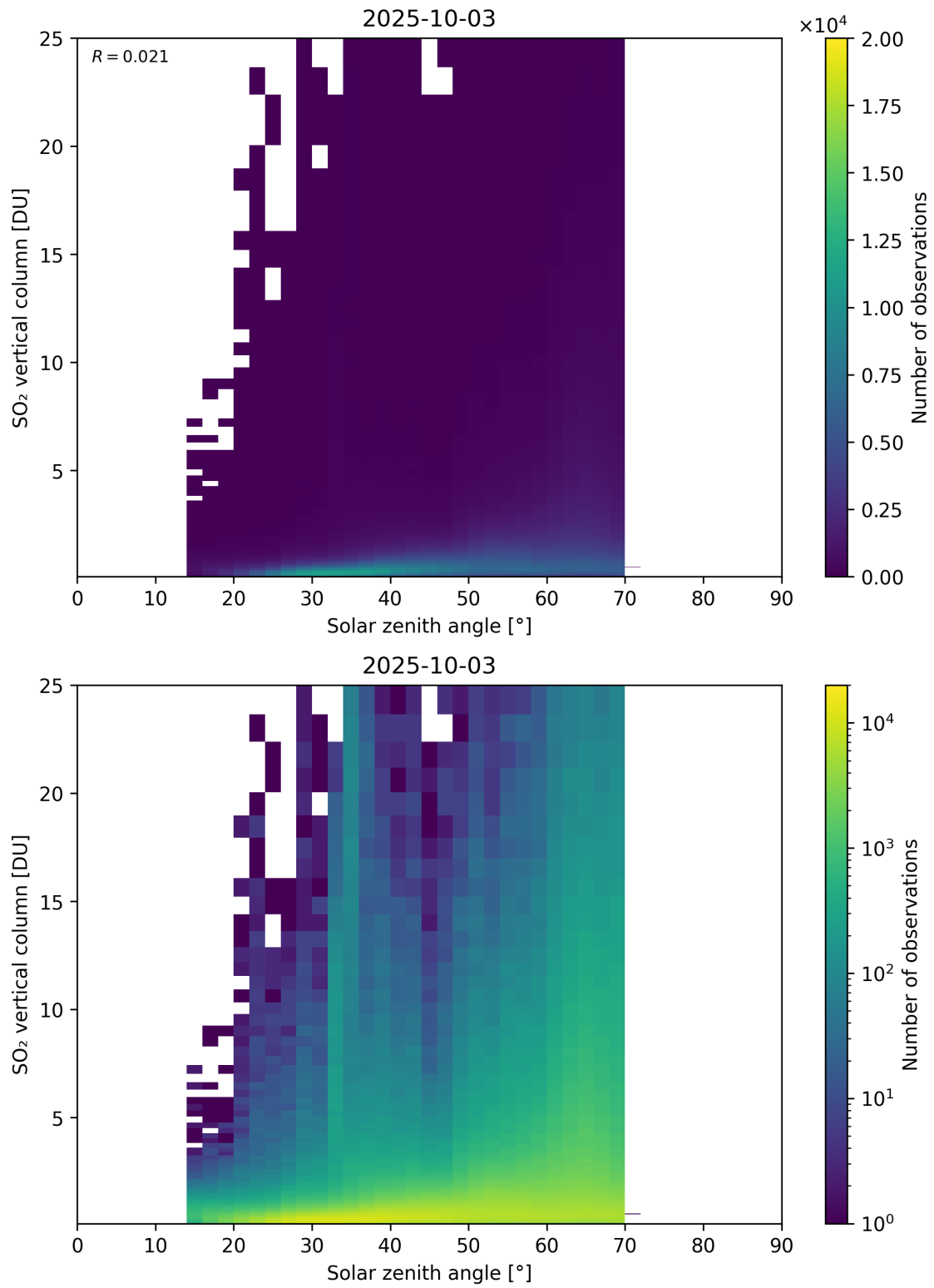
Figure 191: Scatter density plot of “Solar zenith angle” against “SO 2 vertical column” for 2025-10-02 to 2025-10-04.
