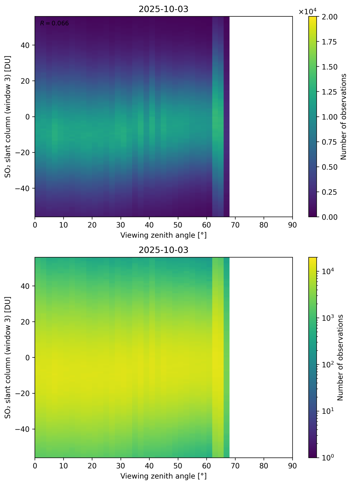
Figure 379: Scatter density plot of “Viewing zenith angle” against “SO 2 slant column (window 3)” for 2025-10-02 to 2025-10-04.
