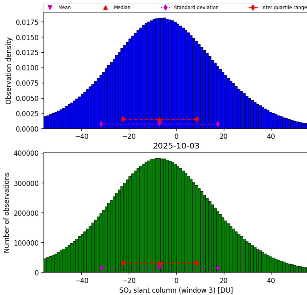
Figure 71: Histogram of “SO 2 slant column (window 3)” for 2025-10-02 to 2025-10-04
