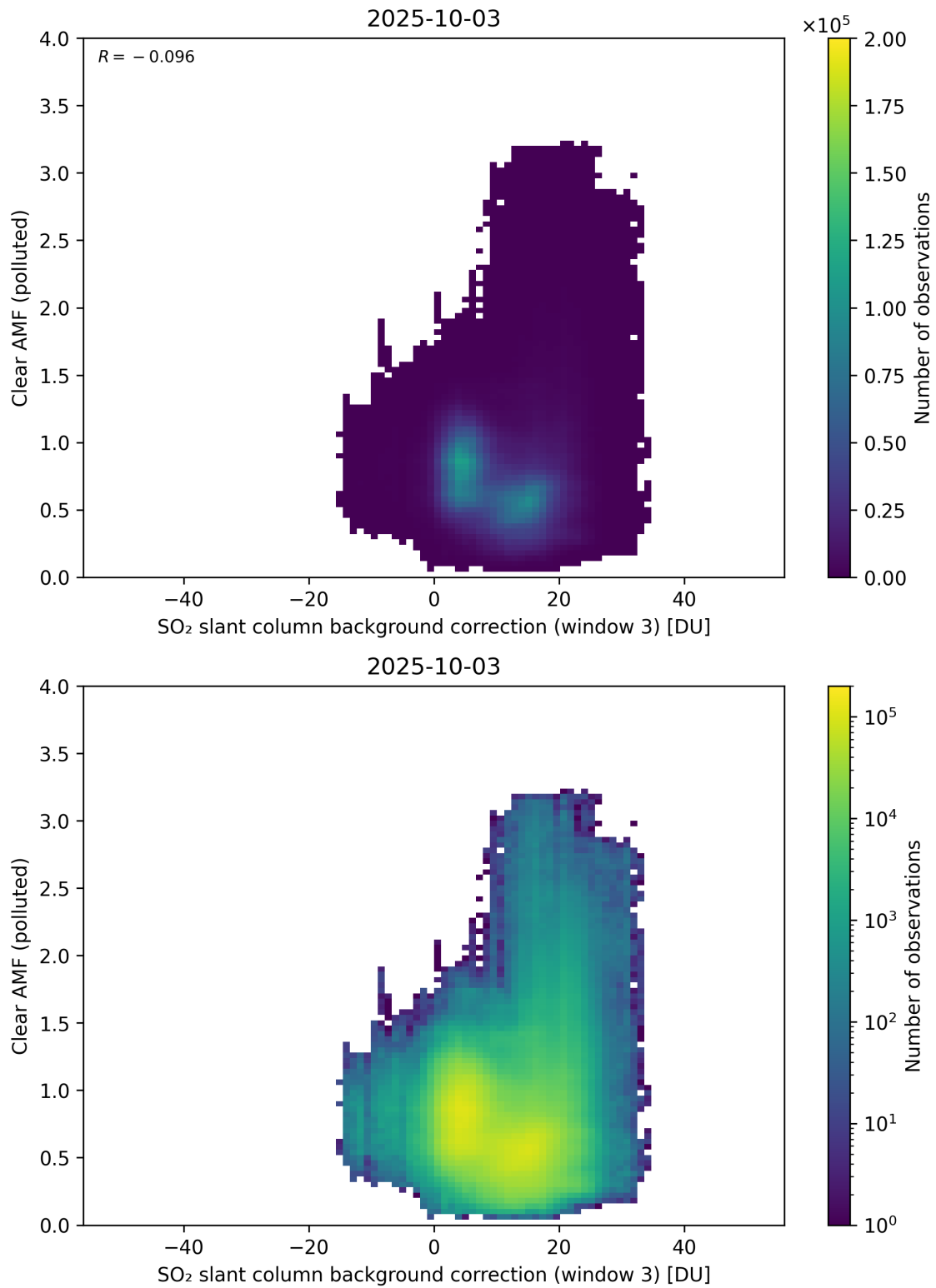
Figure 135: Scatter density plot of “SO 2 slant column background correction (window 3)” against “Clear AMF (polluted)” for 2025-10-02 to 2025-10-04.
