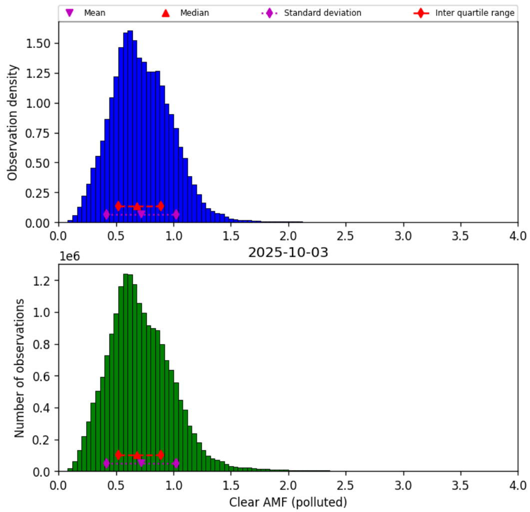
Figure 81: Histogram of “Clear AMF (polluted)” for 2025-10-02 to 2025-10-04
