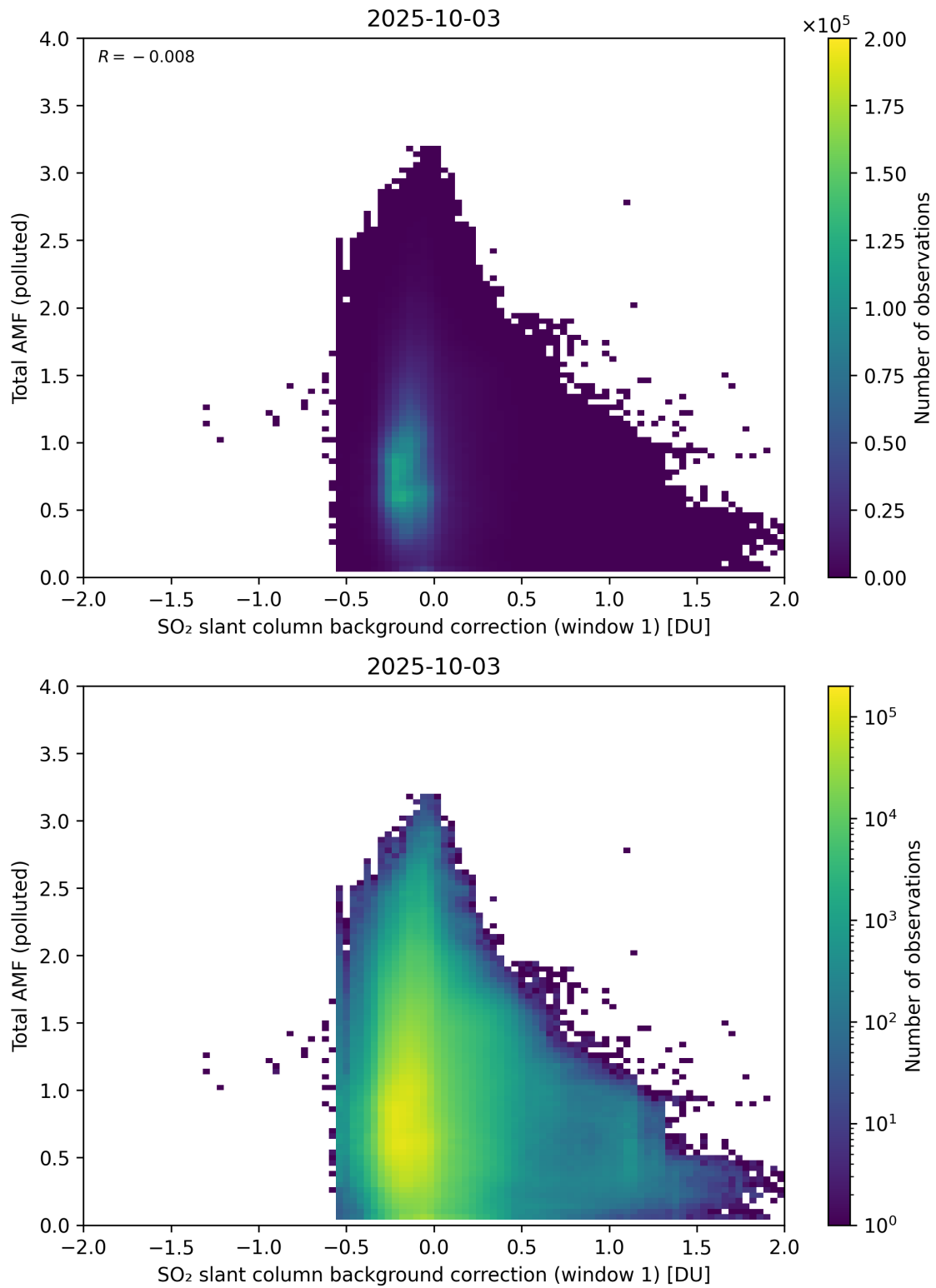
Figure 120: Scatter density plot of “SO 2 slant column background correction (window 1)” against “Total AMF (polluted)” for 2025-10-02 to 2025-10-04.
