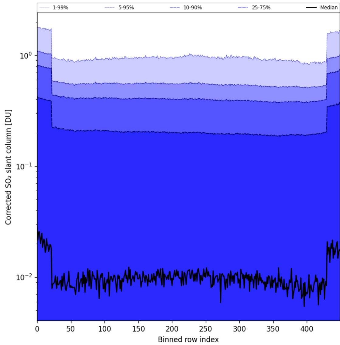
Figure 86: Along track statistics of “Corrected SO 2 slant column” for 2025-10-02 to 2025-10-04
