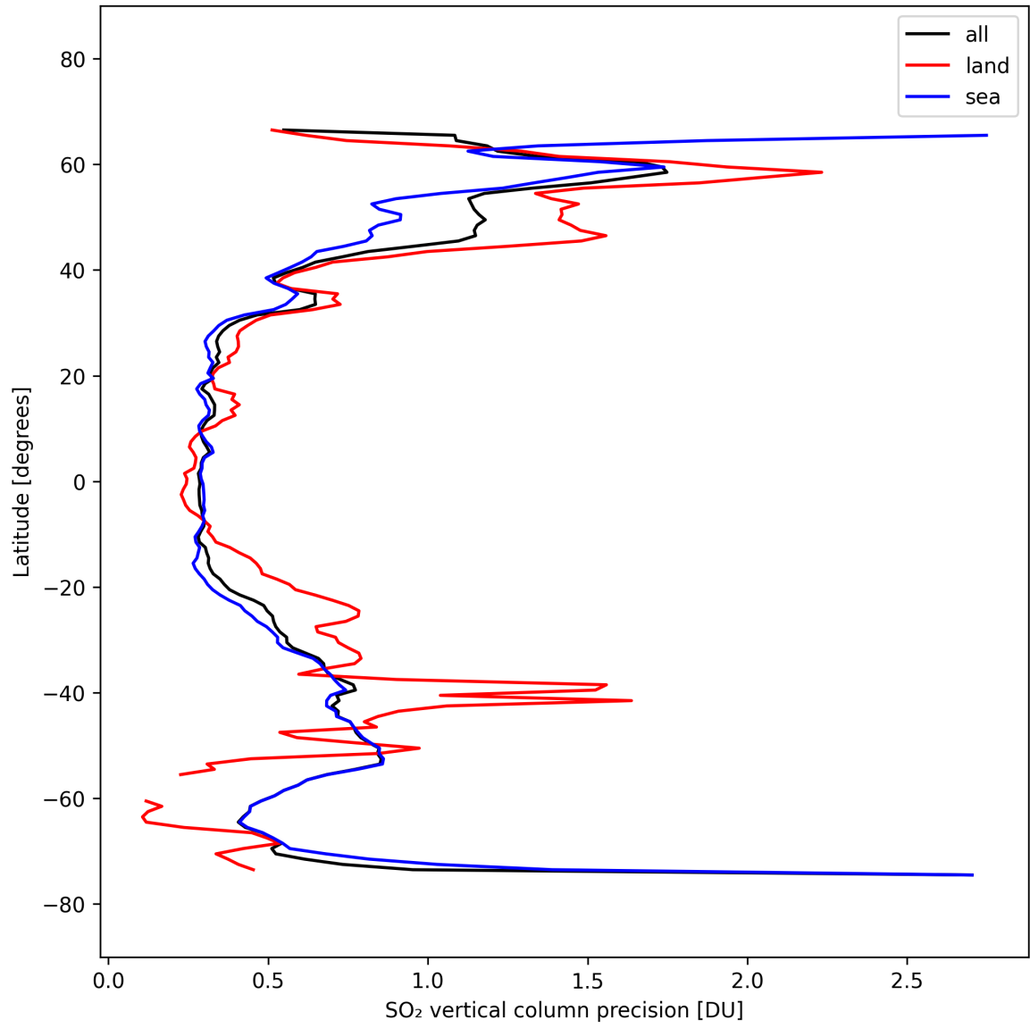
Figure 33: Zonal average of “SO 2 vertical column precision” for 2025-10-02 to 2025-10-04.
