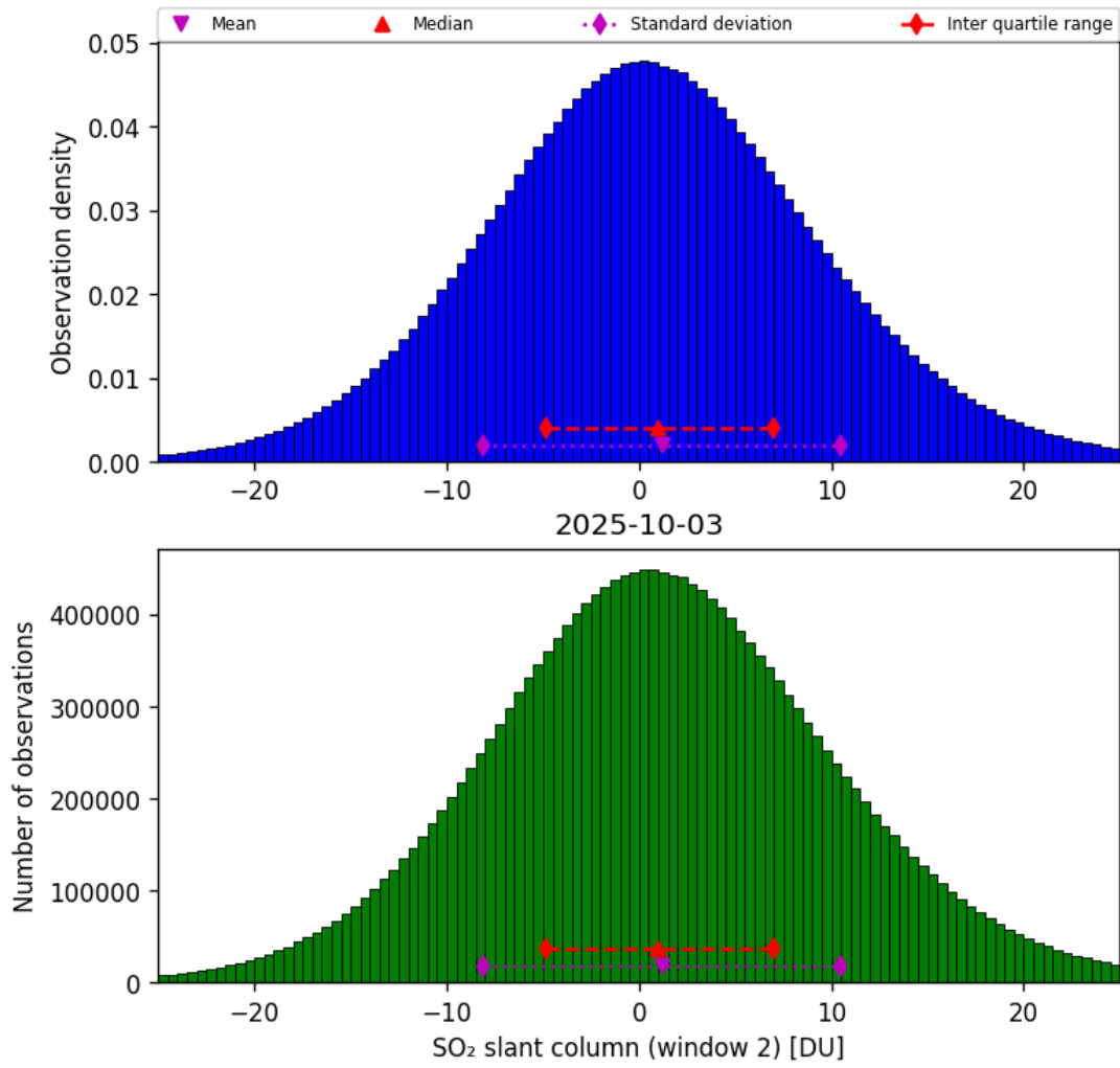
Figure 67: Histogram of “SO 2 slant column (window 2)” for 2025-10-02 to 2025-10-04
