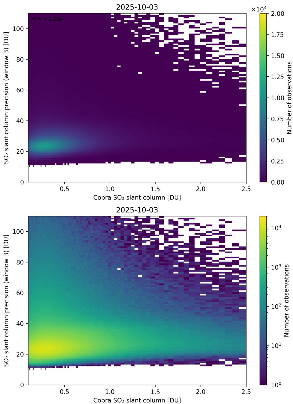
Figure 223: Scatter density plot of “Cobra SO 2 slant column” against “SO 2 slant column precision (window 3)” for 2025-10-02 to 2025-10-04.
