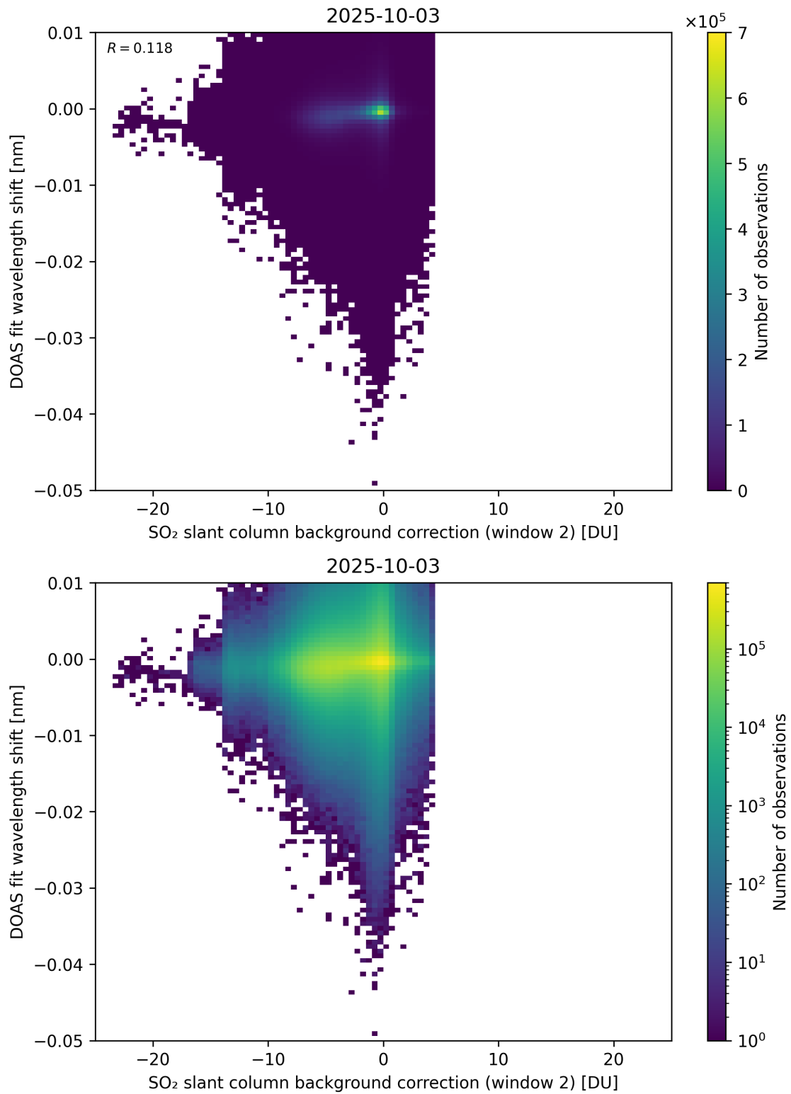
Figure 123: Scatter density plot of “SO 2 slant column background correction (window 2)” against “DOAS fit wavelength shift” for 2025-10-02 to 2025-10-04.
