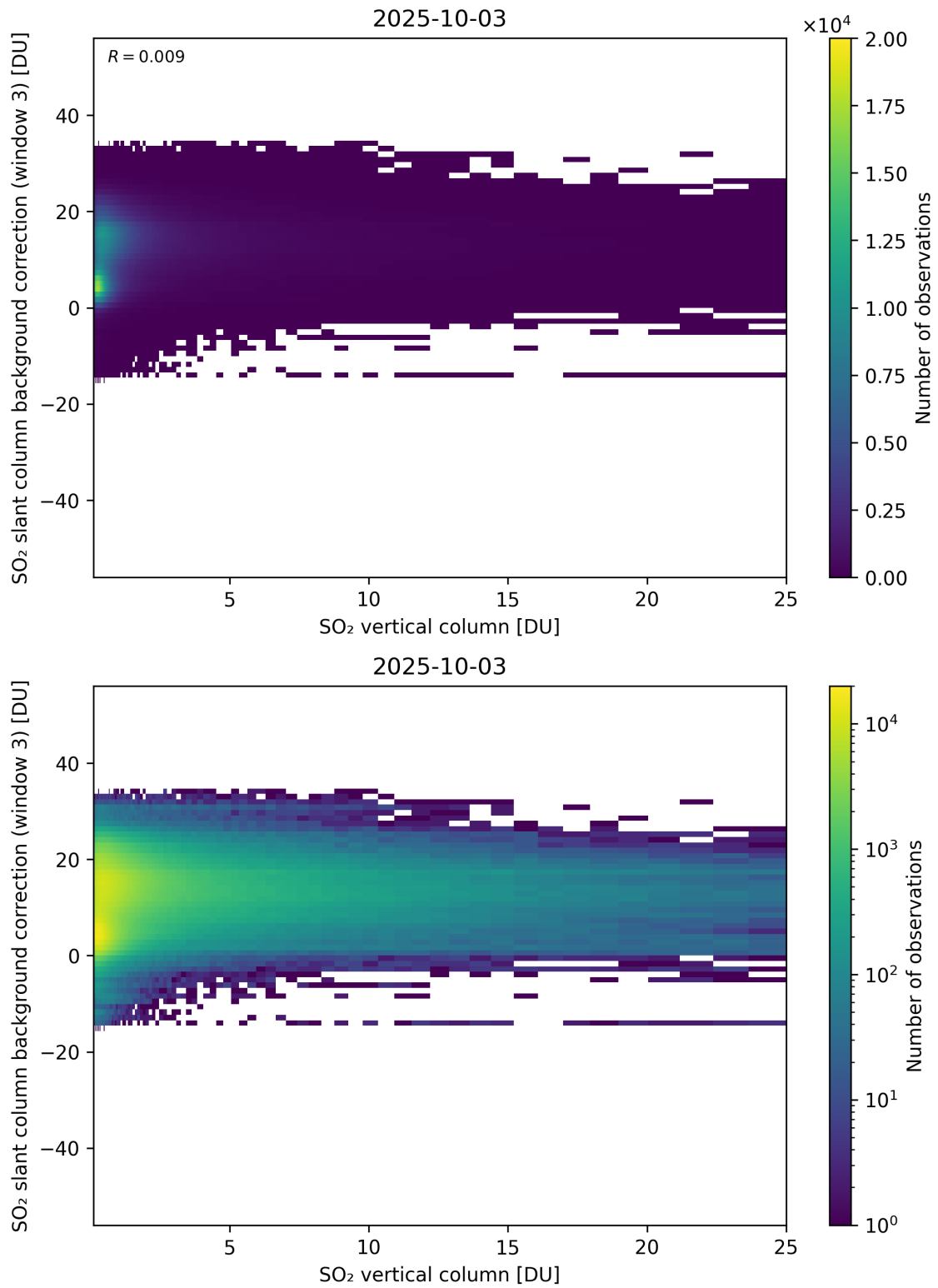
Figure 325: Scatter density plot of “SO 2 vertical column” against “SO 2 slant column background correction (window 3)” for 2025-10-02 to 2025-10-04.
