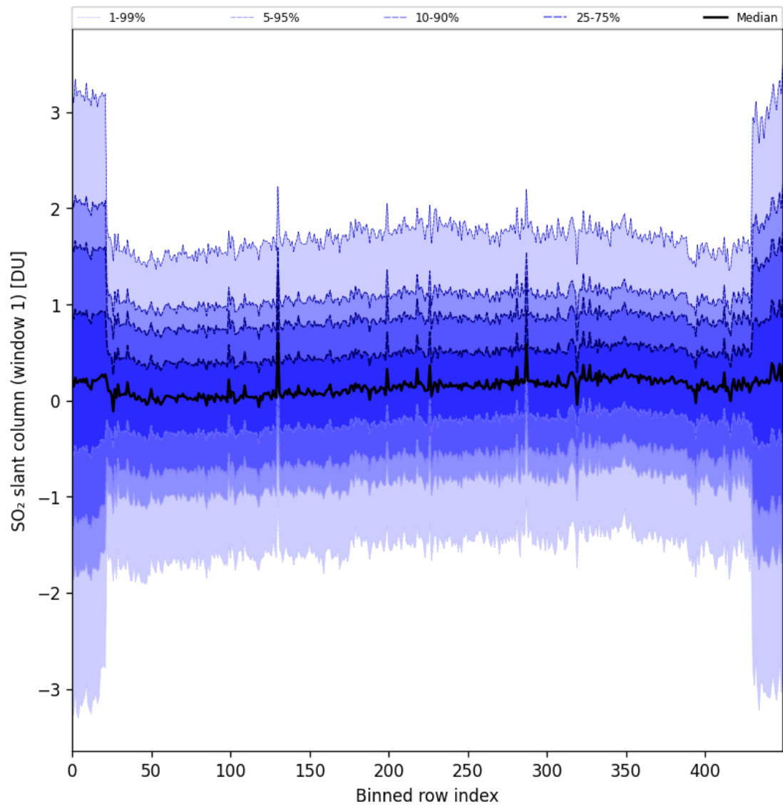
Figure 89: Along track statistics of “SO 2 slant column (window 1)” for 2025-10-02 to 2025-10-04
