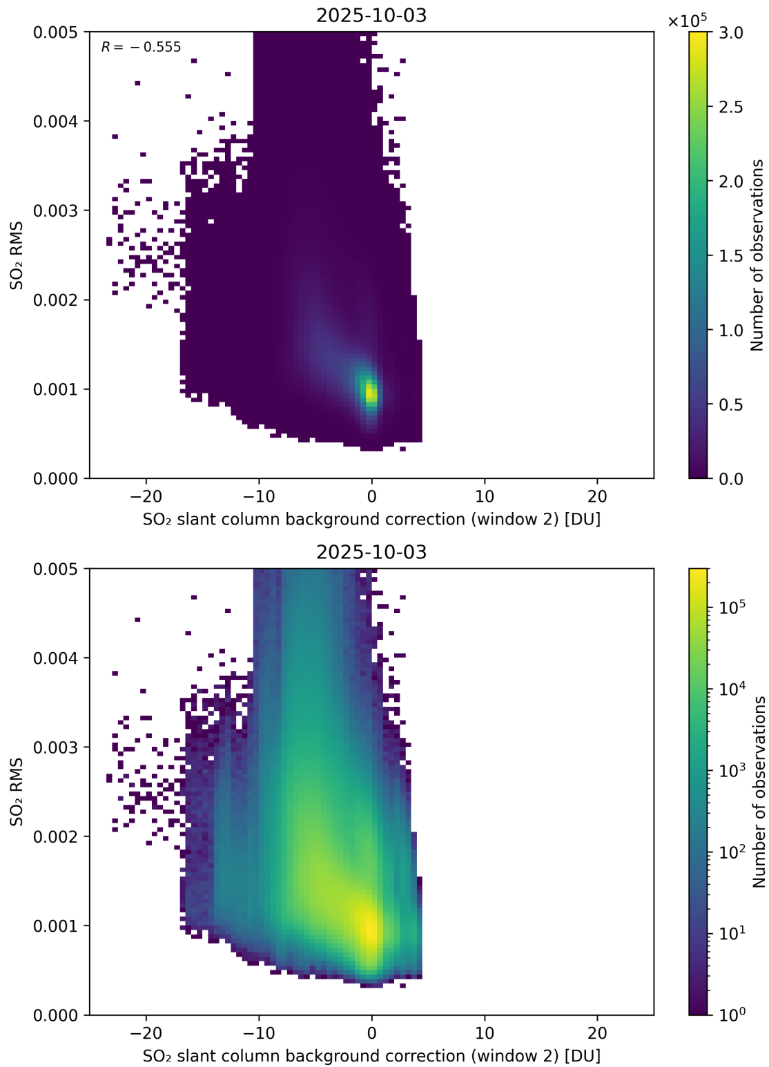
Figure 125: Scatter density plot of “SO 2 slant column background correction (window 2)” against “SO 2 RMS” for 2025-10-02 to 2025-10-04.
