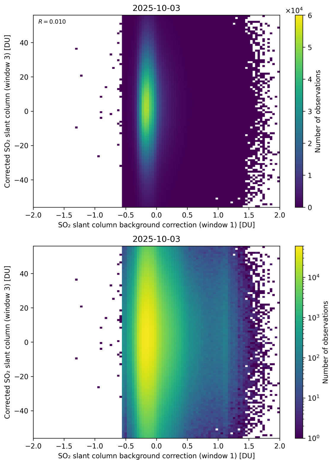
Figure 116: Scatter density plot of “SO 2 slant column background correction (window 1)” against “Corrected SO 2 slant column (window 3)” for 2025-10-02 to 2025-10-04.
