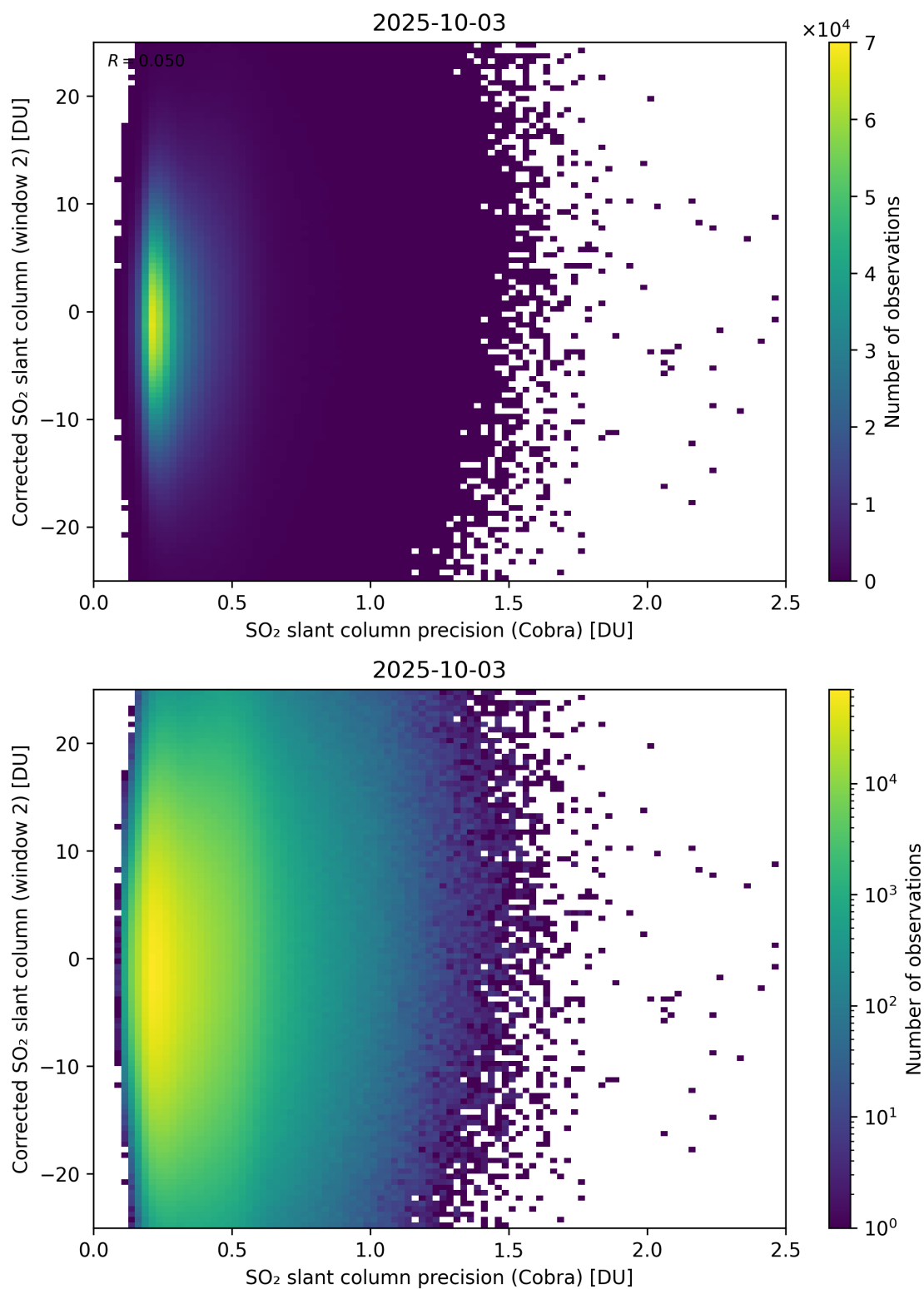
Figure 206: Scatter density plot of “SO 2 slant column precision (Cobra)” against “Corrected SO 2 slant column (window 2)” for 2025-10-02 to 2025-10-04.
