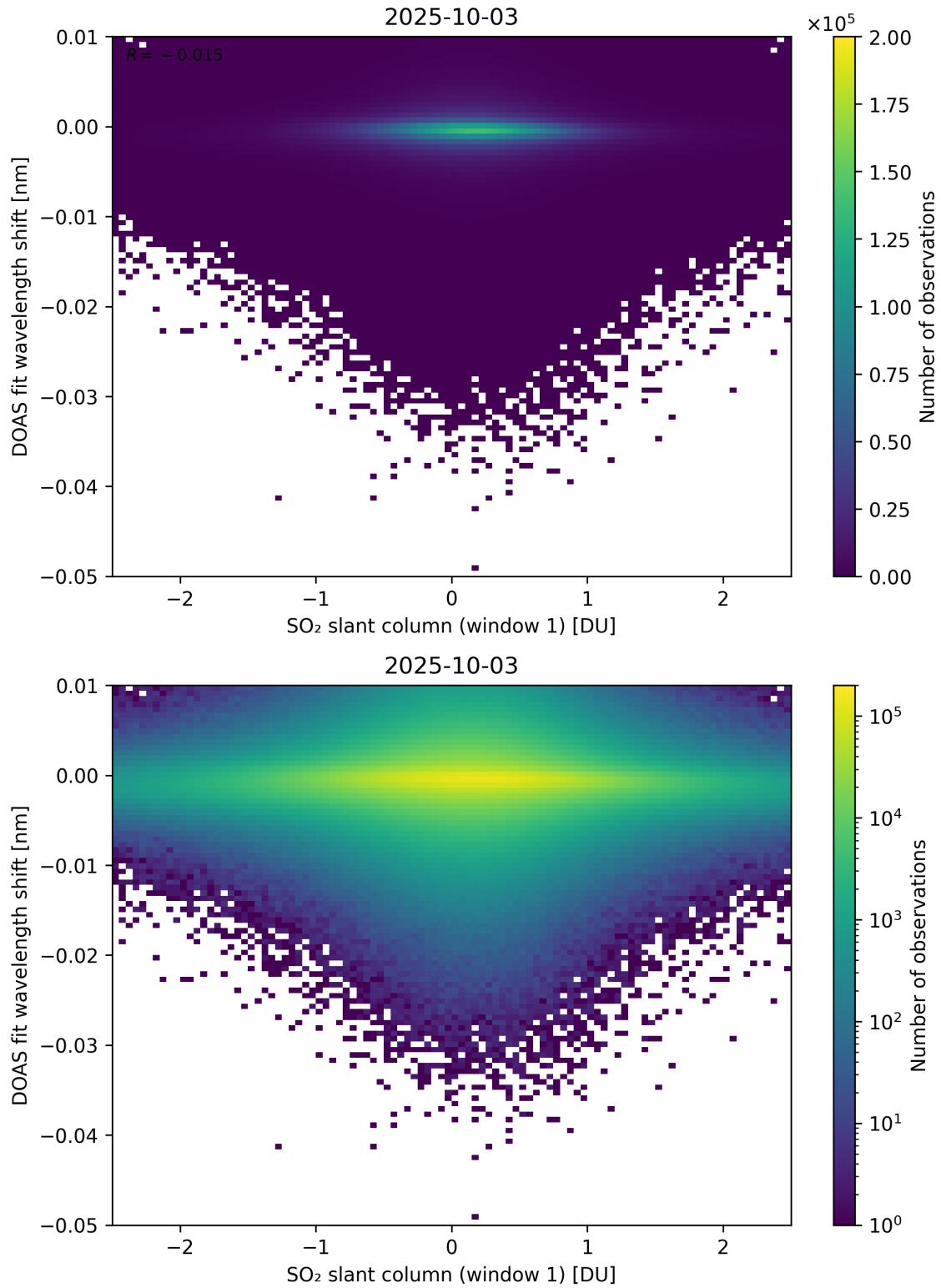
Figure 265: Scatter density plot of “SO 2 slant column (window 1)” against “DOAS fit wavelength shift” for 2025-10-02 to 2025-10-04.
