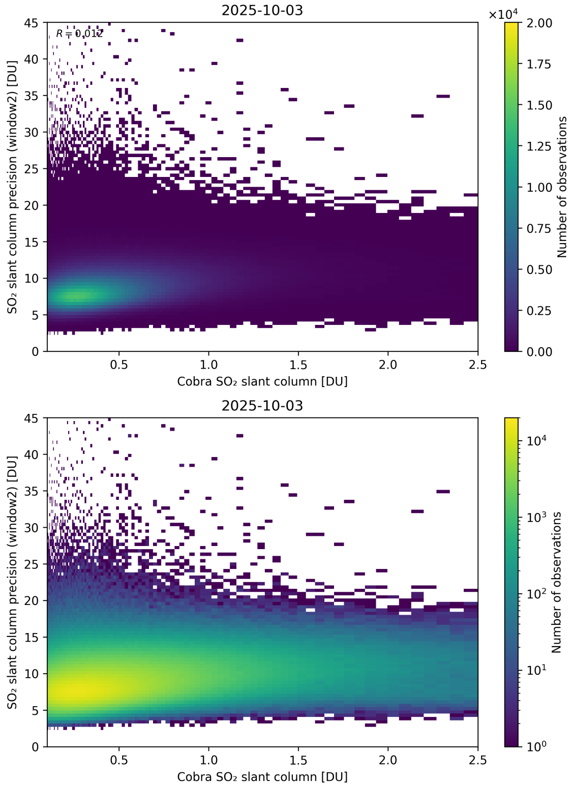
Figure 221: Scatter density plot of “Cobra SO 2 slant column” against “SO 2 slant column precision (window2)” for 2025-10-02 to 2025-10-04.
