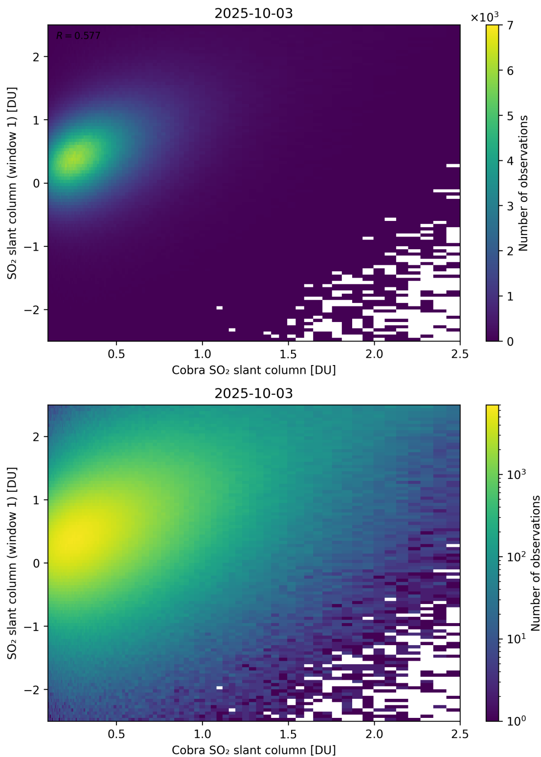
Figure 219: Scatter density plot of “Cobra SO 2 slant column” against “SO 2 slant column (window 1)” for 2025-10-02 to 2025-10-04.
