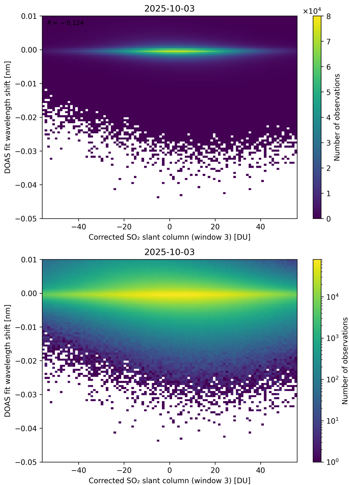
Figure 256: Scatter density plot of “Corrected SO 2 slant column (window 3)” against “DOAS fit wavelength shift” for 2025-10-02 to 2025-10-04.
