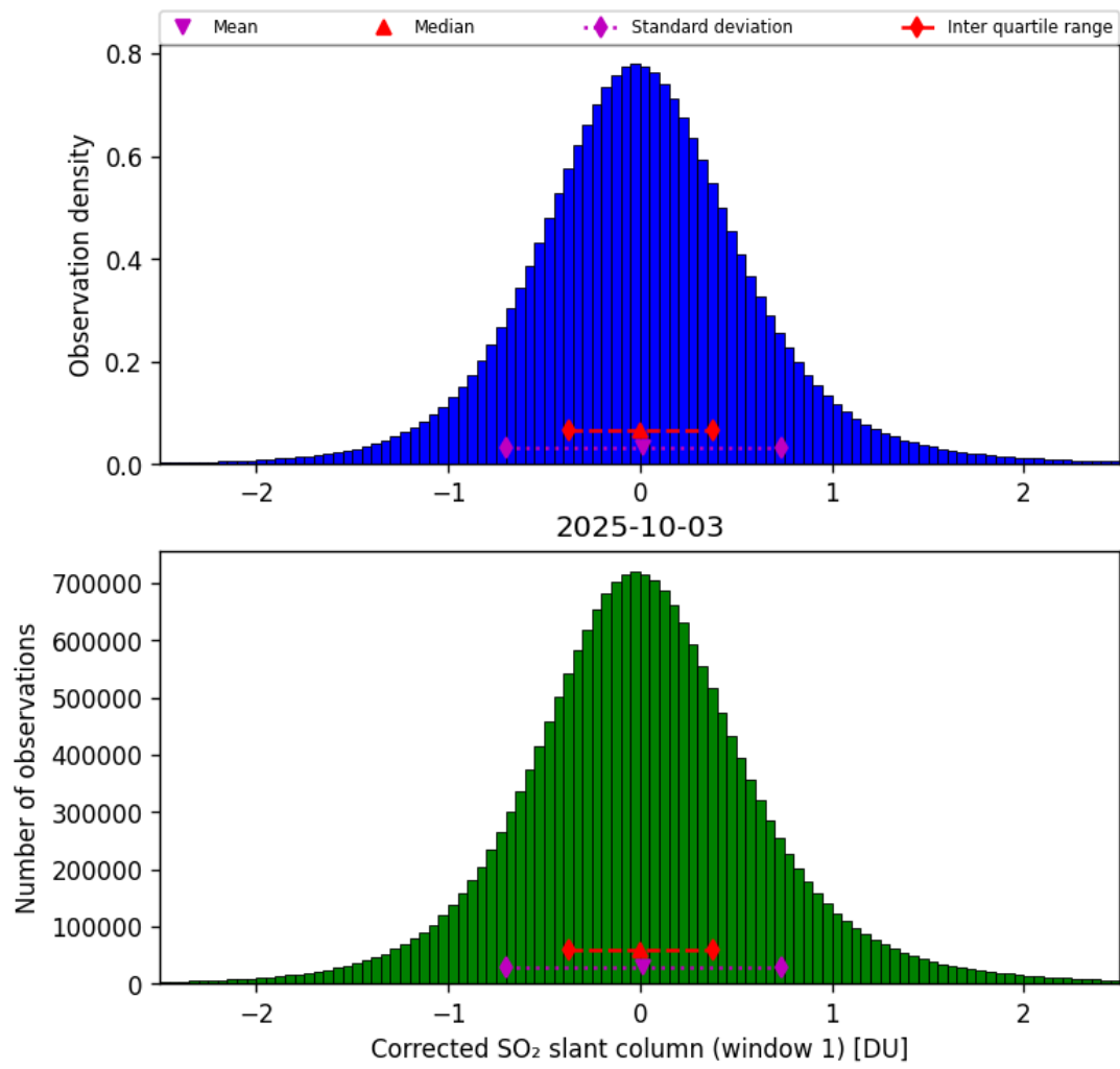
Figure 65: Histogram of “Corrected SO 2 slant column (window 1)” for 2025-10-02 to 2025-10-04
