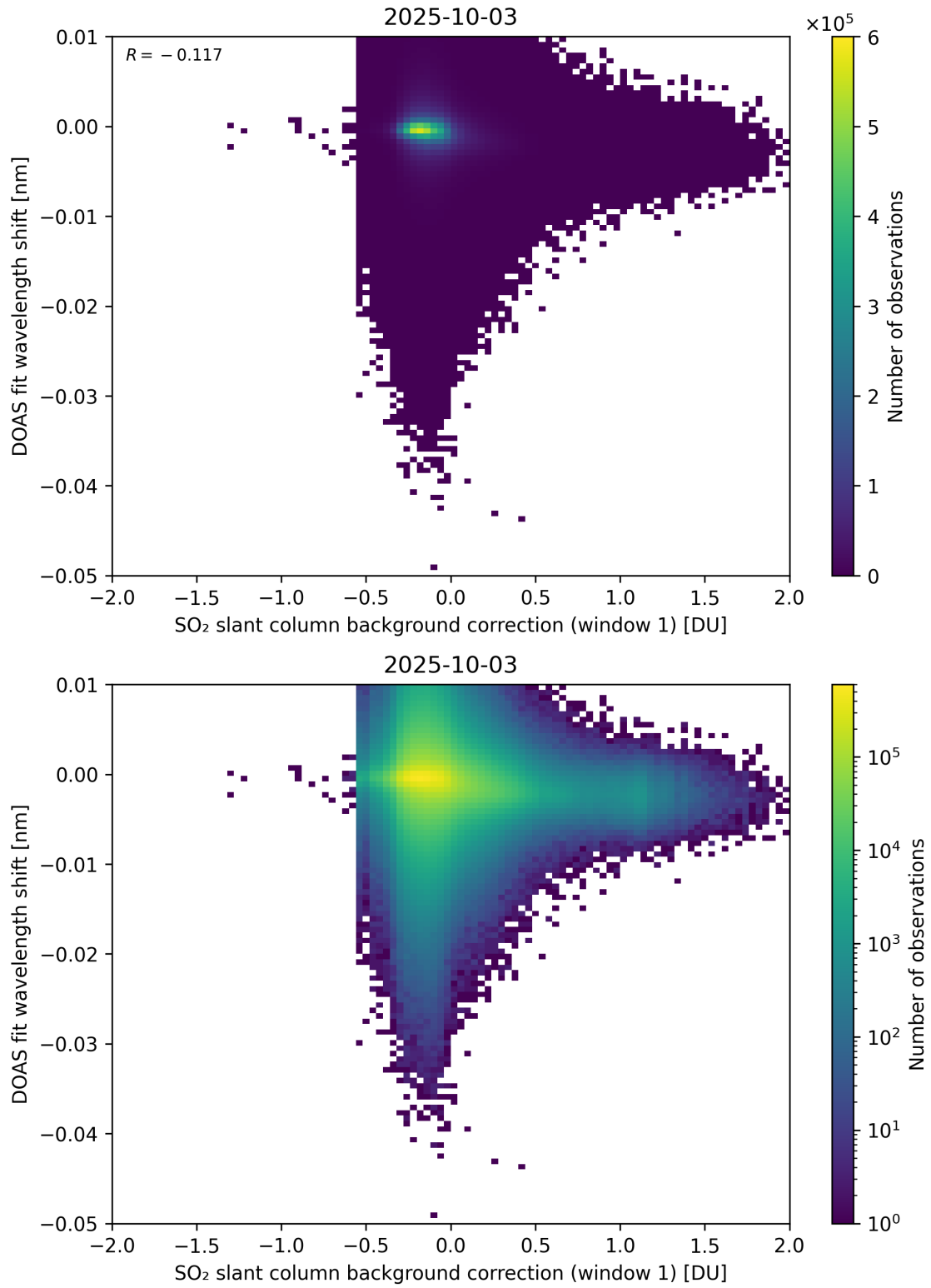
Figure 111: Scatter density plot of “SO 2 slant column background correction (window 1)” against “DOAS fit wavelength shift” for 2025-10-02 to 2025-10-04.
