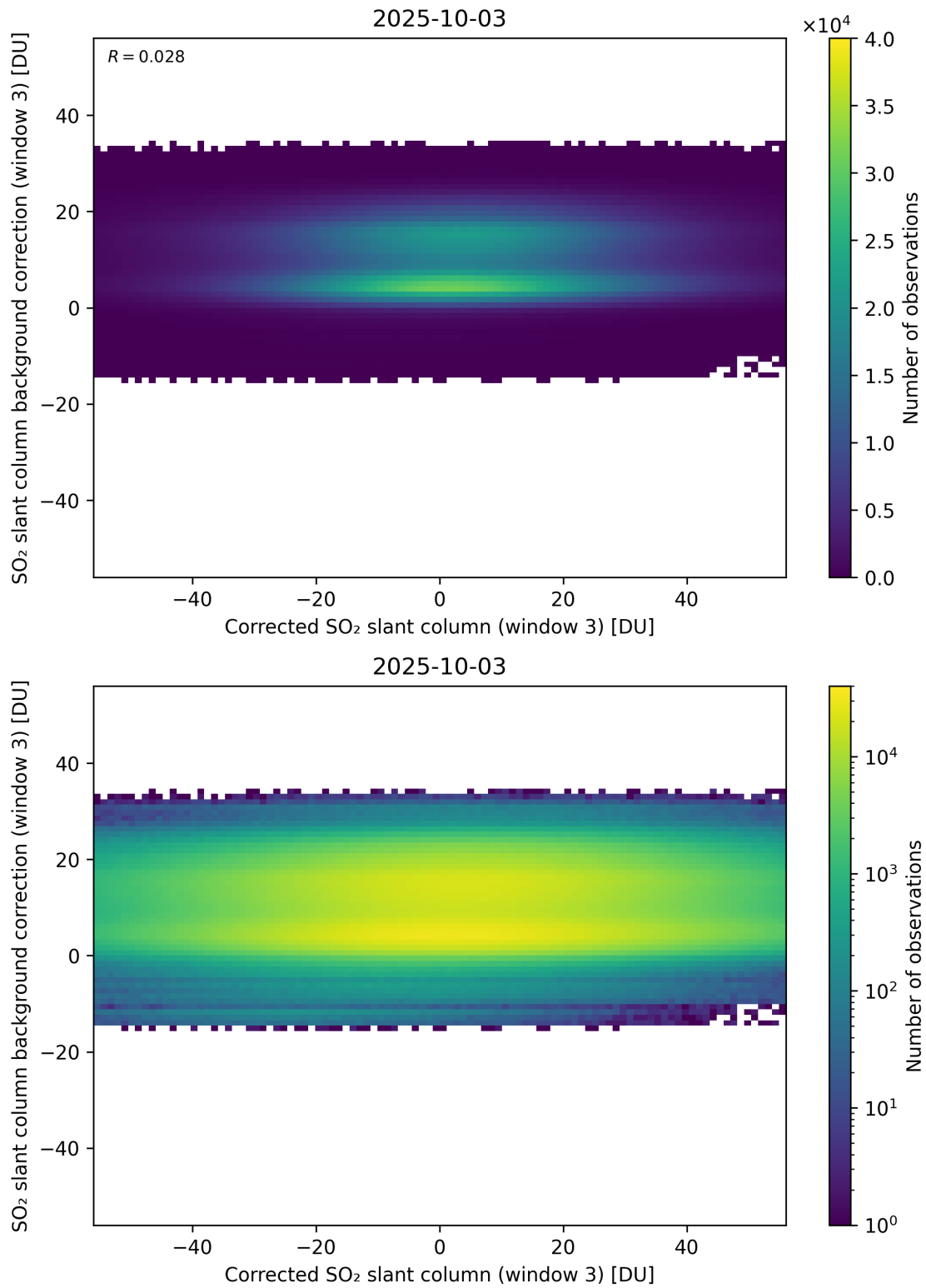
Figure 255: Scatter density plot of “Corrected SO 2 slant column (window 3)” against “SO 2 slant column background correction (window 3)” for 2025-10-02 to 2025-10-04.
