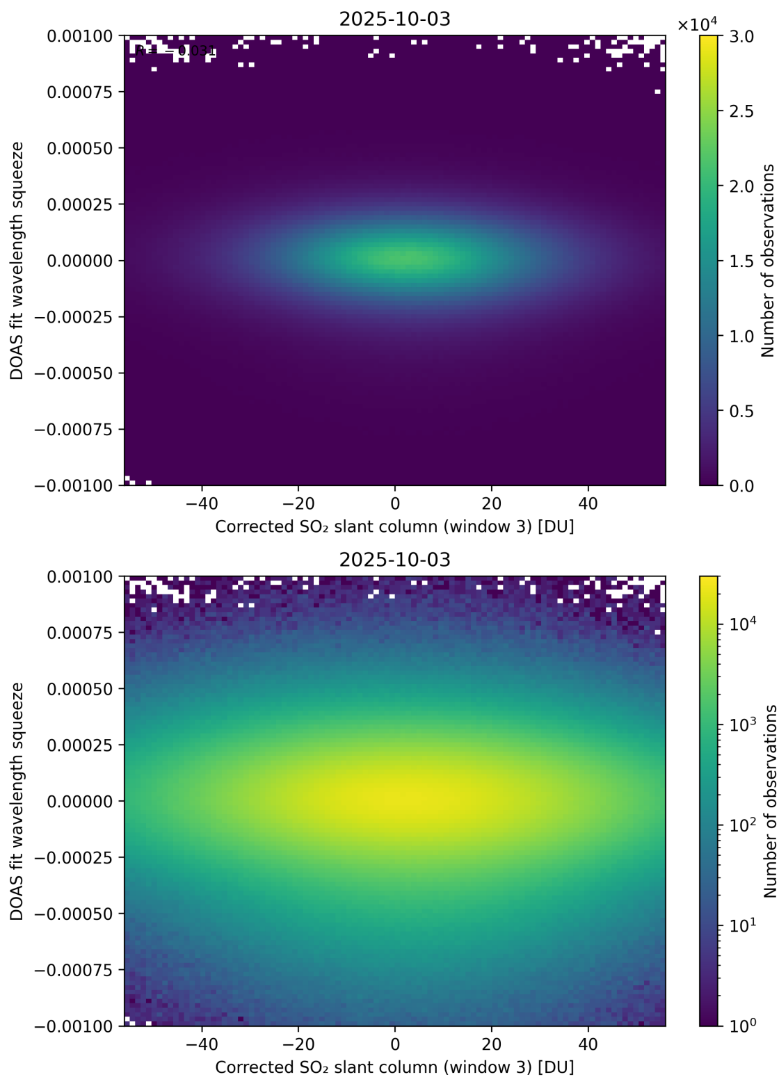
Figure 257: Scatter density plot of “Corrected SO 2 slant column (window 3)” against “DOAS fit wavelength squeeze” for 2025-10-02 to 2025-10-04.
