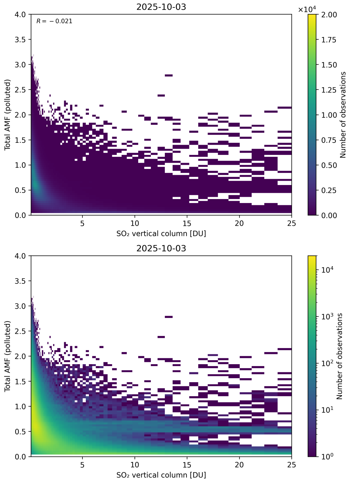
Figure 359: Scatter density plot of “SO 2 vertical column” against “Total AMF (polluted)” for 2025-10-02 to 2025-10-04.
