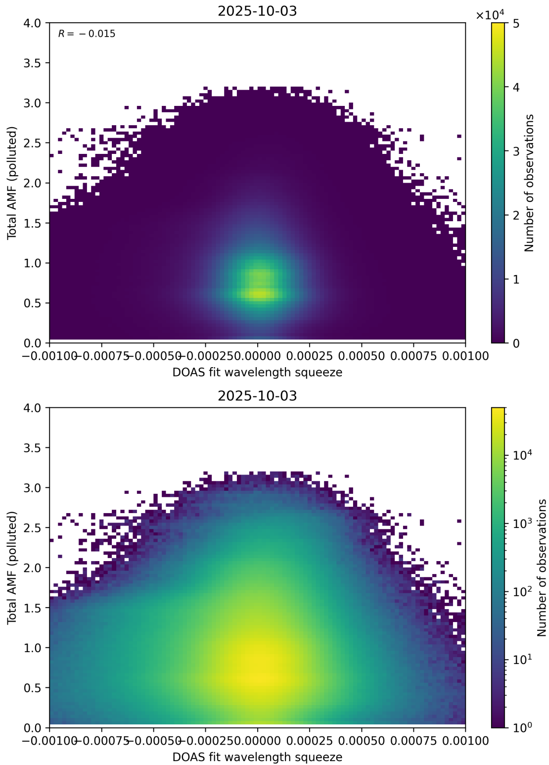
Figure 145: Scatter density plot of “DOAS fit wavelength squeeze” against “Total AMF (polluted)” for 2025-10-02 to 2025-10-04.
