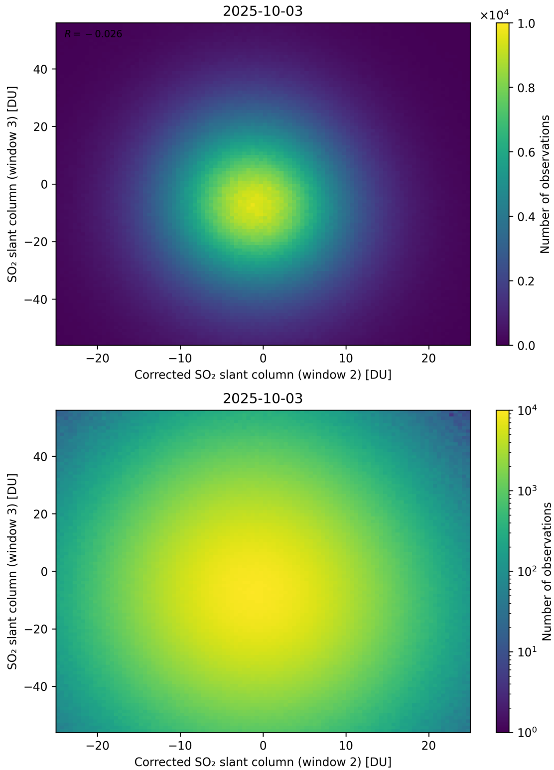
Figure 251: Scatter density plot of “Corrected SO 2 slant column (window 2)” against “SO 2 slant column (window 3)” for 2025-10-02 to 2025-10-04.
