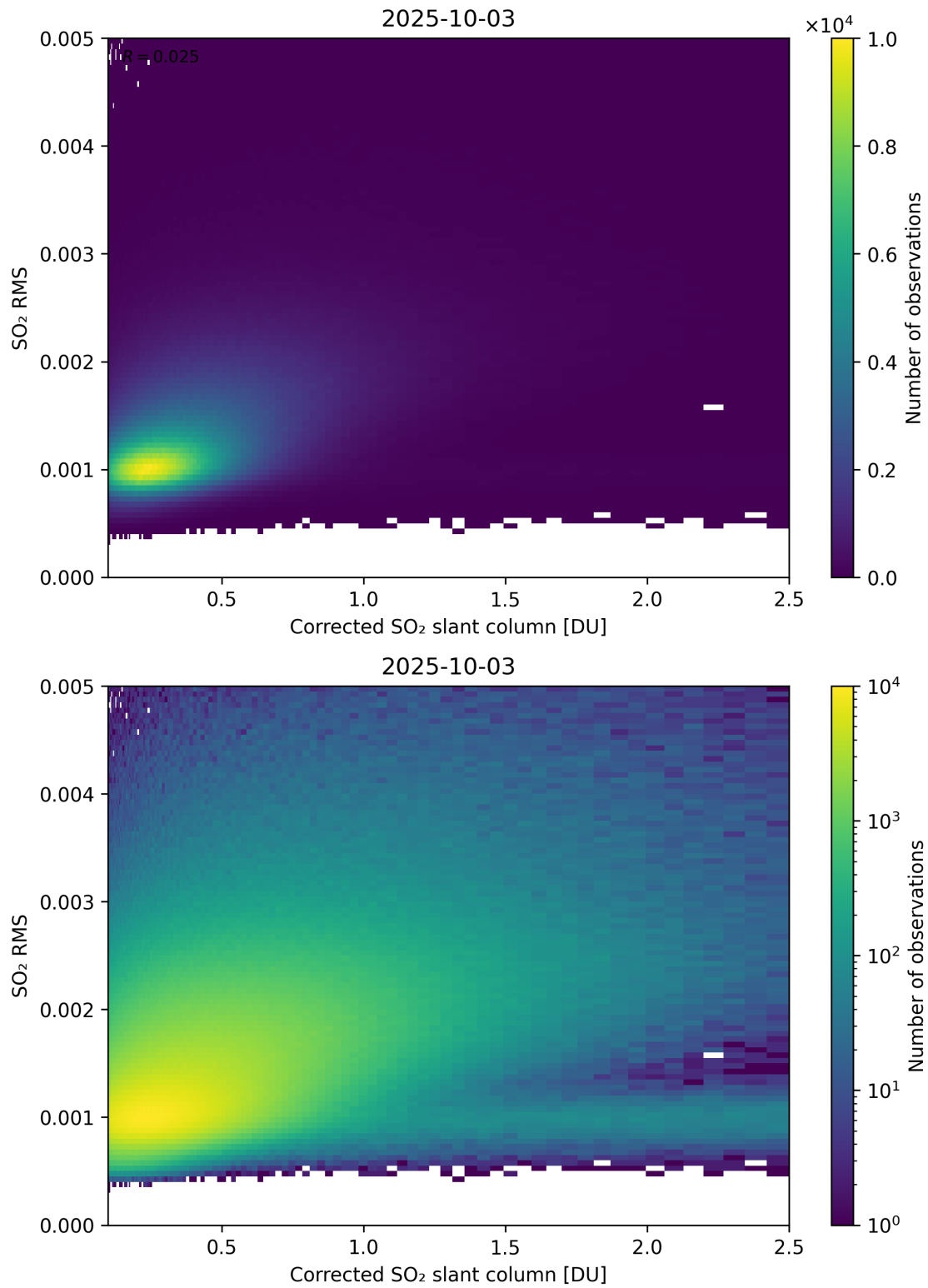
Figure 231: Scatter density plot of “Corrected SO 2 slant column” against “SO 2 RMS” for 2025-10-02 to 2025-10-04.
