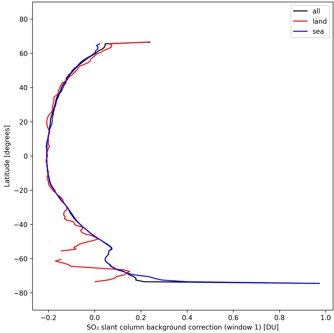
Figure 40: Zonal average of "SO 2 slant column background correction (window 1)" for 2025-10-02 to 2025-10-04.
