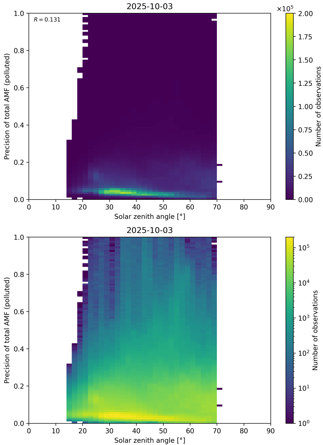
Figure 190: Scatter density plot of “Solar zenith angle” against “Precision of total AMF (polluted)” for 2025-10-02 to 2025-10-04.
