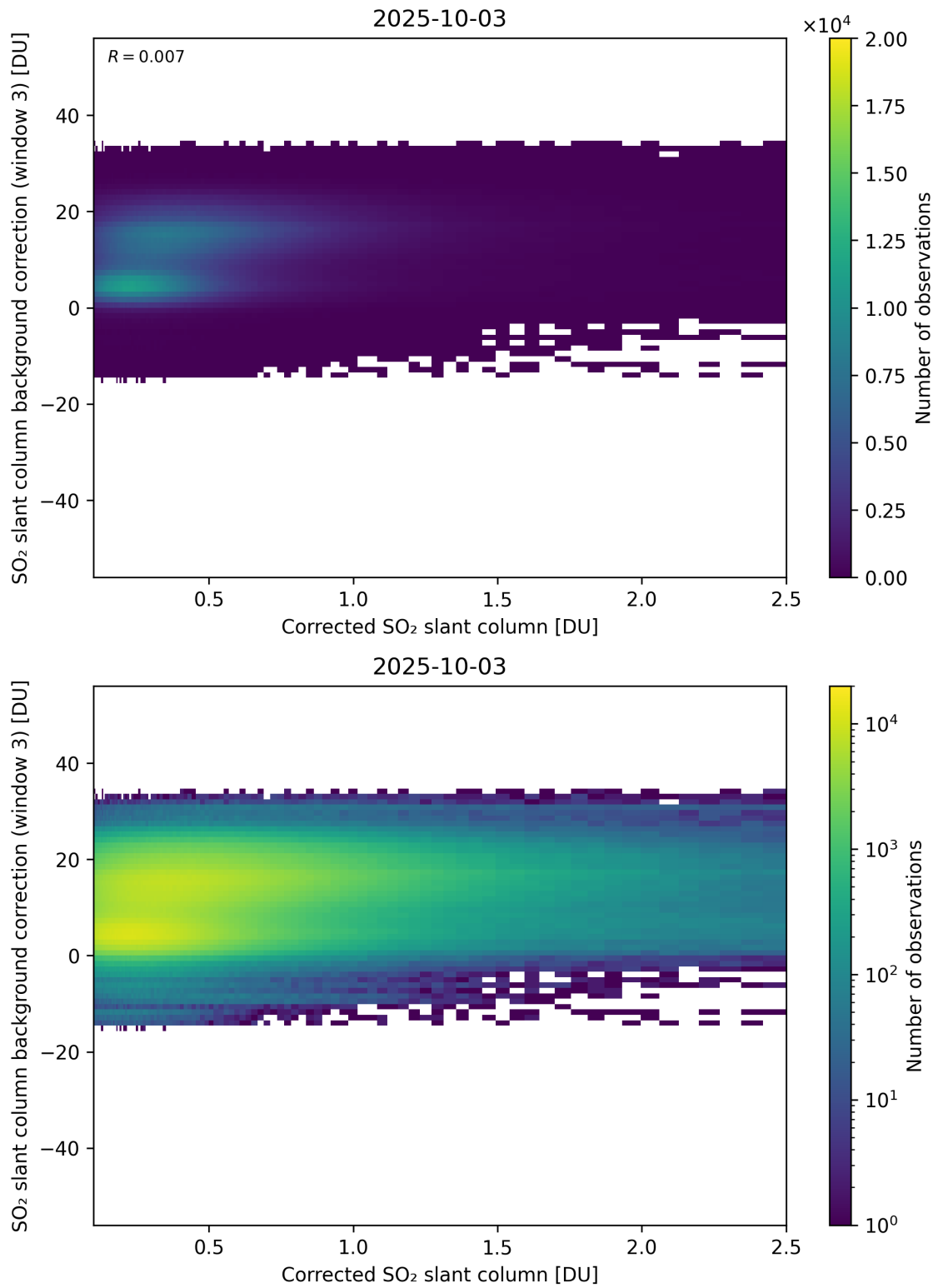
Figure 228: Scatter density plot of “Corrected SO 2 slant column” against “SO 2 slant column background correction (window 3)” for 2025-10-02 to 2025-10-04.
