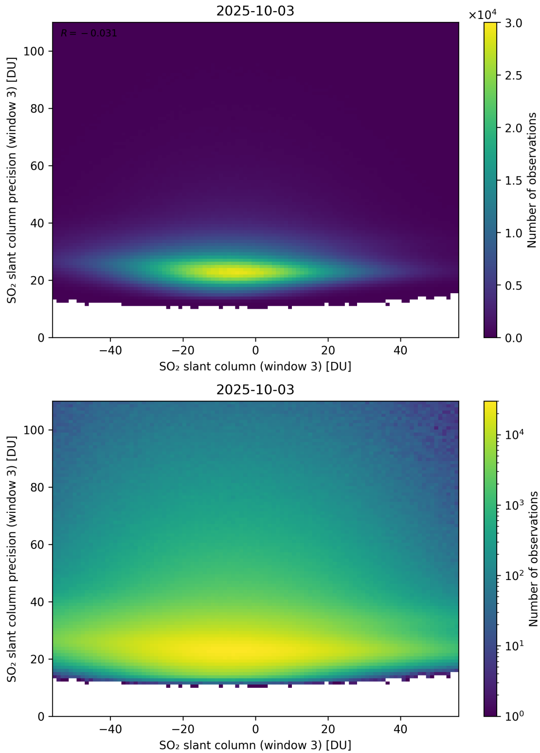
Figure 317: Scatter density plot of “SO 2 slant column (window 3)” against “SO 2 slant column precision (window 3)” for 2025-10-02 to 2025-10-04.
