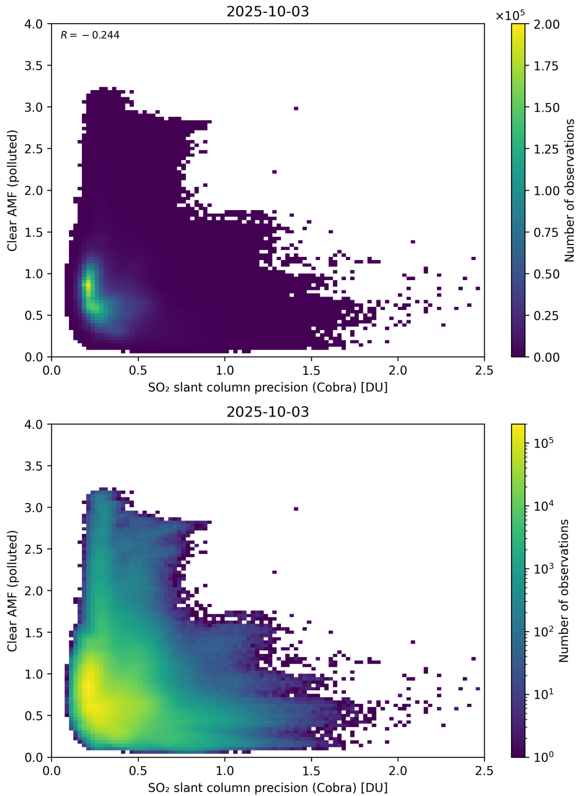
Figure 205: Scatter density plot of “SO 2 slant column precision (Cobra)” against “Clear AMF (polluted)” for 2025-10-02 to 2025-10-04.
