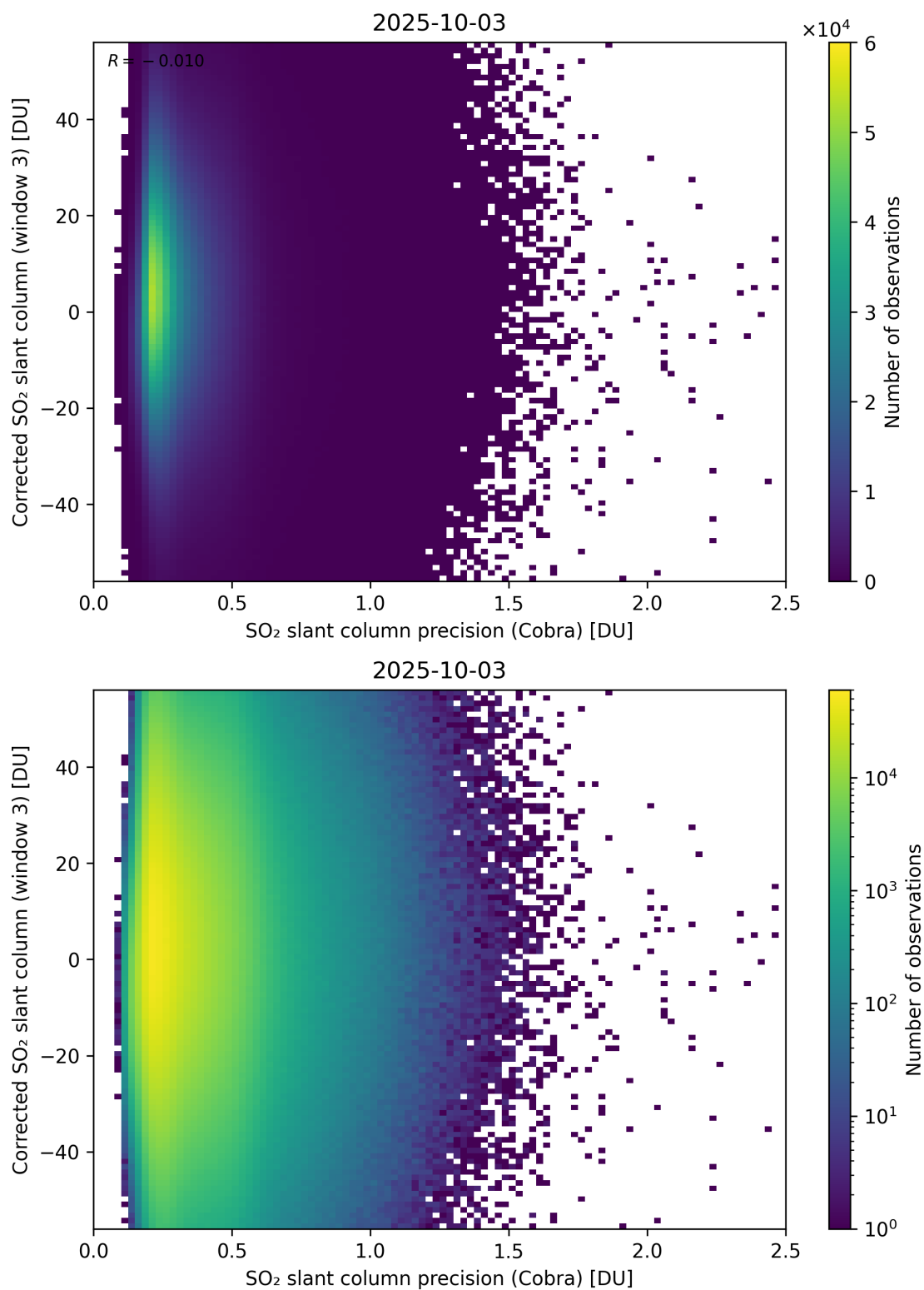
Figure 207: Scatter density plot of “SO 2 slant column precision (Cobra)” against “Corrected SO 2 slant column (window 3)” for 2025-10-02 to 2025-10-04.
