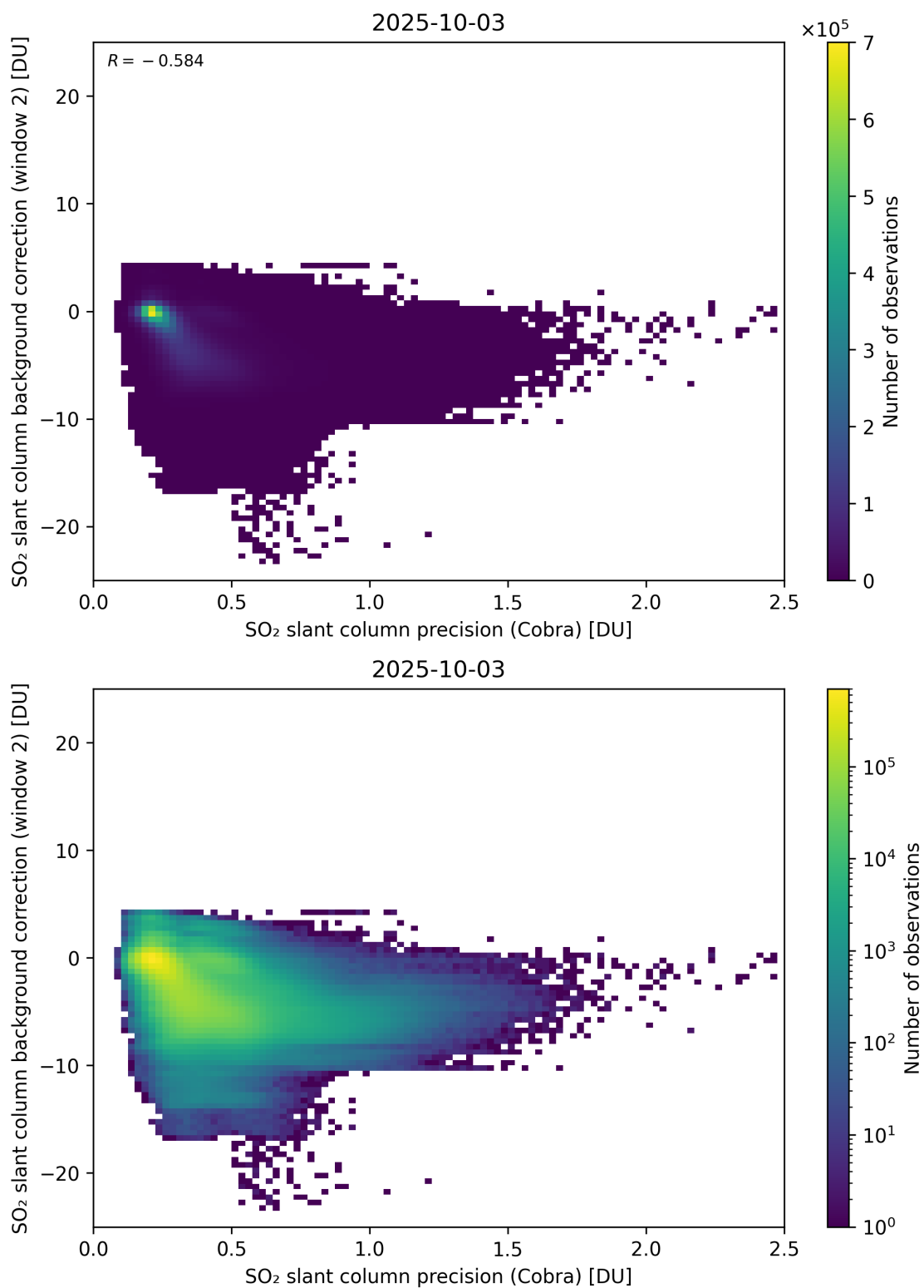
Figure 200: Scatter density plot of “SO 2 slant column precision (Cobra)” against “SO 2 slant column background correction (window 2)” for 2025-10-02 to 2025-10-04.
