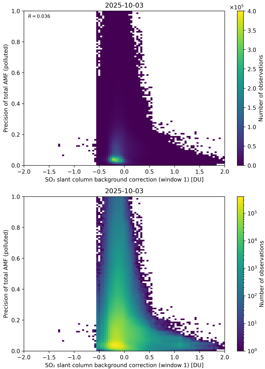
Figure 121: Scatter density plot of “SO 2 slant column background correction (window 1)” against “Precision of total AMF (polluted)” for 2025-10-02 to 2025-10-04.
