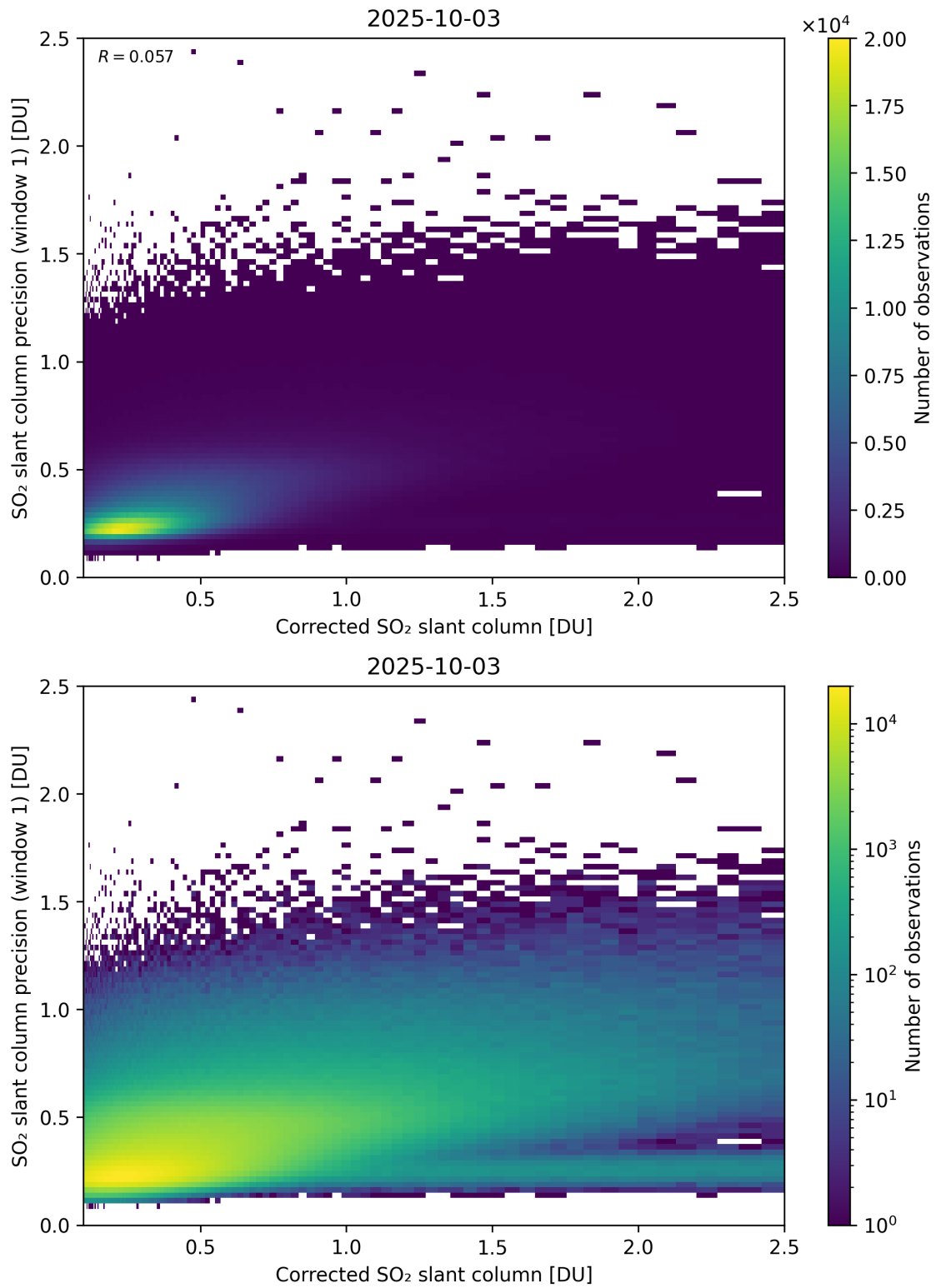
Figure 238: Scatter density plot of “Corrected SO 2 slant column” against “SO 2 slant column precision (window 1)” for 2025-10-02 to 2025-10-04.
