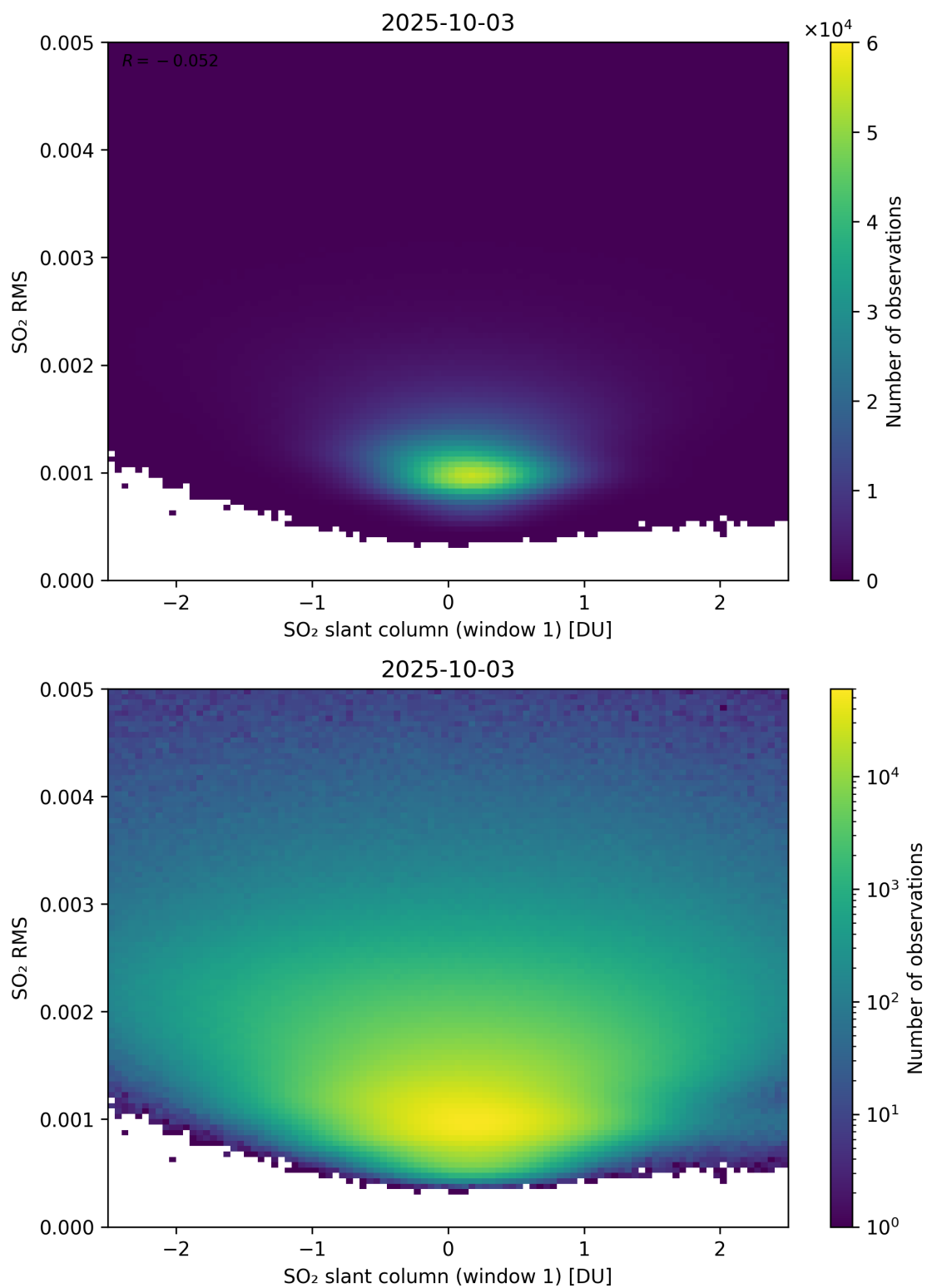
Figure 267: Scatter density plot of “SO 2 slant column (window 1)” against “SO 2 RMS” for 2025-10-02 to 2025-10-04.
