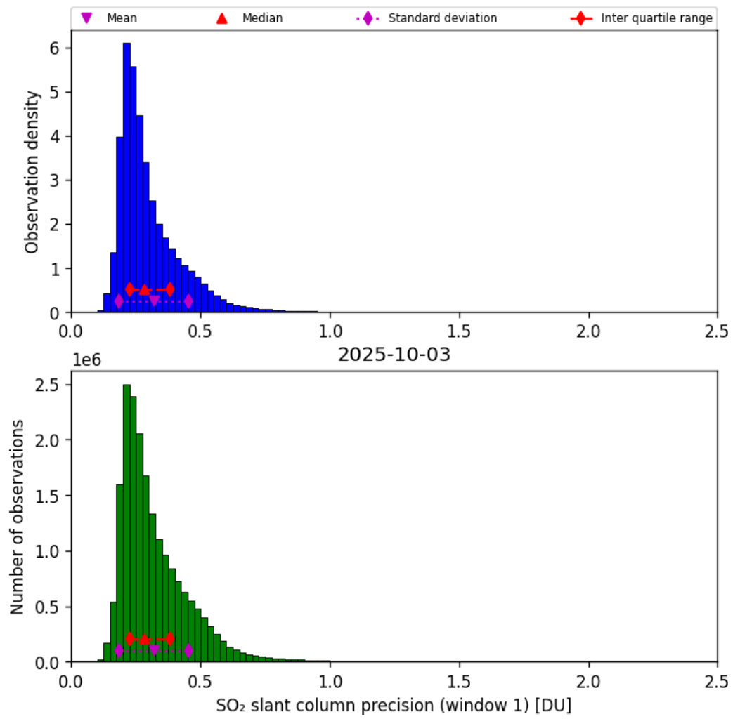
Figure 64: Histogram of “SO 2 slant column precision (window 1)” for 2025-10-02 to 2025-10-04
