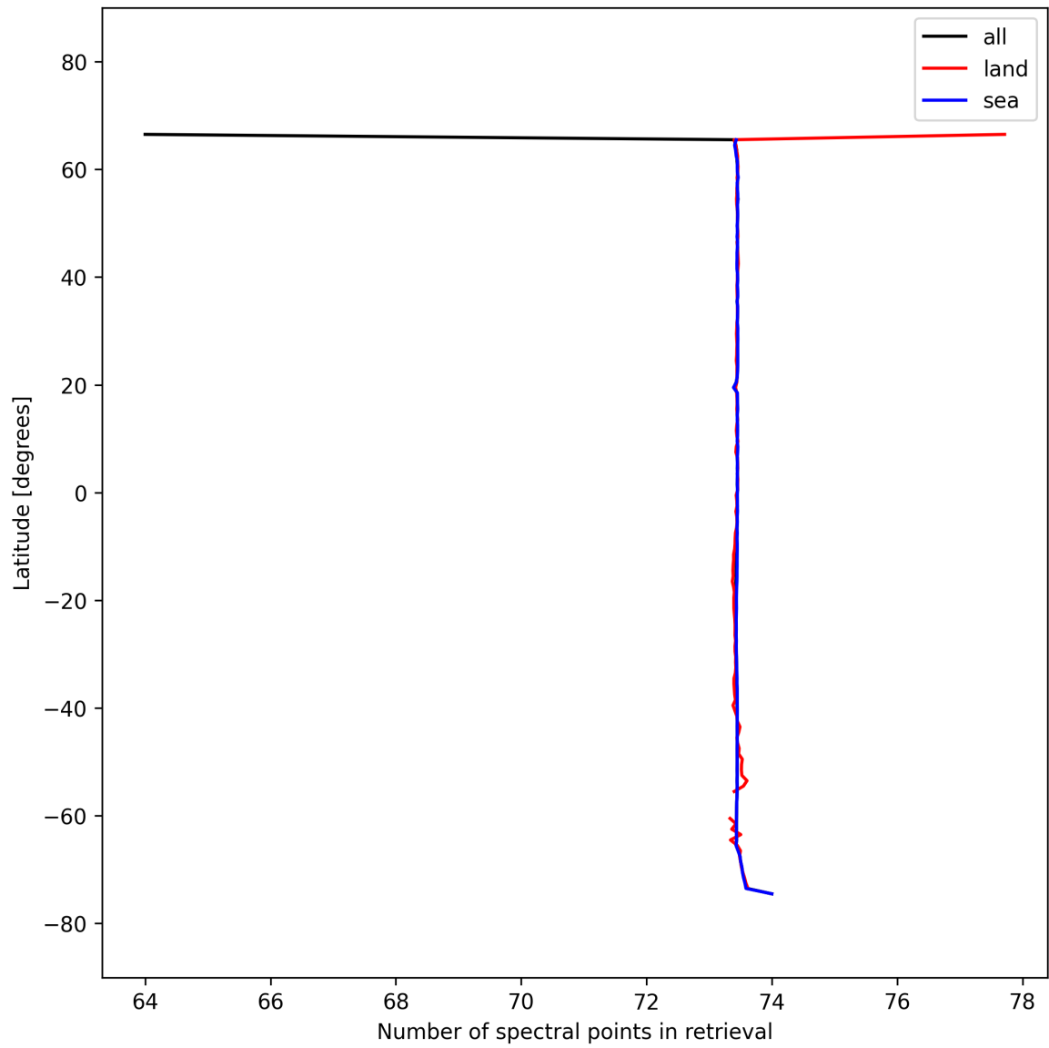
Figure 56: Zonal average of “Number of spectral points in retrieval” for 2025-10-02 to 2025-10-04.
