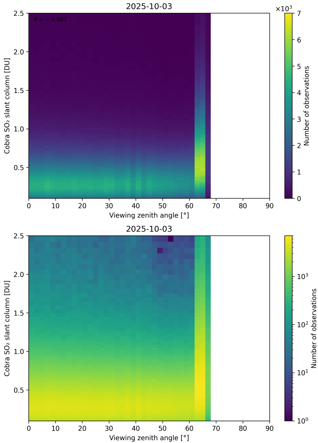
Figure 371: Scatter density plot of “Viewing zenith angle” against “Cobra SO 2 slant column” for 2025-10-02 to 2025-10-04.
