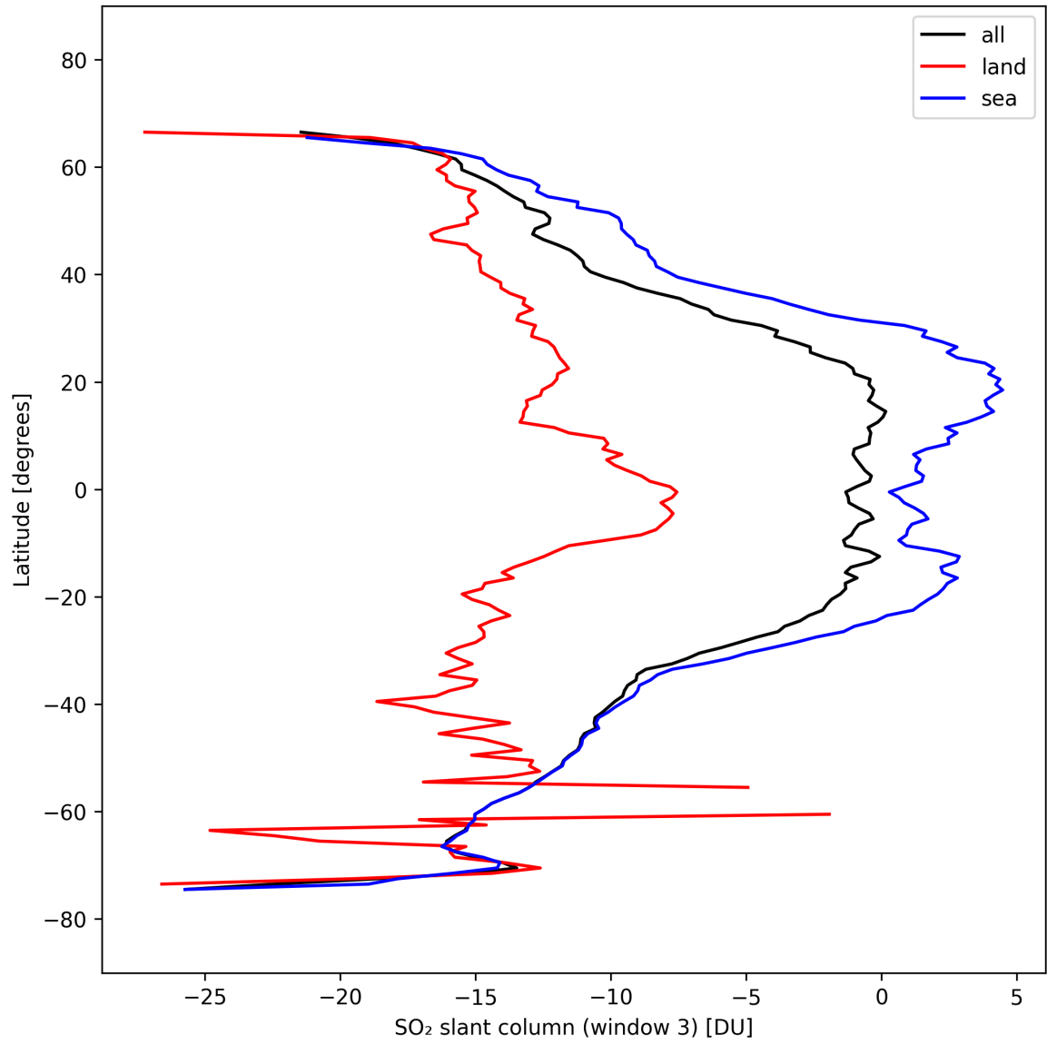
Figure 45: Zonal average of “SO 2 slant column (window 3)” for 2025-10-02 to 2025-10-04.
