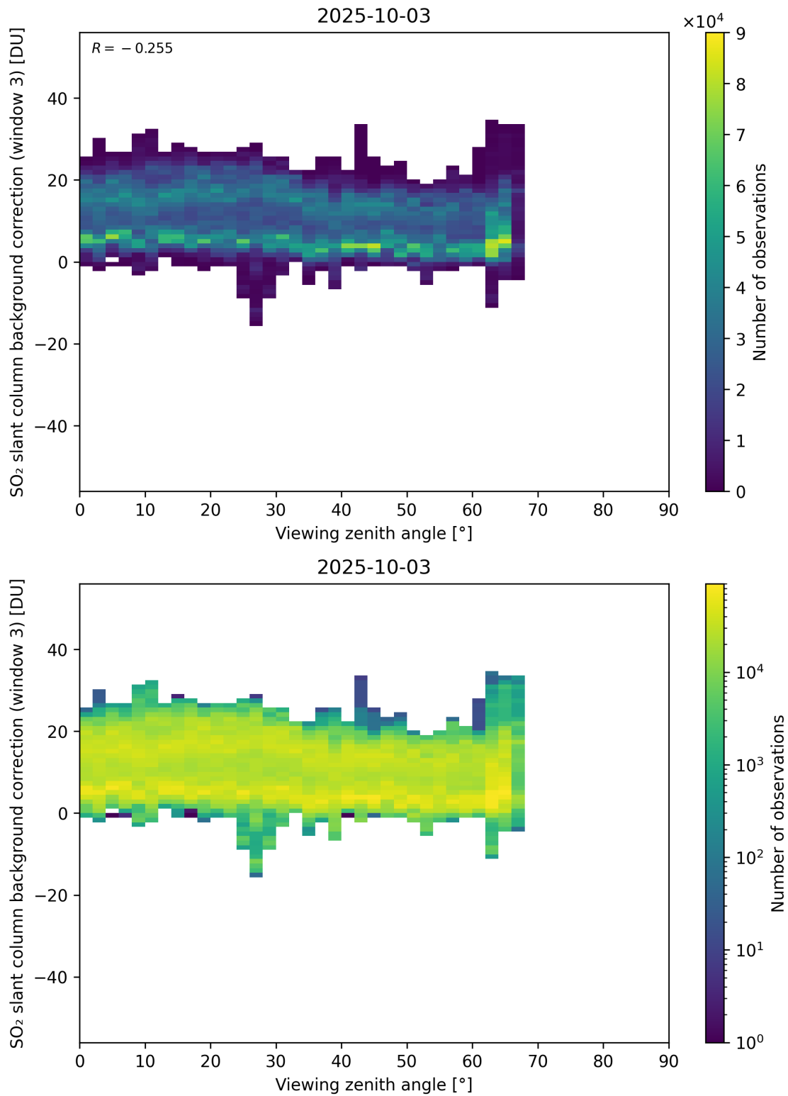
Figure 364: Scatter density plot of “Viewing zenith angle” against “SO 2 slant column background correction (window 3)” for 2025-10-02 to 2025-10-04.
