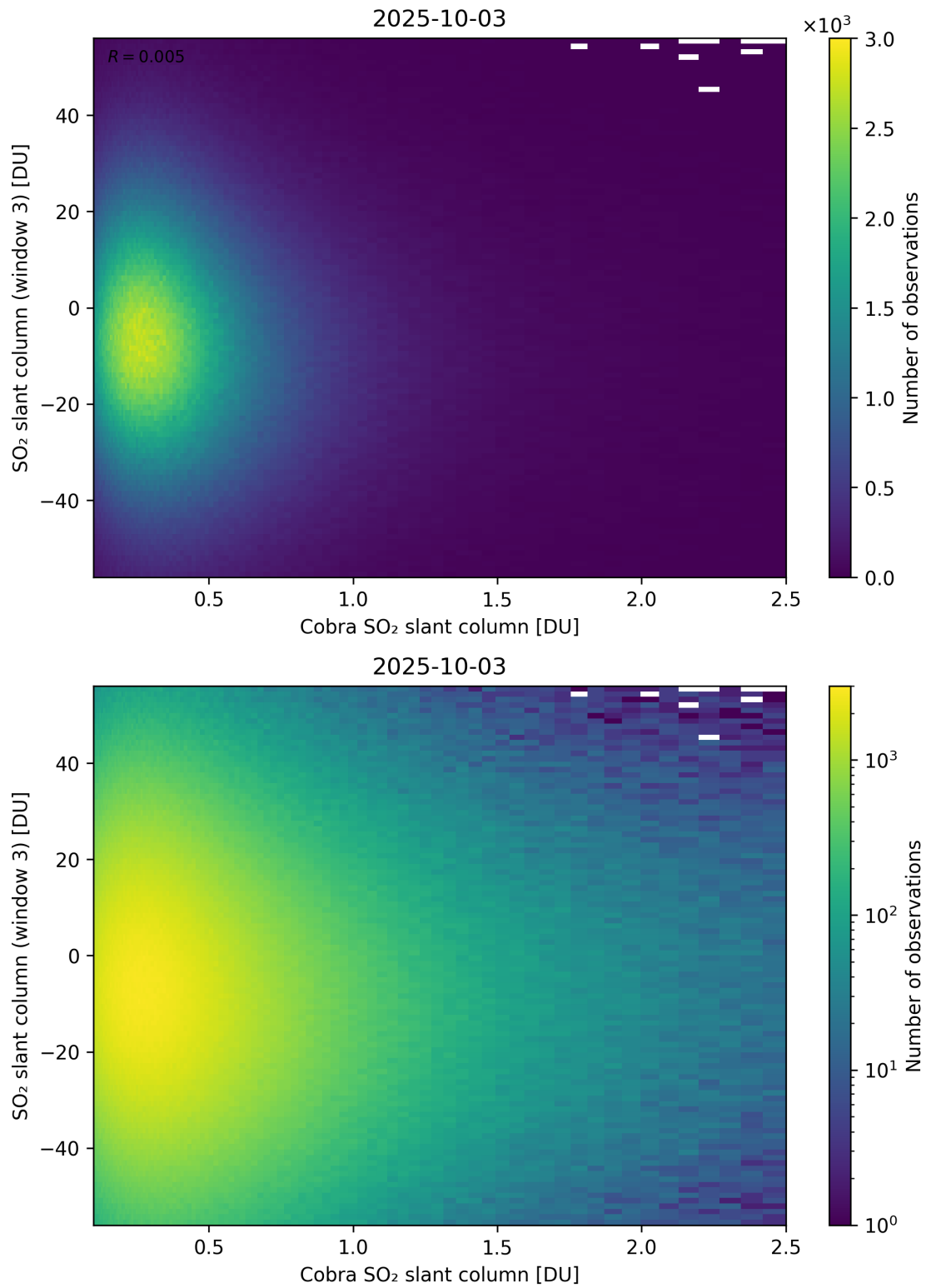
Figure 222: Scatter density plot of “Cobra SO 2 slant column” against “SO 2 slant column (window 3)” for 2025-10-02 to 2025-10-04.
