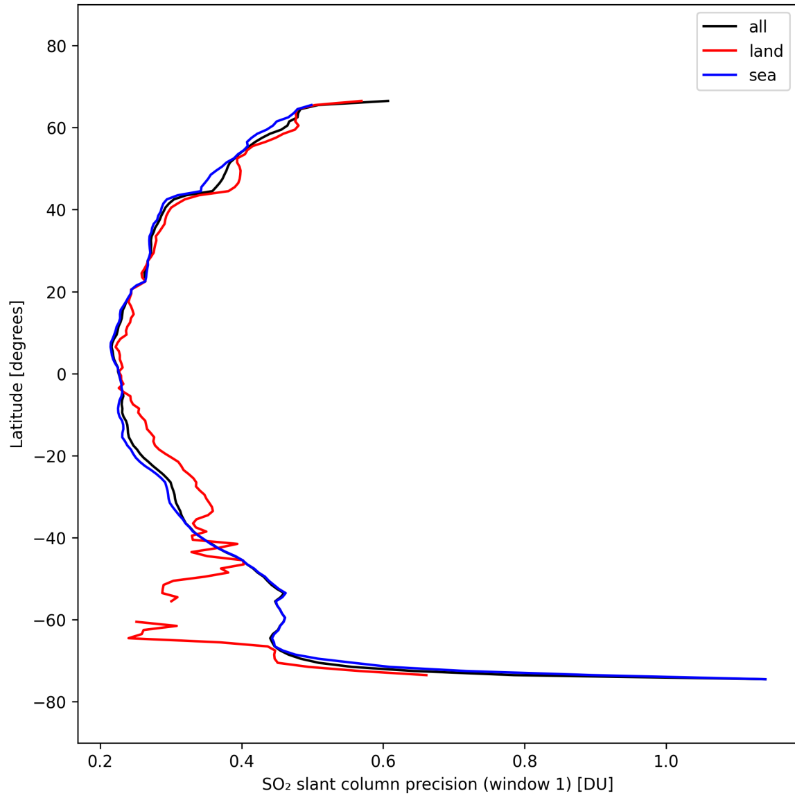
Figure 38: Zonal average of “SO 2 slant column precision (window 1)” for 2025-10-02 to 2025-10-04.
