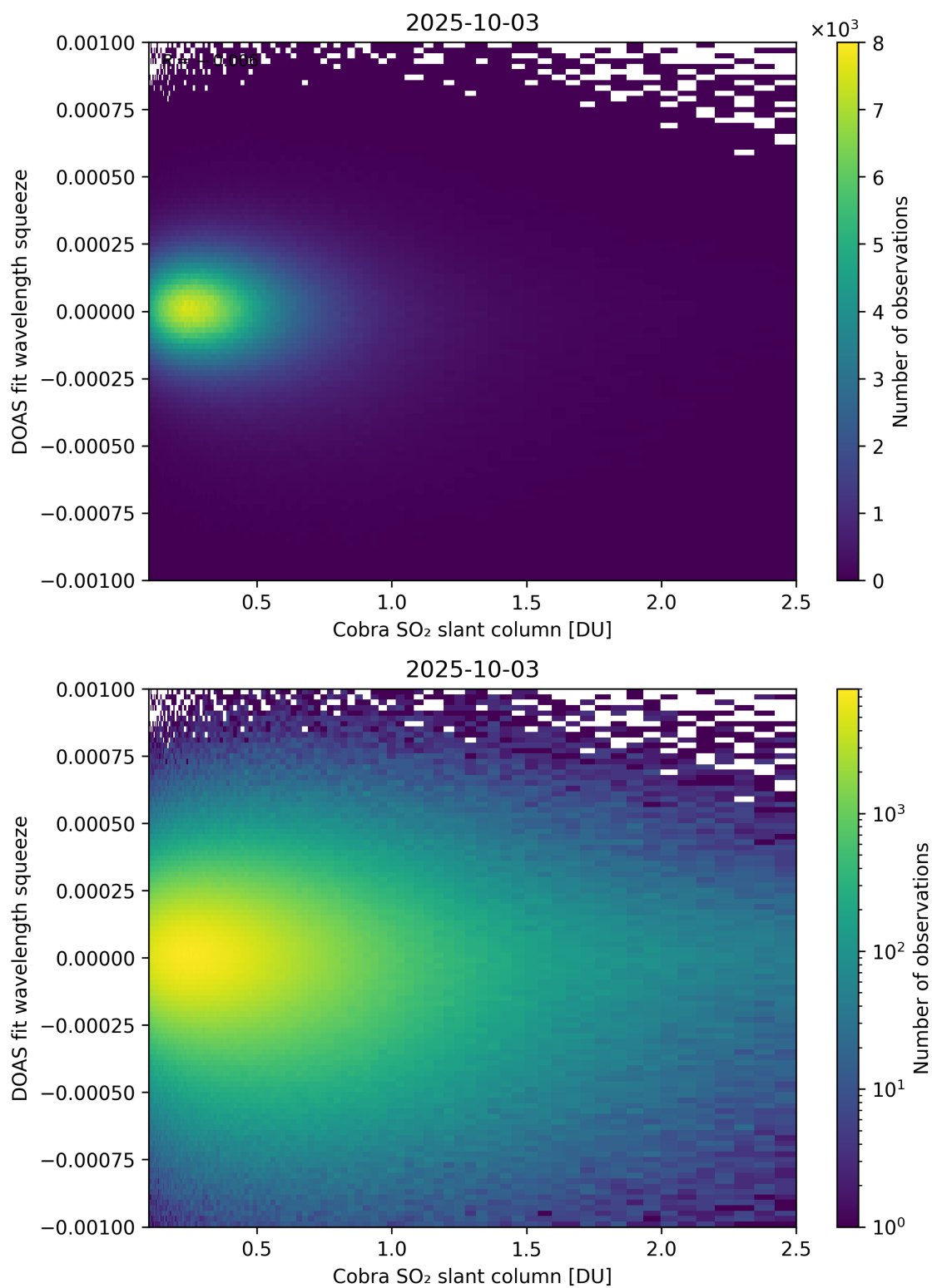
Figure 197: Scatter density plot of “Cobra SO 2 slant column” against “DOAS fit wavelength squeeze” for 2025-10-02 to 2025-10-04.
