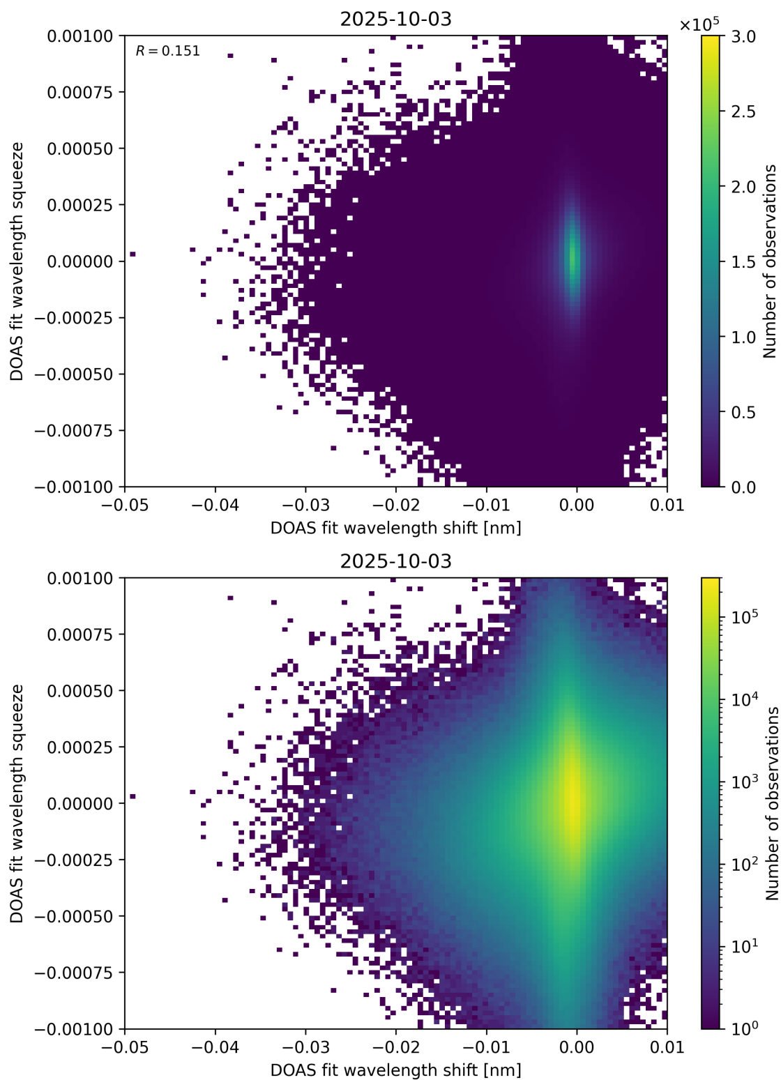
Figure 138: Scatter density plot of “DOAS fit wavelength shift” against “DOAS fit wavelength squeeze” for 2025-10-02 to 2025-10-04.
