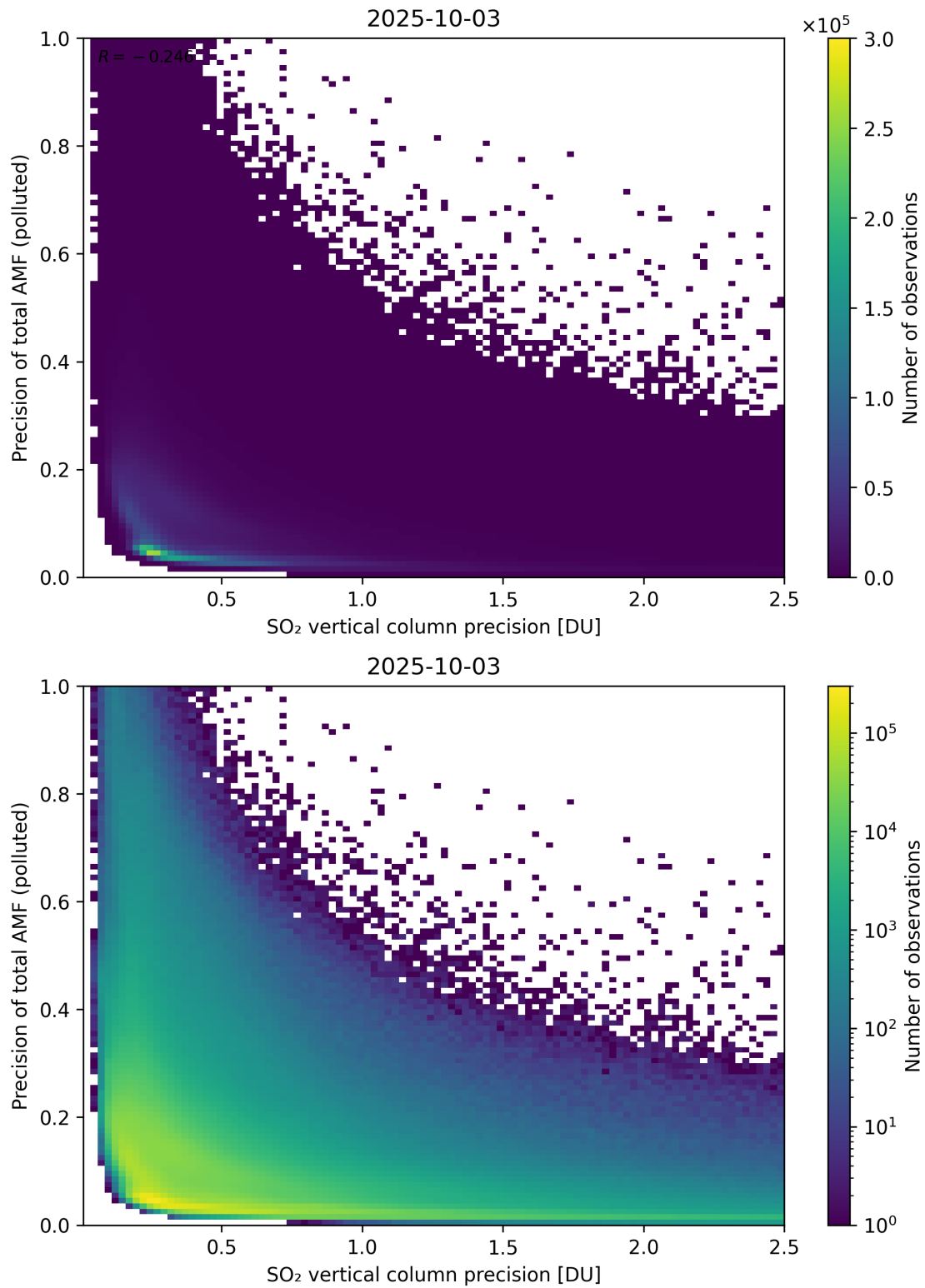
Figure 347: Scatter density plot of “SO 2 vertical column precision” against “Precision of total AMF (polluted)” for 2025-10-02 to 2025-10-04.
