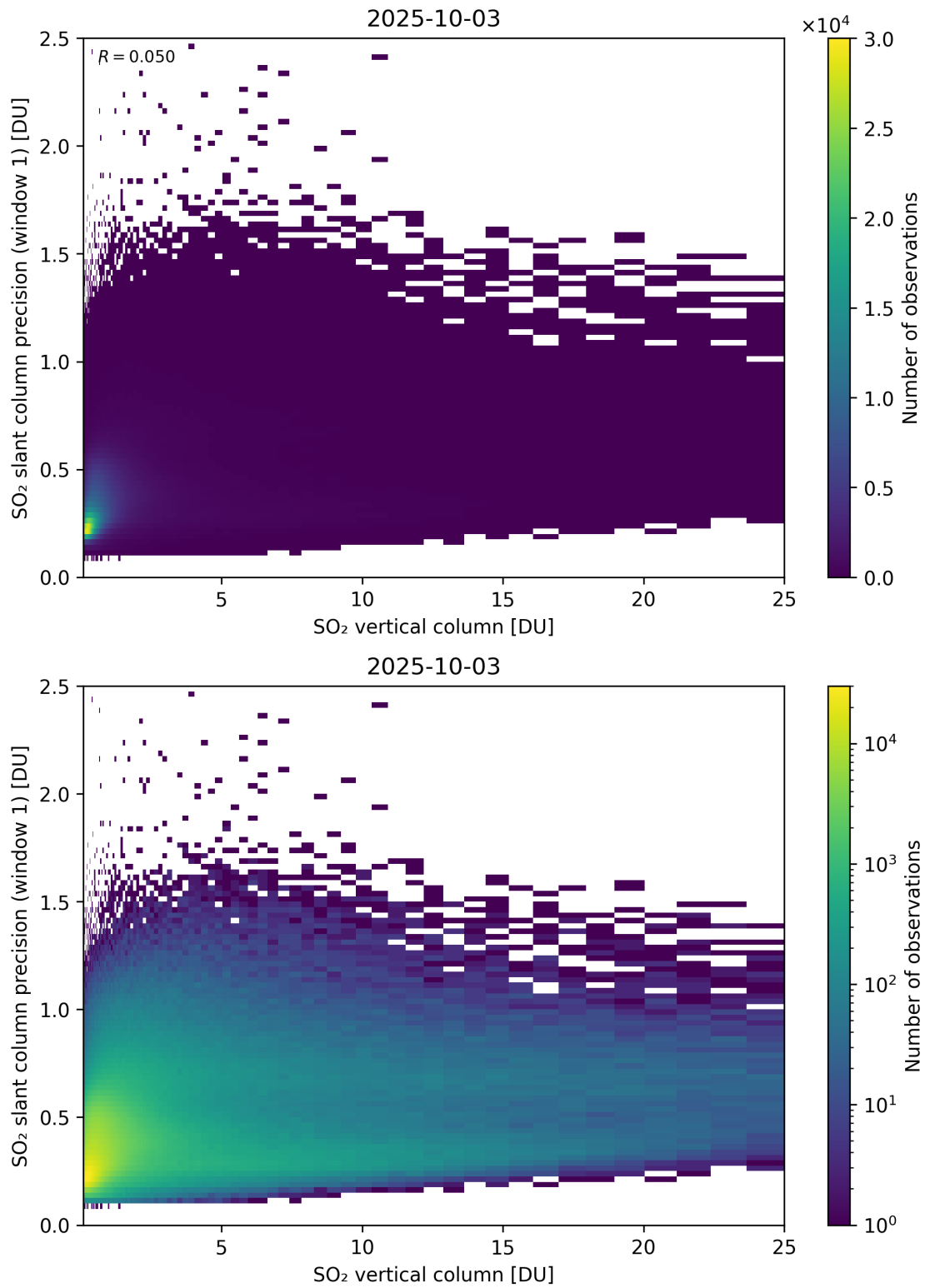
Figure 355: Scatter density plot of “SO 2 vertical column” against “SO 2 slant column precision (window 1)” for 2025-10-02 to 2025-10-04.
