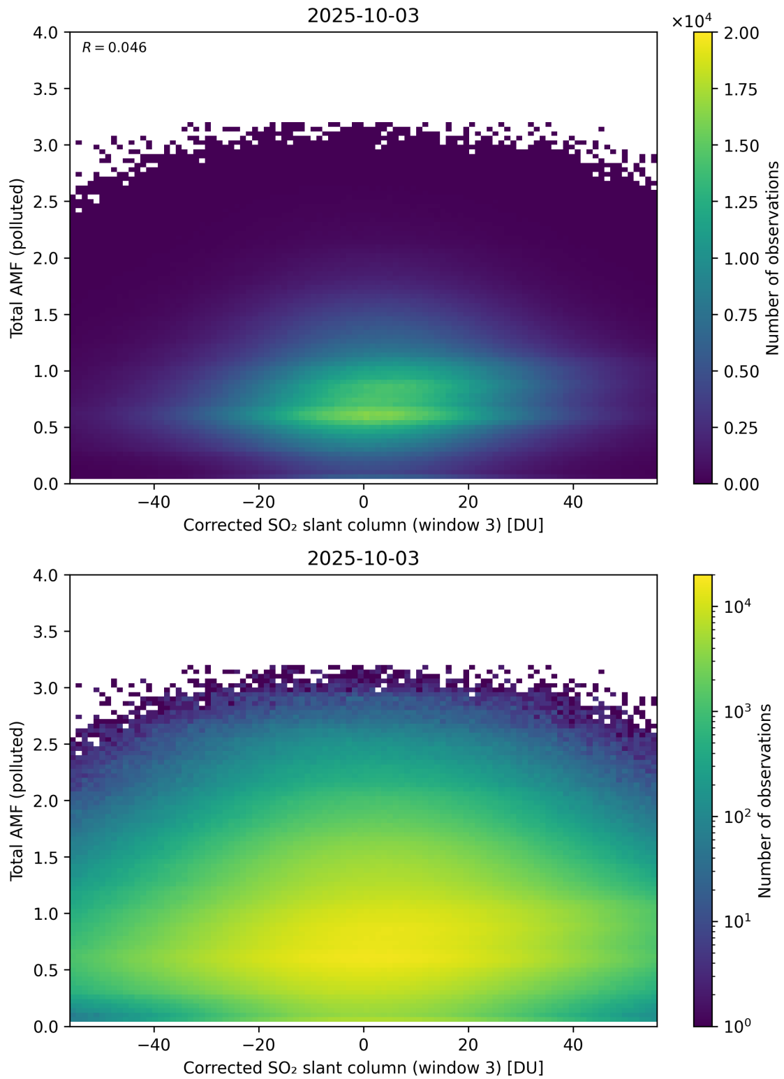
Figure 260: Scatter density plot of “Corrected SO 2 slant column (window 3)” against “Total AMF (polluted)” for 2025-10-02 to 2025-10-04.
