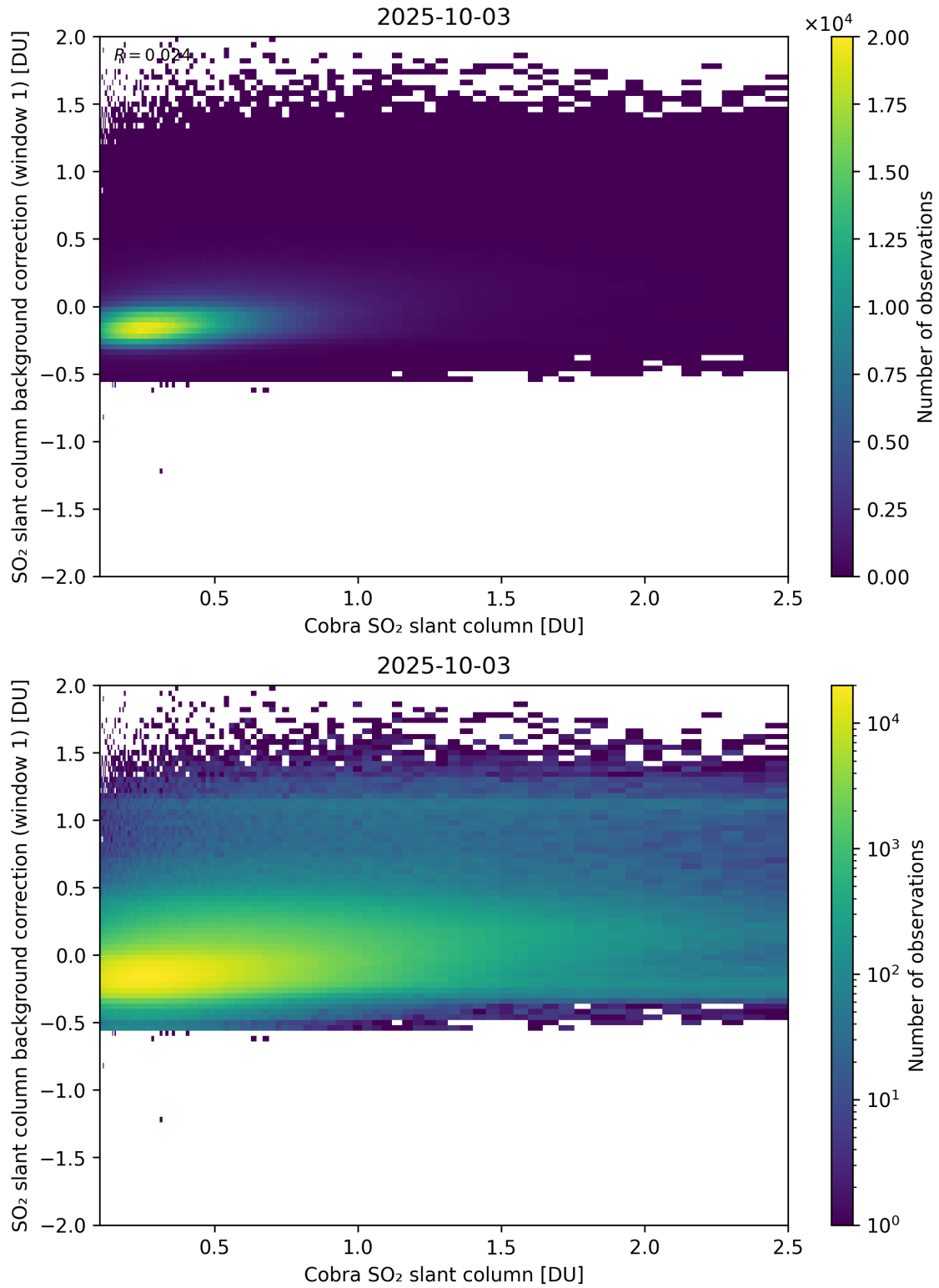
Figure 193: Scatter density plot of “Cobra SO 2 slant column” against “SO 2 slant column background correction (window 1)” for 2025-10-02 to 2025-10-04.
