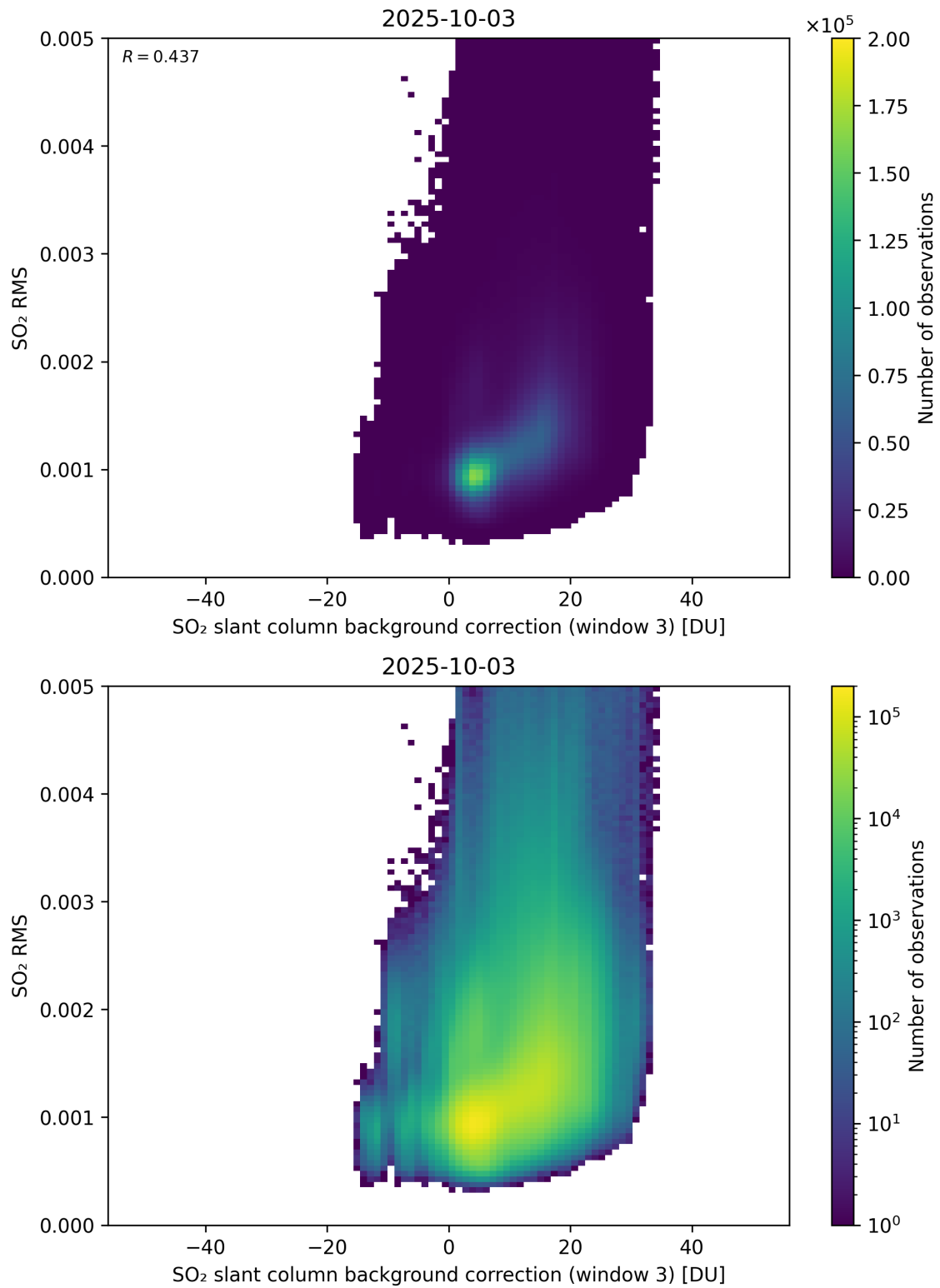
Figure 134: Scatter density plot of “SO 2 slant column background correction (window 3)” against “SO 2 RMS” for 2025-10-02 to 2025-10-04.
