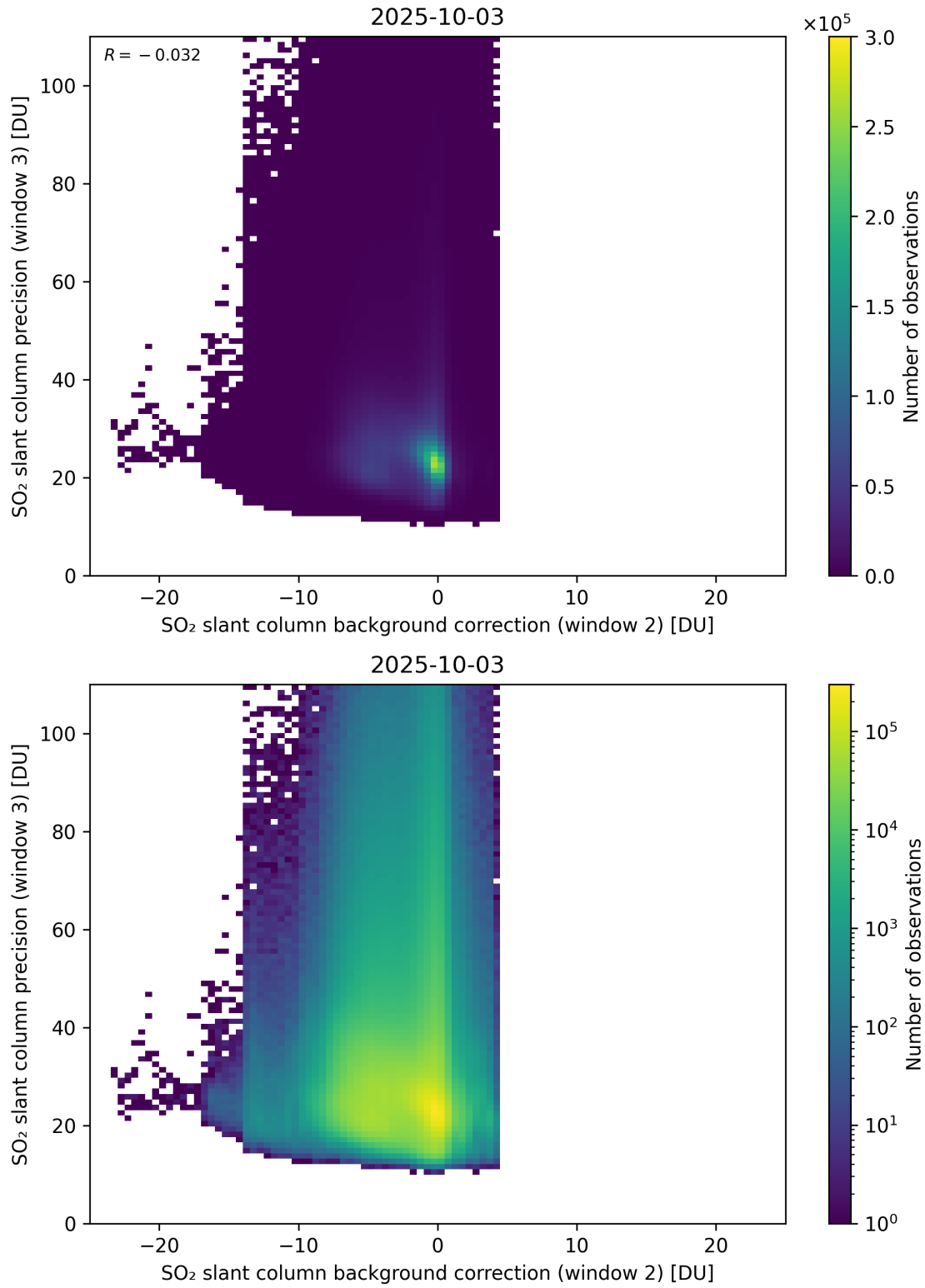
Figure 129: Scatter density plot of “SO 2 slant column background correction (window 2)” against “SO 2 slant column precision (window 3)” for 2025-10-02 to 2025-10-04.
