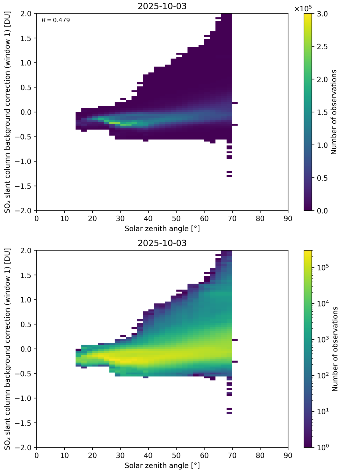
Figure 171: Scatter density plot of “Solar zenith angle” against “SO 2 slant column background correction (window 1)” for 2025-10-02 to 2025-10-04.
