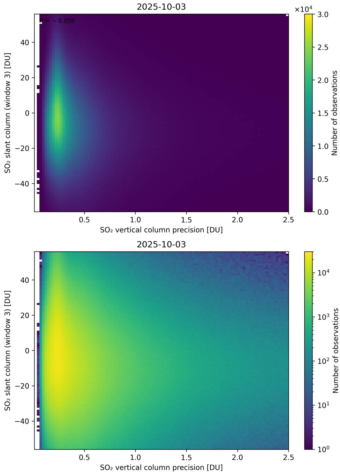
Figure 344: Scatter density plot of “SO 2 vertical column precision” against “SO 2 slant column (window 3)” for 2025-10-02 to 2025-10-04.
