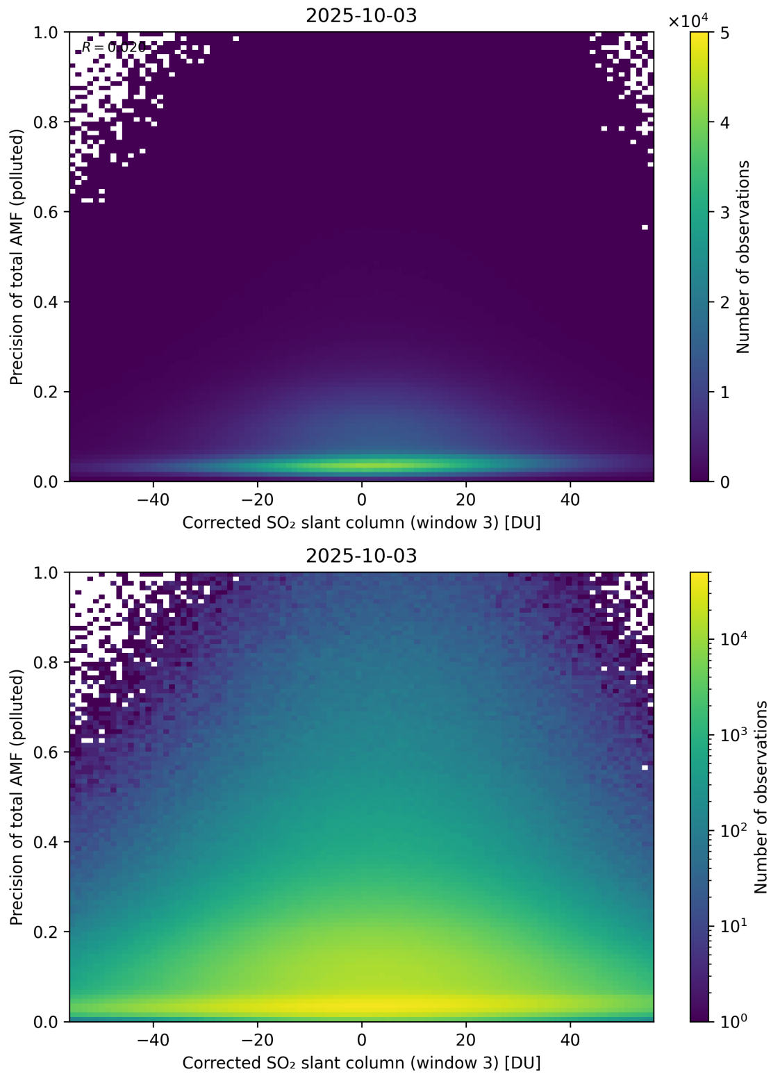
Figure 261: Scatter density plot of “Corrected SO 2 slant column (window 3)” against “Precision of total AMF (polluted)” for 2025-10-02 to 2025-10-04.
