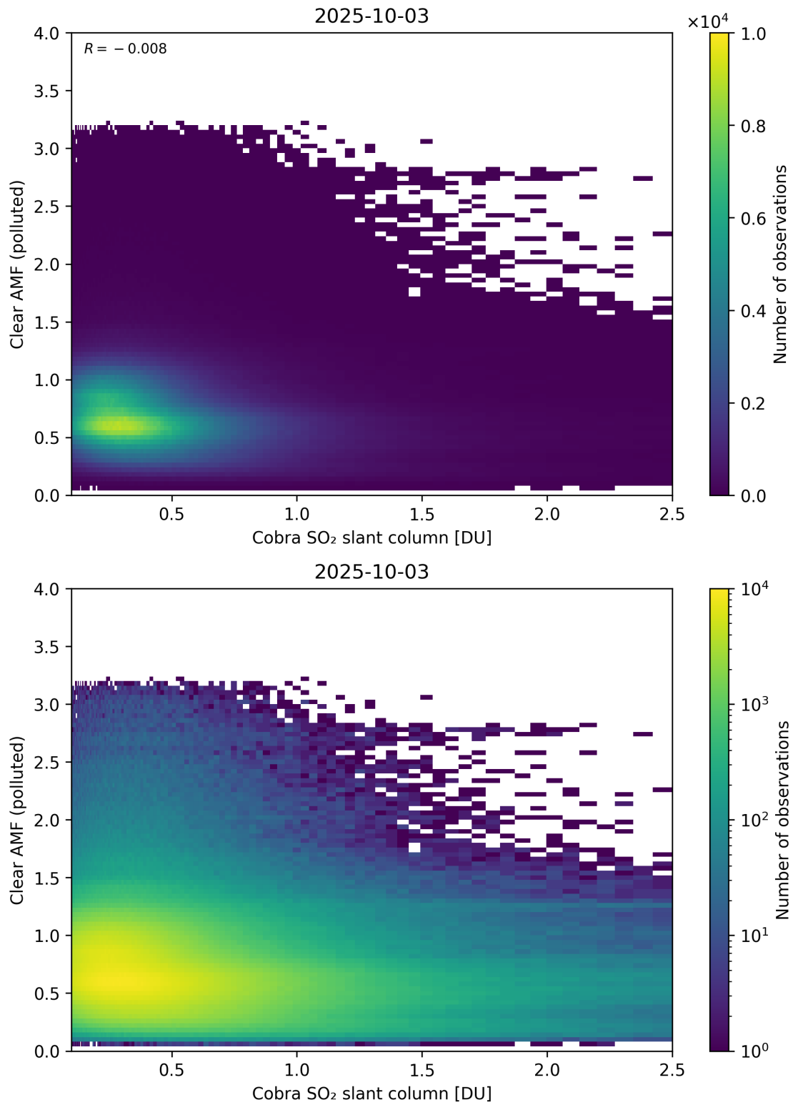
Figure 215: Scatter density plot of “Cobra SO 2 slant column” against “Clear AMF (polluted)” for 2025-10-02 to 2025-10-04.
