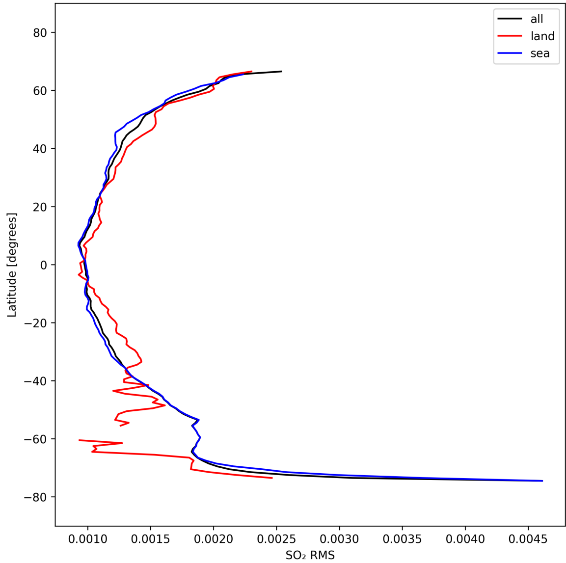
Figure 52: Zonal average of “SO 2 RMS” for 2025-10-02 to 2025-10-04.
