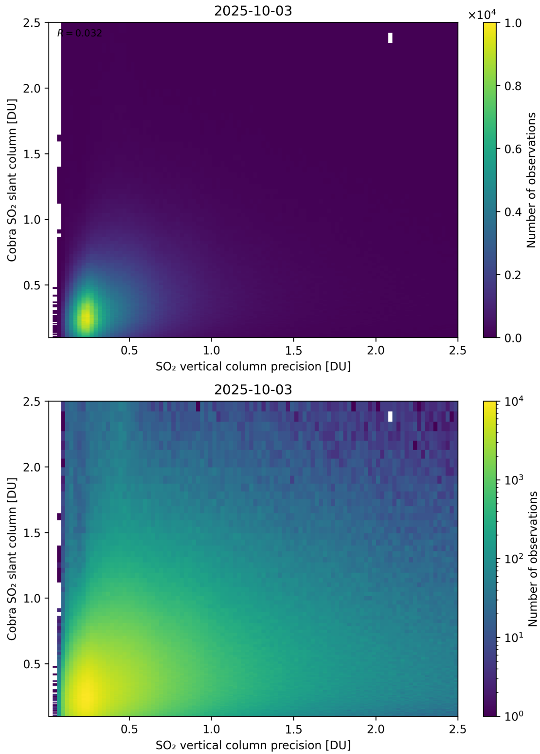
Figure 336: Scatter density plot of “SO 2 vertical column precision” against “Cobra SO 2 slant column” for 2025-10-02 to 2025-10-04.
