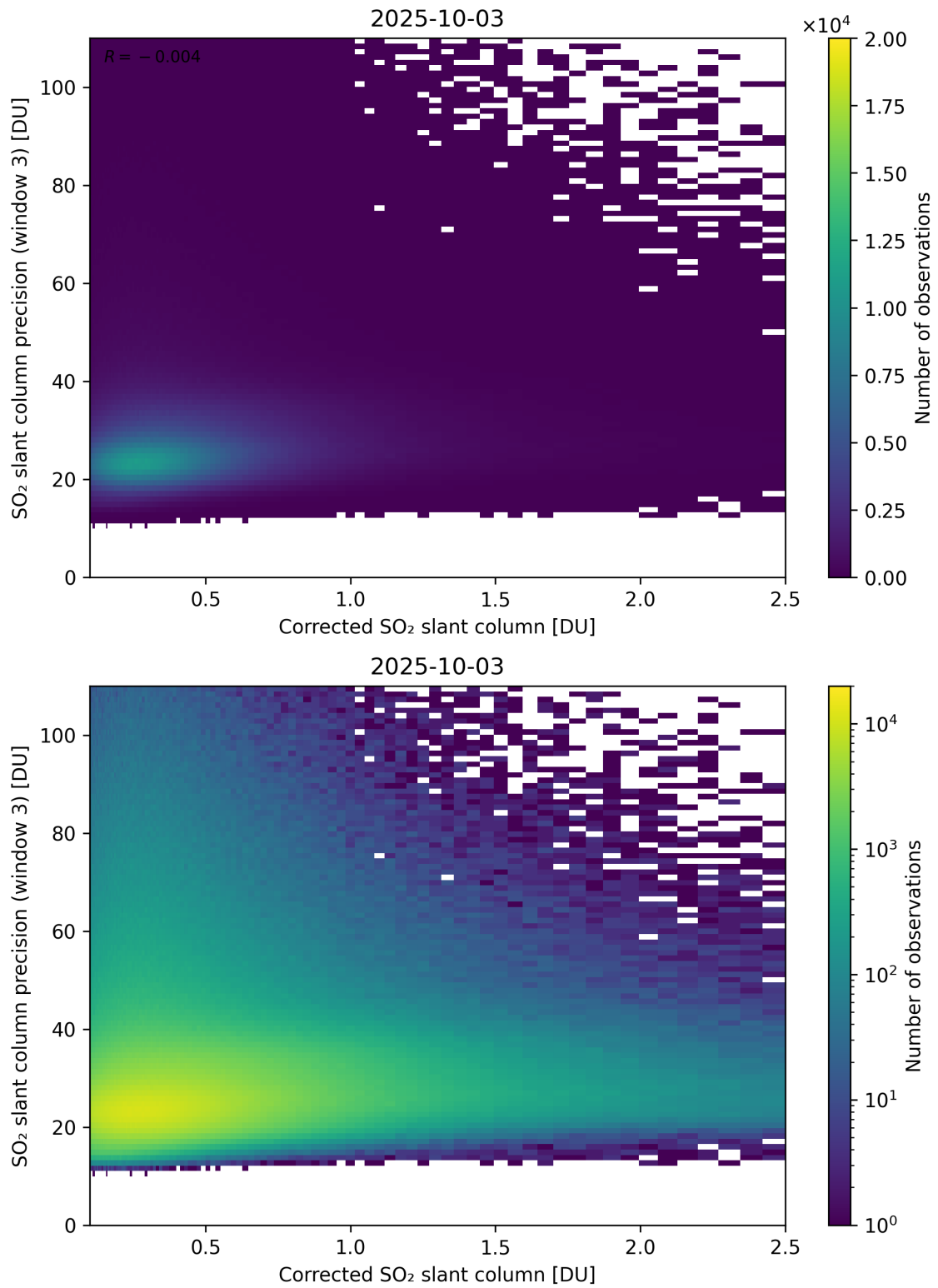
Figure 241: Scatter density plot of “Corrected SO 2 slant column” against “SO 2 slant column precision (window 3)” for 2025-10-02 to 2025-10-04.
