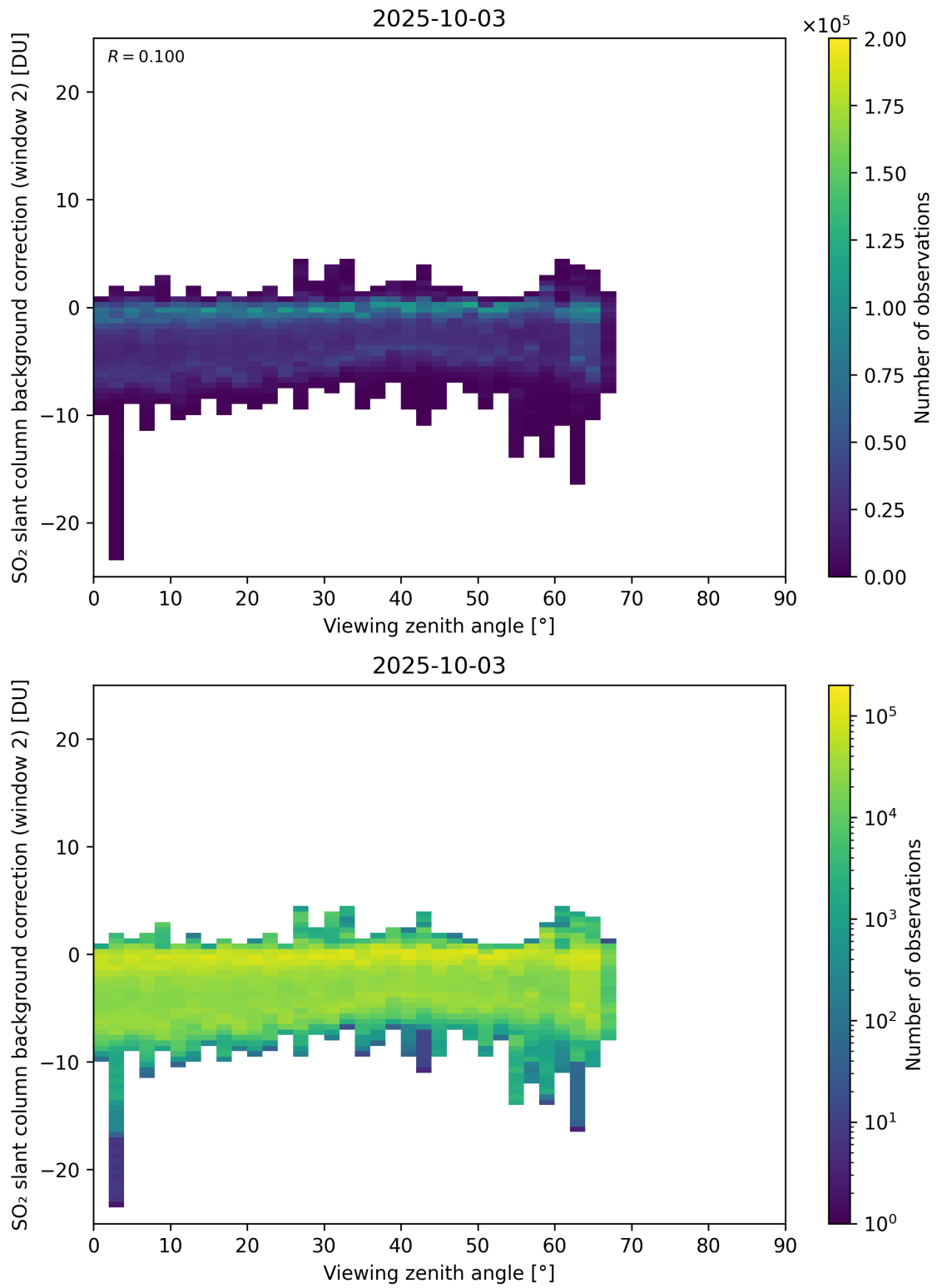
Figure 363: Scatter density plot of “Viewing zenith angle” against “SO 2 slant column background correction (window 2)” for 2025-10-02 to 2025-10-04.
