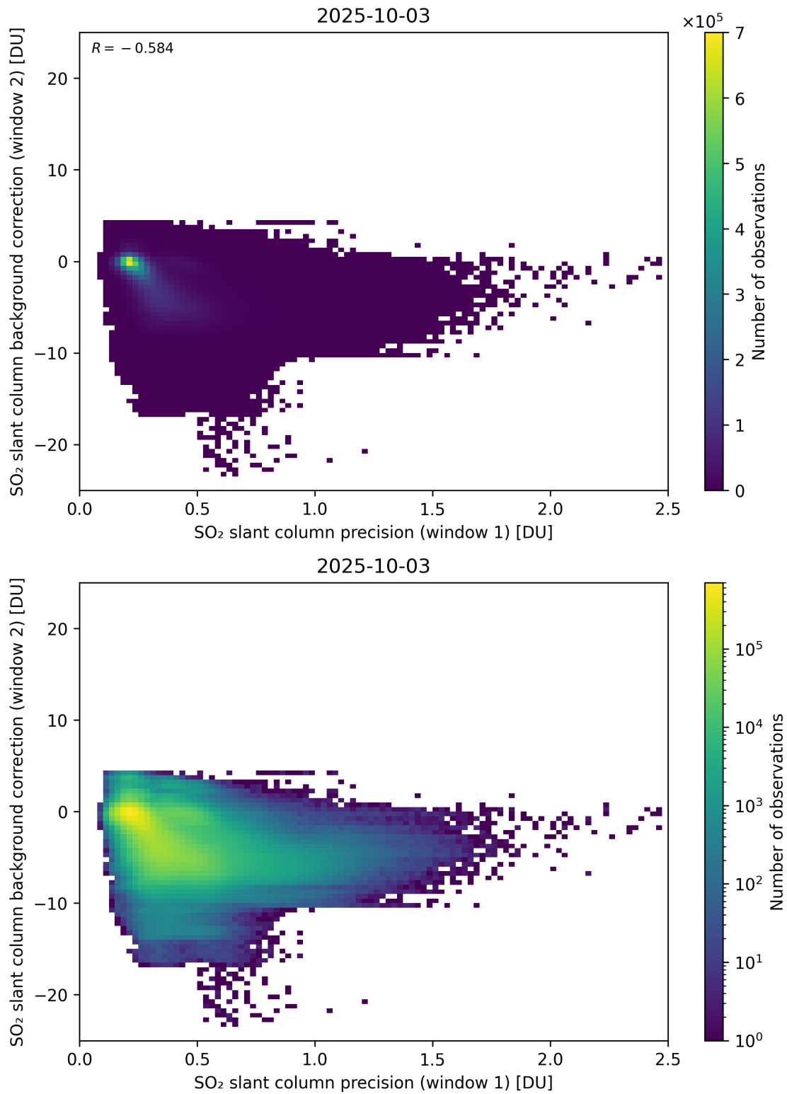
Figure 269: Scatter density plot of “SO 2 slant column precision (window 1)” against “SO 2 slant column background correction (window 2)” for 2025-10-02 to 2025-10-04.
