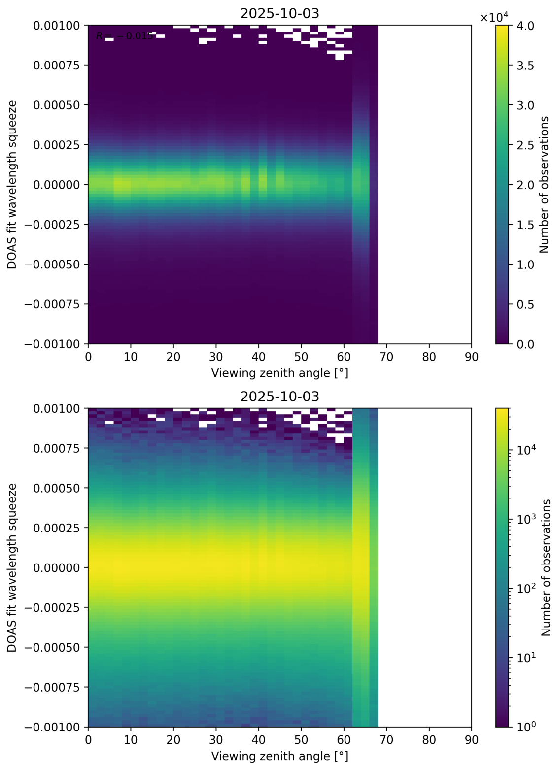
Figure 366: Scatter density plot of “Viewing zenith angle” against “DOAS fit wavelength squeeze” for 2025-10-02 to 2025-10-04.
