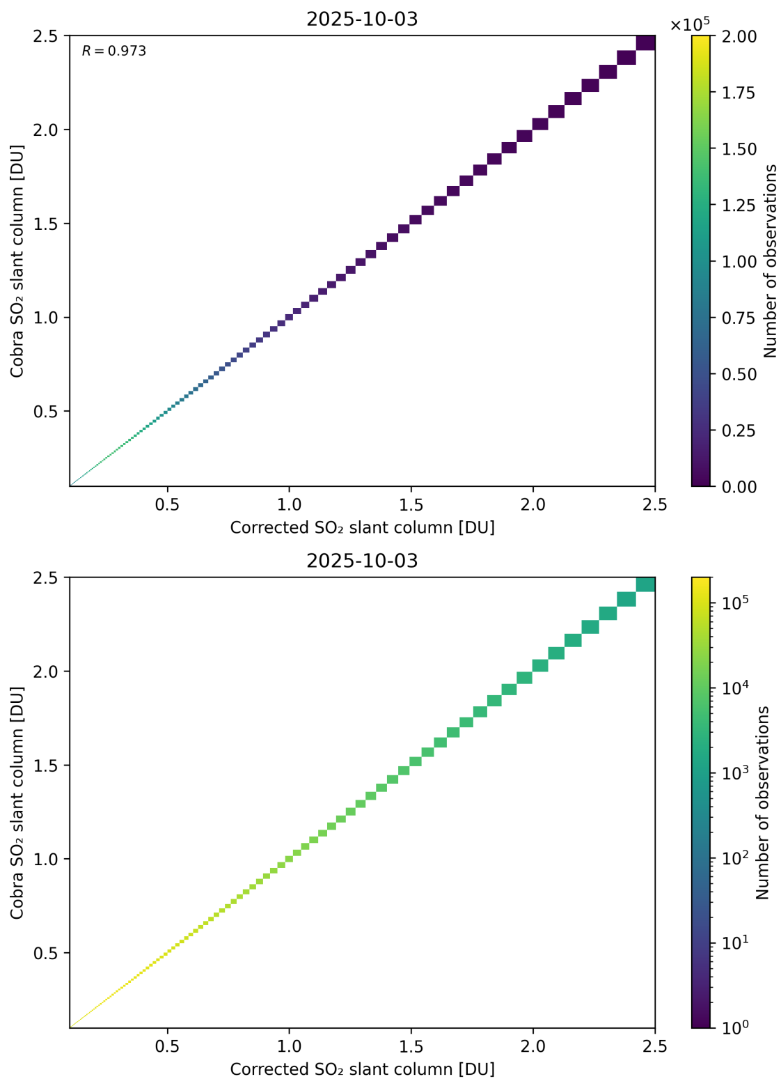
Figure 233: Scatter density plot of “Corrected SO 2 slant column” against “Cobra SO 2 slant column” for 2025-10-02 to 2025-10-04.
