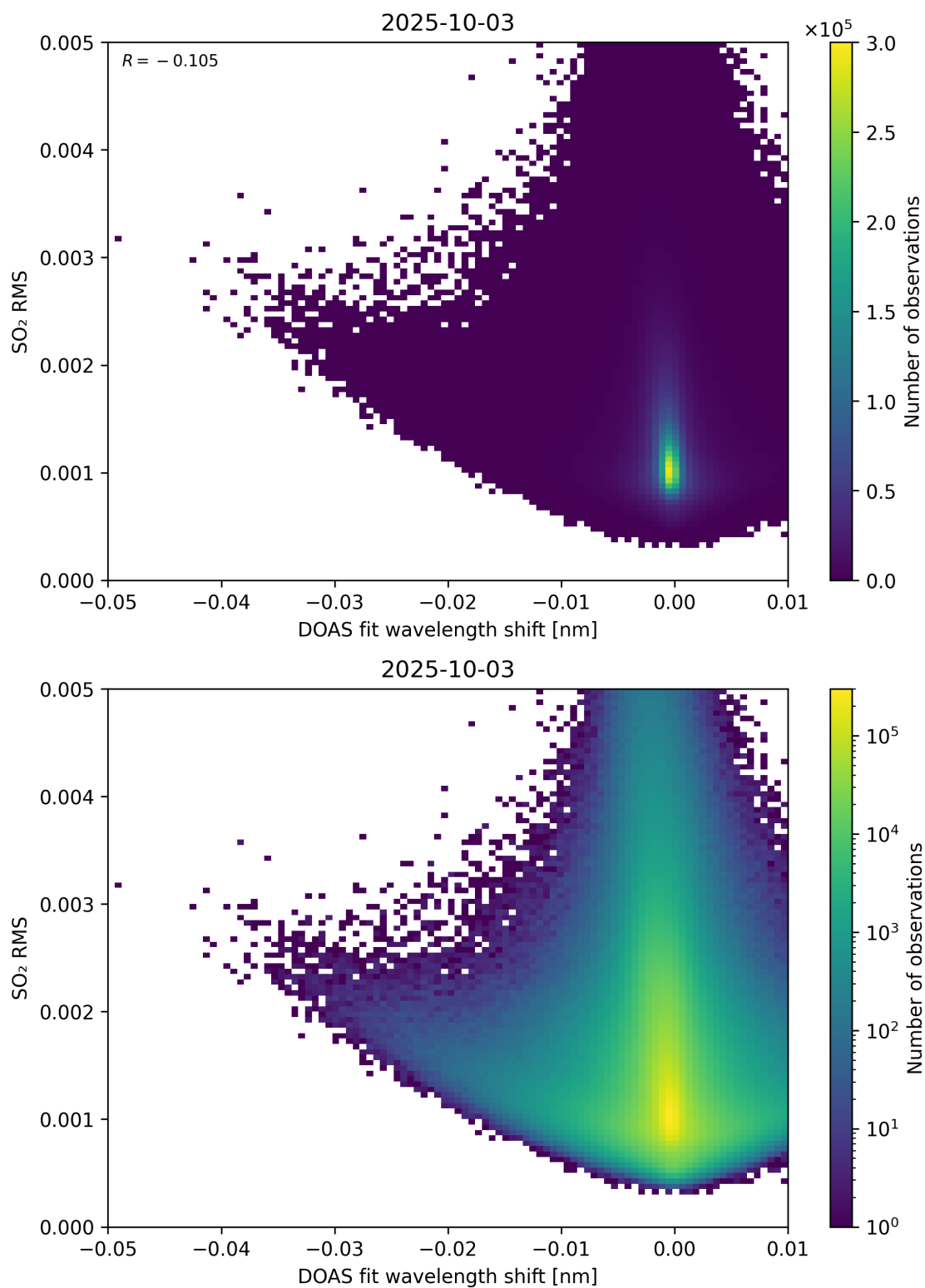
Figure 139: Scatter density plot of “DOAS fit wavelength shift” against “SO 2 RMS” for 2025-10-02 to 2025-10-04.
