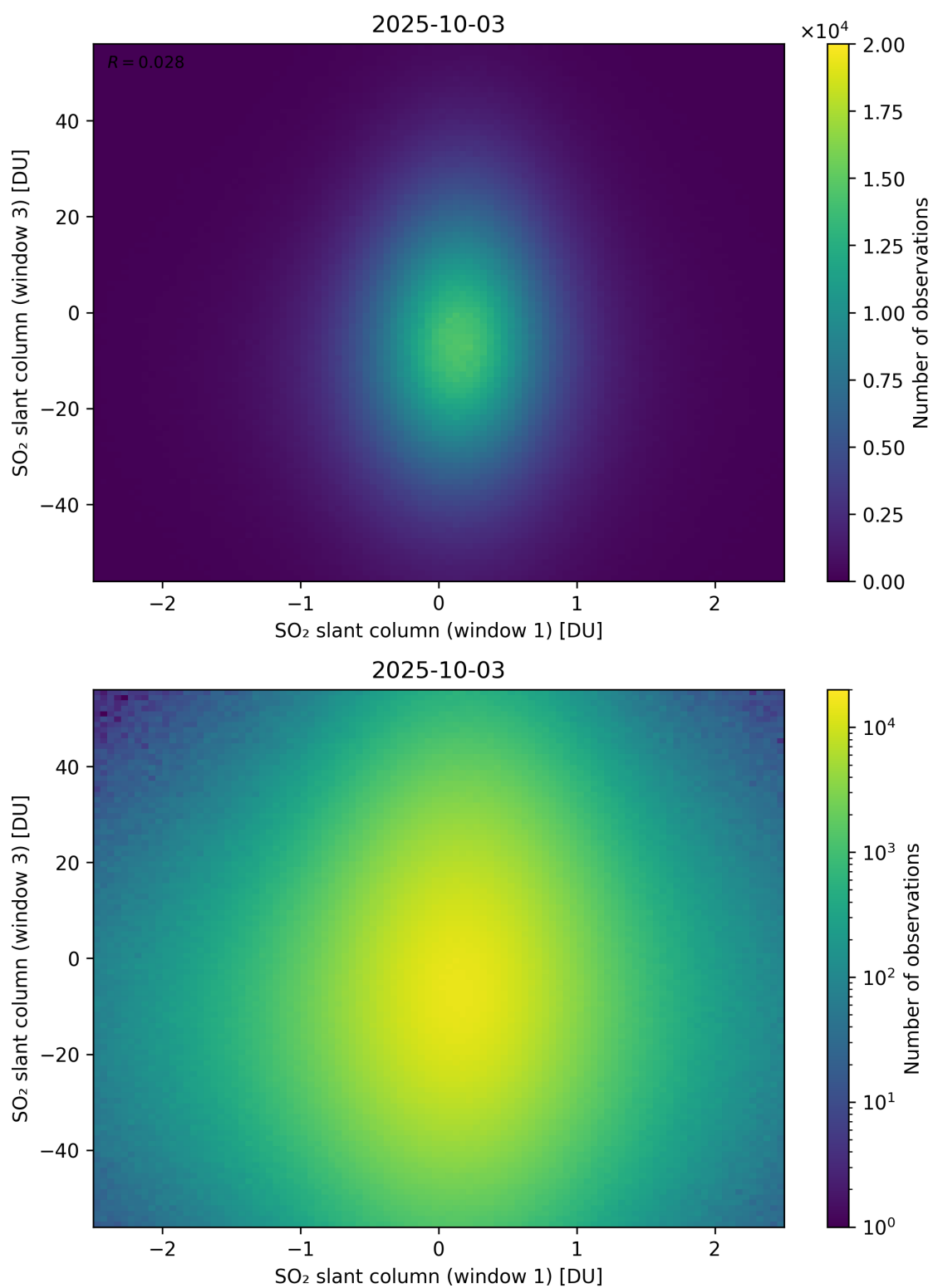
Figure 287: Scatter density plot of “SO 2 slant column (window 1)” against “SO 2 slant column (window 3)” for 2025-10-02 to 2025-10-04.
