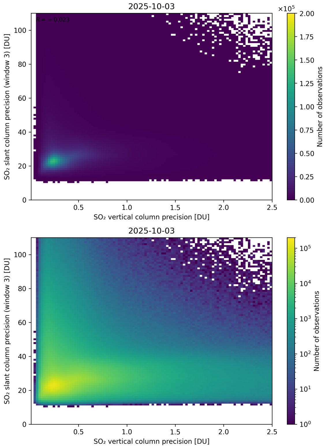
Figure 345: Scatter density plot of “SO 2 vertical column precision” against “SO 2 slant column precision (window 3)” for 2025-10-02 to 2025-10-04.
