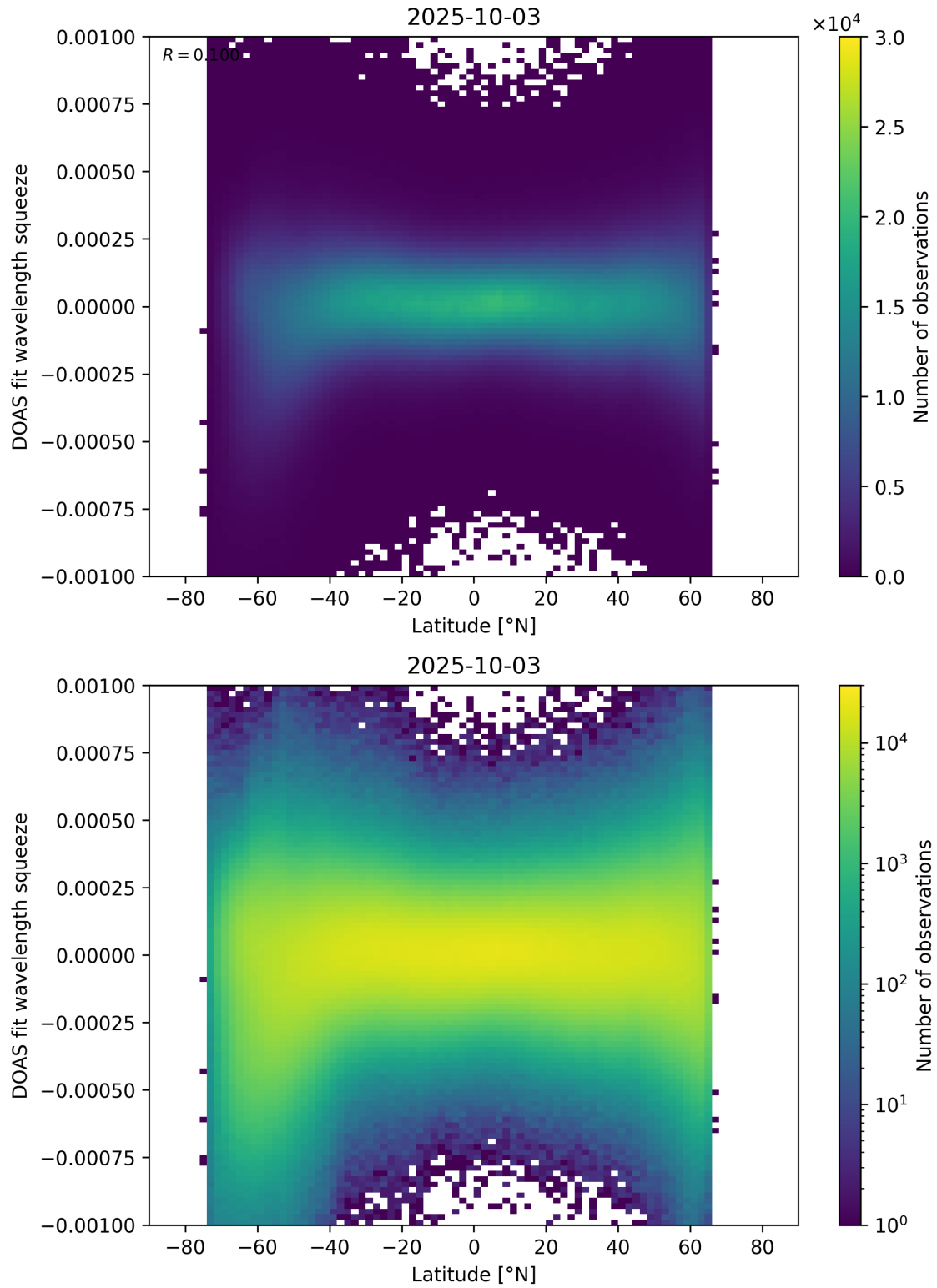
Figure 154: Scatter density plot of “Latitude” against “DOAS fit wavelength squeeze” for 2025-10-02 to 2025-10-04.
