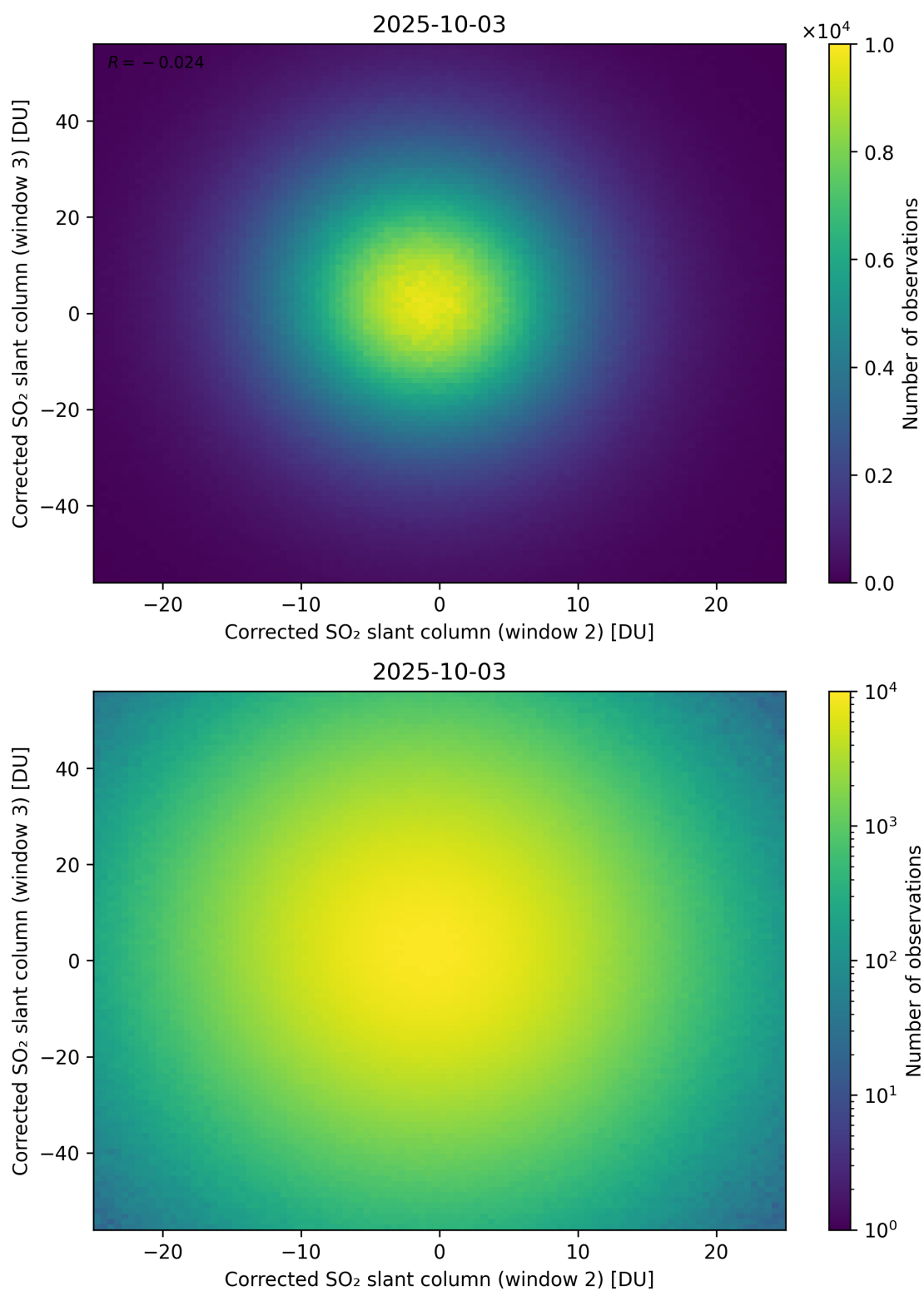
Figure 250: Scatter density plot of “Corrected SO 2 slant column (window 2)” against “Corrected SO 2 slant column (window 3)” for 2025-10-02 to 2025-10-04.
