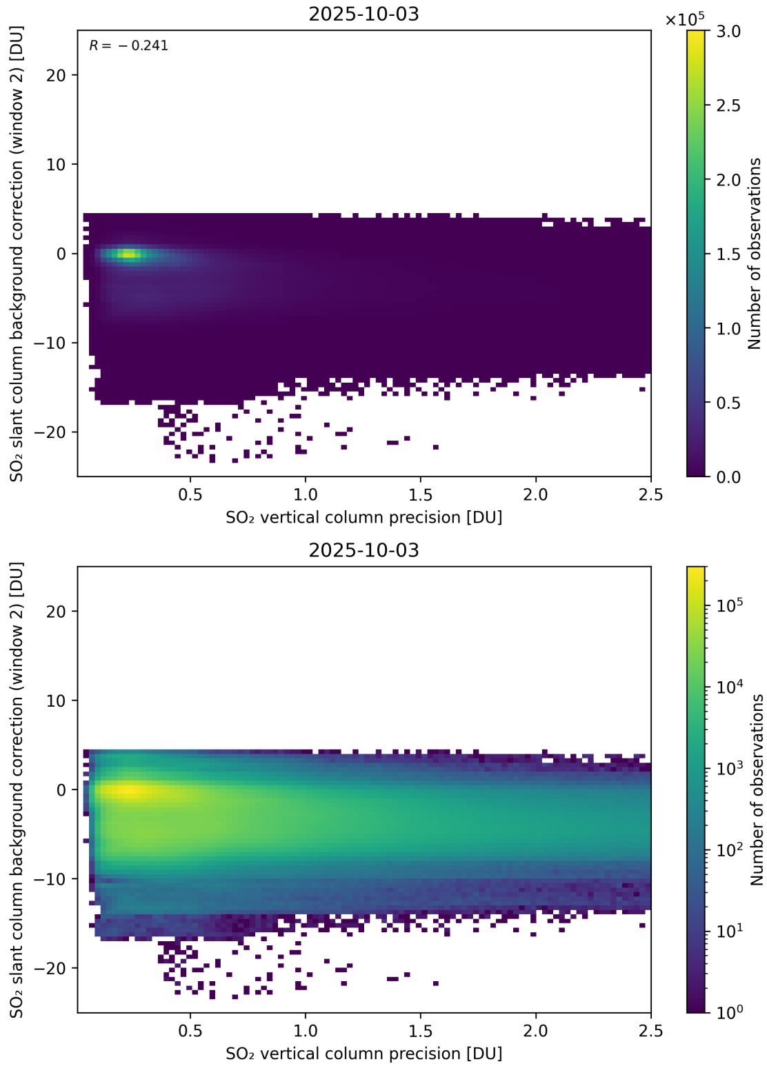
Figure 330: Scatter density plot of “SO 2 vertical column precision” against “SO 2 slant column background correction (window 2)” for 2025-10-02 to 2025-10-04.
