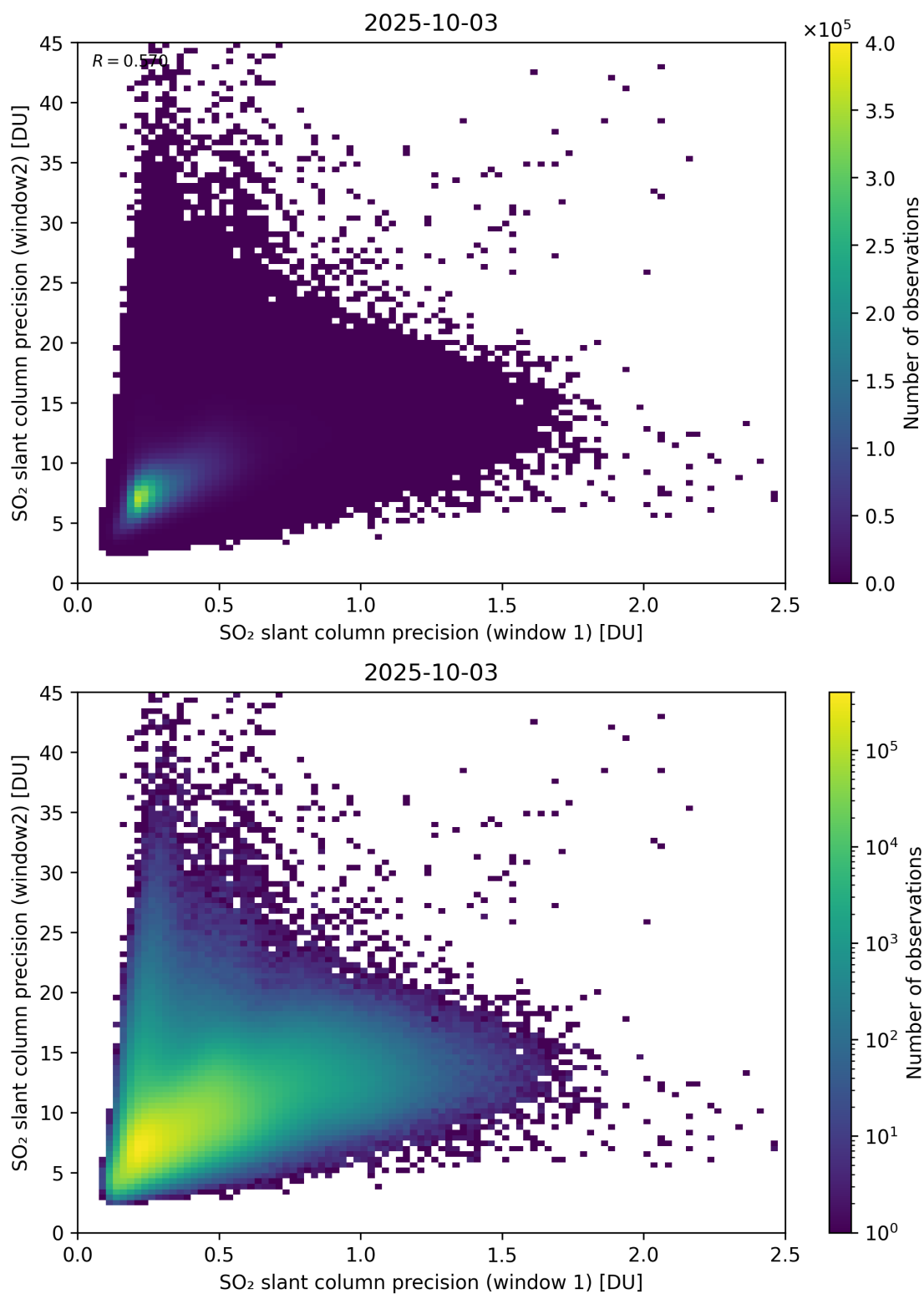
Figure 277: Scatter density plot of “SO 2 slant column precision (window 1)” against “SO 2 slant column precision (window2)” for 2025-10-02 to 2025-10-04.
