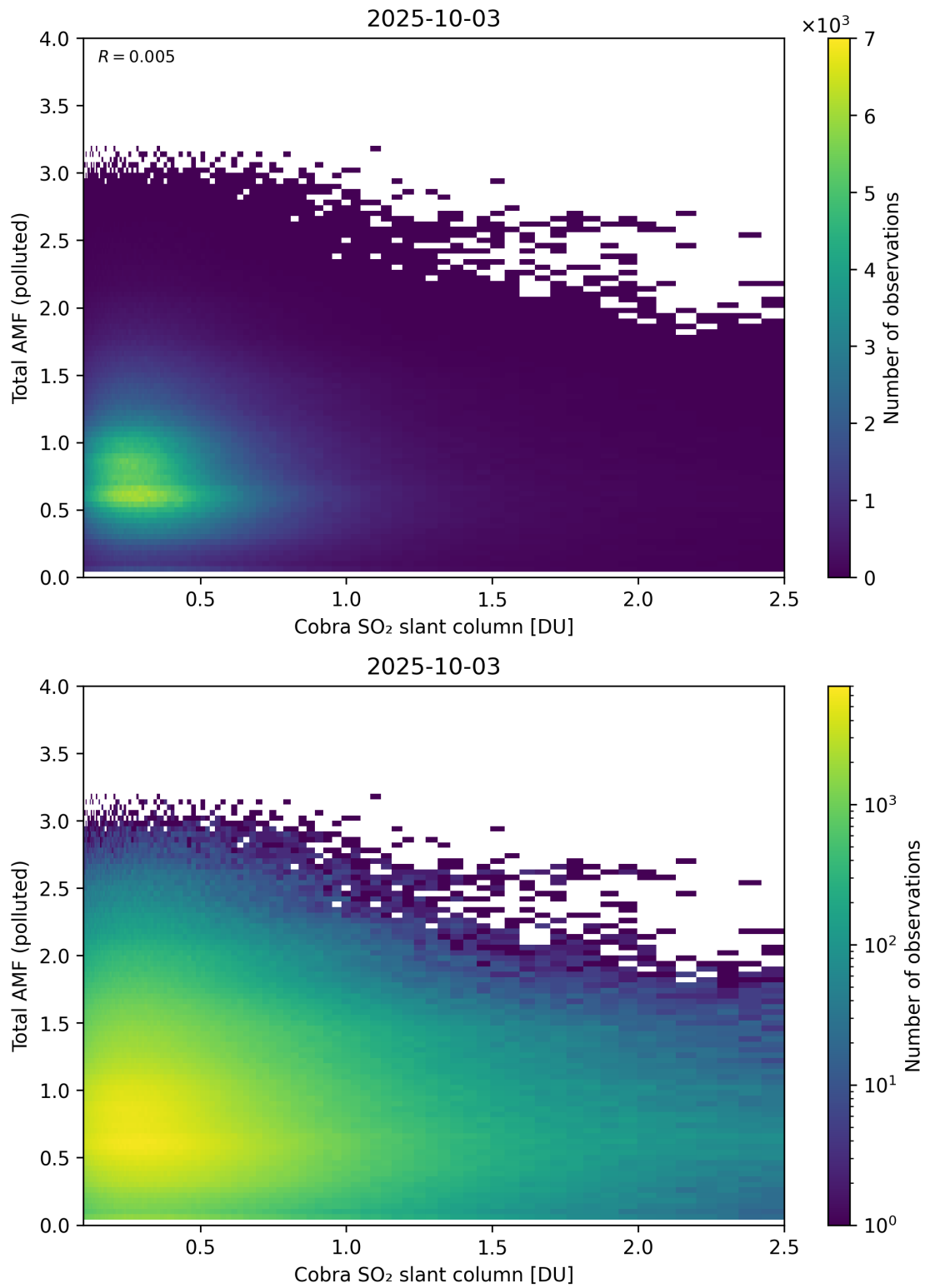
Figure 224: Scatter density plot of “Cobra SO 2 slant column” against “Total AMF (polluted)” for 2025-10-02 to 2025-10-04.
