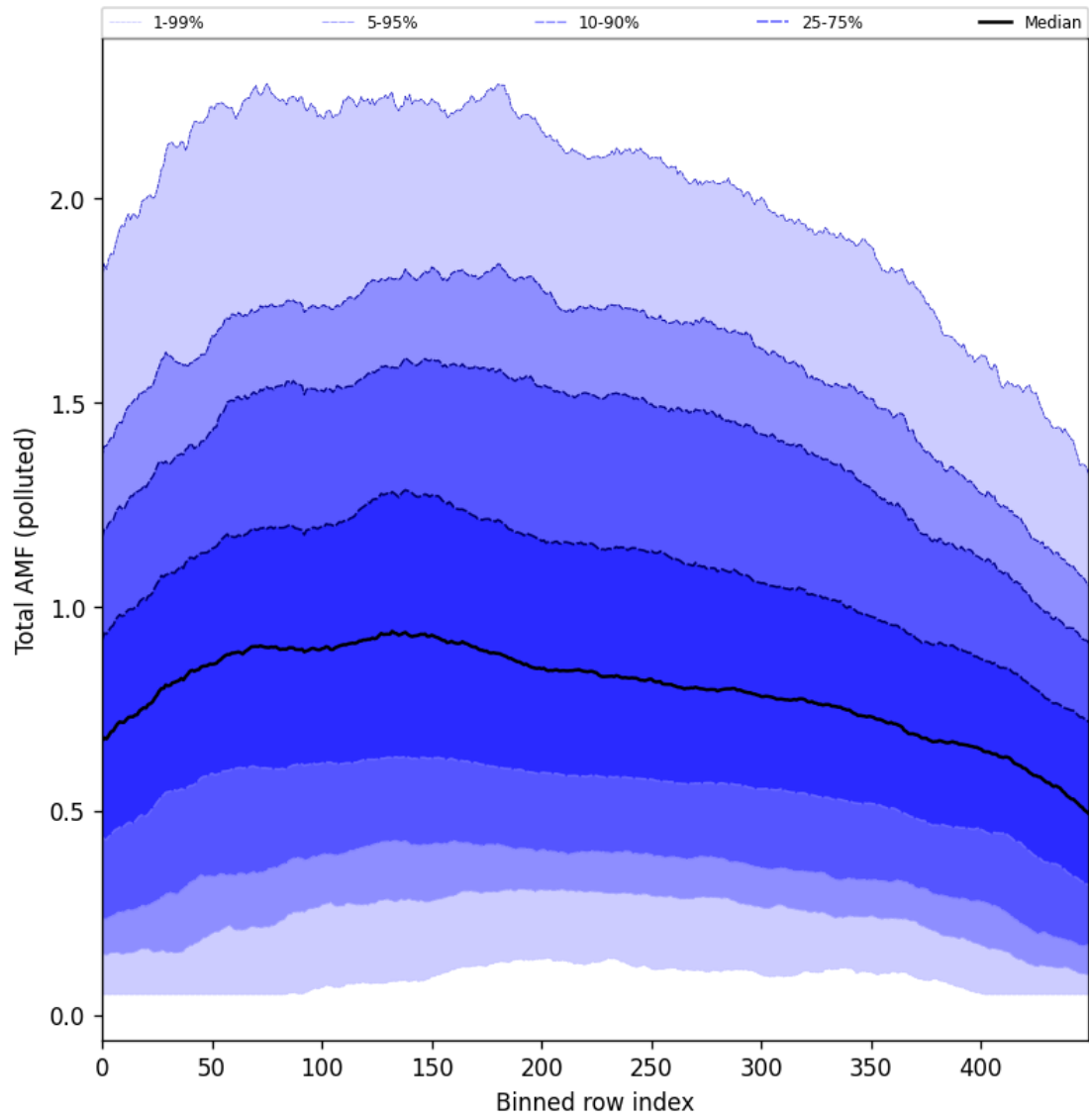
Figure 105: Along track statistics of “Total AMF (polluted)” for 2025-10-02 to 2025-10-04
