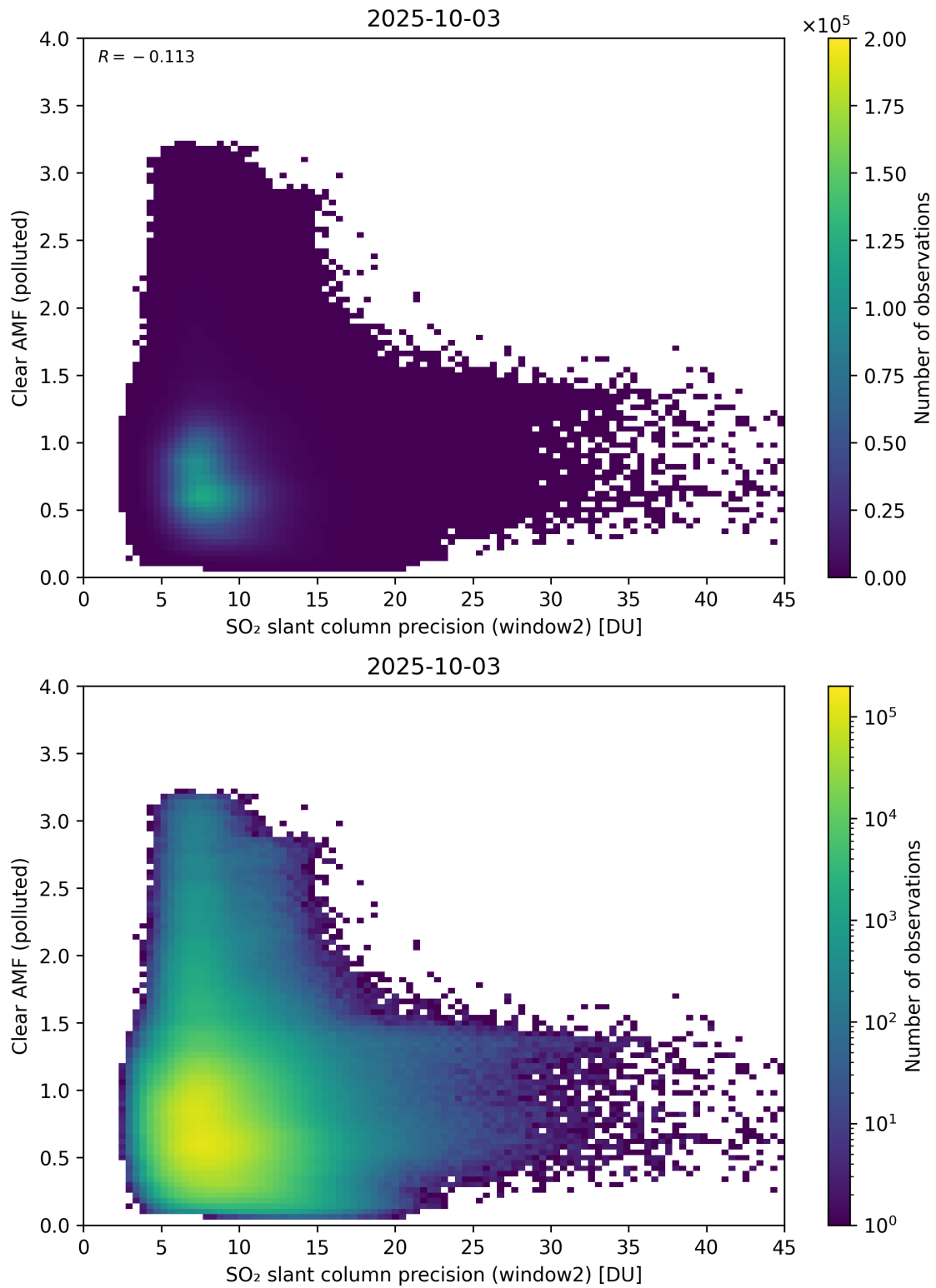
Figure 296: Scatter density plot of “SO 2 slant column precision (window2)” against “Clear AMF (polluted)” for 2025-10-02 to 2025-10-04.
