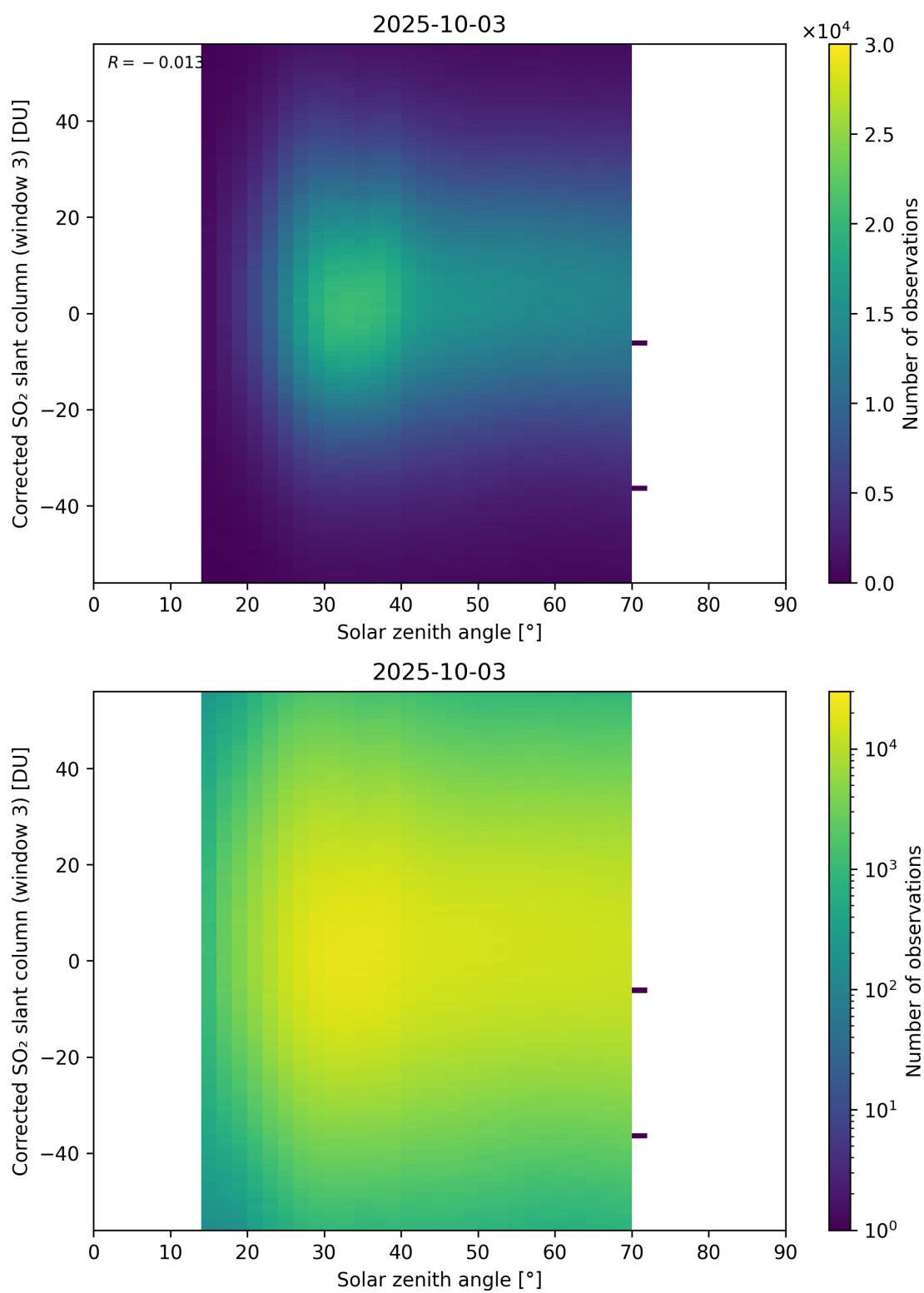
Figure 183: Scatter density plot of “Solar zenith angle” against “Corrected SO 2 slant column (window 3)” for 2025-10-02 to 2025-10-04.
