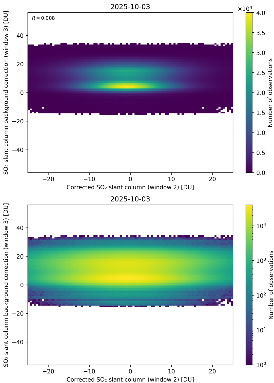
Figure 245: Scatter density plot of “Corrected SO 2 slant column (window 2)” against “SO 2 slant column background correction (window 3)” for 2025-10-02 to 2025-10-04.
