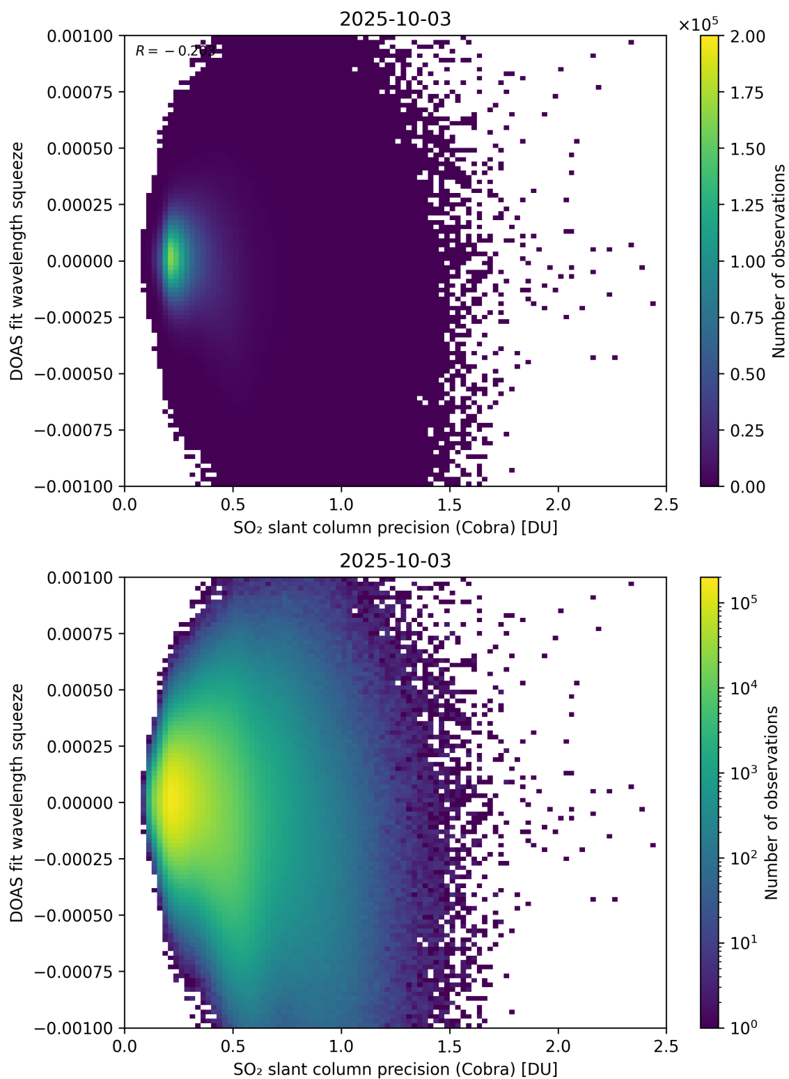
Figure 203: Scatter density plot of “SO 2 slant column precision (Cobra)” against “DOAS fit wavelength squeeze” for 2025-10-02 to 2025-10-04.
