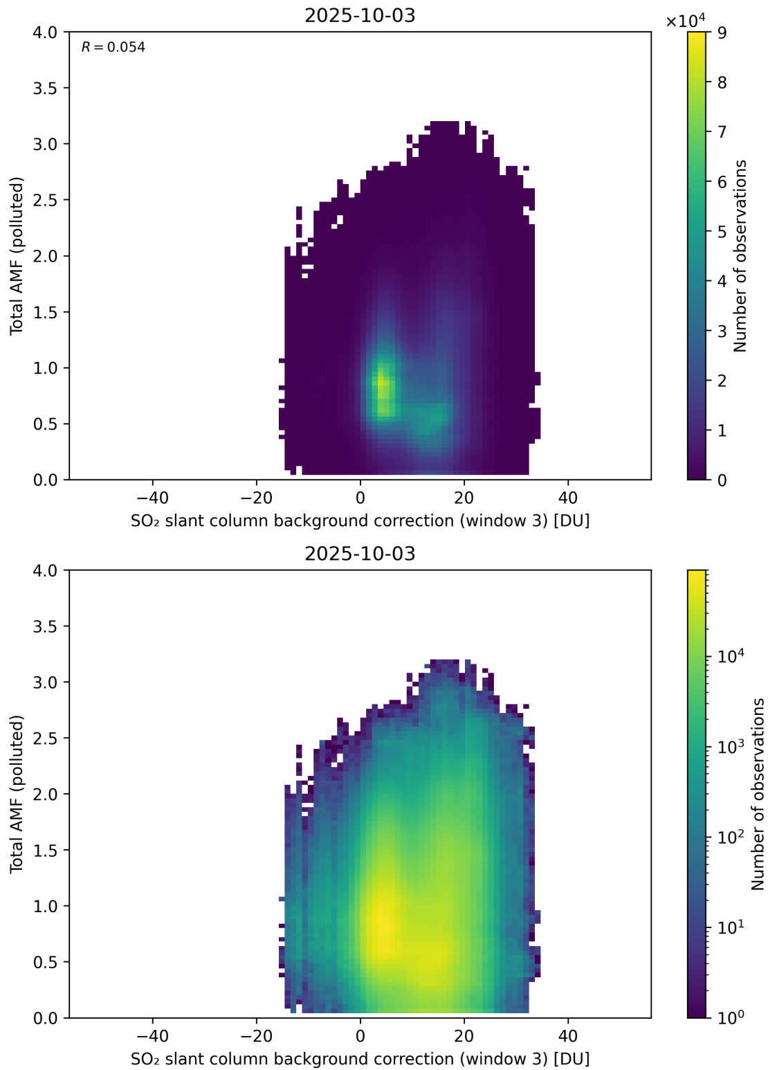
Figure 136: Scatter density plot of “SO 2 slant column background correction (window 3)” against “Total AMF (polluted)” for 2025-10-02 to 2025-10-04.
