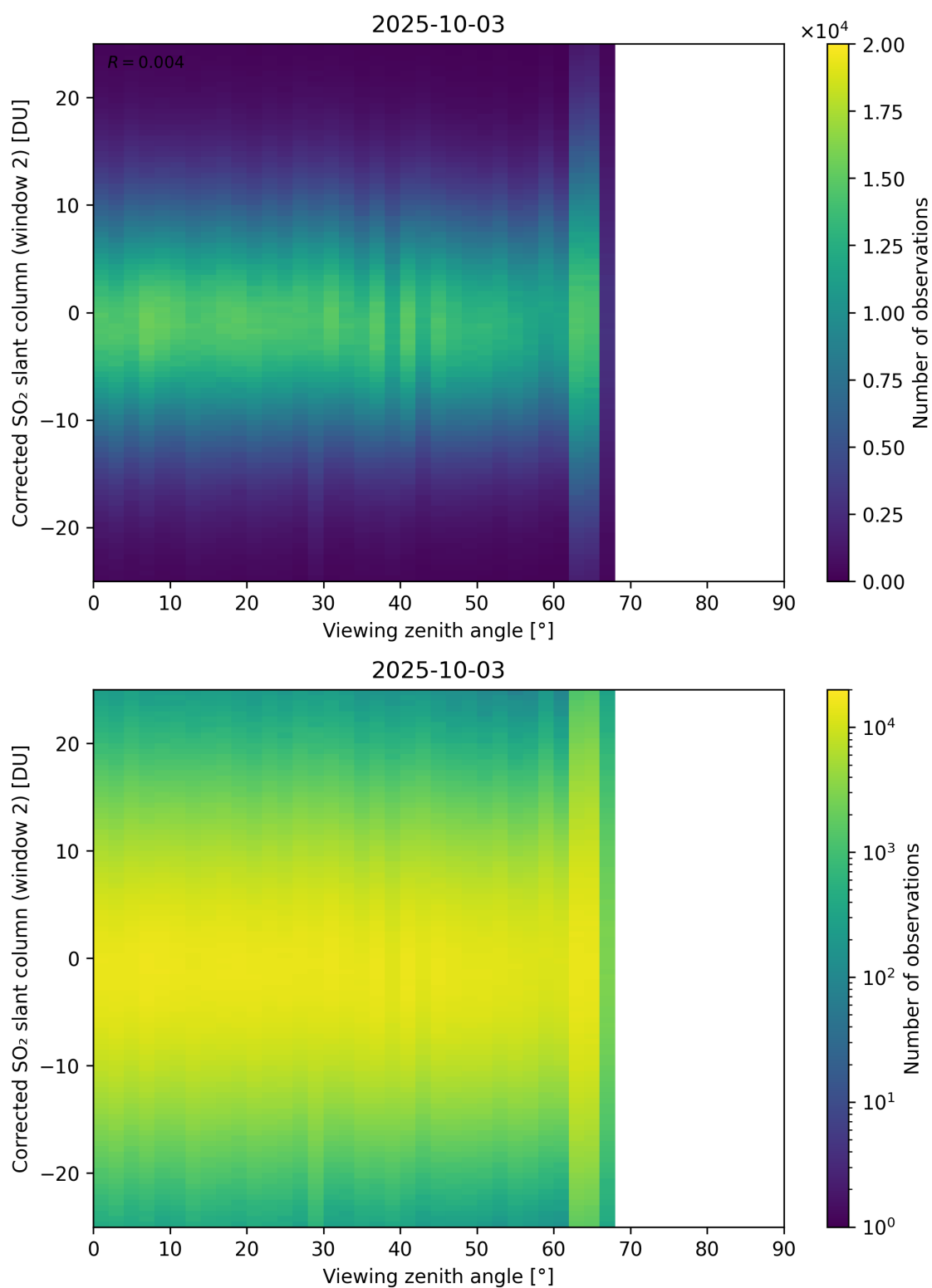
Figure 374: Scatter density plot of “Viewing zenith angle” against “Corrected SO 2 slant column (window 2)” for 2025-10-02 to 2025-10-04.
