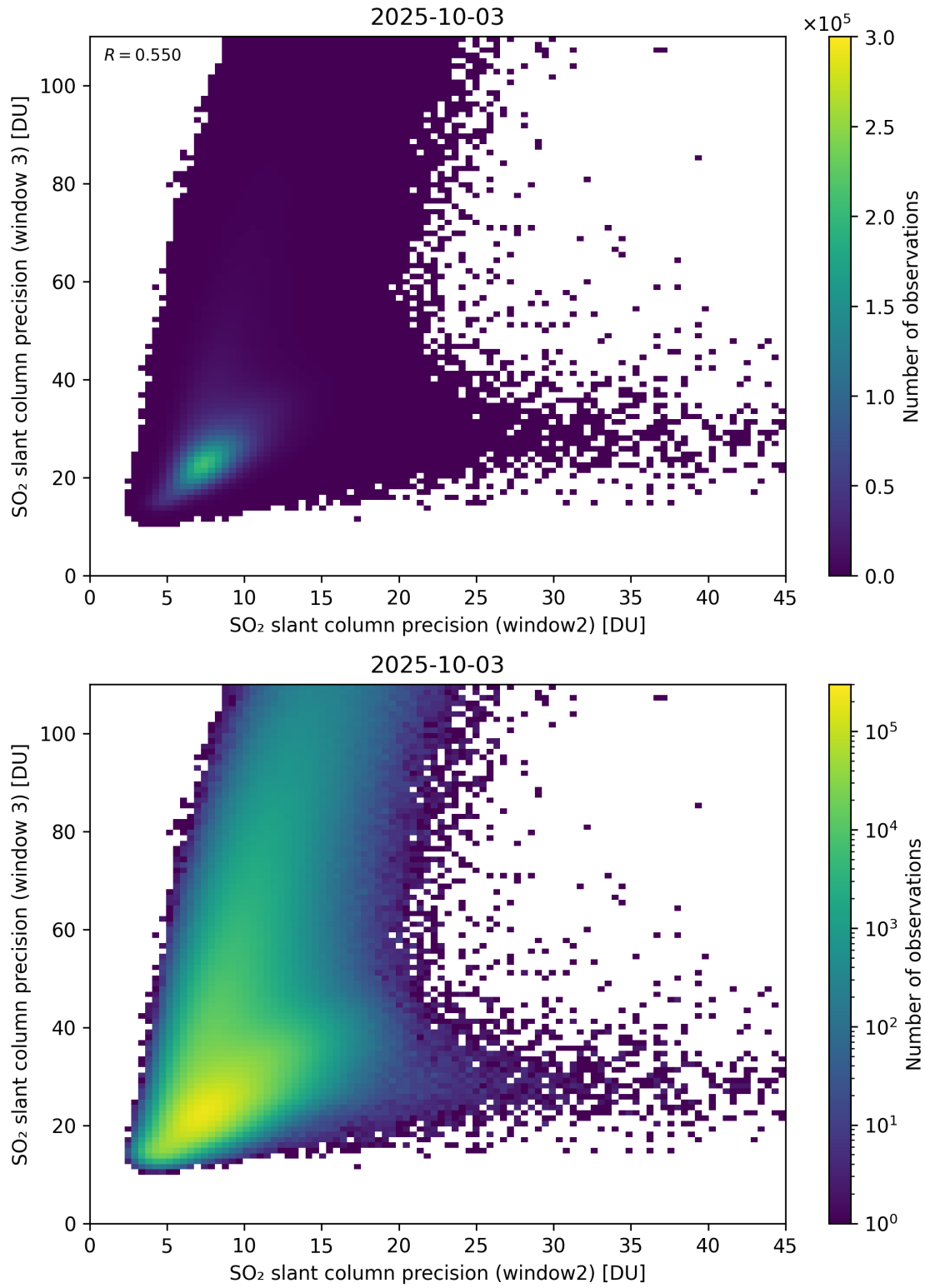
Figure 300: Scatter density plot of “SO 2 slant column precision (window2)” against “SO 2 slant column precision (window 3)” for 2025-10-02 to 2025-10-04.
