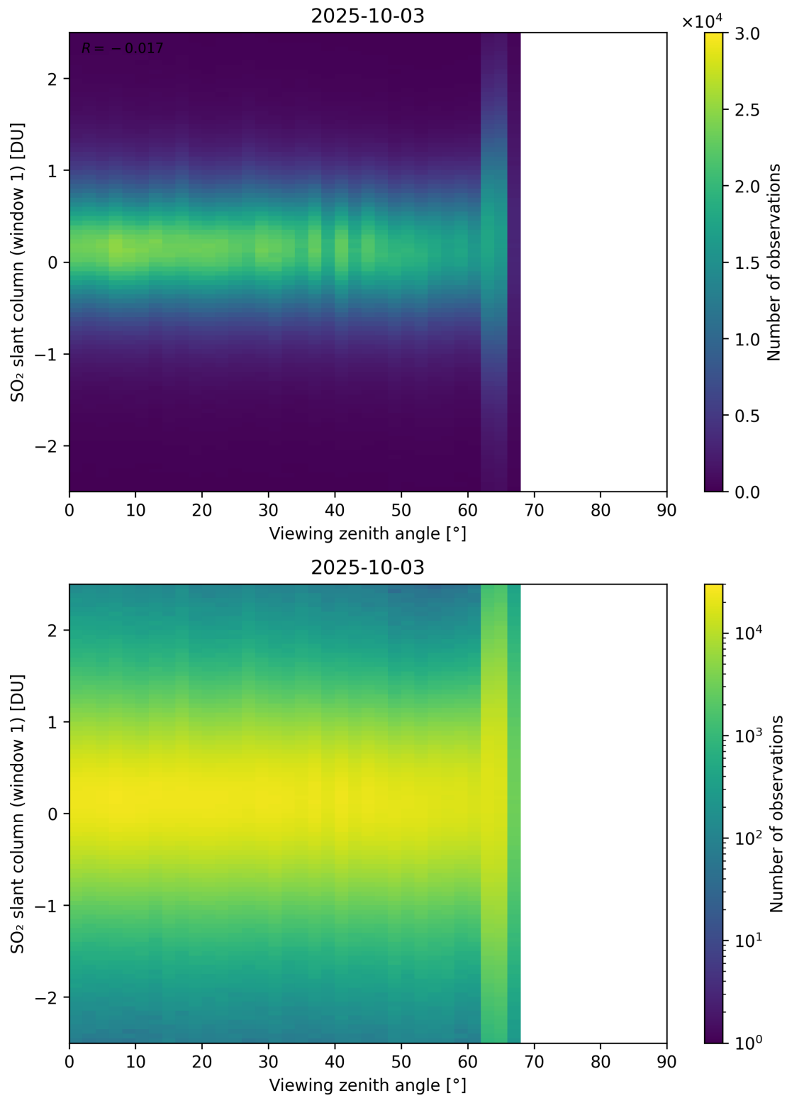
Figure 376: Scatter density plot of “Viewing zenith angle” against “SO 2 slant column (window 1)” for 2025-10-02 to 2025-10-04.
