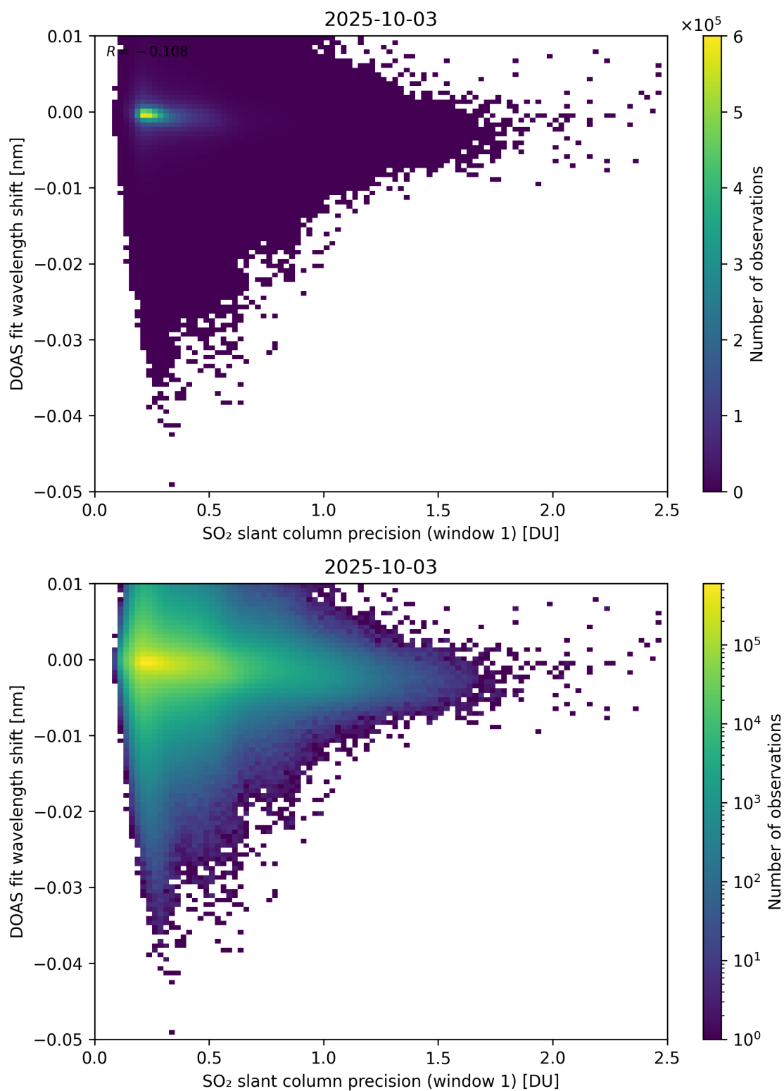
Figure 271: Scatter density plot of “SO 2 slant column precision (window 1)” against “DOAS fit wavelength shift” for 2025-10-02 to 2025-10-04.
