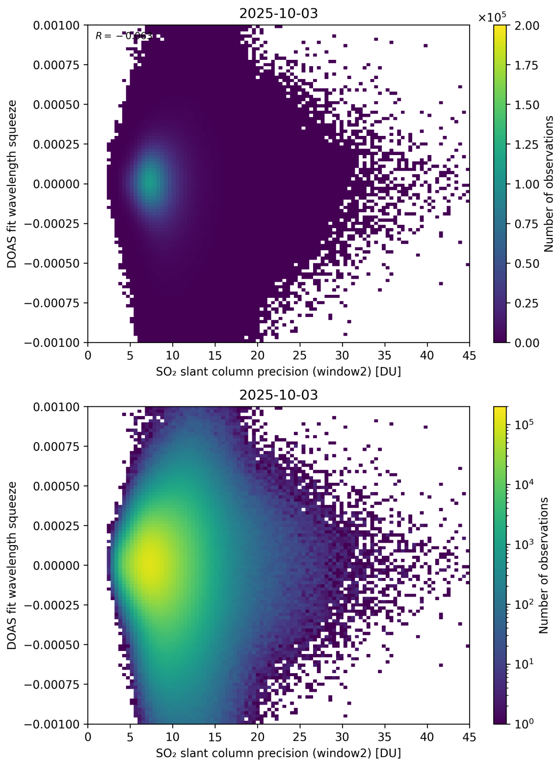
Figure 294: Scatter density plot of “SO 2 slant column precision (window2)” against “DOAS fit wavelength squeeze” for 2025-10-02 to 2025-10-04.
