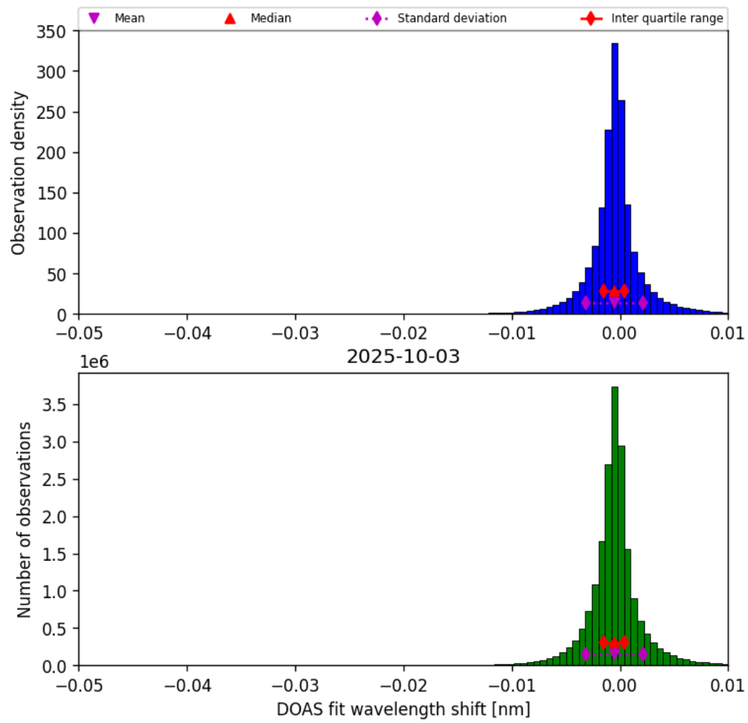
Figure 76: Histogram of “DOAS fit wavelength shift” for 2025-10-02 to 2025-10-04
