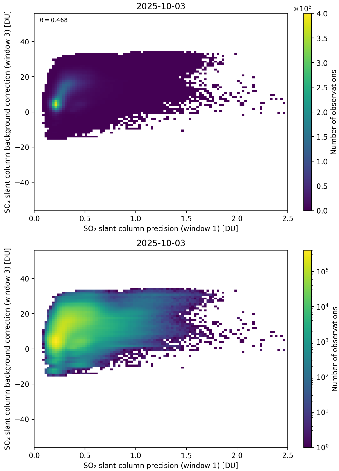
Figure 270: Scatter density plot of “SO 2 slant column precision (window 1)” against “SO 2 slant column background correction (window 3)” for 2025-10-02 to 2025-10-04.
