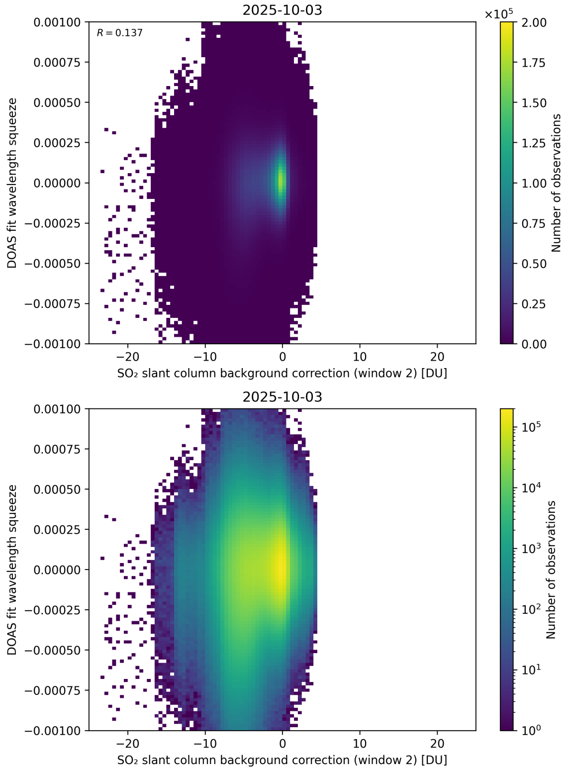
Figure 124: Scatter density plot of “SO 2 slant column background correction (window 2)” against “DOAS fit wavelength squeeze” for 2025-10-02 to 2025-10-04.
