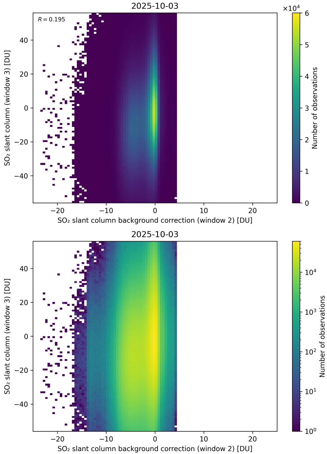
Figure 128: Scatter density plot of “SO 2 slant column background correction (window 2)” against “SO 2 slant column (window 3)” for 2025-10-02 to 2025-10-04.
