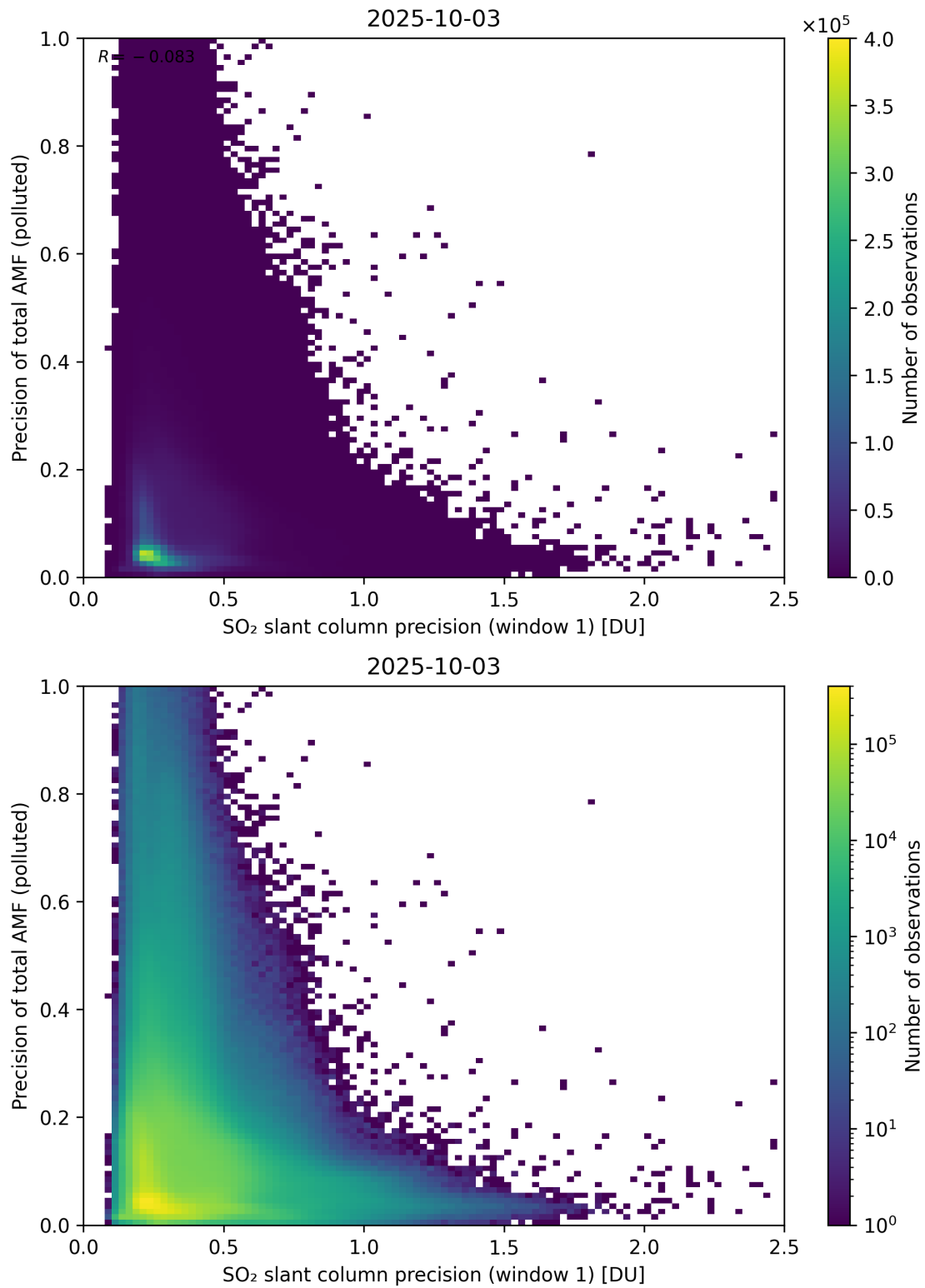
Figure 281: Scatter density plot of “SO 2 slant column precision (window 1)” against “Precision of total AMF (polluted)” for 2025-10-02 to 2025-10-04.
