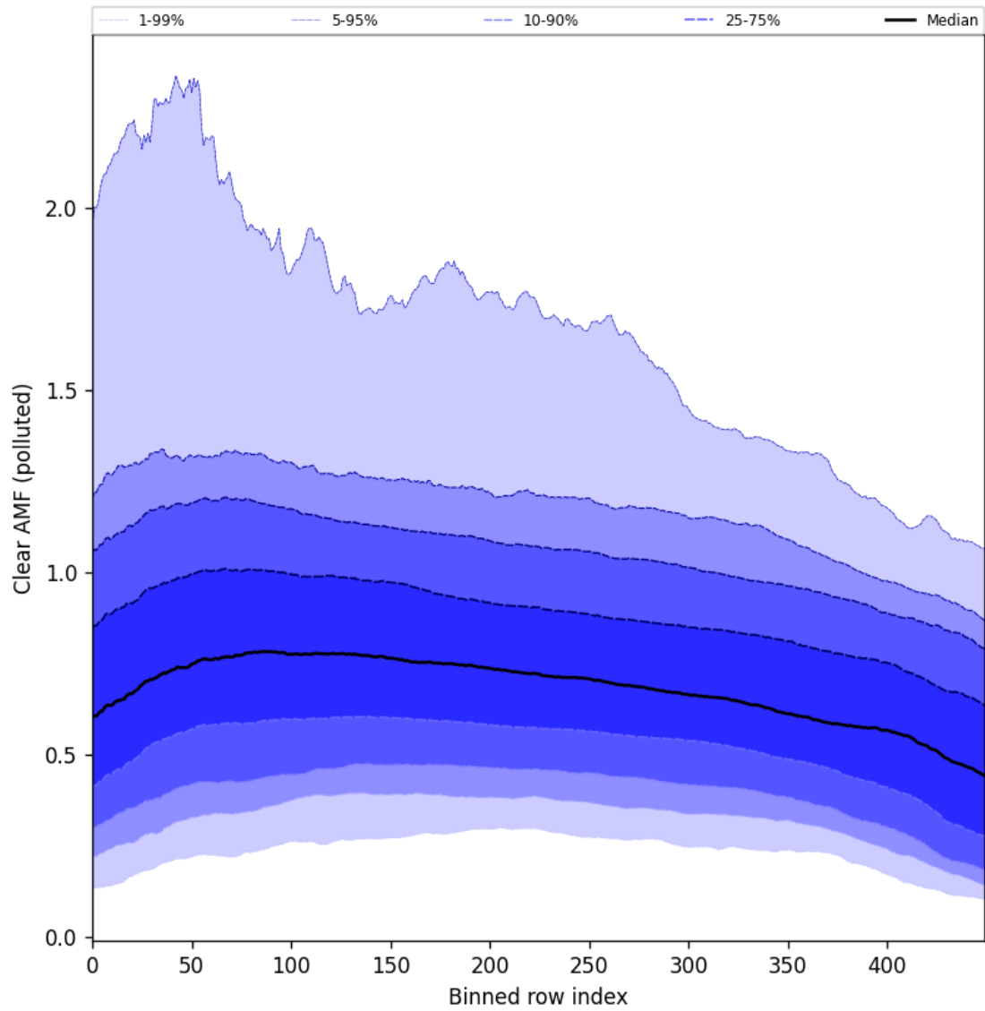
Figure 107: Along track statistics of “Clear AMF (polluted)” for 2025-10-02 to 2025-10-04
