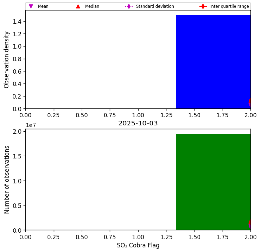
Figure 75: Histogram of “SO 2 Cobra Flag” for 2025-10-02 to 2025-10-04
