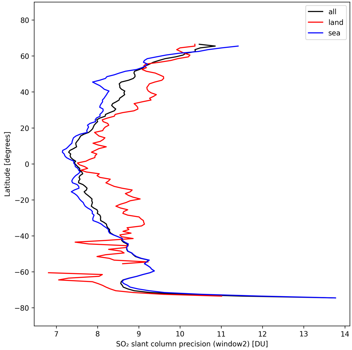
Figure 42: Zonal average of “SO 2 slant column precision (window2)” for 2025-10-02 to 2025-10-04.
