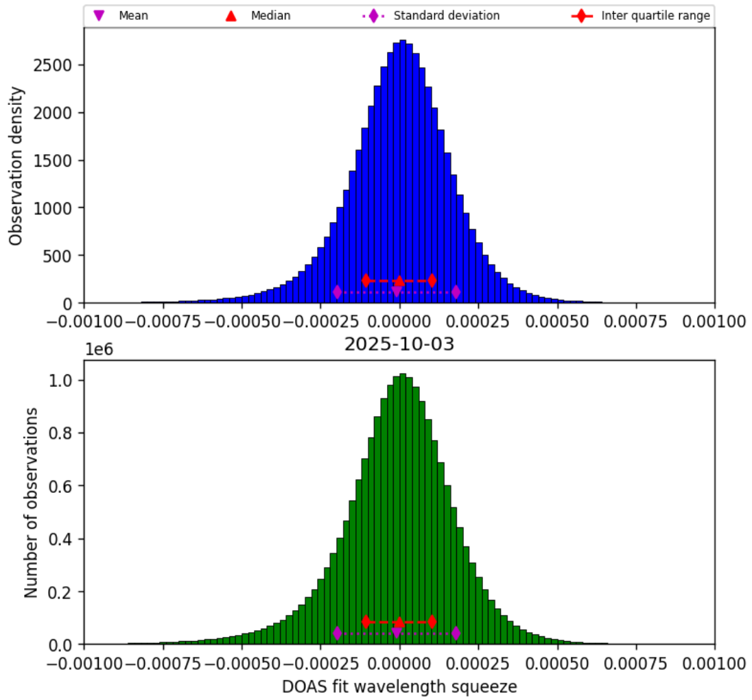
Figure 77: Histogram of “DOAS fit wavelength squeeze” for 2025-10-02 to 2025-10-04
