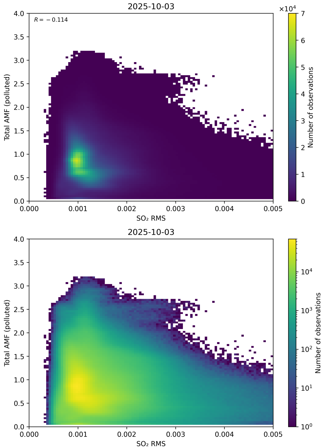
Figure 148: Scatter density plot of “SO 2 RMS” against “Total AMF (polluted)” for 2025-10-02 to 2025-10-04.
