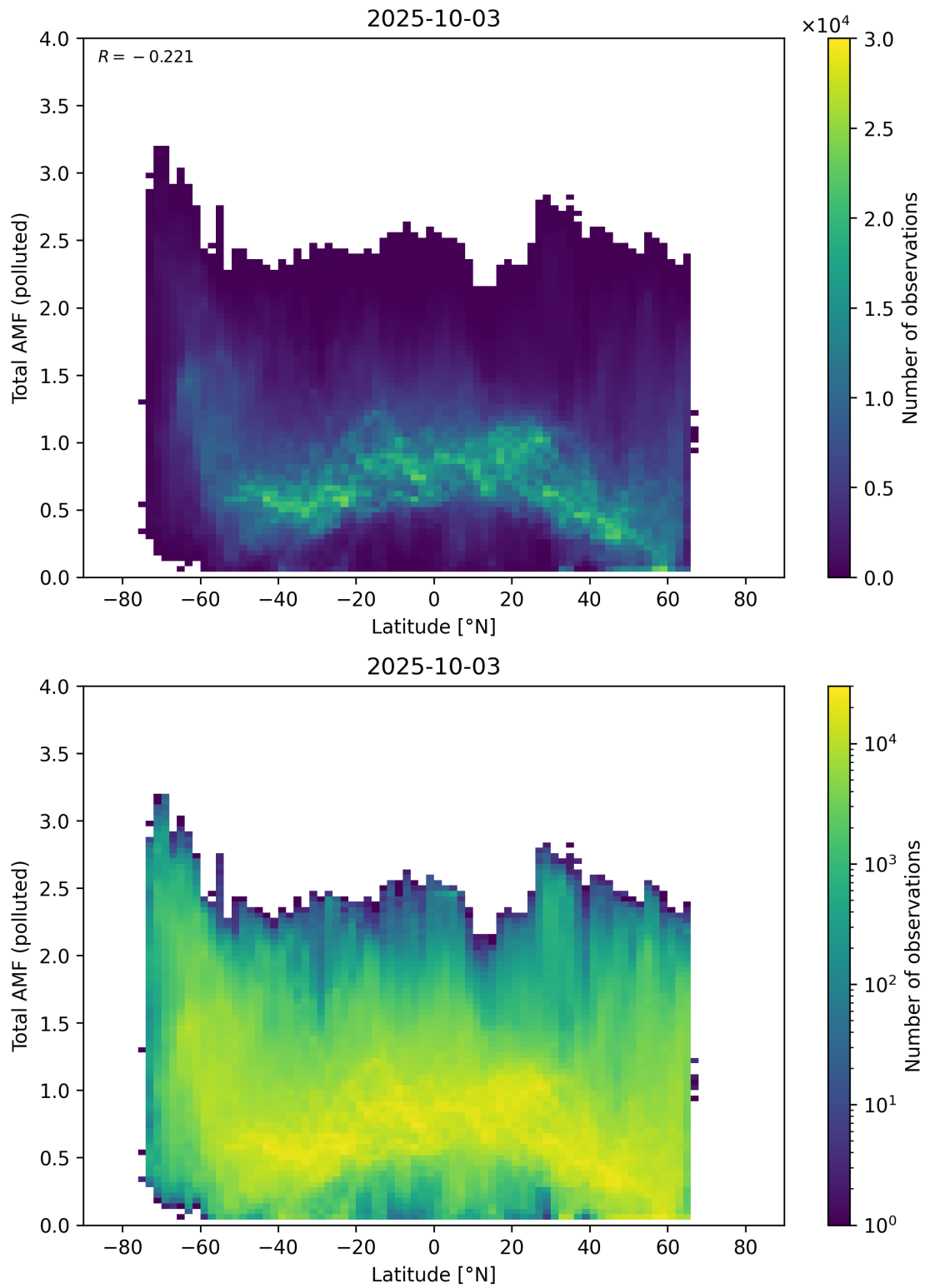
Figure 167: Scatter density plot of “Latitude” against “Total AMF (polluted)” for 2025-10-02 to 2025-10-04.
