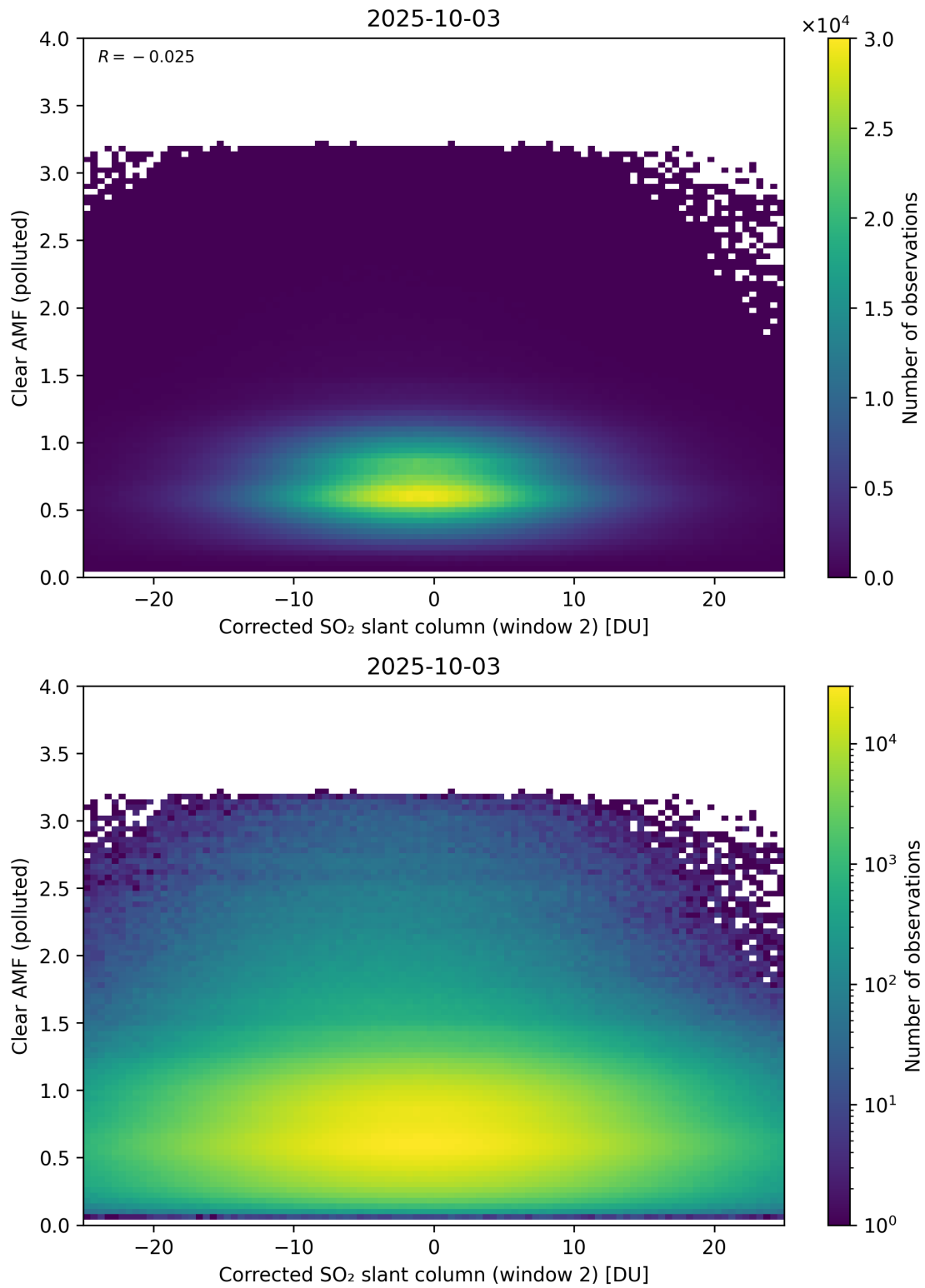
Figure 249: Scatter density plot of “Corrected SO 2 slant column (window 2)” against “Clear AMF (polluted)” for 2025-10-02 to 2025-10-04.
