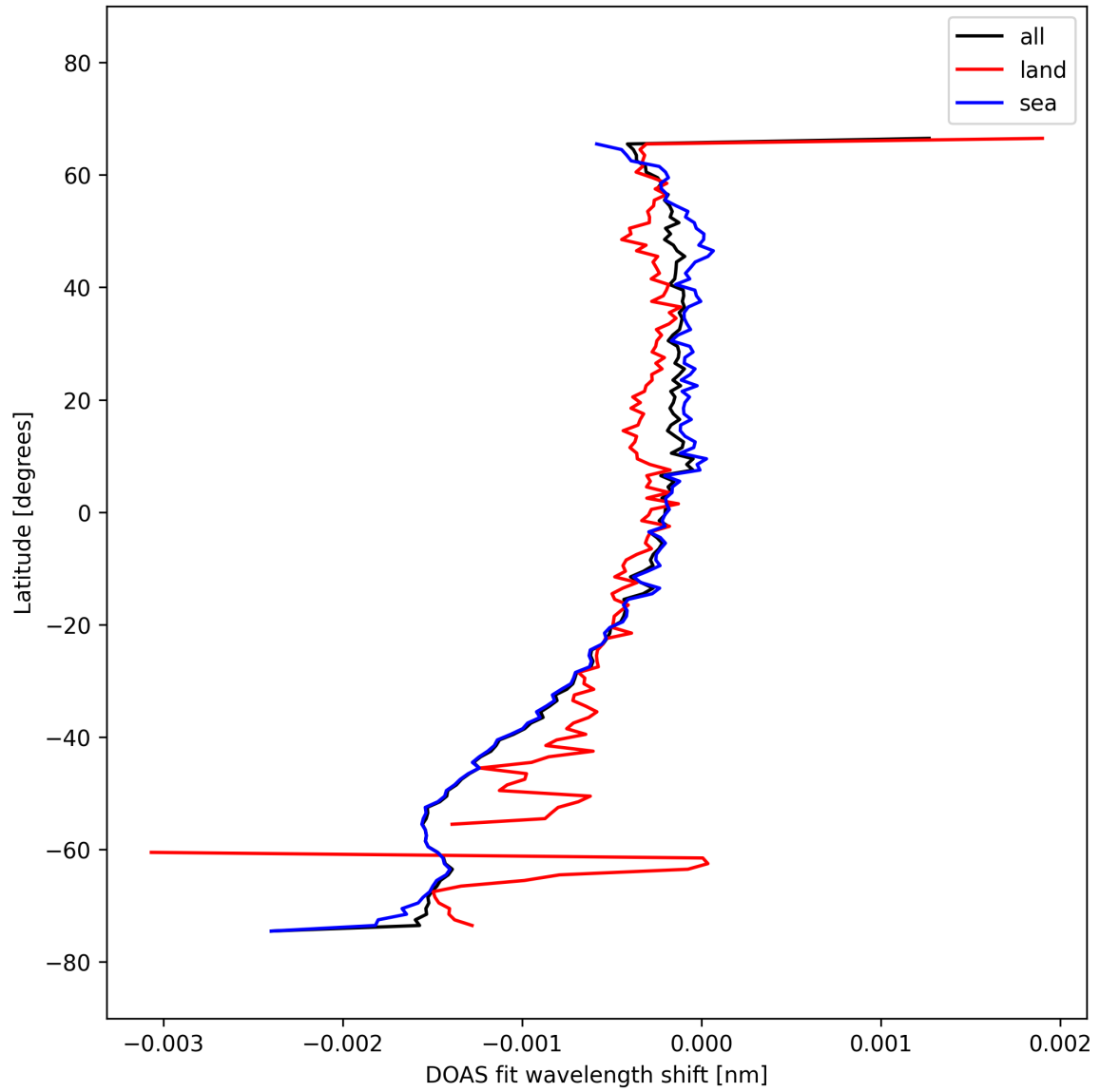
Figure 50: Zonal average of “DOAS fit wavelength shift” for 2025-10-02 to 2025-10-04.
