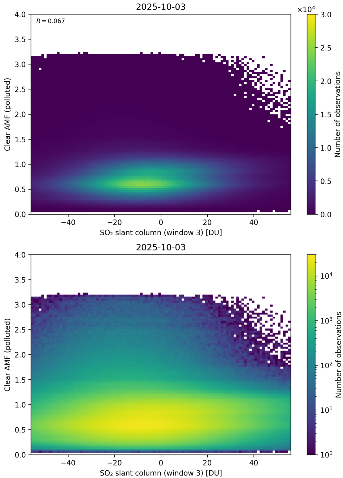
Figure 315: Scatter density plot of “SO 2 slant column (window 3)” against “Clear AMF (polluted)” for 2025-10-02 to 2025-10-04.
