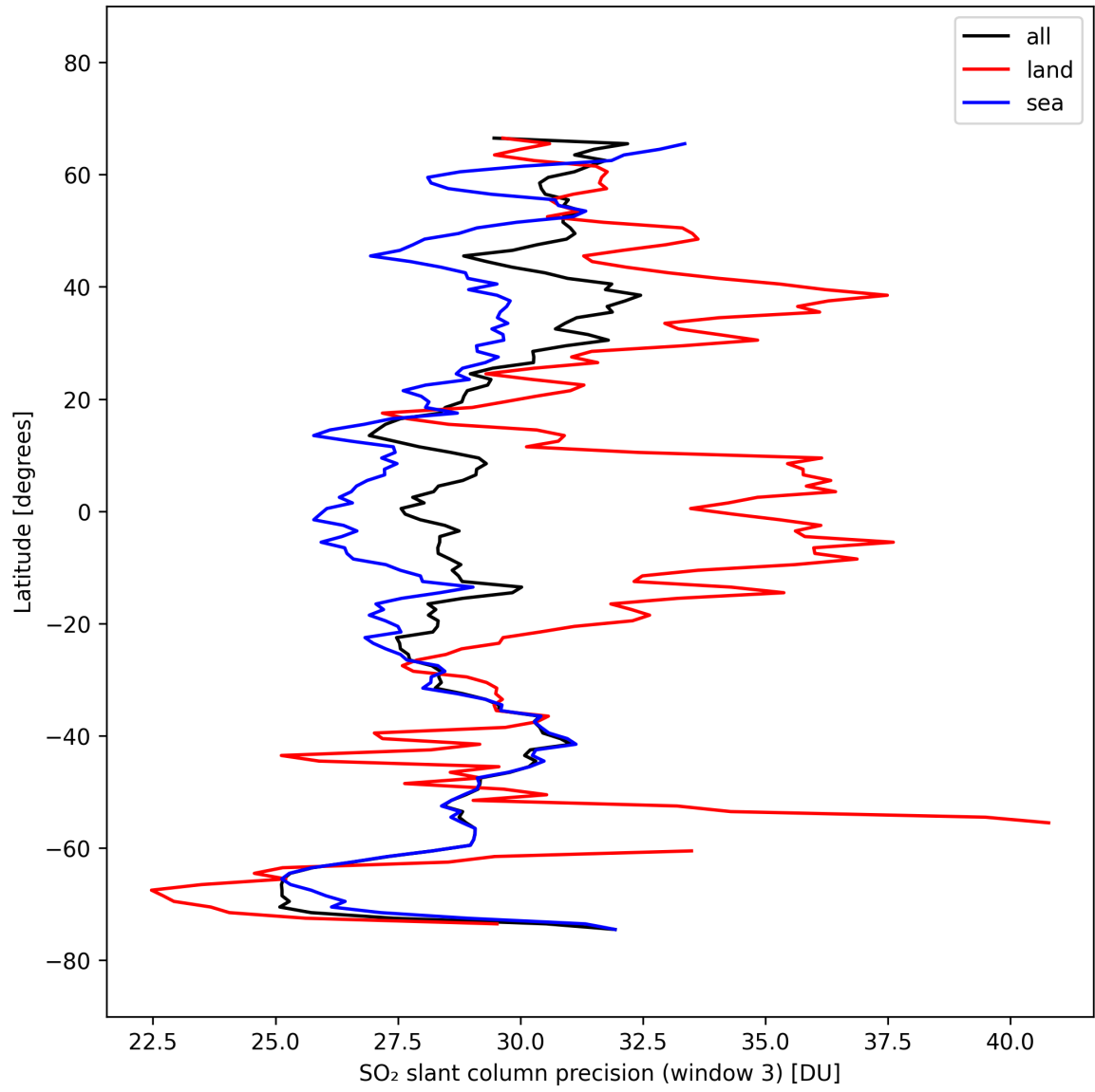
Figure 46: Zonal average of “SO 2 slant column precision (window 3)” for 2025-10-02 to 2025-10-04.
