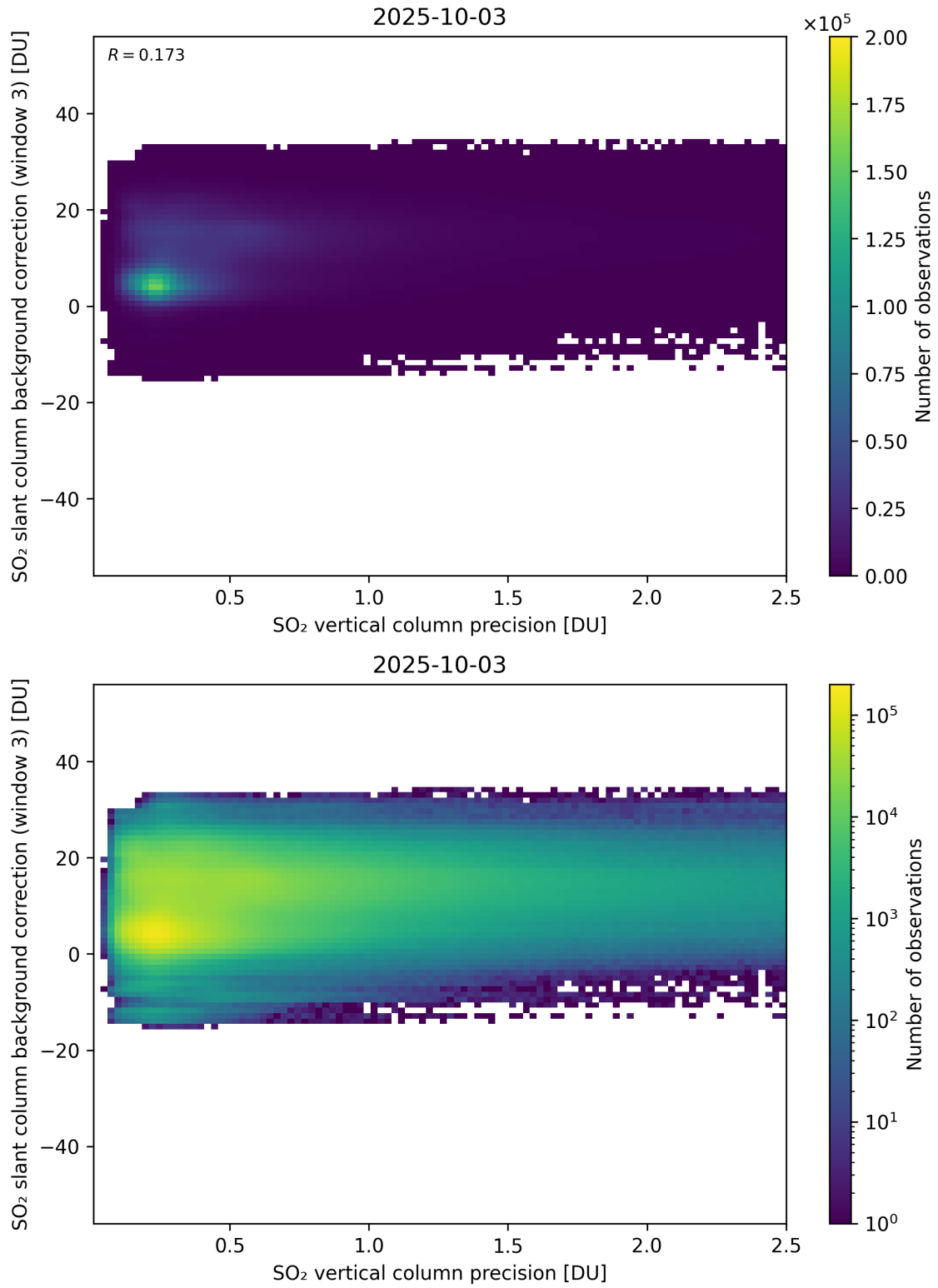
Figure 331: Scatter density plot of “SO 2 vertical column precision” against “SO 2 slant column background correction (window 3)” for 2025-10-02 to 2025-10-04.
