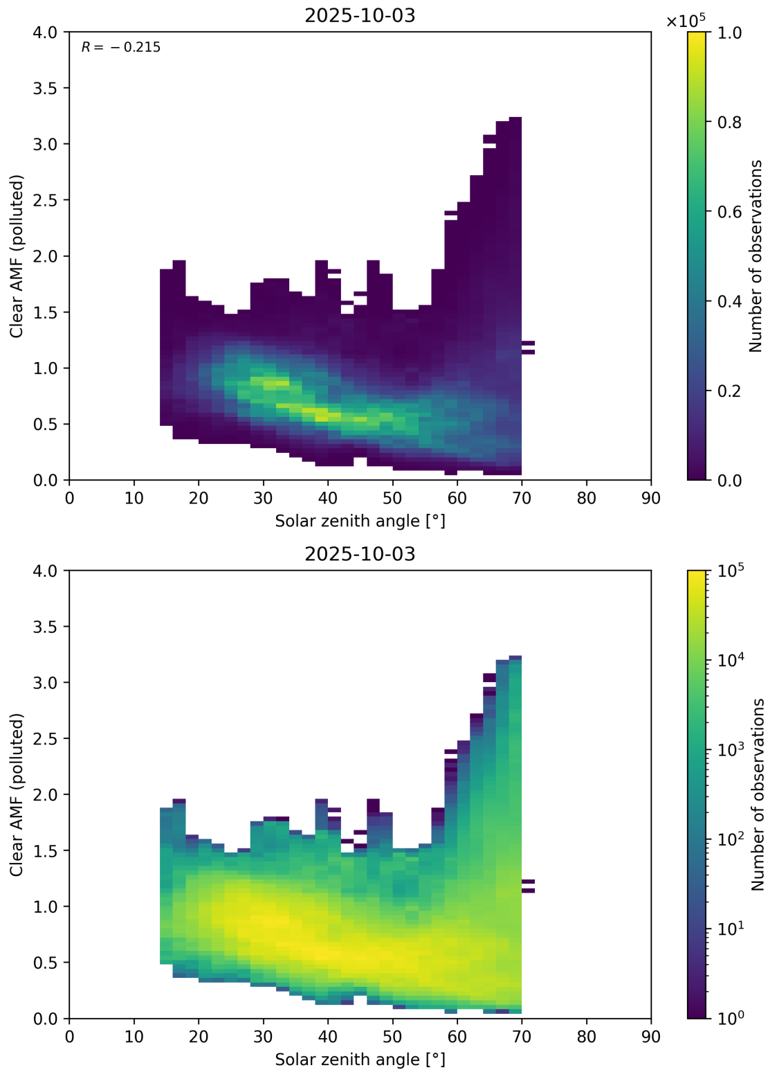
Figure 178: Scatter density plot of “Solar zenith angle” against “Clear AMF (polluted)” for 2025-10-02 to 2025-10-04.
