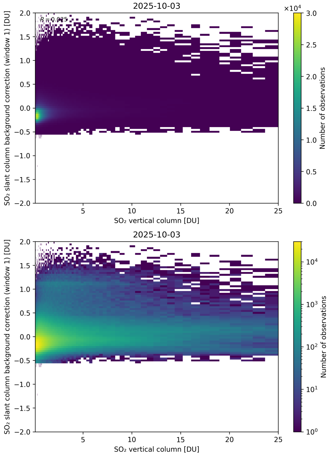
Figure 323: Scatter density plot of “SO 2 vertical column” against “SO 2 slant column background correction (window 1)” for 2025-10-02 to 2025-10-04.
