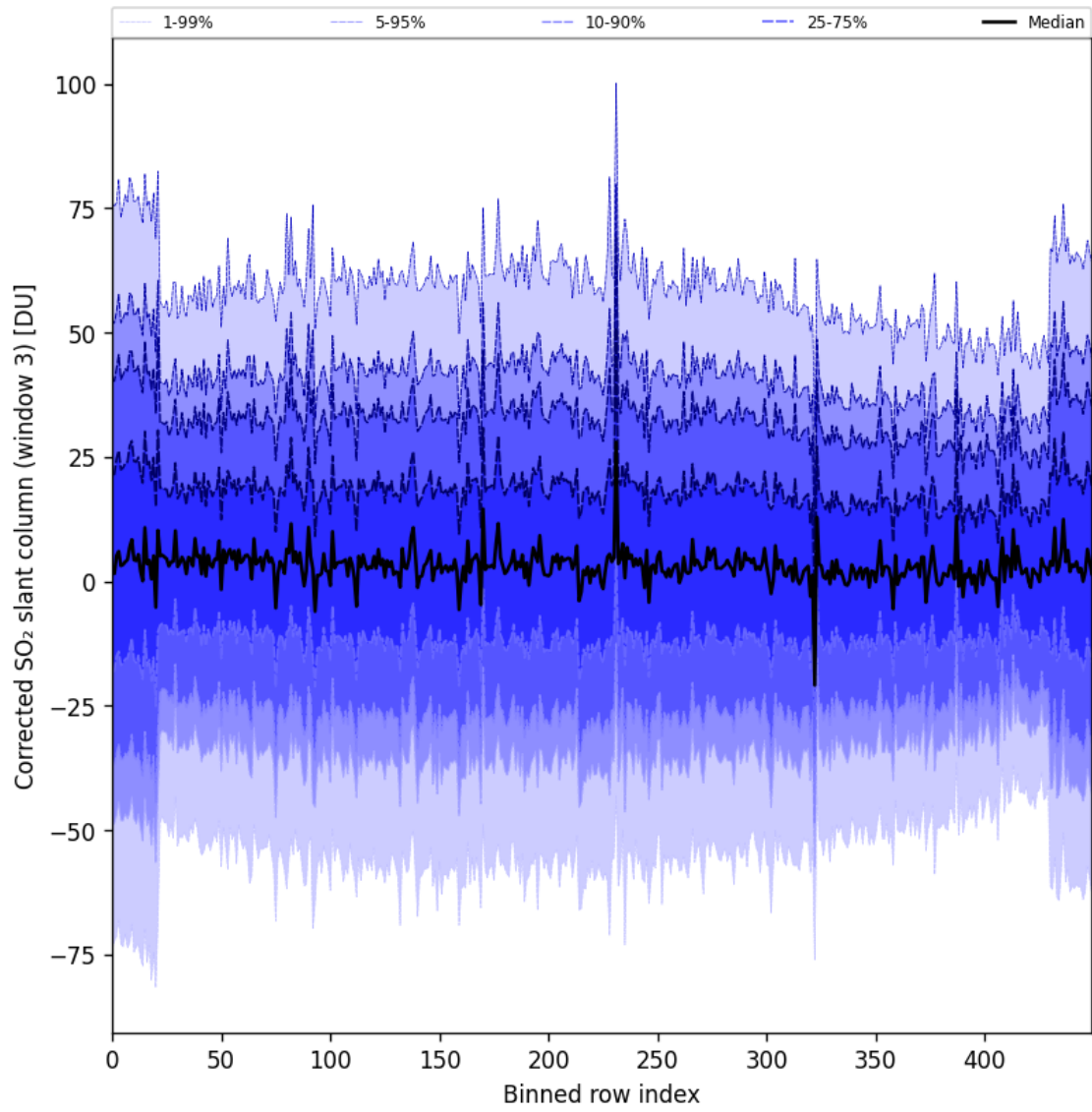
Figure 99: Along track statistics of “Corrected SO 2 slant column (window 3)” for 2025-10-02 to 2025-10-04
