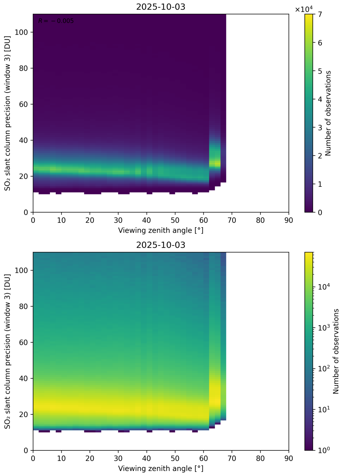
Figure 380: Scatter density plot of “Viewing zenith angle” against “SO 2 slant column precision (window 3)” for 2025-10-02 to 2025-10-04.
