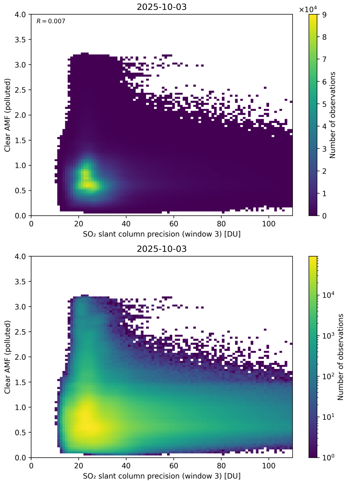
Figure 311: Scatter density plot of “SO 2 slant column precision (window 3)” against “Clear AMF (polluted)” for 2025-10-02 to 2025-10-04.
