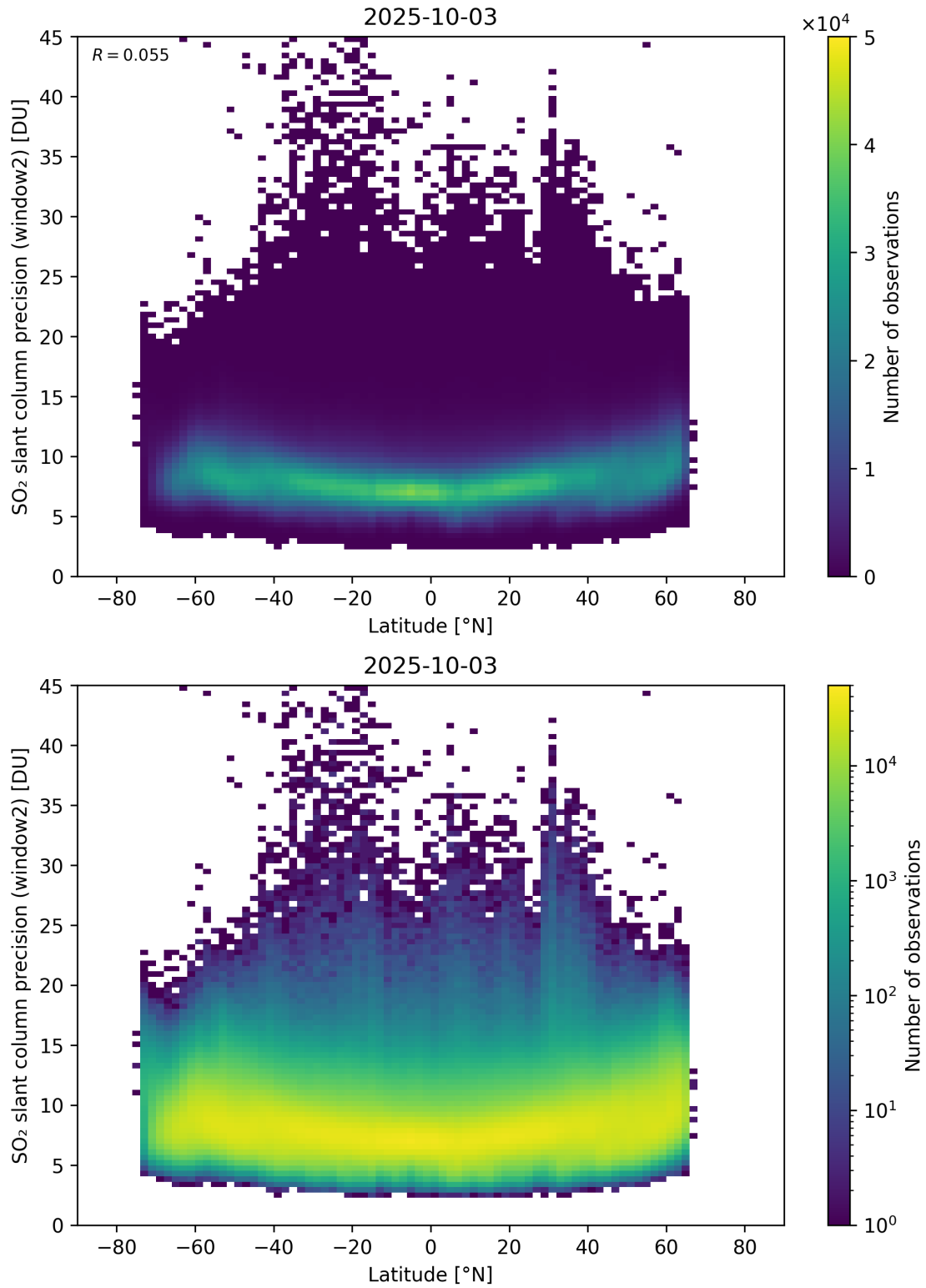
Figure 164: Scatter density plot of “Latitude” against “SO 2 slant column precision (window2)” for 2025-10-02 to 2025-10-04.
