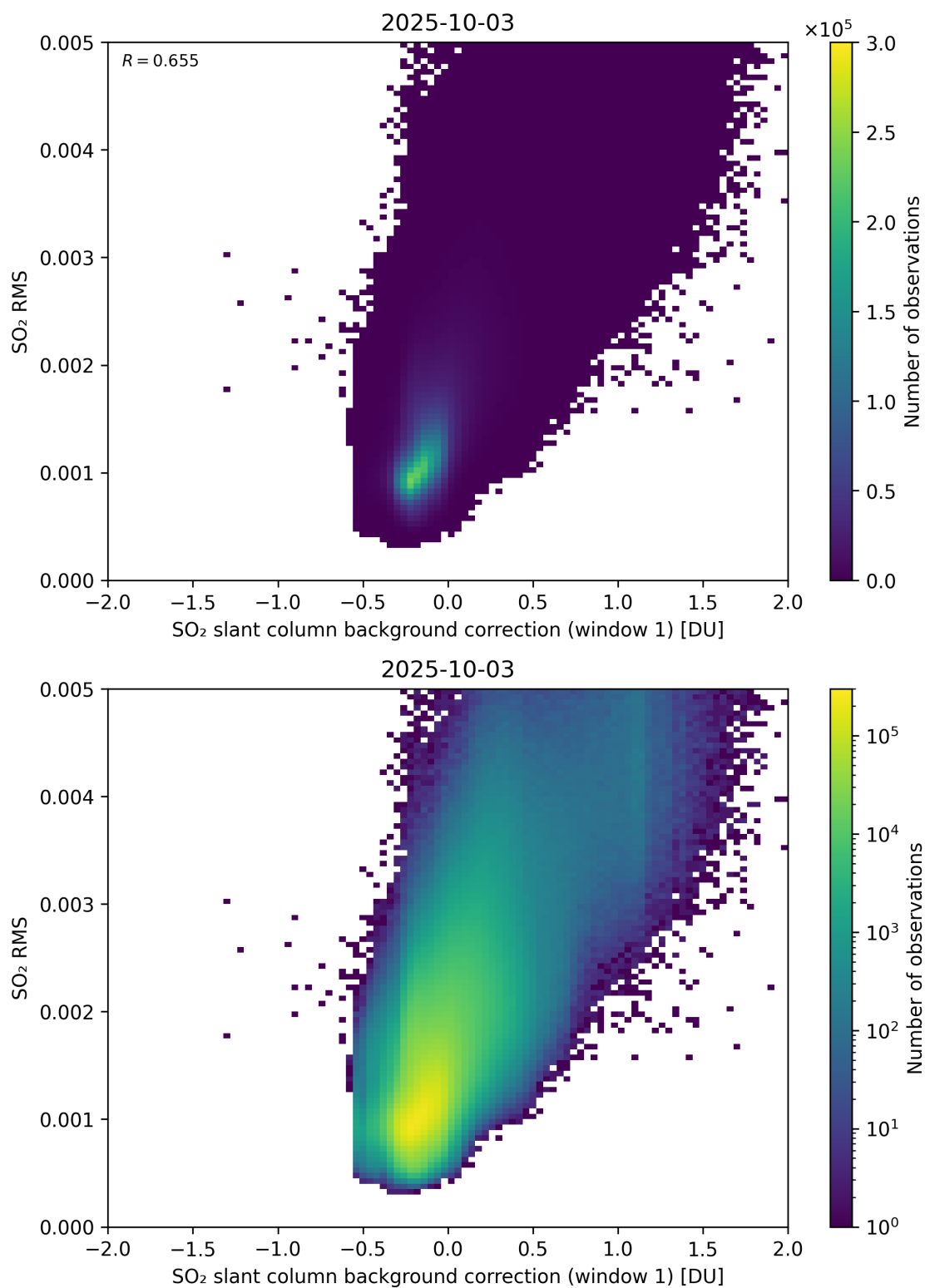
Figure 113: Scatter density plot of “SO 2 slant column background correction (window 1)” against “SO 2 RMS” for 2025-10-02 to 2025-10-04.
