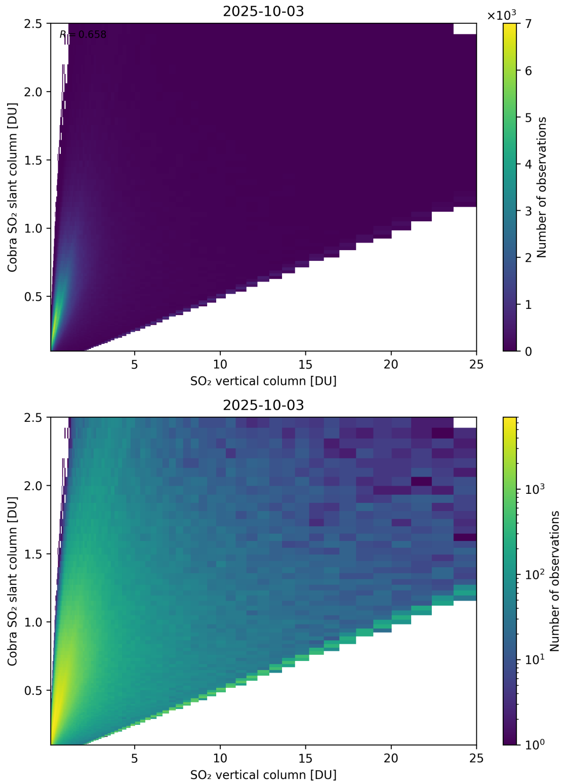
Figure 349: Scatter density plot of “SO 2 vertical column” against “Cobra SO 2 slant column” for 2025-10-02 to 2025-10-04.
