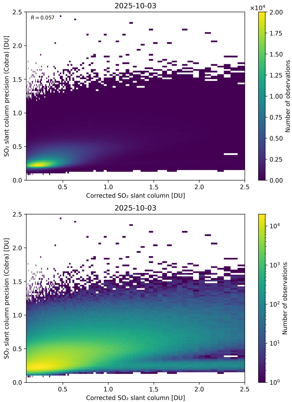
Figure 234: Scatter density plot of “Corrected SO 2 slant column” against “SO 2 slant column precision (Cobra)” for 2025-10-02 to 2025-10-04.
