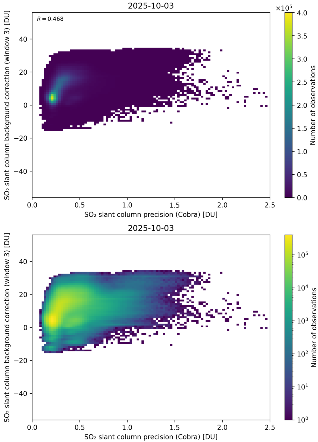
Figure 201: Scatter density plot of “SO 2 slant column precision (Cobra)” against “SO 2 slant column background correction (window 3)” for 2025-10-02 to 2025-10-04.
