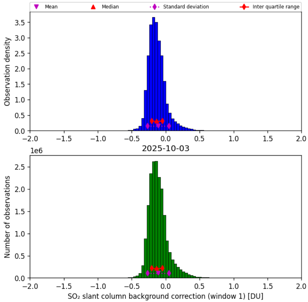
Figure 66: Histogram of “SO 2 slant column background correction (window 1)” for 2025-10-02 to 2025-10-04
