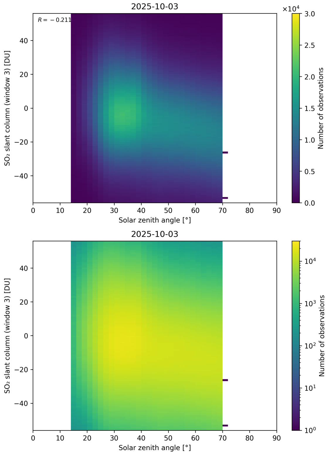
Figure 187: Scatter density plot of “Solar zenith angle” against “SO 2 slant column (window 3)” for 2025-10-02 to 2025-10-04.
