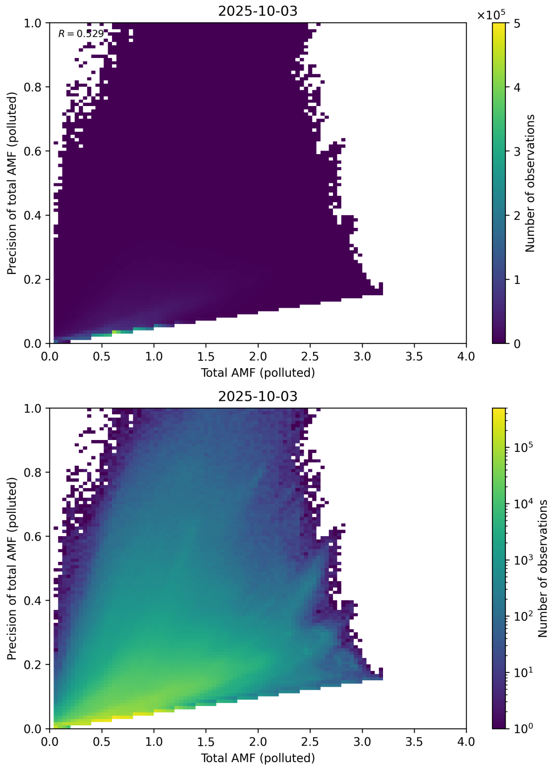
Figure 322: Scatter density plot of “Total AMF (polluted)” against “Precision of total AMF (polluted)” for 2025-10-02 to 2025-10-04.
