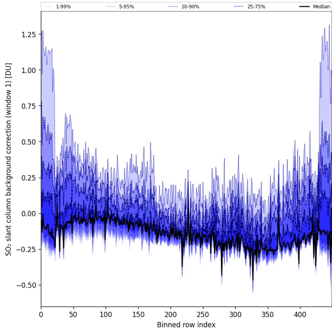
Figure 92: Along track statistics of “SO 2 slant column background correction (window 1)” for 2025-10-02 to 2025-10-04
