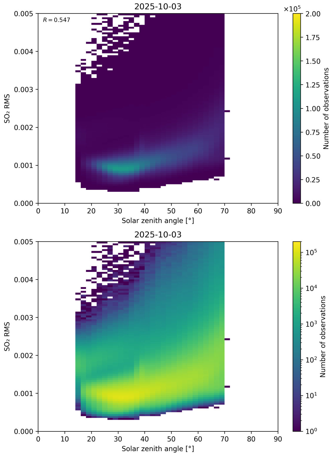
Figure 176: Scatter density plot of “Solar zenith angle” against “SO 2 RMS” for 2025-10-02 to 2025-10-04.
