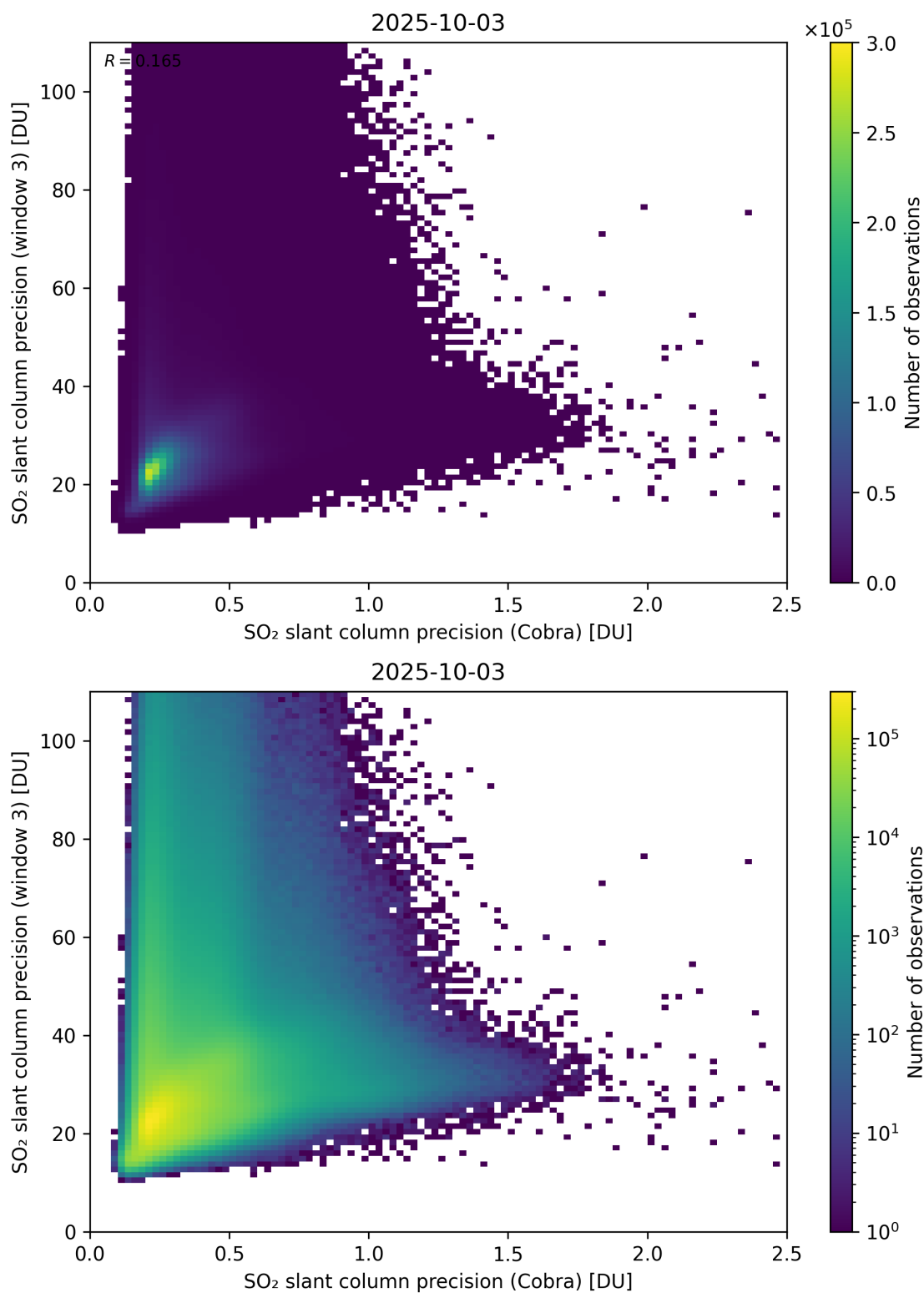
Figure 212: Scatter density plot of “SO 2 slant column precision (Cobra)” against “SO 2 slant column precision (window 3)” for 2025-10-02 to 2025-10-04.
