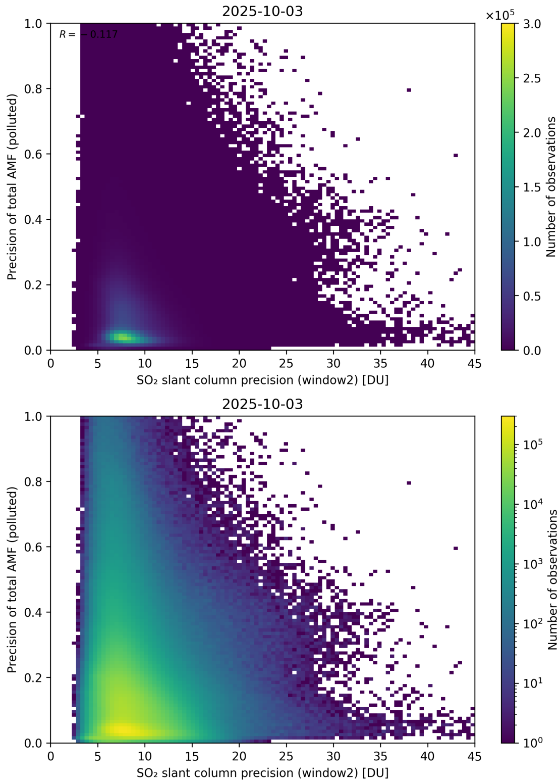
Figure 302: Scatter density plot of “SO 2 slant column precision (window2)” against “Precision of total AMF (polluted)” for 2025-10-02 to 2025-10-04.
