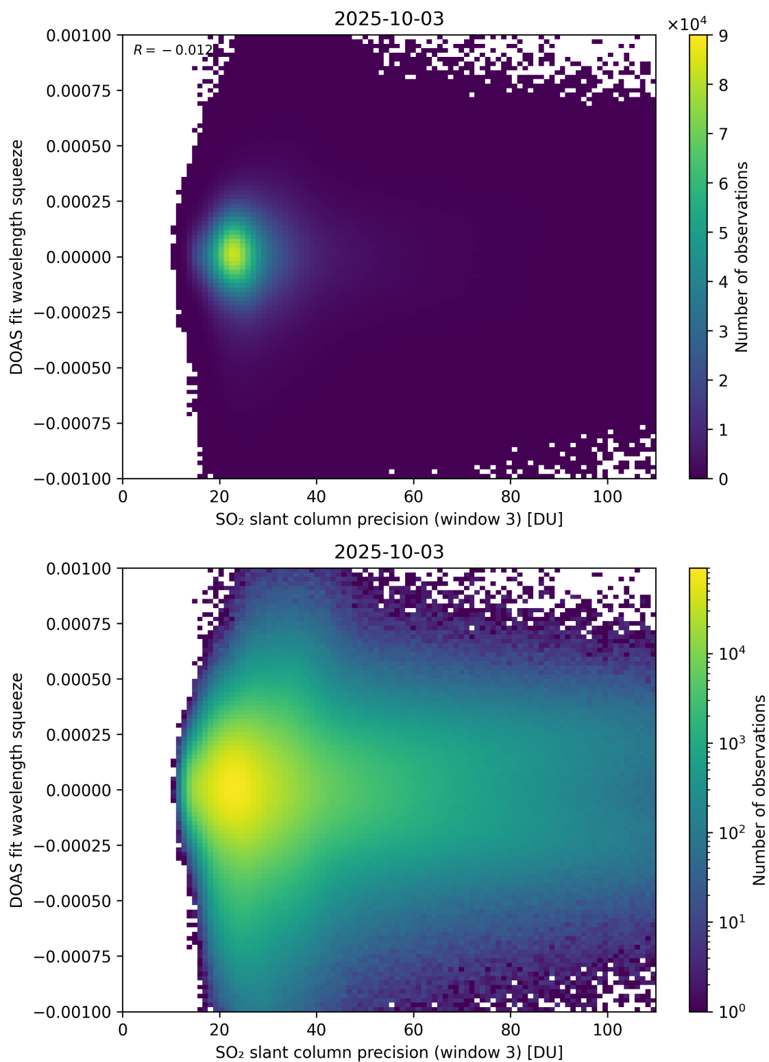
Figure 309: Scatter density plot of “SO 2 slant column precision (window 3)” against “DOAS fit wavelength squeeze” for 2025-10-02 to 2025-10-04.
