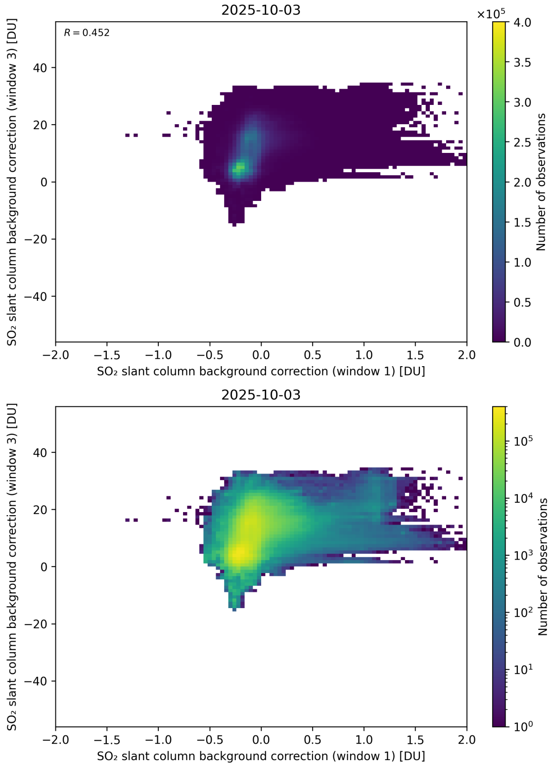
Figure 110: Scatter density plot of “SO 2 slant column background correction (window 1)” against “SO 2 slant column background correction (window 3)” for 2025-10-02 to 2025-10-04.
