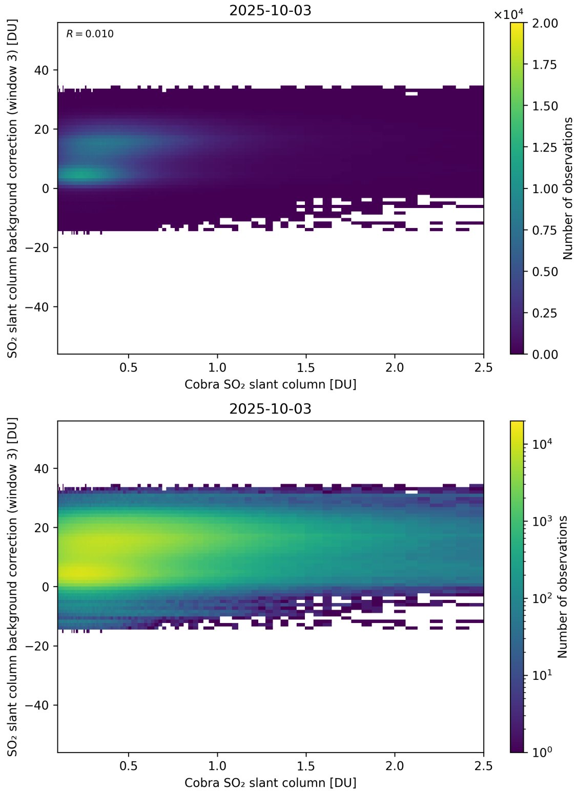
Figure 195: Scatter density plot of “Cobra SO 2 slant column” against “SO 2 slant column background correction (window 3)” for 2025-10-02 to 2025-10-04.
