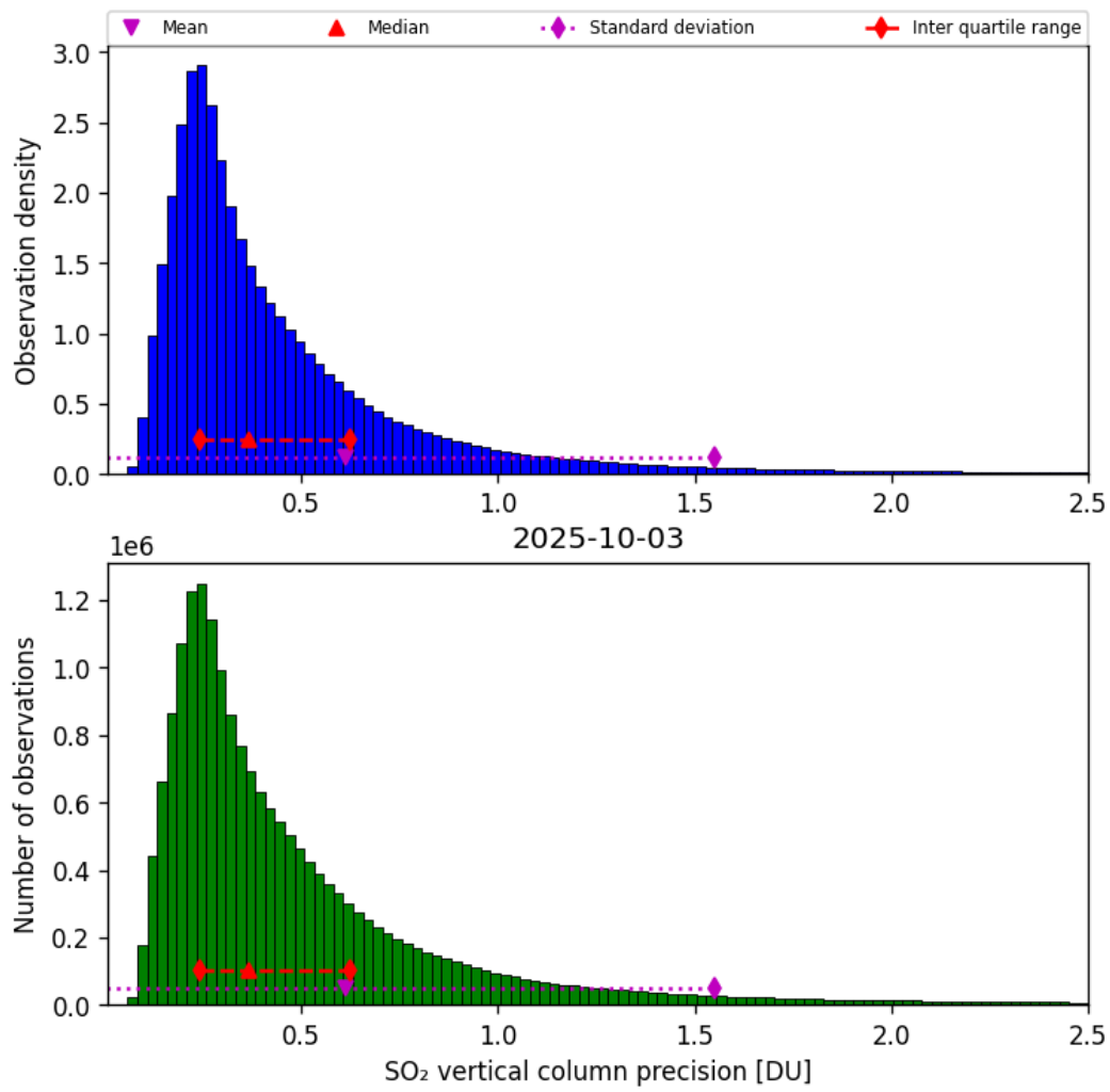
Figure 59: Histogram of “SO 2 vertical column precision” for 2025-10-02 to 2025-10-04
