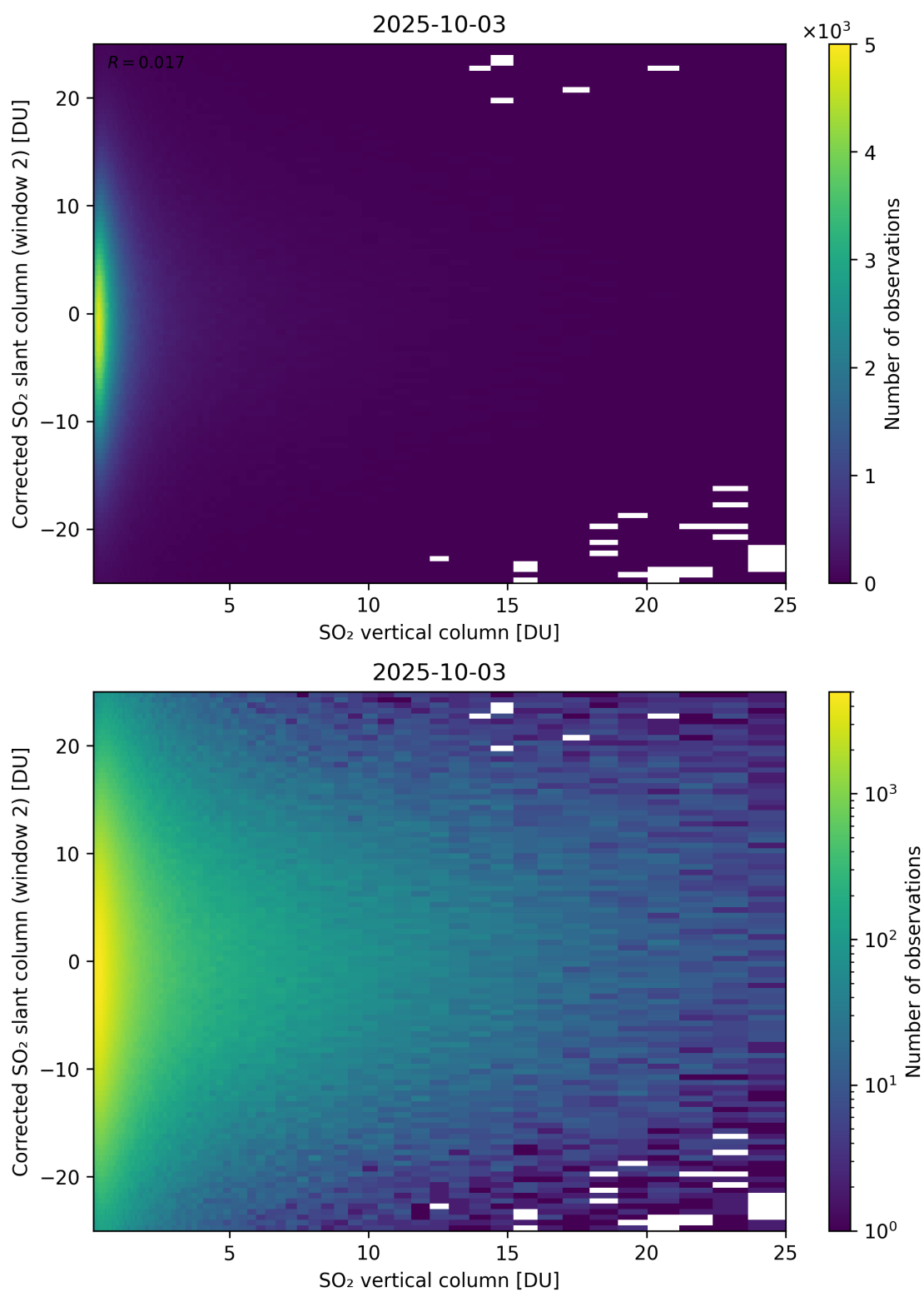
Figure 352: Scatter density plot of “SO 2 vertical column” against “Corrected SO 2 slant column (window 2)” for 2025-10-02 to 2025-10-04.
