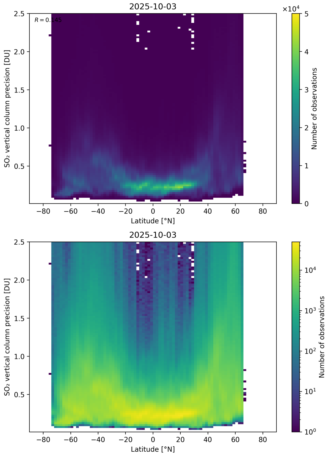
Figure 170: Scatter density plot of “Latitude” against “SO 2 vertical column precision” for 2025-10-02 to 2025-10-04.
