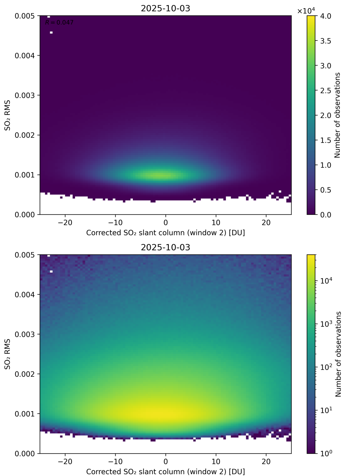
Figure 248: Scatter density plot of “Corrected SO 2 slant column (window 2)” against “SO 2 RMS” for 2025-10-02 to 2025-10-04.
