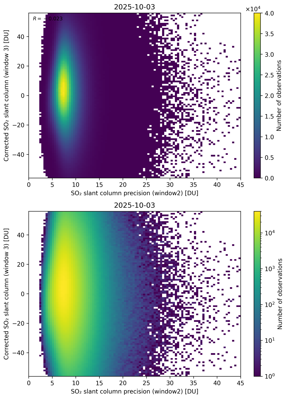
Figure 298: Scatter density plot of “SO 2 slant column precision (window2)” against “Corrected SO 2 slant column (window 3)” for 2025-10-02 to 2025-10-04.
