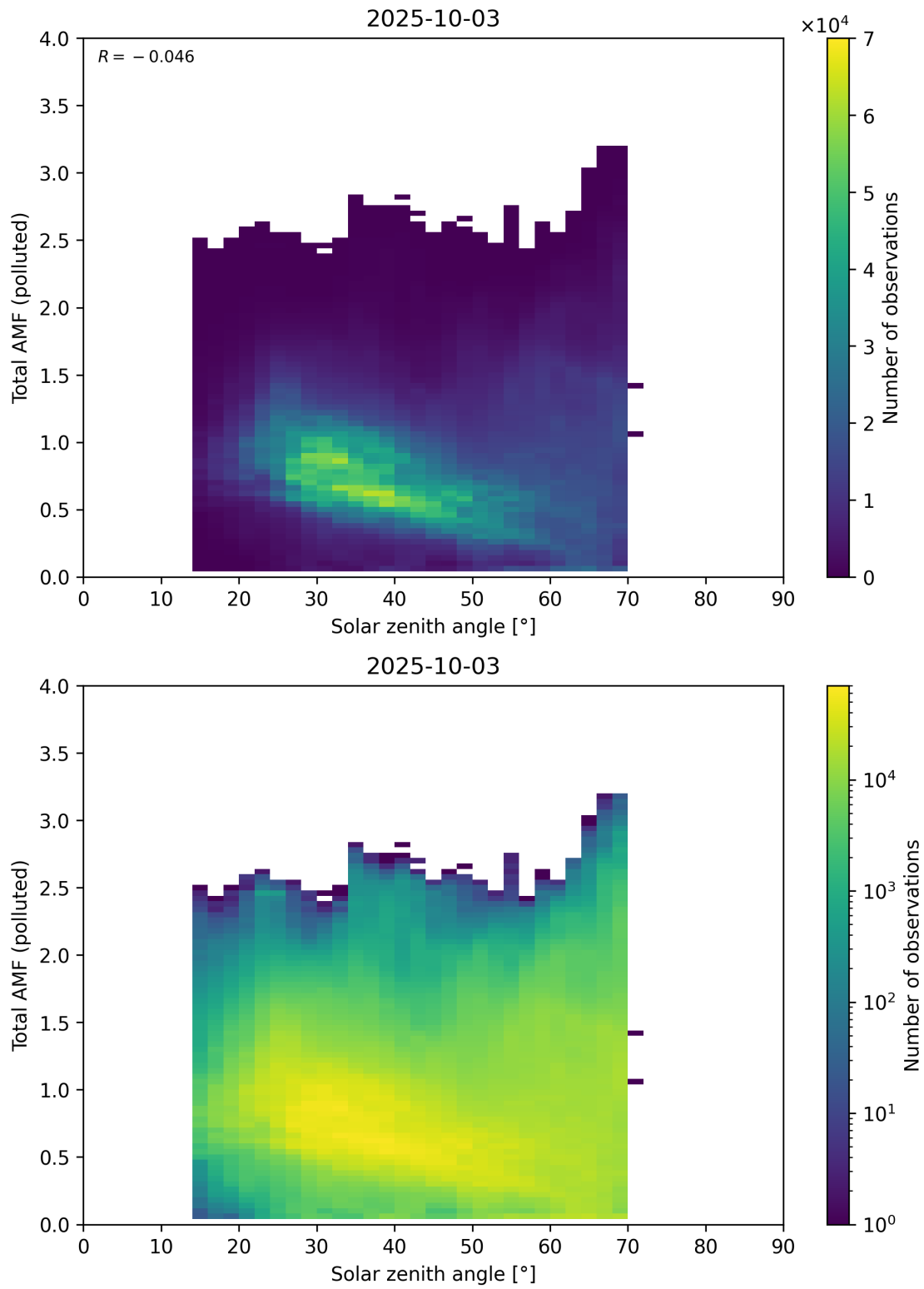
Figure 189: Scatter density plot of “Solar zenith angle” against “Total AMF (polluted)” for 2025-10-02 to 2025-10-04.
