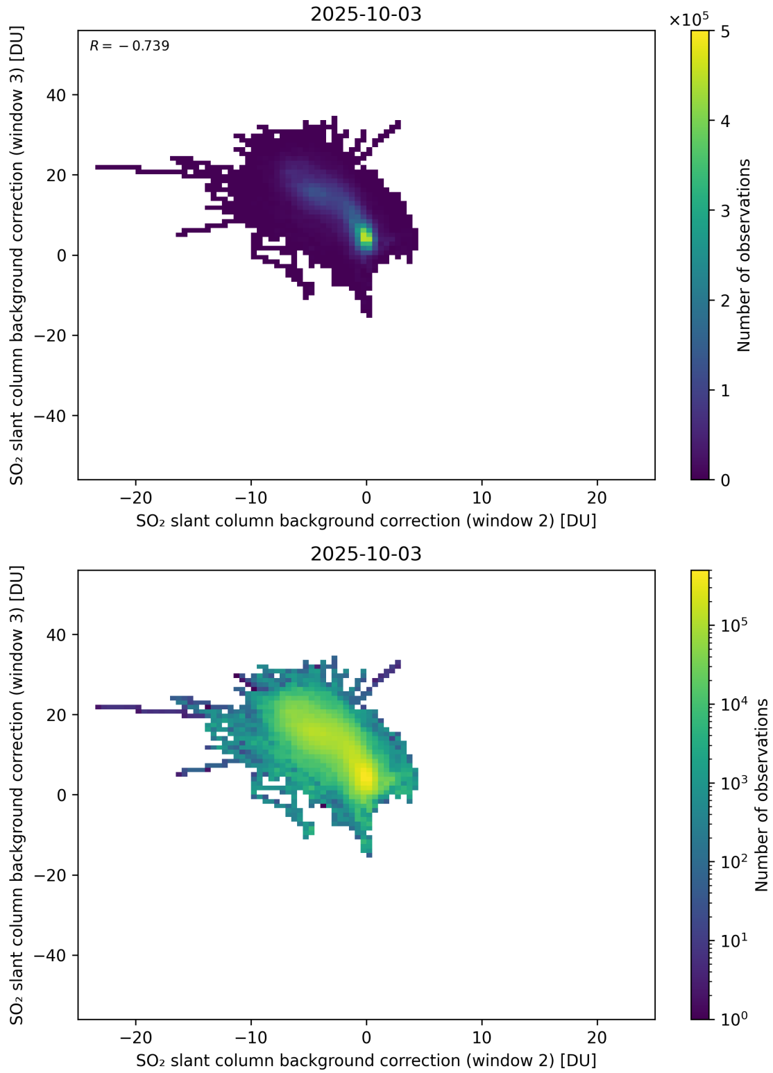
Figure 122: Scatter density plot of “SO 2 slant column background correction (window 2)” against “SO 2 slant column background correction (window 3)” for 2025-10-02 to 2025-10-04.
