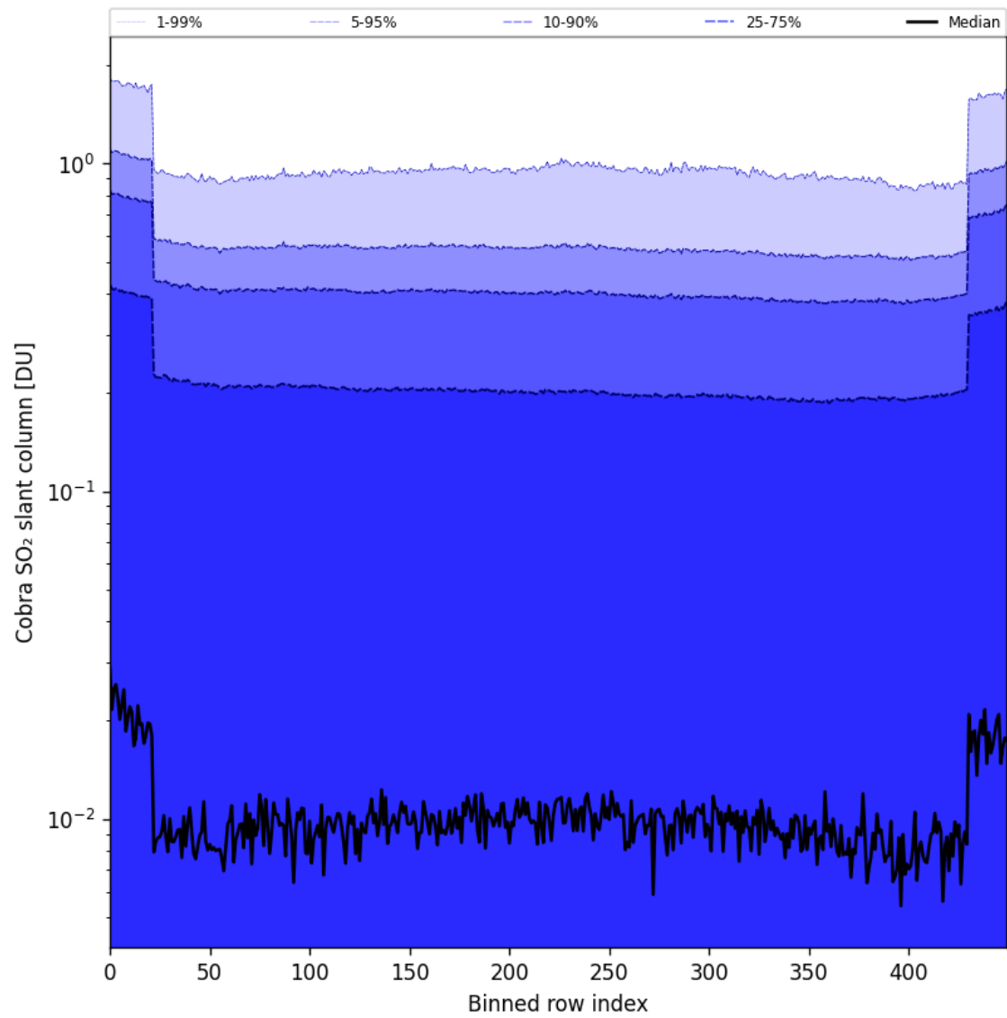
Figure 87: Along track statistics of "Cobra SO 2 slant column" for 2025-10-02 to 2025-10-04
