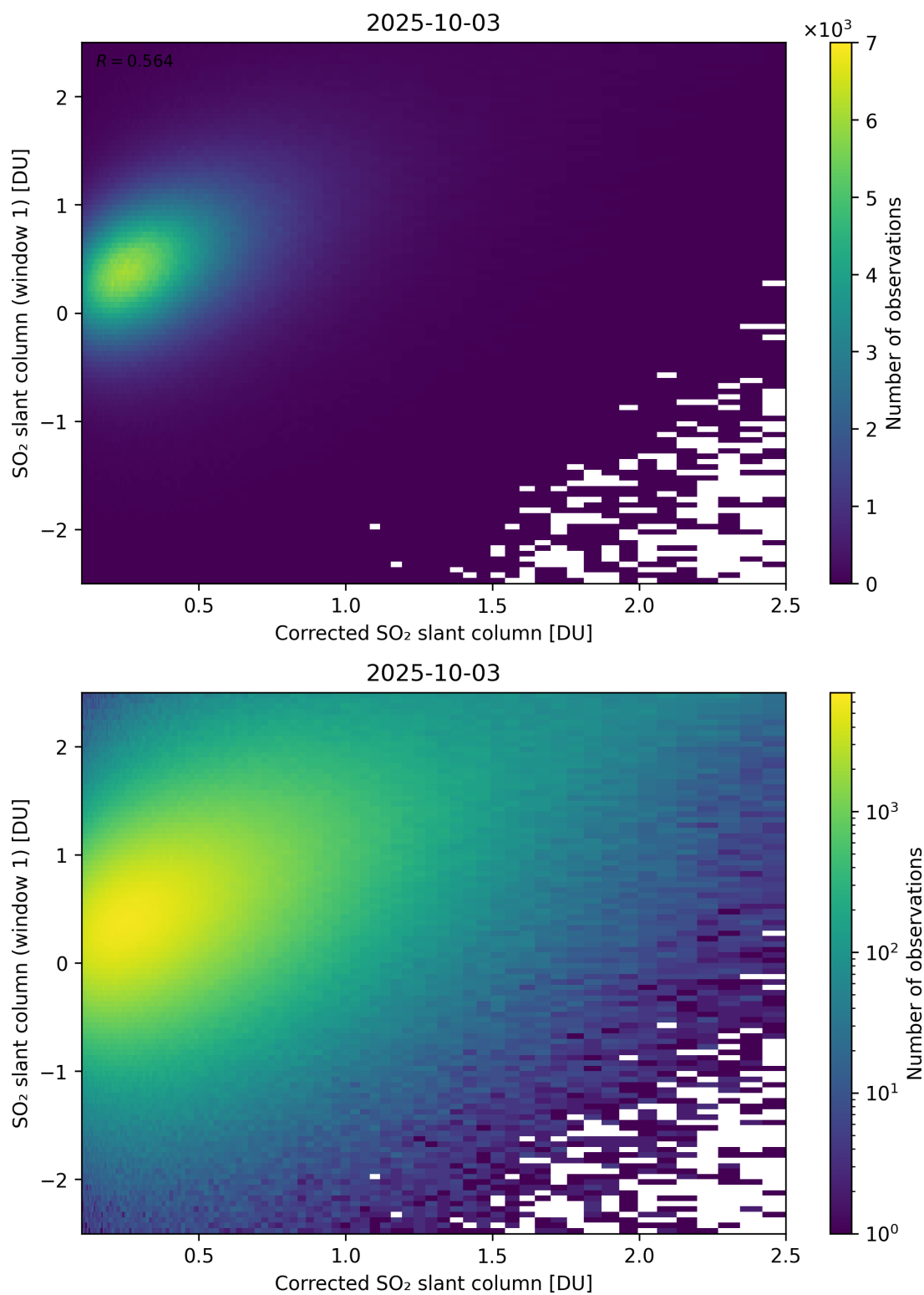
Figure 237: Scatter density plot of “Corrected SO 2 slant column” against “SO 2 slant column (window 1)” for 2025-10-02 to 2025-10-04.
