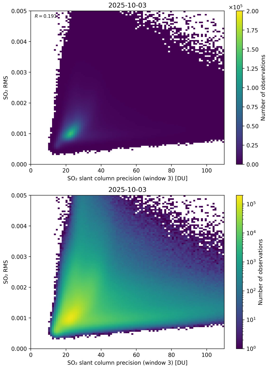
Figure 310: Scatter density plot of “SO 2 slant column precision (window 3)” against “SO 2 RMS” for 2025-10-02 to 2025-10-04.
