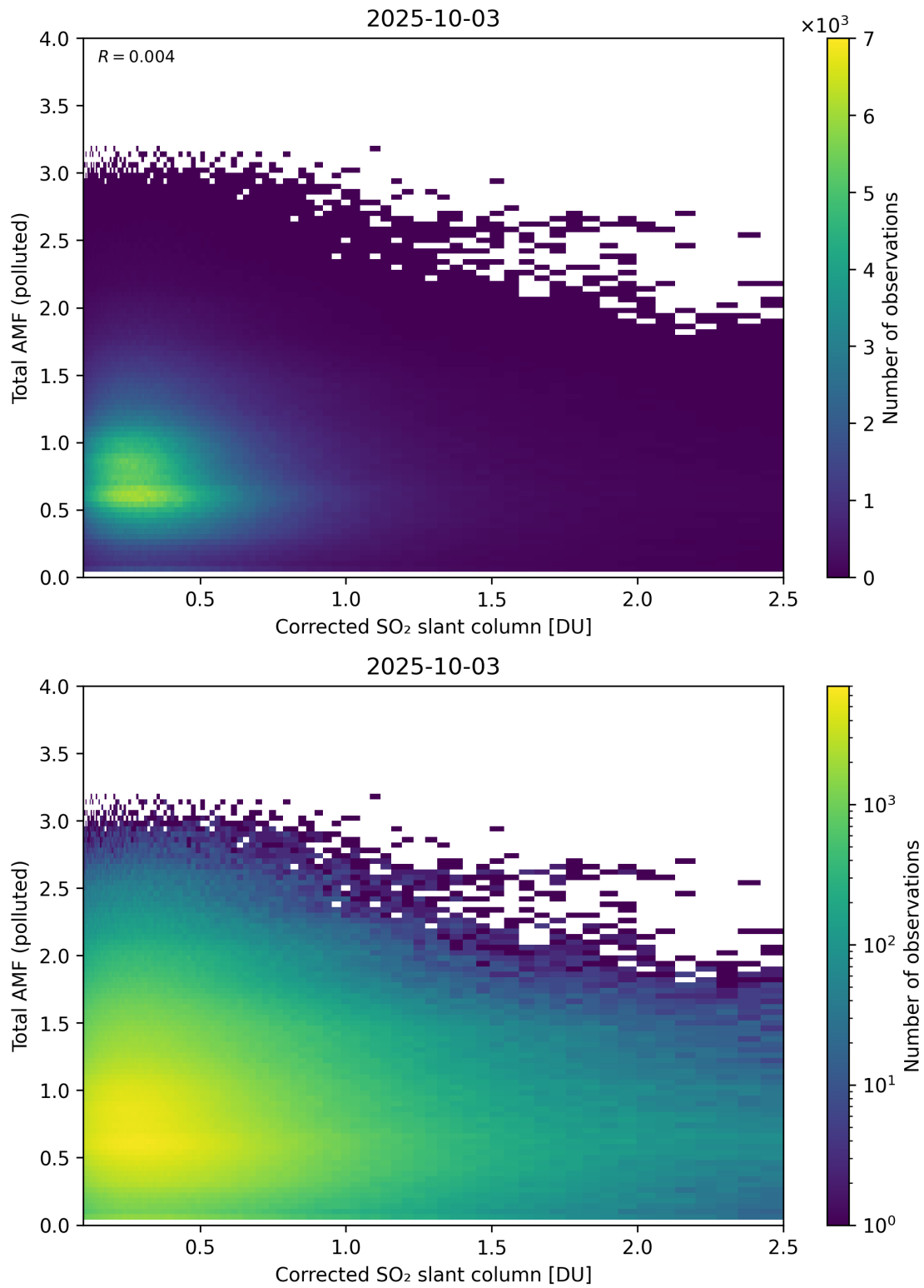
Figure 242: Scatter density plot of “Corrected SO 2 slant column” against “Total AMF (polluted)” for 2025-10-02 to 2025-10-04.
