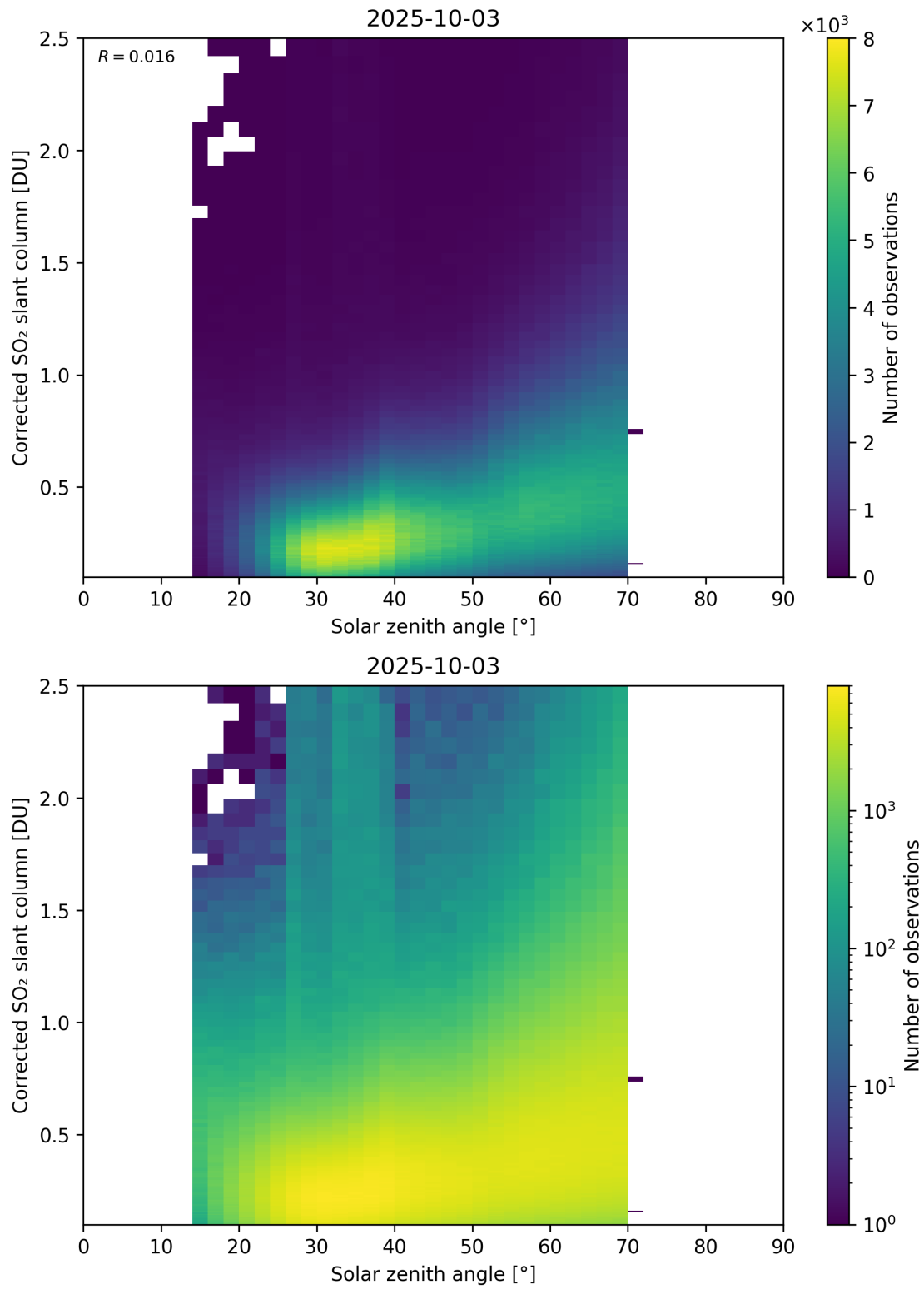
Figure 181: Scatter density plot of “Solar zenith angle” against “Corrected SO 2 slant column” for 2025-10-02 to 2025-10-04.
