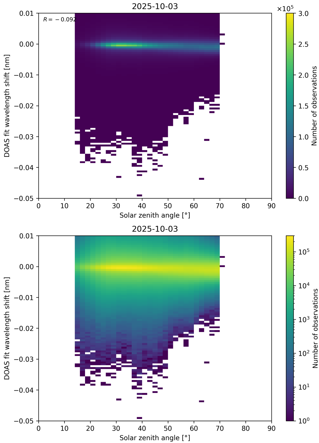
Figure 174: Scatter density plot of “Solar zenith angle” against “DOAS fit wavelength shift” for 2025-10-02 to 2025-10-04.
