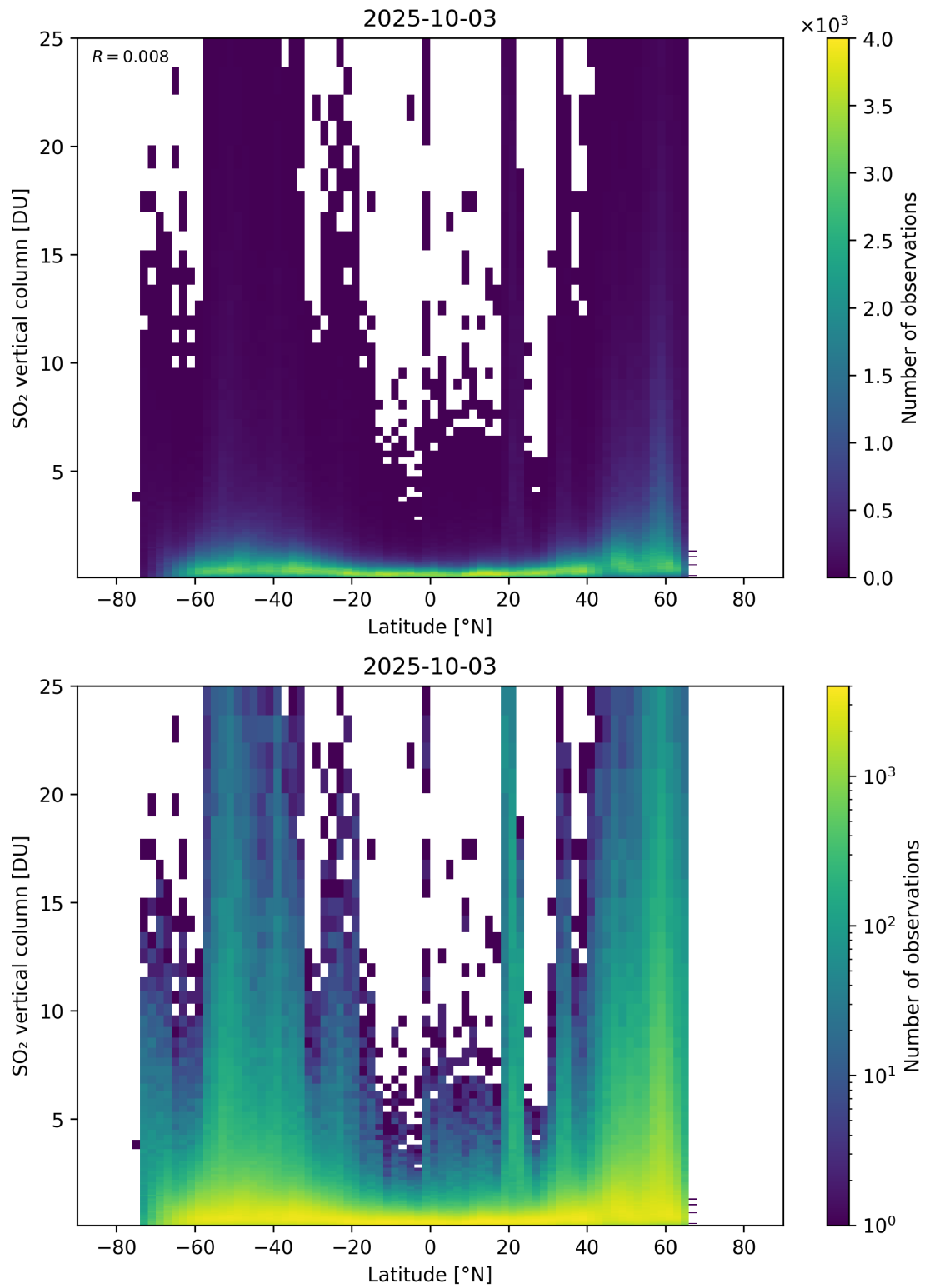
Figure 169: Scatter density plot of “Latitude” against “SO 2 vertical column” for 2025-10-02 to 2025-10-04.
