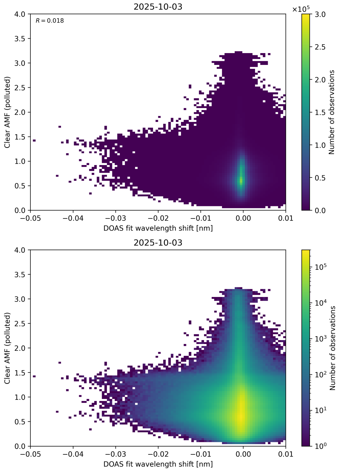
Figure 140: Scatter density plot of “DOAS fit wavelength shift” against “Clear AMF (polluted)” for 2025-10-02 to 2025-10-04.
