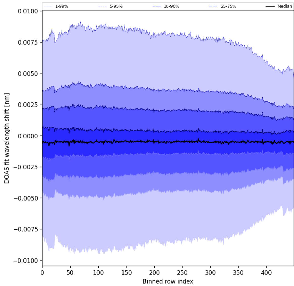
Figure 102: Along track statistics of “DOAS fit wavelength shift” for 2025-10-02 to 2025-10-04
