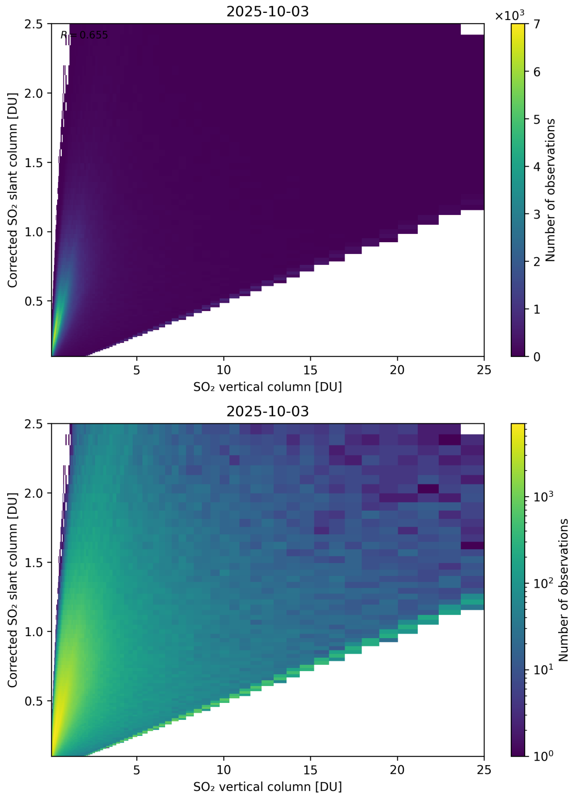
Figure 351: Scatter density plot of “SO 2 vertical column” against “Corrected SO 2 slant column” for 2025-10-02 to 2025-10-04.
