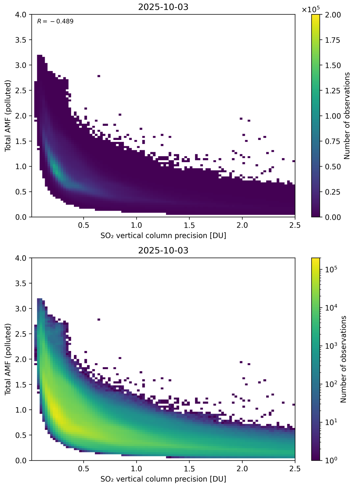
Figure 346: Scatter density plot of “SO 2 vertical column precision” against “Total AMF (polluted)” for 2025-10-02 to 2025-10-04.
