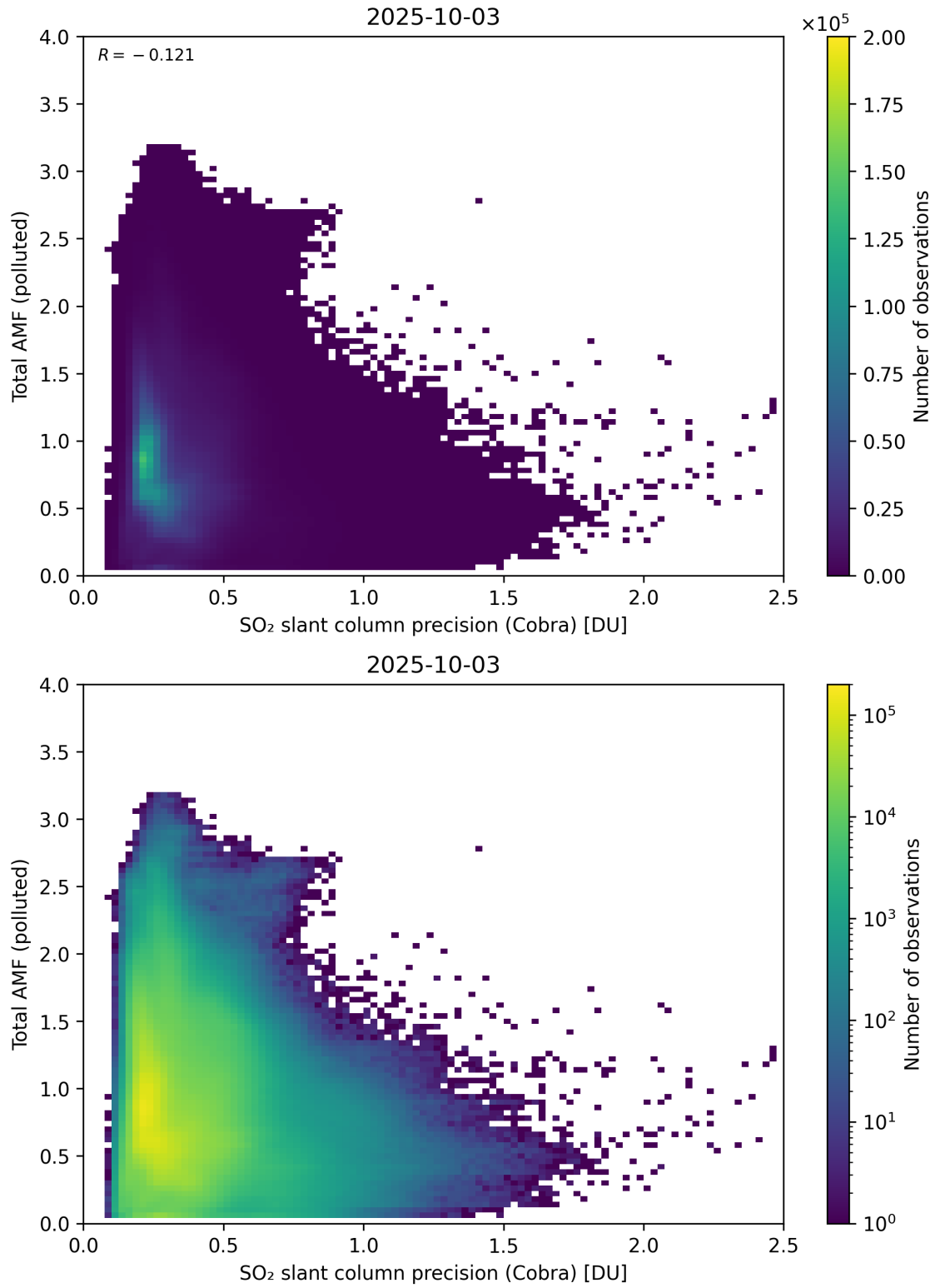
Figure 213: Scatter density plot of “SO 2 slant column precision (Cobra)” against “Total AMF (polluted)” for 2025-10-02 to 2025-10-04.
