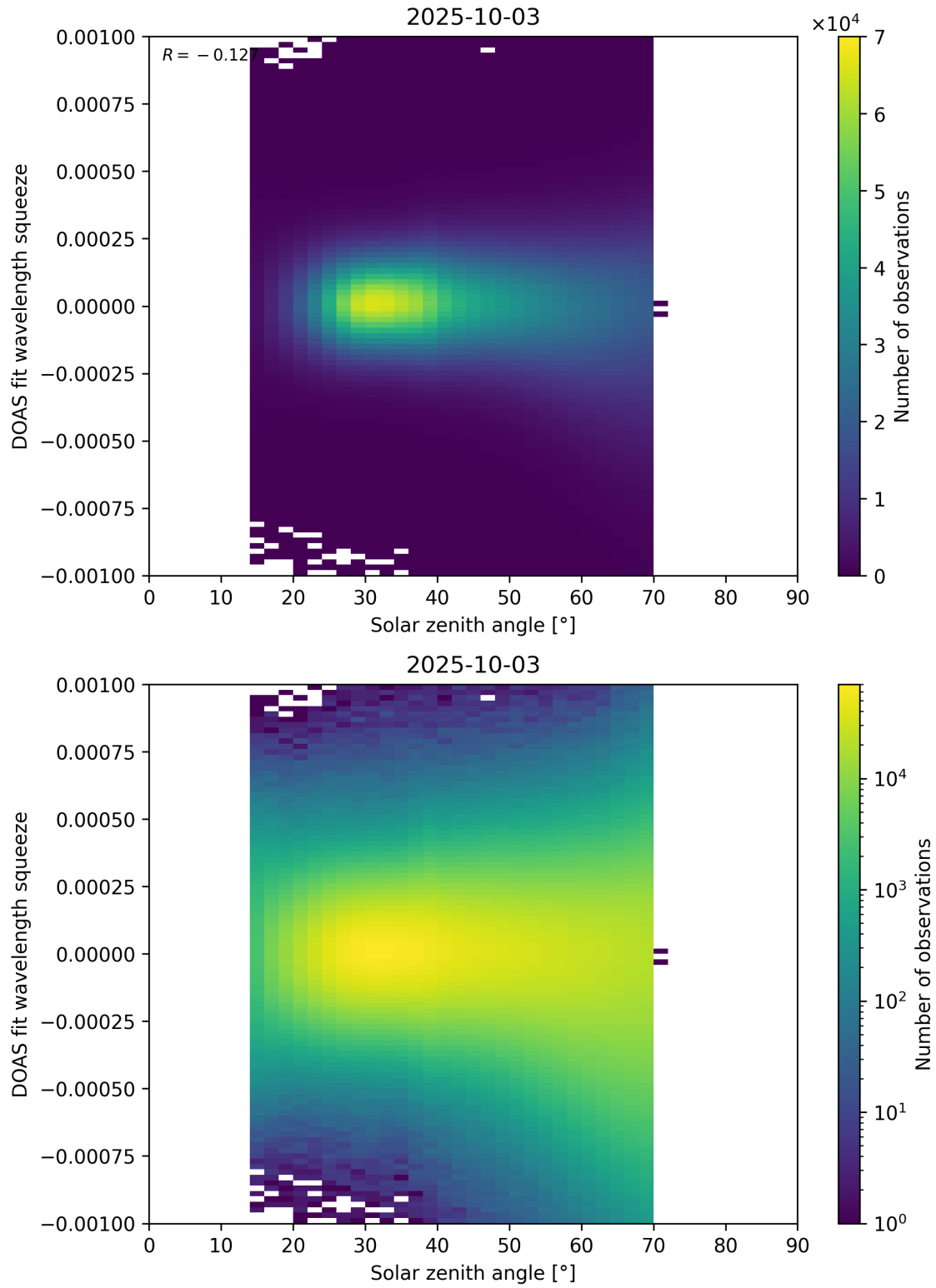
Figure 175: Scatter density plot of “Solar zenith angle” against “DOAS fit wavelength squeeze” for 2025-10-02 to 2025-10-04.
