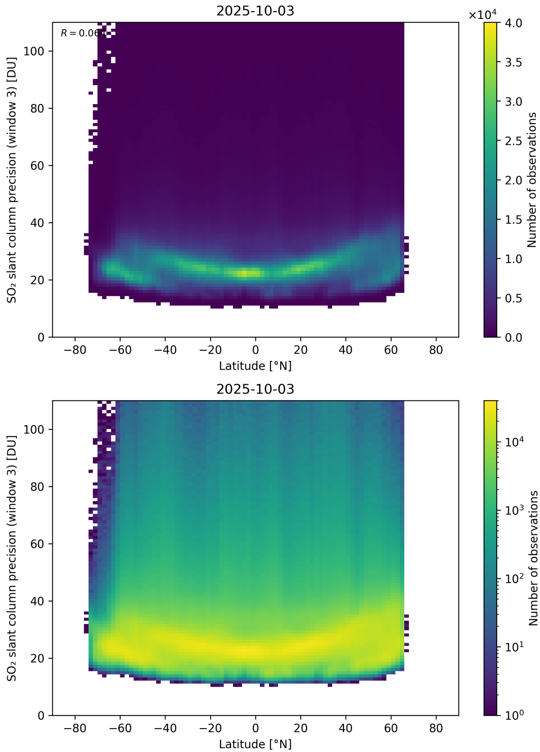
Figure 166: Scatter density plot of “Latitude” against “SO 2 slant column precision (window 3)” for 2025-10-02 to 2025-10-04.
