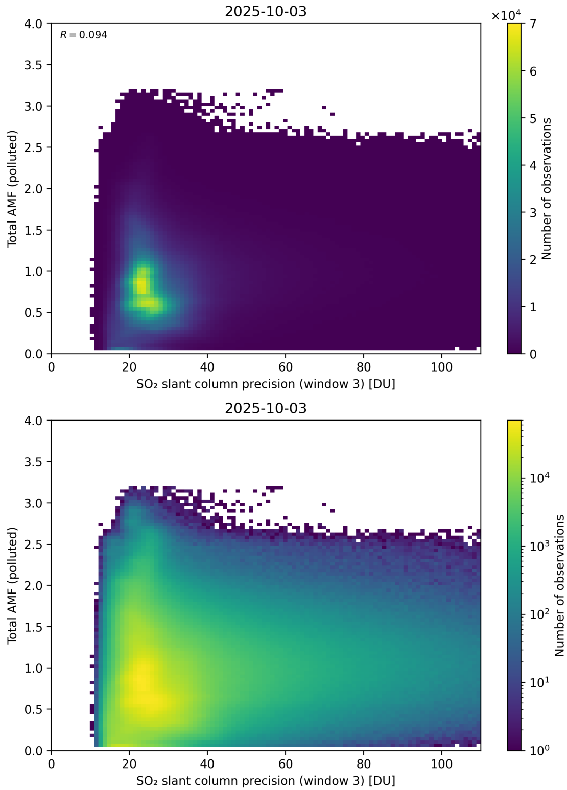
Figure 313: Scatter density plot of “SO 2 slant column precision (window 3)” against “Total AMF (polluted)” for 2025-10-02 to 2025-10-04.
