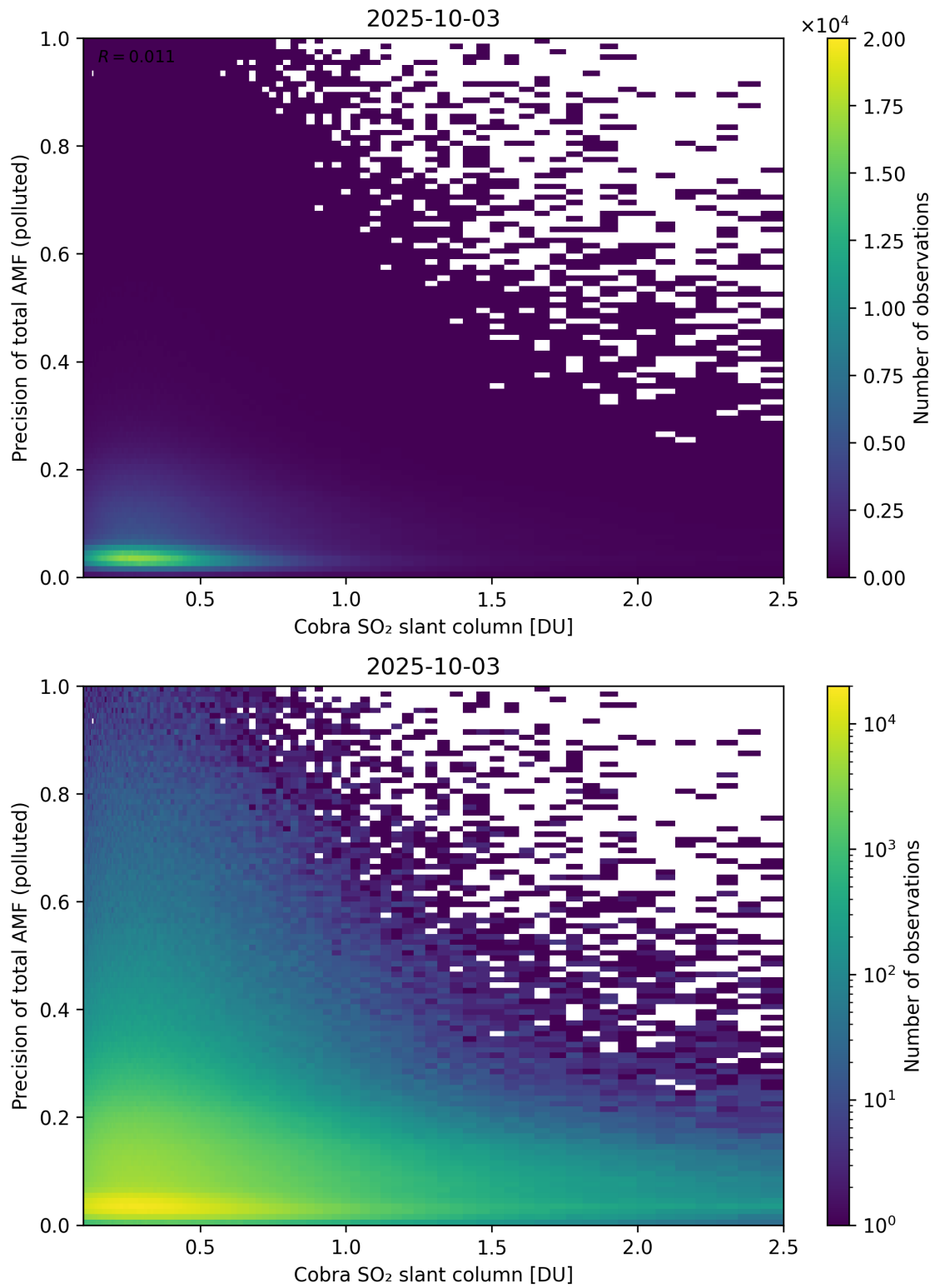
Figure 225: Scatter density plot of “Cobra SO 2 slant column” against “Precision of total AMF (polluted)” for 2025-10-02 to 2025-10-04.
