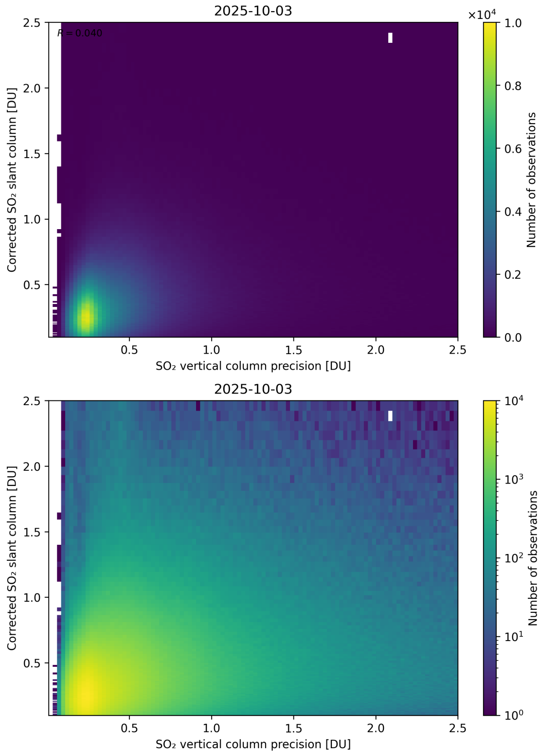
Figure 338: Scatter density plot of “SO 2 vertical column precision” against “Corrected SO 2 slant column” for 2025-10-02 to 2025-10-04.
