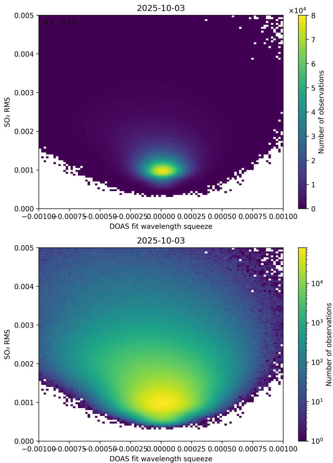
Figure 143: Scatter density plot of “DOAS fit wavelength squeeze” against “SO 2 RMS” for 2025-10-02 to 2025-10-04.
