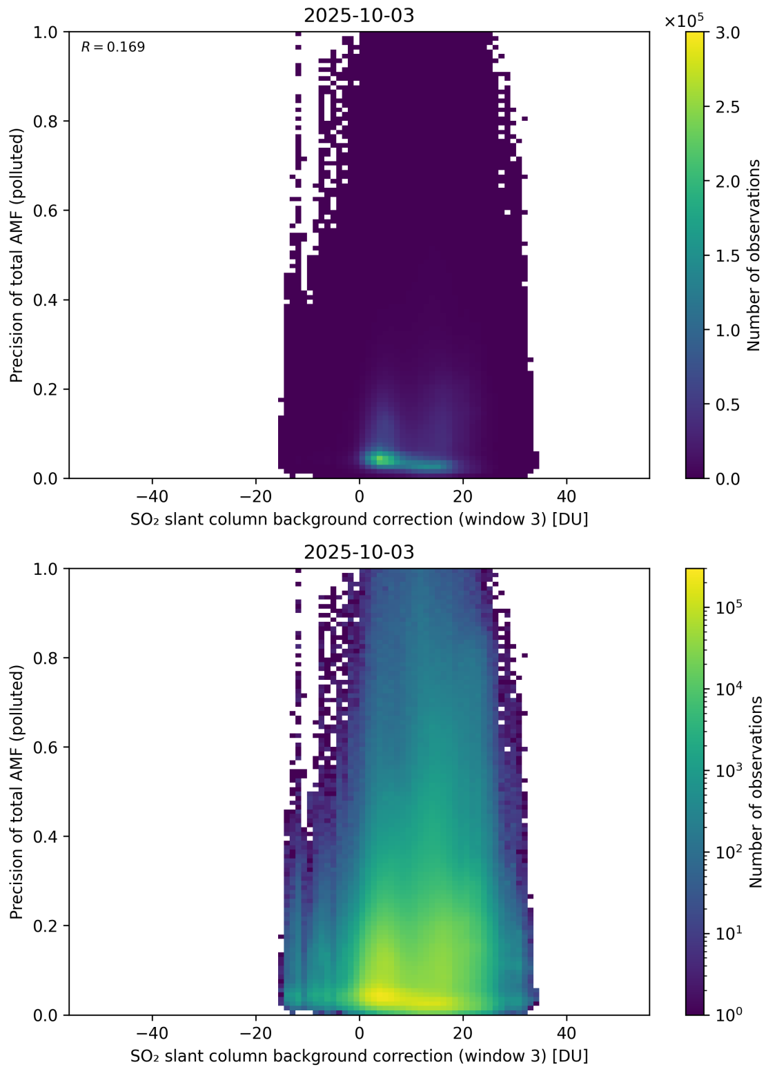
Figure 137: Scatter density plot of “SO 2 slant column background correction (window 3)” against “Precision of total AMF (polluted)” for 2025-10-02 to 2025-10-04.
