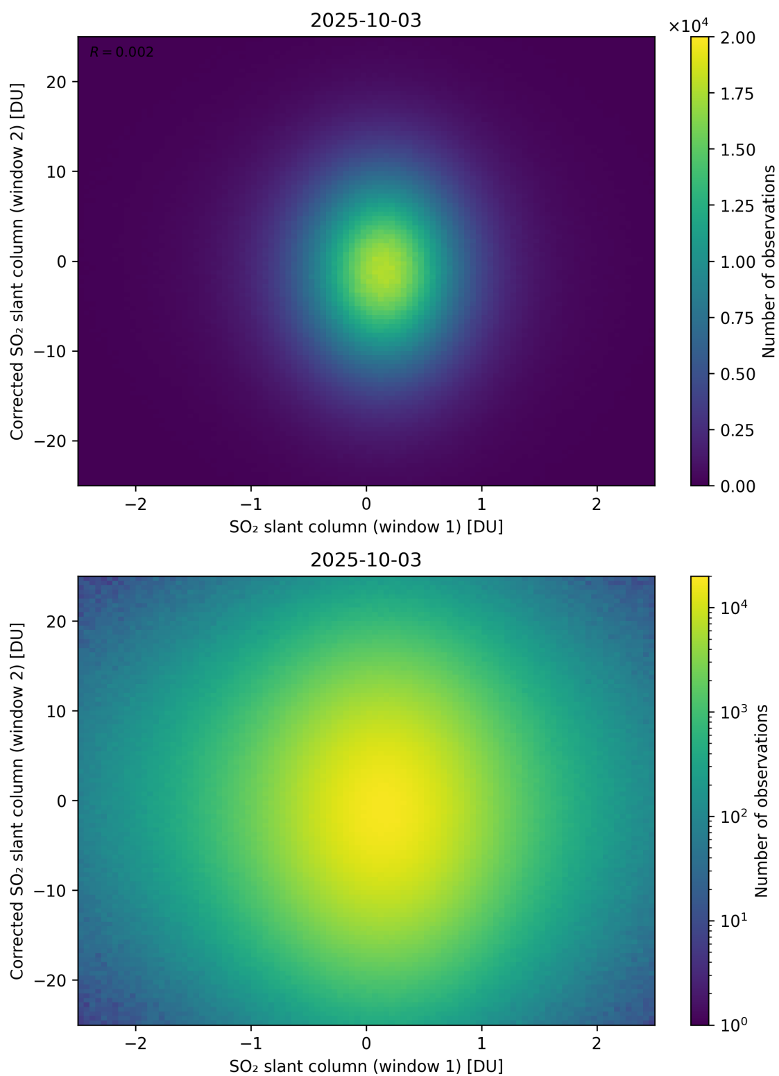
Figure 283: Scatter density plot of “SO 2 slant column (window 1)” against “Corrected SO 2 slant column (window 2)” for 2025-10-02 to 2025-10-04.
