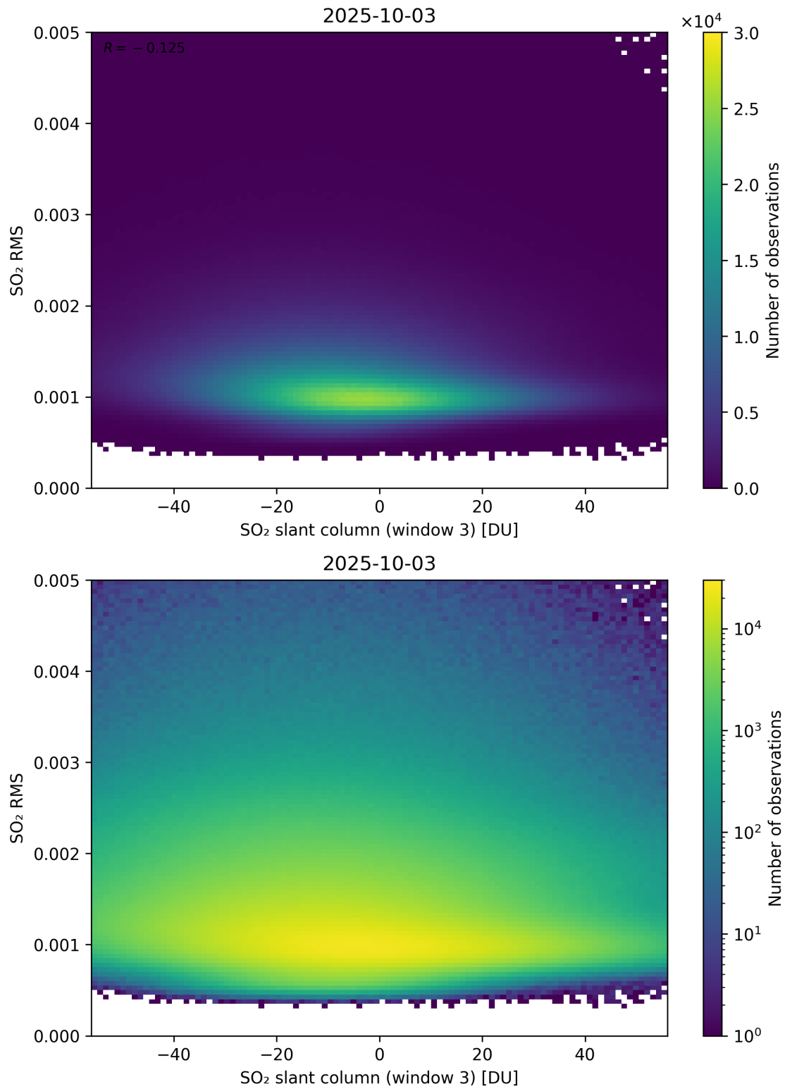
Figure 306: Scatter density plot of “SO 2 slant column (window 3)” against “SO 2 RMS” for 2025-10-02 to 2025-10-04.
