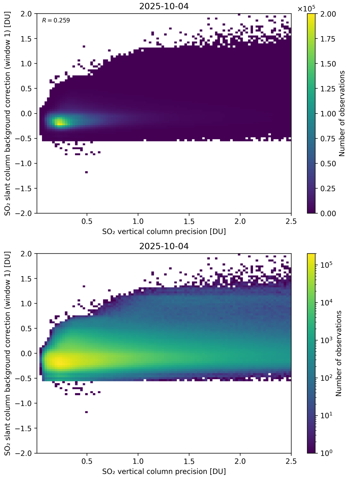
Figure 329: Scatter density plot of “SO 2 vertical column precision” against “SO 2 slant column background correction (window 1)” for 2025-10-03 to 2025-10-05.
