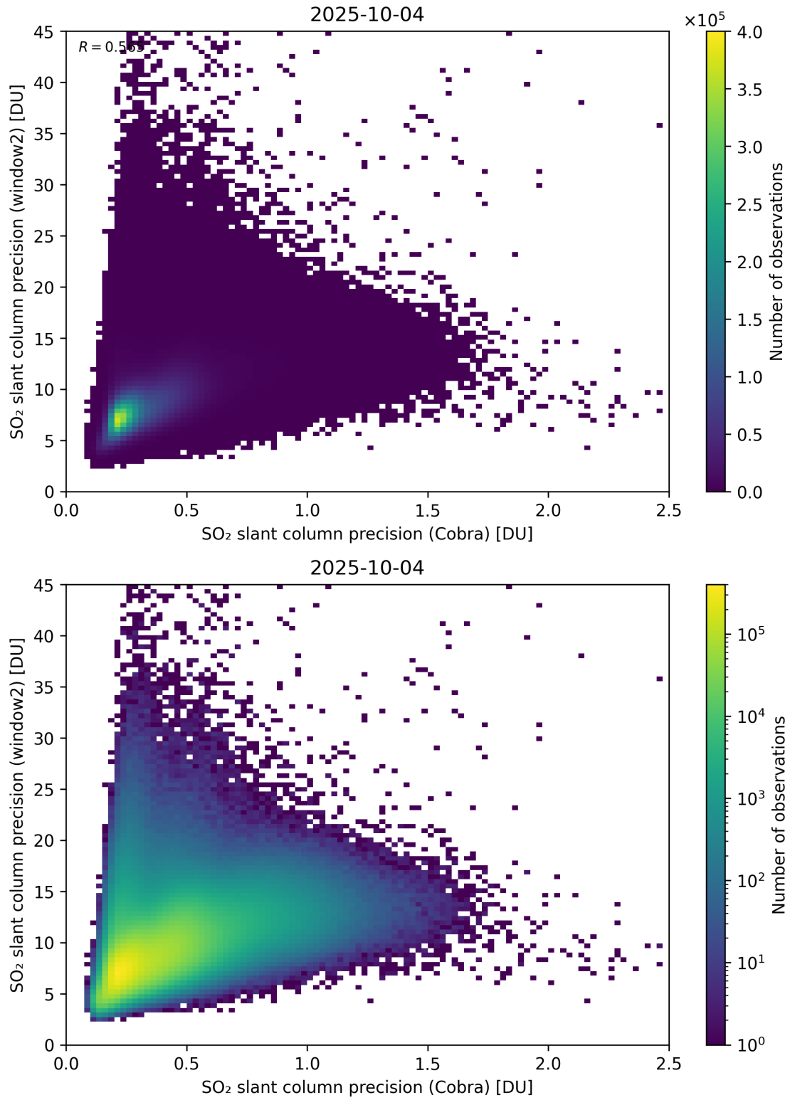
Figure 210: Scatter density plot of “SO 2 slant column precision (Cobra)” against “SO 2 slant column precision (window2)” for 2025-10-03 to 2025-10-05.
