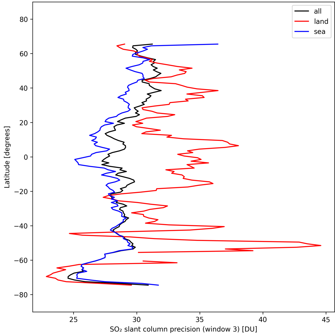
Figure 46: Zonal average of “SO 2 slant column precision (window 3)” for 2025-10-03 to 2025-10-05.
