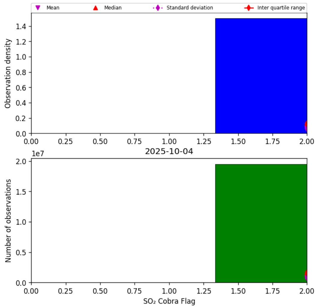
Figure 75: Histogram of “SO 2 Cobra Flag” for 2025-10-03 to 2025-10-05
