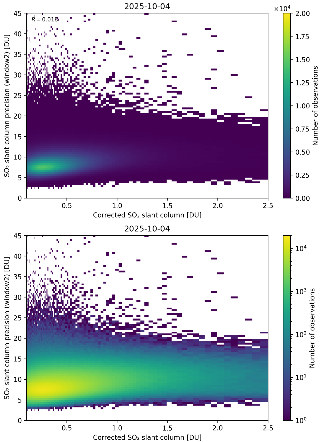
Figure 239: Scatter density plot of “Corrected SO 2 slant column” against “SO 2 slant column precision (window2)” for 2025-10-03 to 2025-10-05.
