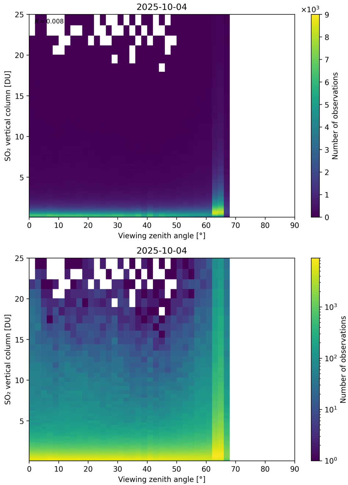
Figure 383: Scatter density plot of “Viewing zenith angle” against “SO 2 vertical column” for 2025-10-03 to 2025-10-05.
