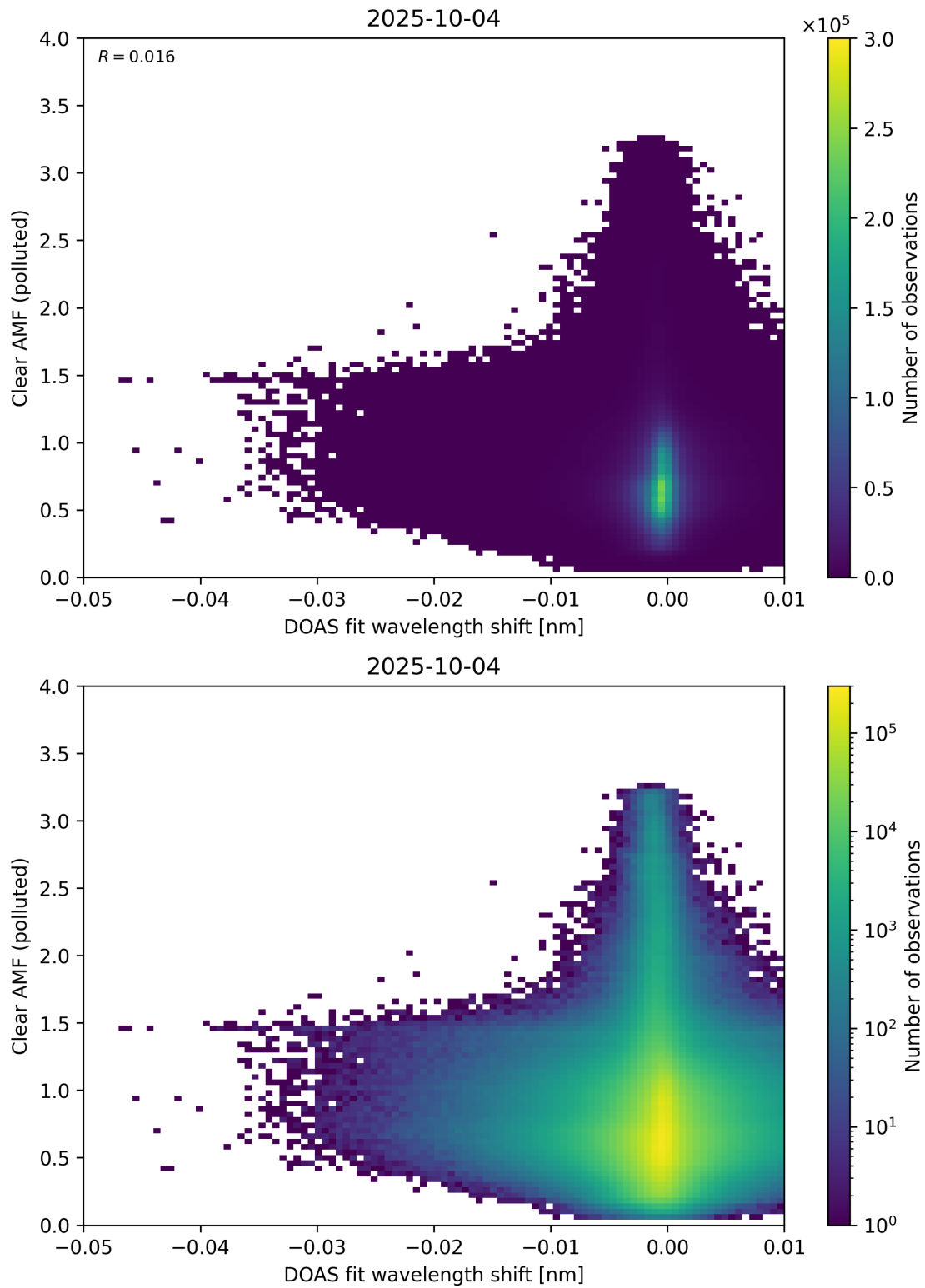
Figure 140: Scatter density plot of “DOAS fit wavelength shift” against “Clear AMF (polluted)” for 2025-10-03 to 2025-10-05.
