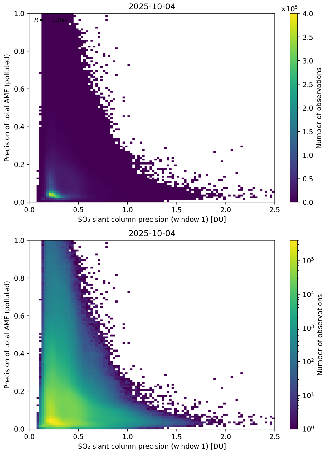
Figure 281: Scatter density plot of “SO 2 slant column precision (window 1)” against “Precision of total AMF (polluted)” for 2025-10-03 to 2025-10-05.
