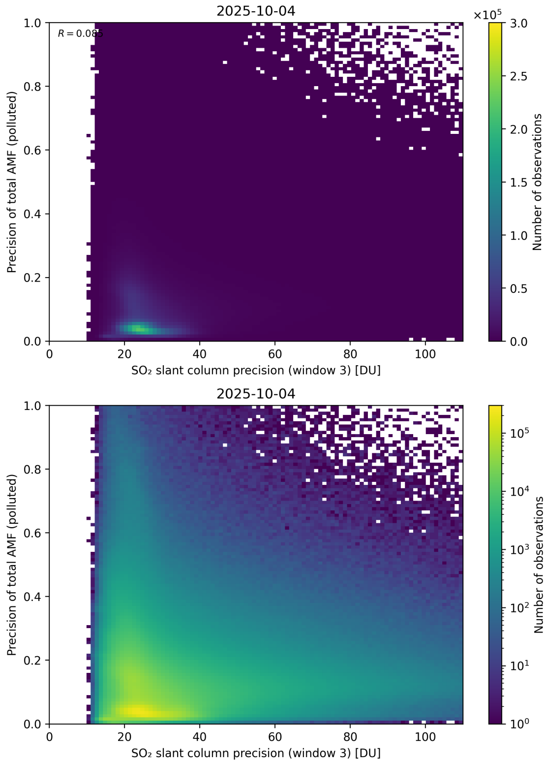
Figure 314: Scatter density plot of “SO 2 slant column precision (window 3)” against “Precision of total AMF (polluted)” for 2025-10-03 to 2025-10-05.
