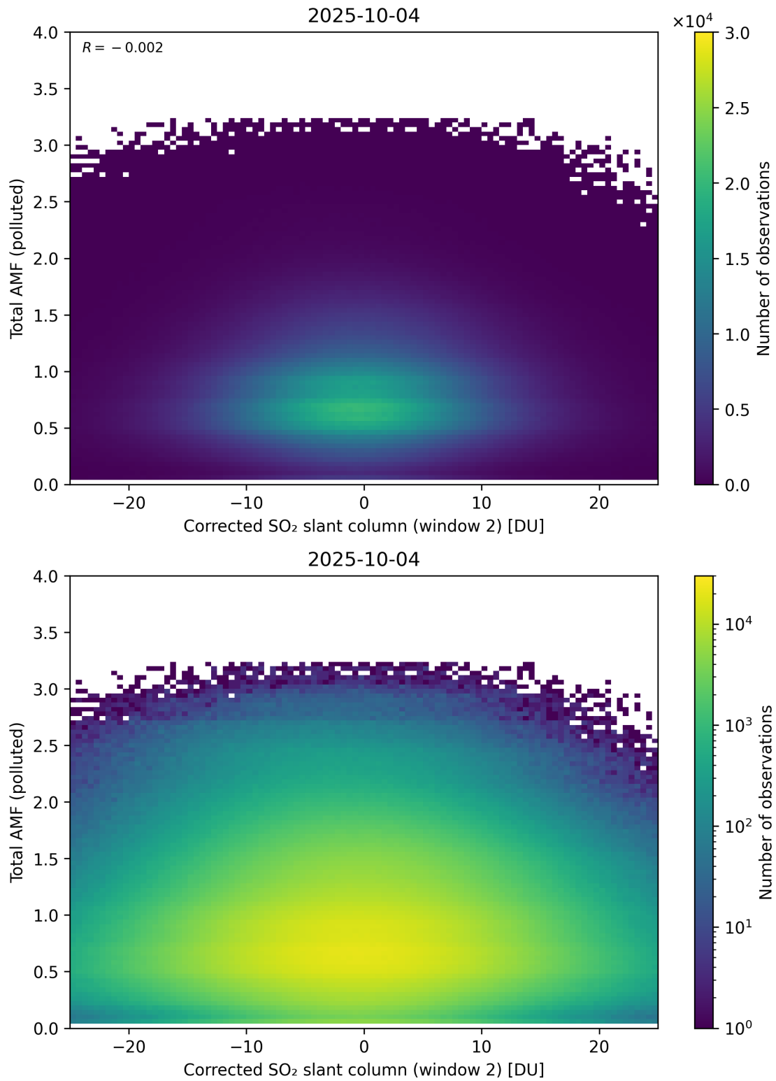
Figure 253: Scatter density plot of “Corrected SO 2 slant column (window 2)” against “Total AMF (polluted)” for 2025-10-03 to 2025-10-05.
