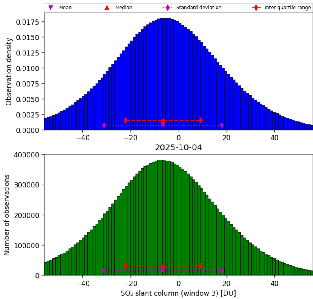
Figure 71: Histogram of “SO 2 slant column (window 3)” for 2025-10-03 to 2025-10-05
