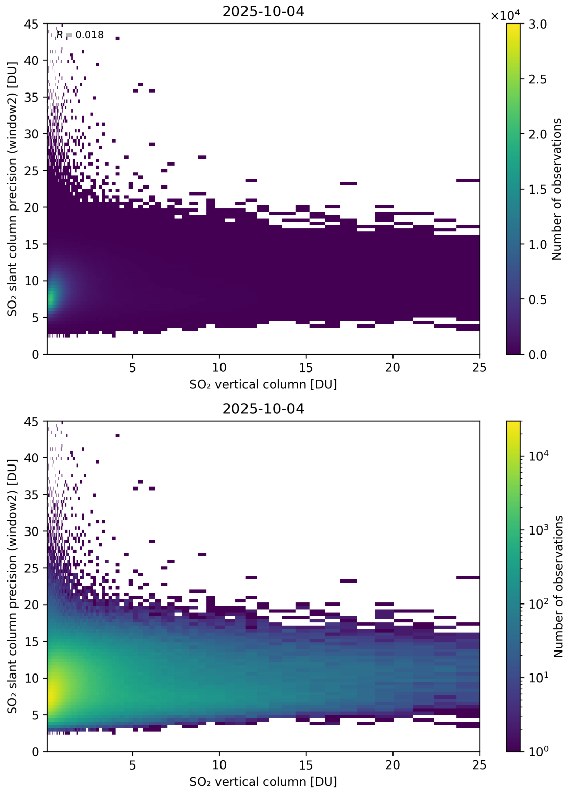
Figure 356: Scatter density plot of “SO 2 vertical column” against “SO 2 slant column precision (window2)” for 2025-10-03 to 2025-10-05.
