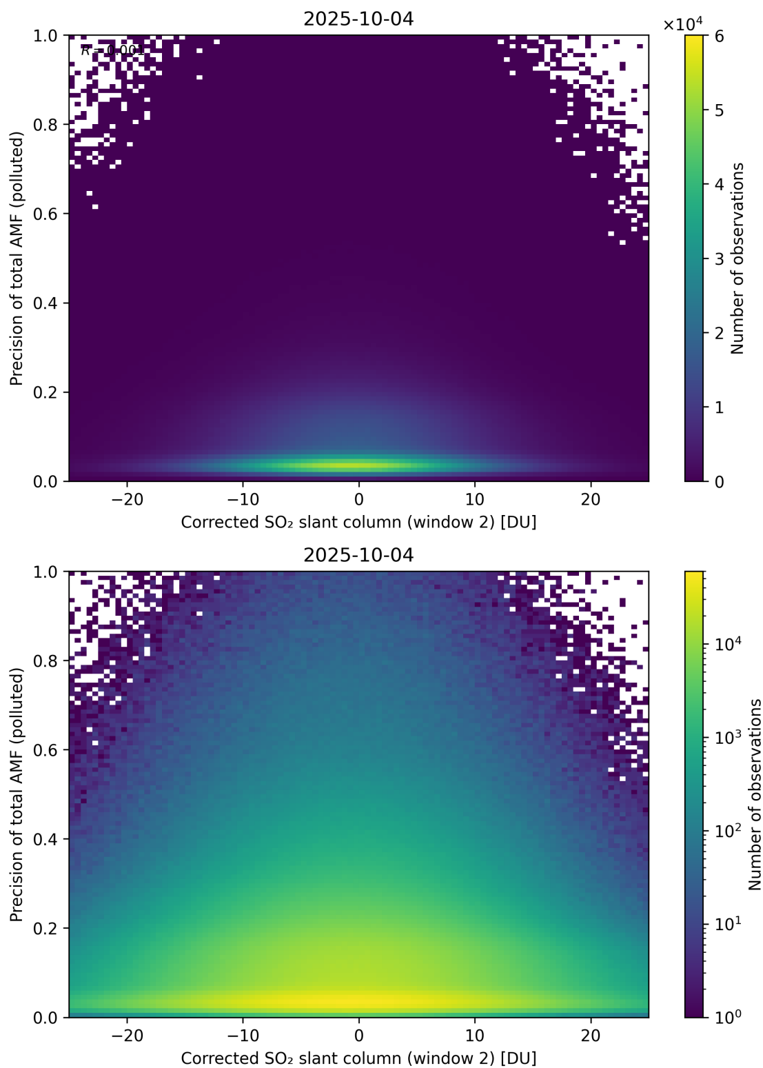
Figure 254: Scatter density plot of “Corrected SO 2 slant column (window 2)” against “Precision of total AMF (polluted)” for 2025-10-03 to 2025-10-05.
