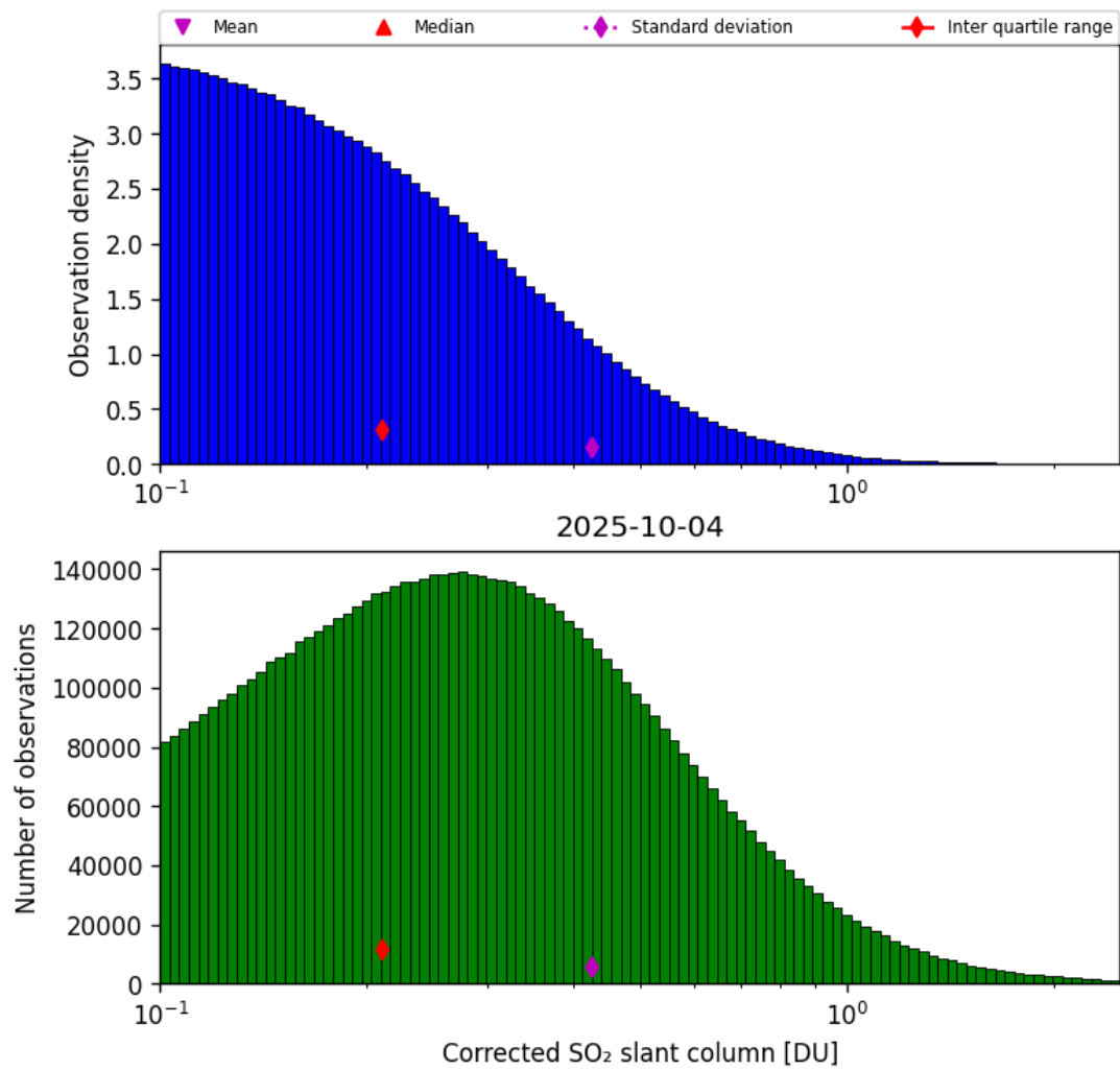
Figure 60: Histogram of "Corrected SO 2 slant column" for 2025-10-03 to 2025-10-05
