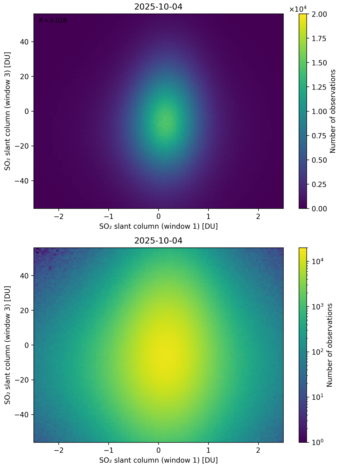
Figure 287: Scatter density plot of “SO 2 slant column (window 1)” against “SO 2 slant column (window 3)” for 2025-10-03 to 2025-10-05.
