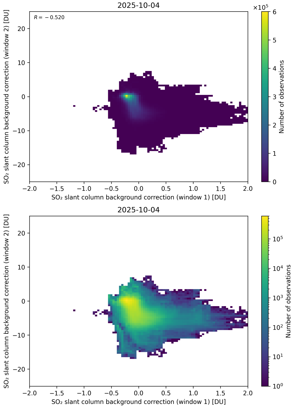
Figure 109: Scatter density plot of “SO 2 slant column background correction (window 1)” against “SO 2 slant column background correction (window 2)” for 2025-10-03 to 2025-10-05.
