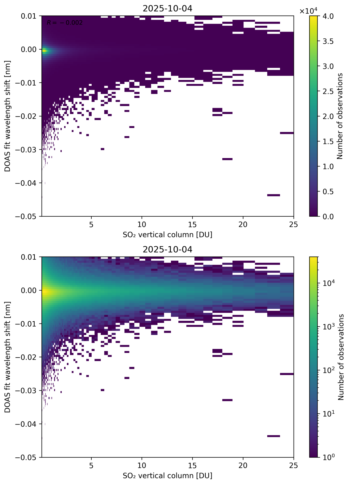
Figure 326: Scatter density plot of “SO 2 vertical column” against “DOAS fit wavelength shift” for 2025-10-03 to 2025-10-05.
