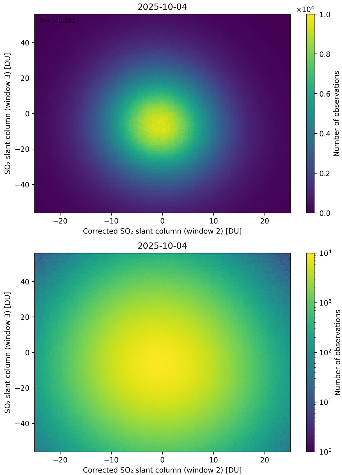
Figure 251: Scatter density plot of “Corrected SO 2 slant column (window 2)” against “SO 2 slant column (window 3)” for 2025-10-03 to 2025-10-05.
