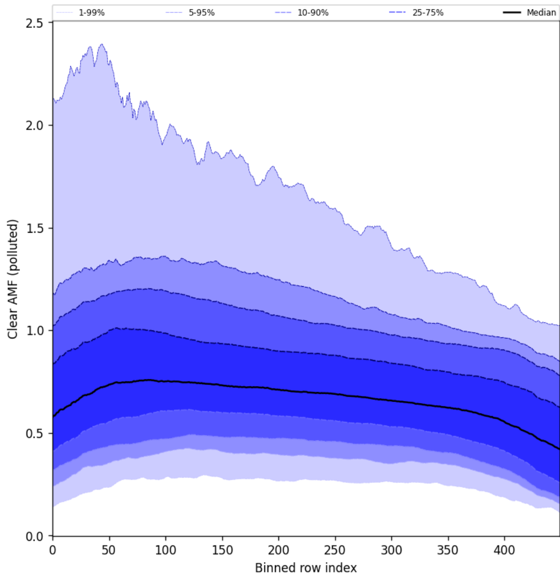
Figure 107: Along track statistics of “Clear AMF (polluted)” for 2025-10-03 to 2025-10-05
