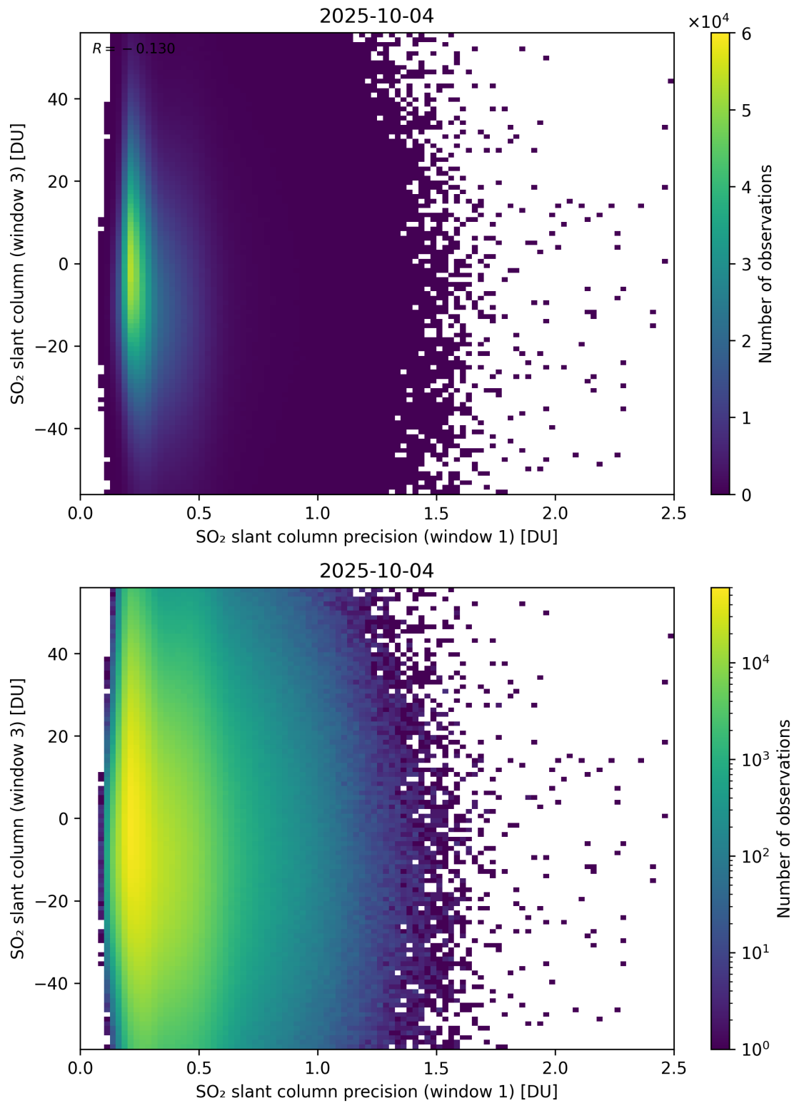
Figure 278: Scatter density plot of “SO 2 slant column precision (window 1)” against “SO 2 slant column (window 3)” for 2025-10-03 to 2025-10-05.
