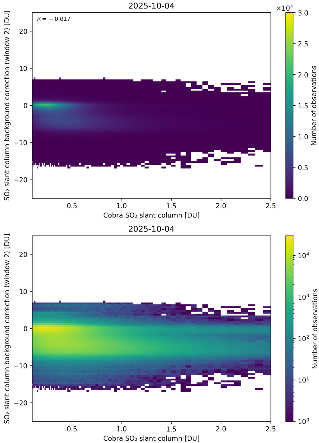
Figure 194: Scatter density plot of “Cobra SO 2 slant column” against “SO 2 slant column background correction (window 2)” for 2025-10-03 to 2025-10-05.
