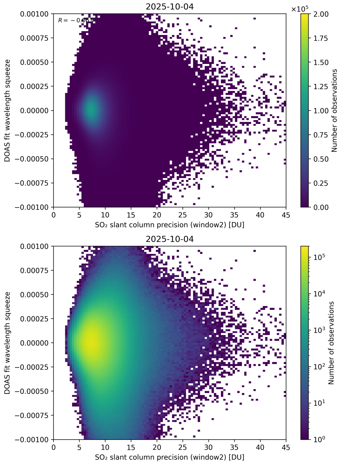
Figure 294: Scatter density plot of “SO 2 slant column precision (window2)” against “DOAS fit wavelength squeeze” for 2025-10-03 to 2025-10-05.
