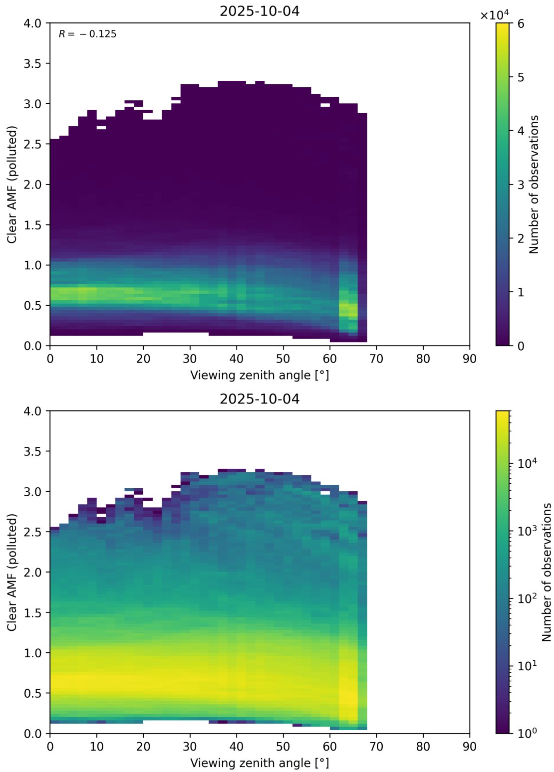
Figure 370: Scatter density plot of “Viewing zenith angle” against “Clear AMF (polluted)” for 2025-10-03 to 2025-10-05.
