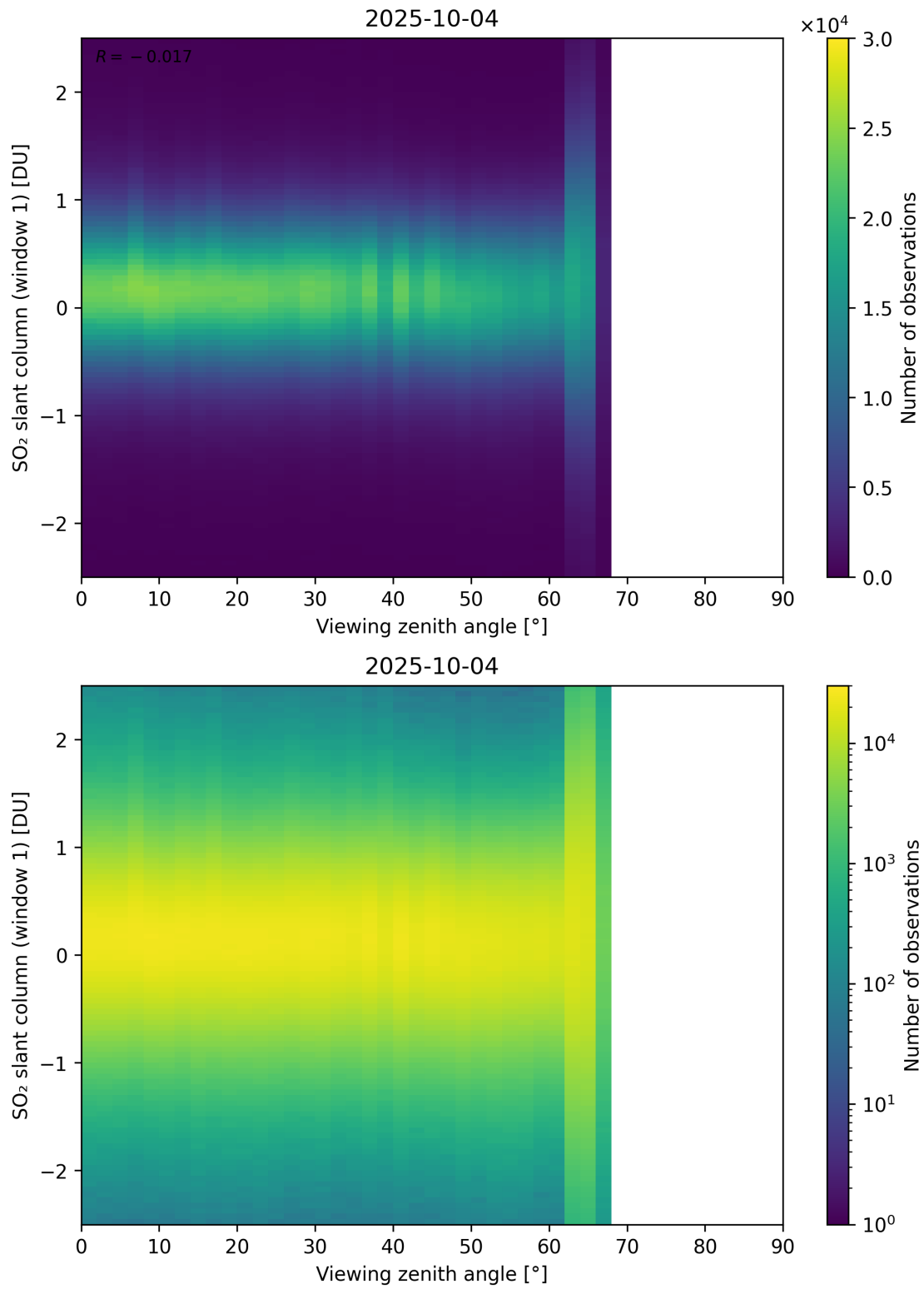
Figure 376: Scatter density plot of “Viewing zenith angle” against “SO 2 slant column (window 1)” for 2025-10-03 to 2025-10-05.
