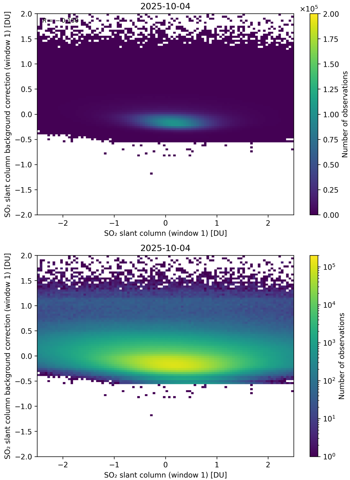
Figure 262: Scatter density plot of “SO 2 slant column (window 1)” against “SO 2 slant column background correction (window 1)” for 2025-10-03 to 2025-10-05.
