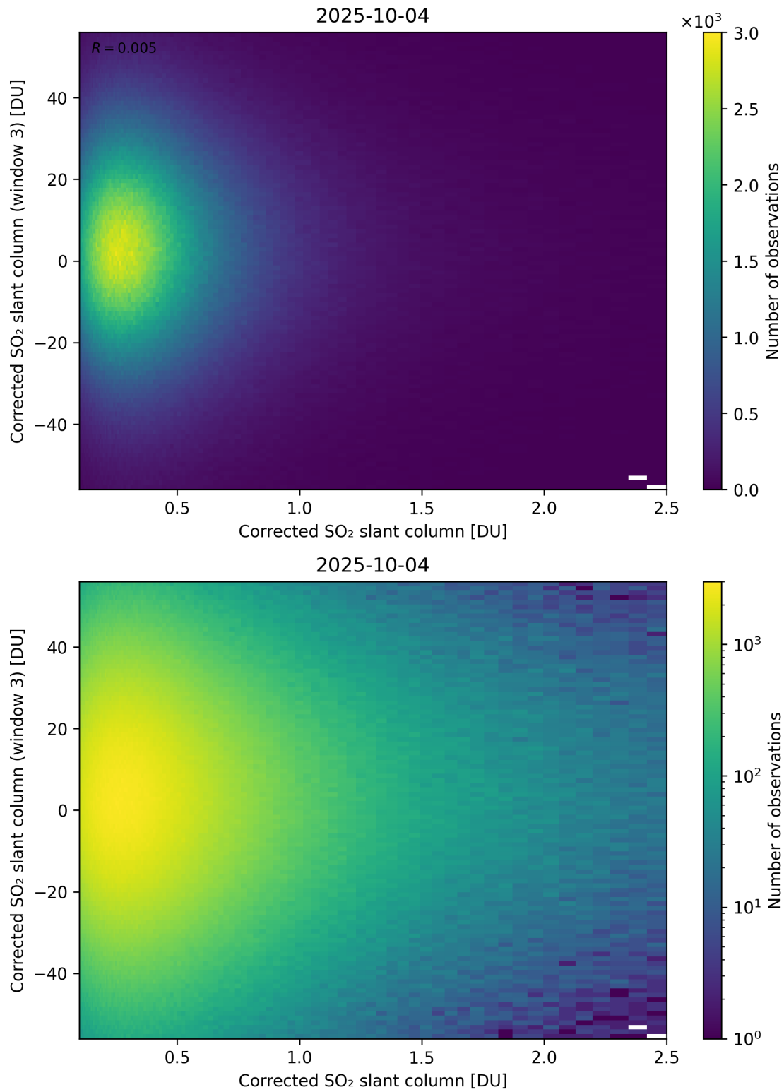
Figure 236: Scatter density plot of “Corrected SO 2 slant column” against “Corrected SO 2 slant column (window 3)” for 2025-10-03 to 2025-10-05.
