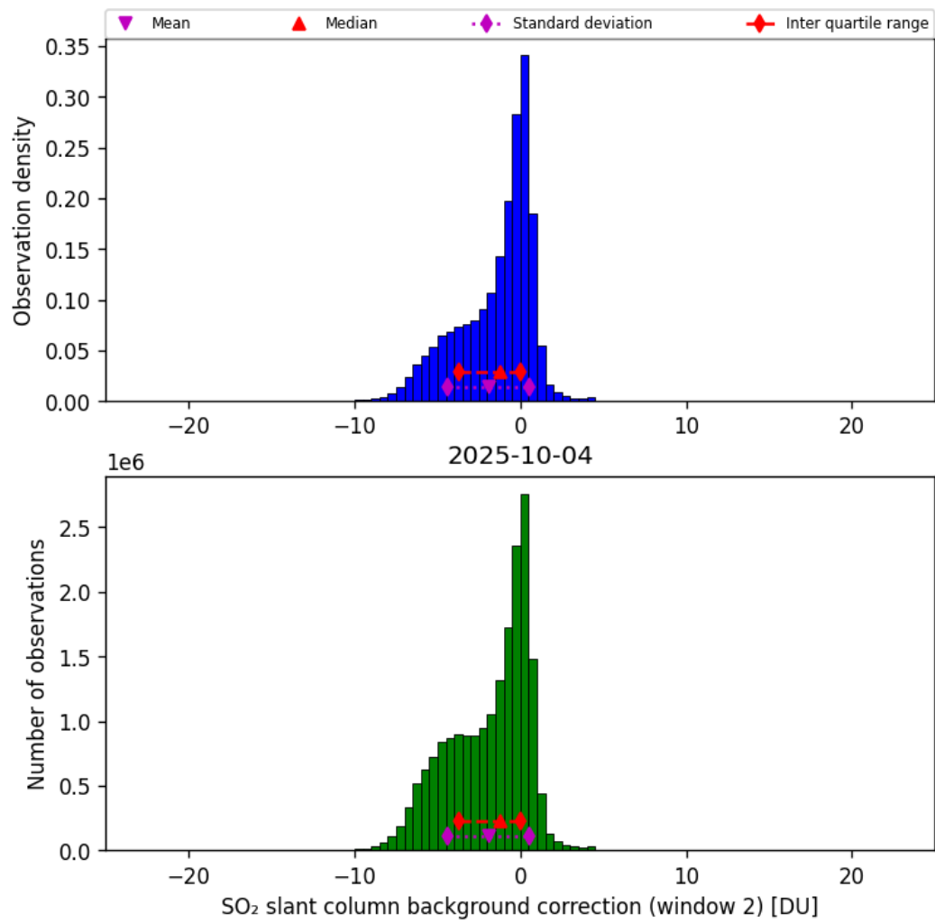
Figure 70: Histogram of “SO 2 slant column background correction (window 2)” for 2025-10-03 to 2025-10-05
