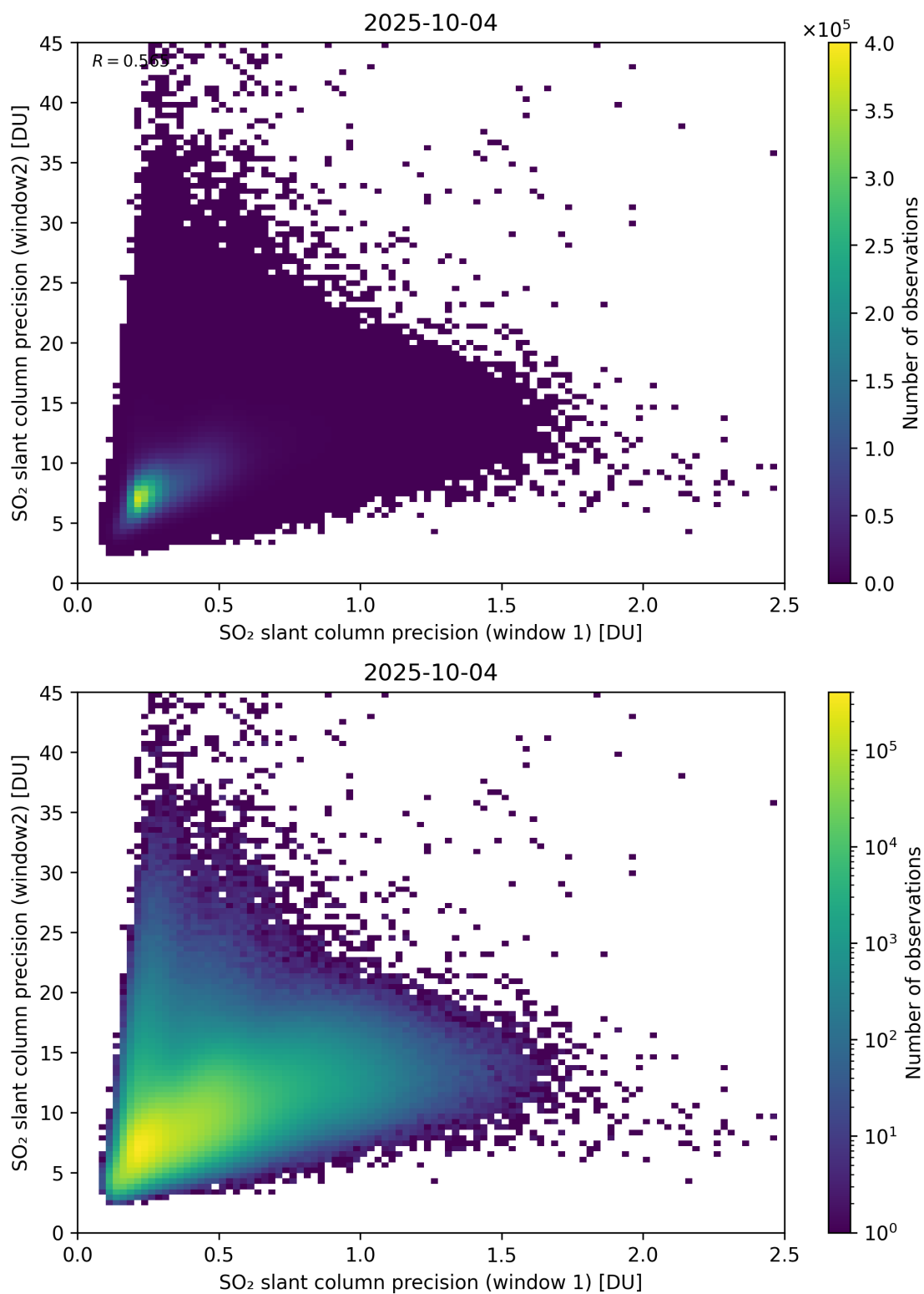
Figure 277: Scatter density plot of “SO 2 slant column precision (window 1)” against “SO 2 slant column precision (window2)” for 2025-10-03 to 2025-10-05.
