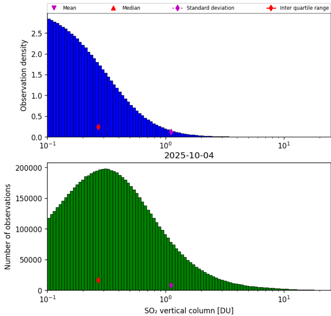
Figure 58: Histogram of “SO 2 vertical column” for 2025-10-03 to 2025-10-05
