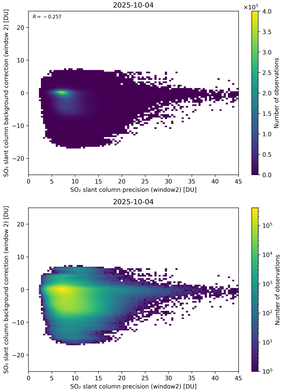
Figure 291: Scatter density plot of “SO 2 slant column precision (window2)” against “SO 2 slant column background correction (window 2)” for 2025-10-03 to 2025-10-05.
