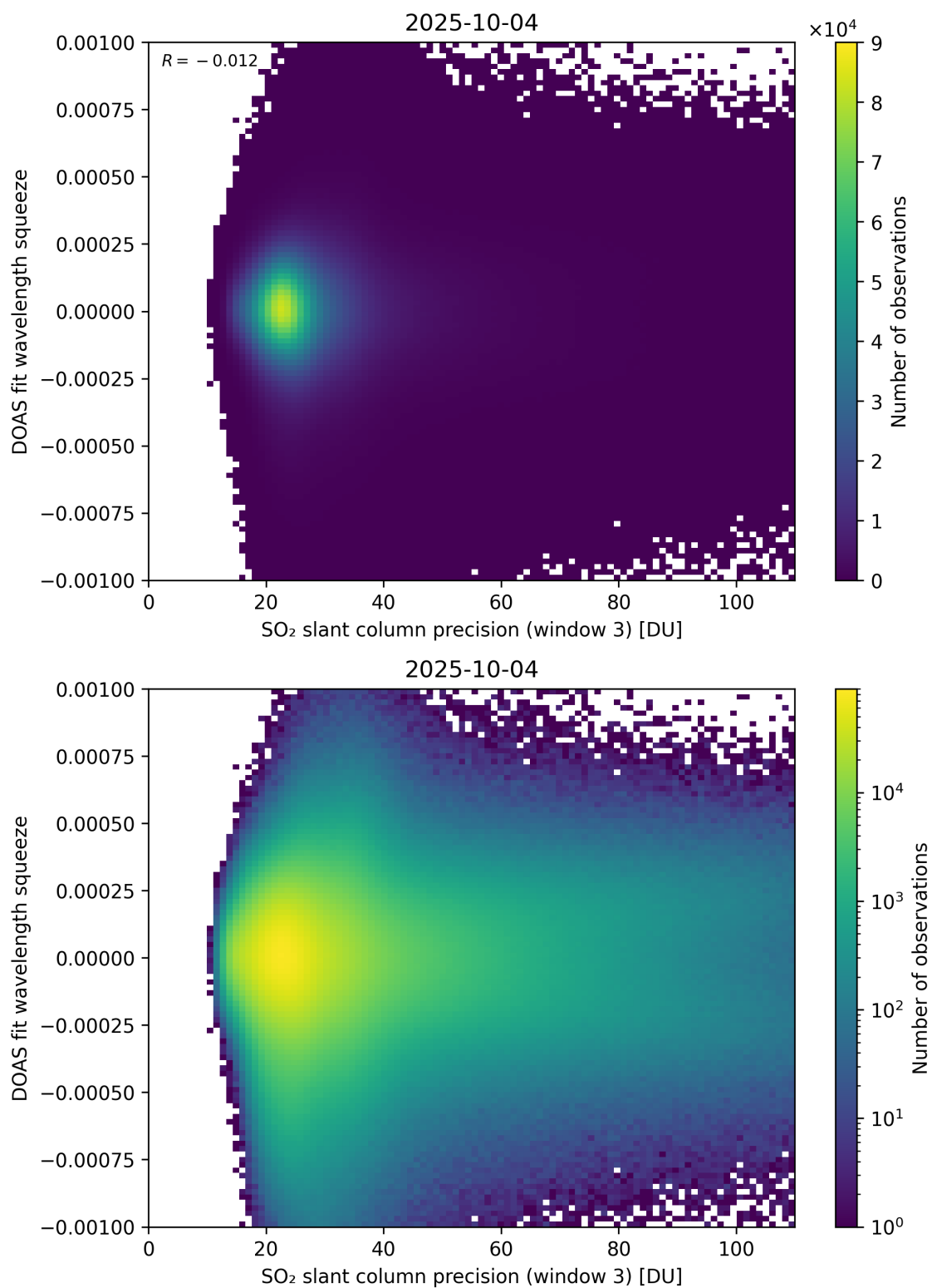
Figure 309: Scatter density plot of “SO 2 slant column precision (window 3)” against “DOAS fit wavelength squeeze” for 2025-10-03 to 2025-10-05.
