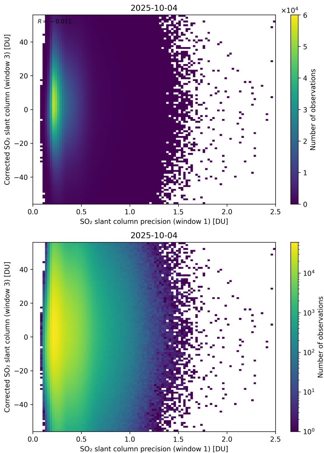
Figure 276: Scatter density plot of “SO 2 slant column precision (window 1)” against “Corrected SO 2 slant column (window 3)” for 2025-10-03 to 2025-10-05.
