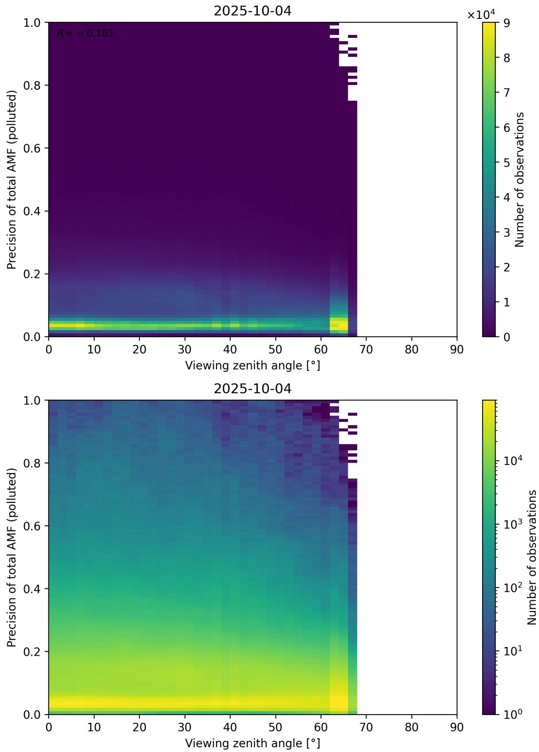
Figure 382: Scatter density plot of “Viewing zenith angle” against “Precision of total AMF (polluted)” for 2025-10-03 to 2025-10-05.
