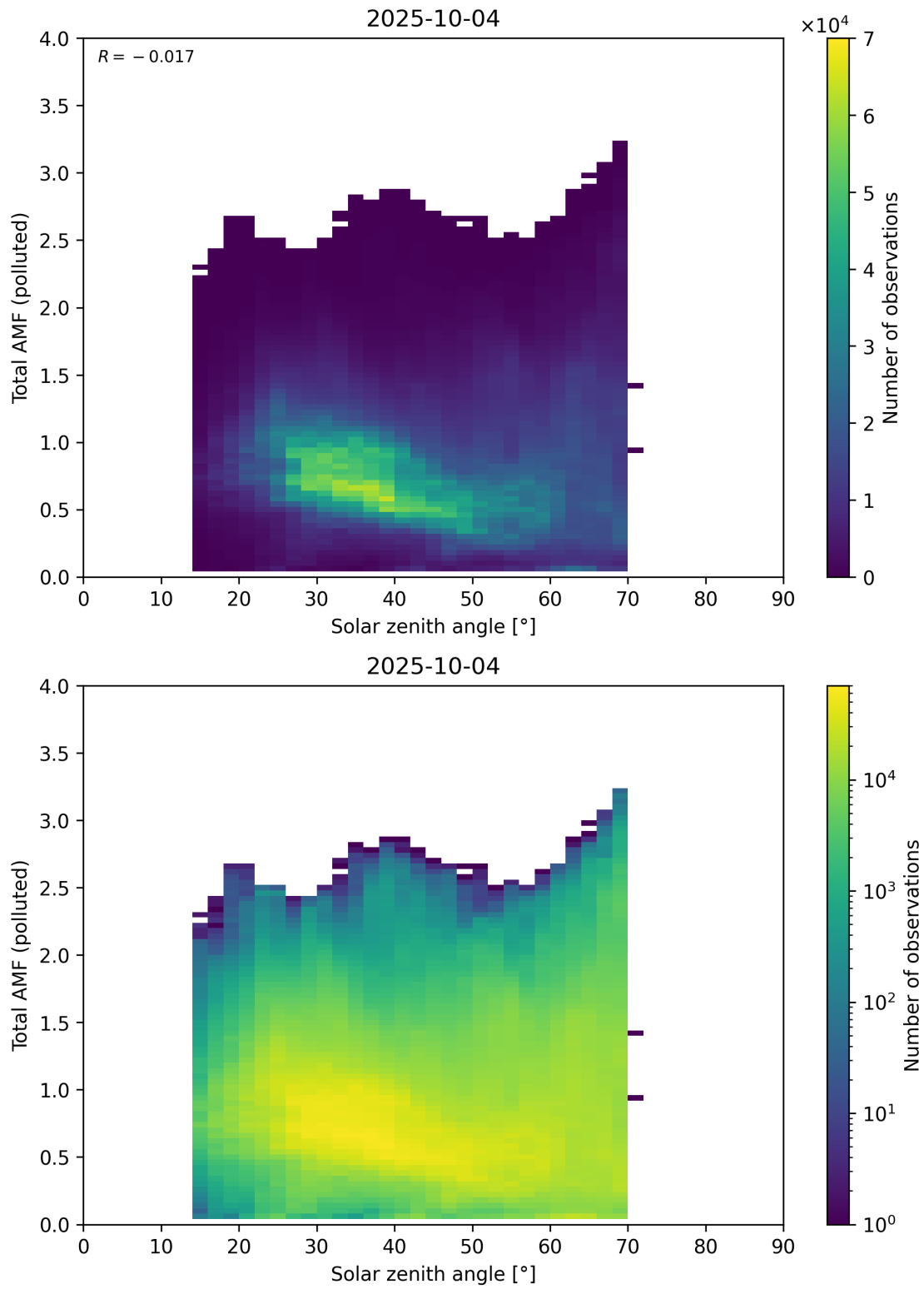
Figure 189: Scatter density plot of “Solar zenith angle” against “Total AMF (polluted)” for 2025-10-03 to 2025-10-05.
