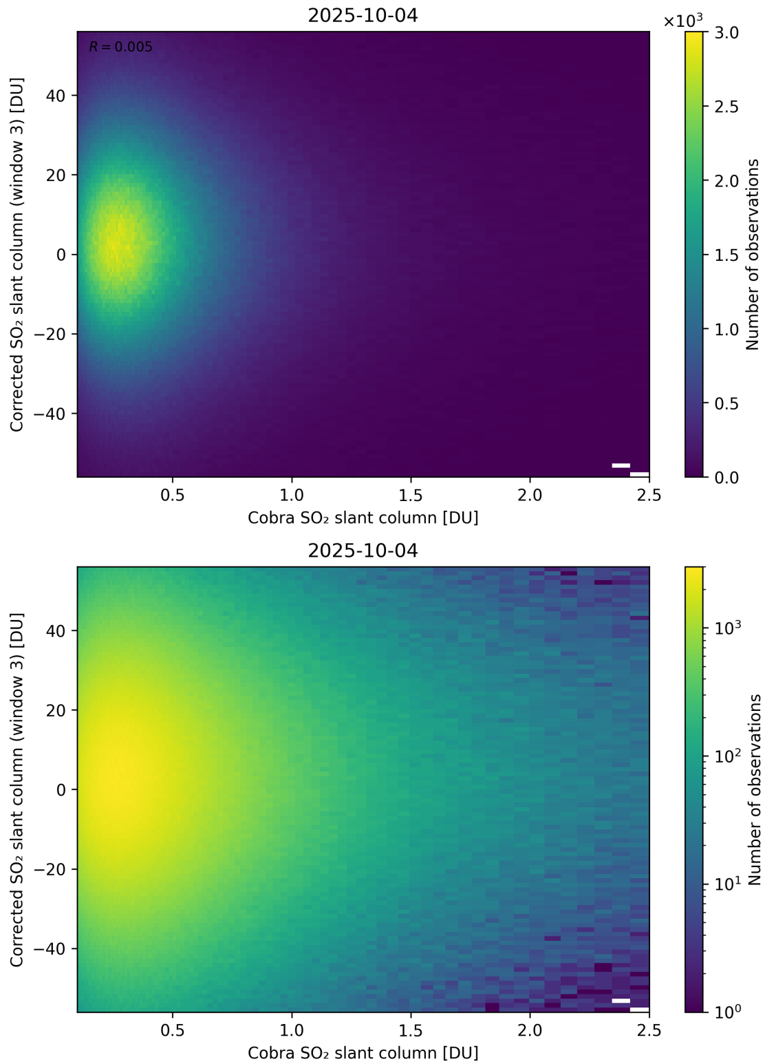
Figure 218: Scatter density plot of “Cobra SO 2 slant column” against “Corrected SO 2 slant column (window 3)” for 2025-10-03 to 2025-10-05.
