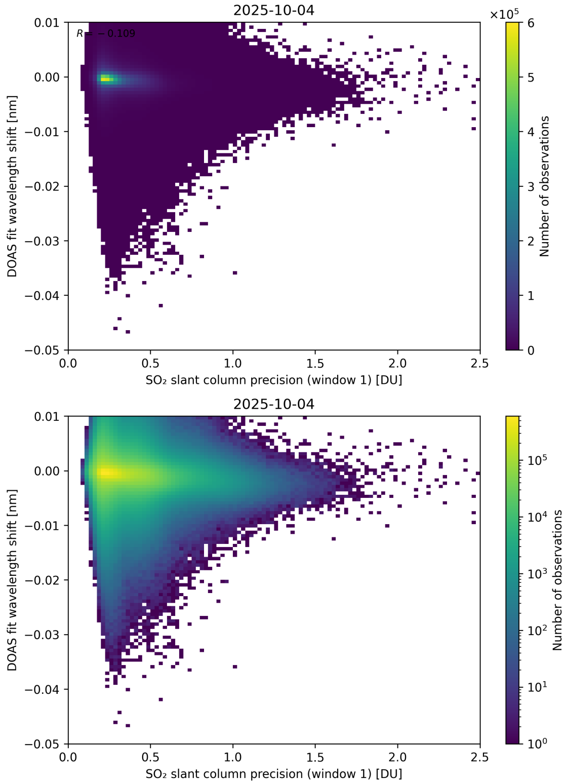
Figure 271: Scatter density plot of “SO 2 slant column precision (window 1)” against “DOAS fit wavelength shift” for 2025-10-03 to 2025-10-05.
