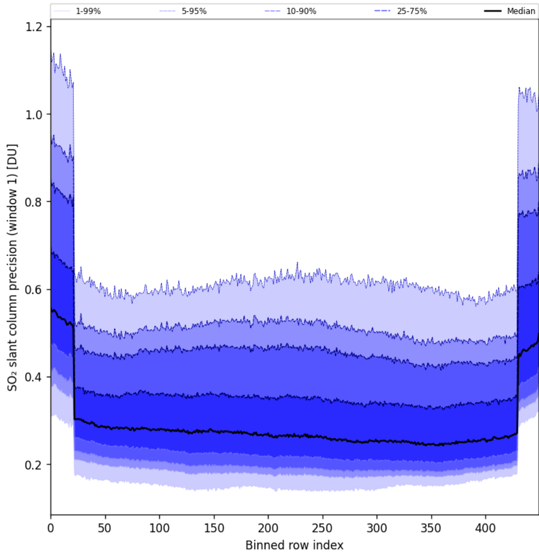
Figure 90: Along track statistics of “SO 2 slant column precision (window 1)” for 2025-10-03 to 2025-10-05
