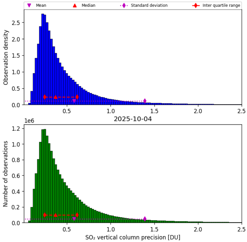
Figure 59: Histogram of “SO 2 vertical column precision” for 2025-10-03 to 2025-10-05
