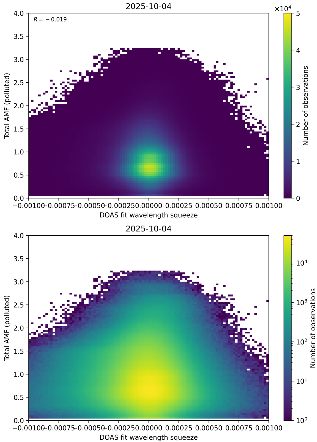
Figure 145: Scatter density plot of “DOAS fit wavelength squeeze” against “Total AMF (polluted)” for 2025-10-03 to 2025-10-05.
