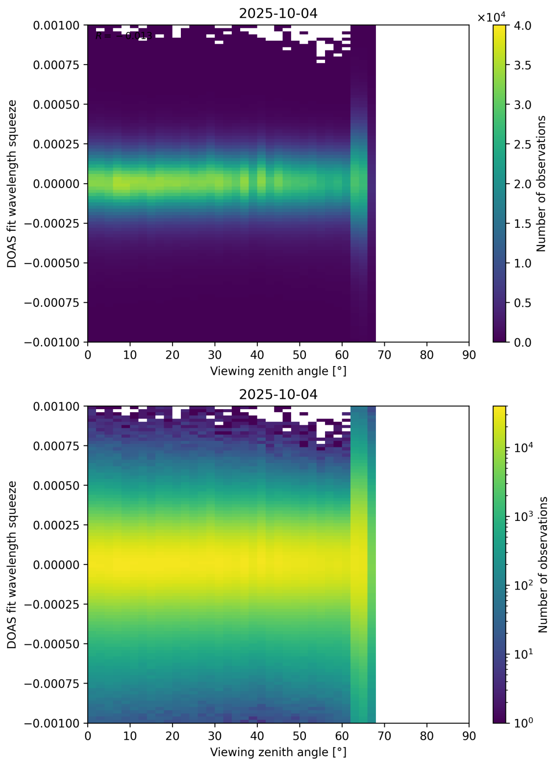
Figure 366: Scatter density plot of “Viewing zenith angle” against “DOAS fit wavelength squeeze” for 2025-10-03 to 2025-10-05.
