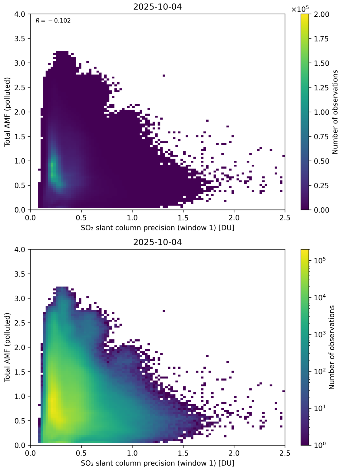
Figure 280: Scatter density plot of “SO 2 slant column precision (window 1)” against “Total AMF (polluted)” for 2025-10-03 to 2025-10-05.
