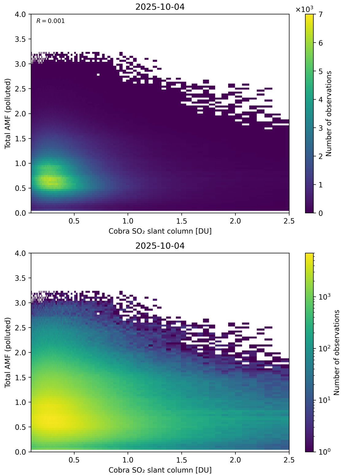
Figure 224: Scatter density plot of “Cobra SO 2 slant column” against “Total AMF (polluted)” for 2025-10-03 to 2025-10-05.
