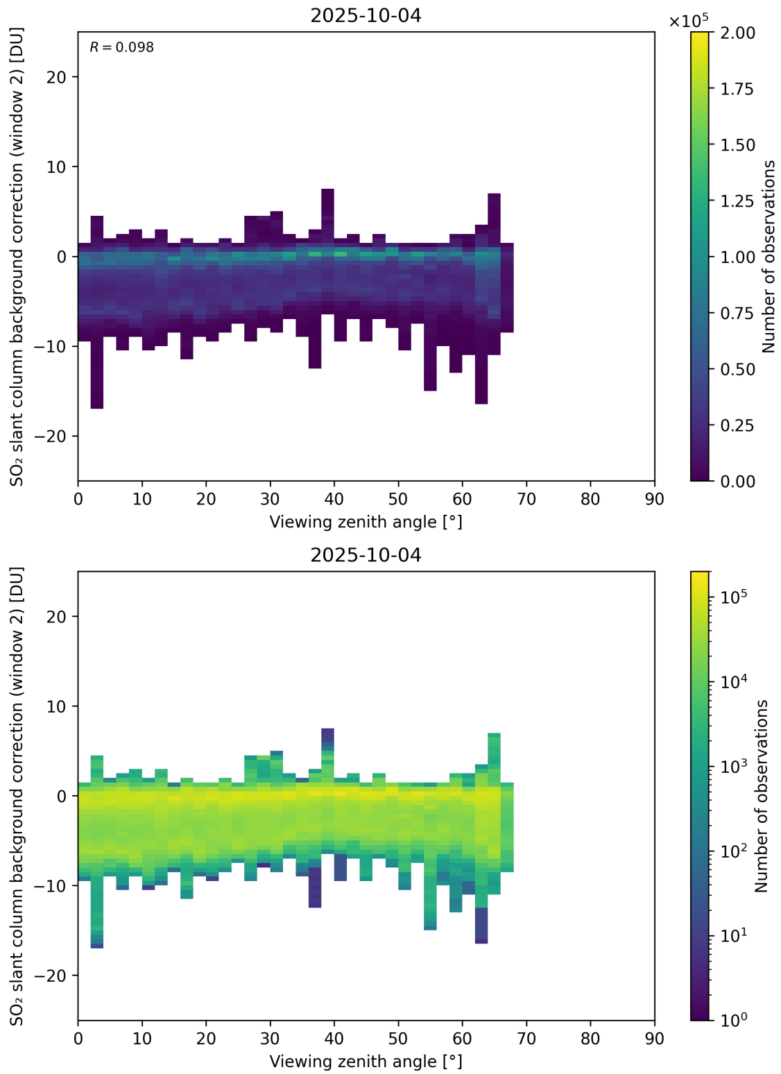
Figure 363: Scatter density plot of “Viewing zenith angle” against “SO 2 slant column background correction (window 2)” for 2025-10-03 to 2025-10-05.
