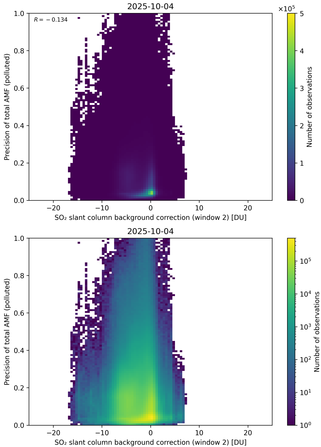
Figure 131: Scatter density plot of “SO 2 slant column background correction (window 2)” against “Precision of total AMF (polluted)” for 2025-10-03 to 2025-10-05.
