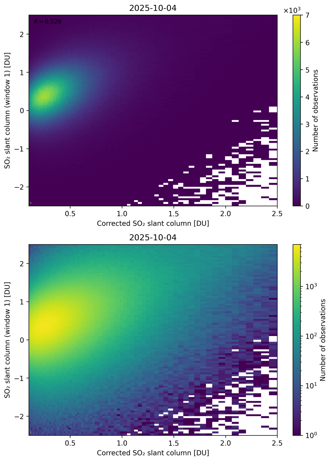
Figure 237: Scatter density plot of “Corrected SO 2 slant column” against “SO 2 slant column (window 1)” for 2025-10-03 to 2025-10-05.
