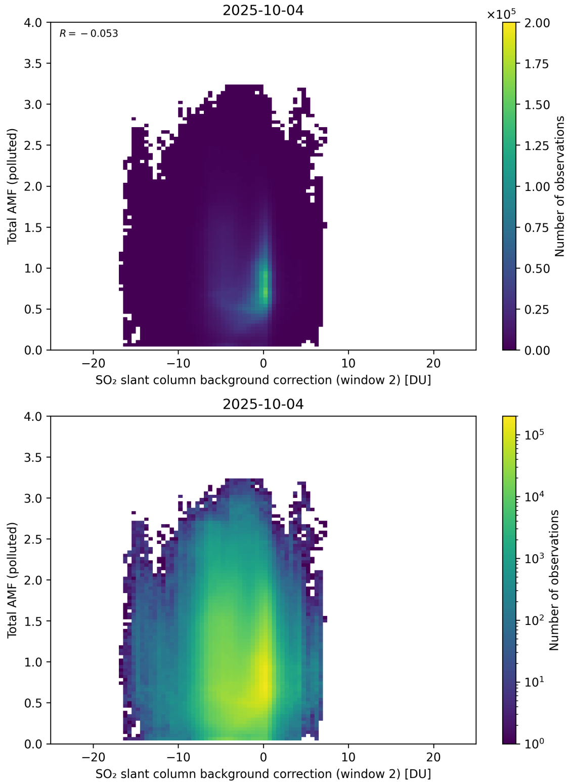
Figure 130: Scatter density plot of “SO 2 slant column background correction (window 2)” against “Total AMF (polluted)” for 2025-10-03 to 2025-10-05.
