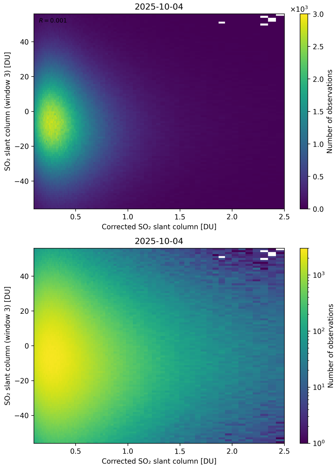
Figure 240: Scatter density plot of “Corrected SO 2 slant column” against “SO 2 slant column (window 3)” for 2025-10-03 to 2025-10-05.
