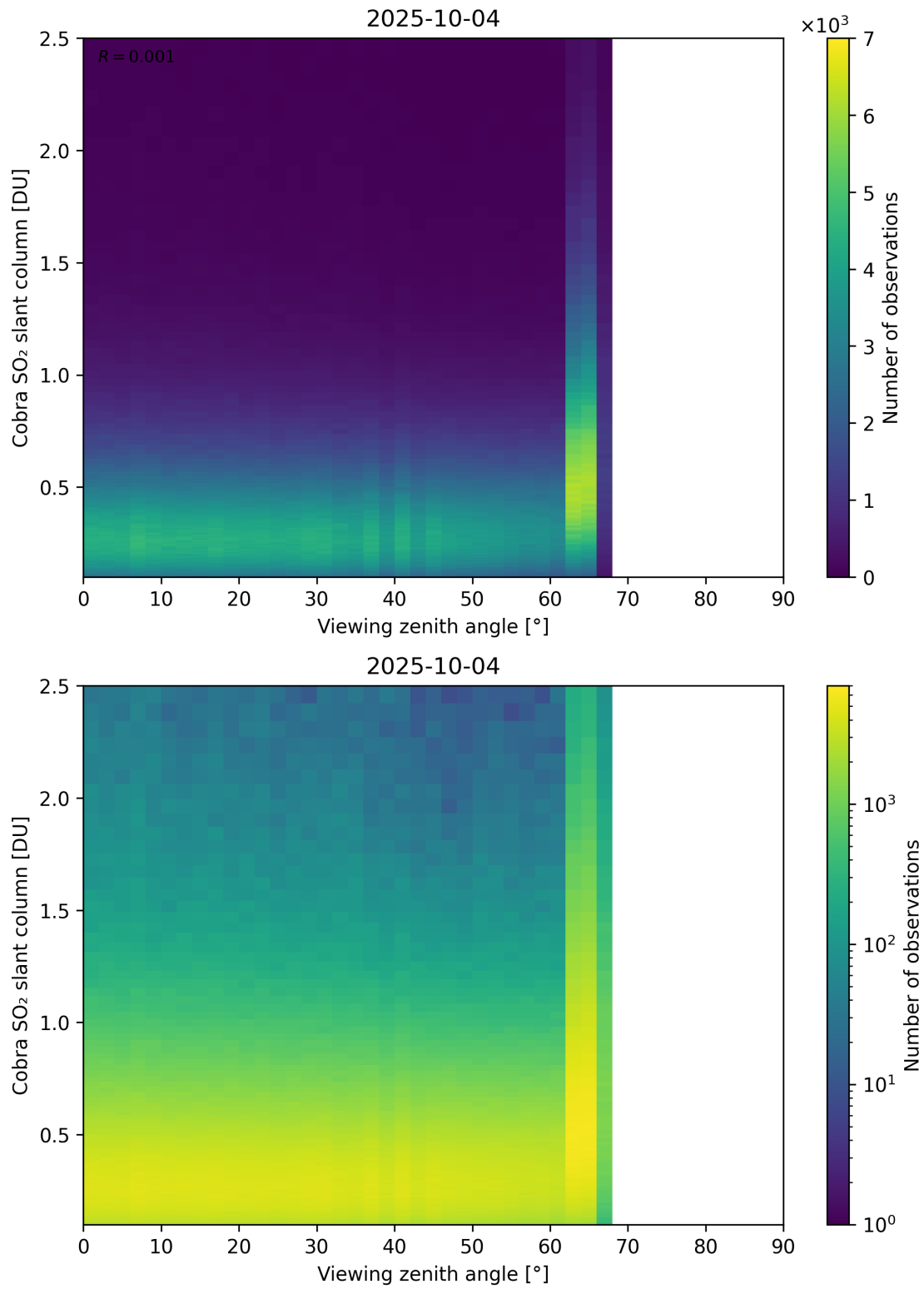
Figure 371: Scatter density plot of “Viewing zenith angle” against “Cobra SO 2 slant column” for 2025-10-03 to 2025-10-05.
