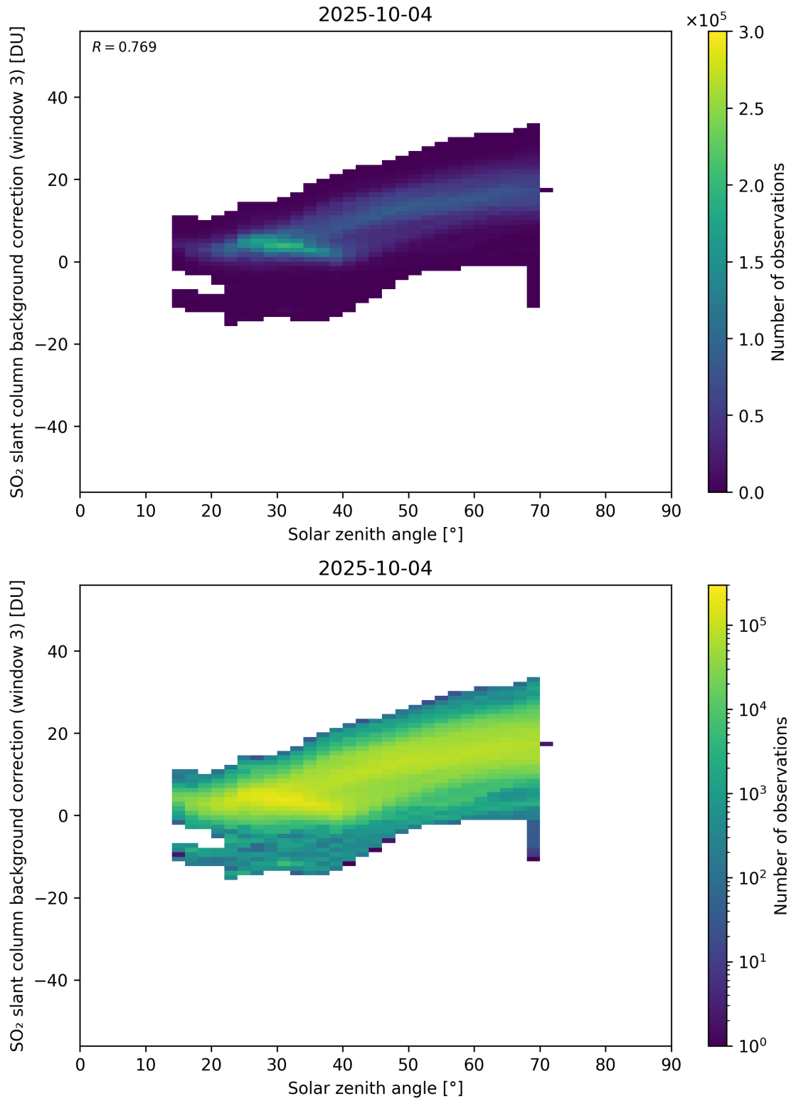
Figure 173: Scatter density plot of “Solar zenith angle” against “SO 2 slant column background correction (window 3)” for 2025-10-03 to 2025-10-05.
