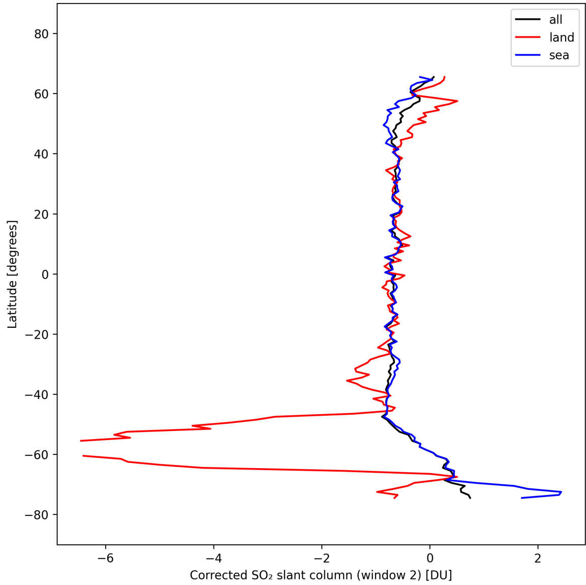
Figure 43: Zonal average of “Corrected SO 2 slant column (window 2)” for 2025-10-03 to 2025-10-05.
