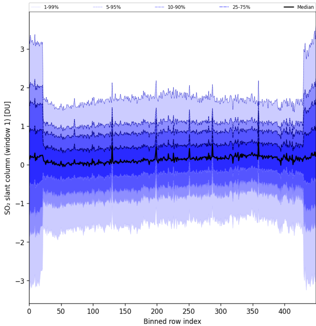
Figure 89: Along track statistics of “SO 2 slant column (window 1)” for 2025-10-03 to 2025-10-05
