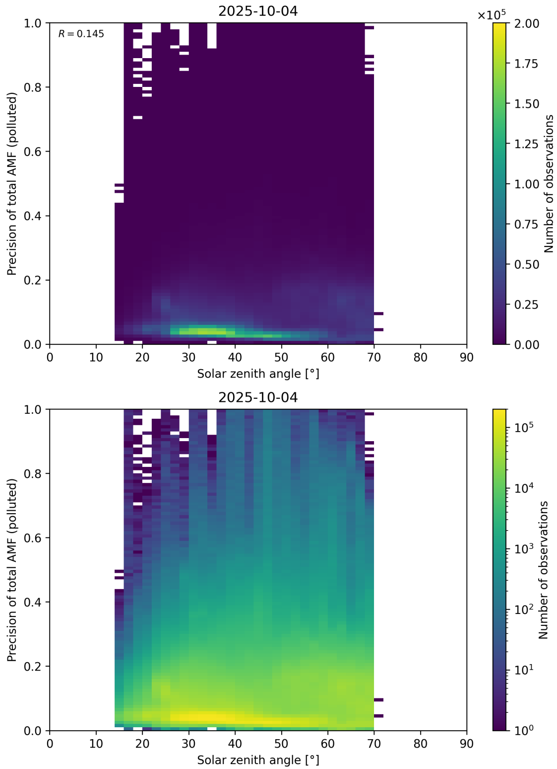
Figure 190: Scatter density plot of “Solar zenith angle” against “Precision of total AMF (polluted)” for 2025-10-03 to 2025-10-05.
