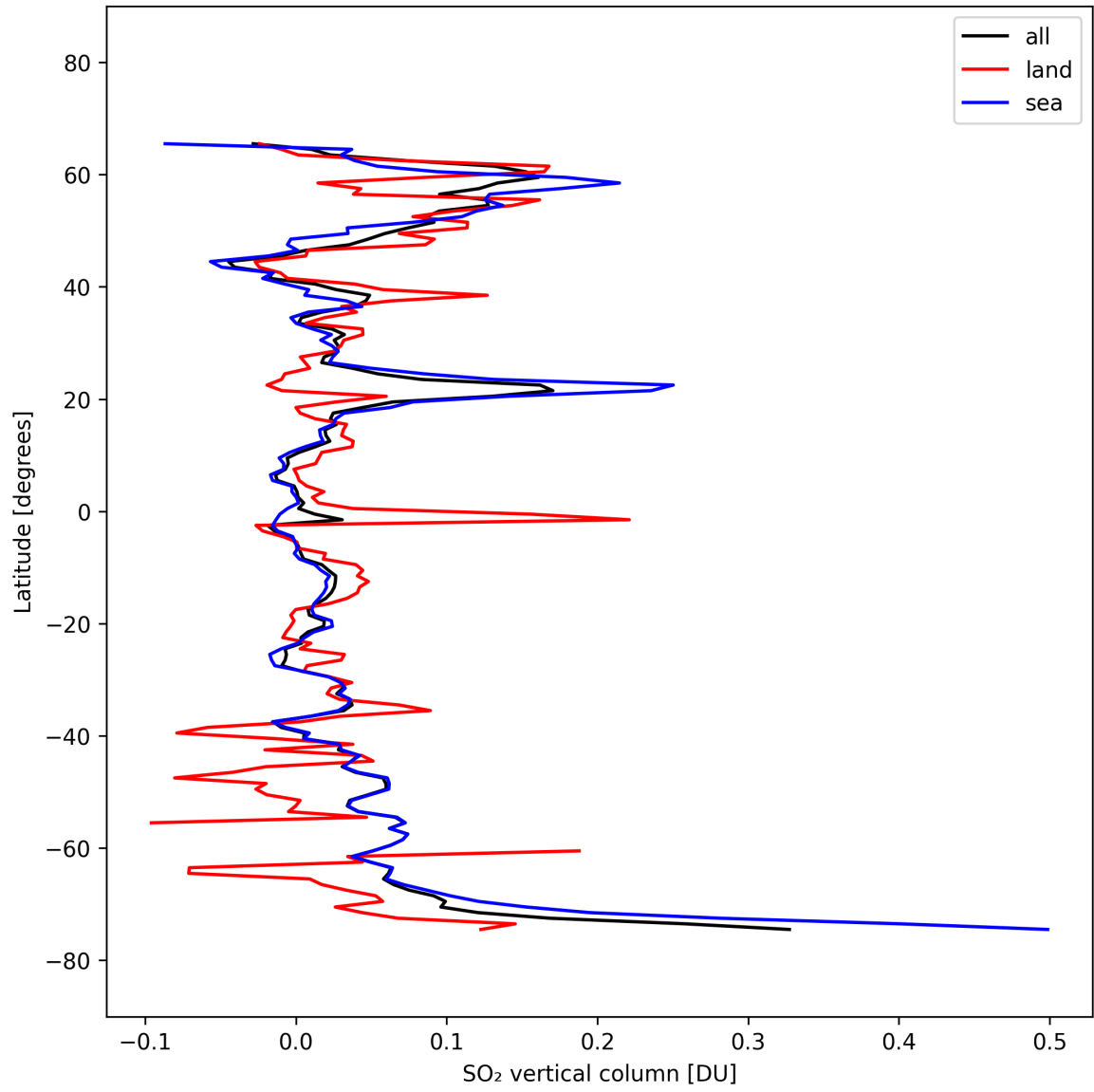
Figure 32: Zonal average of “SO 2 vertical column” for 2025-10-03 to 2025-10-05.
