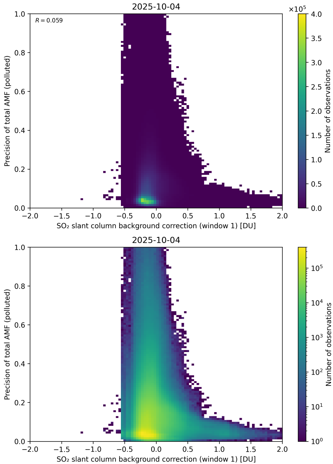
Figure 121: Scatter density plot of “SO 2 slant column background correction (window 1)” against “Precision of total AMF (polluted)” for 2025-10-03 to 2025-10-05.
