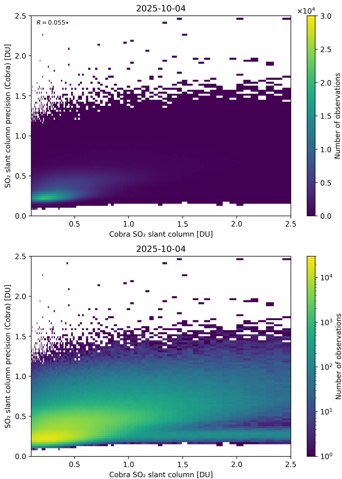
Figure 216: Scatter density plot of “Cobra SO 2 slant column” against “SO 2 slant column precision (Cobra)” for 2025-10-03 to 2025-10-05.
