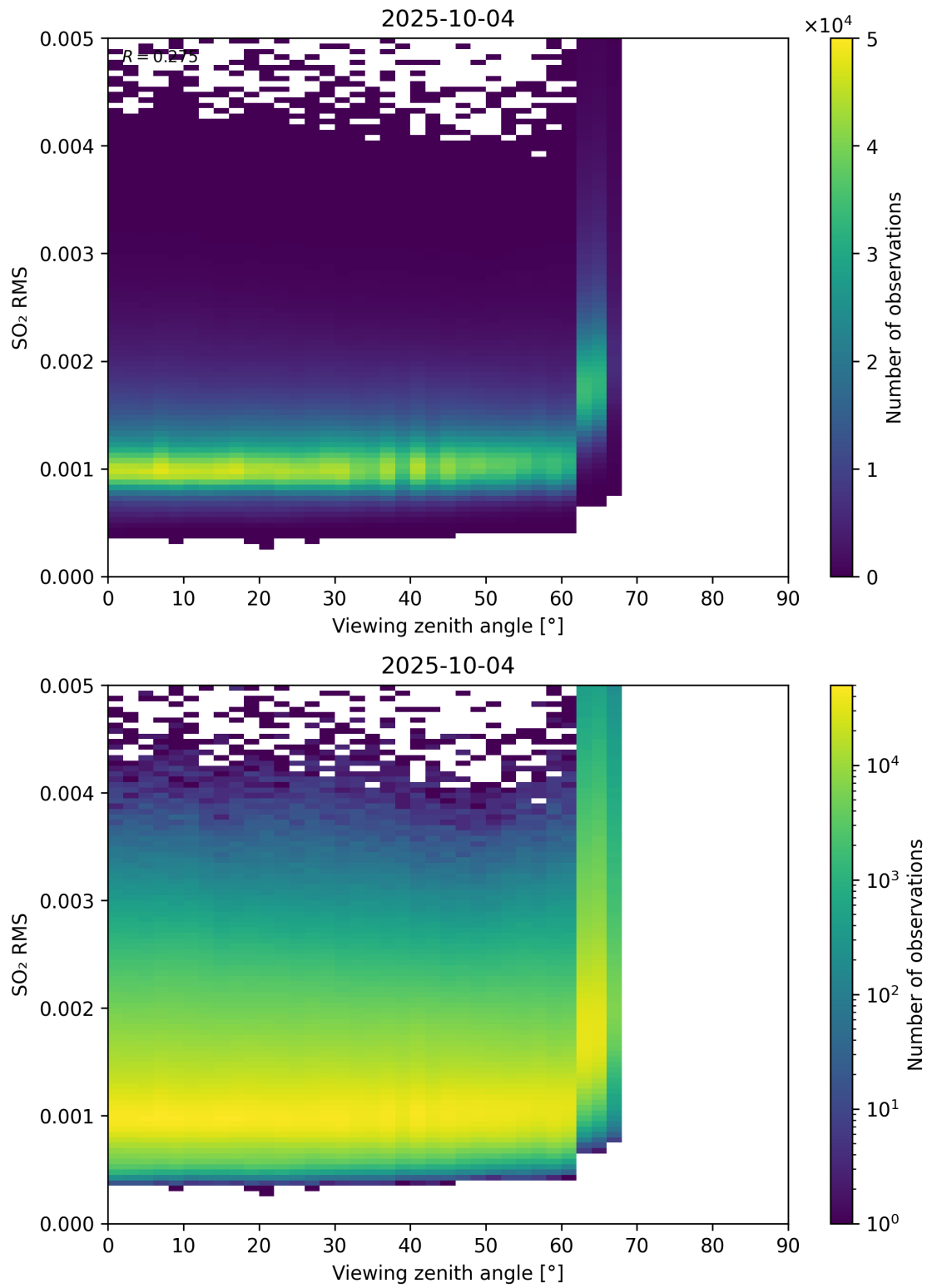
Figure 367: Scatter density plot of “Viewing zenith angle” against “SO 2 RMS” for 2025-10-03 to 2025-10-05.
