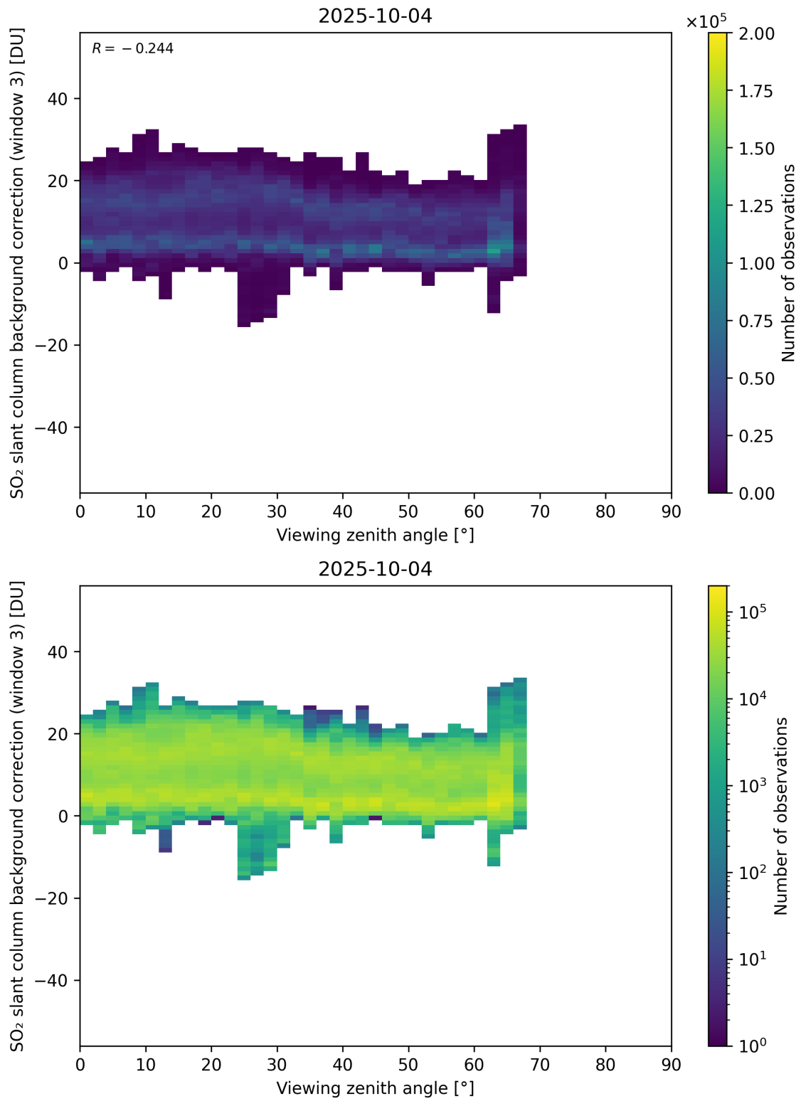
Figure 364: Scatter density plot of “Viewing zenith angle” against “SO 2 slant column background correction (window 3)” for 2025-10-03 to 2025-10-05.
