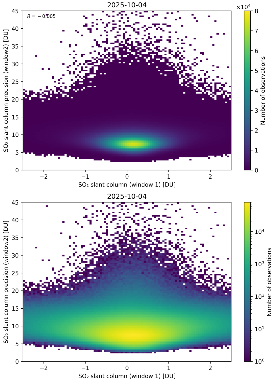
Figure 286: Scatter density plot of “SO 2 slant column (window 1)” against “SO 2 slant column precision (window2)” for 2025-10-03 to 2025-10-05.
