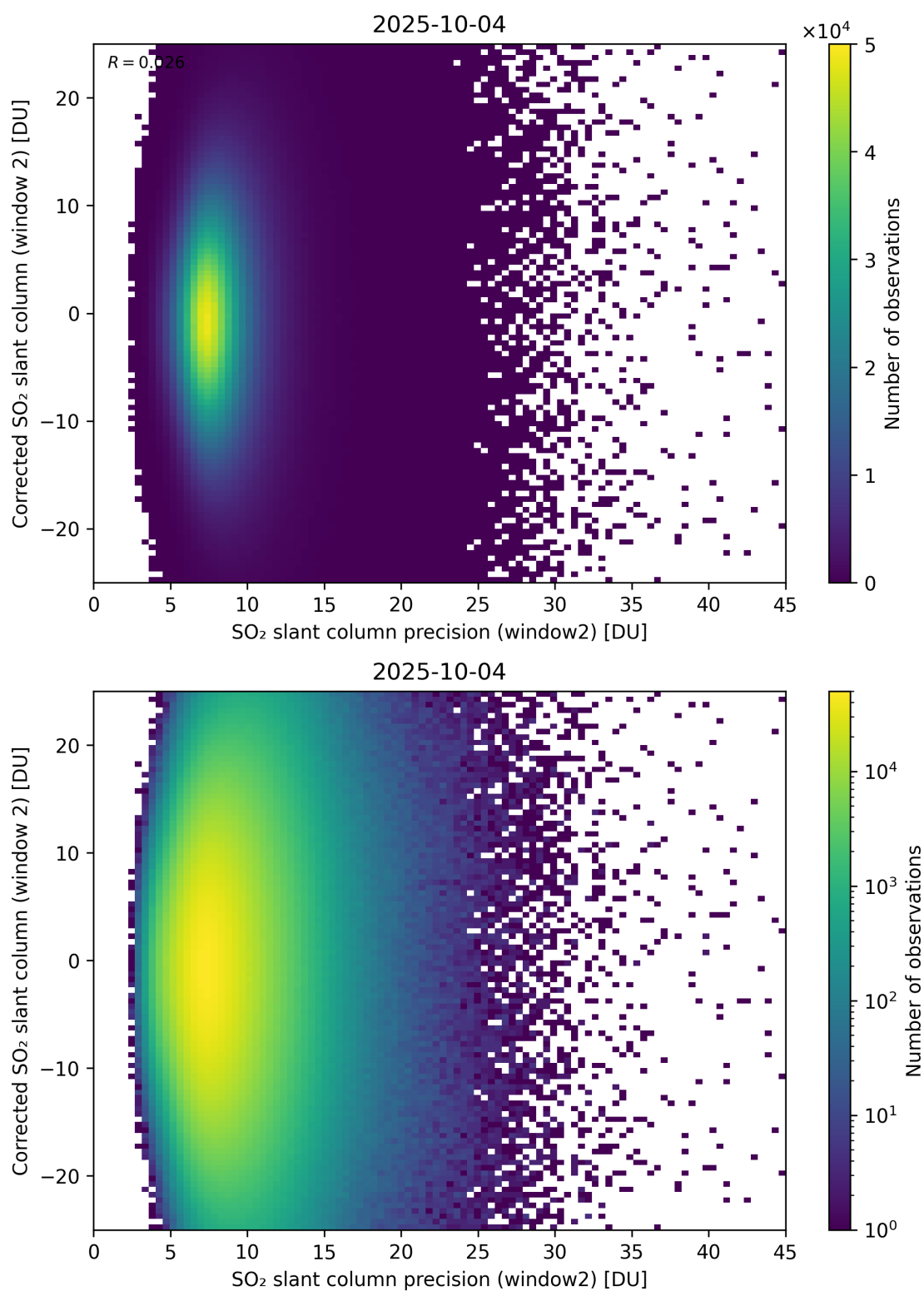
Figure 297: Scatter density plot of “SO 2 slant column precision (window2)” against “Corrected SO 2 slant column (window 2)” for 2025-10-03 to 2025-10-05.
