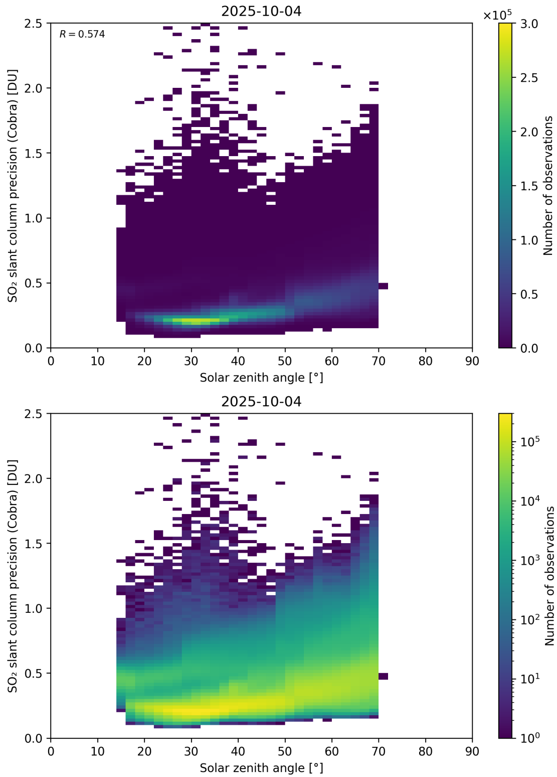
Figure 180: Scatter density plot of “Solar zenith angle” against “SO 2 slant column precision (Cobra)” for 2025-10-03 to 2025-10-05.
