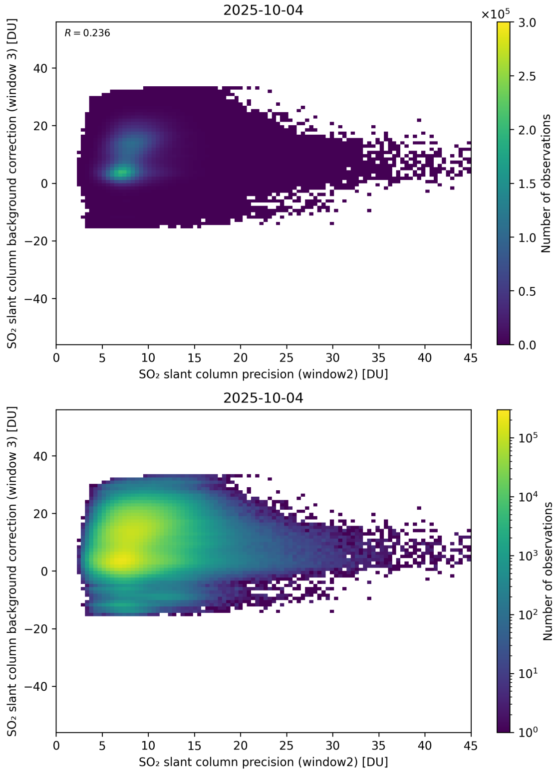
Figure 292: Scatter density plot of “SO 2 slant column precision (window2)” against “SO 2 slant column background correction (window 3)” for 2025-10-03 to 2025-10-05.
