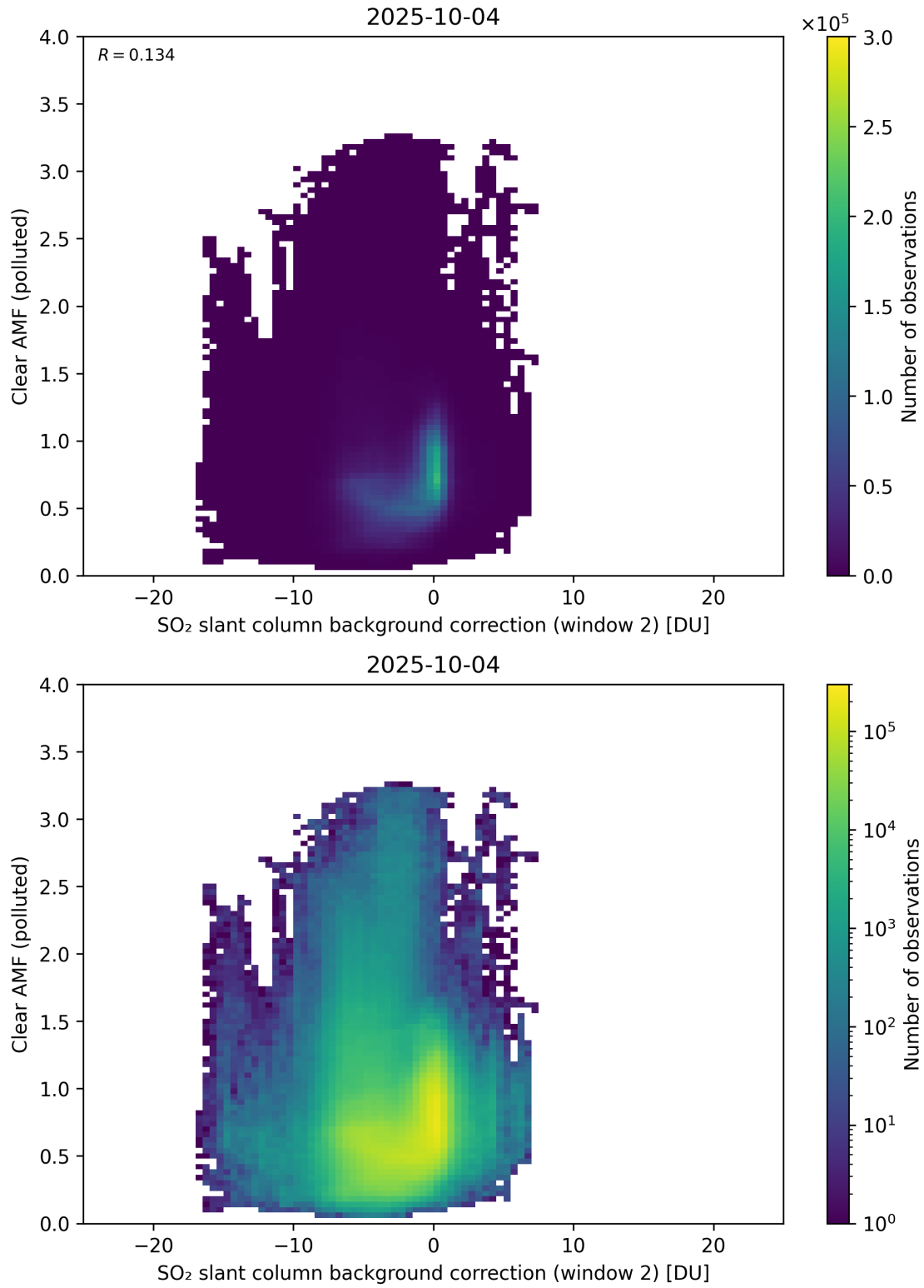
Figure 126: Scatter density plot of “SO 2 slant column background correction (window 2)” against “Clear AMF (polluted)” for 2025-10-03 to 2025-10-05.
