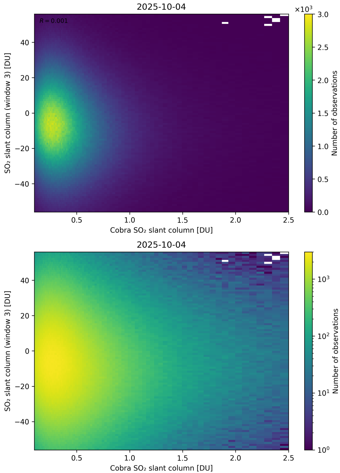
Figure 222: Scatter density plot of “Cobra SO 2 slant column” against “SO 2 slant column (window 3)” for 2025-10-03 to 2025-10-05.
