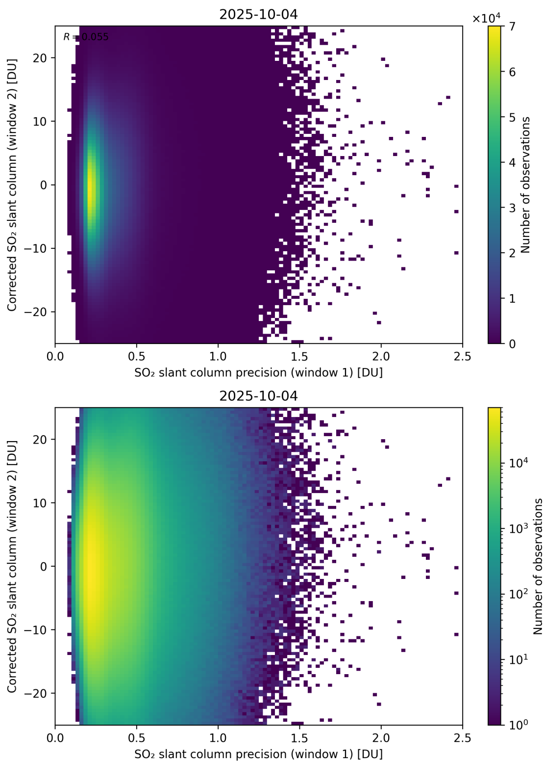
Figure 275: Scatter density plot of “SO 2 slant column precision (window 1)” against “Corrected SO 2 slant column (window 2)” for 2025-10-03 to 2025-10-05.
