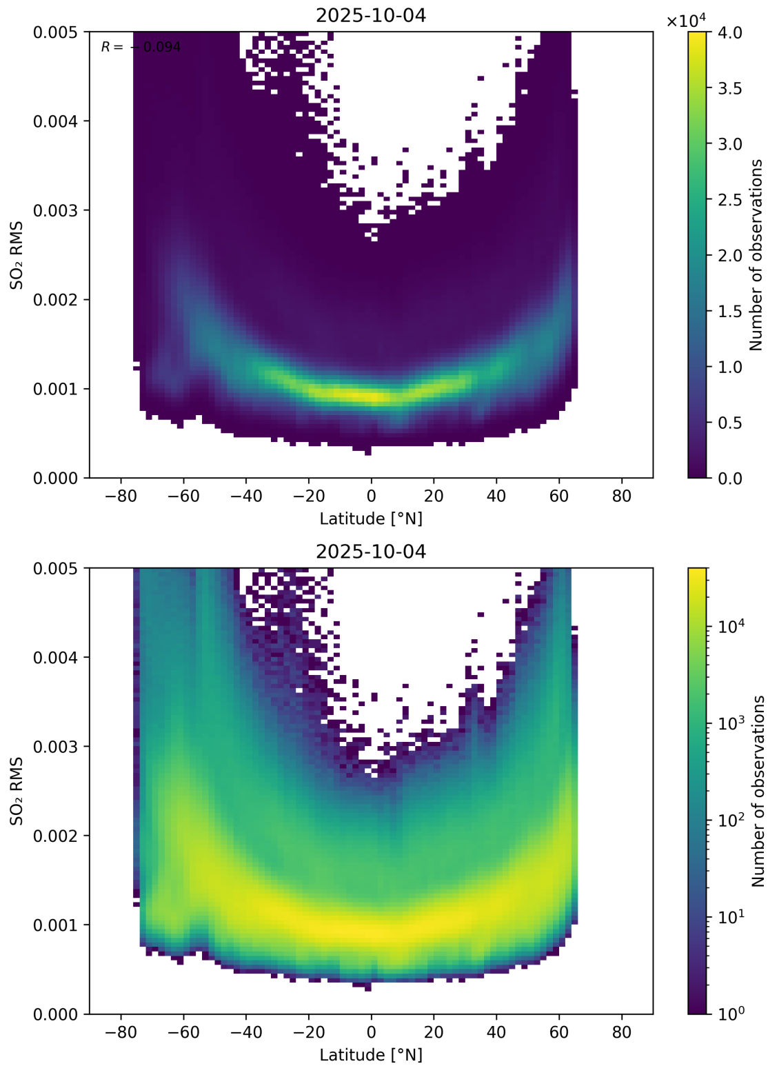
Figure 155: Scatter density plot of “Latitude” against “SO 2 RMS” for 2025-10-03 to 2025-10-05.
