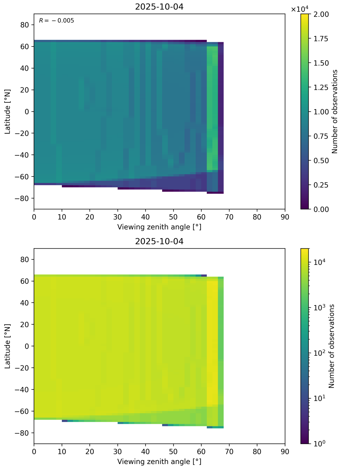
Figure 368: Scatter density plot of “Viewing zenith angle” against “Latitude” for 2025-10-03 to 2025-10-05.
