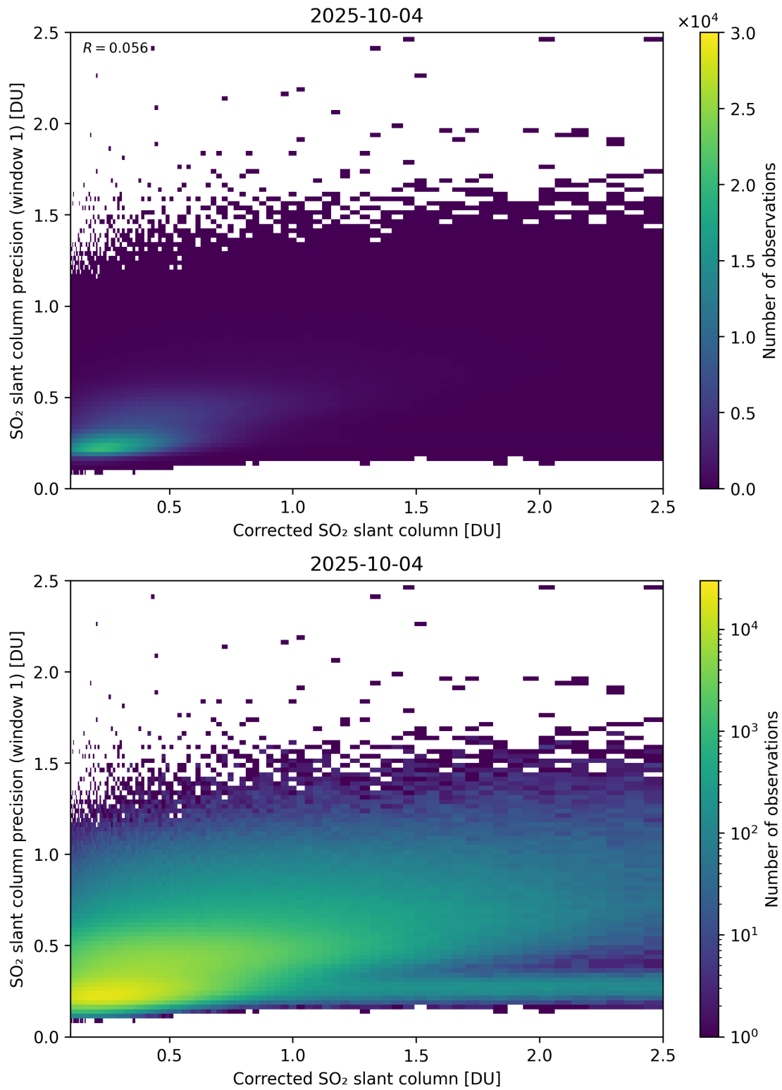
Figure 238: Scatter density plot of “Corrected SO 2 slant column” against “SO 2 slant column precision (window 1)” for 2025-10-03 to 2025-10-05.
