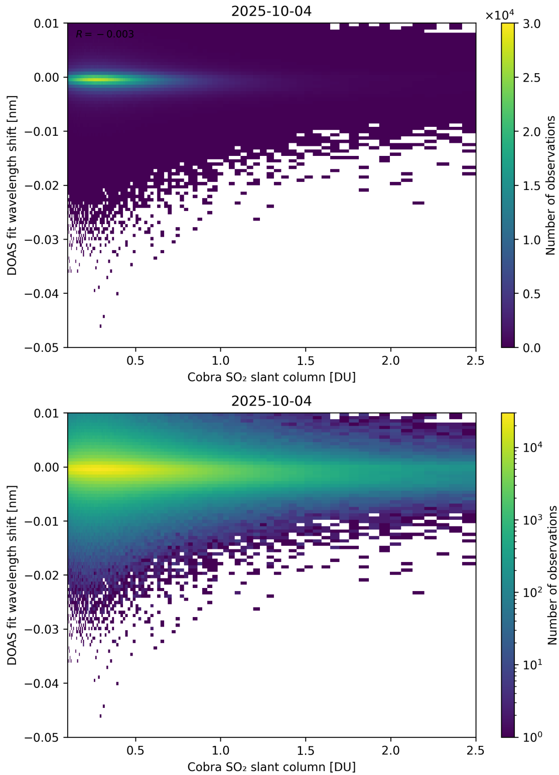
Figure 196: Scatter density plot of “Cobra SO 2 slant column” against “DOAS fit wavelength shift” for 2025-10-03 to 2025-10-05.
