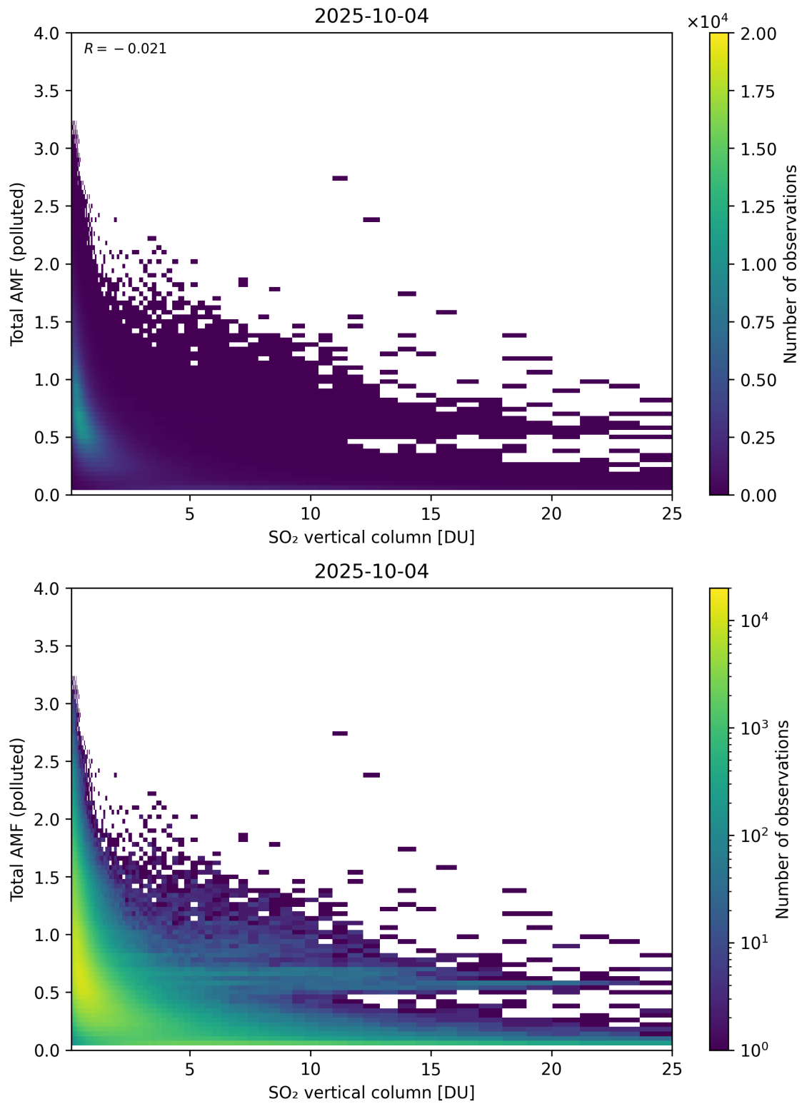
Figure 359: Scatter density plot of “SO 2 vertical column” against “Total AMF (polluted)” for 2025-10-03 to 2025-10-05.
