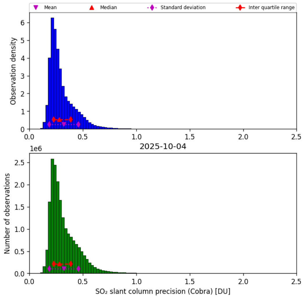
Figure 62: Histogram of “SO 2 slant column precision (Cobra)” for 2025-10-03 to 2025-10-05
