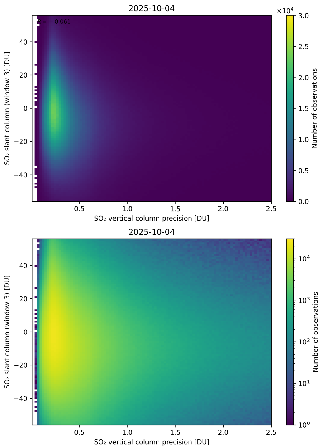
Figure 344: Scatter density plot of “SO 2 vertical column precision” against “SO 2 slant column (window 3)” for 2025-10-03 to 2025-10-05.
