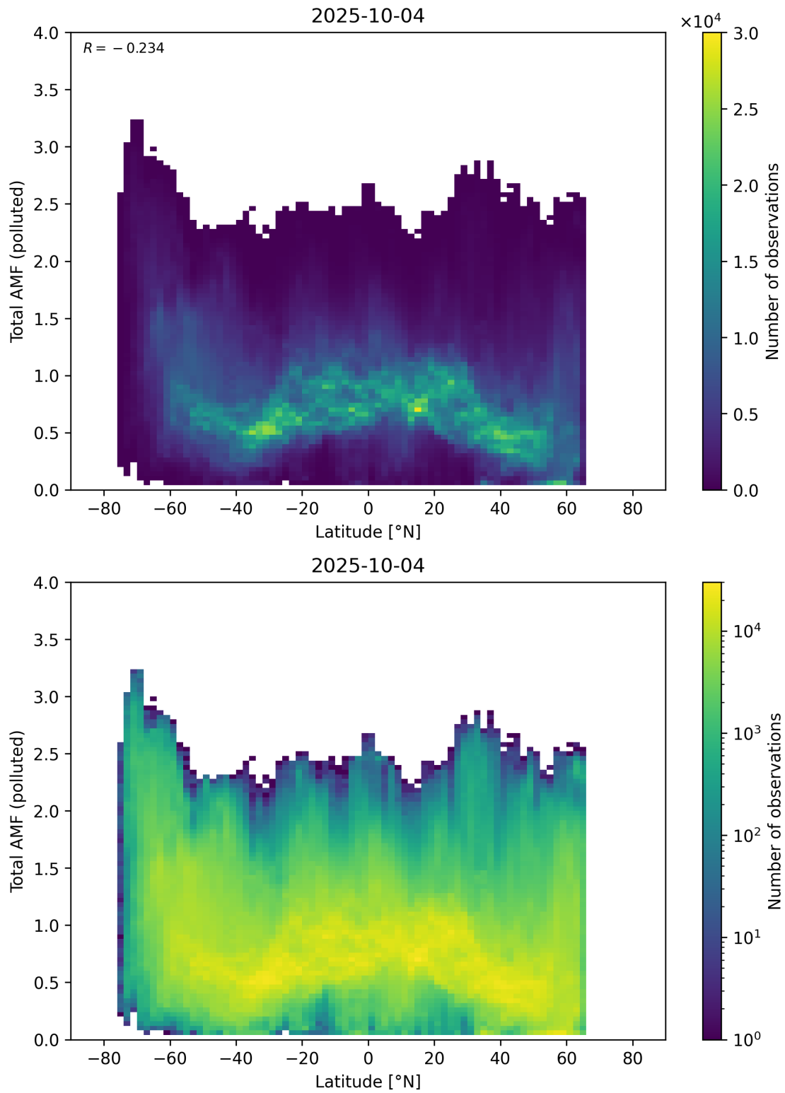
Figure 167: Scatter density plot of “Latitude” against “Total AMF (polluted)” for 2025-10-03 to 2025-10-05.
