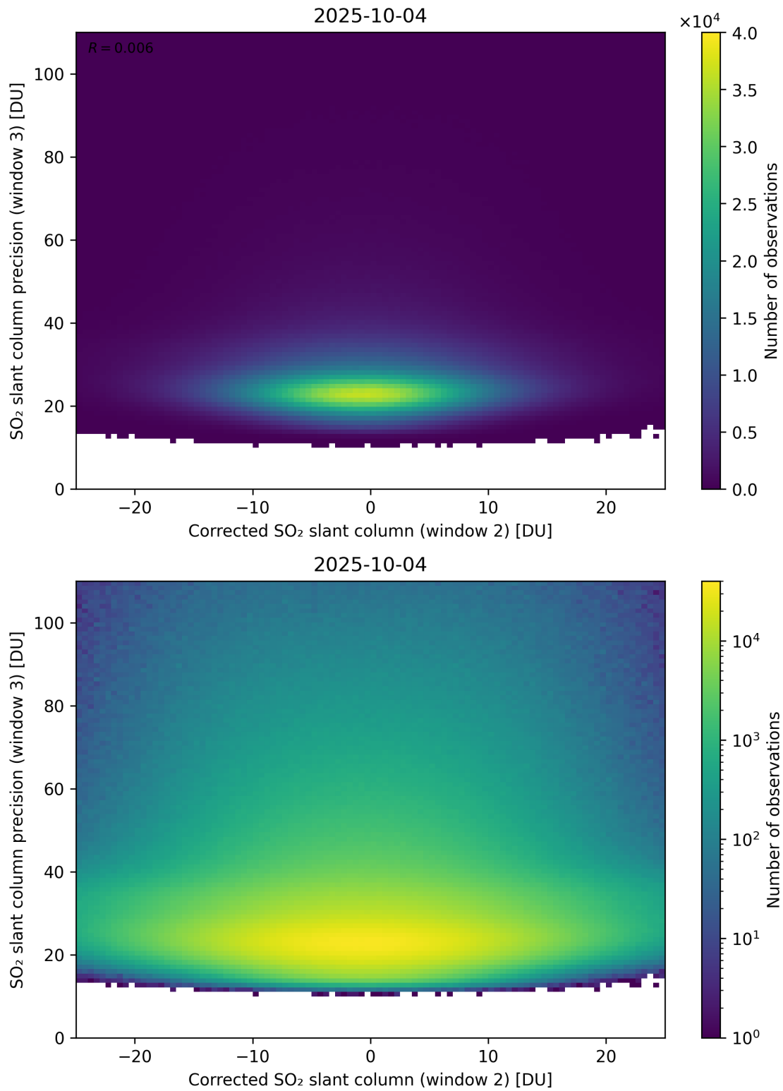
Figure 252: Scatter density plot of “Corrected SO 2 slant column (window 2)” against “SO 2 slant column precision (window 3)” for 2025-10-03 to 2025-10-05.
