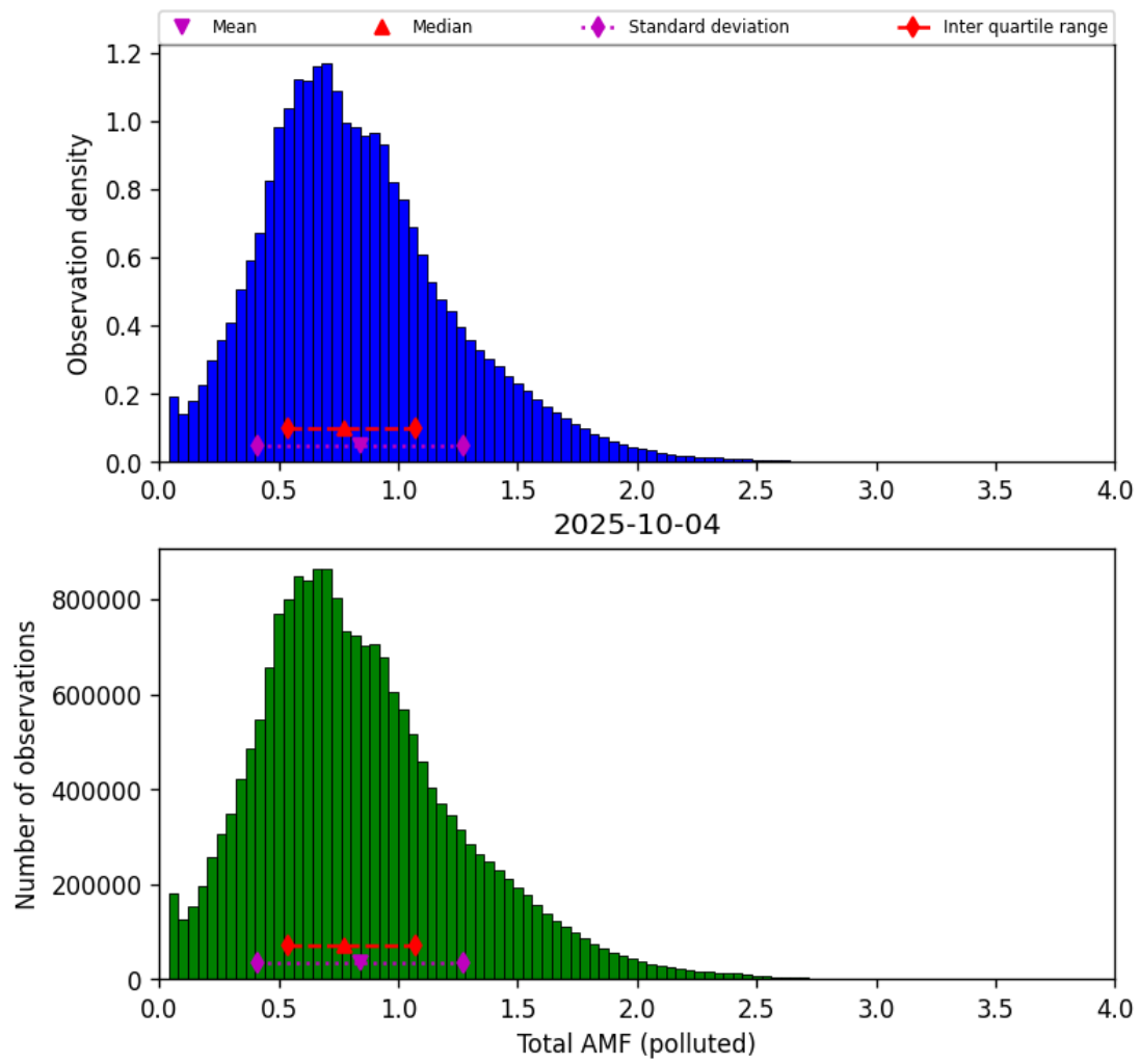
Figure 79: Histogram of “Total AMF (polluted)” for 2025-10-03 to 2025-10-05
