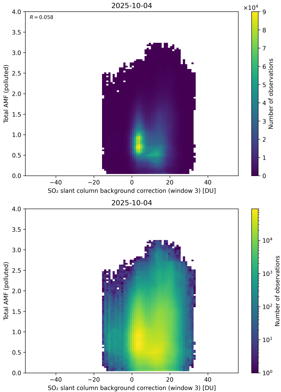
Figure 136: Scatter density plot of “SO 2 slant column background correction (window 3)” against “Total AMF (polluted)” for 2025-10-03 to 2025-10-05.
