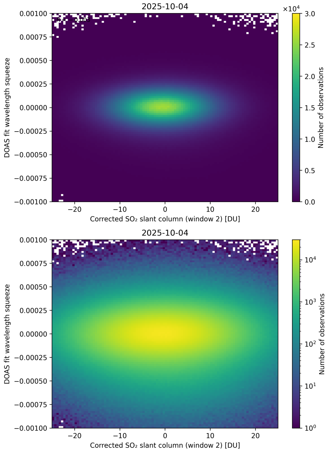
Figure 247: Scatter density plot of “Corrected SO 2 slant column (window 2)” against “DOAS fit wavelength squeeze” for 2025-10-03 to 2025-10-05.
