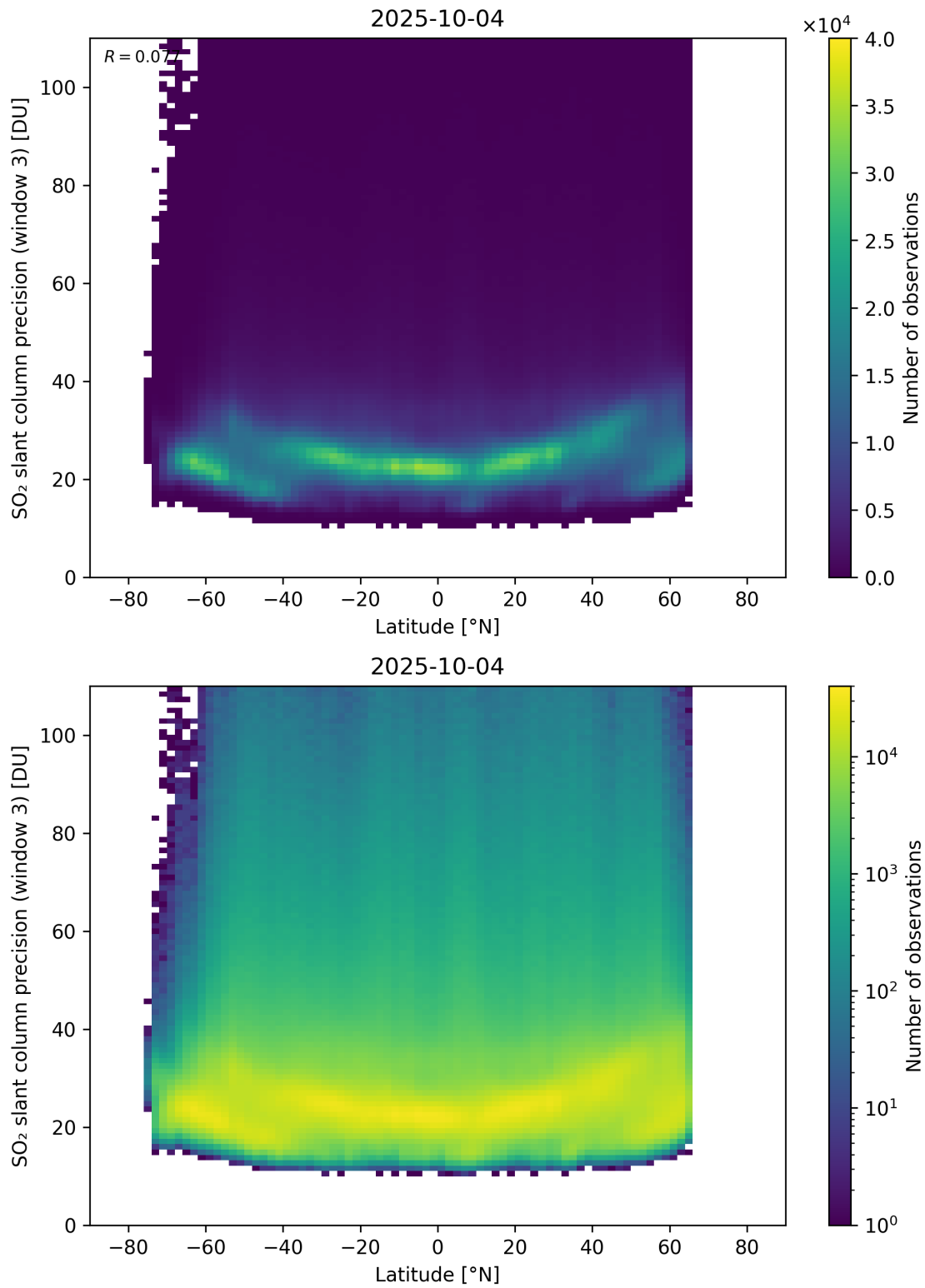
Figure 166: Scatter density plot of “Latitude” against “SO 2 slant column precision (window 3)” for 2025-10-03 to 2025-10-05.
