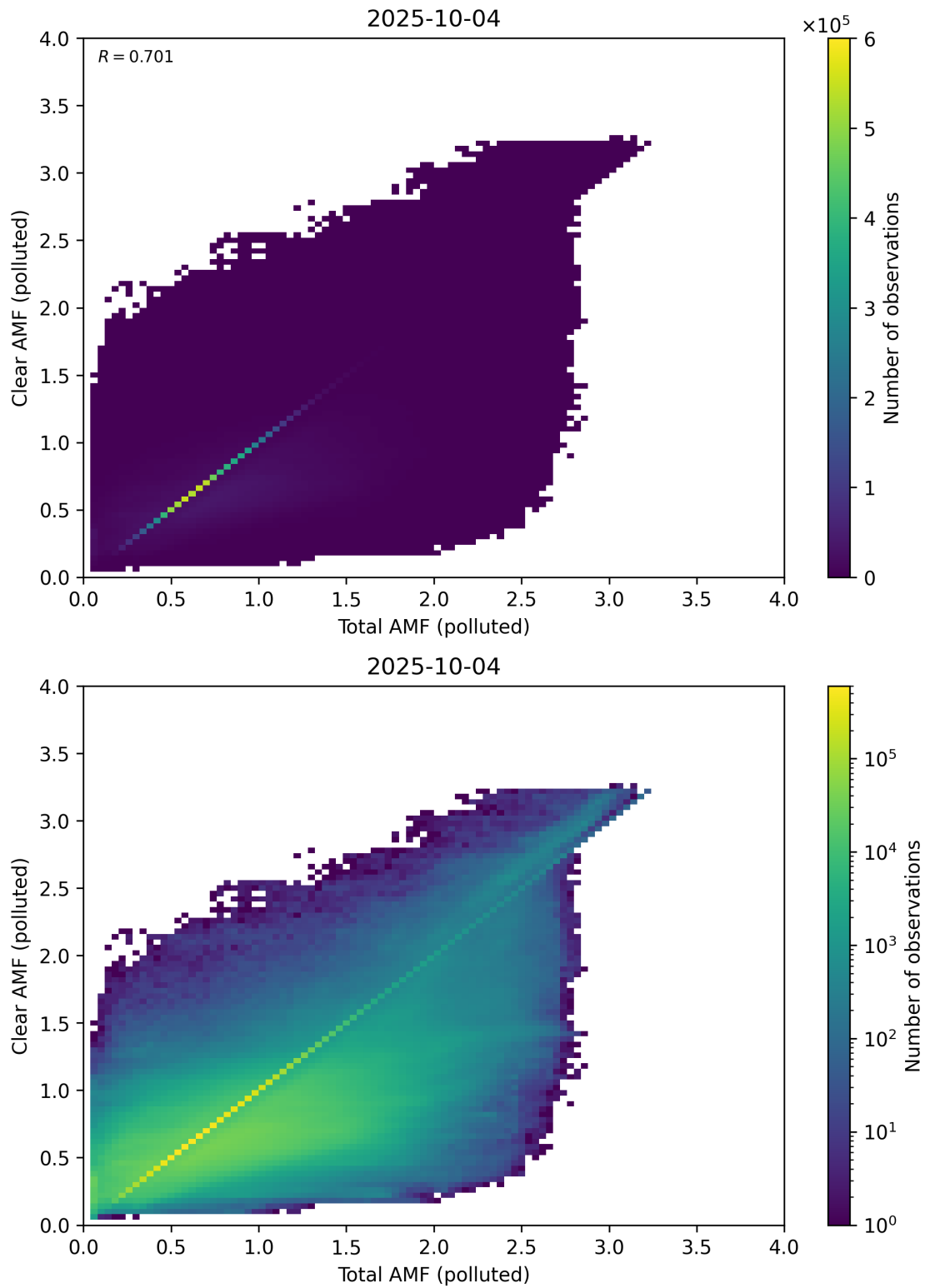
Figure 321: Scatter density plot of “Total AMF (polluted)” against “Clear AMF (polluted)” for 2025-10-03 to 2025-10-05.
