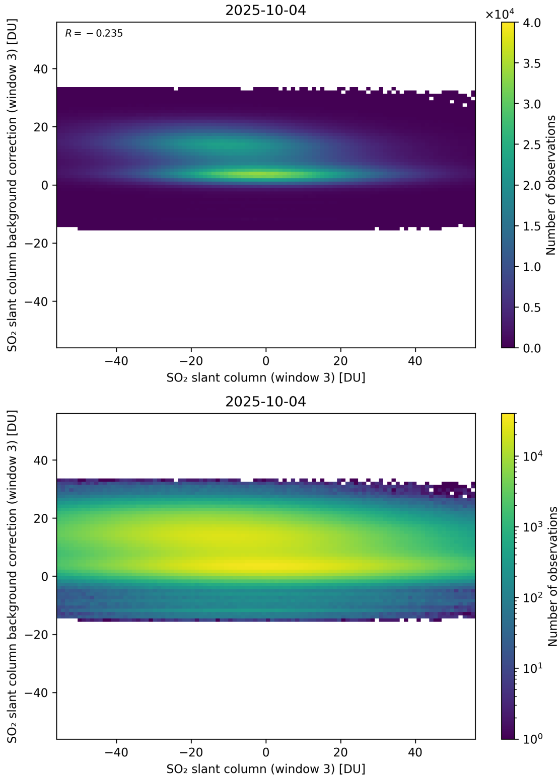
Figure 303: Scatter density plot of “SO 2 slant column (window 3)” against “SO 2 slant column background correction (window 3)” for 2025-10-03 to 2025-10-05.
