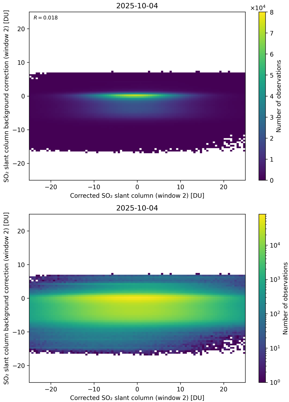
Figure 244: Scatter density plot of “Corrected SO 2 slant column (window 2)” against “SO 2 slant column background correction (window 2)” for 2025-10-03 to 2025-10-05.
