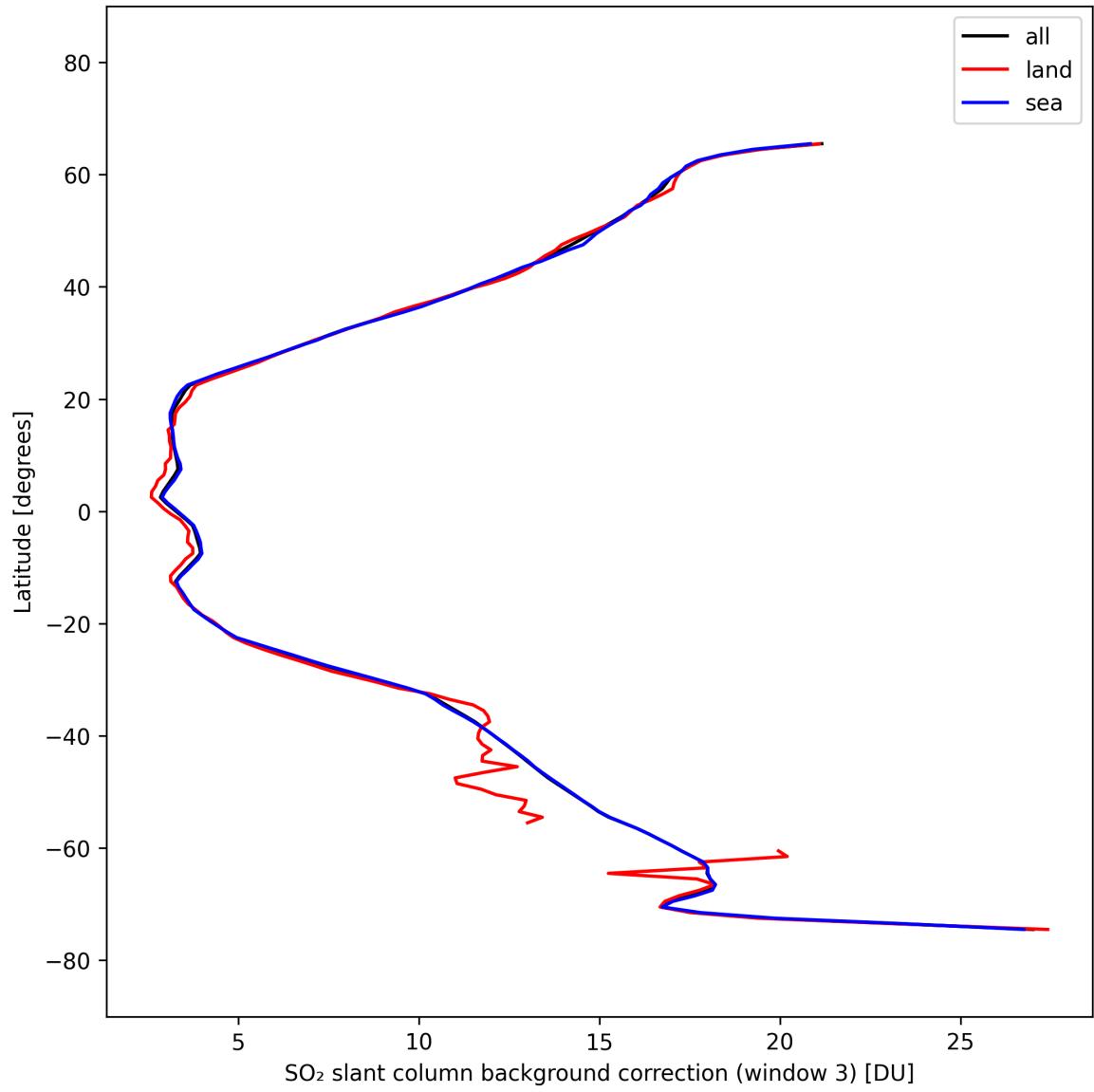
Figure 48: Zonal average of “SO 2 slant column background correction (window 3)” for 2025-10-03 to 2025-10-05.
