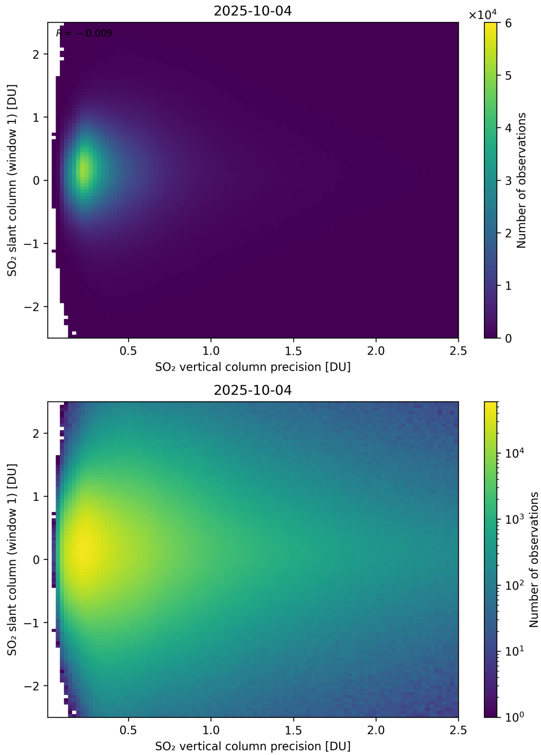
Figure 341: Scatter density plot of “SO 2 vertical column precision” against “SO 2 slant column (window 1)” for 2025-10-03 to 2025-10-05.
