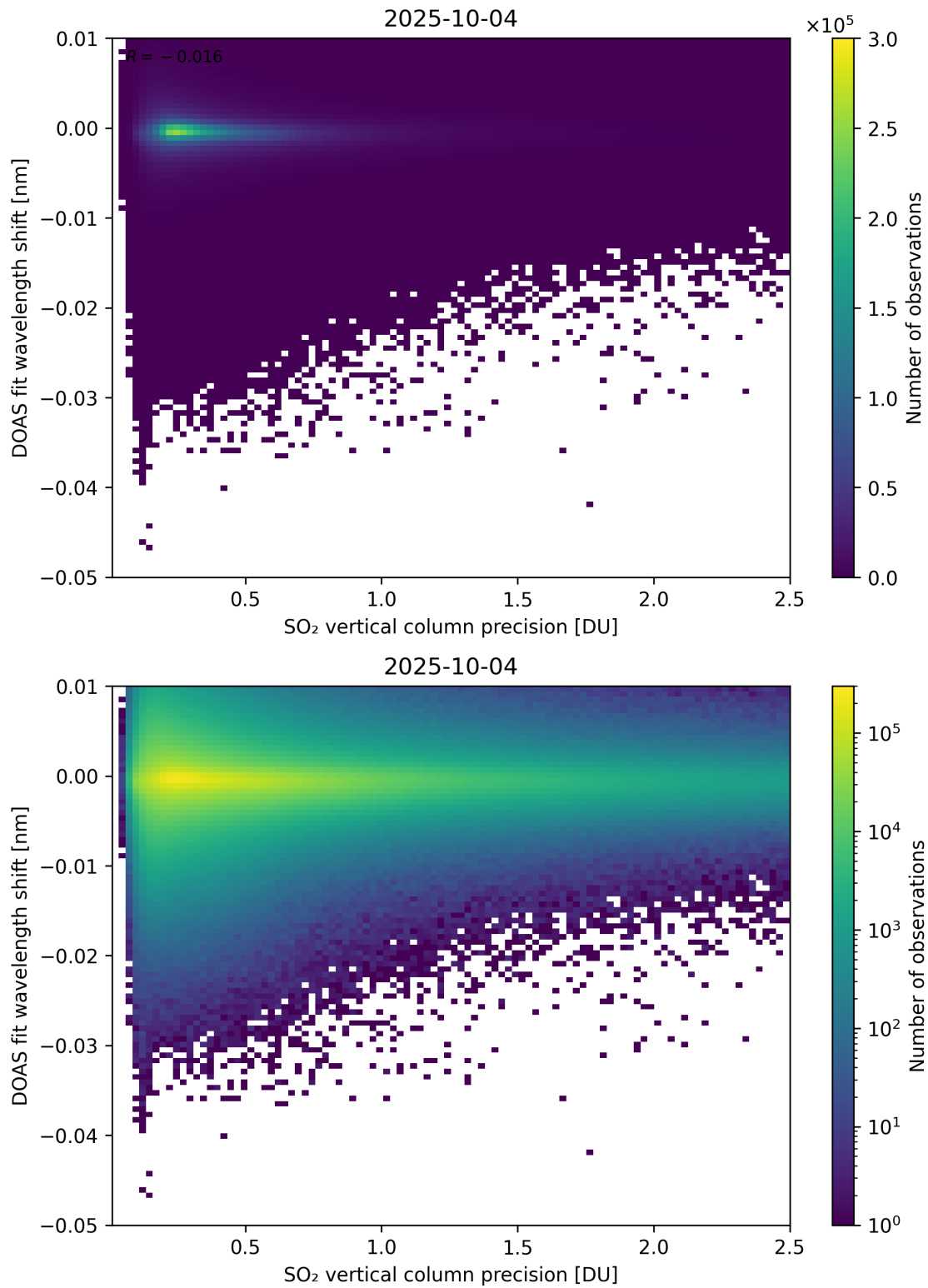
Figure 332: Scatter density plot of “SO 2 vertical column precision” against “DOAS fit wavelength shift” for 2025-10-03 to 2025-10-05.
