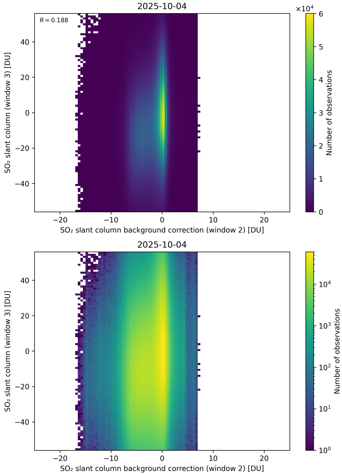
Figure 128: Scatter density plot of “SO 2 slant column background correction (window 2)” against “SO 2 slant column (window 3)” for 2025-10-03 to 2025-10-05.
