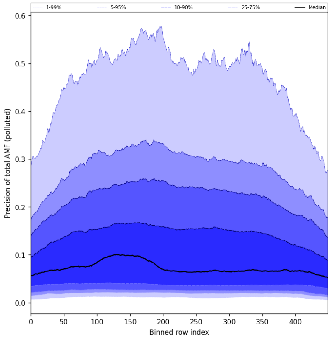
Figure 106: Along track statistics of “Precision of total AMF (polluted)” for 2025-10-03 to 2025-10-05
