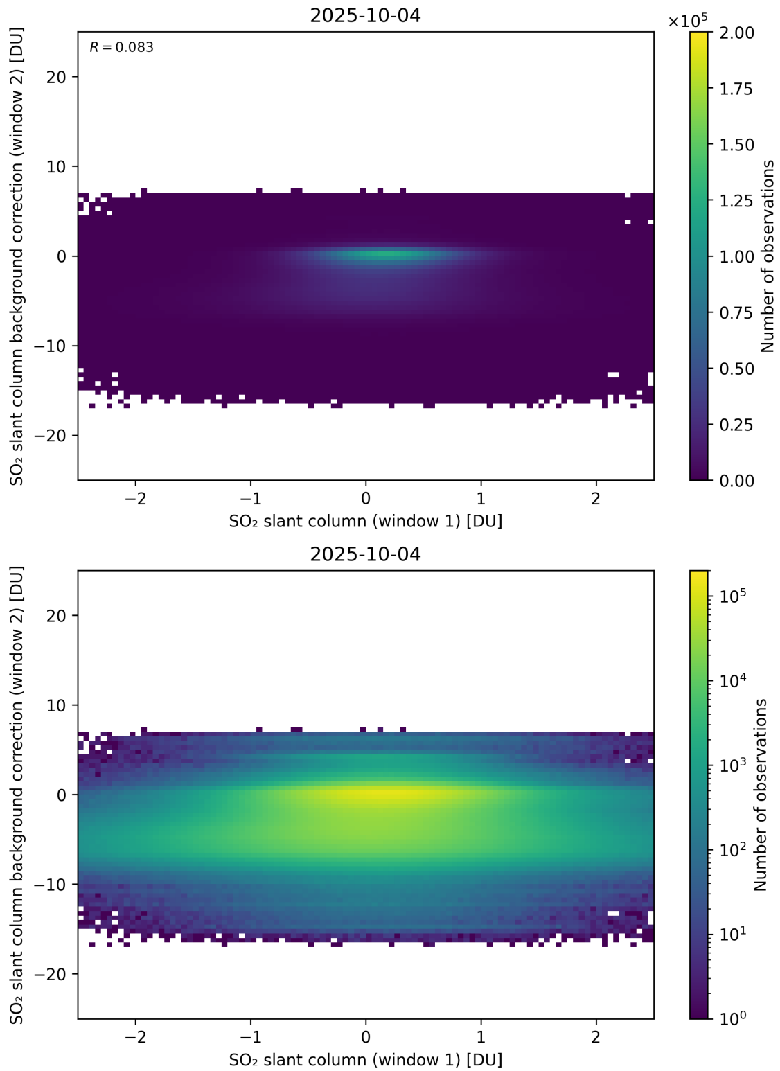
Figure 263: Scatter density plot of “SO 2 slant column (window 1)” against “SO 2 slant column background correction (window 2)” for 2025-10-03 to 2025-10-05.
