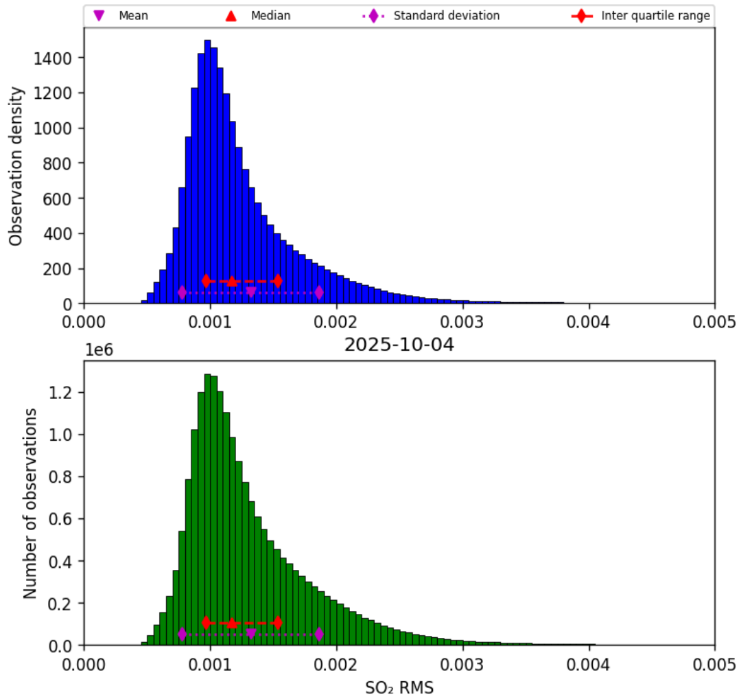
Figure 78: Histogram of “SO 2 RMS” for 2025-10-03 to 2025-10-05
