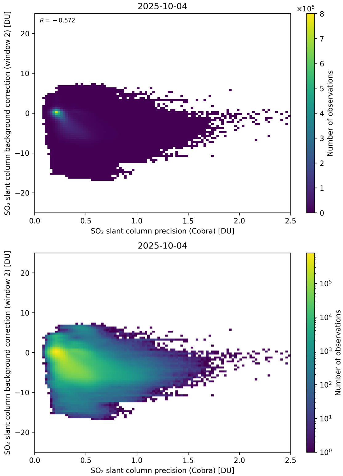
Figure 200: Scatter density plot of “SO 2 slant column precision (Cobra)” against “SO 2 slant column background correction (window 2)” for 2025-10-03 to 2025-10-05.
