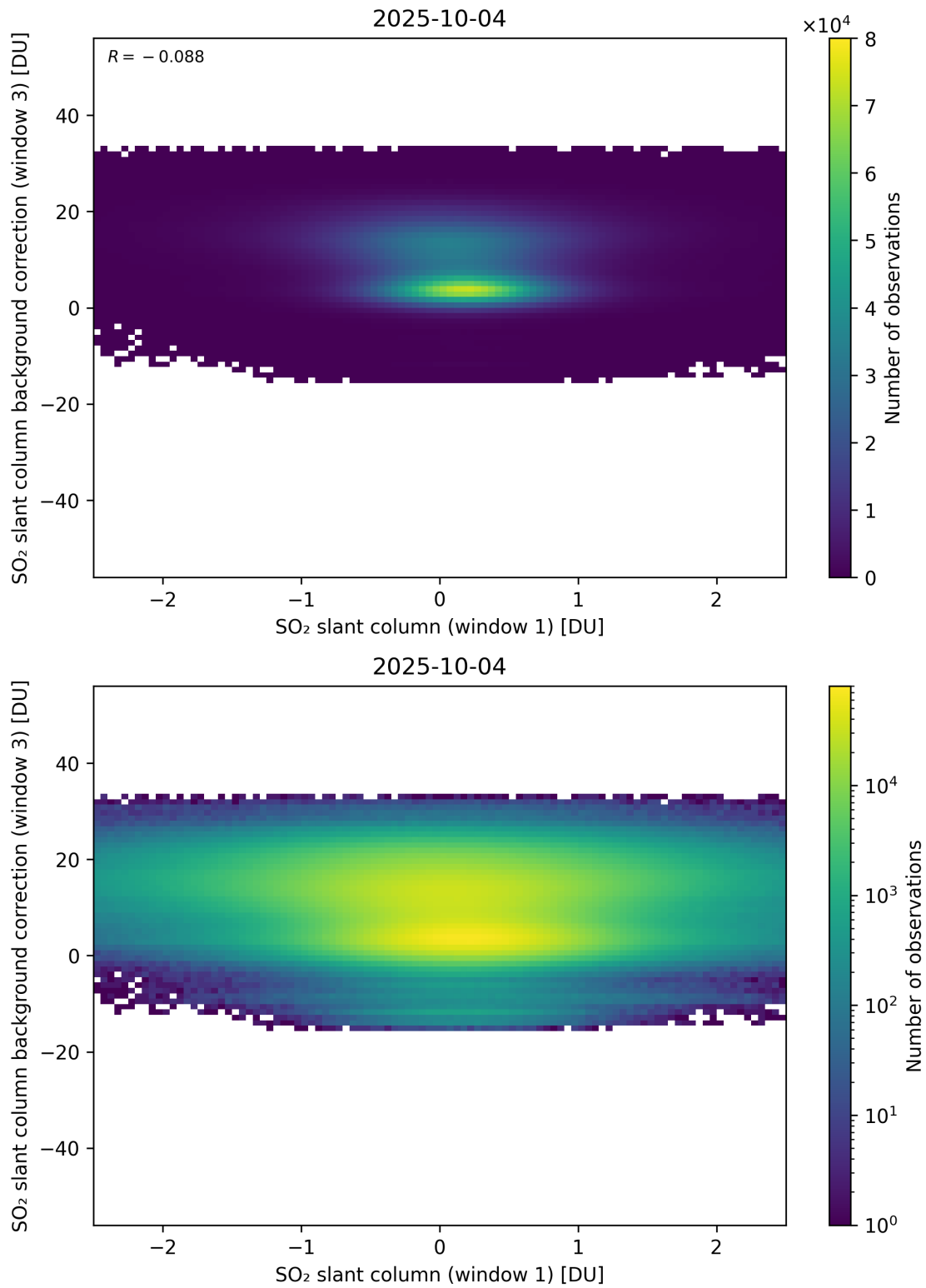
Figure 264: Scatter density plot of “SO 2 slant column (window 1)” against “SO 2 slant column background correction (window 3)” for 2025-10-03 to 2025-10-05.
