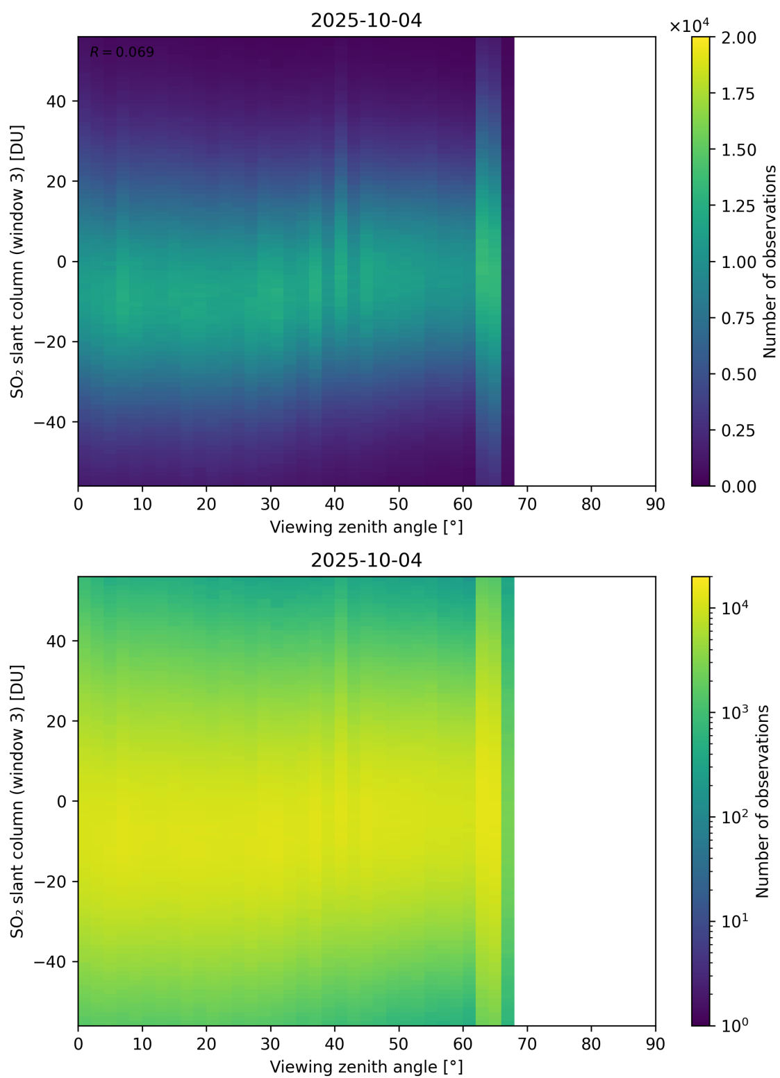
Figure 379: Scatter density plot of “Viewing zenith angle” against “SO 2 slant column (window 3)” for 2025-10-03 to 2025-10-05.
