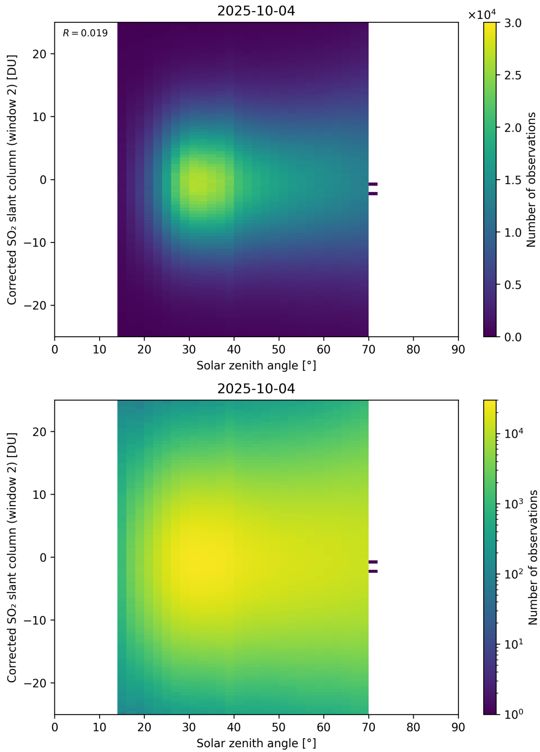
Figure 182: Scatter density plot of “Solar zenith angle” against “Corrected SO 2 slant column (window 2)” for 2025-10-03 to 2025-10-05.
