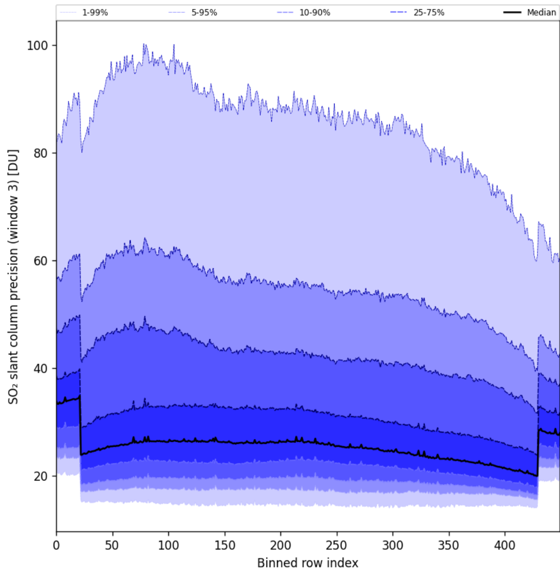
Figure 98: Along track statistics of “SO 2 slant column precision (window 3)” for 2025-10-03 to 2025-10-05
