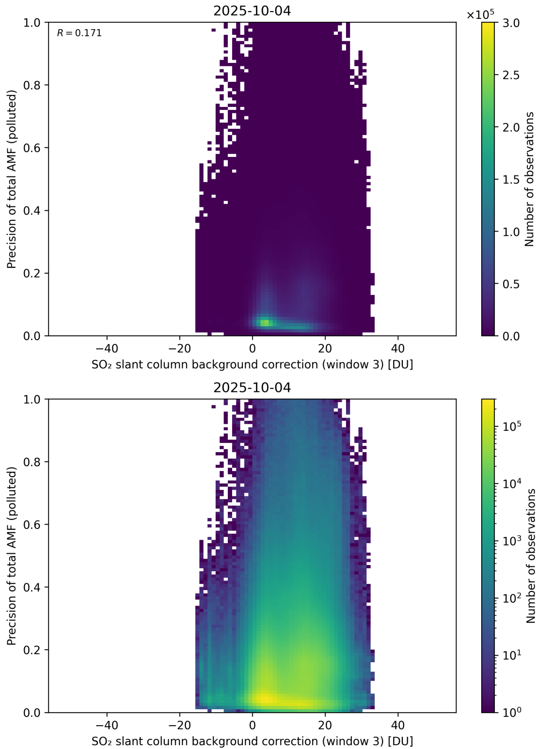
Figure 137: Scatter density plot of “SO 2 slant column background correction (window 3)” against “Precision of total AMF (polluted)” for 2025-10-03 to 2025-10-05.
