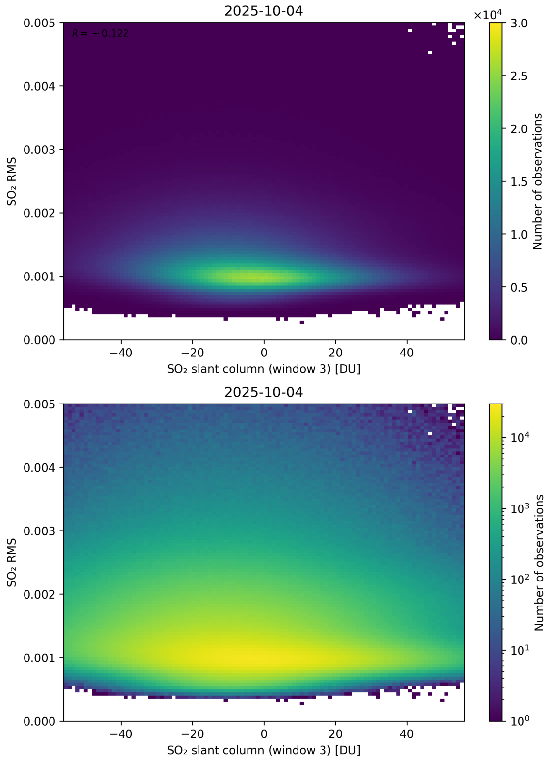
Figure 306: Scatter density plot of “SO 2 slant column (window 3)” against “SO 2 RMS” for 2025-10-03 to 2025-10-05.
