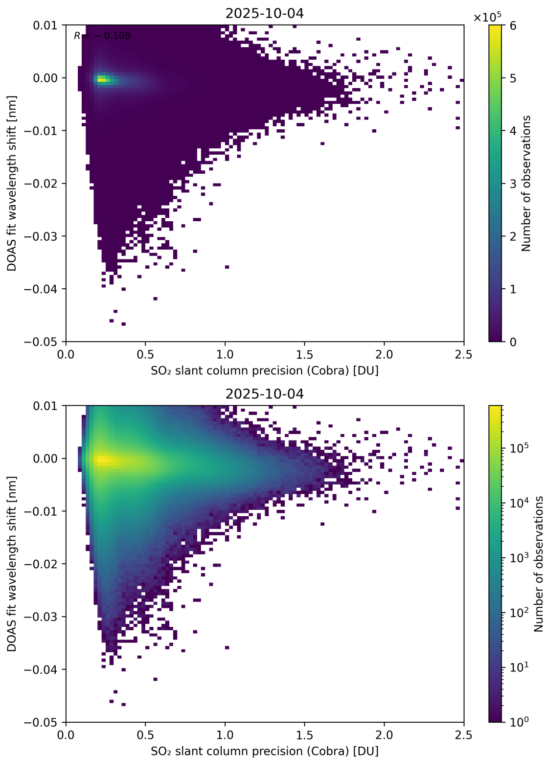
Figure 202: Scatter density plot of “SO 2 slant column precision (Cobra)” against “DOAS fit wavelength shift” for 2025-10-03 to 2025-10-05.
