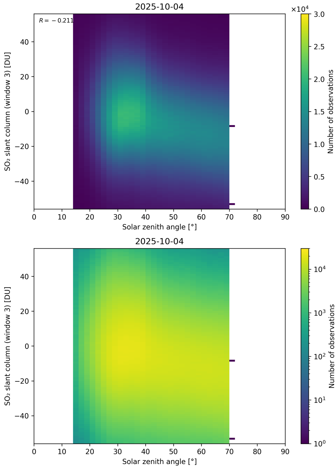
Figure 187: Scatter density plot of “Solar zenith angle” against “SO 2 slant column (window 3)” for 2025-10-03 to 2025-10-05.
