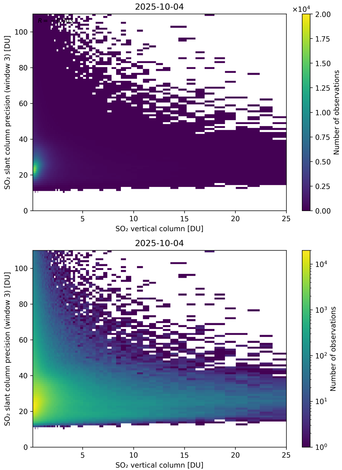
Figure 358: Scatter density plot of “SO 2 vertical column” against “SO 2 slant column precision (window 3)” for 2025-10-03 to 2025-10-05.
