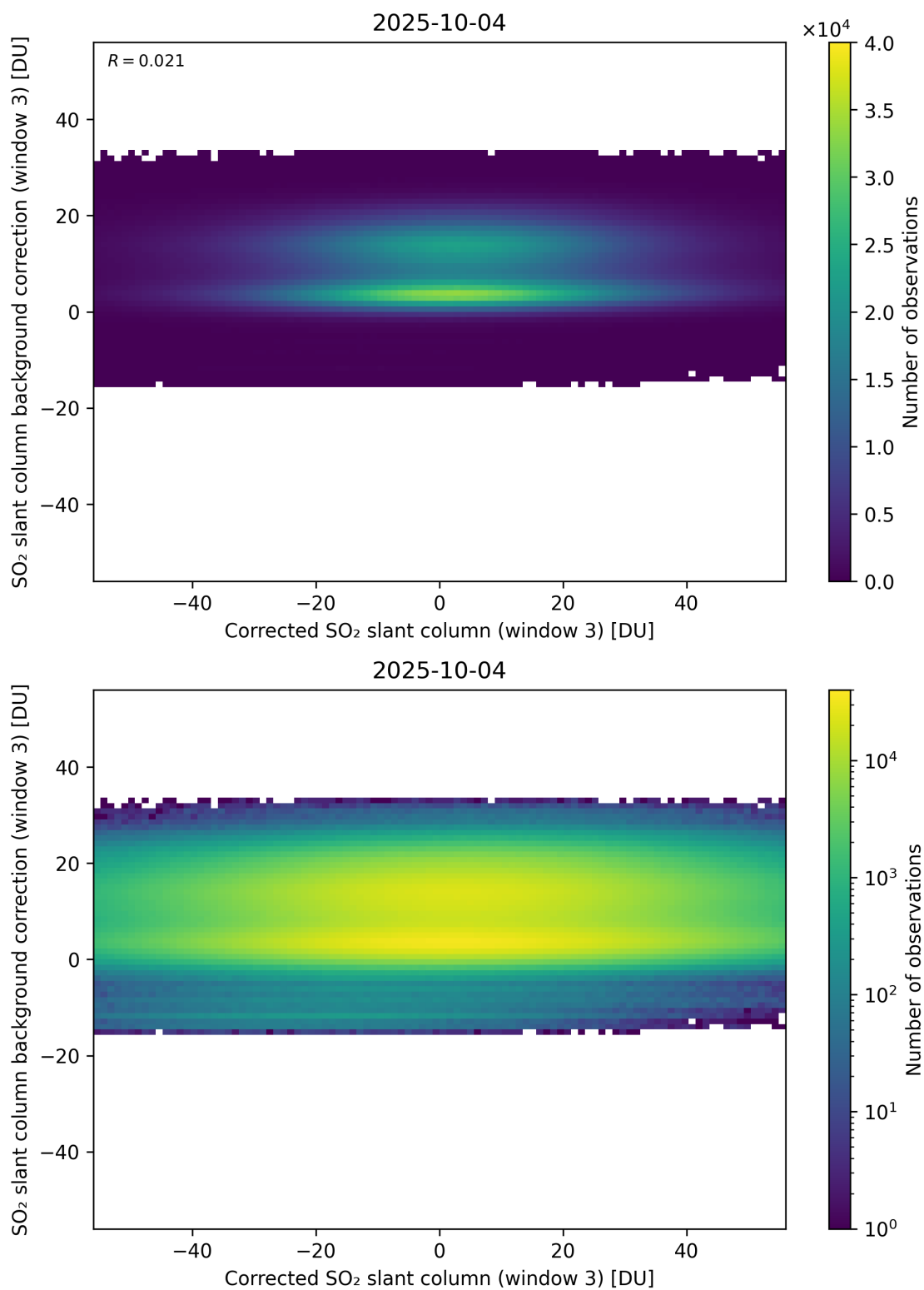
Figure 255: Scatter density plot of “Corrected SO 2 slant column (window 3)” against “SO 2 slant column background correction (window 3)” for 2025-10-03 to 2025-10-05.
