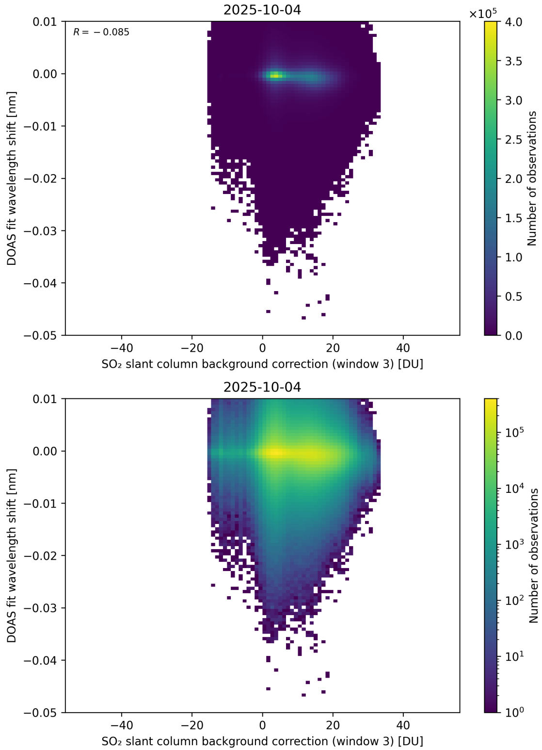
Figure 132: Scatter density plot of “SO 2 slant column background correction (window 3)” against “DOAS fit wavelength shift” for 2025-10-03 to 2025-10-05.
