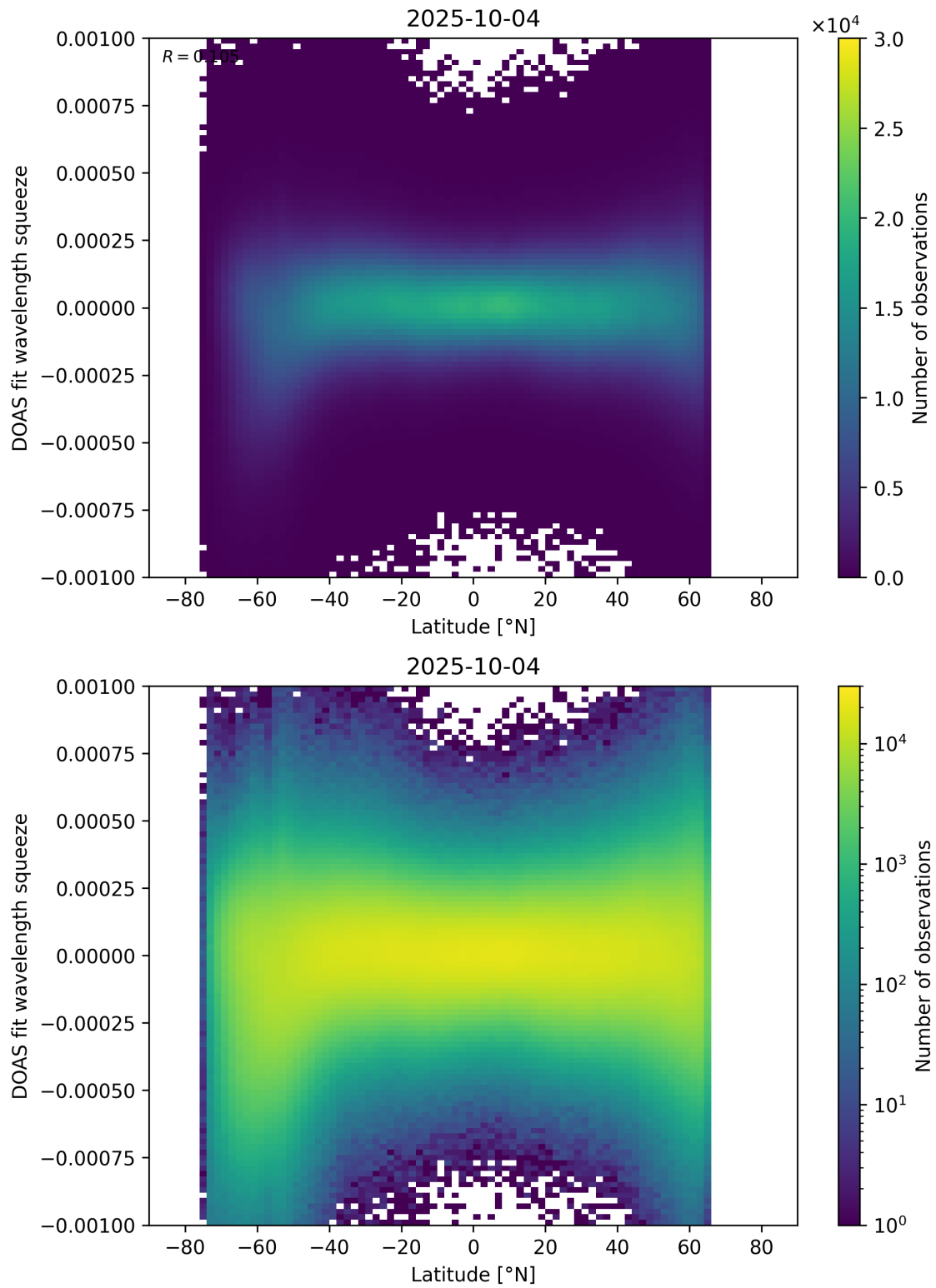
Figure 154: Scatter density plot of “Latitude” against “DOAS fit wavelength squeeze” for 2025-10-03 to 2025-10-05.
