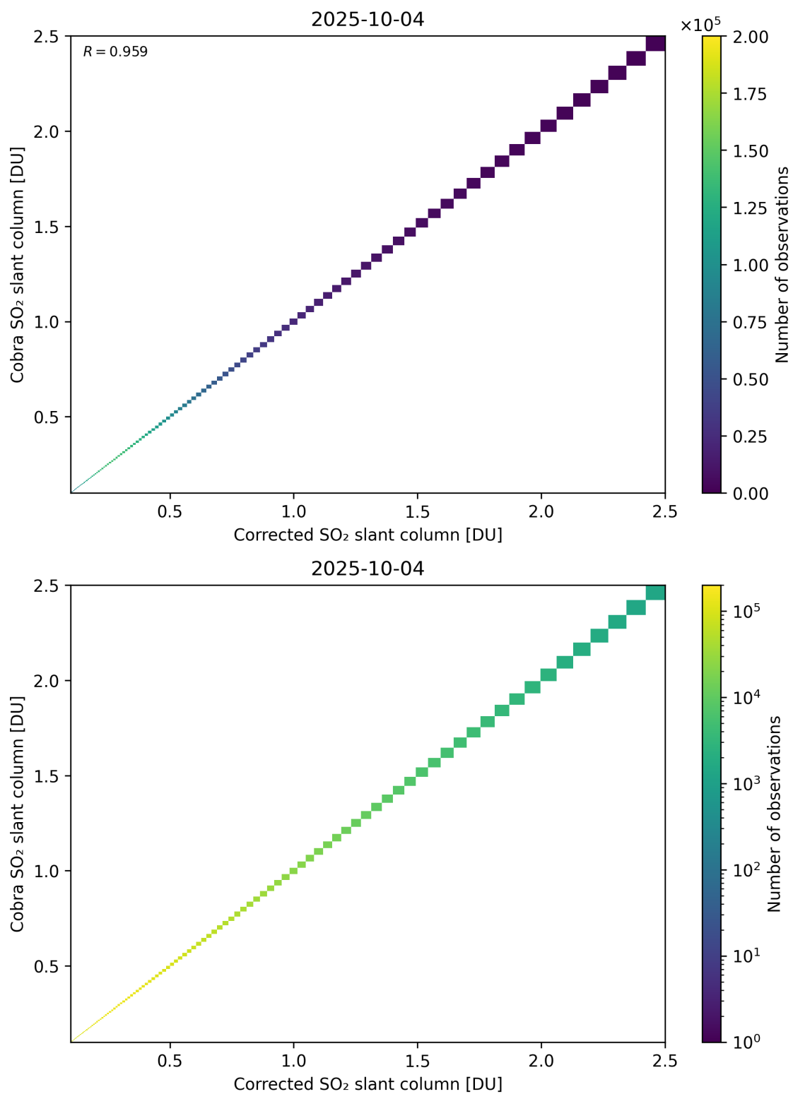
Figure 233: Scatter density plot of “Corrected SO 2 slant column” against “Cobra SO 2 slant column” for 2025-10-03 to 2025-10-05.
