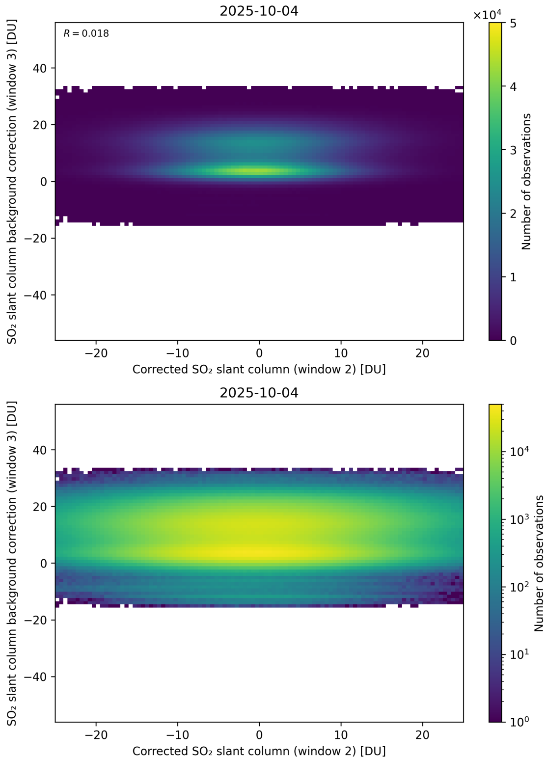
Figure 245: Scatter density plot of “Corrected SO 2 slant column (window 2)” against “SO 2 slant column background correction (window 3)” for 2025-10-03 to 2025-10-05.
