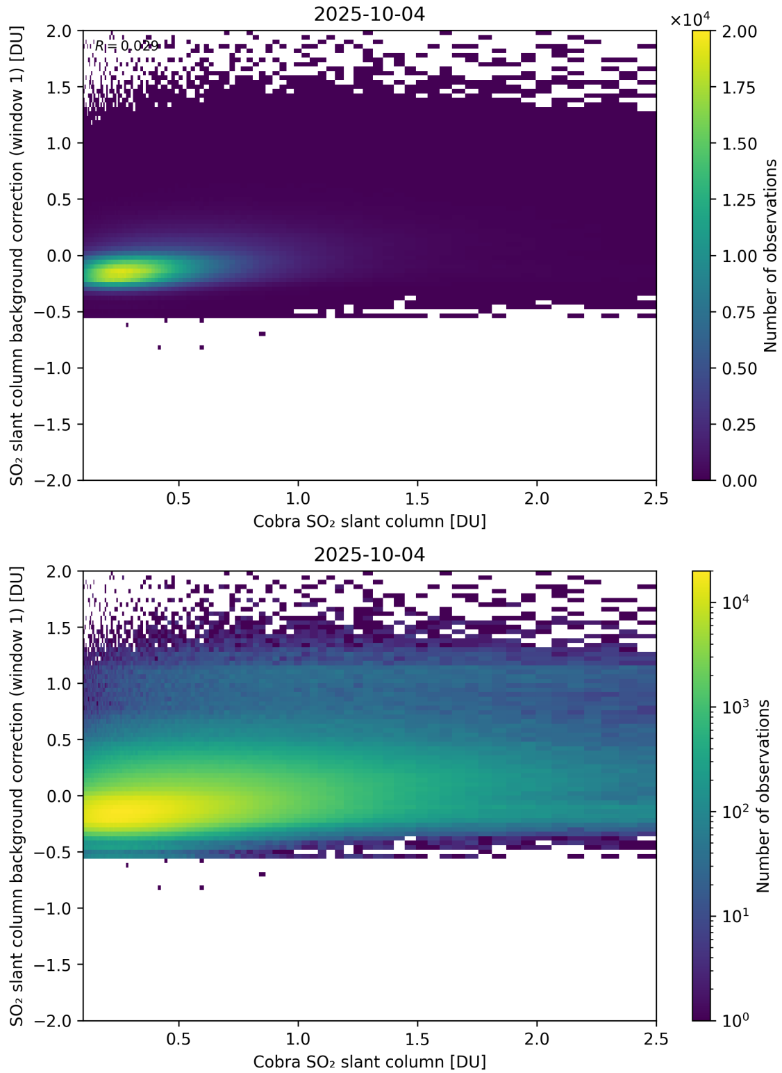
Figure 193: Scatter density plot of “Cobra SO 2 slant column” against “SO 2 slant column background correction (window 1)” for 2025-10-03 to 2025-10-05.
