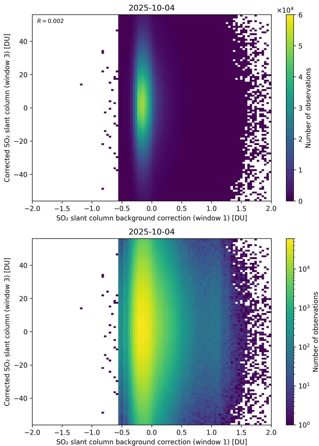
Figure 116: Scatter density plot of “SO 2 slant column background correction (window 1)” against “Corrected SO 2 slant column (window 3)” for 2025-10-03 to 2025-10-05.
