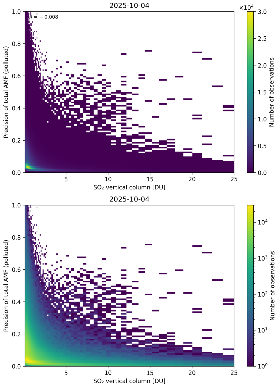
Figure 360: Scatter density plot of “SO 2 vertical column” against “Precision of total AMF (polluted)” for 2025-10-03 to 2025-10-05.
