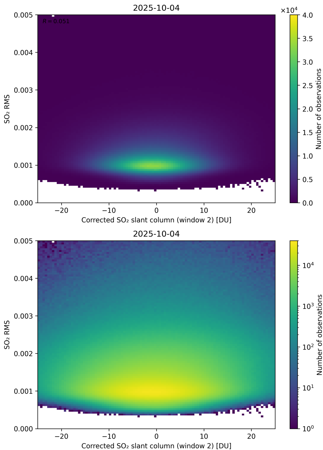
Figure 248: Scatter density plot of “Corrected SO 2 slant column (window 2)” against “SO 2 RMS” for 2025-10-03 to 2025-10-05.
