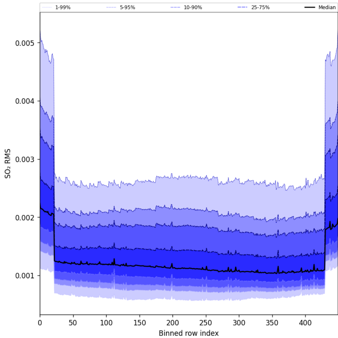
Figure 104: Along track statistics of “SO 2 RMS” for 2025-10-03 to 2025-10-05
