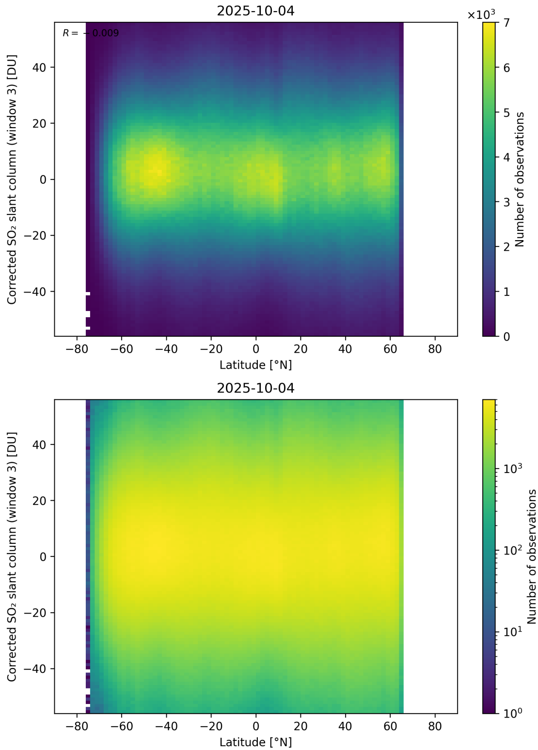
Figure 161: Scatter density plot of “Latitude” against “Corrected SO 2 slant column (window 3)” for 2025-10-03 to 2025-10-05.
