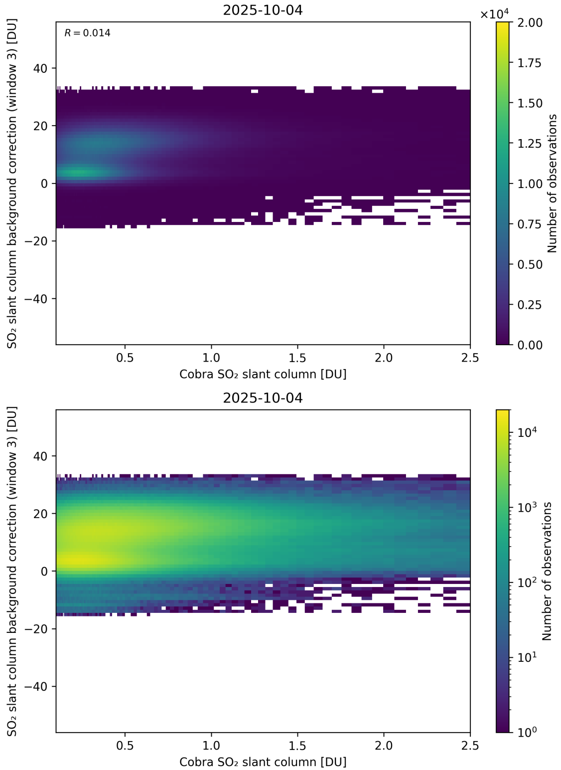
Figure 195: Scatter density plot of “Cobra SO 2 slant column” against “SO 2 slant column background correction (window 3)” for 2025-10-03 to 2025-10-05.
