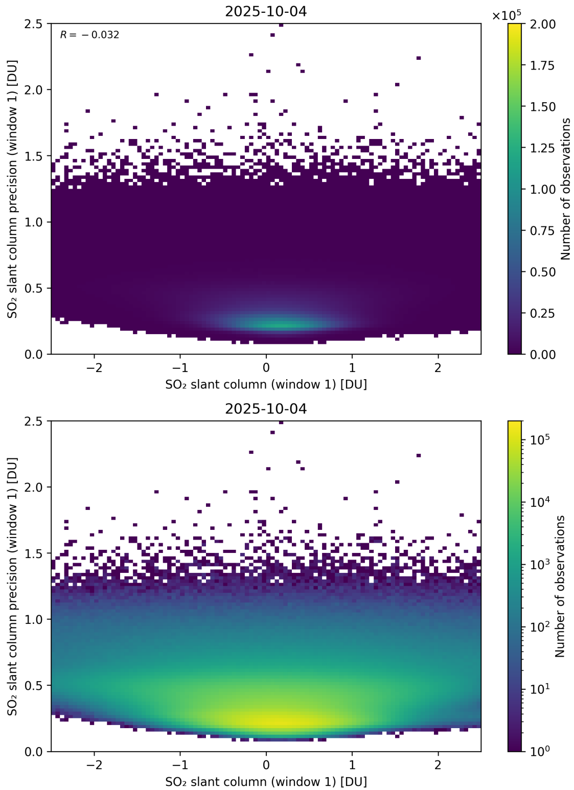
Figure 285: Scatter density plot of “SO 2 slant column (window 1)” against “SO 2 slant column precision (window 1)” for 2025-10-03 to 2025-10-05.
