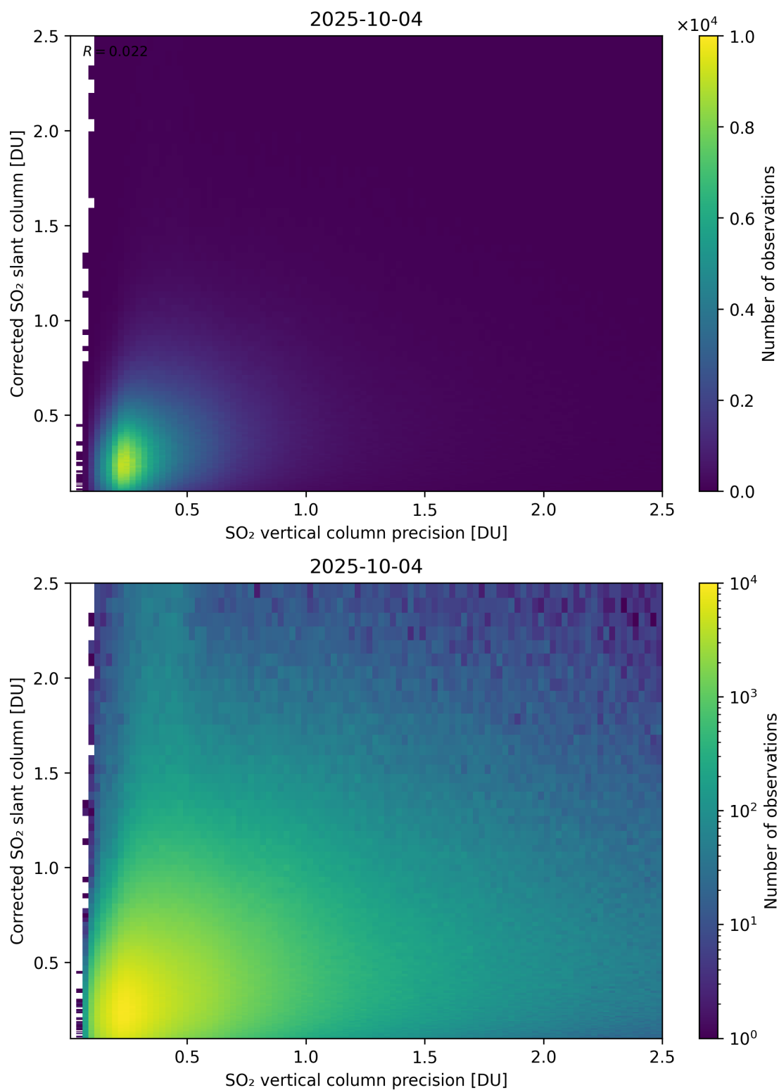
Figure 338: Scatter density plot of “SO 2 vertical column precision” against “Corrected SO 2 slant column” for 2025-10-03 to 2025-10-05.
