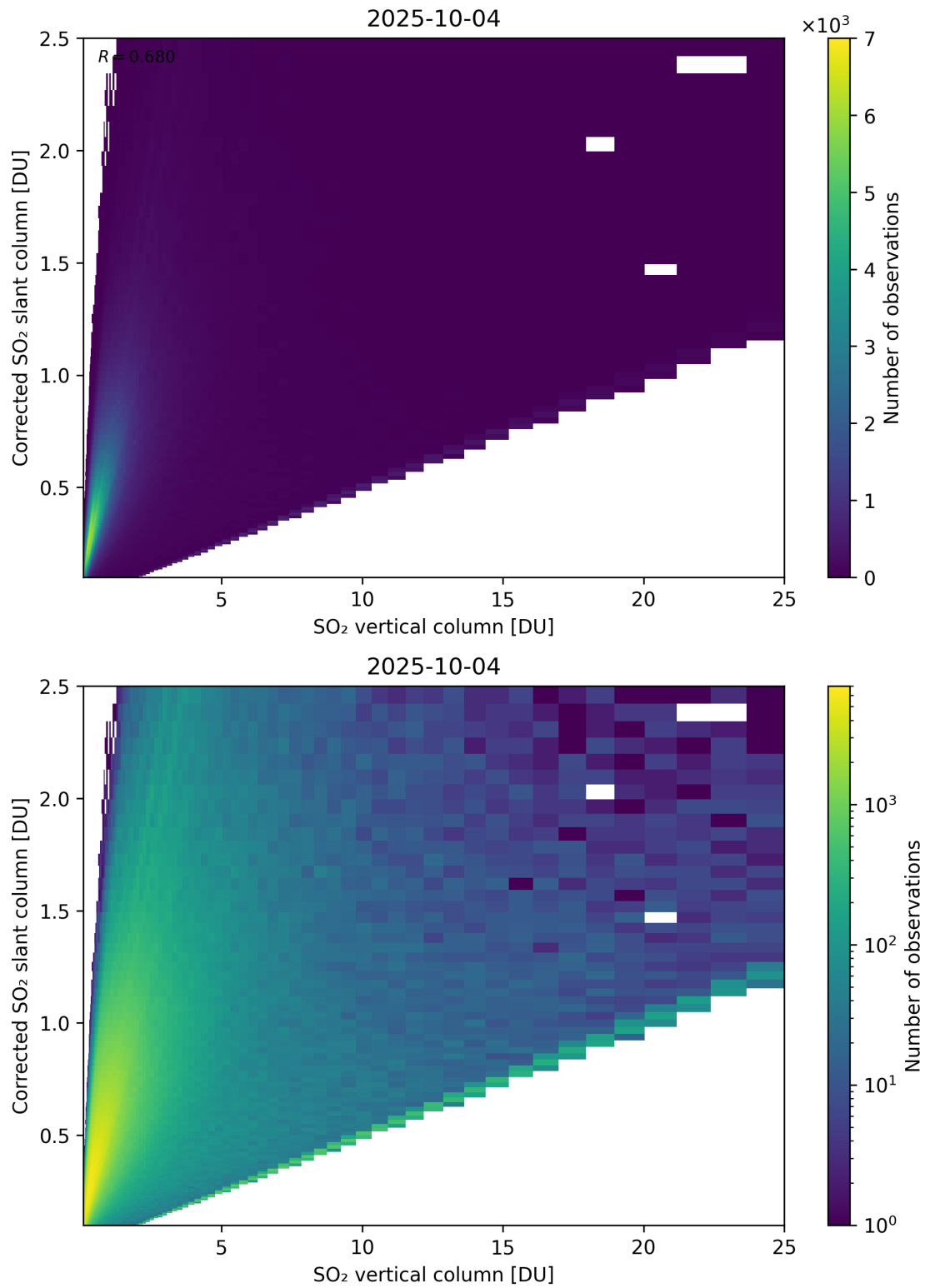
Figure 351: Scatter density plot of “SO 2 vertical column” against “Corrected SO 2 slant column” for 2025-10-03 to 2025-10-05.
