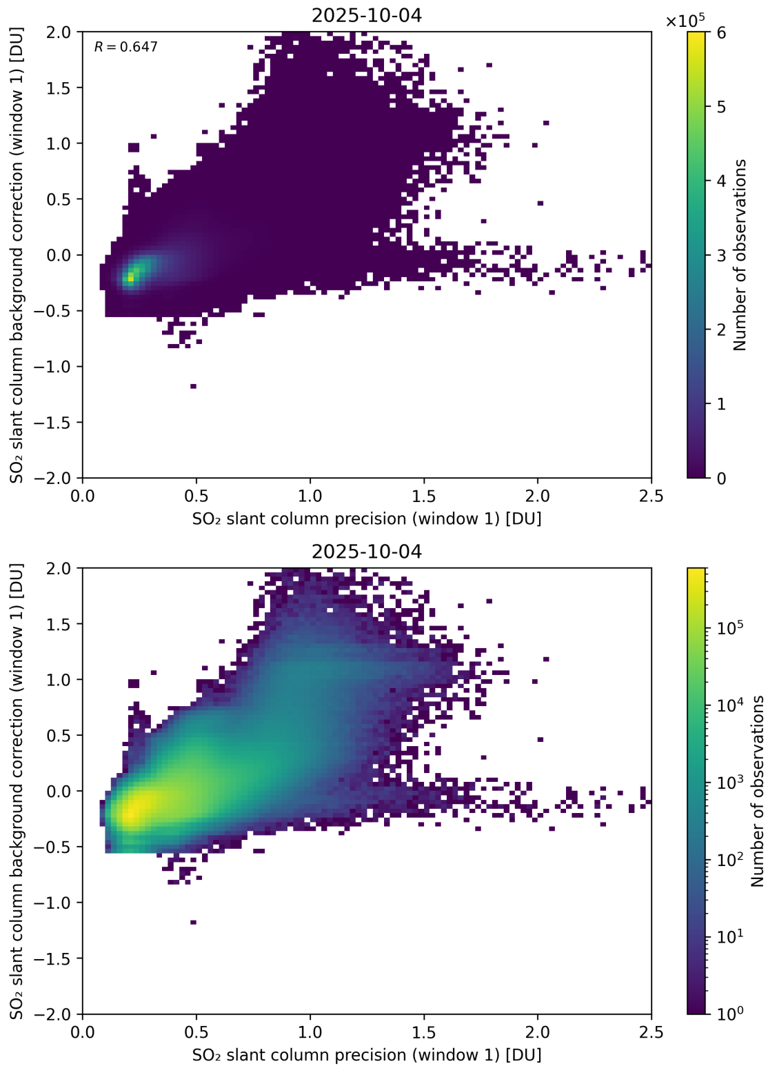
Figure 268: Scatter density plot of “SO 2 slant column precision (window 1)” against “SO 2 slant column background correction (window 1)” for 2025-10-03 to 2025-10-05.
