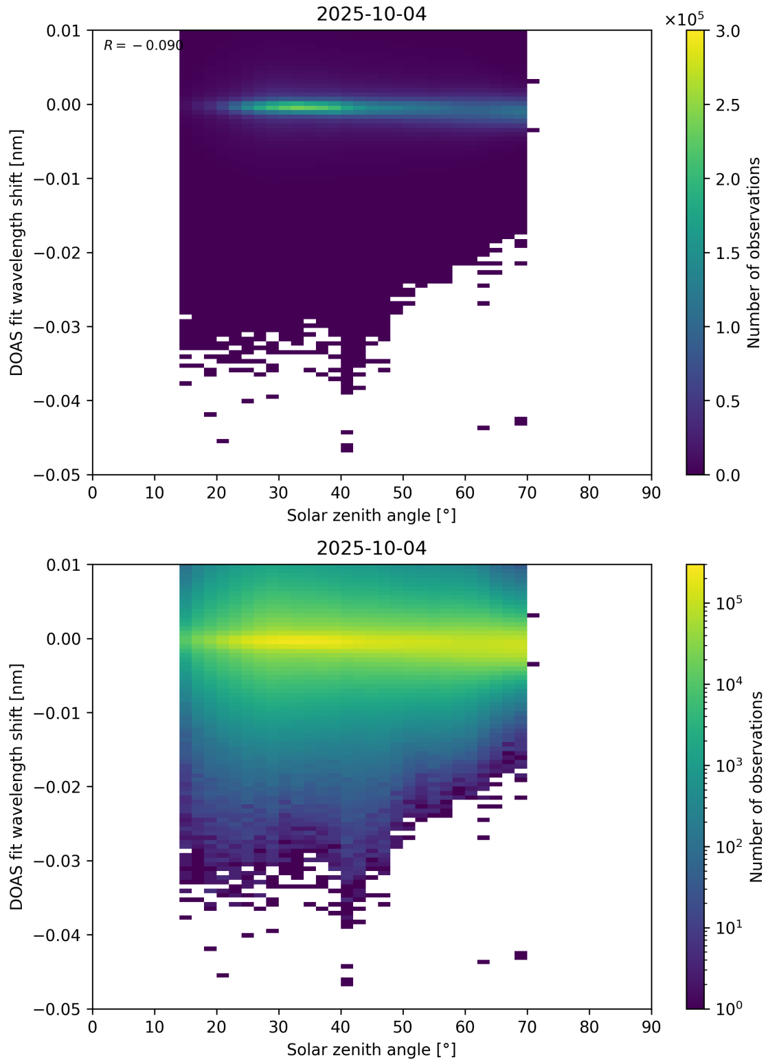
Figure 174: Scatter density plot of “Solar zenith angle” against “DOAS fit wavelength shift” for 2025-10-03 to 2025-10-05.
