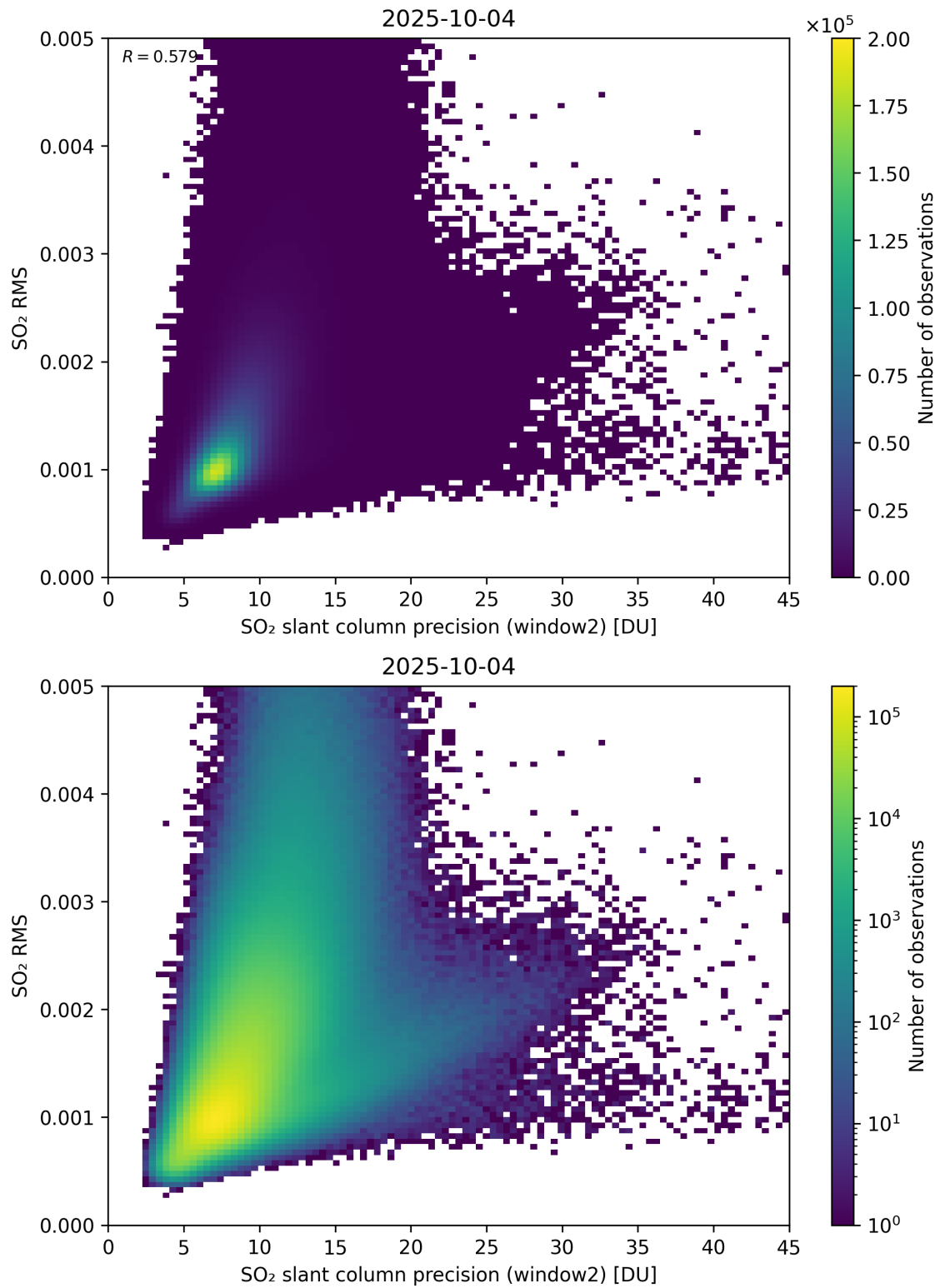
Figure 295: Scatter density plot of “SO 2 slant column precision (window2)” against “SO 2 RMS” for 2025-10-03 to 2025-10-05.
