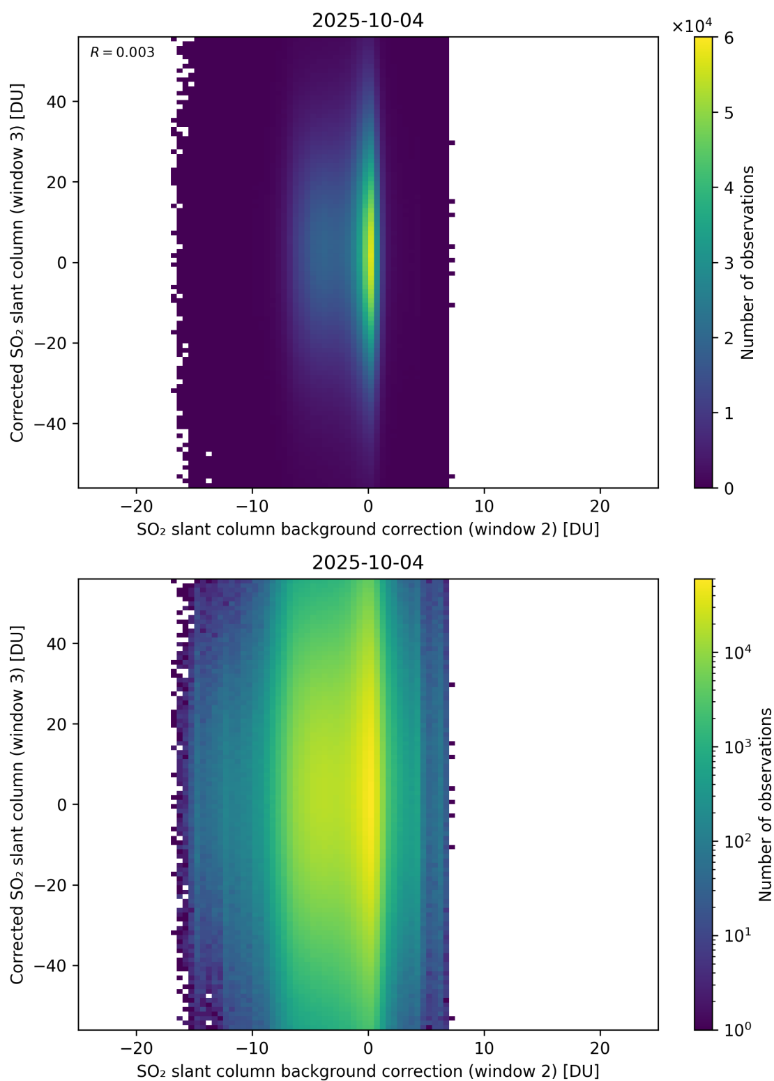
Figure 127: Scatter density plot of “SO 2 slant column background correction (window 2)” against “Corrected SO 2 slant column (window 3)” for 2025-10-03 to 2025-10-05.
