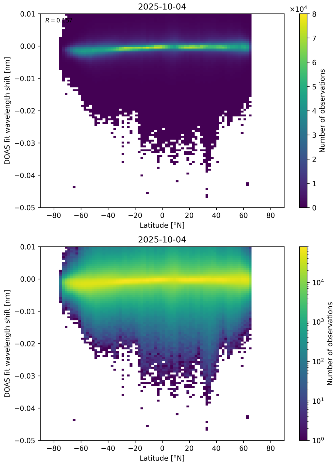
Figure 153: Scatter density plot of “Latitude” against “DOAS fit wavelength shift” for 2025-10-03 to 2025-10-05.
