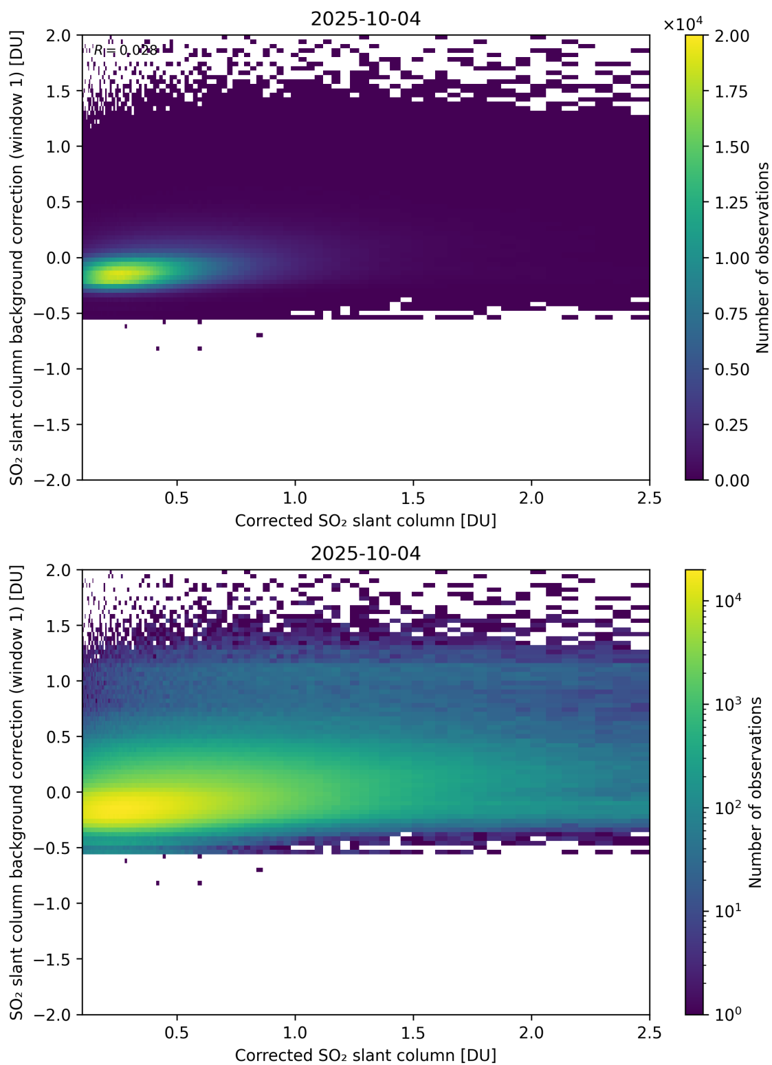
Figure 226: Scatter density plot of “Corrected SO 2 slant column” against “SO 2 slant column background correction (window 1)” for 2025-10-03 to 2025-10-05.
