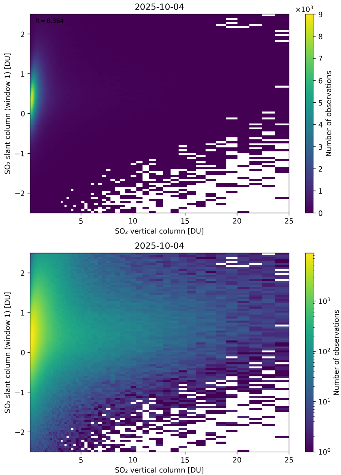
Figure 354: Scatter density plot of “SO 2 vertical column” against “SO 2 slant column (window 1)” for 2025-10-03 to 2025-10-05.
