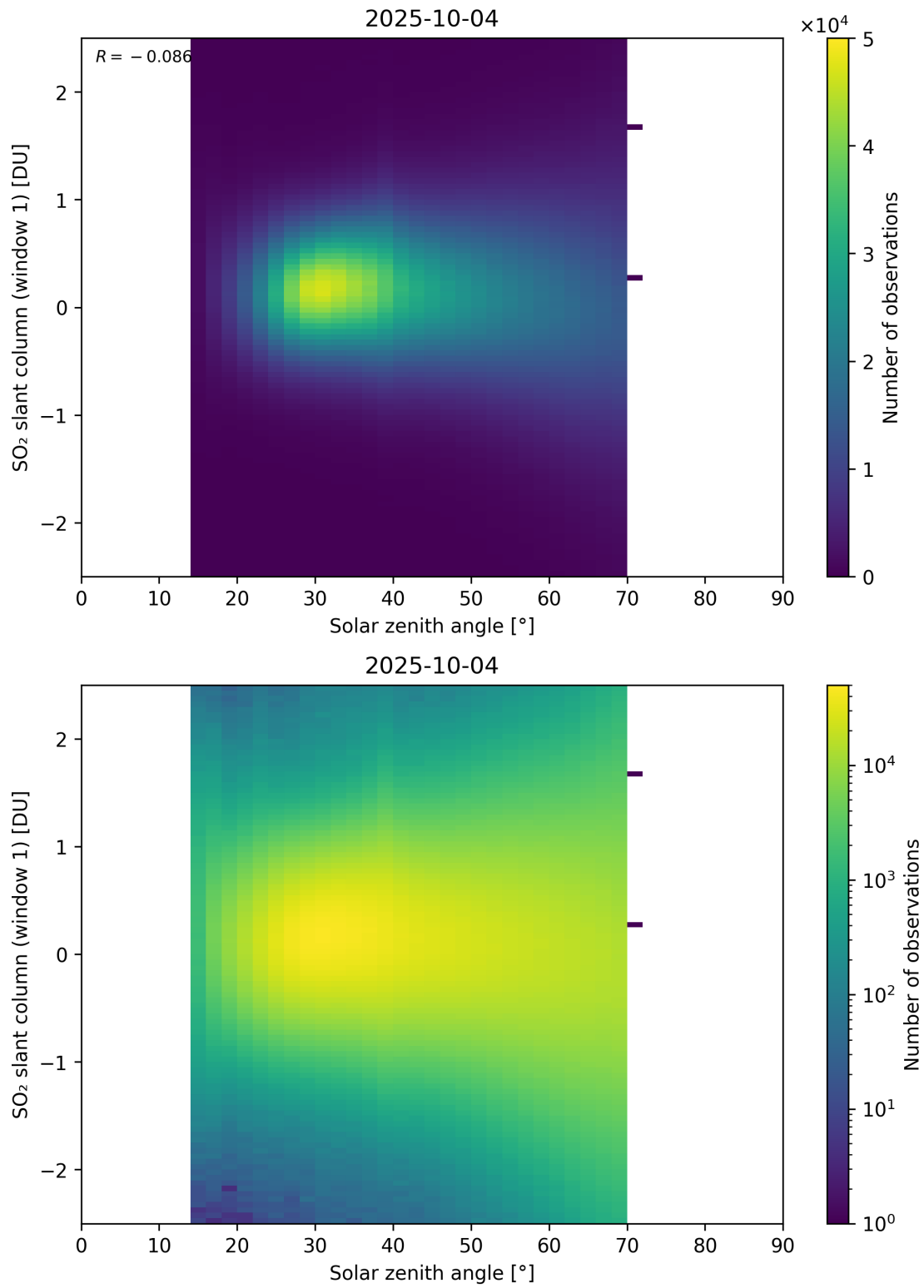
Figure 184: Scatter density plot of “Solar zenith angle” against “SO 2 slant column (window 1)” for 2025-10-03 to 2025-10-05.
