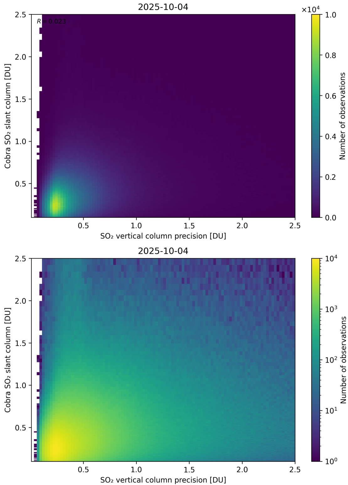
Figure 336: Scatter density plot of “SO 2 vertical column precision” against “Cobra SO 2 slant column” for 2025-10-03 to 2025-10-05.
