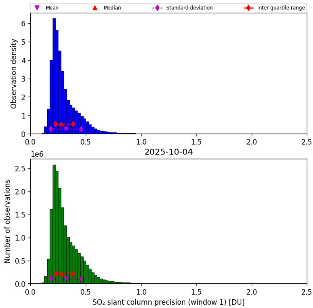
Figure 64: Histogram of “SO 2 slant column precision (window 1)” for 2025-10-03 to 2025-10-05
