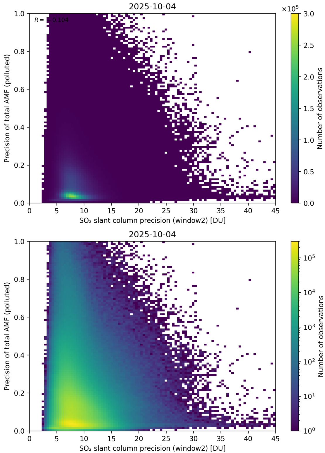
Figure 302: Scatter density plot of “SO 2 slant column precision (window2)” against “Precision of total AMF (polluted)” for 2025-10-03 to 2025-10-05.
