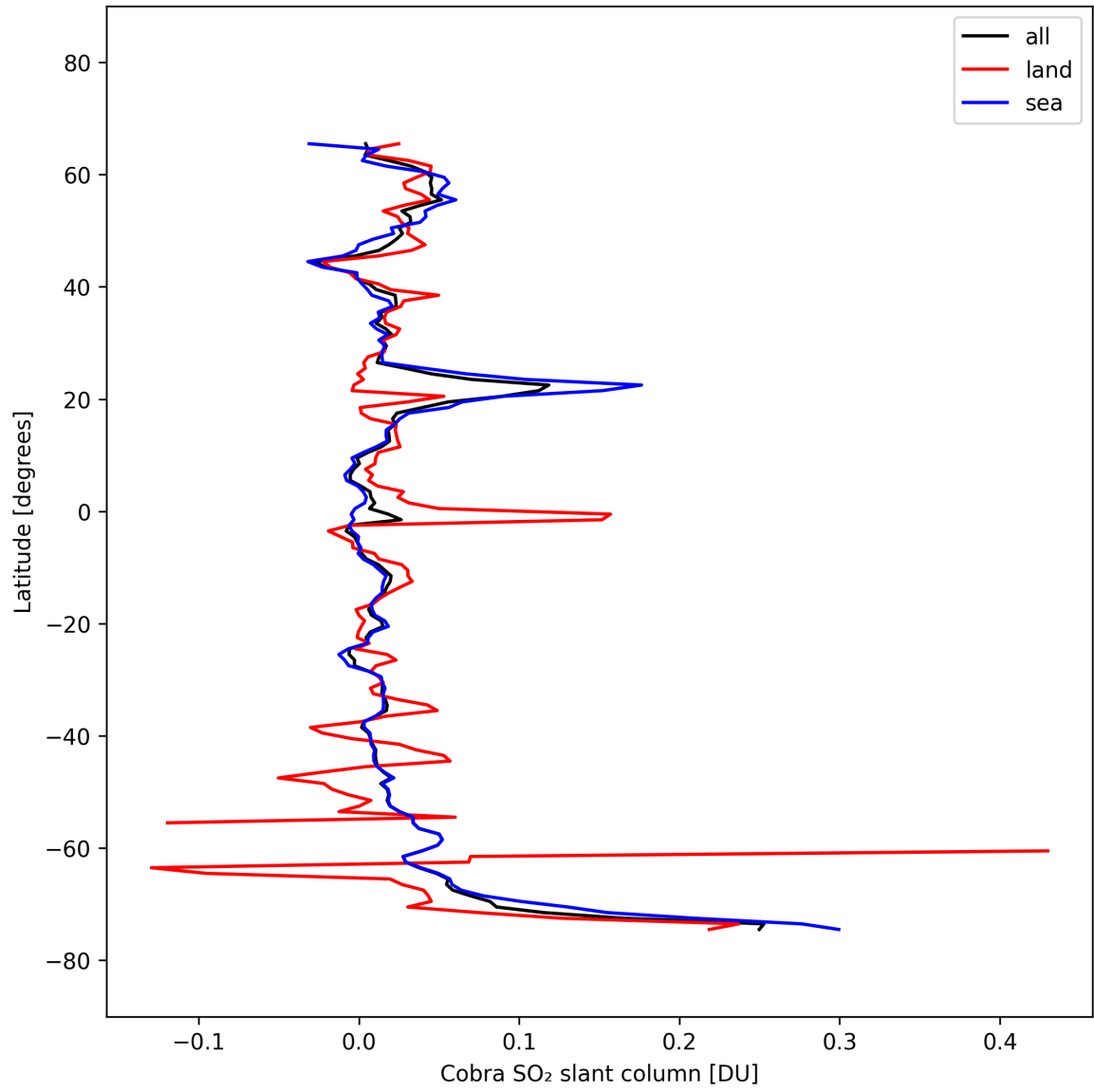
Figure 35: Zonal average of “Cobra SO 2 slant column” for 2025-10-03 to 2025-10-05.
