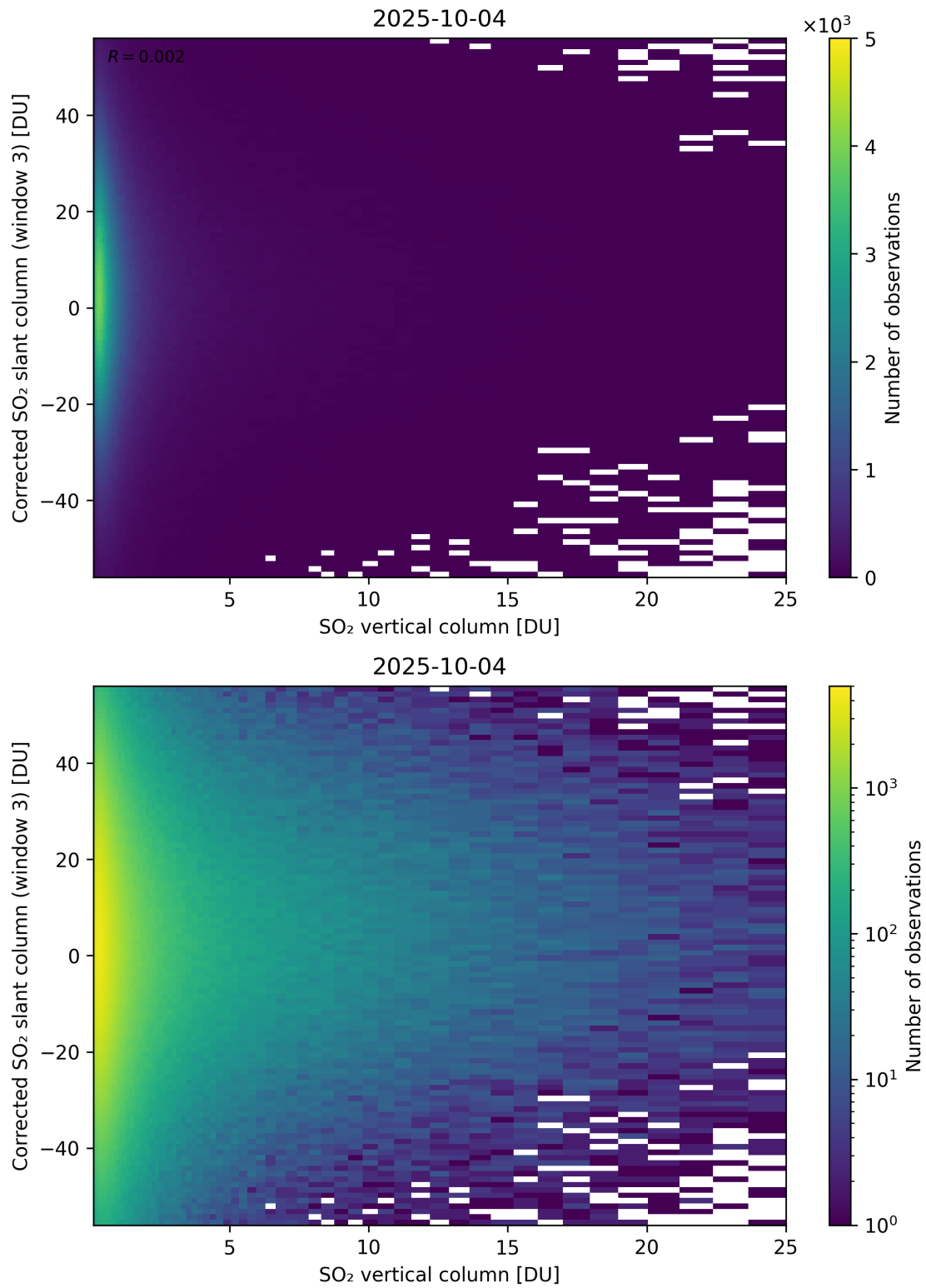
Figure 353: Scatter density plot of “SO 2 vertical column” against “Corrected SO 2 slant column (window 3)” for 2025-10-03 to 2025-10-05.
