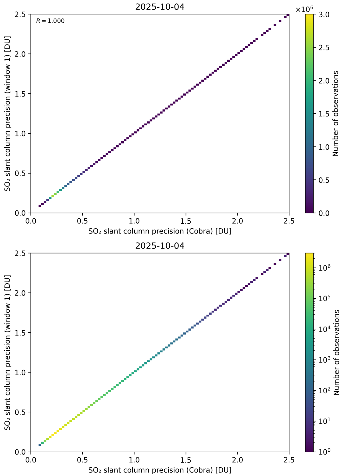
Figure 209: Scatter density plot of “SO 2 slant column precision (Cobra)” against “SO 2 slant column precision (window 1)” for 2025-10-03 to 2025-10-05.
