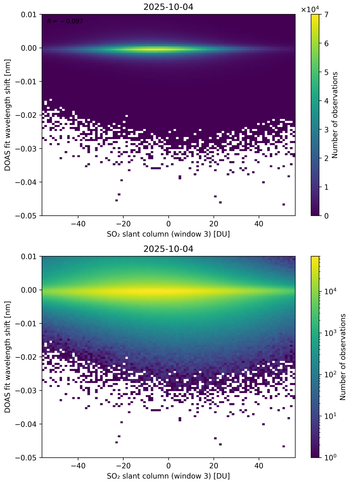
Figure 304: Scatter density plot of “SO 2 slant column (window 3)” against “DOAS fit wavelength shift” for 2025-10-03 to 2025-10-05.
