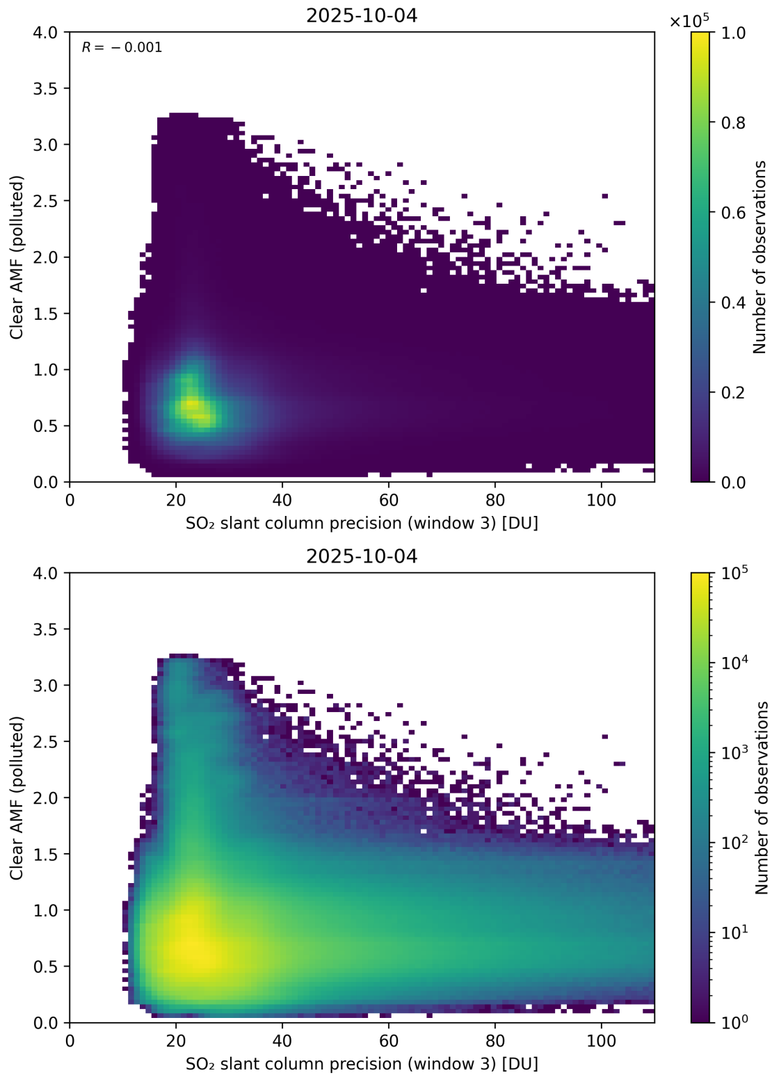
Figure 311: Scatter density plot of “SO 2 slant column precision (window 3)” against “Clear AMF (polluted)” for 2025-10-03 to 2025-10-05.
