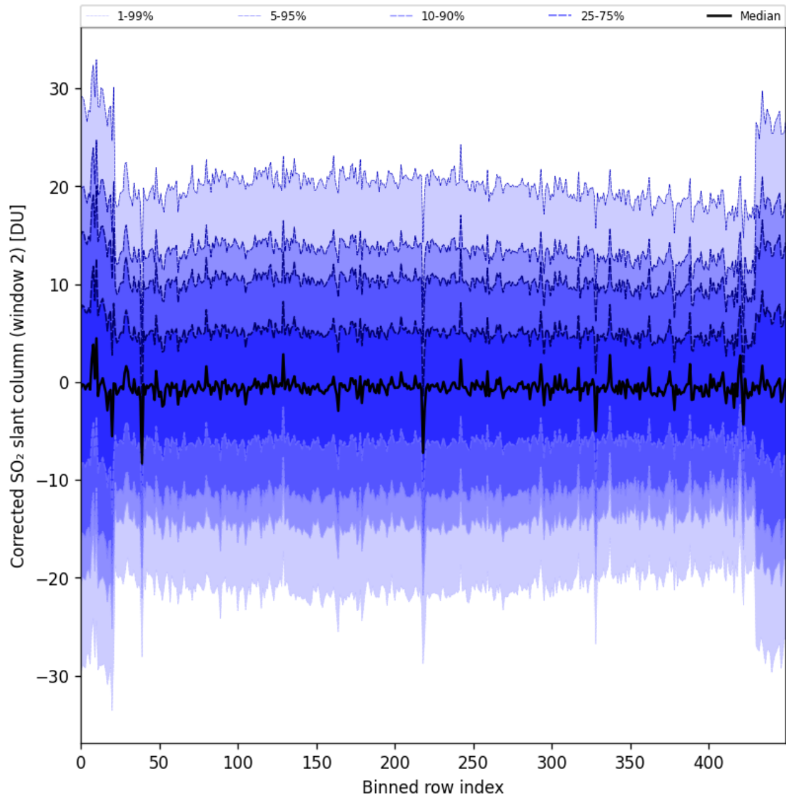
Figure 95: Along track statistics of “Corrected SO 2 slant column (window 2)” for 2025-10-03 to 2025-10-05
