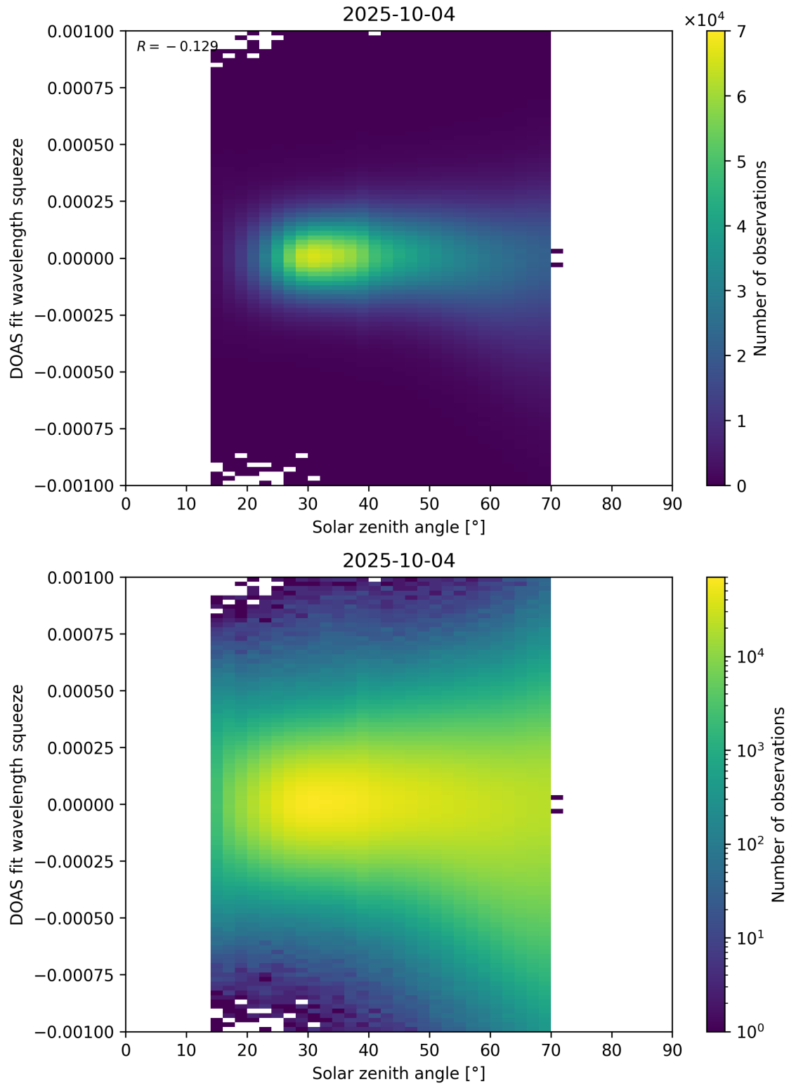
Figure 175: Scatter density plot of “Solar zenith angle” against “DOAS fit wavelength squeeze” for 2025-10-03 to 2025-10-05.
