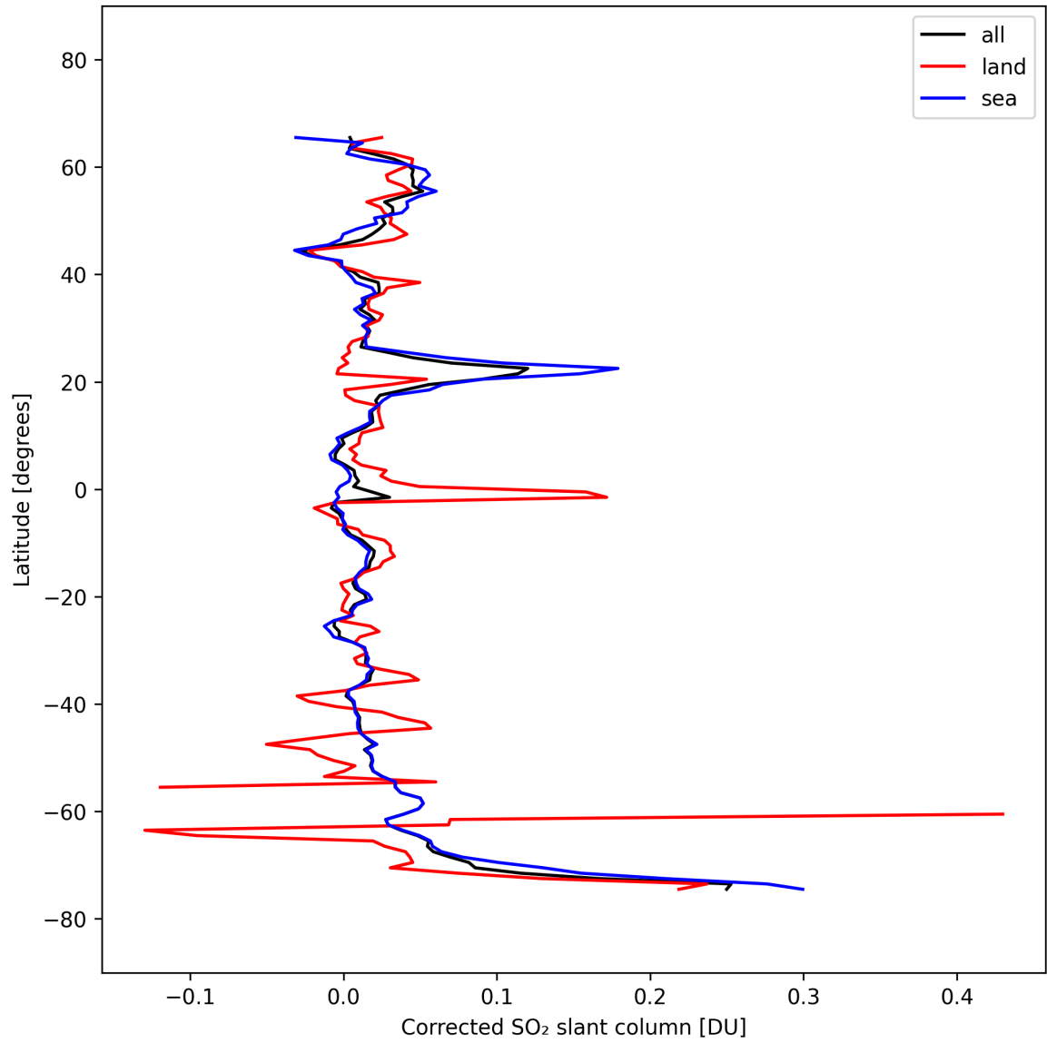
Figure 34: Zonal average of “Corrected SO 2 slant column” for 2025-10-03 to 2025-10-05.
