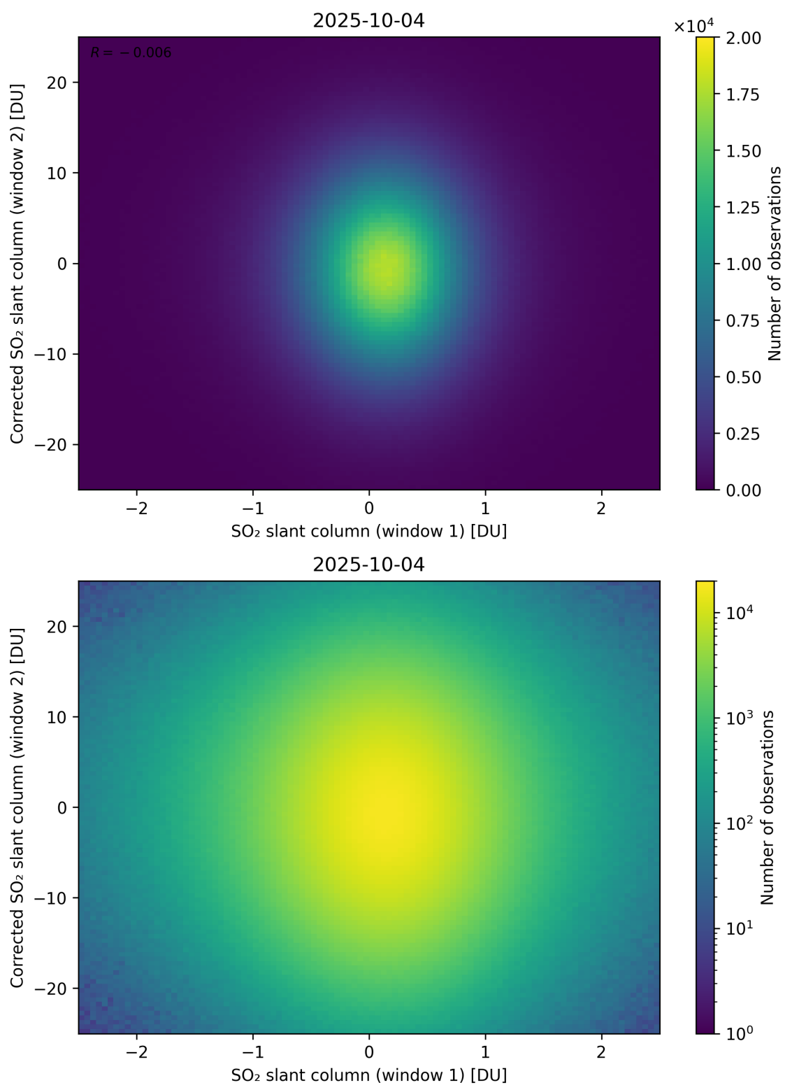
Figure 283: Scatter density plot of “SO 2 slant column (window 1)” against “Corrected SO 2 slant column (window 2)” for 2025-10-03 to 2025-10-05.
