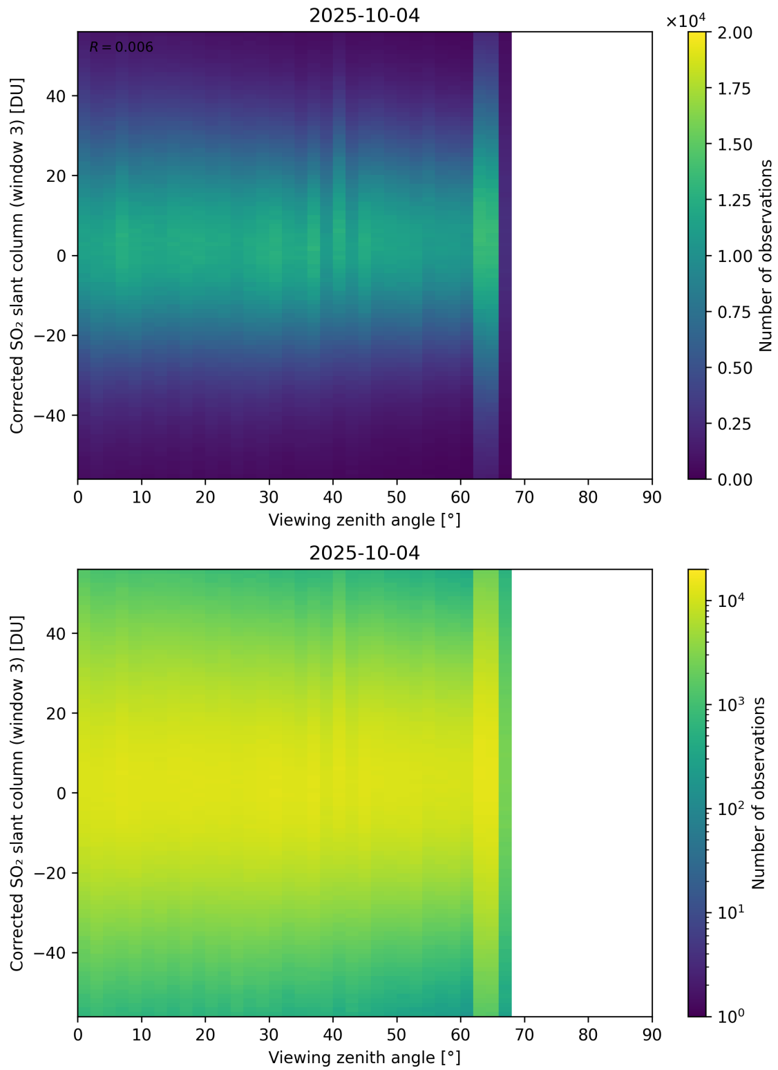
Figure 375: Scatter density plot of “Viewing zenith angle” against “Corrected SO 2 slant column (window 3)” for 2025-10-03 to 2025-10-05.
