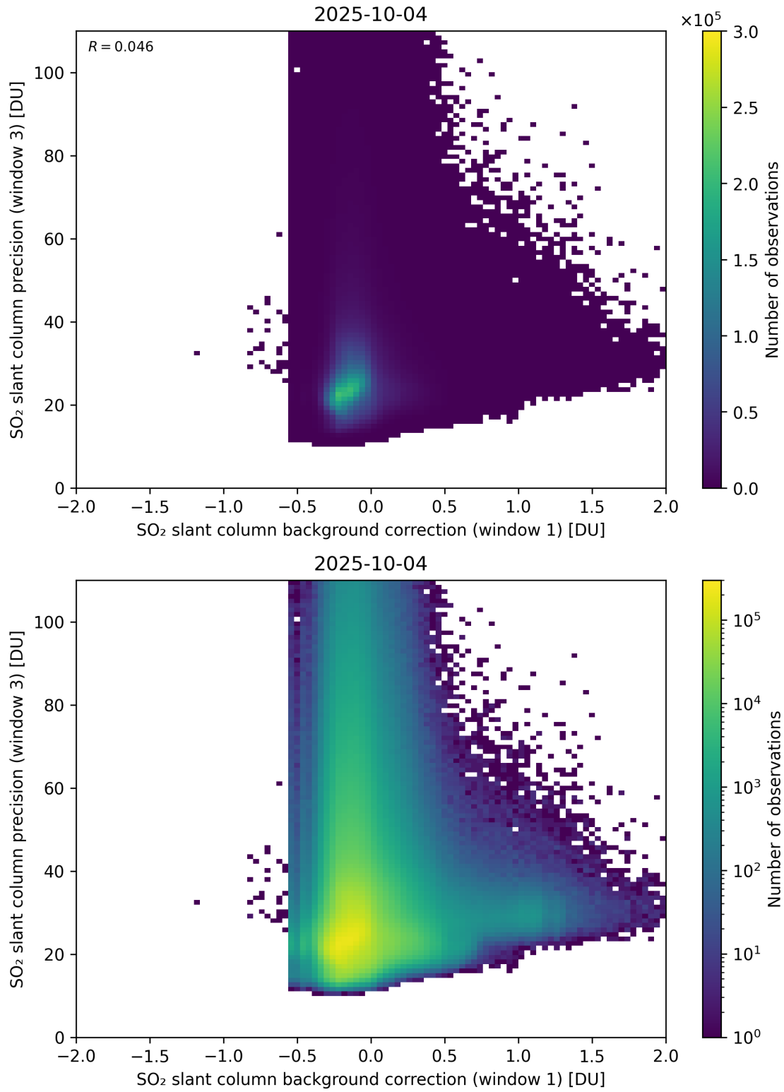
Figure 119: Scatter density plot of “SO 2 slant column background correction (window 1)” against “SO 2 slant column precision (window 3)” for 2025-10-03 to 2025-10-05.
