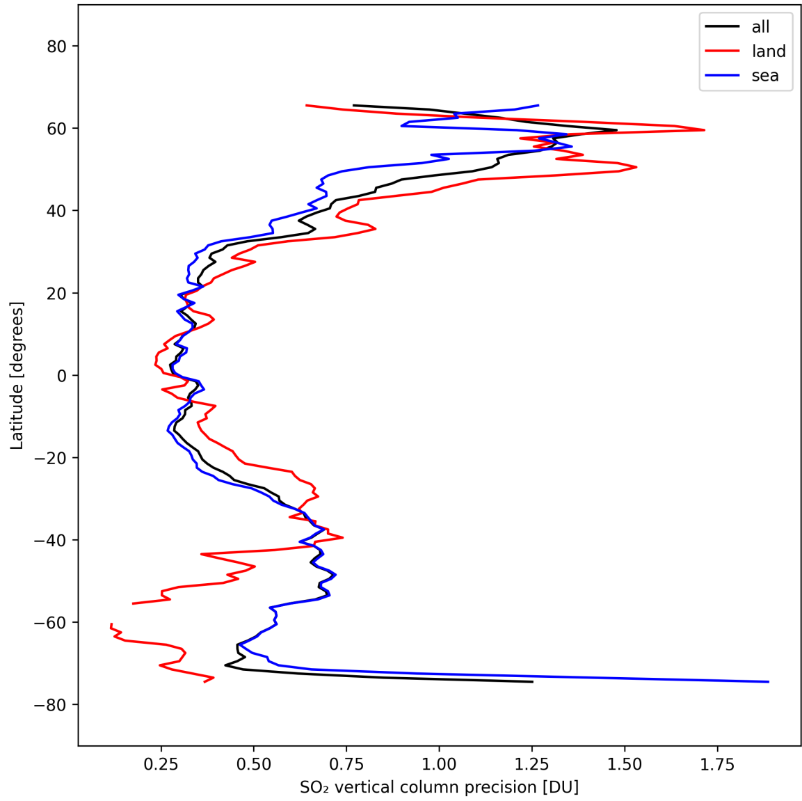
Figure 33: Zonal average of “SO 2 vertical column precision” for 2025-10-03 to 2025-10-05.
