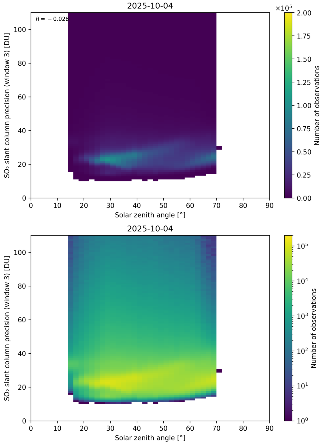
Figure 188: Scatter density plot of “Solar zenith angle” against “SO 2 slant column precision (window 3)” for 2025-10-03 to 2025-10-05.
