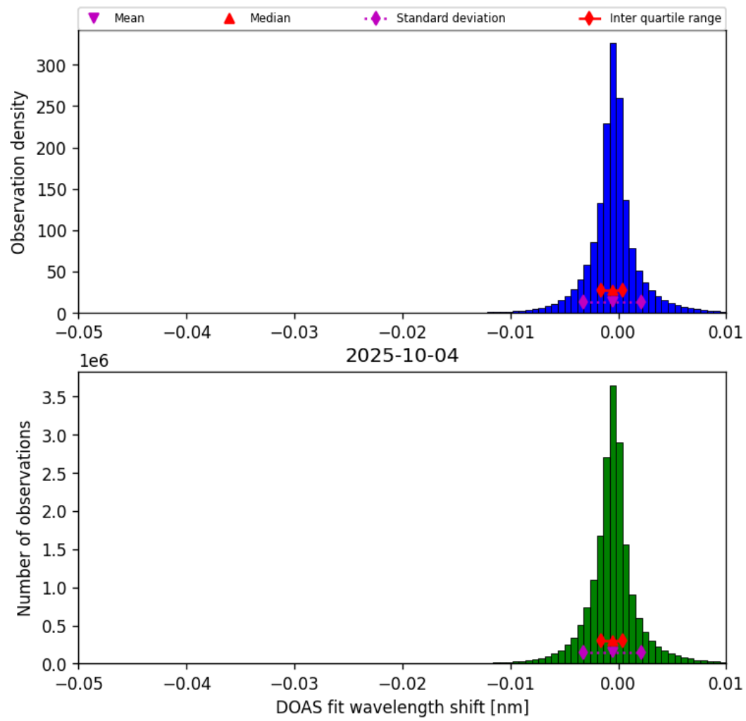
Figure 76: Histogram of “DOAS fit wavelength shift” for 2025-10-03 to 2025-10-05
