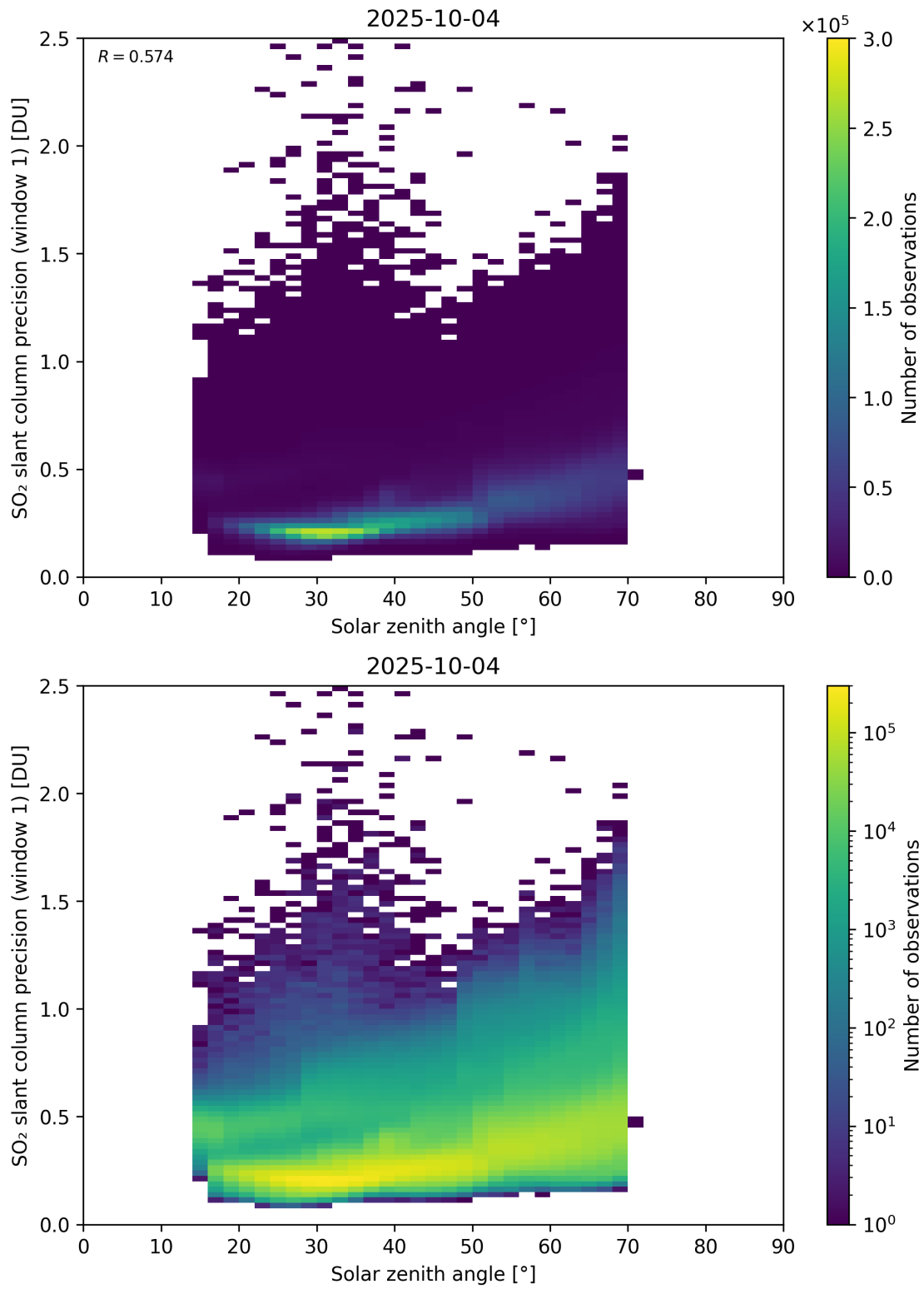
Figure 185: Scatter density plot of “Solar zenith angle” against “SO 2 slant column precision (window 1)” for 2025-10-03 to 2025-10-05.
