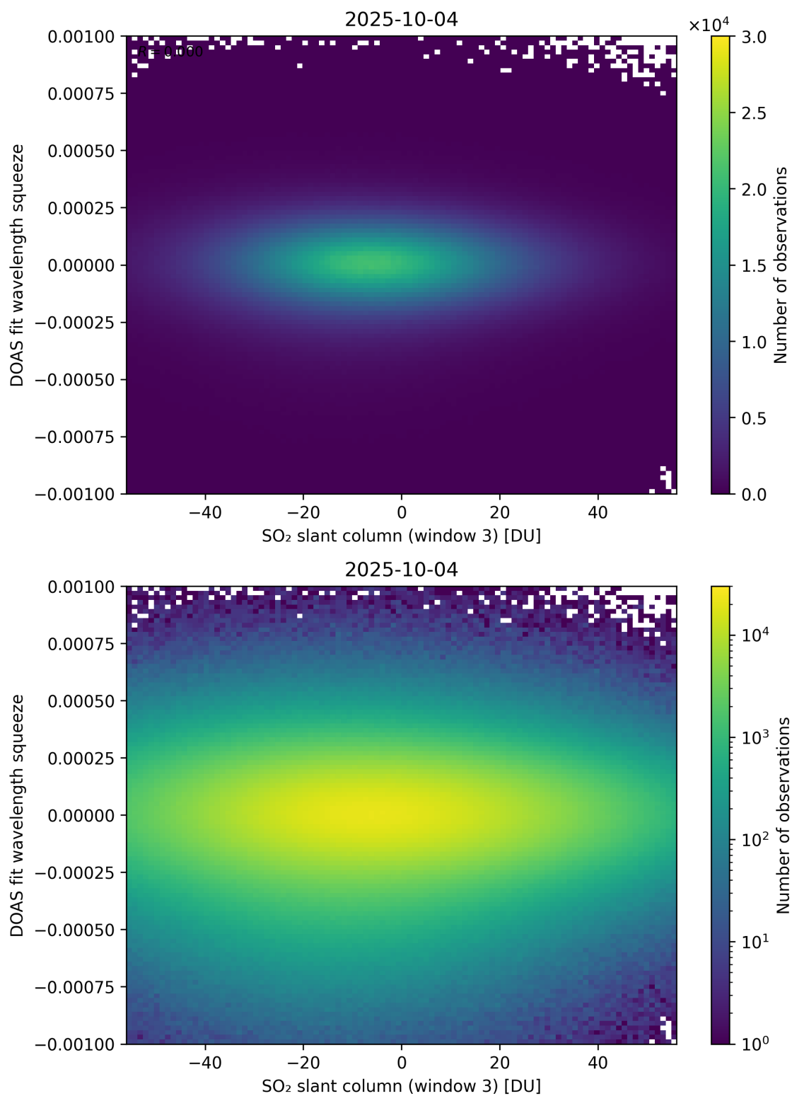
Figure 305: Scatter density plot of “SO 2 slant column (window 3)” against “DOAS fit wavelength squeeze” for 2025-10-03 to 2025-10-05.
