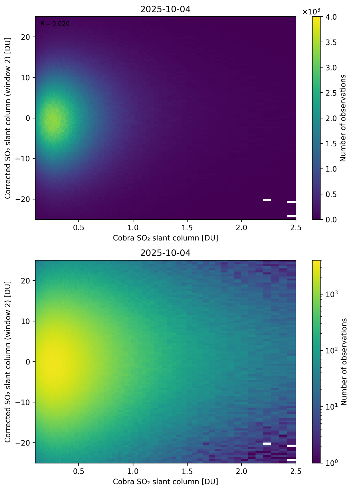
Figure 217: Scatter density plot of “Cobra SO 2 slant column” against “Corrected SO 2 slant column (window 2)” for 2025-10-03 to 2025-10-05.
