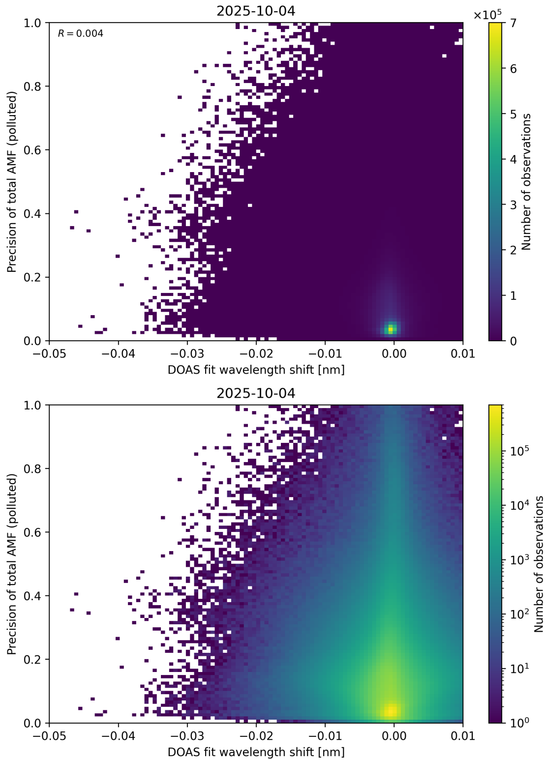
Figure 142: Scatter density plot of “DOAS fit wavelength shift” against “Precision of total AMF (polluted)” for 2025-10-03 to 2025-10-05.
