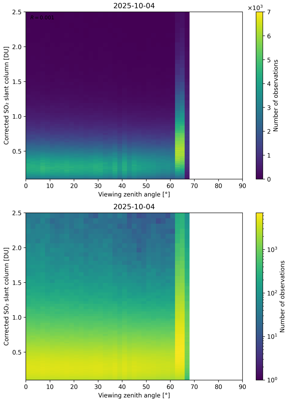
Figure 373: Scatter density plot of “Viewing zenith angle” against “Corrected SO 2 slant column” for 2025-10-03 to 2025-10-05.
