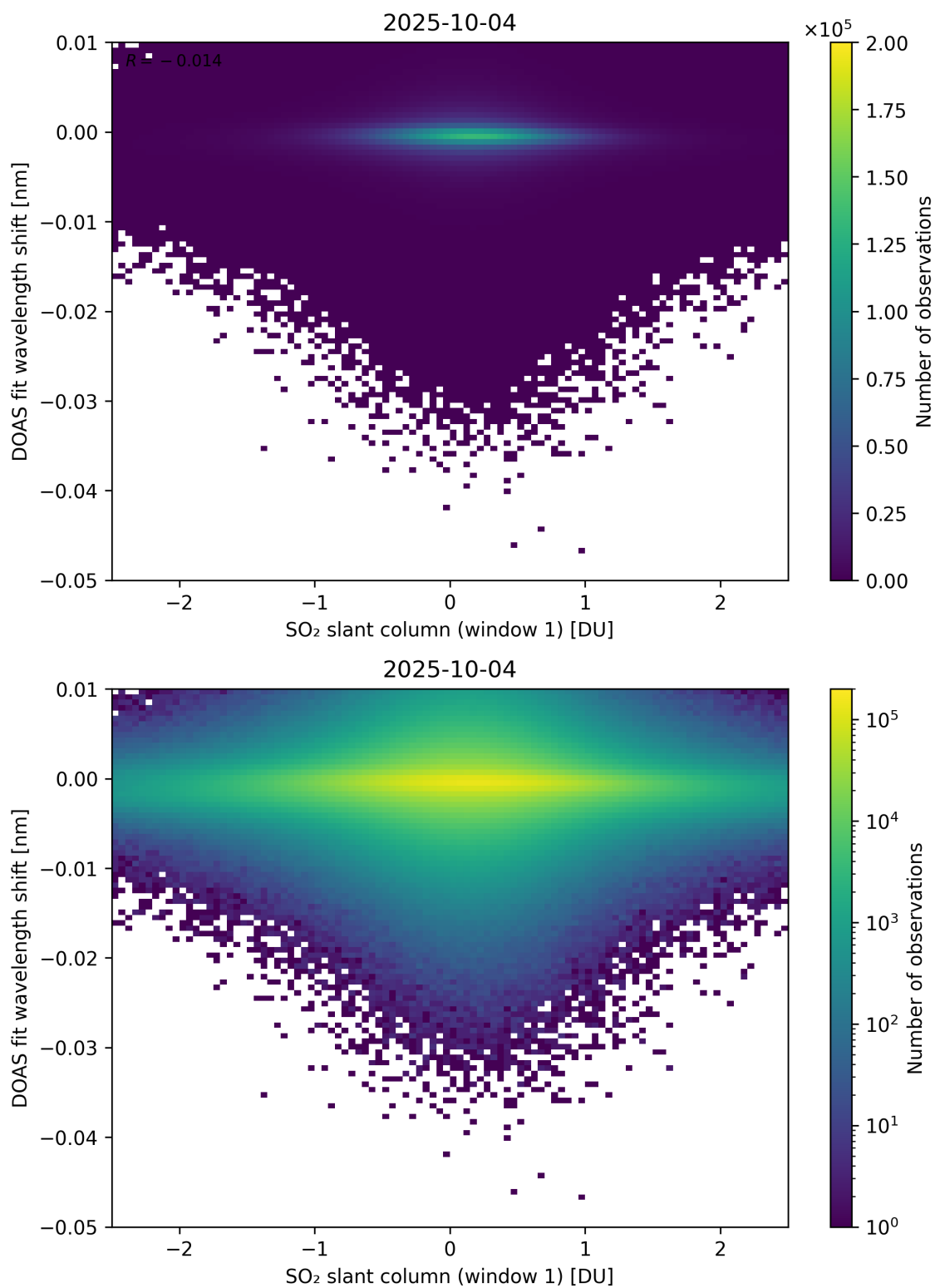
Figure 265: Scatter density plot of “SO 2 slant column (window 1)” against “DOAS fit wavelength shift” for 2025-10-03 to 2025-10-05.
