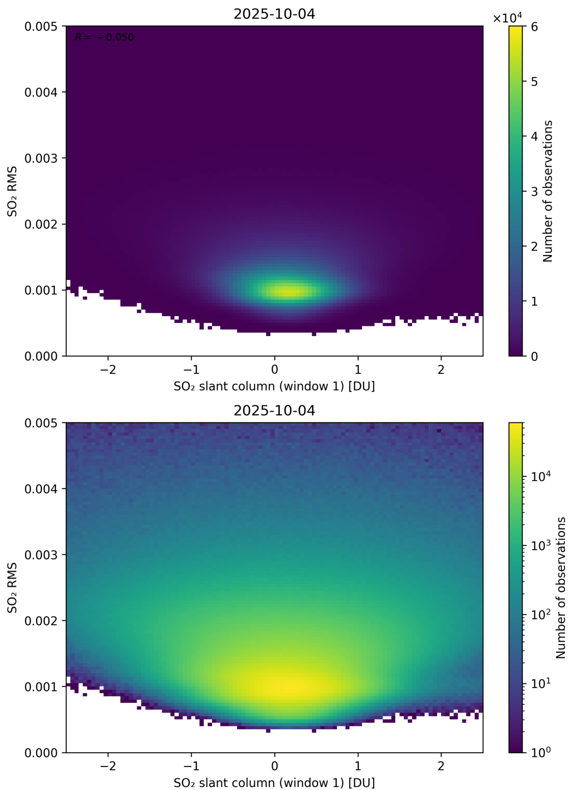
Figure 267: Scatter density plot of “SO 2 slant column (window 1)” against “SO 2 RMS” for 2025-10-03 to 2025-10-05.
