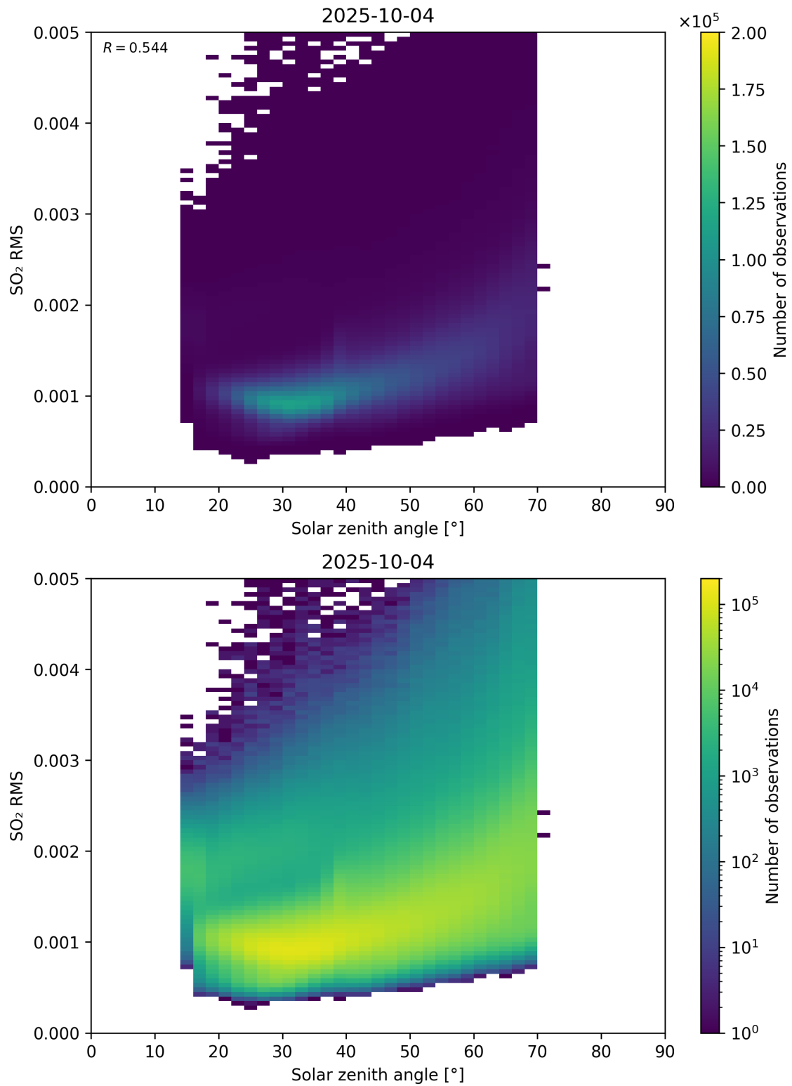
Figure 176: Scatter density plot of “Solar zenith angle” against “SO 2 RMS” for 2025-10-03 to 2025-10-05.
