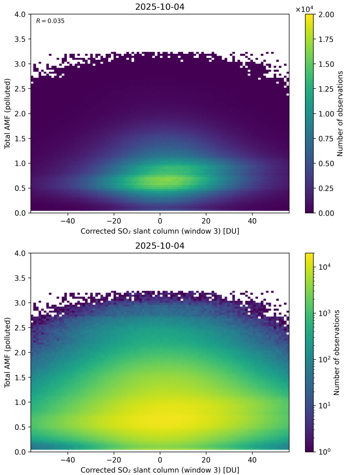
Figure 260: Scatter density plot of “Corrected SO 2 slant column (window 3)” against “Total AMF (polluted)” for 2025-10-03 to 2025-10-05.
