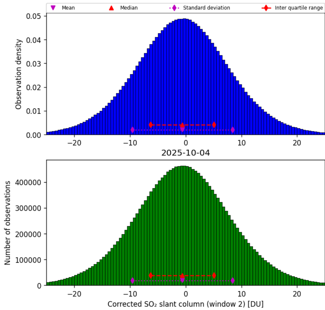
Figure 69: Histogram of “Corrected SO 2 slant column (window 2)” for 2025-10-03 to 2025-10-05
