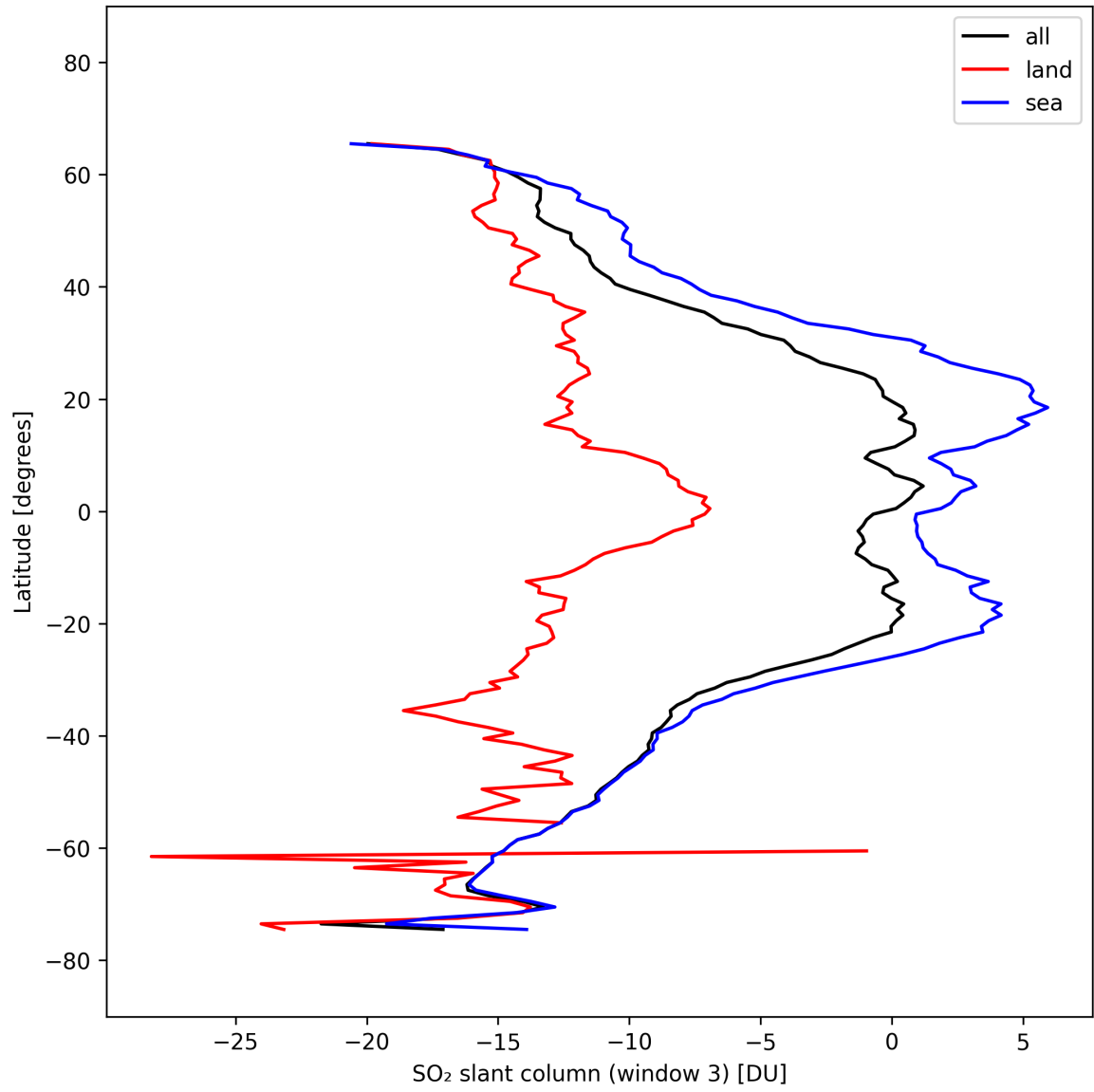
Figure 45: Zonal average of “SO 2 slant column (window 3)” for 2025-10-03 to 2025-10-05.
