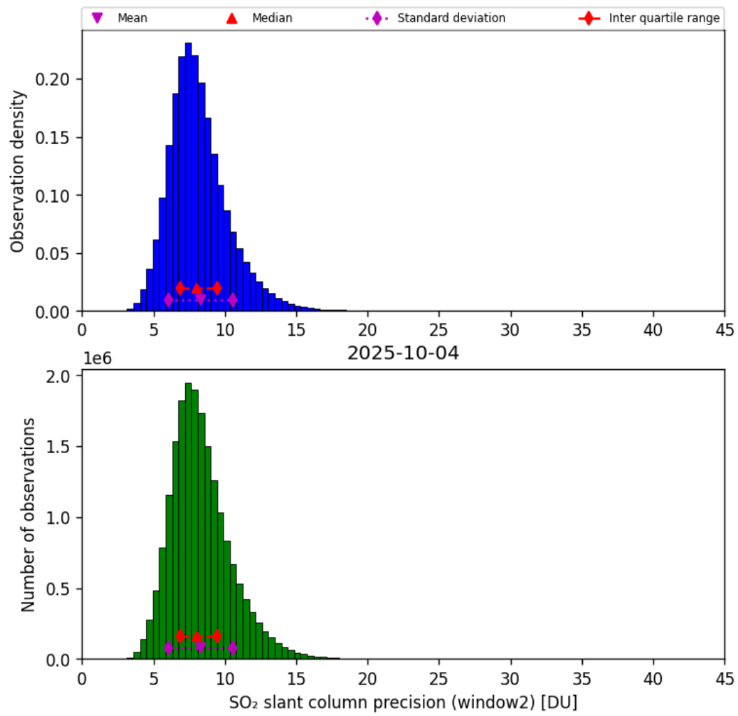
Figure 68: Histogram of “SO 2 slant column precision (window2)” for 2025-10-03 to 2025-10-05
