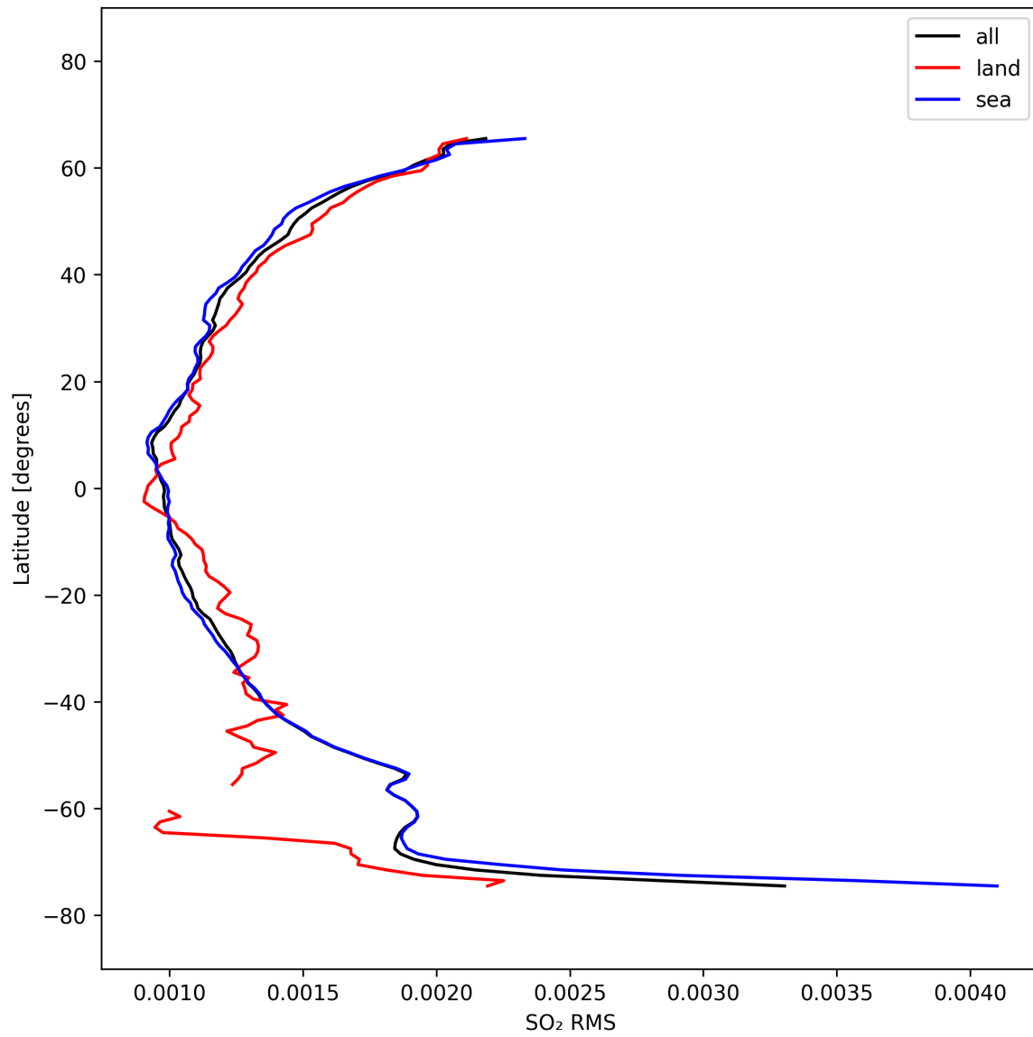
Figure 52: Zonal average of “SO 2 RMS” for 2025-10-03 to 2025-10-05.
