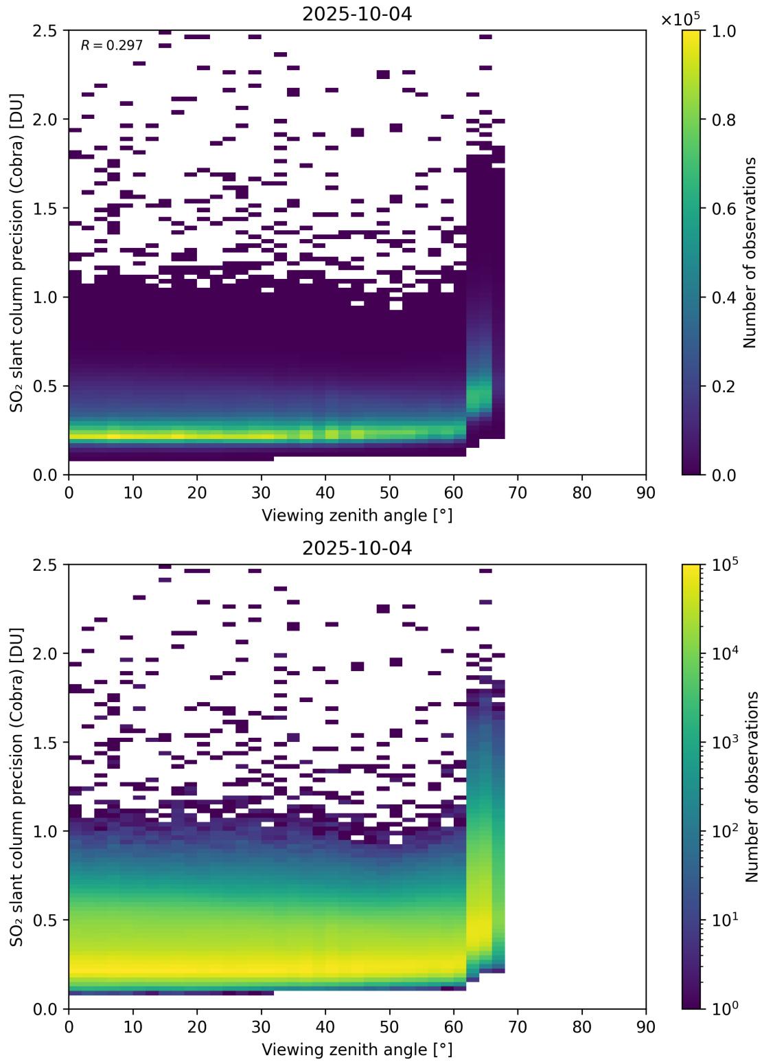
Figure 372: Scatter density plot of “Viewing zenith angle” against “SO 2 slant column precision (Cobra)” for 2025-10-03 to 2025-10-05.
