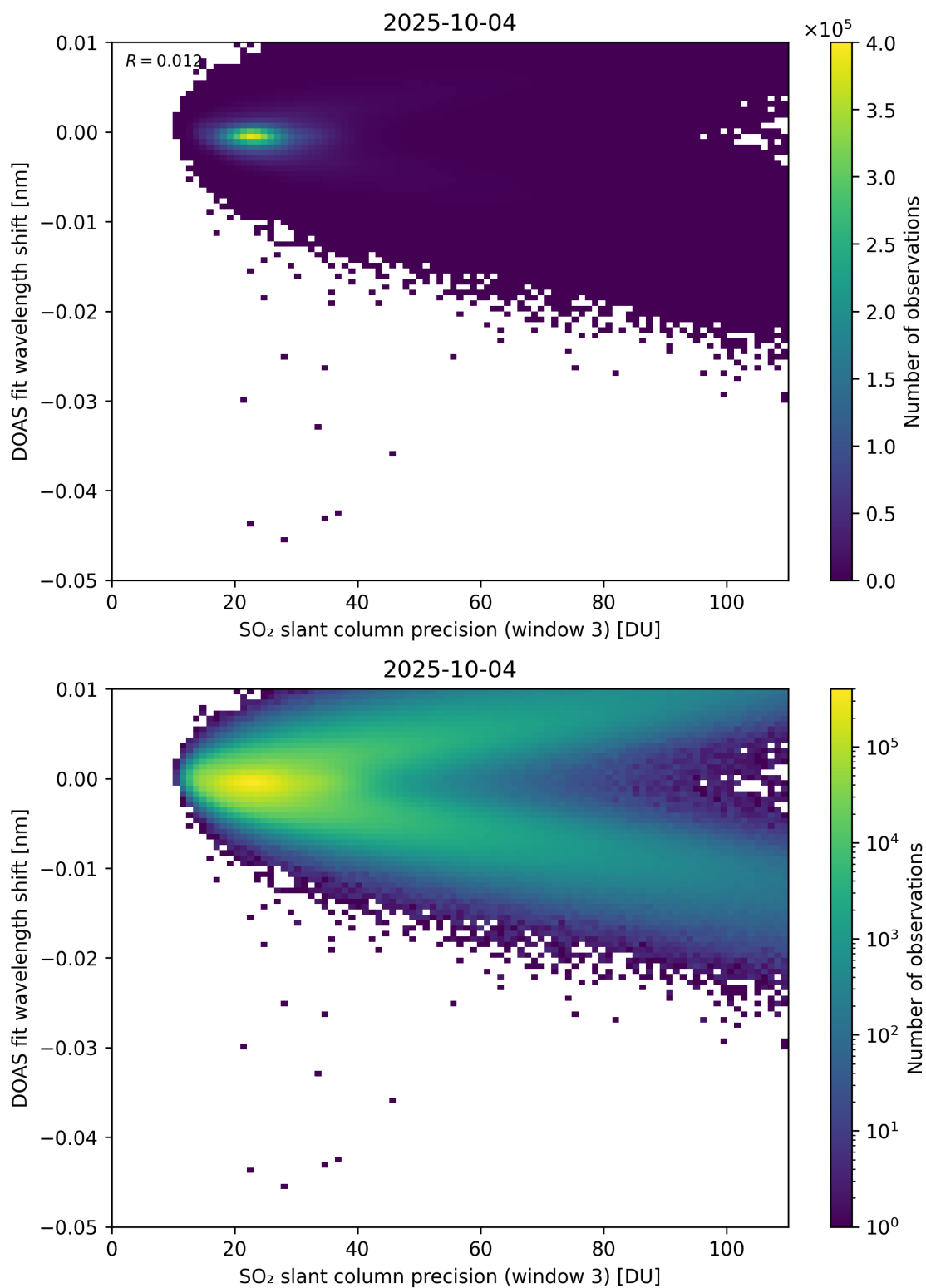
Figure 308: Scatter density plot of “SO 2 slant column precision (window 3)” against “DOAS fit wavelength shift” for 2025-10-03 to 2025-10-05.
