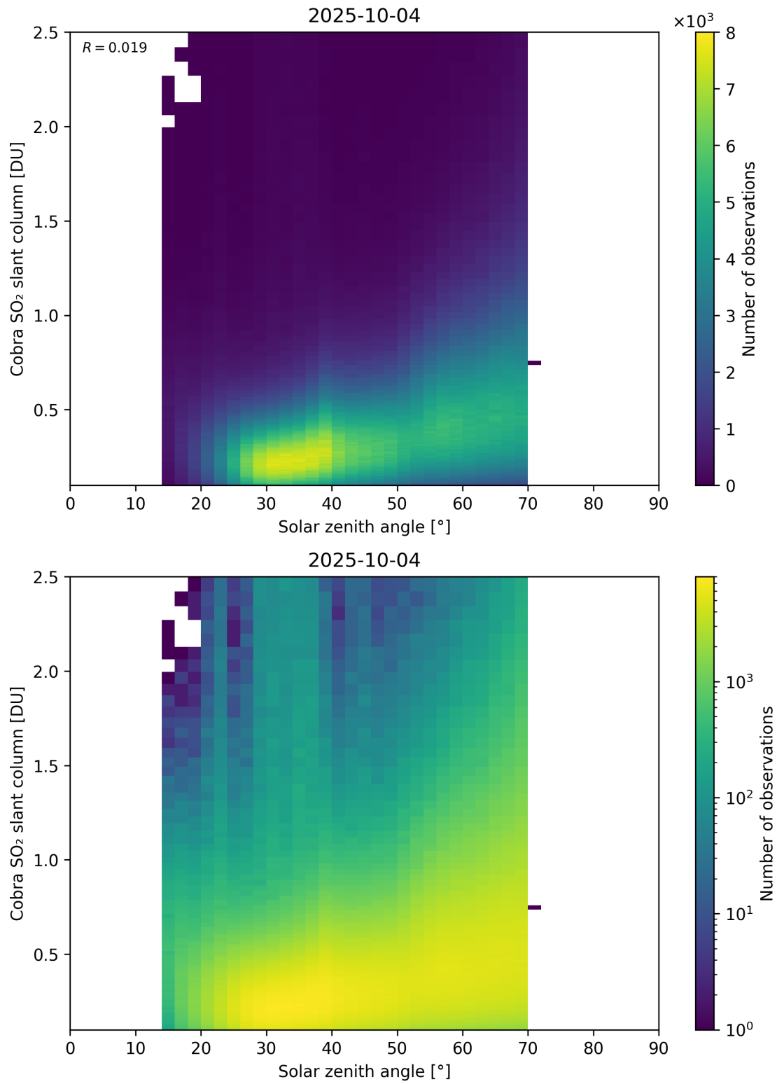
Figure 179: Scatter density plot of “Solar zenith angle” against “Cobra SO 2 slant column” for 2025-10-03 to 2025-10-05.
