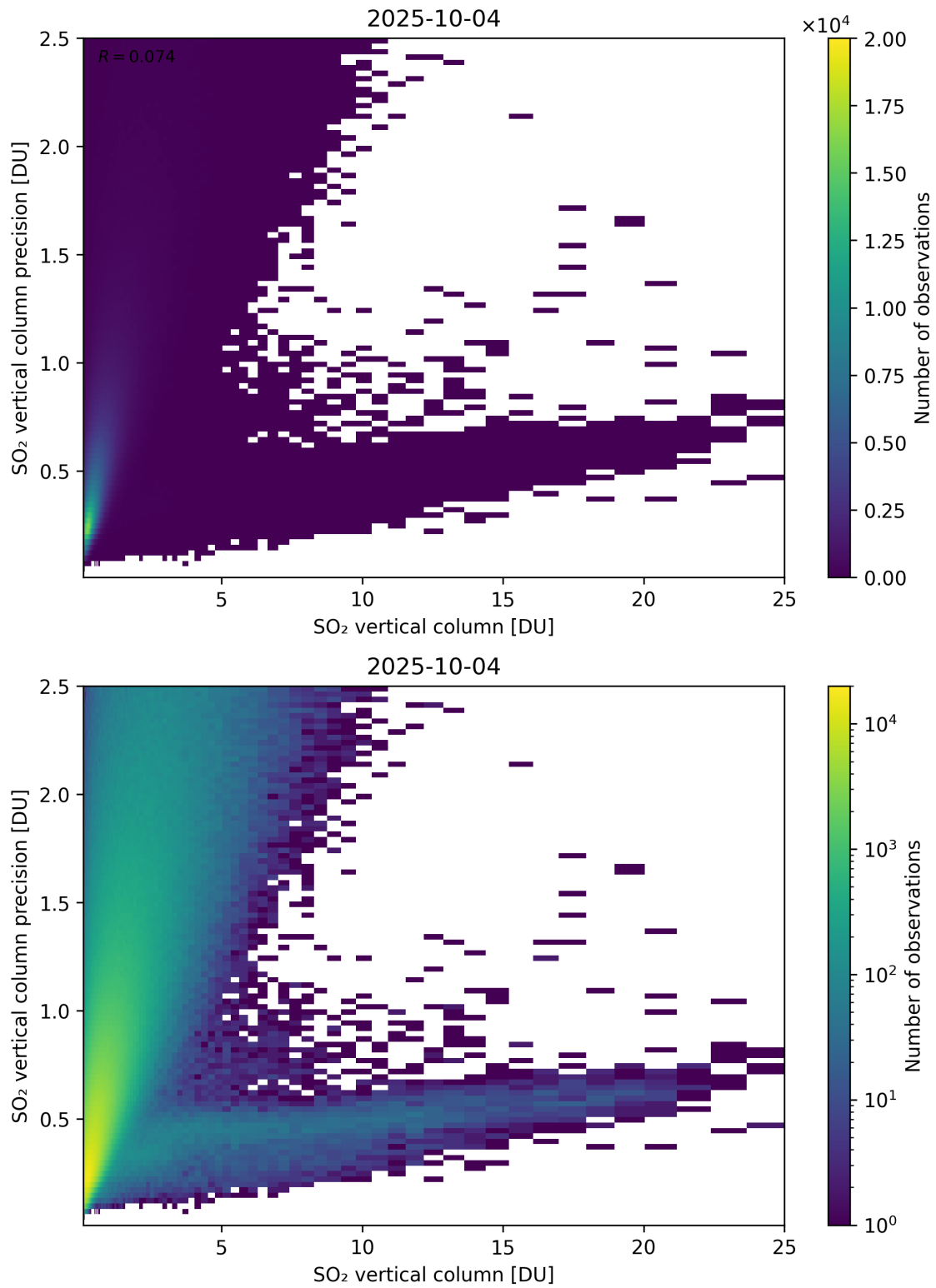
Figure 361: Scatter density plot of “SO 2 vertical column” against “SO 2 vertical column precision” for 2025-10-03 to 2025-10-05.
