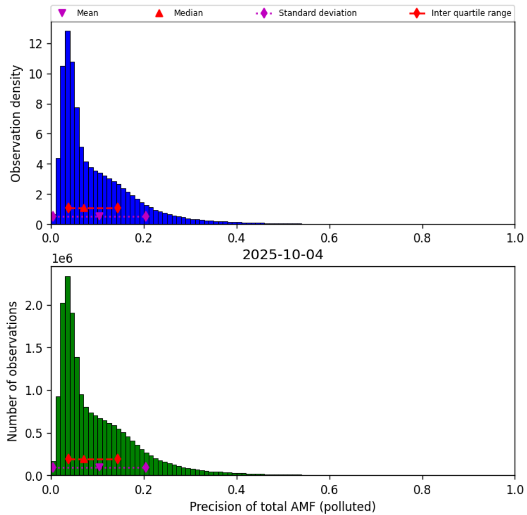
Figure 80: Histogram of “Precision of total AMF (polluted)” for 2025-10-03 to 2025-10-05
