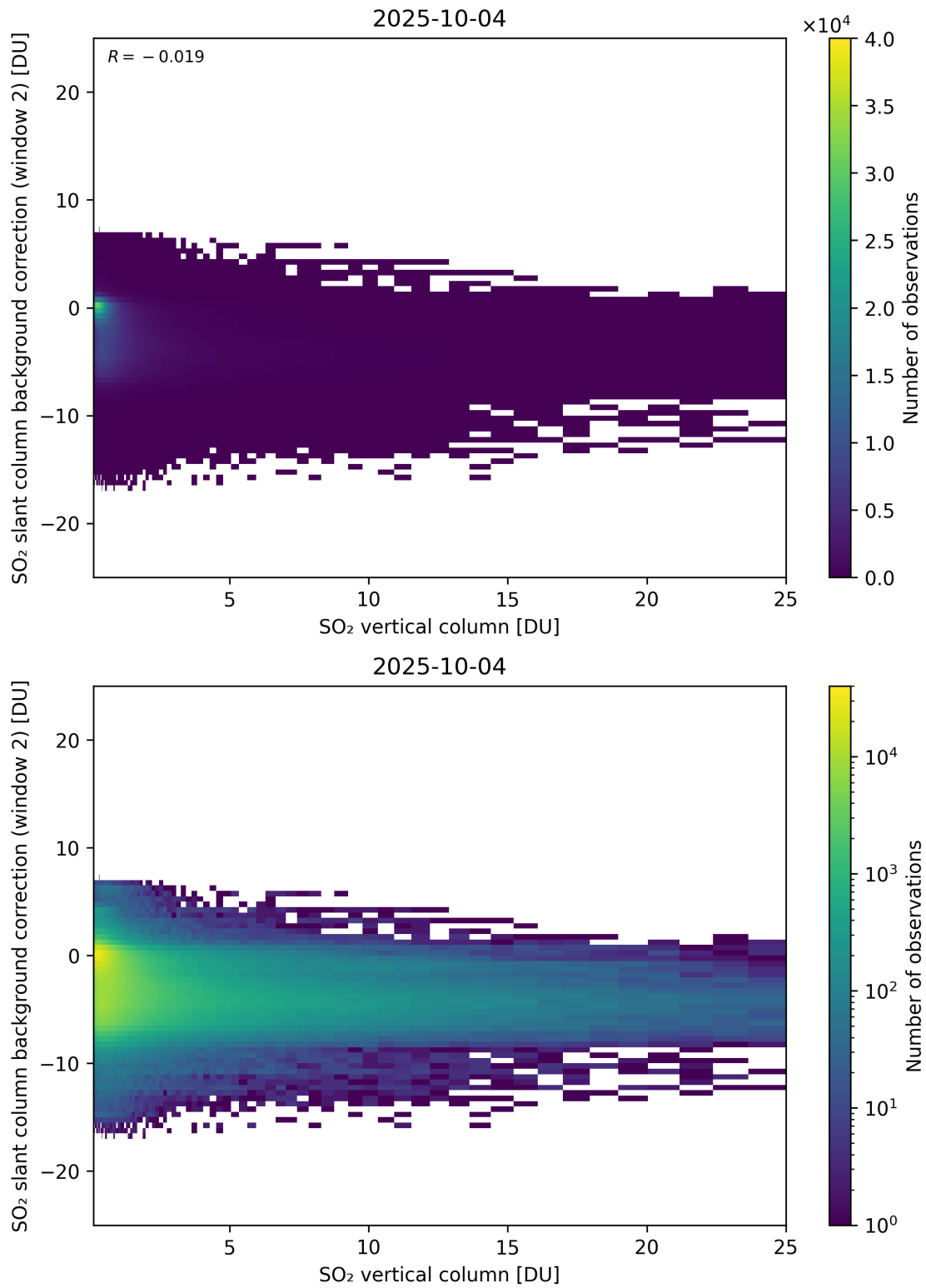
Figure 324: Scatter density plot of “SO 2 vertical column” against “SO 2 slant column background correction (window 2)” for 2025-10-03 to 2025-10-05.
