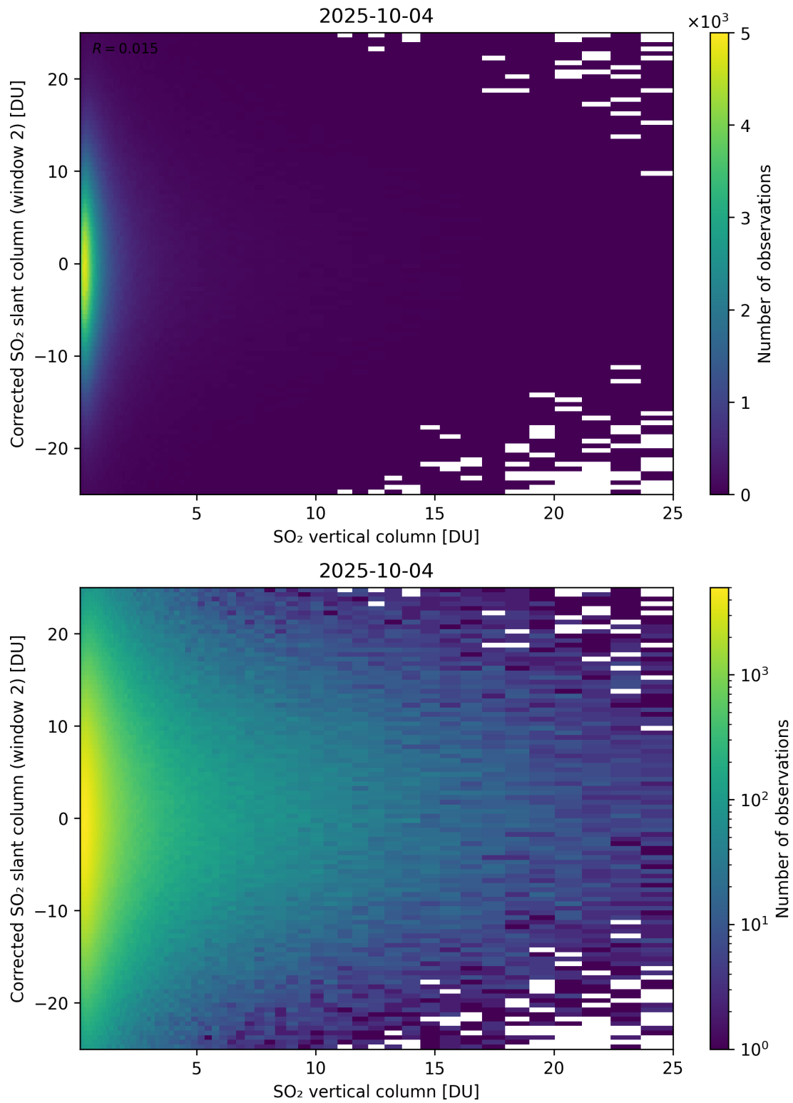
Figure 352: Scatter density plot of “SO 2 vertical column” against “Corrected SO 2 slant column (window 2)” for 2025-10-03 to 2025-10-05.
