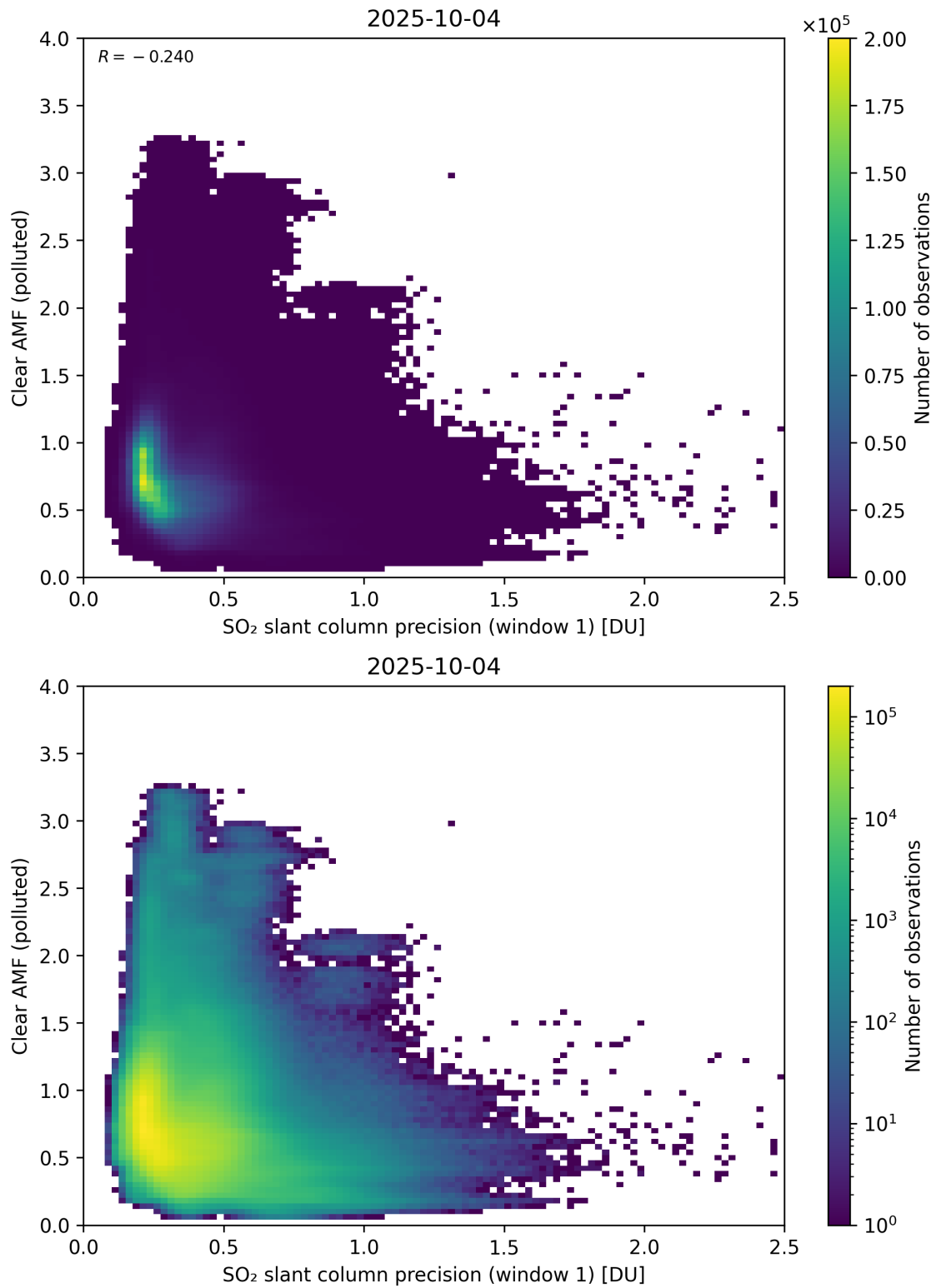
Figure 274: Scatter density plot of “SO 2 slant column precision (window 1)” against “Clear AMF (polluted)” for 2025-10-03 to 2025-10-05.
