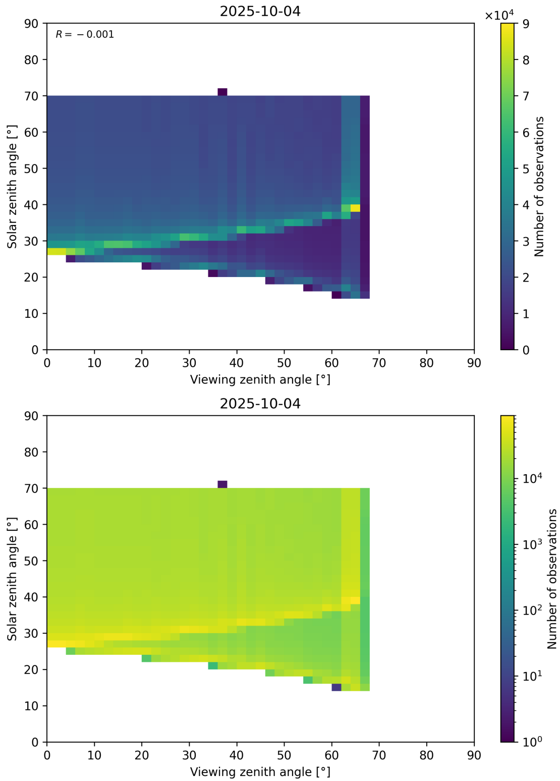
Figure 369: Scatter density plot of “Viewing zenith angle” against “Solar zenith angle” for 2025-10-03 to 2025-10-05.
