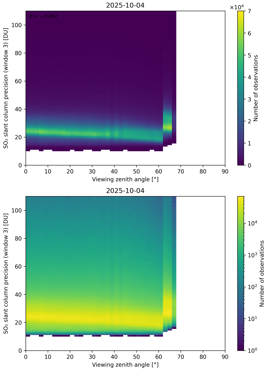
Figure 380: Scatter density plot of “Viewing zenith angle” against “SO 2 slant column precision (window 3)” for 2025-10-03 to 2025-10-05.
