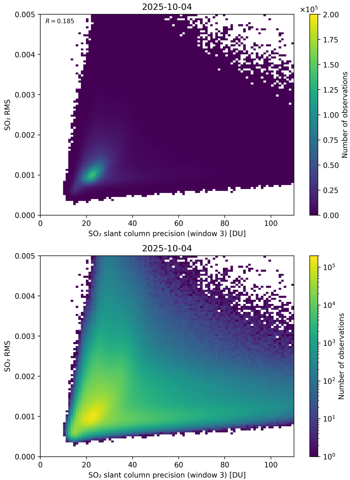
Figure 310: Scatter density plot of “SO 2 slant column precision (window 3)” against “SO 2 RMS” for 2025-10-03 to 2025-10-05.
