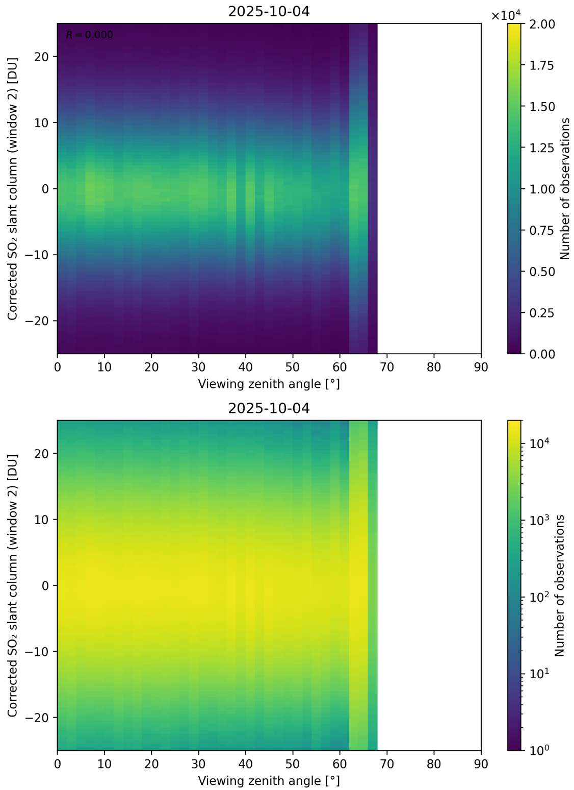
Figure 374: Scatter density plot of “Viewing zenith angle” against “Corrected SO 2 slant column (window 2)” for 2025-10-03 to 2025-10-05.
