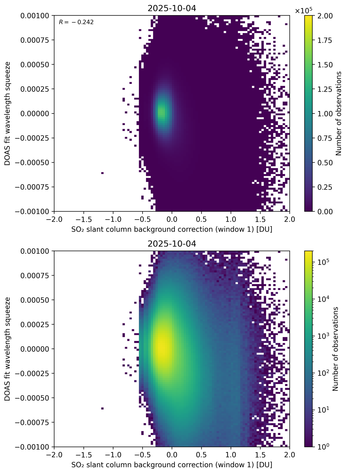
Figure 112: Scatter density plot of “SO 2 slant column background correction (window 1)” against “DOAS fit wavelength squeeze” for 2025-10-03 to 2025-10-05.
