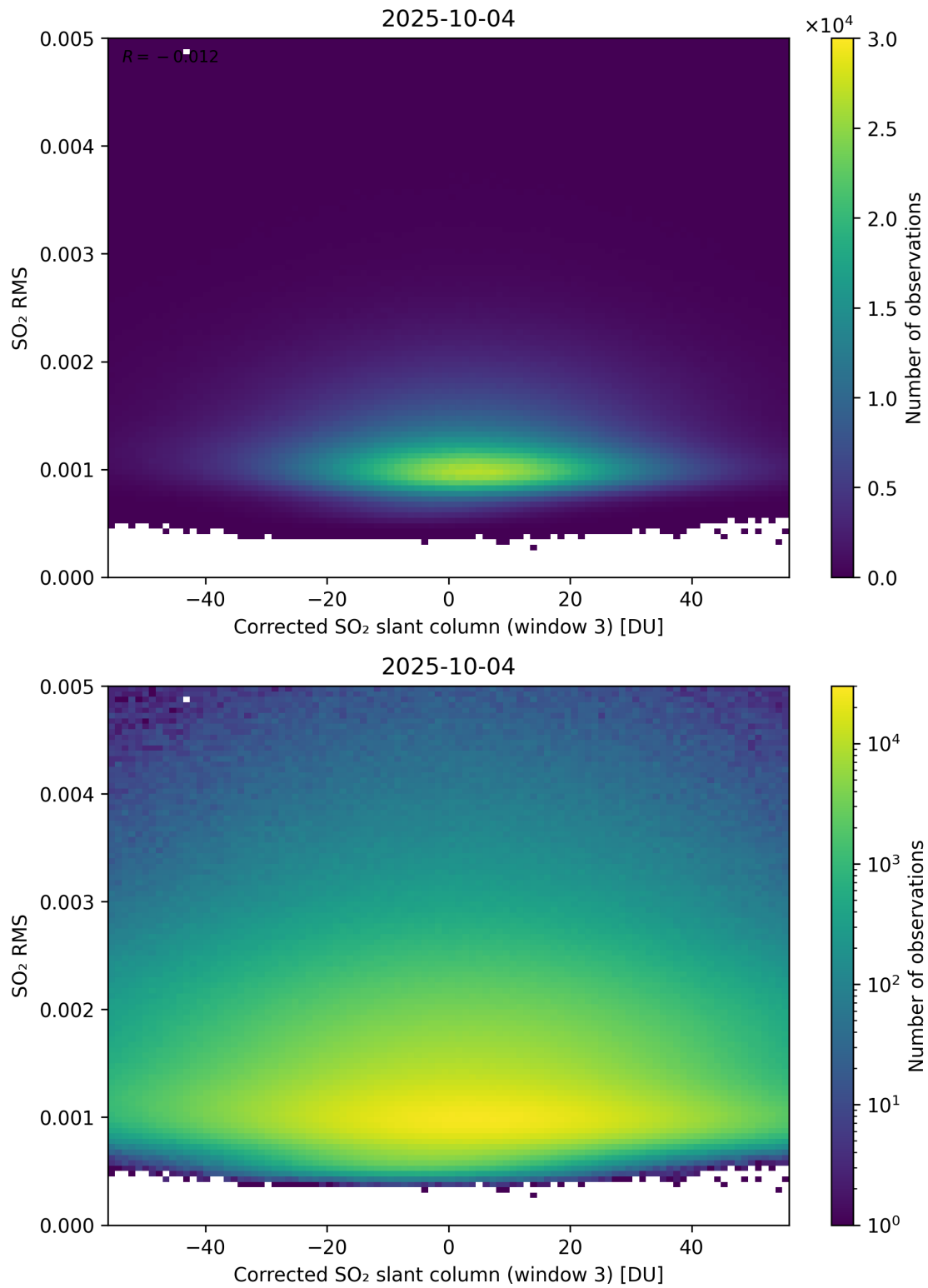
Figure 258: Scatter density plot of “Corrected SO 2 slant column (window 3)” against “SO 2 RMS” for 2025-10-03 to 2025-10-05.
