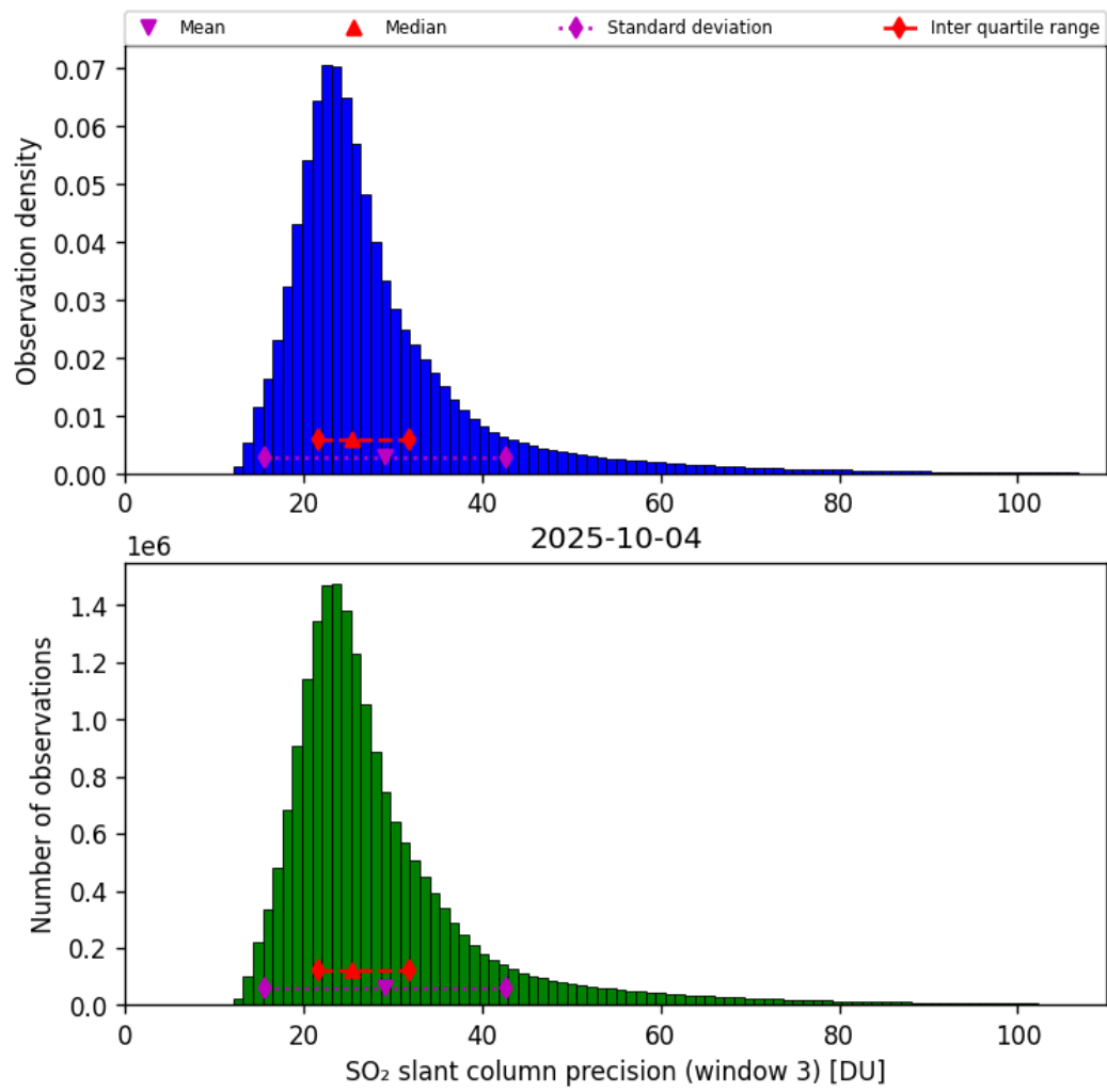
Figure 72: Histogram of “SO 2 slant column precision (window 3)” for 2025-10-03 to 2025-10-05
