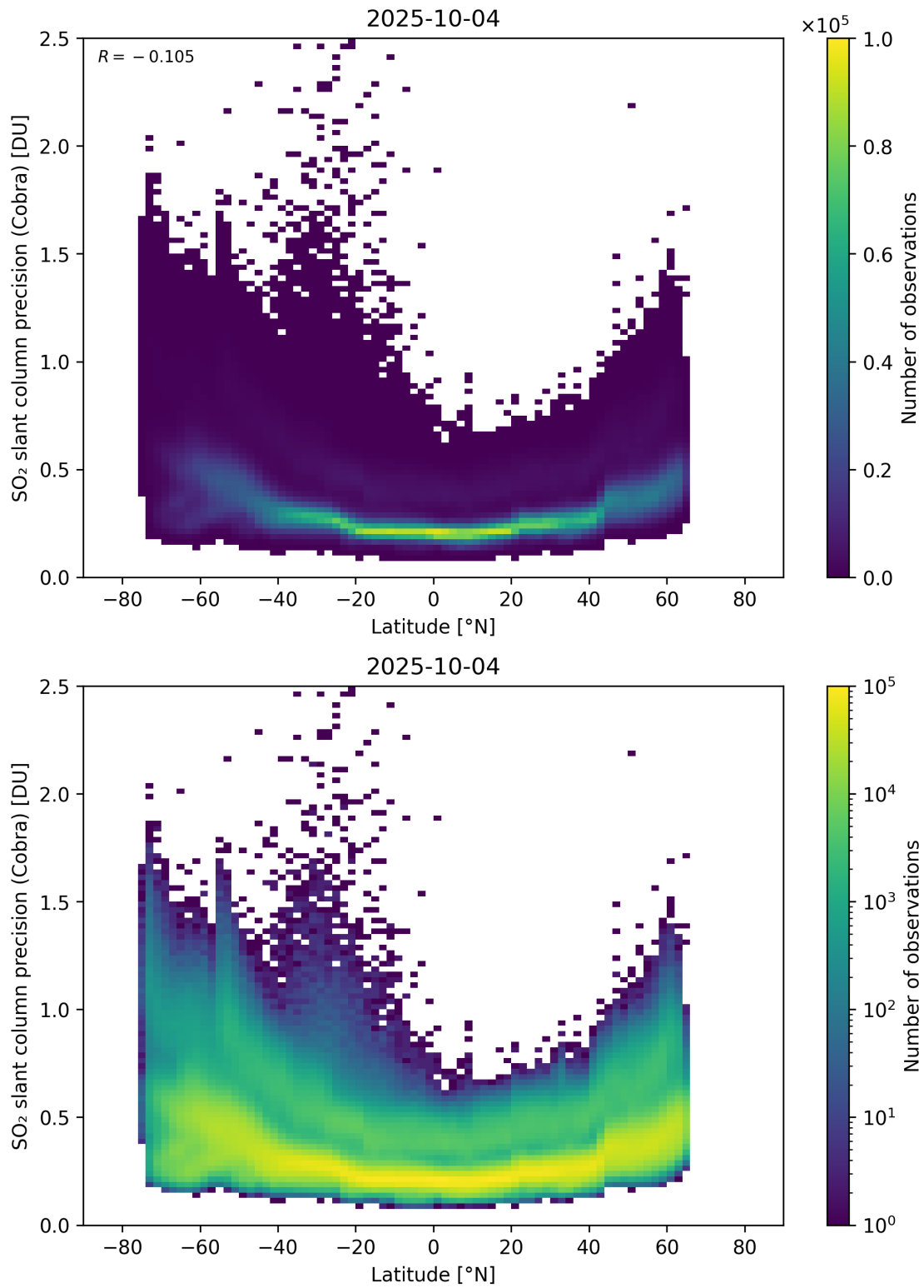
Figure 158: Scatter density plot of “Latitude” against “SO 2 slant column precision (Cobra)” for 2025-10-03 to 2025-10-05.
