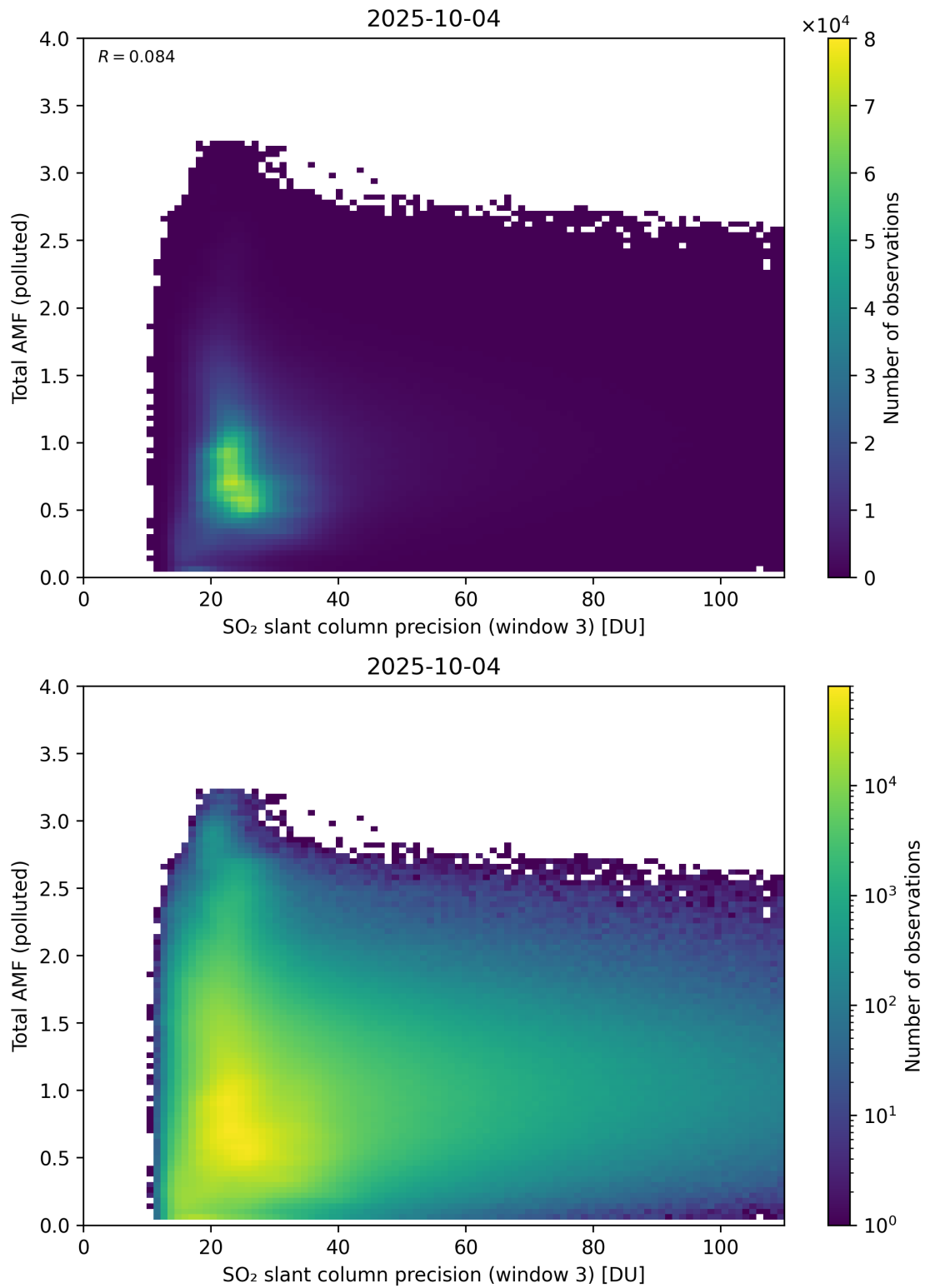
Figure 313: Scatter density plot of “SO 2 slant column precision (window 3)” against “Total AMF (polluted)” for 2025-10-03 to 2025-10-05.
