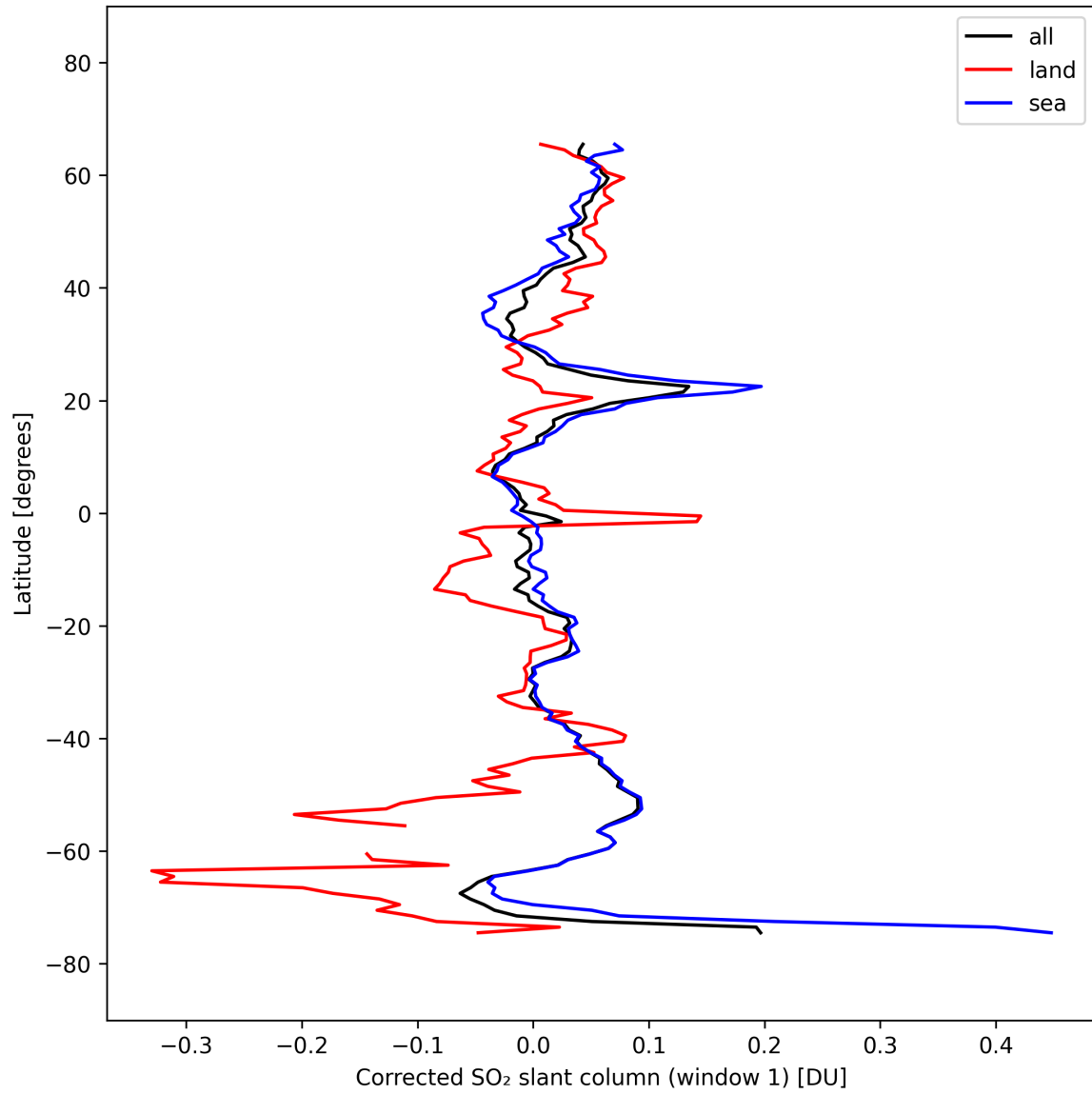
Figure 39: Zonal average of “Corrected SO 2 slant column (window 1)” for 2025-10-03 to 2025-10-05.
