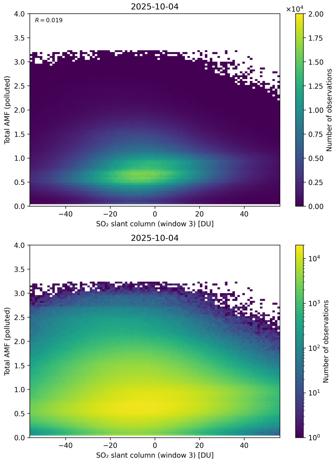
Figure 318: Scatter density plot of “SO 2 slant column (window 3)” against “Total AMF (polluted)” for 2025-10-03 to 2025-10-05.
