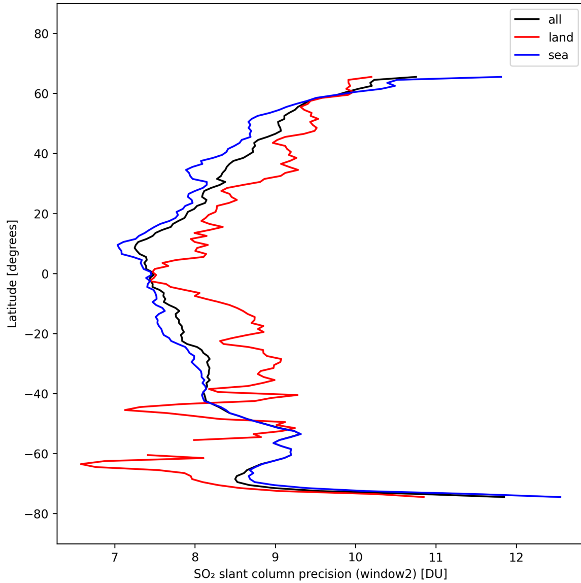
Figure 42: Zonal average of “SO 2 slant column precision (window2)” for 2025-10-03 to 2025-10-05.
