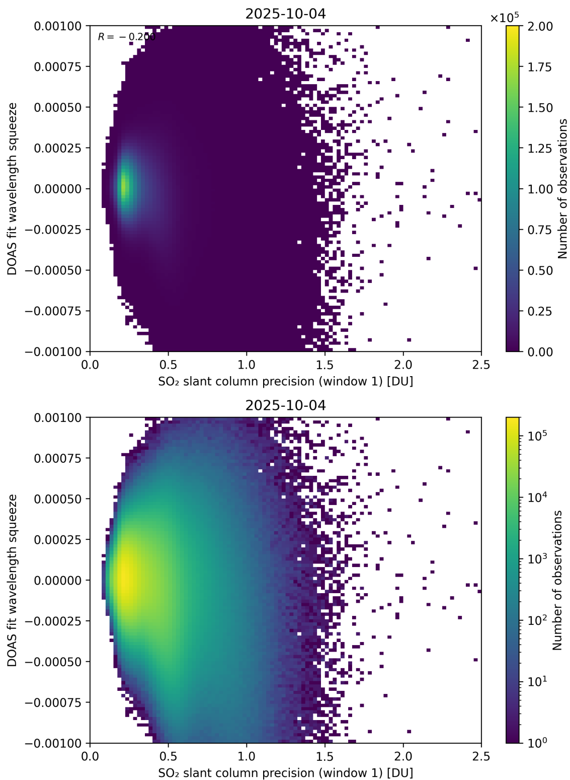
Figure 272: Scatter density plot of “SO 2 slant column precision (window 1)” against “DOAS fit wavelength squeeze” for 2025-10-03 to 2025-10-05.
