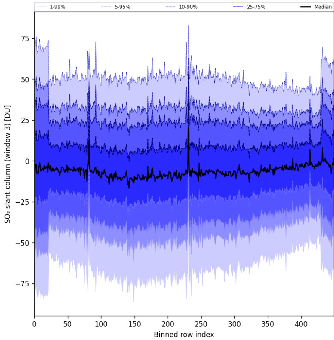
Figure 97: Along track statistics of “SO 2 slant column (window 3)” for 2025-10-03 to 2025-10-05
