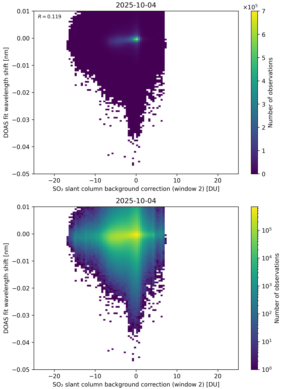
Figure 123: Scatter density plot of “SO 2 slant column background correction (window 2)” against “DOAS fit wavelength shift” for 2025-10-03 to 2025-10-05.
