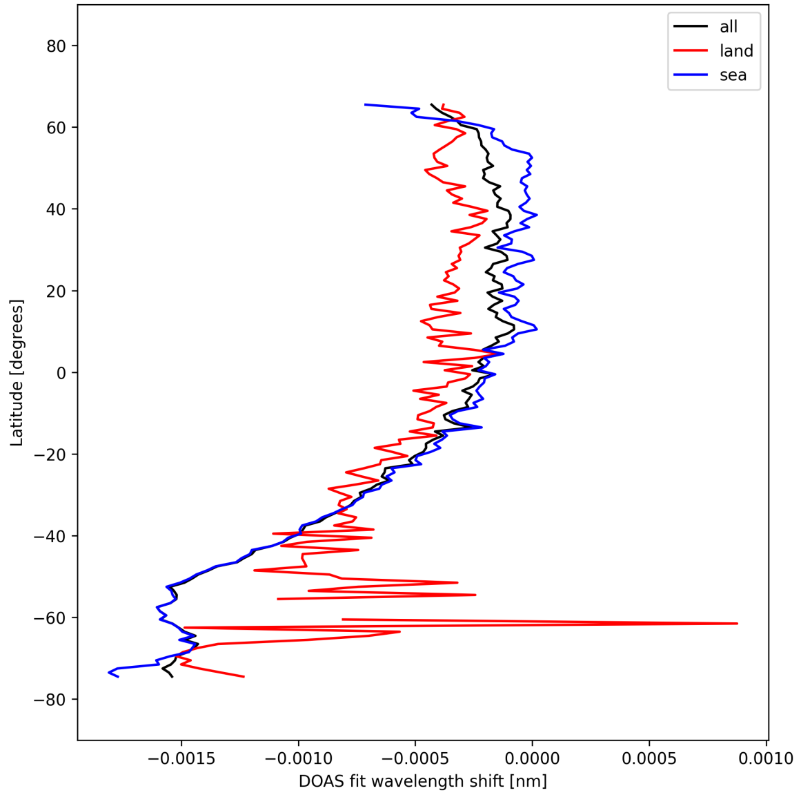
Figure 50: Zonal average of “DOAS fit wavelength shift” for 2025-10-03 to 2025-10-05.
