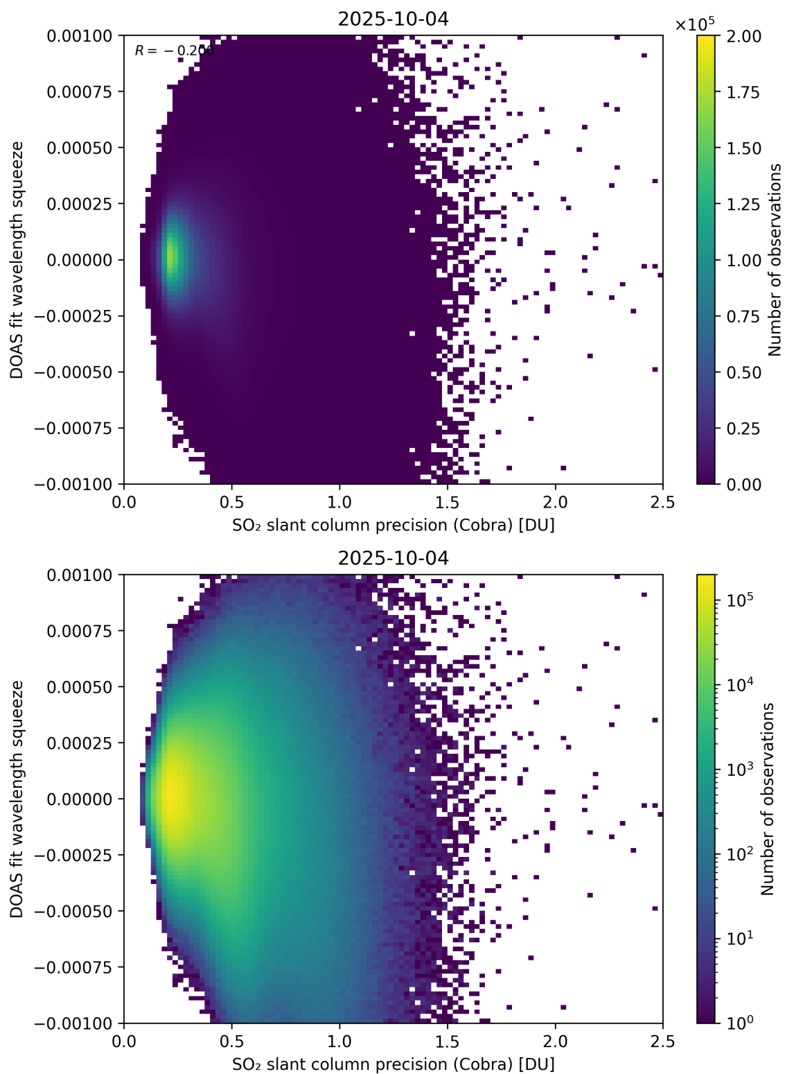
Figure 203: Scatter density plot of “SO 2 slant column precision (Cobra)” against “DOAS fit wavelength squeeze” for 2025-10-03 to 2025-10-05.
