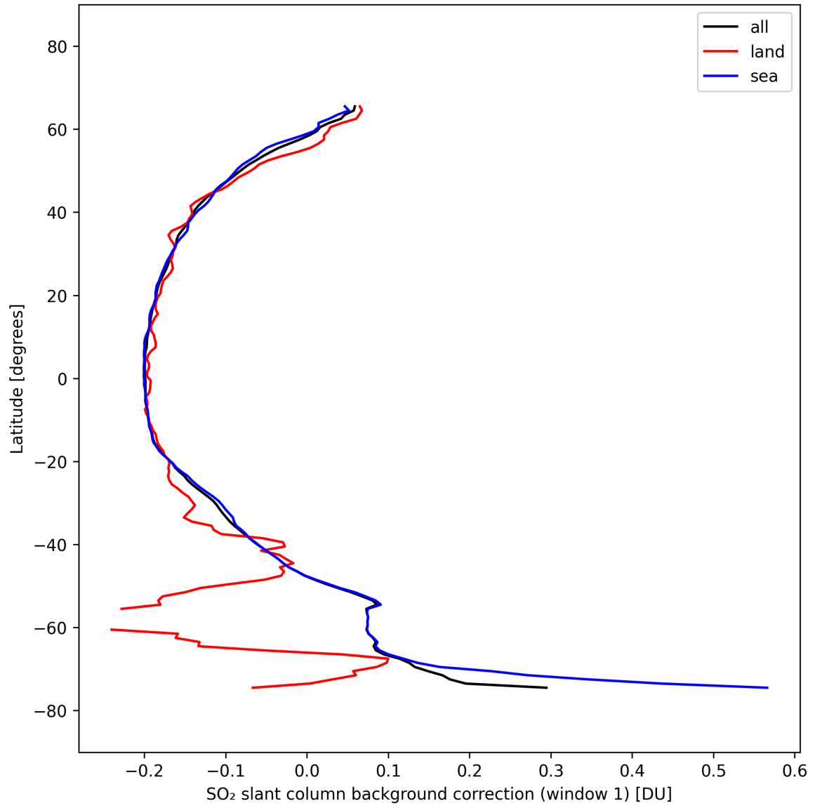
Figure 40: Zonal average of "SO 2 slant column background correction (window 1)" for 2025-10-03 to 2025-10-05.
