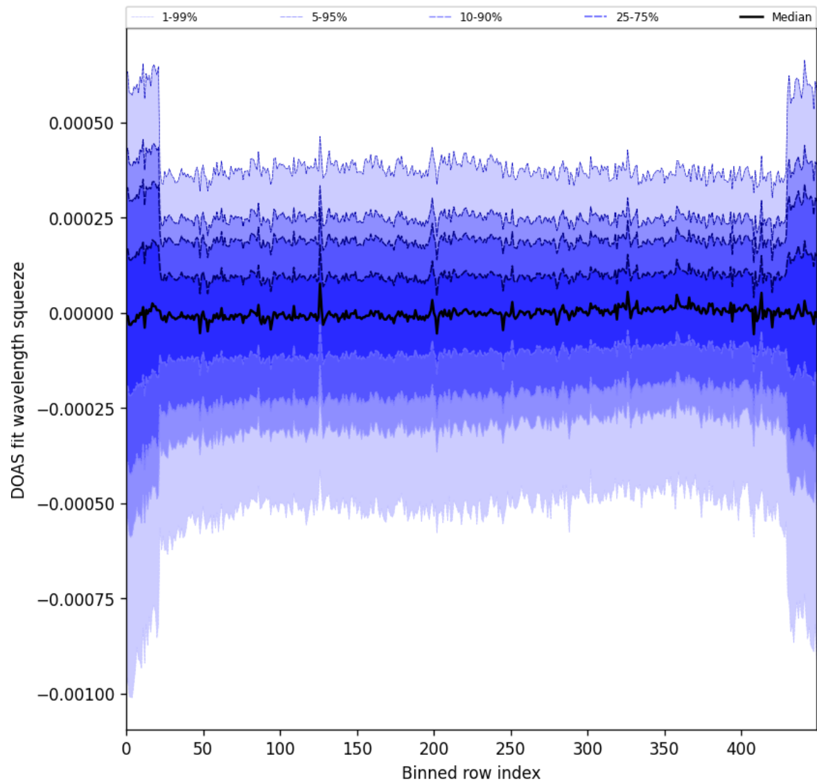
Figure 103: Along track statistics of “DOAS fit wavelength squeeze” for 2025-10-03 to 2025-10-05
