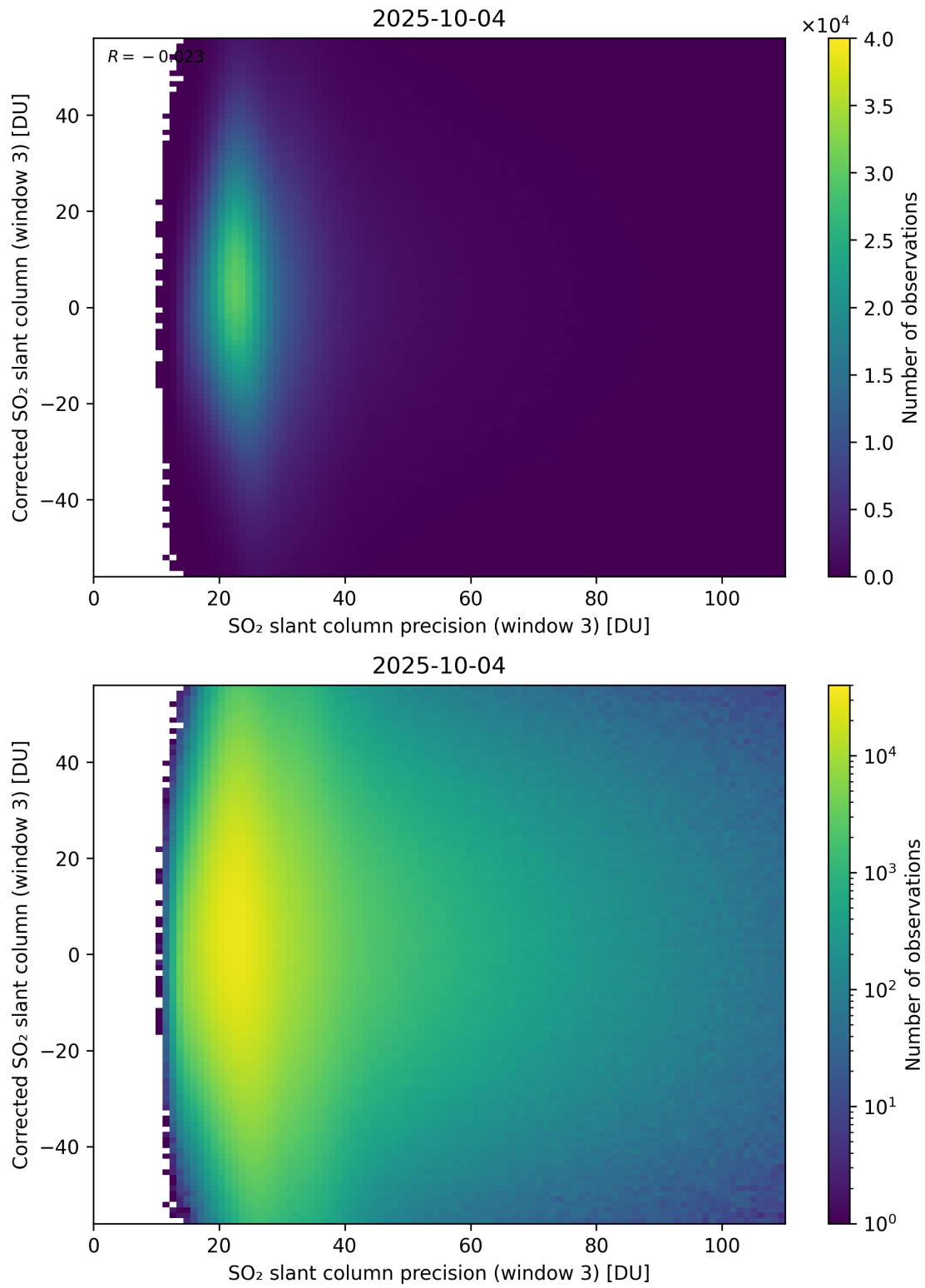
Figure 312: Scatter density plot of “SO 2 slant column precision (window 3)” against “Corrected SO 2 slant column (window 3)” for 2025-10-03 to 2025-10-05.
