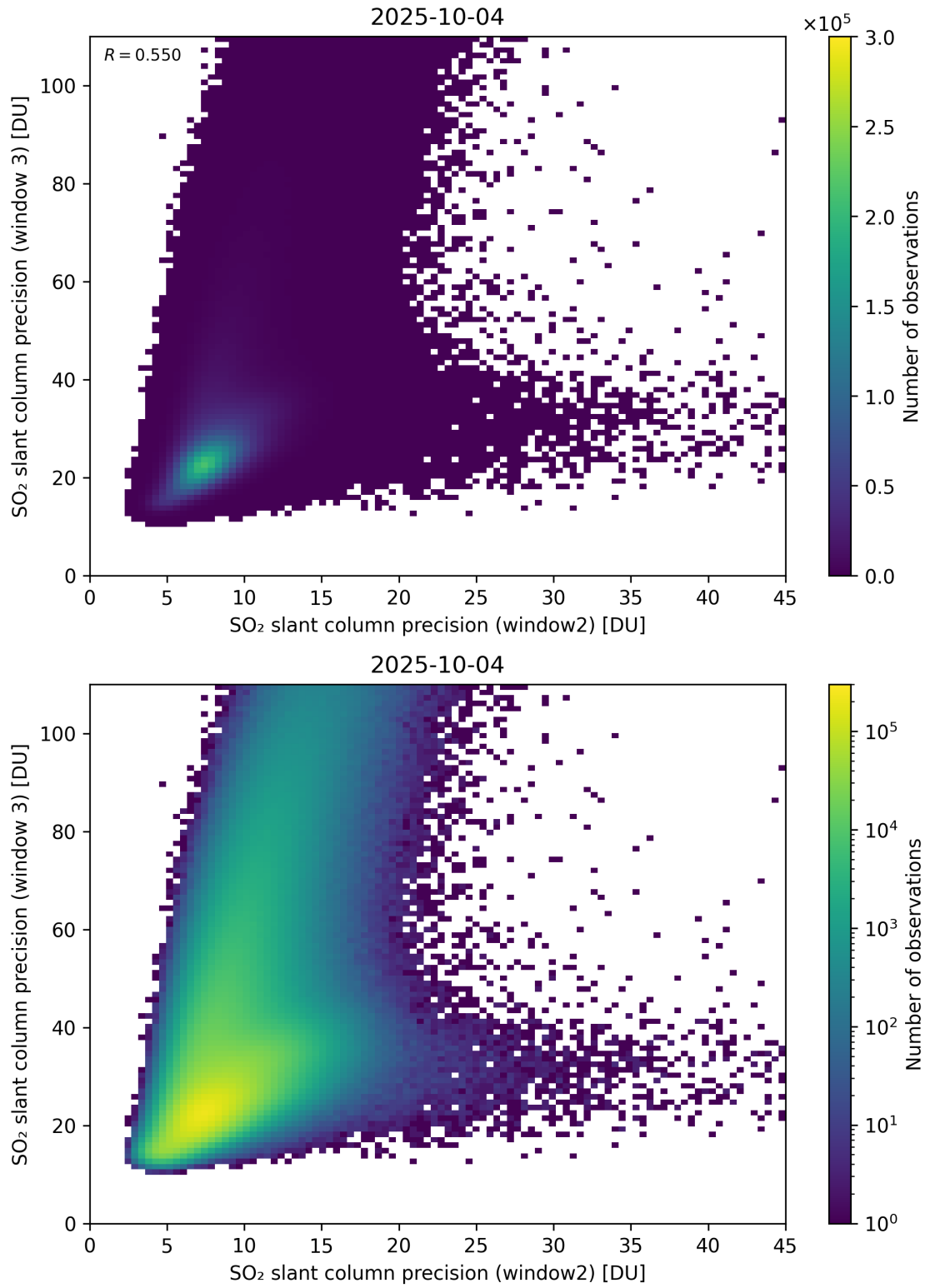
Figure 300: Scatter density plot of “SO 2 slant column precision (window2)” against “SO 2 slant column precision (window 3)” for 2025-10-03 to 2025-10-05.
