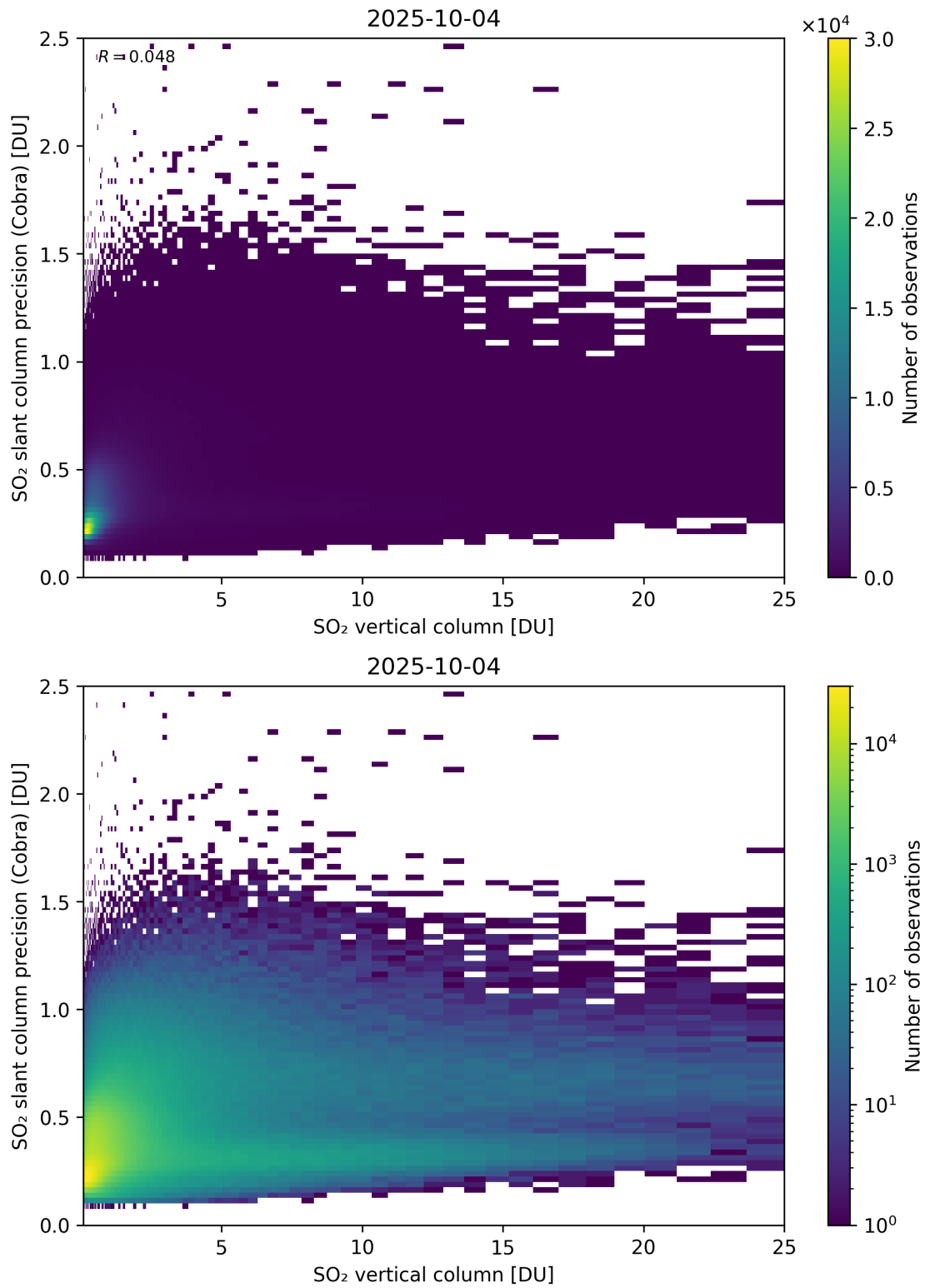
Figure 350: Scatter density plot of “SO 2 vertical column” against “SO 2 slant column precision (Cobra)” for 2025-10-03 to 2025-10-05.
