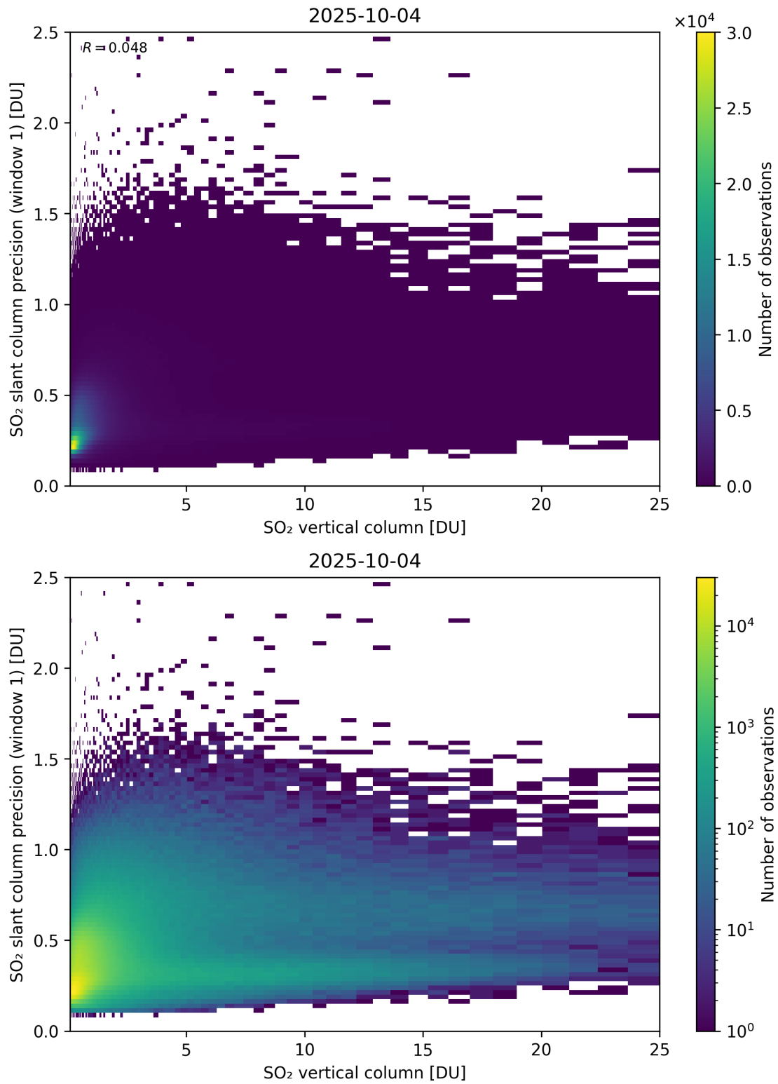
Figure 355: Scatter density plot of “SO 2 vertical column” against “SO 2 slant column precision (window 1)” for 2025-10-03 to 2025-10-05.
