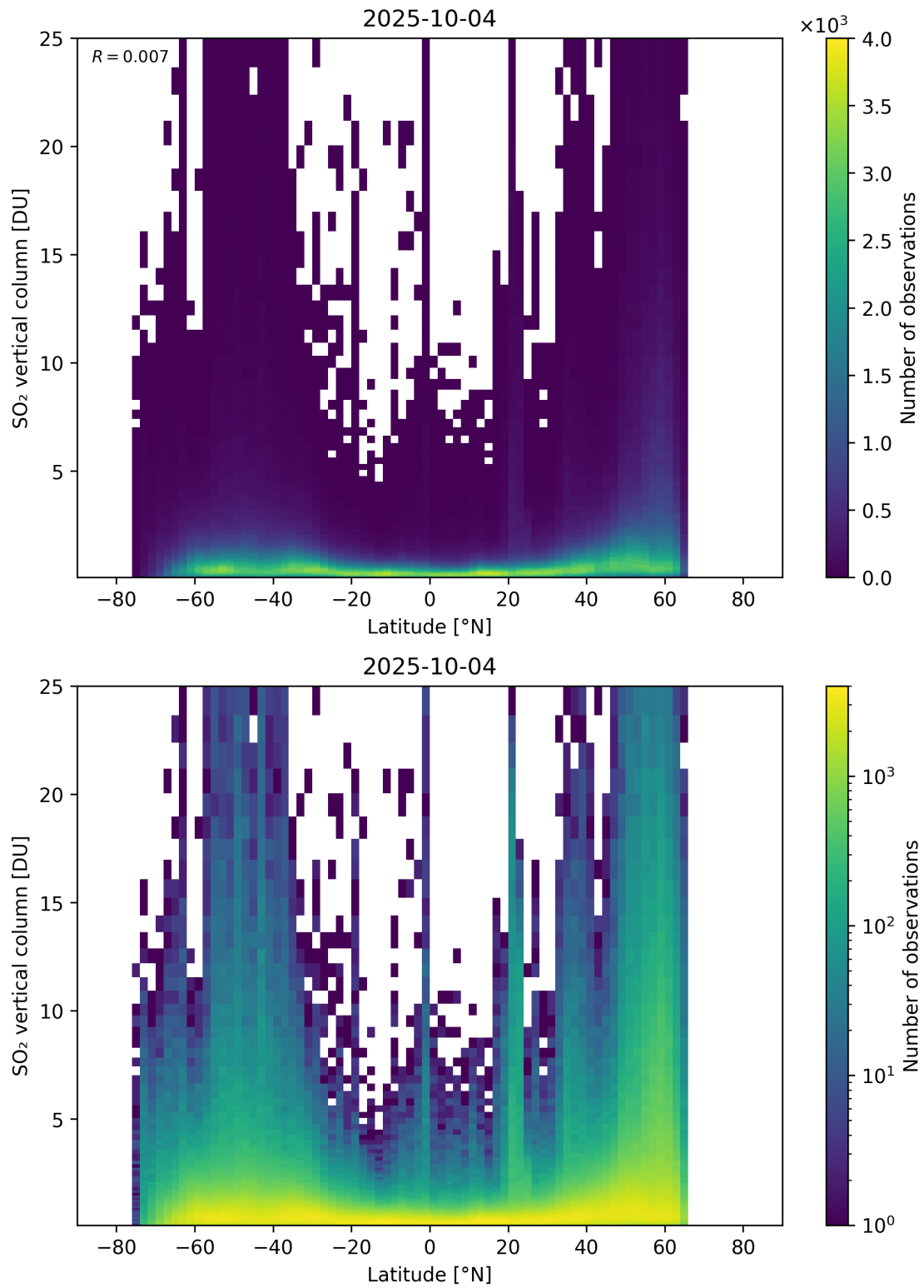
Figure 169: Scatter density plot of “Latitude” against “SO 2 vertical column” for 2025-10-03 to 2025-10-05.
