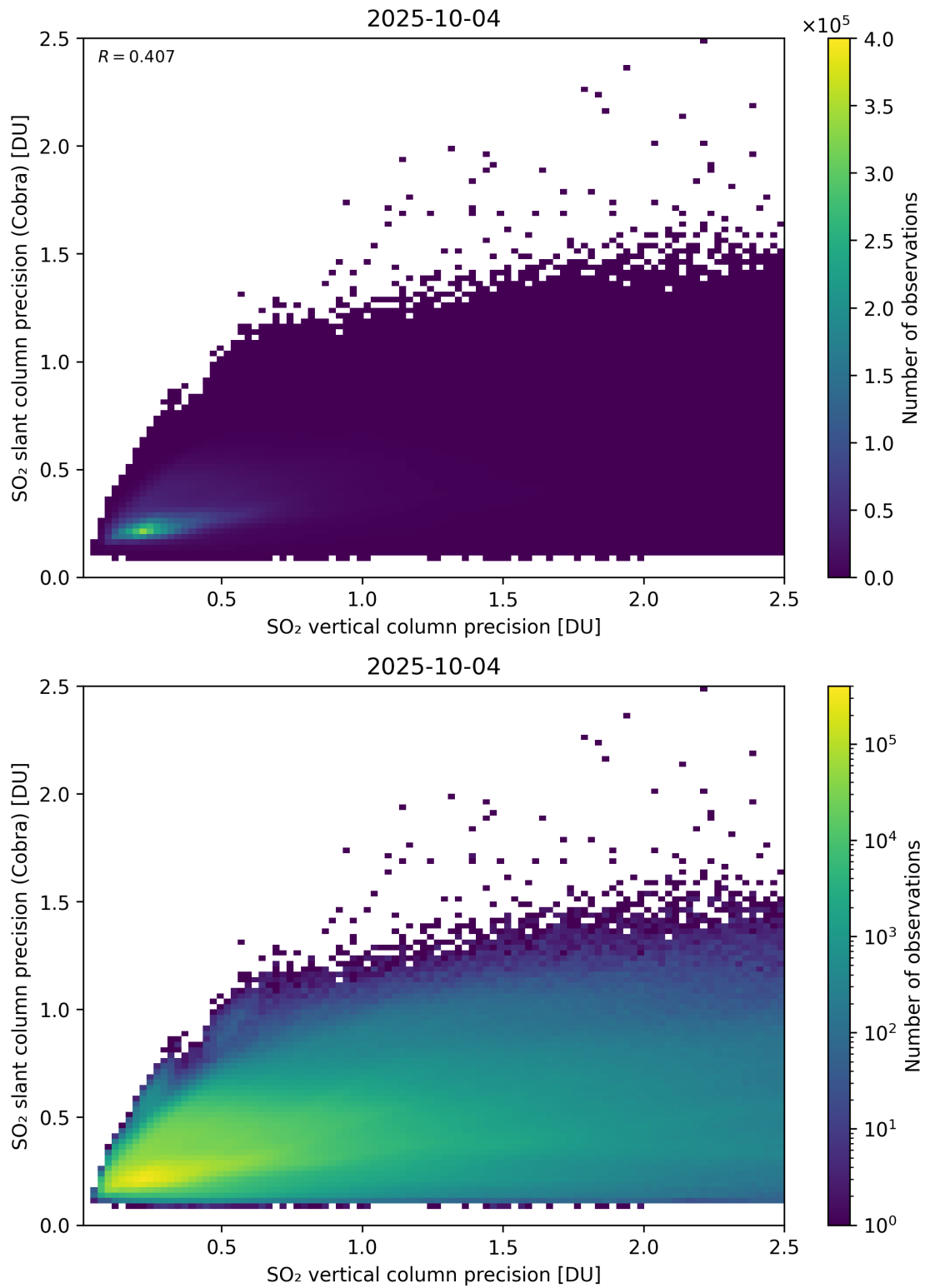
Figure 337: Scatter density plot of “SO 2 vertical column precision” against “SO 2 slant column precision (Cobra)” for 2025-10-03 to 2025-10-05.
