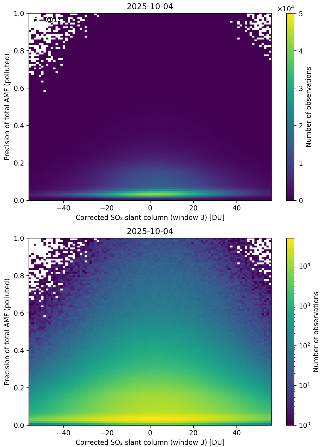
Figure 261: Scatter density plot of “Corrected SO 2 slant column (window 3)” against “Precision of total AMF (polluted)” for 2025-10-03 to 2025-10-05.
