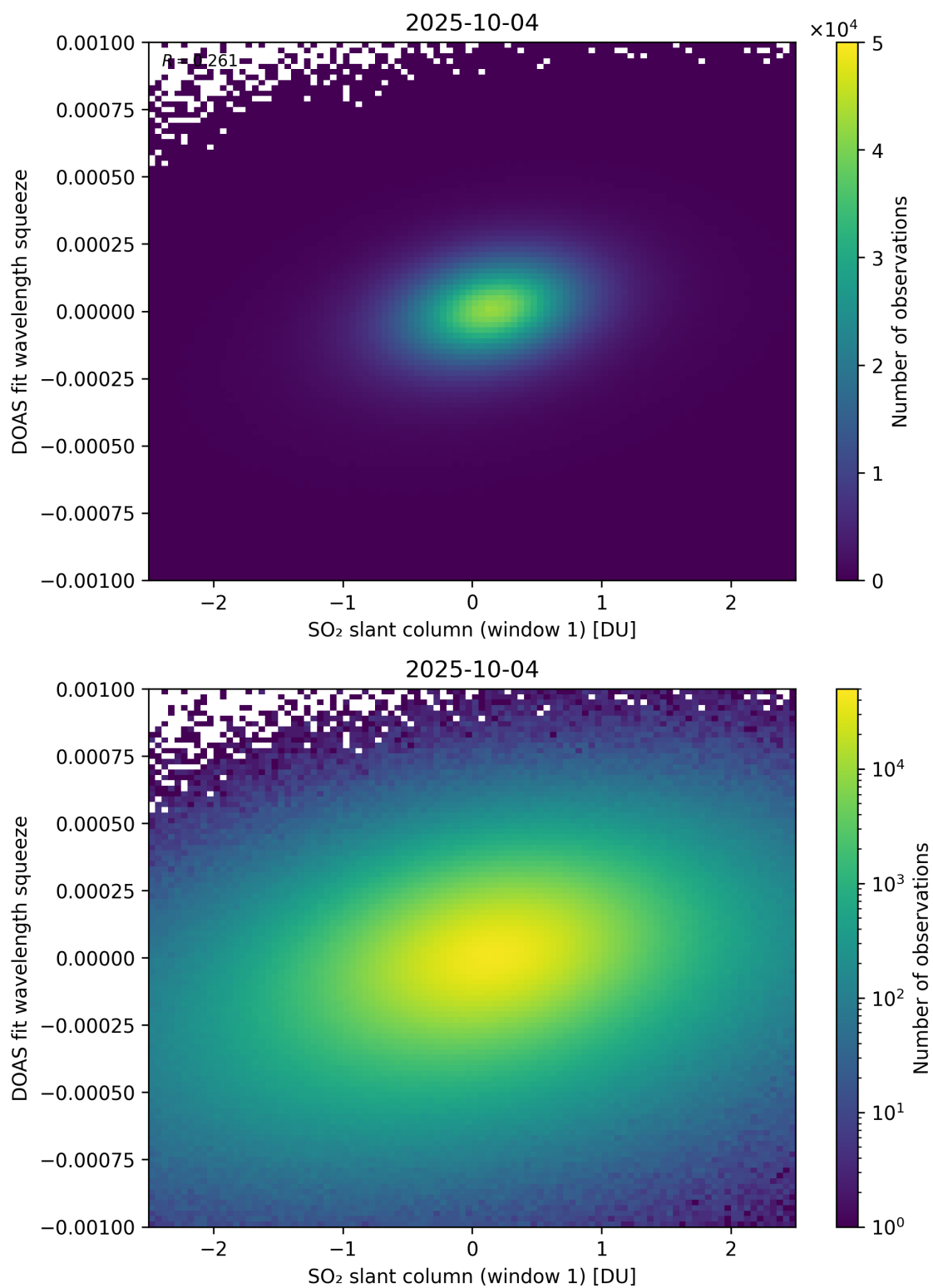
Figure 266: Scatter density plot of “SO 2 slant column (window 1)” against “DOAS fit wavelength squeeze” for 2025-10-03 to 2025-10-05.
