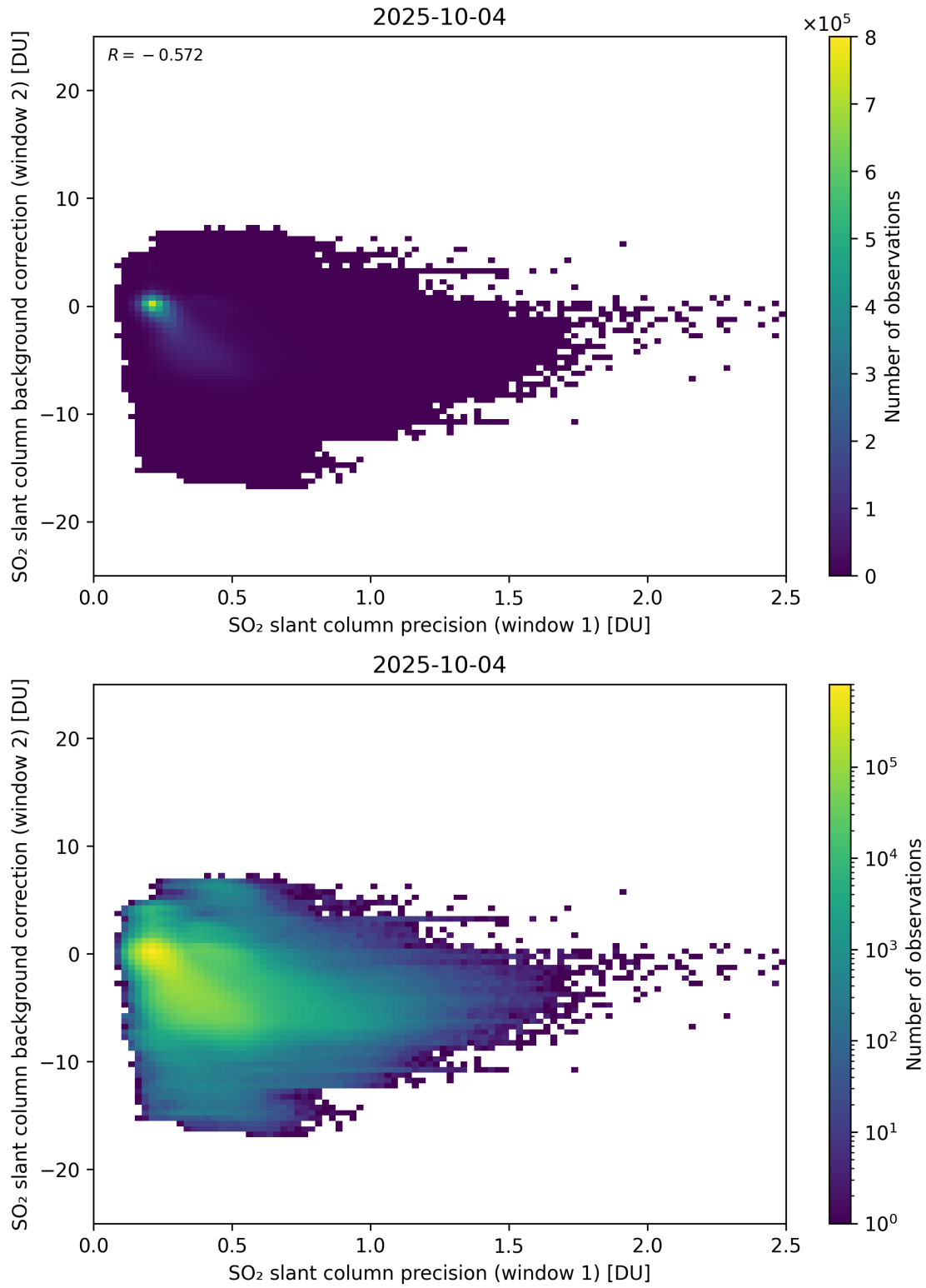
Figure 269: Scatter density plot of “SO 2 slant column precision (window 1)” against “SO 2 slant column background correction (window 2)” for 2025-10-03 to 2025-10-05.
