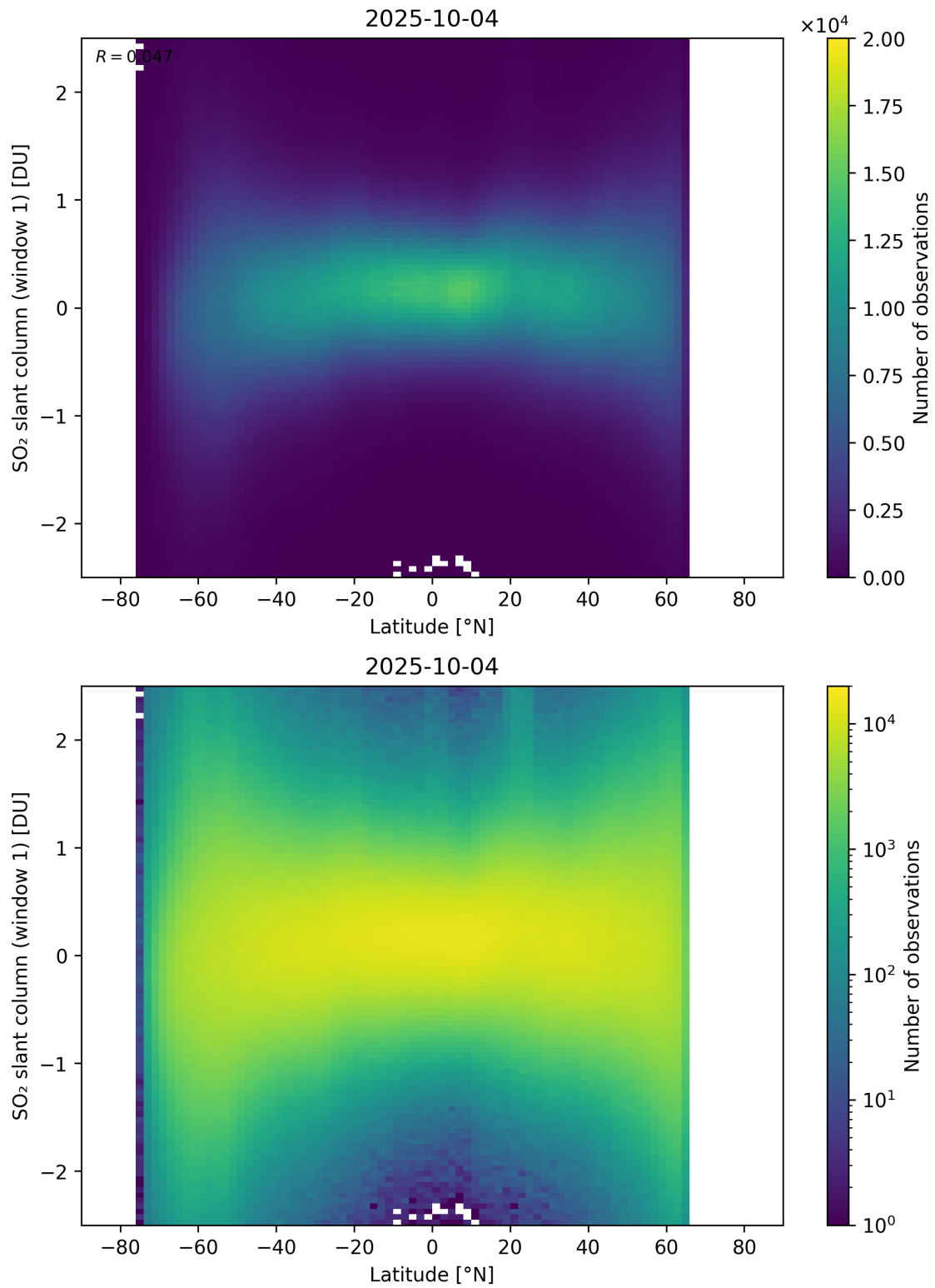
Figure 162: Scatter density plot of “Latitude” against “SO 2 slant column (window 1)” for 2025-10-03 to 2025-10-05.
