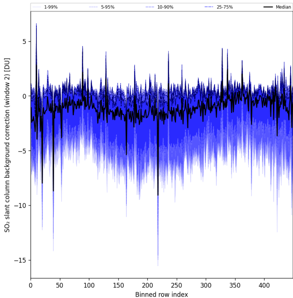
Figure 96: Along track statistics of “SO 2 slant column background correction (window 2)” for 2025-10-03 to 2025-10-05
