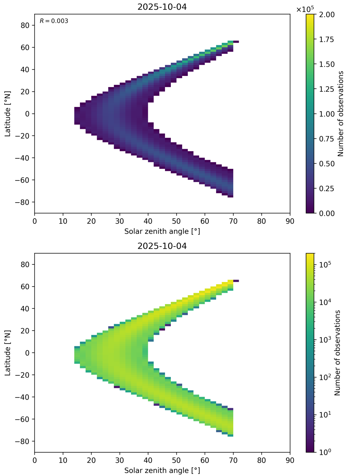
Figure 177: Scatter density plot of “Solar zenith angle” against “Latitude” for 2025-10-03 to 2025-10-05.
