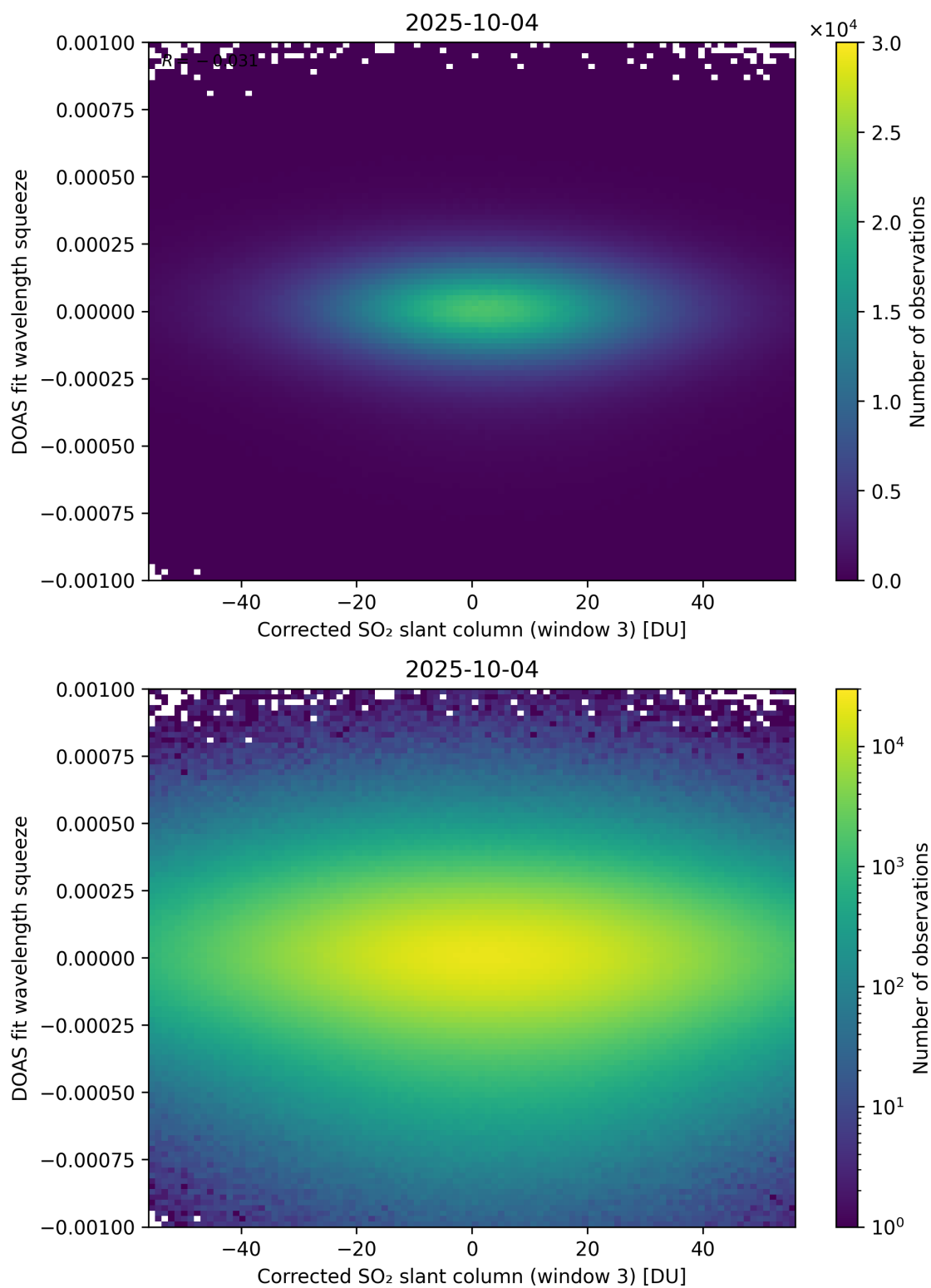
Figure 257: Scatter density plot of “Corrected SO 2 slant column (window 3)” against “DOAS fit wavelength squeeze” for 2025-10-03 to 2025-10-05.
