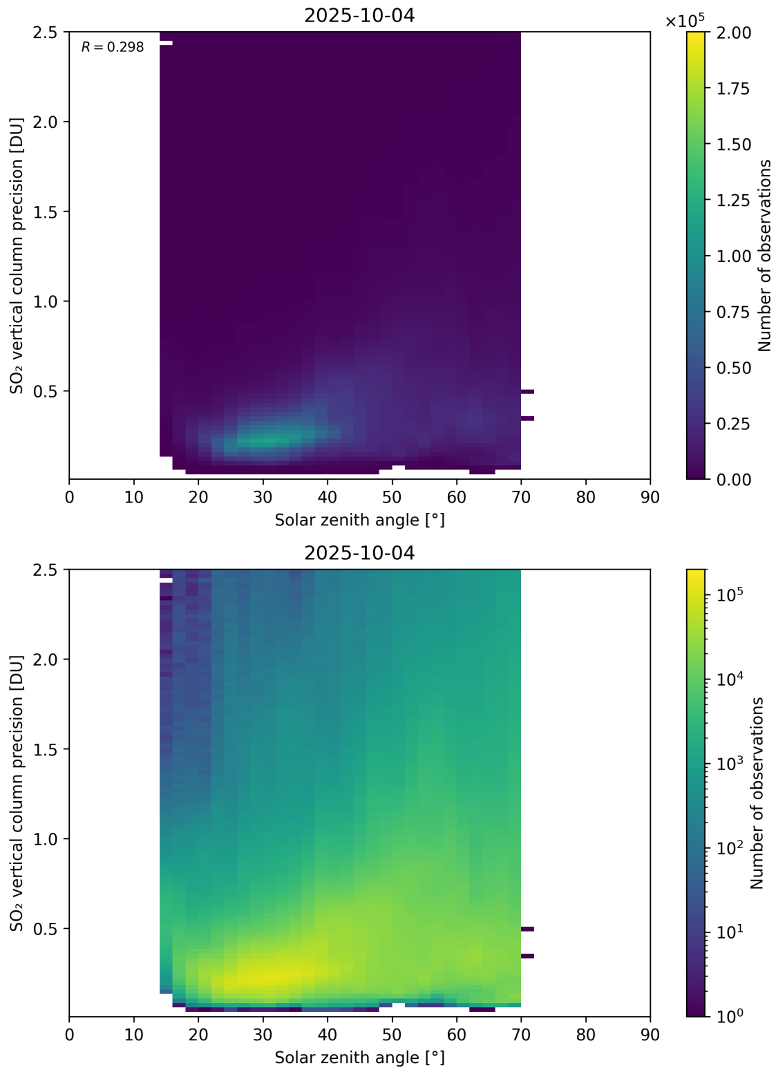
Figure 192: Scatter density plot of “Solar zenith angle” against “SO 2 vertical column precision” for 2025-10-03 to 2025-10-05.
