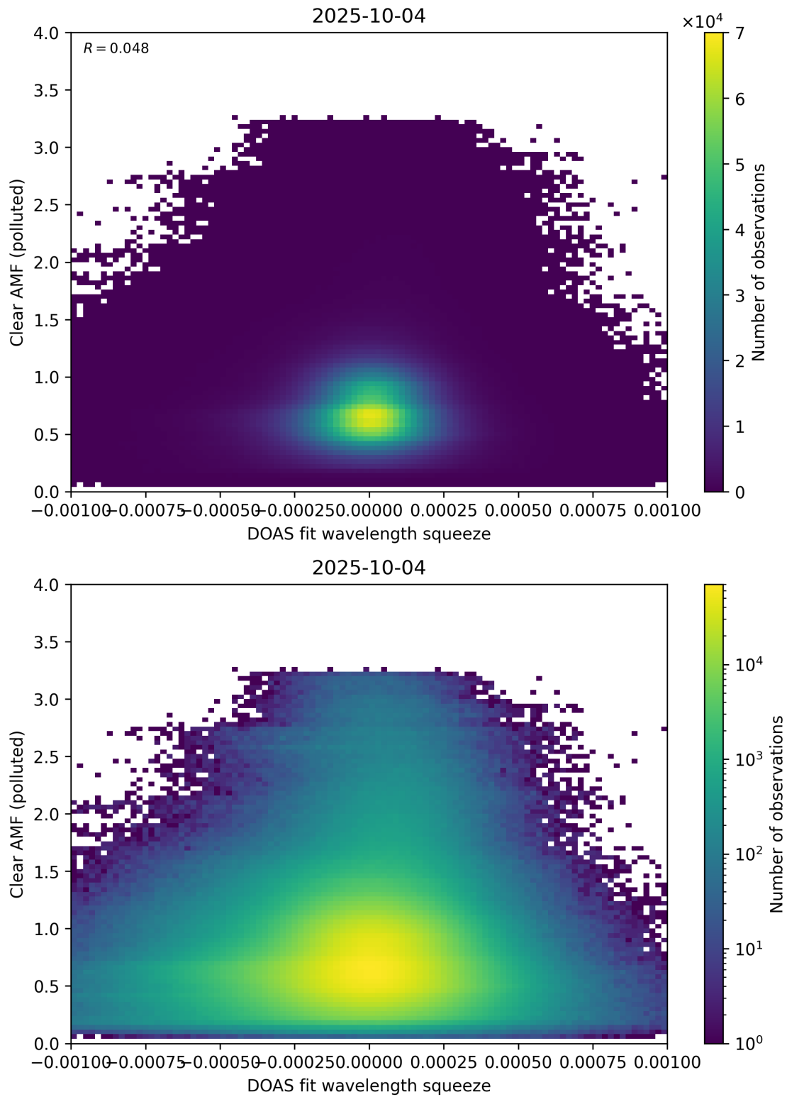
Figure 144: Scatter density plot of “DOAS fit wavelength squeeze” against “Clear AMF (polluted)” for 2025-10-03 to 2025-10-05.
