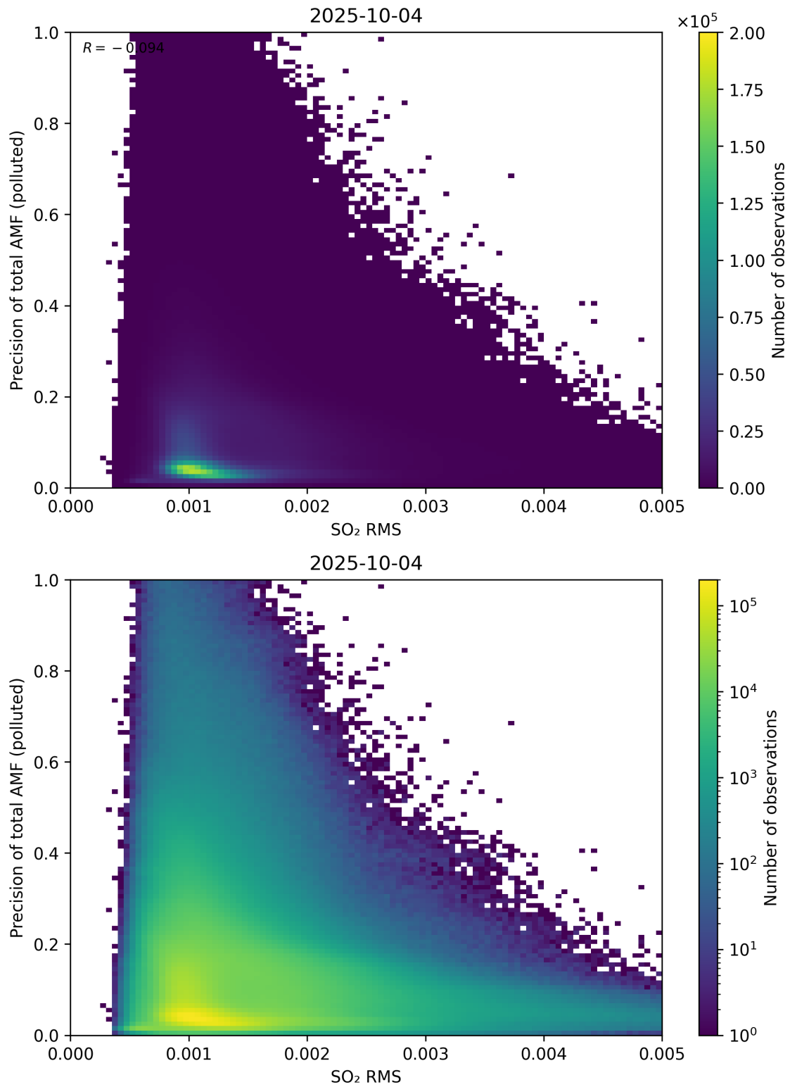
Figure 149: Scatter density plot of “SO 2 RMS” against “Precision of total AMF (polluted)” for 2025-10-03 to 2025-10-05.
