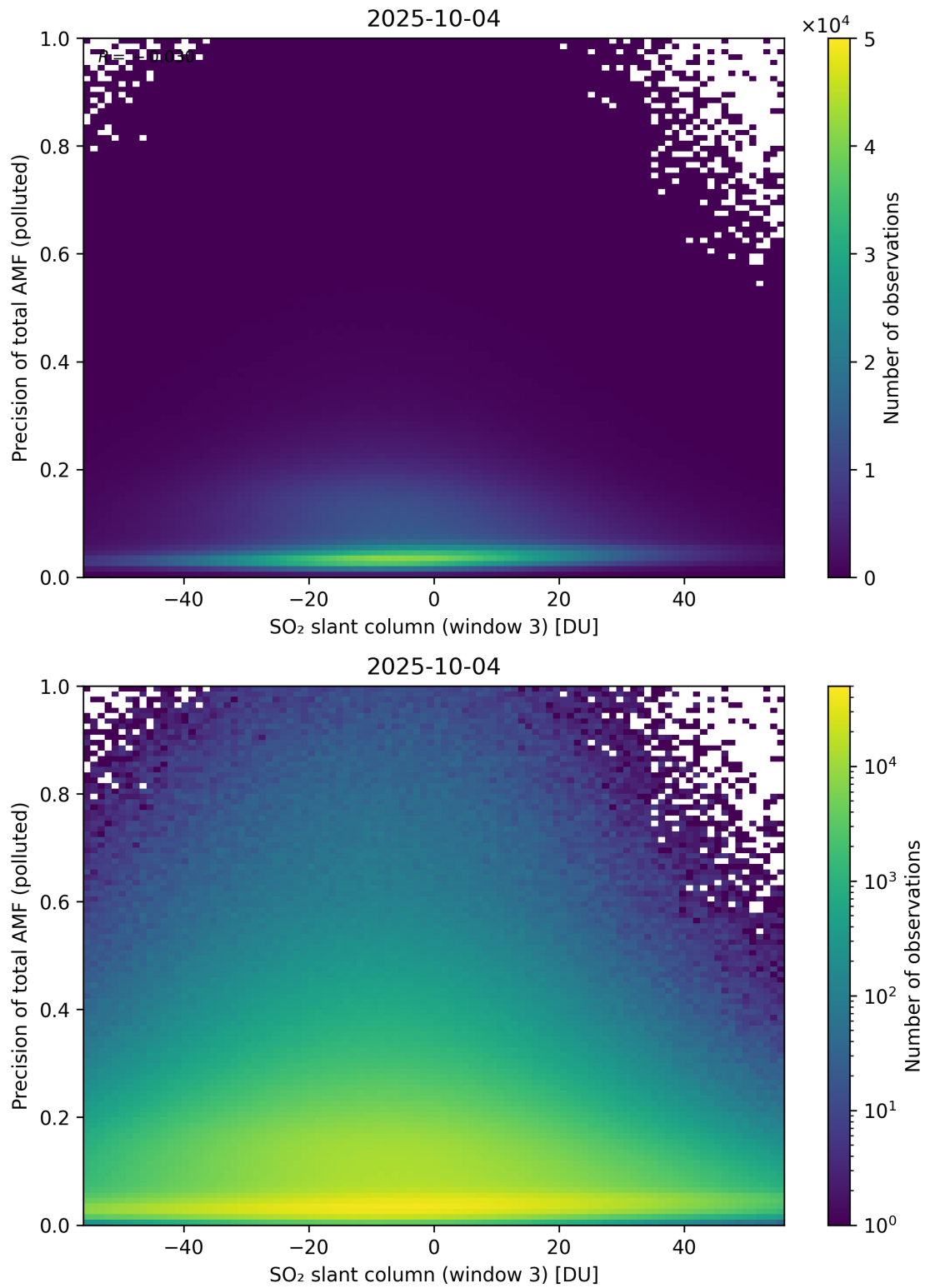
Figure 319: Scatter density plot of “SO 2 slant column (window 3)” against “Precision of total AMF (polluted)” for 2025-10-03 to 2025-10-05.
