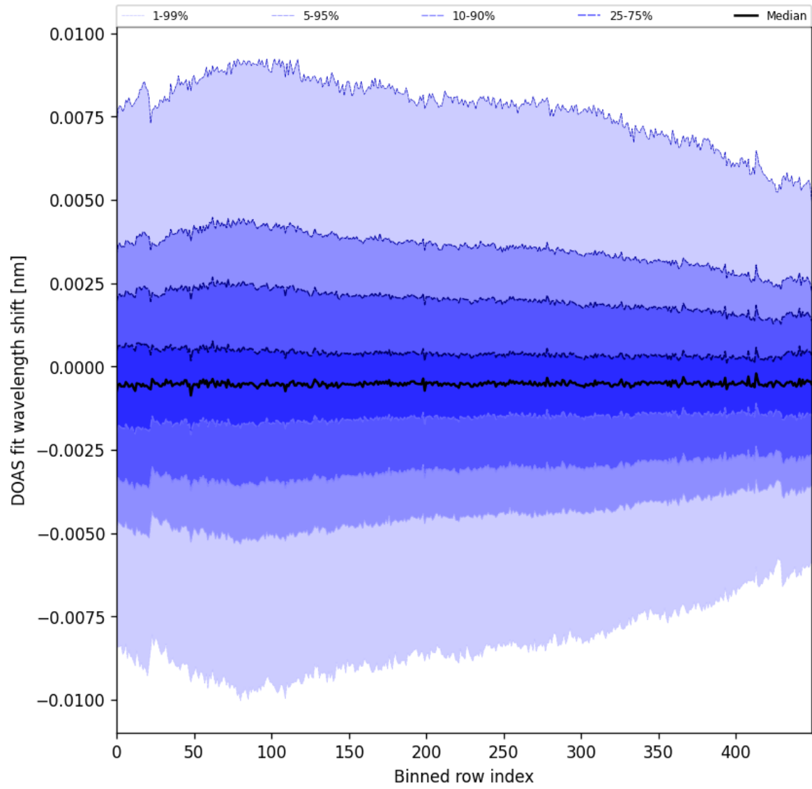
Figure 102: Along track statistics of “DOAS fit wavelength shift” for 2025-10-03 to 2025-10-05
