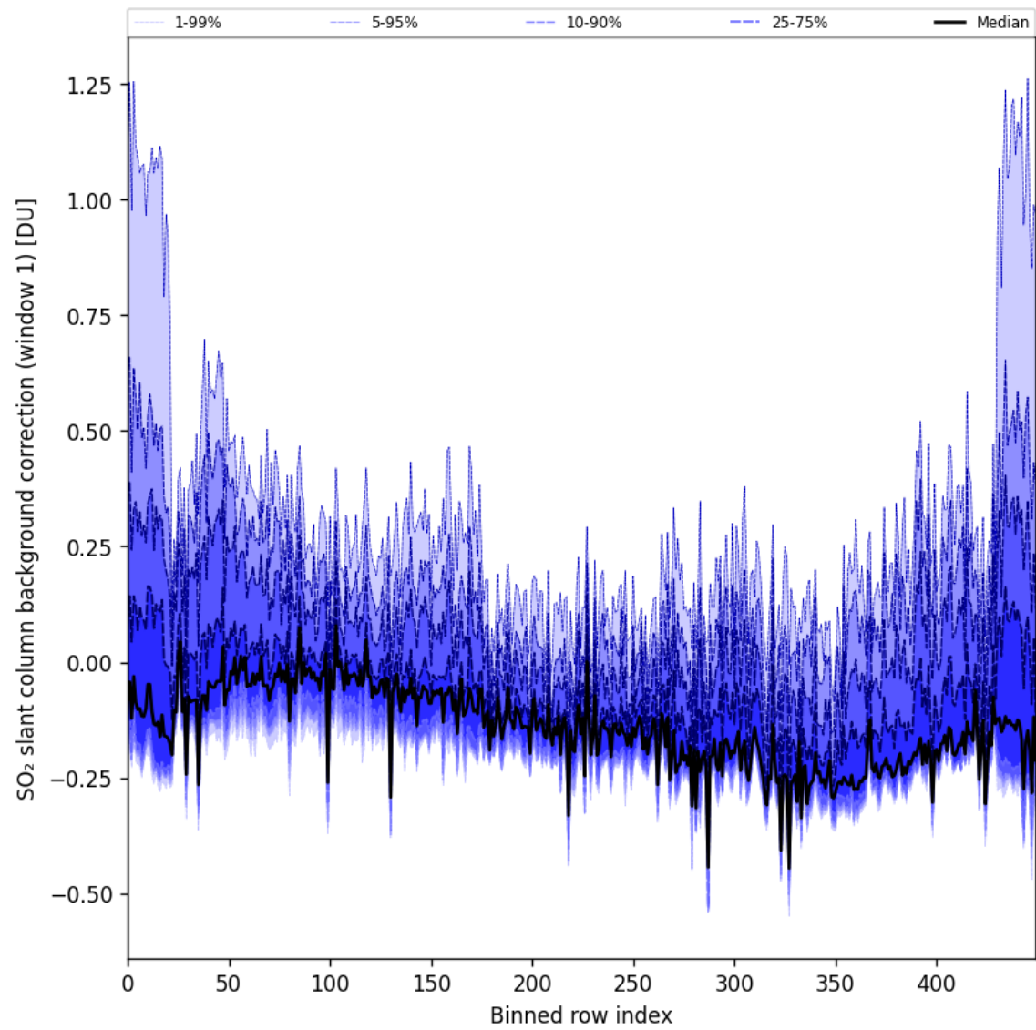
Figure 92: Along track statistics of “SO 2 slant column background correction (window 1)” for 2025-10-03 to 2025-10-05
