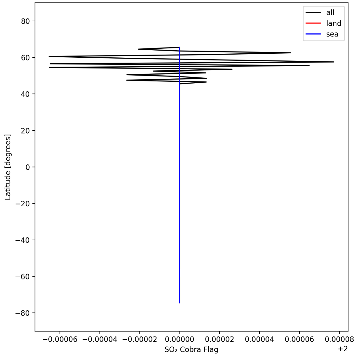
Figure 49: Zonal average of "SO 2 Cobra Flag" for 2025-10-03 to 2025-10-05.
