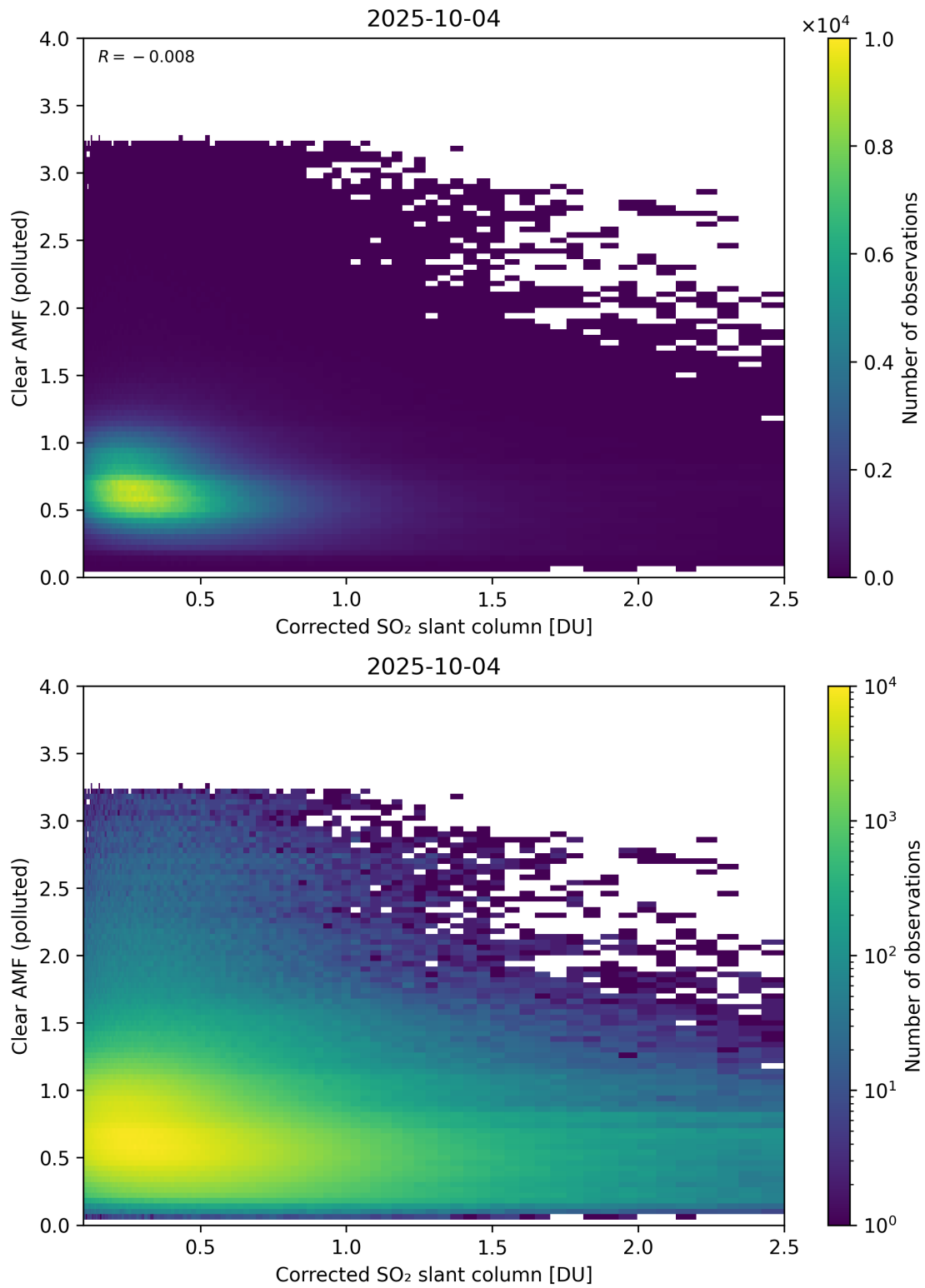
Figure 232: Scatter density plot of “Corrected SO 2 slant column” against “Clear AMF (polluted)” for 2025-10-03 to 2025-10-05.
