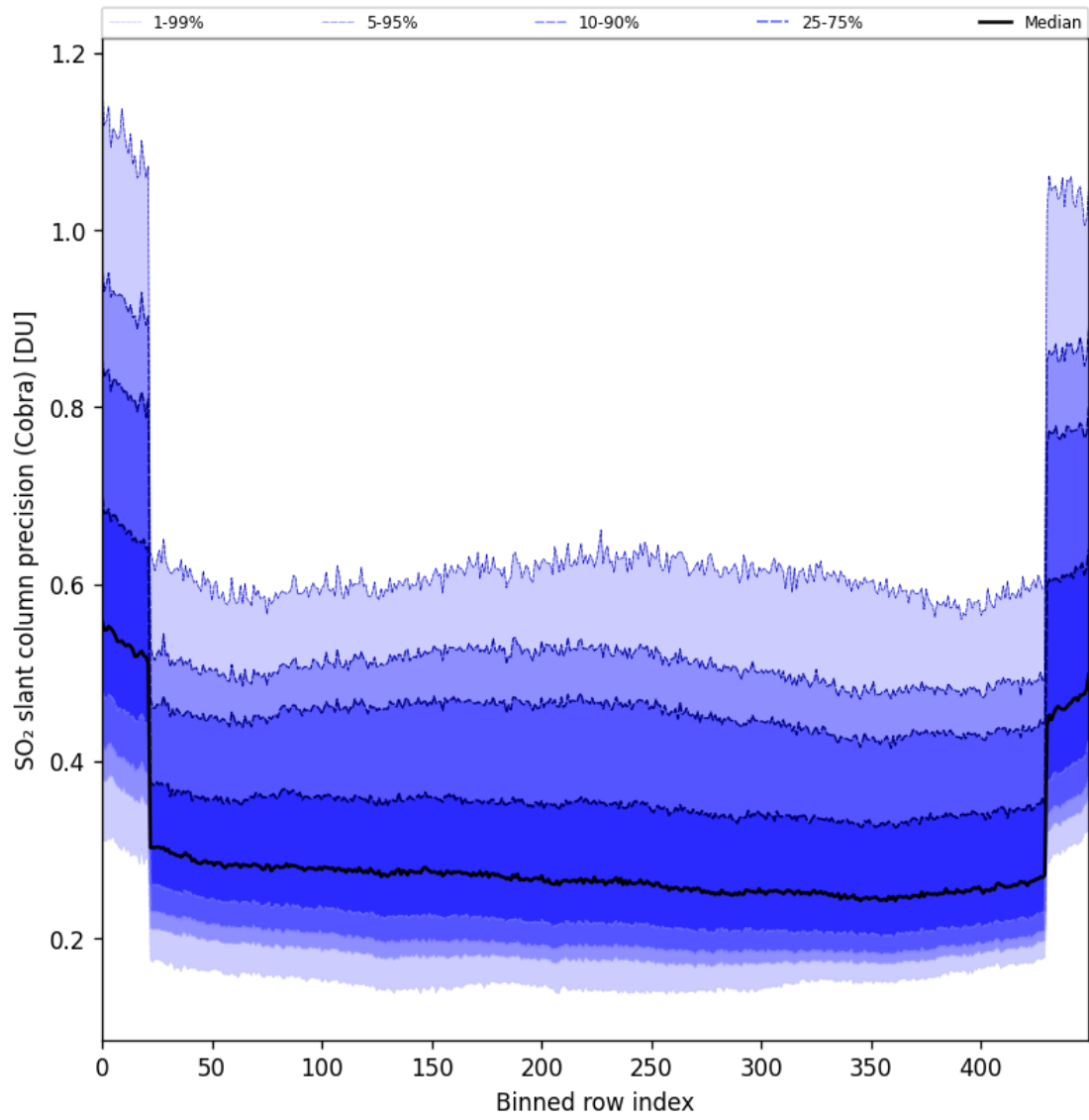
Figure 88: Along track statistics of “SO 2 slant column precision (Cobra)” for 2025-10-03 to 2025-10-05
