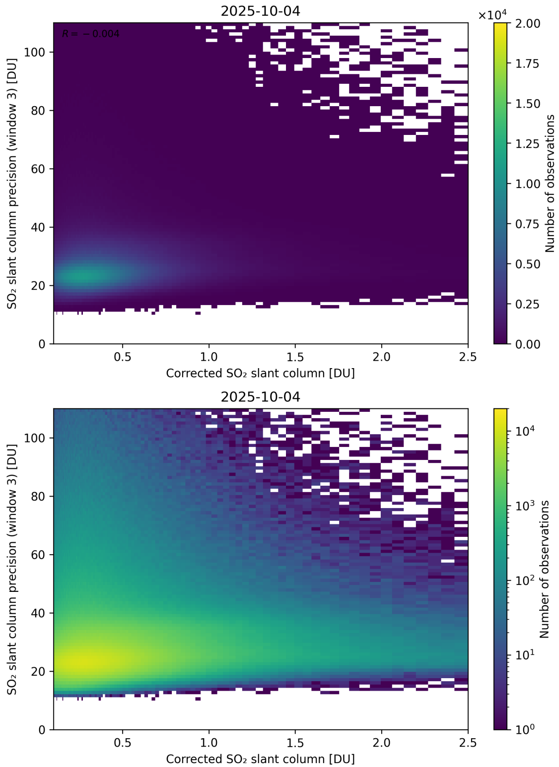
Figure 241: Scatter density plot of “Corrected SO 2 slant column” against “SO 2 slant column precision (window 3)” for 2025-10-03 to 2025-10-05.
