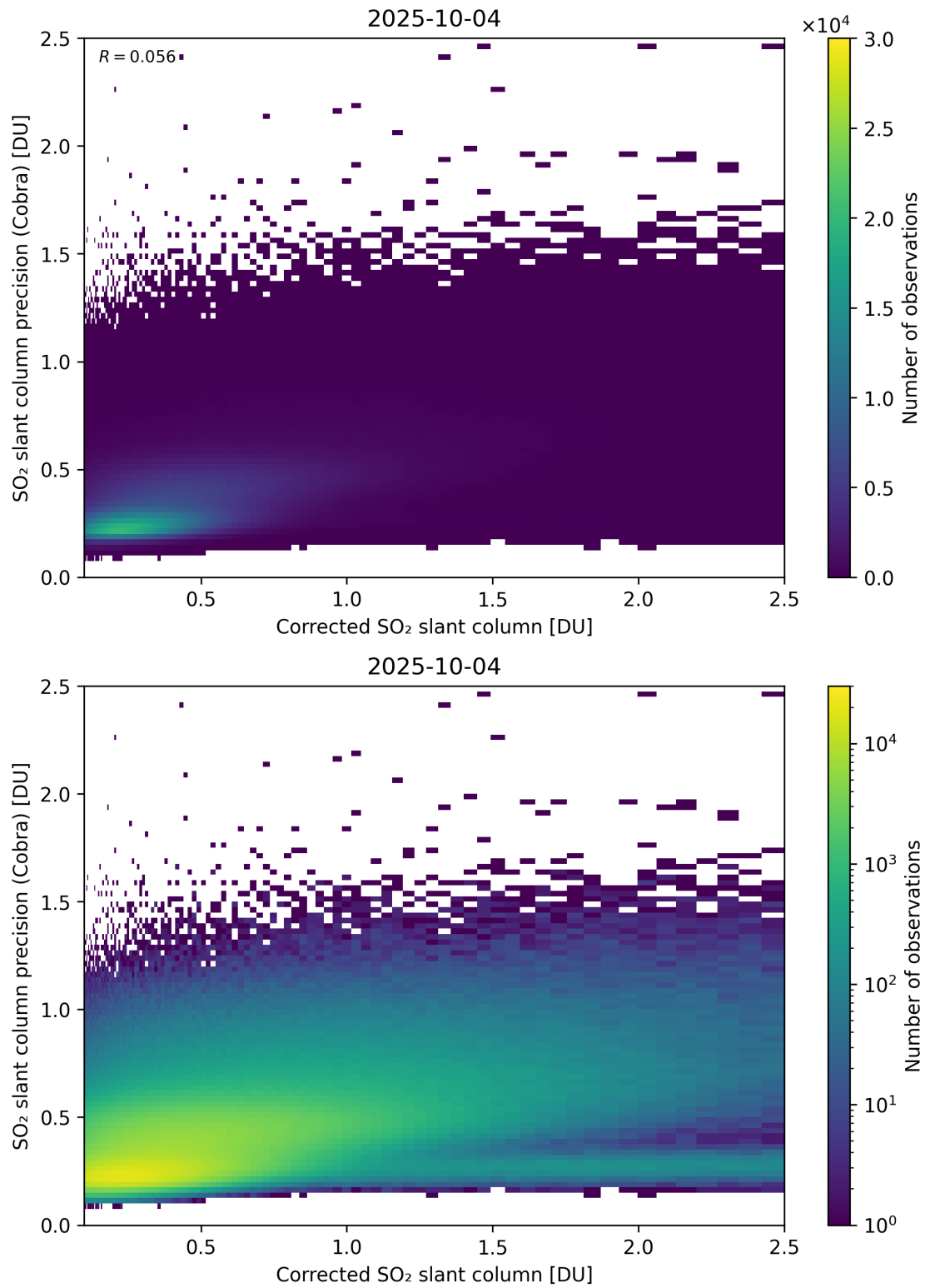
Figure 234: Scatter density plot of “Corrected SO 2 slant column” against “SO 2 slant column precision (Cobra)” for 2025-10-03 to 2025-10-05.
