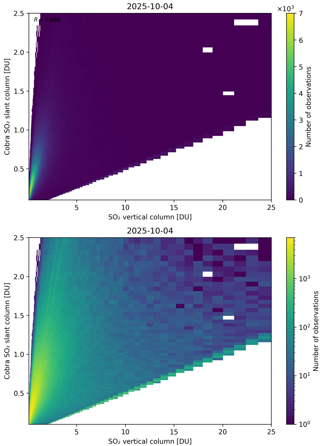
Figure 349: Scatter density plot of “SO 2 vertical column” against “Cobra SO 2 slant column” for 2025-10-03 to 2025-10-05.
