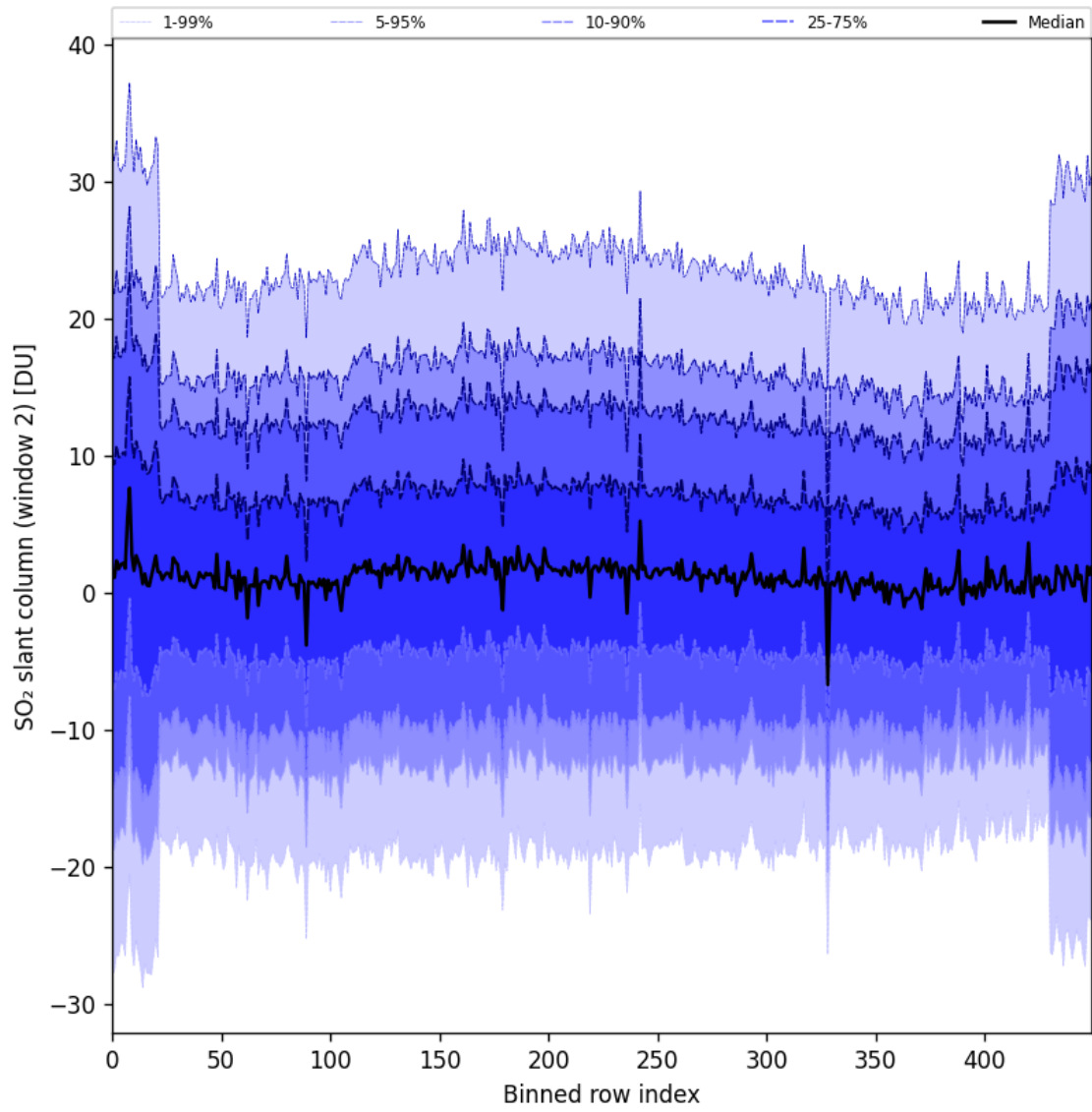
Figure 93: Along track statistics of “SO 2 slant column (window 2)” for 2025-10-03 to 2025-10-05
