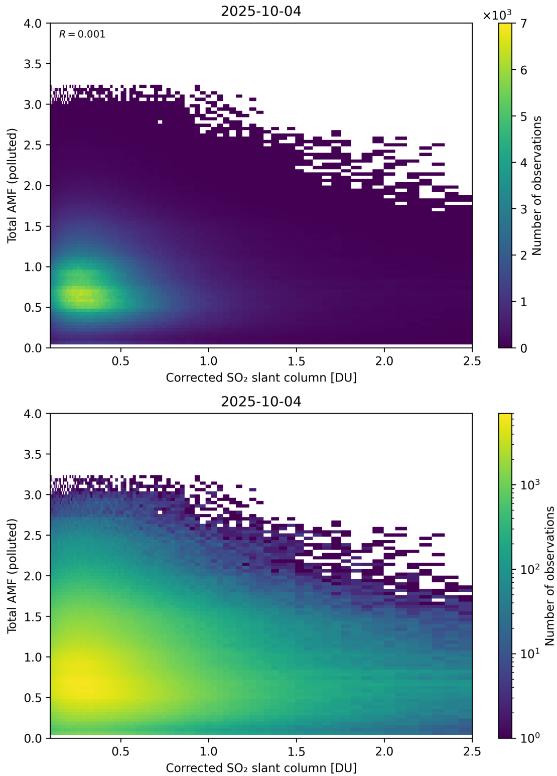
Figure 242: Scatter density plot of “Corrected SO 2 slant column” against “Total AMF (polluted)” for 2025-10-03 to 2025-10-05.
