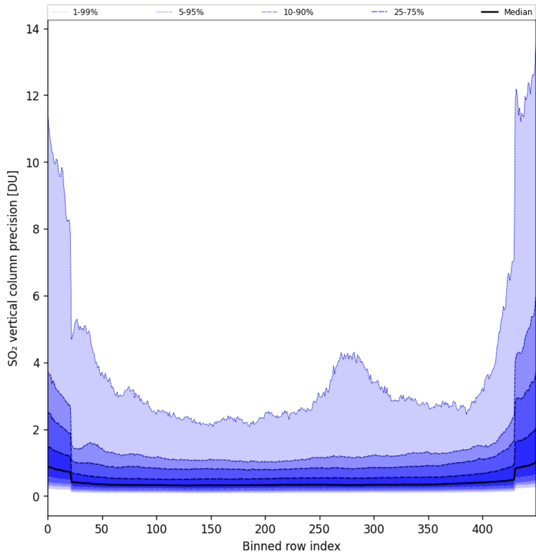
Figure 85: Along track statistics of “SO 2 vertical column precision” for 2025-10-03 to 2025-10-05
