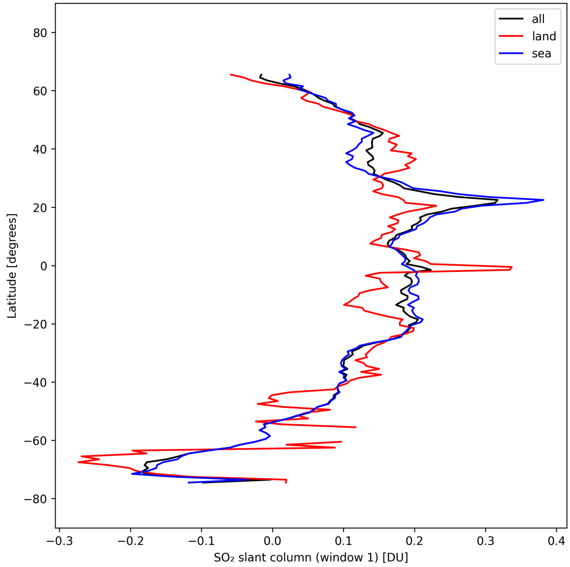
Figure 37: Zonal average of “SO 2 slant column (window 1)” for 2025-10-03 to 2025-10-05.
