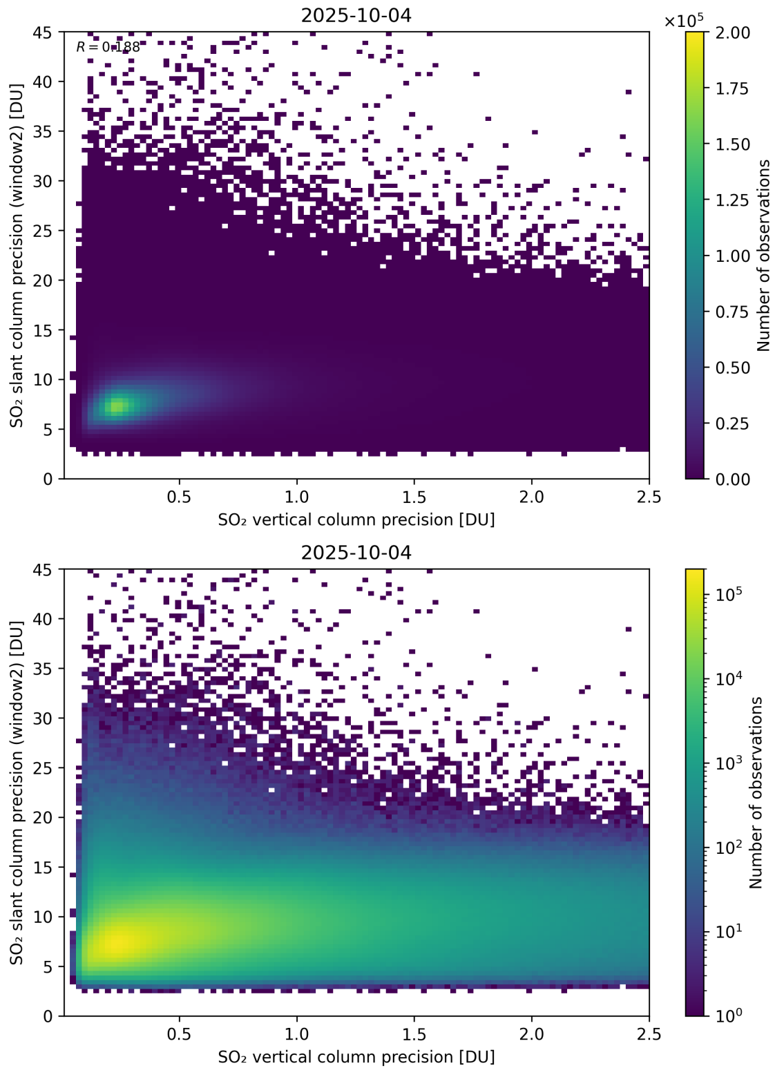
Figure 343: Scatter density plot of “SO 2 vertical column precision” against “SO 2 slant column precision (window2)” for 2025-10-03 to 2025-10-05.
