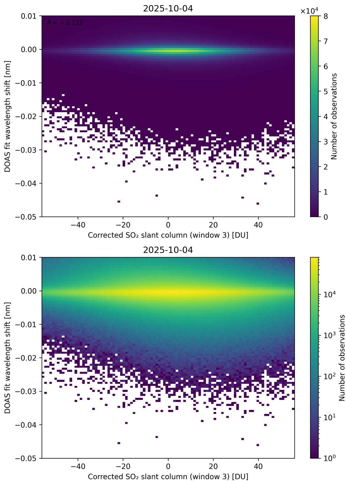
Figure 256: Scatter density plot of “Corrected SO 2 slant column (window 3)” against “DOAS fit wavelength shift” for 2025-10-03 to 2025-10-05.
