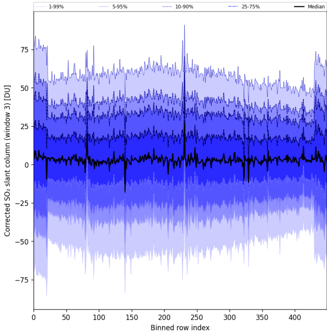
Figure 99: Along track statistics of “Corrected SO 2 slant column (window 3)” for 2025-10-03 to 2025-10-05
