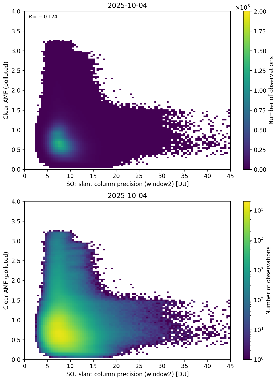
Figure 296: Scatter density plot of “SO 2 slant column precision (window2)” against “Clear AMF (polluted)” for 2025-10-03 to 2025-10-05.
