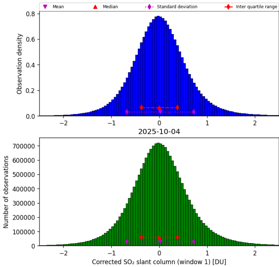
Figure 65: Histogram of “Corrected SO 2 slant column (window 1)” for 2025-10-03 to 2025-10-05
