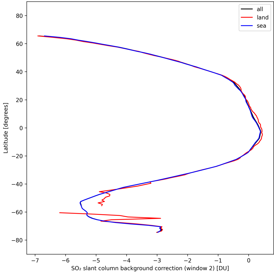
Figure 44: Zonal average of “SO 2 slant column background correction (window 2)” for 2025-10-03 to 2025-10-05.
