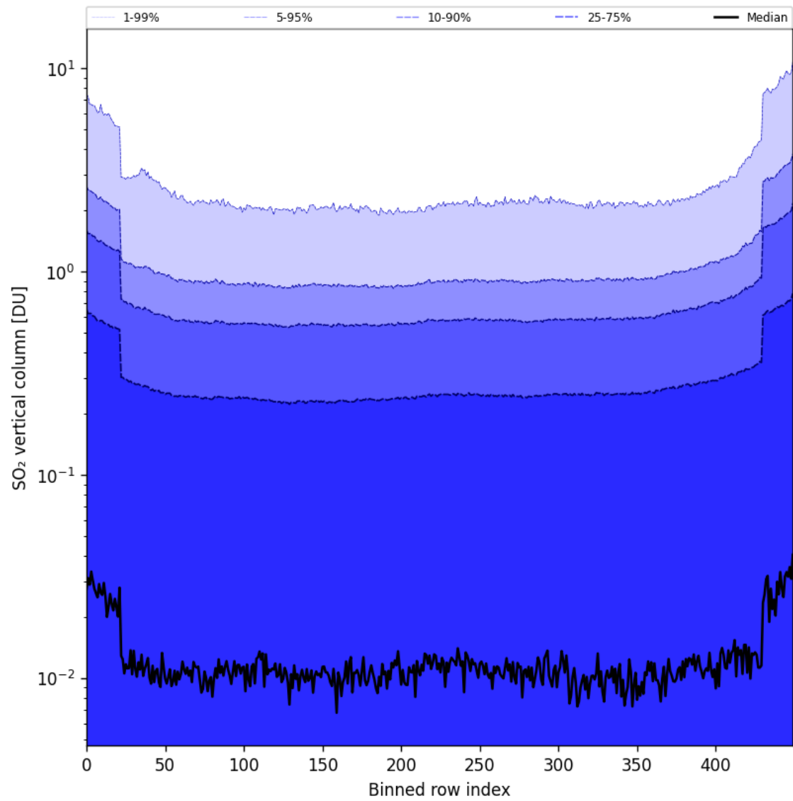
Figure 84: Along track statistics of “SO 2 vertical column” for 2025-10-03 to 2025-10-05
