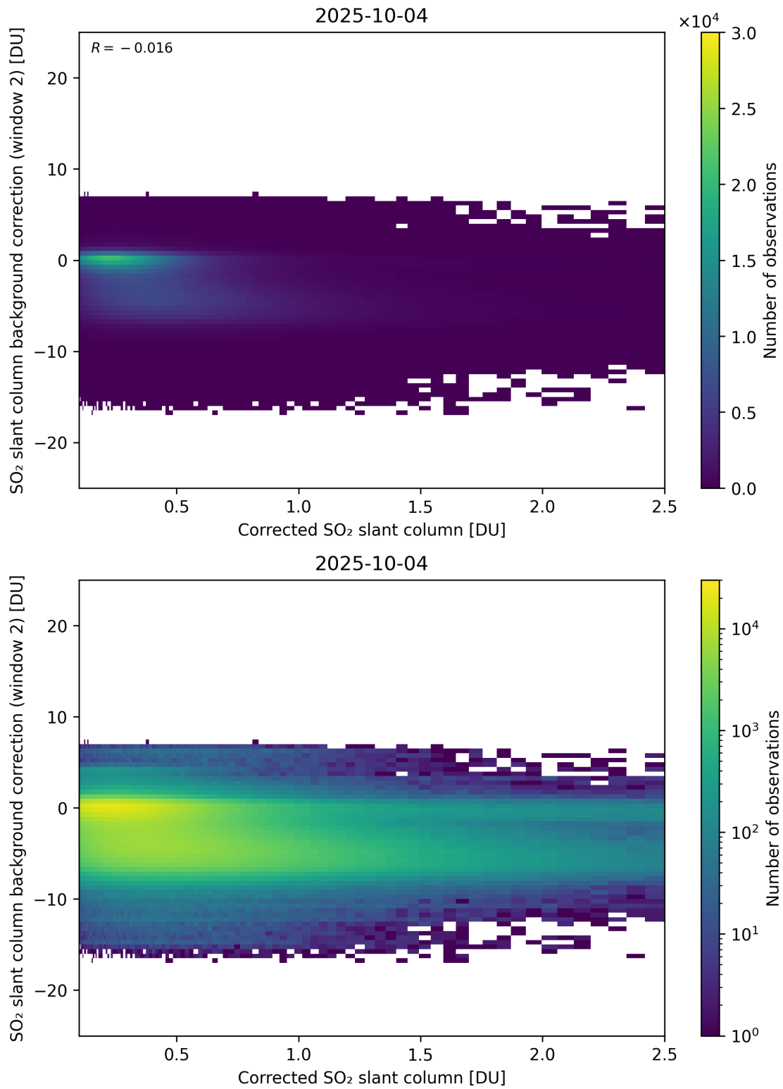
Figure 227: Scatter density plot of “Corrected SO 2 slant column” against “SO 2 slant column background correction (window 2)” for 2025-10-03 to 2025-10-05.
