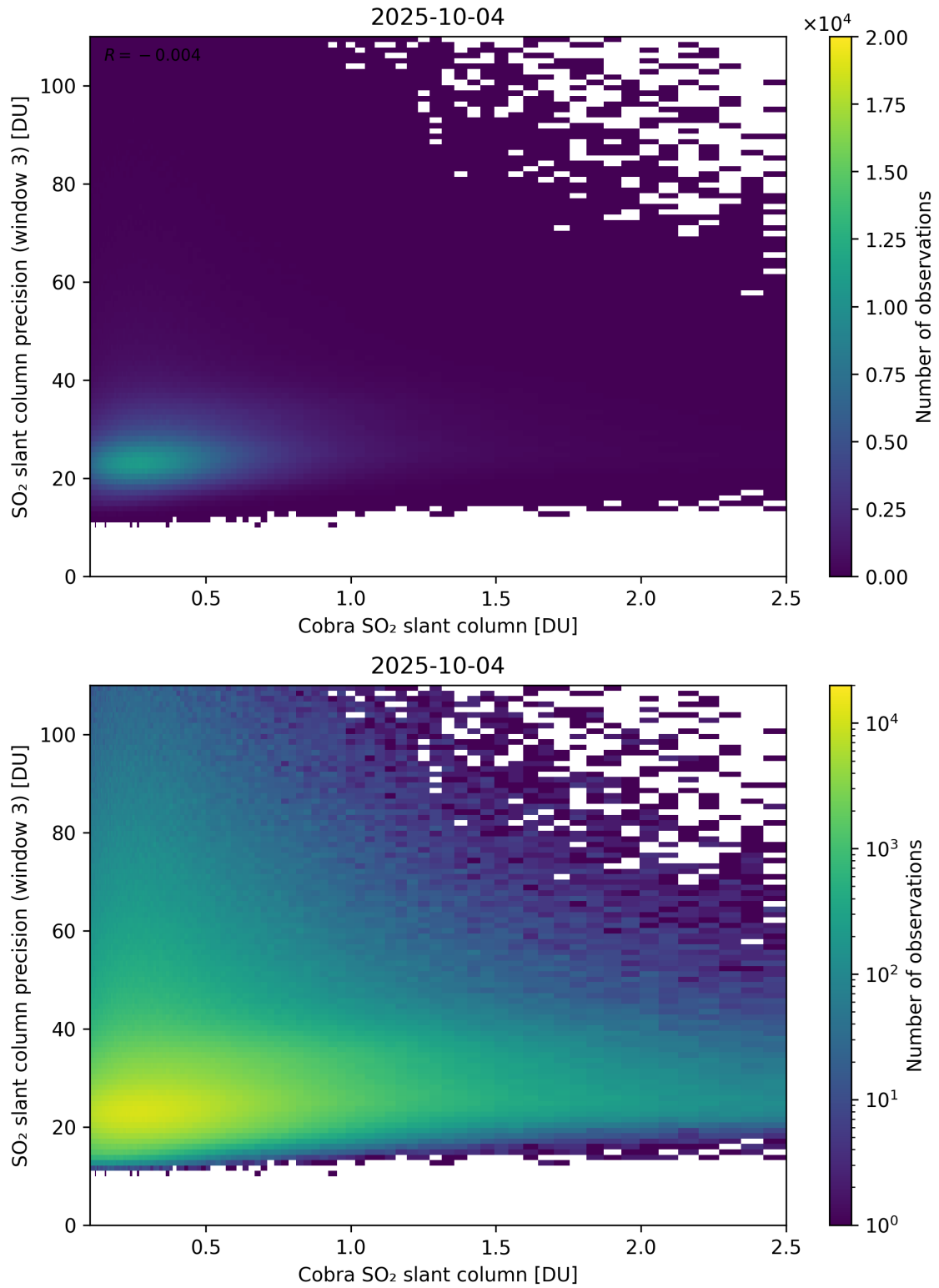
Figure 223: Scatter density plot of “Cobra SO 2 slant column” against “SO 2 slant column precision (window 3)” for 2025-10-03 to 2025-10-05.
