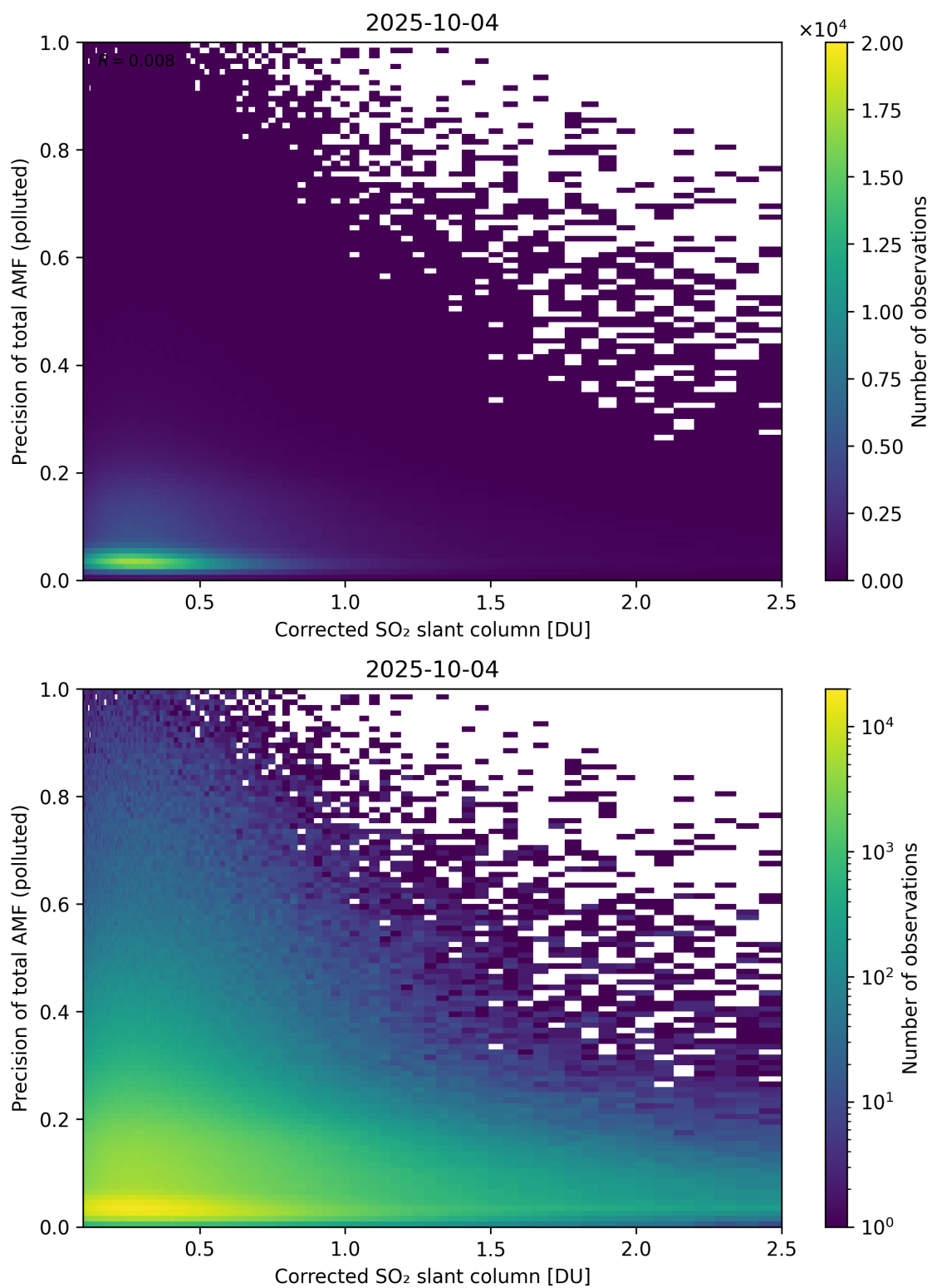
Figure 243: Scatter density plot of “Corrected SO 2 slant column” against “Precision of total AMF (polluted)” for 2025-10-03 to 2025-10-05.
