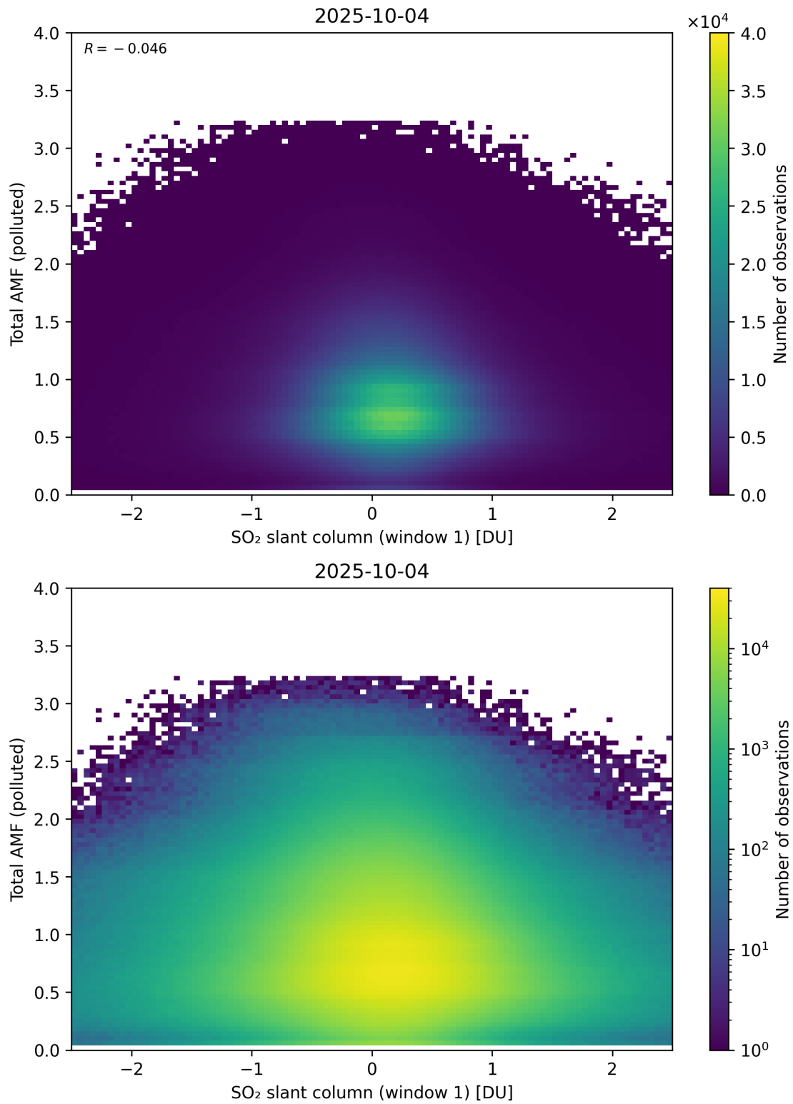
Figure 289: Scatter density plot of “SO 2 slant column (window 1)” against “Total AMF (polluted)” for 2025-10-03 to 2025-10-05.
