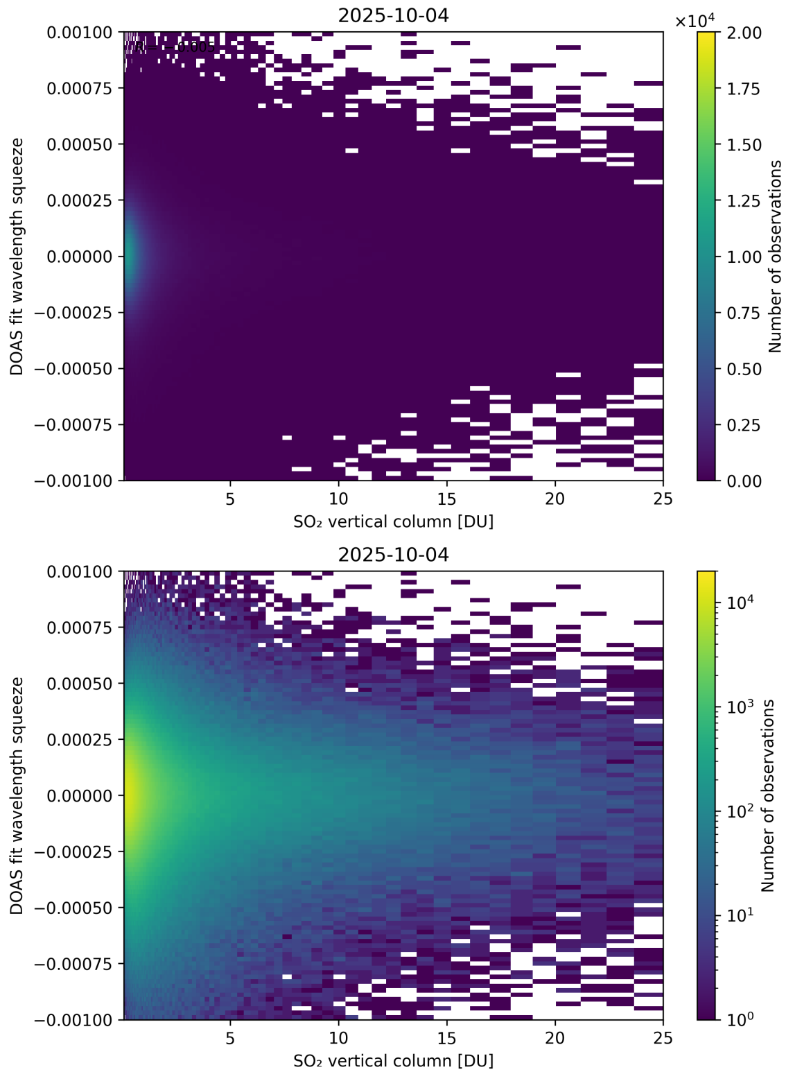
Figure 327: Scatter density plot of “SO 2 vertical column” against “DOAS fit wavelength squeeze” for 2025-10-03 to 2025-10-05.
