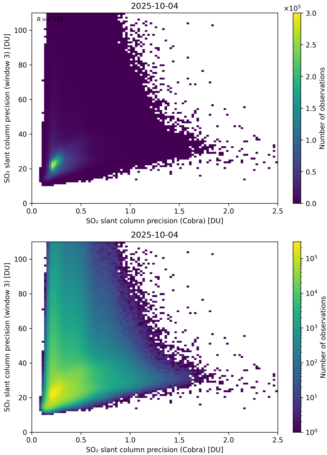
Figure 212: Scatter density plot of “SO 2 slant column precision (Cobra)” against “SO 2 slant column precision (window 3)” for 2025-10-03 to 2025-10-05.
