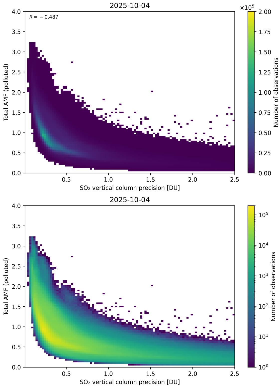
Figure 346: Scatter density plot of “SO 2 vertical column precision” against “Total AMF (polluted)” for 2025-10-03 to 2025-10-05.
