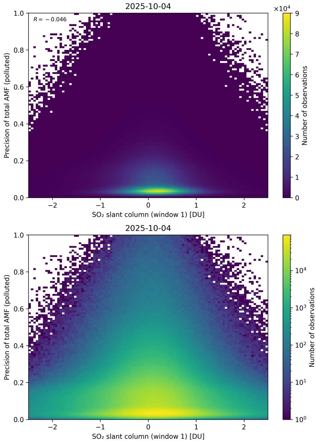
Figure 290: Scatter density plot of “SO 2 slant column (window 1)” against “Precision of total AMF (polluted)” for 2025-10-03 to 2025-10-05.
