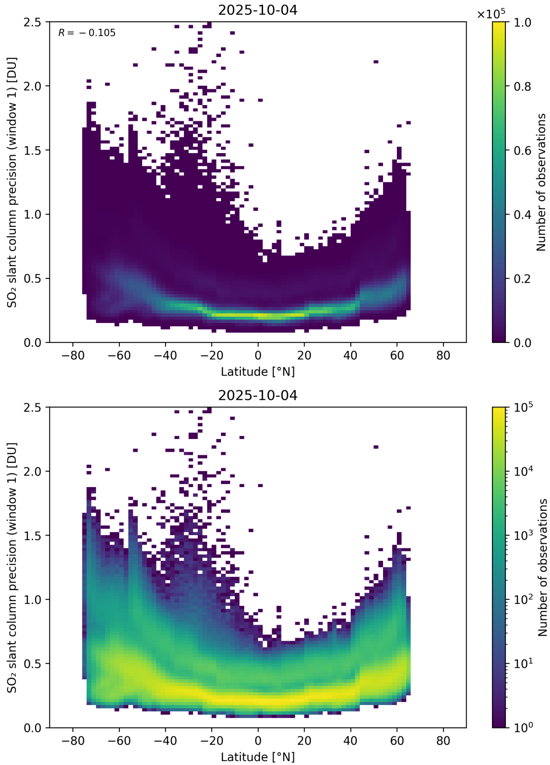
Figure 163: Scatter density plot of “Latitude” against “SO 2 slant column precision (window 1)” for 2025-10-03 to 2025-10-05.
