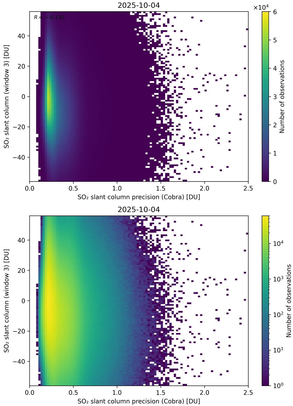
Figure 211: Scatter density plot of “SO 2 slant column precision (Cobra)” against “SO 2 slant column (window 3)” for 2025-10-03 to 2025-10-05.
