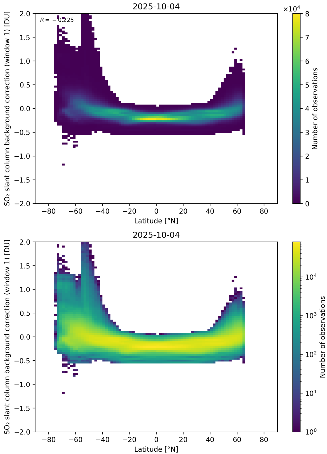
Figure 150: Scatter density plot of “Latitude” against “SO 2 slant column background correction (window 1)” for 2025-10-03 to 2025-10-05.
