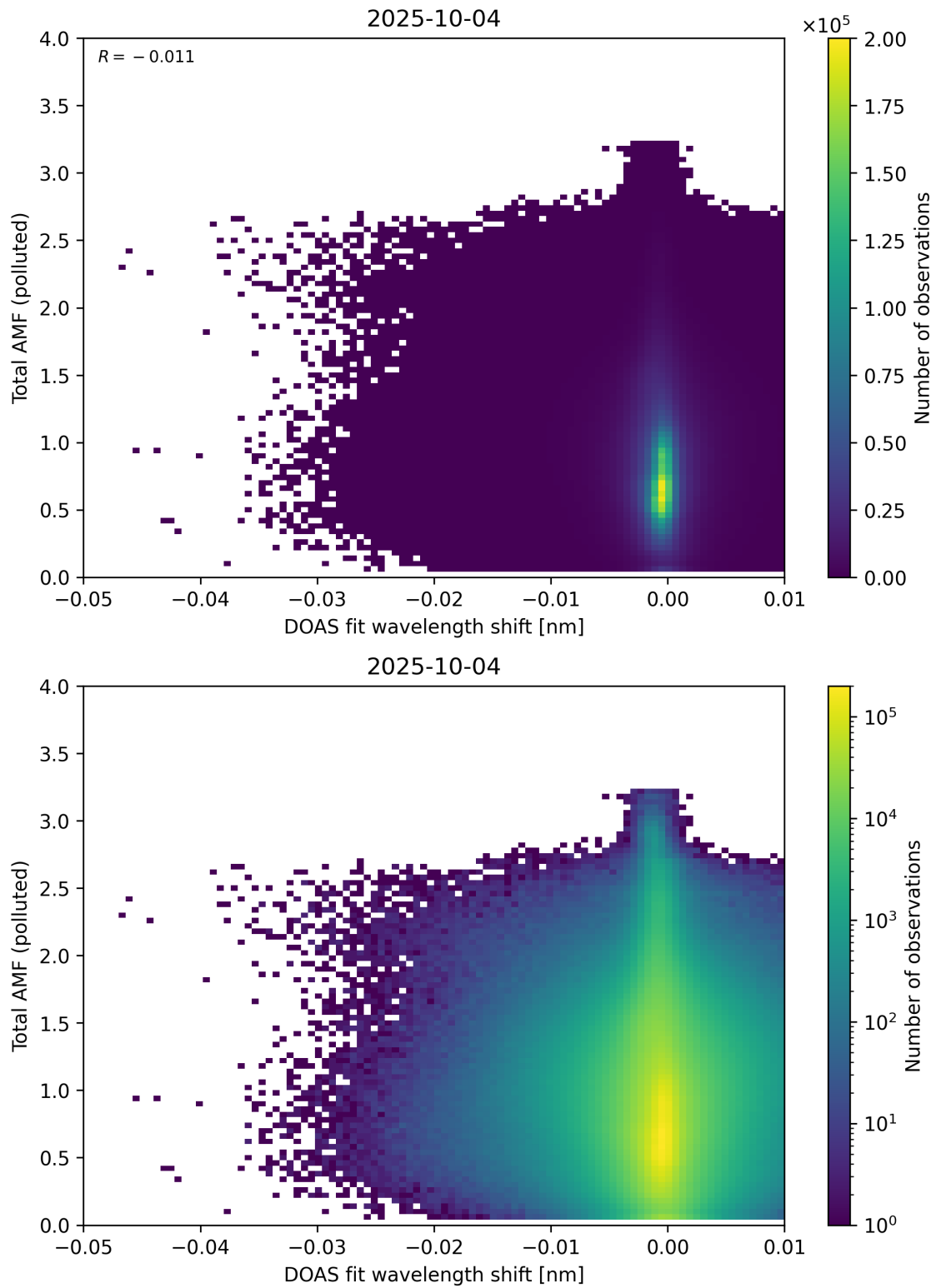
Figure 141: Scatter density plot of “DOAS fit wavelength shift” against “Total AMF (polluted)” for 2025-10-03 to 2025-10-05.
