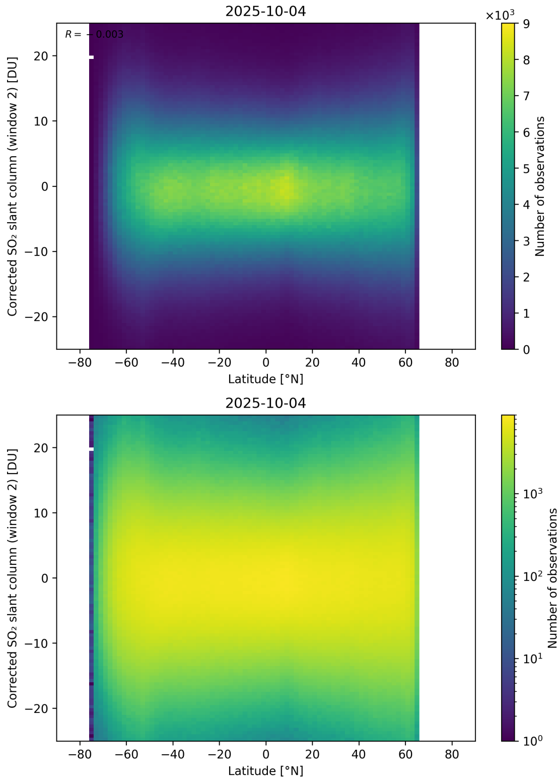
Figure 160: Scatter density plot of “Latitude” against “Corrected SO 2 slant column (window 2)” for 2025-10-03 to 2025-10-05.
