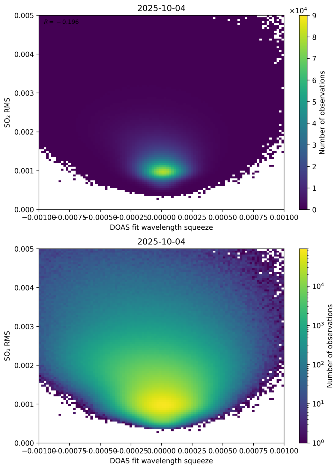
Figure 143: Scatter density plot of “DOAS fit wavelength squeeze” against “SO 2 RMS” for 2025-10-03 to 2025-10-05.
