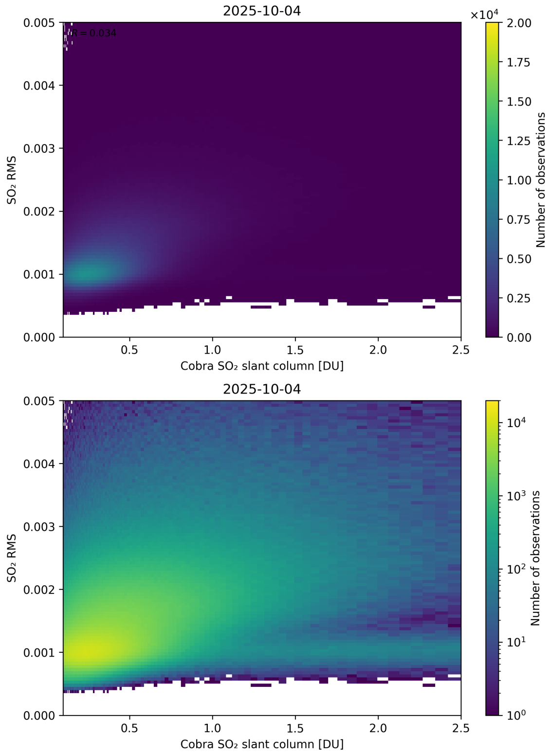
Figure 198: Scatter density plot of “Cobra SO 2 slant column” against “SO 2 RMS” for 2025-10-03 to 2025-10-05.
