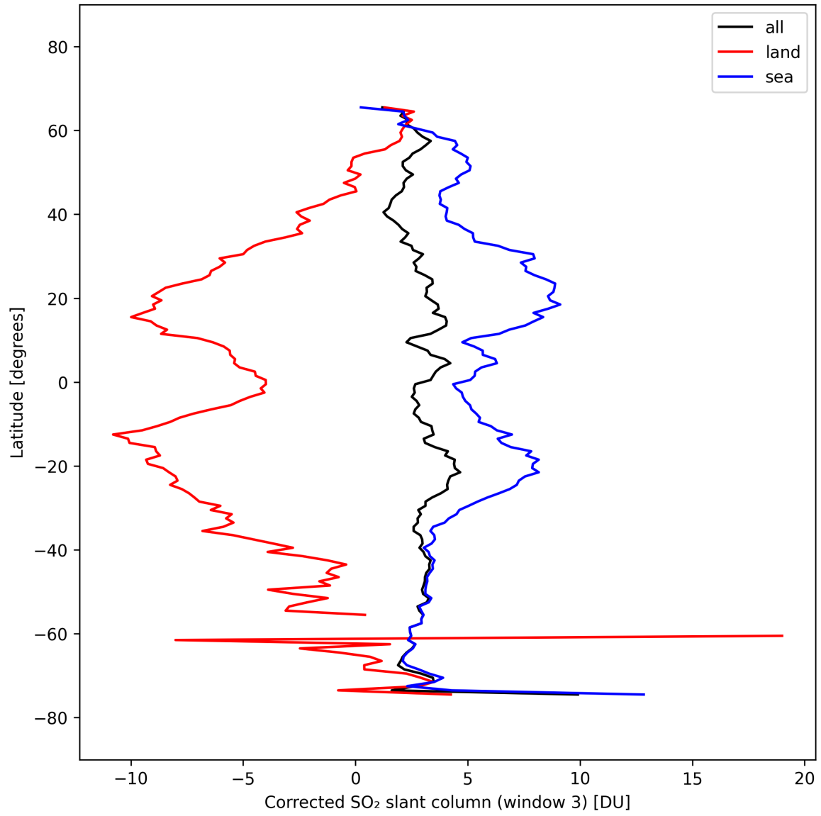
Figure 47: Zonal average of “Corrected SO 2 slant column (window 3)” for 2025-10-03 to 2025-10-05.
