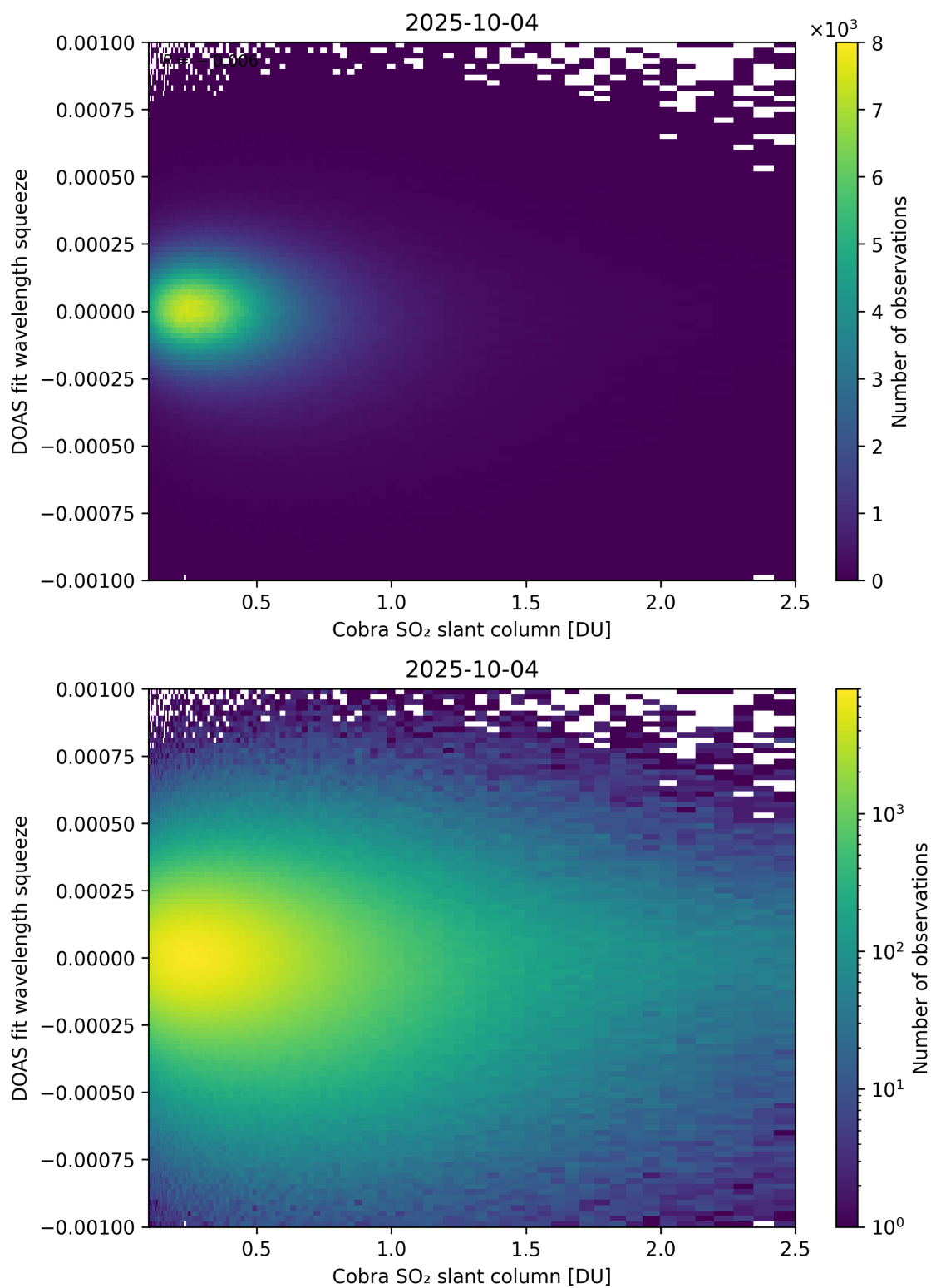
Figure 197: Scatter density plot of “Cobra SO 2 slant column” against “DOAS fit wavelength squeeze” for 2025-10-03 to 2025-10-05.
