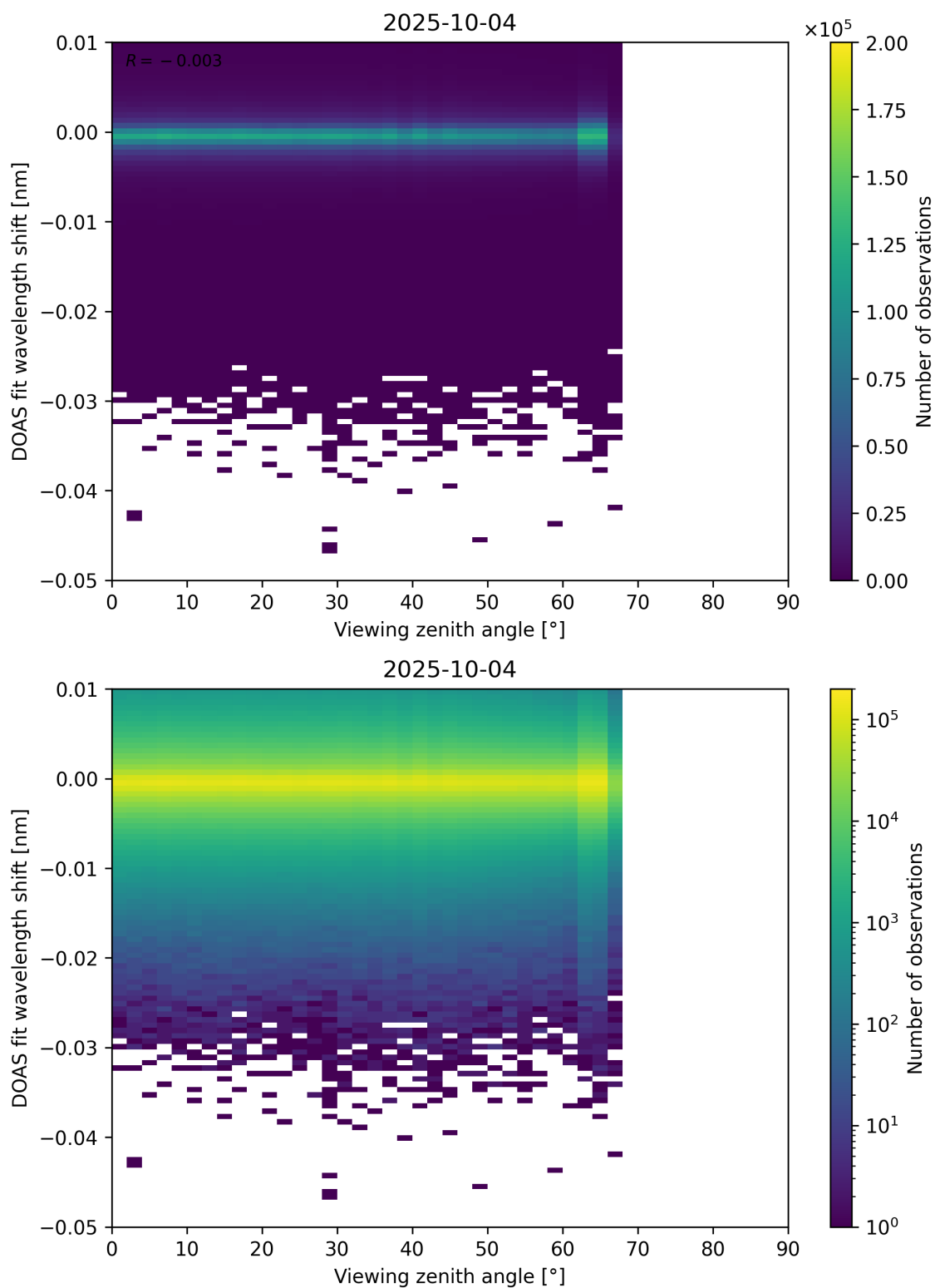
Figure 365: Scatter density plot of “Viewing zenith angle” against “DOAS fit wavelength shift” for 2025-10-03 to 2025-10-05.
