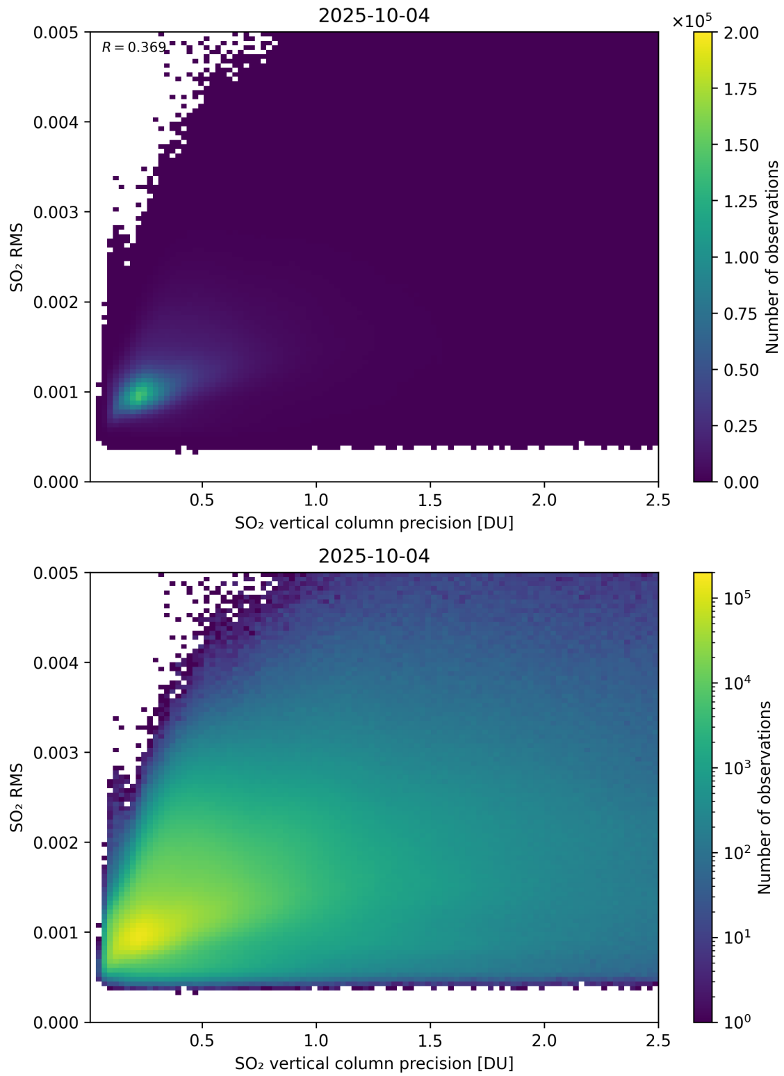
Figure 334: Scatter density plot of “SO 2 vertical column precision” against “SO 2 RMS” for 2025-10-03 to 2025-10-05.
