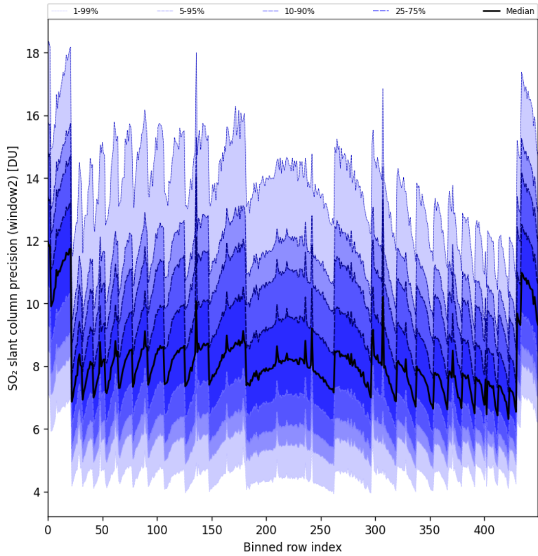
Figure 94: Along track statistics of “SO 2 slant column precision (window2)” for 2025-10-03 to 2025-10-05
