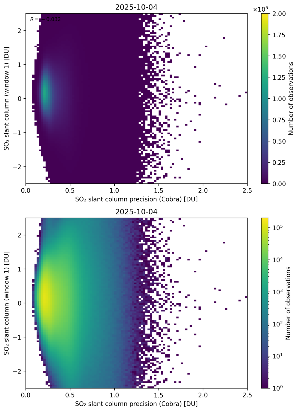
Figure 208: Scatter density plot of “SO 2 slant column precision (Cobra)” against “SO 2 slant column (window 1)” for 2025-10-03 to 2025-10-05.
