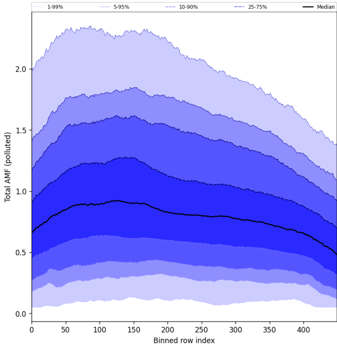
Figure 105: Along track statistics of “Total AMF (polluted)” for 2025-10-03 to 2025-10-05
