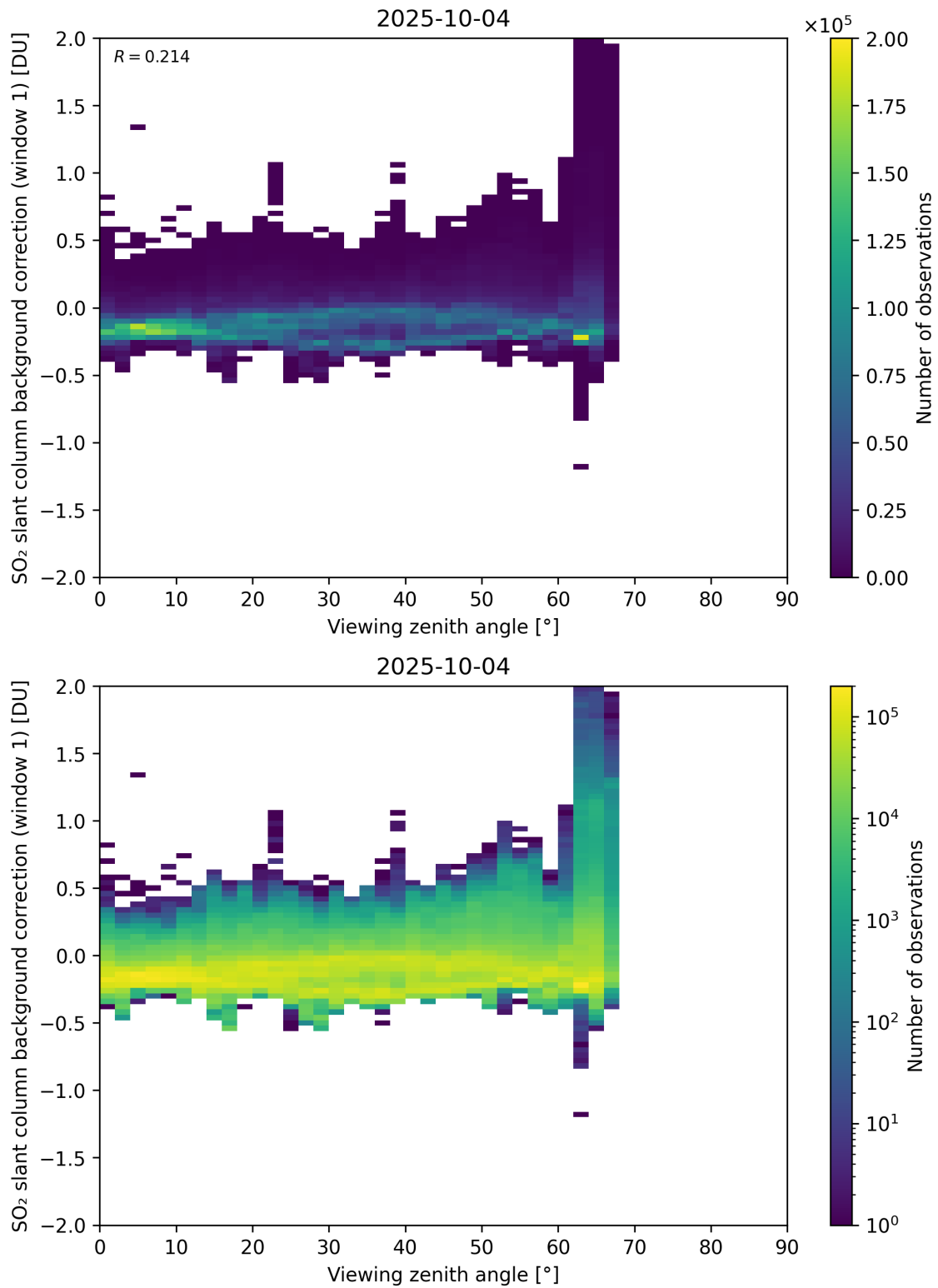
Figure 362: Scatter density plot of “Viewing zenith angle” against “SO 2 slant column background correction (window 1)” for 2025-10-03 to 2025-10-05.
