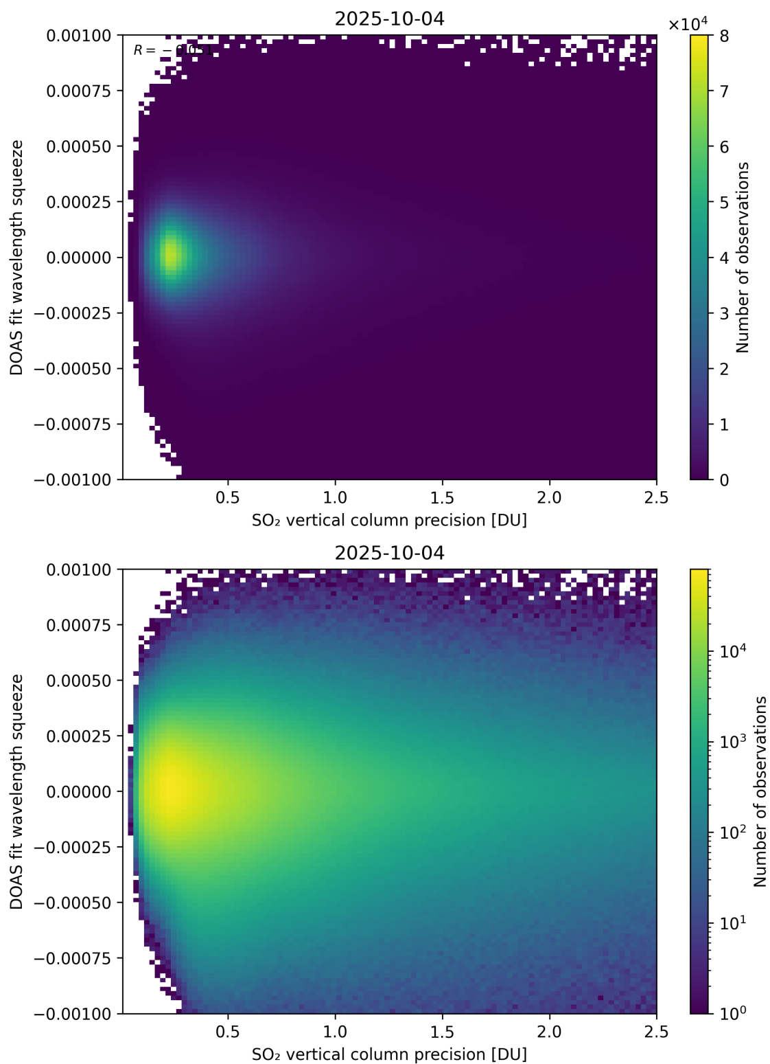
Figure 333: Scatter density plot of “SO 2 vertical column precision” against “DOAS fit wavelength squeeze” for 2025-10-03 to 2025-10-05.
