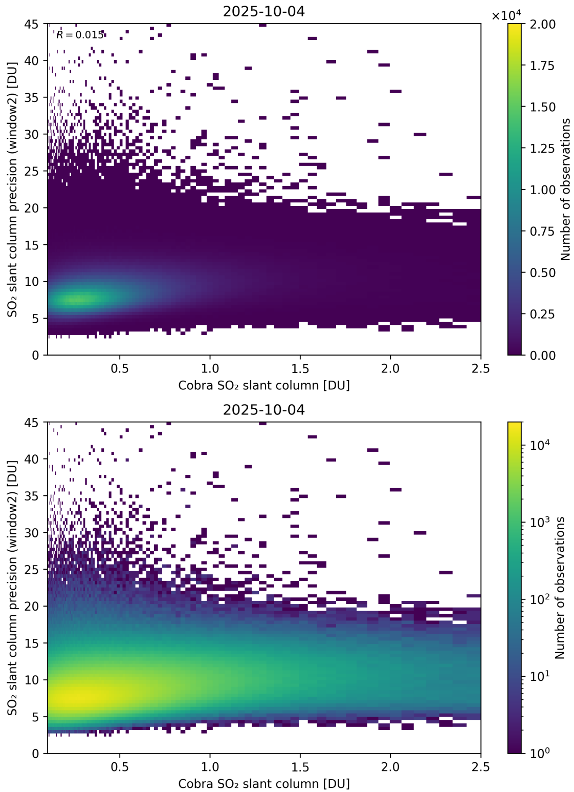
Figure 221: Scatter density plot of “Cobra SO 2 slant column” against “SO 2 slant column precision (window2)” for 2025-10-03 to 2025-10-05.
