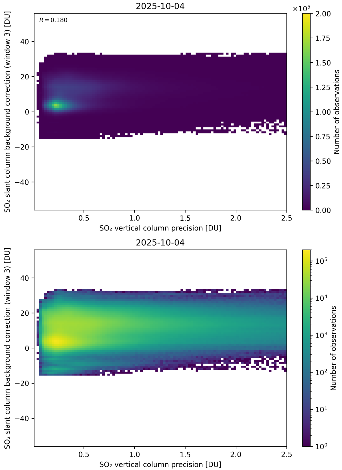
Figure 331: Scatter density plot of “SO 2 vertical column precision” against “SO 2 slant column background correction (window 3)” for 2025-10-03 to 2025-10-05.
