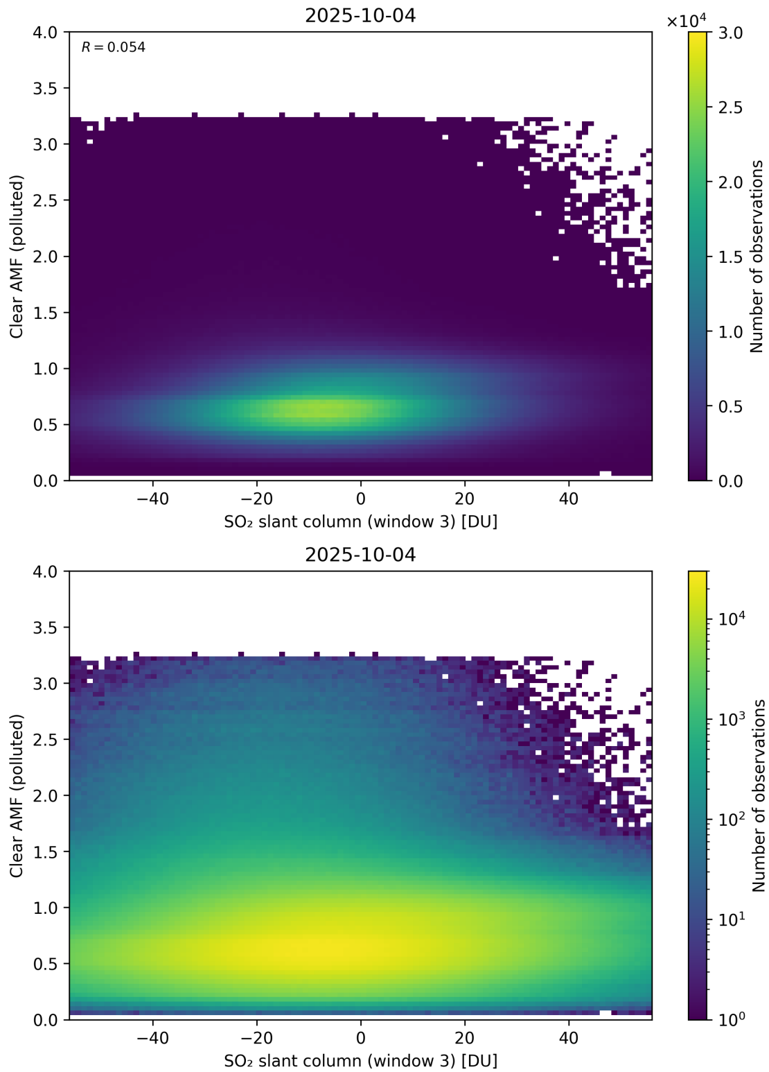
Figure 315: Scatter density plot of “SO 2 slant column (window 3)” against “Clear AMF (polluted)” for 2025-10-03 to 2025-10-05.
