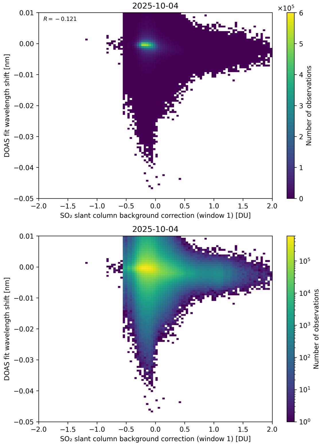
Figure 111: Scatter density plot of “SO 2 slant column background correction (window 1)” against “DOAS fit wavelength shift” for 2025-10-03 to 2025-10-05.
