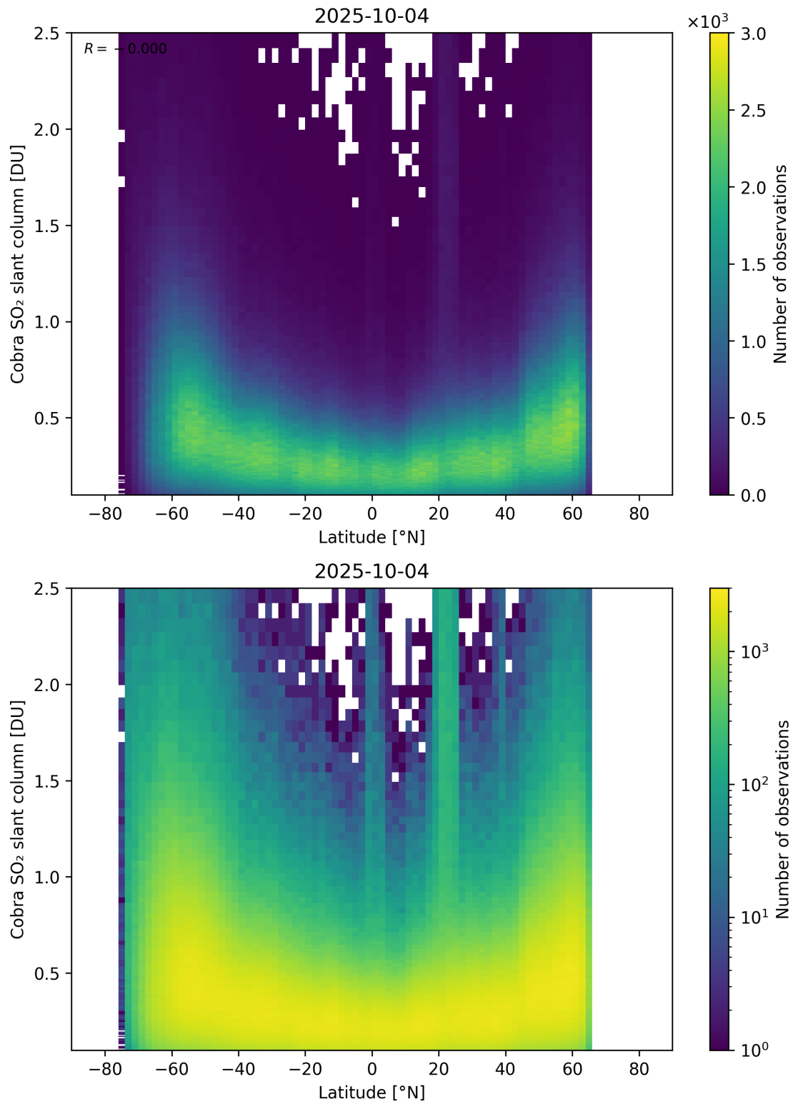
Figure 157: Scatter density plot of “Latitude” against “Cobra SO 2 slant column” for 2025-10-03 to 2025-10-05.
