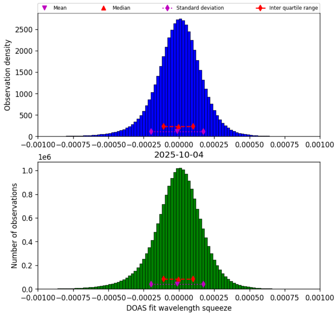
Figure 77: Histogram of “DOAS fit wavelength squeeze” for 2025-10-03 to 2025-10-05
