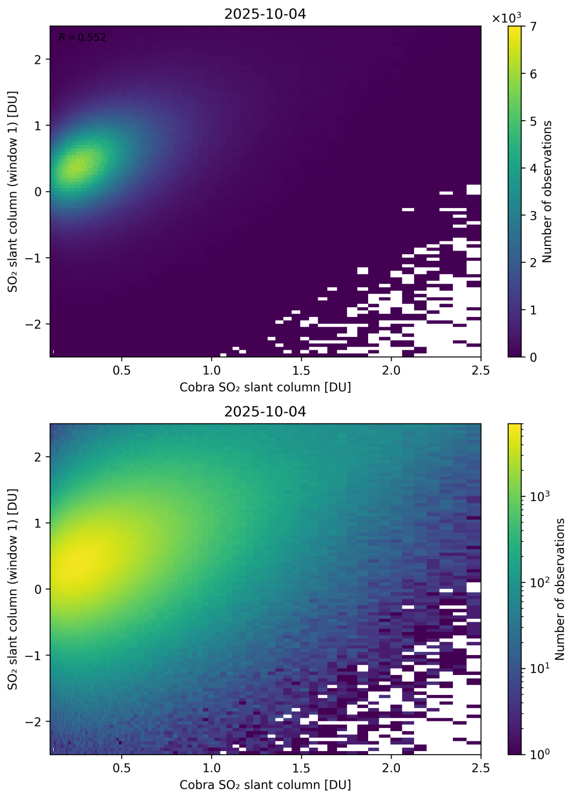
Figure 219: Scatter density plot of “Cobra SO 2 slant column” against “SO 2 slant column (window 1)” for 2025-10-03 to 2025-10-05.
