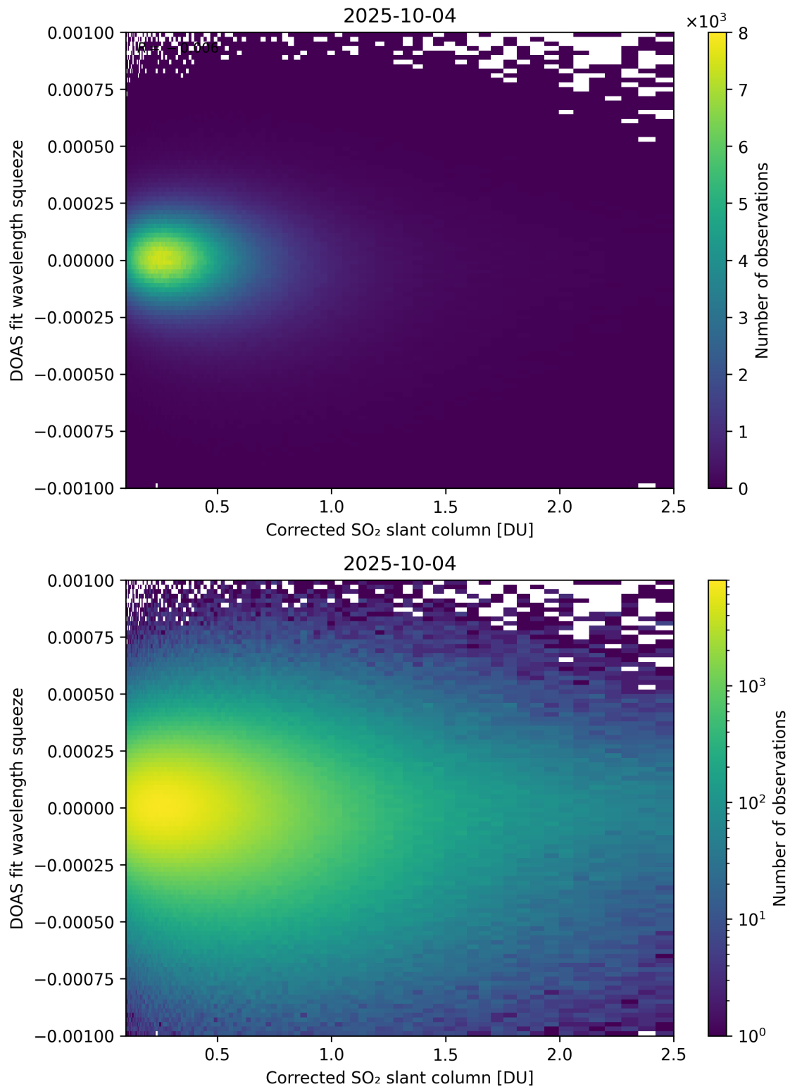
Figure 230: Scatter density plot of “Corrected SO 2 slant column” against “DOAS fit wavelength squeeze” for 2025-10-03 to 2025-10-05.
