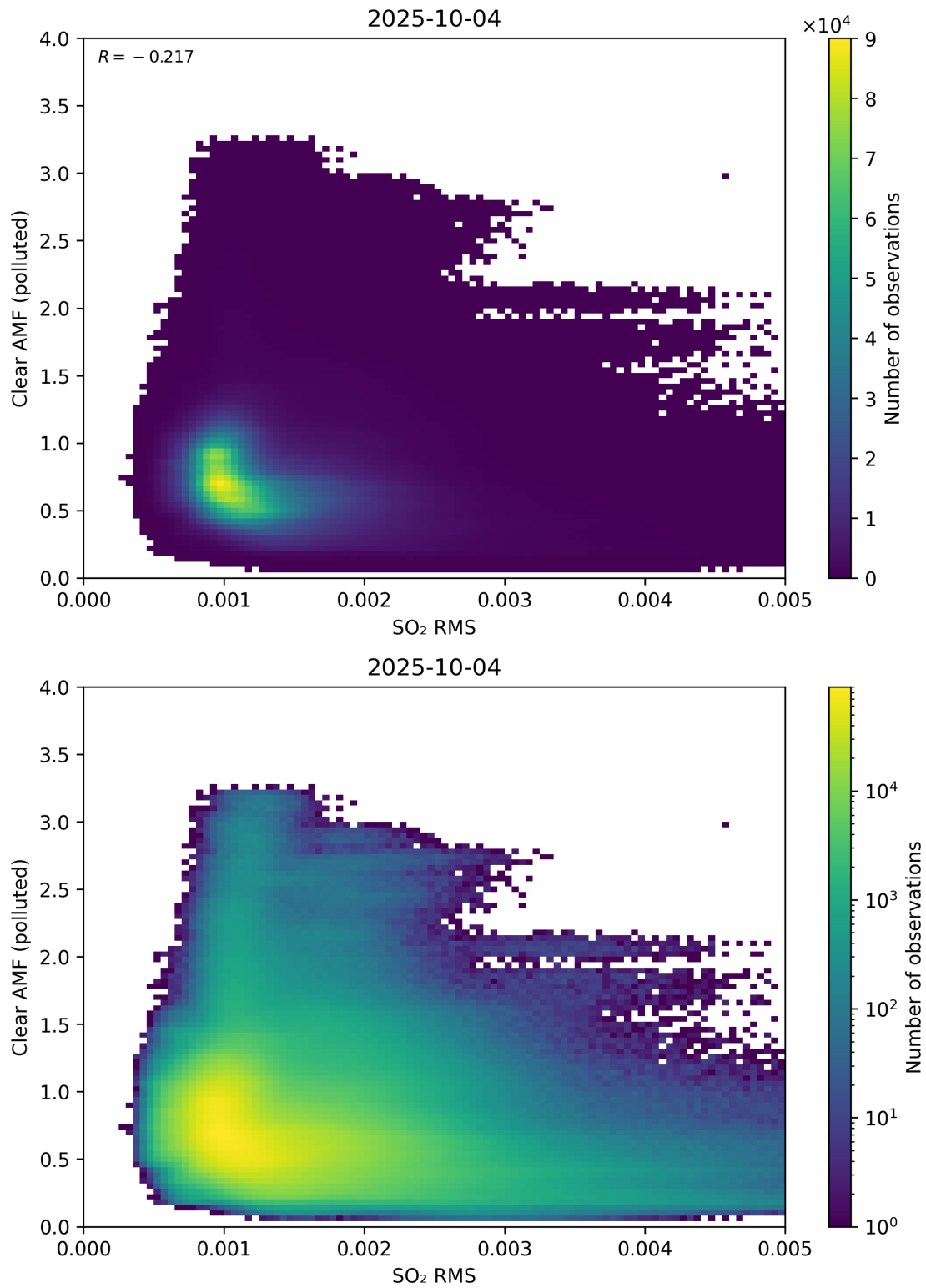
Figure 147: Scatter density plot of “SO 2 RMS” against “Clear AMF (polluted)” for 2025-10-03 to 2025-10-05.
