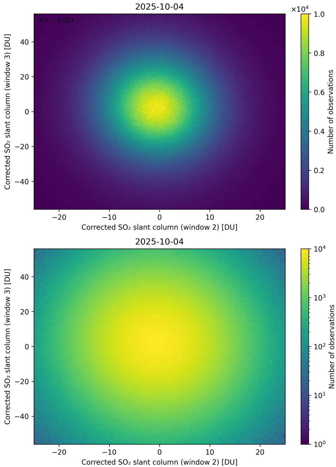
Figure 250: Scatter density plot of “Corrected SO 2 slant column (window 2)” against “Corrected SO 2 slant column (window 3)” for 2025-10-03 to 2025-10-05.
