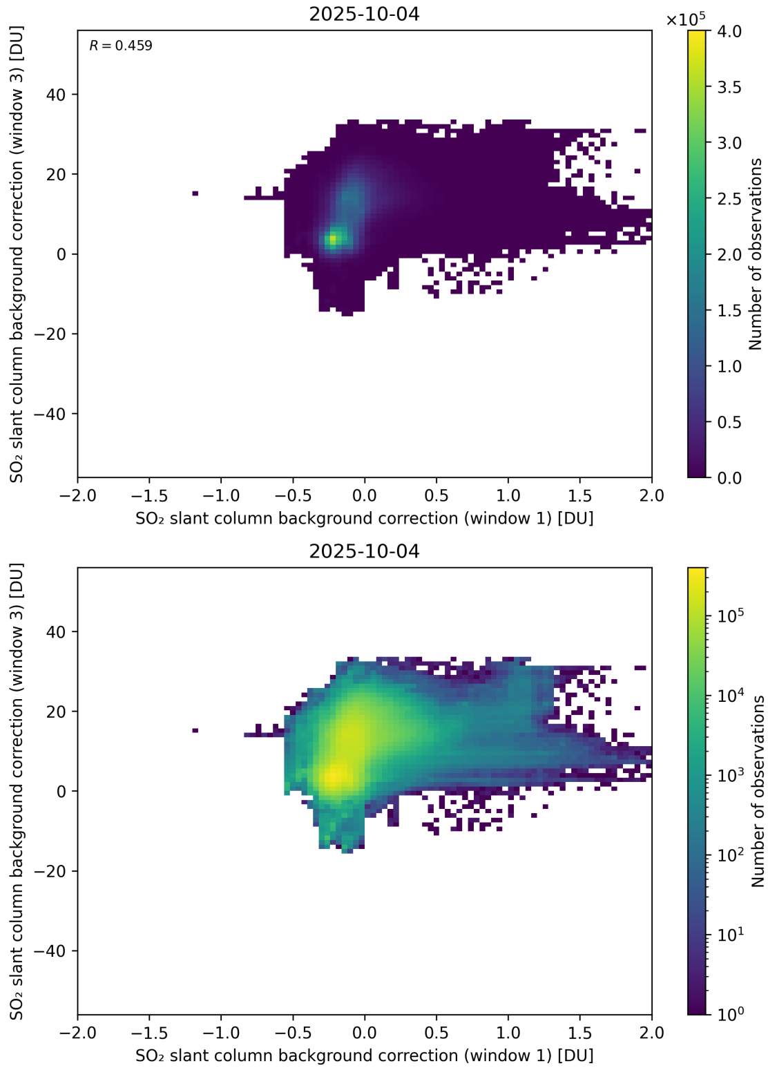
Figure 110: Scatter density plot of “SO 2 slant column background correction (window 1)” against “SO 2 slant column background correction (window 3)” for 2025-10-03 to 2025-10-05.
