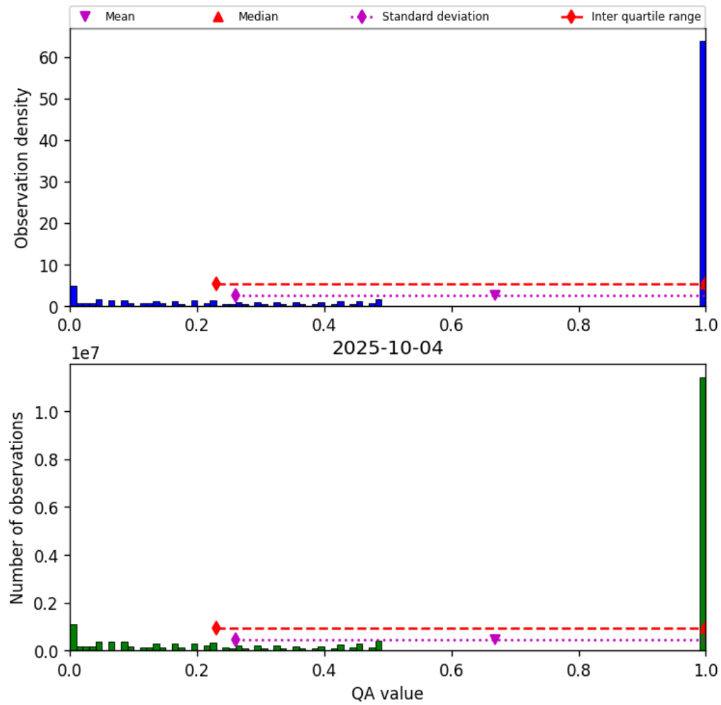
Figure 57: Histogram of “QA value” for 2025-10-03 to 2025-10-05
