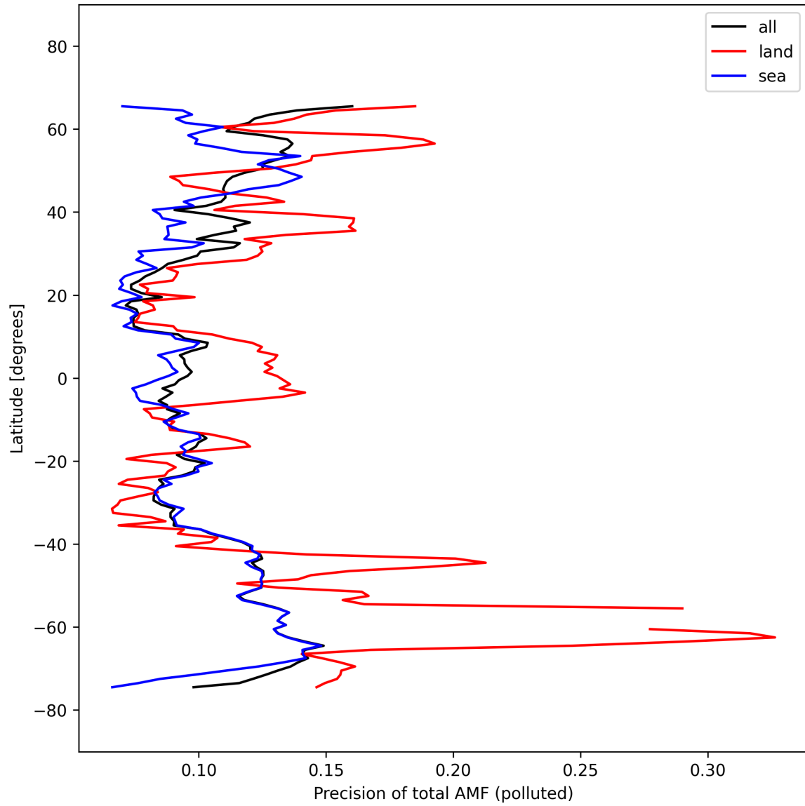
Figure 54: Zonal average of “Precision of total AMF (polluted)” for 2025-10-03 to 2025-10-05.
