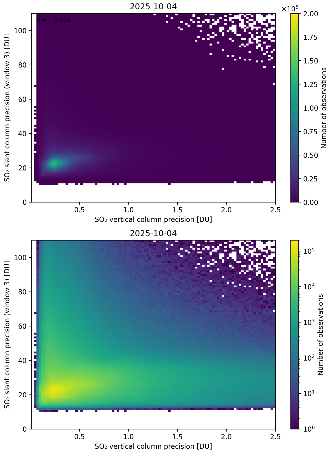
Figure 345: Scatter density plot of “SO 2 vertical column precision” against “SO 2 slant column precision (window 3)” for 2025-10-03 to 2025-10-05.
