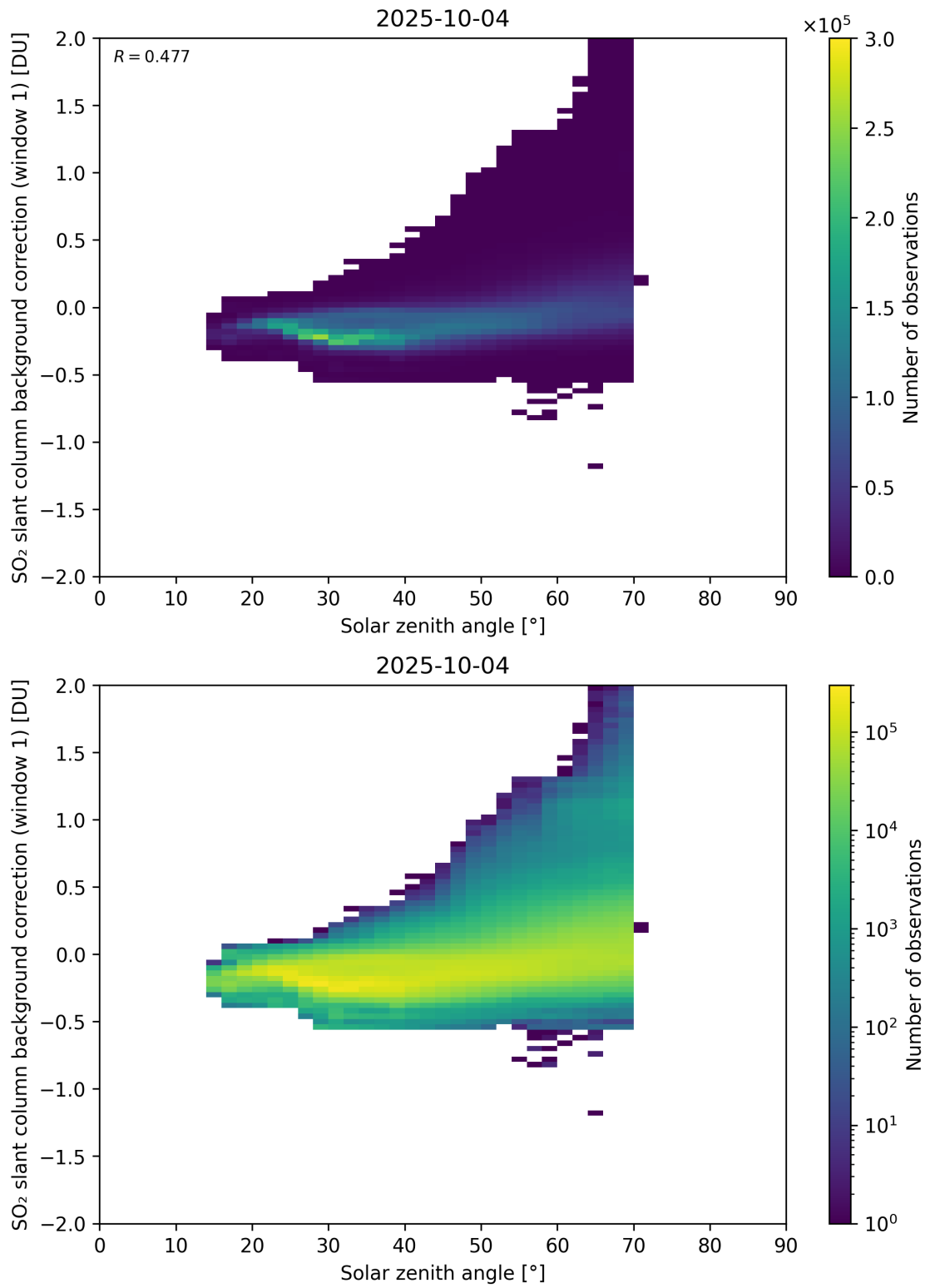
Figure 171: Scatter density plot of “Solar zenith angle” against “SO 2 slant column background correction (window 1)” for 2025-10-03 to 2025-10-05.
