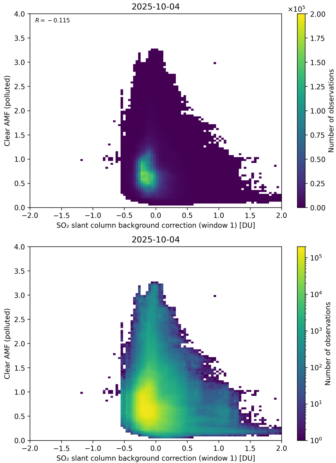
Figure 114: Scatter density plot of “SO 2 slant column background correction (window 1)” against “Clear AMF (polluted)” for 2025-10-03 to 2025-10-05.
