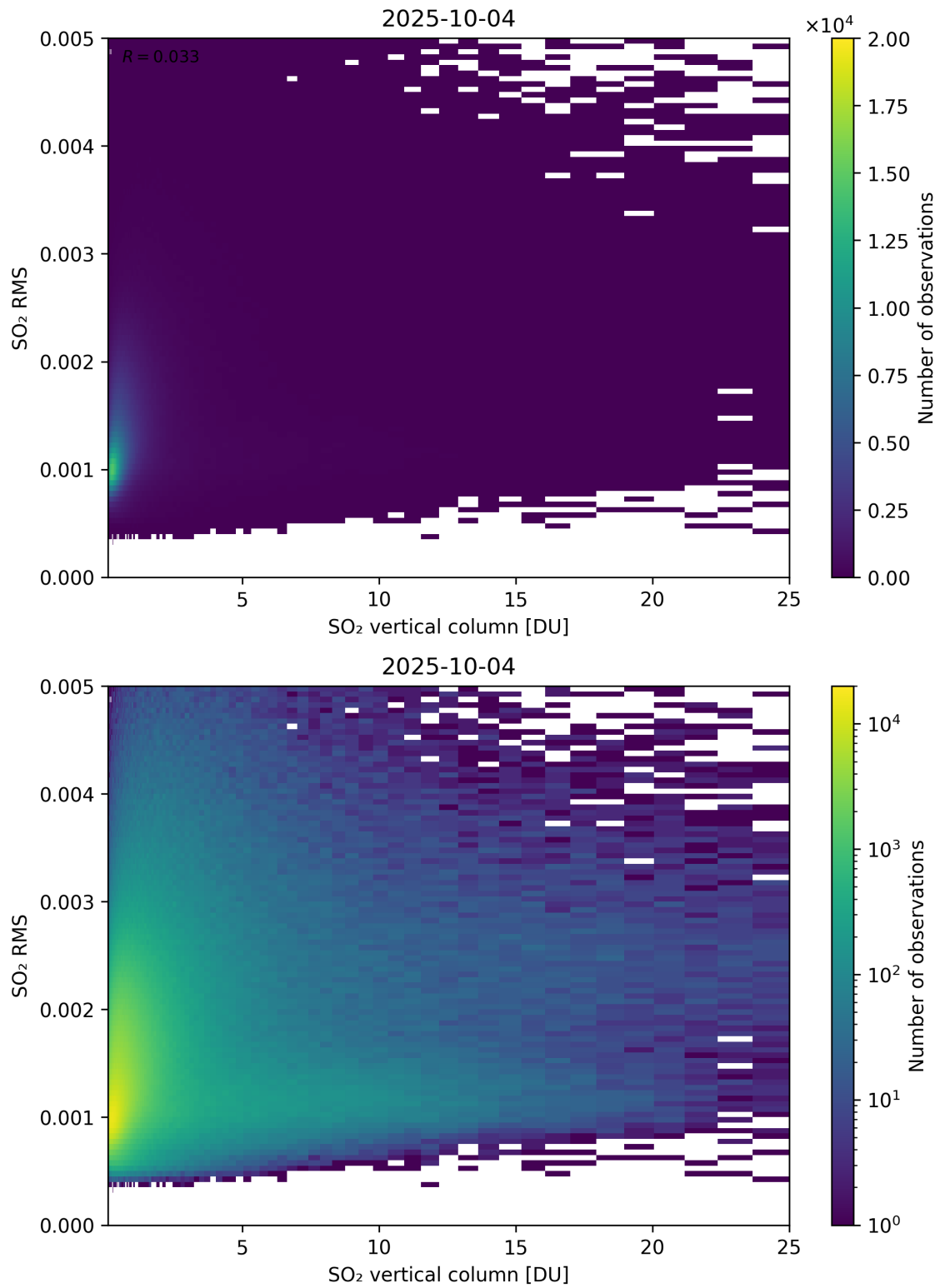
Figure 328: Scatter density plot of “SO 2 vertical column” against “SO 2 RMS” for 2025-10-03 to 2025-10-05.
