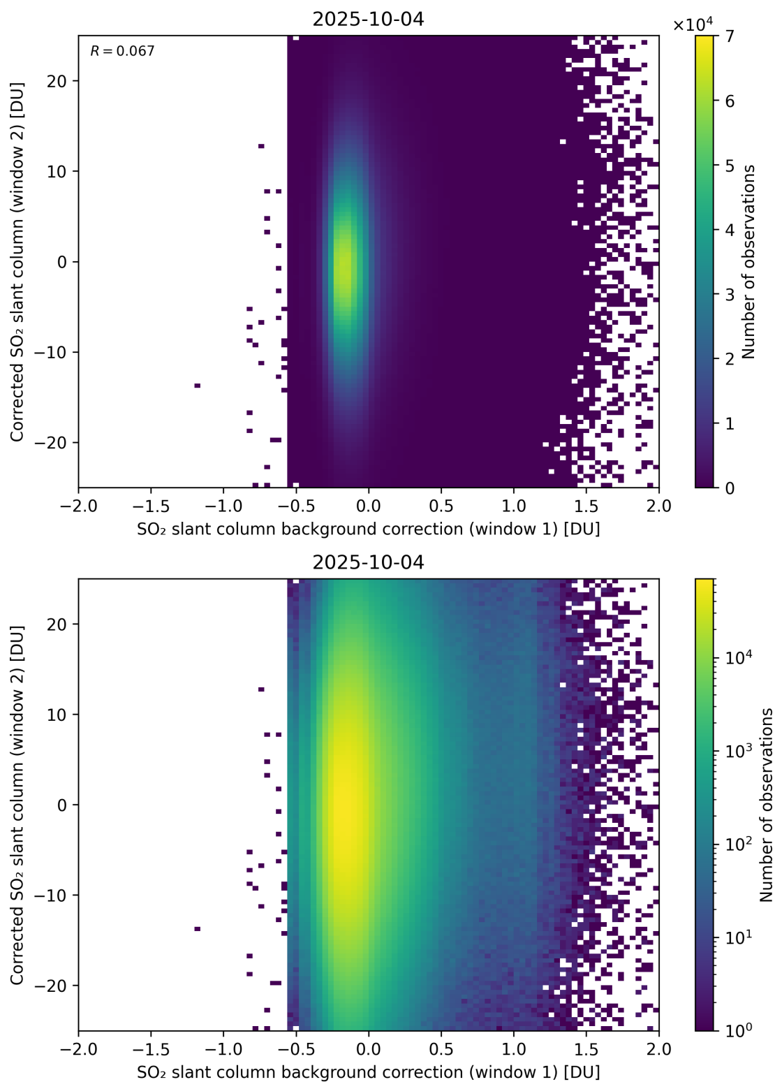
Figure 115: Scatter density plot of “SO 2 slant column background correction (window 1)” against “Corrected SO 2 slant column (window 2)” for 2025-10-03 to 2025-10-05.
