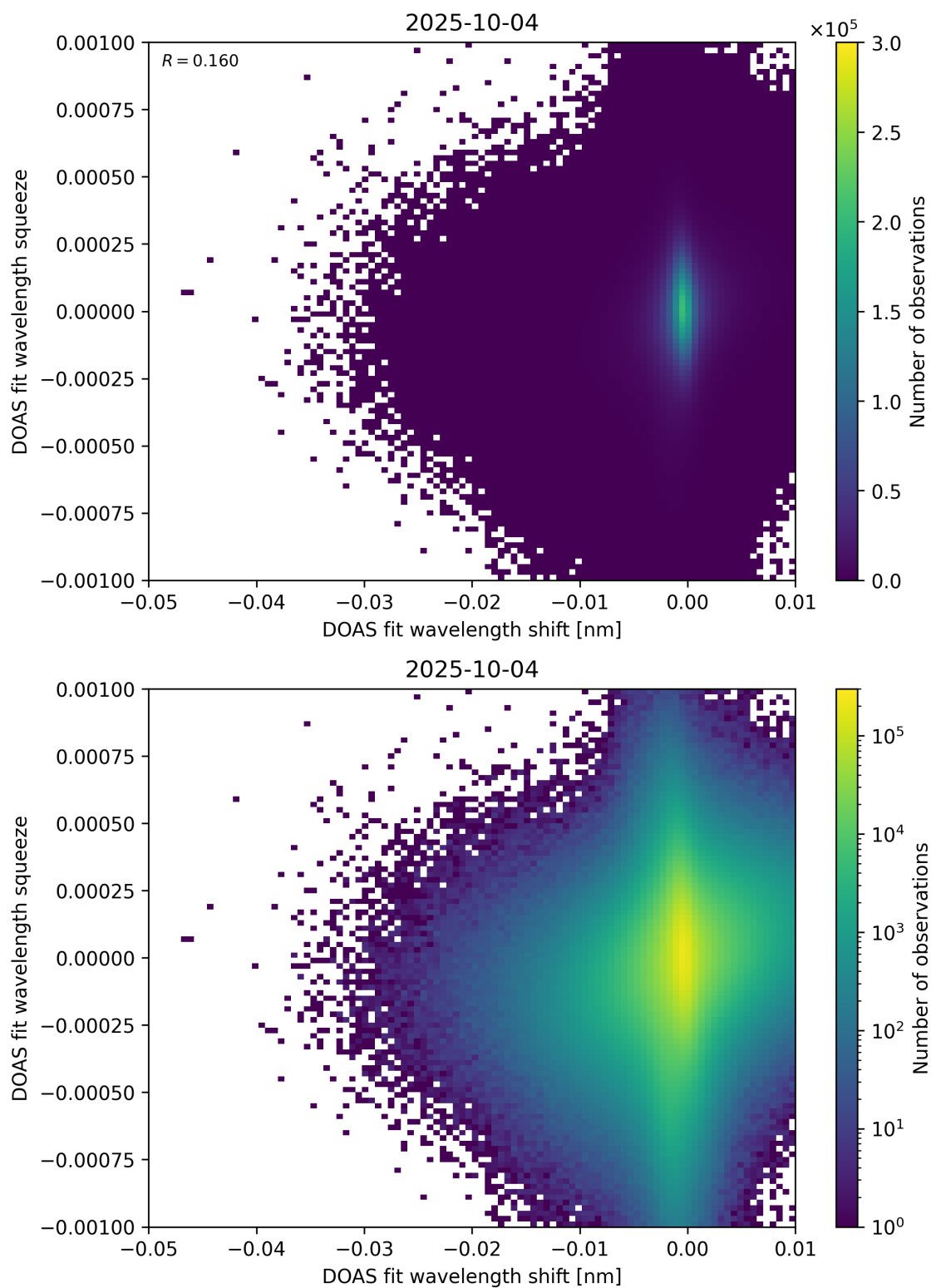
Figure 138: Scatter density plot of “DOAS fit wavelength shift” against “DOAS fit wavelength squeeze” for 2025-10-03 to 2025-10-05.
