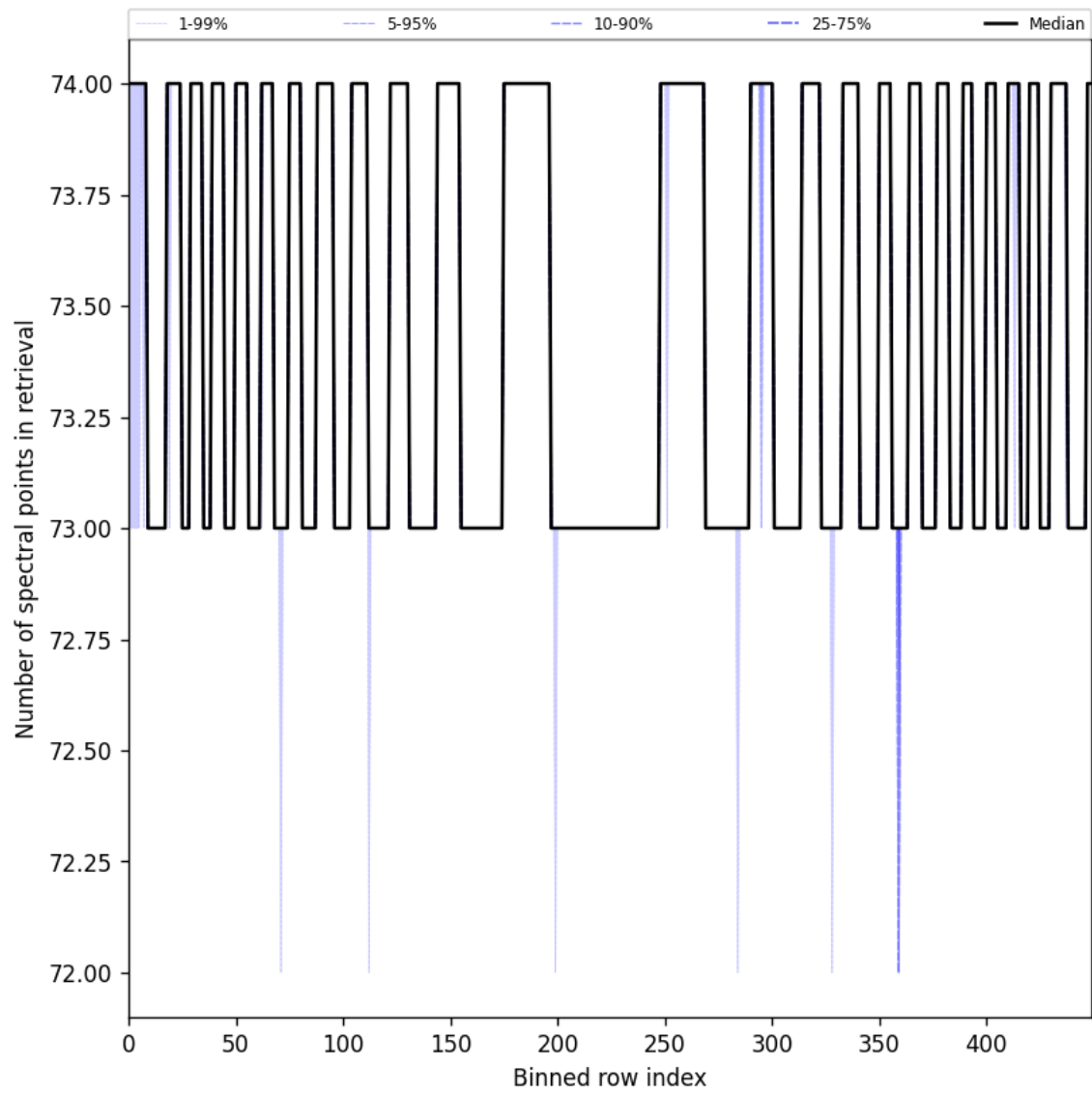
Figure 108: Along track statistics of “Number of spectral points in retrieval” for 2025-10-03 to 2025-10-05
