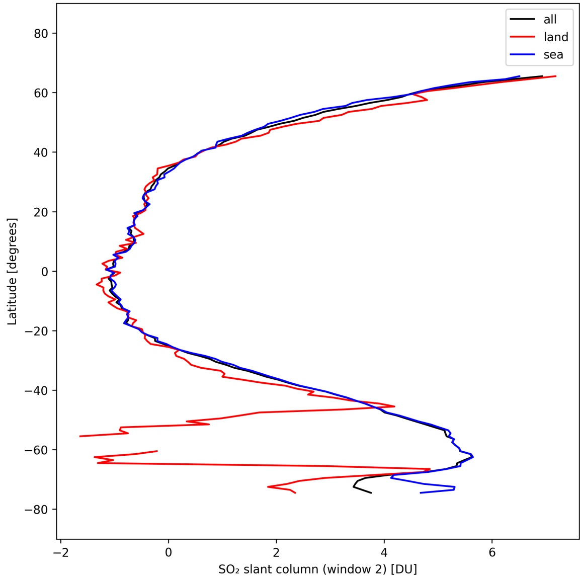
Figure 41: Zonal average of “SO 2 slant column (window 2)” for 2025-10-03 to 2025-10-05.
