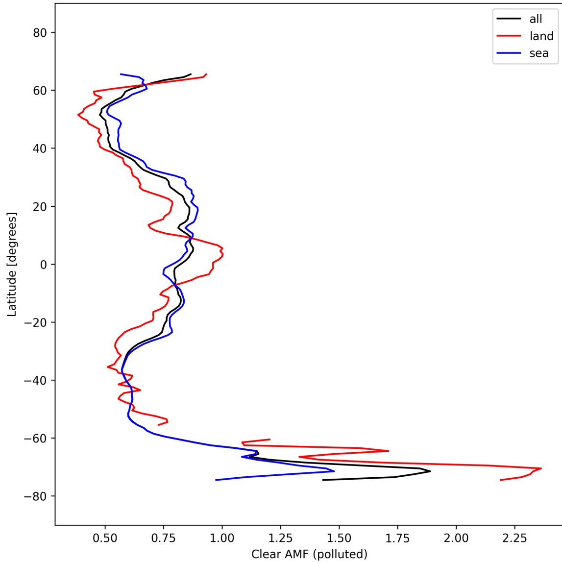
Figure 55: Zonal average of “Clear AMF (polluted)” for 2025-10-03 to 2025-10-05.
