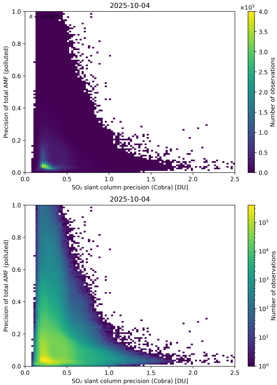
Figure 214: Scatter density plot of “SO 2 slant column precision (Cobra)” against “Precision of total AMF (polluted)” for 2025-10-03 to 2025-10-05.
