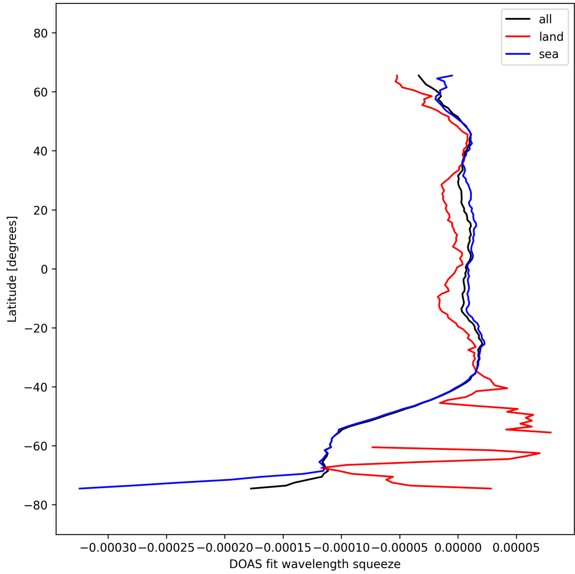
Figure 51: Zonal average of “DOAS fit wavelength squeeze” for 2025-10-03 to 2025-10-05.
