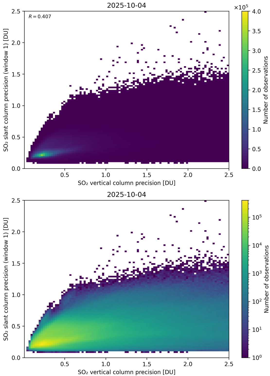
Figure 342: Scatter density plot of “SO 2 vertical column precision” against “SO 2 slant column precision (window 1)” for 2025-10-03 to 2025-10-05.
