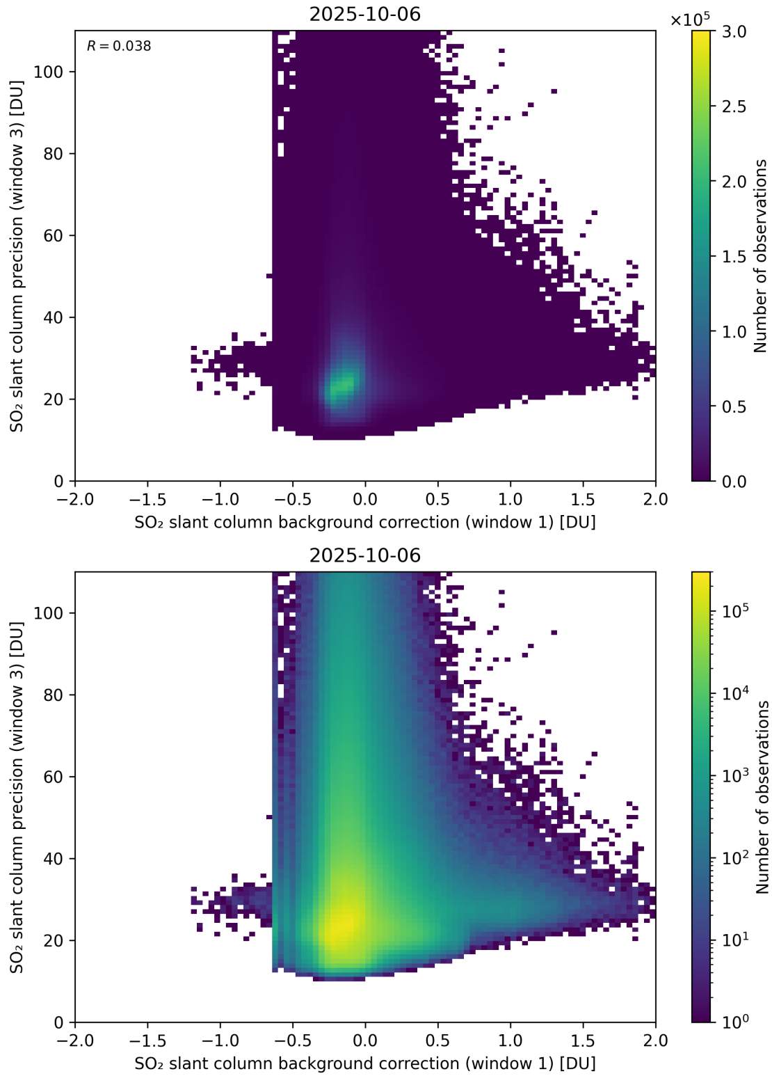
Figure 119: Scatter density plot of “SO 2 slant column background correction (window 1)” against “SO 2 slant column precision (window 3)” for 2025-10-06 to 2025-10-07.
