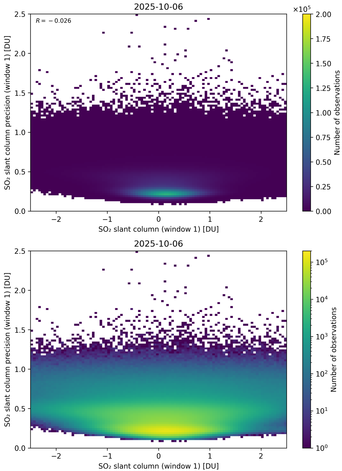
Figure 285: Scatter density plot of “SO 2 slant column (window 1)” against “SO 2 slant column precision (window 1)” for 2025-10-06 to 2025-10-07.
