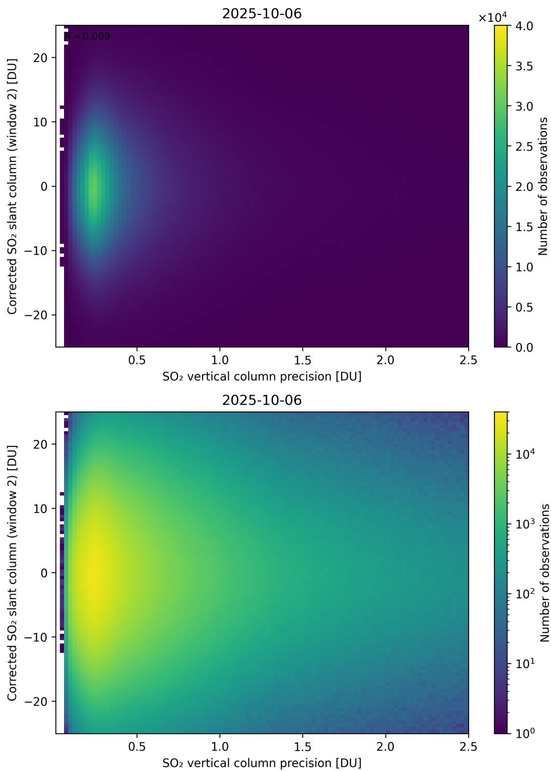
Figure 339: Scatter density plot of “SO 2 vertical column precision” against “Corrected SO 2 slant column (window 2)” for 2025-10-06 to 2025-10-07.
