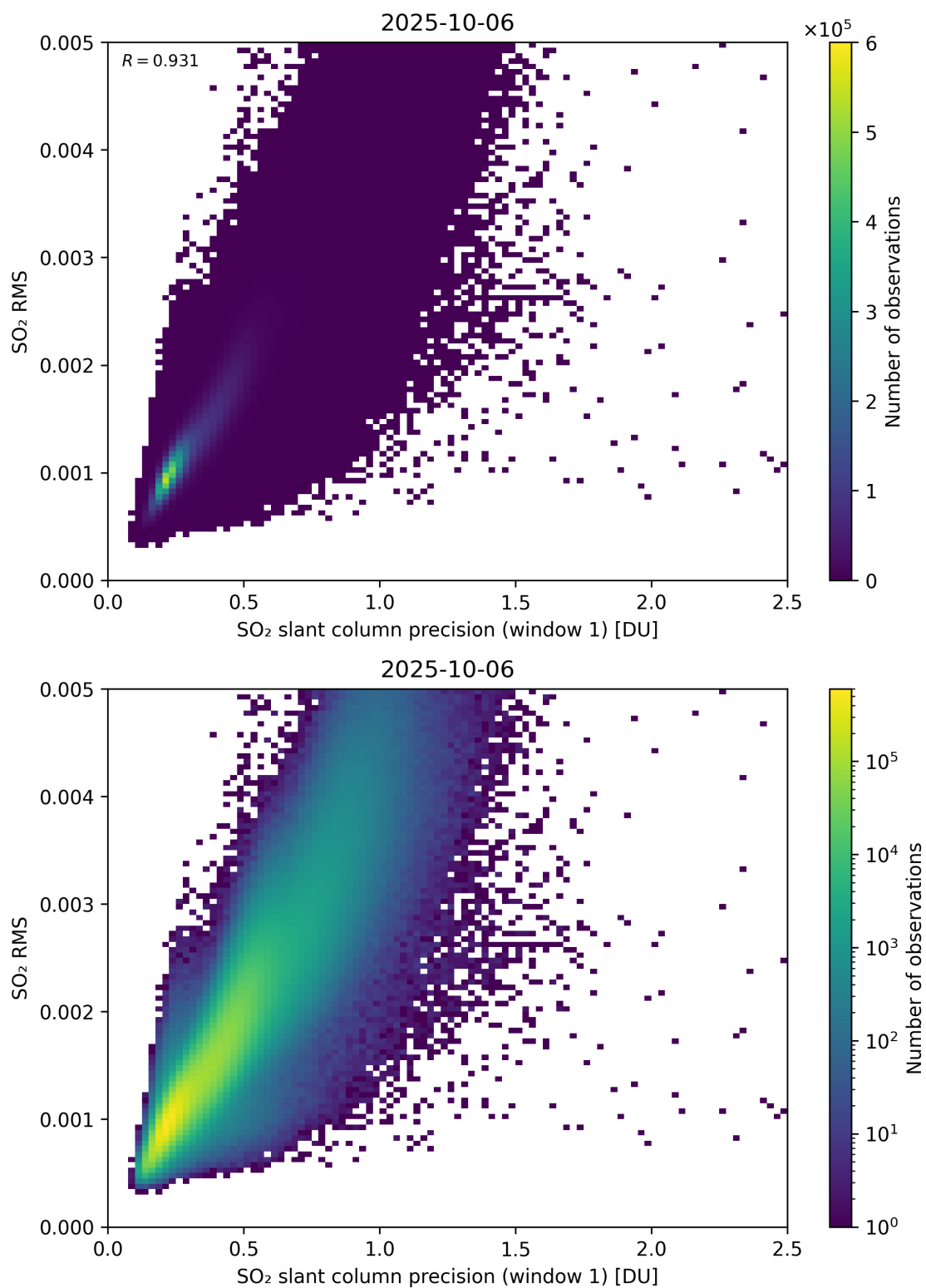
Figure 273: Scatter density plot of “SO 2 slant column precision (window 1)” against “SO 2 RMS” for 2025-10-06 to 2025-10-07.
