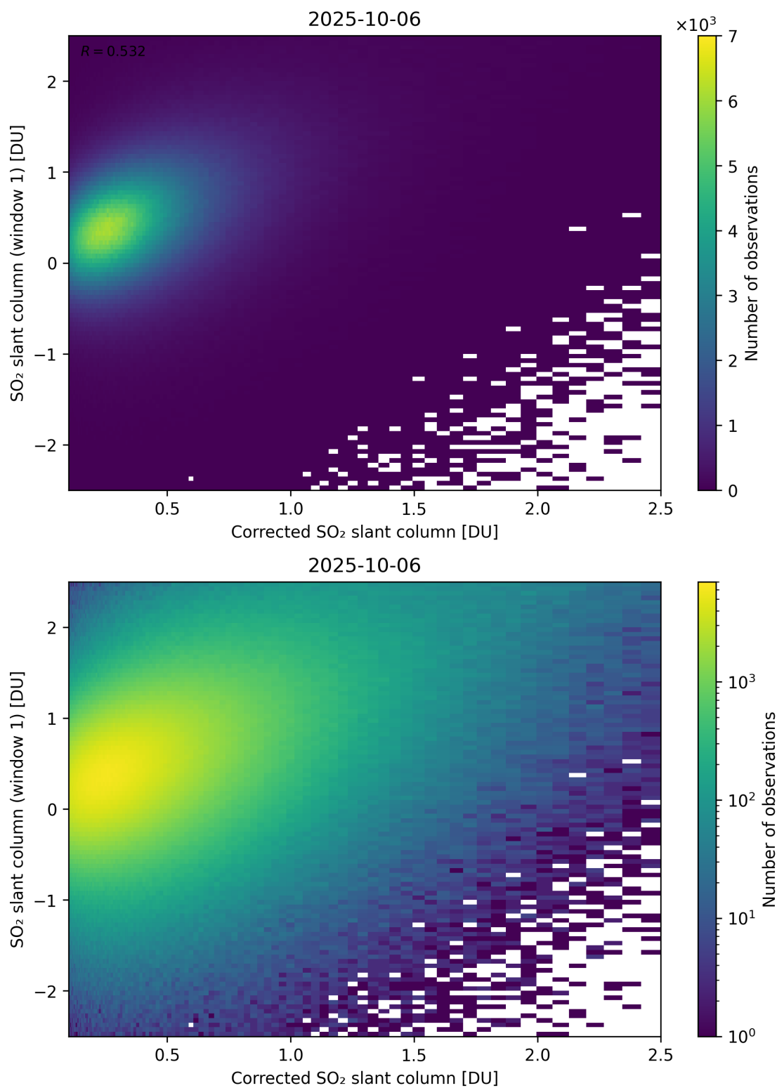
Figure 237: Scatter density plot of “Corrected SO 2 slant column” against “SO 2 slant column (window 1)” for 2025-10-06 to 2025-10-07.
