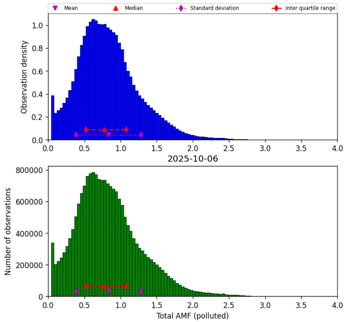
Figure 79: Histogram of “Total AMF (polluted)” for 2025-10-06 to 2025-10-07
