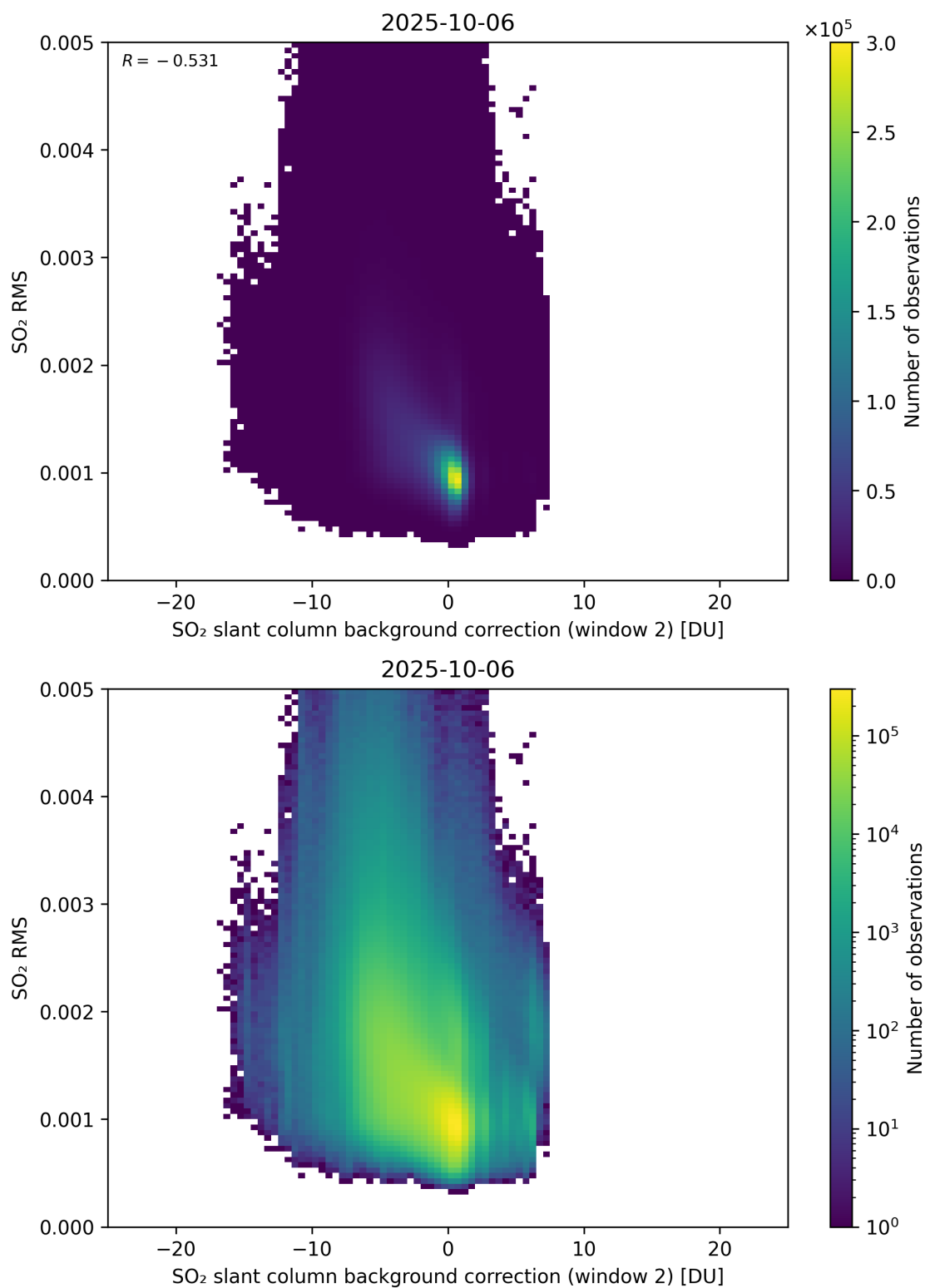
Figure 125: Scatter density plot of “SO 2 slant column background correction (window 2)” against “SO 2 RMS” for 2025-10-06 to 2025-10-07.
