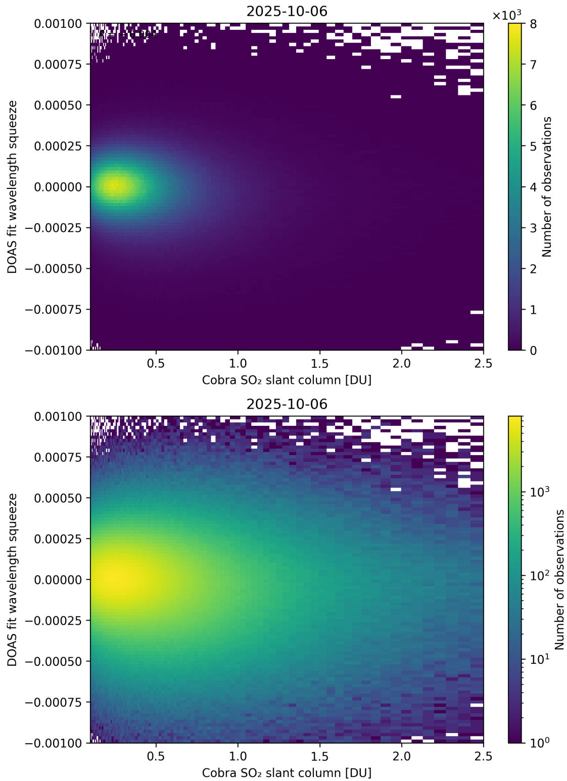
Figure 197: Scatter density plot of “Cobra SO 2 slant column” against “DOAS fit wavelength squeeze” for 2025-10-06 to 2025-10-07.
