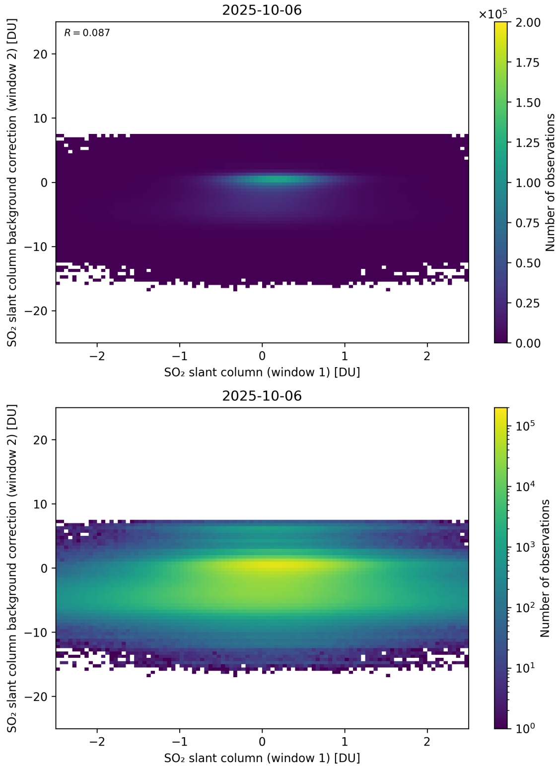
Figure 263: Scatter density plot of “SO 2 slant column (window 1)” against “SO 2 slant column background correction (window 2)” for 2025-10-06 to 2025-10-07.
