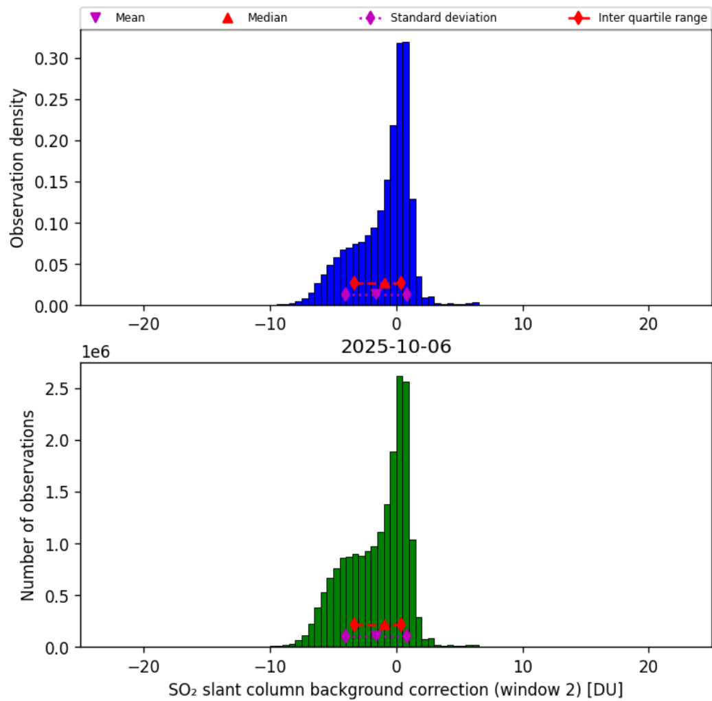
Figure 70: Histogram of “SO 2 slant column background correction (window 2)” for 2025-10-06 to 2025-10-07
