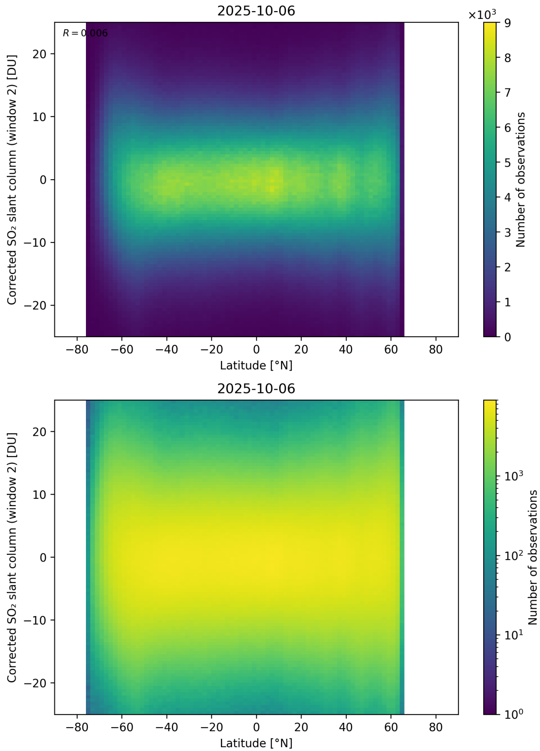
Figure 160: Scatter density plot of “Latitude” against “Corrected SO 2 slant column (window 2)” for 2025-10-06 to 2025-10-07.
