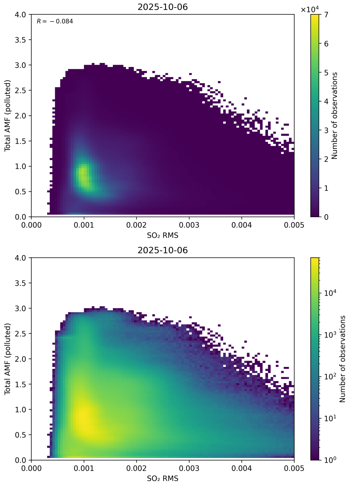
Figure 148: Scatter density plot of “SO 2 RMS” against “Total AMF (polluted)” for 2025-10-06 to 2025-10-07.
