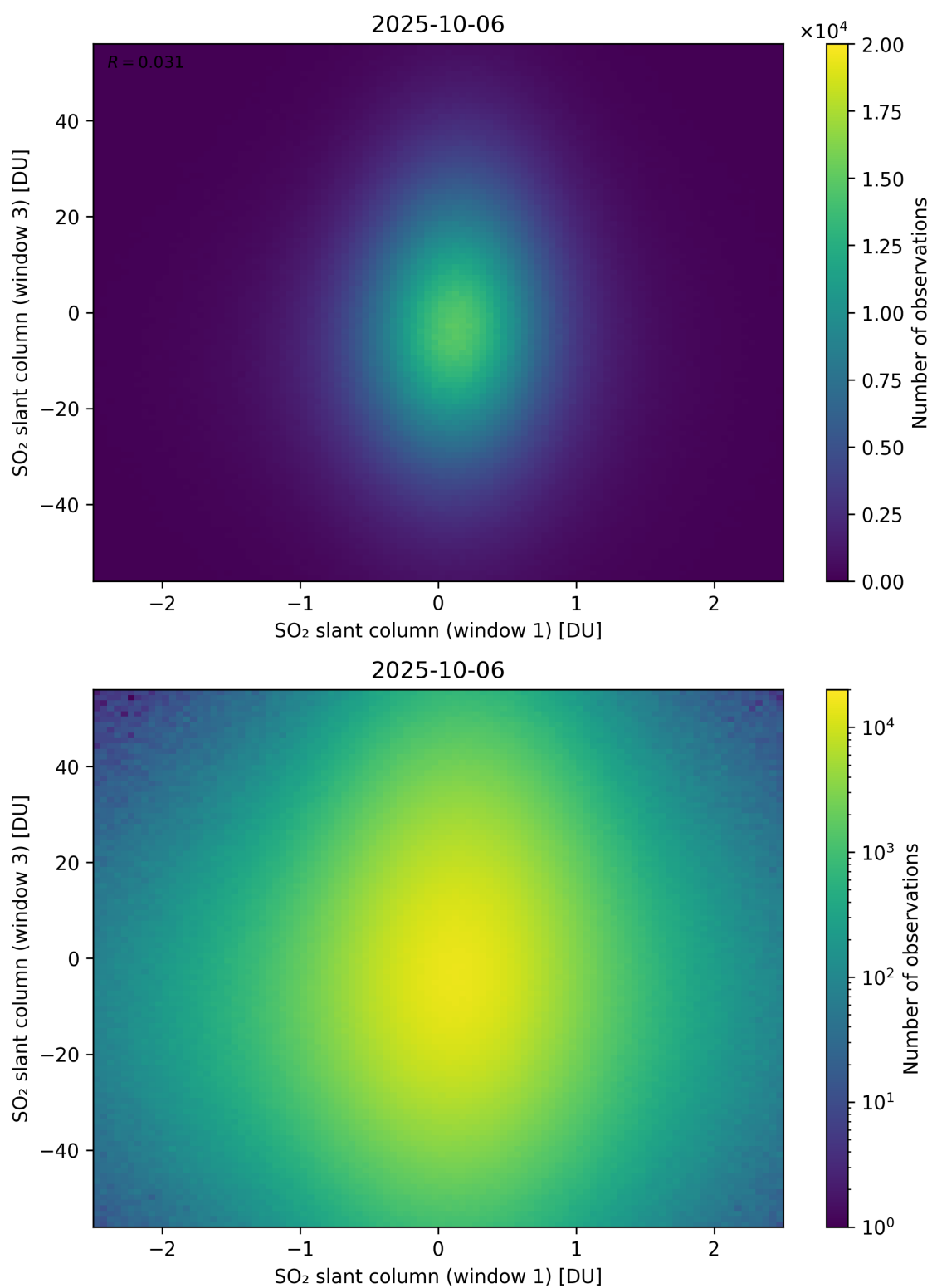
Figure 287: Scatter density plot of “SO 2 slant column (window 1)” against “SO 2 slant column (window 3)” for 2025-10-06 to 2025-10-07.
