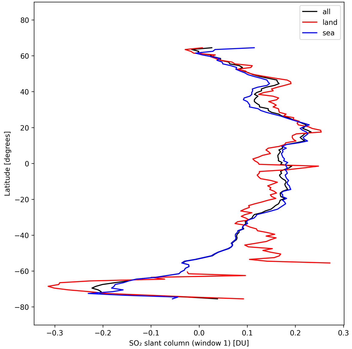
Figure 37: Zonal average of “SO 2 slant column (window 1)” for 2025-10-06 to 2025-10-07.
