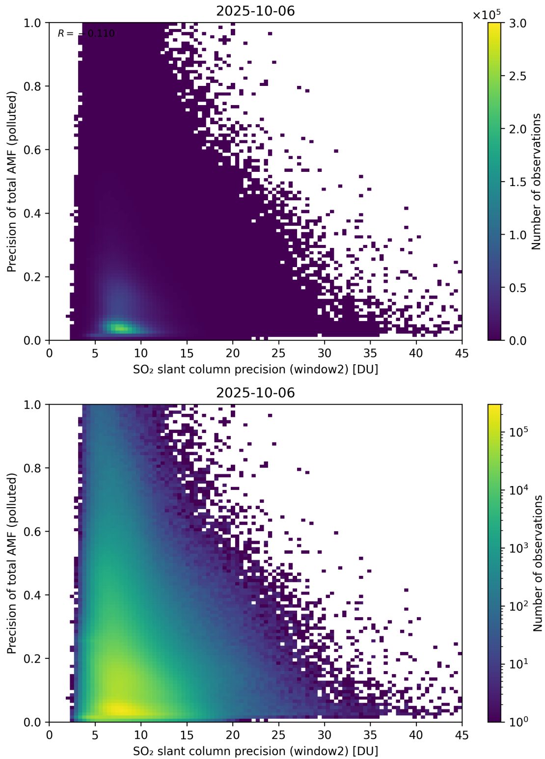
Figure 302: Scatter density plot of “SO 2 slant column precision (window2)” against “Precision of total AMF (polluted)” for 2025-10-06 to 2025-10-07.
