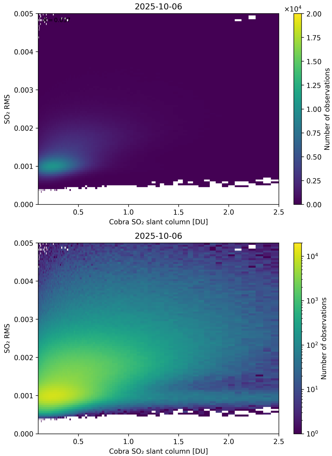
Figure 198: Scatter density plot of “Cobra SO 2 slant column” against “SO 2 RMS” for 2025-10-06 to 2025-10-07.
