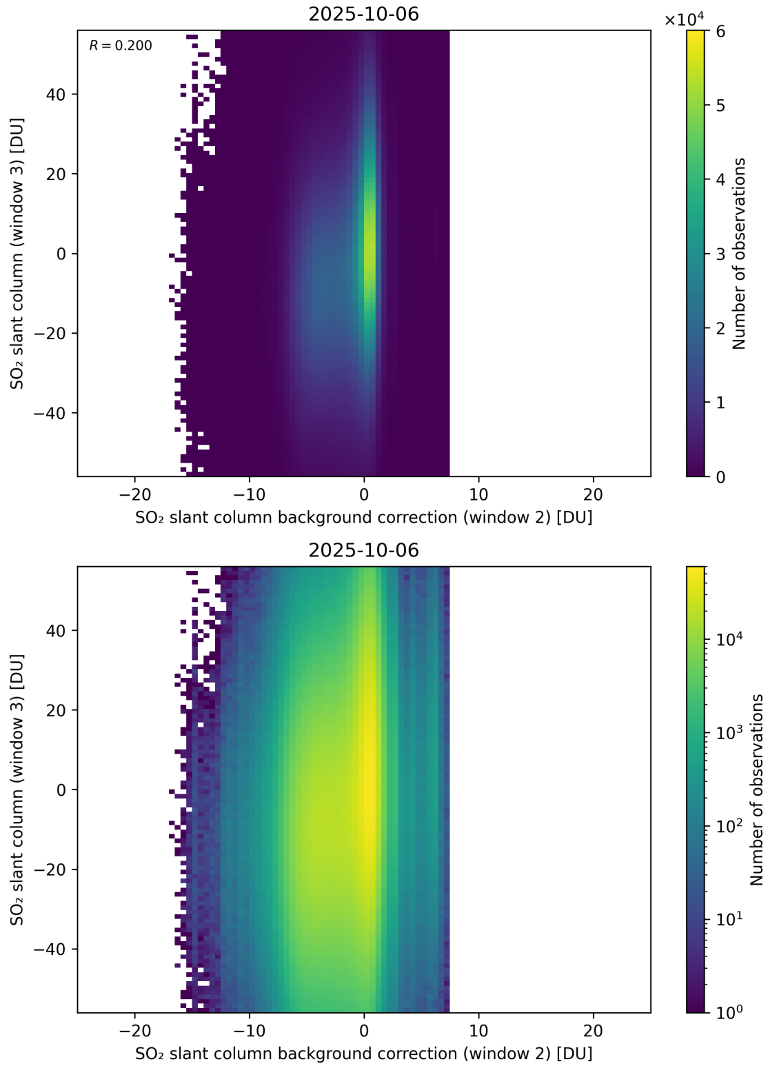
Figure 128: Scatter density plot of “SO 2 slant column background correction (window 2)” against “SO 2 slant column (window 3)” for 2025-10-06 to 2025-10-07.
