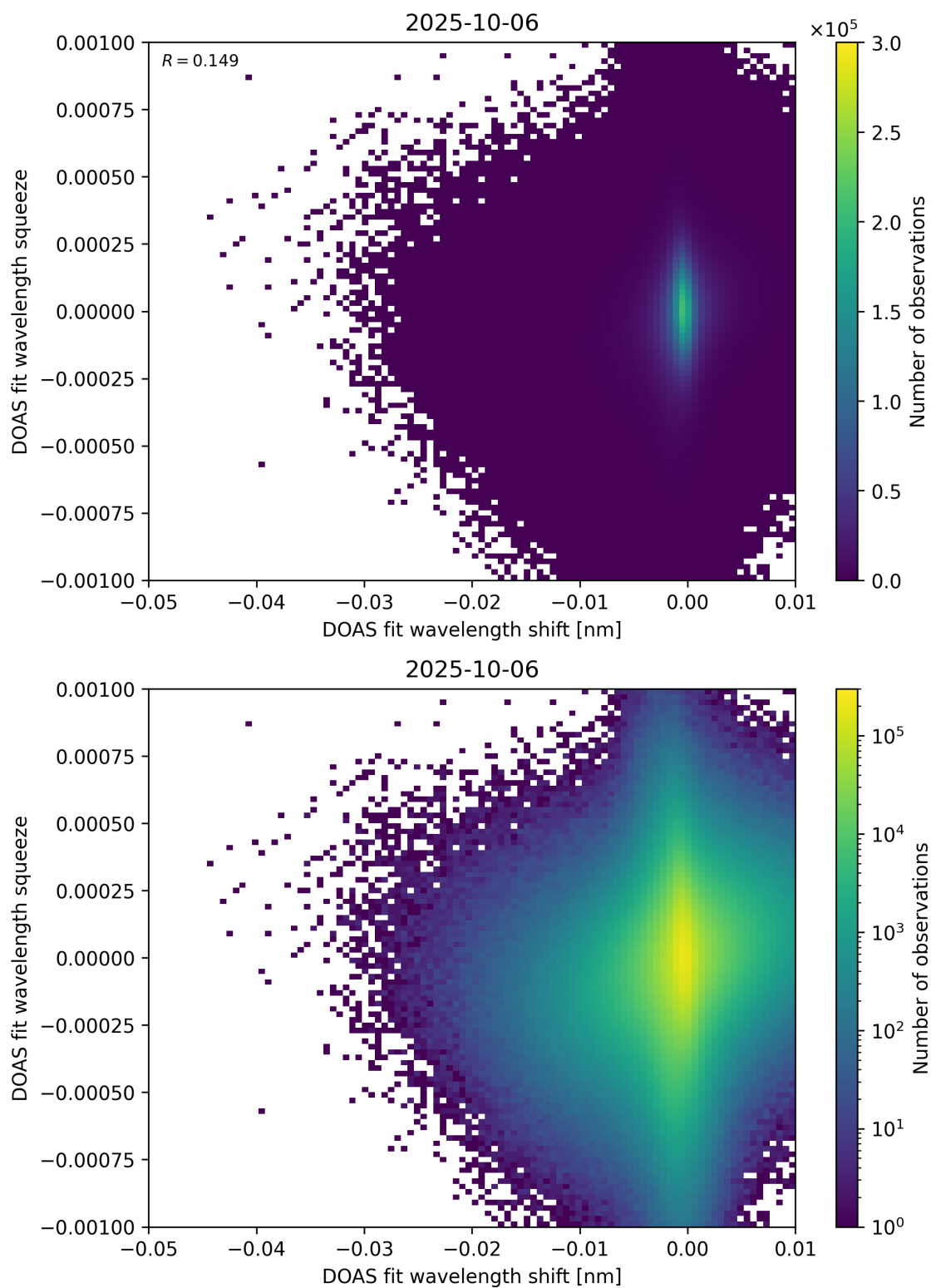
Figure 138: Scatter density plot of “DOAS fit wavelength shift” against “DOAS fit wavelength squeeze” for 2025-10-06 to 2025-10-07.
