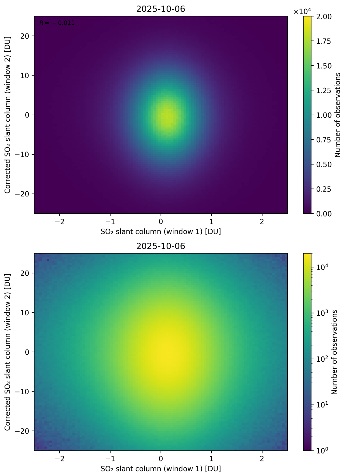
Figure 283: Scatter density plot of “SO 2 slant column (window 1)” against “Corrected SO 2 slant column (window 2)” for 2025-10-06 to 2025-10-07.
