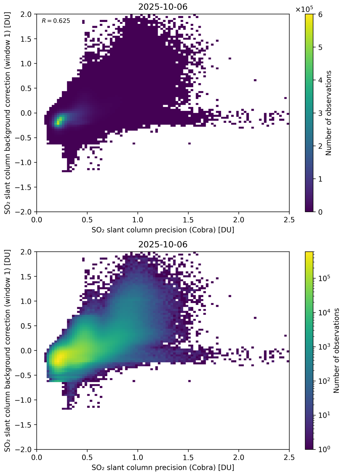
Figure 199: Scatter density plot of “SO 2 slant column precision (Cobra)” against “SO 2 slant column background correction (window 1)” for 2025-10-06 to 2025-10-07.
