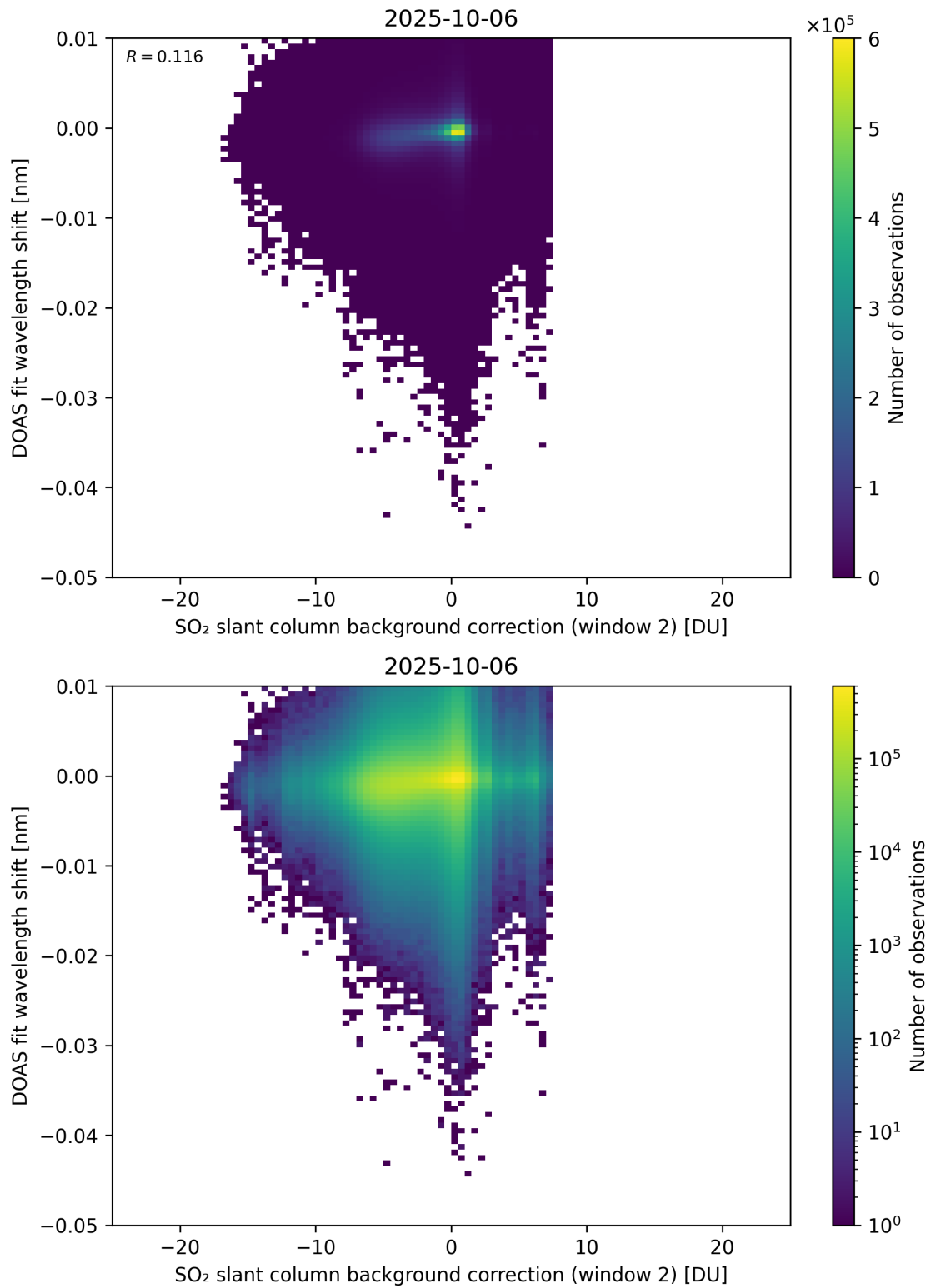
Figure 123: Scatter density plot of “SO 2 slant column background correction (window 2)” against “DOAS fit wavelength shift” for 2025-10-06 to 2025-10-07.
