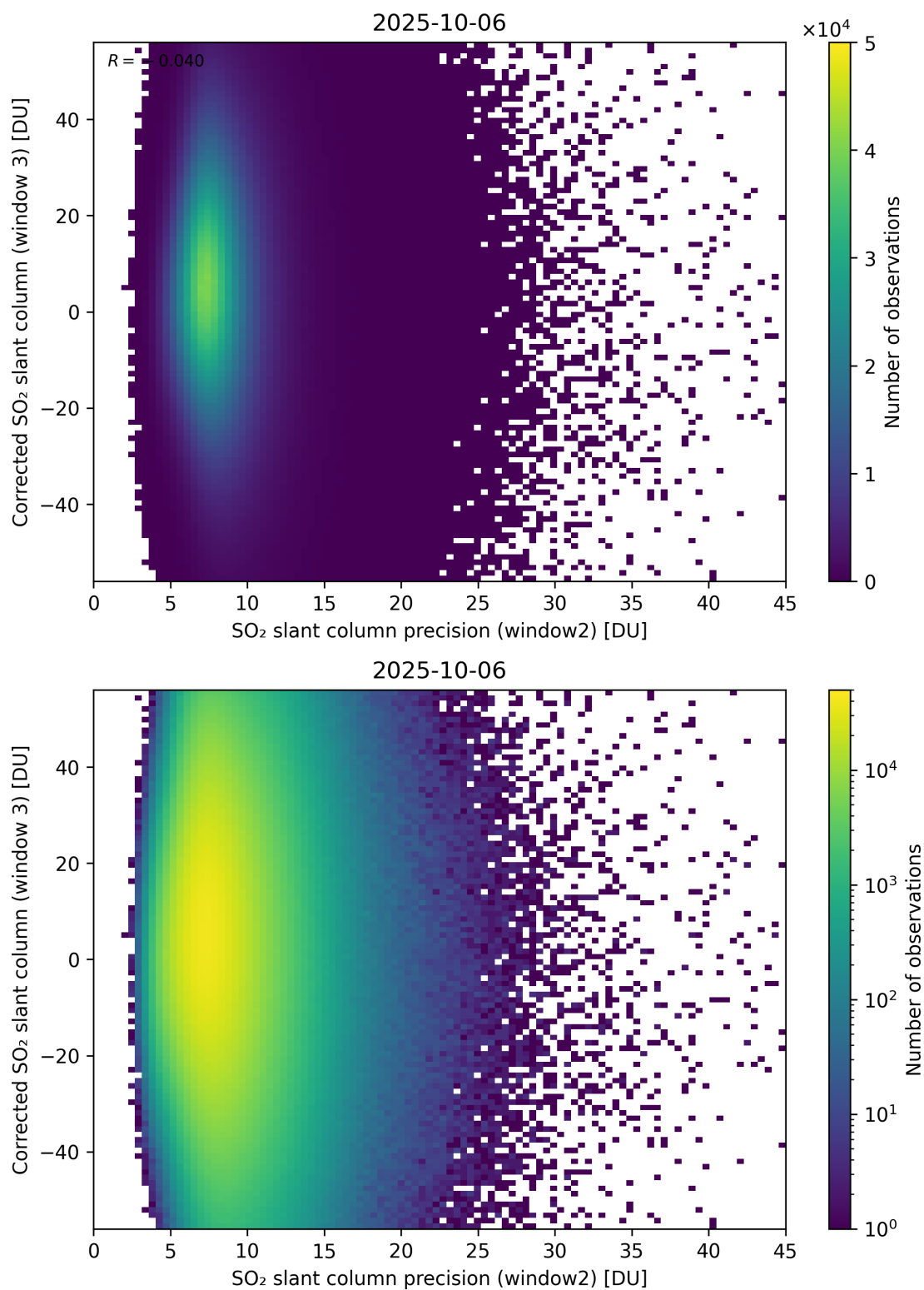
Figure 298: Scatter density plot of “SO 2 slant column precision (window2)” against “Corrected SO 2 slant column (window 3)” for 2025-10-06 to 2025-10-07.
