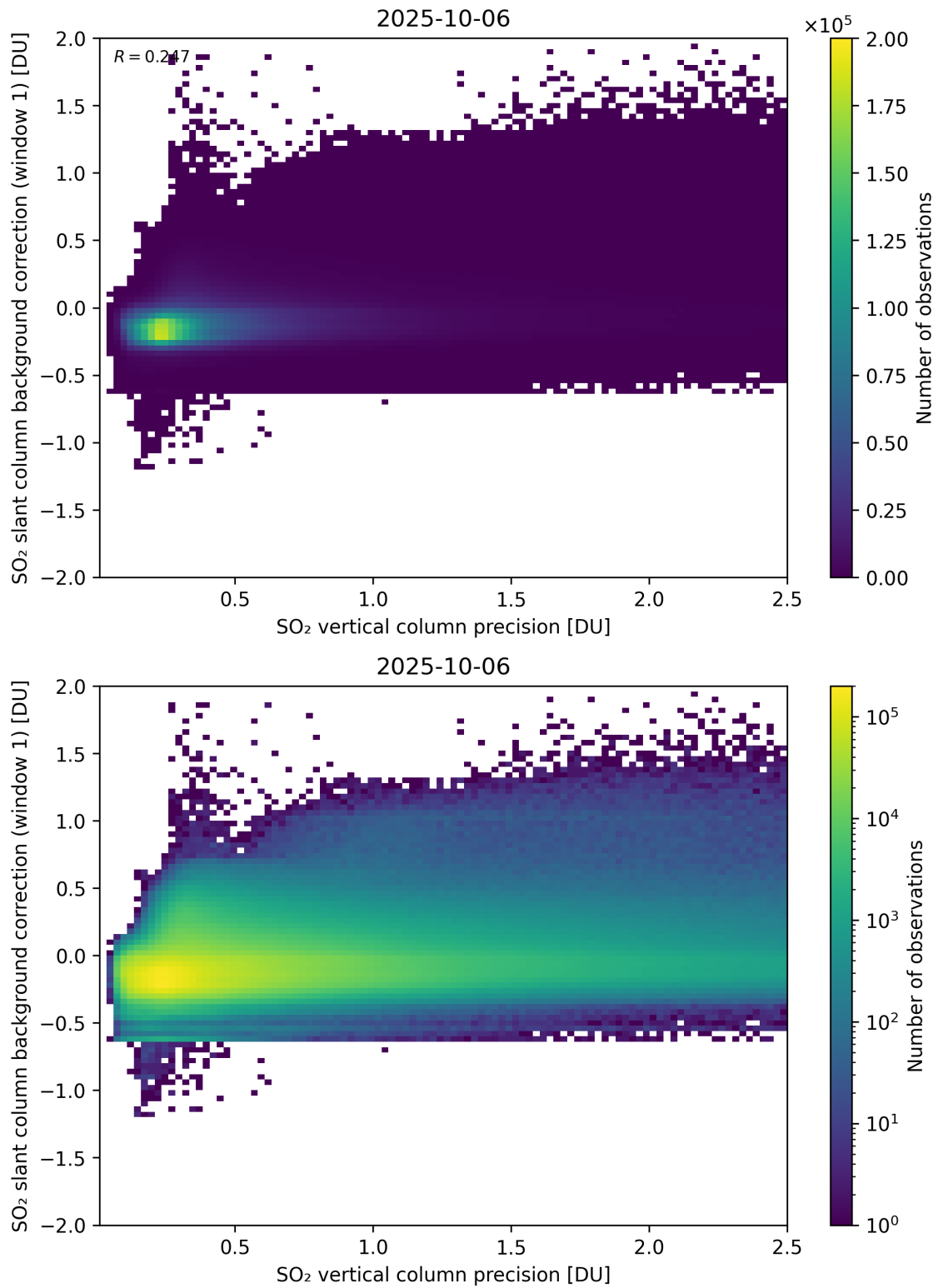
Figure 329: Scatter density plot of “SO 2 vertical column precision” against “SO 2 slant column background correction (window 1)” for 2025-10-06 to 2025-10-07.
