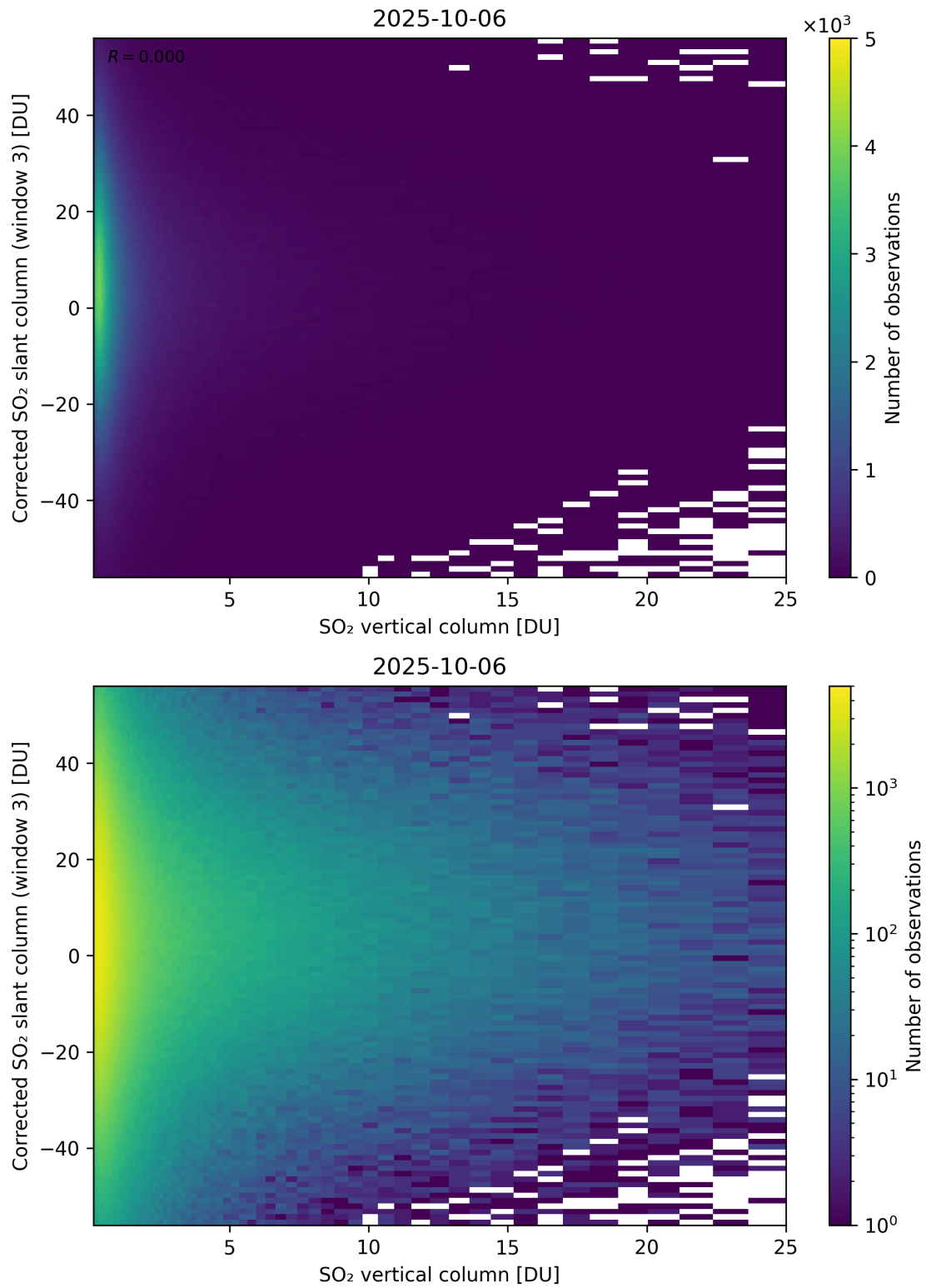
Figure 353: Scatter density plot of “SO 2 vertical column” against “Corrected SO 2 slant column (window 3)” for 2025-10-06 to 2025-10-07.
