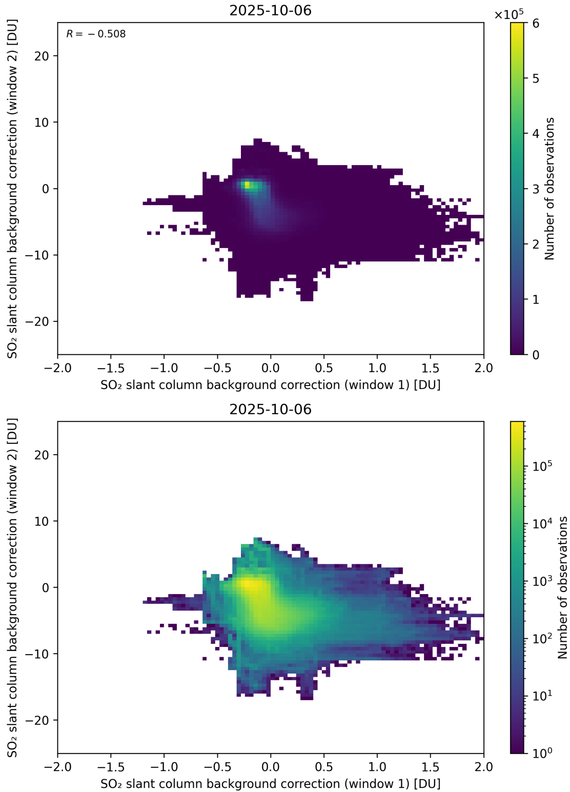
Figure 109: Scatter density plot of “SO 2 slant column background correction (window 1)” against “SO 2 slant column background correction (window 2)” for 2025-10-06 to 2025-10-07.
