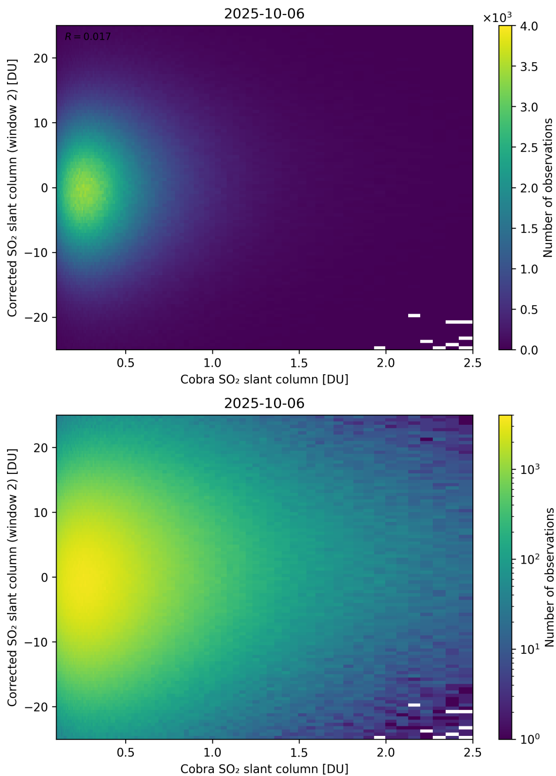
Figure 217: Scatter density plot of “Cobra SO 2 slant column” against “Corrected SO 2 slant column (window 2)” for 2025-10-06 to 2025-10-07.
