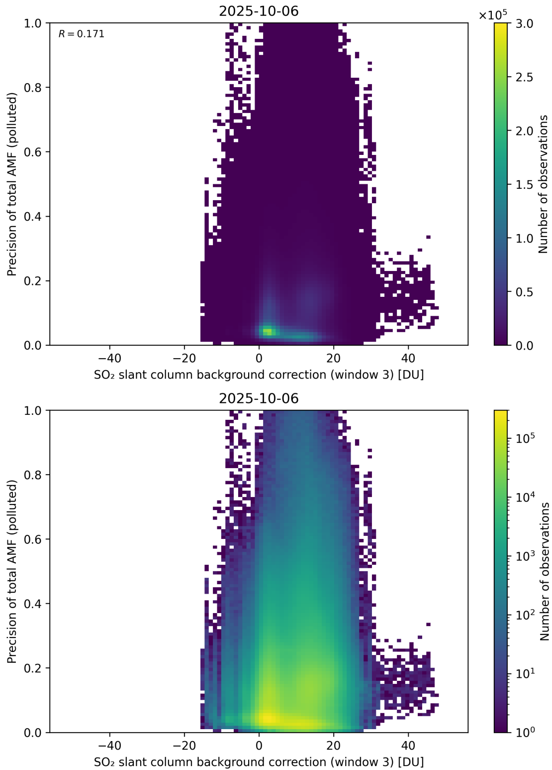
Figure 137: Scatter density plot of “SO 2 slant column background correction (window 3)” against “Precision of total AMF (polluted)” for 2025-10-06 to 2025-10-07.
