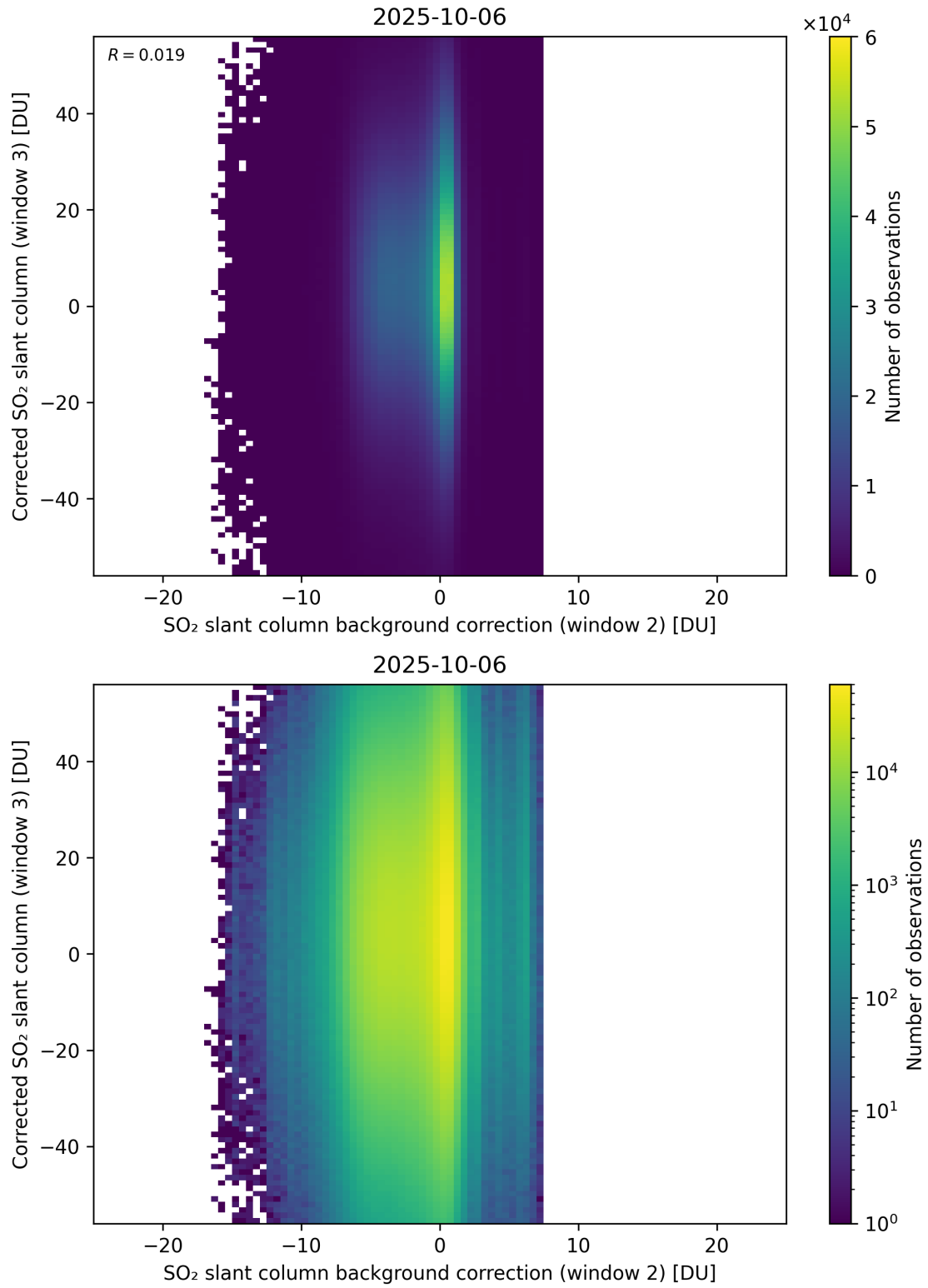
Figure 127: Scatter density plot of “SO 2 slant column background correction (window 2)” against “Corrected SO 2 slant column (window 3)” for 2025-10-06 to 2025-10-07.
