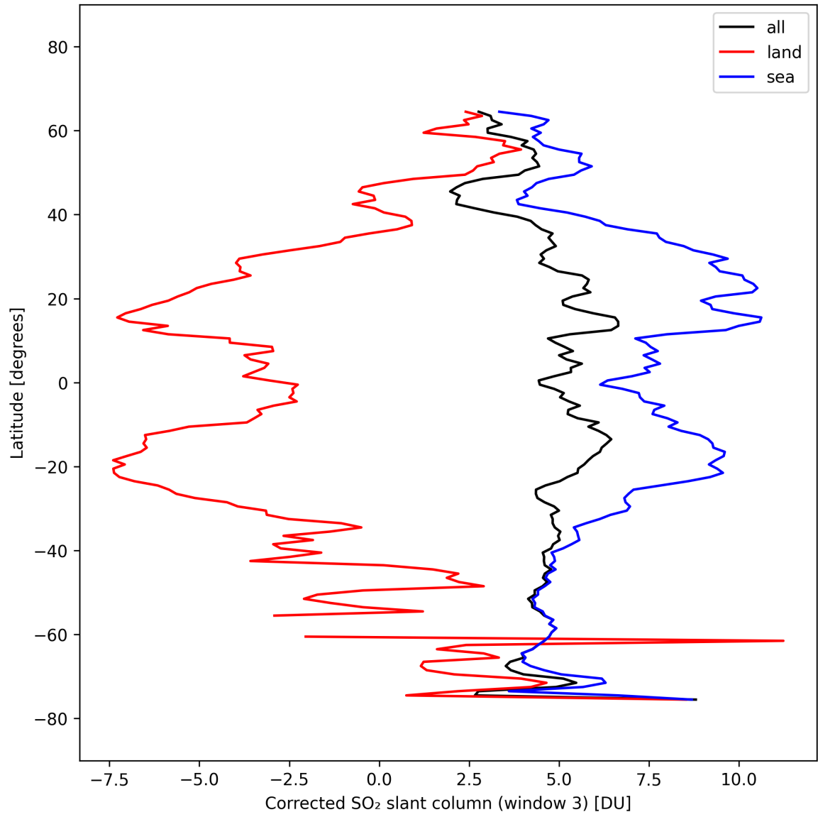
Figure 47: Zonal average of “Corrected SO 2 slant column (window 3)” for 2025-10-06 to 2025-10-07.
