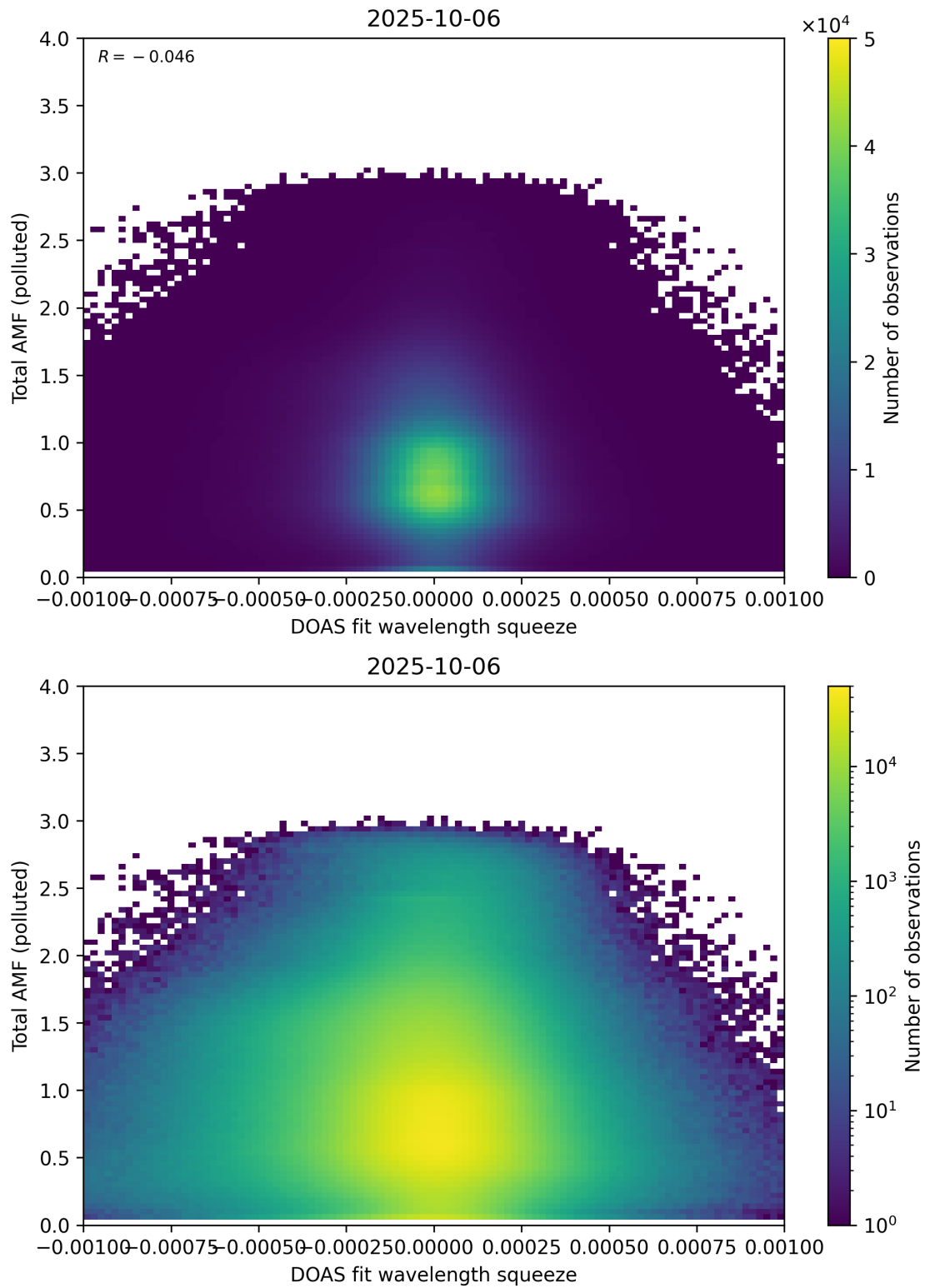
Figure 145: Scatter density plot of “DOAS fit wavelength squeeze” against “Total AMF (polluted)” for 2025-10-06 to 2025-10-07.
