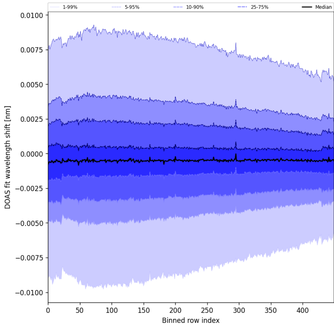
Figure 102: Along track statistics of “DOAS fit wavelength shift” for 2025-10-06 to 2025-10-07
