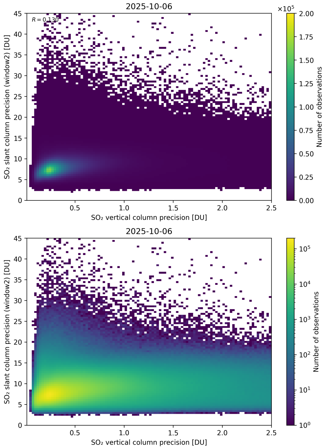
Figure 343: Scatter density plot of “SO 2 vertical column precision” against “SO 2 slant column precision (window2)” for 2025-10-06 to 2025-10-07.
