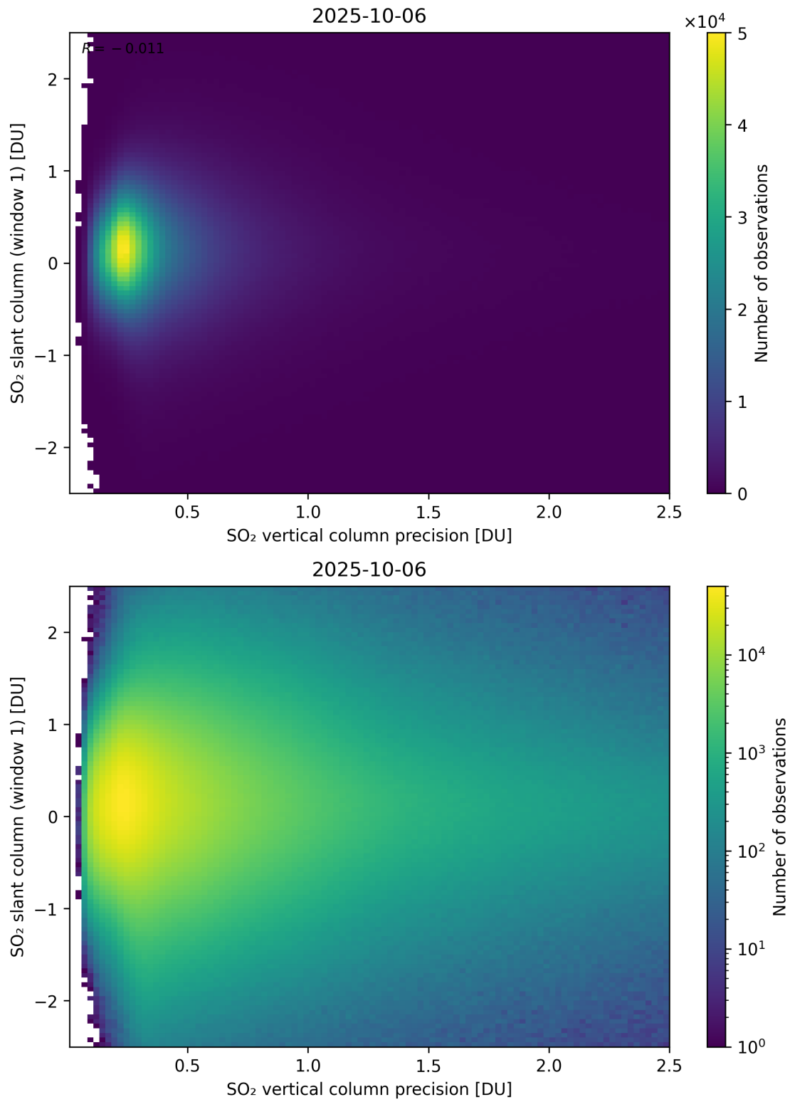
Figure 341: Scatter density plot of “SO 2 vertical column precision” against “SO 2 slant column (window 1)” for 2025-10-06 to 2025-10-07.
