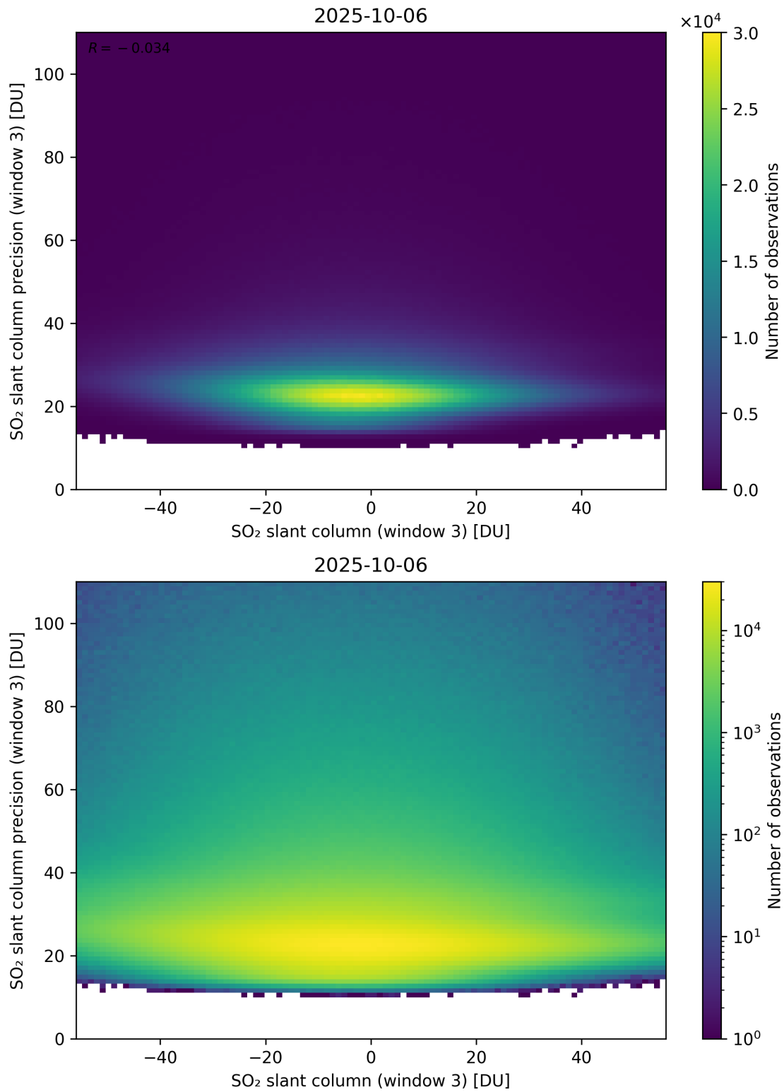
Figure 317: Scatter density plot of “SO 2 slant column (window 3)” against “SO 2 slant column precision (window 3)” for 2025-10-06 to 2025-10-07.
