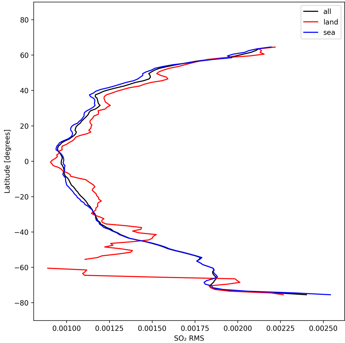
Figure 52: Zonal average of “SO 2 RMS” for 2025-10-06 to 2025-10-07.
