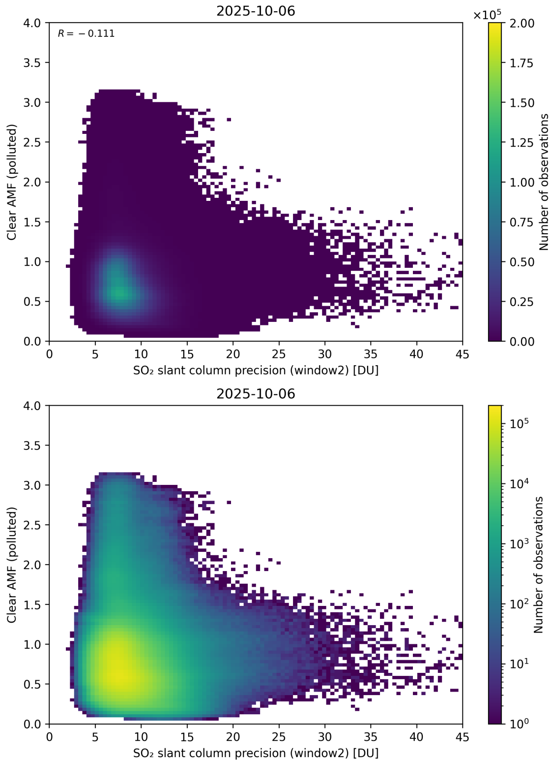
Figure 296: Scatter density plot of “SO 2 slant column precision (window2)” against “Clear AMF (polluted)” for 2025-10-06 to 2025-10-07.
