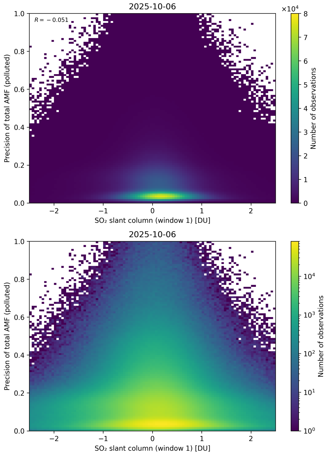
Figure 290: Scatter density plot of “SO 2 slant column (window 1)” against “Precision of total AMF (polluted)” for 2025-10-06 to 2025-10-07.
