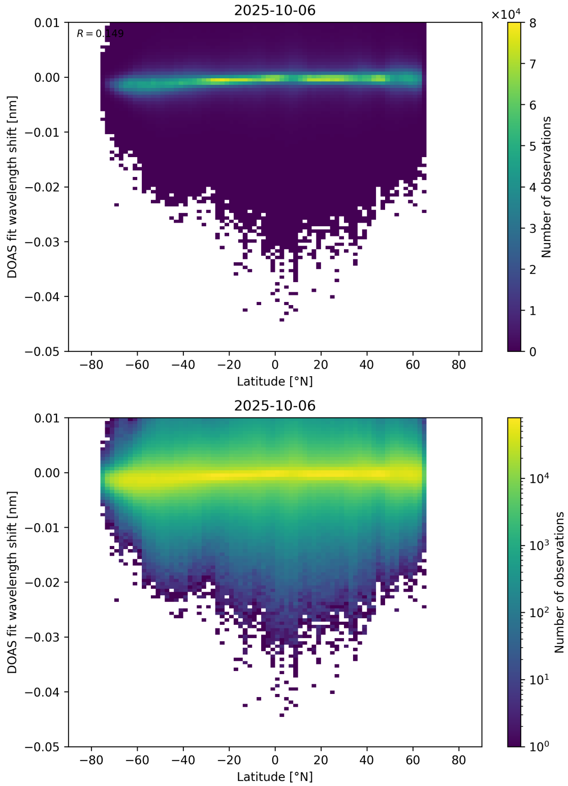
Figure 153: Scatter density plot of “Latitude” against “DOAS fit wavelength shift” for 2025-10-06 to 2025-10-07.
