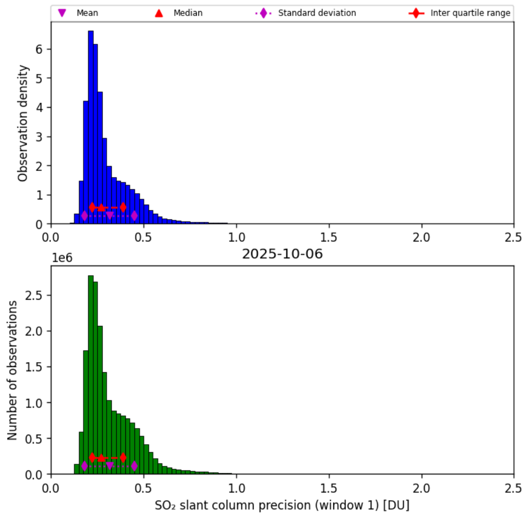
Figure 64: Histogram of “SO 2 slant column precision (window 1)” for 2025-10-06 to 2025-10-07
