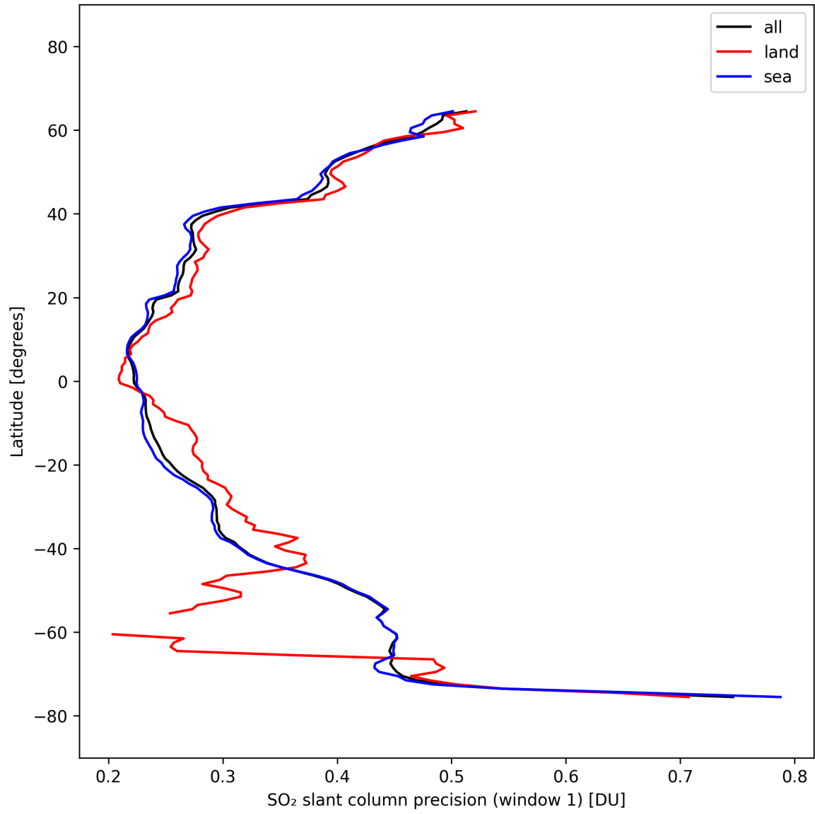
Figure 38: Zonal average of “SO 2 slant column precision (window 1)” for 2025-10-06 to 2025-10-07.
