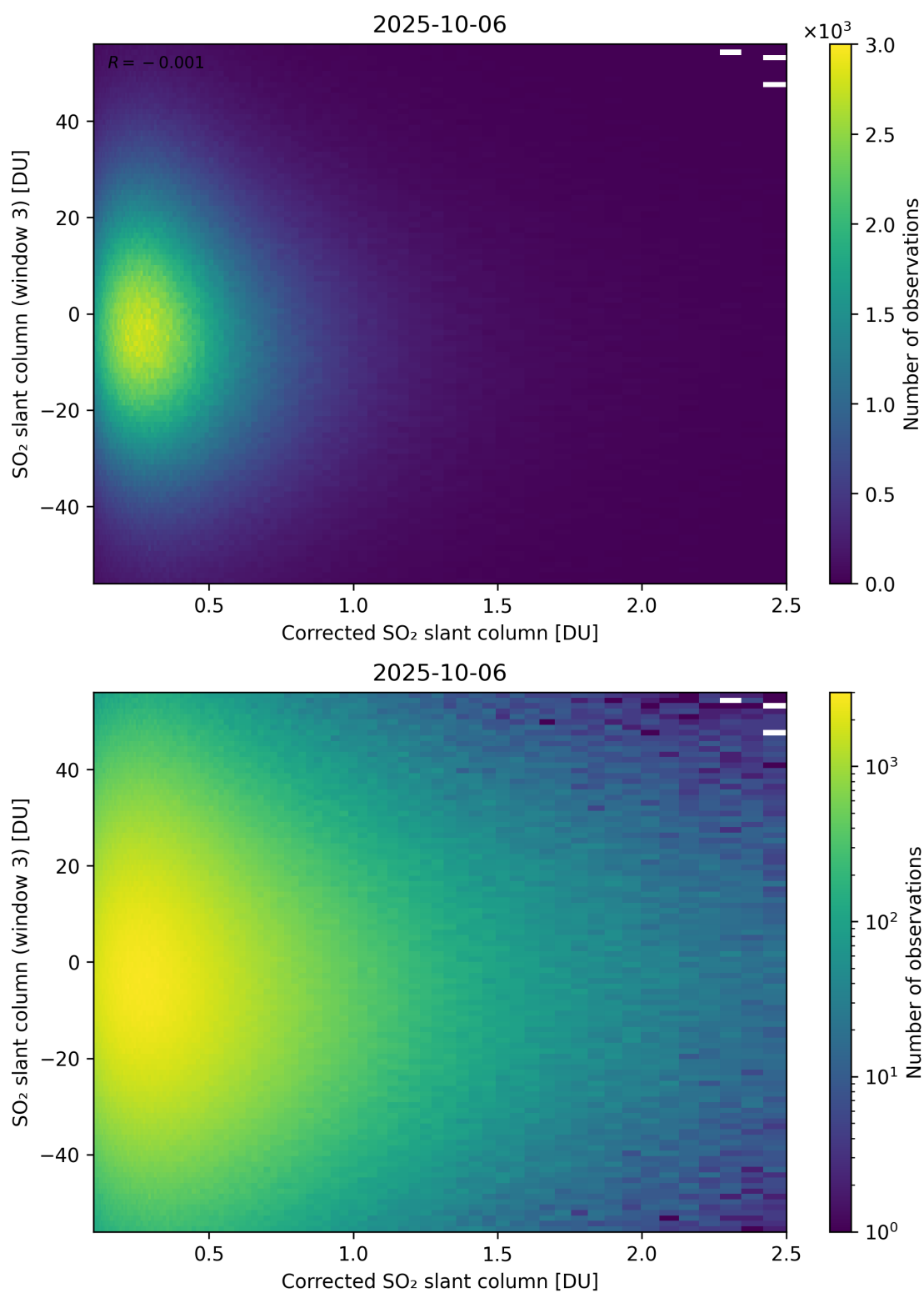
Figure 240: Scatter density plot of “Corrected SO 2 slant column” against “SO 2 slant column (window 3)” for 2025-10-06 to 2025-10-07.
