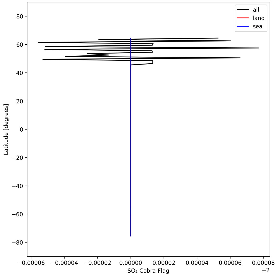
Figure 49: Zonal average of “SO 2 Cobra Flag” for 2025-10-06 to 2025-10-07.
