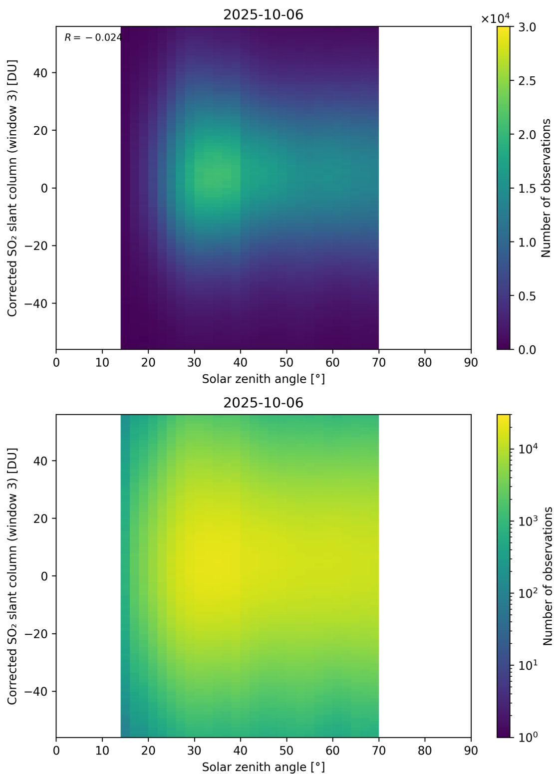
Figure 183: Scatter density plot of “Solar zenith angle” against “Corrected SO 2 slant column (window 3)” for 2025-10-06 to 2025-10-07.
