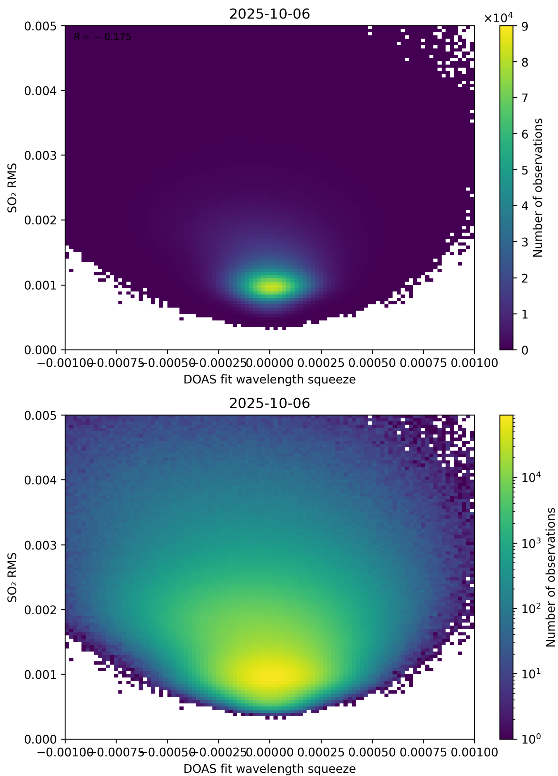
Figure 143: Scatter density plot of “DOAS fit wavelength squeeze” against “SO 2 RMS” for 2025-10-06 to 2025-10-07.
