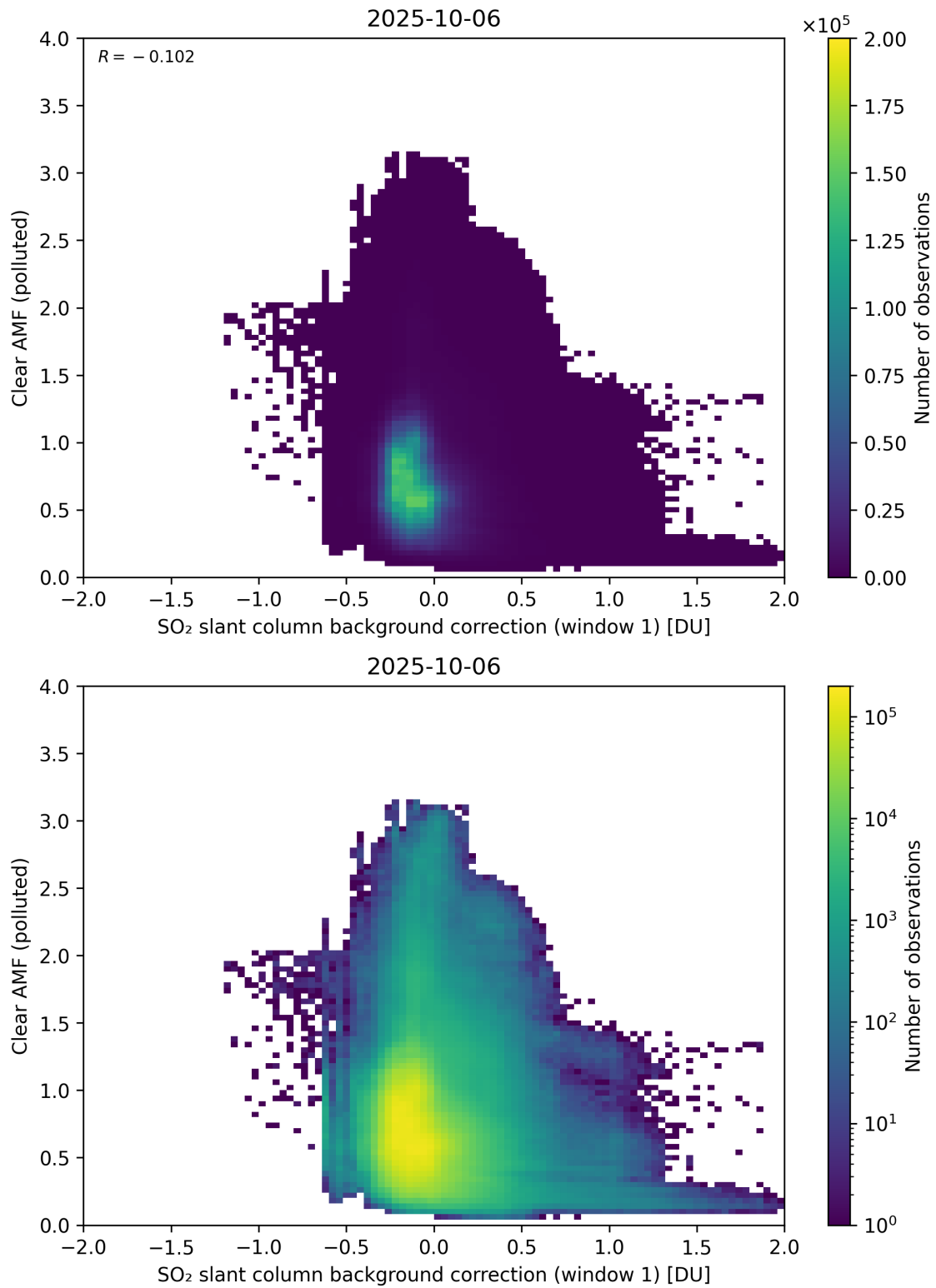
Figure 114: Scatter density plot of “SO 2 slant column background correction (window 1)” against “Clear AMF (polluted)” for 2025-10-06 to 2025-10-07.
