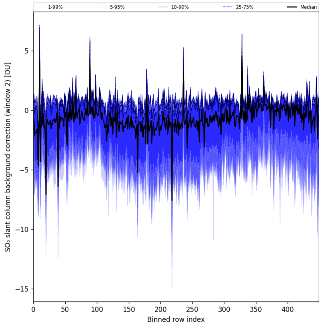
Figure 96: Along track statistics of “SO 2 slant column background correction (window 2)” for 2025-10-06 to 2025-10-07
