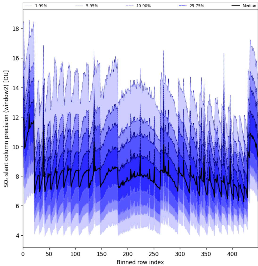
Figure 94: Along track statistics of “SO 2 slant column precision (window2)” for 2025-10-06 to 2025-10-07
