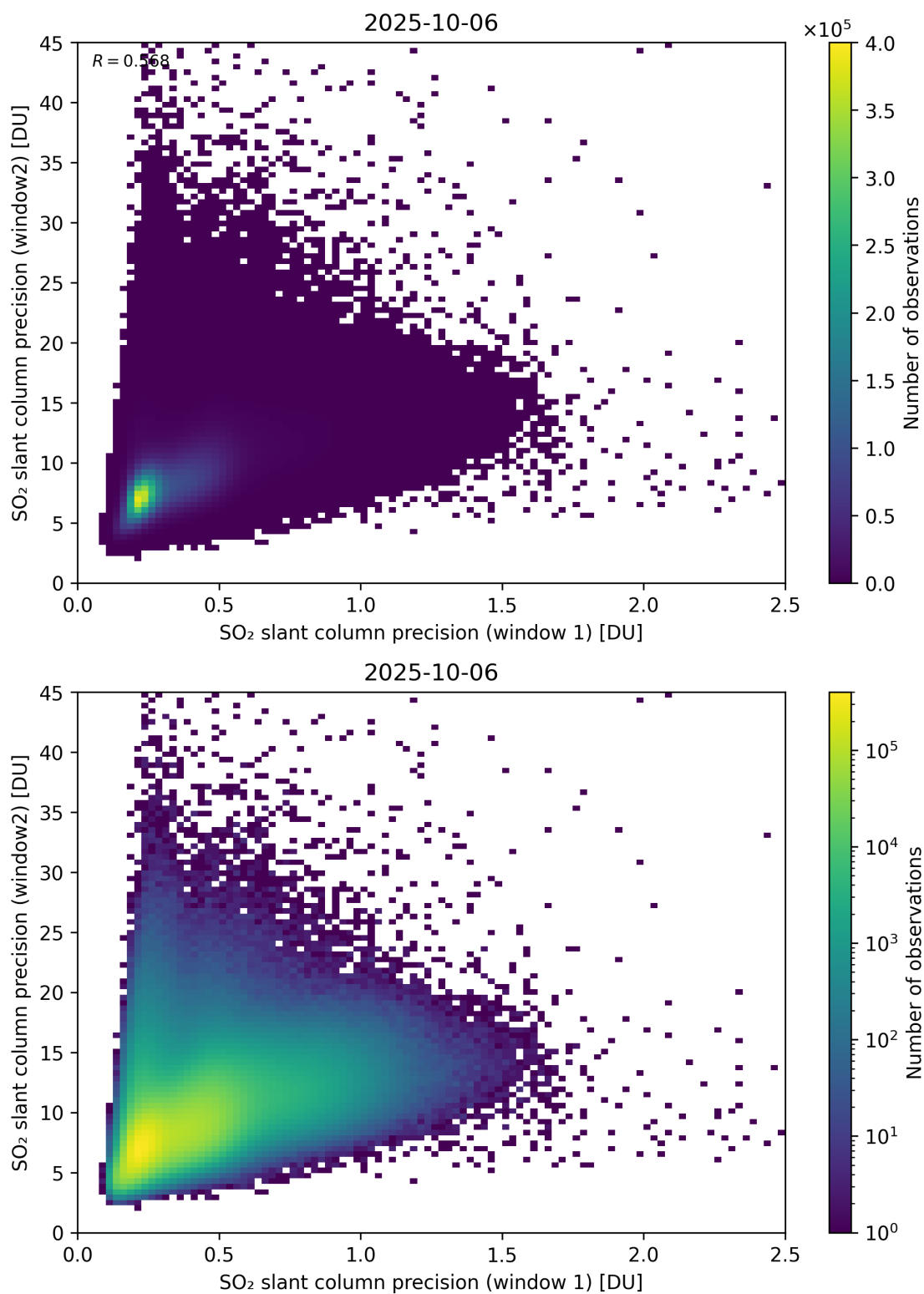
Figure 277: Scatter density plot of “SO 2 slant column precision (window 1)” against “SO 2 slant column precision (window2)” for 2025-10-06 to 2025-10-07.
