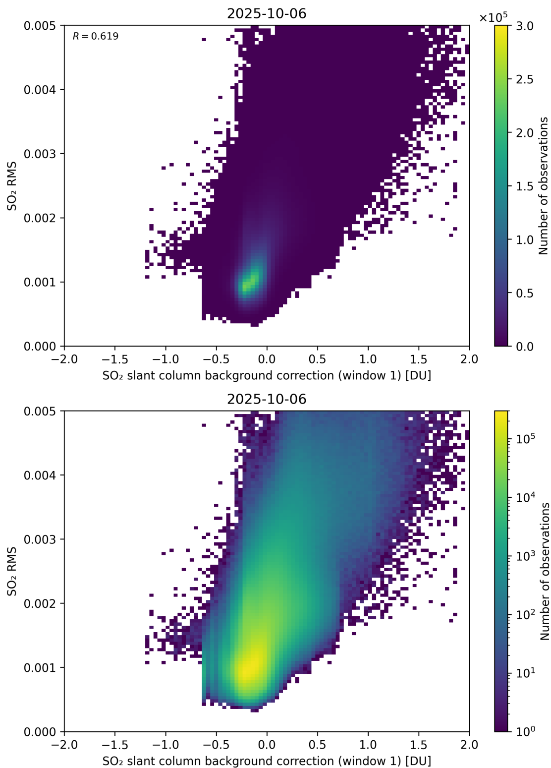
Figure 113: Scatter density plot of “SO 2 slant column background correction (window 1)” against “SO 2 RMS” for 2025-10-06 to 2025-10-07.
