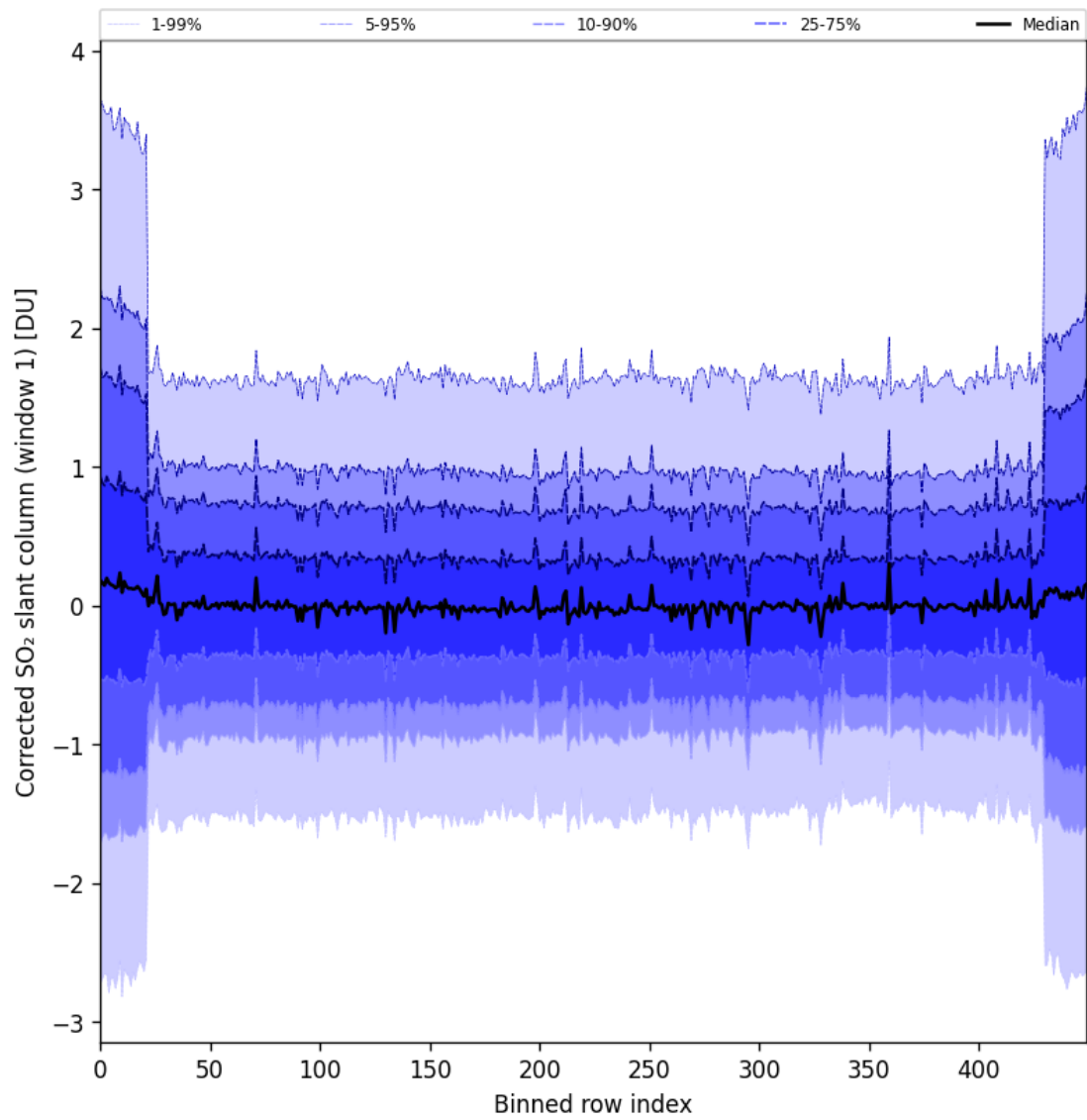
Figure 91: Along track statistics of “Corrected SO 2 slant column (window 1)” for 2025-10-06 to 2025-10-07
