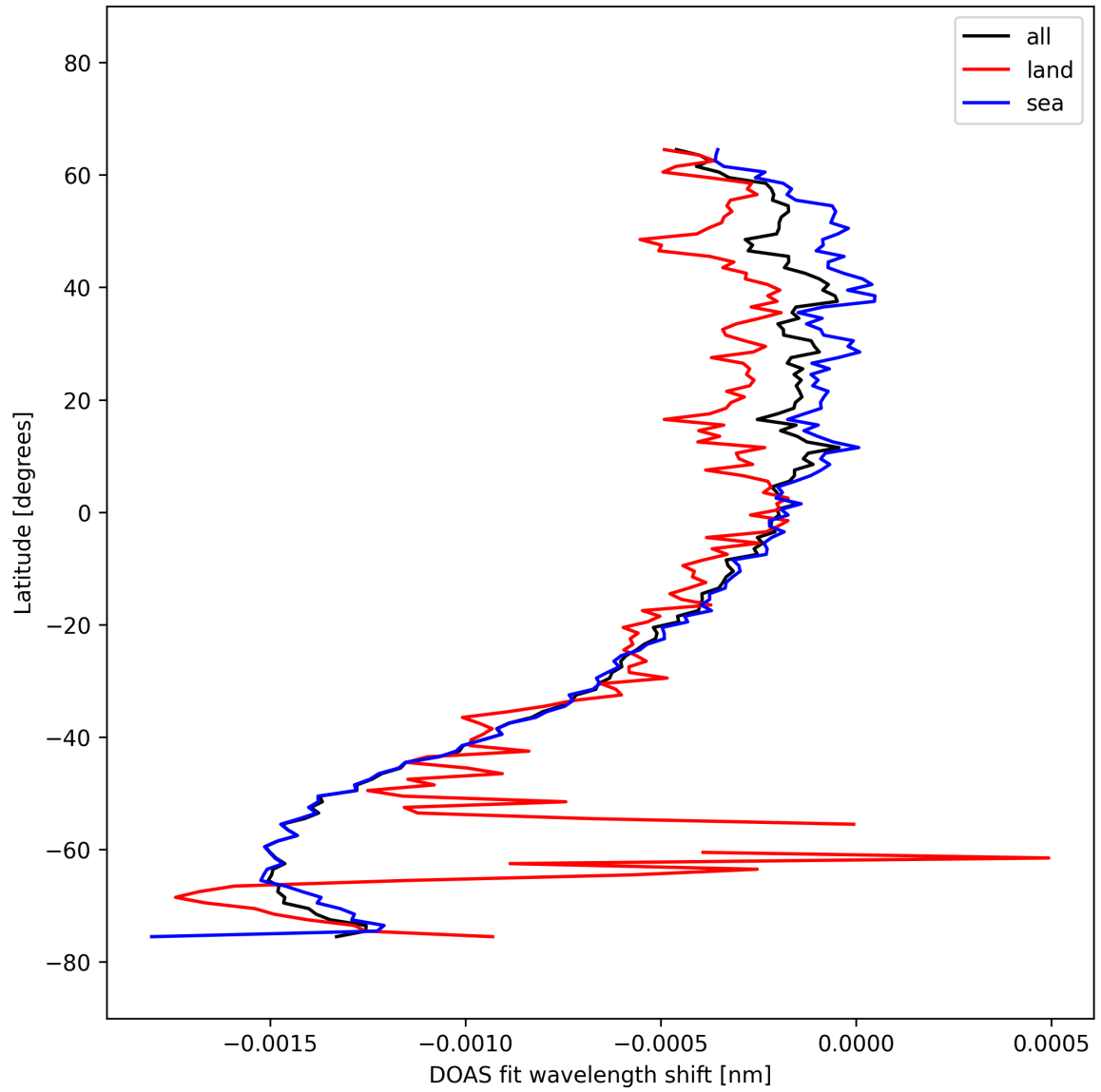
Figure 50: Zonal average of “DOAS fit wavelength shift” for 2025-10-06 to 2025-10-07.
