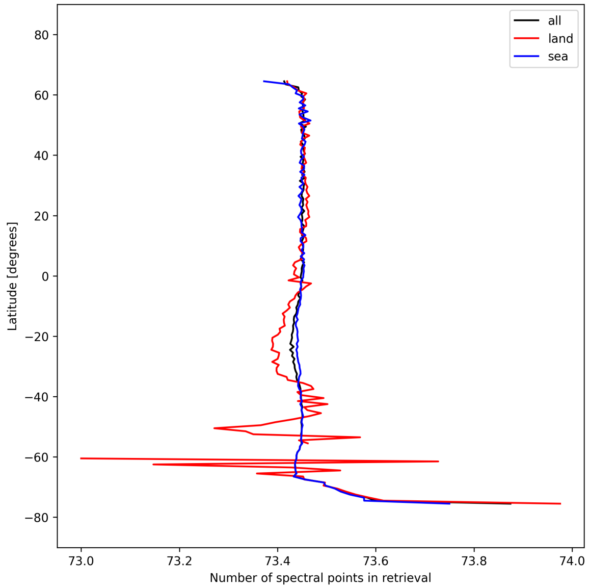
Figure 56: Zonal average of “Number of spectral points in retrieval” for 2025-10-06 to 2025-10-07.
