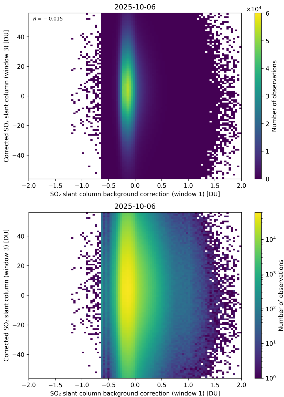
Figure 116: Scatter density plot of “SO 2 slant column background correction (window 1)” against “Corrected SO 2 slant column (window 3)” for 2025-10-06 to 2025-10-07.
