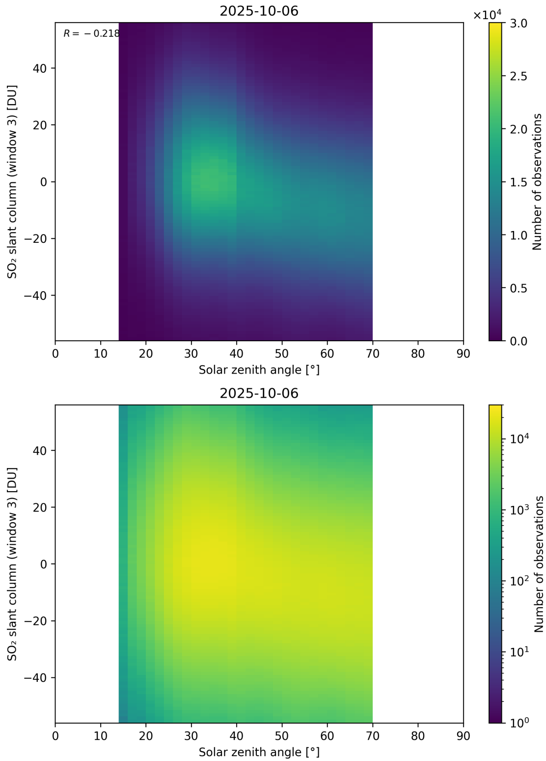
Figure 187: Scatter density plot of “Solar zenith angle” against “SO 2 slant column (window 3)” for 2025-10-06 to 2025-10-07.
