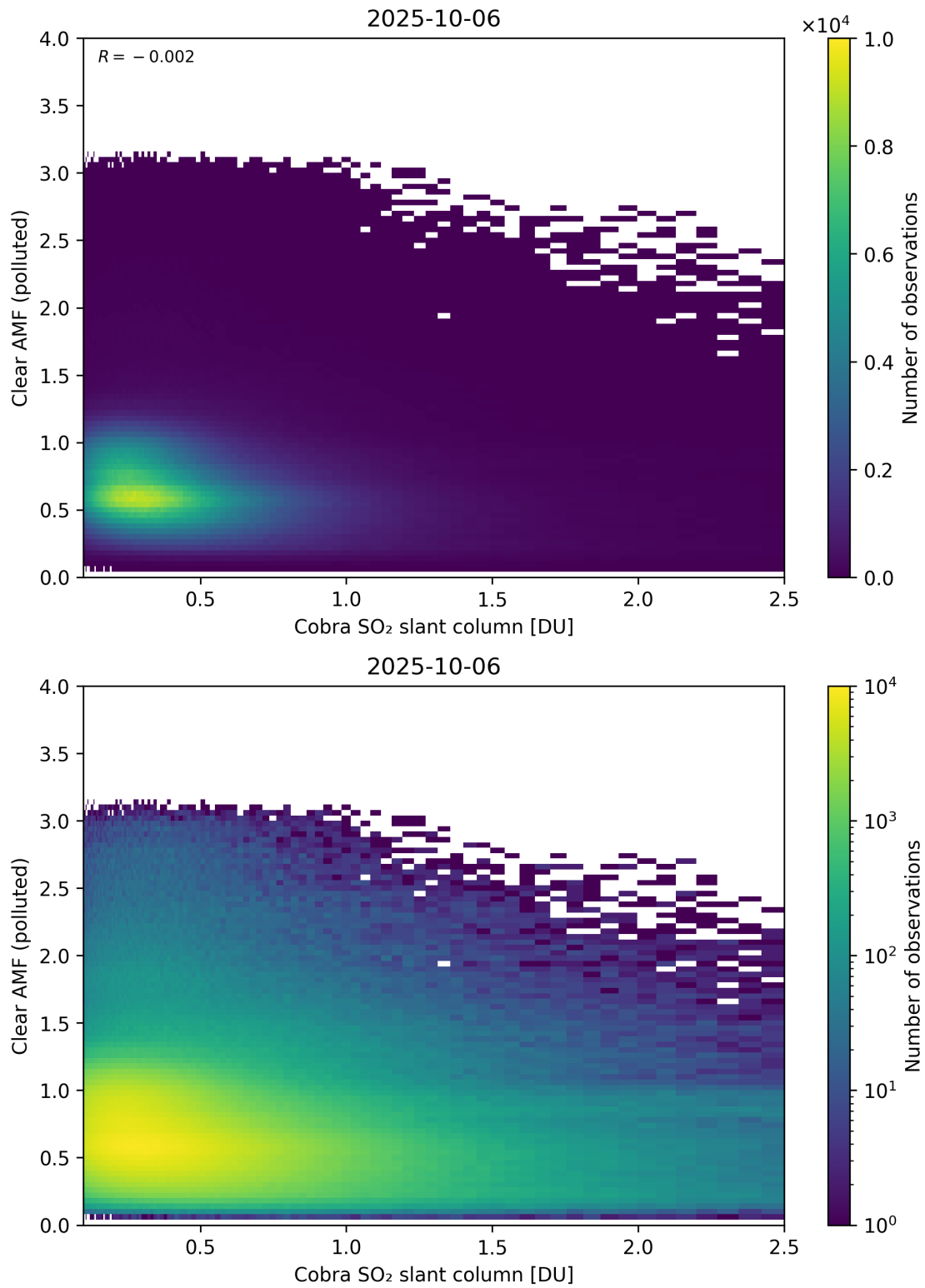
Figure 215: Scatter density plot of “Cobra SO 2 slant column” against “Clear AMF (polluted)” for 2025-10-06 to 2025-10-07.
