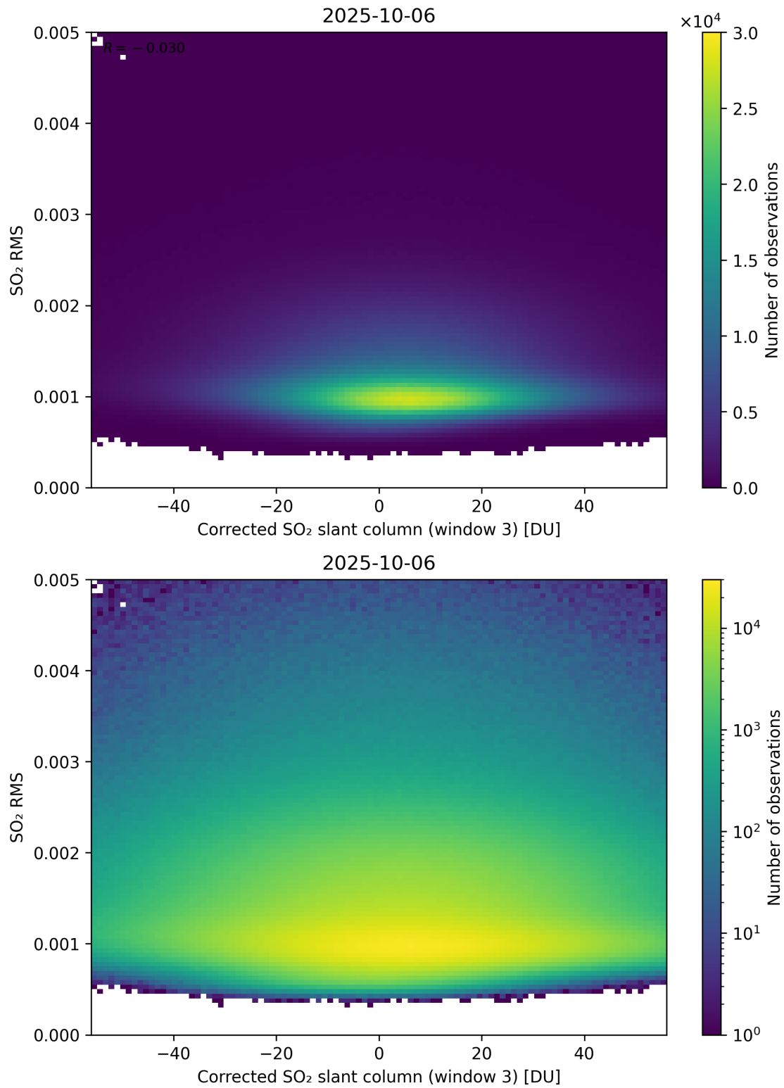
Figure 258: Scatter density plot of “Corrected SO 2 slant column (window 3)” against “SO 2 RMS” for 2025-10-06 to 2025-10-07.
