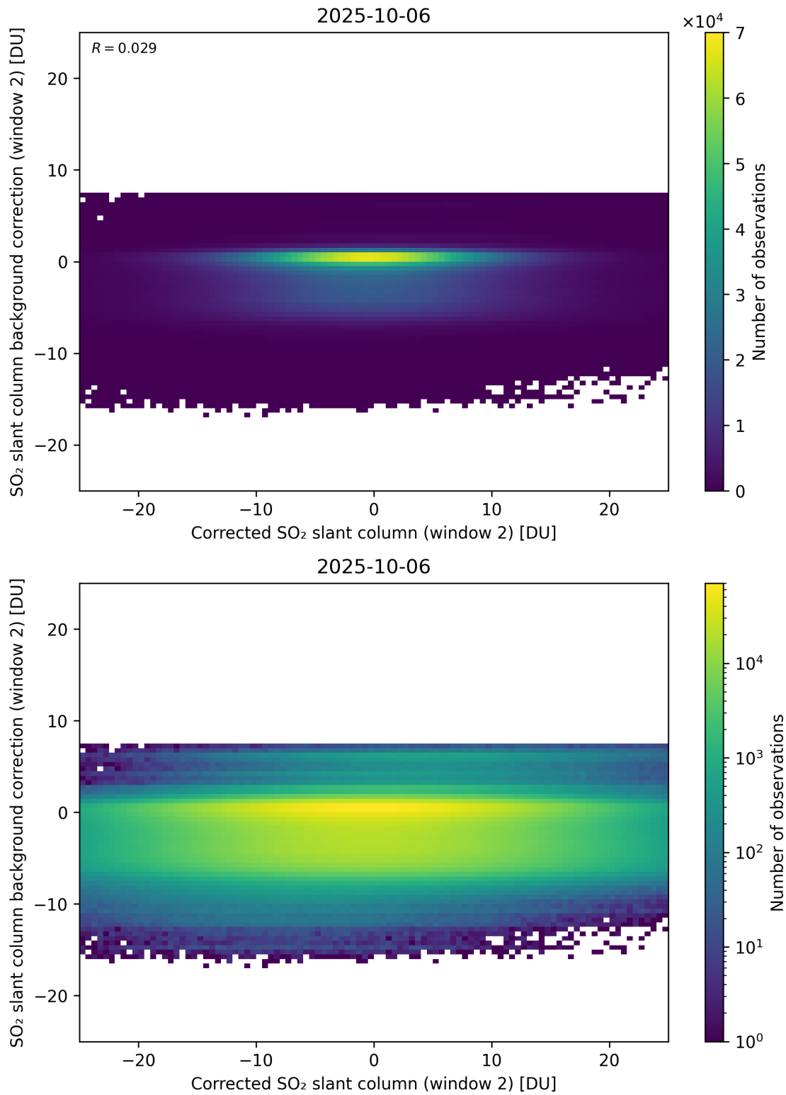
Figure 244: Scatter density plot of “Corrected SO 2 slant column (window 2)” against “SO 2 slant column background correction (window 2)” for 2025-10-06 to 2025-10-07.
