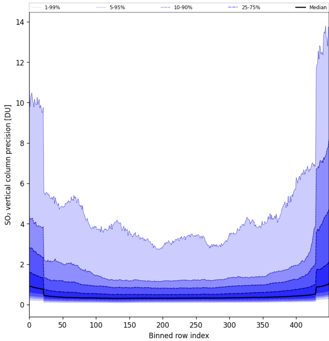
Figure 85: Along track statistics of “SO 2 vertical column precision” for 2025-10-06 to 2025-10-07
