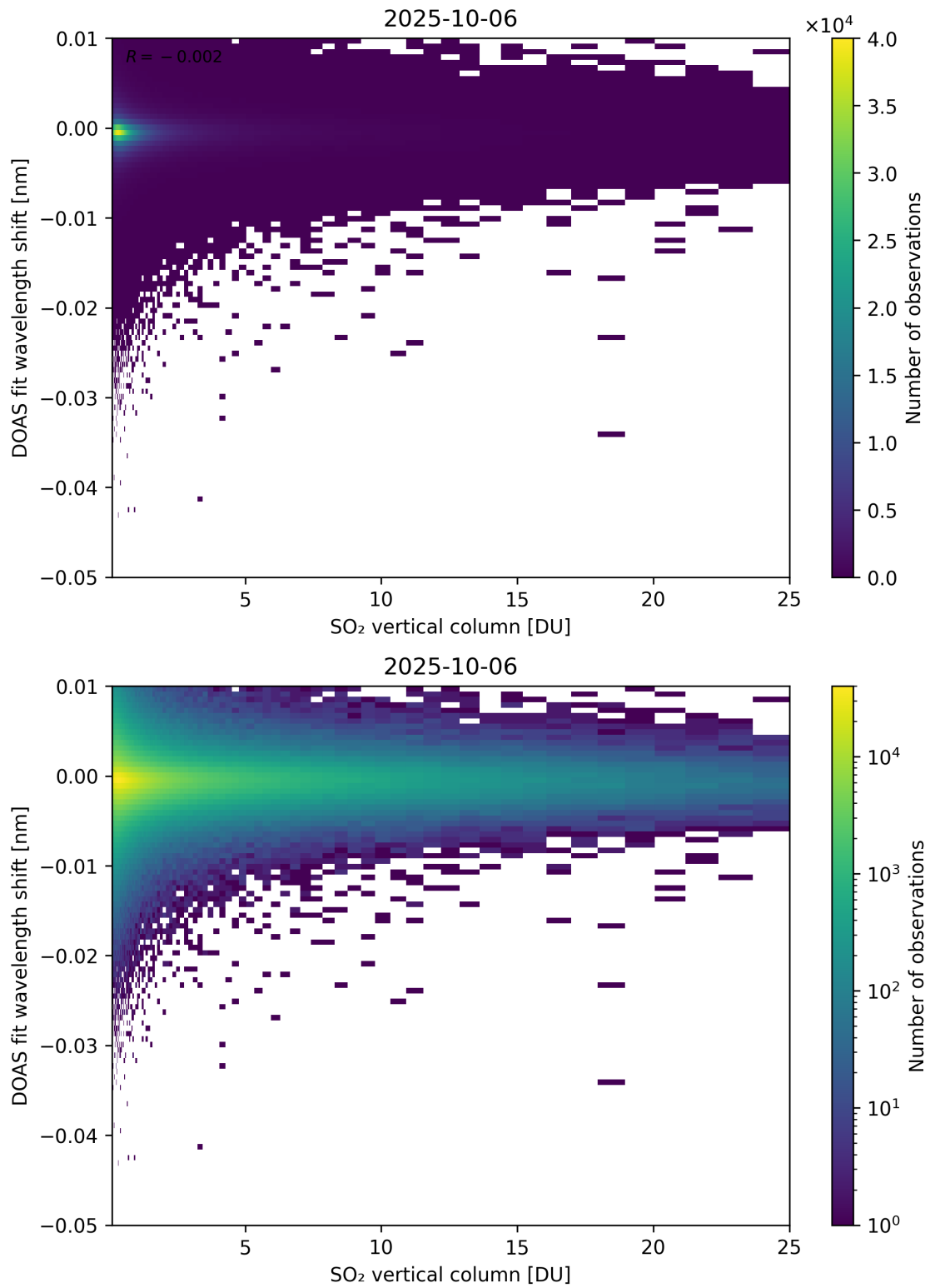
Figure 326: Scatter density plot of “SO 2 vertical column” against “DOAS fit wavelength shift” for 2025-10-06 to 2025-10-07.
