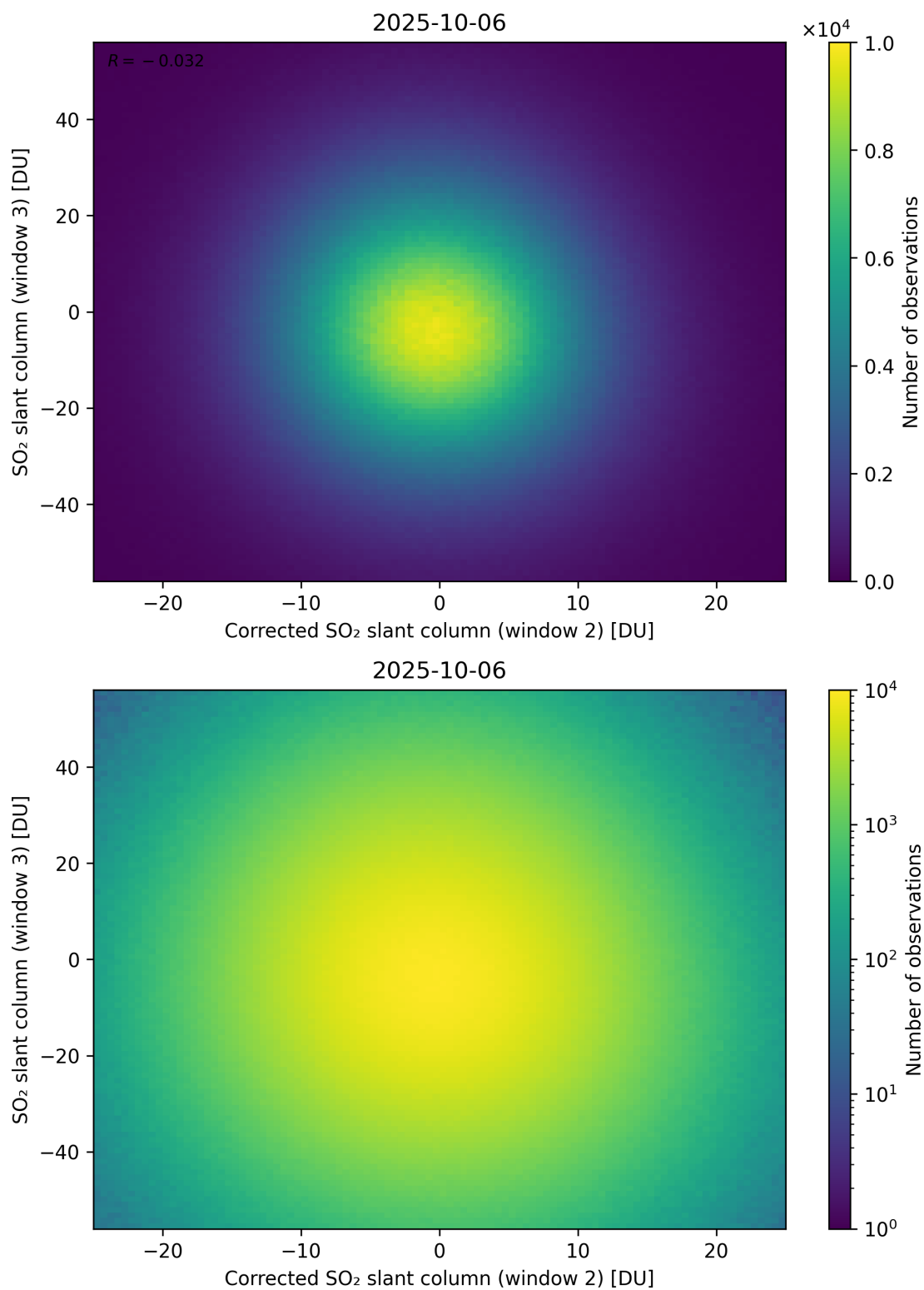
Figure 251: Scatter density plot of “Corrected SO 2 slant column (window 2)” against “SO 2 slant column (window 3)” for 2025-10-06 to 2025-10-07.
