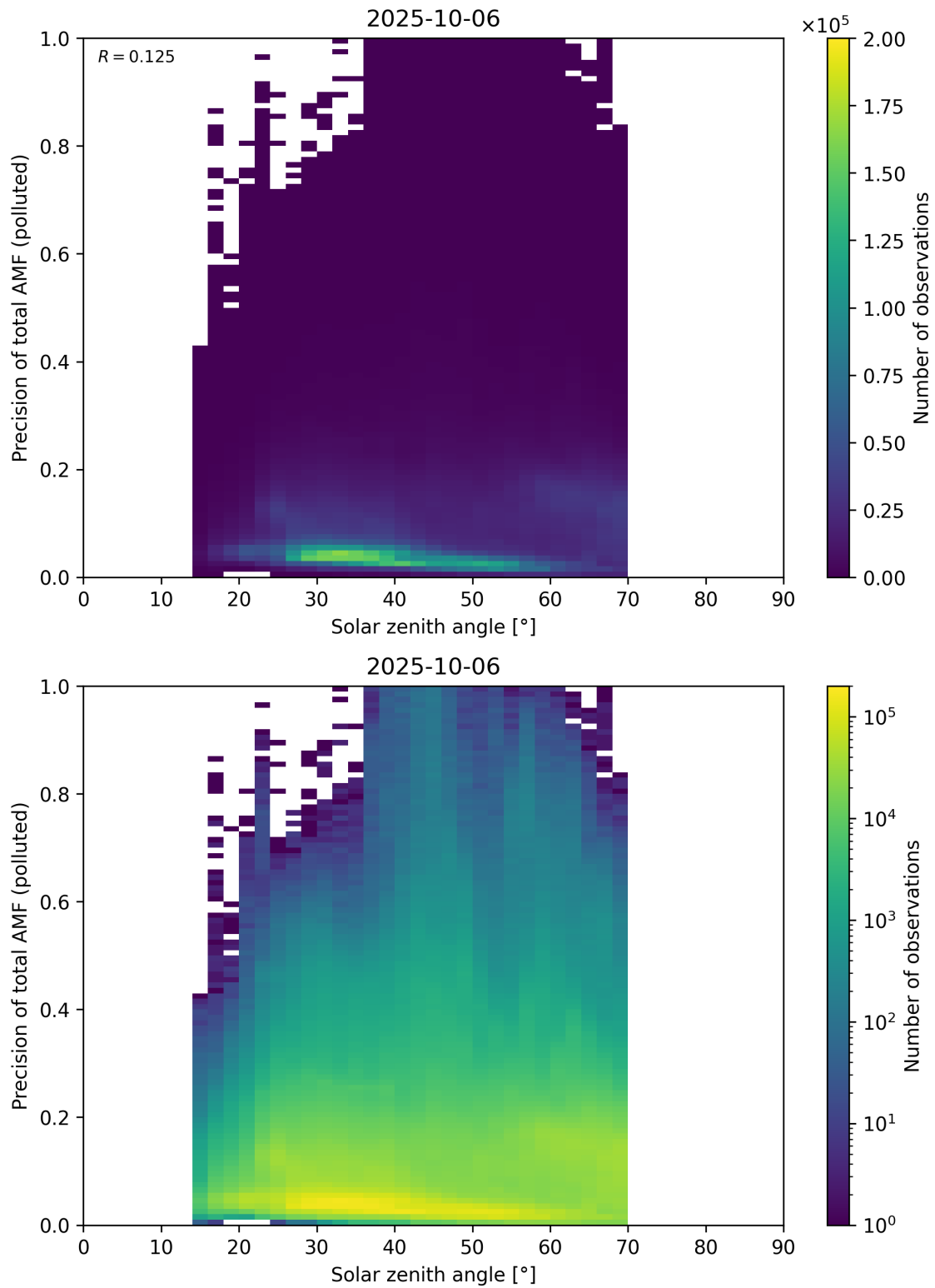
Figure 190: Scatter density plot of “Solar zenith angle” against “Precision of total AMF (polluted)” for 2025-10-06 to 2025-10-07.
