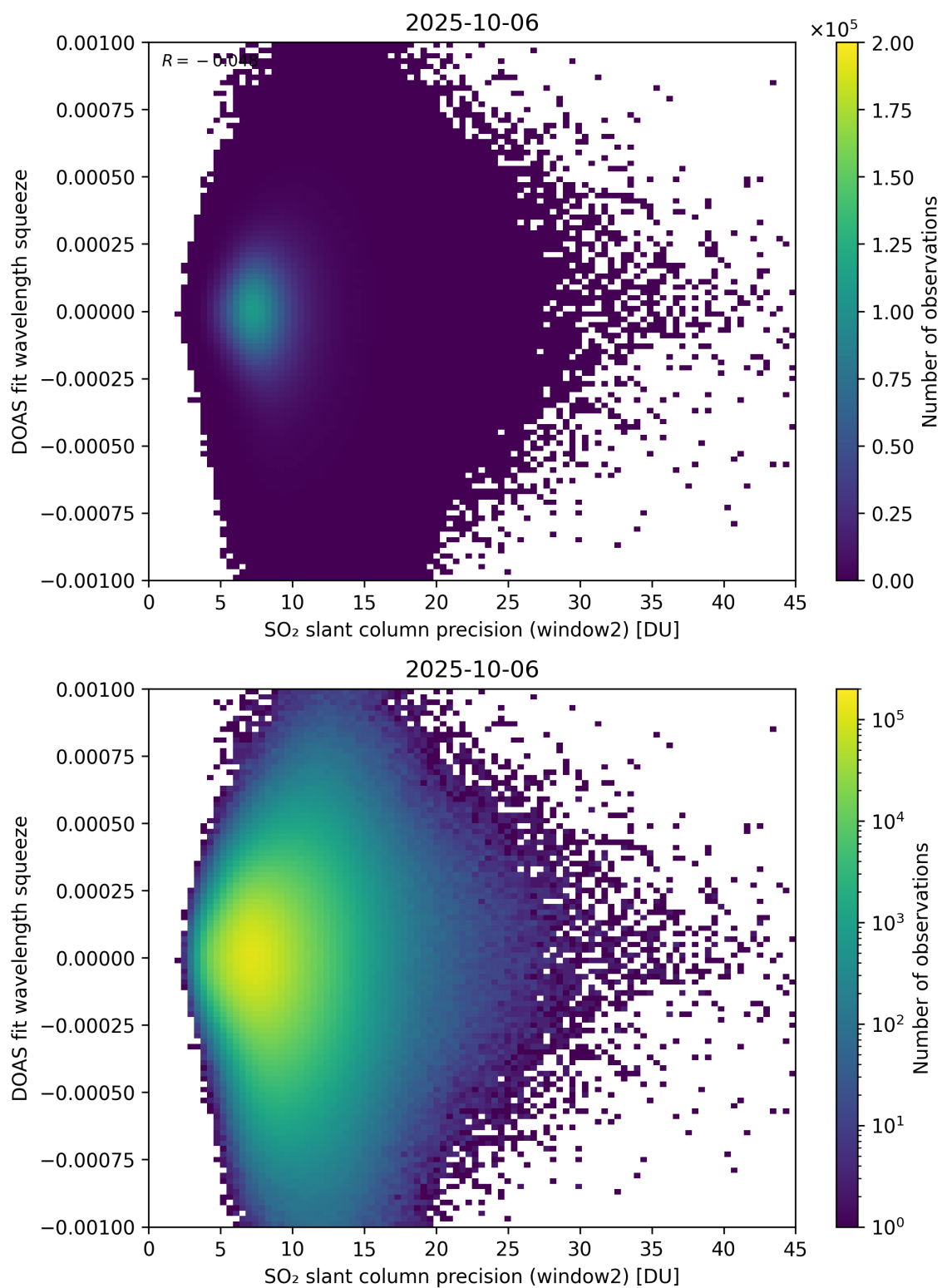
Figure 294: Scatter density plot of “SO 2 slant column precision (window2)” against “DOAS fit wavelength squeeze” for 2025-10-06 to 2025-10-07.
