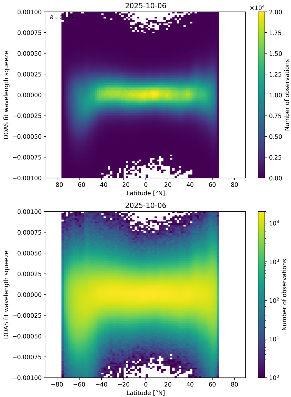
Figure 154: Scatter density plot of “Latitude” against “DOAS fit wavelength squeeze” for 2025-10-06 to 2025-10-07.
