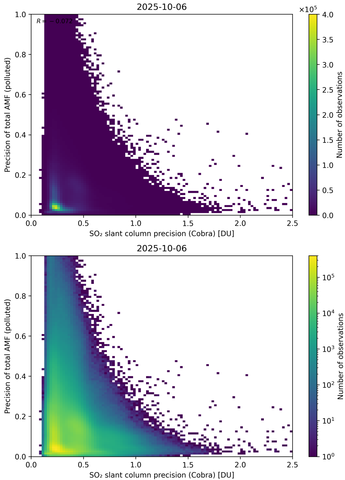
Figure 214: Scatter density plot of “SO 2 slant column precision (Cobra)” against “Precision of total AMF (polluted)” for 2025-10-06 to 2025-10-07.
