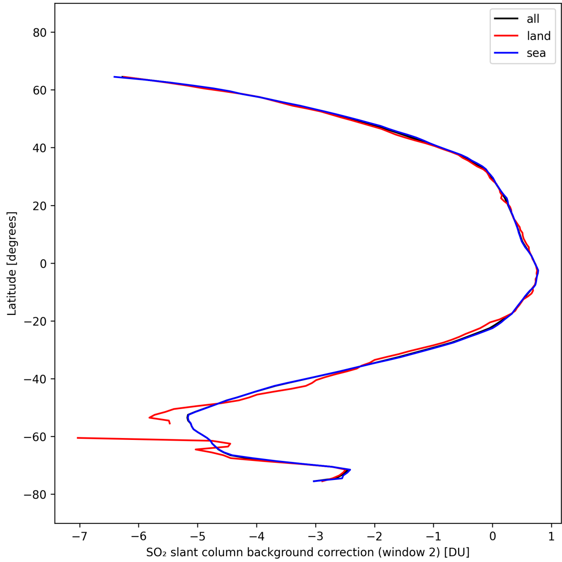
Figure 44: Zonal average of “SO 2 slant column background correction (window 2)” for 2025-10-06 to 2025-10-07.
