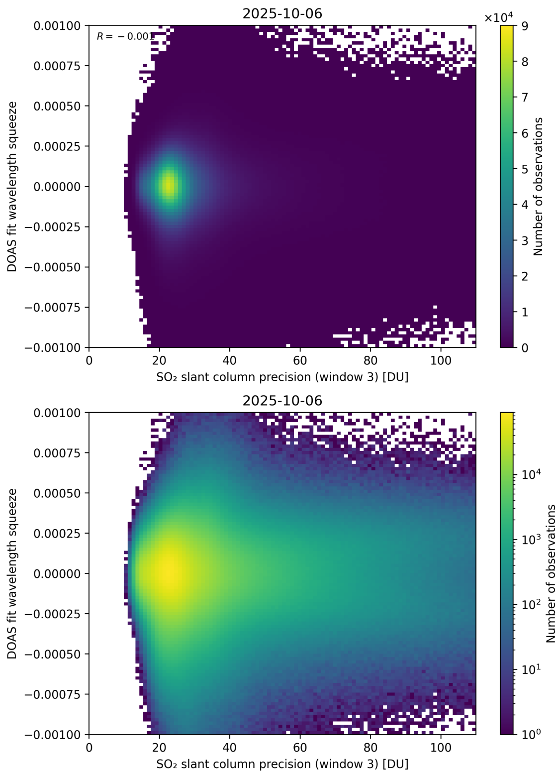
Figure 309: Scatter density plot of “SO 2 slant column precision (window 3)” against “DOAS fit wavelength squeeze” for 2025-10-06 to 2025-10-07.
