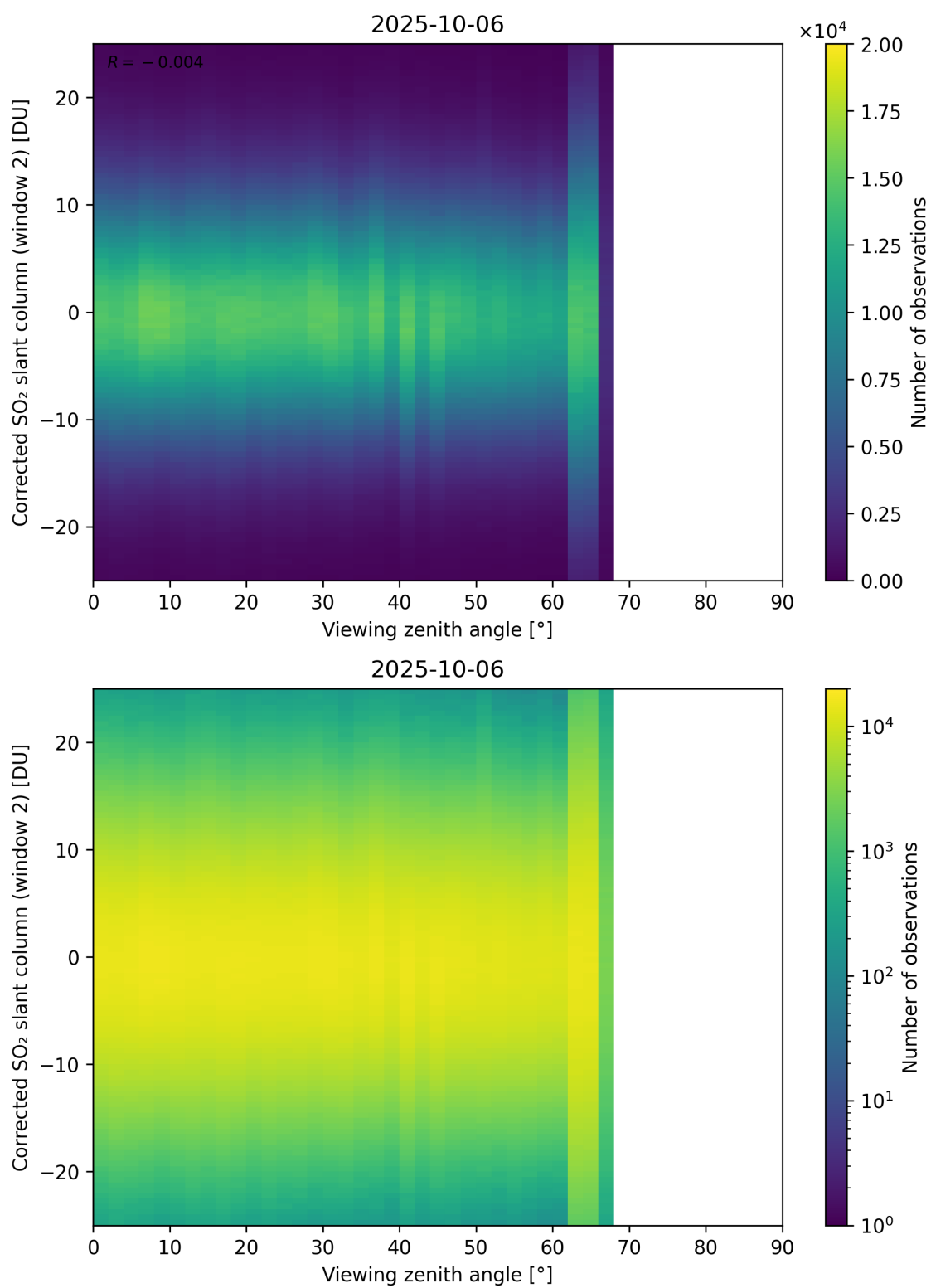
Figure 374: Scatter density plot of “Viewing zenith angle” against “Corrected SO 2 slant column (window 2)” for 2025-10-06 to 2025-10-07.
