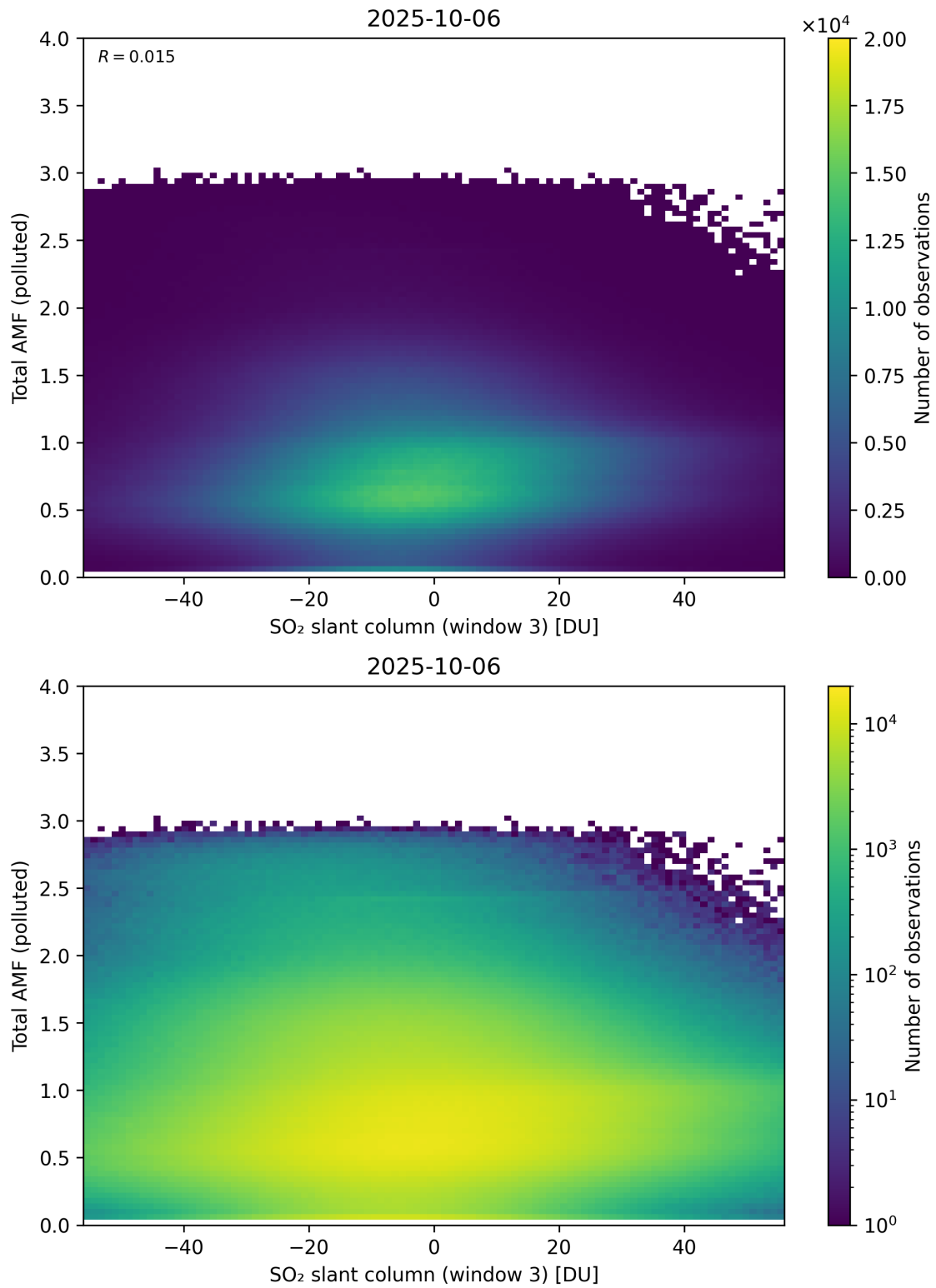
Figure 318: Scatter density plot of “SO 2 slant column (window 3)” against “Total AMF (polluted)” for 2025-10-06 to 2025-10-07.
