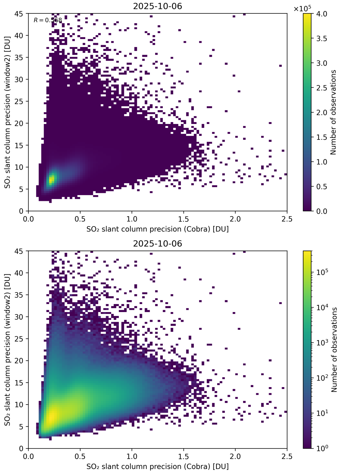
Figure 210: Scatter density plot of “SO 2 slant column precision (Cobra)” against “SO 2 slant column precision (window2)” for 2025-10-06 to 2025-10-07.
