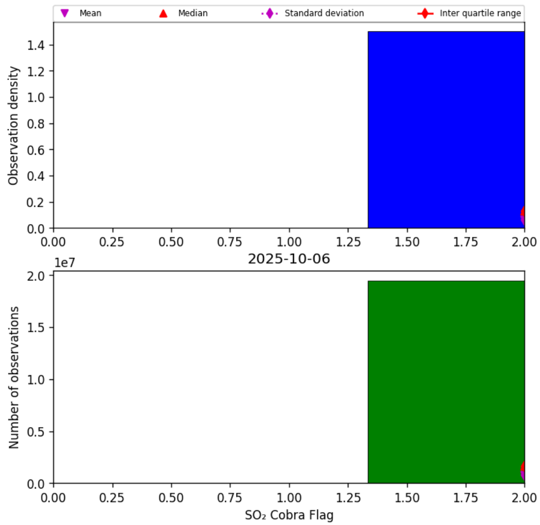
Figure 75: Histogram of “SO 2 Cobra Flag” for 2025-10-06 to 2025-10-07
