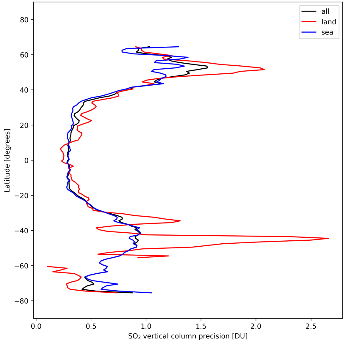
Figure 33: Zonal average of “SO 2 vertical column precision” for 2025-10-06 to 2025-10-07.
