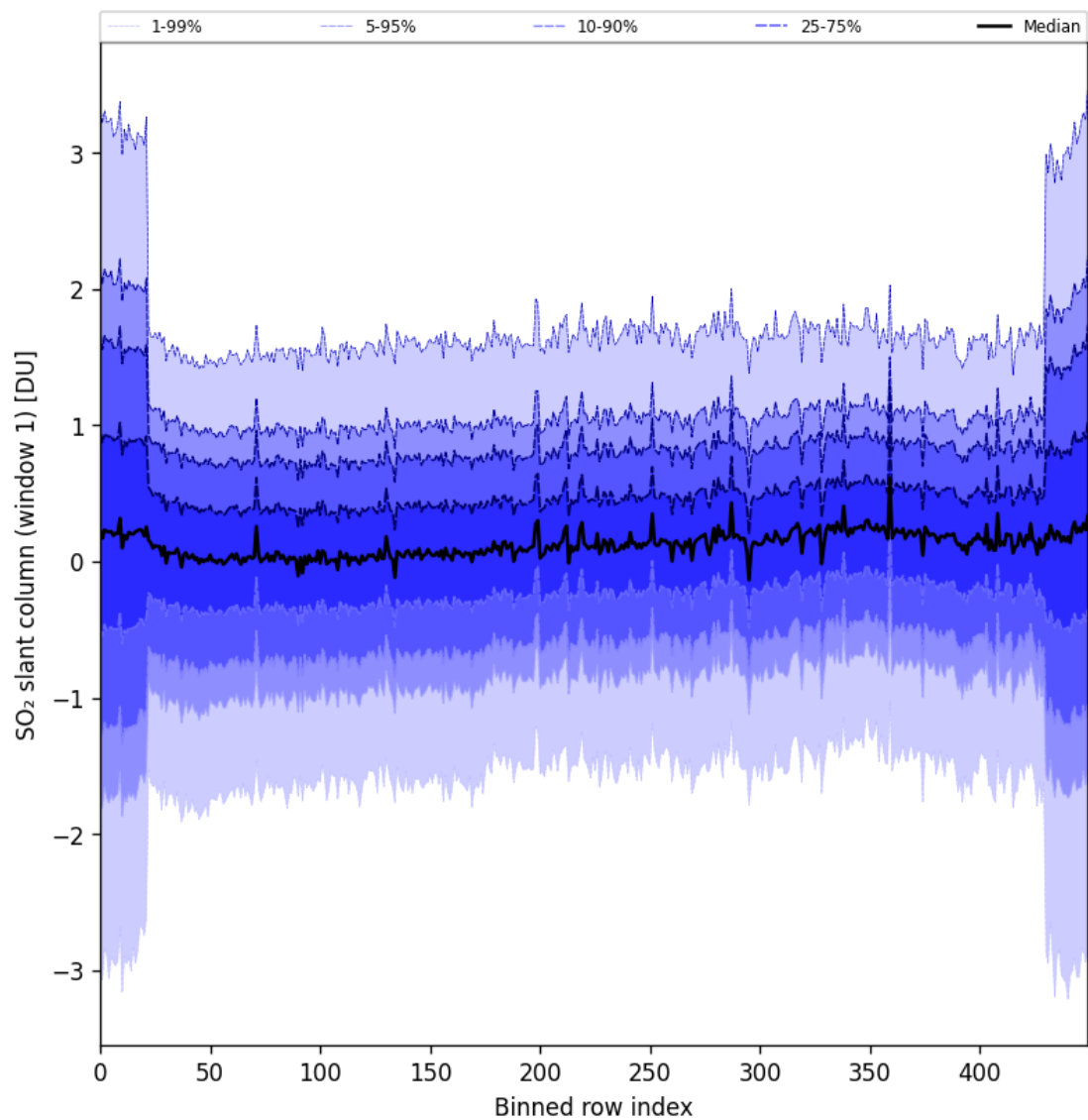
Figure 89: Along track statistics of “SO 2 slant column (window 1)” for 2025-10-06 to 2025-10-07
