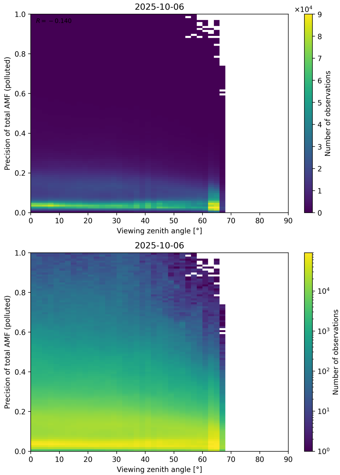
Figure 382: Scatter density plot of “Viewing zenith angle” against “Precision of total AMF (polluted)” for 2025-10-06 to 2025-10-07.
