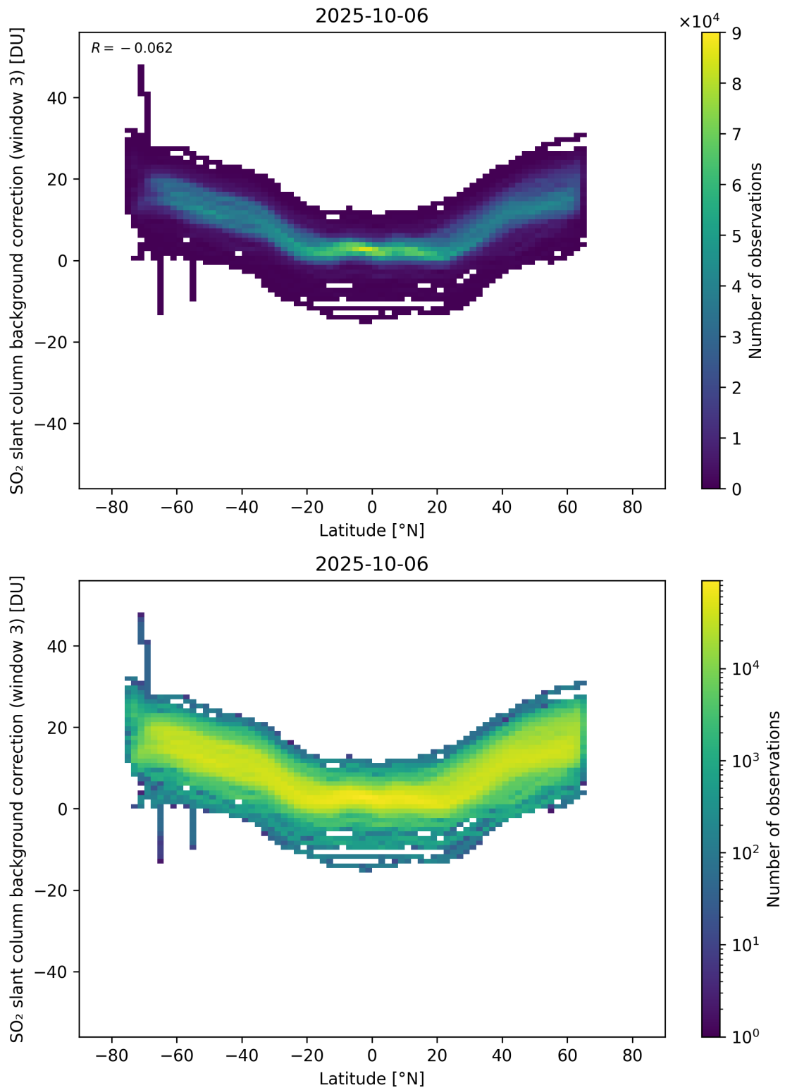
Figure 152: Scatter density plot of “Latitude” against “SO 2 slant column background correction (window 3)” for 2025-10-06 to 2025-10-07.
