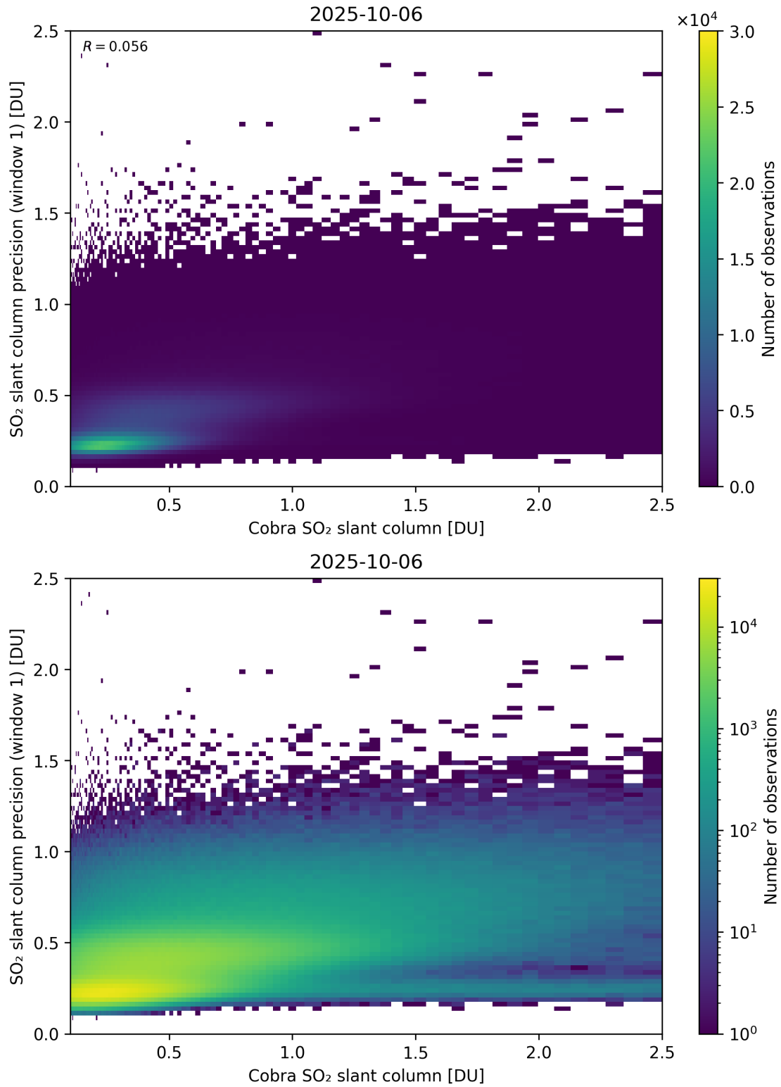
Figure 220: Scatter density plot of “Cobra SO 2 slant column” against “SO 2 slant column precision (window 1)” for 2025-10-06 to 2025-10-07.
