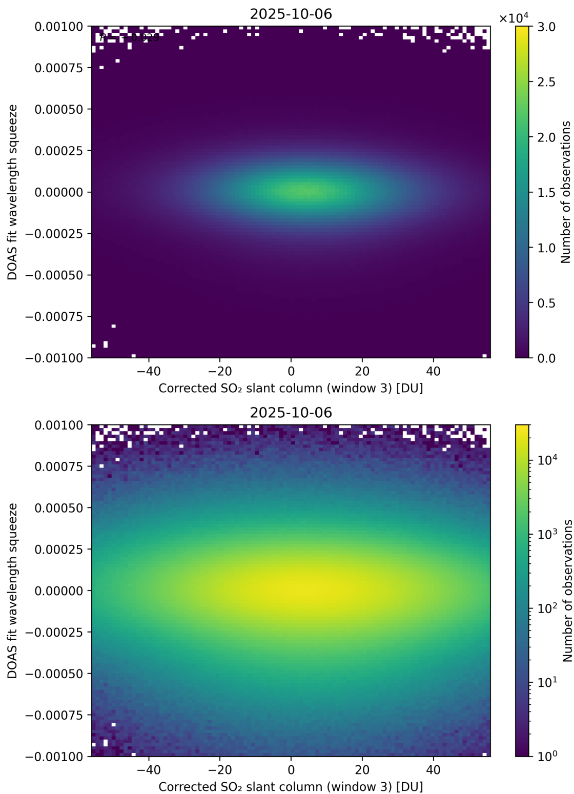
Figure 257: Scatter density plot of “Corrected SO 2 slant column (window 3)” against “DOAS fit wavelength squeeze” for 2025-10-06 to 2025-10-07.
