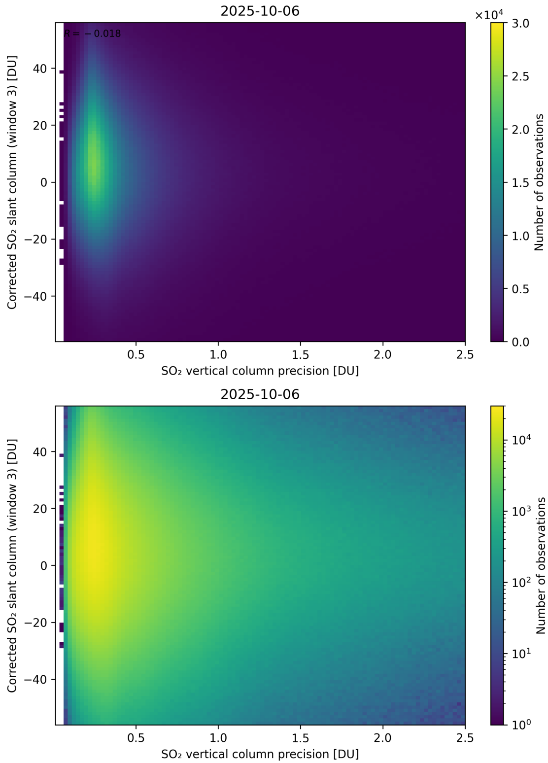
Figure 340: Scatter density plot of “SO 2 vertical column precision” against “Corrected SO 2 slant column (window 3)” for 2025-10-06 to 2025-10-07.
