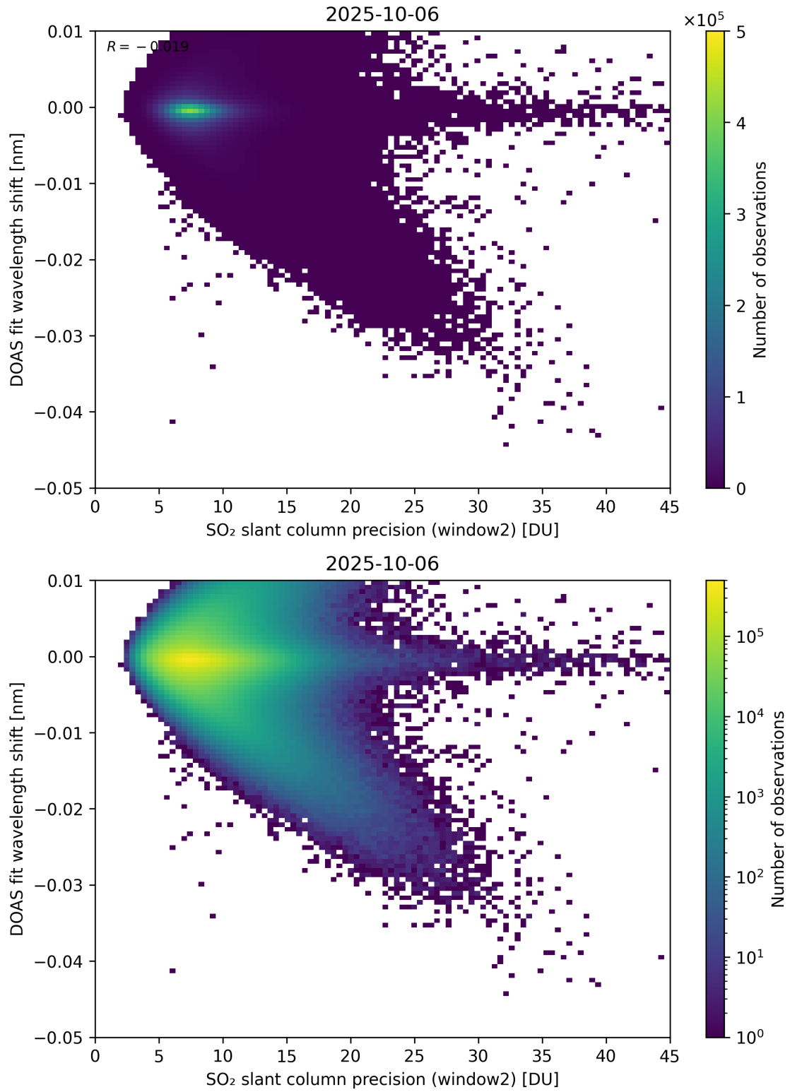
Figure 293: Scatter density plot of “SO 2 slant column precision (window2)” against “DOAS fit wavelength shift” for 2025-10-06 to 2025-10-07.
