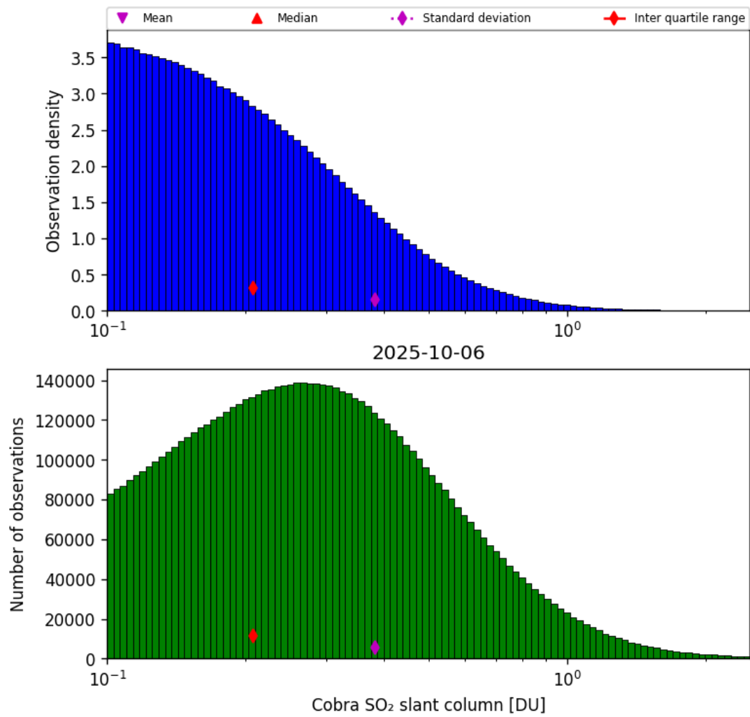
Figure 61: Histogram of “Cobra SO 2 slant column” for 2025-10-06 to 2025-10-07
