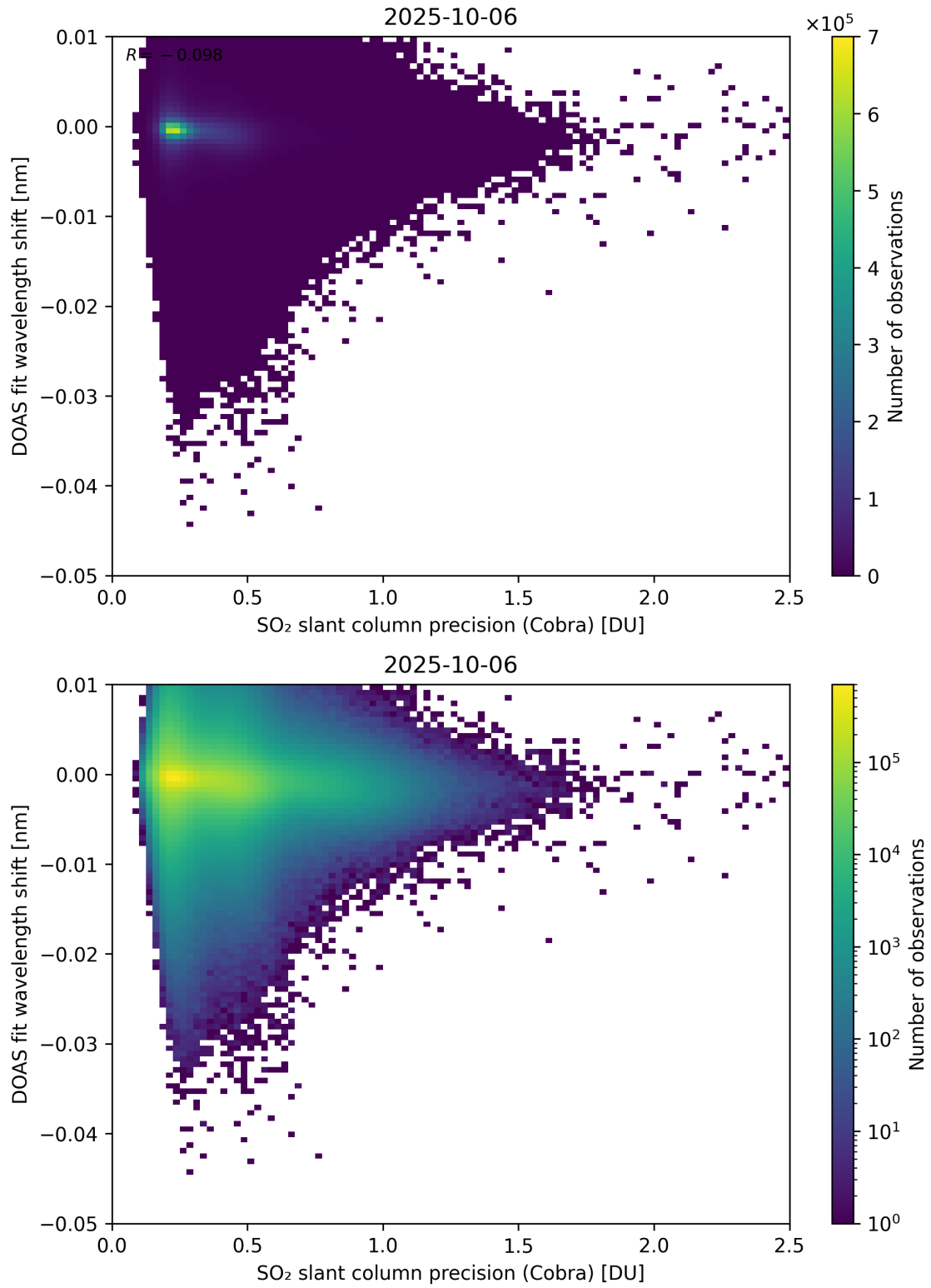
Figure 202: Scatter density plot of “SO 2 slant column precision (Cobra)” against “DOAS fit wavelength shift” for 2025-10-06 to 2025-10-07.
