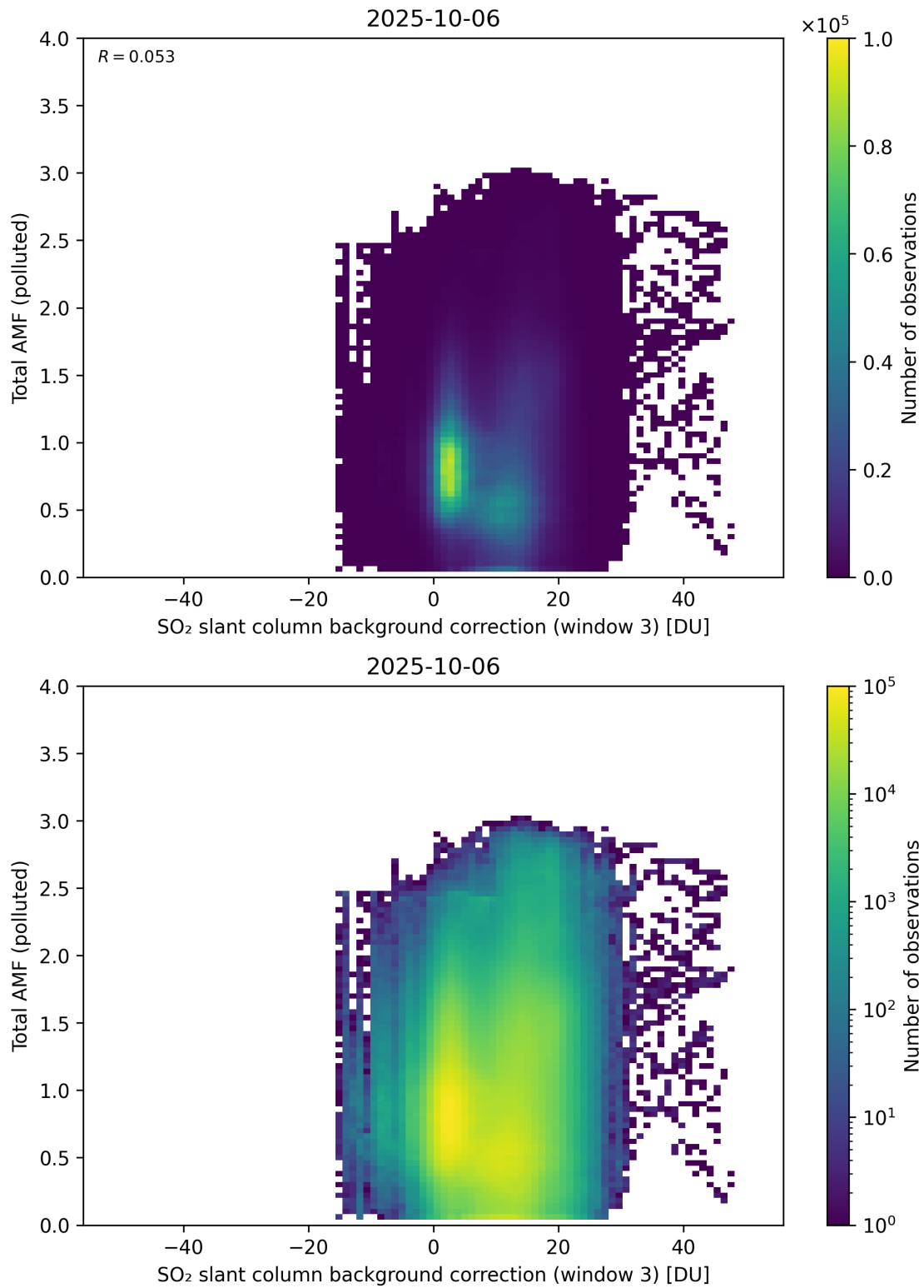
Figure 136: Scatter density plot of “SO 2 slant column background correction (window 3)” against “Total AMF (polluted)” for 2025-10-06 to 2025-10-07.
