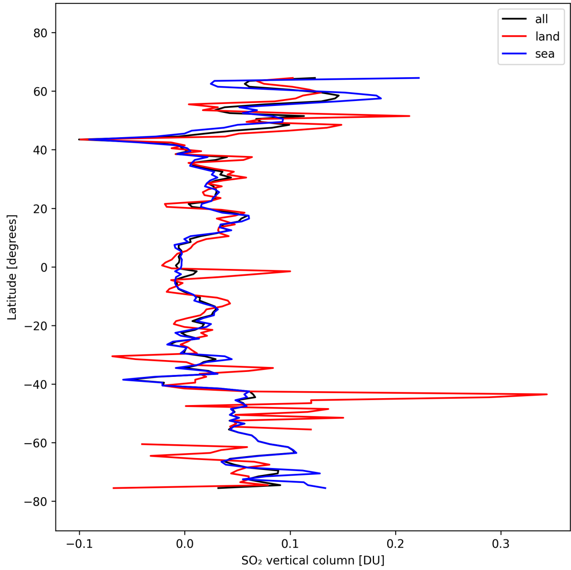
Figure 32: Zonal average of “SO 2 vertical column” for 2025-10-06 to 2025-10-07.
