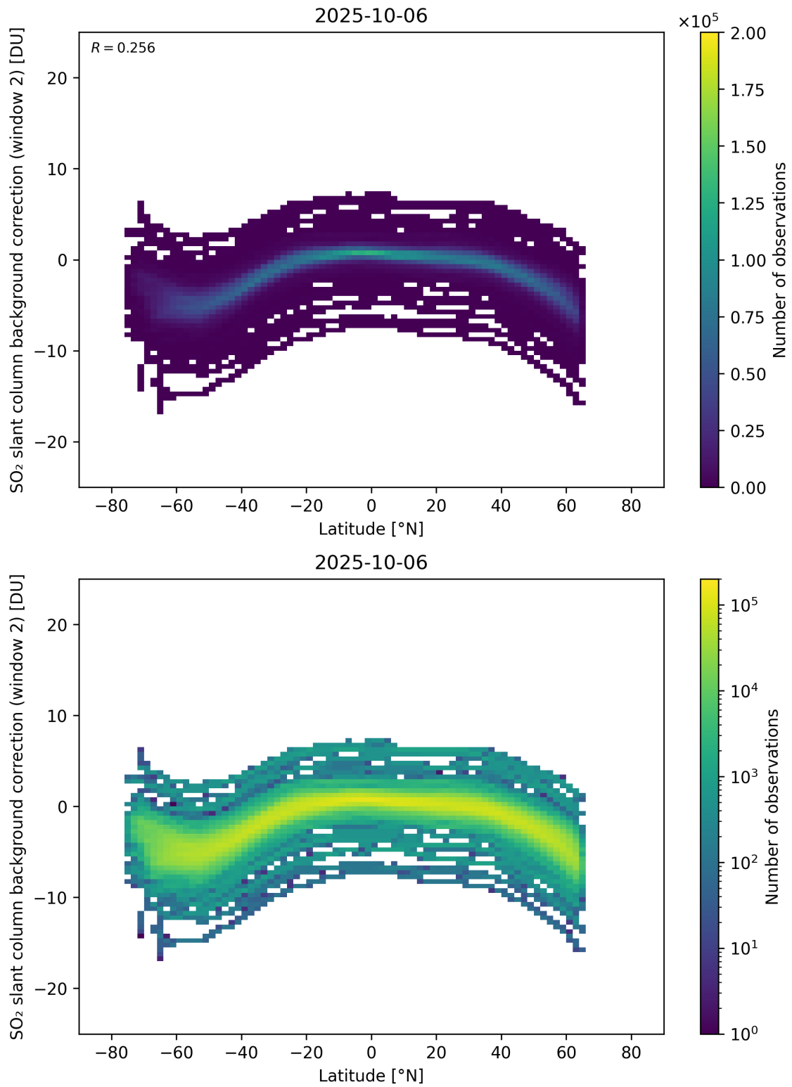
Figure 151: Scatter density plot of “Latitude” against “SO 2 slant column background correction (window 2)” for 2025-10-06 to 2025-10-07.
