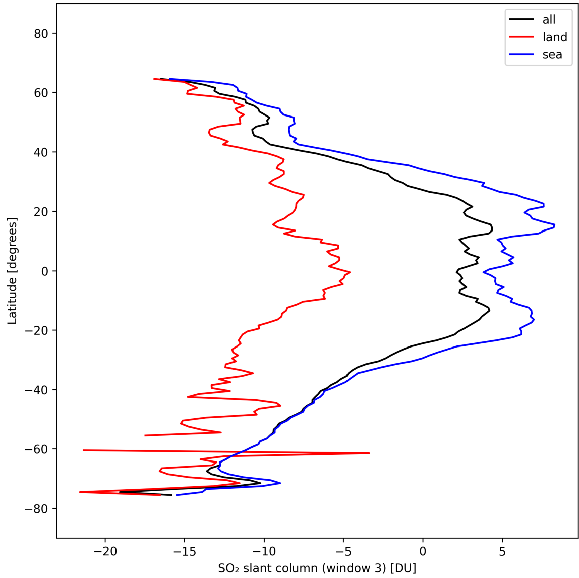
Figure 45: Zonal average of “SO 2 slant column (window 3)” for 2025-10-06 to 2025-10-07.
