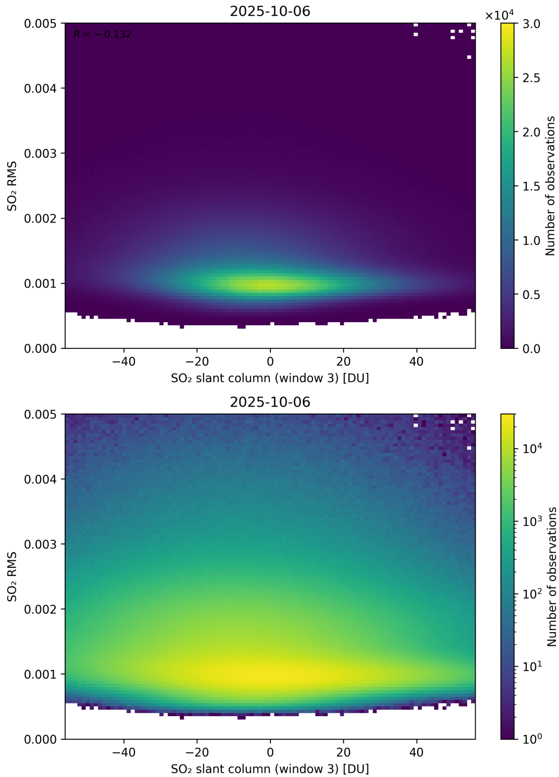
Figure 306: Scatter density plot of “SO 2 slant column (window 3)” against “SO 2 RMS” for 2025-10-06 to 2025-10-07.
