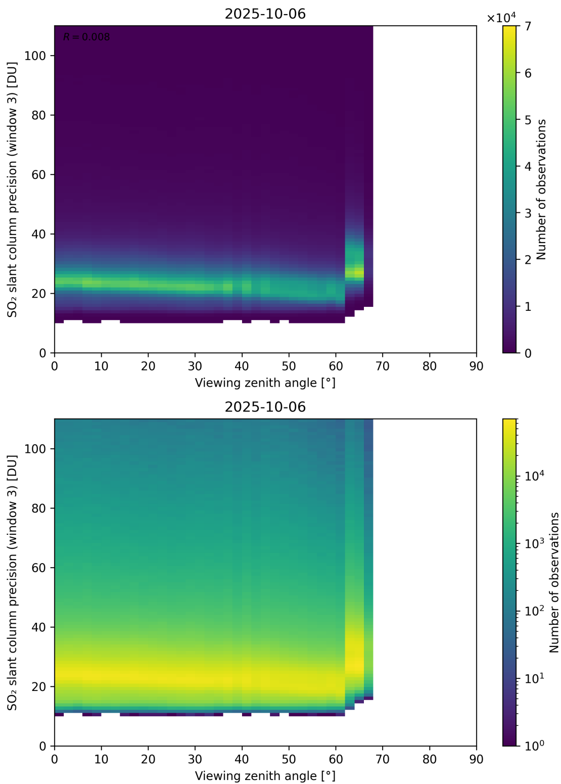
Figure 380: Scatter density plot of “Viewing zenith angle” against “SO 2 slant column precision (window 3)” for 2025-10-06 to 2025-10-07.
