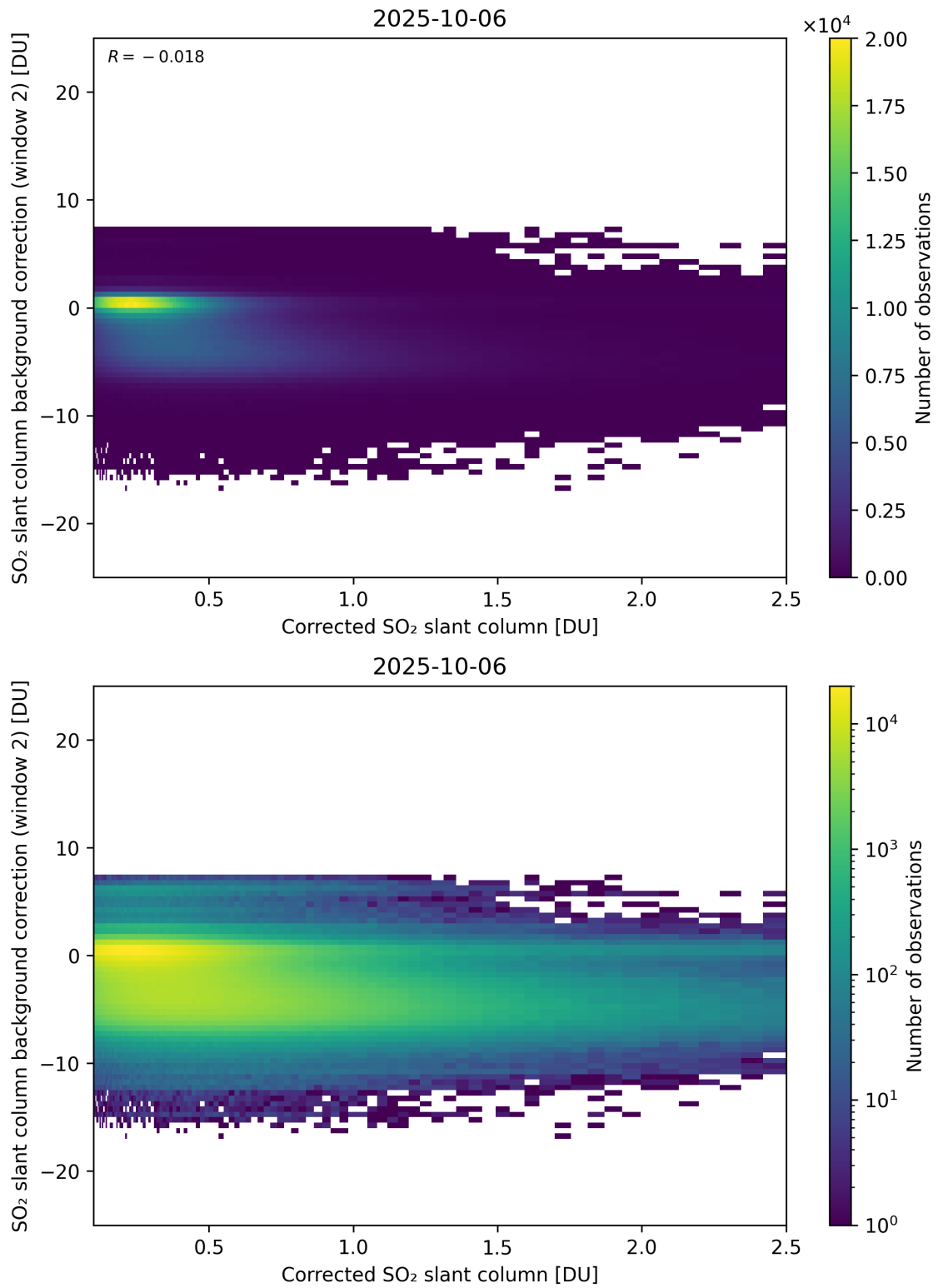
Figure 227: Scatter density plot of “Corrected SO 2 slant column” against “SO 2 slant column background correction (window 2)” for 2025-10-06 to 2025-10-07.
