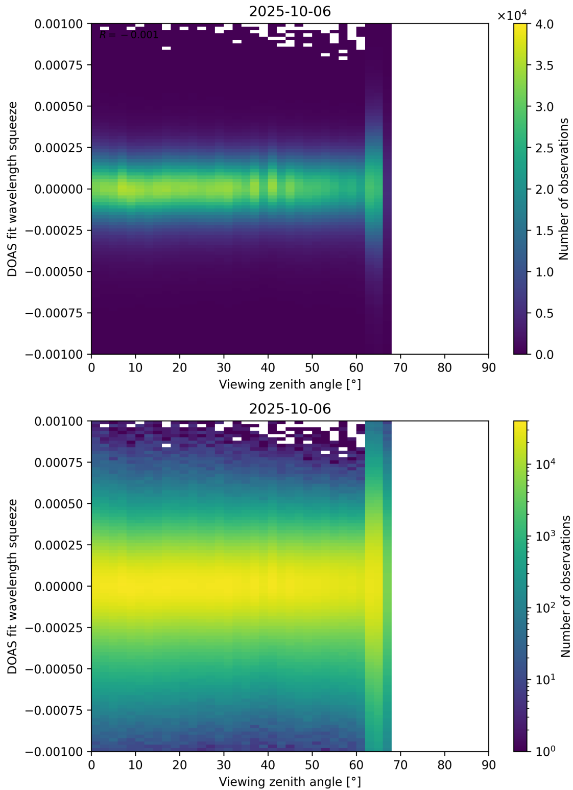
Figure 366: Scatter density plot of “Viewing zenith angle” against “DOAS fit wavelength squeeze” for 2025-10-06 to 2025-10-07.
