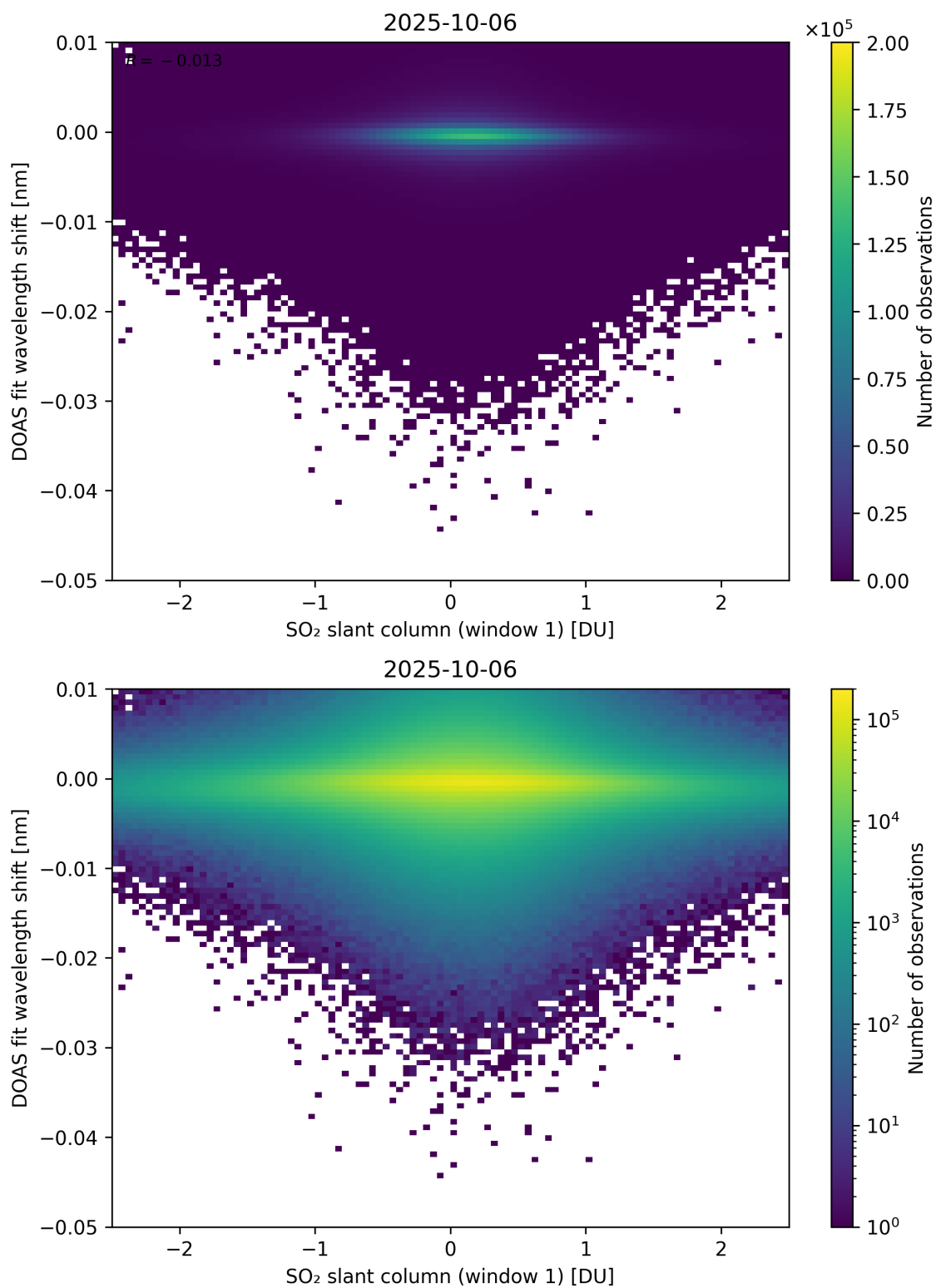
Figure 265: Scatter density plot of “SO 2 slant column (window 1)” against “DOAS fit wavelength shift” for 2025-10-06 to 2025-10-07.
