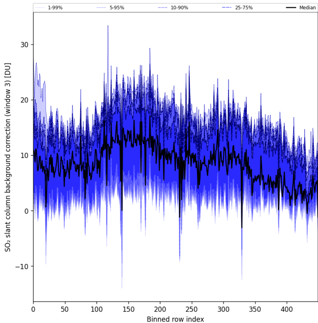
Figure 100: Along track statistics of “SO 2 slant column background correction (window 3)” for 2025-10-06 to 2025-10-07
