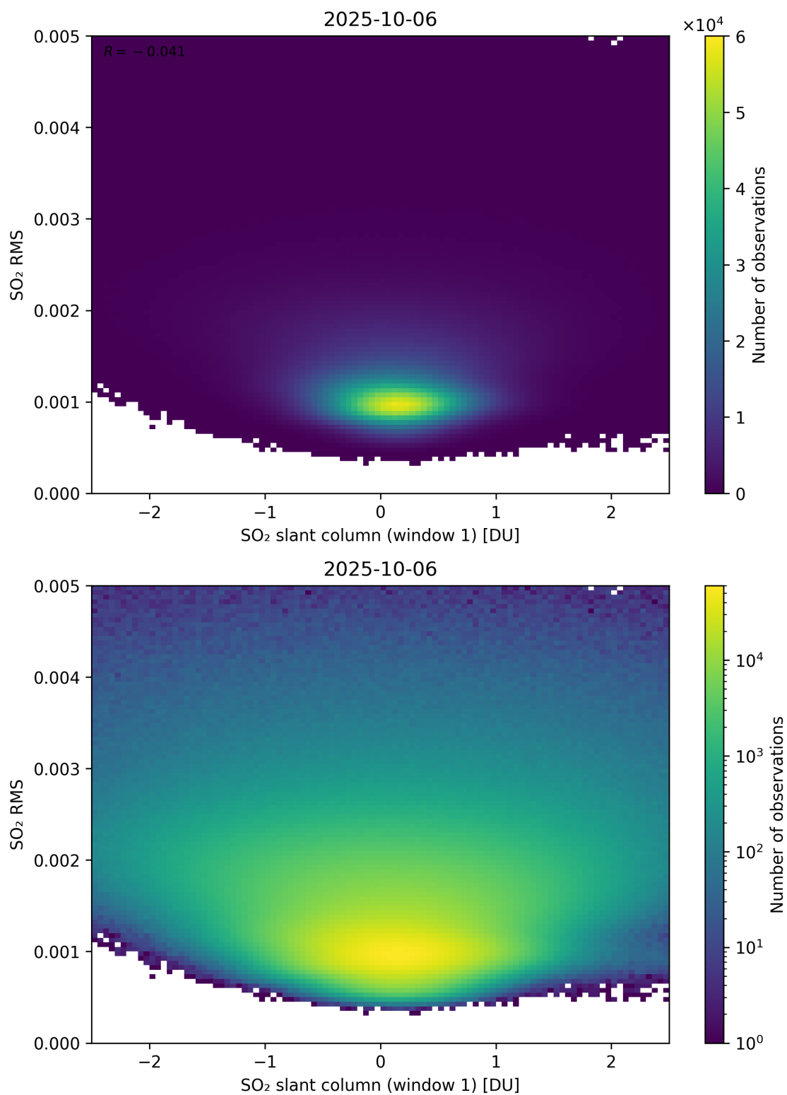
Figure 267: Scatter density plot of “SO 2 slant column (window 1)” against “SO 2 RMS” for 2025-10-06 to 2025-10-07.
