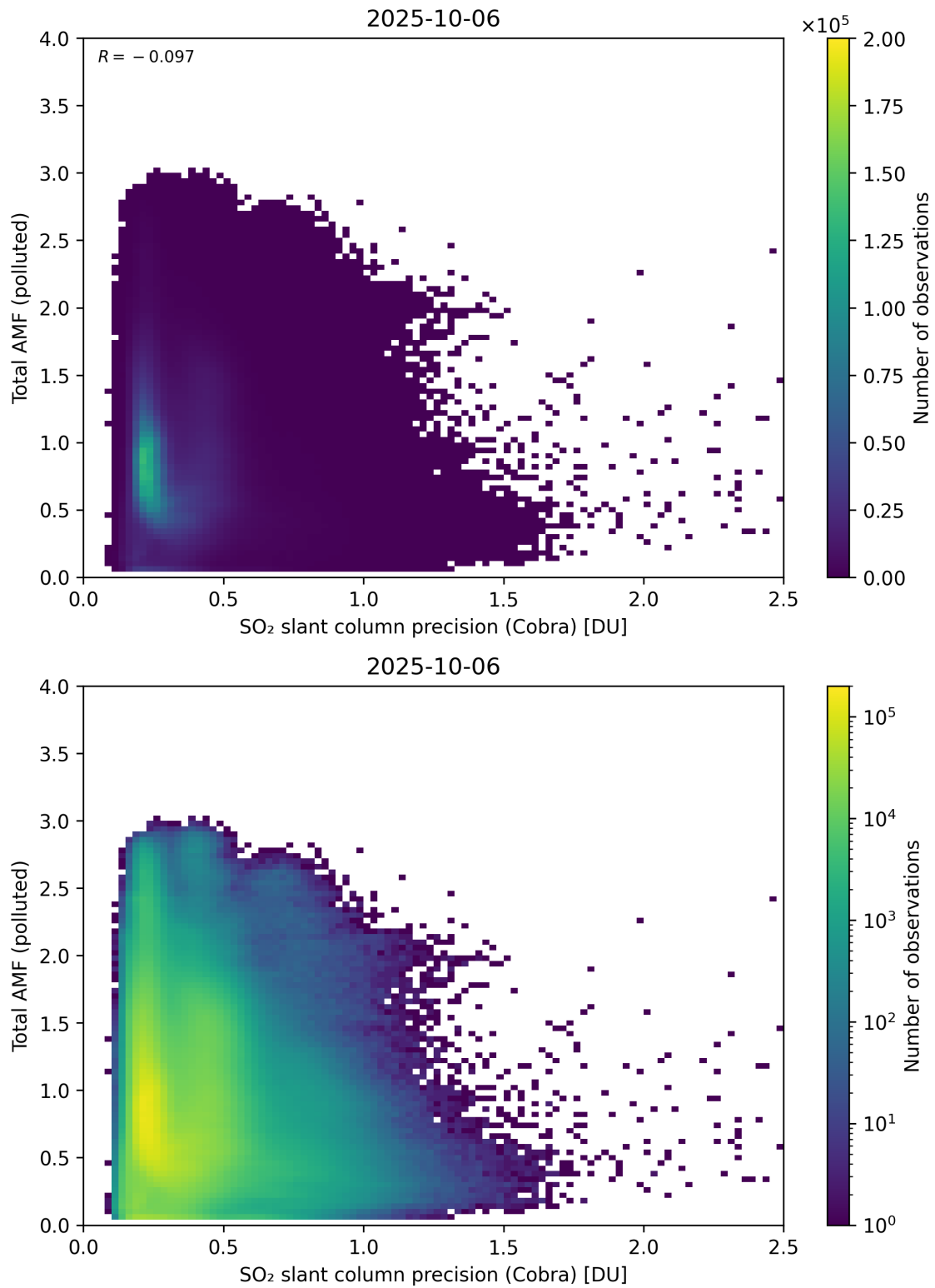
Figure 213: Scatter density plot of “SO 2 slant column precision (Cobra)” against “Total AMF (polluted)” for 2025-10-06 to 2025-10-07.
