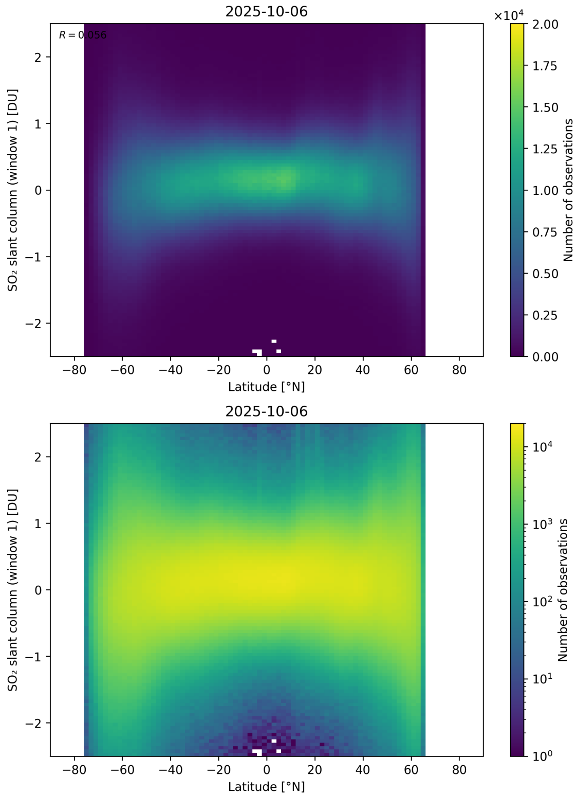
Figure 162: Scatter density plot of “Latitude” against “SO 2 slant column (window 1)” for 2025-10-06 to 2025-10-07.
