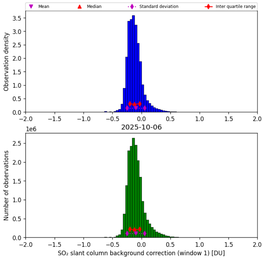
Figure 66: Histogram of “SO 2 slant column background correction (window 1)” for 2025-10-06 to 2025-10-07
