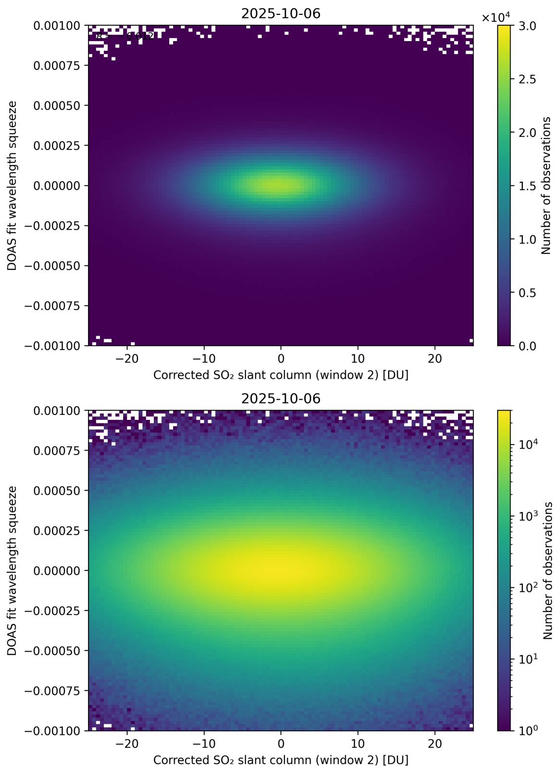
Figure 247: Scatter density plot of “Corrected SO 2 slant column (window 2)” against “DOAS fit wavelength squeeze” for 2025-10-06 to 2025-10-07.
