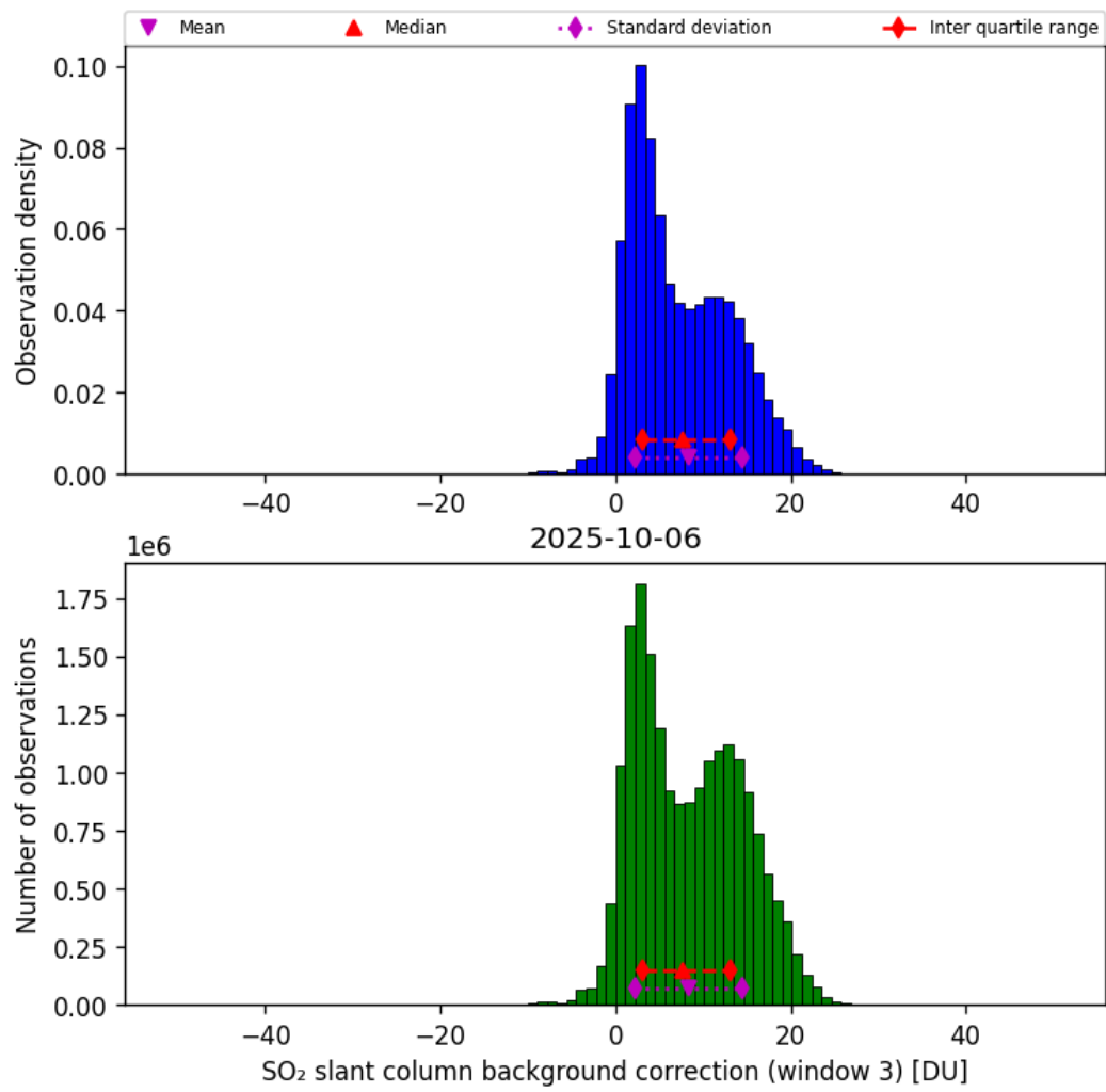
Figure 74: Histogram of “SO 2 slant column background correction (window 3)” for 2025-10-06 to 2025-10-07
