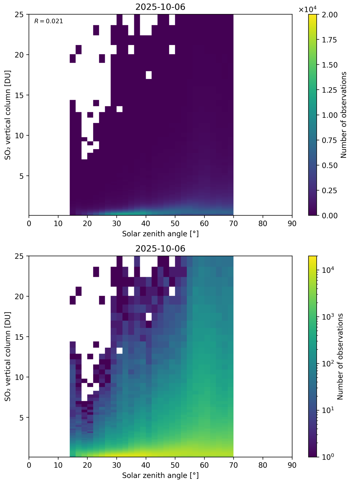
Figure 191: Scatter density plot of “Solar zenith angle” against “SO 2 vertical column” for 2025-10-06 to 2025-10-07.
