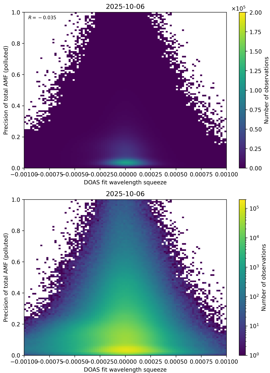
Figure 146: Scatter density plot of “DOAS fit wavelength squeeze” against “Precision of total AMF (polluted)” for 2025-10-06 to 2025-10-07.
