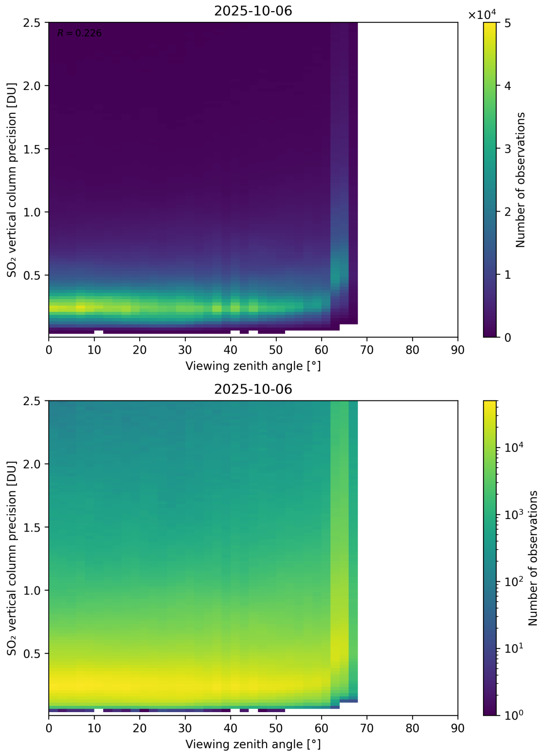
Figure 384: Scatter density plot of “Viewing zenith angle” against “SO 2 vertical column precision” for 2025-10-06 to 2025-10-07.
