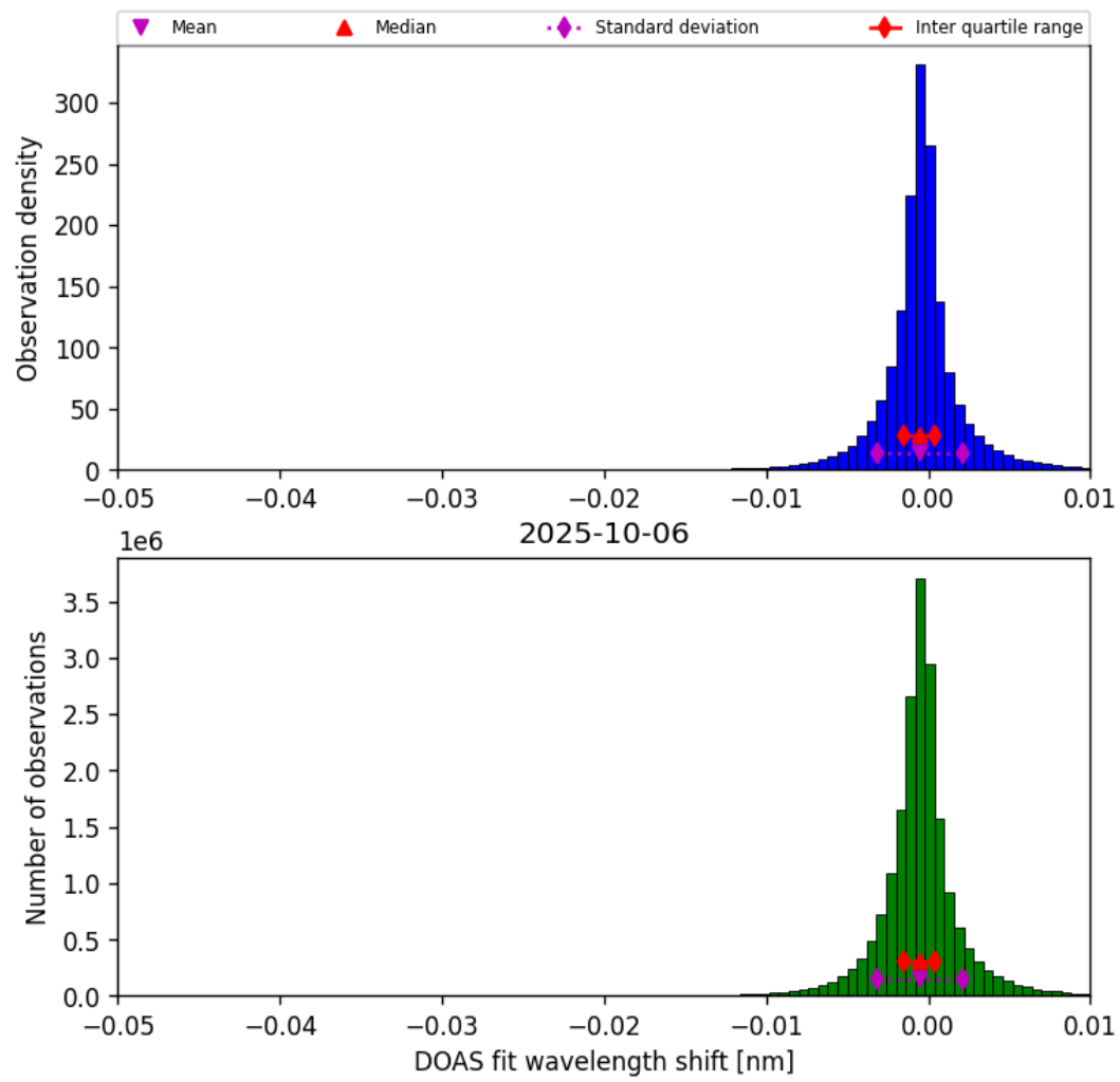
Figure 76: Histogram of “DOAS fit wavelength shift” for 2025-10-06 to 2025-10-07
