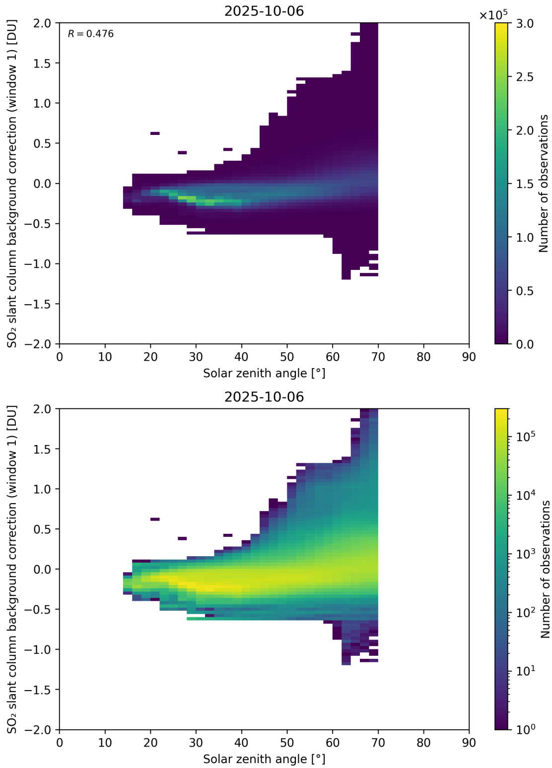
Figure 171: Scatter density plot of “Solar zenith angle” against “SO 2 slant column background correction (window 1)” for 2025-10-06 to 2025-10-07.
