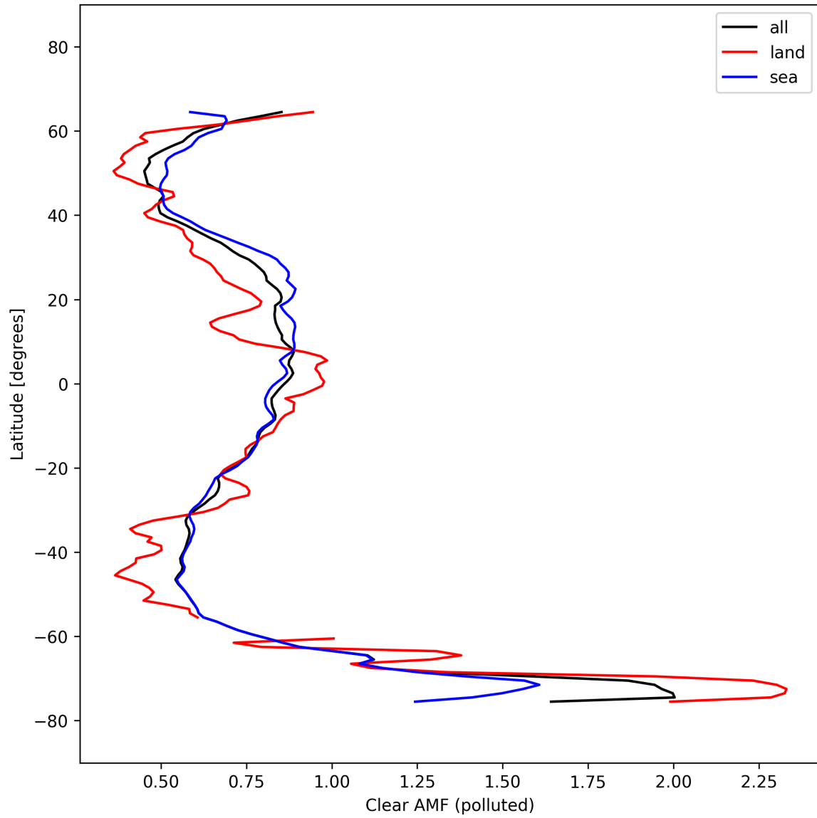
Figure 55: Zonal average of “Clear AMF (polluted)” for 2025-10-06 to 2025-10-07.
