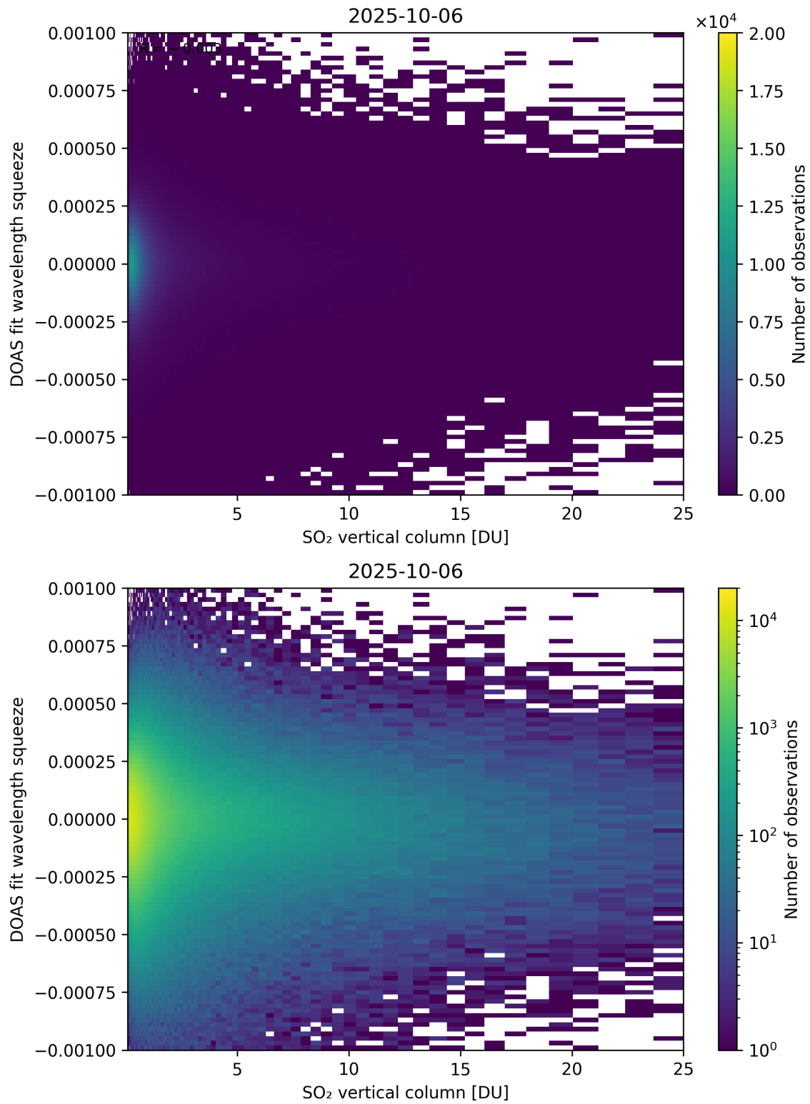
Figure 327: Scatter density plot of “SO 2 vertical column” against “DOAS fit wavelength squeeze” for 2025-10-06 to 2025-10-07.
