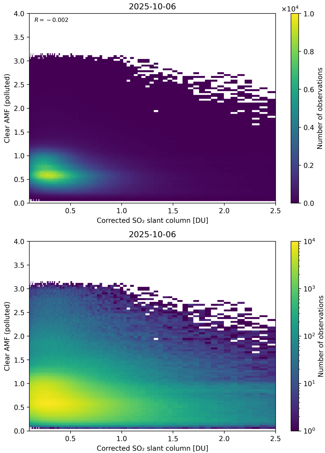
Figure 232: Scatter density plot of “Corrected SO 2 slant column” against “Clear AMF (polluted)” for 2025-10-06 to 2025-10-07.
