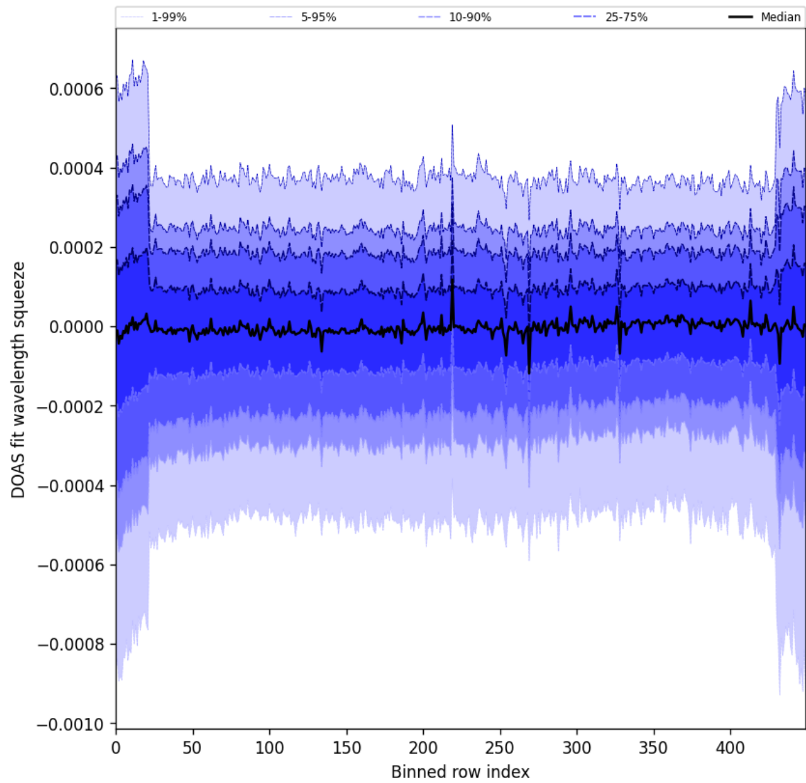
Figure 103: Along track statistics of “DOAS fit wavelength squeeze” for 2025-10-06 to 2025-10-07
