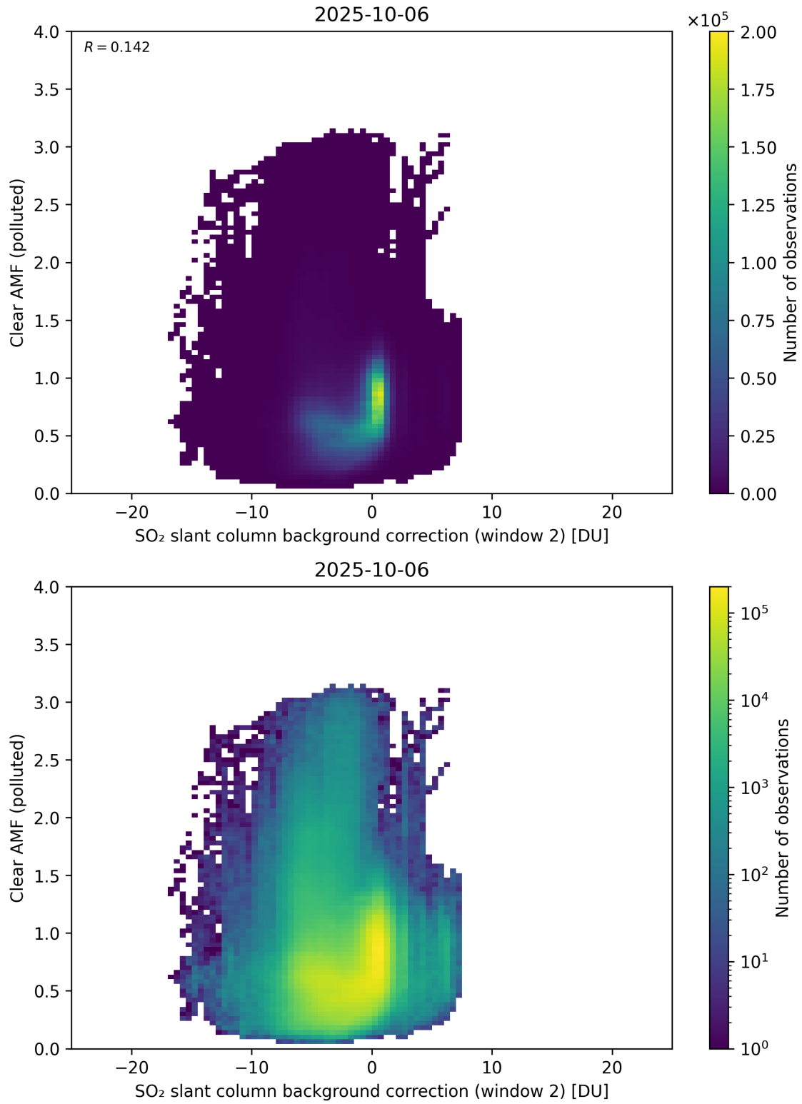
Figure 126: Scatter density plot of “SO 2 slant column background correction (window 2)” against “Clear AMF (polluted)” for 2025-10-06 to 2025-10-07.
