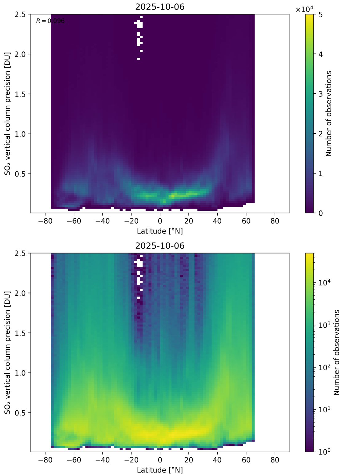
Figure 170: Scatter density plot of “Latitude” against “SO 2 vertical column precision” for 2025-10-06 to 2025-10-07.
