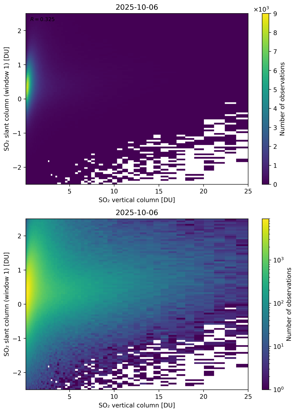
Figure 354: Scatter density plot of “SO 2 vertical column” against “SO 2 slant column (window 1)” for 2025-10-06 to 2025-10-07.
