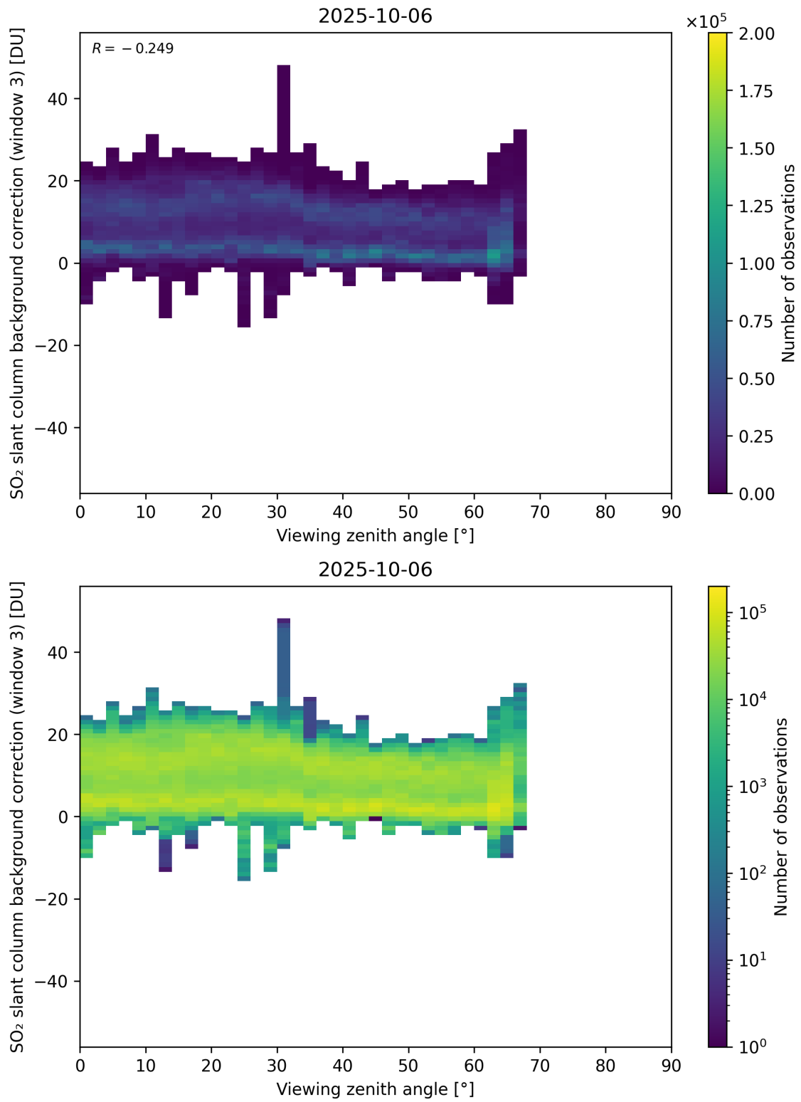
Figure 364: Scatter density plot of “Viewing zenith angle” against “SO 2 slant column background correction (window 3)” for 2025-10-06 to 2025-10-07.
