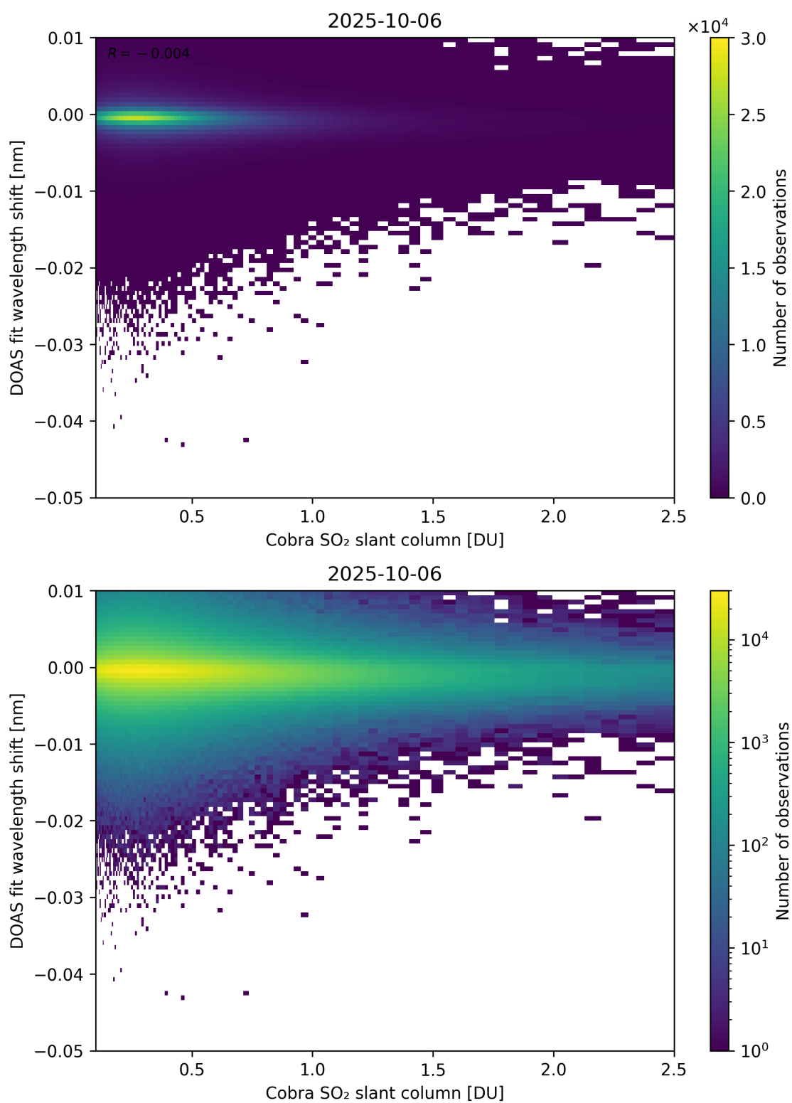
Figure 196: Scatter density plot of “Cobra SO 2 slant column” against “DOAS fit wavelength shift” for 2025-10-06 to 2025-10-07.
