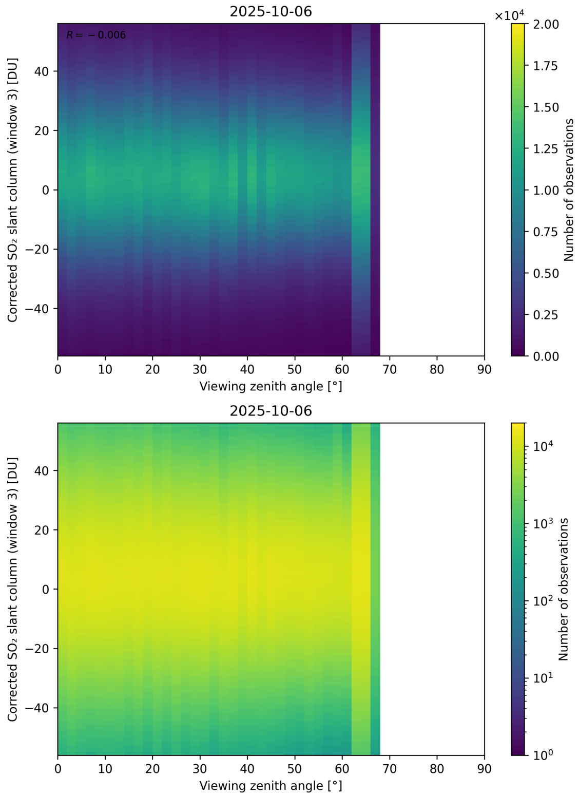
Figure 375: Scatter density plot of “Viewing zenith angle” against “Corrected SO 2 slant column (window 3)” for 2025-10-06 to 2025-10-07.
