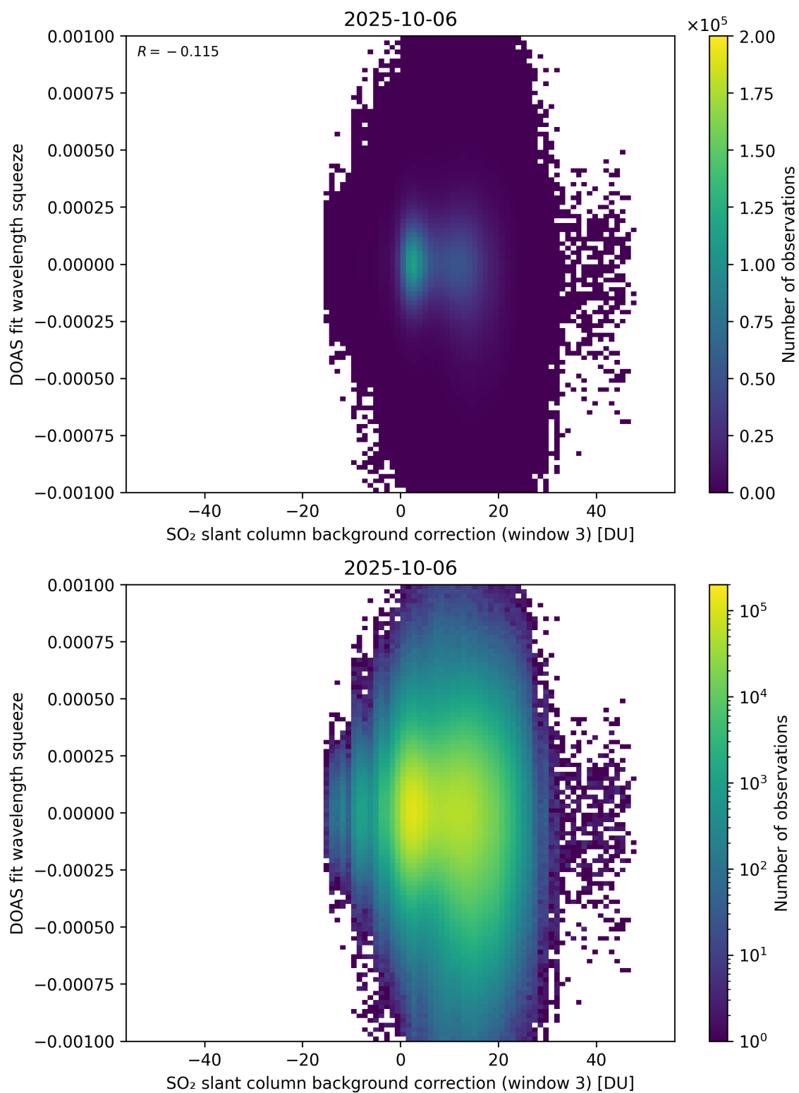
Figure 133: Scatter density plot of “SO 2 slant column background correction (window 3)” against “DOAS fit wavelength squeeze” for 2025-10-06 to 2025-10-07.
