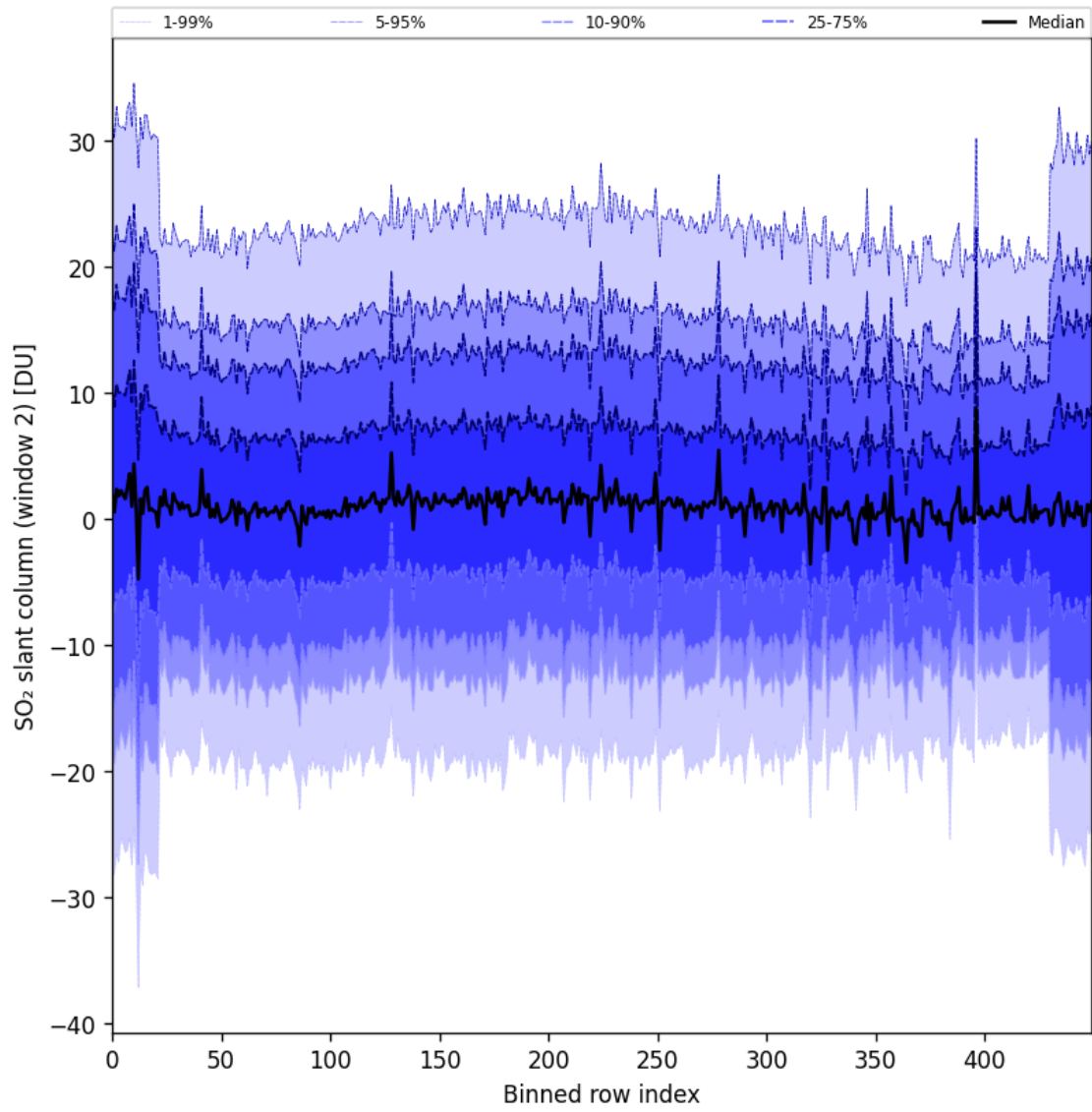
Figure 93: Along track statistics of “SO 2 slant column (window 2)” for 2025-10-06 to 2025-10-07
