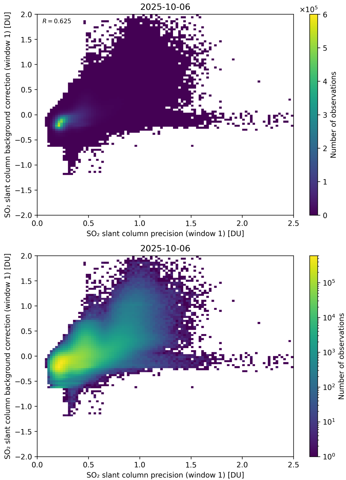
Figure 268: Scatter density plot of “SO 2 slant column precision (window 1)” against “SO 2 slant column background correction (window 1)” for 2025-10-06 to 2025-10-07.
