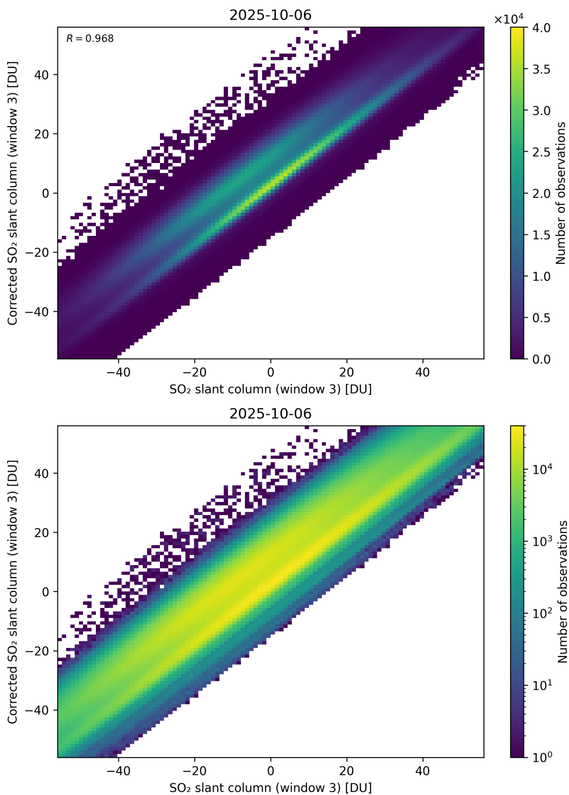
Figure 316: Scatter density plot of “SO 2 slant column (window 3)” against “Corrected SO 2 slant column (window 3)” for 2025-10-06 to 2025-10-07.
