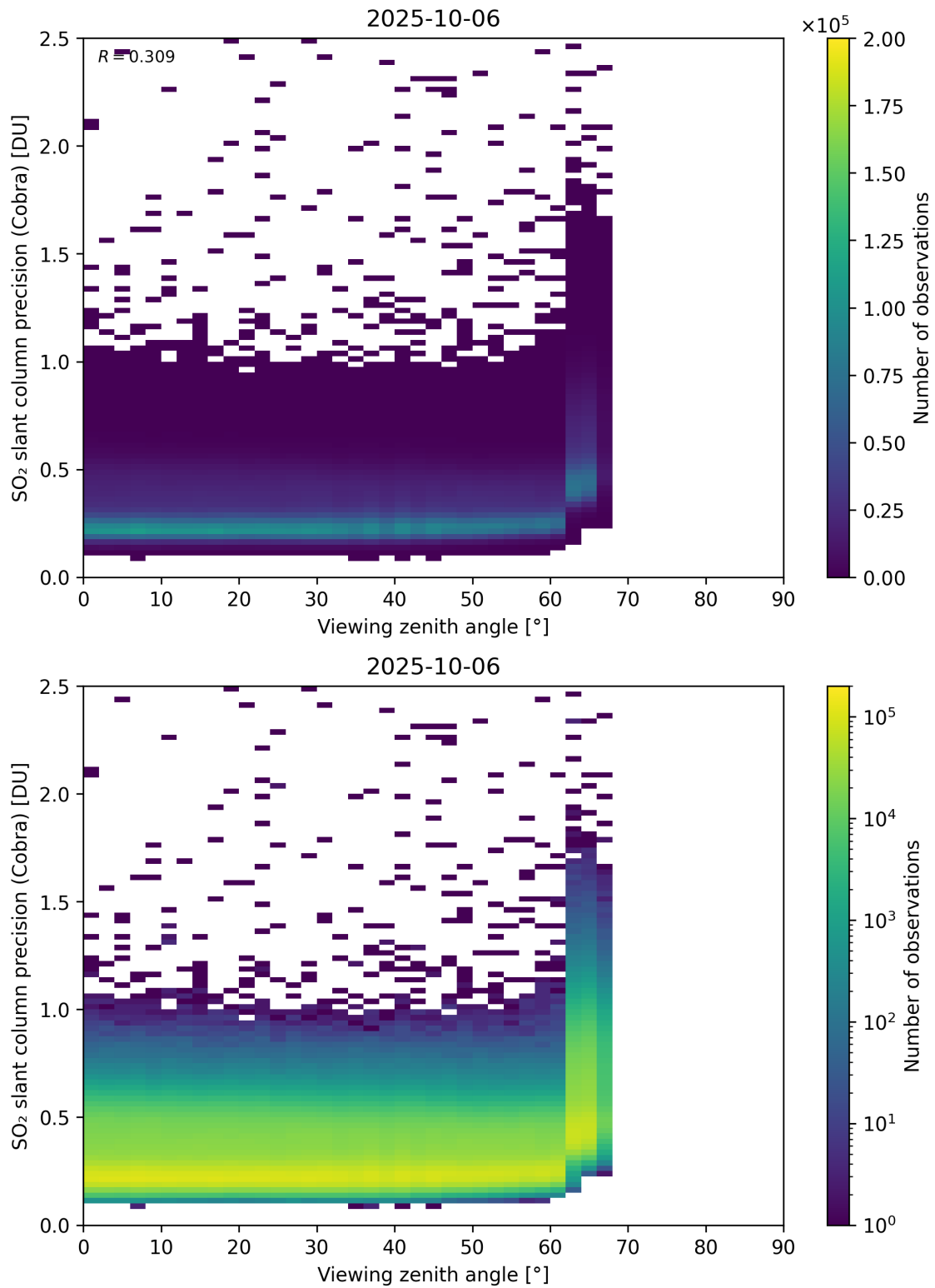
Figure 372: Scatter density plot of “Viewing zenith angle” against “SO 2 slant column precision (Cobra)” for 2025-10-06 to 2025-10-07.
