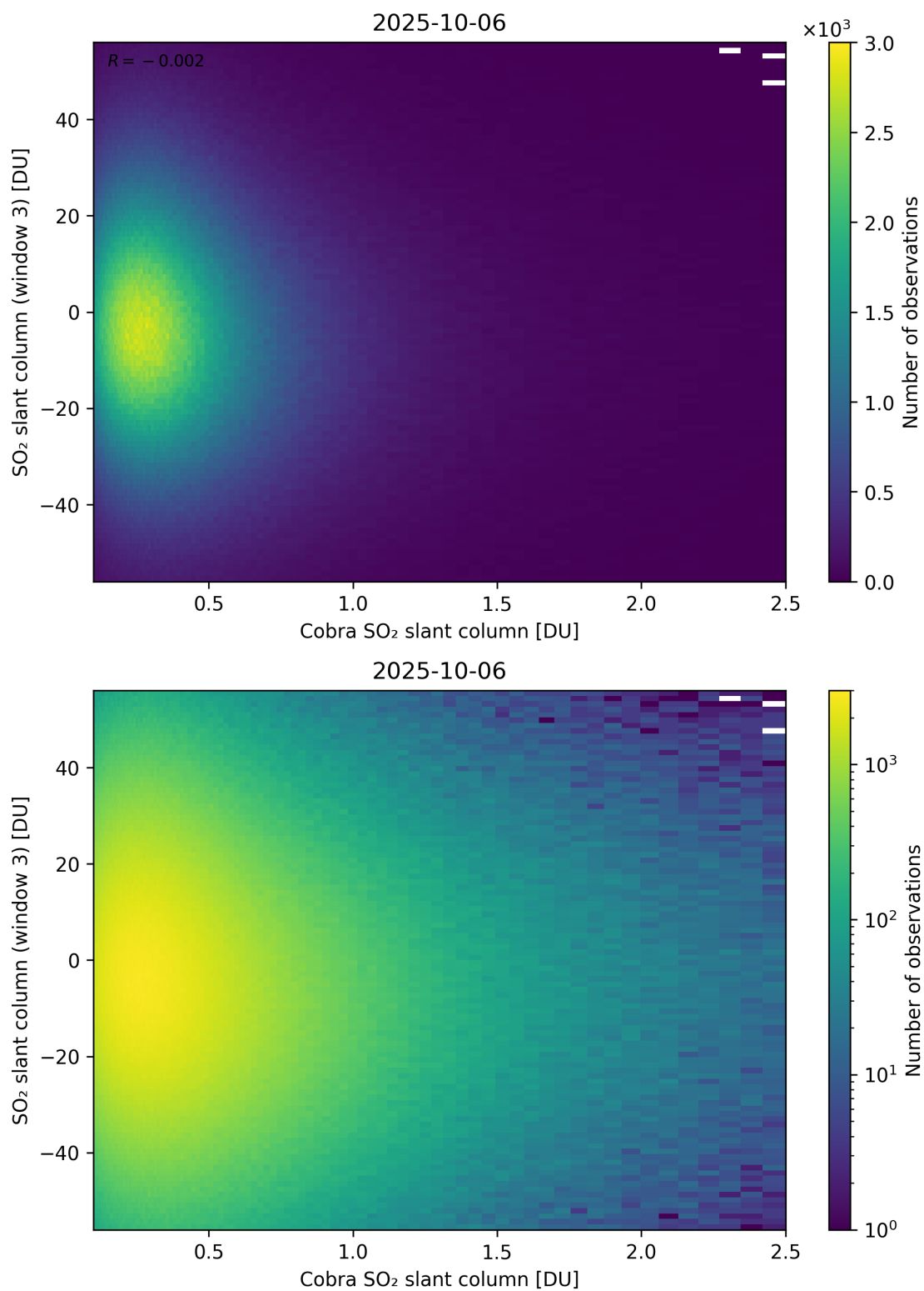
Figure 222: Scatter density plot of “Cobra SO 2 slant column” against “SO 2 slant column (window 3)” for 2025-10-06 to 2025-10-07.
