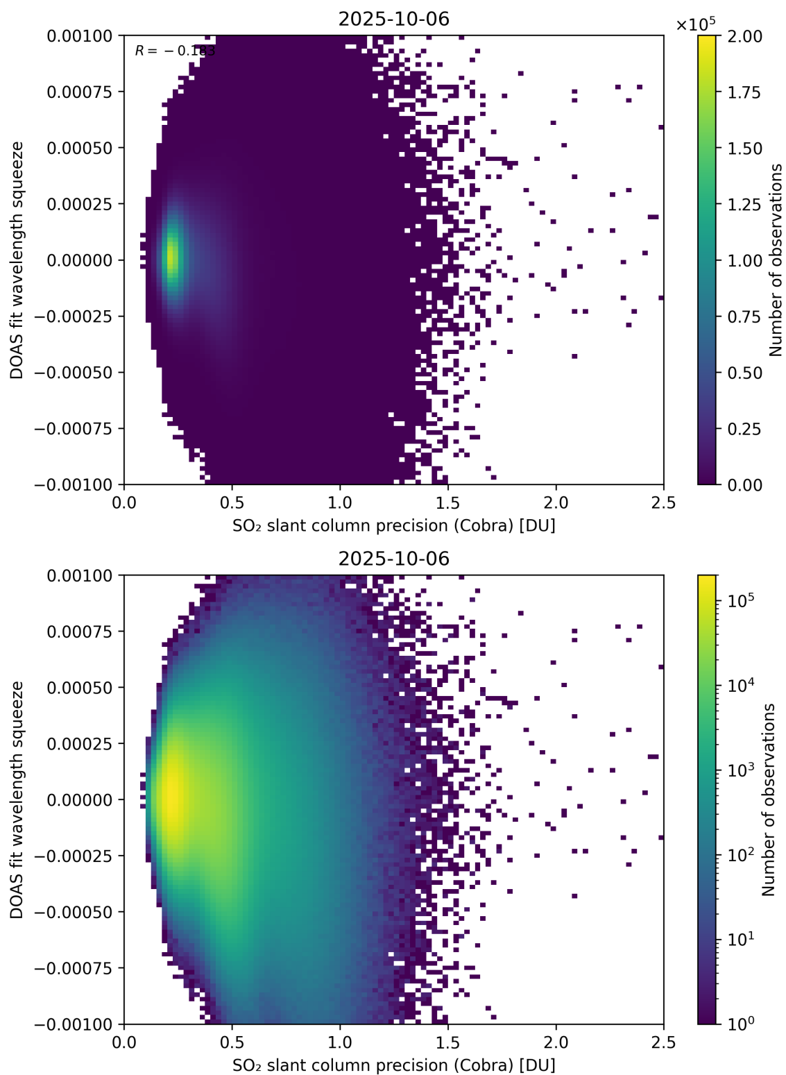
Figure 203: Scatter density plot of “SO 2 slant column precision (Cobra)” against “DOAS fit wavelength squeeze” for 2025-10-06 to 2025-10-07.
