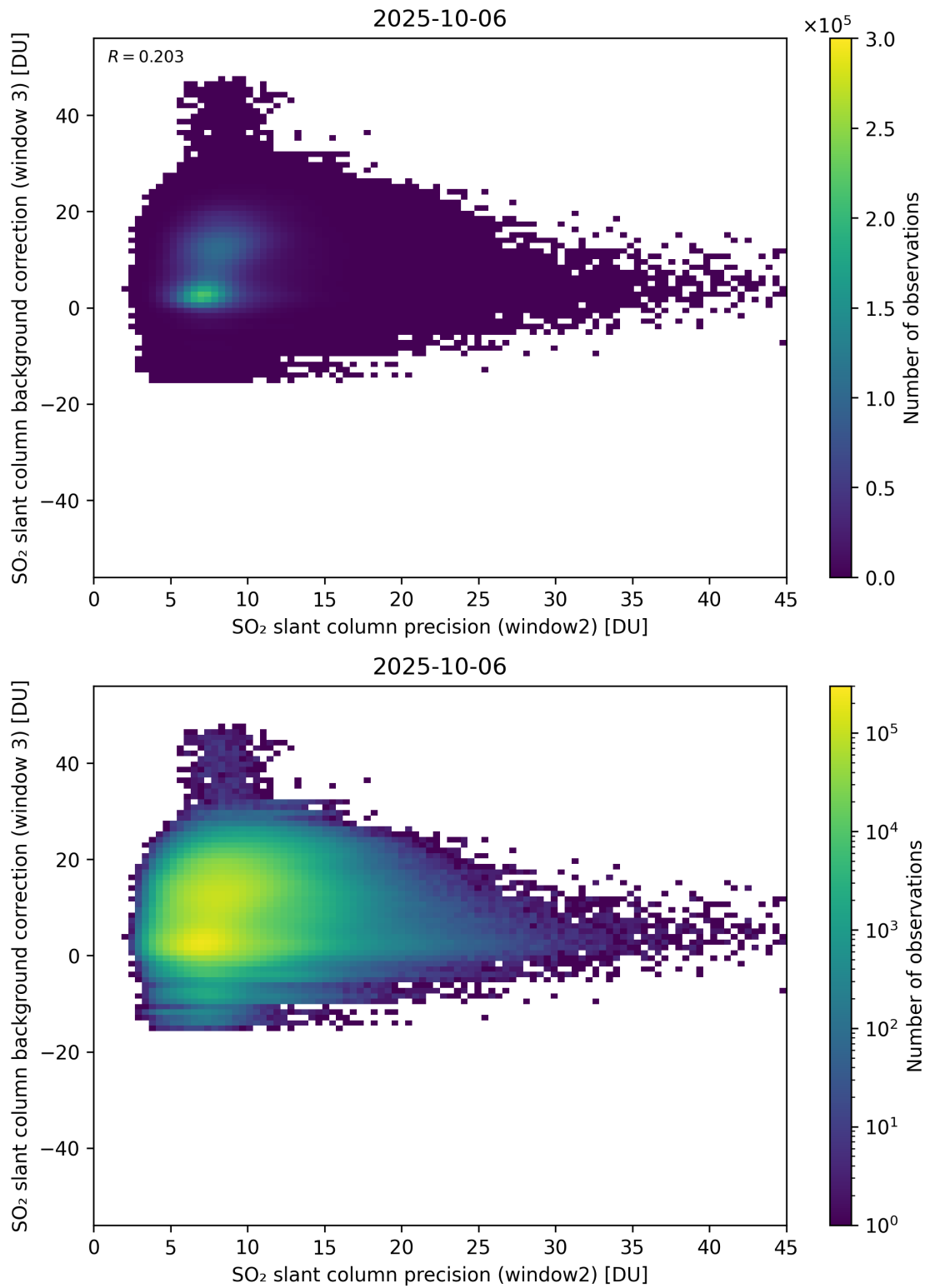
Figure 292: Scatter density plot of “SO 2 slant column precision (window2)” against “SO 2 slant column background correction (window 3)” for 2025-10-06 to 2025-10-07.
