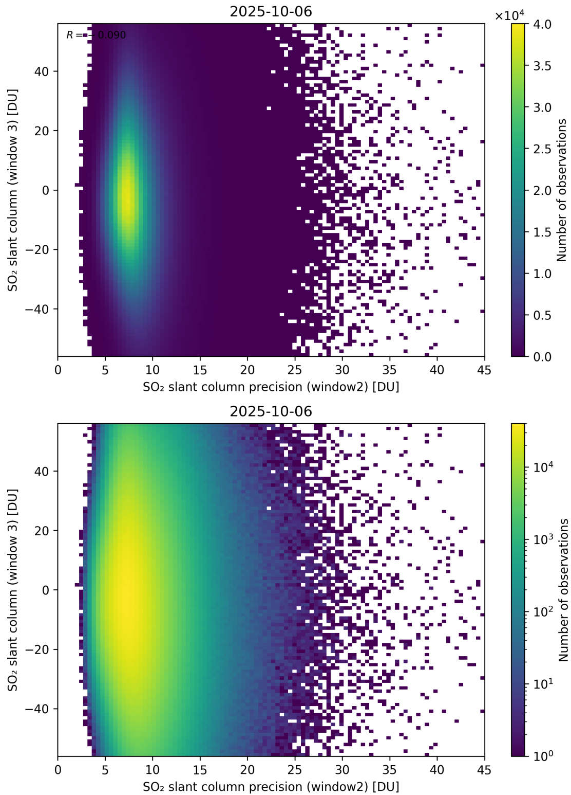
Figure 299: Scatter density plot of “SO 2 slant column precision (window2)” against “SO 2 slant column (window 3)” for 2025-10-06 to 2025-10-07.
