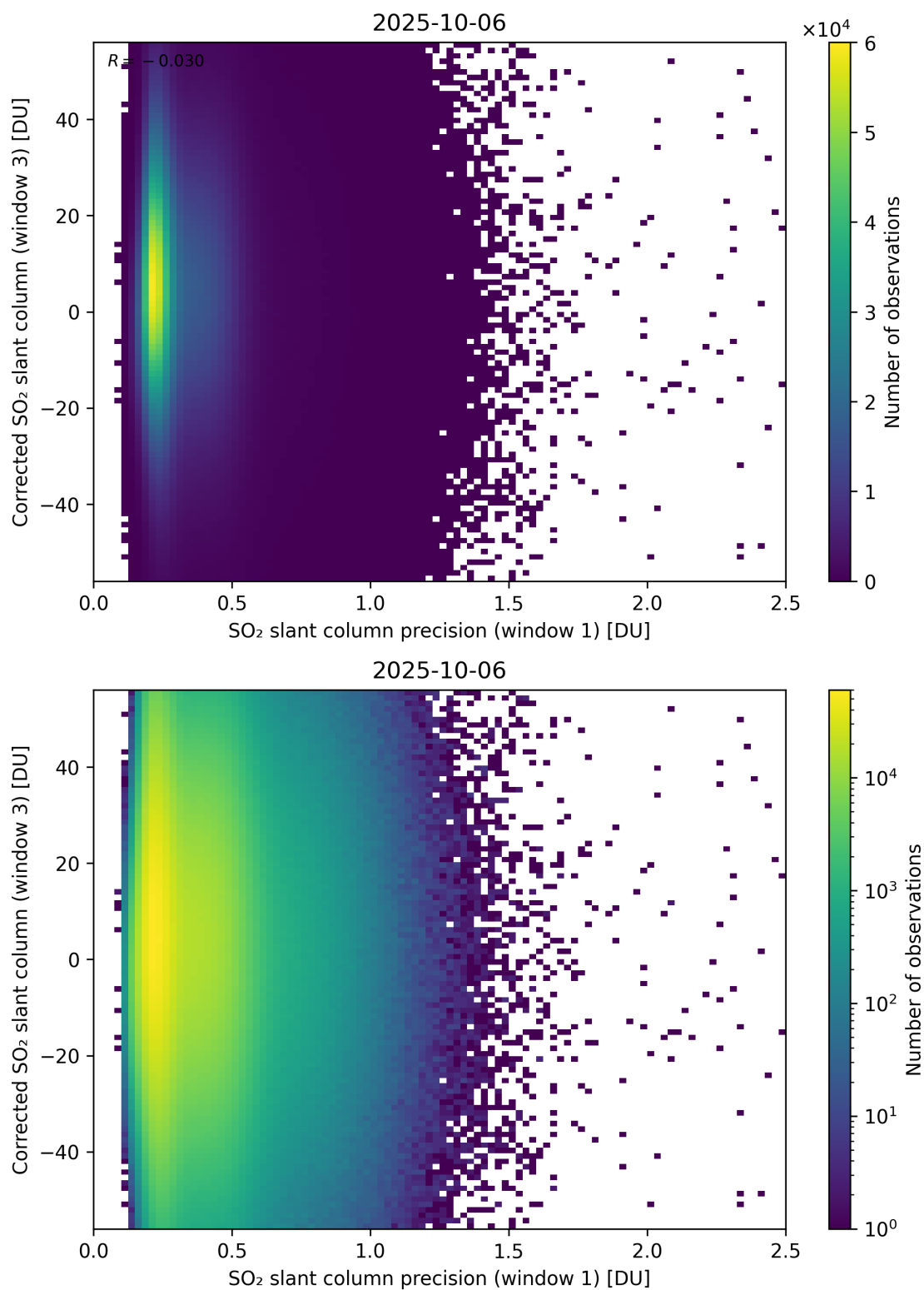
Figure 276: Scatter density plot of “SO 2 slant column precision (window 1)” against “Corrected SO 2 slant column (window 3)” for 2025-10-06 to 2025-10-07.
