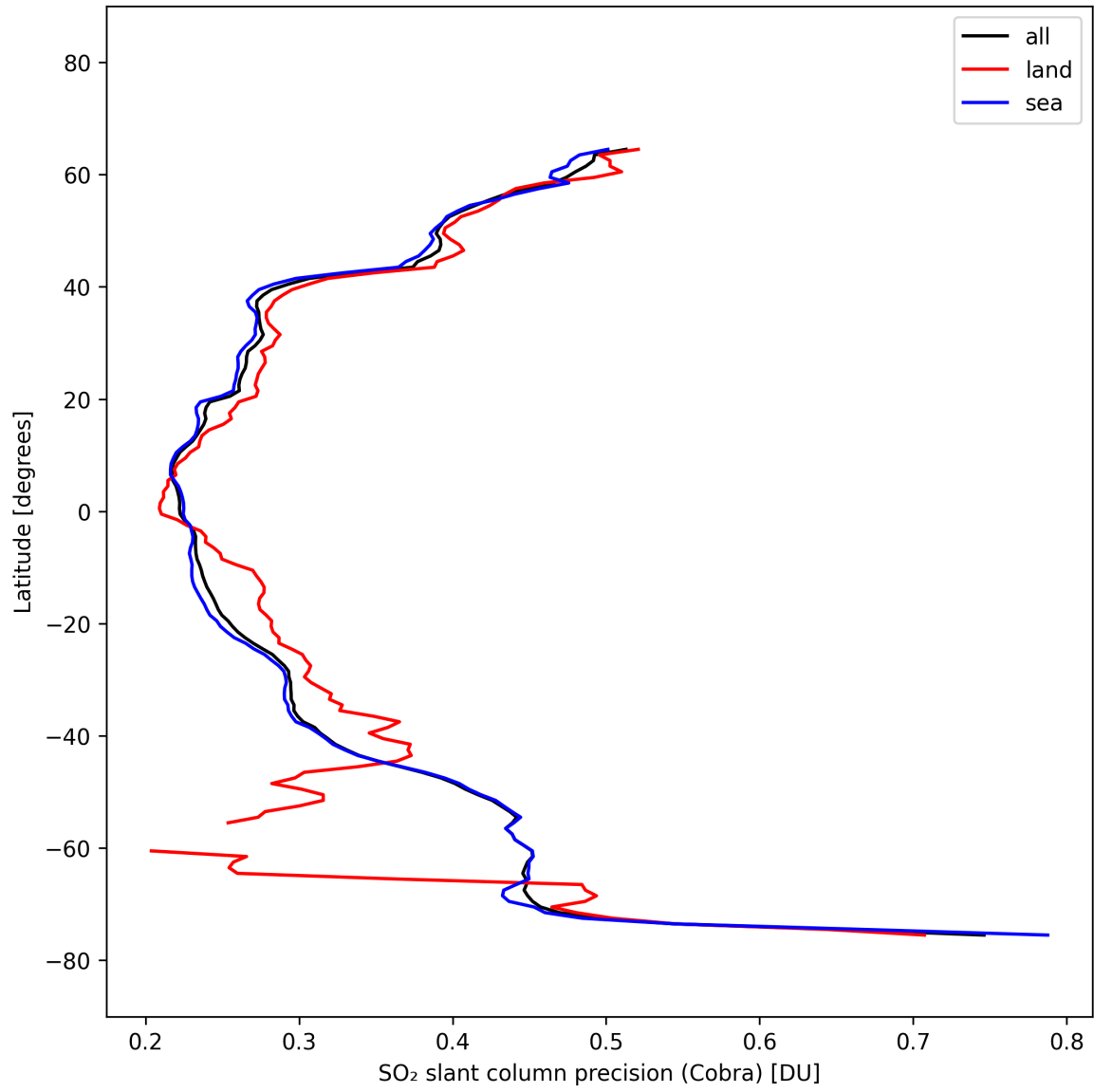
Figure 36: Zonal average of “SO 2 slant column precision (Cobra)” for 2025-10-06 to 2025-10-07.
