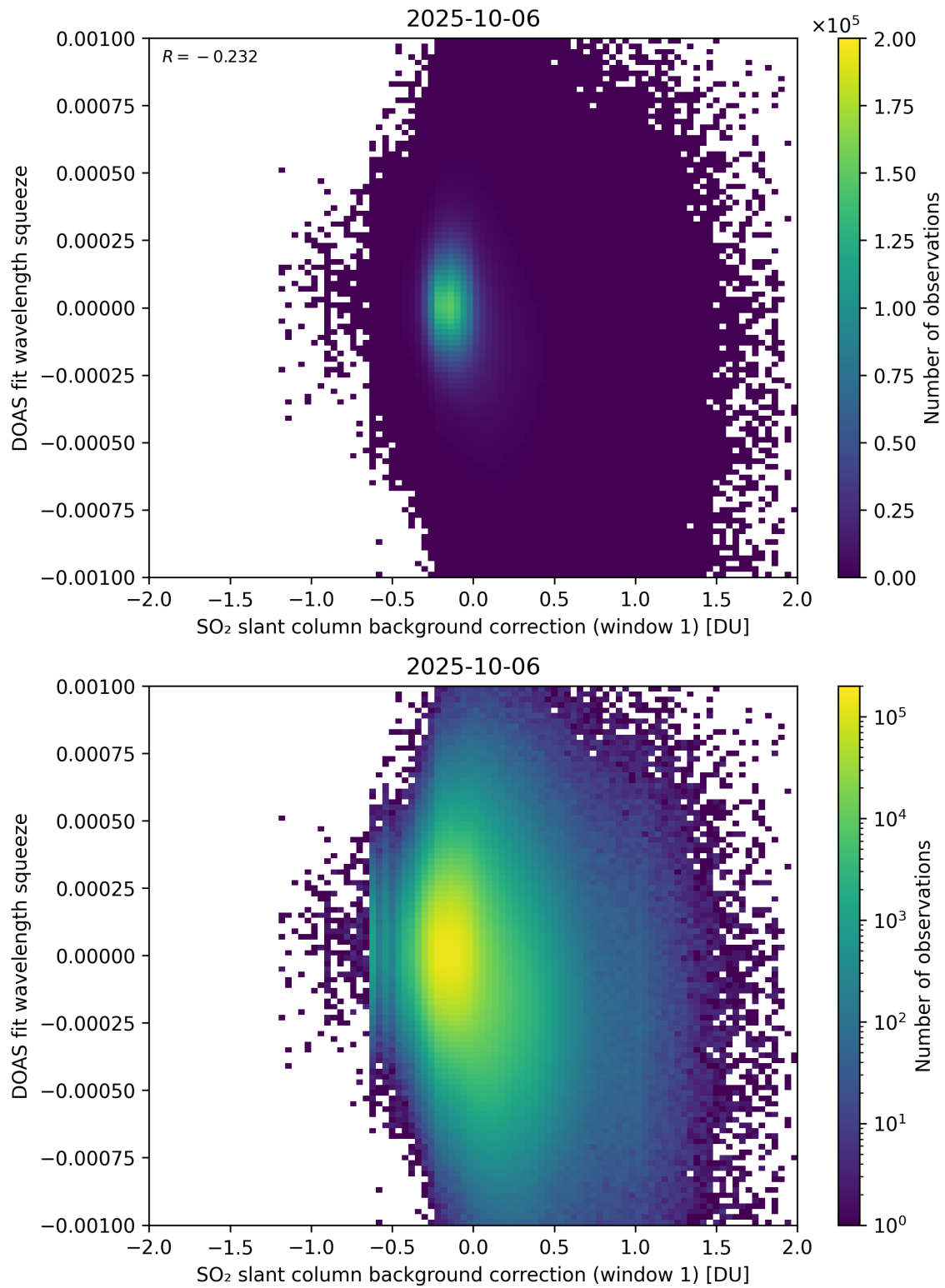
Figure 112: Scatter density plot of “SO 2 slant column background correction (window 1)” against “DOAS fit wavelength squeeze” for 2025-10-06 to 2025-10-07.
