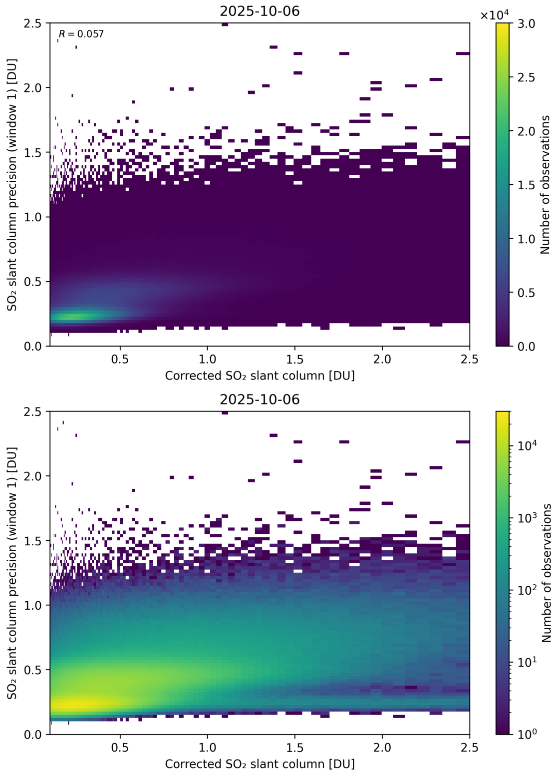
Figure 238: Scatter density plot of “Corrected SO 2 slant column” against “SO 2 slant column precision (window 1)” for 2025-10-06 to 2025-10-07.
