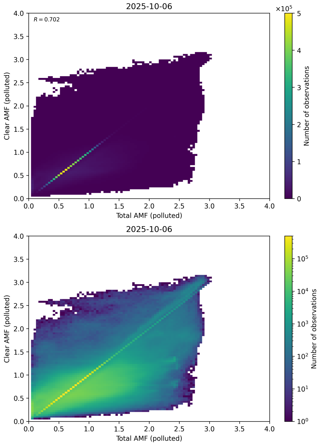
Figure 321: Scatter density plot of “Total AMF (polluted)” against “Clear AMF (polluted)” for 2025-10-06 to 2025-10-07.
