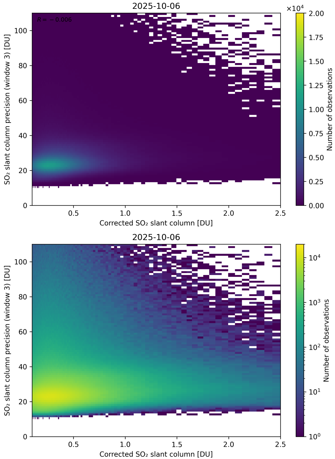
Figure 241: Scatter density plot of “Corrected SO 2 slant column” against “SO 2 slant column precision (window 3)” for 2025-10-06 to 2025-10-07.
