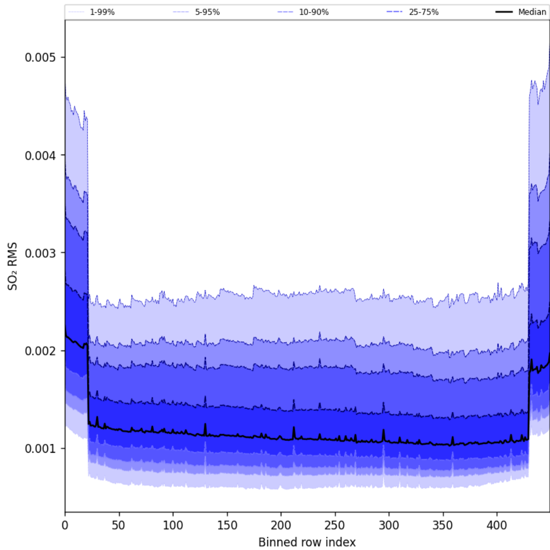
Figure 104: Along track statistics of “SO 2 RMS” for 2025-10-06 to 2025-10-07
