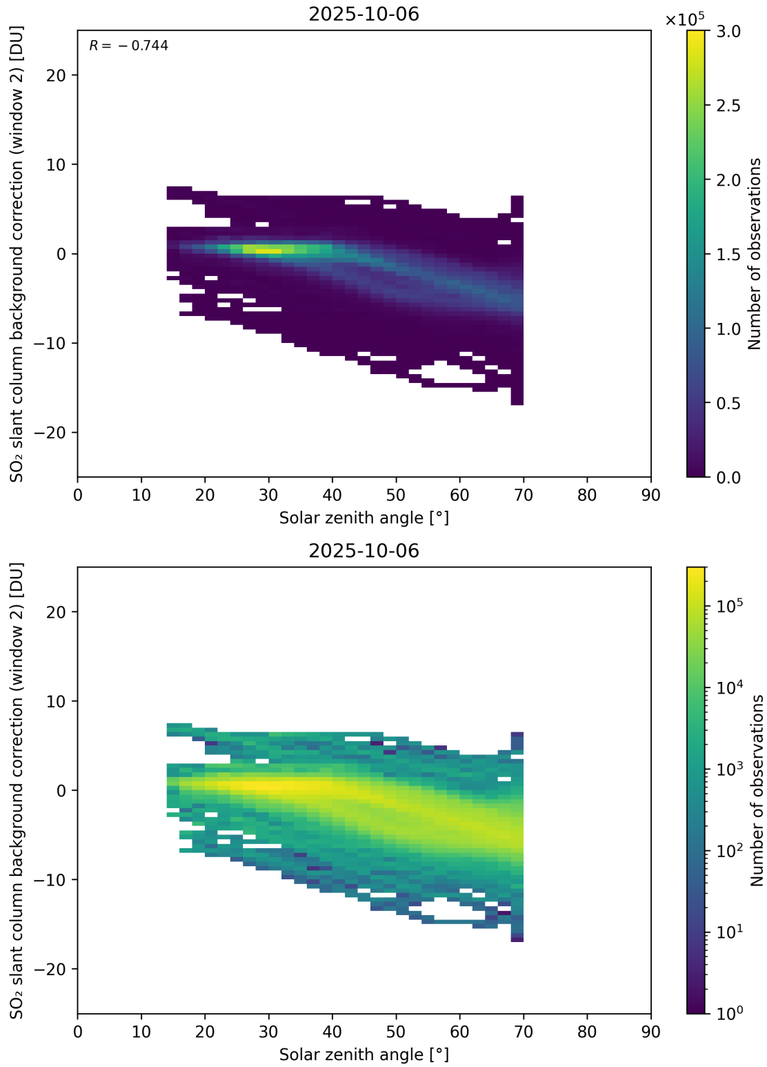
Figure 172: Scatter density plot of “Solar zenith angle” against “SO 2 slant column background correction (window 2)” for 2025-10-06 to 2025-10-07.
