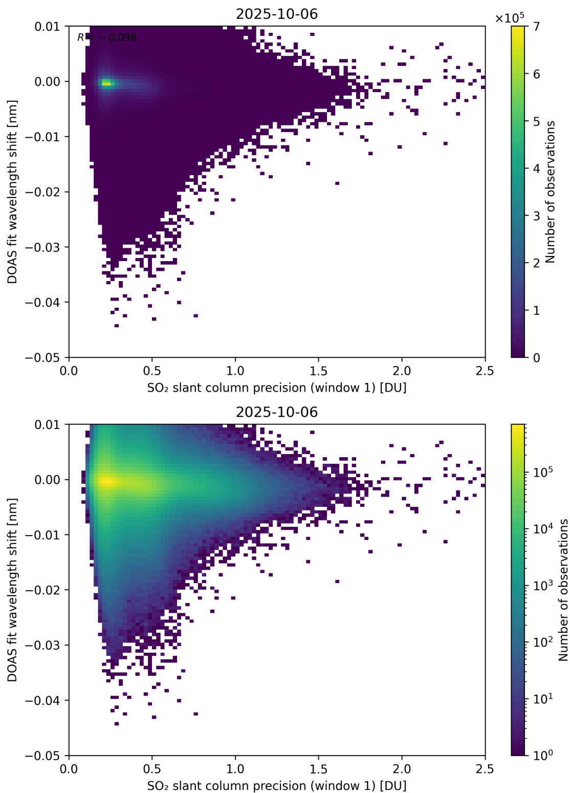
Figure 271: Scatter density plot of “SO 2 slant column precision (window 1)” against “DOAS fit wavelength shift” for 2025-10-06 to 2025-10-07.
