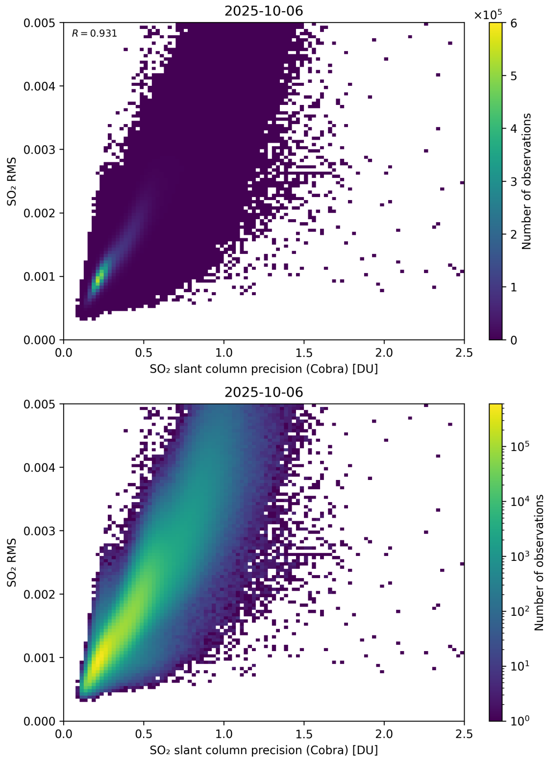
Figure 204: Scatter density plot of “SO 2 slant column precision (Cobra)” against “SO 2 RMS” for 2025-10-06 to 2025-10-07.
