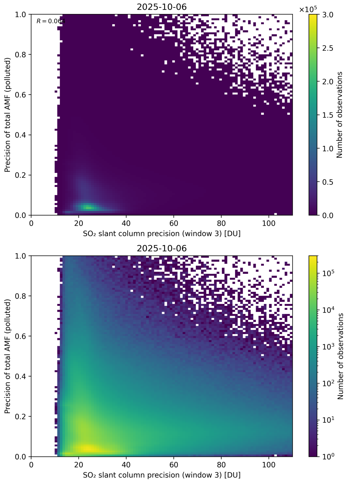
Figure 314: Scatter density plot of “SO 2 slant column precision (window 3)” against “Precision of total AMF (polluted)” for 2025-10-06 to 2025-10-07.
