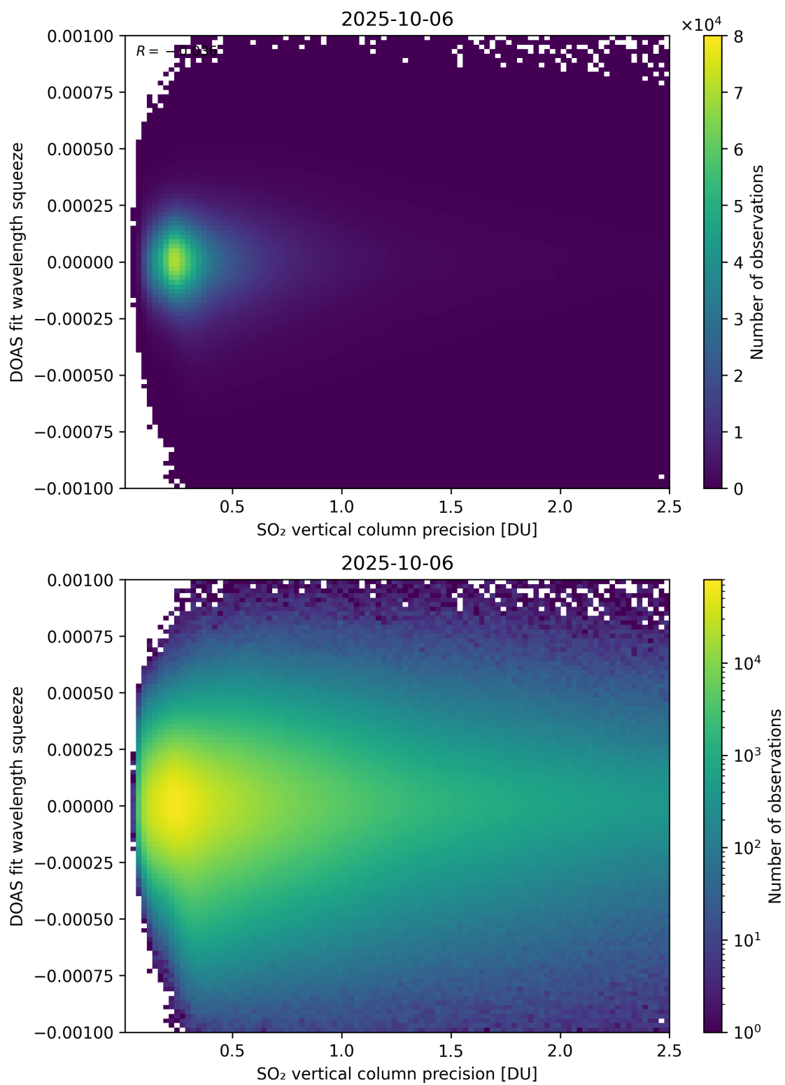
Figure 333: Scatter density plot of “SO 2 vertical column precision” against “DOAS fit wavelength squeeze” for 2025-10-06 to 2025-10-07.
