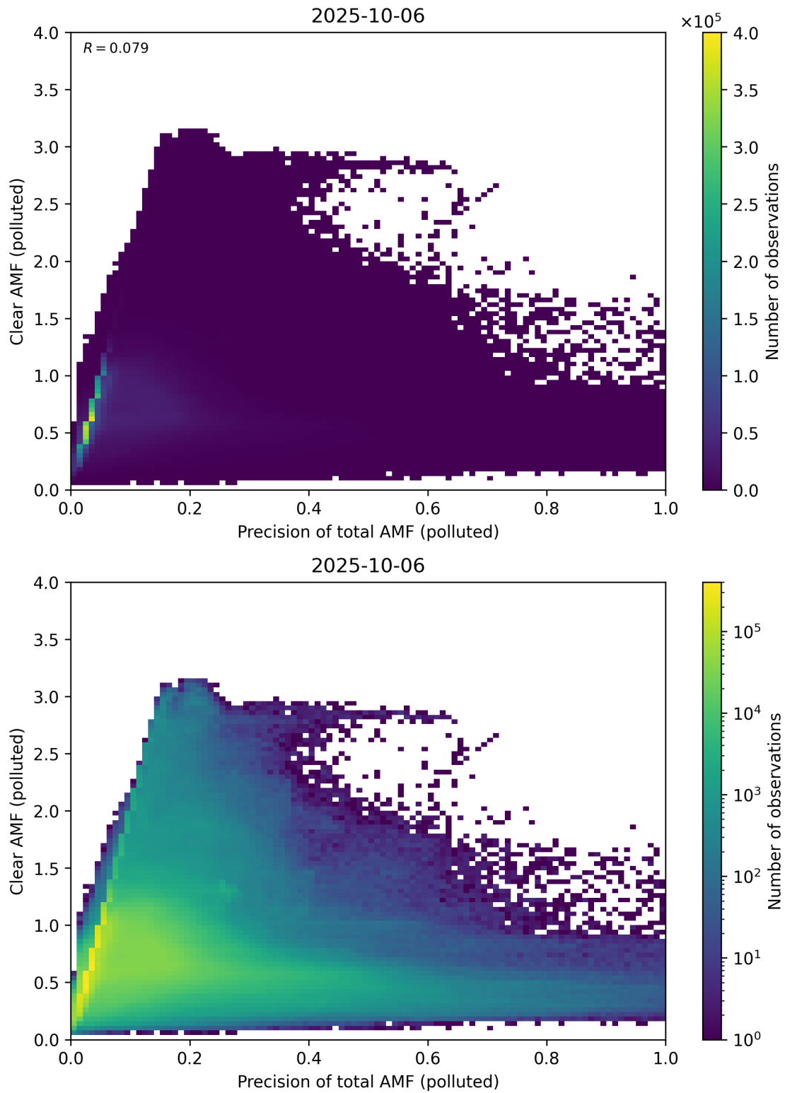
Figure 320: Scatter density plot of “Precision of total AMF (polluted)” against “Clear AMF (polluted)” for 2025-10-06 to 2025-10-07.
