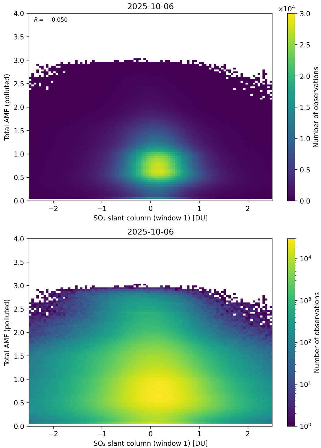
Figure 289: Scatter density plot of “SO 2 slant column (window 1)” against “Total AMF (polluted)” for 2025-10-06 to 2025-10-07.
