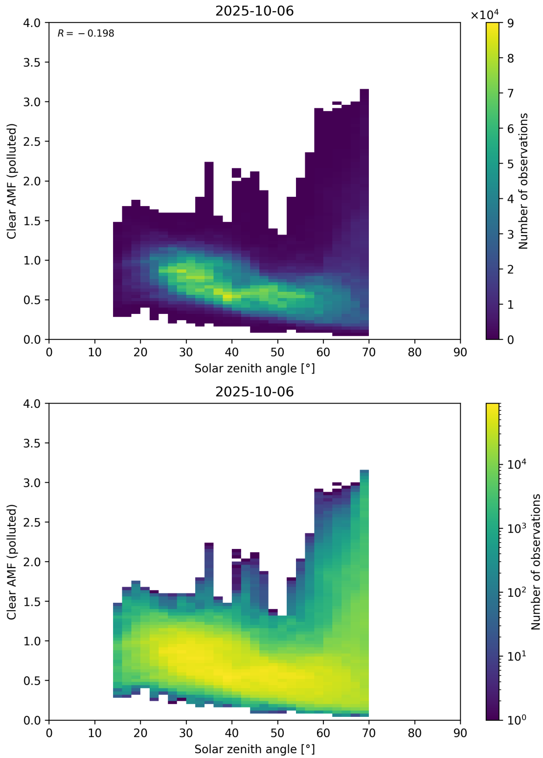
Figure 178: Scatter density plot of “Solar zenith angle” against “Clear AMF (polluted)” for 2025-10-06 to 2025-10-07.
