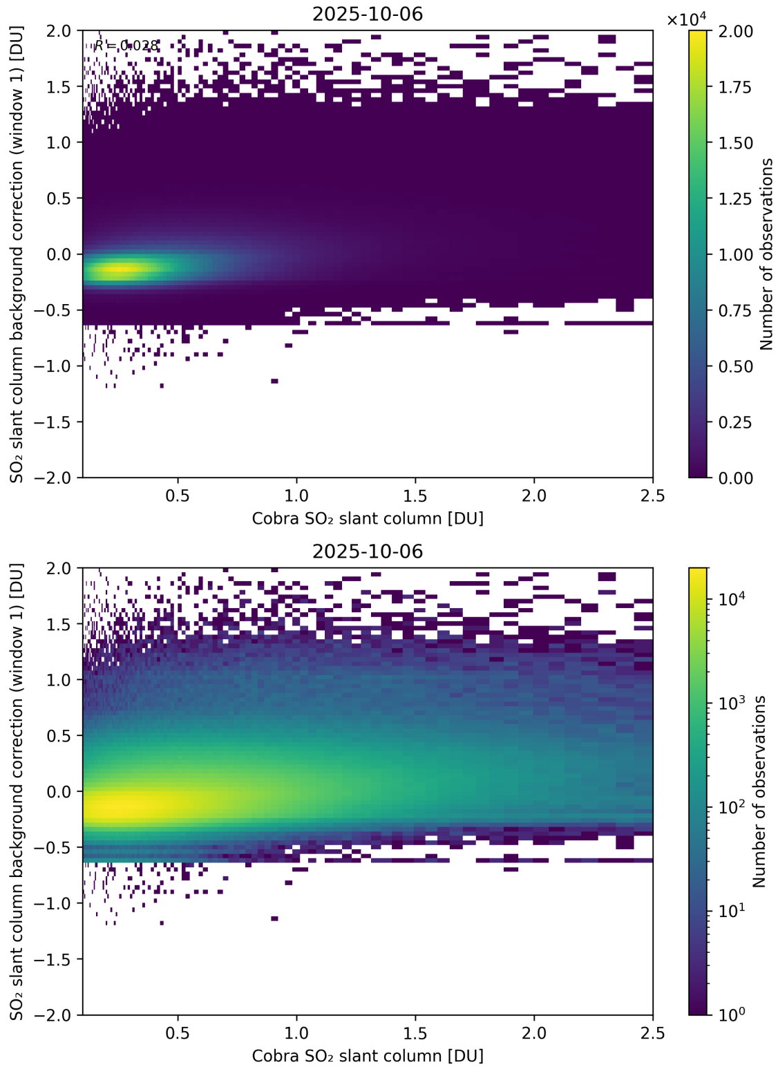
Figure 193: Scatter density plot of “Cobra SO 2 slant column” against “SO 2 slant column background correction (window 1)” for 2025-10-06 to 2025-10-07.
