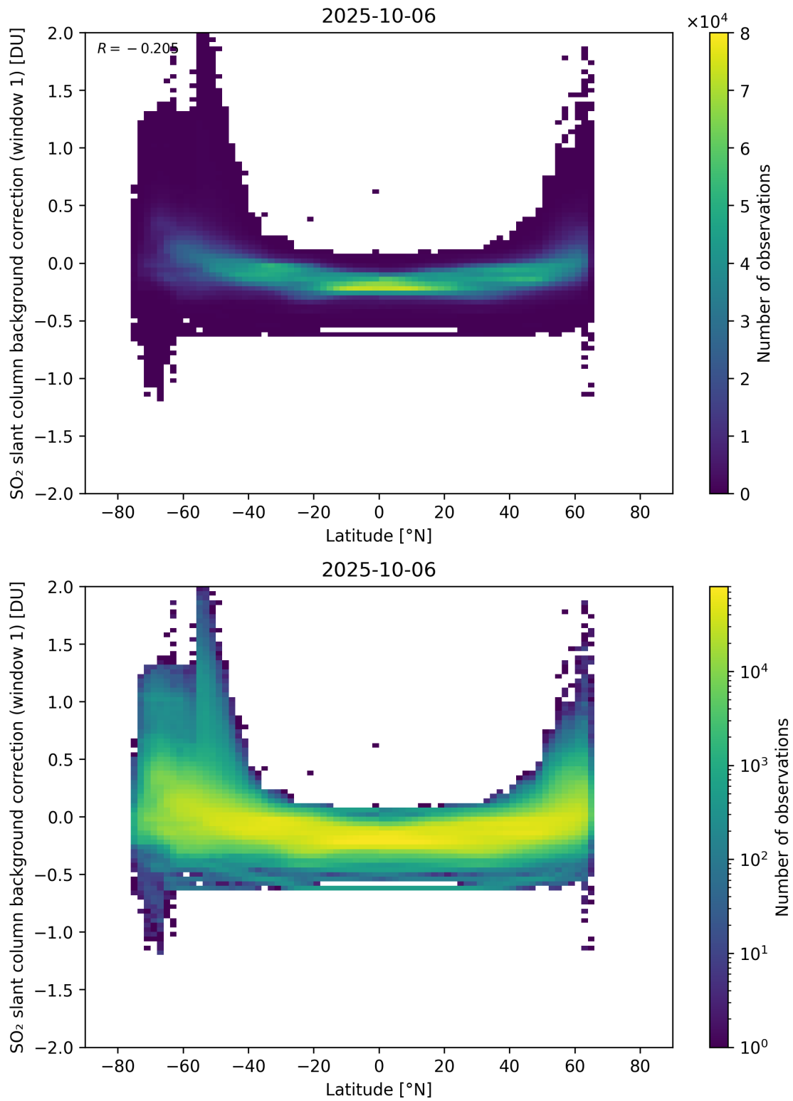
Figure 150: Scatter density plot of “Latitude” against “SO 2 slant column background correction (window 1)” for 2025-10-06 to 2025-10-07.
