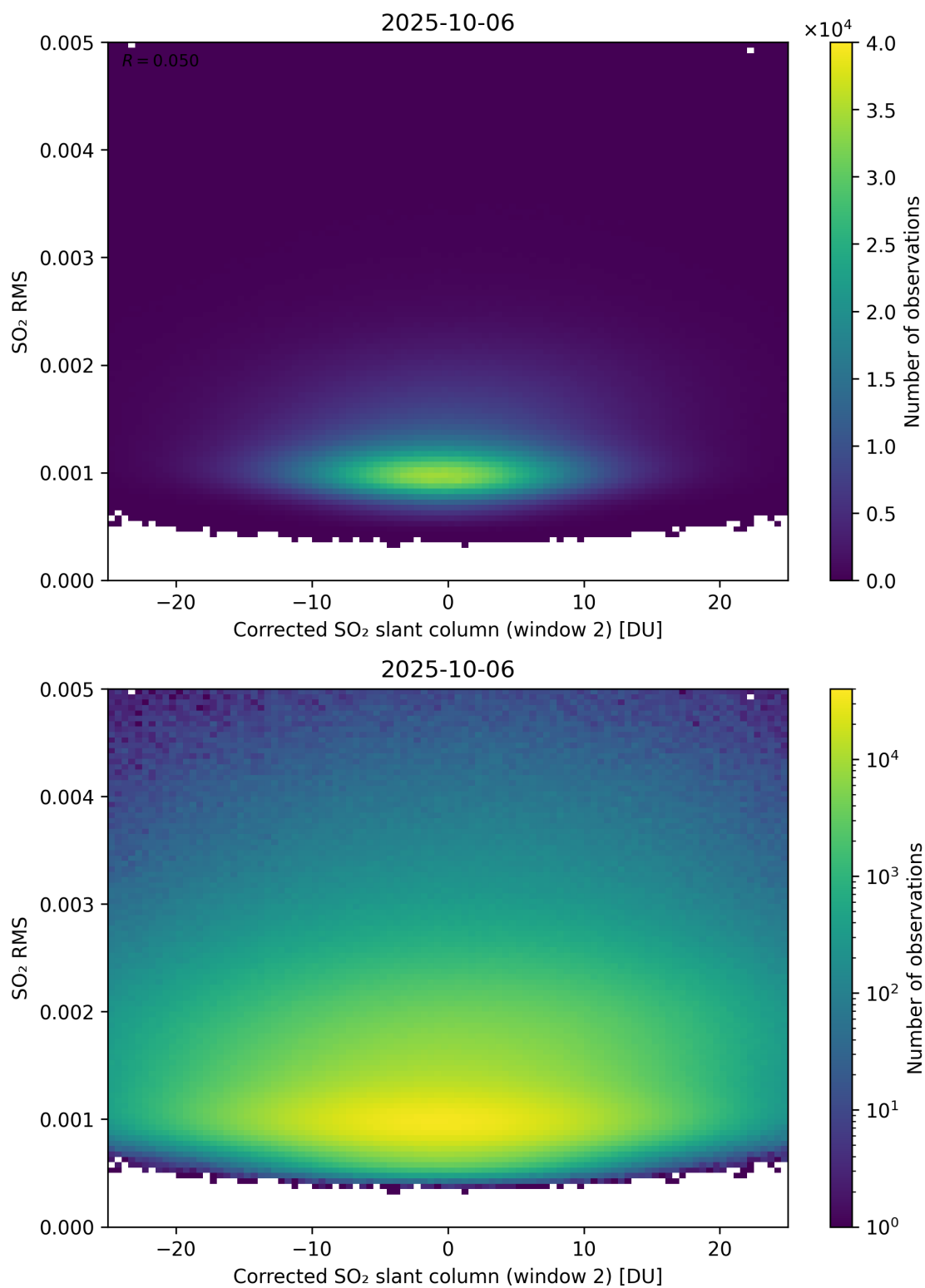
Figure 248: Scatter density plot of “Corrected SO 2 slant column (window 2)” against “SO 2 RMS” for 2025-10-06 to 2025-10-07.
