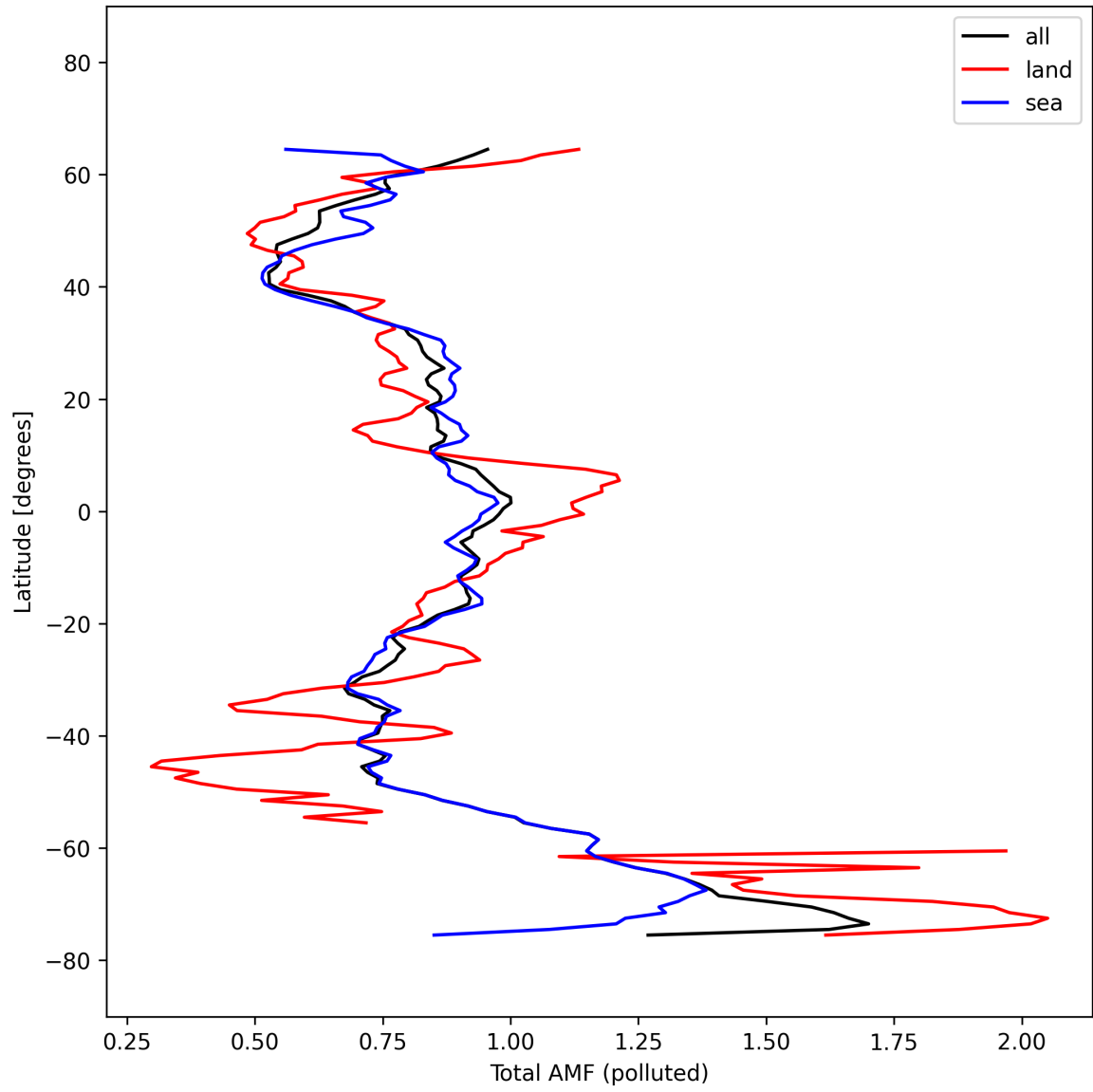
Figure 53: Zonal average of “Total AMF (polluted)” for 2025-10-06 to 2025-10-07.
