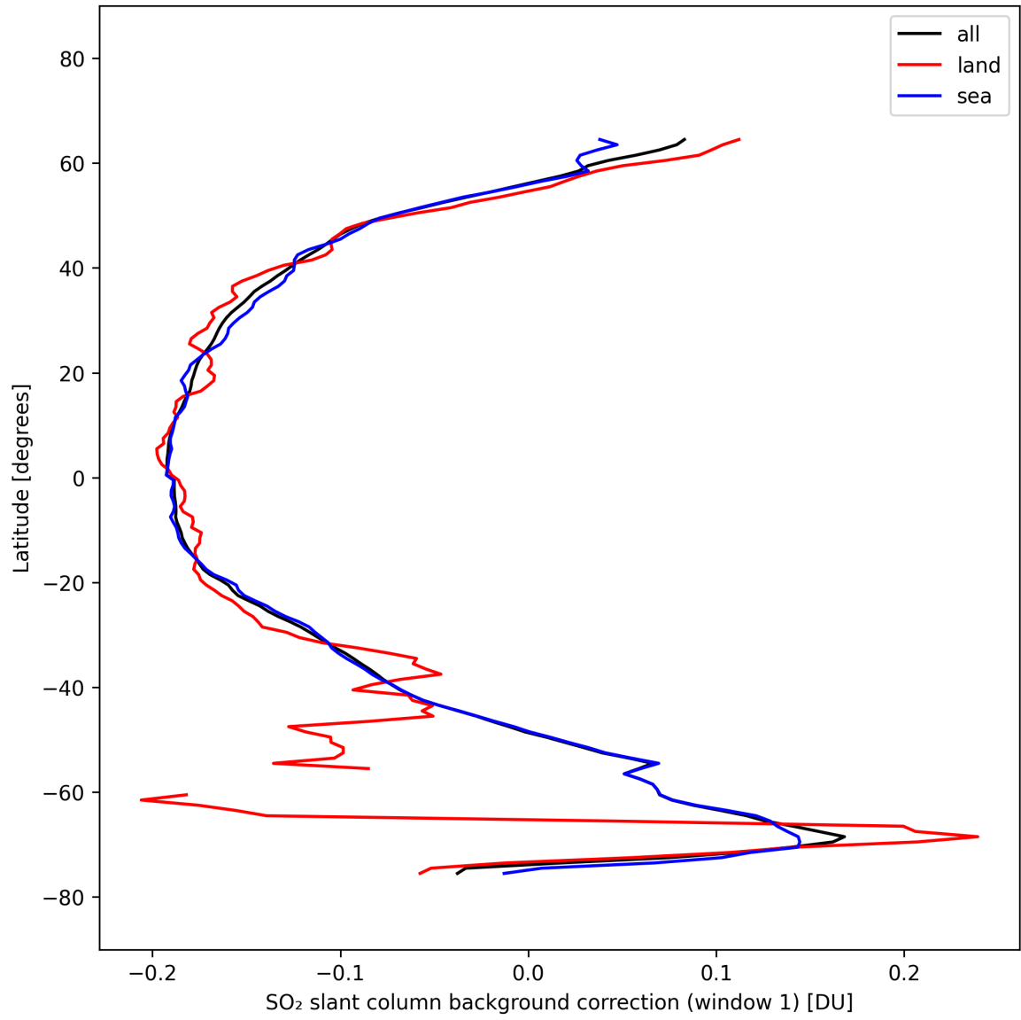
Figure 40: Zonal average of “SO 2 slant column background correction (window 1)” for 2025-10-06 to 2025-10-07.
