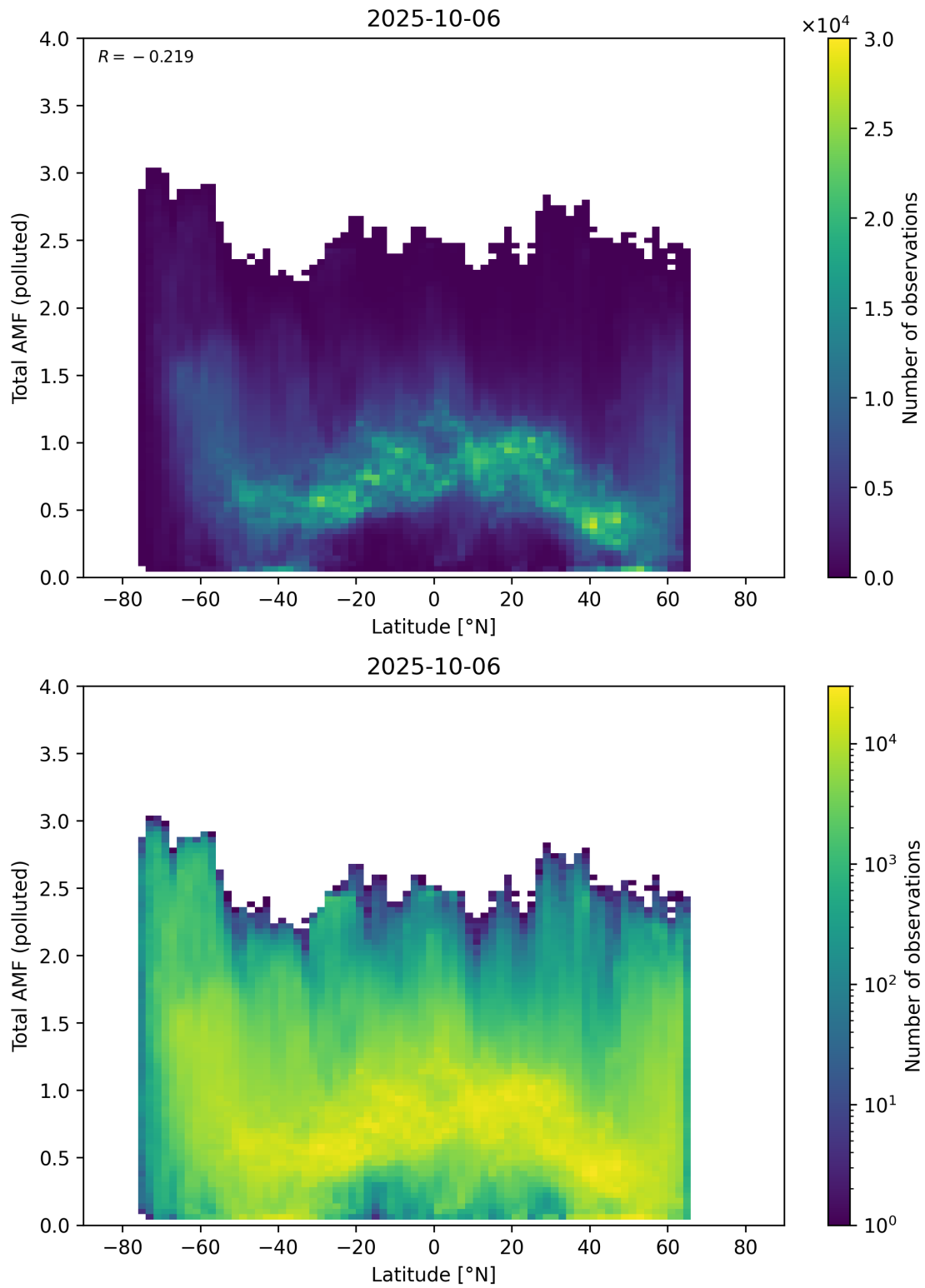
Figure 167: Scatter density plot of “Latitude” against “Total AMF (polluted)” for 2025-10-06 to 2025-10-07.
