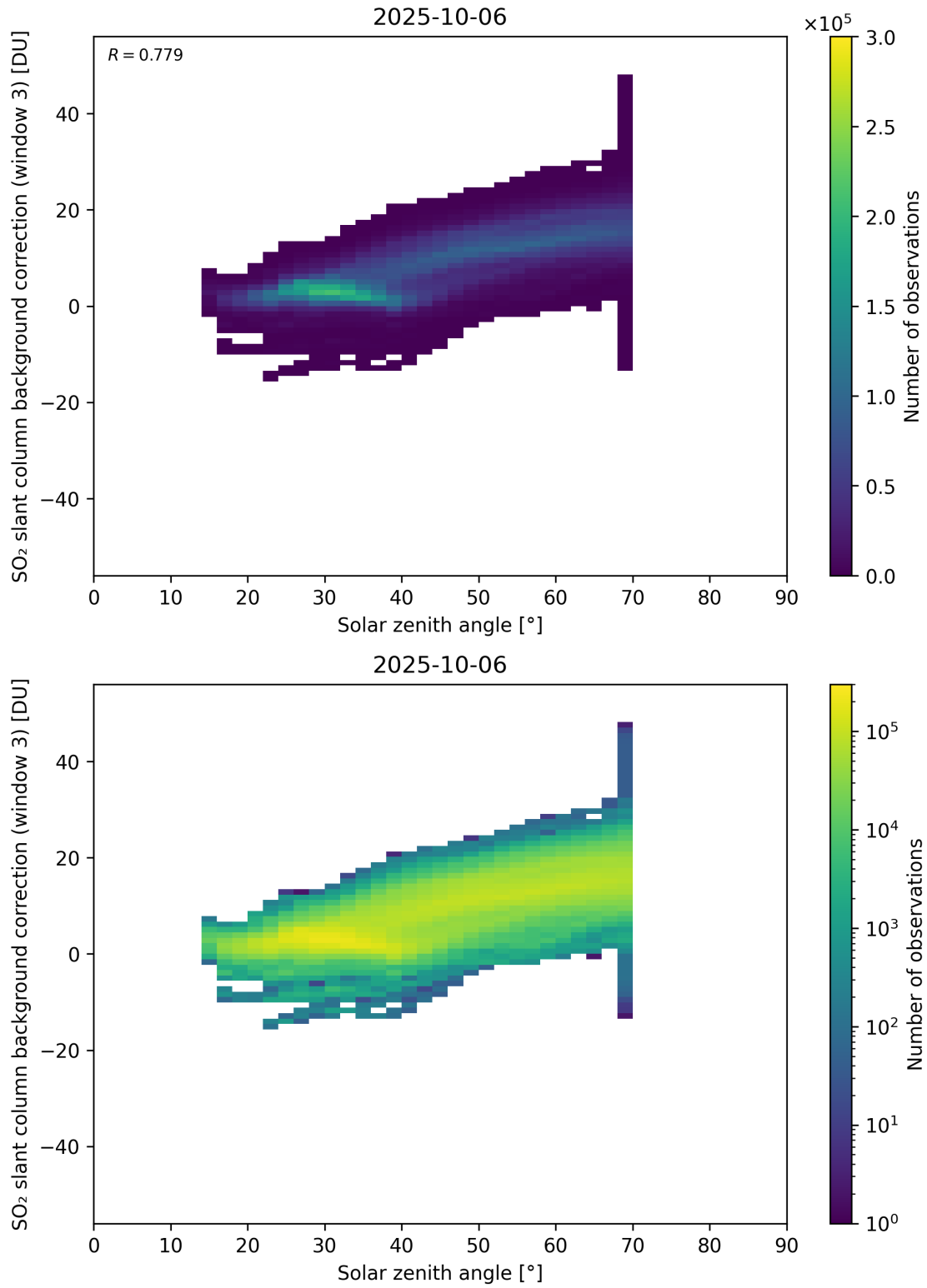
Figure 173: Scatter density plot of “Solar zenith angle” against “SO 2 slant column background correction (window 3)” for 2025-10-06 to 2025-10-07.
