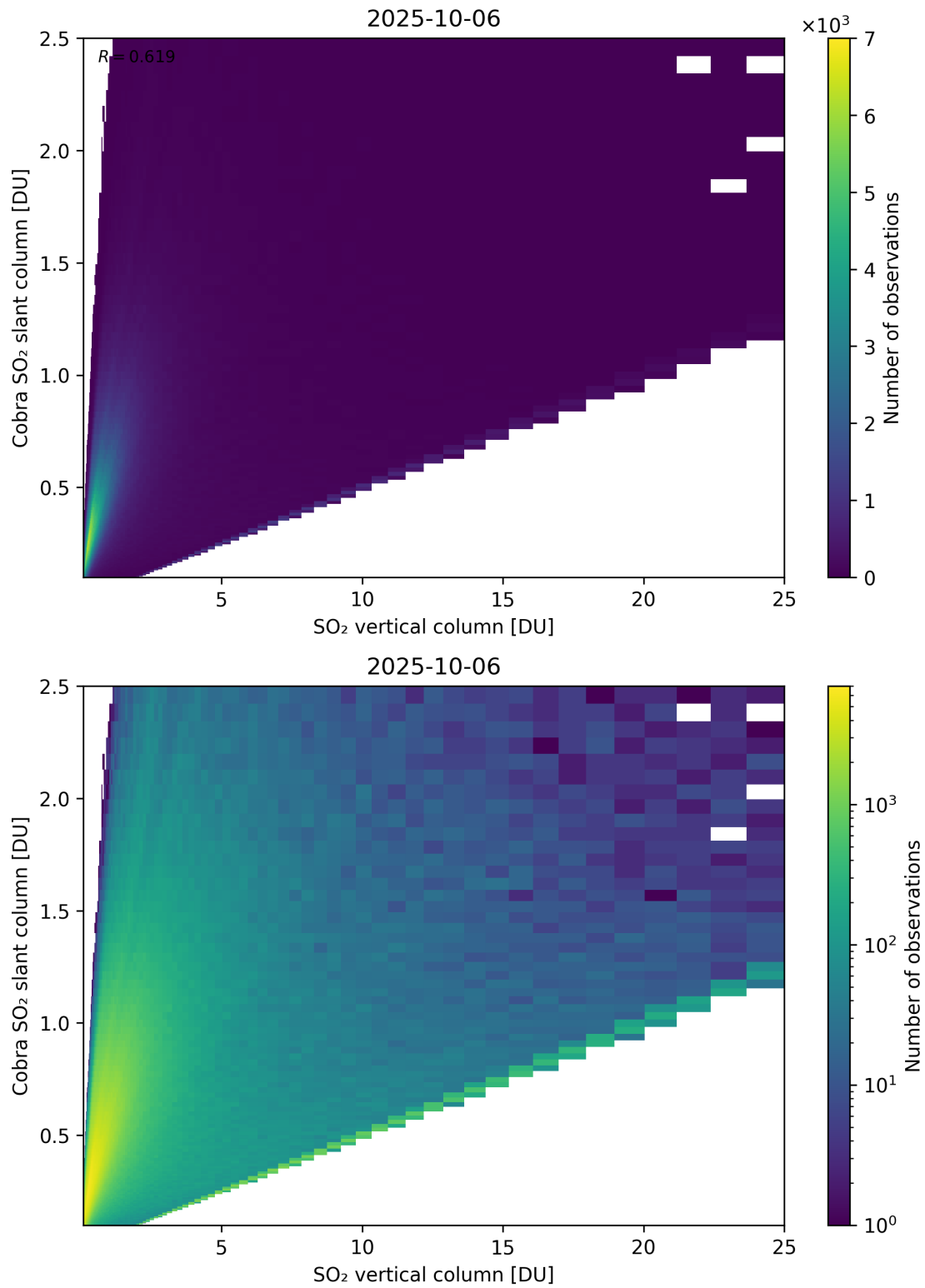
Figure 349: Scatter density plot of “SO 2 vertical column” against “Cobra SO 2 slant column” for 2025-10-06 to 2025-10-07.
