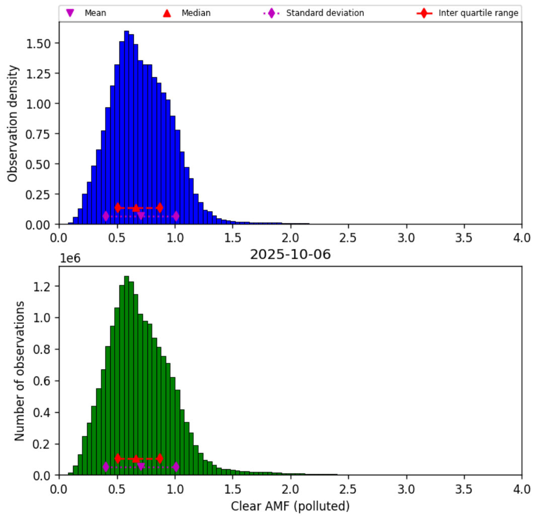
Figure 81: Histogram of “Clear AMF (polluted)” for 2025-10-06 to 2025-10-07
