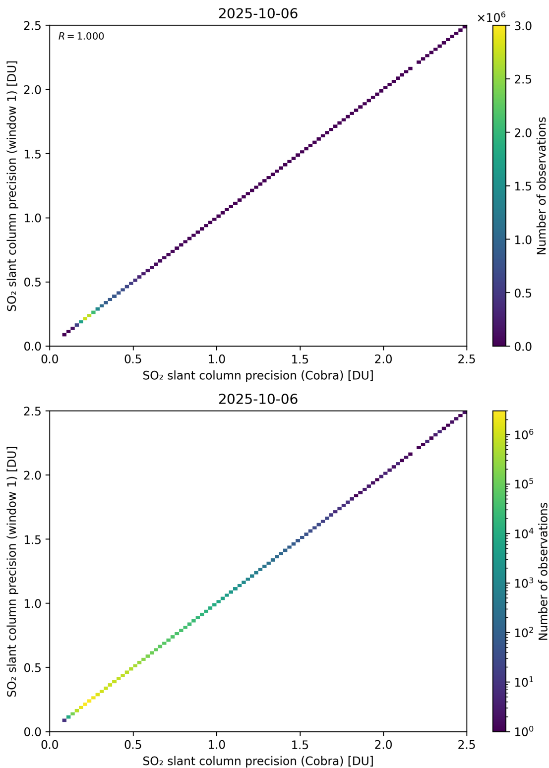
Figure 209: Scatter density plot of “SO 2 slant column precision (Cobra)” against “SO 2 slant column precision (window 1)” for 2025-10-06 to 2025-10-07.
