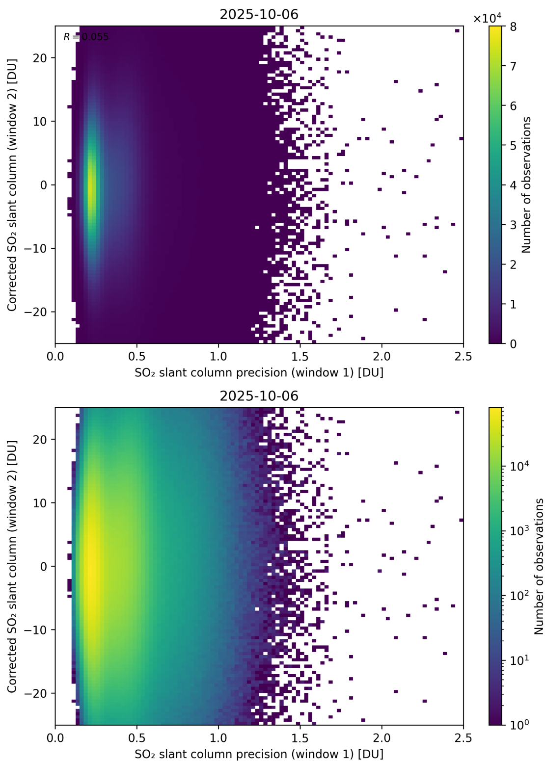
Figure 275: Scatter density plot of “SO 2 slant column precision (window 1)” against “Corrected SO 2 slant column (window 2)” for 2025-10-06 to 2025-10-07.
