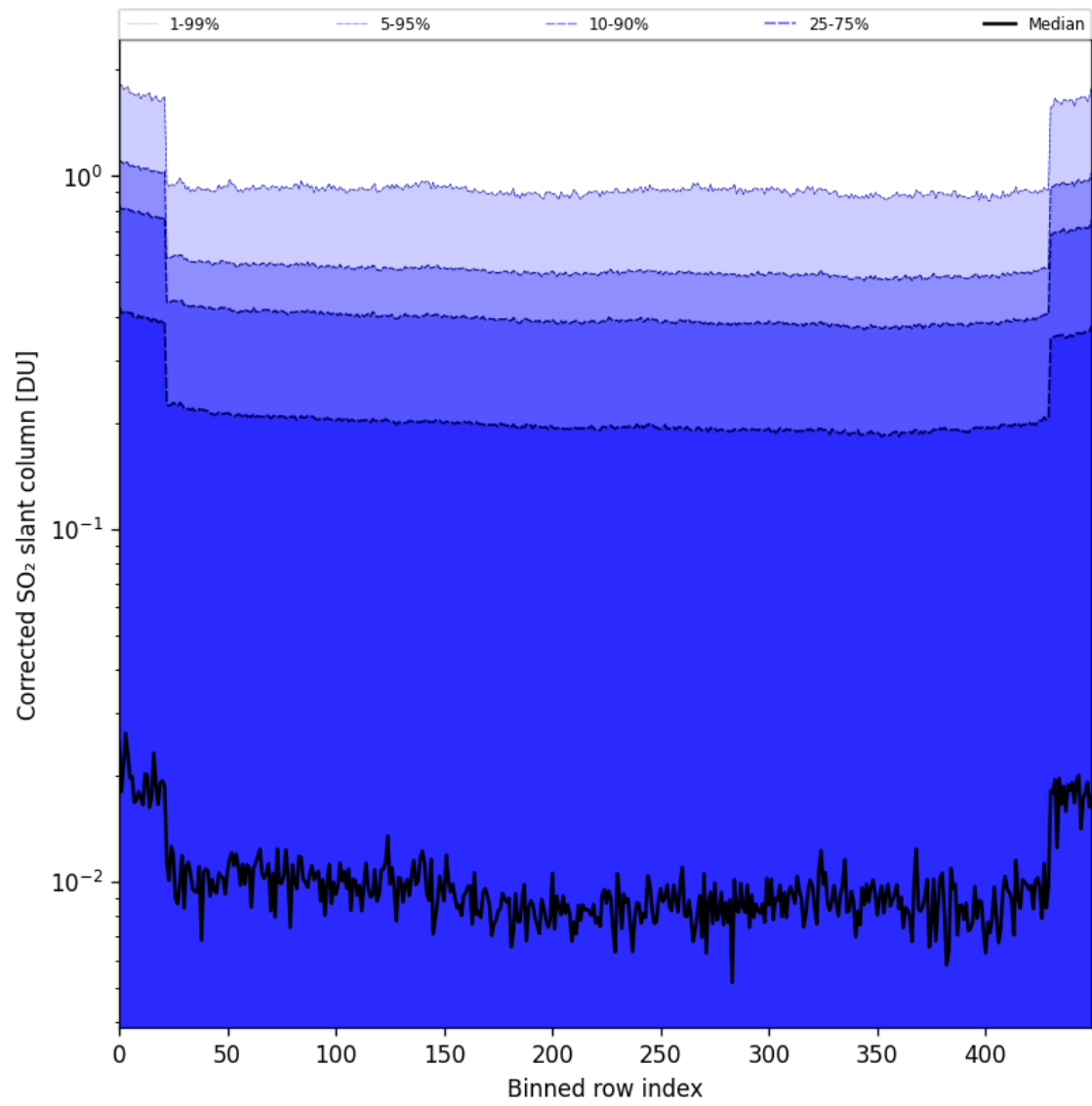
Figure 86: Along track statistics of "Corrected SO 2 slant column" for 2025-10-06 to 2025-10-07
