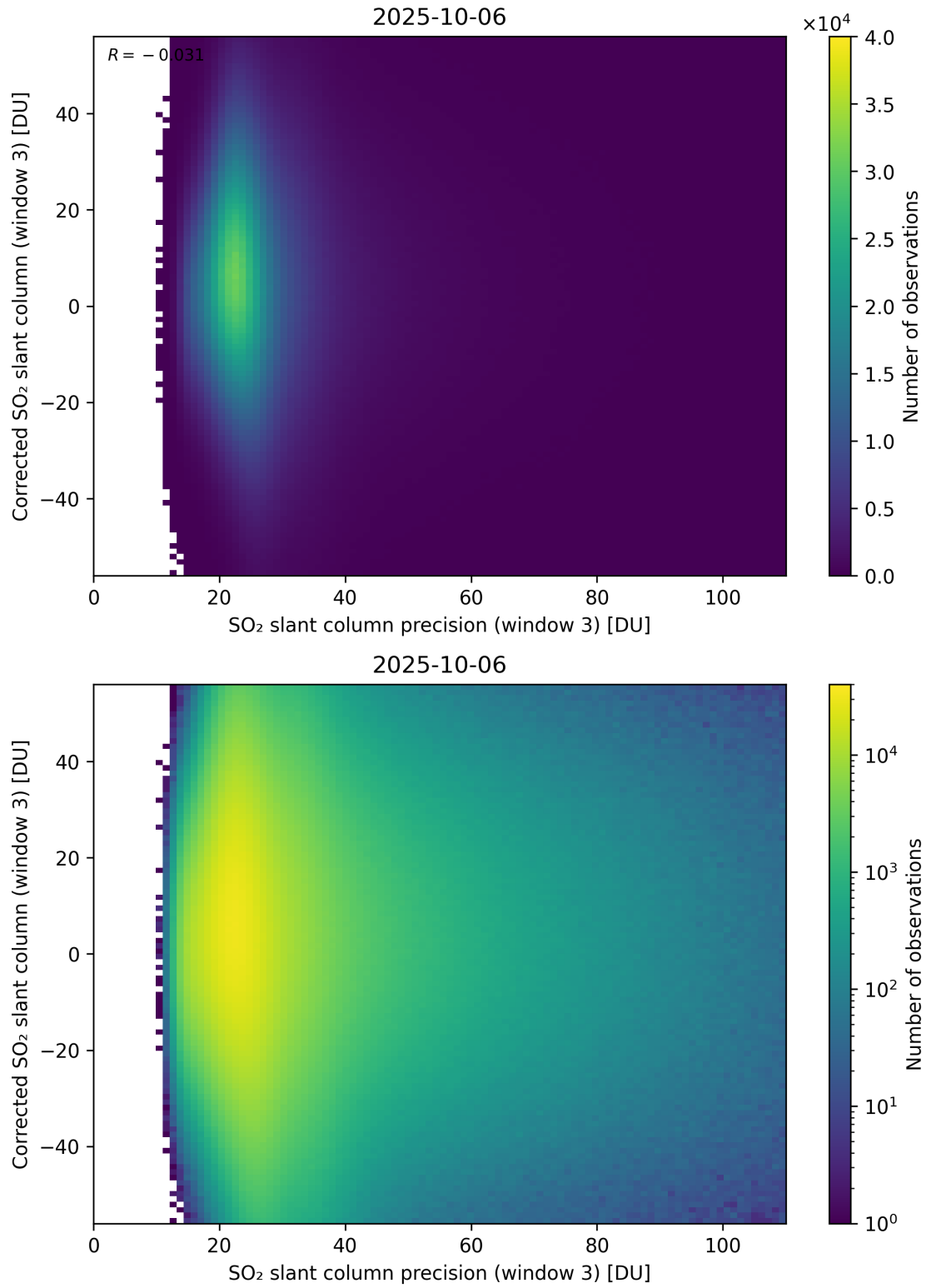
Figure 312: Scatter density plot of “SO 2 slant column precision (window 3)” against “Corrected SO 2 slant column (window 3)” for 2025-10-06 to 2025-10-07.
