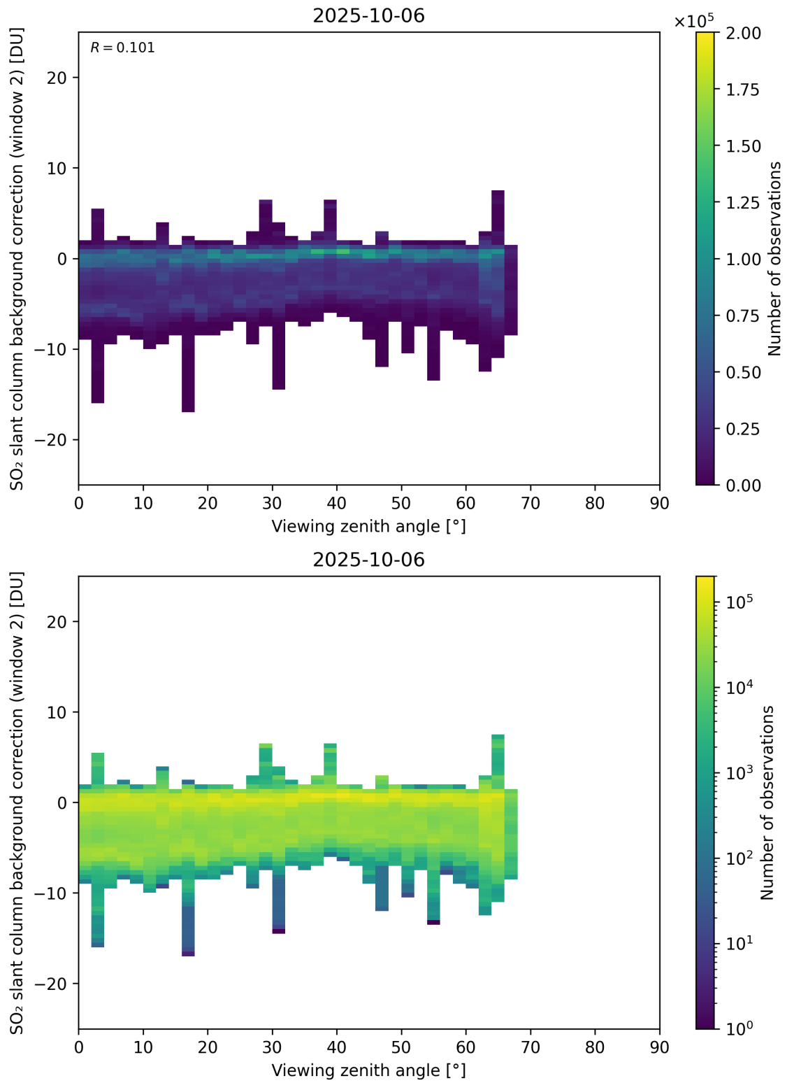
Figure 363: Scatter density plot of “Viewing zenith angle” against “SO 2 slant column background correction (window 2)” for 2025-10-06 to 2025-10-07.
