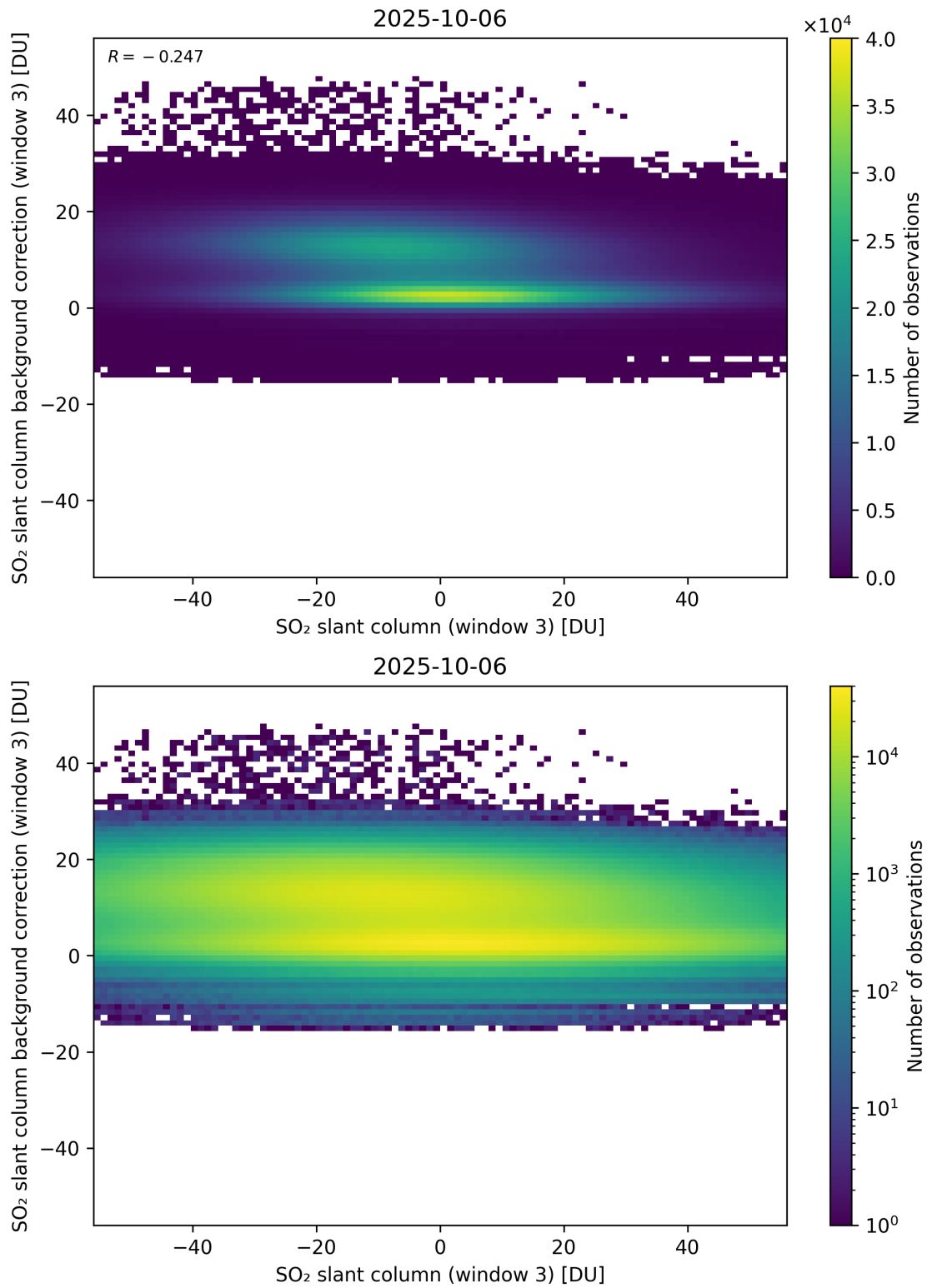
Figure 303: Scatter density plot of “SO 2 slant column (window 3)” against “SO 2 slant column background correction (window 3)” for 2025-10-06 to 2025-10-07.
