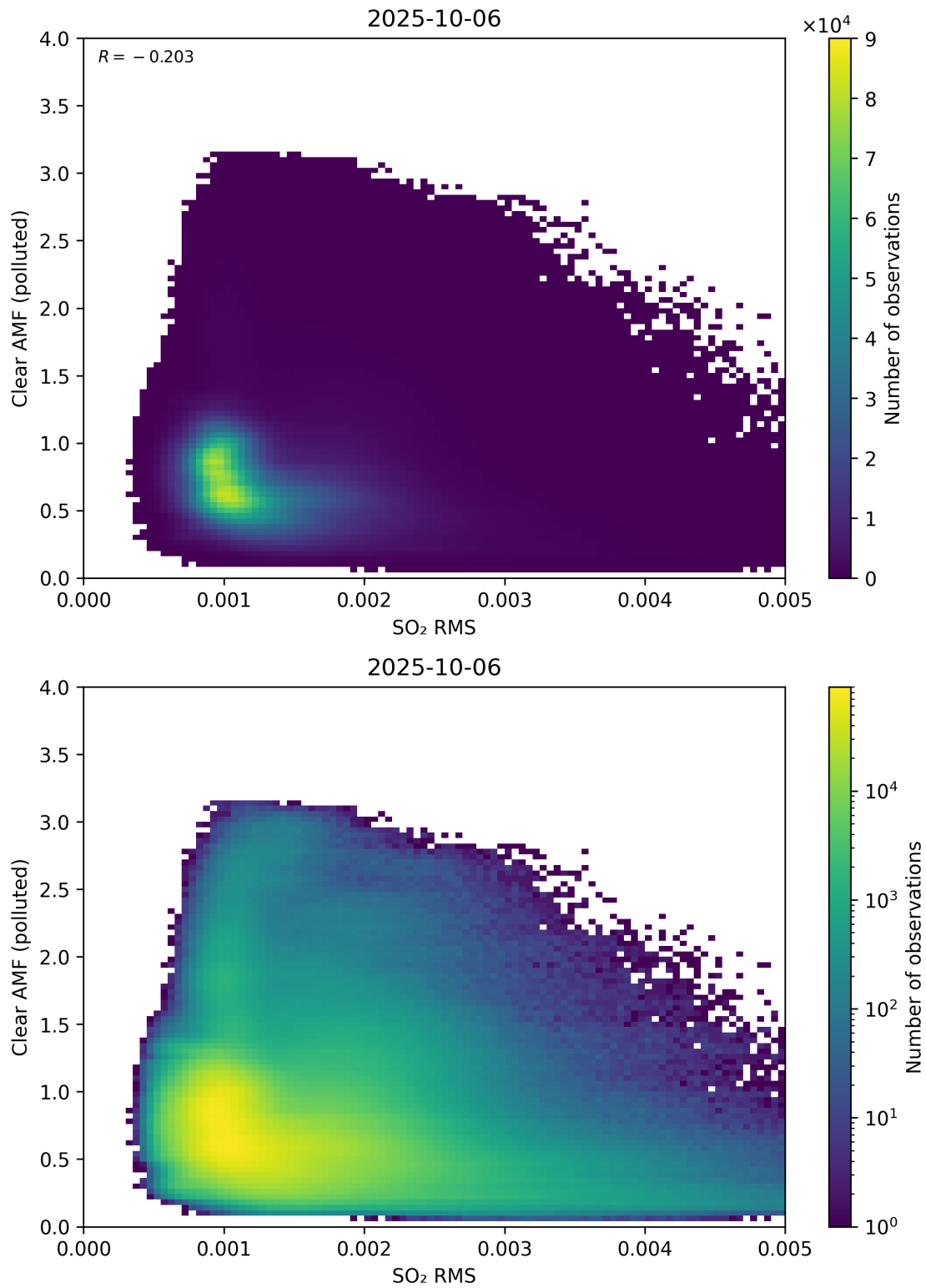
Figure 147: Scatter density plot of “SO 2 RMS” against “Clear AMF (polluted)” for 2025-10-06 to 2025-10-07.
