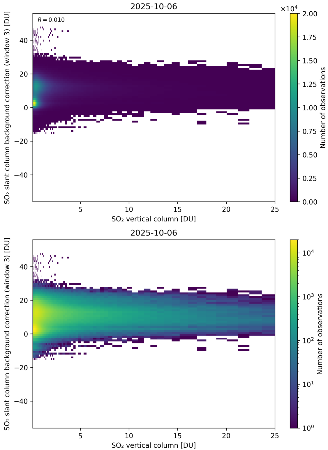
Figure 325: Scatter density plot of “SO 2 vertical column” against “SO 2 slant column background correction (window 3)” for 2025-10-06 to 2025-10-07.
