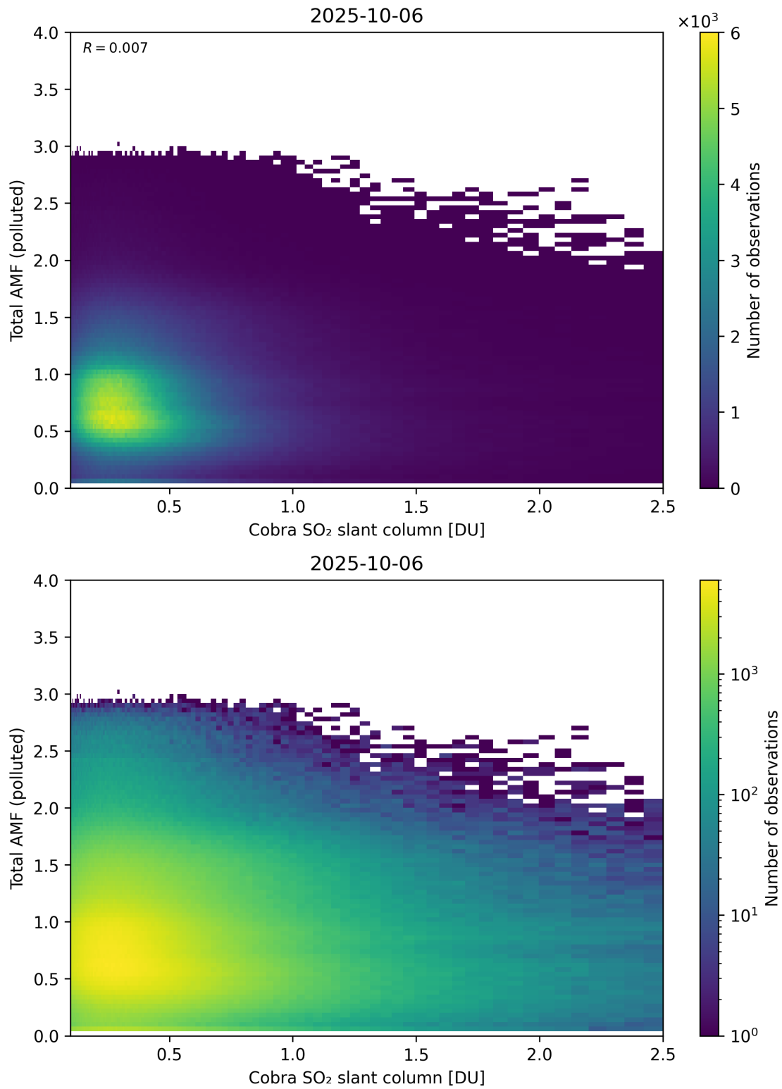
Figure 224: Scatter density plot of “Cobra SO 2 slant column” against “Total AMF (polluted)” for 2025-10-06 to 2025-10-07.
