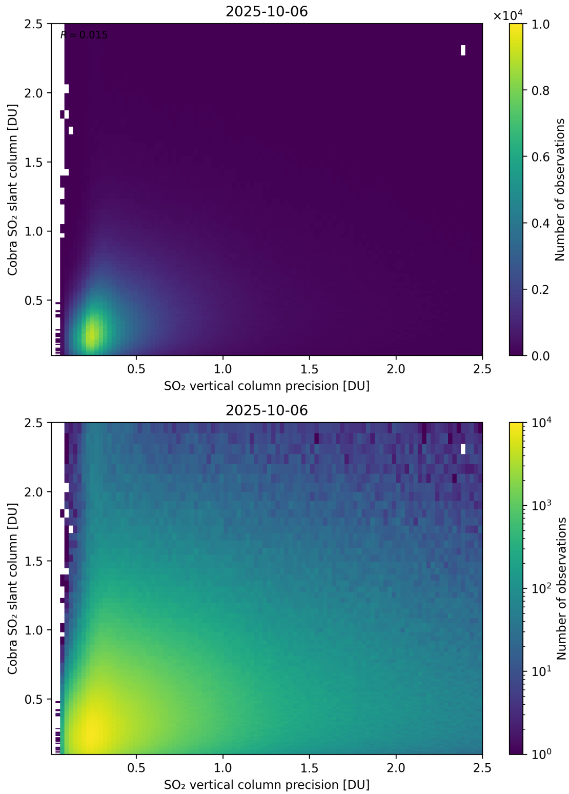
Figure 336: Scatter density plot of “SO 2 vertical column precision” against “Cobra SO 2 slant column” for 2025-10-06 to 2025-10-07.
