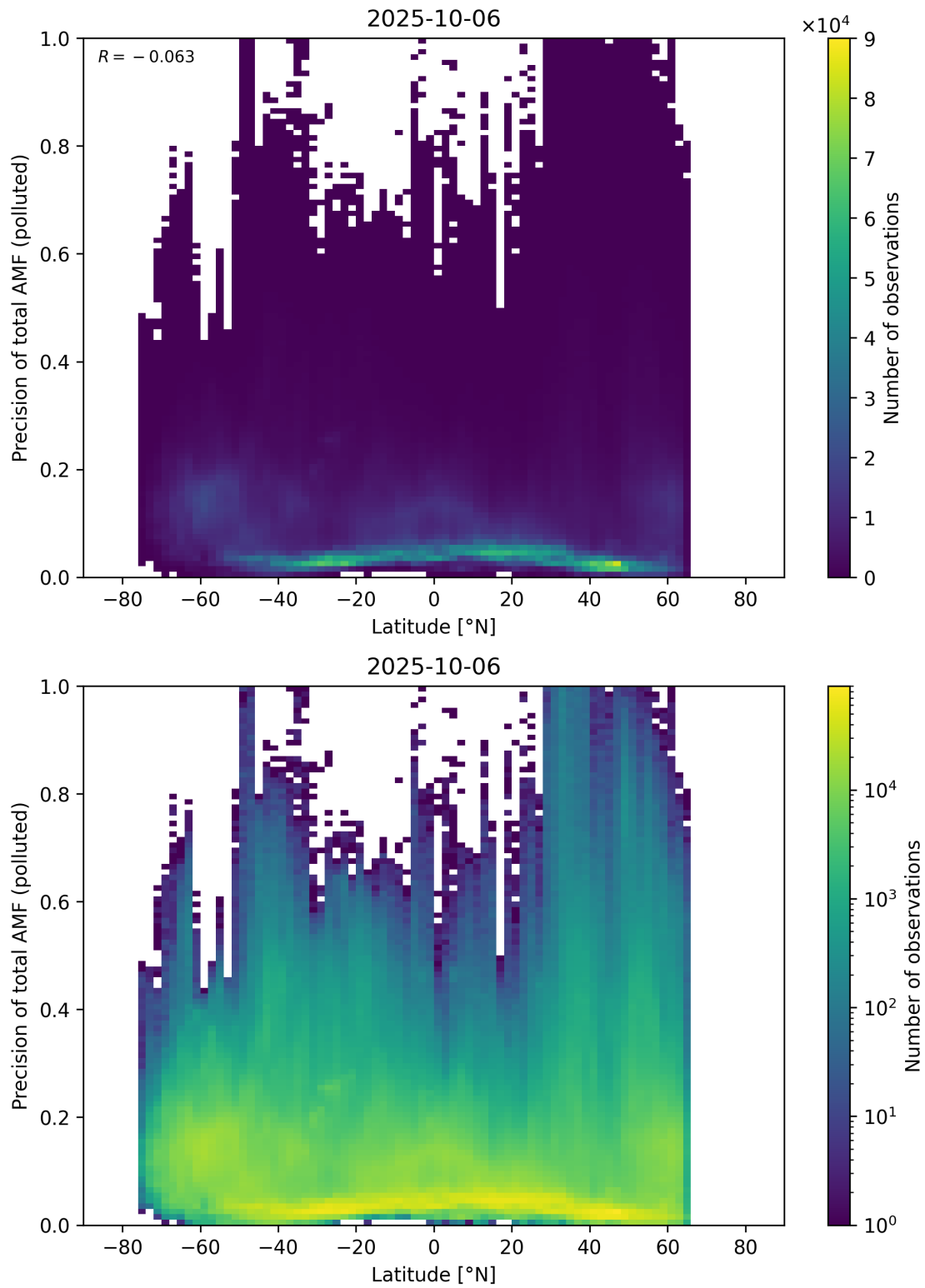
Figure 168: Scatter density plot of “Latitude” against “Precision of total AMF (polluted)” for 2025-10-06 to 2025-10-07.
