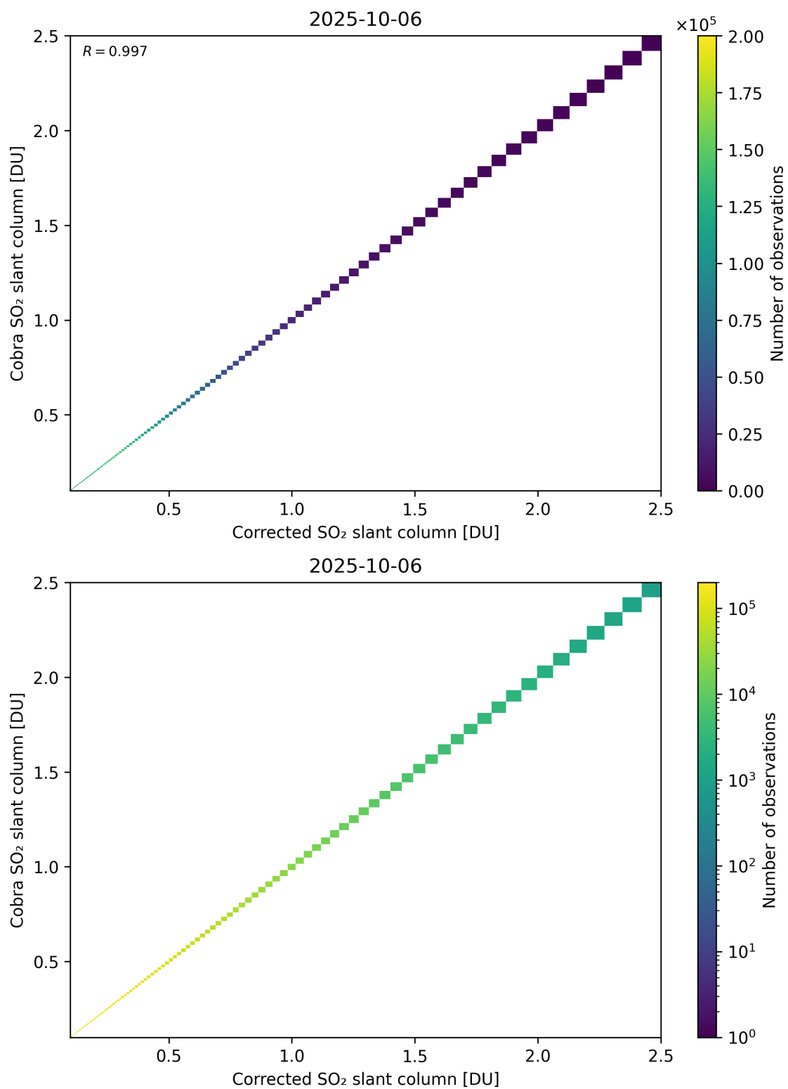
Figure 233: Scatter density plot of “Corrected SO 2 slant column” against “Cobra SO 2 slant column” for 2025-10-06 to 2025-10-07.
