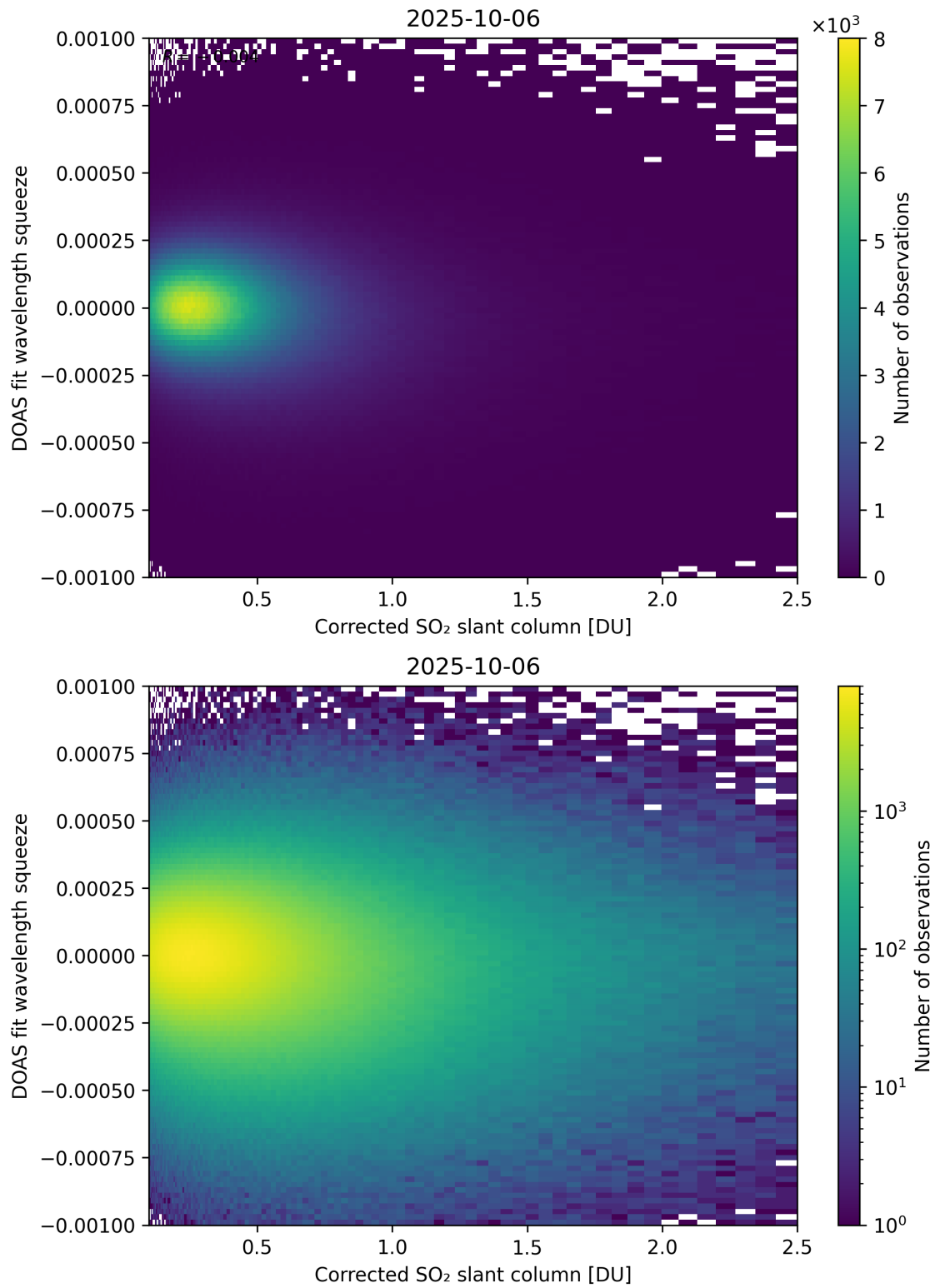
Figure 230: Scatter density plot of “Corrected SO 2 slant column” against “DOAS fit wavelength squeeze” for 2025-10-06 to 2025-10-07.
