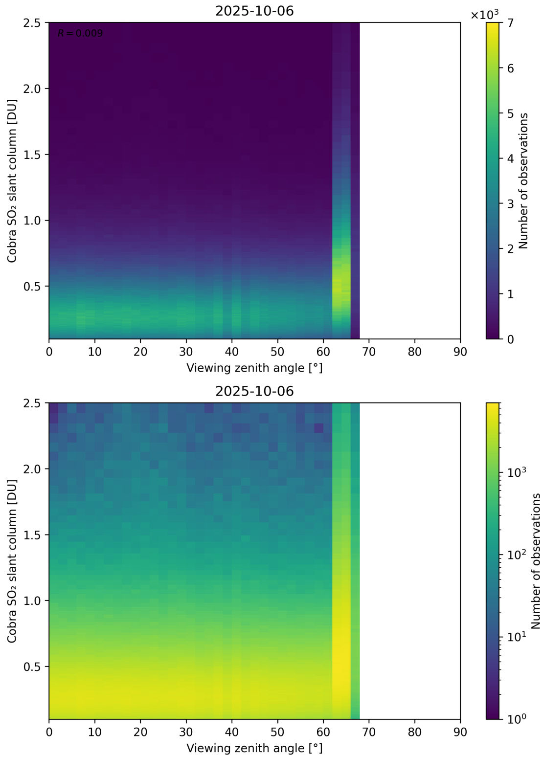
Figure 371: Scatter density plot of “Viewing zenith angle” against “Cobra SO 2 slant column” for 2025-10-06 to 2025-10-07.
