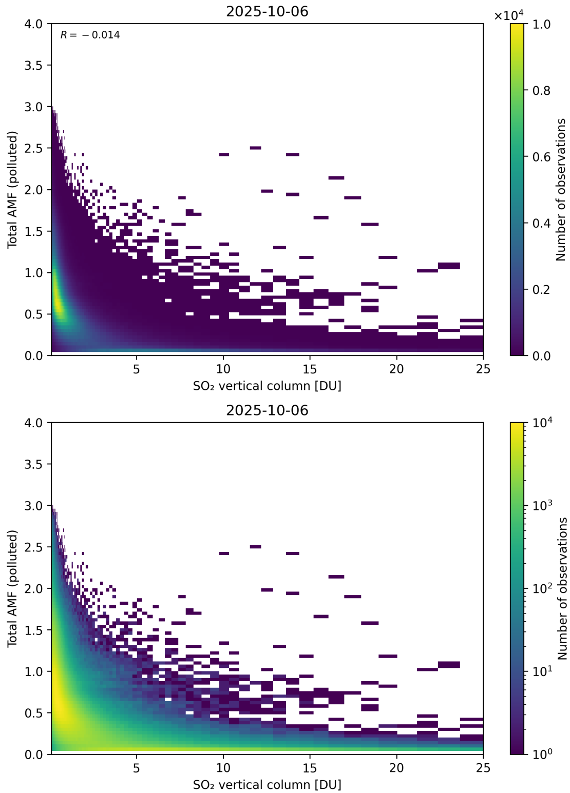
Figure 359: Scatter density plot of “SO 2 vertical column” against “Total AMF (polluted)” for 2025-10-06 to 2025-10-07.
