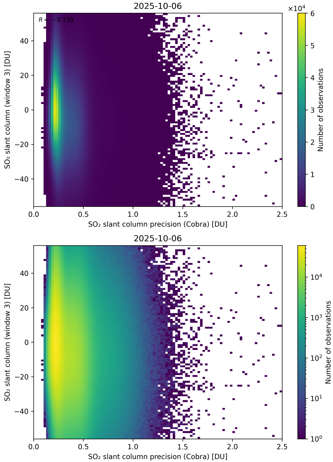
Figure 211: Scatter density plot of “SO 2 slant column precision (Cobra)” against “SO 2 slant column (window 3)” for 2025-10-06 to 2025-10-07.
