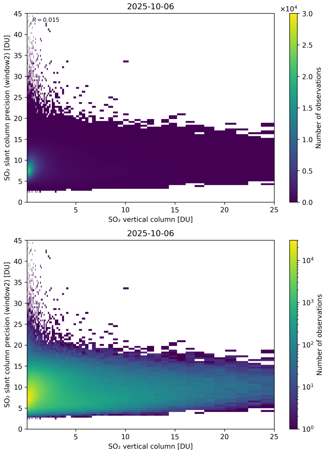
Figure 356: Scatter density plot of “SO 2 vertical column” against “SO 2 slant column precision (window2)” for 2025-10-06 to 2025-10-07.
