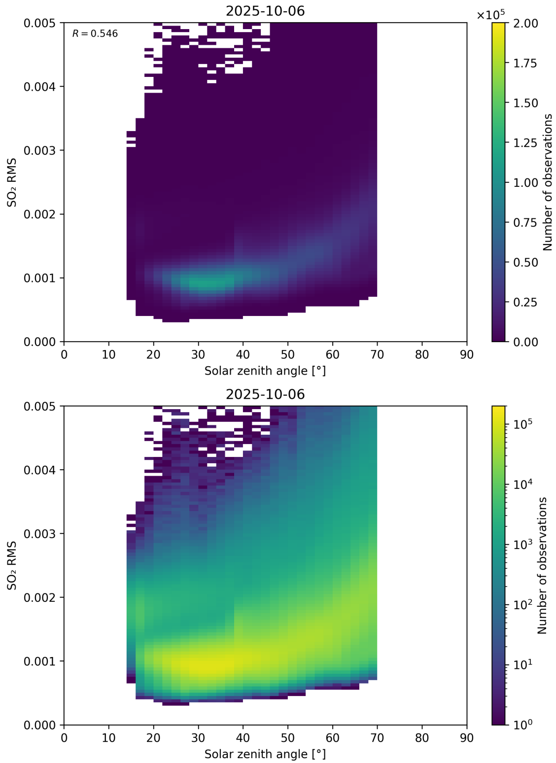
Figure 176: Scatter density plot of “Solar zenith angle” against “SO 2 RMS” for 2025-10-06 to 2025-10-07.
