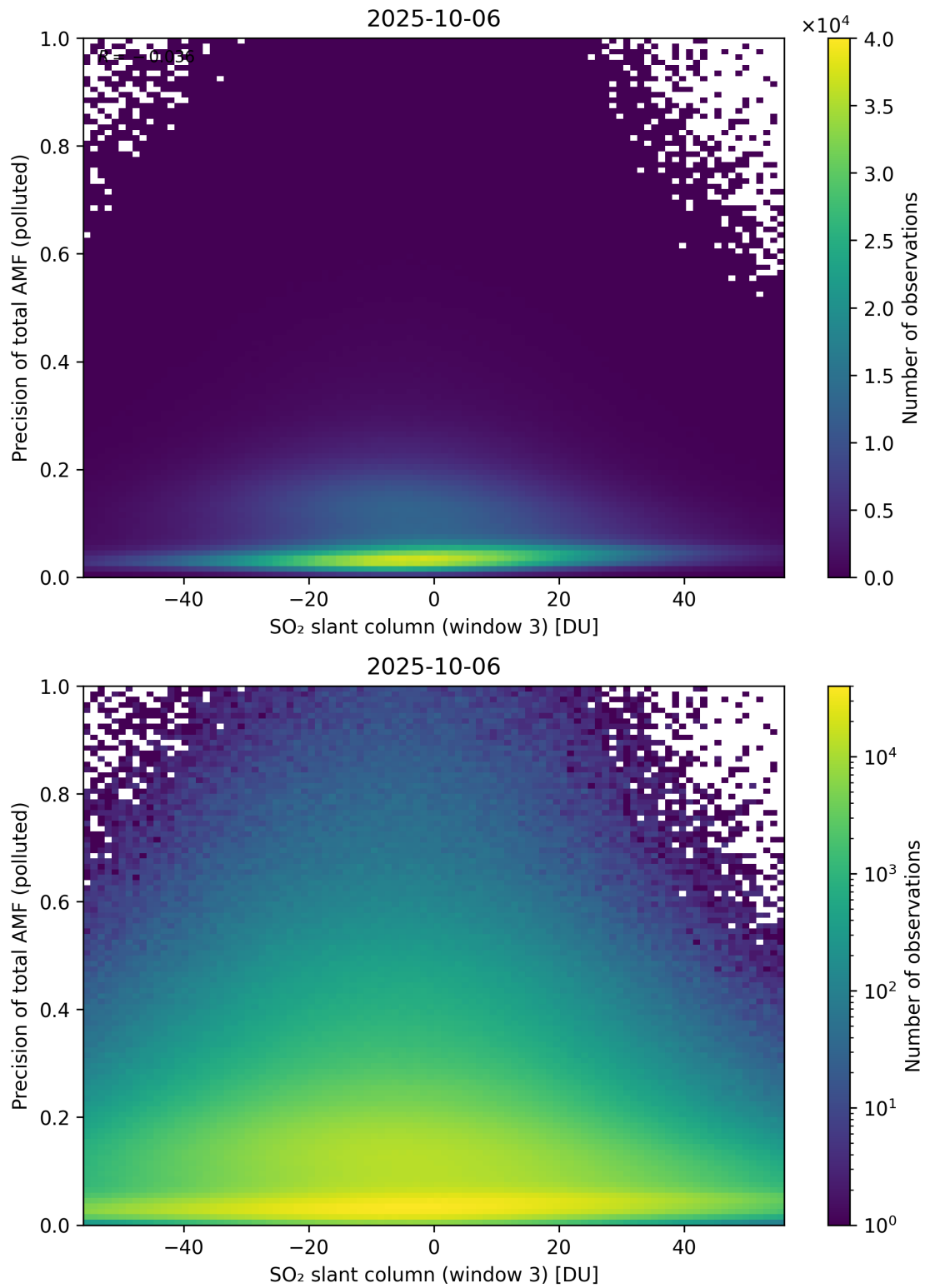
Figure 319: Scatter density plot of “SO 2 slant column (window 3)” against “Precision of total AMF (polluted)” for 2025-10-06 to 2025-10-07.
