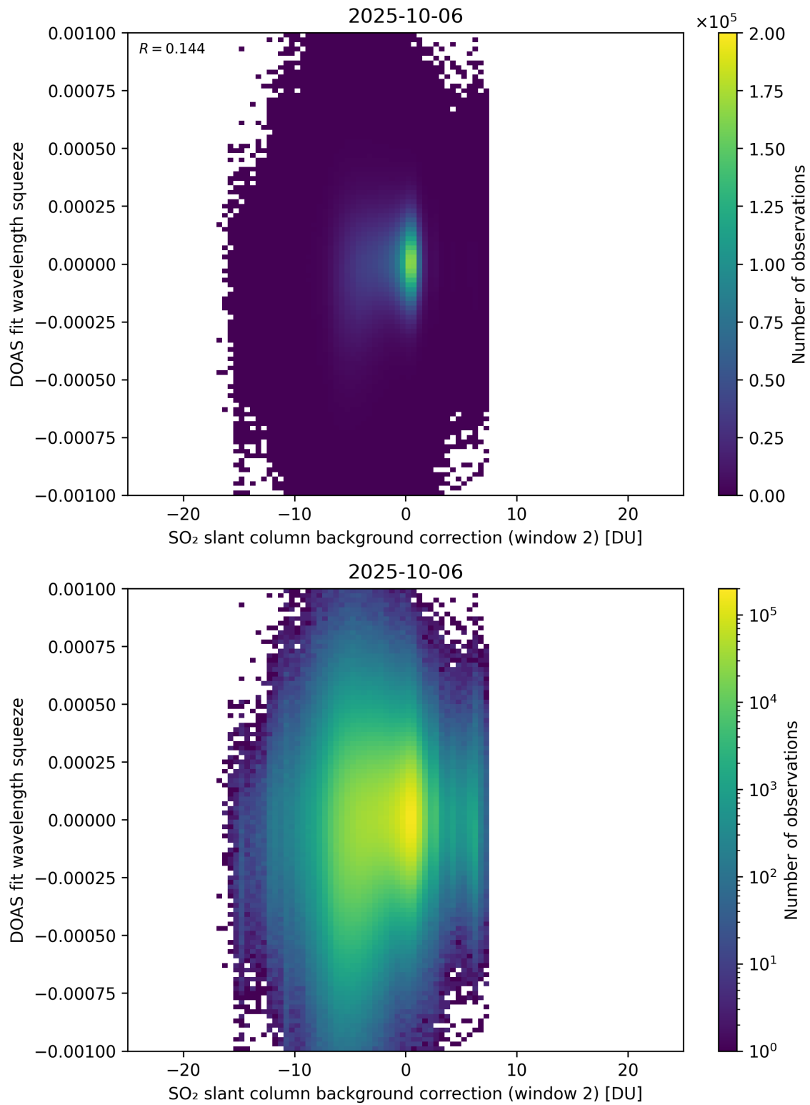
Figure 124: Scatter density plot of “SO 2 slant column background correction (window 2)” against “DOAS fit wavelength squeeze” for 2025-10-06 to 2025-10-07.
