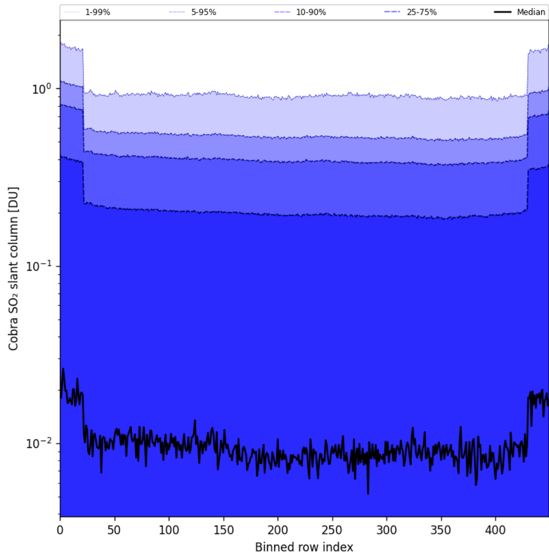
Figure 87: Along track statistics of “Cobra SO 2 slant column” for 2025-10-06 to 2025-10-07
