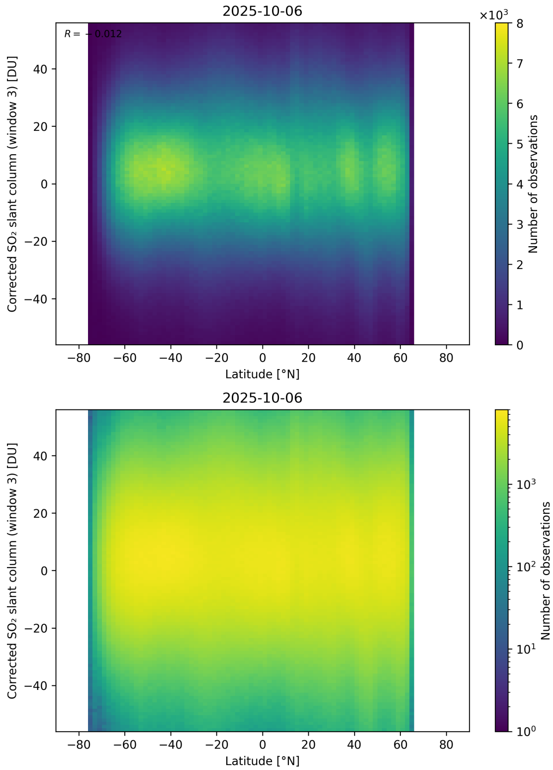
Figure 161: Scatter density plot of “Latitude” against “Corrected SO 2 slant column (window 3)” for 2025-10-06 to 2025-10-07.
