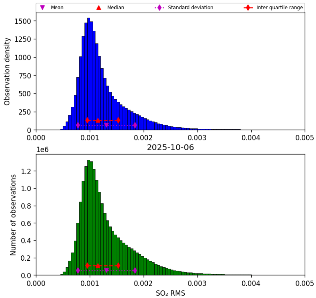
Figure 78: Histogram of “SO 2 RMS” for 2025-10-06 to 2025-10-07
