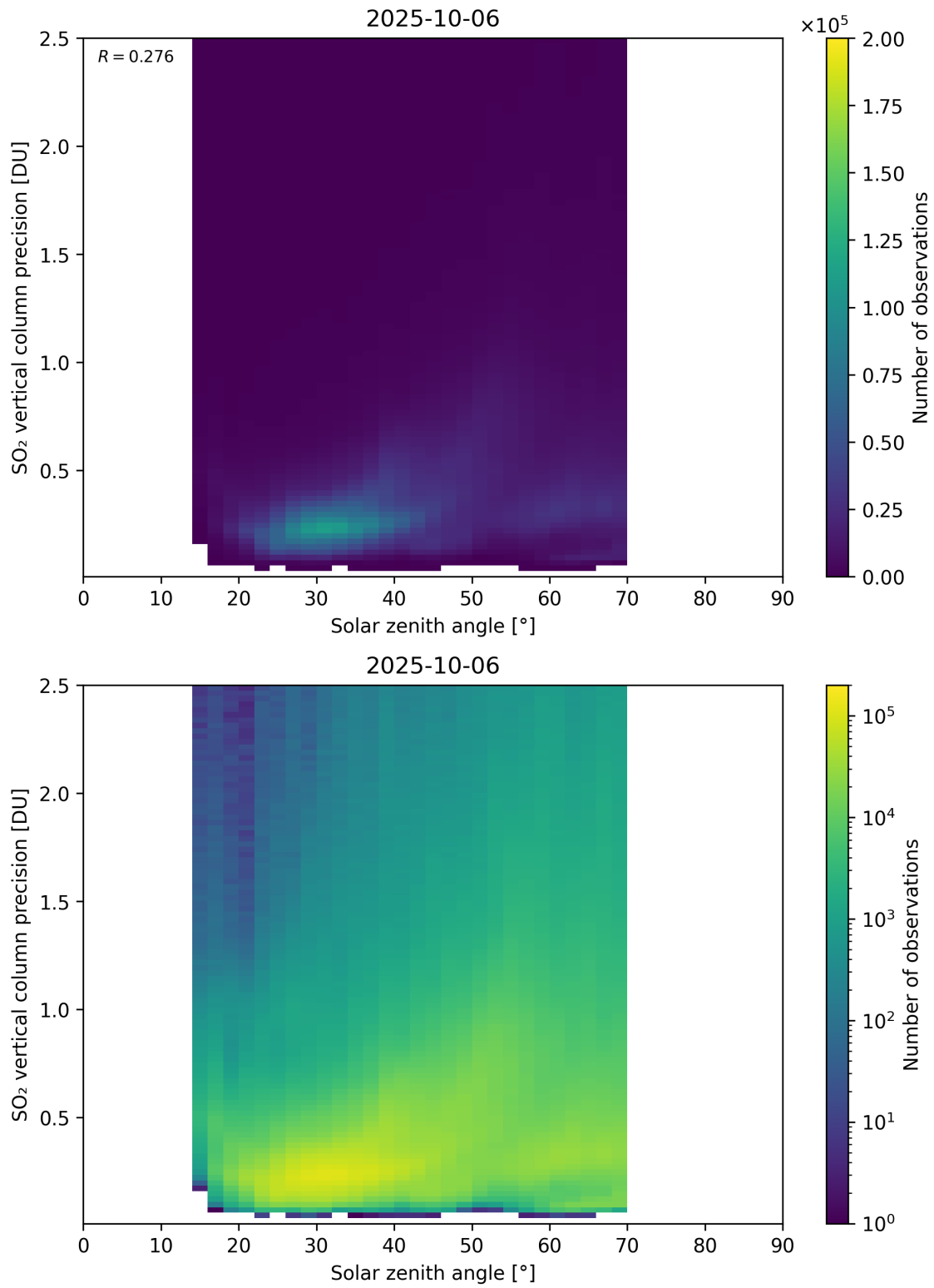
Figure 192: Scatter density plot of “Solar zenith angle” against “SO 2 vertical column precision” for 2025-10-06 to 2025-10-07.
