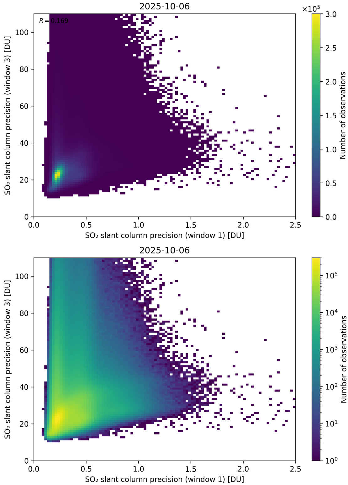
Figure 279: Scatter density plot of “SO 2 slant column precision (window 1)” against “SO 2 slant column precision (window 3)” for 2025-10-06 to 2025-10-07.
