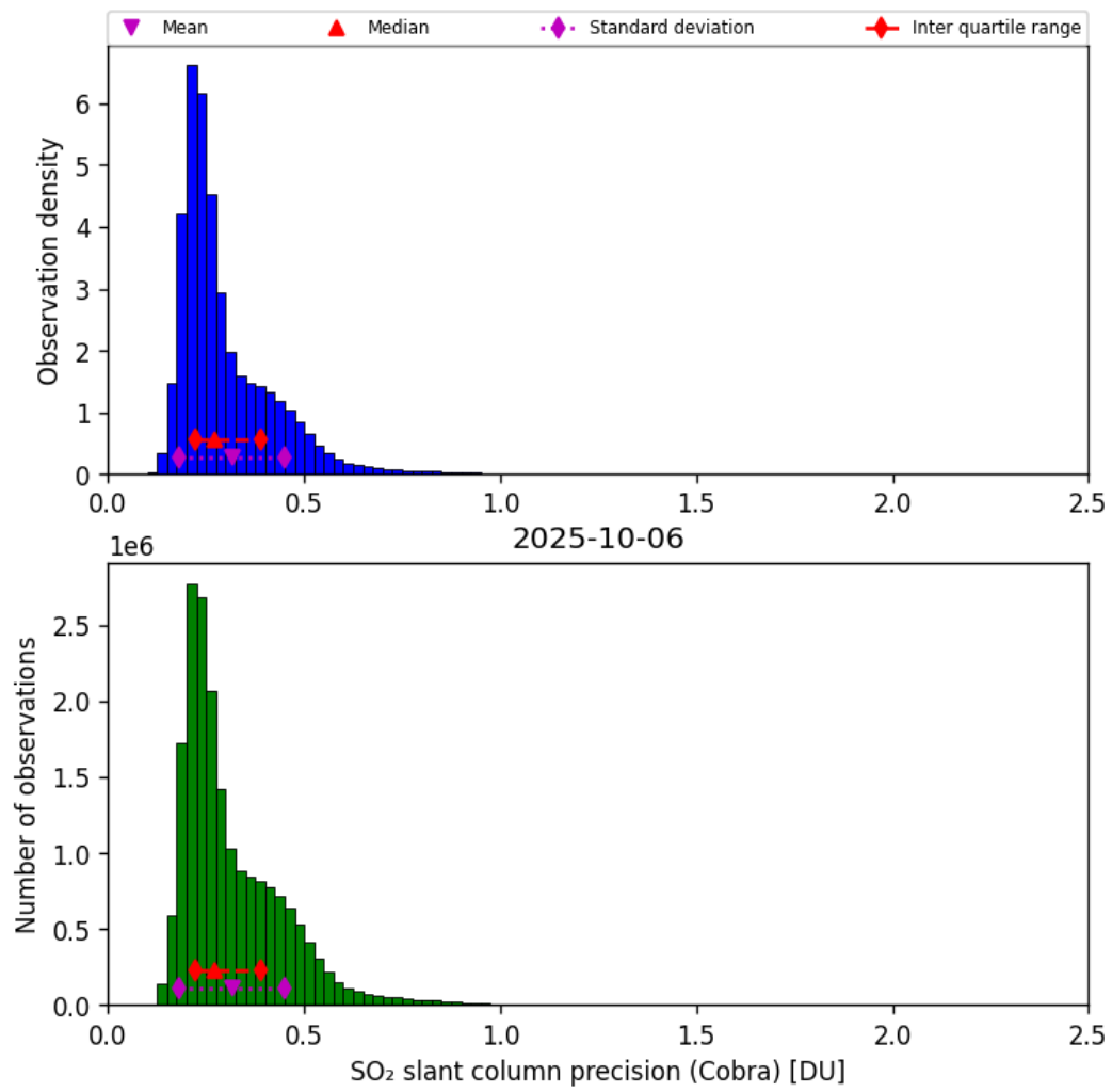
Figure 62: Histogram of “SO 2 slant column precision (Cobra)” for 2025-10-06 to 2025-10-07
