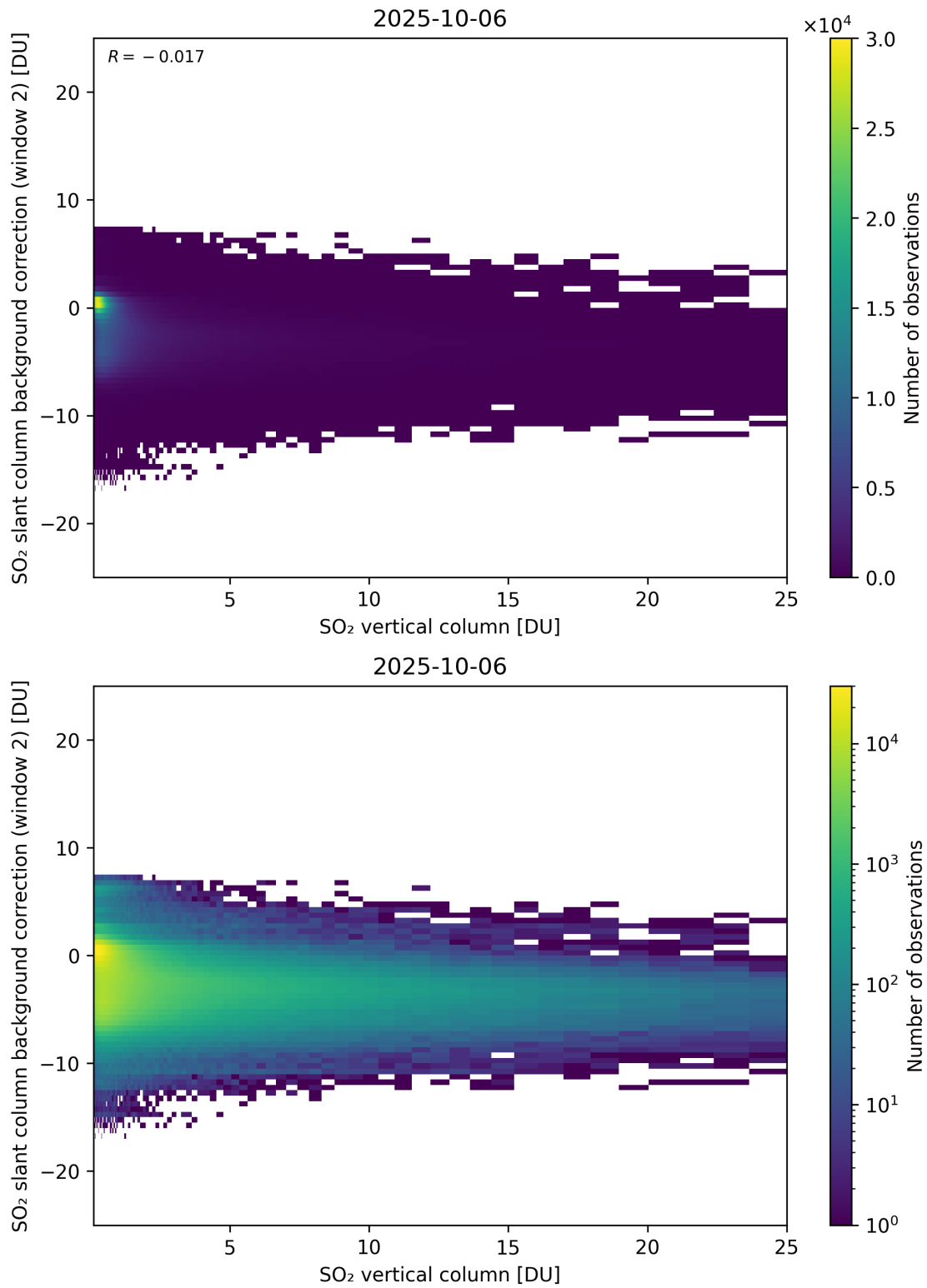
Figure 324: Scatter density plot of “SO 2 vertical column” against “SO 2 slant column background correction (window 2)” for 2025-10-06 to 2025-10-07.
