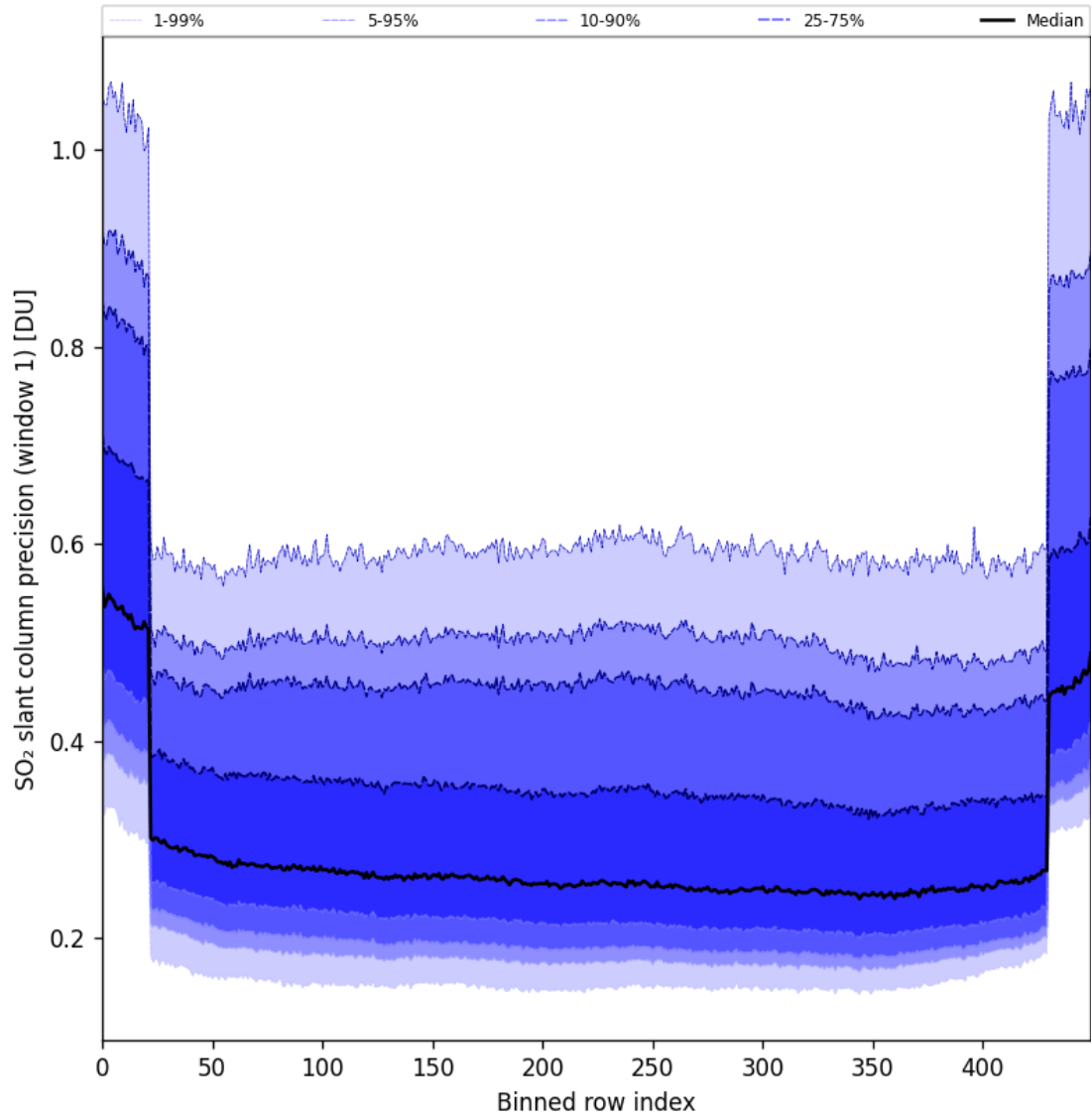
Figure 90: Along track statistics of “SO 2 slant column precision (window 1)” for 2025-10-06 to 2025-10-07
