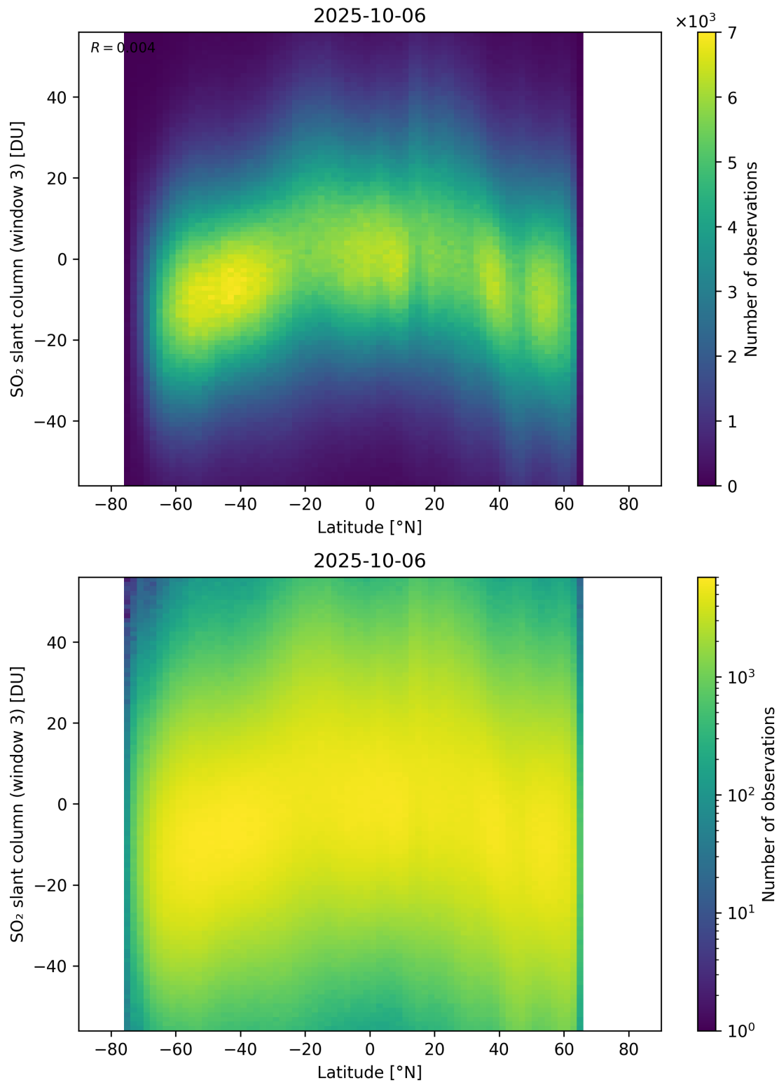
Figure 165: Scatter density plot of “Latitude” against “SO 2 slant column (window 3)” for 2025-10-06 to 2025-10-07.
