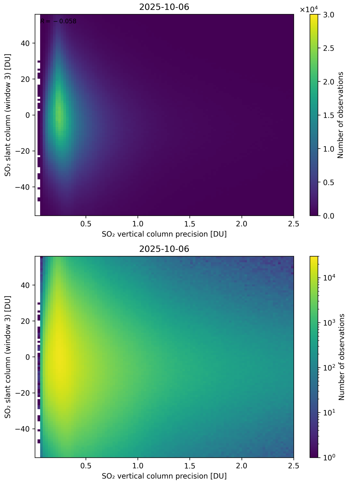
Figure 344: Scatter density plot of “SO 2 vertical column precision” against “SO 2 slant column (window 3)” for 2025-10-06 to 2025-10-07.
