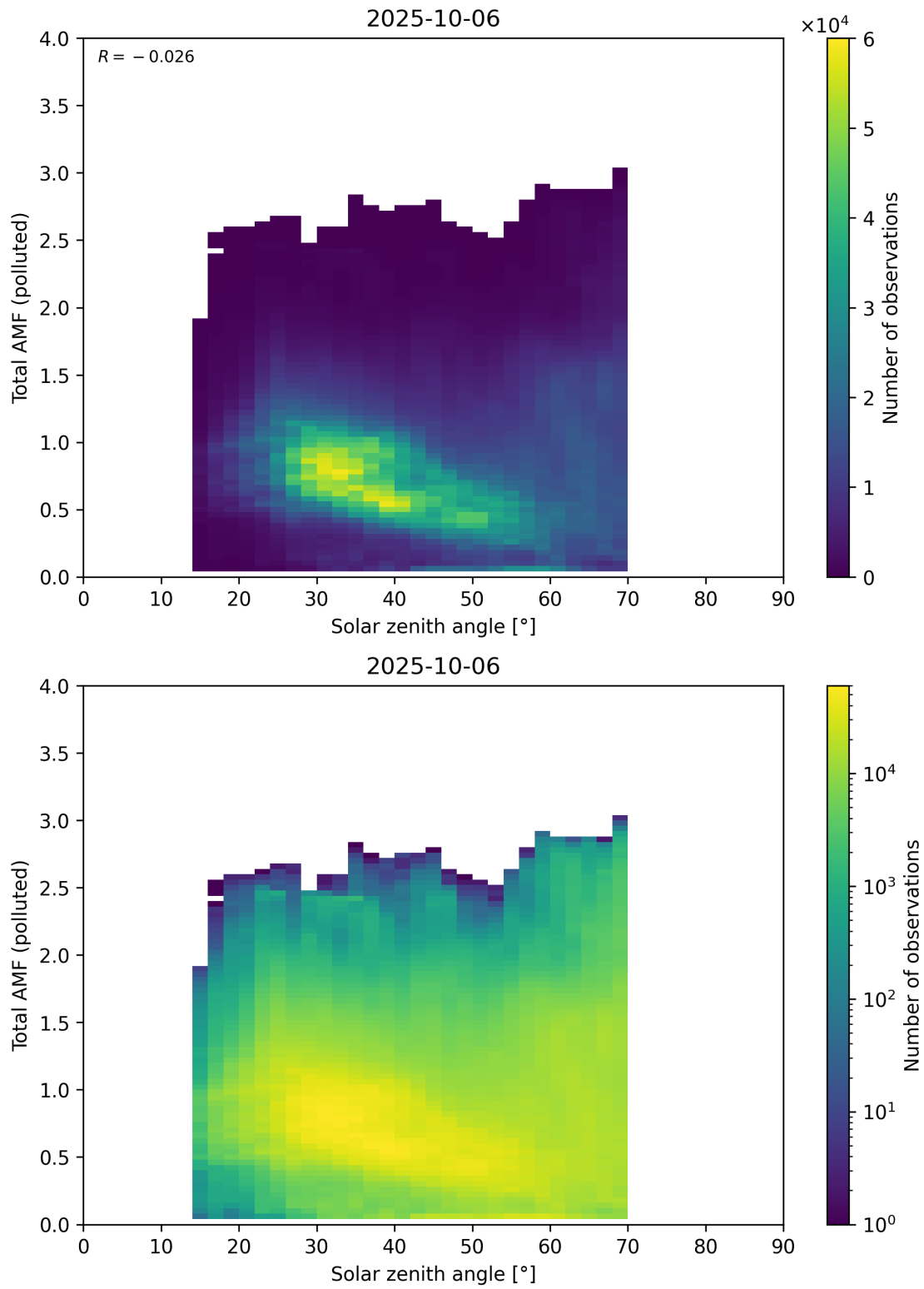
Figure 189: Scatter density plot of “Solar zenith angle” against “Total AMF (polluted)” for 2025-10-06 to 2025-10-07.
