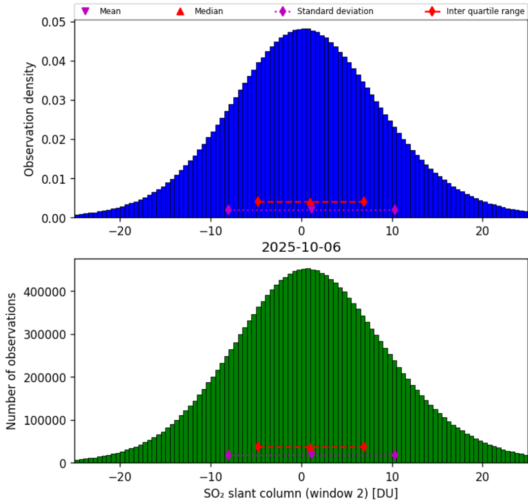
Figure 67: Histogram of “SO 2 slant column (window 2)” for 2025-10-06 to 2025-10-07
