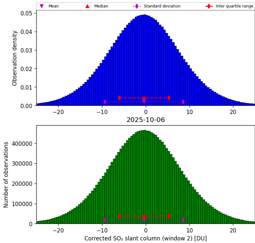
Figure 69: Histogram of “Corrected SO 2 slant column (window 2)” for 2025-10-06 to 2025-10-07
