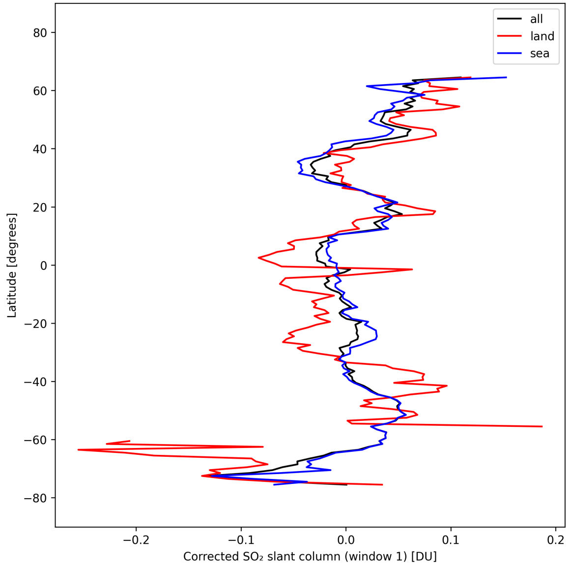
Figure 39: Zonal average of “Corrected SO 2 slant column (window 1)” for 2025-10-06 to 2025-10-07.
