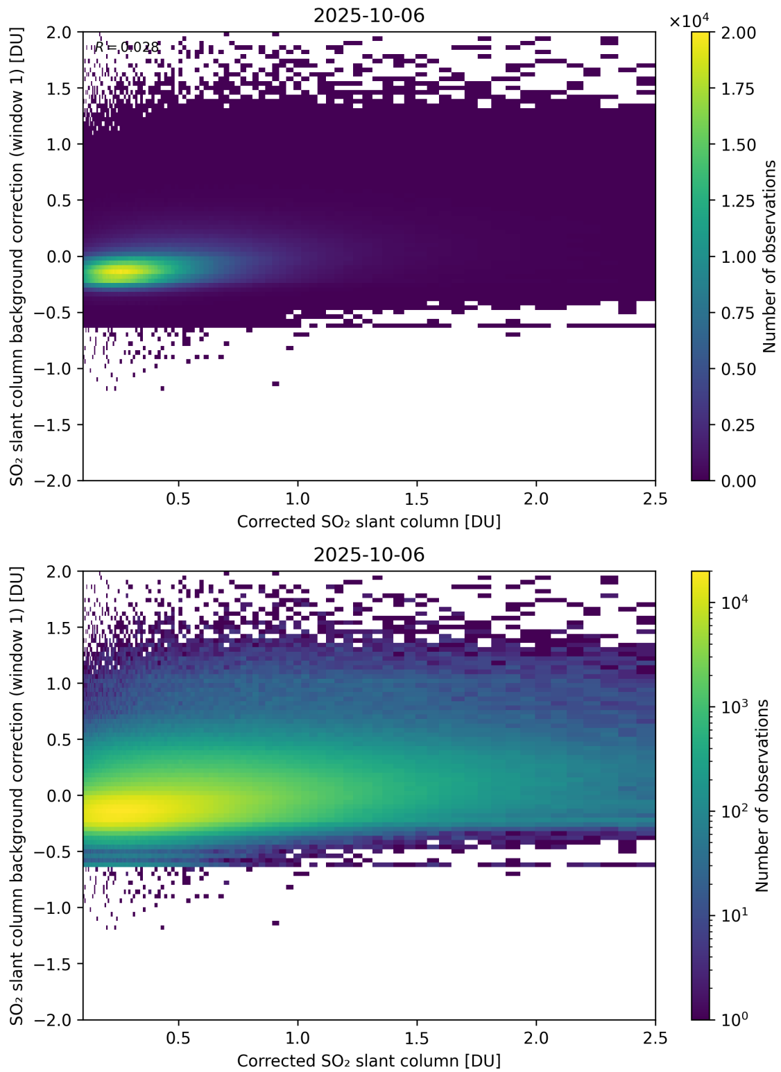
Figure 226: Scatter density plot of “Corrected SO 2 slant column” against “SO 2 slant column background correction (window 1)” for 2025-10-06 to 2025-10-07.
