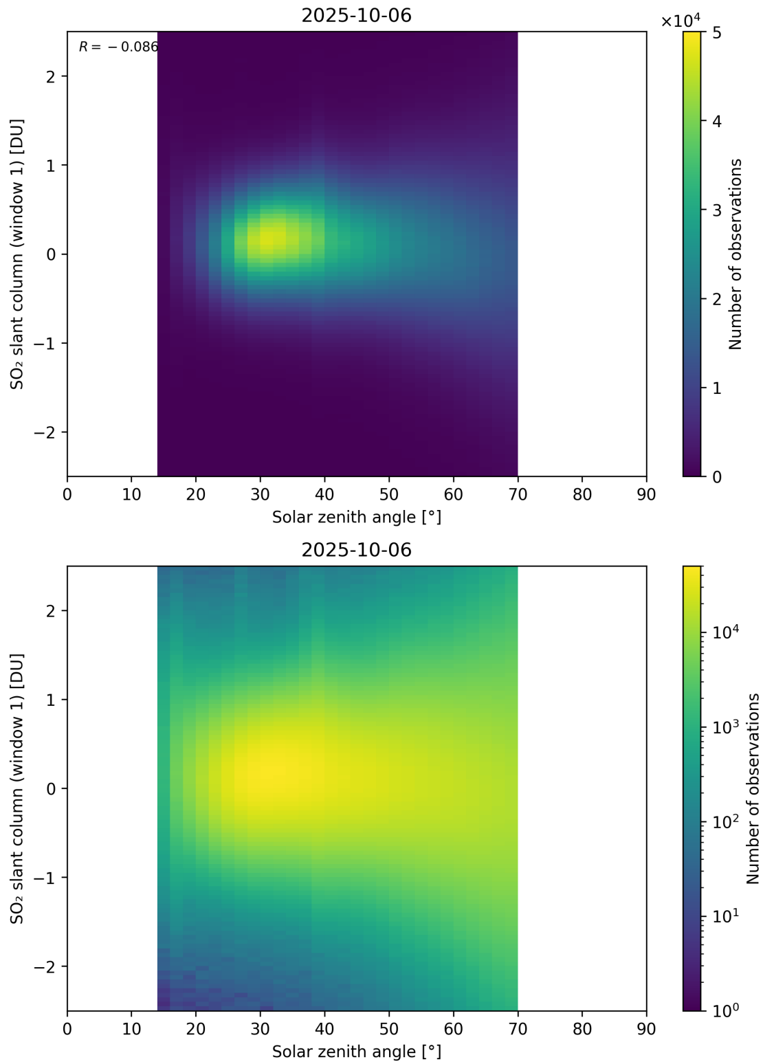
Figure 184: Scatter density plot of “Solar zenith angle” against “SO 2 slant column (window 1)” for 2025-10-06 to 2025-10-07.
