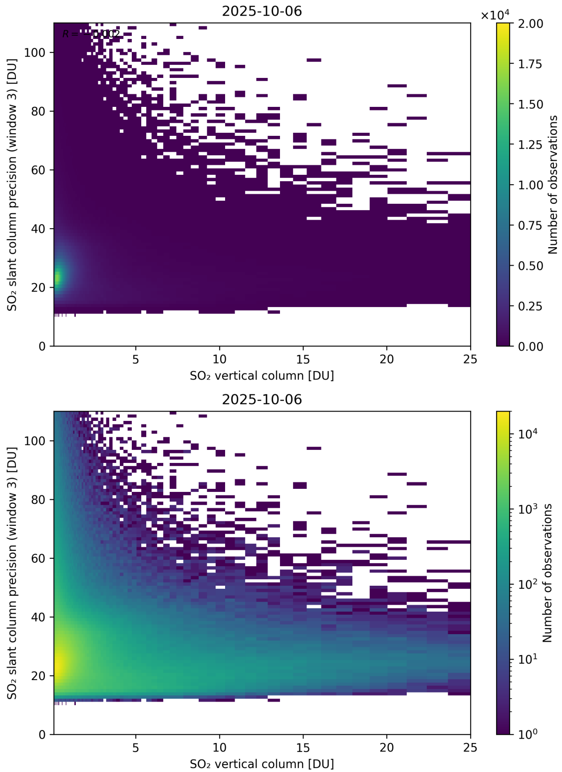
Figure 358: Scatter density plot of “SO 2 vertical column” against “SO 2 slant column precision (window 3)” for 2025-10-06 to 2025-10-07.
