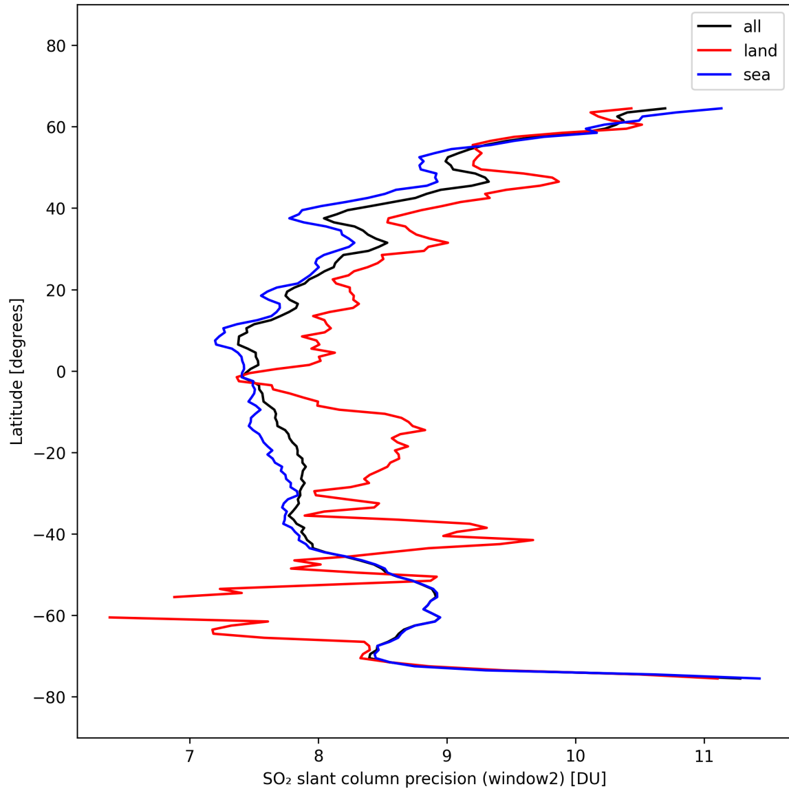
Figure 42: Zonal average of “SO 2 slant column precision (window2)” for 2025-10-06 to 2025-10-07.
