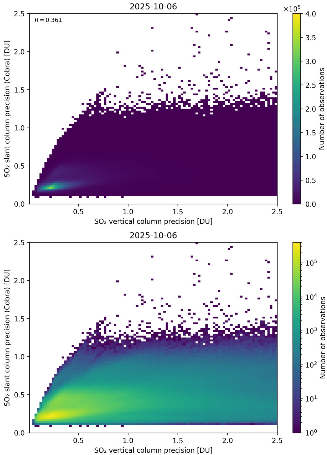
Figure 337: Scatter density plot of “SO 2 vertical column precision” against “SO 2 slant column precision (Cobra)” for 2025-10-06 to 2025-10-07.
