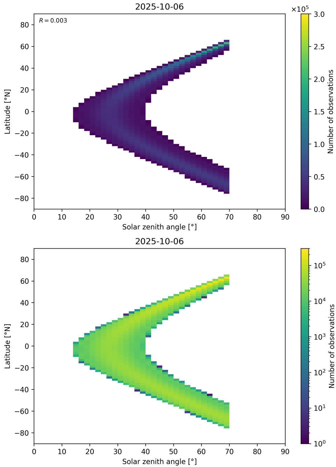
Figure 177: Scatter density plot of “Solar zenith angle” against “Latitude” for 2025-10-06 to 2025-10-07.
