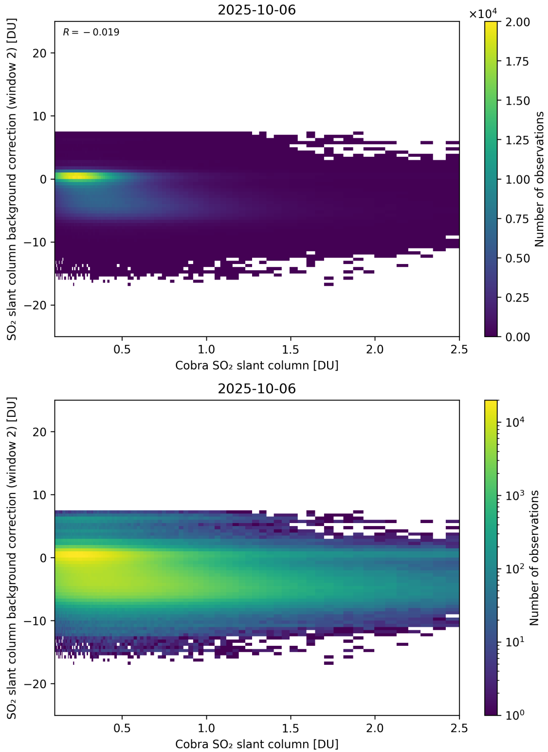
Figure 194: Scatter density plot of “Cobra SO 2 slant column” against “SO 2 slant column background correction (window 2)” for 2025-10-06 to 2025-10-07.
