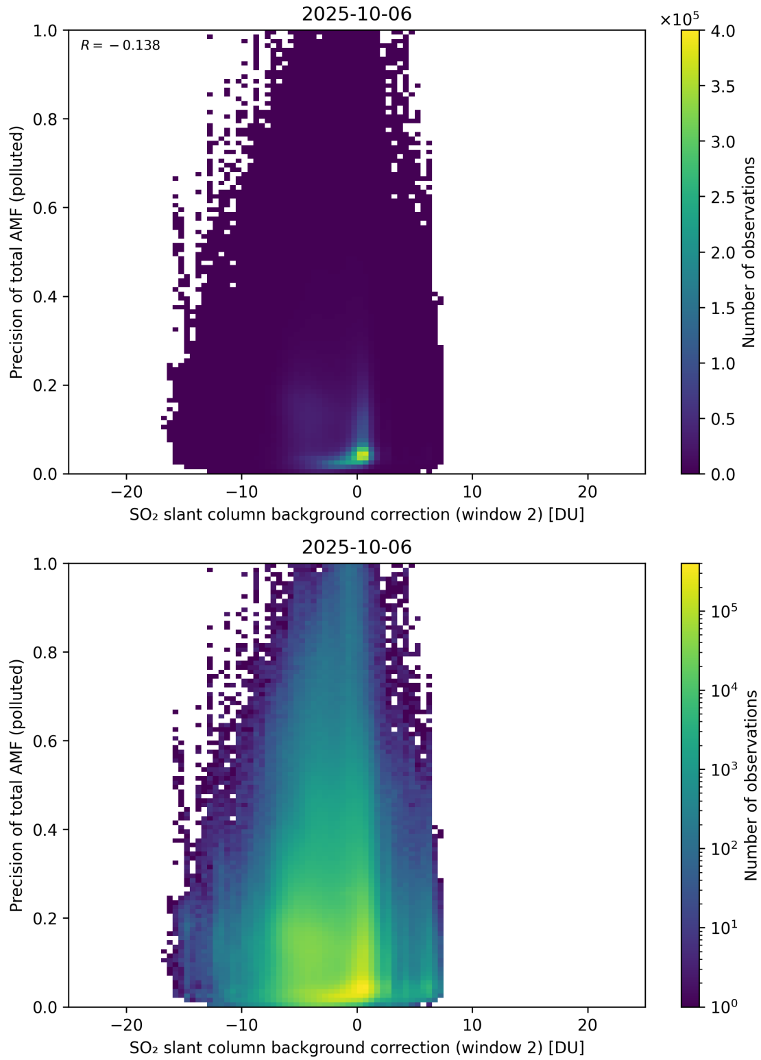
Figure 131: Scatter density plot of “SO 2 slant column background correction (window 2)” against “Precision of total AMF (polluted)” for 2025-10-06 to 2025-10-07.
