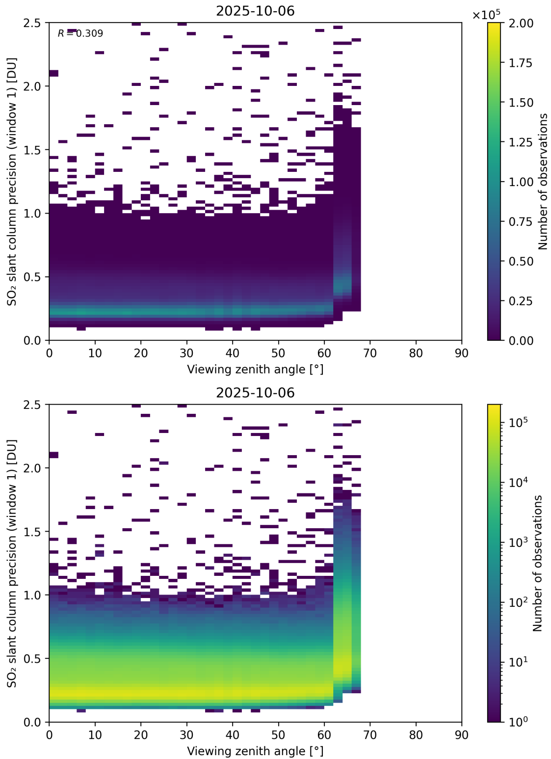
Figure 377: Scatter density plot of “Viewing zenith angle” against “SO 2 slant column precision (window 1)” for 2025-10-06 to 2025-10-07.
