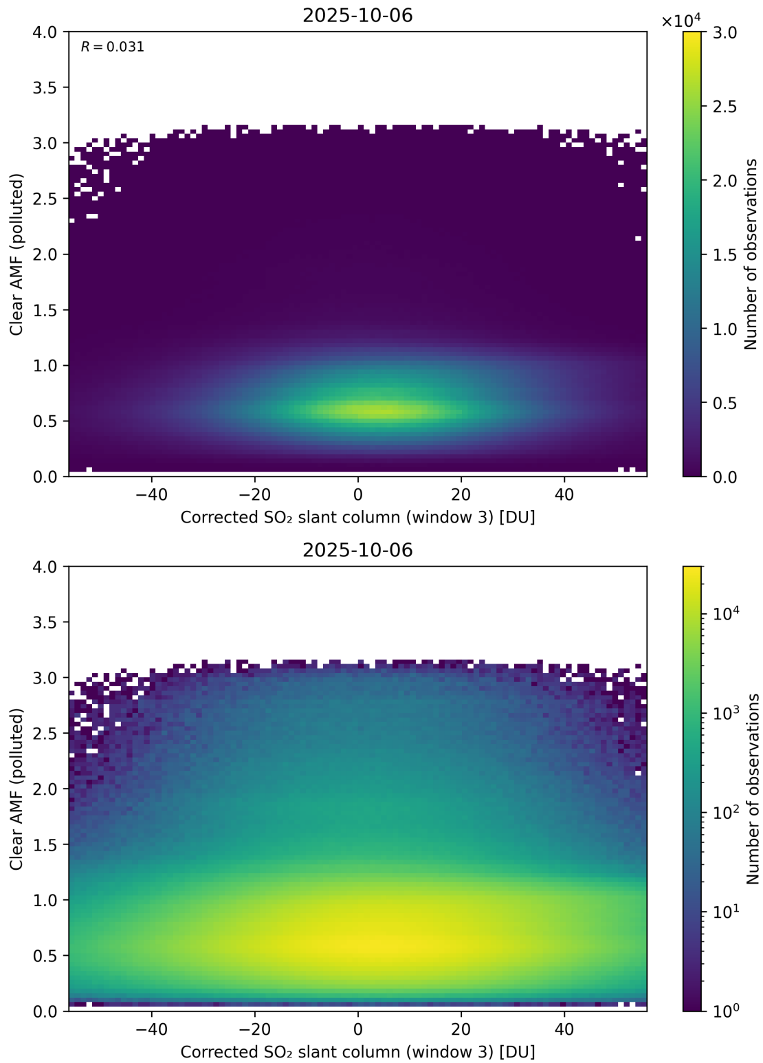
Figure 259: Scatter density plot of “Corrected SO 2 slant column (window 3)” against “Clear AMF (polluted)” for 2025-10-06 to 2025-10-07.
