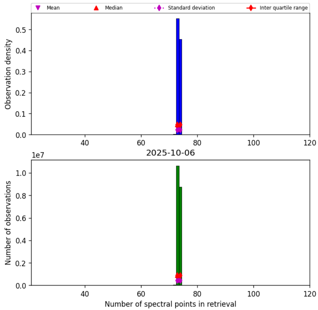
Figure 82: Histogram of “Number of spectral points in retrieval” for 2025-10-06 to 2025-10-07
