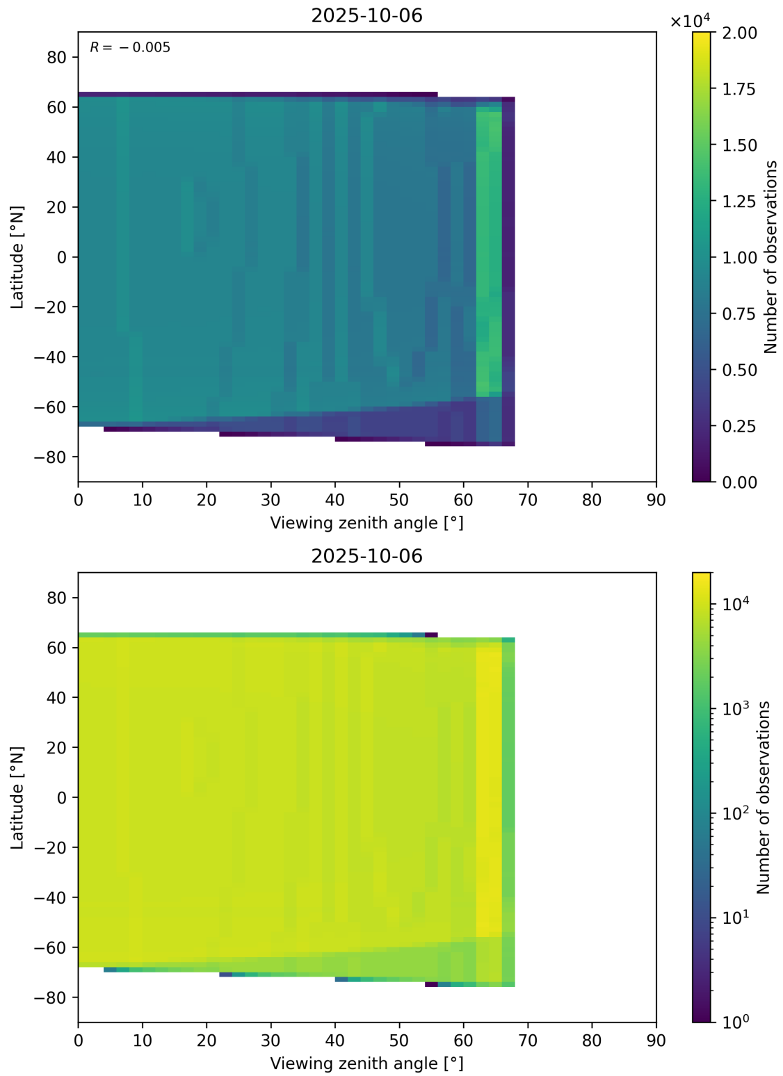
Figure 368: Scatter density plot of “Viewing zenith angle” against “Latitude” for 2025-10-06 to 2025-10-07.
