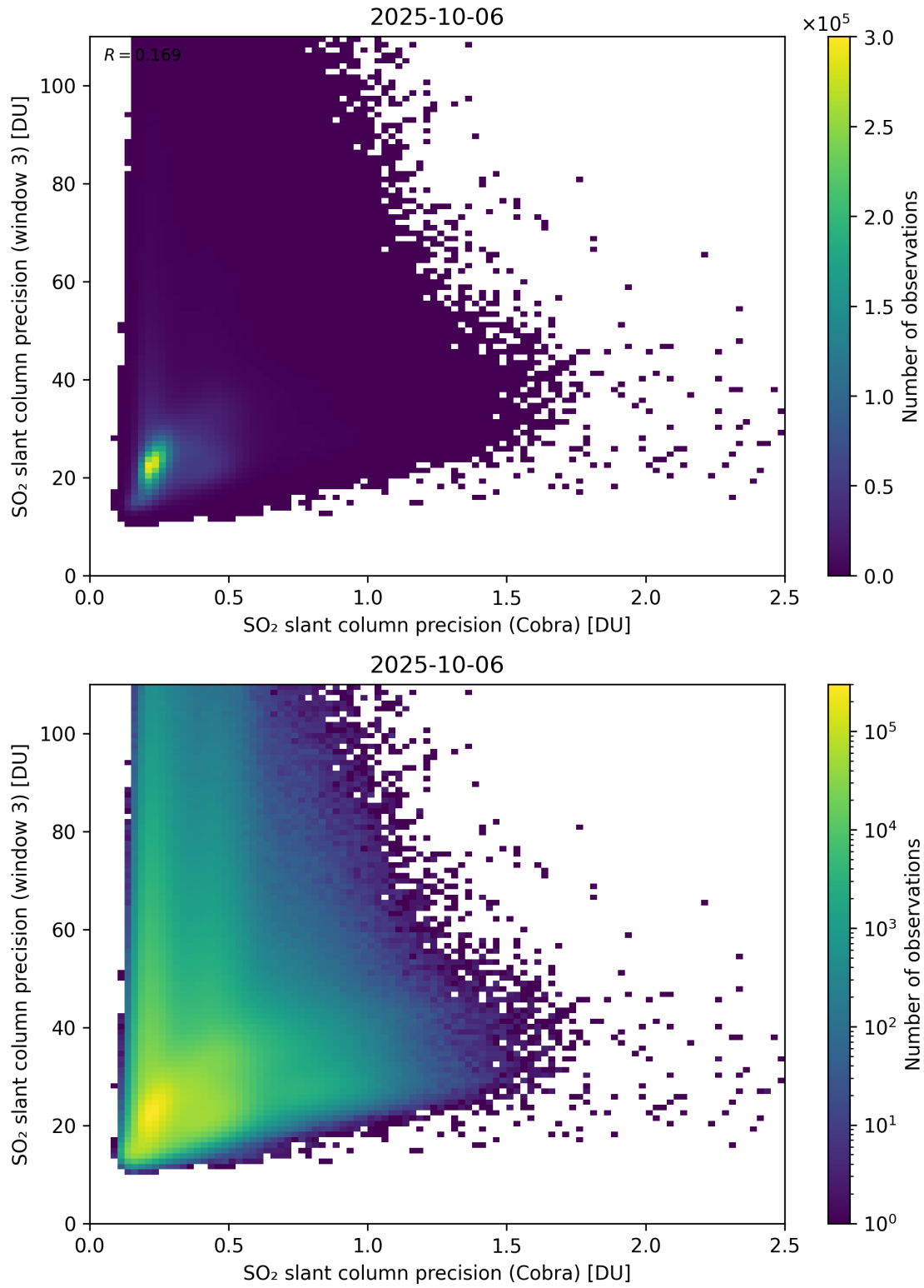
Figure 212: Scatter density plot of “SO 2 slant column precision (Cobra)” against “SO 2 slant column precision (window 3)” for 2025-10-06 to 2025-10-07.
