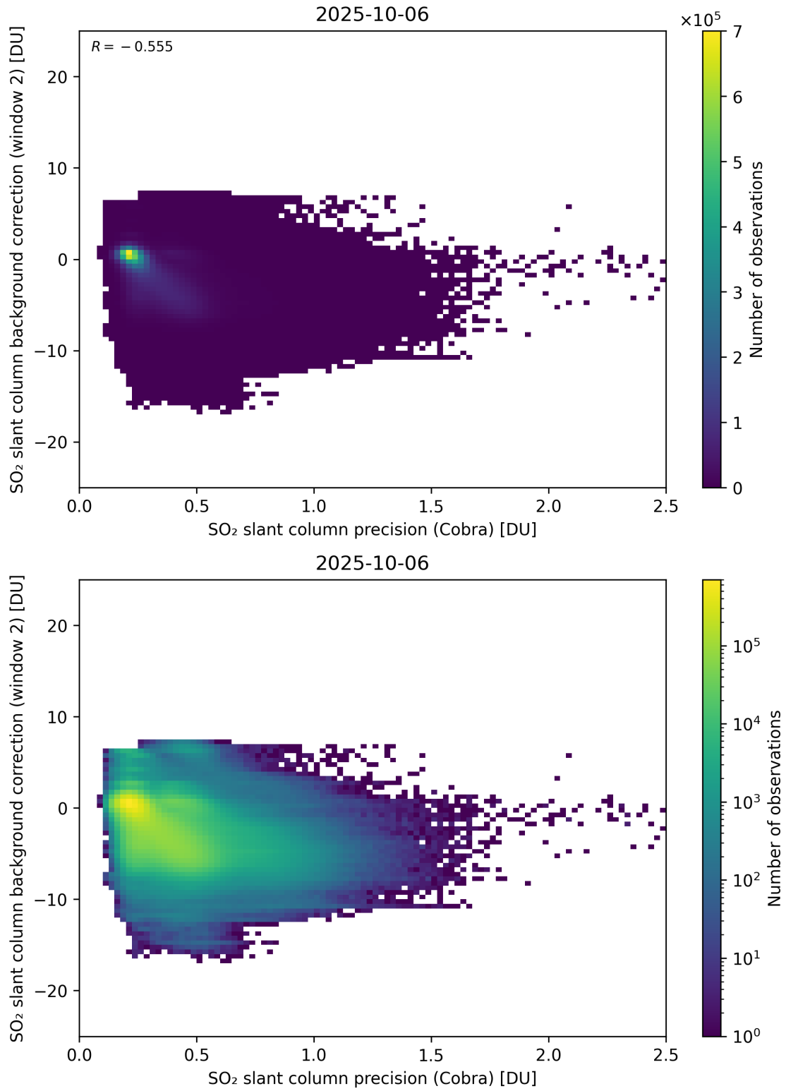
Figure 200: Scatter density plot of “SO 2 slant column precision (Cobra)” against “SO 2 slant column background correction (window 2)” for 2025-10-06 to 2025-10-07.
