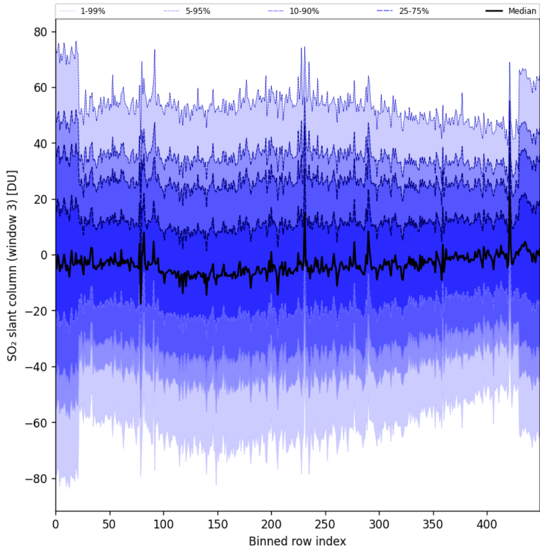
Figure 97: Along track statistics of “SO 2 slant column (window 3)” for 2025-10-06 to 2025-10-07
