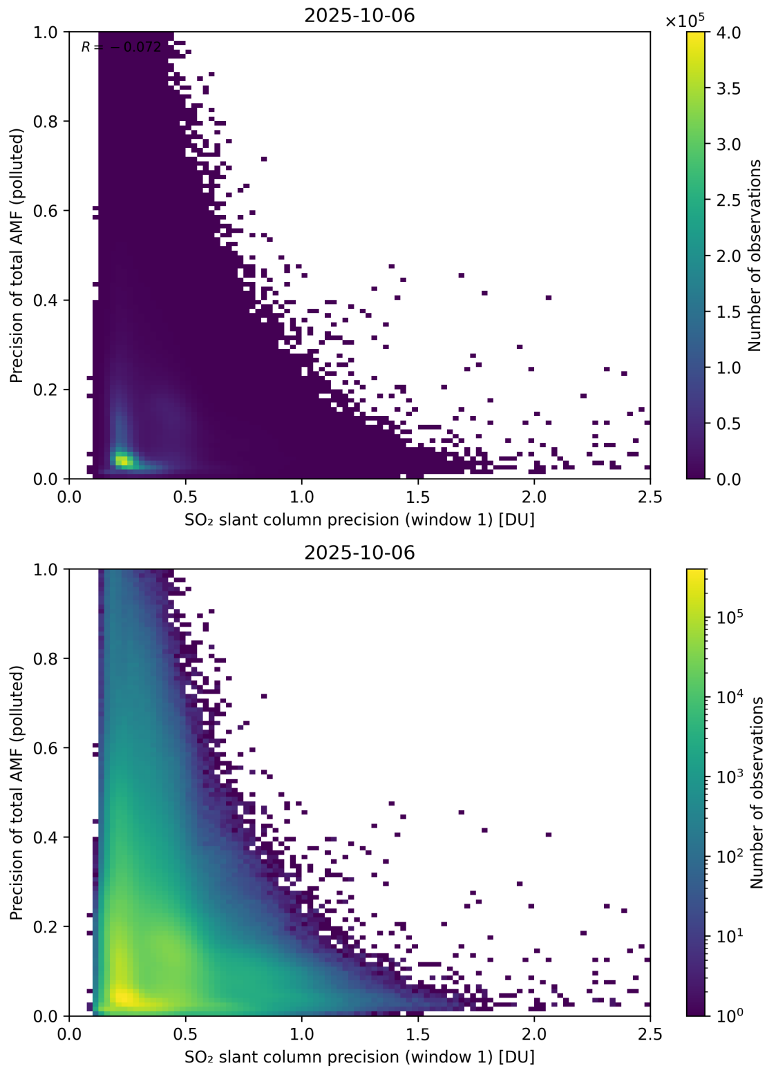
Figure 281: Scatter density plot of “SO 2 slant column precision (window 1)” against “Precision of total AMF (polluted)” for 2025-10-06 to 2025-10-07.
