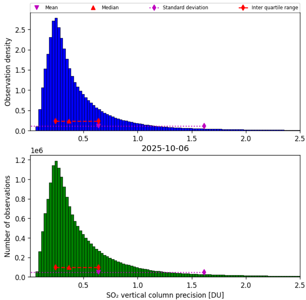
Figure 59: Histogram of “SO 2 vertical column precision” for 2025-10-06 to 2025-10-07
