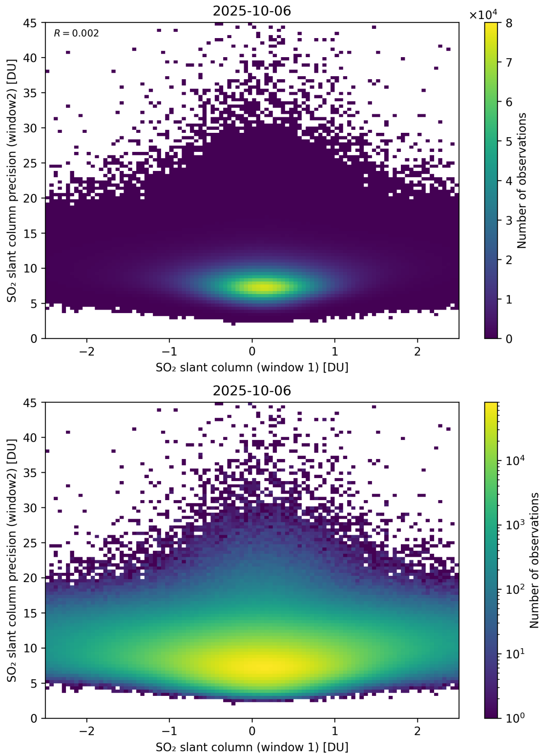
Figure 286: Scatter density plot of “SO 2 slant column (window 1)” against “SO 2 slant column precision (window2)” for 2025-10-06 to 2025-10-07.
