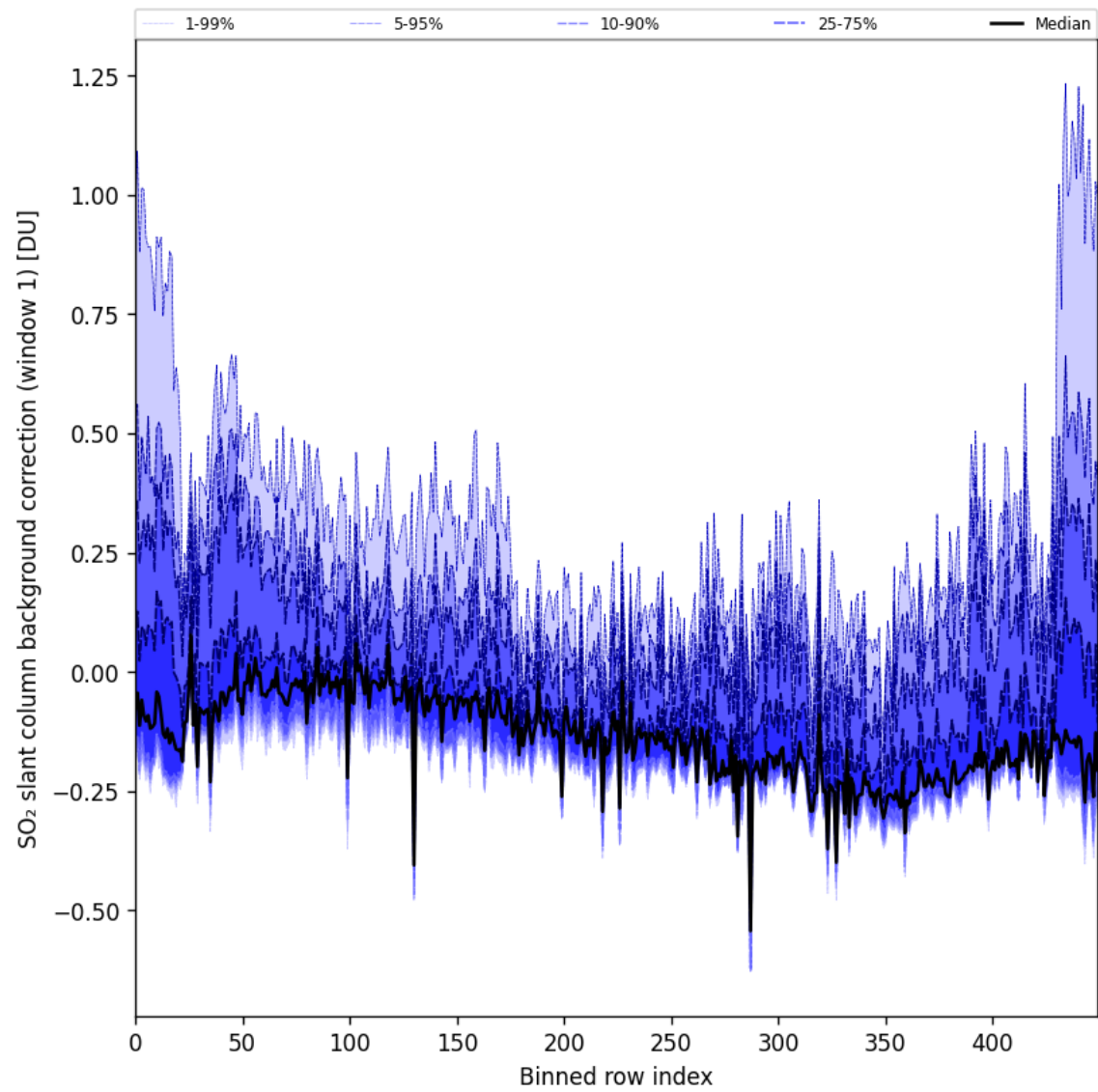
Figure 92: Along track statistics of “SO 2 slant column background correction (window 1)” for 2025-10-06 to 2025-10-07
