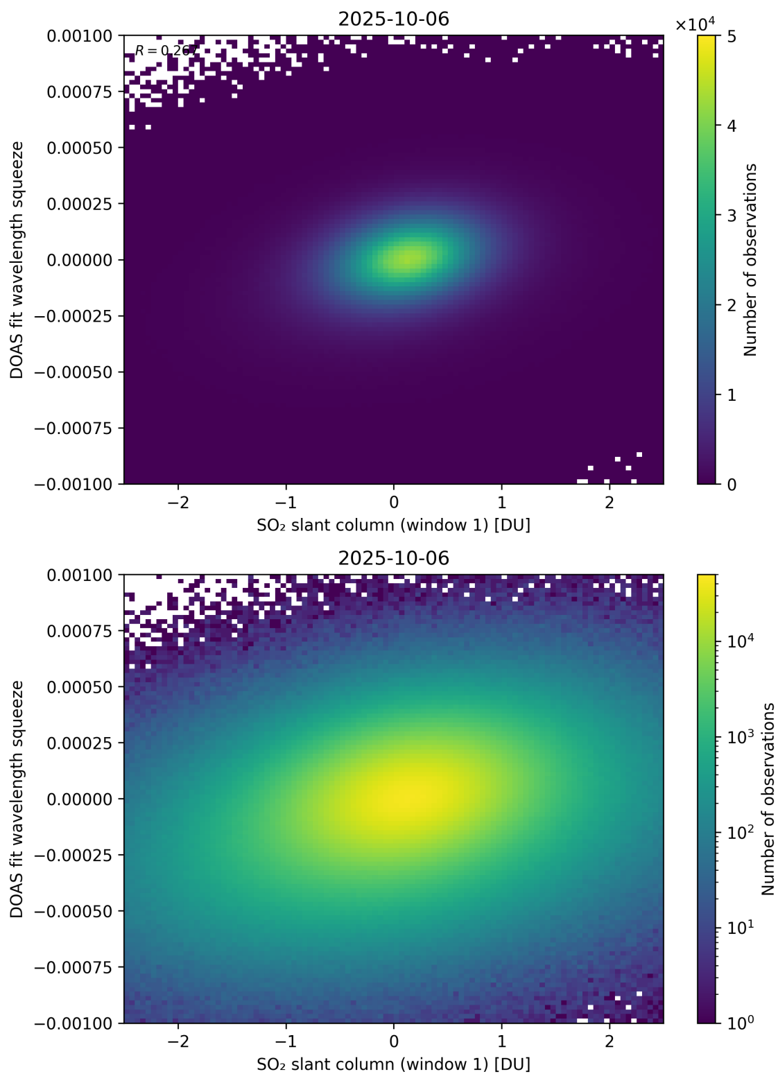
Figure 266: Scatter density plot of “SO 2 slant column (window 1)” against “DOAS fit wavelength squeeze” for 2025-10-06 to 2025-10-07.
