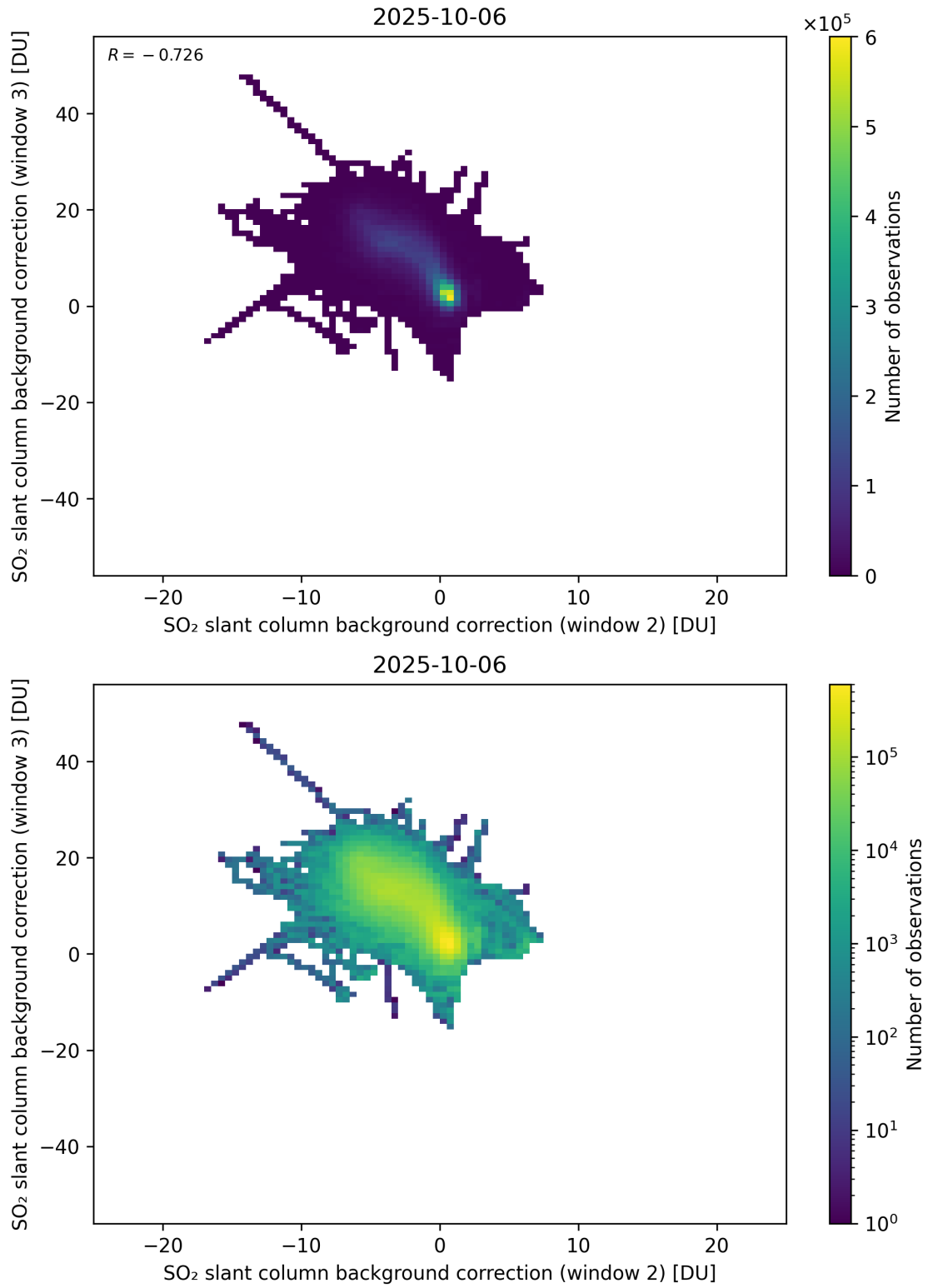
Figure 122: Scatter density plot of “SO 2 slant column background correction (window 2)” against “SO 2 slant column background correction (window 3)” for 2025-10-06 to 2025-10-07.
