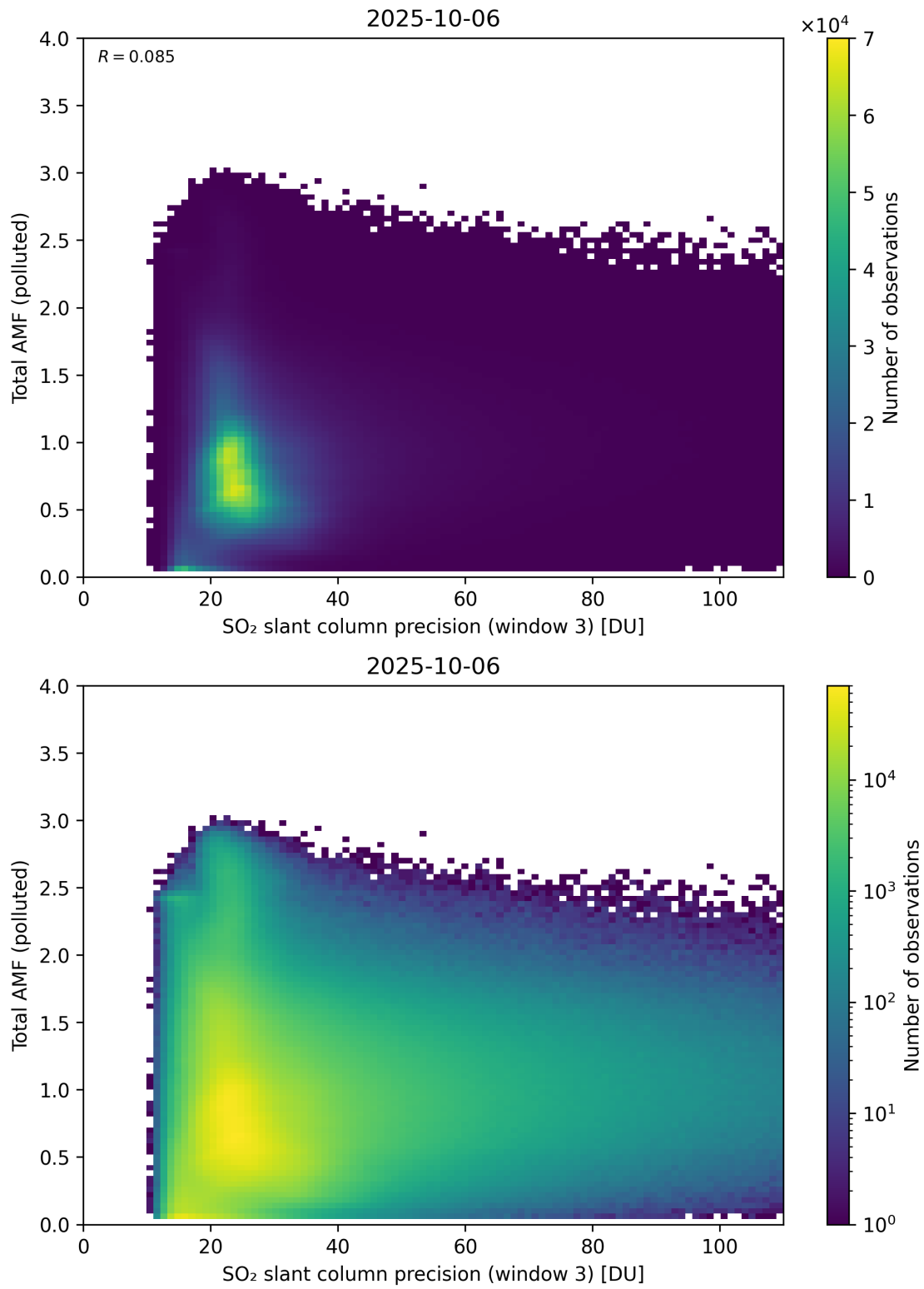
Figure 313: Scatter density plot of “SO 2 slant column precision (window 3)” against “Total AMF (polluted)” for 2025-10-06 to 2025-10-07.
