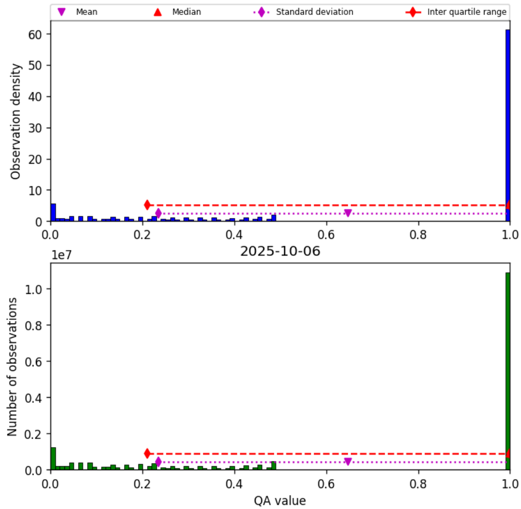
Figure 57: Histogram of “QA value” for 2025-10-06 to 2025-10-07
