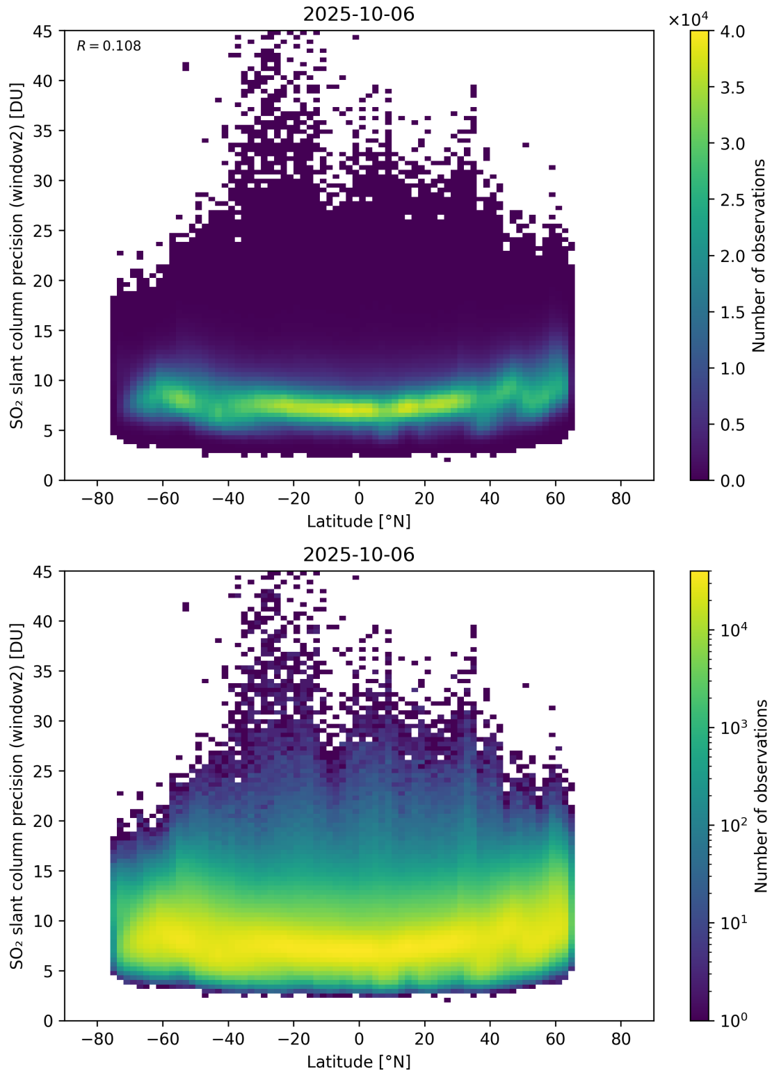
Figure 164: Scatter density plot of “Latitude” against “SO 2 slant column precision (window2)” for 2025-10-06 to 2025-10-07.
