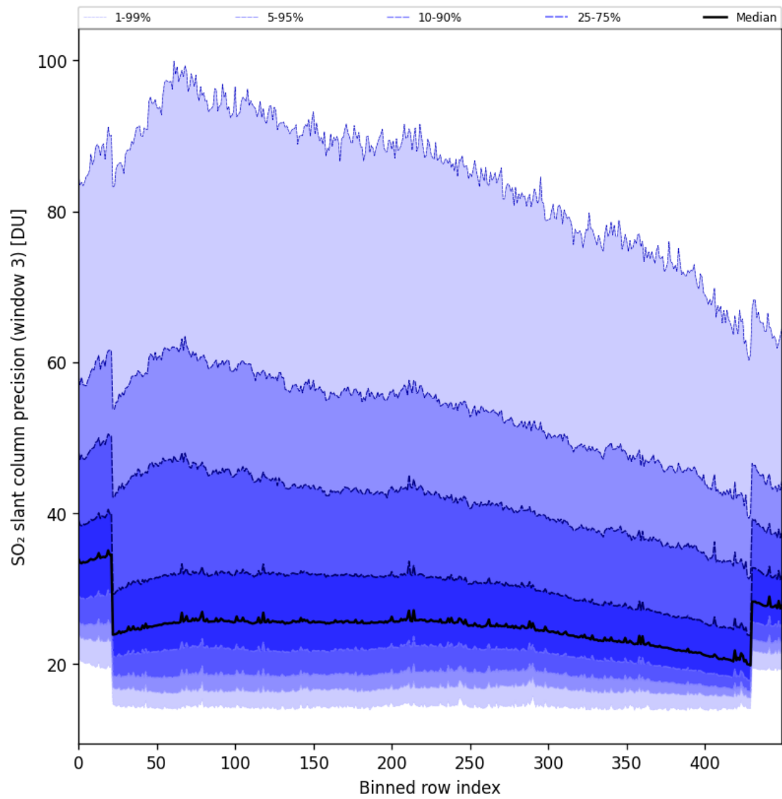
Figure 98: Along track statistics of “SO 2 slant column precision (window 3)” for 2025-10-06 to 2025-10-07
