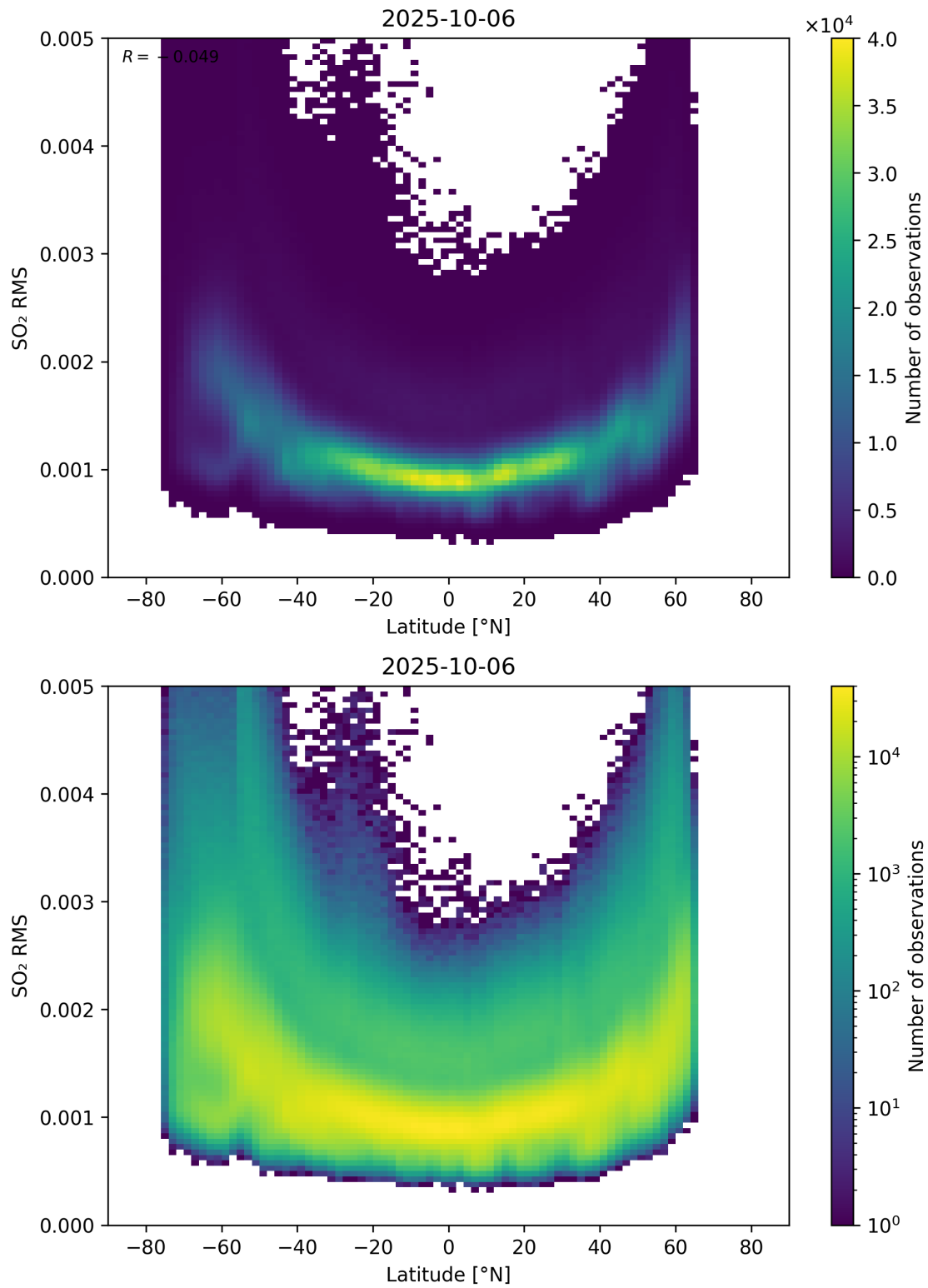
Figure 155: Scatter density plot of “Latitude” against “SO 2 RMS” for 2025-10-06 to 2025-10-07.
