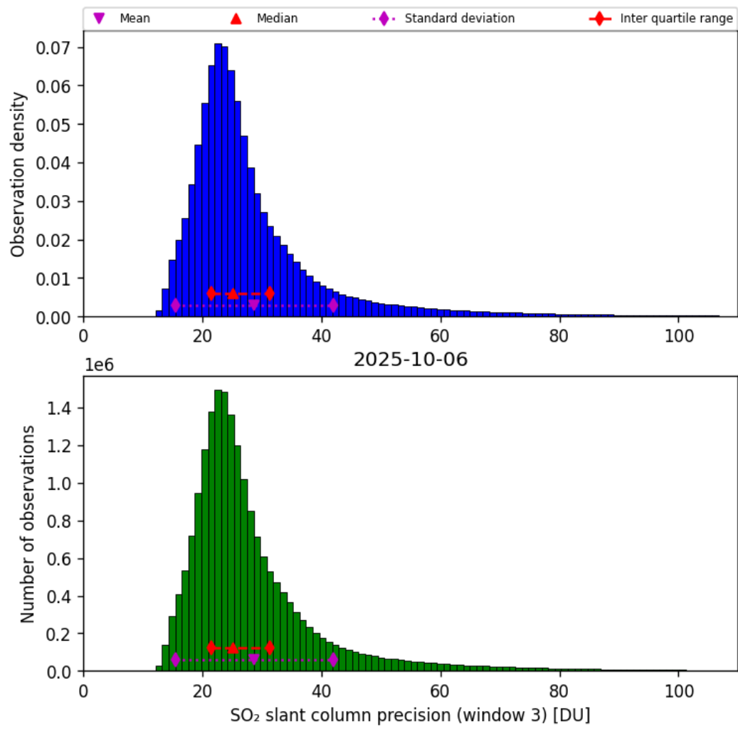
Figure 72: Histogram of “SO 2 slant column precision (window 3)” for 2025-10-06 to 2025-10-07
