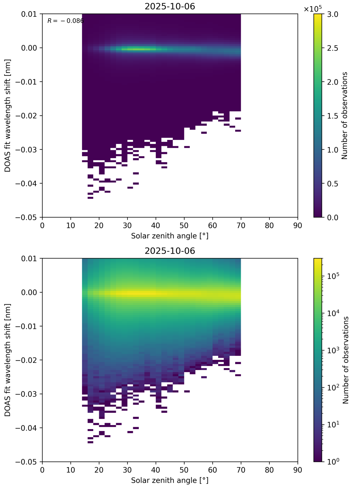
Figure 174: Scatter density plot of “Solar zenith angle” against “DOAS fit wavelength shift” for 2025-10-06 to 2025-10-07.
