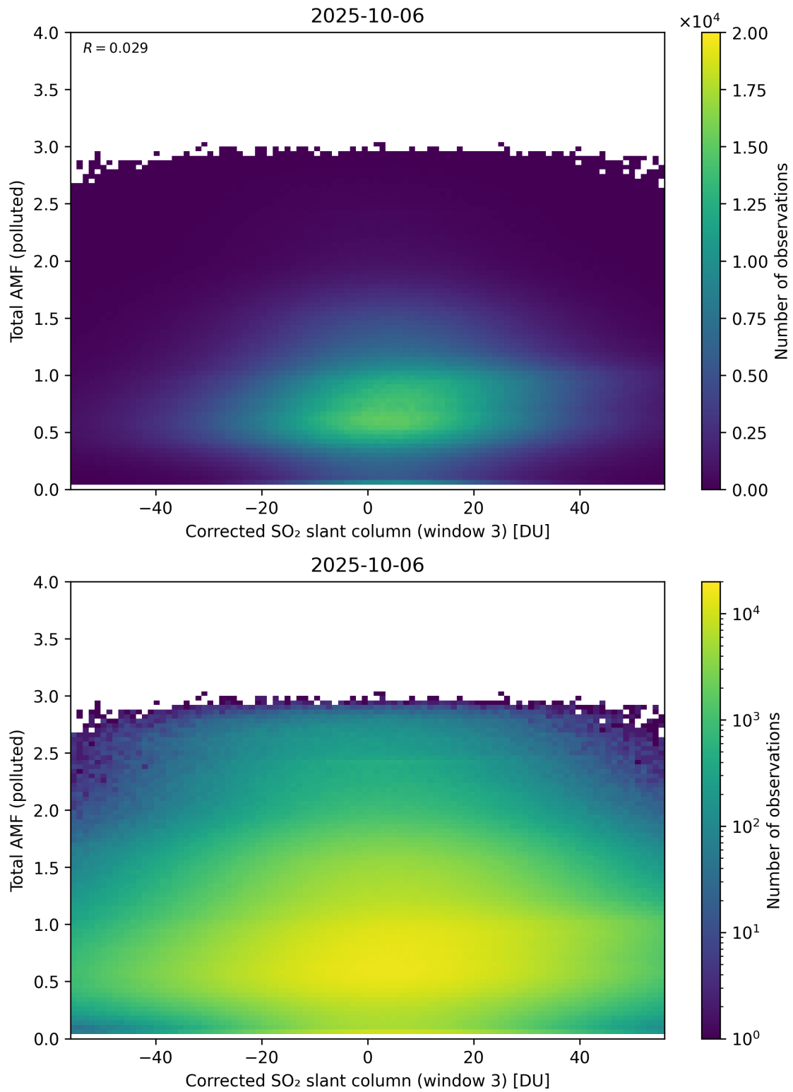
Figure 260: Scatter density plot of “Corrected SO 2 slant column (window 3)” against “Total AMF (polluted)” for 2025-10-06 to 2025-10-07.
