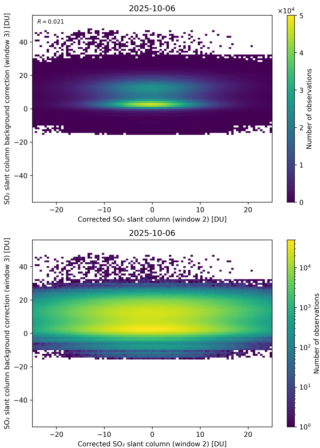
Figure 245: Scatter density plot of “Corrected SO 2 slant column (window 2)” against “SO 2 slant column background correction (window 3)” for 2025-10-06 to 2025-10-07.
