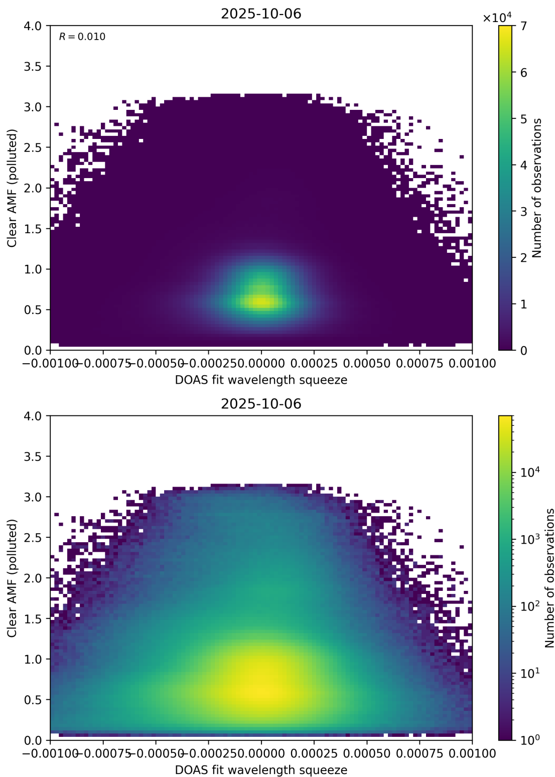
Figure 144: Scatter density plot of “DOAS fit wavelength squeeze” against “Clear AMF (polluted)” for 2025-10-06 to 2025-10-07.
