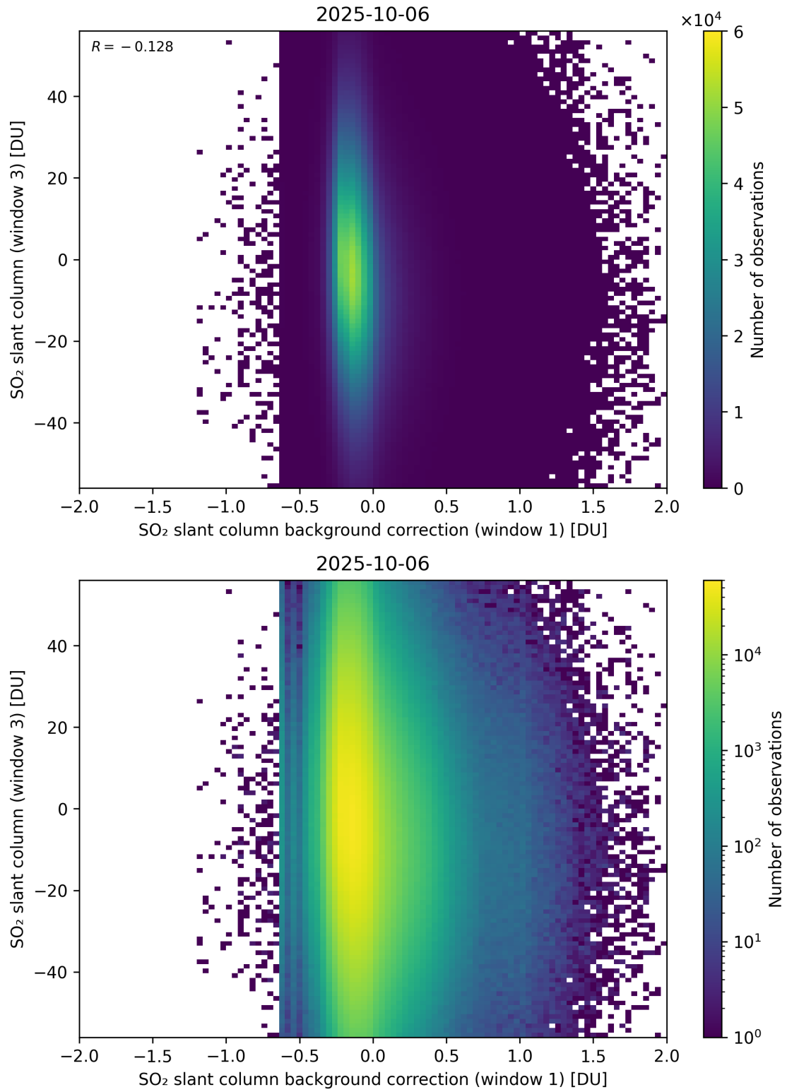
Figure 118: Scatter density plot of “SO 2 slant column background correction (window 1)” against “SO 2 slant column (window 3)” for 2025-10-06 to 2025-10-07.
