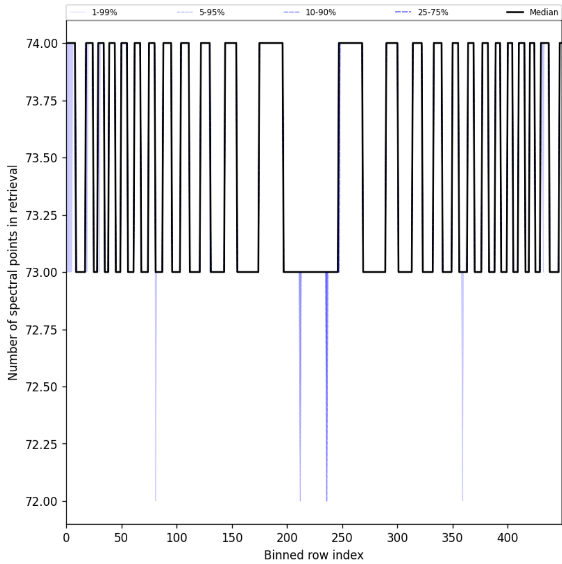
Figure 108: Along track statistics of “Number of spectral points in retrieval” for 2025-10-06 to 2025-10-07
