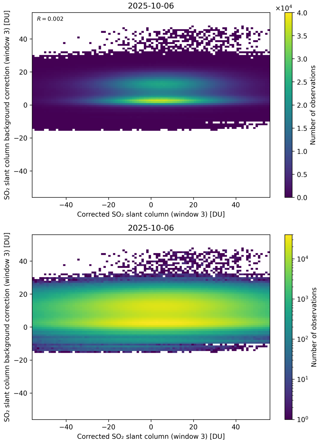
Figure 255: Scatter density plot of “Corrected SO 2 slant column (window 3)” against “SO 2 slant column background correction (window 3)” for 2025-10-06 to 2025-10-07.
