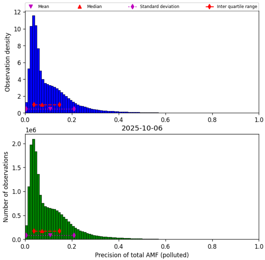
Figure 80: Histogram of “Precision of total AMF (polluted)” for 2025-10-06 to 2025-10-07
