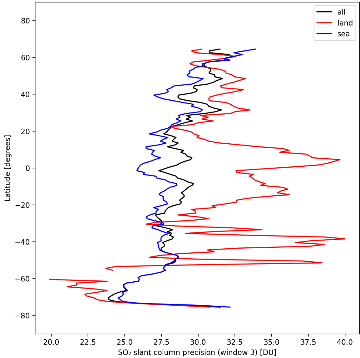
Figure 46: Zonal average of “SO 2 slant column precision (window 3)” for 2025-10-06 to 2025-10-07.
