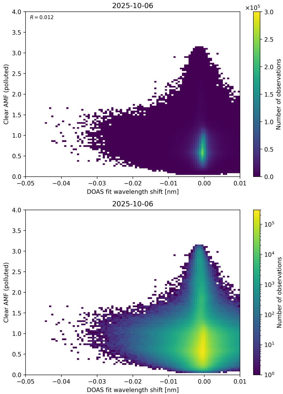
Figure 140: Scatter density plot of “DOAS fit wavelength shift” against “Clear AMF (polluted)” for 2025-10-06 to 2025-10-07.
