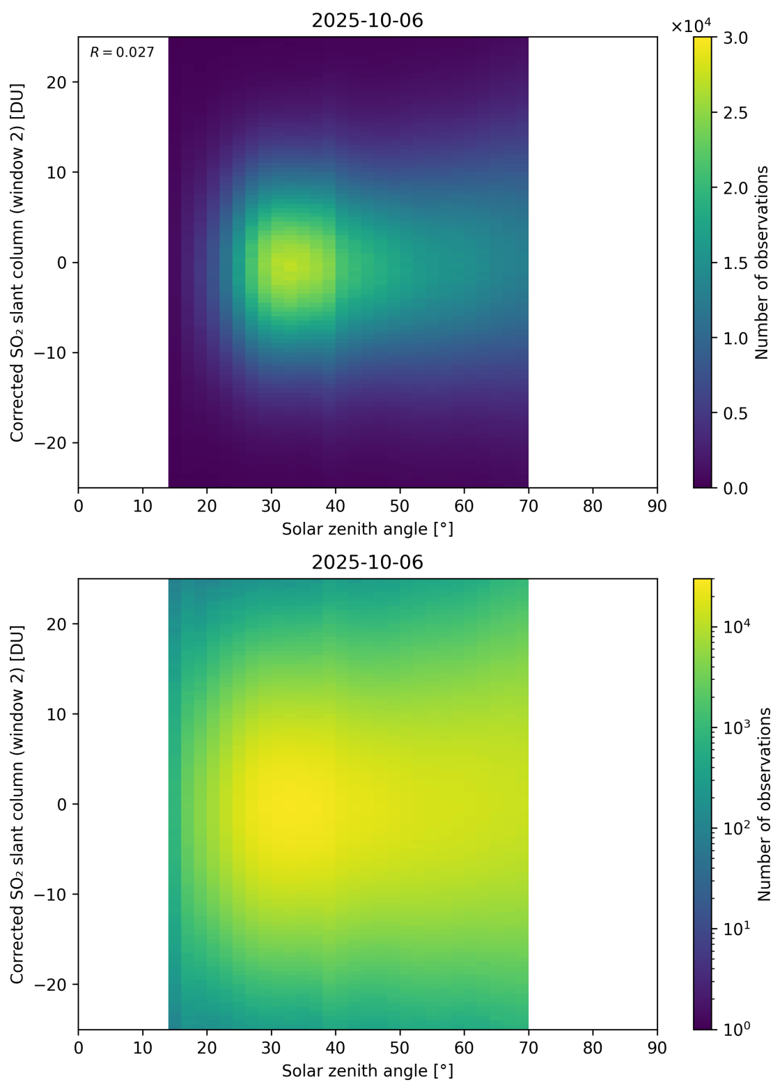
Figure 182: Scatter density plot of “Solar zenith angle” against “Corrected SO 2 slant column (window 2)” for 2025-10-06 to 2025-10-07.
