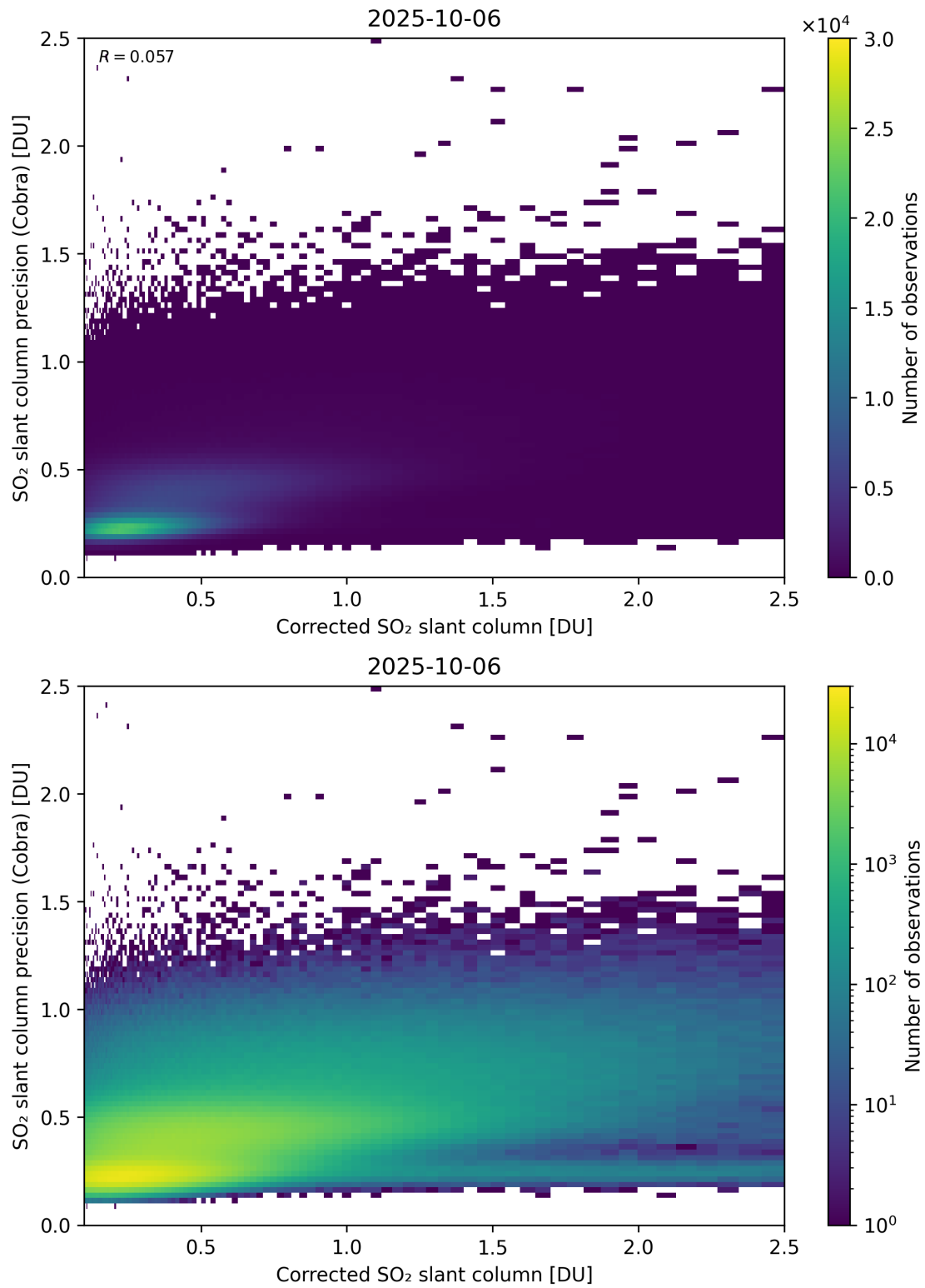
Figure 234: Scatter density plot of “Corrected SO 2 slant column” against “SO 2 slant column precision (Cobra)” for 2025-10-06 to 2025-10-07.
