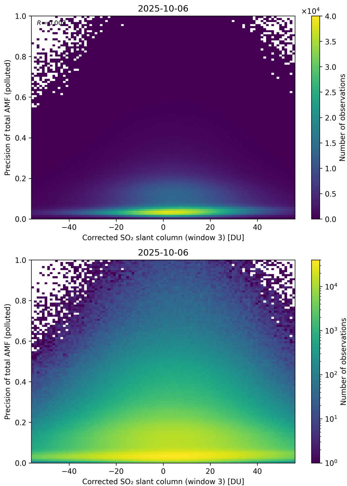
Figure 261: Scatter density plot of “Corrected SO 2 slant column (window 3)” against “Precision of total AMF (polluted)” for 2025-10-06 to 2025-10-07.
