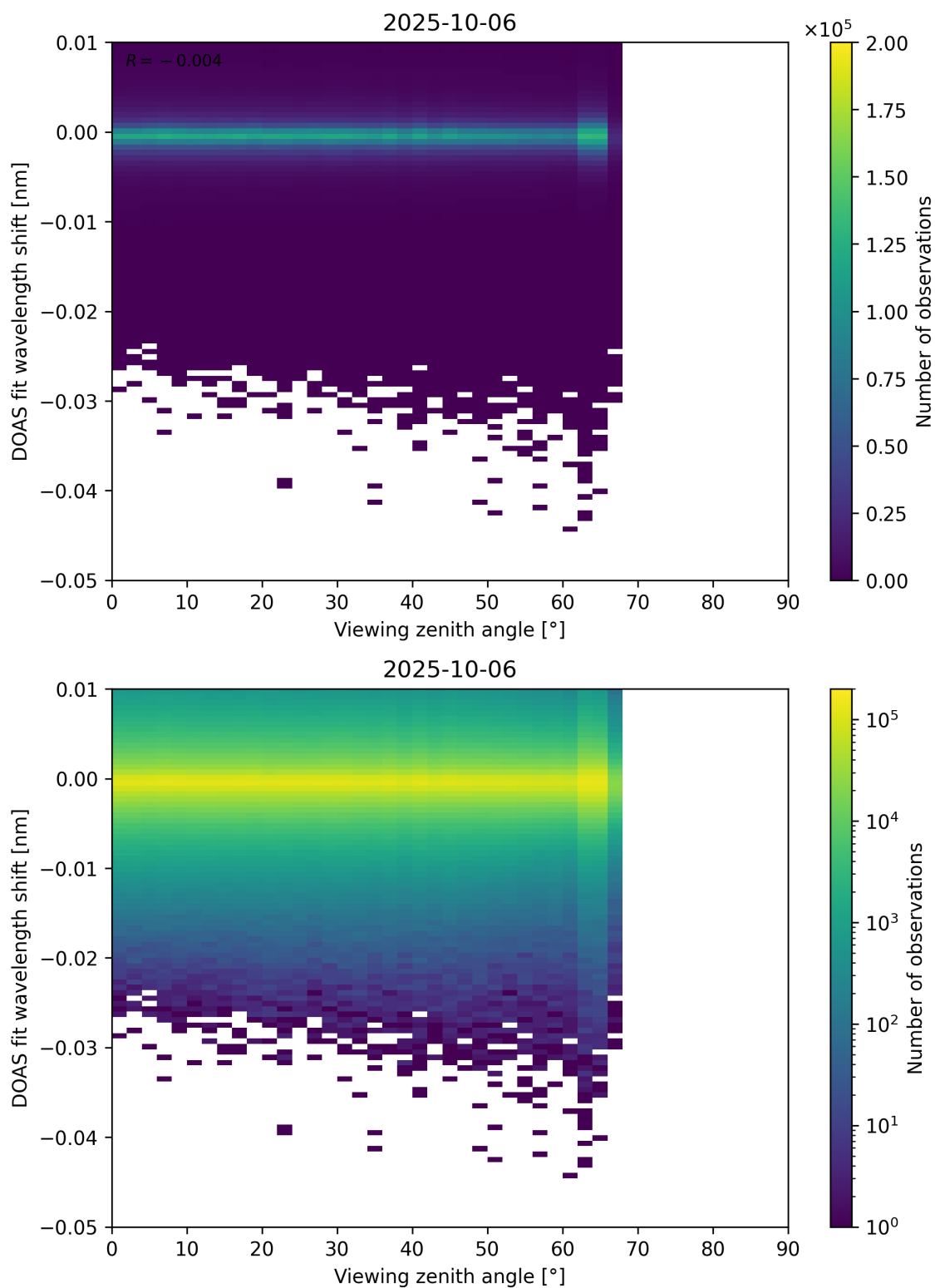
Figure 365: Scatter density plot of “Viewing zenith angle” against “DOAS fit wavelength shift” for 2025-10-06 to 2025-10-07.
