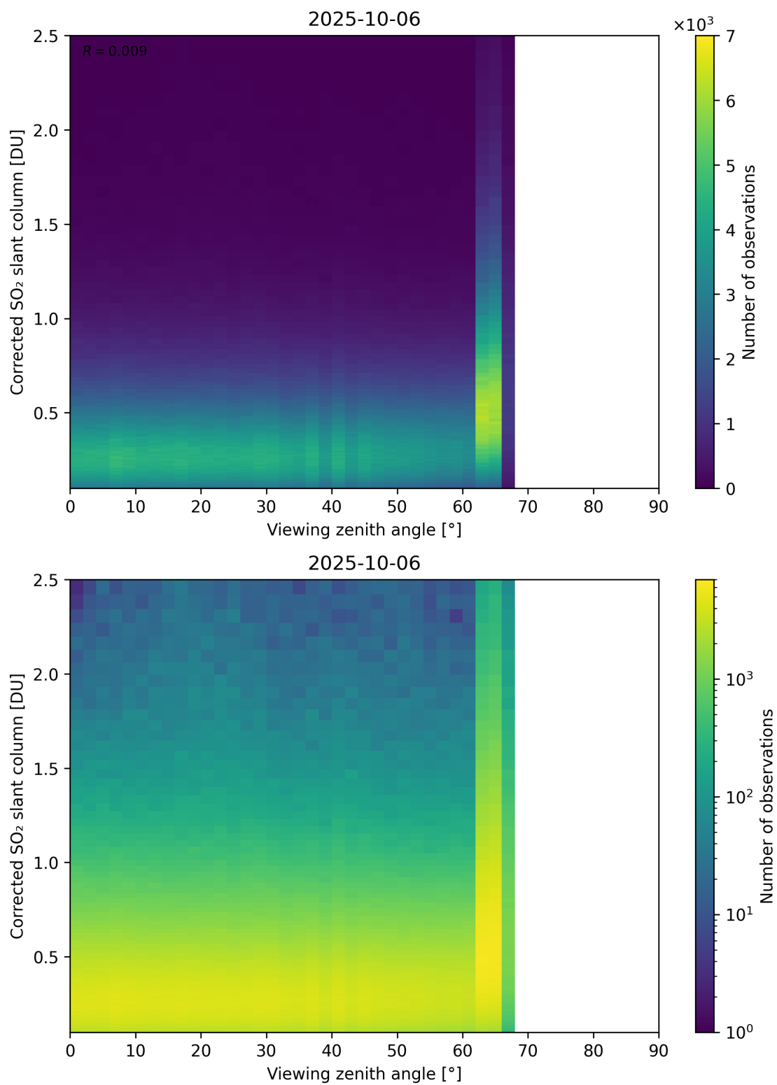
Figure 373: Scatter density plot of “Viewing zenith angle” against “Corrected SO 2 slant column” for 2025-10-06 to 2025-10-07.
