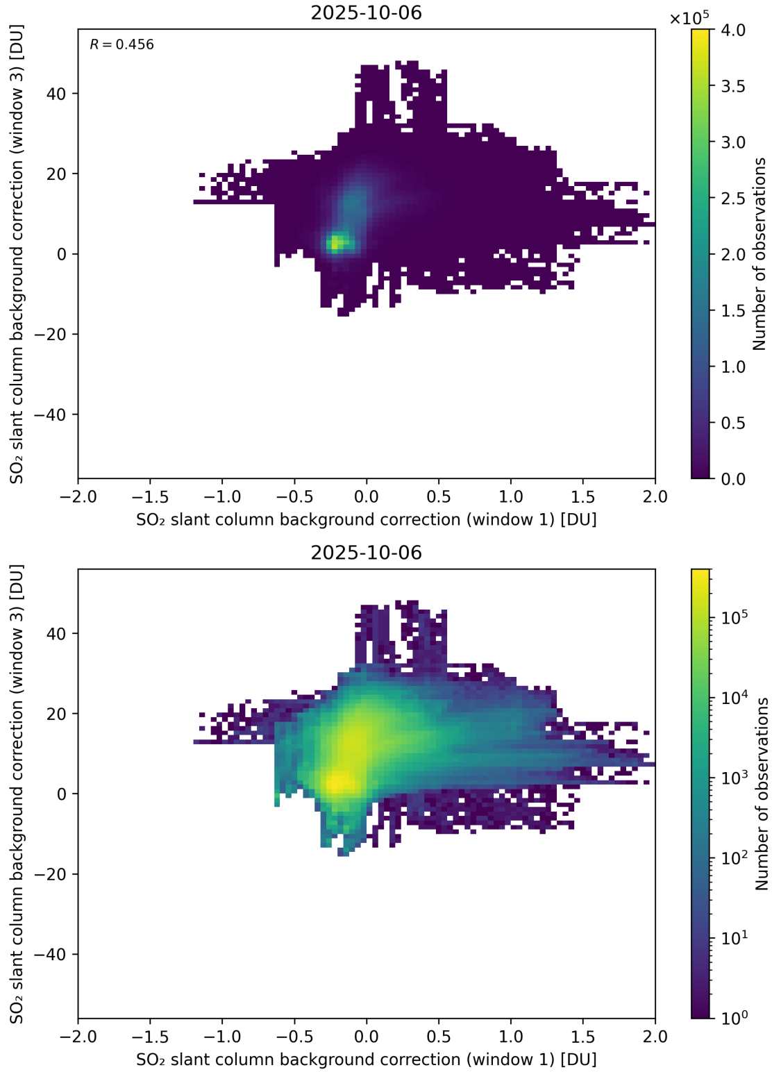
Figure 110: Scatter density plot of “SO 2 slant column background correction (window 1)” against “SO 2 slant column background correction (window 3)” for 2025-10-06 to 2025-10-07.
