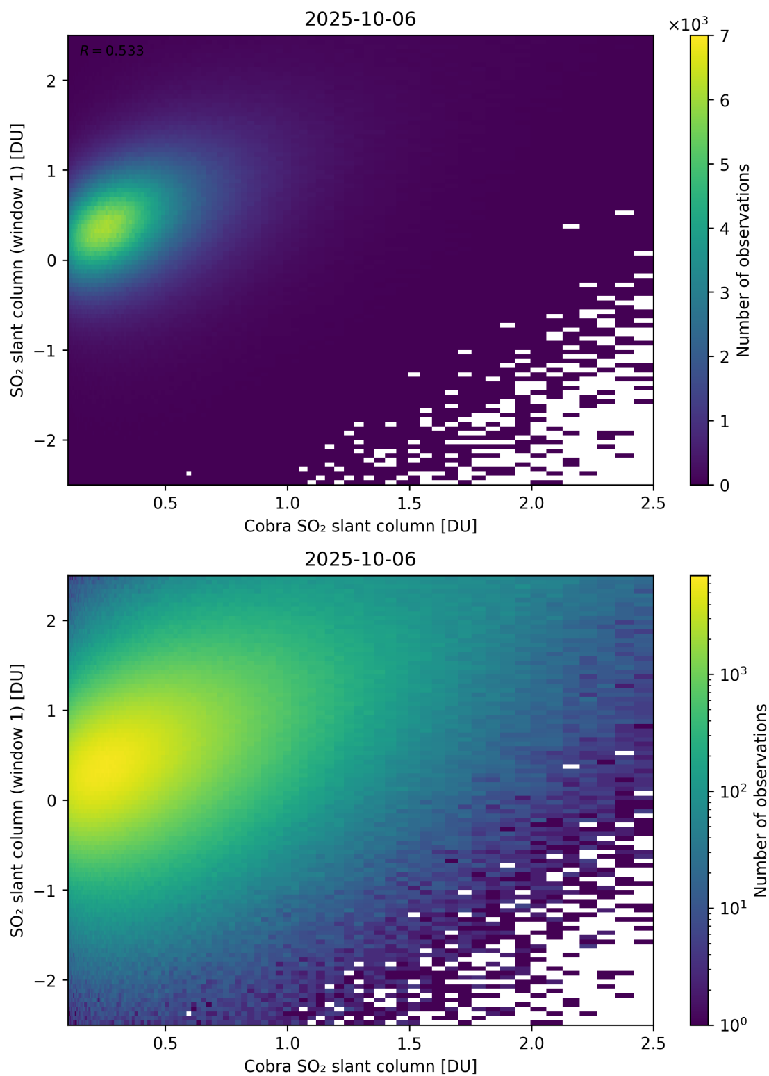
Figure 219: Scatter density plot of “Cobra SO 2 slant column” against “SO 2 slant column (window 1)” for 2025-10-06 to 2025-10-07.
