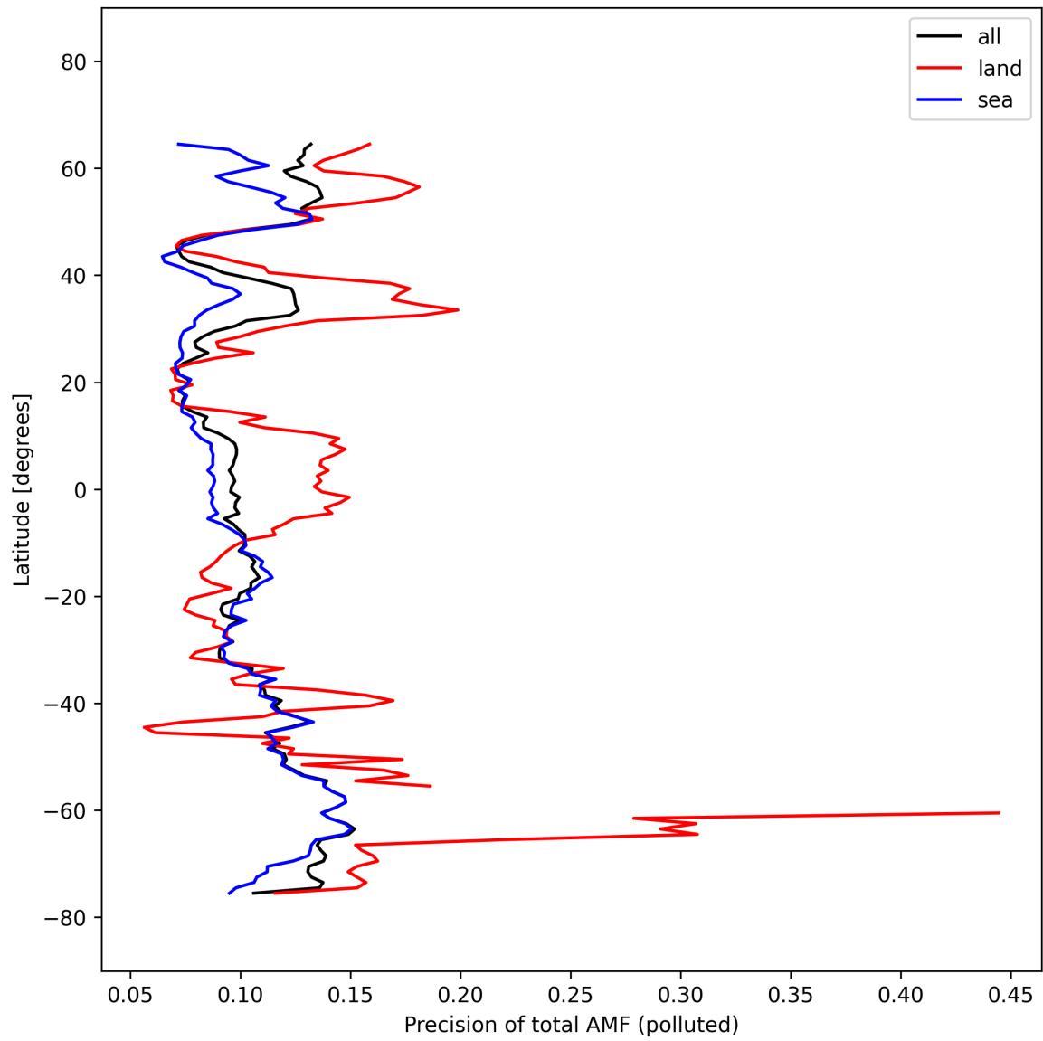
Figure 54: Zonal average of “Precision of total AMF (polluted)” for 2025-10-06 to 2025-10-07.
