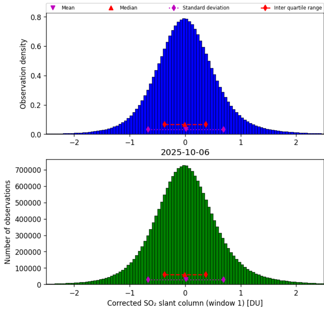
Figure 65: Histogram of “Corrected SO 2 slant column (window 1)” for 2025-10-06 to 2025-10-07
