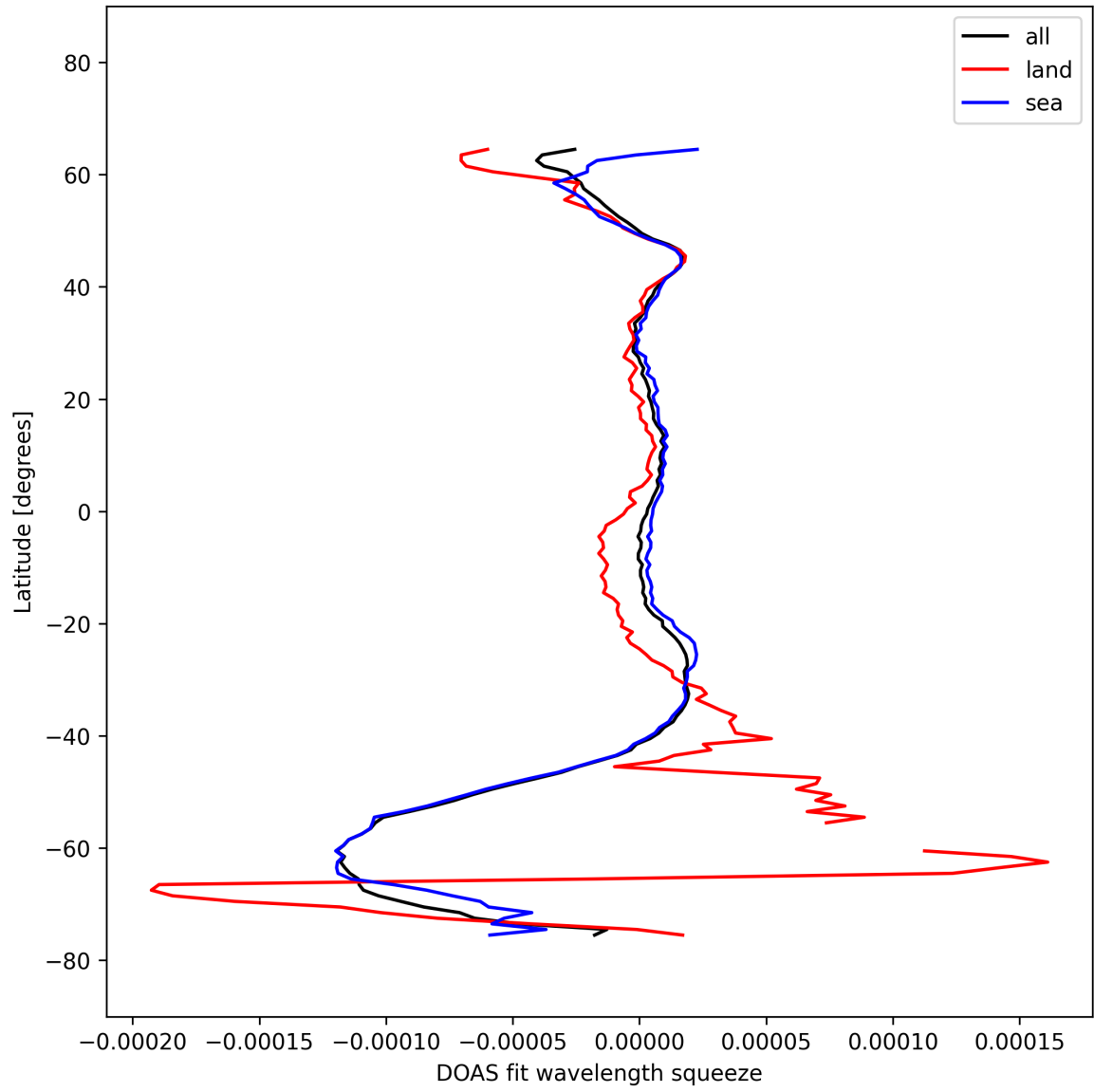
Figure 51: Zonal average of “DOAS fit wavelength squeeze” for 2025-10-06 to 2025-10-07.
