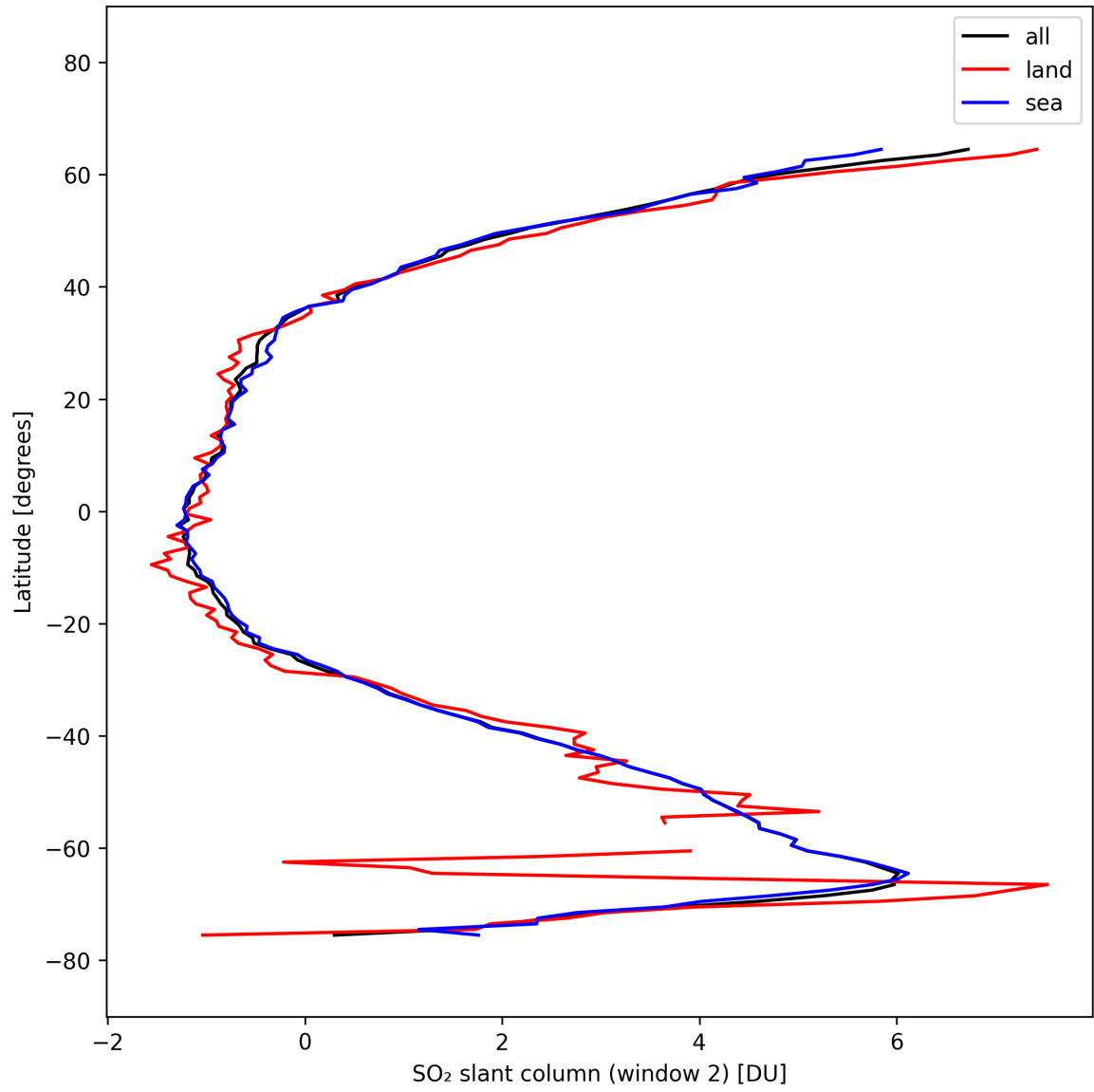
Figure 41: Zonal average of “SO 2 slant column (window 2)” for 2025-10-06 to 2025-10-07.
