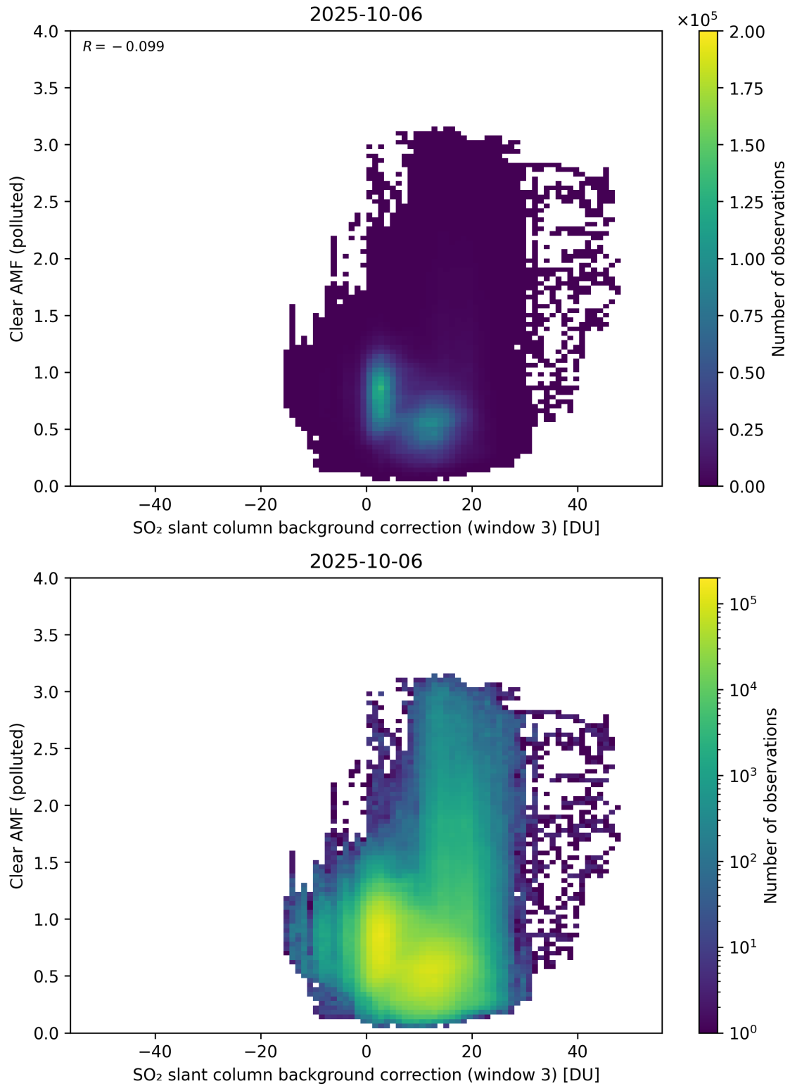
Figure 135: Scatter density plot of “SO 2 slant column background correction (window 3)” against “Clear AMF (polluted)” for 2025-10-06 to 2025-10-07.
