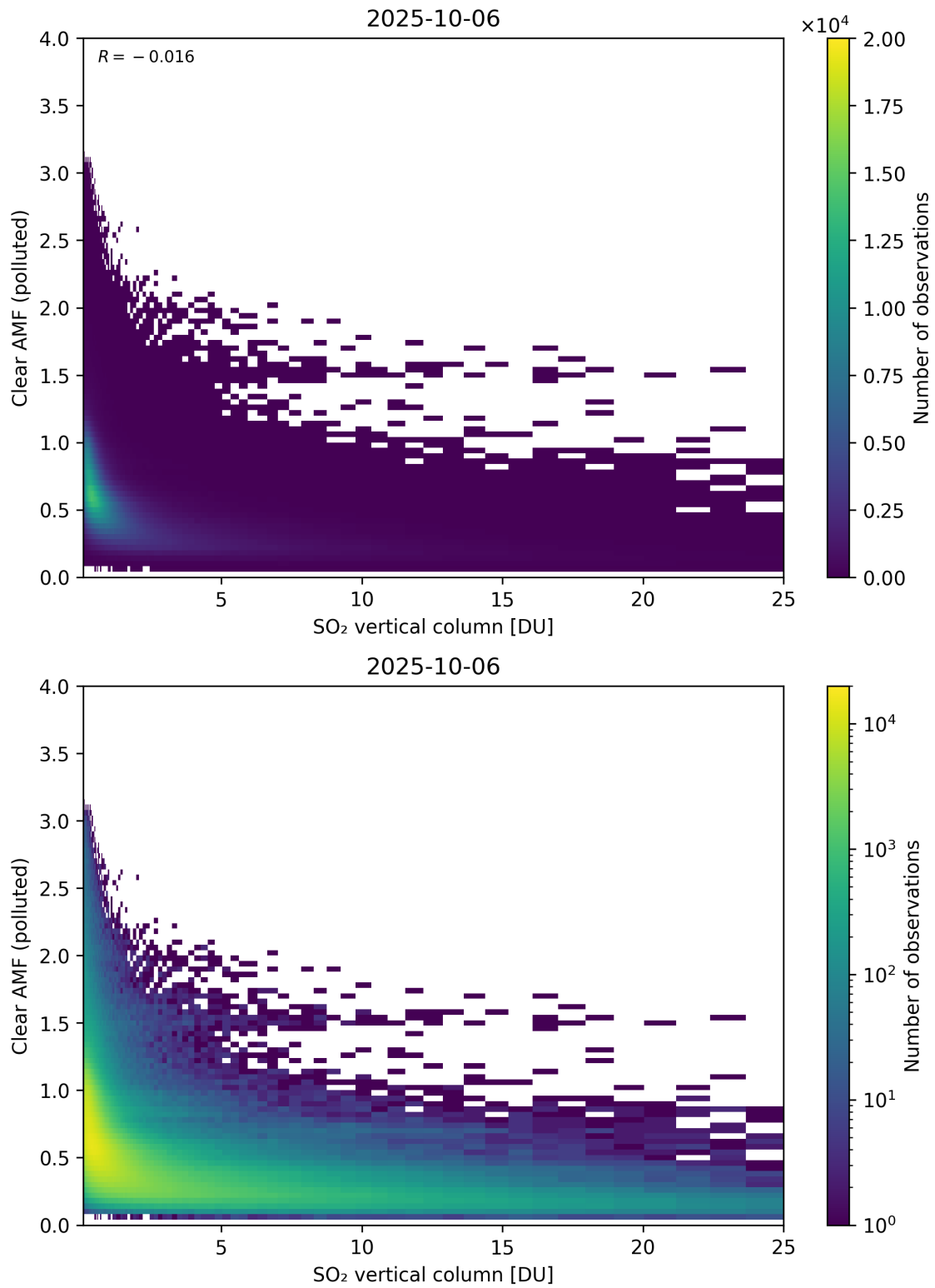
Figure 348: Scatter density plot of “SO 2 vertical column” against “Clear AMF (polluted)” for 2025-10-06 to 2025-10-07.
