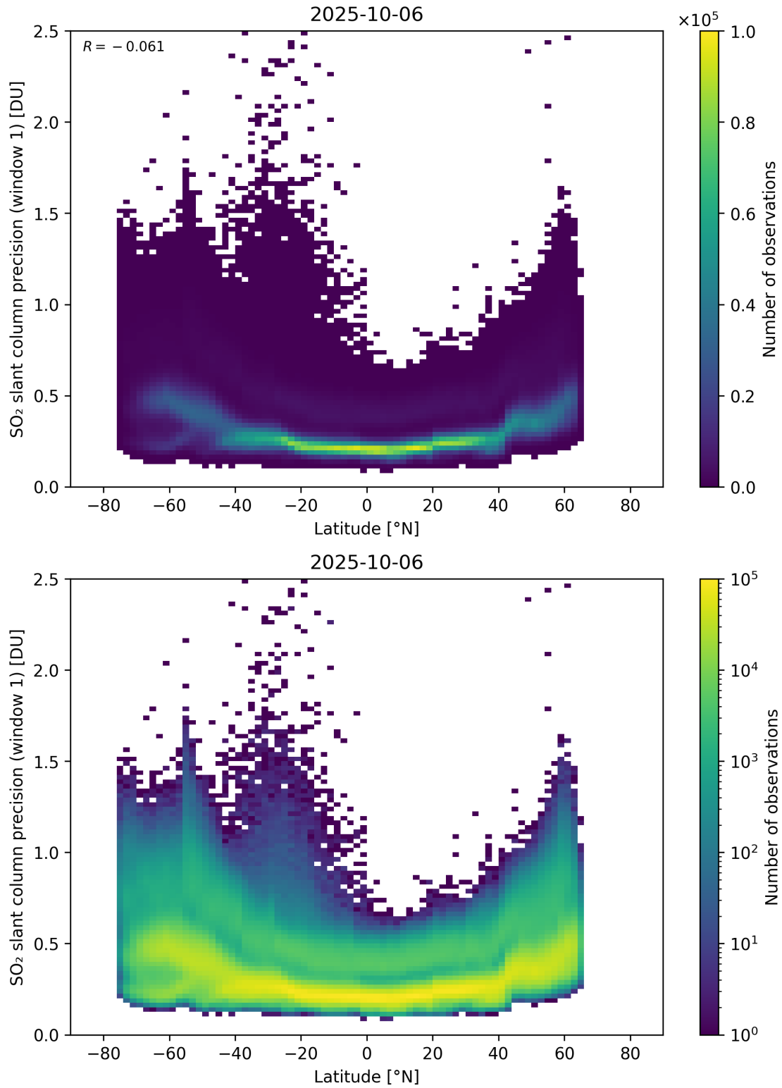
Figure 163: Scatter density plot of “Latitude” against “SO 2 slant column precision (window 1)” for 2025-10-06 to 2025-10-07.
