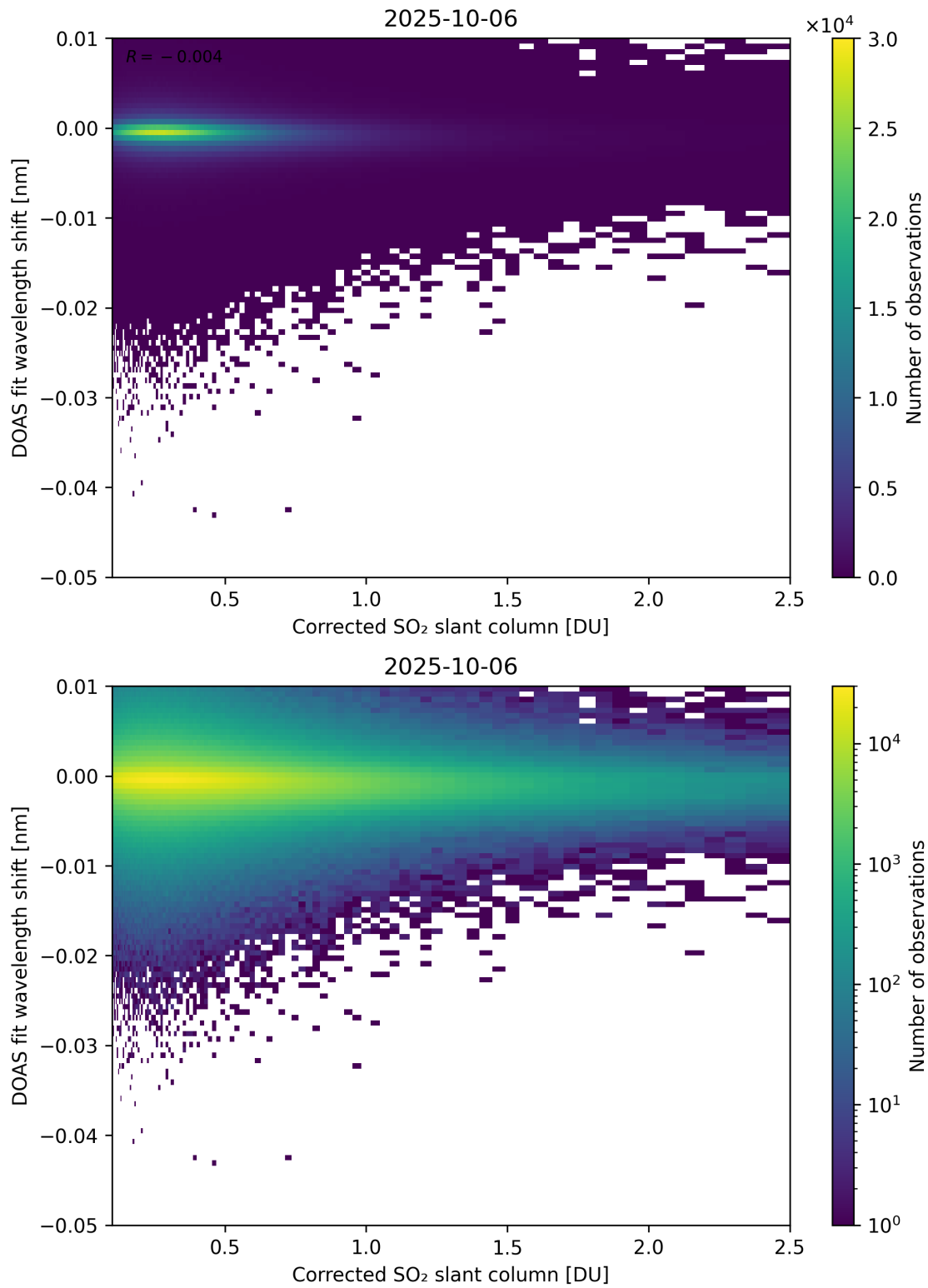
Figure 229: Scatter density plot of “Corrected SO 2 slant column” against “DOAS fit wavelength shift” for 2025-10-06 to 2025-10-07.
