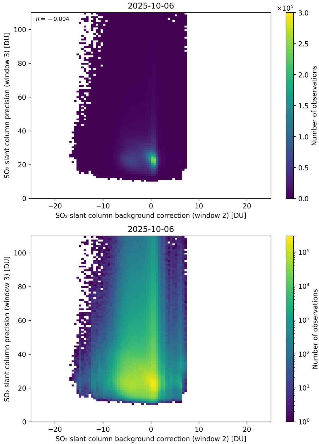
Figure 129: Scatter density plot of “SO 2 slant column background correction (window 2)” against “SO 2 slant column precision (window 3)” for 2025-10-06 to 2025-10-07.
