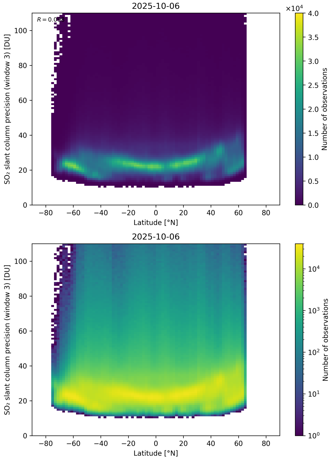
Figure 166: Scatter density plot of “Latitude” against “SO 2 slant column precision (window 3)” for 2025-10-06 to 2025-10-07.
