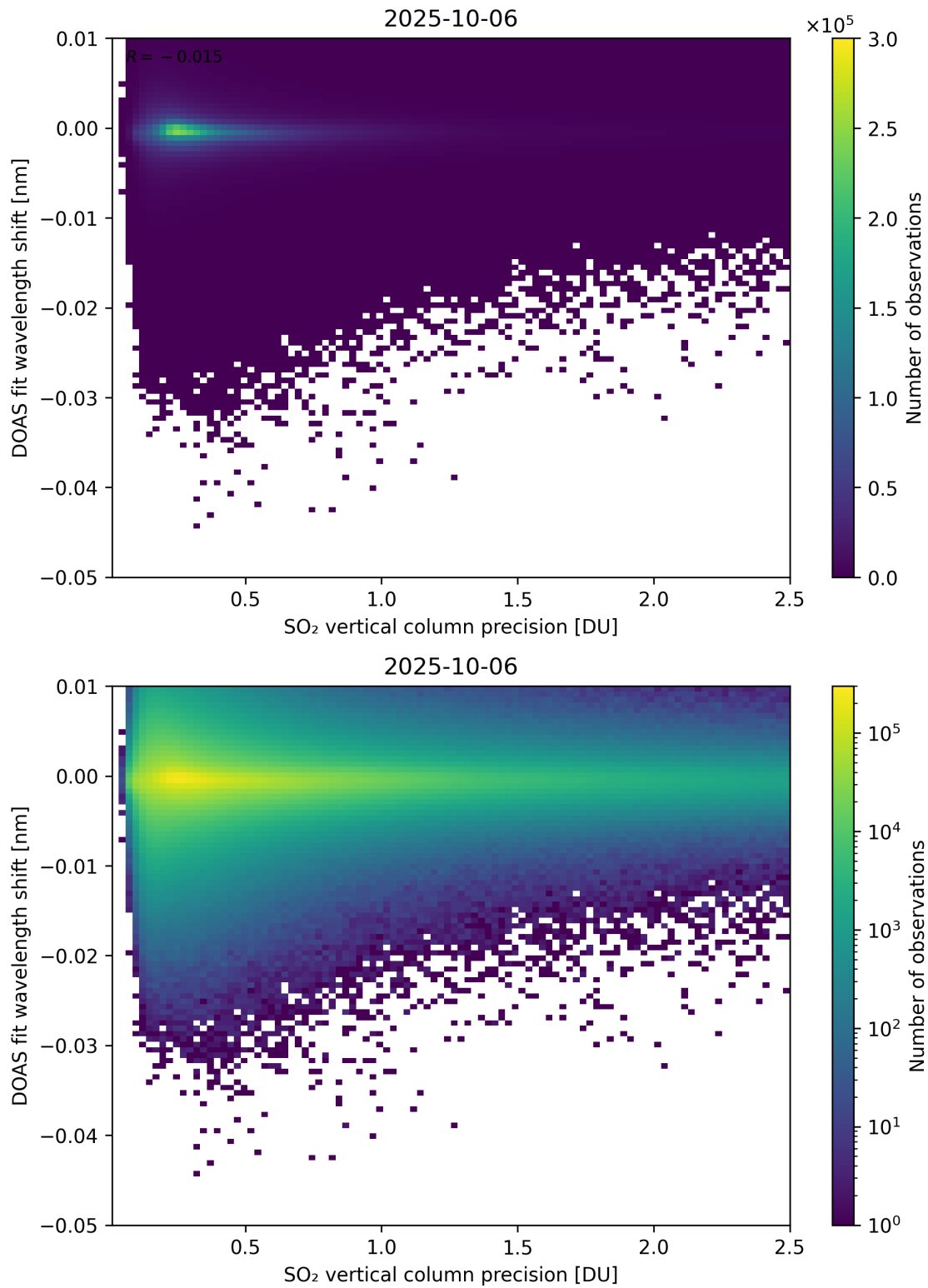
Figure 332: Scatter density plot of “SO 2 vertical column precision” against “DOAS fit wavelength shift” for 2025-10-06 to 2025-10-07.
