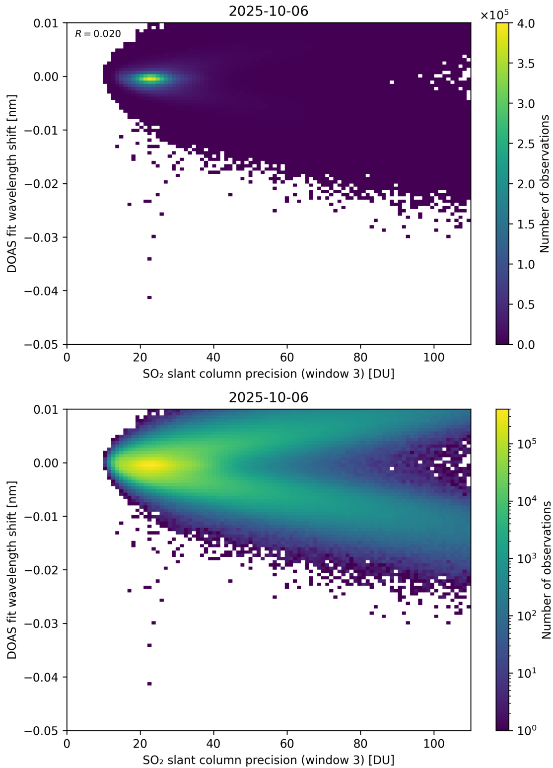
Figure 308: Scatter density plot of “SO 2 slant column precision (window 3)” against “DOAS fit wavelength shift” for 2025-10-06 to 2025-10-07.
