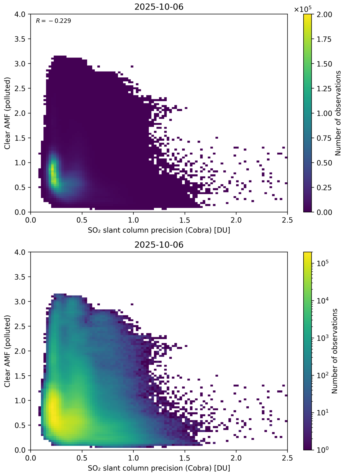
Figure 205: Scatter density plot of “SO 2 slant column precision (Cobra)” against “Clear AMF (polluted)” for 2025-10-06 to 2025-10-07.
