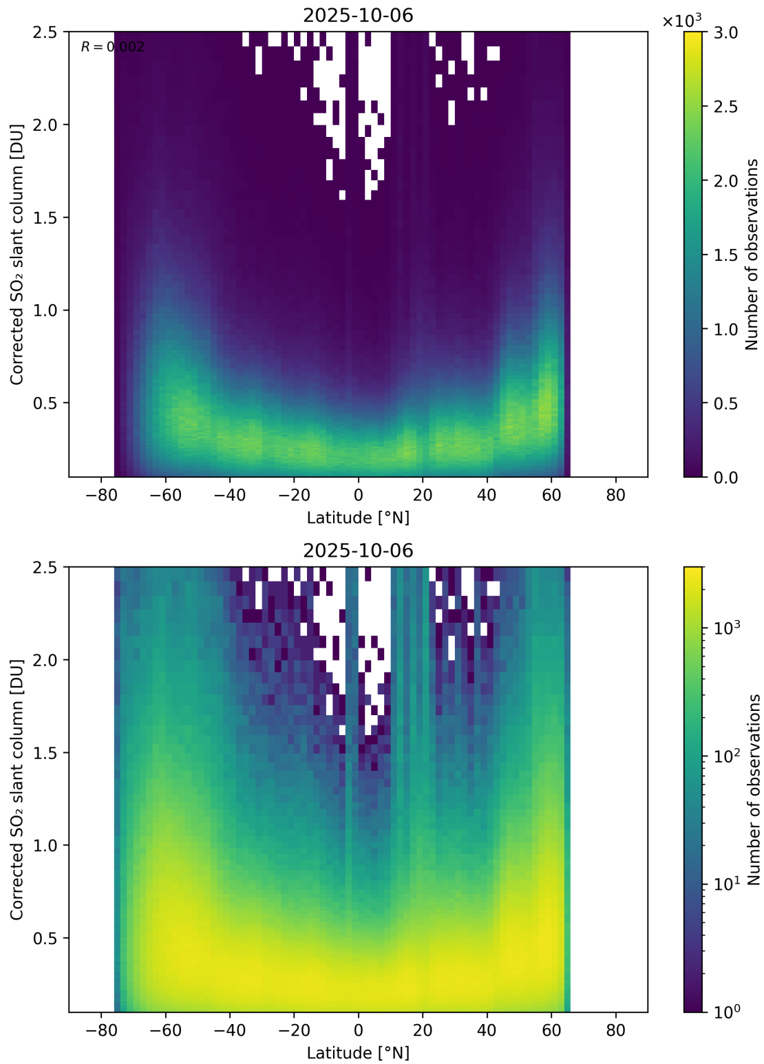
Figure 159: Scatter density plot of “Latitude” against “Corrected SO 2 slant column” for 2025-10-06 to 2025-10-07.
