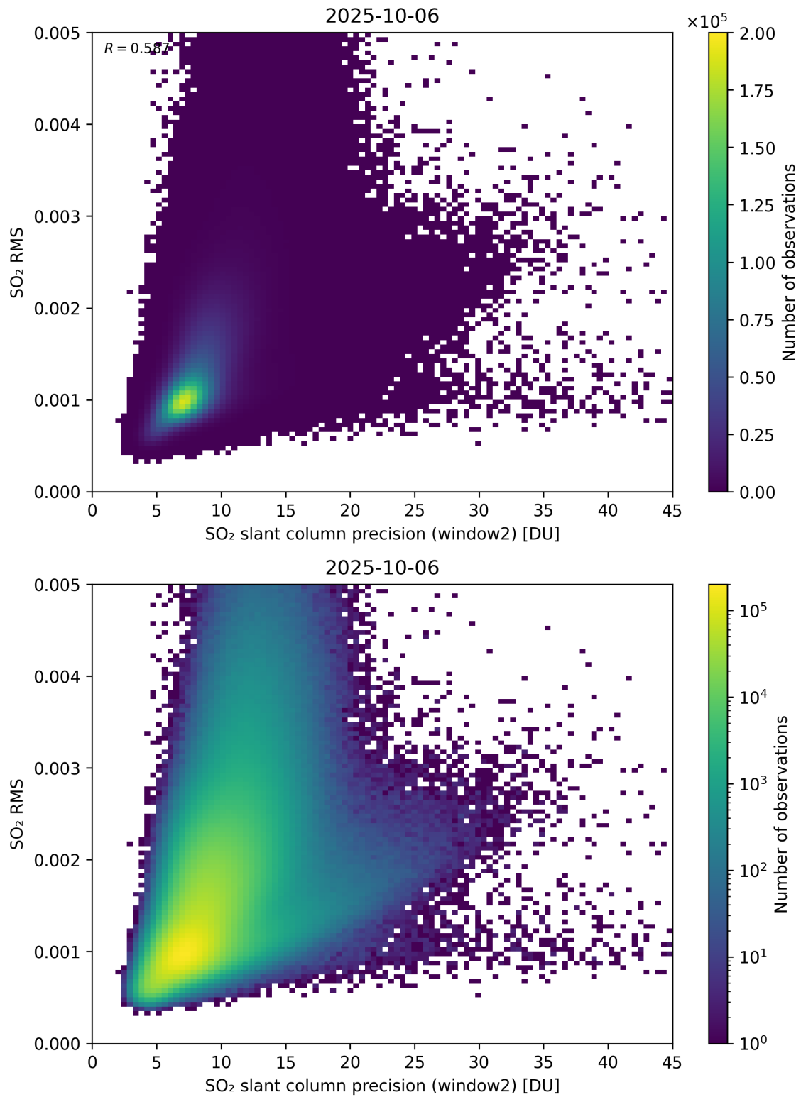
Figure 295: Scatter density plot of “SO 2 slant column precision (window2)” against “SO 2 RMS” for 2025-10-06 to 2025-10-07.
