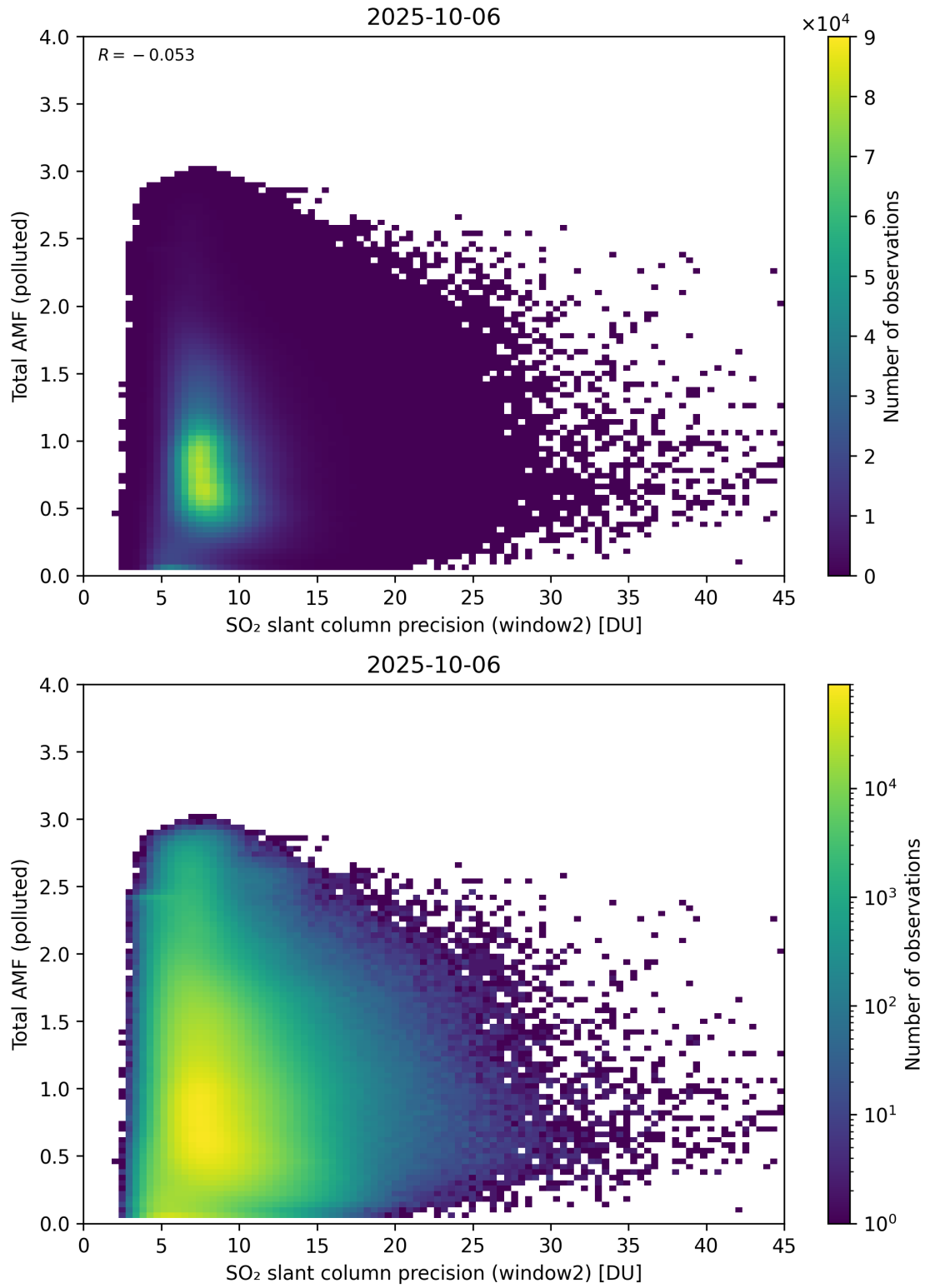
Figure 301: Scatter density plot of “SO 2 slant column precision (window2)” against “Total AMF (polluted)” for 2025-10-06 to 2025-10-07.
