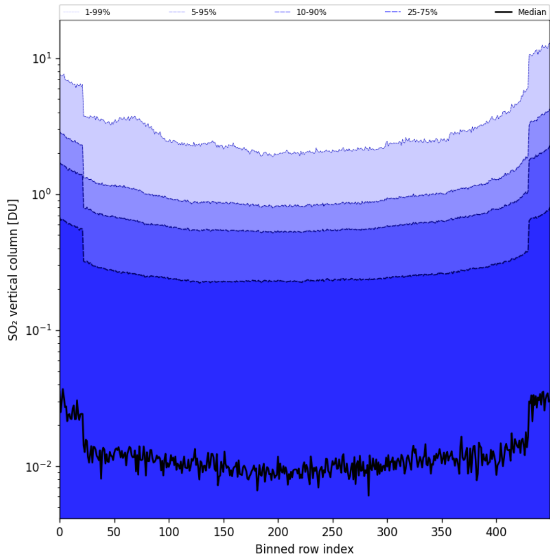
Figure 84: Along track statistics of “SO 2 vertical column” for 2025-10-06 to 2025-10-07
