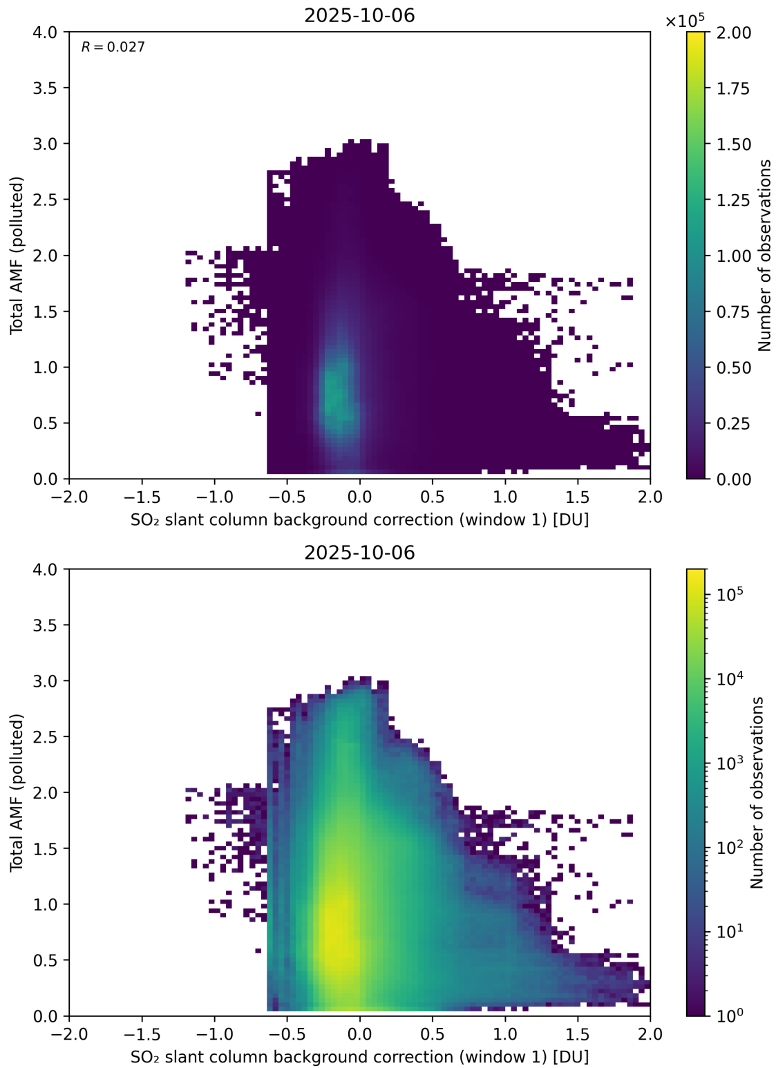
Figure 120: Scatter density plot of “SO 2 slant column background correction (window 1)” against “Total AMF (polluted)” for 2025-10-06 to 2025-10-07.
