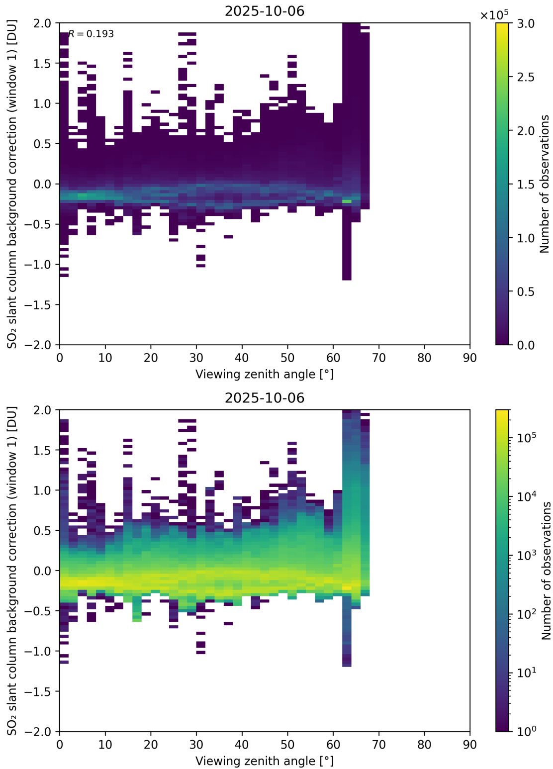
Figure 362: Scatter density plot of “Viewing zenith angle” against “SO 2 slant column background correction (window 1)” for 2025-10-06 to 2025-10-07.
