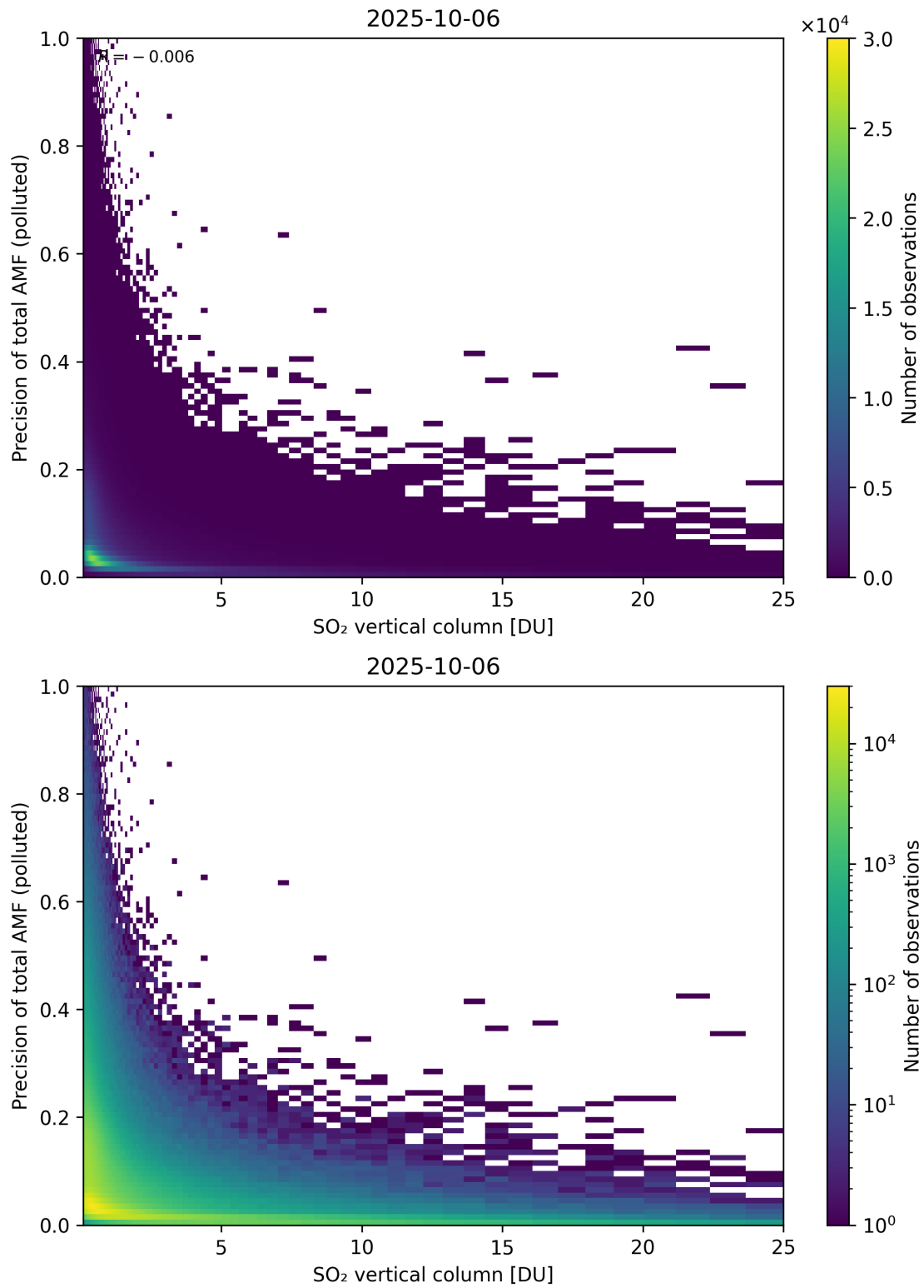
Figure 360: Scatter density plot of “SO 2 vertical column” against “Precision of total AMF (polluted)” for 2025-10-06 to 2025-10-07.
