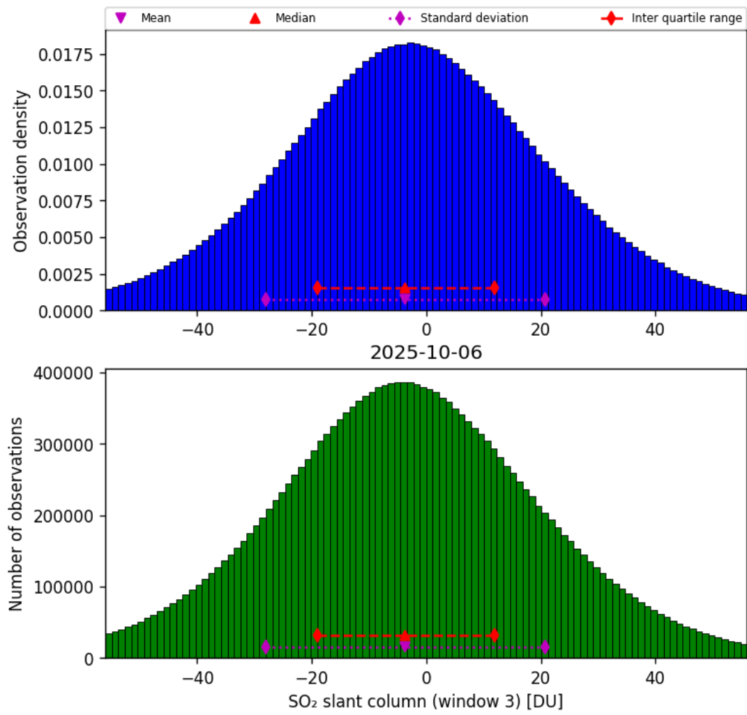
Figure 71: Histogram of “SO 2 slant column (window 3)” for 2025-10-06 to 2025-10-07
