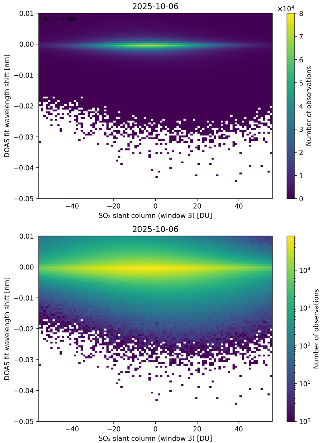
Figure 304: Scatter density plot of “SO 2 slant column (window 3)” against “DOAS fit wavelength shift” for 2025-10-06 to 2025-10-07.
