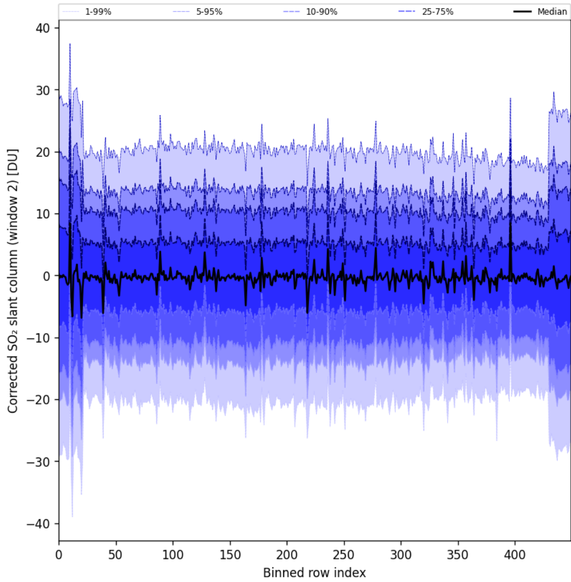
Figure 95: Along track statistics of “Corrected SO 2 slant column (window 2)” for 2025-10-06 to 2025-10-07
