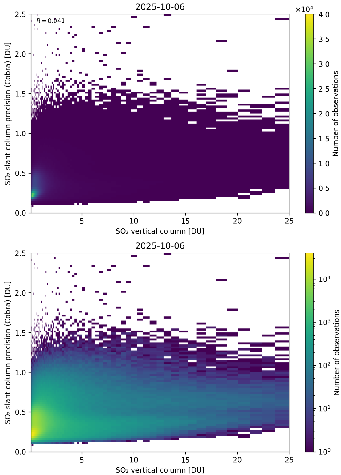
Figure 350: Scatter density plot of “SO 2 vertical column” against “SO 2 slant column precision (Cobra)” for 2025-10-06 to 2025-10-07.
