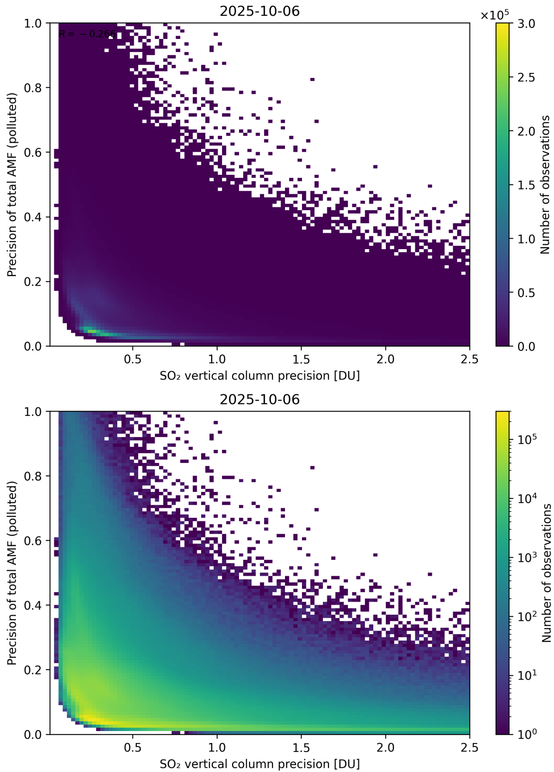
Figure 347: Scatter density plot of “SO 2 vertical column precision” against “Precision of total AMF (polluted)” for 2025-10-06 to 2025-10-07.
