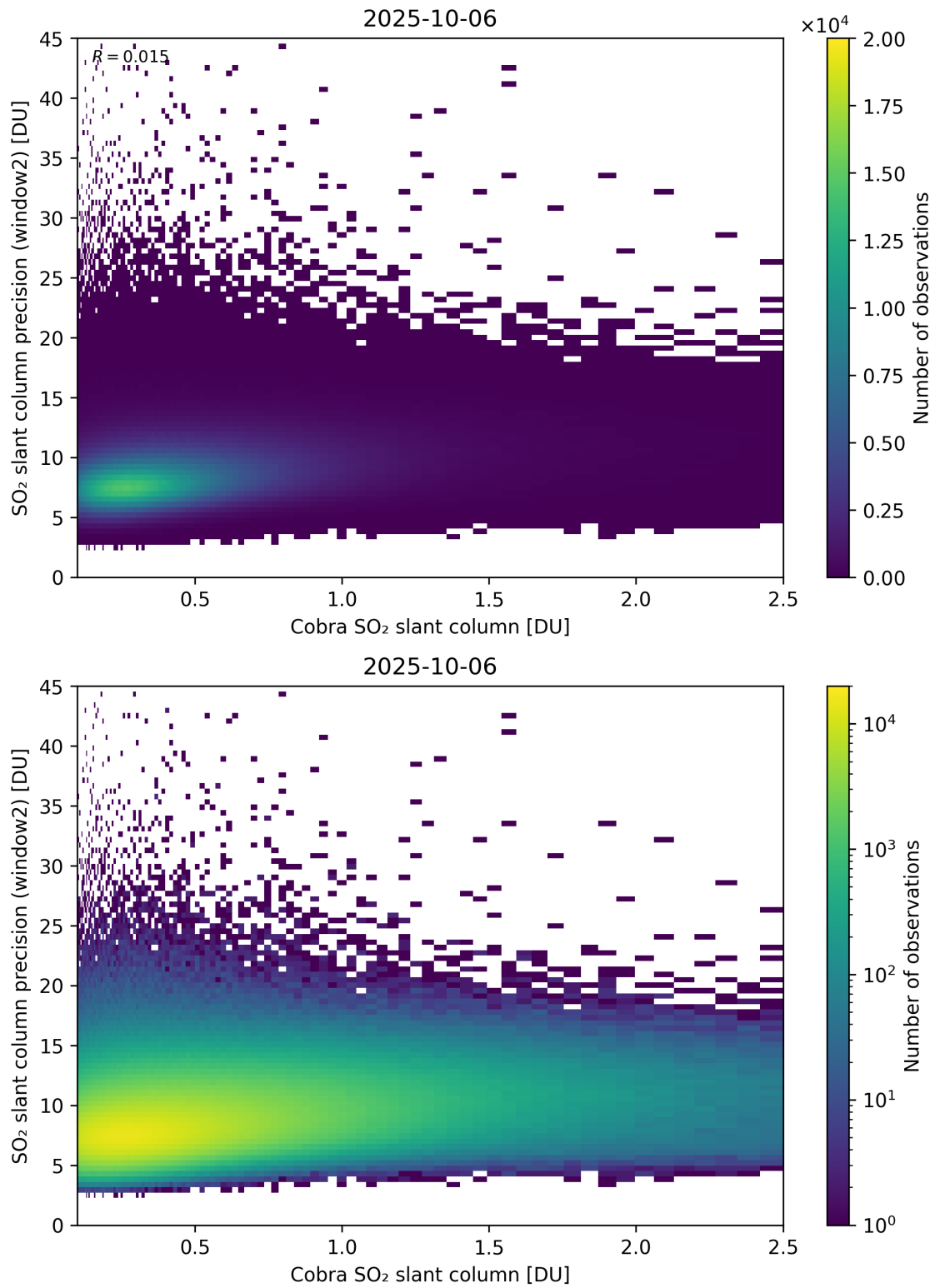
Figure 221: Scatter density plot of “Cobra SO 2 slant column” against “SO 2 slant column precision (window2)” for 2025-10-06 to 2025-10-07.
