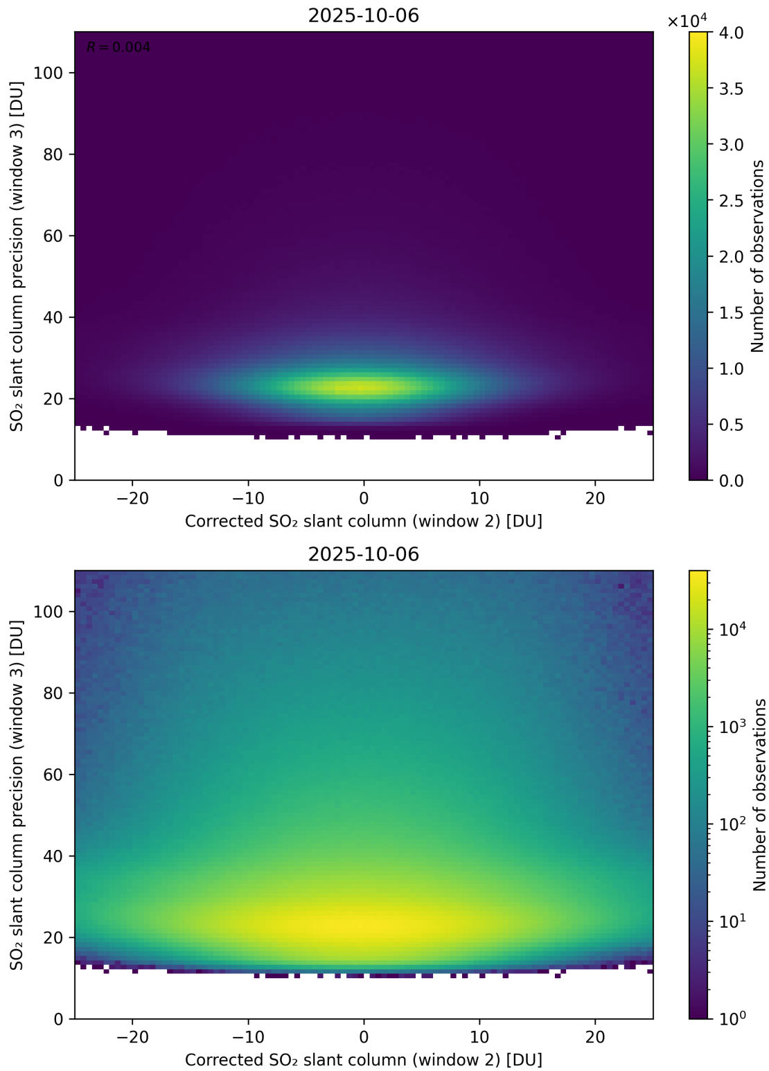
Figure 252: Scatter density plot of “Corrected SO 2 slant column (window 2)” against “SO 2 slant column precision (window 3)” for 2025-10-06 to 2025-10-07.
