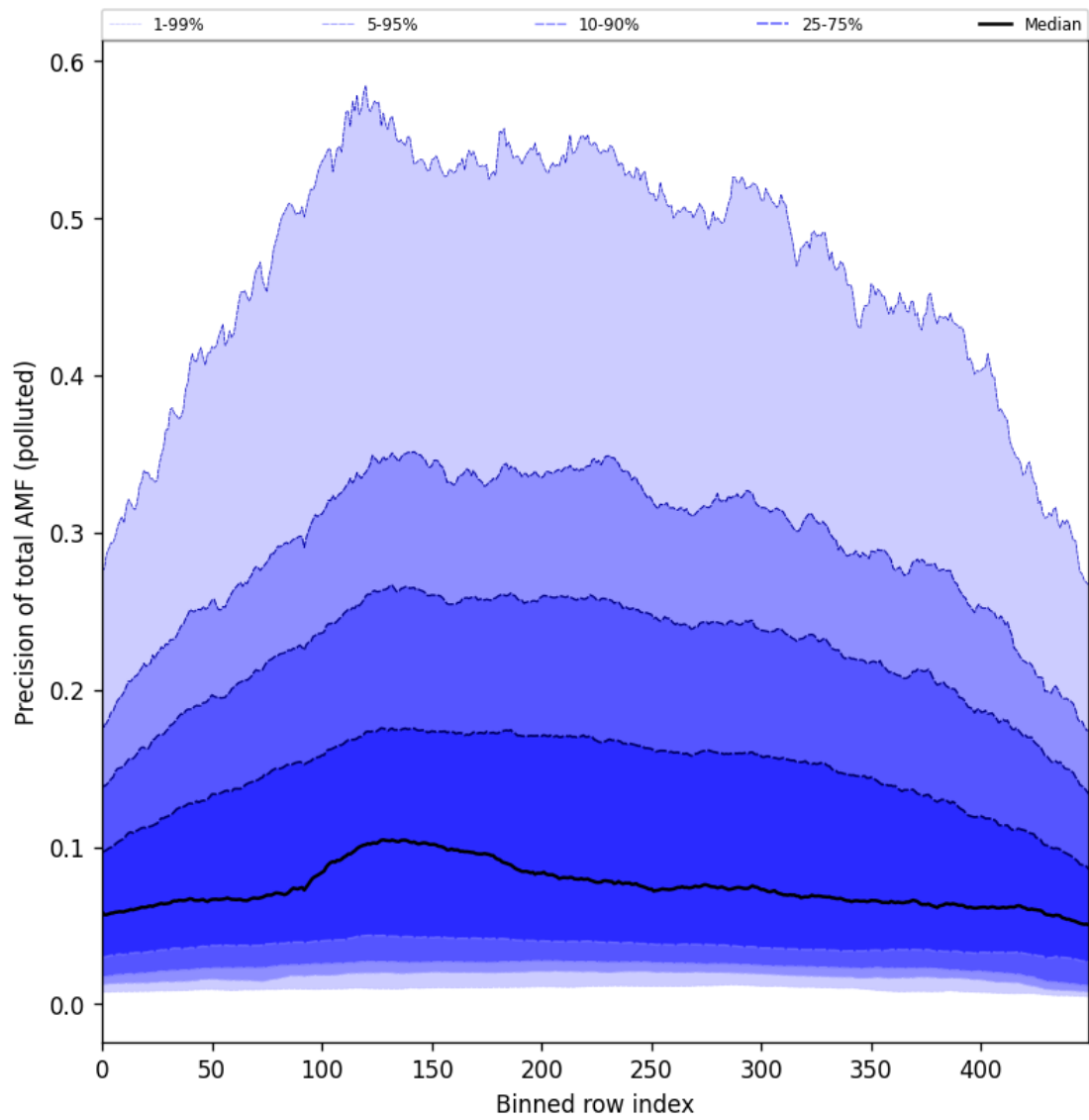
Figure 106: Along track statistics of “Precision of total AMF (polluted)” for 2025-10-06 to 2025-10-07
