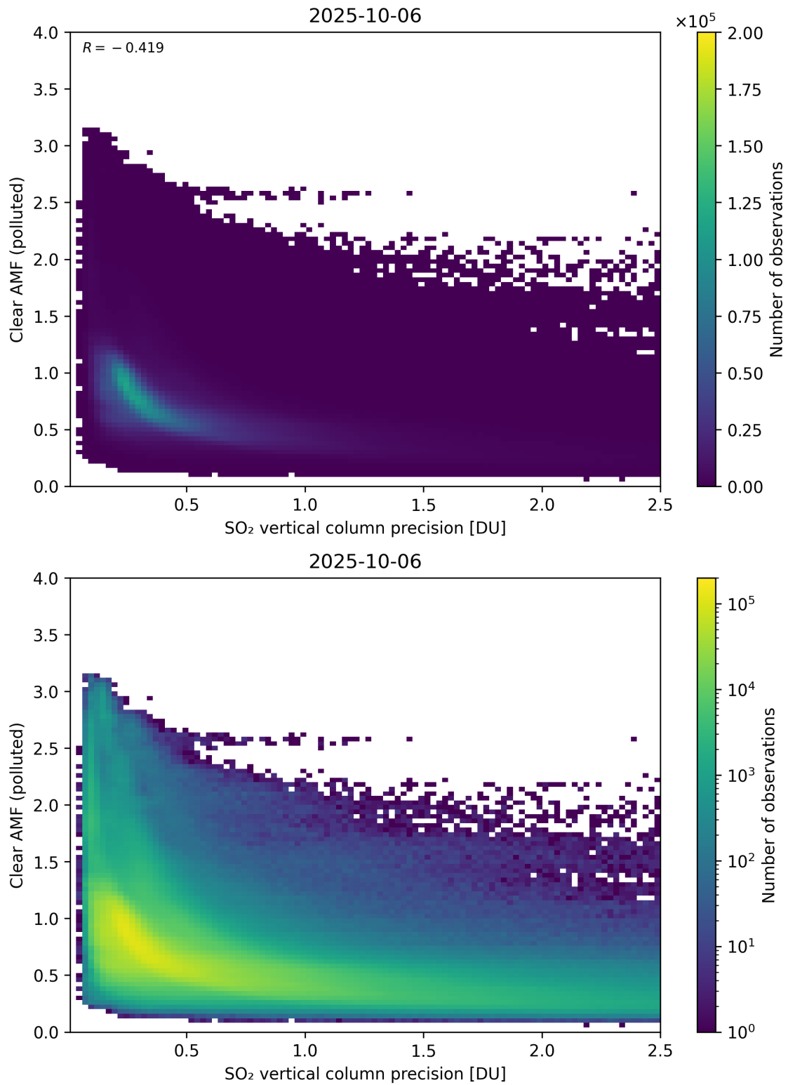
Figure 335: Scatter density plot of “SO 2 vertical column precision” against “Clear AMF (polluted)” for 2025-10-06 to 2025-10-07.
