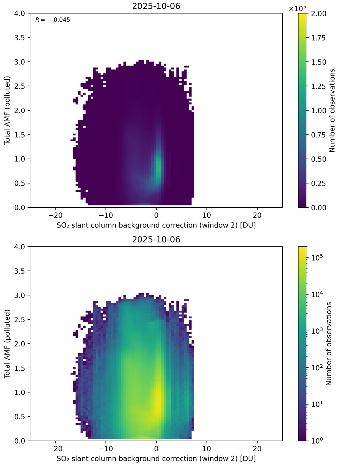
Figure 130: Scatter density plot of “SO 2 slant column background correction (window 2)” against “Total AMF (polluted)” for 2025-10-06 to 2025-10-07.
