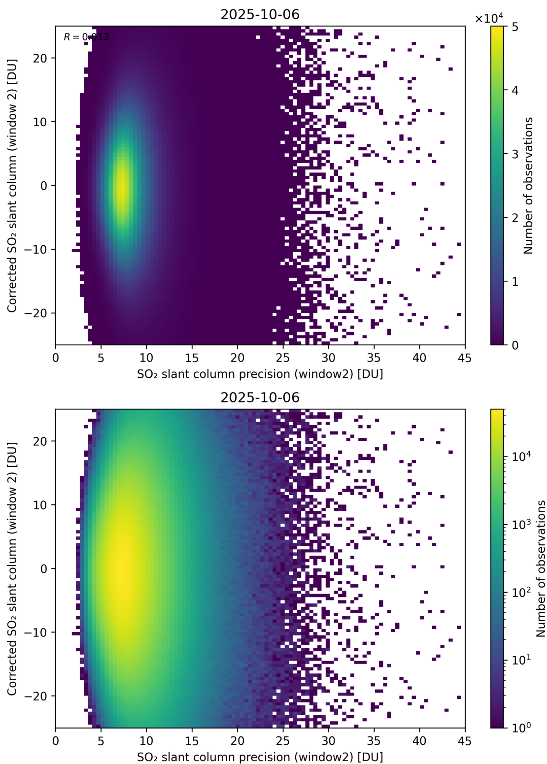
Figure 297: Scatter density plot of “SO 2 slant column precision (window2)” against “Corrected SO 2 slant column (window 2)” for 2025-10-06 to 2025-10-07.
