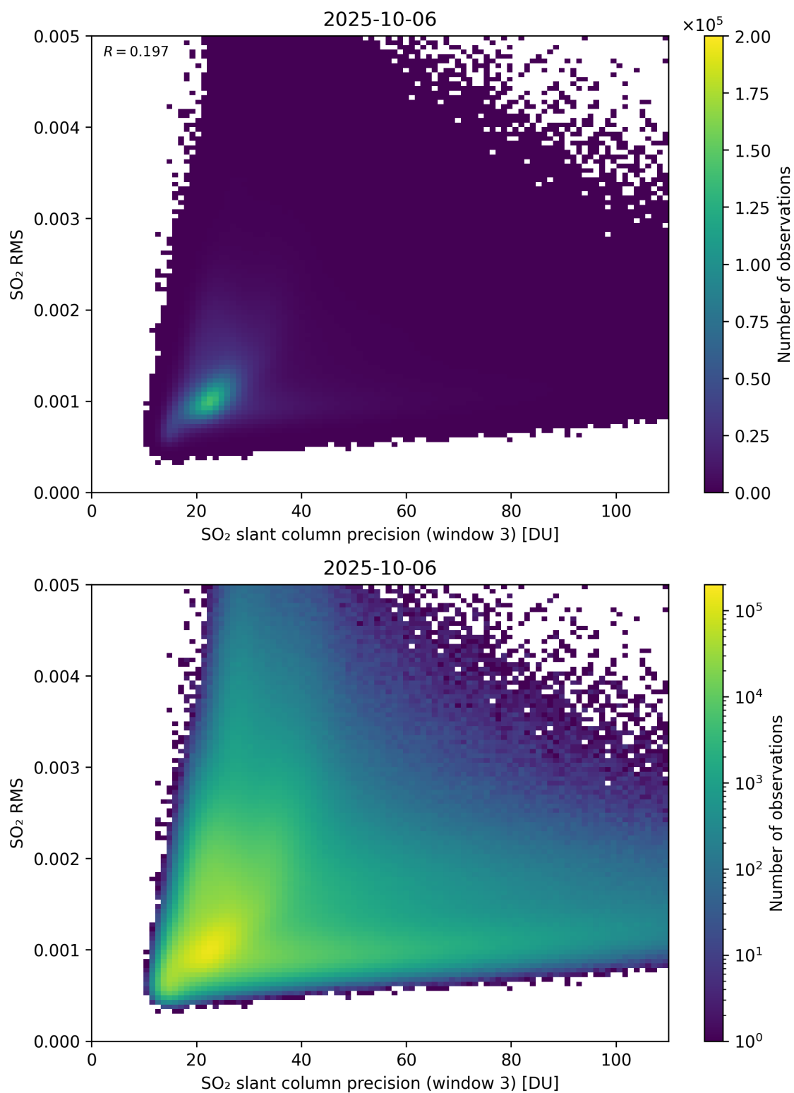
Figure 310: Scatter density plot of “SO 2 slant column precision (window 3)” against “SO 2 RMS” for 2025-10-06 to 2025-10-07.
