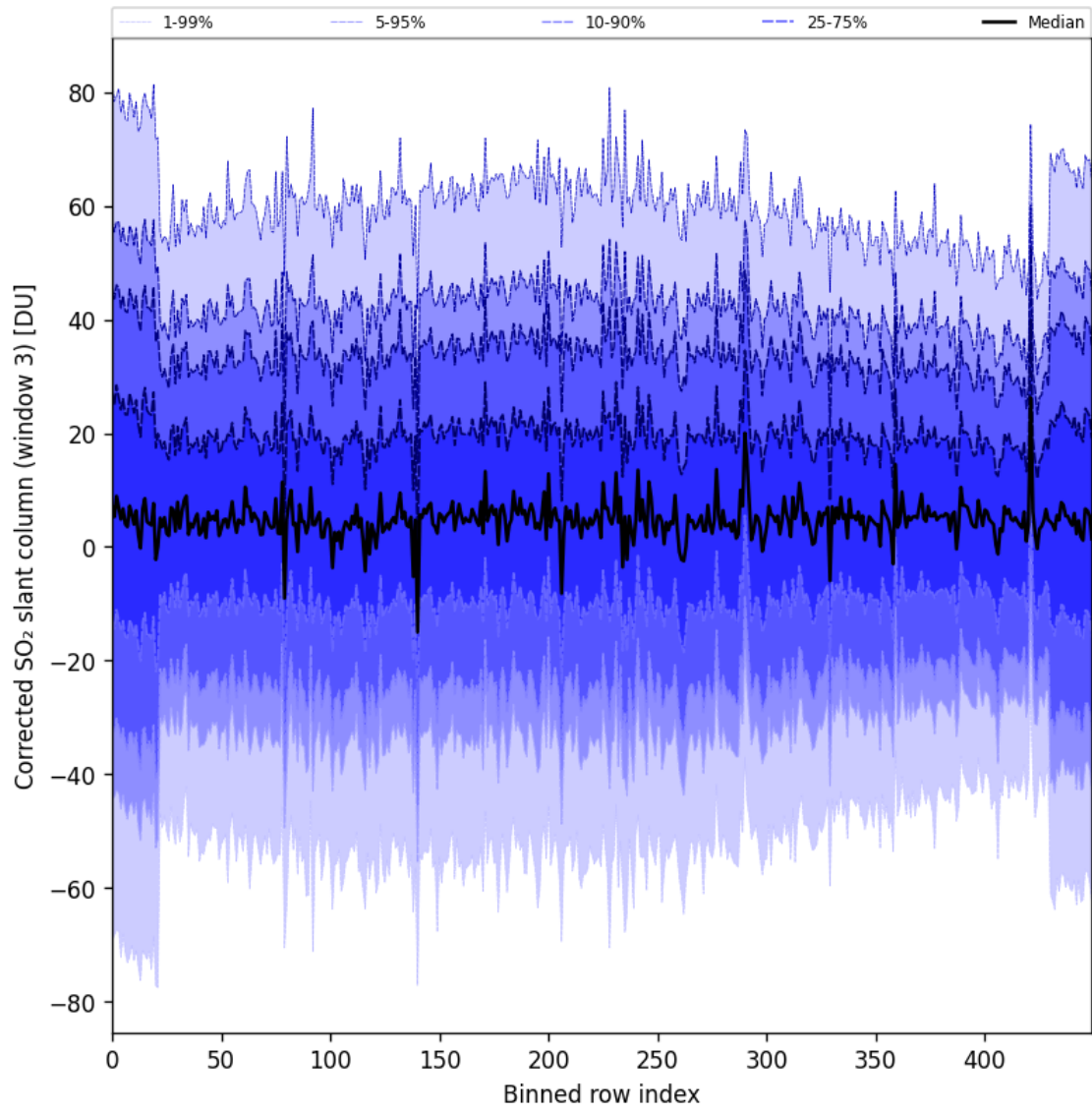
Figure 99: Along track statistics of “Corrected SO 2 slant column (window 3)” for 2025-10-06 to 2025-10-07
