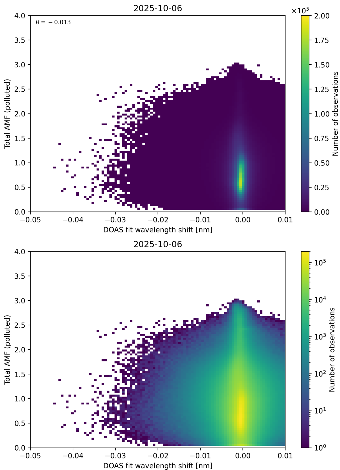
Figure 141: Scatter density plot of “DOAS fit wavelength shift” against “Total AMF (polluted)” for 2025-10-06 to 2025-10-07.
