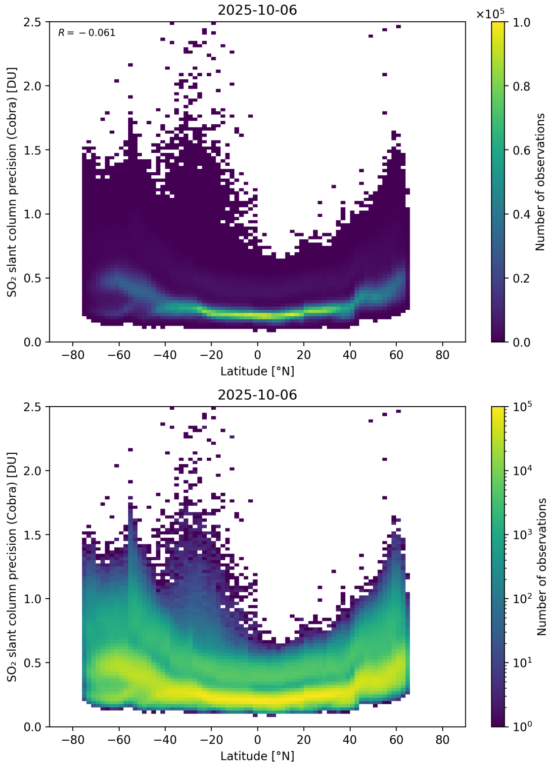
Figure 158: Scatter density plot of “Latitude” against “SO 2 slant column precision (Cobra)” for 2025-10-06 to 2025-10-07.
