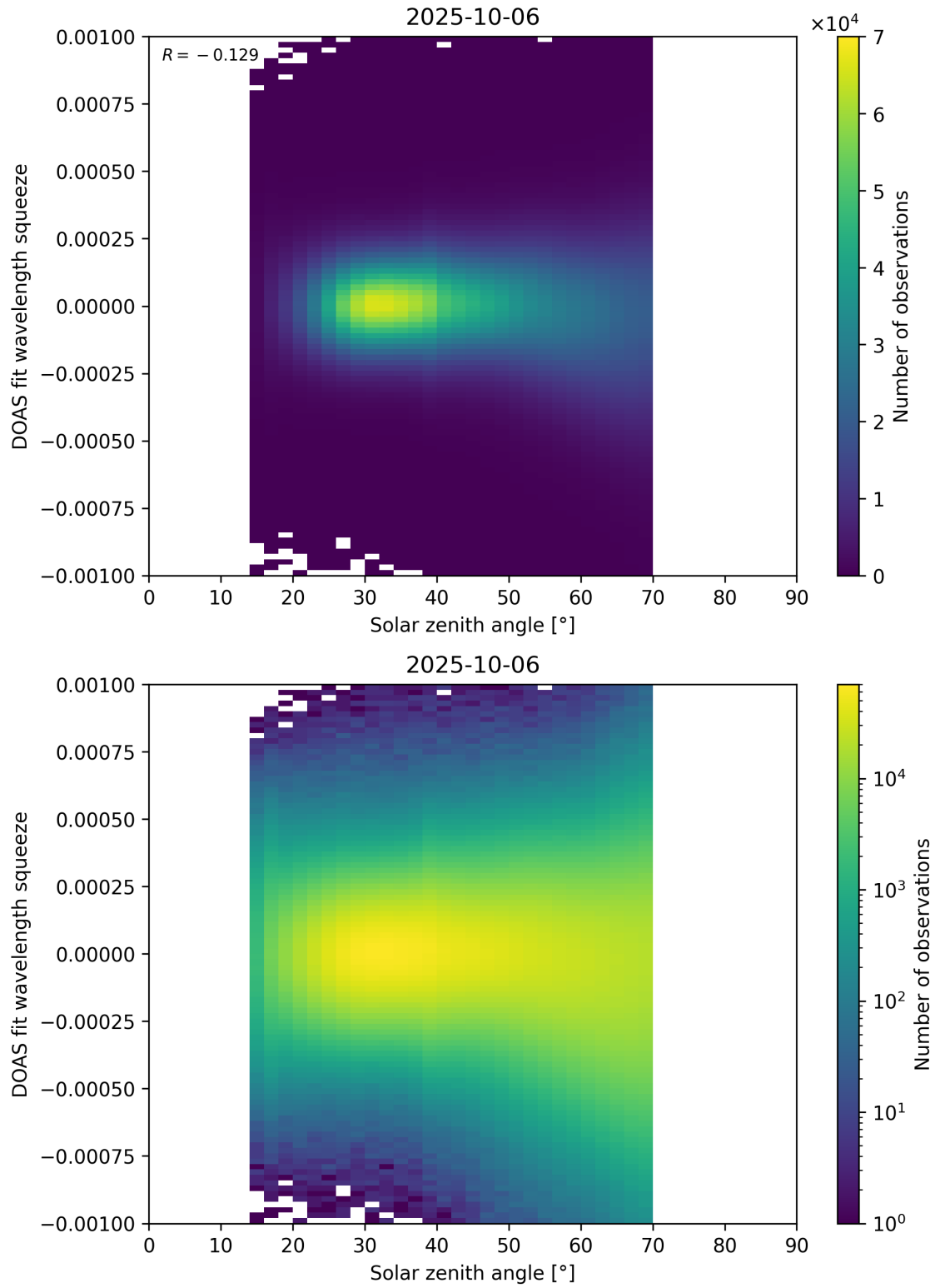
Figure 175: Scatter density plot of “Solar zenith angle” against “DOAS fit wavelength squeeze” for 2025-10-06 to 2025-10-07.
