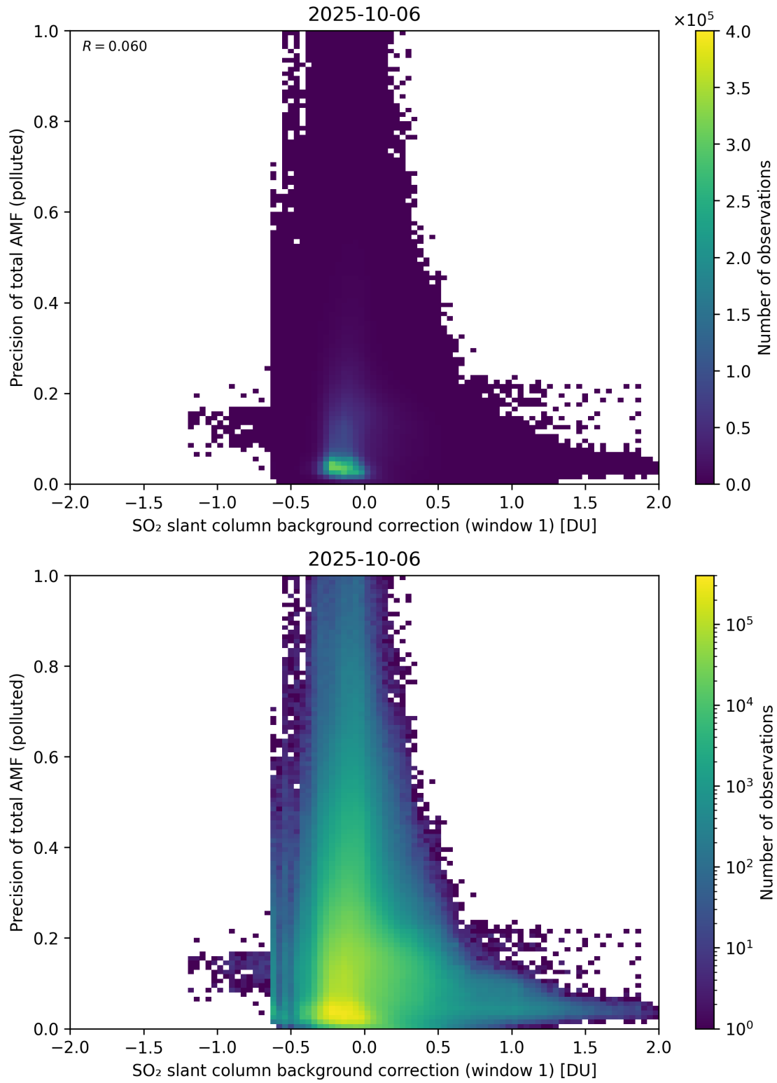
Figure 121: Scatter density plot of “SO 2 slant column background correction (window 1)” against “Precision of total AMF (polluted)” for 2025-10-06 to 2025-10-07.
