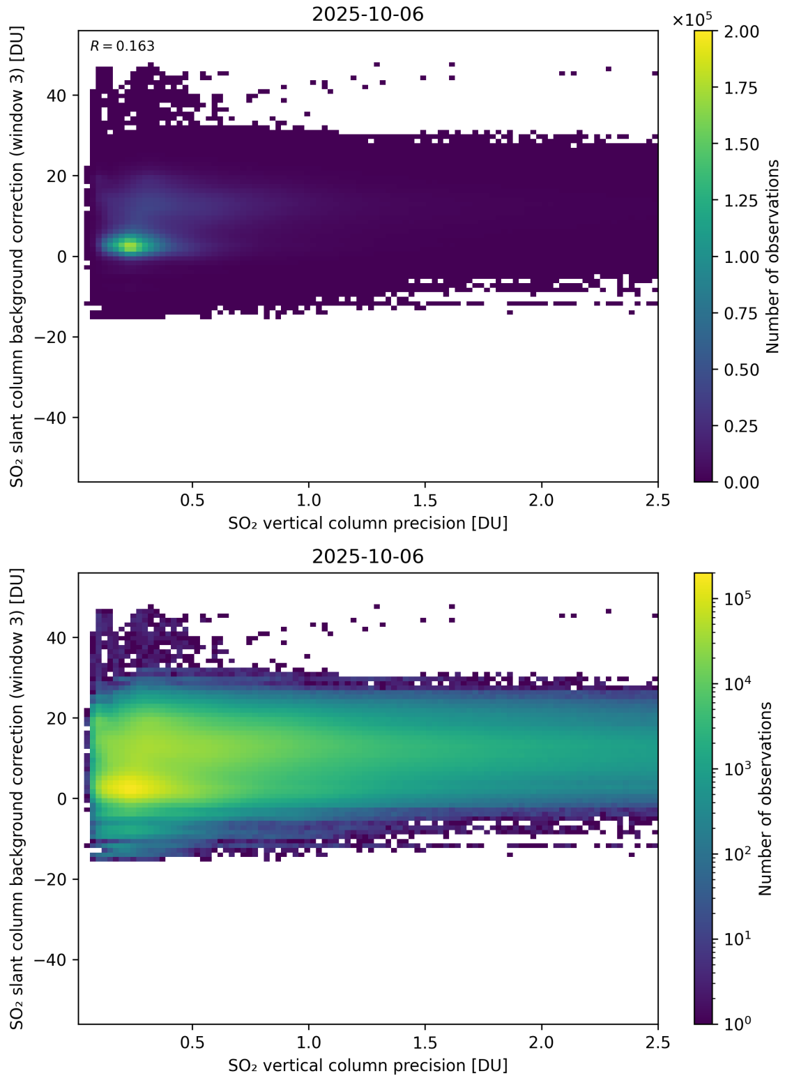
Figure 331: Scatter density plot of “SO 2 vertical column precision” against “SO 2 slant column background correction (window 3)” for 2025-10-06 to 2025-10-07.
