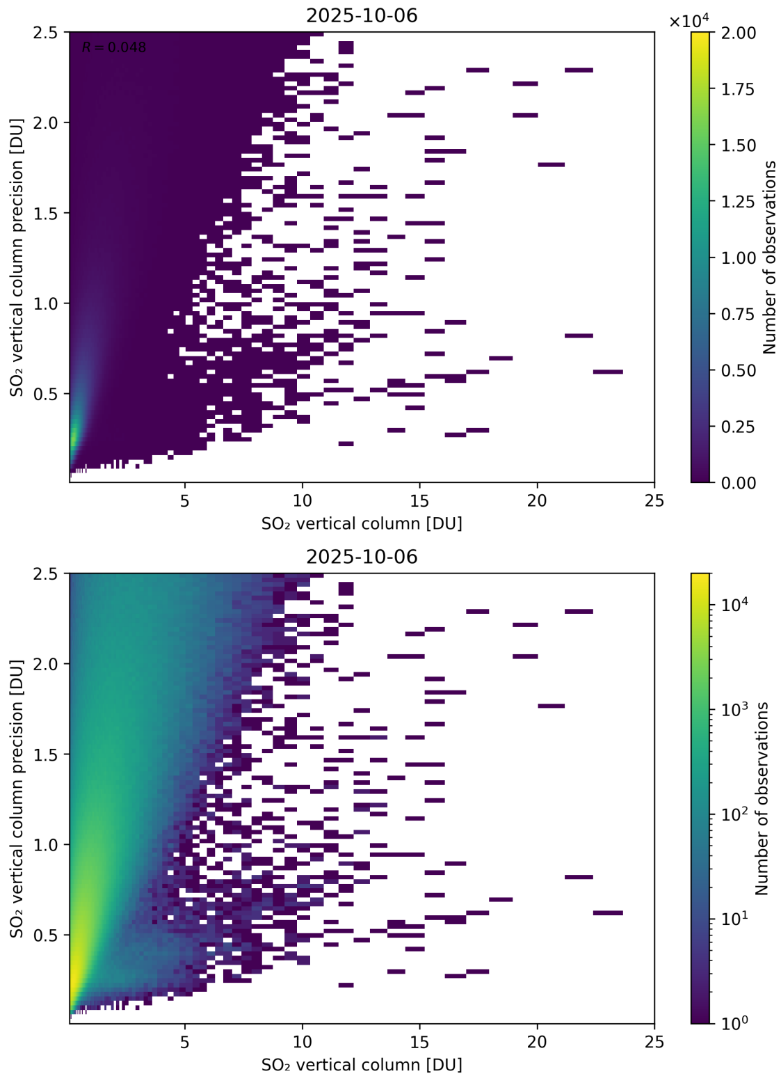
Figure 361: Scatter density plot of “SO 2 vertical column” against “SO 2 vertical column precision” for 2025-10-06 to 2025-10-07.
