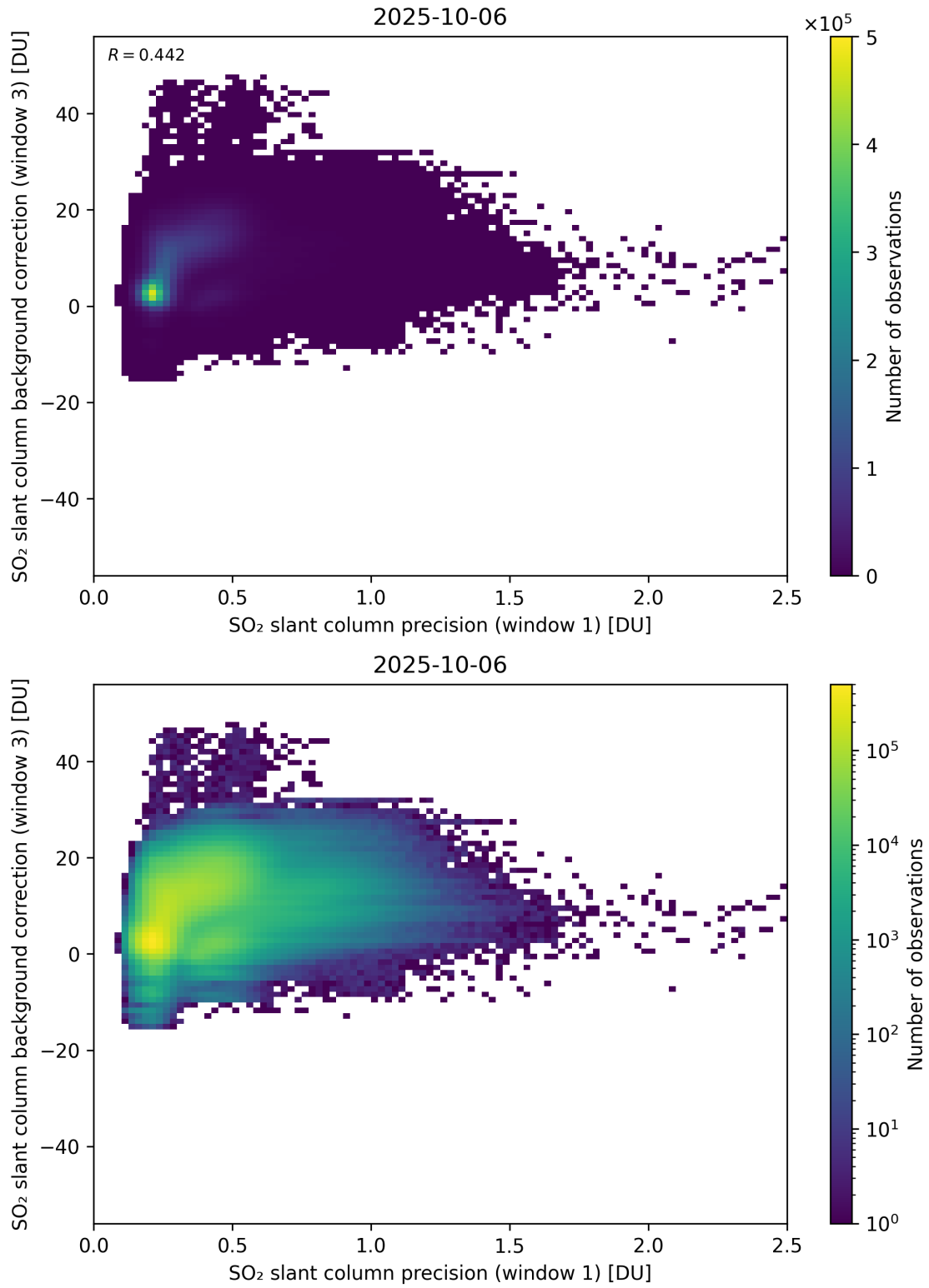
Figure 270: Scatter density plot of “SO 2 slant column precision (window 1)” against “SO 2 slant column background correction (window 3)” for 2025-10-06 to 2025-10-07.
