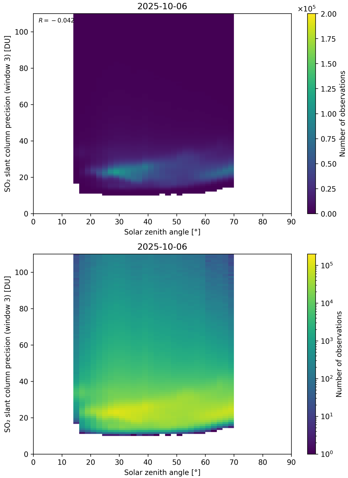
Figure 188: Scatter density plot of “Solar zenith angle” against “SO 2 slant column precision (window 3)” for 2025-10-06 to 2025-10-07.
