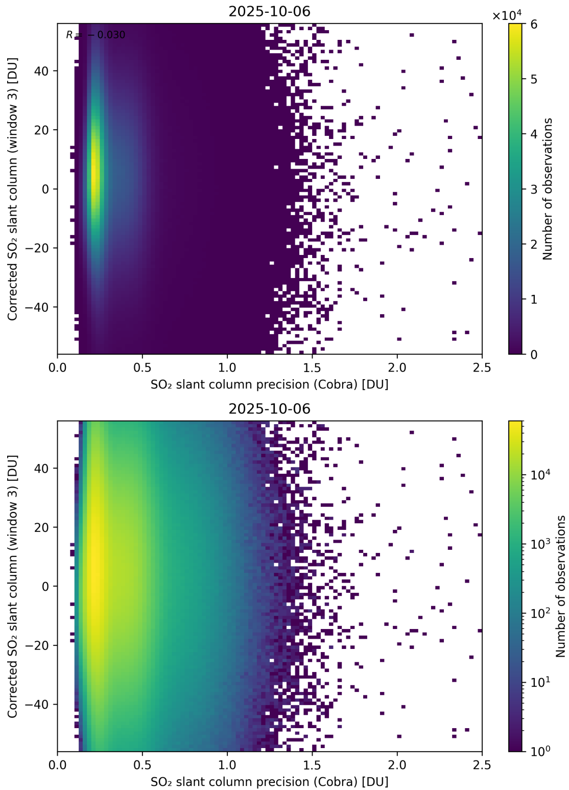
Figure 207: Scatter density plot of “SO 2 slant column precision (Cobra)” against “Corrected SO 2 slant column (window 3)” for 2025-10-06 to 2025-10-07.
