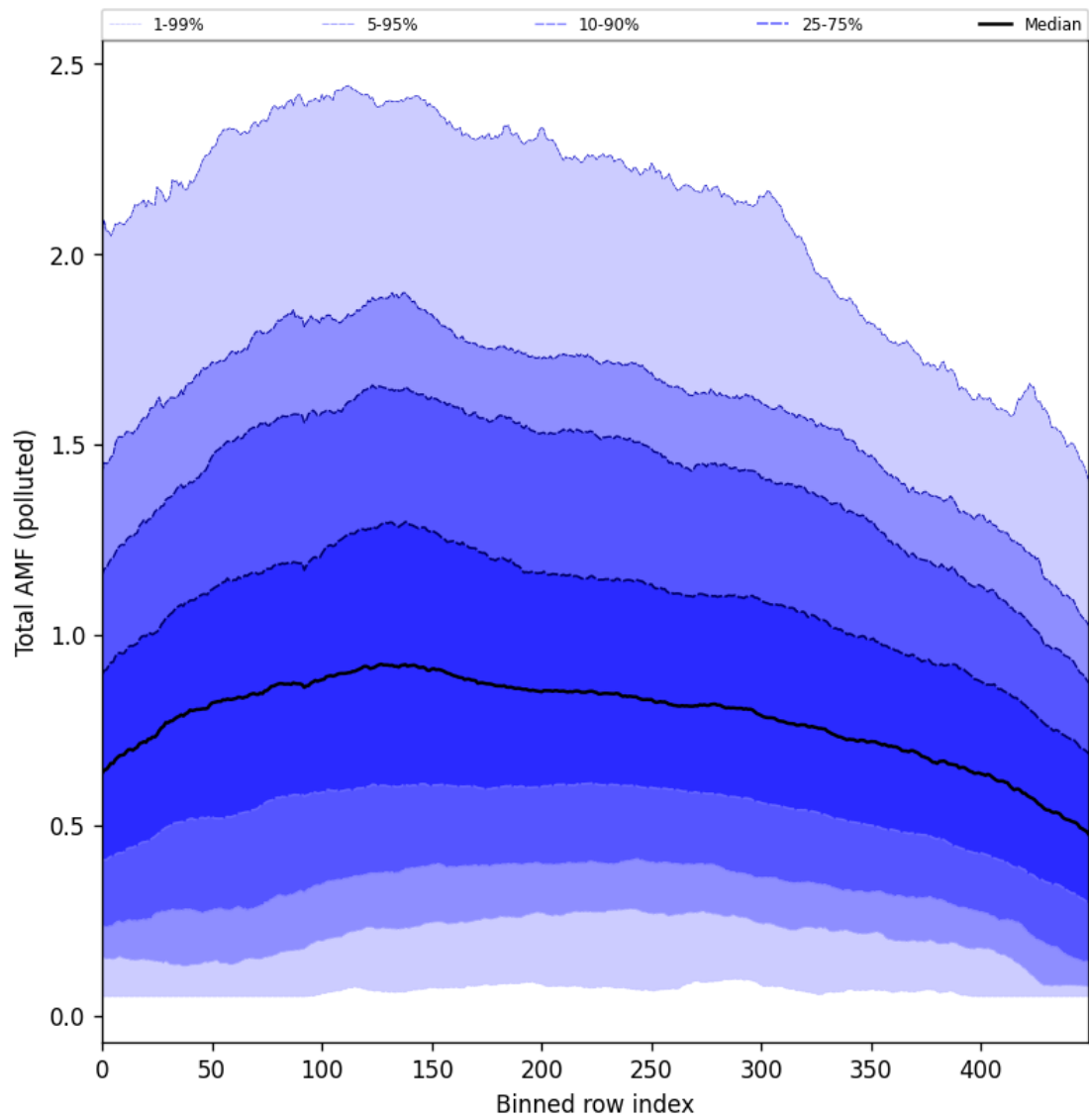
Figure 105: Along track statistics of “Total AMF (polluted)” for 2025-10-06 to 2025-10-07
