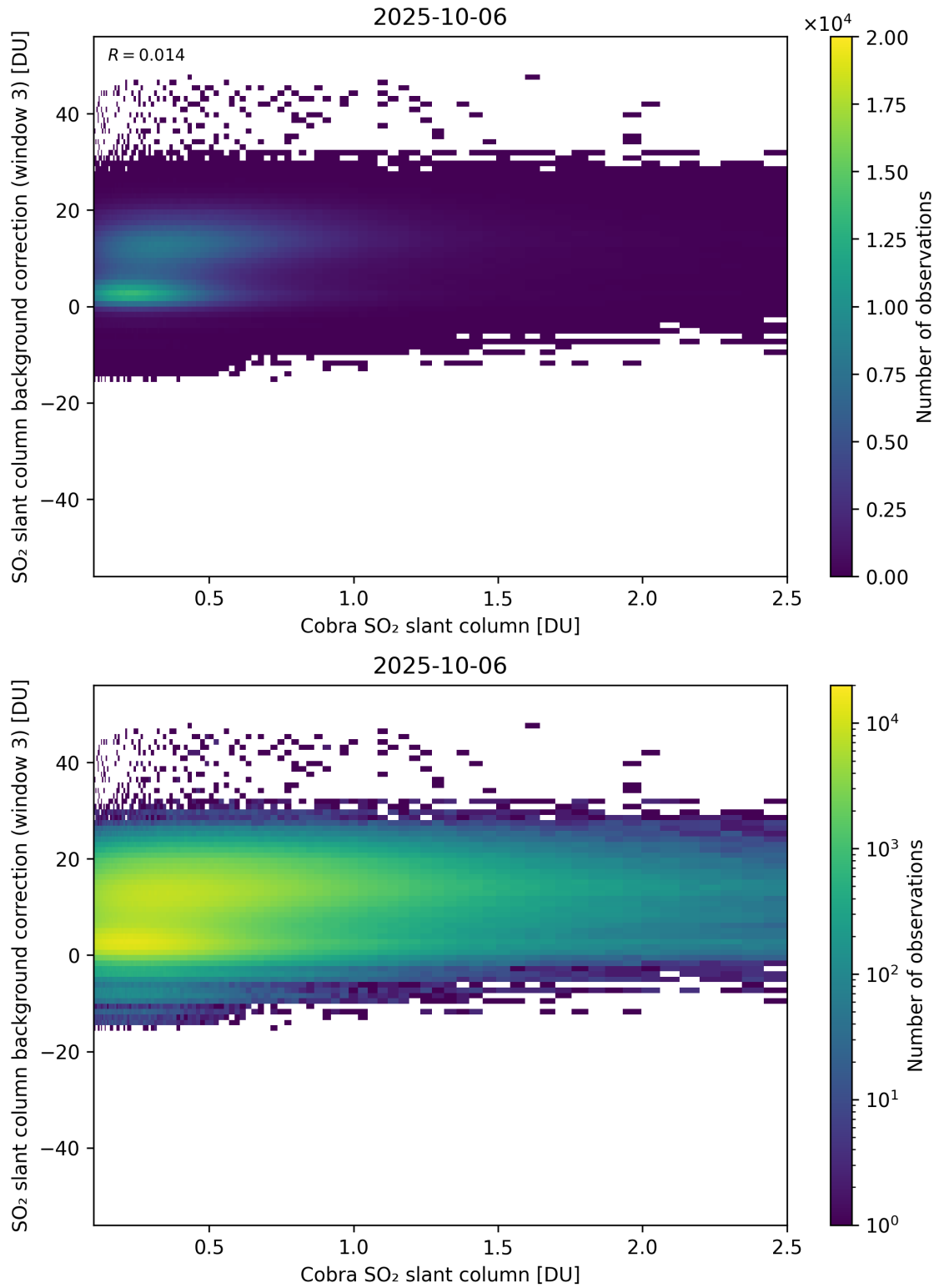
Figure 195: Scatter density plot of “Cobra SO 2 slant column” against “SO 2 slant column background correction (window 3)” for 2025-10-06 to 2025-10-07.
