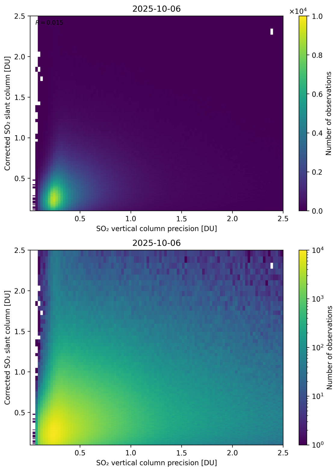
Figure 338: Scatter density plot of “SO 2 vertical column precision” against “Corrected SO 2 slant column” for 2025-10-06 to 2025-10-07.
