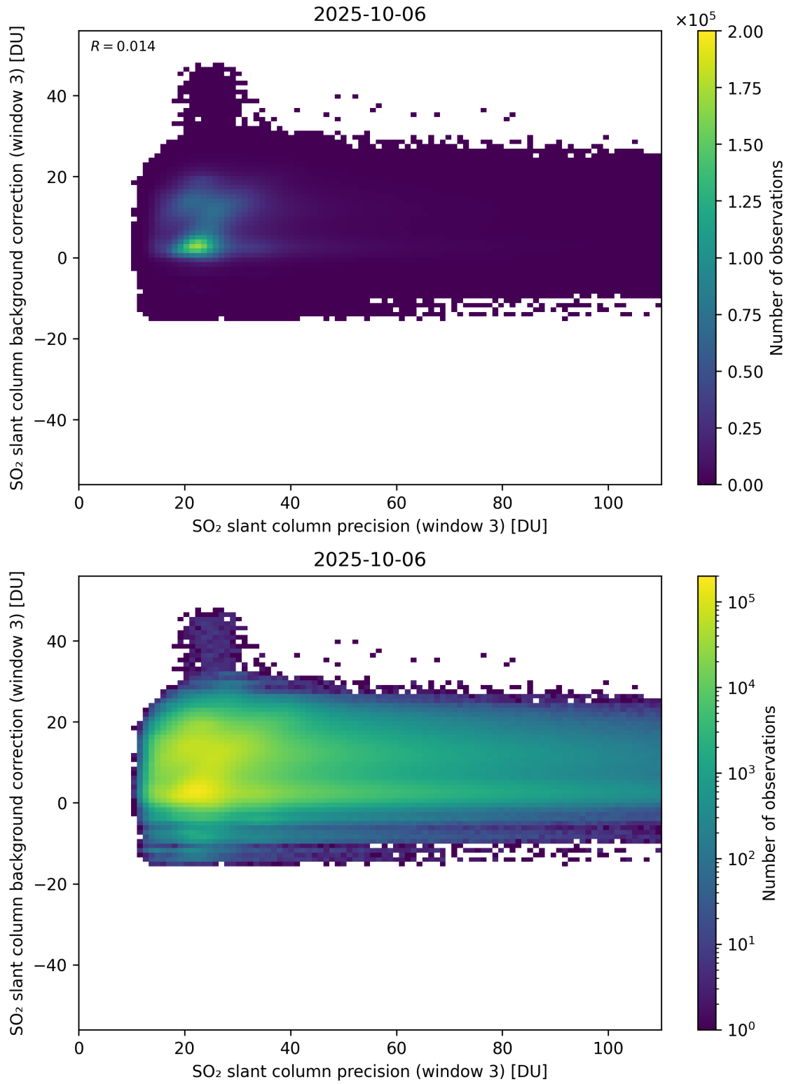
Figure 307: Scatter density plot of “SO 2 slant column precision (window 3)” against “SO 2 slant column background correction (window 3)” for 2025-10-06 to 2025-10-07.
