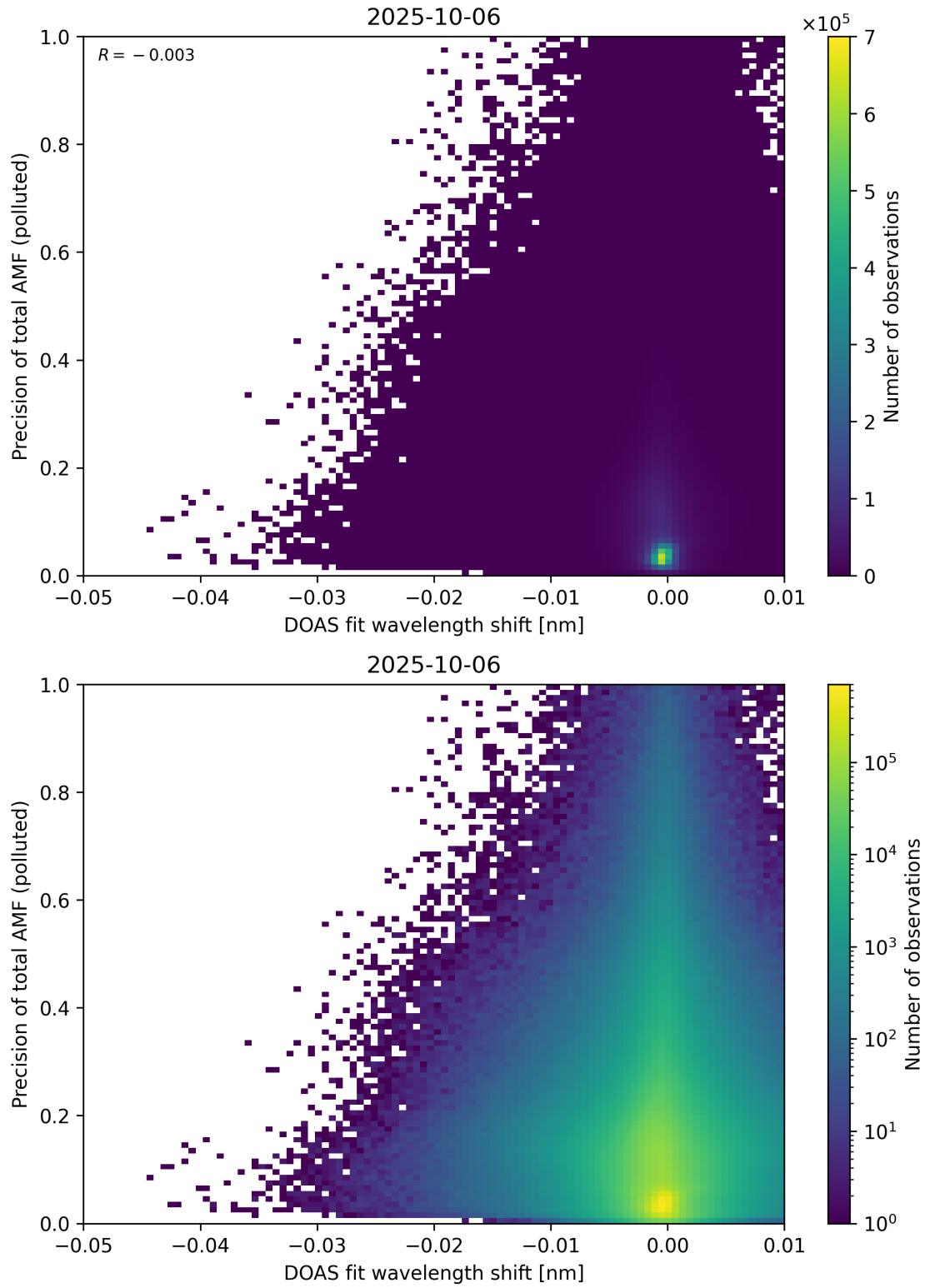
Figure 142: Scatter density plot of “DOAS fit wavelength shift” against “Precision of total AMF (polluted)” for 2025-10-06 to 2025-10-07.
