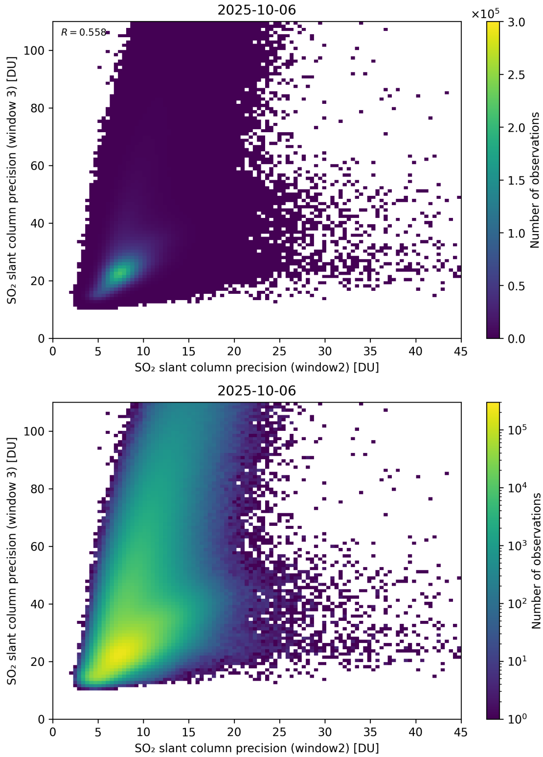
Figure 300: Scatter density plot of “SO 2 slant column precision (window2)” against “SO 2 slant column precision (window 3)” for 2025-10-06 to 2025-10-07.
