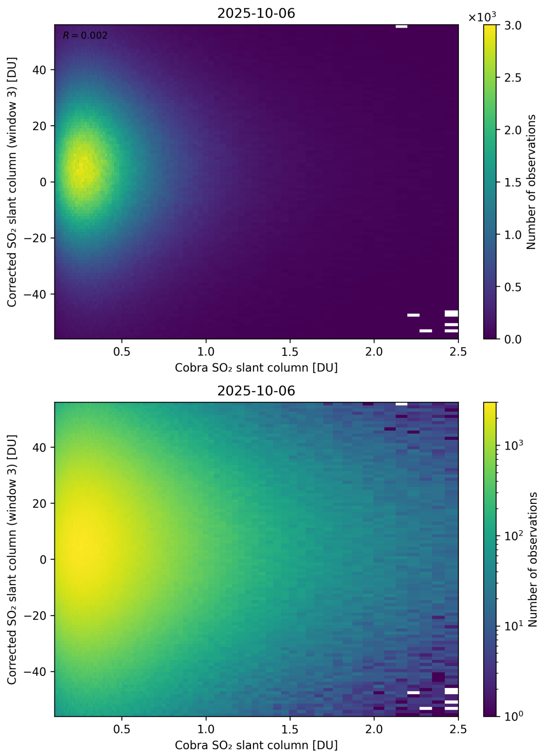
Figure 218: Scatter density plot of “Cobra SO 2 slant column” against “Corrected SO 2 slant column (window 3)” for 2025-10-06 to 2025-10-07.
