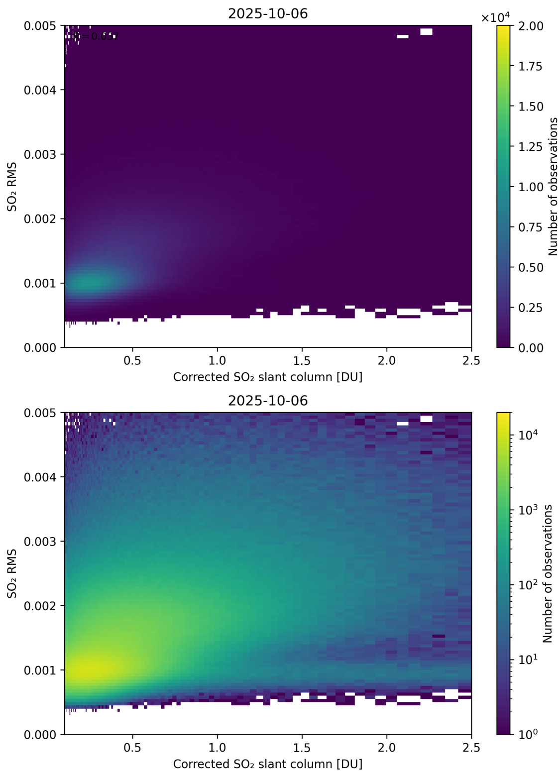
Figure 231: Scatter density plot of “Corrected SO 2 slant column” against “SO 2 RMS” for 2025-10-06 to 2025-10-07.
