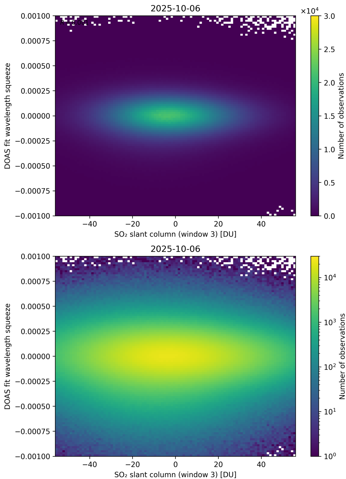
Figure 305: Scatter density plot of “SO 2 slant column (window 3)” against “DOAS fit wavelength squeeze” for 2025-10-06 to 2025-10-07.
