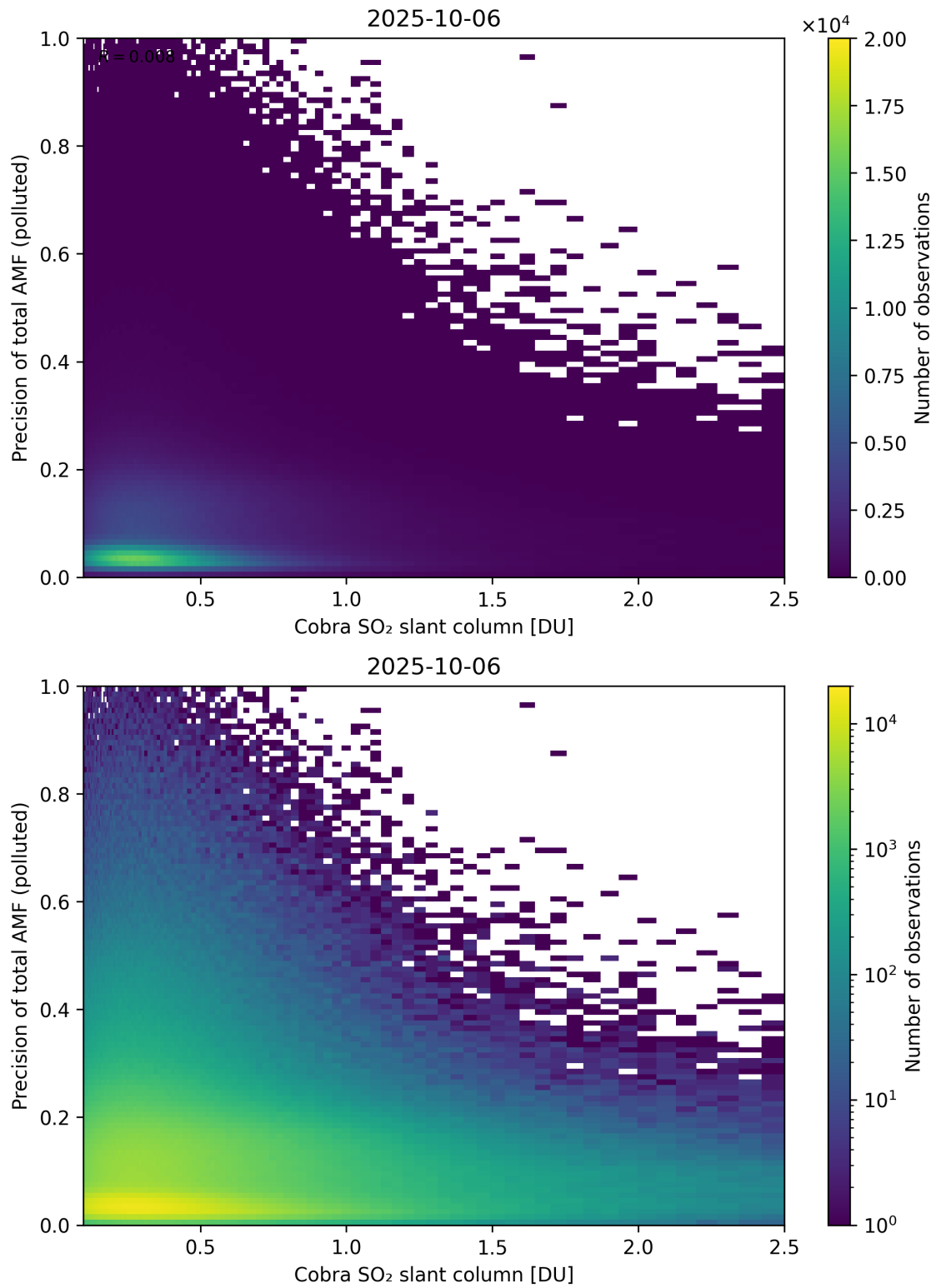
Figure 225: Scatter density plot of “Cobra SO 2 slant column” against “Precision of total AMF (polluted)” for 2025-10-06 to 2025-10-07.
