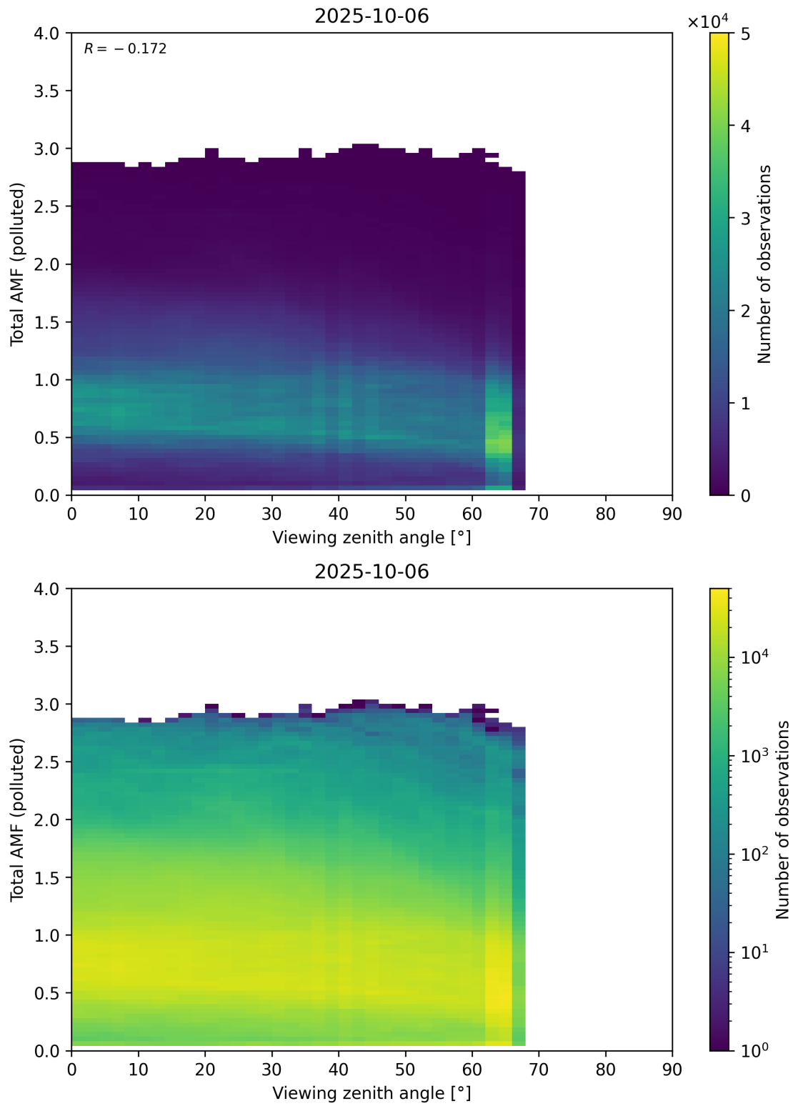
Figure 381: Scatter density plot of “Viewing zenith angle” against “Total AMF (polluted)” for 2025-10-06 to 2025-10-07.
