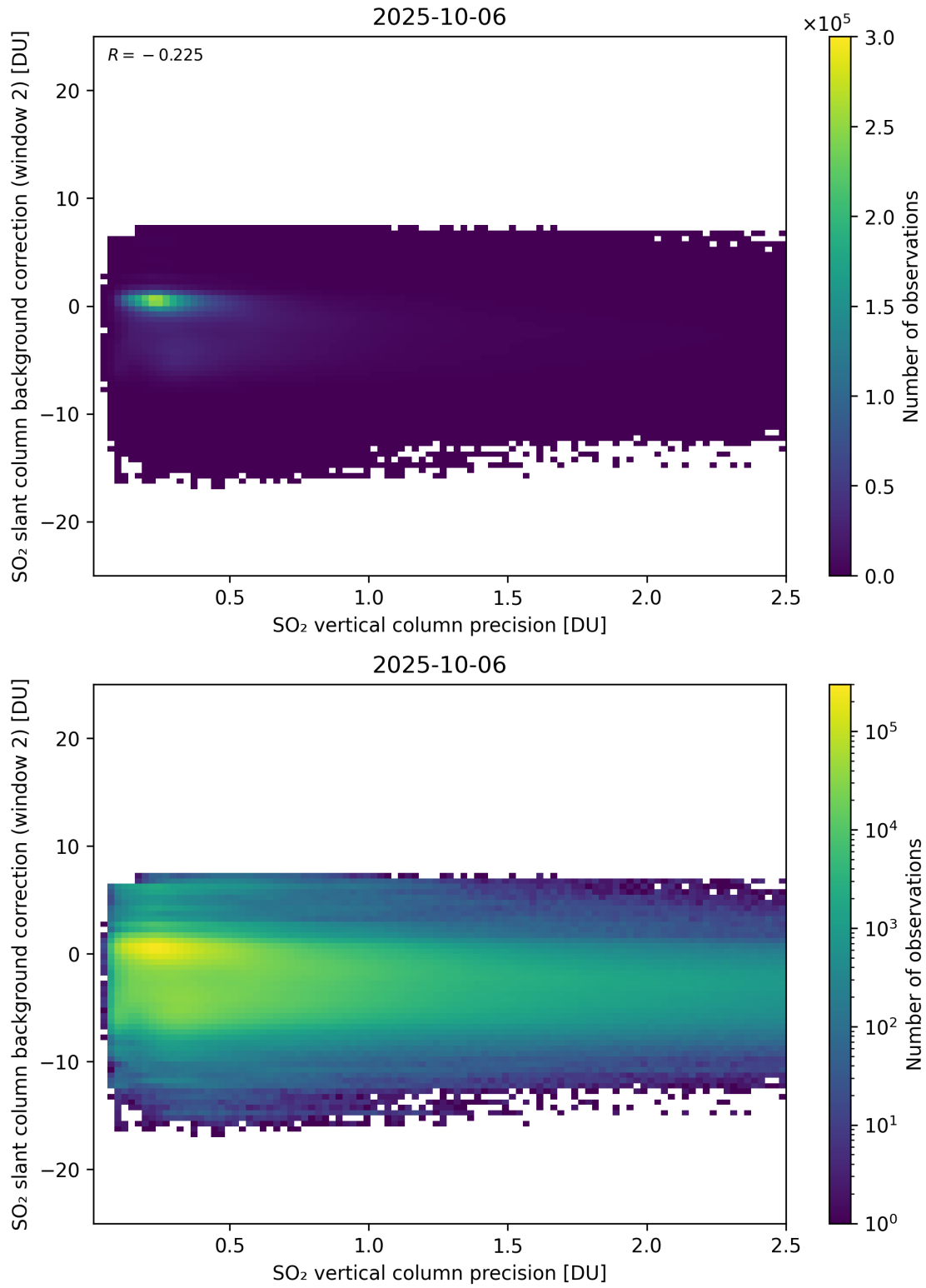
Figure 330: Scatter density plot of “SO 2 vertical column precision” against “SO 2 slant column background correction (window 2)” for 2025-10-06 to 2025-10-07.
