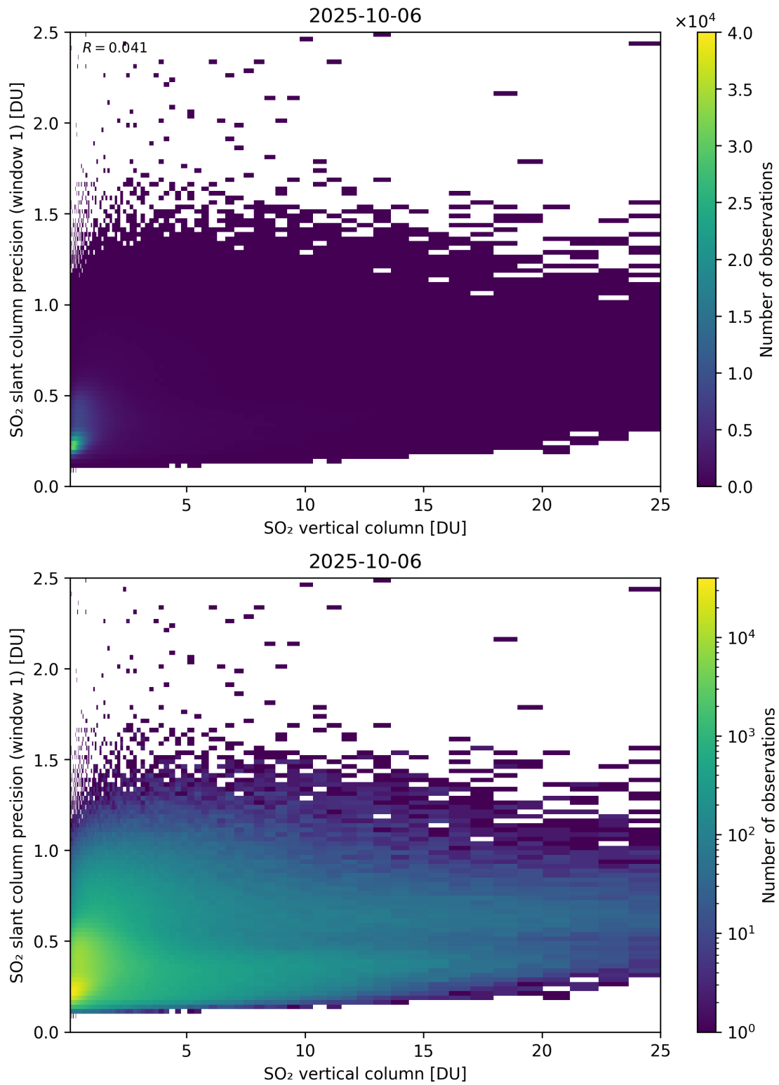
Figure 355: Scatter density plot of “SO 2 vertical column” against “SO 2 slant column precision (window 1)” for 2025-10-06 to 2025-10-07.
