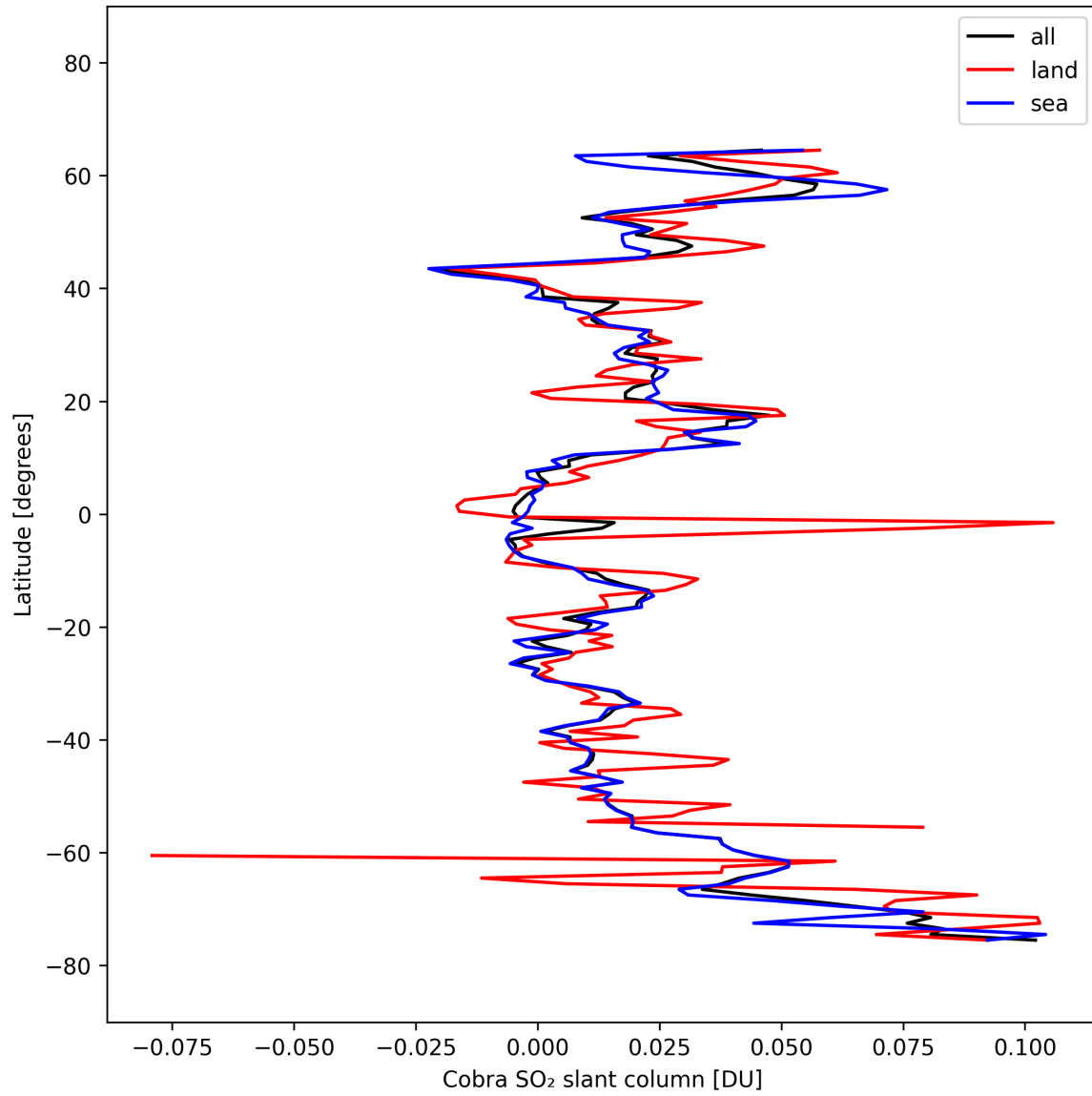
Figure 35: Zonal average of “Cobra SO 2 slant column” for 2025-10-06 to 2025-10-07.
