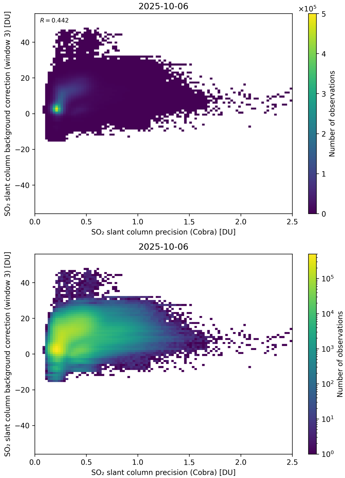
Figure 201: Scatter density plot of “SO 2 slant column precision (Cobra)” against “SO 2 slant column background correction (window 3)” for 2025-10-06 to 2025-10-07.
