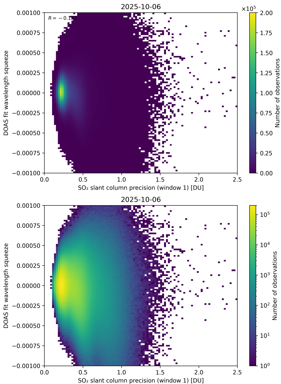
Figure 272: Scatter density plot of “SO 2 slant column precision (window 1)” against “DOAS fit wavelength squeeze” for 2025-10-06 to 2025-10-07.
