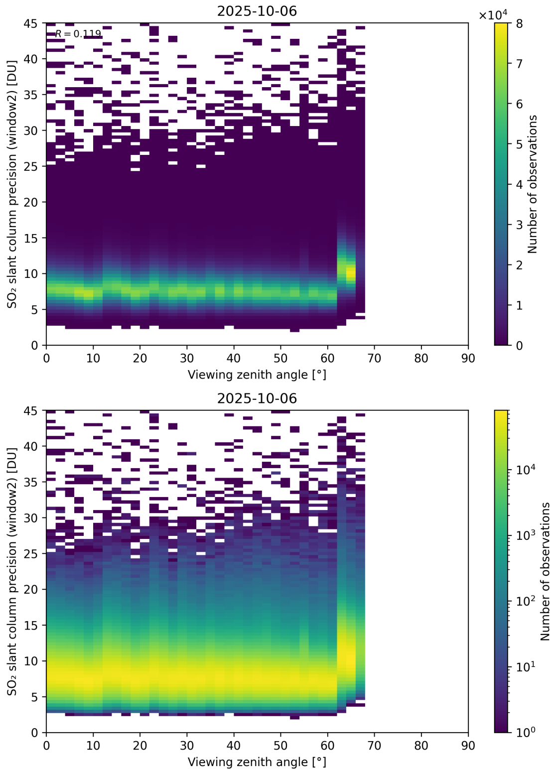
Figure 378: Scatter density plot of “Viewing zenith angle” against “SO 2 slant column precision (window2)” for 2025-10-06 to 2025-10-07.
