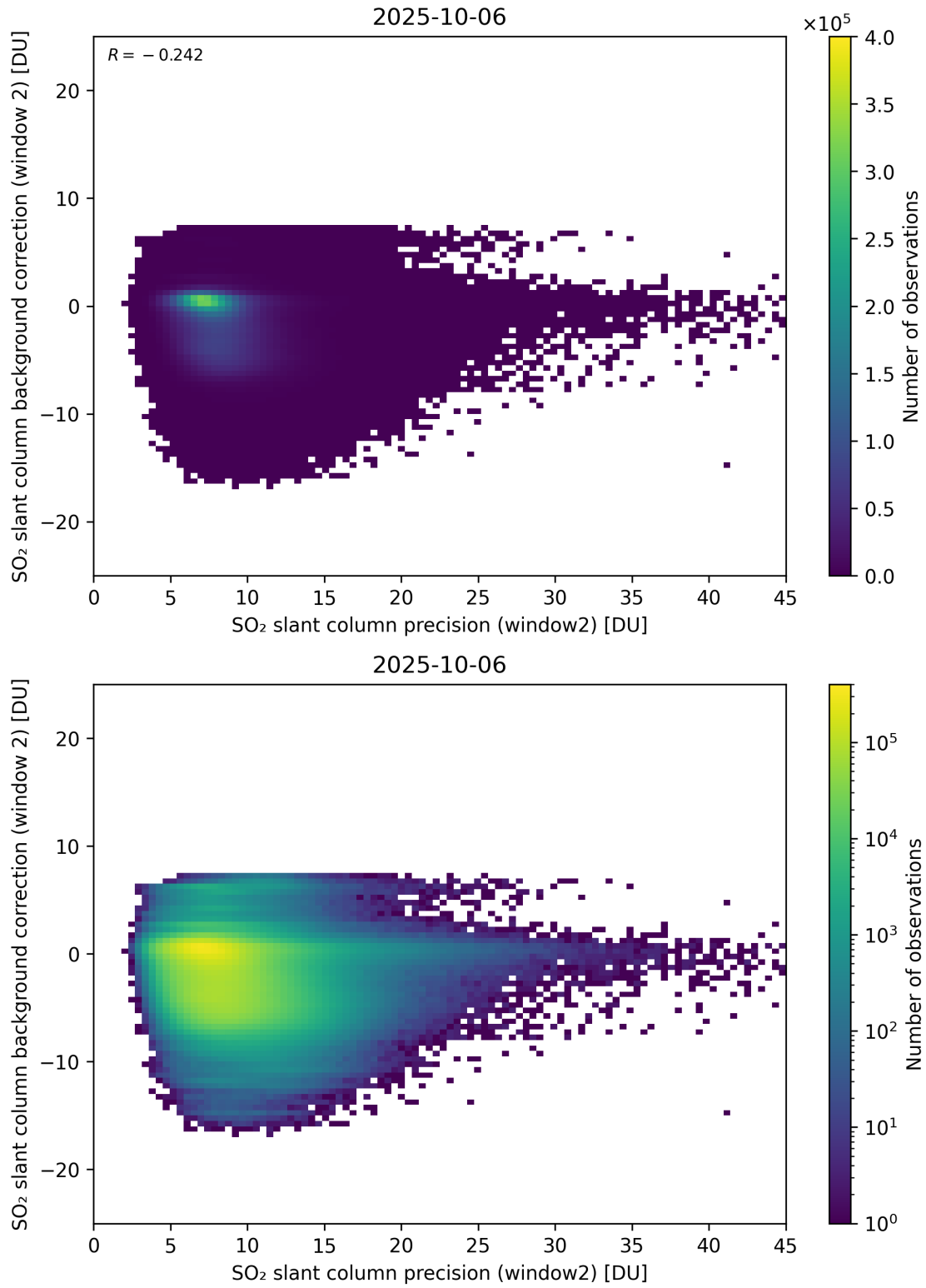
Figure 291: Scatter density plot of “SO 2 slant column precision (window2)” against “SO 2 slant column background correction (window 2)” for 2025-10-06 to 2025-10-07.
