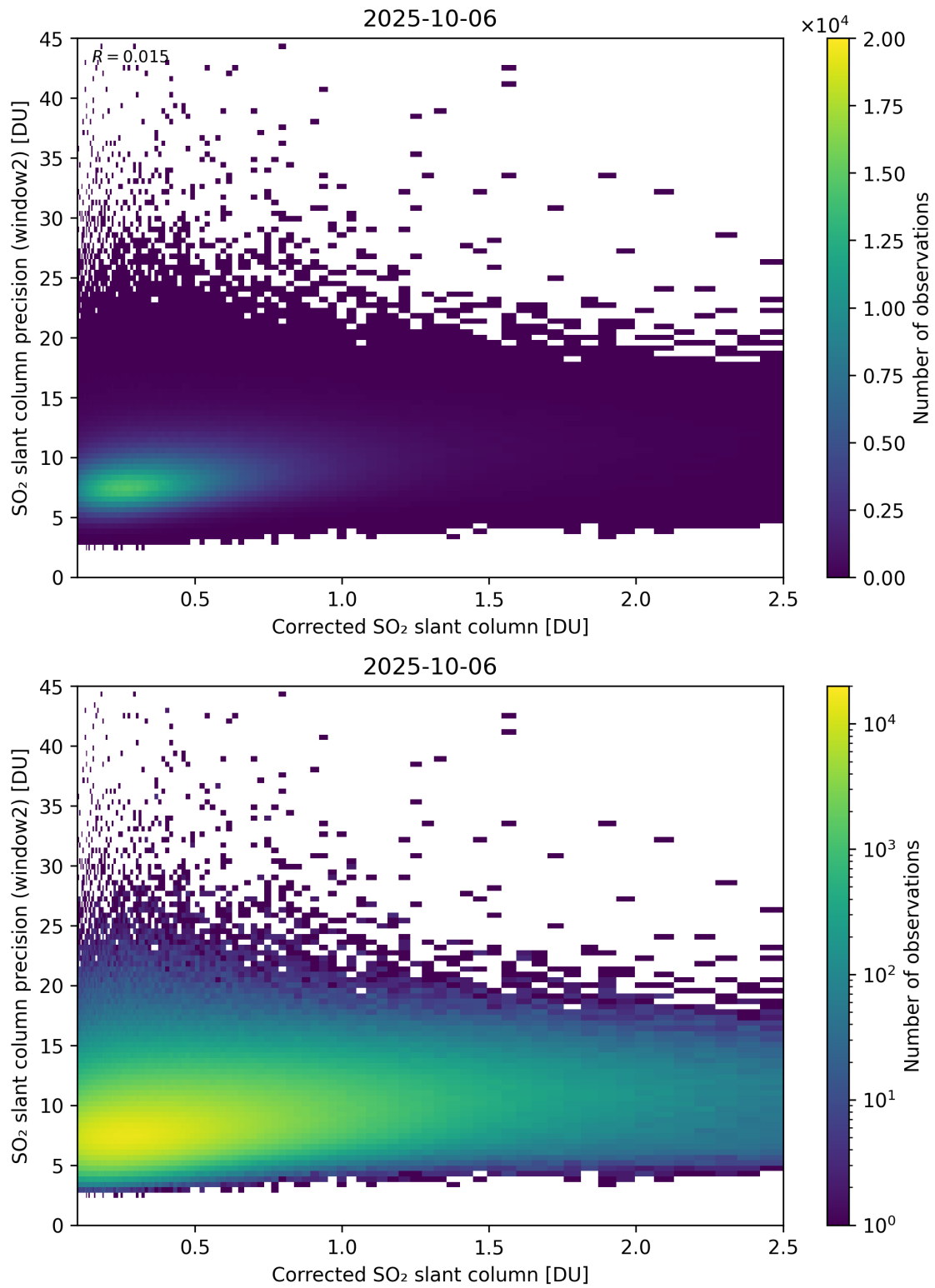
Figure 239: Scatter density plot of “Corrected SO 2 slant column” against “SO 2 slant column precision (window2)” for 2025-10-06 to 2025-10-07.
