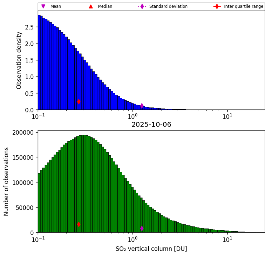
Figure 58: Histogram of “SO 2 vertical column” for 2025-10-06 to 2025-10-07
