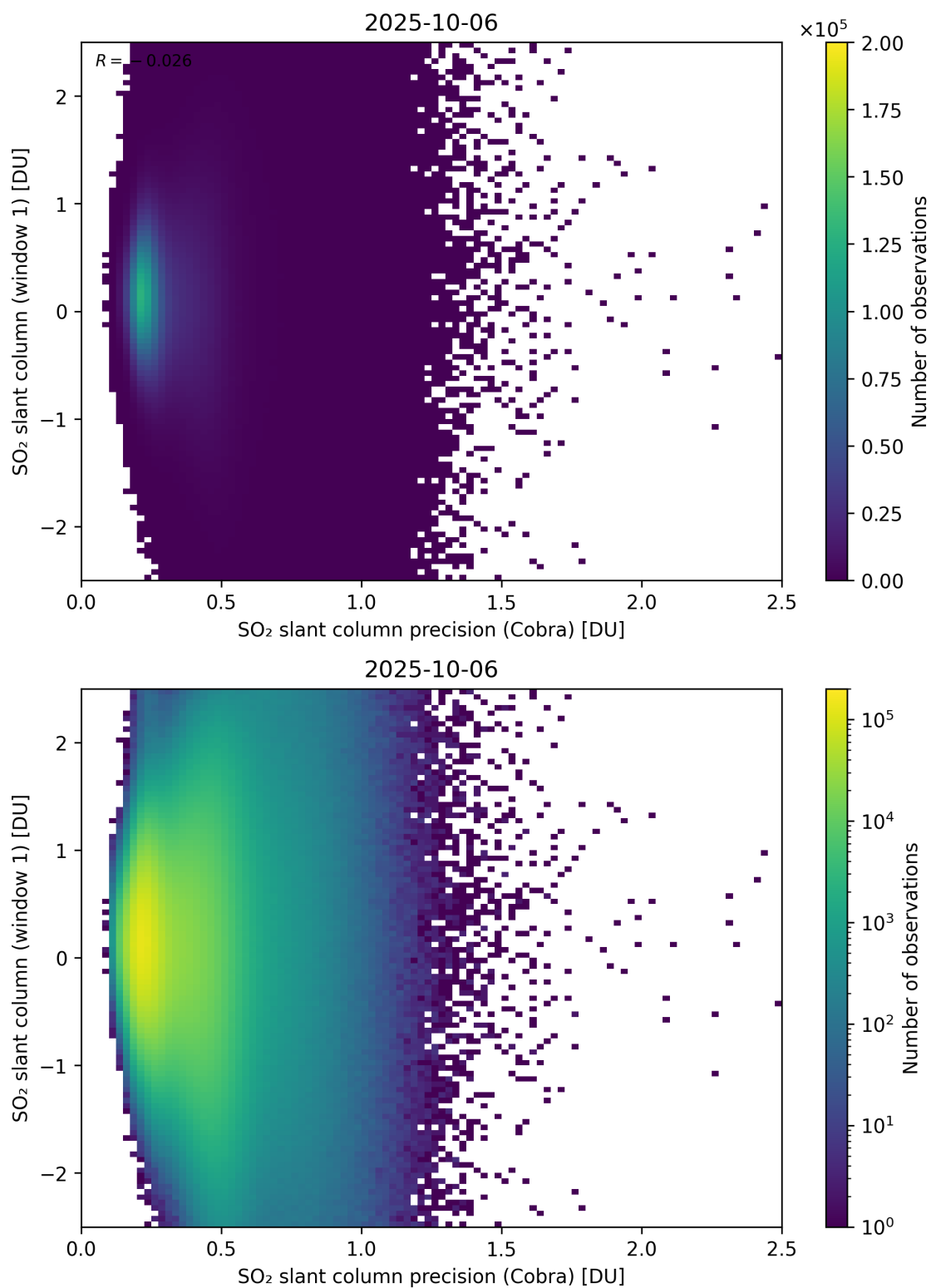
Figure 208: Scatter density plot of “SO 2 slant column precision (Cobra)” against “SO 2 slant column (window 1)” for 2025-10-06 to 2025-10-07.
