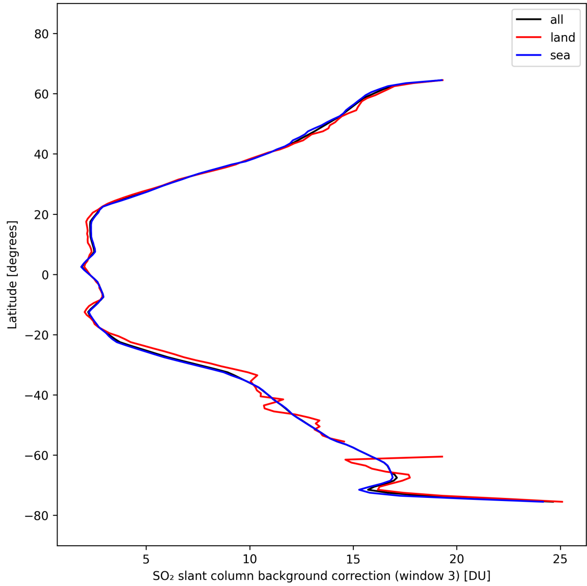
Figure 48: Zonal average of “SO 2 slant column background correction (window 3)” for 2025-10-06 to 2025-10-07.
