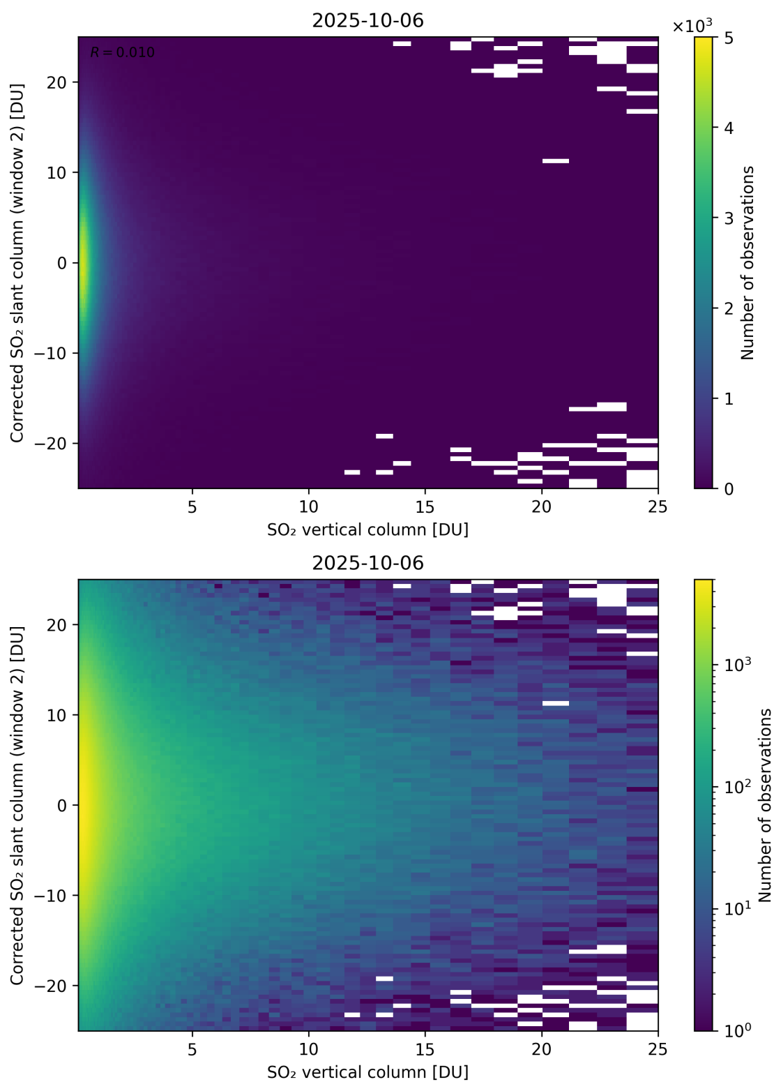
Figure 352: Scatter density plot of “SO 2 vertical column” against “Corrected SO 2 slant column (window 2)” for 2025-10-06 to 2025-10-07.
