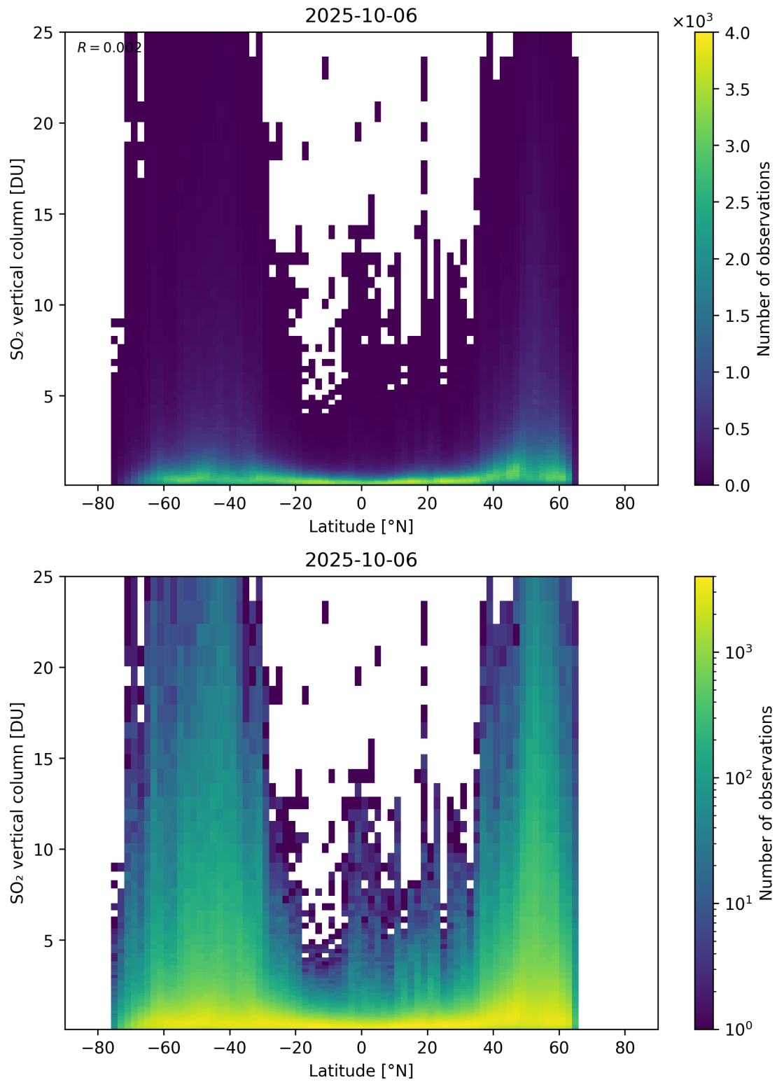
Figure 169: Scatter density plot of “Latitude” against “SO 2 vertical column” for 2025-10-06 to 2025-10-07.
