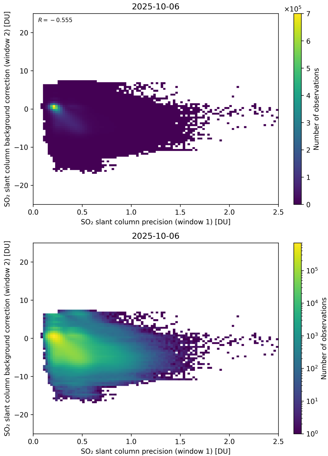
Figure 269: Scatter density plot of “SO 2 slant column precision (window 1)” against “SO 2 slant column background correction (window 2)” for 2025-10-06 to 2025-10-07.
