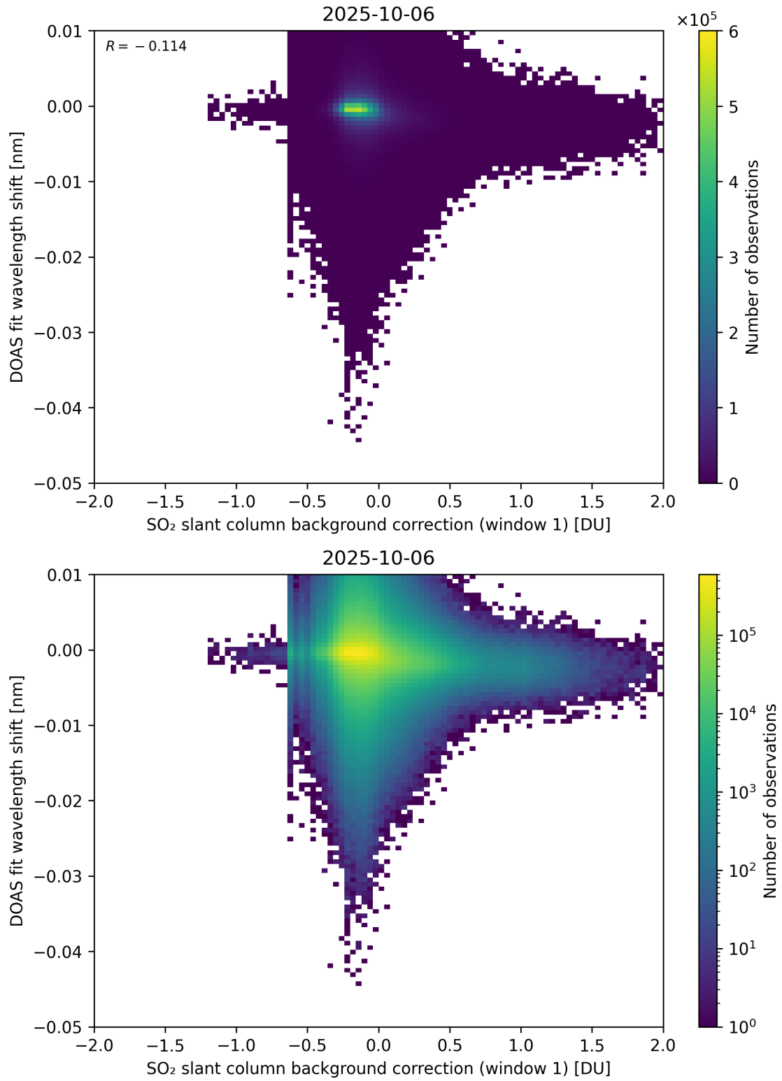
Figure 111: Scatter density plot of “SO 2 slant column background correction (window 1)” against “DOAS fit wavelength shift” for 2025-10-06 to 2025-10-07.
