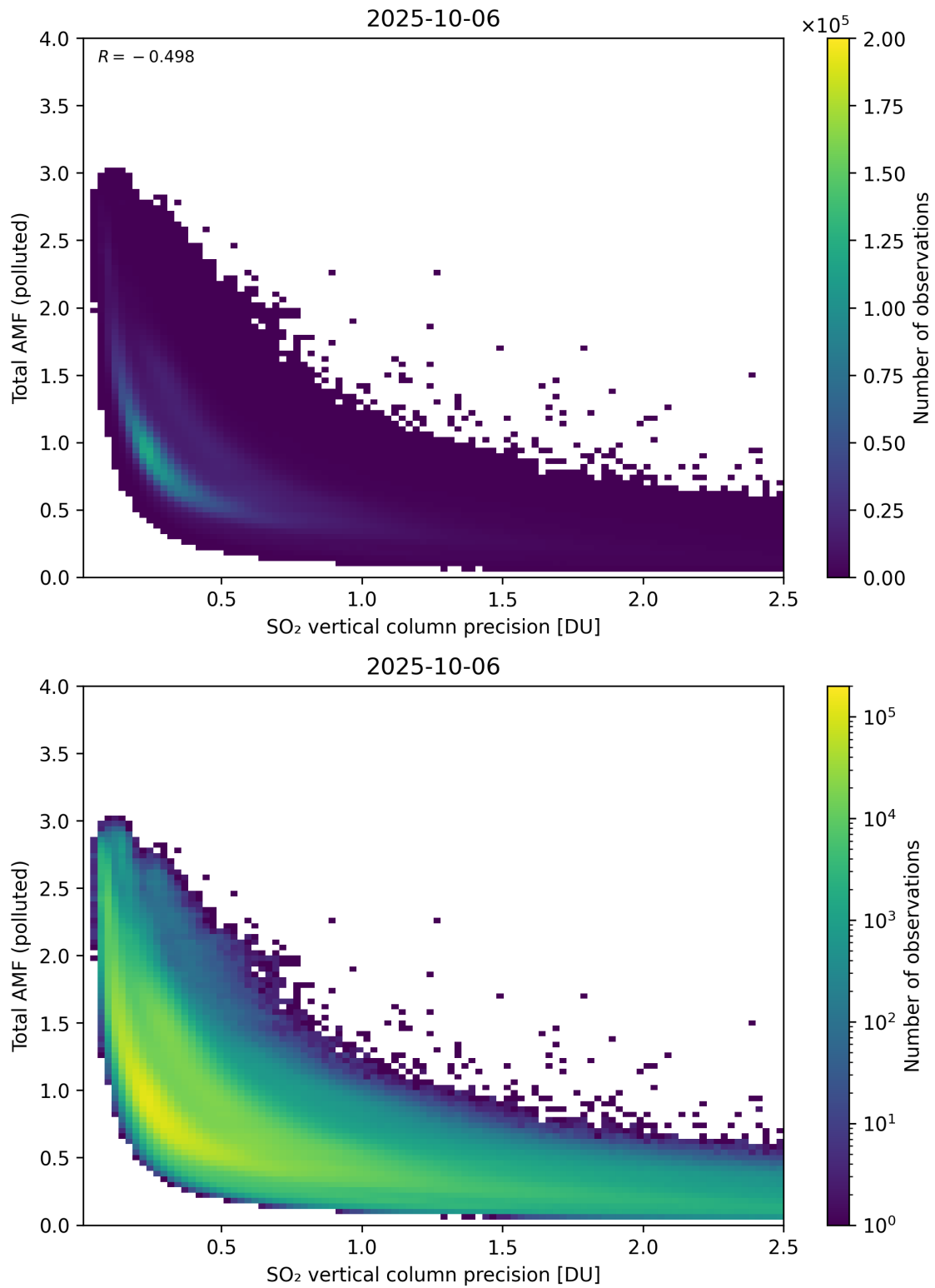
Figure 346: Scatter density plot of “SO 2 vertical column precision” against “Total AMF (polluted)” for 2025-10-06 to 2025-10-07.
