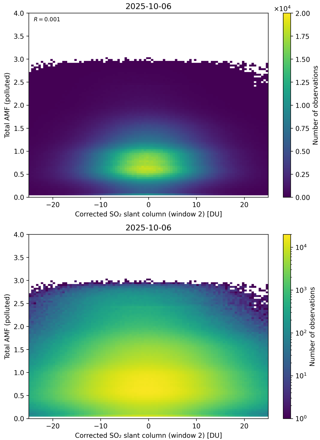
Figure 253: Scatter density plot of “Corrected SO 2 slant column (window 2)” against “Total AMF (polluted)” for 2025-10-06 to 2025-10-07.
