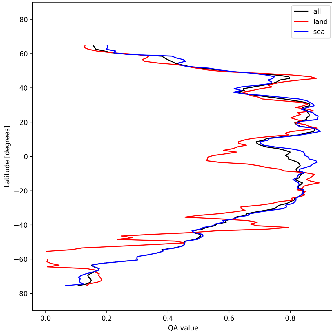
Figure 31: Zonal average of “QA value” for 2025-10-06 to 2025-10-07.
