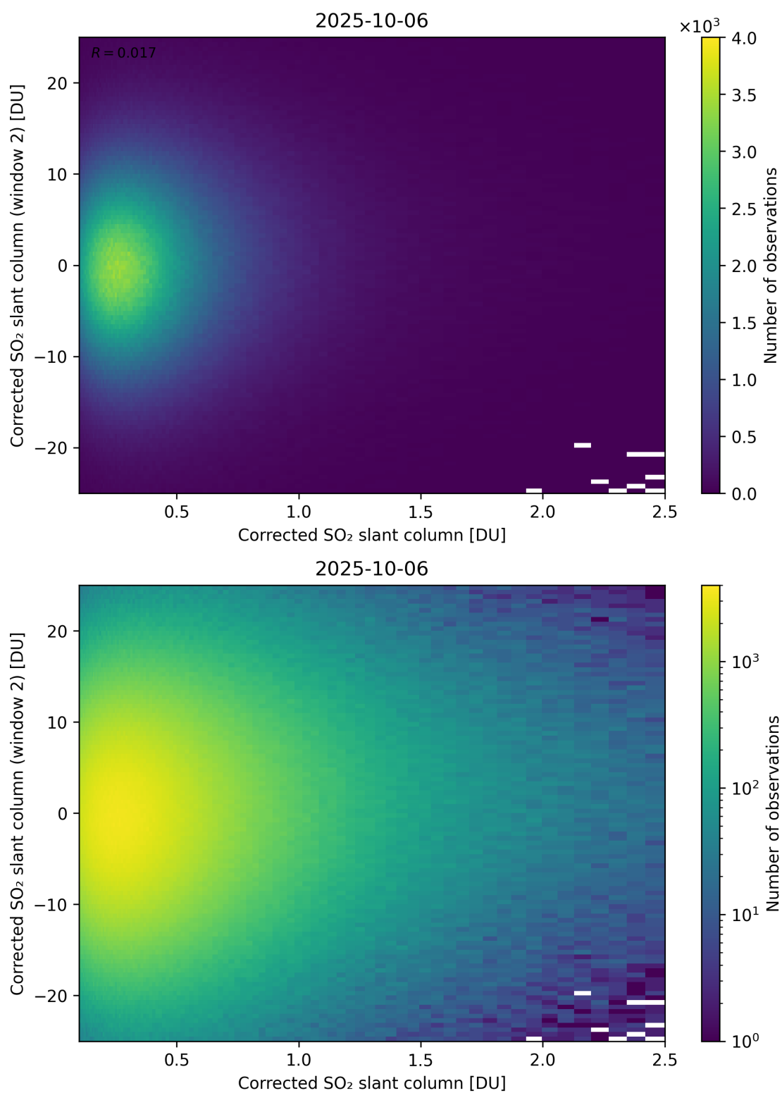
Figure 235: Scatter density plot of “Corrected SO 2 slant column” against “Corrected SO 2 slant column (window 2)” for 2025-10-06 to 2025-10-07.
