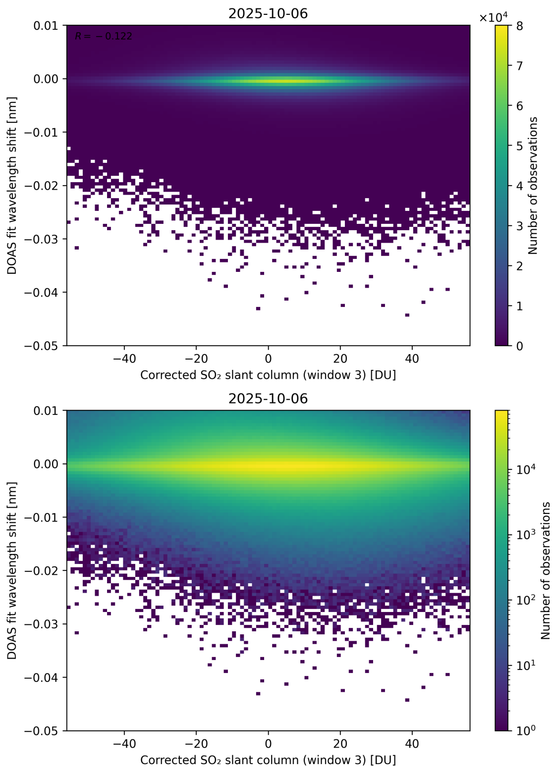
Figure 256: Scatter density plot of “Corrected SO 2 slant column (window 3)” against “DOAS fit wavelength shift” for 2025-10-06 to 2025-10-07.
