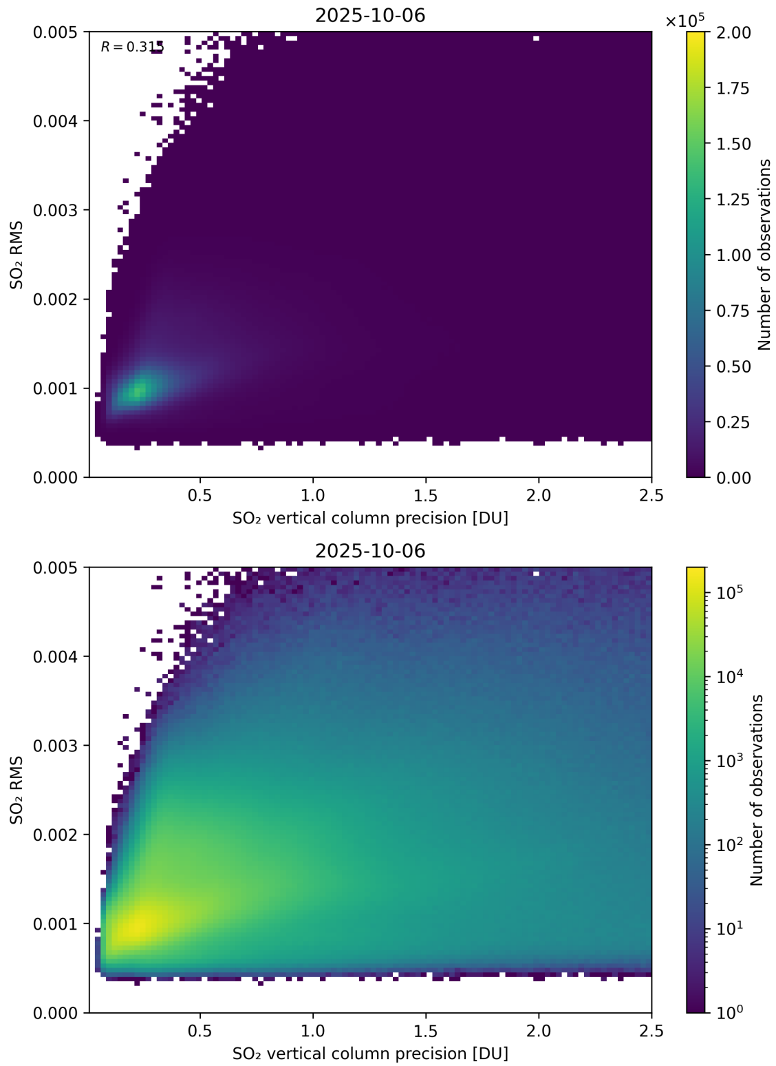
Figure 334: Scatter density plot of “SO 2 vertical column precision” against “SO 2 RMS” for 2025-10-06 to 2025-10-07.
