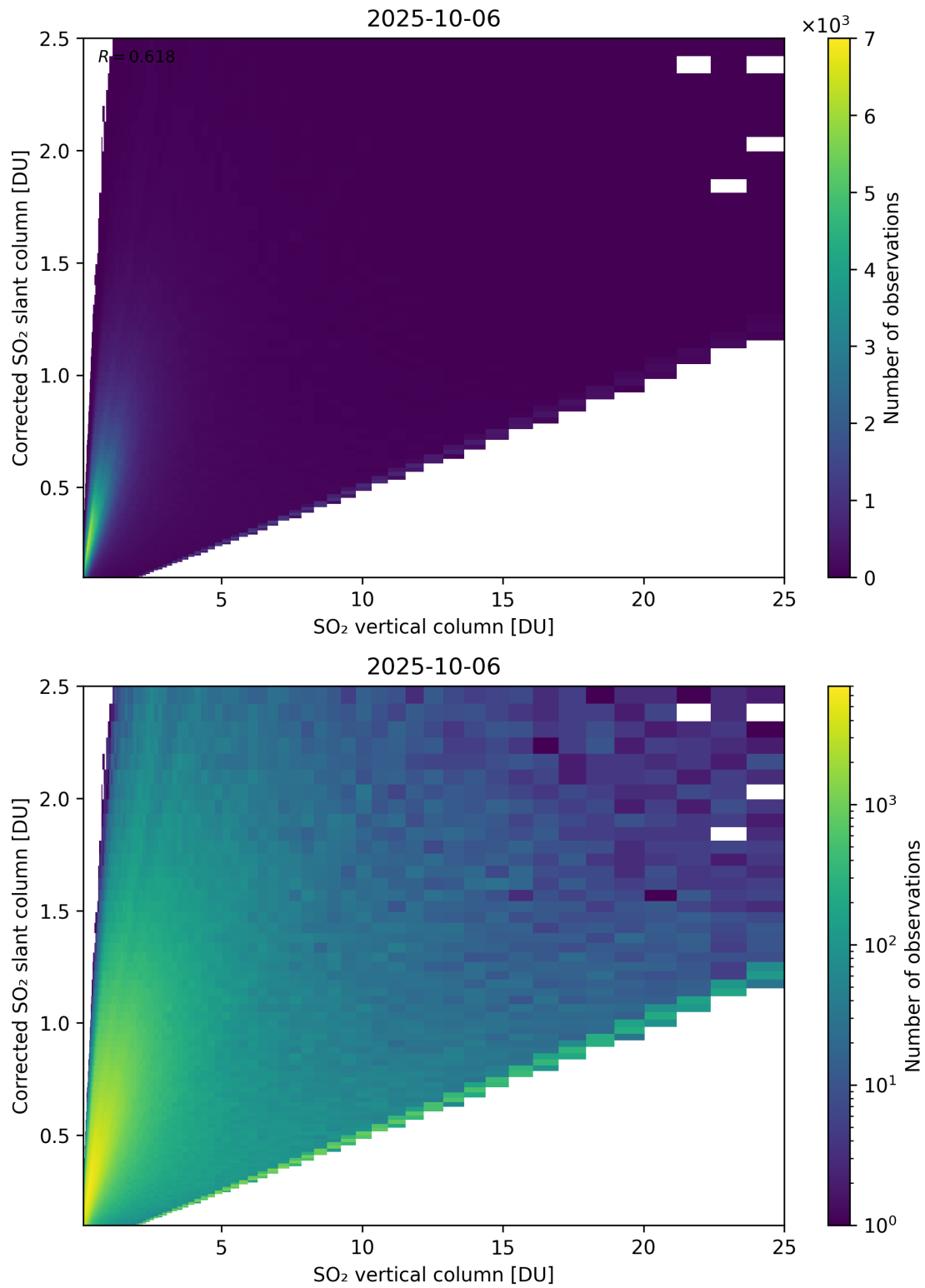
Figure 351: Scatter density plot of “SO 2 vertical column” against “Corrected SO 2 slant column” for 2025-10-06 to 2025-10-07.
