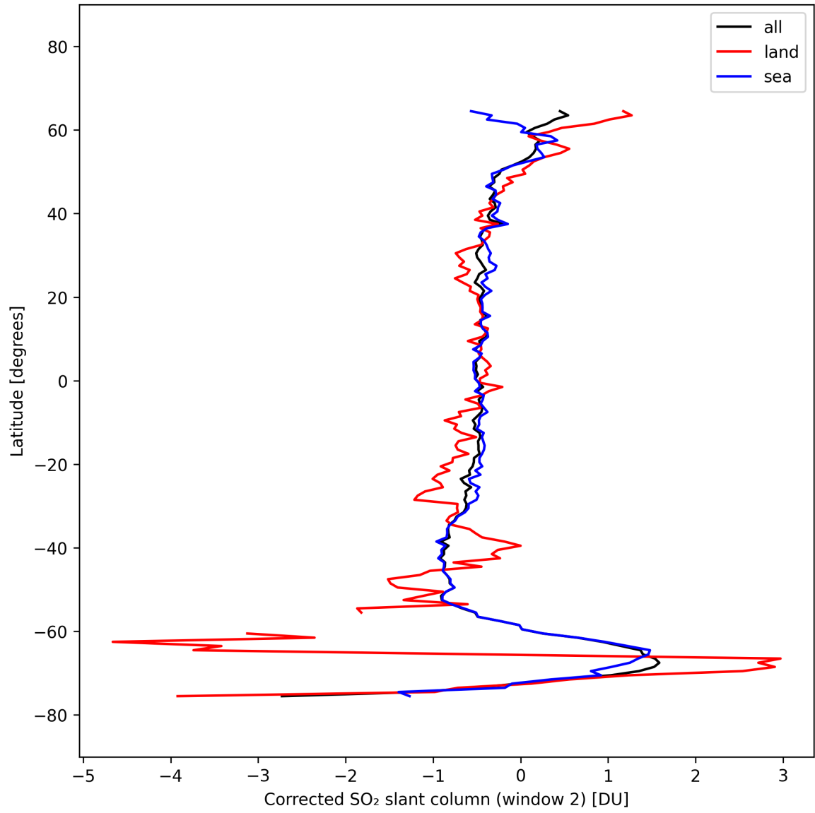
Figure 43: Zonal average of “Corrected SO 2 slant column (window 2)” for 2025-10-06 to 2025-10-07.
