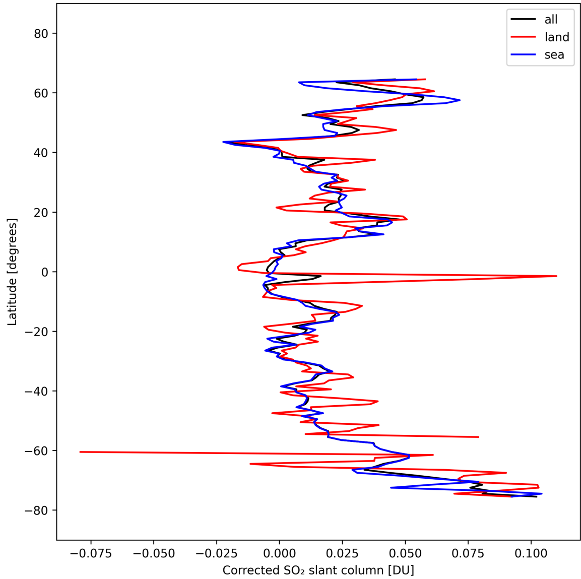
Figure 34: Zonal average of “Corrected SO 2 slant column” for 2025-10-06 to 2025-10-07.
