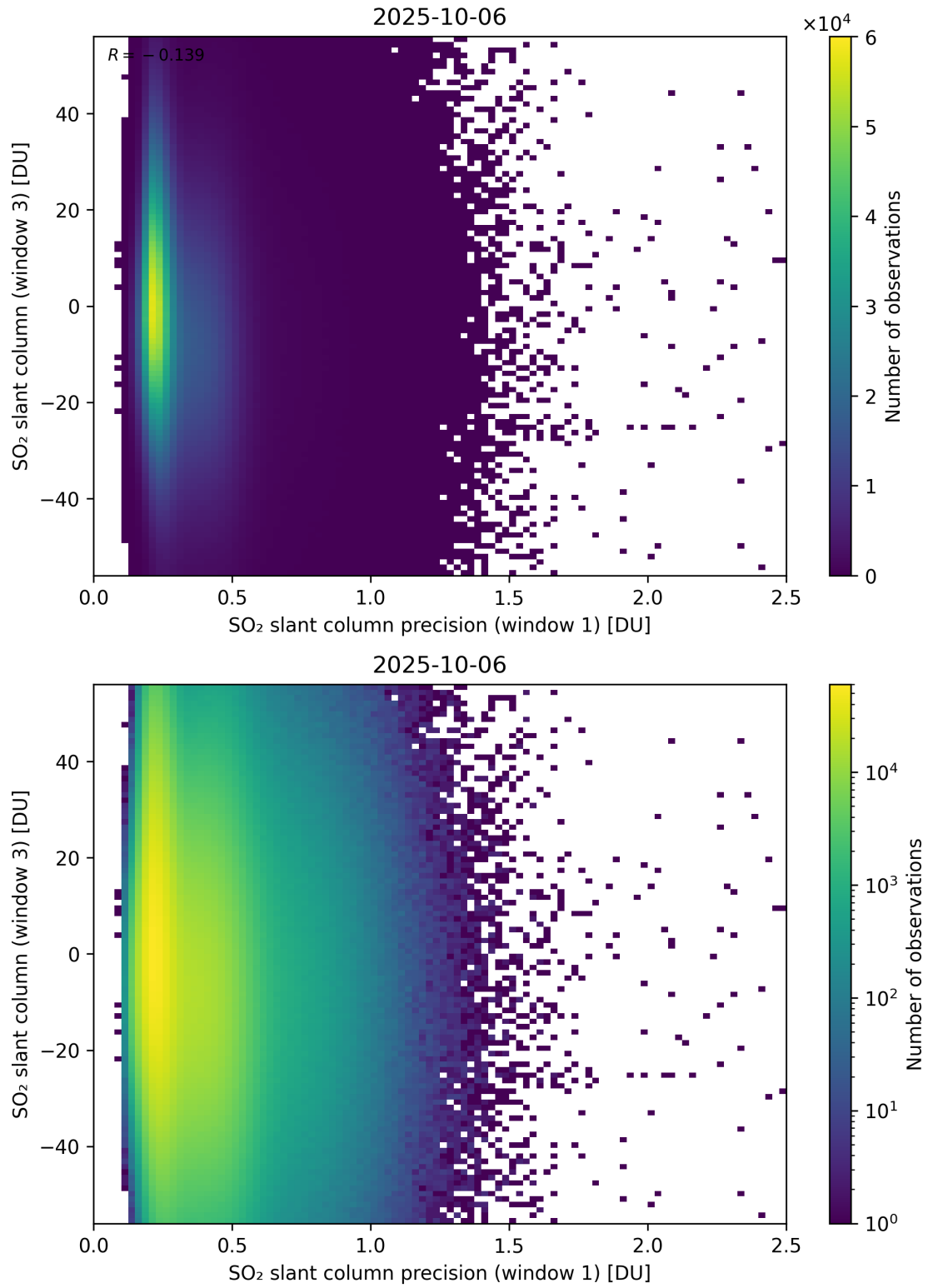
Figure 278: Scatter density plot of “SO 2 slant column precision (window 1)” against “SO 2 slant column (window 3)” for 2025-10-06 to 2025-10-07.
