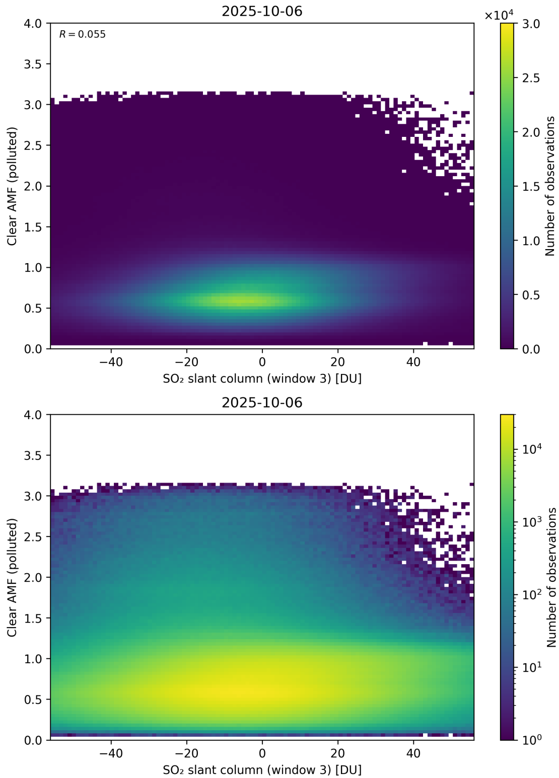
Figure 315: Scatter density plot of “SO 2 slant column (window 3)” against “Clear AMF (polluted)” for 2025-10-06 to 2025-10-07.
