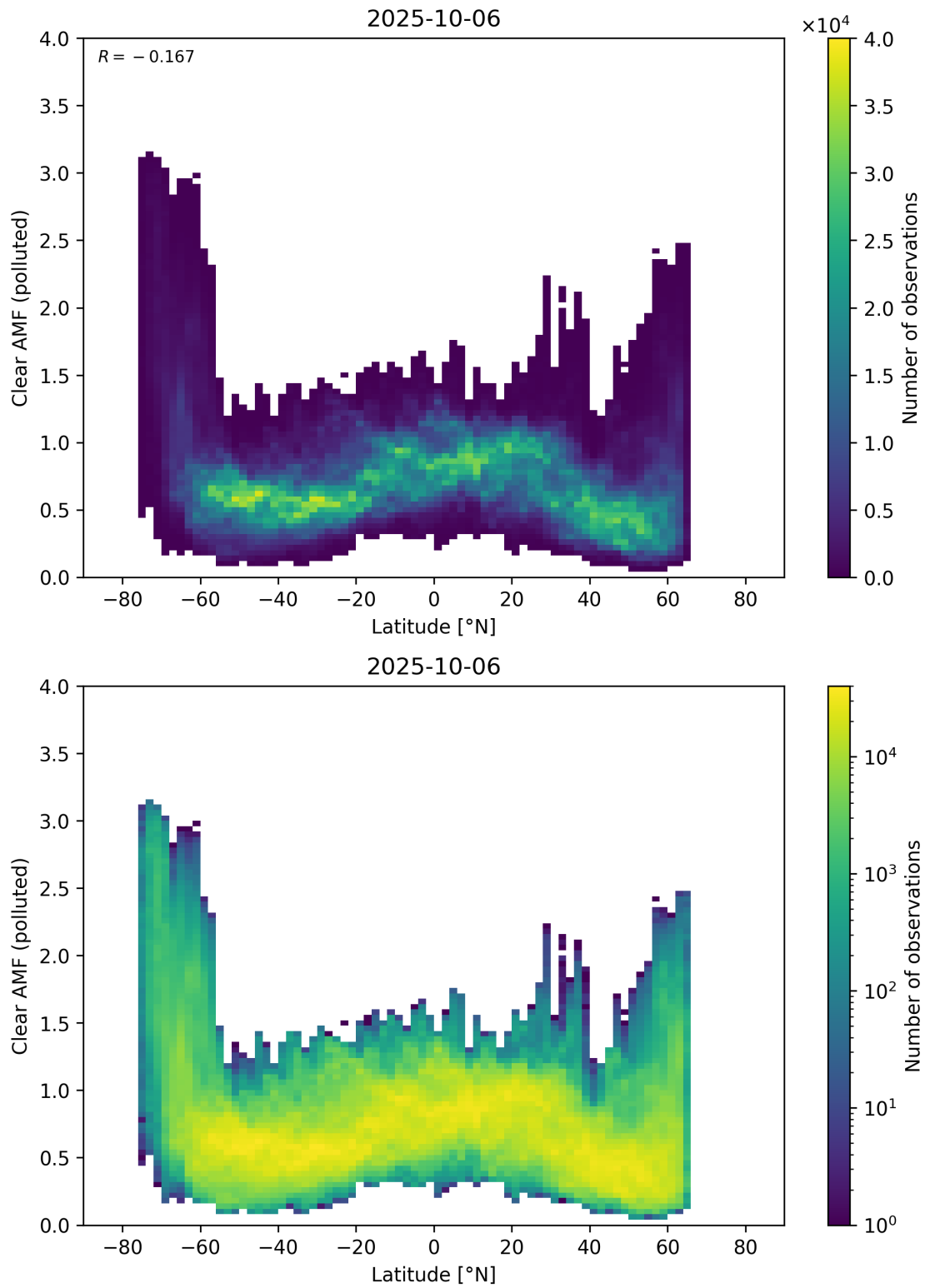
Figure 156: Scatter density plot of “Latitude” against “Clear AMF (polluted)” for 2025-10-06 to 2025-10-07.
