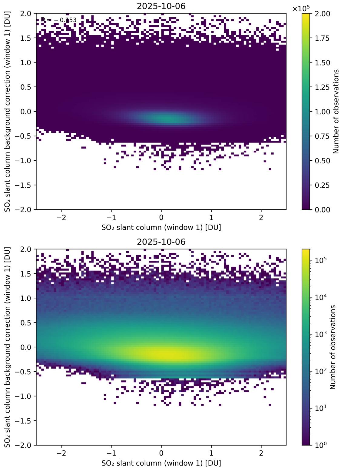
Figure 262: Scatter density plot of “SO 2 slant column (window 1)” against “SO 2 slant column background correction (window 1)” for 2025-10-06 to 2025-10-07.
