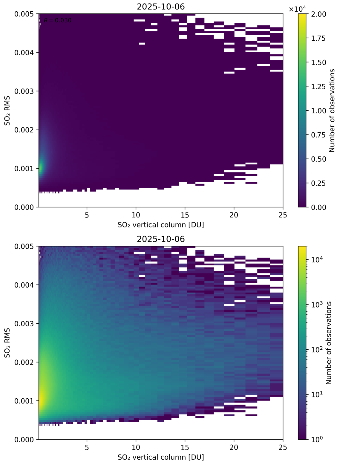
Figure 328: Scatter density plot of “SO 2 vertical column” against “SO 2 RMS” for 2025-10-06 to 2025-10-07.
