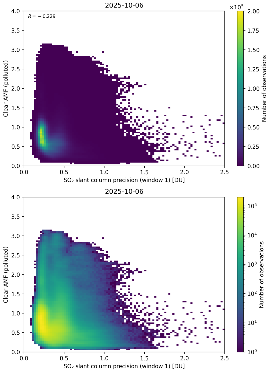
Figure 274: Scatter density plot of “SO 2 slant column precision (window 1)” against “Clear AMF (polluted)” for 2025-10-06 to 2025-10-07.
