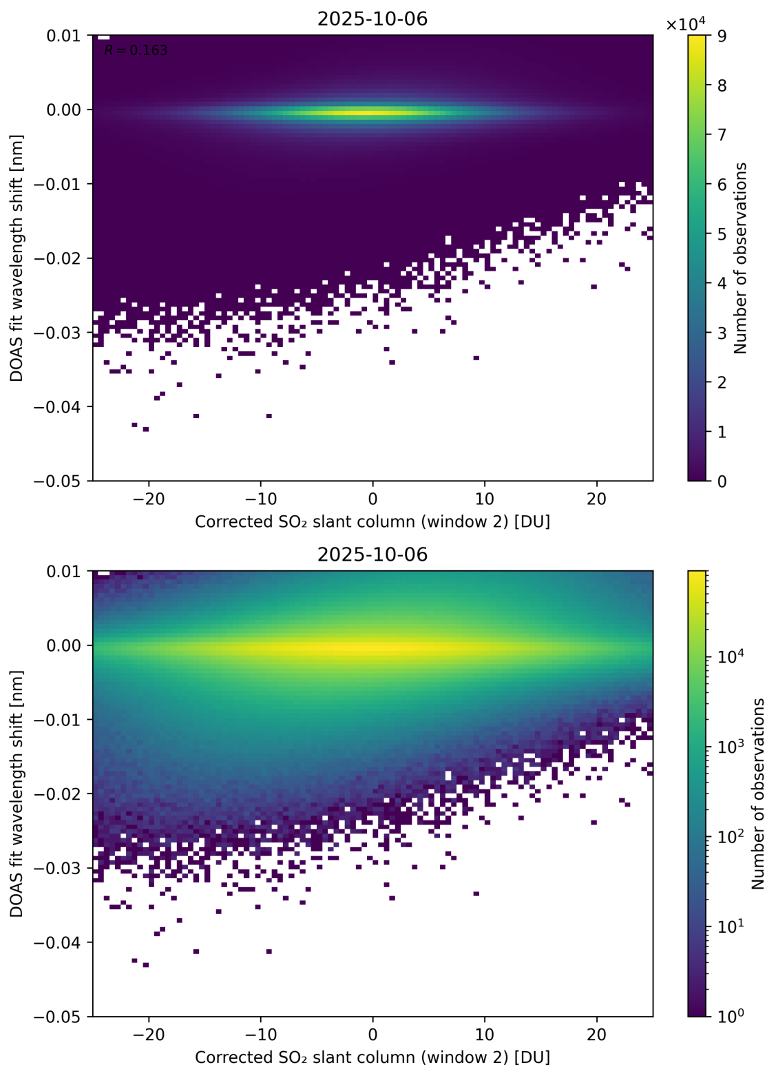
Figure 246: Scatter density plot of “Corrected SO 2 slant column (window 2)” against “DOAS fit wavelength shift” for 2025-10-06 to 2025-10-07.
