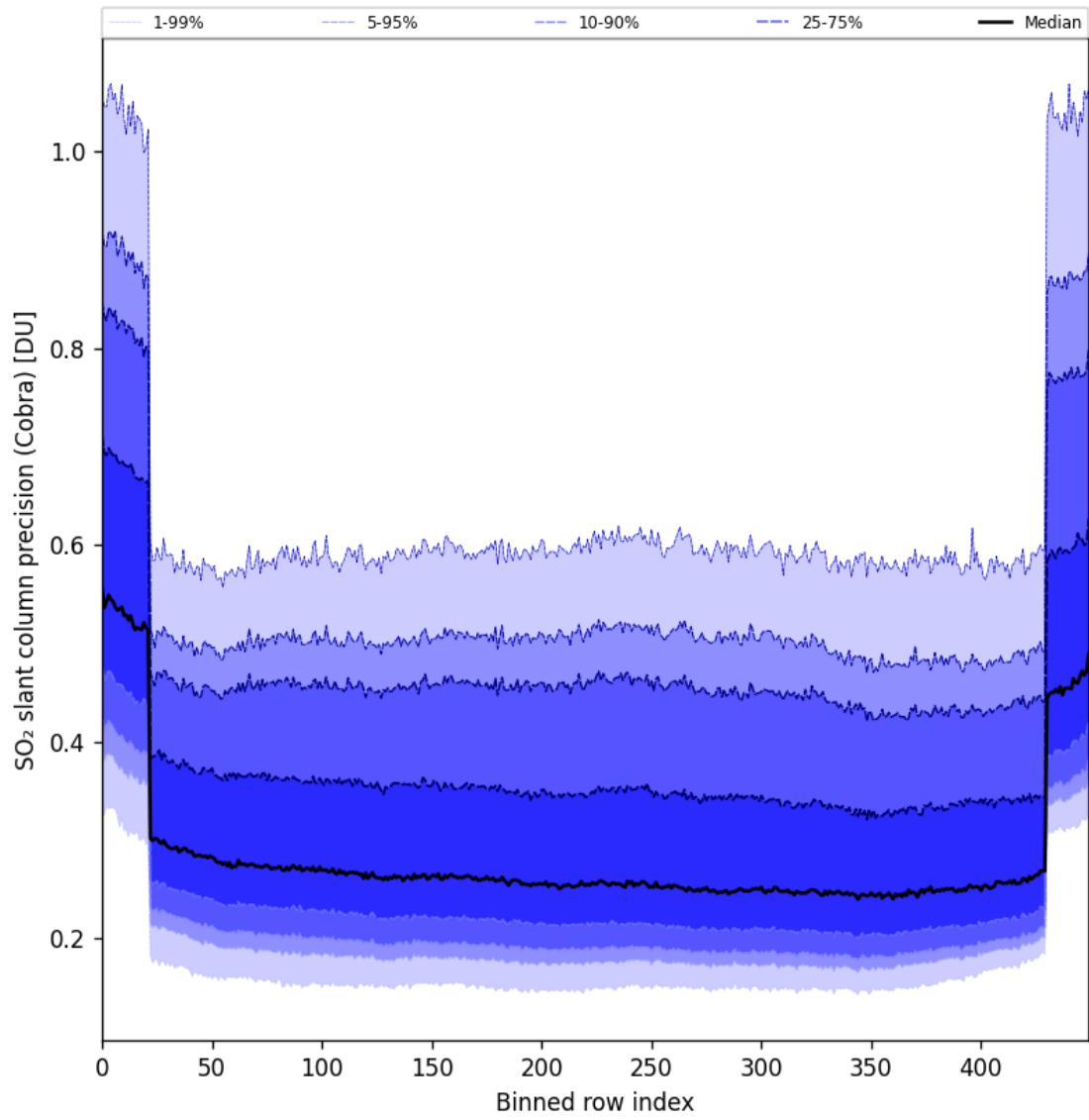
Figure 88: Along track statistics of “SO 2 slant column precision (Cobra)” for 2025-10-06 to 2025-10-07
