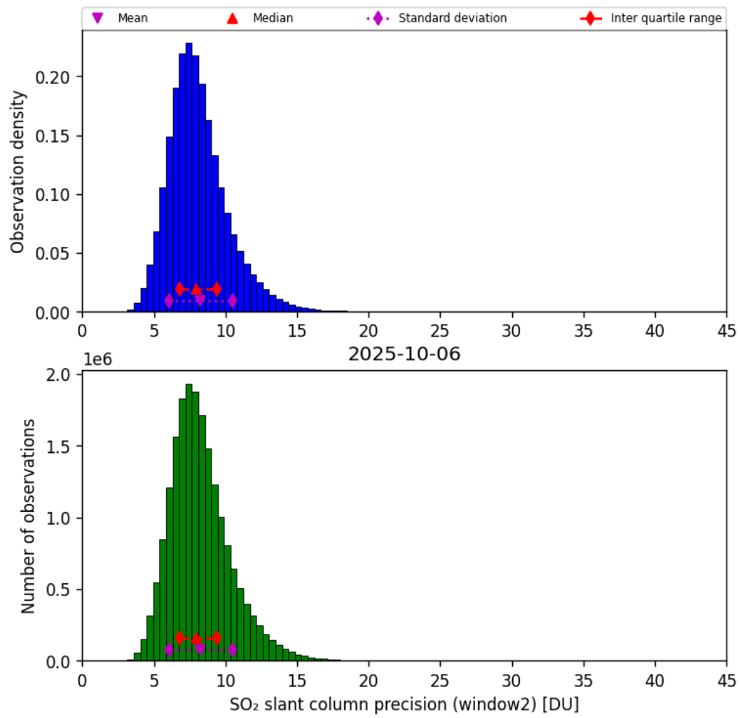
Figure 68: Histogram of “SO 2 slant column precision (window2)” for 2025-10-06 to 2025-10-07
