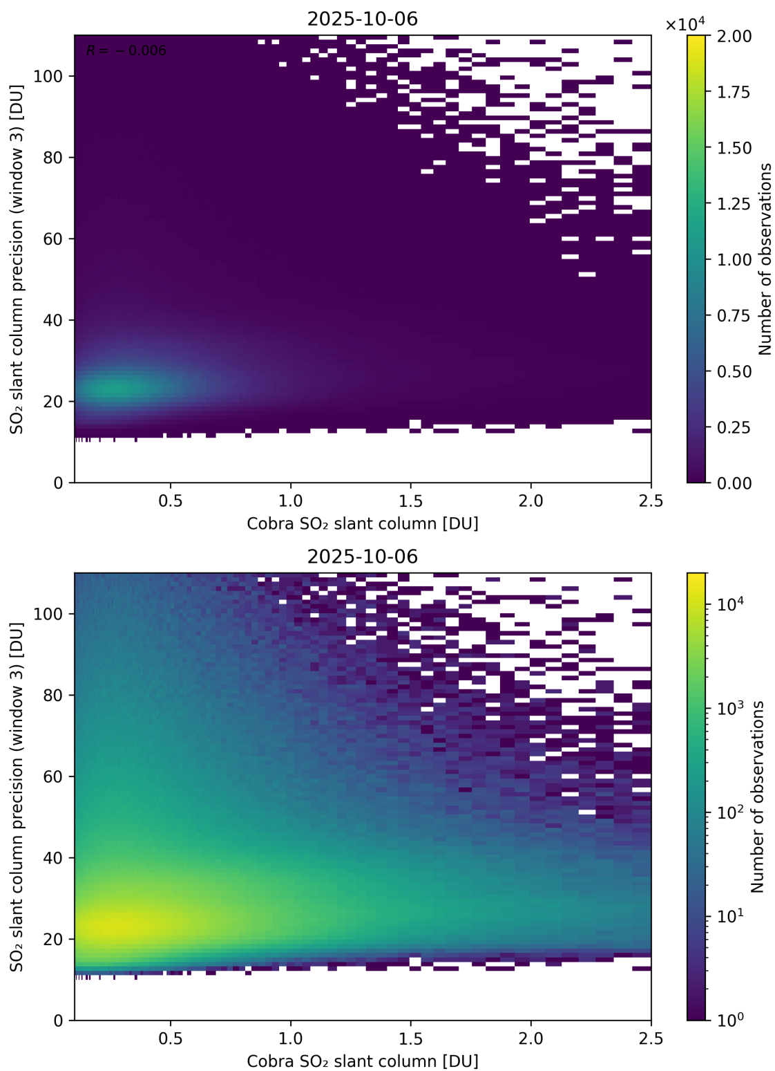
Figure 223: Scatter density plot of “Cobra SO 2 slant column” against “SO 2 slant column precision (window 3)” for 2025-10-06 to 2025-10-07.
