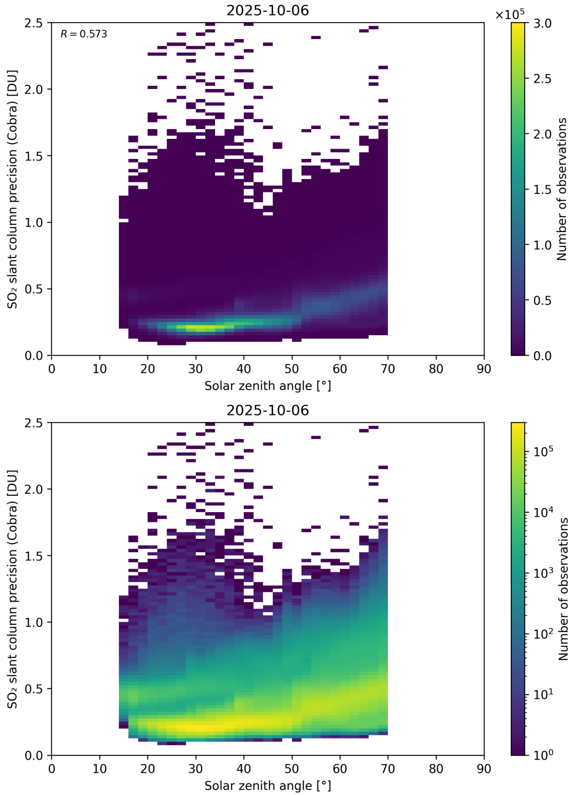
Figure 180: Scatter density plot of “Solar zenith angle” against “SO 2 slant column precision (Cobra)” for 2025-10-06 to 2025-10-07.
