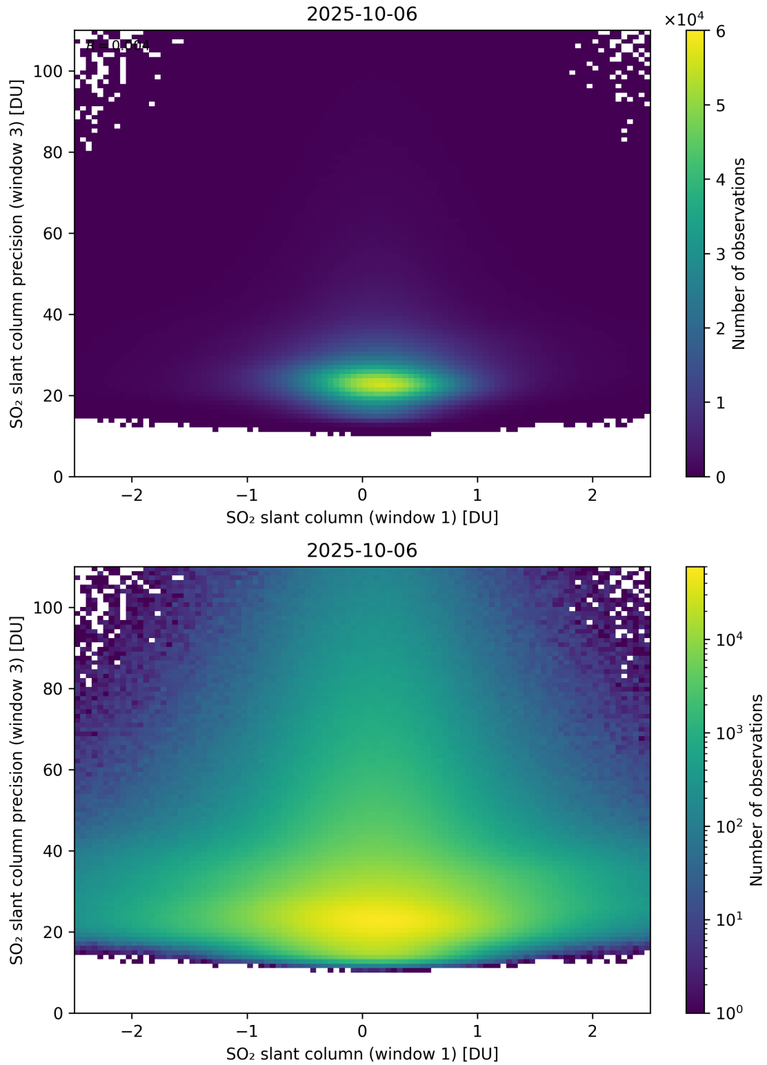
Figure 288: Scatter density plot of “SO 2 slant column (window 1)” against “SO 2 slant column precision (window 3)” for 2025-10-06 to 2025-10-07.
