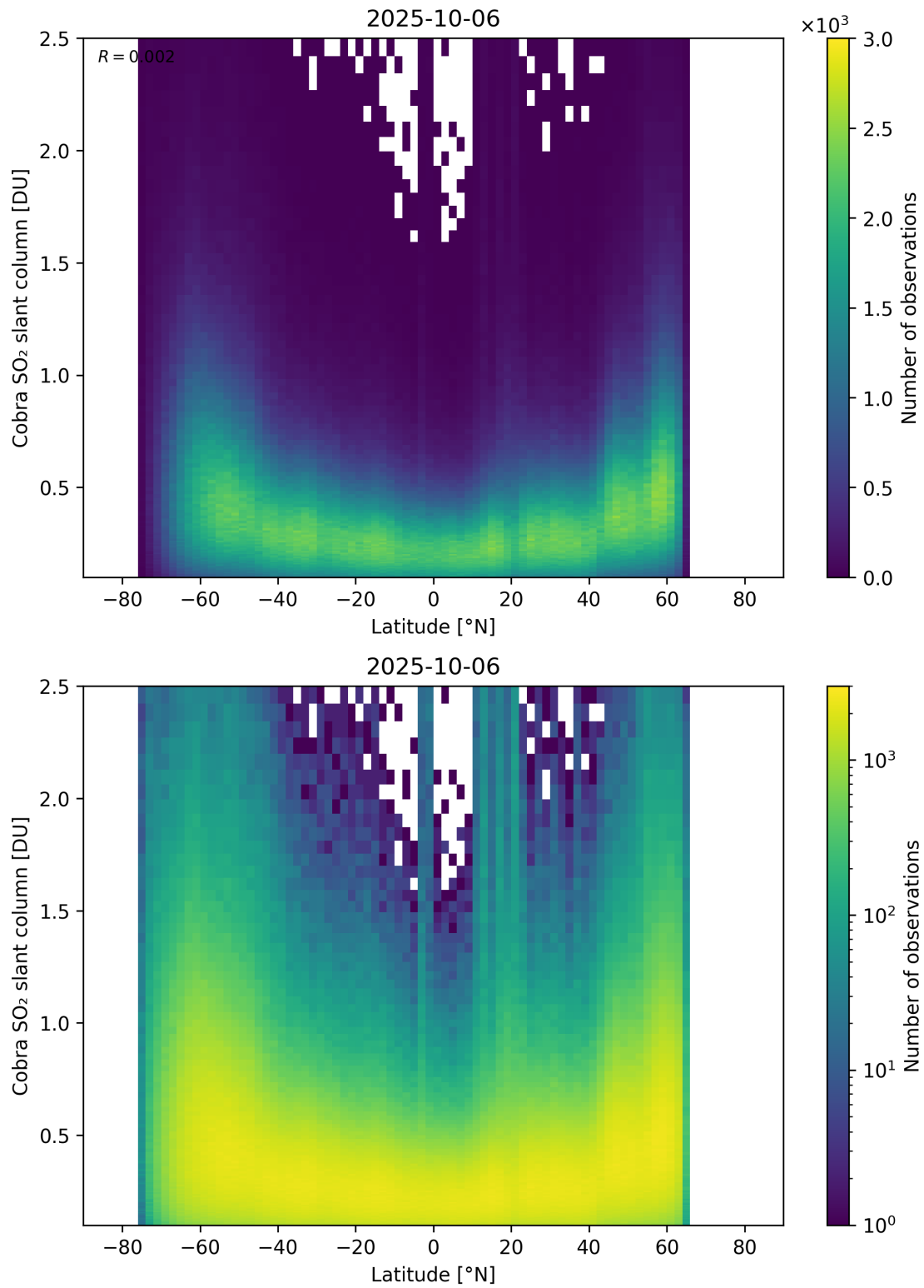
Figure 157: Scatter density plot of “Latitude” against “Cobra SO 2 slant column” for 2025-10-06 to 2025-10-07.
