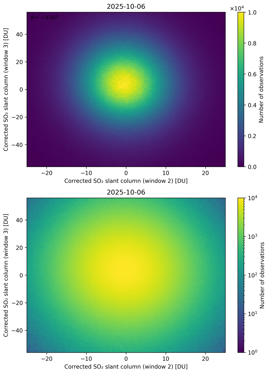
Figure 250: Scatter density plot of “Corrected SO 2 slant column (window 2)” against “Corrected SO 2 slant column (window 3)” for 2025-10-06 to 2025-10-07.
