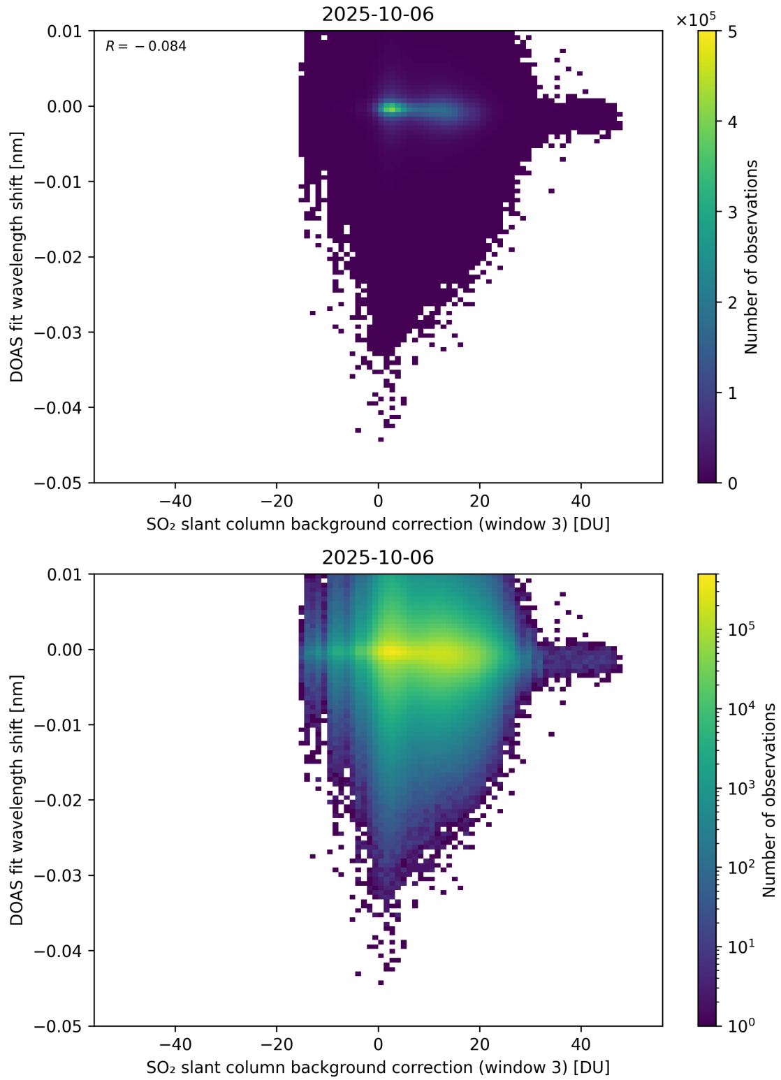
Figure 132: Scatter density plot of “SO 2 slant column background correction (window 3)” against “DOAS fit wavelength shift” for 2025-10-06 to 2025-10-07.
