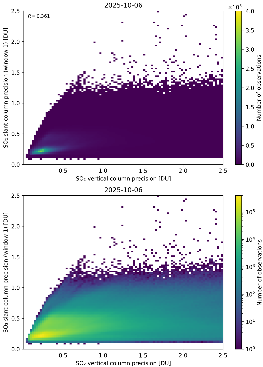
Figure 342: Scatter density plot of “SO 2 vertical column precision” against “SO 2 slant column precision (window 1)” for 2025-10-06 to 2025-10-07.
