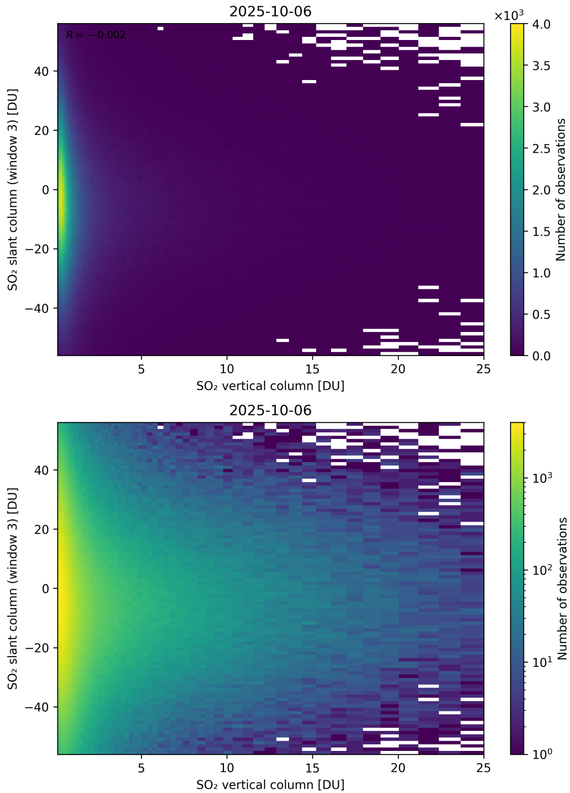
Figure 357: Scatter density plot of “SO 2 vertical column” against “SO 2 slant column (window 3)” for 2025-10-06 to 2025-10-07.
