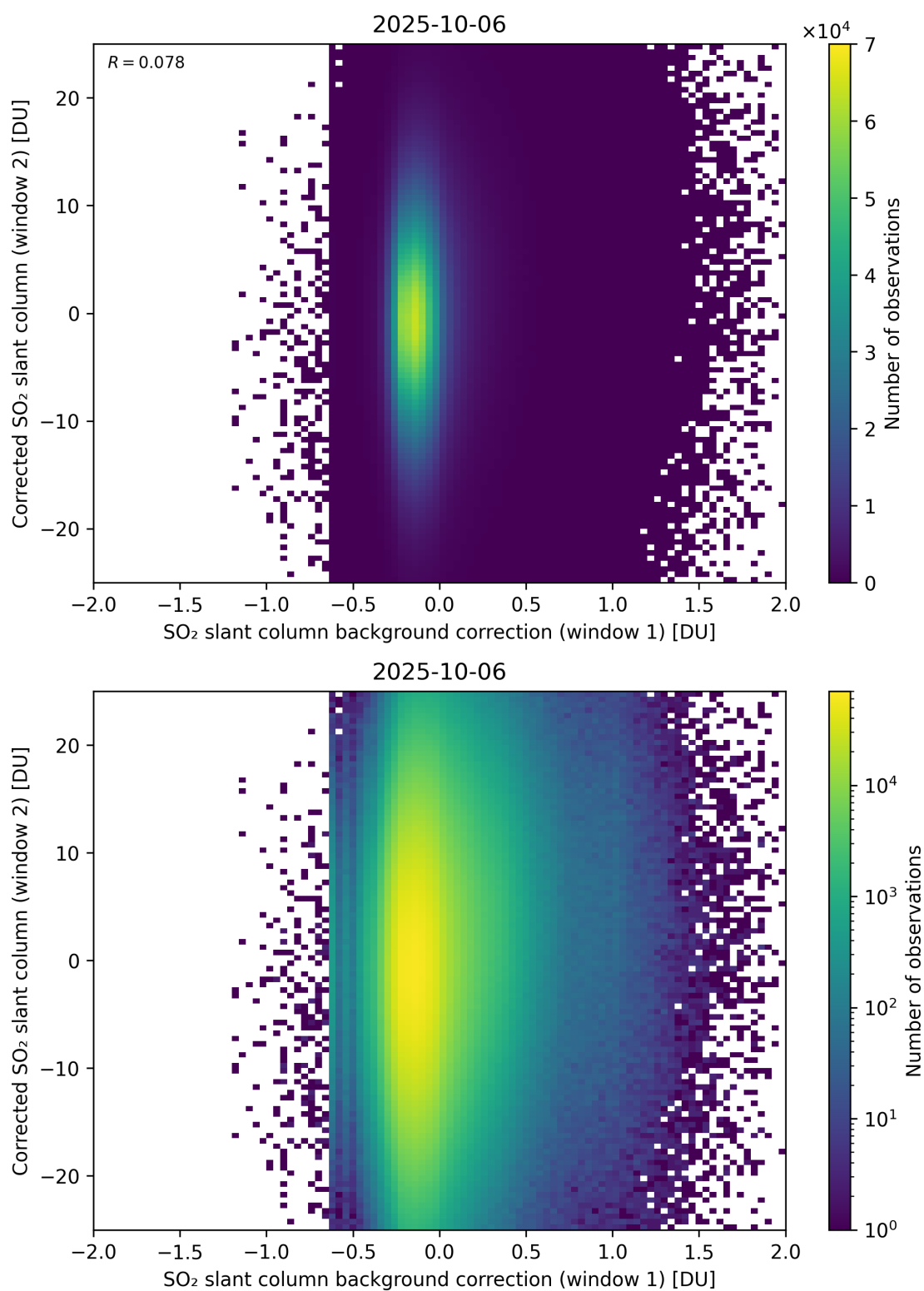
Figure 115: Scatter density plot of “SO 2 slant column background correction (window 1)” against “Corrected SO 2 slant column (window 2)” for 2025-10-06 to 2025-10-07.
