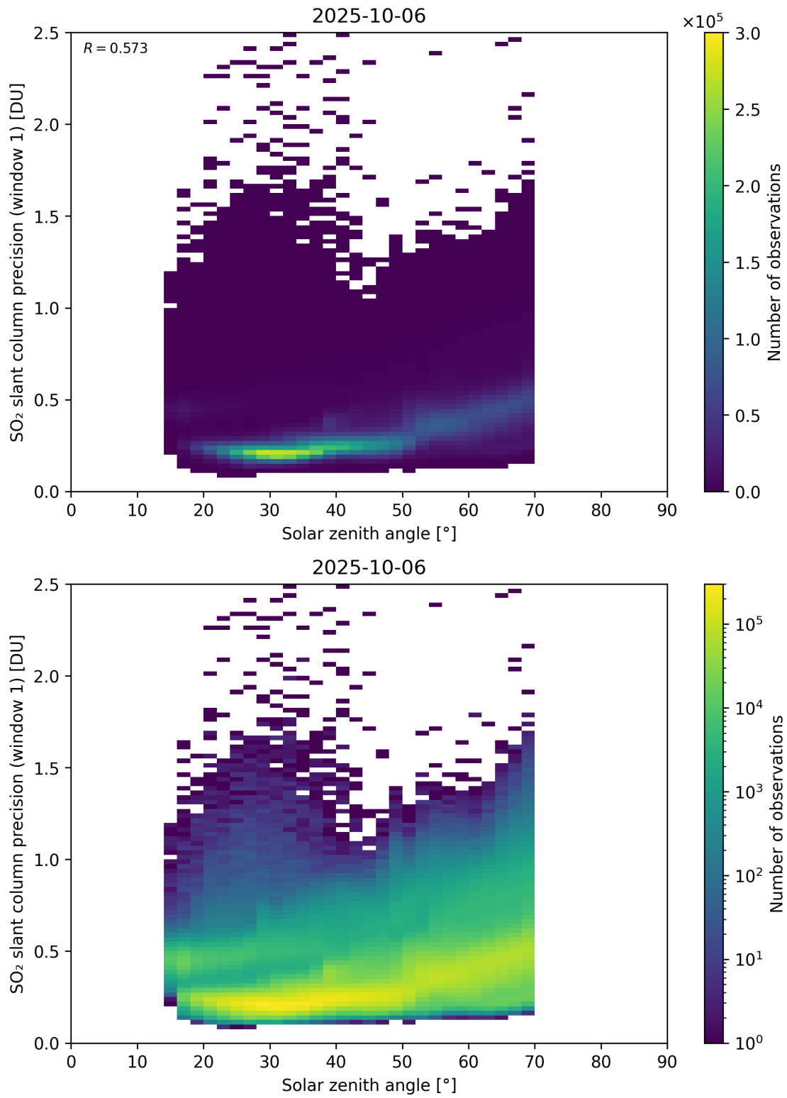
Figure 185: Scatter density plot of “Solar zenith angle” against “SO 2 slant column precision (window 1)” for 2025-10-06 to 2025-10-07.
