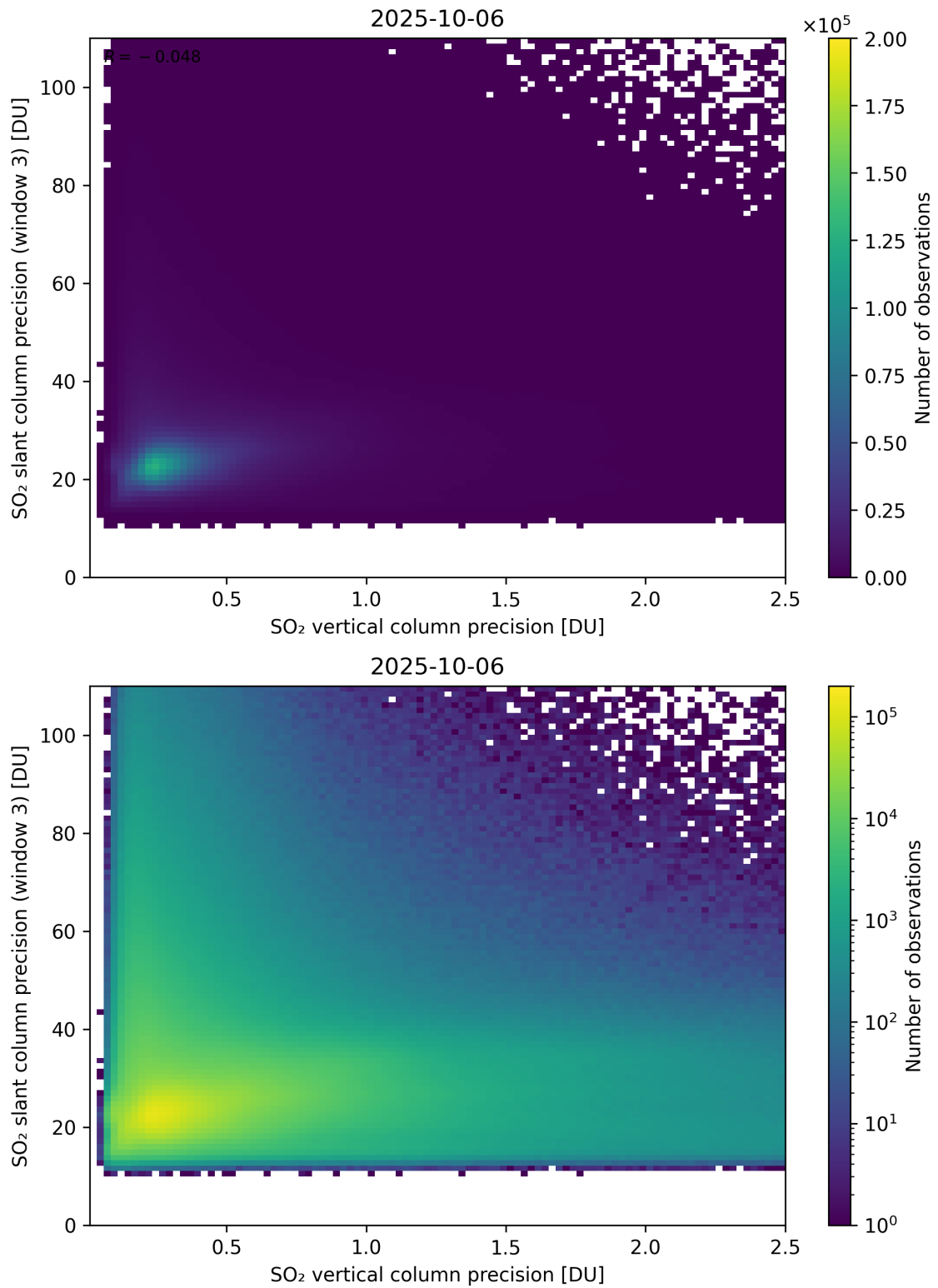
Figure 345: Scatter density plot of “SO 2 vertical column precision” against “SO 2 slant column precision (window 3)” for 2025-10-06 to 2025-10-07.
