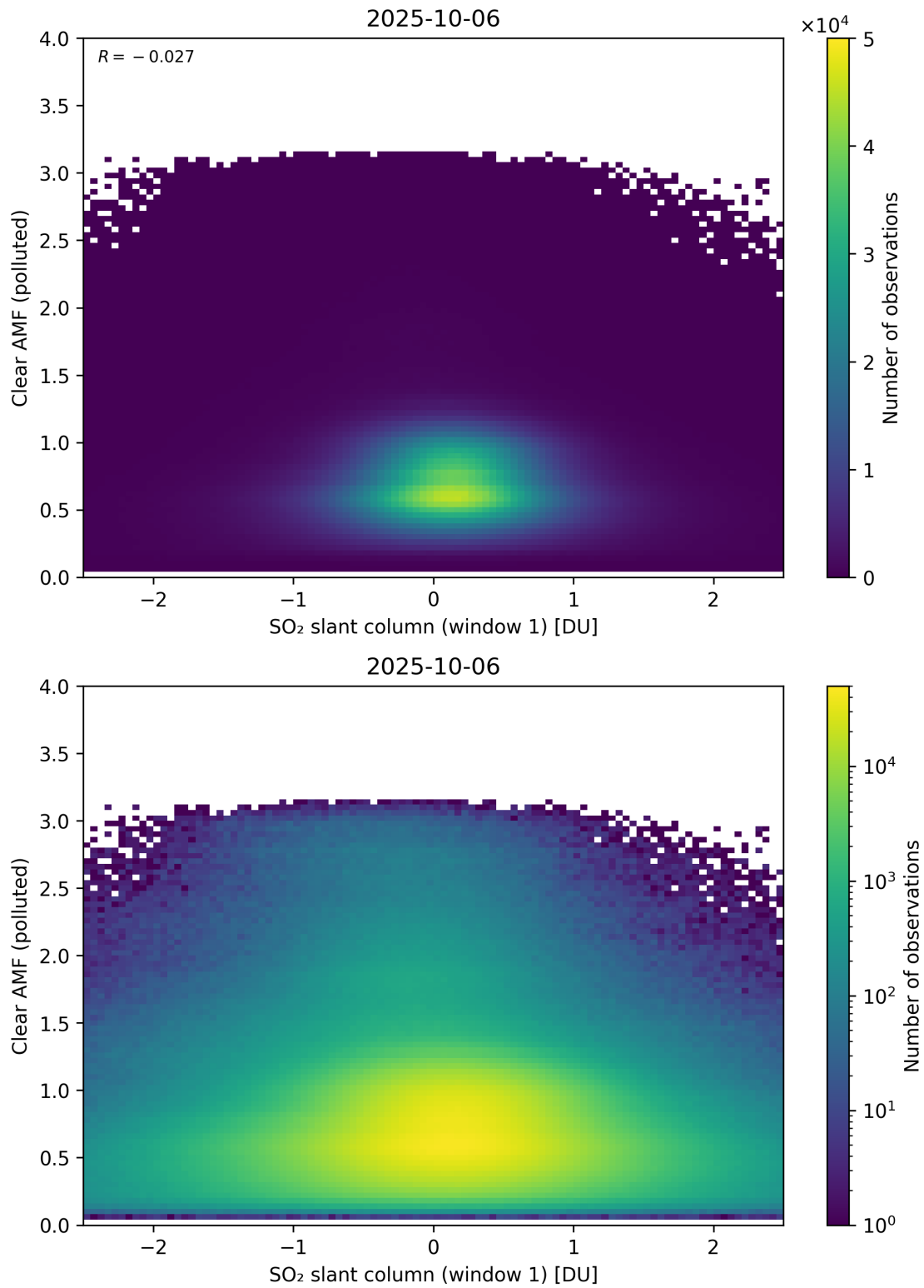
Figure 282: Scatter density plot of “SO 2 slant column (window 1)” against “Clear AMF (polluted)” for 2025-10-06 to 2025-10-07.
