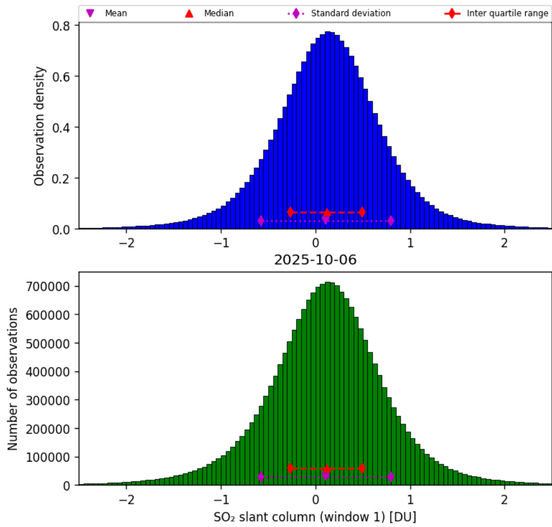
Figure 63: Histogram of “SO 2 slant column (window 1)” for 2025-10-06 to 2025-10-07
