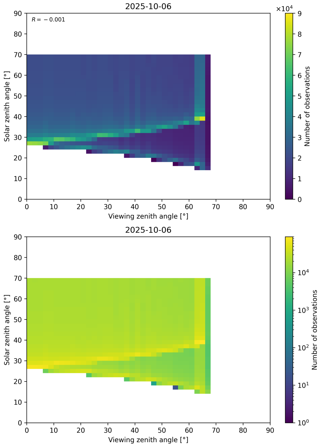
Figure 369: Scatter density plot of “Viewing zenith angle” against “Solar zenith angle” for 2025-10-06 to 2025-10-07.
