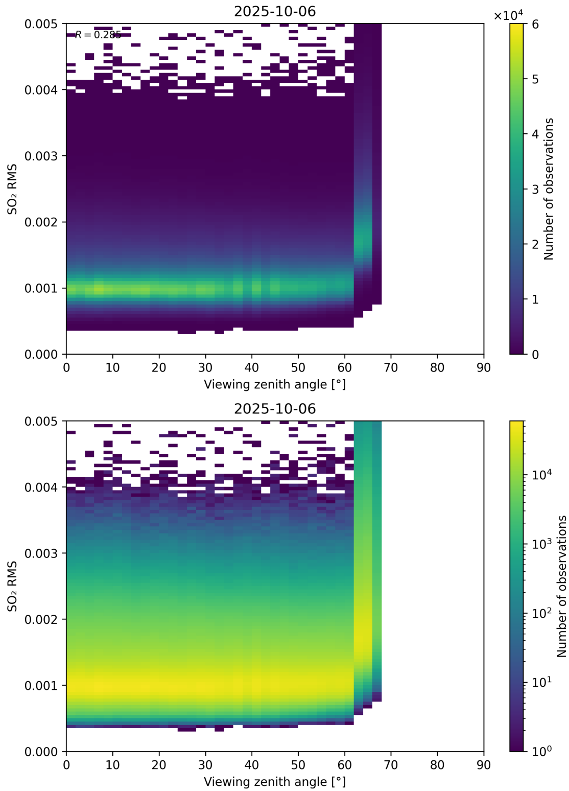
Figure 367: Scatter density plot of “Viewing zenith angle” against “SO 2 RMS” for 2025-10-06 to 2025-10-07.
