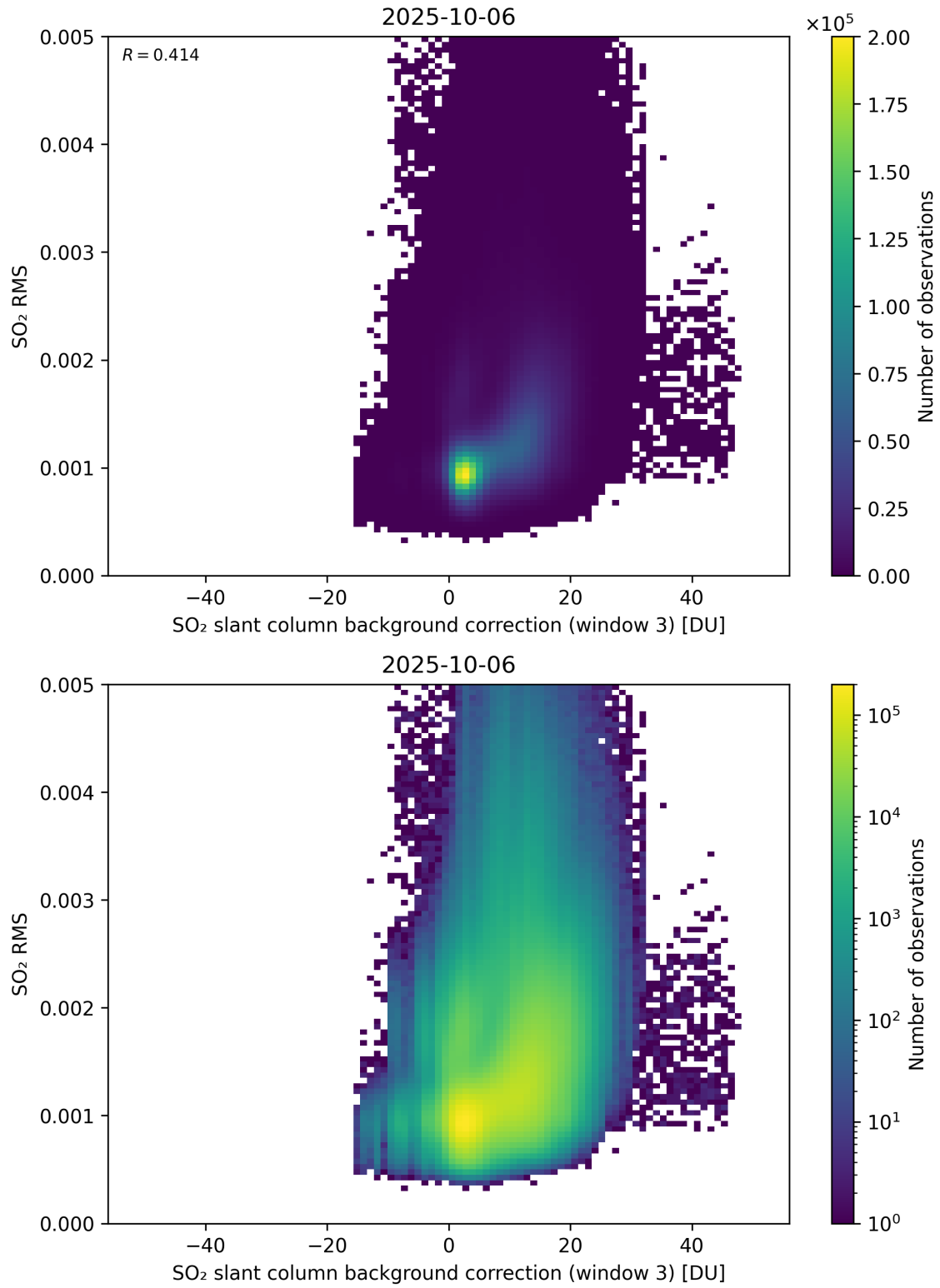
Figure 134: Scatter density plot of “SO 2 slant column background correction (window 3)” against “SO 2 RMS” for 2025-10-06 to 2025-10-07.
