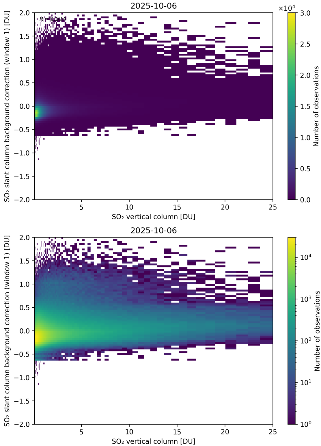
Figure 323: Scatter density plot of “SO 2 vertical column” against “SO 2 slant column background correction (window 1)” for 2025-10-06 to 2025-10-07.
