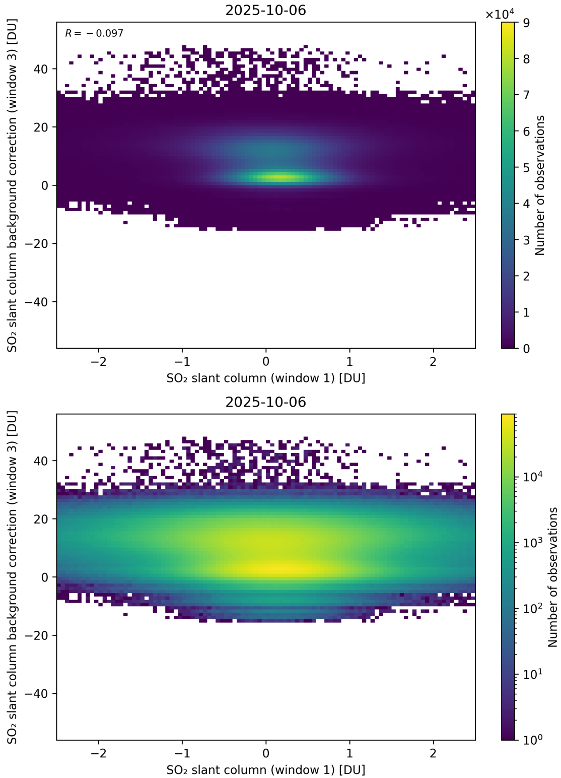
Figure 264: Scatter density plot of “SO 2 slant column (window 1)” against “SO 2 slant column background correction (window 3)” for 2025-10-06 to 2025-10-07.
