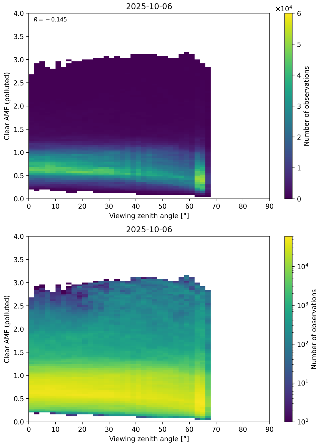
Figure 370: Scatter density plot of “Viewing zenith angle” against “Clear AMF (polluted)” for 2025-10-06 to 2025-10-07.
