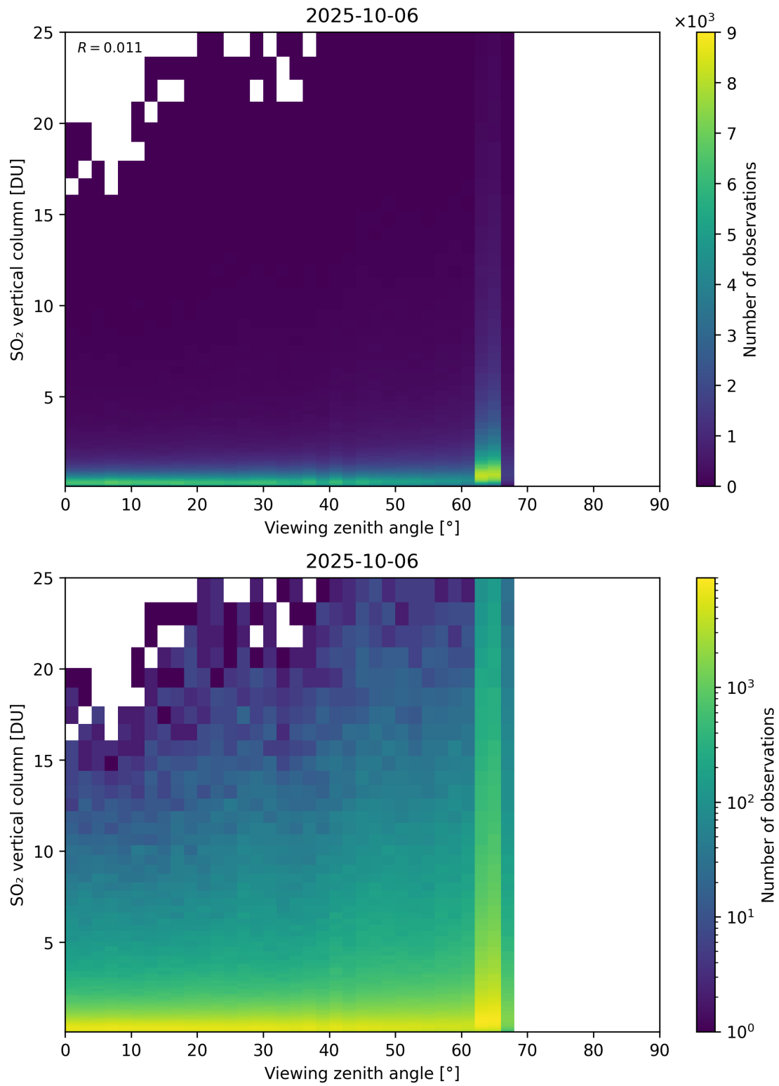
Figure 383: Scatter density plot of “Viewing zenith angle” against “SO 2 vertical column” for 2025-10-06 to 2025-10-07.
