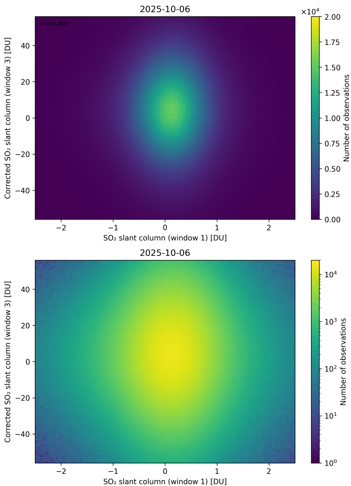
Figure 284: Scatter density plot of “SO 2 slant column (window 1)” against “Corrected SO 2 slant column (window 3)” for 2025-10-06 to 2025-10-07.
