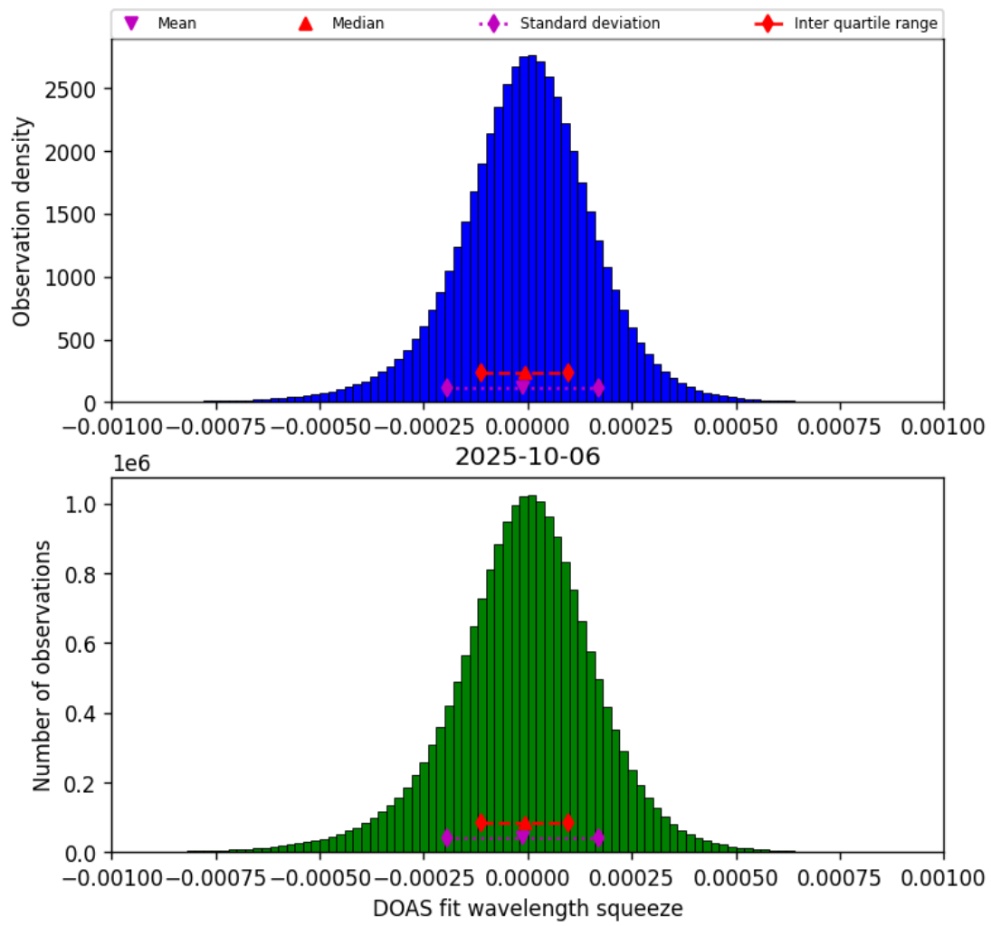
Figure 77: Histogram of “DOAS fit wavelength squeeze” for 2025-10-06 to 2025-10-07
