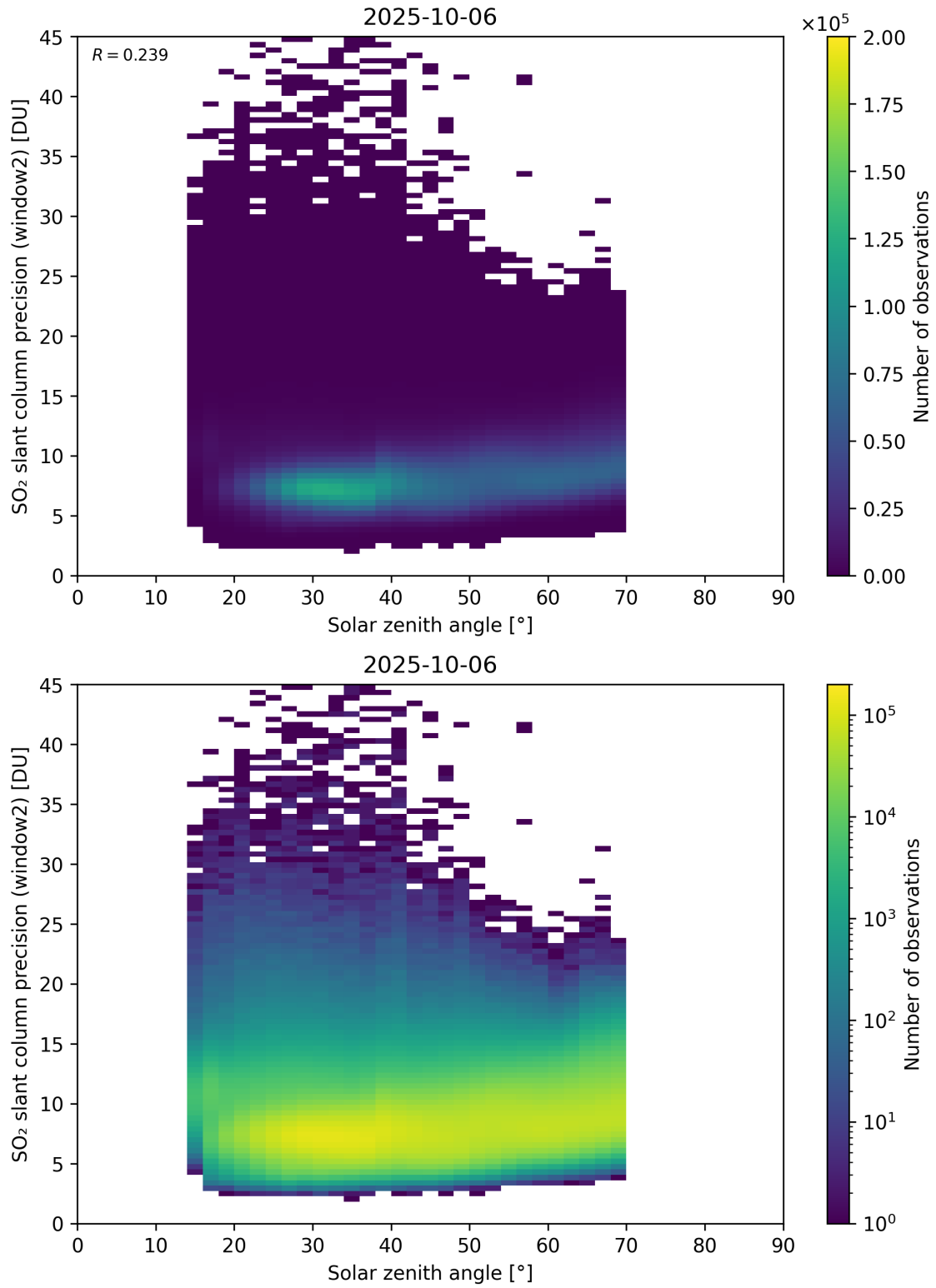
Figure 186: Scatter density plot of “Solar zenith angle” against “SO 2 slant column precision (window2)” for 2025-10-06 to 2025-10-07.
