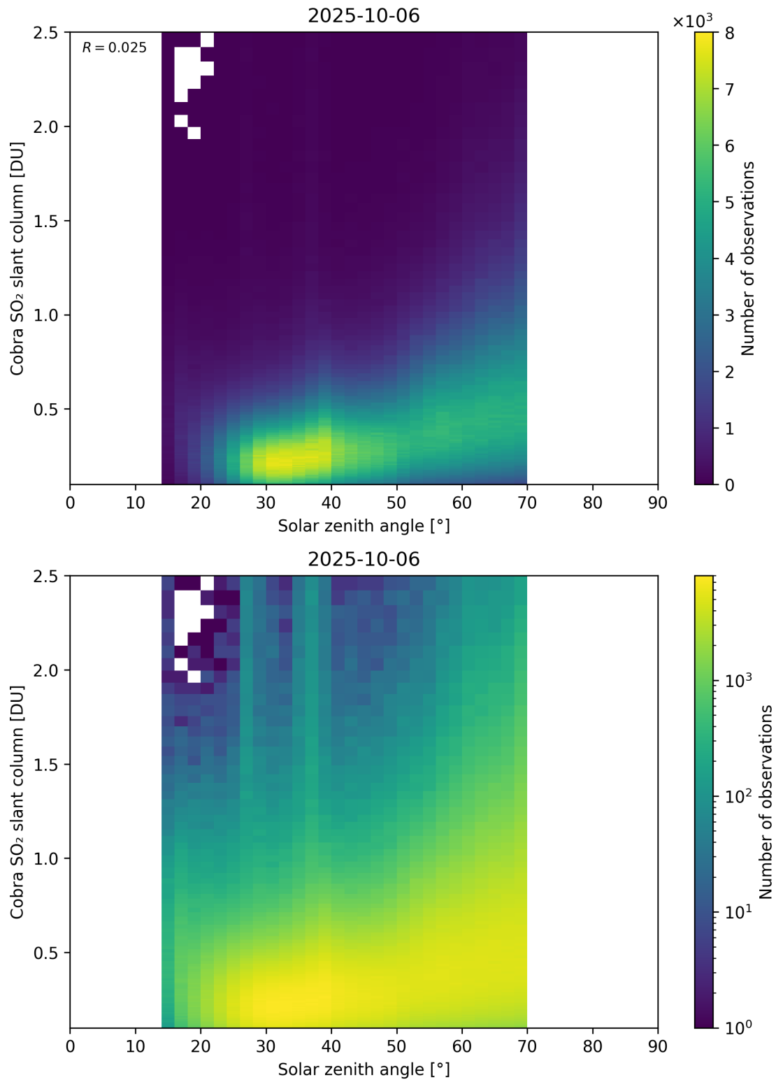
Figure 179: Scatter density plot of “Solar zenith angle” against “Cobra SO 2 slant column” for 2025-10-06 to 2025-10-07.
