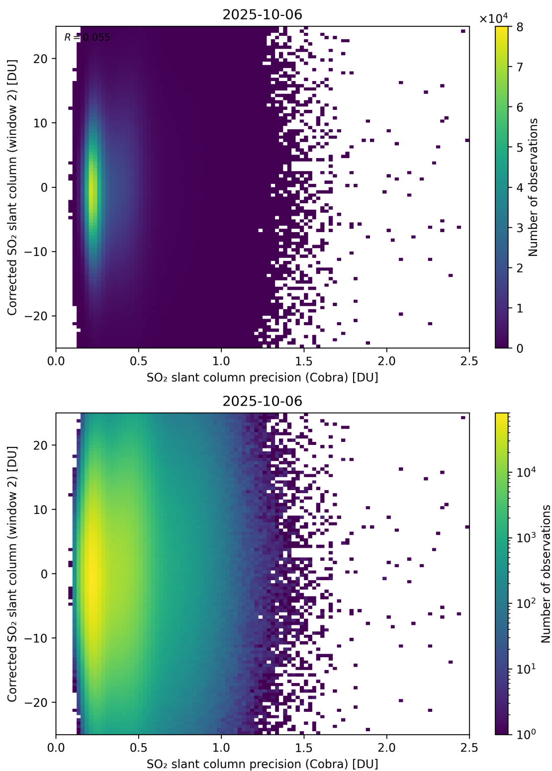
Figure 206: Scatter density plot of “SO 2 slant column precision (Cobra)” against “Corrected SO 2 slant column (window 2)” for 2025-10-06 to 2025-10-07.
