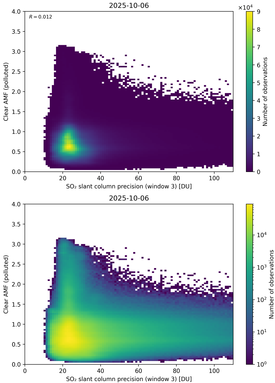
Figure 311: Scatter density plot of “SO 2 slant column precision (window 3)” against “Clear AMF (polluted)” for 2025-10-06 to 2025-10-07.
