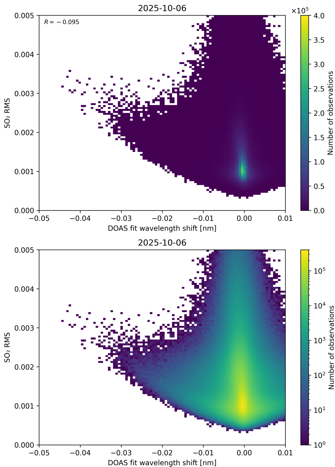
Figure 139: Scatter density plot of “DOAS fit wavelength shift” against “SO 2 RMS” for 2025-10-06 to 2025-10-07.
