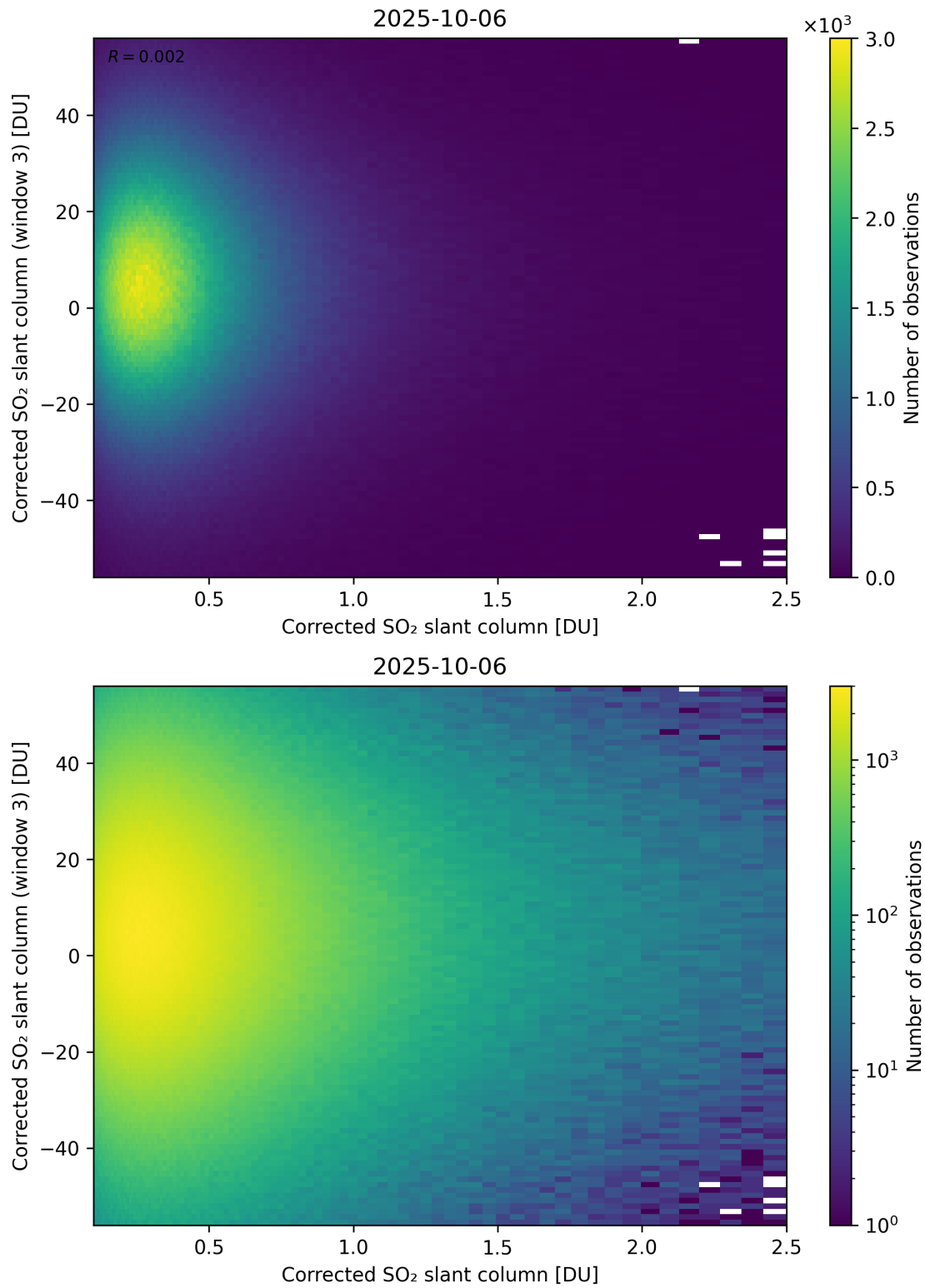
Figure 236: Scatter density plot of “Corrected SO 2 slant column” against “Corrected SO 2 slant column (window 3)” for 2025-10-06 to 2025-10-07.
