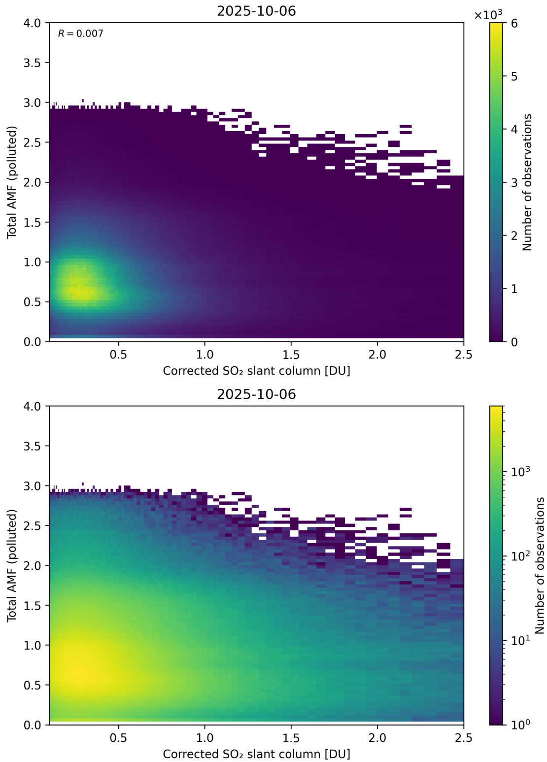
Figure 242: Scatter density plot of “Corrected SO 2 slant column” against “Total AMF (polluted)” for 2025-10-06 to 2025-10-07.
