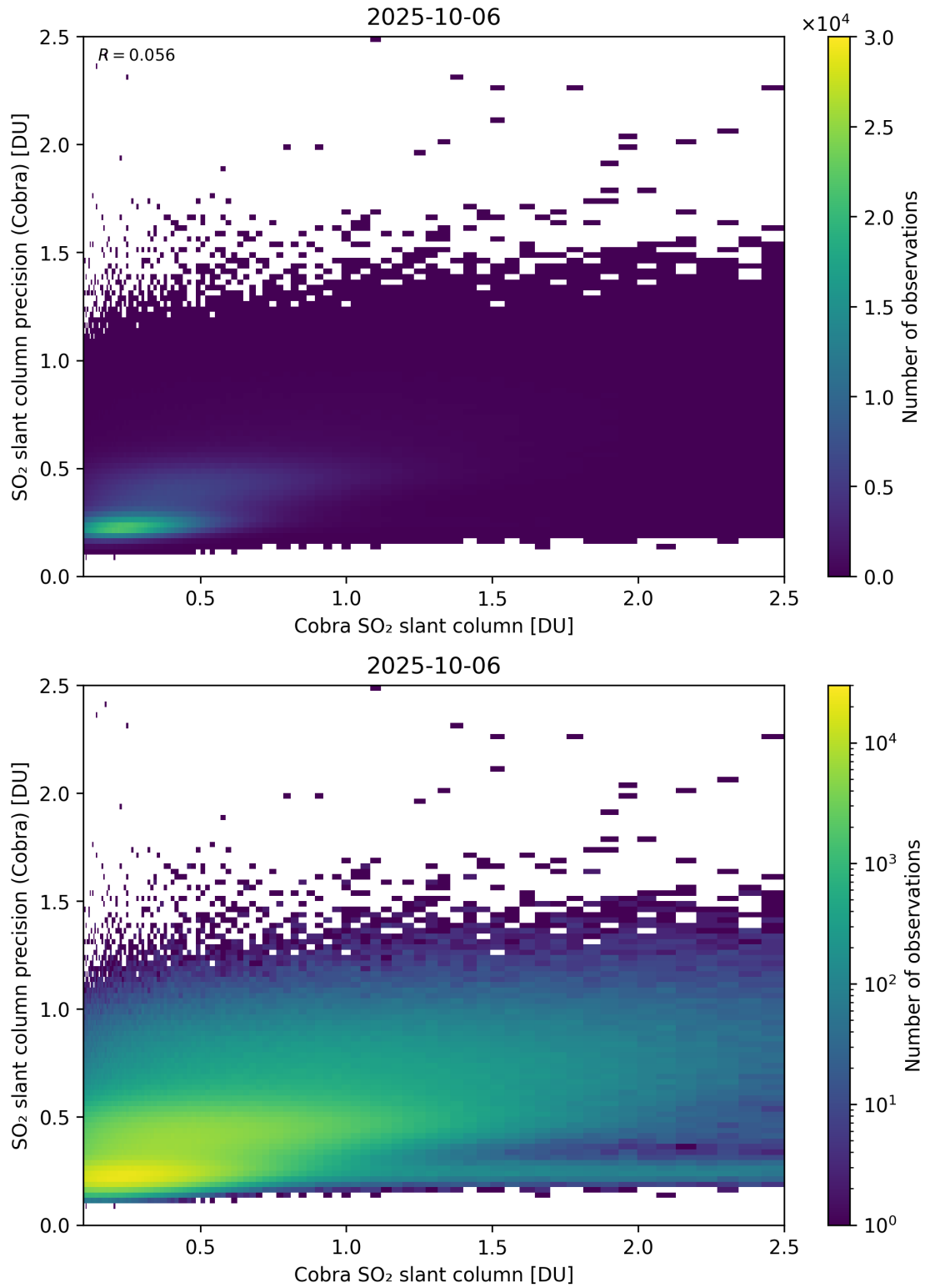
Figure 216: Scatter density plot of “Cobra SO 2 slant column” against “SO 2 slant column precision (Cobra)” for 2025-10-06 to 2025-10-07.
