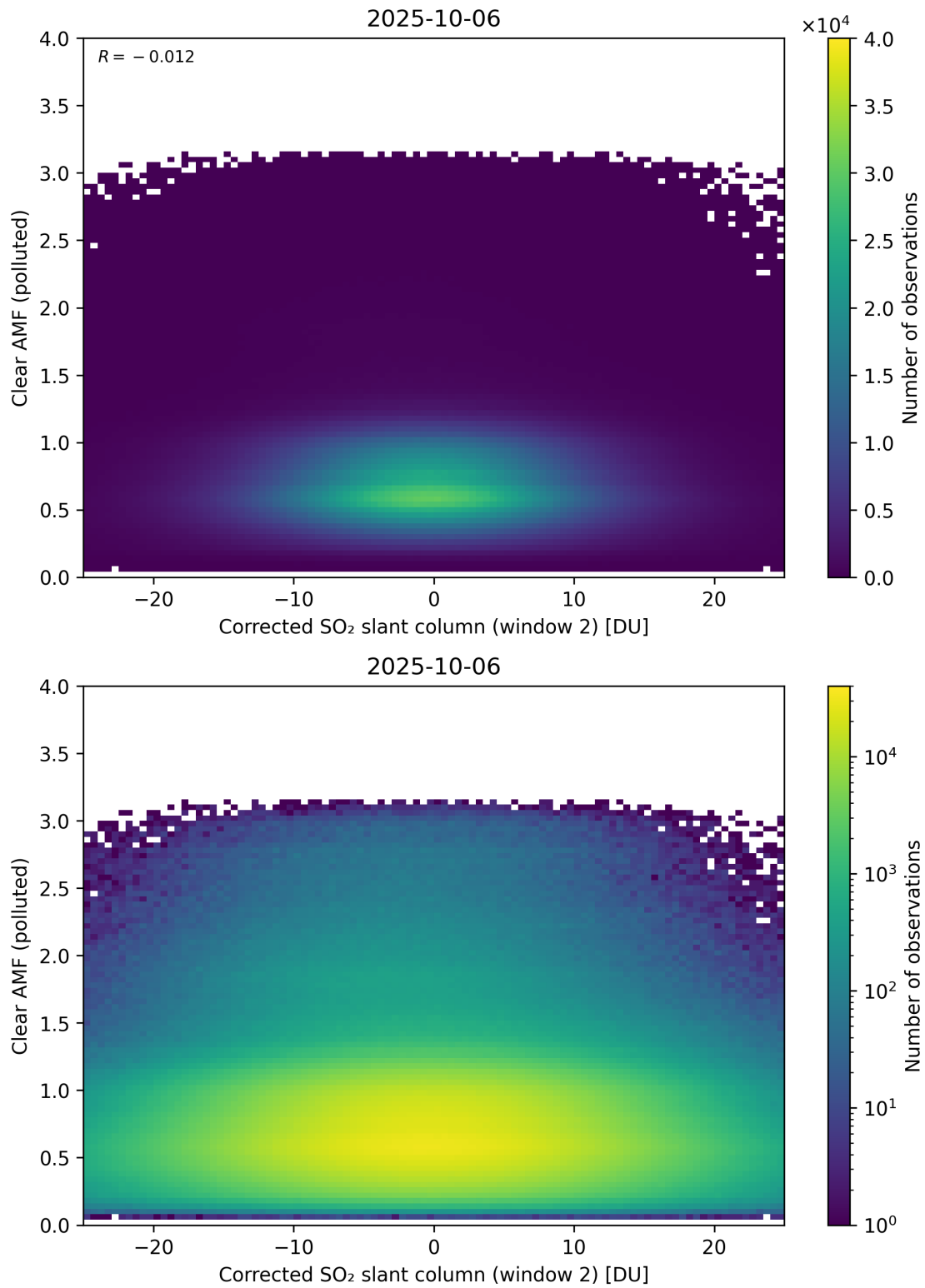
Figure 249: Scatter density plot of “Corrected SO 2 slant column (window 2)” against “Clear AMF (polluted)” for 2025-10-06 to 2025-10-07.
