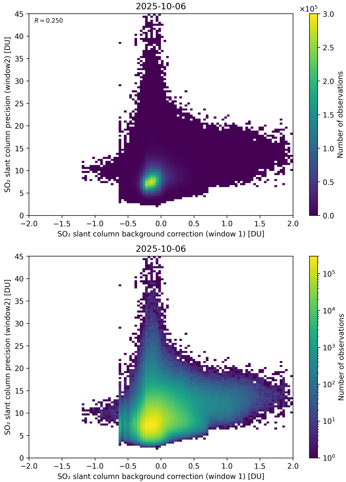
Figure 117: Scatter density plot of “SO 2 slant column background correction (window 1)” against “SO 2 slant column precision (window2)” for 2025-10-06 to 2025-10-07.
