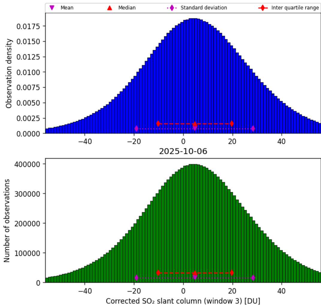
Figure 73: Histogram of “Corrected SO 2 slant column (window 3)” for 2025-10-06 to 2025-10-07
