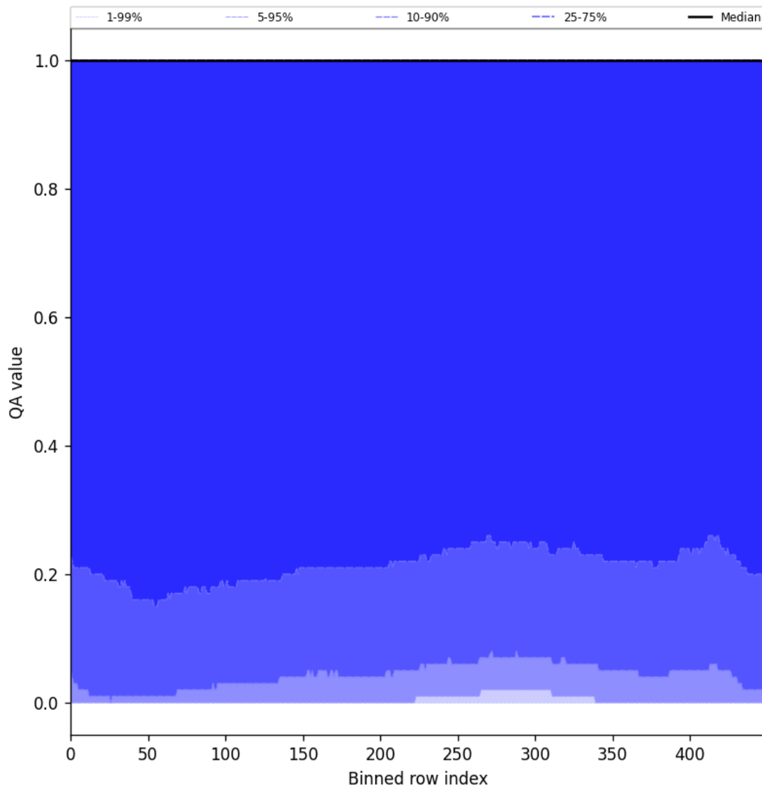
Figure 83: Along track statistics of “QA value” for 2025-10-06 to 2025-10-07
