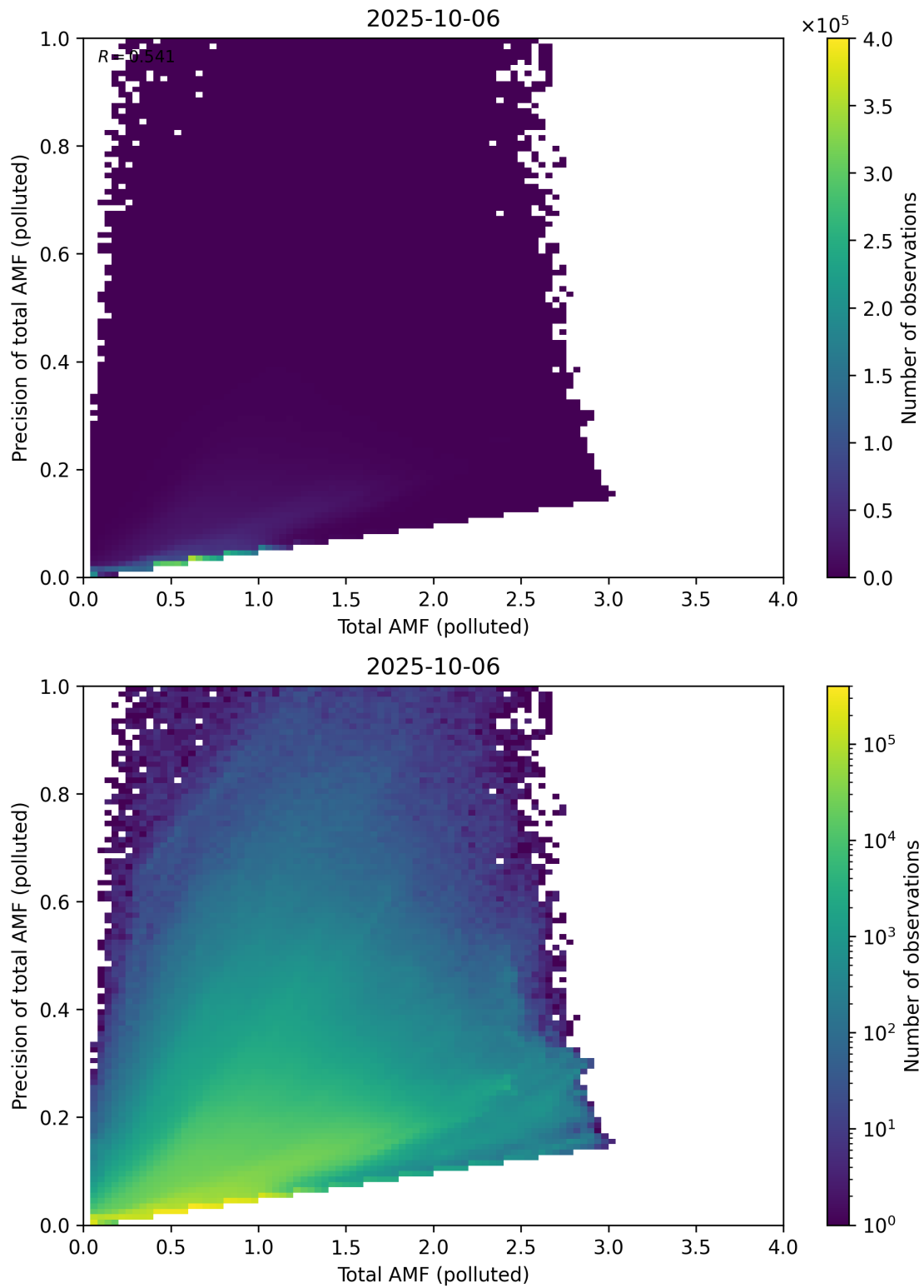
Figure 322: Scatter density plot of “Total AMF (polluted)” against “Precision of total AMF (polluted)” for 2025-10-06 to 2025-10-07.
