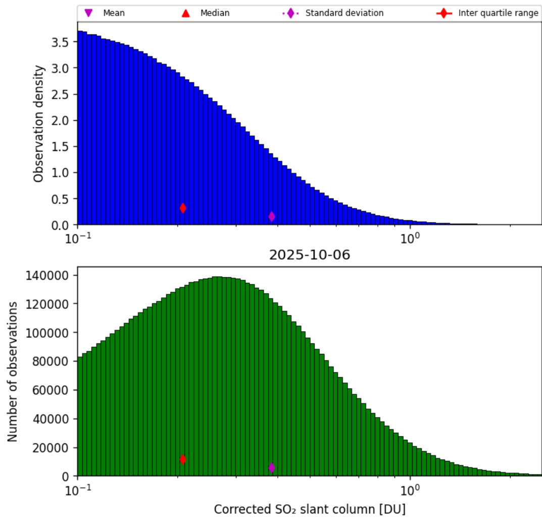
Figure 60: Histogram of “Corrected SO 2 slant column” for 2025-10-06 to 2025-10-07
