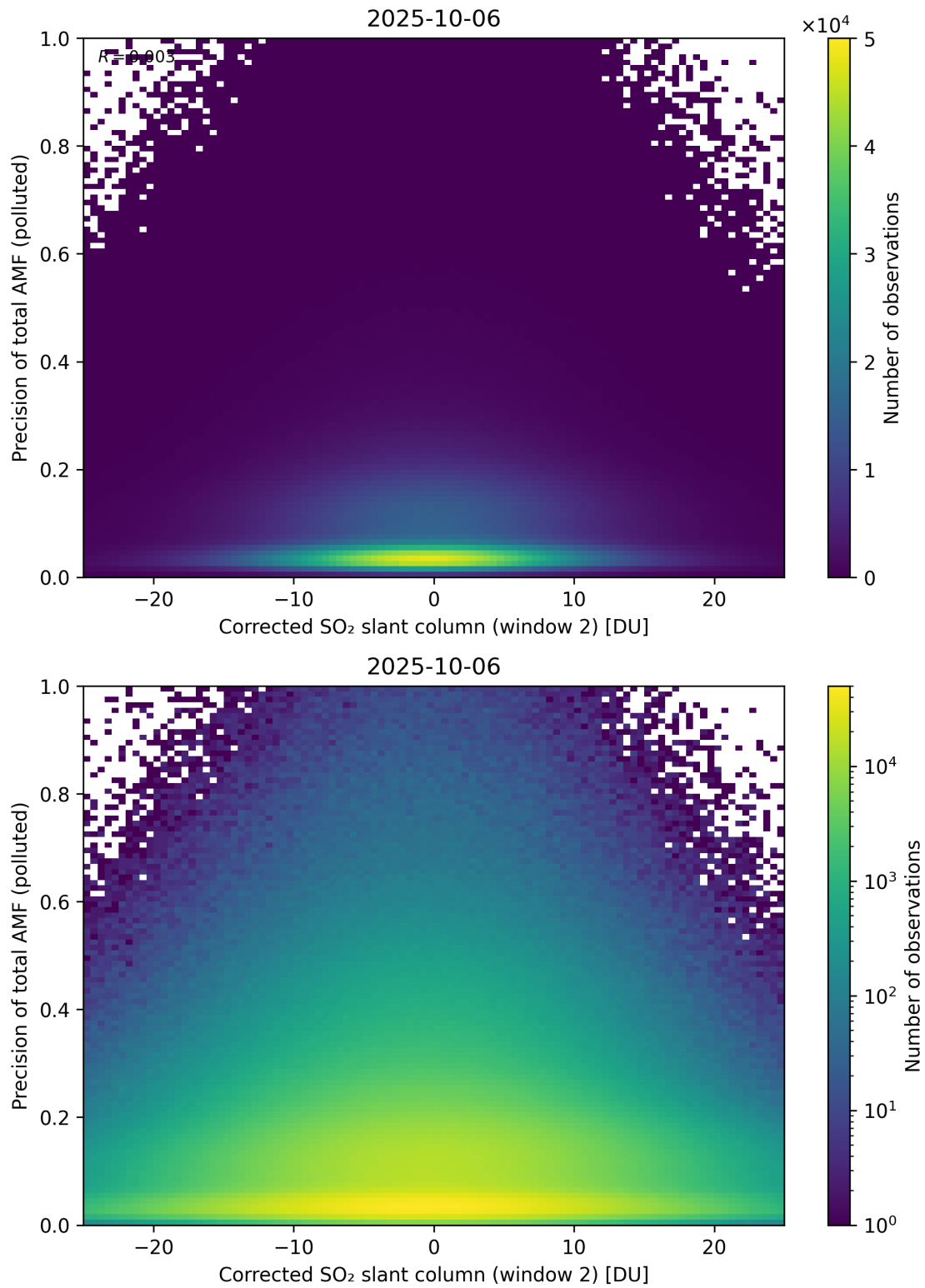
Figure 254: Scatter density plot of “Corrected SO 2 slant column (window 2)” against “Precision of total AMF (polluted)” for 2025-10-06 to 2025-10-07.
