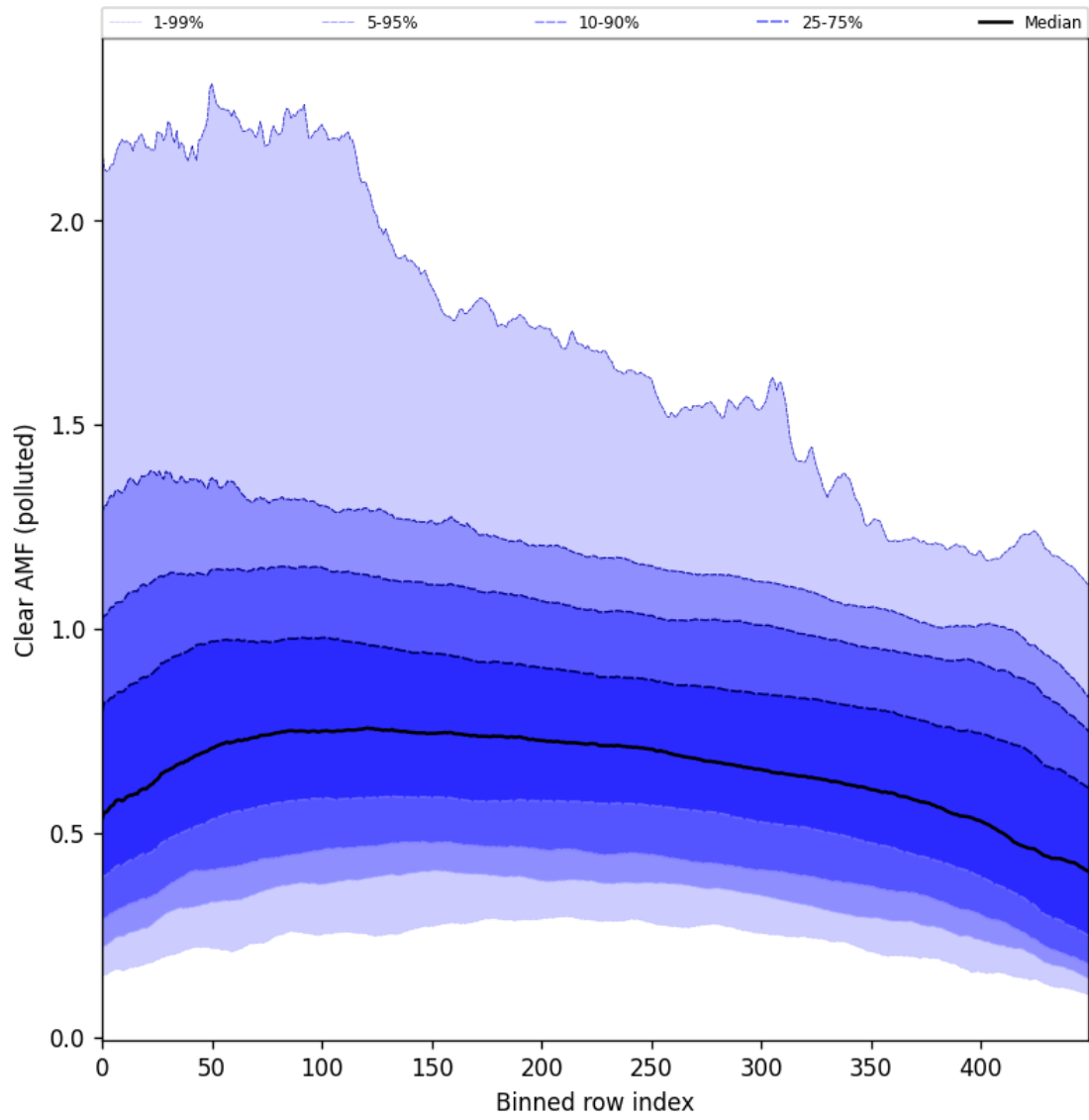
Figure 107: Along track statistics of “Clear AMF (polluted)” for 2025-10-06 to 2025-10-07
