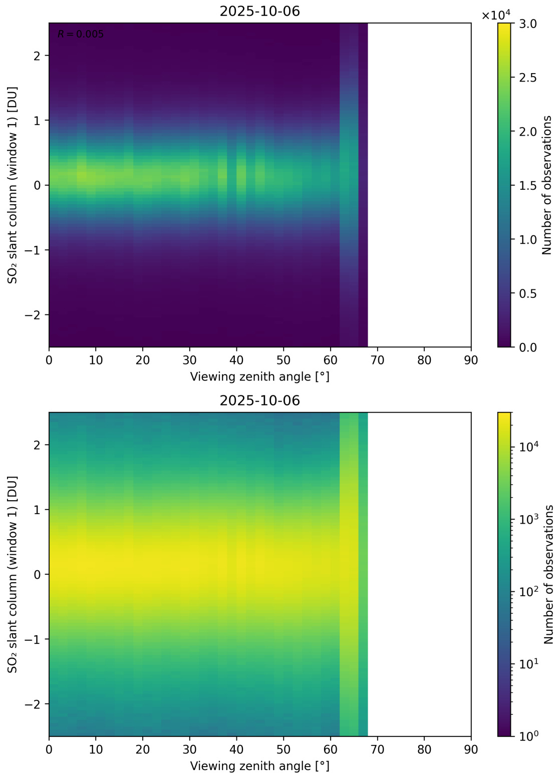
Figure 376: Scatter density plot of “Viewing zenith angle” against “SO 2 slant column (window 1)” for 2025-10-06 to 2025-10-07.
