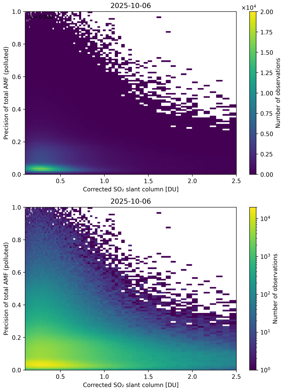
Figure 243: Scatter density plot of “Corrected SO 2 slant column” against “Precision of total AMF (polluted)” for 2025-10-06 to 2025-10-07.
