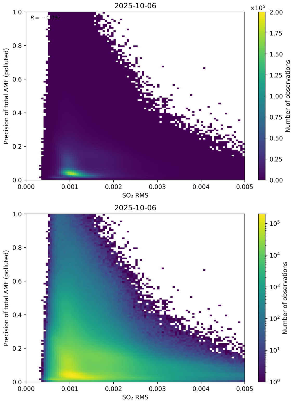
Figure 149: Scatter density plot of “SO 2 RMS” against “Precision of total AMF (polluted)” for 2025-10-06 to 2025-10-07.
