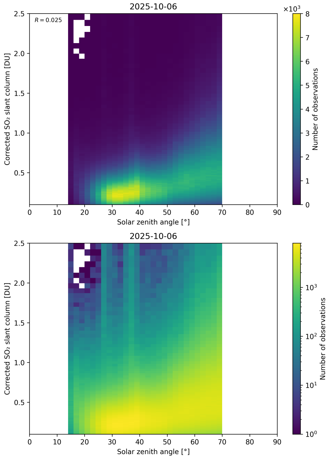
Figure 181: Scatter density plot of “Solar zenith angle” against “Corrected SO 2 slant column” for 2025-10-06 to 2025-10-07.
