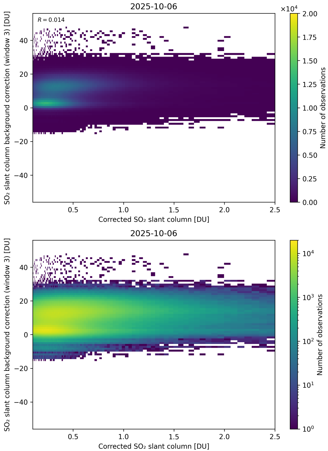
Figure 228: Scatter density plot of “Corrected SO 2 slant column” against “SO 2 slant column background correction (window 3)” for 2025-10-06 to 2025-10-07.
