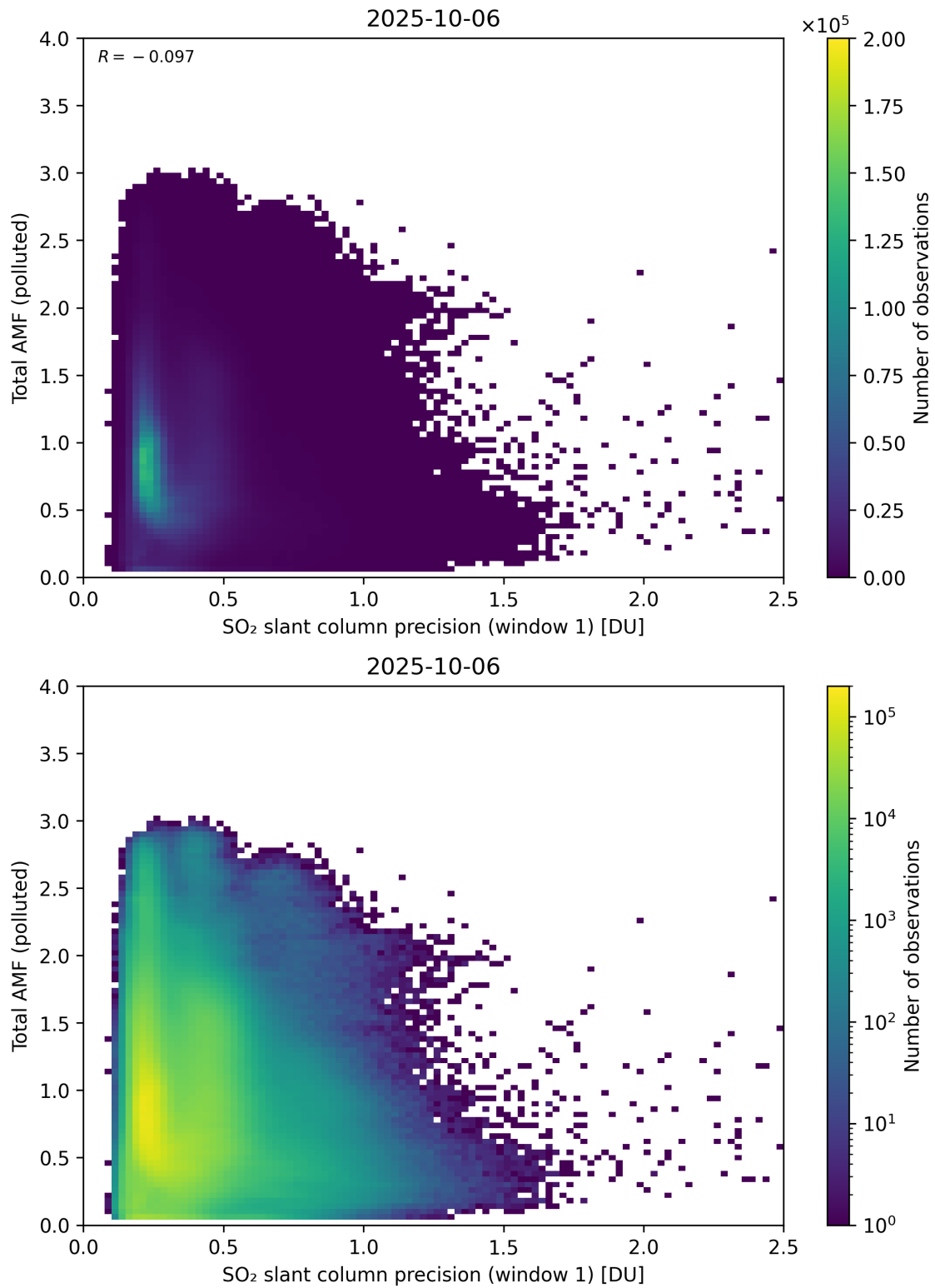
Figure 280: Scatter density plot of “SO 2 slant column precision (window 1)” against “Total AMF (polluted)” for 2025-10-06 to 2025-10-07.
