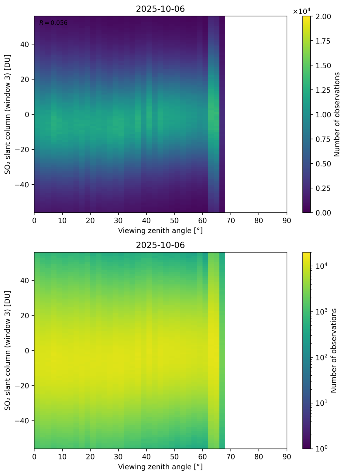
Figure 379: Scatter density plot of “Viewing zenith angle” against “SO 2 slant column (window 3)” for 2025-10-06 to 2025-10-07.
