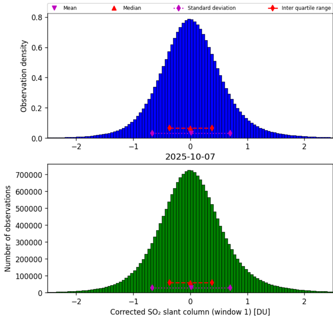
Figure 65: Histogram of “Corrected SO 2 slant column (window 1)” for 2025-10-06 to 2025-10-08
