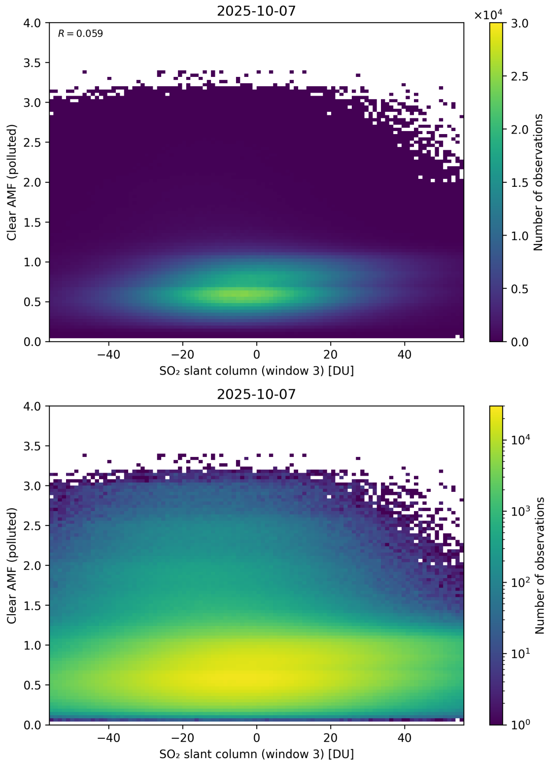
Figure 315: Scatter density plot of “SO 2 slant column (window 3)” against “Clear AMF (polluted)” for 2025-10-06 to 2025-10-08.
