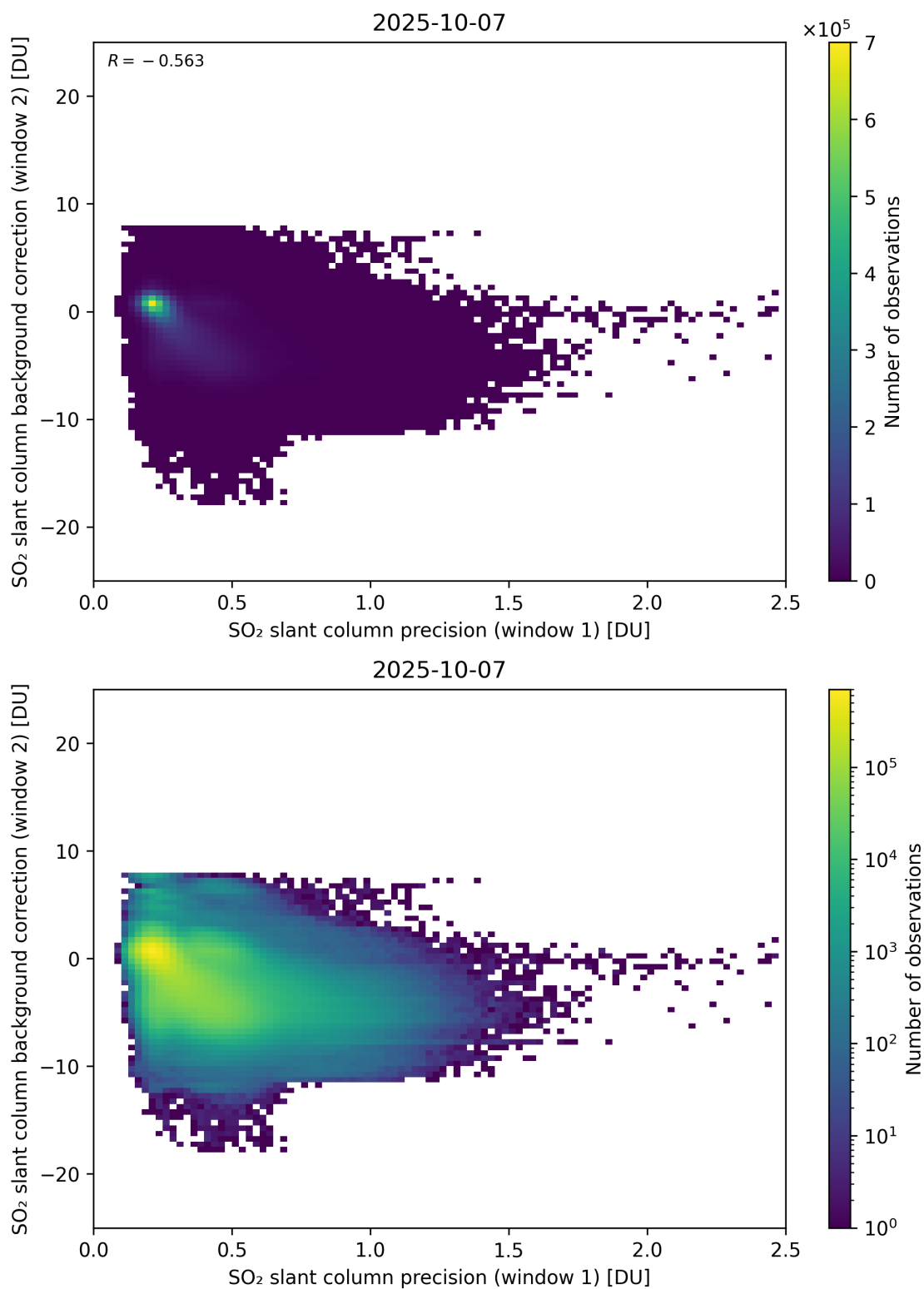
Figure 269: Scatter density plot of “SO 2 slant column precision (window 1)” against “SO 2 slant column background correction (window 2)” for 2025-10-06 to 2025-10-08.
