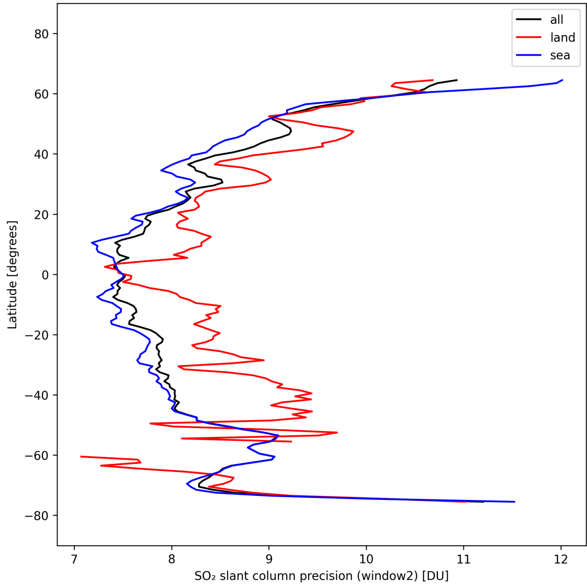
Figure 42: Zonal average of “SO 2 slant column precision (window2)” for 2025-10-06 to 2025-10-08.
