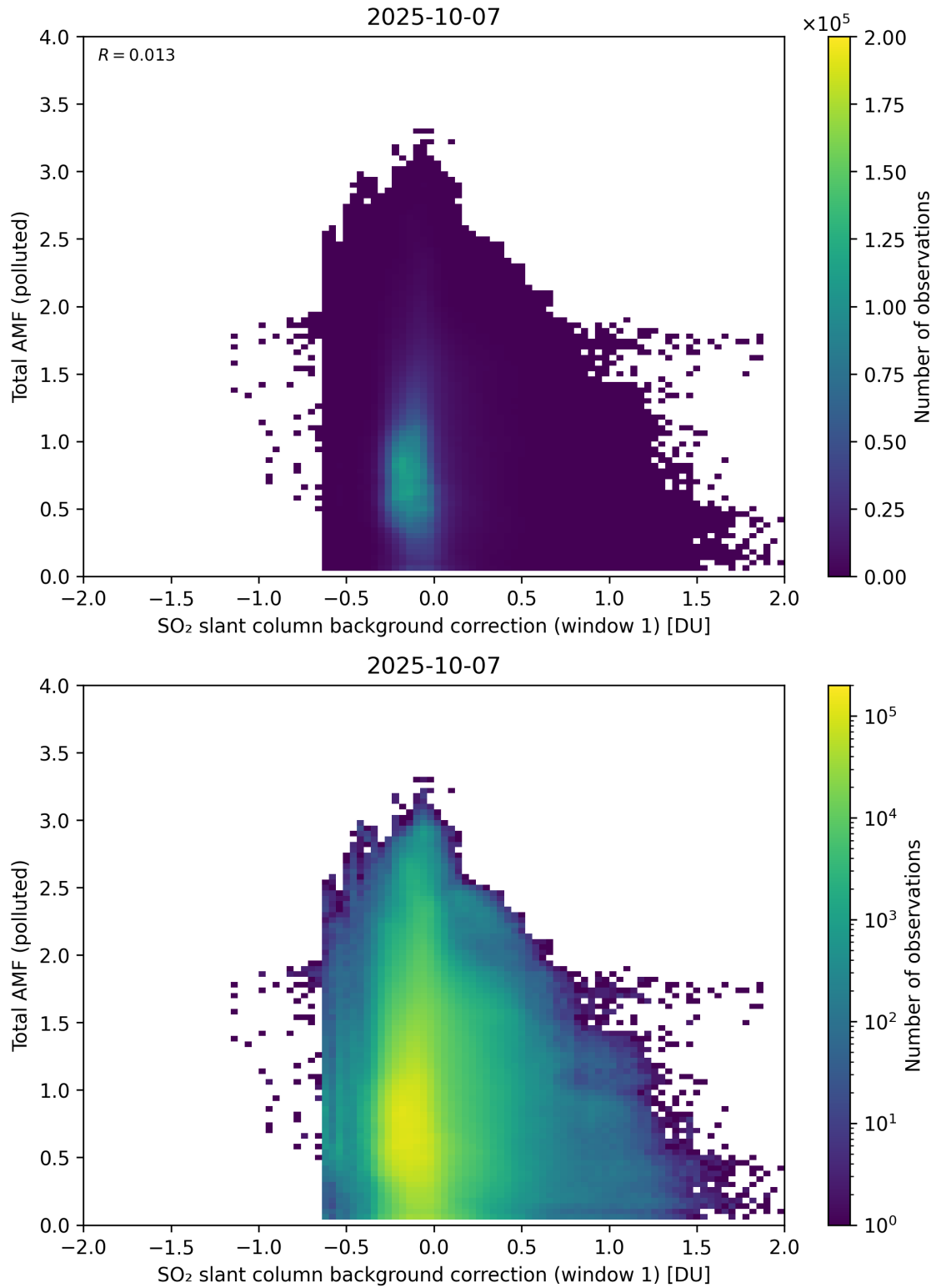
Figure 120: Scatter density plot of “SO 2 slant column background correction (window 1)” against “Total AMF (polluted)” for 2025-10-06 to 2025-10-08.
