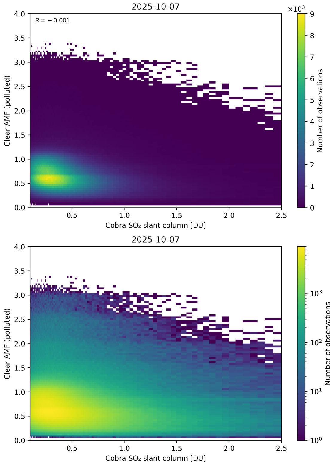
Figure 215: Scatter density plot of “Cobra SO 2 slant column” against “Clear AMF (polluted)” for 2025-10-06 to 2025-10-08.
