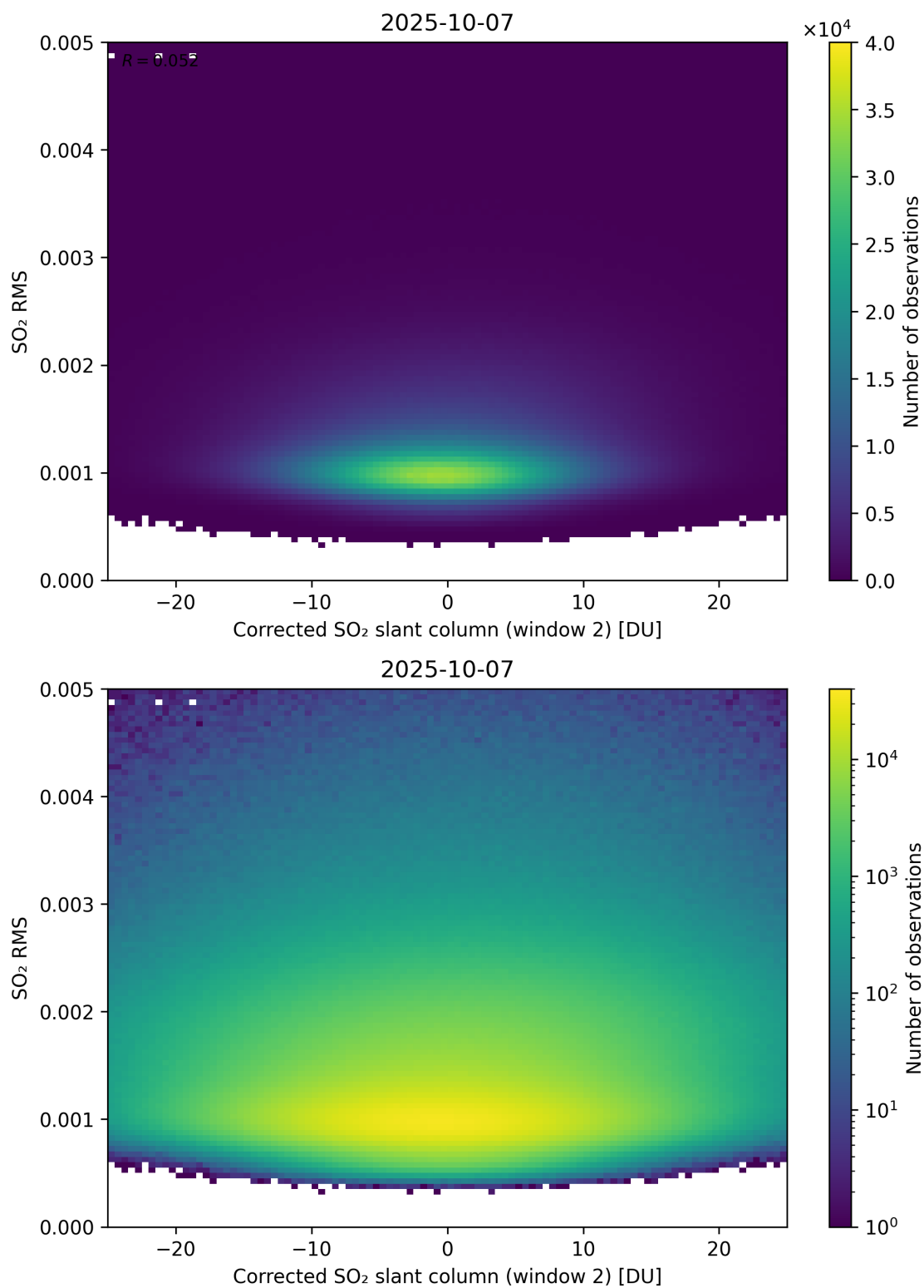
Figure 248: Scatter density plot of “Corrected SO 2 slant column (window 2)” against “SO 2 RMS” for 2025-10-06 to 2025-10-08.
