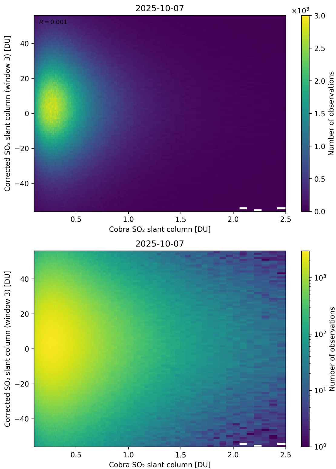
Figure 218: Scatter density plot of “Cobra SO 2 slant column” against “Corrected SO 2 slant column (window 3)” for 2025-10-06 to 2025-10-08.
