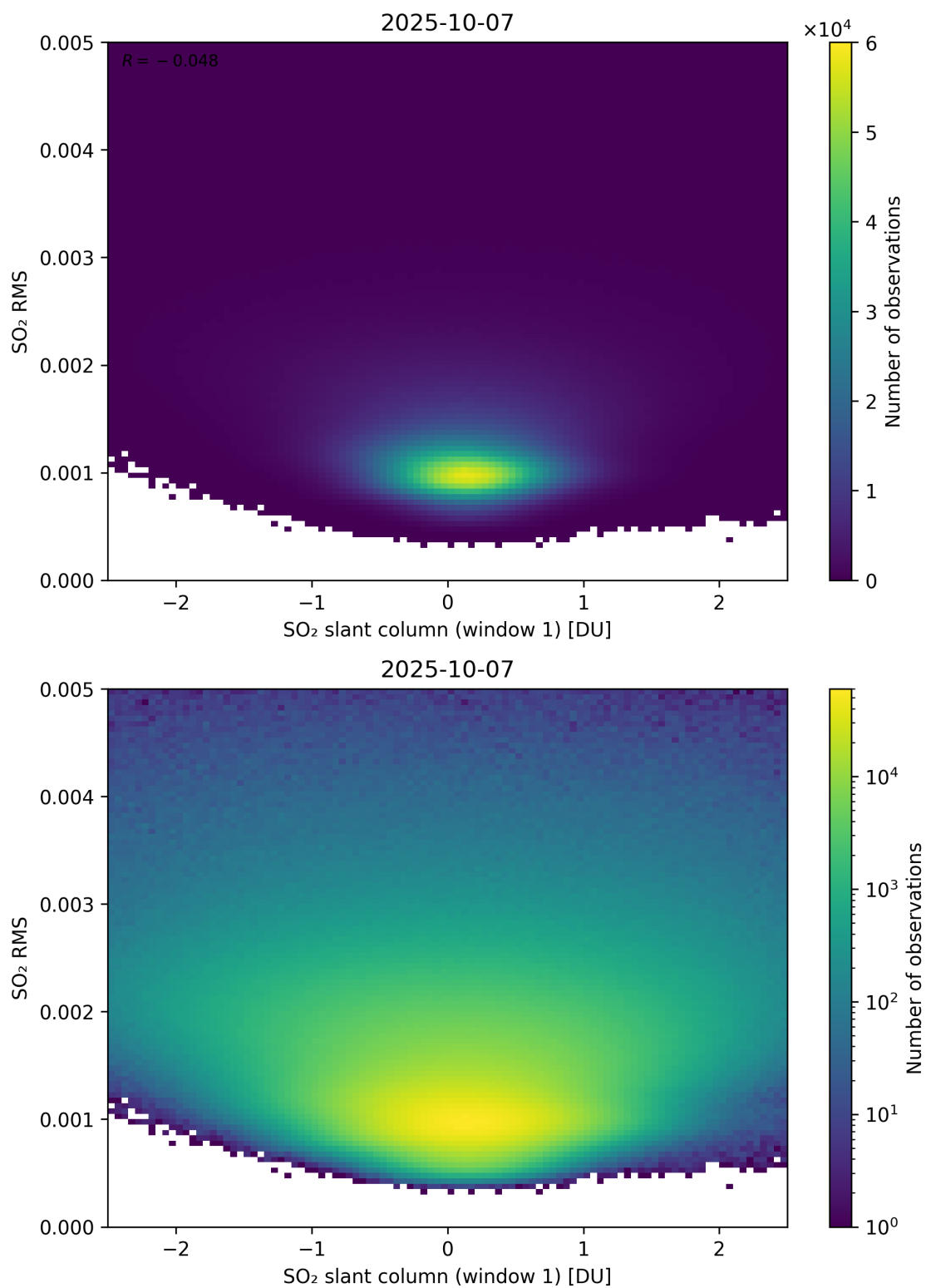
Figure 267: Scatter density plot of “SO 2 slant column (window 1)” against “SO 2 RMS” for 2025-10-06 to 2025-10-08.
