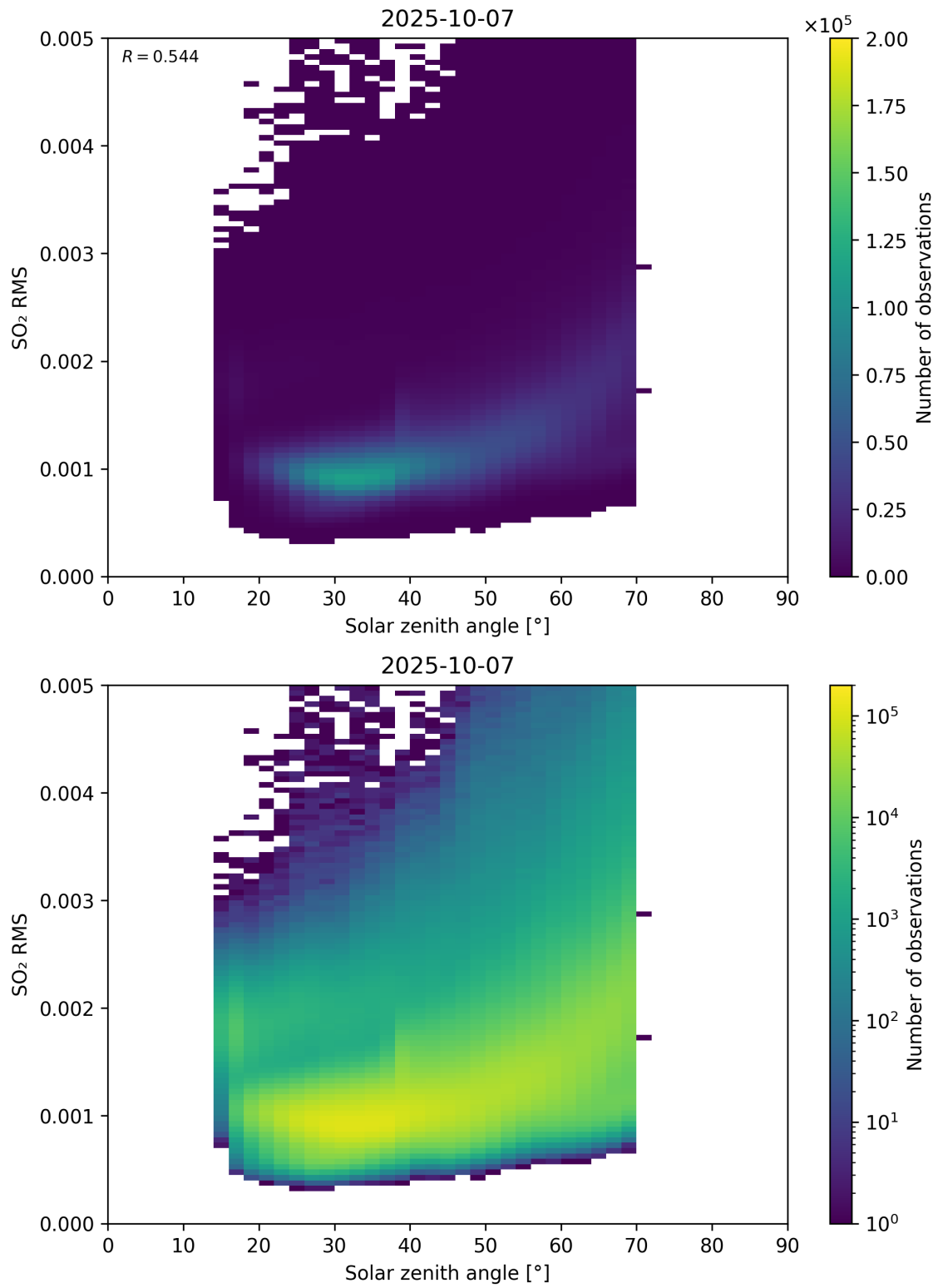
Figure 176: Scatter density plot of “Solar zenith angle” against “SO 2 RMS” for 2025-10-06 to 2025-10-08.
