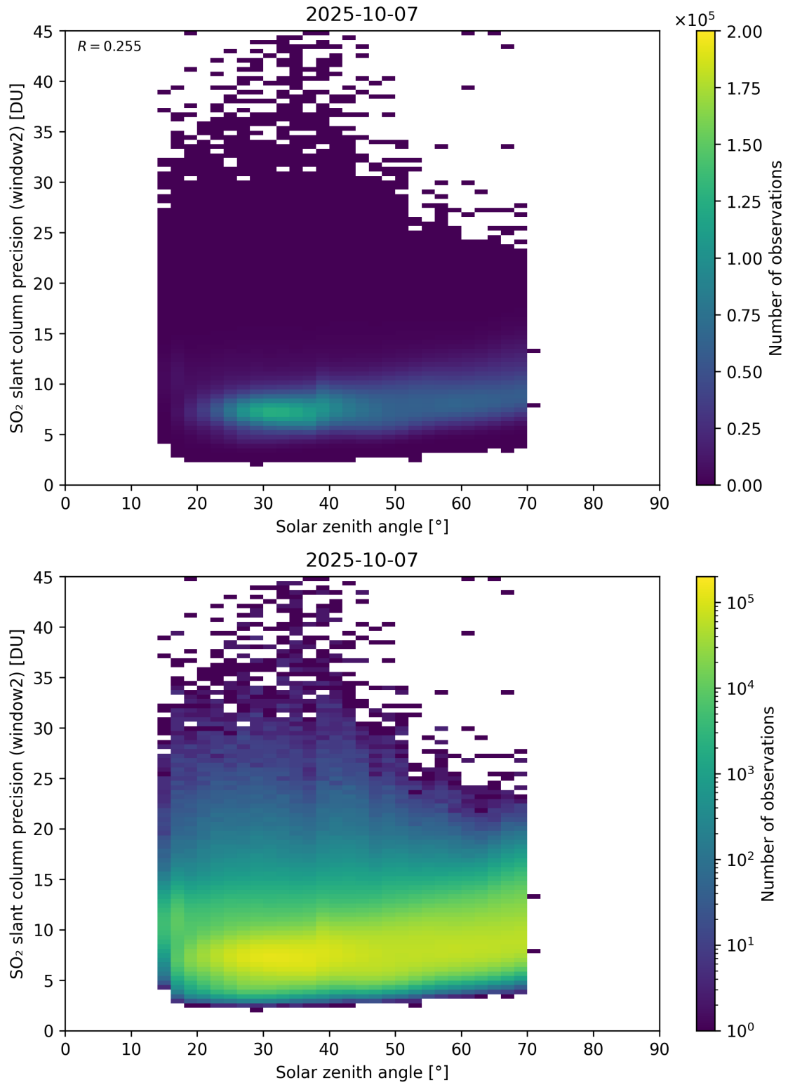
Figure 186: Scatter density plot of “Solar zenith angle” against “SO 2 slant column precision (window2)” for 2025-10-06 to 2025-10-08.
