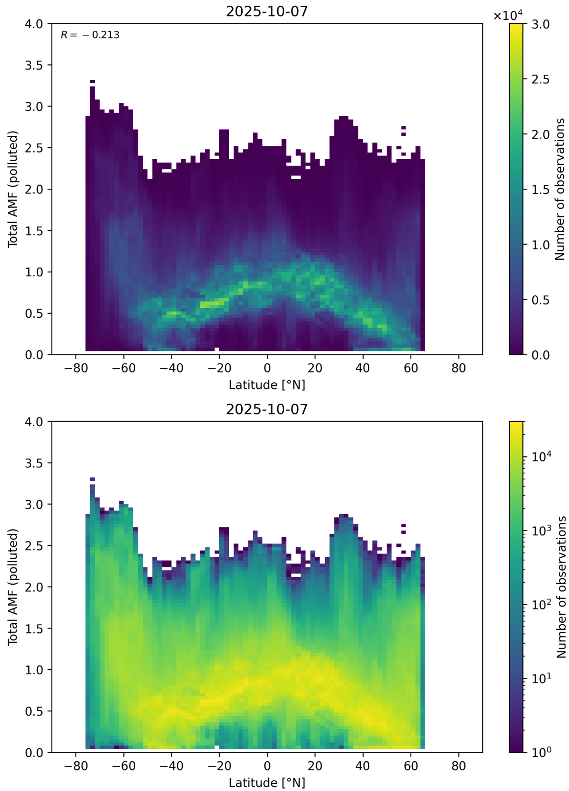
Figure 167: Scatter density plot of “Latitude” against “Total AMF (polluted)” for 2025-10-06 to 2025-10-08.
