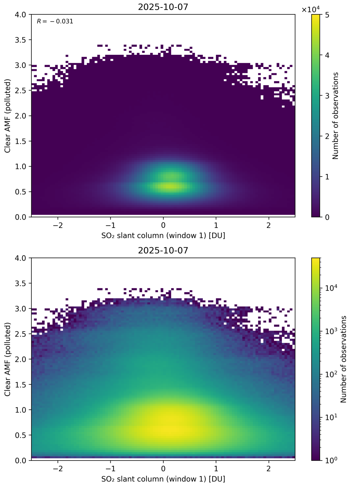
Figure 282: Scatter density plot of “SO 2 slant column (window 1)” against “Clear AMF (polluted)” for 2025-10-06 to 2025-10-08.
