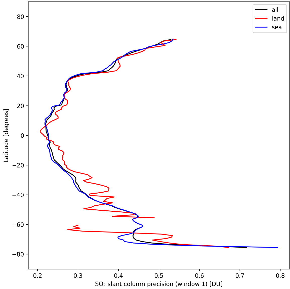
Figure 38: Zonal average of “SO 2 slant column precision (window 1)” for 2025-10-06 to 2025-10-08.
