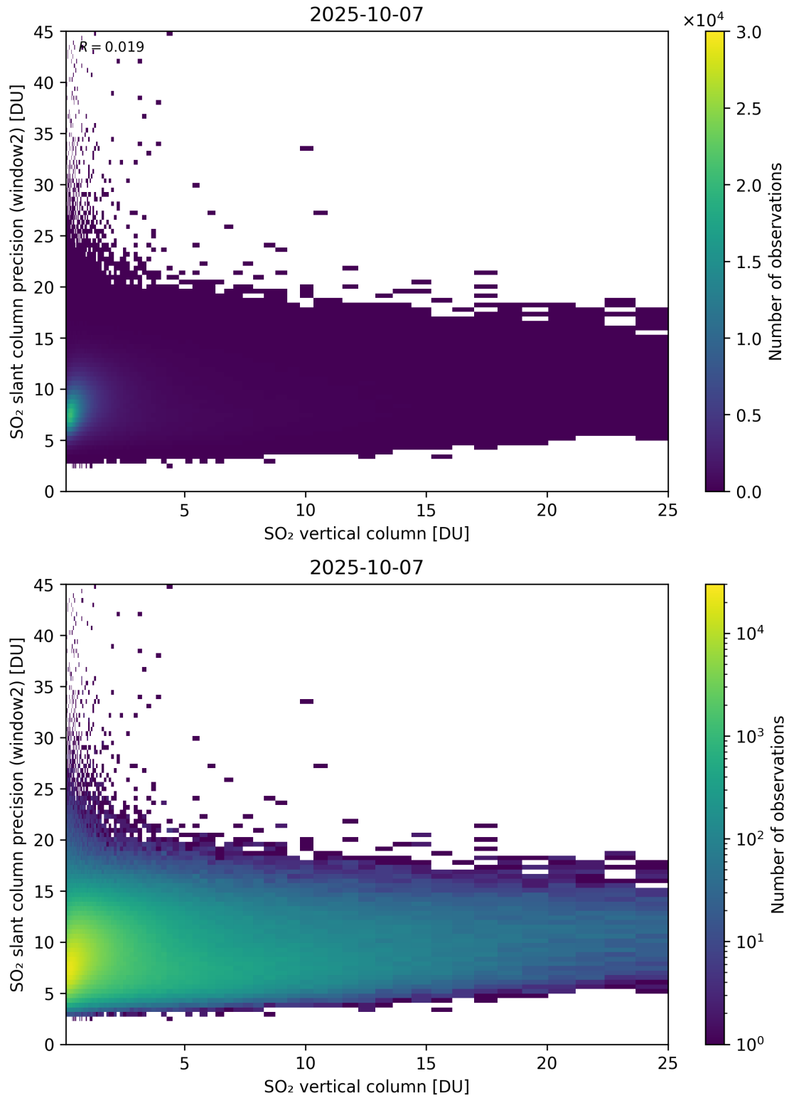
Figure 356: Scatter density plot of “SO 2 vertical column” against “SO 2 slant column precision (window2)” for 2025-10-06 to 2025-10-08.
