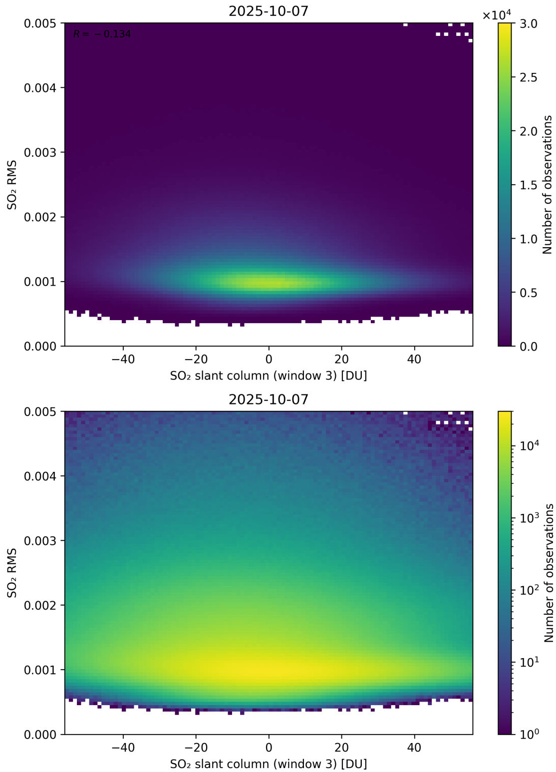
Figure 306: Scatter density plot of “SO 2 slant column (window 3)” against “SO 2 RMS” for 2025-10-06 to 2025-10-08.
