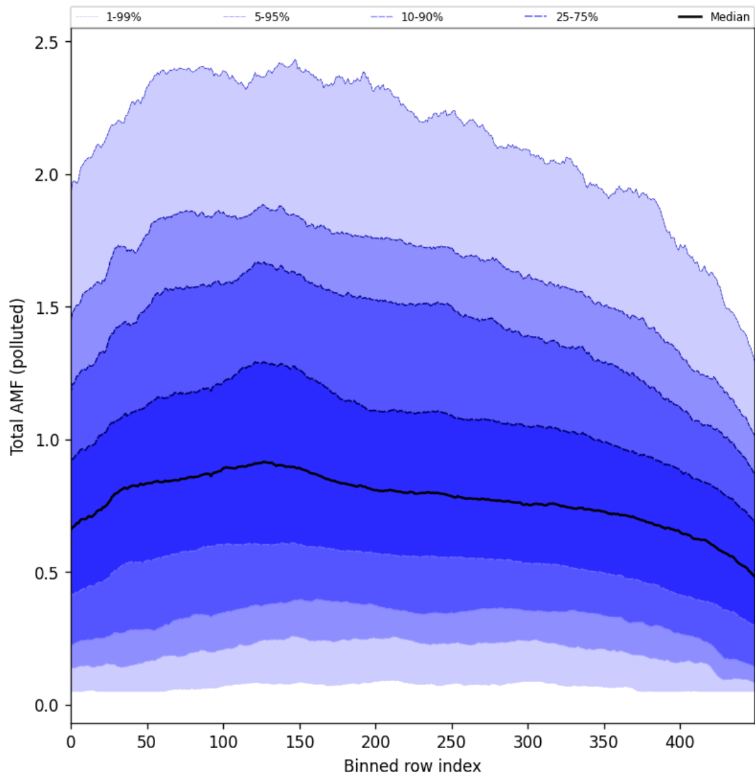
Figure 105: Along track statistics of “Total AMF (polluted)” for 2025-10-06 to 2025-10-08
