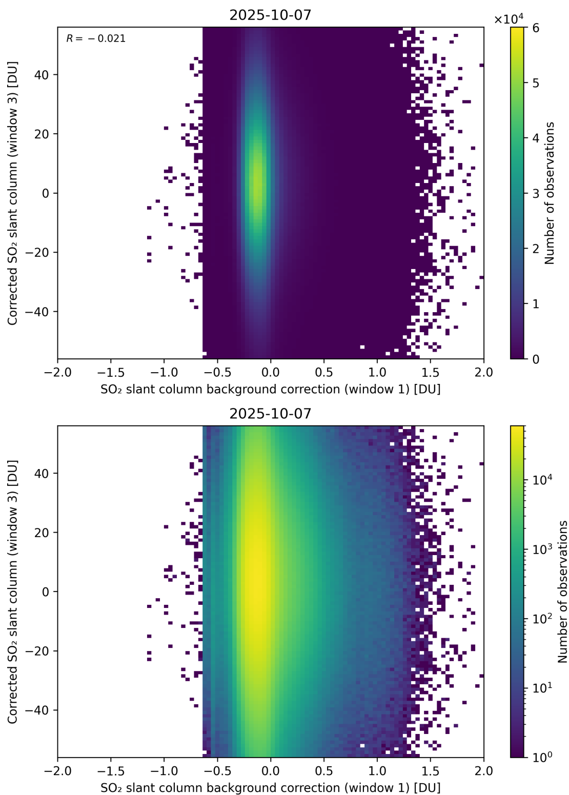
Figure 116: Scatter density plot of “SO 2 slant column background correction (window 1)” against “Corrected SO 2 slant column (window 3)” for 2025-10-06 to 2025-10-08.
