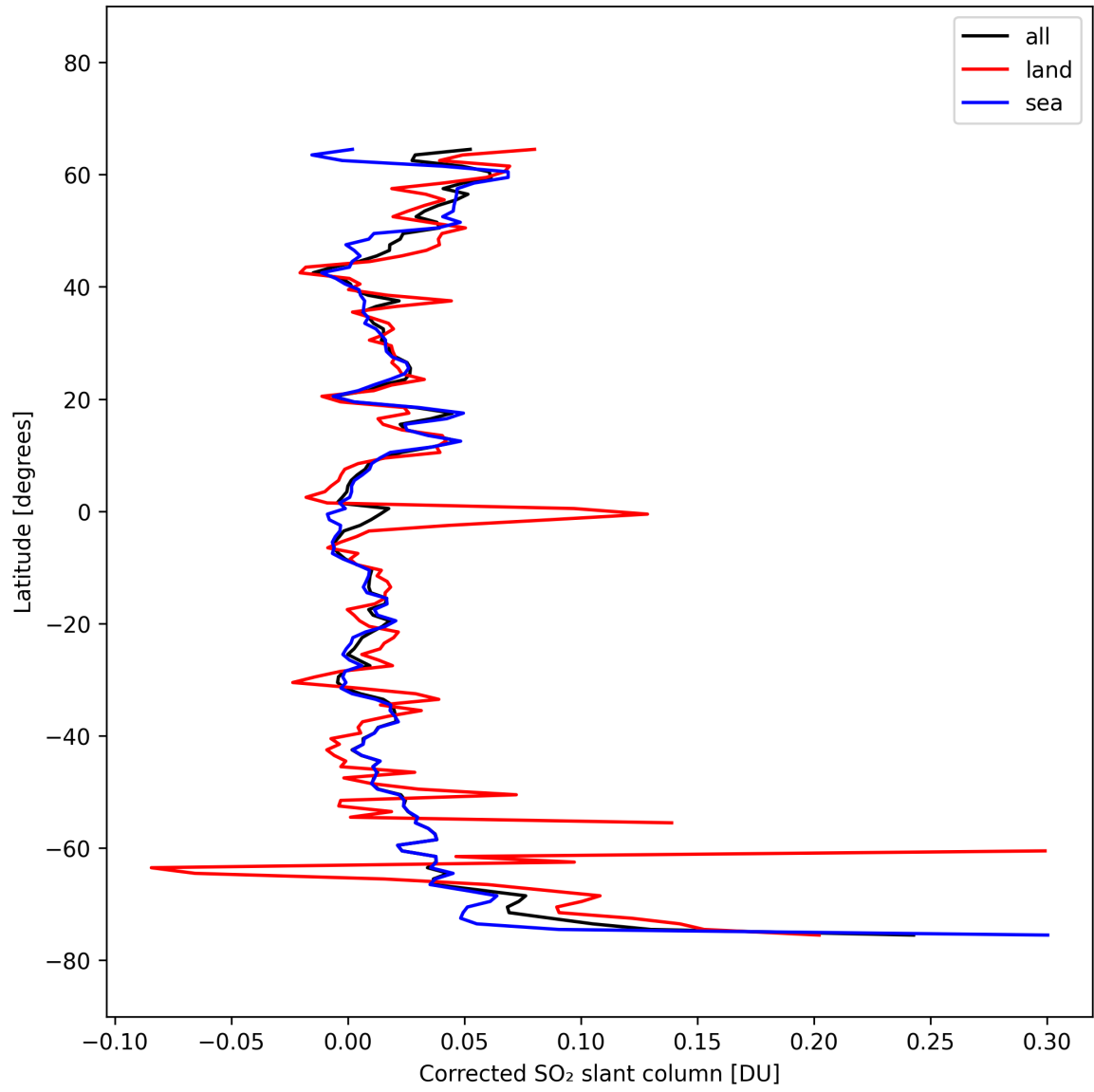
Figure 34: Zonal average of “Corrected SO 2 slant column” for 2025-10-06 to 2025-10-08.
