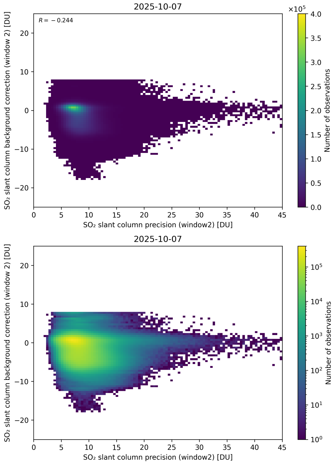
Figure 291: Scatter density plot of “SO 2 slant column precision (window2)” against “SO 2 slant column background correction (window 2)” for 2025-10-06 to 2025-10-08.
