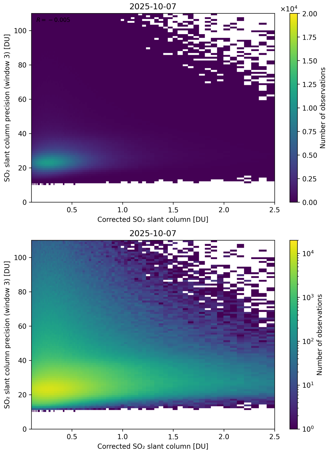
Figure 241: Scatter density plot of “Corrected SO 2 slant column” against “SO 2 slant column precision (window 3)” for 2025-10-06 to 2025-10-08.
