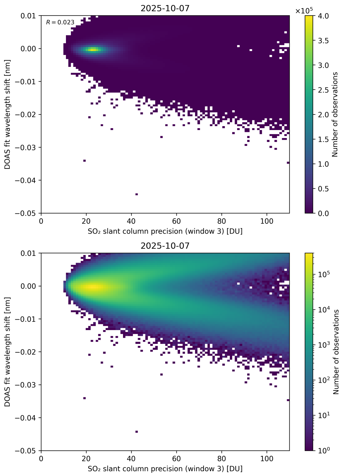
Figure 308: Scatter density plot of “SO 2 slant column precision (window 3)” against “DOAS fit wavelength shift” for 2025-10-06 to 2025-10-08.
