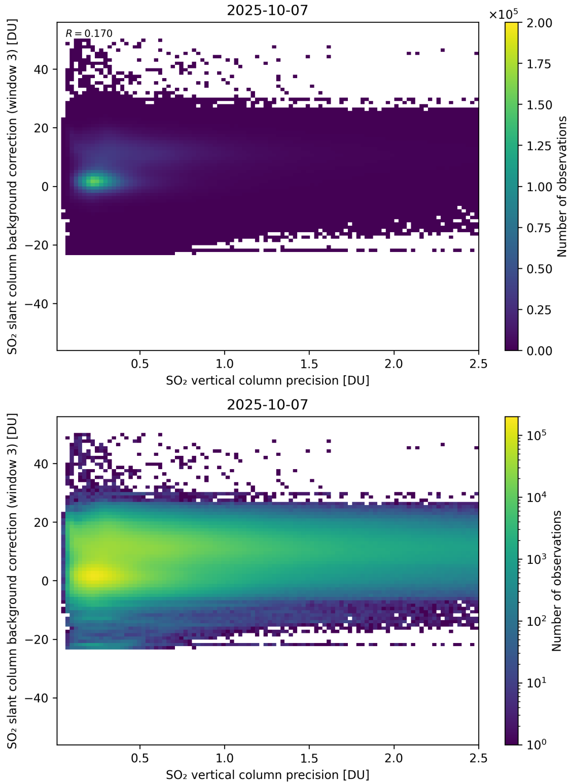
Figure 331: Scatter density plot of “SO 2 vertical column precision” against “SO 2 slant column background correction (window 3)” for 2025-10-06 to 2025-10-08.
