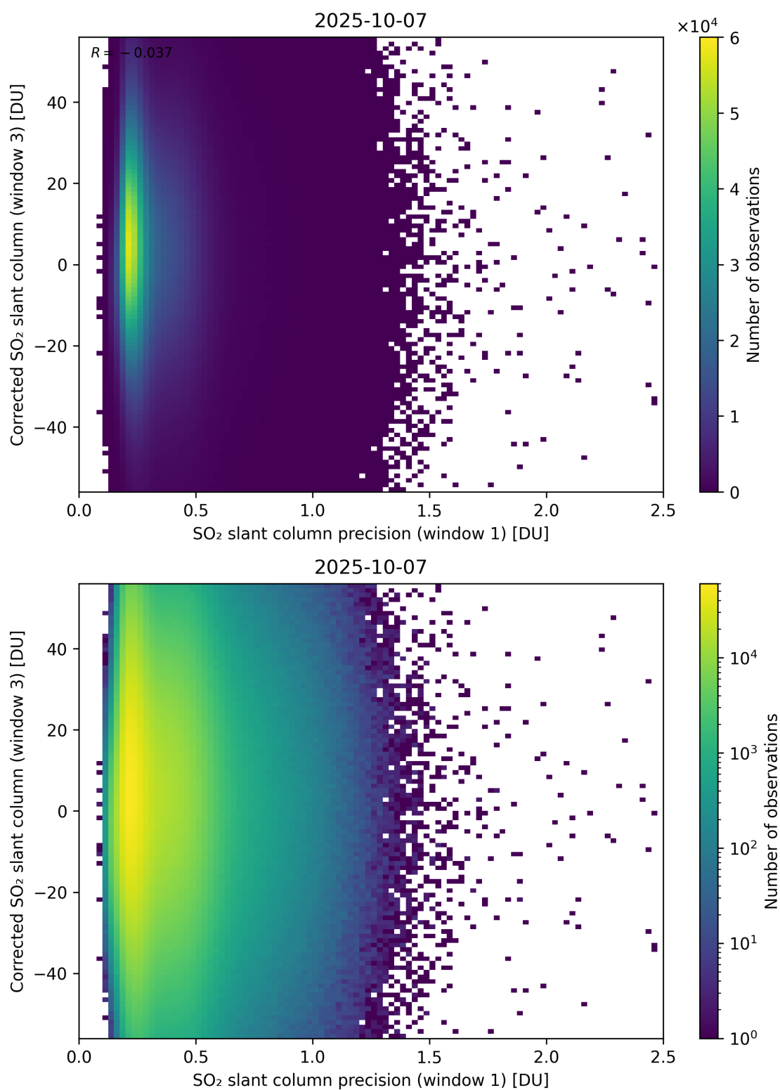
Figure 276: Scatter density plot of “SO 2 slant column precision (window 1)” against “Corrected SO 2 slant column (window 3)” for 2025-10-06 to 2025-10-08.
