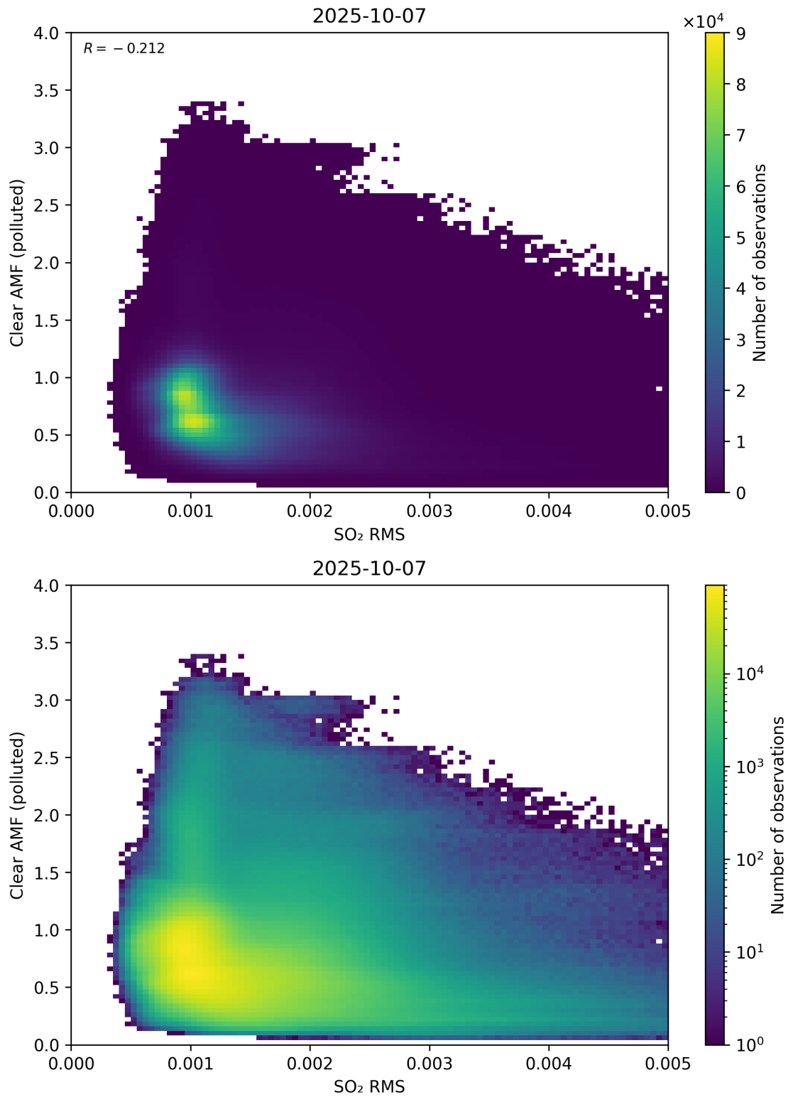
Figure 147: Scatter density plot of “SO 2 RMS” against “Clear AMF (polluted)” for 2025-10-06 to 2025-10-08.
