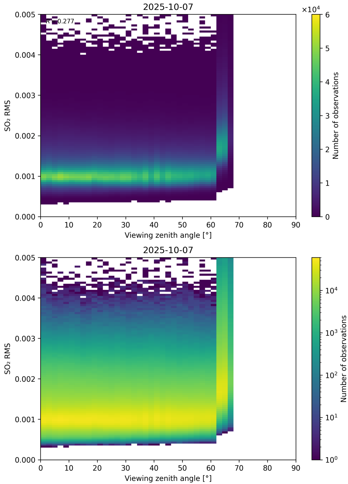
Figure 367: Scatter density plot of “Viewing zenith angle” against “SO 2 RMS” for 2025-10-06 to 2025-10-08.
