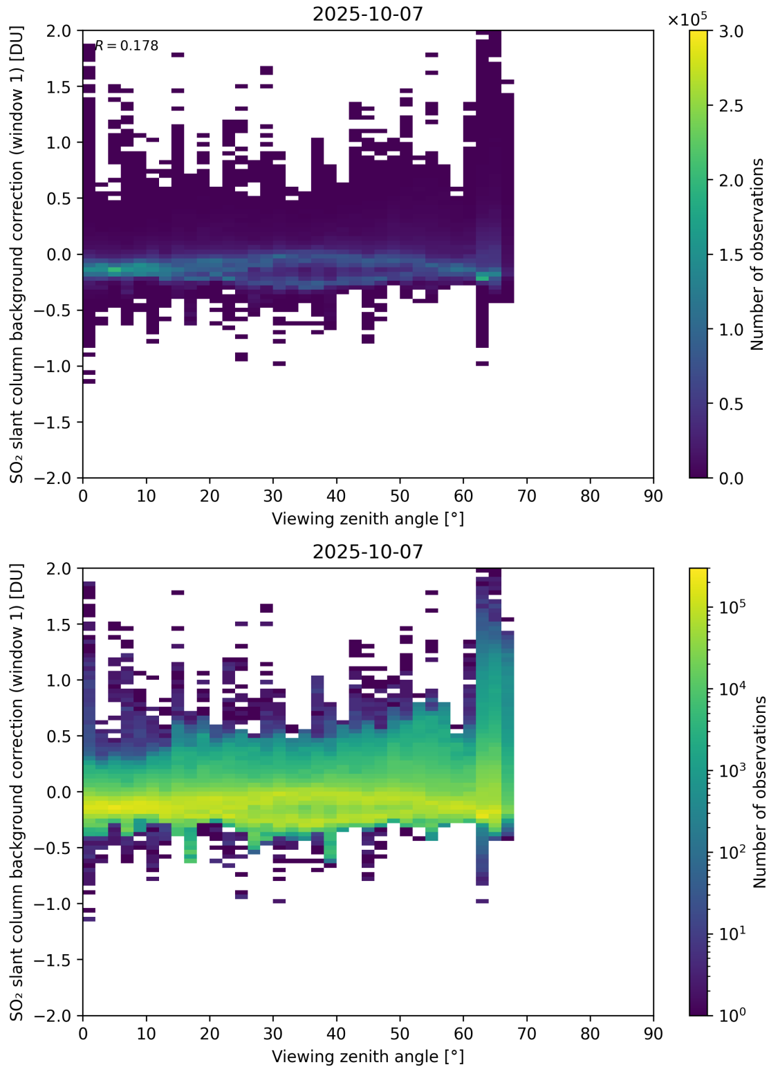
Figure 362: Scatter density plot of “Viewing zenith angle” against “SO 2 slant column background correction (window 1)” for 2025-10-06 to 2025-10-08.
