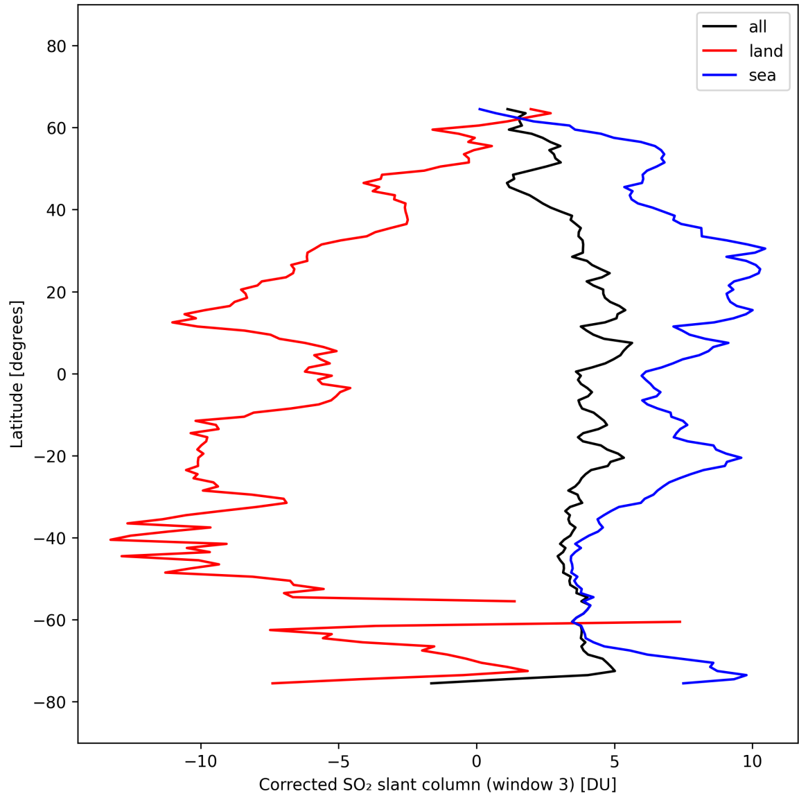
Figure 47: Zonal average of “Corrected SO 2 slant column (window 3)” for 2025-10-06 to 2025-10-08.
