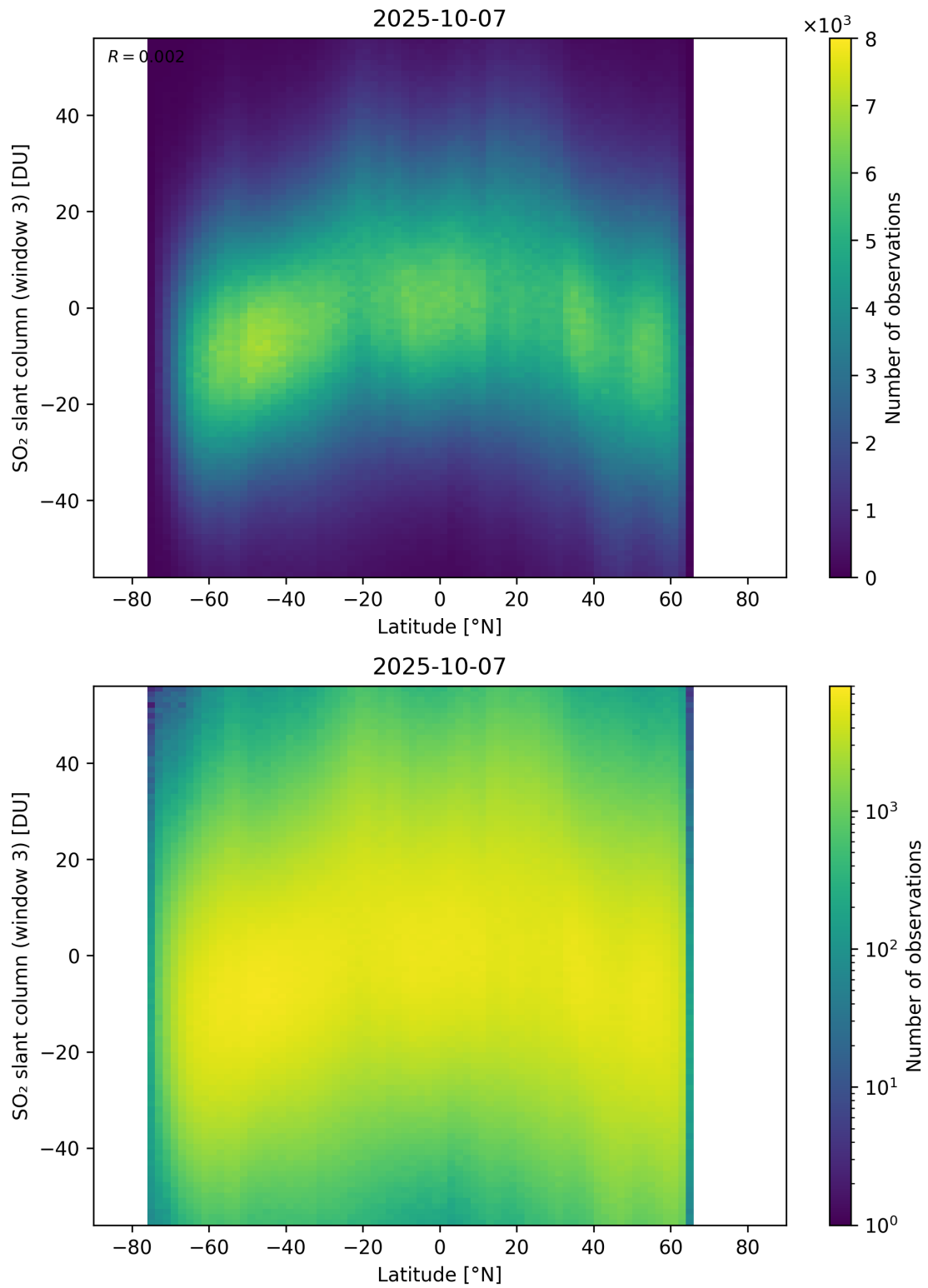
Figure 165: Scatter density plot of “Latitude” against “SO 2 slant column (window 3)” for 2025-10-06 to 2025-10-08.
