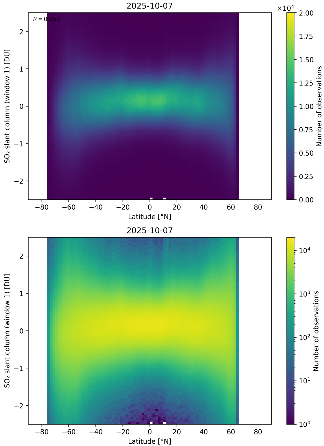
Figure 162: Scatter density plot of “Latitude” against “SO 2 slant column (window 1)” for 2025-10-06 to 2025-10-08.
