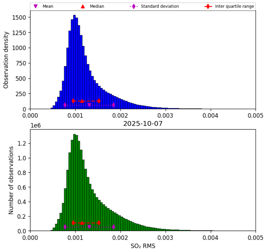
Figure 78: Histogram of “SO 2 RMS” for 2025-10-06 to 2025-10-08
