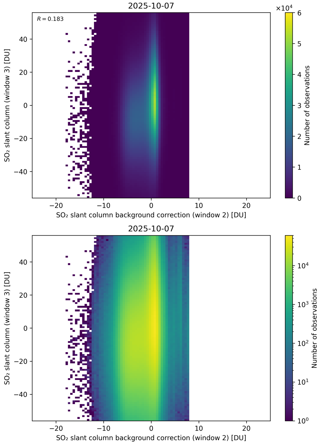
Figure 128: Scatter density plot of “SO 2 slant column background correction (window 2)” against “SO 2 slant column (window 3)” for 2025-10-06 to 2025-10-08.
