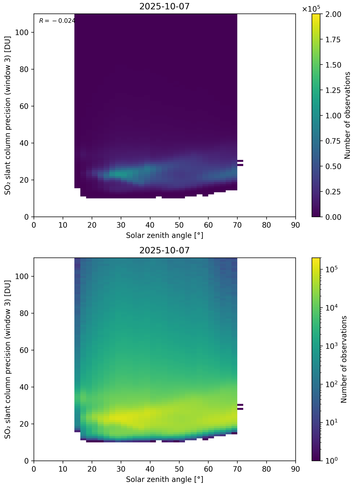
Figure 188: Scatter density plot of “Solar zenith angle” against “SO 2 slant column precision (window 3)” for 2025-10-06 to 2025-10-08.
