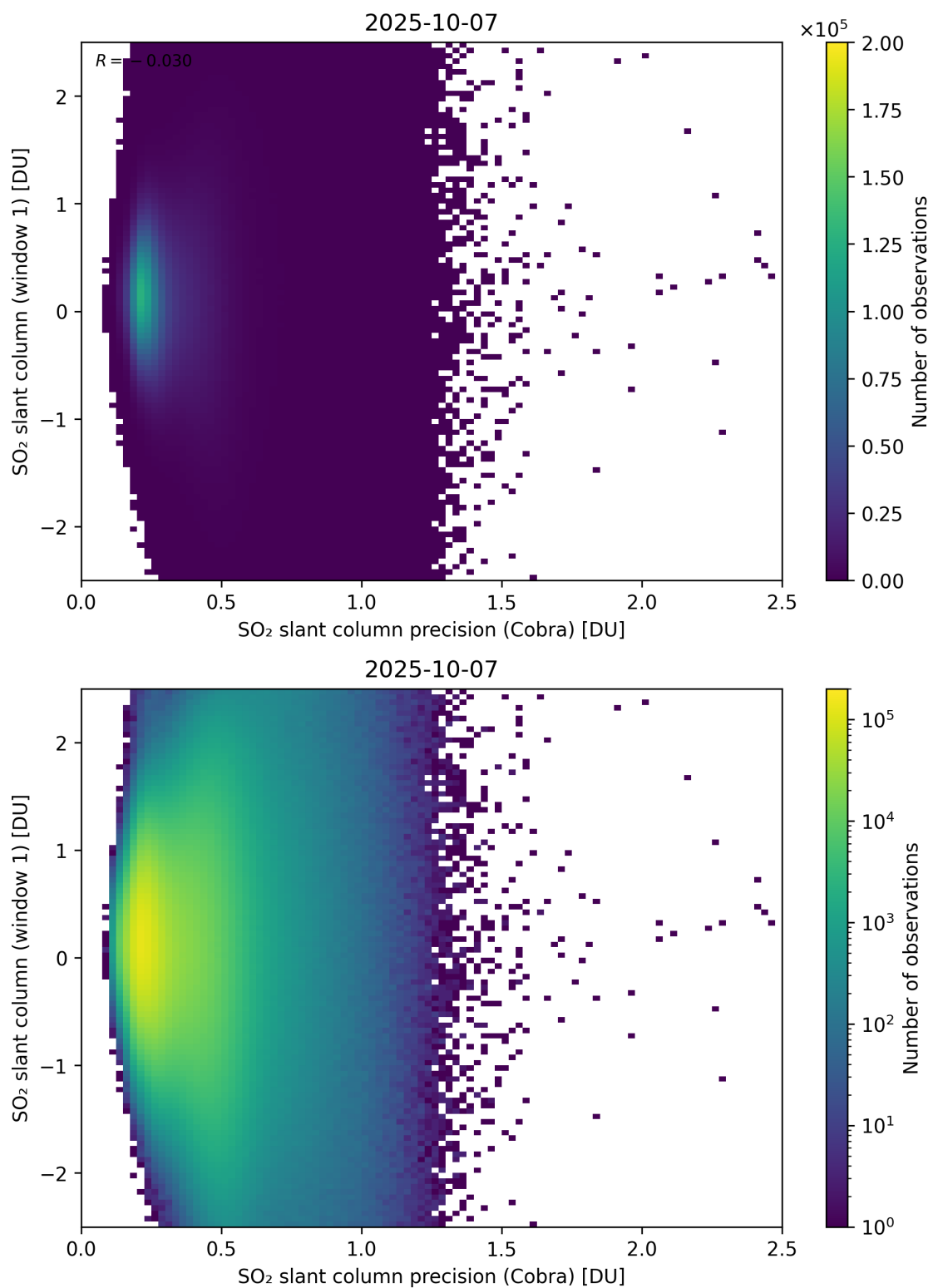
Figure 208: Scatter density plot of “SO 2 slant column precision (Cobra)” against “SO 2 slant column (window 1)” for 2025-10-06 to 2025-10-08.
