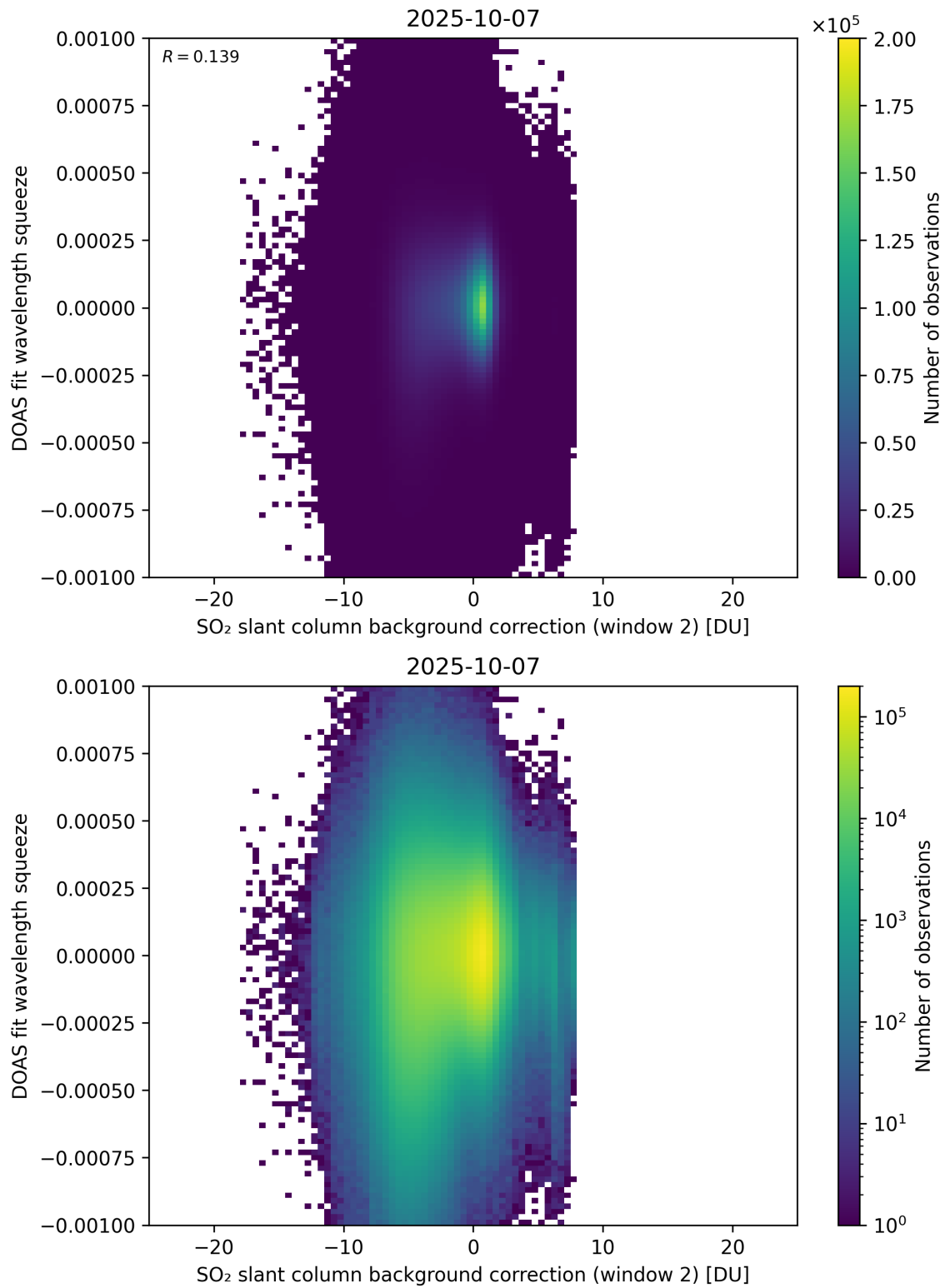
Figure 124: Scatter density plot of “SO 2 slant column background correction (window 2)” against “DOAS fit wavelength squeeze” for 2025-10-06 to 2025-10-08.
