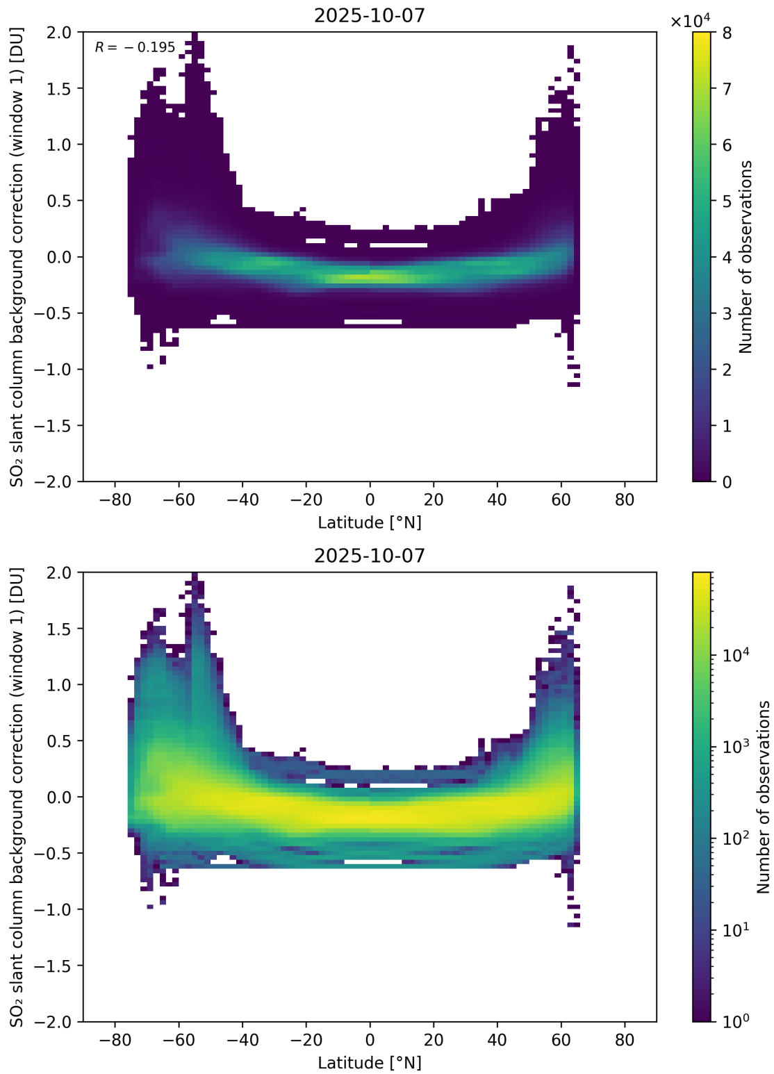
Figure 150: Scatter density plot of “Latitude” against “SO 2 slant column background correction (window 1)” for 2025-10-06 to 2025-10-08.
