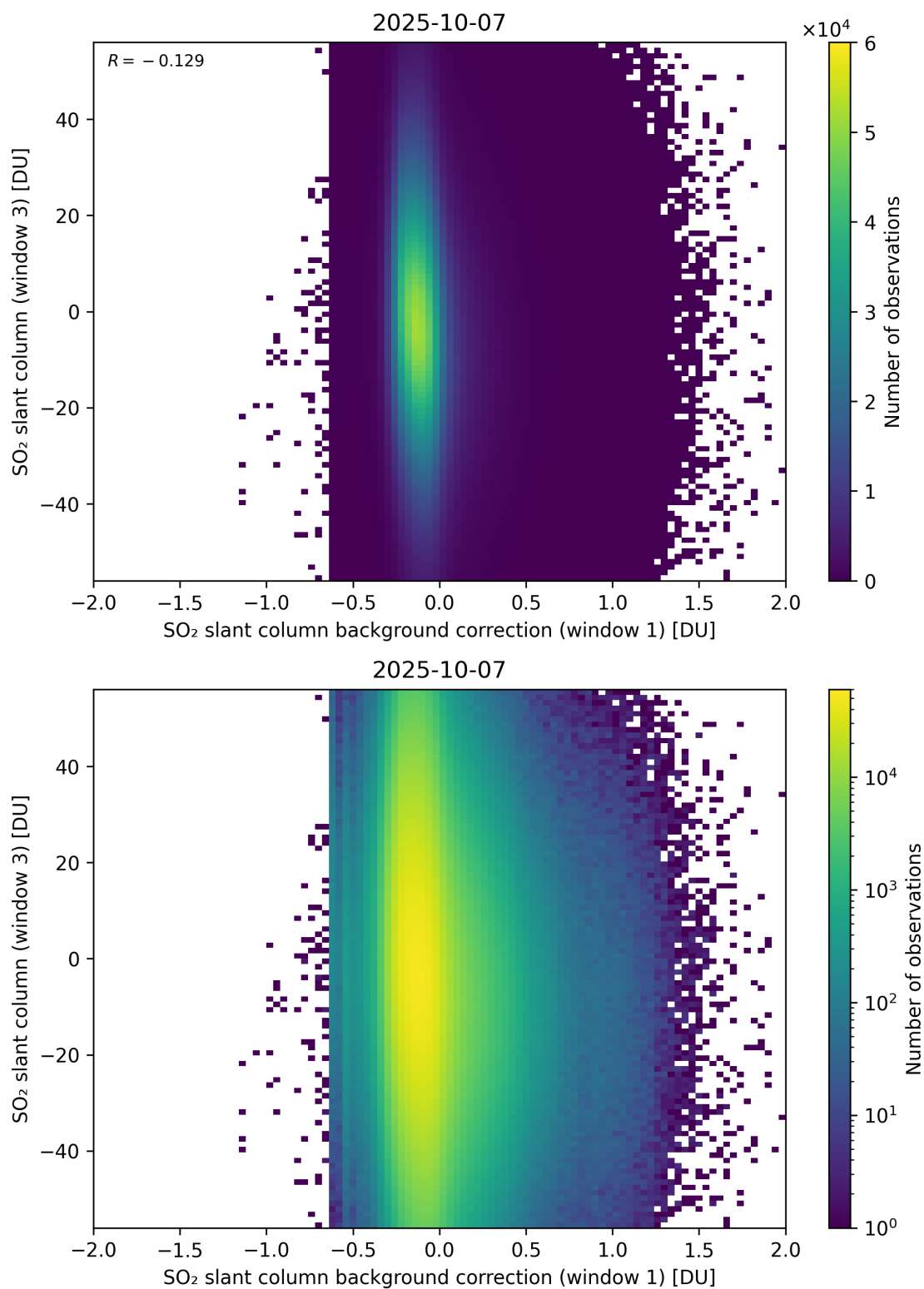
Figure 118: Scatter density plot of “SO 2 slant column background correction (window 1)” against “SO 2 slant column (window 3)” for 2025-10-06 to 2025-10-08.
