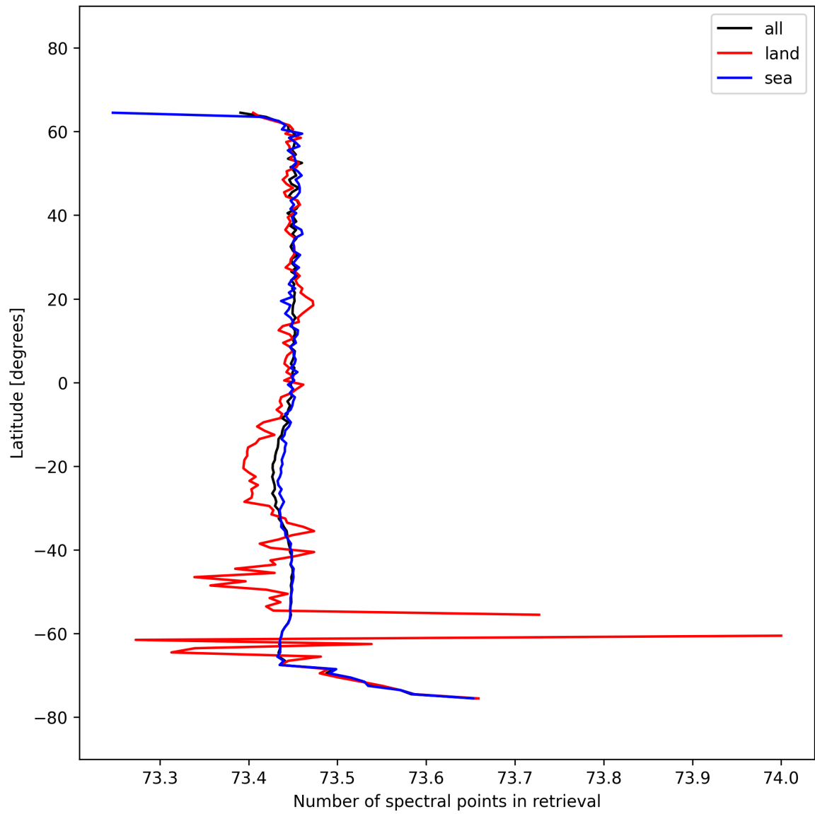
Figure 56: Zonal average of “Number of spectral points in retrieval” for 2025-10-06 to 2025-10-08.
