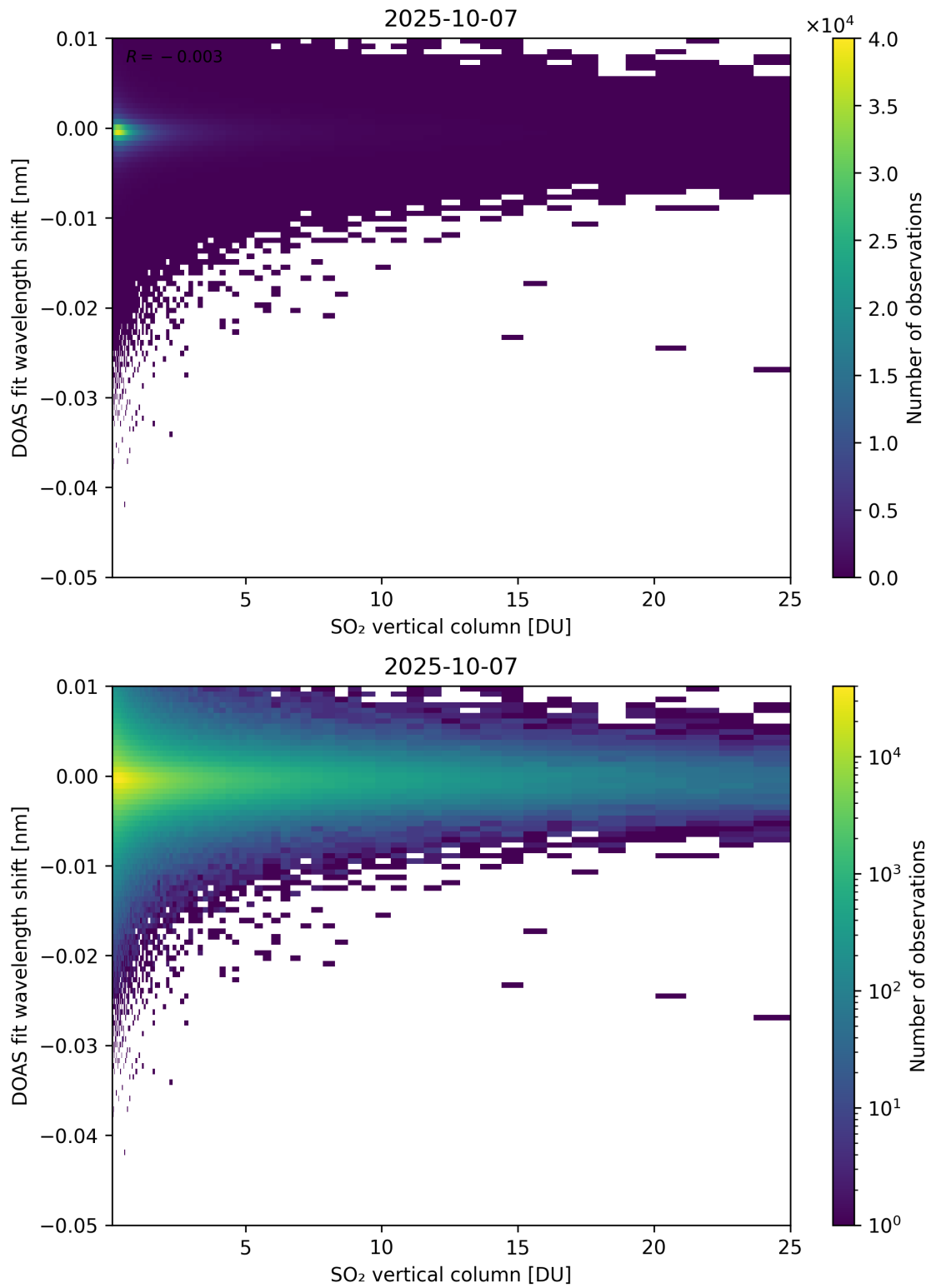
Figure 326: Scatter density plot of “SO 2 vertical column” against “DOAS fit wavelength shift” for 2025-10-06 to 2025-10-08.
