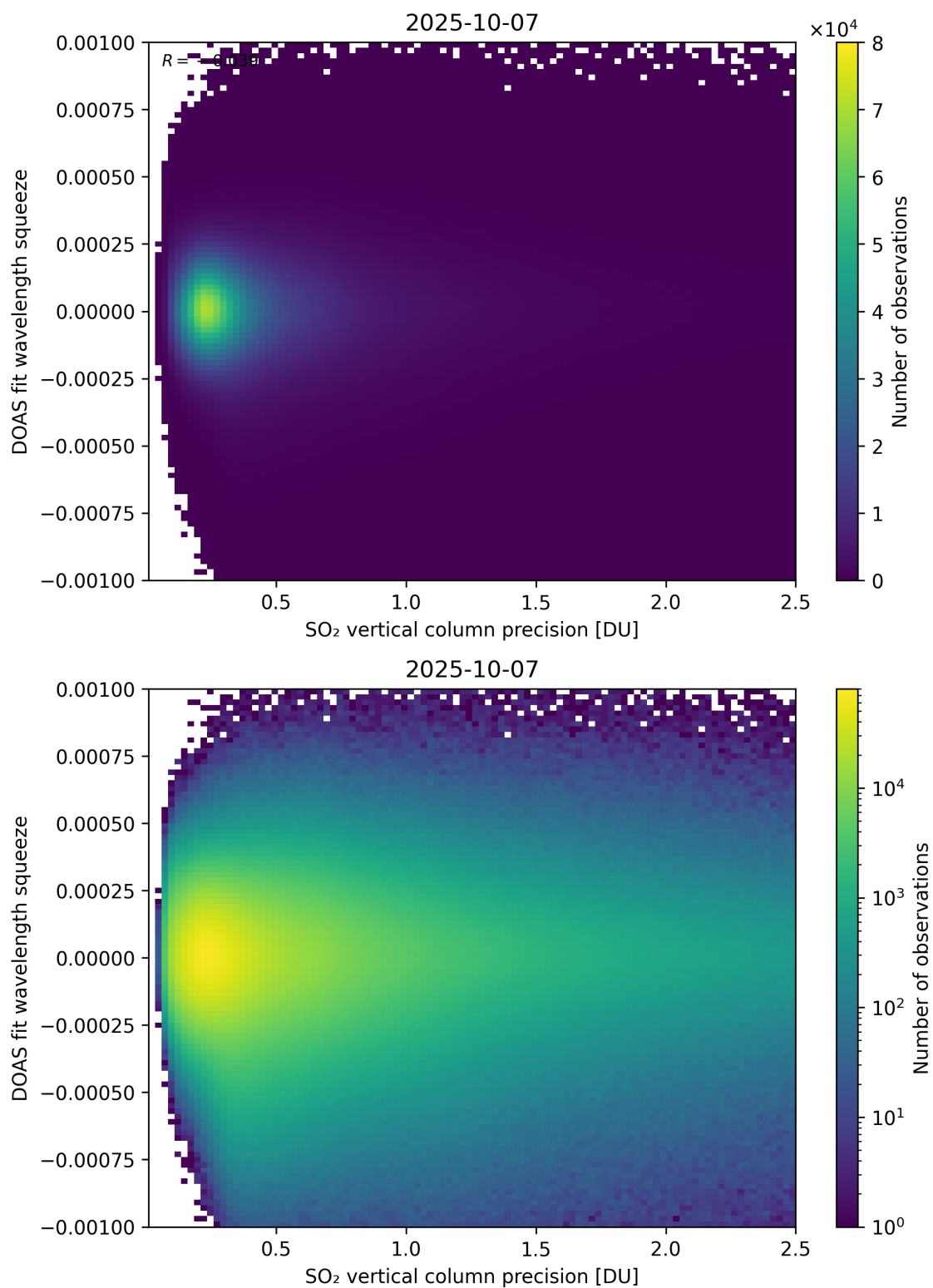
Figure 333: Scatter density plot of “SO 2 vertical column precision” against “DOAS fit wavelength squeeze” for 2025-10-06 to 2025-10-08.
