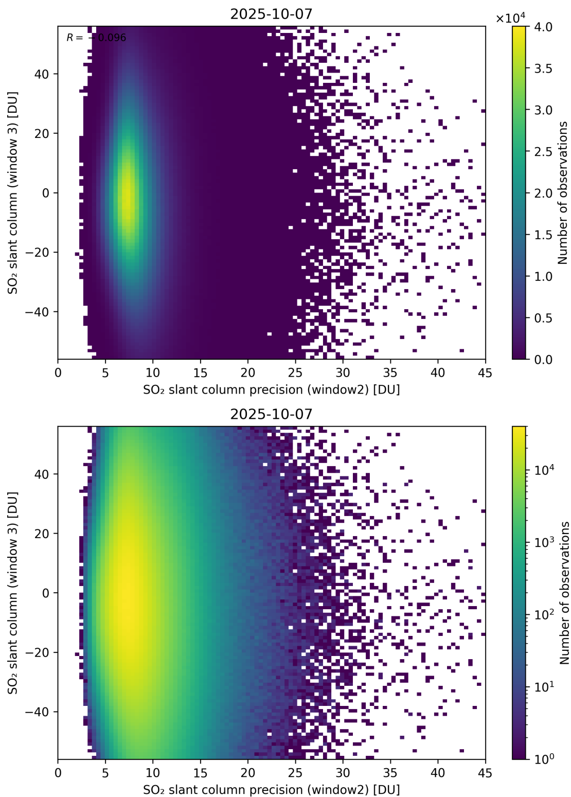
Figure 299: Scatter density plot of “SO 2 slant column precision (window2)” against “SO 2 slant column (window 3)” for 2025-10-06 to 2025-10-08.
