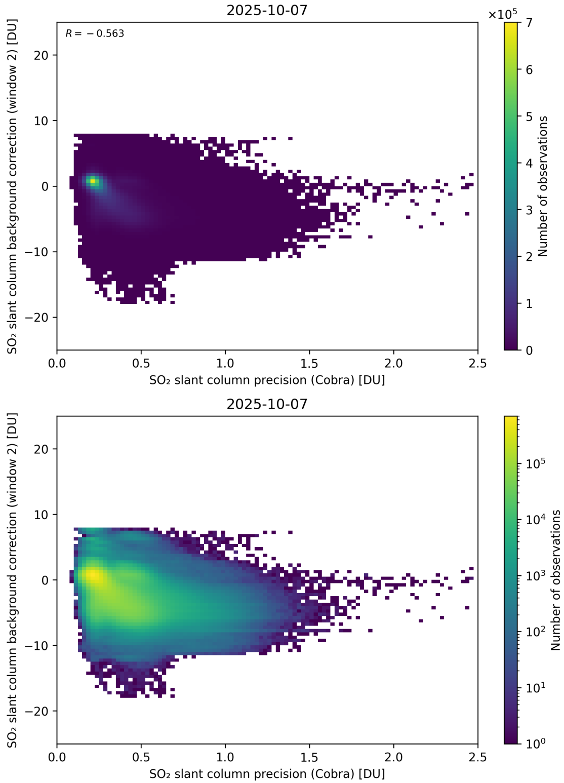
Figure 200: Scatter density plot of “SO 2 slant column precision (Cobra)” against “SO 2 slant column background correction (window 2)” for 2025-10-06 to 2025-10-08.
