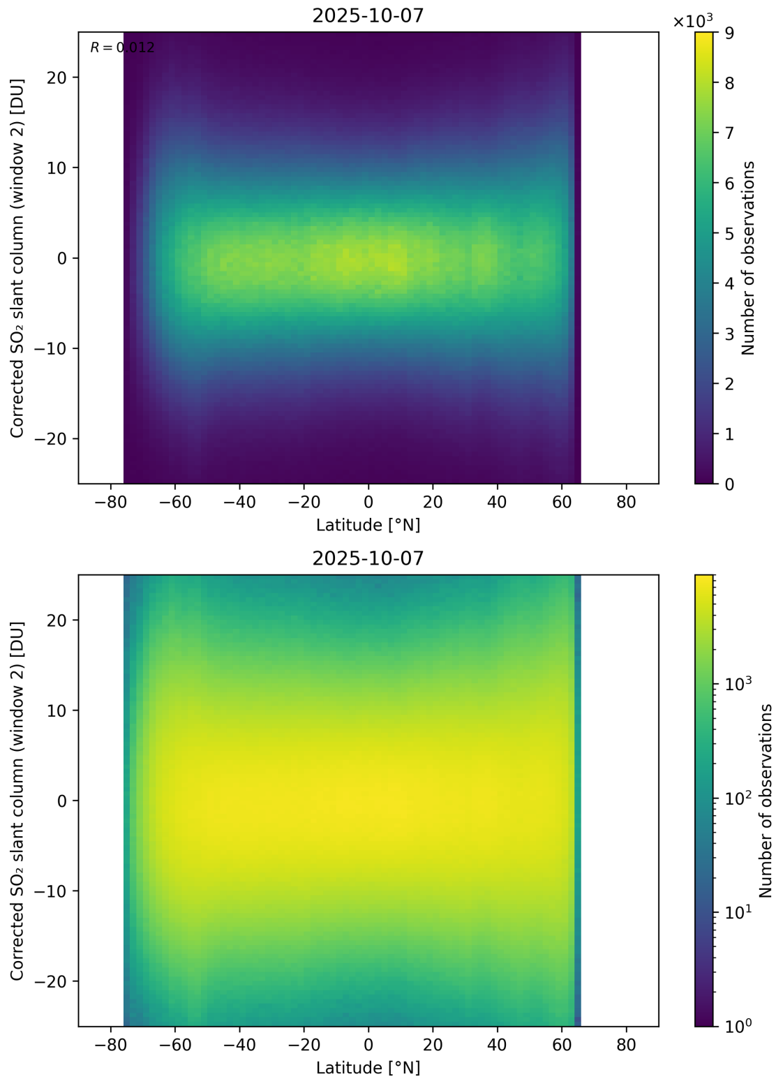
Figure 160: Scatter density plot of “Latitude” against “Corrected SO 2 slant column (window 2)” for 2025-10-06 to 2025-10-08.
