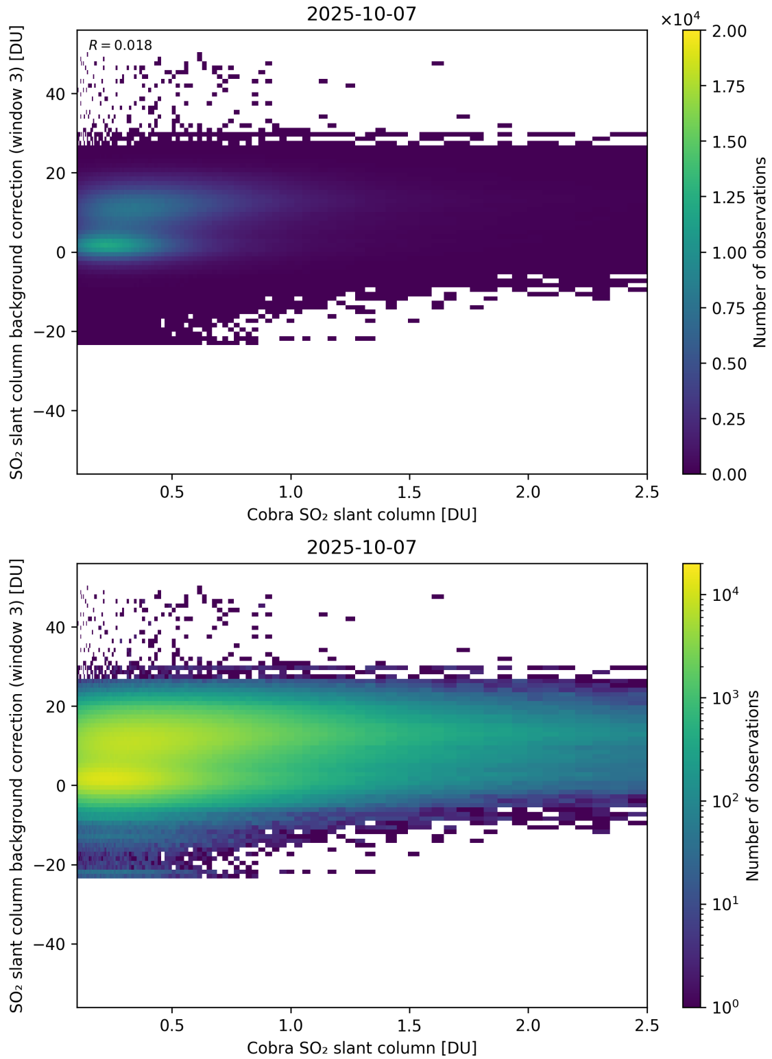
Figure 195: Scatter density plot of “Cobra SO 2 slant column” against “SO 2 slant column background correction (window 3)” for 2025-10-06 to 2025-10-08.
