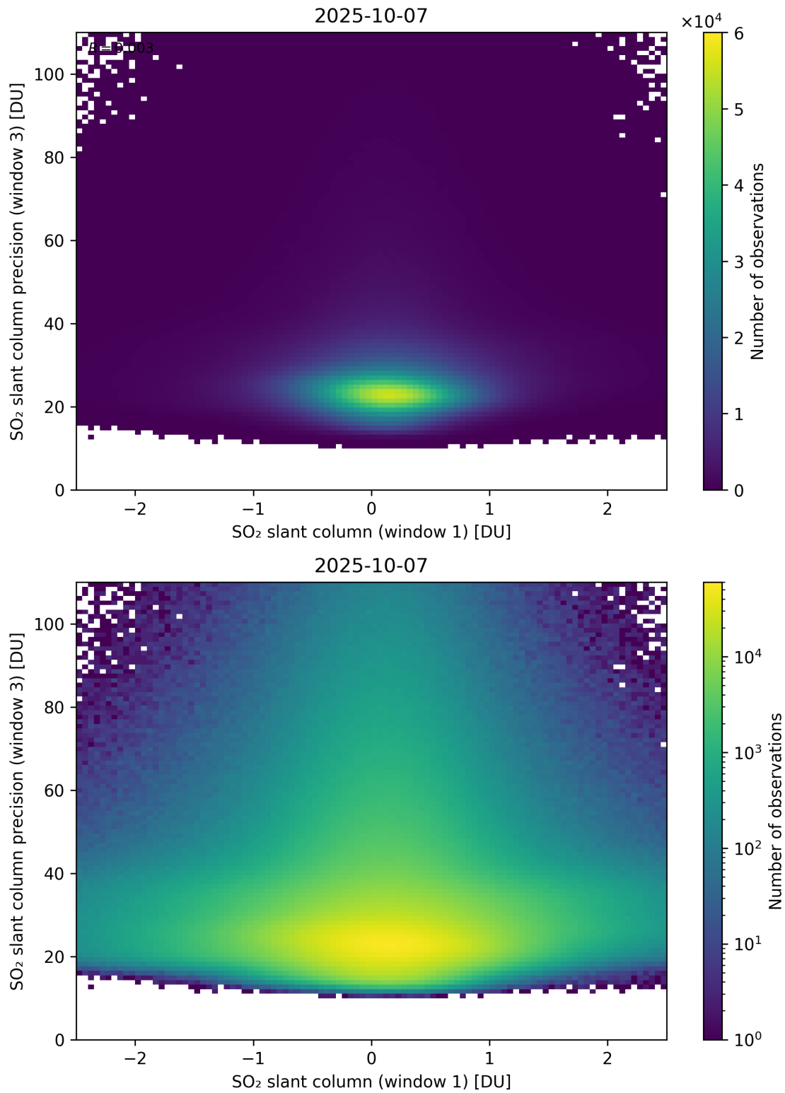
Figure 288: Scatter density plot of “SO 2 slant column (window 1)” against “SO 2 slant column precision (window 3)” for 2025-10-06 to 2025-10-08.
