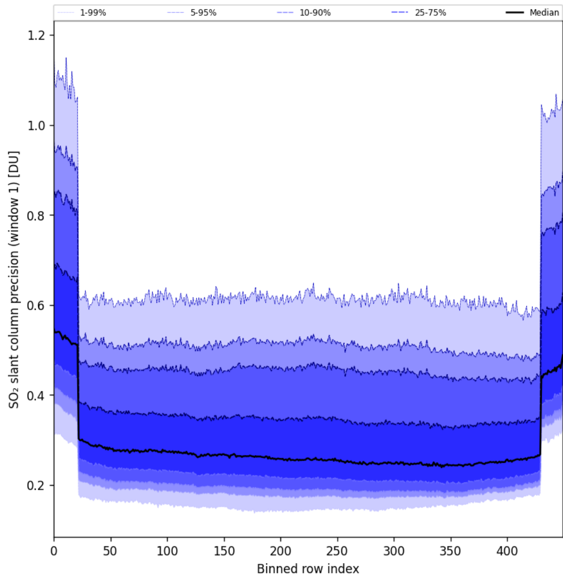
Figure 90: Along track statistics of “SO 2 slant column precision (window 1)” for 2025-10-06 to 2025-10-08
