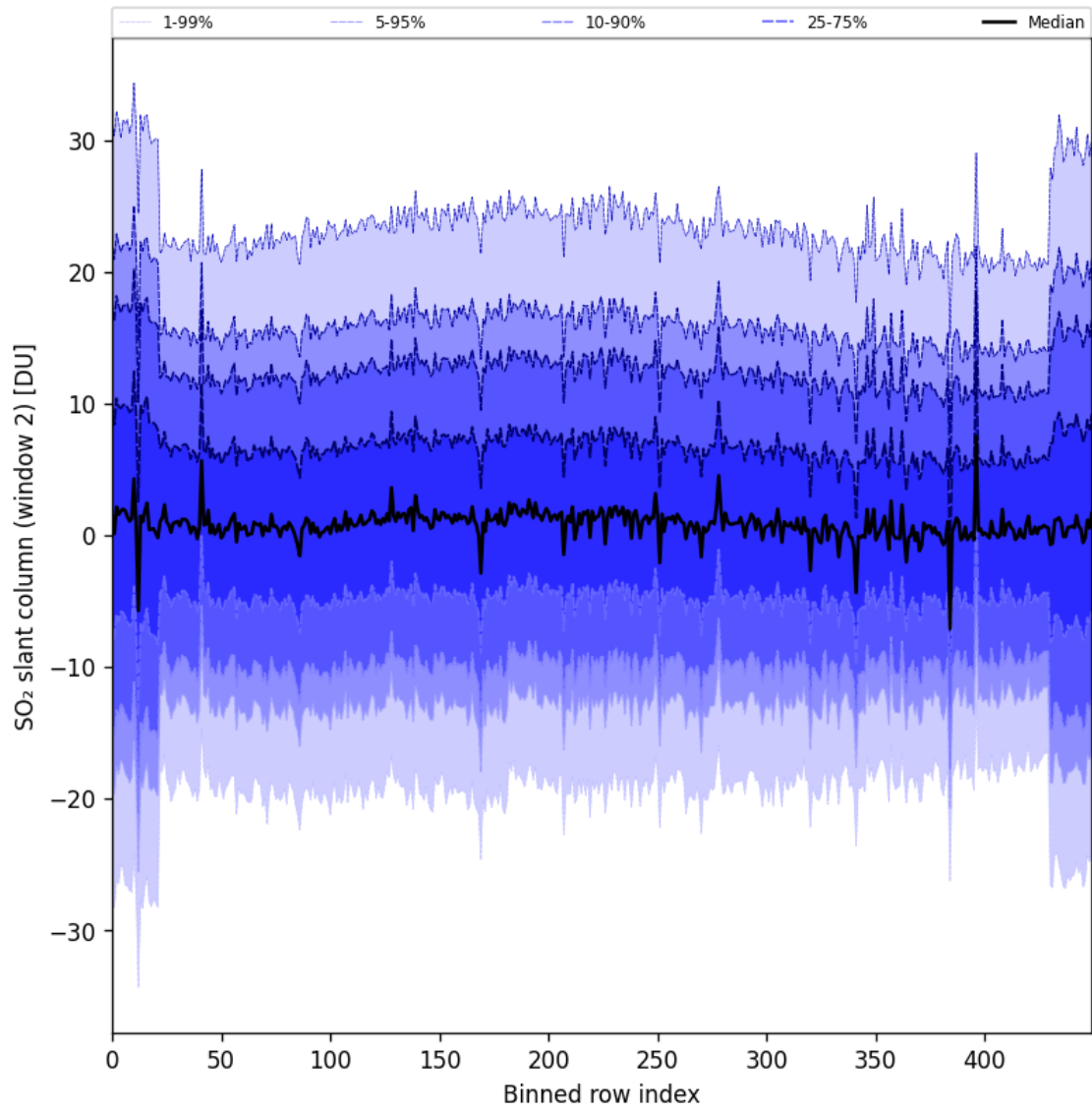
Figure 93: Along track statistics of “SO 2 slant column (window 2)” for 2025-10-06 to 2025-10-08
