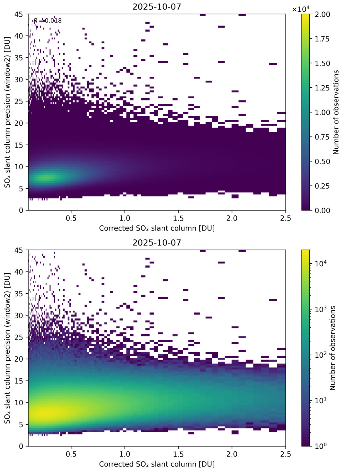
Figure 239: Scatter density plot of “Corrected SO 2 slant column” against “SO 2 slant column precision (window2)” for 2025-10-06 to 2025-10-08.
