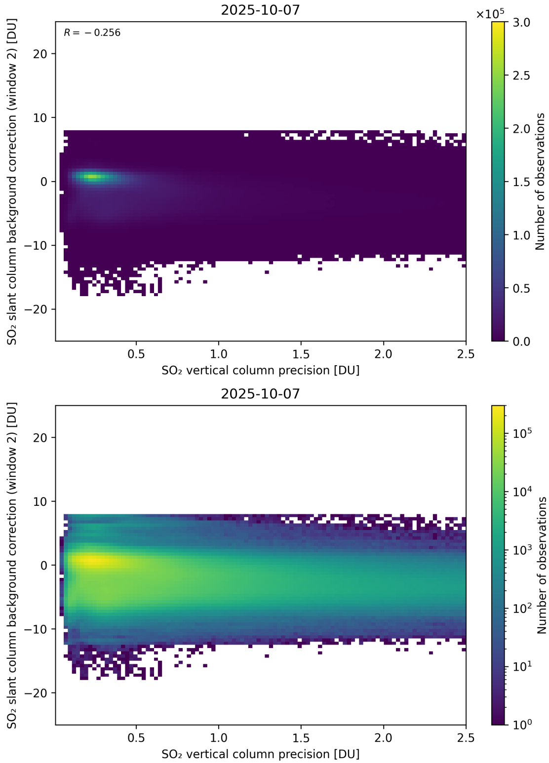
Figure 330: Scatter density plot of “SO 2 vertical column precision” against “SO 2 slant column background correction (window 2)” for 2025-10-06 to 2025-10-08.
