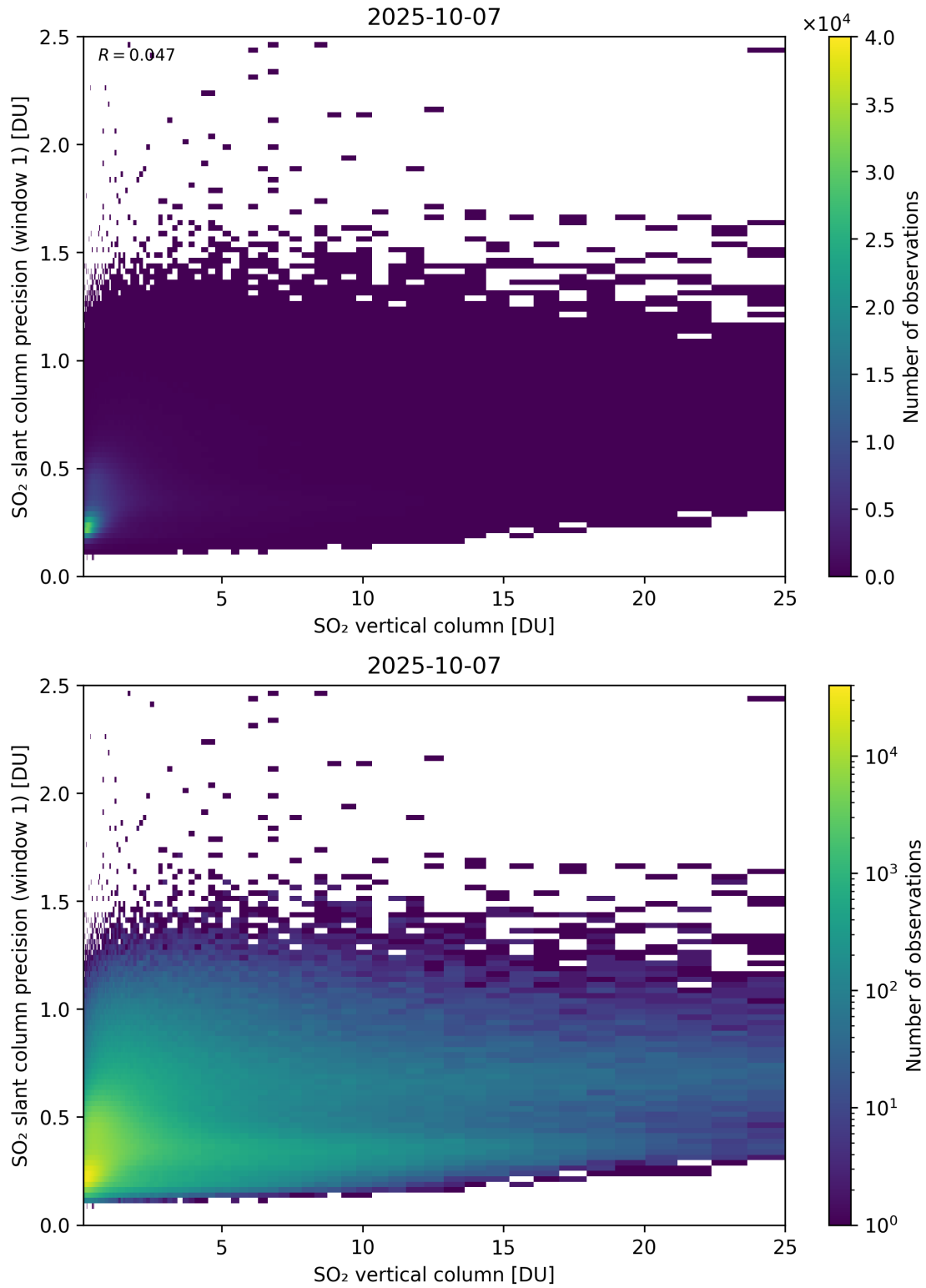
Figure 355: Scatter density plot of “SO 2 vertical column” against “SO 2 slant column precision (window 1)” for 2025-10-06 to 2025-10-08.
