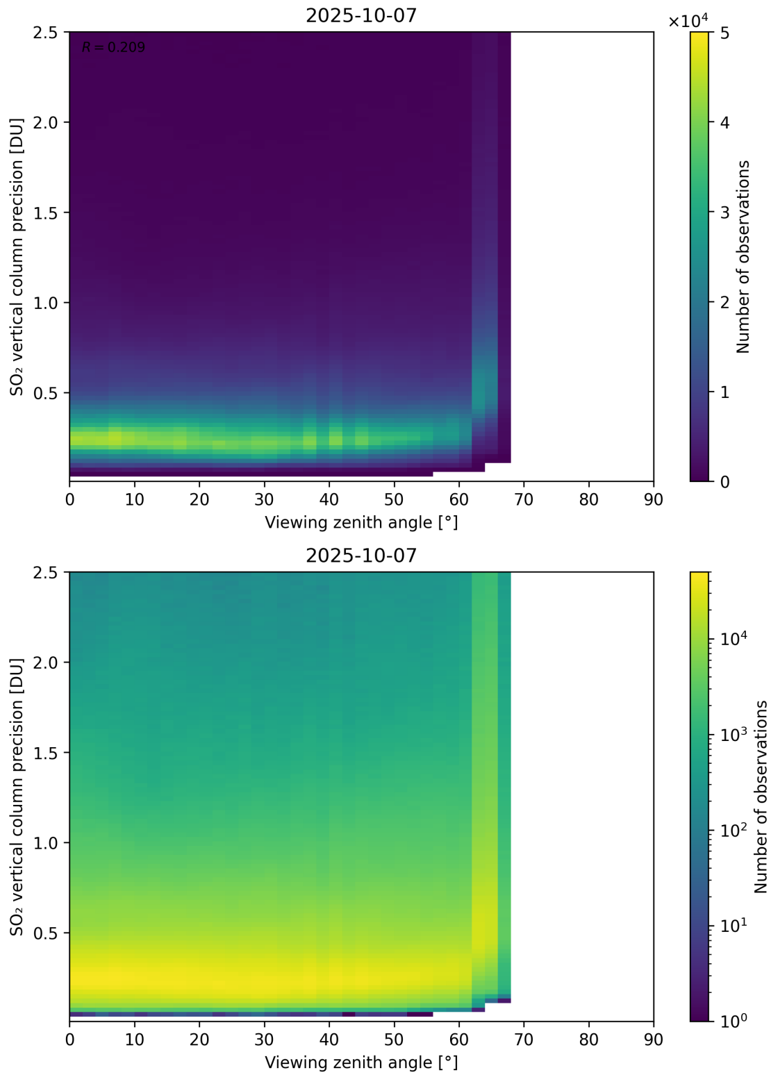
Figure 384: Scatter density plot of “Viewing zenith angle” against “SO 2 vertical column precision” for 2025-10-06 to 2025-10-08.
