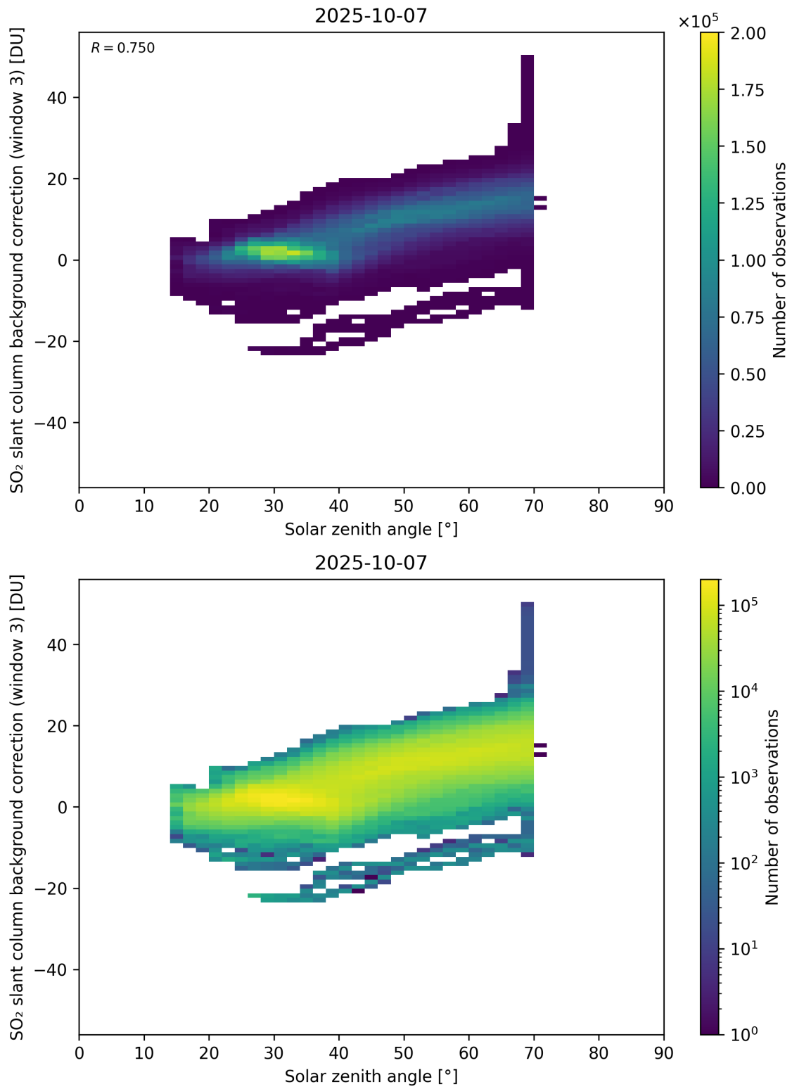
Figure 173: Scatter density plot of “Solar zenith angle” against “SO 2 slant column background correction (window 3)” for 2025-10-06 to 2025-10-08.
