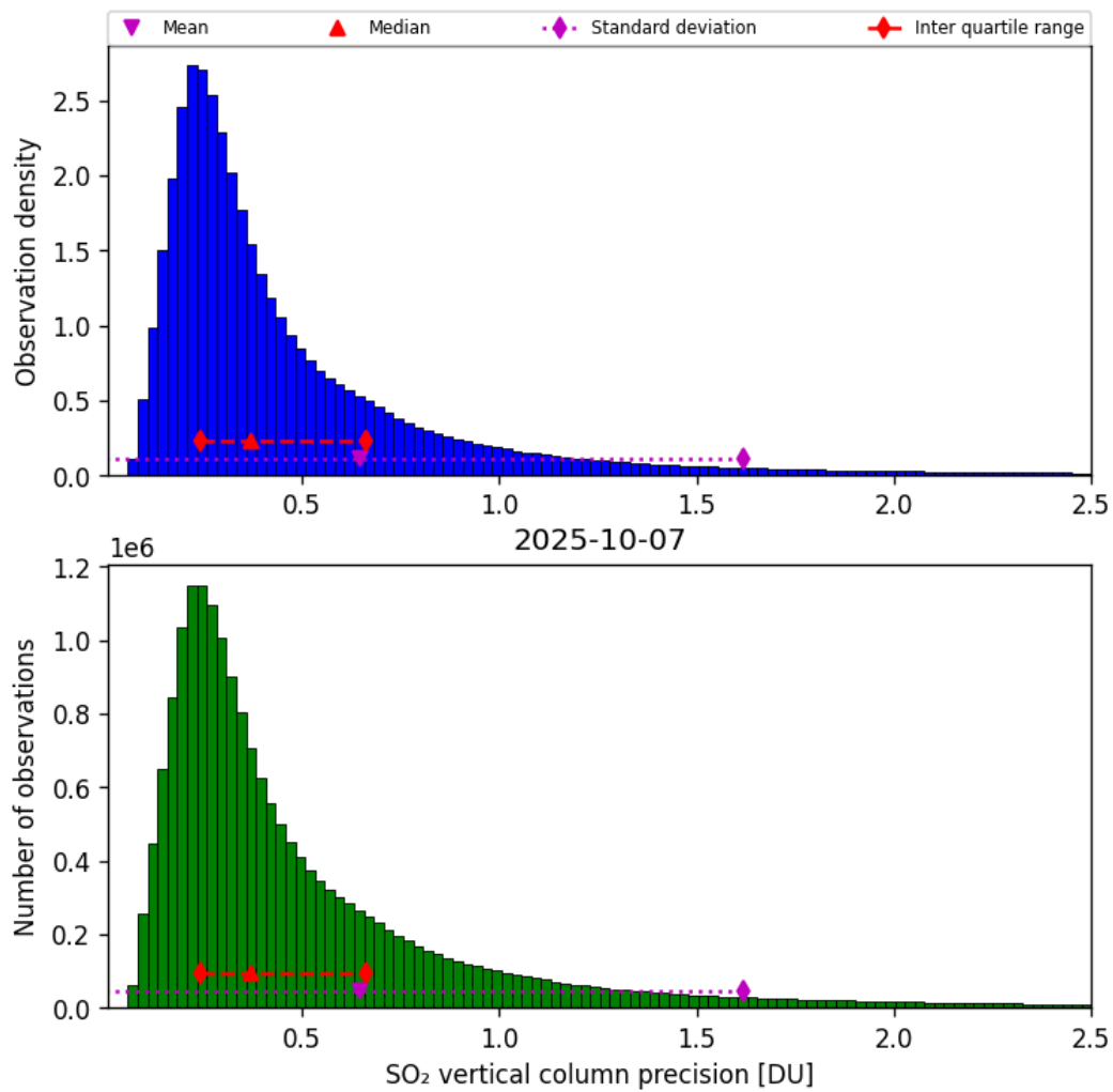
Figure 59: Histogram of “SO 2 vertical column precision” for 2025-10-06 to 2025-10-08
