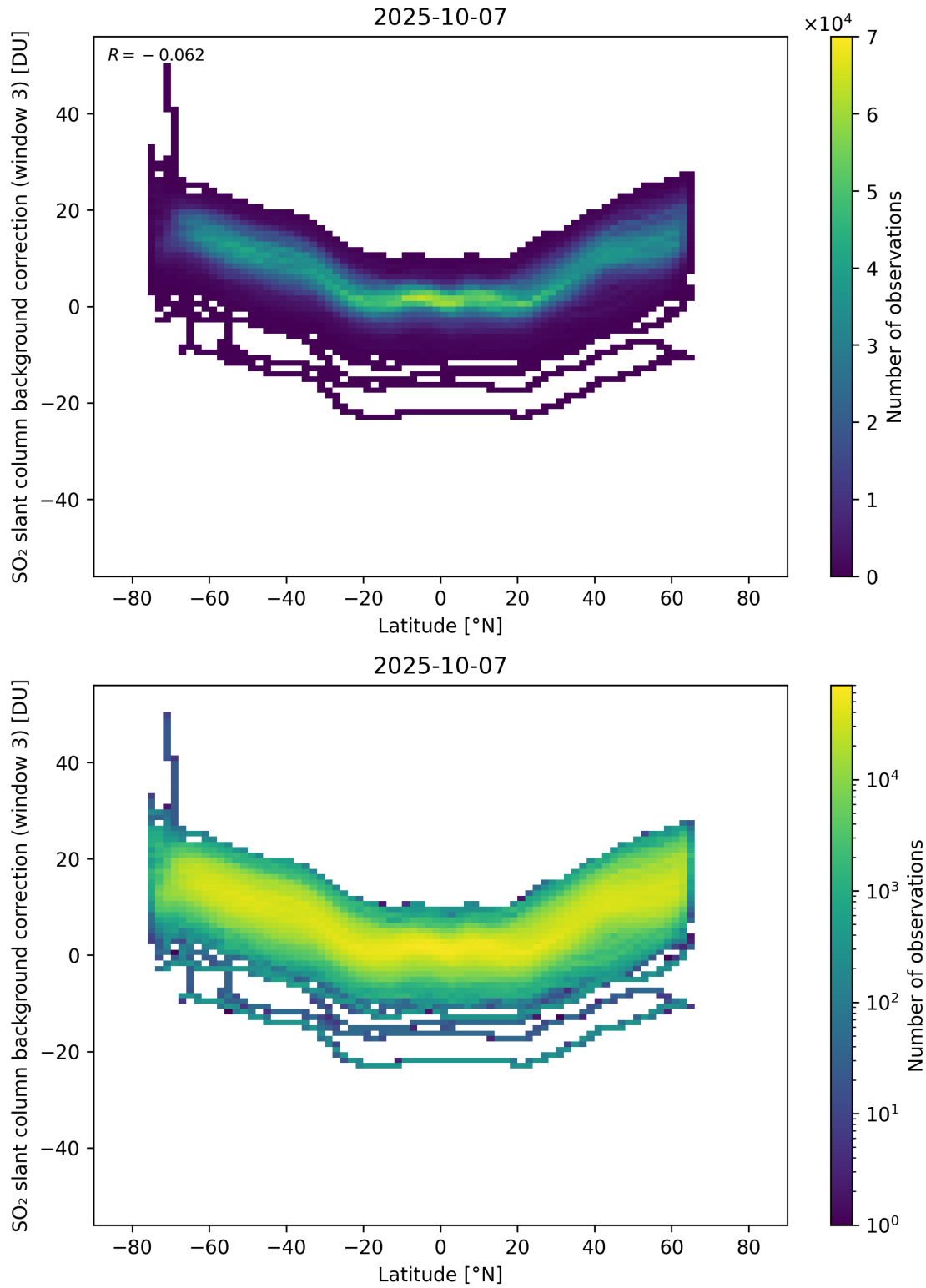
Figure 152: Scatter density plot of “Latitude” against “SO 2 slant column background correction (window 3)” for 2025-10-06 to 2025-10-08.
