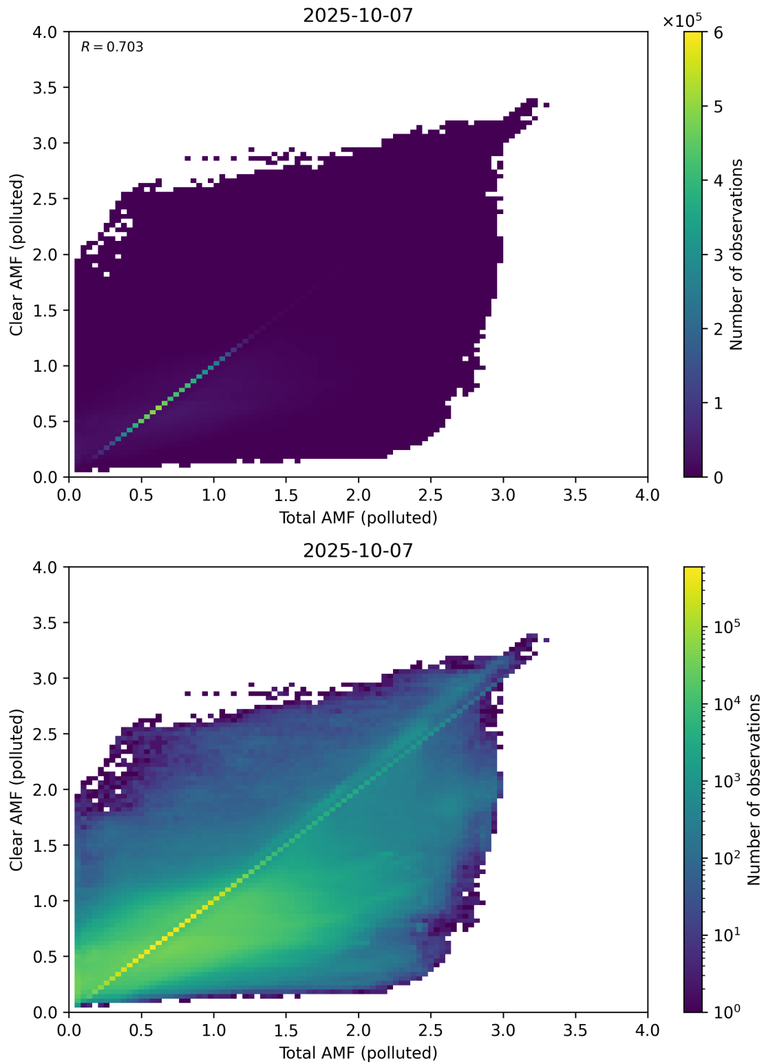
Figure 321: Scatter density plot of “Total AMF (polluted)” against “Clear AMF (polluted)” for 2025-10-06 to 2025-10-08.
