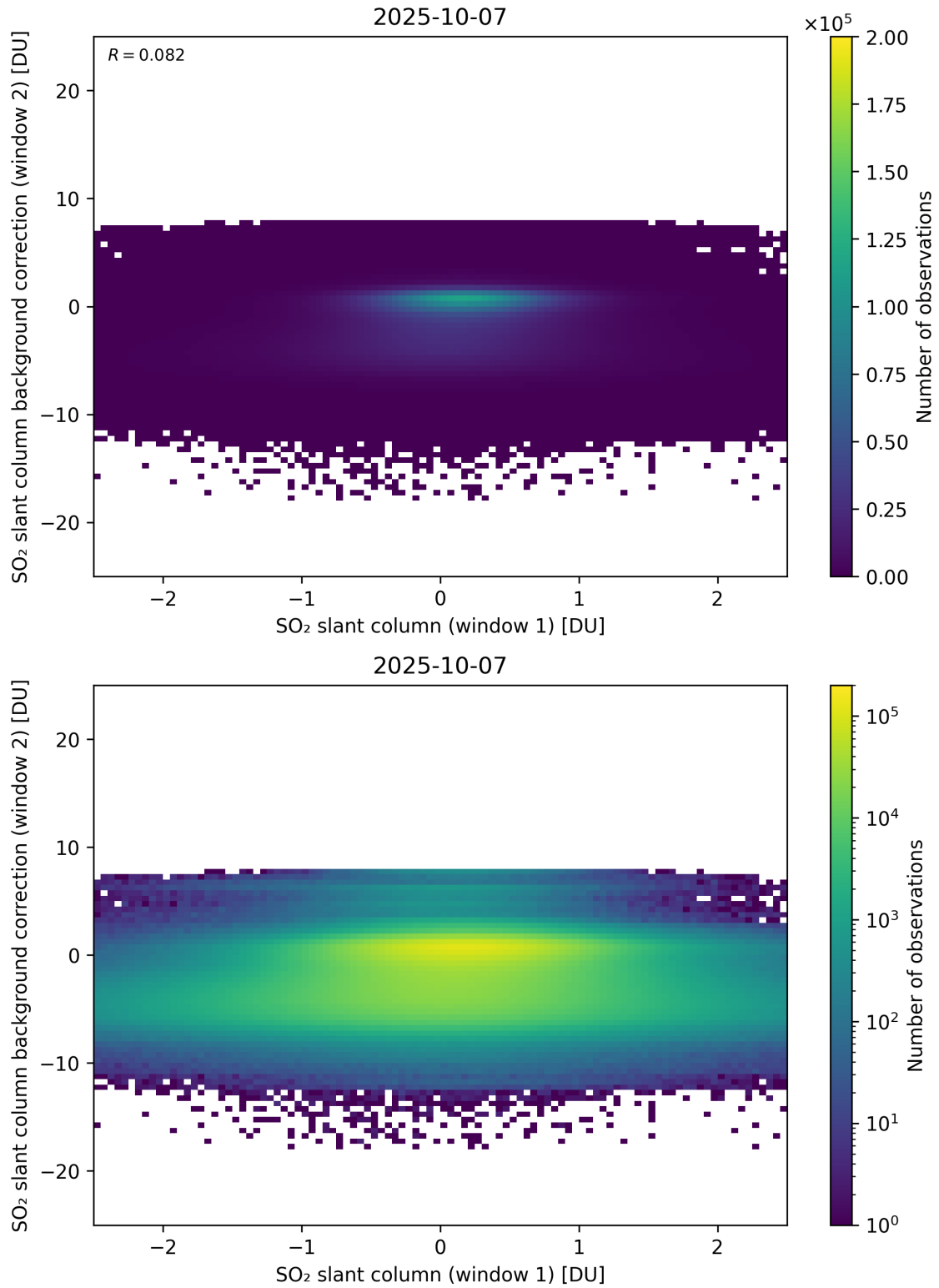
Figure 263: Scatter density plot of “SO 2 slant column (window 1)” against “SO 2 slant column background correction (window 2)” for 2025-10-06 to 2025-10-08.
