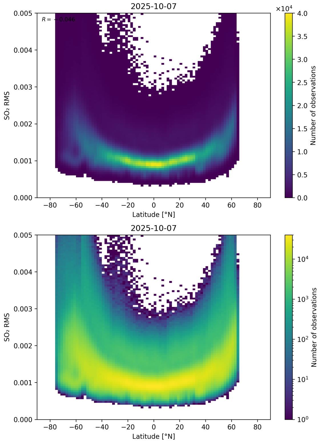
Figure 155: Scatter density plot of “Latitude” against “SO 2 RMS” for 2025-10-06 to 2025-10-08.
