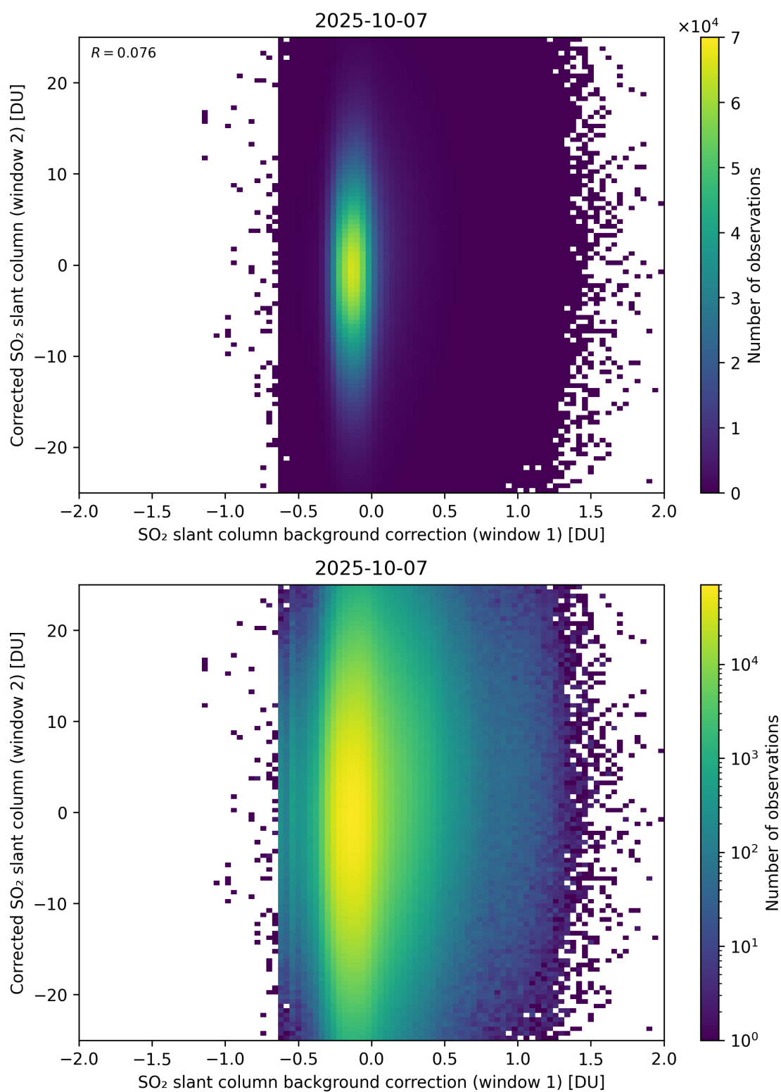
Figure 115: Scatter density plot of “SO 2 slant column background correction (window 1)” against “Corrected SO 2 slant column (window 2)” for 2025-10-06 to 2025-10-08.
