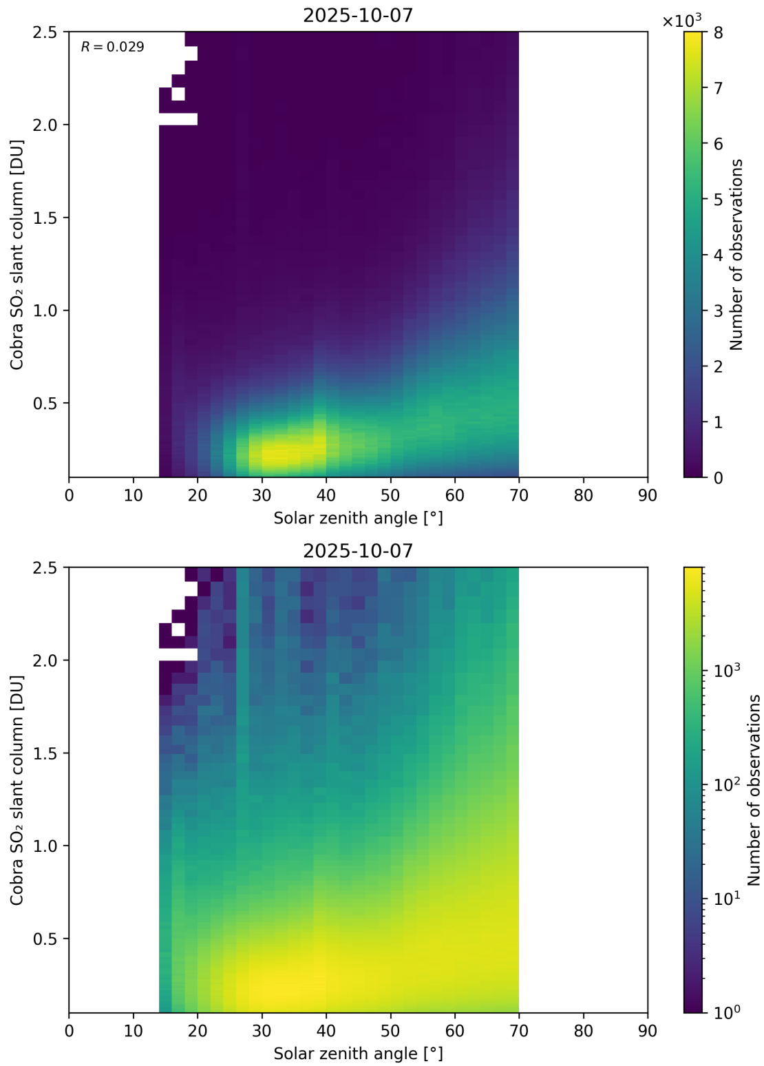
Figure 179: Scatter density plot of “Solar zenith angle” against “Cobra SO 2 slant column” for 2025-10-06 to 2025-10-08.
