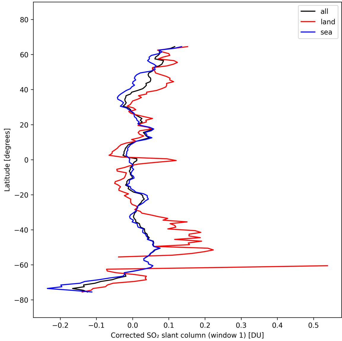
Figure 39: Zonal average of “Corrected SO 2 slant column (window 1)” for 2025-10-06 to 2025-10-08.
