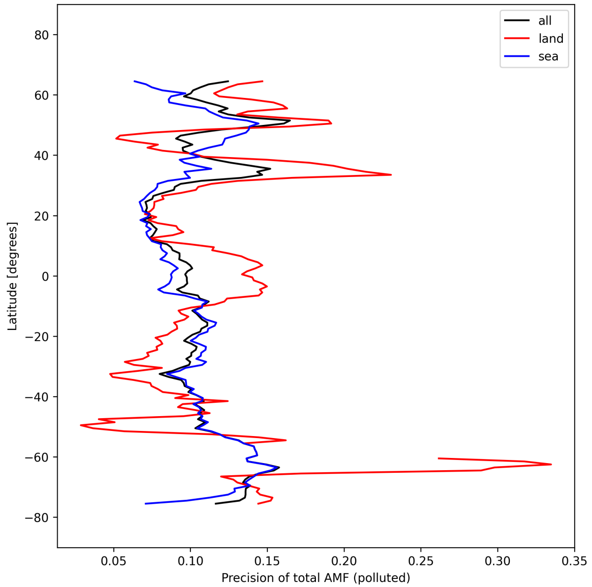
Figure 54: Zonal average of “Precision of total AMF (polluted)” for 2025-10-06 to 2025-10-08.
