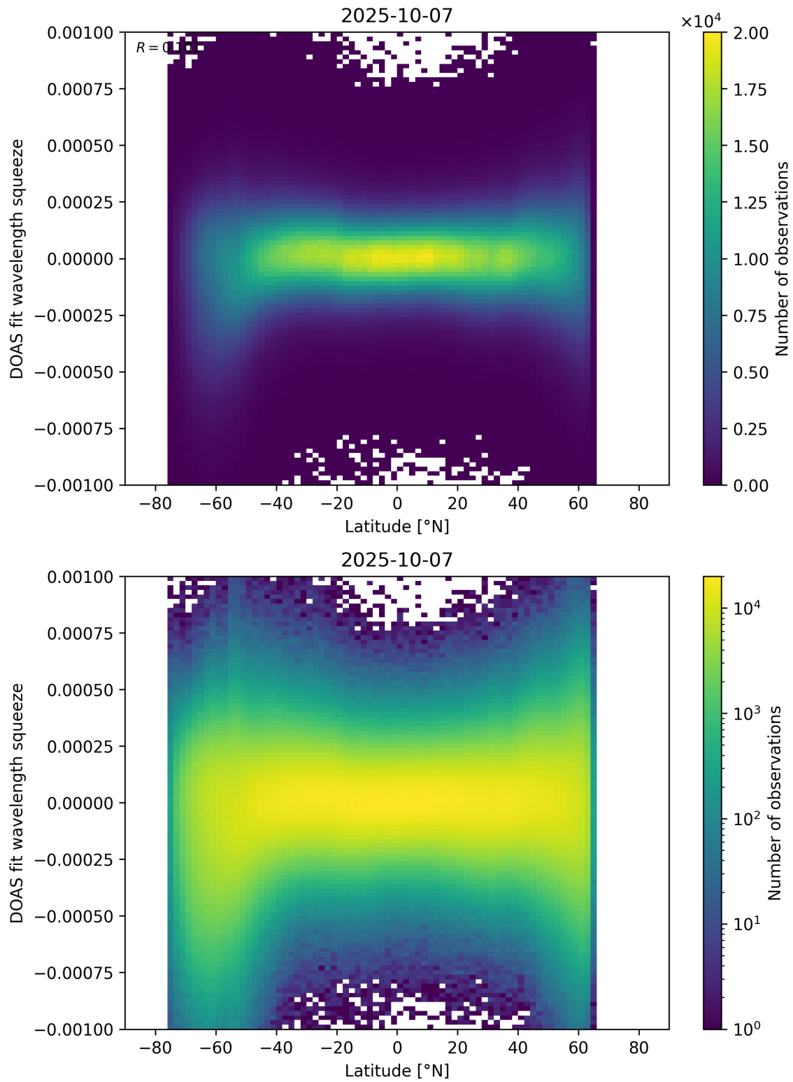
Figure 154: Scatter density plot of “Latitude” against “DOAS fit wavelength squeeze” for 2025-10-06 to 2025-10-08.
