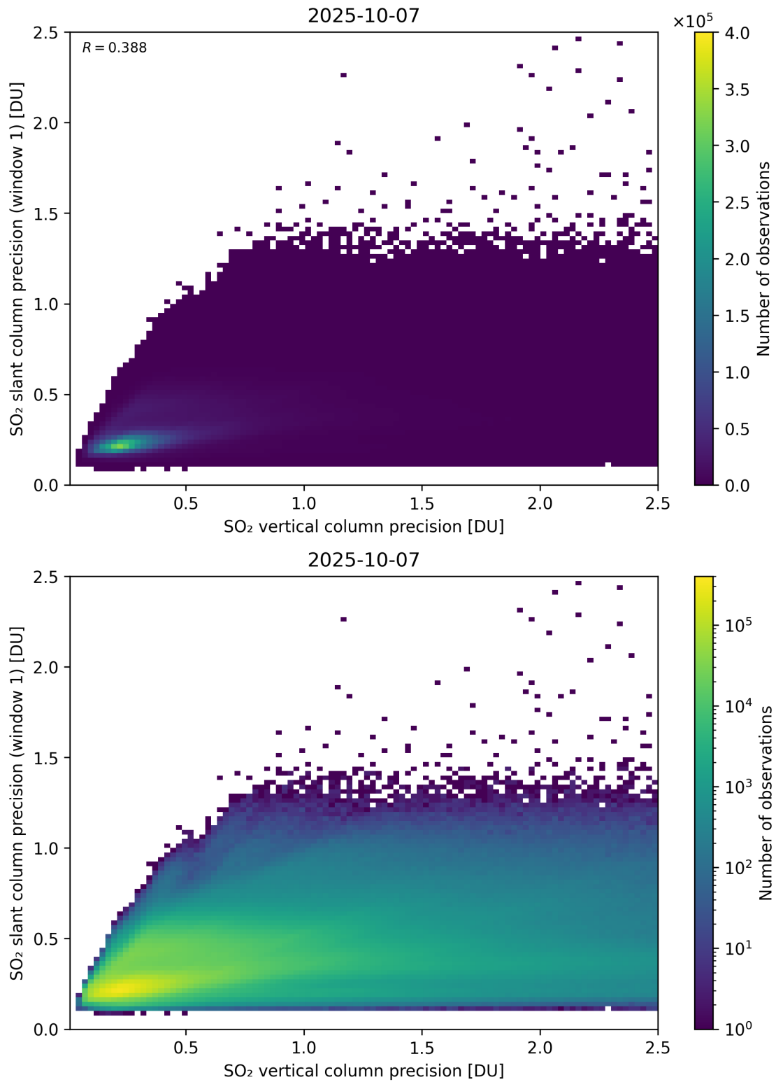
Figure 342: Scatter density plot of “SO 2 vertical column precision” against “SO 2 slant column precision (window 1)” for 2025-10-06 to 2025-10-08.
