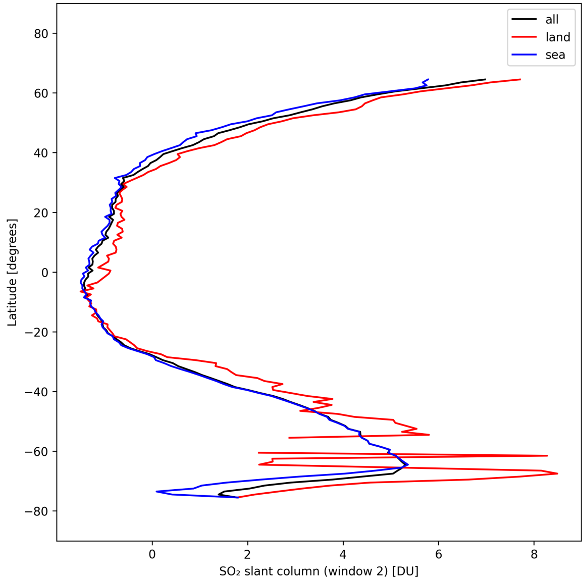
Figure 41: Zonal average of “SO 2 slant column (window 2)” for 2025-10-06 to 2025-10-08.
