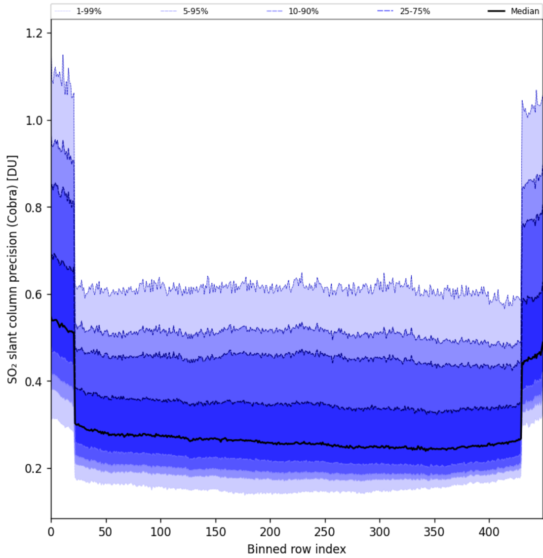
Figure 88: Along track statistics of “SO 2 slant column precision (Cobra)” for 2025-10-06 to 2025-10-08
