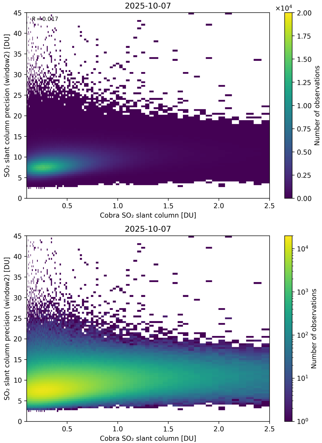
Figure 221: Scatter density plot of “Cobra SO 2 slant column” against “SO 2 slant column precision (window2)” for 2025-10-06 to 2025-10-08.
