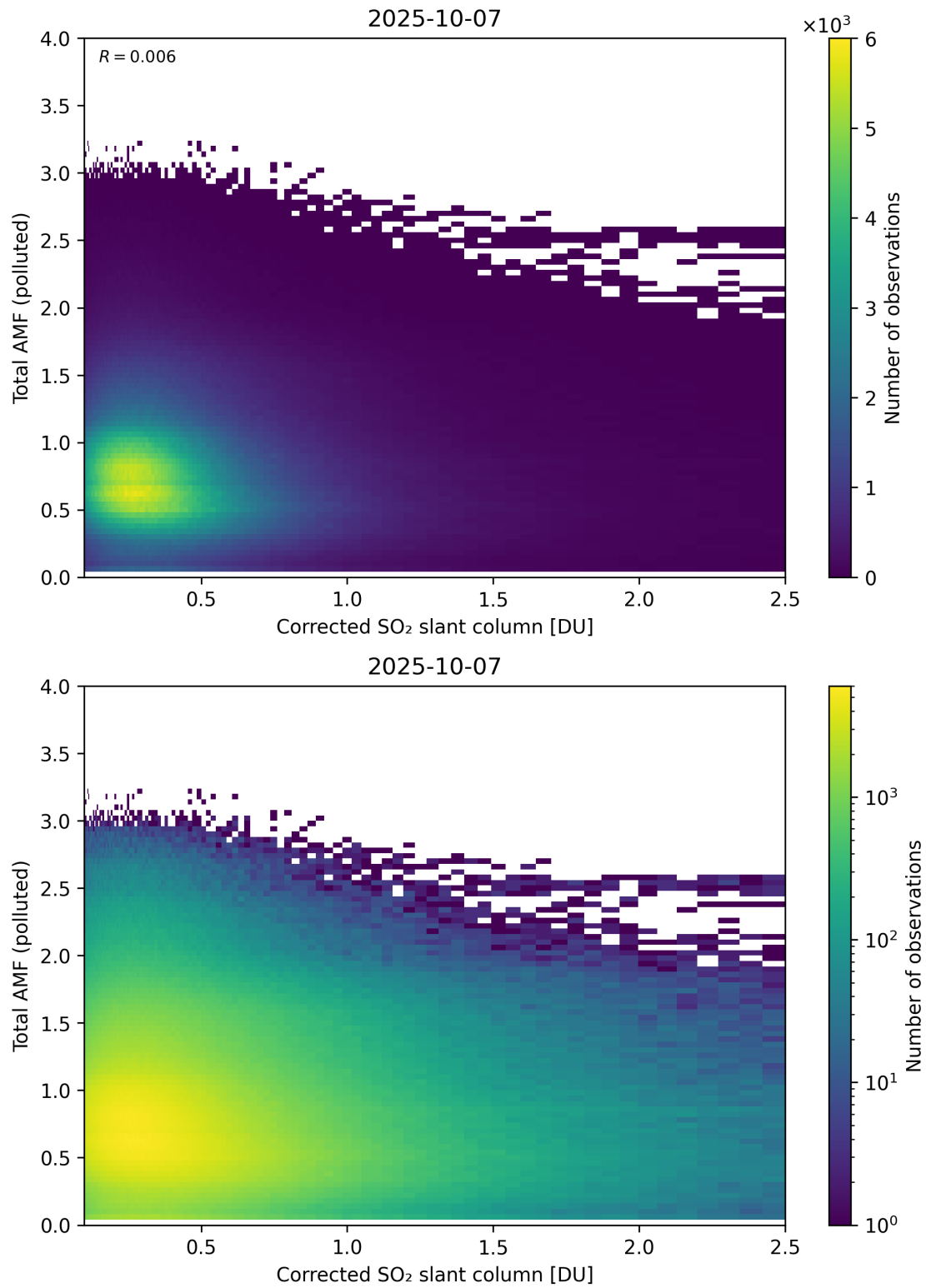
Figure 242: Scatter density plot of “Corrected SO 2 slant column” against “Total AMF (polluted)” for 2025-10-06 to 2025-10-08.
