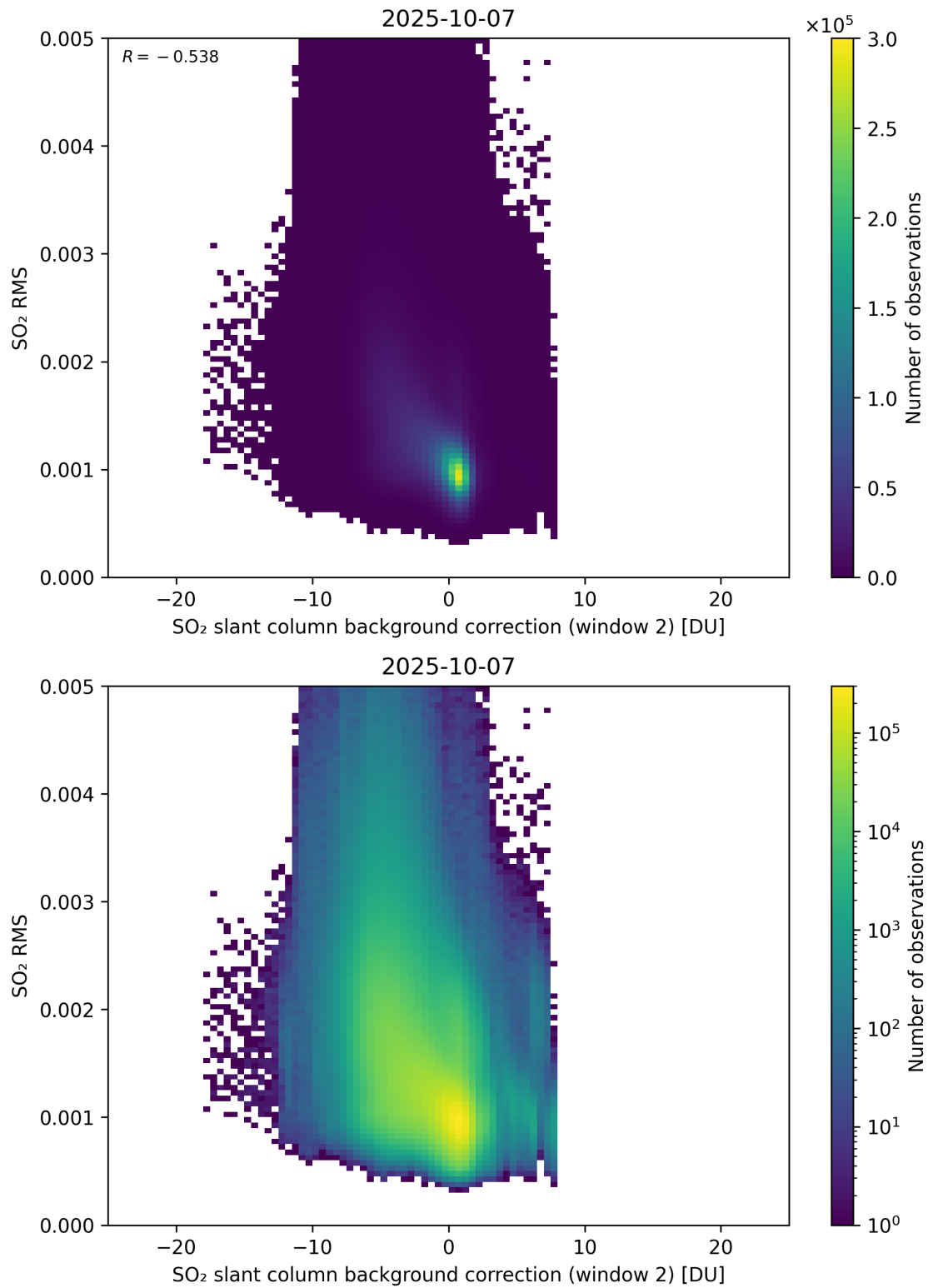
Figure 125: Scatter density plot of “SO 2 slant column background correction (window 2)” against “SO 2 RMS” for 2025-10-06 to 2025-10-08.
