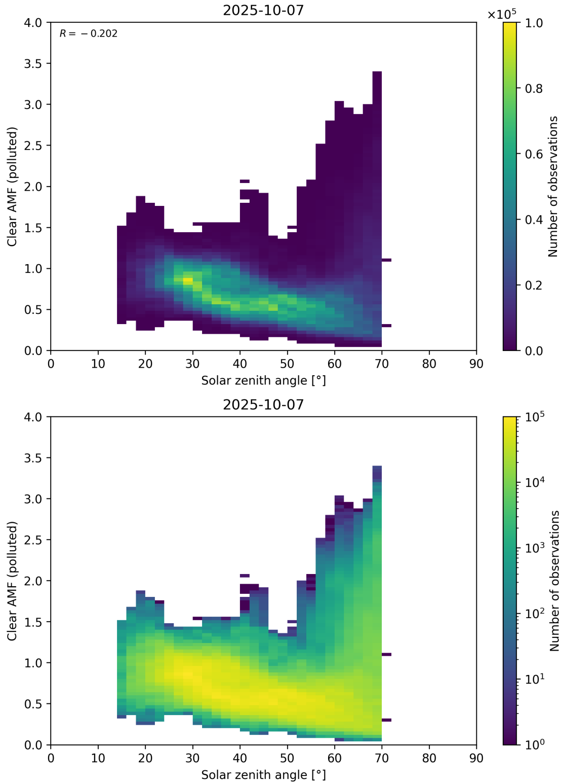
Figure 178: Scatter density plot of “Solar zenith angle” against “Clear AMF (polluted)” for 2025-10-06 to 2025-10-08.
