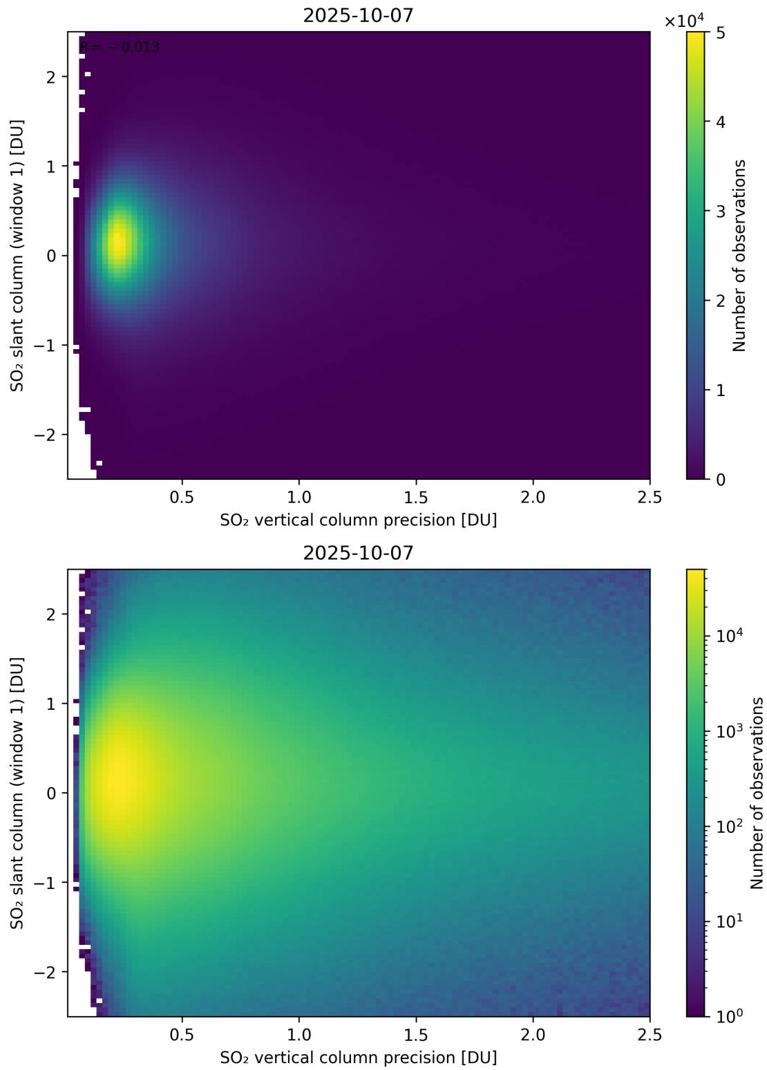
Figure 341: Scatter density plot of “SO 2 vertical column precision” against “SO 2 slant column (window 1)” for 2025-10-06 to 2025-10-08.
