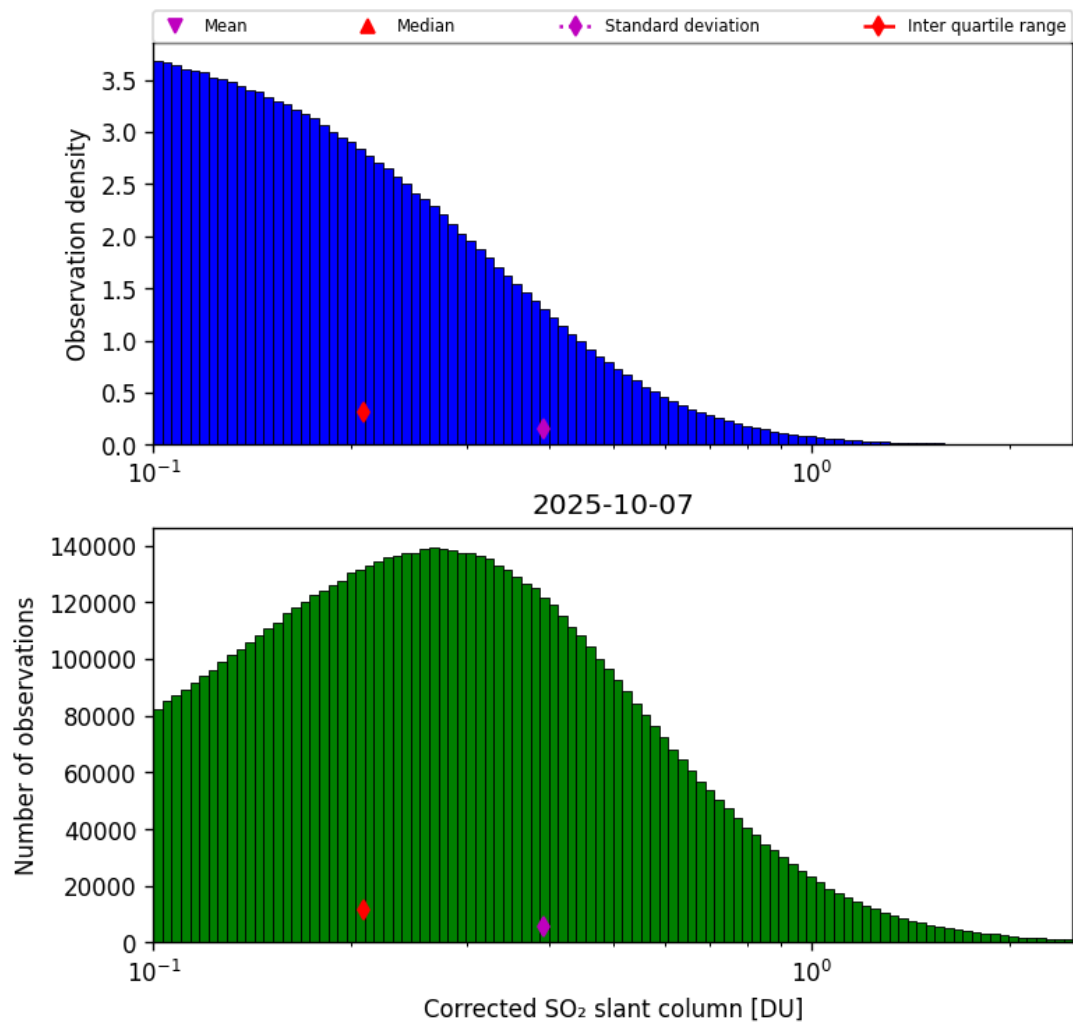
Figure 60: Histogram of "Corrected SO 2 slant column" for 2025-10-06 to 2025-10-08
