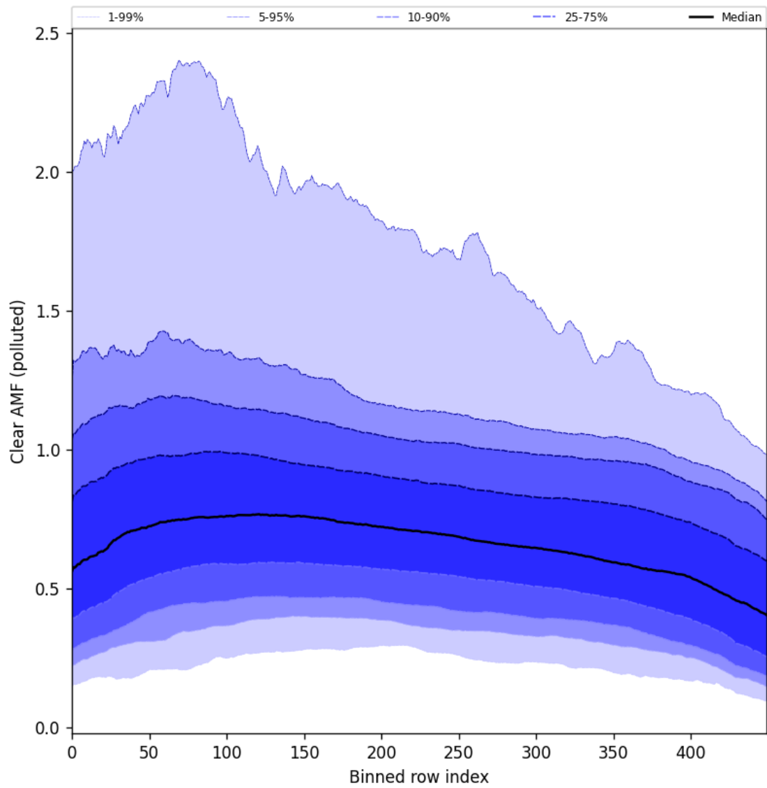
Figure 107: Along track statistics of “Clear AMF (polluted)” for 2025-10-06 to 2025-10-08
