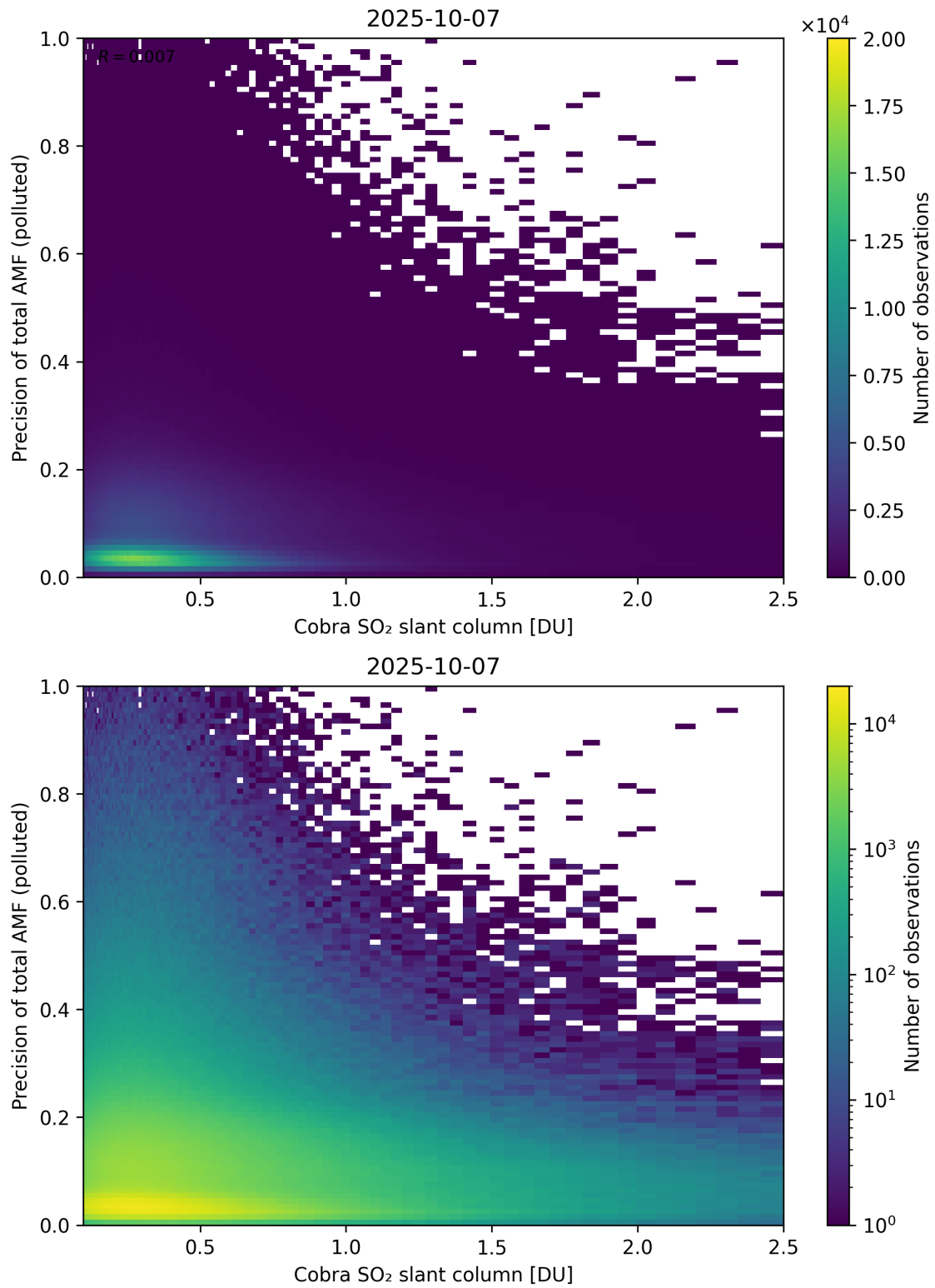
Figure 225: Scatter density plot of “Cobra SO 2 slant column” against “Precision of total AMF (polluted)” for 2025-10-06 to 2025-10-08.
