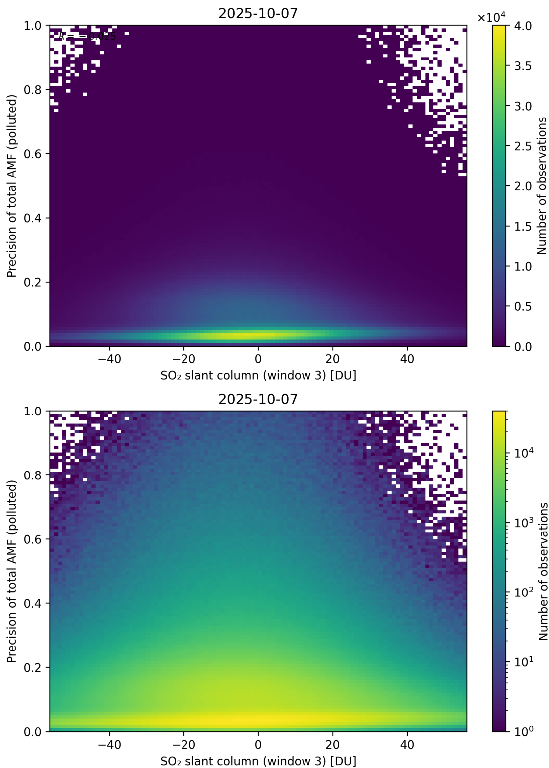
Figure 319: Scatter density plot of “SO 2 slant column (window 3)” against “Precision of total AMF (polluted)” for 2025-10-06 to 2025-10-08.
