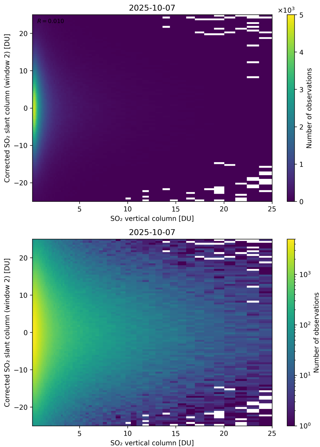
Figure 352: Scatter density plot of “SO 2 vertical column” against “Corrected SO 2 slant column (window 2)” for 2025-10-06 to 2025-10-08.
