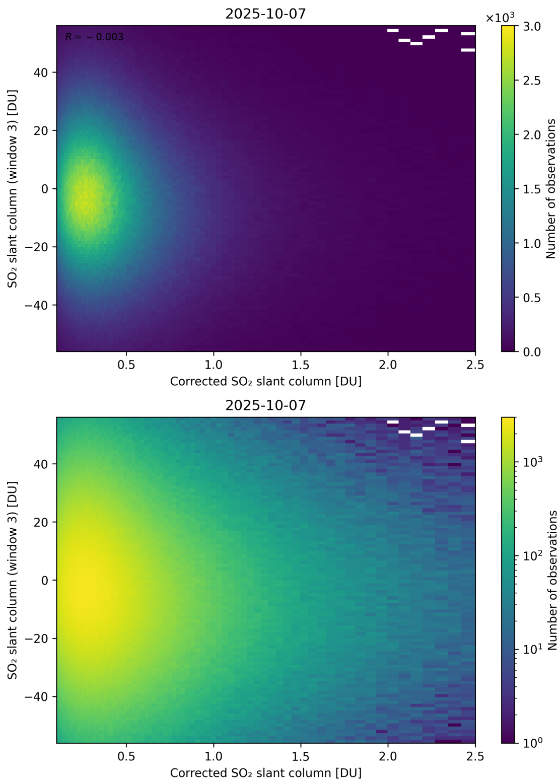
Figure 240: Scatter density plot of “Corrected SO 2 slant column” against “SO 2 slant column (window 3)” for 2025-10-06 to 2025-10-08.
