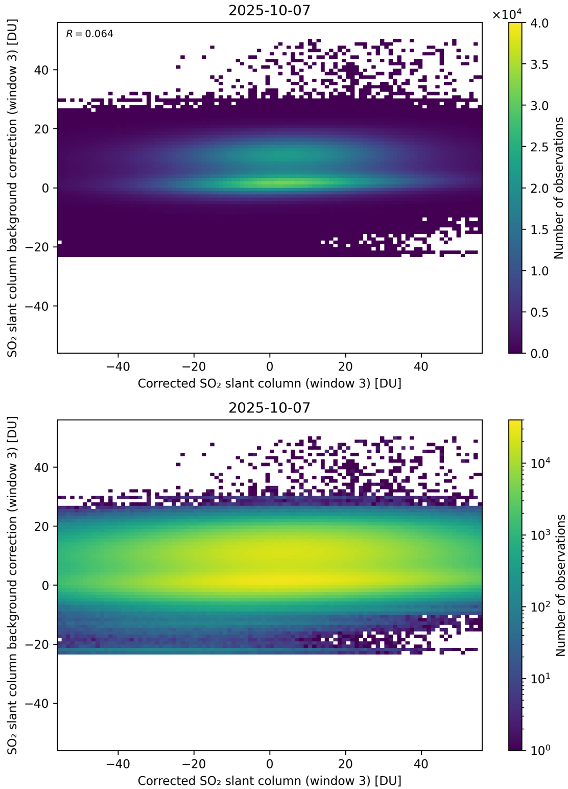
Figure 255: Scatter density plot of “Corrected SO 2 slant column (window 3)” against “SO 2 slant column background correction (window 3)” for 2025-10-06 to 2025-10-08.
