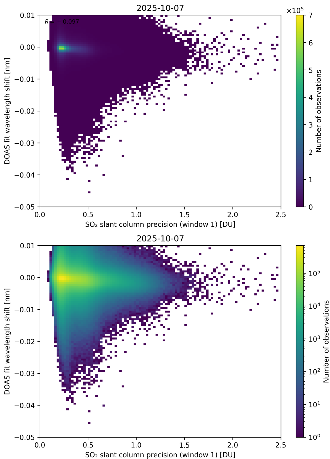
Figure 271: Scatter density plot of “SO 2 slant column precision (window 1)” against “DOAS fit wavelength shift” for 2025-10-06 to 2025-10-08.
