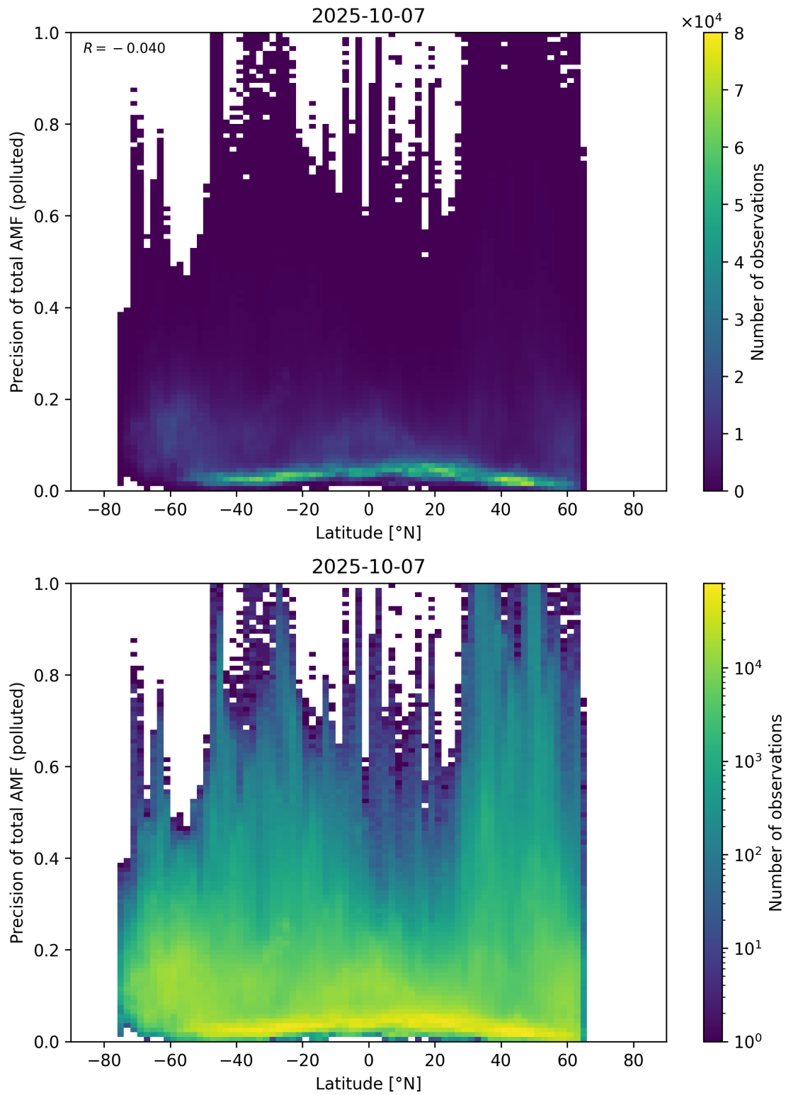
Figure 168: Scatter density plot of “Latitude” against “Precision of total AMF (polluted)” for 2025-10-06 to 2025-10-08.
