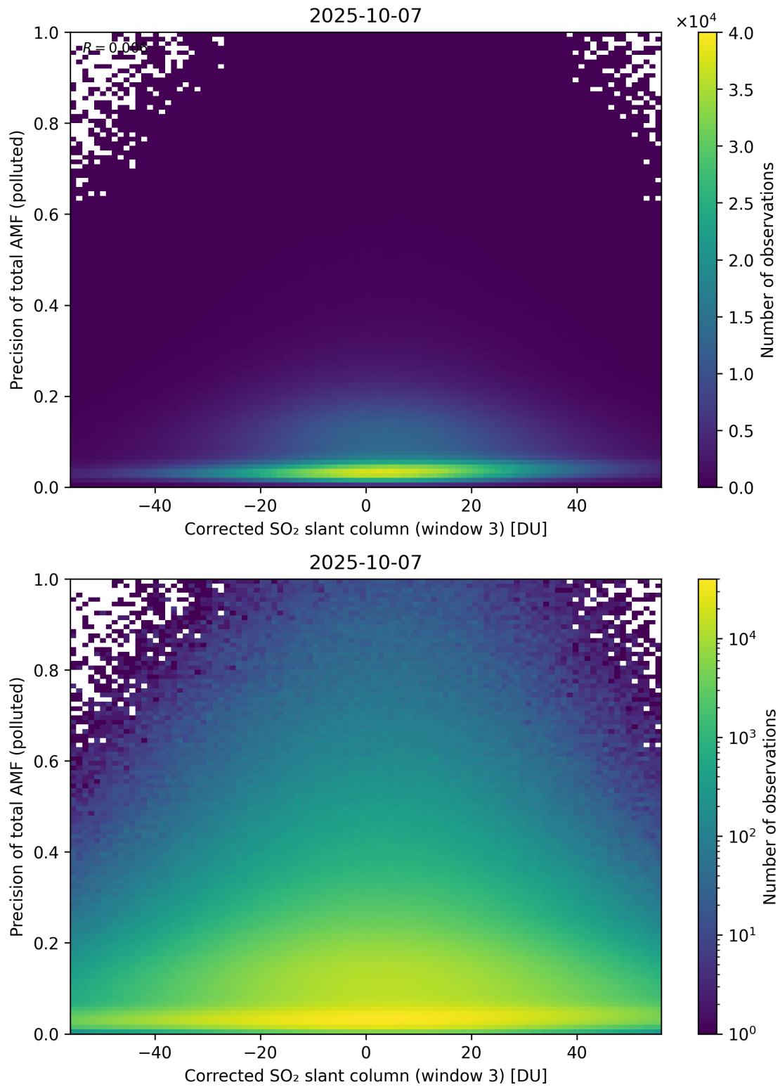
Figure 261: Scatter density plot of “Corrected SO 2 slant column (window 3)” against “Precision of total AMF (polluted)” for 2025-10-06 to 2025-10-08.
