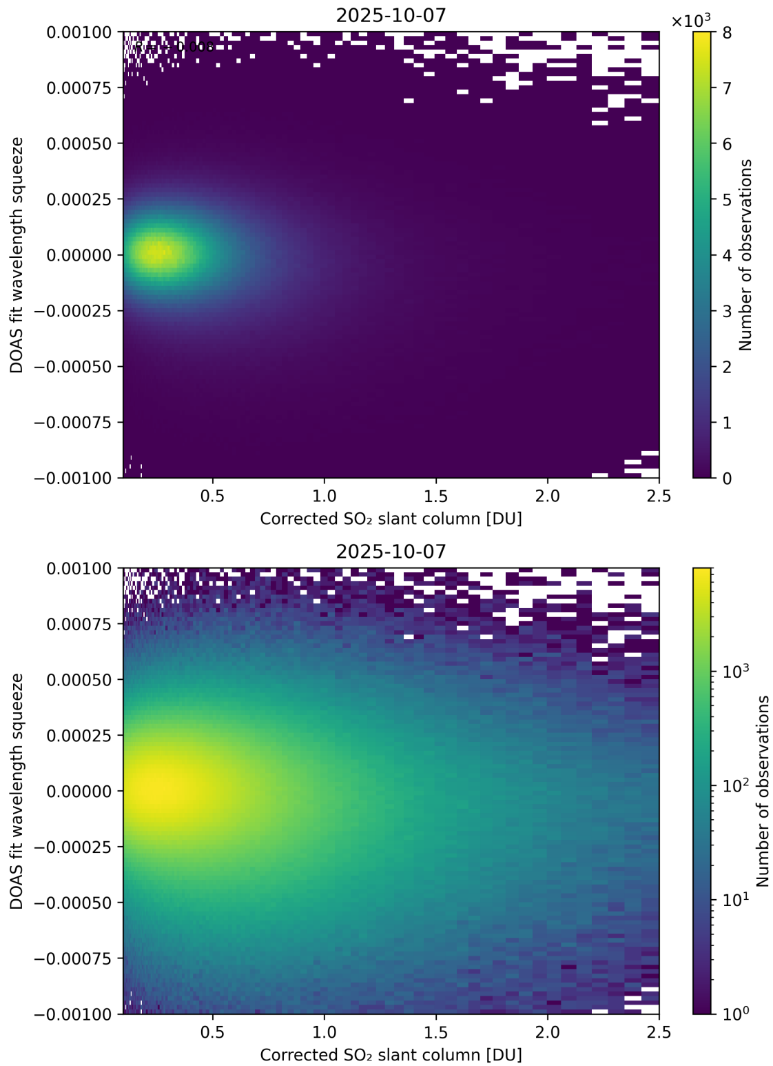
Figure 230: Scatter density plot of "Corrected SO 2 slant column" against "DOAS fit wavelength squeeze" for 2025-10-06 to 2025-10-08.
