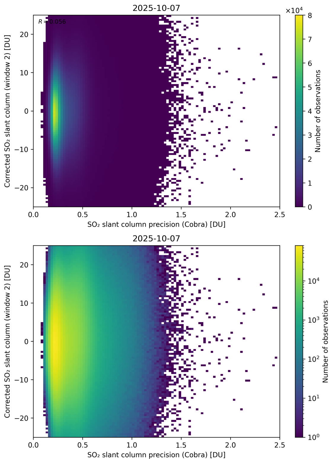
Figure 206: Scatter density plot of “SO 2 slant column precision (Cobra)” against “Corrected SO 2 slant column (window 2)” for 2025-10-06 to 2025-10-08.
