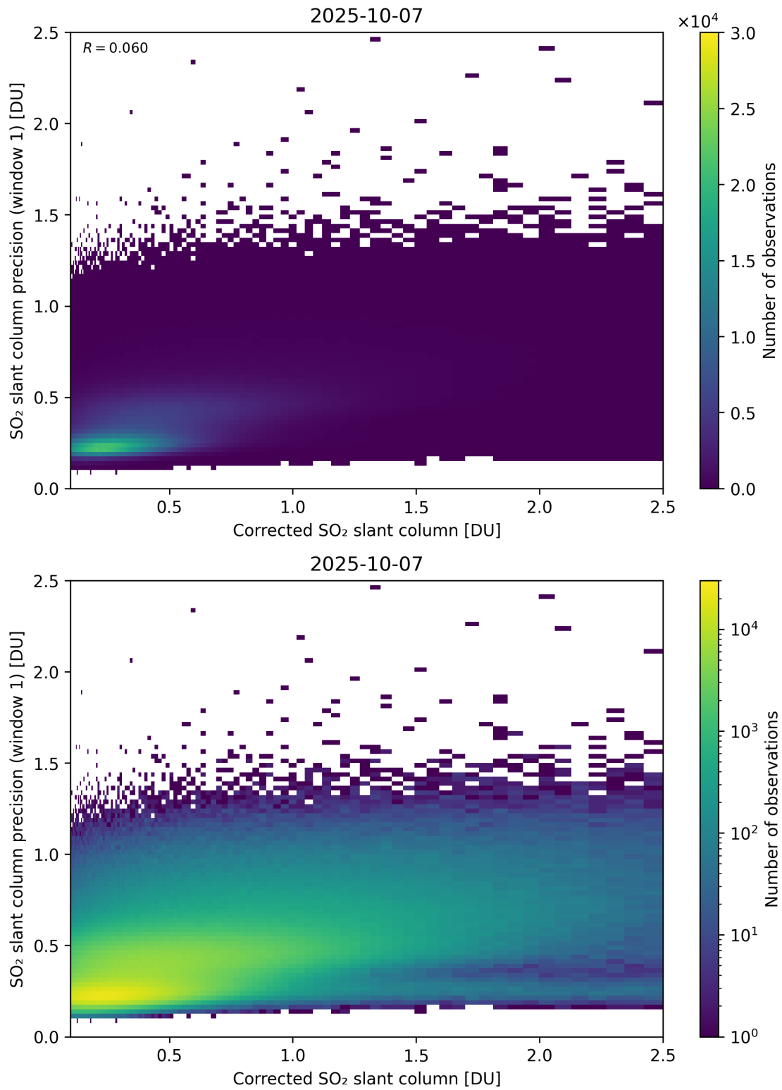
Figure 238: Scatter density plot of “Corrected SO 2 slant column” against “SO 2 slant column precision (window 1)” for 2025-10-06 to 2025-10-08.
