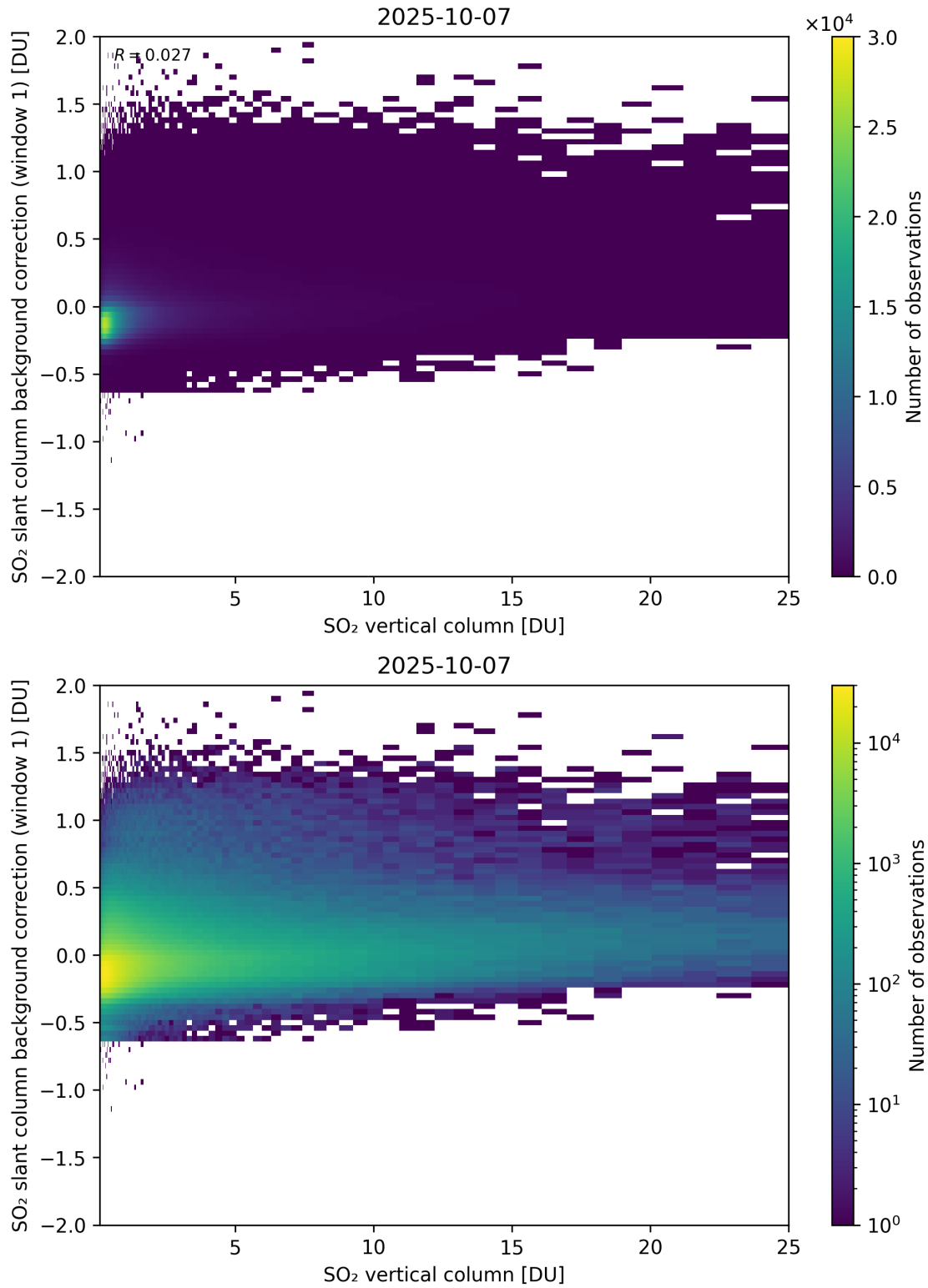
Figure 323: Scatter density plot of “SO 2 vertical column” against “SO 2 slant column background correction (window 1)” for 2025-10-06 to 2025-10-08.
