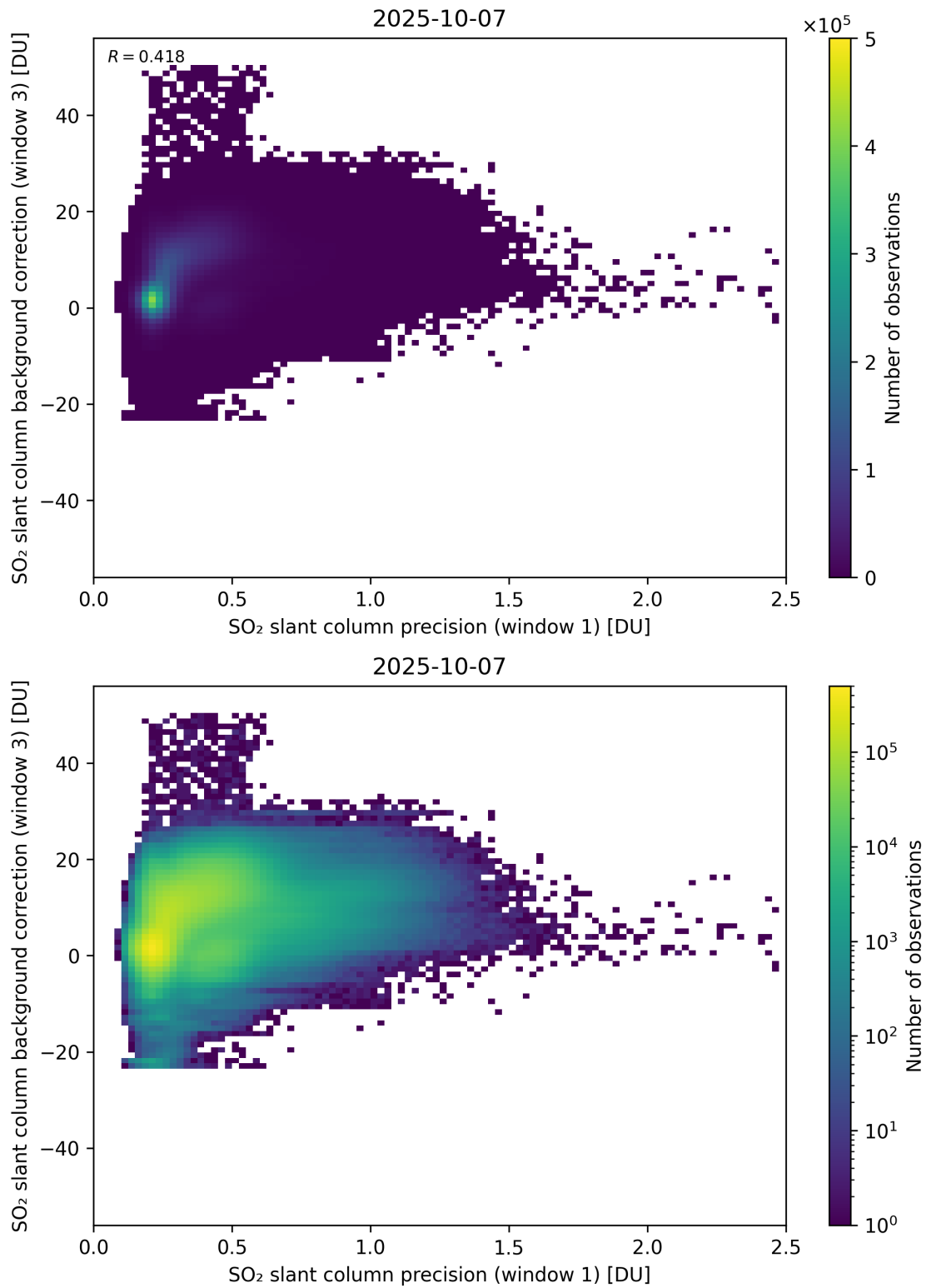
Figure 270: Scatter density plot of “SO 2 slant column precision (window 1)” against “SO 2 slant column background correction (window 3)” for 2025-10-06 to 2025-10-08.
