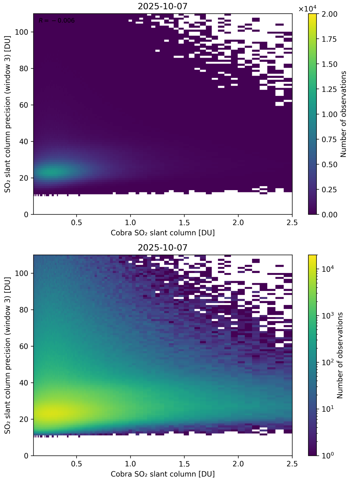
Figure 223: Scatter density plot of “Cobra SO 2 slant column” against “SO 2 slant column precision (window 3)” for 2025-10-06 to 2025-10-08.
