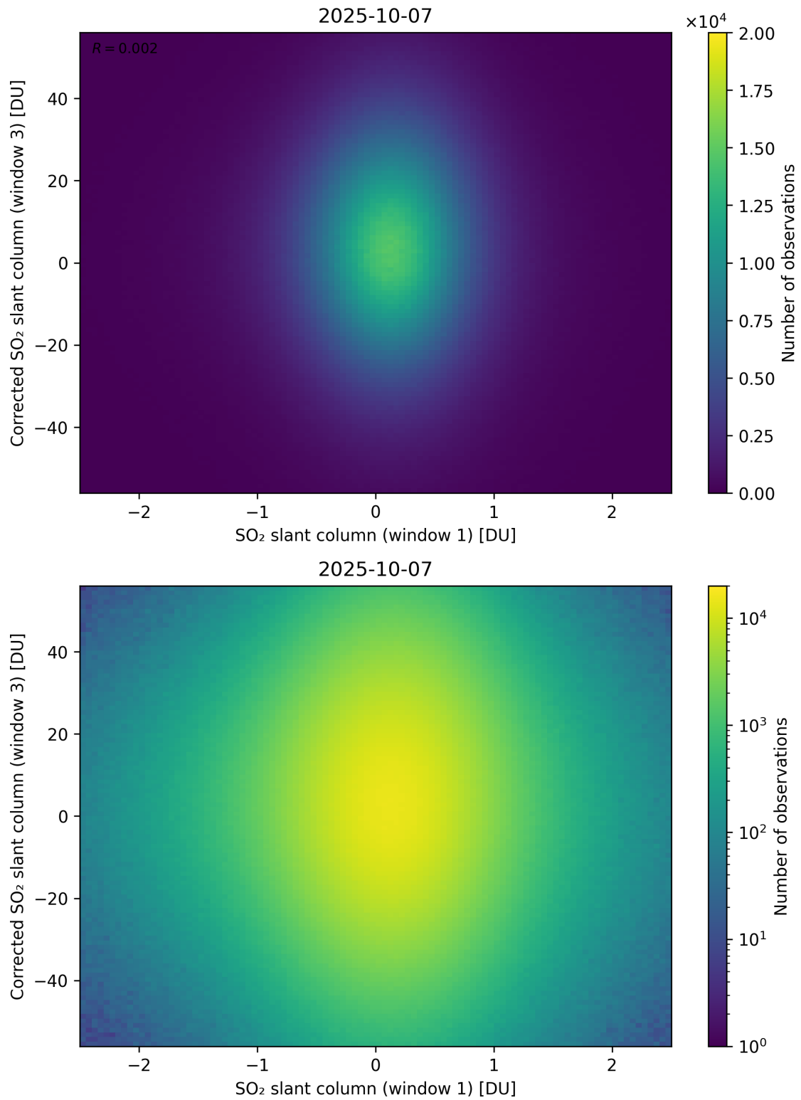
Figure 284: Scatter density plot of “SO 2 slant column (window 1)” against “Corrected SO 2 slant column (window 3)” for 2025-10-06 to 2025-10-08.
