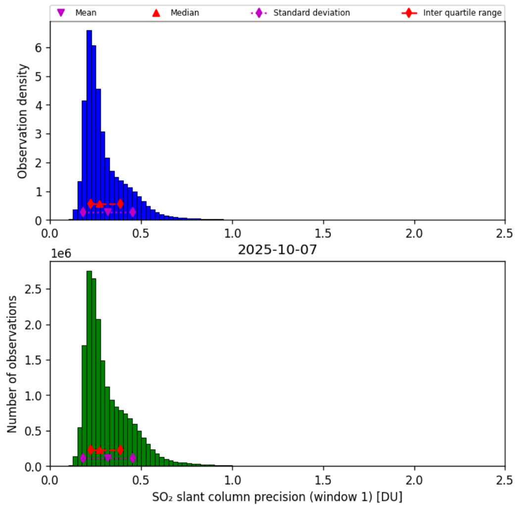
Figure 64: Histogram of “SO 2 slant column precision (window 1)” for 2025-10-06 to 2025-10-08
