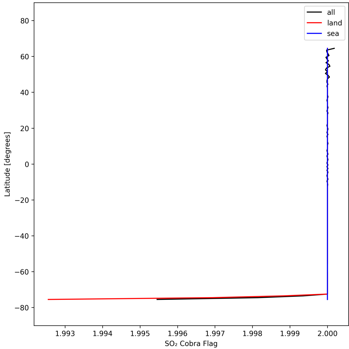
Figure 49: Zonal average of “SO 2 Cobra Flag” for 2025-10-06 to 2025-10-08.
