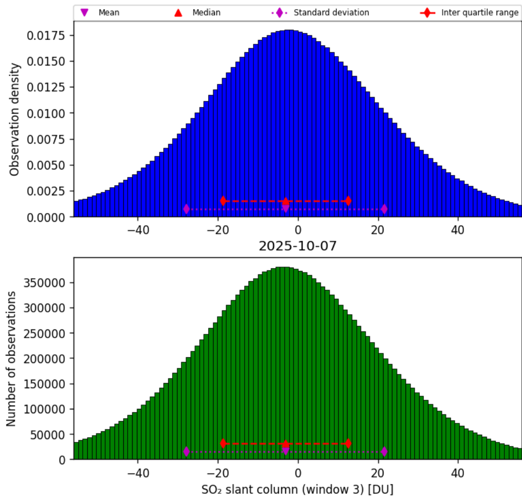
Figure 71: Histogram of “SO 2 slant column (window 3)” for 2025-10-06 to 2025-10-08
