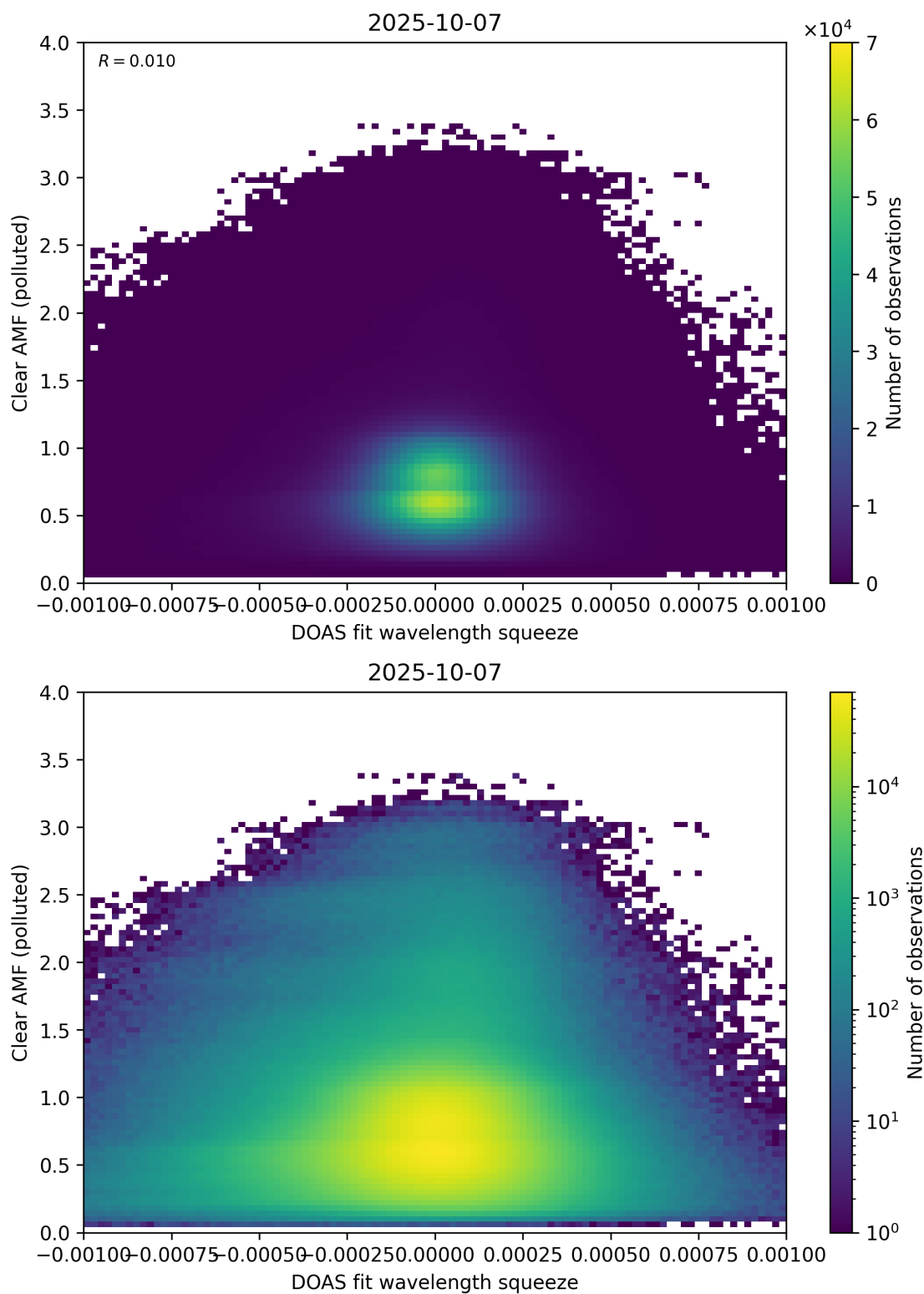
Figure 144: Scatter density plot of “DOAS fit wavelength squeeze” against “Clear AMF (polluted)” for 2025-10-06 to 2025-10-08.
