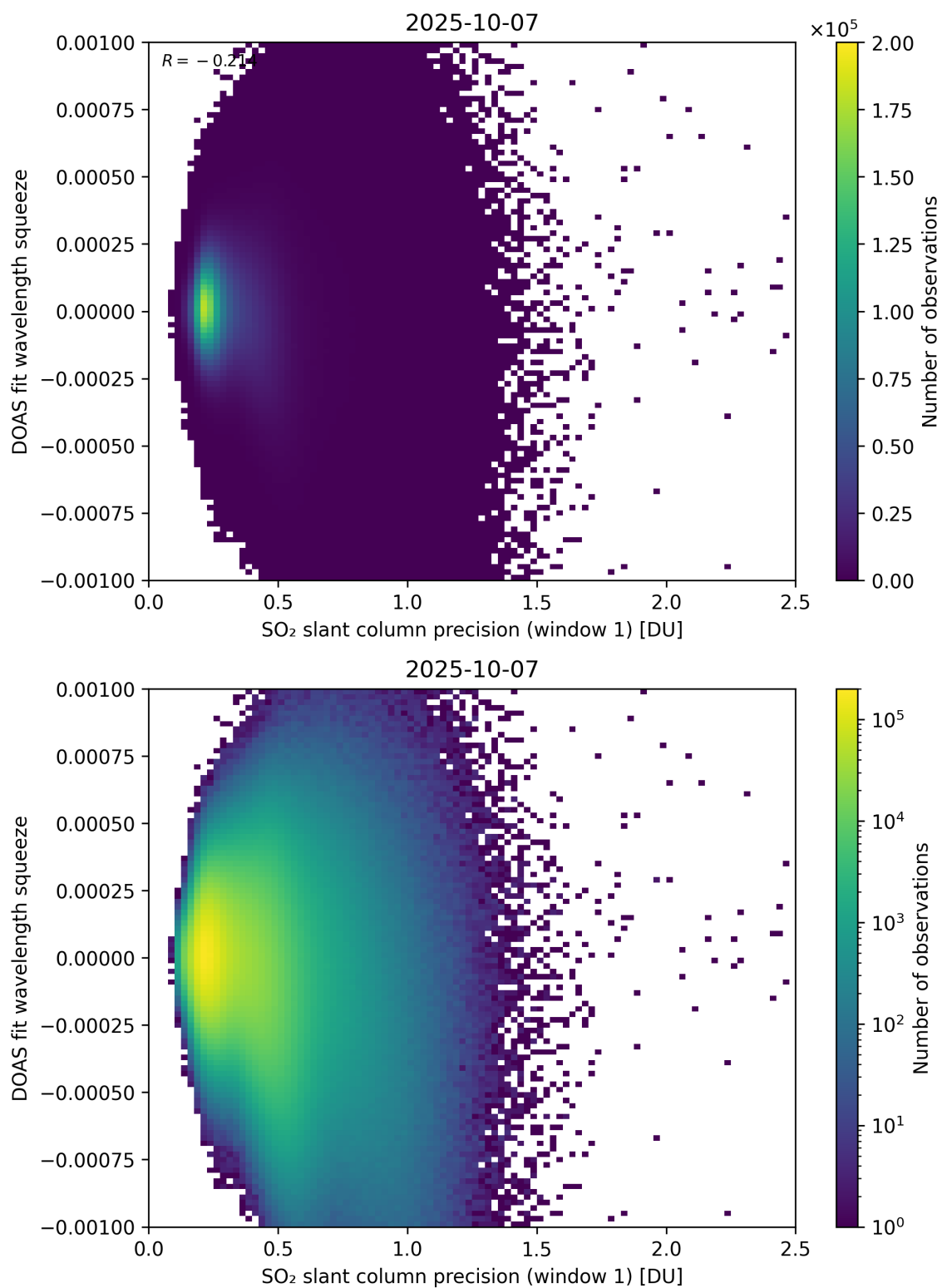
Figure 272: Scatter density plot of “SO 2 slant column precision (window 1)” against “DOAS fit wavelength squeeze” for 2025-10-06 to 2025-10-08.
