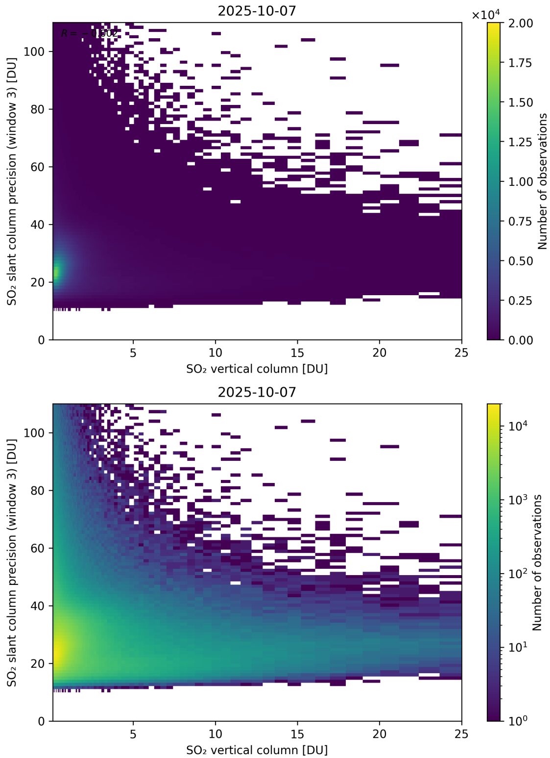
Figure 358: Scatter density plot of “SO 2 vertical column” against “SO 2 slant column precision (window 3)” for 2025-10-06 to 2025-10-08.
