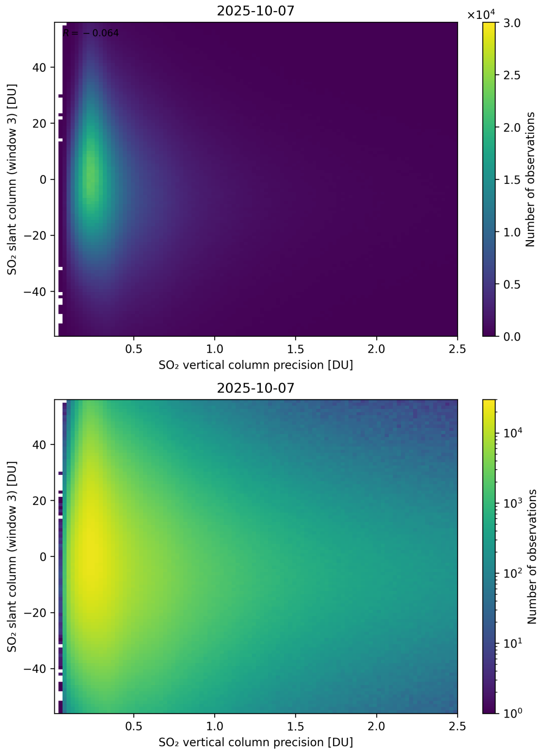
Figure 344: Scatter density plot of “SO 2 vertical column precision” against “SO 2 slant column (window 3)” for 2025-10-06 to 2025-10-08.
