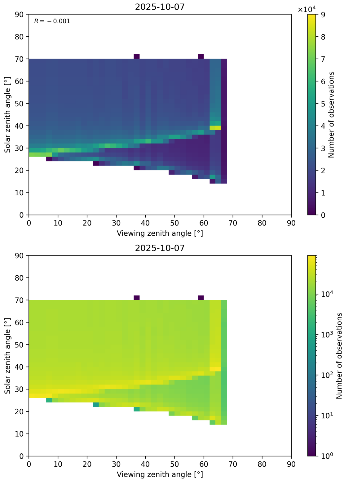
Figure 369: Scatter density plot of “Viewing zenith angle” against “Solar zenith angle” for 2025-10-06 to 2025-10-08.
