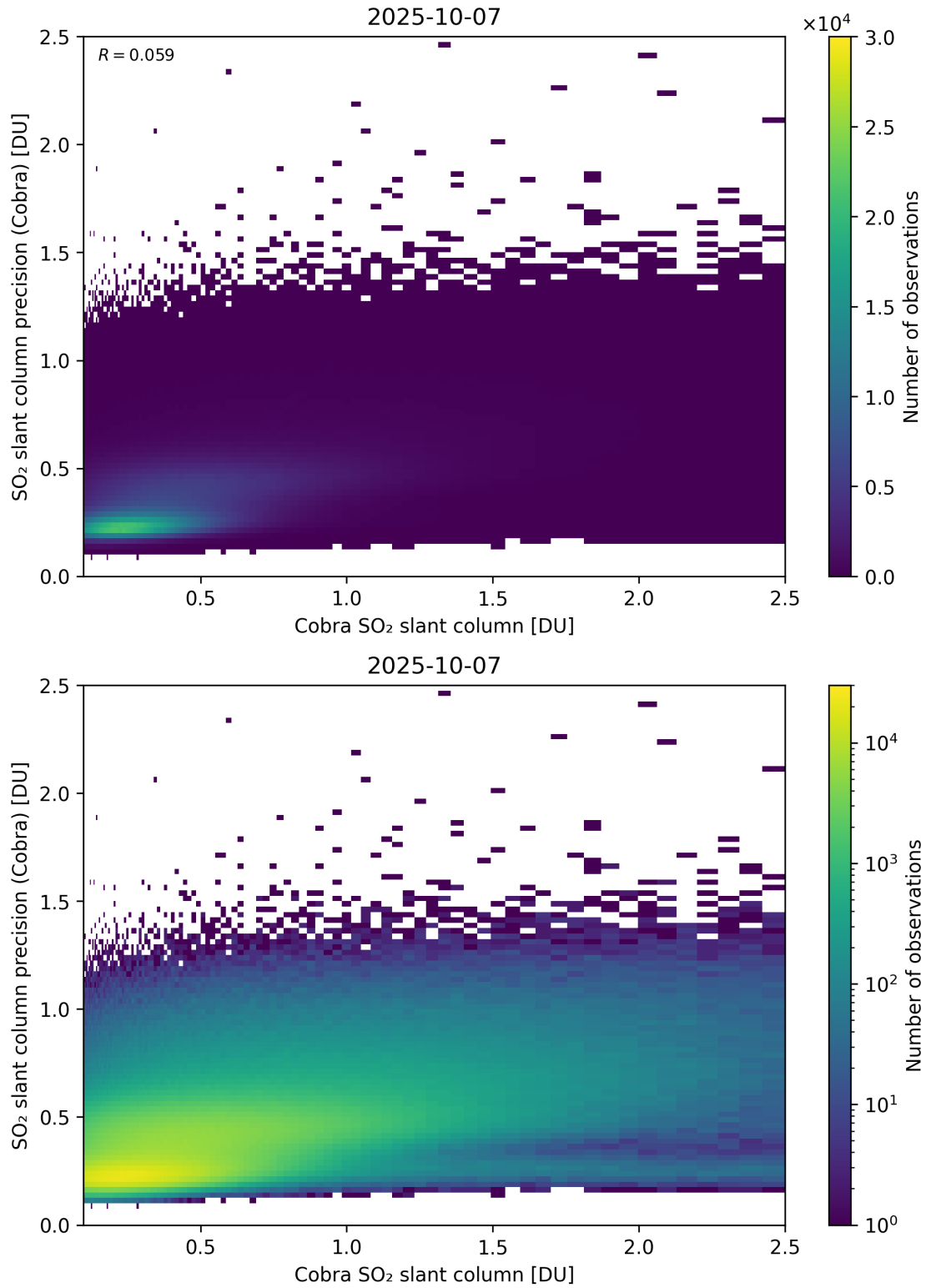
Figure 216: Scatter density plot of “Cobra SO 2 slant column” against “SO 2 slant column precision (Cobra)” for 2025-10-06 to 2025-10-08.
