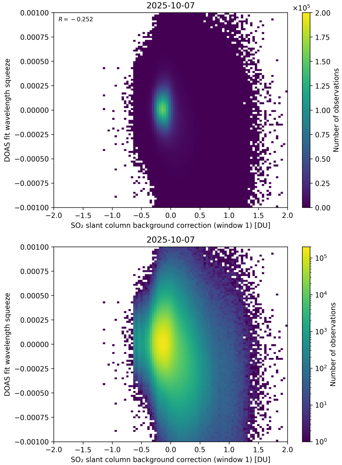
Figure 112: Scatter density plot of “SO 2 slant column background correction (window 1)” against “DOAS fit wavelength squeeze” for 2025-10-06 to 2025-10-08.
