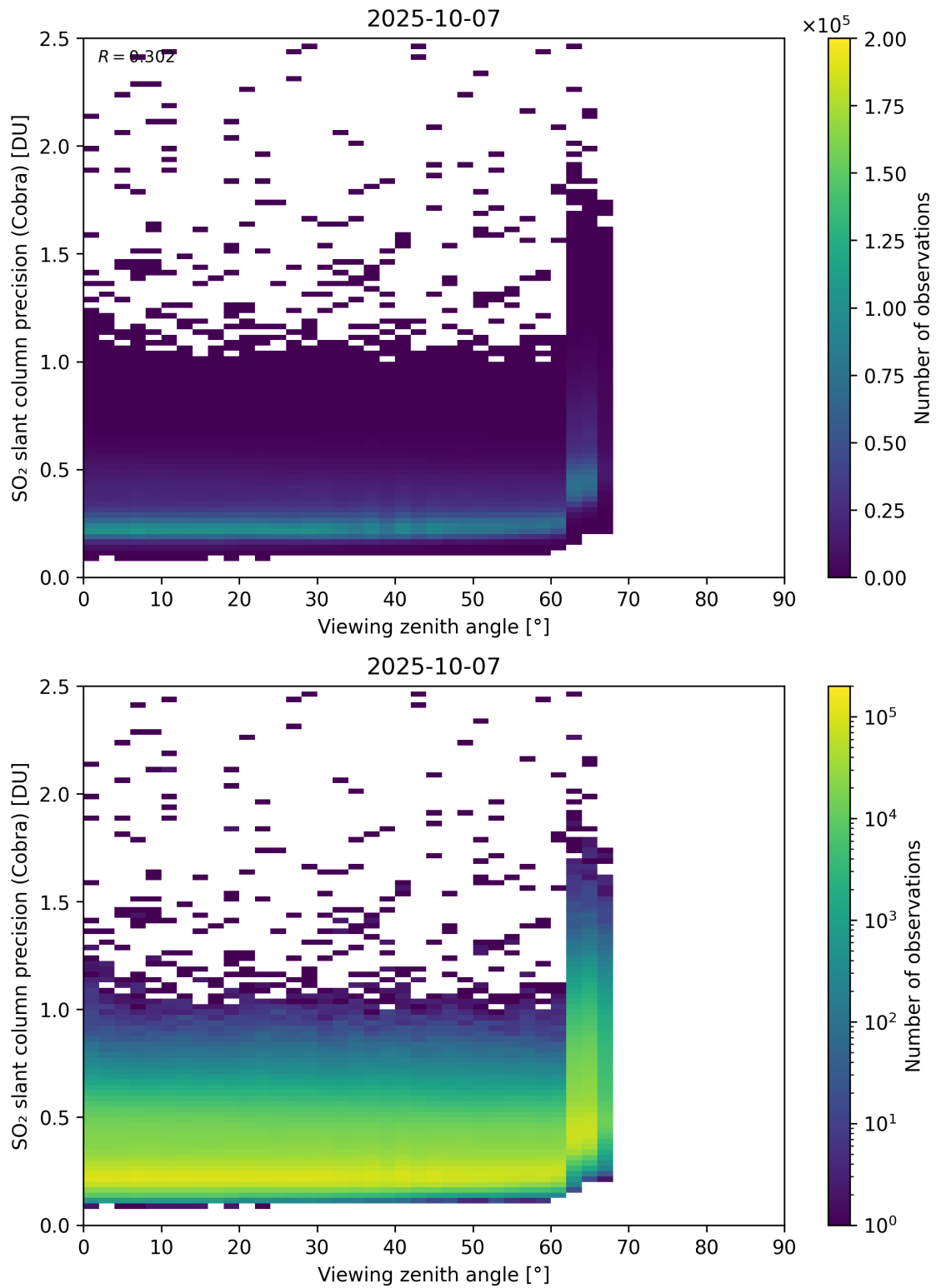
Figure 372: Scatter density plot of “Viewing zenith angle” against “SO 2 slant column precision (Cobra)” for 2025-10-06 to 2025-10-08.
