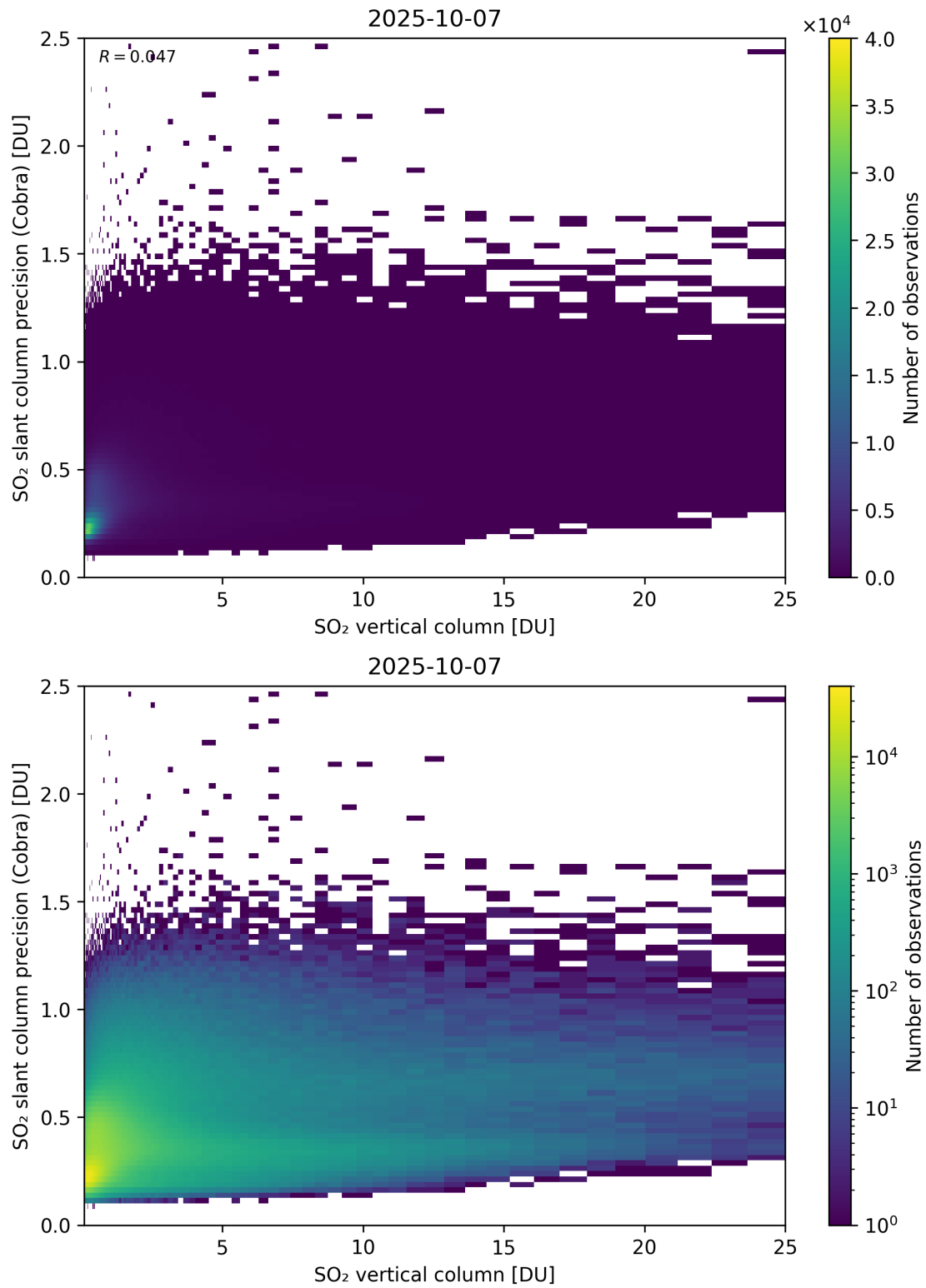
Figure 350: Scatter density plot of “SO 2 vertical column” against “SO 2 slant column precision (Cobra)” for 2025-10-06 to 2025-10-08.
