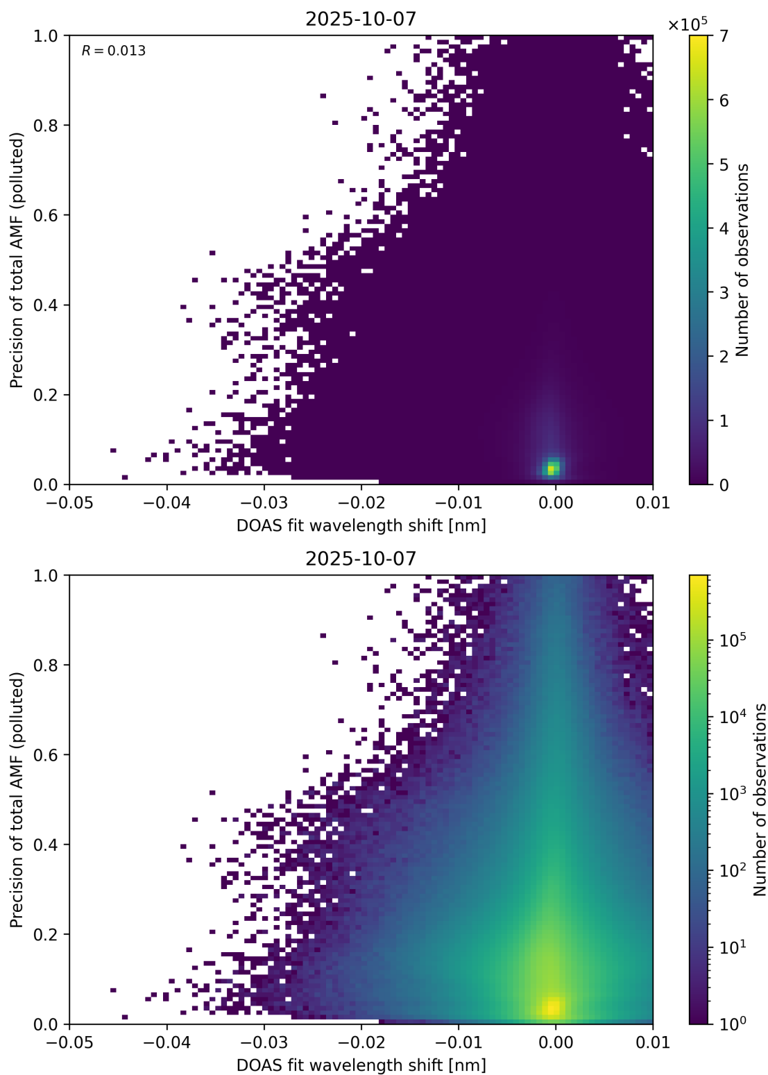
Figure 142: Scatter density plot of “DOAS fit wavelength shift” against “Precision of total AMF (polluted)” for 2025-10-06 to 2025-10-08.
