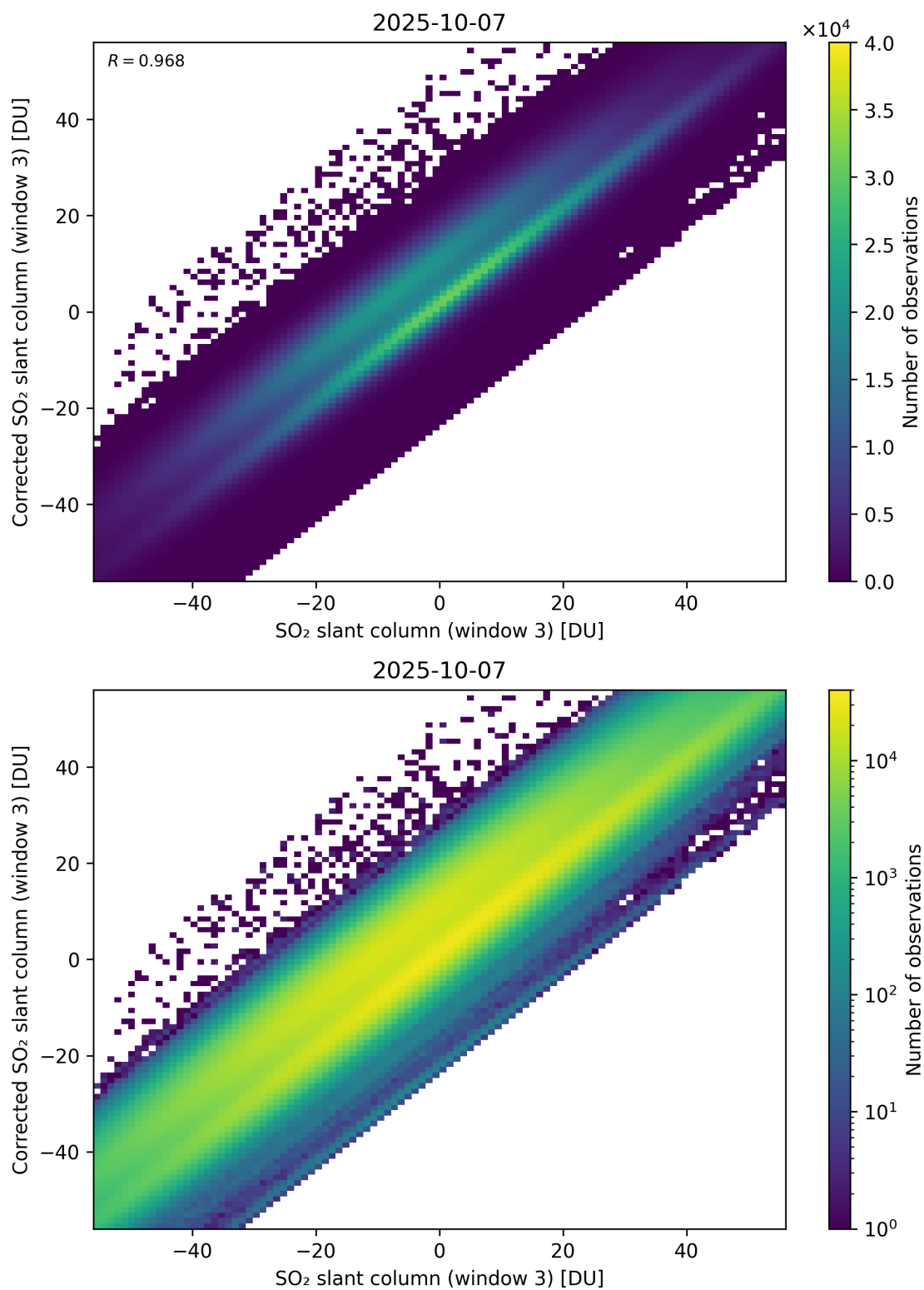
Figure 316: Scatter density plot of “SO 2 slant column (window 3)” against “Corrected SO 2 slant column (window 3)” for 2025-10-06 to 2025-10-08.
