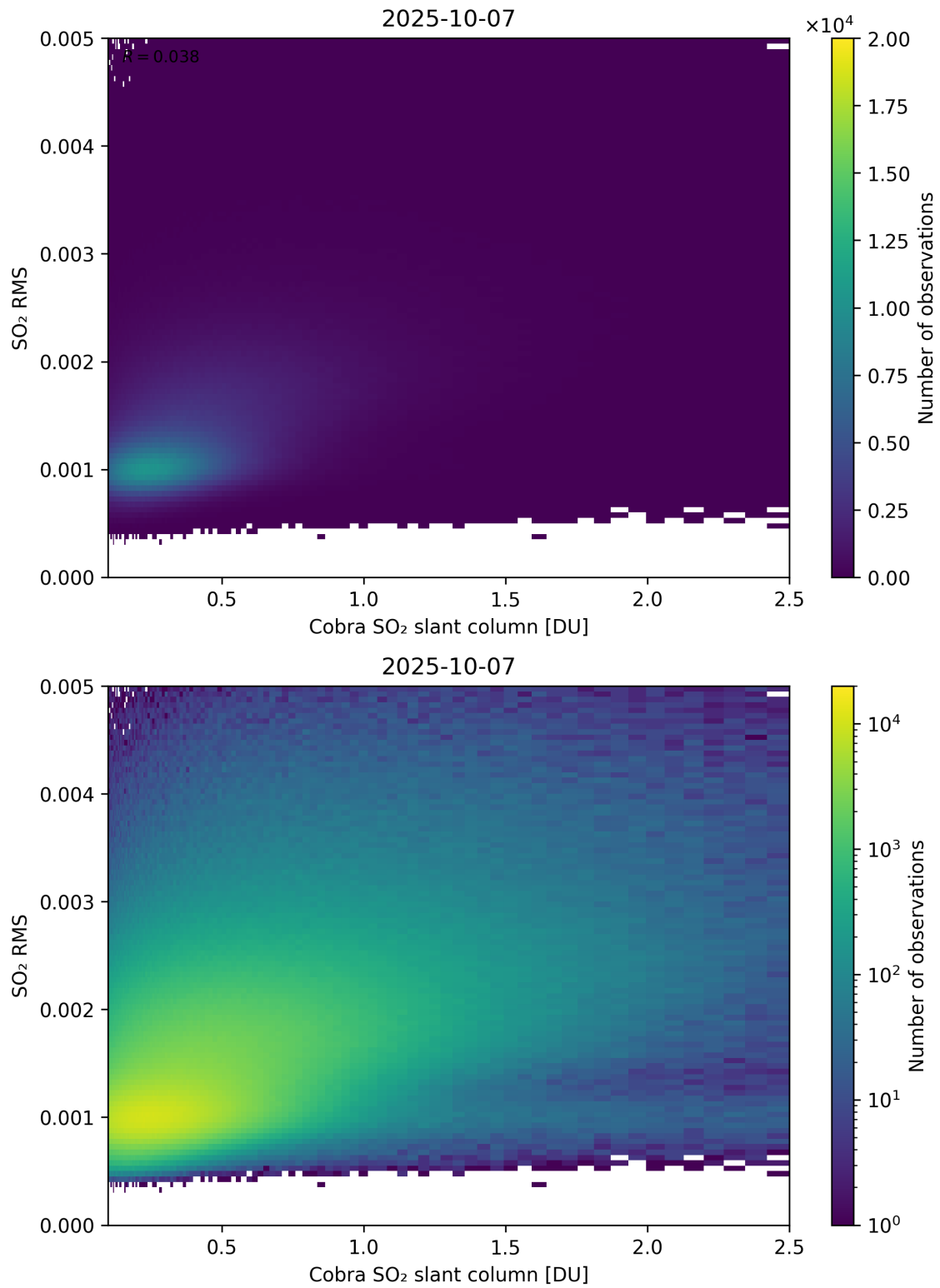
Figure 198: Scatter density plot of “Cobra SO 2 slant column” against “SO 2 RMS” for 2025-10-06 to 2025-10-08.
