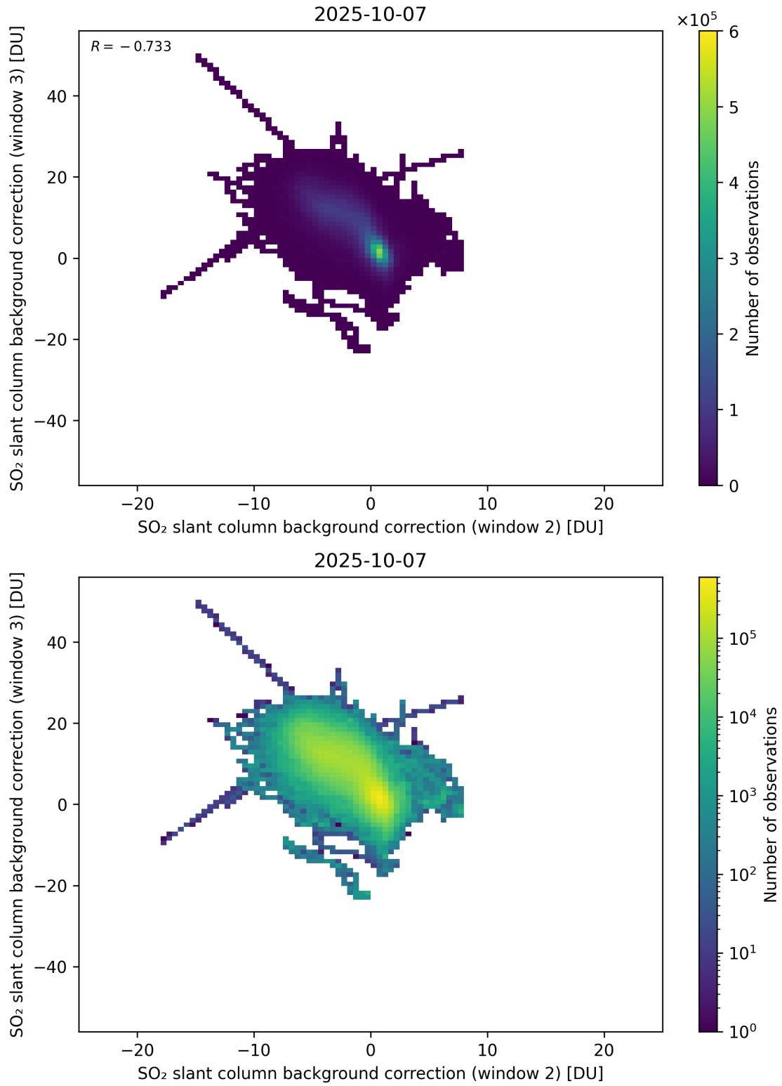
Figure 122: Scatter density plot of “SO 2 slant column background correction (window 2)” against “SO 2 slant column background correction (window 3)” for 2025-10-06 to 2025-10-08.
