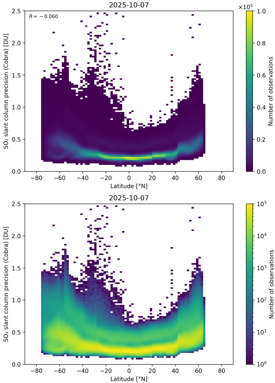
Figure 158: Scatter density plot of “Latitude” against “SO 2 slant column precision (Cobra)” for 2025-10-06 to 2025-10-08.
