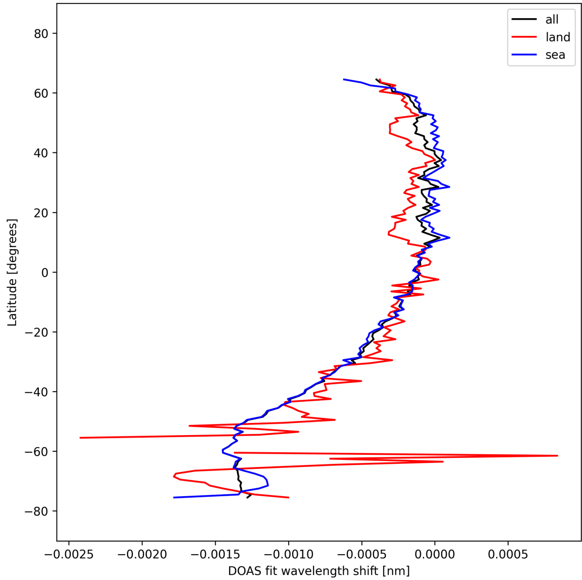
Figure 50: Zonal average of "DOAS fit wavelength shift" for 2025-10-06 to 2025-10-08.
