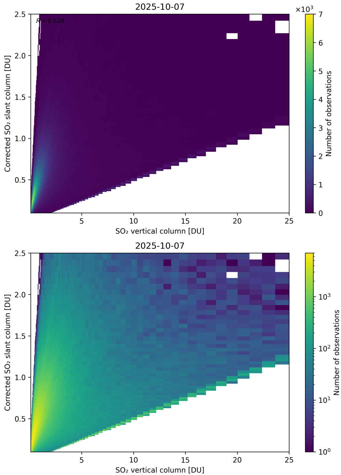
Figure 351: Scatter density plot of “SO 2 vertical column” against “Corrected SO 2 slant column” for 2025-10-06 to 2025-10-08.
