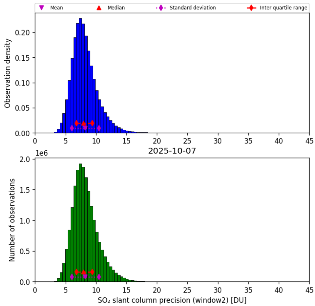
Figure 68: Histogram of “SO 2 slant column precision (window2)” for 2025-10-06 to 2025-10-08
