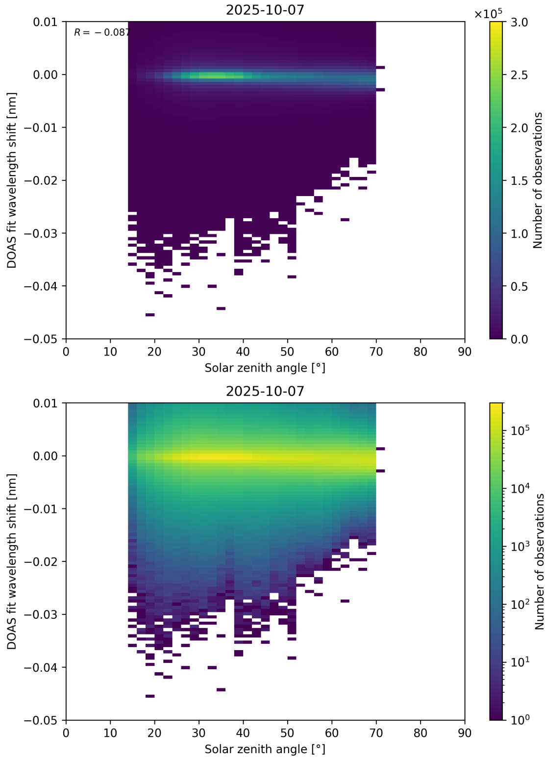
Figure 174: Scatter density plot of “Solar zenith angle” against “DOAS fit wavelength shift” for 2025-10-06 to 2025-10-08.
