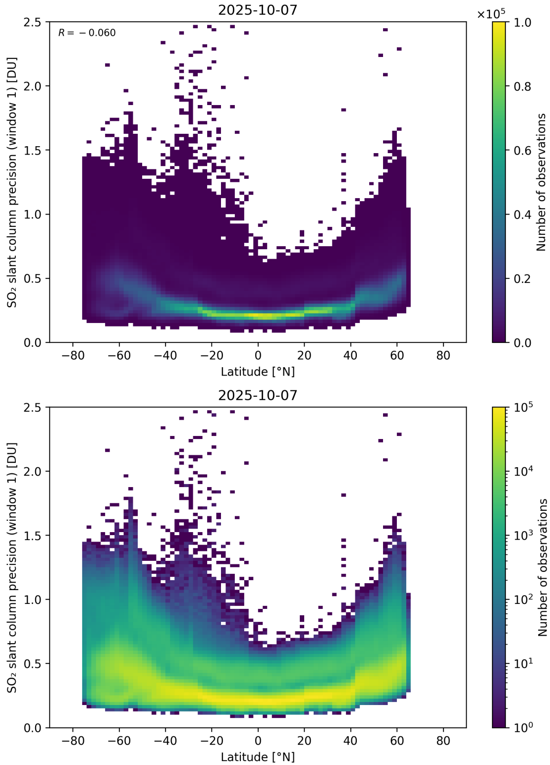
Figure 163: Scatter density plot of “Latitude” against “SO 2 slant column precision (window 1)” for 2025-10-06 to 2025-10-08.
