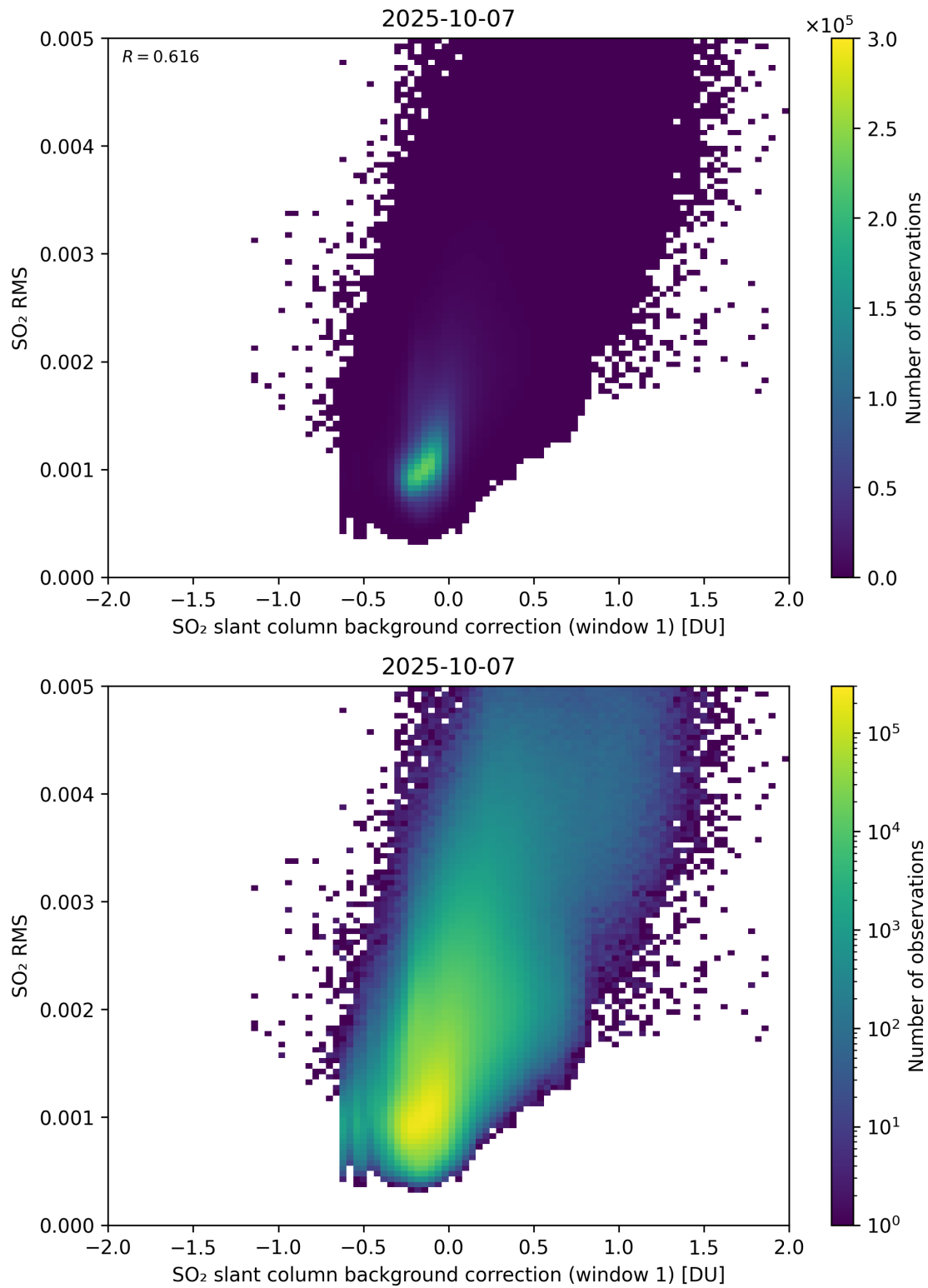
Figure 113: Scatter density plot of “SO 2 slant column background correction (window 1)” against “SO 2 RMS” for 2025-10-06 to 2025-10-08.
