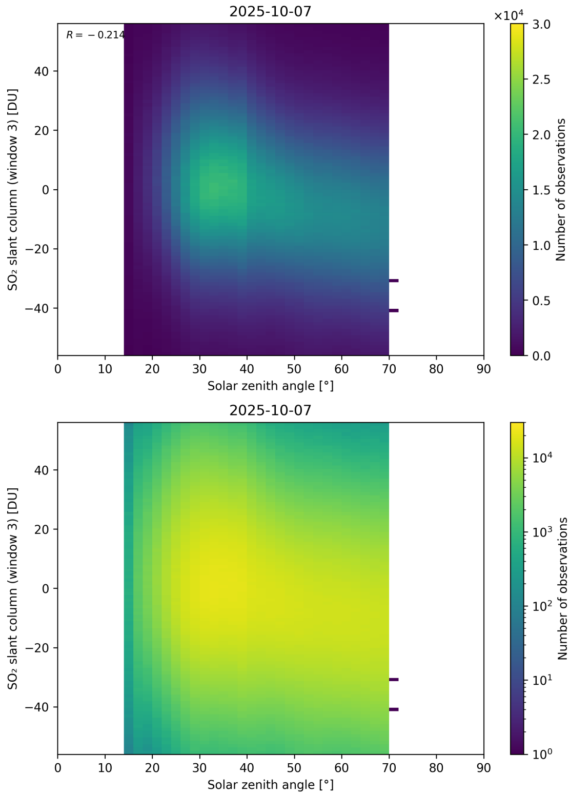
Figure 187: Scatter density plot of “Solar zenith angle” against “SO 2 slant column (window 3)” for 2025-10-06 to 2025-10-08.
