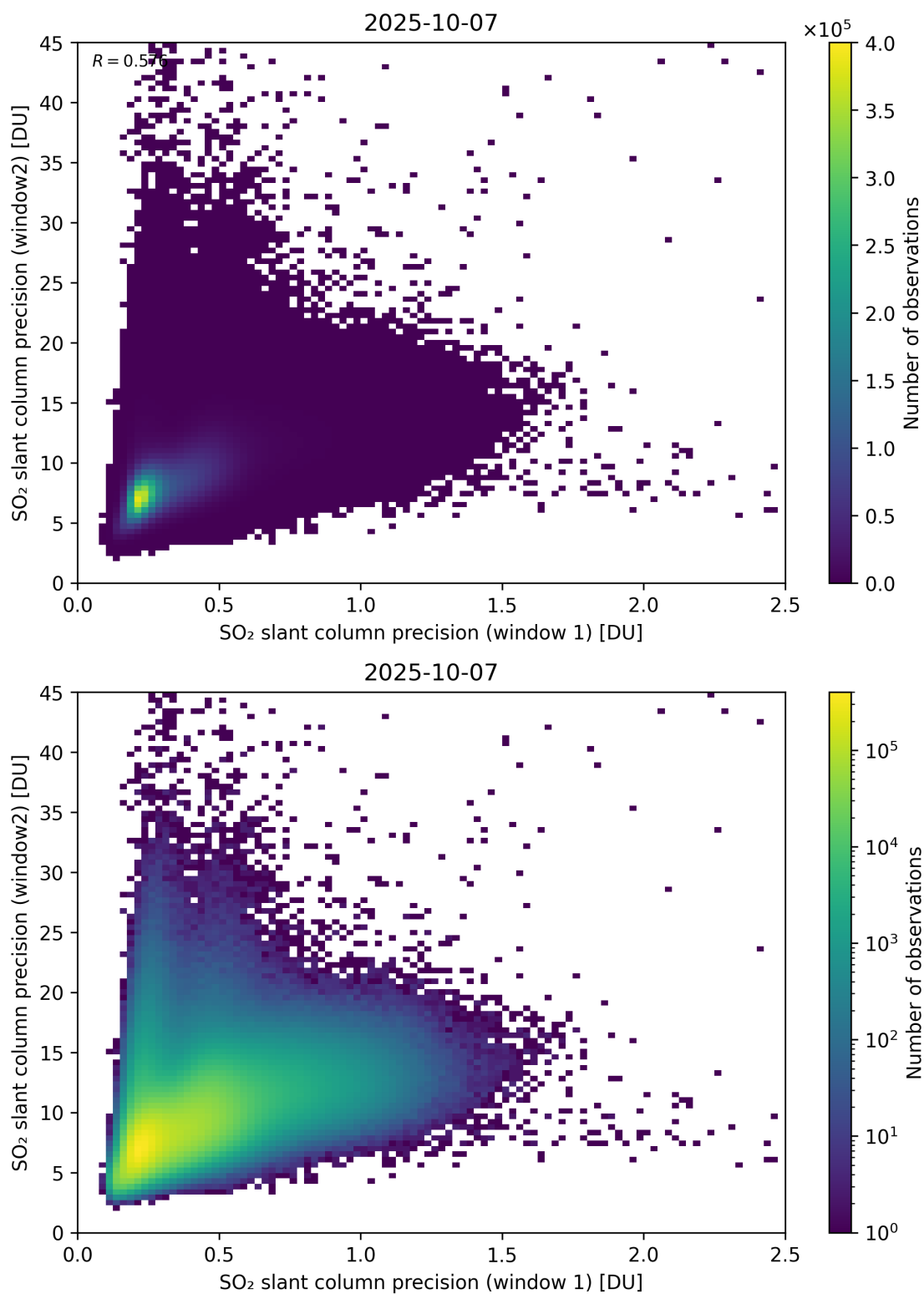
Figure 277: Scatter density plot of “SO 2 slant column precision (window 1)” against “SO 2 slant column precision (window2)” for 2025-10-06 to 2025-10-08.
