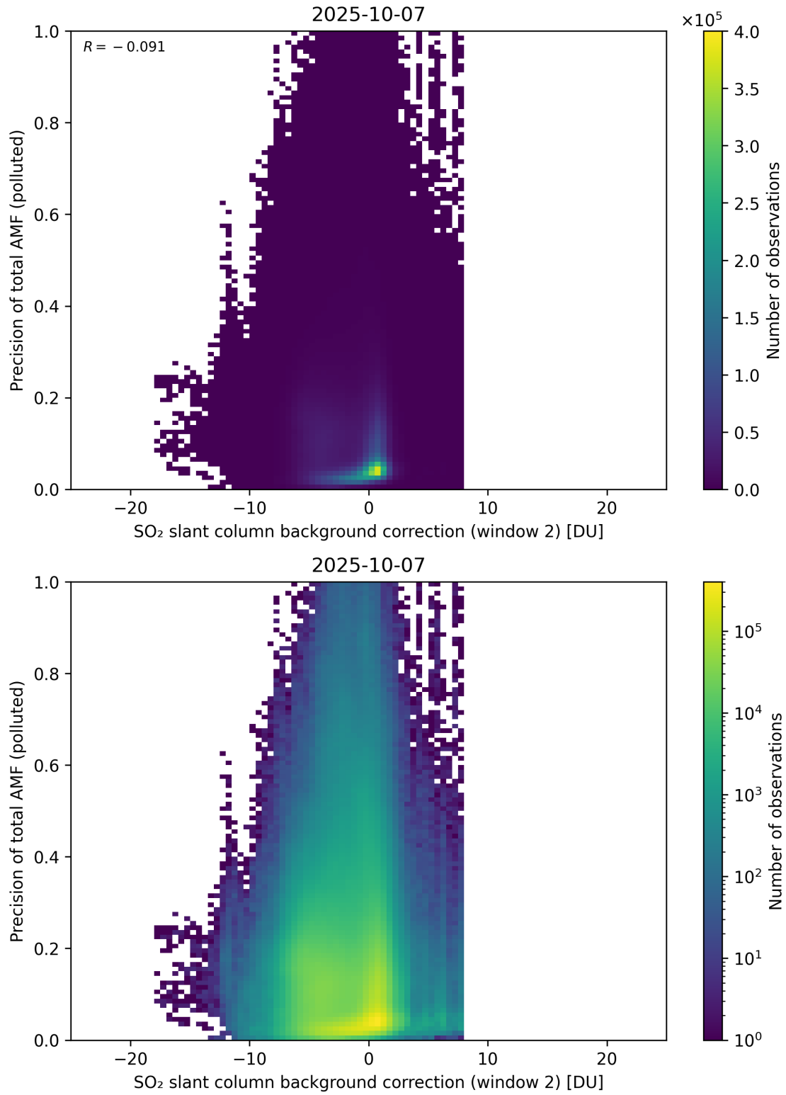
Figure 131: Scatter density plot of “SO 2 slant column background correction (window 2)” against “Precision of total AMF (polluted)” for 2025-10-06 to 2025-10-08.
