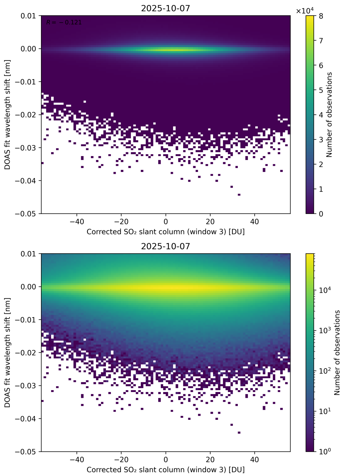
Figure 256: Scatter density plot of “Corrected SO 2 slant column (window 3)” against “DOAS fit wavelength shift” for 2025-10-06 to 2025-10-08.
