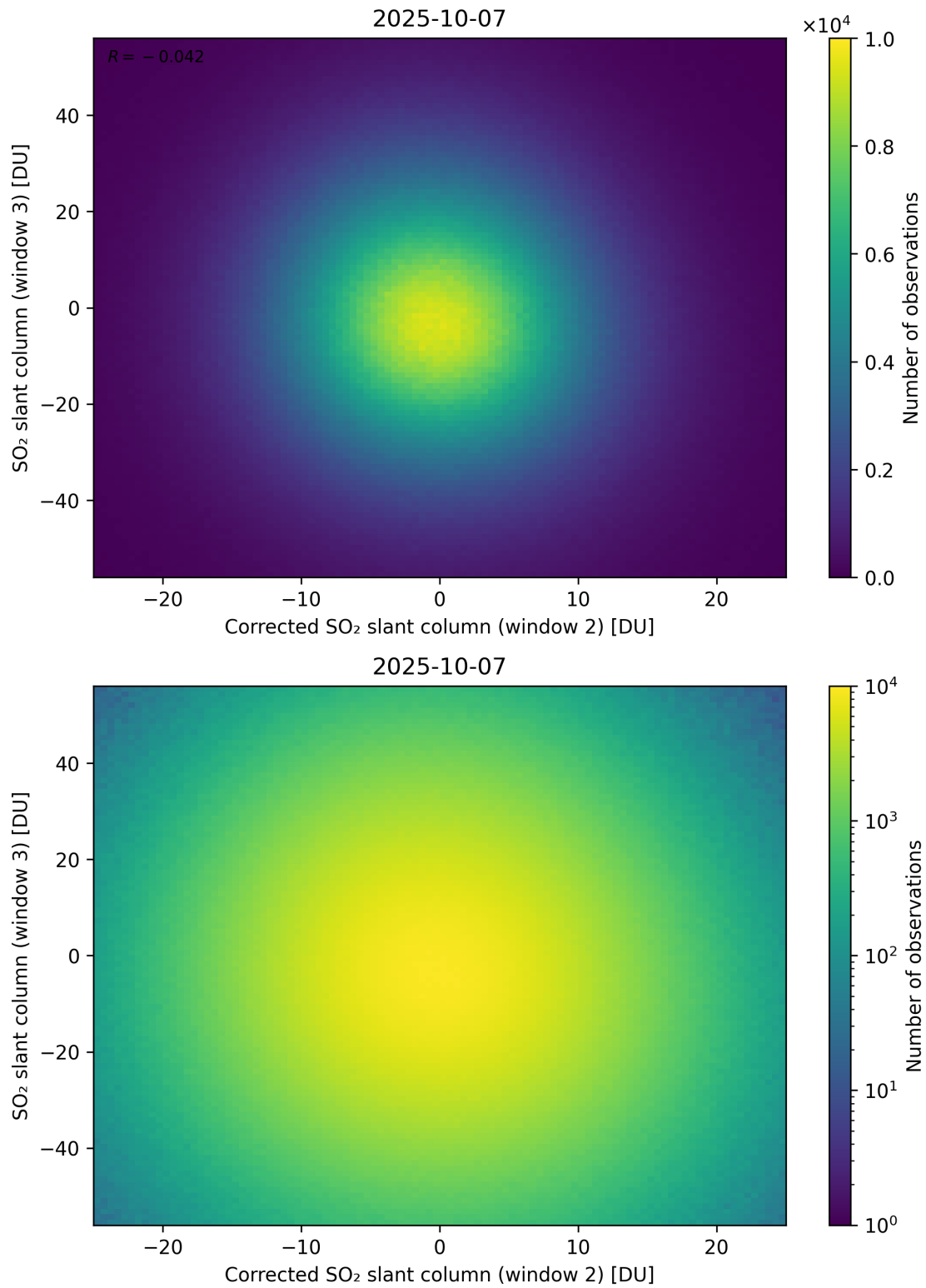
Figure 251: Scatter density plot of “Corrected SO 2 slant column (window 2)” against “SO 2 slant column (window 3)” for 2025-10-06 to 2025-10-08.
