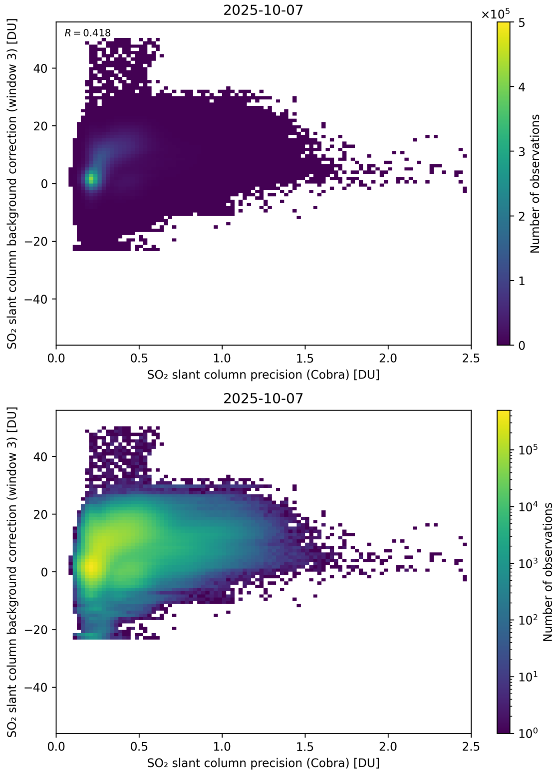
Figure 201: Scatter density plot of “SO 2 slant column precision (Cobra)” against “SO 2 slant column background correction (window 3)” for 2025-10-06 to 2025-10-08.
