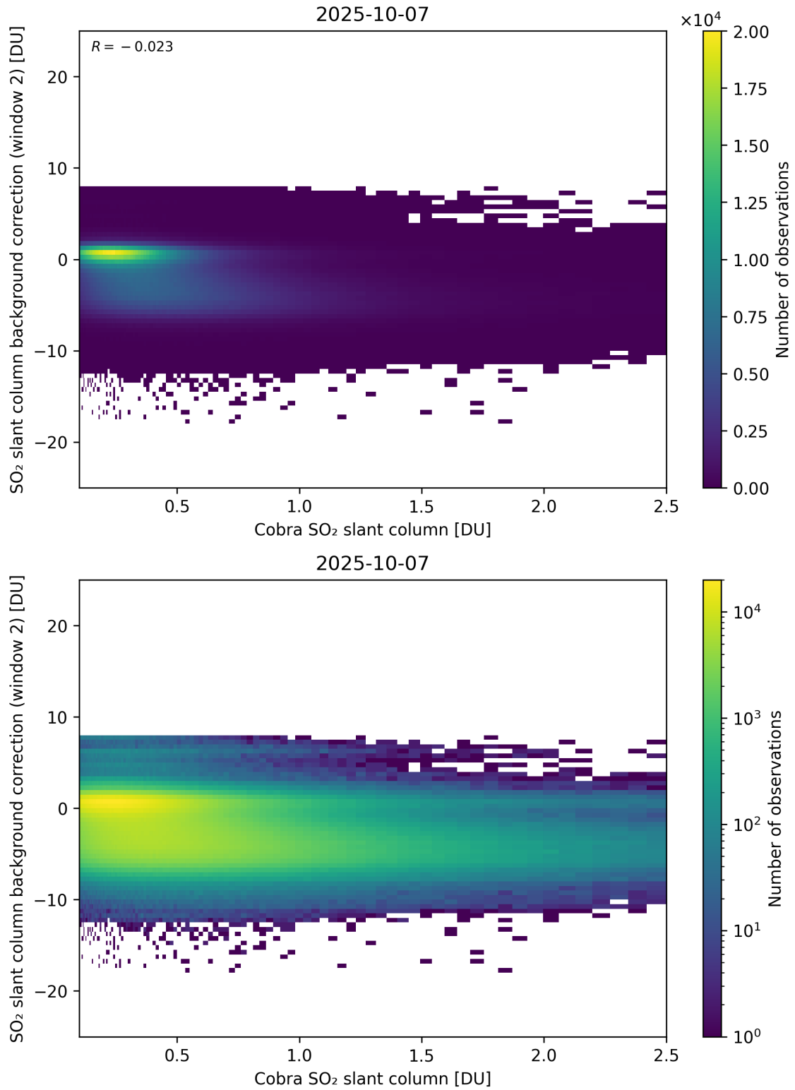
Figure 194: Scatter density plot of “Cobra SO 2 slant column” against “SO 2 slant column background correction (window 2)” for 2025-10-06 to 2025-10-08.
