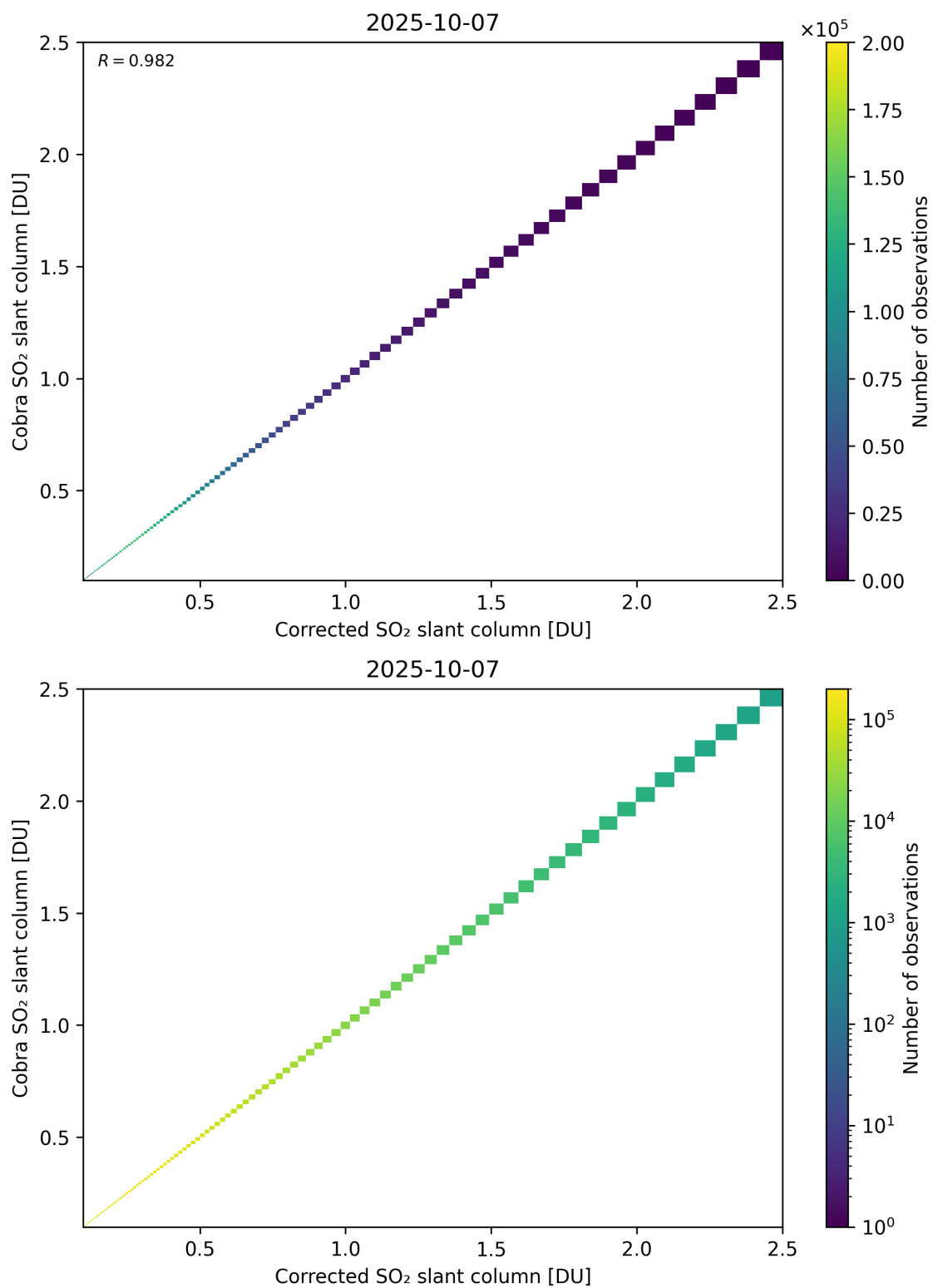
Figure 233: Scatter density plot of “Corrected SO 2 slant column” against “Cobra SO 2 slant column” for 2025-10-06 to 2025-10-08.
