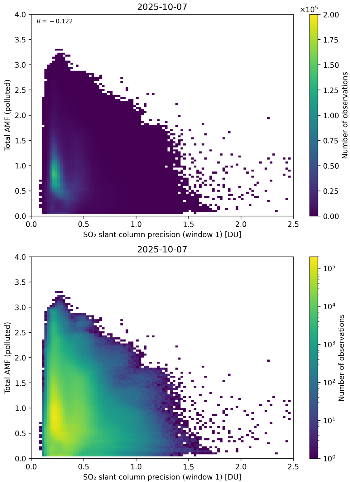
Figure 280: Scatter density plot of “SO 2 slant column precision (window 1)” against “Total AMF (polluted)” for 2025-10-06 to 2025-10-08.
