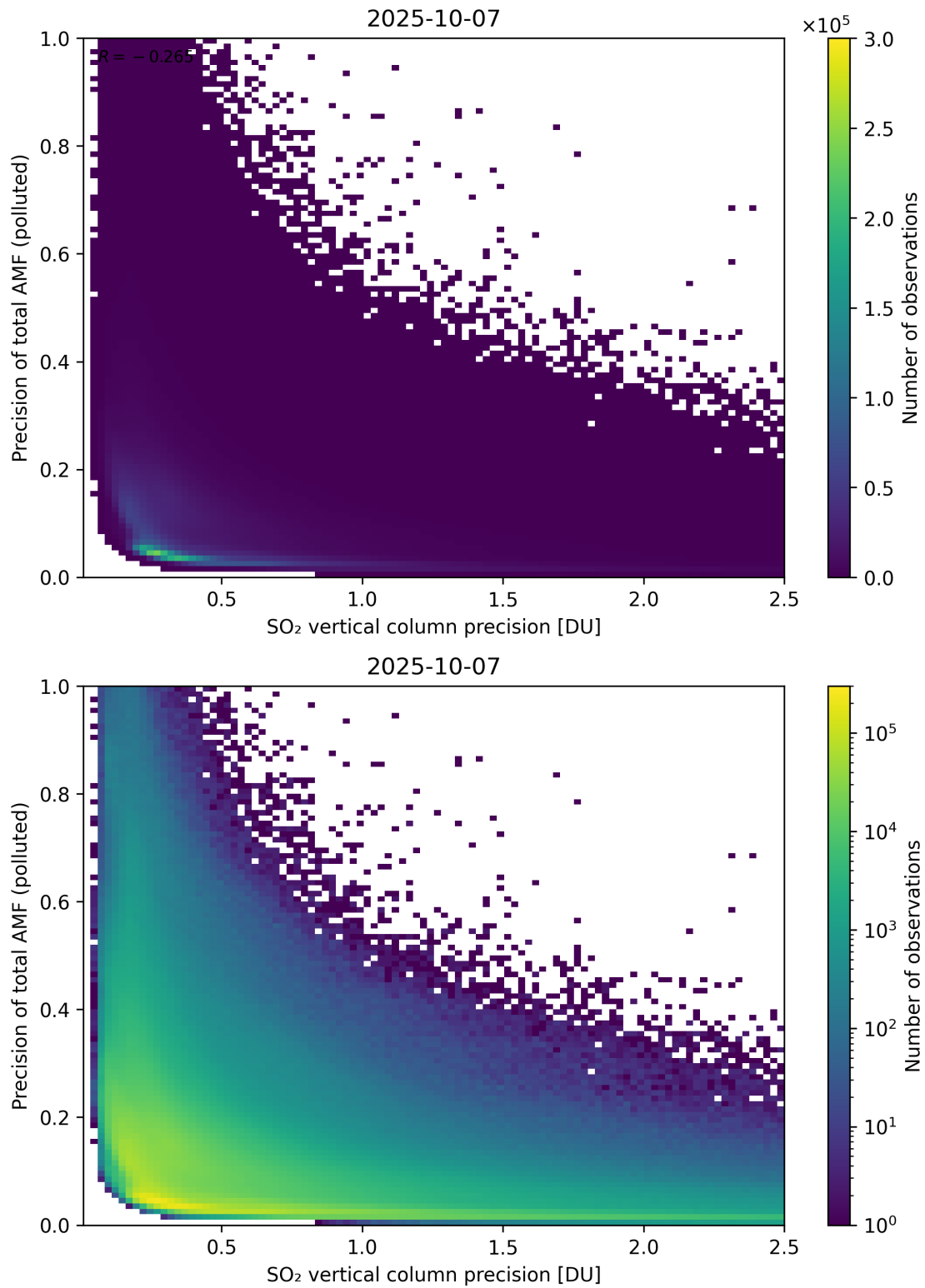
Figure 347: Scatter density plot of “SO 2 vertical column precision” against “Precision of total AMF (polluted)” for 2025-10-06 to 2025-10-08.
