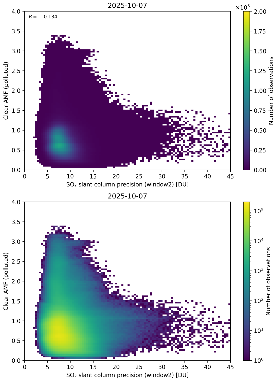
Figure 296: Scatter density plot of “SO 2 slant column precision (window2)” against “Clear AMF (polluted)” for 2025-10-06 to 2025-10-08.
