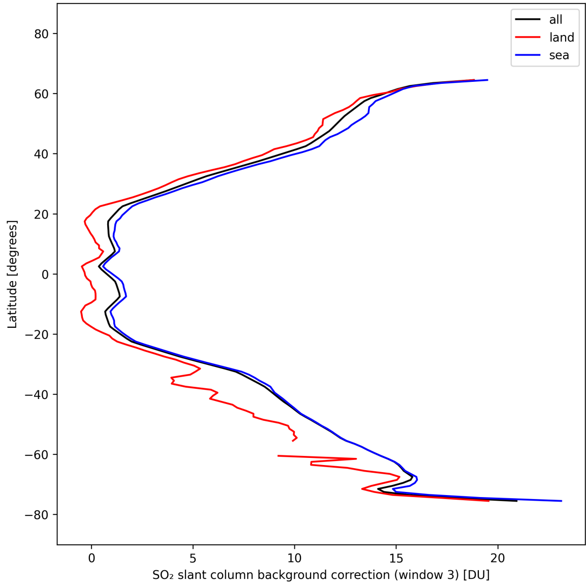
Figure 48: Zonal average of “SO 2 slant column background correction (window 3)” for 2025-10-06 to 2025-10-08.
