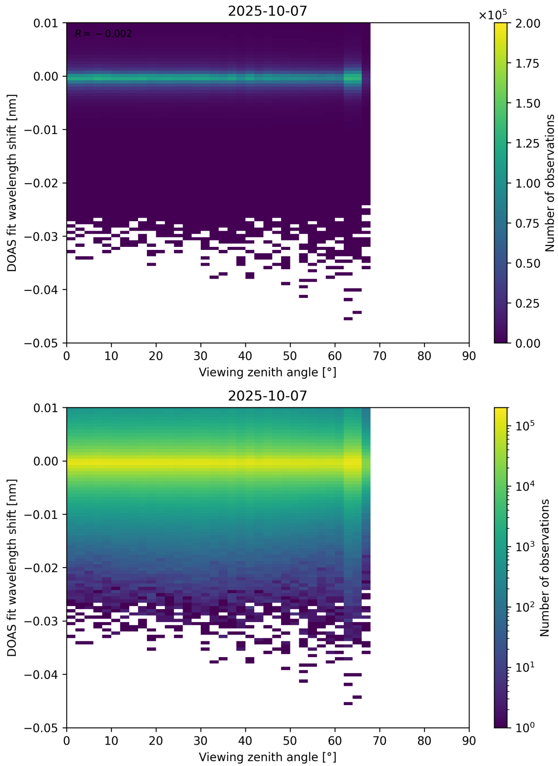
Figure 365: Scatter density plot of “Viewing zenith angle” against “DOAS fit wavelength shift” for 2025-10-06 to 2025-10-08.
