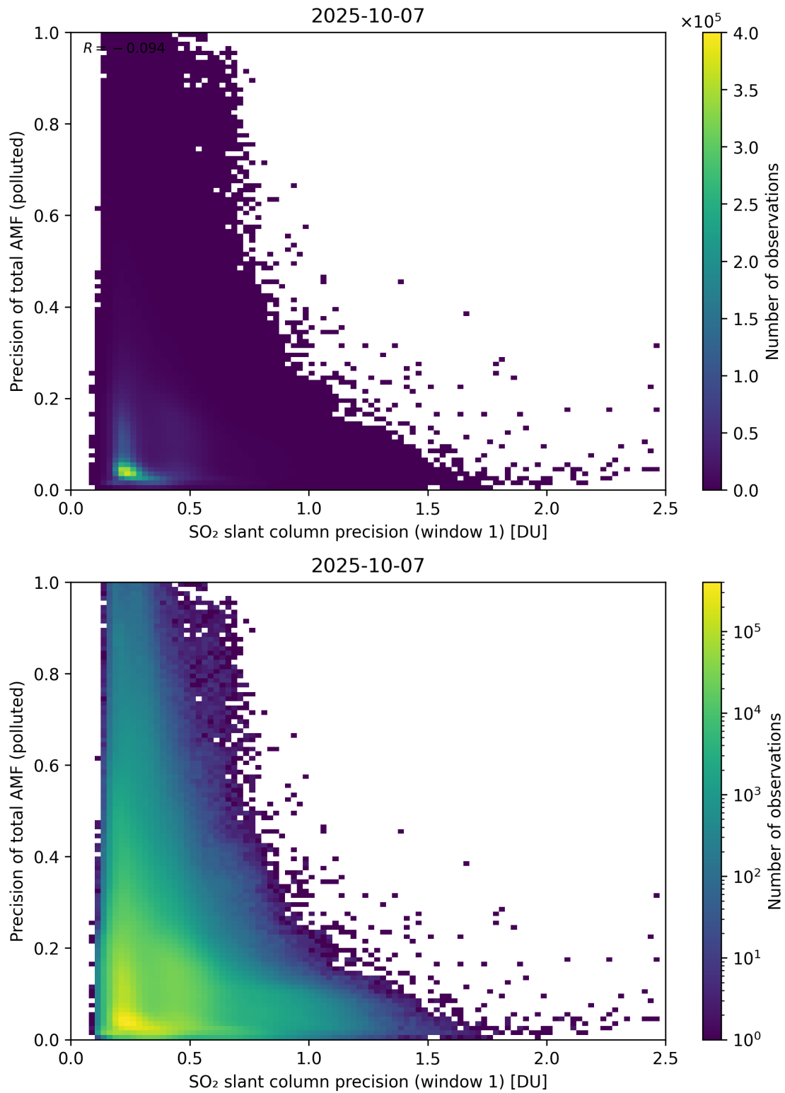
Figure 281: Scatter density plot of “SO 2 slant column precision (window 1)” against “Precision of total AMF (polluted)” for 2025-10-06 to 2025-10-08.
