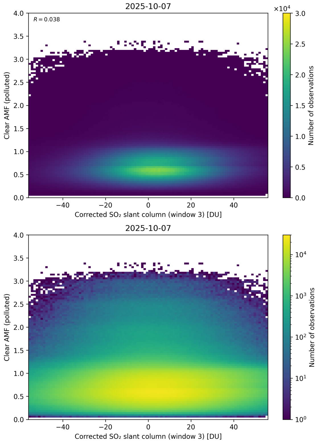
Figure 259: Scatter density plot of “Corrected SO 2 slant column (window 3)” against “Clear AMF (polluted)” for 2025-10-06 to 2025-10-08.
