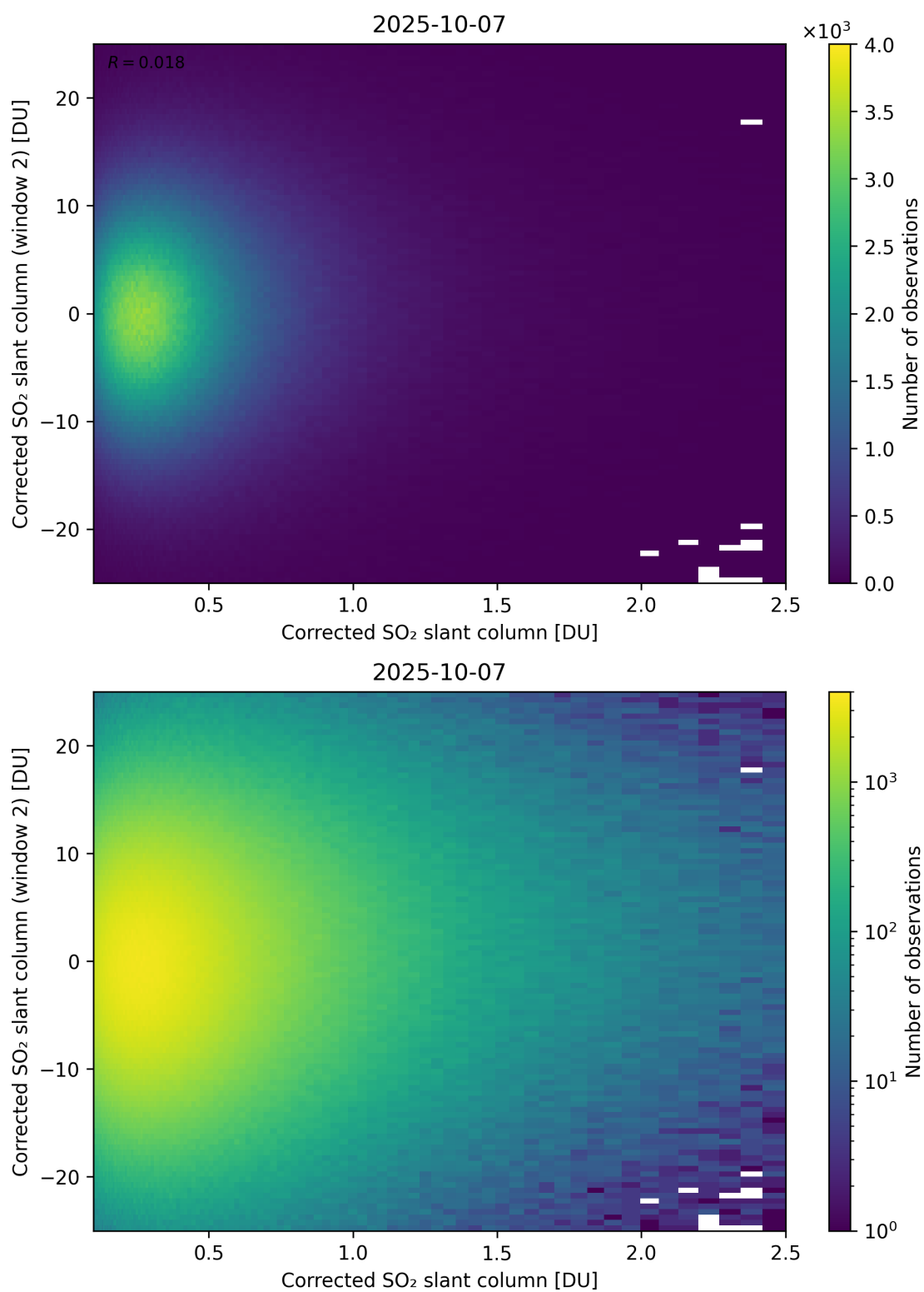
Figure 235: Scatter density plot of “Corrected SO 2 slant column” against “Corrected SO 2 slant column (window 2)” for 2025-10-06 to 2025-10-08.
