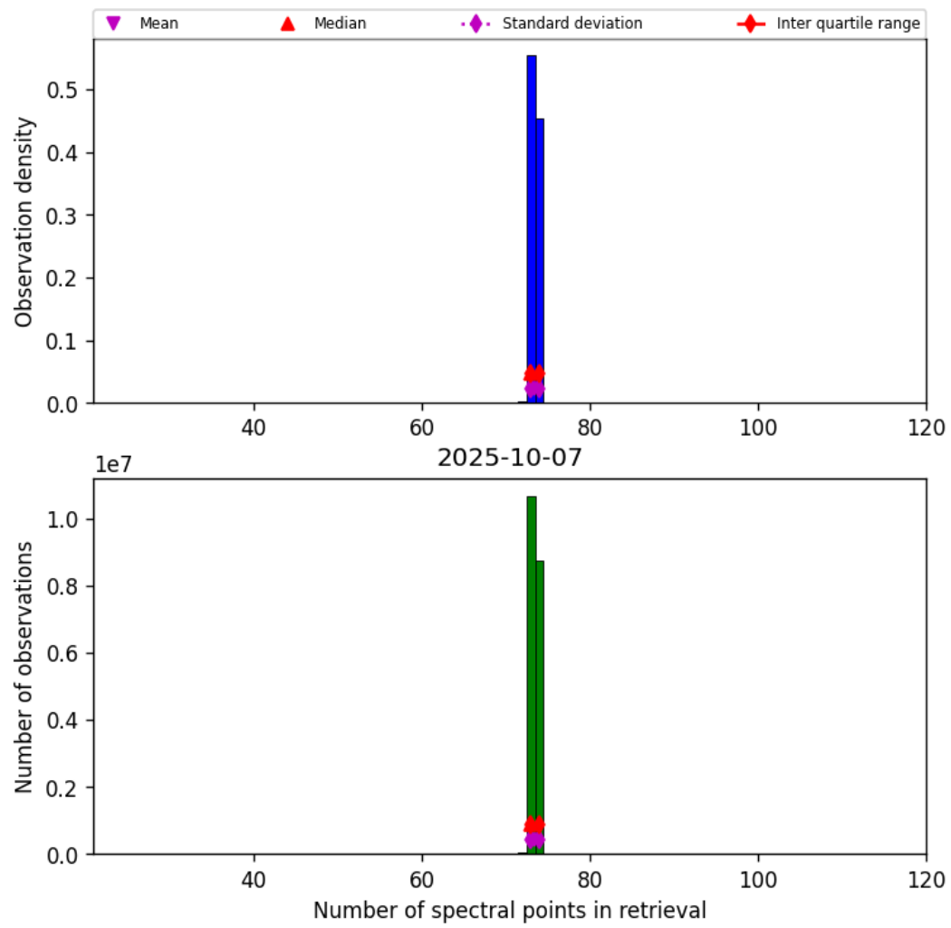
Figure 82: Histogram of “Number of spectral points in retrieval” for 2025-10-06 to 2025-10-08
