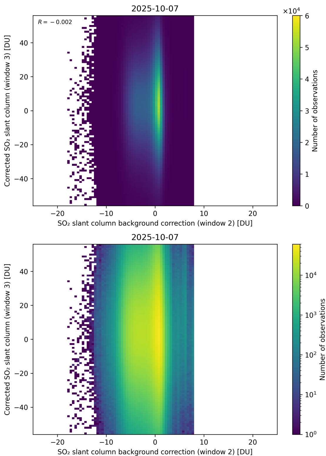
Figure 127: Scatter density plot of “SO 2 slant column background correction (window 2)” against “Corrected SO 2 slant column (window 3)” for 2025-10-06 to 2025-10-08.
