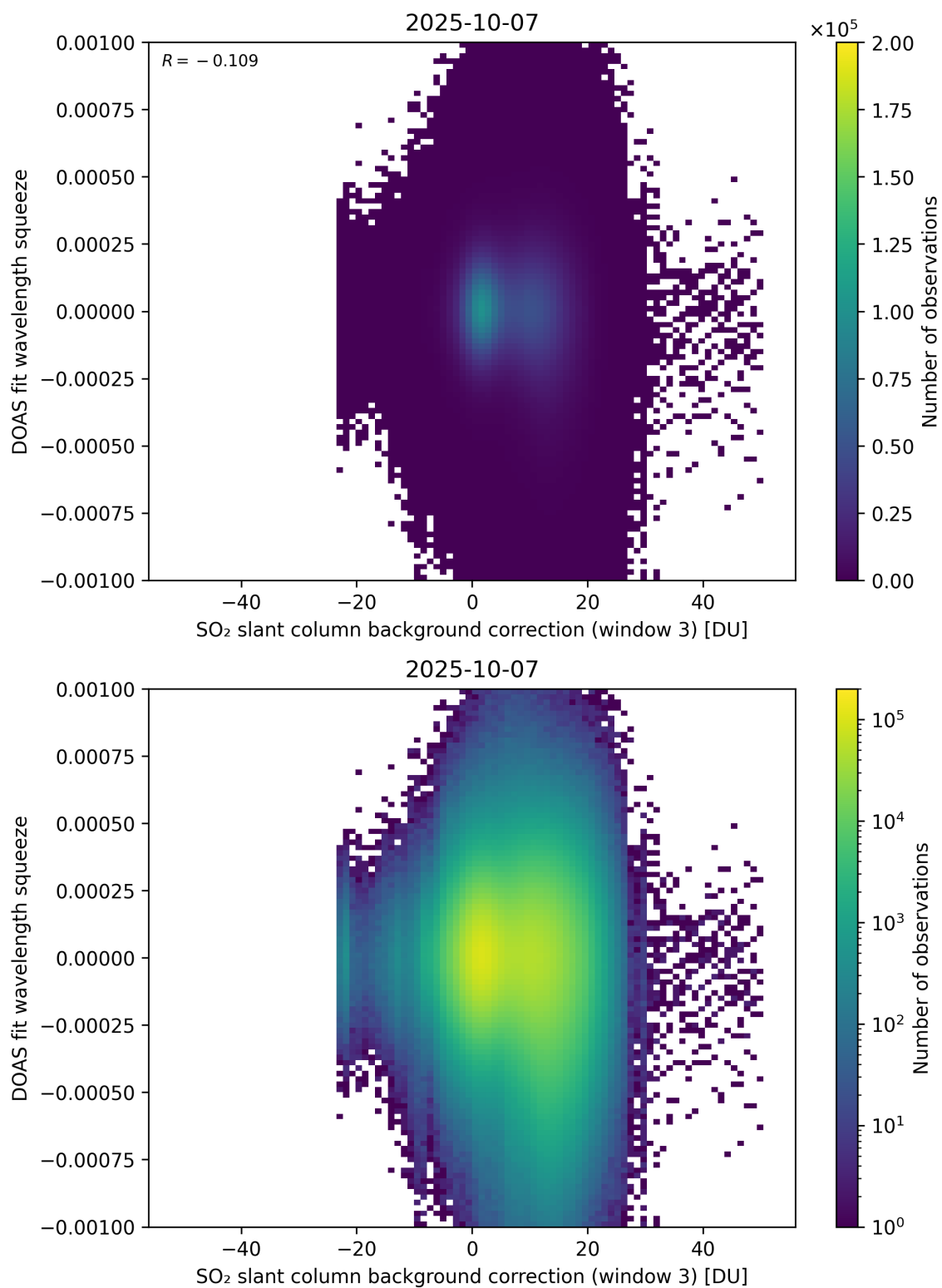
Figure 133: Scatter density plot of “SO 2 slant column background correction (window 3)” against “DOAS fit wavelength squeeze” for 2025-10-06 to 2025-10-08.
