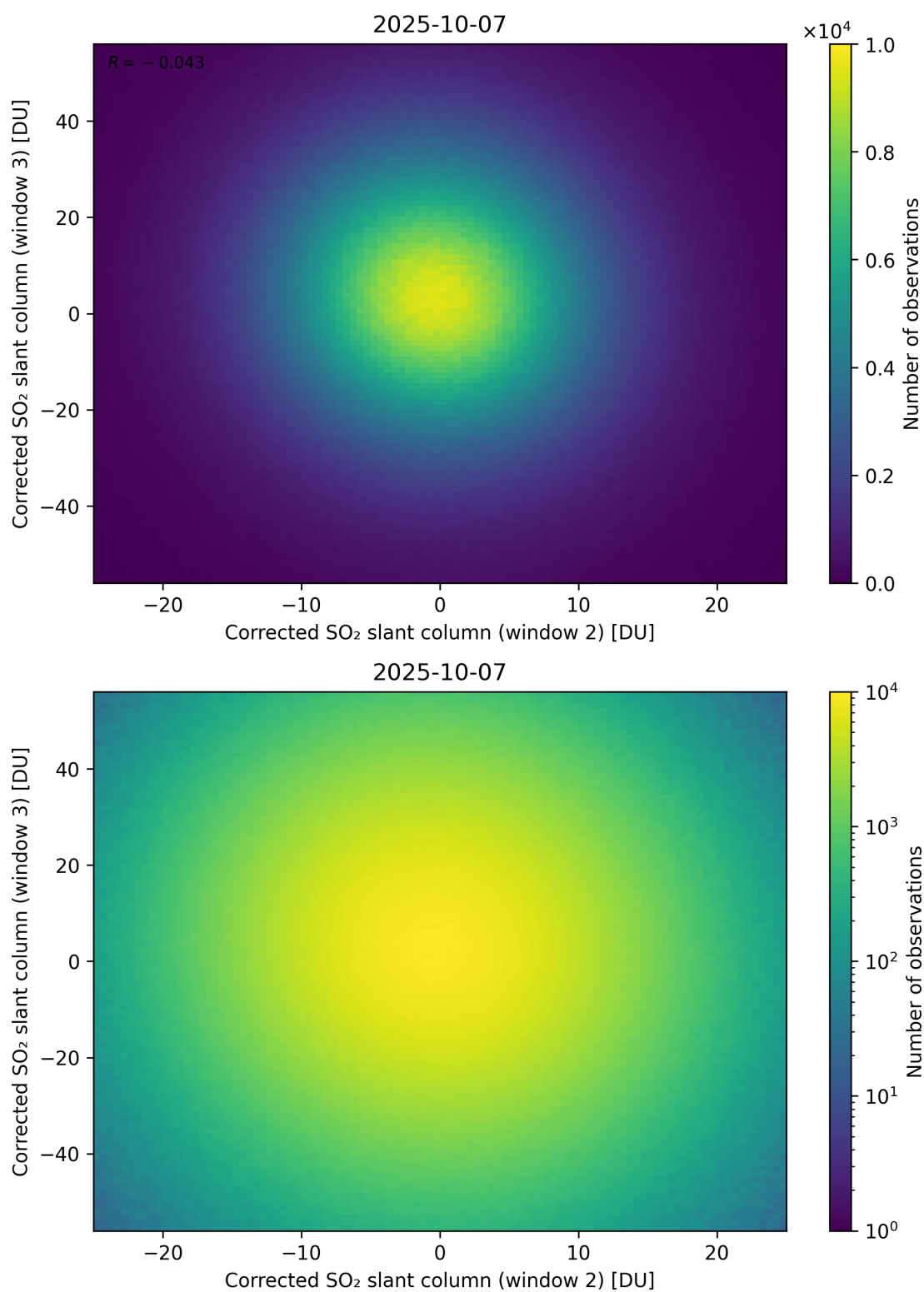
Figure 250: Scatter density plot of “Corrected SO 2 slant column (window 2)” against “Corrected SO 2 slant column (window 3)” for 2025-10-06 to 2025-10-08.
