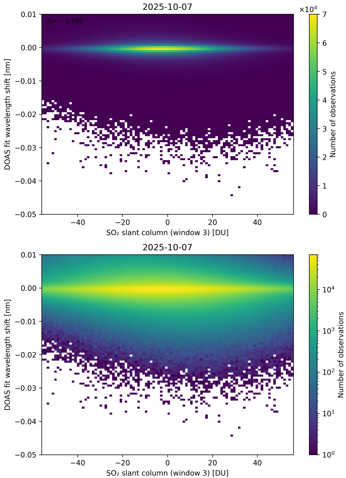
Figure 304: Scatter density plot of “SO 2 slant column (window 3)” against “DOAS fit wavelength shift” for 2025-10-06 to 2025-10-08.
