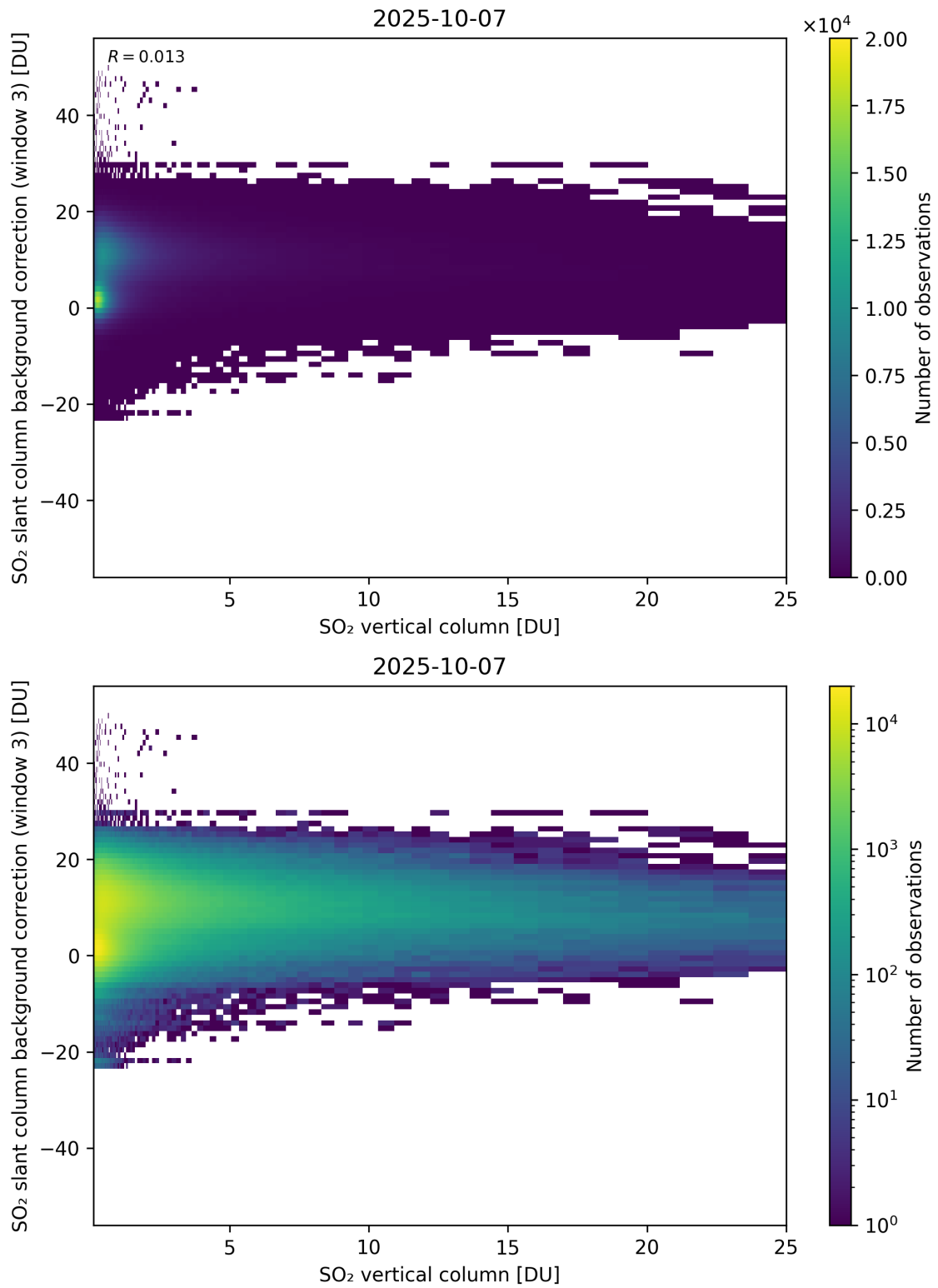
Figure 325: Scatter density plot of “SO 2 vertical column” against “SO 2 slant column background correction (window 3)” for 2025-10-06 to 2025-10-08.
