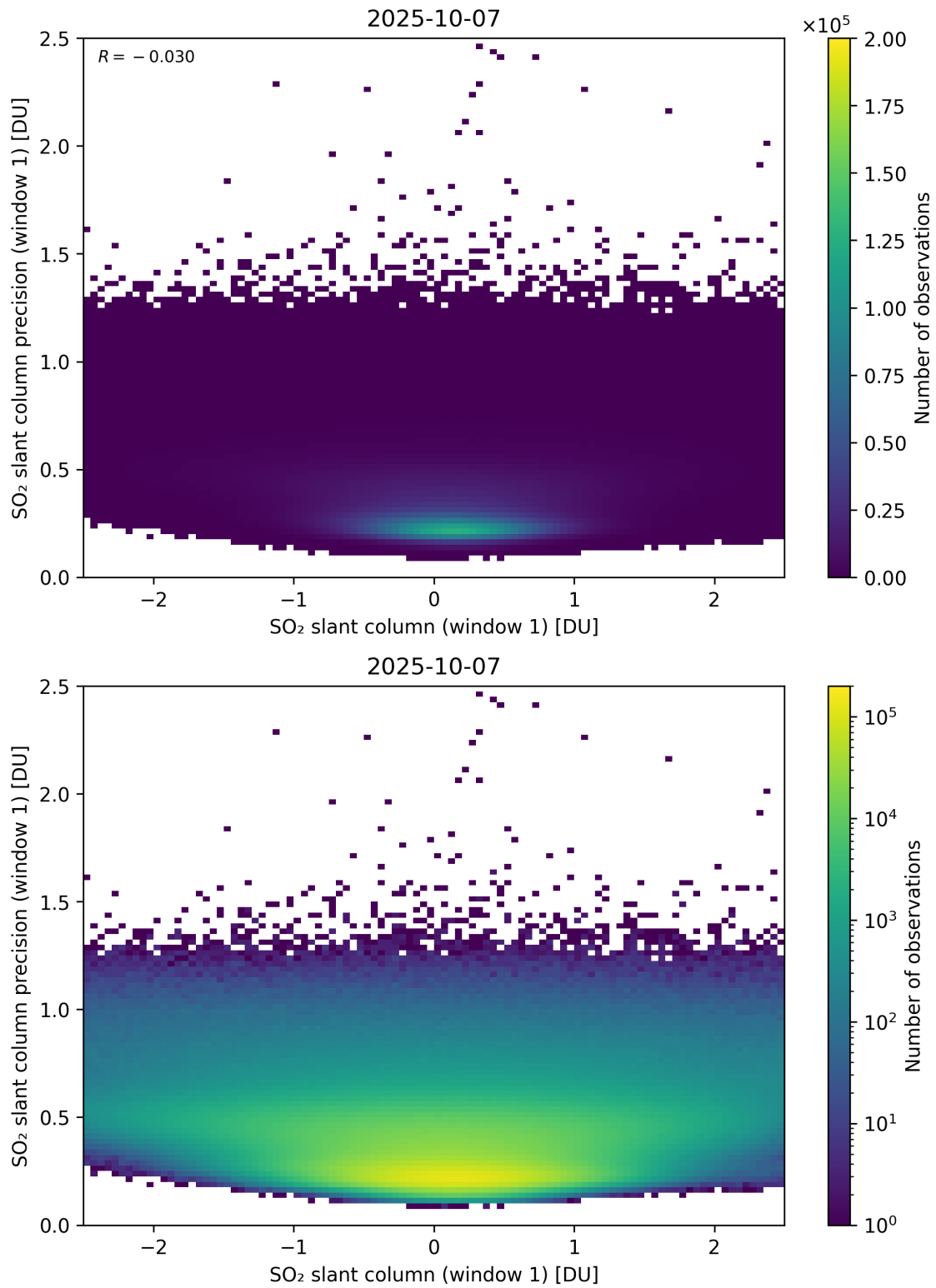
Figure 285: Scatter density plot of “SO 2 slant column (window 1)” against “SO 2 slant column precision (window 1)” for 2025-10-06 to 2025-10-08.
