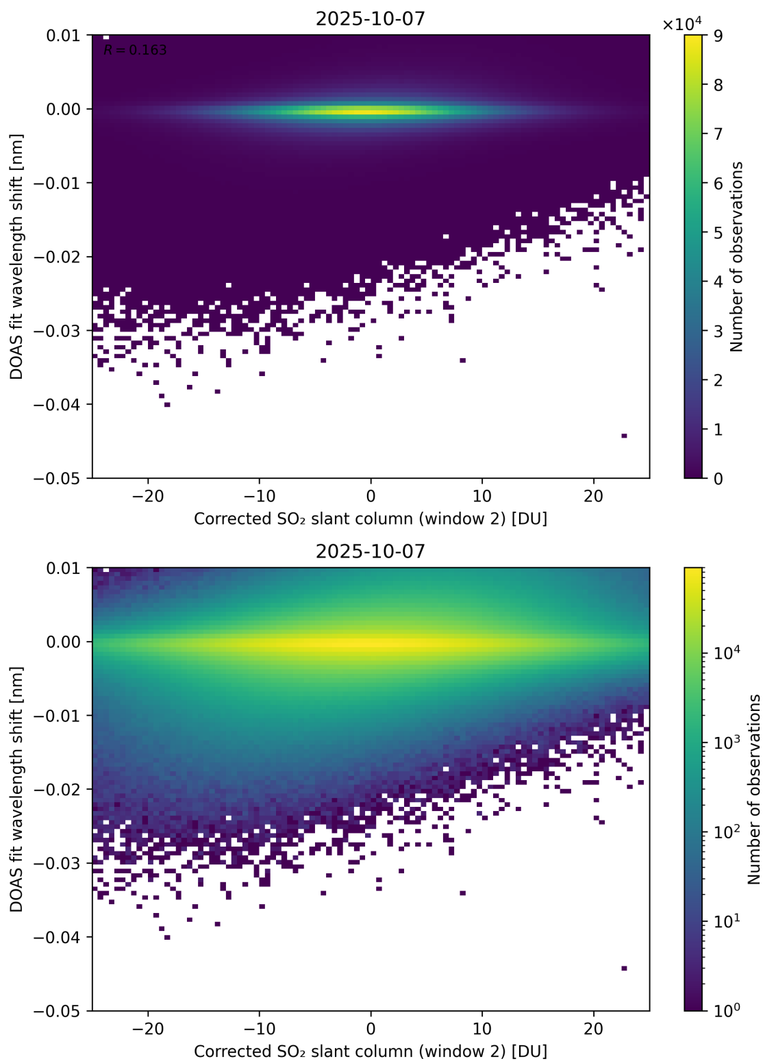
Figure 246: Scatter density plot of “Corrected SO 2 slant column (window 2)” against “DOAS fit wavelength shift” for 2025-10-06 to 2025-10-08.
