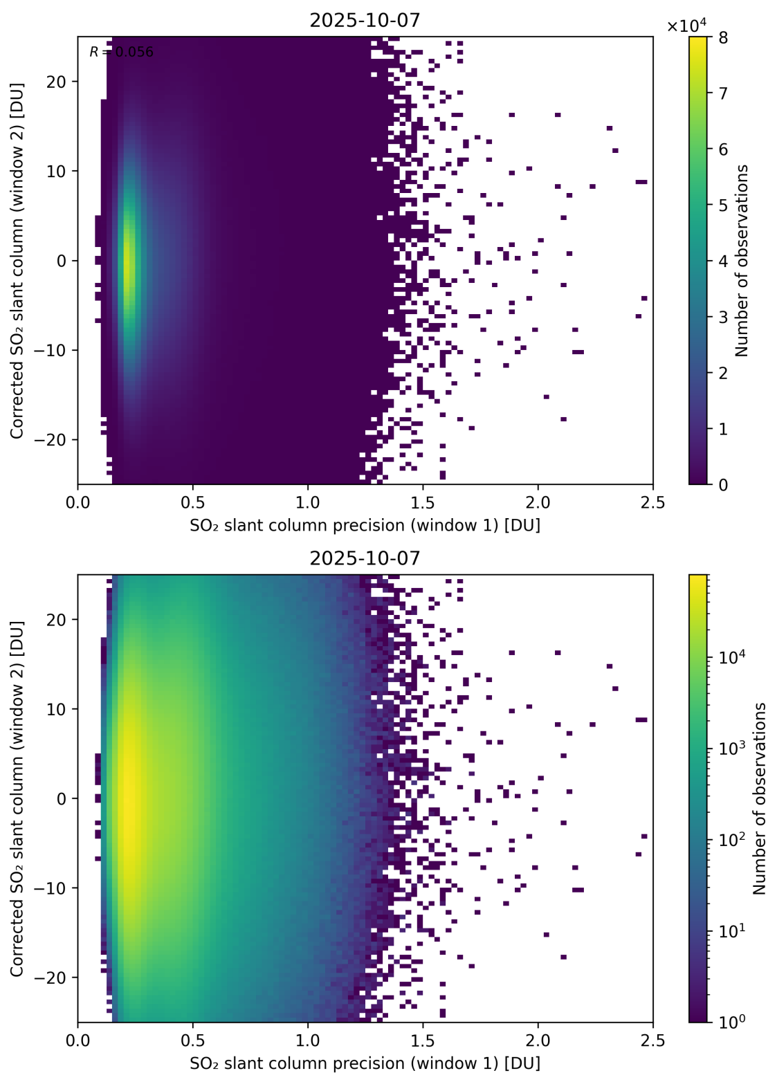
Figure 275: Scatter density plot of “SO 2 slant column precision (window 1)” against “Corrected SO 2 slant column (window 2)” for 2025-10-06 to 2025-10-08.
