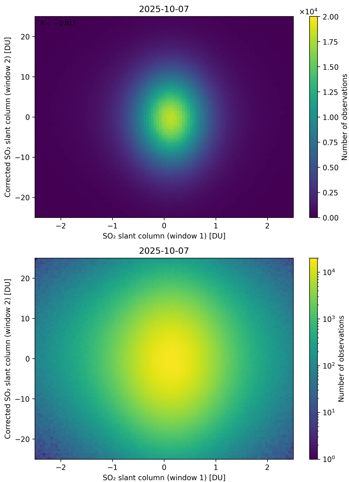
Figure 283: Scatter density plot of “SO 2 slant column (window 1)” against “Corrected SO 2 slant column (window 2)” for 2025-10-06 to 2025-10-08.
