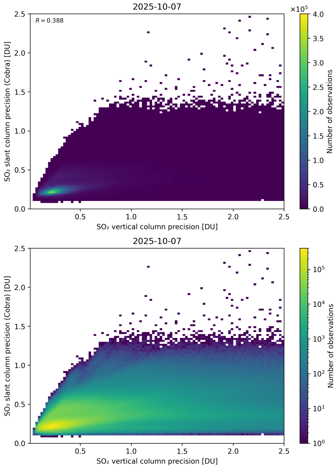
Figure 337: Scatter density plot of “SO 2 vertical column precision” against “SO 2 slant column precision (Cobra)” for 2025-10-06 to 2025-10-08.
