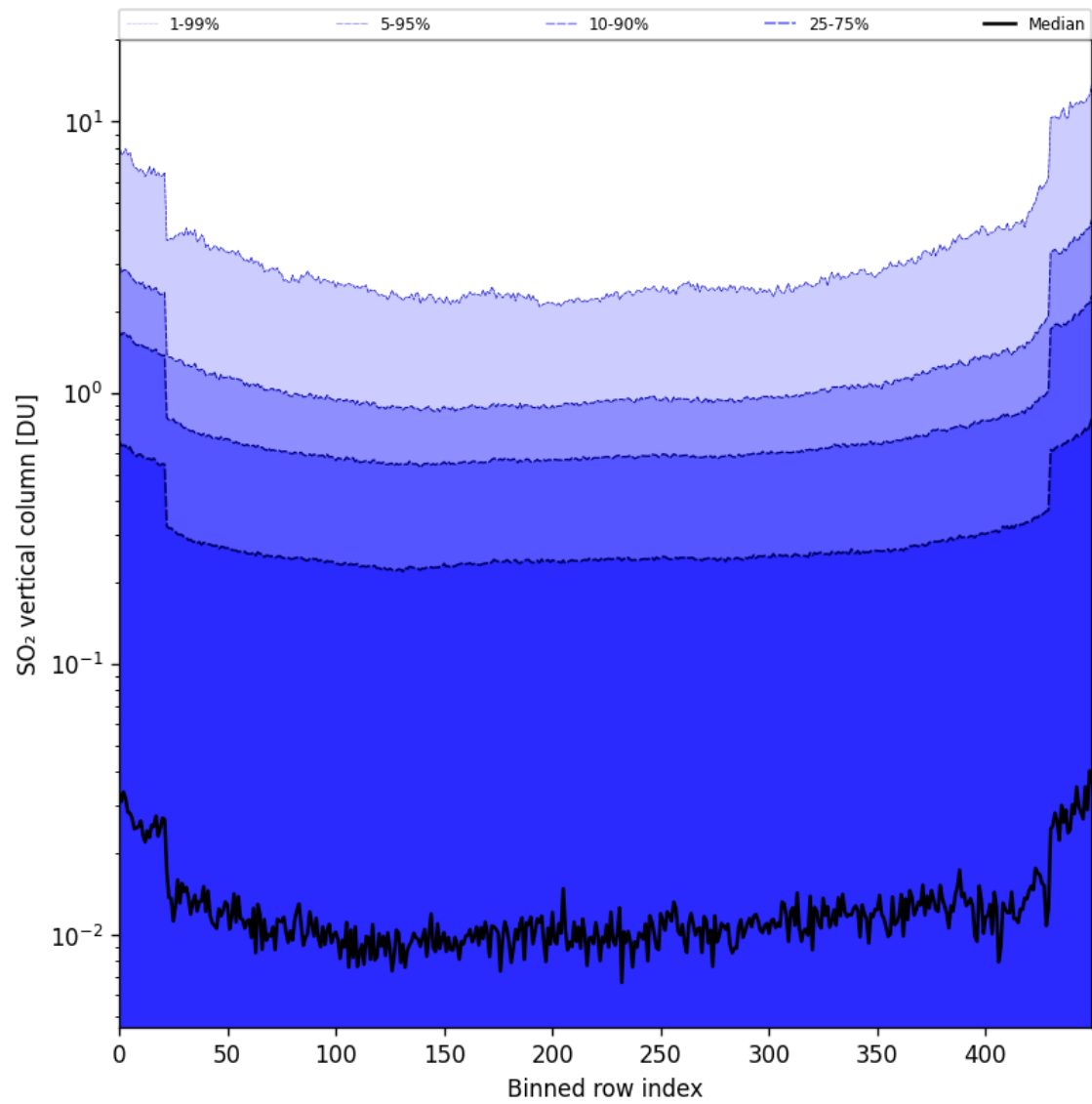
Figure 84: Along track statistics of “SO 2 vertical column” for 2025-10-06 to 2025-10-08
