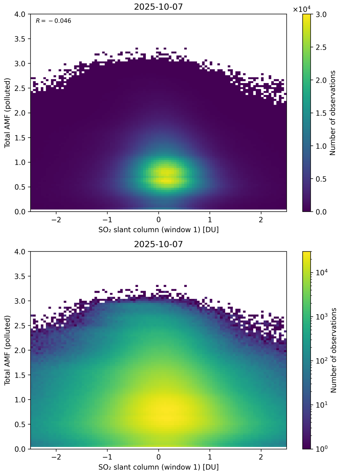
Figure 289: Scatter density plot of “SO 2 slant column (window 1)” against “Total AMF (polluted)” for 2025-10-06 to 2025-10-08.
