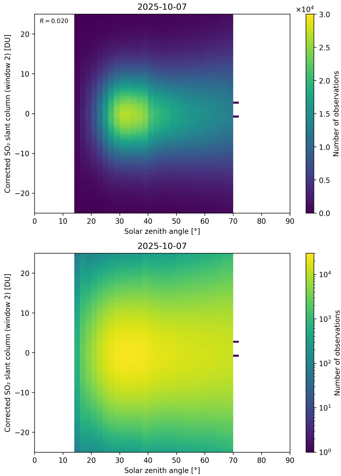
Figure 182: Scatter density plot of “Solar zenith angle” against “Corrected SO 2 slant column (window 2)” for 2025-10-06 to 2025-10-08.
