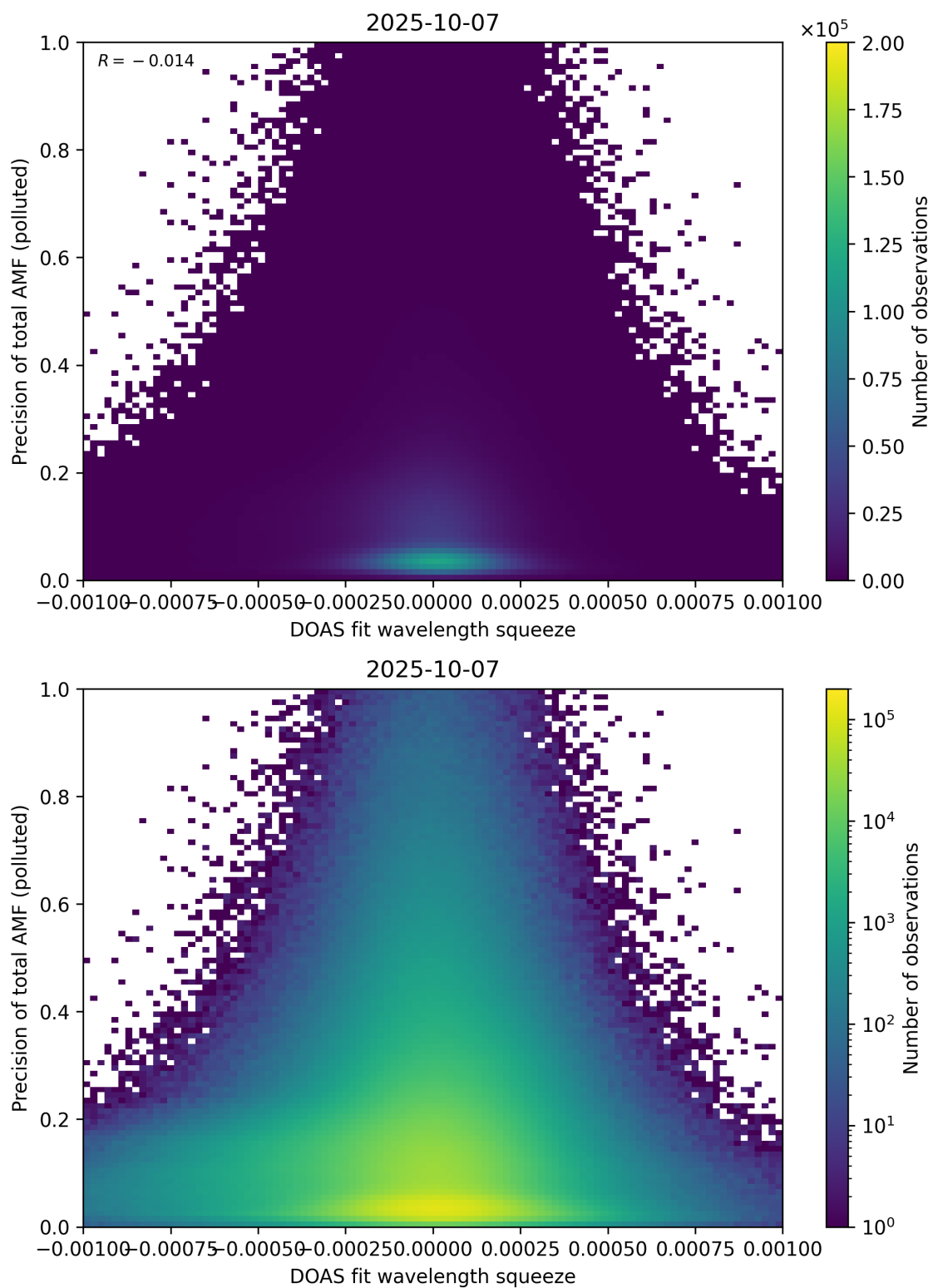
Figure 146: Scatter density plot of “DOAS fit wavelength squeeze” against “Precision of total AMF (polluted)” for 2025-10-06 to 2025-10-08.
