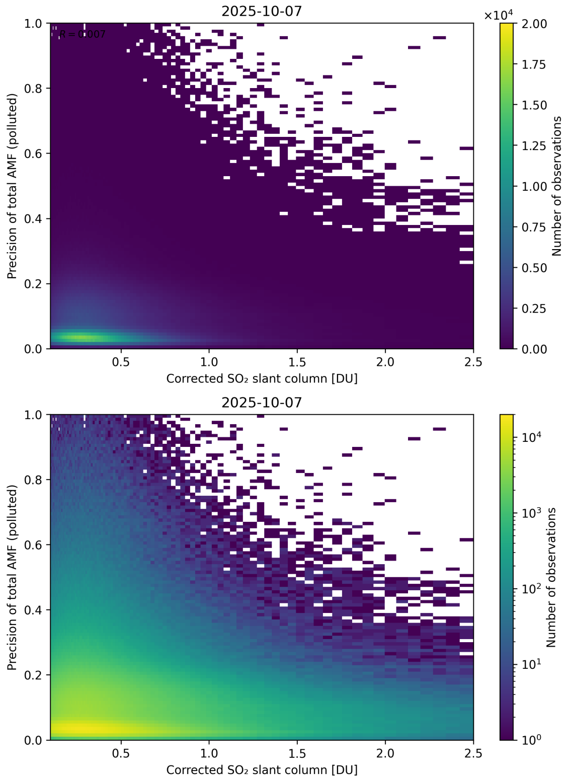
Figure 243: Scatter density plot of “Corrected SO 2 slant column” against “Precision of total AMF (polluted)” for 2025-10-06 to 2025-10-08.
