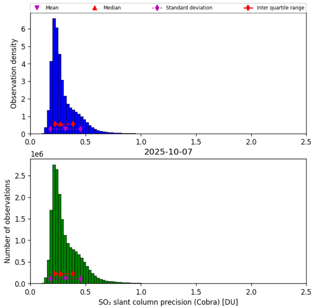
Figure 62: Histogram of “SO 2 slant column precision (Cobra)” for 2025-10-06 to 2025-10-08
