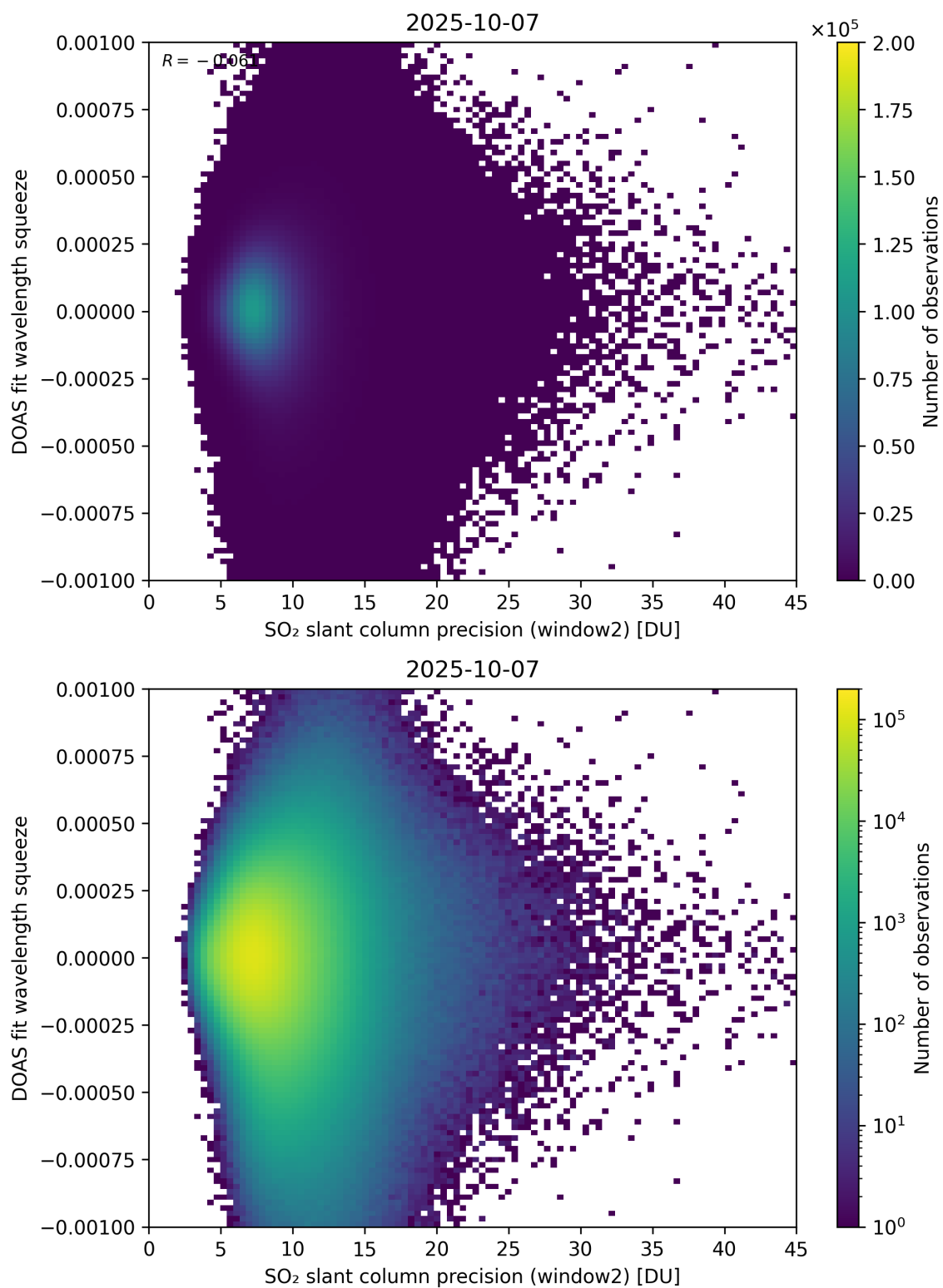
Figure 294: Scatter density plot of “SO 2 slant column precision (window2)” against “DOAS fit wavelength squeeze” for 2025-10-06 to 2025-10-08.
