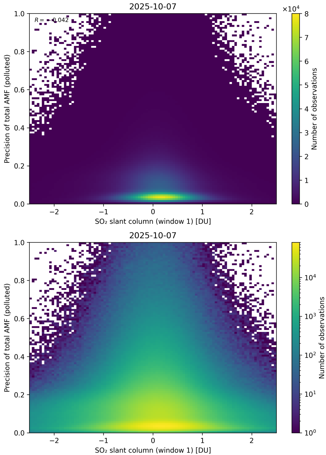
Figure 290: Scatter density plot of “SO 2 slant column (window 1)” against “Precision of total AMF (polluted)” for 2025-10-06 to 2025-10-08.
