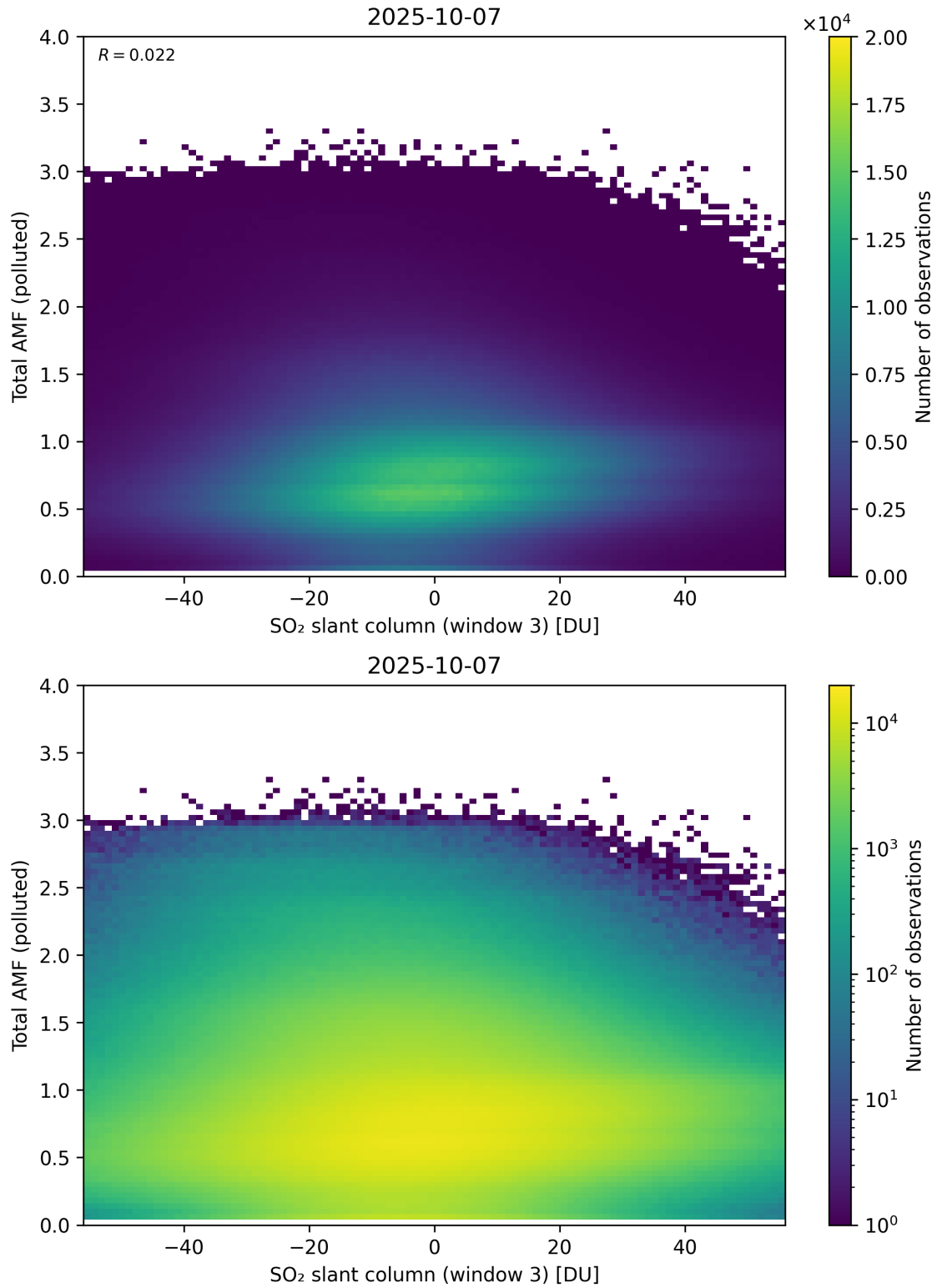
Figure 318: Scatter density plot of “SO 2 slant column (window 3)” against “Total AMF (polluted)” for 2025-10-06 to 2025-10-08.
