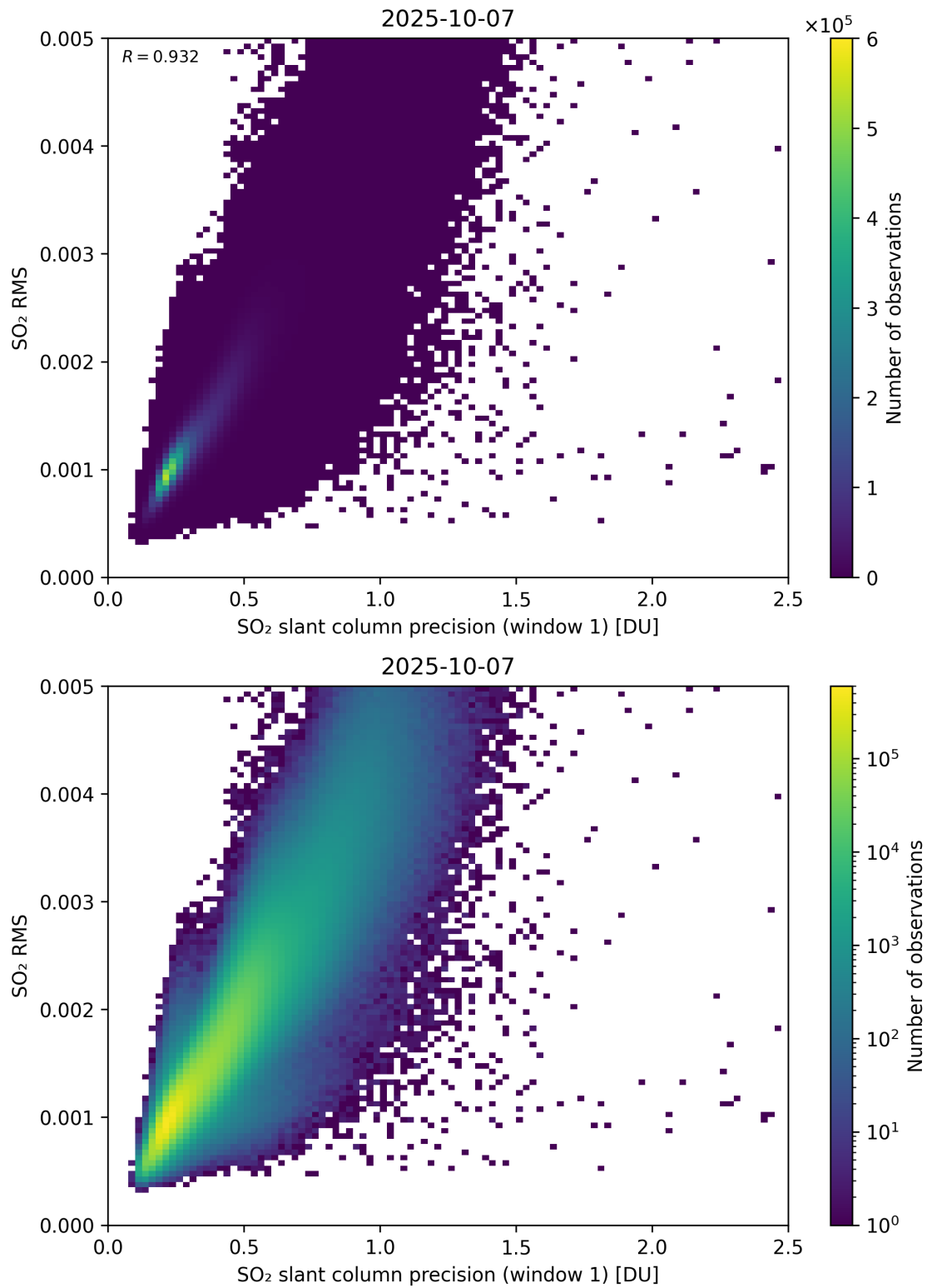
Figure 273: Scatter density plot of “SO 2 slant column precision (window 1)” against “SO 2 RMS” for 2025-10-06 to 2025-10-08.
