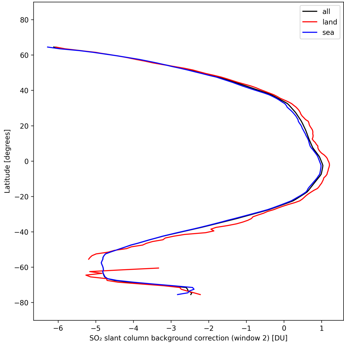
Figure 44: Zonal average of “SO 2 slant column background correction (window 2)” for 2025-10-06 to 2025-10-08.
