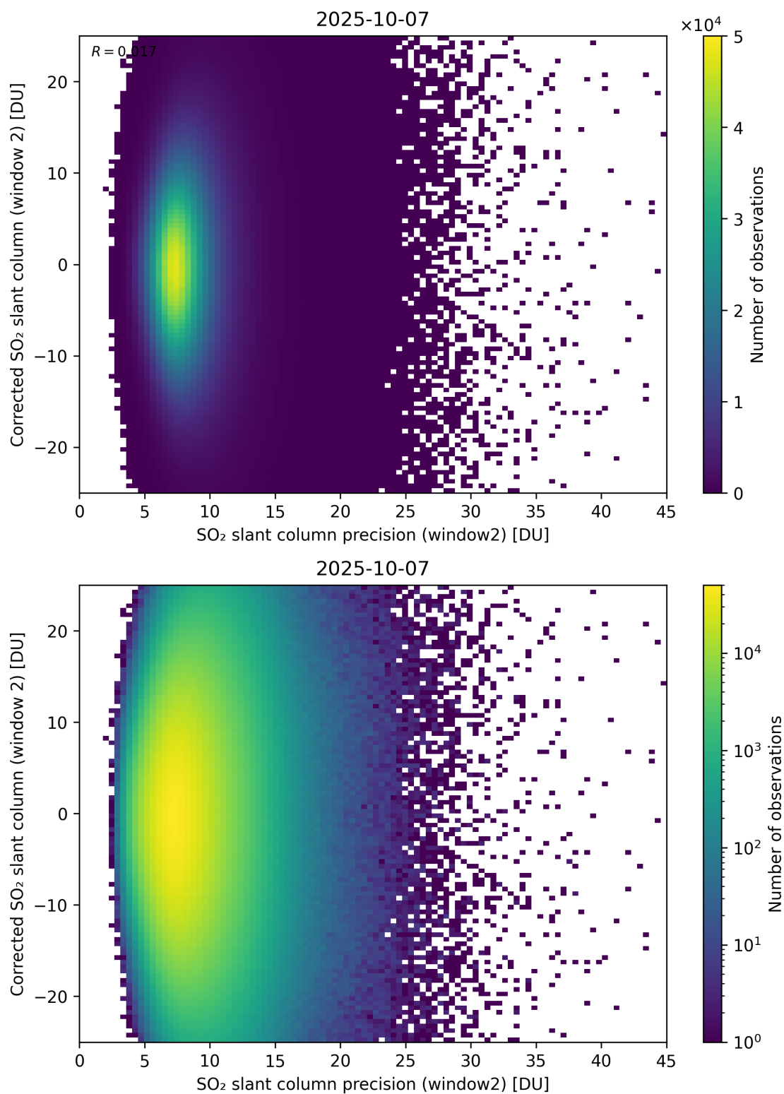
Figure 297: Scatter density plot of “SO 2 slant column precision (window2)” against “Corrected SO 2 slant column (window 2)” for 2025-10-06 to 2025-10-08.
