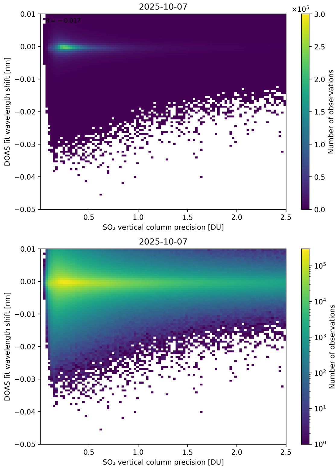
Figure 332: Scatter density plot of “SO 2 vertical column precision” against “DOAS fit wavelength shift” for 2025-10-06 to 2025-10-08.
