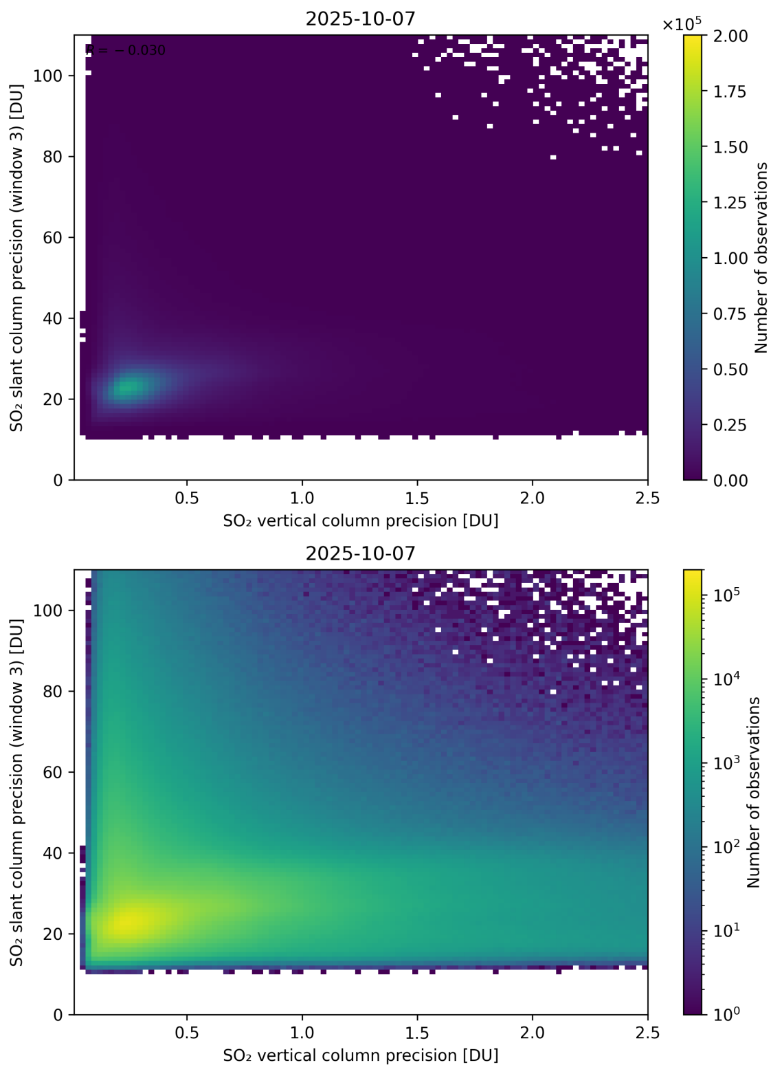
Figure 345: Scatter density plot of “SO 2 vertical column precision” against “SO 2 slant column precision (window 3)” for 2025-10-06 to 2025-10-08.
