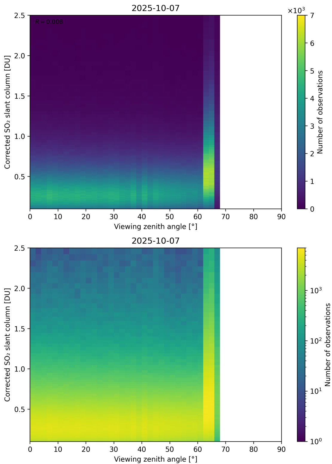
Figure 373: Scatter density plot of “Viewing zenith angle” against “Corrected SO 2 slant column” for 2025-10-06 to 2025-10-08.
