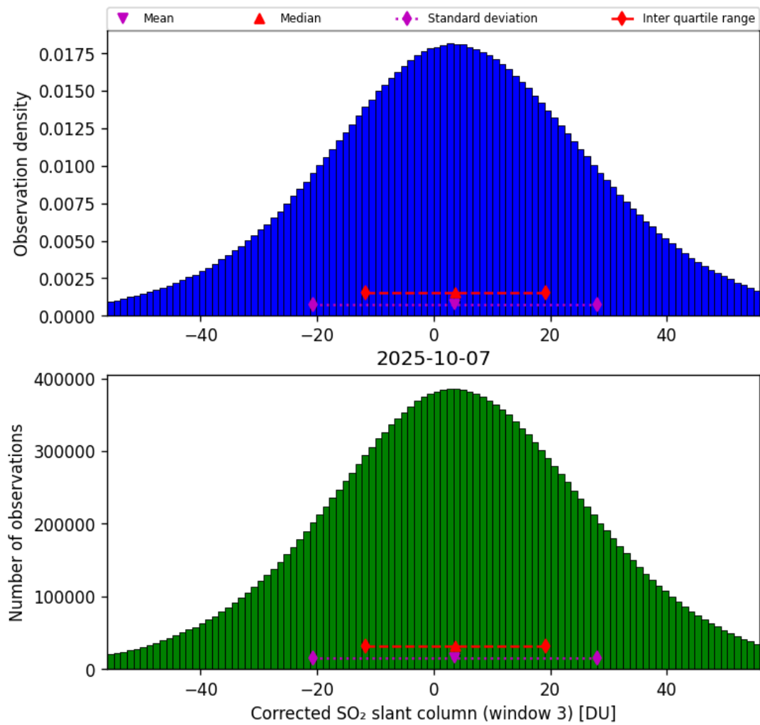
Figure 73: Histogram of “Corrected SO 2 slant column (window 3)” for 2025-10-06 to 2025-10-08
