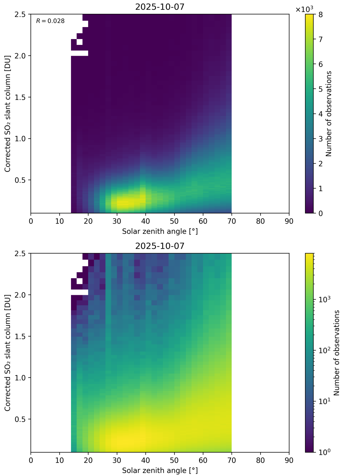
Figure 181: Scatter density plot of “Solar zenith angle” against “Corrected SO 2 slant column” for 2025-10-06 to 2025-10-08.
