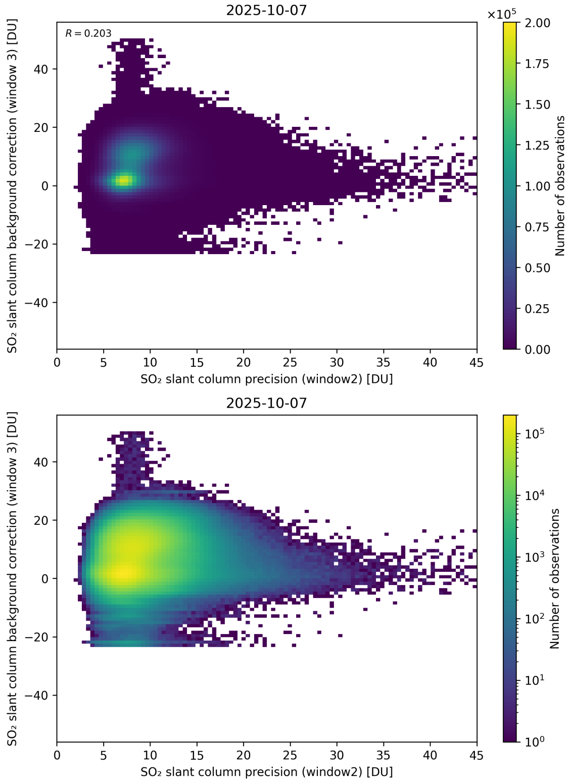
Figure 292: Scatter density plot of “SO 2 slant column precision (window2)” against “SO 2 slant column background correction (window 3)” for 2025-10-06 to 2025-10-08.
