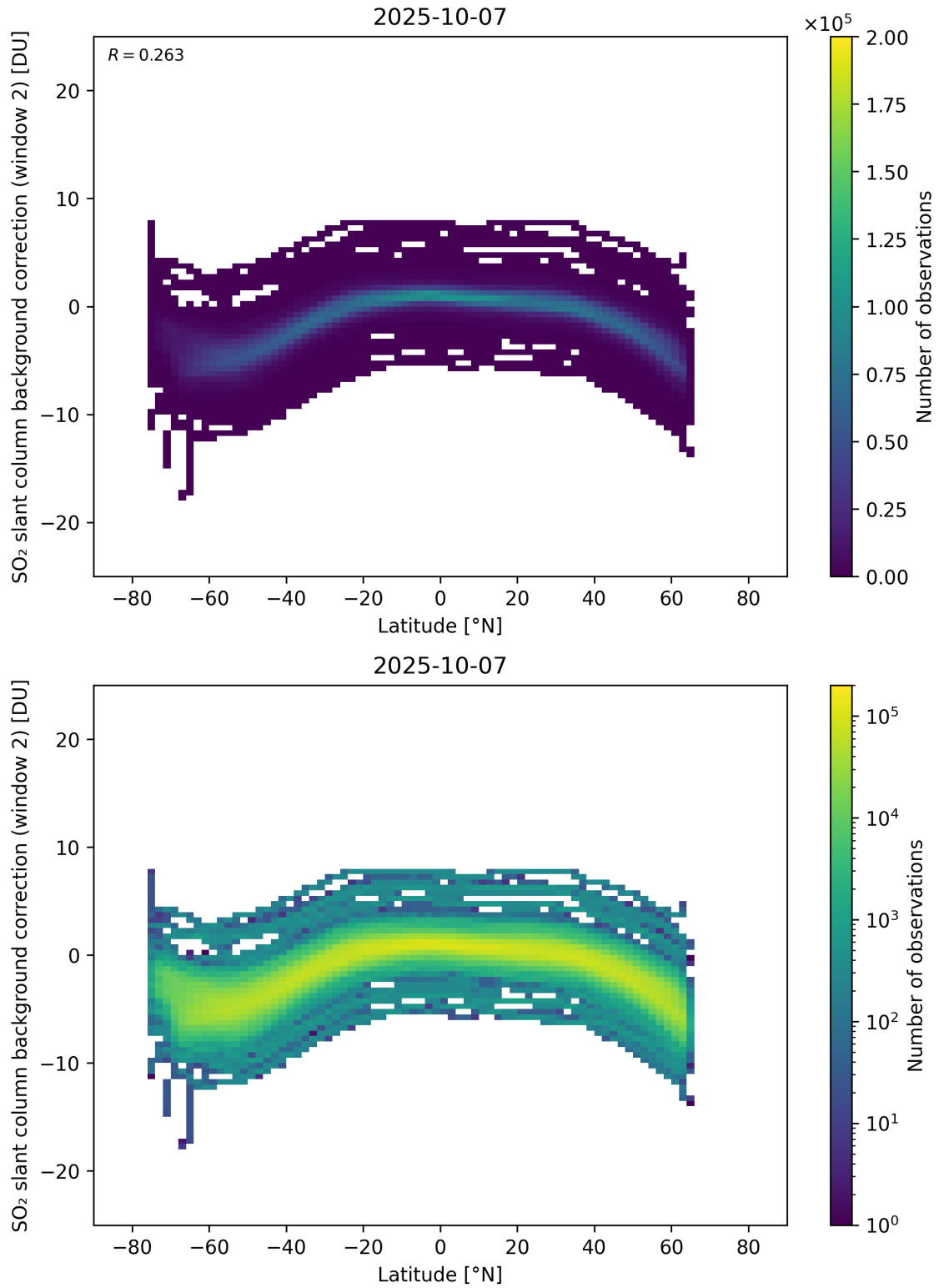
Figure 151: Scatter density plot of “Latitude” against “SO 2 slant column background correction (window 2)” for 2025-10-06 to 2025-10-08.
