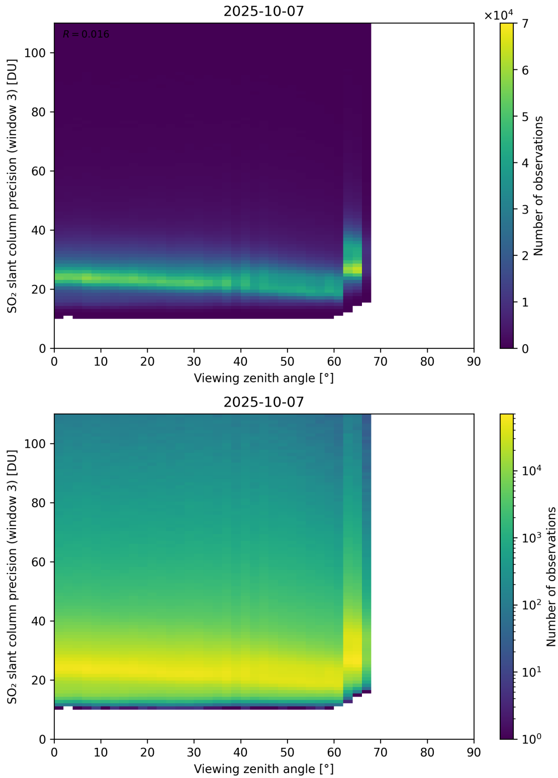
Figure 380: Scatter density plot of “Viewing zenith angle” against “SO 2 slant column precision (window 3)” for 2025-10-06 to 2025-10-08.
