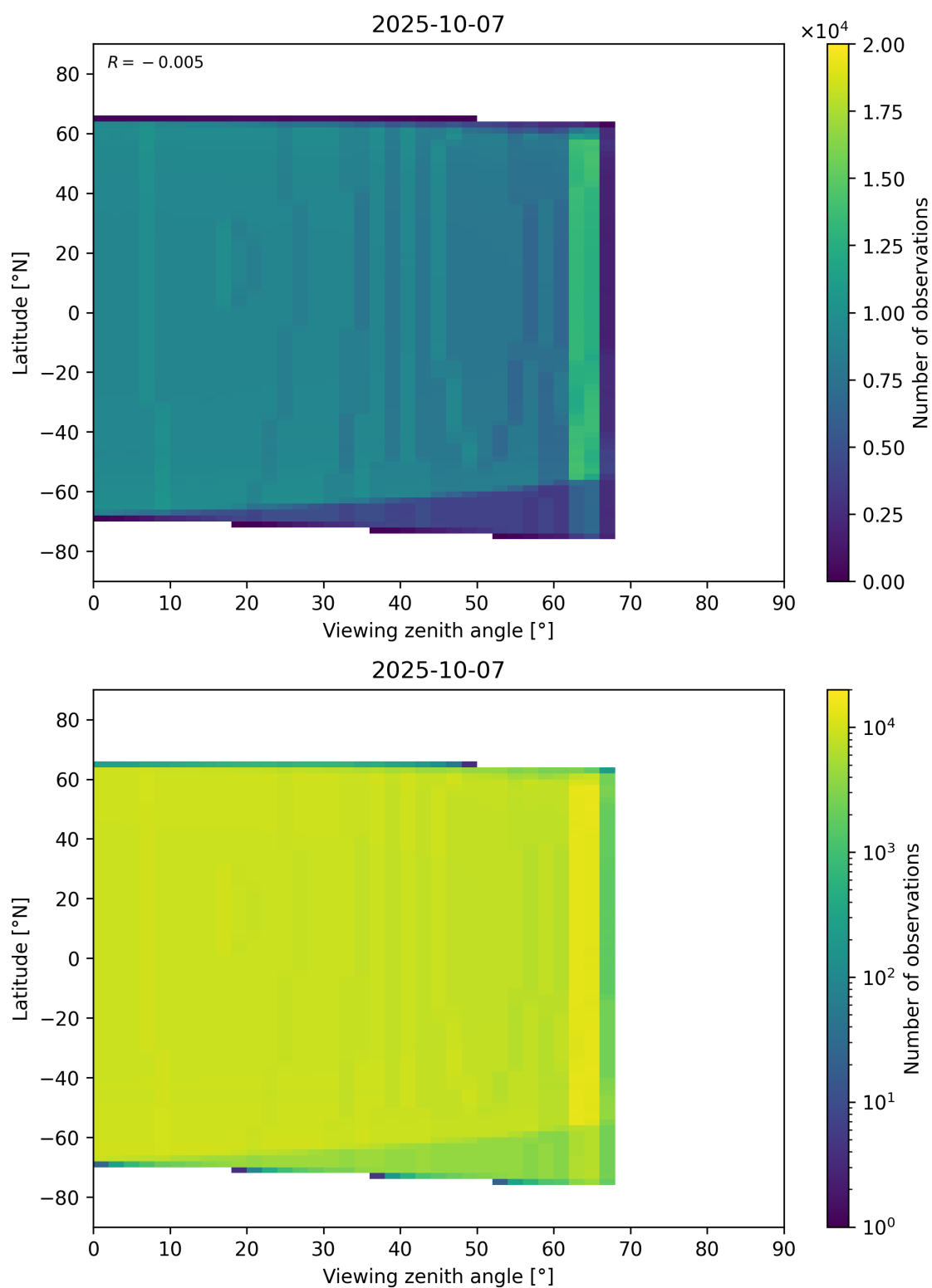
Figure 368: Scatter density plot of “Viewing zenith angle” against “Latitude” for 2025-10-06 to 2025-10-08.
