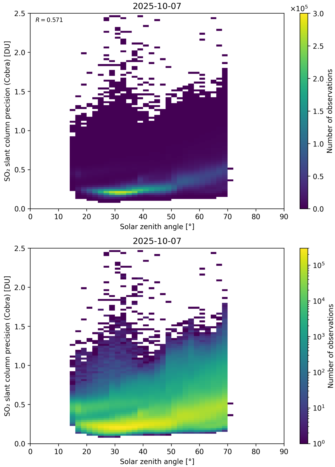
Figure 180: Scatter density plot of “Solar zenith angle” against “SO 2 slant column precision (Cobra)” for 2025-10-06 to 2025-10-08.
