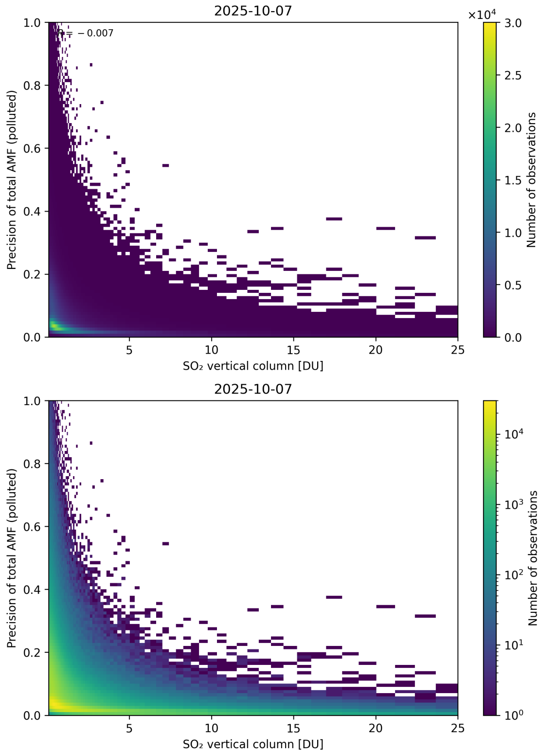
Figure 360: Scatter density plot of “SO 2 vertical column” against “Precision of total AMF (polluted)” for 2025-10-06 to 2025-10-08.
