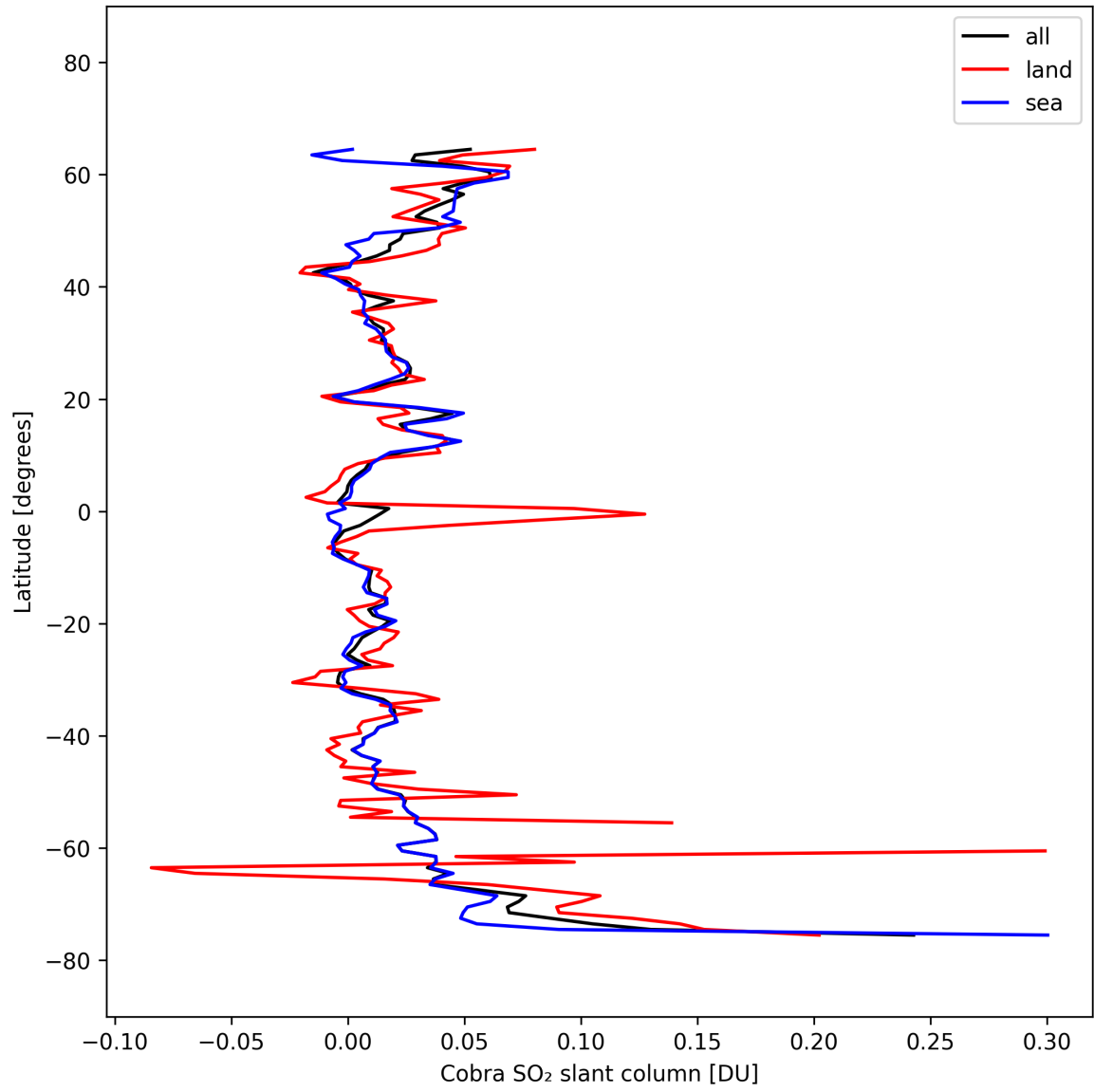
Figure 35: Zonal average of “Cobra SO 2 slant column” for 2025-10-06 to 2025-10-08.
