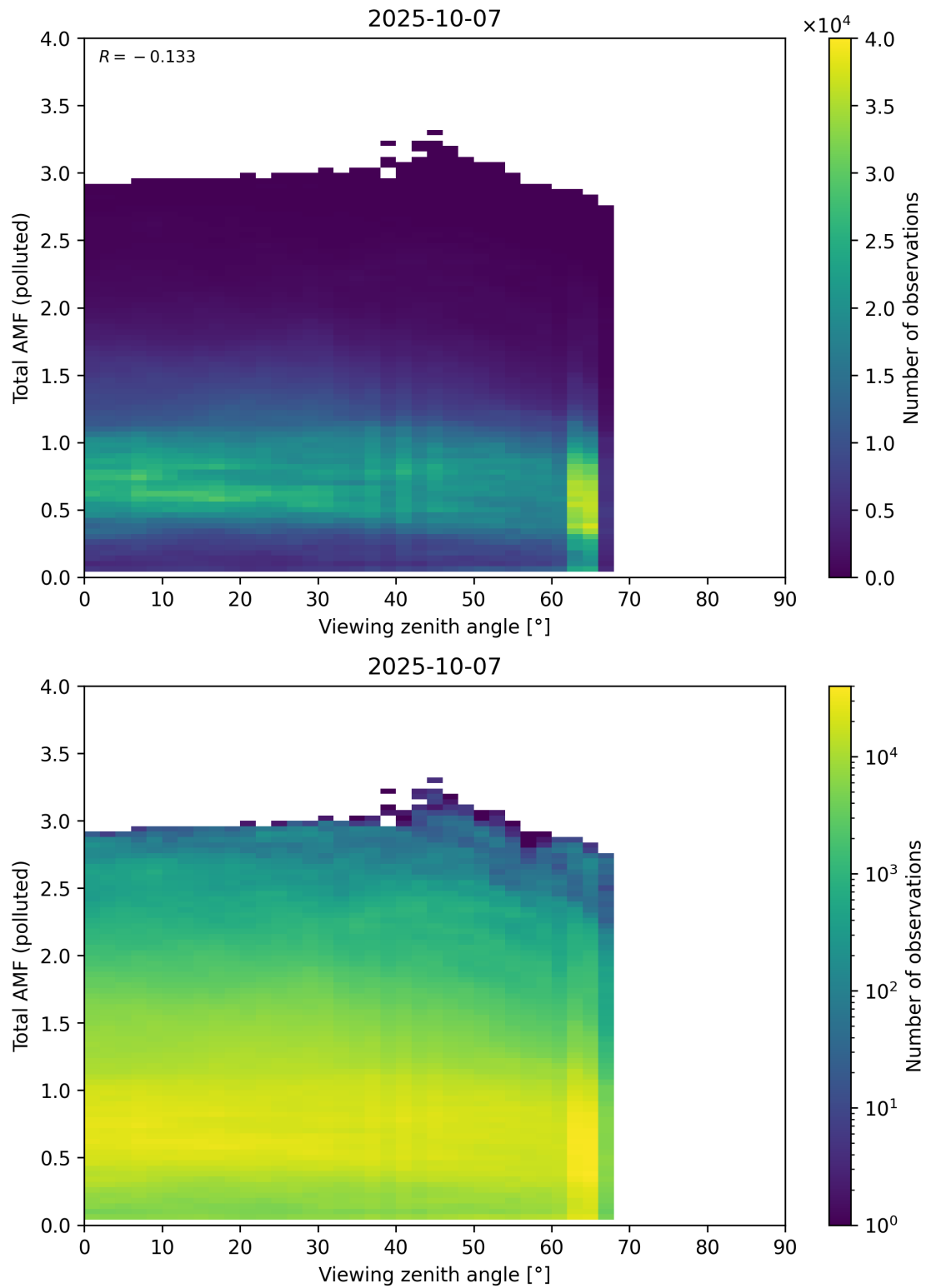
Figure 381: Scatter density plot of “Viewing zenith angle” against “Total AMF (polluted)” for 2025-10-06 to 2025-10-08.
