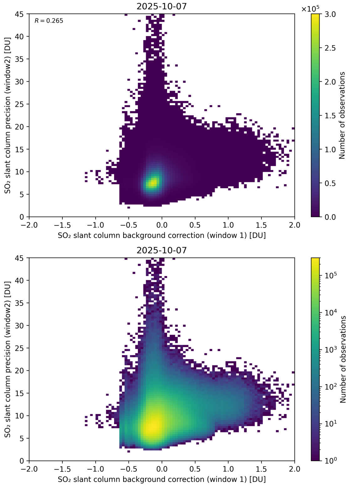
Figure 117: Scatter density plot of “SO 2 slant column background correction (window 1)” against “SO 2 slant column precision (window2)” for 2025-10-06 to 2025-10-08.
