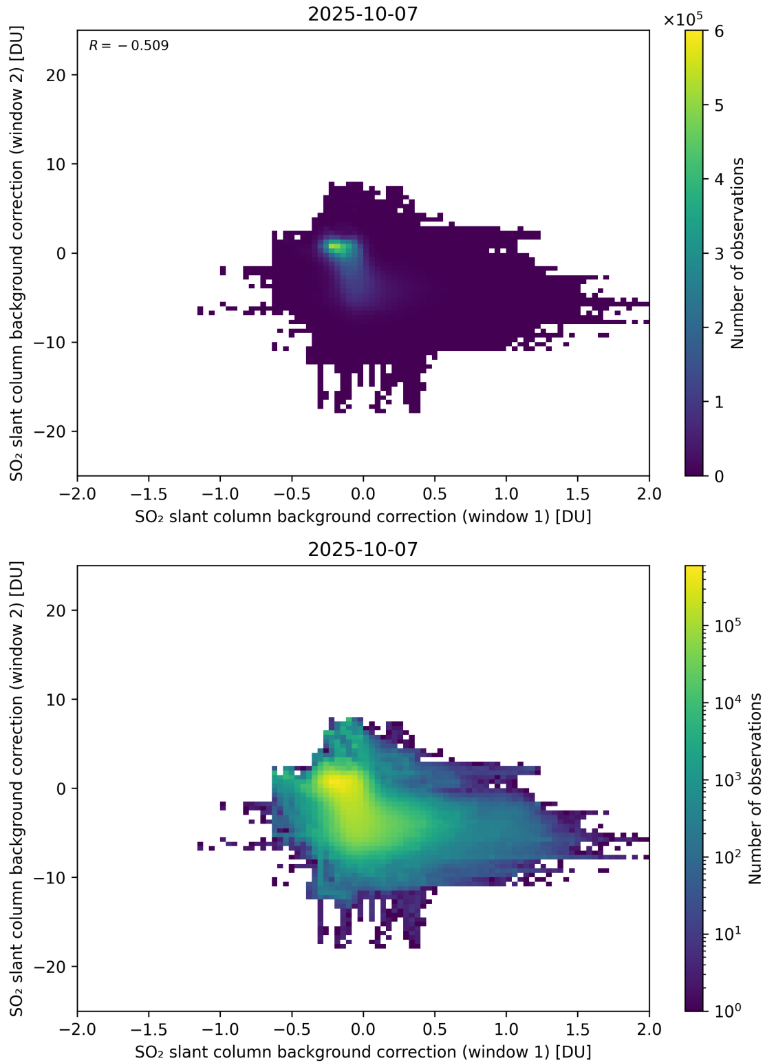
Figure 109: Scatter density plot of “SO 2 slant column background correction (window 1)” against “SO 2 slant column background correction (window 2)” for 2025-10-06 to 2025-10-08.
