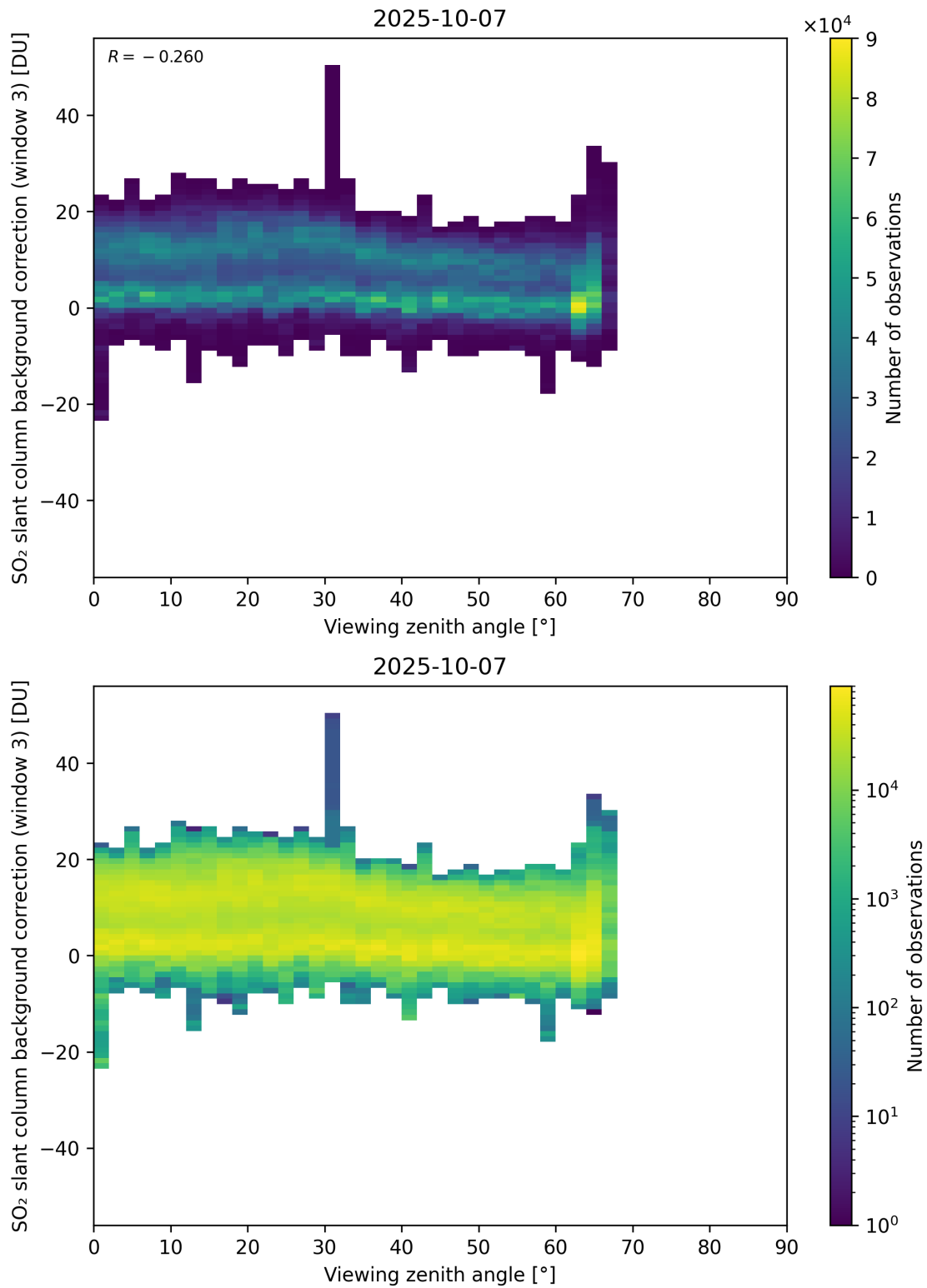
Figure 364: Scatter density plot of “Viewing zenith angle” against “SO 2 slant column background correction (window 3)” for 2025-10-06 to 2025-10-08.
