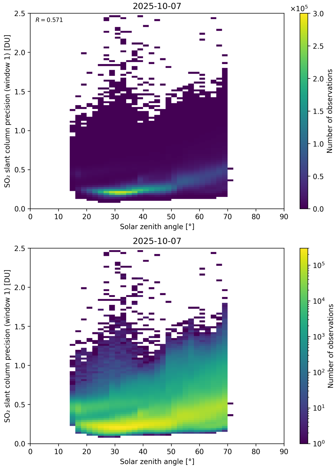
Figure 185: Scatter density plot of “Solar zenith angle” against “SO 2 slant column precision (window 1)” for 2025-10-06 to 2025-10-08.
