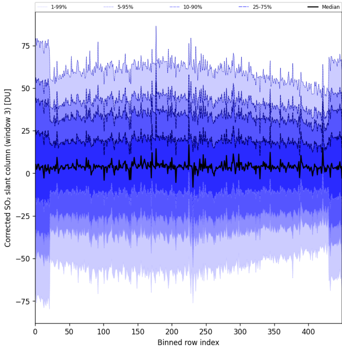
Figure 99: Along track statistics of “Corrected SO 2 slant column (window 3)” for 2025-10-06 to 2025-10-08
