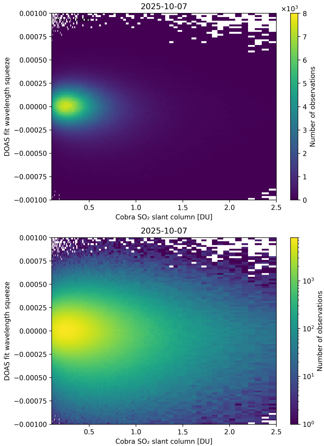
Figure 197: Scatter density plot of “Cobra SO 2 slant column” against “DOAS fit wavelength squeeze” for 2025-10-06 to 2025-10-08.
