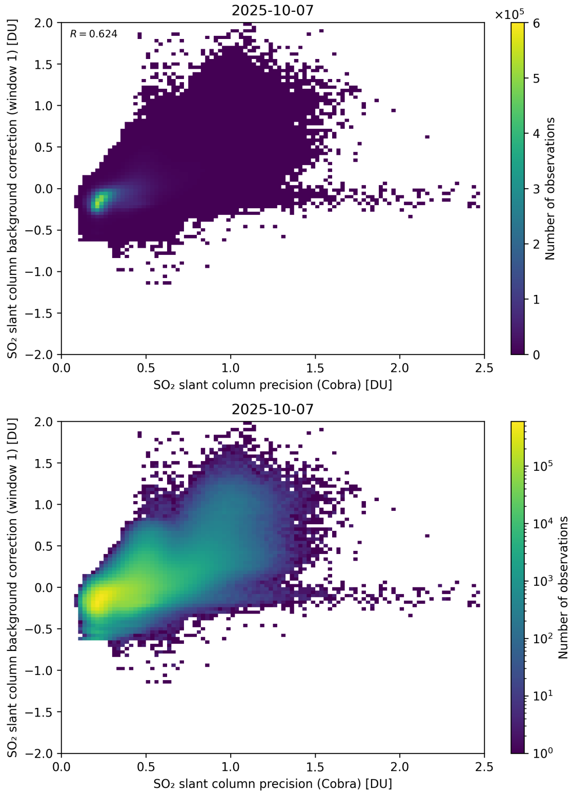
Figure 199: Scatter density plot of “SO 2 slant column precision (Cobra)” against “SO 2 slant column background correction (window 1)” for 2025-10-06 to 2025-10-08.
