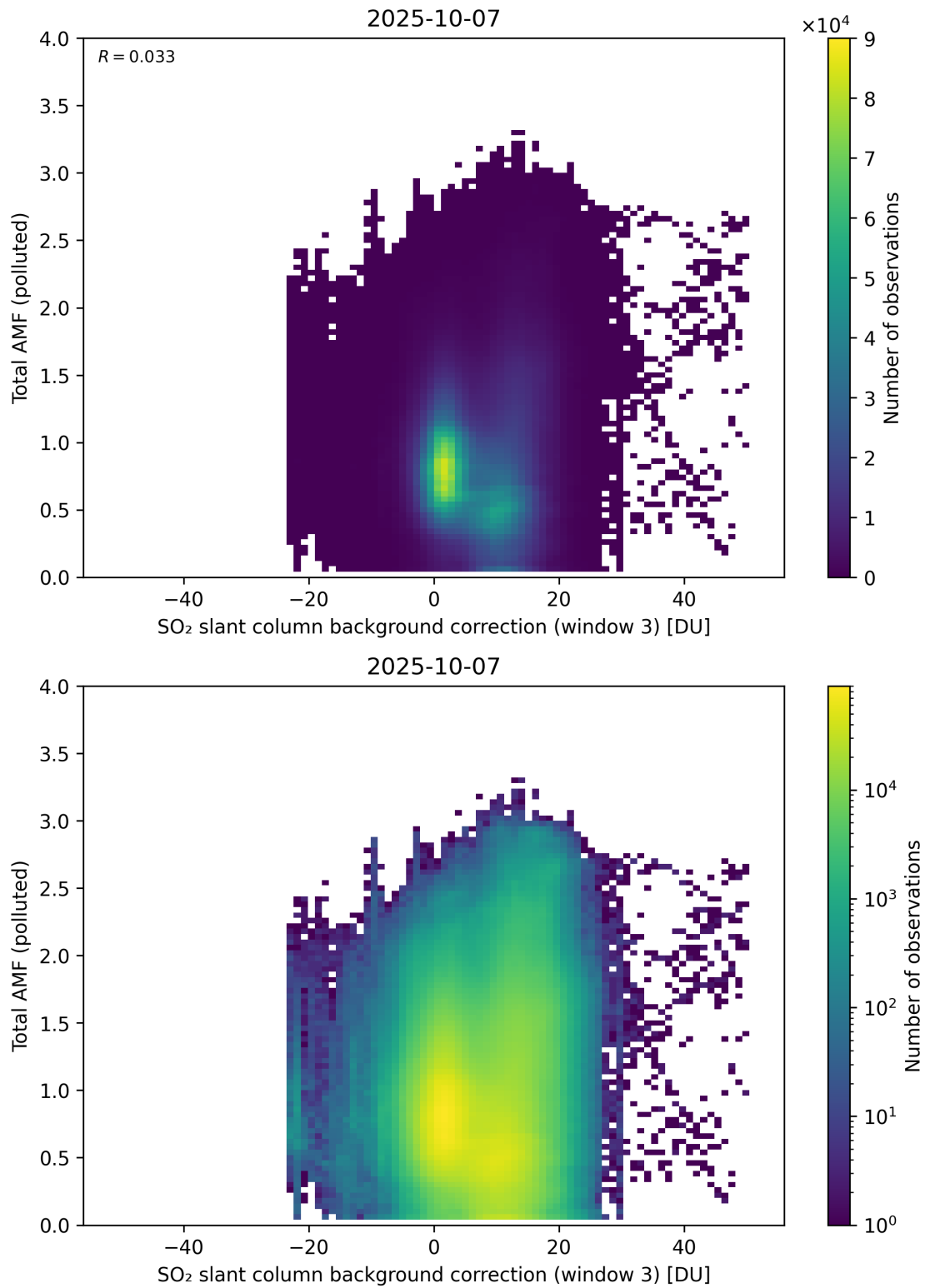
Figure 136: Scatter density plot of “SO 2 slant column background correction (window 3)” against “Total AMF (polluted)” for 2025-10-06 to 2025-10-08.
