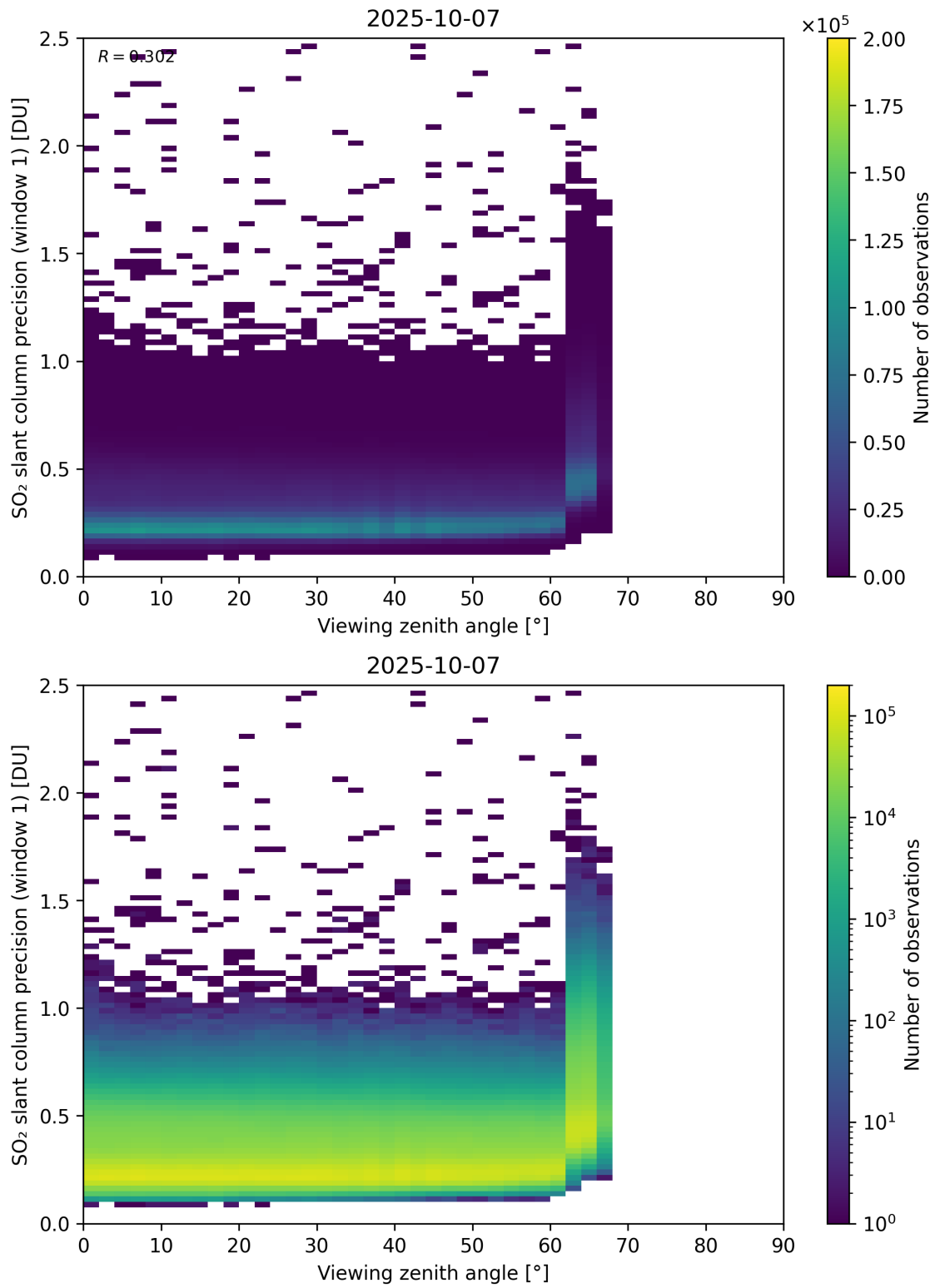
Figure 377: Scatter density plot of “Viewing zenith angle” against “SO 2 slant column precision (window 1)” for 2025-10-06 to 2025-10-08.
