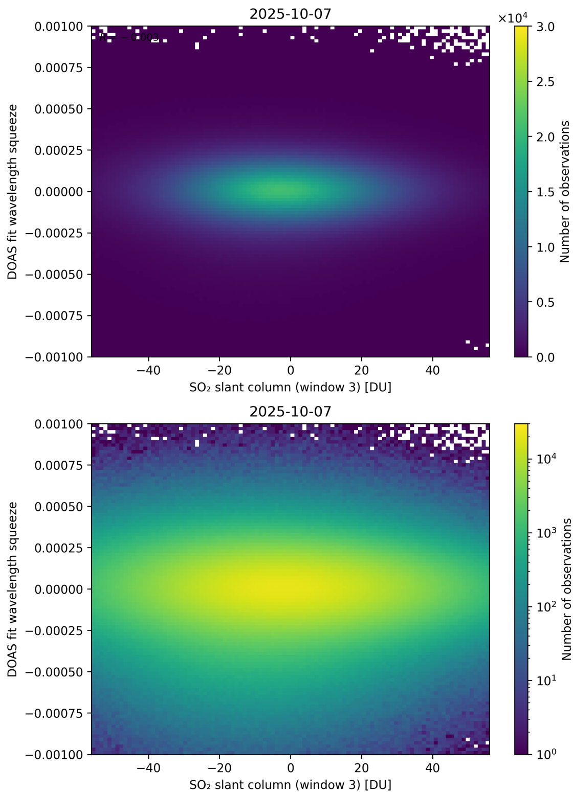
Figure 305: Scatter density plot of “SO 2 slant column (window 3)” against “DOAS fit wavelength squeeze” for 2025-10-06 to 2025-10-08.
