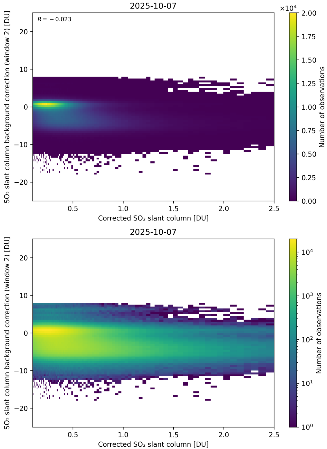
Figure 227: Scatter density plot of “Corrected SO 2 slant column” against “SO 2 slant column background correction (window 2)” for 2025-10-06 to 2025-10-08.
