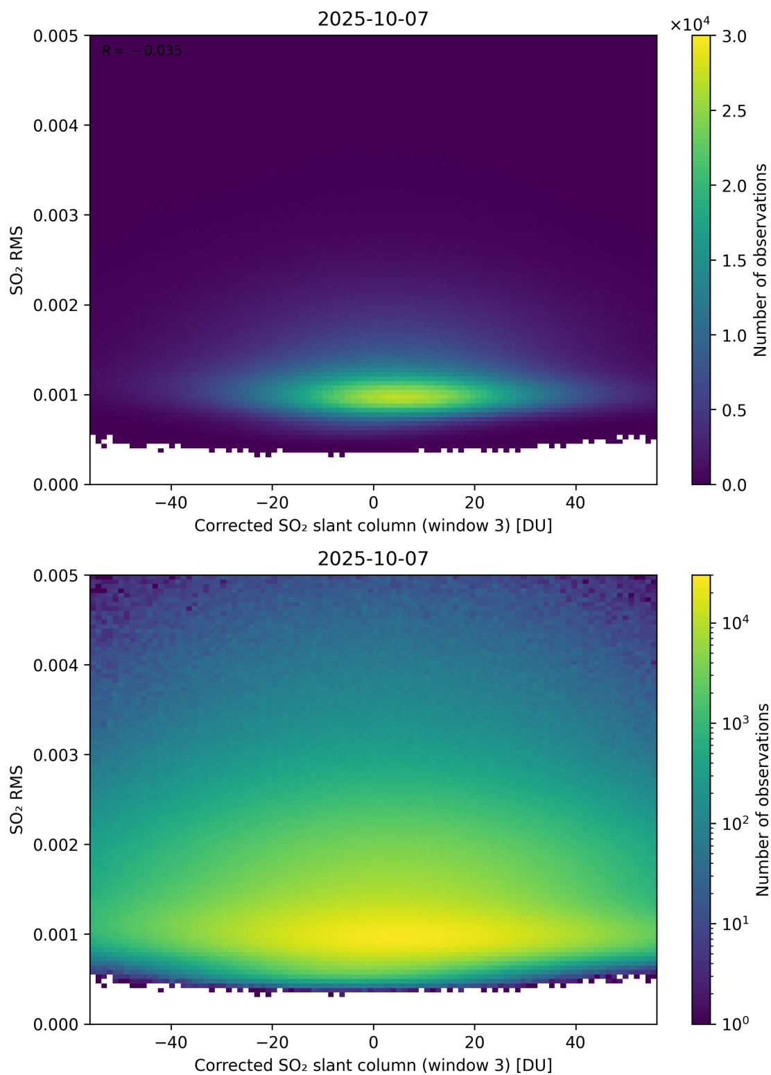
Figure 258: Scatter density plot of “Corrected SO 2 slant column (window 3)” against “SO 2 RMS” for 2025-10-06 to 2025-10-08.
