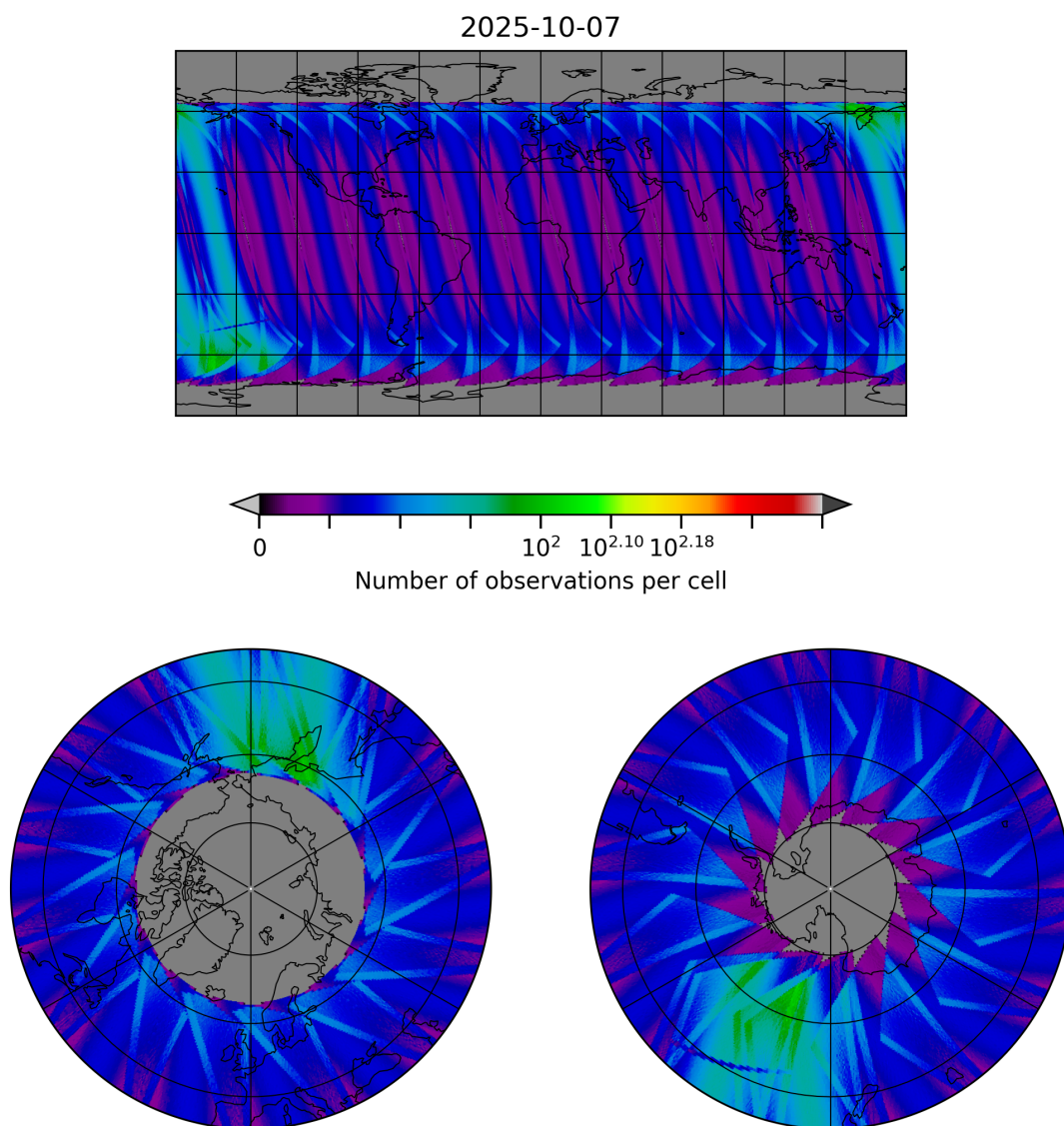
Figure 30: Map of the number of observations for 2025-10-06 to 2025-10-08
