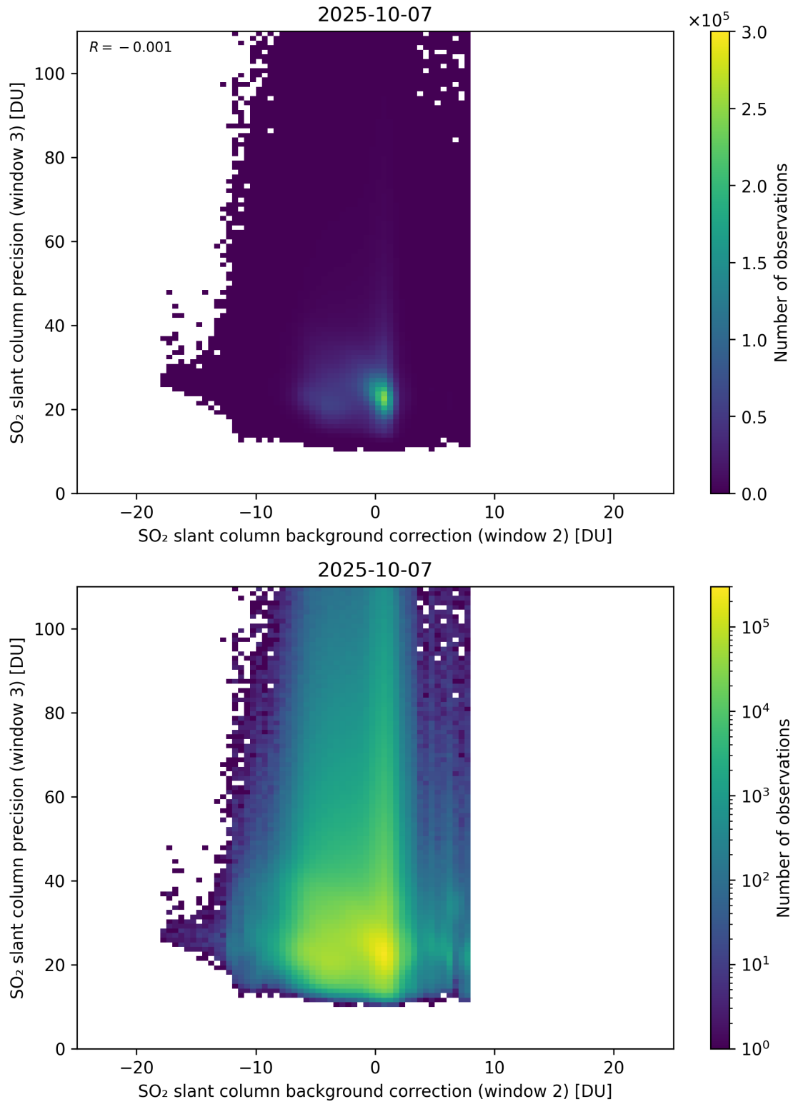
Figure 129: Scatter density plot of “SO 2 slant column background correction (window 2)” against “SO 2 slant column precision (window 3)” for 2025-10-06 to 2025-10-08.
