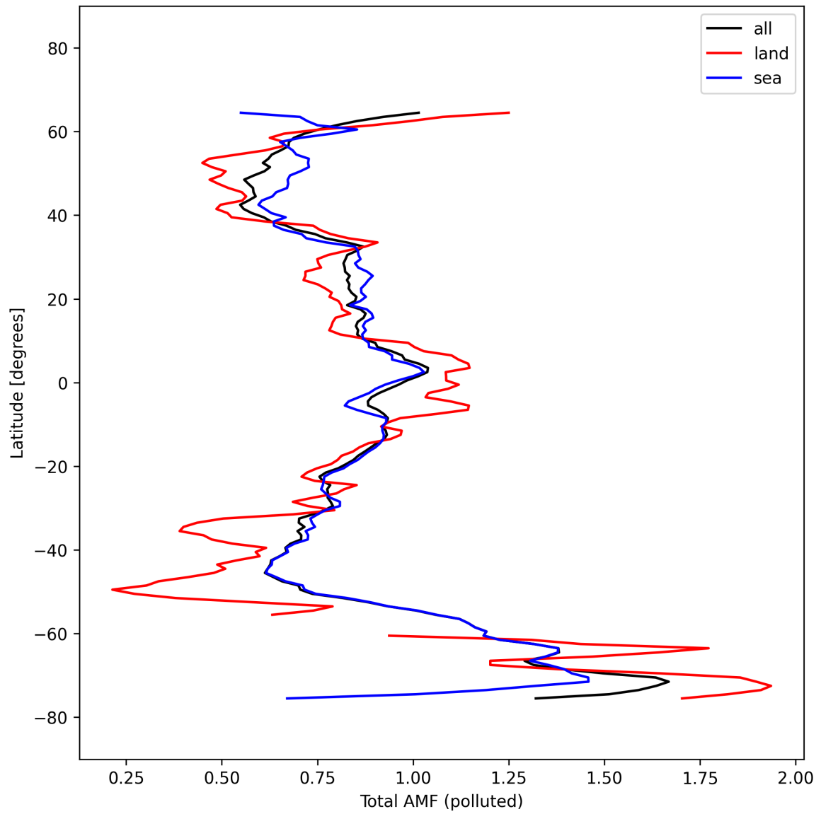
Figure 53: Zonal average of “Total AMF (polluted)” for 2025-10-06 to 2025-10-08.
