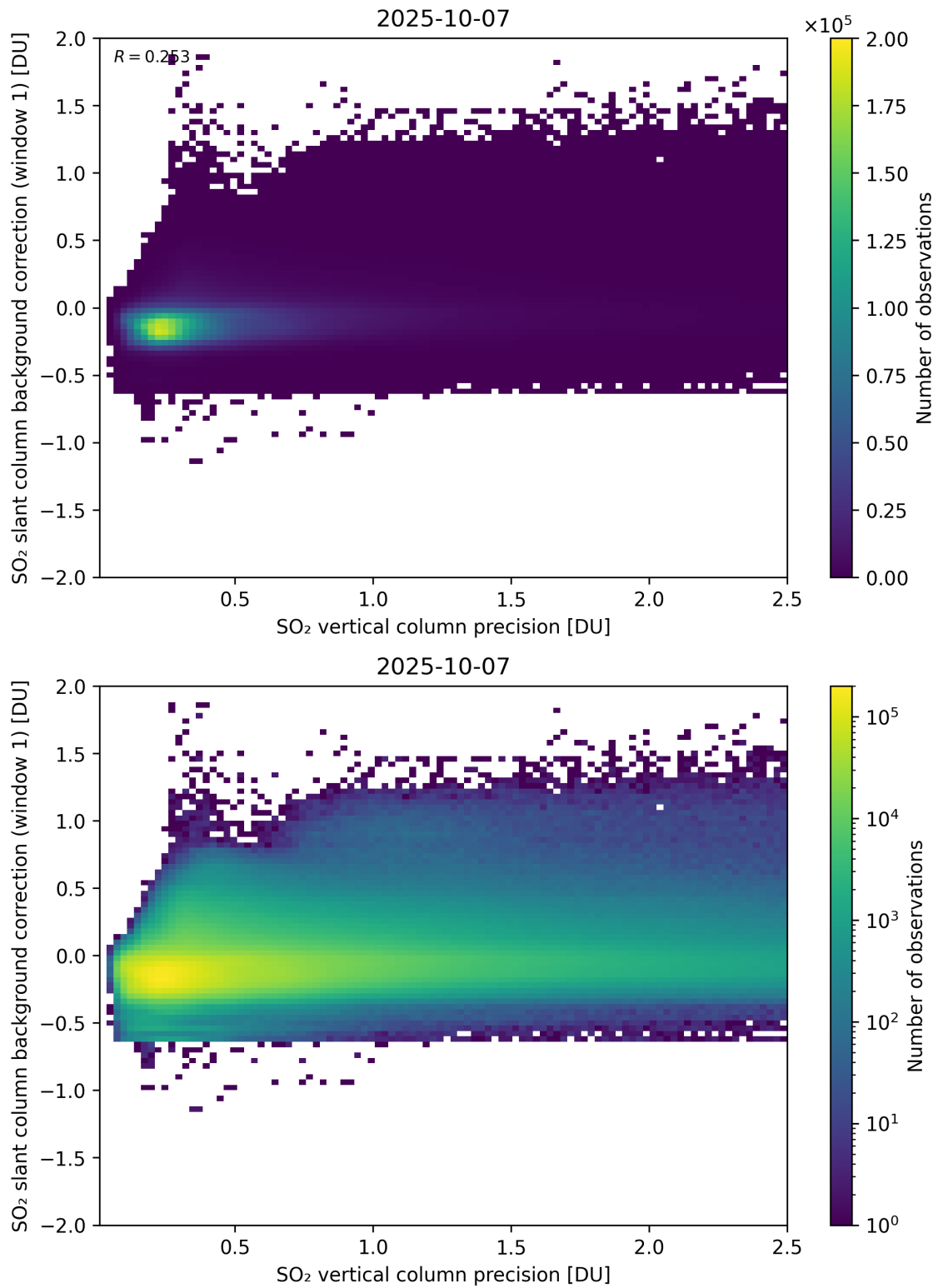
Figure 329: Scatter density plot of “SO 2 vertical column precision” against “SO 2 slant column background correction (window 1)” for 2025-10-06 to 2025-10-08.
