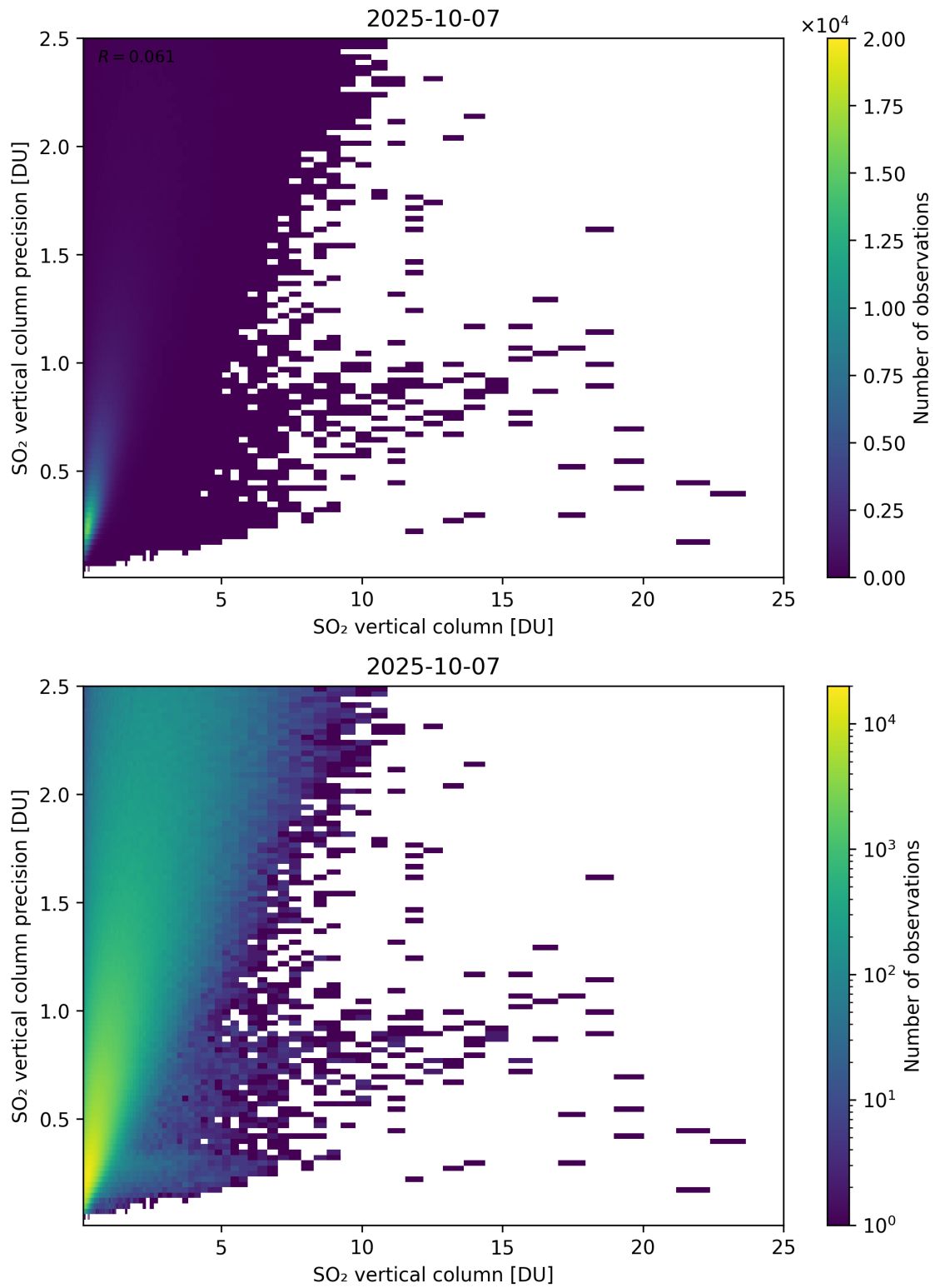
Figure 361: Scatter density plot of “SO 2 vertical column” against “SO 2 vertical column precision” for 2025-10-06 to 2025-10-08.
