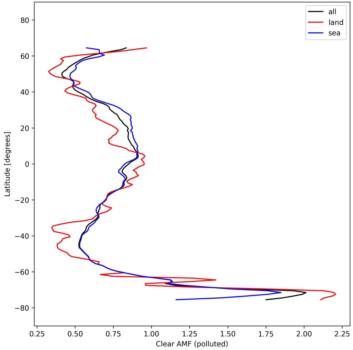
Figure 55: Zonal average of “Clear AMF (polluted)” for 2025-10-06 to 2025-10-08.
