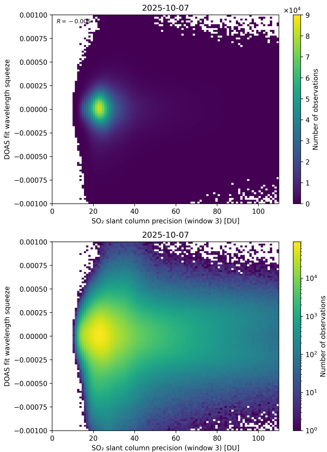
Figure 309: Scatter density plot of “SO 2 slant column precision (window 3)” against “DOAS fit wavelength squeeze” for 2025-10-06 to 2025-10-08.
