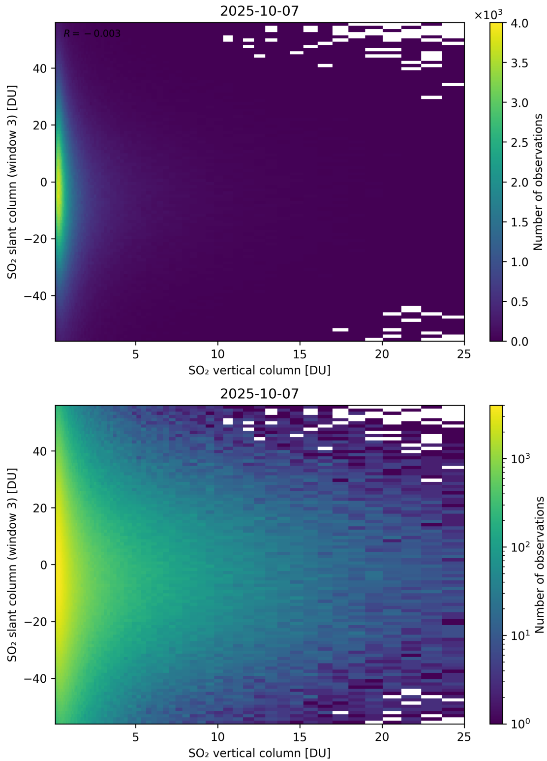
Figure 357: Scatter density plot of “SO 2 vertical column” against “SO 2 slant column (window 3)” for 2025-10-06 to 2025-10-08.
