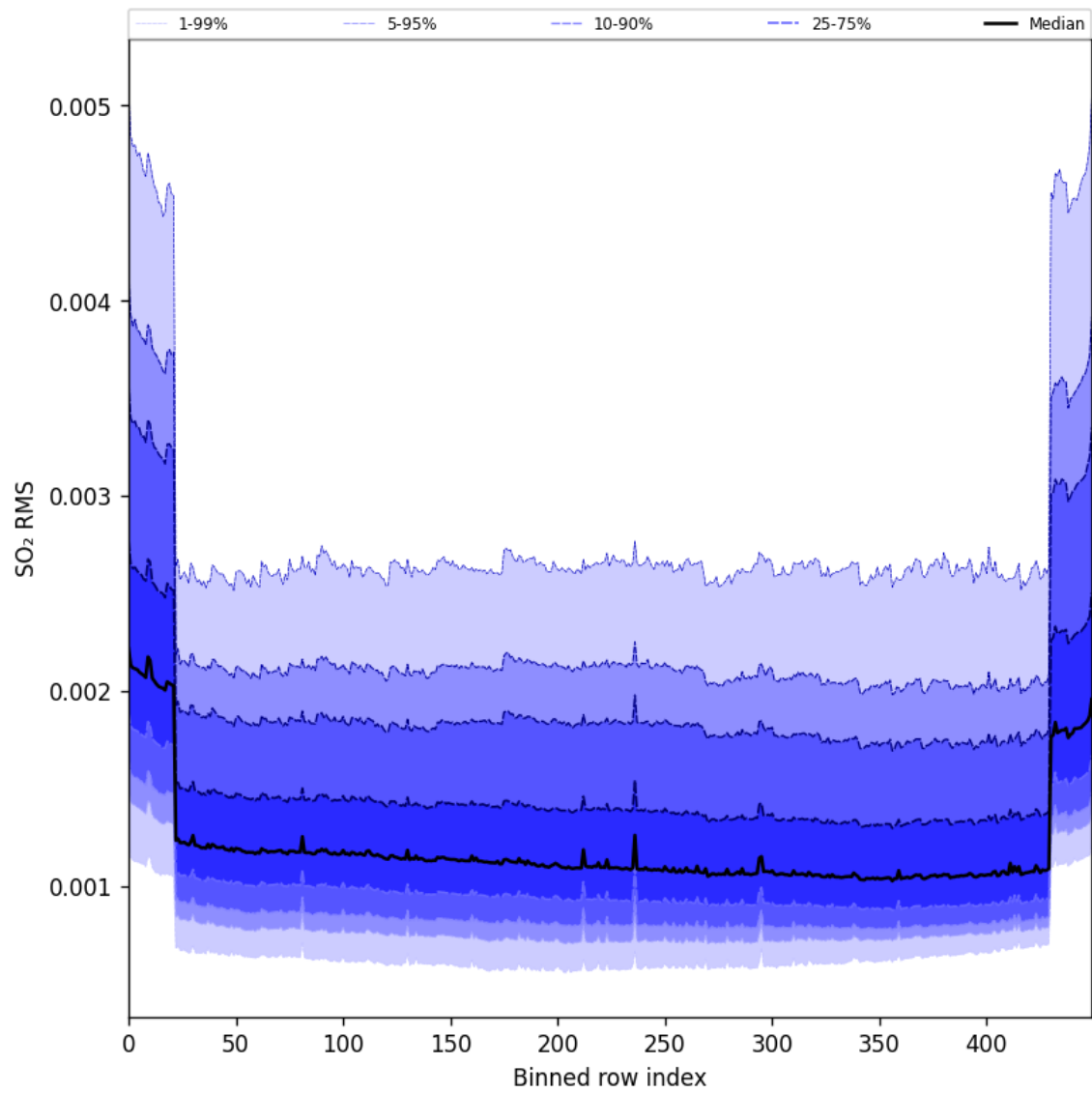
Figure 104: Along track statistics of “SO 2 RMS” for 2025-10-06 to 2025-10-08
