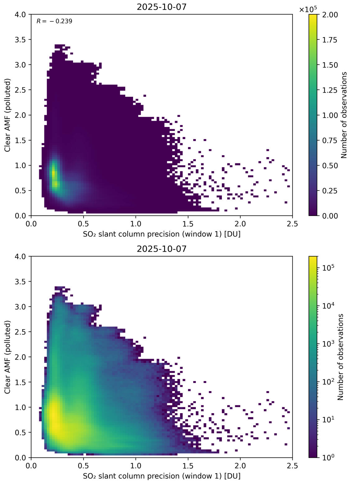
Figure 274: Scatter density plot of “SO 2 slant column precision (window 1)” against “Clear AMF (polluted)” for 2025-10-06 to 2025-10-08.
