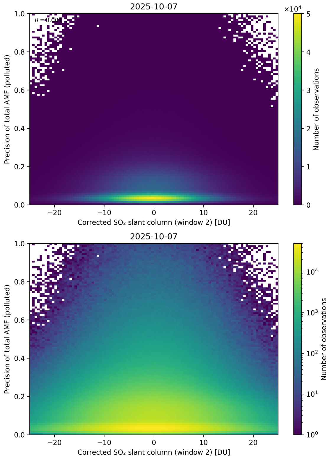
Figure 254: Scatter density plot of “Corrected SO 2 slant column (window 2)” against “Precision of total AMF (polluted)” for 2025-10-06 to 2025-10-08.
