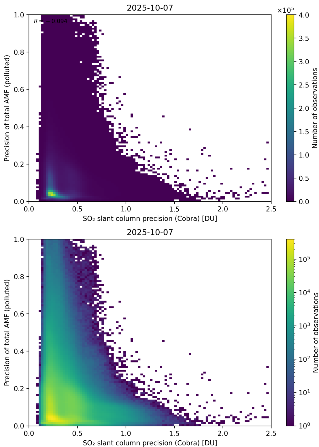
Figure 214: Scatter density plot of “SO 2 slant column precision (Cobra)” against “Precision of total AMF (polluted)” for 2025-10-06 to 2025-10-08.
