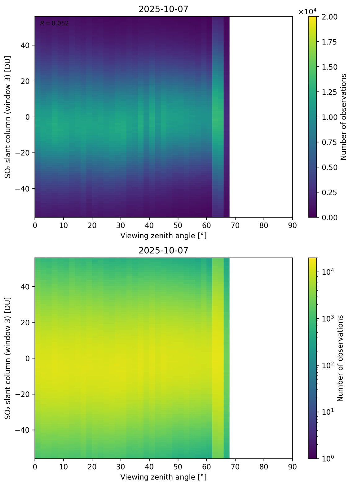
Figure 379: Scatter density plot of “Viewing zenith angle” against “SO 2 slant column (window 3)” for 2025-10-06 to 2025-10-08.
