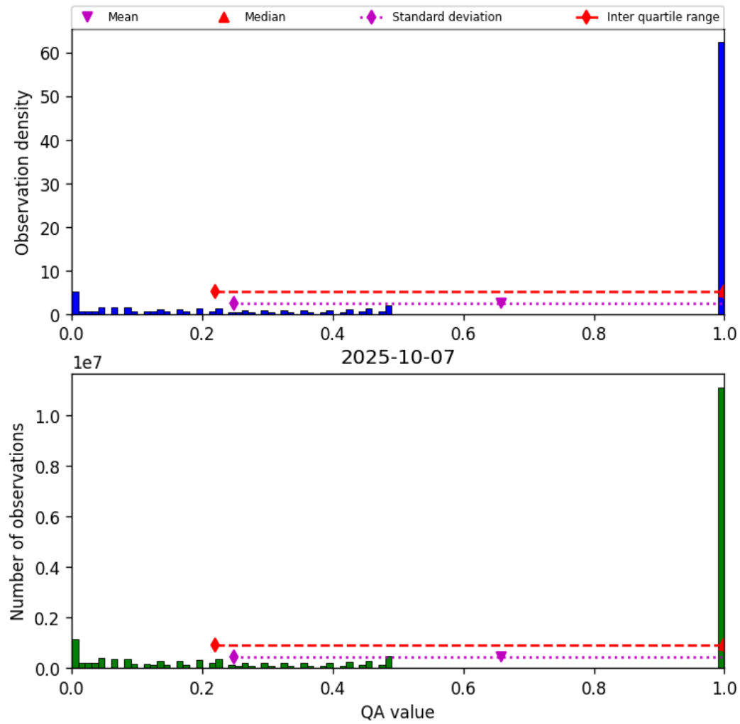
Figure 57: Histogram of “QA value” for 2025-10-06 to 2025-10-08
