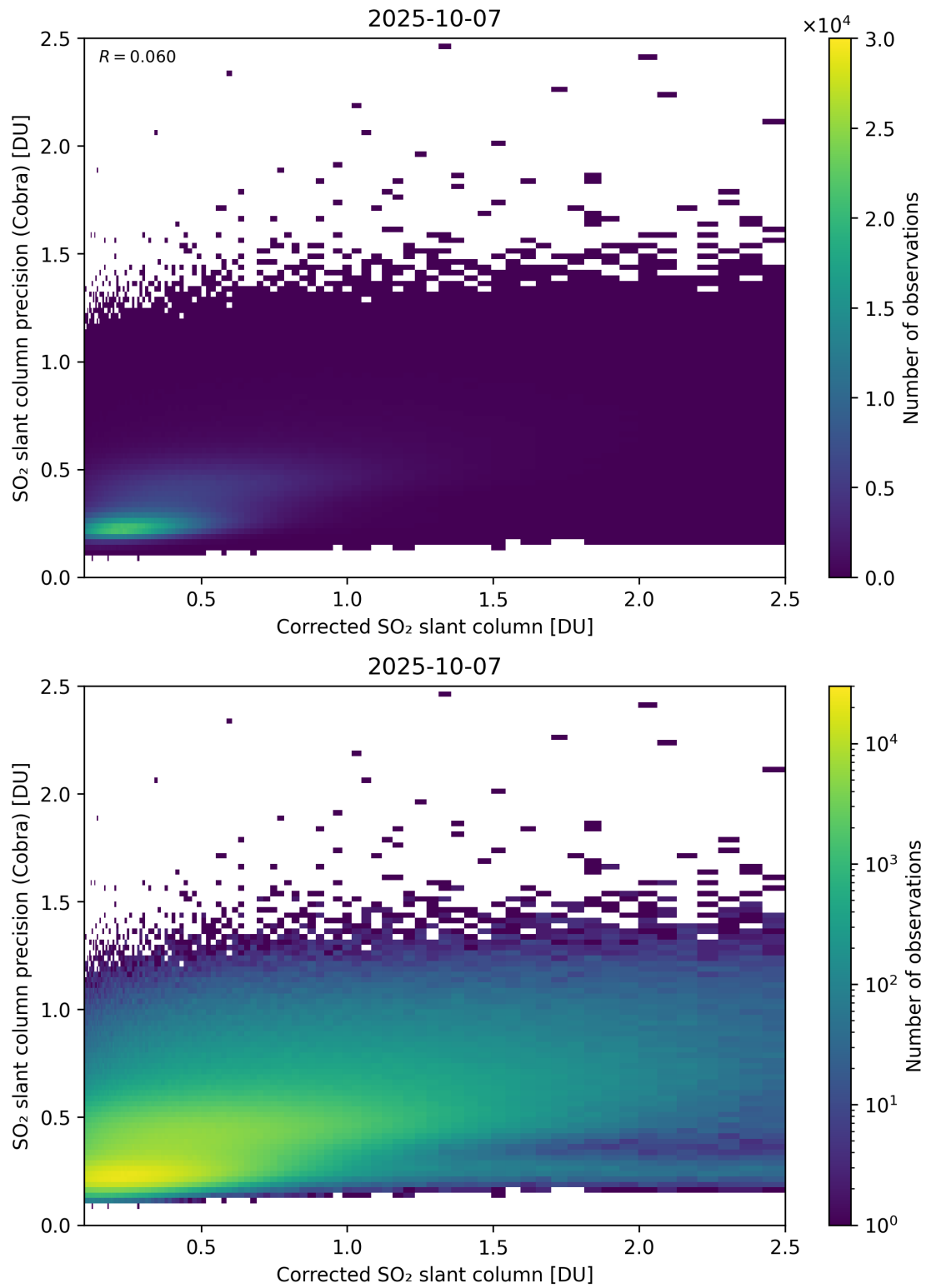
Figure 234: Scatter density plot of “Corrected SO 2 slant column” against “SO 2 slant column precision (Cobra)” for 2025-10-06 to 2025-10-08.
