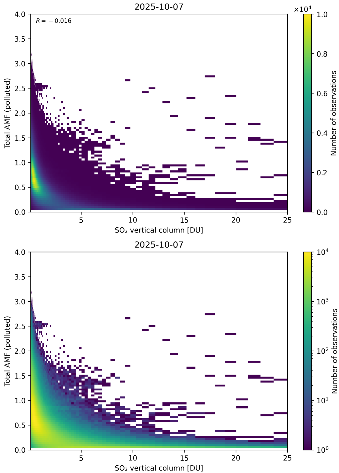
Figure 359: Scatter density plot of “SO 2 vertical column” against “Total AMF (polluted)” for 2025-10-06 to 2025-10-08.
