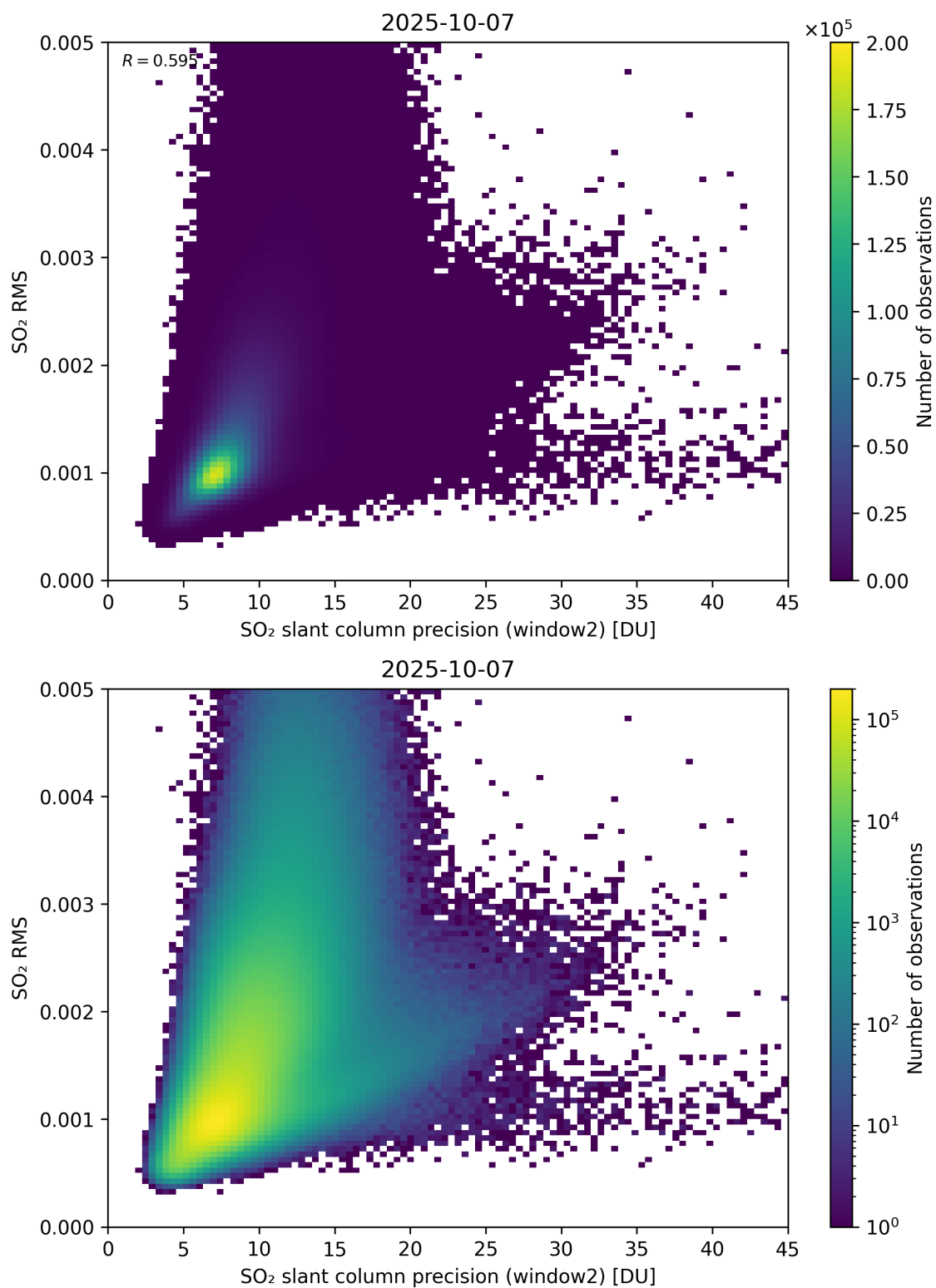
Figure 295: Scatter density plot of “SO 2 slant column precision (window2)” against “SO 2 RMS” for 2025-10-06 to 2025-10-08.
