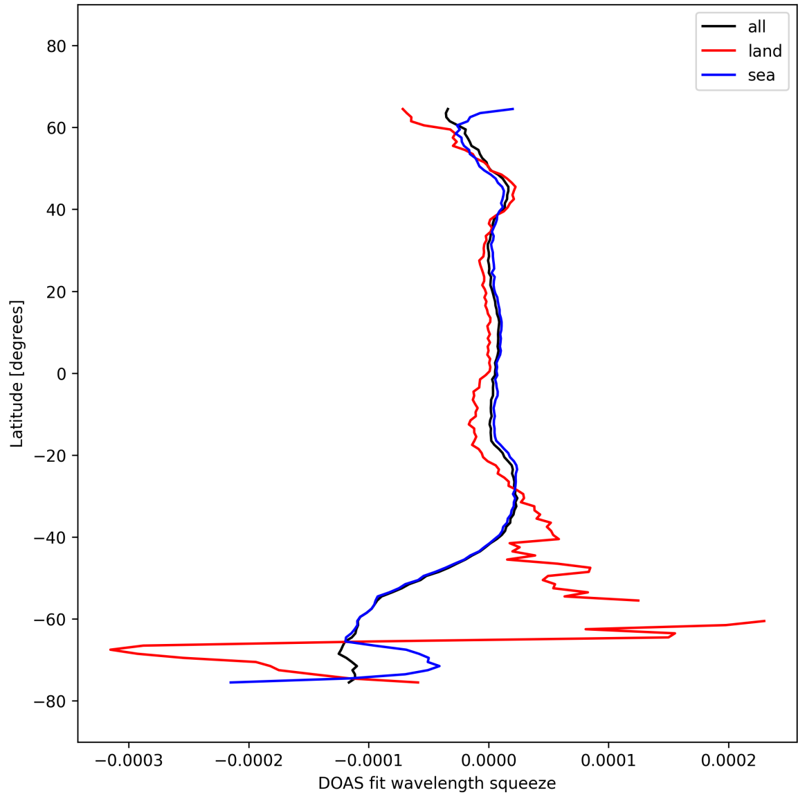
Figure 51: Zonal average of “DOAS fit wavelength squeeze” for 2025-10-06 to 2025-10-08.
