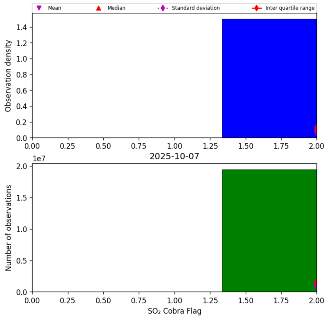
Figure 75: Histogram of “SO 2 Cobra Flag” for 2025-10-06 to 2025-10-08
