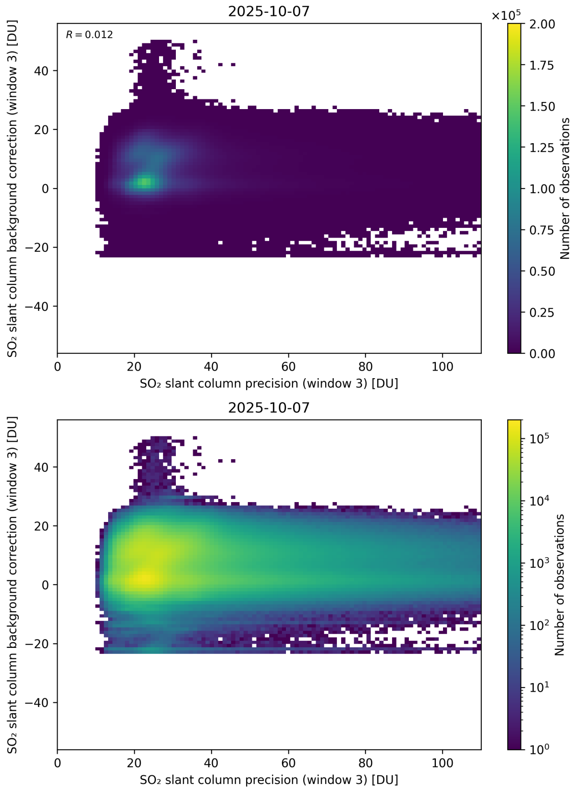
Figure 307: Scatter density plot of “SO 2 slant column precision (window 3)” against “SO 2 slant column background correction (window 3)” for 2025-10-06 to 2025-10-08.
