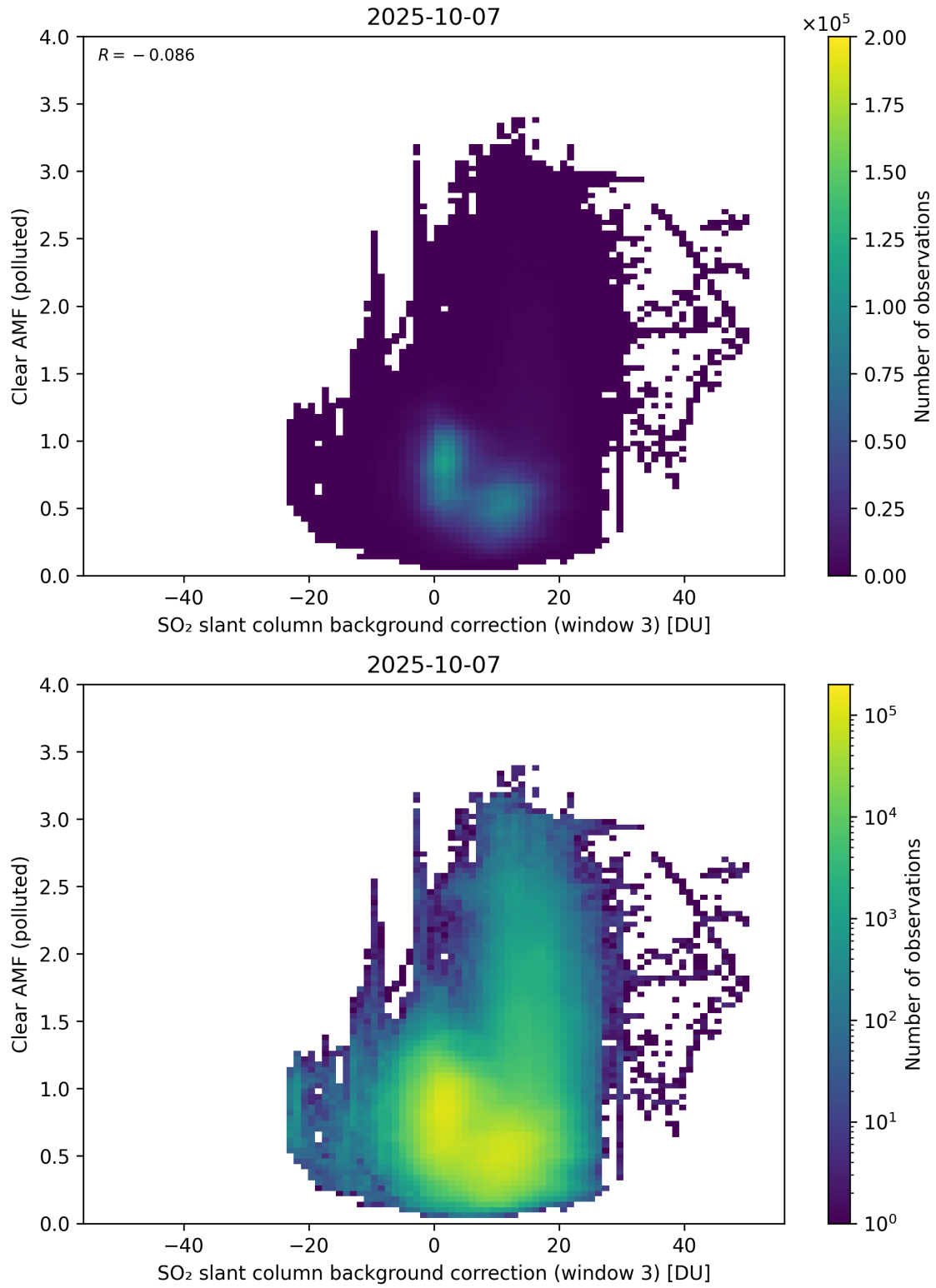
Figure 135: Scatter density plot of “SO 2 slant column background correction (window 3)” against “Clear AMF (polluted)” for 2025-10-06 to 2025-10-08.
