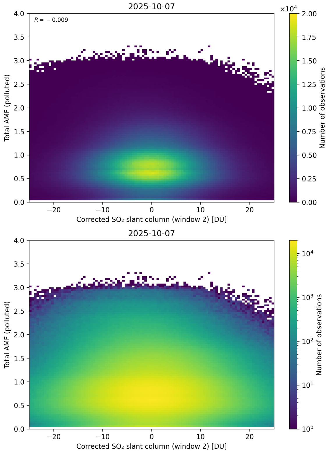
Figure 253: Scatter density plot of “Corrected SO 2 slant column (window 2)” against “Total AMF (polluted)” for 2025-10-06 to 2025-10-08.
