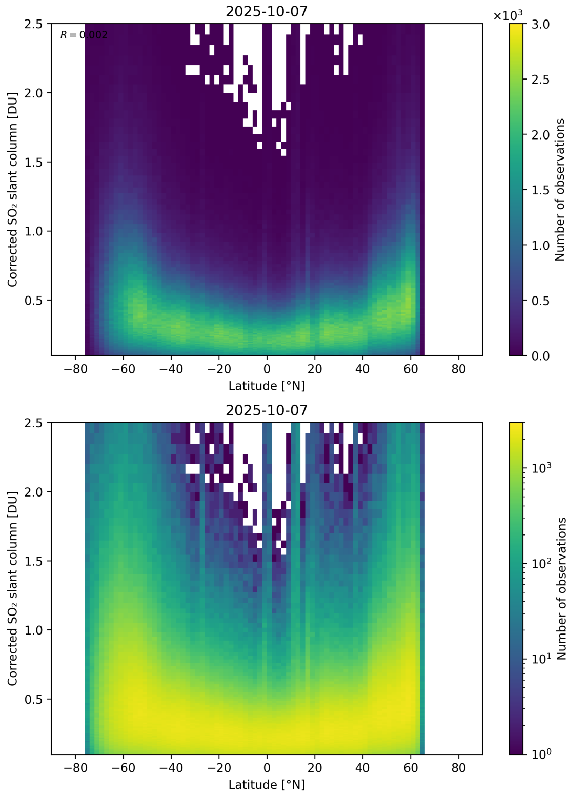
Figure 159: Scatter density plot of “Latitude” against “Corrected SO 2 slant column” for 2025-10-06 to 2025-10-08.
