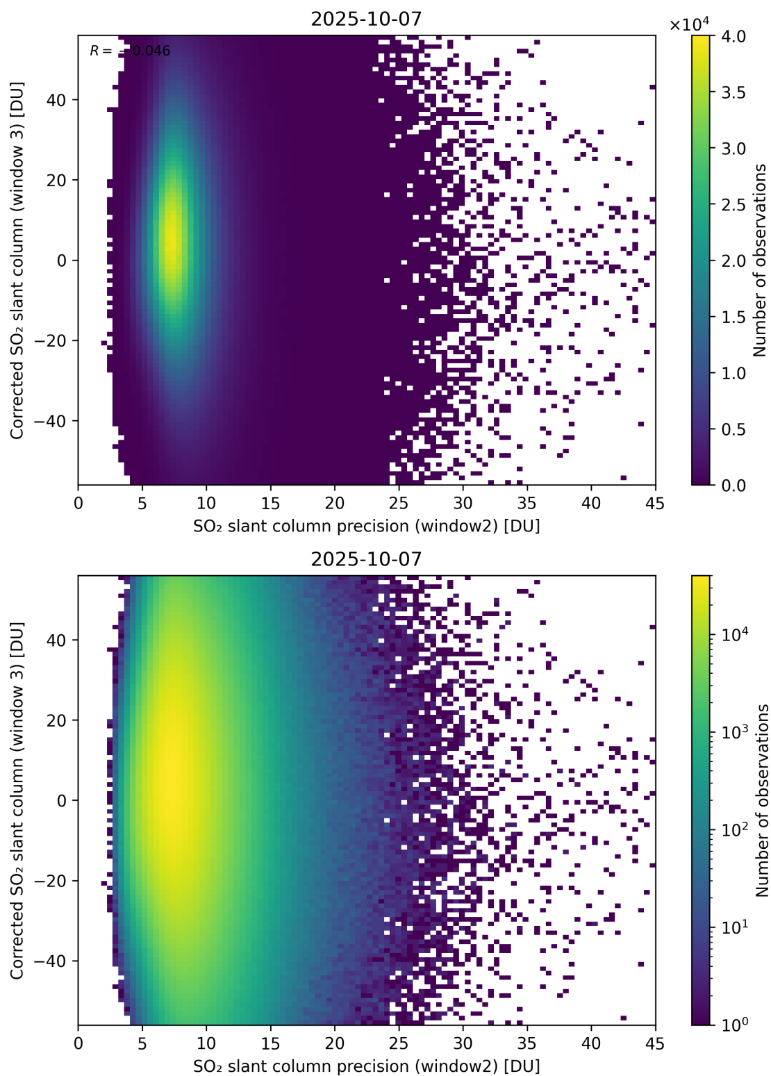
Figure 298: Scatter density plot of “SO 2 slant column precision (window2)” against “Corrected SO 2 slant column (window 3)” for 2025-10-06 to 2025-10-08.
