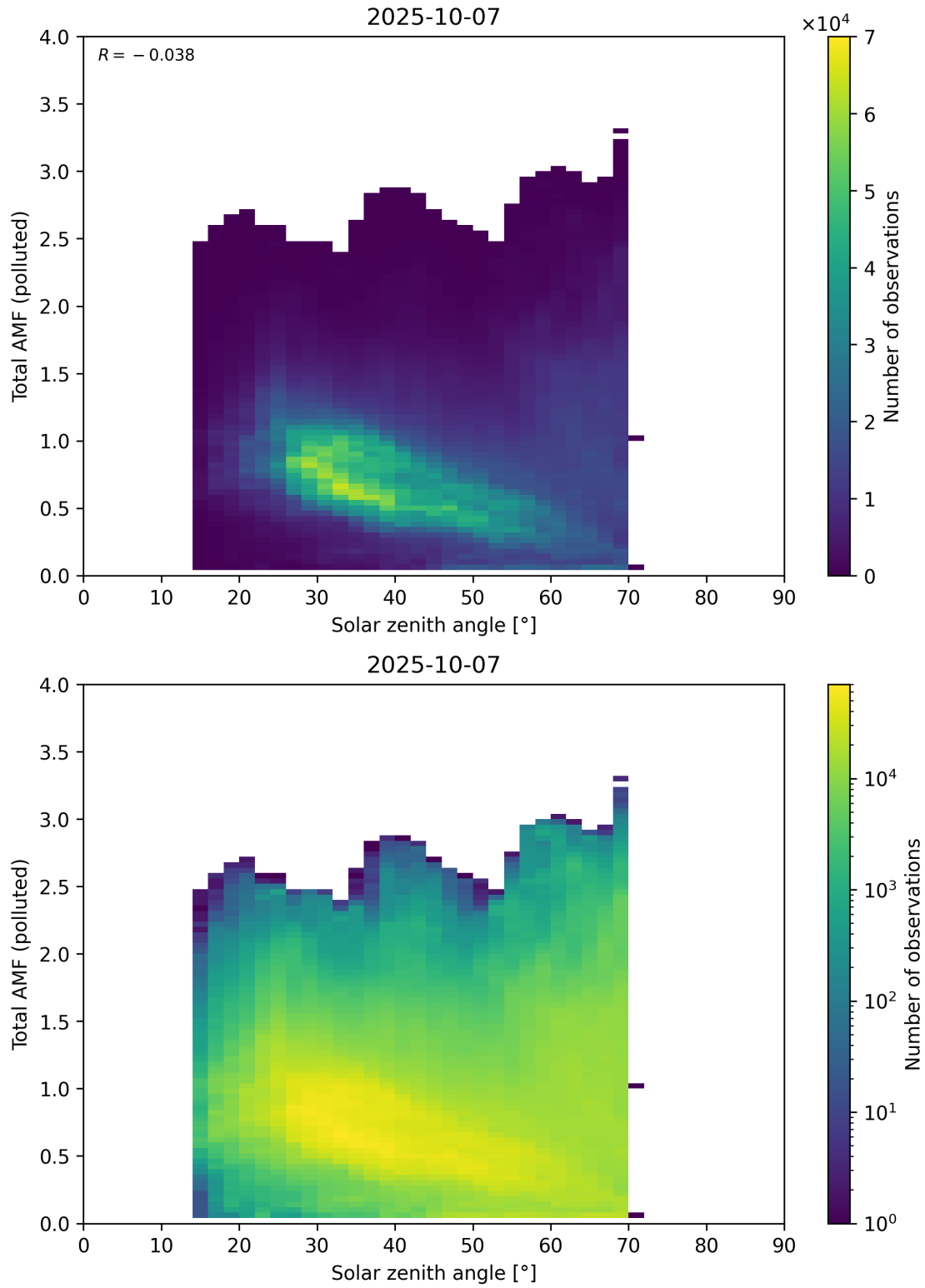
Figure 189: Scatter density plot of “Solar zenith angle” against “Total AMF (polluted)” for 2025-10-06 to 2025-10-08.
