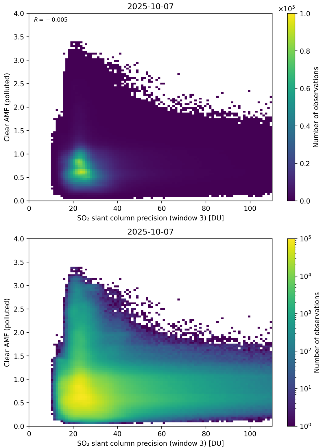
Figure 311: Scatter density plot of “SO 2 slant column precision (window 3)” against “Clear AMF (polluted)” for 2025-10-06 to 2025-10-08.
