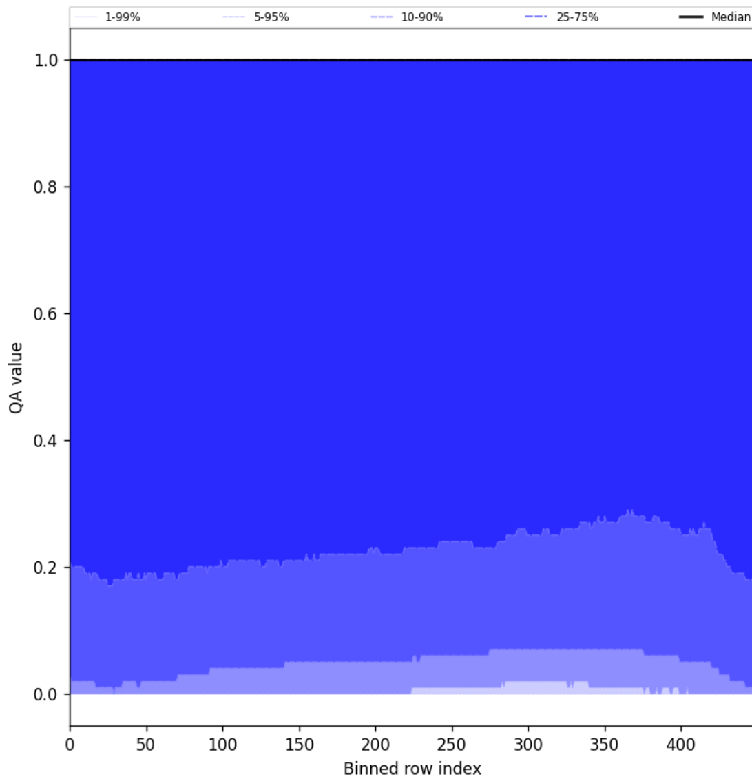
Figure 83: Along track statistics of “QA value” for 2025-10-06 to 2025-10-08
