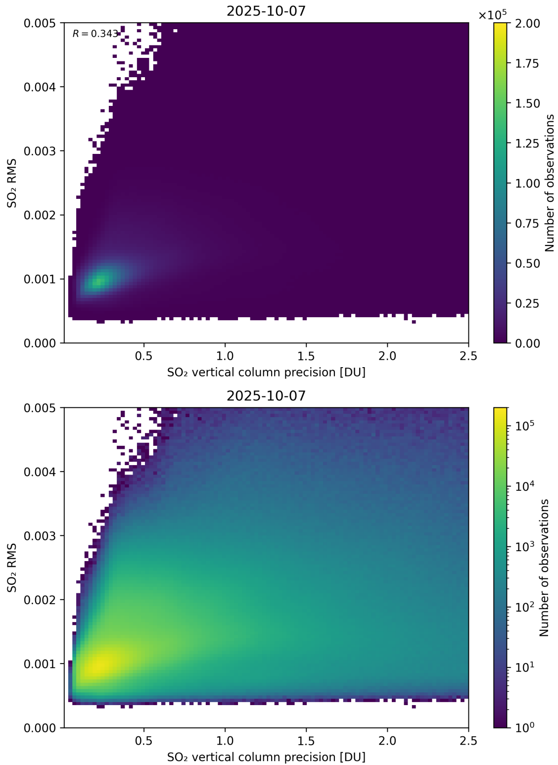
Figure 334: Scatter density plot of “SO 2 vertical column precision” against “SO 2 RMS” for 2025-10-06 to 2025-10-08.
