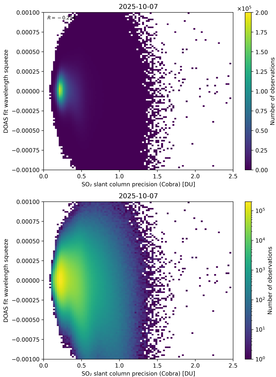
Figure 203: Scatter density plot of “SO 2 slant column precision (Cobra)” against “DOAS fit wavelength squeeze” for 2025-10-06 to 2025-10-08.
