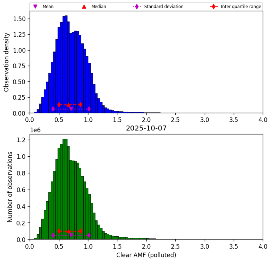
Figure 81: Histogram of “Clear AMF (polluted)” for 2025-10-06 to 2025-10-08
