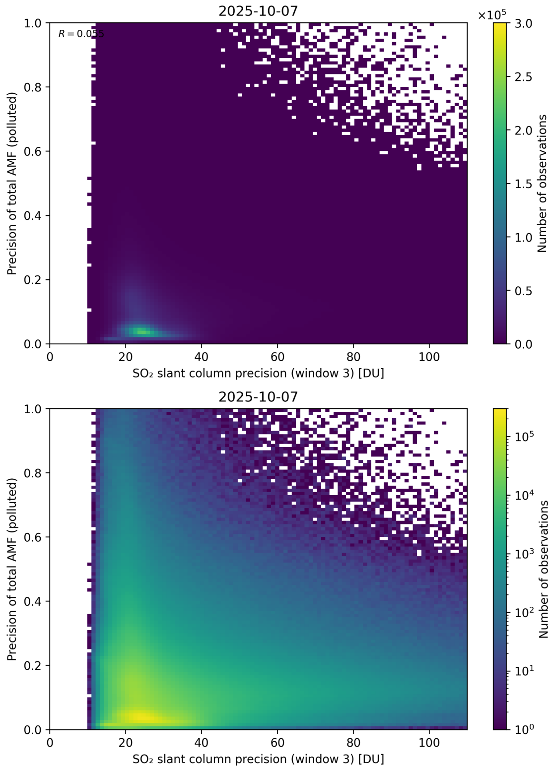
Figure 314: Scatter density plot of “SO 2 slant column precision (window 3)” against “Precision of total AMF (polluted)” for 2025-10-06 to 2025-10-08.
