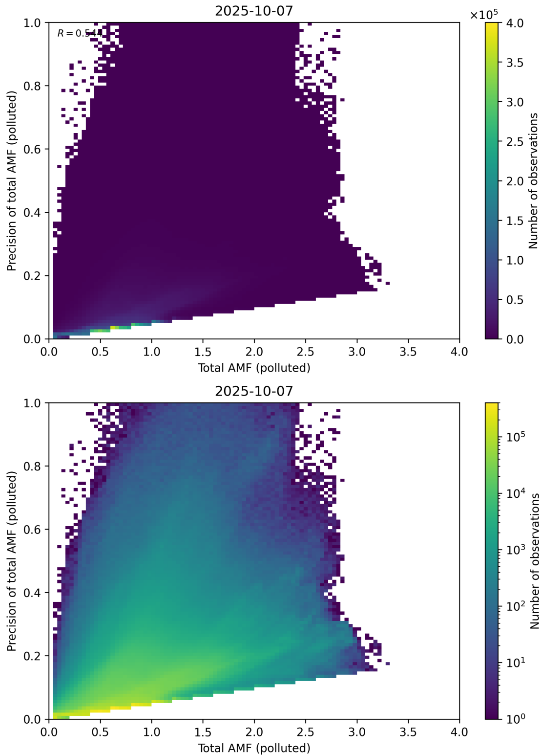
Figure 322: Scatter density plot of “Total AMF (polluted)” against “Precision of total AMF (polluted)” for 2025-10-06 to 2025-10-08.
