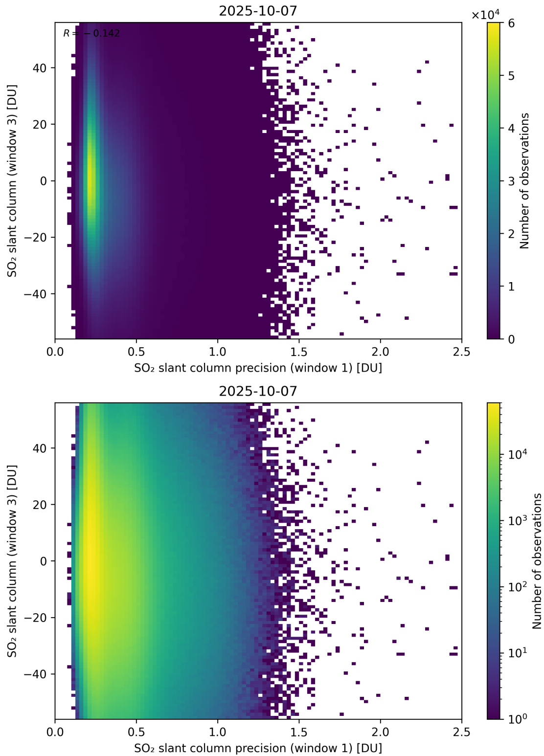
Figure 278: Scatter density plot of “SO 2 slant column precision (window 1)” against “SO 2 slant column (window 3)” for 2025-10-06 to 2025-10-08.
