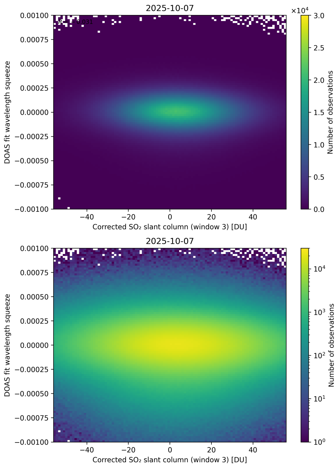
Figure 257: Scatter density plot of “Corrected SO 2 slant column (window 3)” against “DOAS fit wavelength squeeze” for 2025-10-06 to 2025-10-08.
