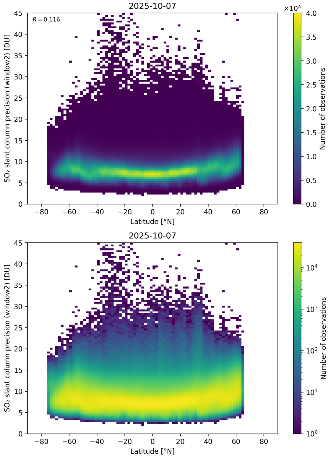
Figure 164: Scatter density plot of “Latitude” against “SO 2 slant column precision (window2)” for 2025-10-06 to 2025-10-08.
