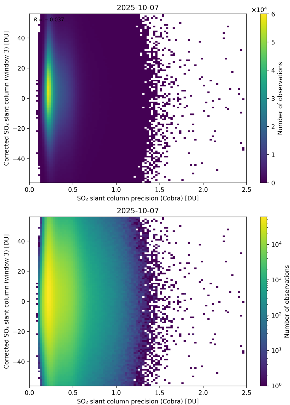
Figure 207: Scatter density plot of “SO 2 slant column precision (Cobra)” against “Corrected SO 2 slant column (window 3)” for 2025-10-06 to 2025-10-08.
