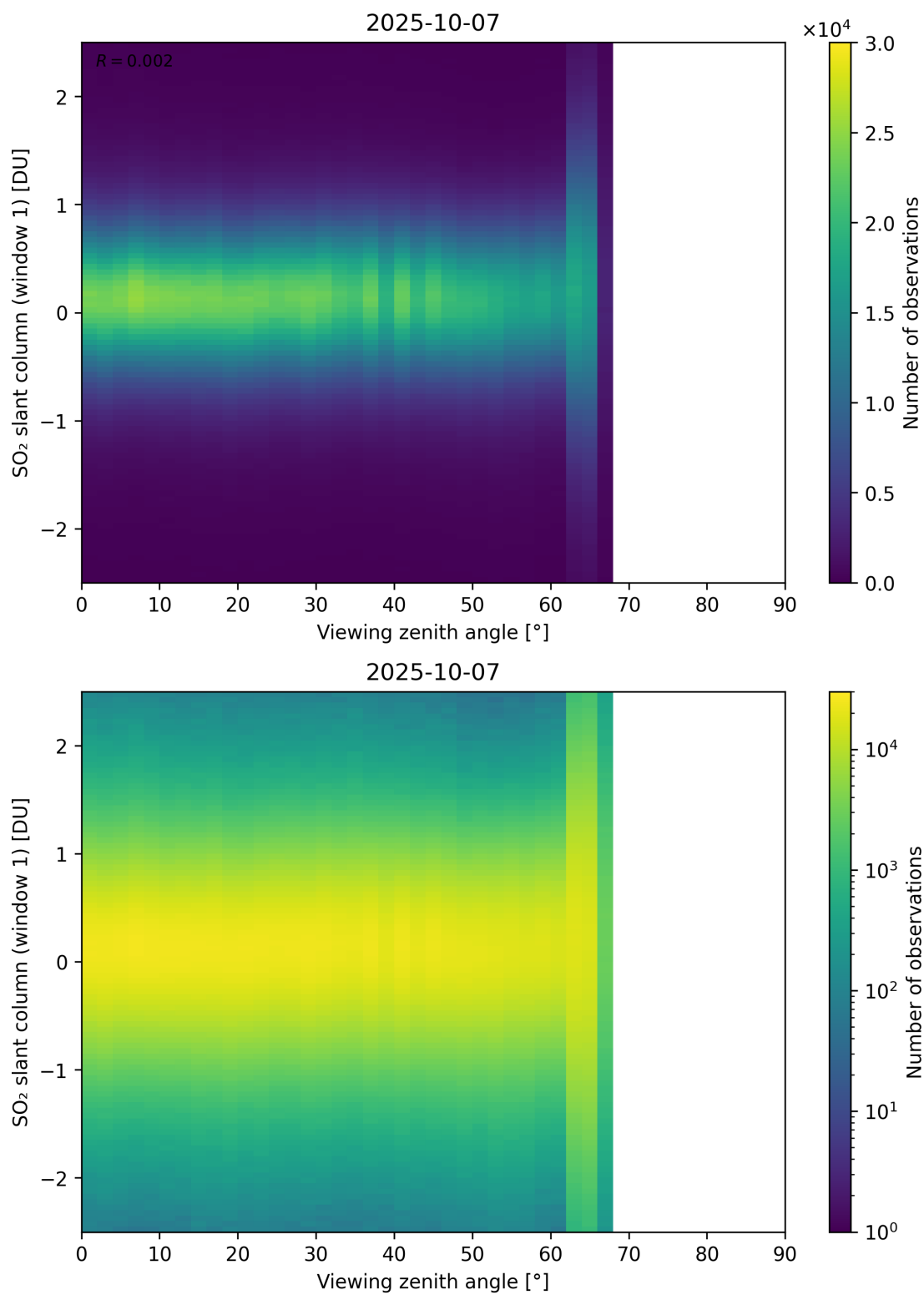
Figure 376: Scatter density plot of “Viewing zenith angle” against “SO 2 slant column (window 1)” for 2025-10-06 to 2025-10-08.
