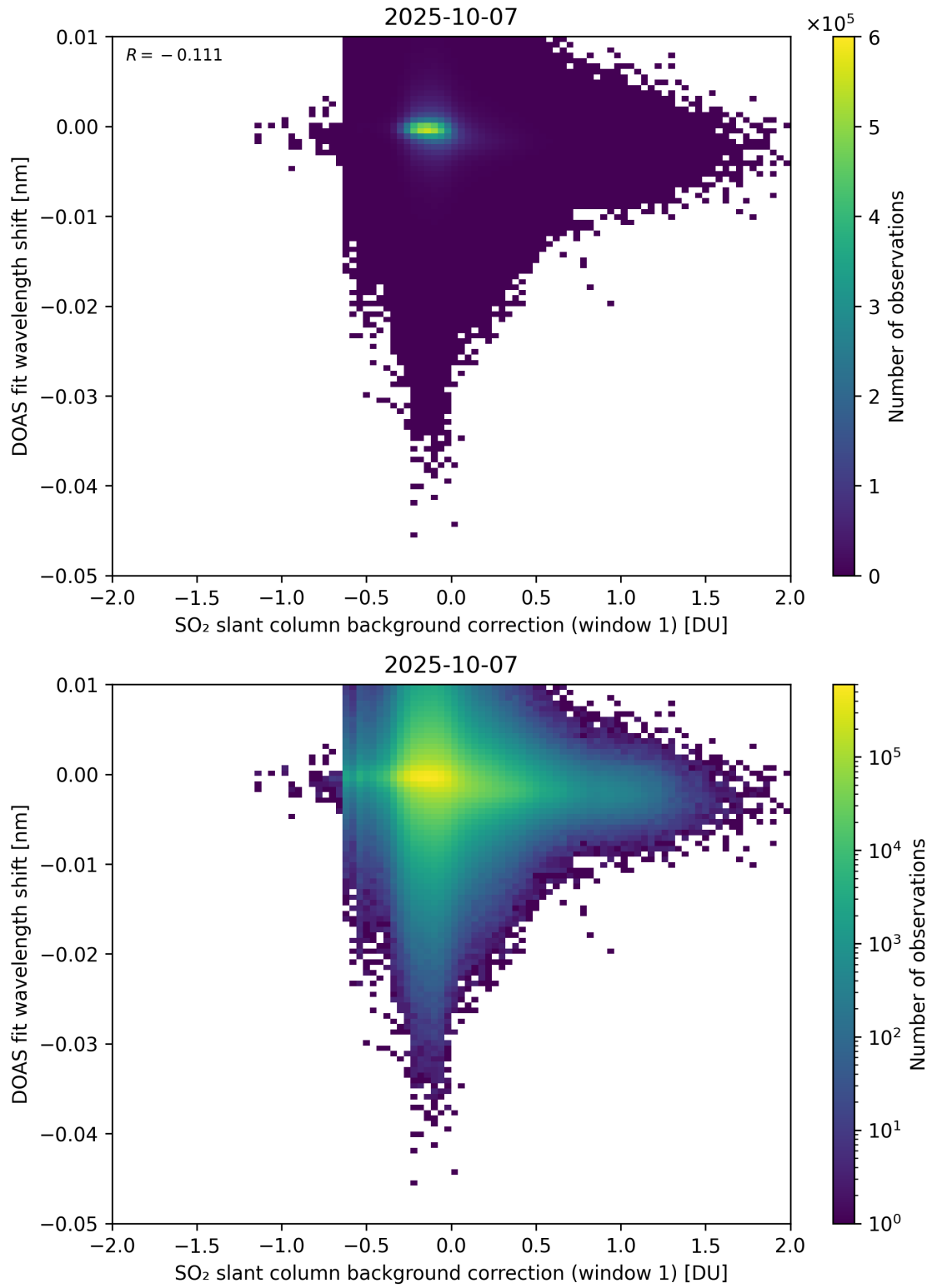
Figure 111: Scatter density plot of “SO 2 slant column background correction (window 1)” against “DOAS fit wavelength shift” for 2025-10-06 to 2025-10-08.
