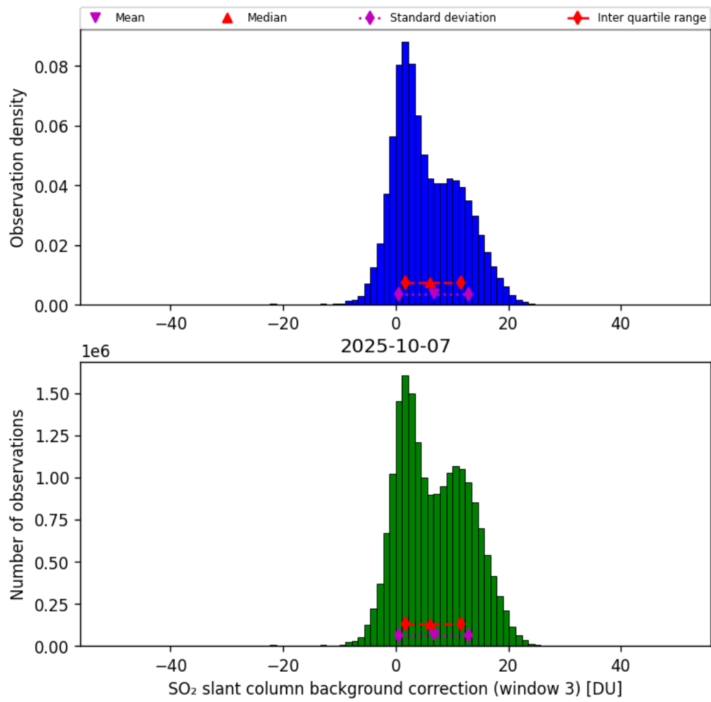
Figure 74: Histogram of “SO 2 slant column background correction (window 3)” for 2025-10-06 to 2025-10-08
