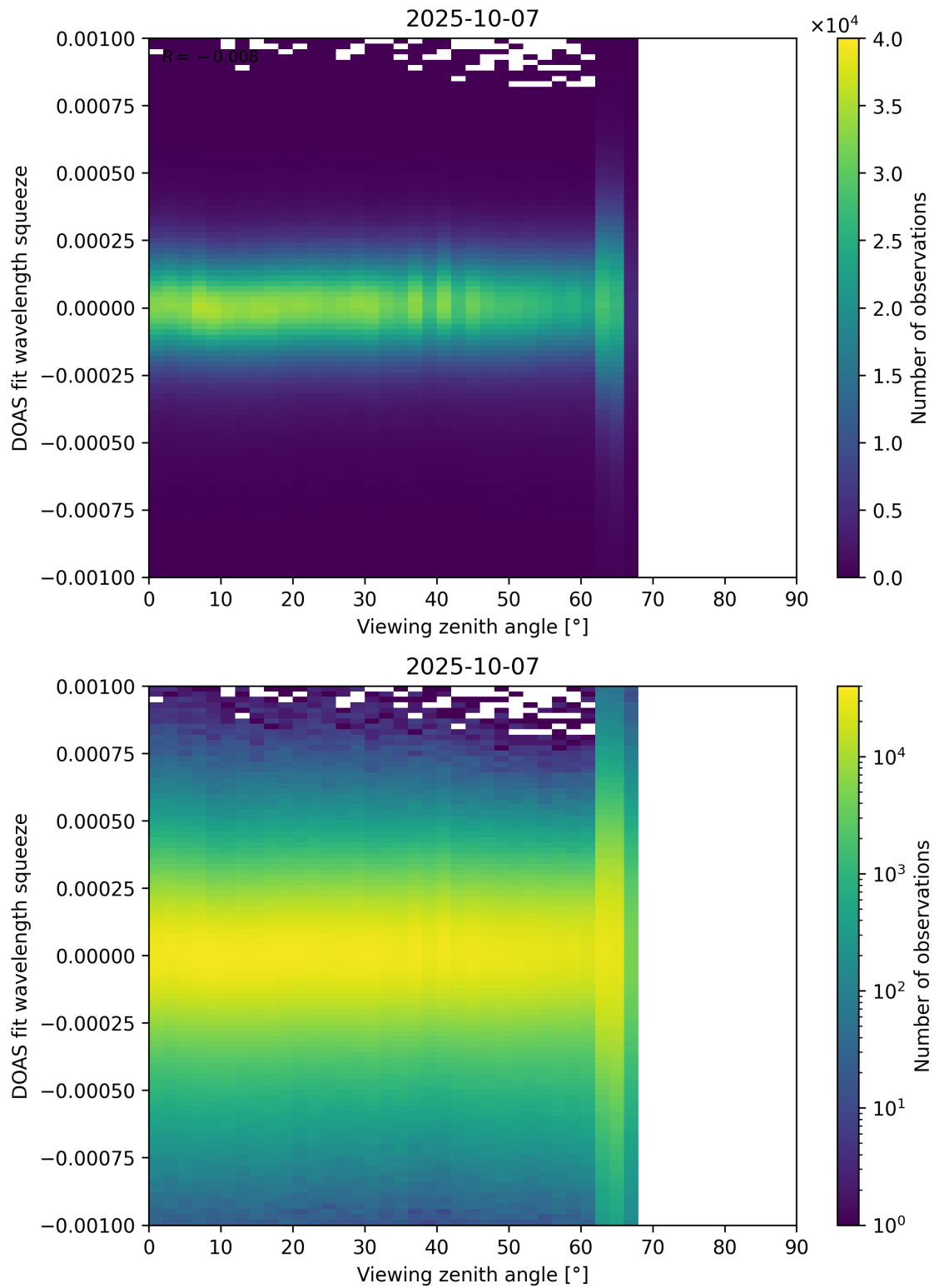
Figure 366: Scatter density plot of “Viewing zenith angle” against “DOAS fit wavelength squeeze” for 2025-10-06 to 2025-10-08.
