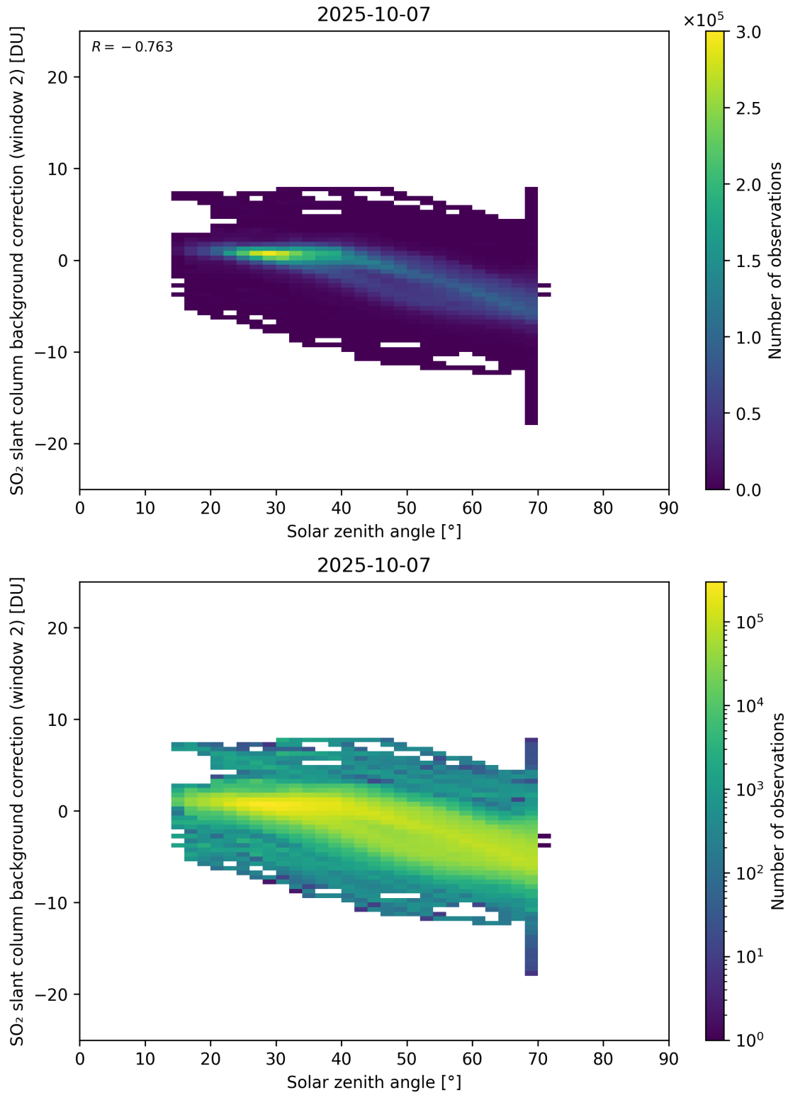
Figure 172: Scatter density plot of “Solar zenith angle” against “SO 2 slant column background correction (window 2)” for 2025-10-06 to 2025-10-08.
