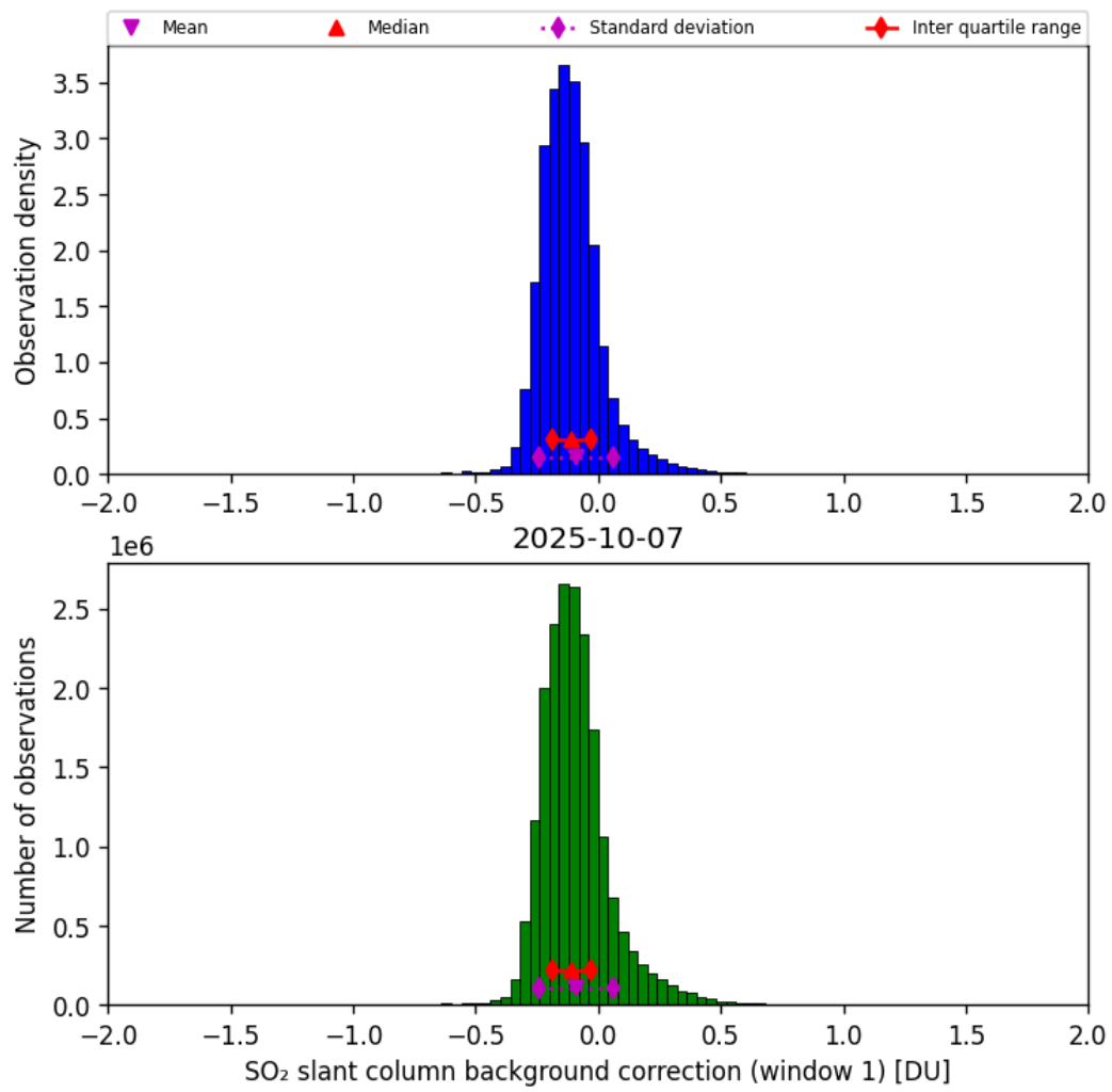
Figure 66: Histogram of “SO 2 slant column background correction (window 1)” for 2025-10-06 to 2025-10-08
