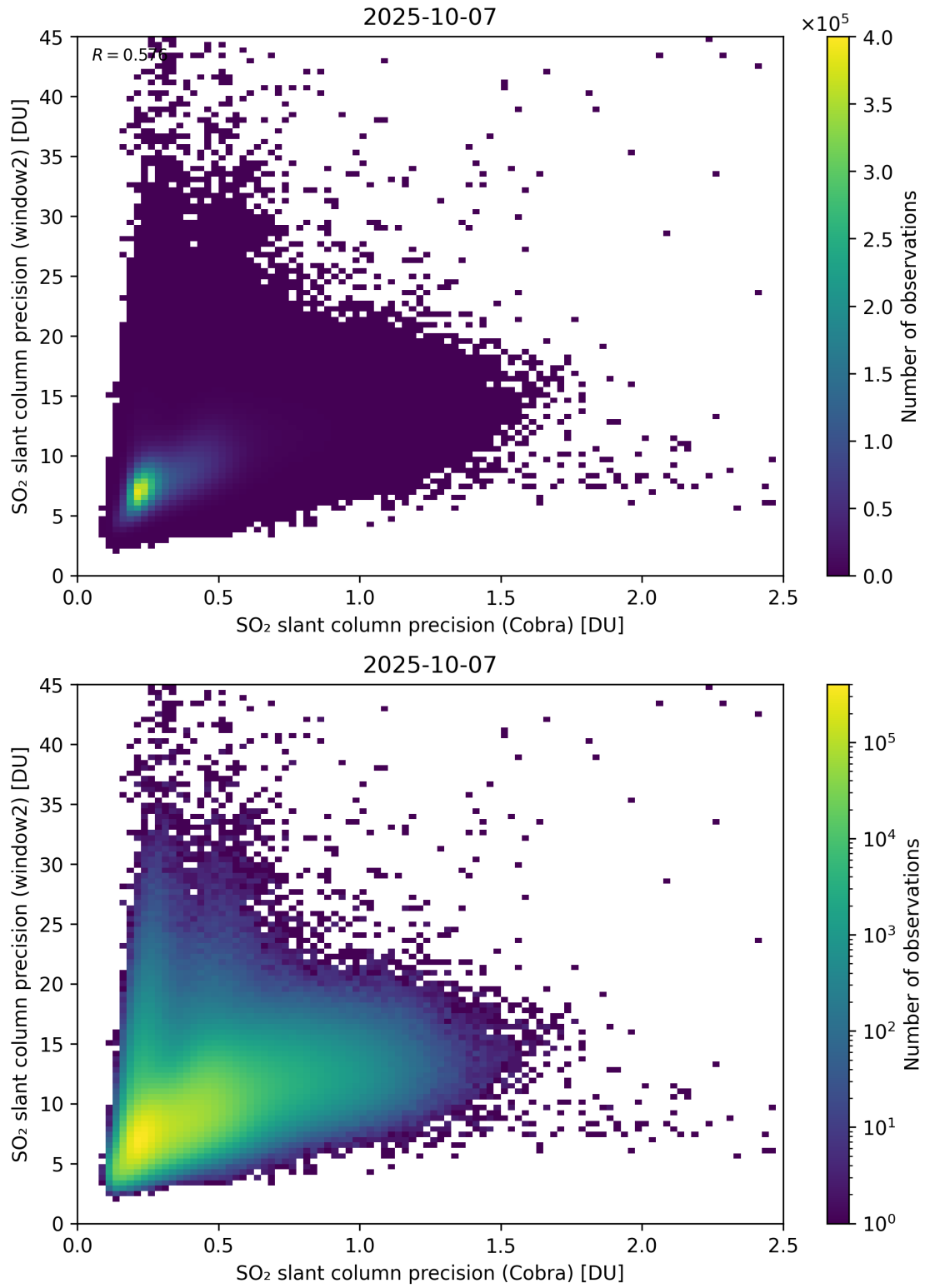
Figure 210: Scatter density plot of “SO 2 slant column precision (Cobra)” against “SO 2 slant column precision (window2)” for 2025-10-06 to 2025-10-08.
