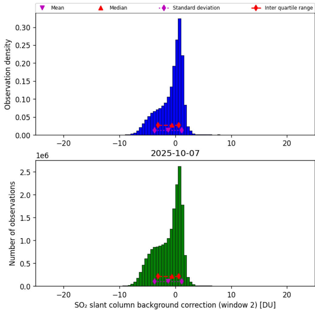
Figure 70: Histogram of “SO 2 slant column background correction (window 2)” for 2025-10-06 to 2025-10-08
