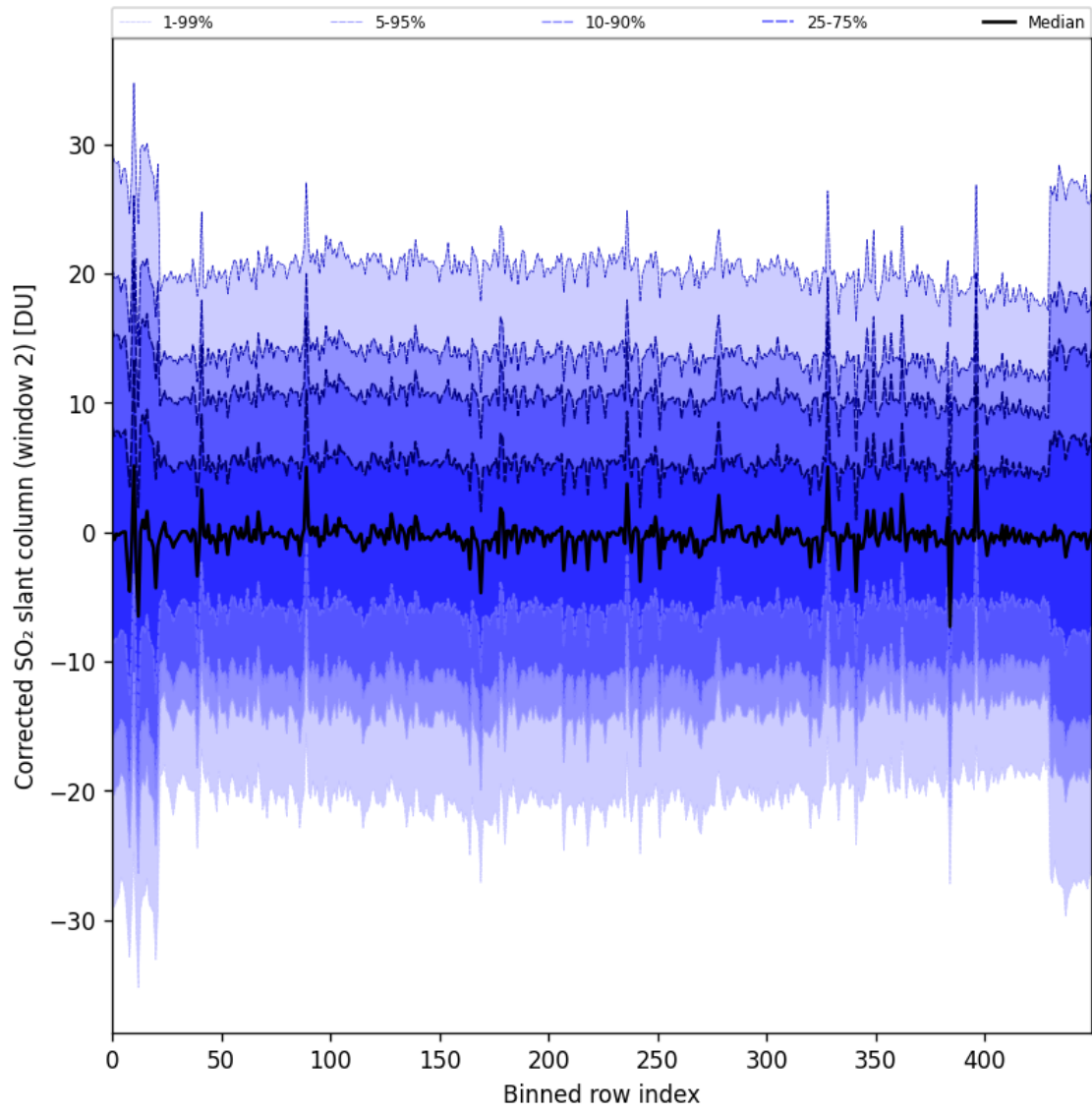
Figure 95: Along track statistics of "Corrected SO 2 slant column (window 2)" for 2025-10-06 to 2025-10-08
