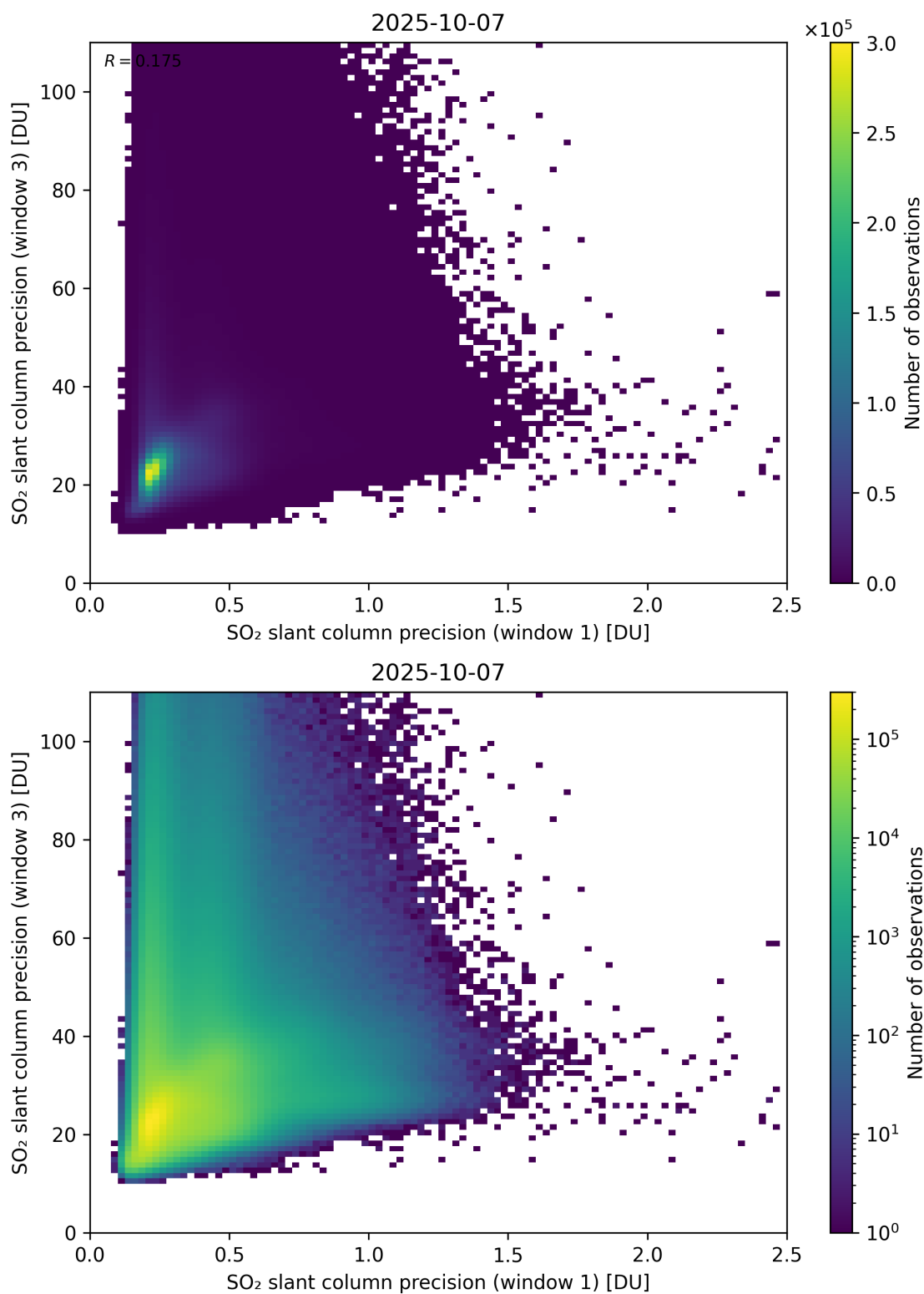
Figure 279: Scatter density plot of “SO 2 slant column precision (window 1)” against “SO 2 slant column precision (window 3)” for 2025-10-06 to 2025-10-08.
