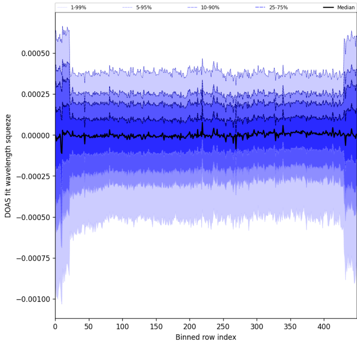
Figure 103: Along track statistics of “DOAS fit wavelength squeeze” for 2025-10-06 to 2025-10-08
