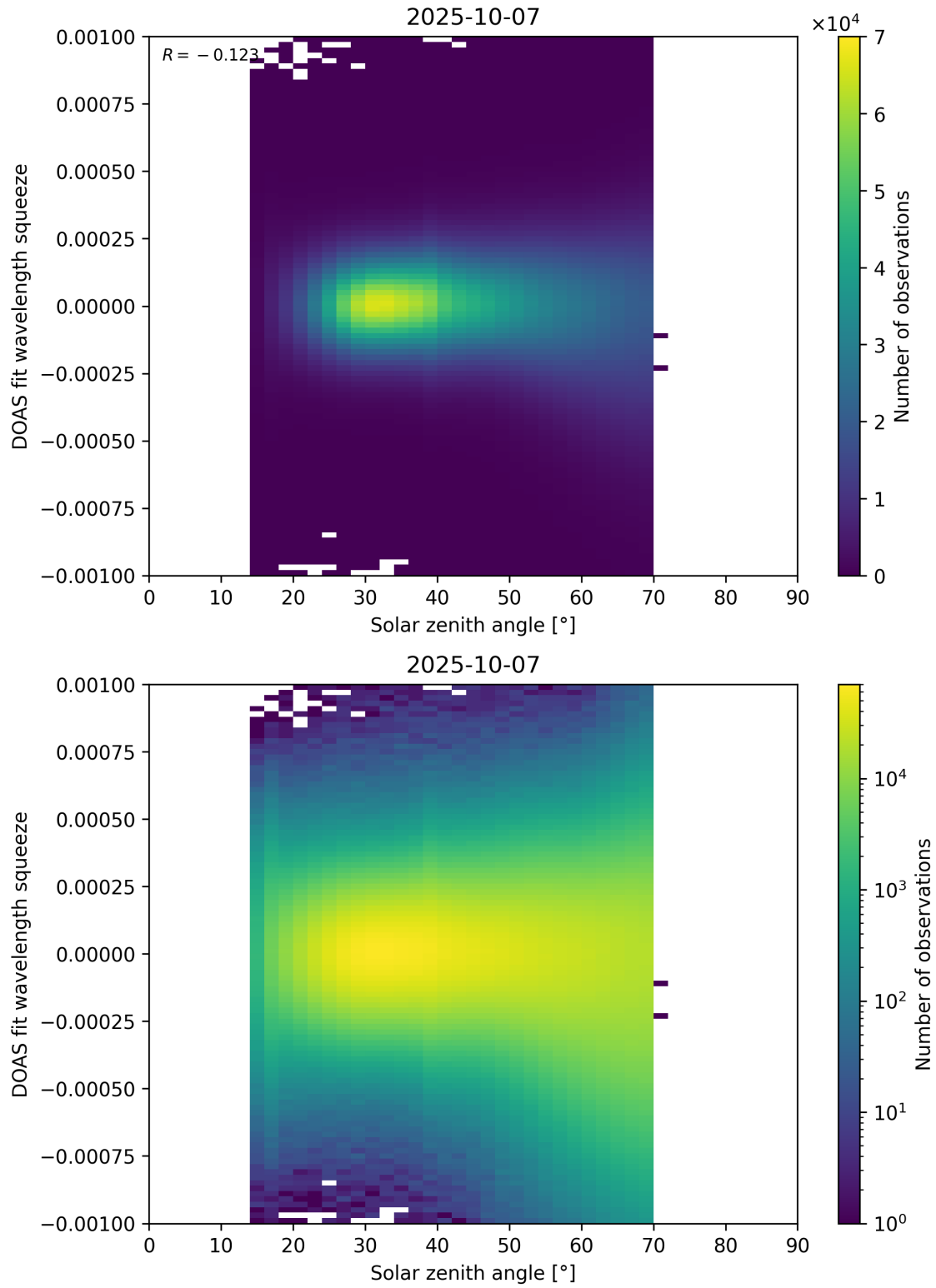
Figure 175: Scatter density plot of “Solar zenith angle” against “DOAS fit wavelength squeeze” for 2025-10-06 to 2025-10-08.
