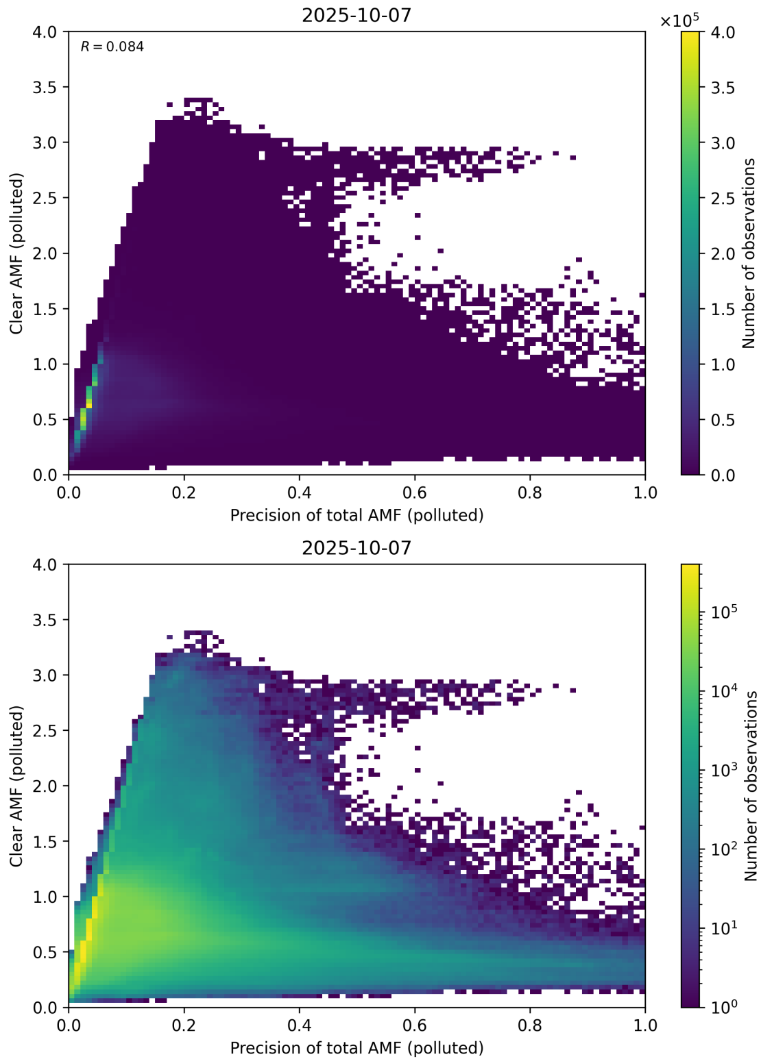
Figure 320: Scatter density plot of “Precision of total AMF (polluted)” against “Clear AMF (polluted)” for 2025-10-06 to 2025-10-08.
