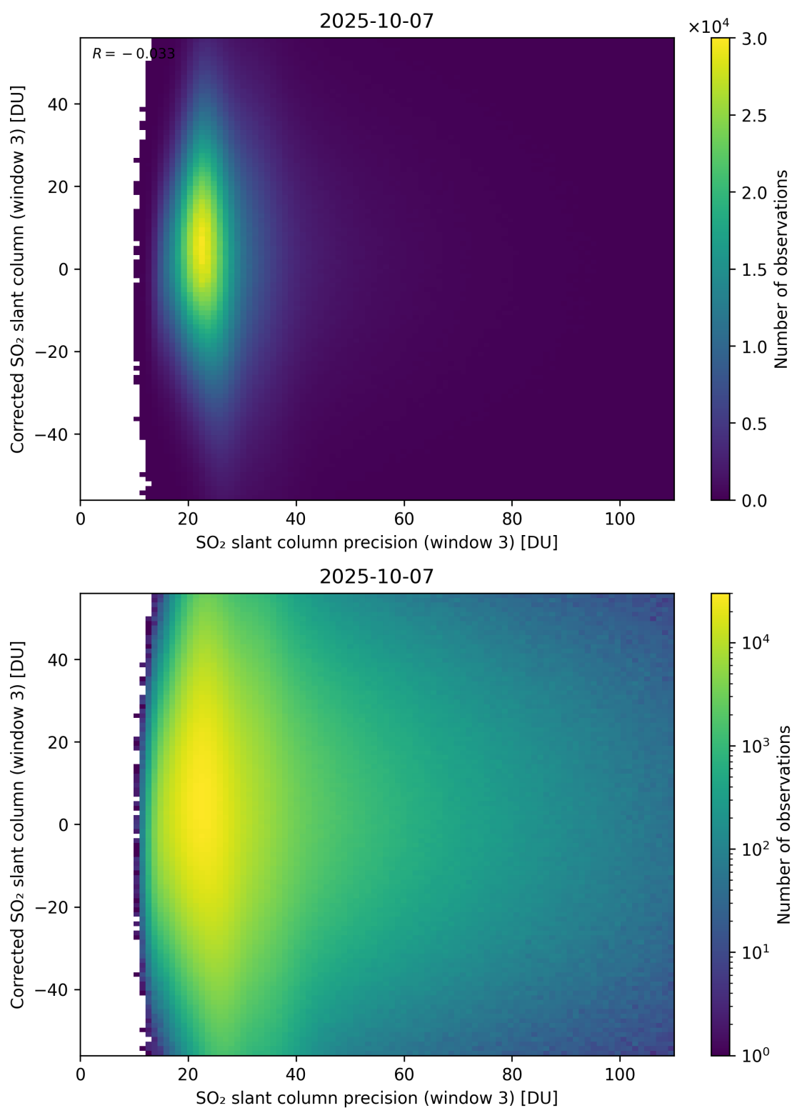
Figure 312: Scatter density plot of “SO 2 slant column precision (window 3)” against “Corrected SO 2 slant column (window 3)” for 2025-10-06 to 2025-10-08.
