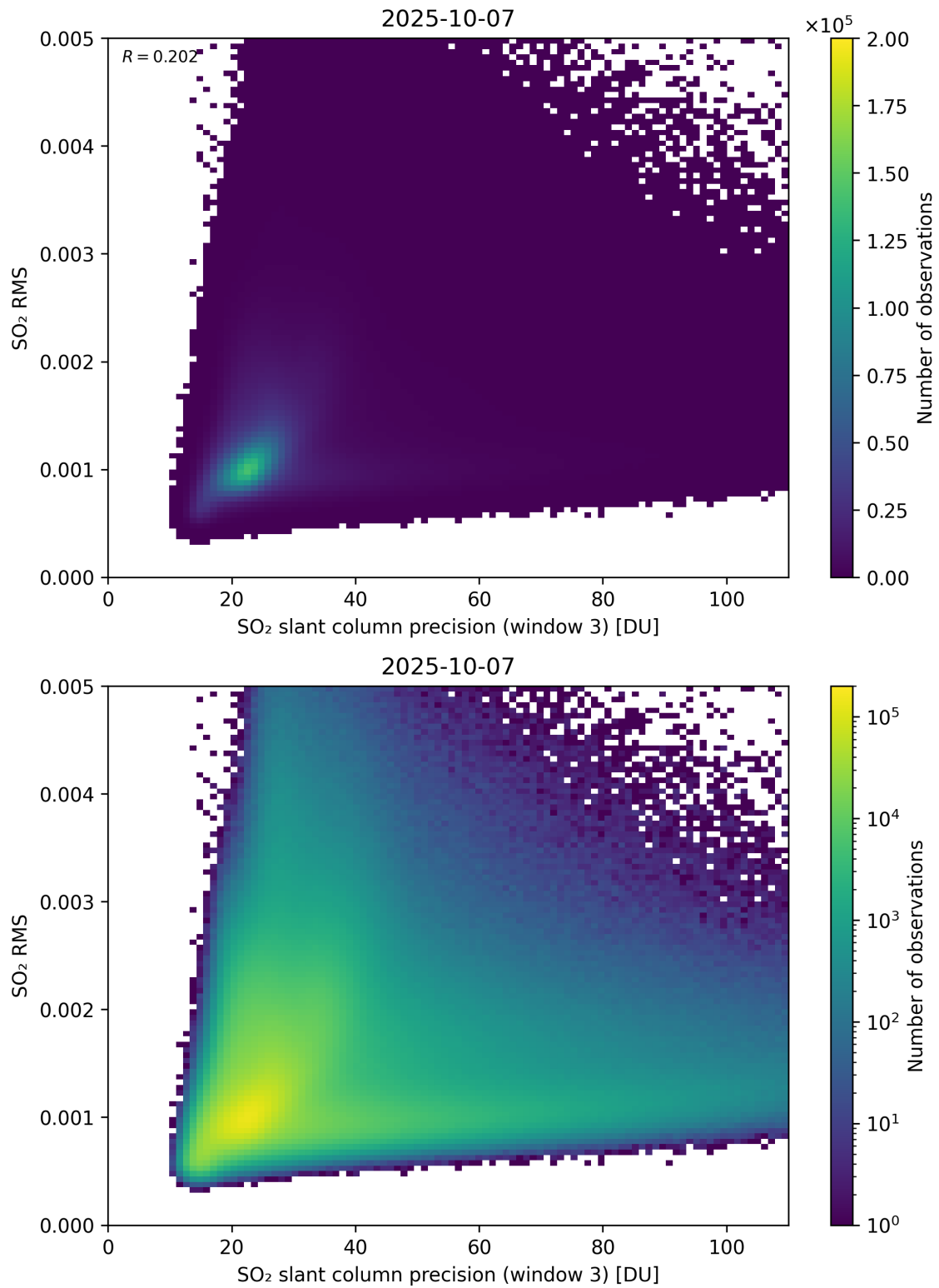
Figure 310: Scatter density plot of “SO 2 slant column precision (window 3)” against “SO 2 RMS” for 2025-10-06 to 2025-10-08.
