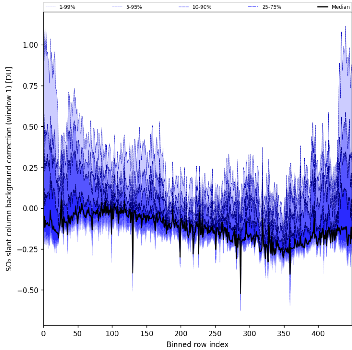
Figure 92: Along track statistics of “SO 2 slant column background correction (window 1)” for 2025-10-06 to 2025-10-08
