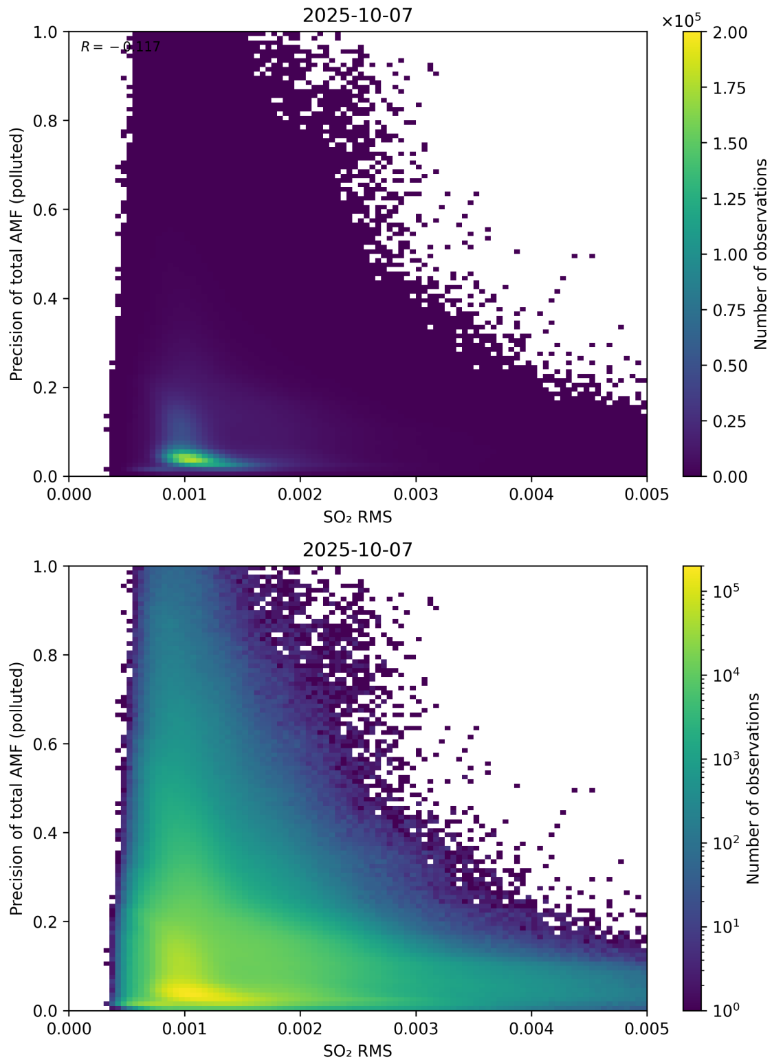
Figure 149: Scatter density plot of “SO 2 RMS” against “Precision of total AMF (polluted)” for 2025-10-06 to 2025-10-08.
