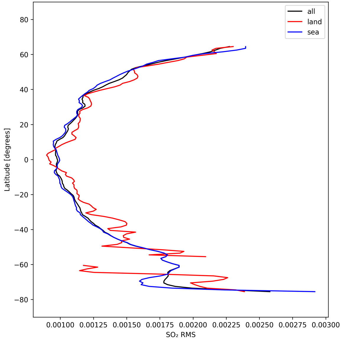
Figure 52: Zonal average of “SO 2 RMS” for 2025-10-06 to 2025-10-08.
