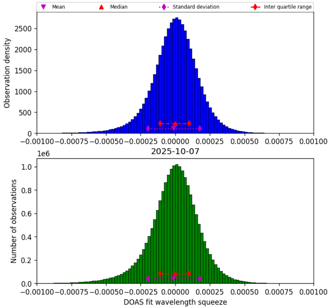
Figure 77: Histogram of “DOAS fit wavelength squeeze” for 2025-10-06 to 2025-10-08
