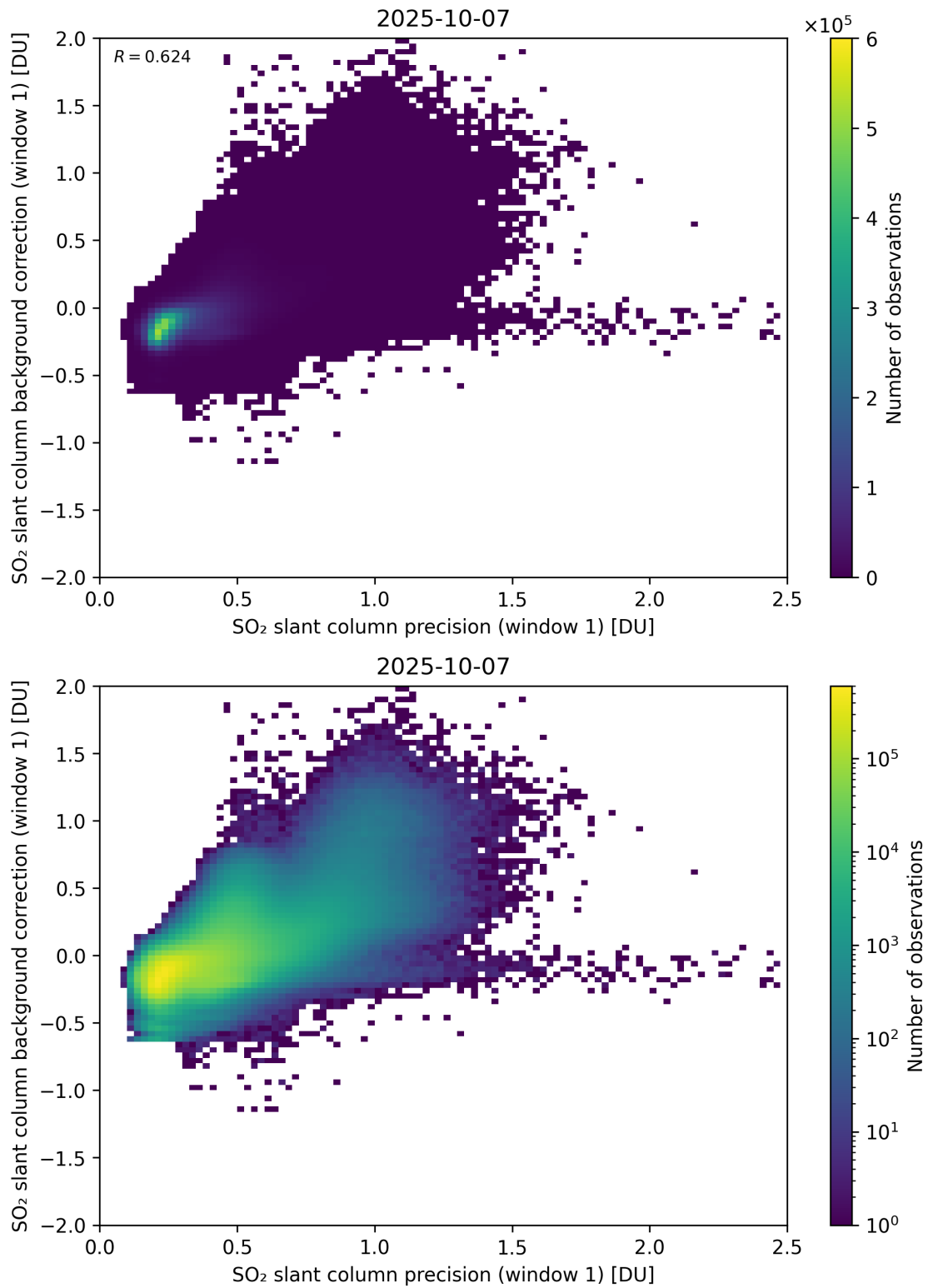
Figure 268: Scatter density plot of “SO 2 slant column precision (window 1)” against “SO 2 slant column background correction (window 1)” for 2025-10-06 to 2025-10-08.
