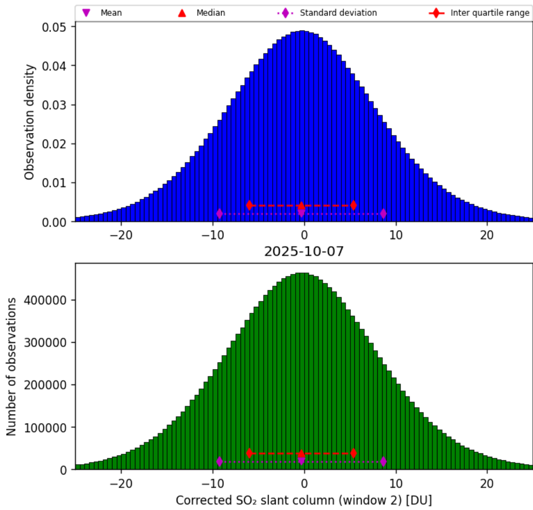
Figure 69: Histogram of “Corrected SO 2 slant column (window 2)” for 2025-10-06 to 2025-10-08
