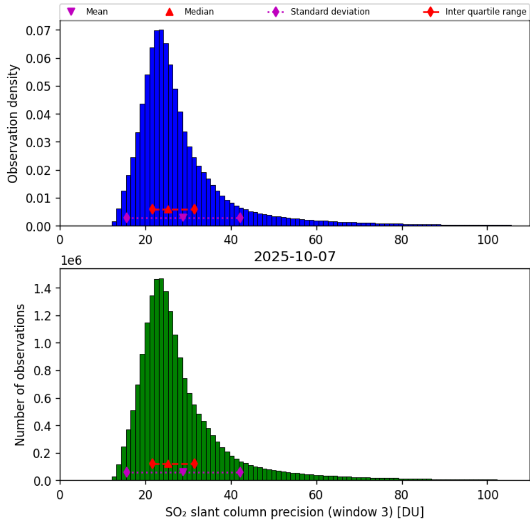
Figure 72: Histogram of “SO 2 slant column precision (window 3)” for 2025-10-06 to 2025-10-08
