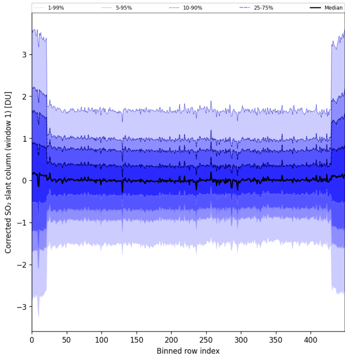
Figure 91: Along track statistics of “Corrected SO 2 slant column (window 1)” for 2025-10-06 to 2025-10-08
