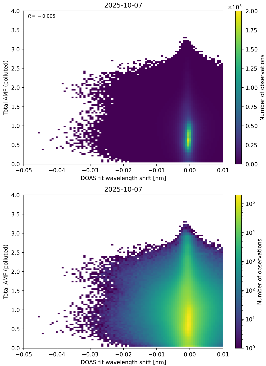
Figure 141: Scatter density plot of “DOAS fit wavelength shift” against “Total AMF (polluted)” for 2025-10-06 to 2025-10-08.
