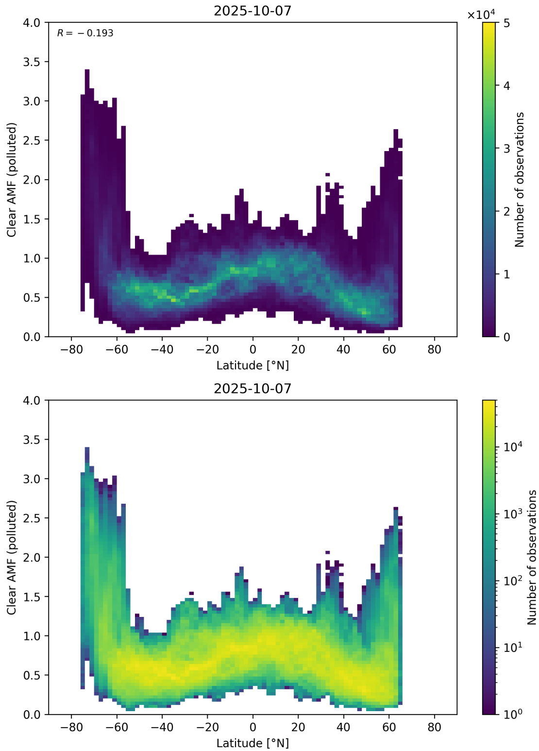
Figure 156: Scatter density plot of “Latitude” against “Clear AMF (polluted)” for 2025-10-06 to 2025-10-08.
