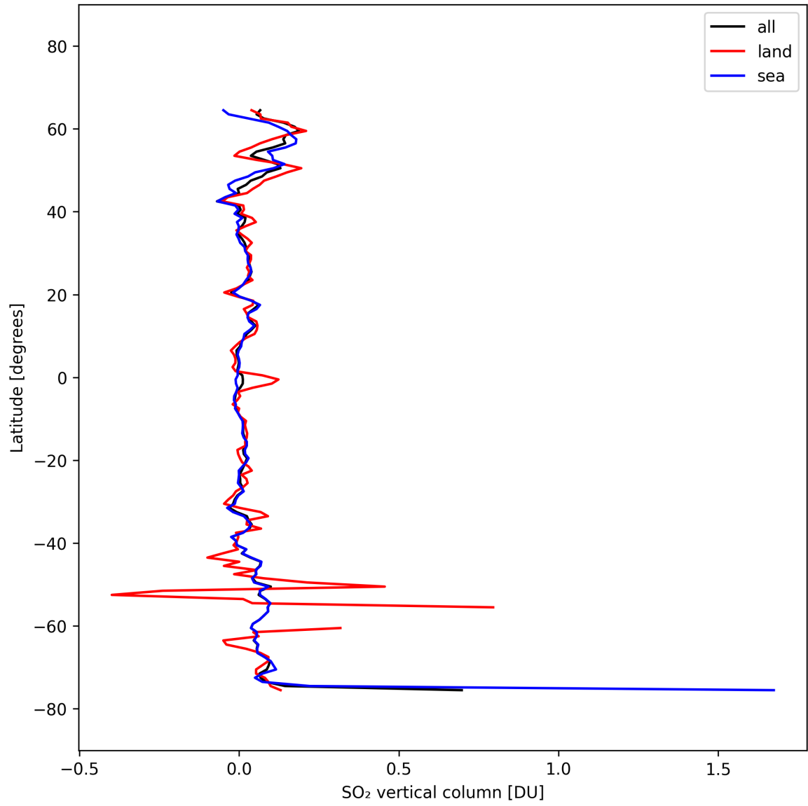
Figure 32: Zonal average of “SO 2 vertical column” for 2025-10-06 to 2025-10-08.
