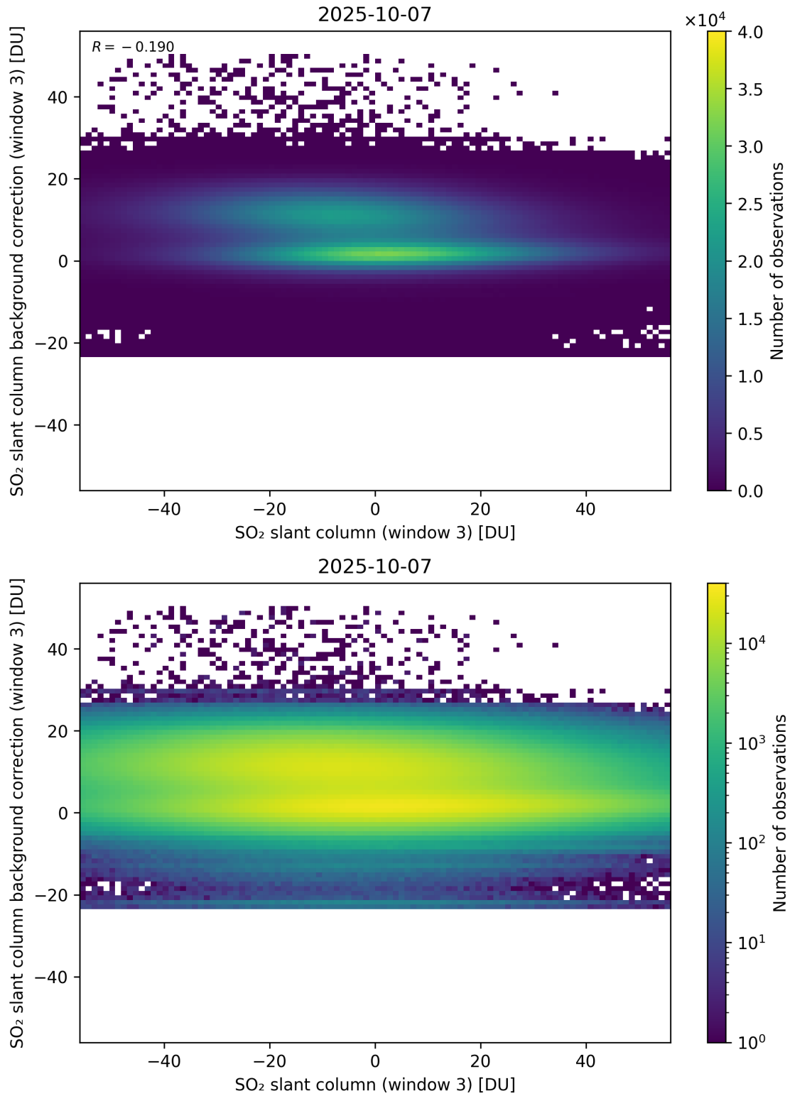
Figure 303: Scatter density plot of “SO 2 slant column (window 3)” against “SO 2 slant column background correction (window 3)” for 2025-10-06 to 2025-10-08.
