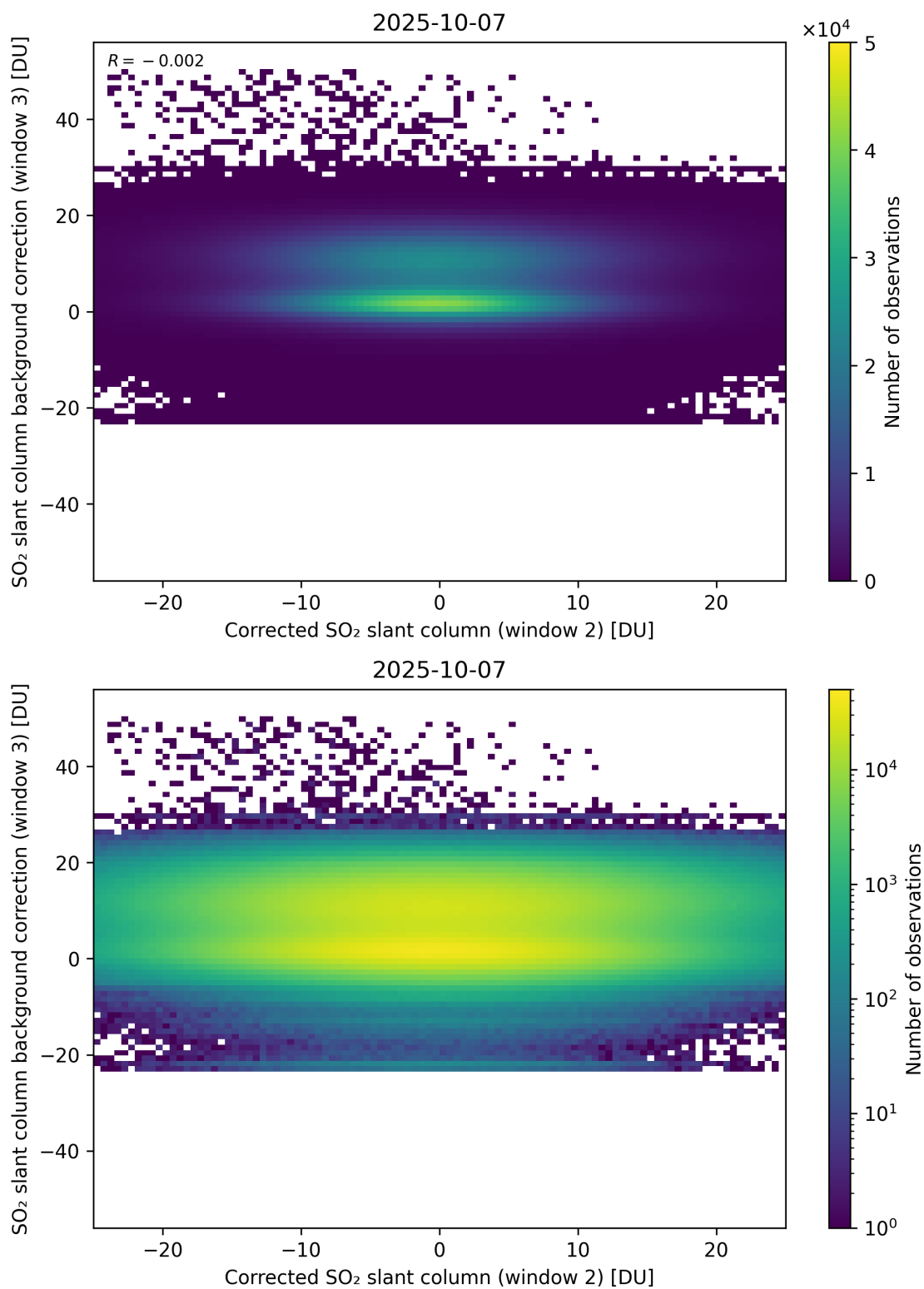
Figure 245: Scatter density plot of “Corrected SO 2 slant column (window 2)” against “SO 2 slant column background correction (window 3)” for 2025-10-06 to 2025-10-08.
