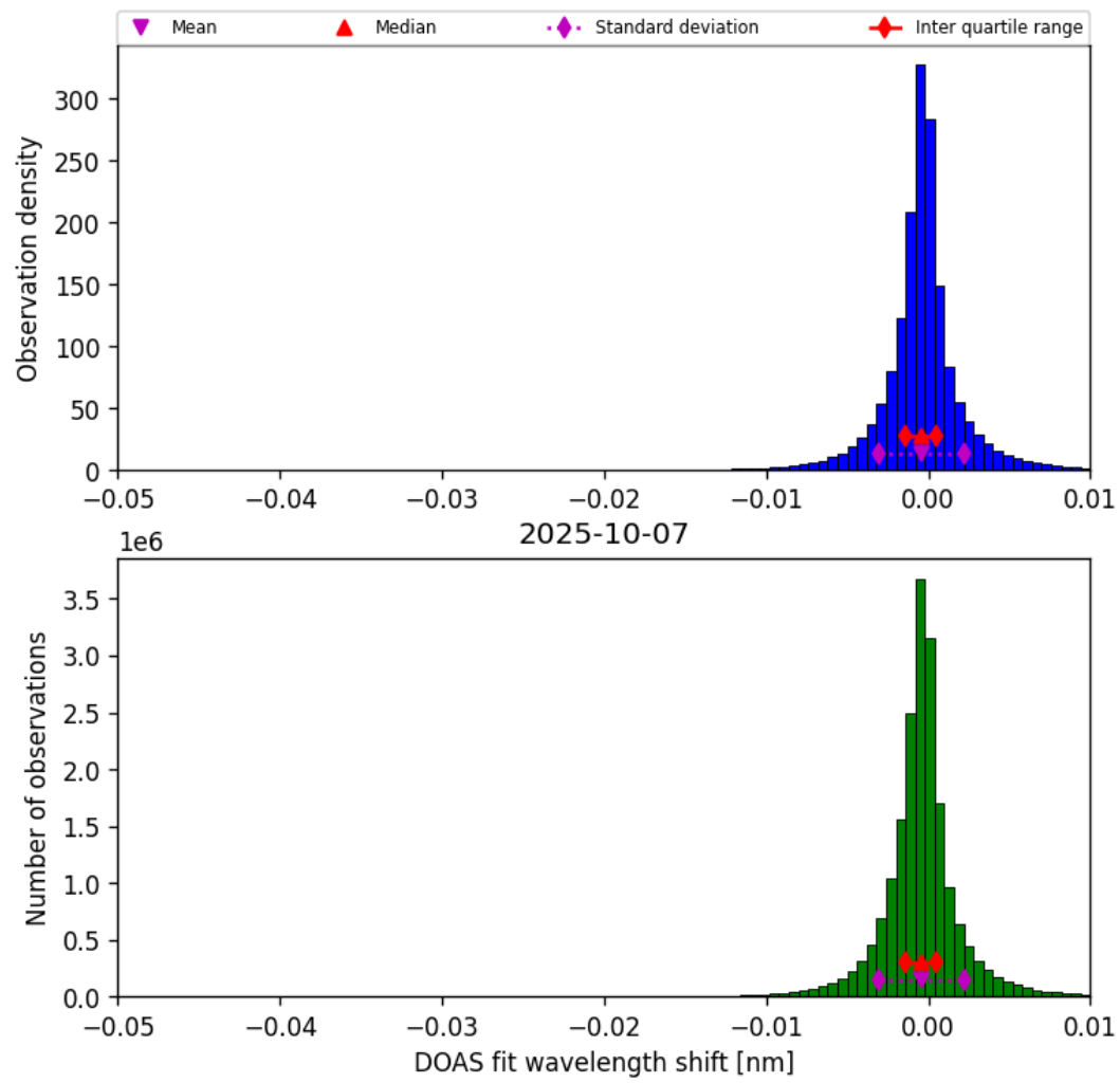
Figure 76: Histogram of “DOAS fit wavelength shift” for 2025-10-06 to 2025-10-08
