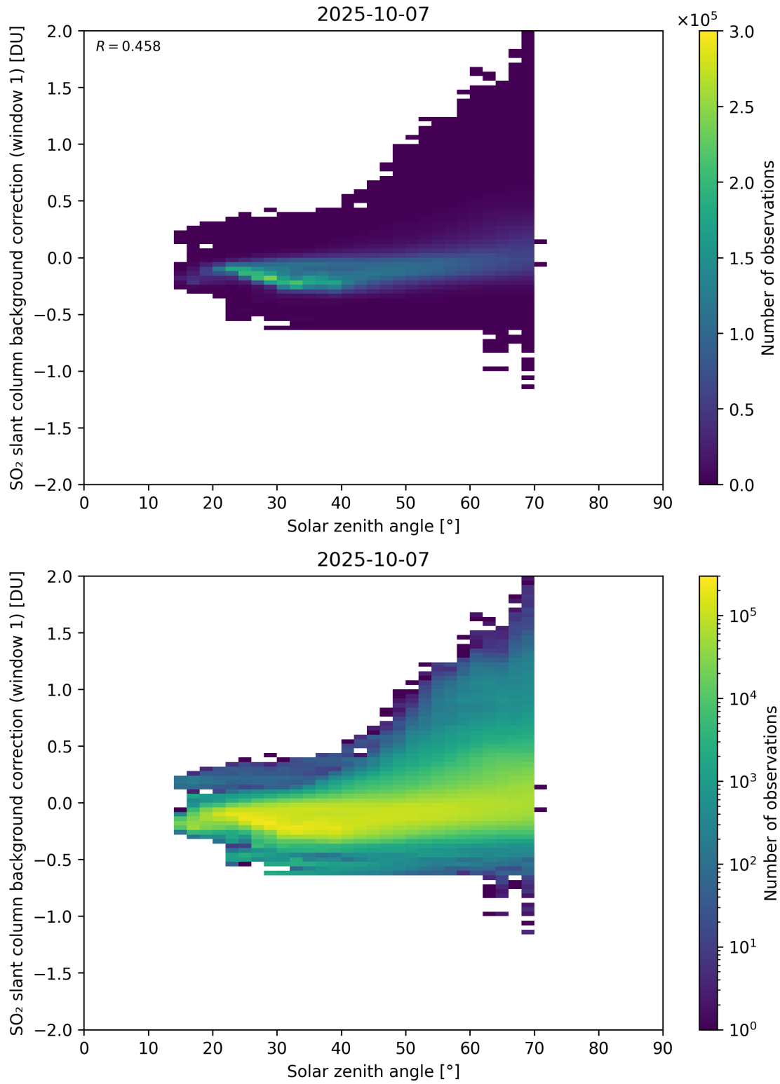
Figure 171: Scatter density plot of “Solar zenith angle” against “SO 2 slant column background correction (window 1)” for 2025-10-06 to 2025-10-08.
