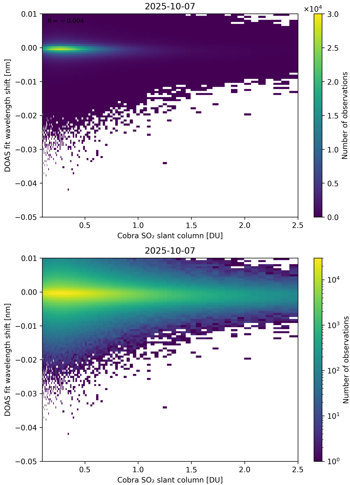
Figure 196: Scatter density plot of “Cobra SO 2 slant column” against “DOAS fit wavelength shift” for 2025-10-06 to 2025-10-08.
