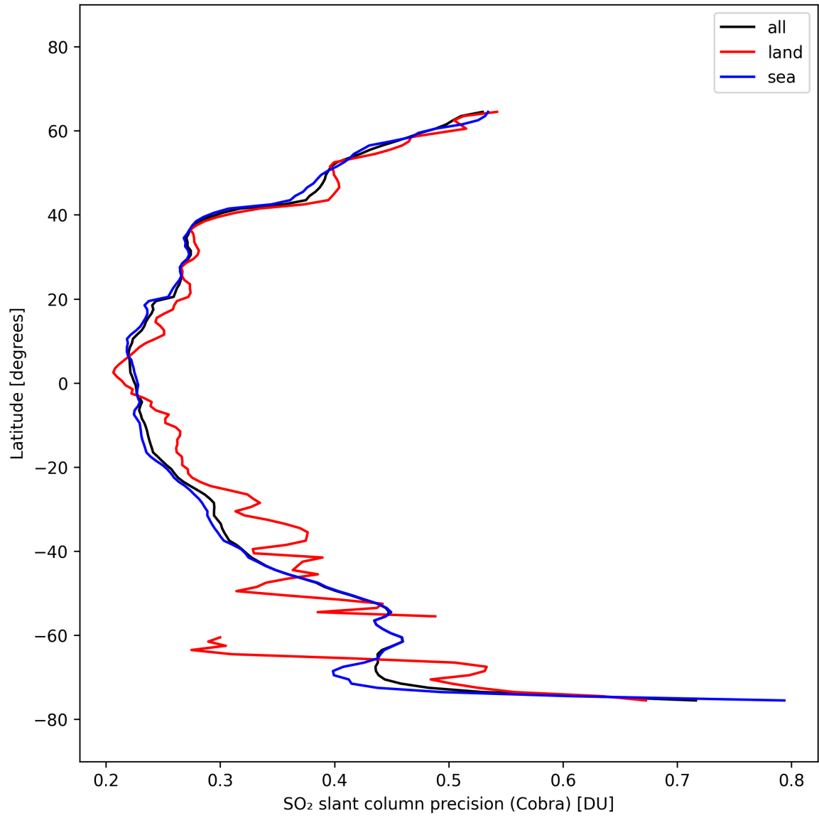
Figure 36: Zonal average of “SO 2 slant column precision (Cobra)” for 2025-10-06 to 2025-10-08.
