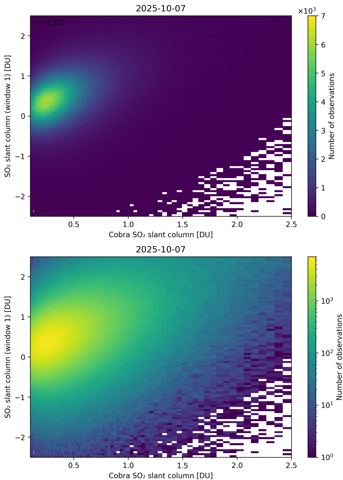
Figure 219: Scatter density plot of “Cobra SO 2 slant column” against “SO 2 slant column (window 1)” for 2025-10-06 to 2025-10-08.
