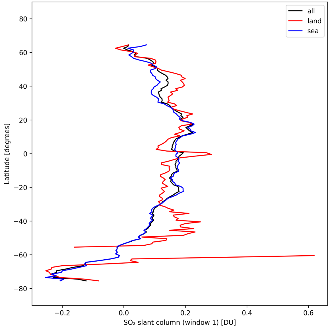
Figure 37: Zonal average of “SO 2 slant column (window 1)” for 2025-10-06 to 2025-10-08.
