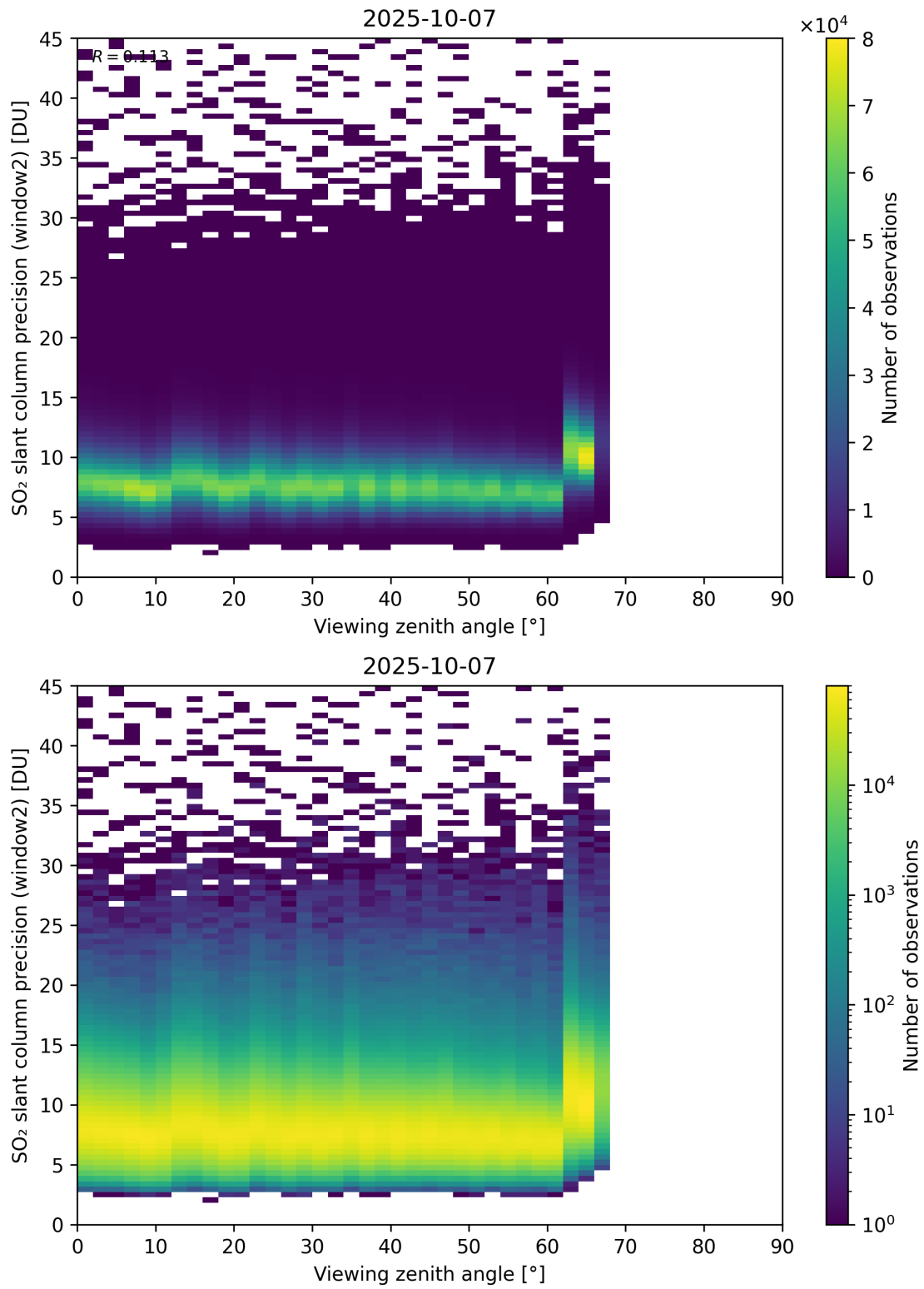
Figure 378: Scatter density plot of “Viewing zenith angle” against “SO 2 slant column precision (window2)” for 2025-10-06 to 2025-10-08.
