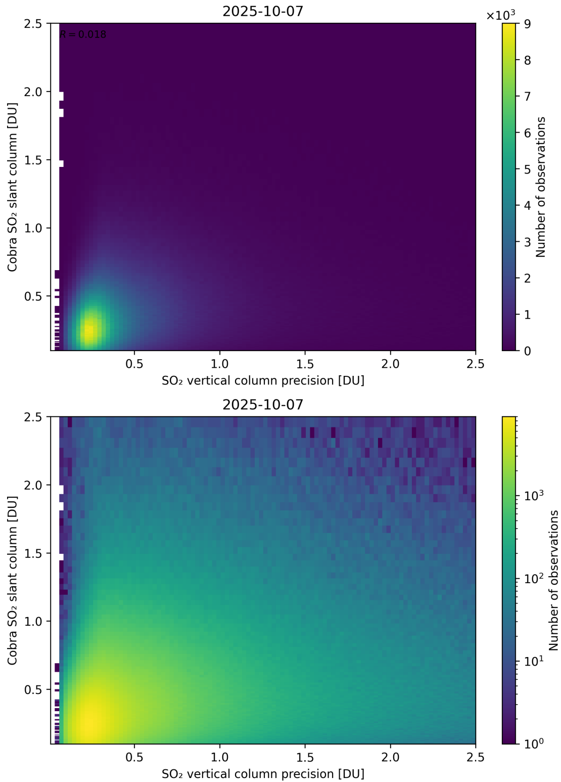
Figure 336: Scatter density plot of “SO 2 vertical column precision” against “Cobra SO 2 slant column” for 2025-10-06 to 2025-10-08.
