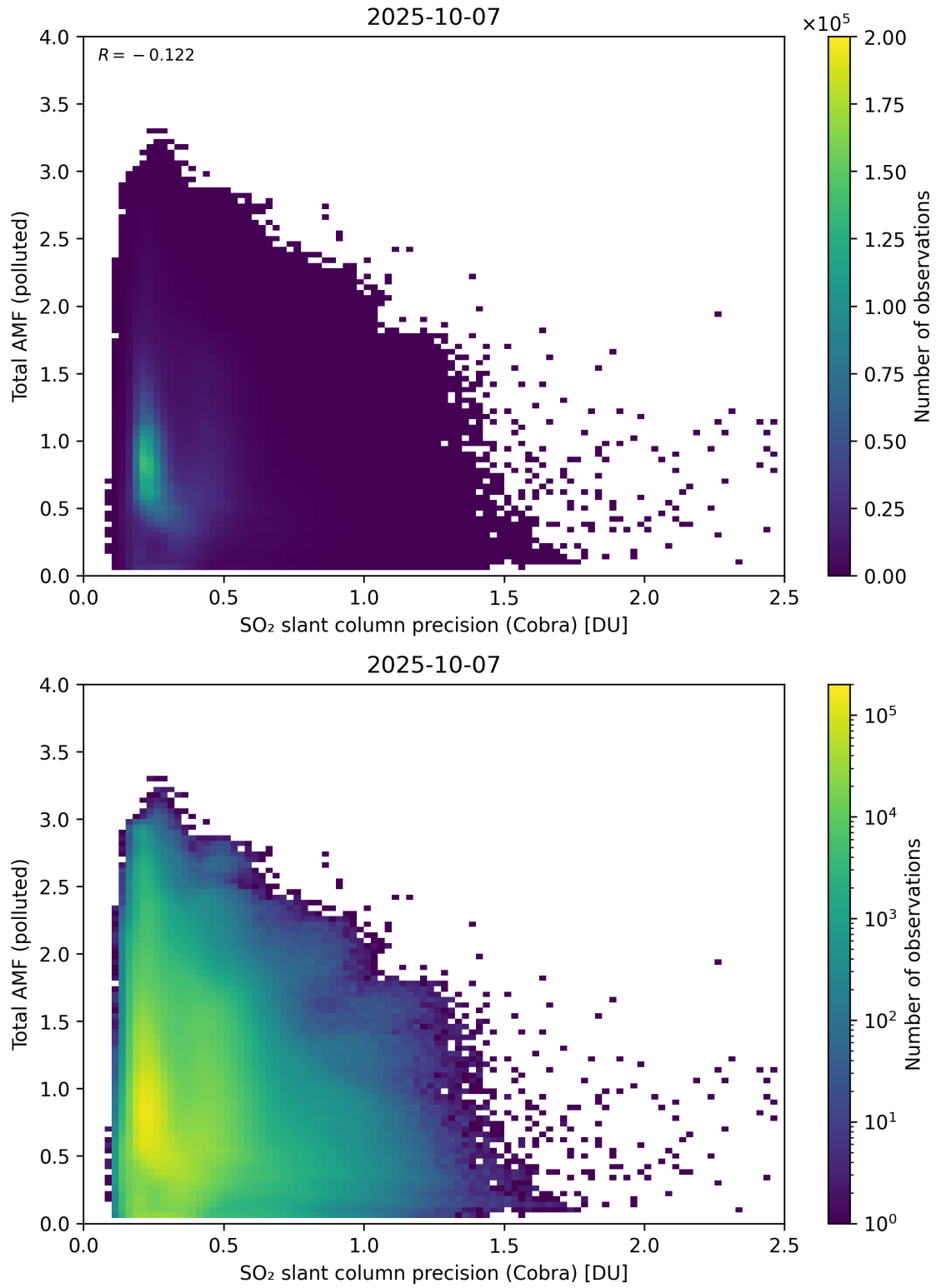
Figure 213: Scatter density plot of “SO 2 slant column precision (Cobra)” against “Total AMF (polluted)” for 2025-10-06 to 2025-10-08.
