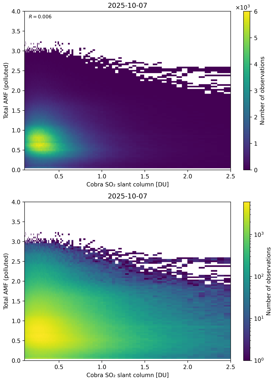
Figure 224: Scatter density plot of “Cobra SO 2 slant column” against “Total AMF (polluted)” for 2025-10-06 to 2025-10-08.
