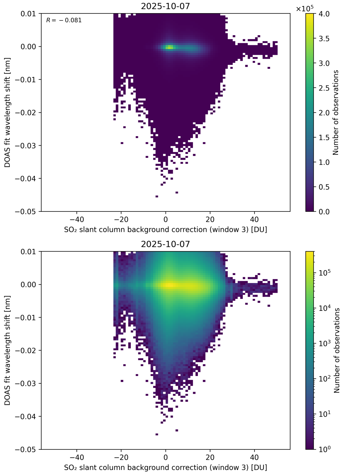
Figure 132: Scatter density plot of “SO 2 slant column background correction (window 3)” against “DOAS fit wavelength shift” for 2025-10-06 to 2025-10-08.
