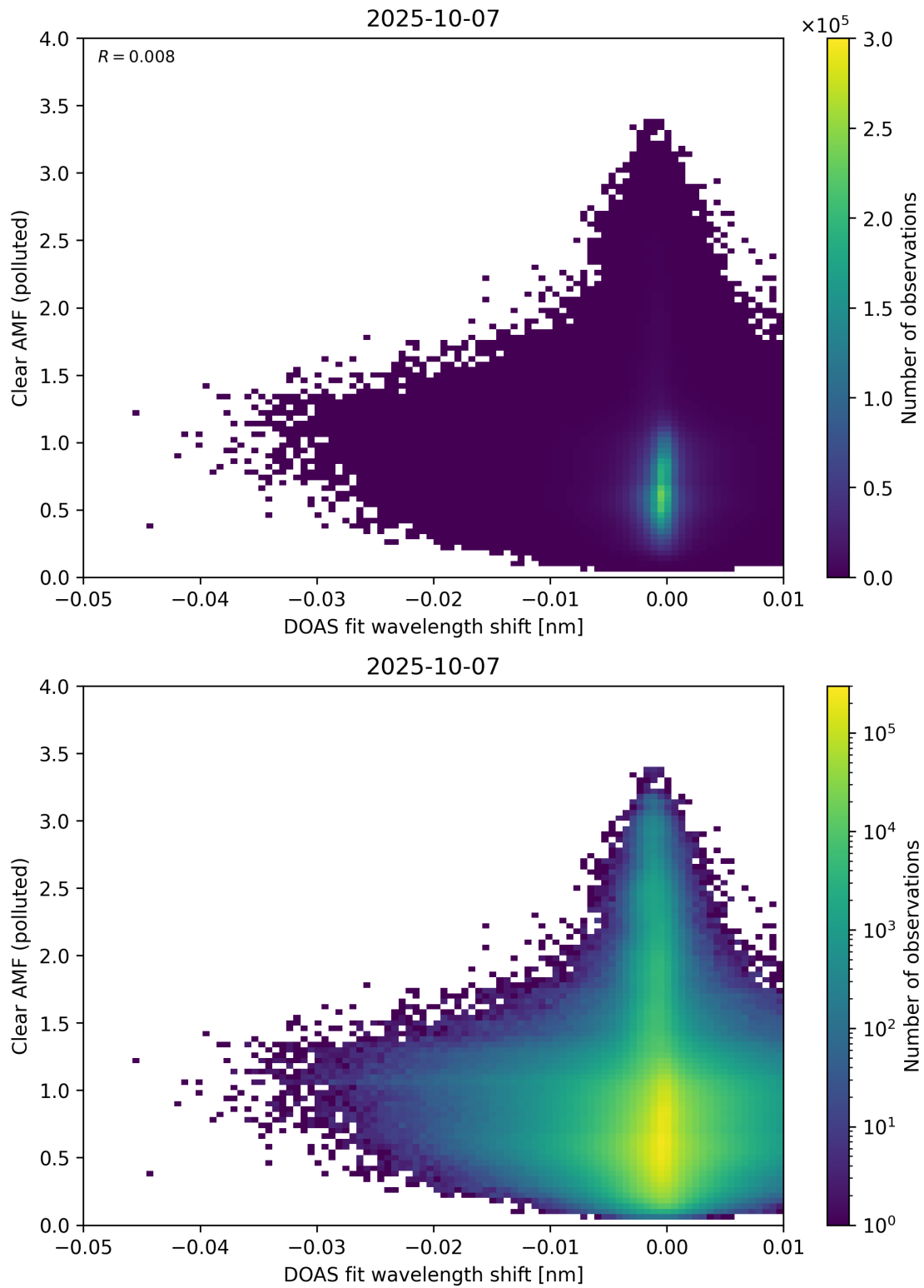
Figure 140: Scatter density plot of “DOAS fit wavelength shift” against “Clear AMF (polluted)” for 2025-10-06 to 2025-10-08.
