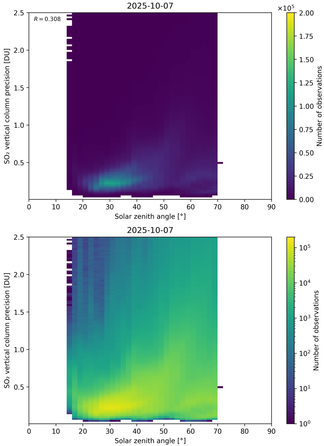
Figure 192: Scatter density plot of “Solar zenith angle” against “SO 2 vertical column precision” for 2025-10-06 to 2025-10-08.
