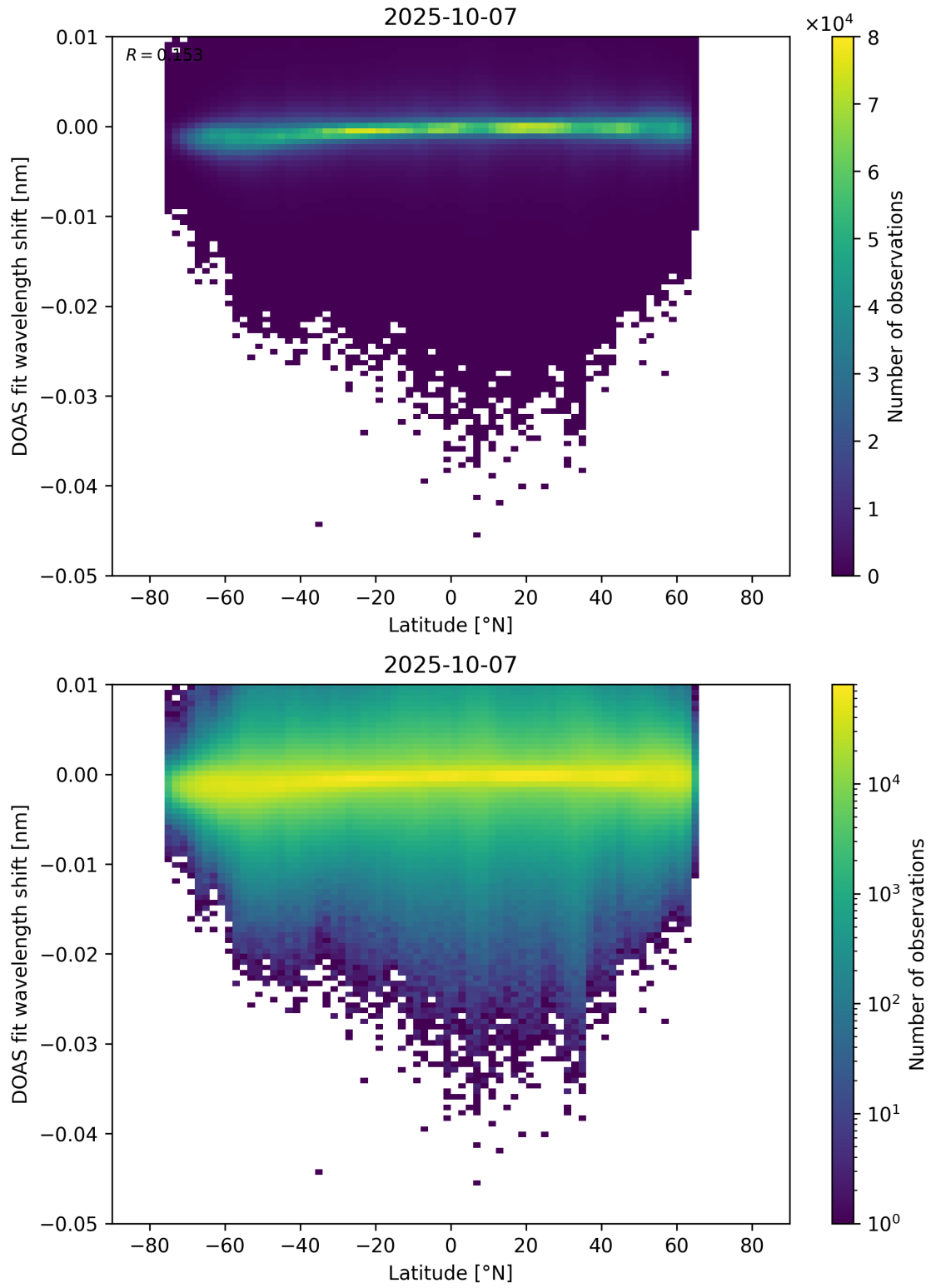
Figure 153: Scatter density plot of “Latitude” against “DOAS fit wavelength shift” for 2025-10-06 to 2025-10-08.
