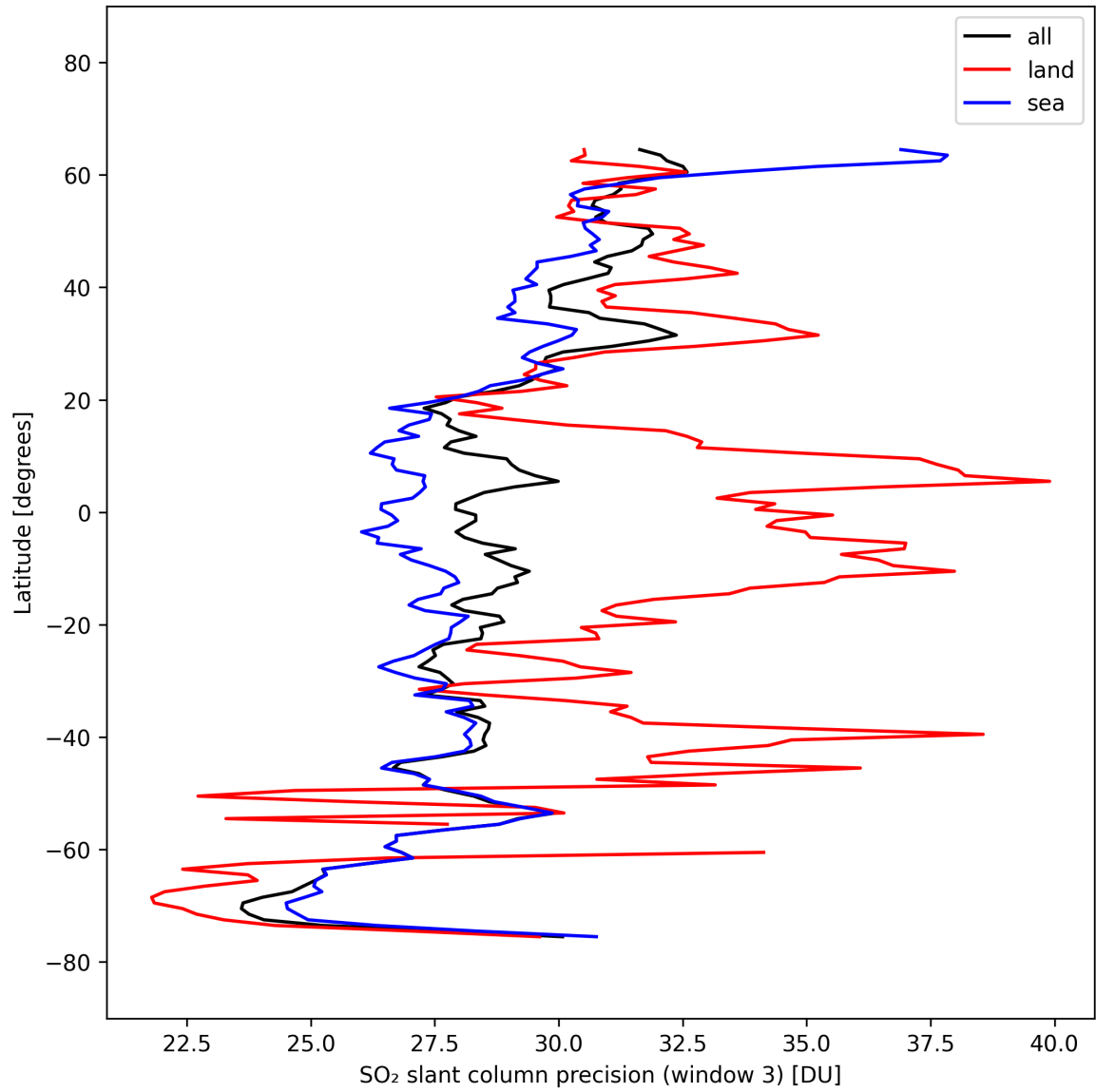
Figure 46: Zonal average of “SO 2 slant column precision (window 3)” for 2025-10-06 to 2025-10-08.
