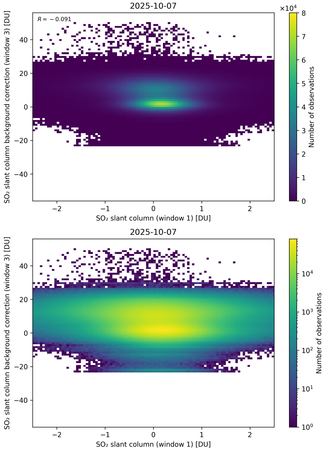
Figure 264: Scatter density plot of “SO 2 slant column (window 1)” against “SO 2 slant column background correction (window 3)” for 2025-10-06 to 2025-10-08.
