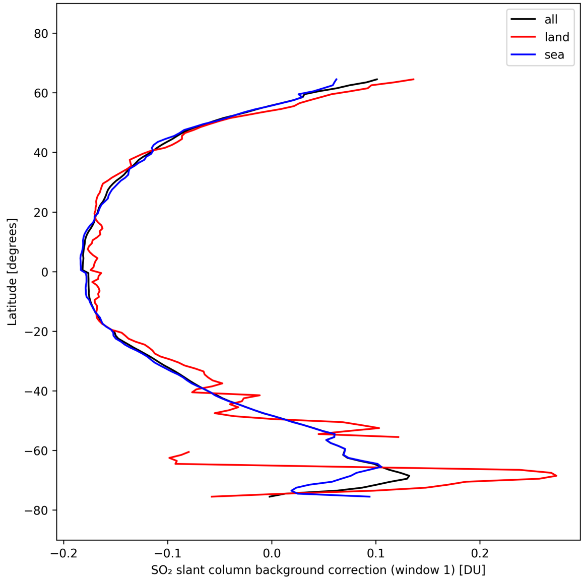
Figure 40: Zonal average of “SO 2 slant column background correction (window 1)” for 2025-10-06 to 2025-10-08.
