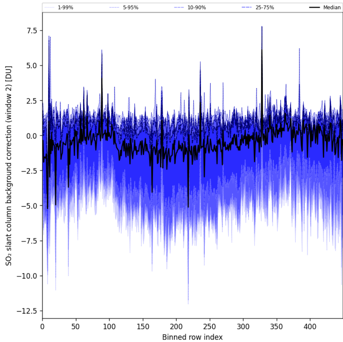
Figure 96: Along track statistics of “SO 2 slant column background correction (window 2)” for 2025-10-06 to 2025-10-08
