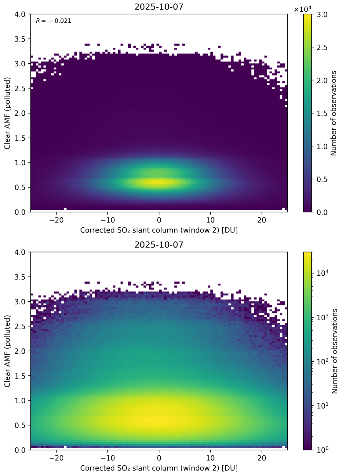
Figure 249: Scatter density plot of “Corrected SO 2 slant column (window 2)” against “Clear AMF (polluted)” for 2025-10-06 to 2025-10-08.
