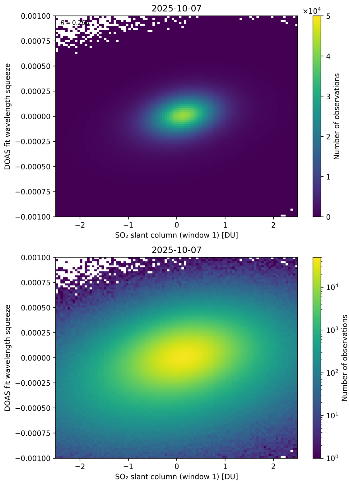
Figure 266: Scatter density plot of “SO 2 slant column (window 1)” against “DOAS fit wavelength squeeze” for 2025-10-06 to 2025-10-08.
