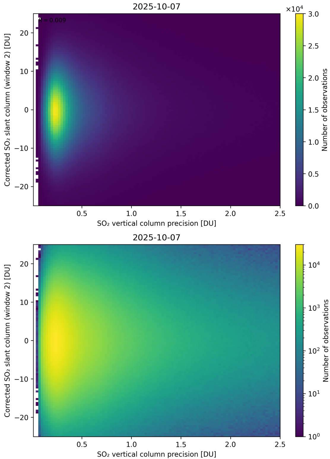
Figure 339: Scatter density plot of “SO 2 vertical column precision” against “Corrected SO 2 slant column (window 2)” for 2025-10-06 to 2025-10-08.
