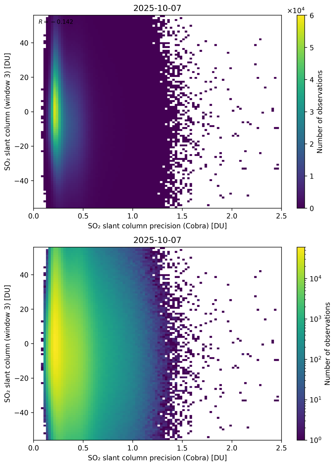
Figure 211: Scatter density plot of “SO 2 slant column precision (Cobra)” against “SO 2 slant column (window 3)” for 2025-10-06 to 2025-10-08.
