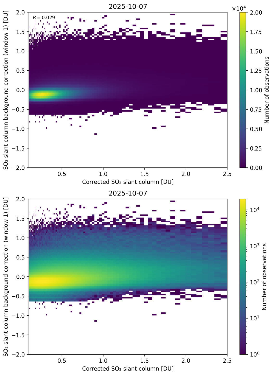
Figure 226: Scatter density plot of “Corrected SO 2 slant column” against “SO 2 slant column background correction (window 1)” for 2025-10-06 to 2025-10-08.
