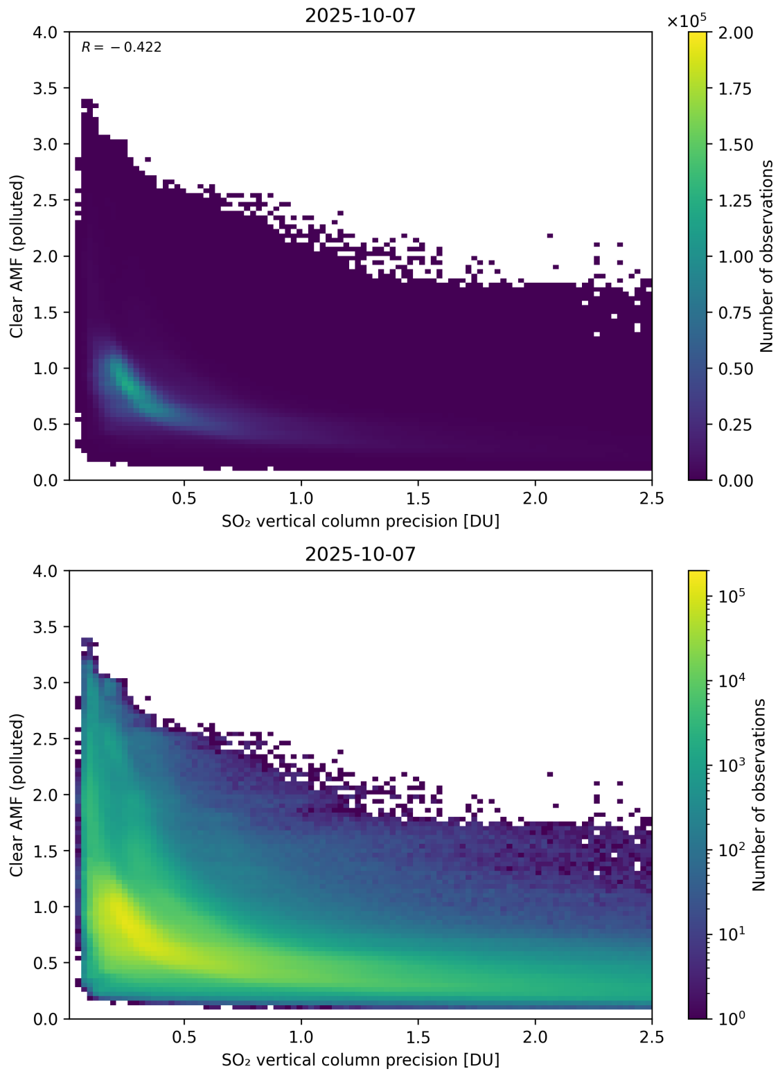
Figure 335: Scatter density plot of “SO 2 vertical column precision” against “Clear AMF (polluted)” for 2025-10-06 to 2025-10-08.
