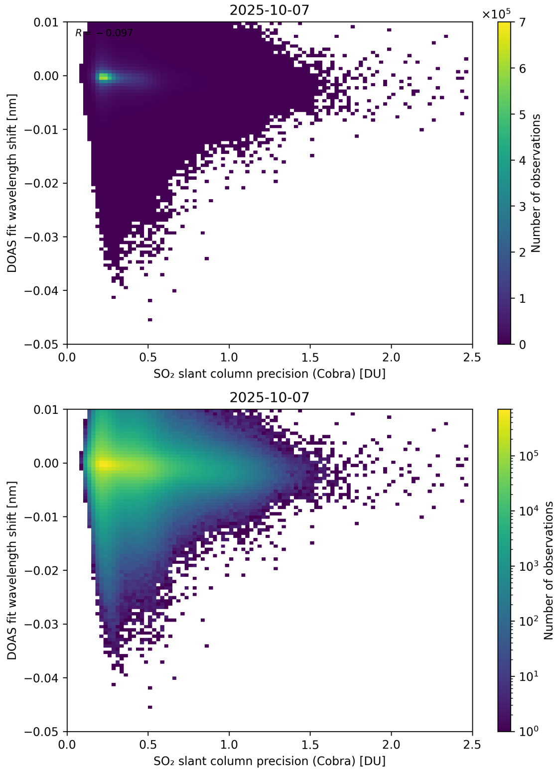
Figure 202: Scatter density plot of “SO 2 slant column precision (Cobra)” against “DOAS fit wavelength shift” for 2025-10-06 to 2025-10-08.
