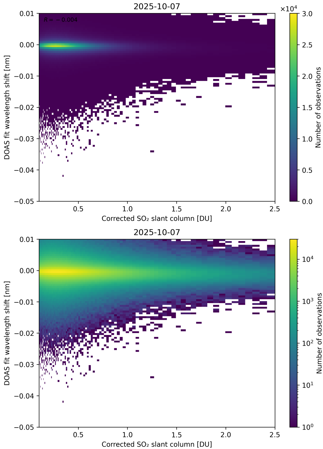
Figure 229: Scatter density plot of “Corrected SO 2 slant column” against “DOAS fit wavelength shift” for 2025-10-06 to 2025-10-08.
