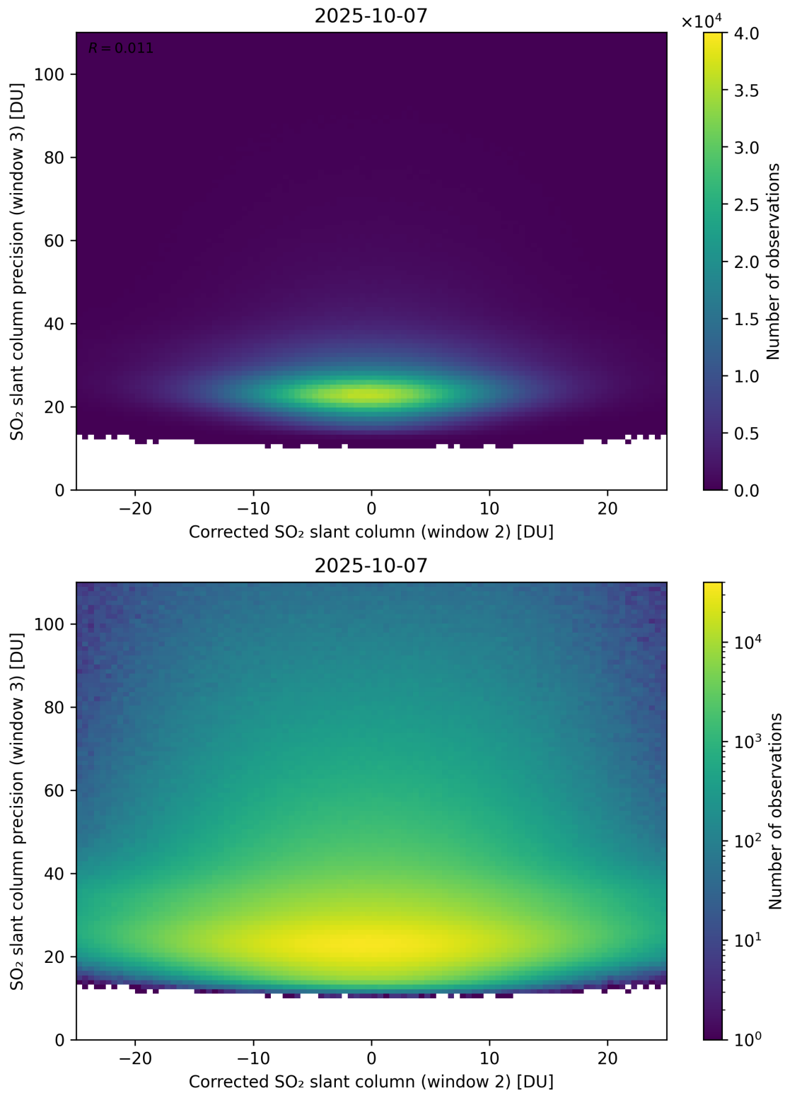
Figure 252: Scatter density plot of “Corrected SO 2 slant column (window 2)” against “SO 2 slant column precision (window 3)” for 2025-10-06 to 2025-10-08.
