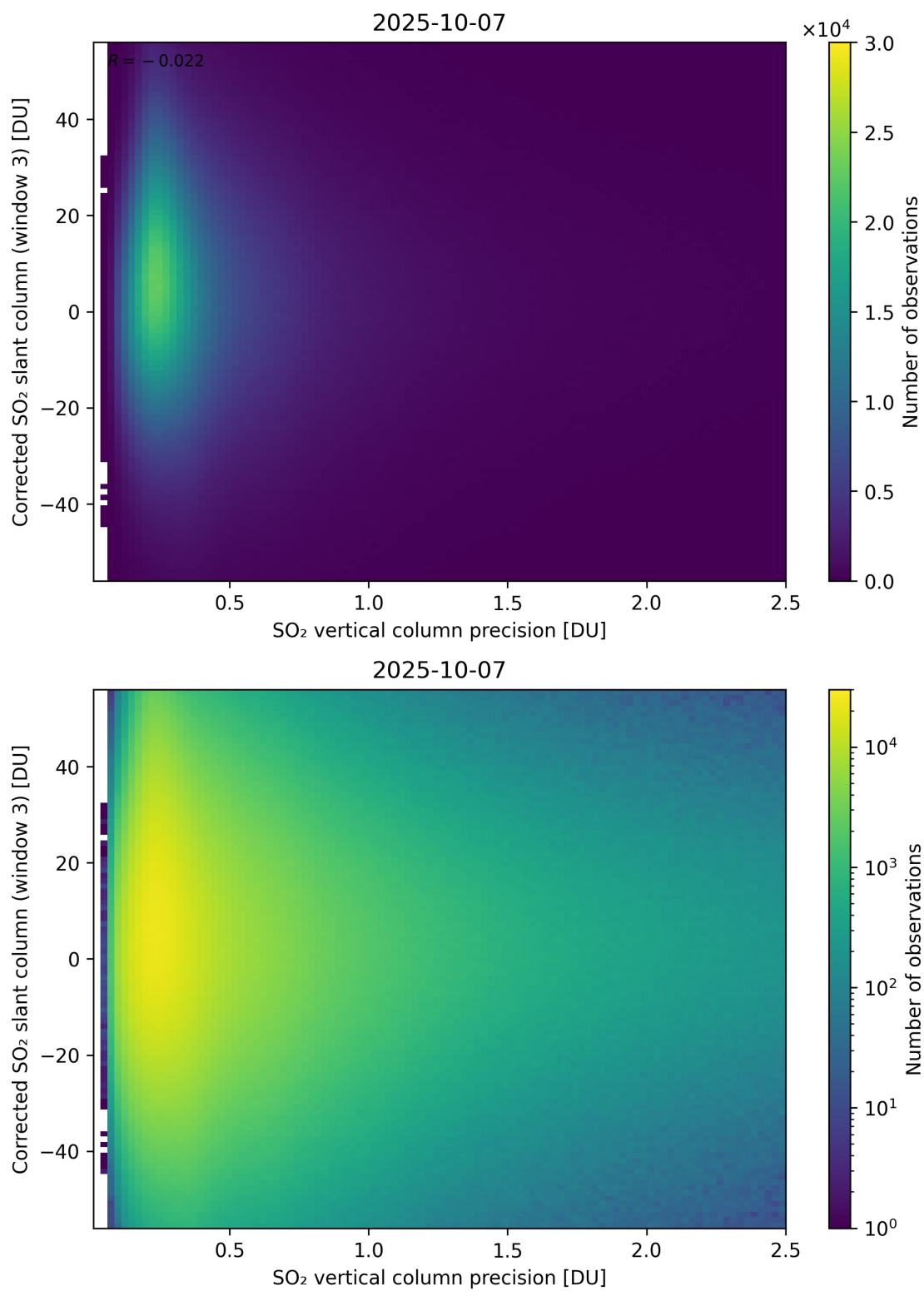
Figure 340: Scatter density plot of “SO 2 vertical column precision” against “Corrected SO 2 slant column (window 3)” for 2025-10-06 to 2025-10-08.
