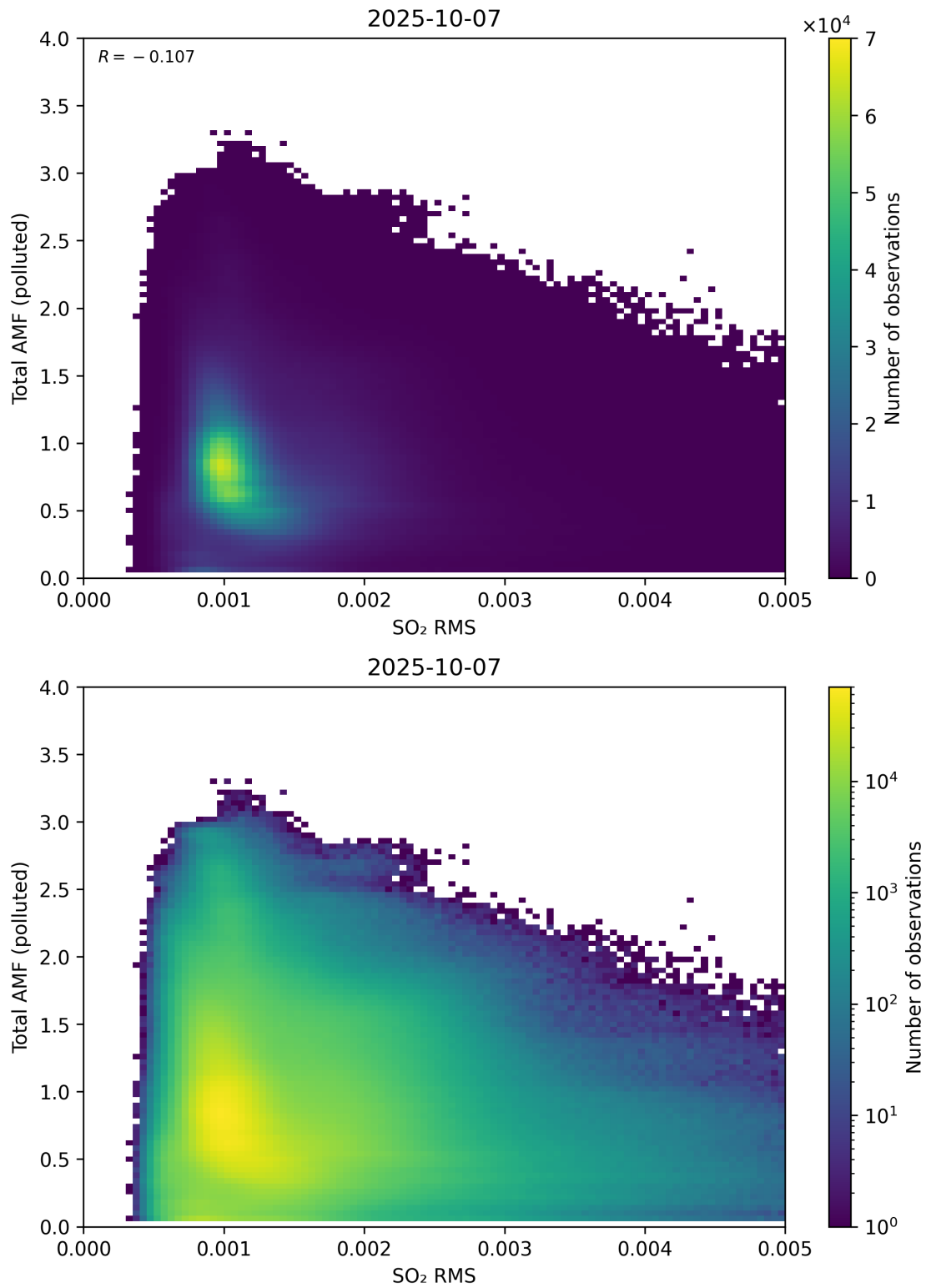
Figure 148: Scatter density plot of “SO 2 RMS” against “Total AMF (polluted)” for 2025-10-06 to 2025-10-08.
