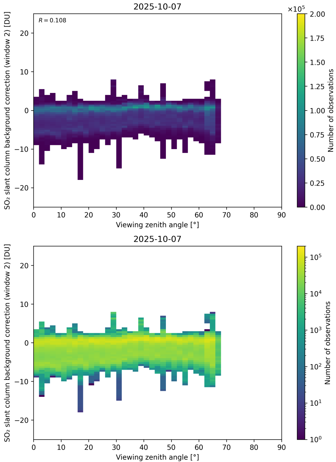
Figure 363: Scatter density plot of “Viewing zenith angle” against “SO 2 slant column background correction (window 2)” for 2025-10-06 to 2025-10-08.
