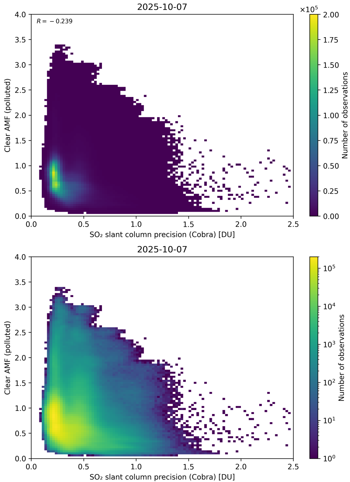
Figure 205: Scatter density plot of “SO 2 slant column precision (Cobra)” against “Clear AMF (polluted)” for 2025-10-06 to 2025-10-08.
