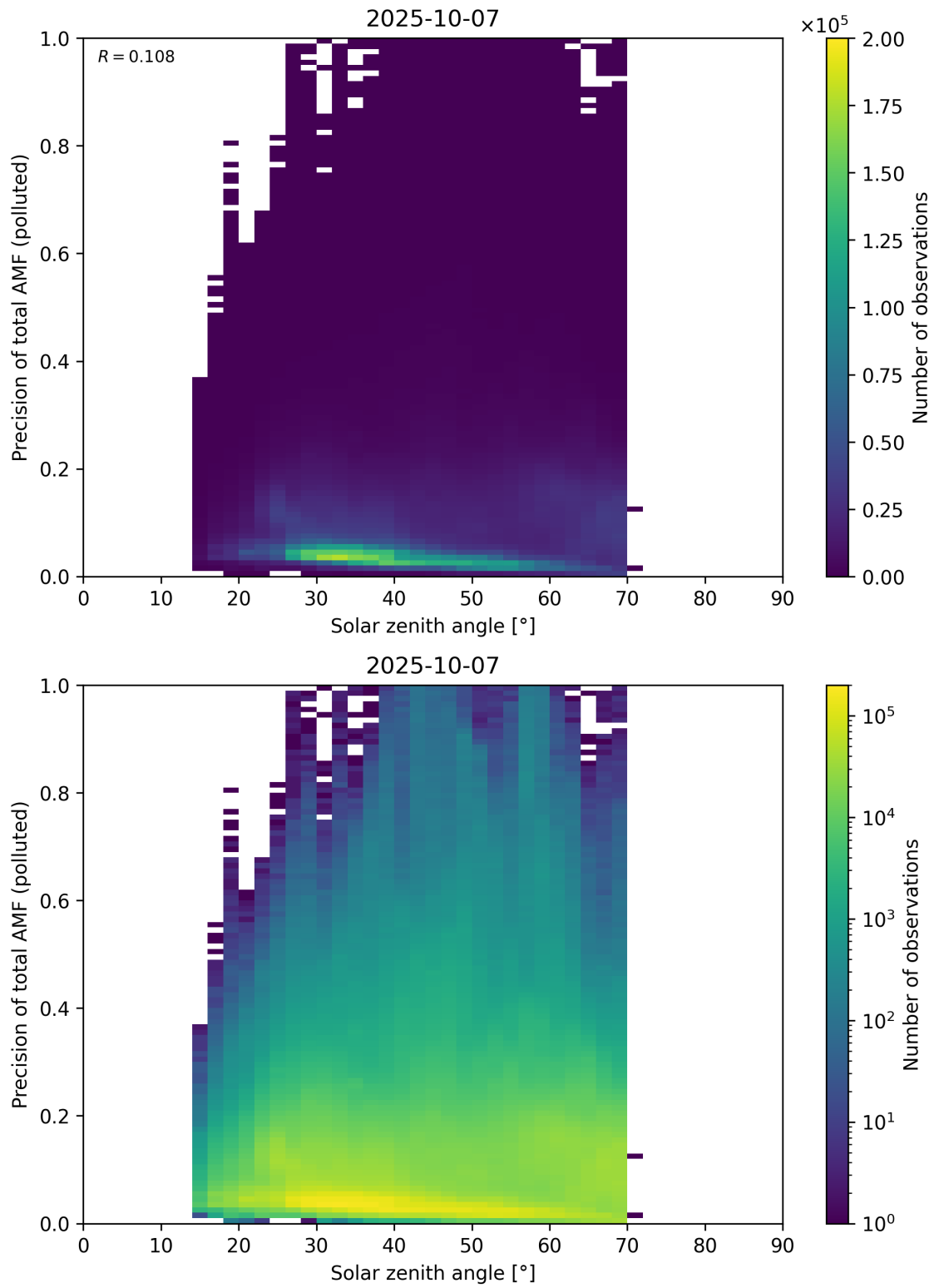
Figure 190: Scatter density plot of “Solar zenith angle” against “Precision of total AMF (polluted)” for 2025-10-06 to 2025-10-08.
