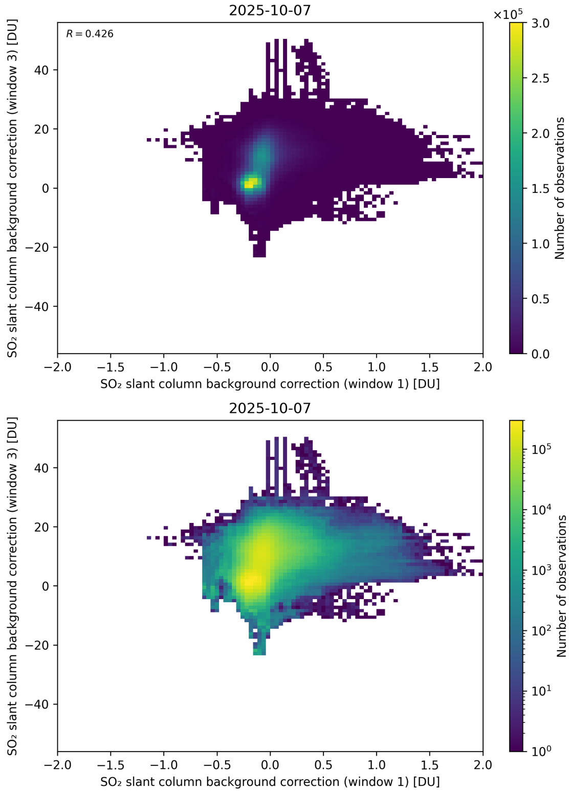
Figure 110: Scatter density plot of “SO 2 slant column background correction (window 1)” against “SO 2 slant column background correction (window 3)” for 2025-10-06 to 2025-10-08.
