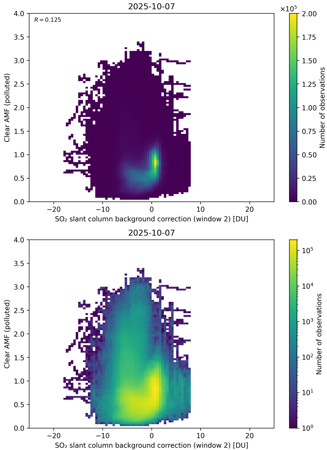
Figure 126: Scatter density plot of “SO 2 slant column background correction (window 2)” against “Clear AMF (polluted)” for 2025-10-06 to 2025-10-08.
