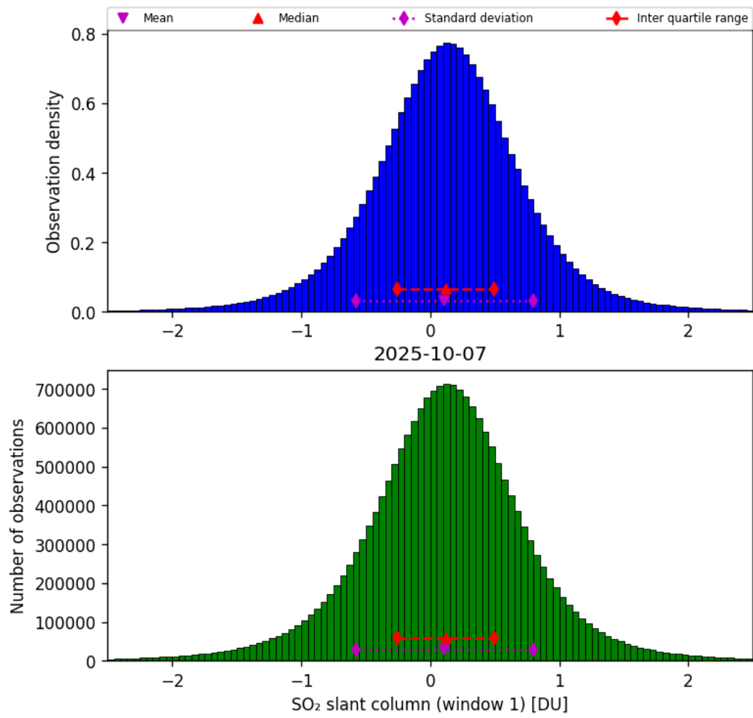
Figure 63: Histogram of “SO 2 slant column (window 1)” for 2025-10-06 to 2025-10-08
