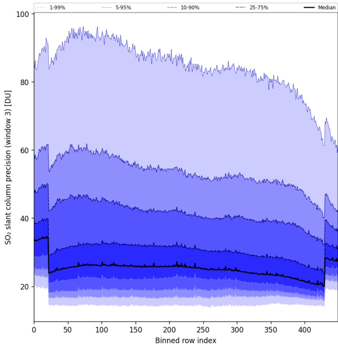
Figure 98: Along track statistics of “SO 2 slant column precision (window 3)” for 2025-10-06 to 2025-10-08
