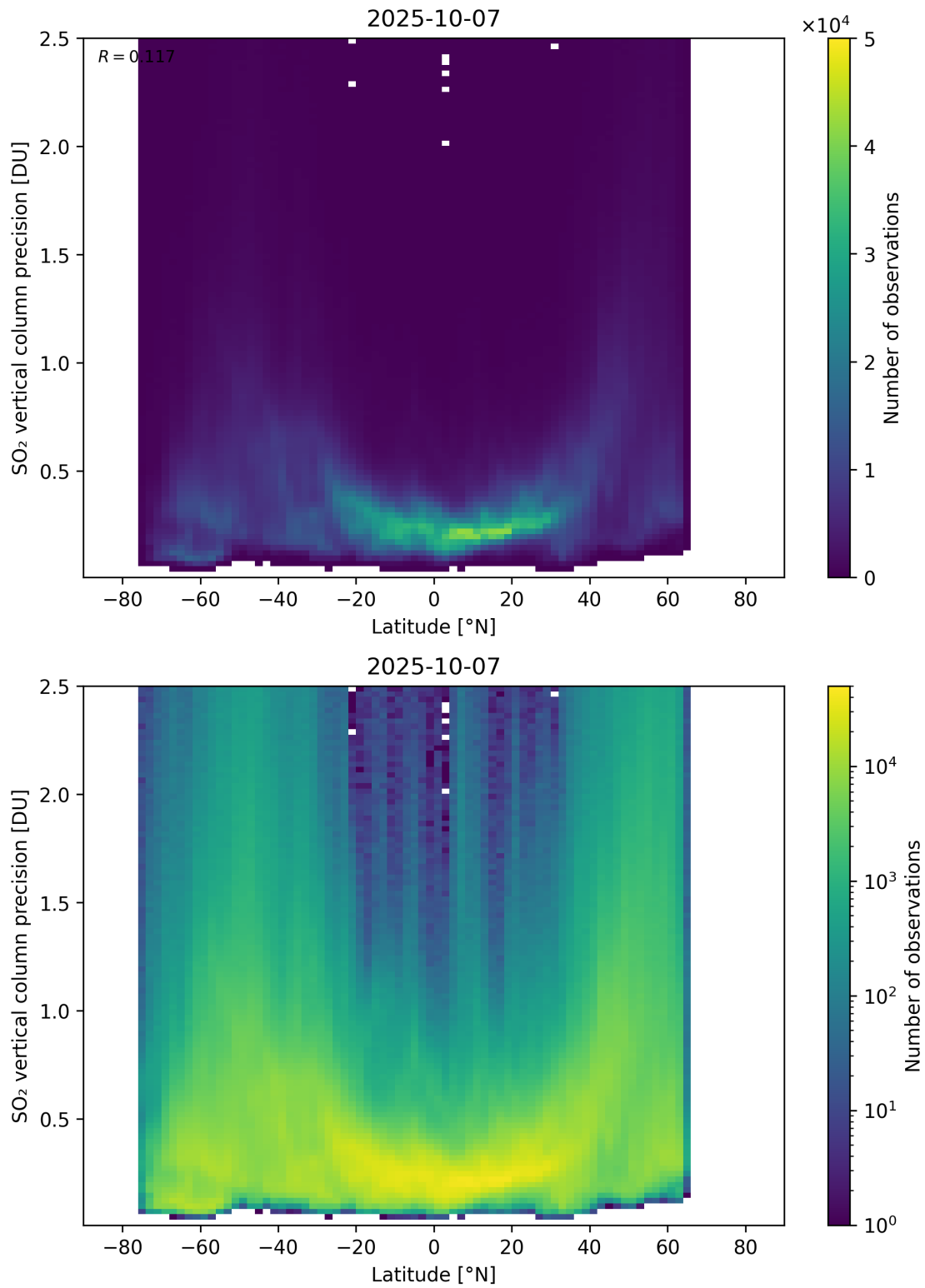
Figure 170: Scatter density plot of “Latitude” against “SO 2 vertical column precision” for 2025-10-06 to 2025-10-08.
