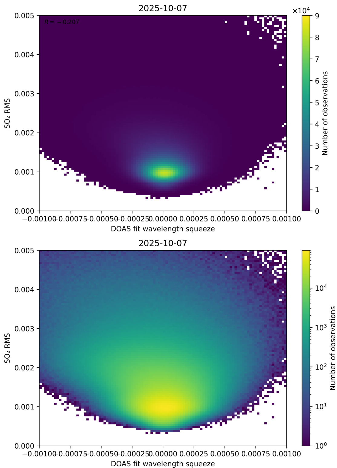
Figure 143: Scatter density plot of “DOAS fit wavelength squeeze” against “SO 2 RMS” for 2025-10-06 to 2025-10-08.
