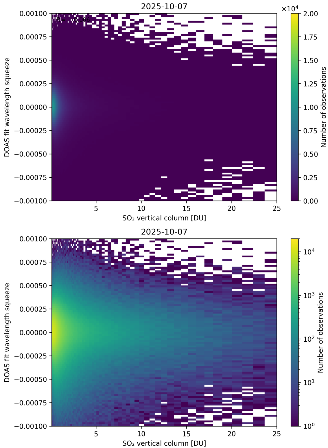
Figure 327: Scatter density plot of “SO 2 vertical column” against “DOAS fit wavelength squeeze” for 2025-10-06 to 2025-10-08.
