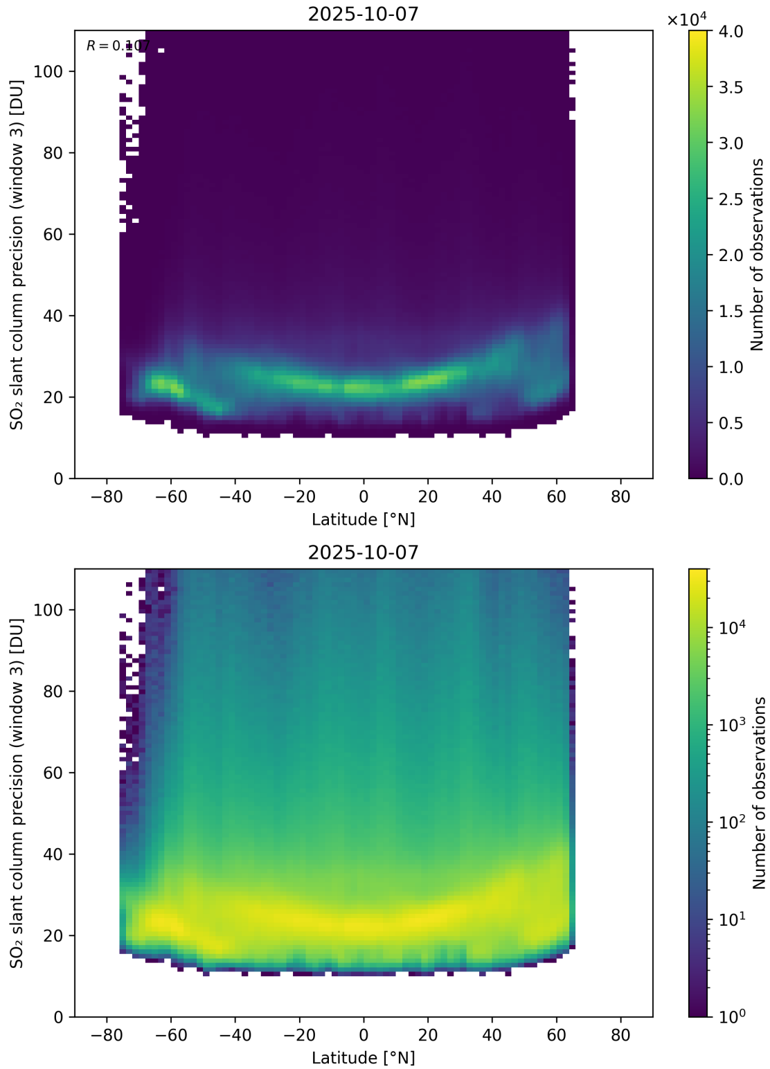
Figure 166: Scatter density plot of “Latitude” against “SO 2 slant column precision (window 3)” for 2025-10-06 to 2025-10-08.
