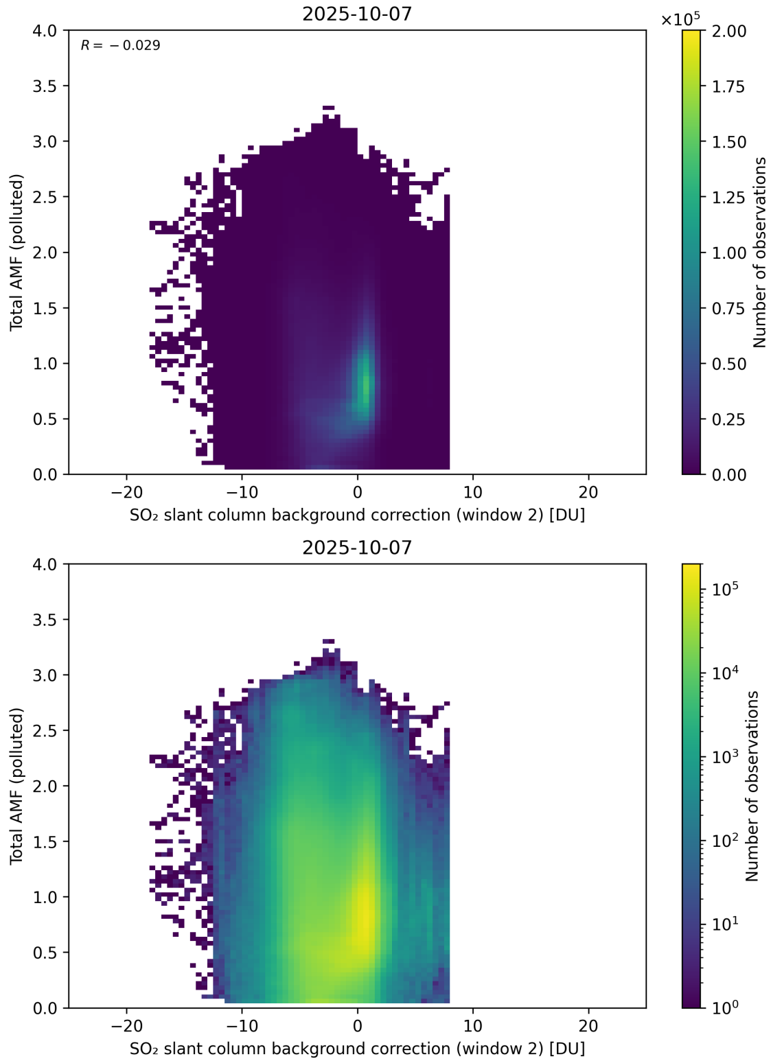
Figure 130: Scatter density plot of “SO 2 slant column background correction (window 2)” against “Total AMF (polluted)” for 2025-10-06 to 2025-10-08.
