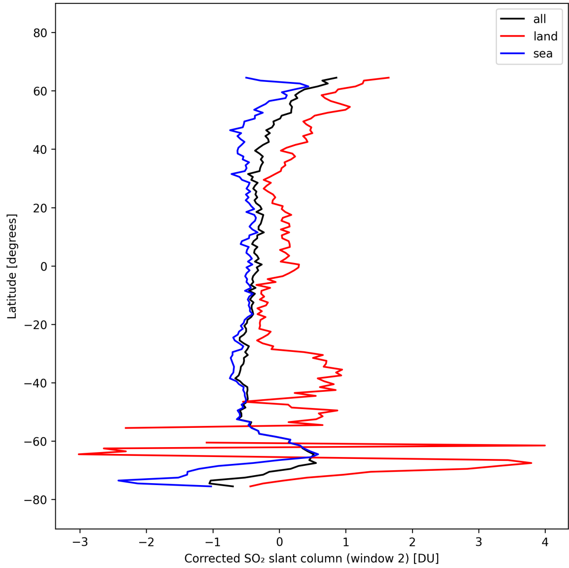
Figure 43: Zonal average of "Corrected SO 2 slant column (window 2)" for 2025-10-06 to 2025-10-08.
