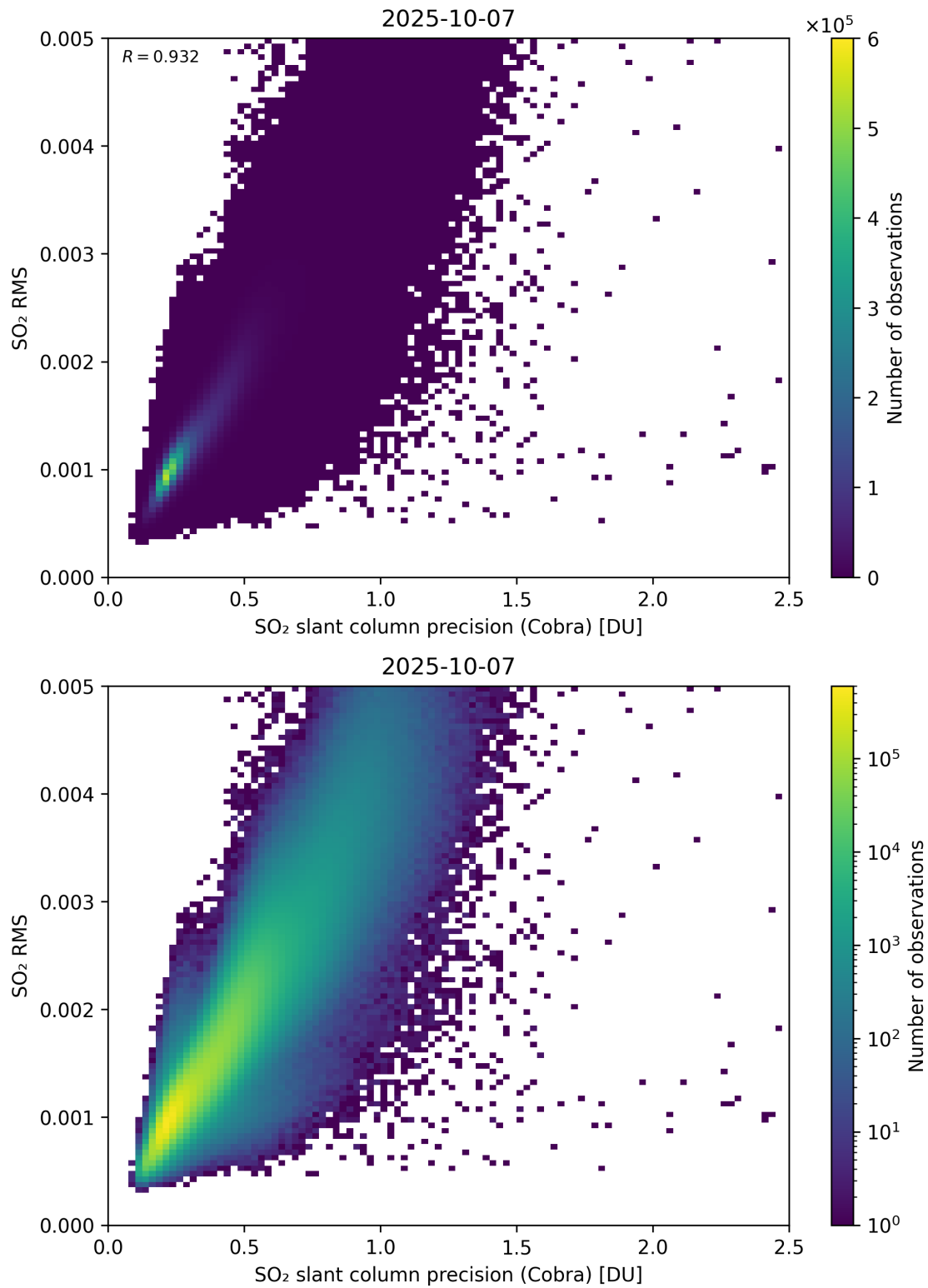
Figure 204: Scatter density plot of “SO 2 slant column precision (Cobra)” against “SO 2 RMS” for 2025-10-06 to 2025-10-08.
