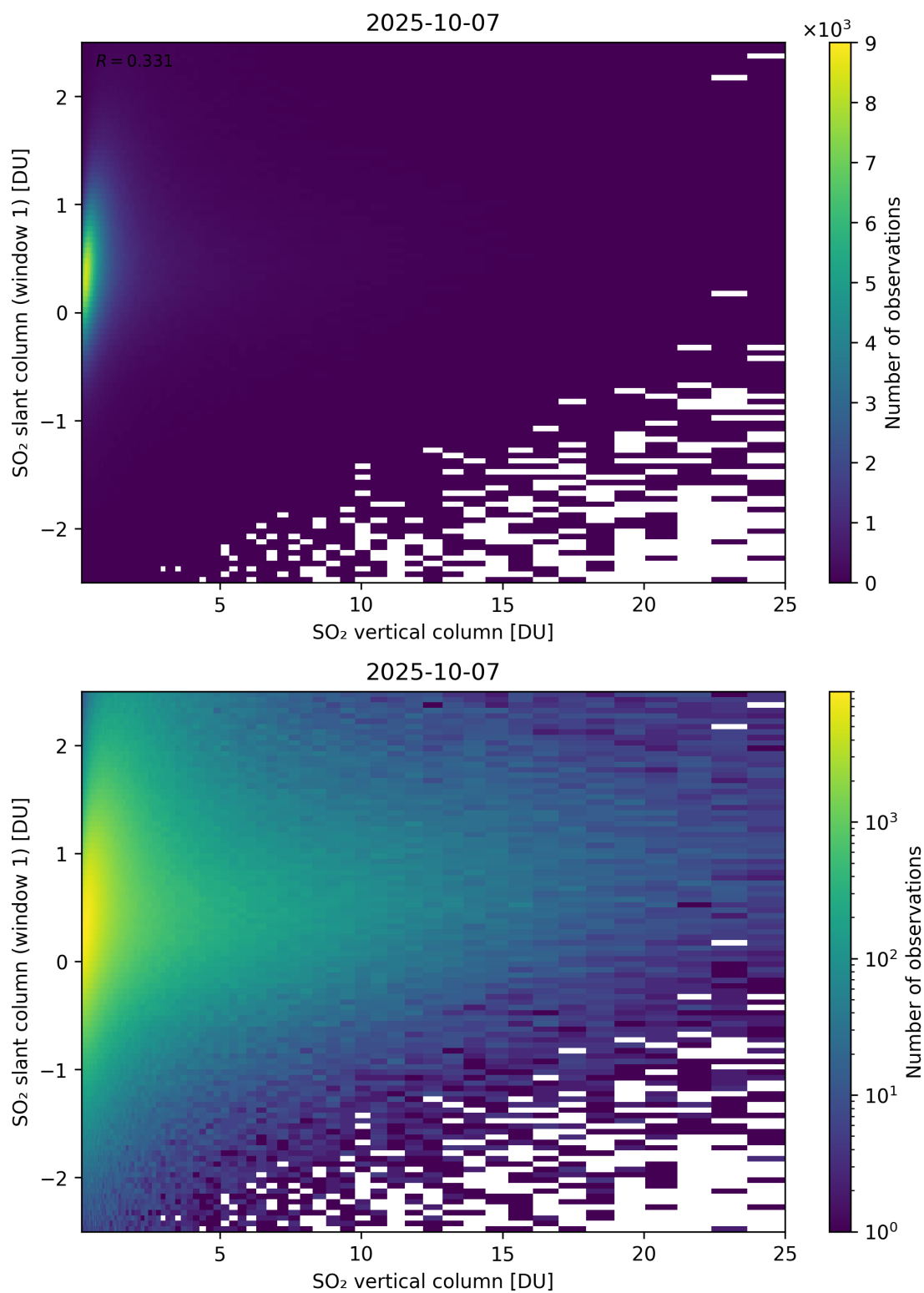
Figure 354: Scatter density plot of “SO 2 vertical column” against “SO 2 slant column (window 1)” for 2025-10-06 to 2025-10-08.
