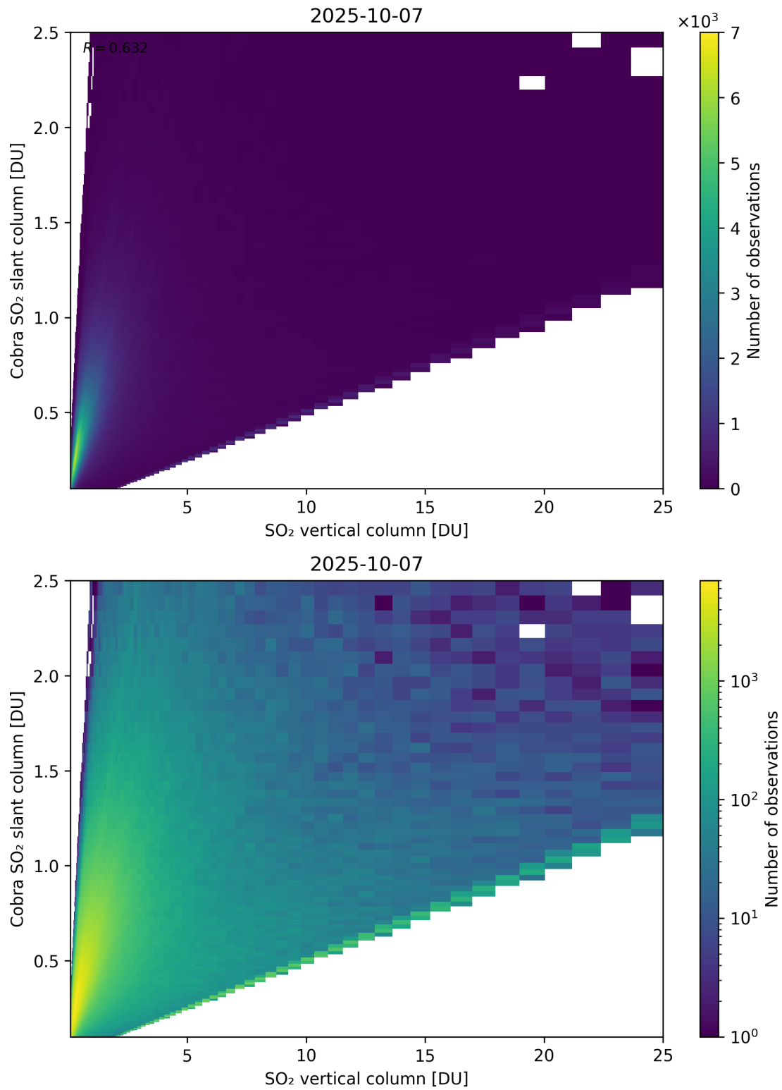
Figure 349: Scatter density plot of “SO 2 vertical column” against “Cobra SO 2 slant column” for 2025-10-06 to 2025-10-08.
