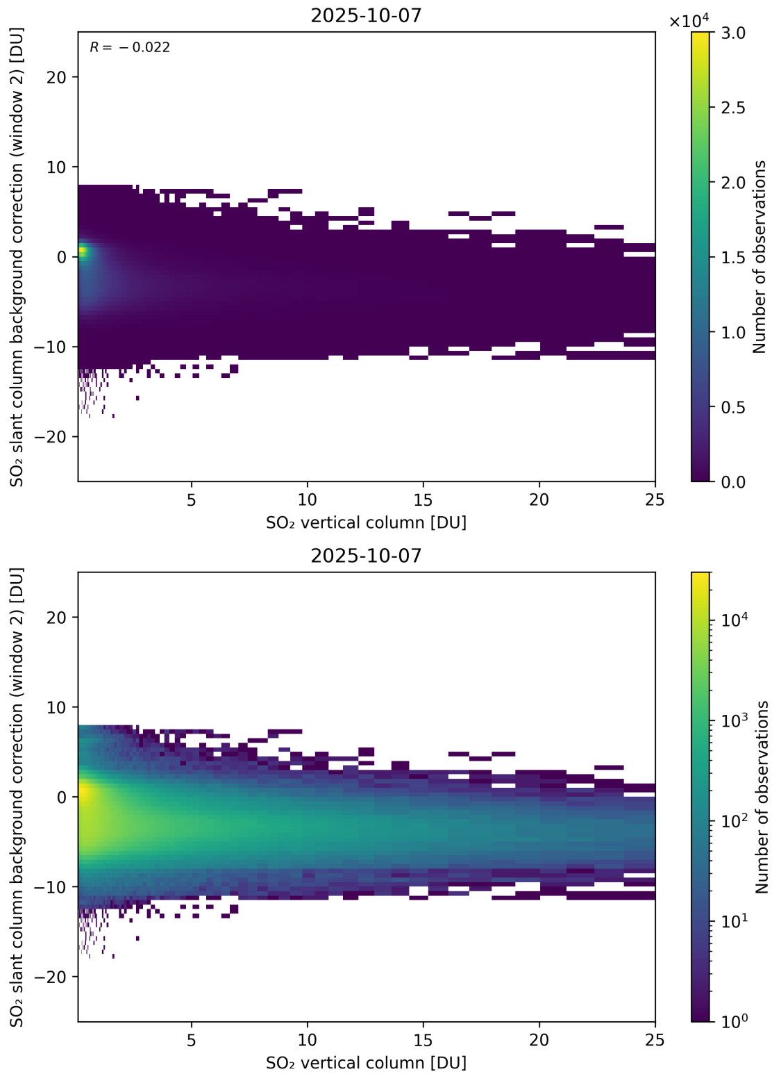
Figure 324: Scatter density plot of “SO 2 vertical column” against “SO 2 slant column background correction (window 2)” for 2025-10-06 to 2025-10-08.
