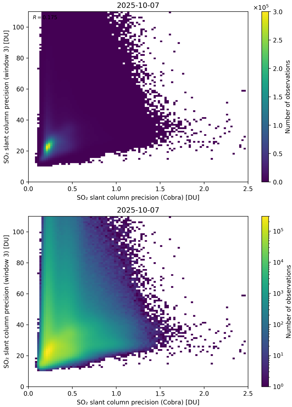
Figure 212: Scatter density plot of “SO 2 slant column precision (Cobra)” against “SO 2 slant column precision (window 3)” for 2025-10-06 to 2025-10-08.
