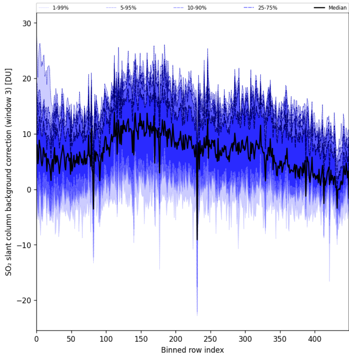
Figure 100: Along track statistics of “SO 2 slant column background correction (window 3)” for 2025-10-06 to 2025-10-08
