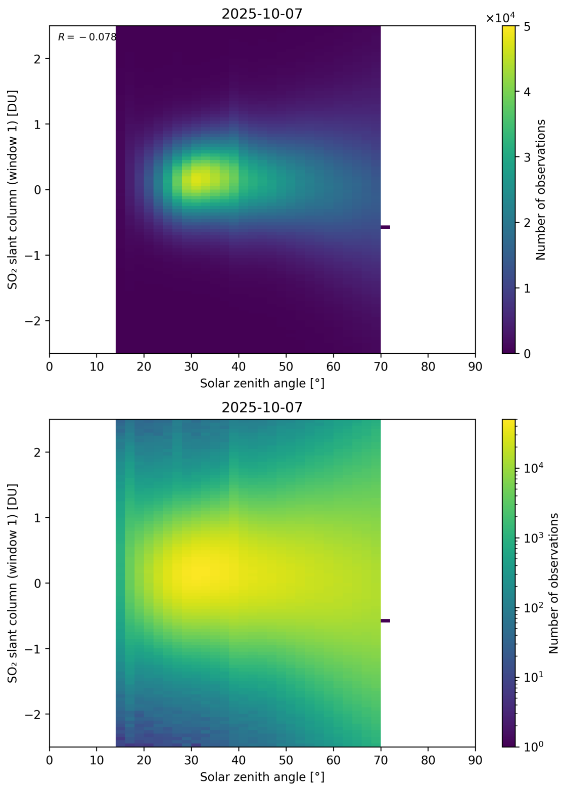
Figure 184: Scatter density plot of “Solar zenith angle” against “SO 2 slant column (window 1)” for 2025-10-06 to 2025-10-08.
