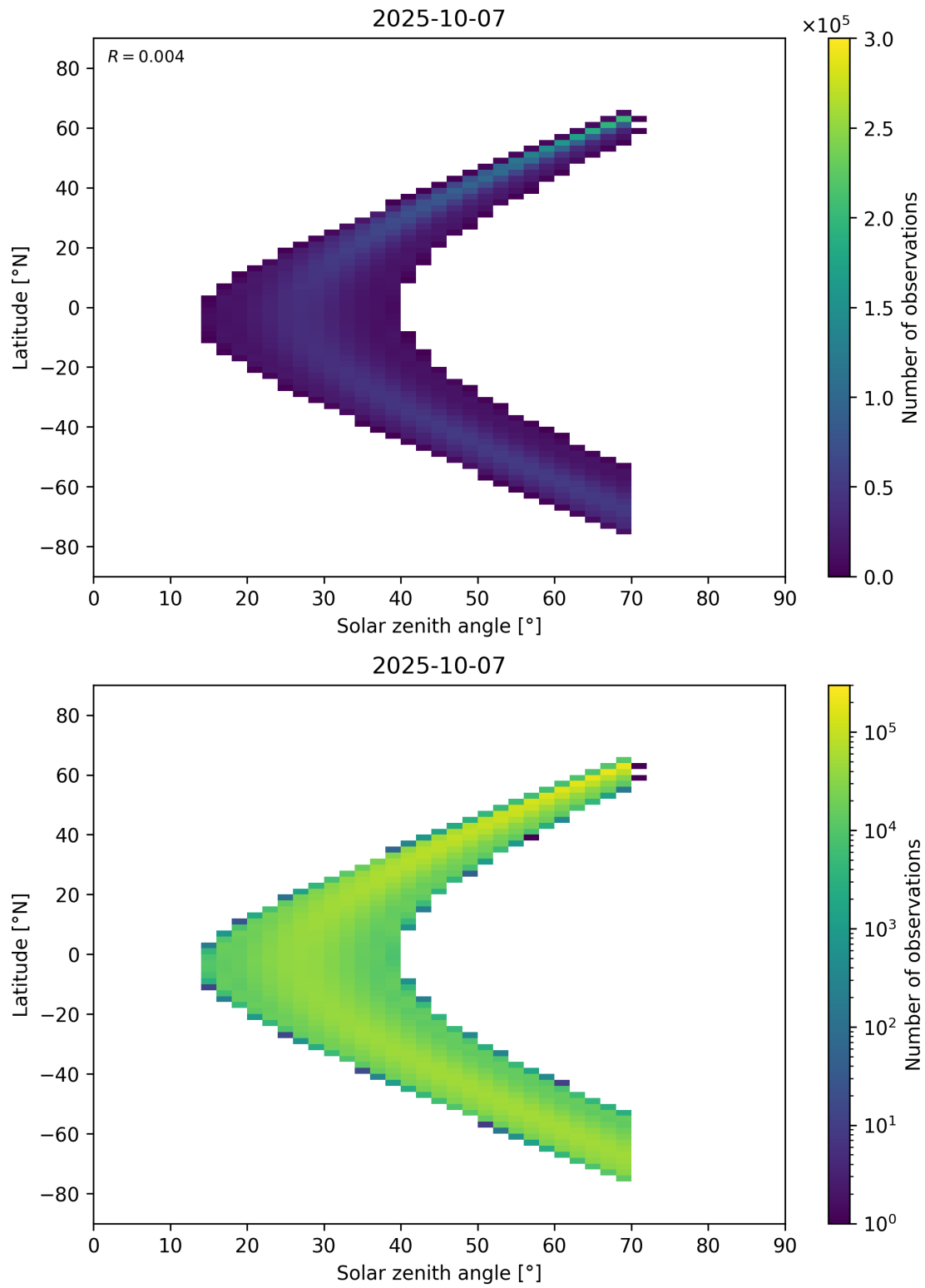
Figure 177: Scatter density plot of “Solar zenith angle” against “Latitude” for 2025-10-06 to 2025-10-08.
