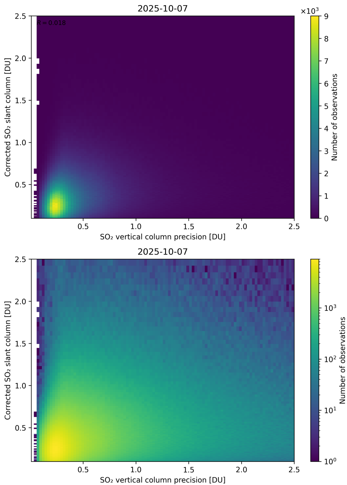
Figure 338: Scatter density plot of “SO 2 vertical column precision” against “Corrected SO 2 slant column” for 2025-10-06 to 2025-10-08.
