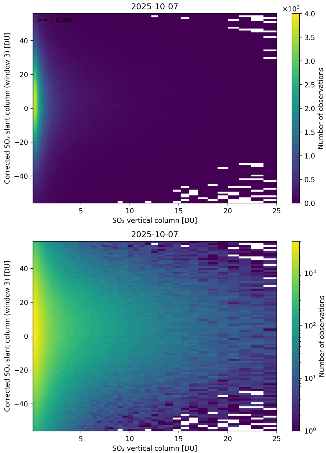
Figure 353: Scatter density plot of “SO 2 vertical column” against “Corrected SO 2 slant column (window 3)” for 2025-10-06 to 2025-10-08.
