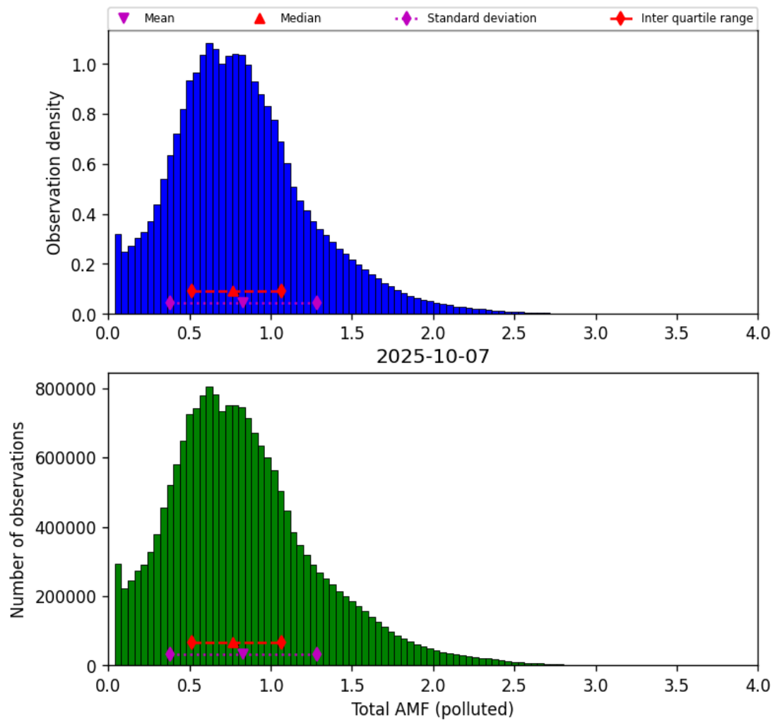
Figure 79: Histogram of “Total AMF (polluted)” for 2025-10-06 to 2025-10-08
