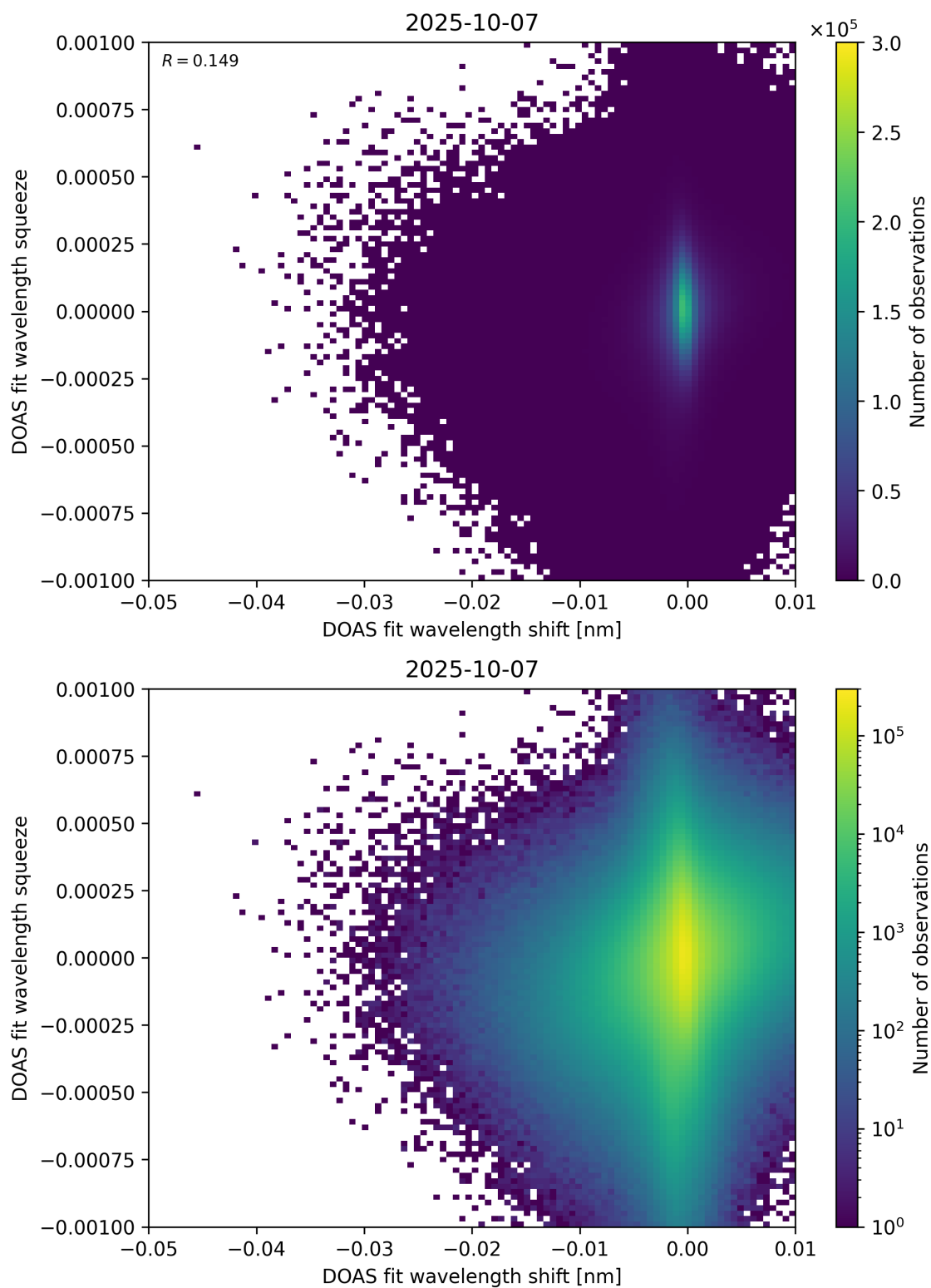
Figure 138: Scatter density plot of “DOAS fit wavelength shift” against “DOAS fit wavelength squeeze” for 2025-10-06 to 2025-10-08.
