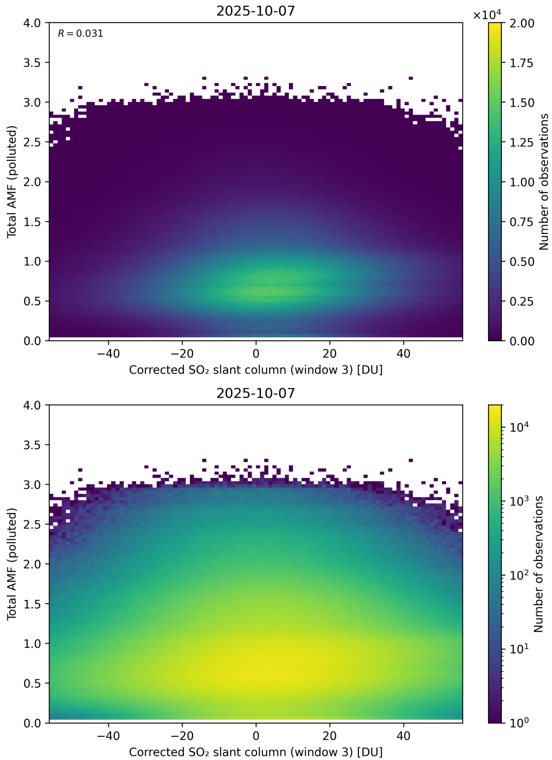
Figure 260: Scatter density plot of “Corrected SO 2 slant column (window 3)” against “Total AMF (polluted)” for 2025-10-06 to 2025-10-08.
