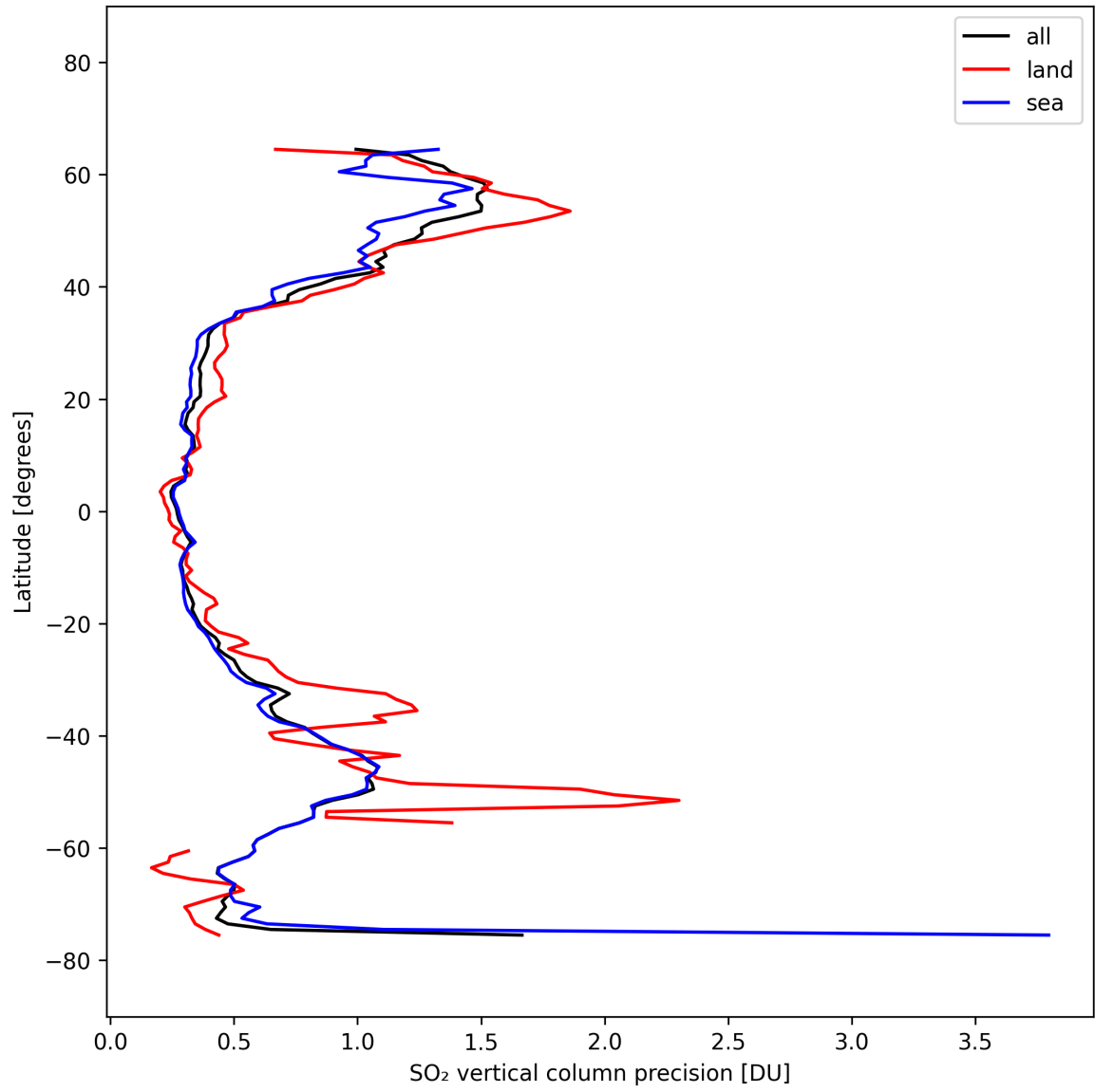
Figure 33: Zonal average of “SO 2 vertical column precision” for 2025-10-06 to 2025-10-08.
