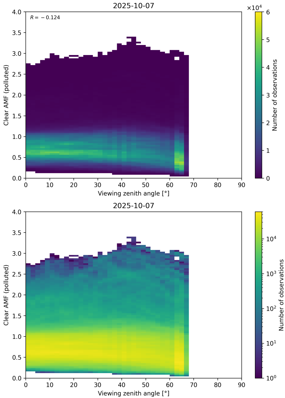
Figure 370: Scatter density plot of “Viewing zenith angle” against “Clear AMF (polluted)” for 2025-10-06 to 2025-10-08.
