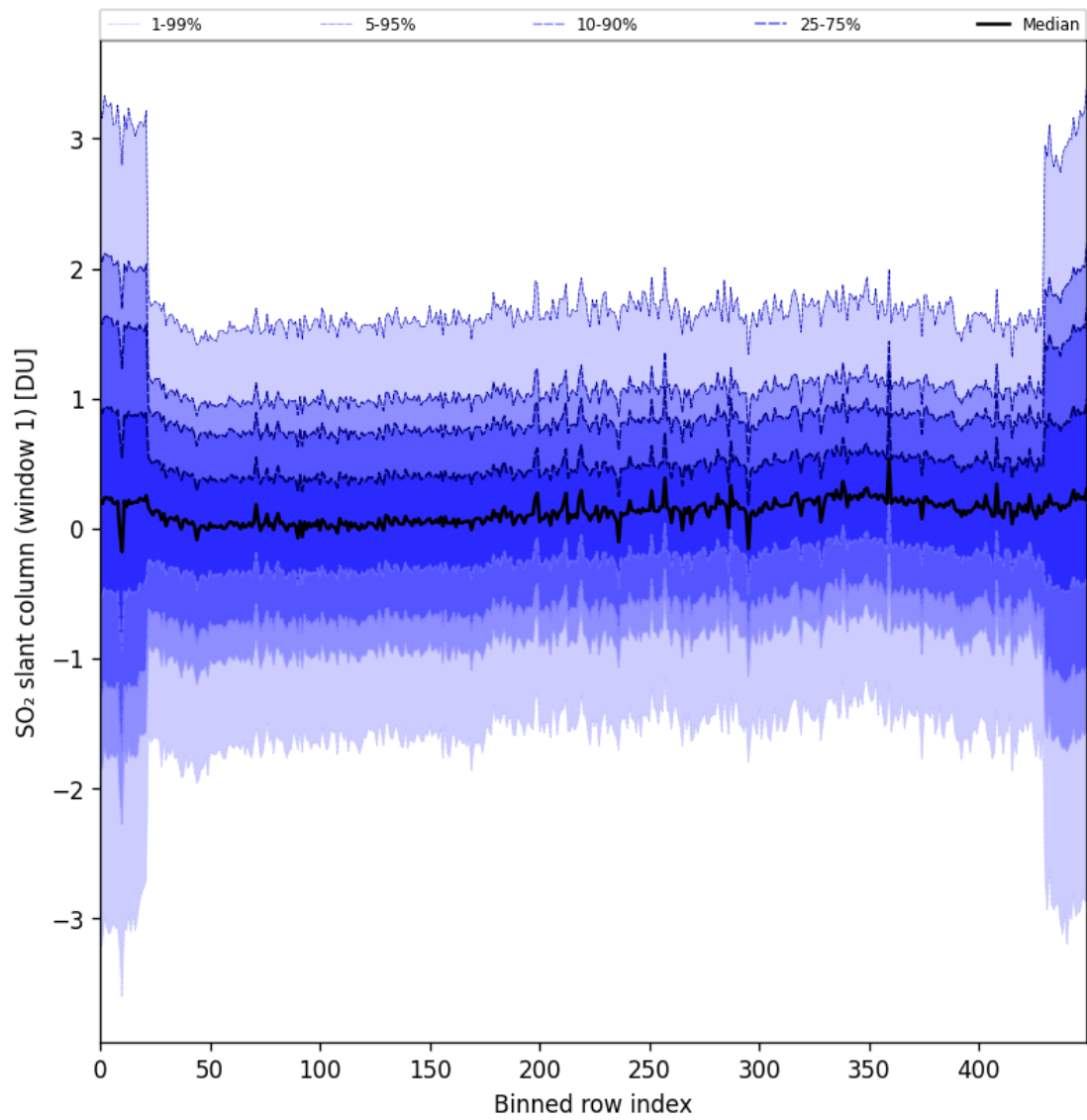
Figure 89: Along track statistics of “SO 2 slant column (window 1)” for 2025-10-06 to 2025-10-08
