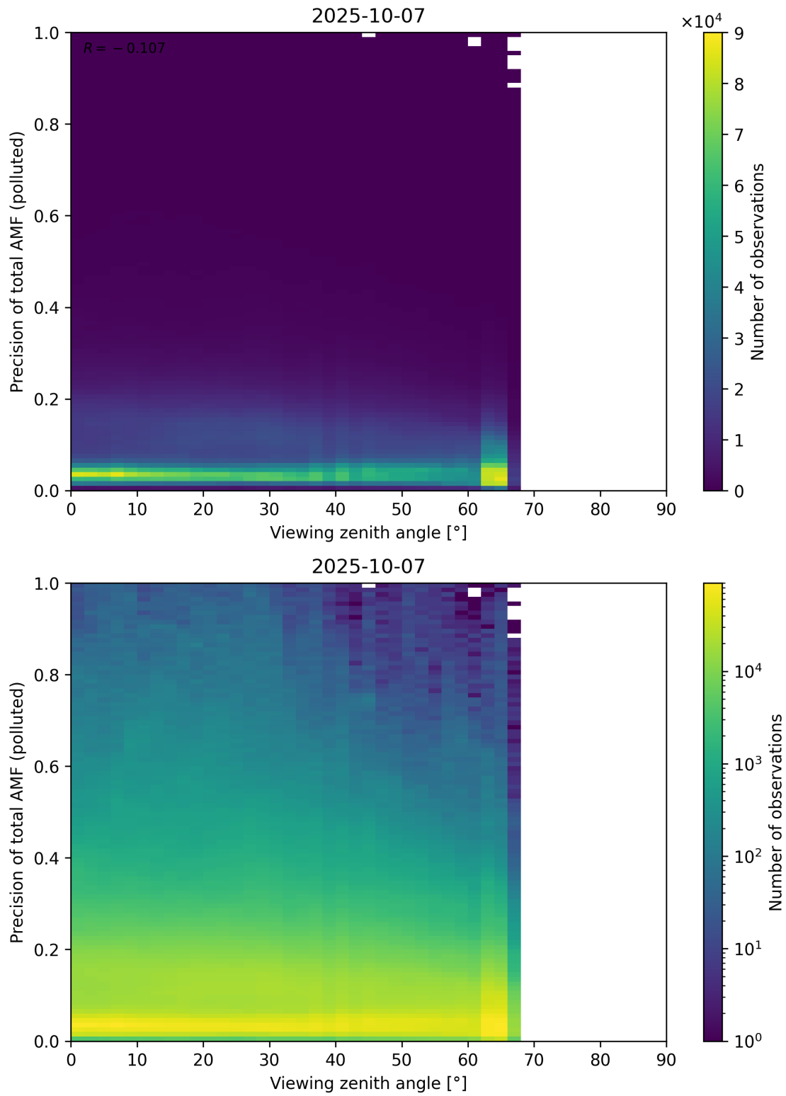
Figure 382: Scatter density plot of “Viewing zenith angle” against “Precision of total AMF (polluted)” for 2025-10-06 to 2025-10-08.
