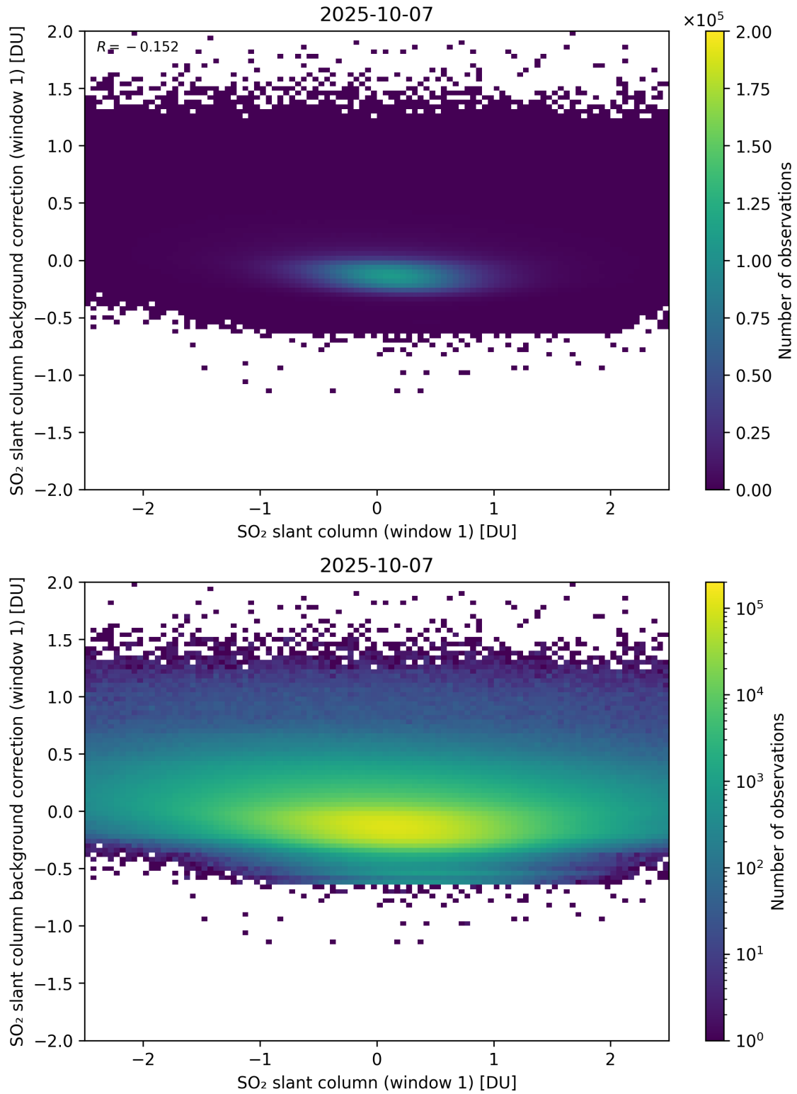
Figure 262: Scatter density plot of “SO 2 slant column (window 1)” against “SO 2 slant column background correction (window 1)” for 2025-10-06 to 2025-10-08.
