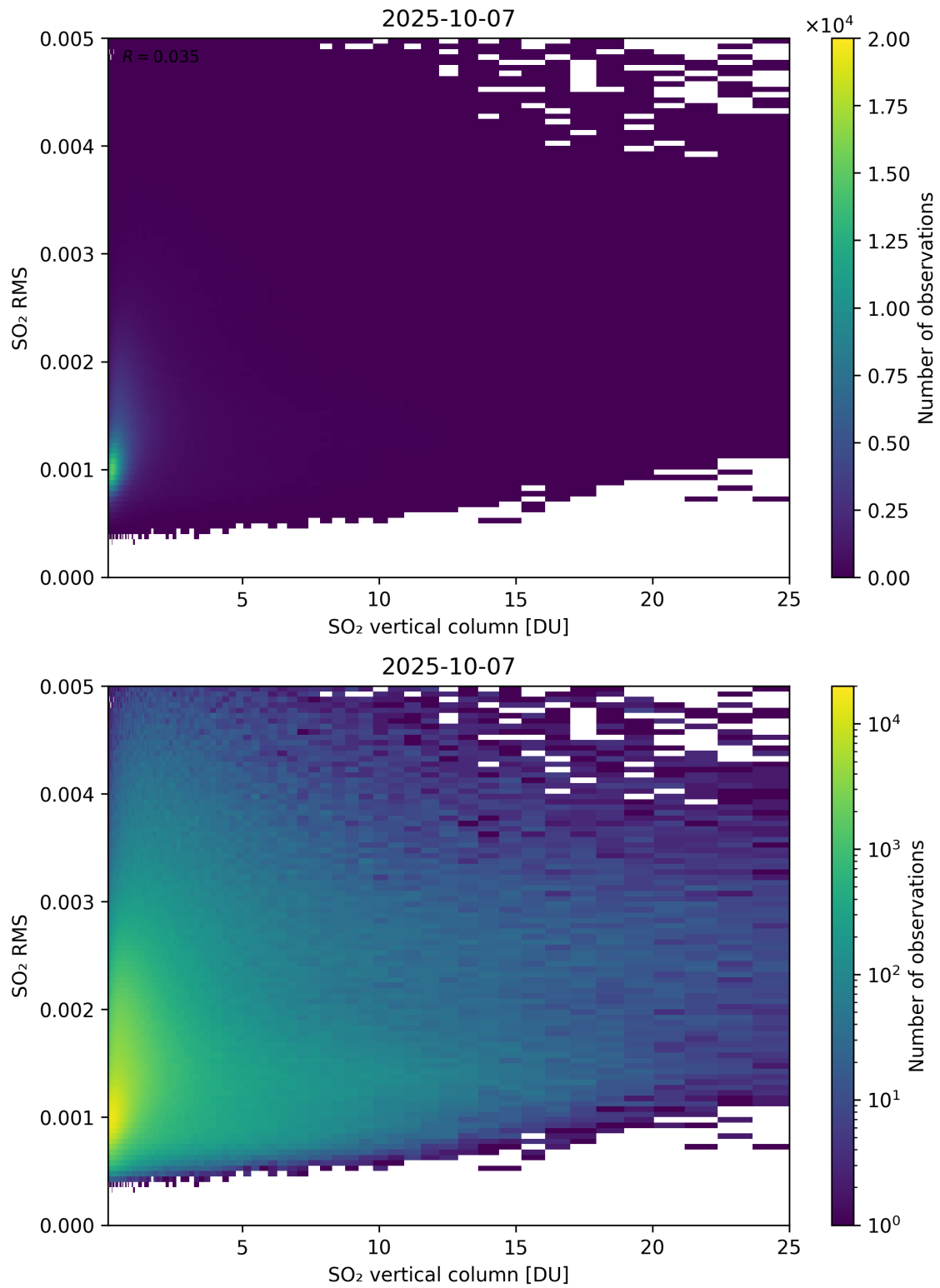
Figure 328: Scatter density plot of “SO 2 vertical column” against “SO 2 RMS” for 2025-10-06 to 2025-10-08.
