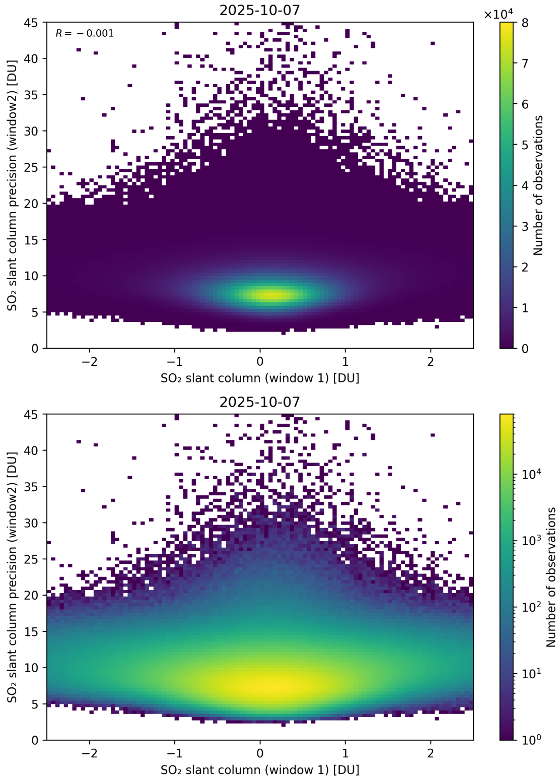
Figure 286: Scatter density plot of “SO 2 slant column (window 1)” against “SO 2 slant column precision (window2)” for 2025-10-06 to 2025-10-08.
