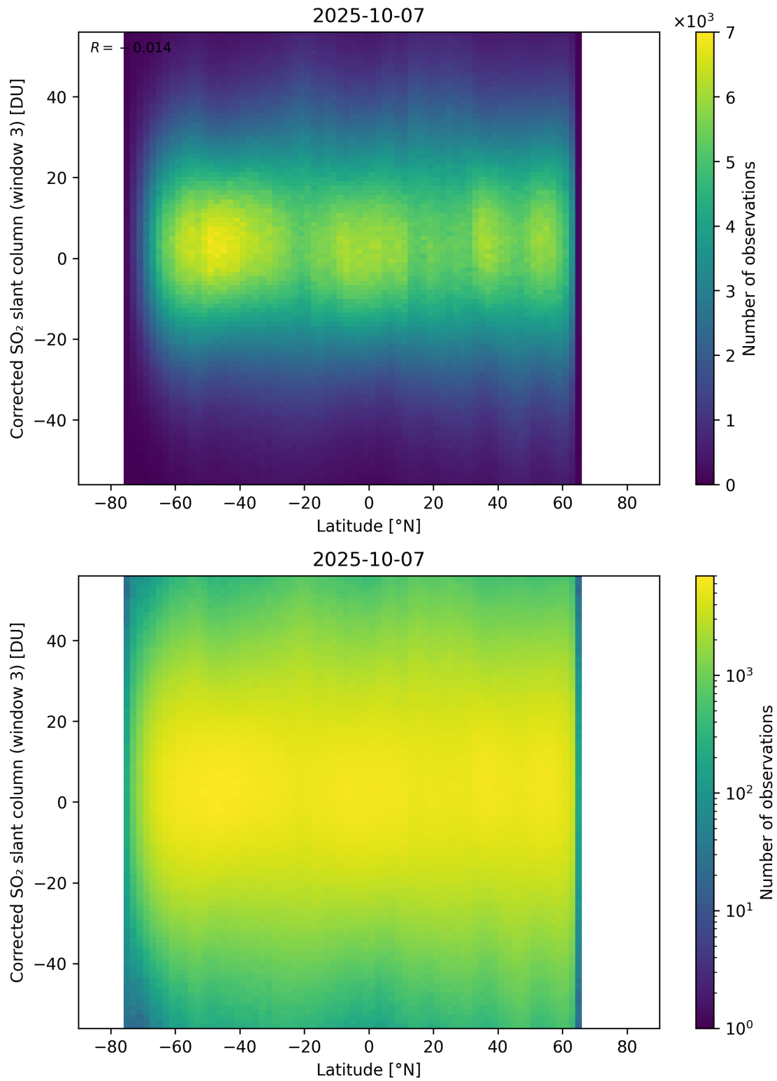
Figure 161: Scatter density plot of “Latitude” against “Corrected SO 2 slant column (window 3)” for 2025-10-06 to 2025-10-08.
