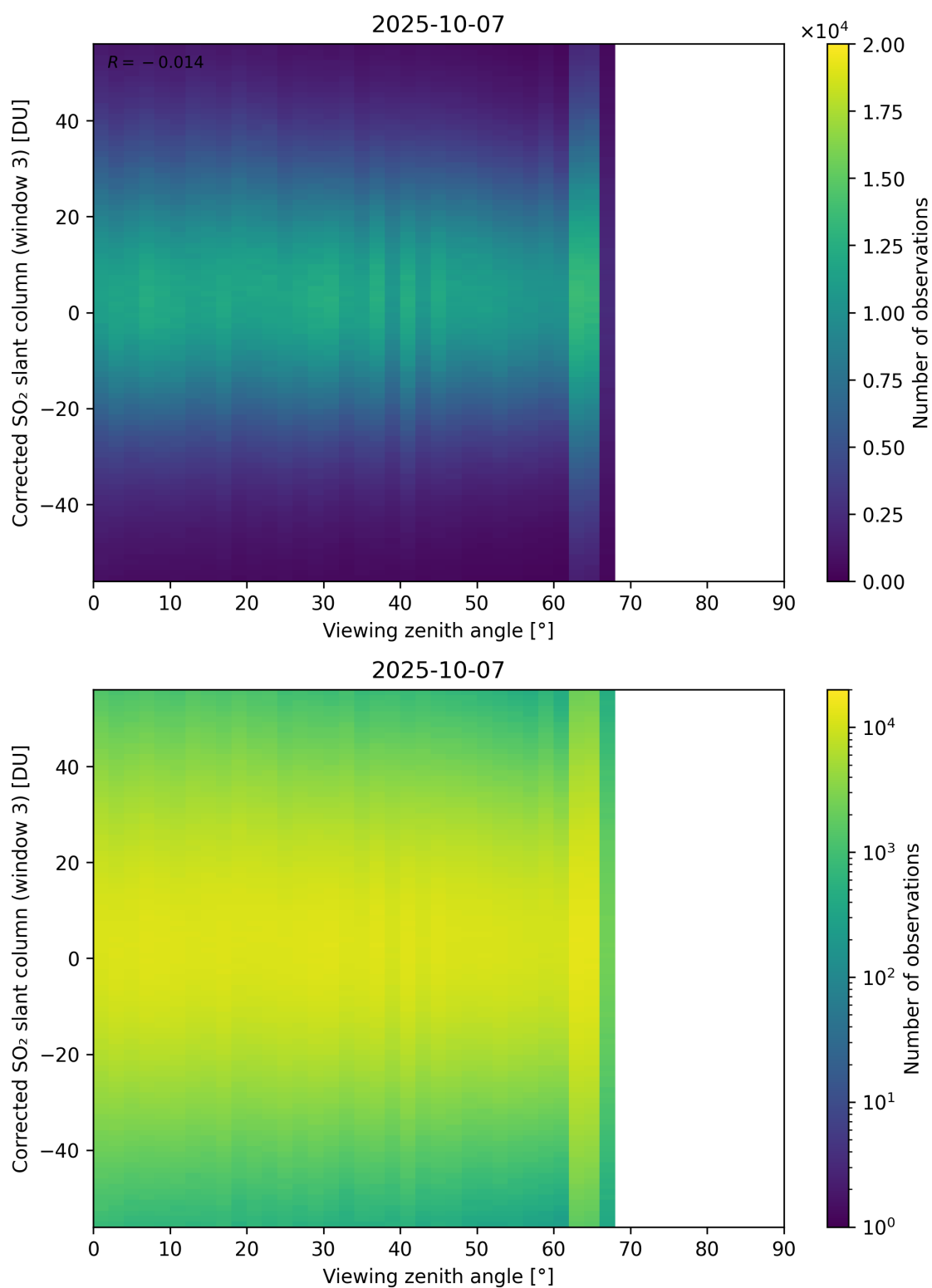
Figure 375: Scatter density plot of “Viewing zenith angle” against “Corrected SO 2 slant column (window 3)” for 2025-10-06 to 2025-10-08.
