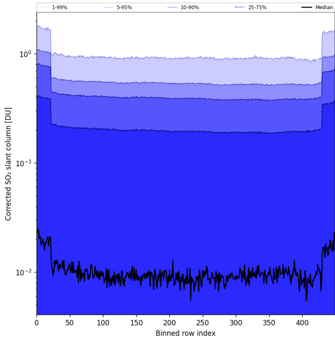
Figure 86: Along track statistics of “Corrected SO 2 slant column” for 2025-10-06 to 2025-10-08
