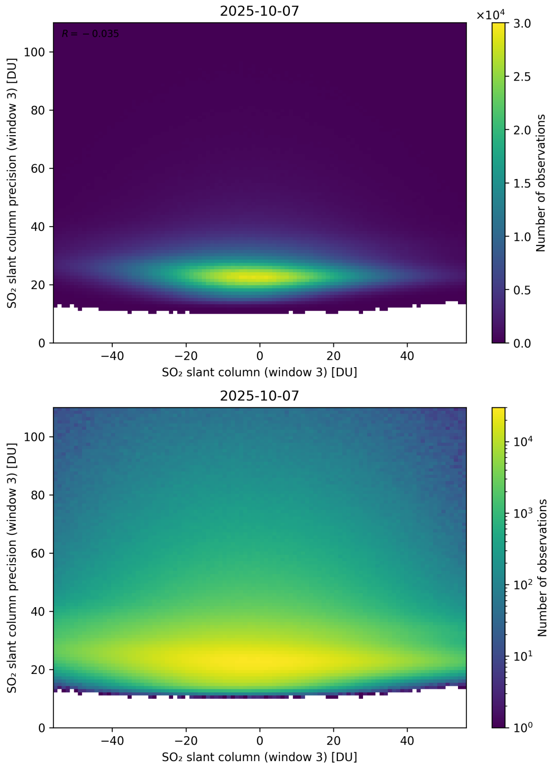
Figure 317: Scatter density plot of “SO 2 slant column (window 3)” against “SO 2 slant column precision (window 3)” for 2025-10-06 to 2025-10-08.
