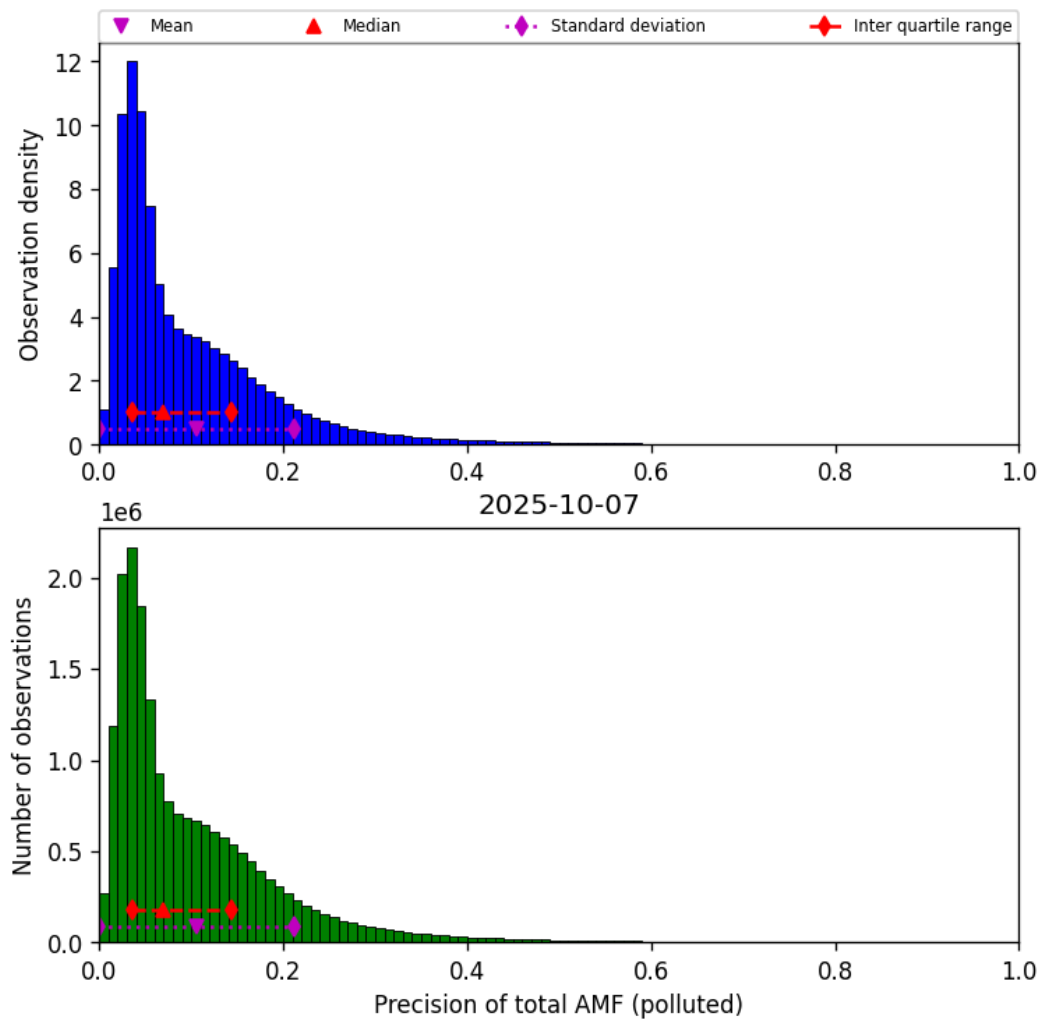
Figure 80: Histogram of “Precision of total AMF (polluted)” for 2025-10-06 to 2025-10-08
