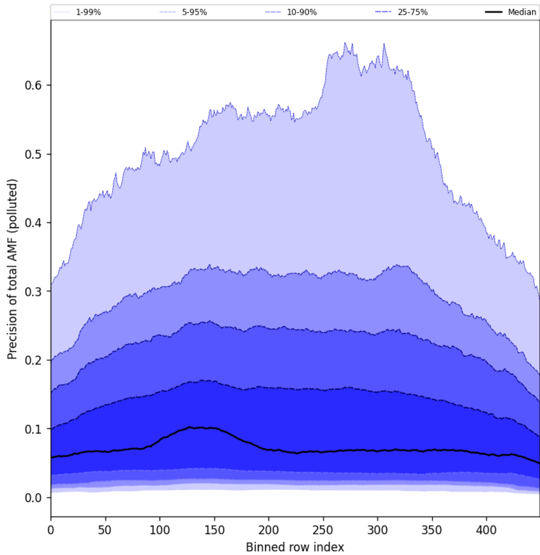
Figure 106: Along track statistics of “Precision of total AMF (polluted)” for 2025-10-06 to 2025-10-08
