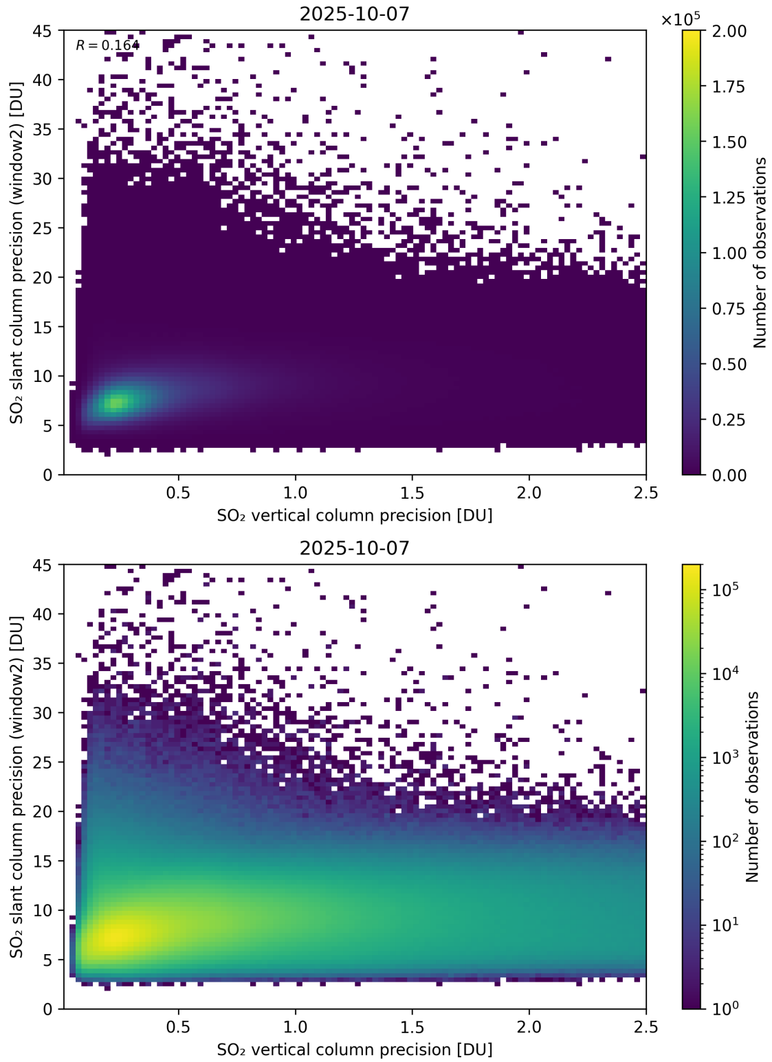
Figure 343: Scatter density plot of “SO 2 vertical column precision” against “SO 2 slant column precision (window2)” for 2025-10-06 to 2025-10-08.
