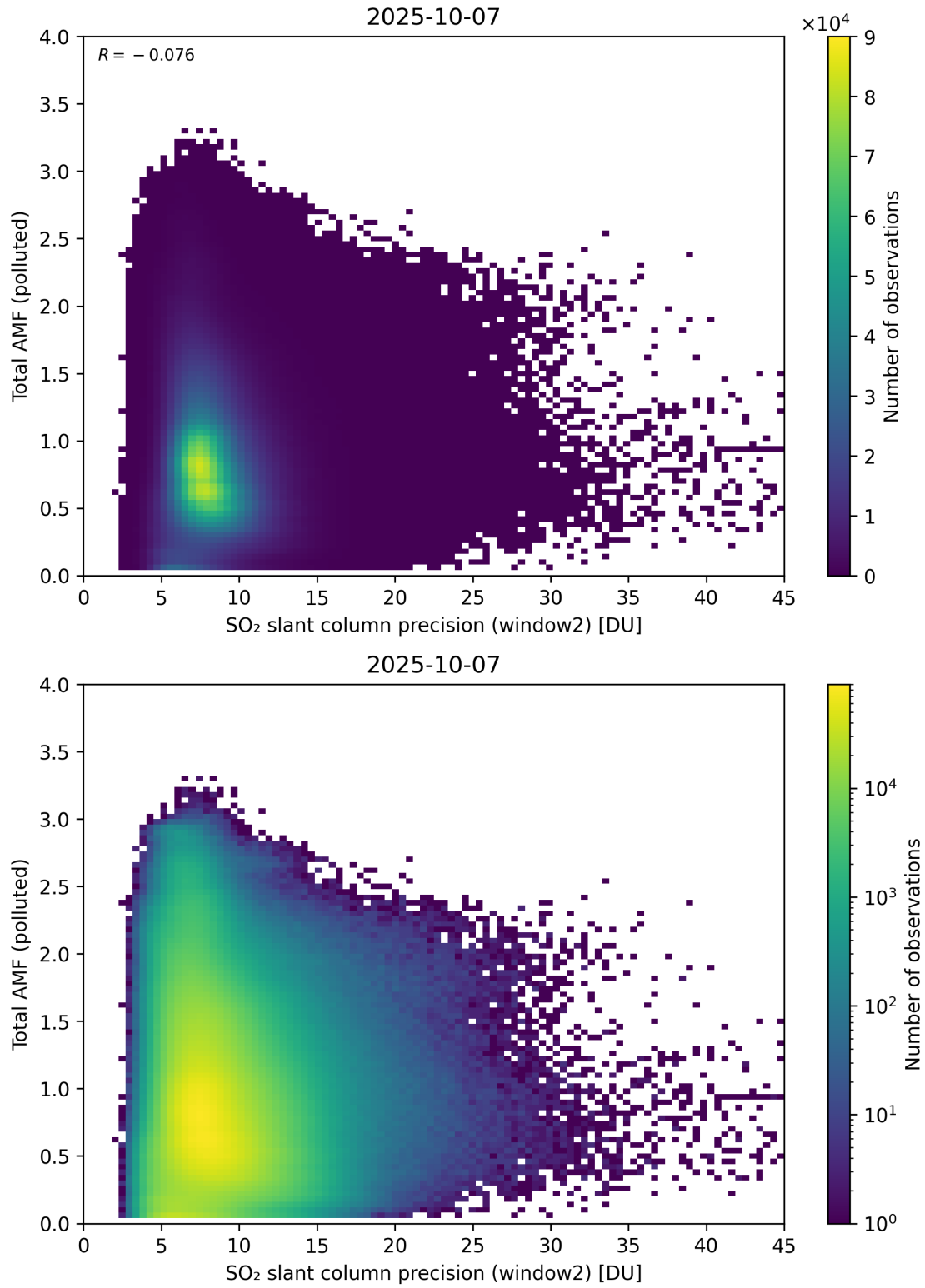
Figure 301: Scatter density plot of “SO 2 slant column precision (window2)” against “Total AMF (polluted)” for 2025-10-06 to 2025-10-08.
