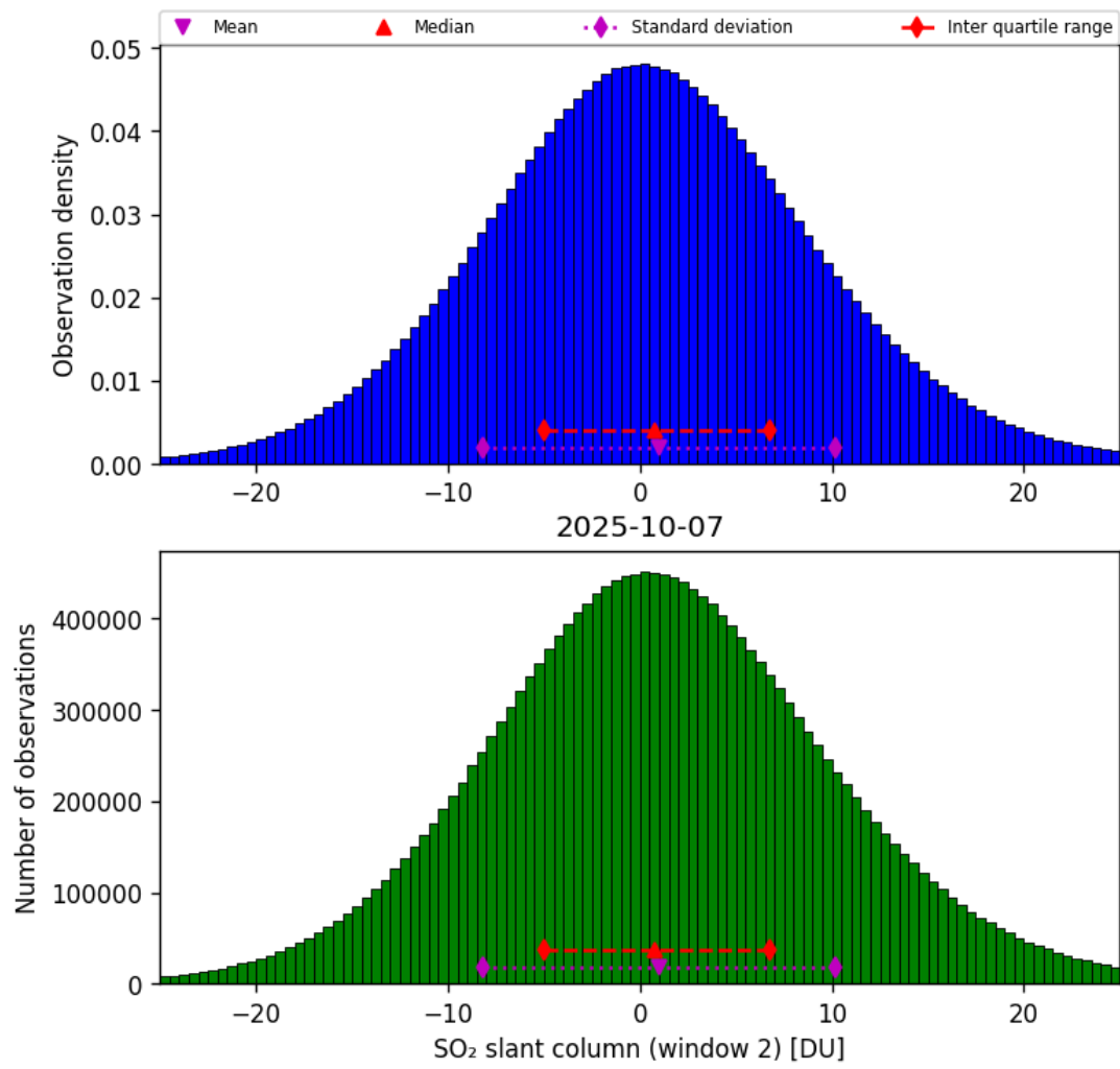
Figure 67: Histogram of “SO 2 slant column (window 2)” for 2025-10-06 to 2025-10-08
