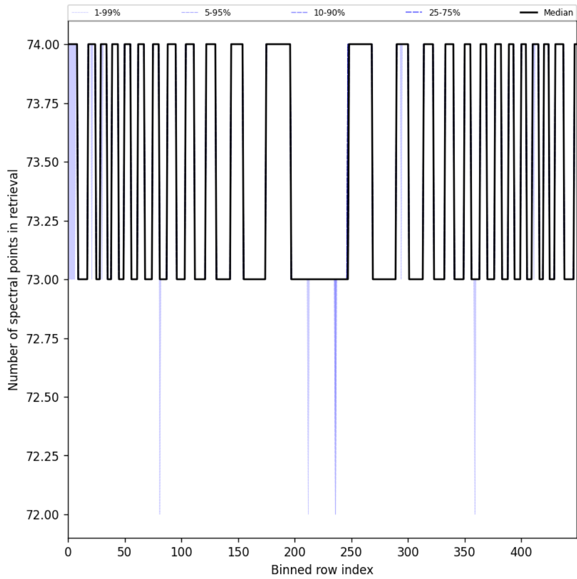
Figure 108: Along track statistics of “Number of spectral points in retrieval” for 2025-10-06 to 2025-10-08
