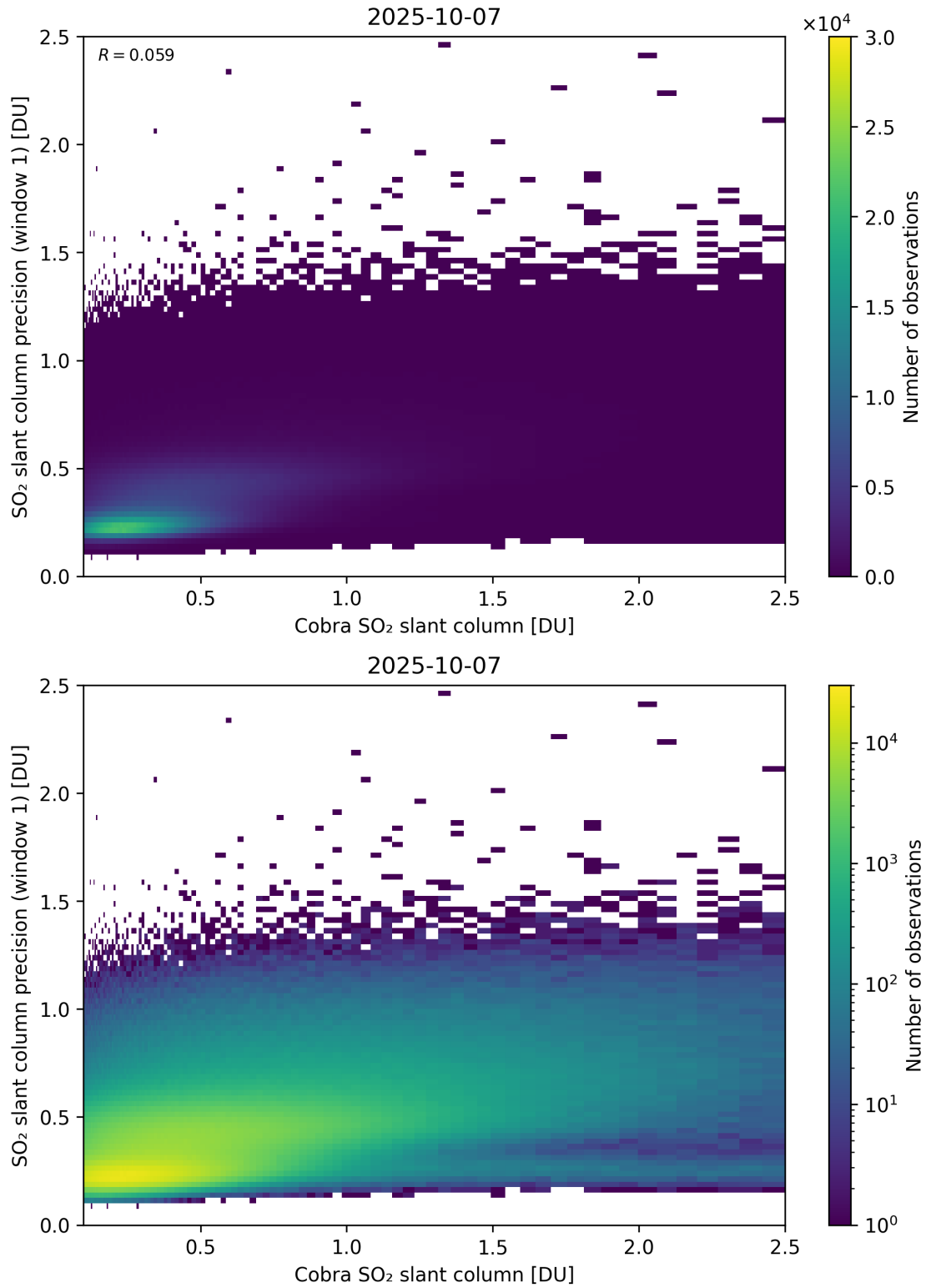
Figure 220: Scatter density plot of “Cobra SO 2 slant column” against “SO 2 slant column precision (window 1)” for 2025-10-06 to 2025-10-08.
