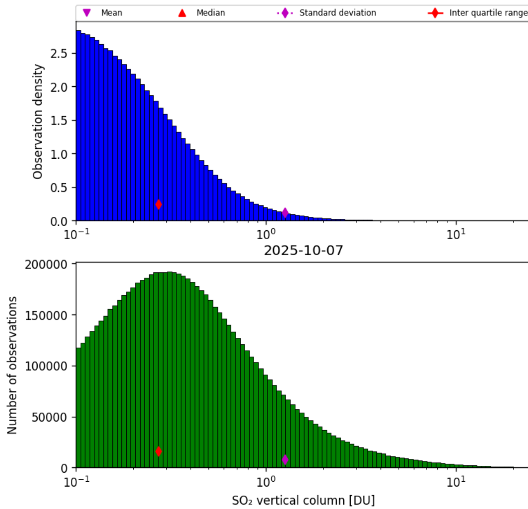
Figure 58: Histogram of “SO 2 vertical column” for 2025-10-06 to 2025-10-08
