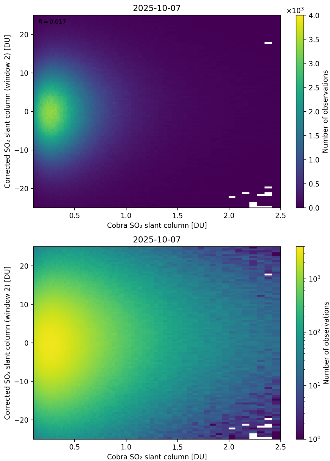
Figure 217: Scatter density plot of “Cobra SO 2 slant column” against “Corrected SO 2 slant column (window 2)” for 2025-10-06 to 2025-10-08.
