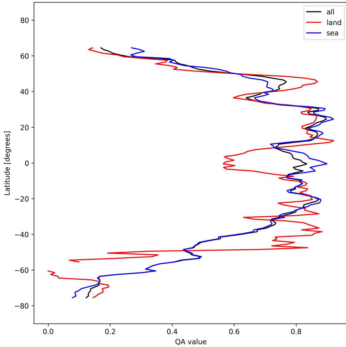
Figure 31: Zonal average of “QA value” for 2025-10-06 to 2025-10-08.
