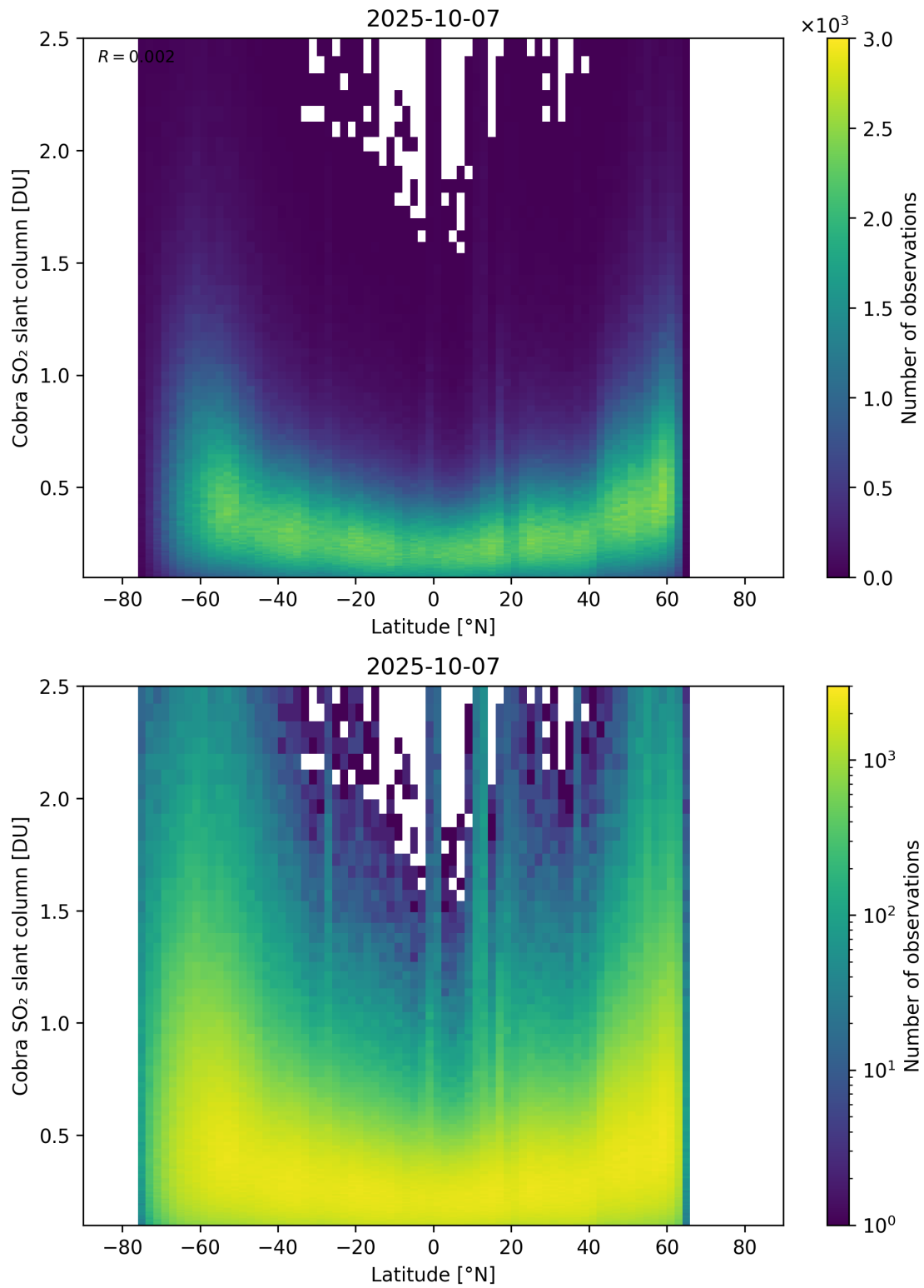
Figure 157: Scatter density plot of “Latitude” against “Cobra SO 2 slant column” for 2025-10-06 to 2025-10-08.
