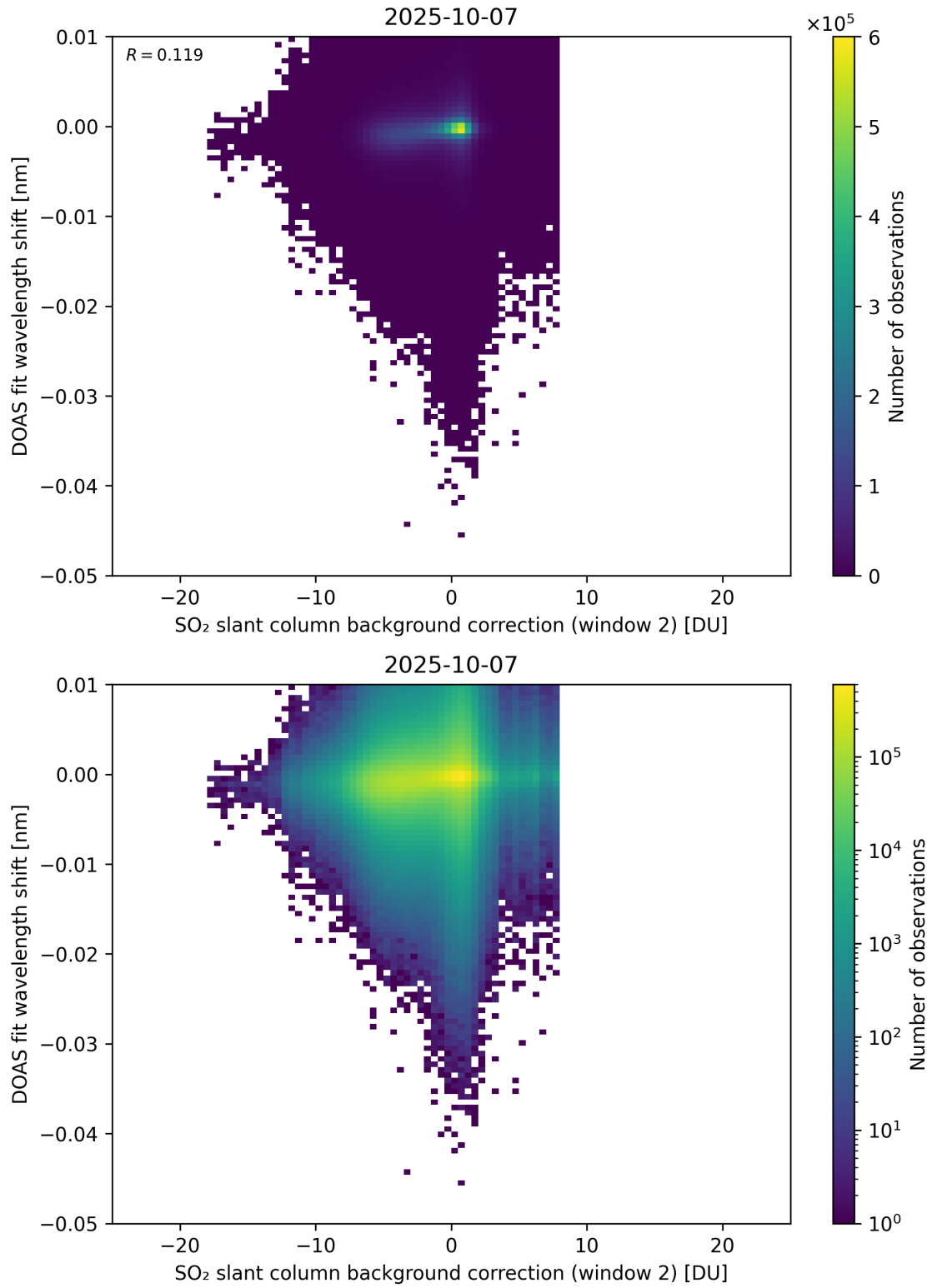
Figure 123: Scatter density plot of “SO 2 slant column background correction (window 2)” against “DOAS fit wavelength shift” for 2025-10-06 to 2025-10-08.
