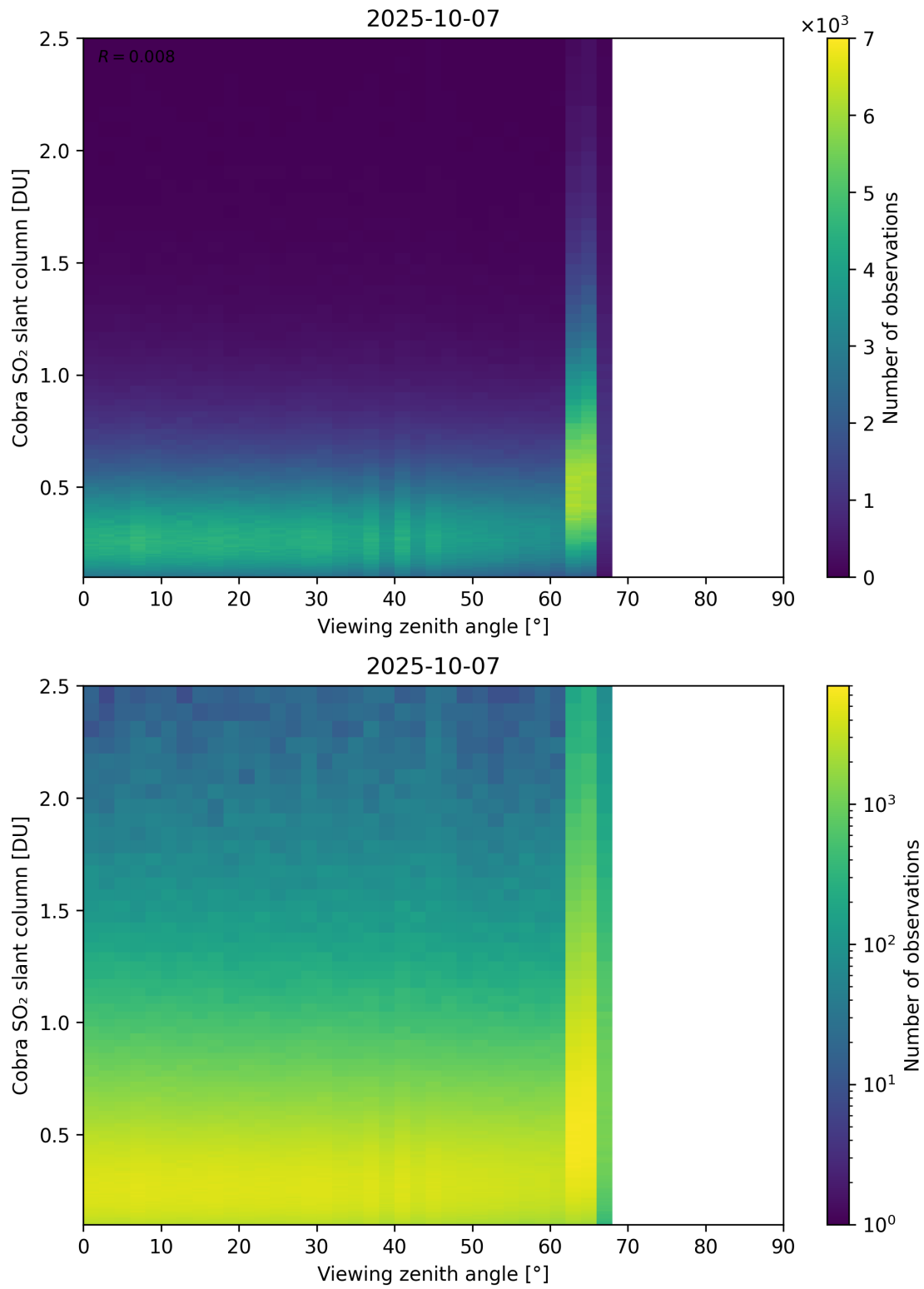
Figure 371: Scatter density plot of “Viewing zenith angle” against “Cobra SO 2 slant column” for 2025-10-06 to 2025-10-08.
