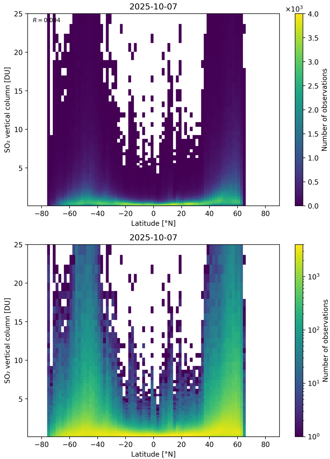
Figure 169: Scatter density plot of “Latitude” against “SO 2 vertical column” for 2025-10-06 to 2025-10-08.
