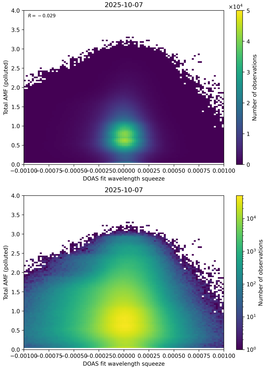
Figure 145: Scatter density plot of “DOAS fit wavelength squeeze” against “Total AMF (polluted)” for 2025-10-06 to 2025-10-08.
