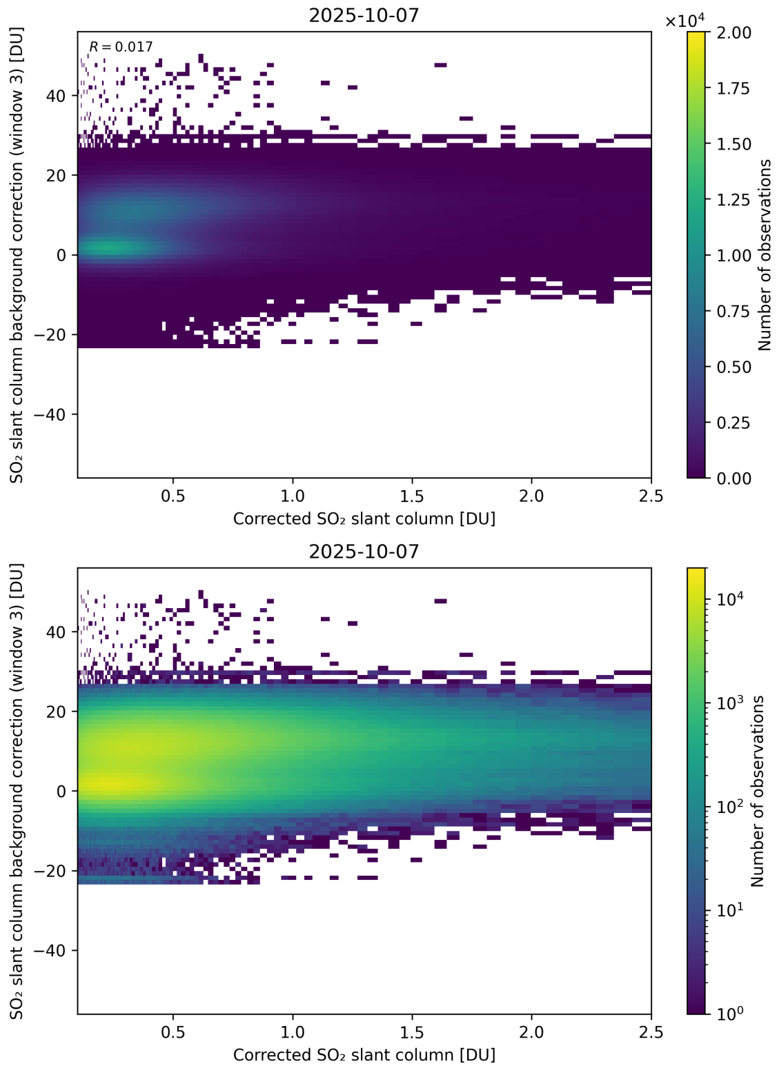
Figure 228: Scatter density plot of “Corrected SO 2 slant column” against “SO 2 slant column background correction (window 3)” for 2025-10-06 to 2025-10-08.
