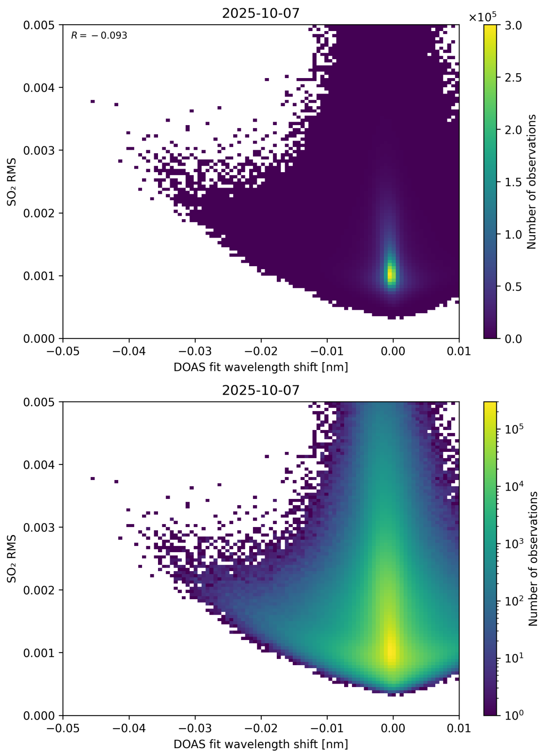
Figure 139: Scatter density plot of “DOAS fit wavelength shift” against “SO 2 RMS” for 2025-10-06 to 2025-10-08.
