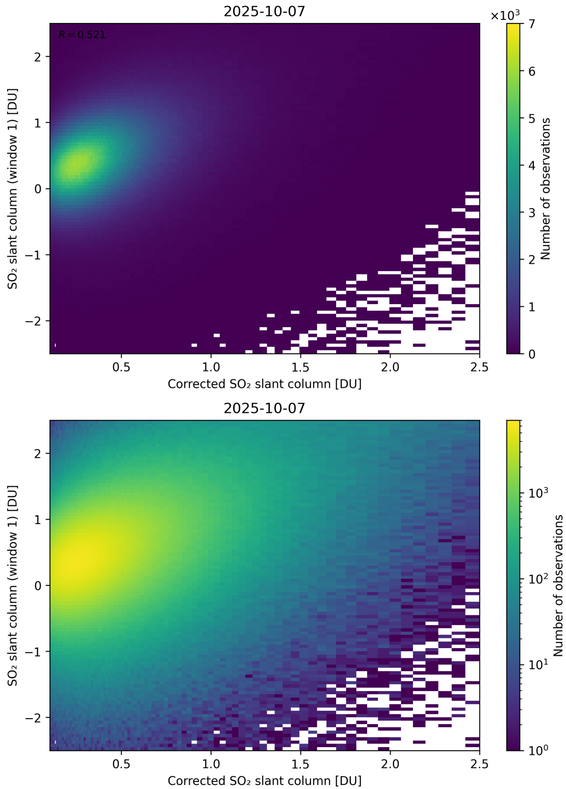
Figure 237: Scatter density plot of “Corrected SO 2 slant column” against “SO 2 slant column (window 1)” for 2025-10-06 to 2025-10-08.
