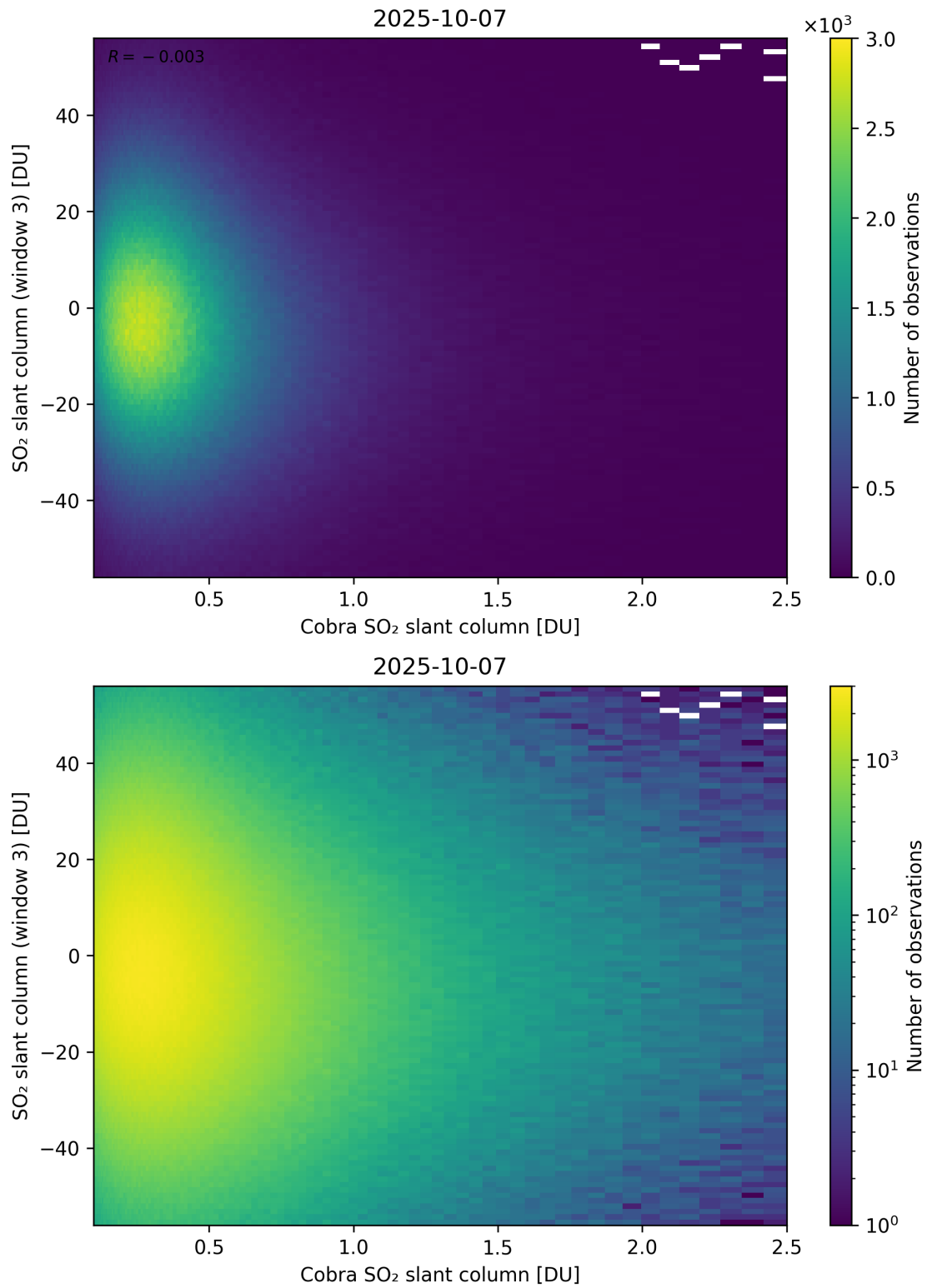
Figure 222: Scatter density plot of “Cobra SO 2 slant column” against “SO 2 slant column (window 3)” for 2025-10-06 to 2025-10-08.
