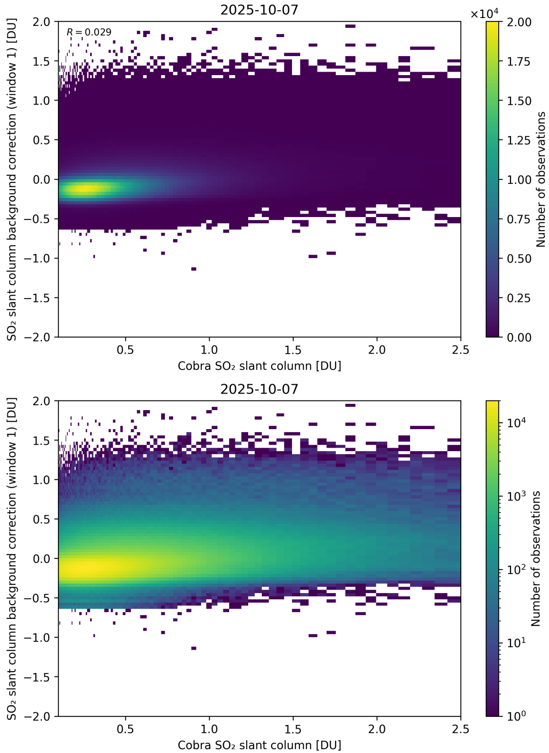
Figure 193: Scatter density plot of “Cobra SO 2 slant column” against “SO 2 slant column background correction (window 1)” for 2025-10-06 to 2025-10-08.
