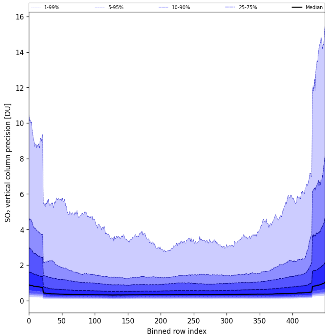
Figure 85: Along track statistics of “SO 2 vertical column precision” for 2025-10-06 to 2025-10-08
