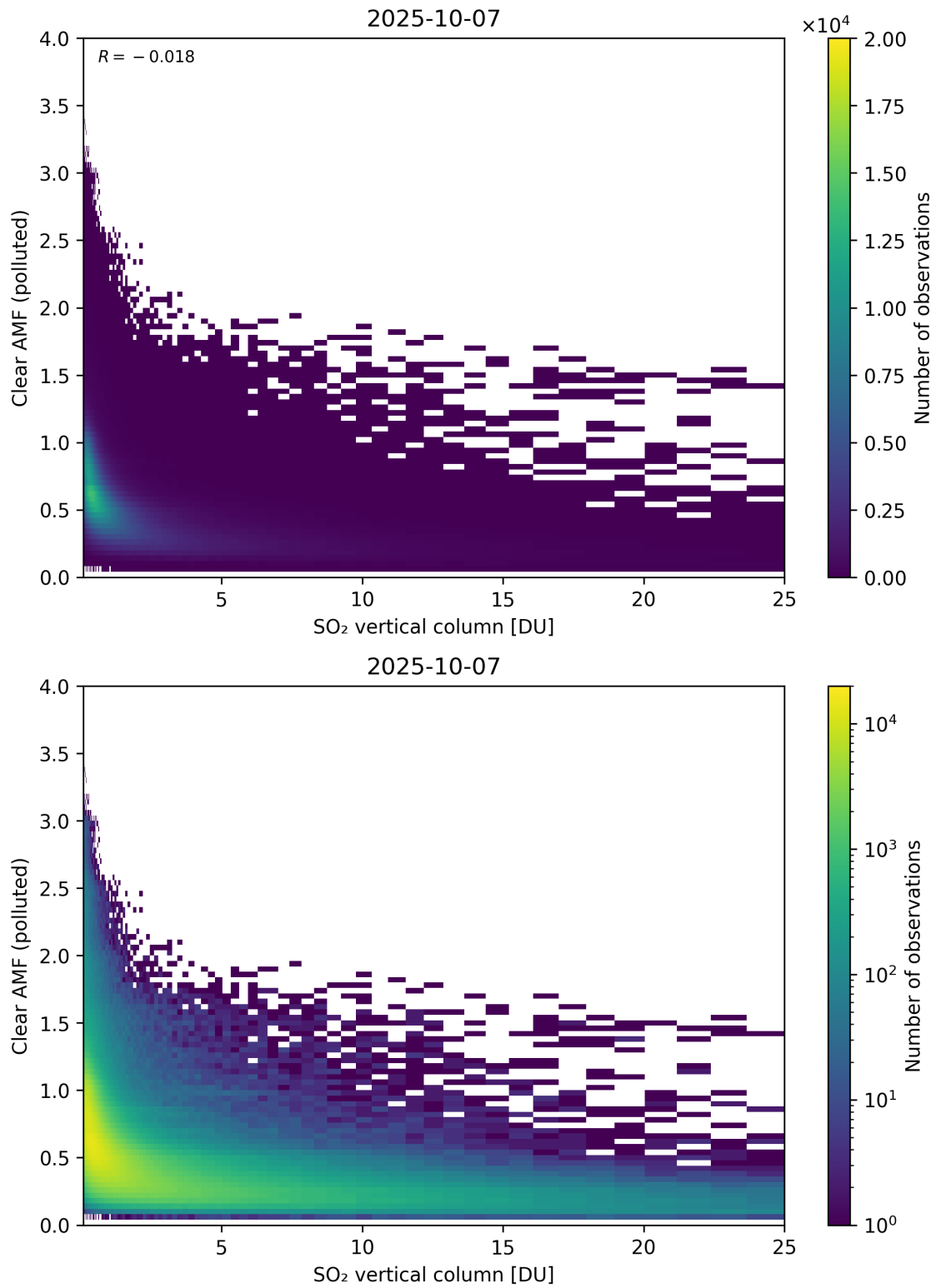
Figure 348: Scatter density plot of “SO 2 vertical column” against “Clear AMF (polluted)” for 2025-10-06 to 2025-10-08.
