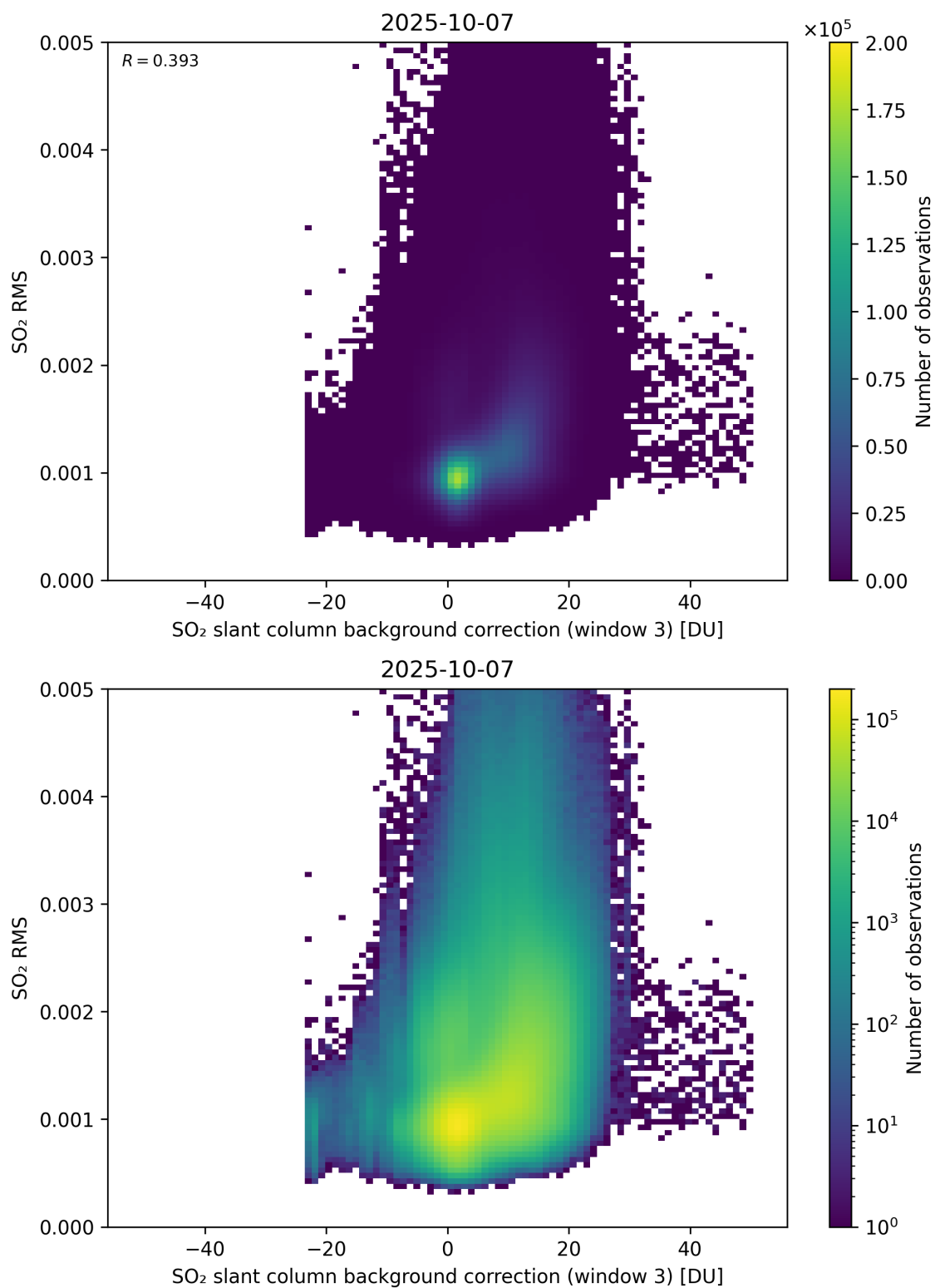
Figure 134: Scatter density plot of “SO 2 slant column background correction (window 3)” against “SO 2 RMS” for 2025-10-06 to 2025-10-08.
