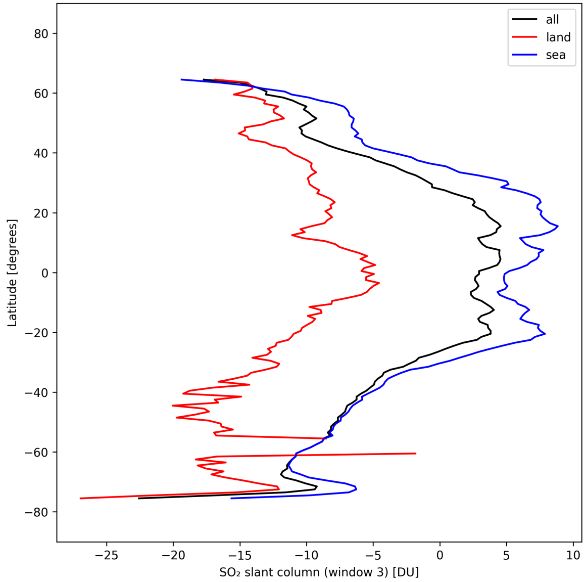
Figure 45: Zonal average of “SO 2 slant column (window 3)” for 2025-10-06 to 2025-10-08.
