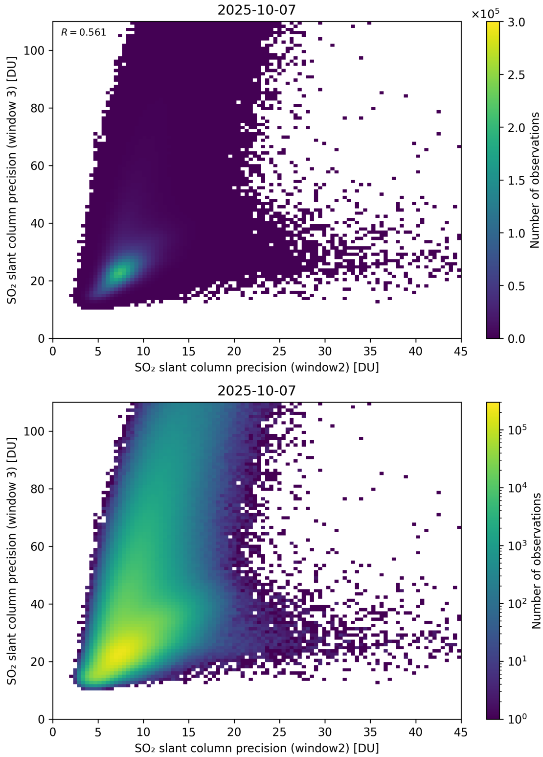
Figure 300: Scatter density plot of “SO 2 slant column precision (window2)” against “SO 2 slant column precision (window 3)” for 2025-10-06 to 2025-10-08.
