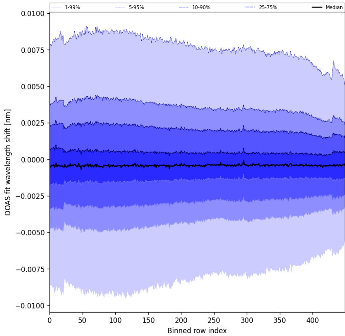
Figure 102: Along track statistics of “DOAS fit wavelength shift” for 2025-10-06 to 2025-10-08
