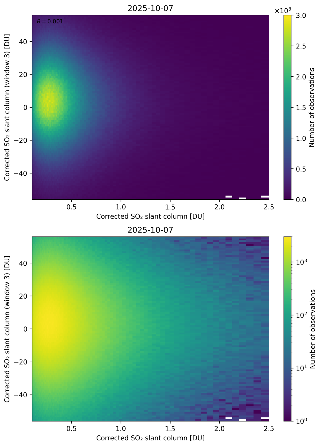
Figure 236: Scatter density plot of “Corrected SO 2 slant column” against “Corrected SO 2 slant column (window 3)” for 2025-10-06 to 2025-10-08.
