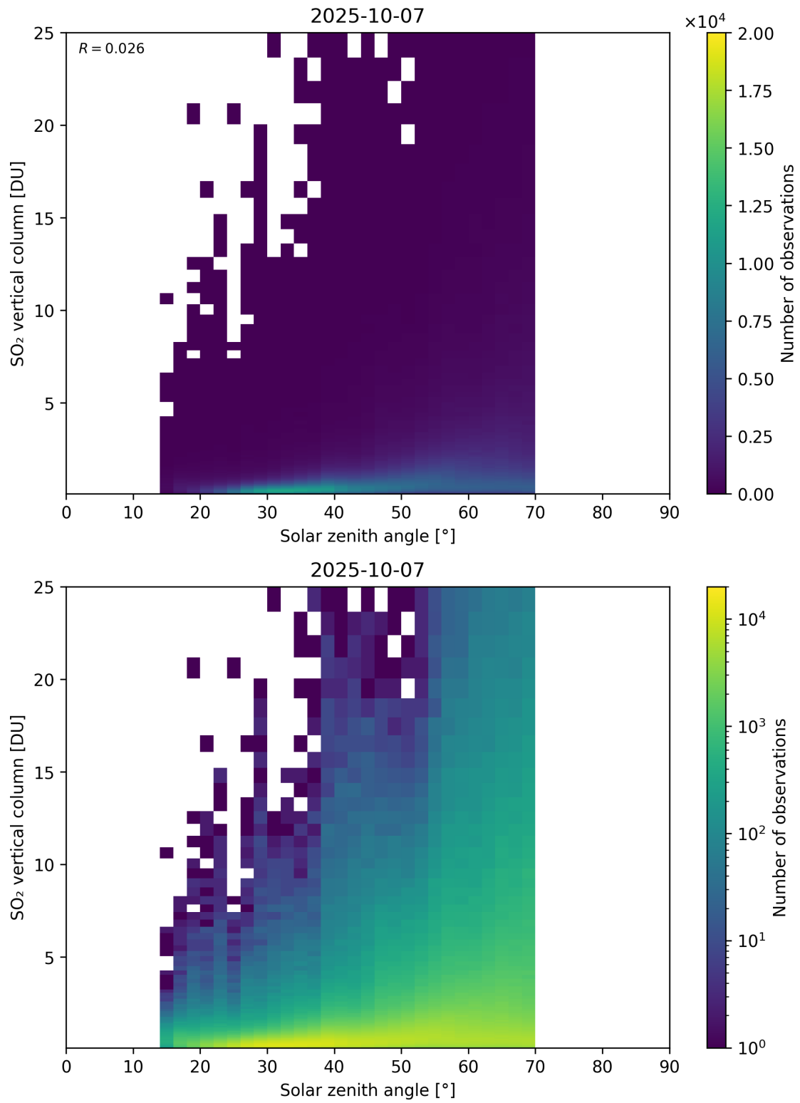
Figure 191: Scatter density plot of “Solar zenith angle” against “SO 2 vertical column” for 2025-10-06 to 2025-10-08.
