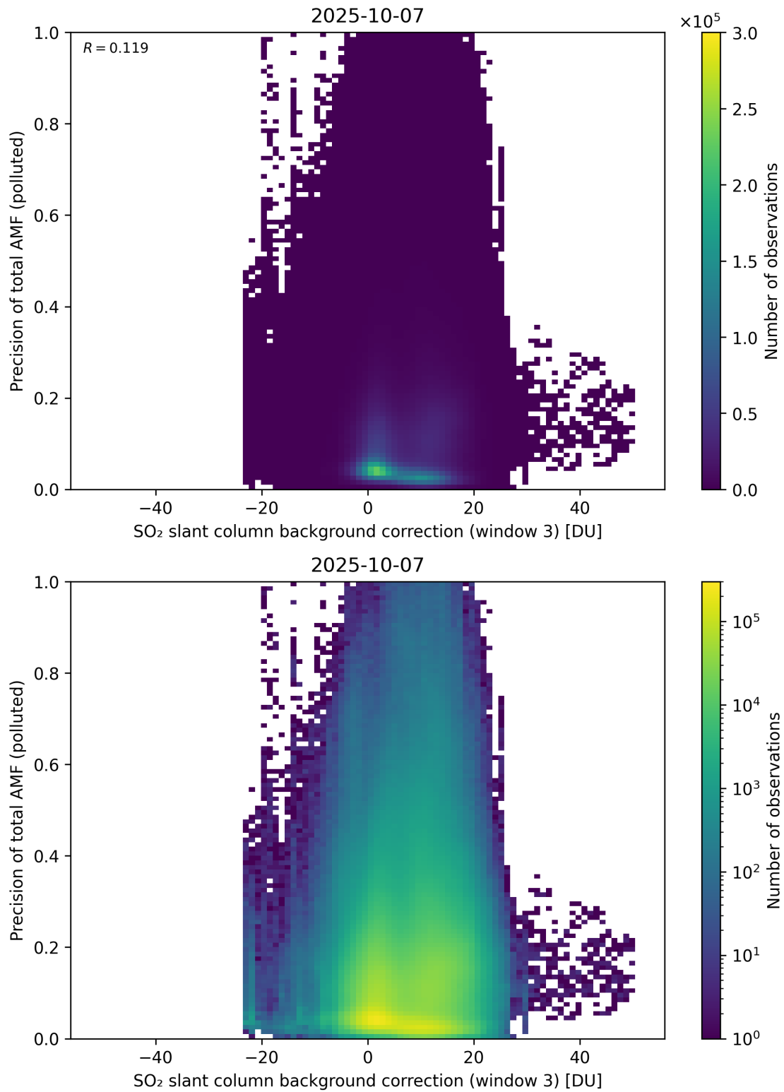
Figure 137: Scatter density plot of “SO 2 slant column background correction (window 3)” against “Precision of total AMF (polluted)” for 2025-10-06 to 2025-10-08.
