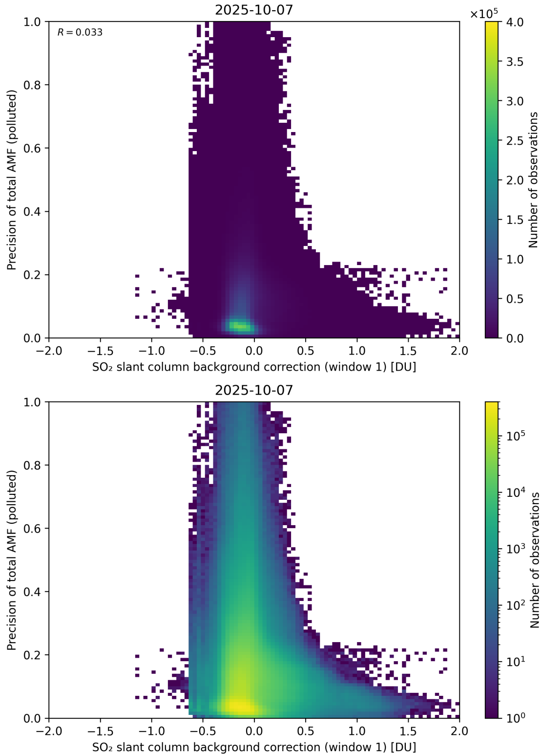
Figure 121: Scatter density plot of “SO 2 slant column background correction (window 1)” against “Precision of total AMF (polluted)” for 2025-10-06 to 2025-10-08.
