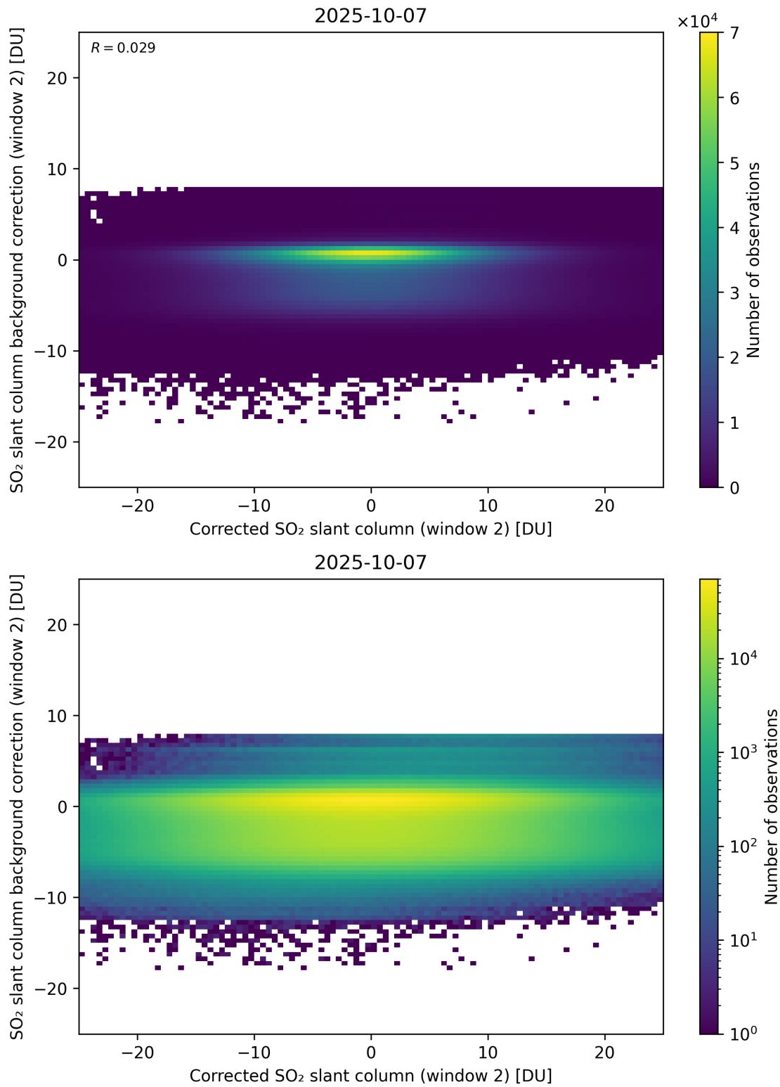
Figure 244: Scatter density plot of “Corrected SO 2 slant column (window 2)” against “SO 2 slant column background correction (window 2)” for 2025-10-06 to 2025-10-08.
