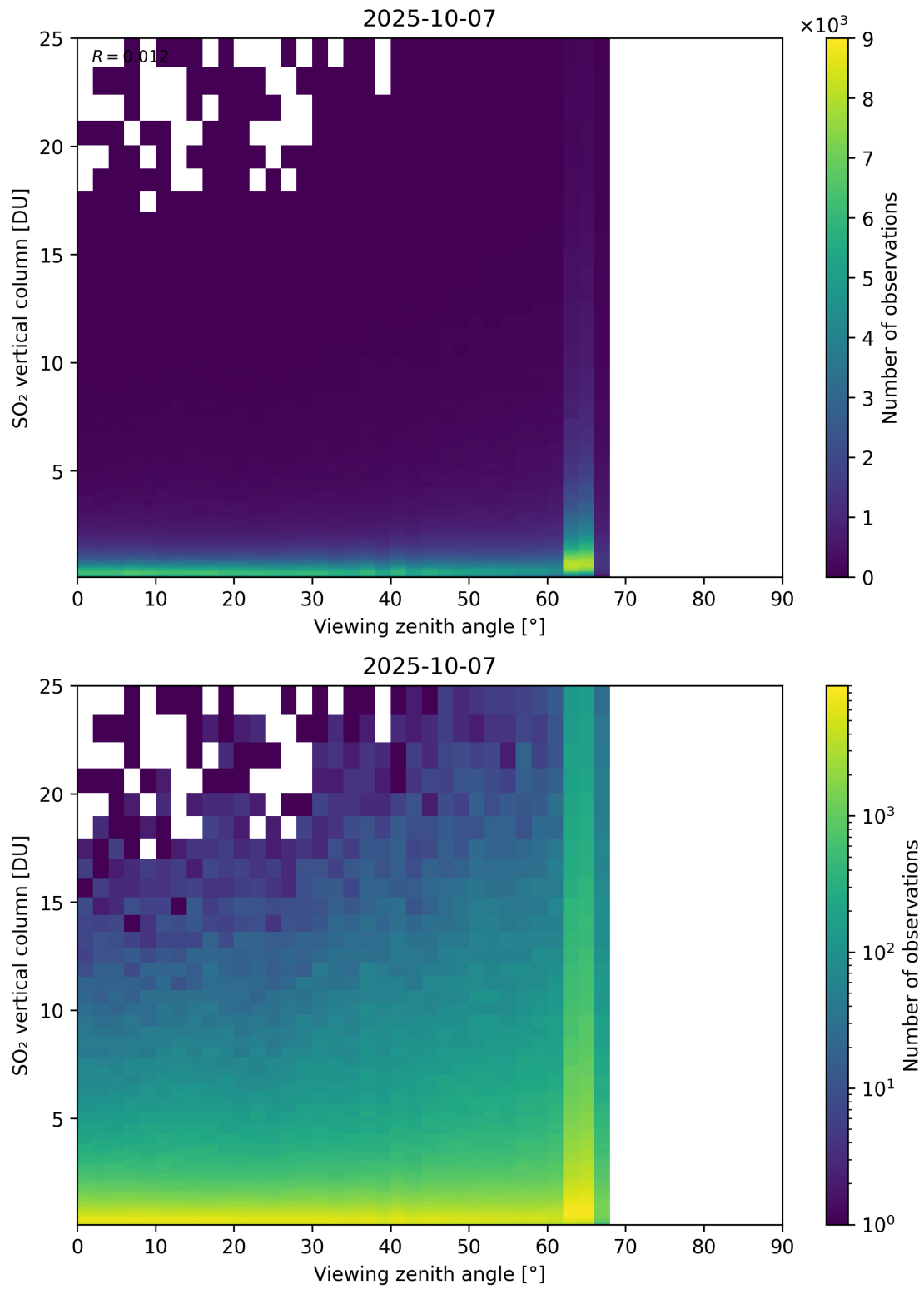
Figure 383: Scatter density plot of “Viewing zenith angle” against “SO 2 vertical column” for 2025-10-06 to 2025-10-08.
