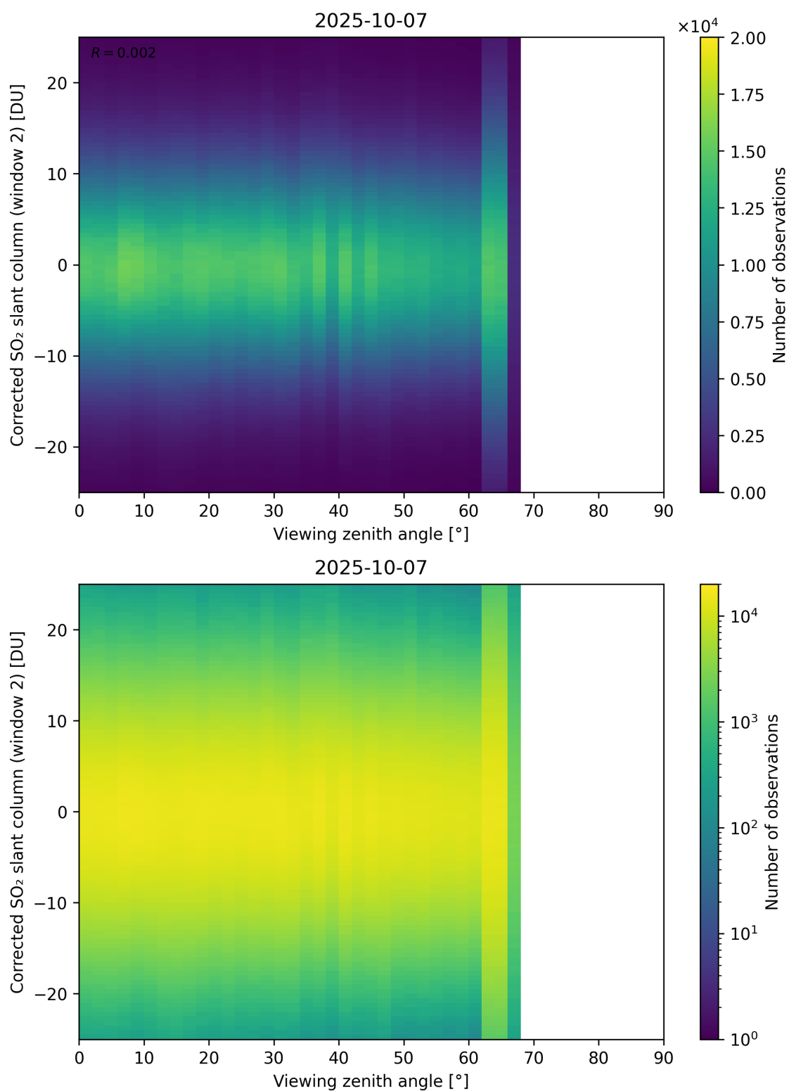
Figure 374: Scatter density plot of “Viewing zenith angle” against “Corrected SO 2 slant column (window 2)” for 2025-10-06 to 2025-10-08.
