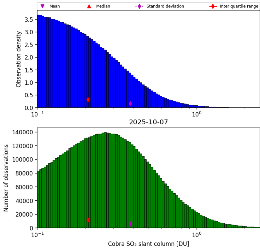
Figure 61: Histogram of “Cobra SO 2 slant column” for 2025-10-06 to 2025-10-08
