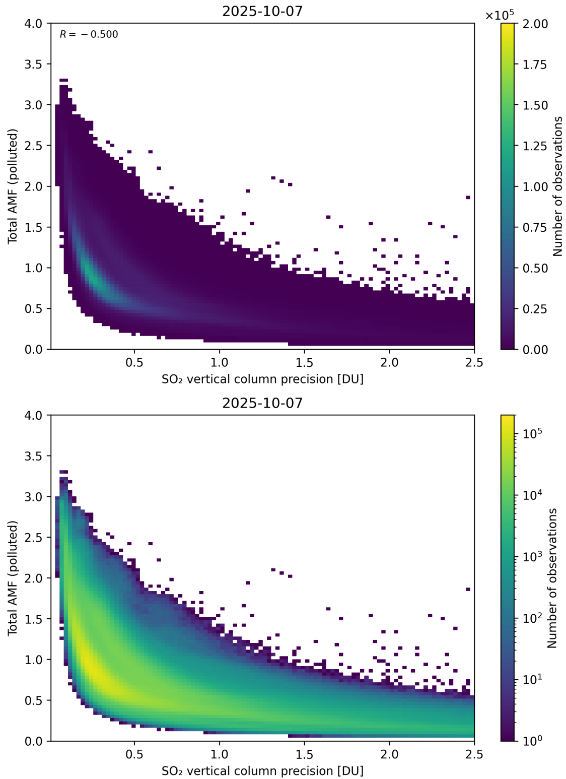
Figure 346: Scatter density plot of “SO 2 vertical column precision” against “Total AMF (polluted)” for 2025-10-06 to 2025-10-08.
