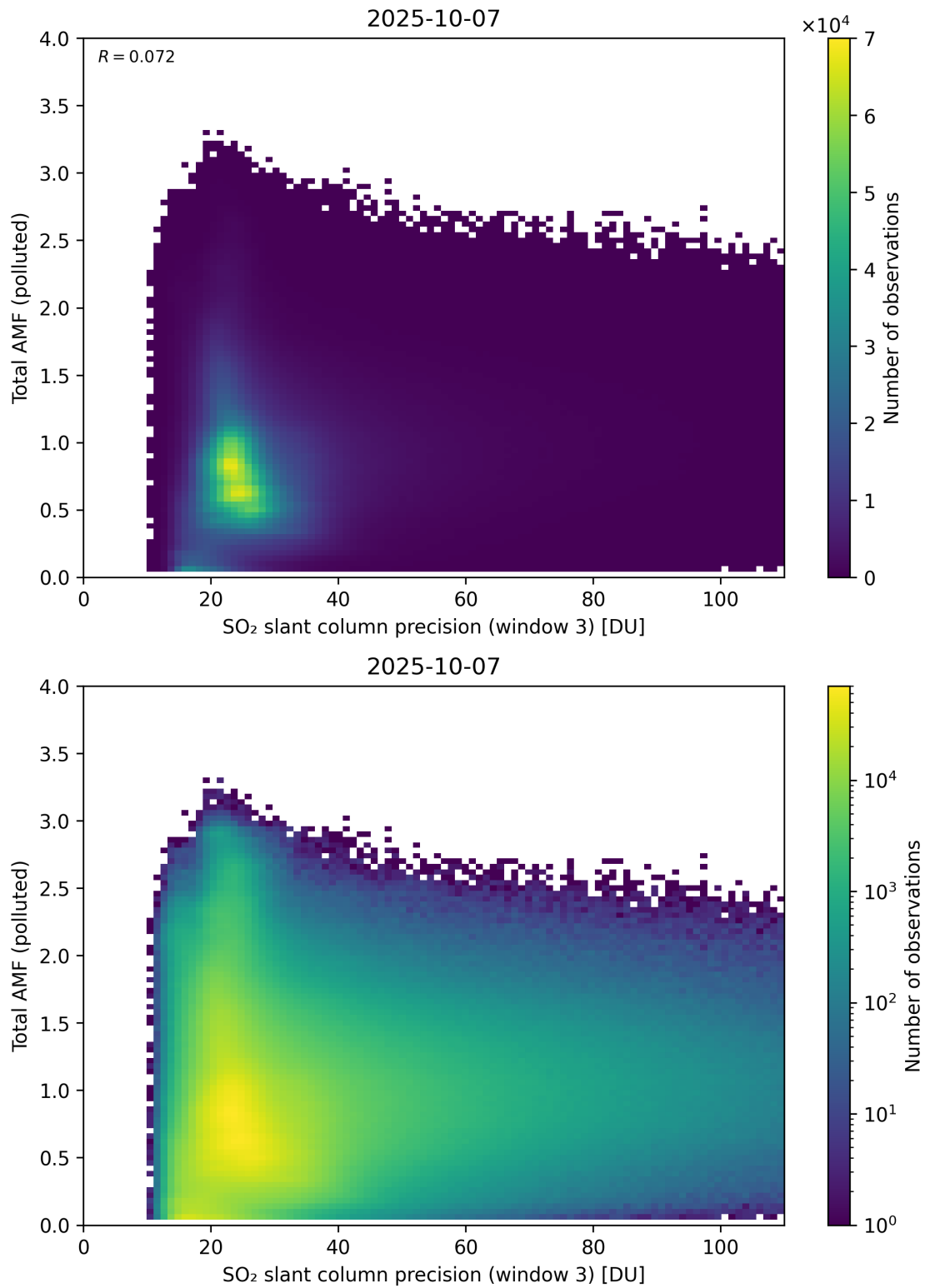
Figure 313: Scatter density plot of “SO 2 slant column precision (window 3)” against “Total AMF (polluted)” for 2025-10-06 to 2025-10-08.
