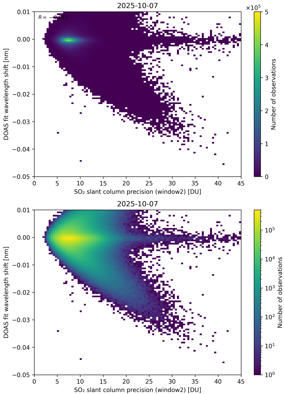
Figure 293: Scatter density plot of “SO 2 slant column precision (window2)” against “DOAS fit wavelength shift” for 2025-10-06 to 2025-10-08.
