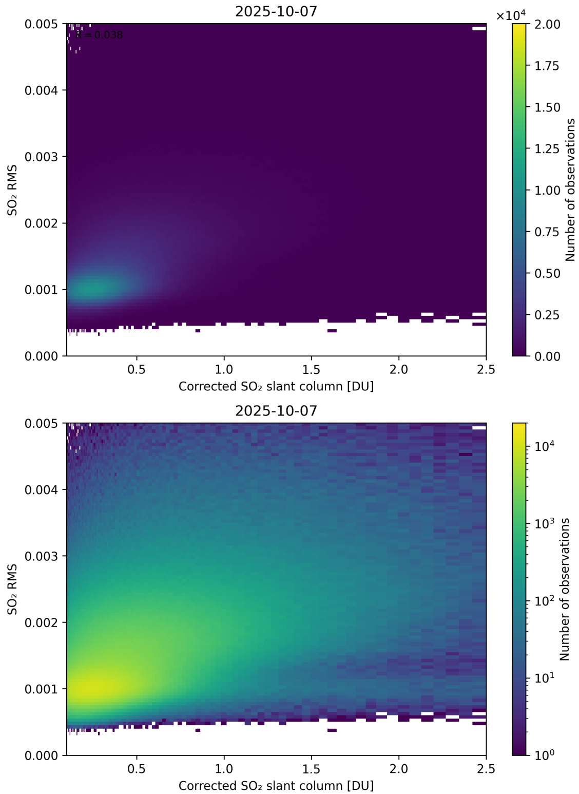
Figure 231: Scatter density plot of “Corrected SO 2 slant column” against “SO 2 RMS” for 2025-10-06 to 2025-10-08.
