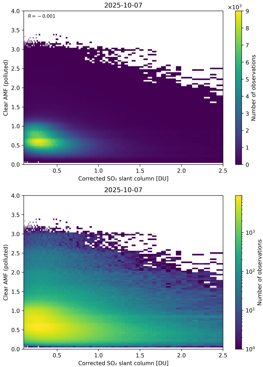
Figure 232: Scatter density plot of “Corrected SO 2 slant column” against “Clear AMF (polluted)” for 2025-10-06 to 2025-10-08.
