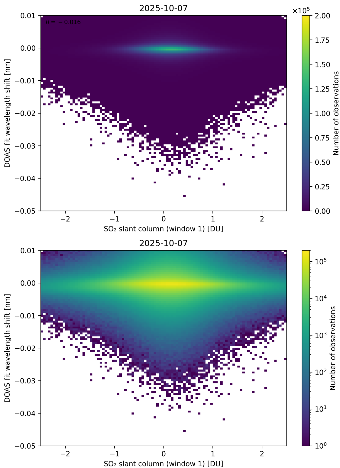
Figure 265: Scatter density plot of “SO 2 slant column (window 1)” against “DOAS fit wavelength shift” for 2025-10-06 to 2025-10-08.
