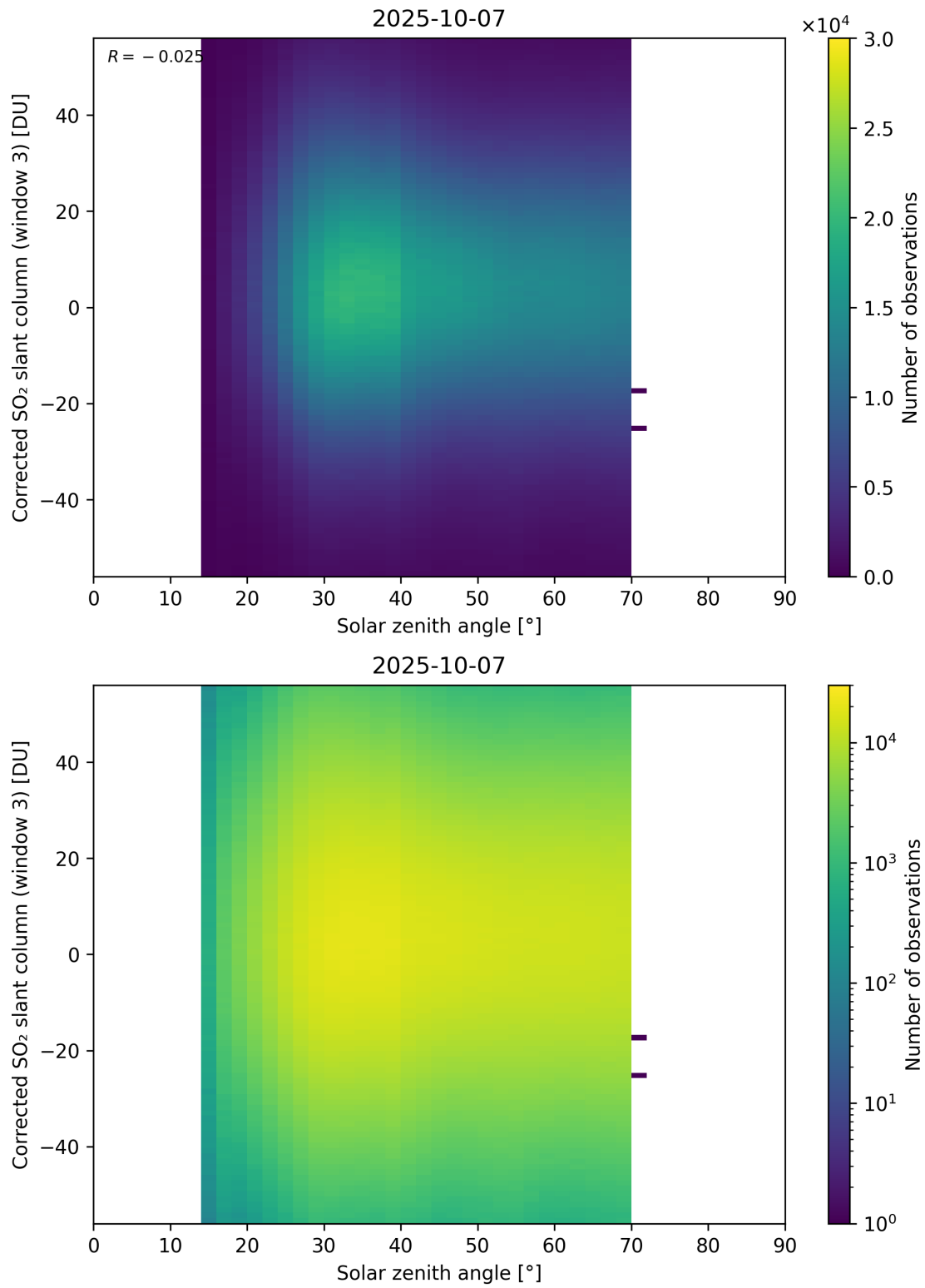
Figure 183: Scatter density plot of “Solar zenith angle” against “Corrected SO 2 slant column (window 3)” for 2025-10-06 to 2025-10-08.
