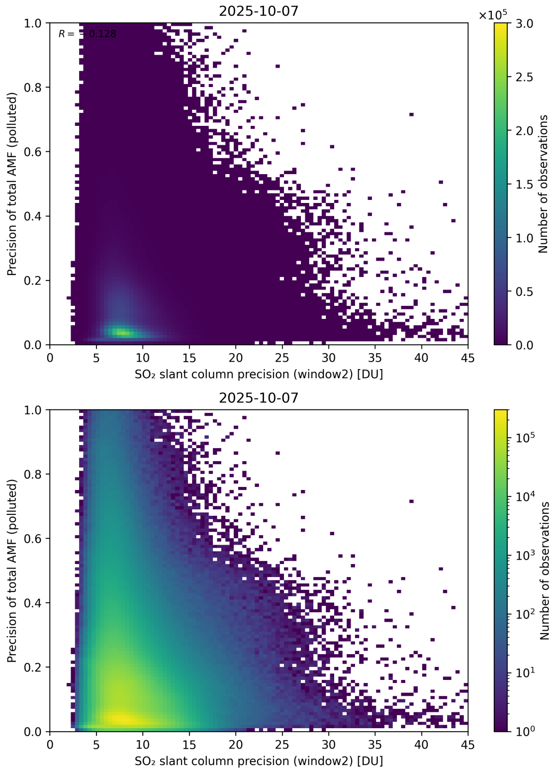
Figure 302: Scatter density plot of “SO 2 slant column precision (window2)” against “Precision of total AMF (polluted)” for 2025-10-06 to 2025-10-08.
