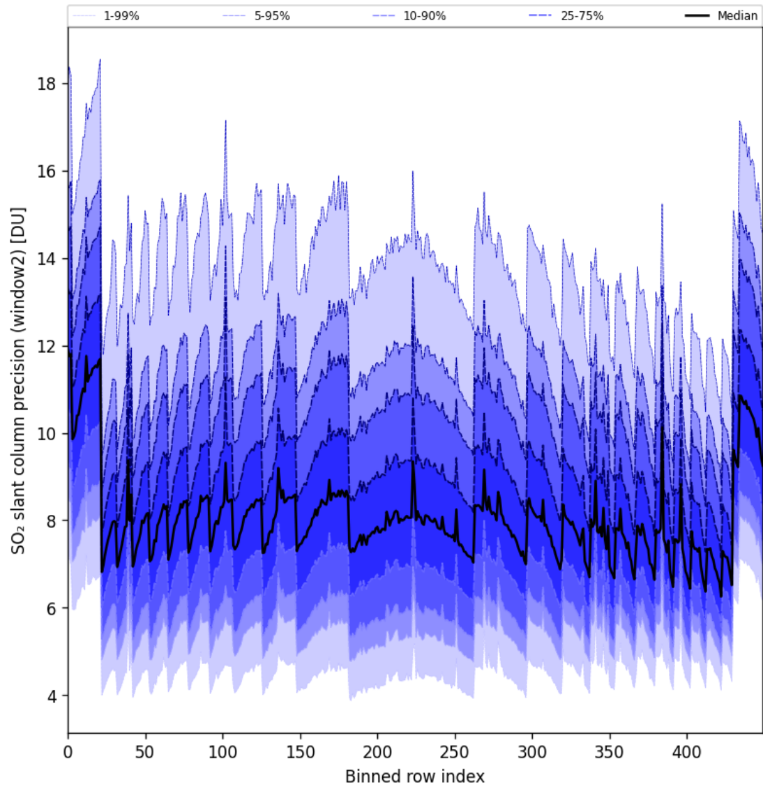
Figure 94: Along track statistics of “SO 2 slant column precision (window2)” for 2025-10-06 to 2025-10-08
