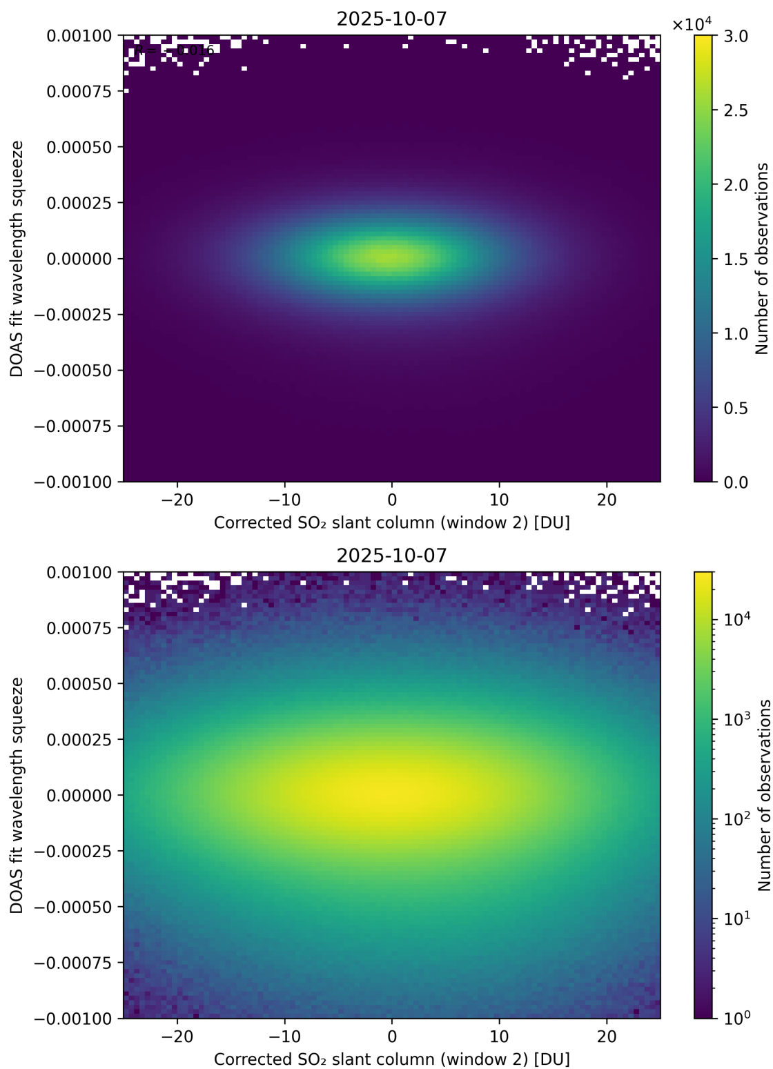
Figure 247: Scatter density plot of “Corrected SO 2 slant column (window 2)” against “DOAS fit wavelength squeeze” for 2025-10-06 to 2025-10-08.
