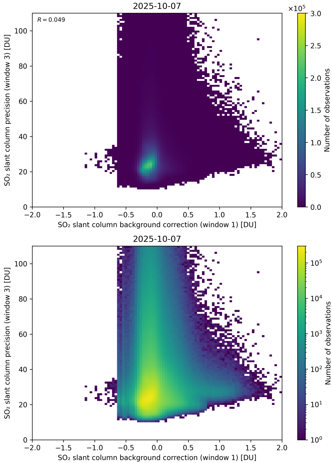
Figure 119: Scatter density plot of “SO 2 slant column background correction (window 1)” against “SO 2 slant column precision (window 3)” for 2025-10-06 to 2025-10-08.
