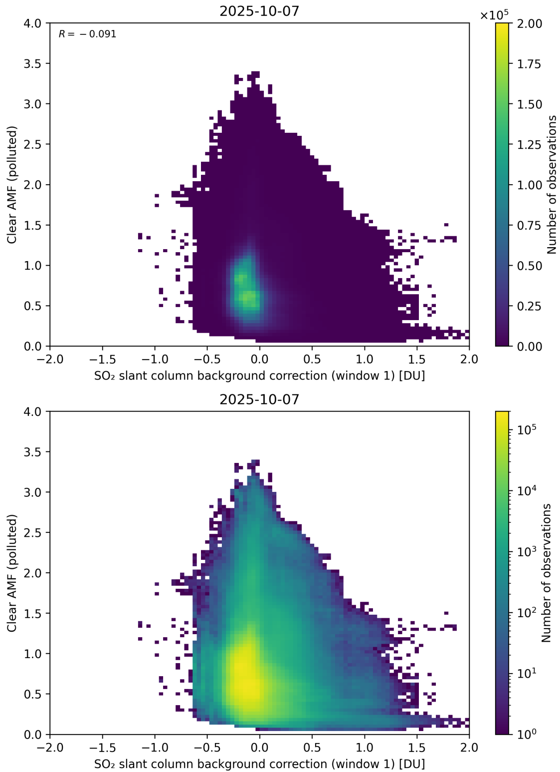
Figure 114: Scatter density plot of “SO 2 slant column background correction (window 1)” against “Clear AMF (polluted)” for 2025-10-06 to 2025-10-08.
