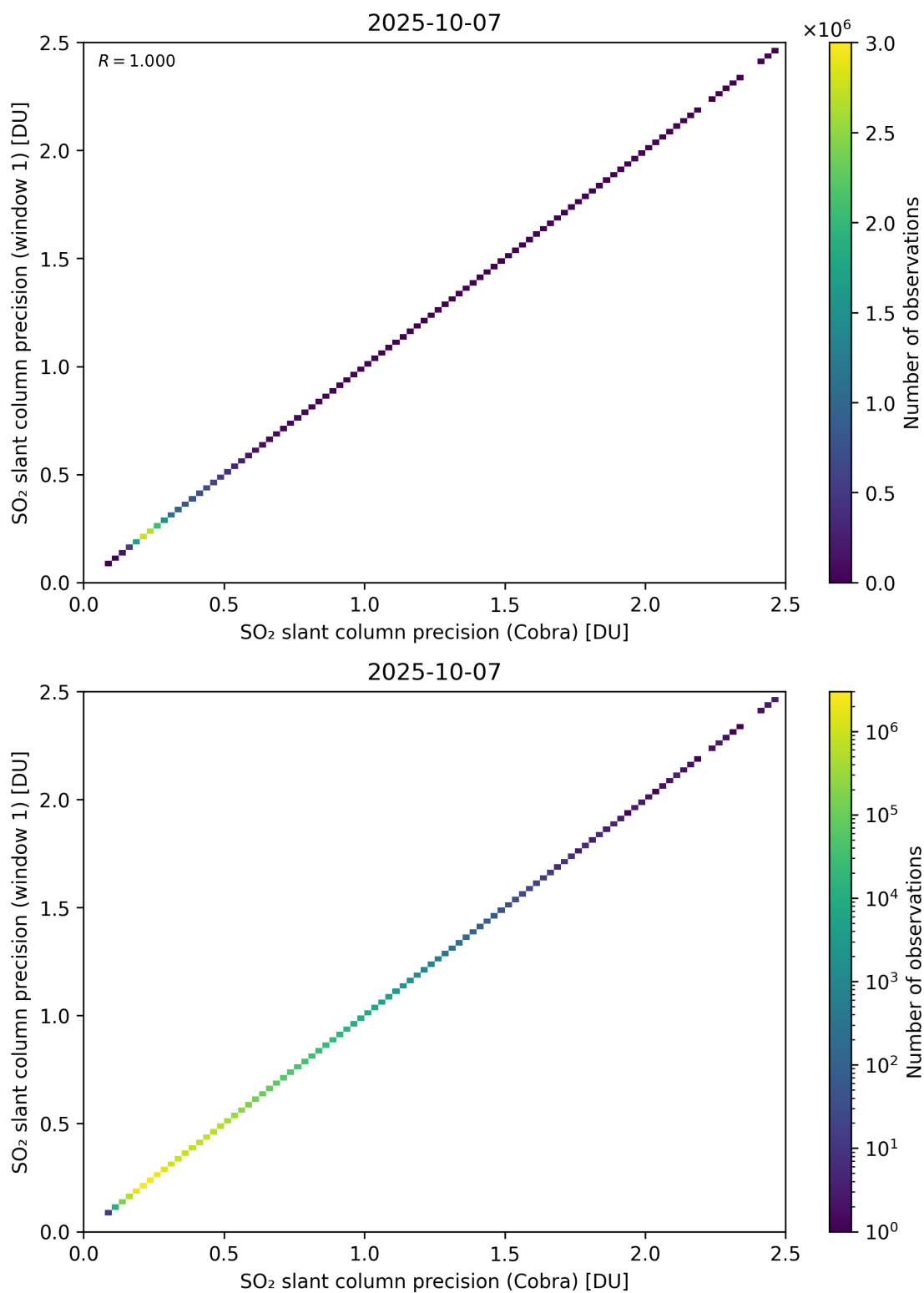
Figure 209: Scatter density plot of “SO 2 slant column precision (Cobra)” against “SO 2 slant column precision (window 1)” for 2025-10-06 to 2025-10-08.
