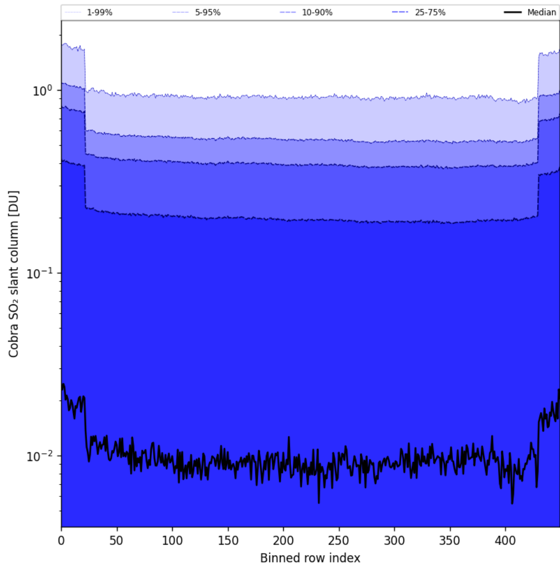
Figure 87: Along track statistics of "Cobra SO 2 slant column" for 2025-10-06 to 2025-10-08
