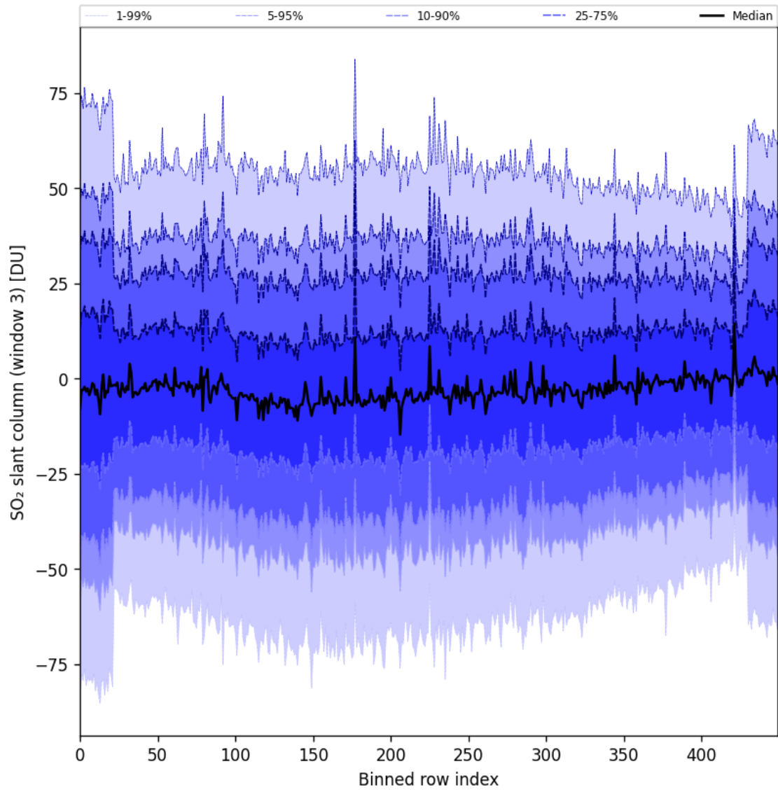
Figure 97: Along track statistics of “SO 2 slant column (window 3)” for 2025-10-06 to 2025-10-08
