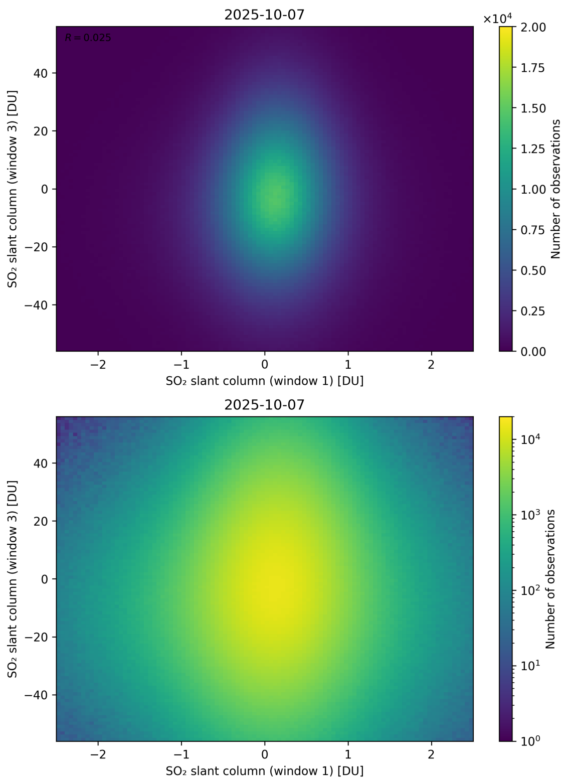
Figure 287: Scatter density plot of “SO 2 slant column (window 1)” against “SO 2 slant column (window 3)” for 2025-10-06 to 2025-10-08.
