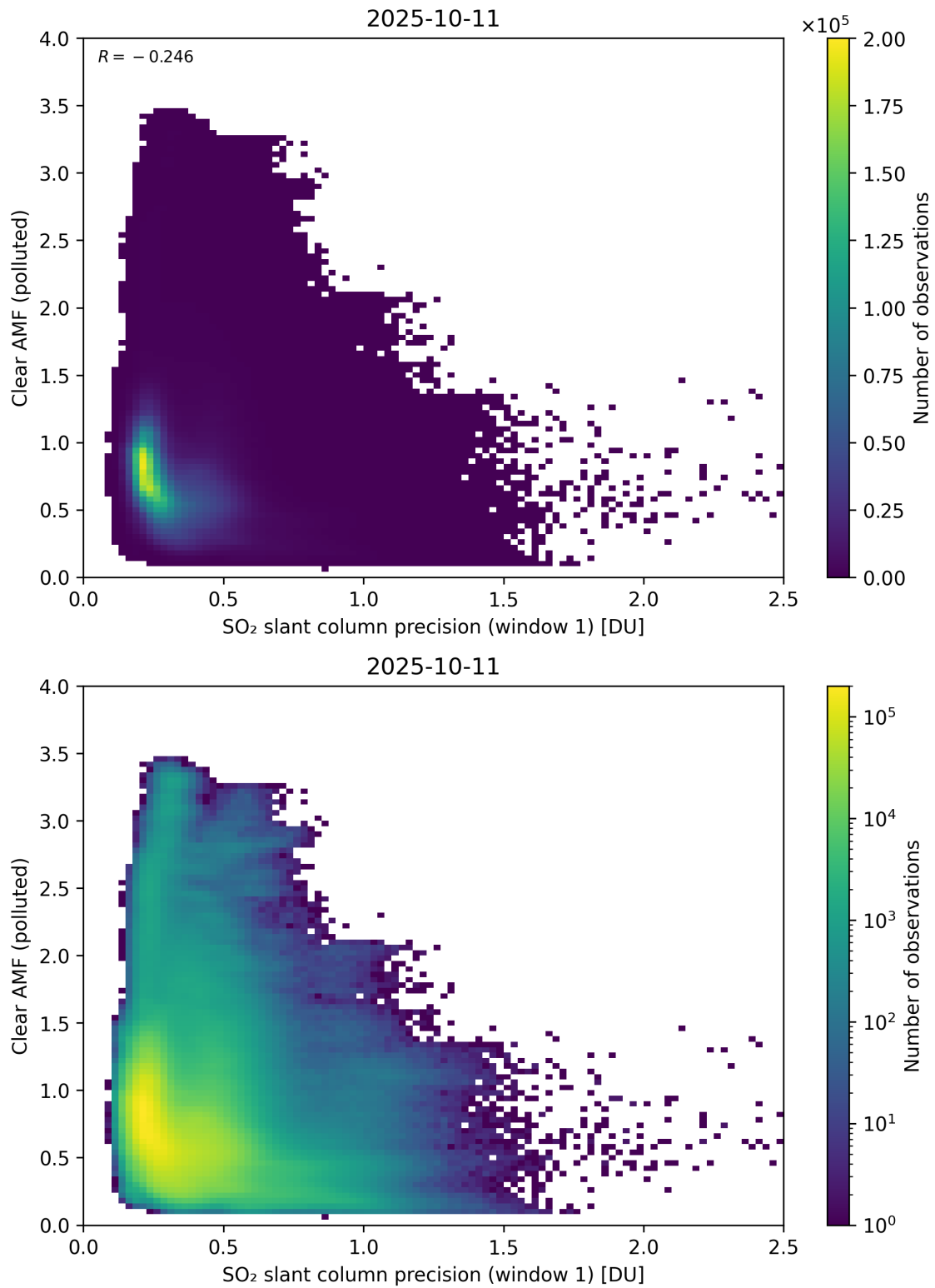
Figure 274: Scatter density plot of “SO 2 slant column precision (window 1)” against “Clear AMF (polluted)” for 2025-10-11 to 2025-10-12.
