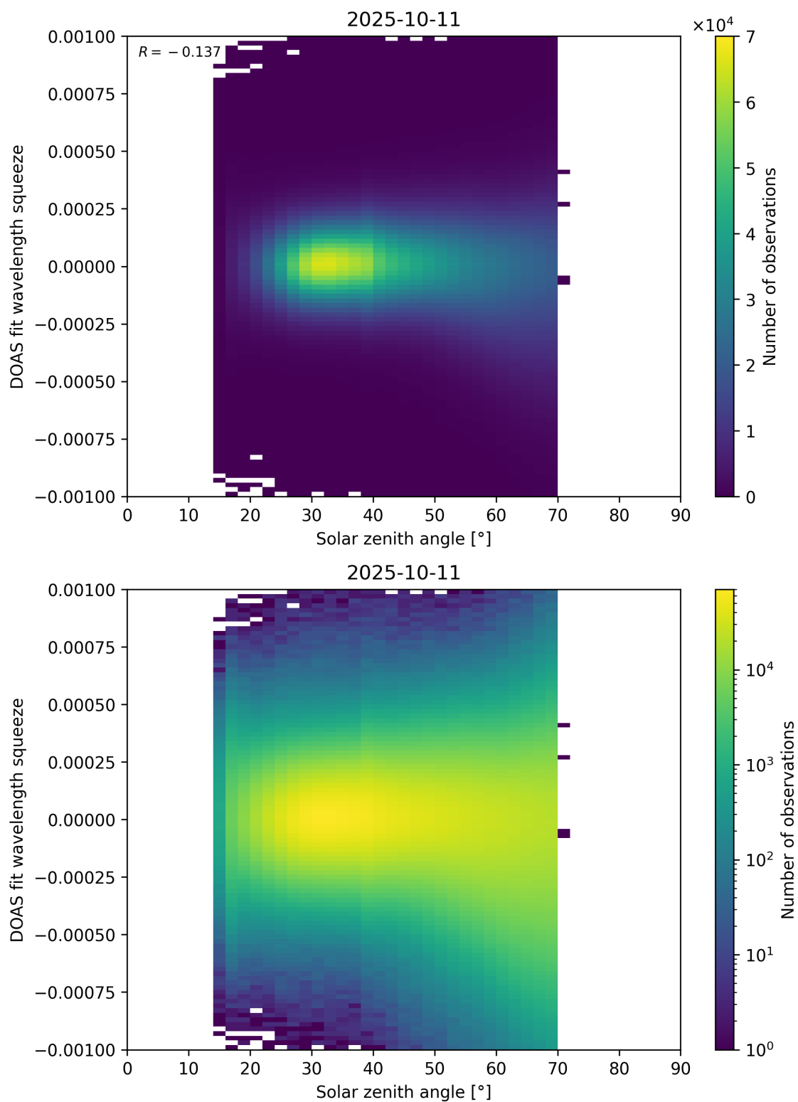
Figure 175: Scatter density plot of “Solar zenith angle” against “DOAS fit wavelength squeeze” for 2025-10-11 to 2025-10-12.
