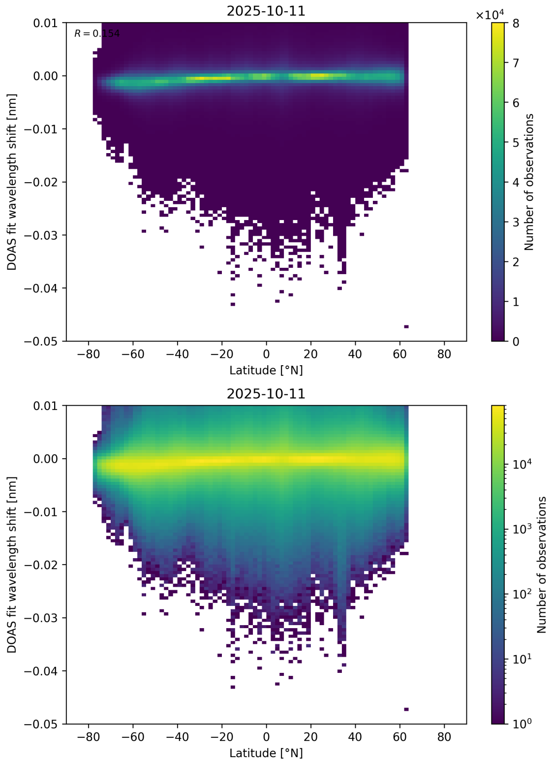
Figure 153: Scatter density plot of “Latitude” against “DOAS fit wavelength shift” for 2025-10-11 to 2025-10-12.
