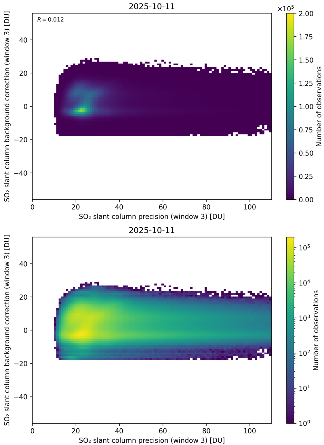
Figure 307: Scatter density plot of “SO 2 slant column precision (window 3)” against “SO 2 slant column background correction (window 3)” for 2025-10-11 to 2025-10-12.
