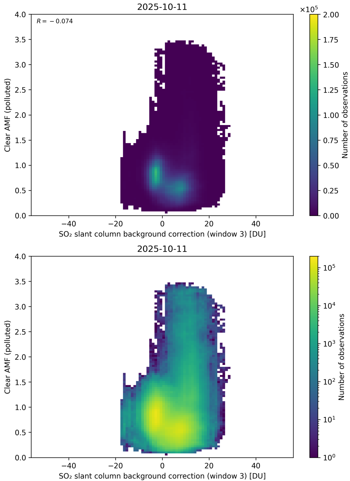
Figure 135: Scatter density plot of “SO 2 slant column background correction (window 3)” against “Clear AMF (polluted)” for 2025-10-11 to 2025-10-12.
