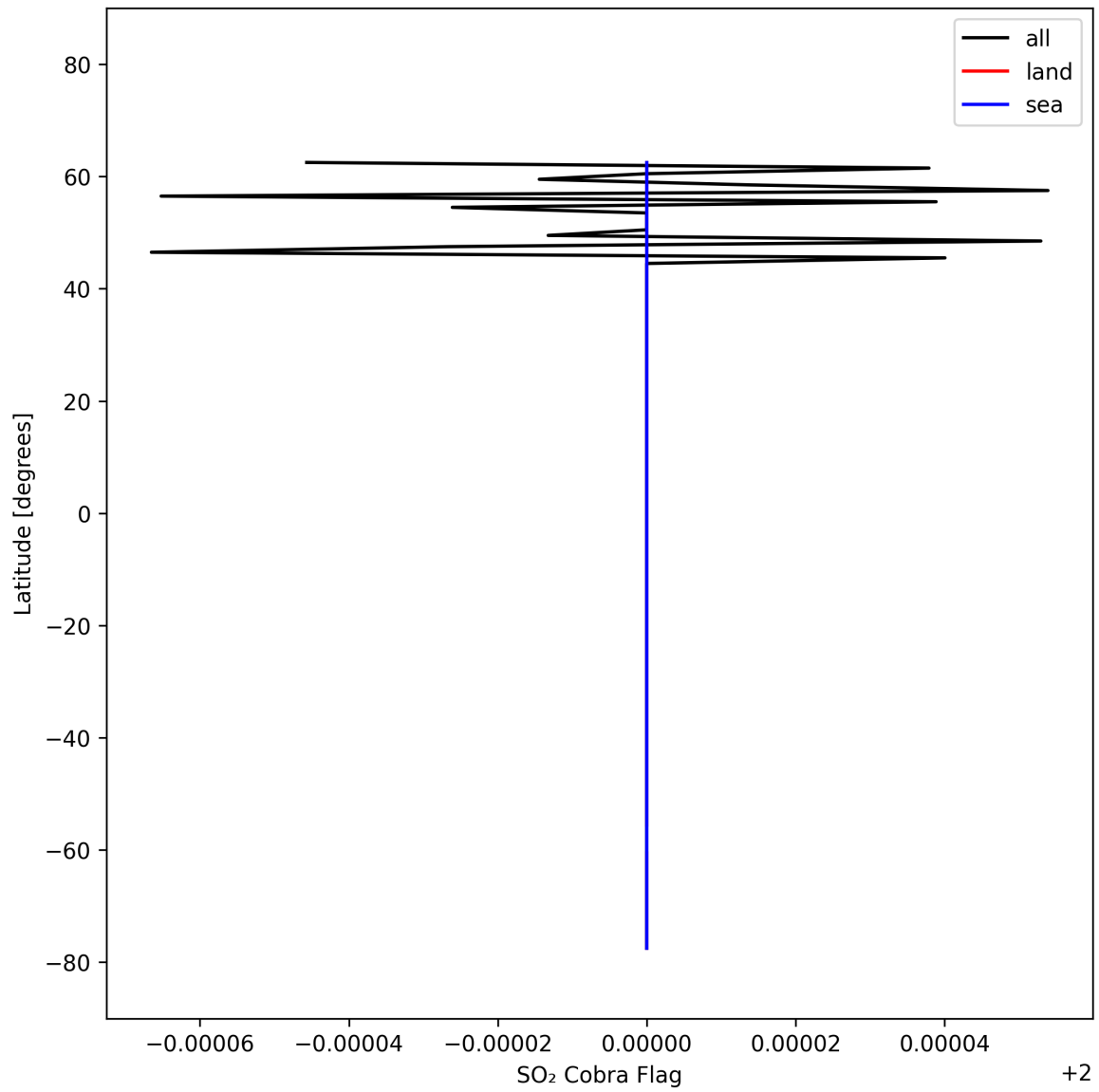
Figure 49: Zonal average of "SO 2 Cobra Flag" for 2025-10-11 to 2025-10-12.
