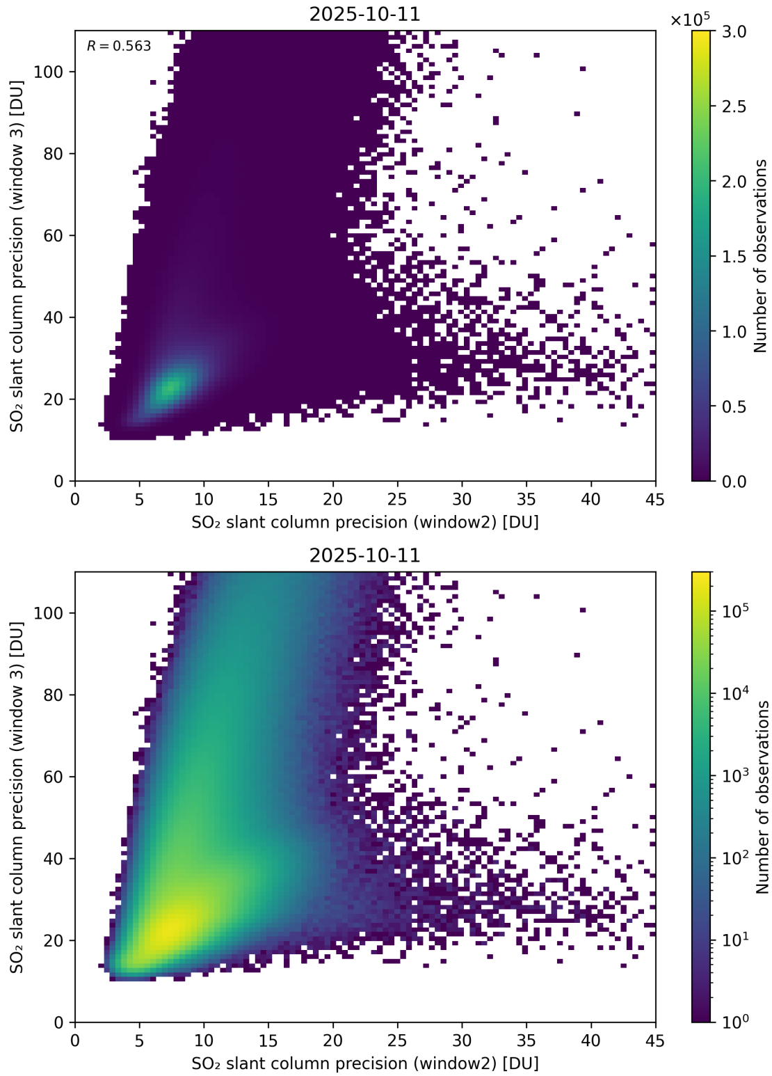
Figure 300: Scatter density plot of “SO 2 slant column precision (window2)” against “SO 2 slant column precision (window 3)” for 2025-10-11 to 2025-10-12.
