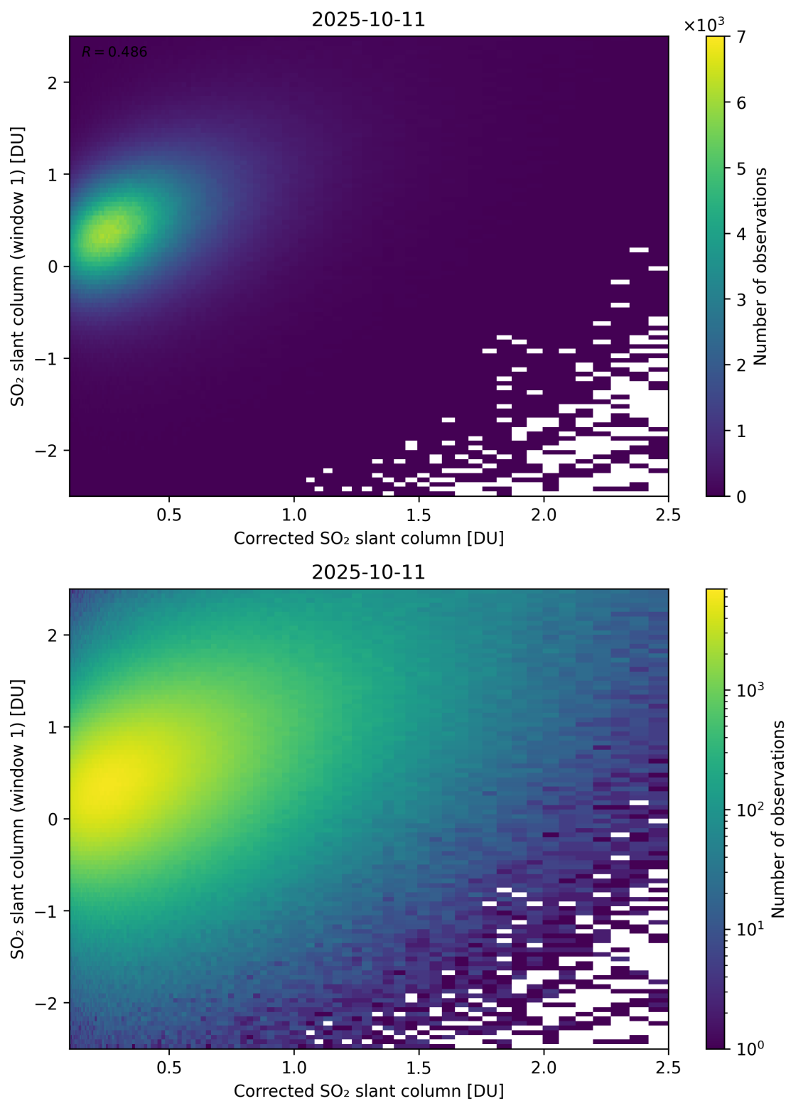
Figure 237: Scatter density plot of “Corrected SO 2 slant column” against “SO 2 slant column (window 1)” for 2025-10-11 to 2025-10-12.
