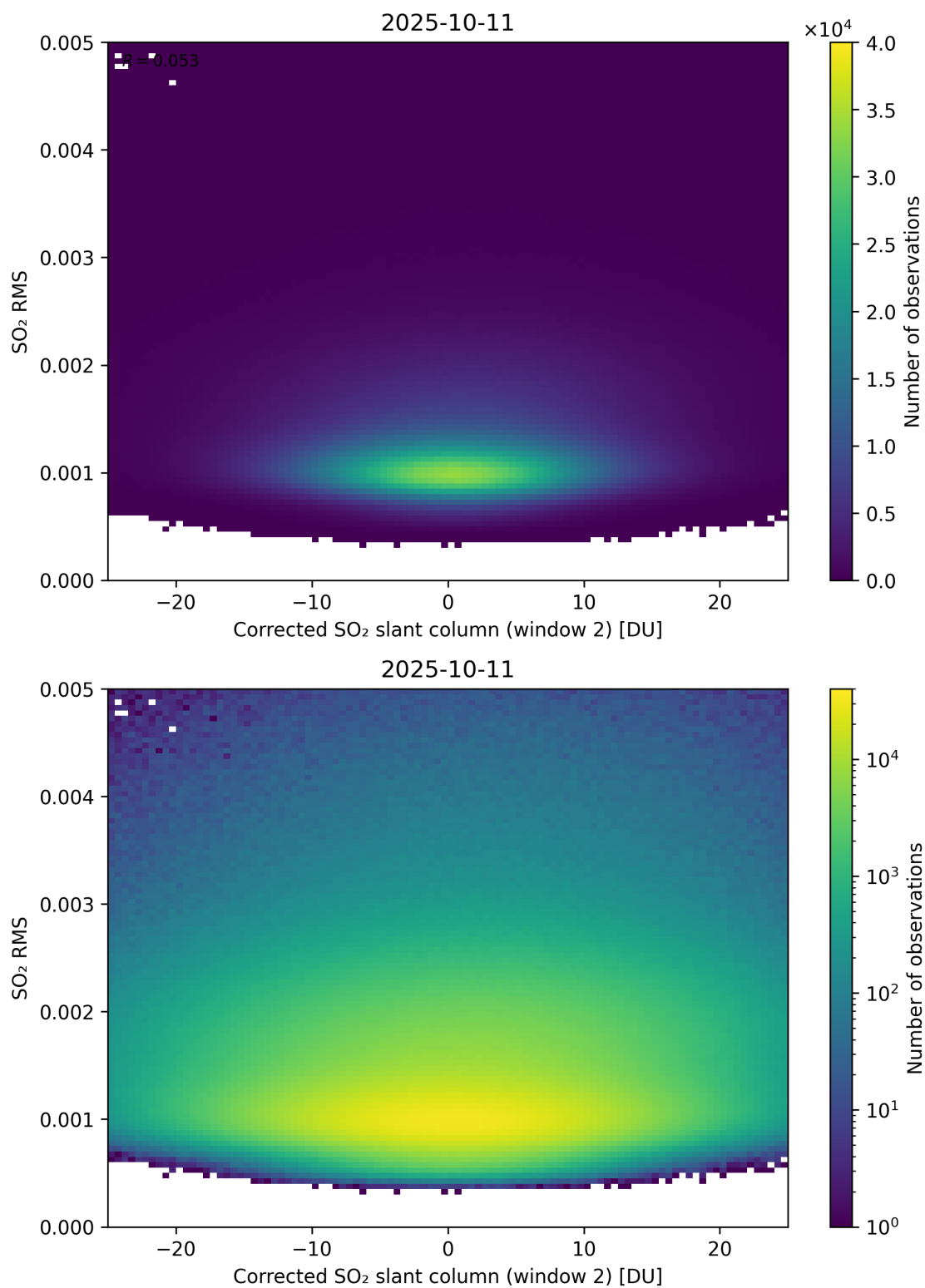
Figure 248: Scatter density plot of “Corrected SO 2 slant column (window 2)” against “SO 2 RMS” for 2025-10-11 to 2025-10-12.
