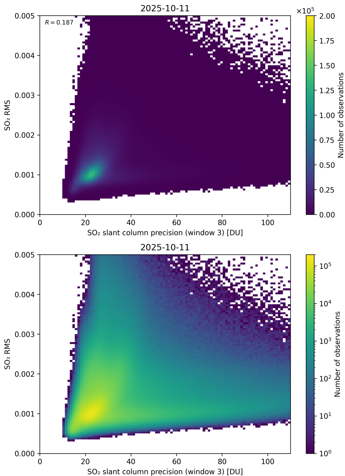
Figure 310: Scatter density plot of “SO 2 slant column precision (window 3)” against “SO 2 RMS” for 2025-10-11 to 2025-10-12.
