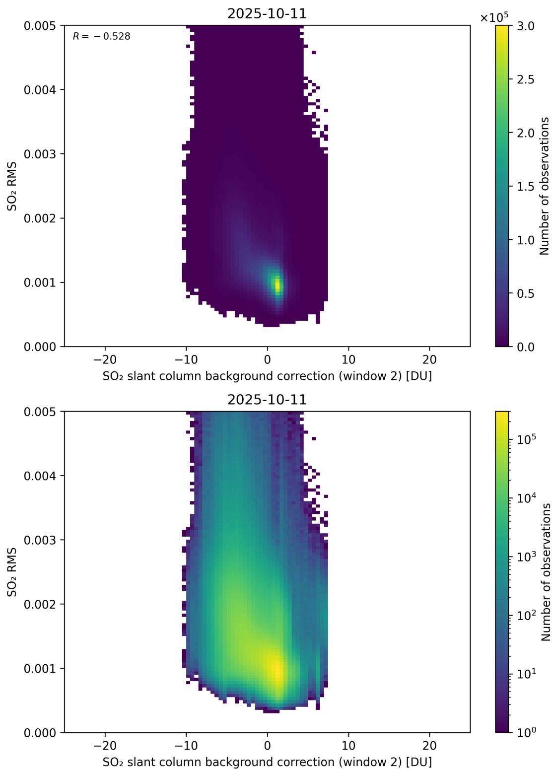
Figure 125: Scatter density plot of “SO 2 slant column background correction (window 2)” against “SO 2 RMS” for 2025-10-11 to 2025-10-12.
