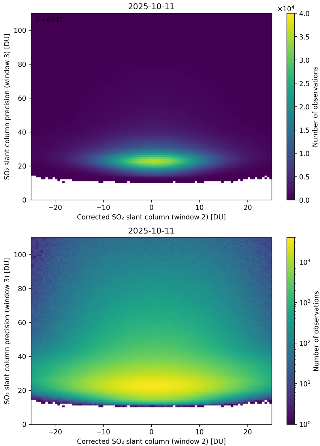
Figure 252: Scatter density plot of “Corrected SO 2 slant column (window 2)” against “SO 2 slant column precision (window 3)” for 2025-10-11 to 2025-10-12.
