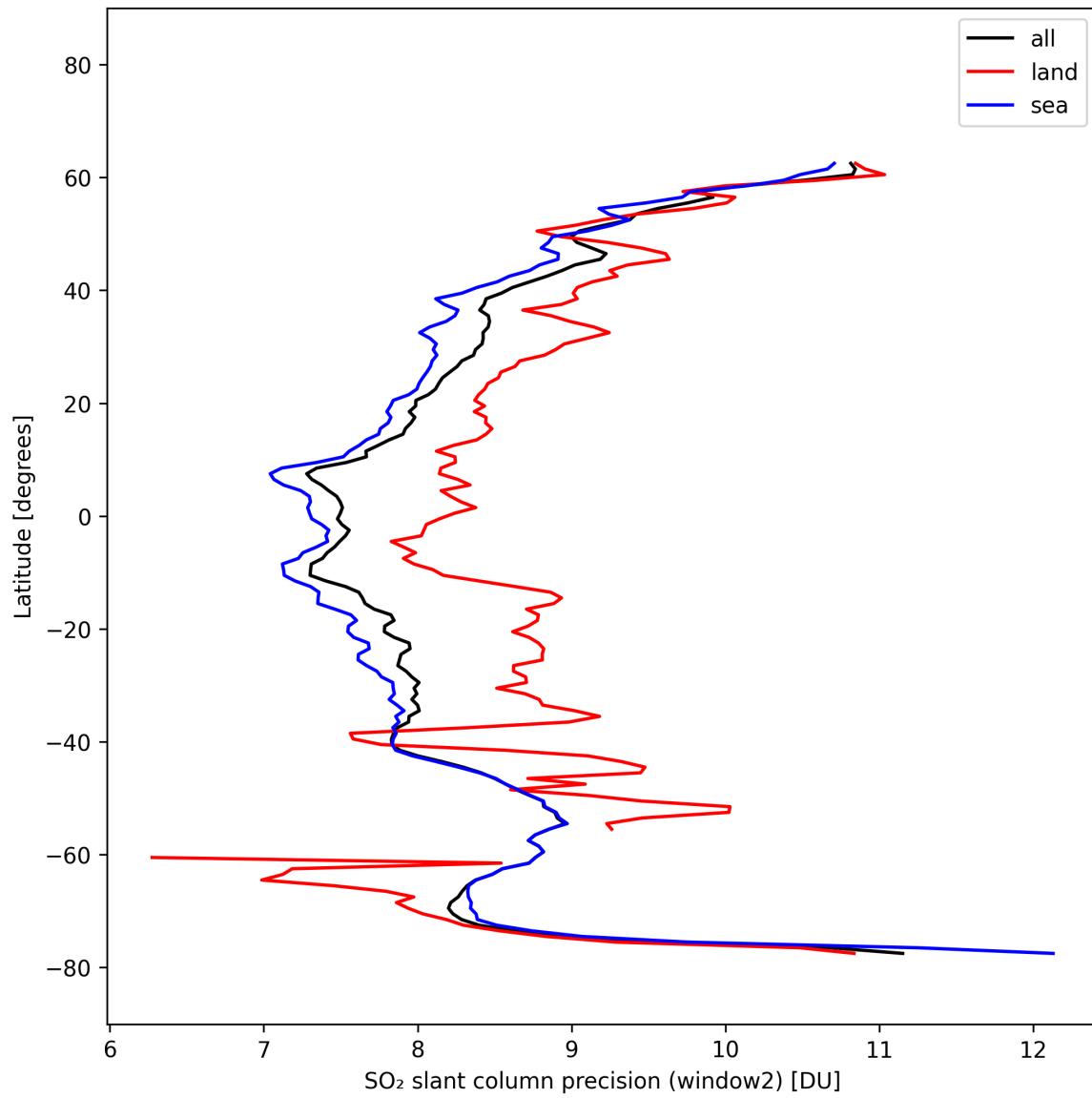
Figure 42: Zonal average of “SO 2 slant column precision (window2)” for 2025-10-11 to 2025-10-12.
