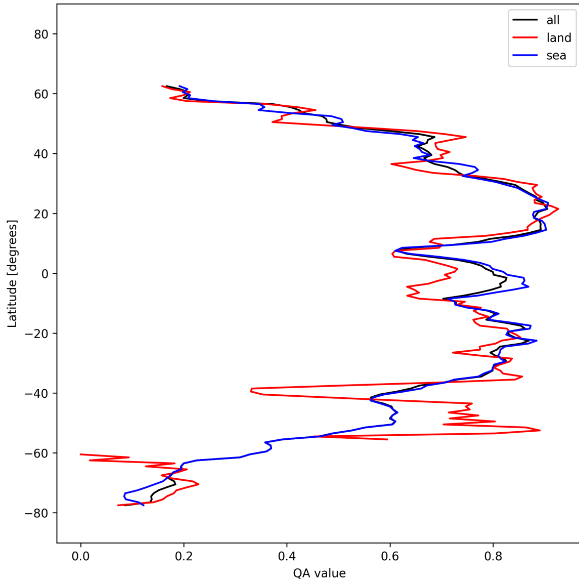
Figure 31: Zonal average of “QA value” for 2025-10-11 to 2025-10-12.
