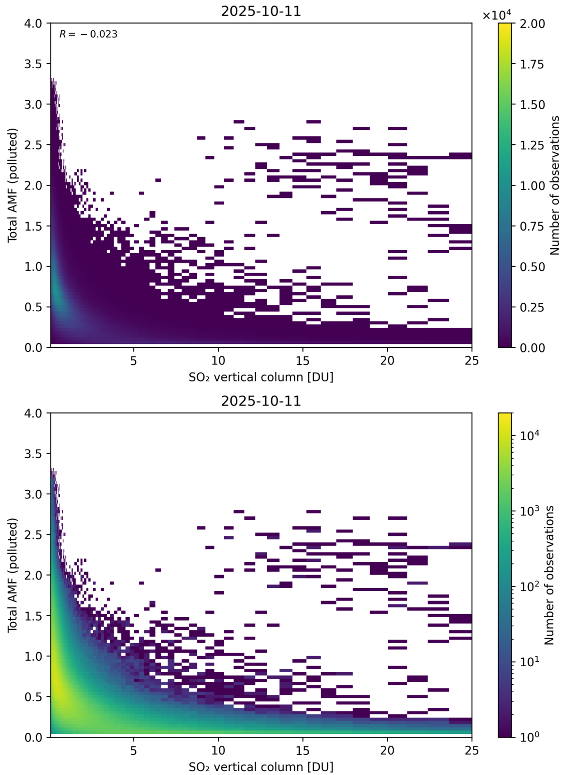
Figure 359: Scatter density plot of “SO 2 vertical column” against “Total AMF (polluted)” for 2025-10-11 to 2025-10-12.
