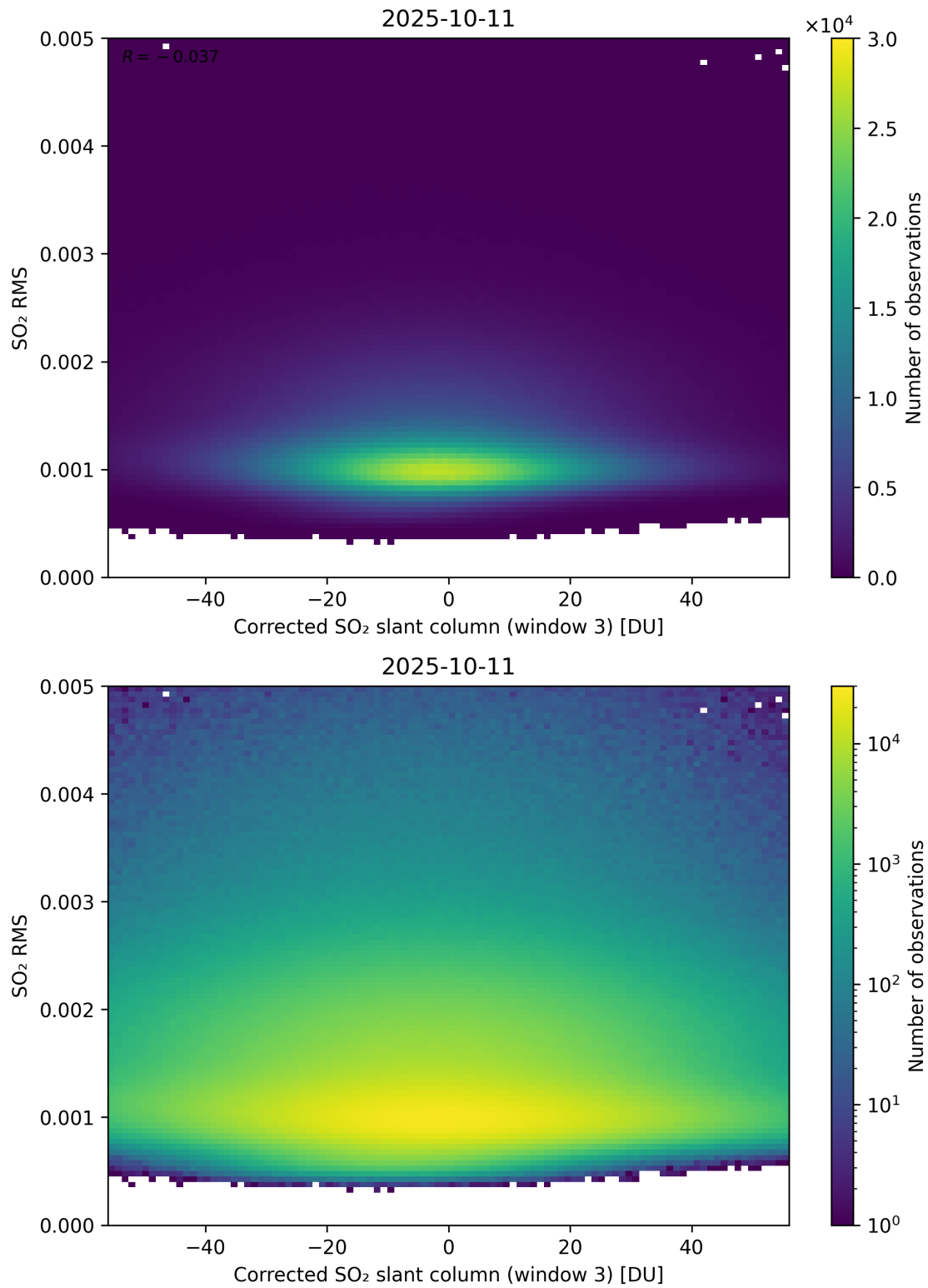
Figure 258: Scatter density plot of “Corrected SO 2 slant column (window 3)” against “SO 2 RMS” for 2025-10-11 to 2025-10-12.
