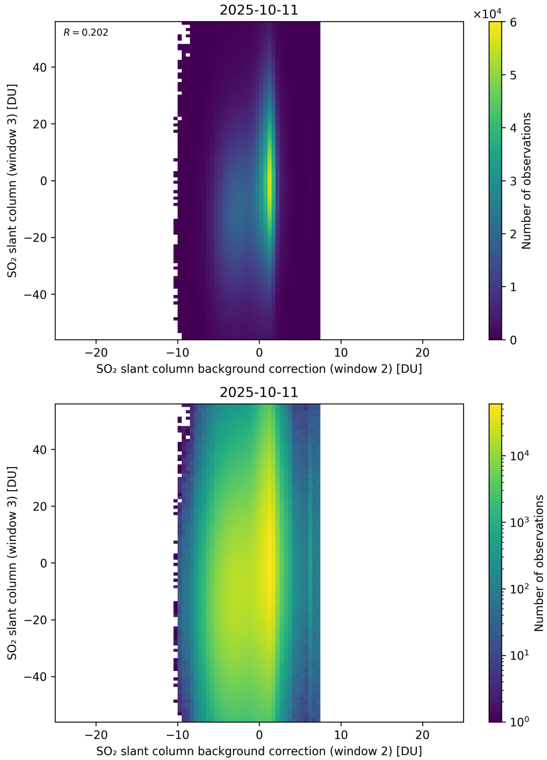
Figure 128: Scatter density plot of “SO 2 slant column background correction (window 2)” against “SO 2 slant column (window 3)” for 2025-10-11 to 2025-10-12.
