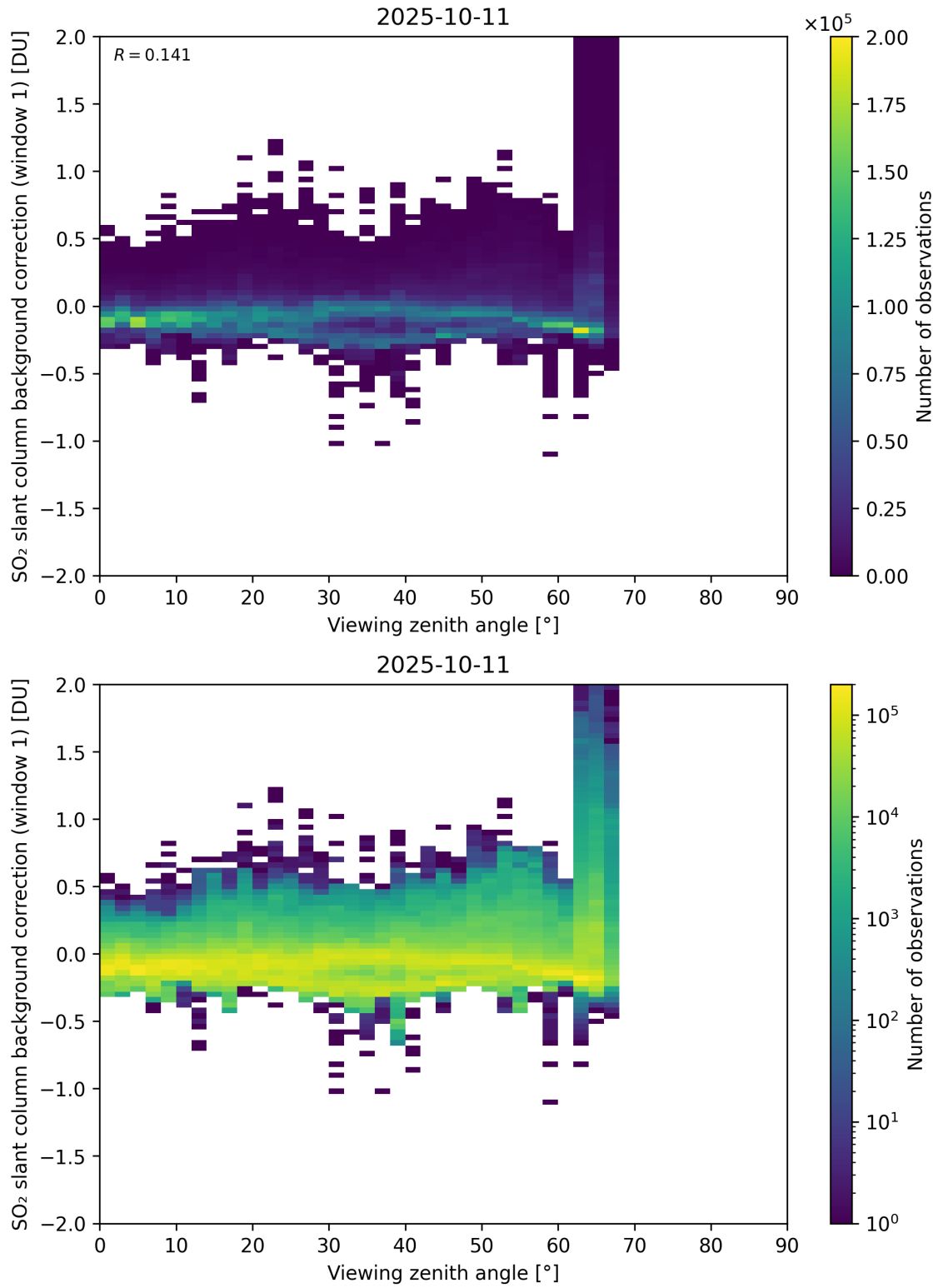
Figure 362: Scatter density plot of “Viewing zenith angle” against “SO 2 slant column background correction (window 1)” for 2025-10-11 to 2025-10-12.
