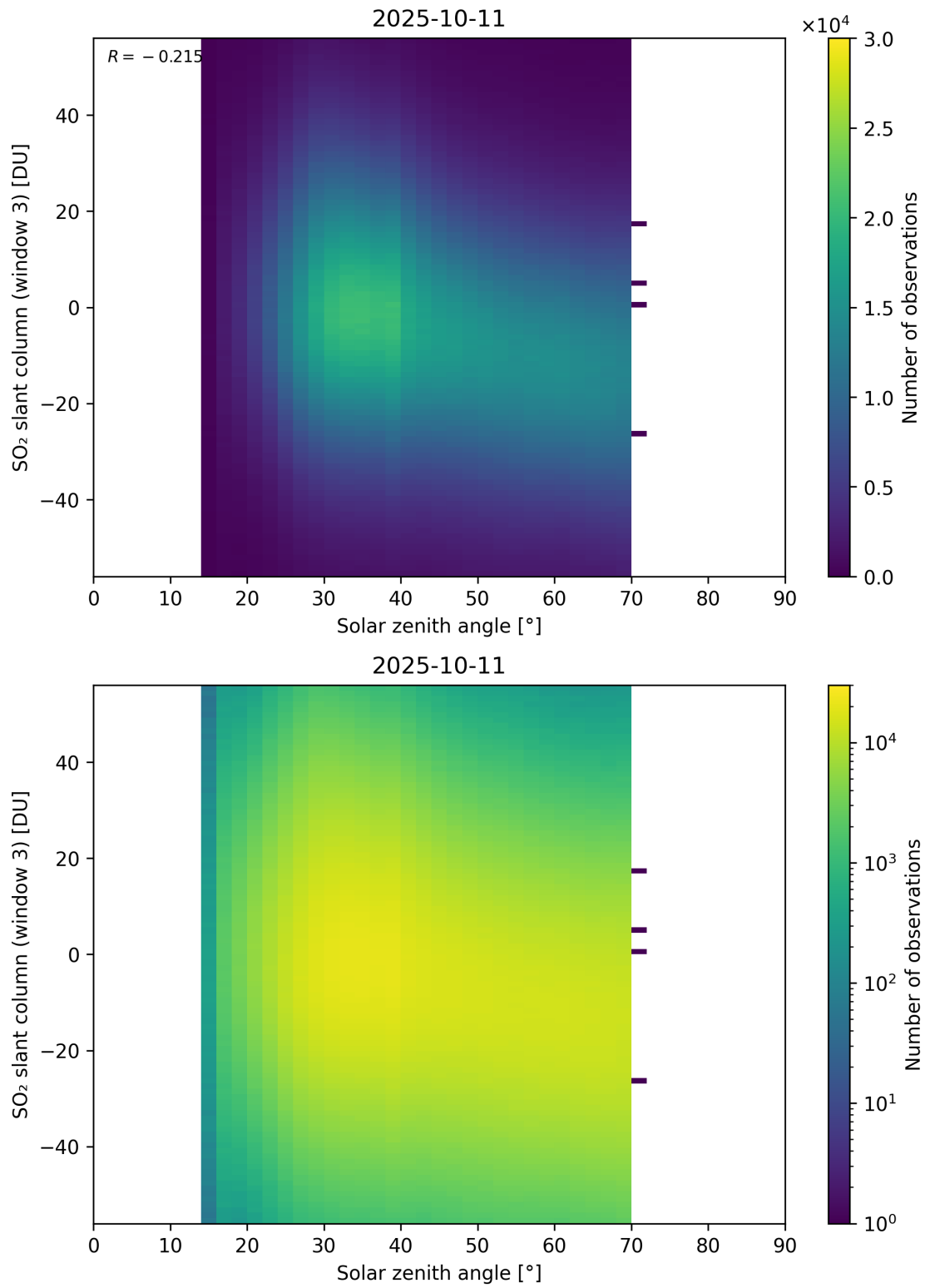
Figure 187: Scatter density plot of “Solar zenith angle” against “SO 2 slant column (window 3)” for 2025-10-11 to 2025-10-12.
