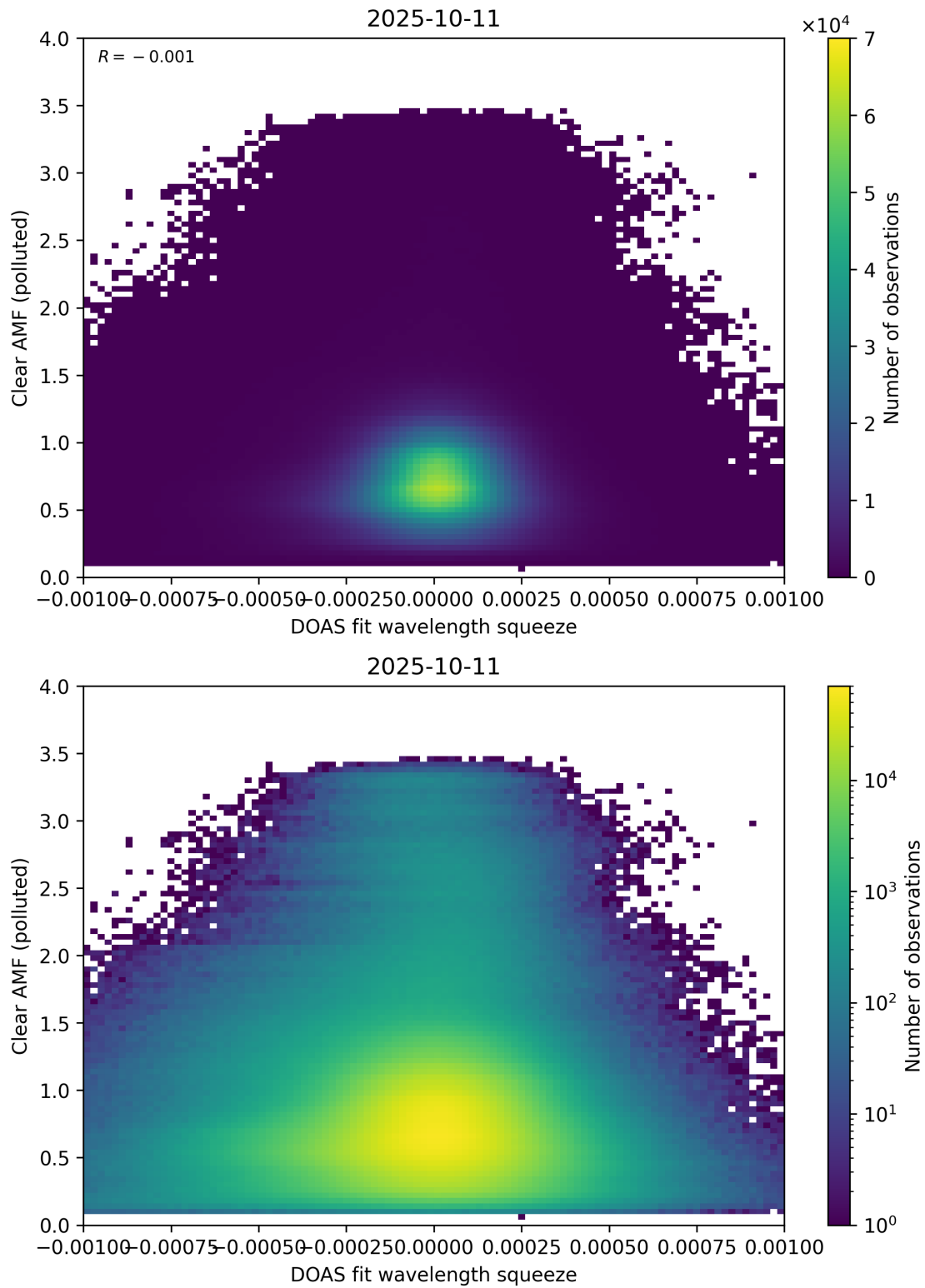
Figure 144: Scatter density plot of “DOAS fit wavelength squeeze” against “Clear AMF (polluted)” for 2025-10-11 to 2025-10-12.
