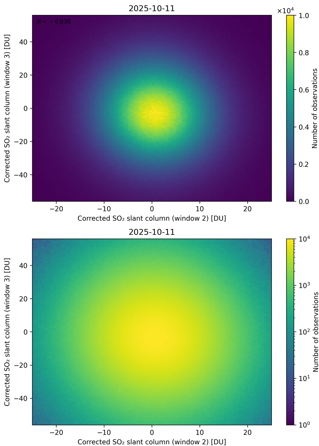
Figure 250: Scatter density plot of “Corrected SO 2 slant column (window 2)” against “Corrected SO 2 slant column (window 3)” for 2025-10-11 to 2025-10-12.
