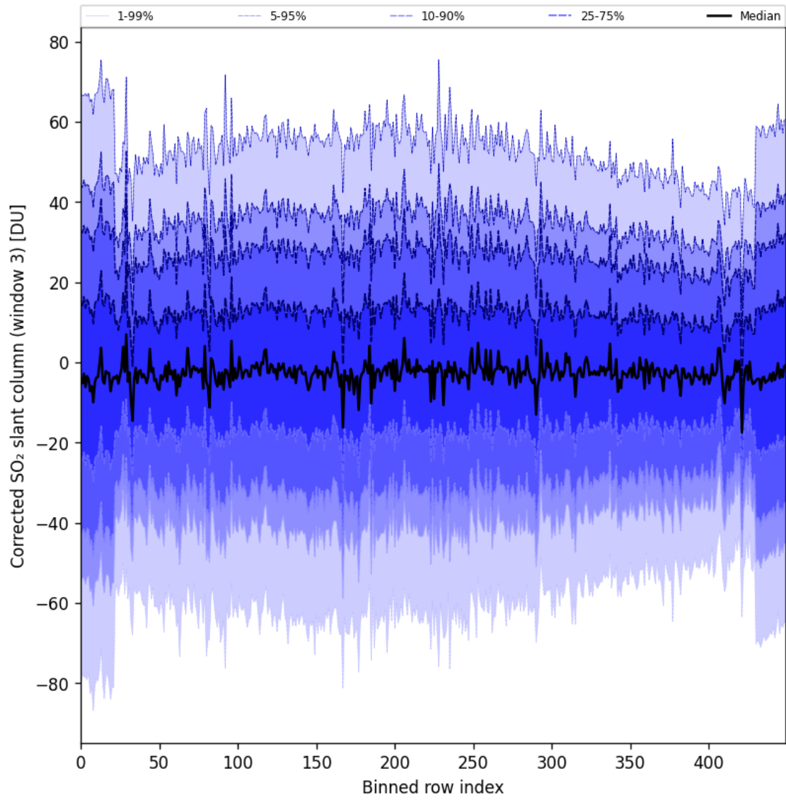
Figure 99: Along track statistics of “Corrected SO 2 slant column (window 3)” for 2025-10-11 to 2025-10-12
