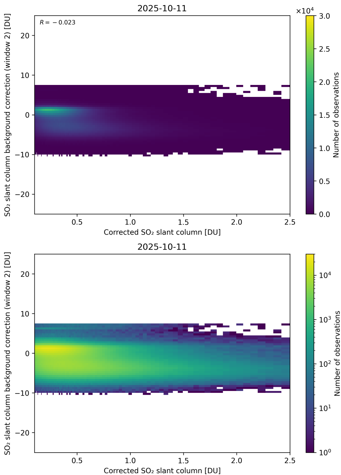
Figure 227: Scatter density plot of “Corrected SO 2 slant column” against “SO 2 slant column background correction (window 2)” for 2025-10-11 to 2025-10-12.
