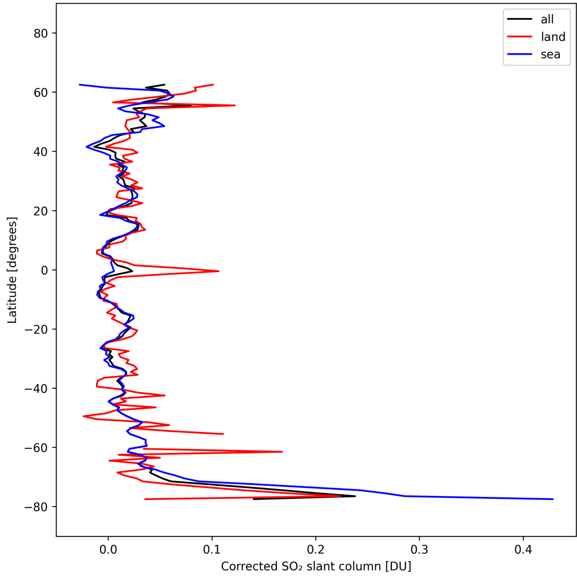
Figure 34: Zonal average of “Corrected SO 2 slant column” for 2025-10-11 to 2025-10-12.
