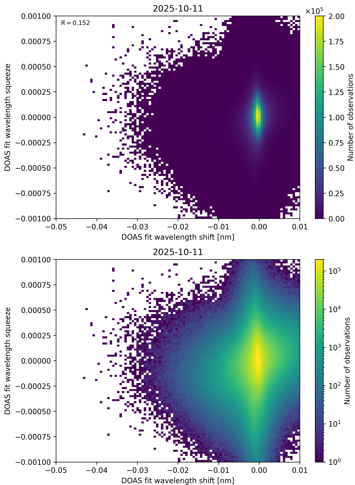
Figure 138: Scatter density plot of “DOAS fit wavelength shift” against “DOAS fit wavelength squeeze” for 2025-10-11 to 2025-10-12.
