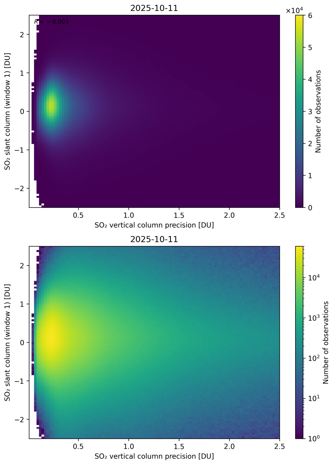
Figure 341: Scatter density plot of “SO 2 vertical column precision” against “SO 2 slant column (window 1)” for 2025-10-11 to 2025-10-12.
