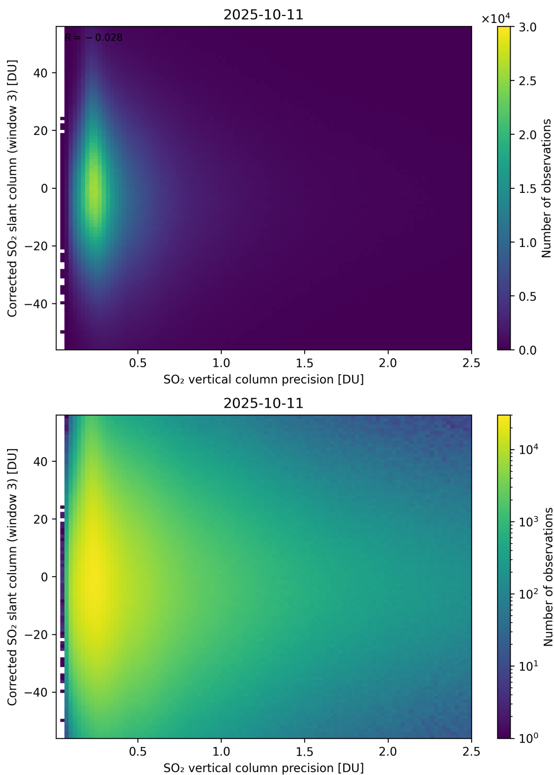
Figure 340: Scatter density plot of “SO 2 vertical column precision” against “Corrected SO 2 slant column (window 3)” for 2025-10-11 to 2025-10-12.
