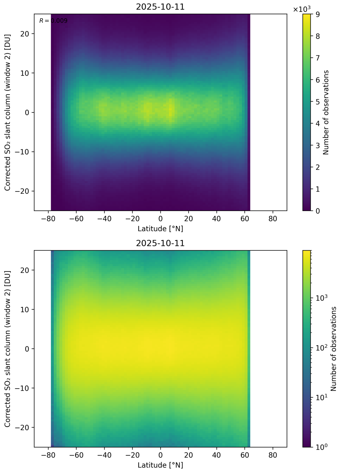
Figure 160: Scatter density plot of “Latitude” against “Corrected SO 2 slant column (window 2)” for 2025-10-11 to 2025-10-12.
