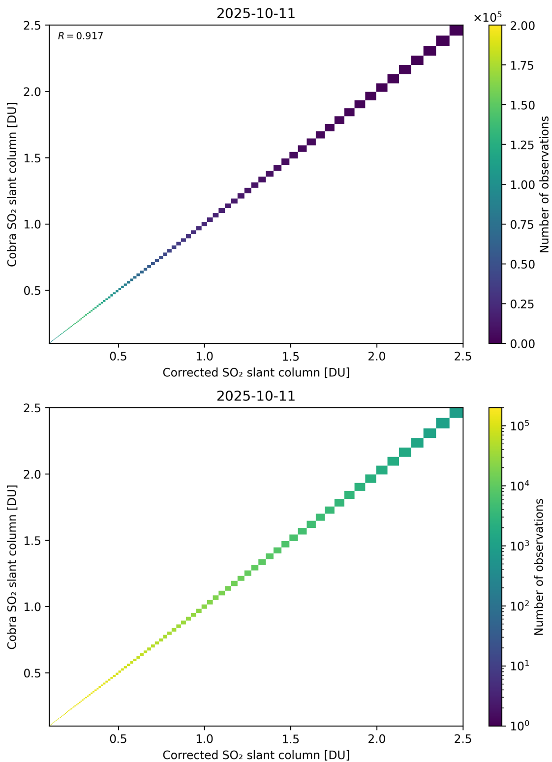
Figure 233: Scatter density plot of “Corrected SO 2 slant column” against “Cobra SO 2 slant column” for 2025-10-11 to 2025-10-12.
