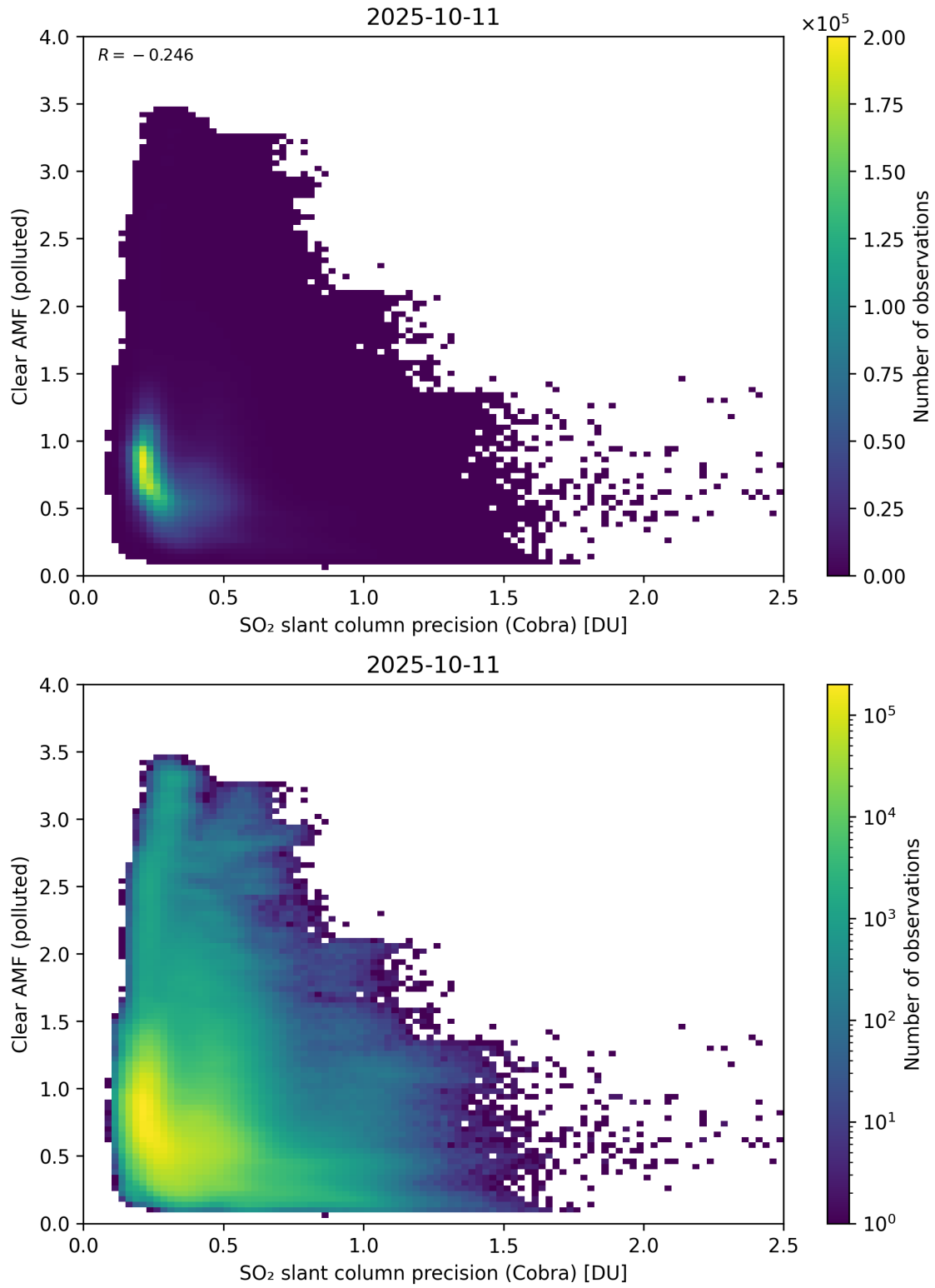
Figure 205: Scatter density plot of “SO 2 slant column precision (Cobra)” against “Clear AMF (polluted)” for 2025-10-11 to 2025-10-12.
