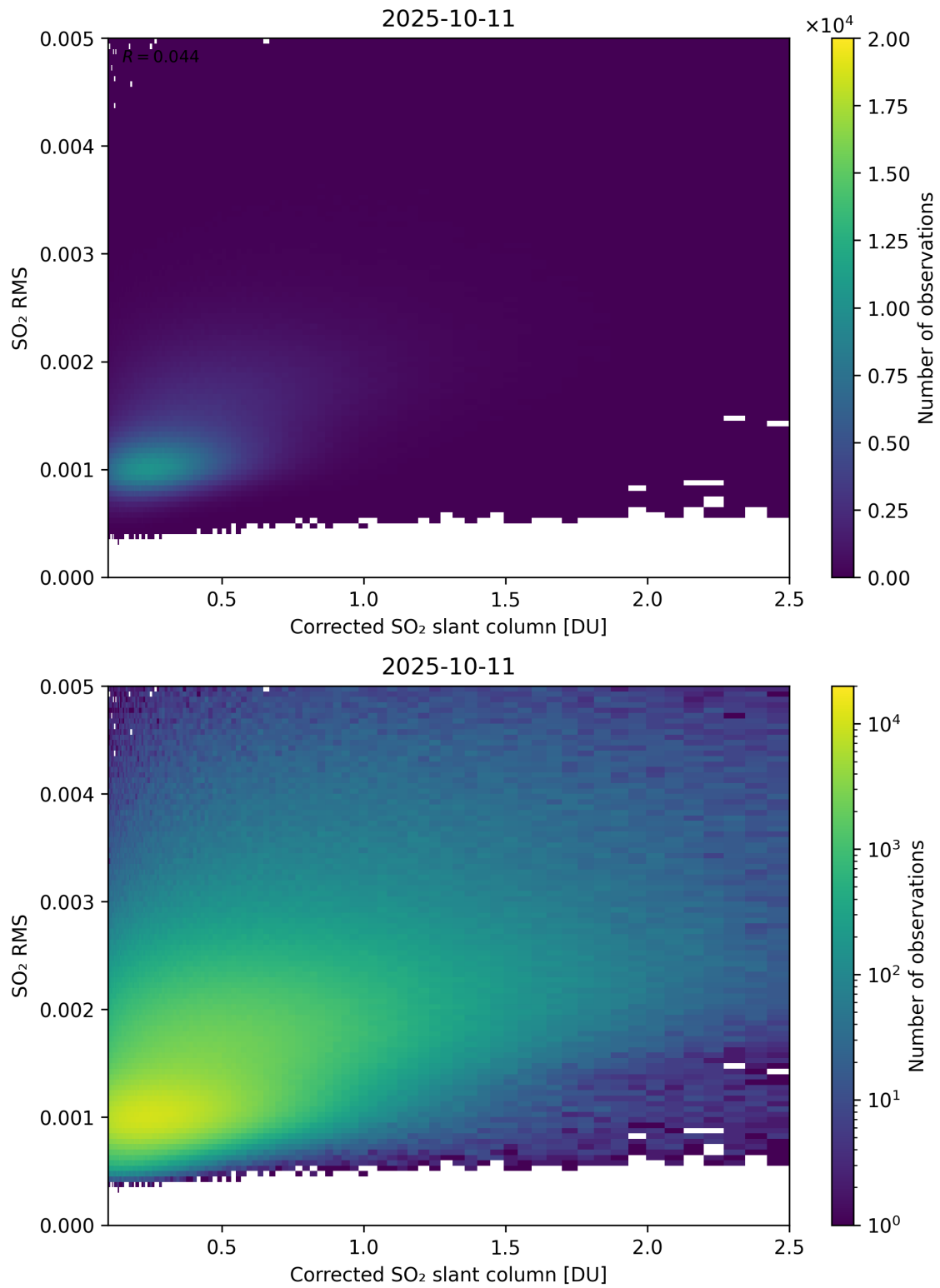
Figure 231: Scatter density plot of “Corrected SO 2 slant column” against “SO 2 RMS” for 2025-10-11 to 2025-10-12.
