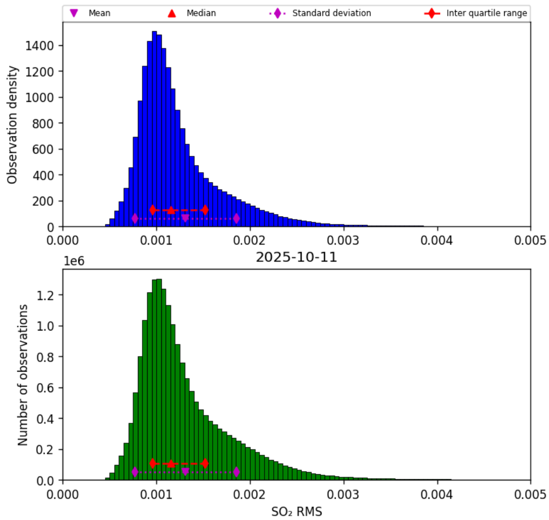
Figure 78: Histogram of “SO 2 RMS” for 2025-10-11 to 2025-10-12
