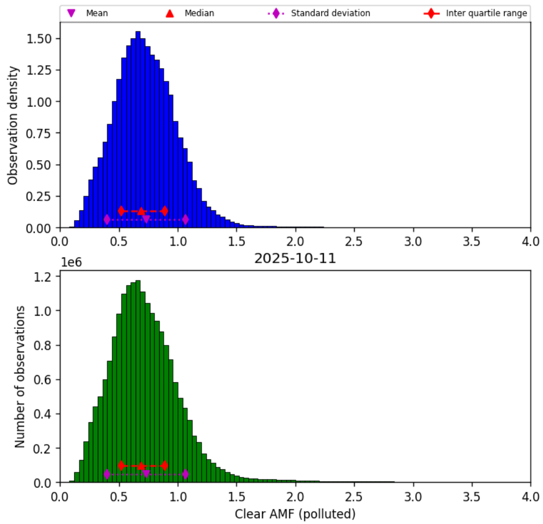
Figure 81: Histogram of “Clear AMF (polluted)” for 2025-10-11 to 2025-10-12
