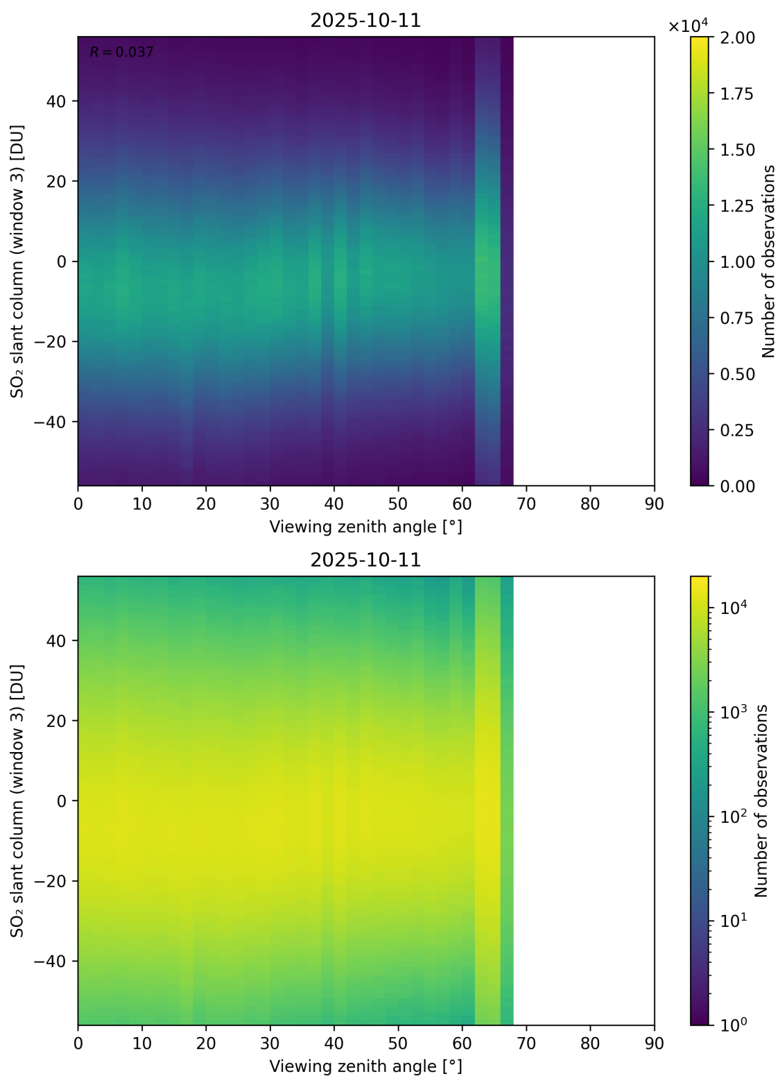
Figure 379: Scatter density plot of “Viewing zenith angle” against “SO 2 slant column (window 3)” for 2025-10-11 to 2025-10-12.
