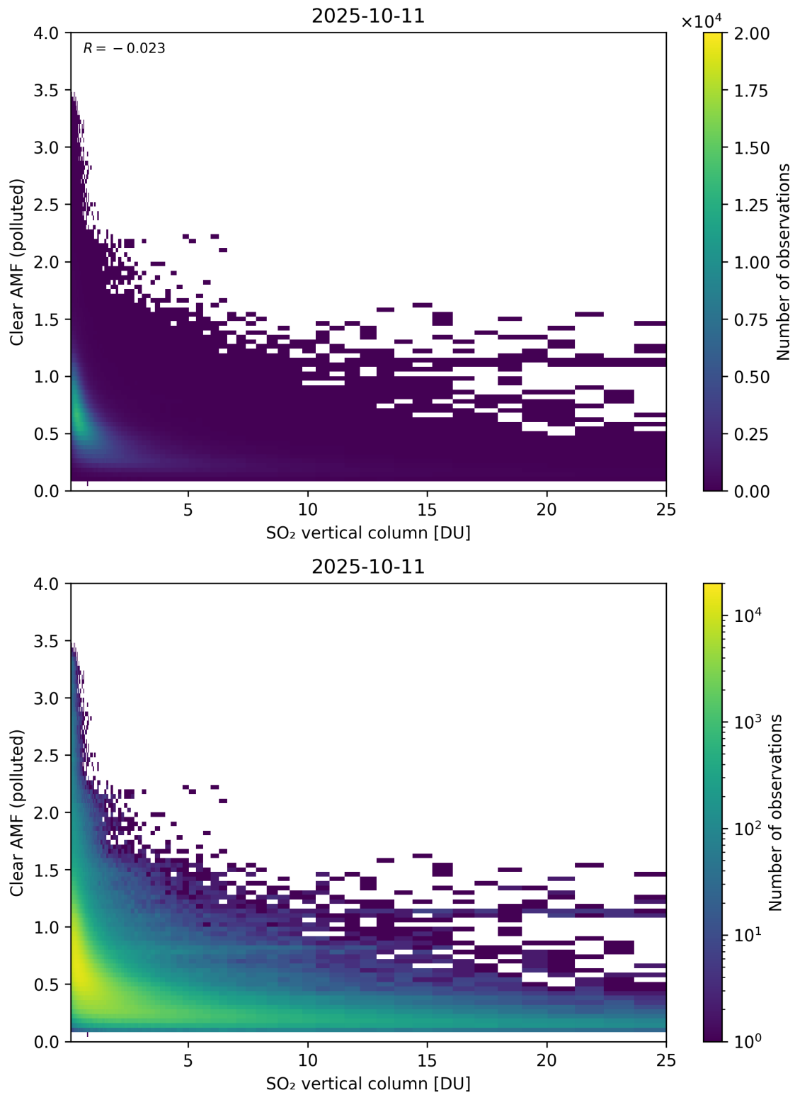
Figure 348: Scatter density plot of “SO 2 vertical column” against “Clear AMF (polluted)” for 2025-10-11 to 2025-10-12.
