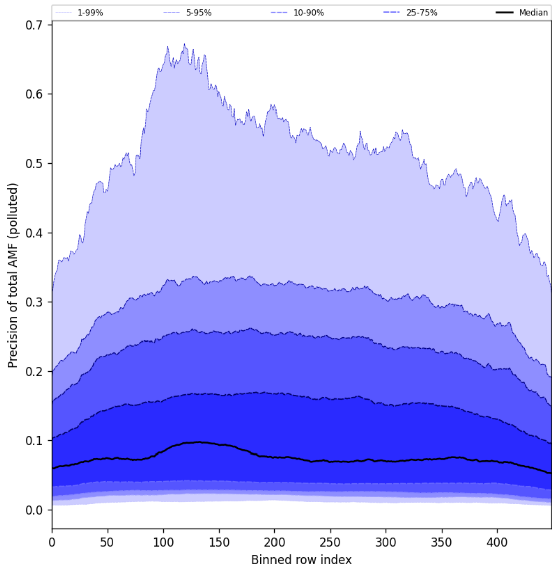
Figure 106: Along track statistics of “Precision of total AMF (polluted)” for 2025-10-11 to 2025-10-12
