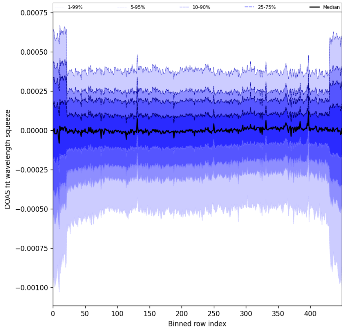
Figure 103: Along track statistics of “DOAS fit wavelength squeeze” for 2025-10-11 to 2025-10-12
