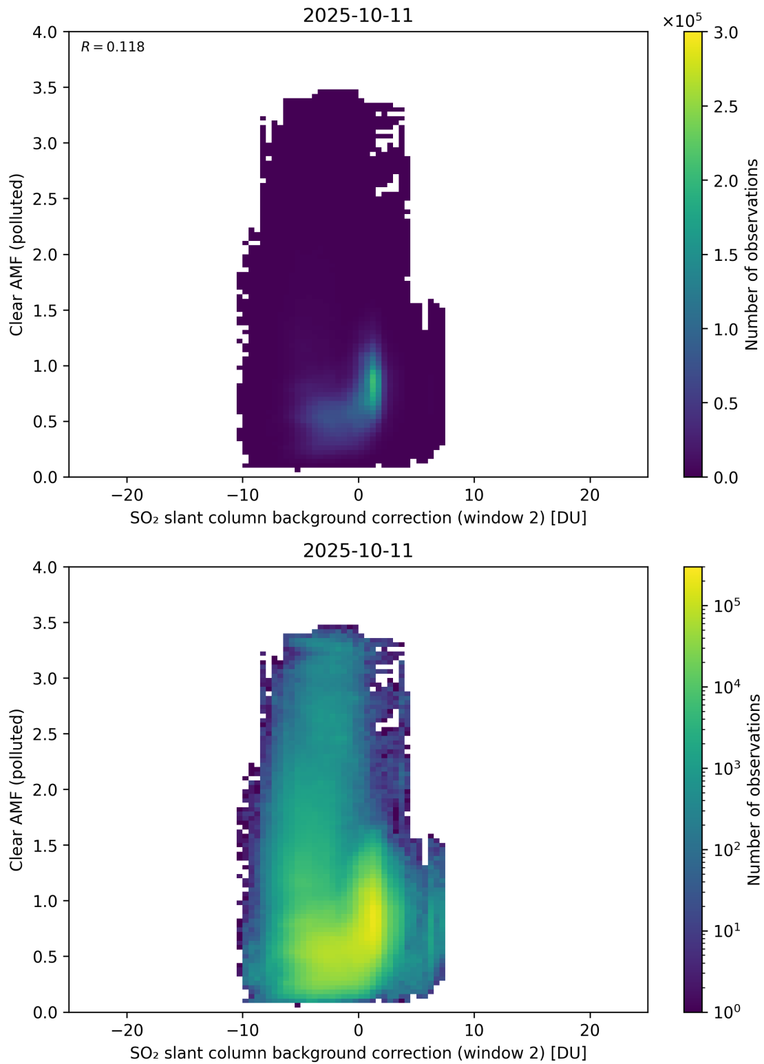
Figure 126: Scatter density plot of “SO 2 slant column background correction (window 2)” against “Clear AMF (polluted)” for 2025-10-11 to 2025-10-12.
