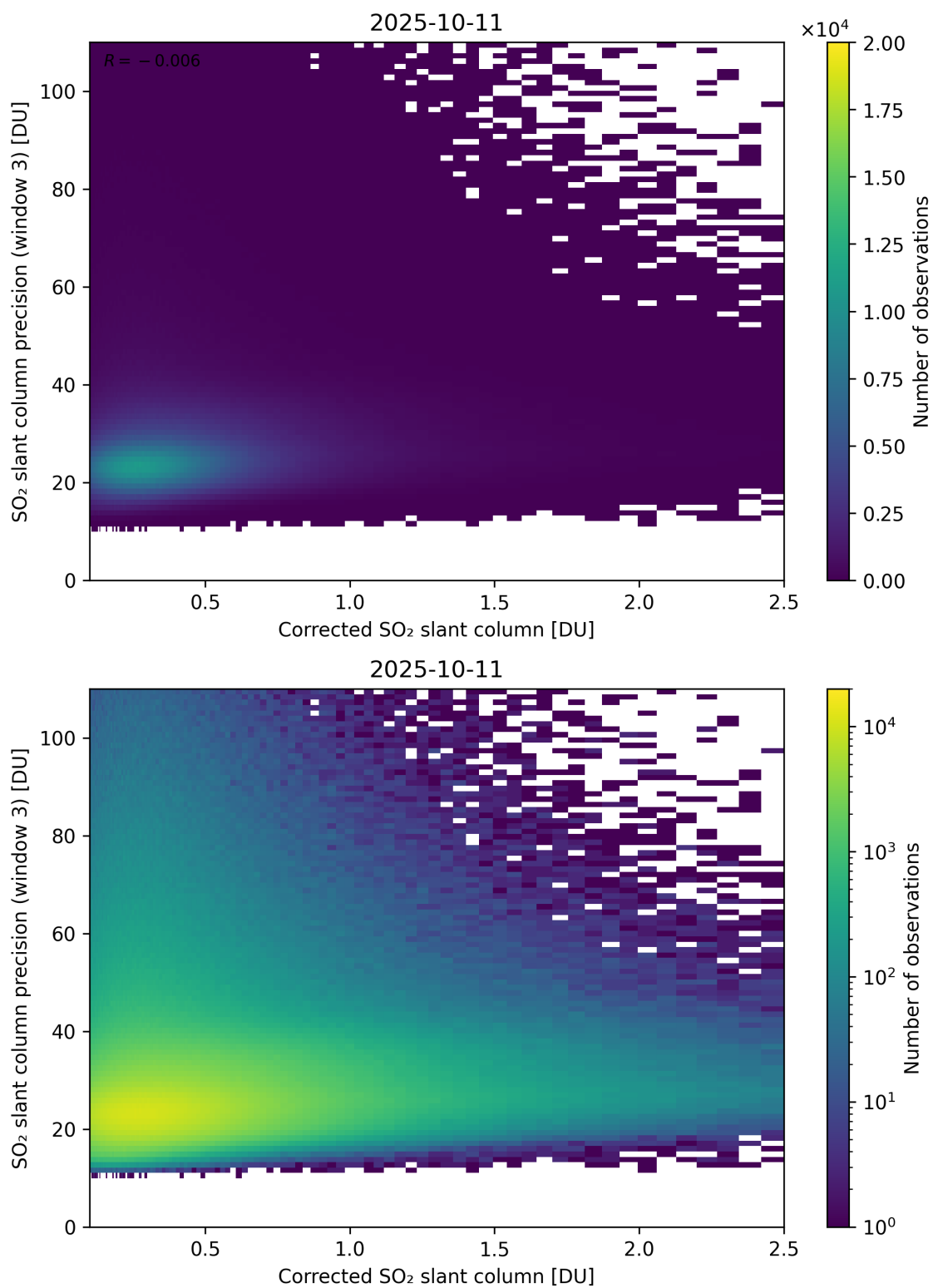
Figure 241: Scatter density plot of “Corrected SO 2 slant column” against “SO 2 slant column precision (window 3)” for 2025-10-11 to 2025-10-12.
