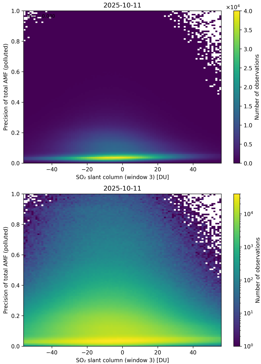
Figure 319: Scatter density plot of “SO 2 slant column (window 3)” against “Precision of total AMF (polluted)” for 2025-10-11 to 2025-10-12.
