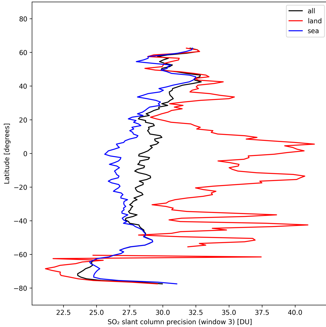
Figure 46: Zonal average of “SO 2 slant column precision (window 3)” for 2025-10-11 to 2025-10-12.
