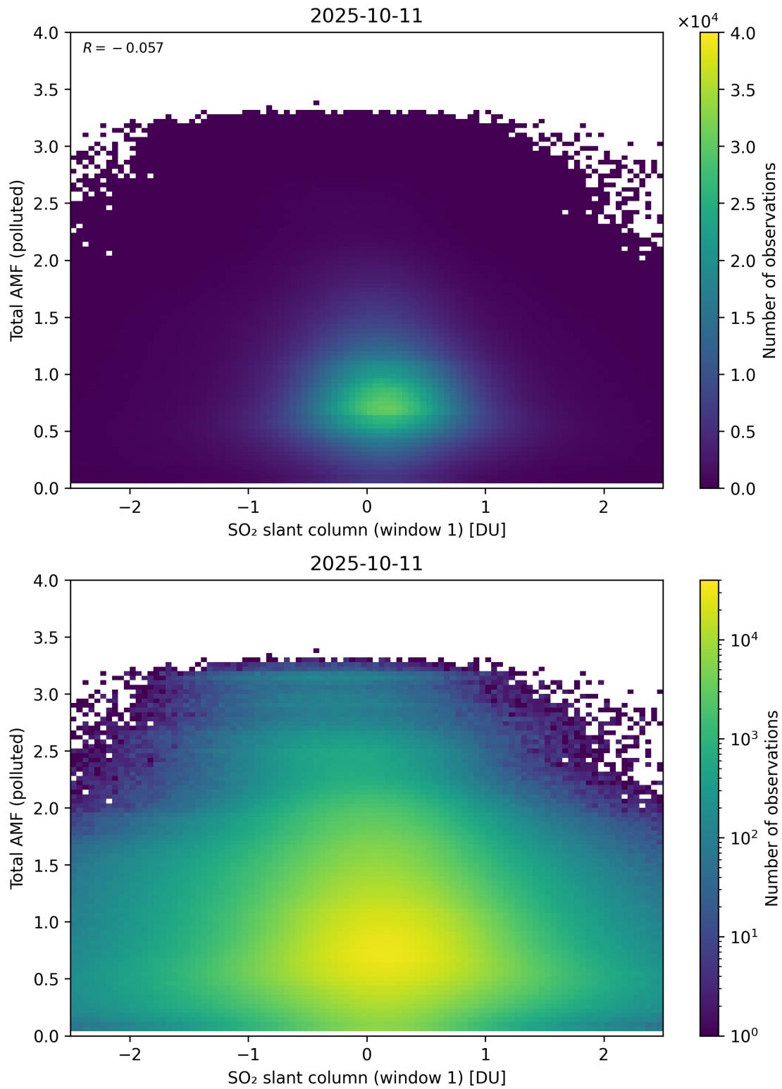
Figure 289: Scatter density plot of “SO 2 slant column (window 1)” against “Total AMF (polluted)” for 2025-10-11 to 2025-10-12.
