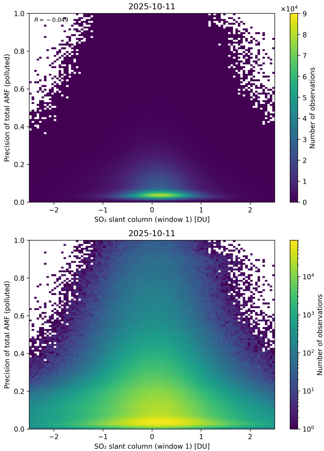
Figure 290: Scatter density plot of “SO 2 slant column (window 1)” against “Precision of total AMF (polluted)” for 2025-10-11 to 2025-10-12.
