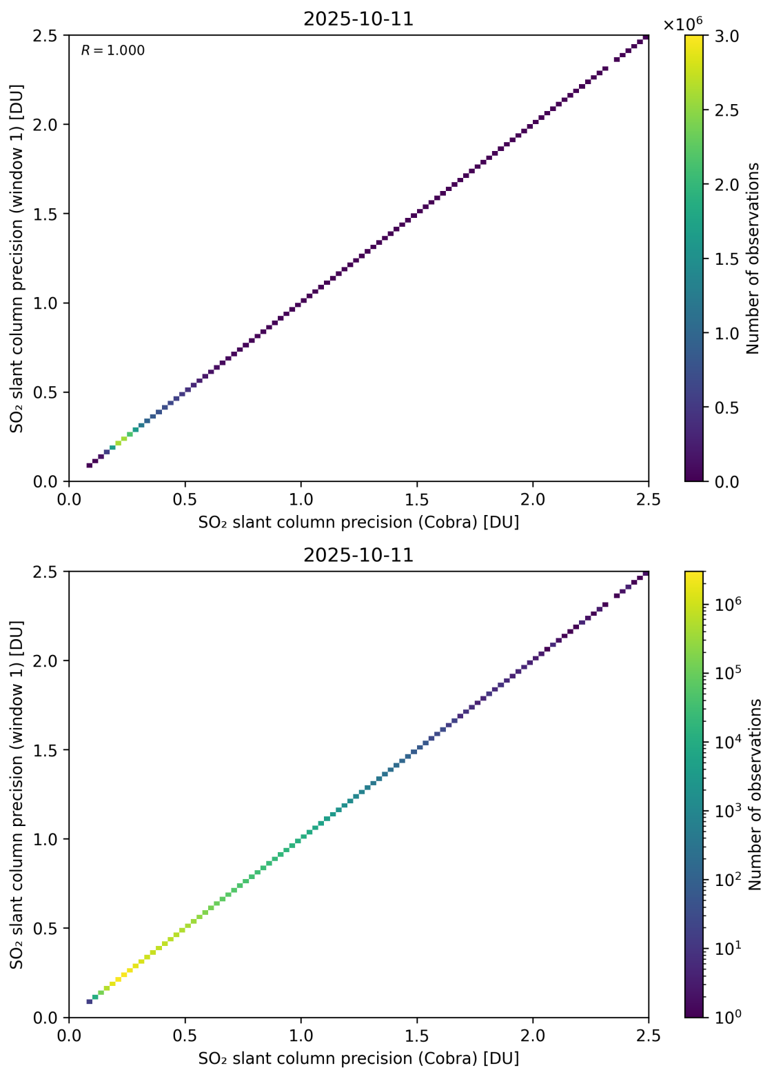
Figure 209: Scatter density plot of “SO 2 slant column precision (Cobra)” against “SO 2 slant column precision (window 1)” for 2025-10-11 to 2025-10-12.
