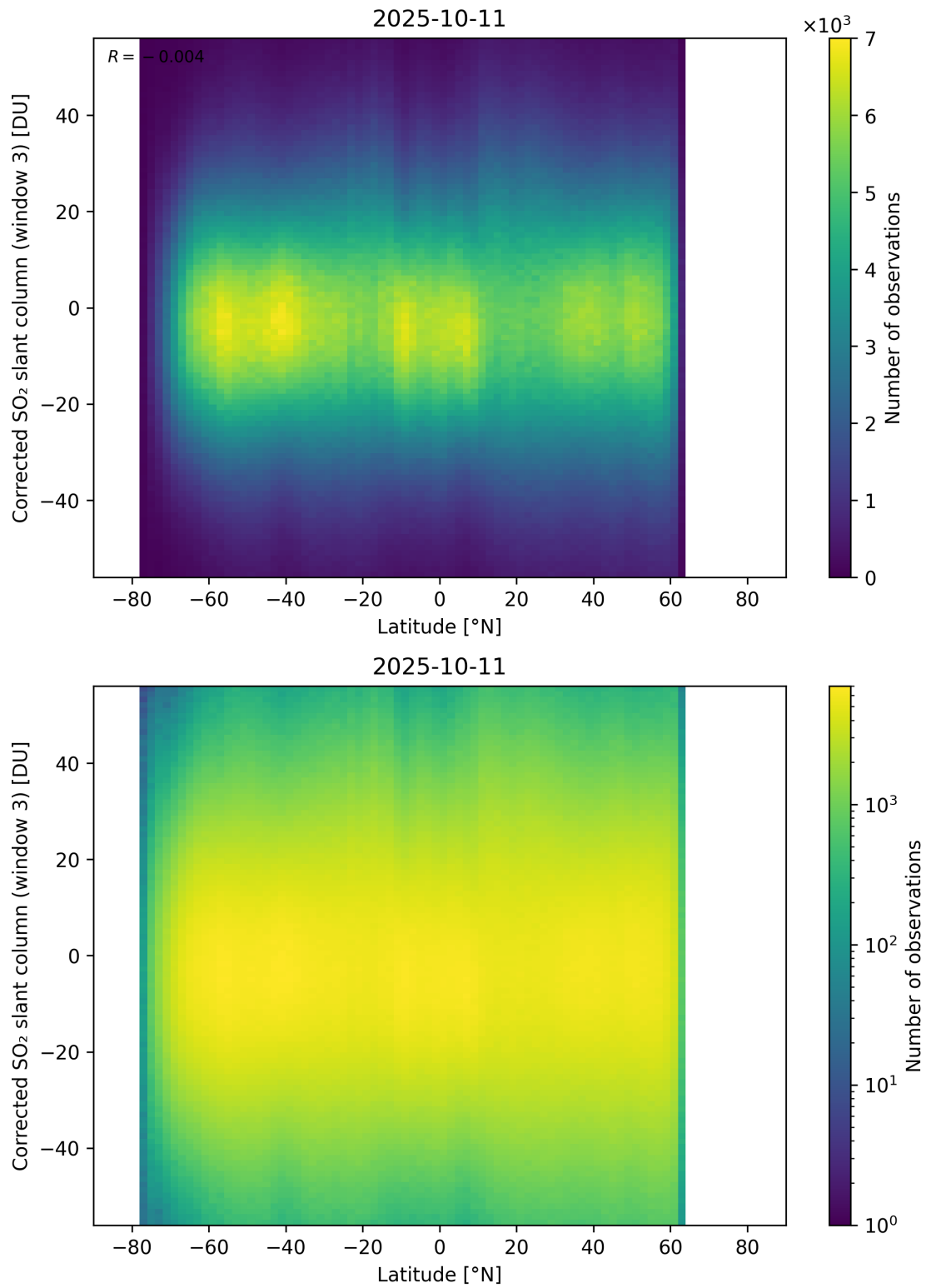
Figure 161: Scatter density plot of “Latitude” against “Corrected SO 2 slant column (window 3)” for 2025-10-11 to 2025-10-12.
