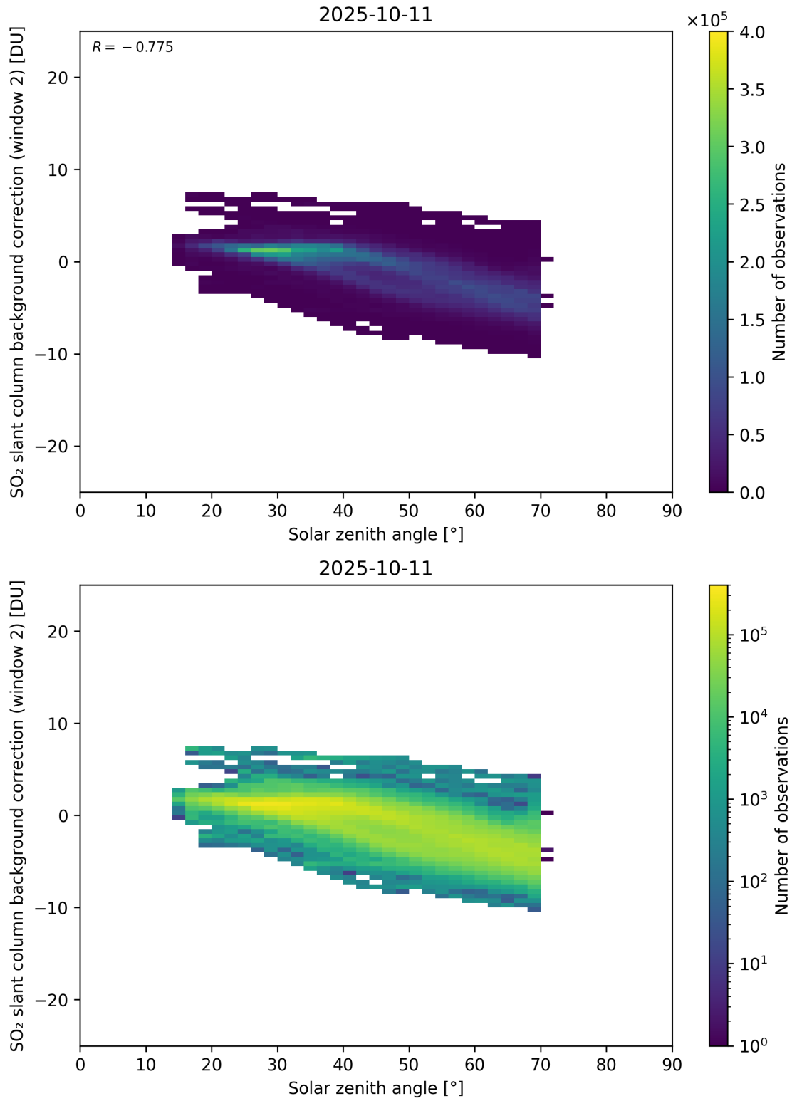
Figure 172: Scatter density plot of “Solar zenith angle” against “SO 2 slant column background correction (window 2)” for 2025-10-11 to 2025-10-12.
