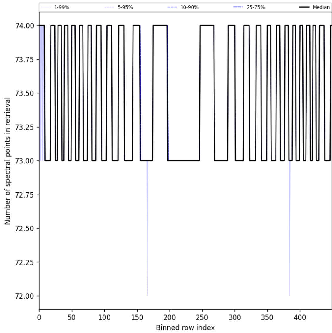
Figure 108: Along track statistics of “Number of spectral points in retrieval” for 2025-10-11 to 2025-10-12
