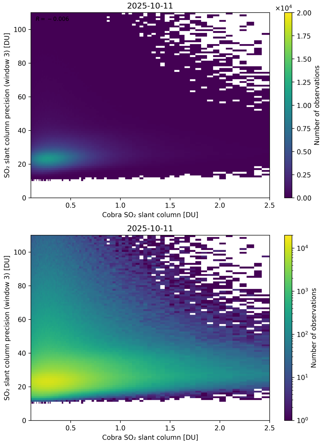
Figure 223: Scatter density plot of “Cobra SO 2 slant column” against “SO 2 slant column precision (window 3)” for 2025-10-11 to 2025-10-12.
