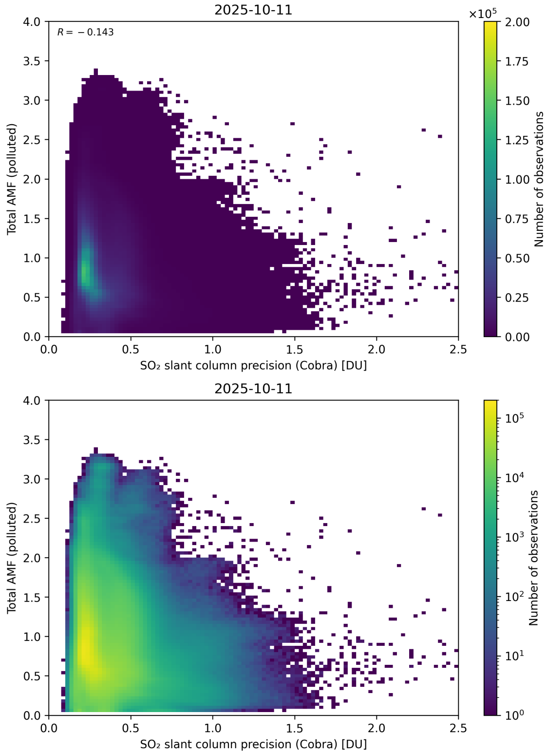
Figure 213: Scatter density plot of “SO 2 slant column precision (Cobra)” against “Total AMF (polluted)” for 2025-10-11 to 2025-10-12.
