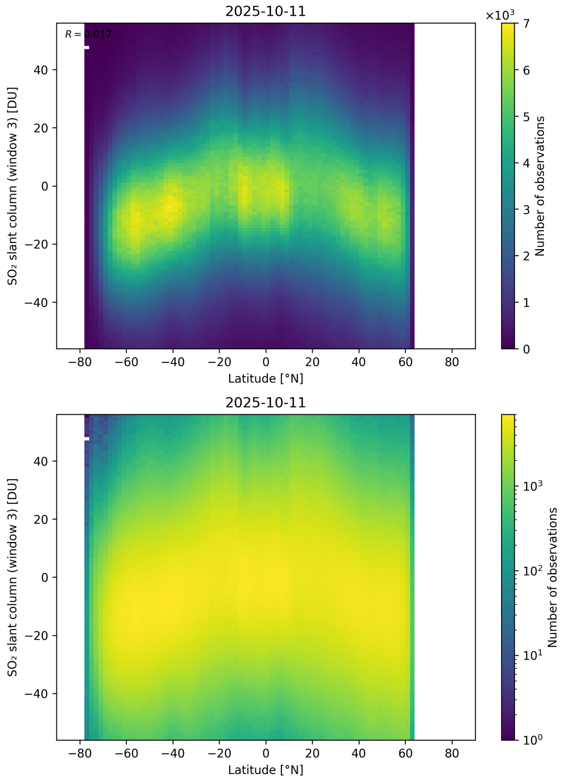
Figure 165: Scatter density plot of “Latitude” against “SO 2 slant column (window 3)” for 2025-10-11 to 2025-10-12.
