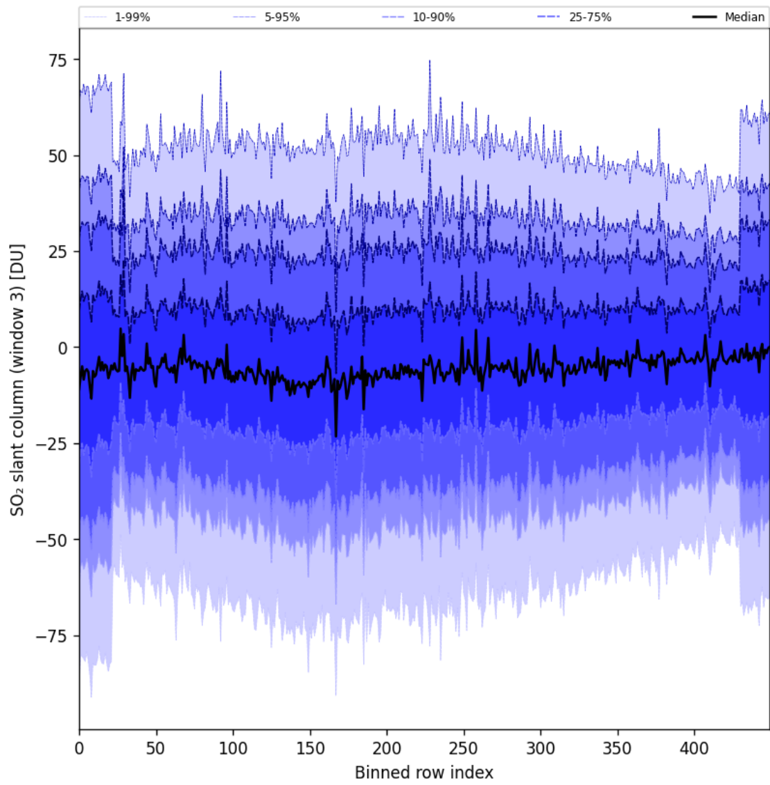
Figure 97: Along track statistics of “SO 2 slant column (window 3)” for 2025-10-11 to 2025-10-12
