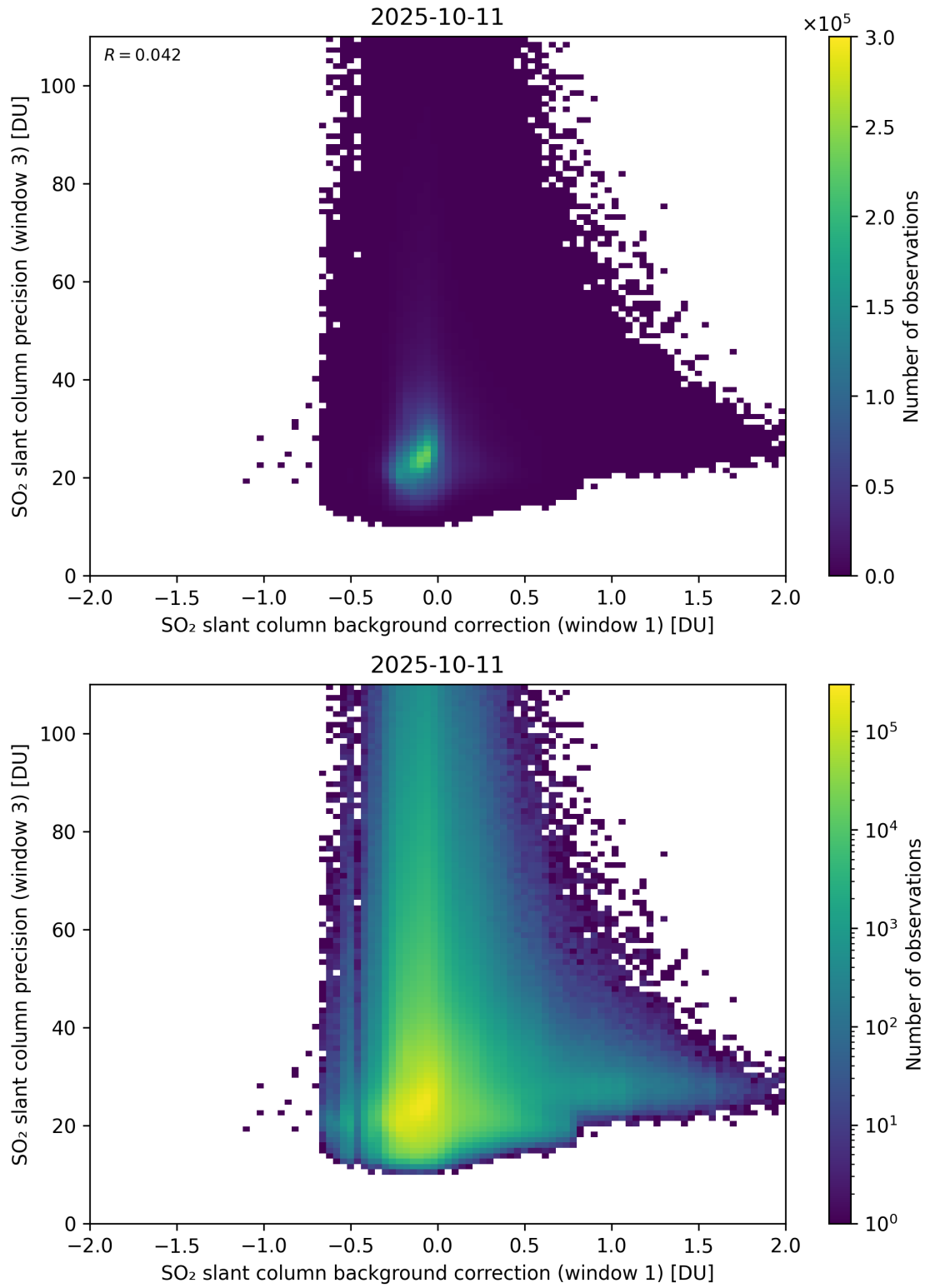
Figure 119: Scatter density plot of “SO 2 slant column background correction (window 1)” against “SO 2 slant column precision (window 3)” for 2025-10-11 to 2025-10-12.
