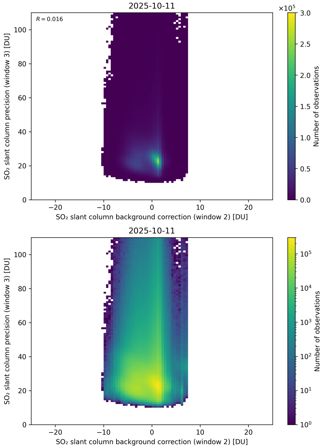
Figure 129: Scatter density plot of “SO 2 slant column background correction (window 2)” against “SO 2 slant column precision (window 3)” for 2025-10-11 to 2025-10-12.
