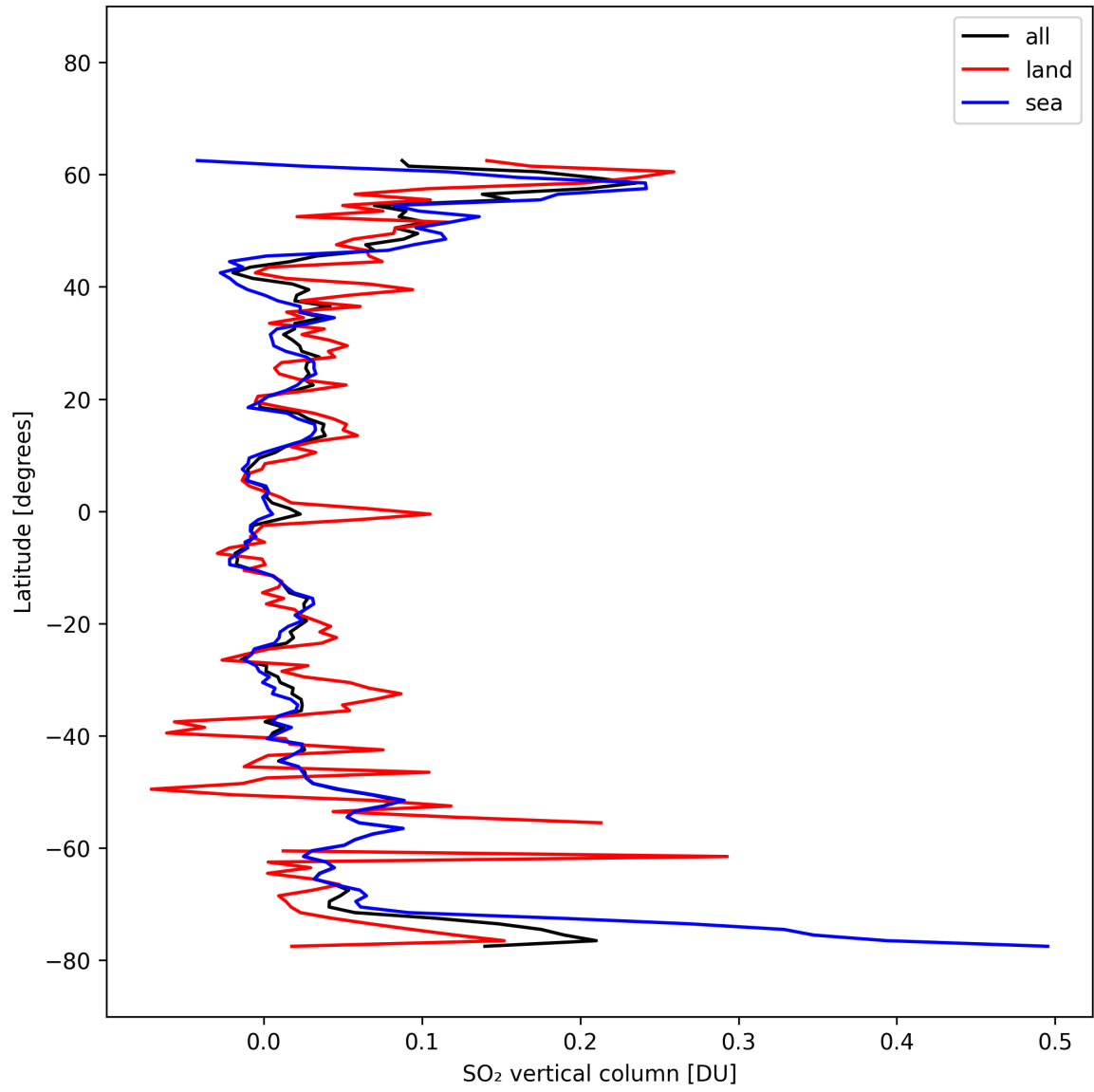
Figure 32: Zonal average of “SO 2 vertical column” for 2025-10-11 to 2025-10-12.
