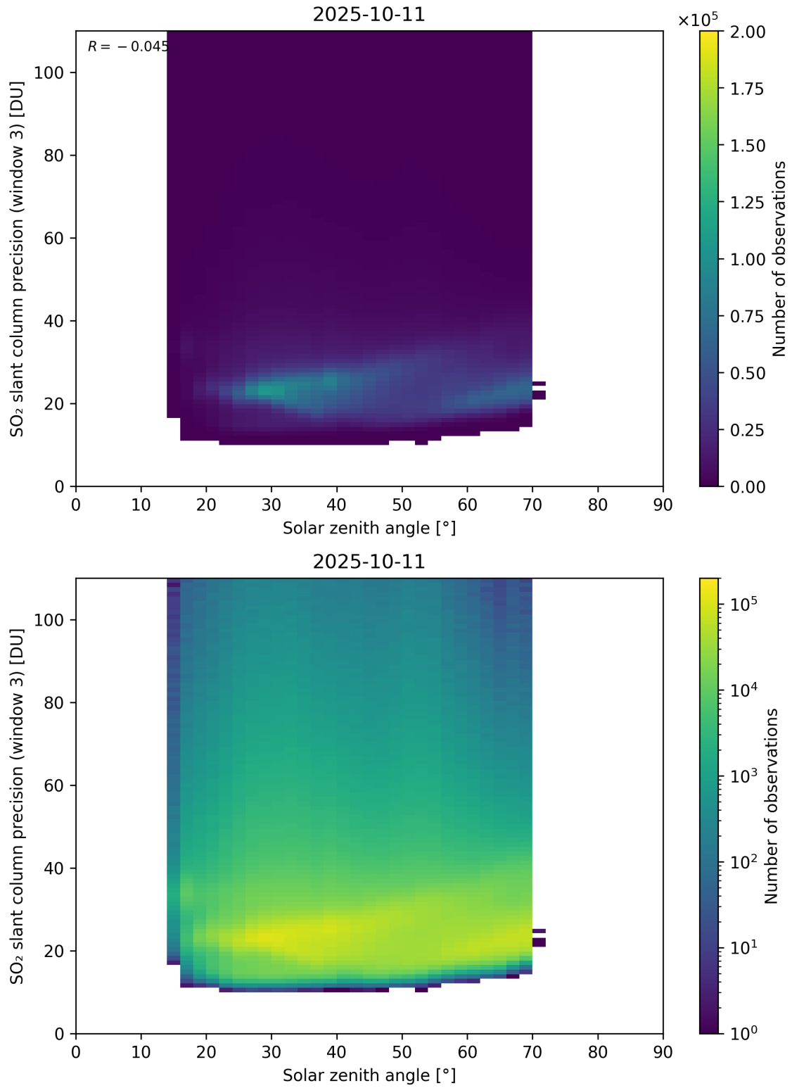
Figure 188: Scatter density plot of “Solar zenith angle” against “SO 2 slant column precision (window 3)” for 2025-10-11 to 2025-10-12.
