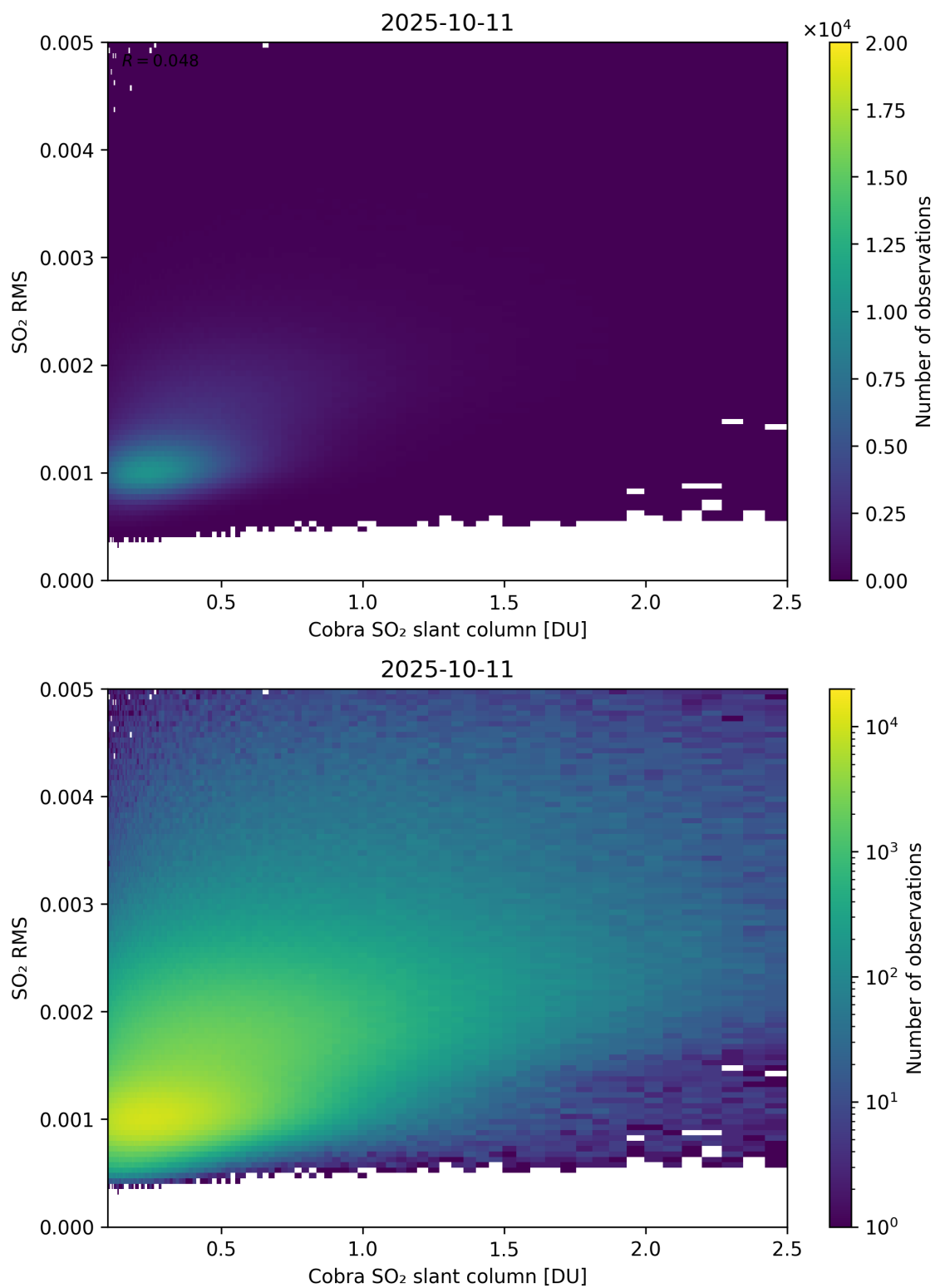
Figure 198: Scatter density plot of “Cobra SO 2 slant column” against “SO 2 RMS” for 2025-10-11 to 2025-10-12.
