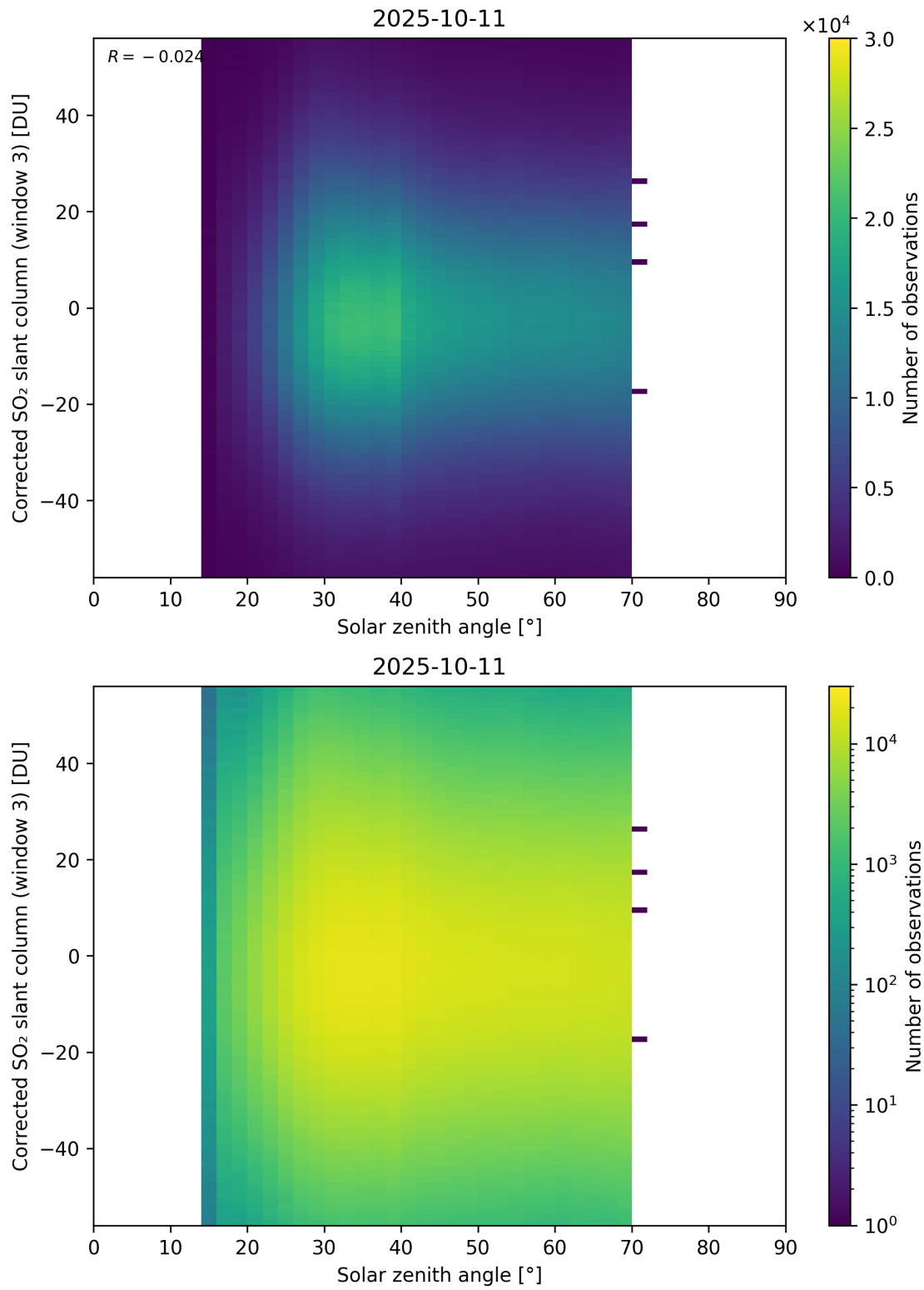
Figure 183: Scatter density plot of “Solar zenith angle” against “Corrected SO 2 slant column (window 3)” for 2025-10-11 to 2025-10-12.
