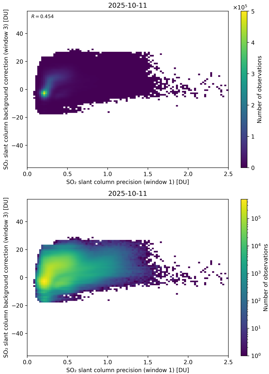
Figure 270: Scatter density plot of “SO 2 slant column precision (window 1)” against “SO 2 slant column background correction (window 3)” for 2025-10-11 to 2025-10-12.
