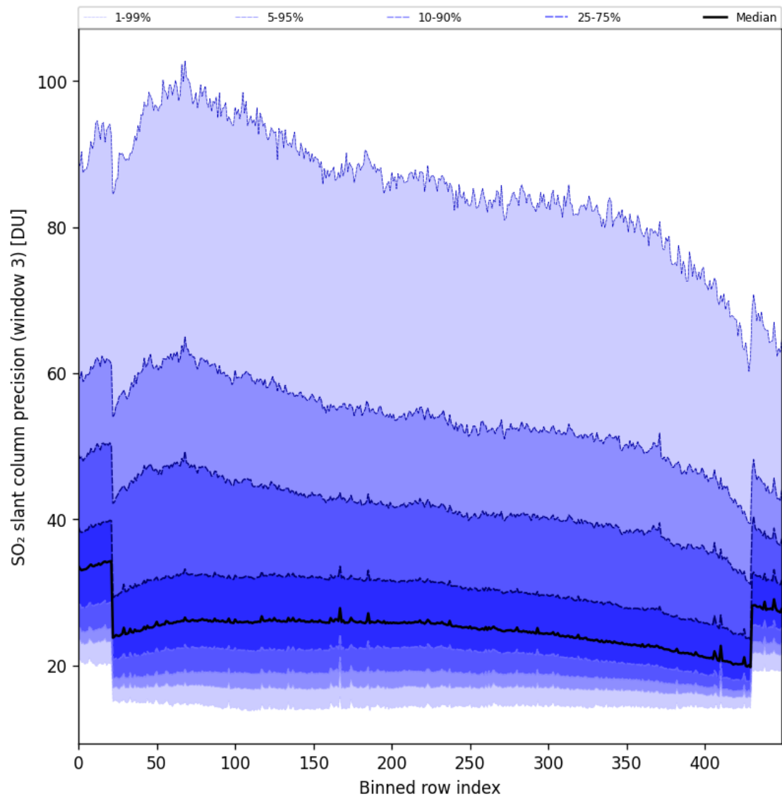
Figure 98: Along track statistics of “SO 2 slant column precision (window 3)” for 2025-10-11 to 2025-10-12
