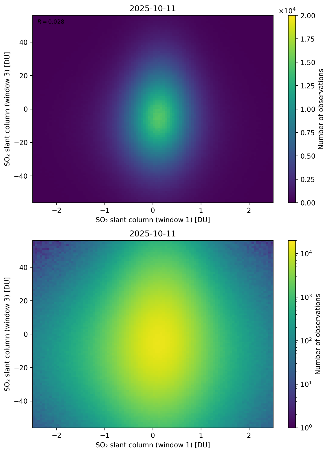
Figure 287: Scatter density plot of “SO 2 slant column (window 1)” against “SO 2 slant column (window 3)” for 2025-10-11 to 2025-10-12.
