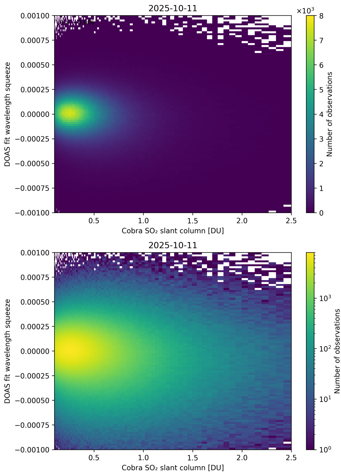
Figure 197: Scatter density plot of “Cobra SO 2 slant column” against “DOAS fit wavelength squeeze” for 2025-10-11 to 2025-10-12.
