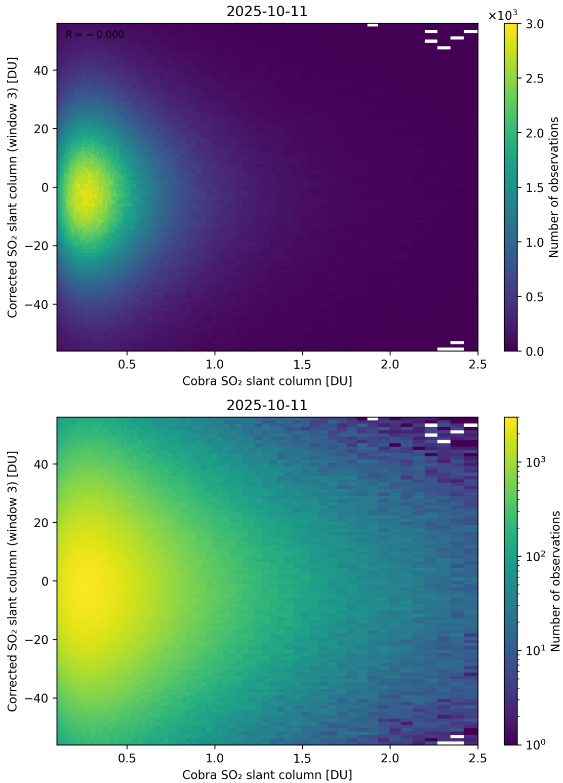
Figure 218: Scatter density plot of “Cobra SO 2 slant column” against “Corrected SO 2 slant column (window 3)” for 2025-10-11 to 2025-10-12.
