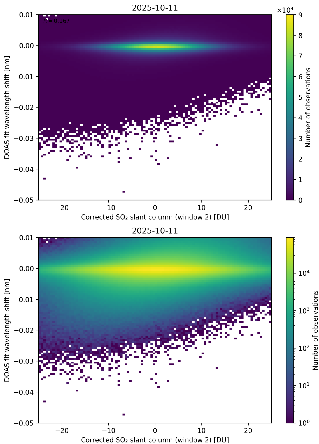
Figure 246: Scatter density plot of “Corrected SO 2 slant column (window 2)” against “DOAS fit wavelength shift” for 2025-10-11 to 2025-10-12.
