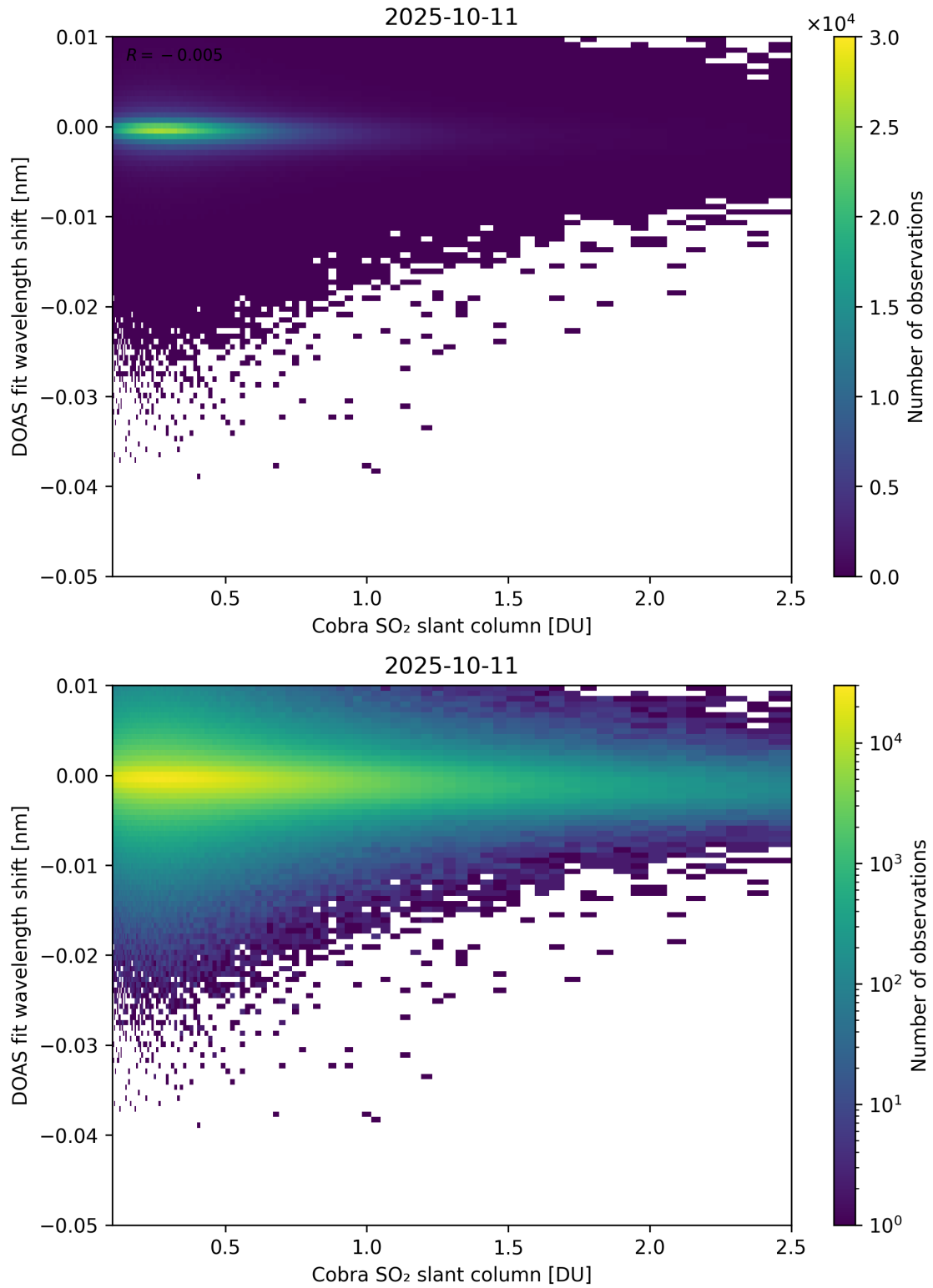
Figure 196: Scatter density plot of “Cobra SO 2 slant column” against “DOAS fit wavelength shift” for 2025-10-11 to 2025-10-12.
