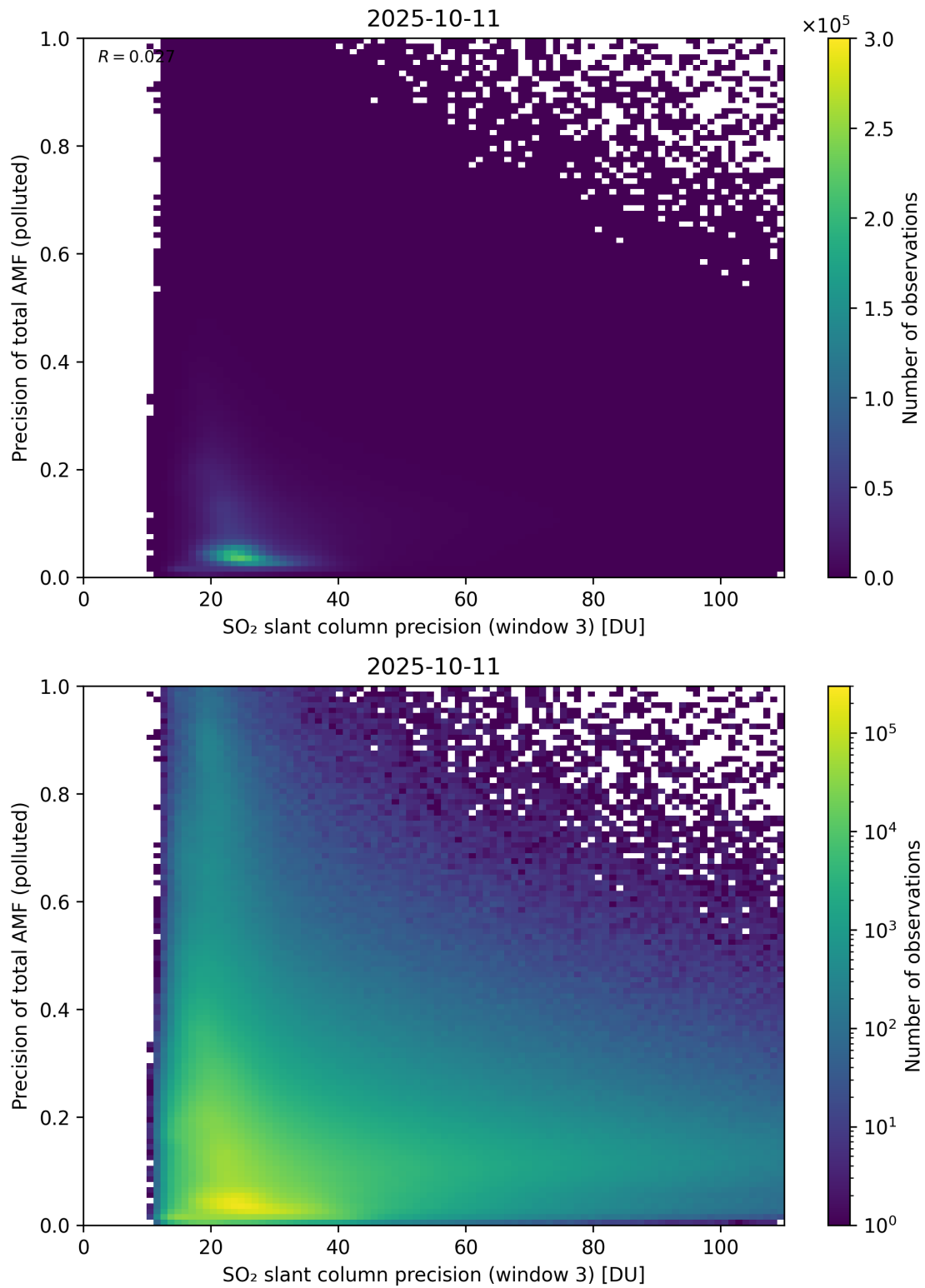
Figure 314: Scatter density plot of “SO 2 slant column precision (window 3)” against “Precision of total AMF (polluted)” for 2025-10-11 to 2025-10-12.
