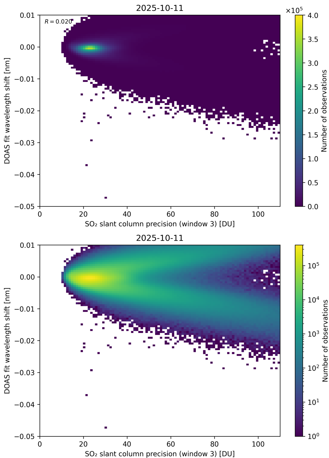
Figure 308: Scatter density plot of “SO 2 slant column precision (window 3)” against “DOAS fit wavelength shift” for 2025-10-11 to 2025-10-12.
