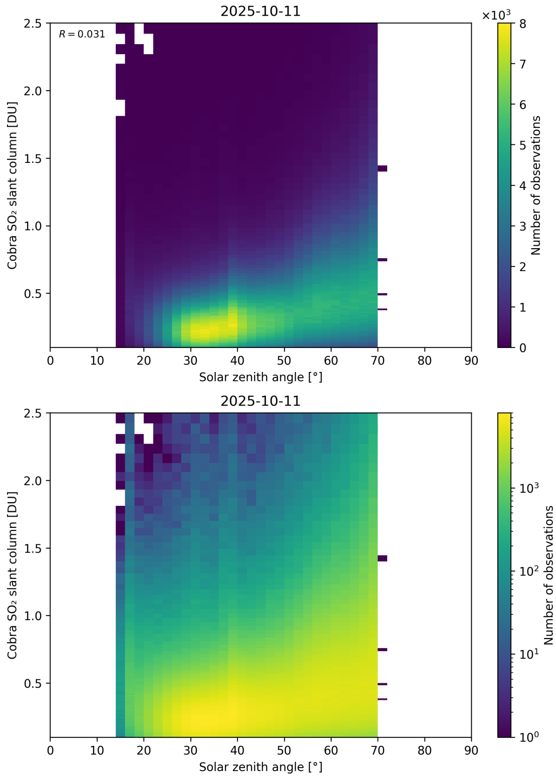
Figure 179: Scatter density plot of “Solar zenith angle” against “Cobra SO 2 slant column” for 2025-10-11 to 2025-10-12.
