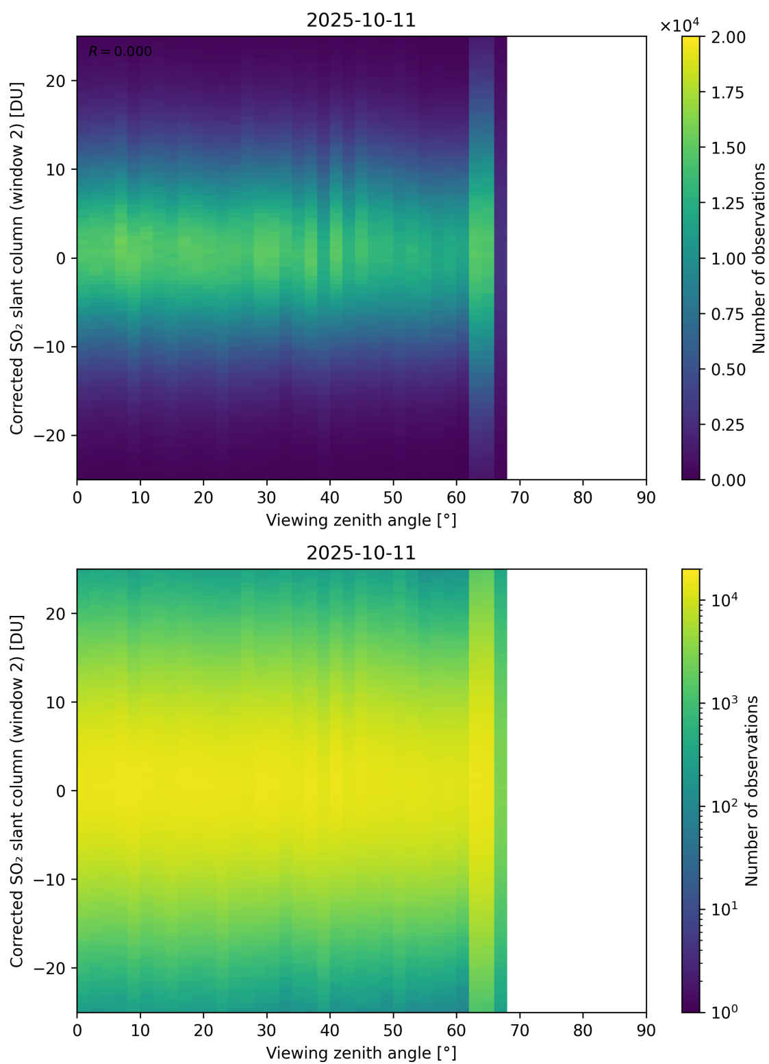
Figure 374: Scatter density plot of “Viewing zenith angle” against “Corrected SO 2 slant column (window 2)” for 2025-10-11 to 2025-10-12.
