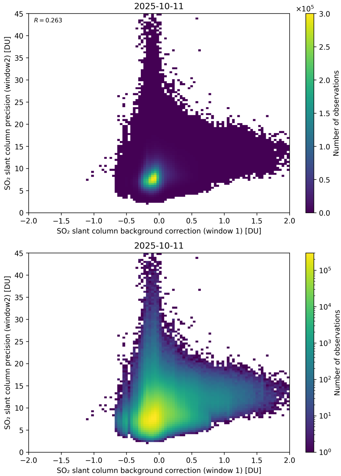
Figure 117: Scatter density plot of “SO 2 slant column background correction (window 1)” against “SO 2 slant column precision (window2)” for 2025-10-11 to 2025-10-12.
