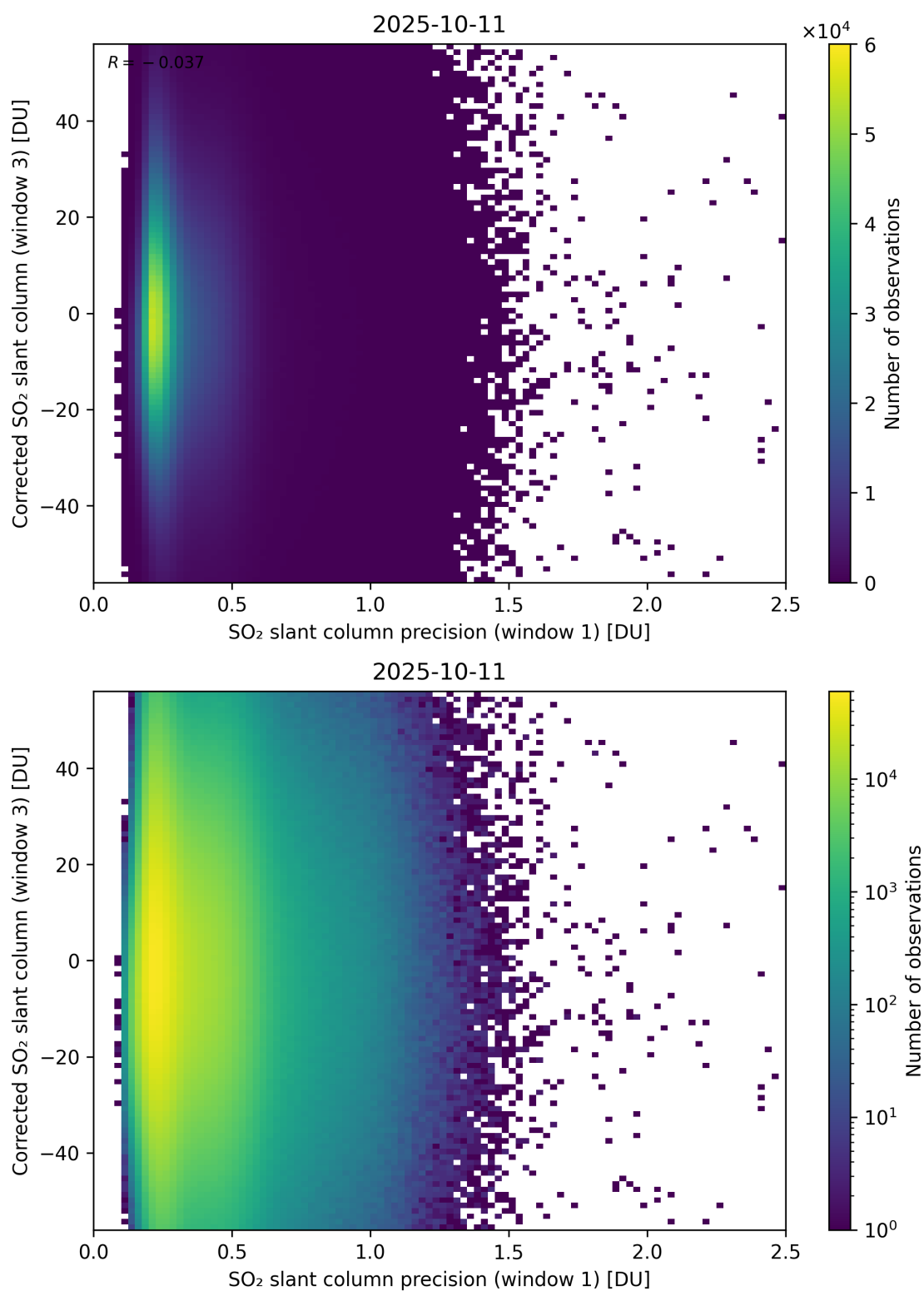
Figure 276: Scatter density plot of “SO 2 slant column precision (window 1)” against “Corrected SO 2 slant column (window 3)” for 2025-10-11 to 2025-10-12.
