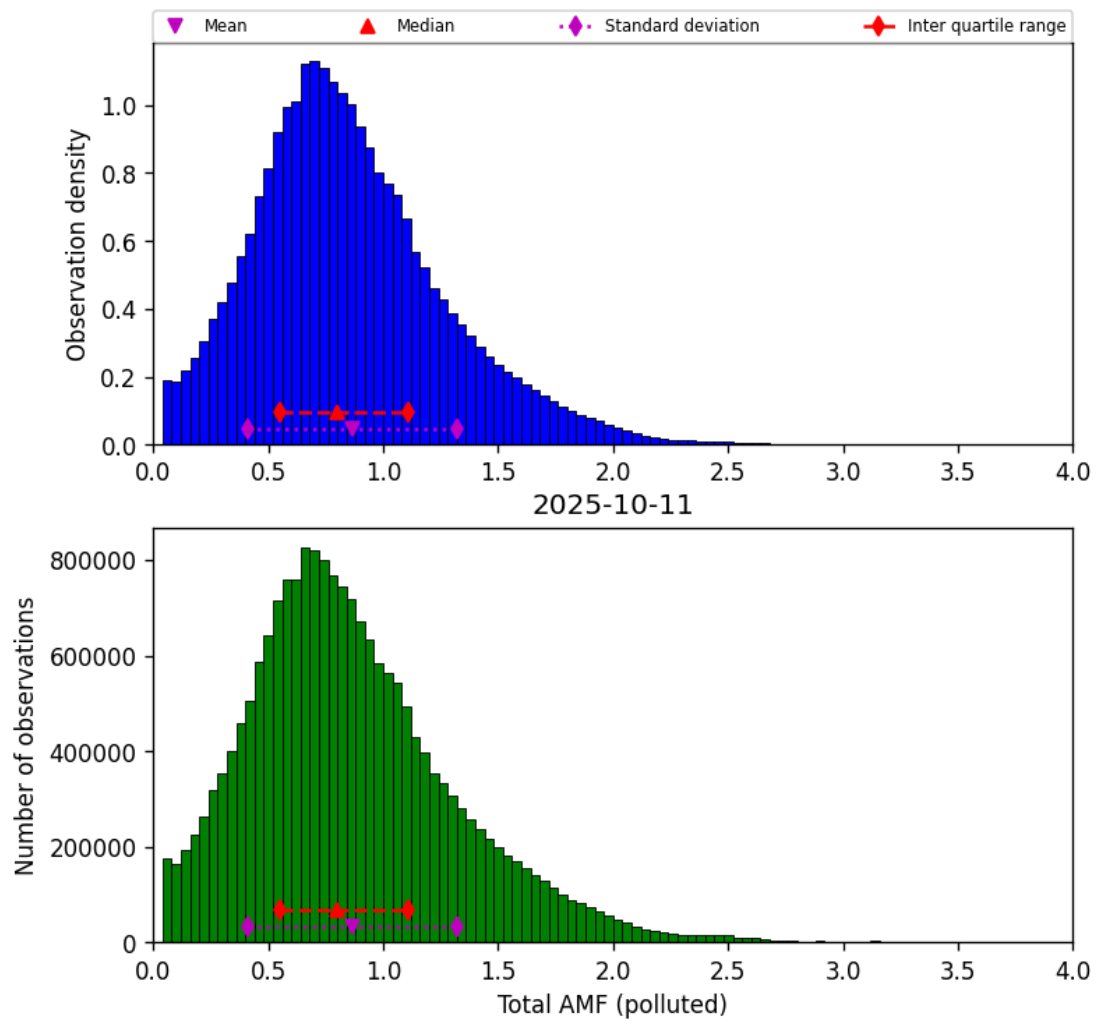
Figure 79: Histogram of “Total AMF (polluted)” for 2025-10-11 to 2025-10-12
