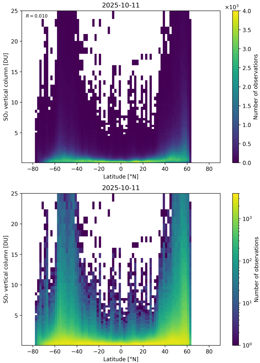
Figure 169: Scatter density plot of “Latitude” against “SO 2 vertical column” for 2025-10-11 to 2025-10-12.
