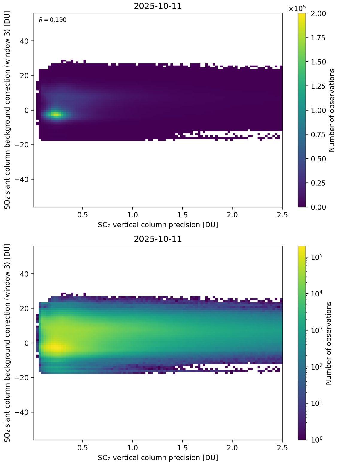
Figure 331: Scatter density plot of “SO 2 vertical column precision” against “SO 2 slant column background correction (window 3)” for 2025-10-11 to 2025-10-12.
