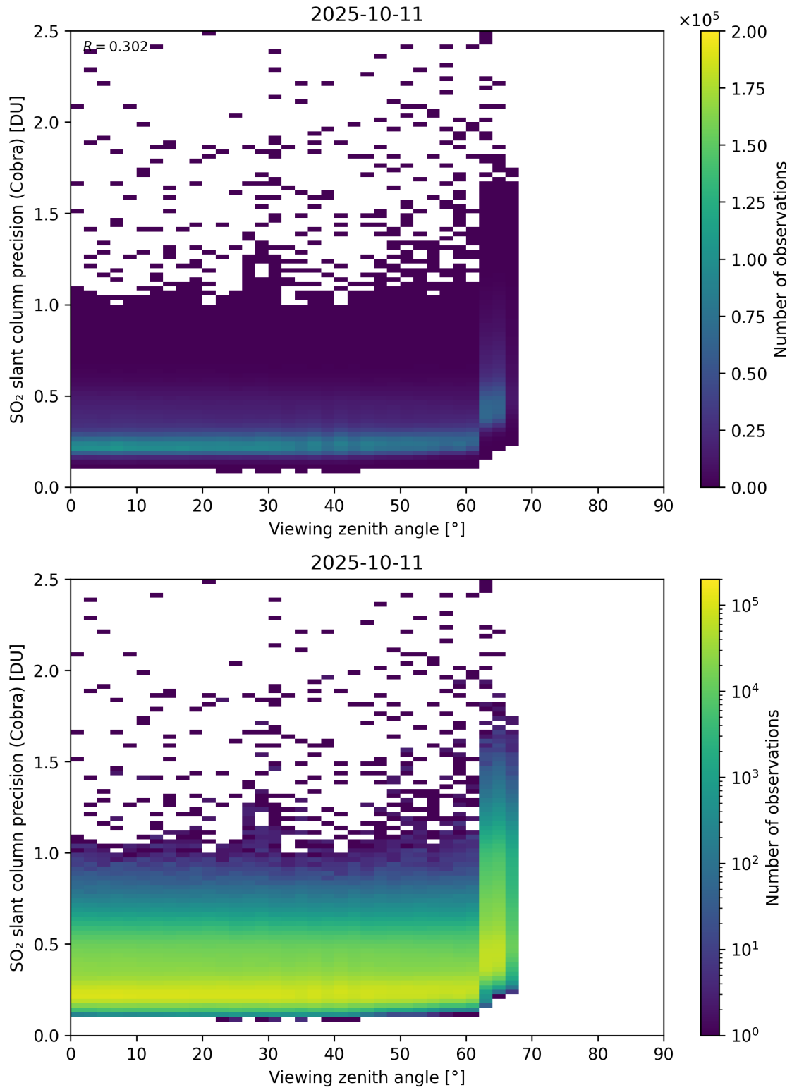
Figure 372: Scatter density plot of “Viewing zenith angle” against “SO 2 slant column precision (Cobra)” for 2025-10-11 to 2025-10-12.
