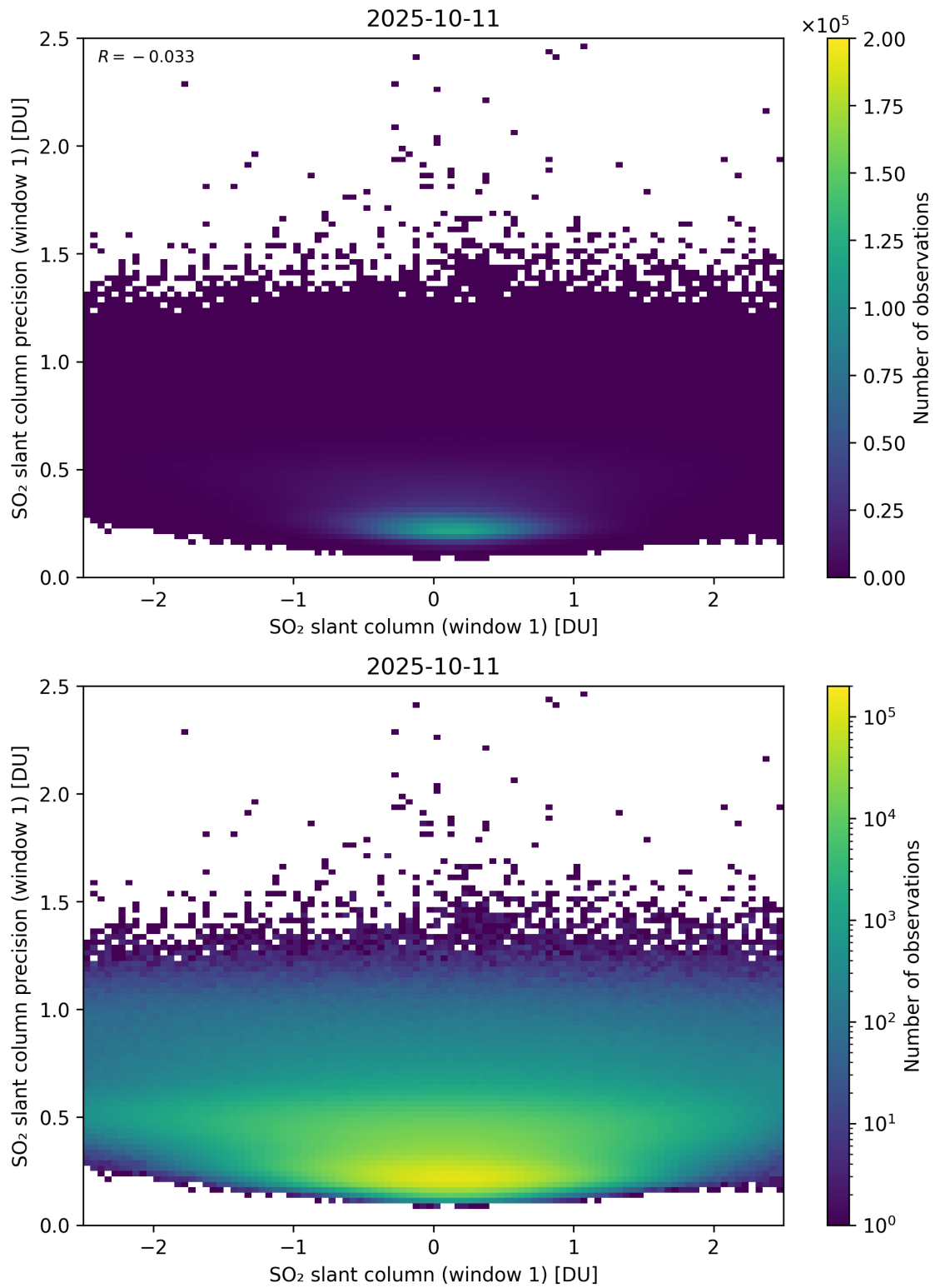
Figure 285: Scatter density plot of “SO 2 slant column (window 1)” against “SO 2 slant column precision (window 1)” for 2025-10-11 to 2025-10-12.
