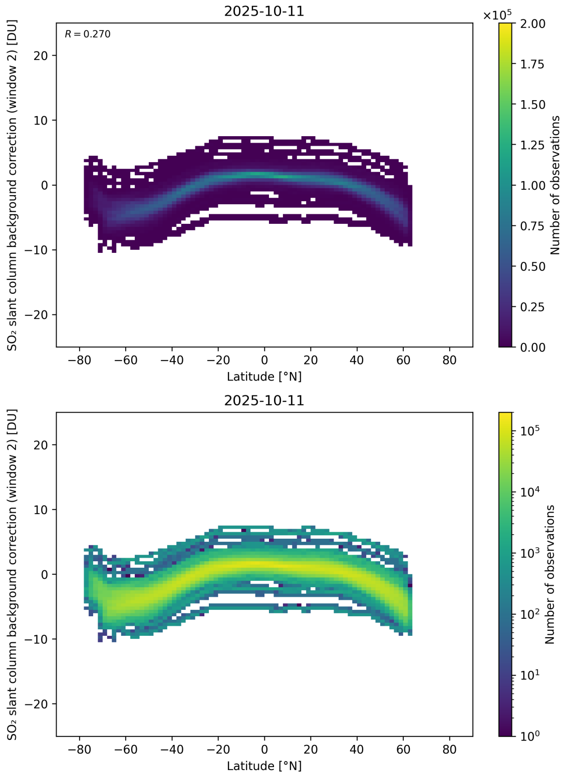
Figure 151: Scatter density plot of “Latitude” against “SO 2 slant column background correction (window 2)” for 2025-10-11 to 2025-10-12.
