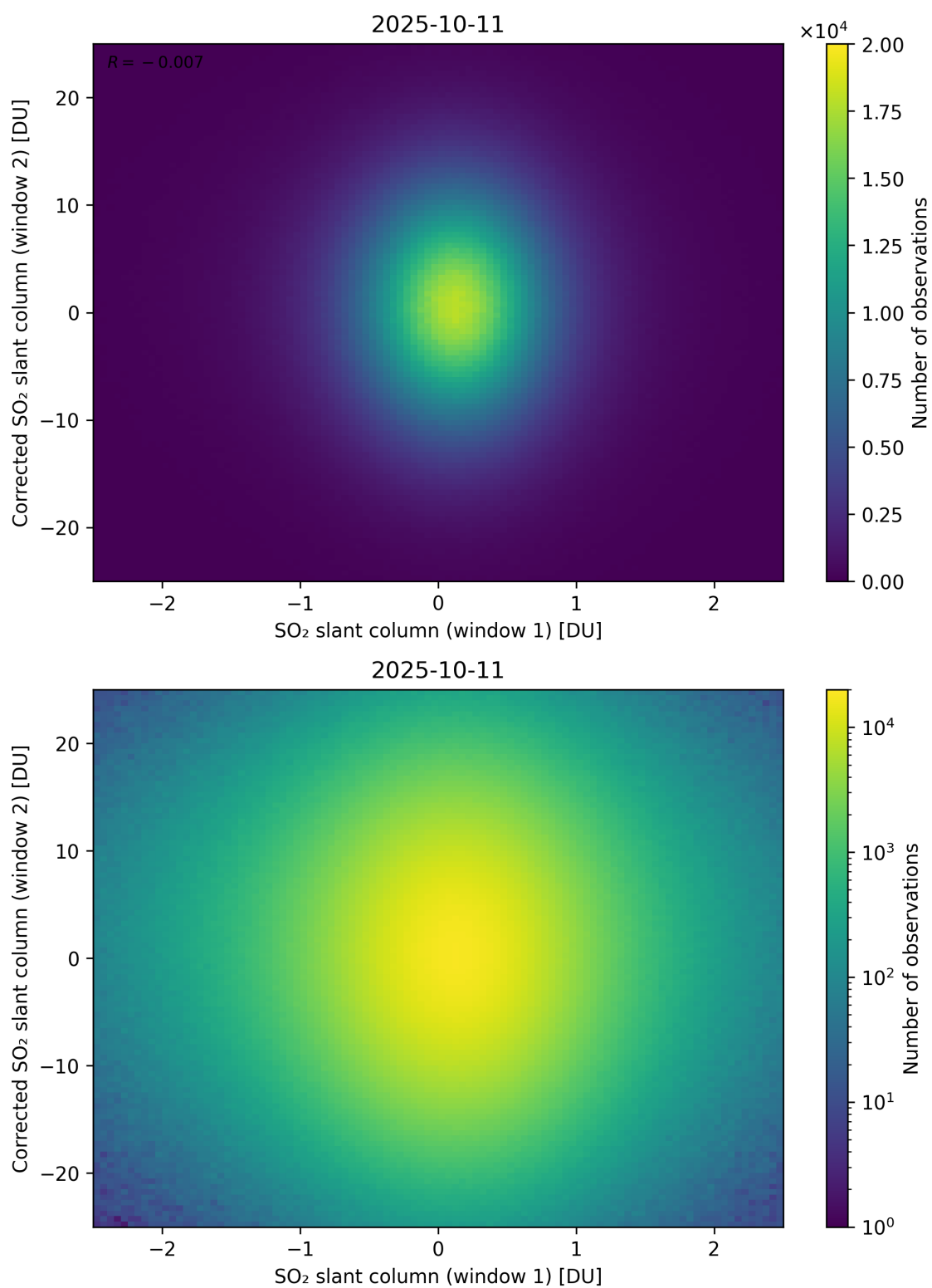
Figure 283: Scatter density plot of “SO 2 slant column (window 1)” against “Corrected SO 2 slant column (window 2)” for 2025-10-11 to 2025-10-12.
