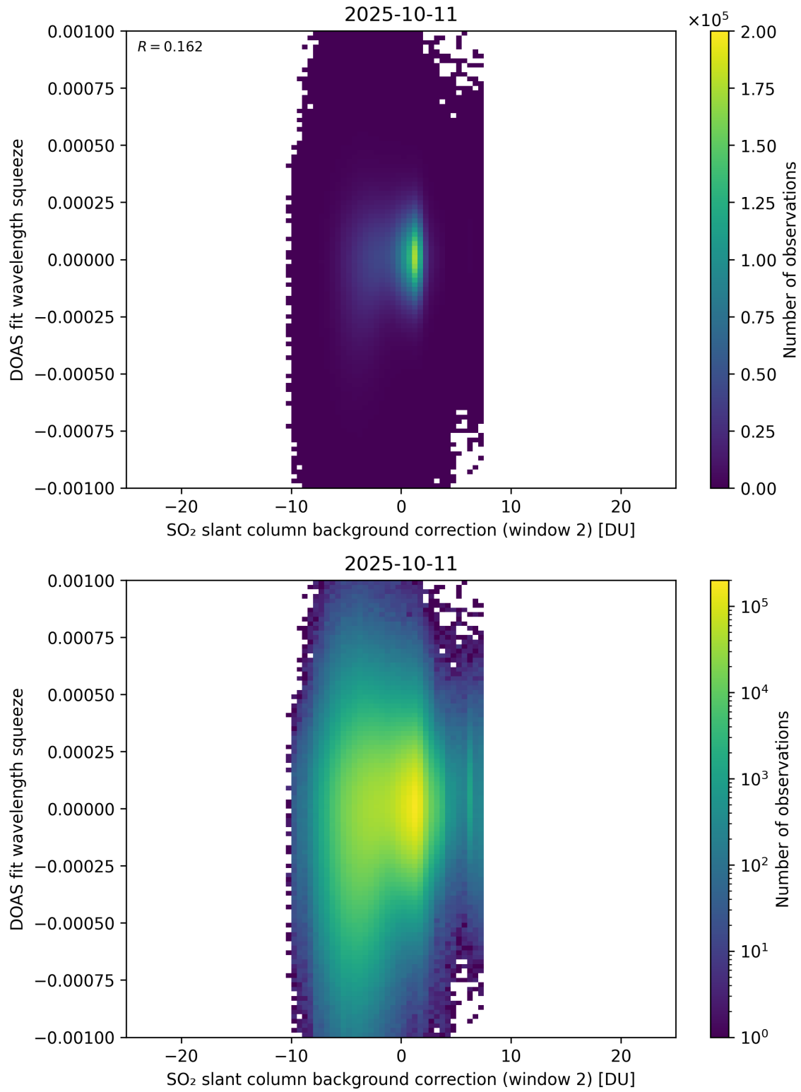
Figure 124: Scatter density plot of “SO 2 slant column background correction (window 2)” against “DOAS fit wavelength squeeze” for 2025-10-11 to 2025-10-12.
