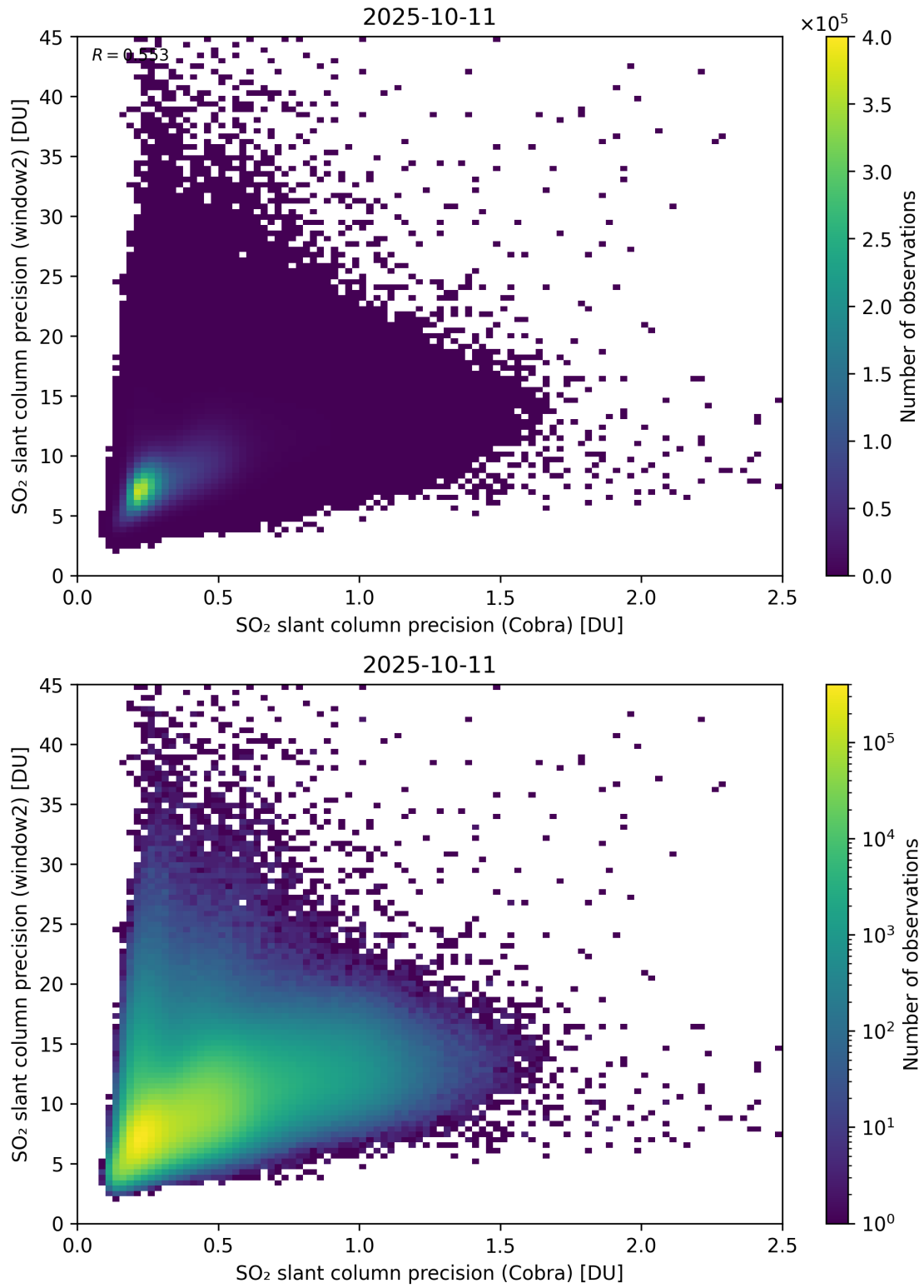
Figure 210: Scatter density plot of “SO 2 slant column precision (Cobra)” against “SO 2 slant column precision (window2)” for 2025-10-11 to 2025-10-12.
