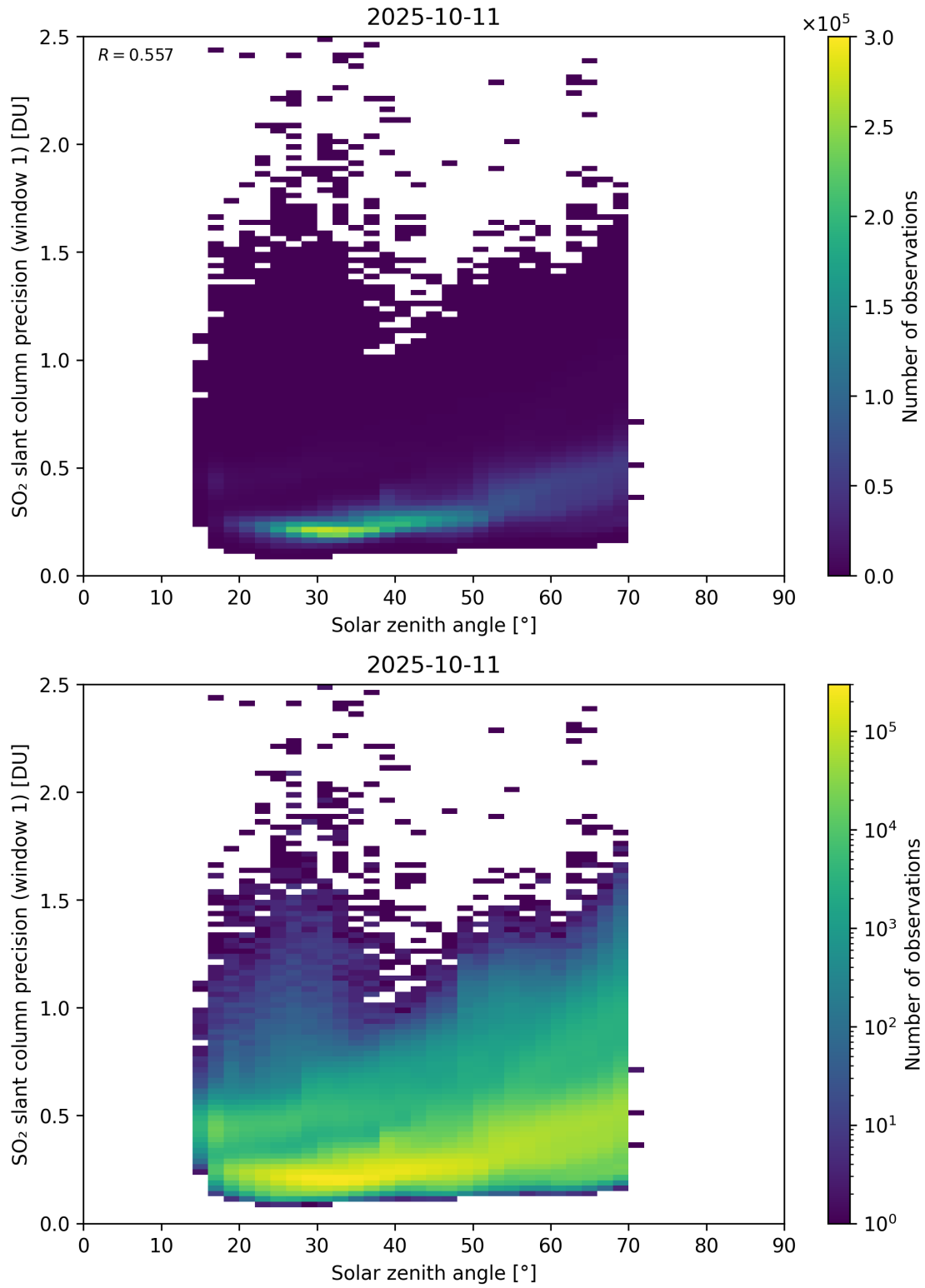
Figure 185: Scatter density plot of “Solar zenith angle” against “SO 2 slant column precision (window 1)” for 2025-10-11 to 2025-10-12.
