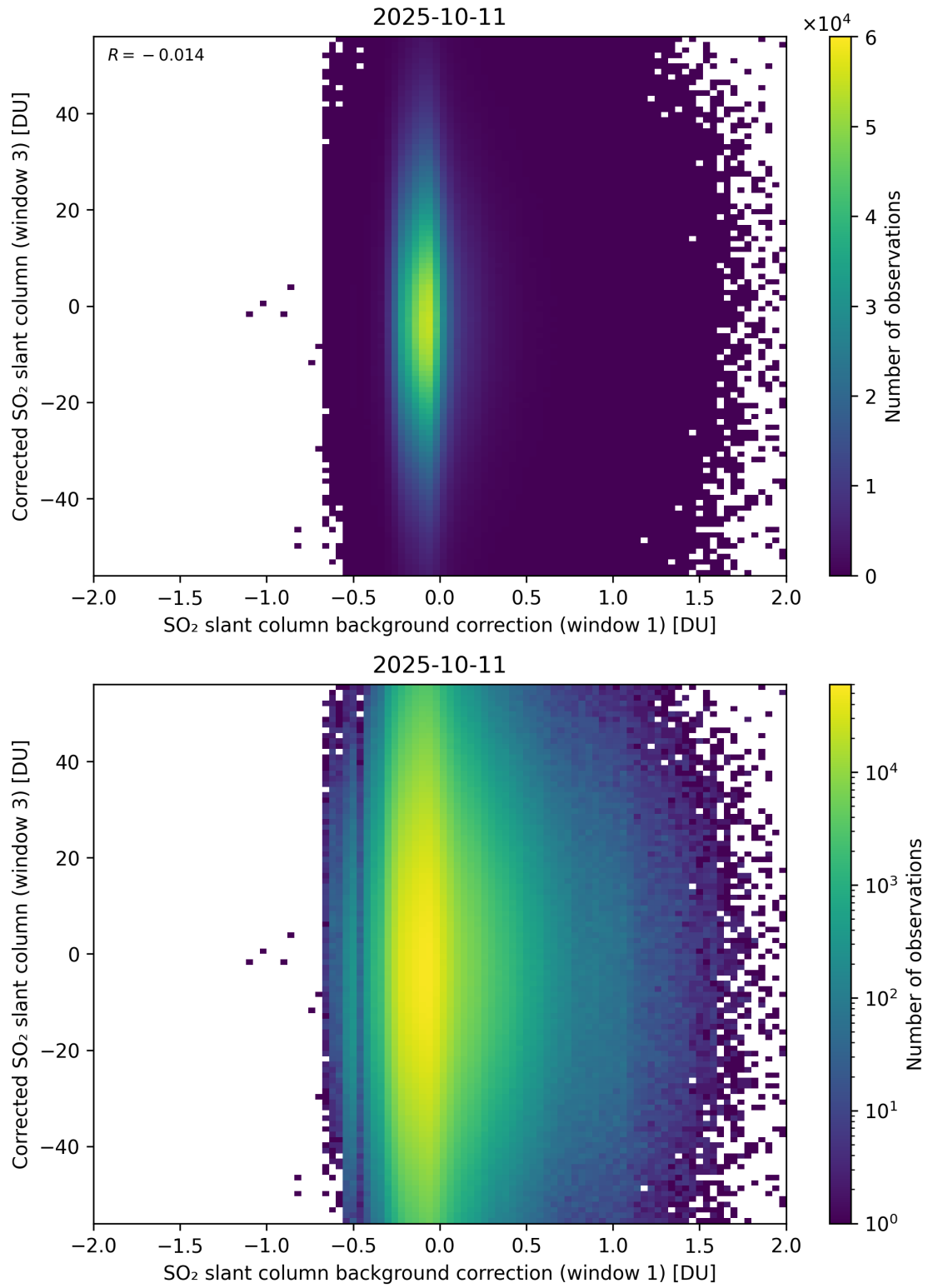
Figure 116: Scatter density plot of “SO 2 slant column background correction (window 1)” against “Corrected SO 2 slant column (window 3)” for 2025-10-11 to 2025-10-12.
