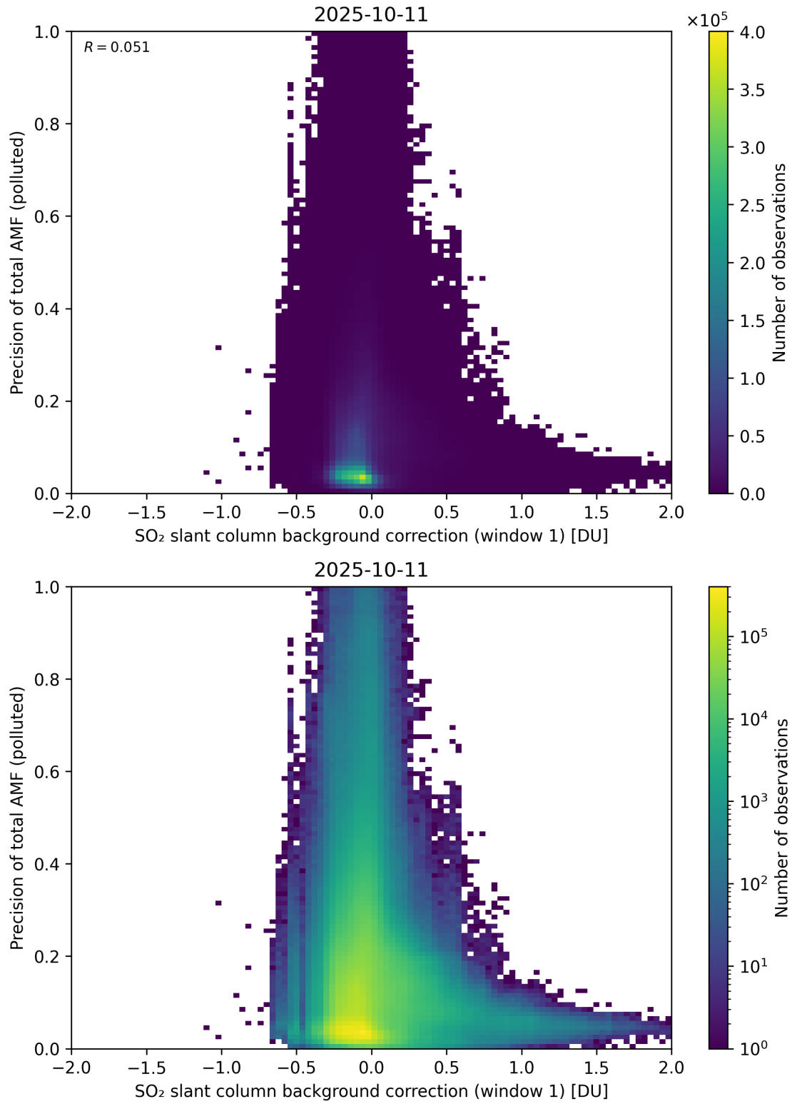
Figure 121: Scatter density plot of “SO 2 slant column background correction (window 1)” against “Precision of total AMF (polluted)” for 2025-10-11 to 2025-10-12.
