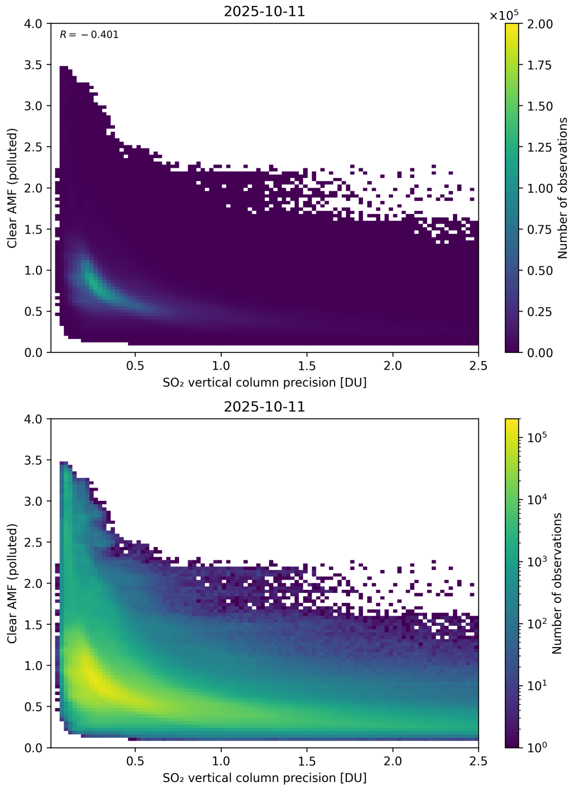
Figure 335: Scatter density plot of “SO 2 vertical column precision” against “Clear AMF (polluted)” for 2025-10-11 to 2025-10-12.
