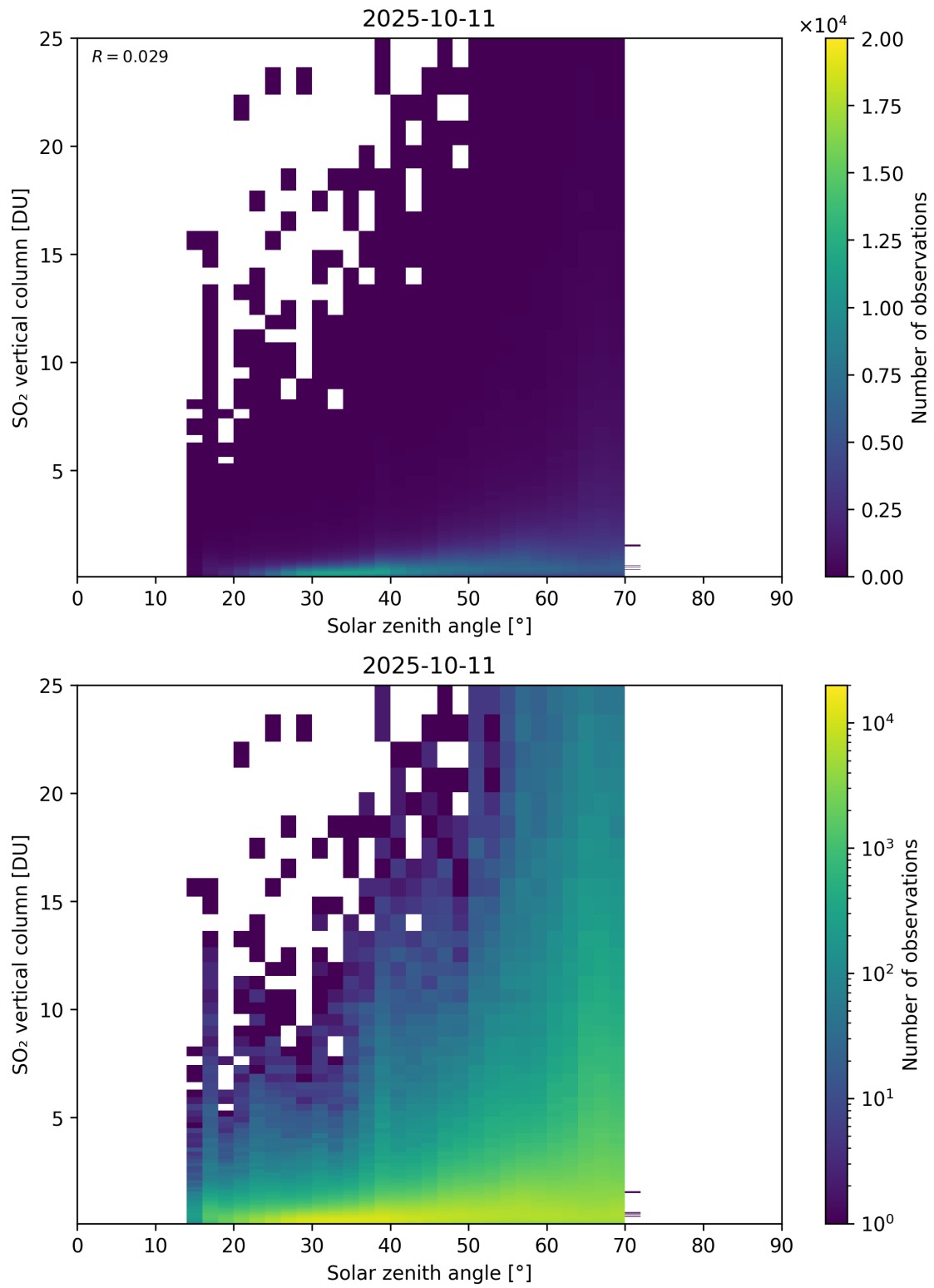
Figure 191: Scatter density plot of “Solar zenith angle” against “SO 2 vertical column” for 2025-10-11 to 2025-10-12.
