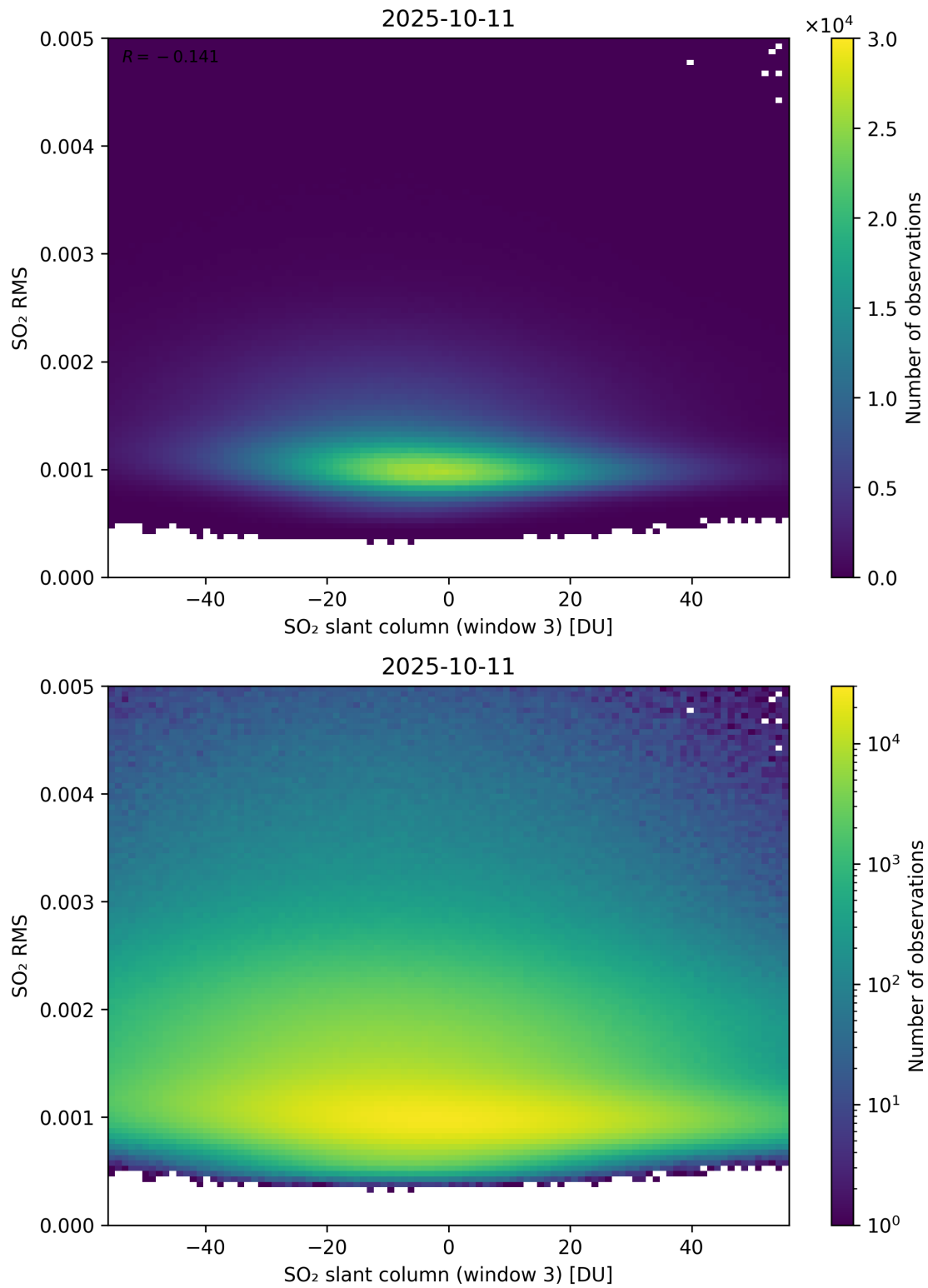
Figure 306: Scatter density plot of “SO 2 slant column (window 3)” against “SO 2 RMS” for 2025-10-11 to 2025-10-12.
