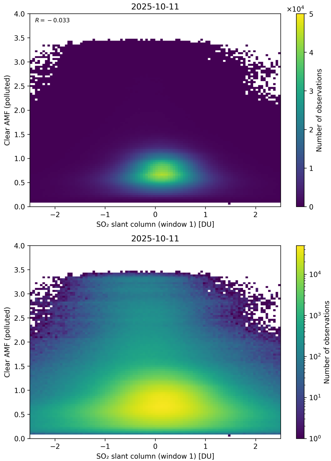
Figure 282: Scatter density plot of “SO 2 slant column (window 1)” against “Clear AMF (polluted)” for 2025-10-11 to 2025-10-12.
