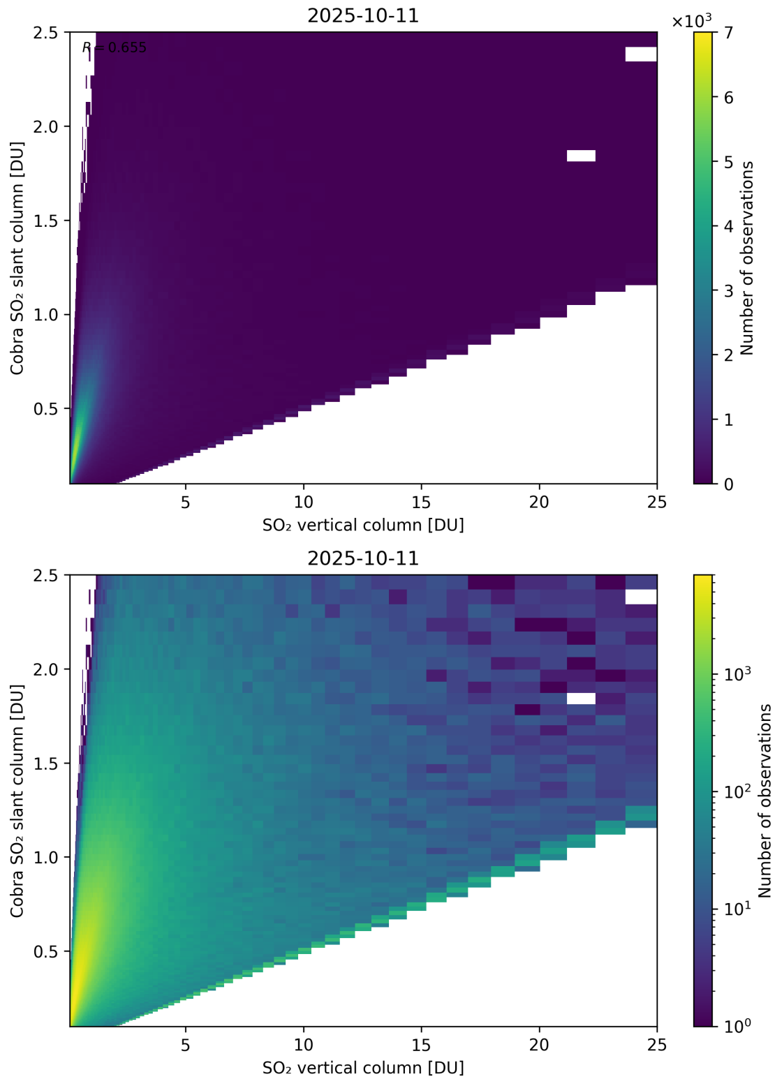
Figure 349: Scatter density plot of “SO 2 vertical column” against “Cobra SO 2 slant column” for 2025-10-11 to 2025-10-12.
