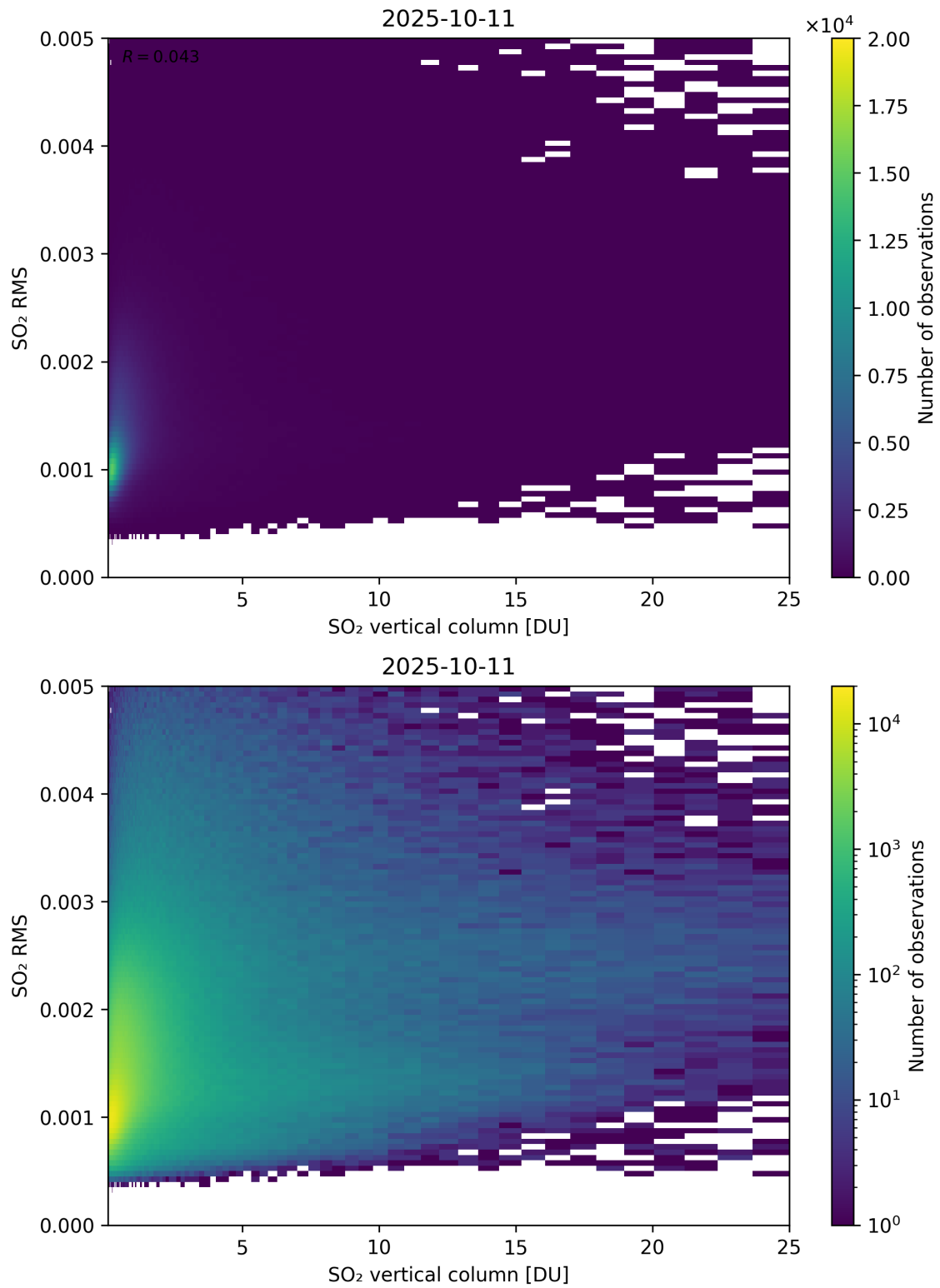
Figure 328: Scatter density plot of “SO 2 vertical column” against “SO 2 RMS” for 2025-10-11 to 2025-10-12.
