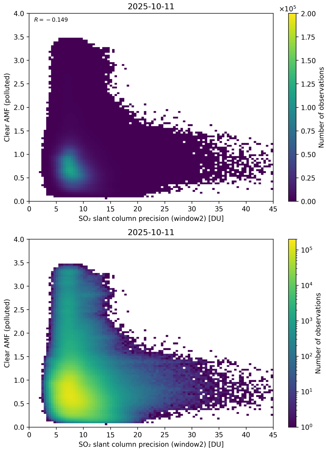
Figure 296: Scatter density plot of “SO 2 slant column precision (window2)” against “Clear AMF (polluted)” for 2025-10-11 to 2025-10-12.
