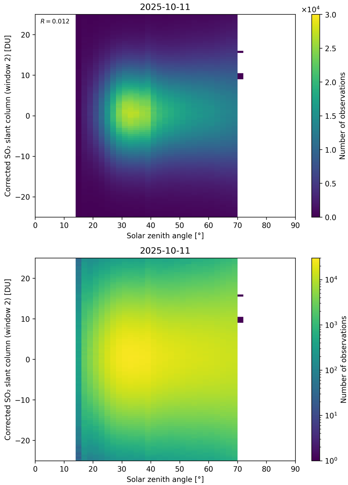
Figure 182: Scatter density plot of “Solar zenith angle” against “Corrected SO 2 slant column (window 2)” for 2025-10-11 to 2025-10-12.
