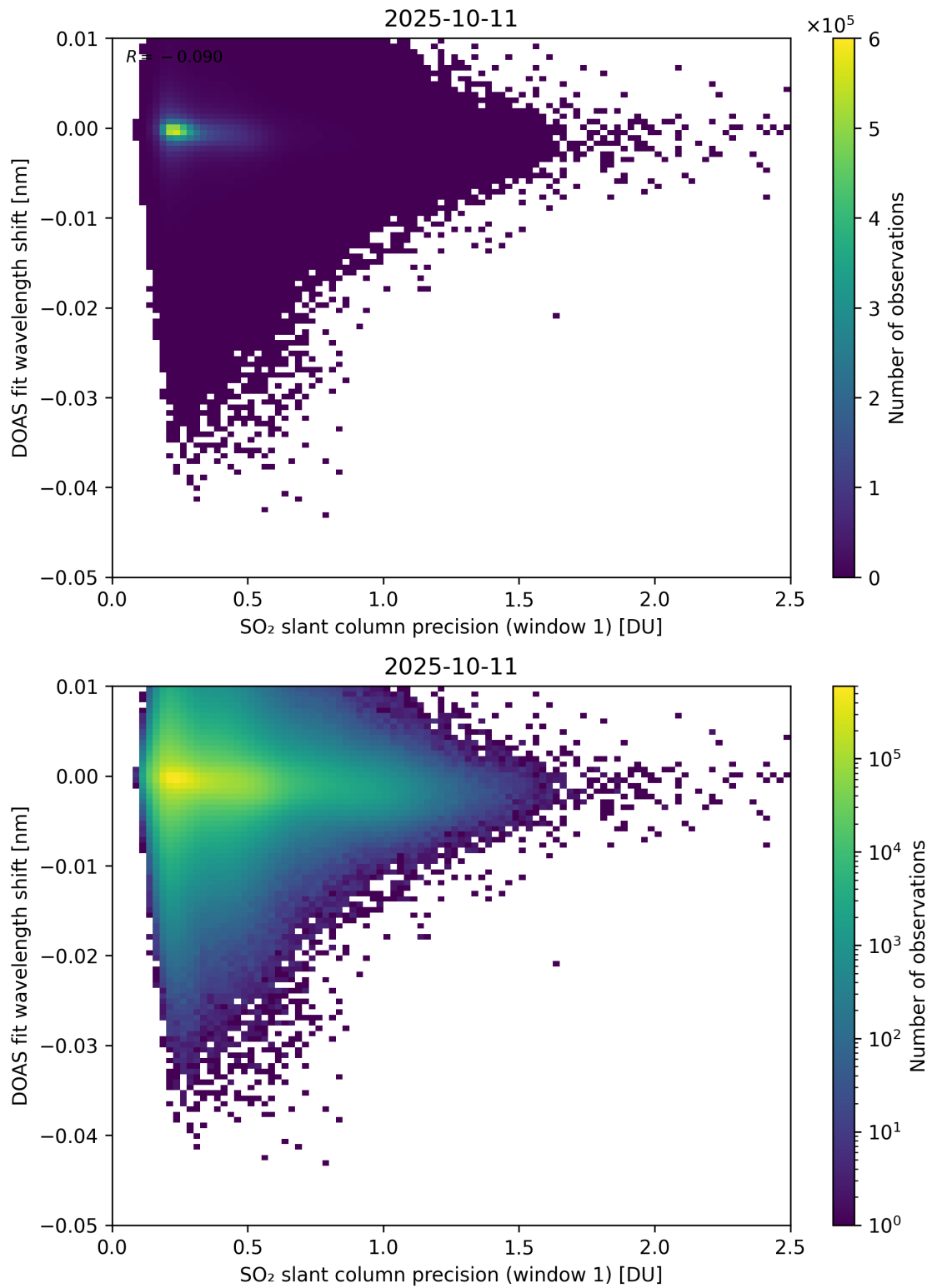
Figure 271: Scatter density plot of “SO 2 slant column precision (window 1)” against “DOAS fit wavelength shift” for 2025-10-11 to 2025-10-12.
