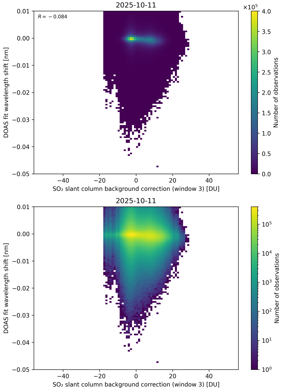
Figure 132: Scatter density plot of “SO 2 slant column background correction (window 3)” against “DOAS fit wavelength shift” for 2025-10-11 to 2025-10-12.
