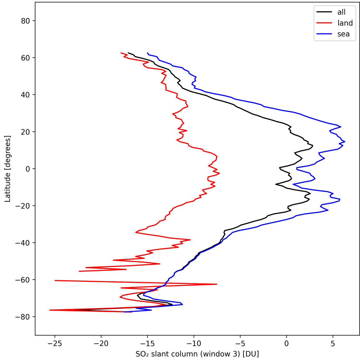
Figure 45: Zonal average of “SO 2 slant column (window 3)” for 2025-10-11 to 2025-10-12.
