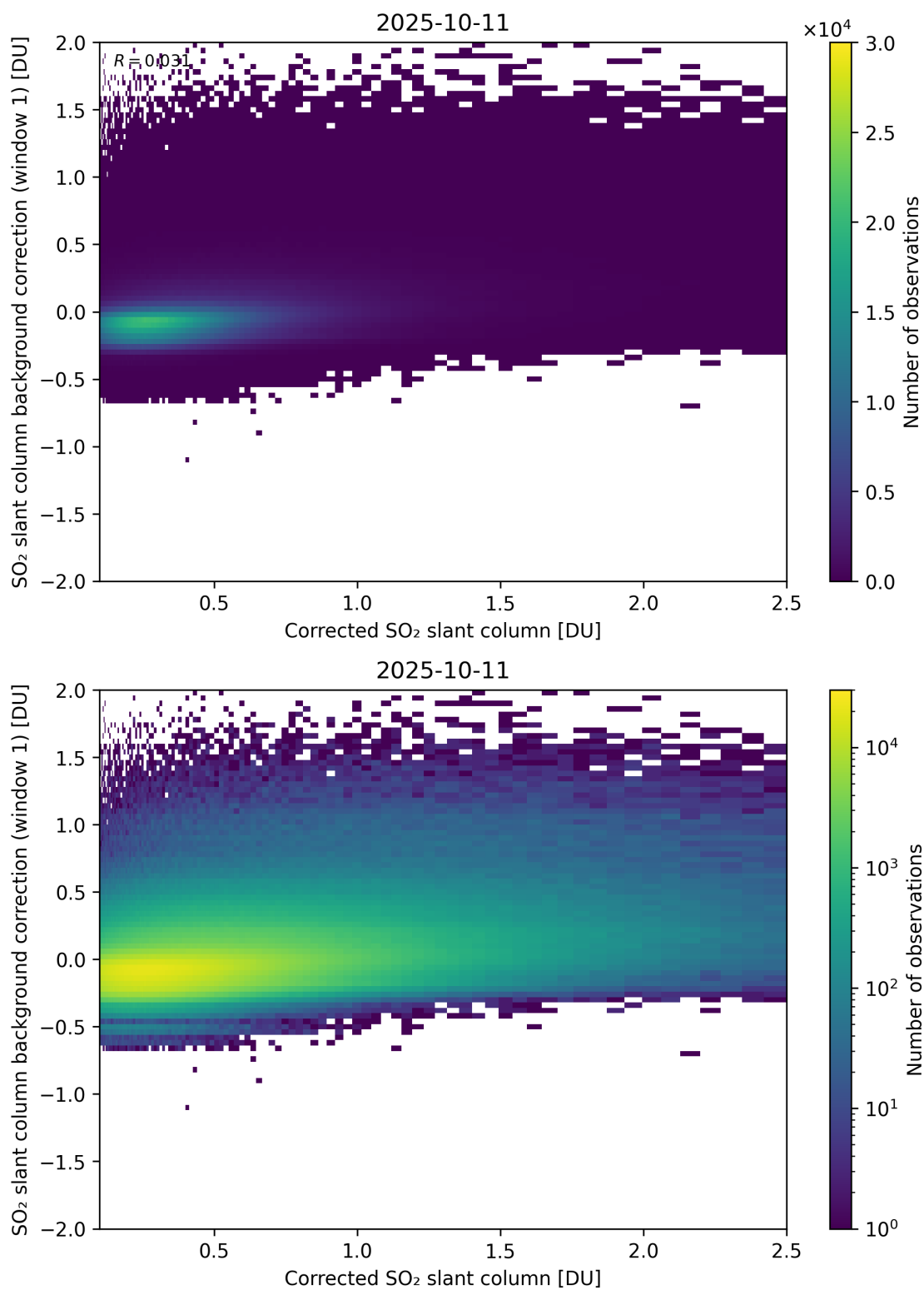
Figure 226: Scatter density plot of “Corrected SO 2 slant column” against “SO 2 slant column background correction (window 1)” for 2025-10-11 to 2025-10-12.
