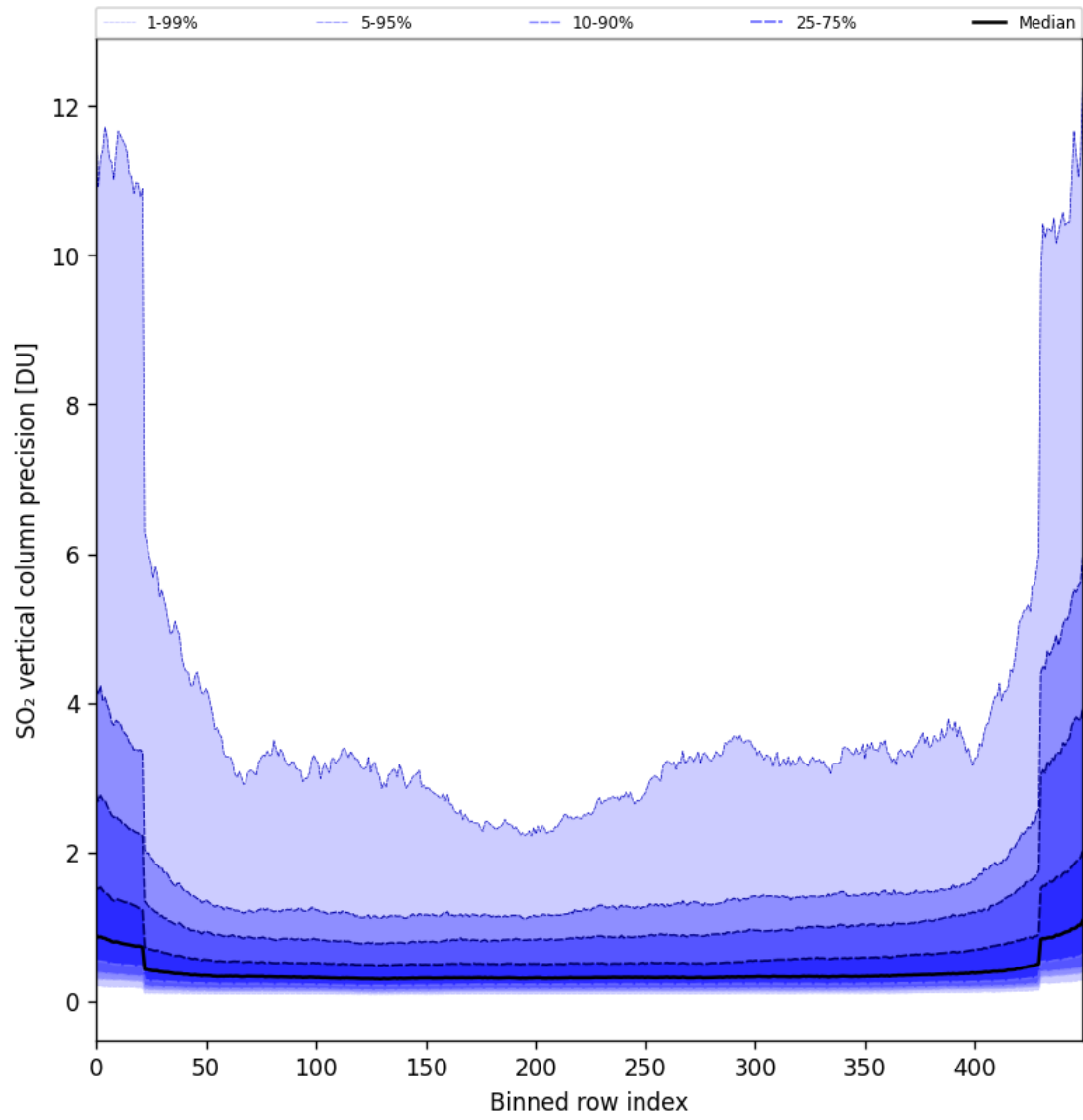
Figure 85: Along track statistics of “SO 2 vertical column precision” for 2025-10-11 to 2025-10-12
