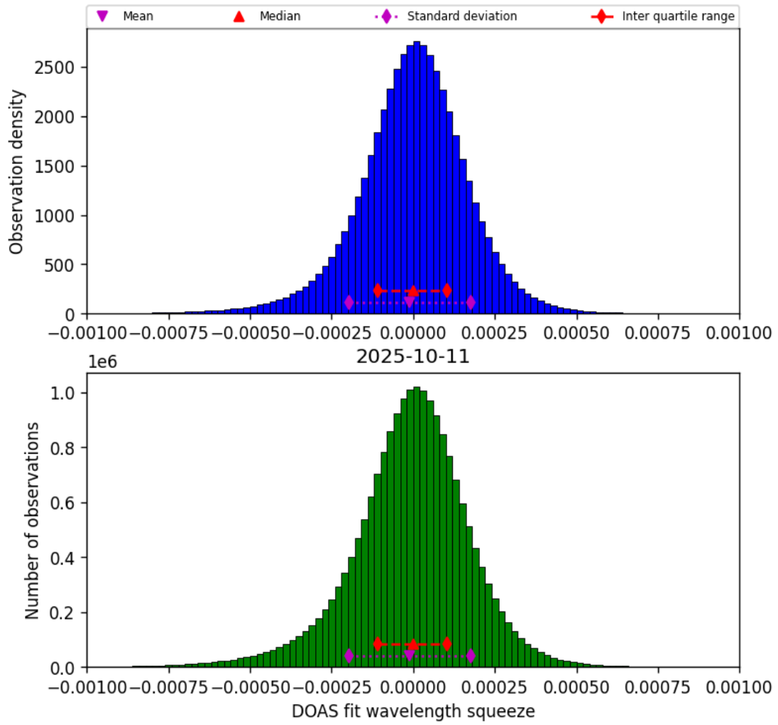
Figure 77: Histogram of “DOAS fit wavelength squeeze” for 2025-10-11 to 2025-10-12
