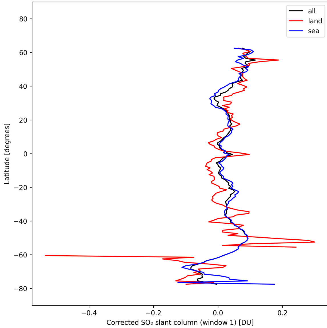
Figure 39: Zonal average of “Corrected SO 2 slant column (window 1)” for 2025-10-11 to 2025-10-12.
