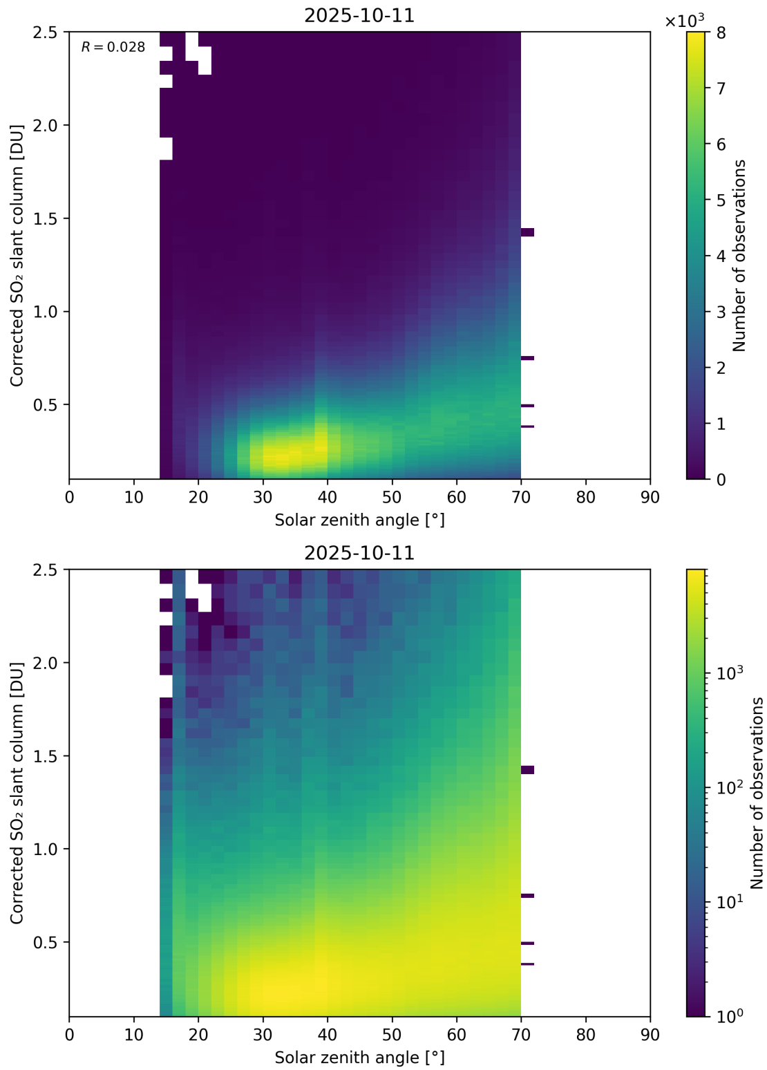
Figure 181: Scatter density plot of “Solar zenith angle” against “Corrected SO 2 slant column” for 2025-10-11 to 2025-10-12.
