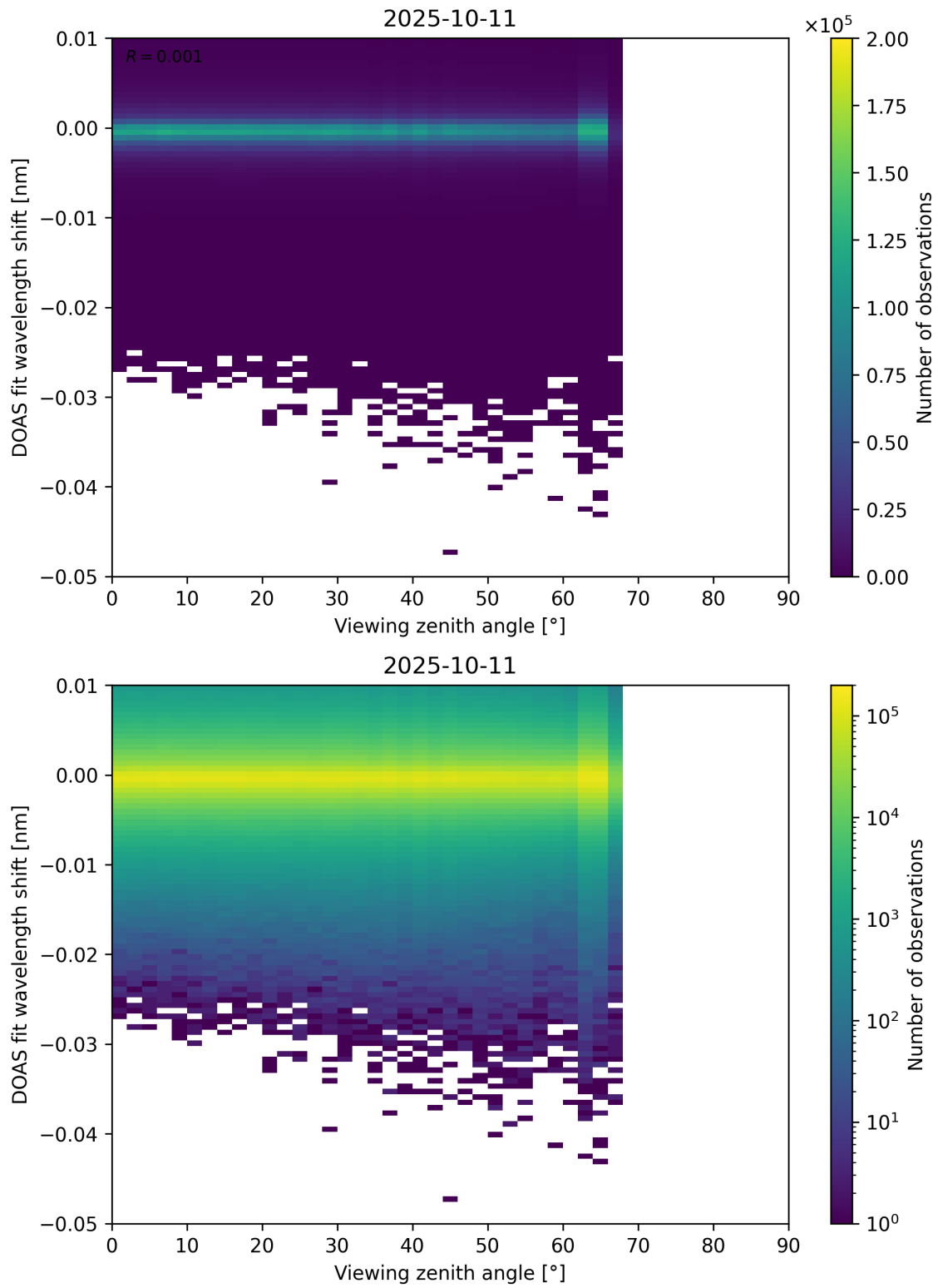
Figure 365: Scatter density plot of “Viewing zenith angle” against “DOAS fit wavelength shift” for 2025-10-11 to 2025-10-12.
