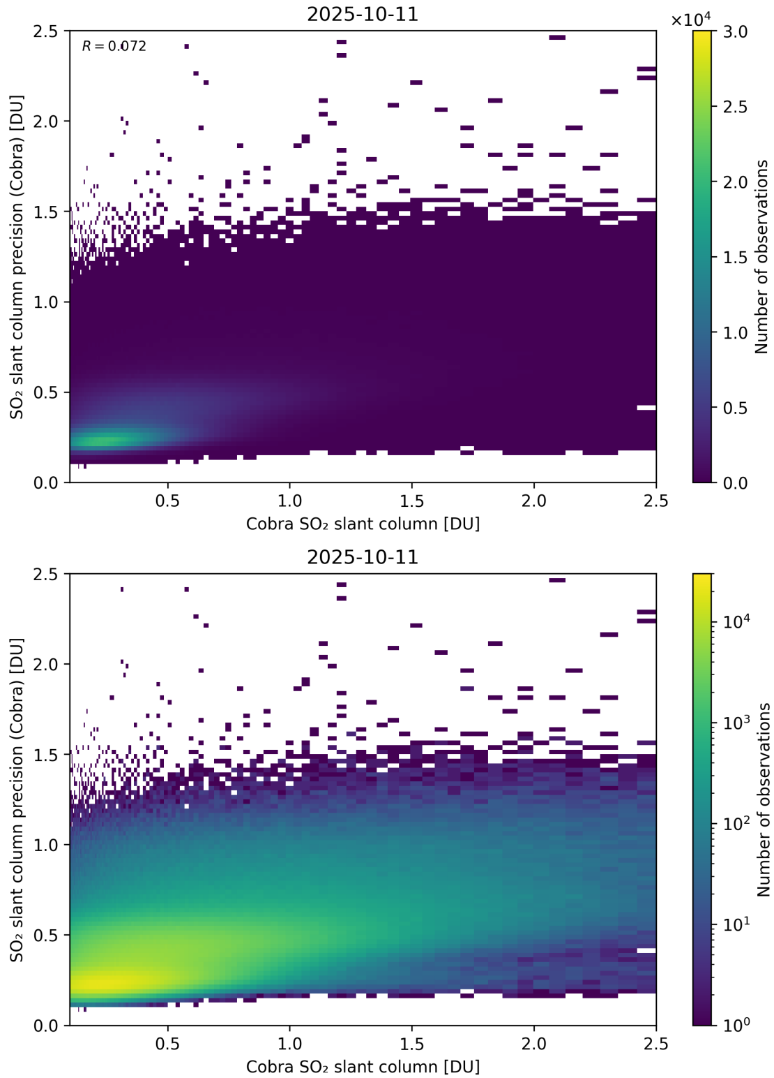
Figure 216: Scatter density plot of “Cobra SO 2 slant column” against “SO 2 slant column precision (Cobra)” for 2025-10-11 to 2025-10-12.
