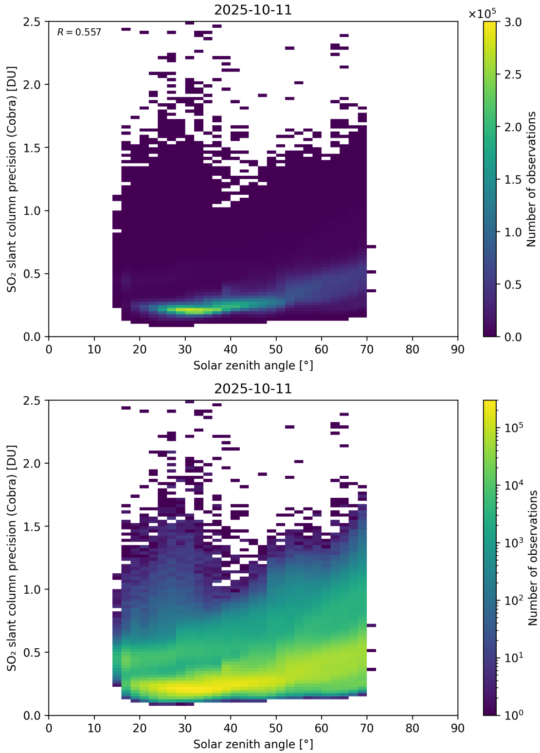
Figure 180: Scatter density plot of “Solar zenith angle” against “SO 2 slant column precision (Cobra)” for 2025-10-11 to 2025-10-12.
