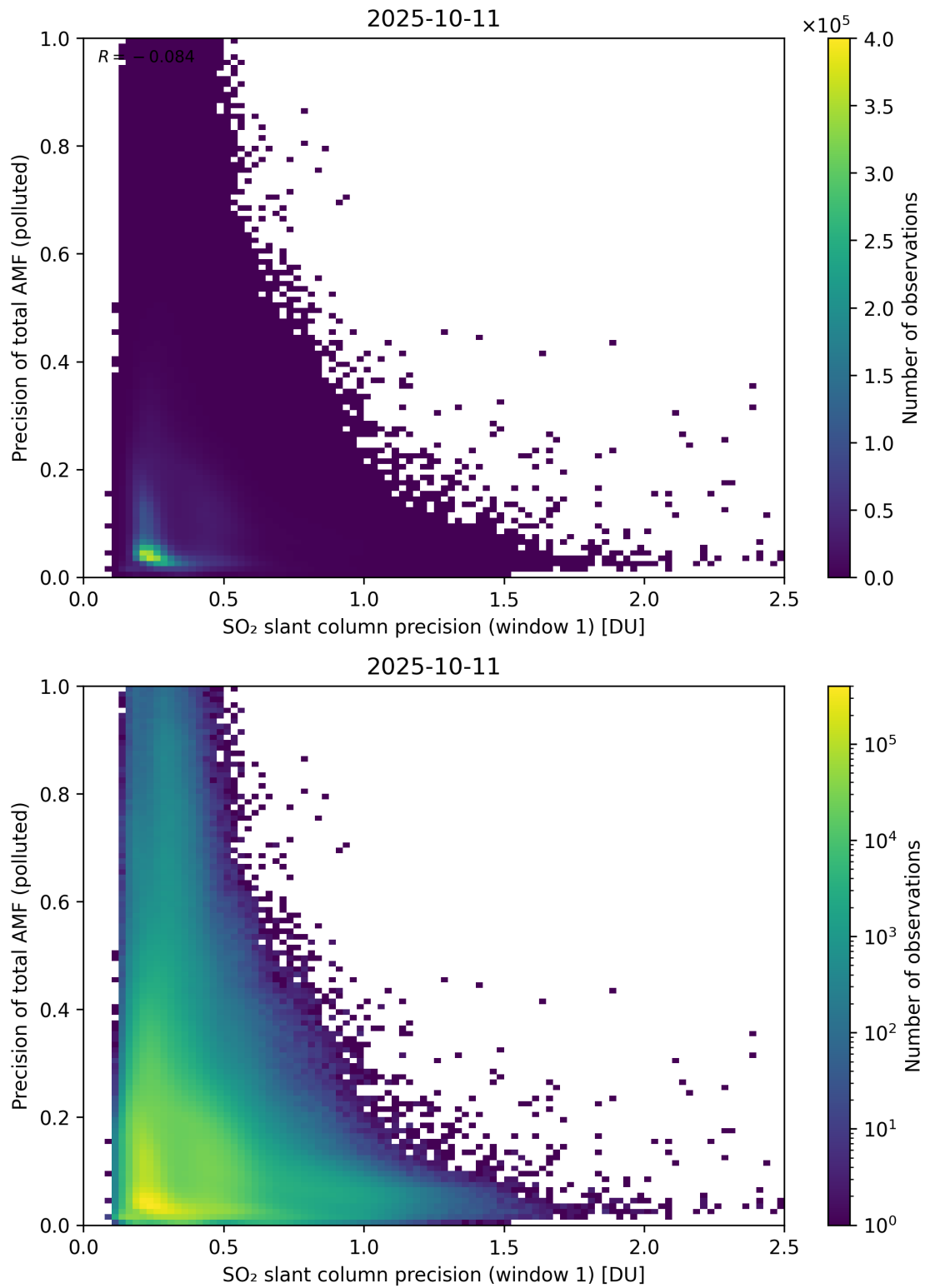
Figure 281: Scatter density plot of “SO 2 slant column precision (window 1)” against “Precision of total AMF (polluted)” for 2025-10-11 to 2025-10-12.
