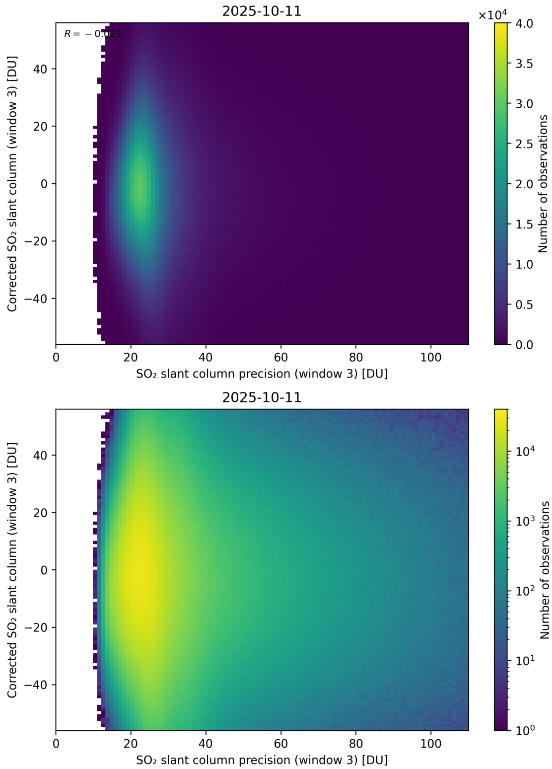
Figure 312: Scatter density plot of “SO 2 slant column precision (window 3)” against “Corrected SO 2 slant column (window 3)” for 2025-10-11 to 2025-10-12.
