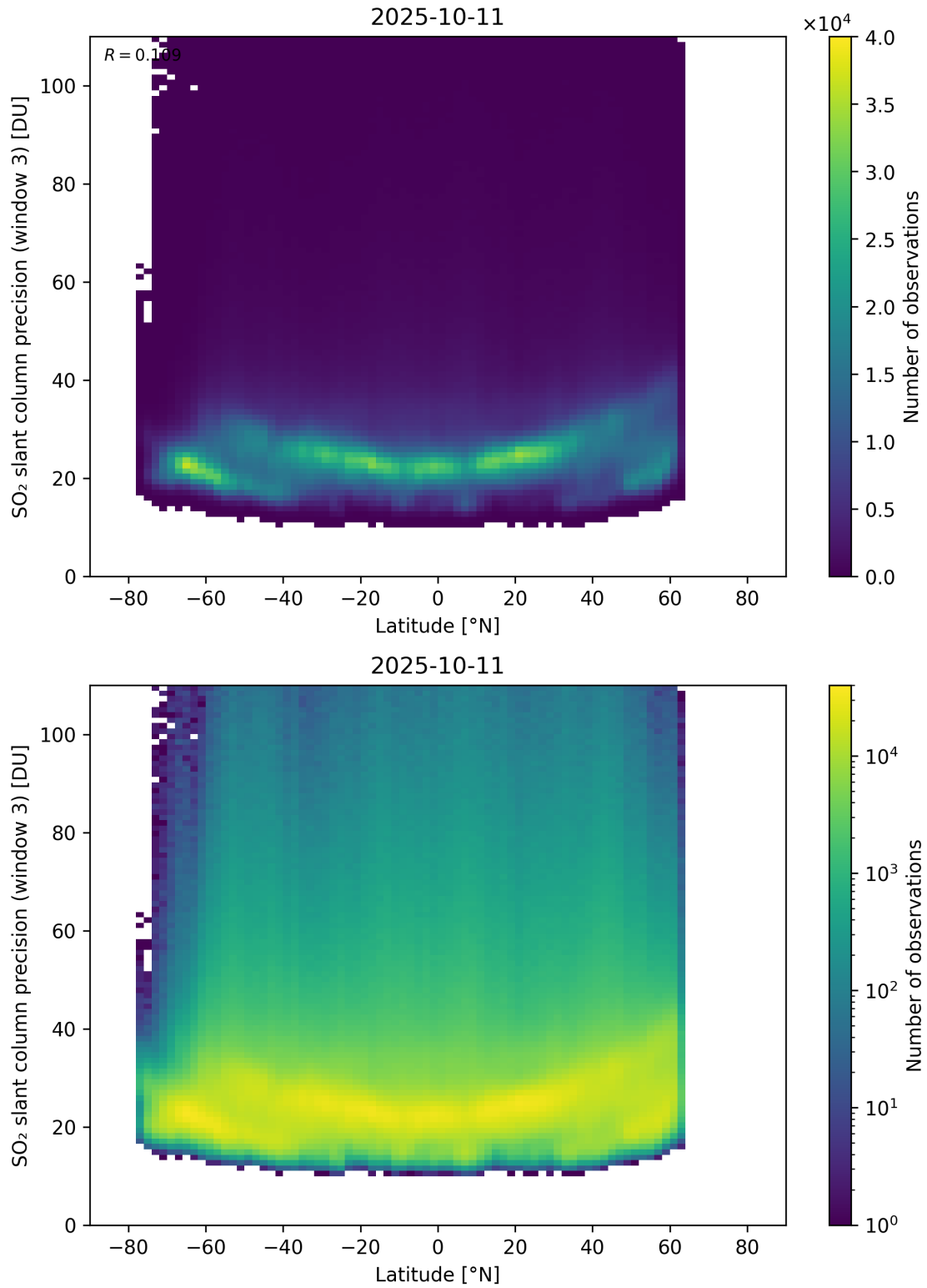
Figure 166: Scatter density plot of “Latitude” against “SO 2 slant column precision (window 3)” for 2025-10-11 to 2025-10-12.
