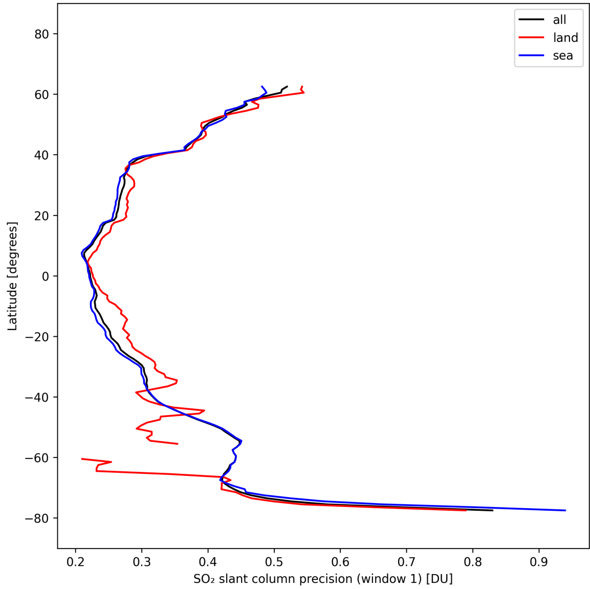
Figure 38: Zonal average of “SO 2 slant column precision (window 1)” for 2025-10-11 to 2025-10-12.
