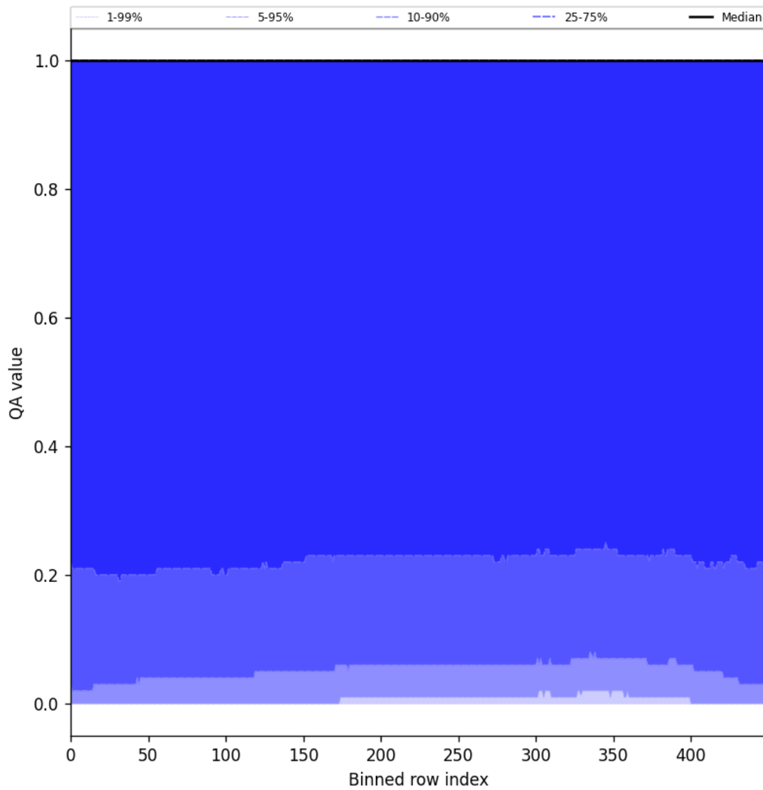
Figure 83: Along track statistics of “QA value” for 2025-10-11 to 2025-10-12
