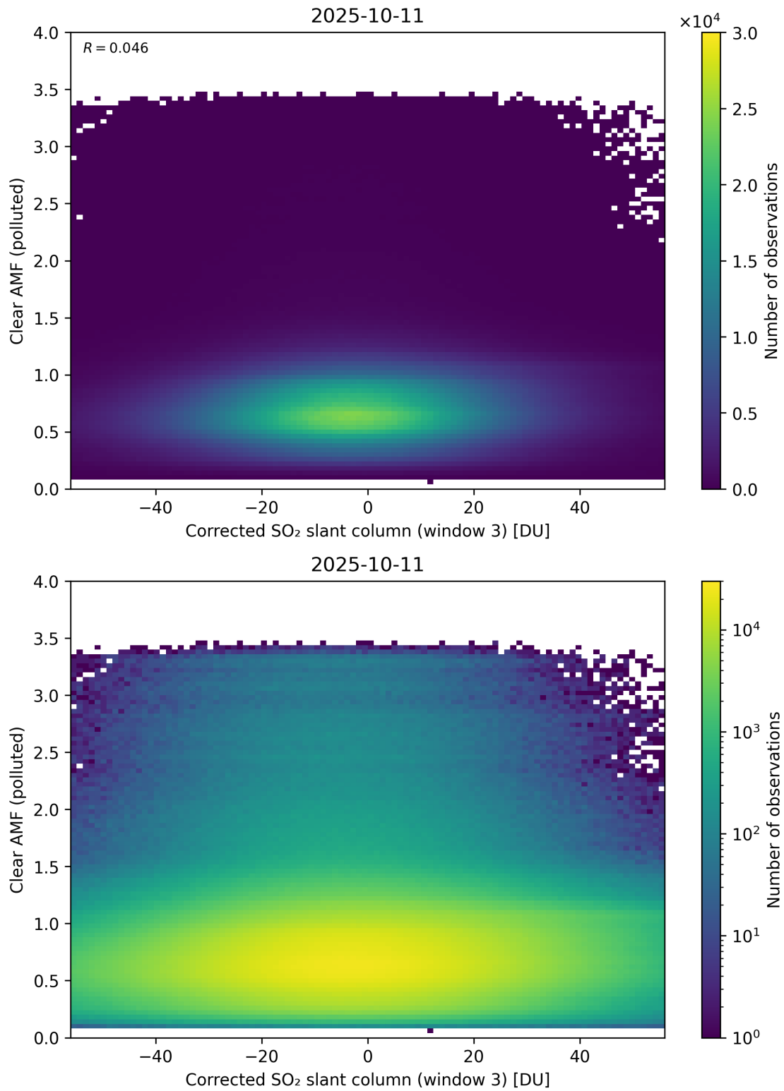
Figure 259: Scatter density plot of “Corrected SO 2 slant column (window 3)” against “Clear AMF (polluted)” for 2025-10-11 to 2025-10-12.
