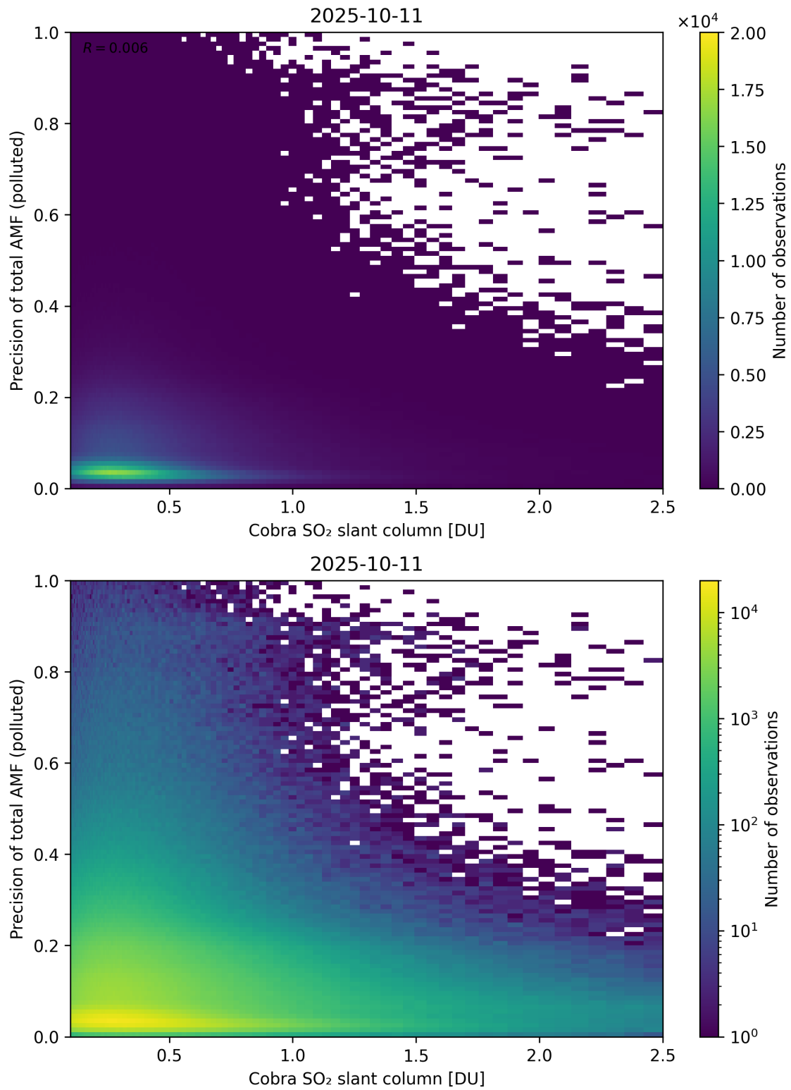
Figure 225: Scatter density plot of “Cobra SO 2 slant column” against “Precision of total AMF (polluted)” for 2025-10-11 to 2025-10-12.
