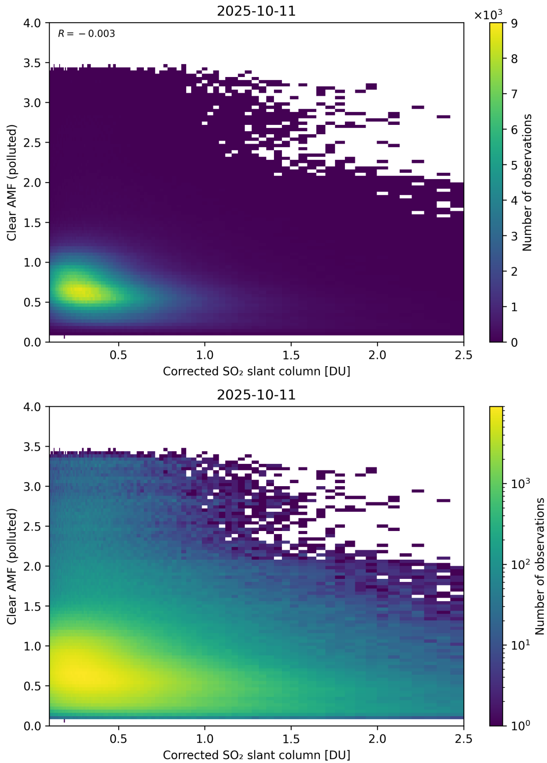
Figure 232: Scatter density plot of “Corrected SO 2 slant column” against “Clear AMF (polluted)” for 2025-10-11 to 2025-10-12.
