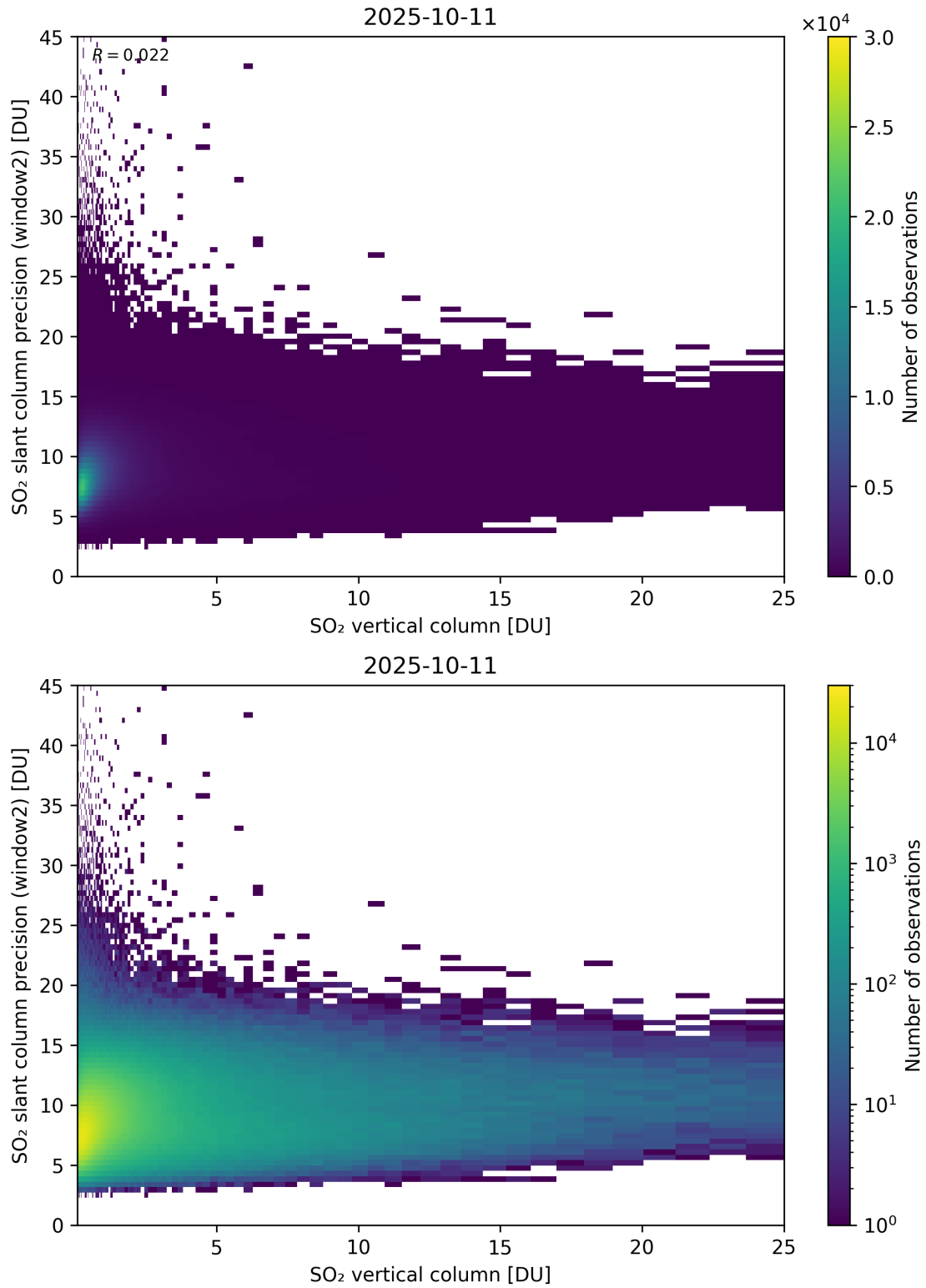
Figure 356: Scatter density plot of “SO 2 vertical column” against “SO 2 slant column precision (window2)” for 2025-10-11 to 2025-10-12.
