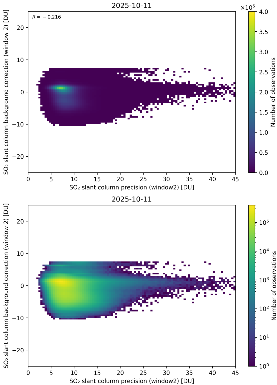
Figure 291: Scatter density plot of “SO 2 slant column precision (window2)” against “SO 2 slant column background correction (window 2)” for 2025-10-11 to 2025-10-12.
