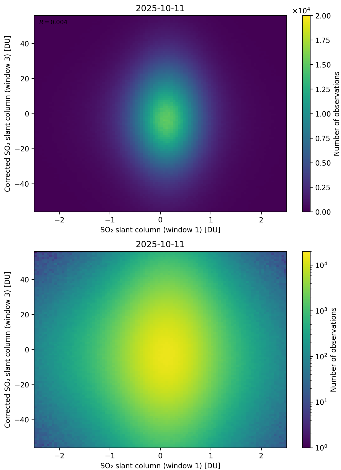
Figure 284: Scatter density plot of “SO 2 slant column (window 1)” against “Corrected SO 2 slant column (window 3)” for 2025-10-11 to 2025-10-12.
