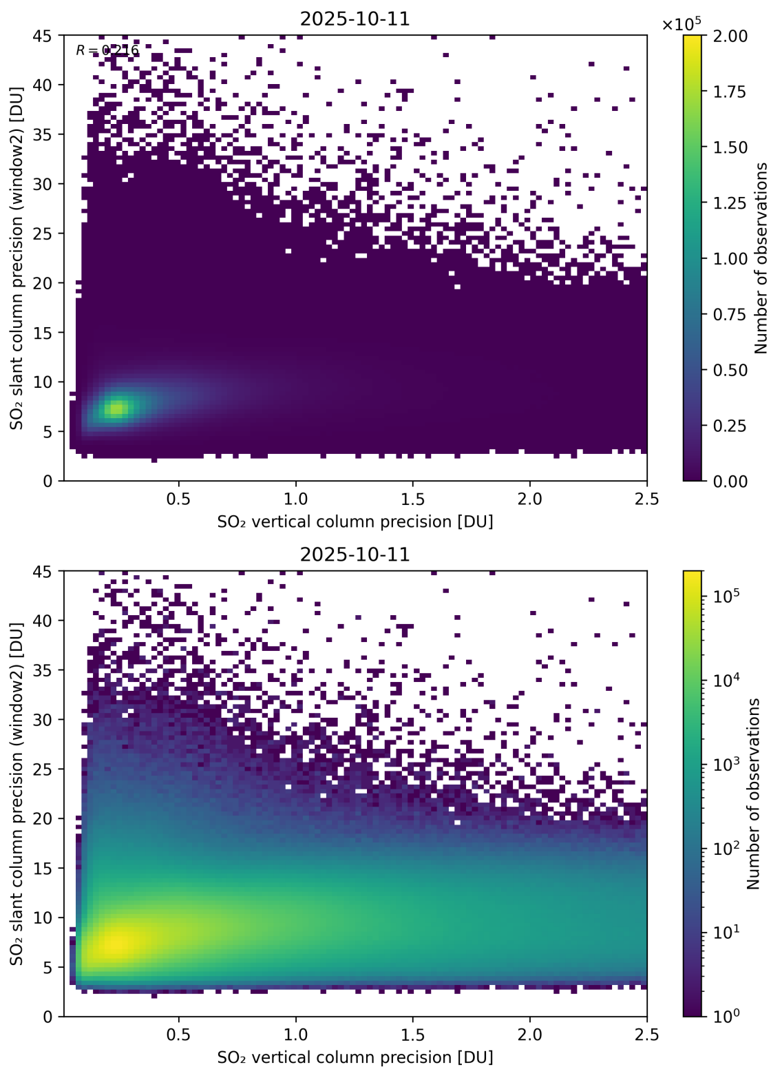
Figure 343: Scatter density plot of “SO 2 vertical column precision” against “SO 2 slant column precision (window2)” for 2025-10-11 to 2025-10-12.
