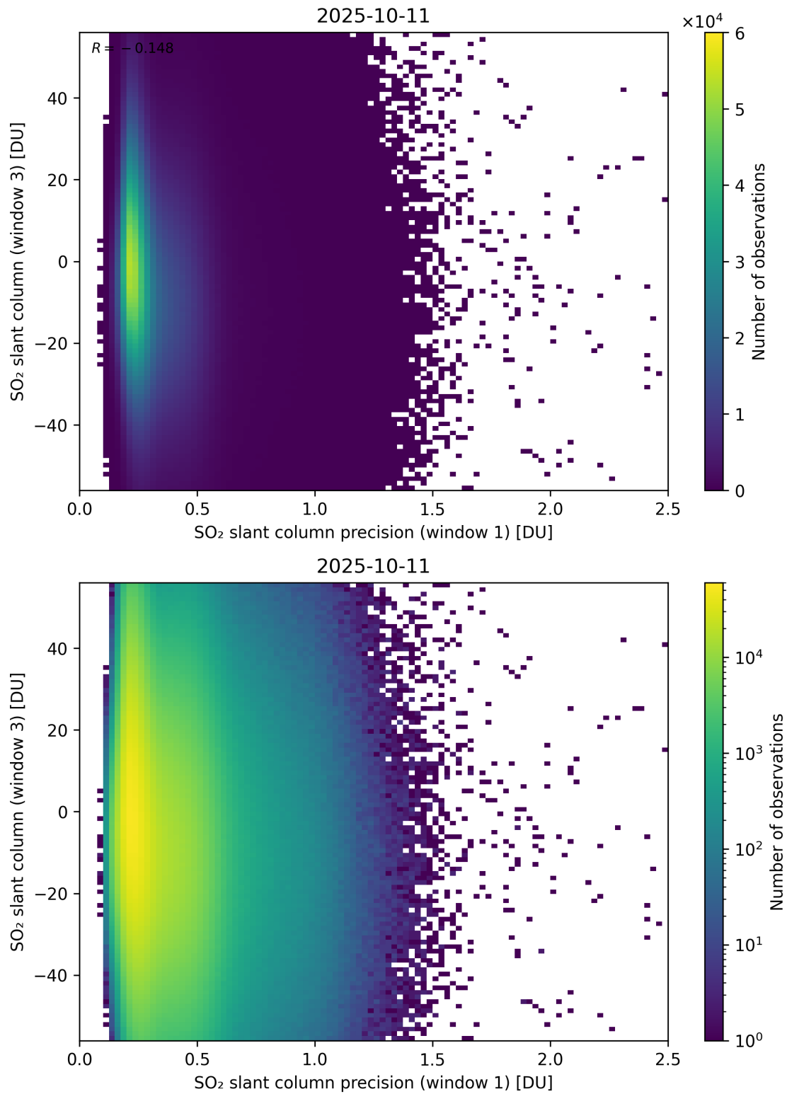
Figure 278: Scatter density plot of “SO 2 slant column precision (window 1)” against “SO 2 slant column (window 3)” for 2025-10-11 to 2025-10-12.
