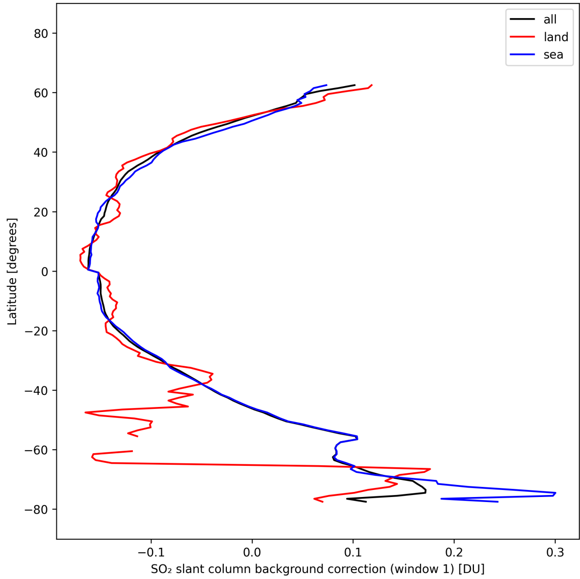
Figure 40: Zonal average of “SO 2 slant column background correction (window 1)” for 2025-10-11 to 2025-10-12.
