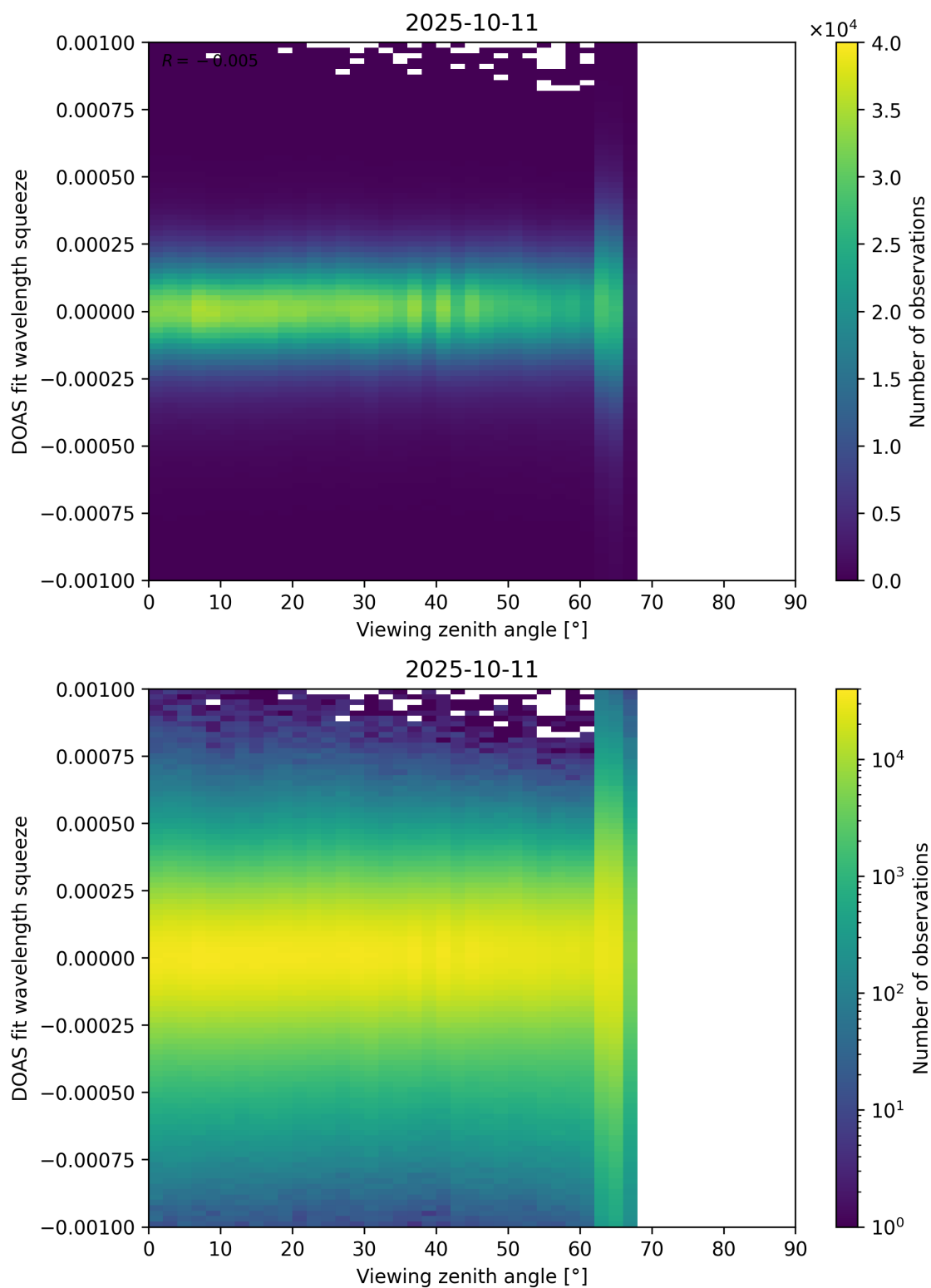
Figure 366: Scatter density plot of “Viewing zenith angle” against “DOAS fit wavelength squeeze” for 2025-10-11 to 2025-10-12.
