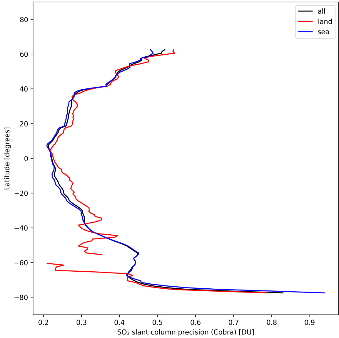
Figure 36: Zonal average of “SO 2 slant column precision (Cobra)” for 2025-10-11 to 2025-10-12.
