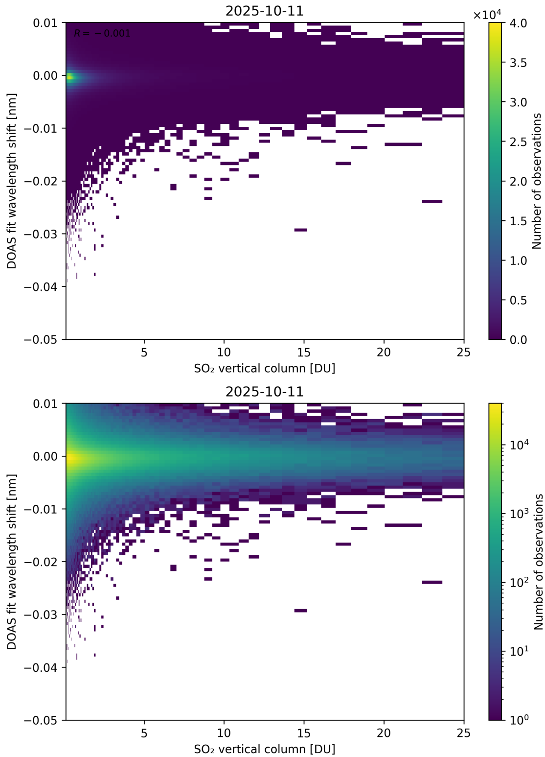
Figure 326: Scatter density plot of “SO 2 vertical column” against “DOAS fit wavelength shift” for 2025-10-11 to 2025-10-12.
