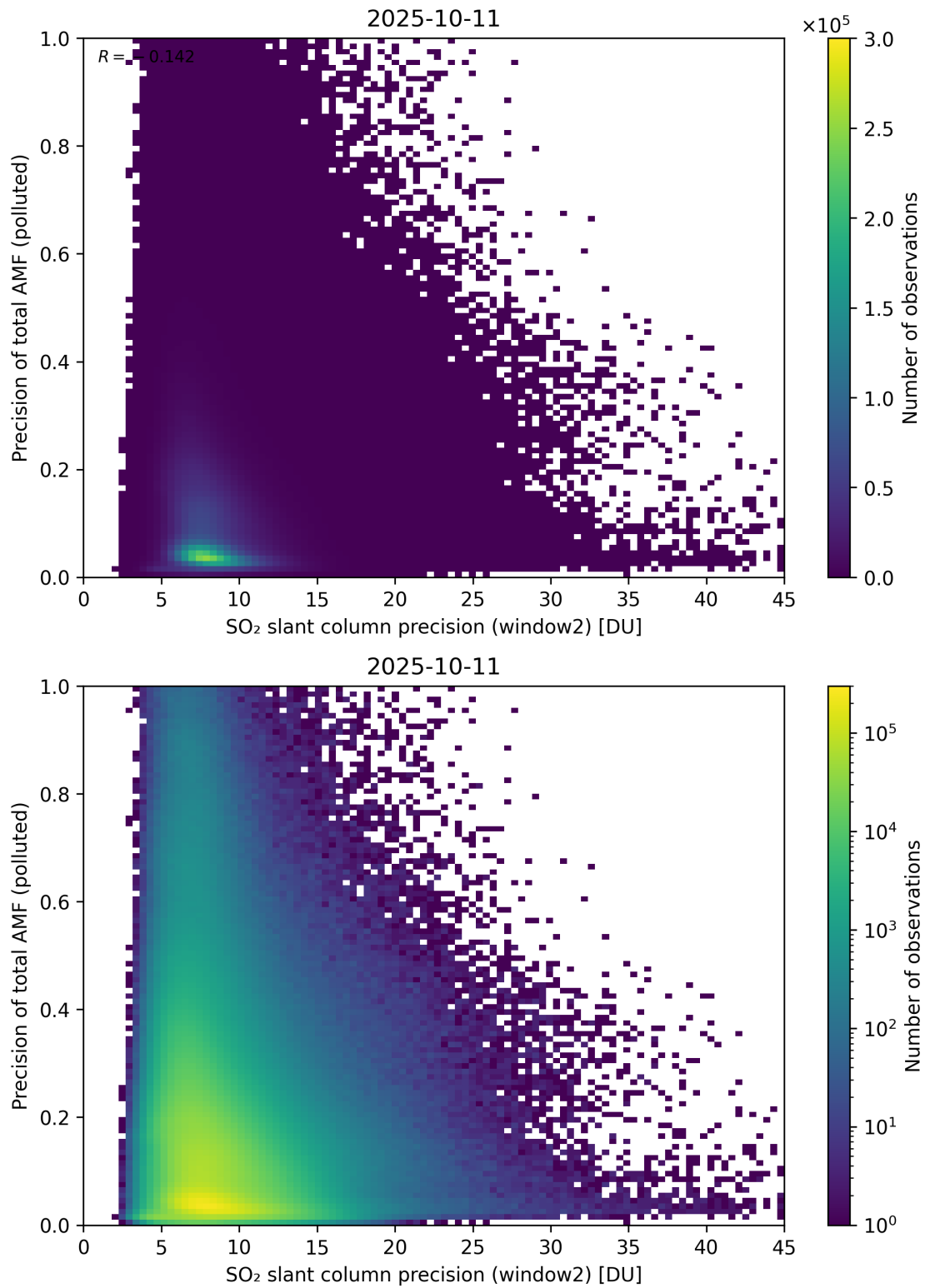
Figure 302: Scatter density plot of “SO 2 slant column precision (window2)” against “Precision of total AMF (polluted)” for 2025-10-11 to 2025-10-12.
