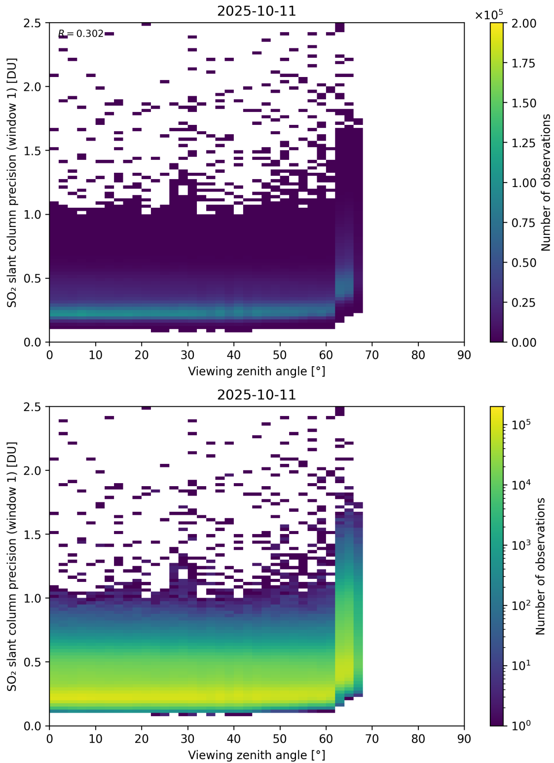
Figure 377: Scatter density plot of “Viewing zenith angle” against “SO 2 slant column precision (window 1)” for 2025-10-11 to 2025-10-12.
