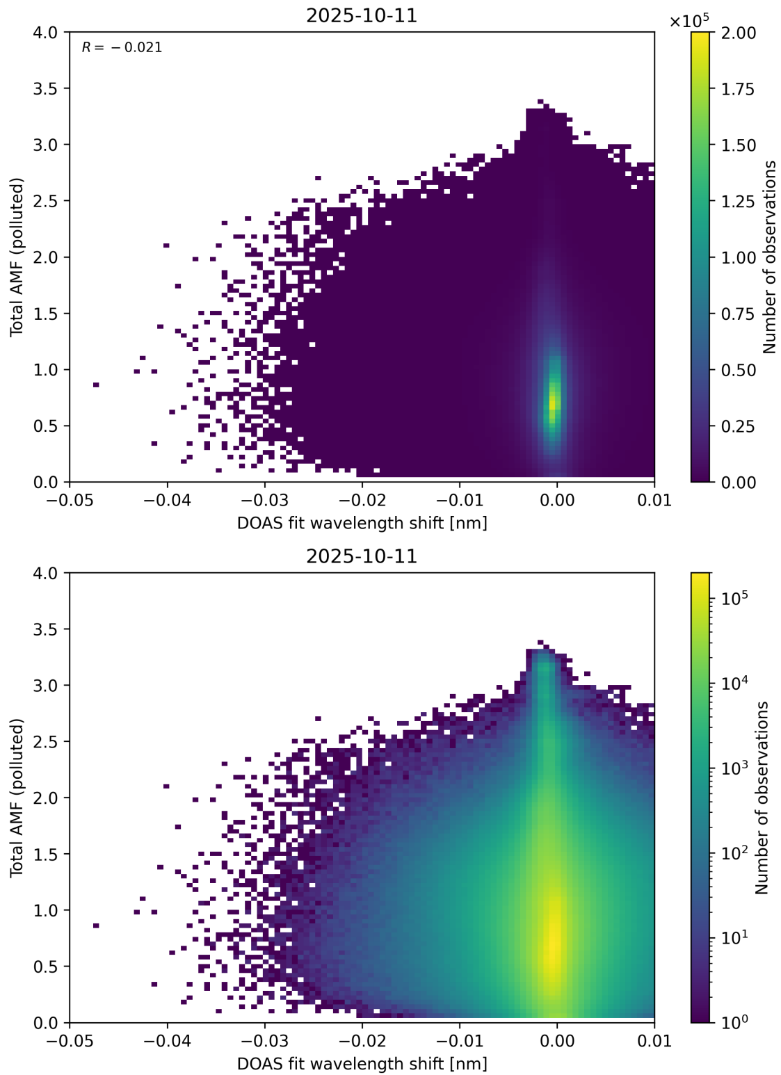
Figure 141: Scatter density plot of “DOAS fit wavelength shift” against “Total AMF (polluted)” for 2025-10-11 to 2025-10-12.
