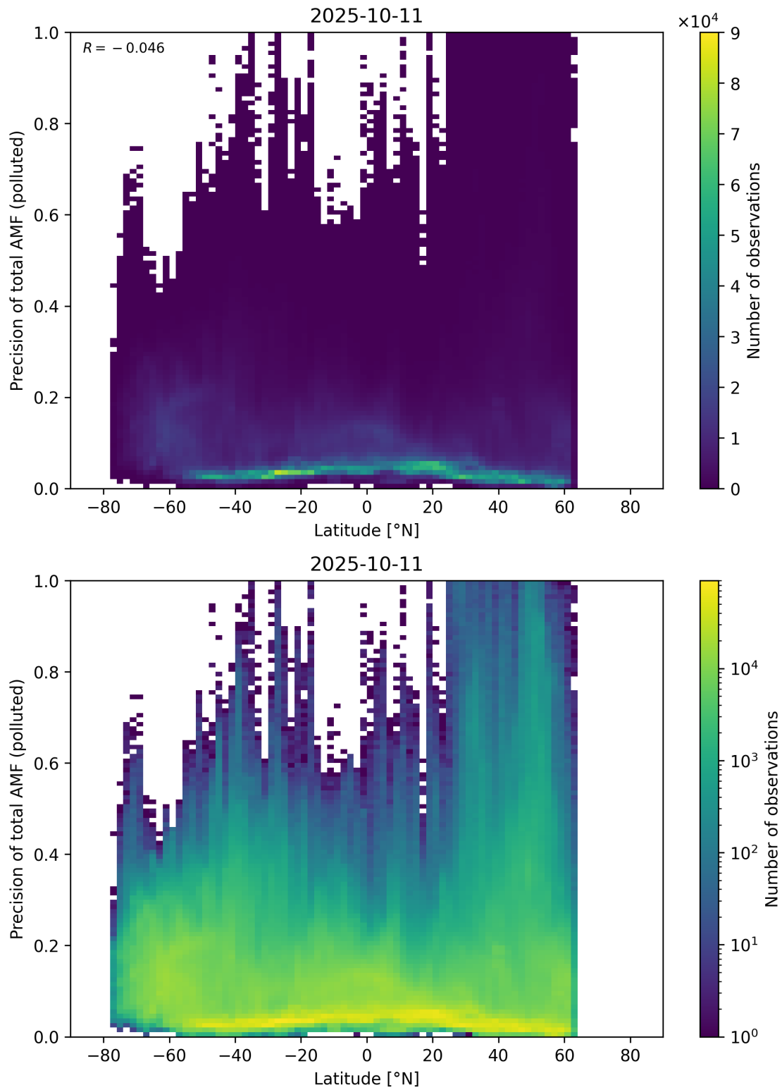
Figure 168: Scatter density plot of “Latitude” against “Precision of total AMF (polluted)” for 2025-10-11 to 2025-10-12.
