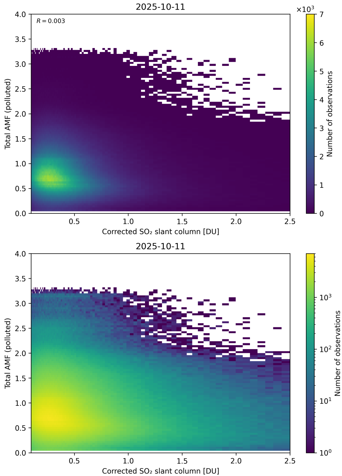
Figure 242: Scatter density plot of “Corrected SO 2 slant column” against “Total AMF (polluted)” for 2025-10-11 to 2025-10-12.
