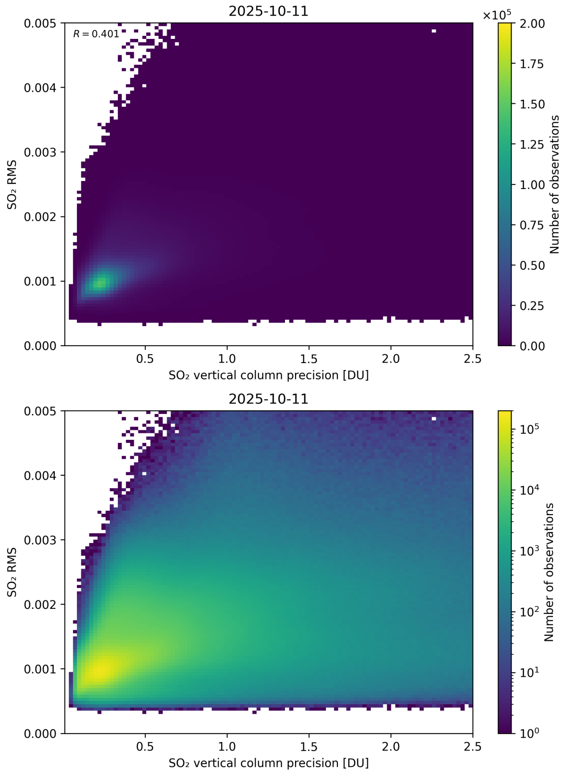
Figure 334: Scatter density plot of “SO 2 vertical column precision” against “SO 2 RMS” for 2025-10-11 to 2025-10-12.
