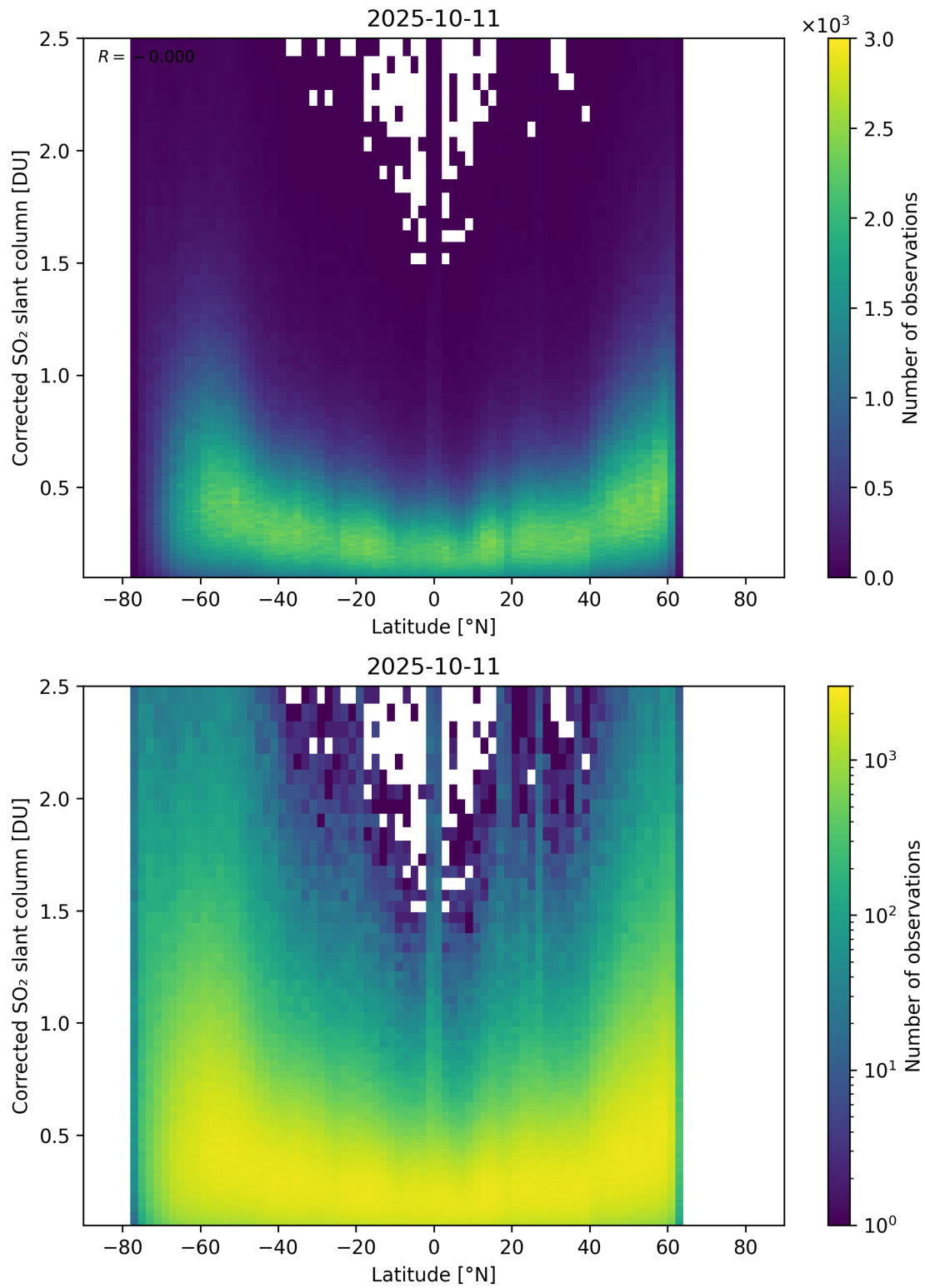
Figure 159: Scatter density plot of “Latitude” against “Corrected SO 2 slant column” for 2025-10-11 to 2025-10-12.
