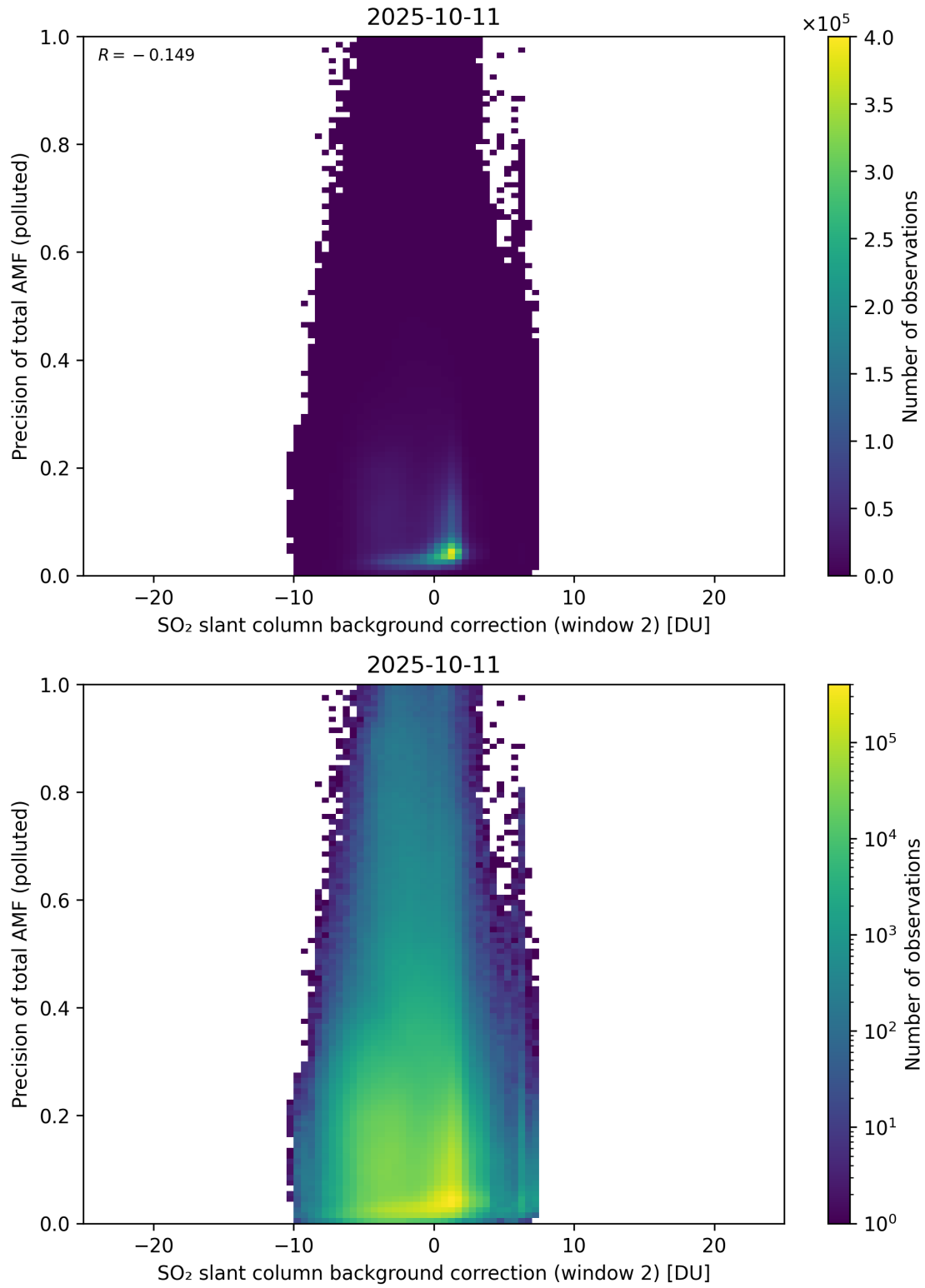
Figure 131: Scatter density plot of “SO 2 slant column background correction (window 2)” against “Precision of total AMF (polluted)” for 2025-10-11 to 2025-10-12.
