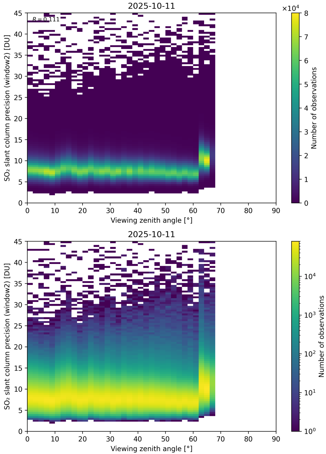
Figure 378: Scatter density plot of “Viewing zenith angle” against “SO 2 slant column precision (window2)” for 2025-10-11 to 2025-10-12.
