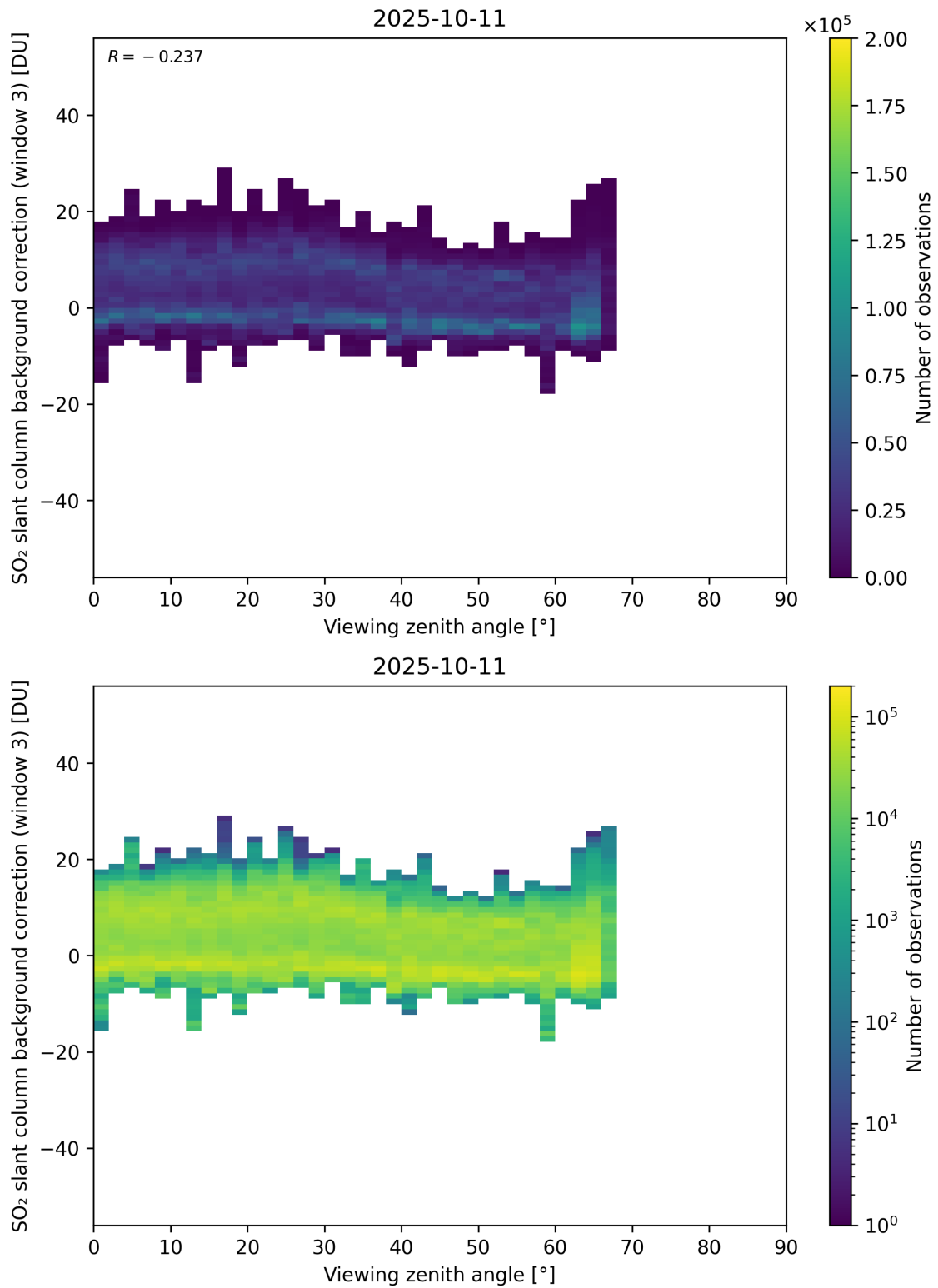
Figure 364: Scatter density plot of “Viewing zenith angle” against “SO 2 slant column background correction (window 3)” for 2025-10-11 to 2025-10-12.
