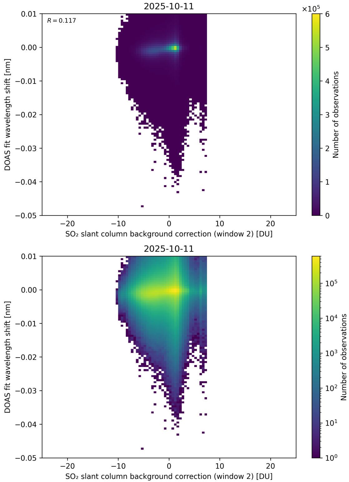
Figure 123: Scatter density plot of “SO 2 slant column background correction (window 2)” against “DOAS fit wavelength shift” for 2025-10-11 to 2025-10-12.
