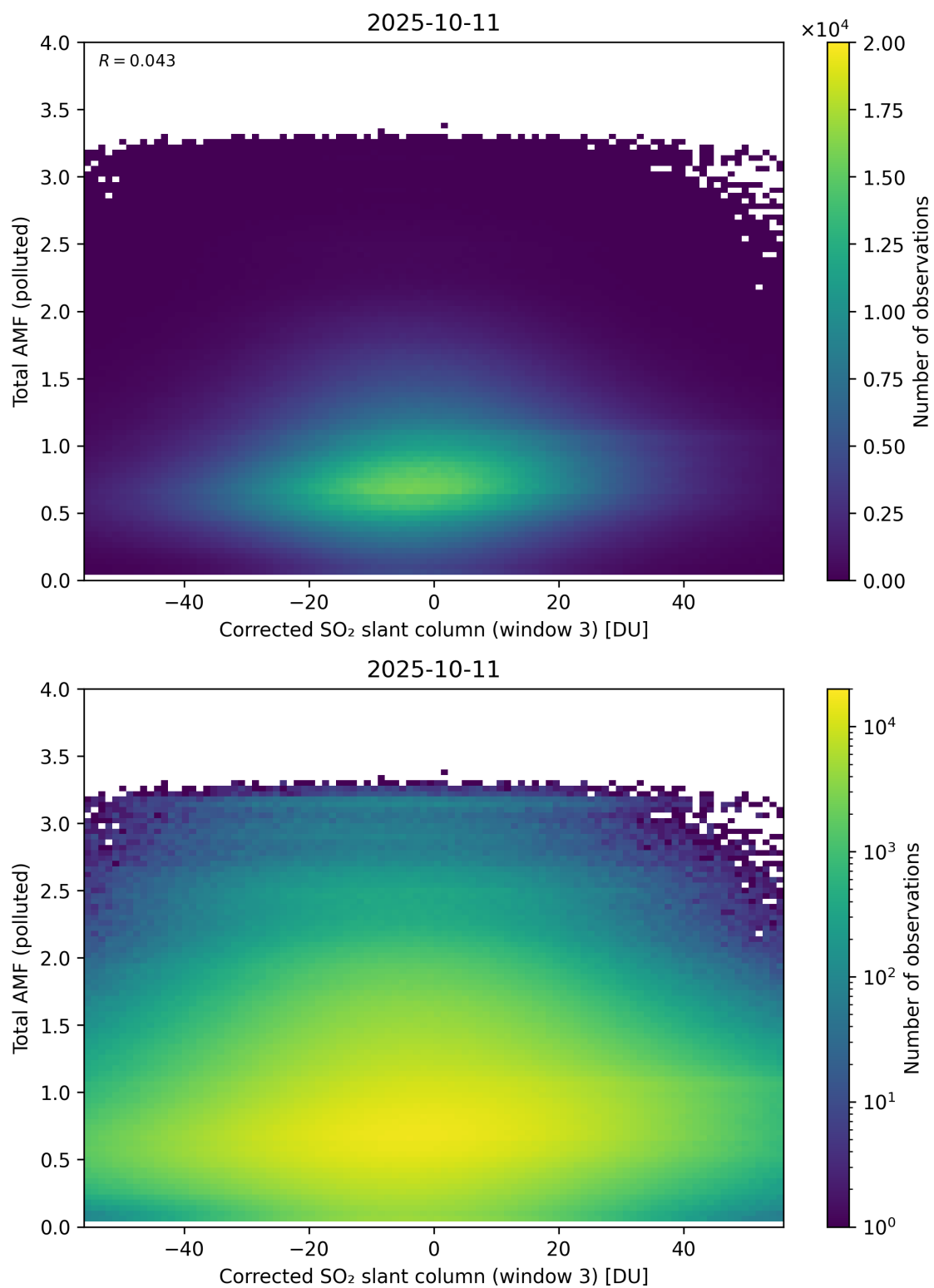
Figure 260: Scatter density plot of “Corrected SO 2 slant column (window 3)” against “Total AMF (polluted)” for 2025-10-11 to 2025-10-12.
