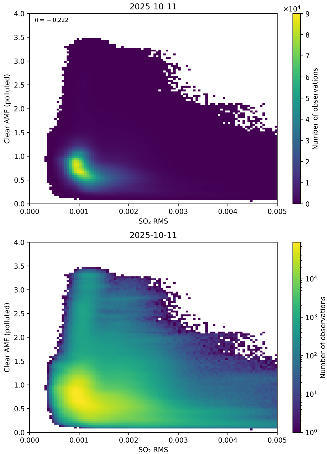
Figure 147: Scatter density plot of “SO 2 RMS” against “Clear AMF (polluted)” for 2025-10-11 to 2025-10-12.
