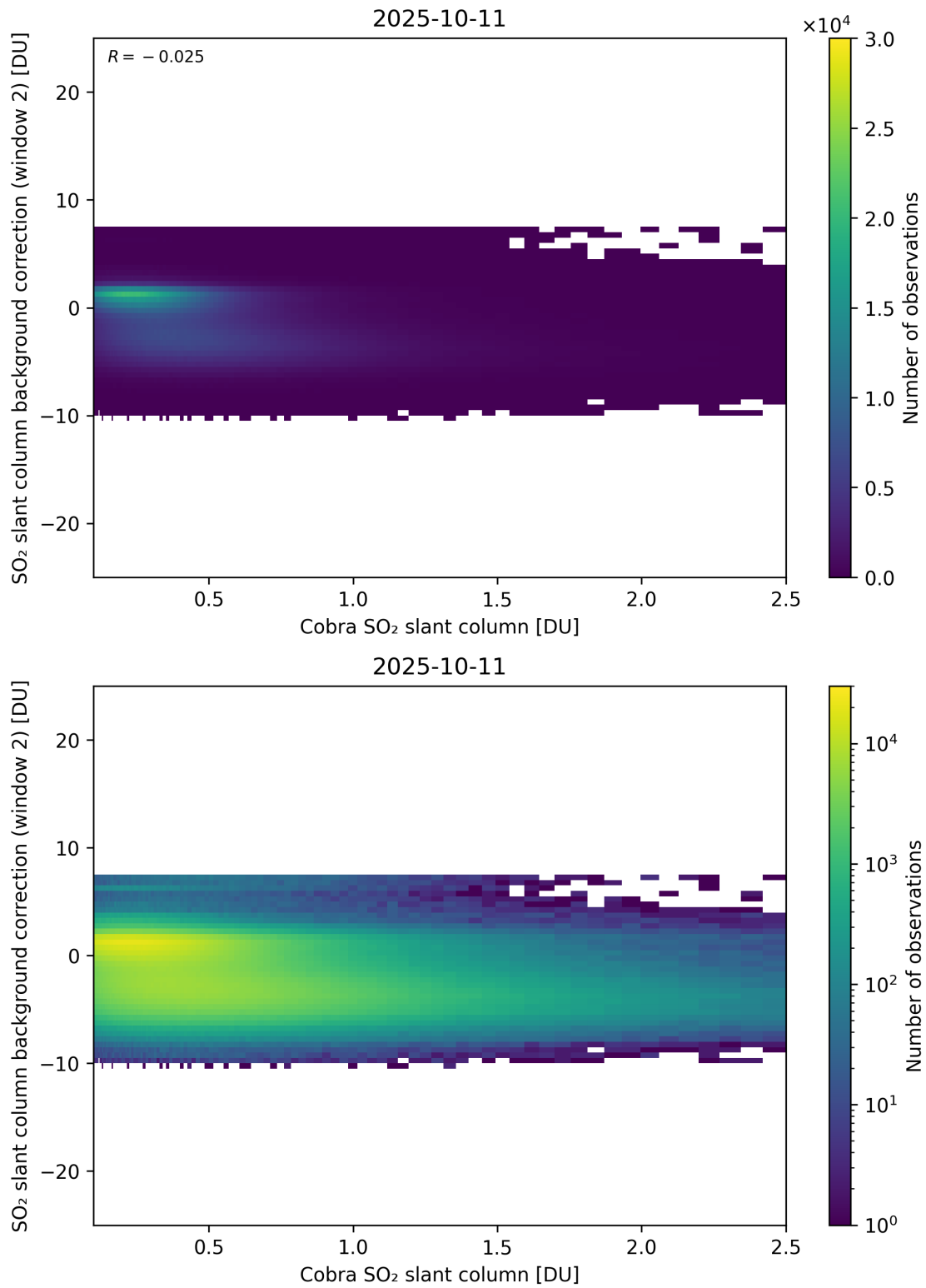
Figure 194: Scatter density plot of “Cobra SO 2 slant column” against “SO 2 slant column background correction (window 2)” for 2025-10-11 to 2025-10-12.
