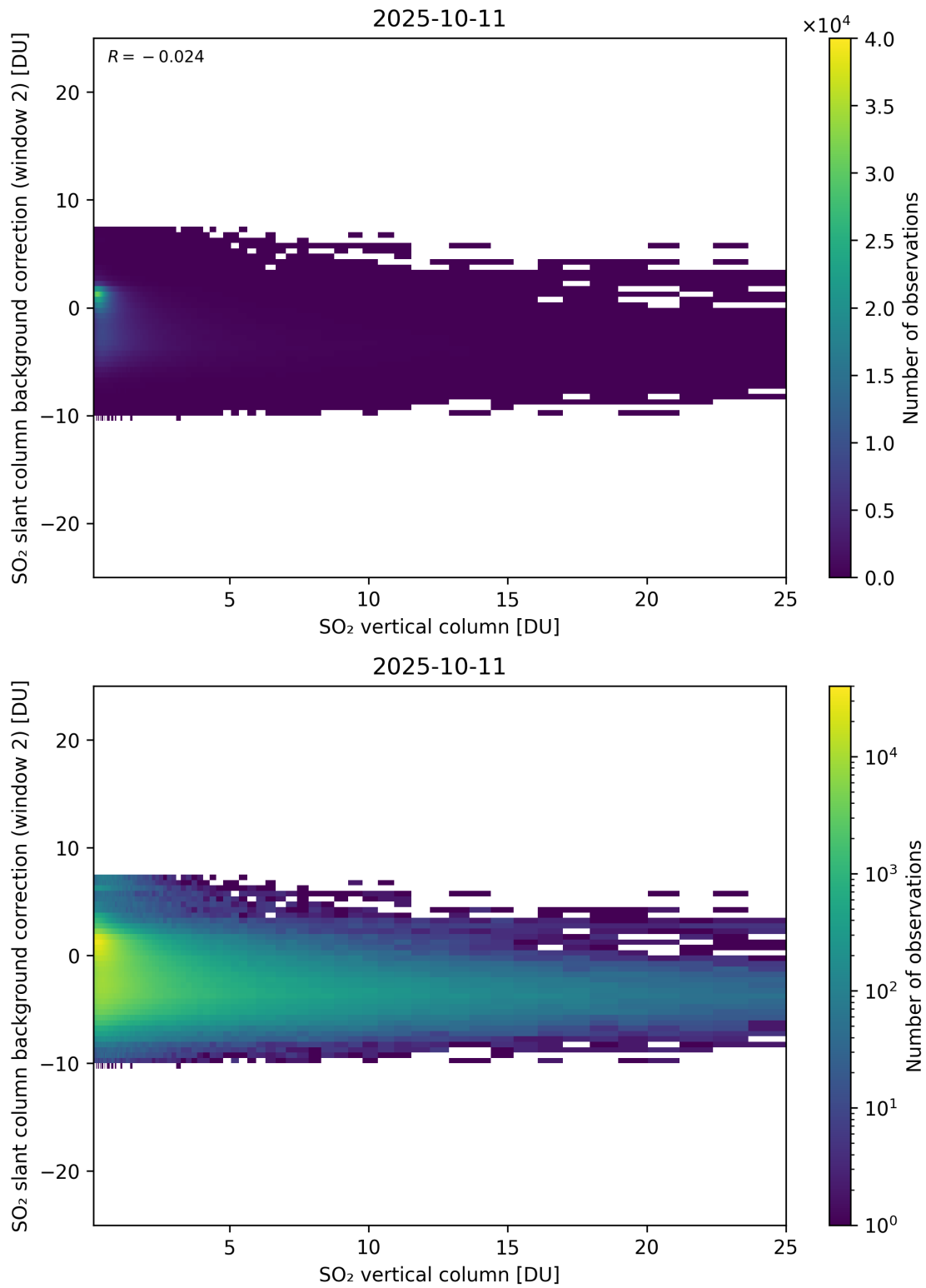
Figure 324: Scatter density plot of “SO 2 vertical column” against “SO 2 slant column background correction (window 2)” for 2025-10-11 to 2025-10-12.
