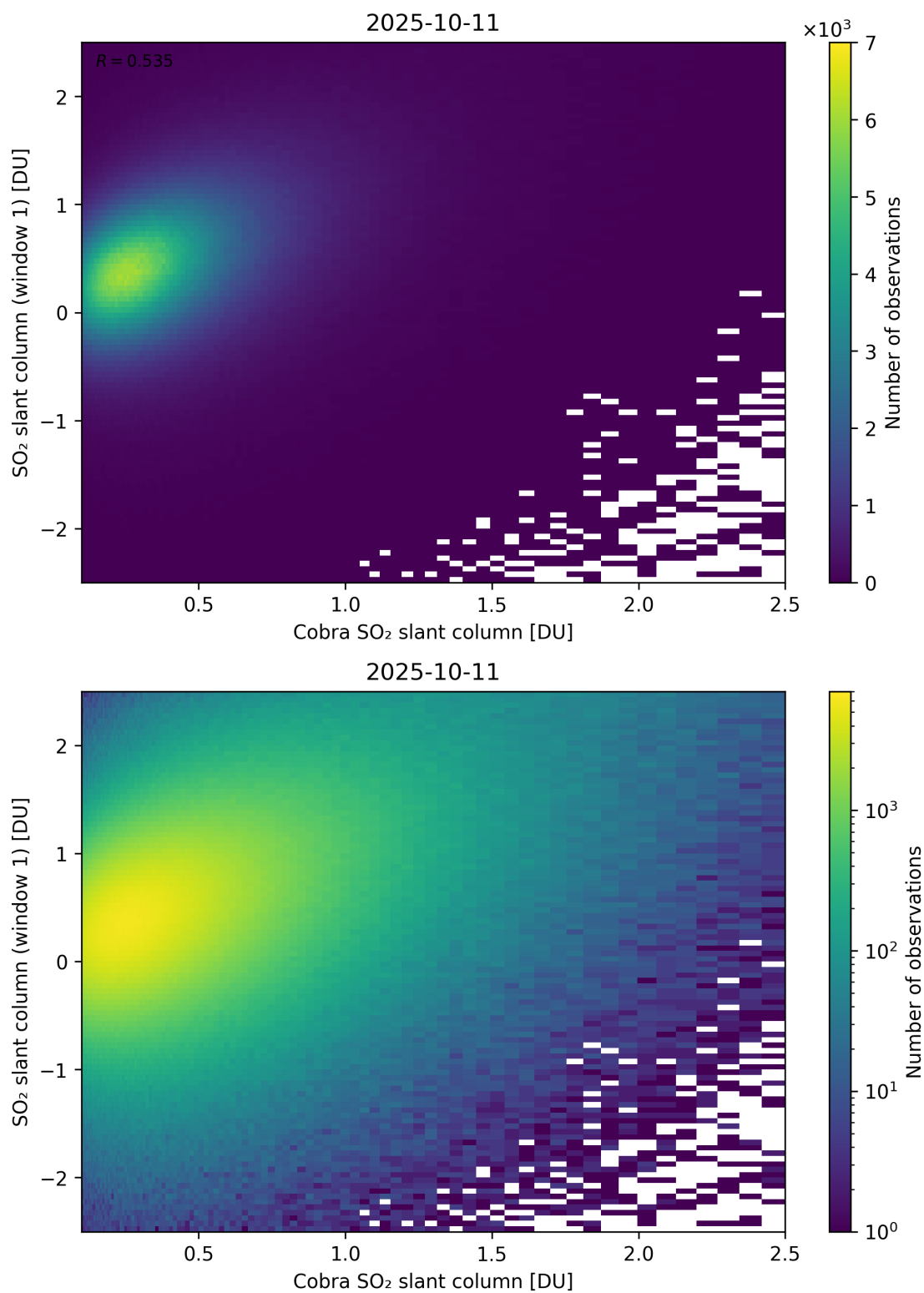
Figure 219: Scatter density plot of “Cobra SO 2 slant column” against “SO 2 slant column (window 1)” for 2025-10-11 to 2025-10-12.
