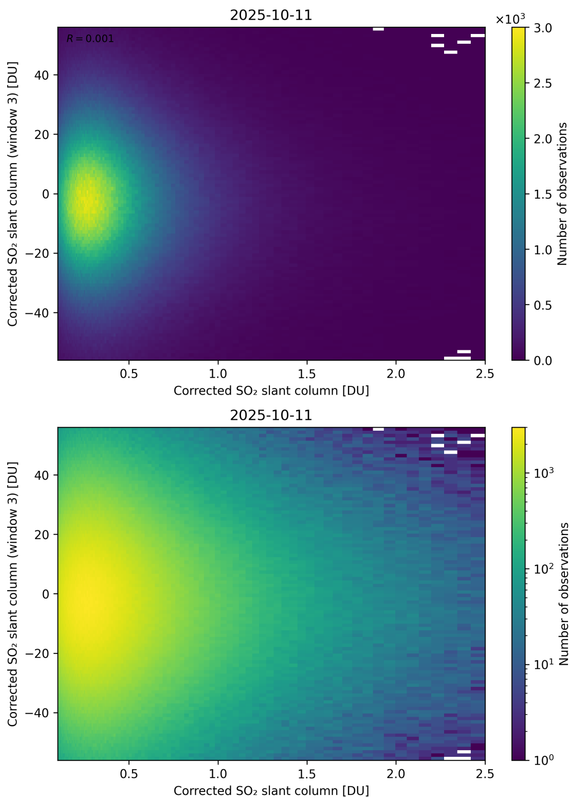
Figure 236: Scatter density plot of “Corrected SO 2 slant column” against “Corrected SO 2 slant column (window 3)” for 2025-10-11 to 2025-10-12.
