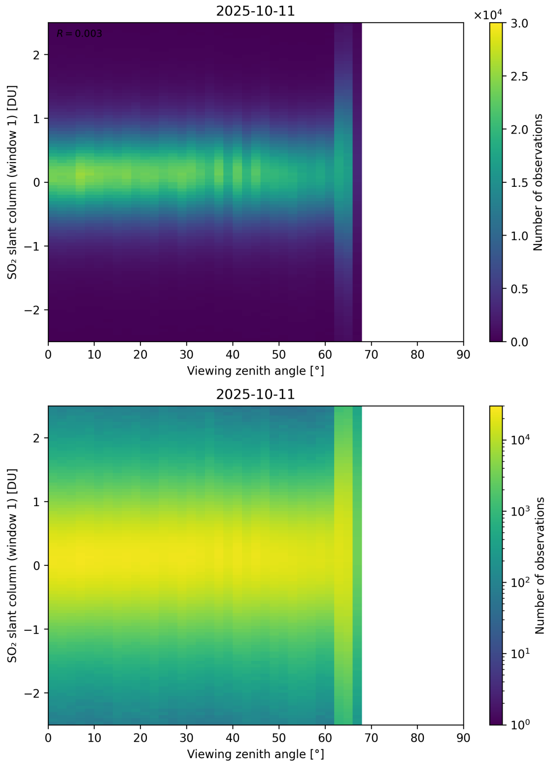
Figure 376: Scatter density plot of “Viewing zenith angle” against “SO 2 slant column (window 1)” for 2025-10-11 to 2025-10-12.
