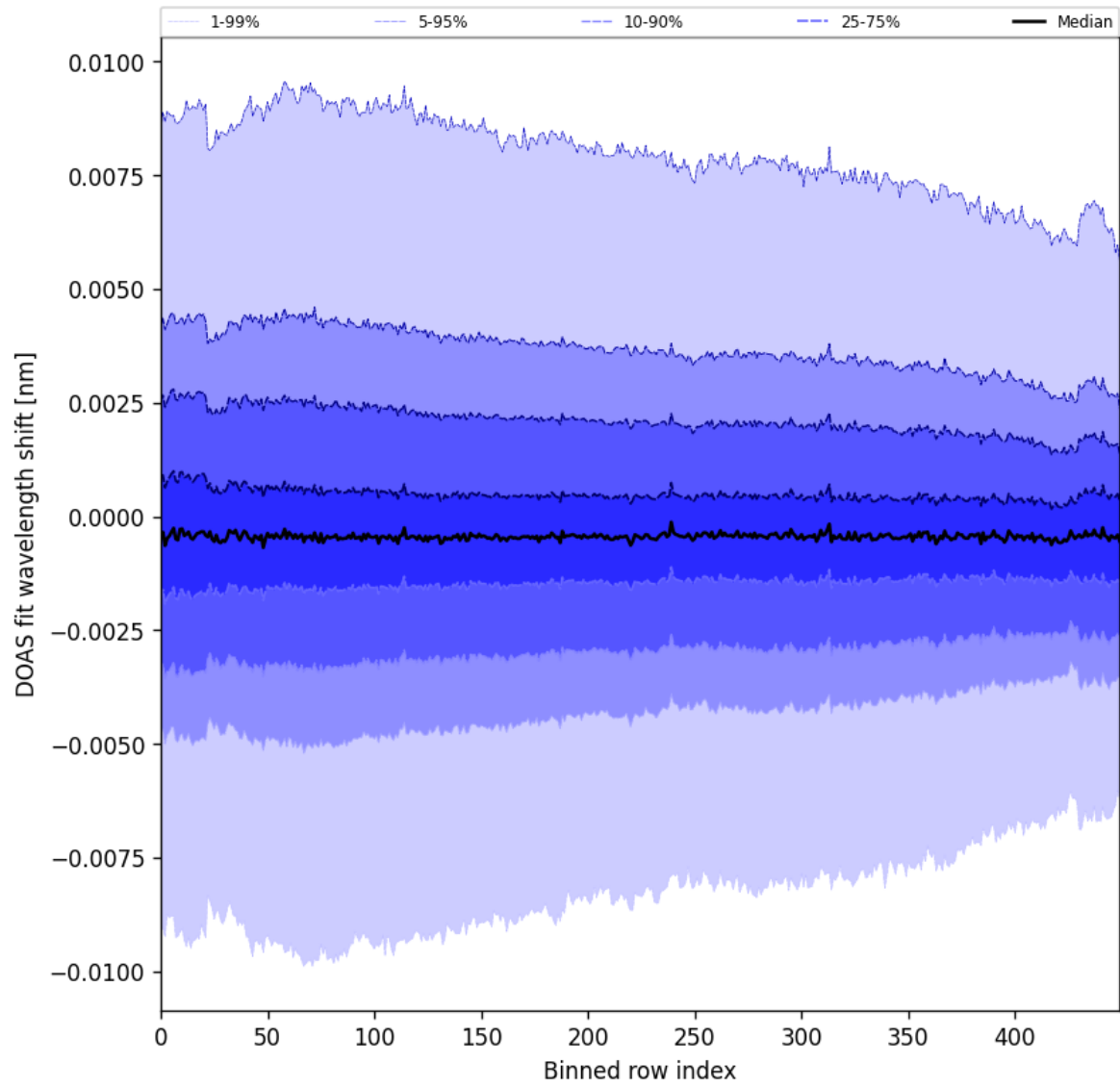
Figure 102: Along track statistics of “DOAS fit wavelength shift” for 2025-10-11 to 2025-10-12
