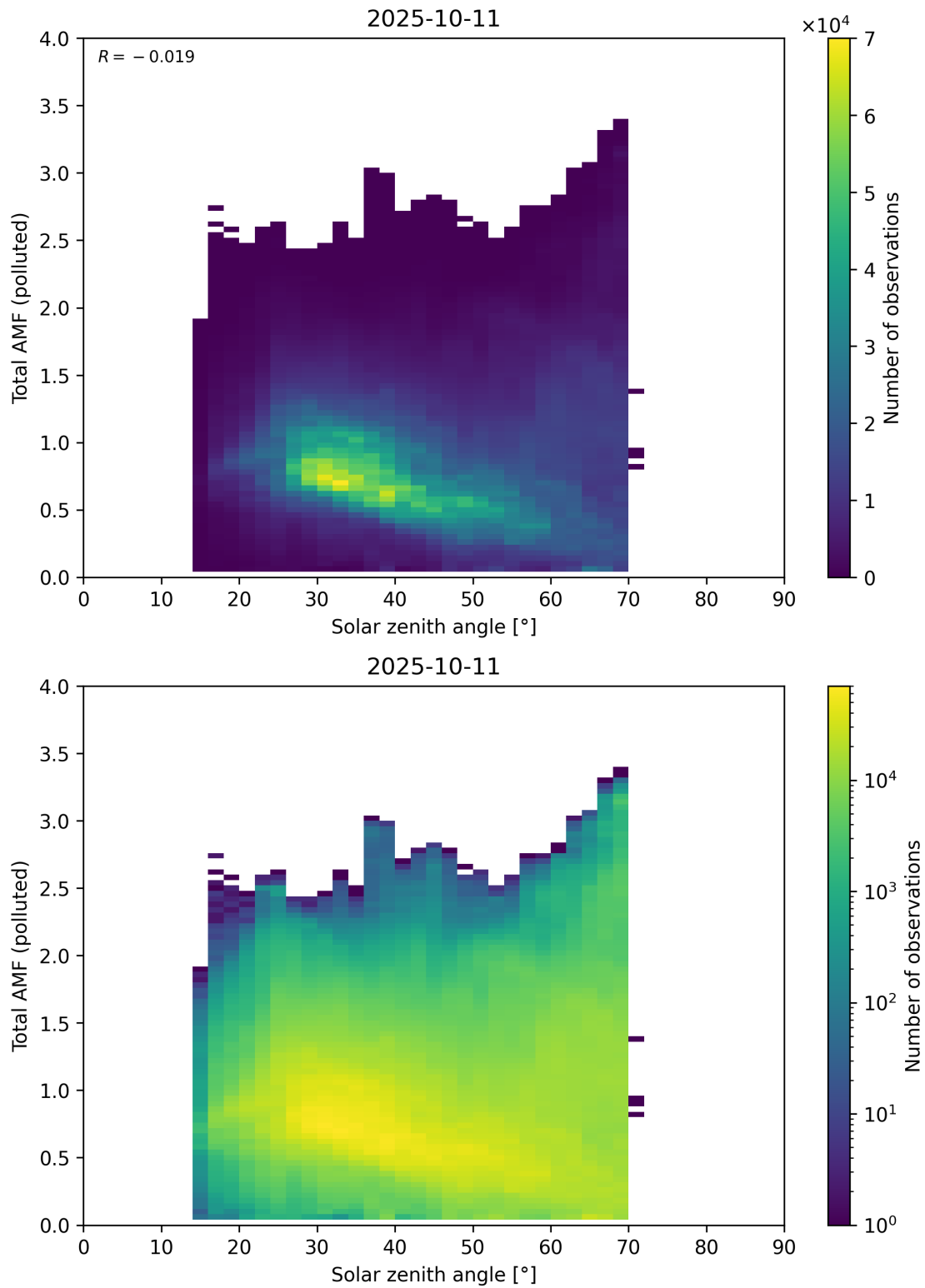
Figure 189: Scatter density plot of “Solar zenith angle” against “Total AMF (polluted)” for 2025-10-11 to 2025-10-12.
