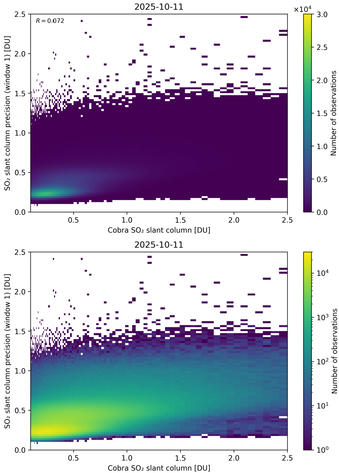
Figure 220: Scatter density plot of “Cobra SO 2 slant column” against “SO 2 slant column precision (window 1)” for 2025-10-11 to 2025-10-12.
