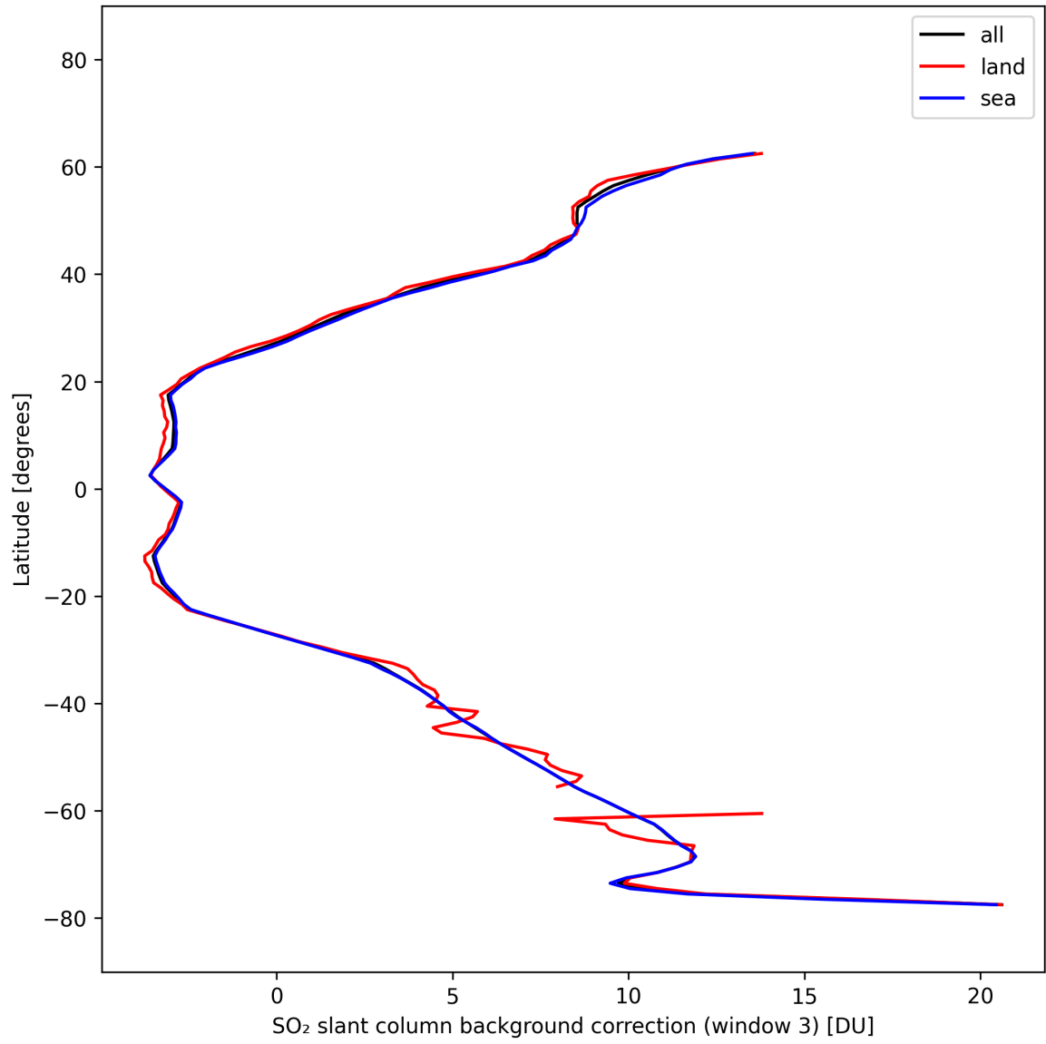
Figure 48: Zonal average of “SO 2 slant column background correction (window 3)” for 2025-10-11 to 2025-10-12.
