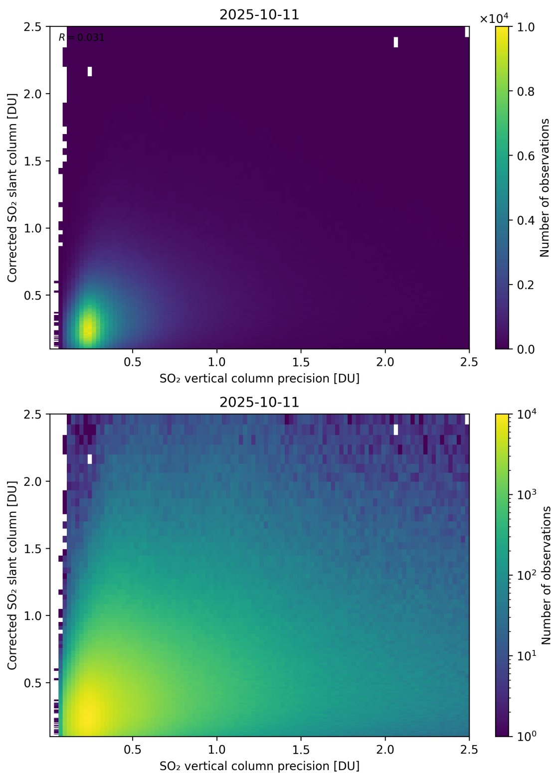
Figure 338: Scatter density plot of “SO 2 vertical column precision” against “Corrected SO 2 slant column” for 2025-10-11 to 2025-10-12.
