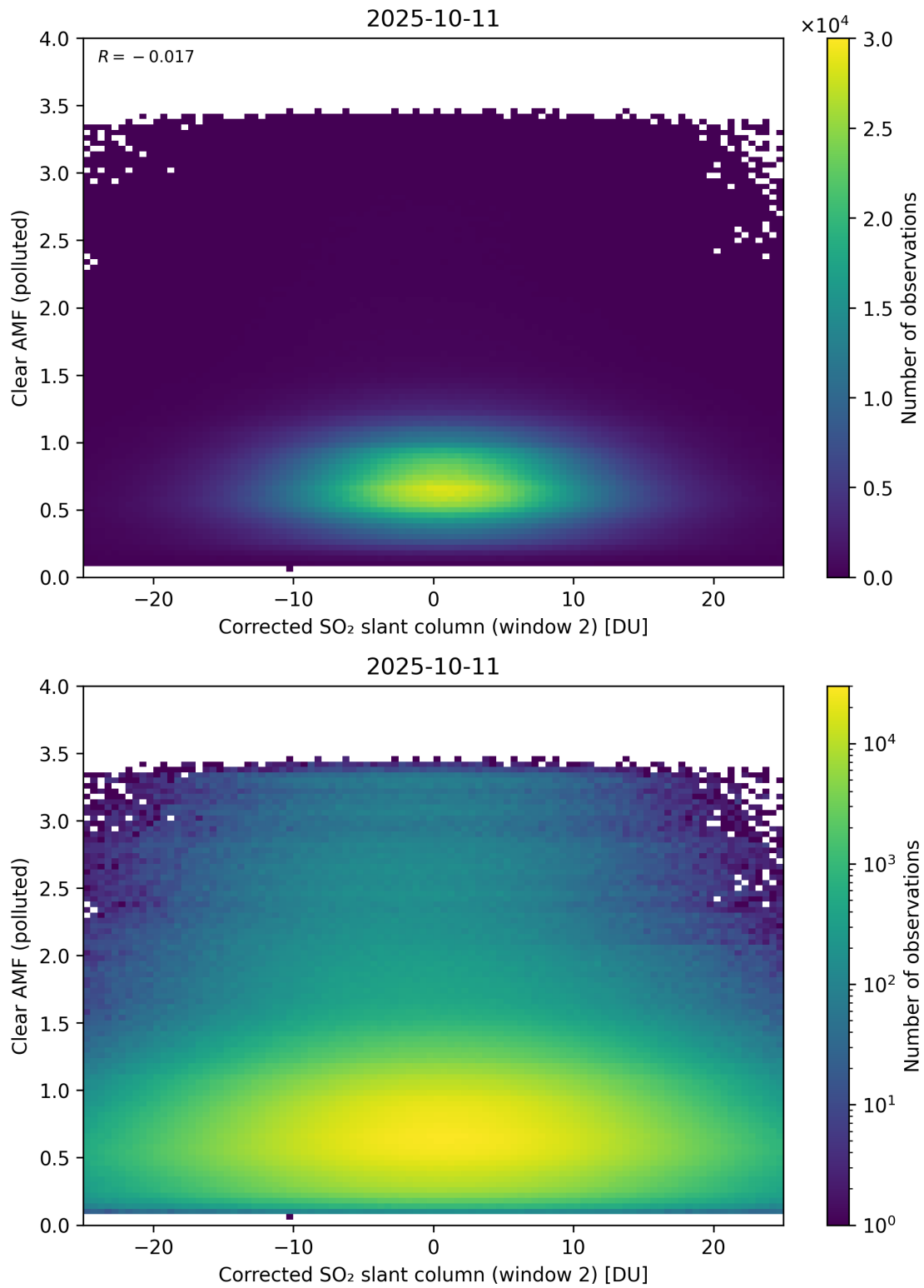
Figure 249: Scatter density plot of “Corrected SO 2 slant column (window 2)” against “Clear AMF (polluted)” for 2025-10-11 to 2025-10-12.
