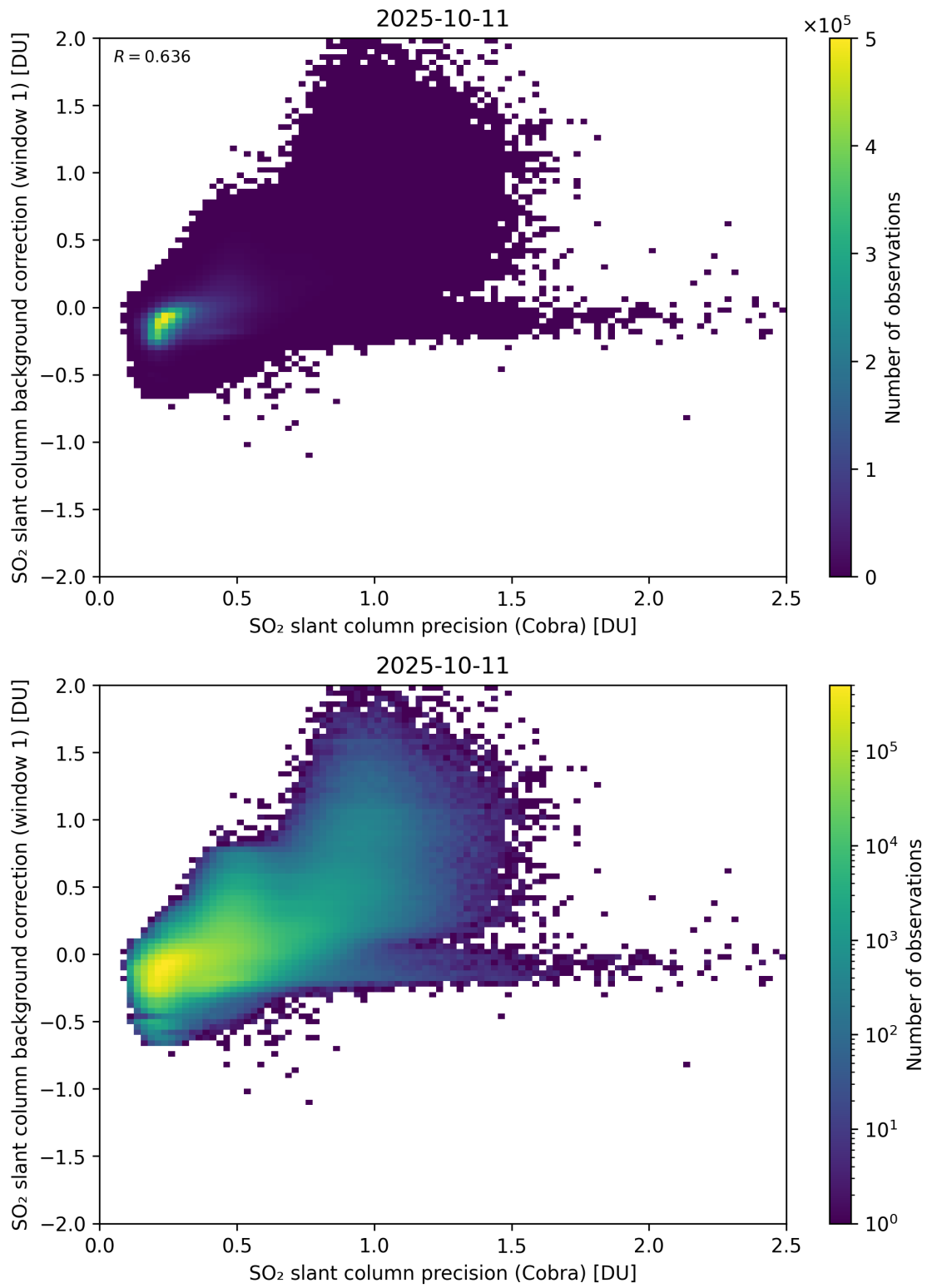
Figure 199: Scatter density plot of “SO 2 slant column precision (Cobra)” against “SO 2 slant column background correction (window 1)” for 2025-10-11 to 2025-10-12.
