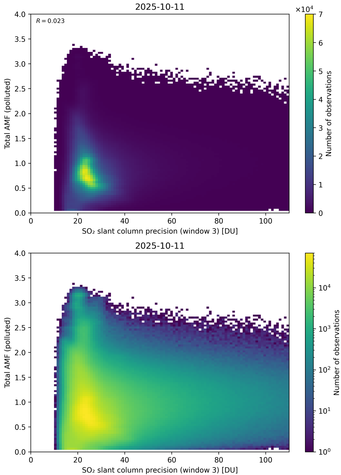
Figure 313: Scatter density plot of “SO 2 slant column precision (window 3)” against “Total AMF (polluted)” for 2025-10-11 to 2025-10-12.
