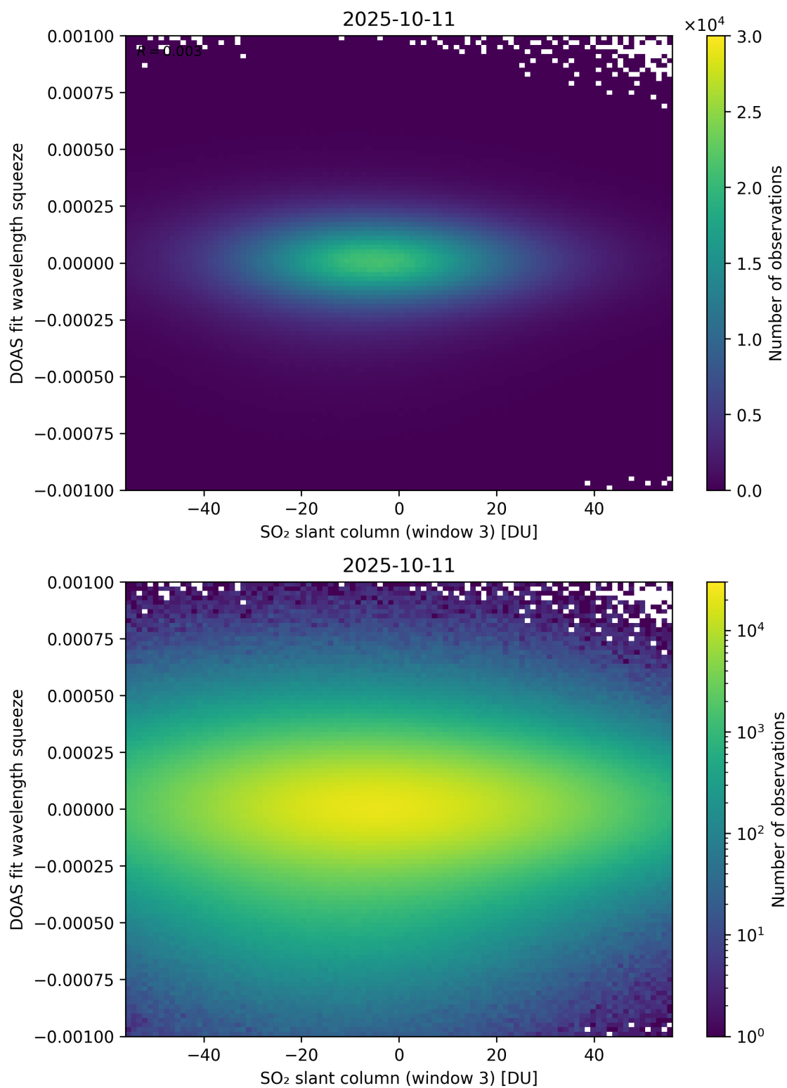
Figure 305: Scatter density plot of “SO 2 slant column (window 3)” against “DOAS fit wavelength squeeze” for 2025-10-11 to 2025-10-12.
