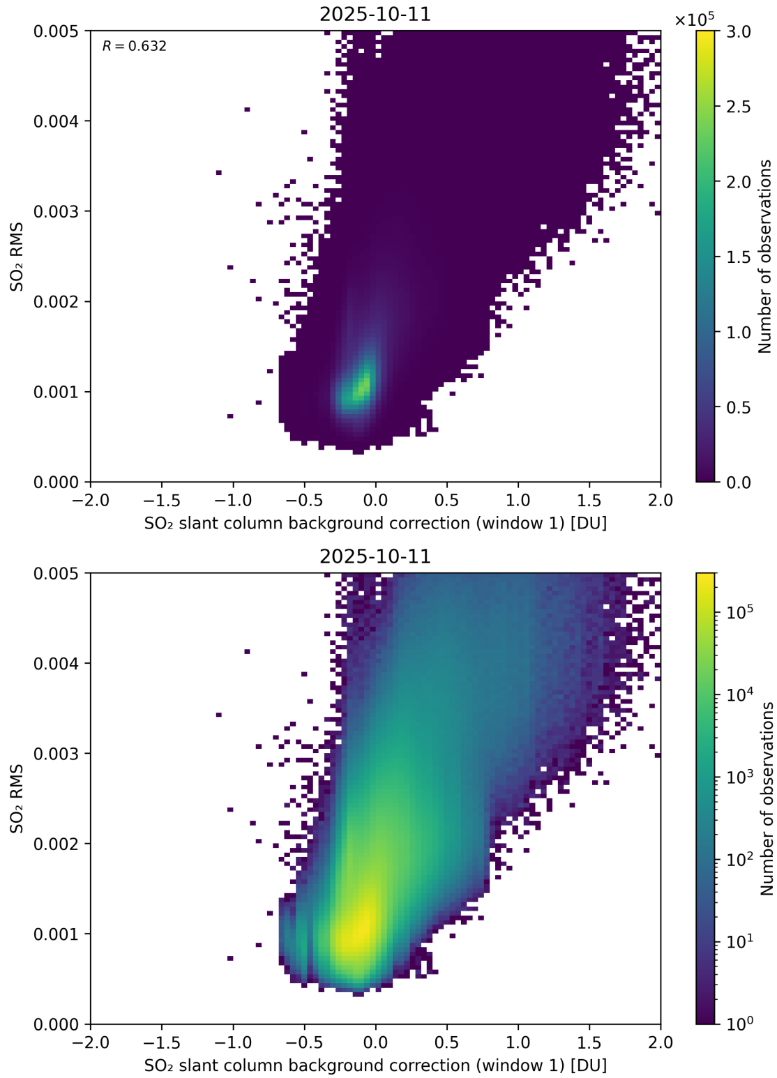
Figure 113: Scatter density plot of “SO 2 slant column background correction (window 1)” against “SO 2 RMS” for 2025-10-11 to 2025-10-12.
