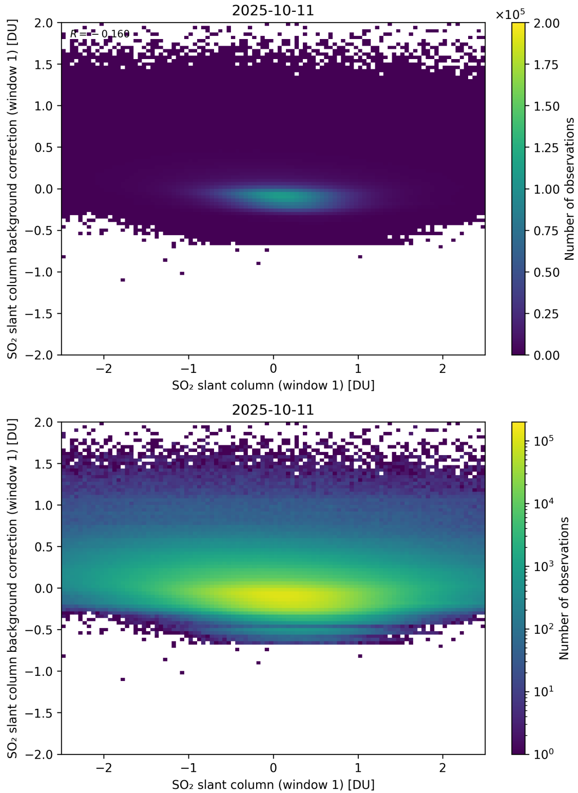
Figure 262: Scatter density plot of “SO 2 slant column (window 1)” against “SO 2 slant column background correction (window 1)” for 2025-10-11 to 2025-10-12.
