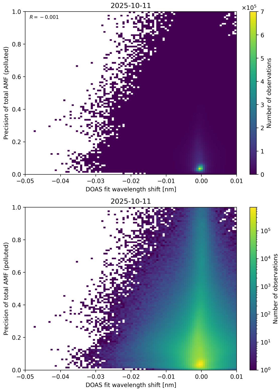
Figure 142: Scatter density plot of “DOAS fit wavelength shift” against “Precision of total AMF (polluted)” for 2025-10-11 to 2025-10-12.
