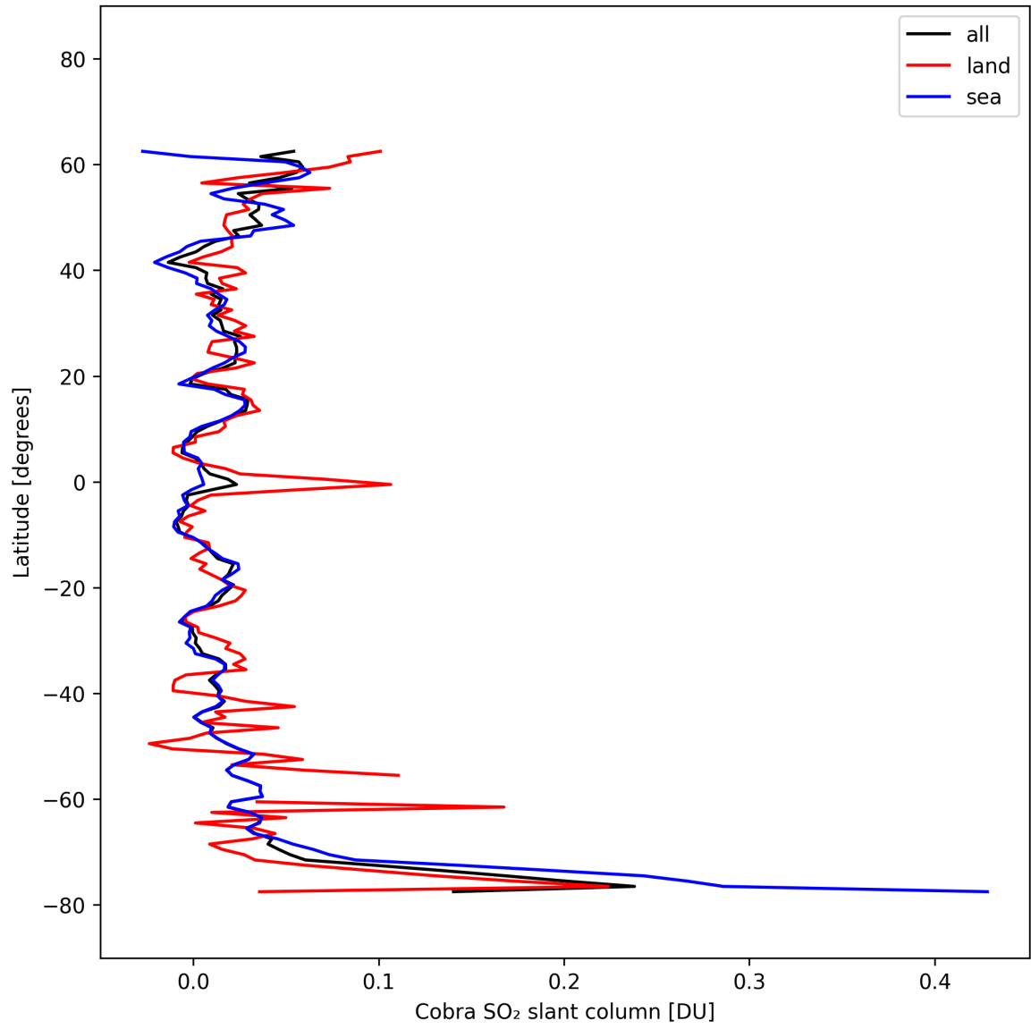
Figure 35: Zonal average of “Cobra SO 2 slant column” for 2025-10-11 to 2025-10-12.
