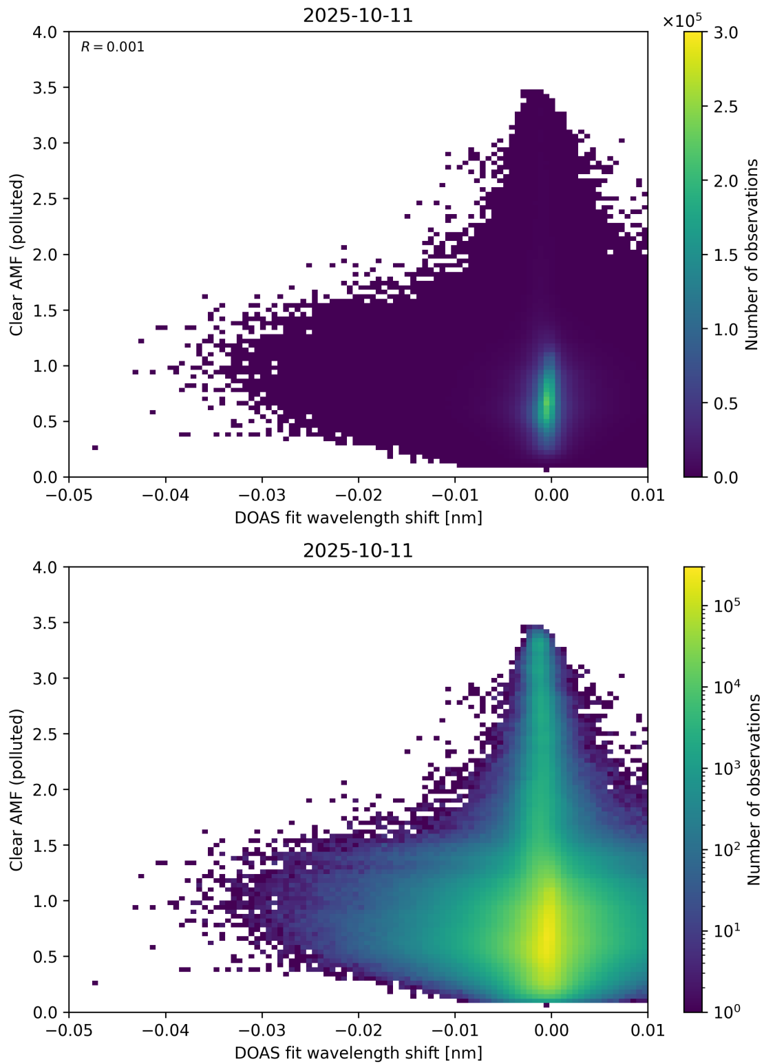
Figure 140: Scatter density plot of “DOAS fit wavelength shift” against “Clear AMF (polluted)” for 2025-10-11 to 2025-10-12.
