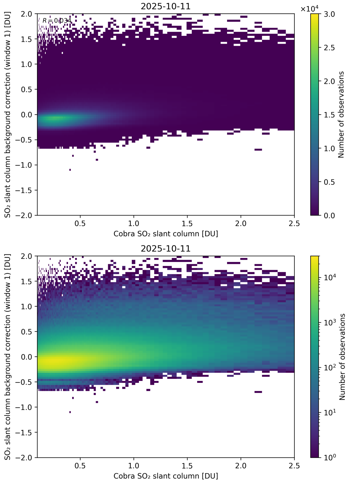
Figure 193: Scatter density plot of “Cobra SO 2 slant column” against “SO 2 slant column background correction (window 1)” for 2025-10-11 to 2025-10-12.
