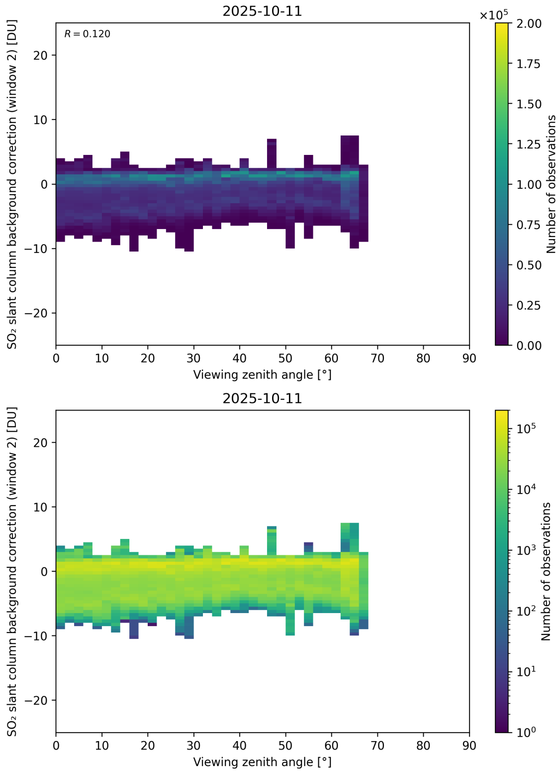
Figure 363: Scatter density plot of “Viewing zenith angle” against “SO 2 slant column background correction (window 2)” for 2025-10-11 to 2025-10-12.
