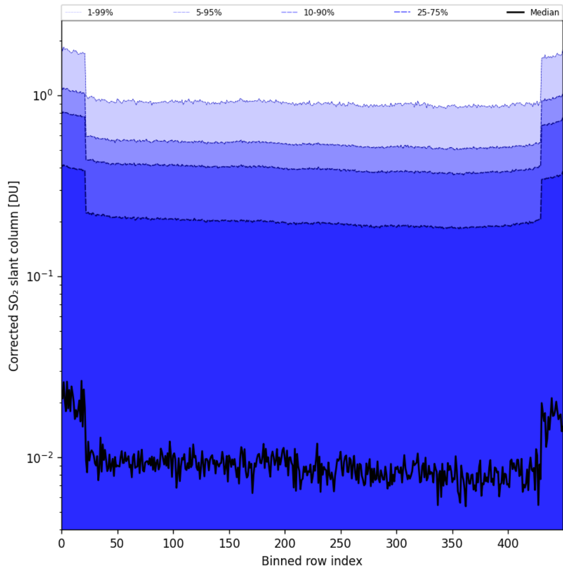
Figure 86: Along track statistics of “Corrected SO 2 slant column” for 2025-10-11 to 2025-10-12
