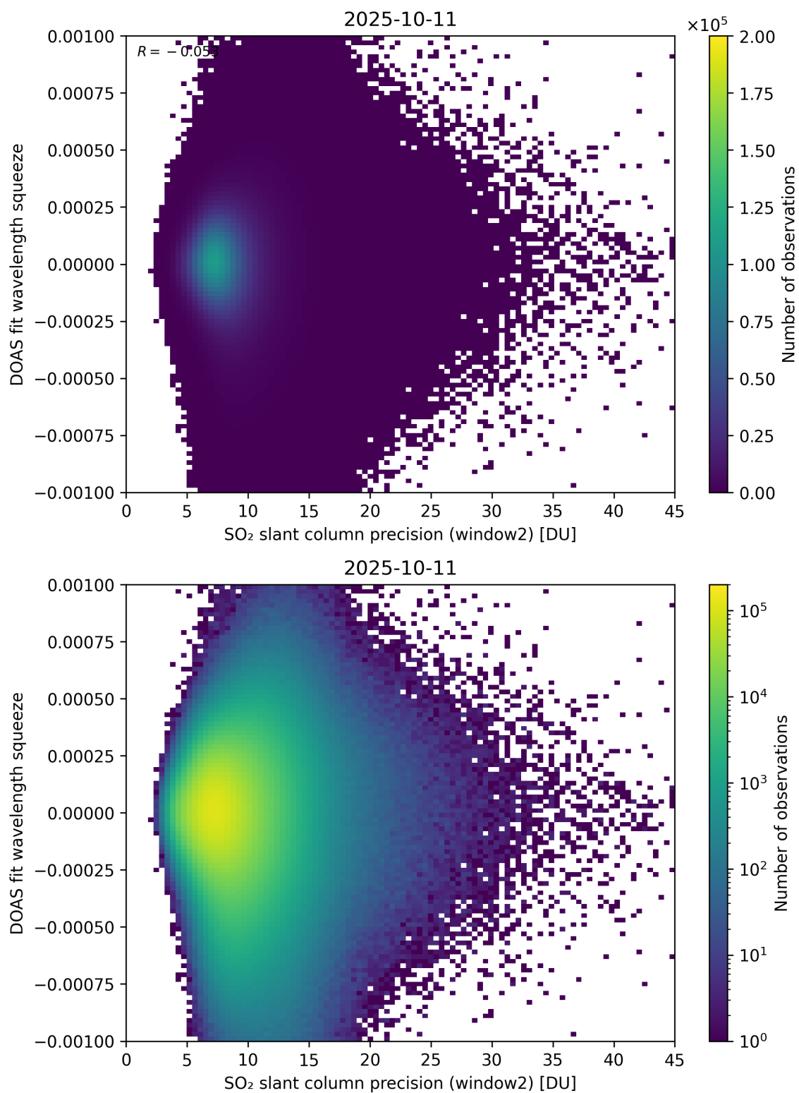
Figure 294: Scatter density plot of “SO 2 slant column precision (window2)” against “DOAS fit wavelength squeeze” for 2025-10-11 to 2025-10-12.
