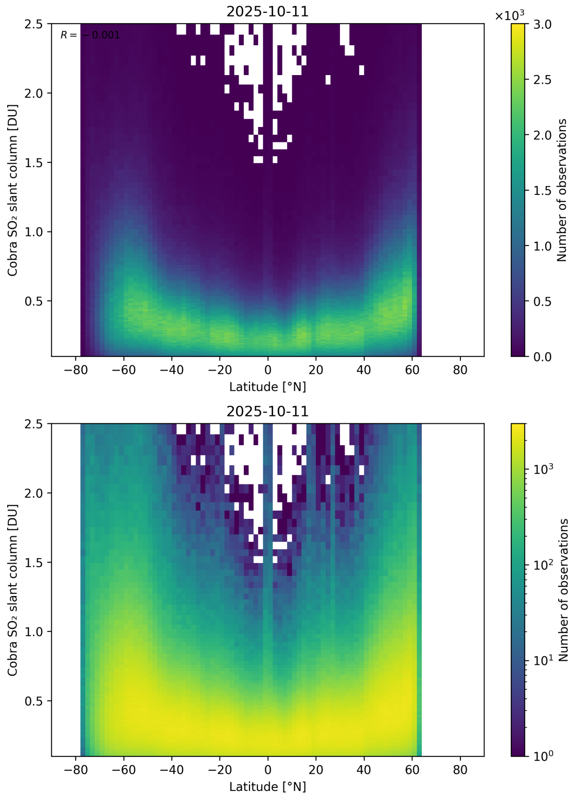
Figure 157: Scatter density plot of “Latitude” against “Cobra SO 2 slant column” for 2025-10-11 to 2025-10-12.
