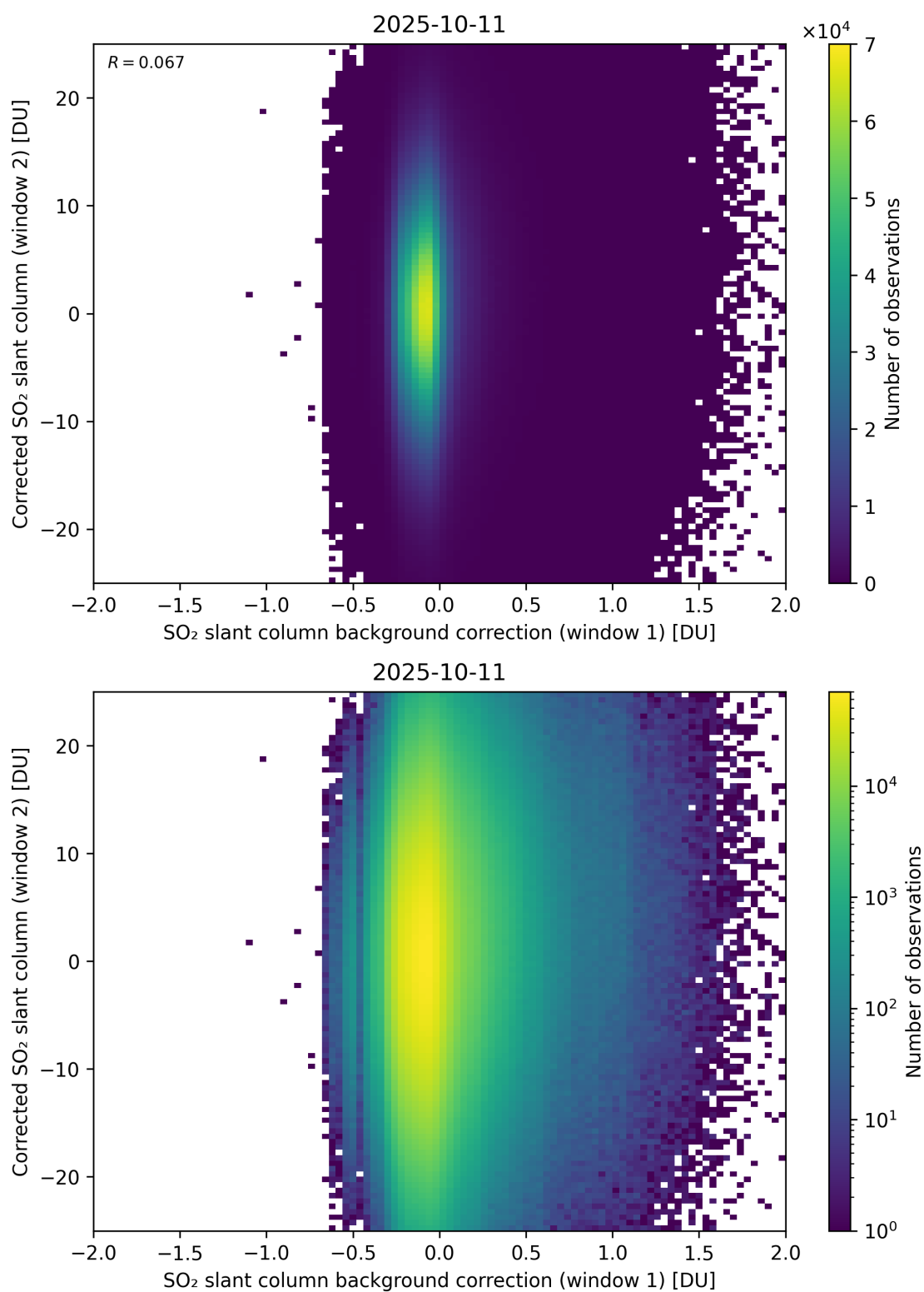
Figure 115: Scatter density plot of “SO 2 slant column background correction (window 1)” against “Corrected SO 2 slant column (window 2)” for 2025-10-11 to 2025-10-12.
