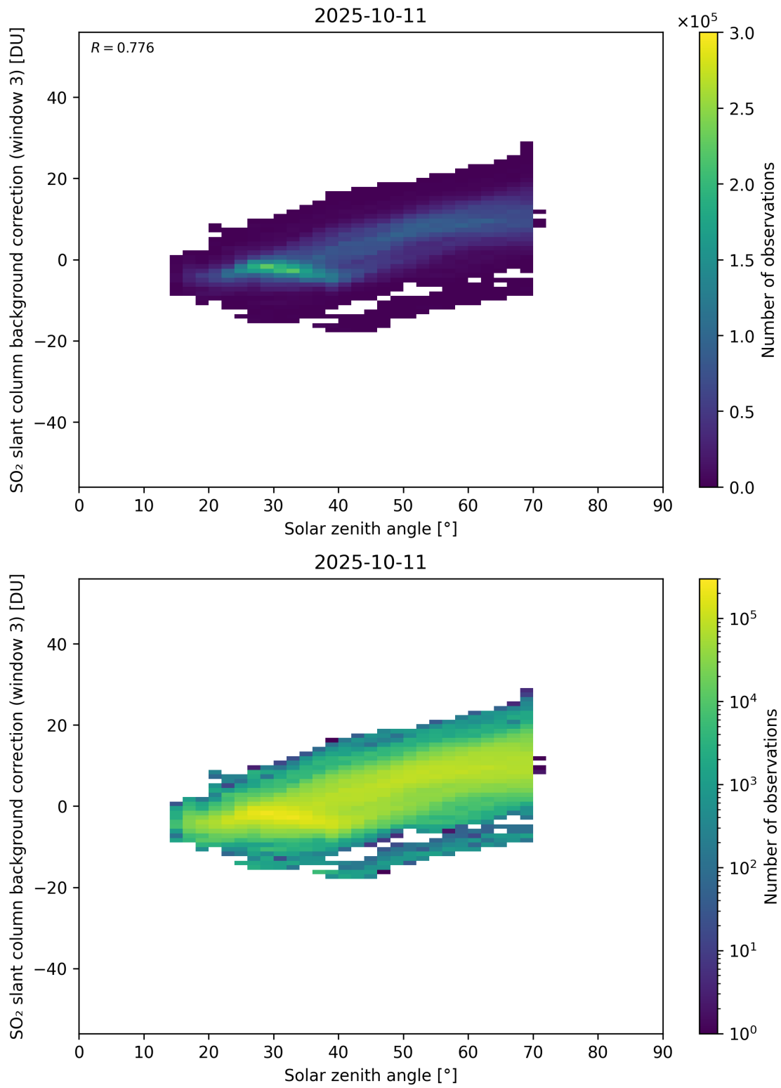
Figure 173: Scatter density plot of “Solar zenith angle” against “SO 2 slant column background correction (window 3)” for 2025-10-11 to 2025-10-12.
