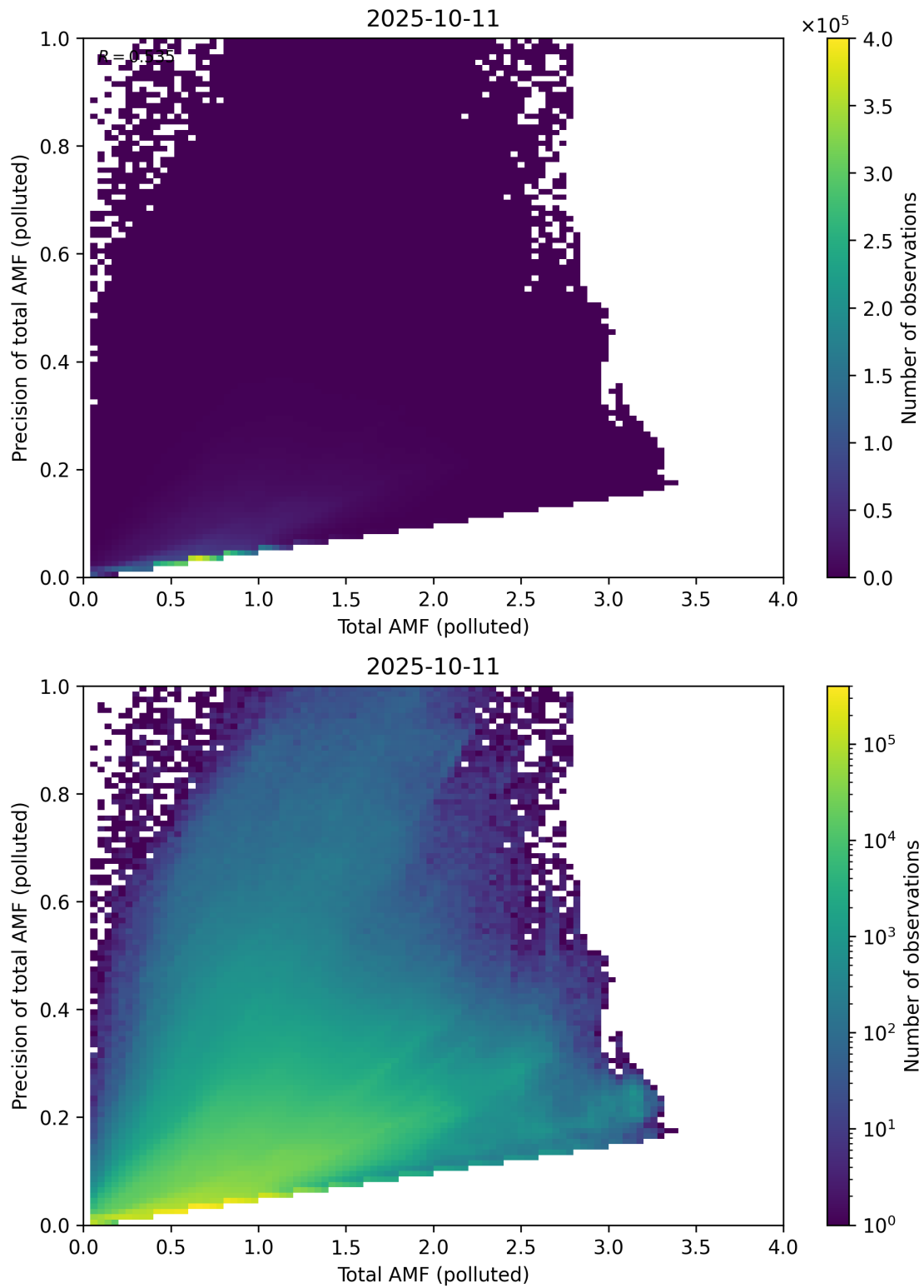
Figure 322: Scatter density plot of “Total AMF (polluted)” against “Precision of total AMF (polluted)” for 2025-10-11 to 2025-10-12.
