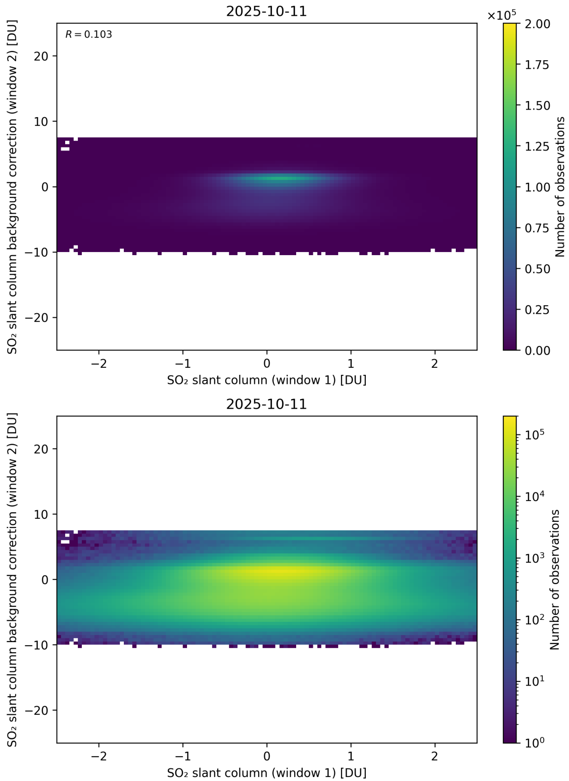
Figure 263: Scatter density plot of “SO 2 slant column (window 1)” against “SO 2 slant column background correction (window 2)” for 2025-10-11 to 2025-10-12.
