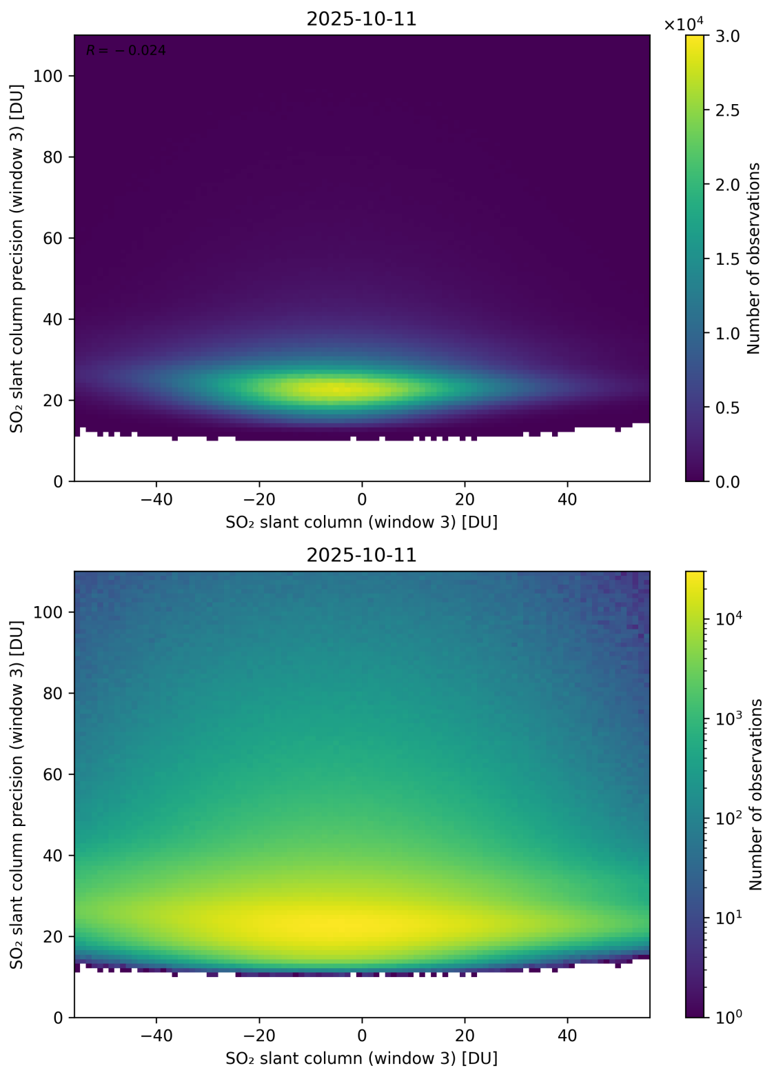
Figure 317: Scatter density plot of “SO 2 slant column (window 3)” against “SO 2 slant column precision (window 3)” for 2025-10-11 to 2025-10-12.
