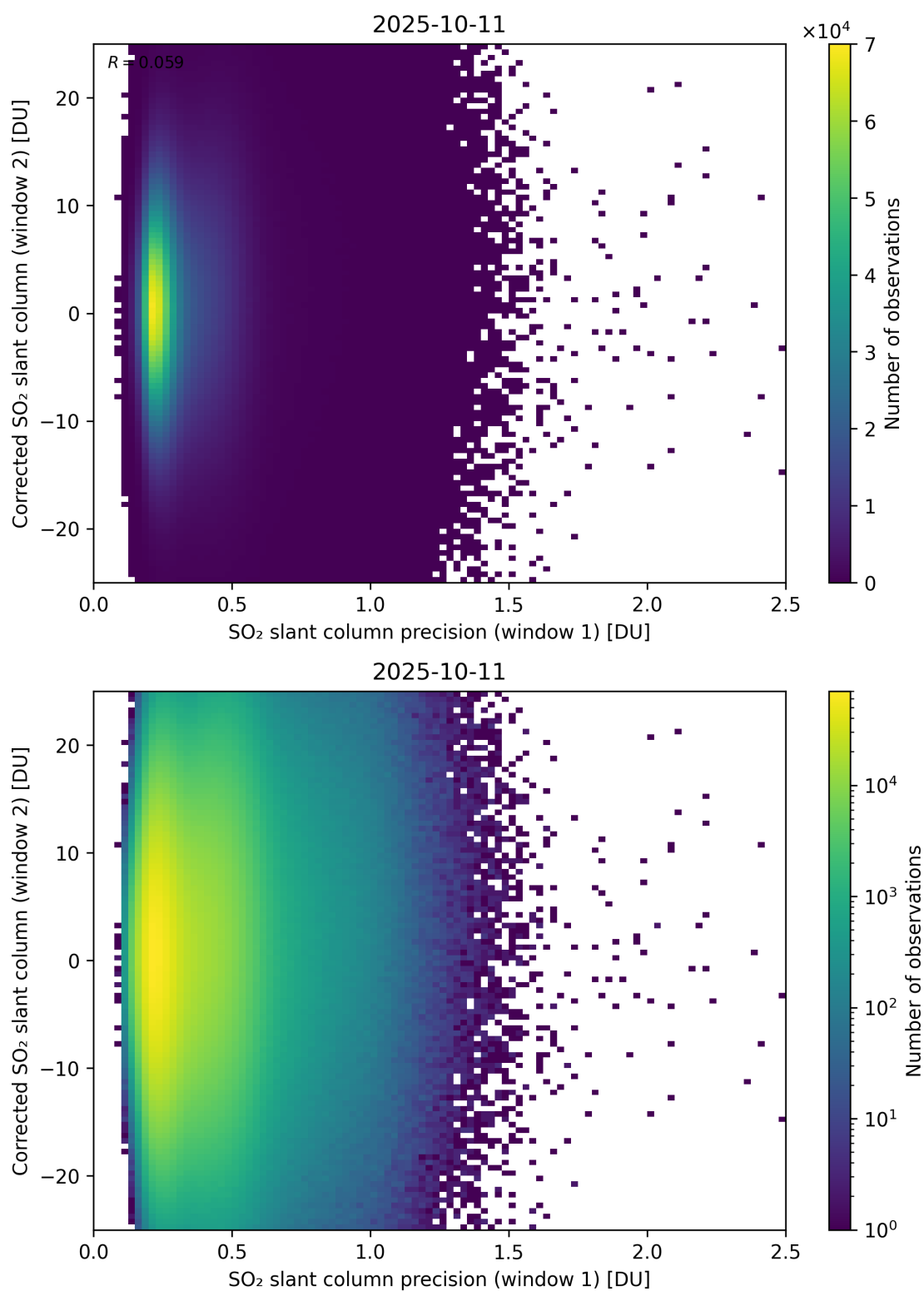
Figure 275: Scatter density plot of “SO 2 slant column precision (window 1)” against “Corrected SO 2 slant column (window 2)” for 2025-10-11 to 2025-10-12.
