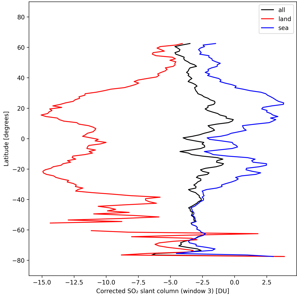
Figure 47: Zonal average of “Corrected SO 2 slant column (window 3)” for 2025-10-11 to 2025-10-12.
