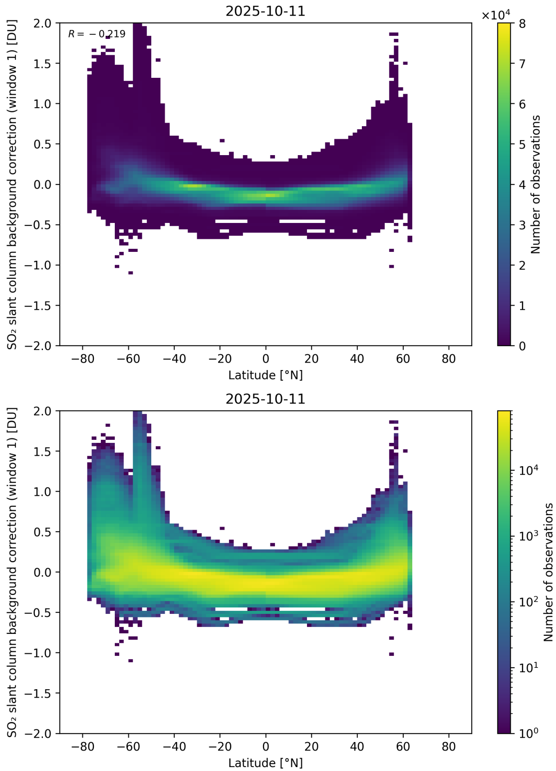
Figure 150: Scatter density plot of “Latitude” against “SO 2 slant column background correction (window 1)” for 2025-10-11 to 2025-10-12.
