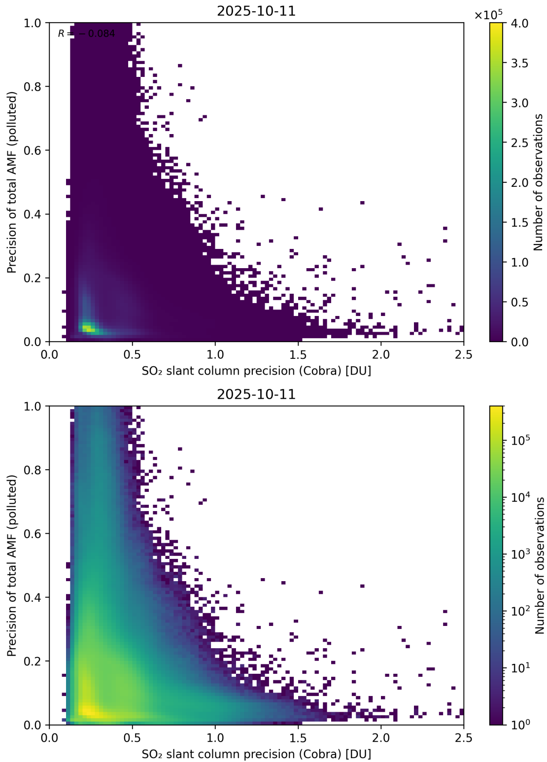
Figure 214: Scatter density plot of “SO 2 slant column precision (Cobra)” against “Precision of total AMF (polluted)” for 2025-10-11 to 2025-10-12.
