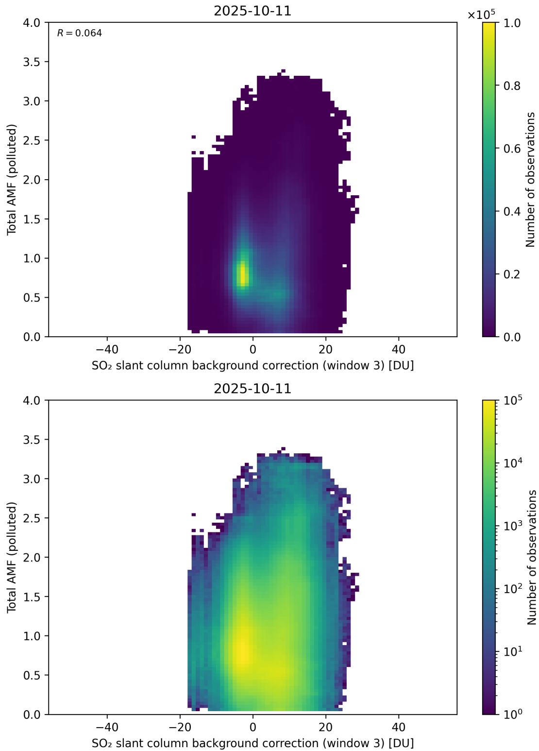
Figure 136: Scatter density plot of “SO 2 slant column background correction (window 3)” against “Total AMF (polluted)” for 2025-10-11 to 2025-10-12.
