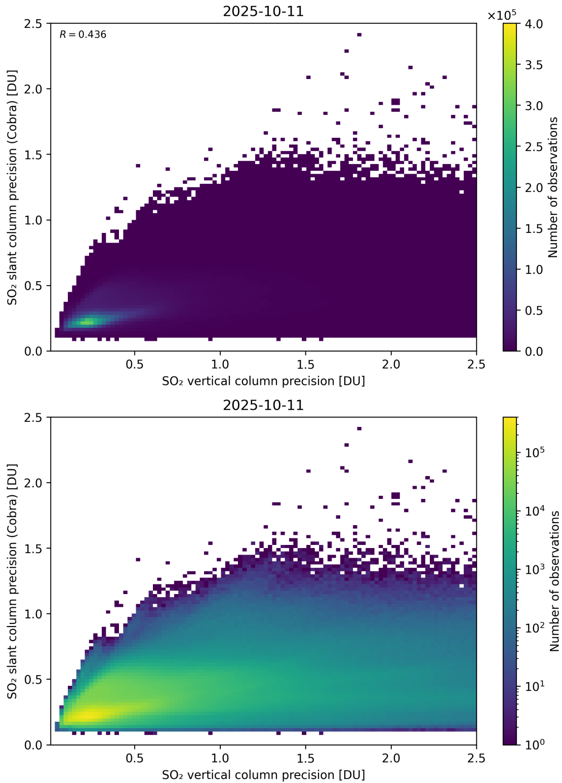
Figure 337: Scatter density plot of “SO 2 vertical column precision” against “SO 2 slant column precision (Cobra)” for 2025-10-11 to 2025-10-12.
