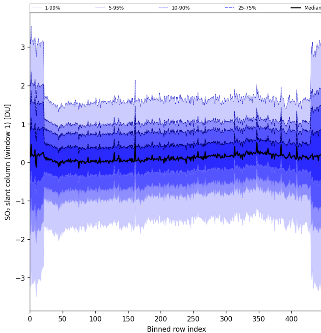
Figure 89: Along track statistics of “SO 2 slant column (window 1)” for 2025-10-11 to 2025-10-12
