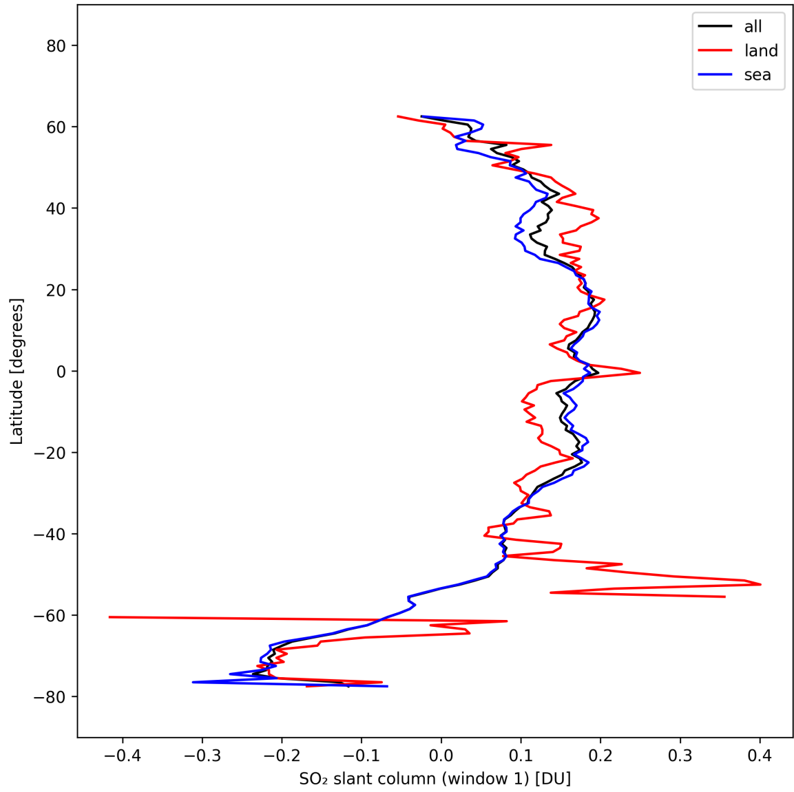
Figure 37: Zonal average of “SO 2 slant column (window 1)” for 2025-10-11 to 2025-10-12.
