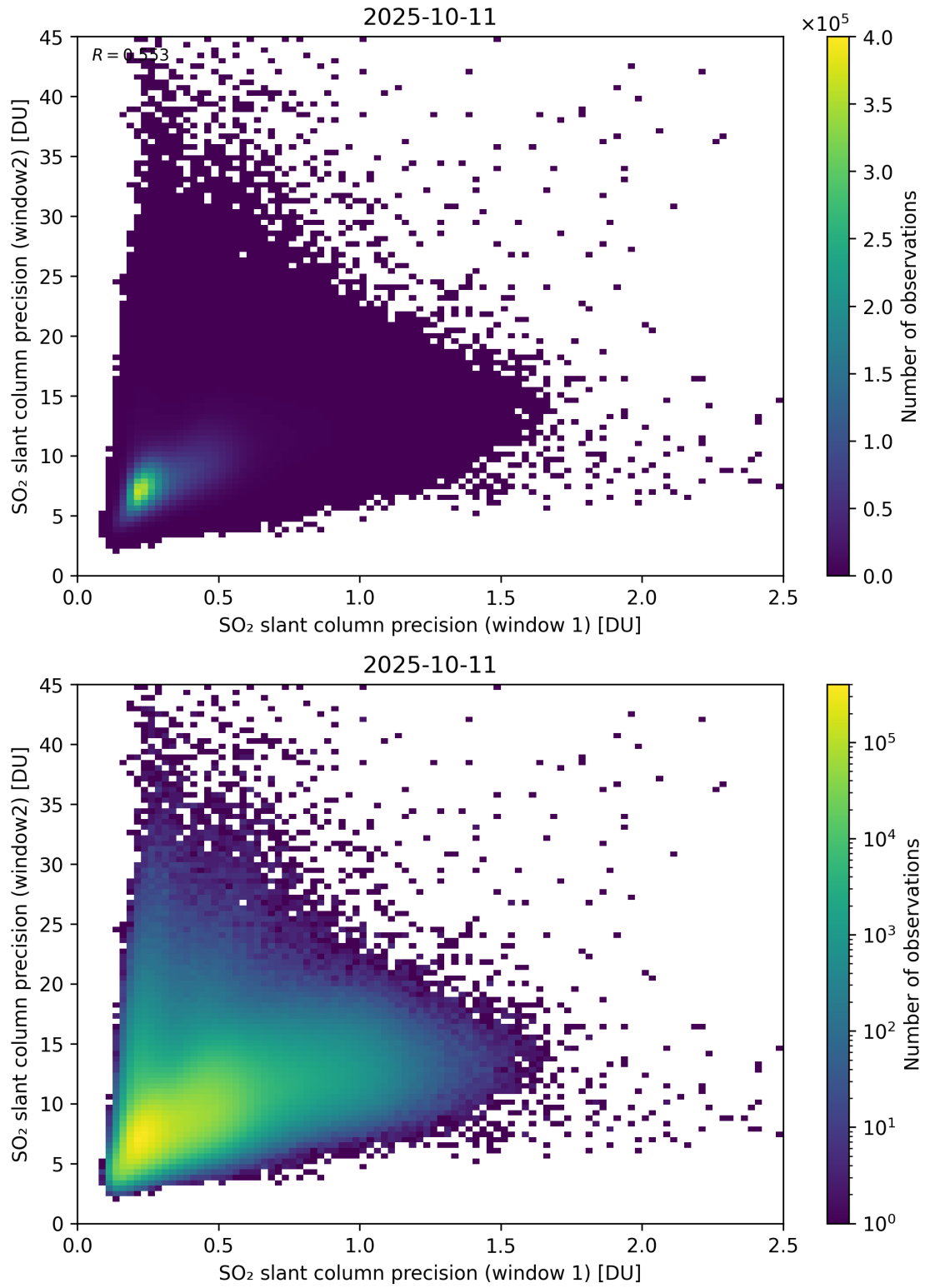
Figure 277: Scatter density plot of “SO 2 slant column precision (window 1)” against “SO 2 slant column precision (window2)” for 2025-10-11 to 2025-10-12.
