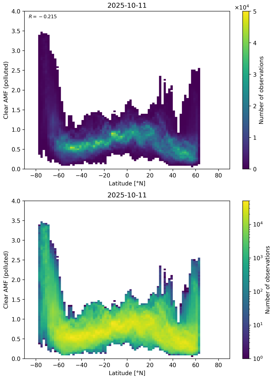
Figure 156: Scatter density plot of “Latitude” against “Clear AMF (polluted)” for 2025-10-11 to 2025-10-12.
