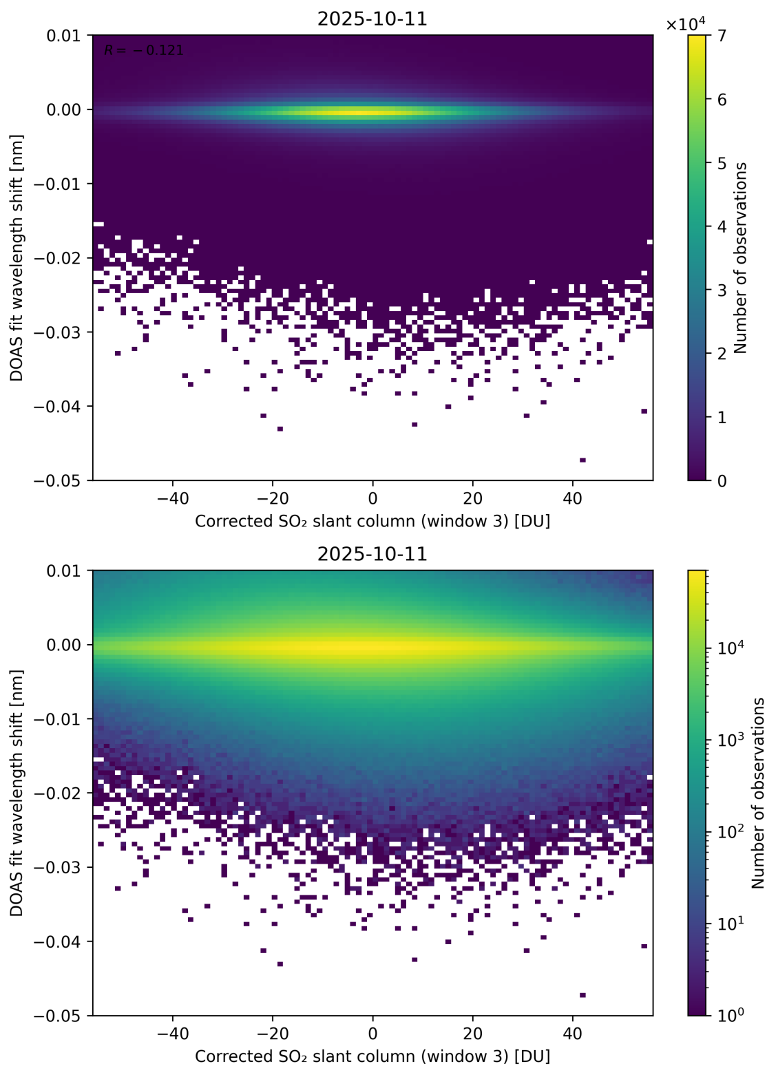
Figure 256: Scatter density plot of “Corrected SO 2 slant column (window 3)” against “DOAS fit wavelength shift” for 2025-10-11 to 2025-10-12.
