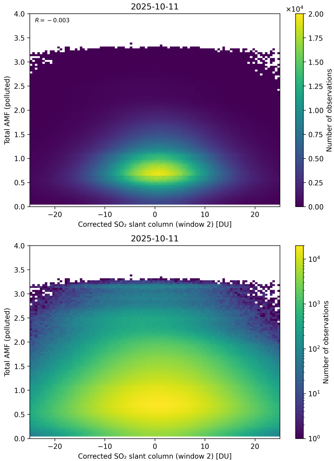
Figure 253: Scatter density plot of “Corrected SO 2 slant column (window 2)” against “Total AMF (polluted)” for 2025-10-11 to 2025-10-12.
