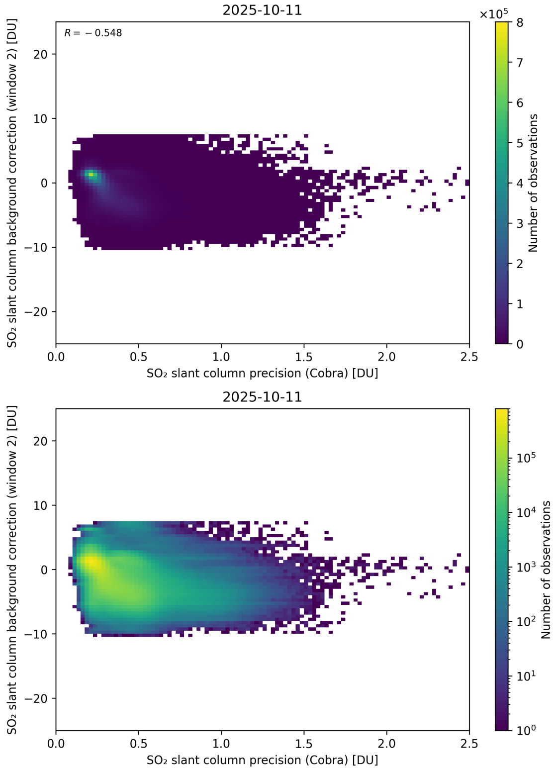
Figure 200: Scatter density plot of “SO 2 slant column precision (Cobra)” against “SO 2 slant column background correction (window 2)” for 2025-10-11 to 2025-10-12.
