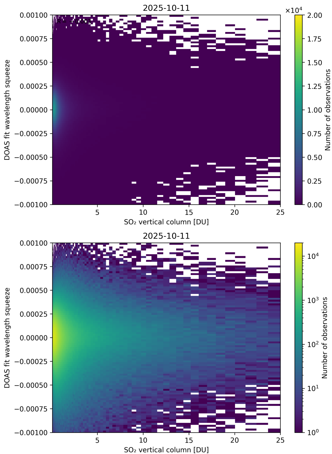
Figure 327: Scatter density plot of “SO 2 vertical column” against “DOAS fit wavelength squeeze” for 2025-10-11 to 2025-10-12.
