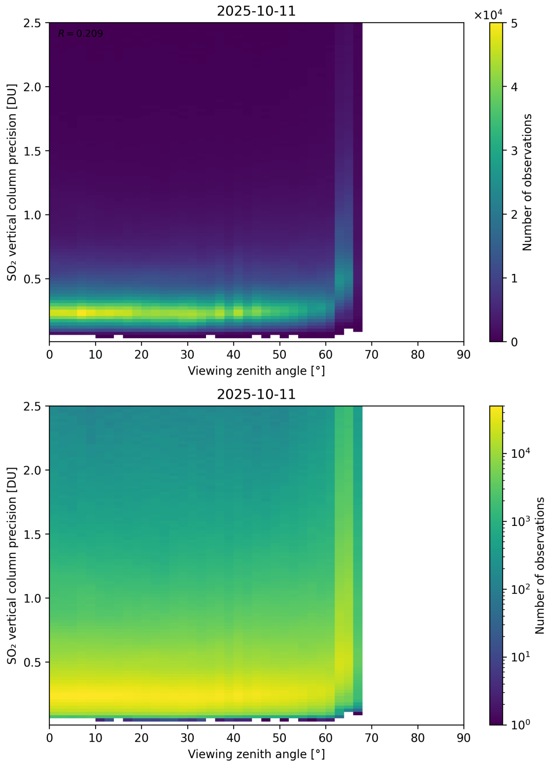
Figure 384: Scatter density plot of “Viewing zenith angle” against “SO 2 vertical column precision” for 2025-10-11 to 2025-10-12.
