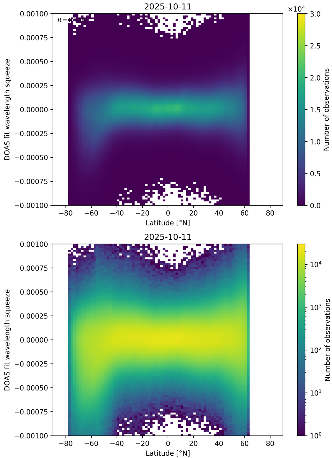
Figure 154: Scatter density plot of “Latitude” against “DOAS fit wavelength squeeze” for 2025-10-11 to 2025-10-12.
