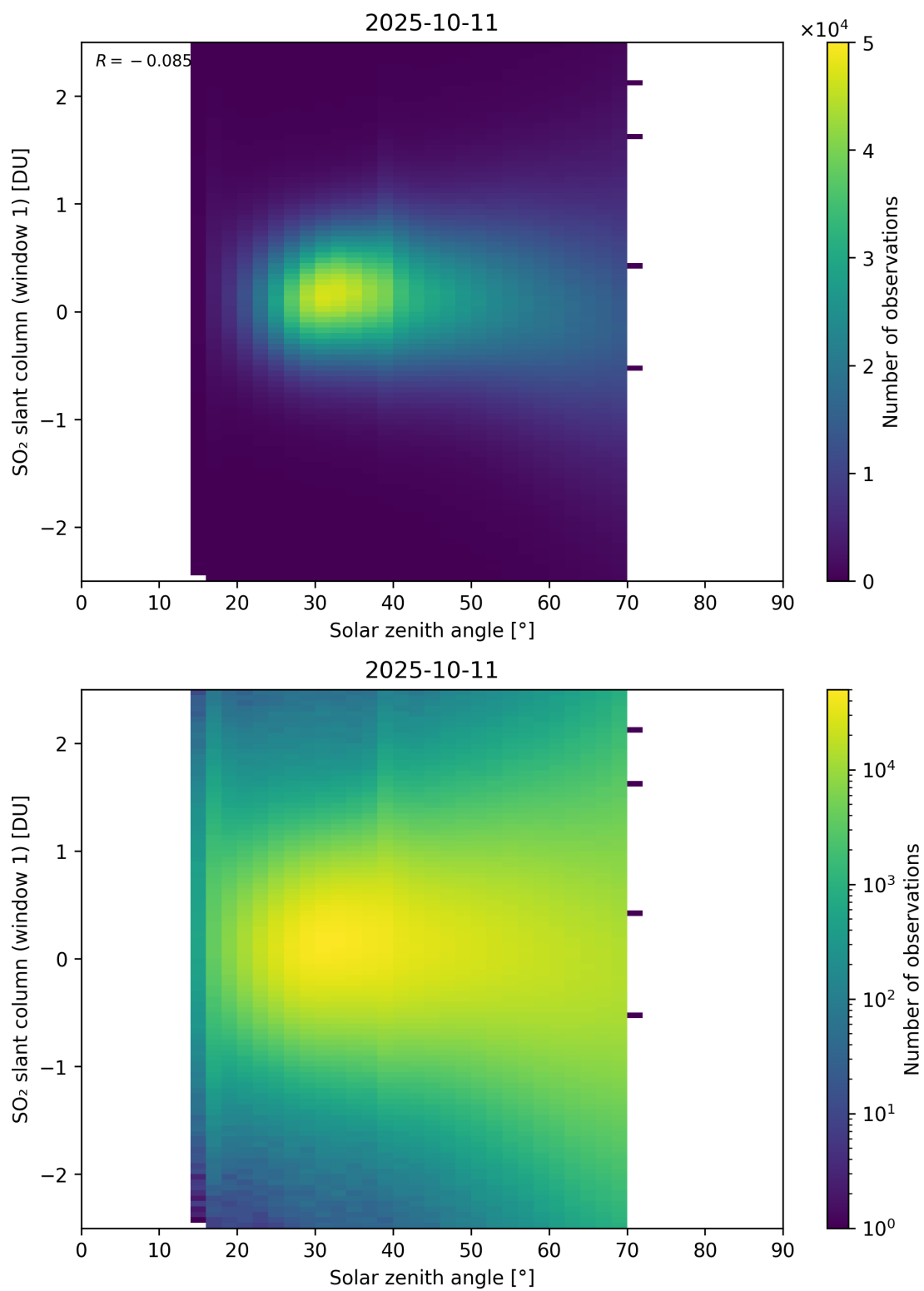
Figure 184: Scatter density plot of “Solar zenith angle” against “SO 2 slant column (window 1)” for 2025-10-11 to 2025-10-12.
