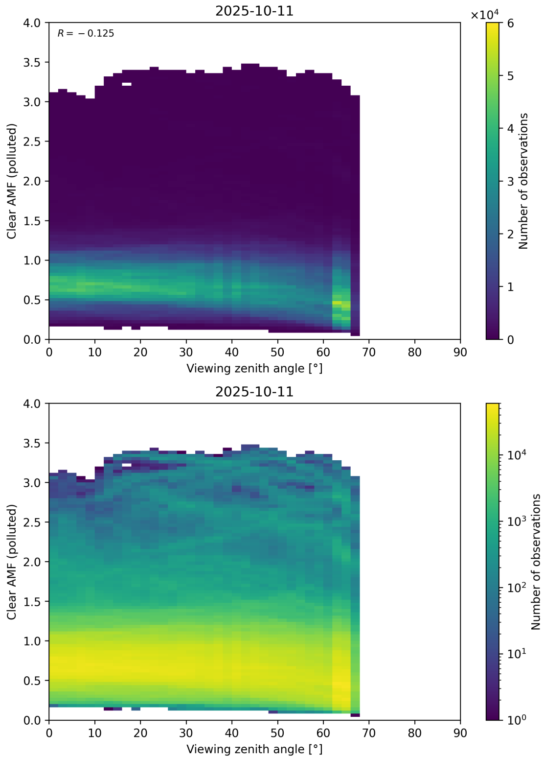
Figure 370: Scatter density plot of “Viewing zenith angle” against “Clear AMF (polluted)” for 2025-10-11 to 2025-10-12.
