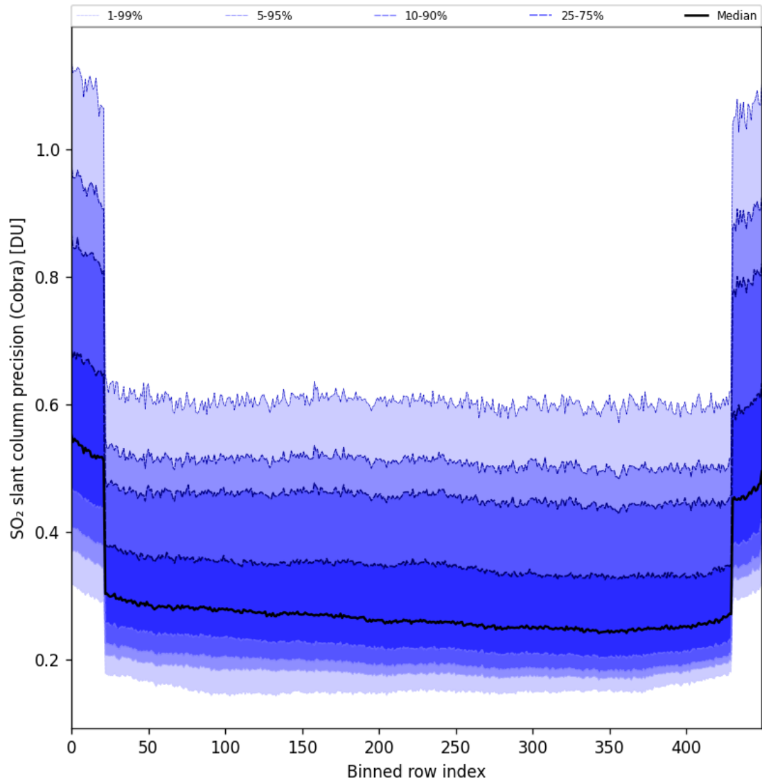
Figure 88: Along track statistics of “SO 2 slant column precision (Cobra)” for 2025-10-11 to 2025-10-12
