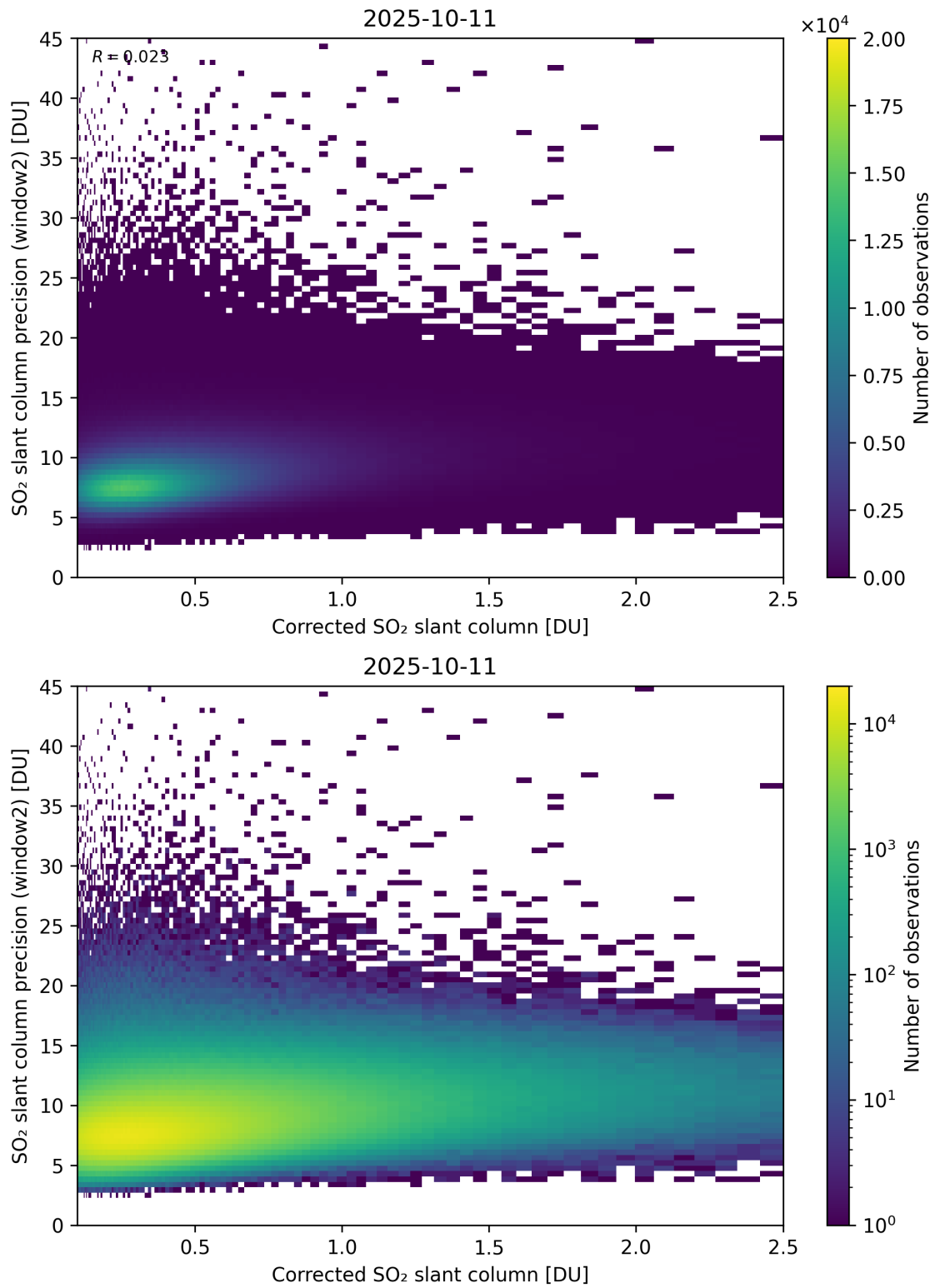
Figure 239: Scatter density plot of “Corrected SO 2 slant column” against “SO 2 slant column precision (window2)” for 2025-10-11 to 2025-10-12.
