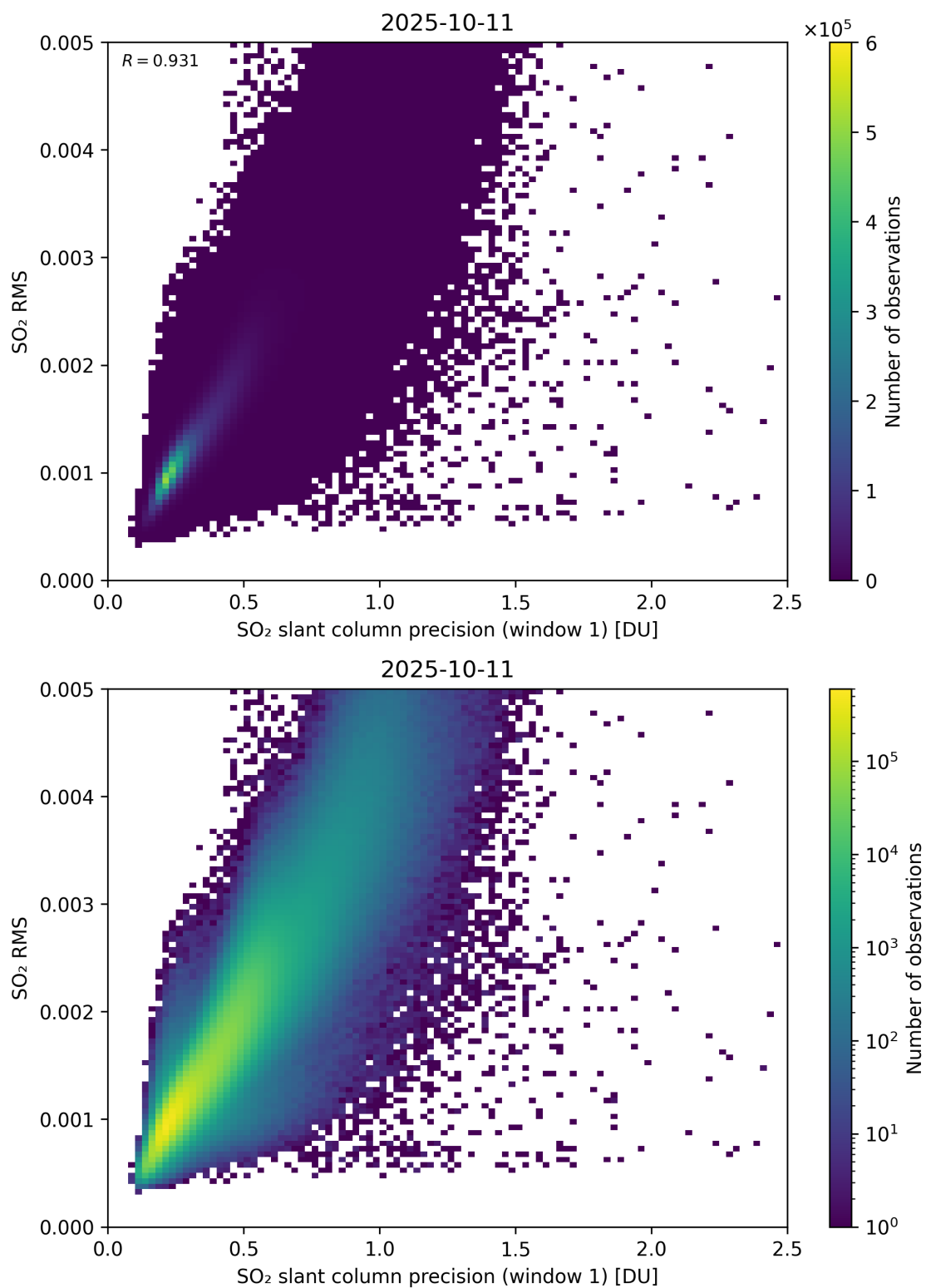
Figure 273: Scatter density plot of “SO 2 slant column precision (window 1)” against “SO 2 RMS” for 2025-10-11 to 2025-10-12.
