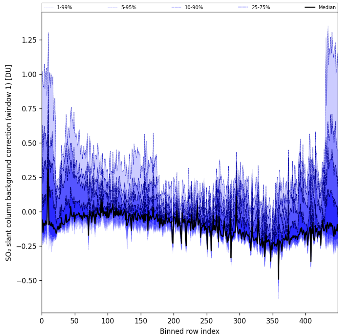
Figure 92: Along track statistics of “SO 2 slant column background correction (window 1)” for 2025-10-11 to 2025-10-12
