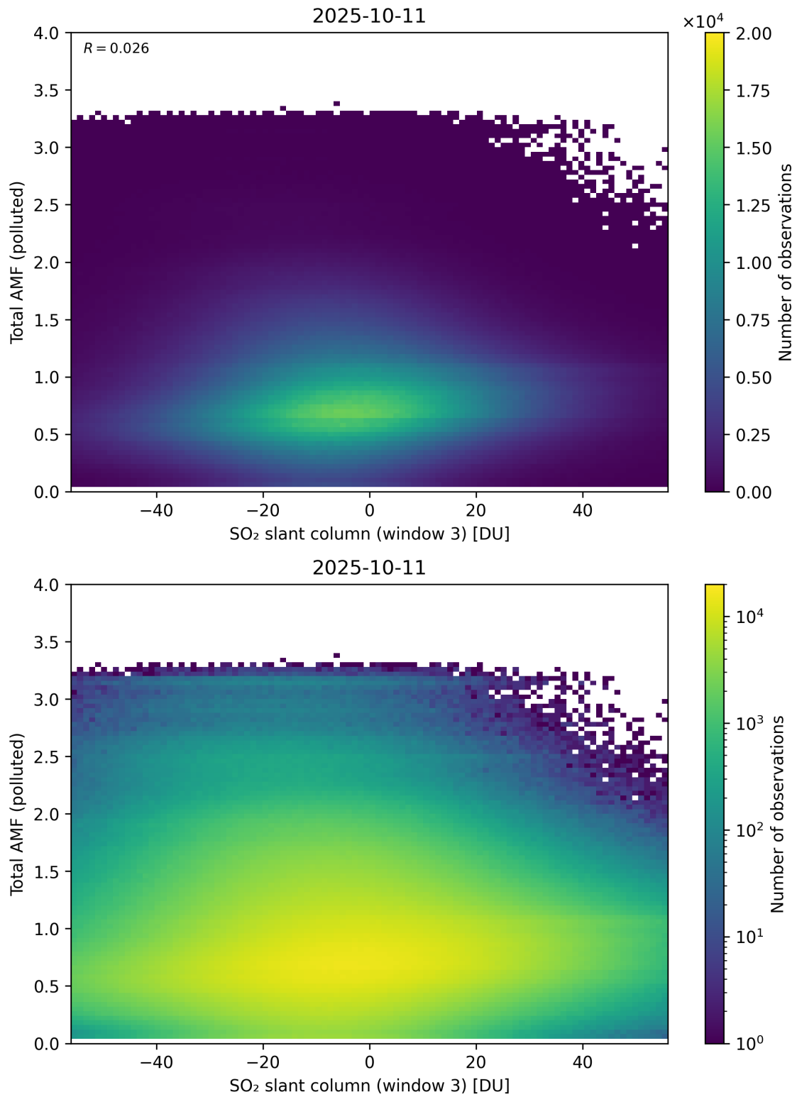
Figure 318: Scatter density plot of “SO 2 slant column (window 3)” against “Total AMF (polluted)” for 2025-10-11 to 2025-10-12.
