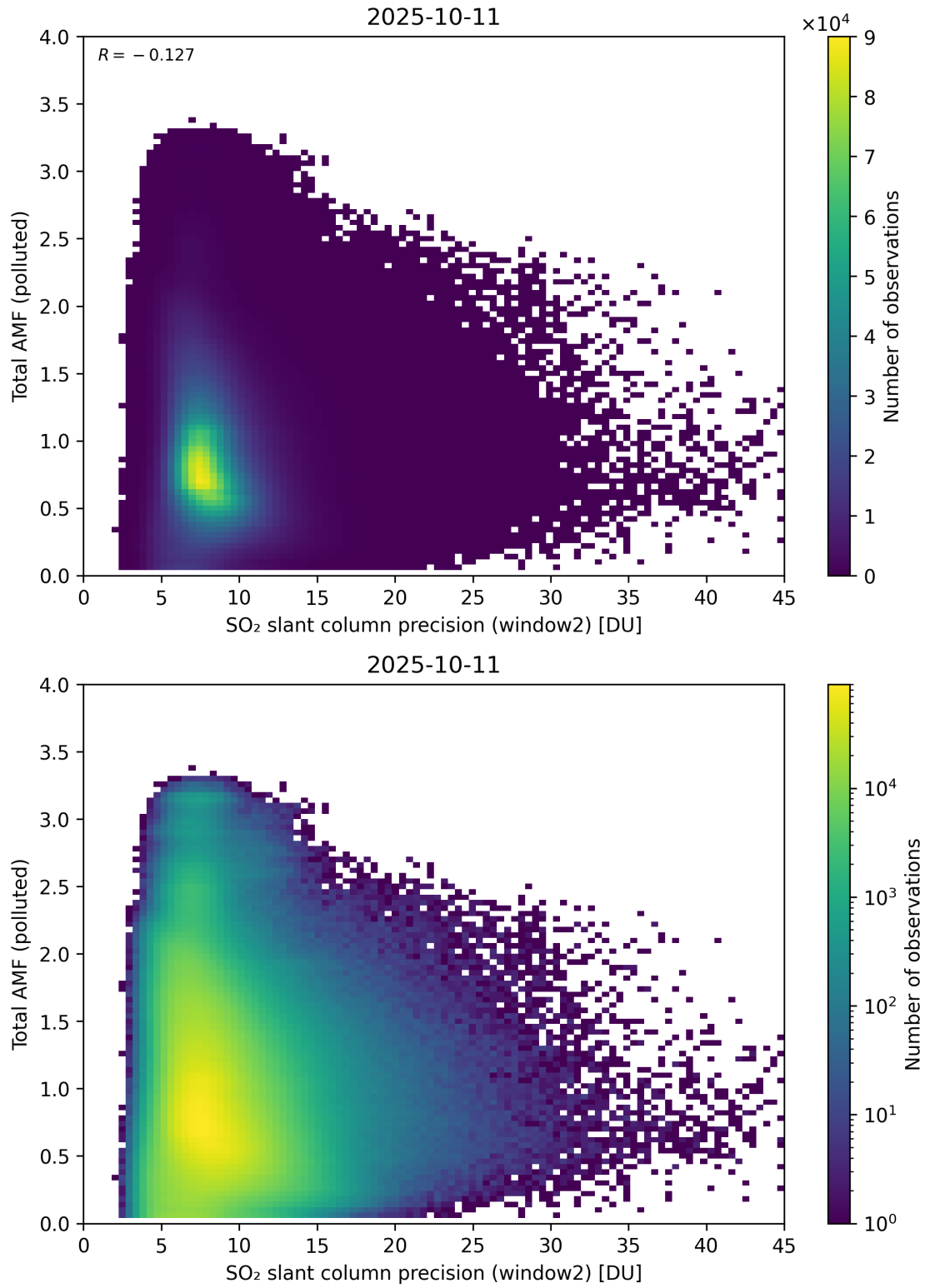
Figure 301: Scatter density plot of “SO 2 slant column precision (window2)” against “Total AMF (polluted)” for 2025-10-11 to 2025-10-12.
