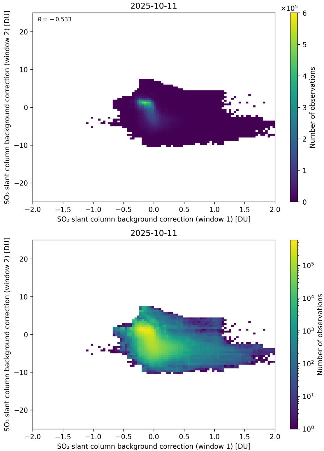
Figure 109: Scatter density plot of “SO 2 slant column background correction (window 1)” against “SO 2 slant column background correction (window 2)” for 2025-10-11 to 2025-10-12.
