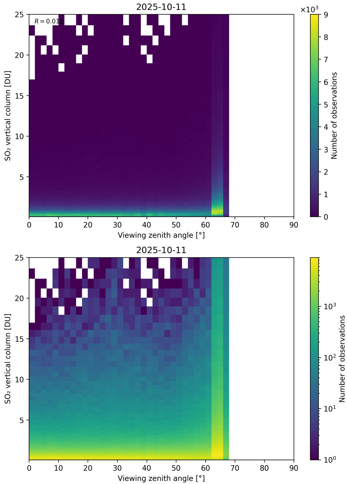
Figure 383: Scatter density plot of “Viewing zenith angle” against “SO 2 vertical column” for 2025-10-11 to 2025-10-12.
