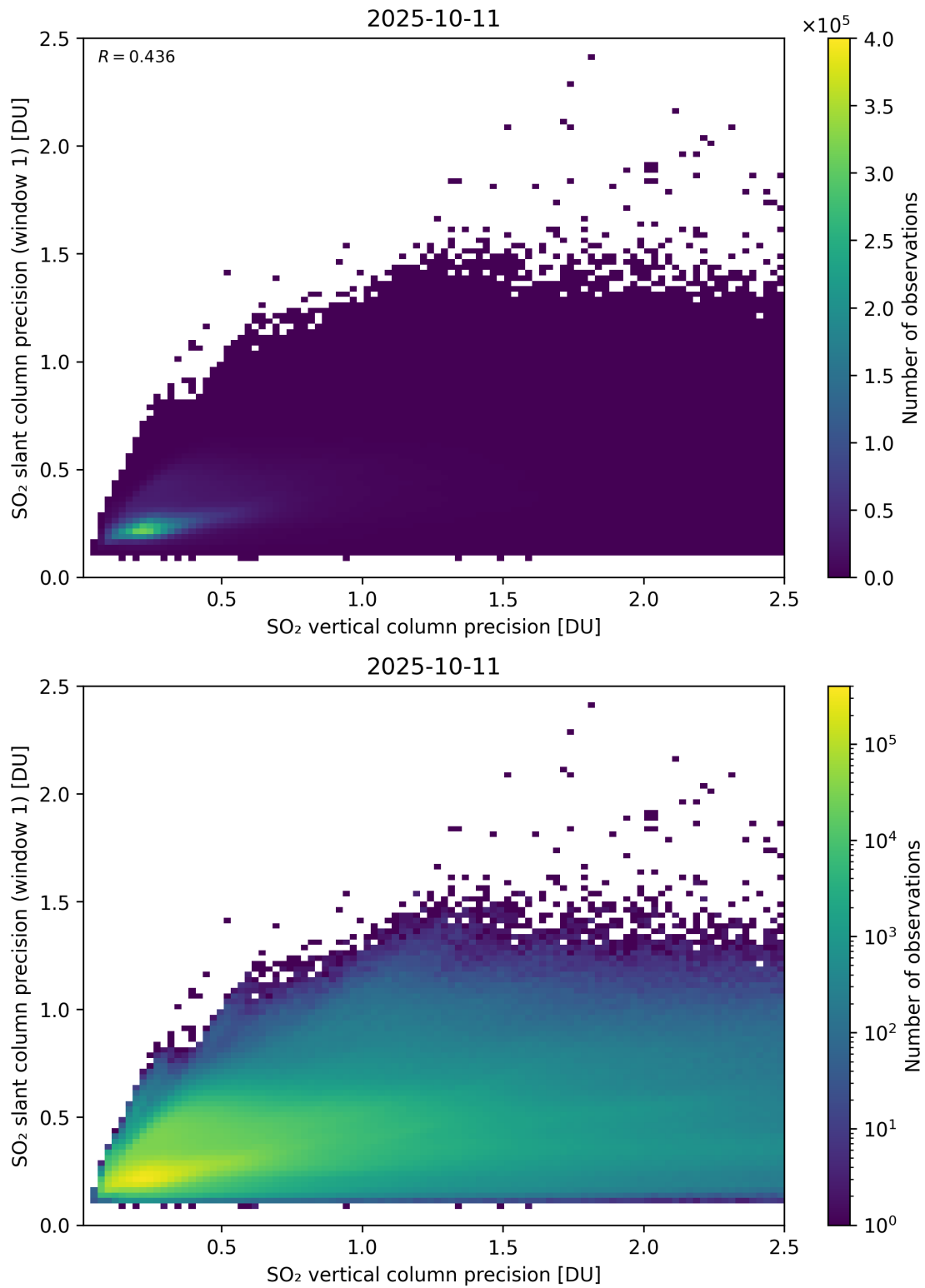
Figure 342: Scatter density plot of “SO 2 vertical column precision” against “SO 2 slant column precision (window 1)” for 2025-10-11 to 2025-10-12.
