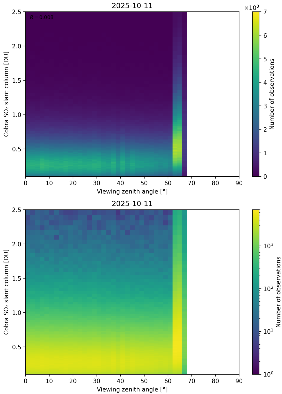
Figure 371: Scatter density plot of “Viewing zenith angle” against “Cobra SO 2 slant column” for 2025-10-11 to 2025-10-12.
