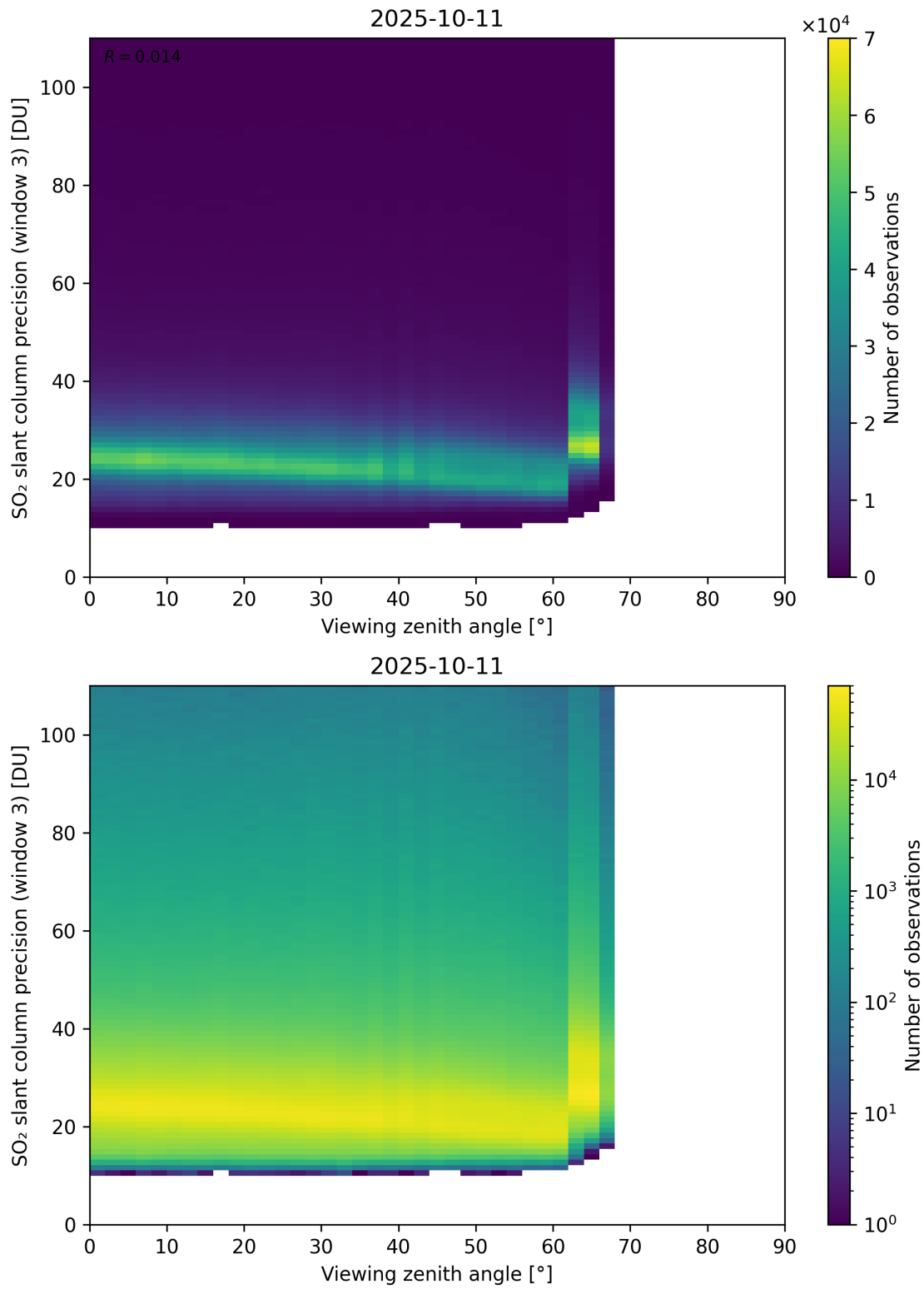
Figure 380: Scatter density plot of “Viewing zenith angle” against “SO 2 slant column precision (window 3)” for 2025-10-11 to 2025-10-12.
