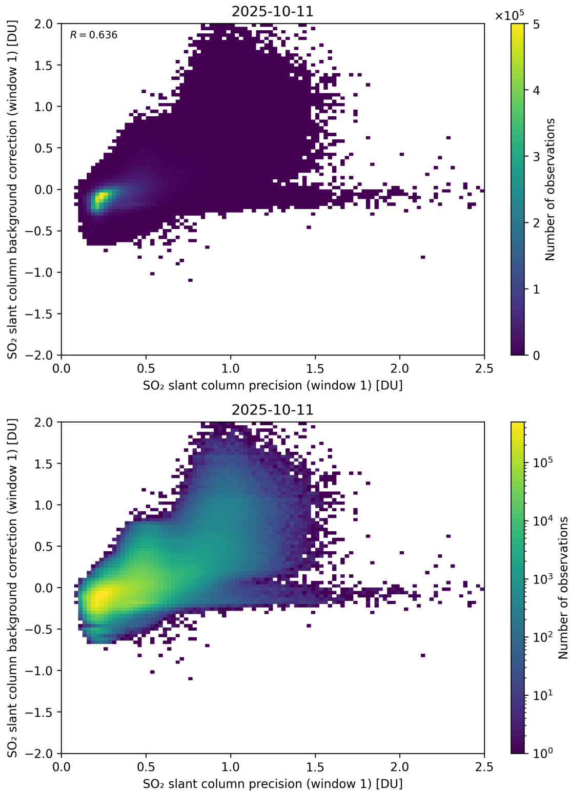
Figure 268: Scatter density plot of “SO 2 slant column precision (window 1)” against “SO 2 slant column background correction (window 1)” for 2025-10-11 to 2025-10-12.
