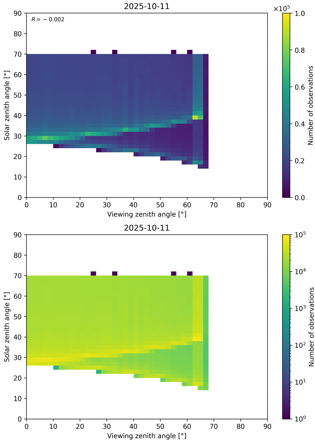
Figure 369: Scatter density plot of “Viewing zenith angle” against “Solar zenith angle” for 2025-10-11 to 2025-10-12.
