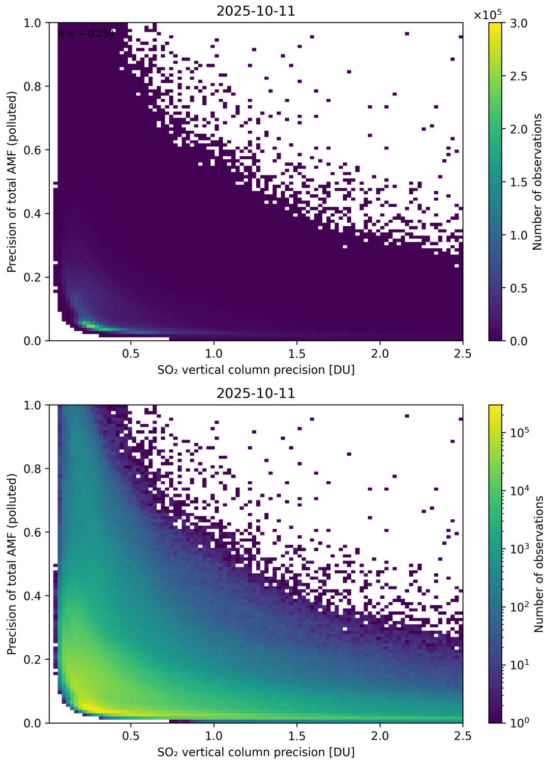
Figure 347: Scatter density plot of “SO 2 vertical column precision” against “Precision of total AMF (polluted)” for 2025-10-11 to 2025-10-12.
