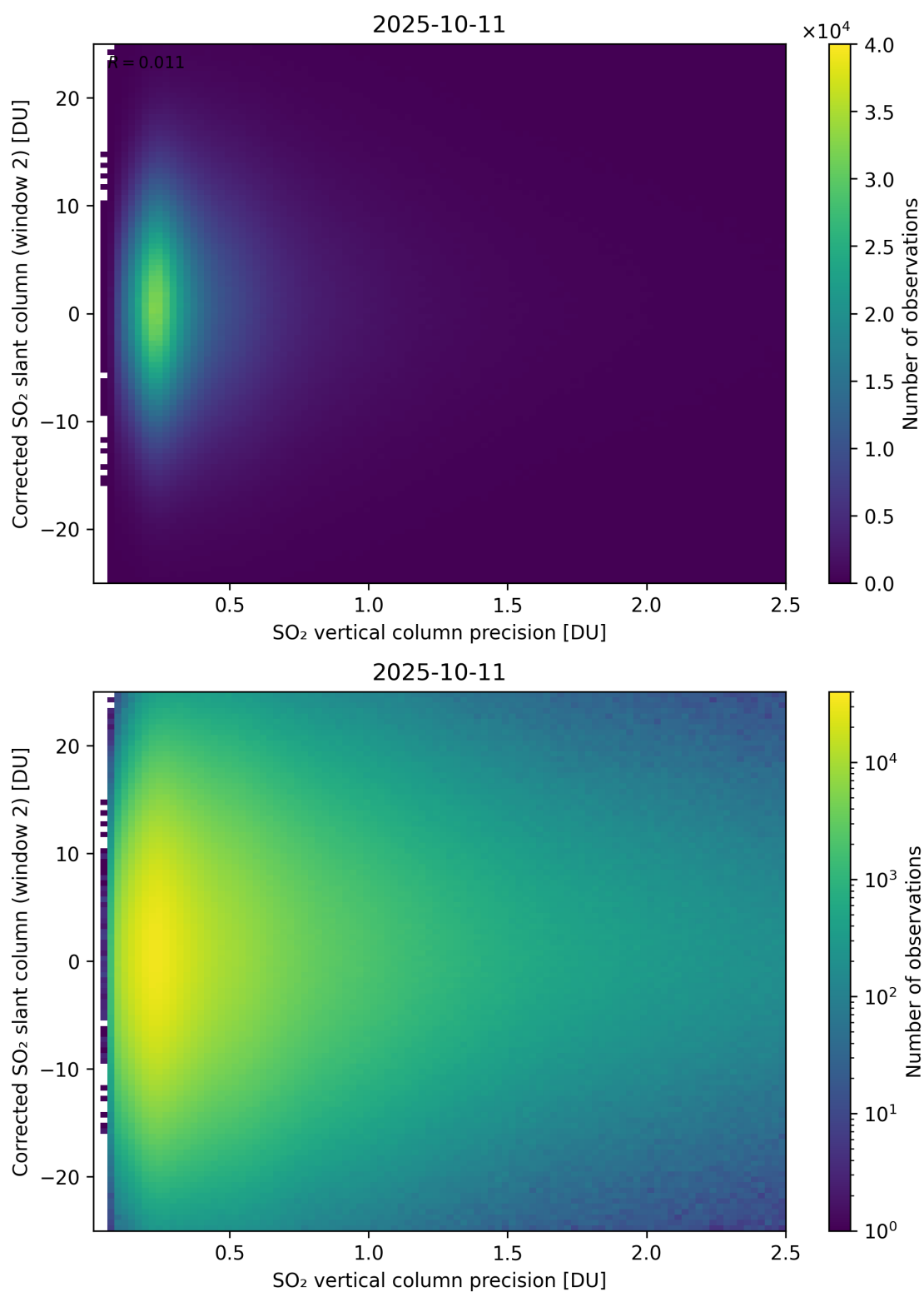
Figure 339: Scatter density plot of “SO 2 vertical column precision” against “Corrected SO 2 slant column (window 2)” for 2025-10-11 to 2025-10-12.
