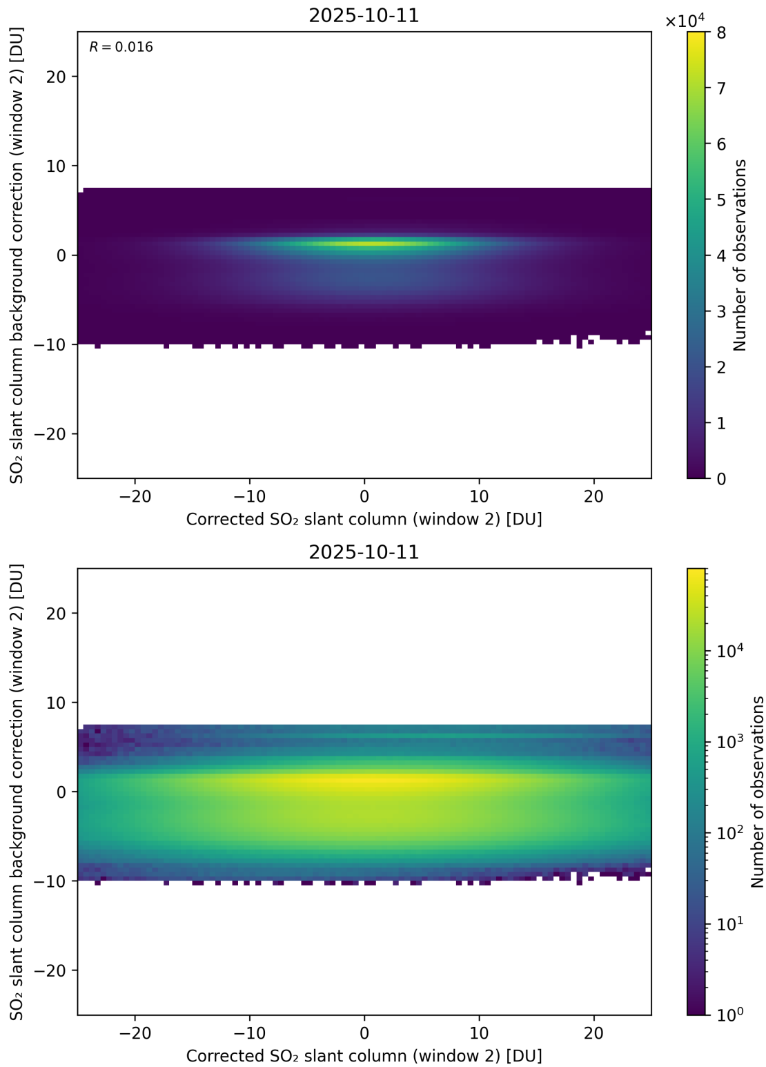
Figure 244: Scatter density plot of “Corrected SO 2 slant column (window 2)” against “SO 2 slant column background correction (window 2)” for 2025-10-11 to 2025-10-12.
