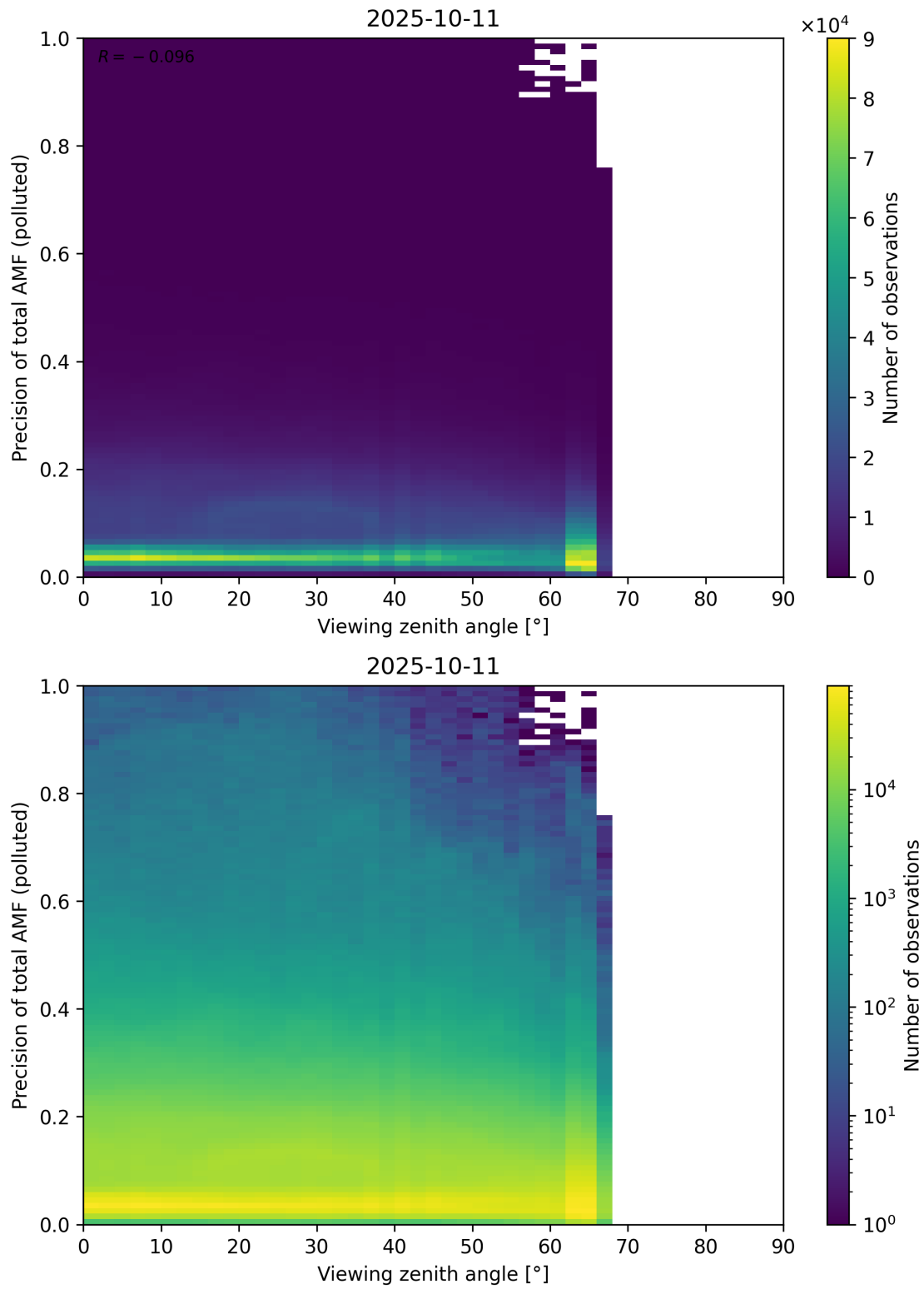
Figure 382: Scatter density plot of “Viewing zenith angle” against “Precision of total AMF (polluted)” for 2025-10-11 to 2025-10-12.
