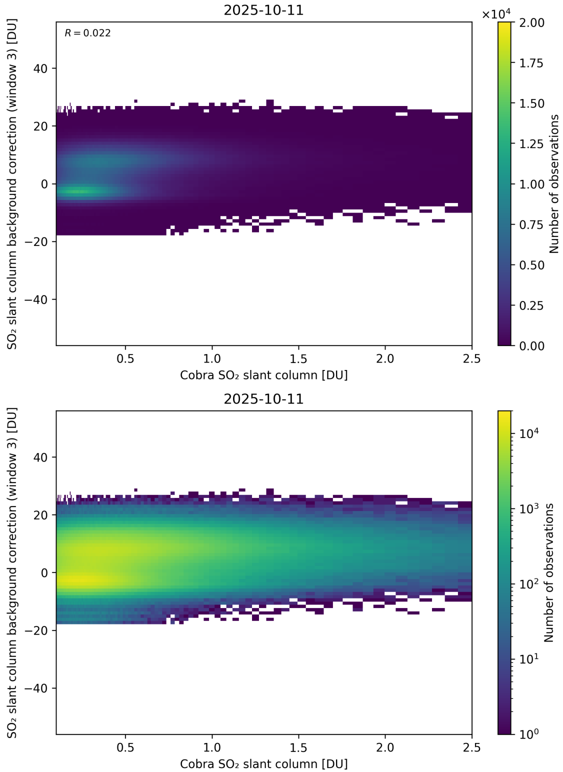
Figure 195: Scatter density plot of “Cobra SO 2 slant column” against “SO 2 slant column background correction (window 3)” for 2025-10-11 to 2025-10-12.
