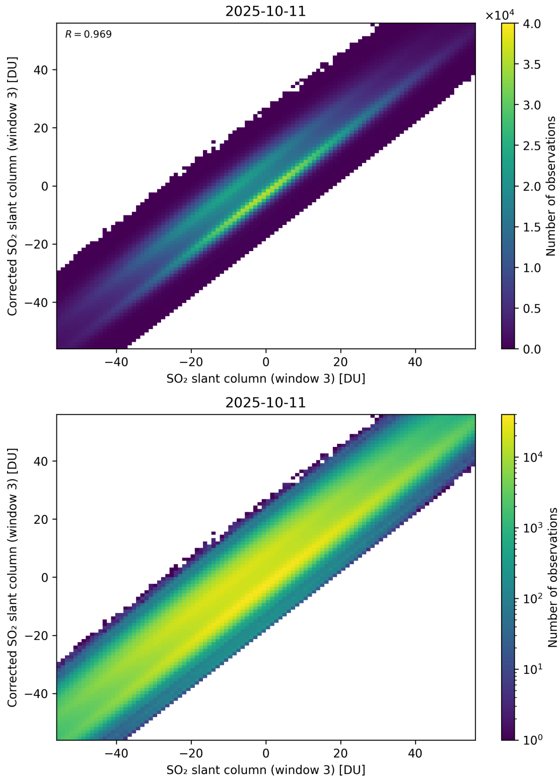
Figure 316: Scatter density plot of “SO 2 slant column (window 3)” against “Corrected SO 2 slant column (window 3)” for 2025-10-11 to 2025-10-12.
