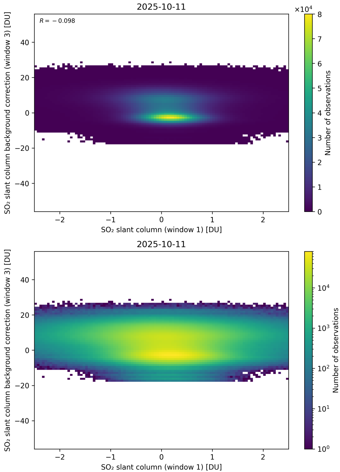
Figure 264: Scatter density plot of “SO 2 slant column (window 1)” against “SO 2 slant column background correction (window 3)” for 2025-10-11 to 2025-10-12.
