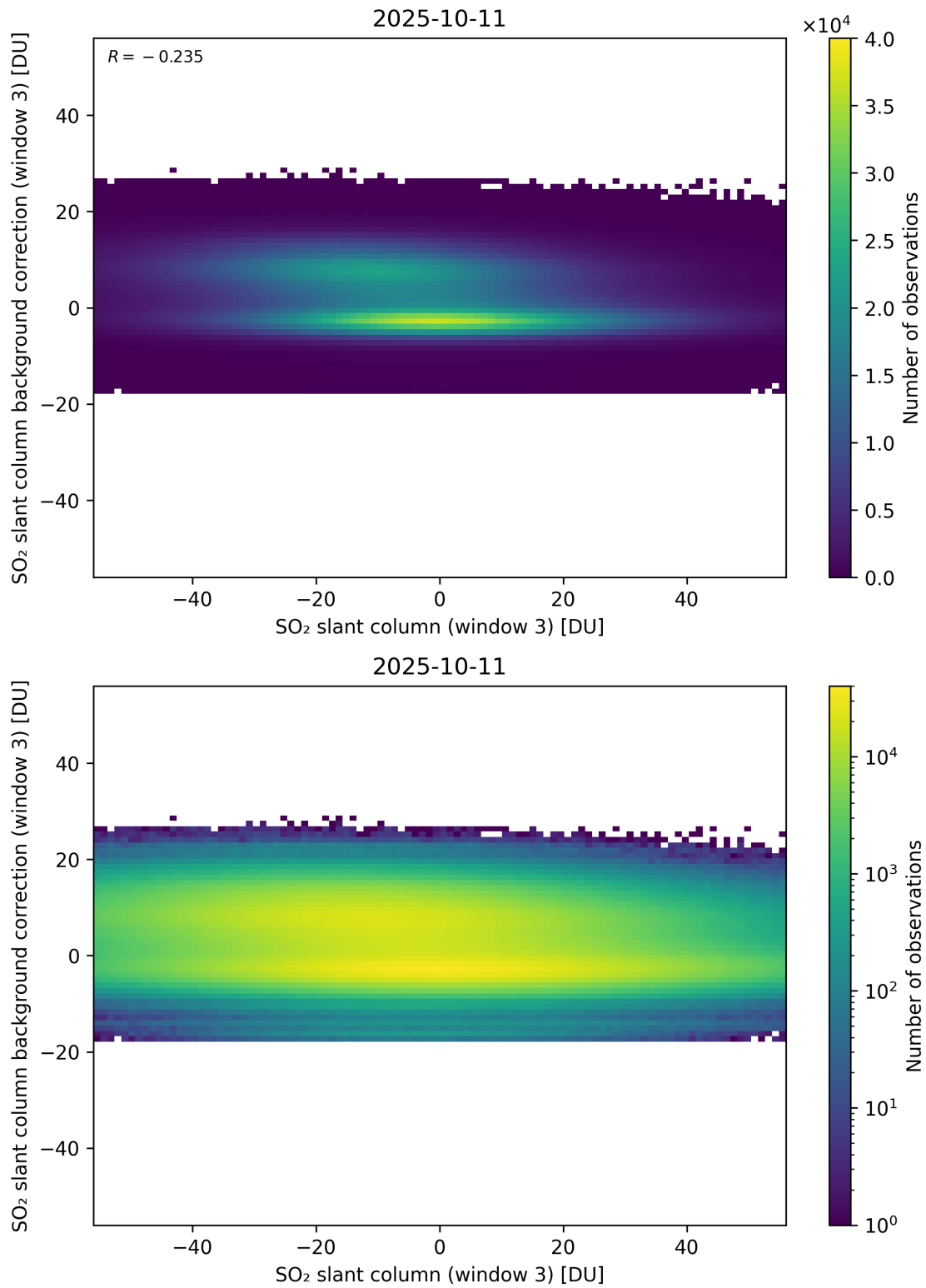
Figure 303: Scatter density plot of “SO 2 slant column (window 3)” against “SO 2 slant column background correction (window 3)” for 2025-10-11 to 2025-10-12.
