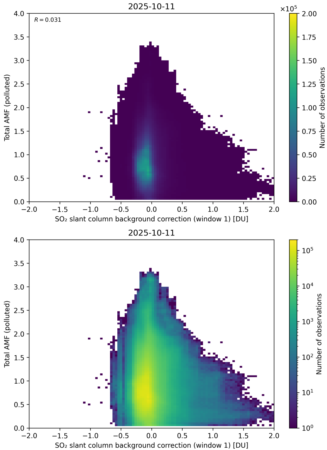
Figure 120: Scatter density plot of “SO 2 slant column background correction (window 1)” against “Total AMF (polluted)” for 2025-10-11 to 2025-10-12.
