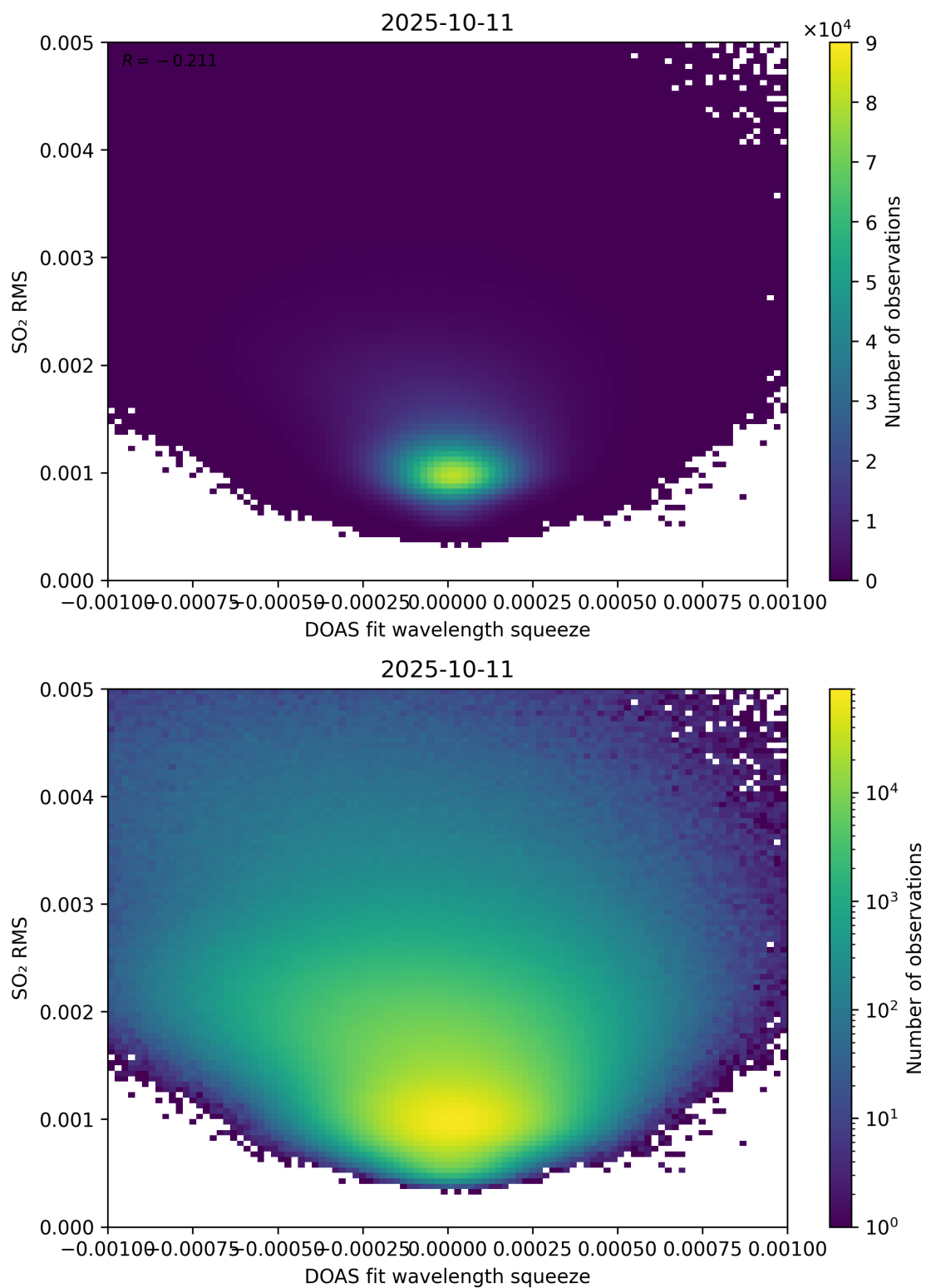
Figure 143: Scatter density plot of “DOAS fit wavelength squeeze” against “SO 2 RMS” for 2025-10-11 to 2025-10-12.
