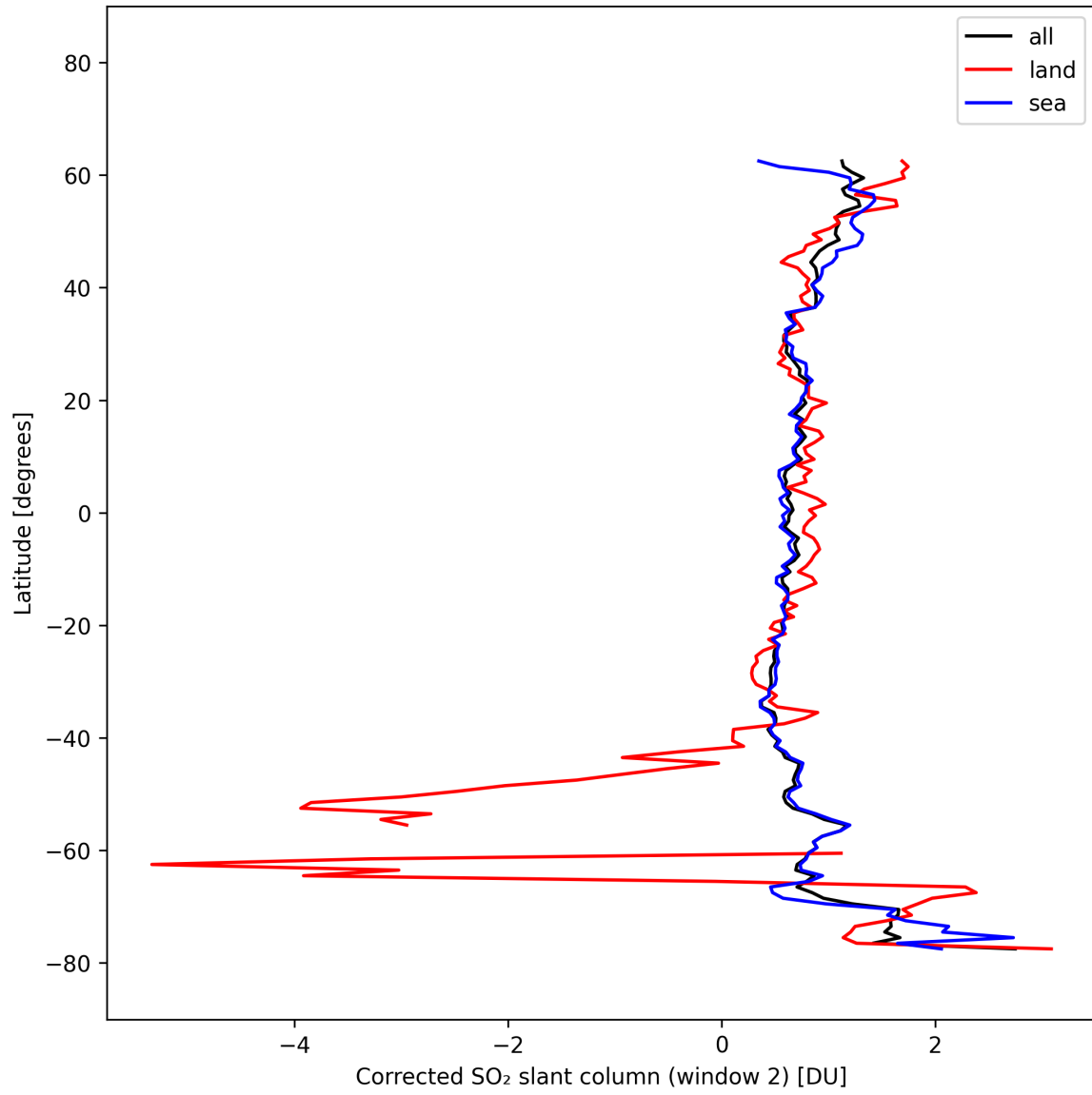
Figure 43: Zonal average of “Corrected SO 2 slant column (window 2)” for 2025-10-11 to 2025-10-12.
