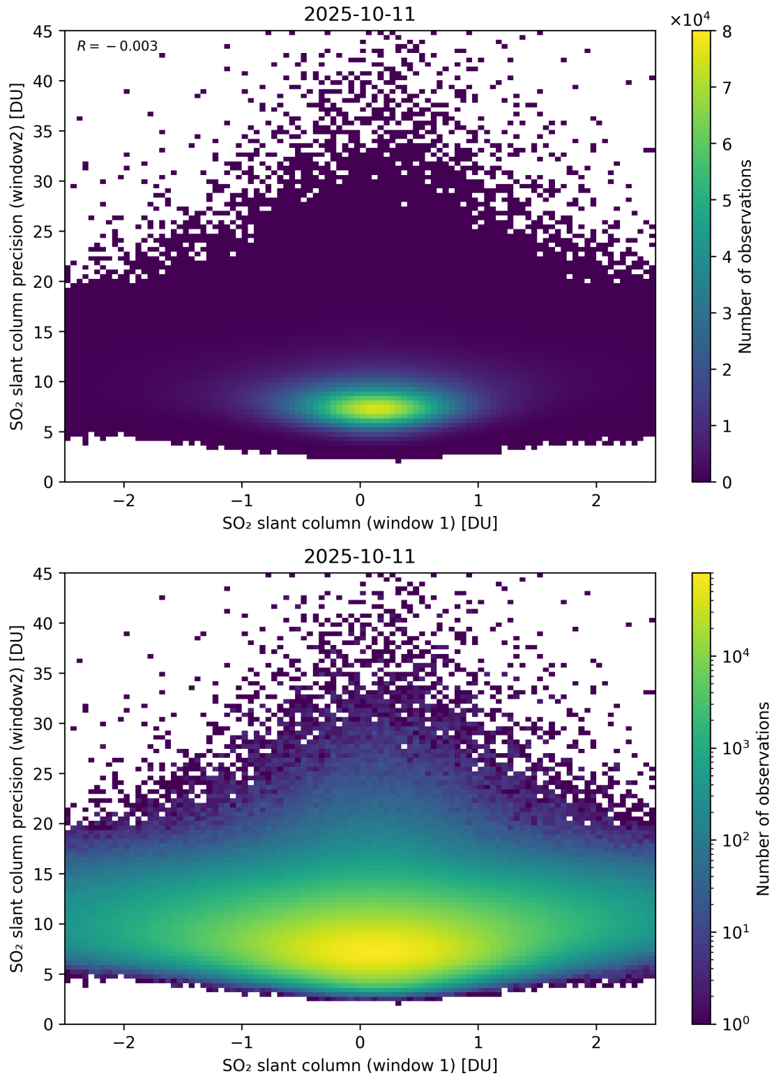
Figure 286: Scatter density plot of “SO 2 slant column (window 1)” against “SO 2 slant column precision (window2)” for 2025-10-11 to 2025-10-12.
