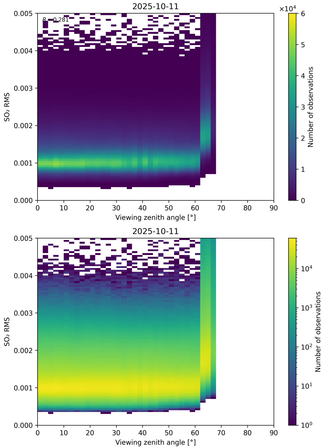
Figure 367: Scatter density plot of “Viewing zenith angle” against “SO 2 RMS” for 2025-10-11 to 2025-10-12.
