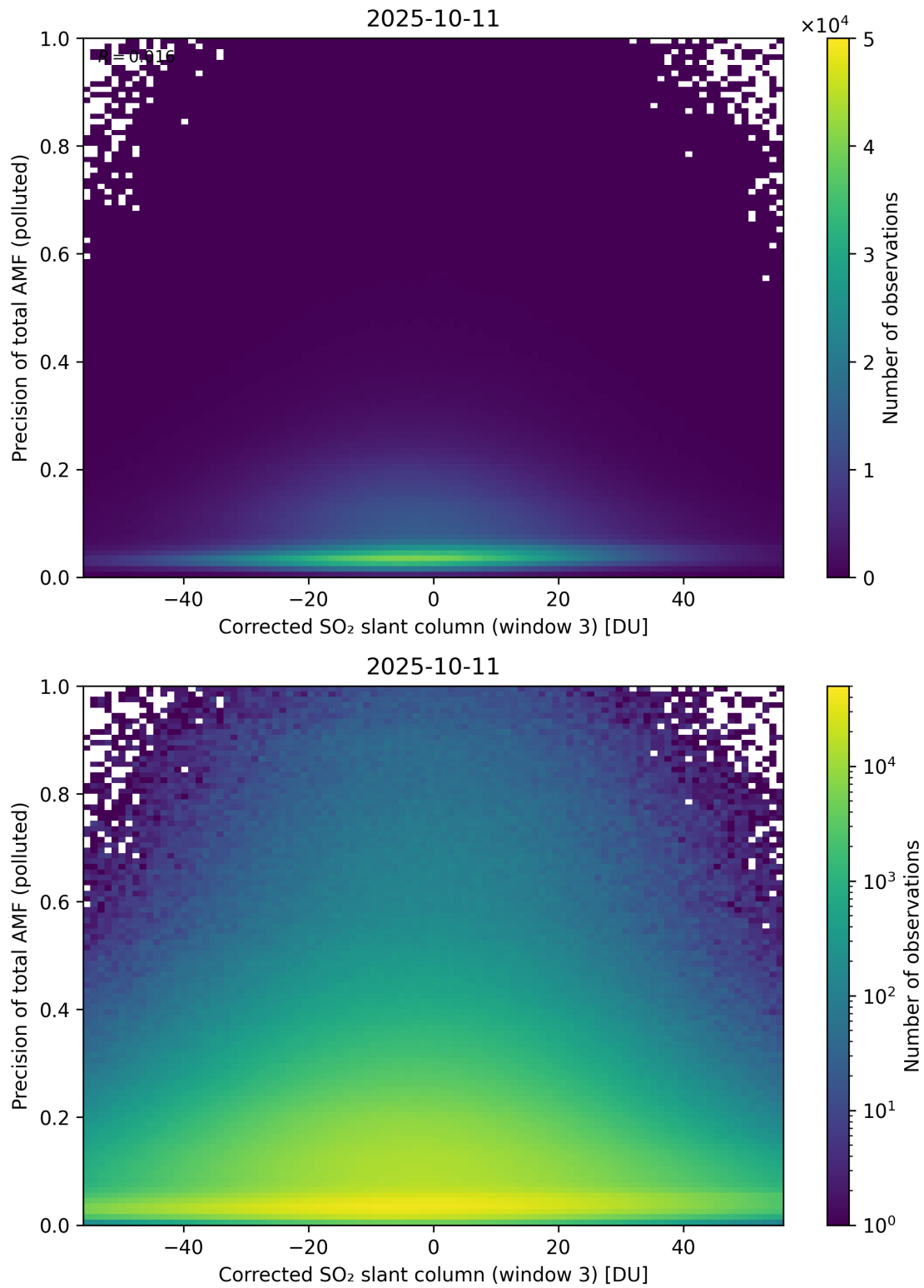
Figure 261: Scatter density plot of “Corrected SO 2 slant column (window 3)” against “Precision of total AMF (polluted)” for 2025-10-11 to 2025-10-12.
