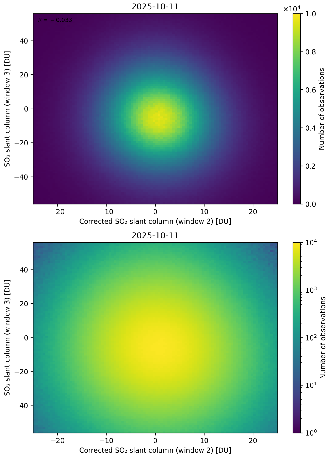
Figure 251: Scatter density plot of “Corrected SO 2 slant column (window 2)” against “SO 2 slant column (window 3)” for 2025-10-11 to 2025-10-12.
