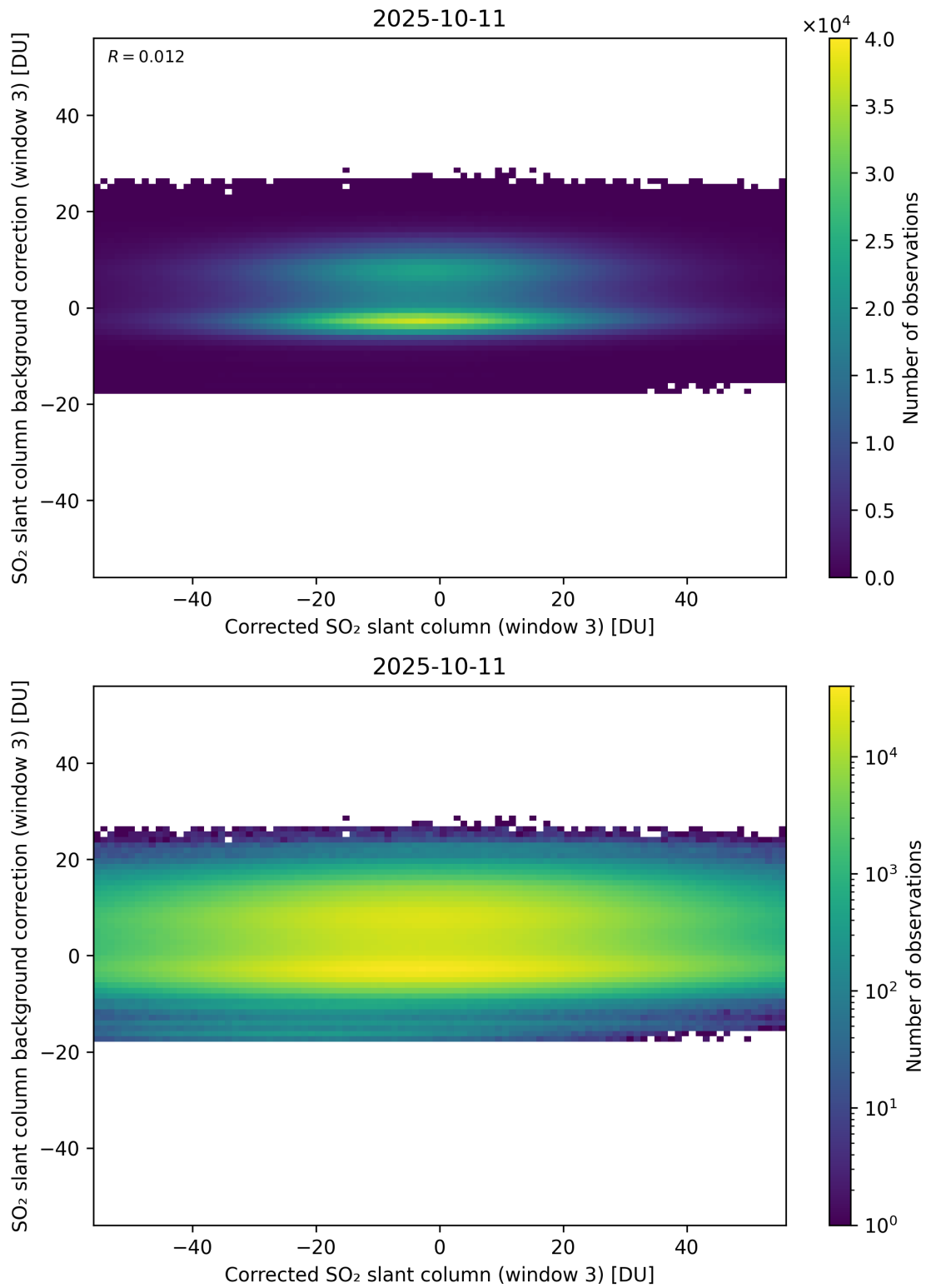
Figure 255: Scatter density plot of “Corrected SO 2 slant column (window 3)” against “SO 2 slant column background correction (window 3)” for 2025-10-11 to 2025-10-12.
