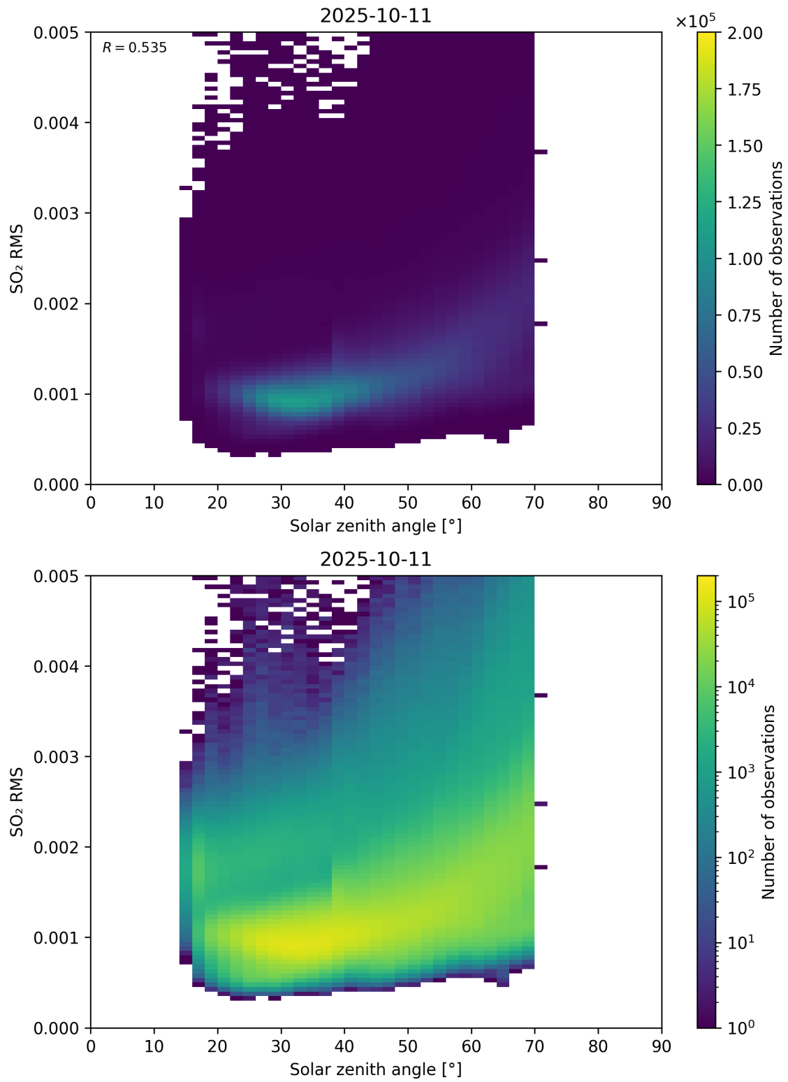
Figure 176: Scatter density plot of “Solar zenith angle” against “SO 2 RMS” for 2025-10-11 to 2025-10-12.
