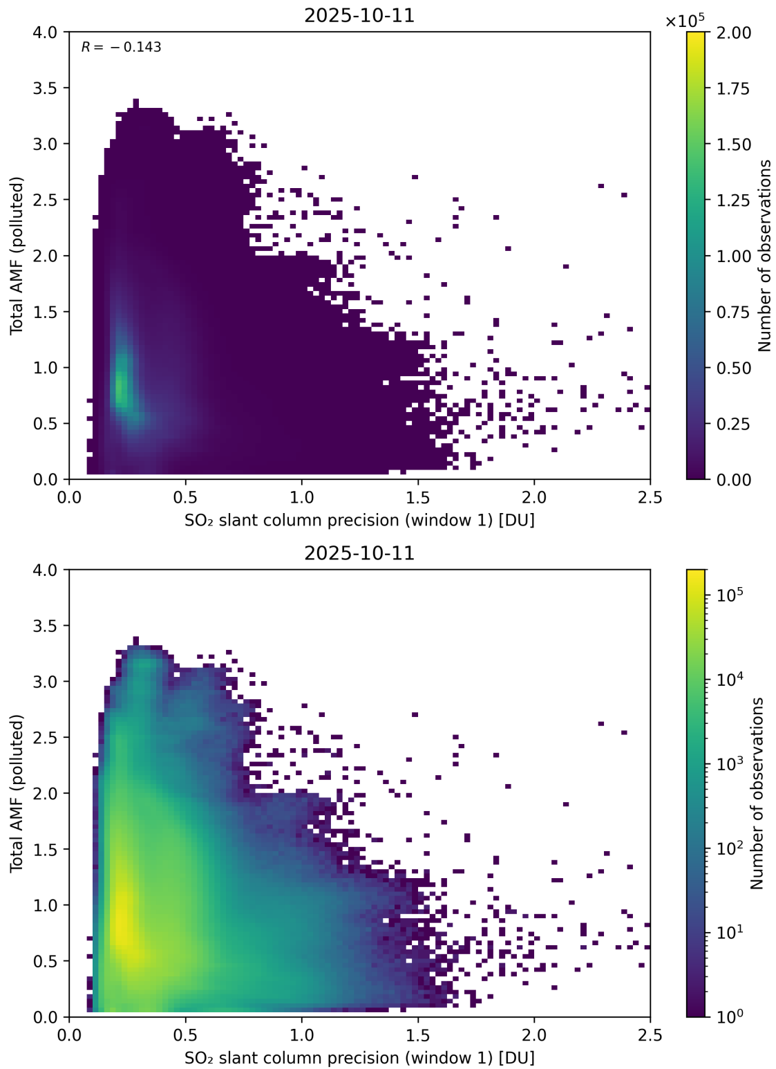
Figure 280: Scatter density plot of “SO 2 slant column precision (window 1)” against “Total AMF (polluted)” for 2025-10-11 to 2025-10-12.
