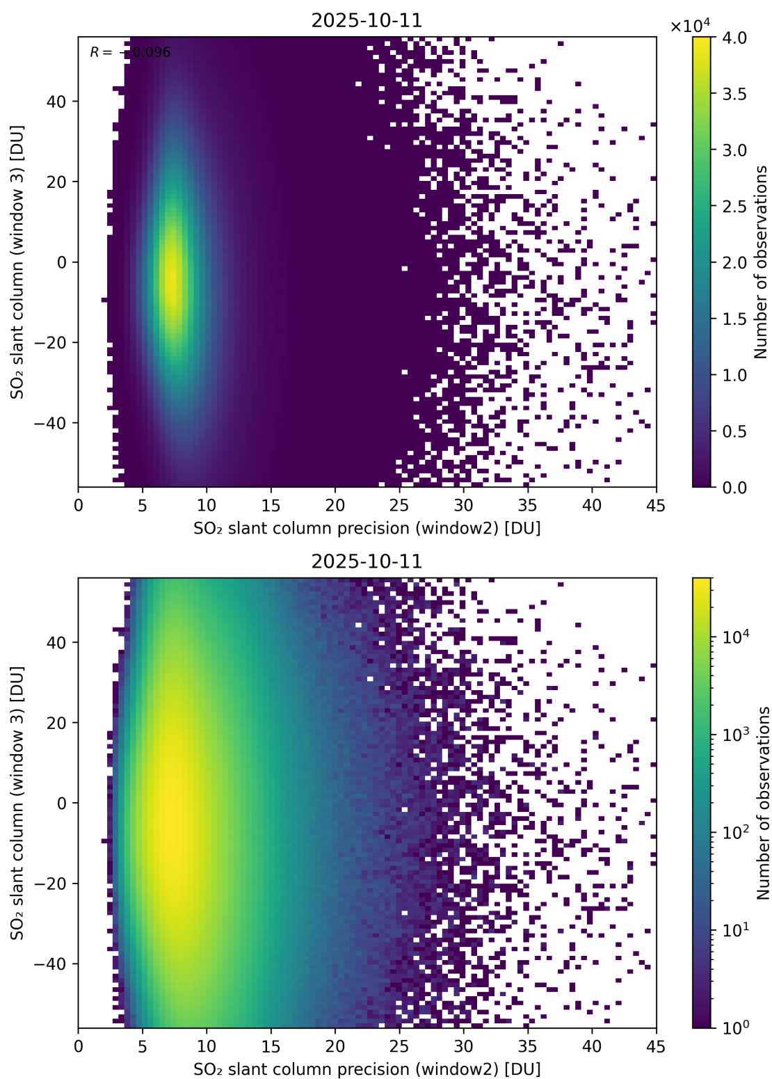
Figure 299: Scatter density plot of “SO 2 slant column precision (window2)” against “SO 2 slant column (window 3)” for 2025-10-11 to 2025-10-12.
