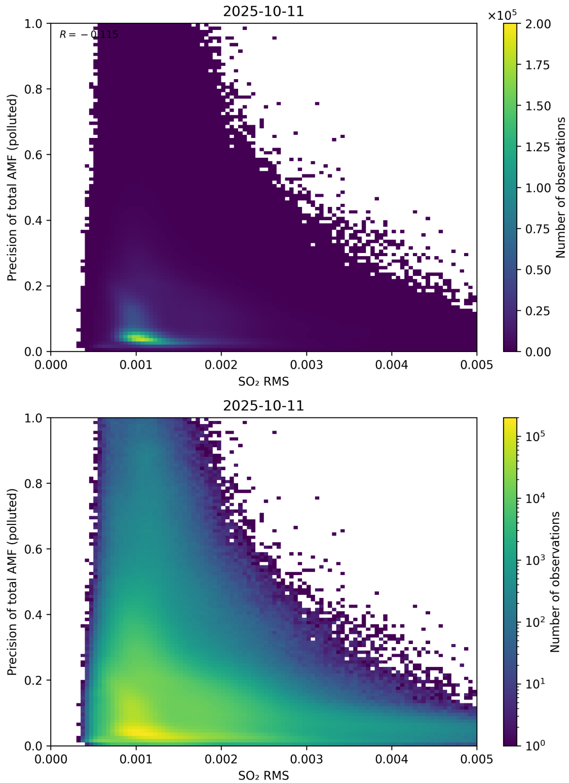
Figure 149: Scatter density plot of “SO 2 RMS” against “Precision of total AMF (polluted)” for 2025-10-11 to 2025-10-12.
