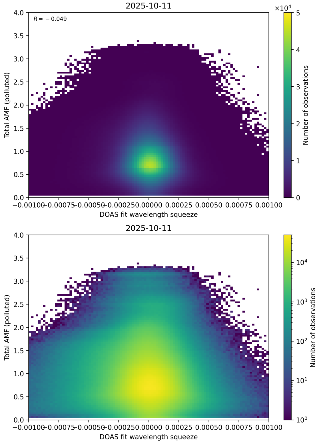
Figure 145: Scatter density plot of “DOAS fit wavelength squeeze” against “Total AMF (polluted)” for 2025-10-11 to 2025-10-12.
