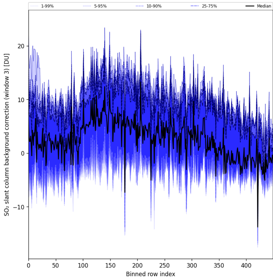
Figure 100: Along track statistics of “SO 2 slant column background correction (window 3)” for 2025-10-11 to 2025-10-12
