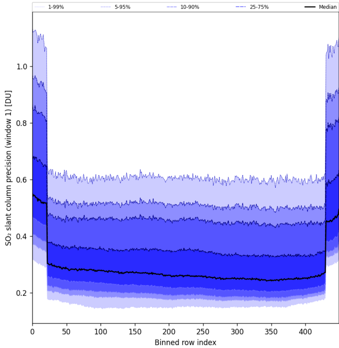
Figure 90: Along track statistics of “SO 2 slant column precision (window 1)” for 2025-10-11 to 2025-10-12
