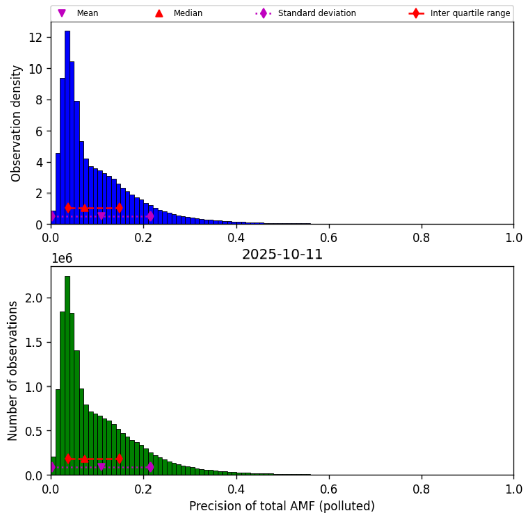
Figure 80: Histogram of “Precision of total AMF (polluted)” for 2025-10-11 to 2025-10-12
