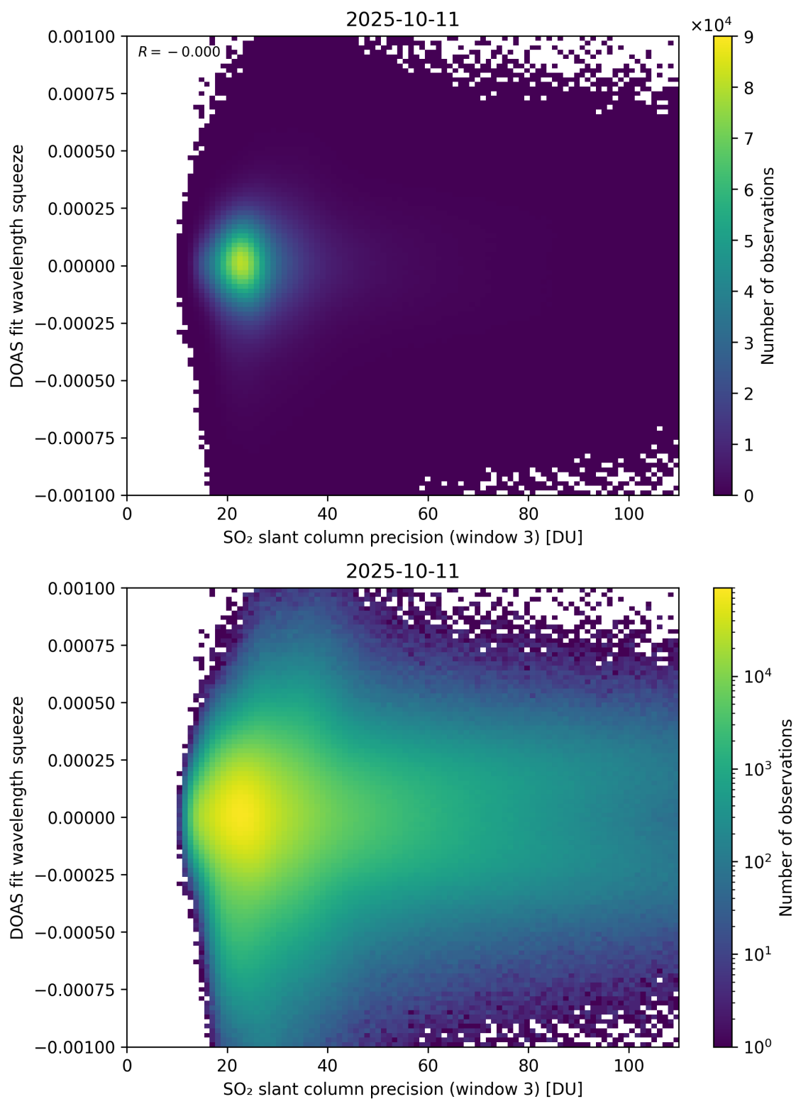
Figure 309: Scatter density plot of “SO 2 slant column precision (window 3)” against “DOAS fit wavelength squeeze” for 2025-10-11 to 2025-10-12.
