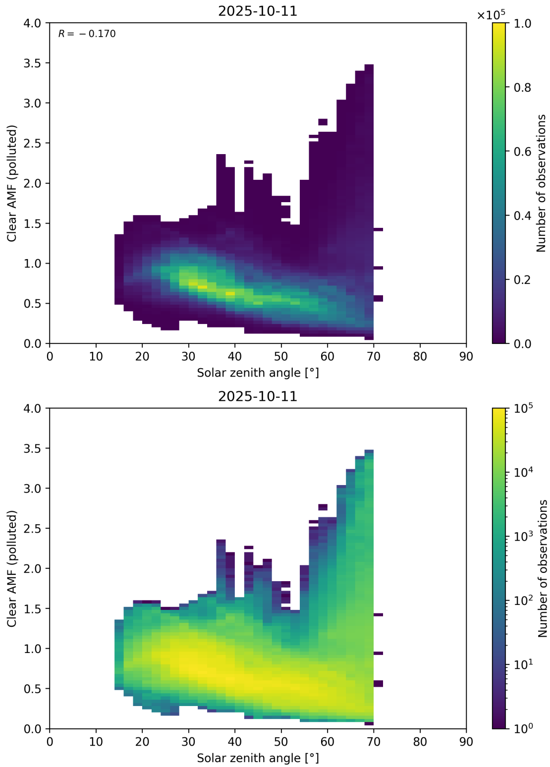
Figure 178: Scatter density plot of “Solar zenith angle” against “Clear AMF (polluted)” for 2025-10-11 to 2025-10-12.
