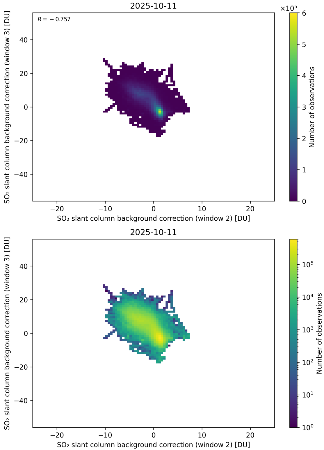
Figure 122: Scatter density plot of “SO 2 slant column background correction (window 2)” against “SO 2 slant column background correction (window 3)” for 2025-10-11 to 2025-10-12.
