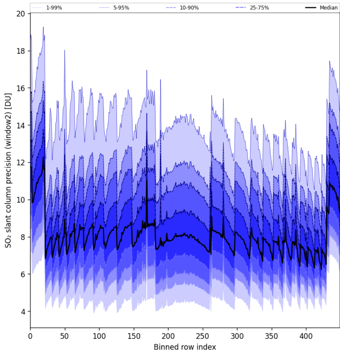
Figure 94: Along track statistics of “SO 2 slant column precision (window2)” for 2025-10-11 to 2025-10-12
