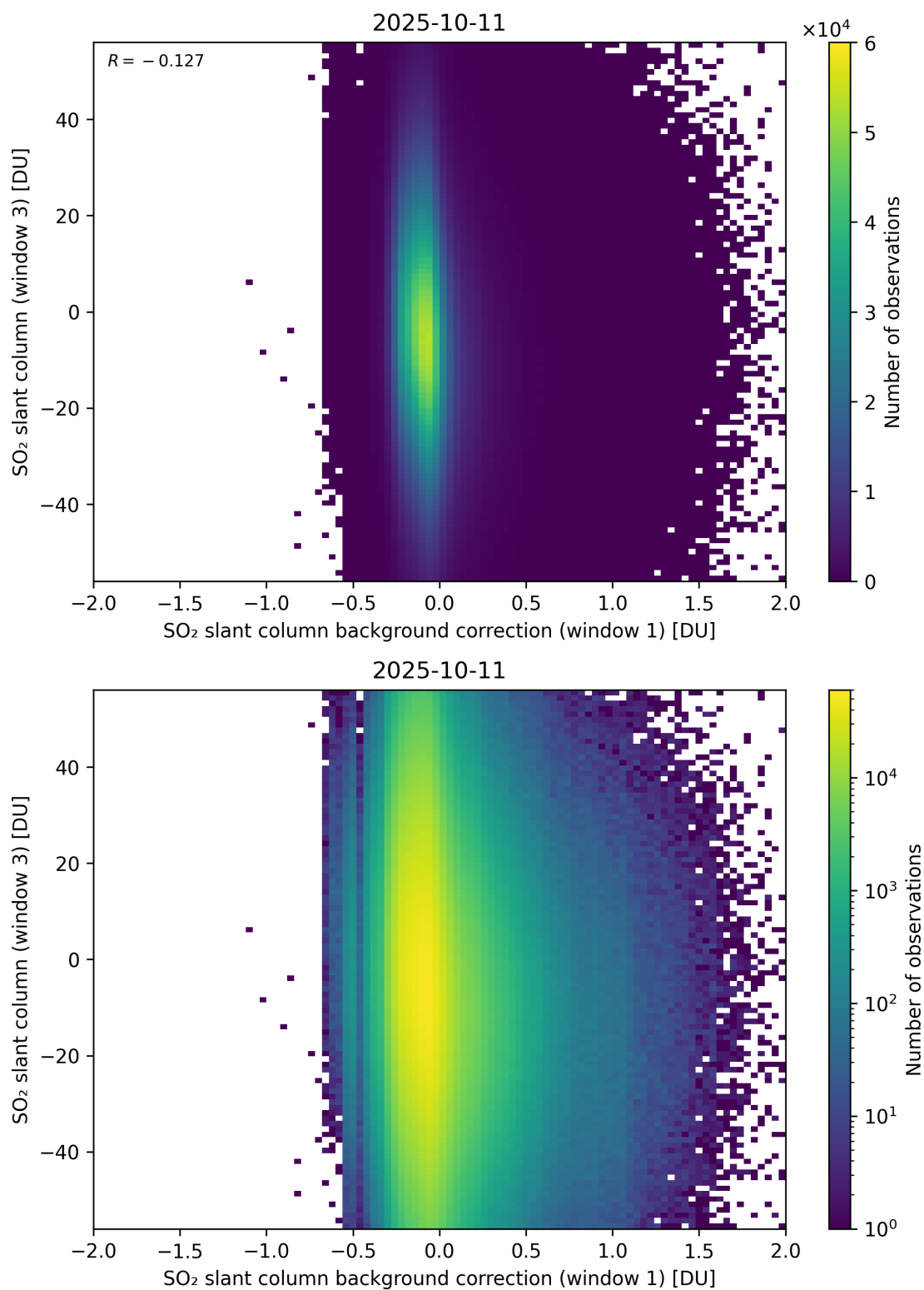
Figure 118: Scatter density plot of “SO 2 slant column background correction (window 1)” against “SO 2 slant column (window 3)” for 2025-10-11 to 2025-10-12.
