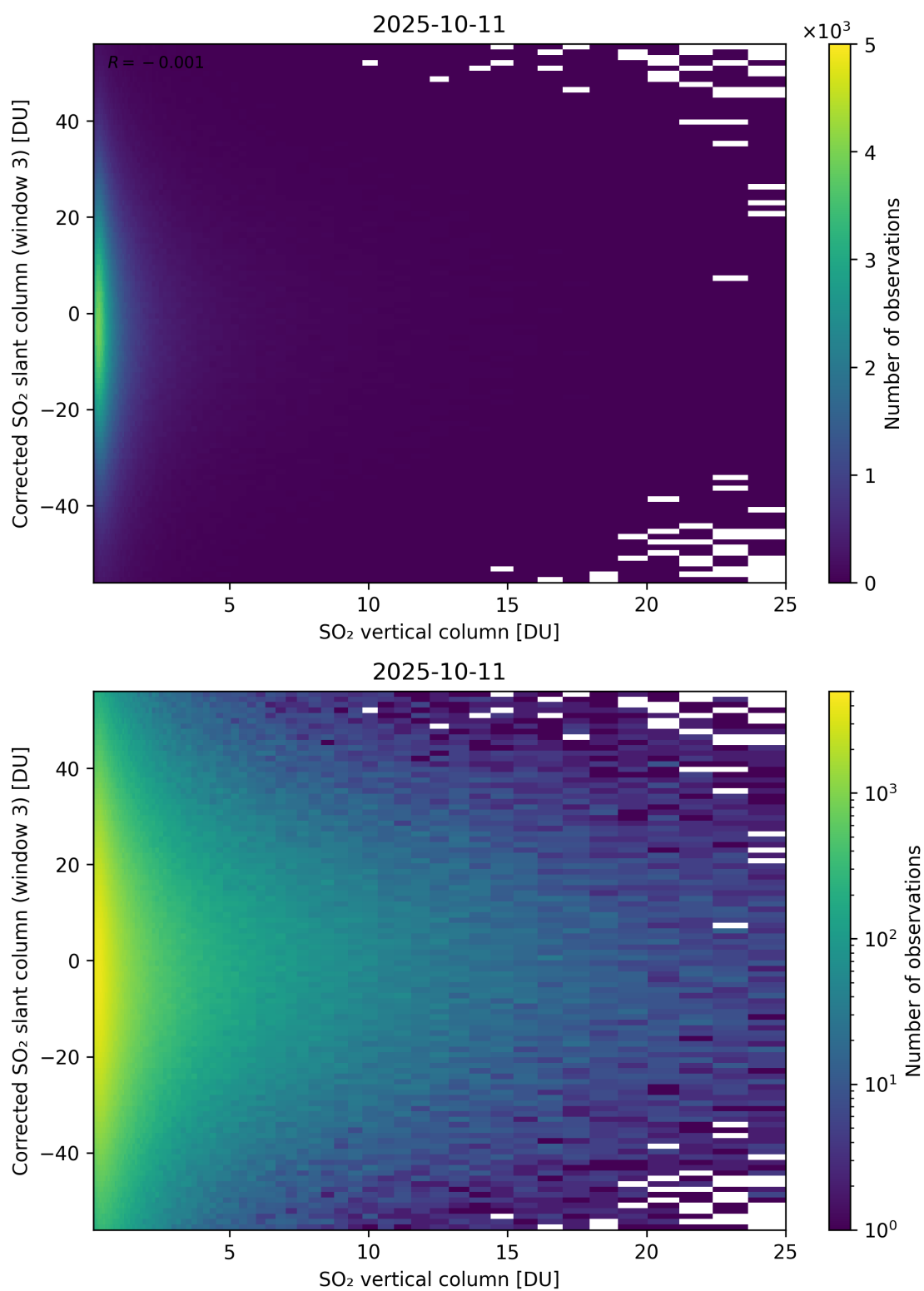
Figure 353: Scatter density plot of “SO 2 vertical column” against “Corrected SO 2 slant column (window 3)” for 2025-10-11 to 2025-10-12.
