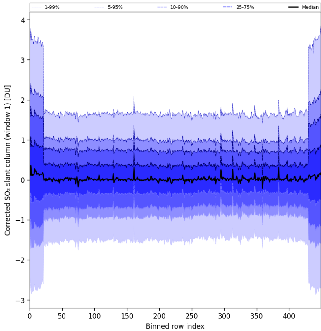
Figure 91: Along track statistics of "Corrected SO 2 slant column (window 1)" for 2025-10-11 to 2025-10-12
