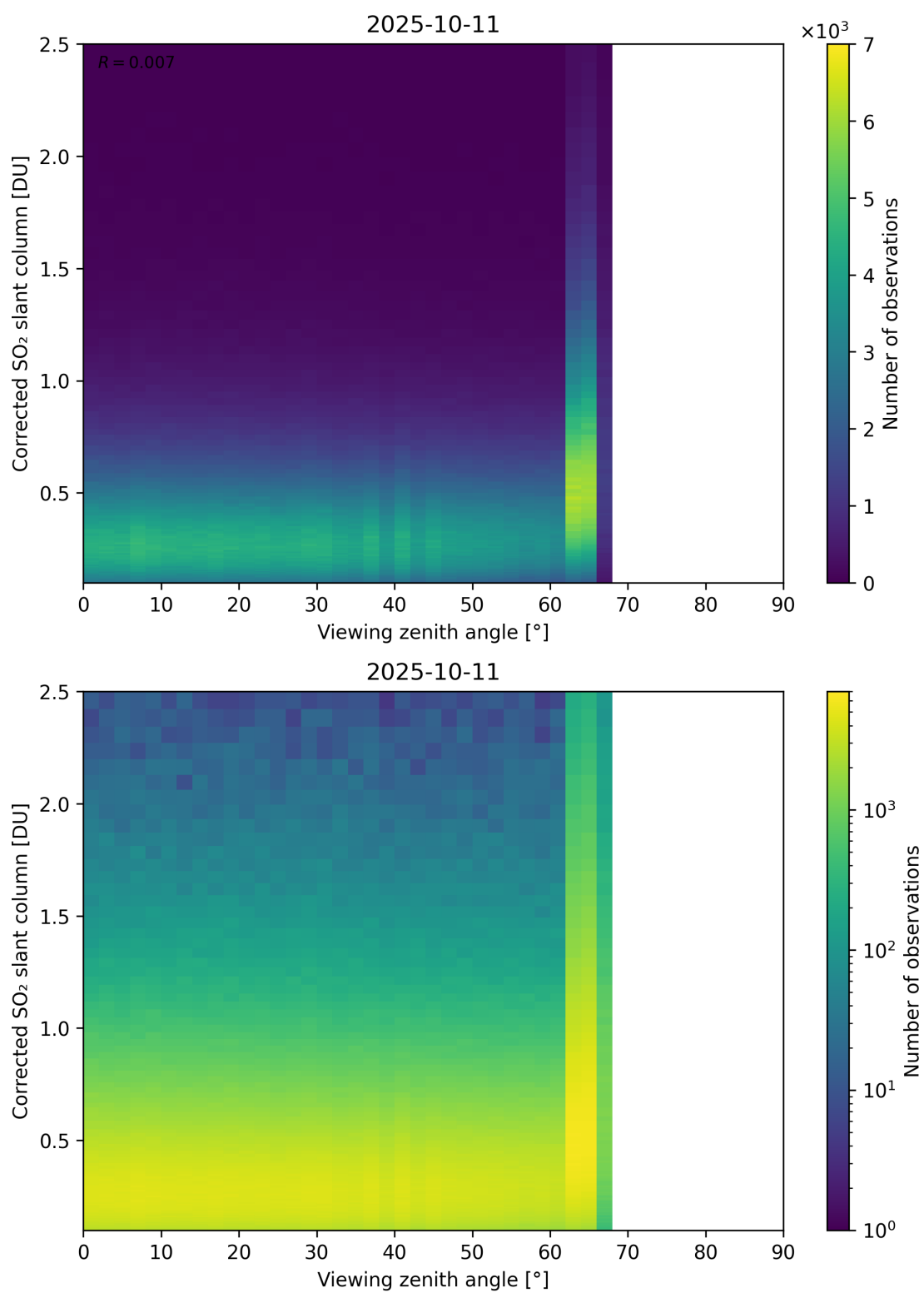
Figure 373: Scatter density plot of “Viewing zenith angle” against “Corrected SO 2 slant column” for 2025-10-11 to 2025-10-12.
