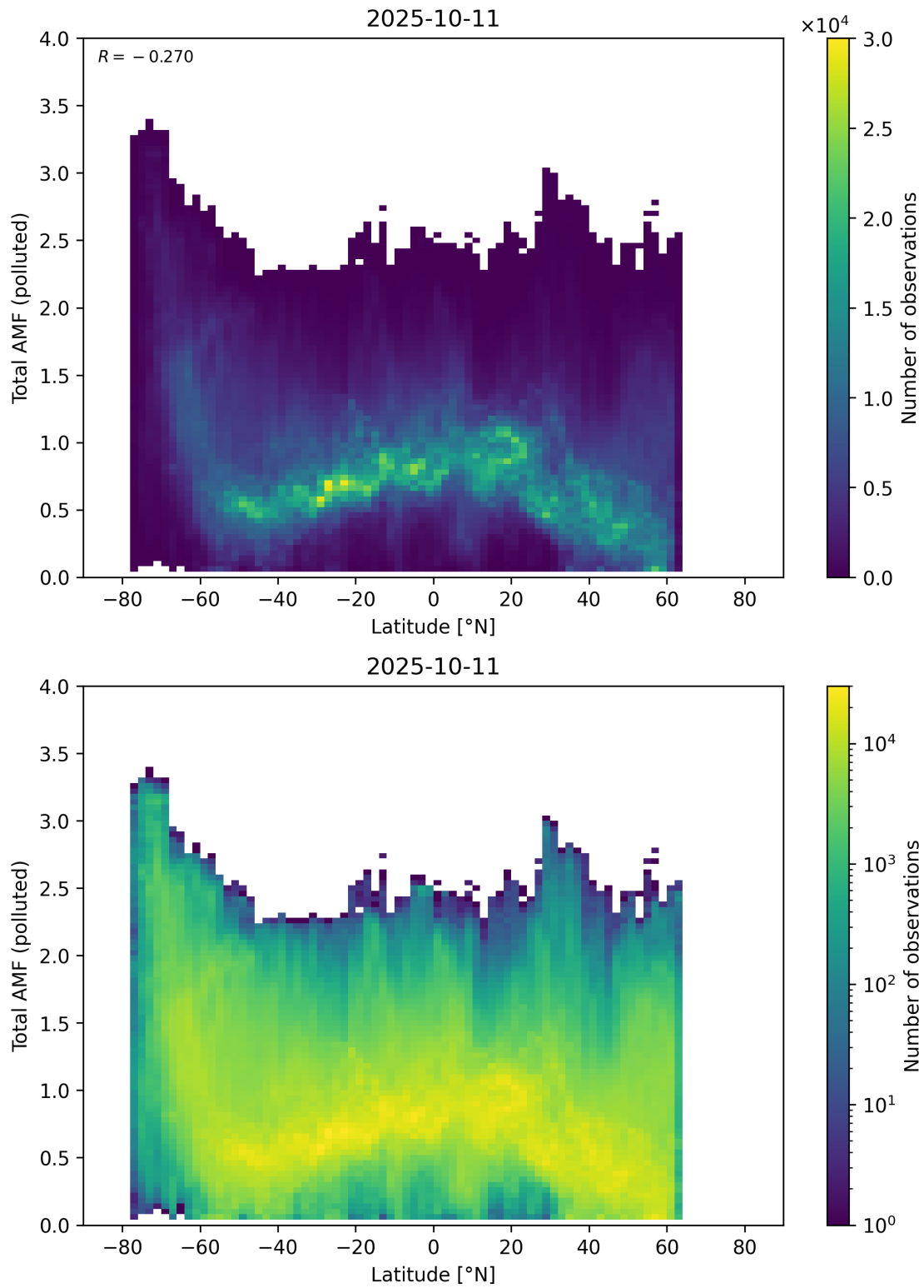
Figure 167: Scatter density plot of “Latitude” against “Total AMF (polluted)” for 2025-10-11 to 2025-10-12.
