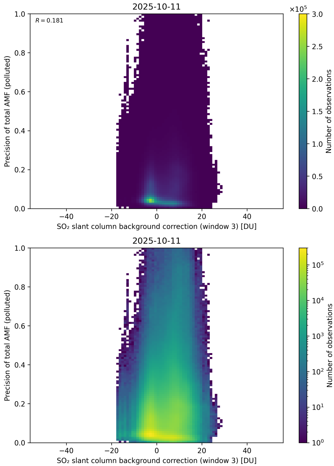
Figure 137: Scatter density plot of “SO 2 slant column background correction (window 3)” against “Precision of total AMF (polluted)” for 2025-10-11 to 2025-10-12.
