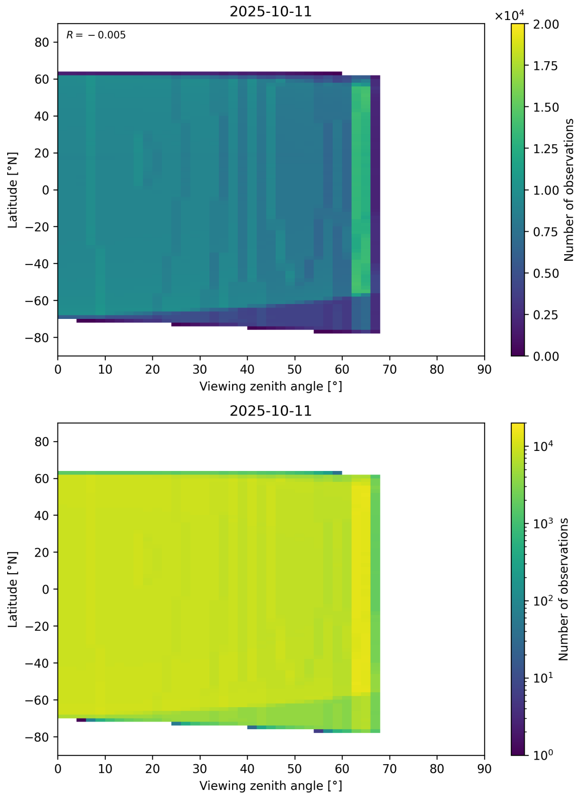
Figure 368: Scatter density plot of “Viewing zenith angle” against “Latitude” for 2025-10-11 to 2025-10-12.
