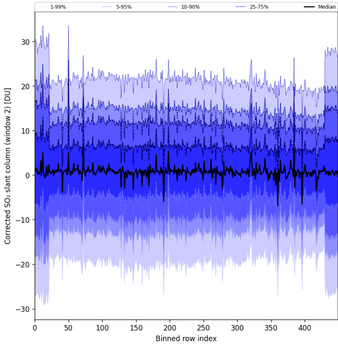
Figure 95: Along track statistics of “Corrected SO 2 slant column (window 2)” for 2025-10-11 to 2025-10-12
