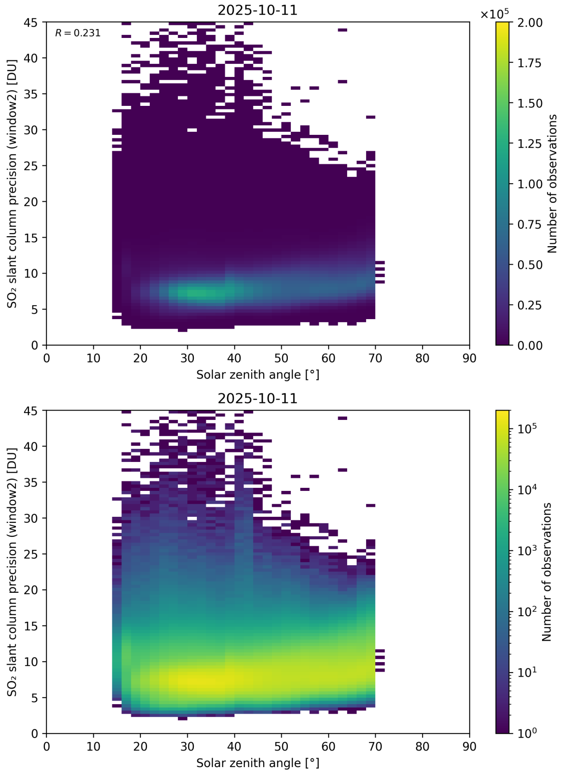
Figure 186: Scatter density plot of “Solar zenith angle” against “SO 2 slant column precision (window2)” for 2025-10-11 to 2025-10-12.
