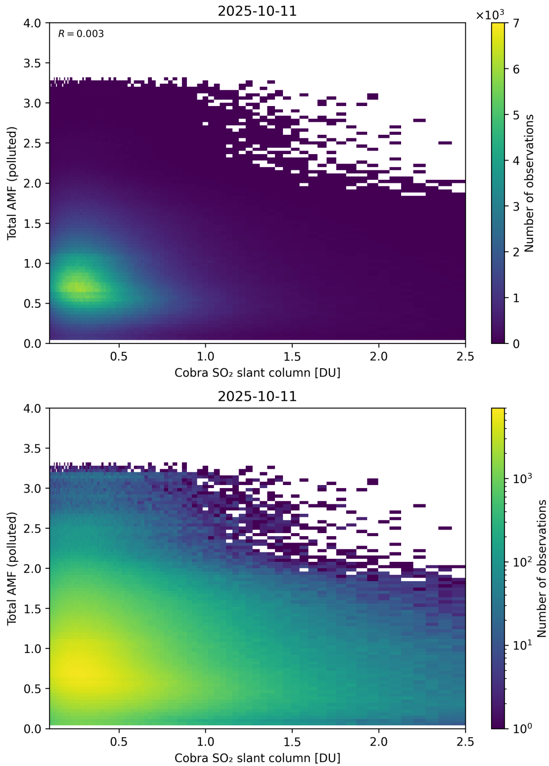
Figure 224: Scatter density plot of “Cobra SO 2 slant column” against “Total AMF (polluted)” for 2025-10-11 to 2025-10-12.
