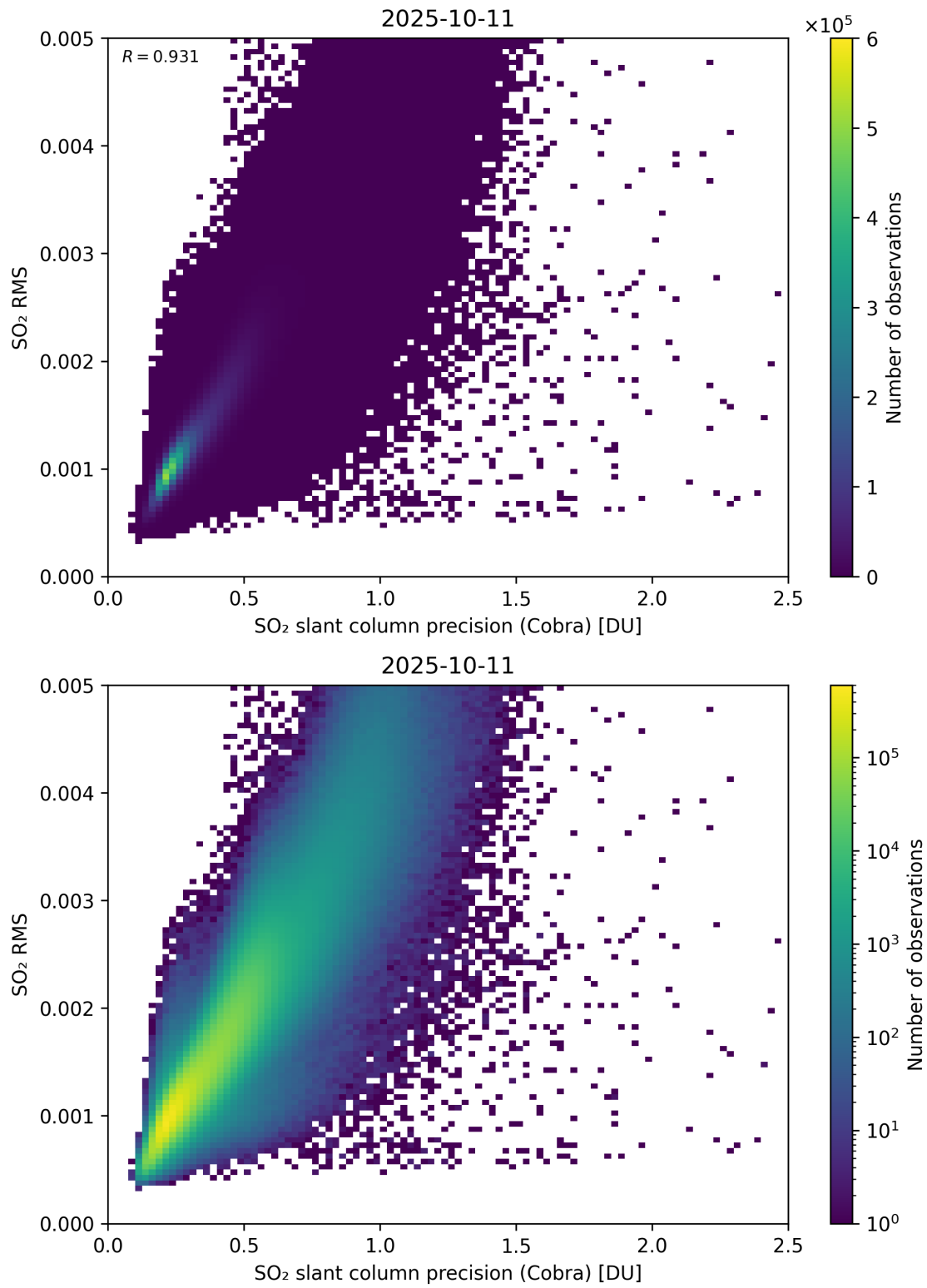
Figure 204: Scatter density plot of “SO 2 slant column precision (Cobra)” against “SO 2 RMS” for 2025-10-11 to 2025-10-12.
