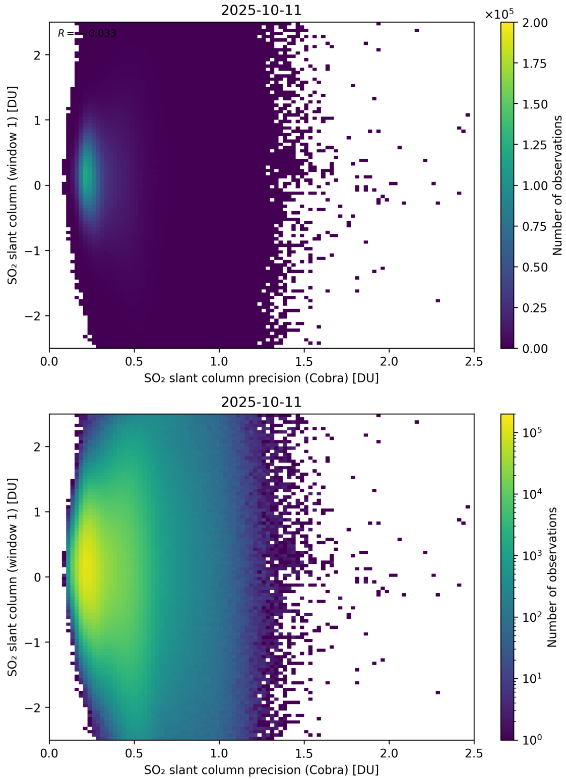
Figure 208: Scatter density plot of “SO 2 slant column precision (Cobra)” against “SO 2 slant column (window 1)” for 2025-10-11 to 2025-10-12.
