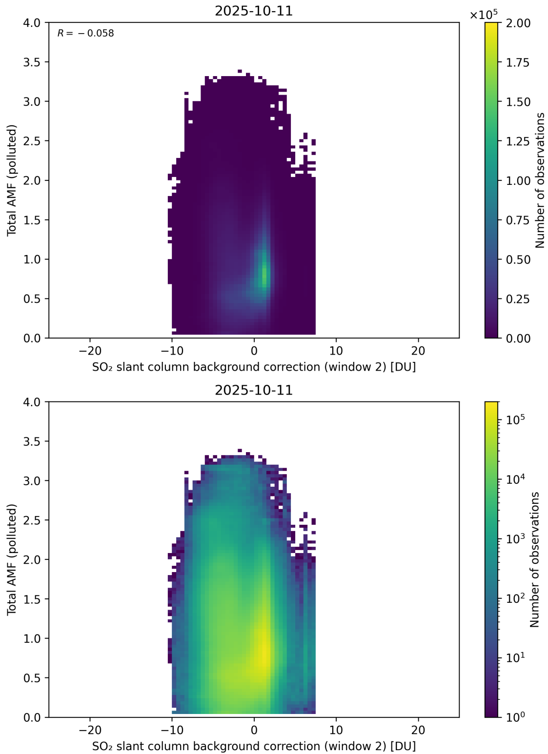
Figure 130: Scatter density plot of “SO 2 slant column background correction (window 2)” against “Total AMF (polluted)” for 2025-10-11 to 2025-10-12.
