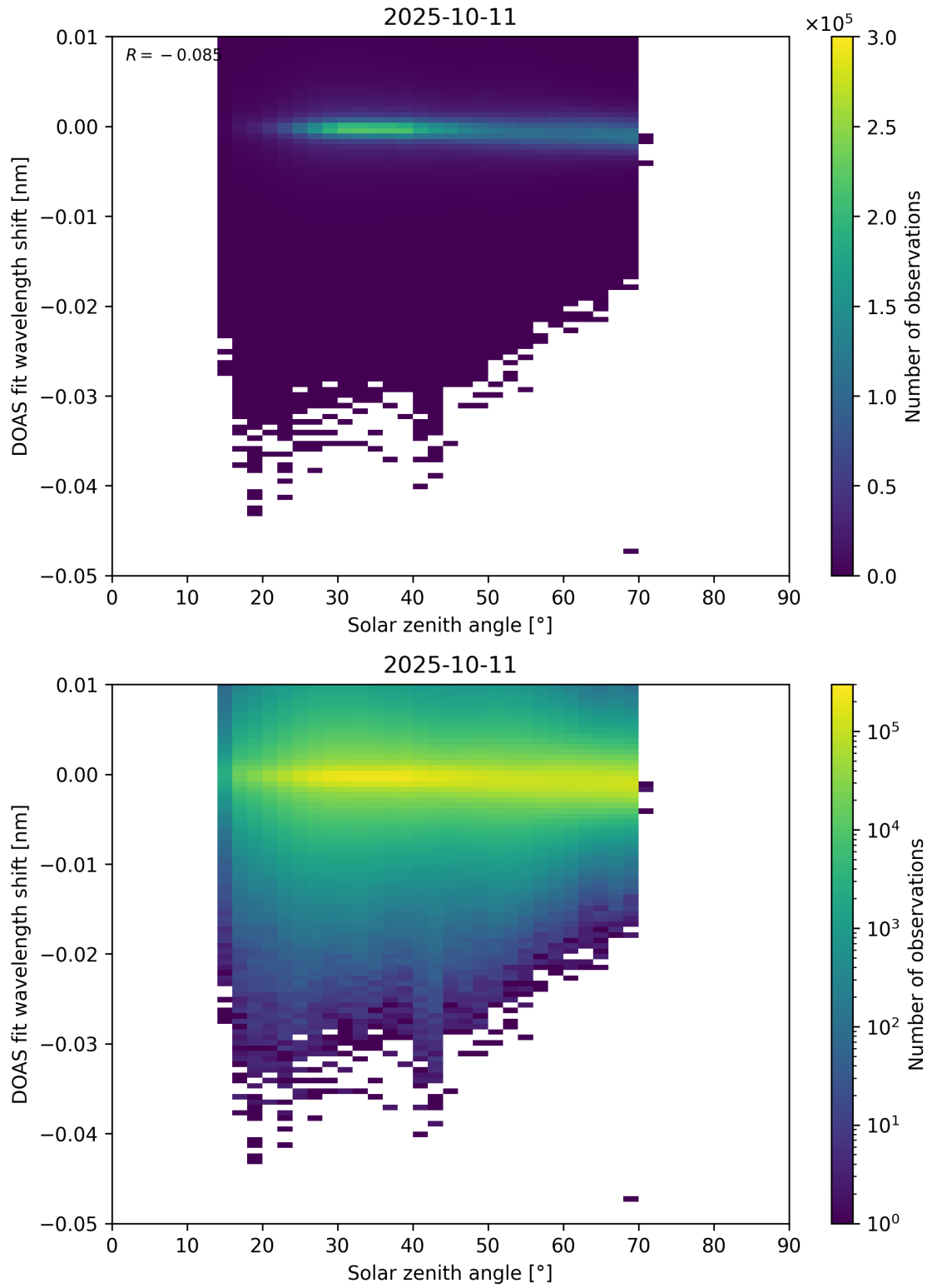
Figure 174: Scatter density plot of “Solar zenith angle” against “DOAS fit wavelength shift” for 2025-10-11 to 2025-10-12.
