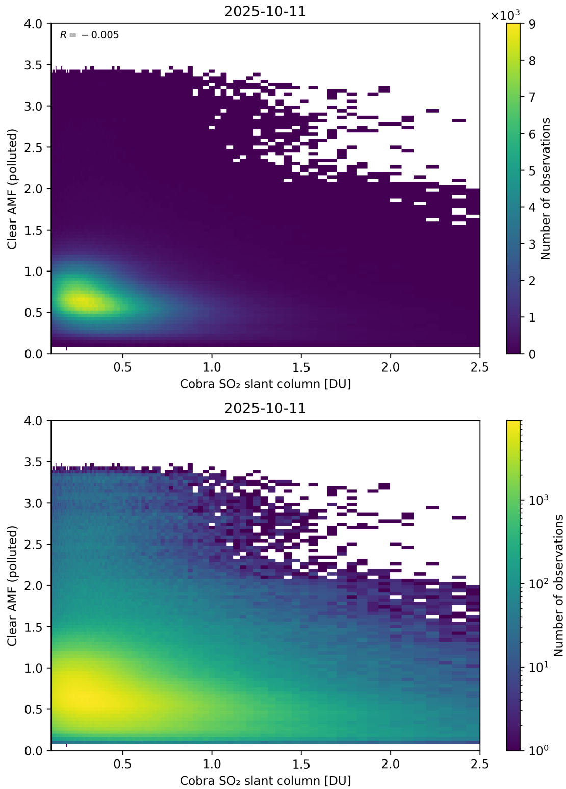
Figure 215: Scatter density plot of “Cobra SO 2 slant column” against “Clear AMF (polluted)” for 2025-10-11 to 2025-10-12.
