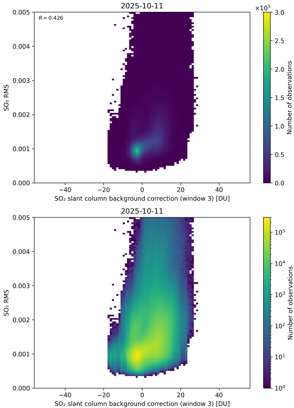
Figure 134: Scatter density plot of “SO 2 slant column background correction (window 3)” against “SO 2 RMS” for 2025-10-11 to 2025-10-12.
