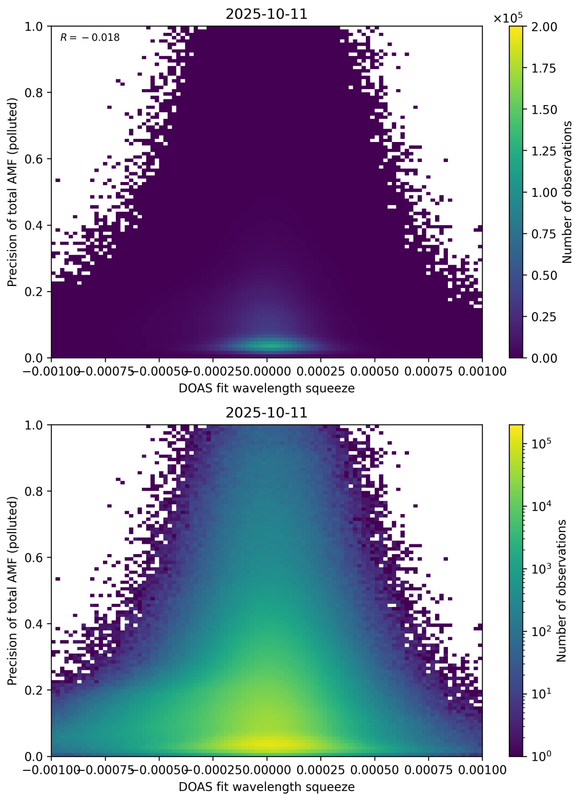
Figure 146: Scatter density plot of “DOAS fit wavelength squeeze” against “Precision of total AMF (polluted)” for 2025-10-11 to 2025-10-12.
