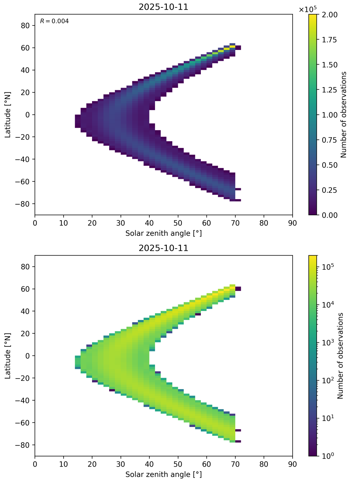
Figure 177: Scatter density plot of “Solar zenith angle” against “Latitude” for 2025-10-11 to 2025-10-12.
