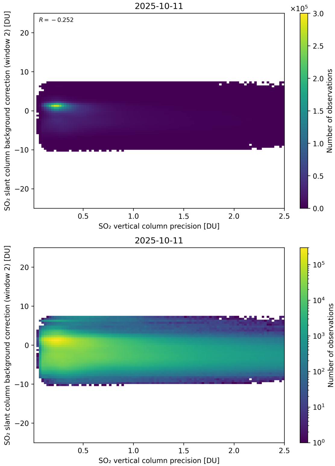
Figure 330: Scatter density plot of “SO 2 vertical column precision” against “SO 2 slant column background correction (window 2)” for 2025-10-11 to 2025-10-12.
