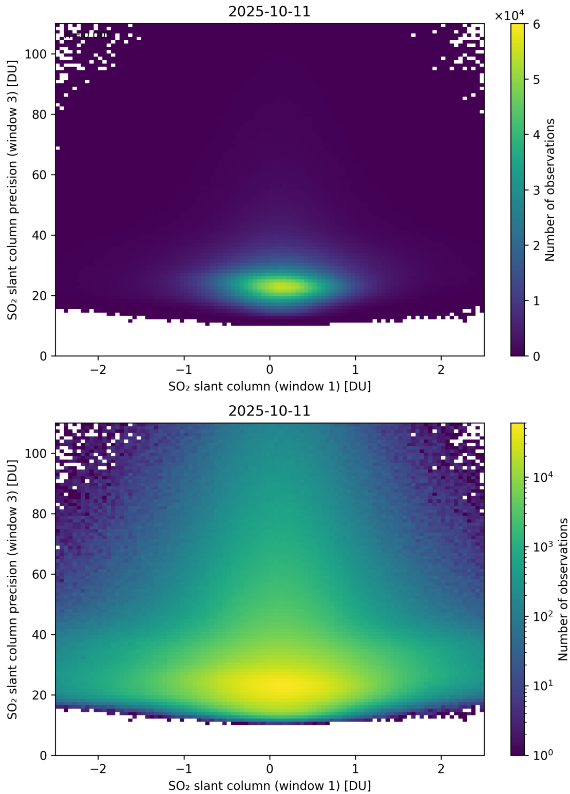
Figure 288: Scatter density plot of “SO 2 slant column (window 1)” against “SO 2 slant column precision (window 3)” for 2025-10-11 to 2025-10-12.
