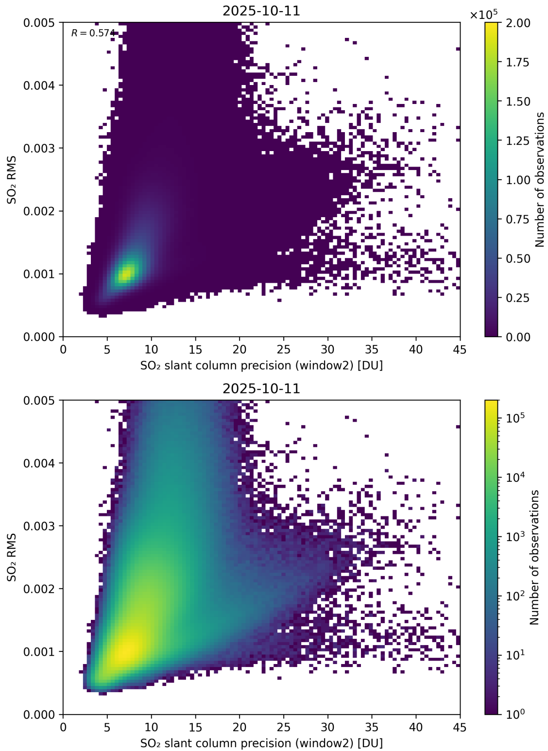
Figure 295: Scatter density plot of “SO 2 slant column precision (window2)” against “SO 2 RMS” for 2025-10-11 to 2025-10-12.
