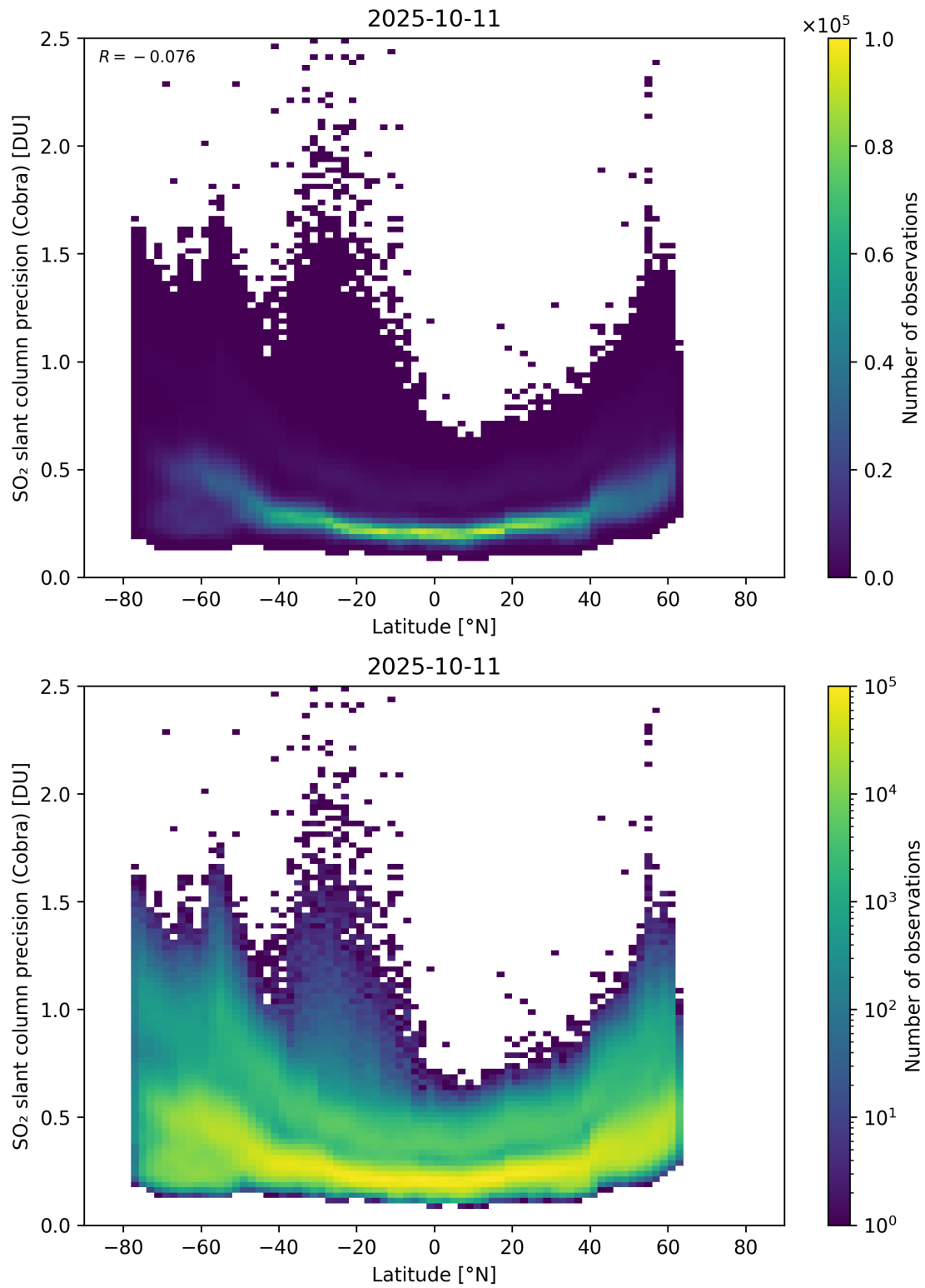
Figure 158: Scatter density plot of “Latitude” against “SO 2 slant column precision (Cobra)” for 2025-10-11 to 2025-10-12.
