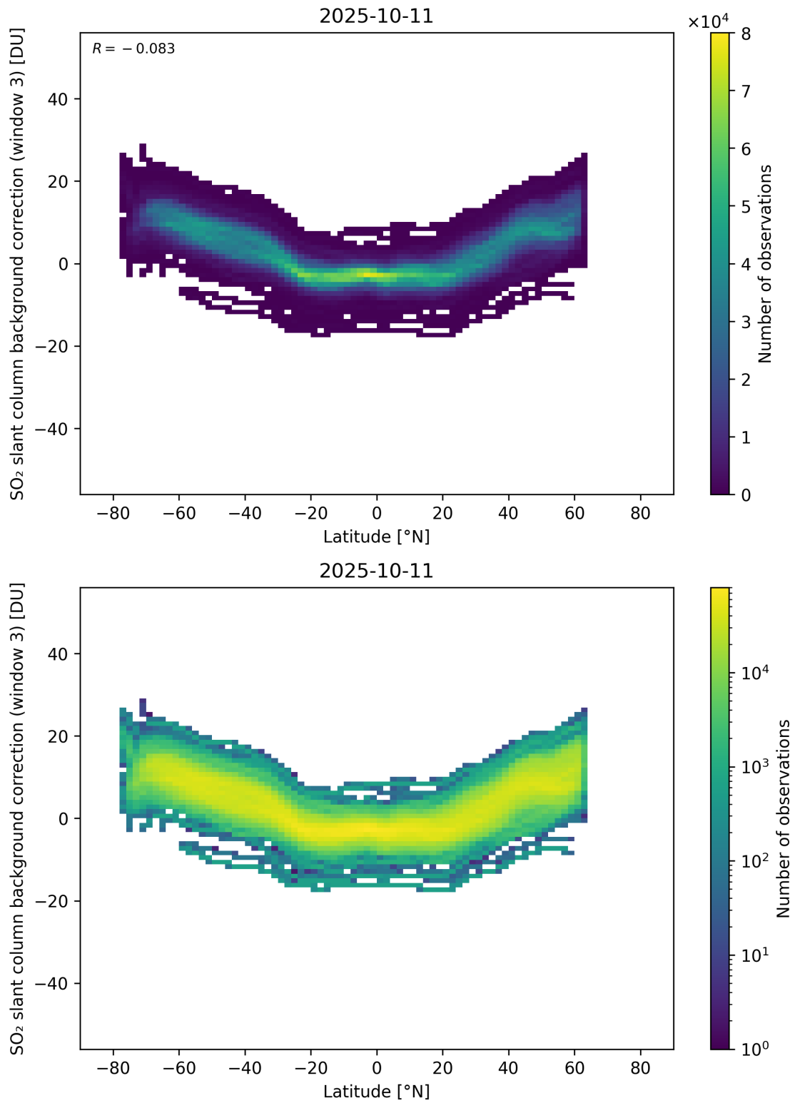
Figure 152: Scatter density plot of “Latitude” against “SO 2 slant column background correction (window 3)” for 2025-10-11 to 2025-10-12.
