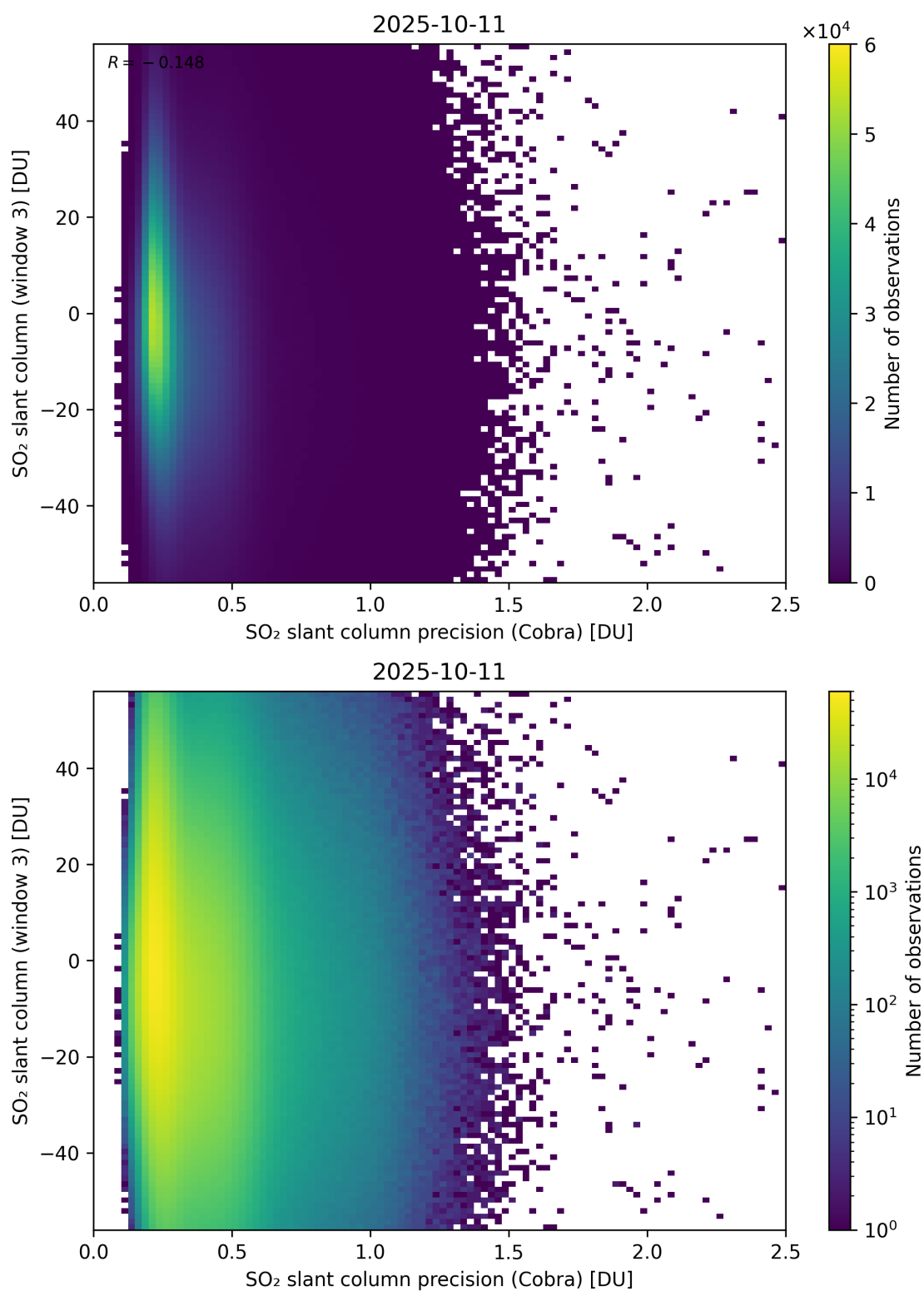
Figure 211: Scatter density plot of “SO 2 slant column precision (Cobra)” against “SO 2 slant column (window 3)” for 2025-10-11 to 2025-10-12.
