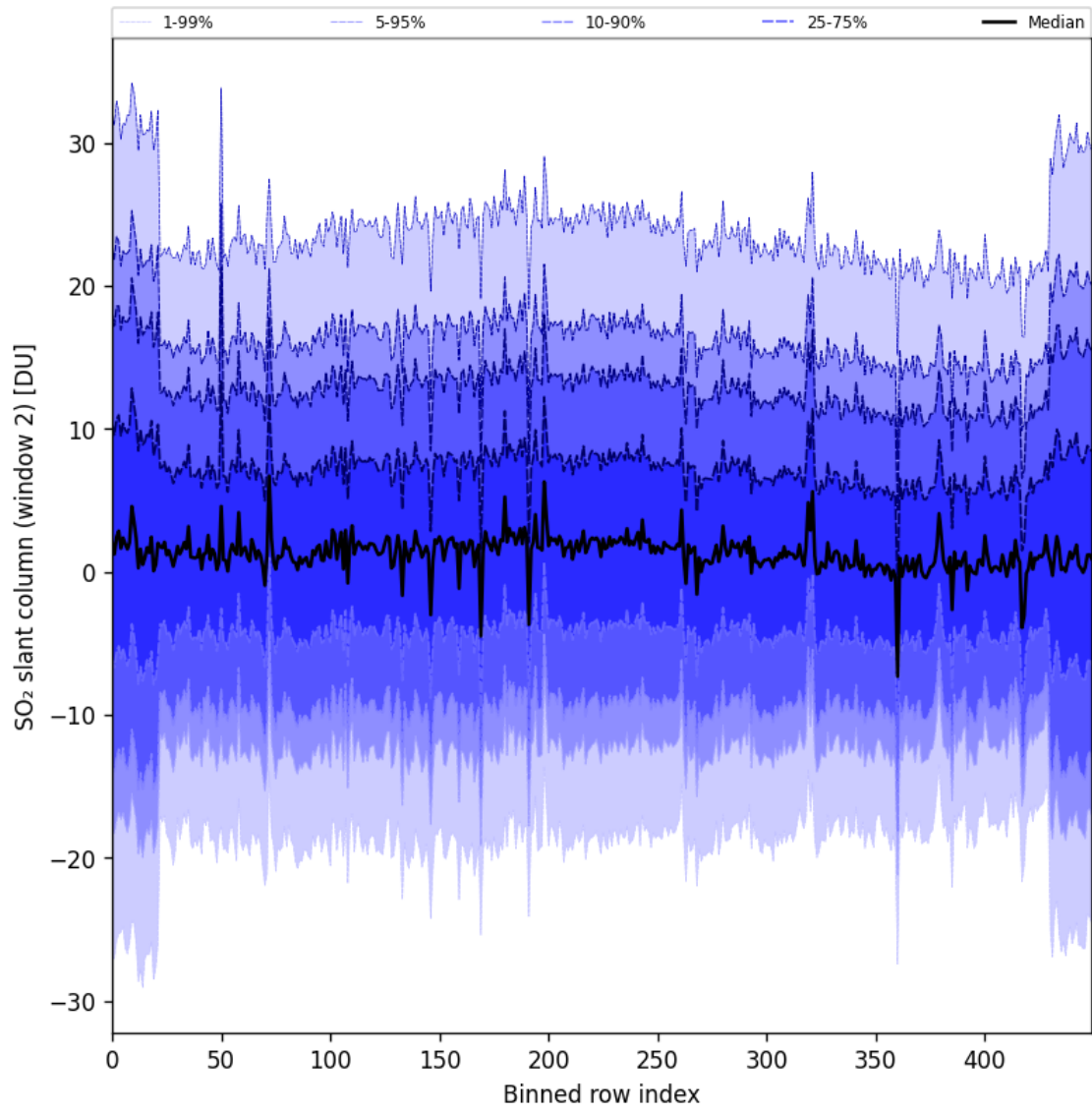
Figure 93: Along track statistics of “SO 2 slant column (window 2)” for 2025-10-11 to 2025-10-12
