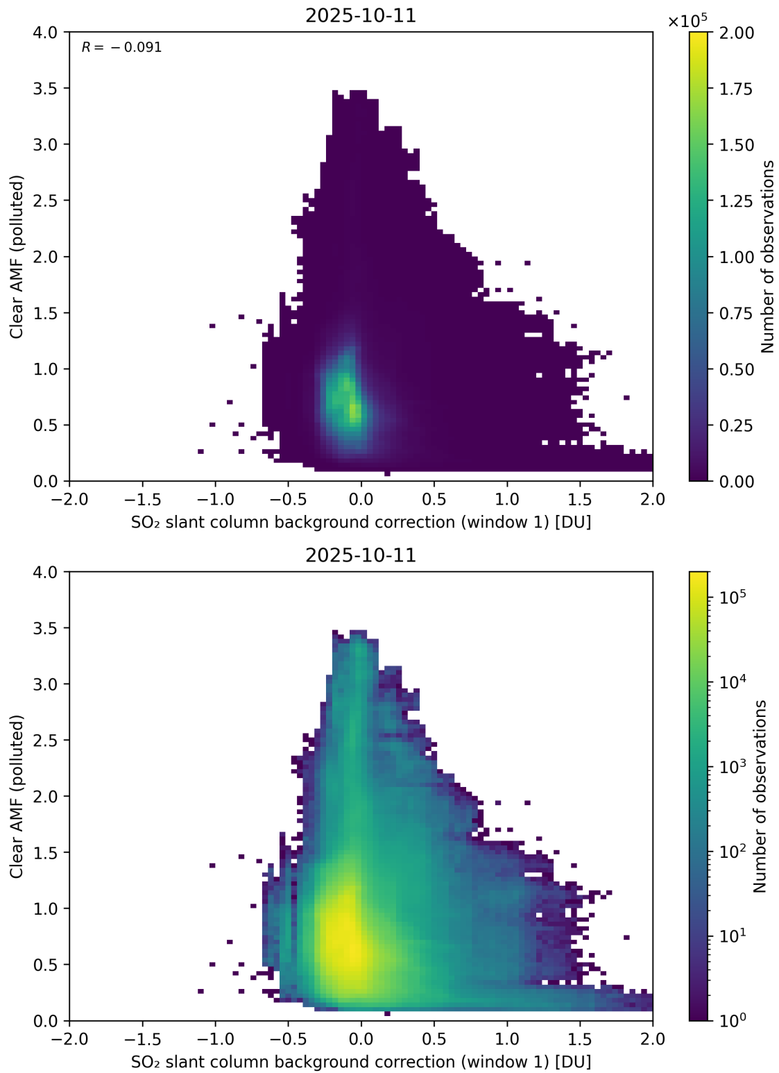
Figure 114: Scatter density plot of “SO 2 slant column background correction (window 1)” against “Clear AMF (polluted)” for 2025-10-11 to 2025-10-12.
