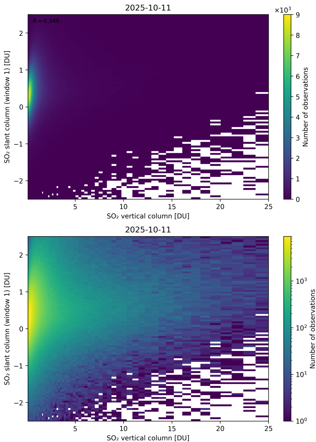
Figure 354: Scatter density plot of “SO 2 vertical column” against “SO 2 slant column (window 1)” for 2025-10-11 to 2025-10-12.
