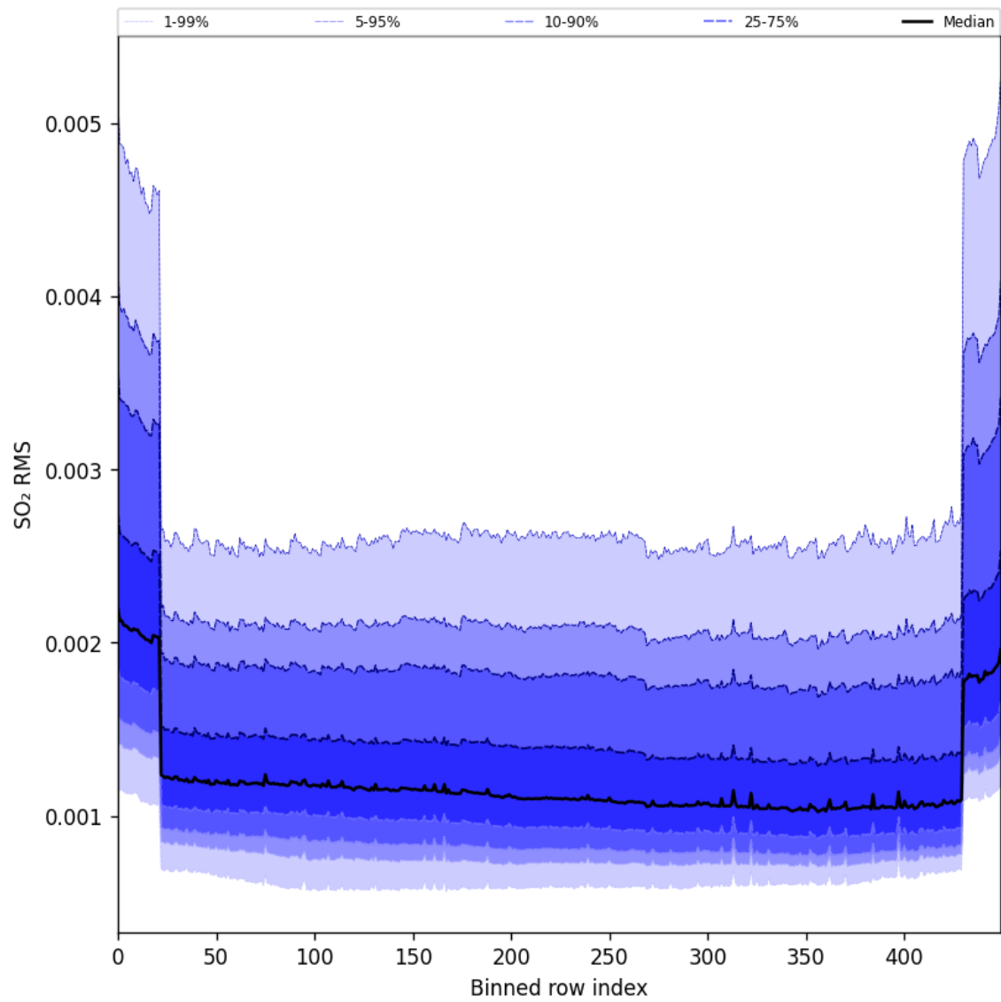
Figure 104: Along track statistics of “SO 2 RMS” for 2025-10-11 to 2025-10-12
