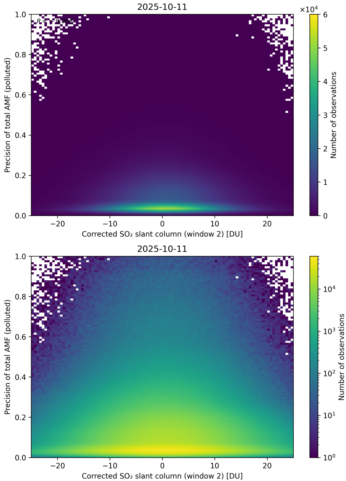
Figure 254: Scatter density plot of “Corrected SO 2 slant column (window 2)” against “Precision of total AMF (polluted)” for 2025-10-11 to 2025-10-12.
