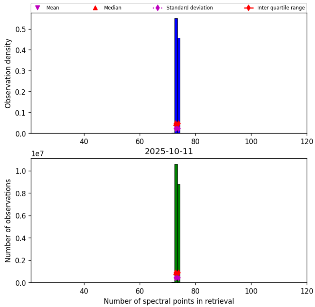
Figure 82: Histogram of “Number of spectral points in retrieval” for 2025-10-11 to 2025-10-12
