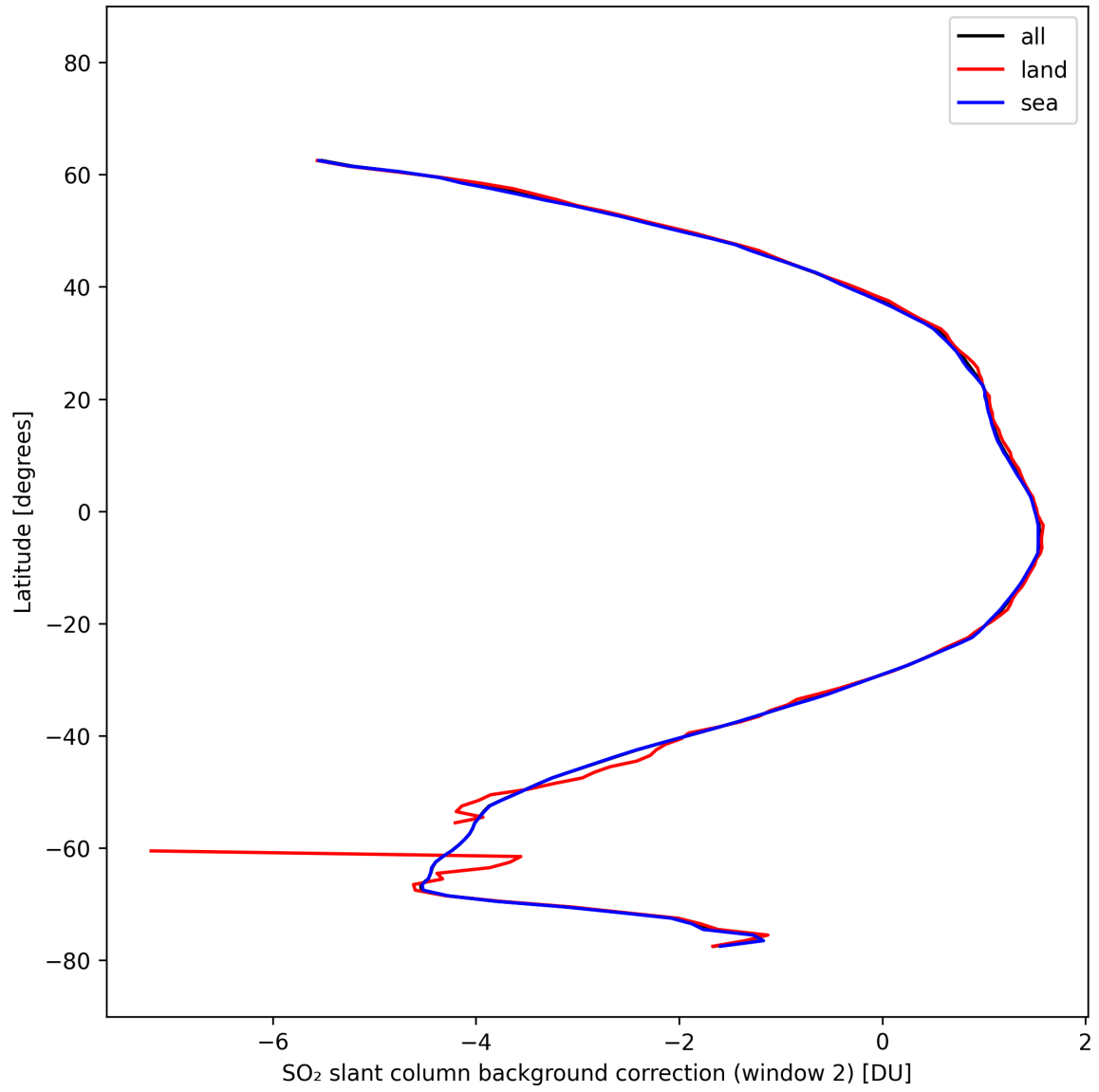
Figure 44: Zonal average of “SO 2 slant column background correction (window 2)” for 2025-10-11 to 2025-10-12.
