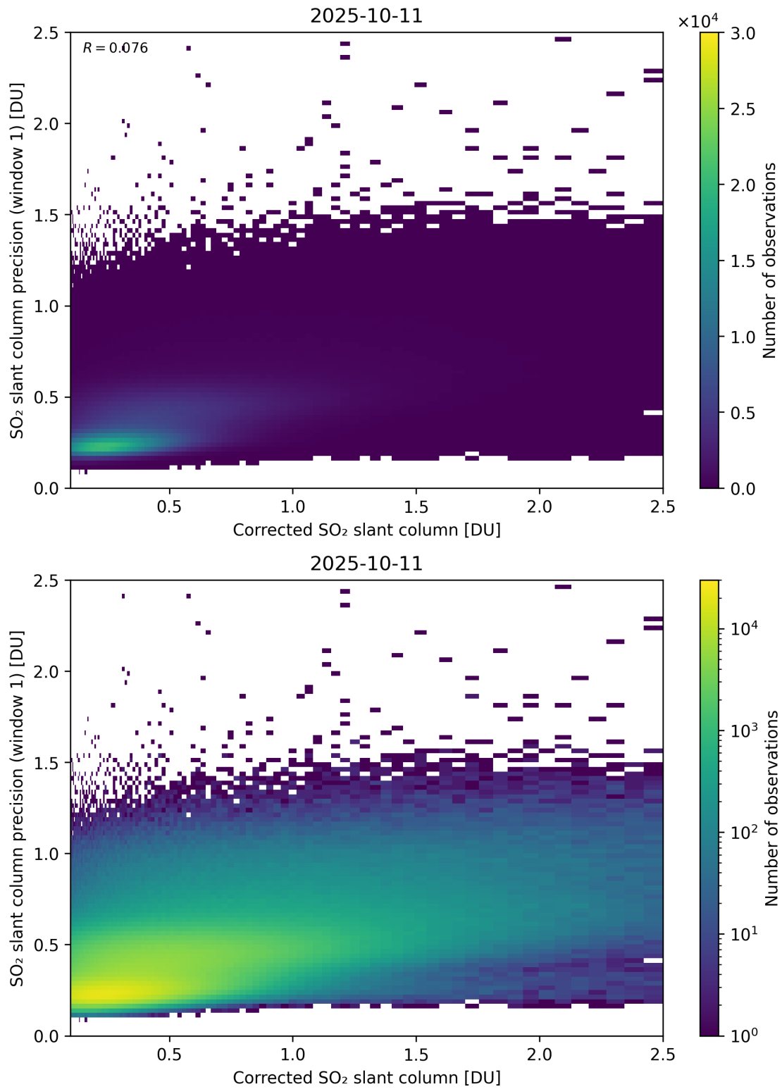
Figure 238: Scatter density plot of “Corrected SO 2 slant column” against “SO 2 slant column precision (window 1)” for 2025-10-11 to 2025-10-12.
