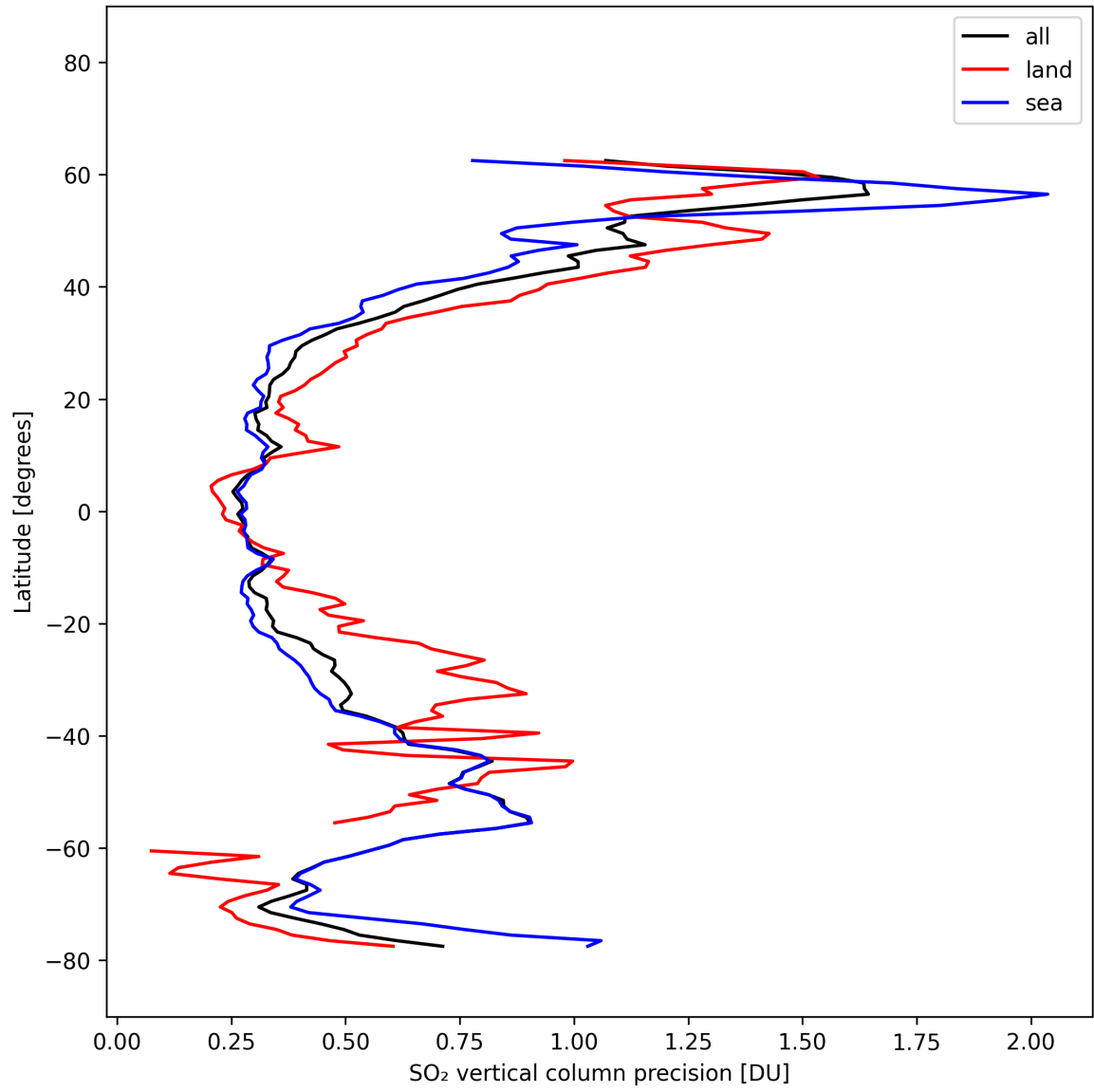
Figure 33: Zonal average of “SO 2 vertical column precision” for 2025-10-11 to 2025-10-12.
