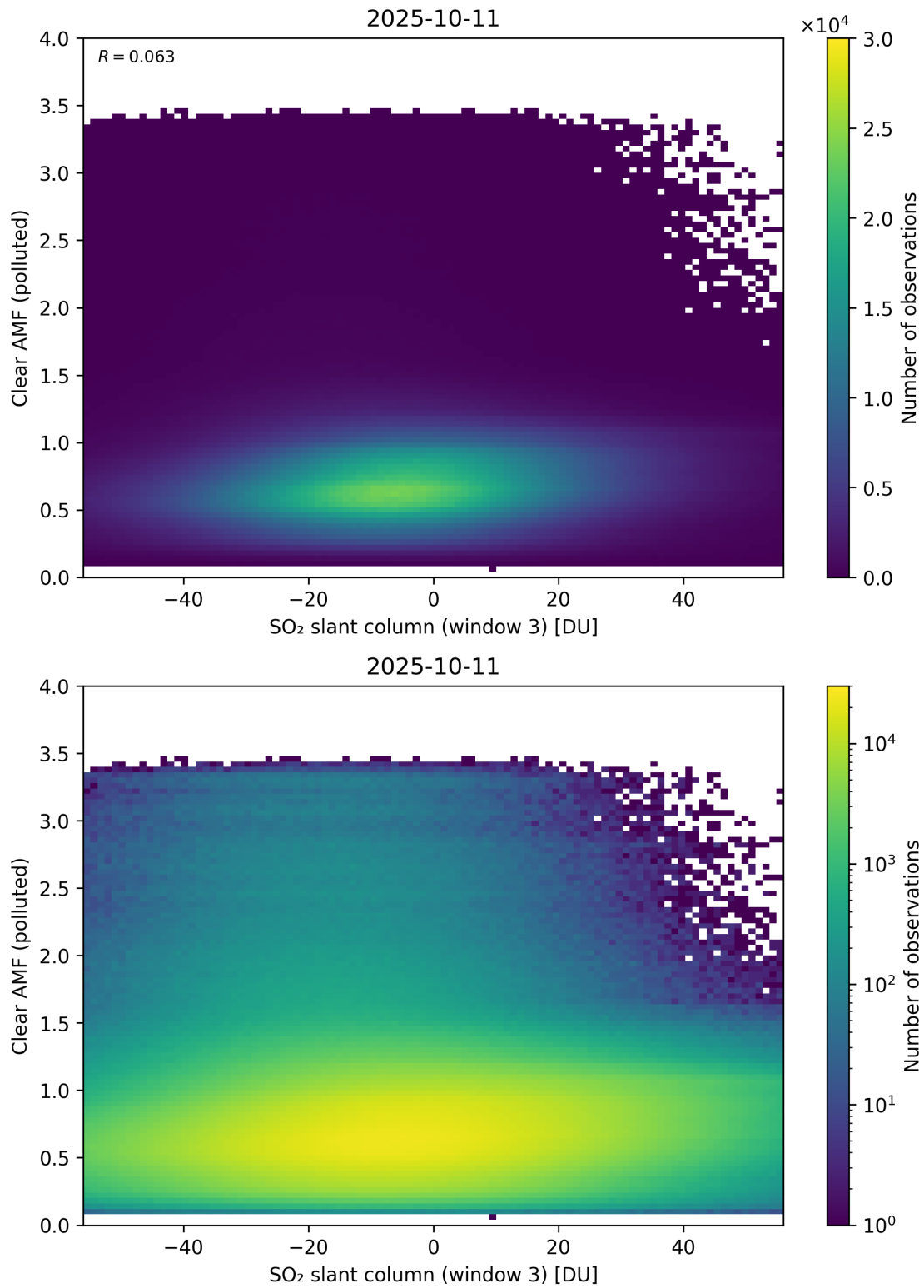
Figure 315: Scatter density plot of “SO 2 slant column (window 3)” against “Clear AMF (polluted)” for 2025-10-11 to 2025-10-12.
