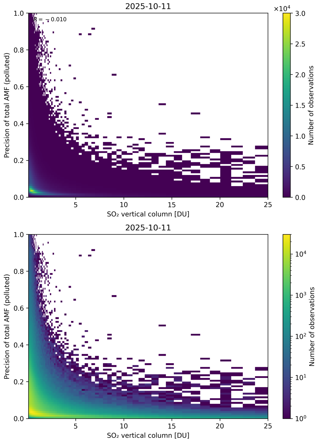
Figure 360: Scatter density plot of “SO 2 vertical column” against “Precision of total AMF (polluted)” for 2025-10-11 to 2025-10-12.
