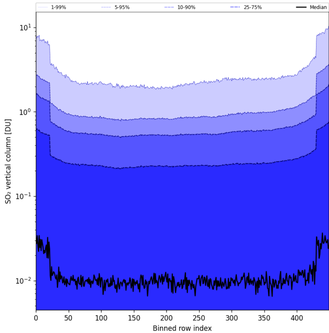
Figure 84: Along track statistics of “SO 2 vertical column” for 2025-10-11 to 2025-10-12
