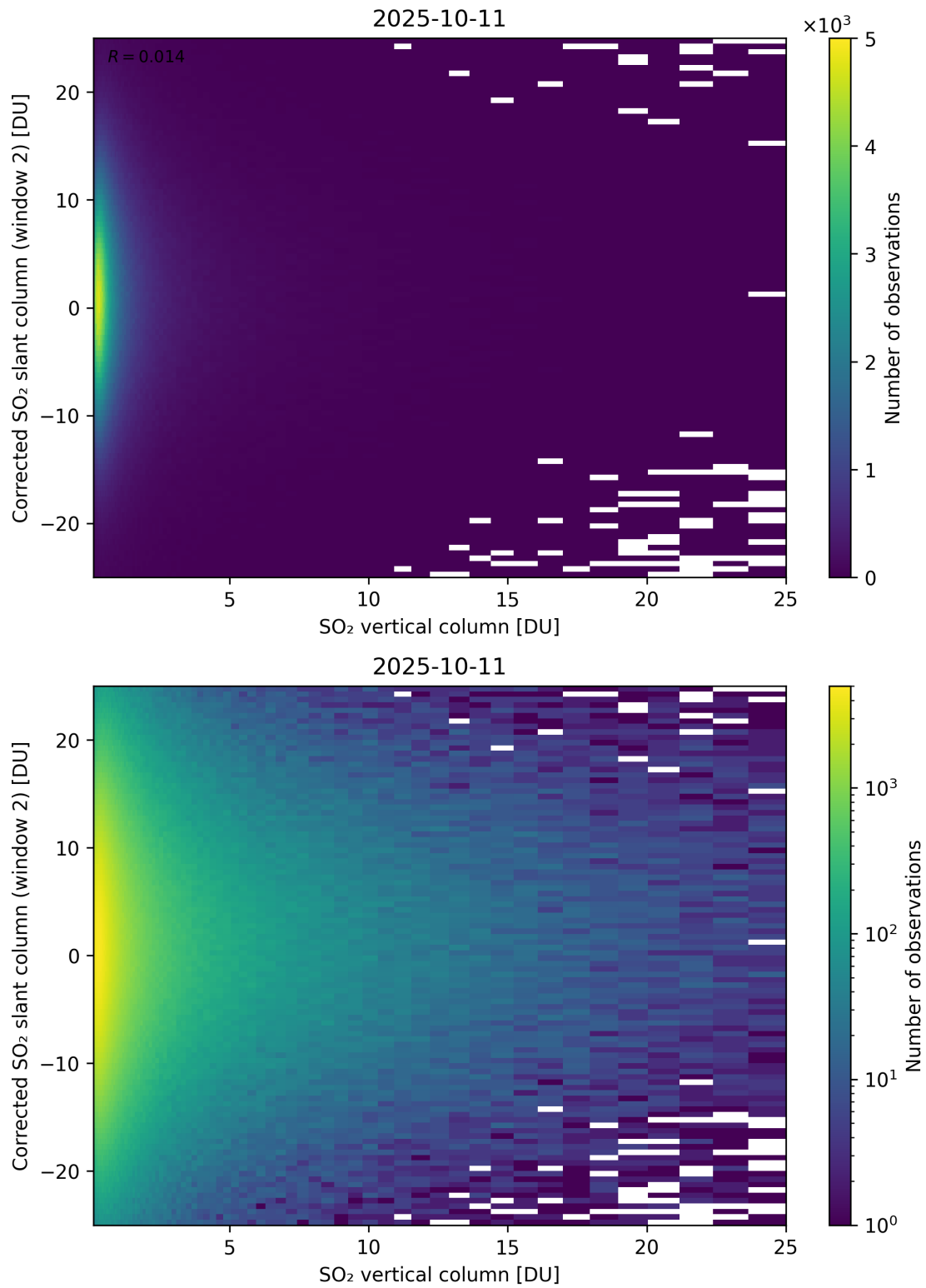
Figure 352: Scatter density plot of “SO 2 vertical column” against “Corrected SO 2 slant column (window 2)” for 2025-10-11 to 2025-10-12.
