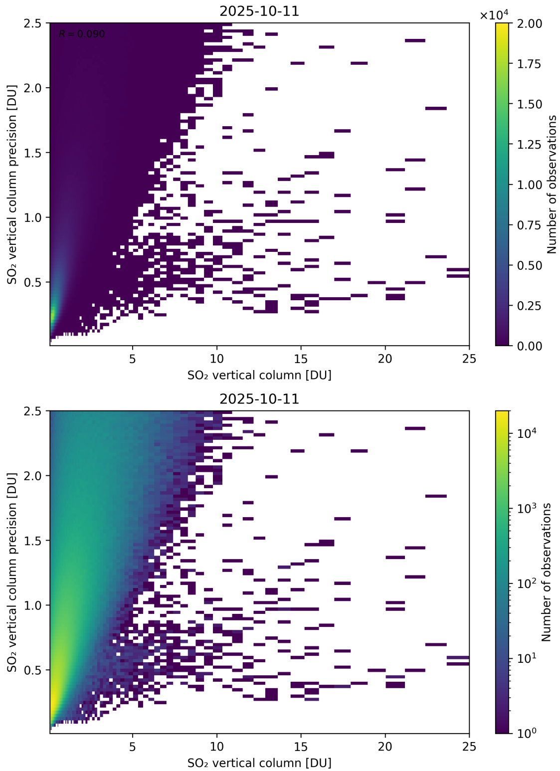
Figure 361: Scatter density plot of “SO 2 vertical column” against “SO 2 vertical column precision” for 2025-10-11 to 2025-10-12.
