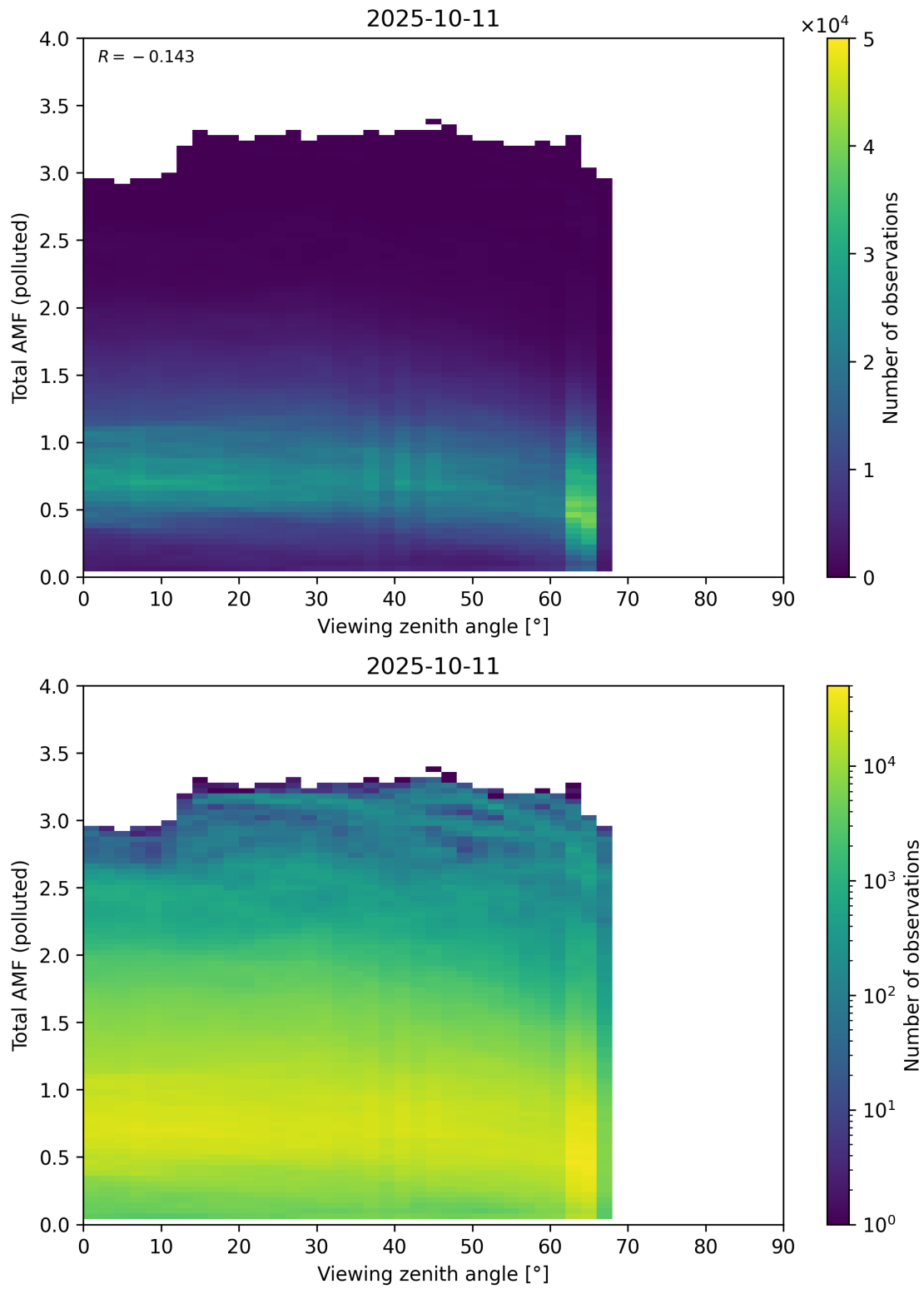
Figure 381: Scatter density plot of “Viewing zenith angle” against “Total AMF (polluted)” for 2025-10-11 to 2025-10-12.
