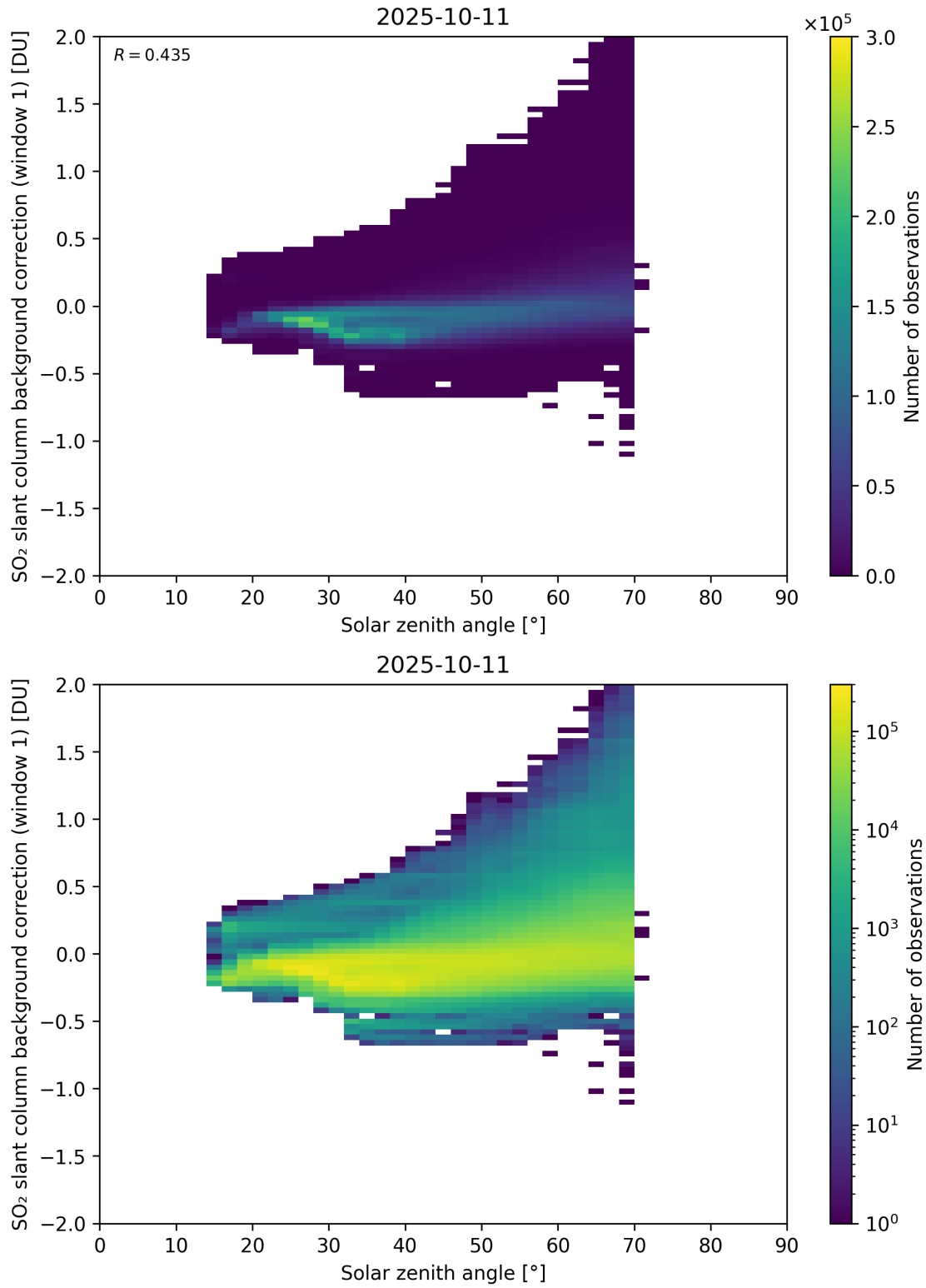
Figure 171: Scatter density plot of “Solar zenith angle” against “SO 2 slant column background correction (window 1)” for 2025-10-11 to 2025-10-12.
