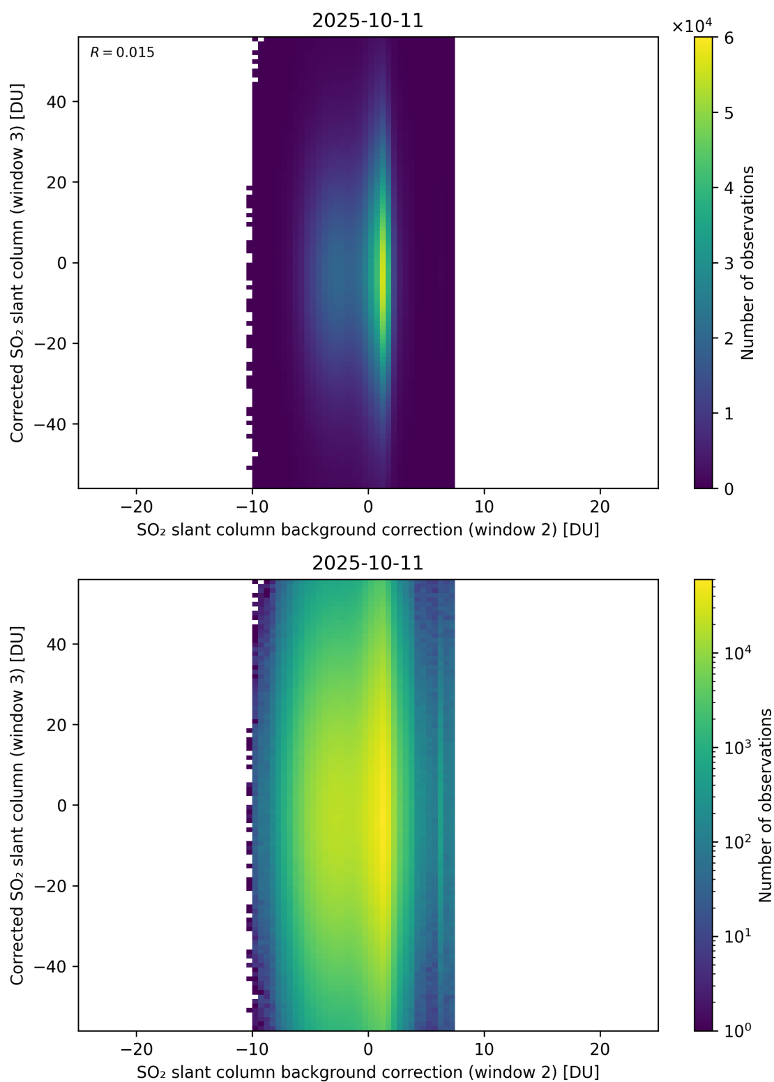
Figure 127: Scatter density plot of “SO 2 slant column background correction (window 2)” against “Corrected SO 2 slant column (window 3)” for 2025-10-11 to 2025-10-12.
