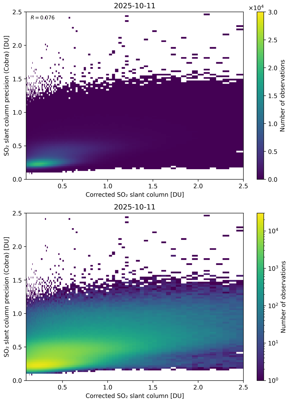
Figure 234: Scatter density plot of “Corrected SO 2 slant column” against “SO 2 slant column precision (Cobra)” for 2025-10-11 to 2025-10-12.
