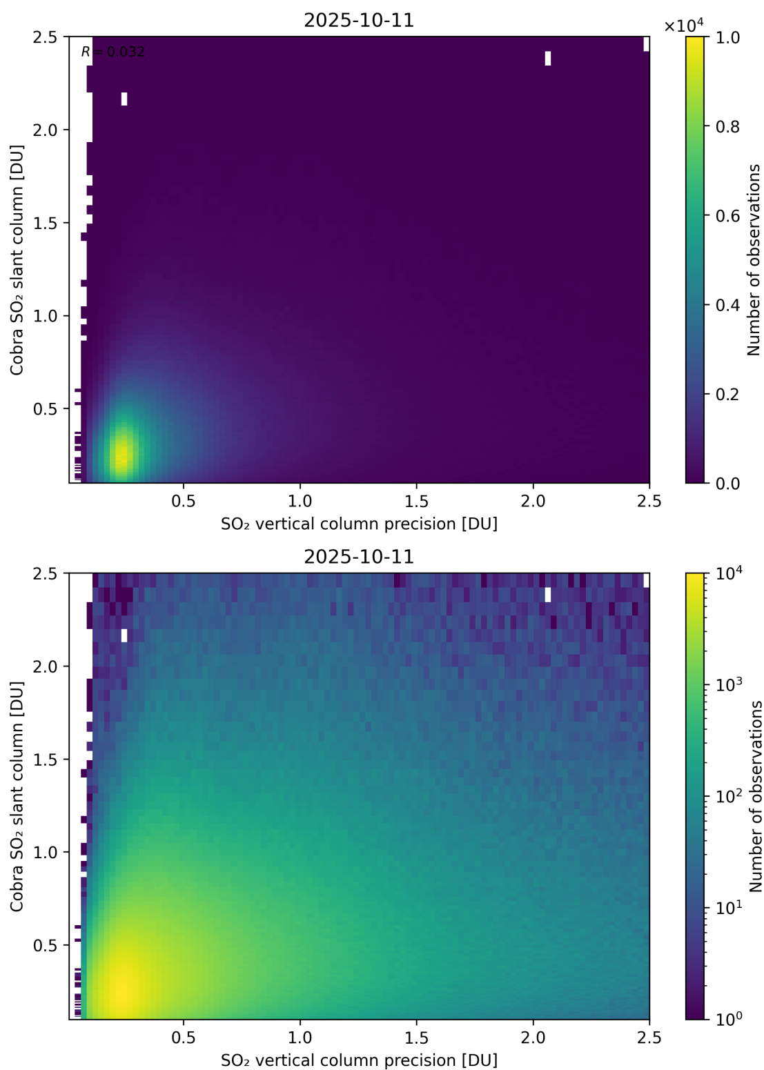
Figure 336: Scatter density plot of “SO 2 vertical column precision” against “Cobra SO 2 slant column” for 2025-10-11 to 2025-10-12.
