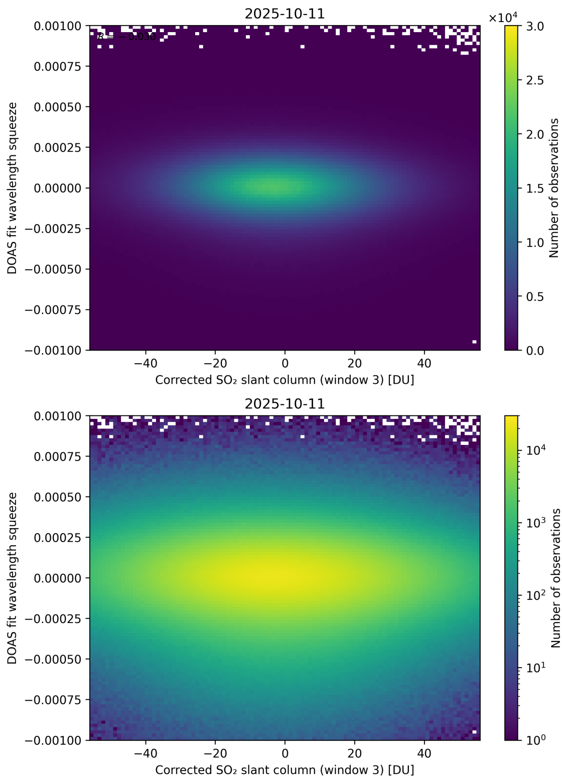
Figure 257: Scatter density plot of “Corrected SO 2 slant column (window 3)” against “DOAS fit wavelength squeeze” for 2025-10-11 to 2025-10-12.
