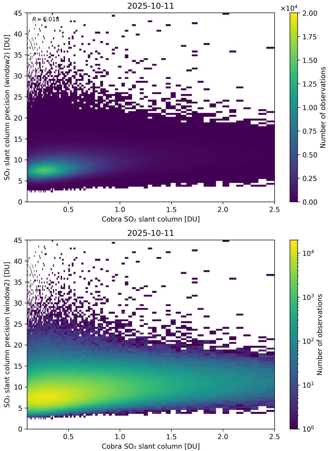
Figure 221: Scatter density plot of “Cobra SO 2 slant column” against “SO 2 slant column precision (window2)” for 2025-10-11 to 2025-10-12.
