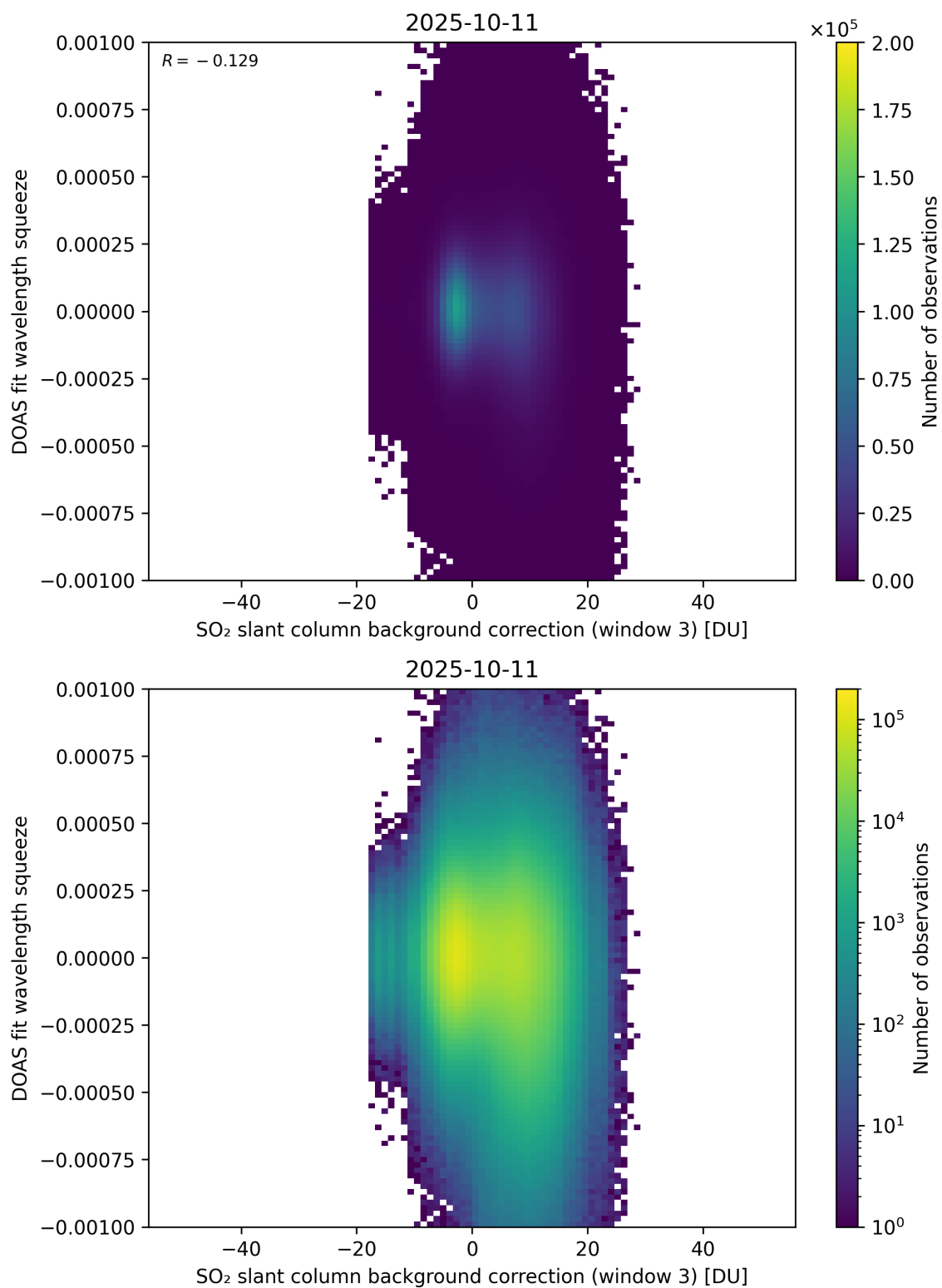
Figure 133: Scatter density plot of “SO 2 slant column background correction (window 3)” against “DOAS fit wavelength squeeze” for 2025-10-11 to 2025-10-12.
