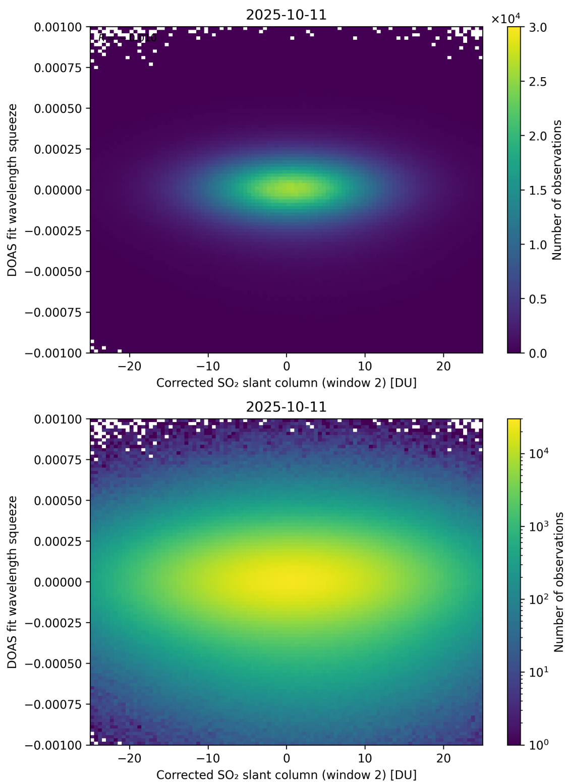
Figure 247: Scatter density plot of “Corrected SO 2 slant column (window 2)” against “DOAS fit wavelength squeeze” for 2025-10-11 to 2025-10-12.
