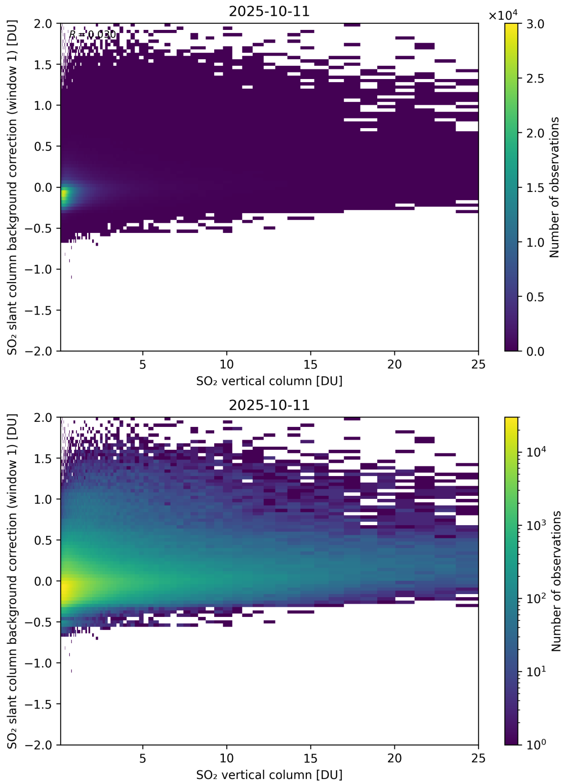
Figure 323: Scatter density plot of “SO 2 vertical column” against “SO 2 slant column background correction (window 1)” for 2025-10-11 to 2025-10-12.
