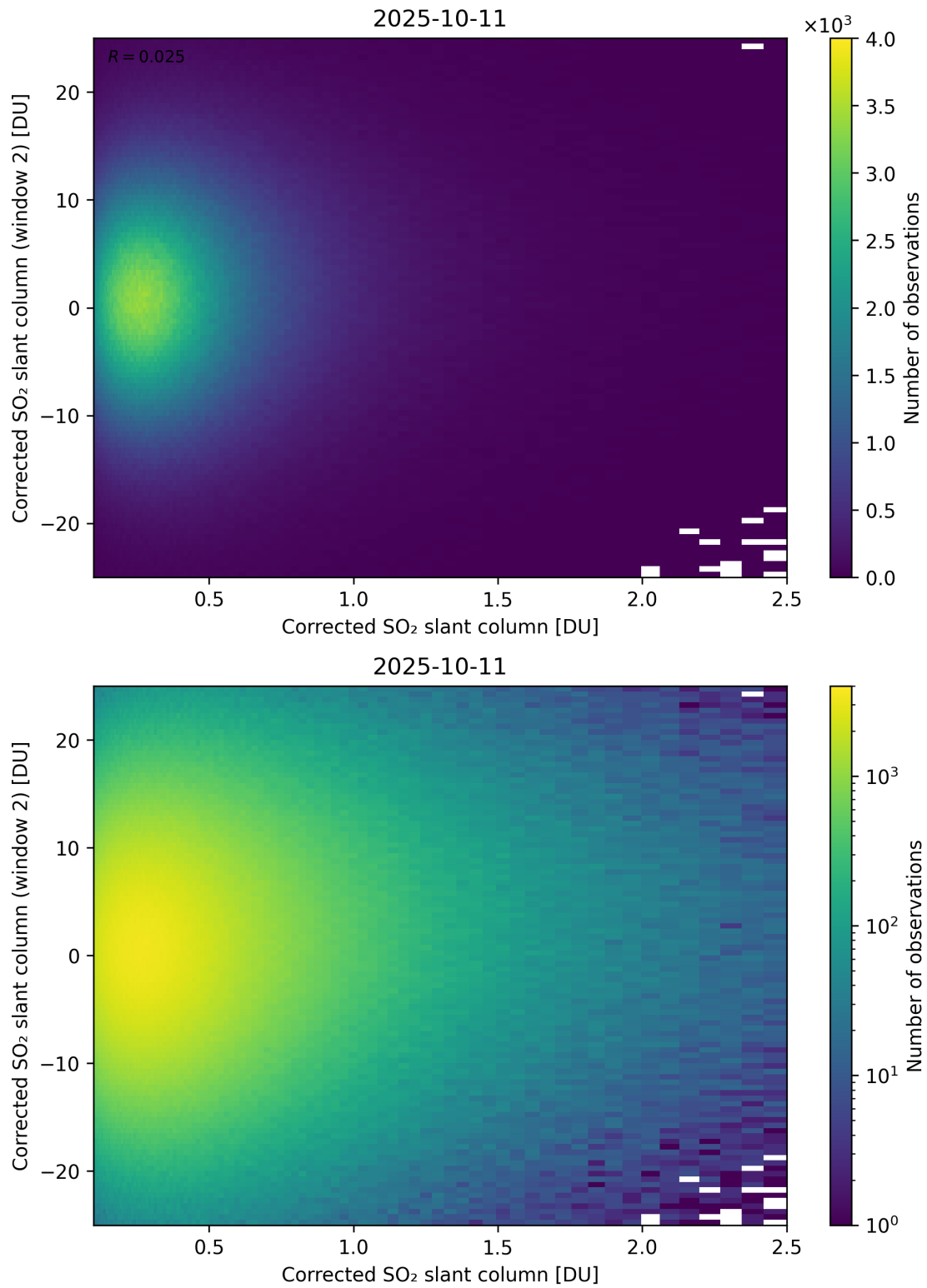
Figure 235: Scatter density plot of “Corrected SO 2 slant column” against “Corrected SO 2 slant column (window 2)” for 2025-10-11 to 2025-10-12.
