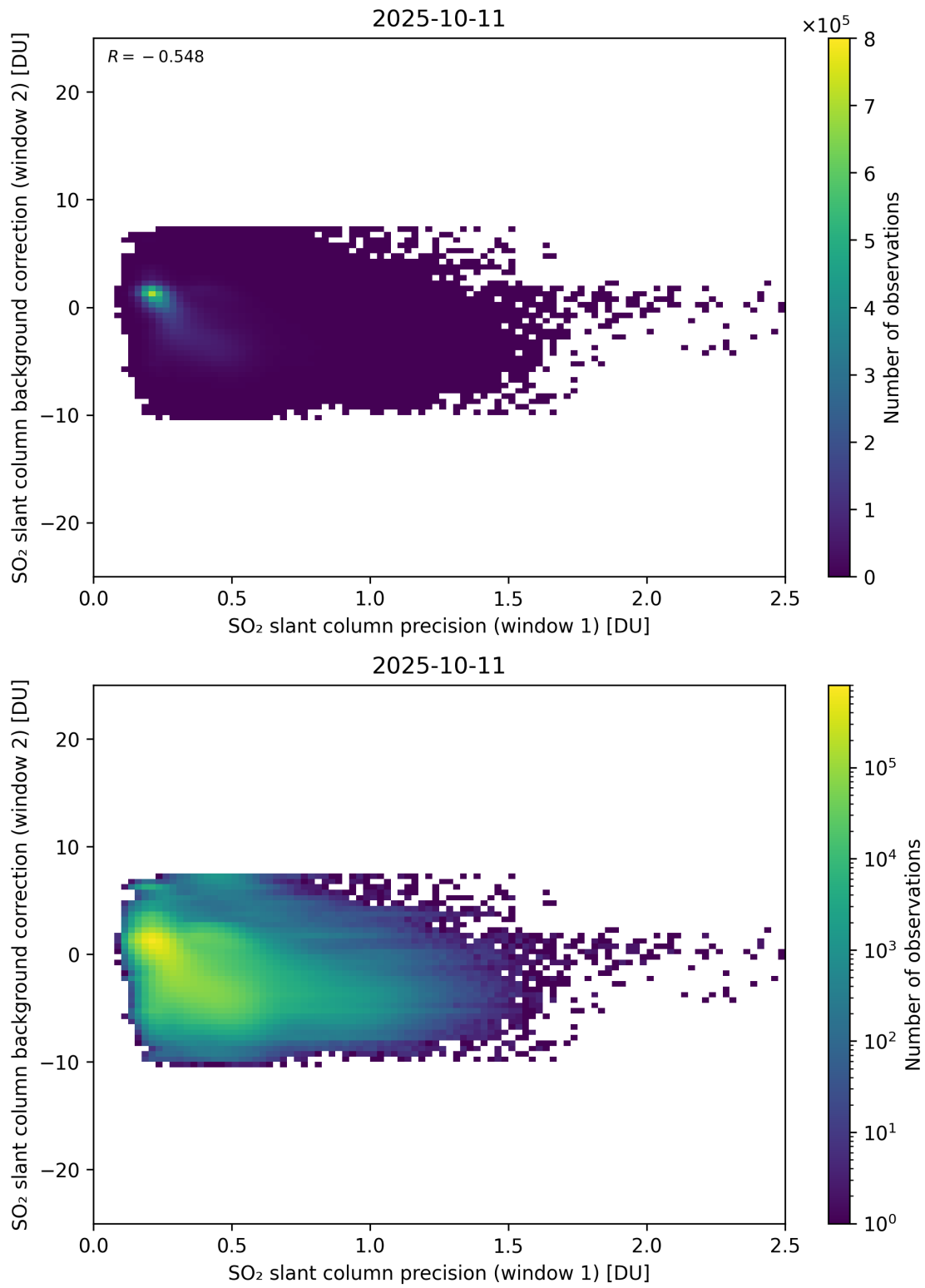
Figure 269: Scatter density plot of “SO 2 slant column precision (window 1)” against “SO 2 slant column background correction (window 2)” for 2025-10-11 to 2025-10-12.
