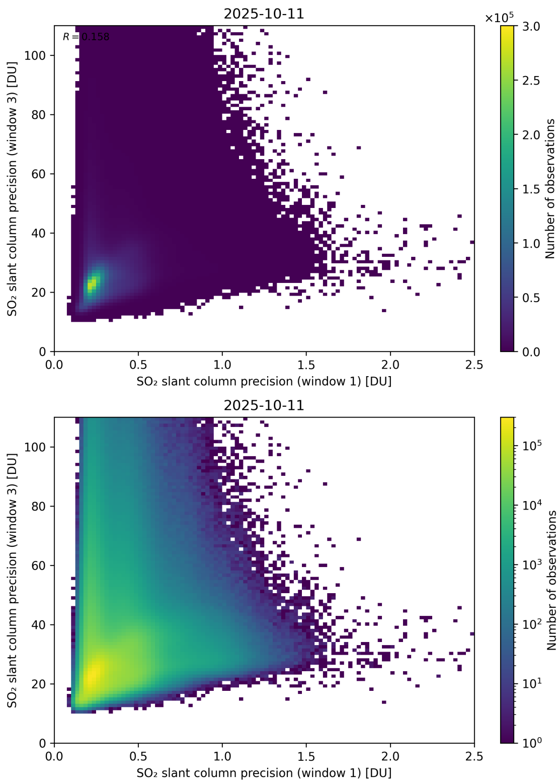
Figure 279: Scatter density plot of “SO 2 slant column precision (window 1)” against “SO 2 slant column precision (window 3)” for 2025-10-11 to 2025-10-12.
