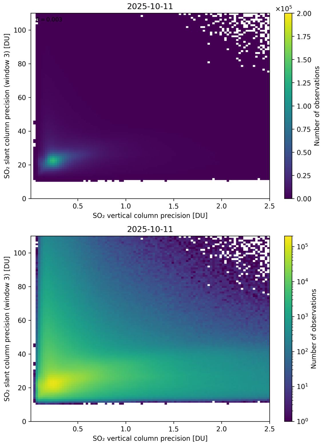
Figure 345: Scatter density plot of “SO 2 vertical column precision” against “SO 2 slant column precision (window 3)” for 2025-10-11 to 2025-10-12.
