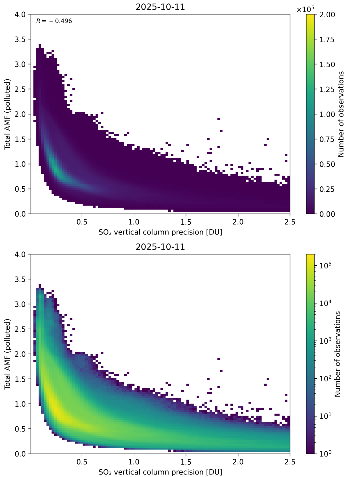
Figure 346: Scatter density plot of “SO 2 vertical column precision” against “Total AMF (polluted)” for 2025-10-11 to 2025-10-12.
