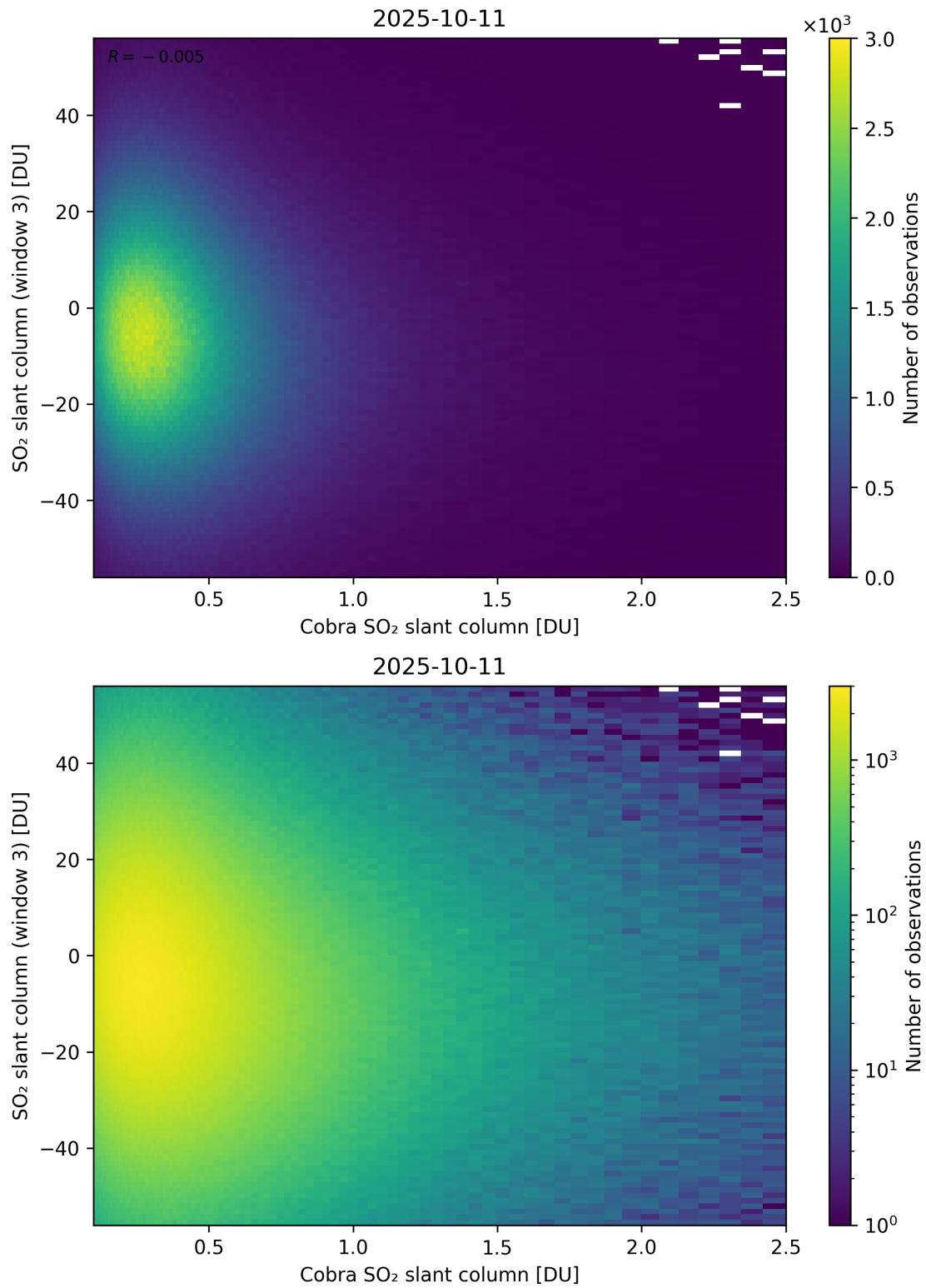
Figure 222: Scatter density plot of “Cobra SO 2 slant column” against “SO 2 slant column (window 3)” for 2025-10-11 to 2025-10-12.
