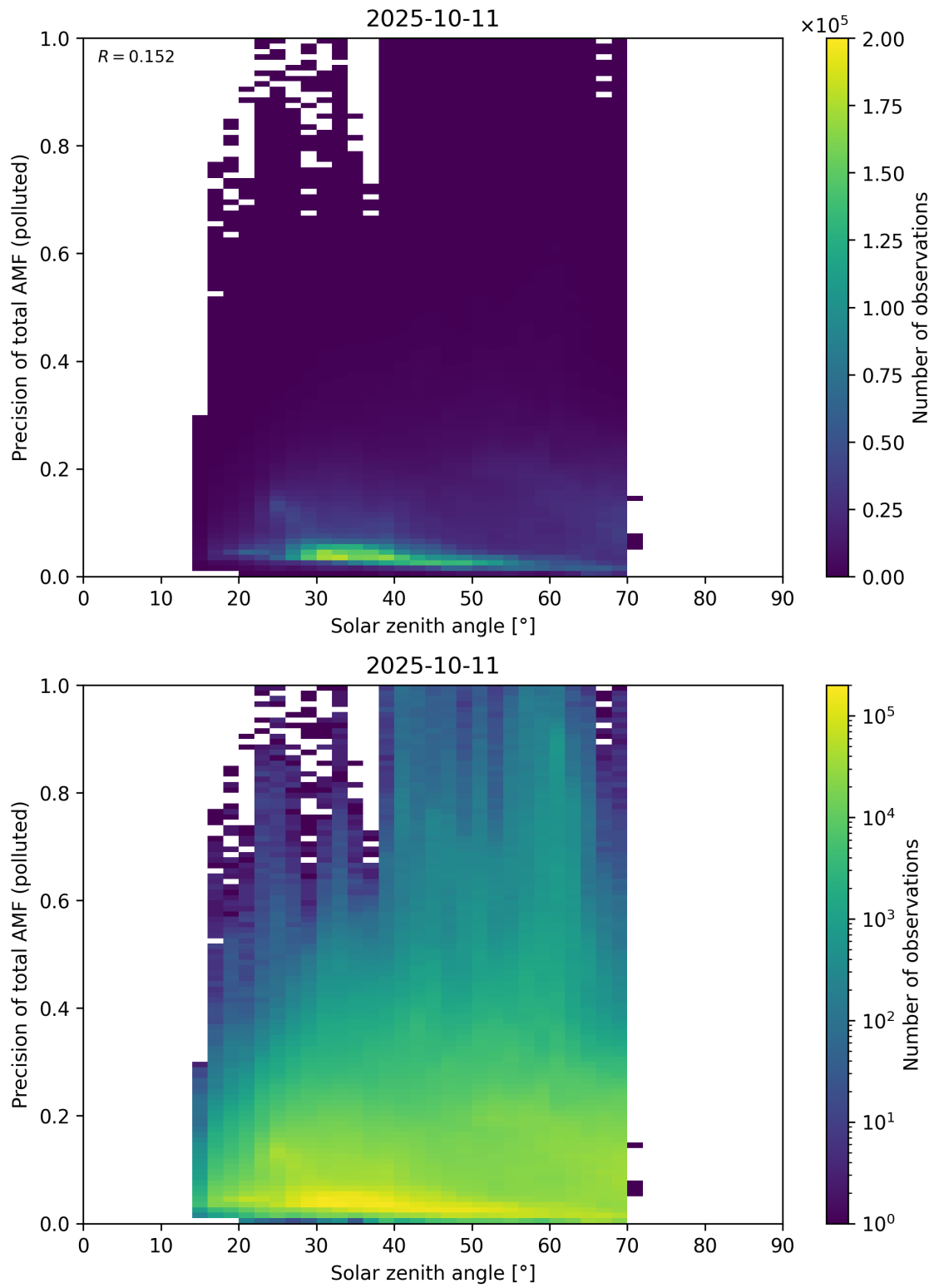
Figure 190: Scatter density plot of “Solar zenith angle” against “Precision of total AMF (polluted)” for 2025-10-11 to 2025-10-12.
