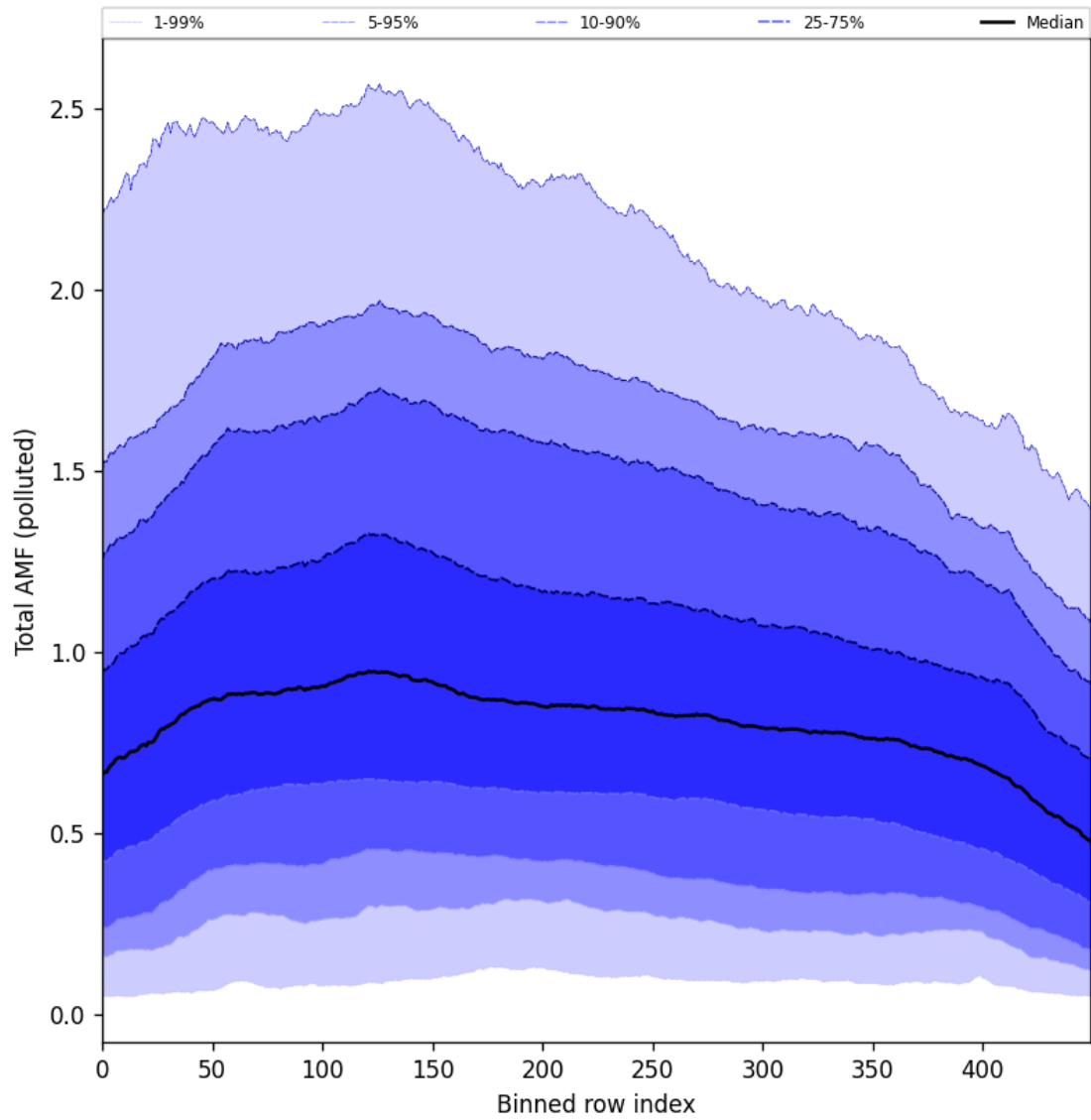
Figure 105: Along track statistics of “Total AMF (polluted)” for 2025-10-11 to 2025-10-12
