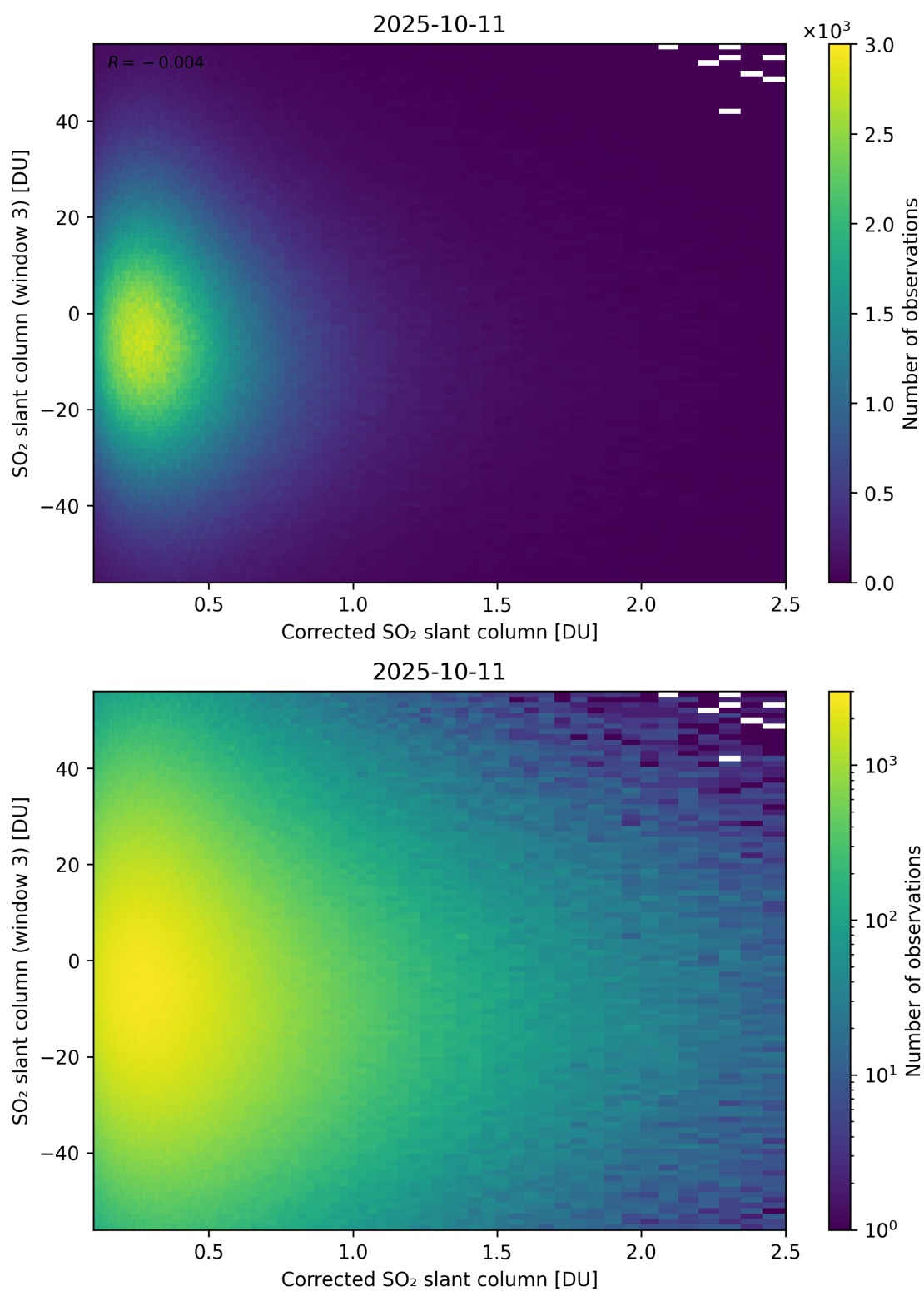
Figure 240: Scatter density plot of “Corrected SO 2 slant column” against “SO 2 slant column (window 3)” for 2025-10-11 to 2025-10-12.
