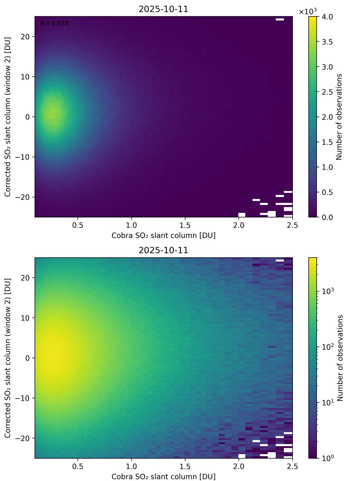
Figure 217: Scatter density plot of “Cobra SO 2 slant column” against “Corrected SO 2 slant column (window 2)” for 2025-10-11 to 2025-10-12.
