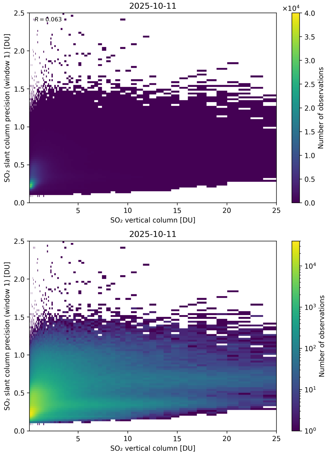
Figure 355: Scatter density plot of “SO 2 vertical column” against “SO 2 slant column precision (window 1)” for 2025-10-11 to 2025-10-12.
