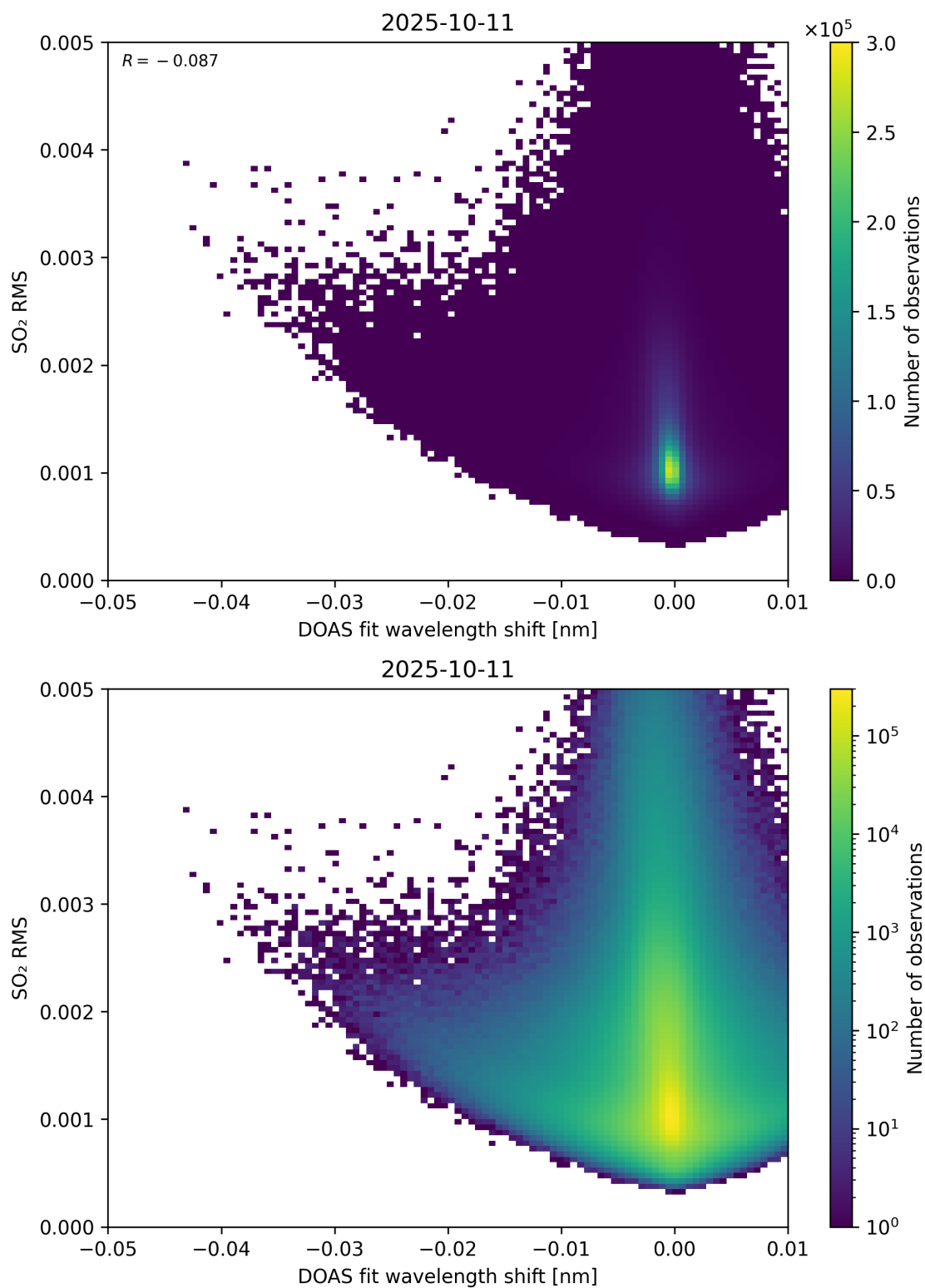
Figure 139: Scatter density plot of “DOAS fit wavelength shift” against “SO 2 RMS” for 2025-10-11 to 2025-10-12.
