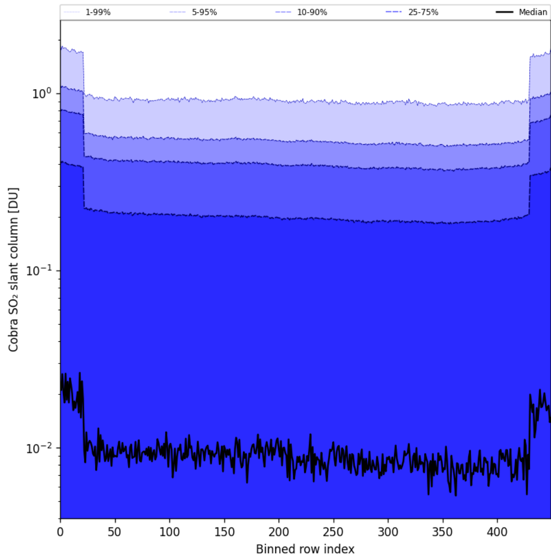
Figure 87: Along track statistics of “Cobra SO 2 slant column” for 2025-10-11 to 2025-10-12
