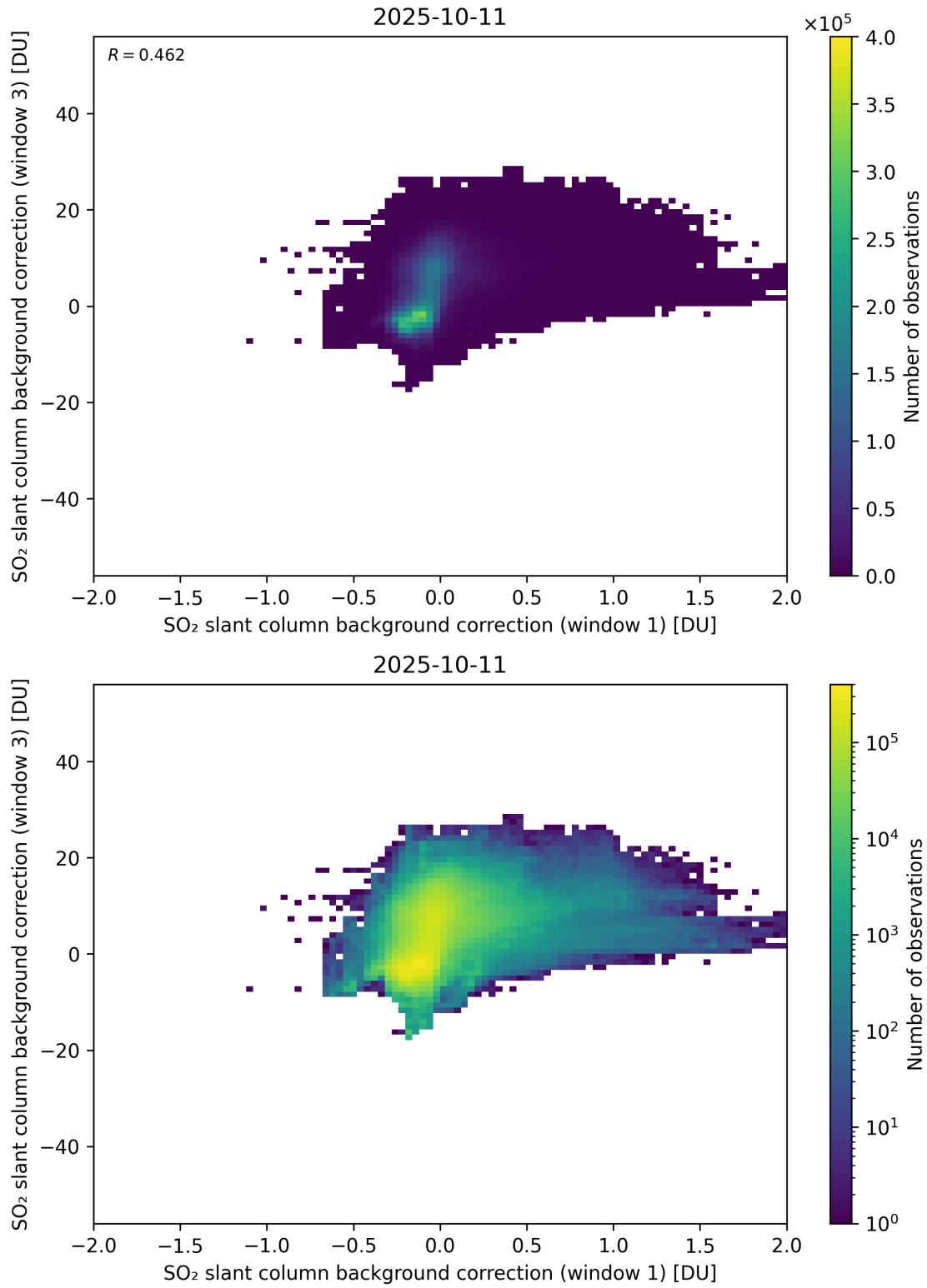
Figure 110: Scatter density plot of “SO 2 slant column background correction (window 1)” against “SO 2 slant column background correction (window 3)” for 2025-10-11 to 2025-10-12.
