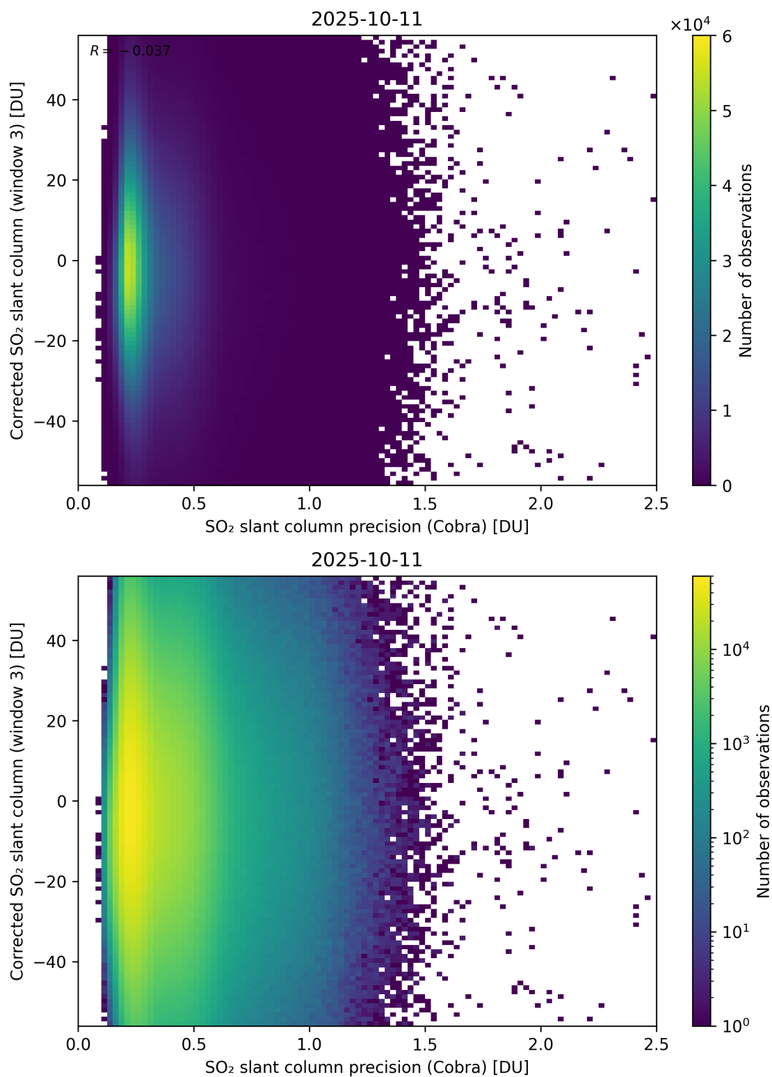
Figure 207: Scatter density plot of “SO 2 slant column precision (Cobra)” against “Corrected SO 2 slant column (window 3)” for 2025-10-11 to 2025-10-12.
