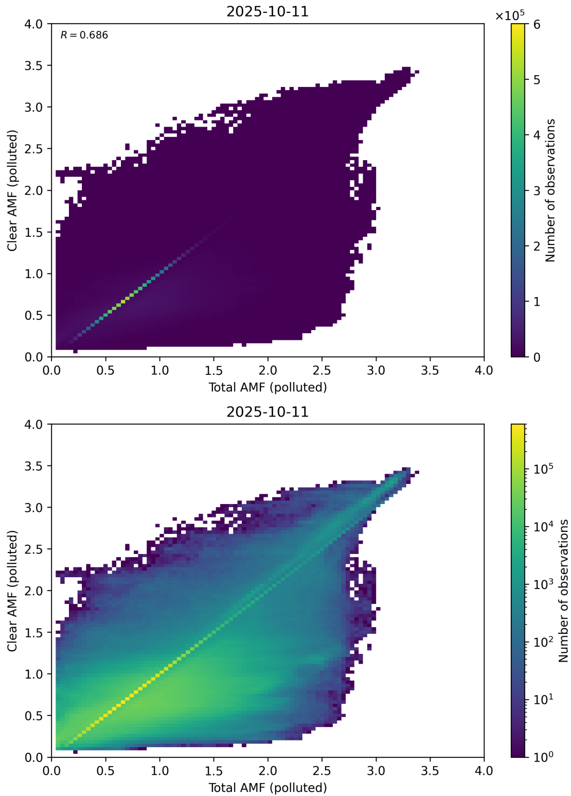
Figure 321: Scatter density plot of “Total AMF (polluted)” against “Clear AMF (polluted)” for 2025-10-11 to 2025-10-12.
