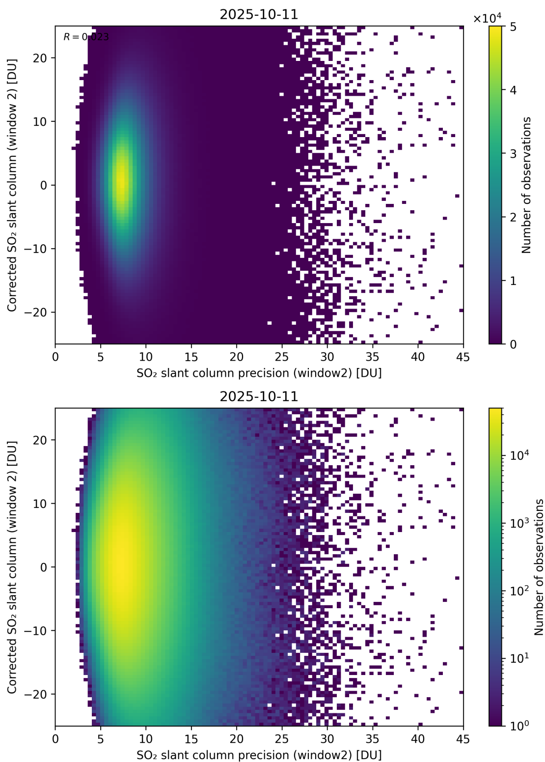
Figure 297: Scatter density plot of “SO 2 slant column precision (window2)” against “Corrected SO 2 slant column (window 2)” for 2025-10-11 to 2025-10-12.
