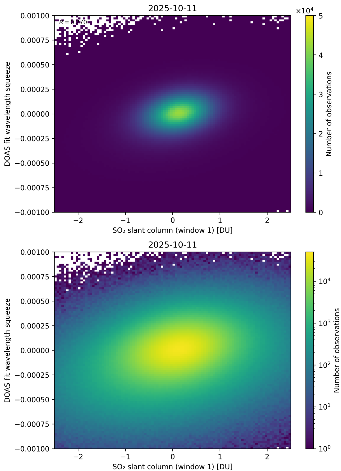
Figure 266: Scatter density plot of “SO 2 slant column (window 1)” against “DOAS fit wavelength squeeze” for 2025-10-11 to 2025-10-12.
