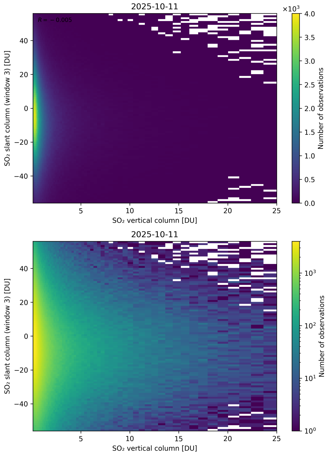
Figure 357: Scatter density plot of “SO 2 vertical column” against “SO 2 slant column (window 3)” for 2025-10-11 to 2025-10-12.
