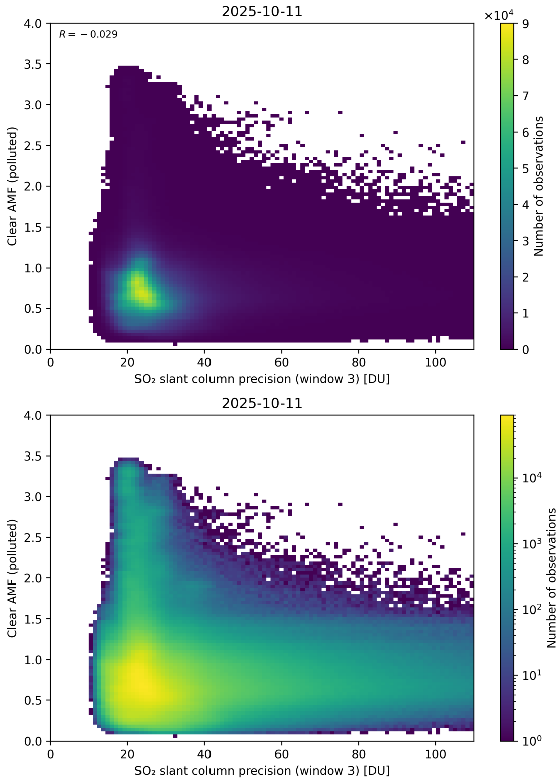
Figure 311: Scatter density plot of “SO 2 slant column precision (window 3)” against “Clear AMF (polluted)” for 2025-10-11 to 2025-10-12.
