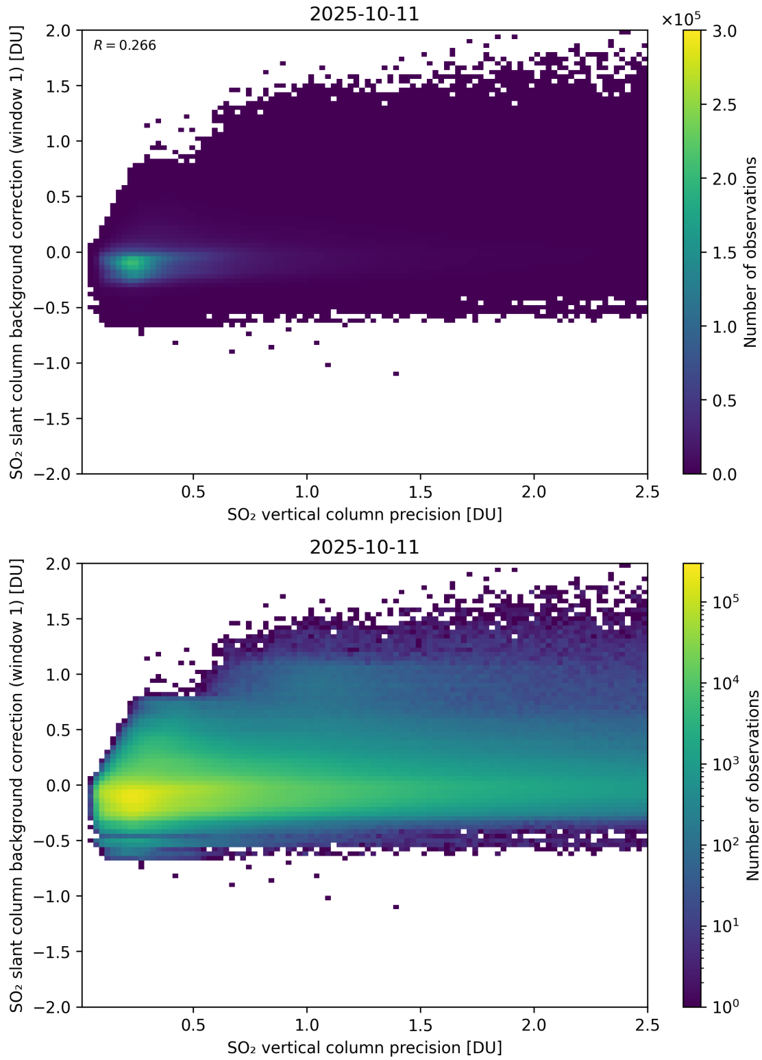
Figure 329: Scatter density plot of “SO 2 vertical column precision” against “SO 2 slant column background correction (window 1)” for 2025-10-11 to 2025-10-12.
