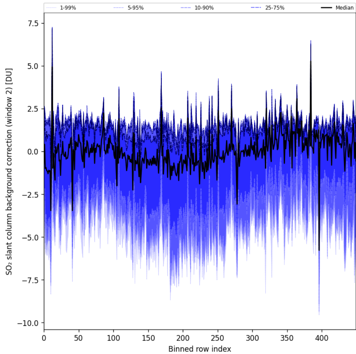
Figure 96: Along track statistics of “SO 2 slant column background correction (window 2)” for 2025-10-11 to 2025-10-12
