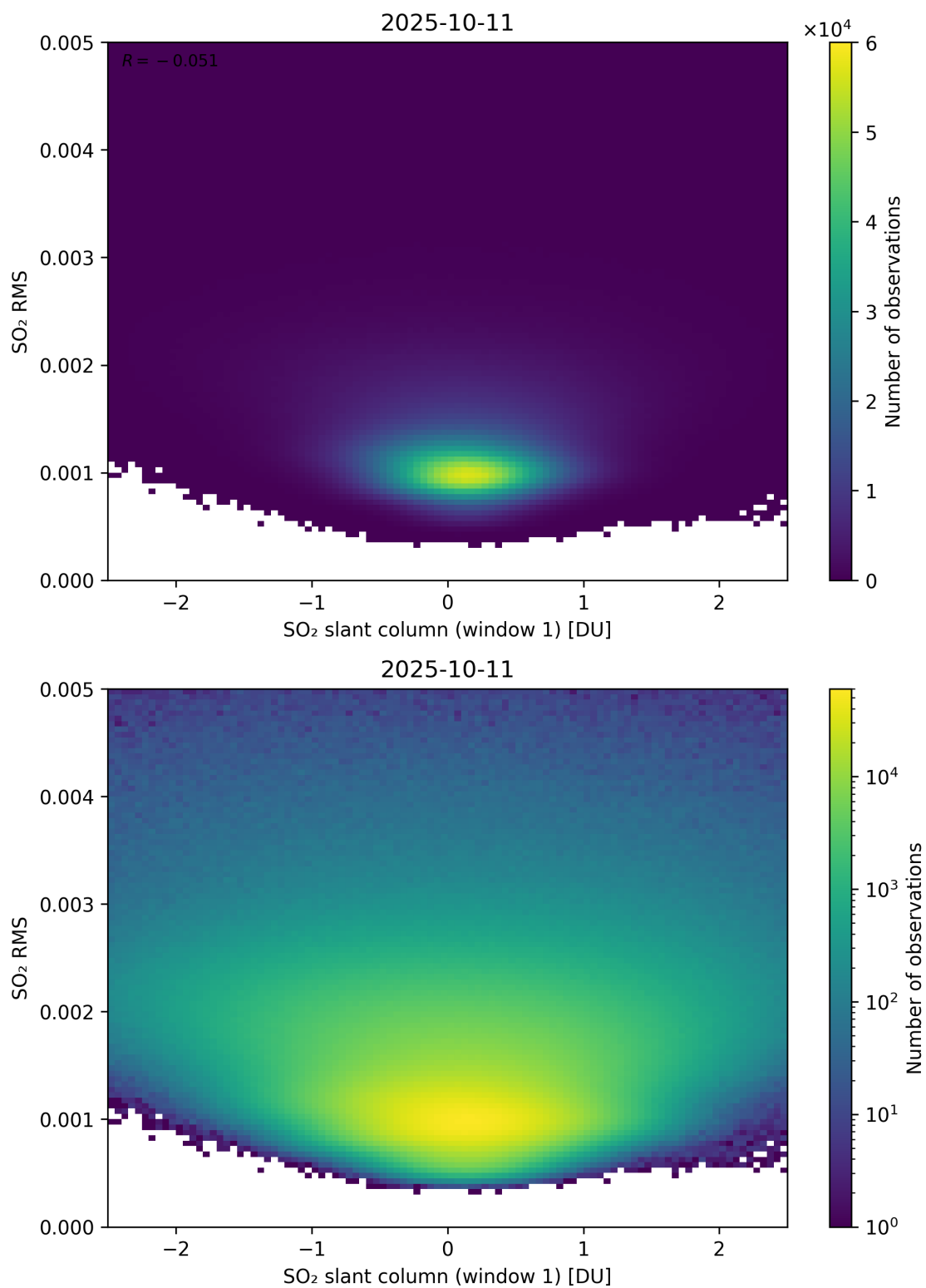
Figure 267: Scatter density plot of “SO 2 slant column (window 1)” against “SO 2 RMS” for 2025-10-11 to 2025-10-12.
