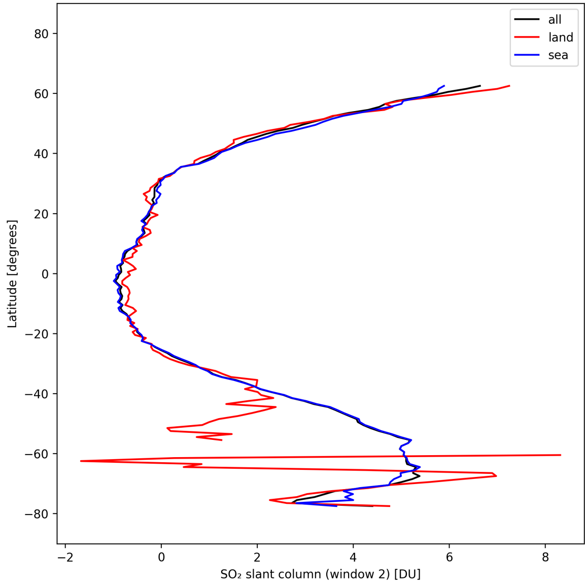
Figure 41: Zonal average of “SO 2 slant column (window 2)” for 2025-10-11 to 2025-10-12.
