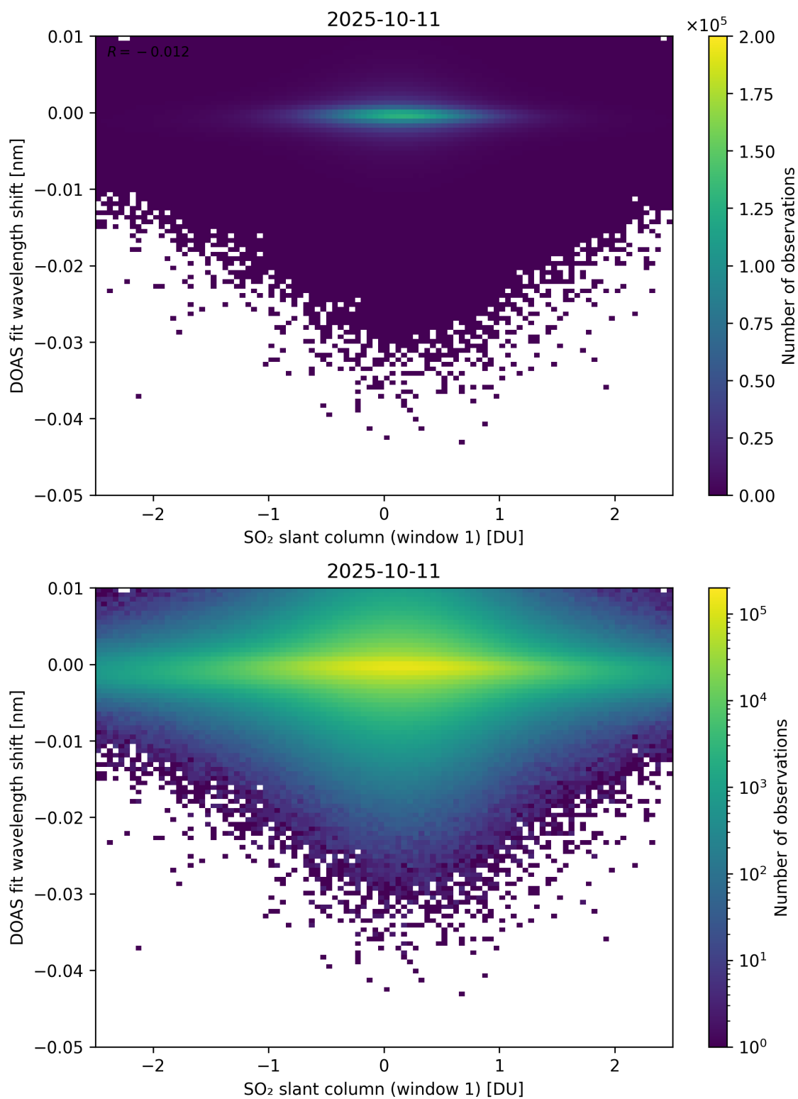
Figure 265: Scatter density plot of “SO 2 slant column (window 1)” against “DOAS fit wavelength shift” for 2025-10-11 to 2025-10-12.
