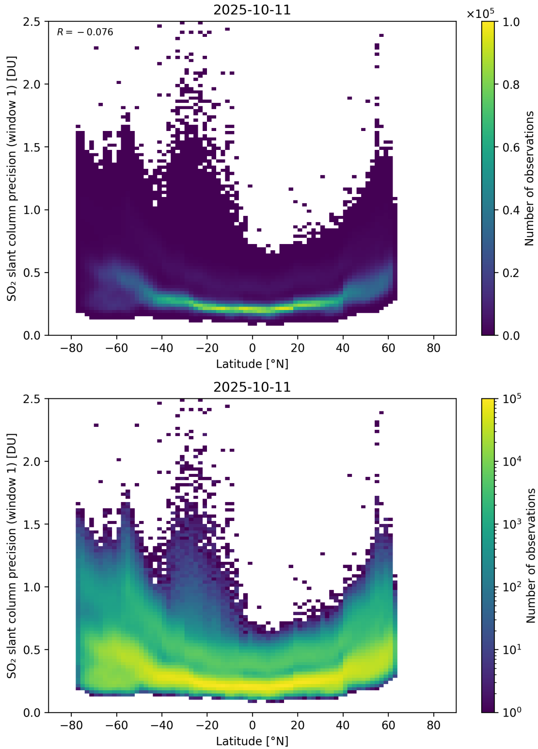
Figure 163: Scatter density plot of “Latitude” against “SO 2 slant column precision (window 1)” for 2025-10-11 to 2025-10-12.
