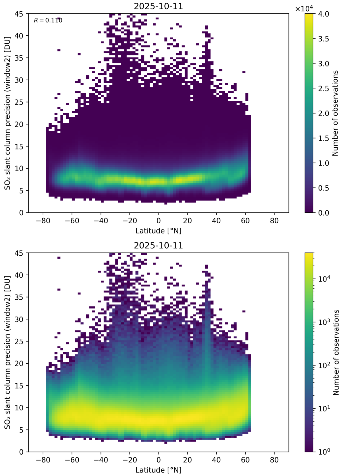
Figure 164: Scatter density plot of “Latitude” against “SO 2 slant column precision (window2)” for 2025-10-11 to 2025-10-12.
