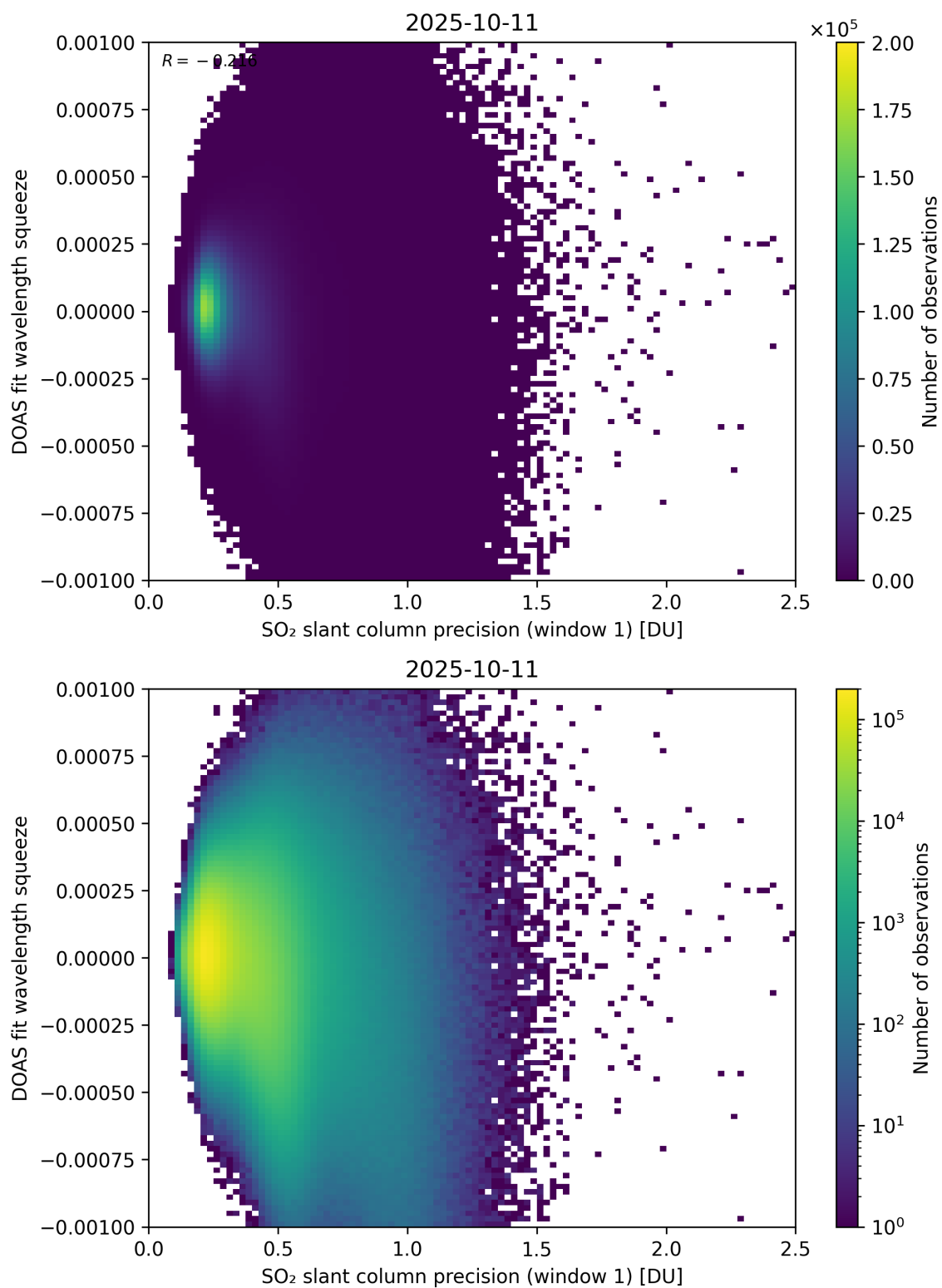
Figure 272: Scatter density plot of “SO 2 slant column precision (window 1)” against “DOAS fit wavelength squeeze” for 2025-10-11 to 2025-10-12.
