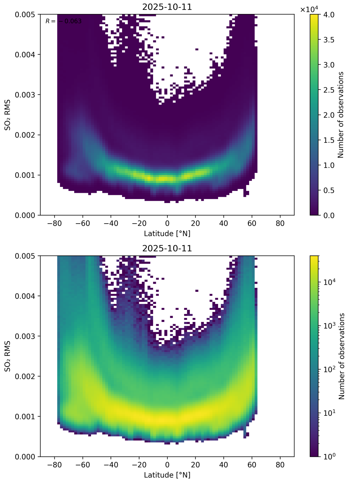
Figure 155: Scatter density plot of “Latitude” against “SO 2 RMS” for 2025-10-11 to 2025-10-12.
