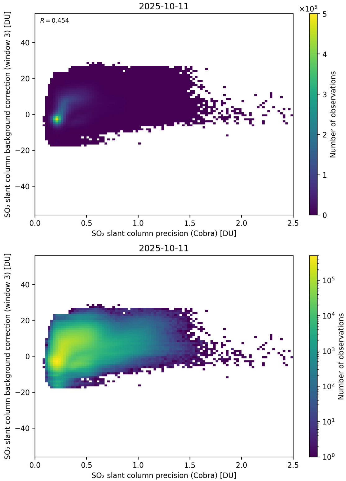
Figure 201: Scatter density plot of “SO 2 slant column precision (Cobra)” against “SO 2 slant column background correction (window 3)” for 2025-10-11 to 2025-10-12.
