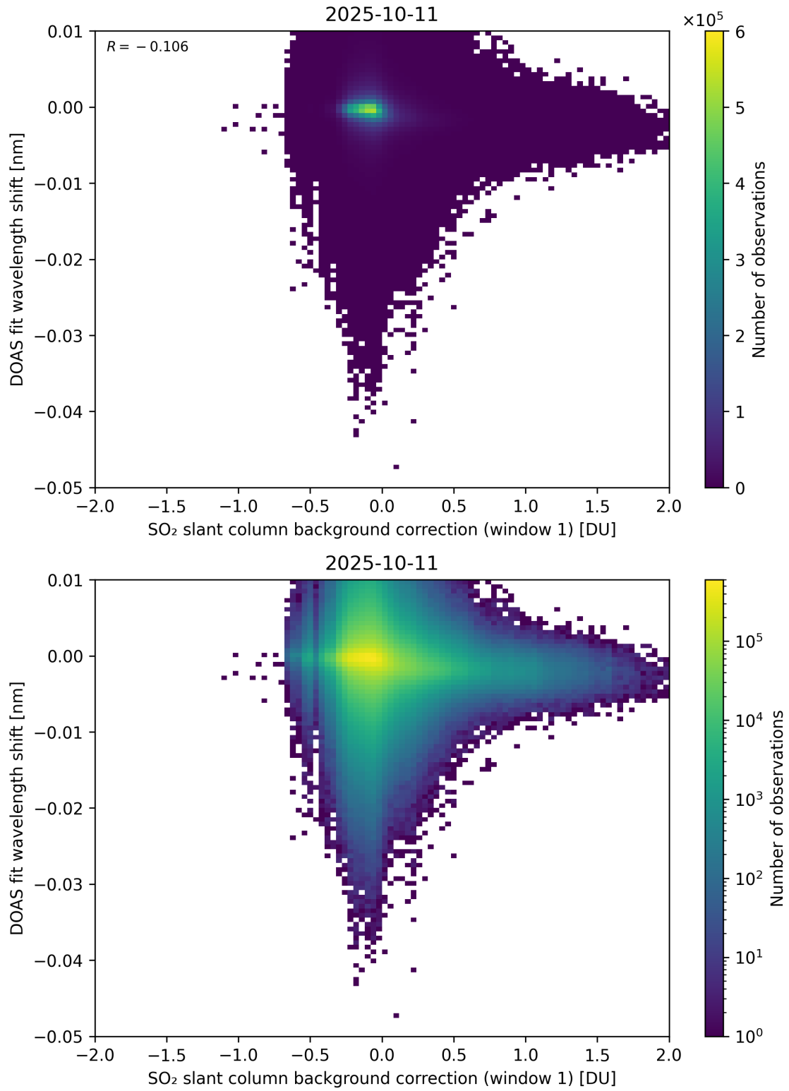
Figure 111: Scatter density plot of “SO 2 slant column background correction (window 1)” against “DOAS fit wavelength shift” for 2025-10-11 to 2025-10-12.
