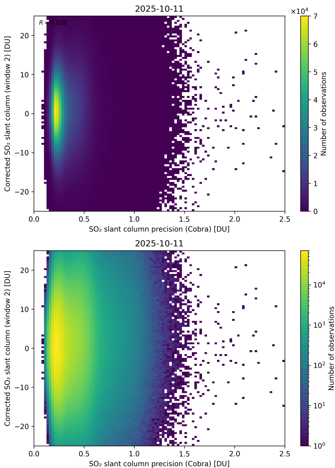
Figure 206: Scatter density plot of “SO 2 slant column precision (Cobra)” against “Corrected SO 2 slant column (window 2)” for 2025-10-11 to 2025-10-12.
