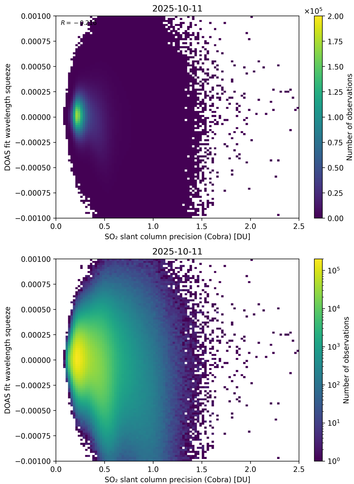
Figure 203: Scatter density plot of “SO 2 slant column precision (Cobra)” against “DOAS fit wavelength squeeze” for 2025-10-11 to 2025-10-12.
