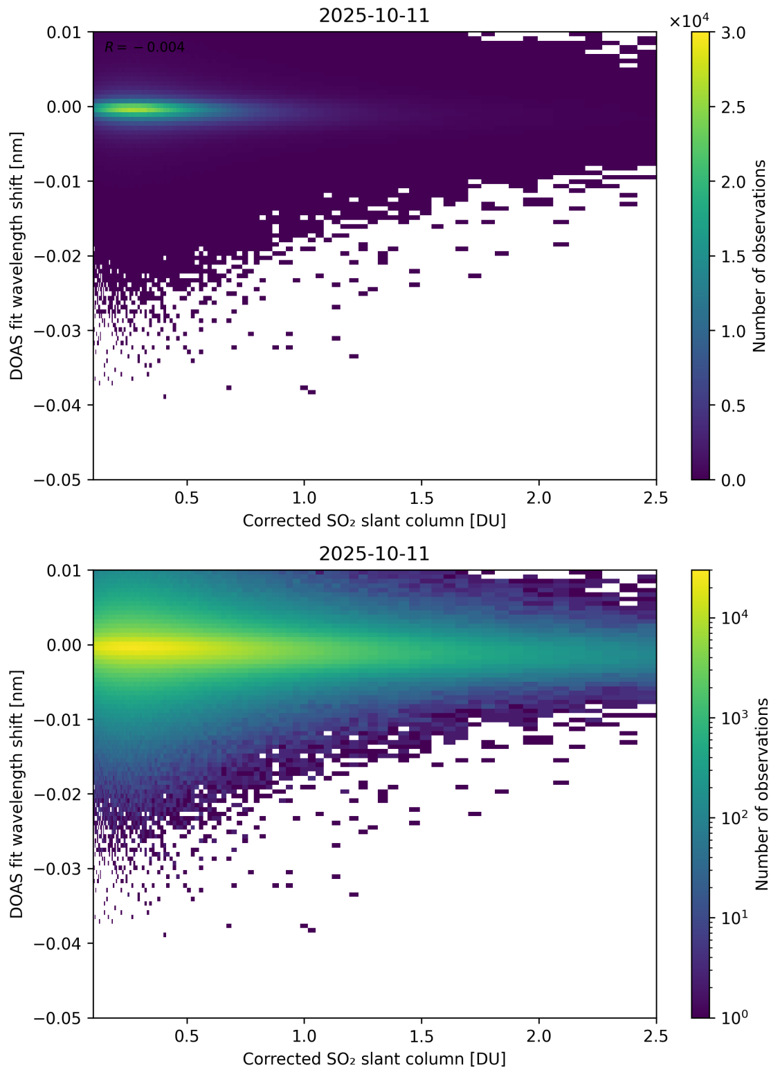
Figure 229: Scatter density plot of “Corrected SO 2 slant column” against “DOAS fit wavelength shift” for 2025-10-11 to 2025-10-12.
