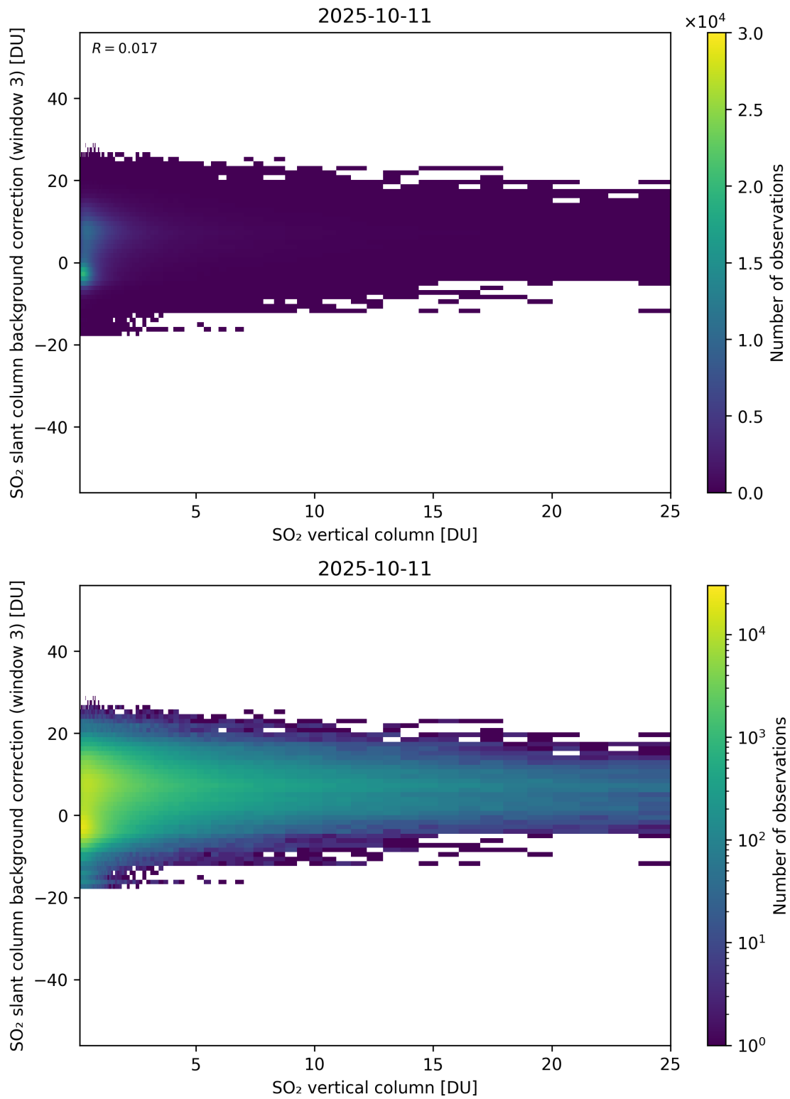
Figure 325: Scatter density plot of “SO 2 vertical column” against “SO 2 slant column background correction (window 3)” for 2025-10-11 to 2025-10-12.
