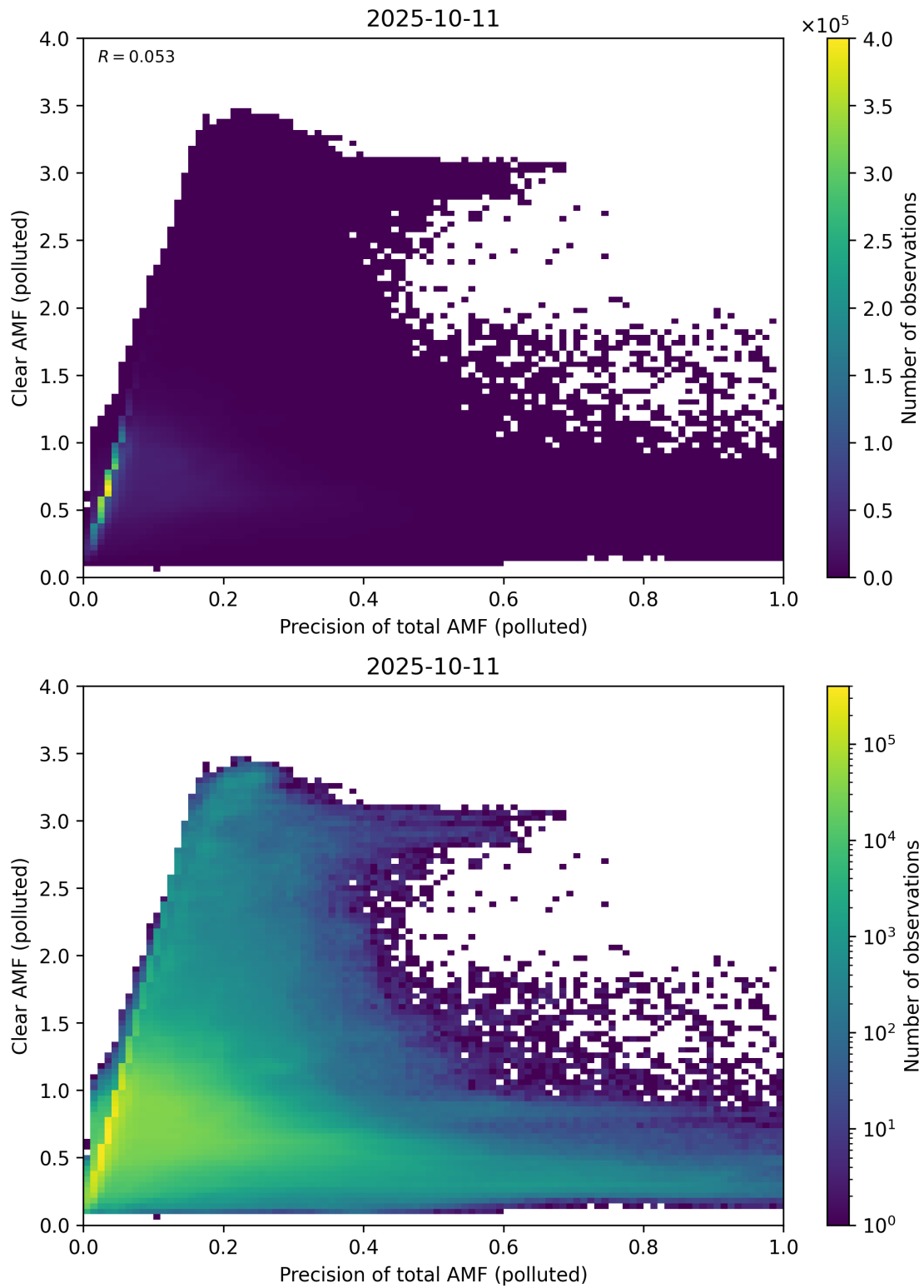
Figure 320: Scatter density plot of “Precision of total AMF (polluted)” against “Clear AMF (polluted)” for 2025-10-11 to 2025-10-12.
