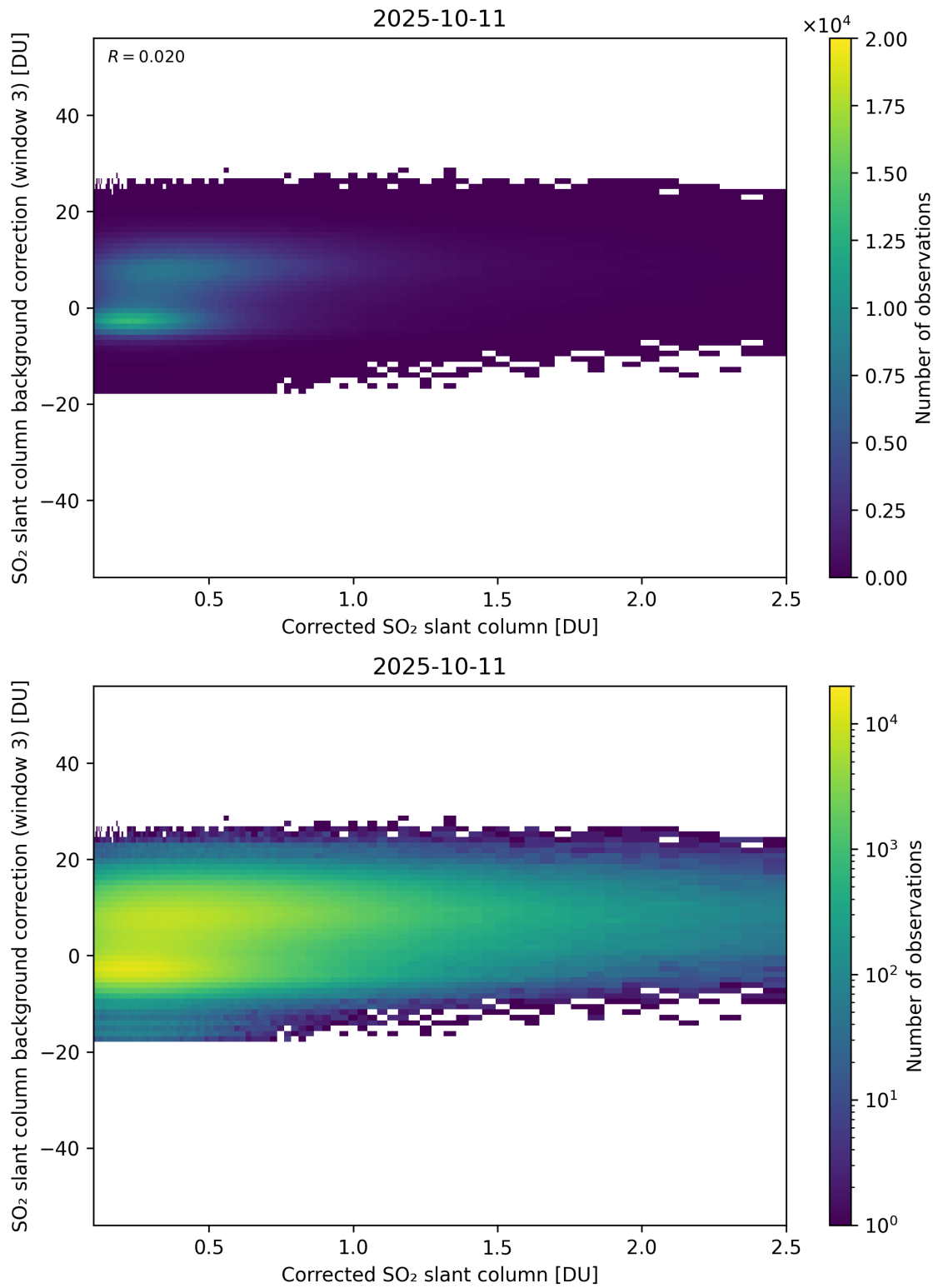
Figure 228: Scatter density plot of “Corrected SO 2 slant column” against “SO 2 slant column background correction (window 3)” for 2025-10-11 to 2025-10-12.
