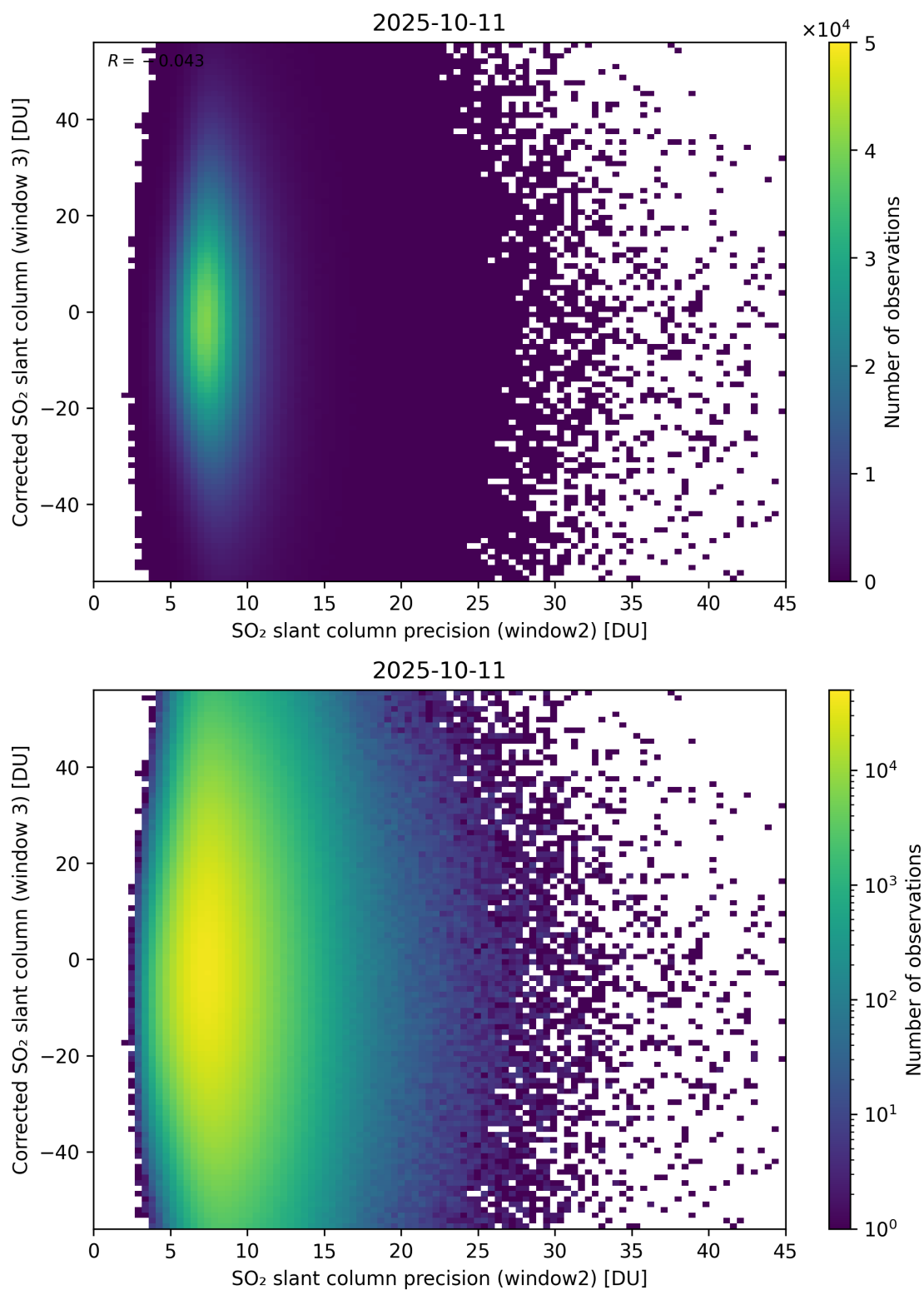
Figure 298: Scatter density plot of “SO 2 slant column precision (window2)” against “Corrected SO 2 slant column (window 3)” for 2025-10-11 to 2025-10-12.
