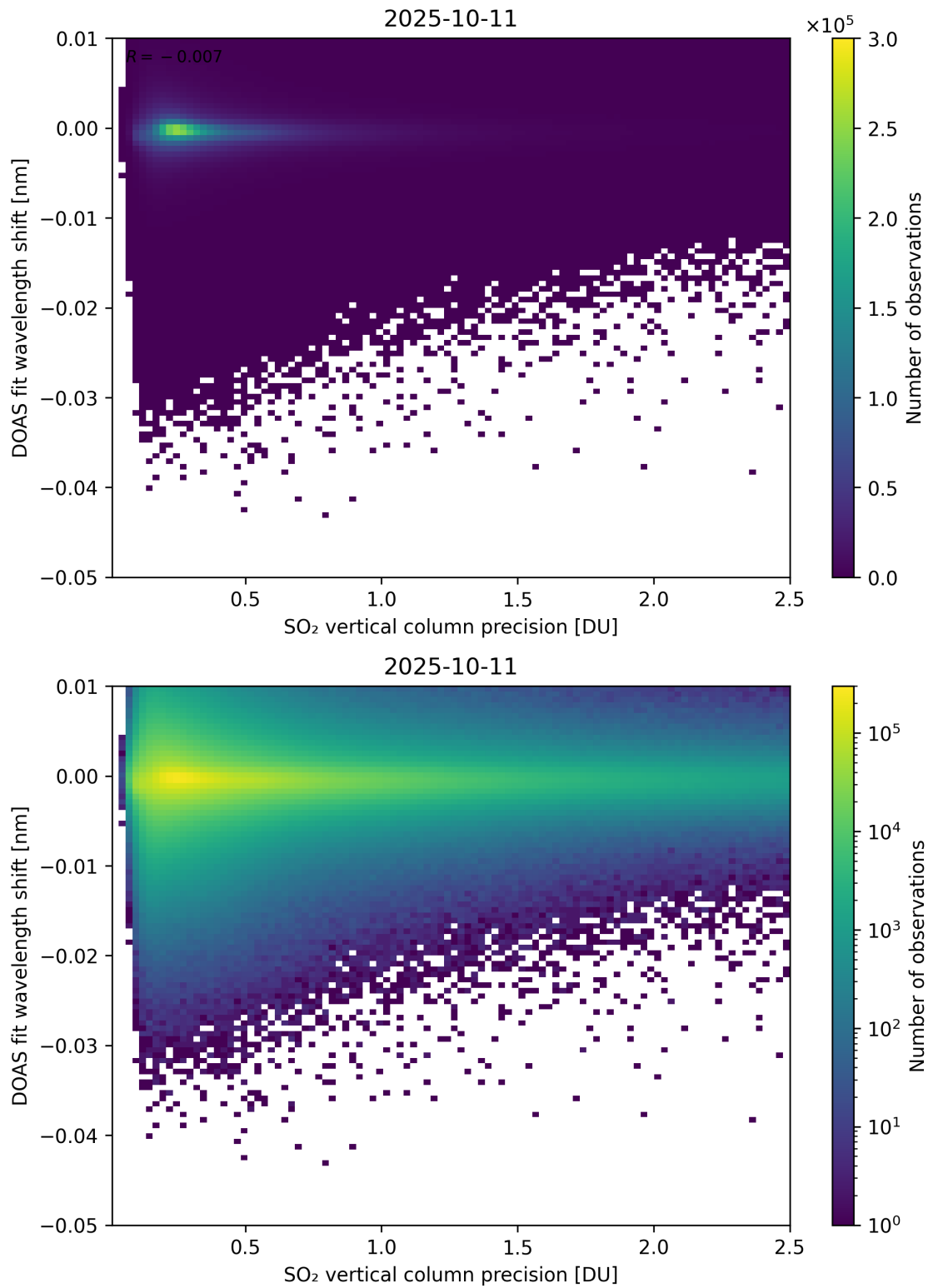
Figure 332: Scatter density plot of “SO 2 vertical column precision” against “DOAS fit wavelength shift” for 2025-10-11 to 2025-10-12.
