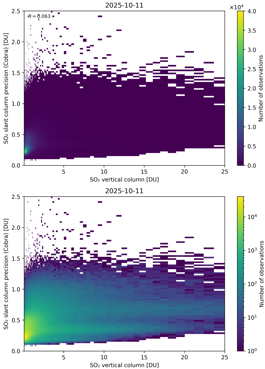
Figure 350: Scatter density plot of “SO 2 vertical column” against “SO 2 slant column precision (Cobra)” for 2025-10-11 to 2025-10-12.
