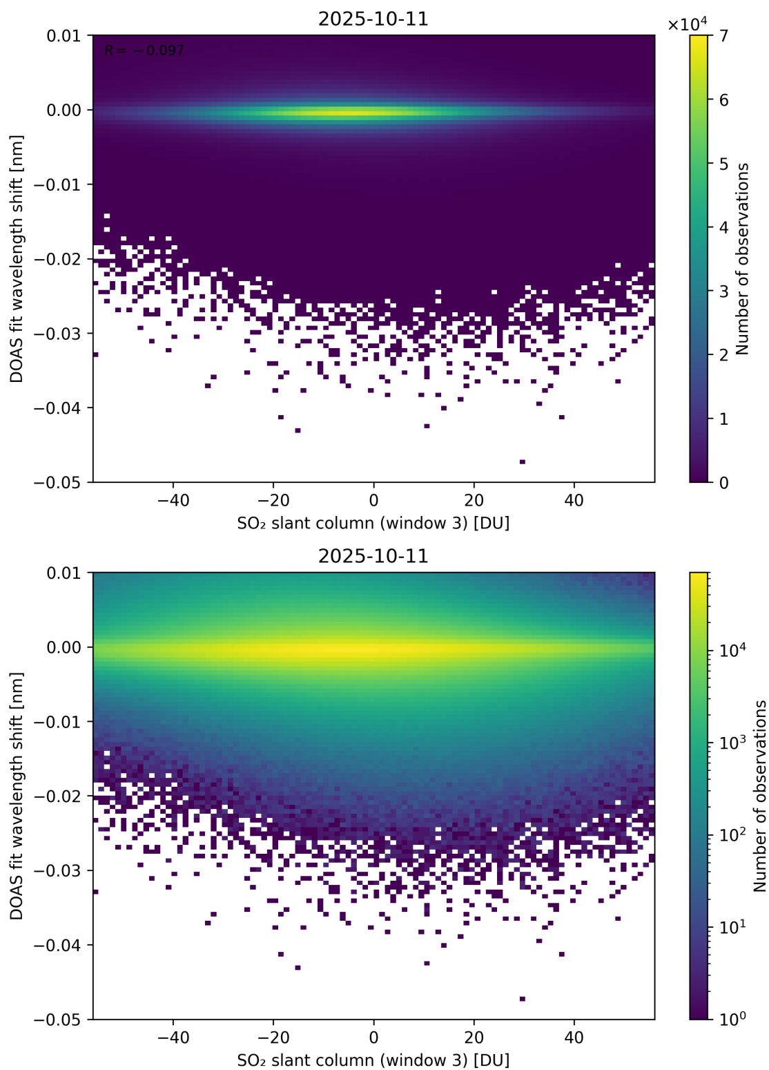
Figure 304: Scatter density plot of “SO 2 slant column (window 3)” against “DOAS fit wavelength shift” for 2025-10-11 to 2025-10-12.
