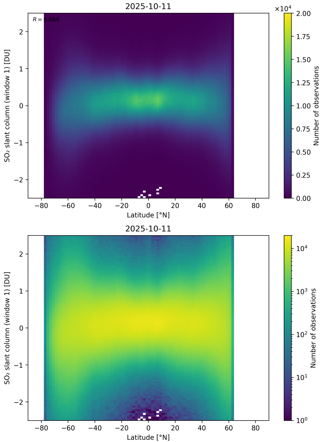
Figure 162: Scatter density plot of “Latitude” against “SO 2 slant column (window 1)” for 2025-10-11 to 2025-10-12.
