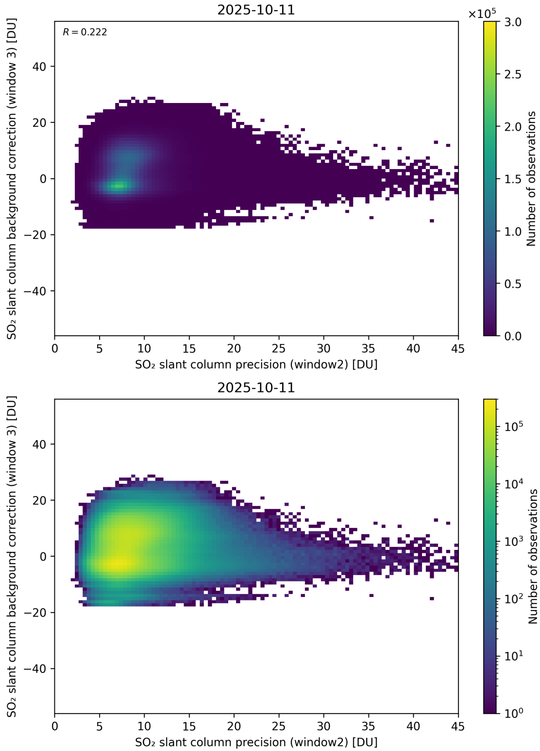
Figure 292: Scatter density plot of “SO 2 slant column precision (window2)” against “SO 2 slant column background correction (window 3)” for 2025-10-11 to 2025-10-12.
