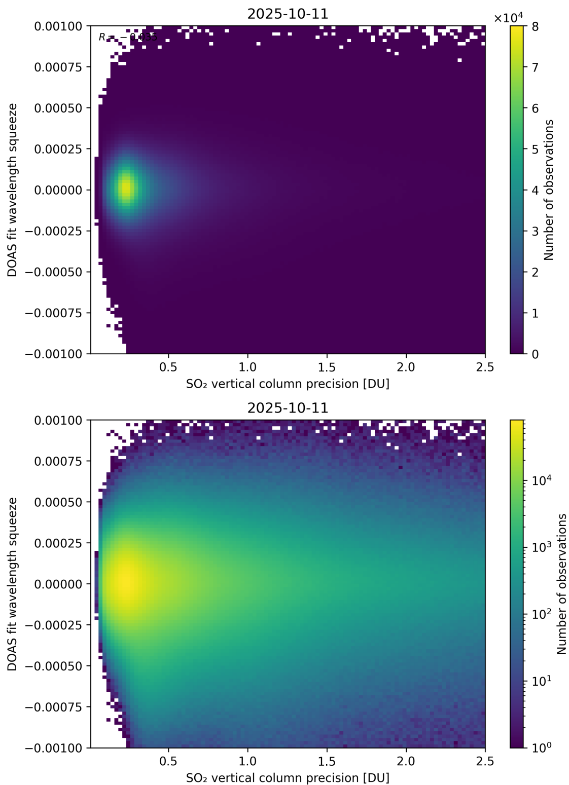
Figure 333: Scatter density plot of “SO 2 vertical column precision” against “DOAS fit wavelength squeeze” for 2025-10-11 to 2025-10-12.
