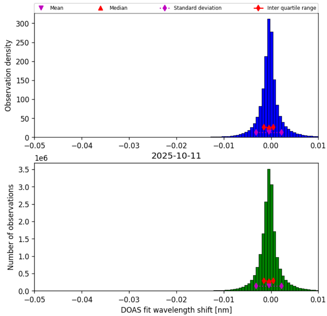
Figure 76: Histogram of “DOAS fit wavelength shift” for 2025-10-11 to 2025-10-12
