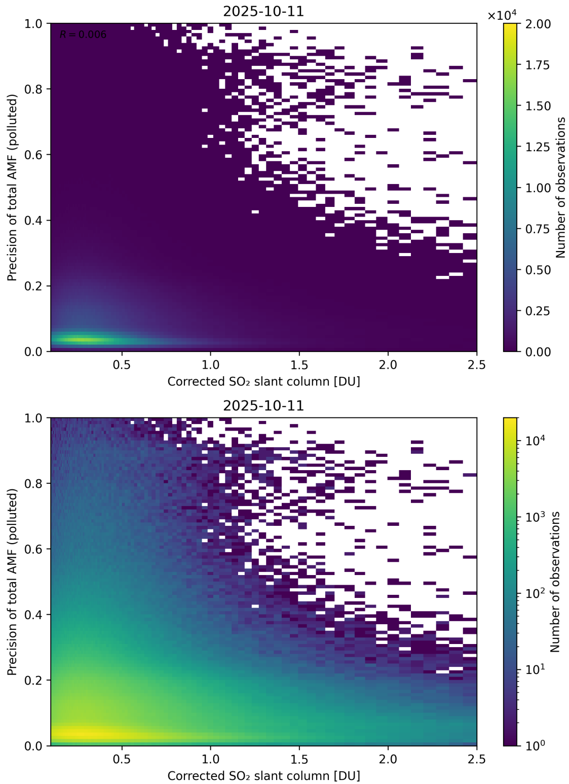
Figure 243: Scatter density plot of “Corrected SO 2 slant column” against “Precision of total AMF (polluted)” for 2025-10-11 to 2025-10-12.
