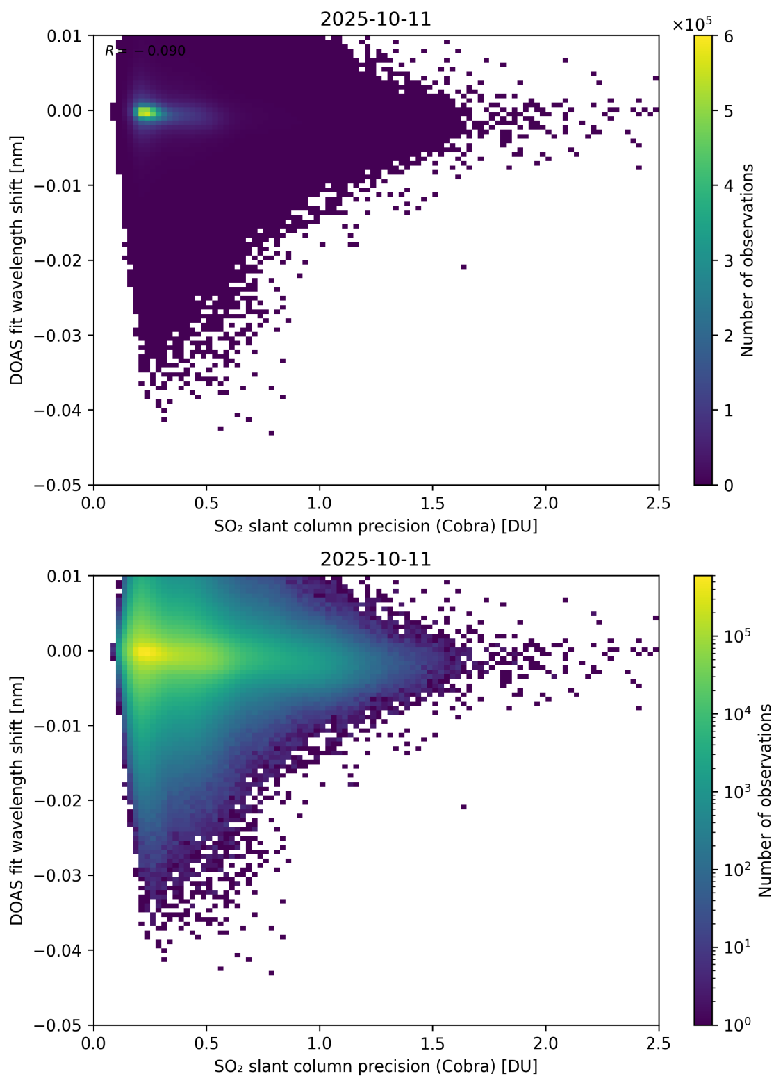
Figure 202: Scatter density plot of “SO 2 slant column precision (Cobra)” against “DOAS fit wavelength shift” for 2025-10-11 to 2025-10-12.
