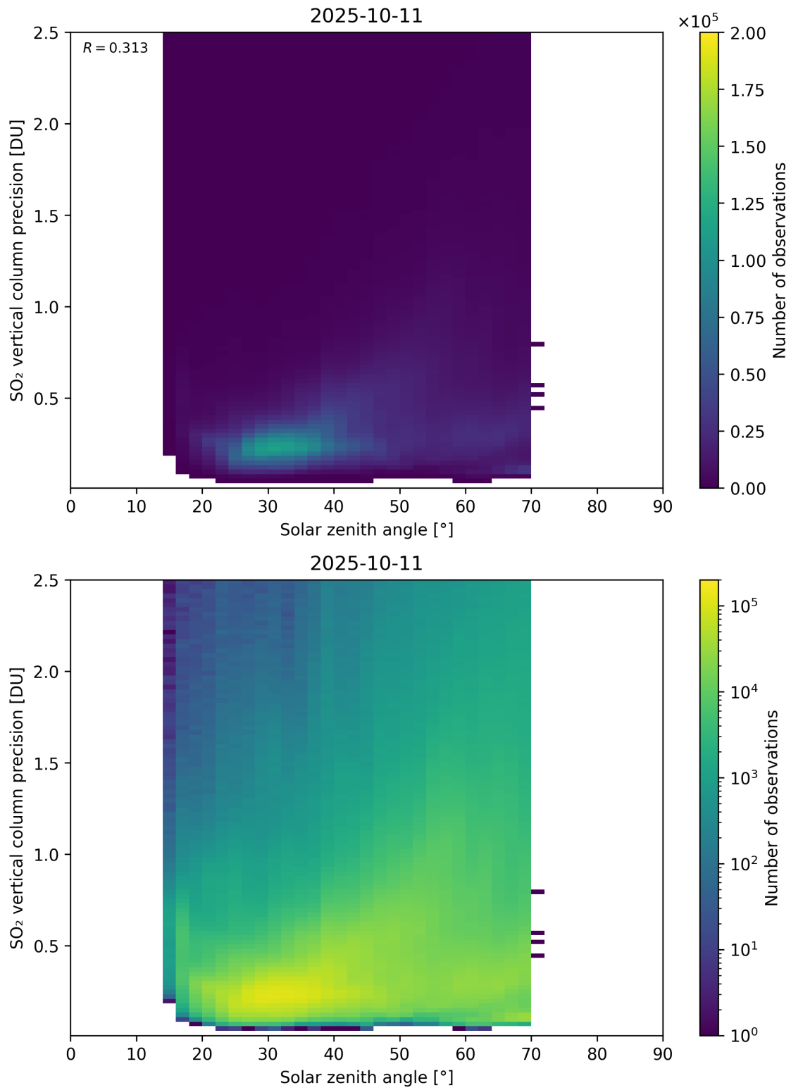
Figure 192: Scatter density plot of “Solar zenith angle” against “SO 2 vertical column precision” for 2025-10-11 to 2025-10-12.
