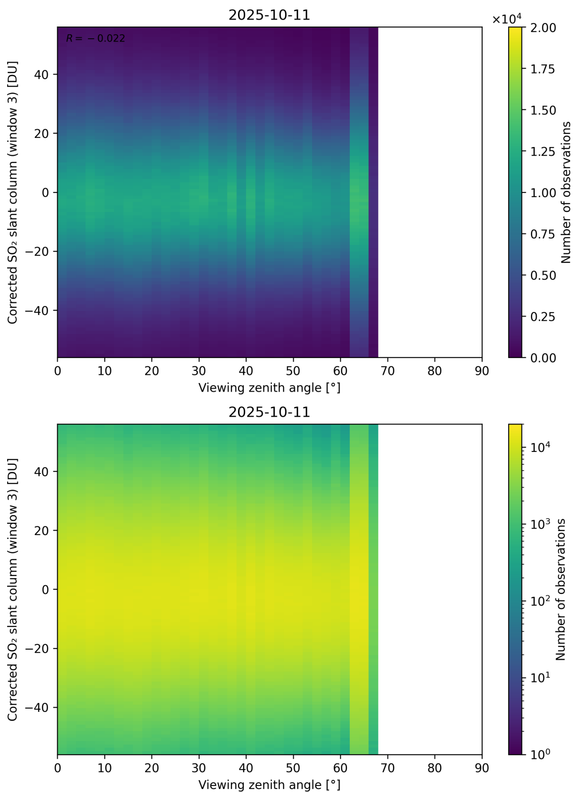
Figure 375: Scatter density plot of “Viewing zenith angle” against “Corrected SO 2 slant column (window 3)” for 2025-10-11 to 2025-10-12.
