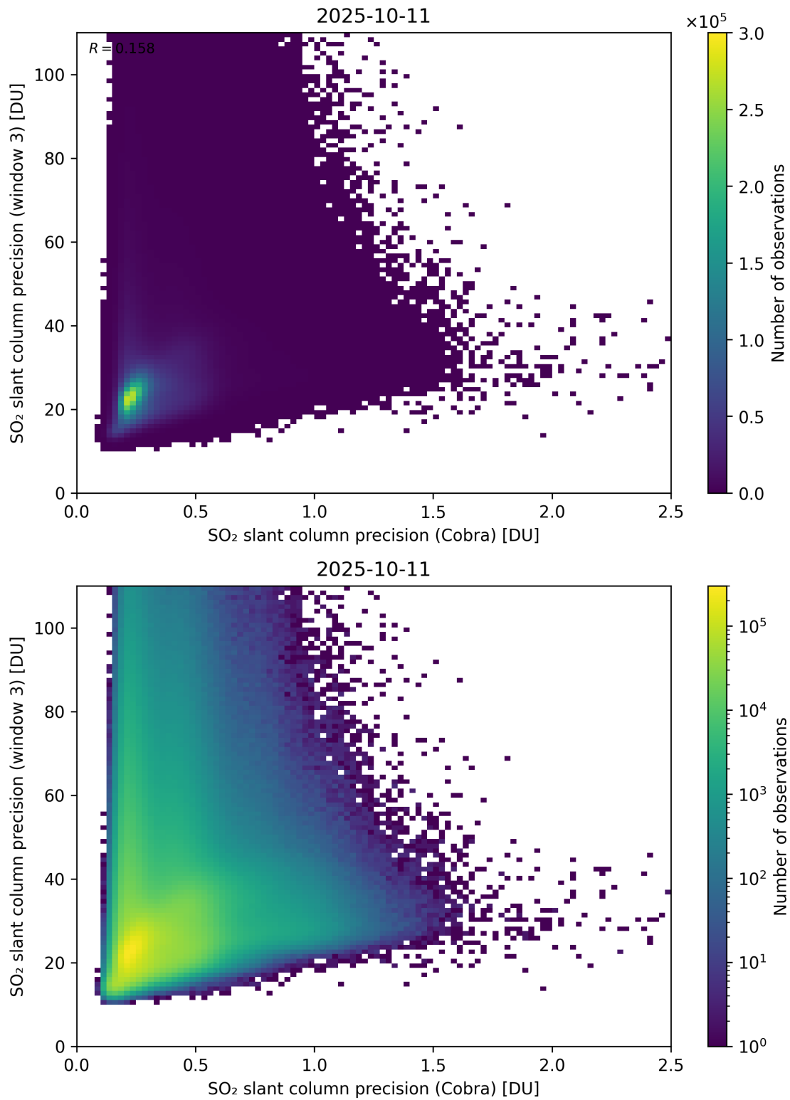
Figure 212: Scatter density plot of “SO 2 slant column precision (Cobra)” against “SO 2 slant column precision (window 3)” for 2025-10-11 to 2025-10-12.
