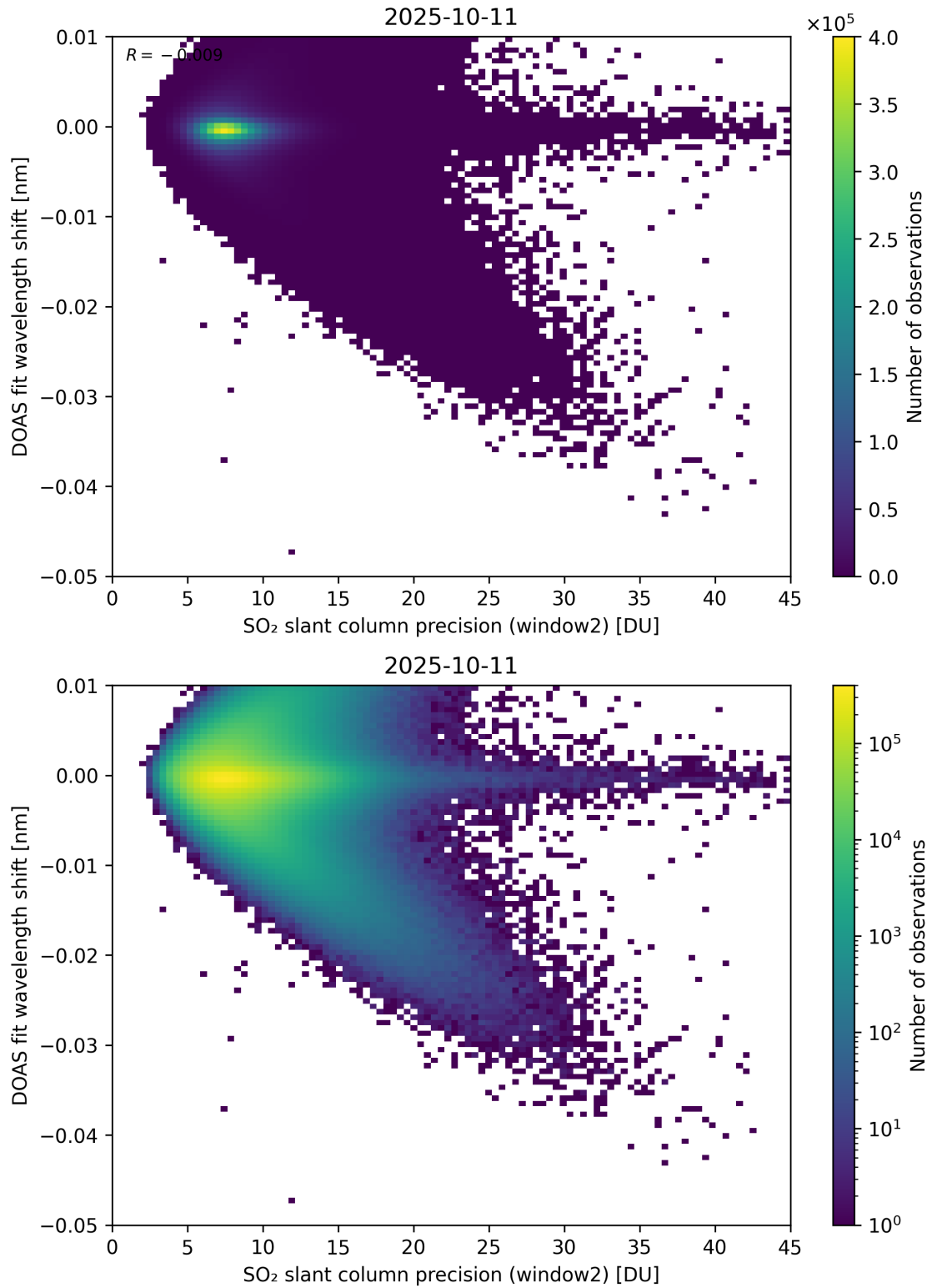
Figure 293: Scatter density plot of “SO 2 slant column precision (window2)” against “DOAS fit wavelength shift” for 2025-10-11 to 2025-10-12.
