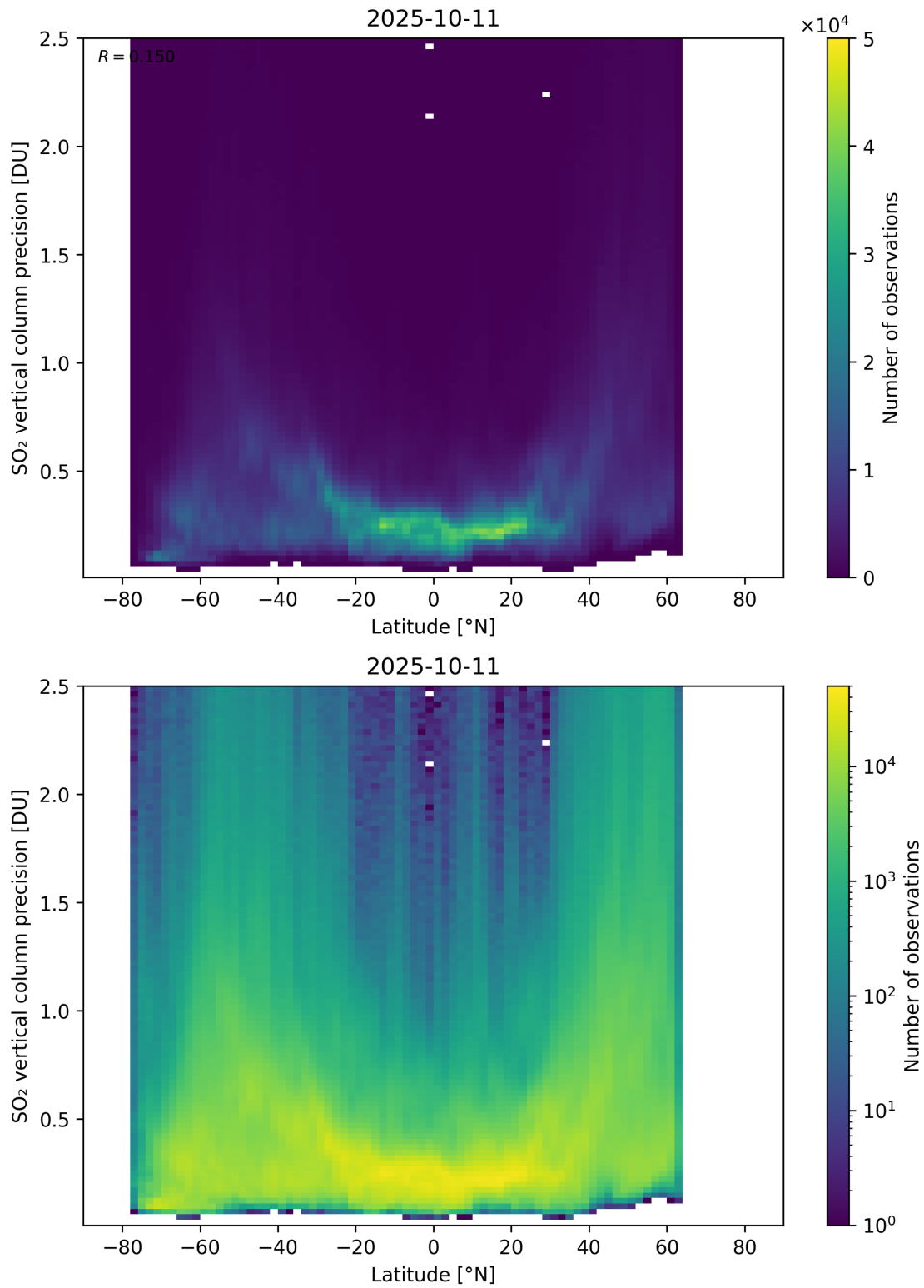
Figure 170: Scatter density plot of “Latitude” against “SO 2 vertical column precision” for 2025-10-11 to 2025-10-12.
