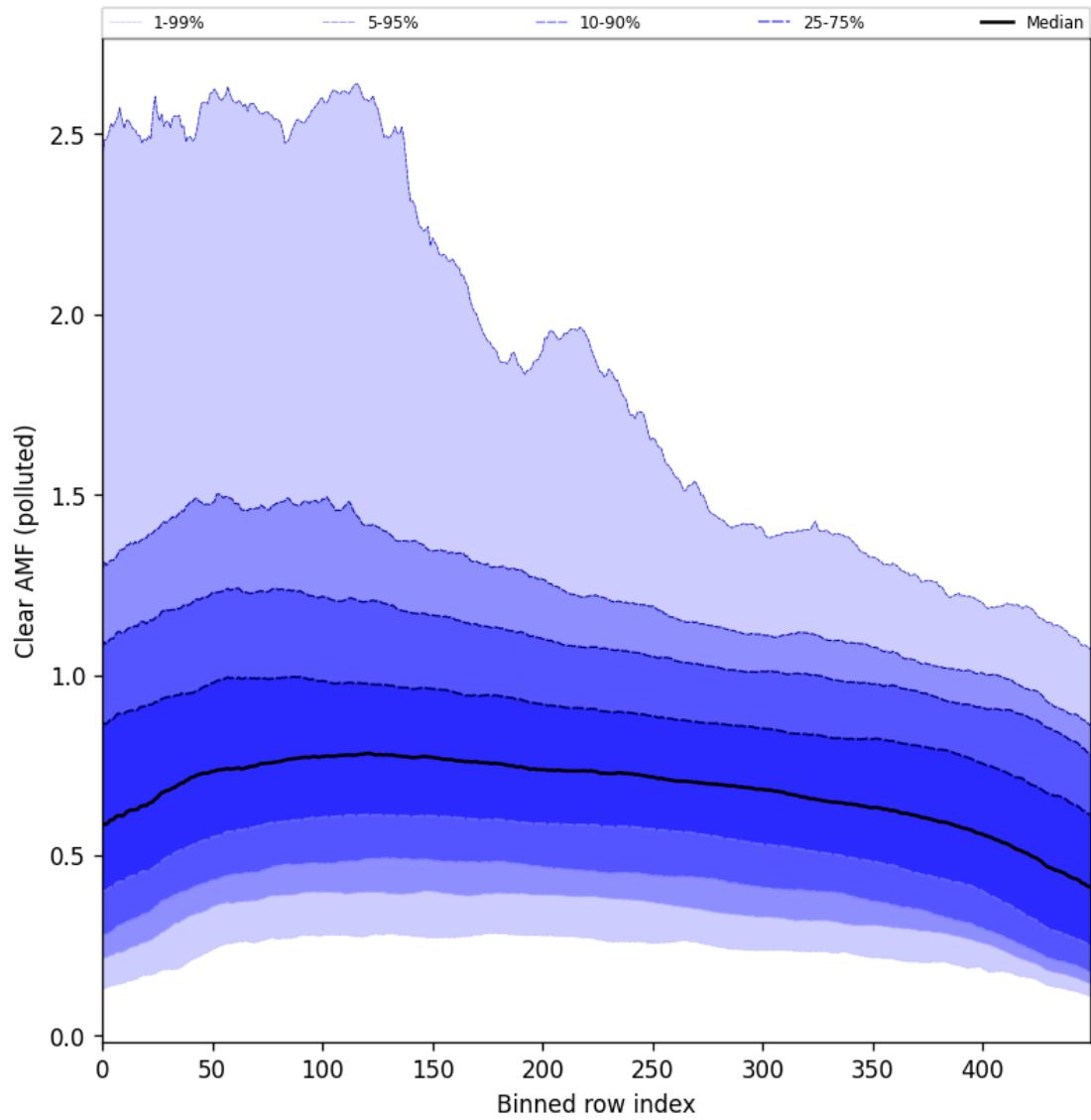
Figure 107: Along track statistics of “Clear AMF (polluted)” for 2025-10-11 to 2025-10-12
