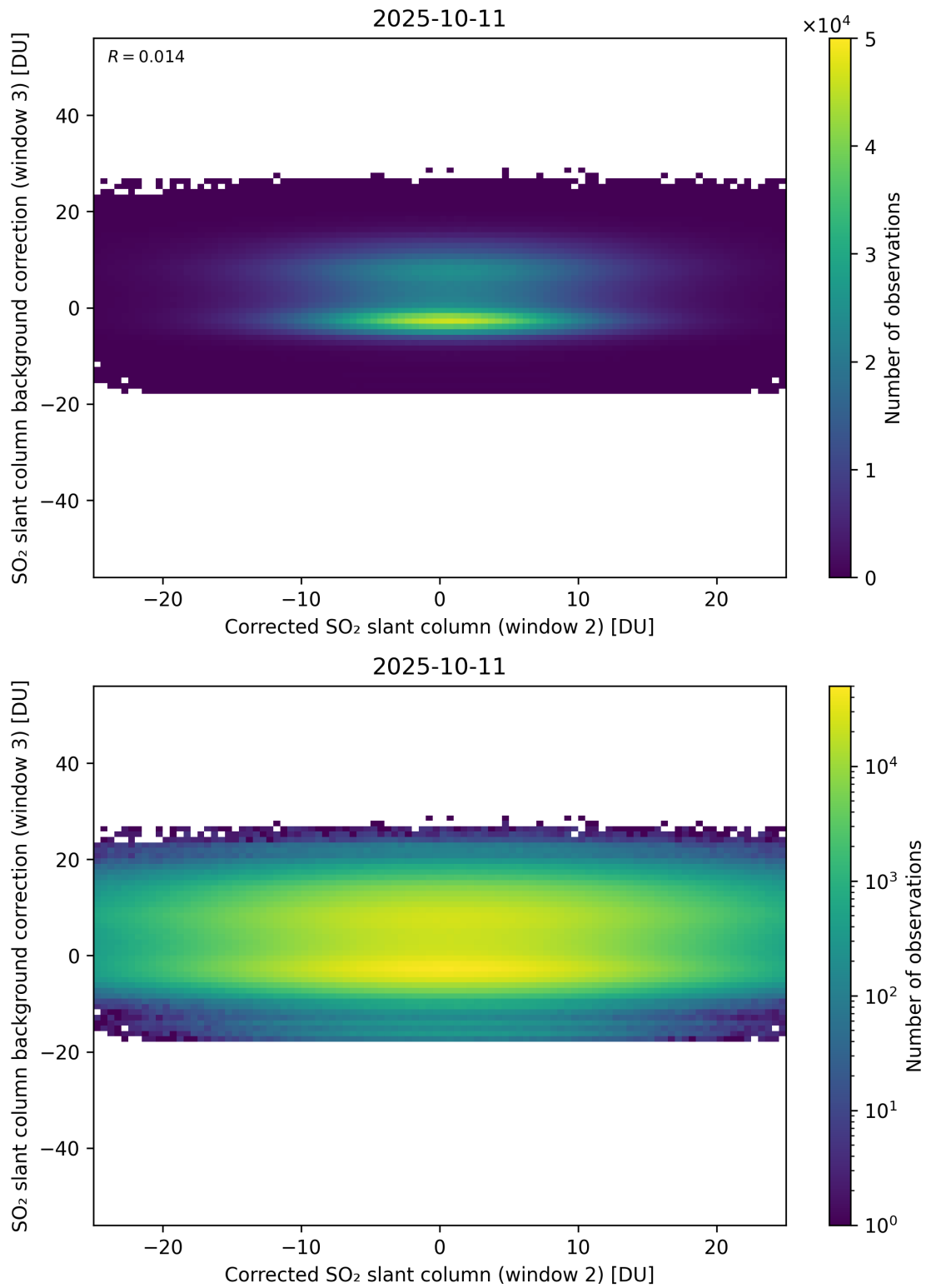
Figure 245: Scatter density plot of “Corrected SO 2 slant column (window 2)” against “SO 2 slant column background correction (window 3)” for 2025-10-11 to 2025-10-12.
