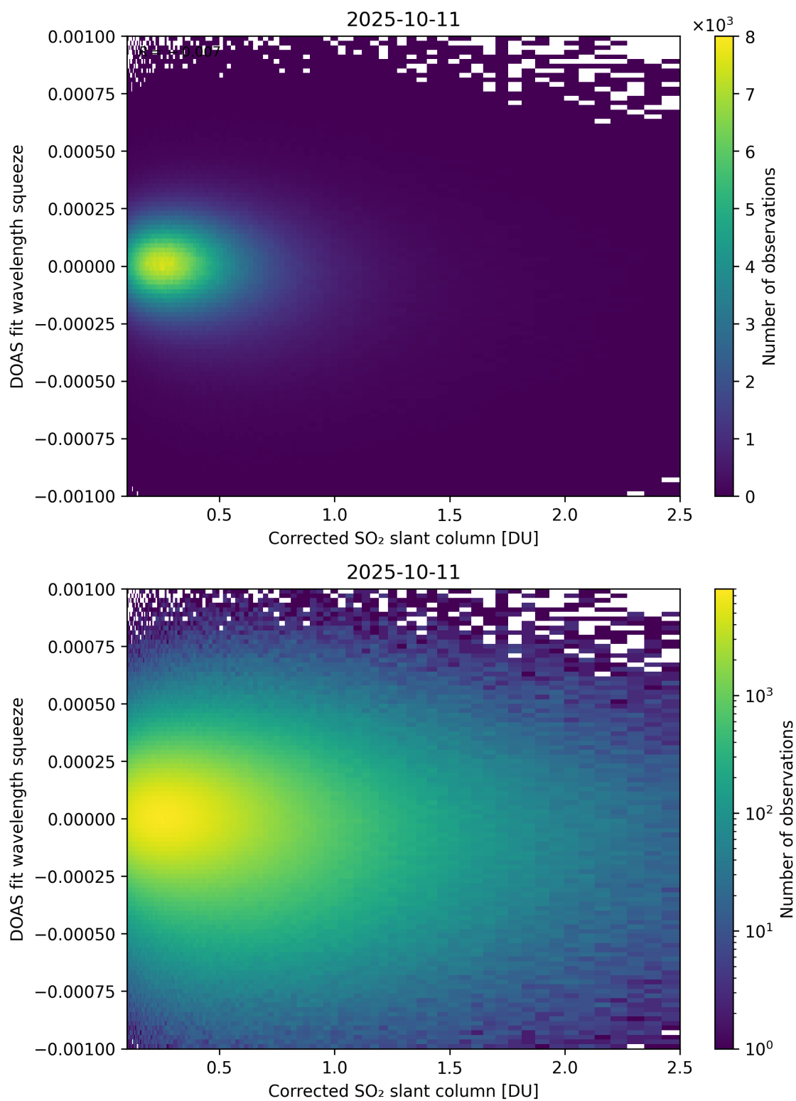
Figure 230: Scatter density plot of “Corrected SO 2 slant column” against “DOAS fit wavelength squeeze” for 2025-10-11 to 2025-10-12.
