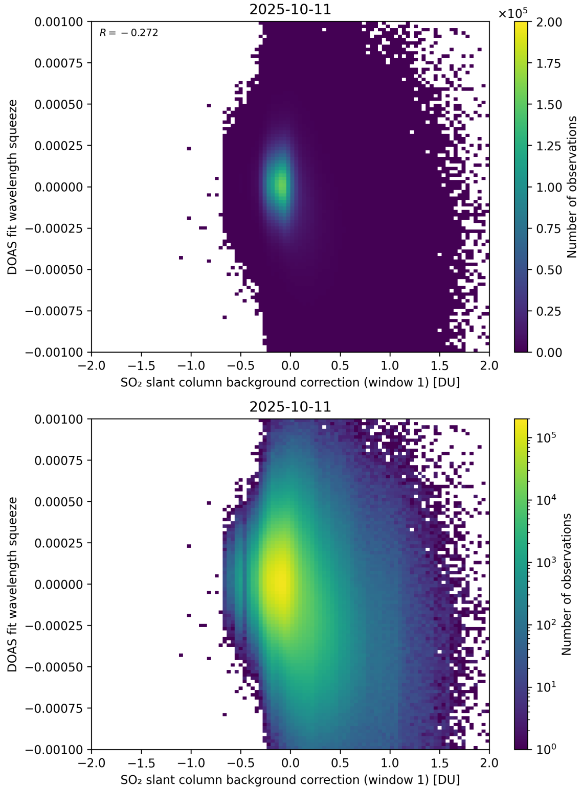
Figure 112: Scatter density plot of “SO 2 slant column background correction (window 1)” against “DOAS fit wavelength squeeze” for 2025-10-11 to 2025-10-12.
