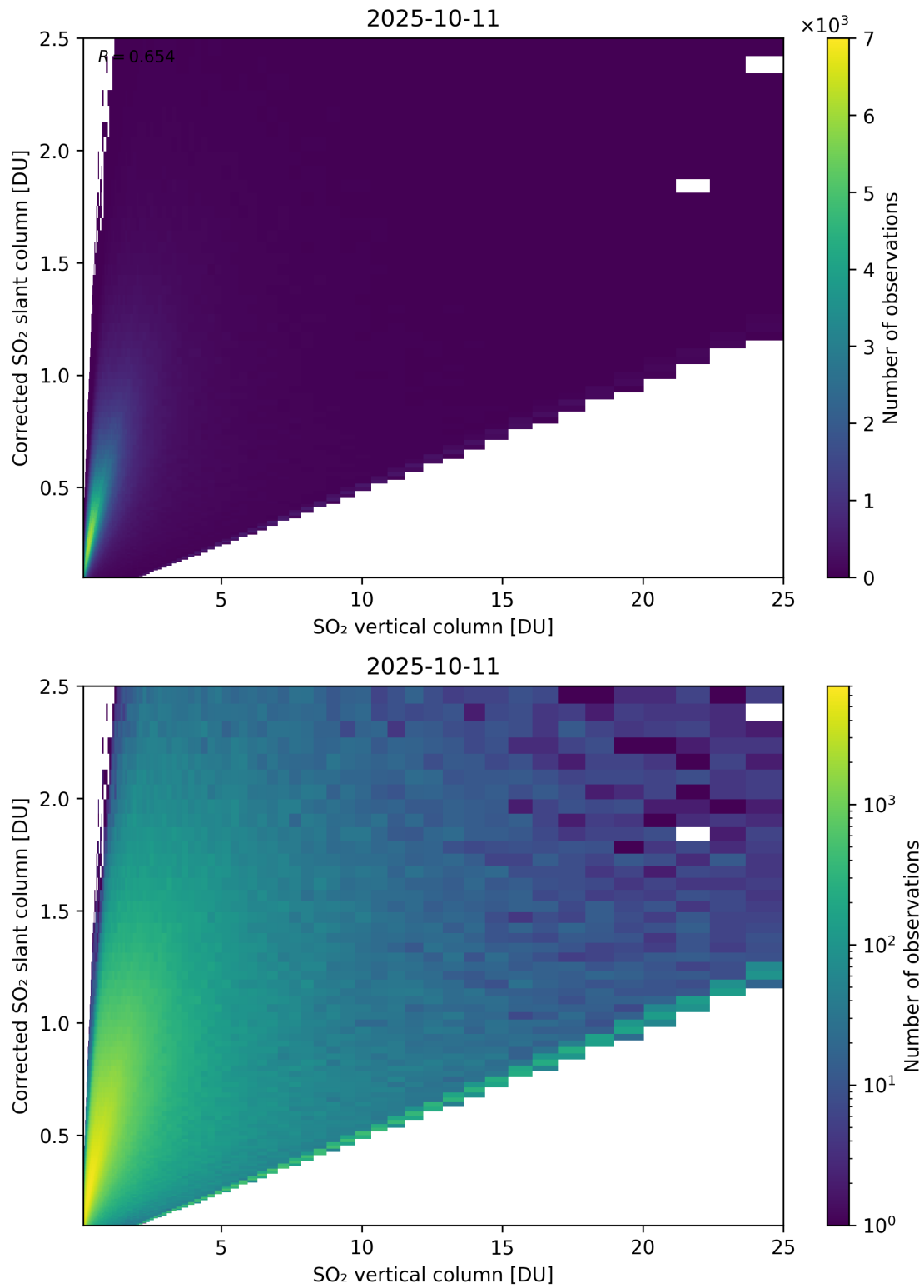
Figure 351: Scatter density plot of “SO 2 vertical column” against “Corrected SO 2 slant column” for 2025-10-11 to 2025-10-12.
