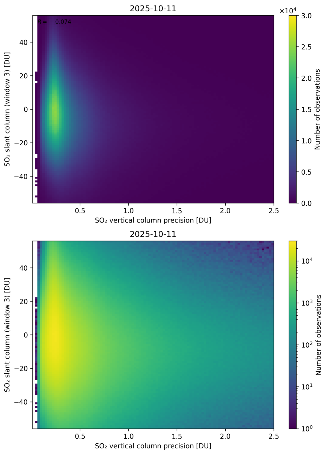
Figure 344: Scatter density plot of “SO 2 vertical column precision” against “SO 2 slant column (window 3)” for 2025-10-11 to 2025-10-12.
