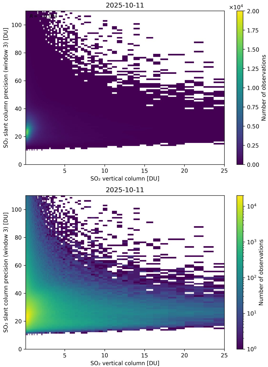
Figure 358: Scatter density plot of “SO 2 vertical column” against “SO 2 slant column precision (window 3)” for 2025-10-11 to 2025-10-12.
