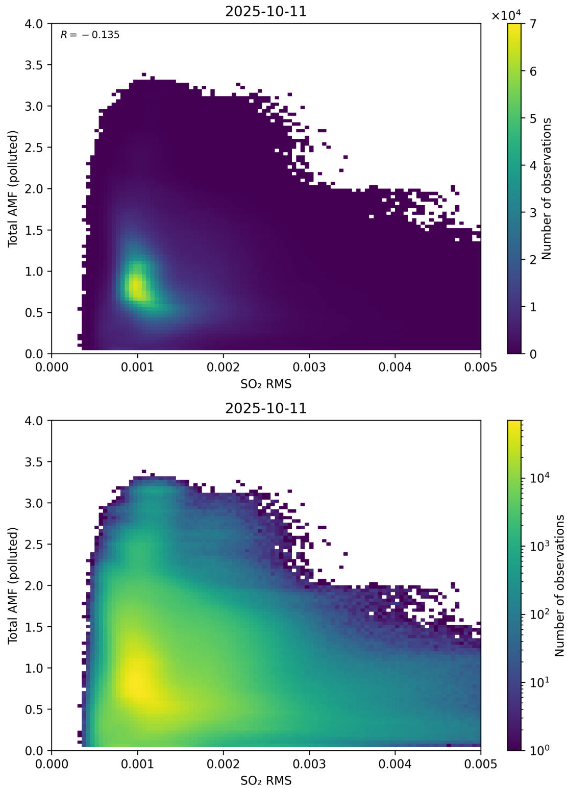
Figure 148: Scatter density plot of “SO 2 RMS” against “Total AMF (polluted)” for 2025-10-11 to 2025-10-12.
