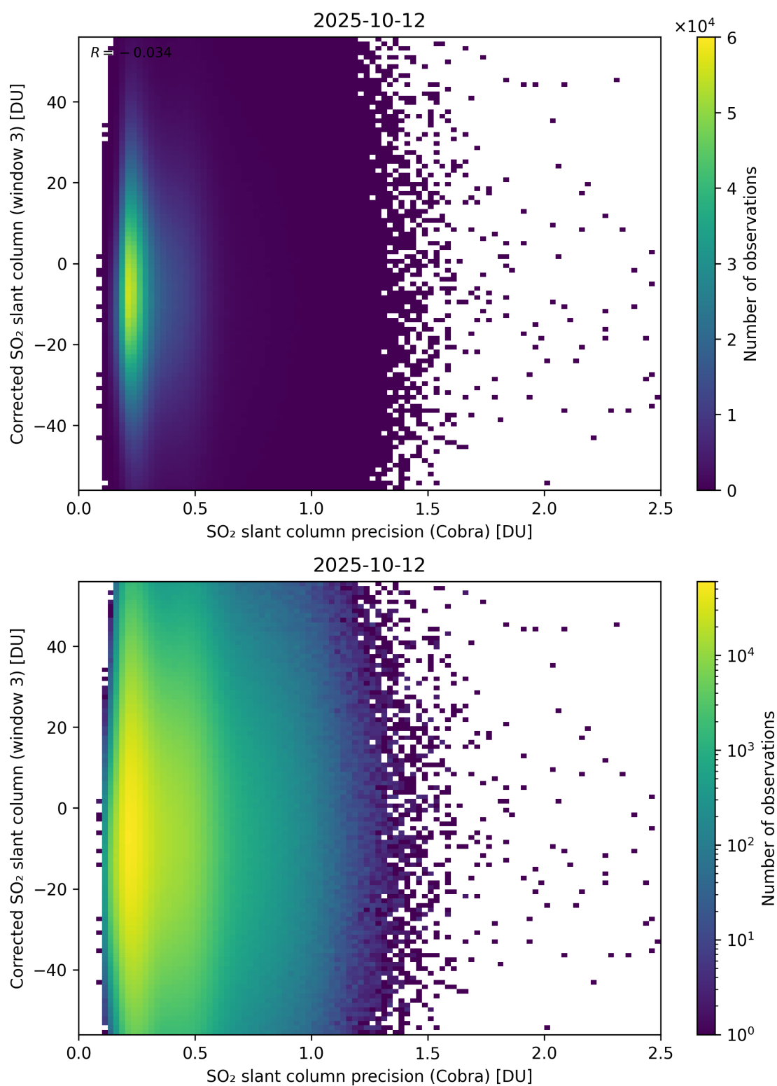
Figure 207: Scatter density plot of “SO 2 slant column precision (Cobra)” against “Corrected SO 2 slant column (window 3)” for 2025-10-11 to 2025-10-13.
