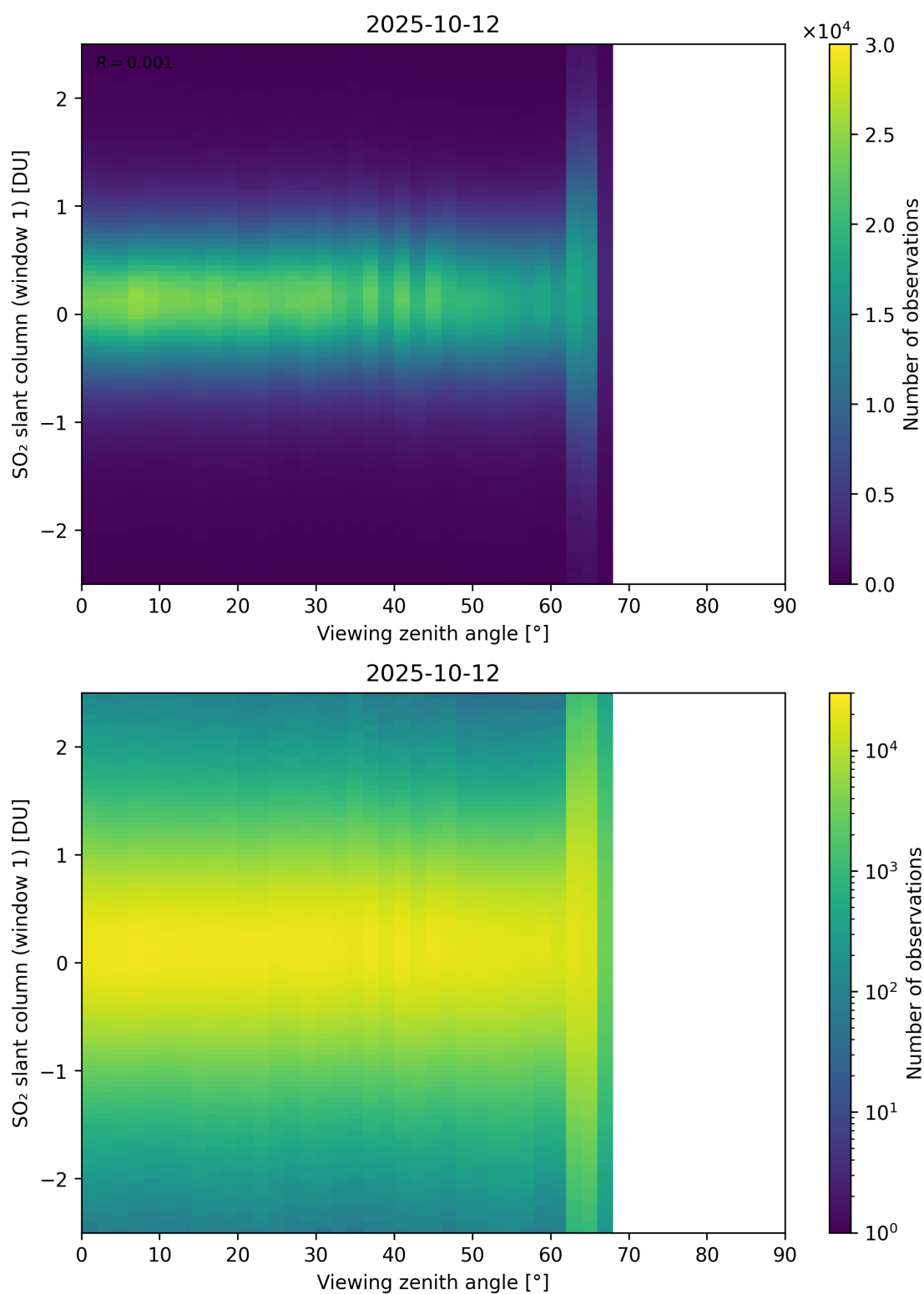
Figure 376: Scatter density plot of “Viewing zenith angle” against “SO 2 slant column (window 1)” for 2025-10-11 to 2025-10-13.
