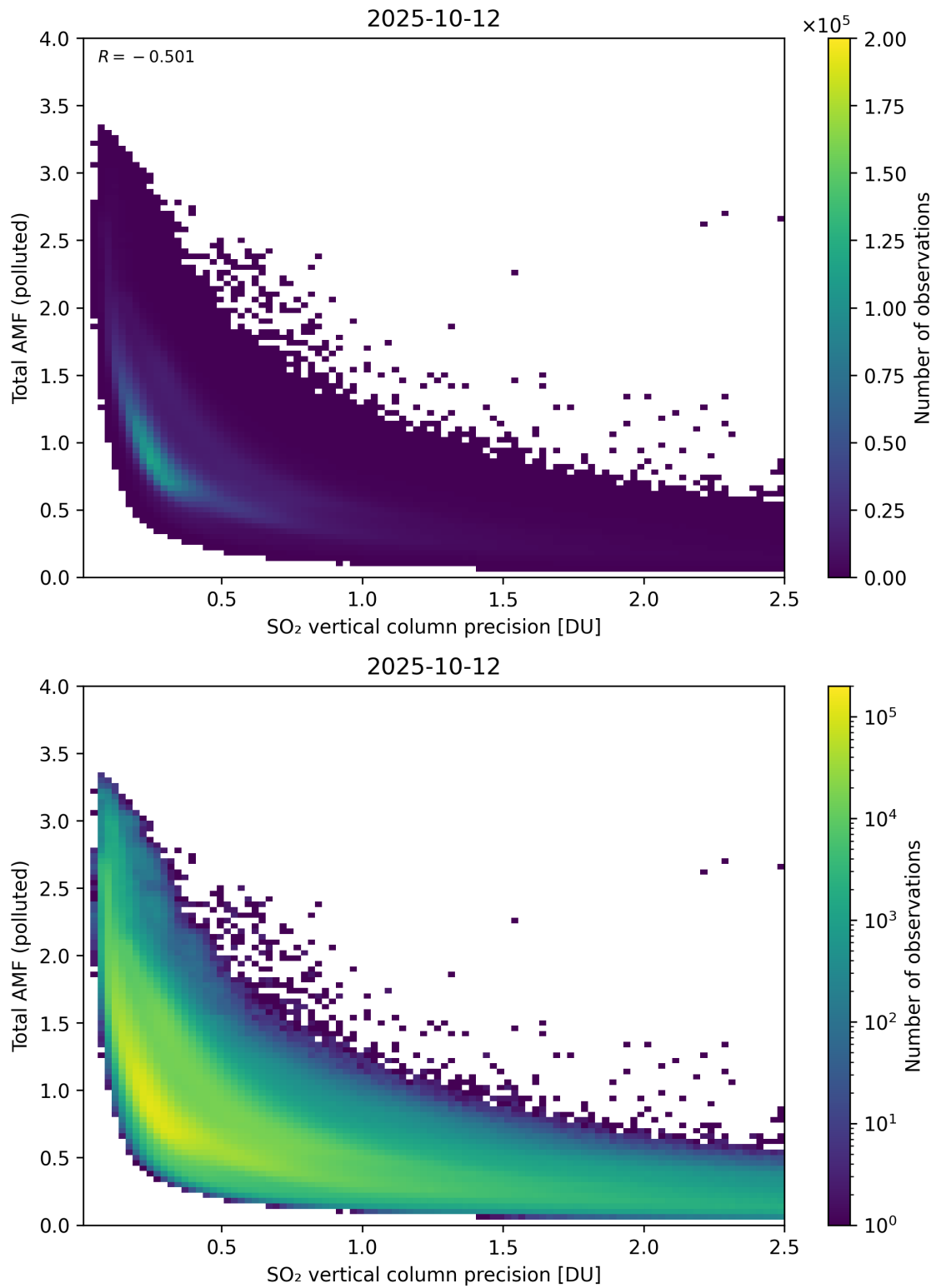
Figure 346: Scatter density plot of “SO 2 vertical column precision” against “Total AMF (polluted)” for 2025-10-11 to 2025-10-13.
