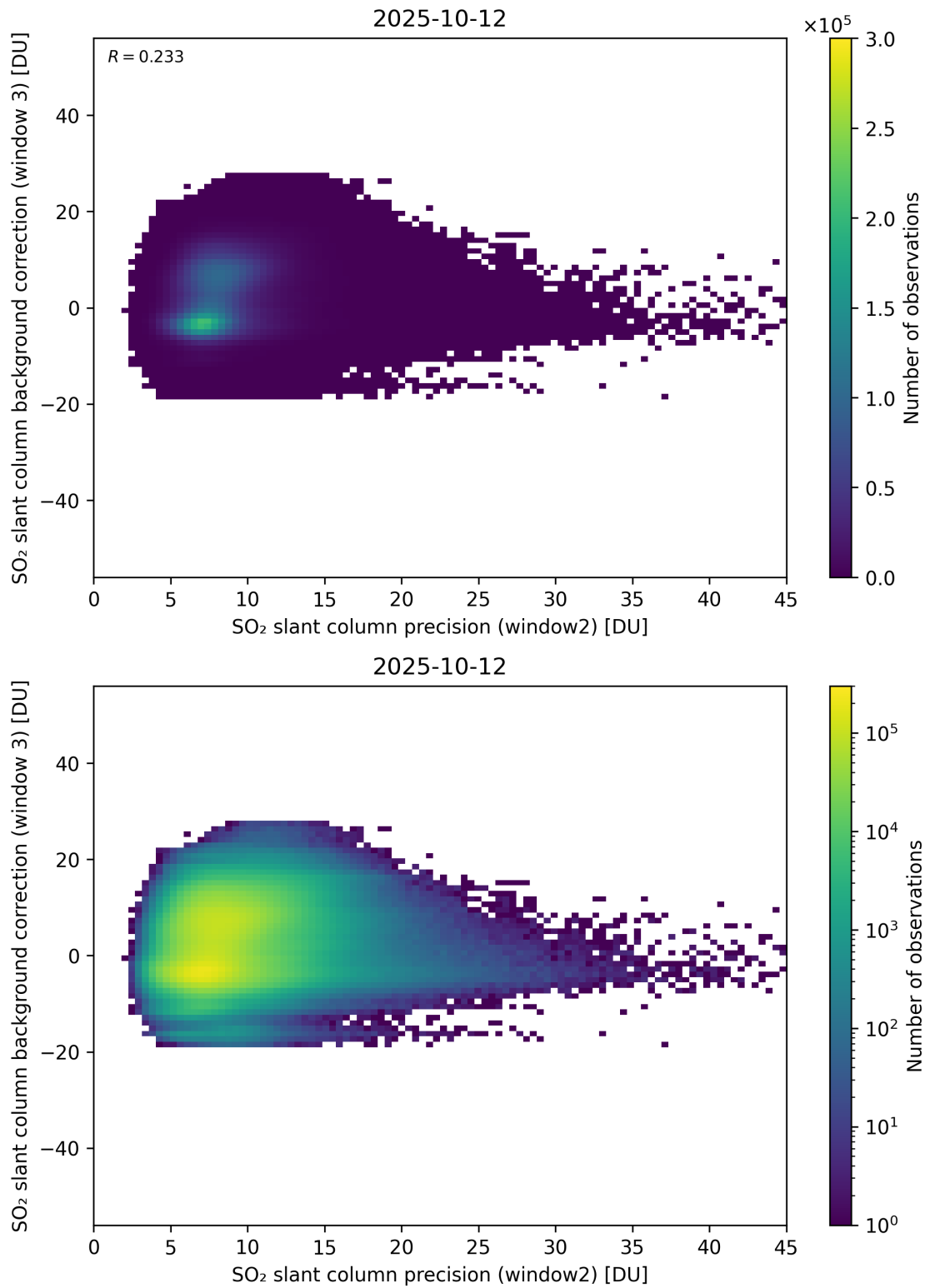
Figure 292: Scatter density plot of “SO 2 slant column precision (window2)” against “SO 2 slant column background correction (window 3)” for 2025-10-11 to 2025-10-13.
