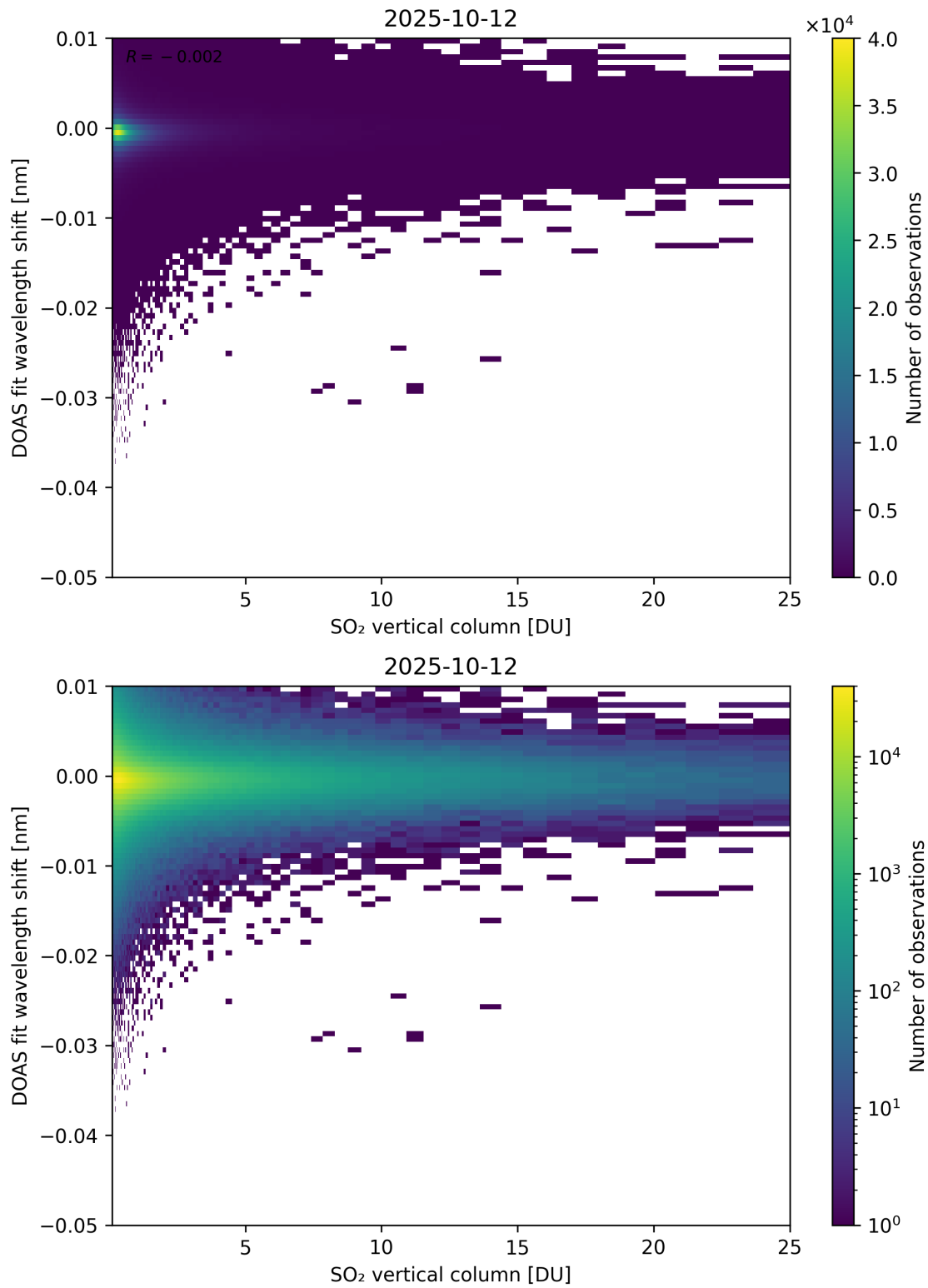
Figure 326: Scatter density plot of “SO 2 vertical column” against “DOAS fit wavelength shift” for 2025-10-11 to 2025-10-13.
