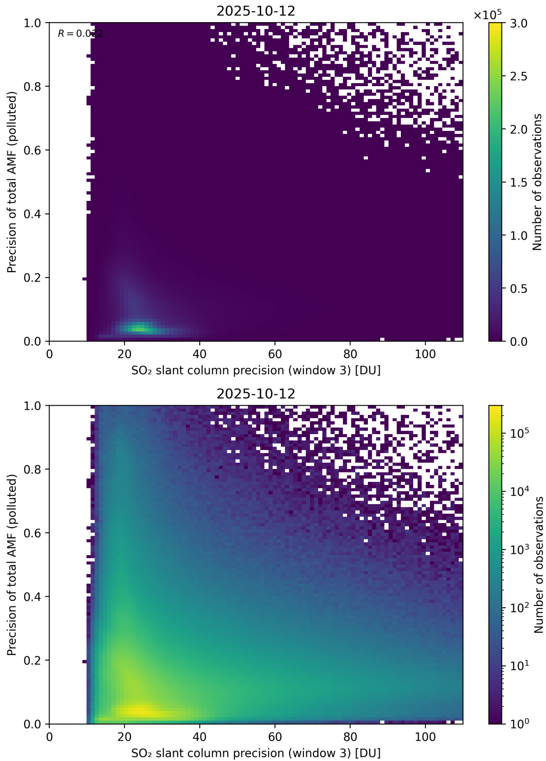
Figure 314: Scatter density plot of “SO 2 slant column precision (window 3)” against “Precision of total AMF (polluted)” for 2025-10-11 to 2025-10-13.
