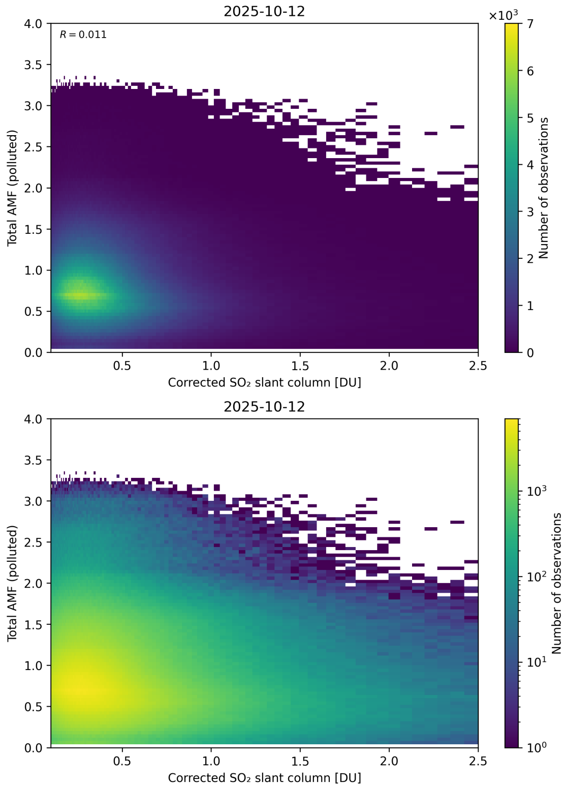
Figure 242: Scatter density plot of “Corrected SO 2 slant column” against “Total AMF (polluted)” for 2025-10-11 to 2025-10-13.
