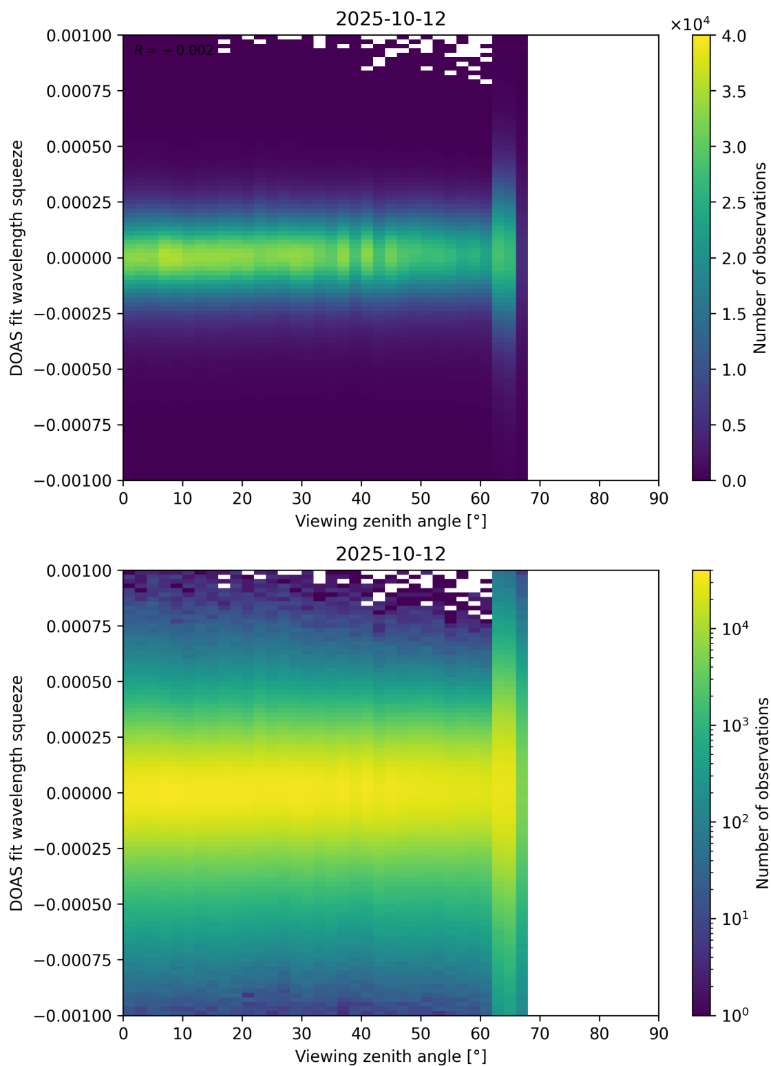
Figure 366: Scatter density plot of “Viewing zenith angle” against “DOAS fit wavelength squeeze” for 2025-10-11 to 2025-10-13.
