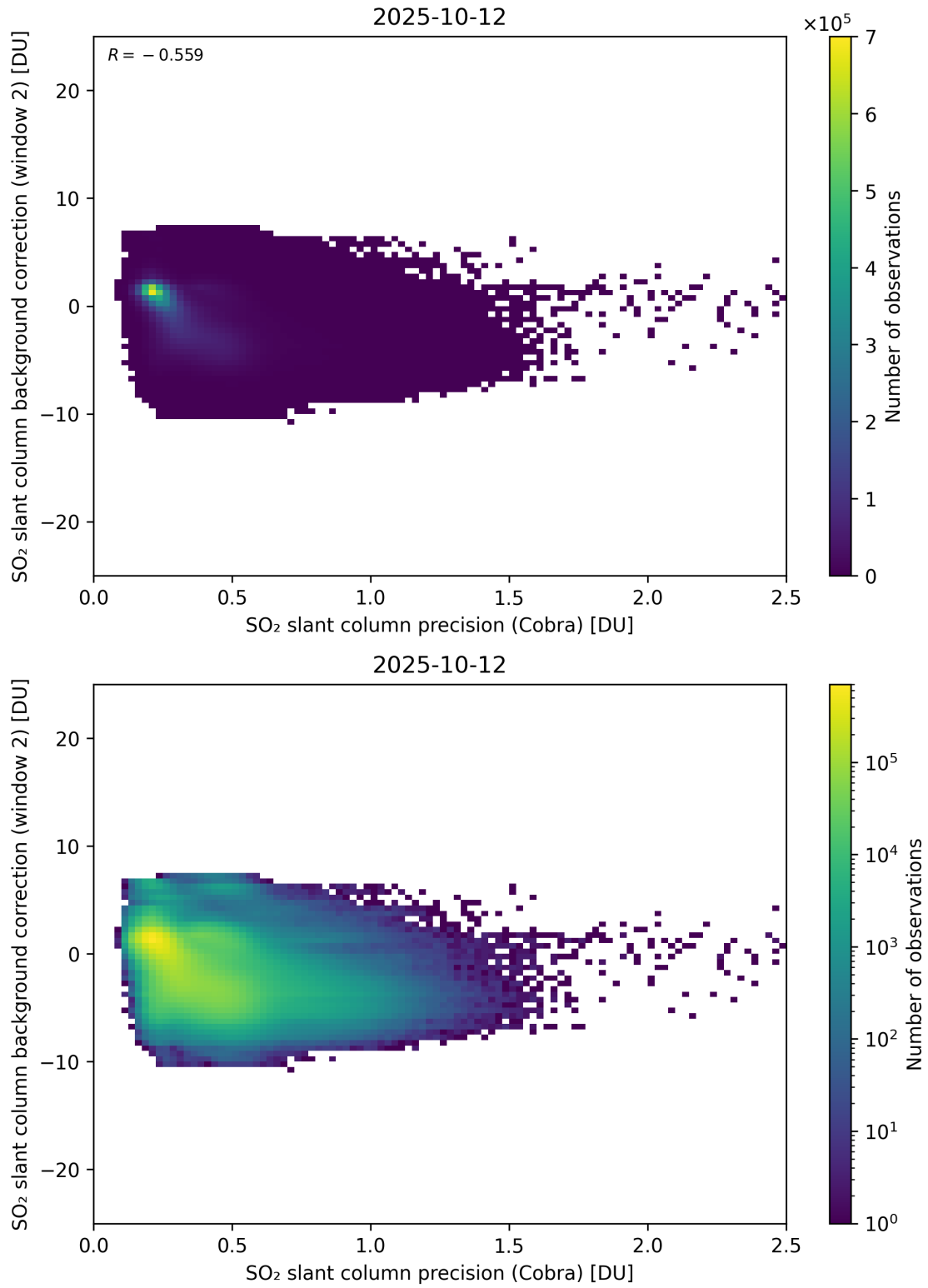
Figure 200: Scatter density plot of “SO 2 slant column precision (Cobra)” against “SO 2 slant column background correction (window 2)” for 2025-10-11 to 2025-10-13.
