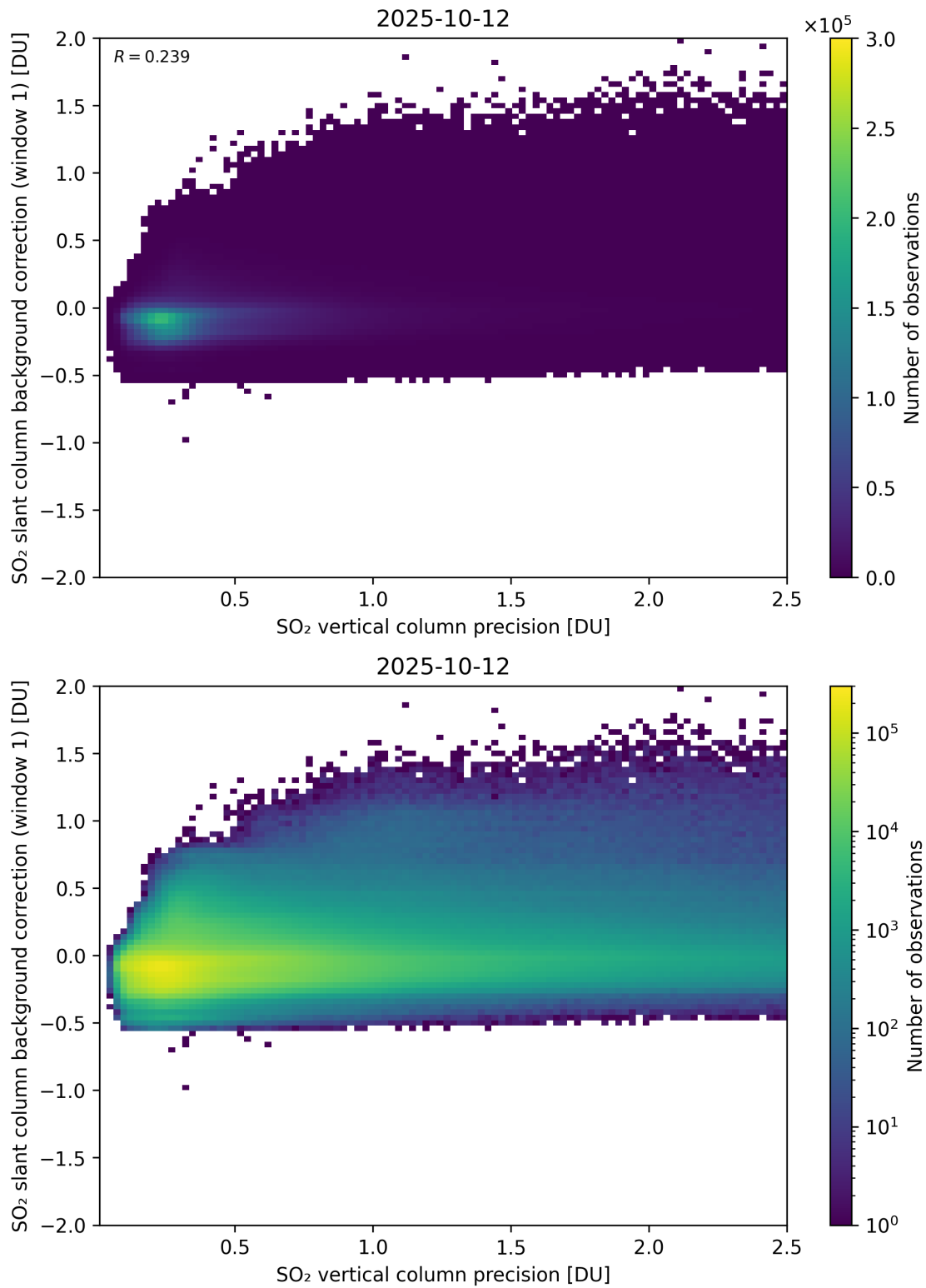
Figure 329: Scatter density plot of “SO 2 vertical column precision” against “SO 2 slant column background correction (window 1)” for 2025-10-11 to 2025-10-13.
