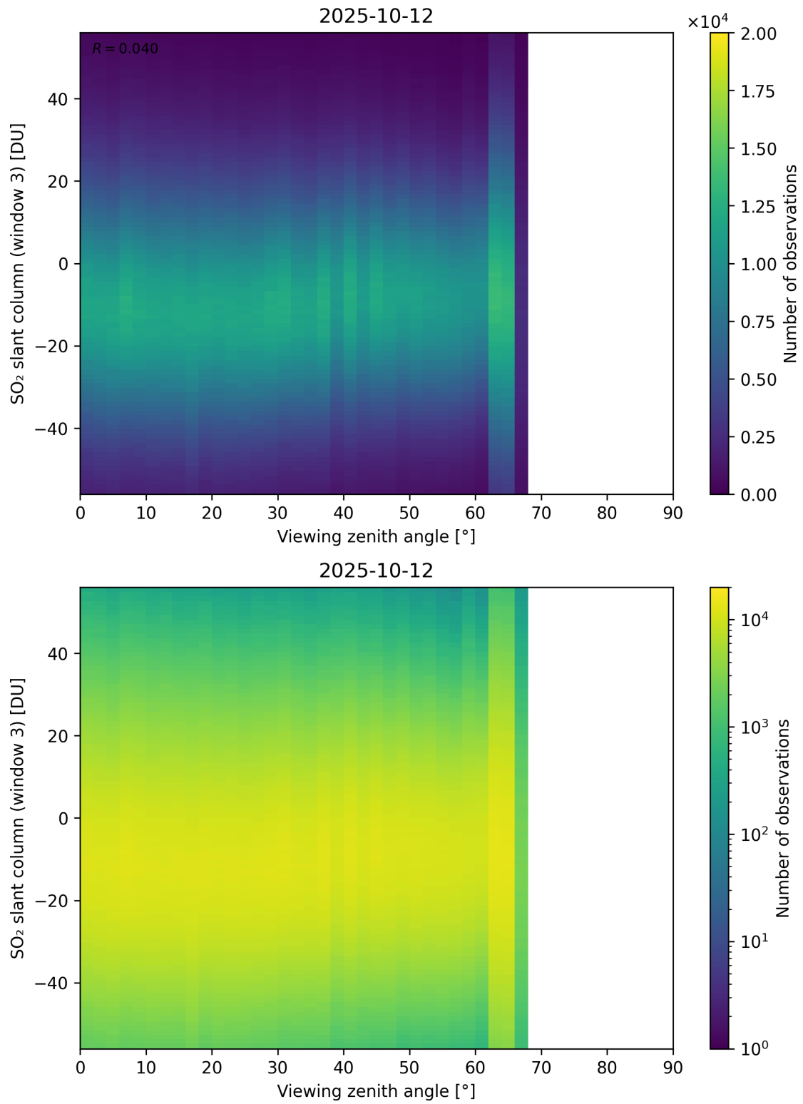
Figure 379: Scatter density plot of “Viewing zenith angle” against “SO 2 slant column (window 3)” for 2025-10-11 to 2025-10-13.
