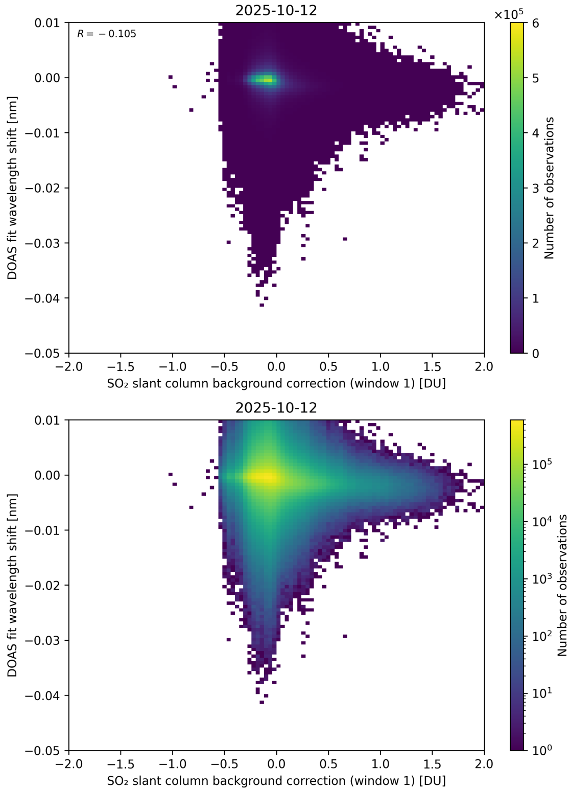
Figure 111: Scatter density plot of “SO 2 slant column background correction (window 1)” against “DOAS fit wavelength shift” for 2025-10-11 to 2025-10-13.
