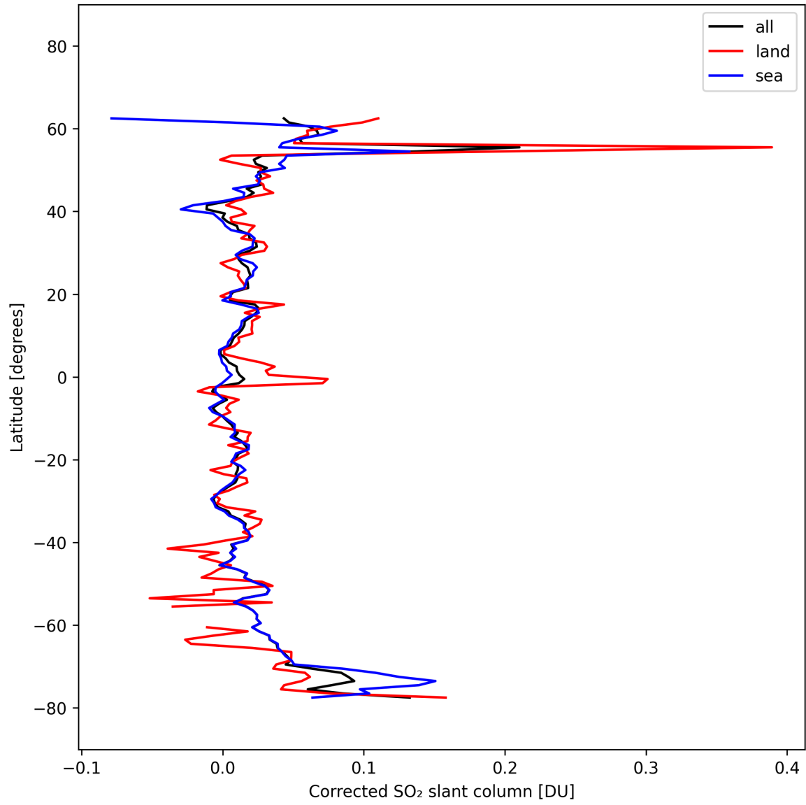
Figure 34: Zonal average of “Corrected SO 2 slant column” for 2025-10-11 to 2025-10-13.
