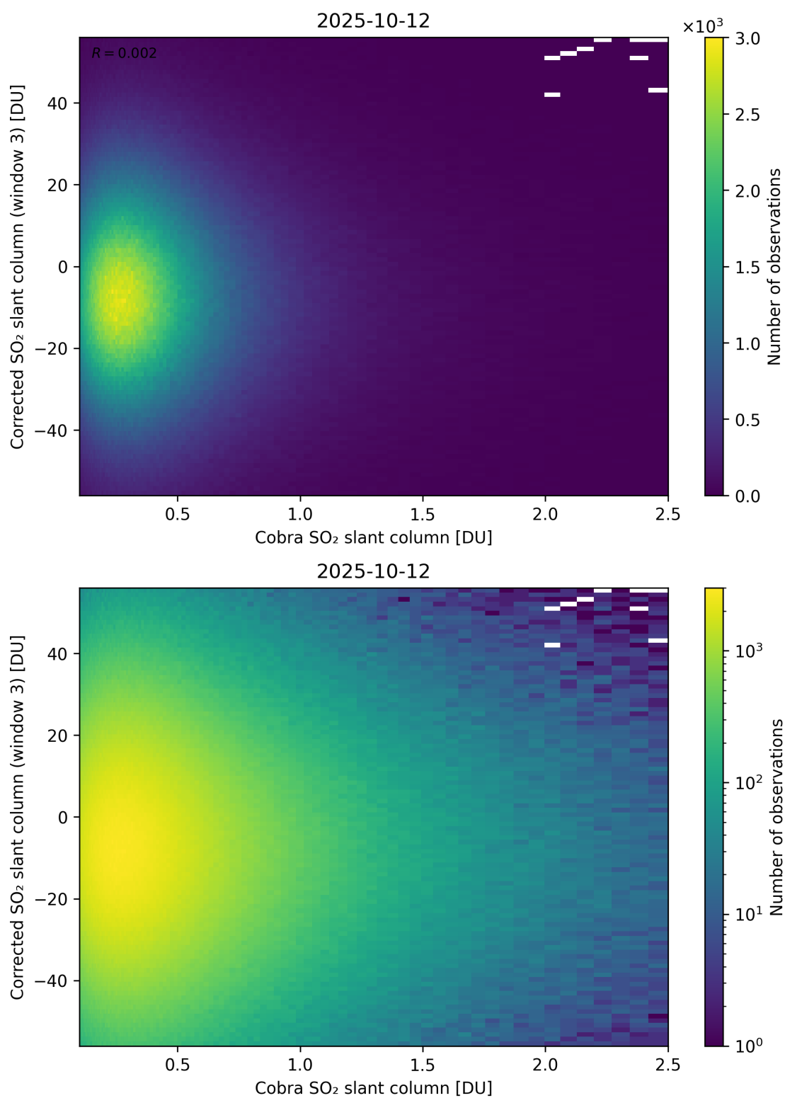
Figure 218: Scatter density plot of “Cobra SO 2 slant column” against “Corrected SO 2 slant column (window 3)” for 2025-10-11 to 2025-10-13.
