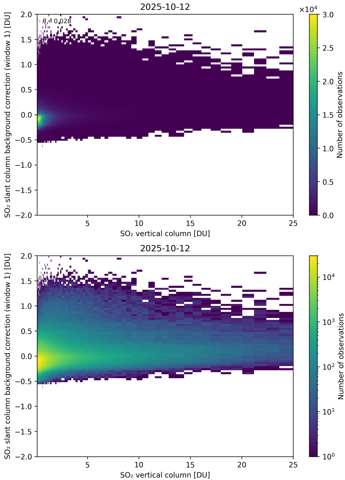
Figure 323: Scatter density plot of “SO 2 vertical column” against “SO 2 slant column background correction (window 1)” for 2025-10-11 to 2025-10-13.
