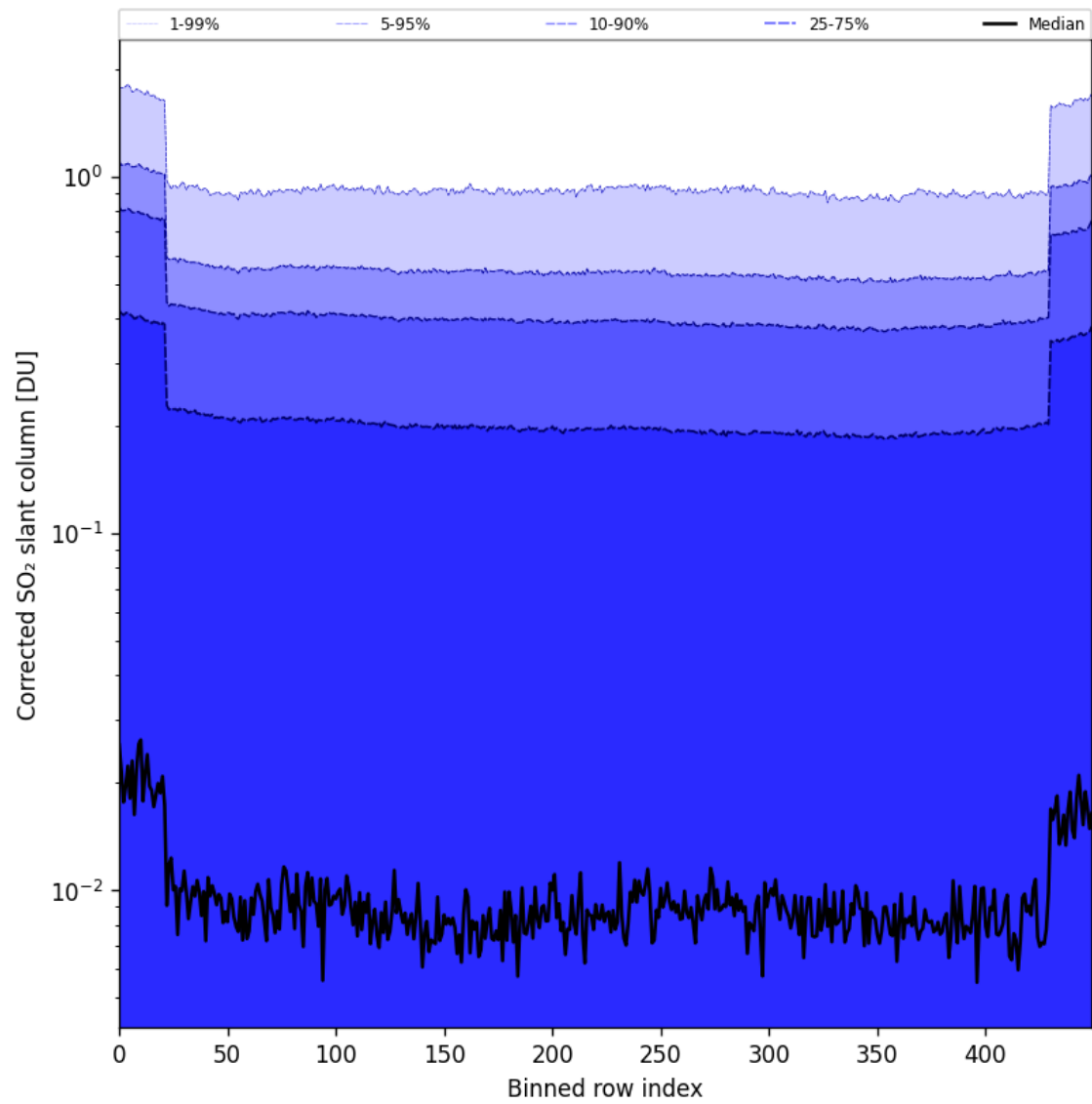
Figure 86: Along track statistics of “Corrected SO 2 slant column” for 2025-10-11 to 2025-10-13
