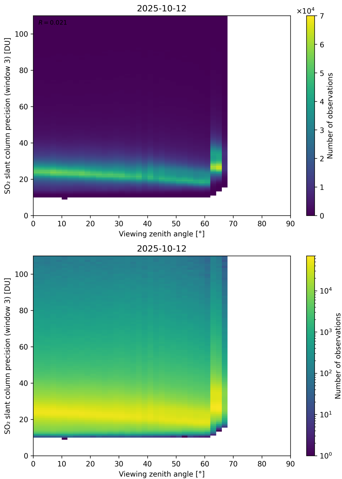
Figure 380: Scatter density plot of “Viewing zenith angle” against “SO 2 slant column precision (window 3)” for 2025-10-11 to 2025-10-13.
