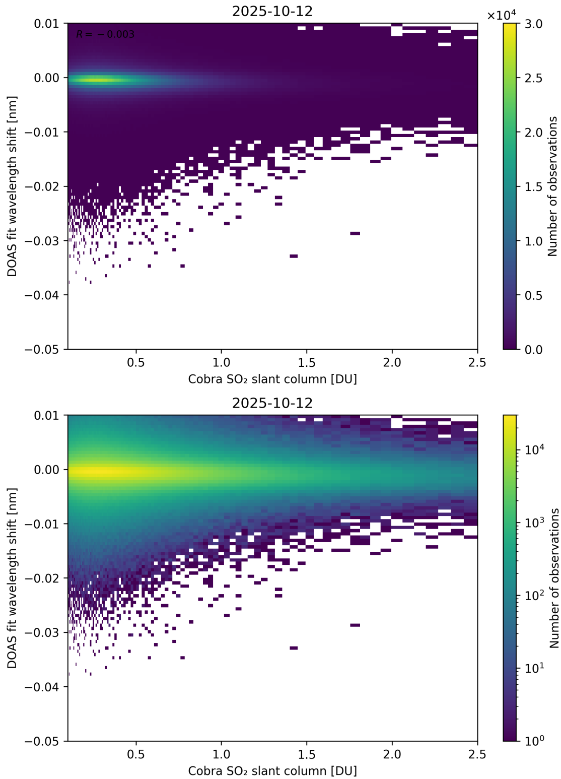
Figure 196: Scatter density plot of “Cobra SO 2 slant column” against “DOAS fit wavelength shift” for 2025-10-11 to 2025-10-13.
