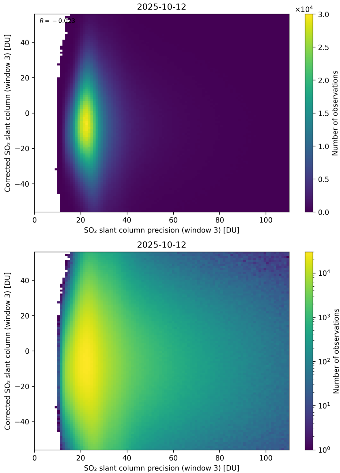
Figure 312: Scatter density plot of “SO 2 slant column precision (window 3)” against “Corrected SO 2 slant column (window 3)” for 2025-10-11 to 2025-10-13.
