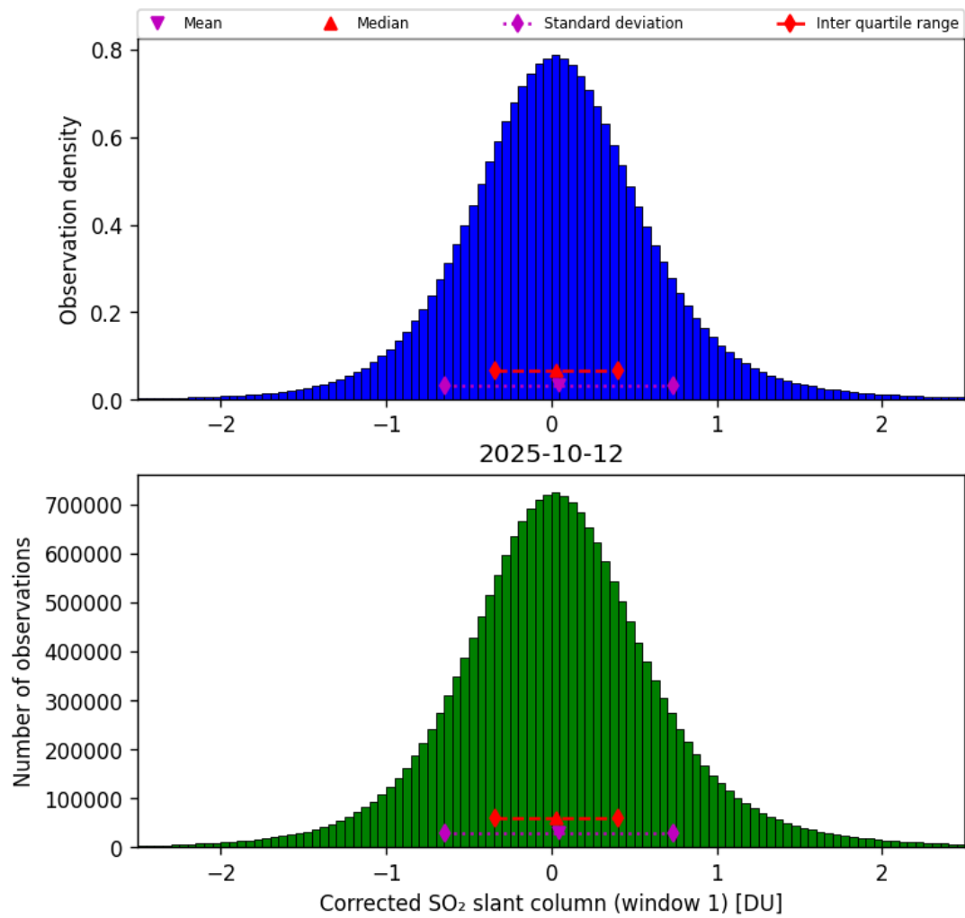
Figure 65: Histogram of “Corrected SO 2 slant column (window 1)” for 2025-10-11 to 2025-10-13
