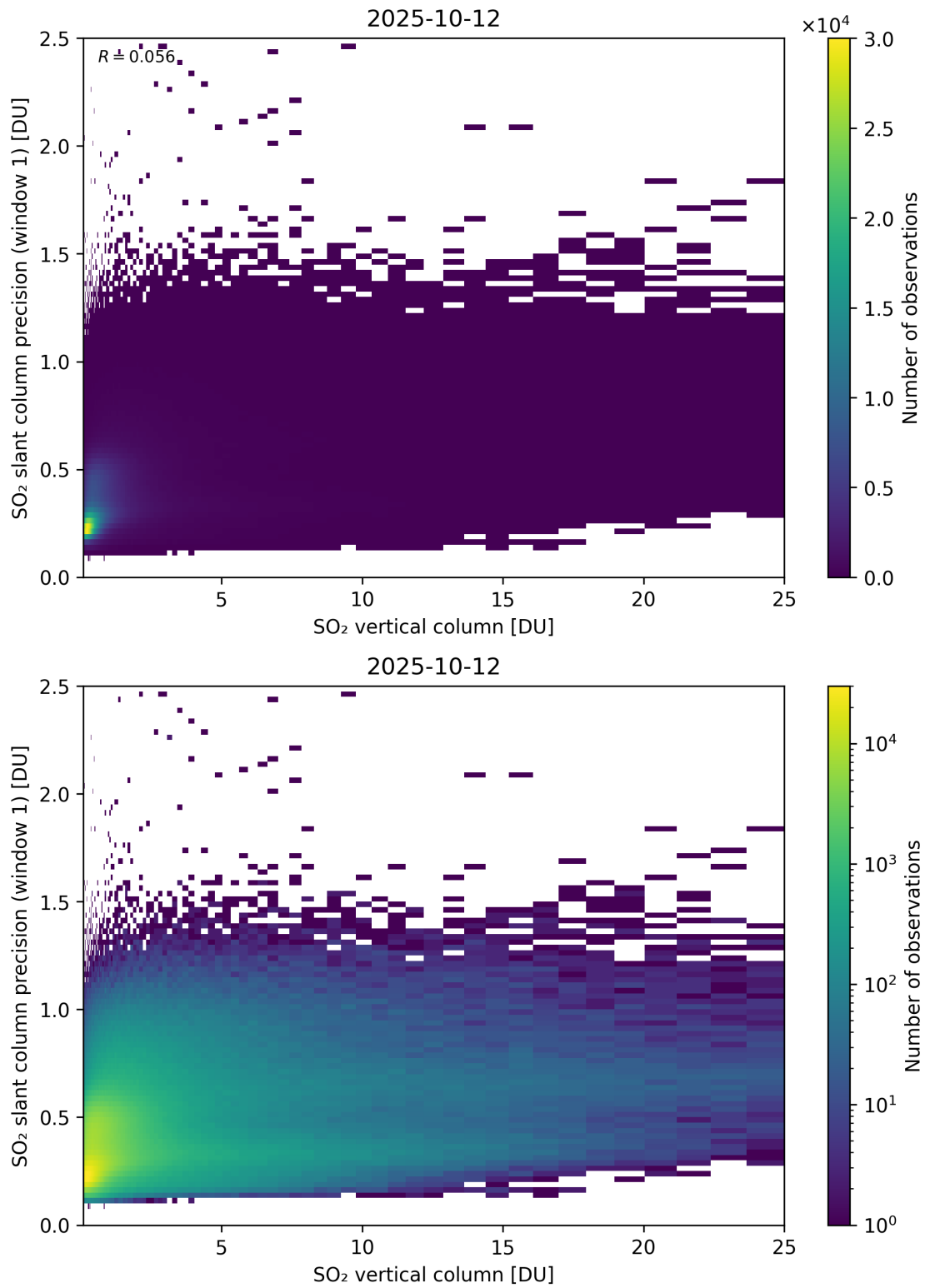
Figure 355: Scatter density plot of “SO 2 vertical column” against “SO 2 slant column precision (window 1)” for 2025-10-11 to 2025-10-13.
