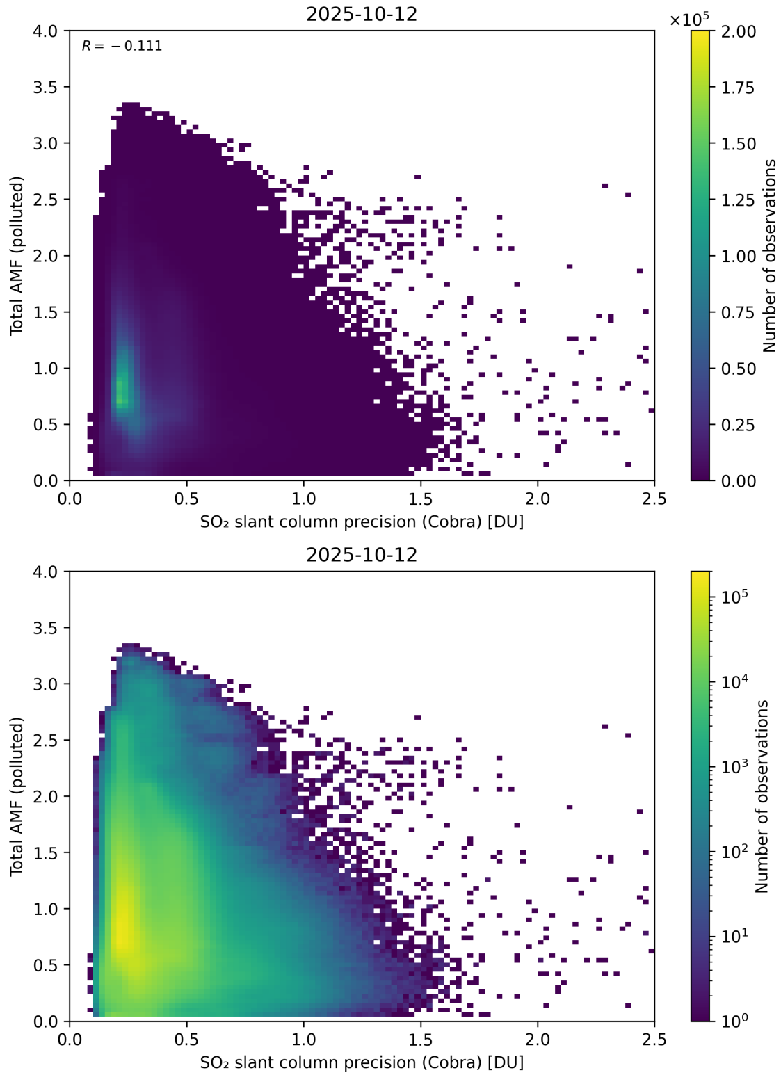
Figure 213: Scatter density plot of “SO 2 slant column precision (Cobra)” against “Total AMF (polluted)” for 2025-10-11 to 2025-10-13.
