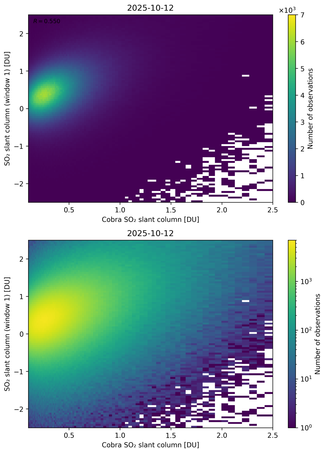
Figure 219: Scatter density plot of “Cobra SO 2 slant column” against “SO 2 slant column (window 1)” for 2025-10-11 to 2025-10-13.
