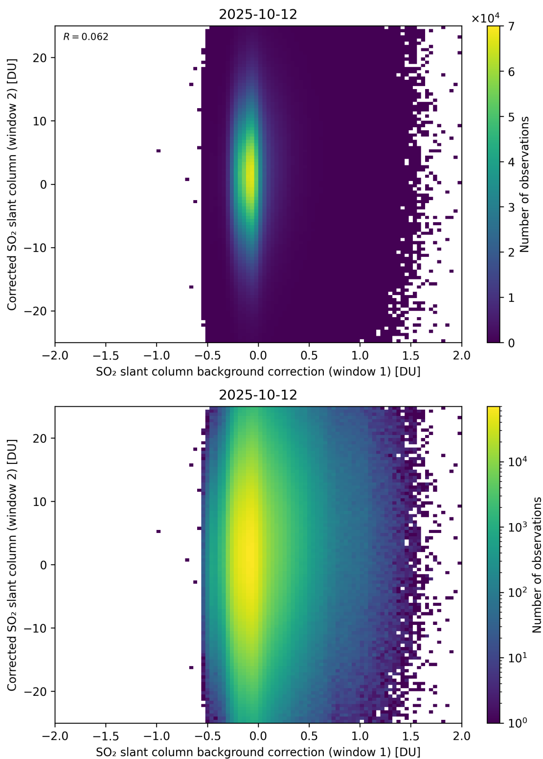
Figure 115: Scatter density plot of “SO 2 slant column background correction (window 1)” against “Corrected SO 2 slant column (window 2)” for 2025-10-11 to 2025-10-13.
