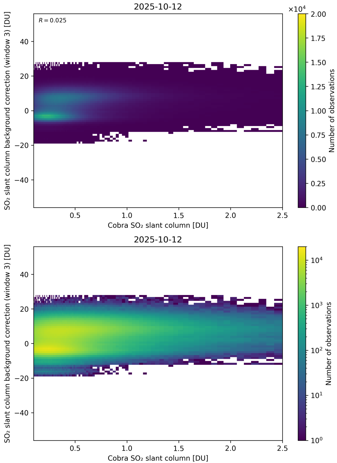
Figure 195: Scatter density plot of “Cobra SO 2 slant column” against “SO 2 slant column background correction (window 3)” for 2025-10-11 to 2025-10-13.
