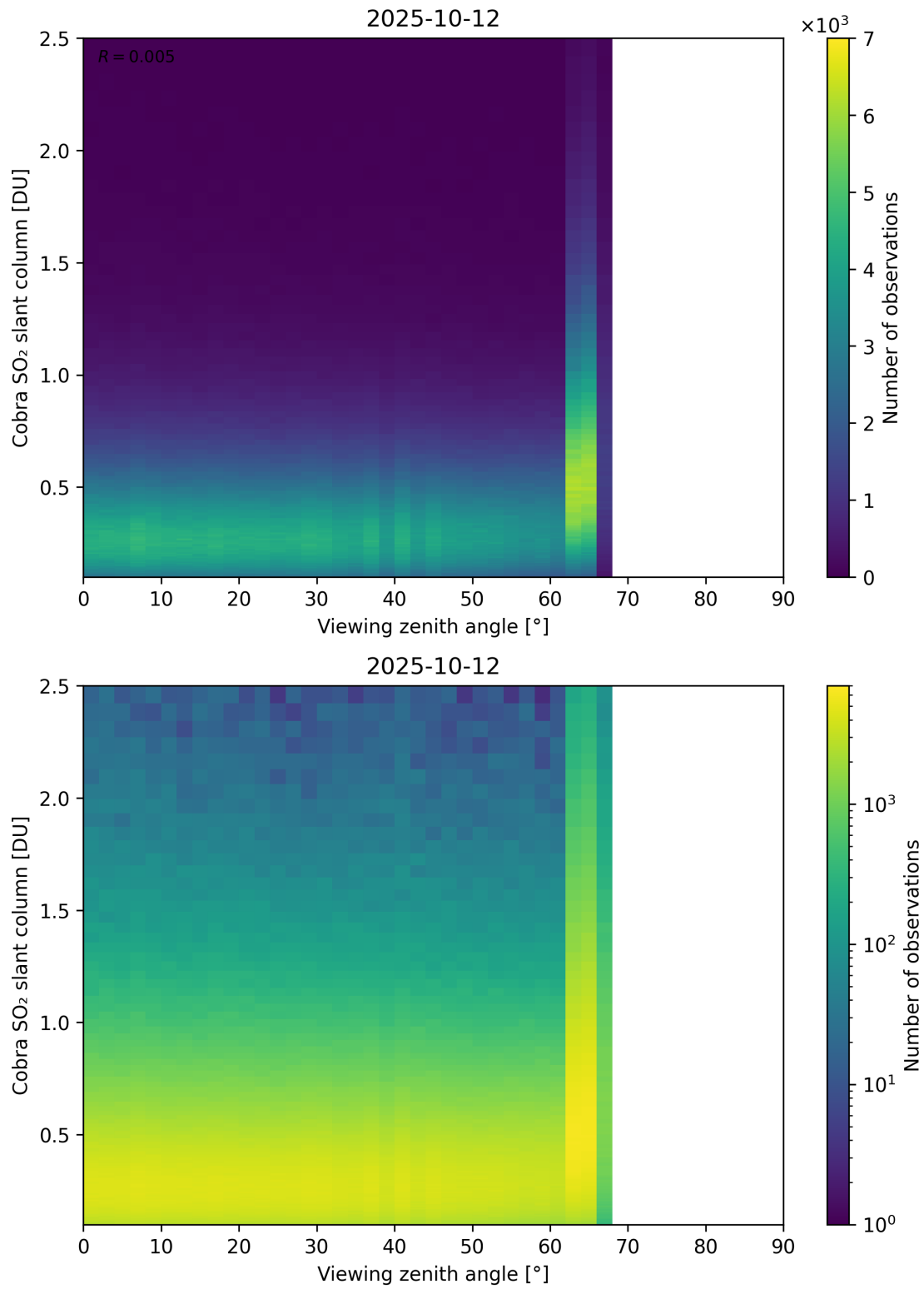
Figure 371: Scatter density plot of “Viewing zenith angle” against “Cobra SO 2 slant column” for 2025-10-11 to 2025-10-13.
