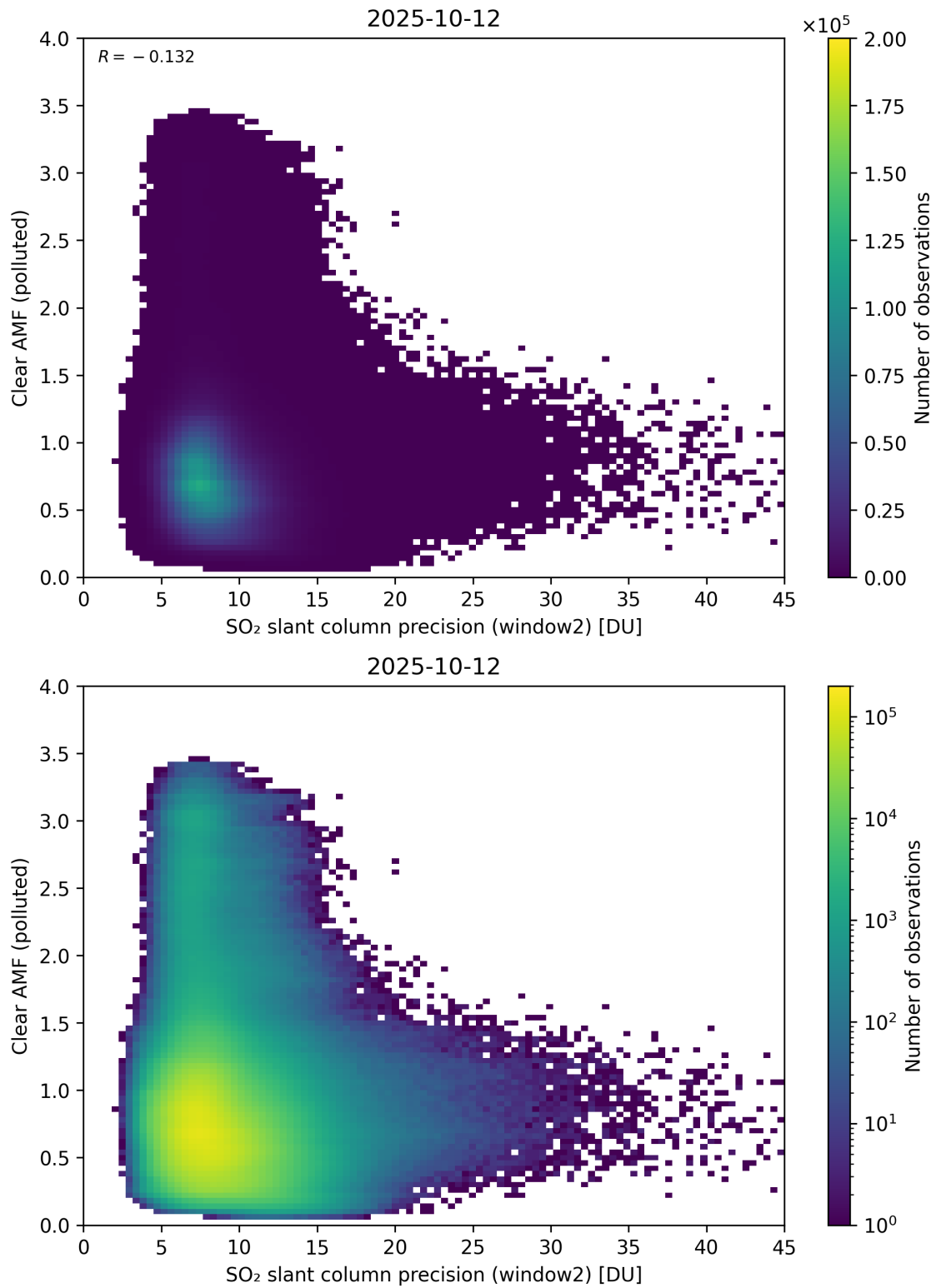
Figure 296: Scatter density plot of “SO 2 slant column precision (window2)” against “Clear AMF (polluted)” for 2025-10-11 to 2025-10-13.
