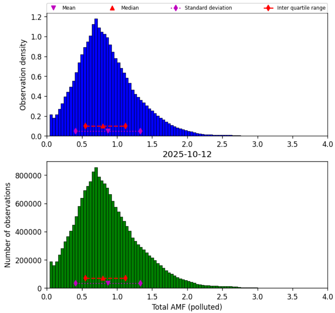
Figure 79: Histogram of “Total AMF (polluted)” for 2025-10-11 to 2025-10-13
