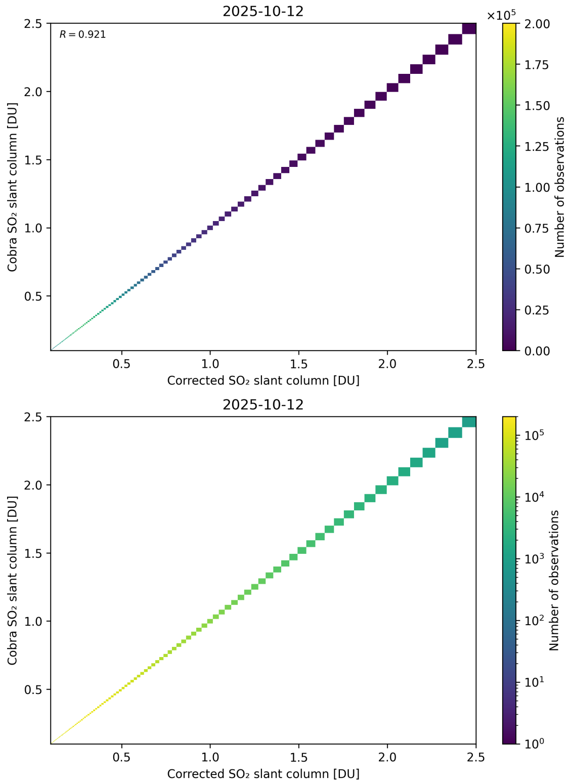
Figure 233: Scatter density plot of “Corrected SO 2 slant column” against “Cobra SO 2 slant column” for 2025-10-11 to 2025-10-13.
