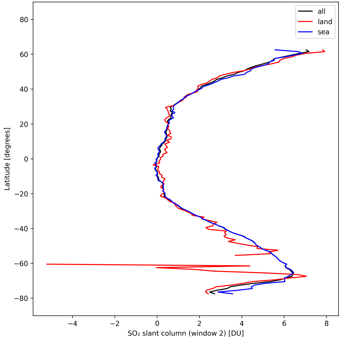
Figure 41: Zonal average of “SO 2 slant column (window 2)” for 2025-10-11 to 2025-10-13.
