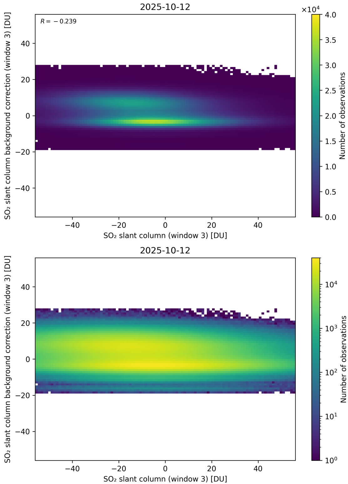
Figure 303: Scatter density plot of “SO 2 slant column (window 3)” against “SO 2 slant column background correction (window 3)” for 2025-10-11 to 2025-10-13.
