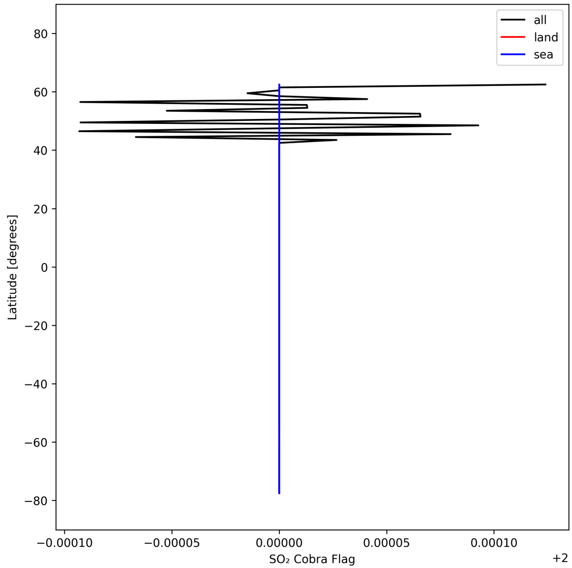
Figure 49: Zonal average of “SO 2 Cobra Flag” for 2025-10-11 to 2025-10-13.
