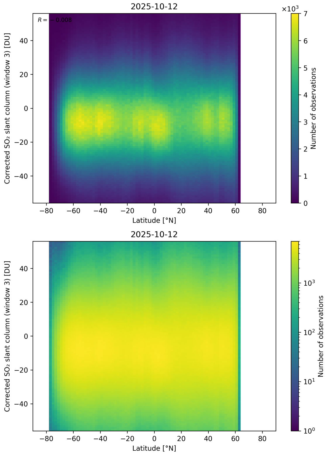
Figure 161: Scatter density plot of “Latitude” against “Corrected SO 2 slant column (window 3)” for 2025-10-11 to 2025-10-13.
