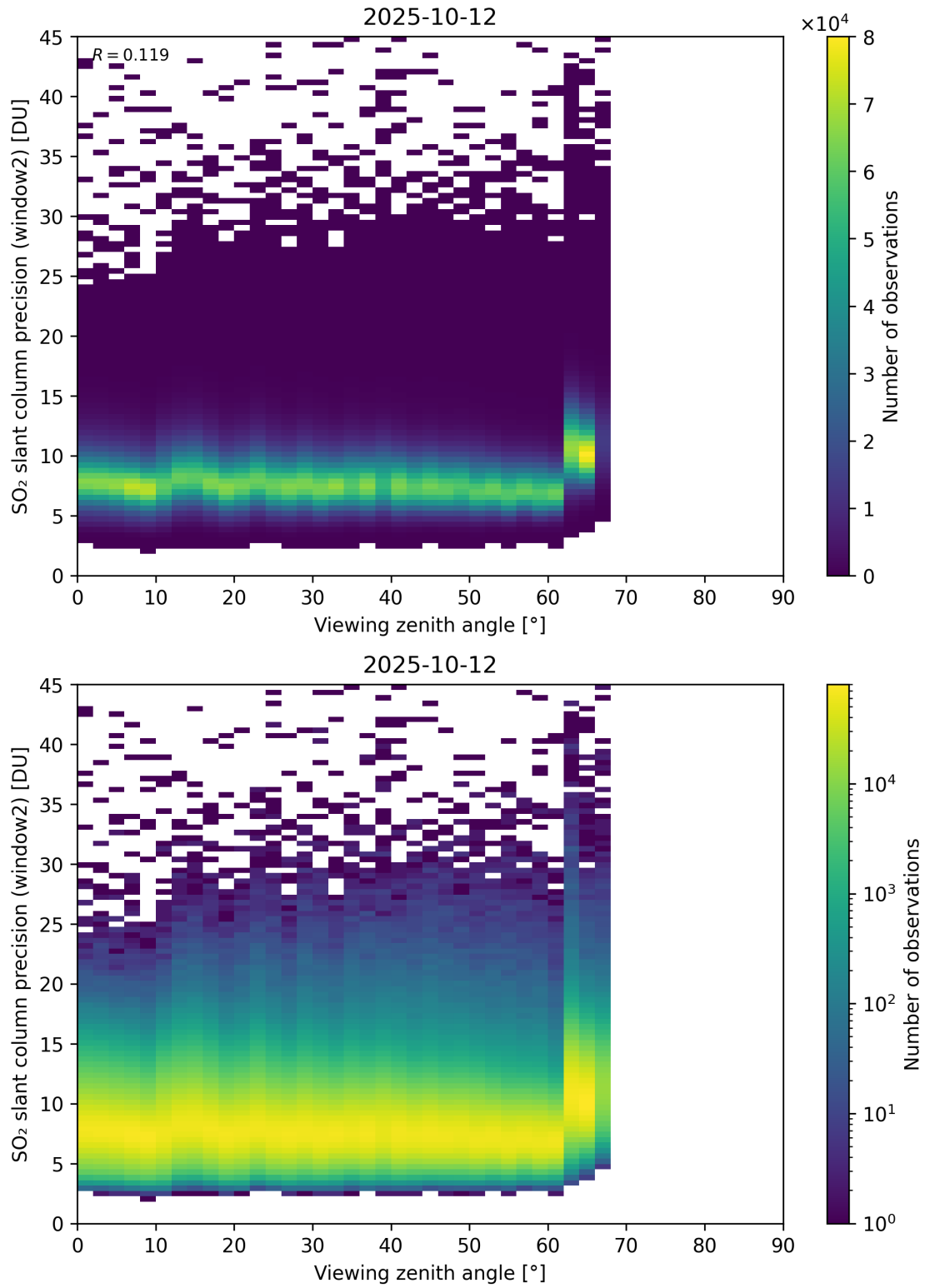
Figure 378: Scatter density plot of “Viewing zenith angle” against “SO 2 slant column precision (window2)” for 2025-10-11 to 2025-10-13.
