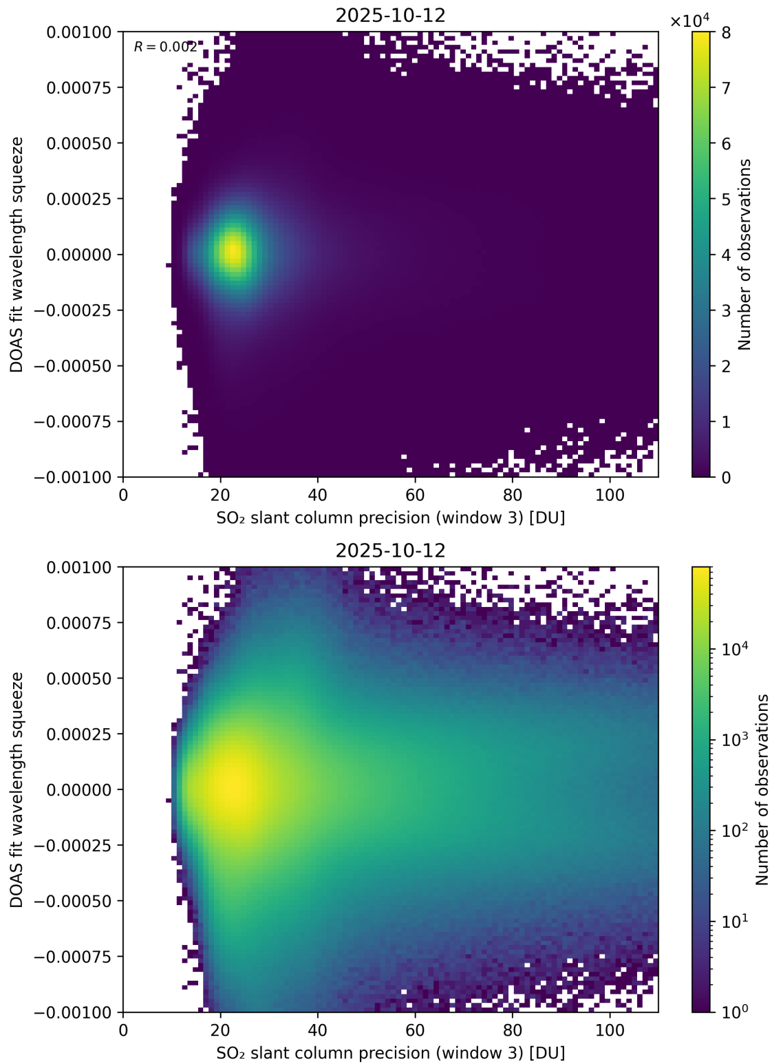
Figure 309: Scatter density plot of “SO 2 slant column precision (window 3)” against “DOAS fit wavelength squeeze” for 2025-10-11 to 2025-10-13.
