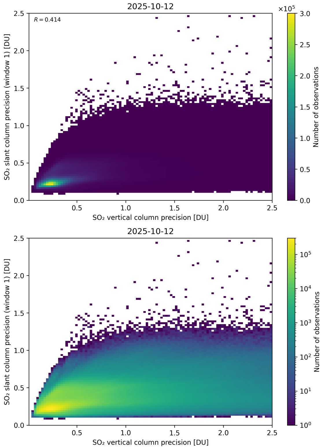
Figure 342: Scatter density plot of “SO 2 vertical column precision” against “SO 2 slant column precision (window 1)” for 2025-10-11 to 2025-10-13.
