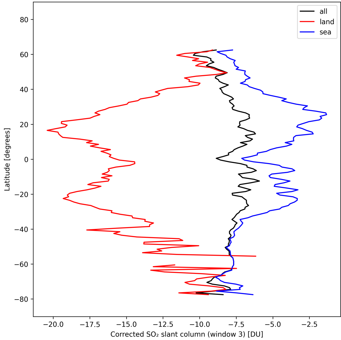
Figure 47: Zonal average of “Corrected SO 2 slant column (window 3)” for 2025-10-11 to 2025-10-13.
