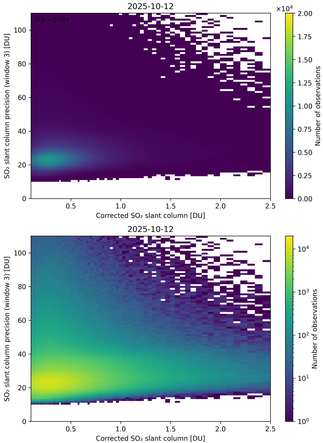
Figure 241: Scatter density plot of “Corrected SO 2 slant column” against “SO 2 slant column precision (window 3)” for 2025-10-11 to 2025-10-13.
