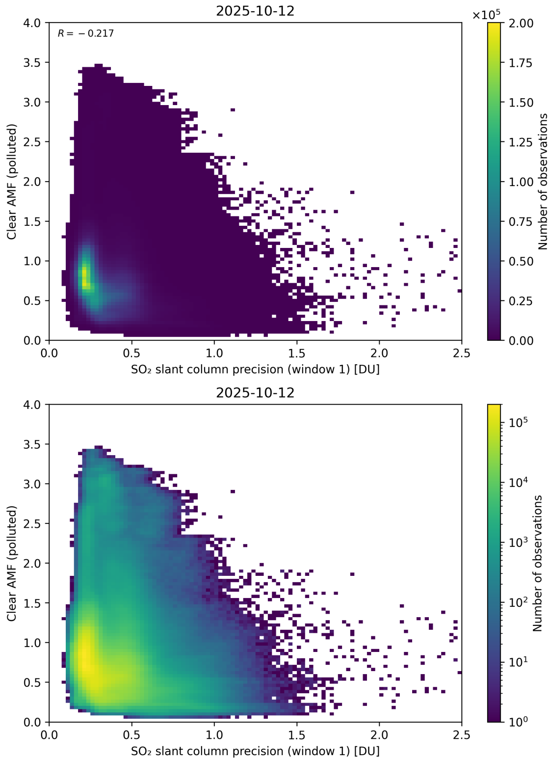
Figure 274: Scatter density plot of “SO 2 slant column precision (window 1)” against “Clear AMF (polluted)” for 2025-10-11 to 2025-10-13.
