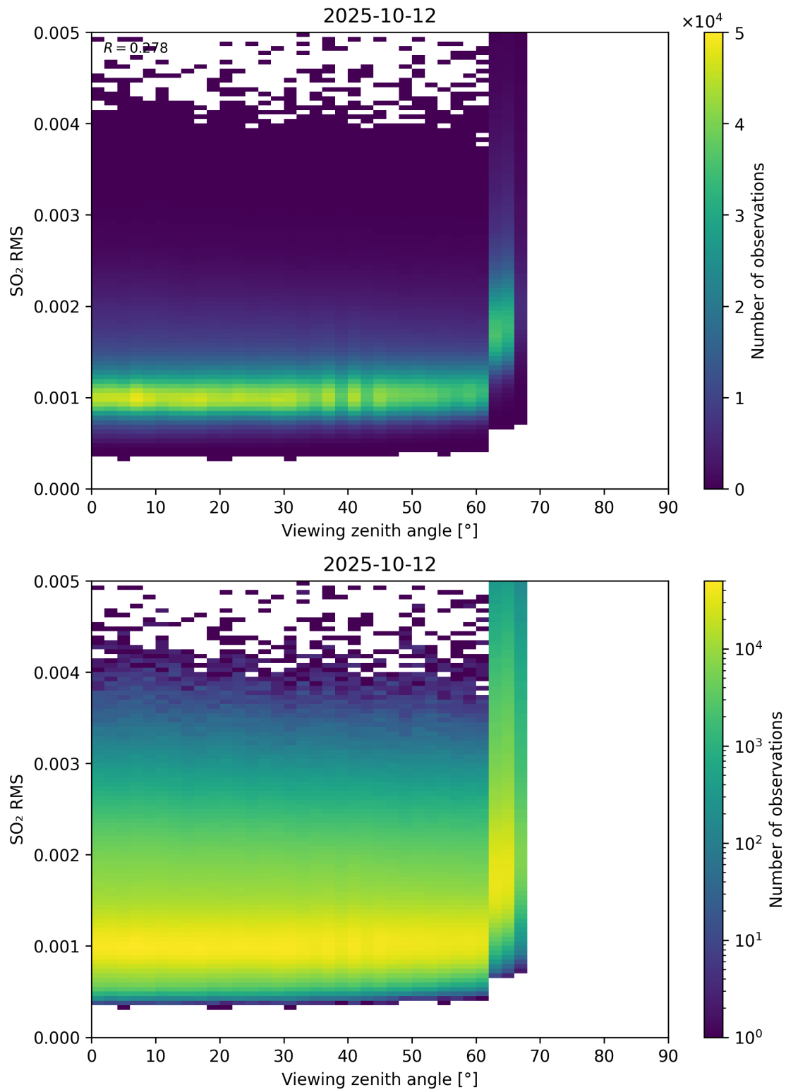
Figure 367: Scatter density plot of “Viewing zenith angle” against “SO 2 RMS” for 2025-10-11 to 2025-10-13.
