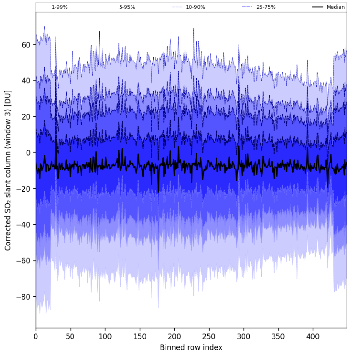
Figure 99: Along track statistics of “Corrected SO 2 slant column (window 3)” for 2025-10-11 to 2025-10-13
