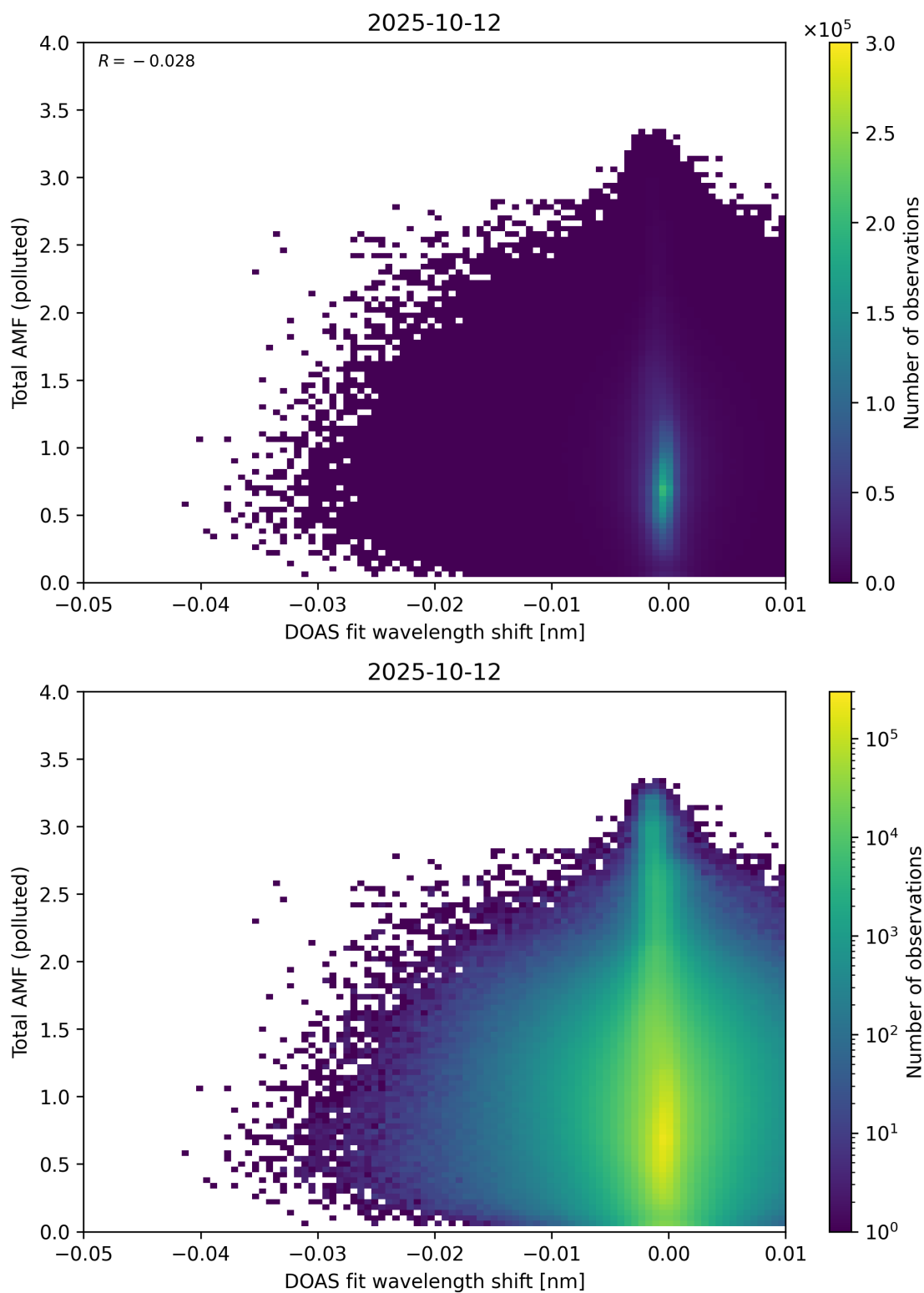
Figure 141: Scatter density plot of “DOAS fit wavelength shift” against “Total AMF (polluted)” for 2025-10-11 to 2025-10-13.
