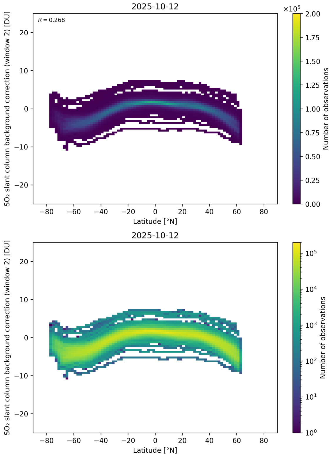
Figure 151: Scatter density plot of “Latitude” against “SO 2 slant column background correction (window 2)” for 2025-10-11 to 2025-10-13.
