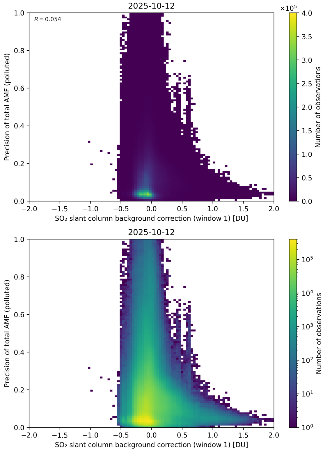
Figure 121: Scatter density plot of “SO 2 slant column background correction (window 1)” against “Precision of total AMF (polluted)” for 2025-10-11 to 2025-10-13.
