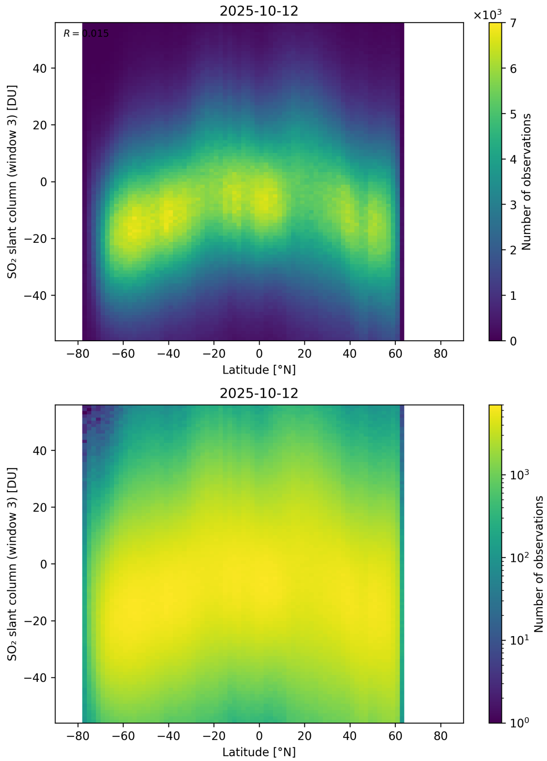
Figure 165: Scatter density plot of “Latitude” against “SO 2 slant column (window 3)” for 2025-10-11 to 2025-10-13.
