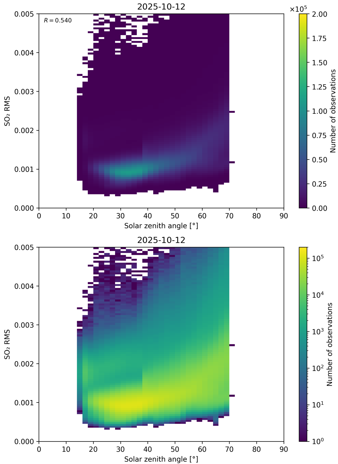
Figure 176: Scatter density plot of “Solar zenith angle” against “SO 2 RMS” for 2025-10-11 to 2025-10-13.
