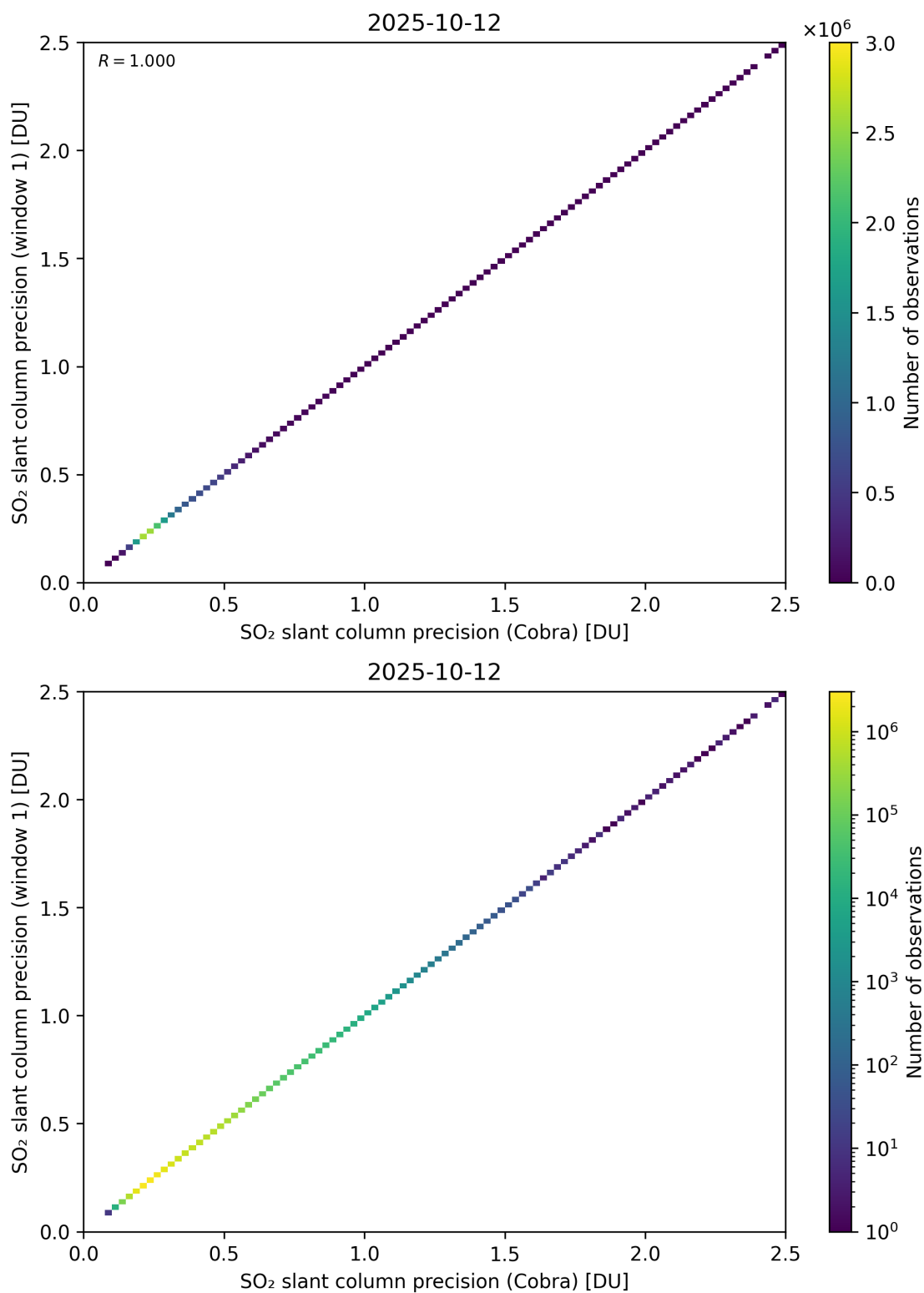
Figure 209: Scatter density plot of “SO 2 slant column precision (Cobra)” against “SO 2 slant column precision (window 1)” for 2025-10-11 to 2025-10-13.
