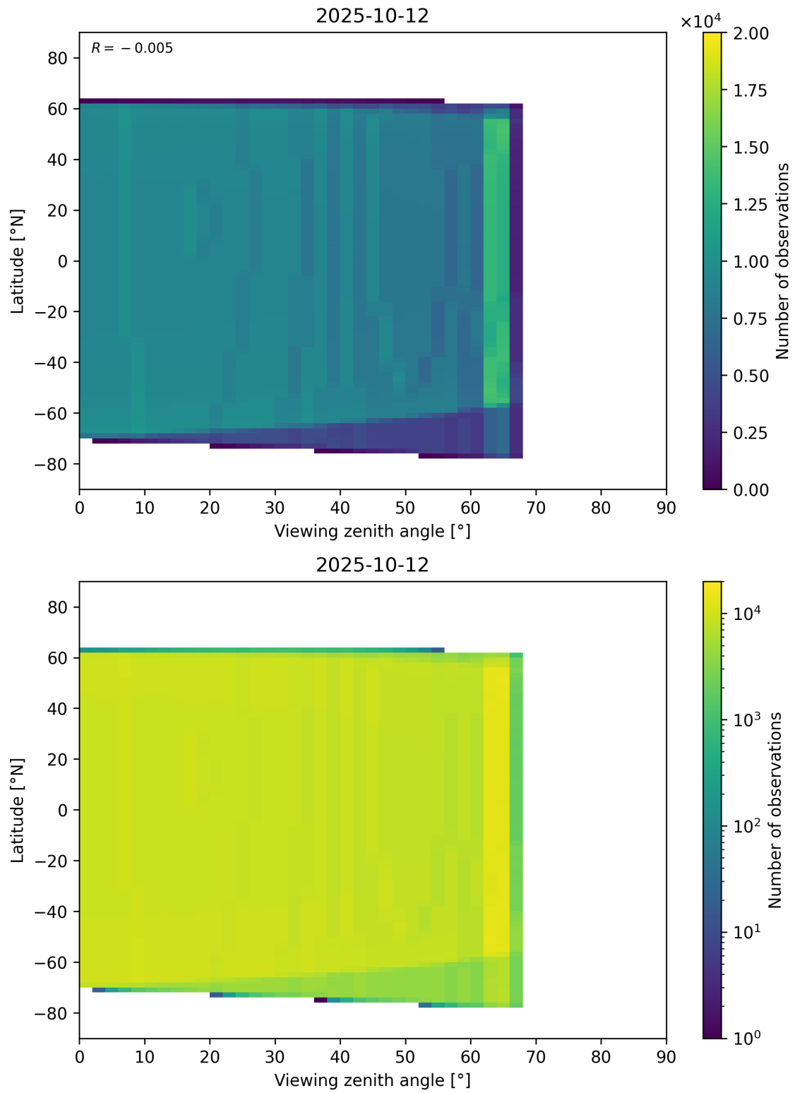
Figure 368: Scatter density plot of “Viewing zenith angle” against “Latitude” for 2025-10-11 to 2025-10-13.
