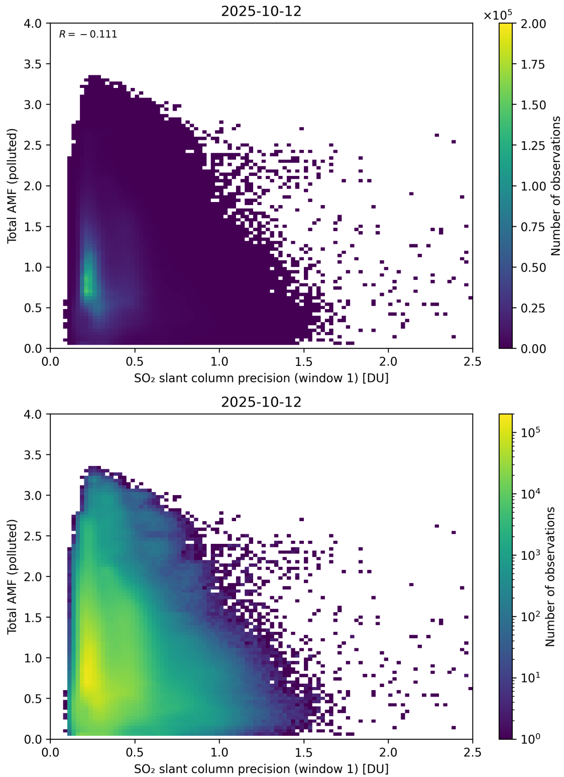
Figure 280: Scatter density plot of “SO 2 slant column precision (window 1)” against “Total AMF (polluted)” for 2025-10-11 to 2025-10-13.
