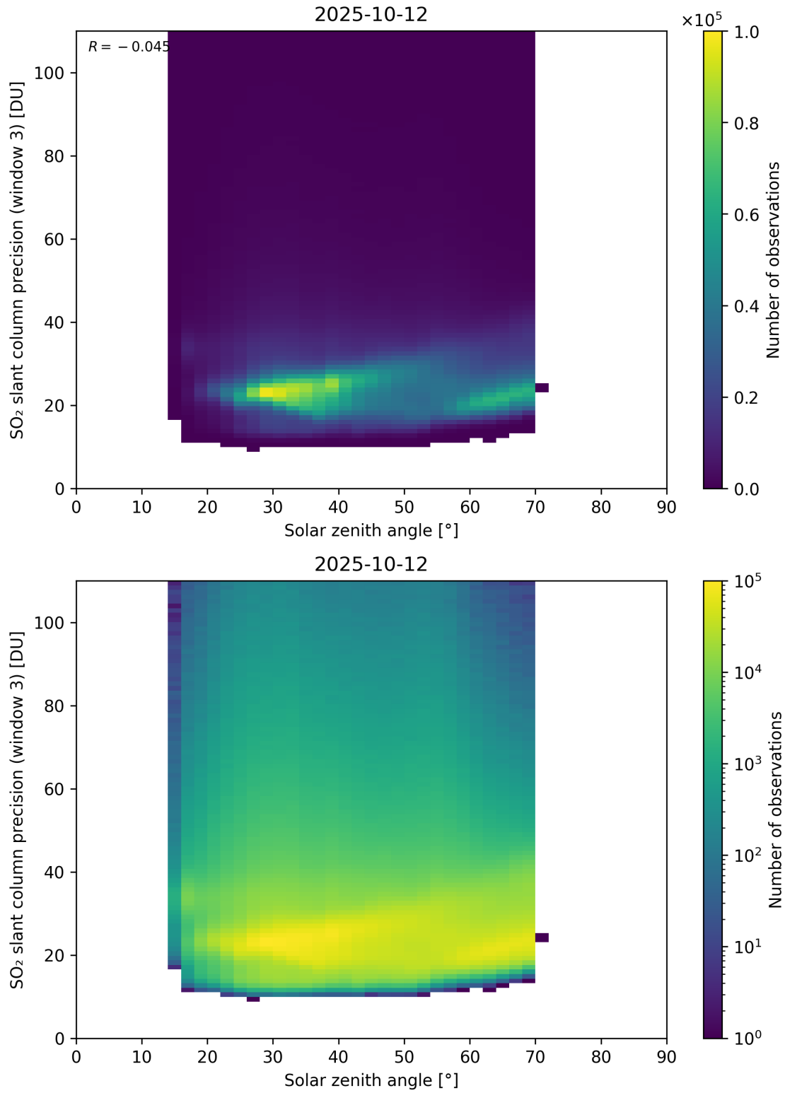
Figure 188: Scatter density plot of “Solar zenith angle” against “SO 2 slant column precision (window 3)” for 2025-10-11 to 2025-10-13.
