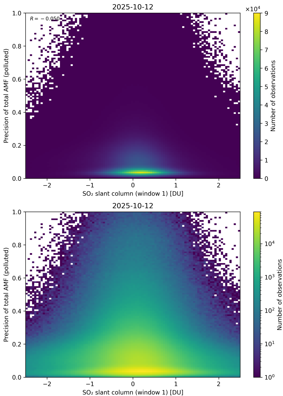
Figure 290: Scatter density plot of “SO 2 slant column (window 1)” against “Precision of total AMF (polluted)” for 2025-10-11 to 2025-10-13.
