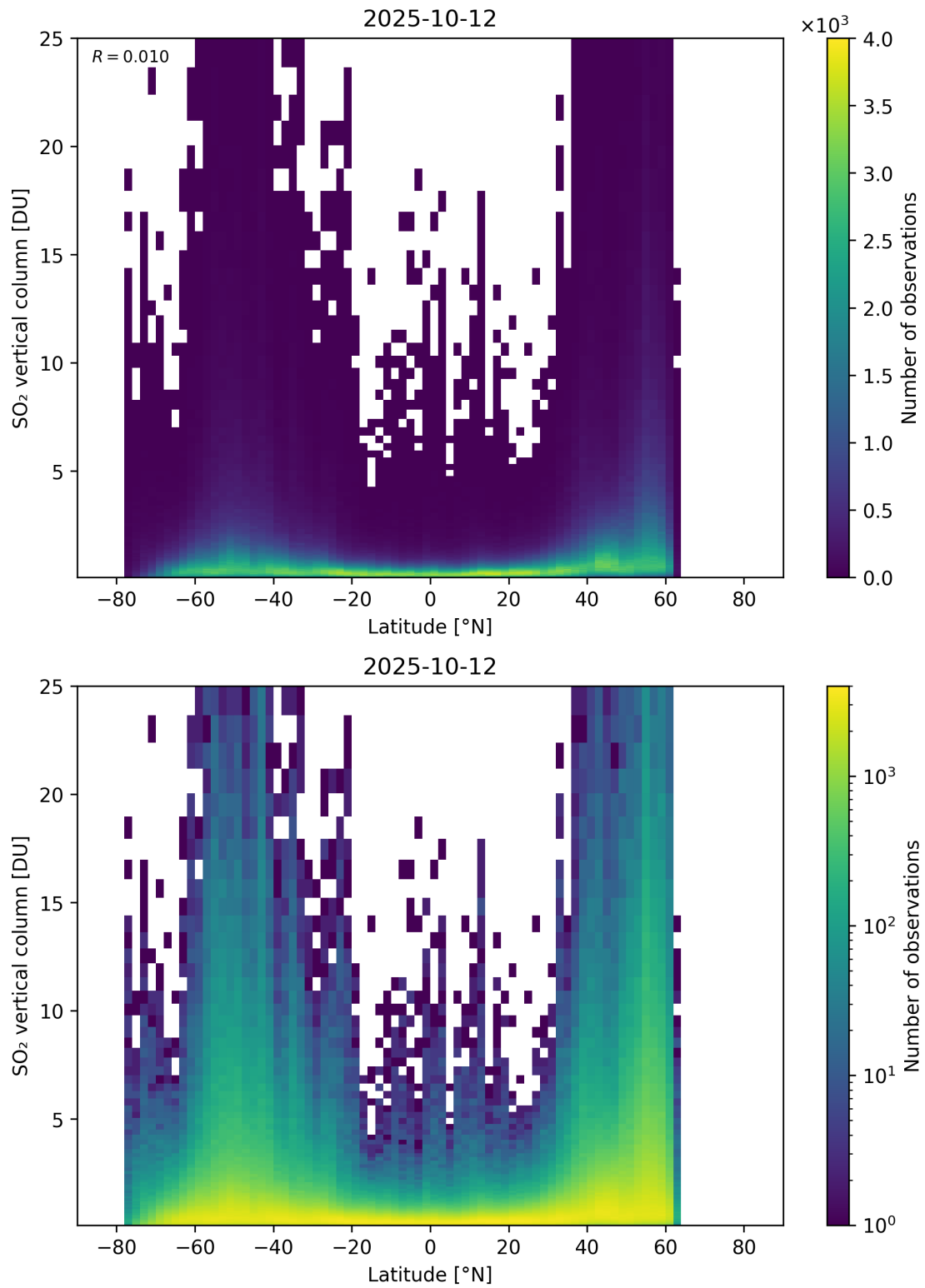
Figure 169: Scatter density plot of “Latitude” against “SO 2 vertical column” for 2025-10-11 to 2025-10-13.
