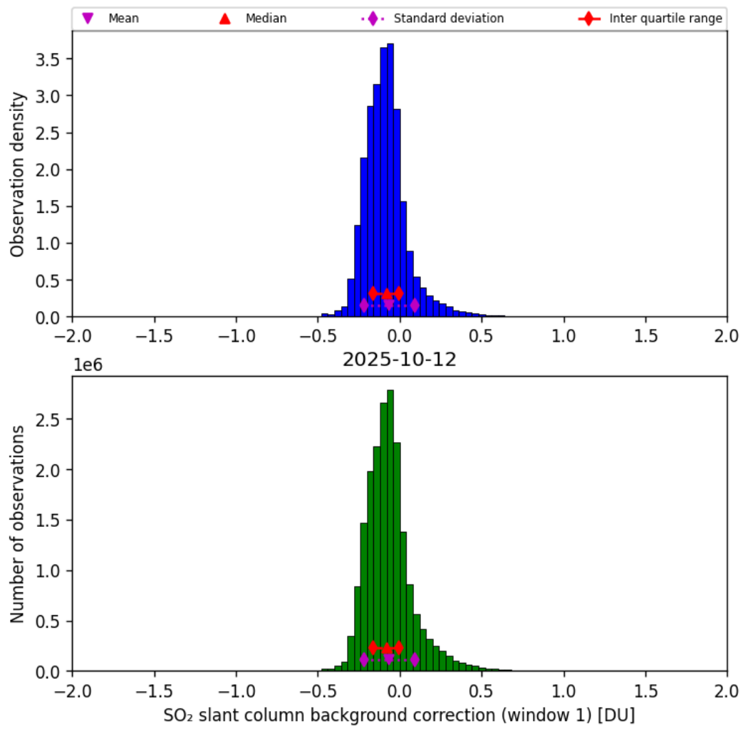
Figure 66: Histogram of “SO 2 slant column background correction (window 1)” for 2025-10-11 to 2025-10-13
