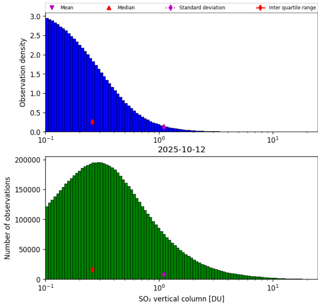
Figure 58: Histogram of “SO 2 vertical column” for 2025-10-11 to 2025-10-13
