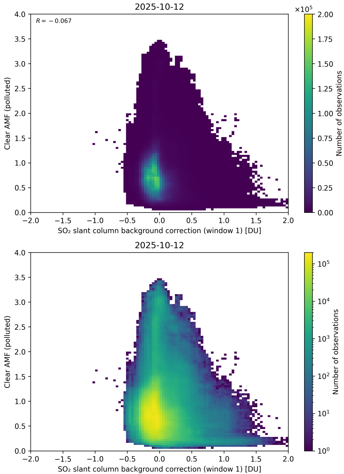
Figure 114: Scatter density plot of “SO 2 slant column background correction (window 1)” against “Clear AMF (polluted)” for 2025-10-11 to 2025-10-13.
