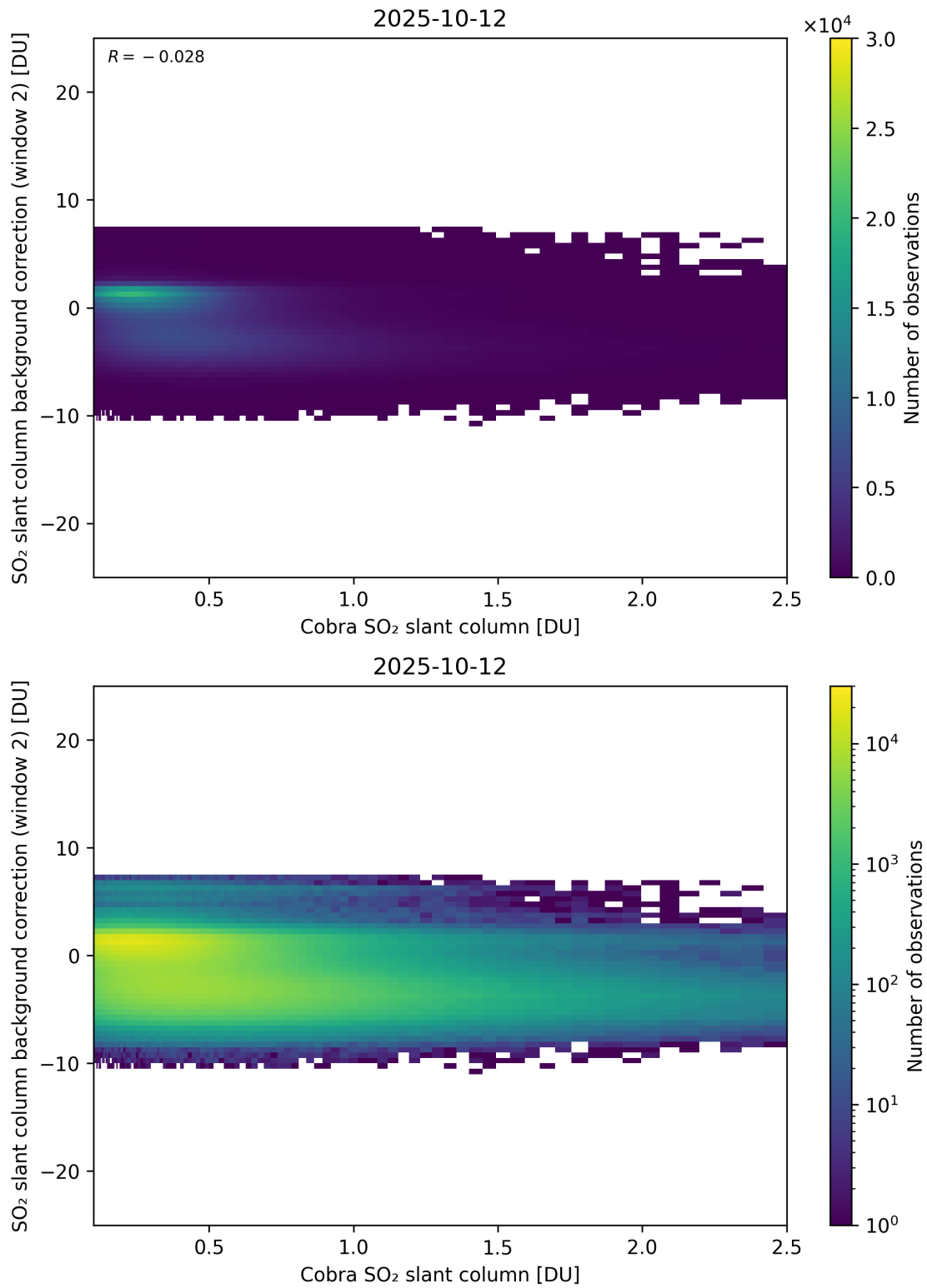
Figure 194: Scatter density plot of “Cobra SO 2 slant column” against “SO 2 slant column background correction (window 2)” for 2025-10-11 to 2025-10-13.
