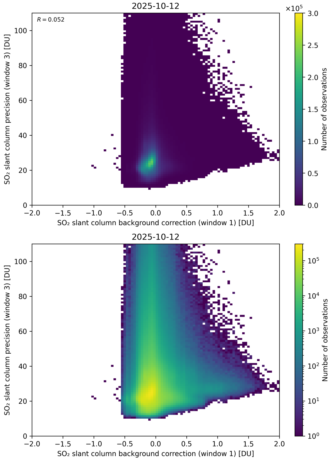
Figure 119: Scatter density plot of “SO 2 slant column background correction (window 1)” against “SO 2 slant column precision (window 3)” for 2025-10-11 to 2025-10-13.
