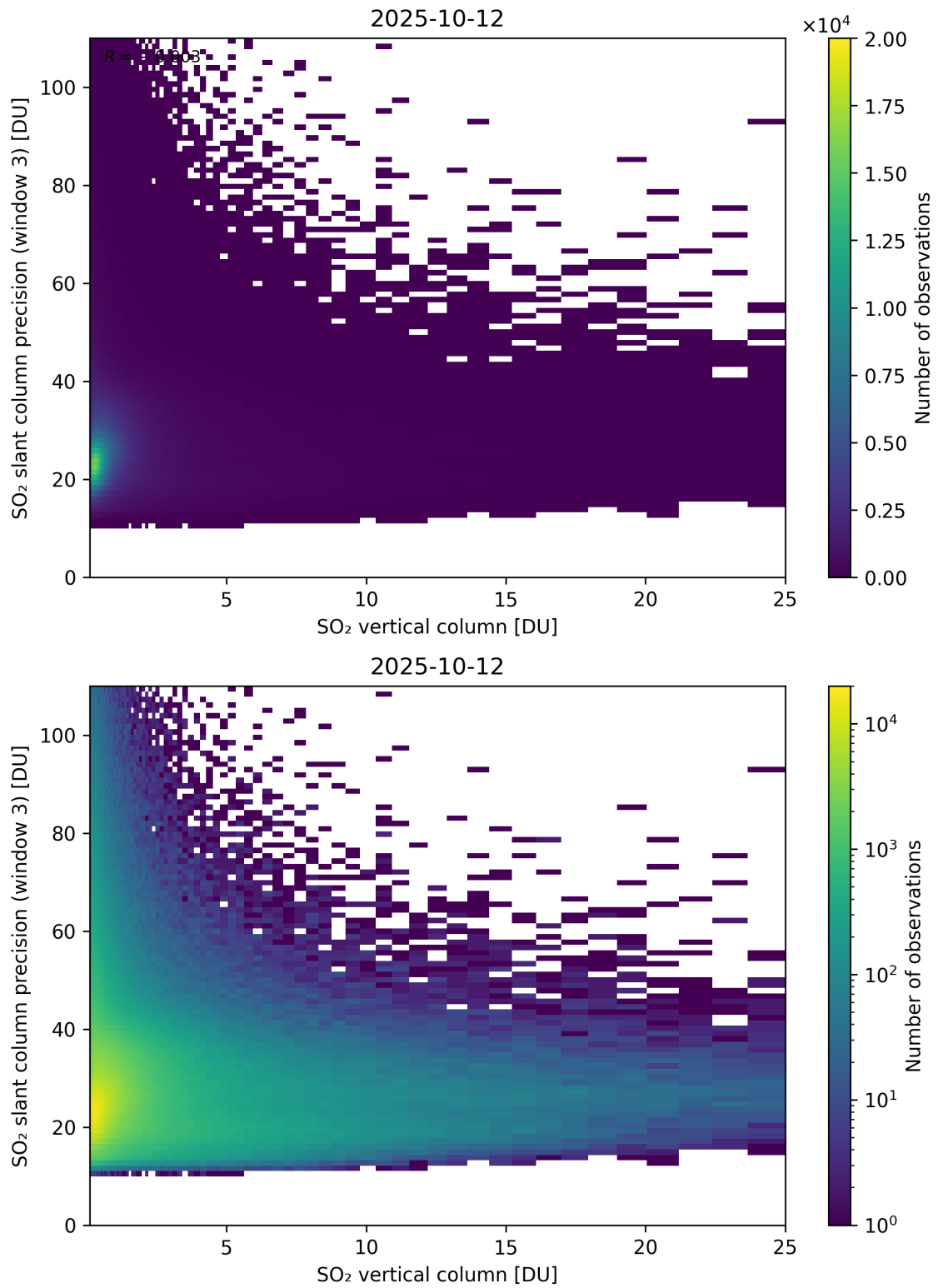
Figure 358: Scatter density plot of “SO 2 vertical column” against “SO 2 slant column precision (window 3)” for 2025-10-11 to 2025-10-13.
