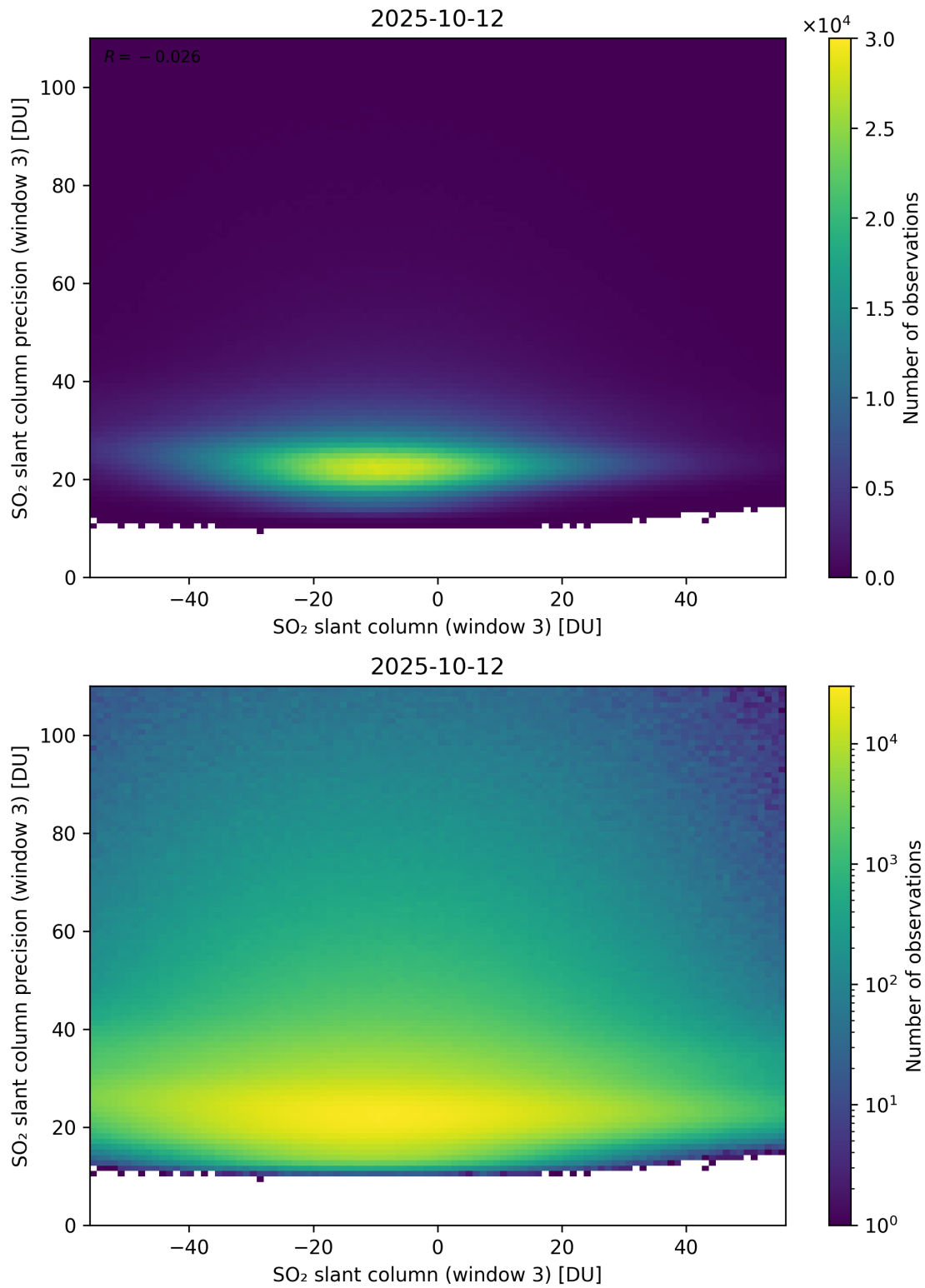
Figure 317: Scatter density plot of “SO 2 slant column (window 3)” against “SO 2 slant column precision (window 3)” for 2025-10-11 to 2025-10-13.
