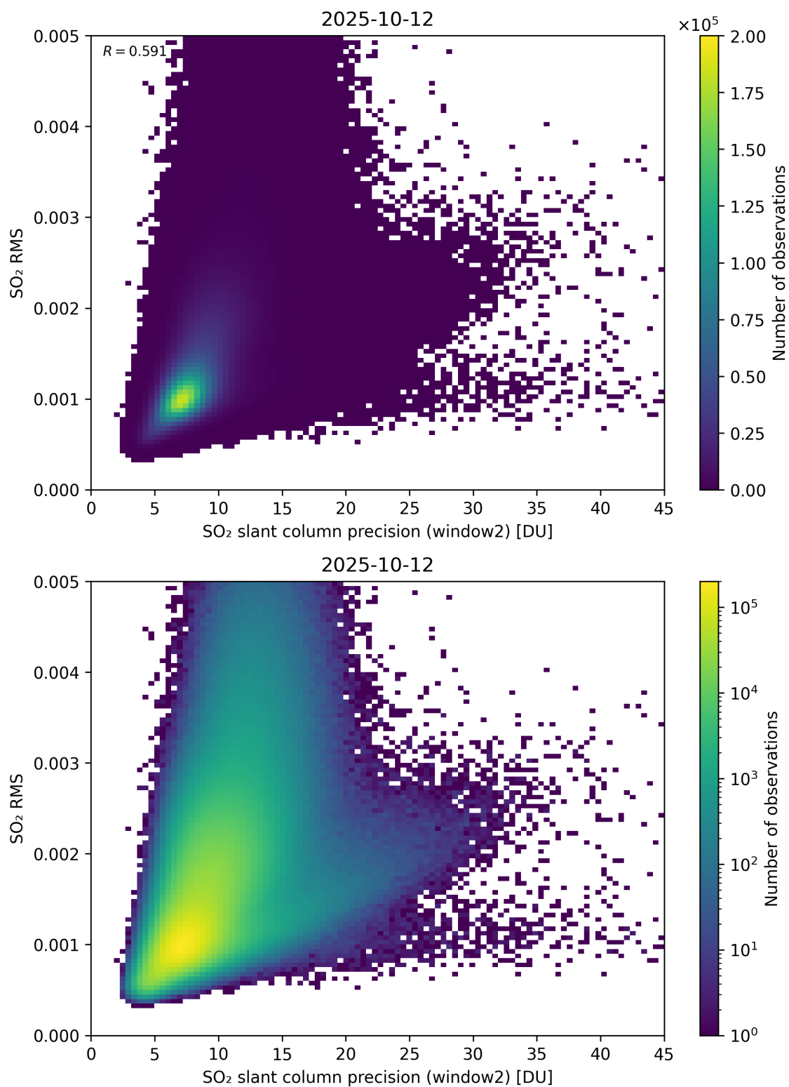
Figure 295: Scatter density plot of “SO 2 slant column precision (window2)” against “SO 2 RMS” for 2025-10-11 to 2025-10-13.
