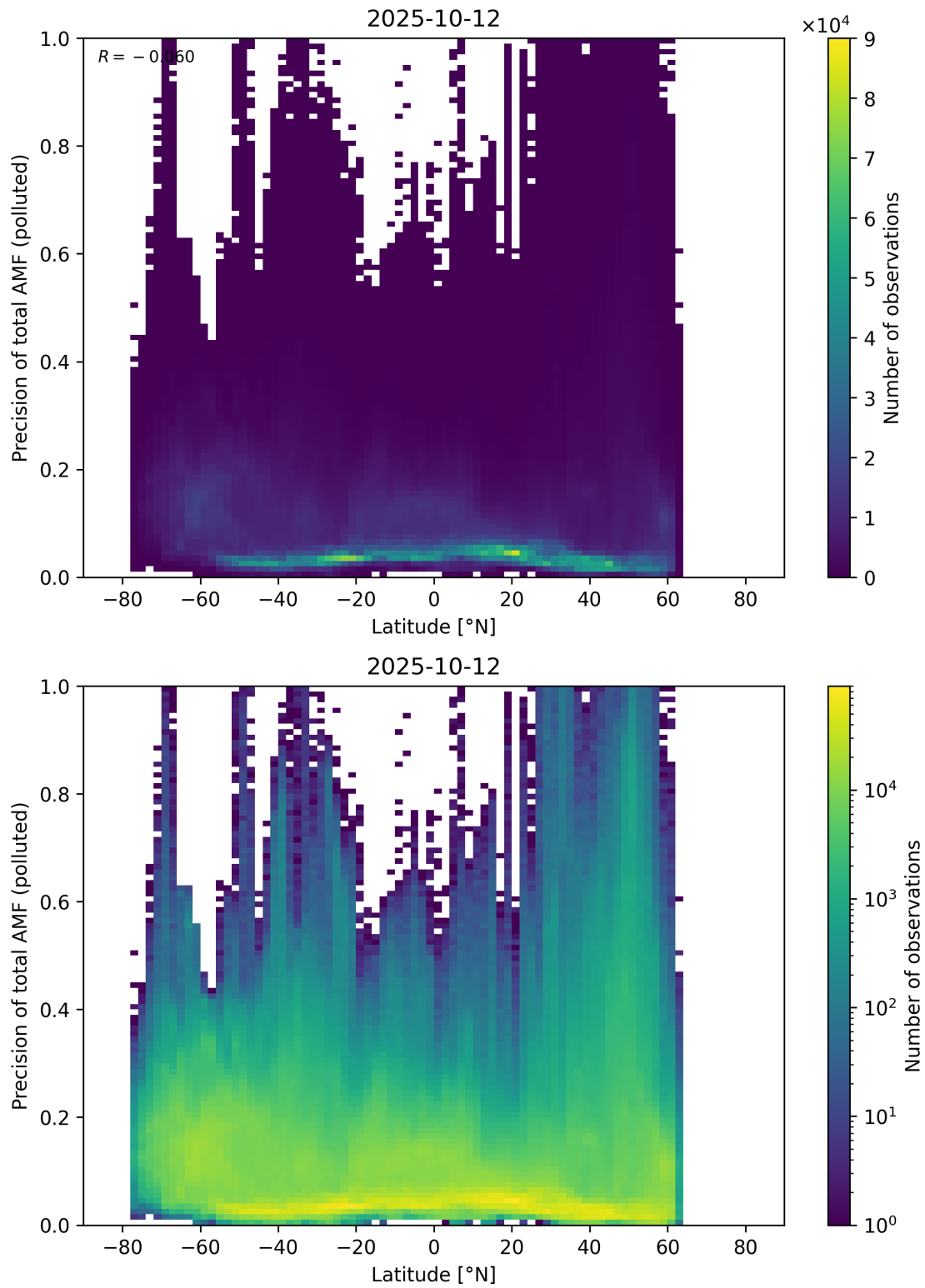
Figure 168: Scatter density plot of “Latitude” against “Precision of total AMF (polluted)” for 2025-10-11 to 2025-10-13.
