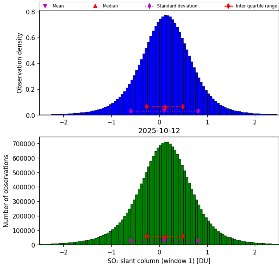
Figure 63: Histogram of “SO 2 slant column (window 1)” for 2025-10-11 to 2025-10-13
