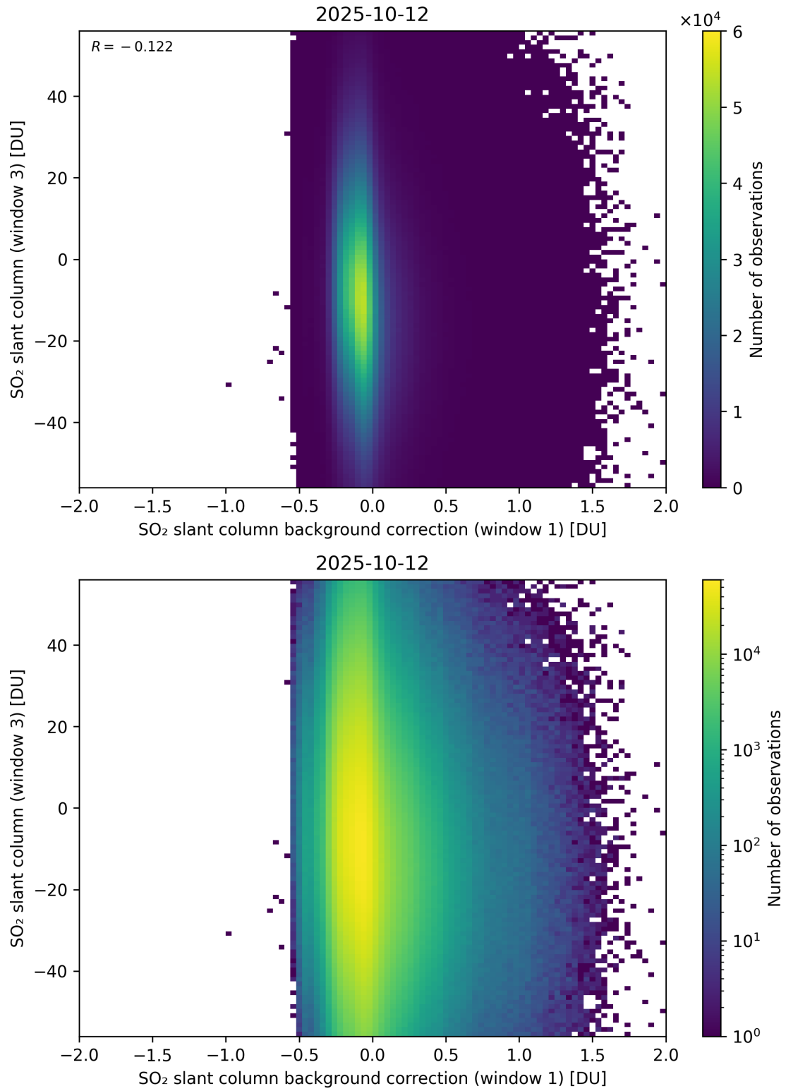
Figure 118: Scatter density plot of “SO 2 slant column background correction (window 1)” against “SO 2 slant column (window 3)” for 2025-10-11 to 2025-10-13.
