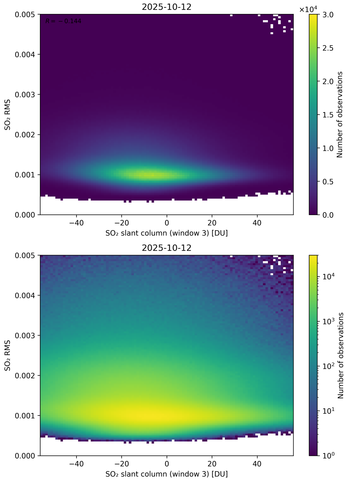
Figure 306: Scatter density plot of “SO 2 slant column (window 3)” against “SO 2 RMS” for 2025-10-11 to 2025-10-13.
