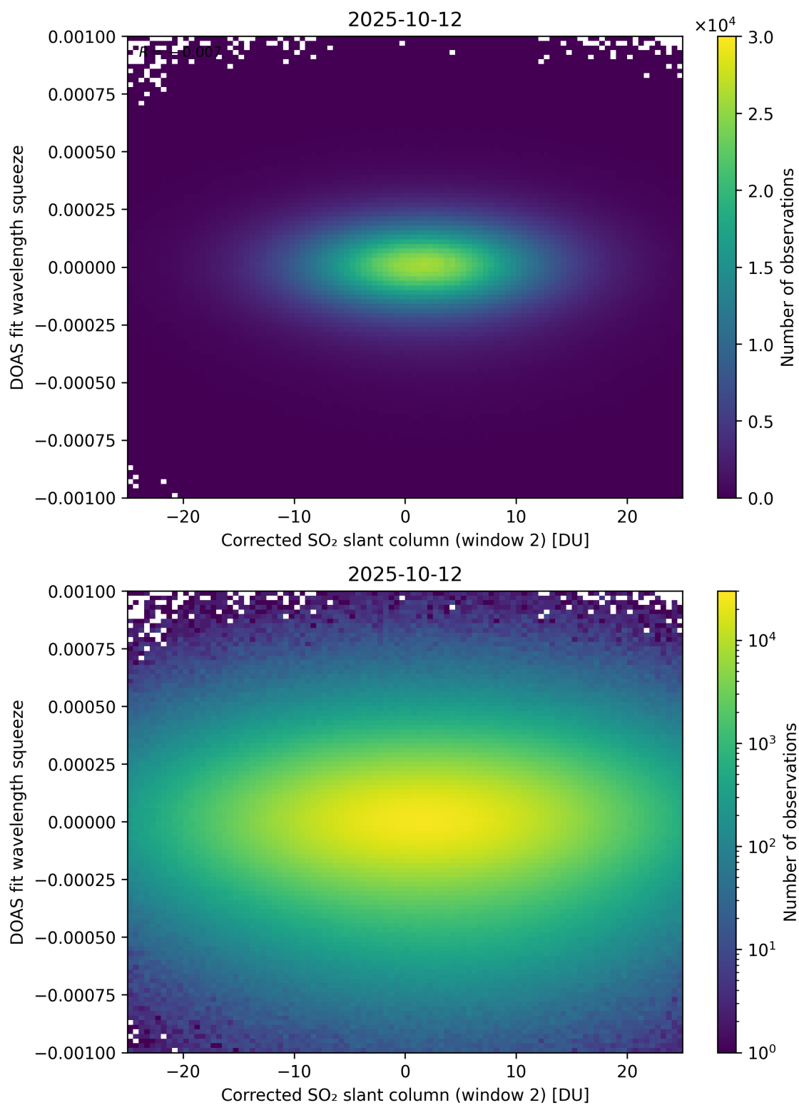
Figure 247: Scatter density plot of “Corrected SO 2 slant column (window 2)” against “DOAS fit wavelength squeeze” for 2025-10-11 to 2025-10-13.
