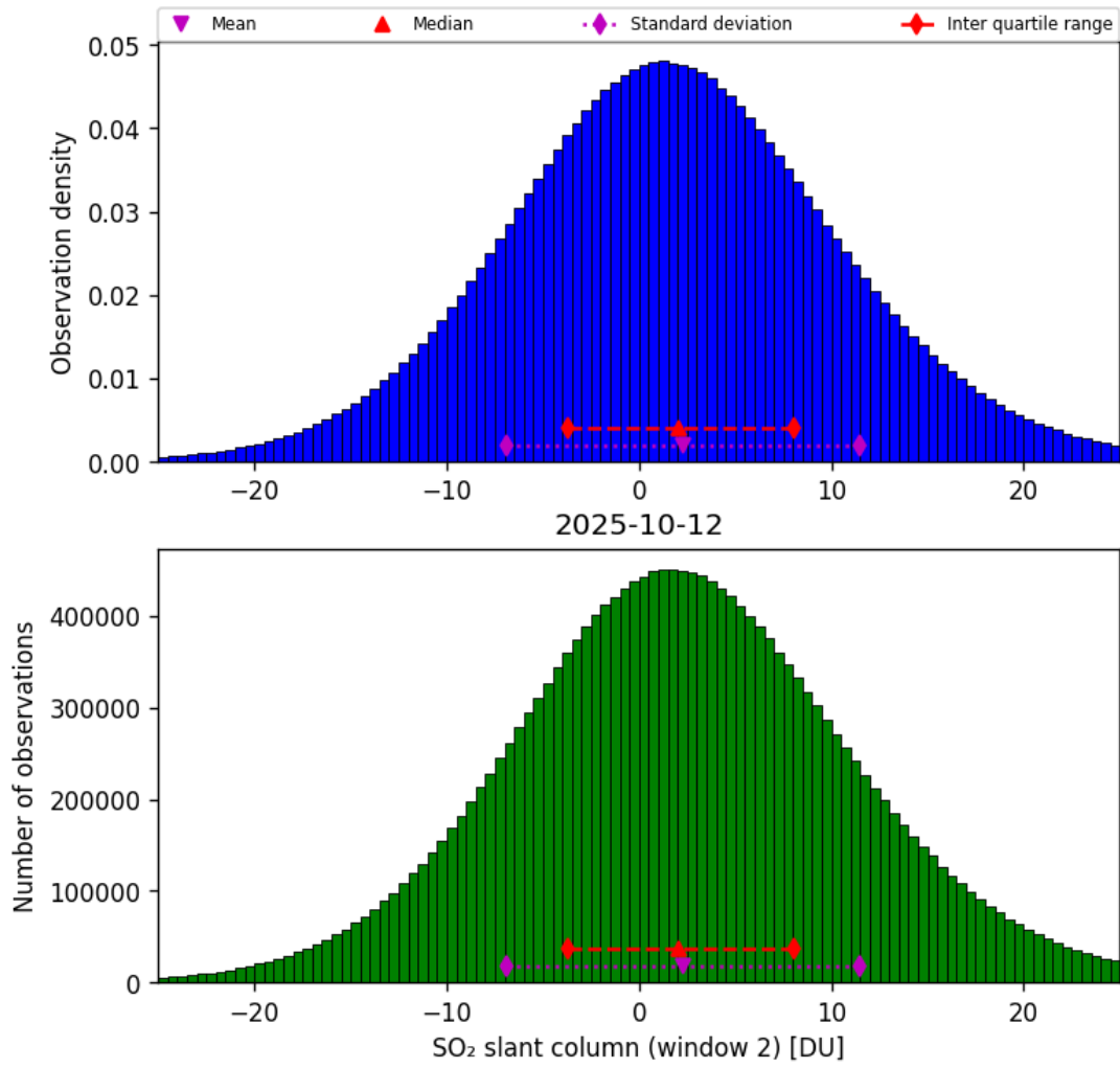
Figure 67: Histogram of “SO 2 slant column (window 2)” for 2025-10-11 to 2025-10-13
