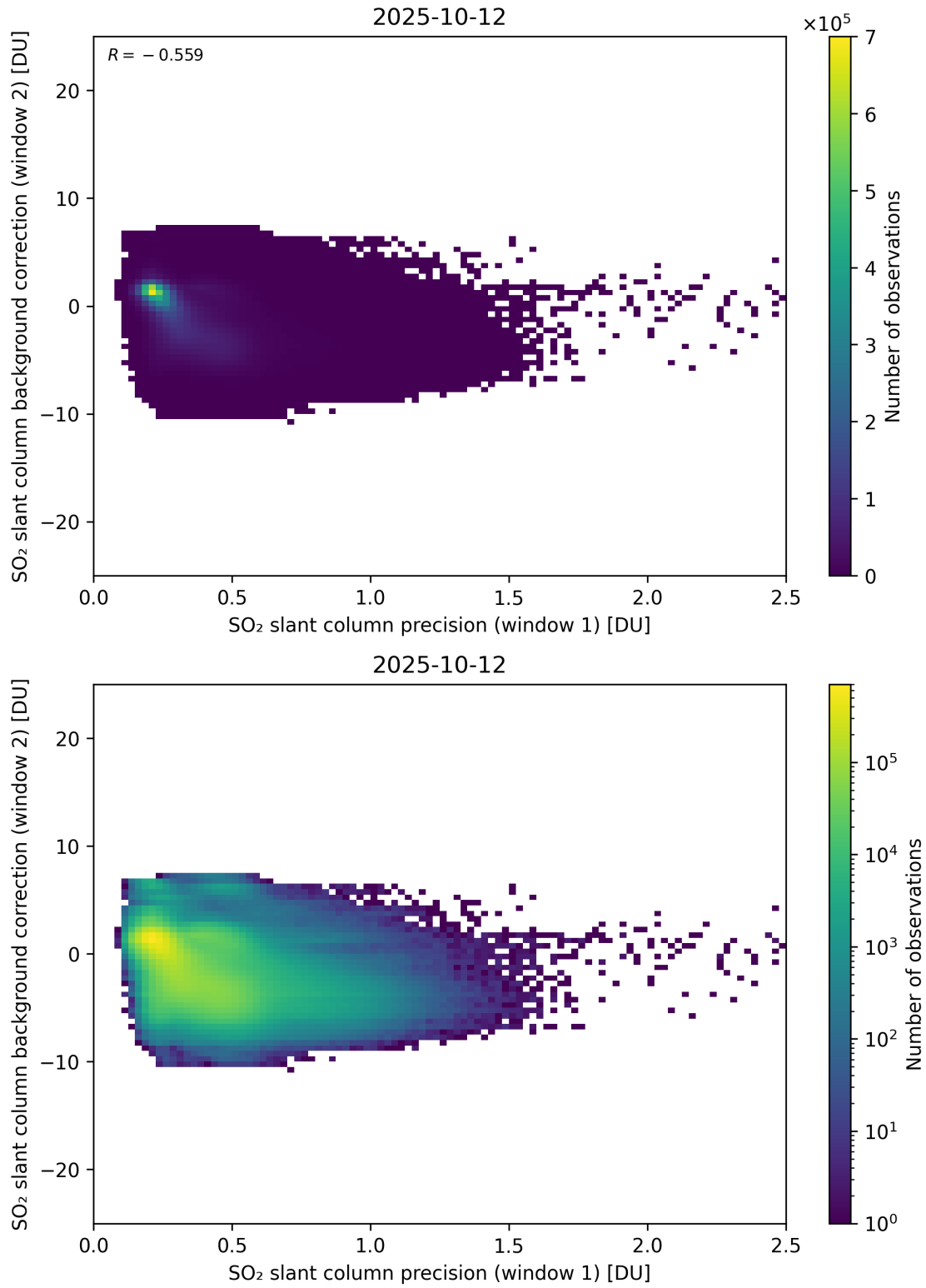
Figure 269: Scatter density plot of “SO 2 slant column precision (window 1)” against “SO 2 slant column background correction (window 2)” for 2025-10-11 to 2025-10-13.
