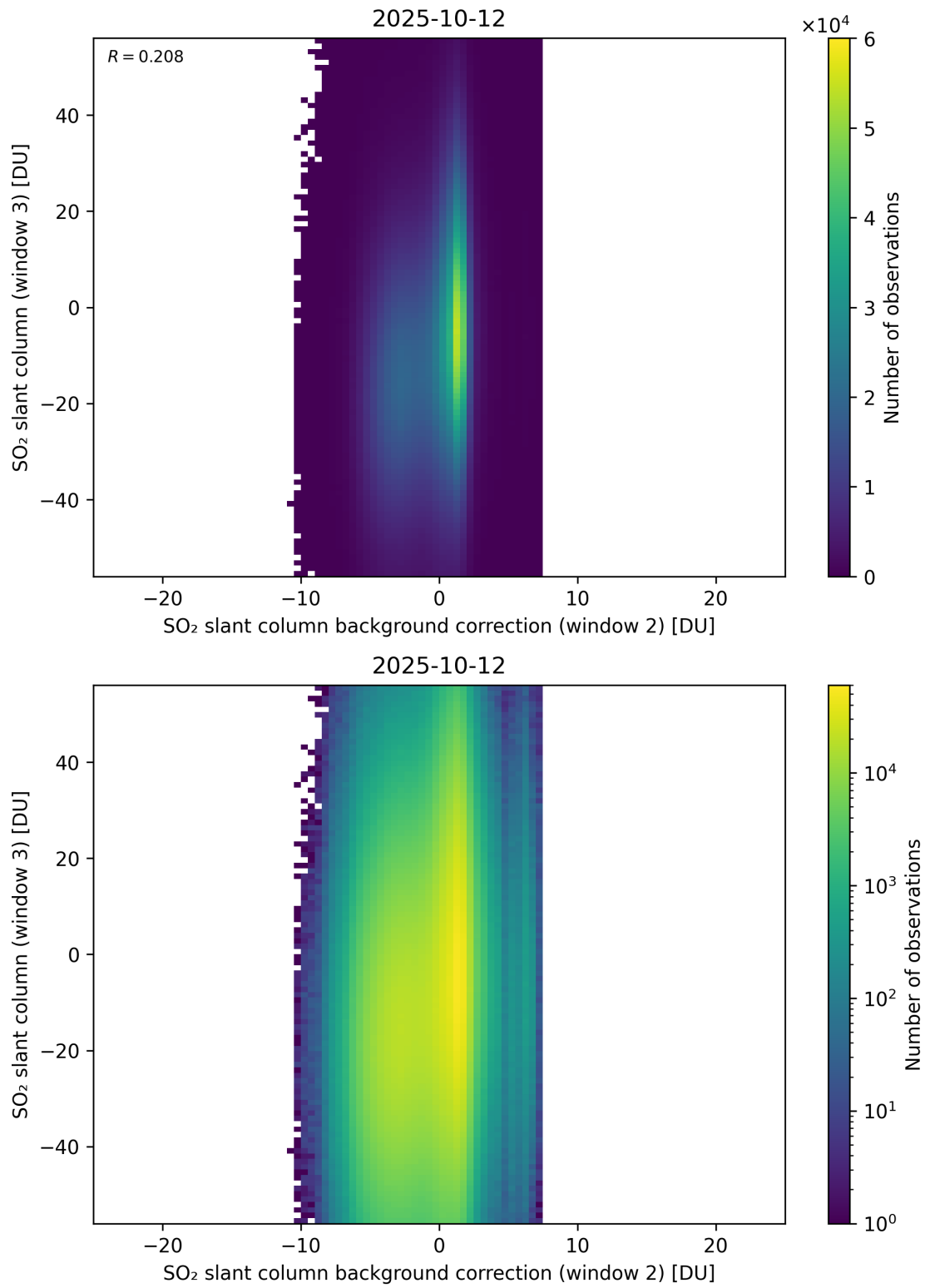
Figure 128: Scatter density plot of “SO 2 slant column background correction (window 2)” against “SO 2 slant column (window 3)” for 2025-10-11 to 2025-10-13.
