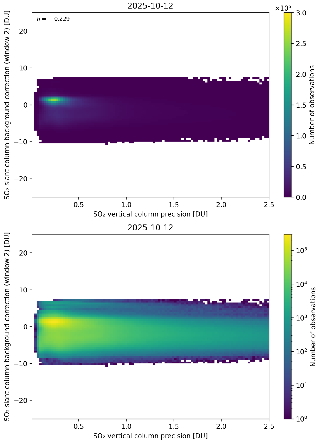
Figure 330: Scatter density plot of “SO 2 vertical column precision” against “SO 2 slant column background correction (window 2)” for 2025-10-11 to 2025-10-13.
