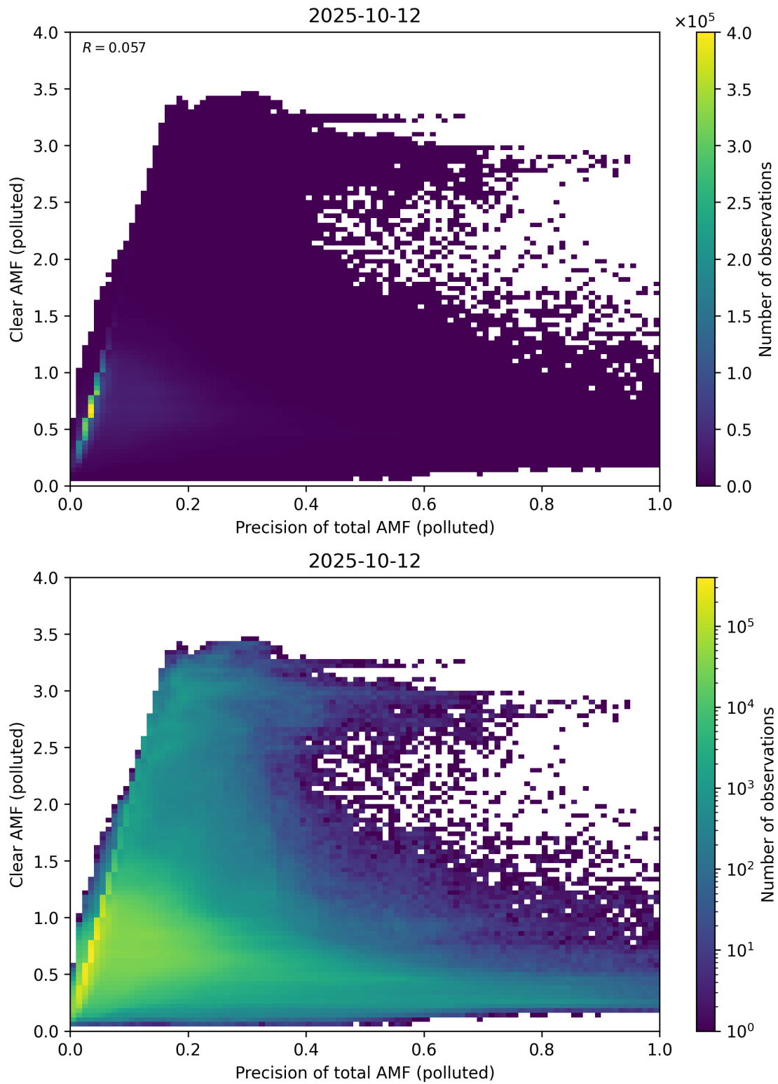
Figure 320: Scatter density plot of “Precision of total AMF (polluted)” against “Clear AMF (polluted)” for 2025-10-11 to 2025-10-13.
