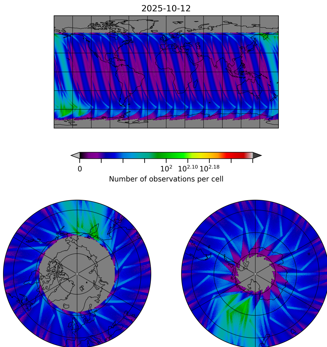
Figure 30: Map of the number of observations for 2025-10-11 to 2025-10-13
