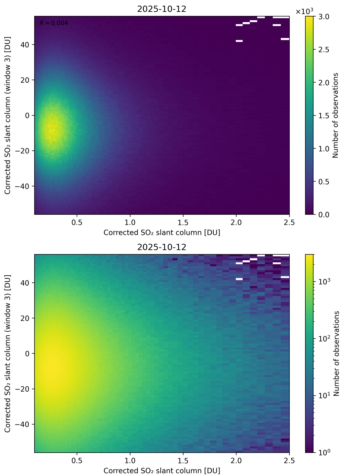
Figure 236: Scatter density plot of “Corrected SO 2 slant column” against “Corrected SO 2 slant column (window 3)” for 2025-10-11 to 2025-10-13.
