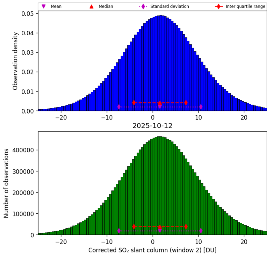
Figure 69: Histogram of “Corrected SO 2 slant column (window 2)” for 2025-10-11 to 2025-10-13
