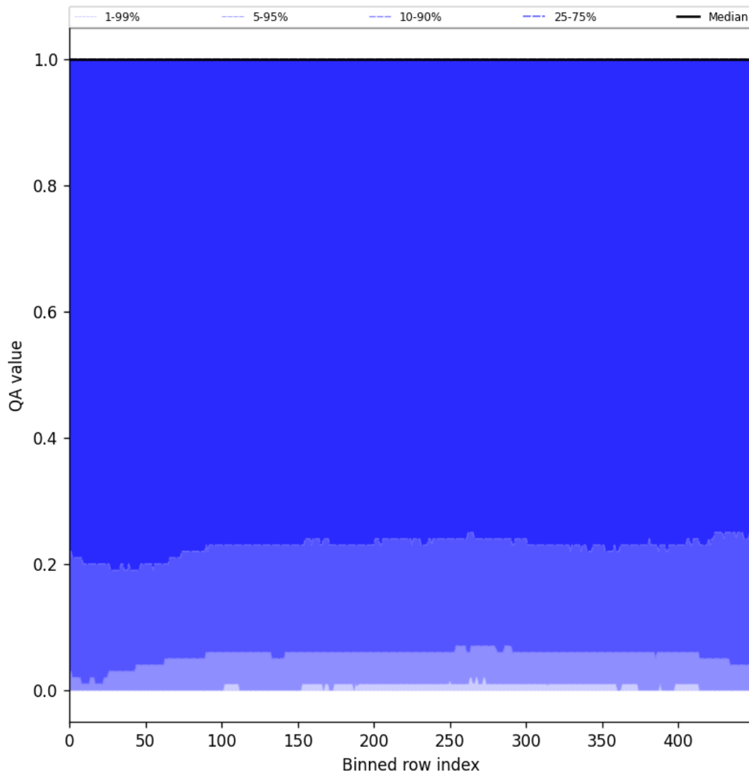
Figure 83: Along track statistics of “QA value” for 2025-10-11 to 2025-10-13
