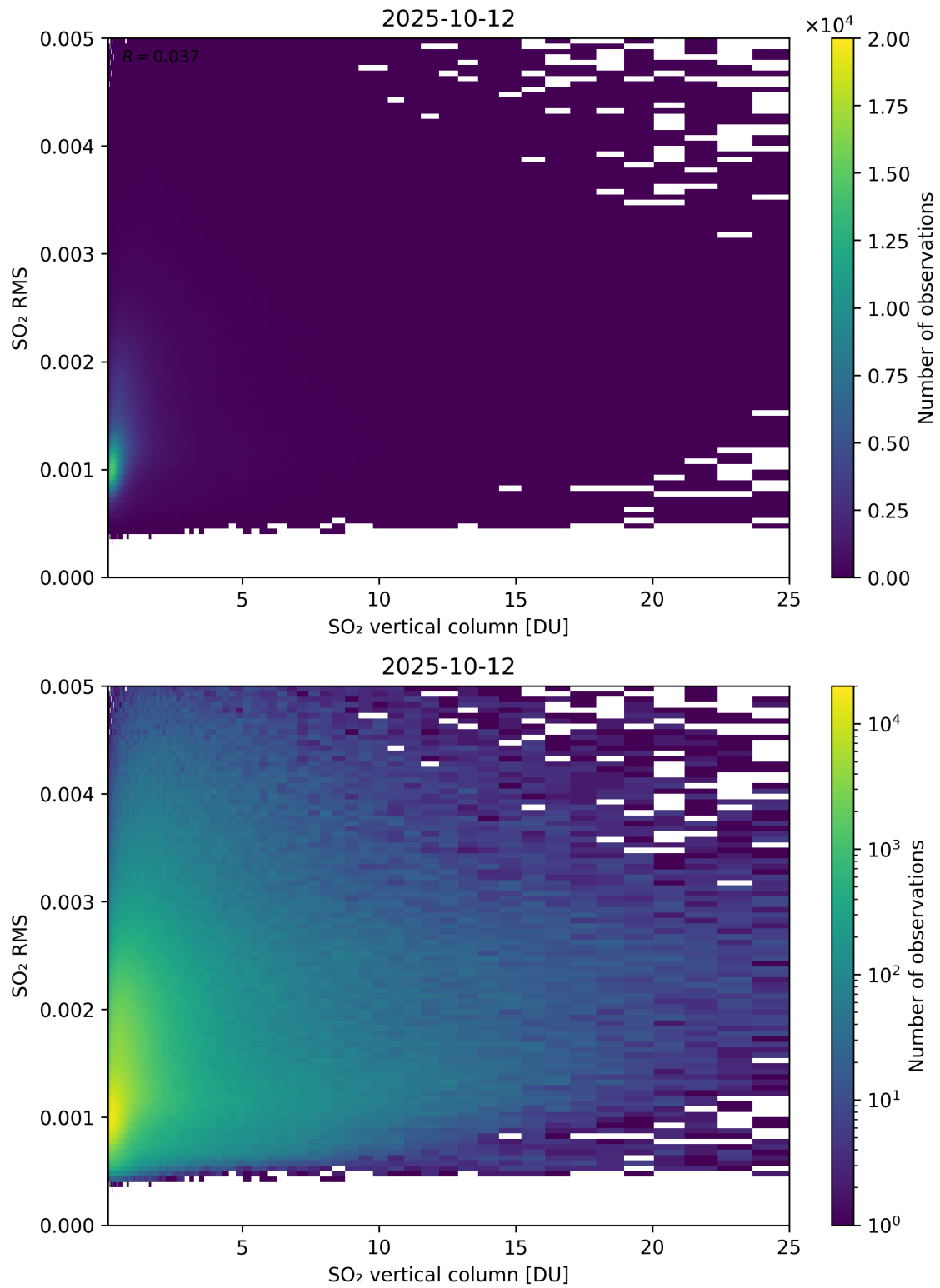
Figure 328: Scatter density plot of “SO 2 vertical column” against “SO 2 RMS” for 2025-10-11 to 2025-10-13.
