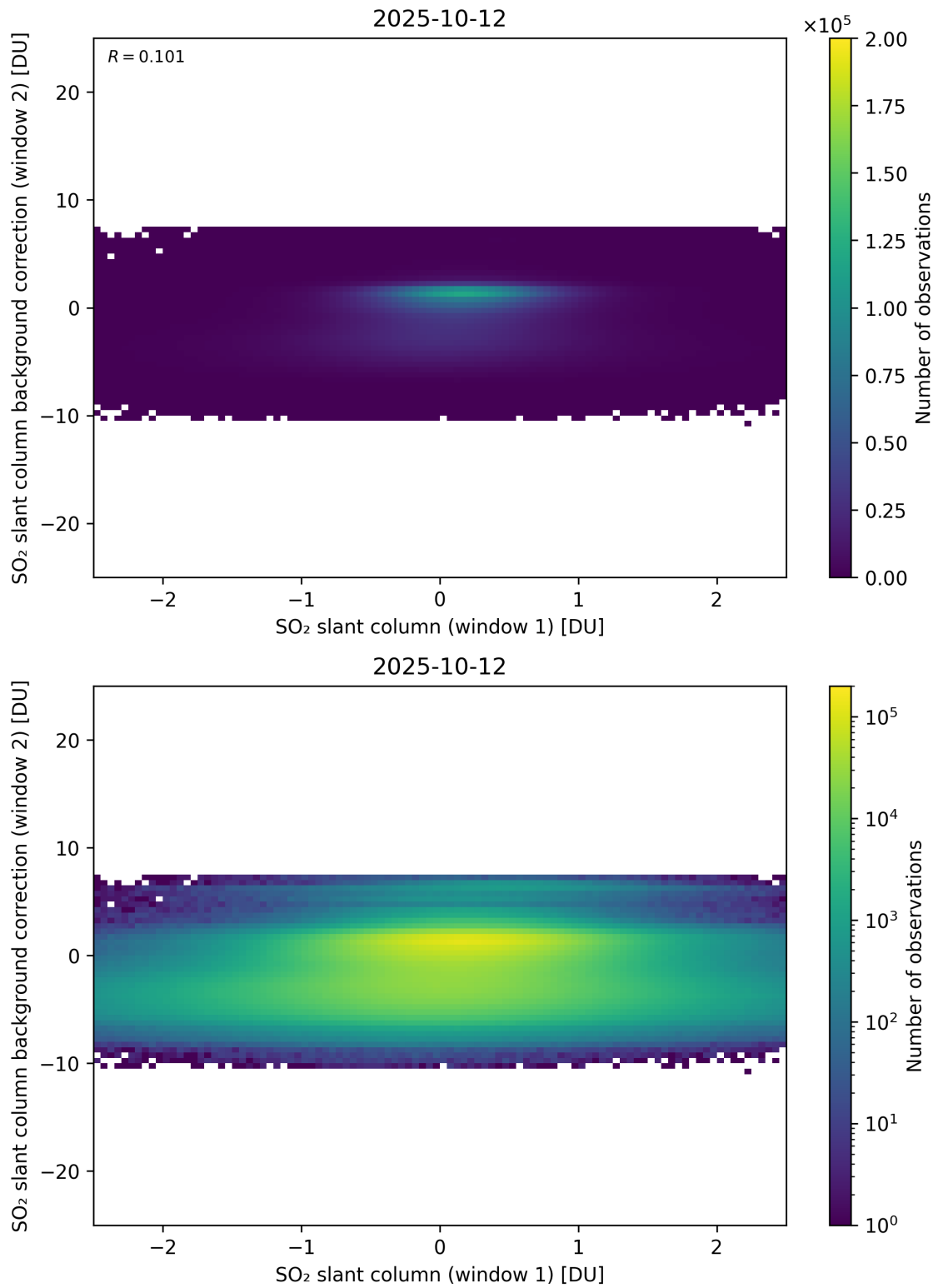
Figure 263: Scatter density plot of “SO 2 slant column (window 1)” against “SO 2 slant column background correction (window 2)” for 2025-10-11 to 2025-10-13.
