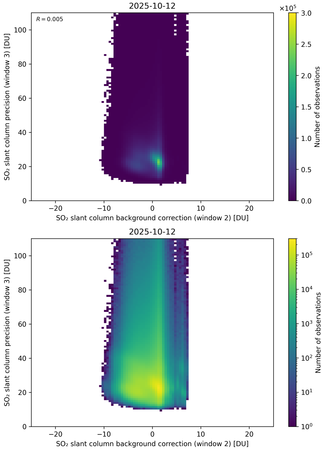
Figure 129: Scatter density plot of “SO 2 slant column background correction (window 2)” against “SO 2 slant column precision (window 3)” for 2025-10-11 to 2025-10-13.
