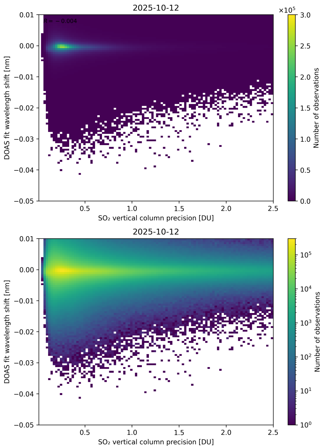
Figure 332: Scatter density plot of “SO 2 vertical column precision” against “DOAS fit wavelength shift” for 2025-10-11 to 2025-10-13.
