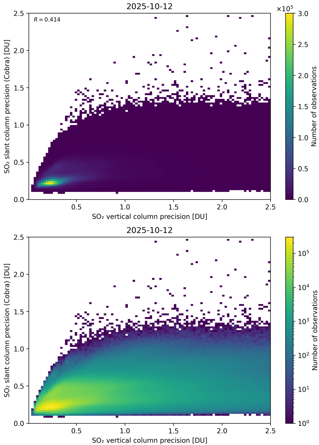
Figure 337: Scatter density plot of “SO 2 vertical column precision” against “SO 2 slant column precision (Cobra)” for 2025-10-11 to 2025-10-13.
