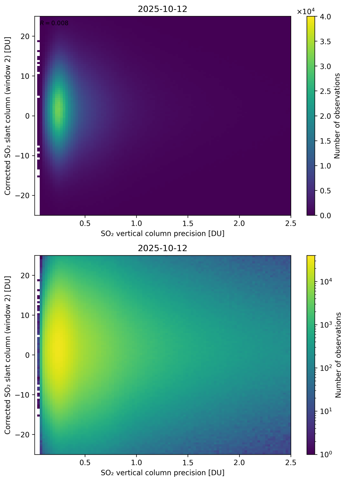
Figure 339: Scatter density plot of “SO 2 vertical column precision” against “Corrected SO 2 slant column (window 2)” for 2025-10-11 to 2025-10-13.
