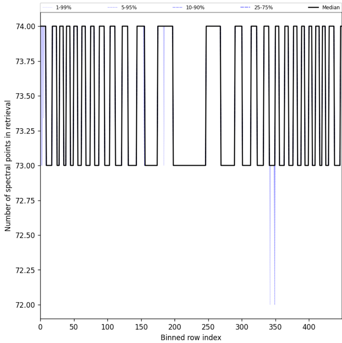
Figure 108: Along track statistics of “Number of spectral points in retrieval” for 2025-10-11 to 2025-10-13
