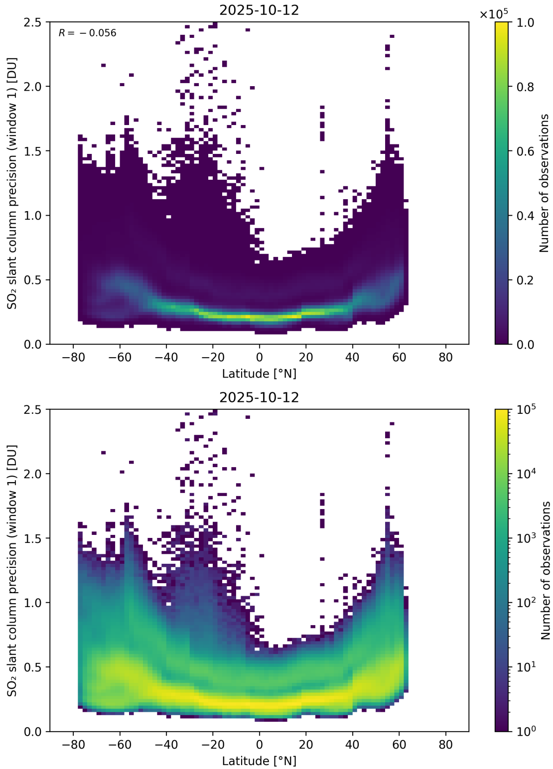
Figure 163: Scatter density plot of “Latitude” against “SO 2 slant column precision (window 1)” for 2025-10-11 to 2025-10-13.
