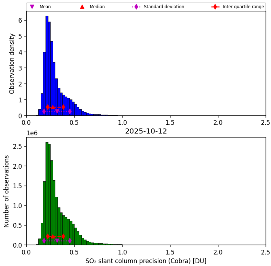
Figure 62: Histogram of “SO 2 slant column precision (Cobra)” for 2025-10-11 to 2025-10-13
