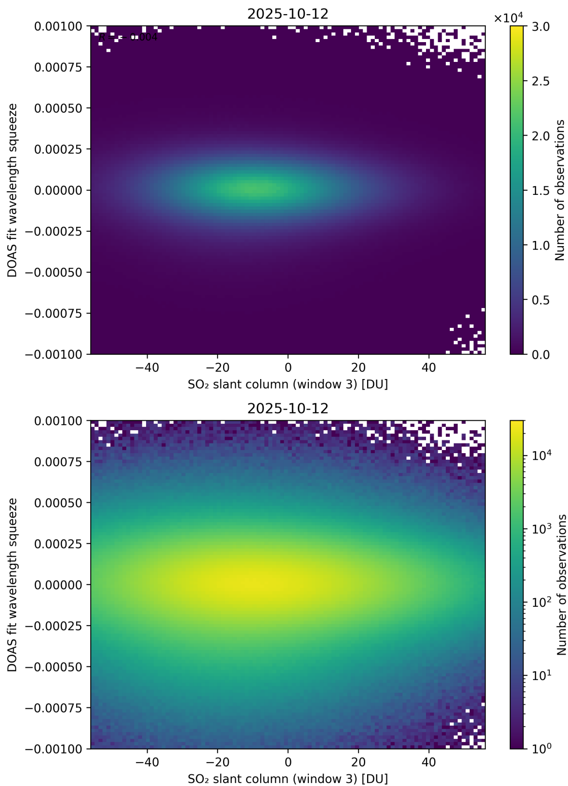
Figure 305: Scatter density plot of “SO 2 slant column (window 3)” against “DOAS fit wavelength squeeze” for 2025-10-11 to 2025-10-13.
