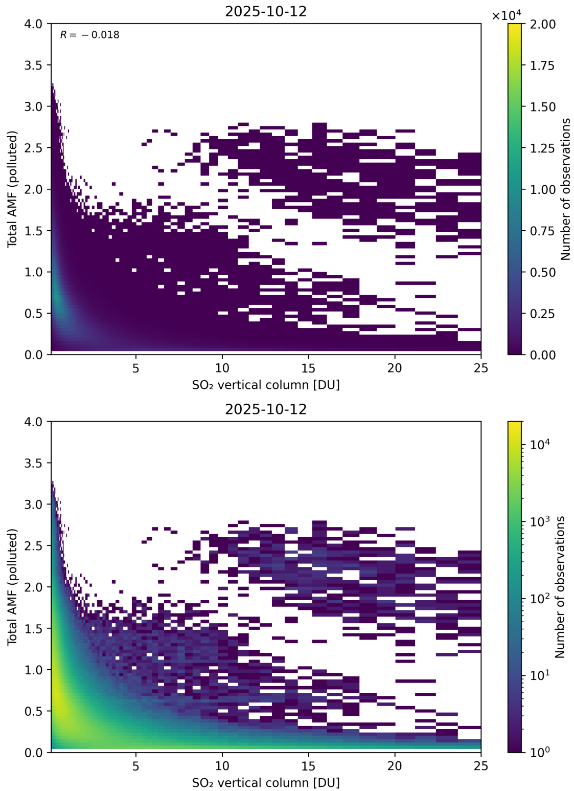
Figure 359: Scatter density plot of “SO 2 vertical column” against “Total AMF (polluted)” for 2025-10-11 to 2025-10-13.
