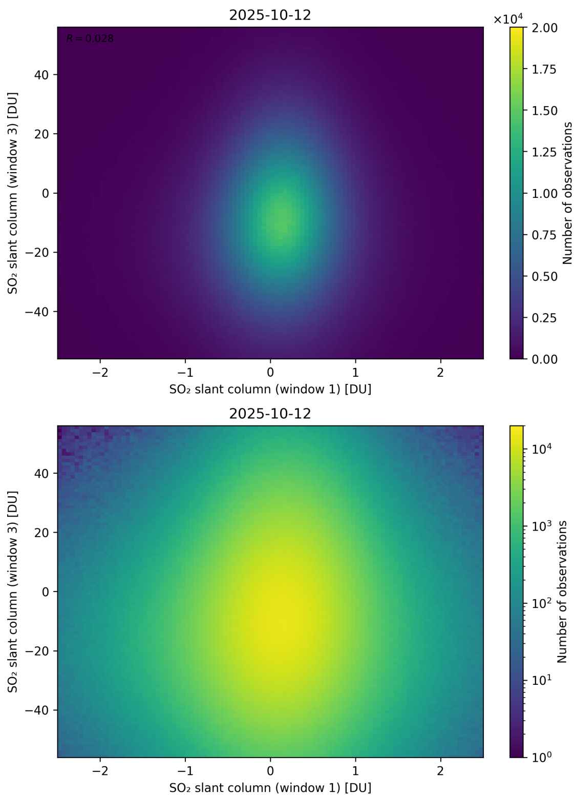
Figure 287: Scatter density plot of “SO 2 slant column (window 1)” against “SO 2 slant column (window 3)” for 2025-10-11 to 2025-10-13.
