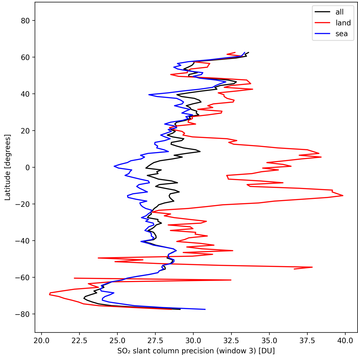
Figure 46: Zonal average of “SO 2 slant column precision (window 3)” for 2025-10-11 to 2025-10-13.
