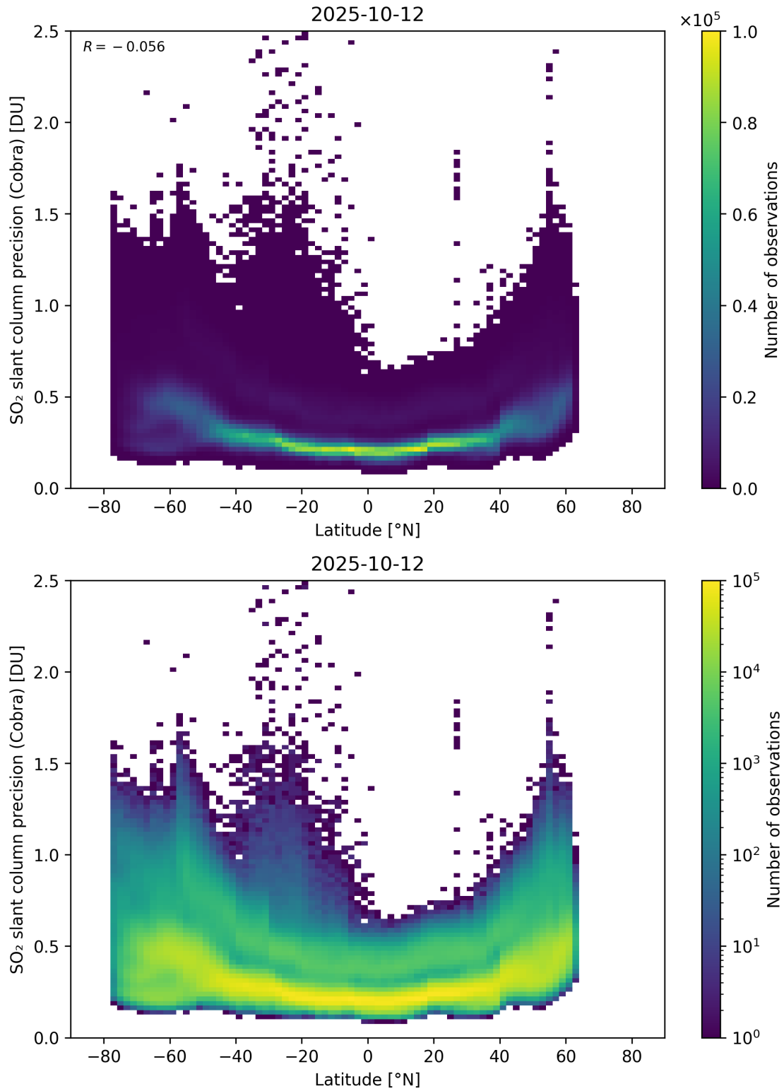
Figure 158: Scatter density plot of “Latitude” against “SO 2 slant column precision (Cobra)” for 2025-10-11 to 2025-10-13.
