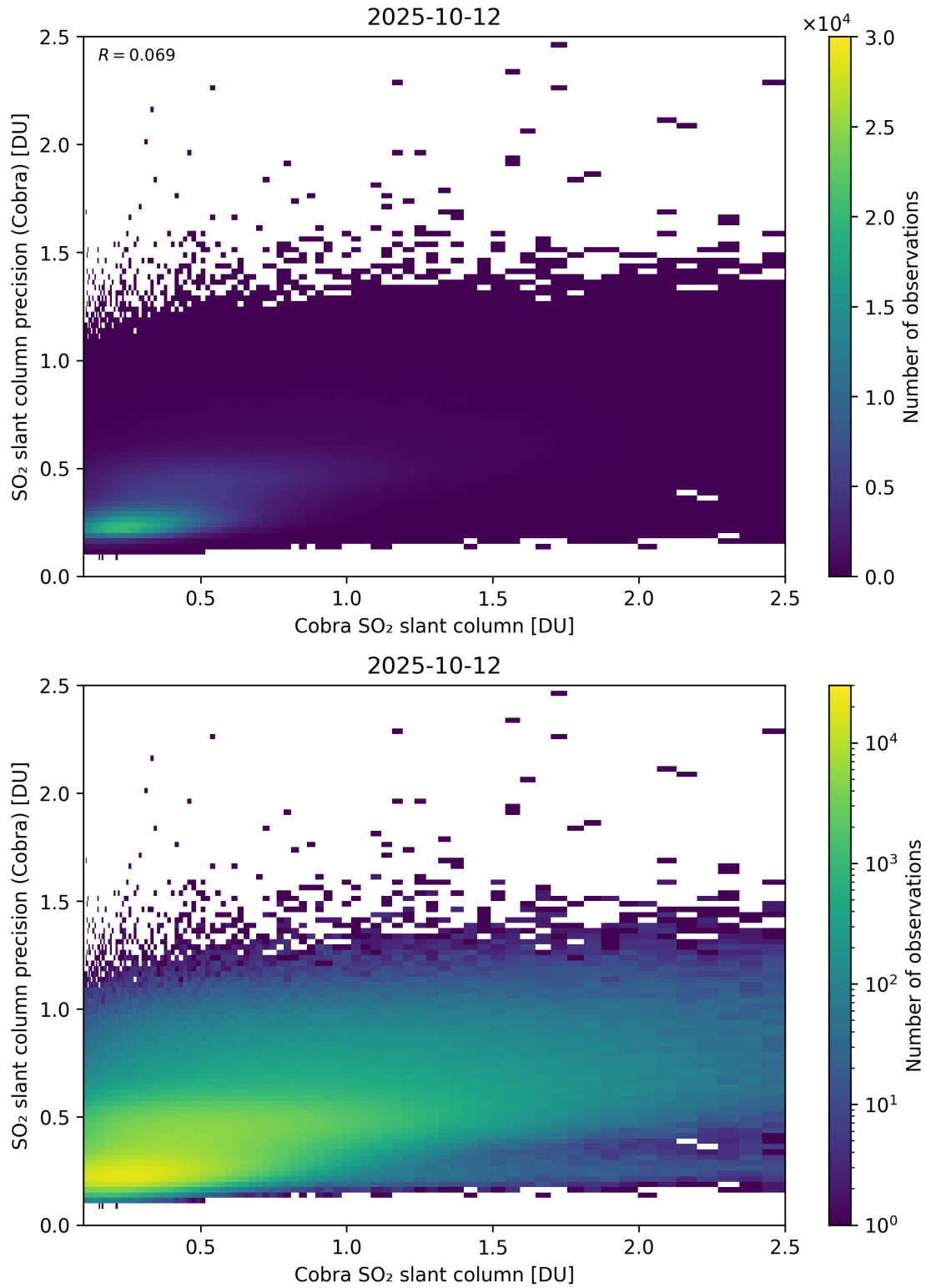
Figure 216: Scatter density plot of “Cobra SO 2 slant column” against “SO 2 slant column precision (Cobra)” for 2025-10-11 to 2025-10-13.
