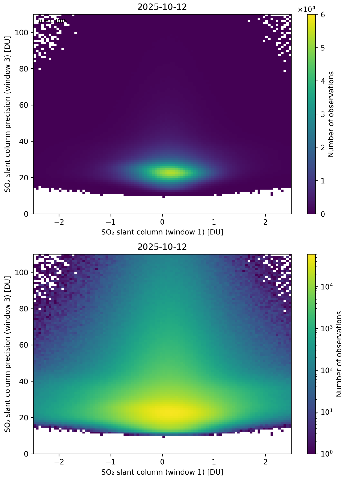
Figure 288: Scatter density plot of “SO 2 slant column (window 1)” against “SO 2 slant column precision (window 3)” for 2025-10-11 to 2025-10-13.
