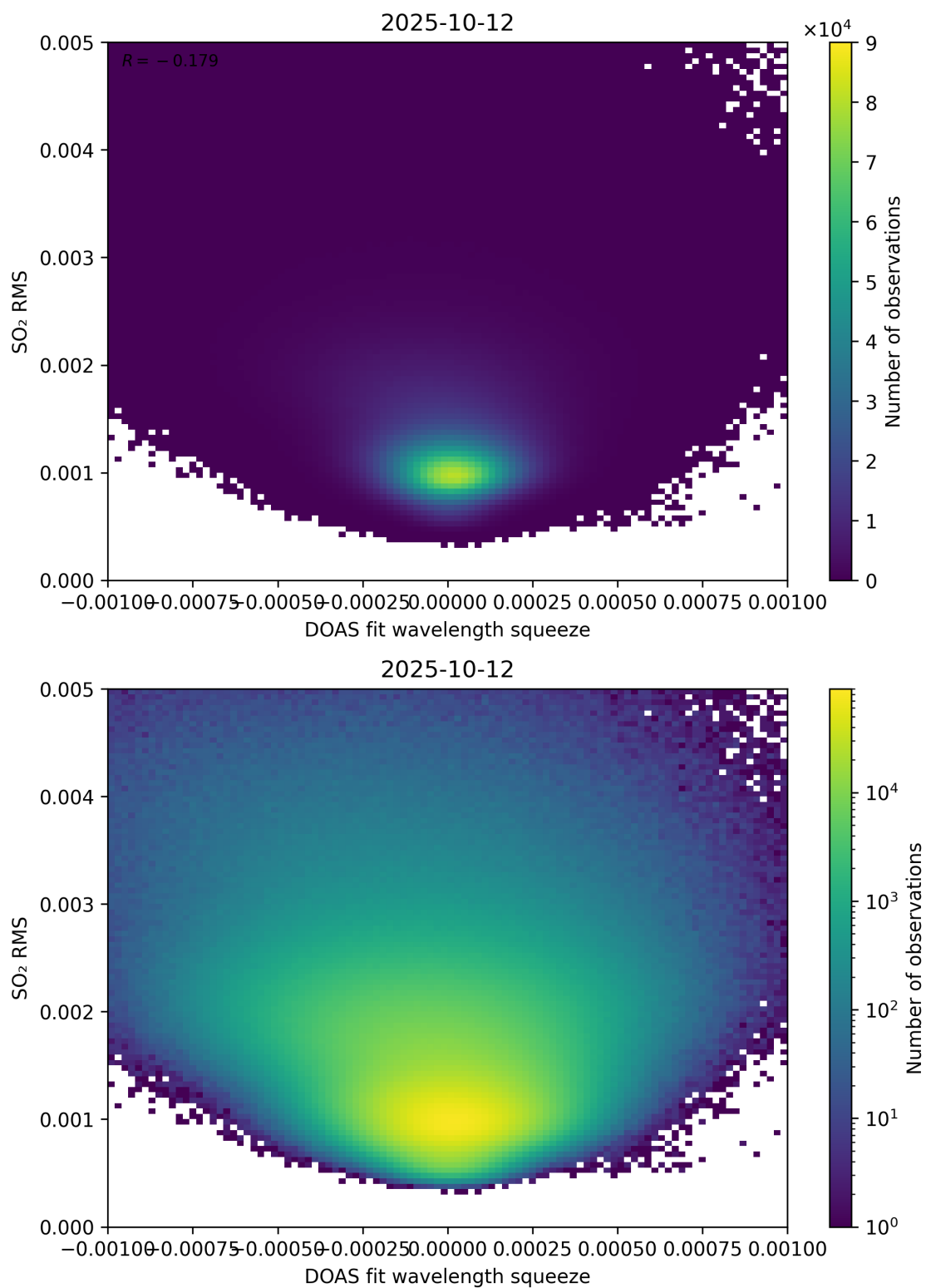
Figure 143: Scatter density plot of “DOAS fit wavelength squeeze” against “SO 2 RMS” for 2025-10-11 to 2025-10-13.
