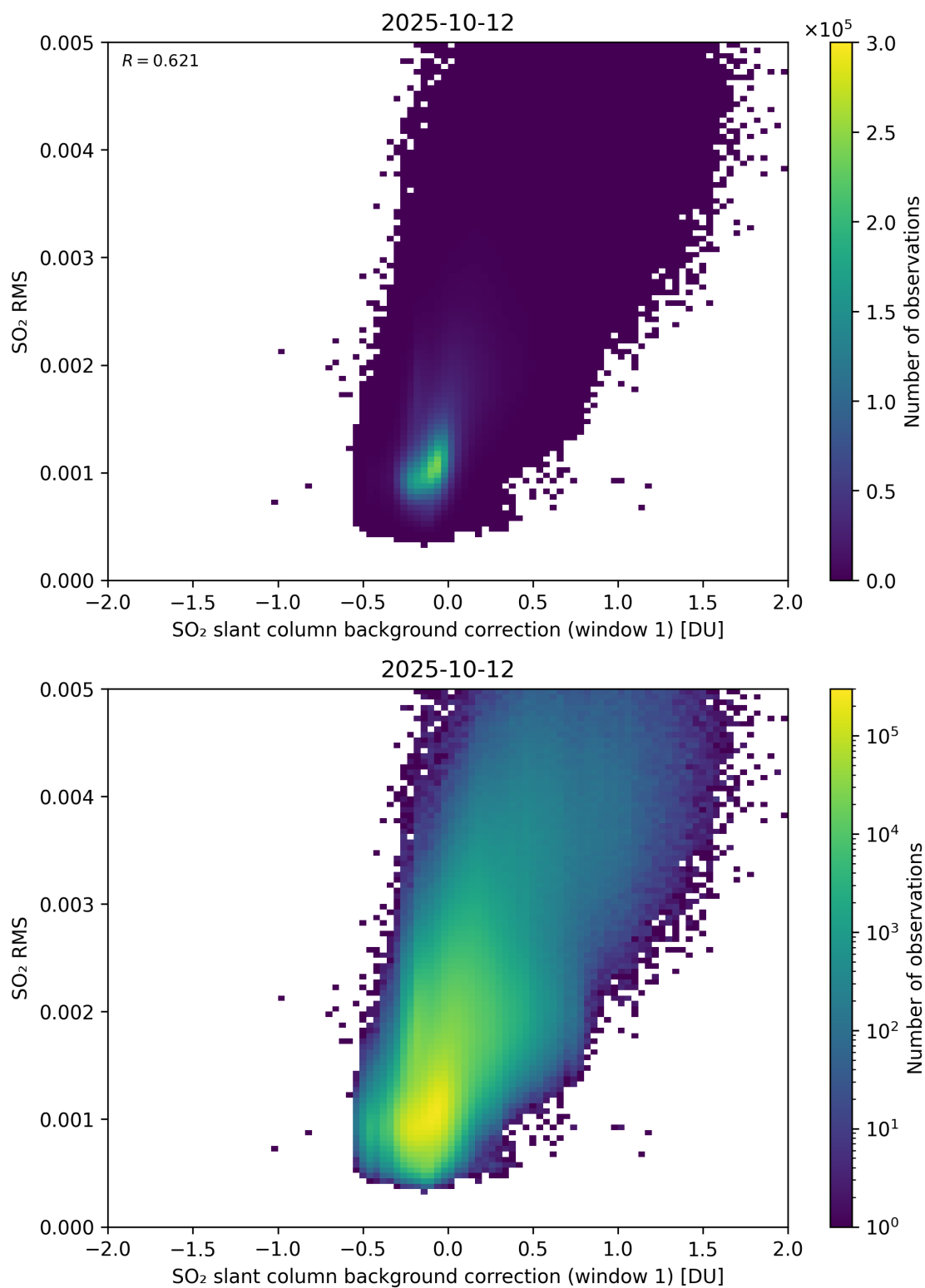
Figure 113: Scatter density plot of “SO 2 slant column background correction (window 1)” against “SO 2 RMS” for 2025-10-11 to 2025-10-13.
