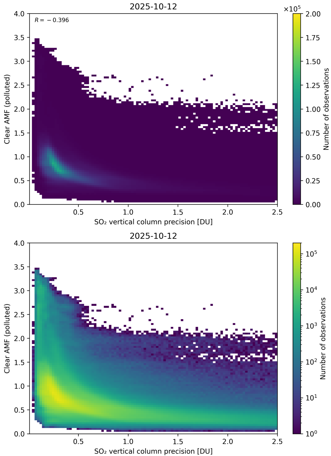
Figure 335: Scatter density plot of “SO 2 vertical column precision” against “Clear AMF (polluted)” for 2025-10-11 to 2025-10-13.
