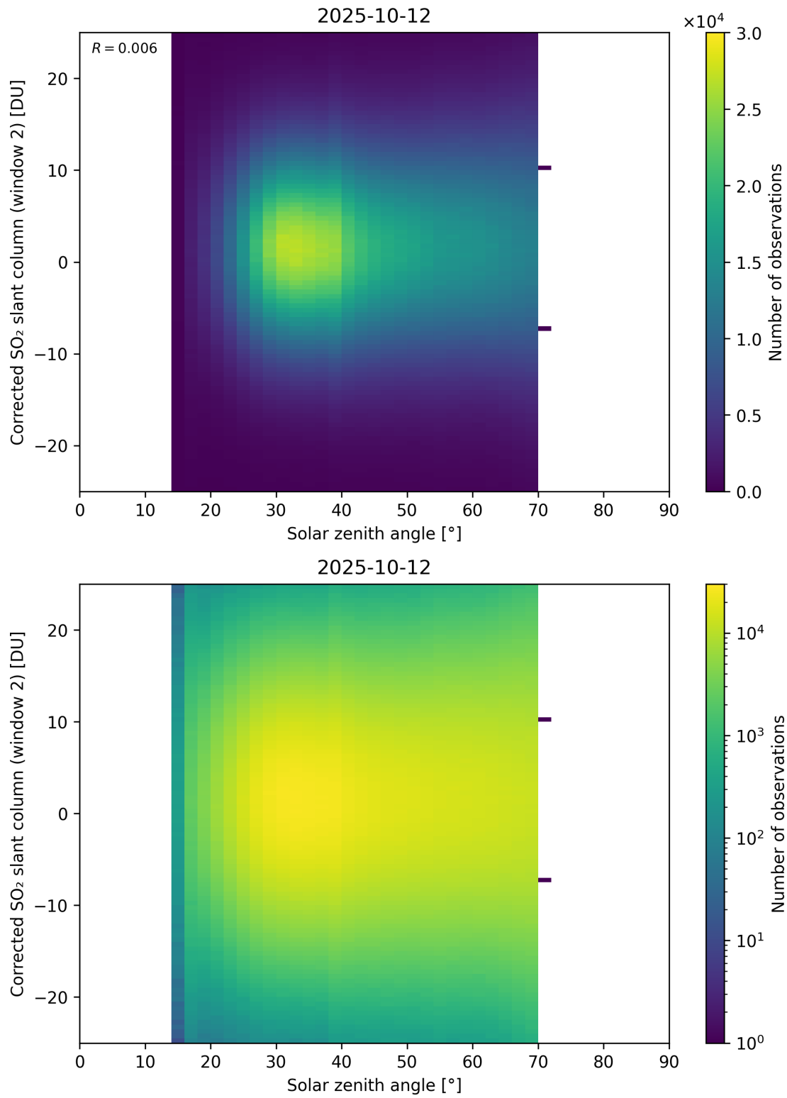
Figure 182: Scatter density plot of “Solar zenith angle” against “Corrected SO 2 slant column (window 2)” for 2025-10-11 to 2025-10-13.
