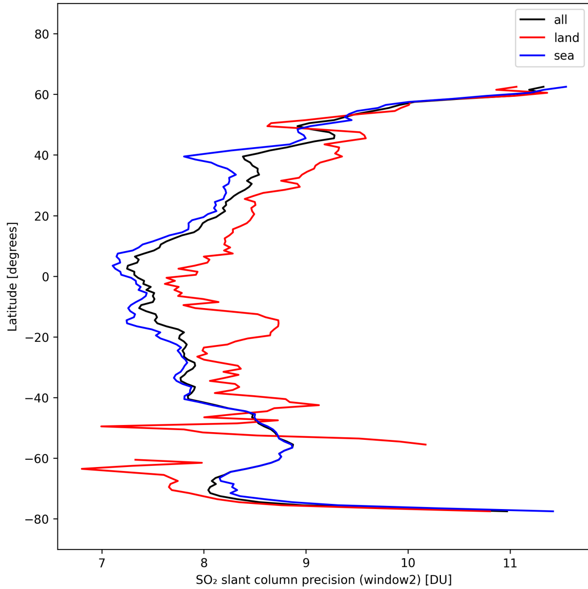
Figure 42: Zonal average of “SO 2 slant column precision (window2)” for 2025-10-11 to 2025-10-13.
