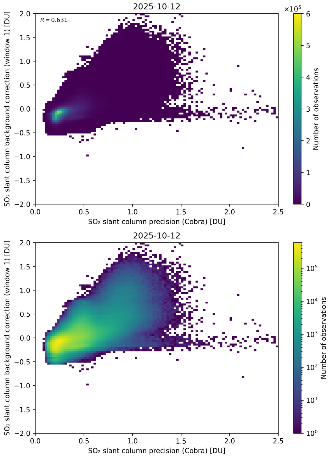
Figure 199: Scatter density plot of “SO 2 slant column precision (Cobra)” against “SO 2 slant column background correction (window 1)” for 2025-10-11 to 2025-10-13.
