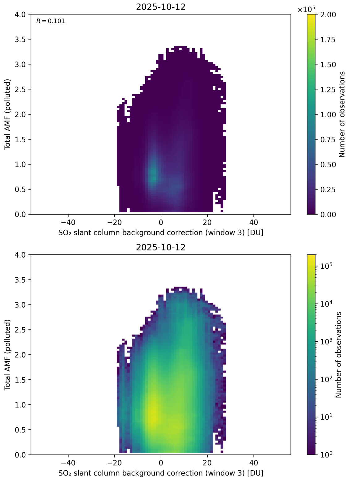
Figure 136: Scatter density plot of “SO 2 slant column background correction (window 3)” against “Total AMF (polluted)” for 2025-10-11 to 2025-10-13.
