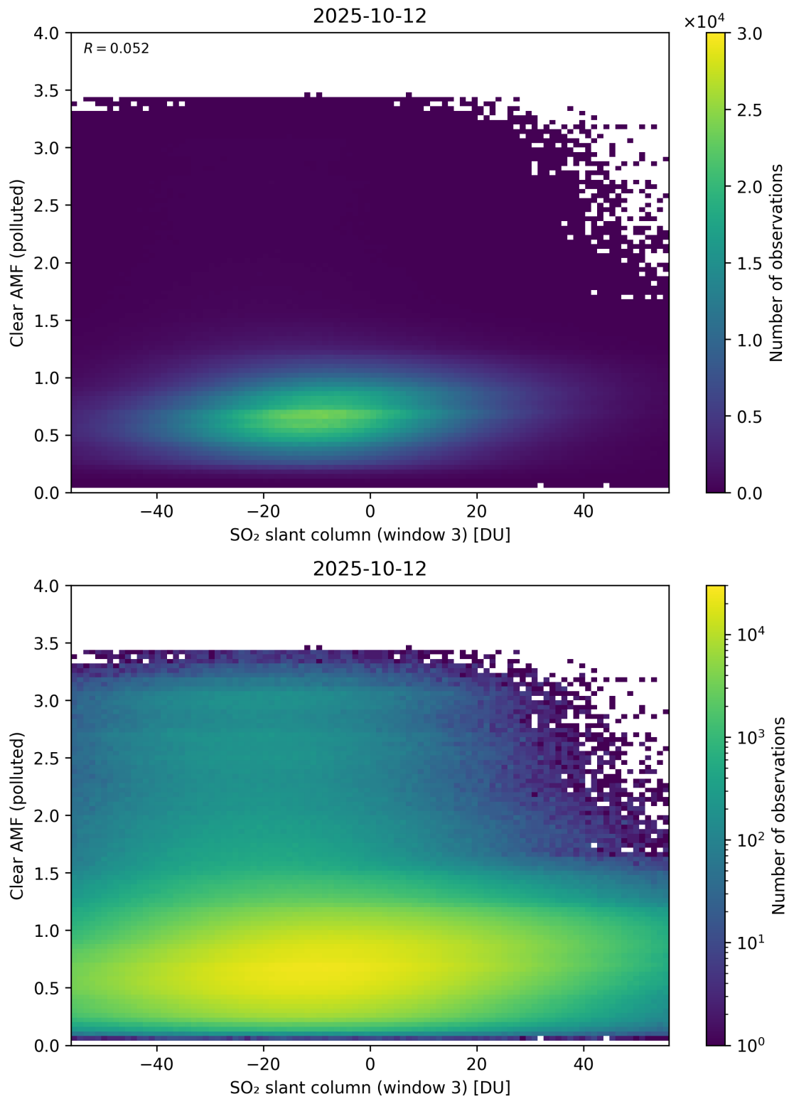
Figure 315: Scatter density plot of “SO 2 slant column (window 3)” against “Clear AMF (polluted)” for 2025-10-11 to 2025-10-13.
