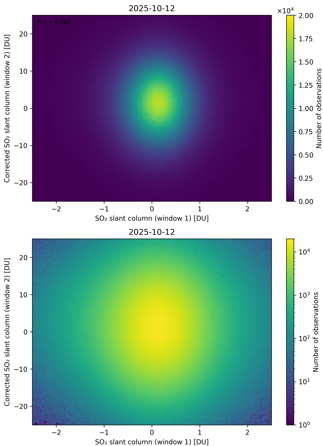
Figure 283: Scatter density plot of “SO 2 slant column (window 1)” against “Corrected SO 2 slant column (window 2)” for 2025-10-11 to 2025-10-13.
