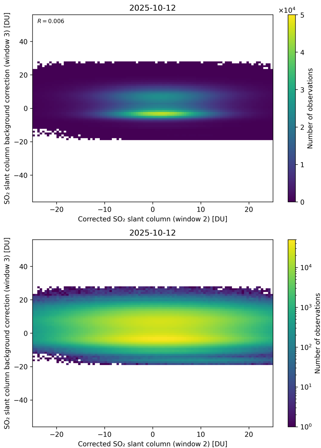
Figure 245: Scatter density plot of “Corrected SO 2 slant column (window 2)” against “SO 2 slant column background correction (window 3)” for 2025-10-11 to 2025-10-13.
