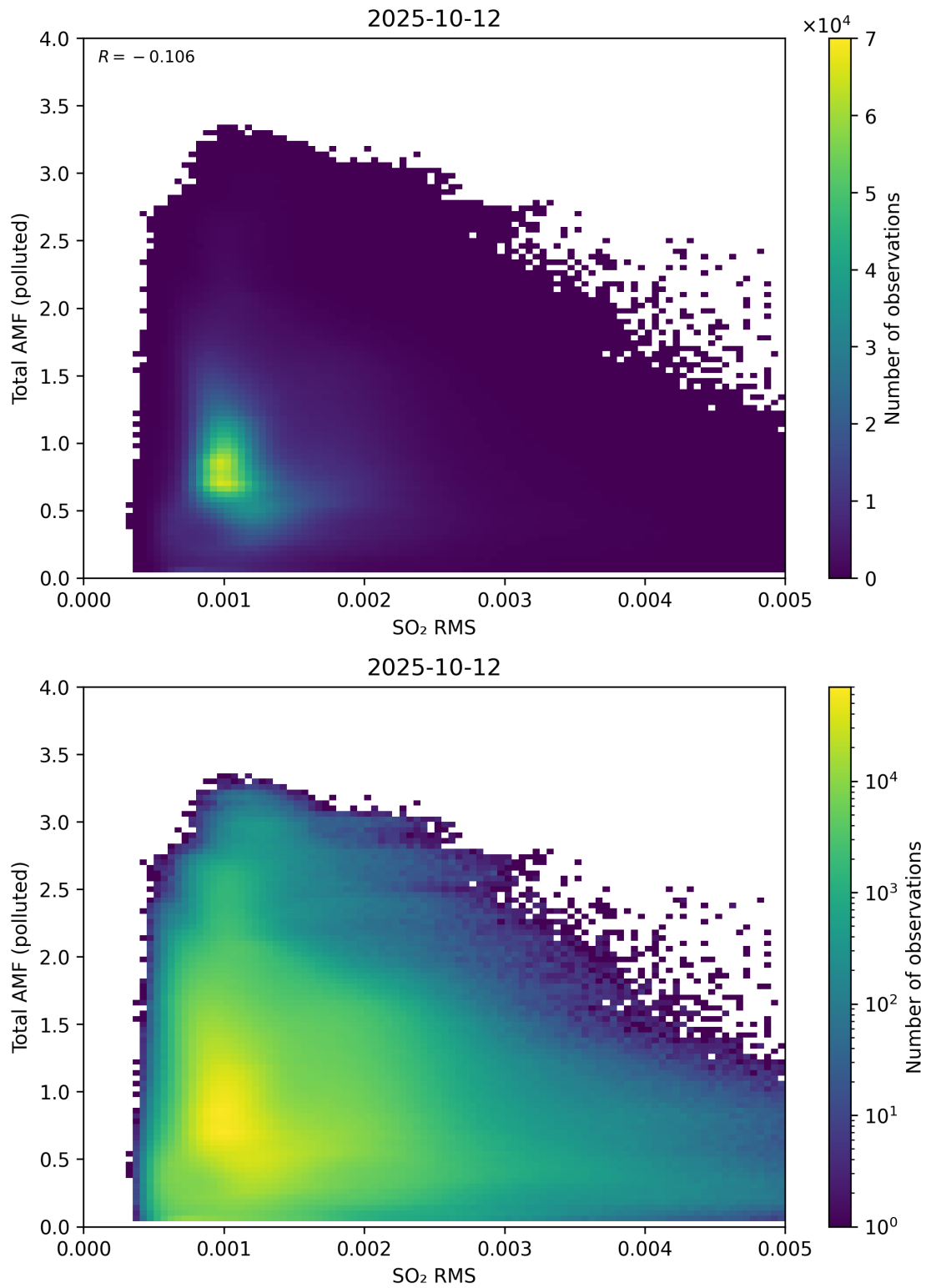
Figure 148: Scatter density plot of “SO 2 RMS” against “Total AMF (polluted)” for 2025-10-11 to 2025-10-13.
