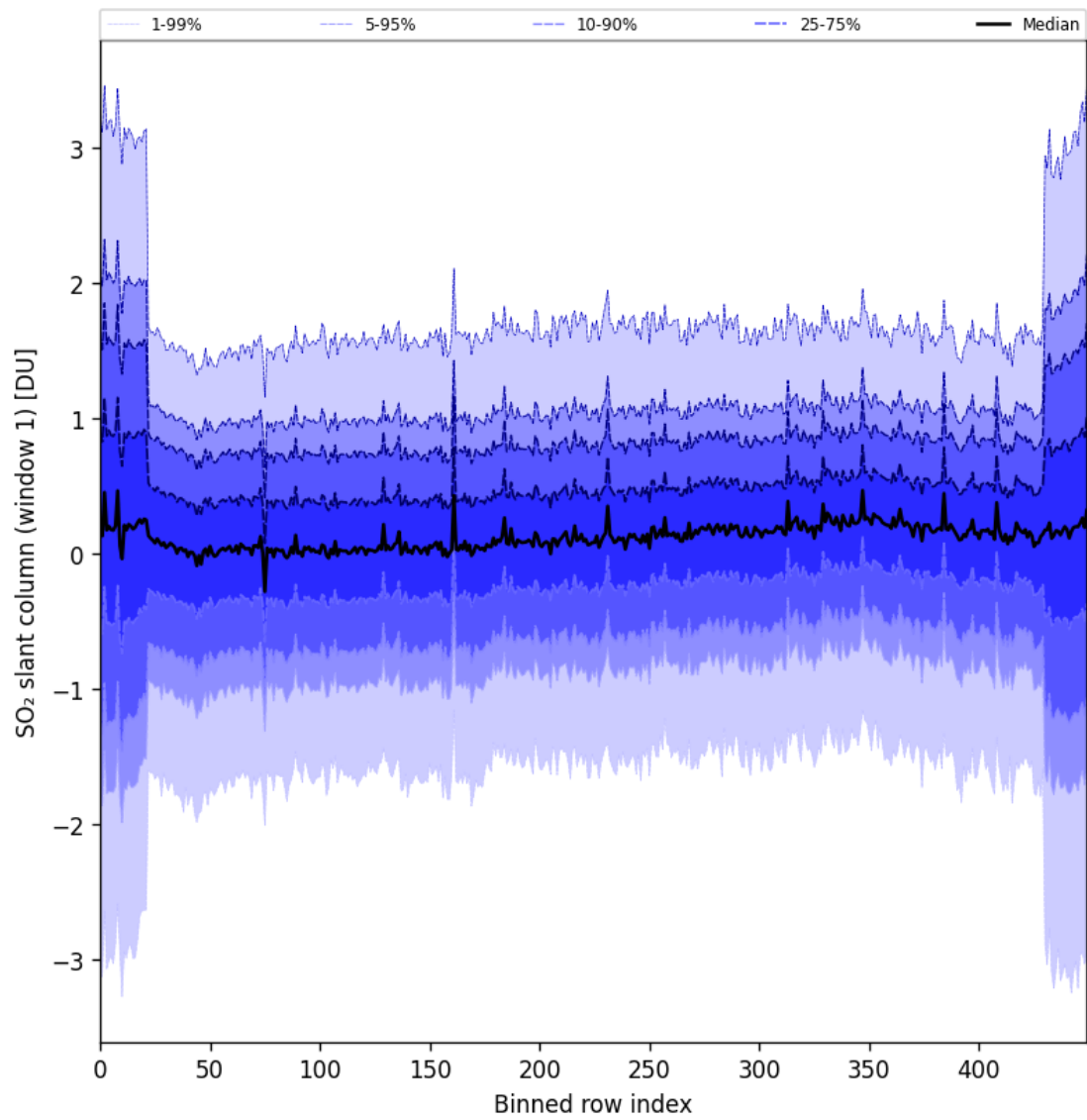
Figure 89: Along track statistics of “SO 2 slant column (window 1)” for 2025-10-11 to 2025-10-13
