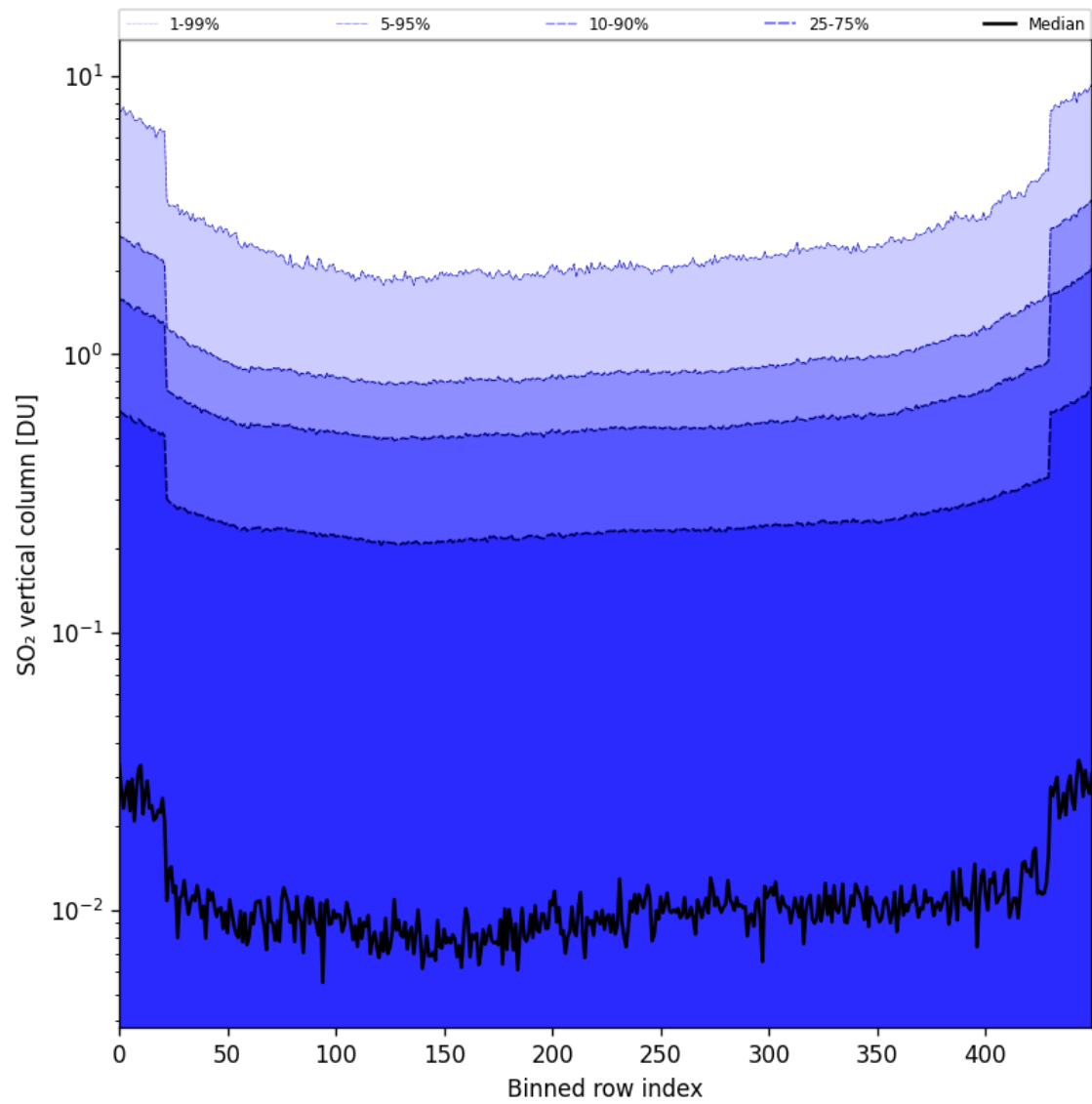
Figure 84: Along track statistics of “SO 2 vertical column” for 2025-10-11 to 2025-10-13
