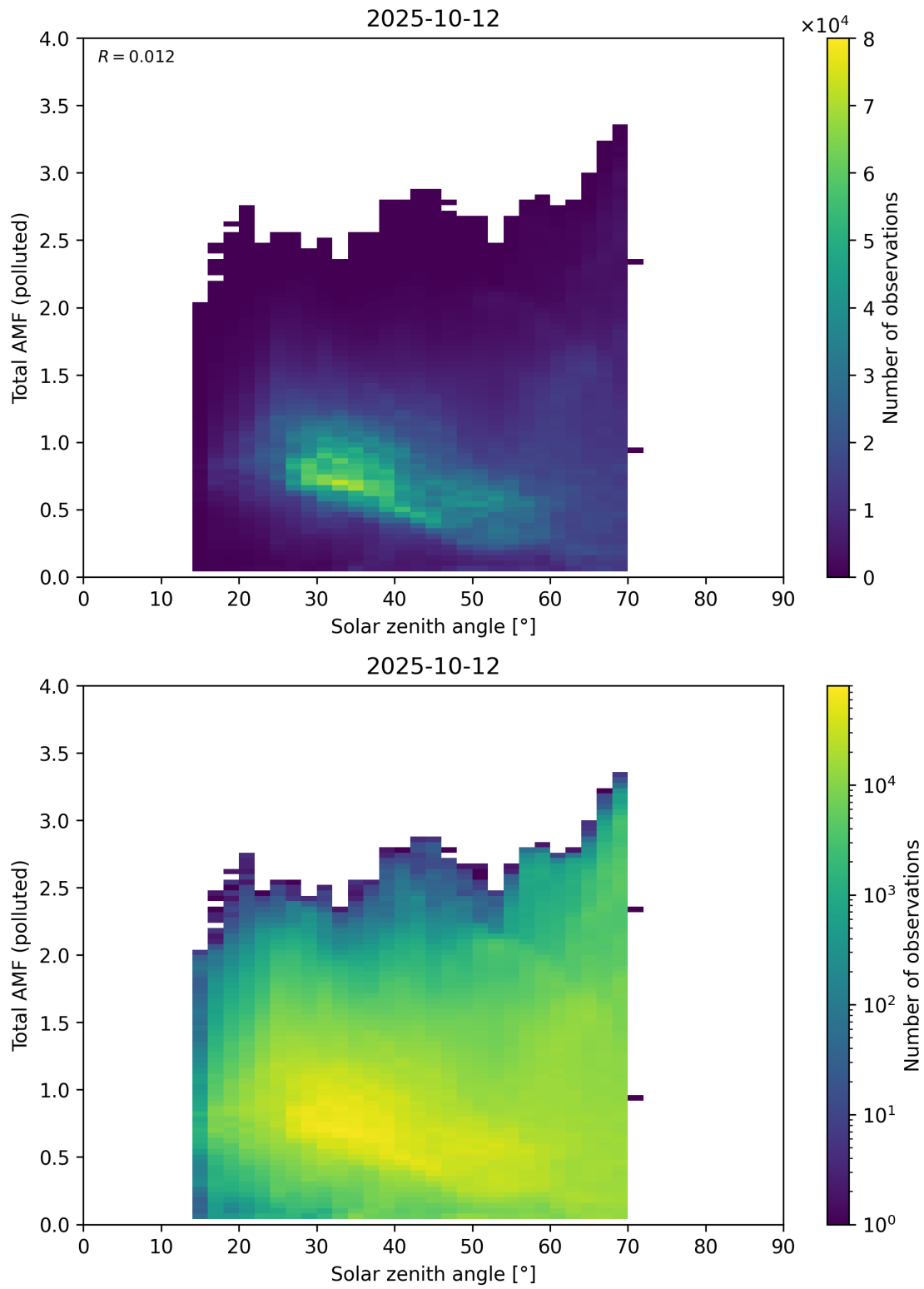
Figure 189: Scatter density plot of “Solar zenith angle” against “Total AMF (polluted)” for 2025-10-11 to 2025-10-13.
