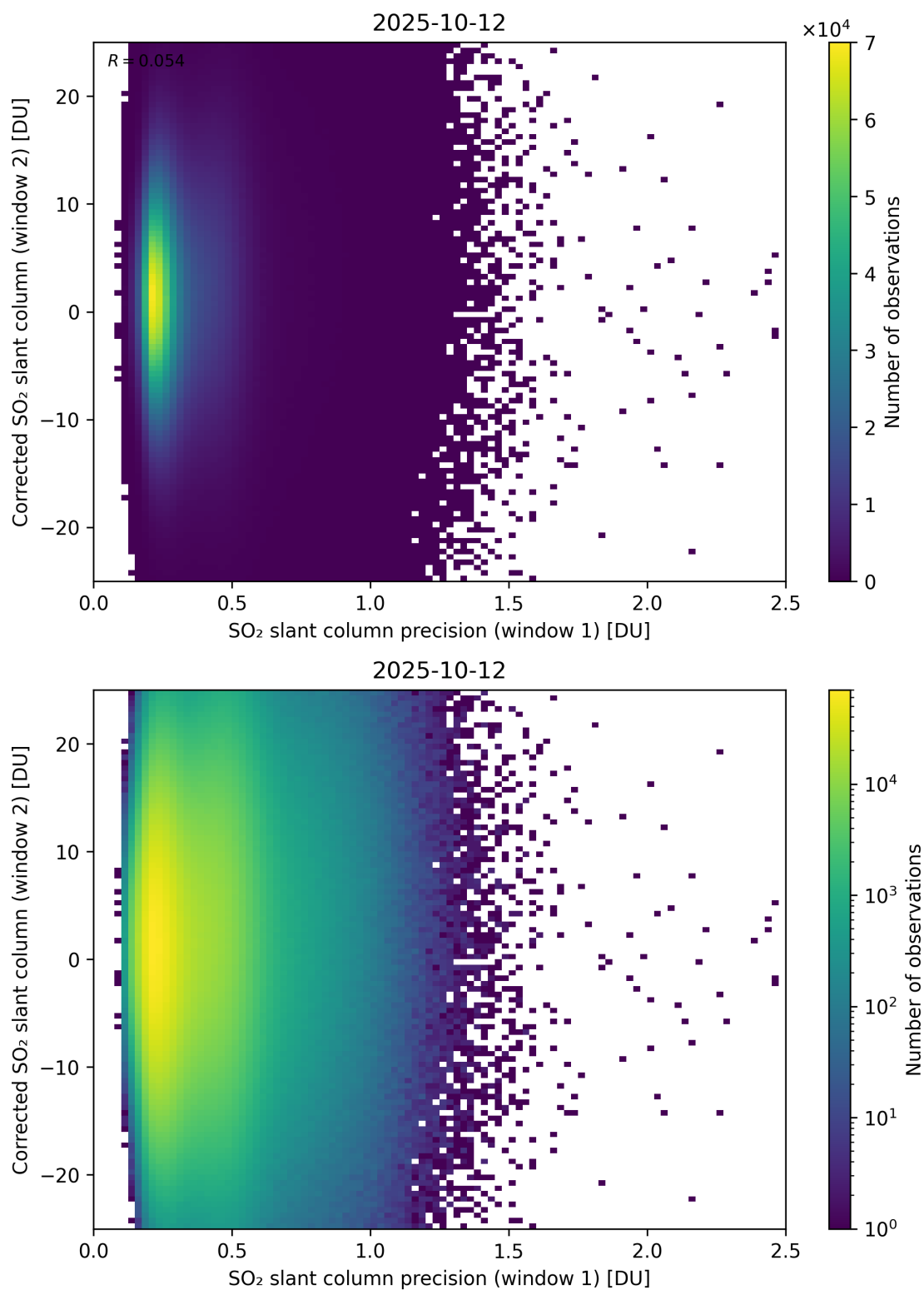
Figure 275: Scatter density plot of “SO 2 slant column precision (window 1)” against “Corrected SO 2 slant column (window 2)” for 2025-10-11 to 2025-10-13.
