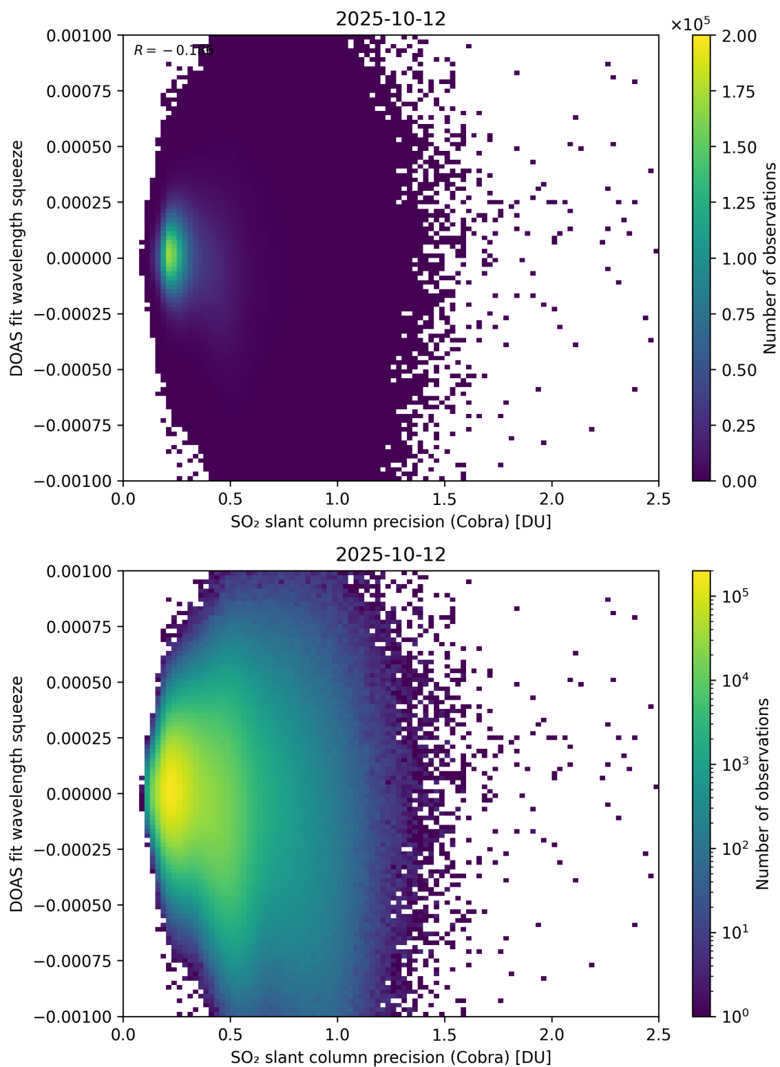
Figure 203: Scatter density plot of “SO 2 slant column precision (Cobra)” against “DOAS fit wavelength squeeze” for 2025-10-11 to 2025-10-13.
