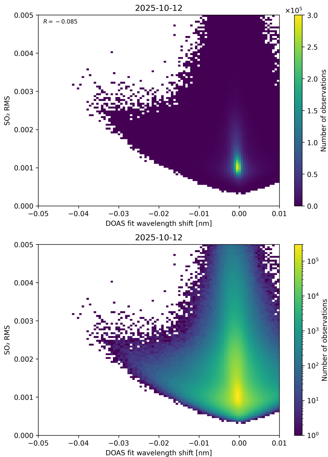
Figure 139: Scatter density plot of “DOAS fit wavelength shift” against “SO 2 RMS” for 2025-10-11 to 2025-10-13.
