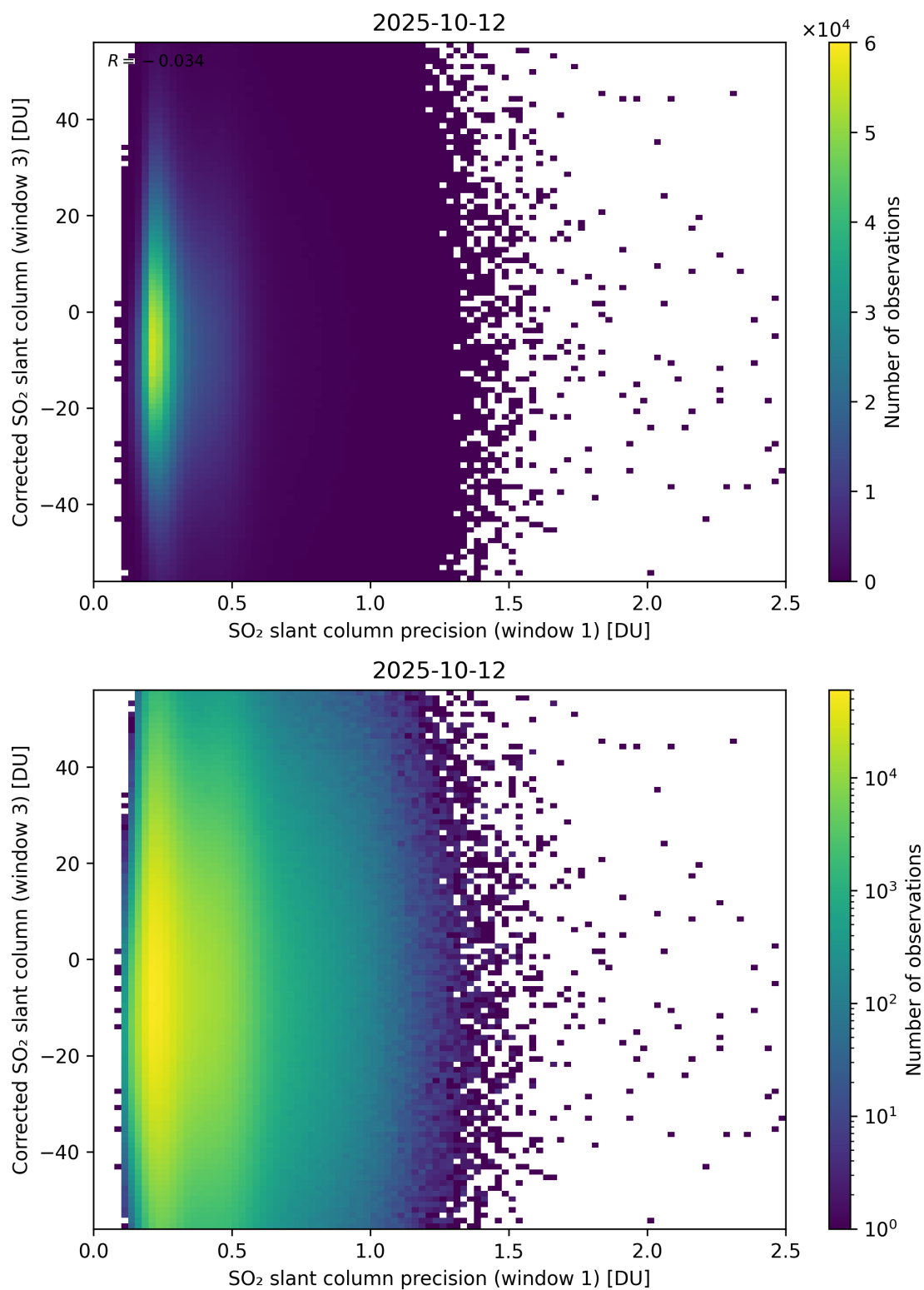
Figure 276: Scatter density plot of “SO 2 slant column precision (window 1)” against “Corrected SO 2 slant column (window 3)” for 2025-10-11 to 2025-10-13.
