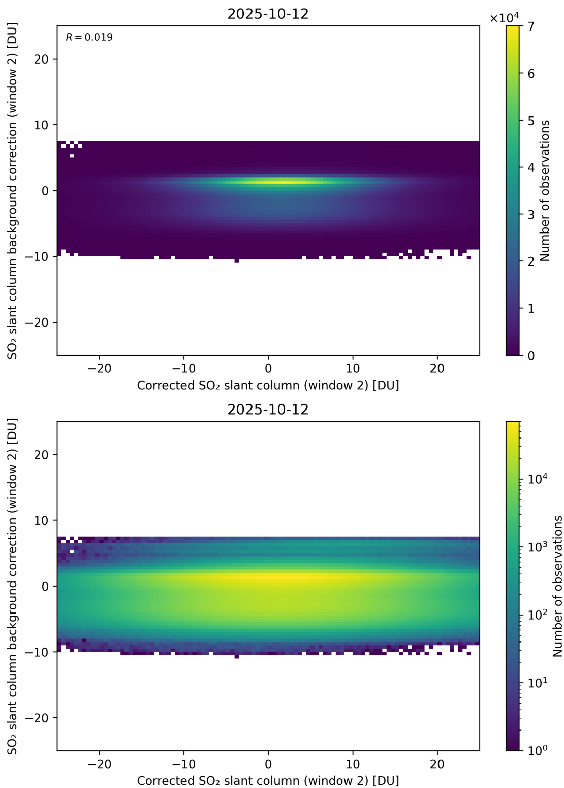
Figure 244: Scatter density plot of “Corrected SO 2 slant column (window 2)” against “SO 2 slant column background correction (window 2)” for 2025-10-11 to 2025-10-13.
