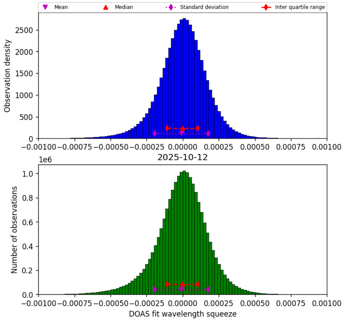
Figure 77: Histogram of “DOAS fit wavelength squeeze” for 2025-10-11 to 2025-10-13
