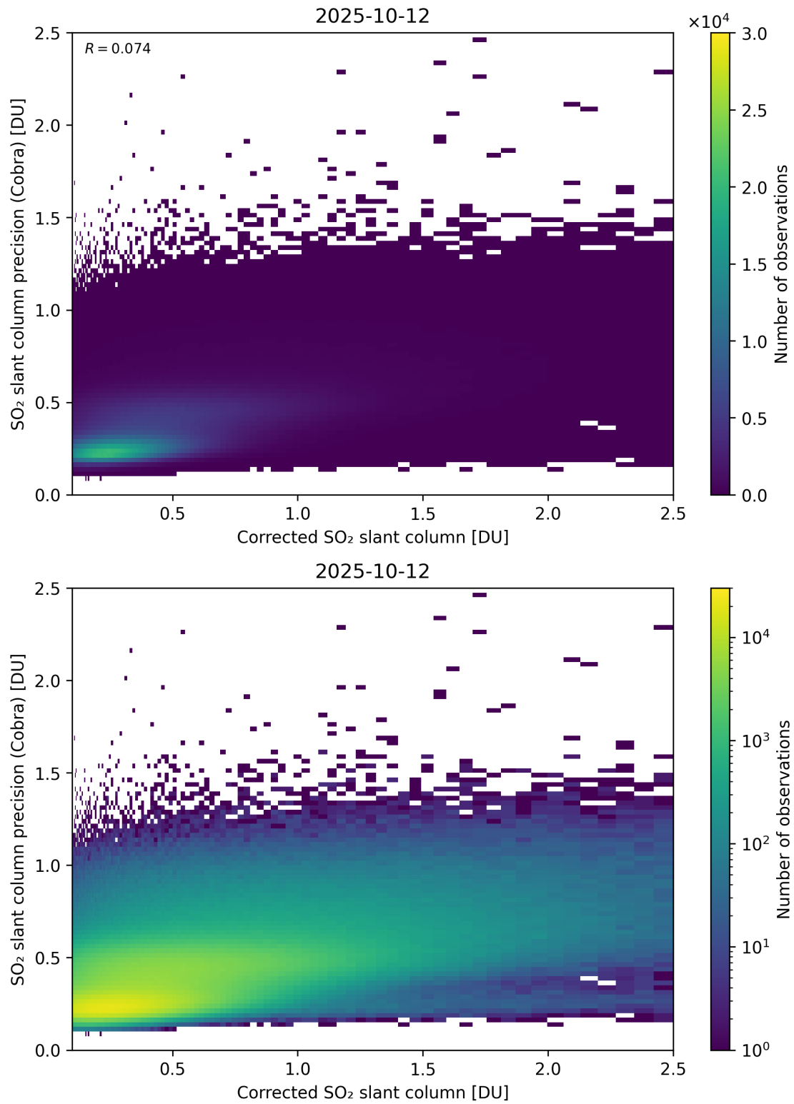
Figure 234: Scatter density plot of “Corrected SO 2 slant column” against “SO 2 slant column precision (Cobra)” for 2025-10-11 to 2025-10-13.
