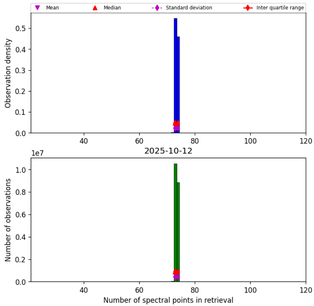
Figure 82: Histogram of “Number of spectral points in retrieval” for 2025-10-11 to 2025-10-13
