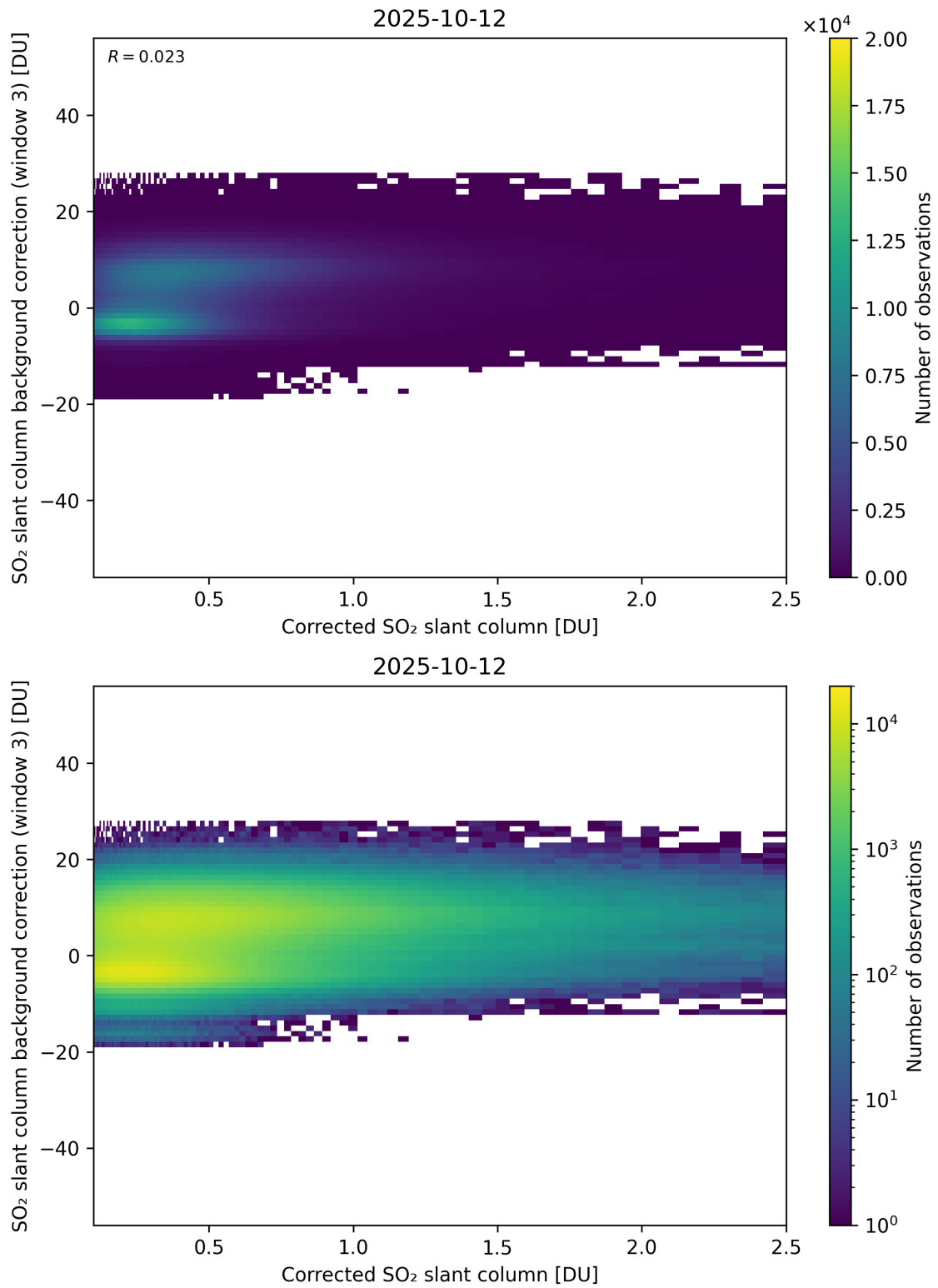
Figure 228: Scatter density plot of “Corrected SO 2 slant column” against “SO 2 slant column background correction (window 3)” for 2025-10-11 to 2025-10-13.
