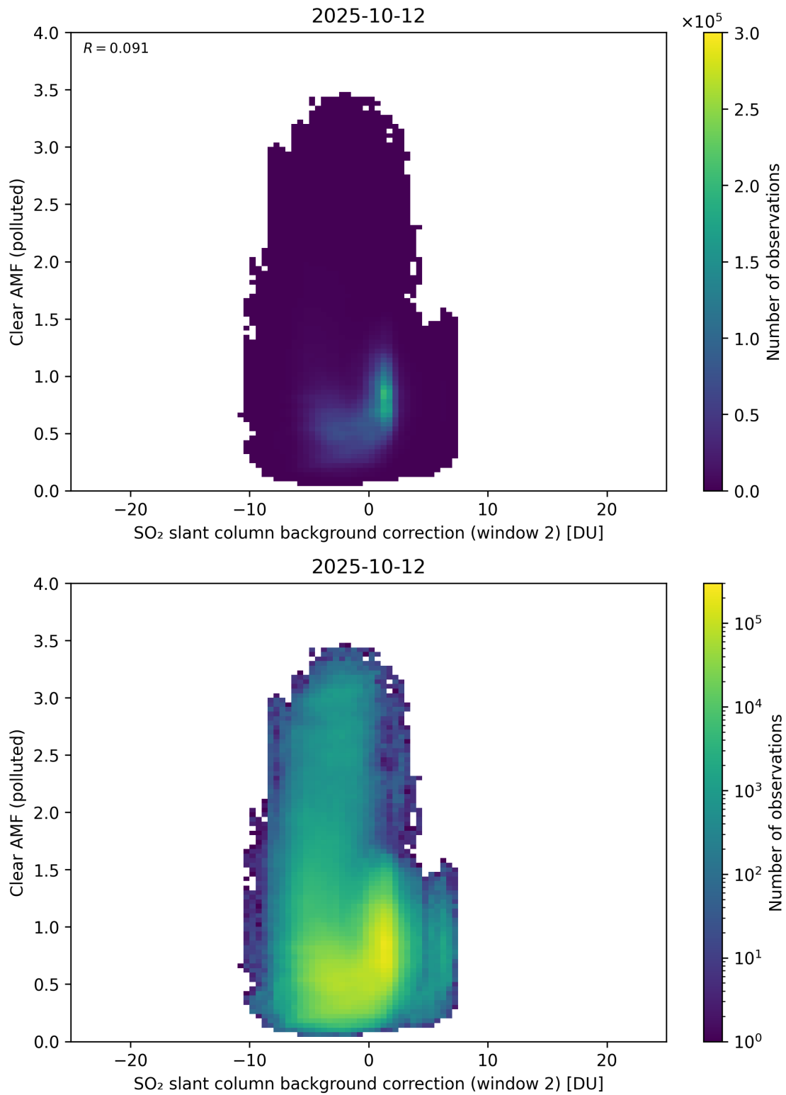
Figure 126: Scatter density plot of “SO 2 slant column background correction (window 2)” against “Clear AMF (polluted)” for 2025-10-11 to 2025-10-13.
