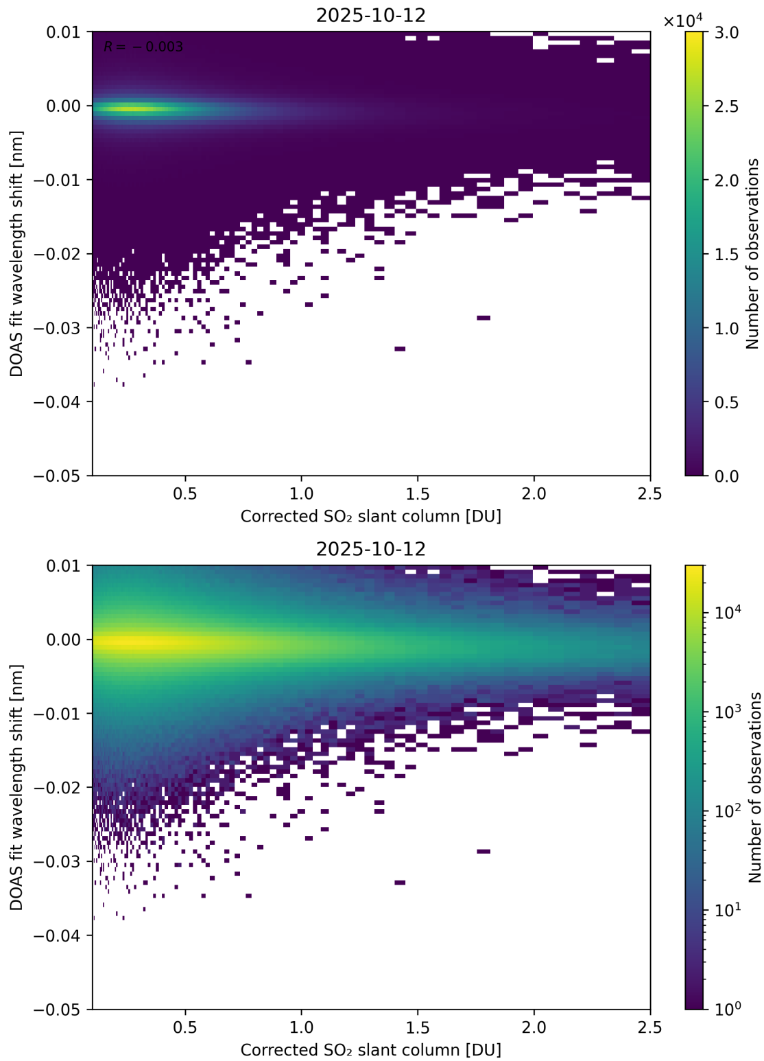
Figure 229: Scatter density plot of “Corrected SO 2 slant column” against “DOAS fit wavelength shift” for 2025-10-11 to 2025-10-13.
