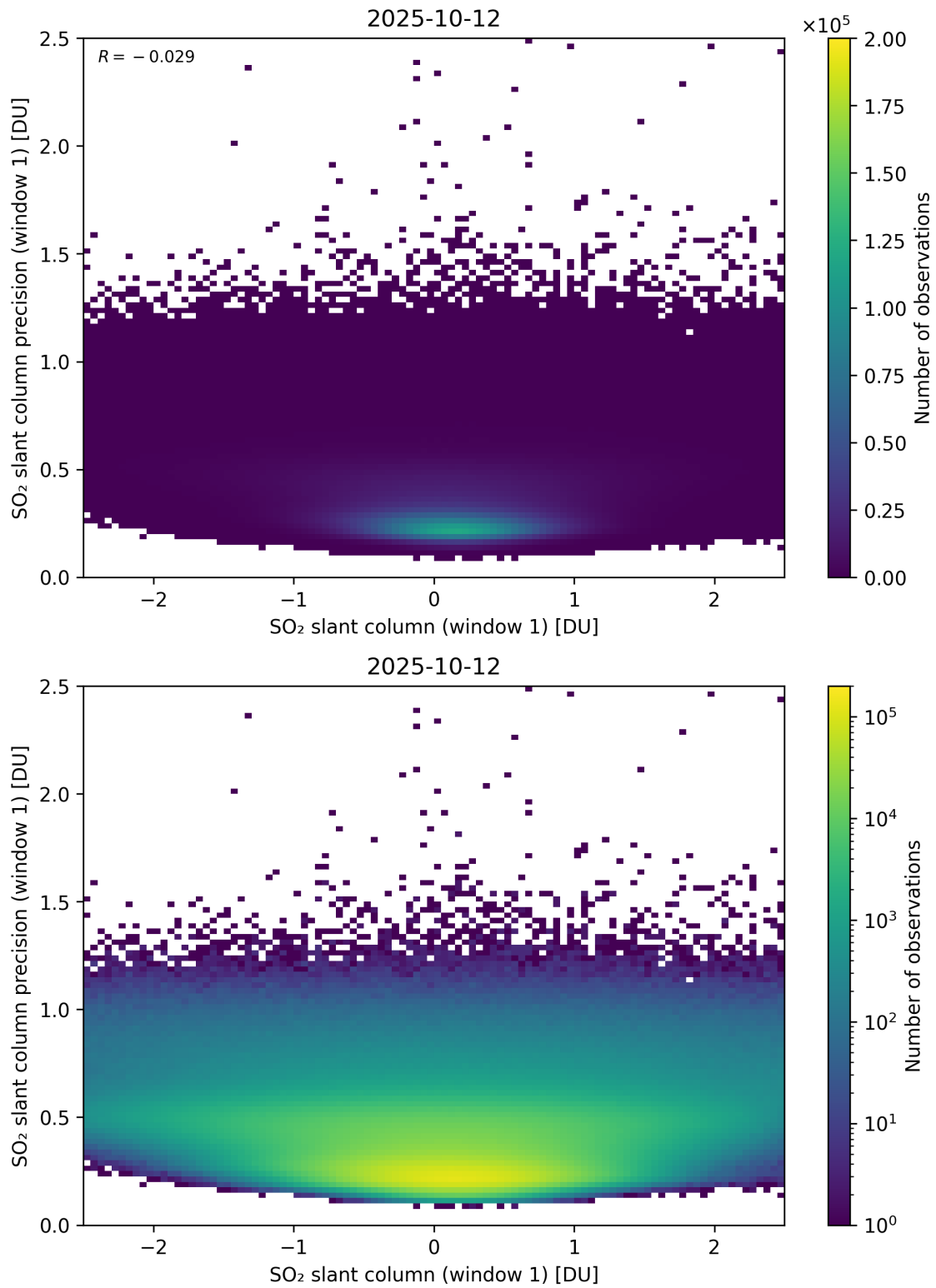
Figure 285: Scatter density plot of “SO 2 slant column (window 1)” against “SO 2 slant column precision (window 1)” for 2025-10-11 to 2025-10-13.
