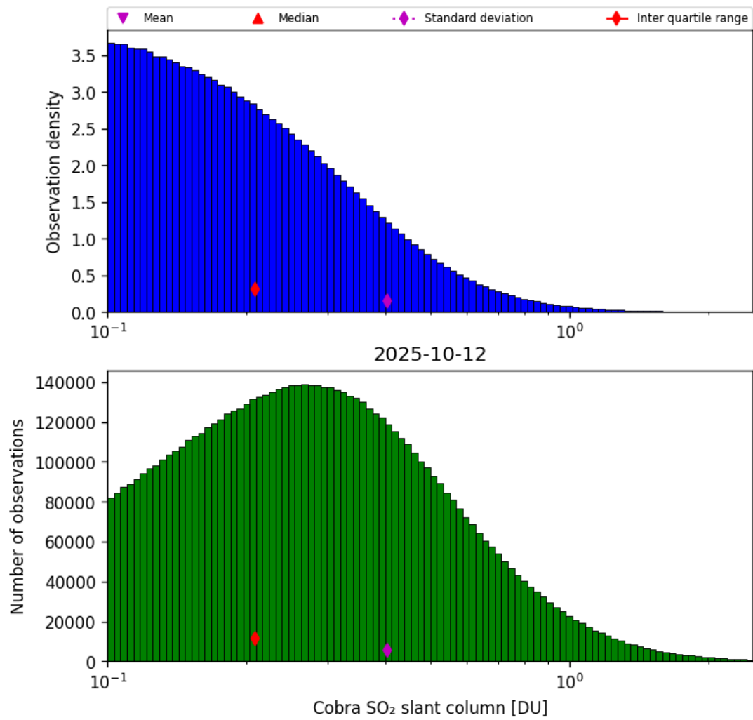
Figure 61: Histogram of “Cobra SO 2 slant column” for 2025-10-11 to 2025-10-13
