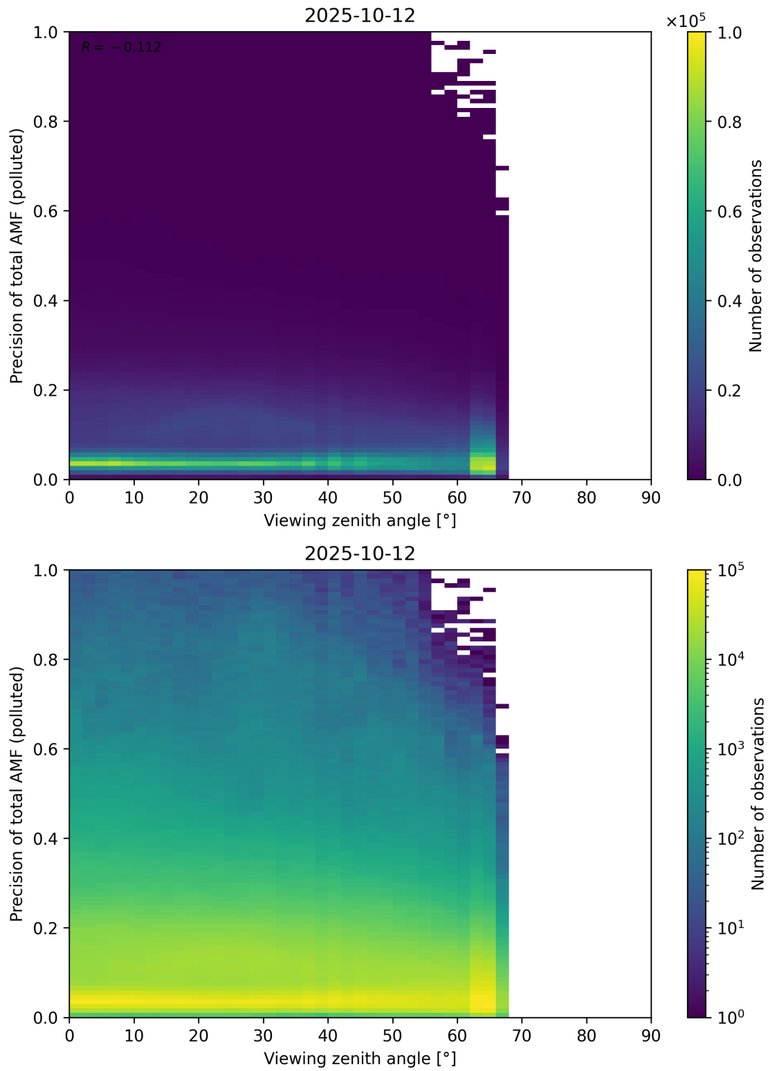
Figure 382: Scatter density plot of “Viewing zenith angle” against “Precision of total AMF (polluted)” for 2025-10-11 to 2025-10-13.
