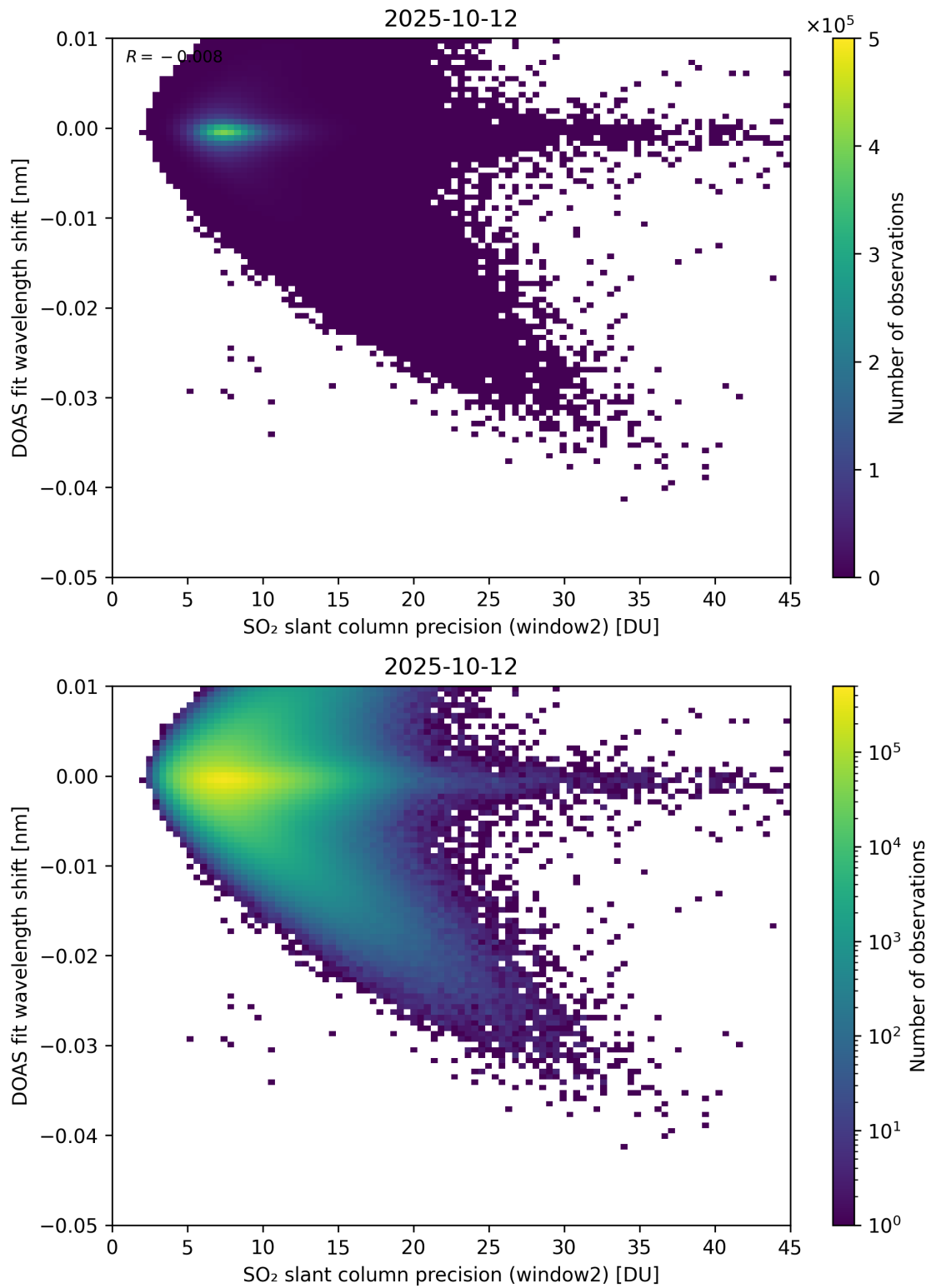
Figure 293: Scatter density plot of “SO 2 slant column precision (window2)” against “DOAS fit wavelength shift” for 2025-10-11 to 2025-10-13.
