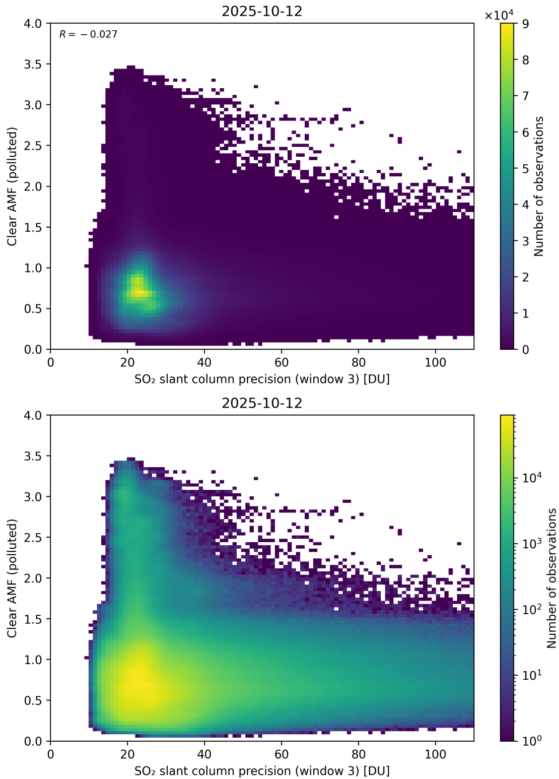
Figure 311: Scatter density plot of “SO 2 slant column precision (window 3)” against “Clear AMF (polluted)” for 2025-10-11 to 2025-10-13.
