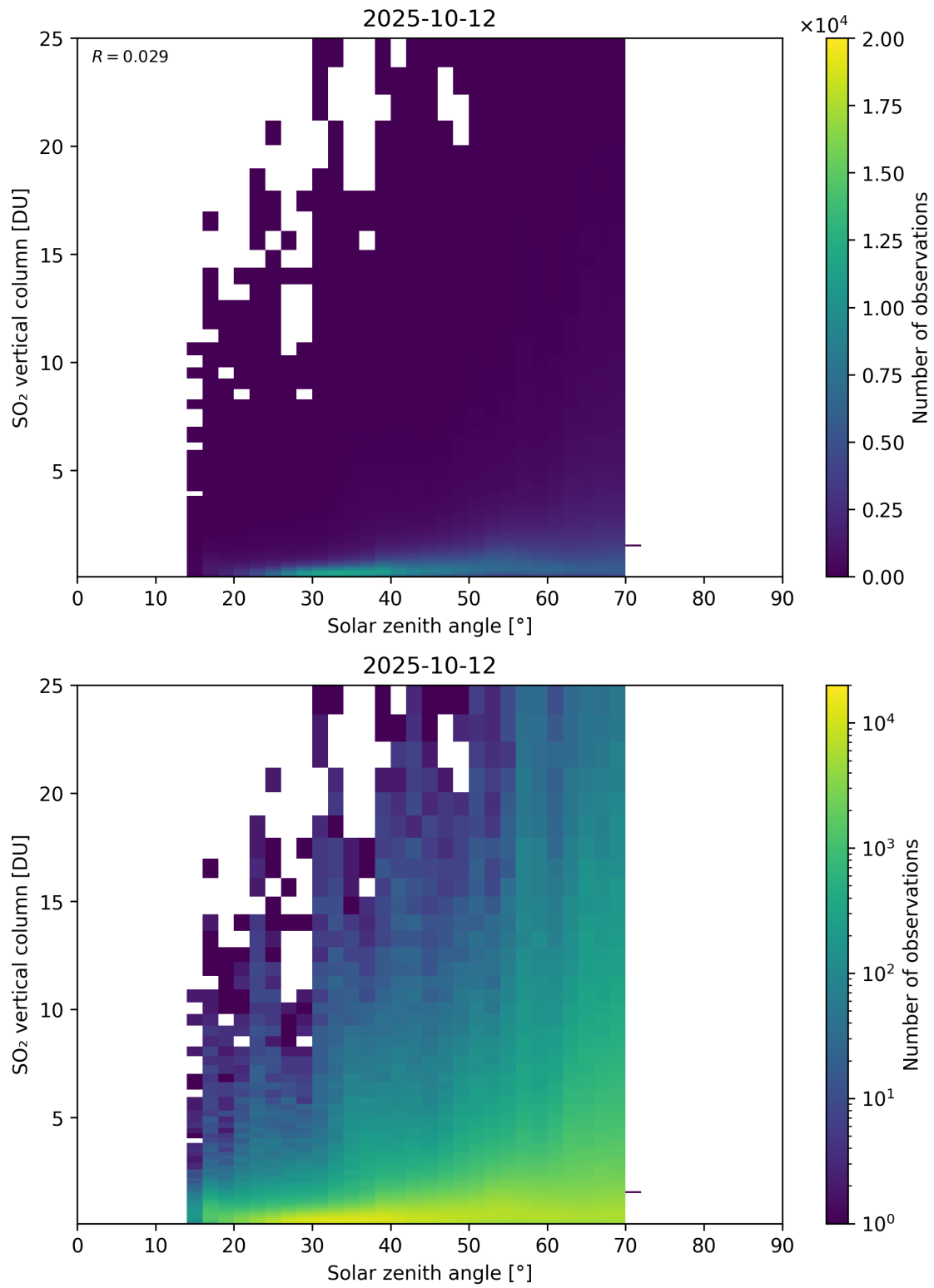
Figure 191: Scatter density plot of “Solar zenith angle” against “SO 2 vertical column” for 2025-10-11 to 2025-10-13.
