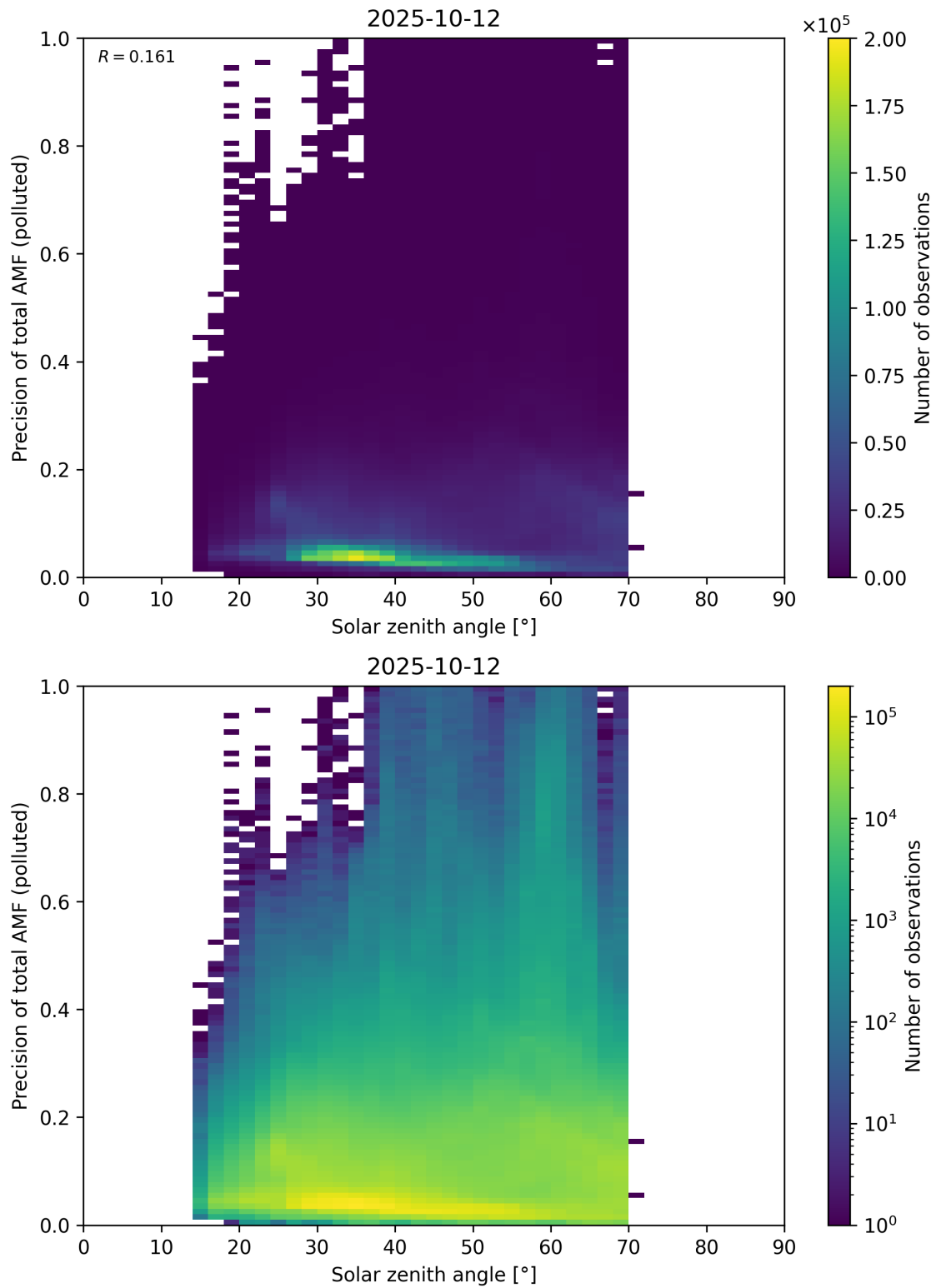
Figure 190: Scatter density plot of “Solar zenith angle” against “Precision of total AMF (polluted)” for 2025-10-11 to 2025-10-13.
