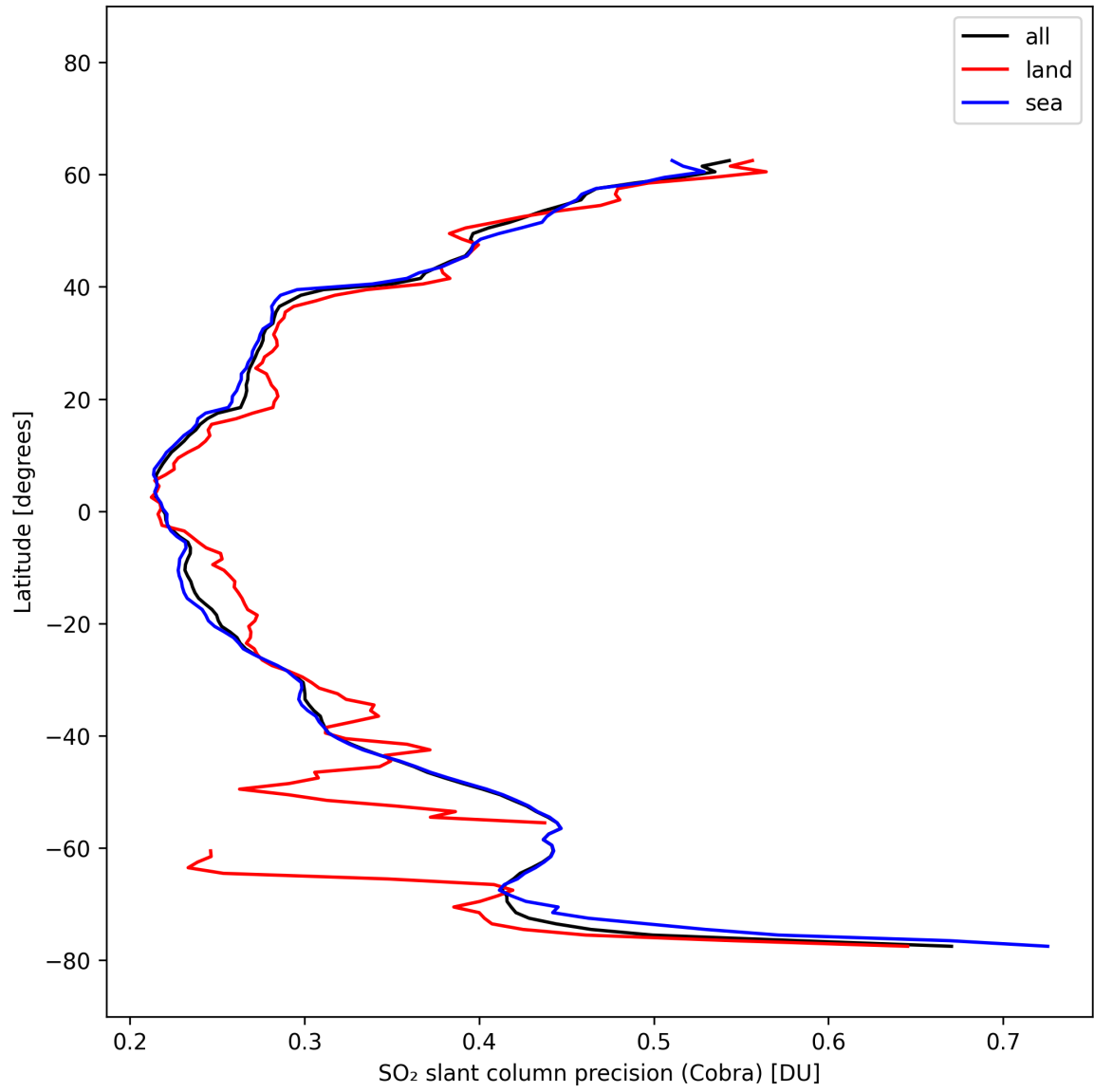
Figure 36: Zonal average of “SO 2 slant column precision (Cobra)” for 2025-10-11 to 2025-10-13.
