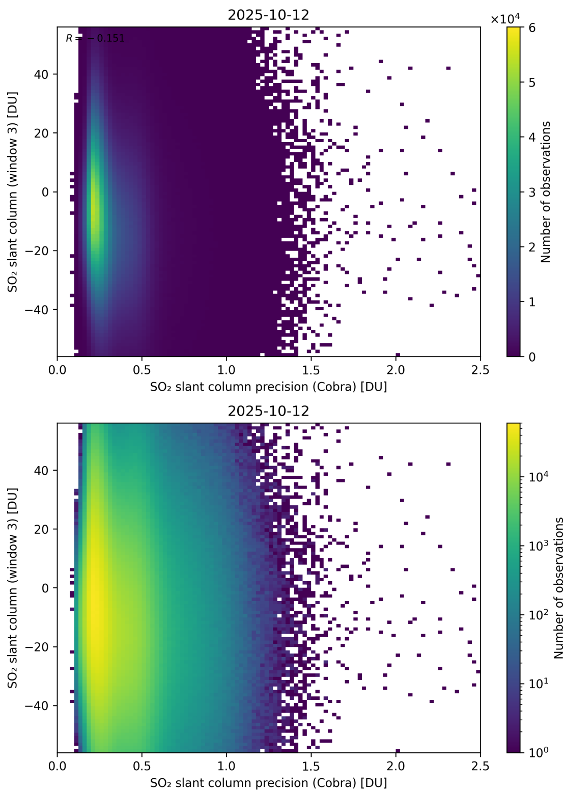
Figure 211: Scatter density plot of “SO 2 slant column precision (Cobra)” against “SO 2 slant column (window 3)” for 2025-10-11 to 2025-10-13.
