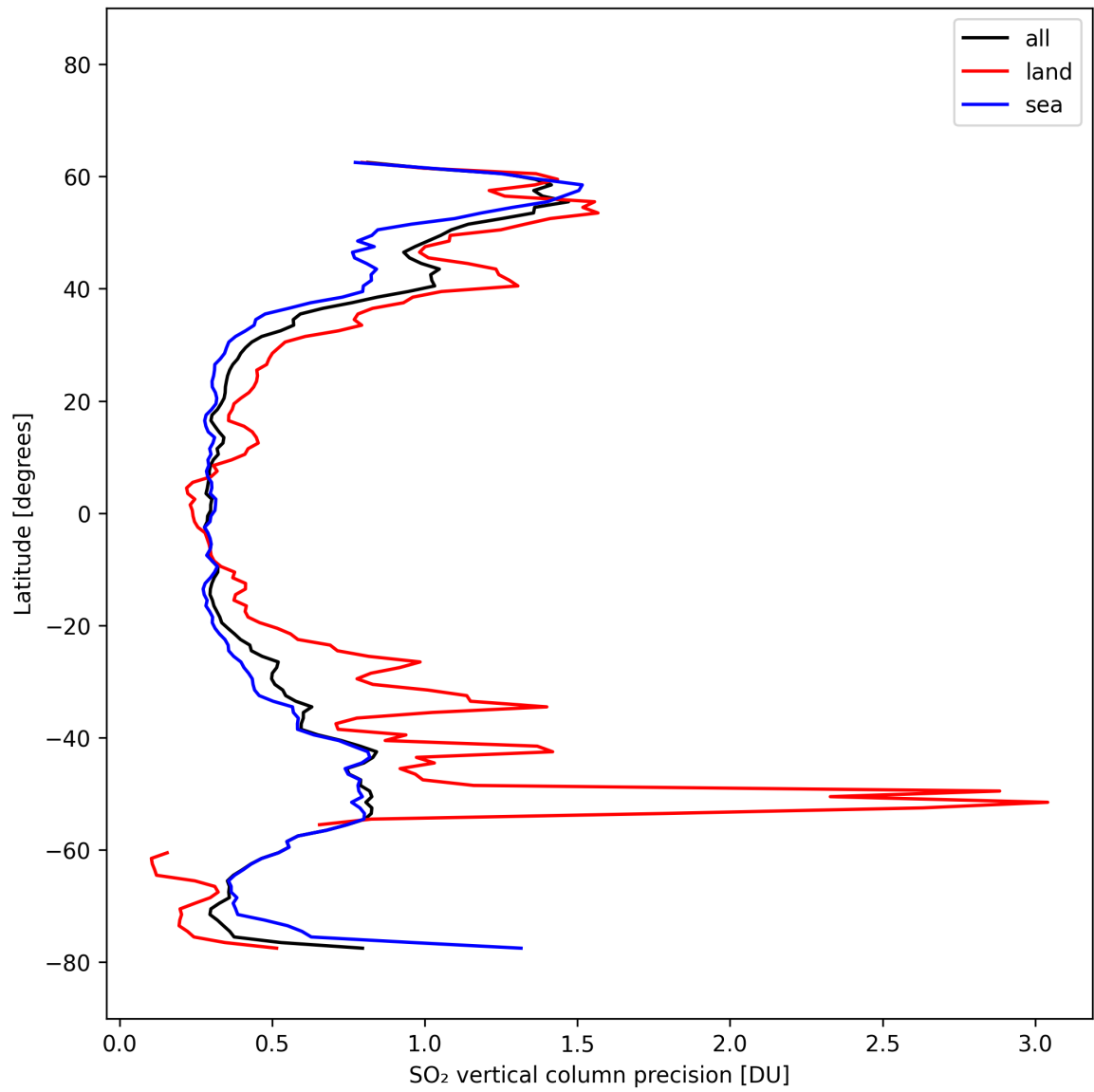
Figure 33: Zonal average of “SO 2 vertical column precision” for 2025-10-11 to 2025-10-13.
