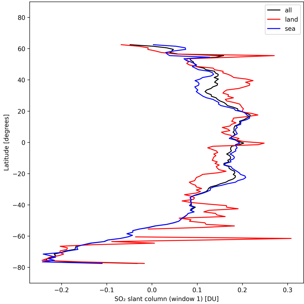
Figure 37: Zonal average of “SO 2 slant column (window 1)” for 2025-10-11 to 2025-10-13.
