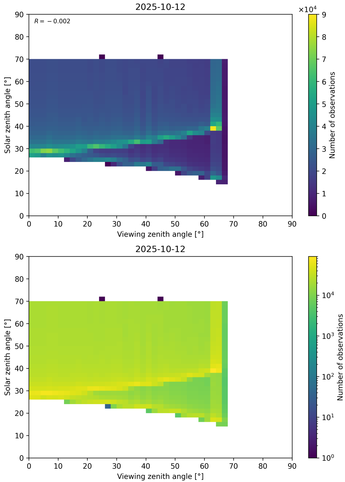
Figure 369: Scatter density plot of “Viewing zenith angle” against “Solar zenith angle” for 2025-10-11 to 2025-10-13.
