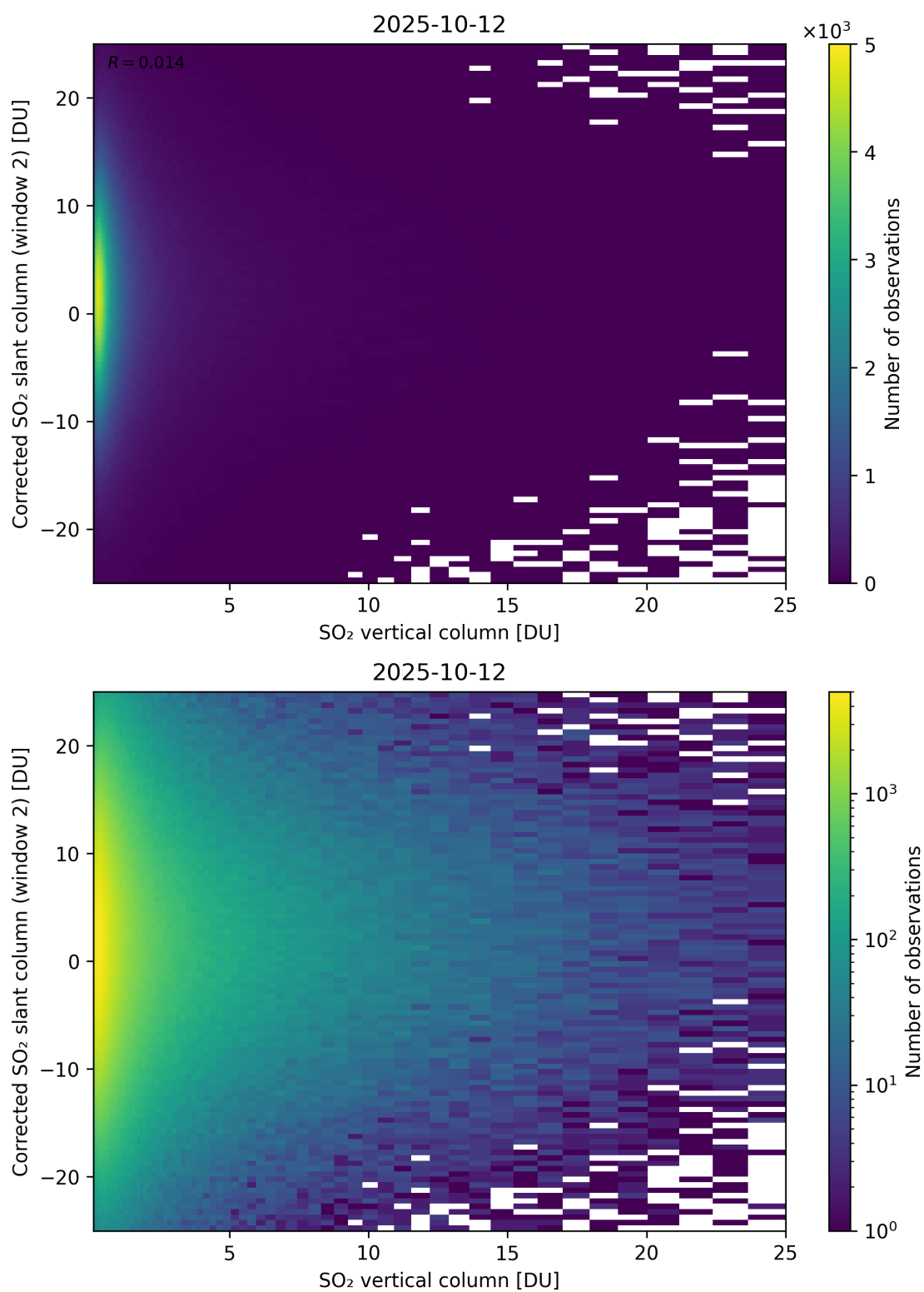
Figure 352: Scatter density plot of “SO 2 vertical column” against “Corrected SO 2 slant column (window 2)” for 2025-10-11 to 2025-10-13.
