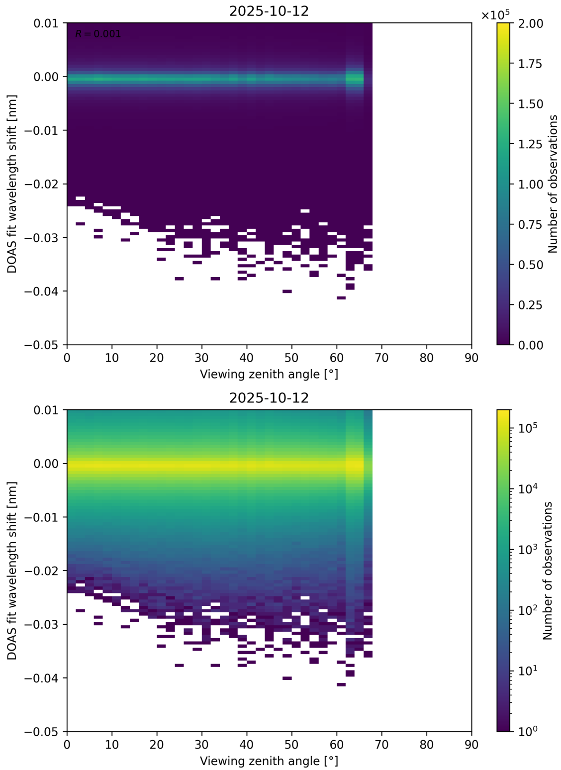
Figure 365: Scatter density plot of “Viewing zenith angle” against “DOAS fit wavelength shift” for 2025-10-11 to 2025-10-13.
