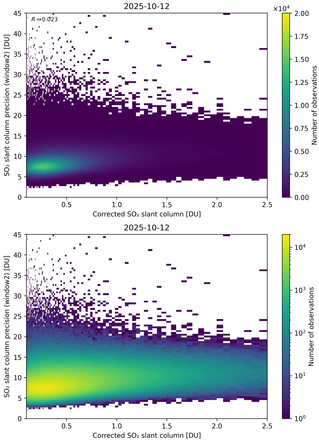
Figure 239: Scatter density plot of “Corrected SO 2 slant column” against “SO 2 slant column precision (window2)” for 2025-10-11 to 2025-10-13.
