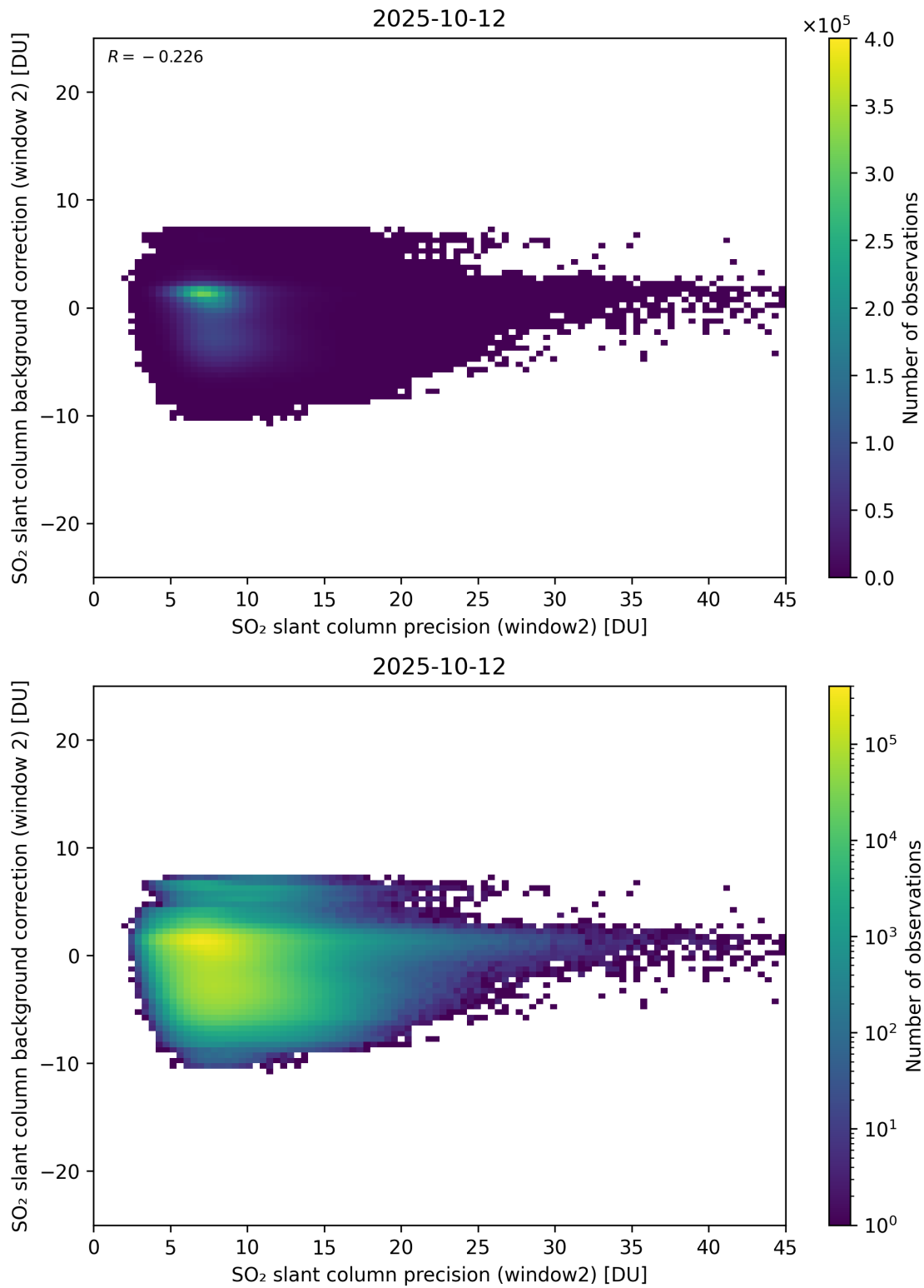
Figure 291: Scatter density plot of “SO 2 slant column precision (window2)” against “SO 2 slant column background correction (window 2)” for 2025-10-11 to 2025-10-13.
