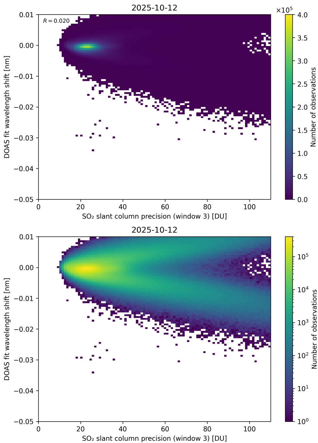
Figure 308: Scatter density plot of “SO 2 slant column precision (window 3)” against “DOAS fit wavelength shift” for 2025-10-11 to 2025-10-13.
