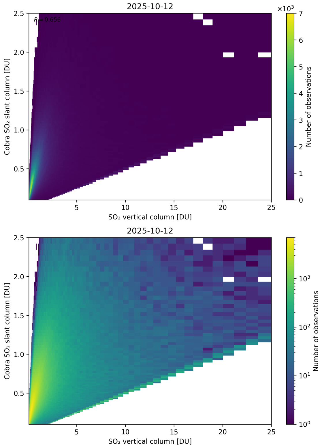
Figure 349: Scatter density plot of “SO 2 vertical column” against “Cobra SO 2 slant column” for 2025-10-11 to 2025-10-13.
