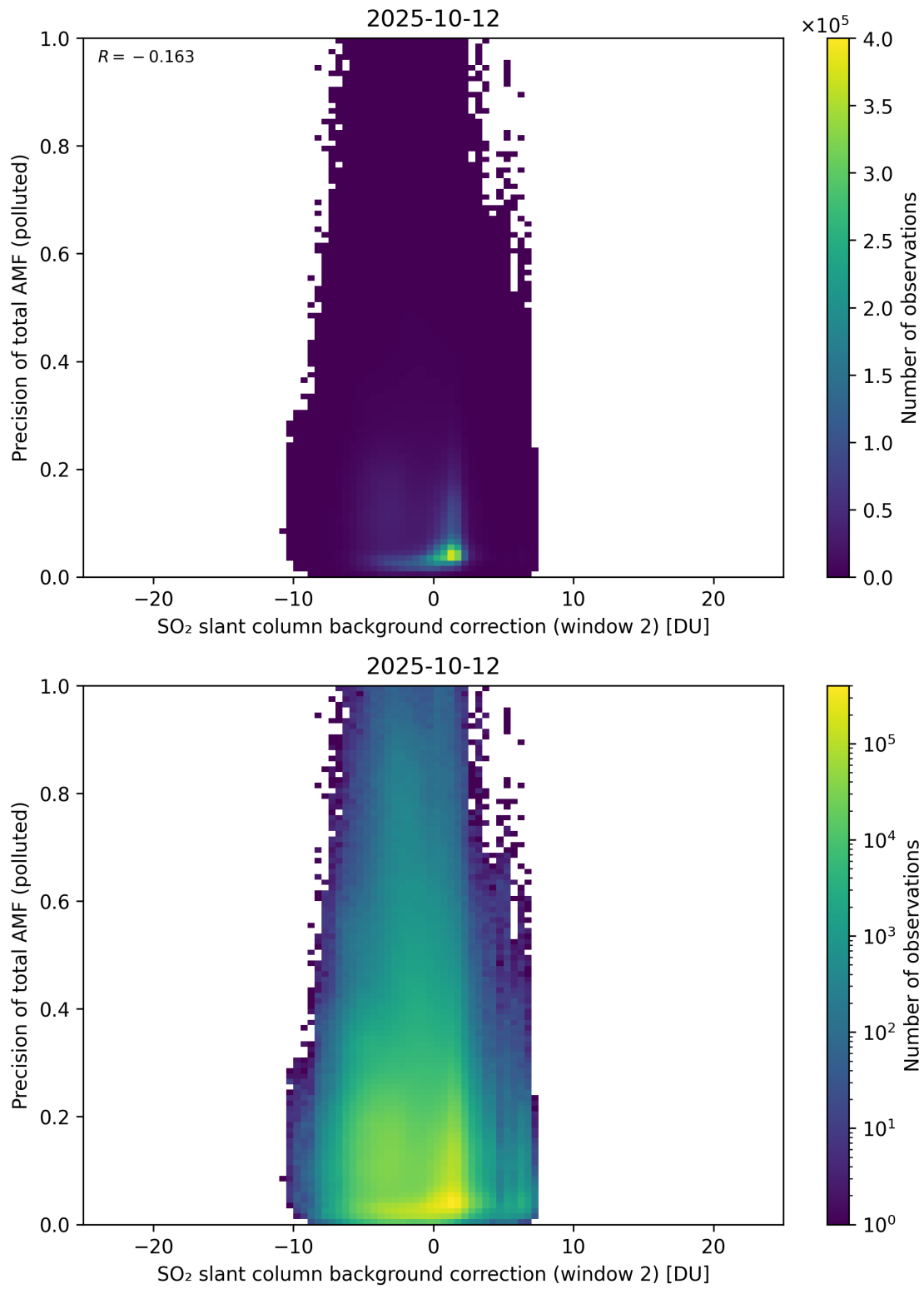
Figure 131: Scatter density plot of “SO 2 slant column background correction (window 2)” against “Precision of total AMF (polluted)” for 2025-10-11 to 2025-10-13.
