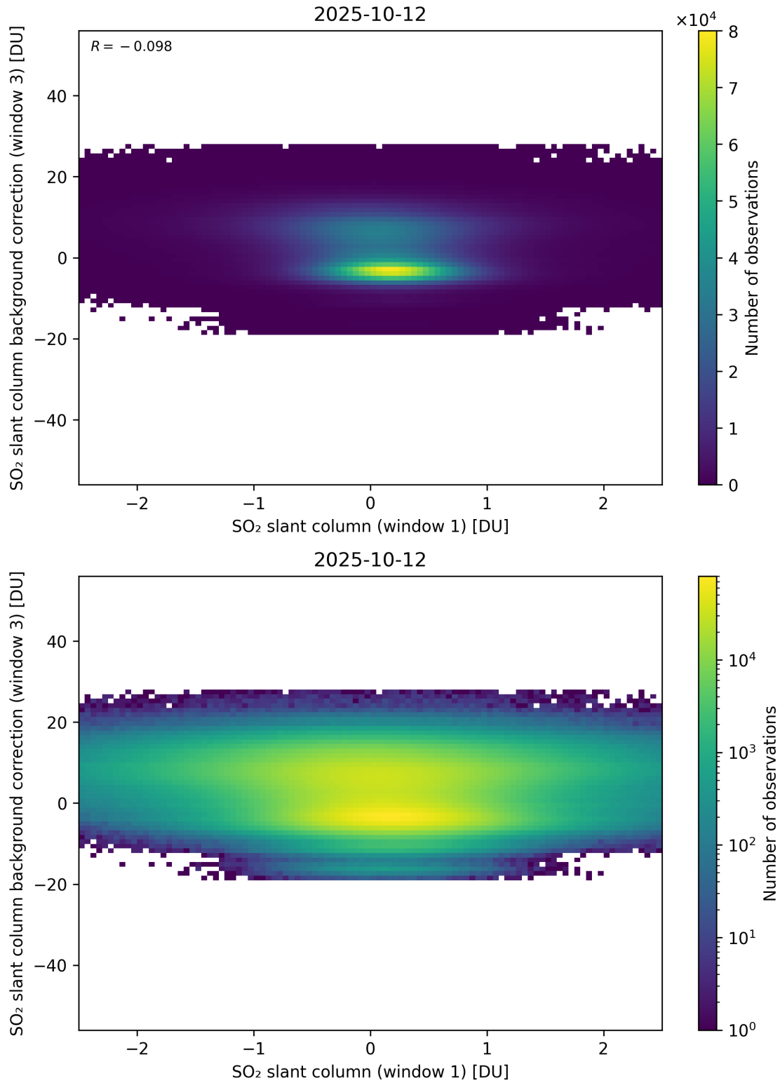
Figure 264: Scatter density plot of “SO 2 slant column (window 1)” against “SO 2 slant column background correction (window 3)” for 2025-10-11 to 2025-10-13.
