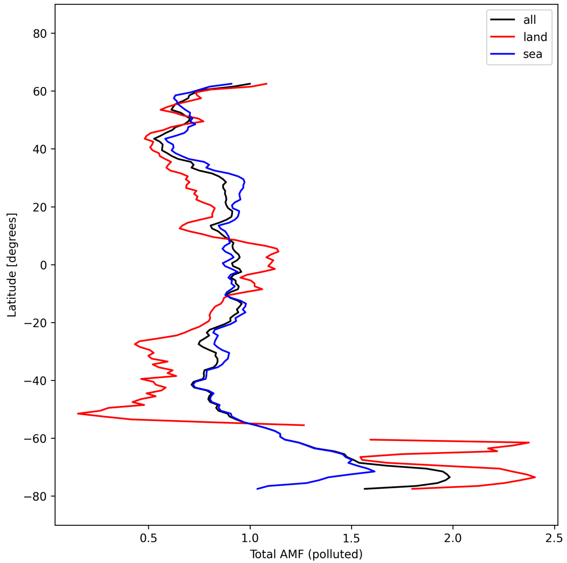
Figure 53: Zonal average of “Total AMF (polluted)” for 2025-10-11 to 2025-10-13.
