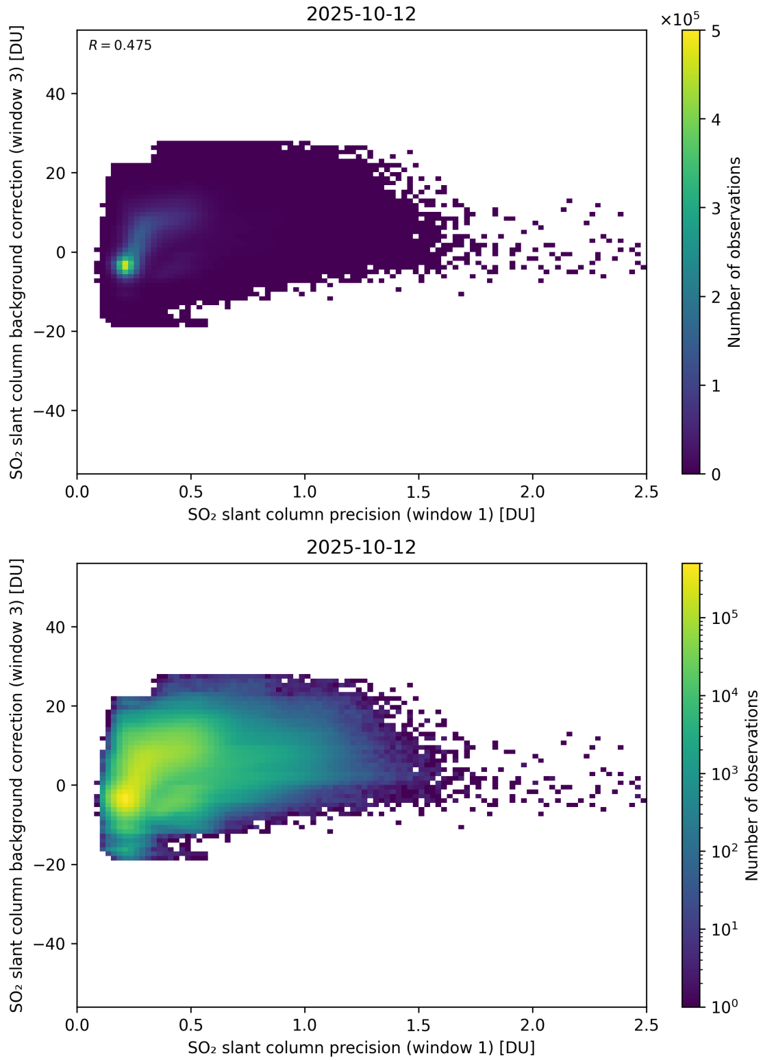
Figure 270: Scatter density plot of “SO 2 slant column precision (window 1)” against “SO 2 slant column background correction (window 3)” for 2025-10-11 to 2025-10-13.
