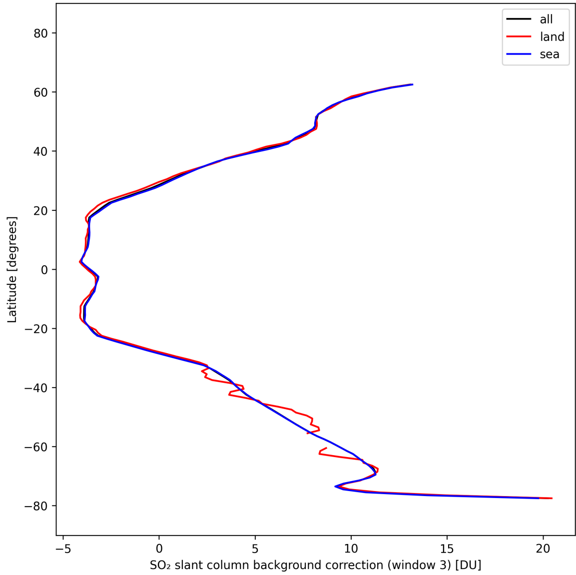
Figure 48: Zonal average of “SO 2 slant column background correction (window 3)” for 2025-10-11 to 2025-10-13.
