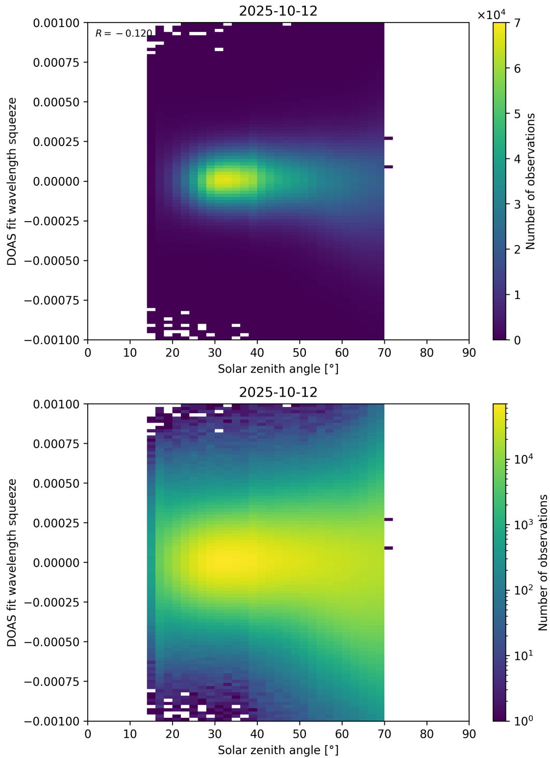
Figure 175: Scatter density plot of “Solar zenith angle” against “DOAS fit wavelength squeeze” for 2025-10-11 to 2025-10-13.
