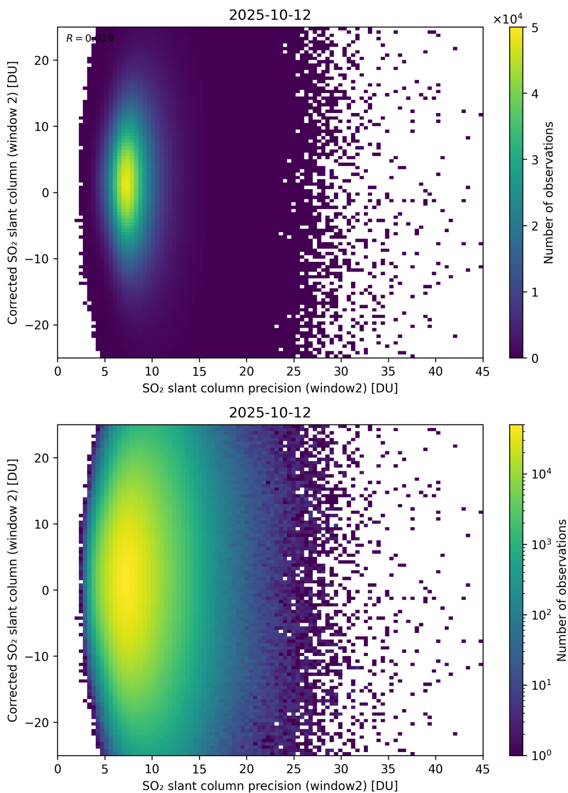
Figure 297: Scatter density plot of “SO 2 slant column precision (window2)” against “Corrected SO 2 slant column (window 2)” for 2025-10-11 to 2025-10-13.
