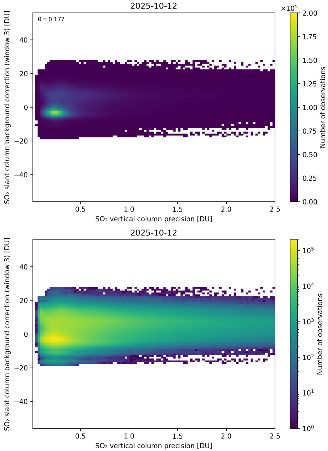
Figure 331: Scatter density plot of “SO 2 vertical column precision” against “SO 2 slant column background correction (window 3)” for 2025-10-11 to 2025-10-13.
