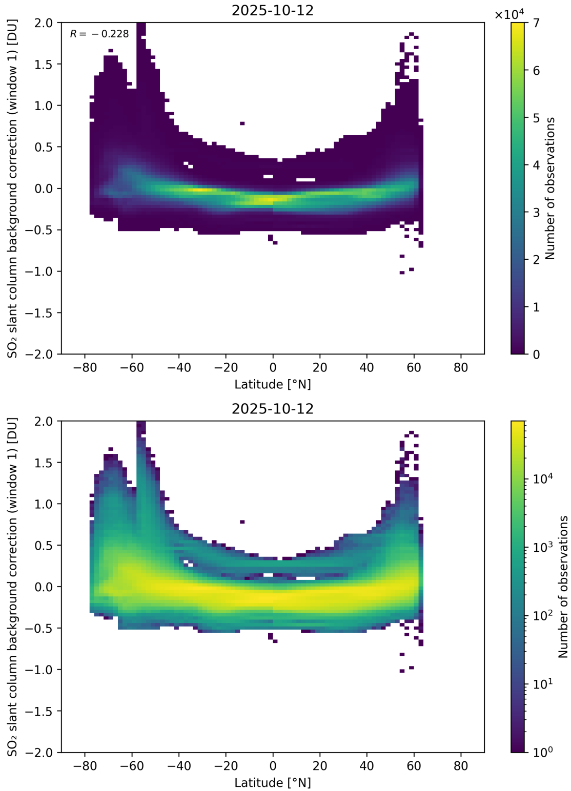
Figure 150: Scatter density plot of “Latitude” against “SO 2 slant column background correction (window 1)” for 2025-10-11 to 2025-10-13.
