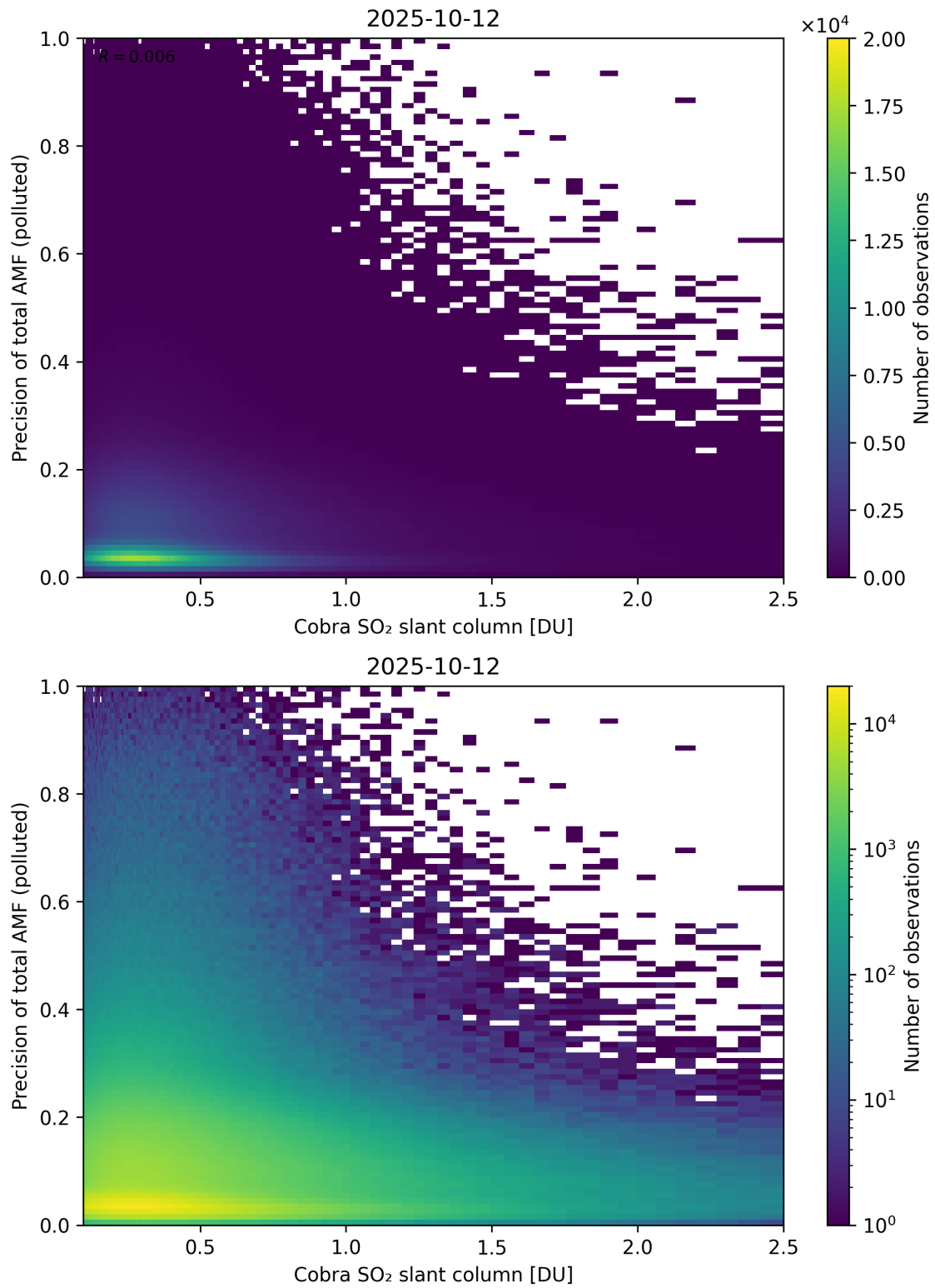
Figure 225: Scatter density plot of “Cobra SO 2 slant column” against “Precision of total AMF (polluted)” for 2025-10-11 to 2025-10-13.
