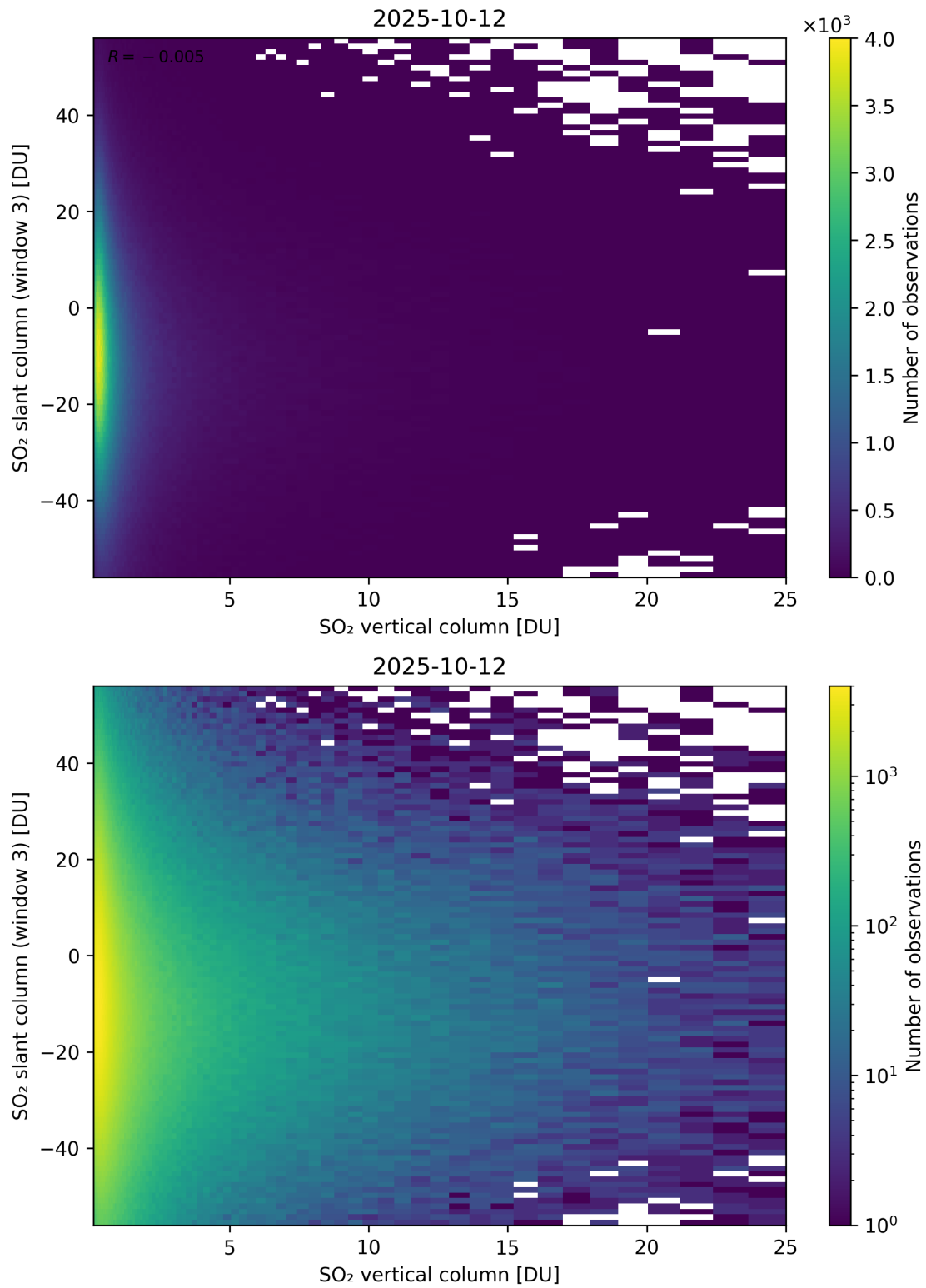
Figure 357: Scatter density plot of “SO 2 vertical column” against “SO 2 slant column (window 3)” for 2025-10-11 to 2025-10-13.
