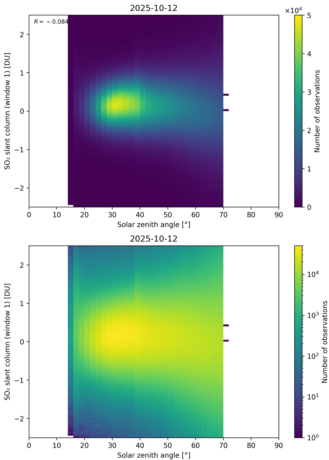
Figure 184: Scatter density plot of “Solar zenith angle” against “SO 2 slant column (window 1)” for 2025-10-11 to 2025-10-13.
