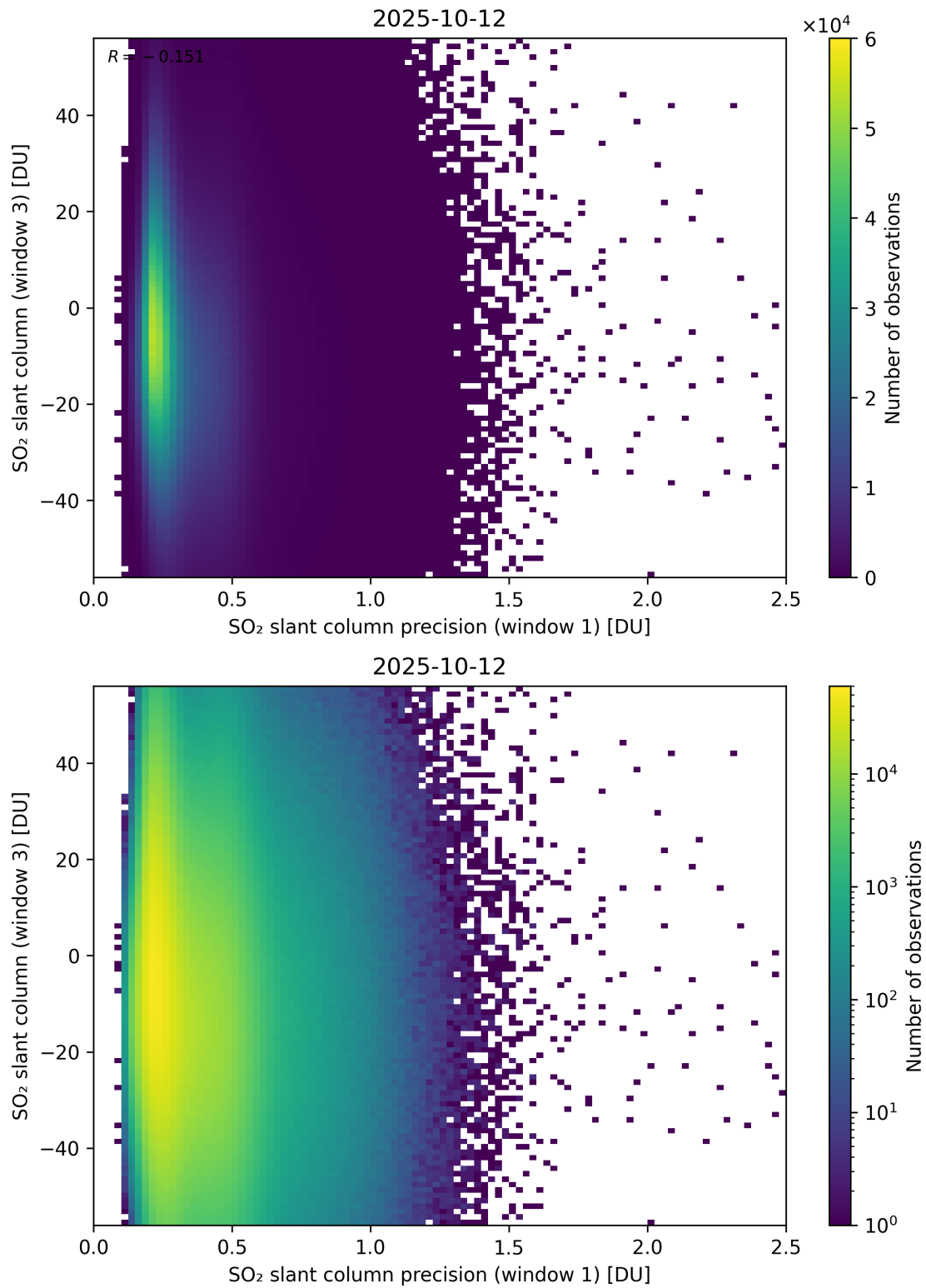
Figure 278: Scatter density plot of “SO 2 slant column precision (window 1)” against “SO 2 slant column (window 3)” for 2025-10-11 to 2025-10-13.
