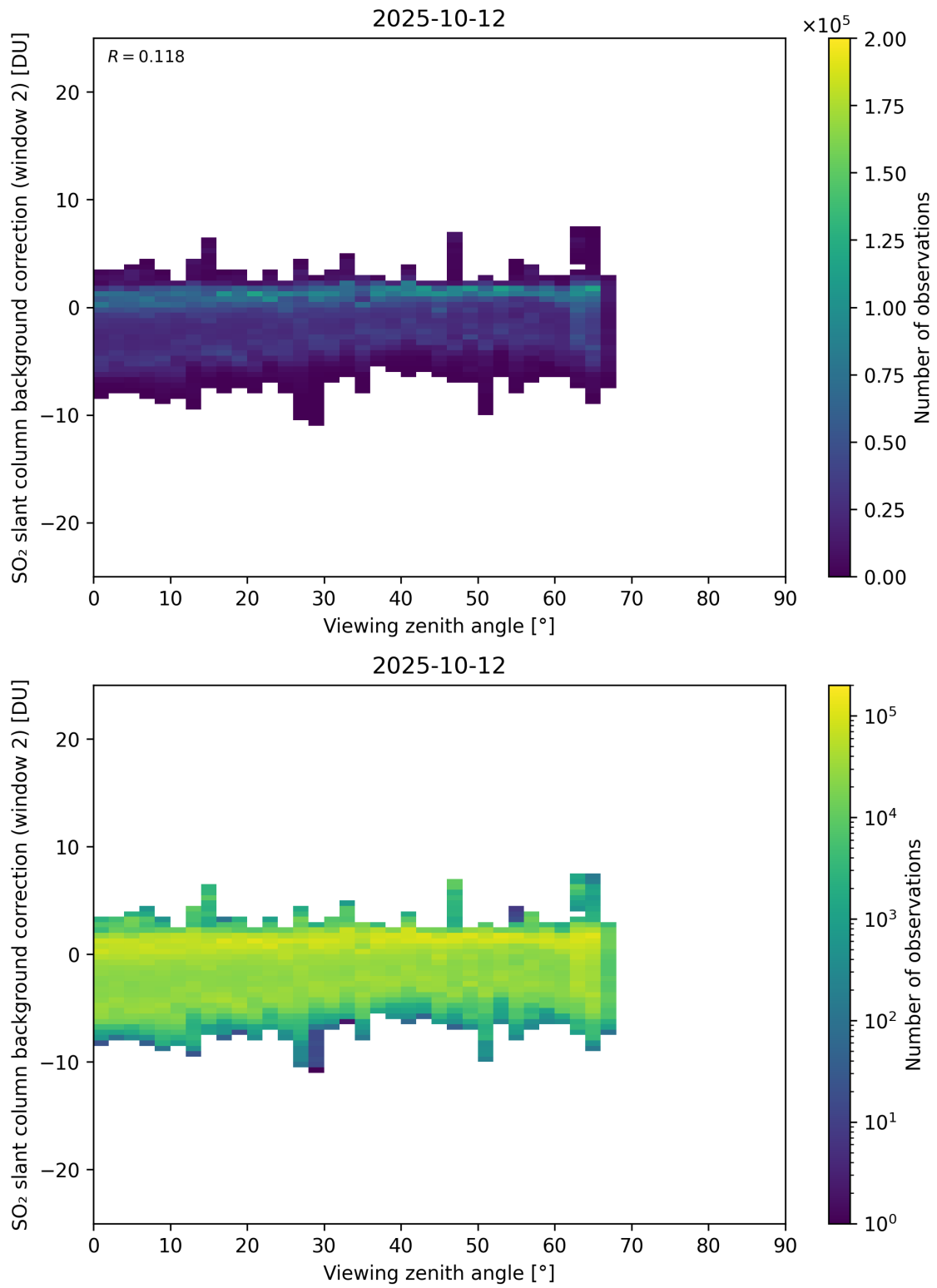
Figure 363: Scatter density plot of “Viewing zenith angle” against “SO 2 slant column background correction (window 2)” for 2025-10-11 to 2025-10-13.
