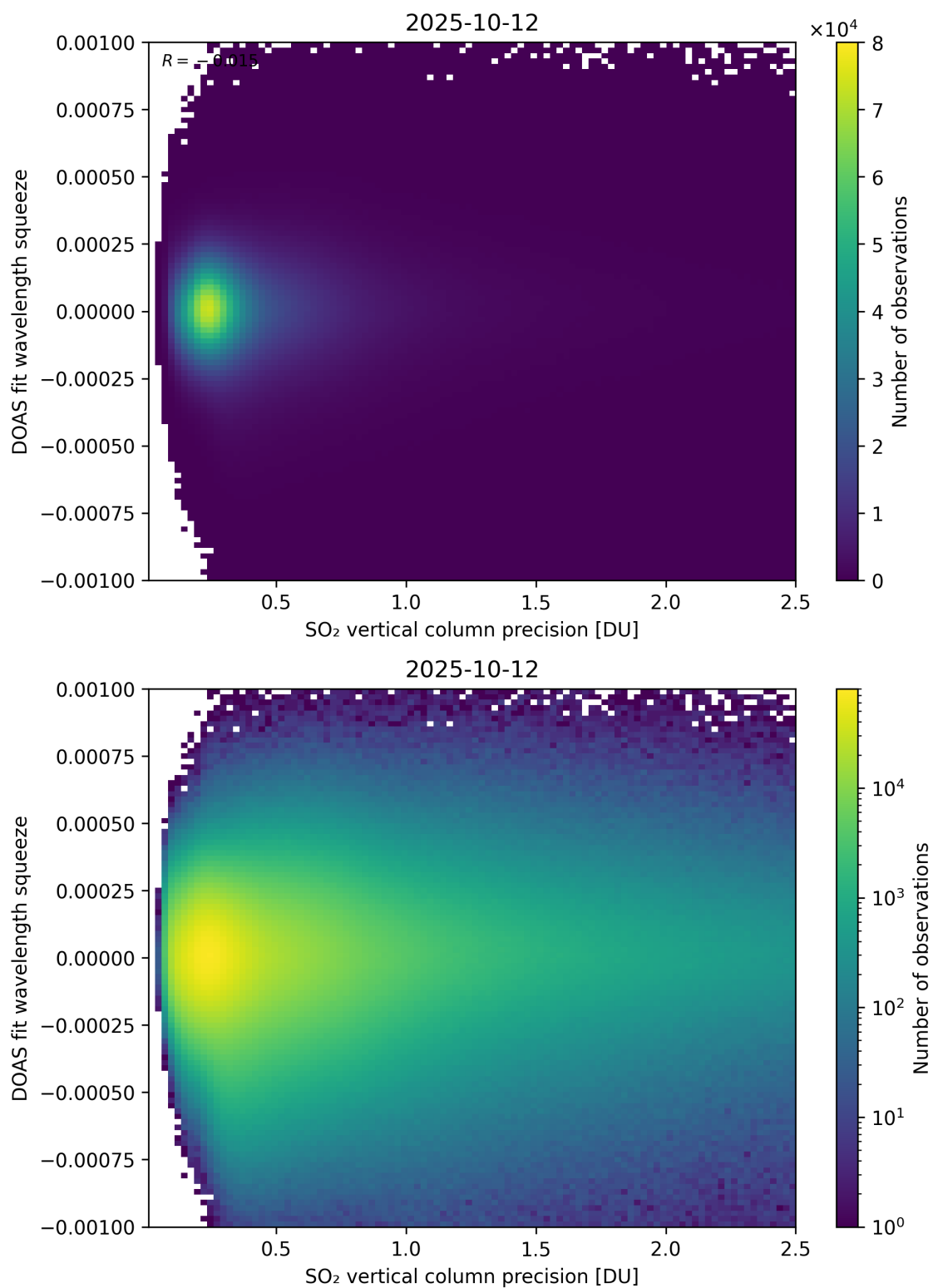
Figure 333: Scatter density plot of “SO 2 vertical column precision” against “DOAS fit wavelength squeeze” for 2025-10-11 to 2025-10-13.
