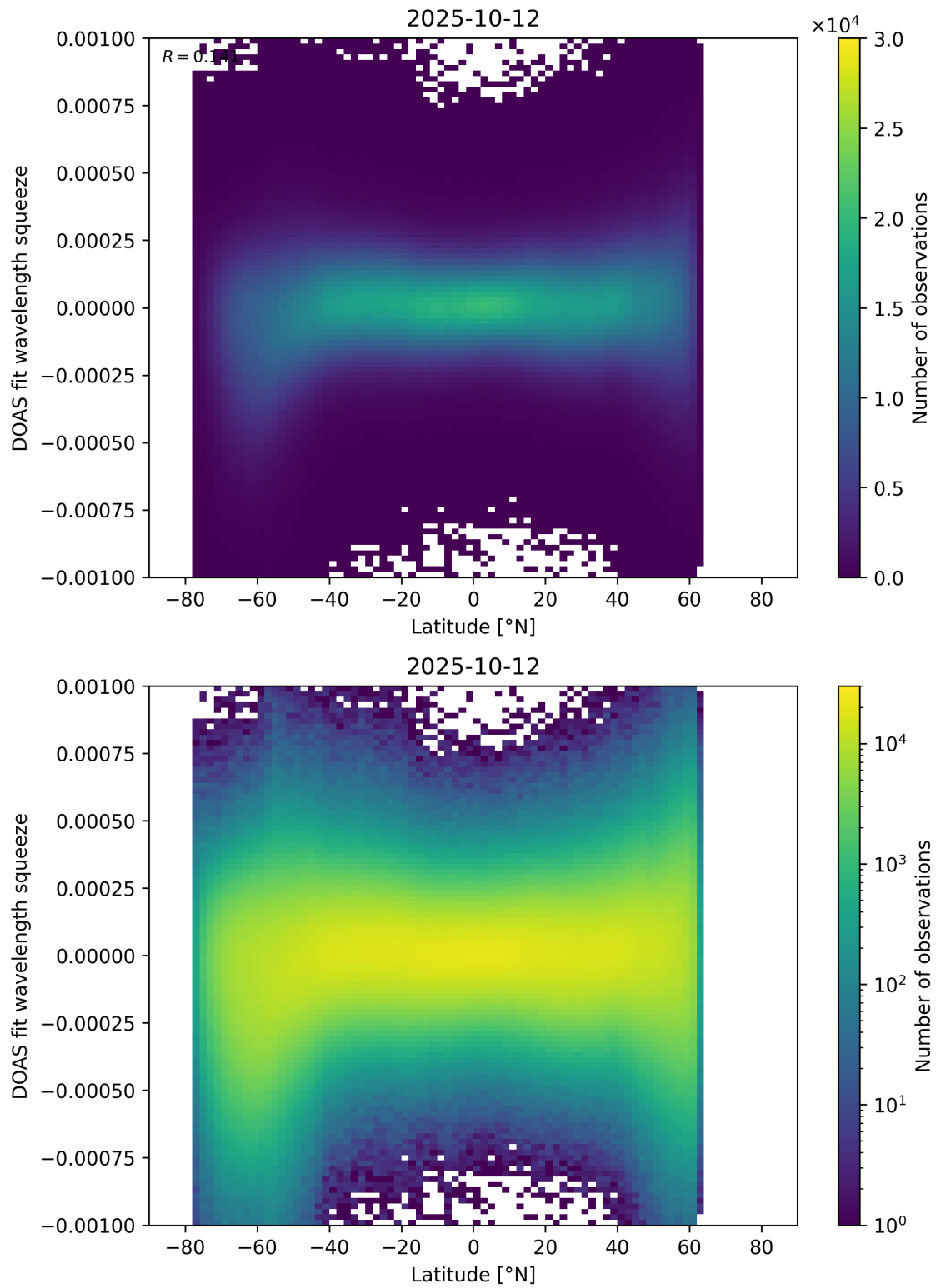
Figure 154: Scatter density plot of “Latitude” against “DOAS fit wavelength squeeze” for 2025-10-11 to 2025-10-13.
