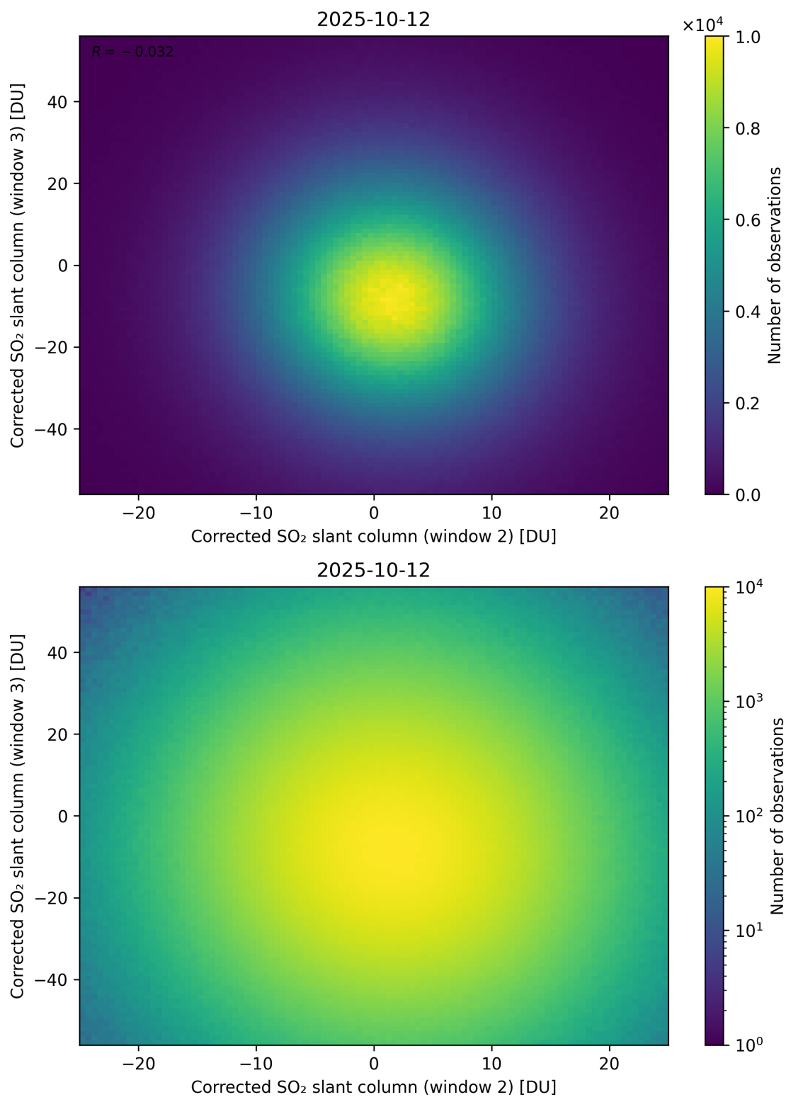
Figure 250: Scatter density plot of “Corrected SO 2 slant column (window 2)” against “Corrected SO 2 slant column (window 3)” for 2025-10-11 to 2025-10-13.
