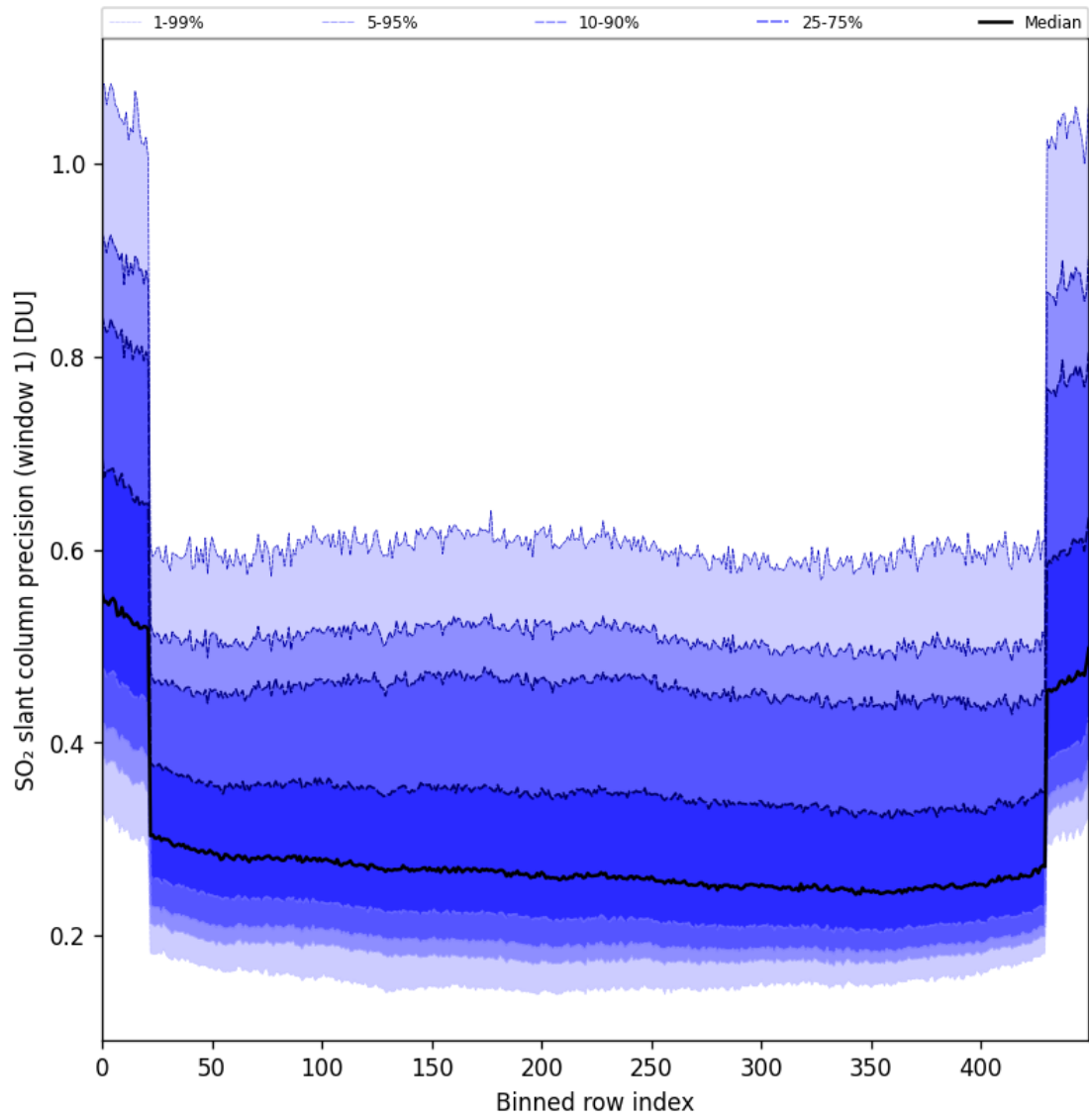
Figure 90: Along track statistics of “SO 2 slant column precision (window 1)” for 2025-10-11 to 2025-10-13
