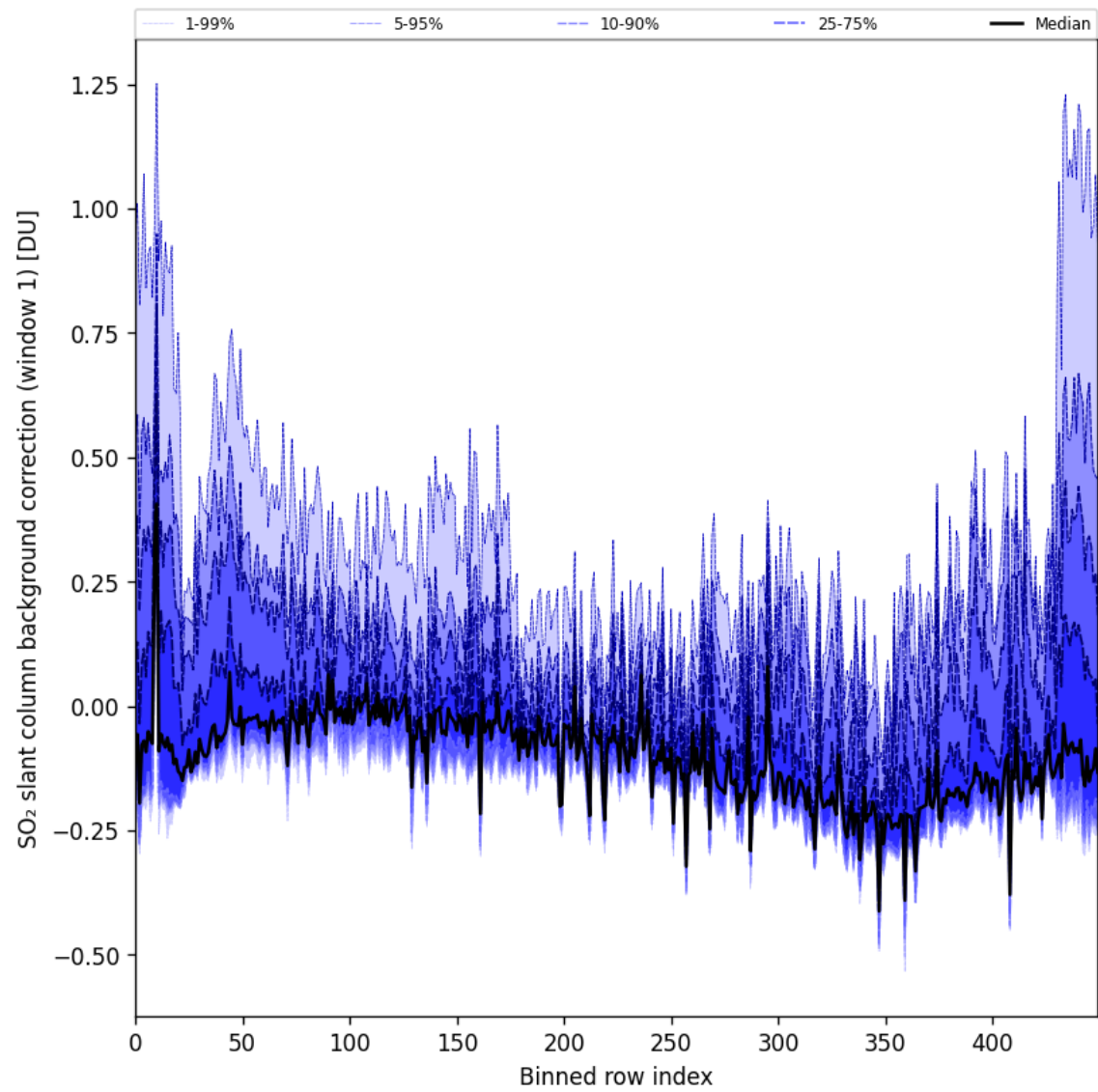
Figure 92: Along track statistics of “SO 2 slant column background correction (window 1)” for 2025-10-11 to 2025-10-13
