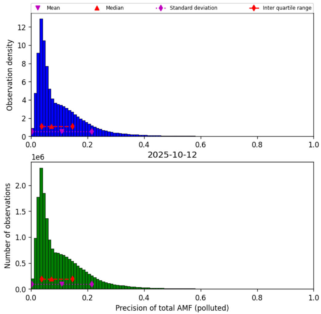
Figure 80: Histogram of “Precision of total AMF (polluted)” for 2025-10-11 to 2025-10-13
