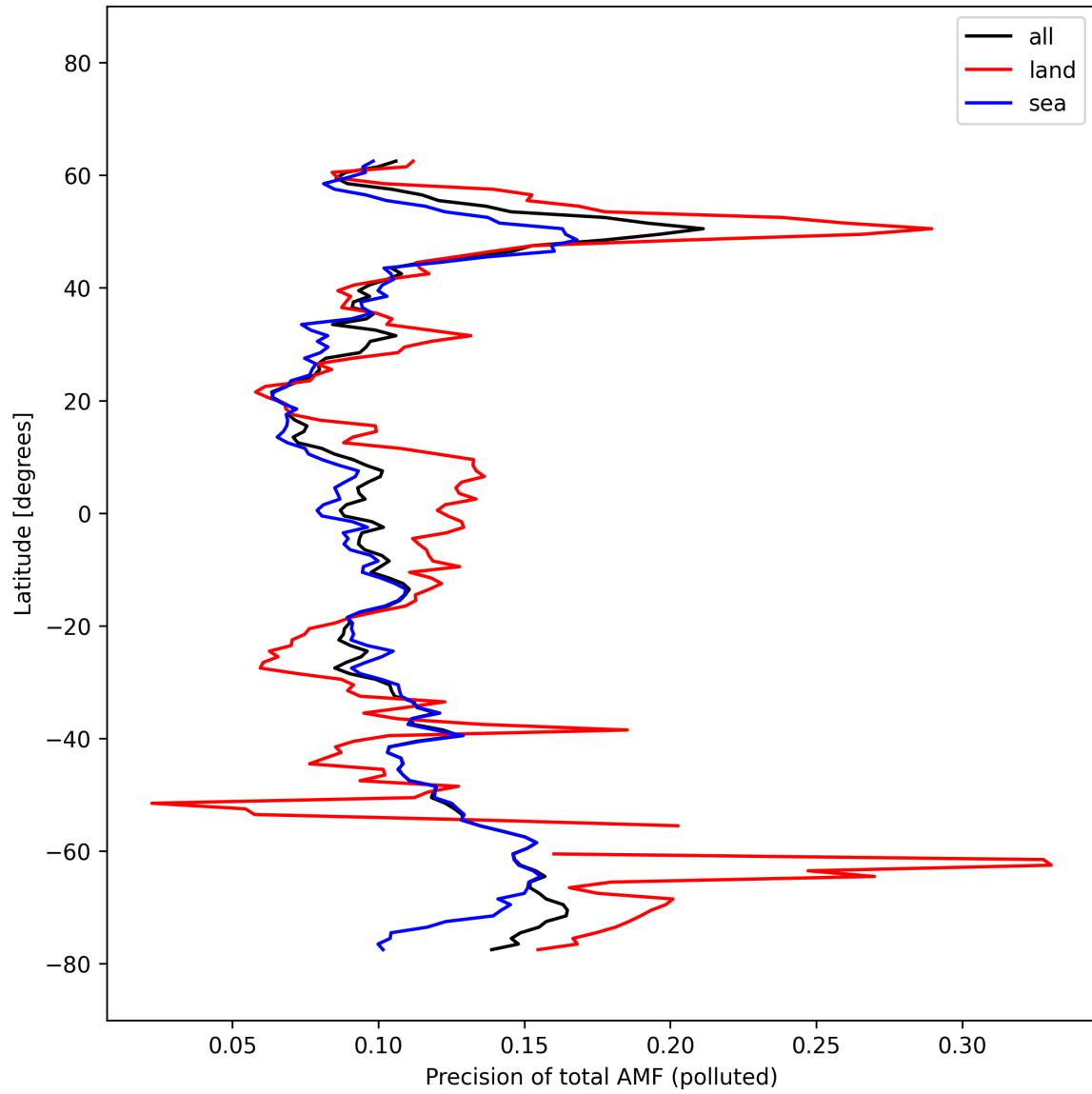
Figure 54: Zonal average of “Precision of total AMF (polluted)” for 2025-10-11 to 2025-10-13.
