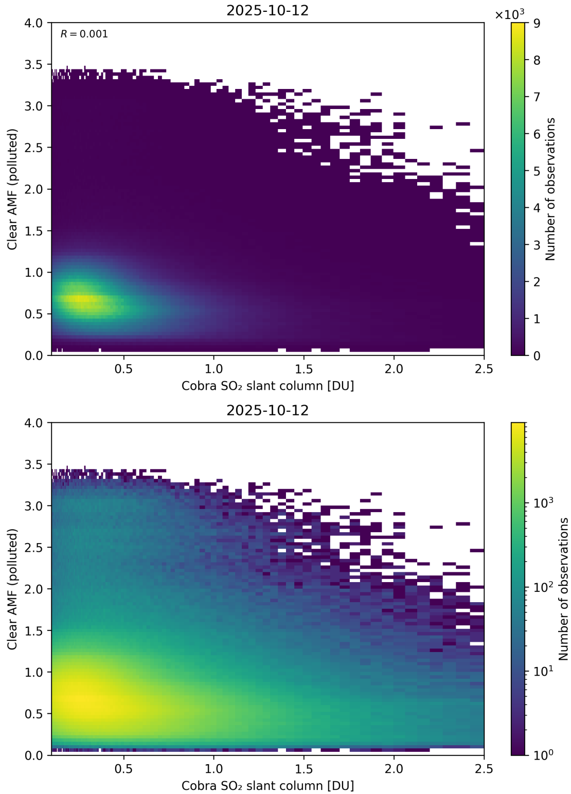
Figure 215: Scatter density plot of “Cobra SO 2 slant column” against “Clear AMF (polluted)” for 2025-10-11 to 2025-10-13.
