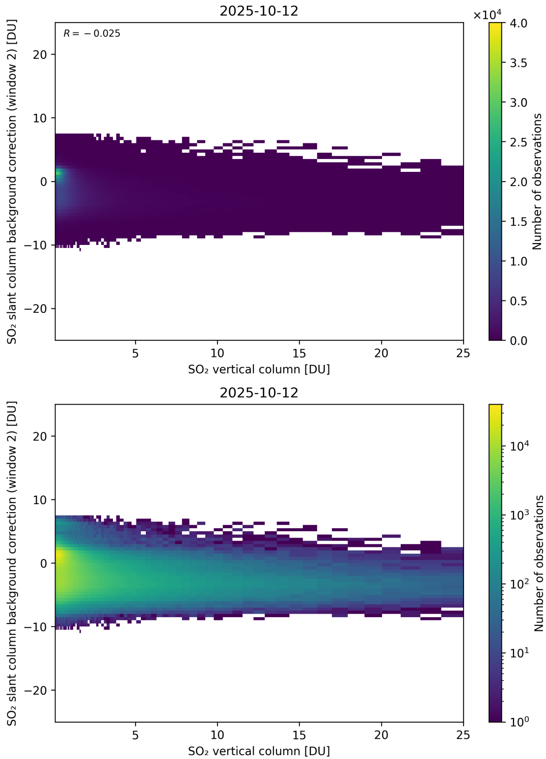
Figure 324: Scatter density plot of “SO 2 vertical column” against “SO 2 slant column background correction (window 2)” for 2025-10-11 to 2025-10-13.
