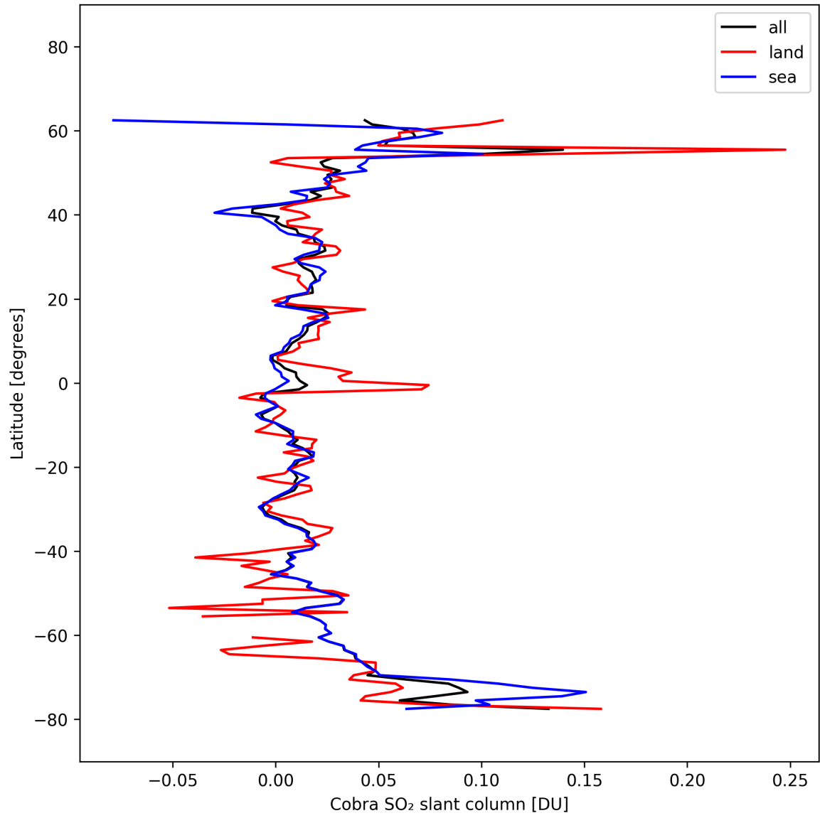
Figure 35: Zonal average of “Cobra SO 2 slant column” for 2025-10-11 to 2025-10-13.
