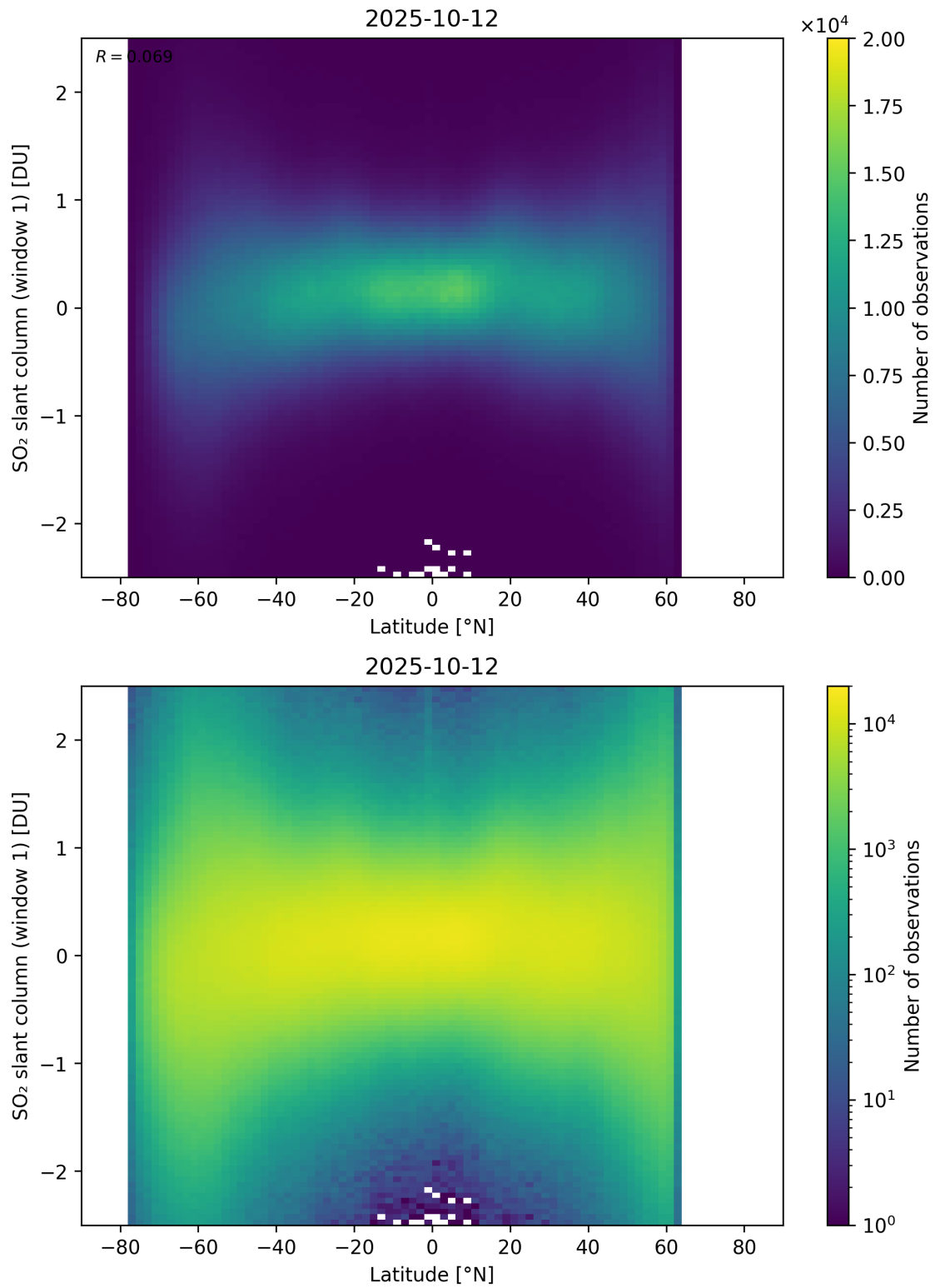
Figure 162: Scatter density plot of “Latitude” against “SO 2 slant column (window 1)” for 2025-10-11 to 2025-10-13.
