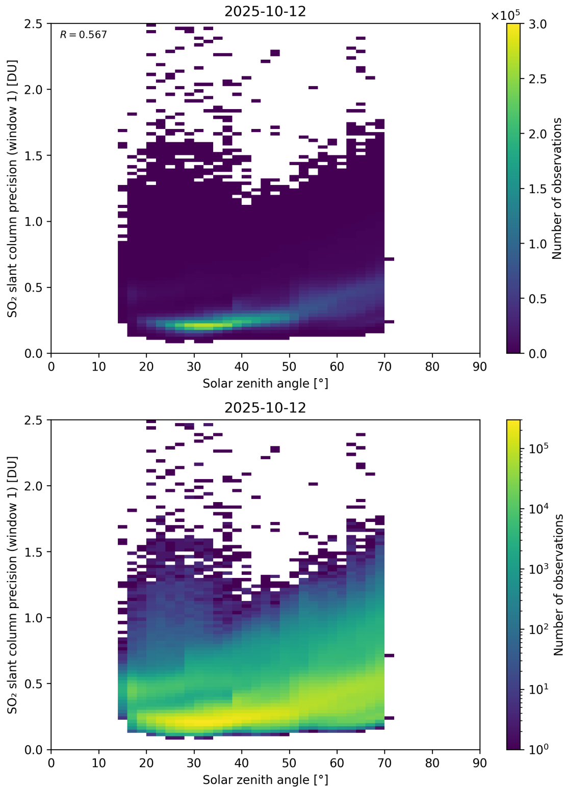
Figure 185: Scatter density plot of “Solar zenith angle” against “SO 2 slant column precision (window 1)” for 2025-10-11 to 2025-10-13.
