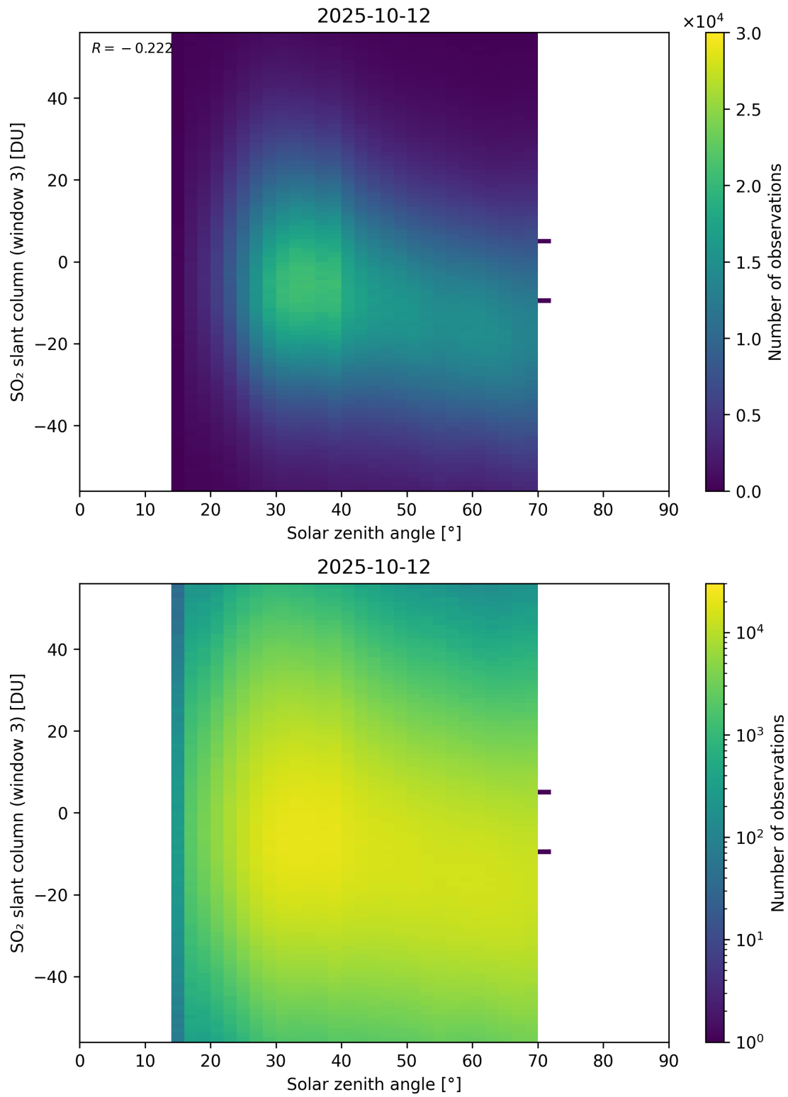
Figure 187: Scatter density plot of “Solar zenith angle” against “SO 2 slant column (window 3)” for 2025-10-11 to 2025-10-13.
