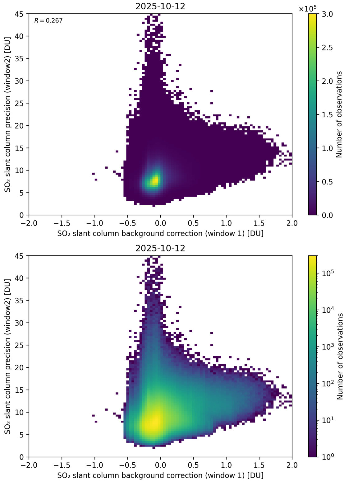
Figure 117: Scatter density plot of “SO 2 slant column background correction (window 1)” against “SO 2 slant column precision (window2)” for 2025-10-11 to 2025-10-13.
