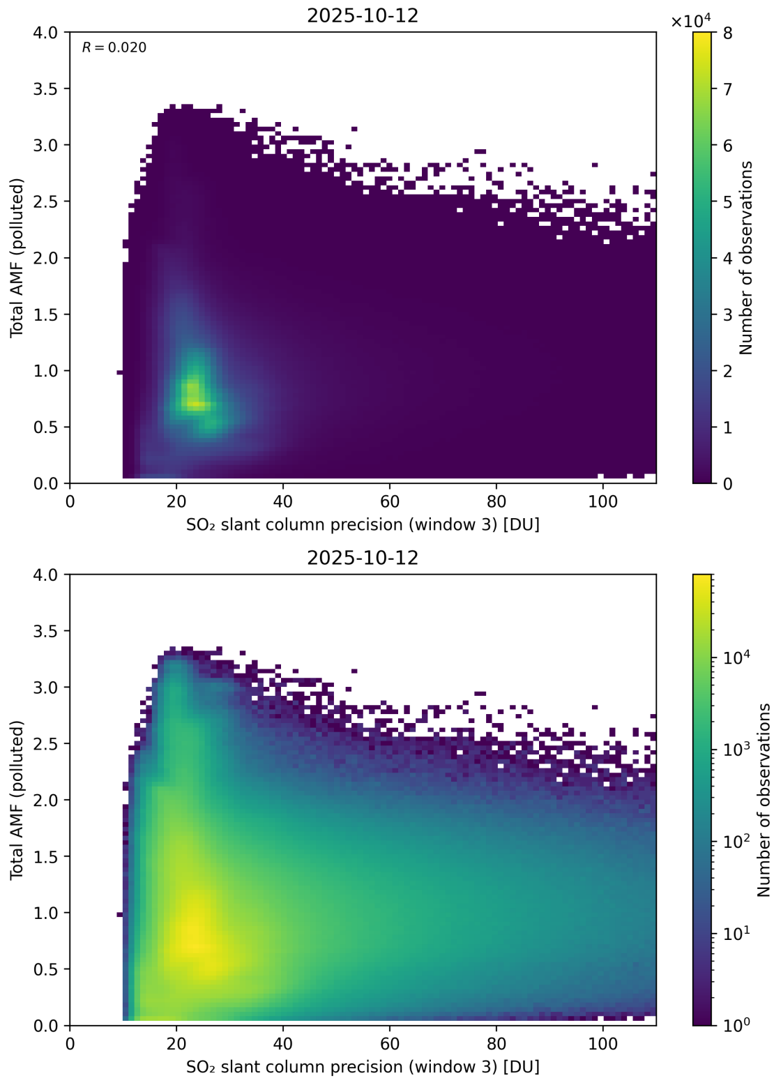
Figure 313: Scatter density plot of “SO 2 slant column precision (window 3)” against “Total AMF (polluted)” for 2025-10-11 to 2025-10-13.
