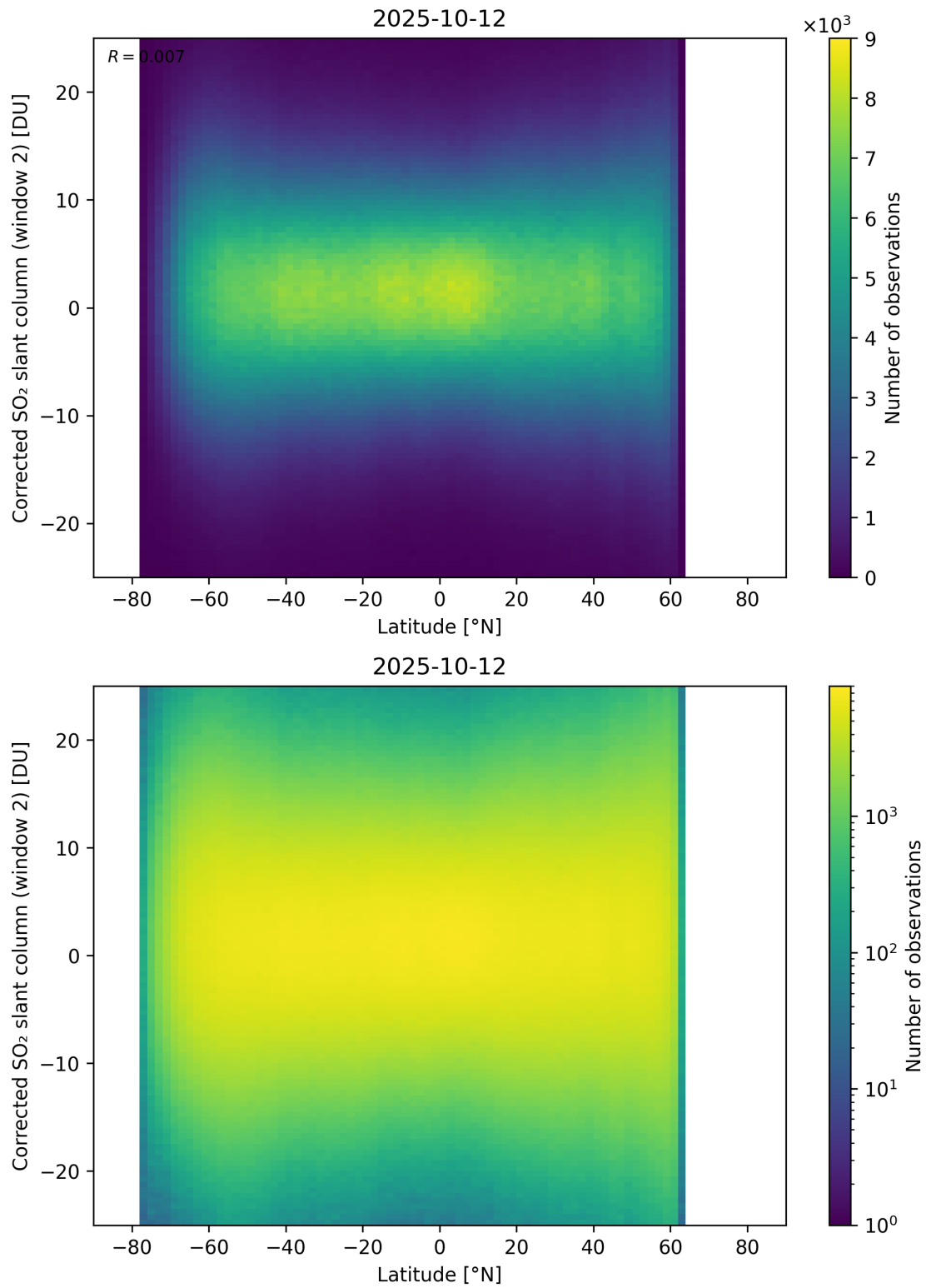
Figure 160: Scatter density plot of “Latitude” against “Corrected SO 2 slant column (window 2)” for 2025-10-11 to 2025-10-13.
