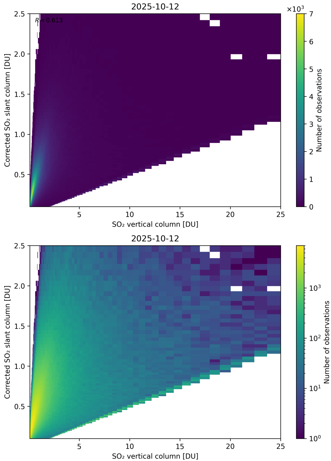
Figure 351: Scatter density plot of “SO 2 vertical column” against “Corrected SO 2 slant column” for 2025-10-11 to 2025-10-13.
