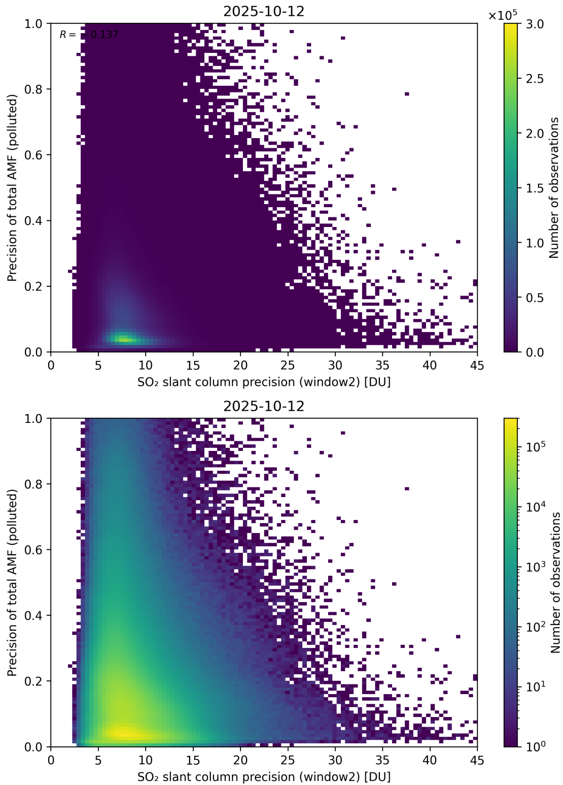
Figure 302: Scatter density plot of “SO 2 slant column precision (window2)” against “Precision of total AMF (polluted)” for 2025-10-11 to 2025-10-13.
