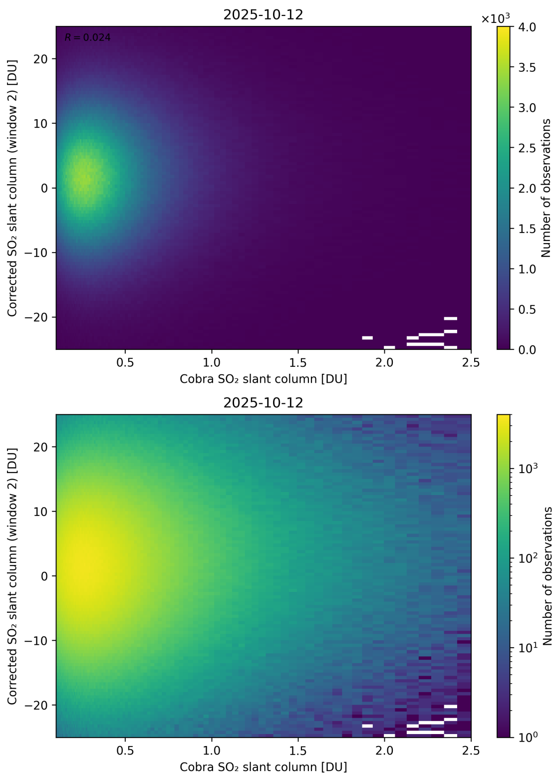
Figure 217: Scatter density plot of “Cobra SO 2 slant column” against “Corrected SO 2 slant column (window 2)” for 2025-10-11 to 2025-10-13.
