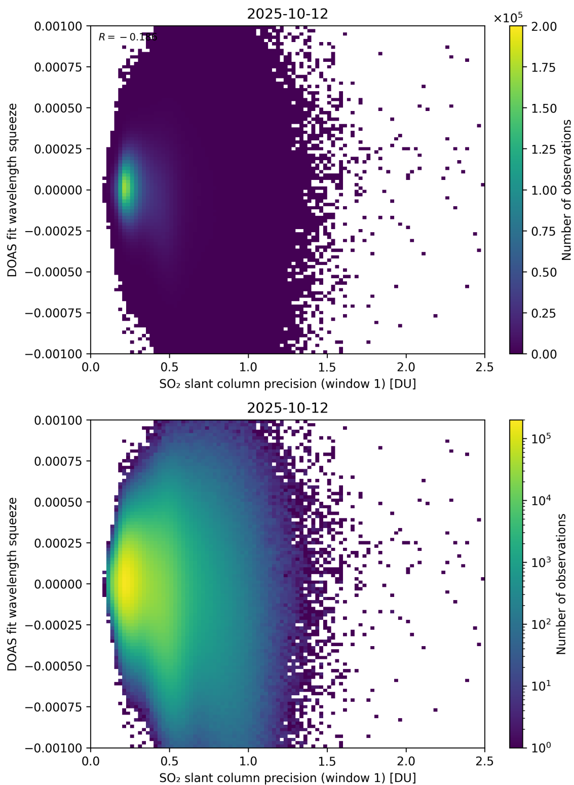
Figure 272: Scatter density plot of “SO 2 slant column precision (window 1)” against “DOAS fit wavelength squeeze” for 2025-10-11 to 2025-10-13.
