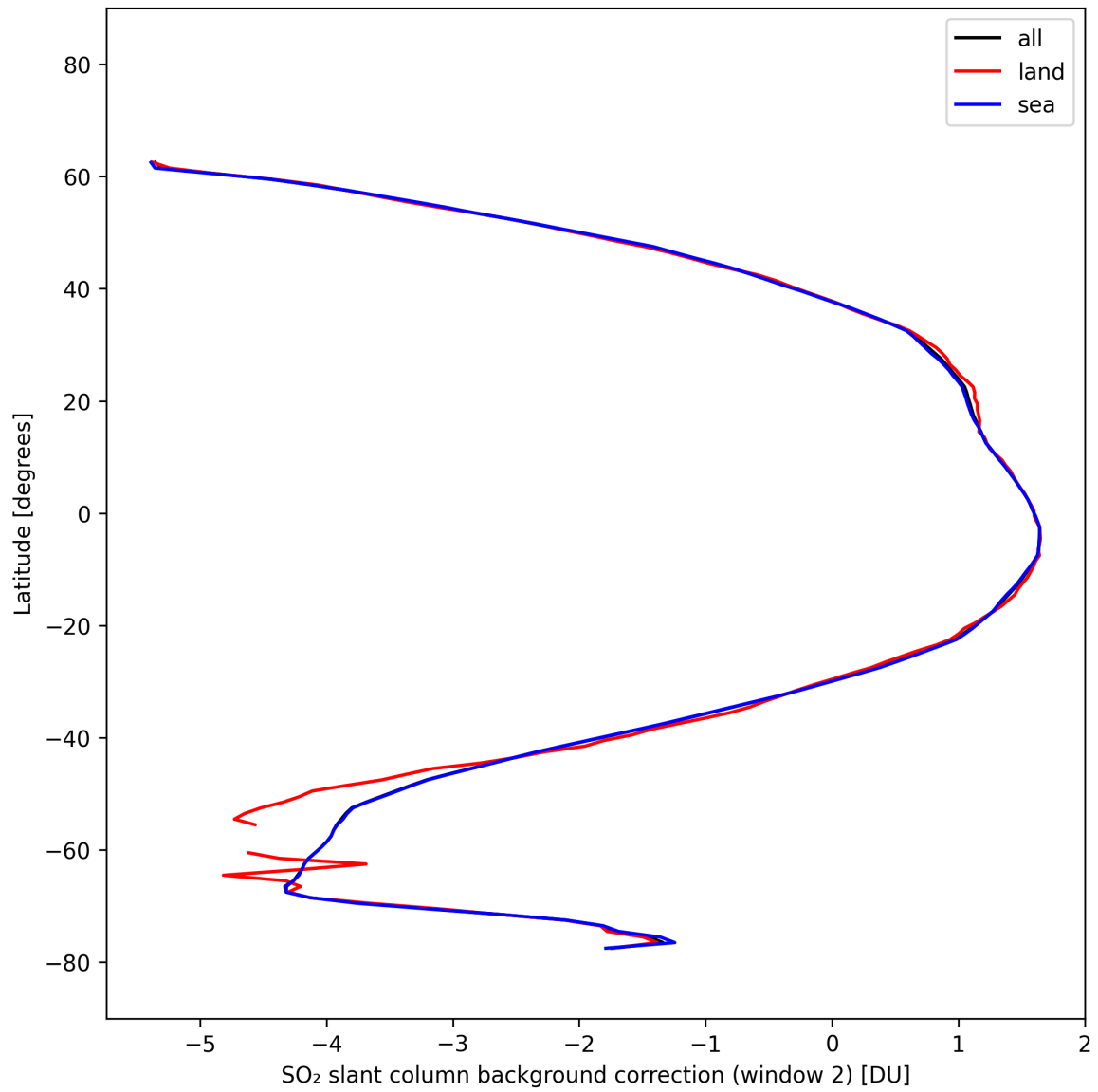
Figure 44: Zonal average of “SO 2 slant column background correction (window 2)” for 2025-10-11 to 2025-10-13.
