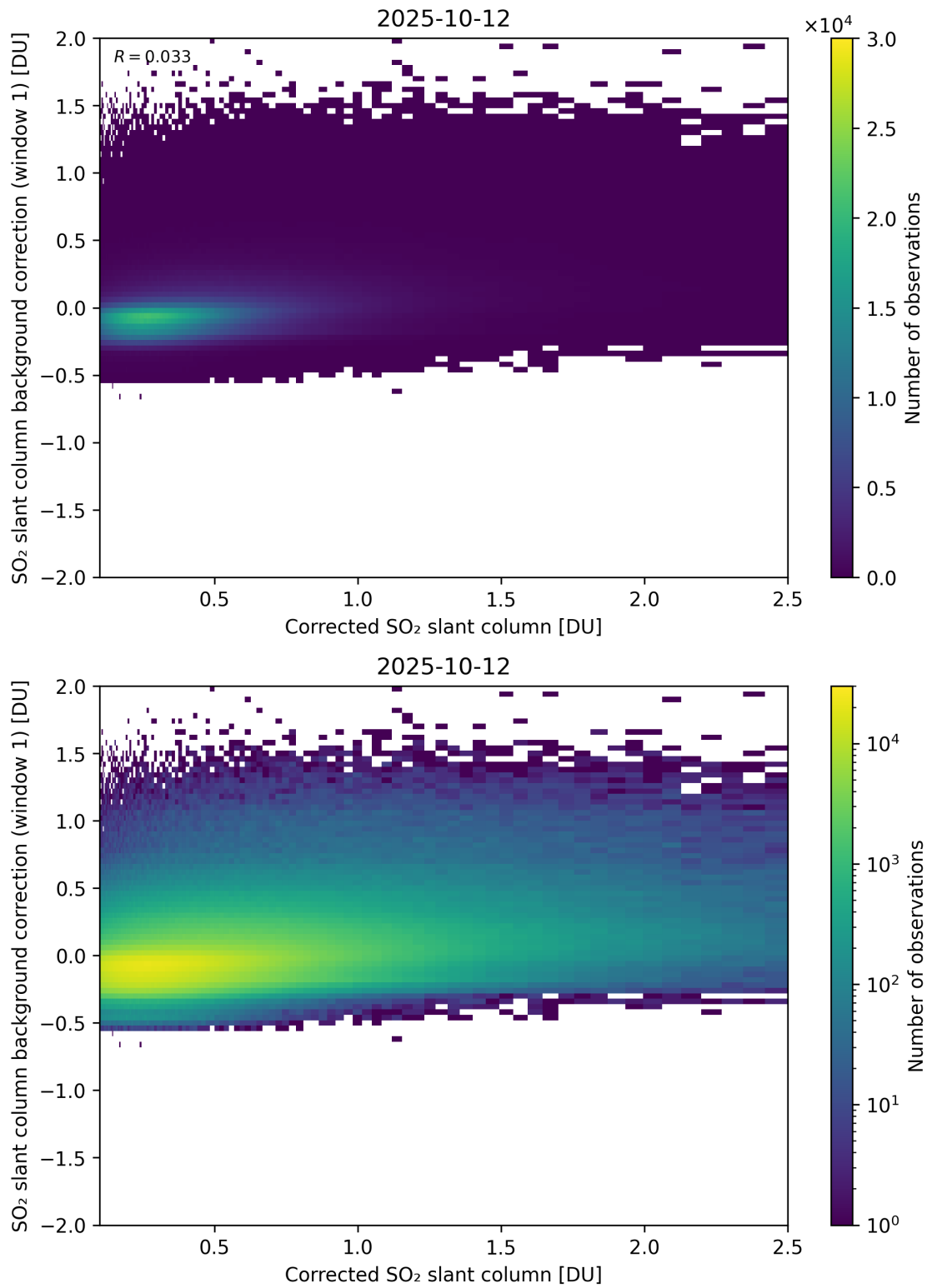
Figure 226: Scatter density plot of “Corrected SO 2 slant column” against “SO 2 slant column background correction (window 1)” for 2025-10-11 to 2025-10-13.
