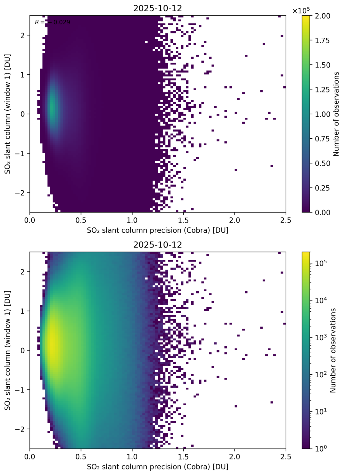
Figure 208: Scatter density plot of “SO 2 slant column precision (Cobra)” against “SO 2 slant column (window 1)” for 2025-10-11 to 2025-10-13.
