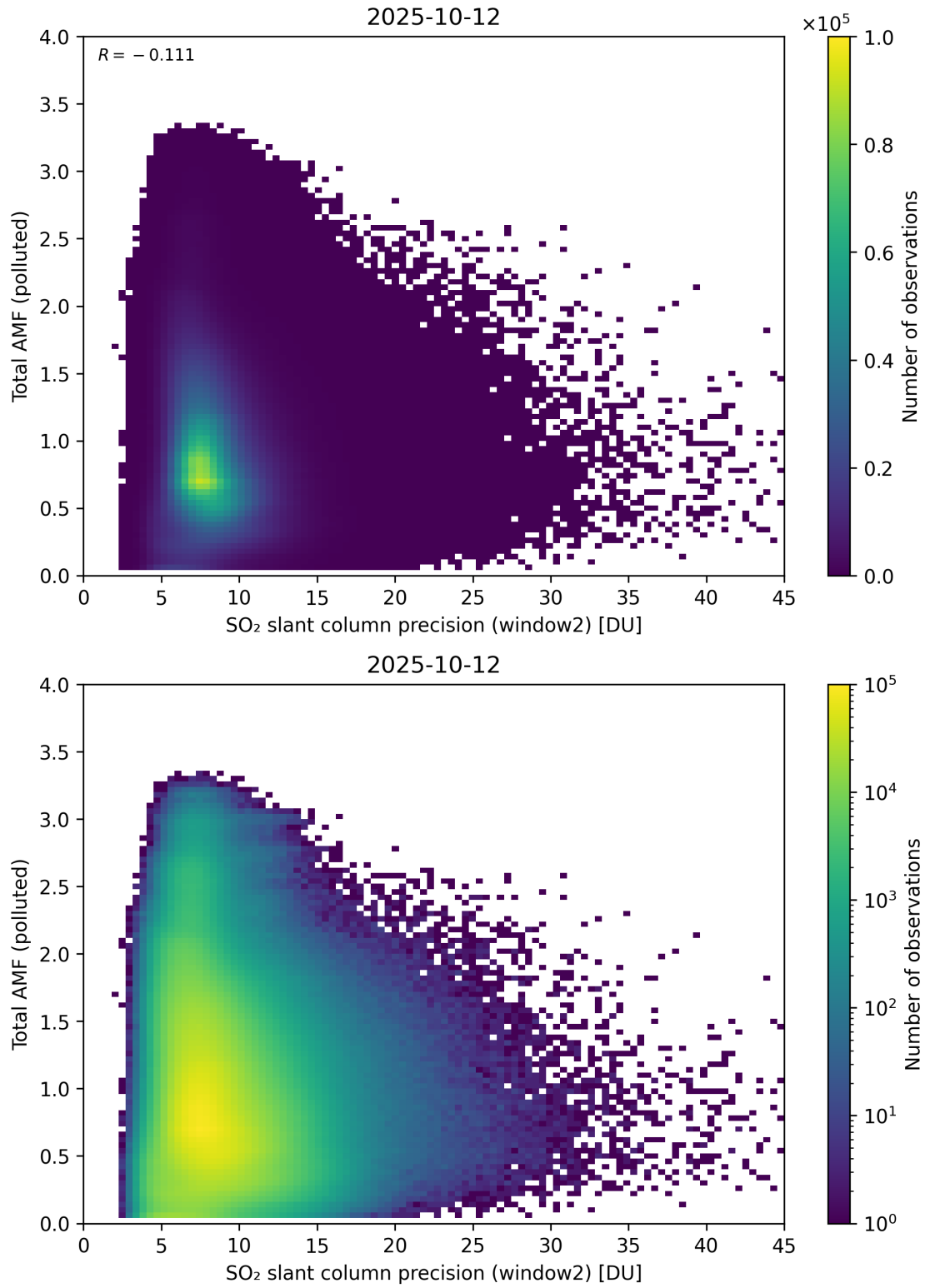
Figure 301: Scatter density plot of “SO 2 slant column precision (window2)” against “Total AMF (polluted)” for 2025-10-11 to 2025-10-13.
