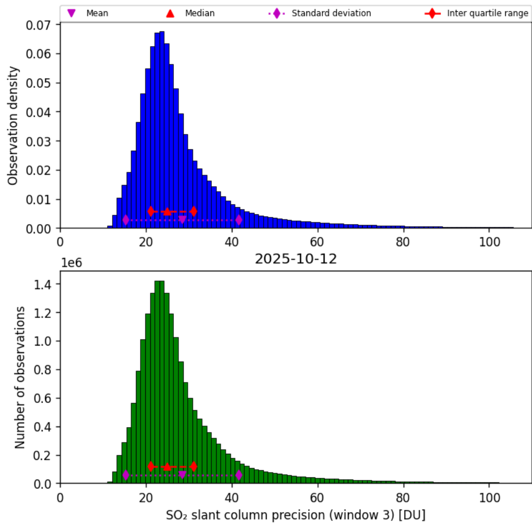
Figure 72: Histogram of “SO 2 slant column precision (window 3)” for 2025-10-11 to 2025-10-13
