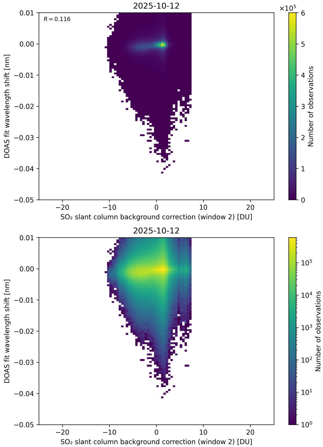
Figure 123: Scatter density plot of “SO 2 slant column background correction (window 2)” against “DOAS fit wavelength shift” for 2025-10-11 to 2025-10-13.
