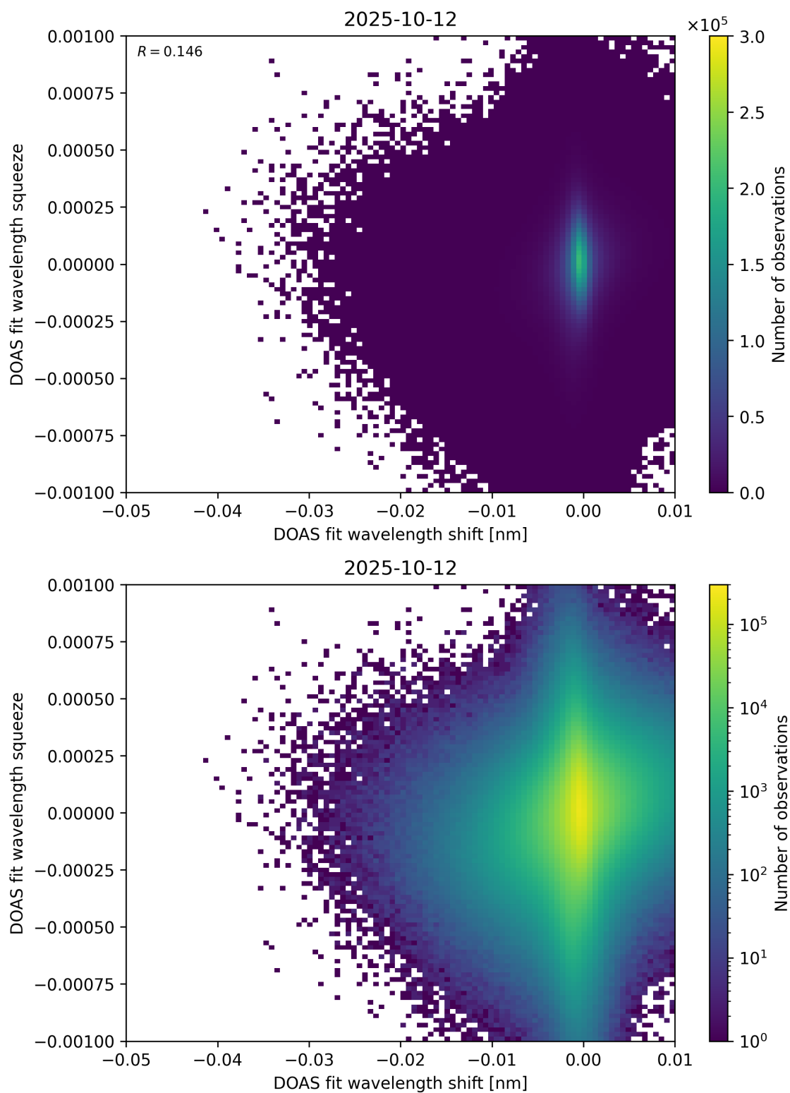
Figure 138: Scatter density plot of “DOAS fit wavelength shift” against “DOAS fit wavelength squeeze” for 2025-10-11 to 2025-10-13.
