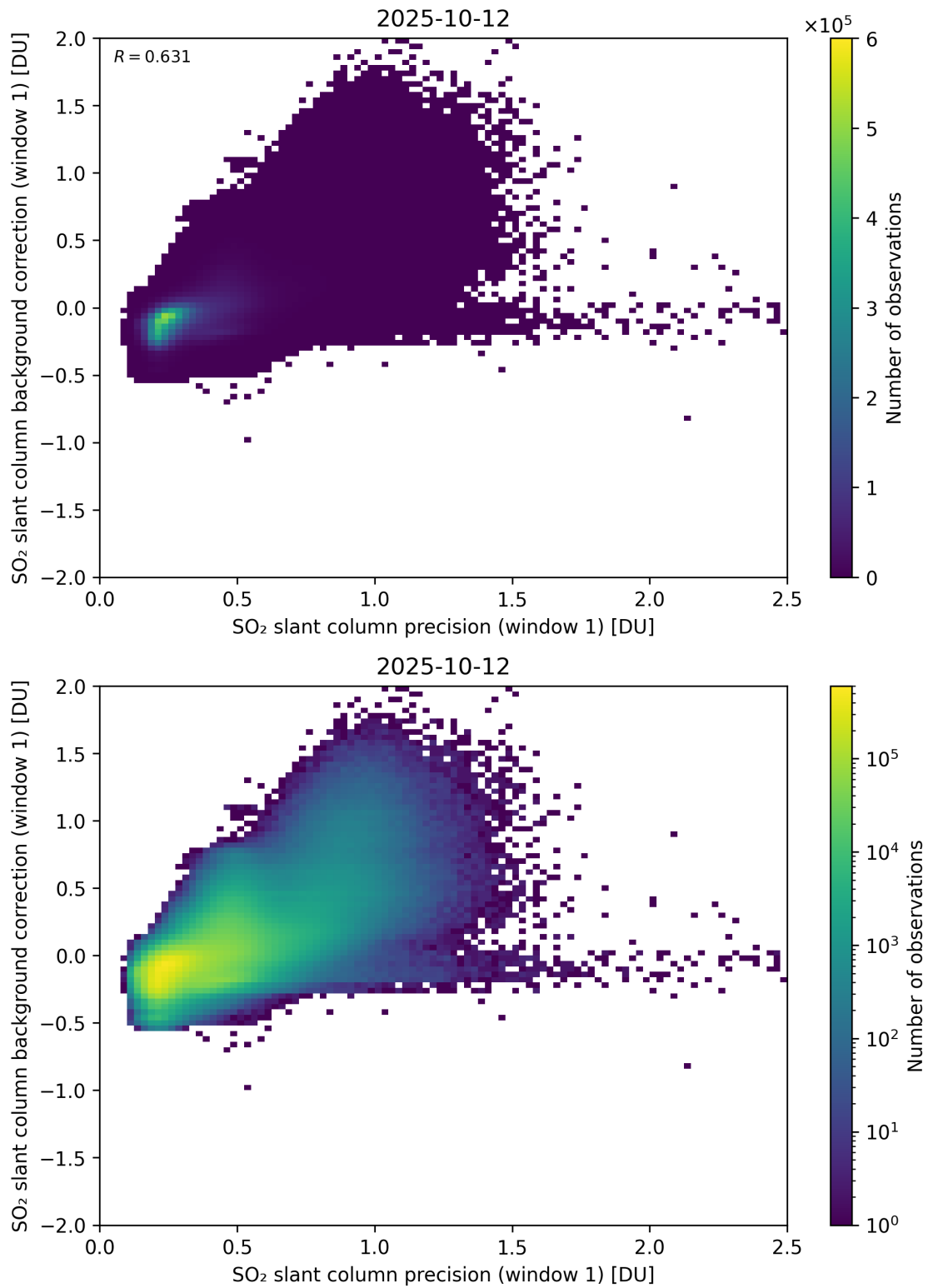
Figure 268: Scatter density plot of “SO 2 slant column precision (window 1)” against “SO 2 slant column background correction (window 1)” for 2025-10-11 to 2025-10-13.
