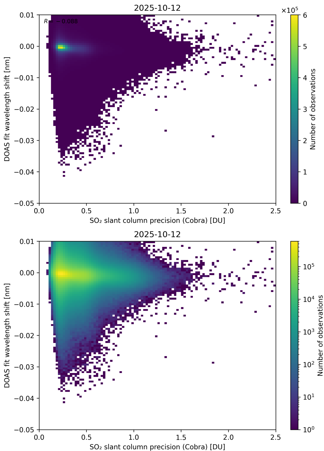
Figure 202: Scatter density plot of “SO 2 slant column precision (Cobra)” against “DOAS fit wavelength shift” for 2025-10-11 to 2025-10-13.
