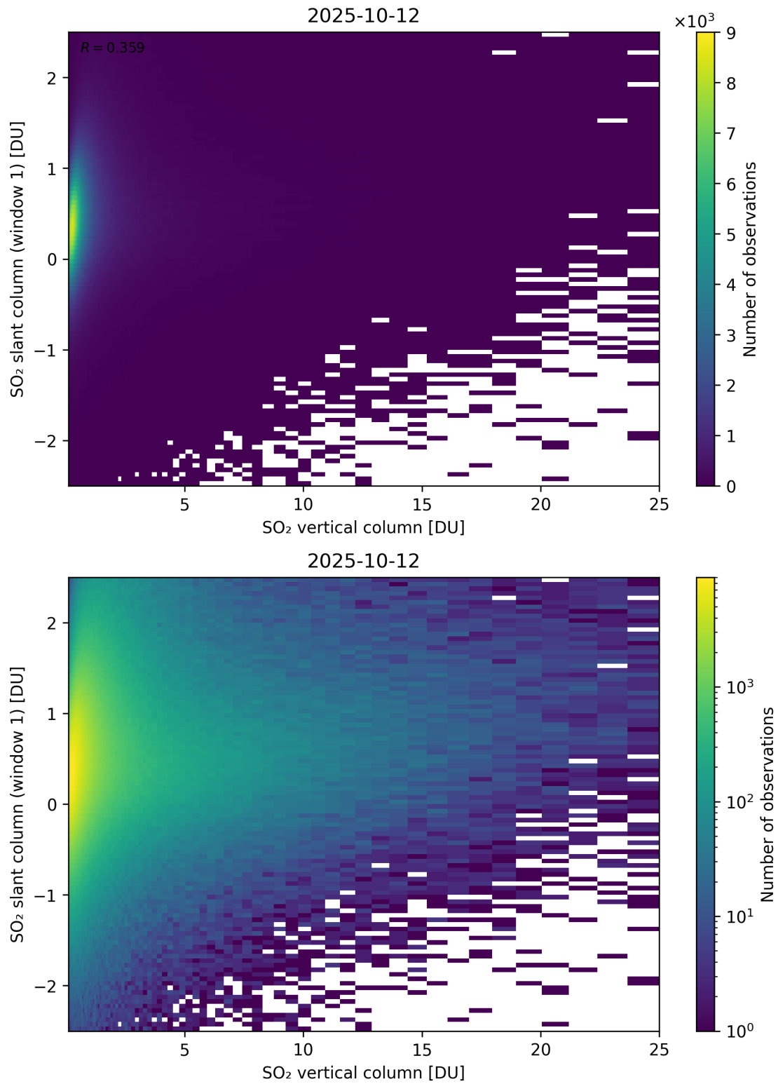
Figure 354: Scatter density plot of “SO 2 vertical column” against “SO 2 slant column (window 1)” for 2025-10-11 to 2025-10-13.
