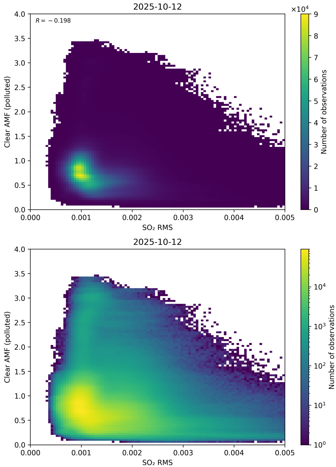
Figure 147: Scatter density plot of “SO 2 RMS” against “Clear AMF (polluted)” for 2025-10-11 to 2025-10-13.
