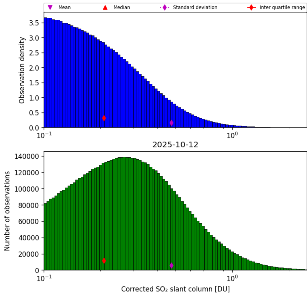
Figure 60: Histogram of "Corrected SO 2 slant column" for 2025-10-11 to 2025-10-13
