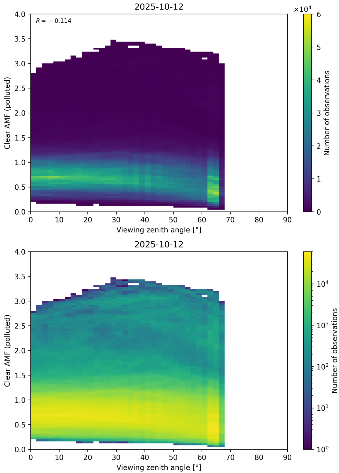
Figure 370: Scatter density plot of “Viewing zenith angle” against “Clear AMF (polluted)” for 2025-10-11 to 2025-10-13.
