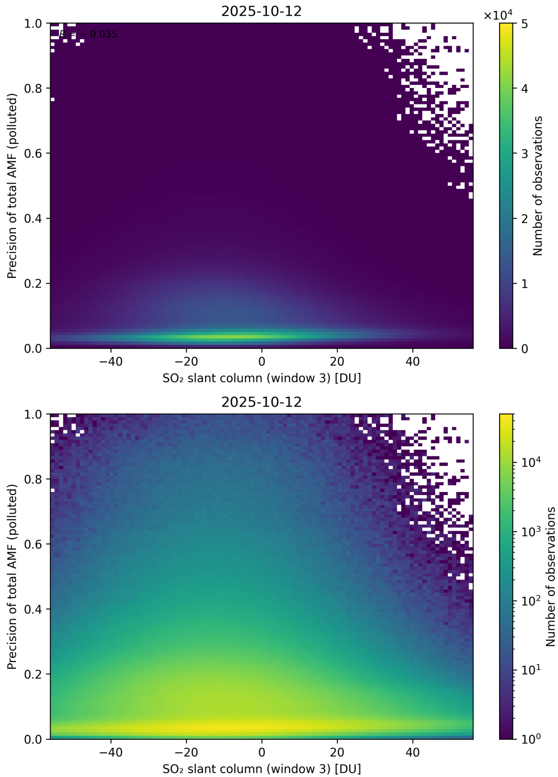
Figure 319: Scatter density plot of “SO 2 slant column (window 3)” against “Precision of total AMF (polluted)” for 2025-10-11 to 2025-10-13.
