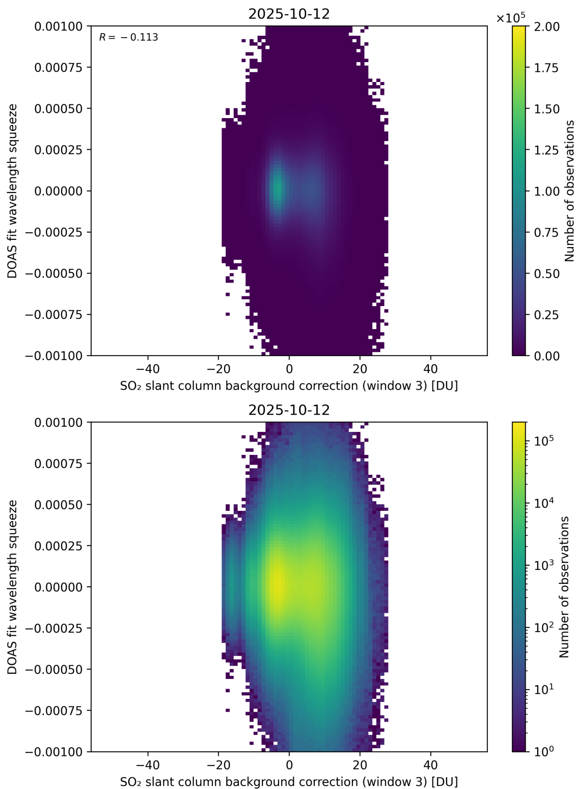
Figure 133: Scatter density plot of “SO 2 slant column background correction (window 3)” against “DOAS fit wavelength squeeze” for 2025-10-11 to 2025-10-13.
