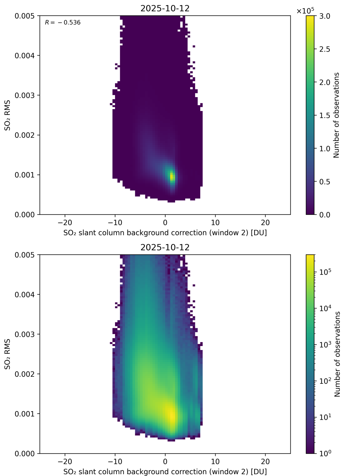
Figure 125: Scatter density plot of “SO 2 slant column background correction (window 2)” against “SO 2 RMS” for 2025-10-11 to 2025-10-13.
