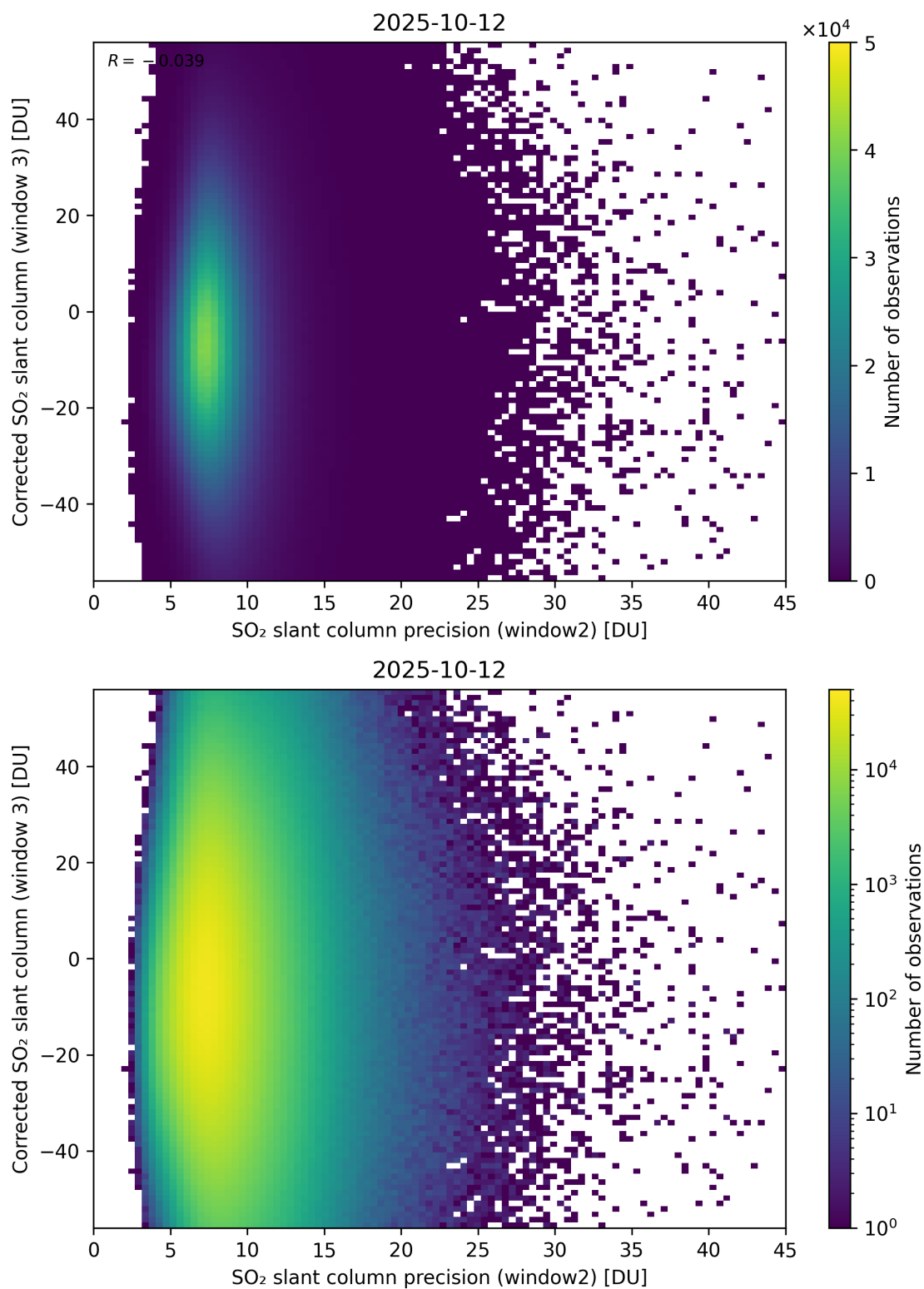
Figure 298: Scatter density plot of “SO 2 slant column precision (window2)” against “Corrected SO 2 slant column (window 3)” for 2025-10-11 to 2025-10-13.
