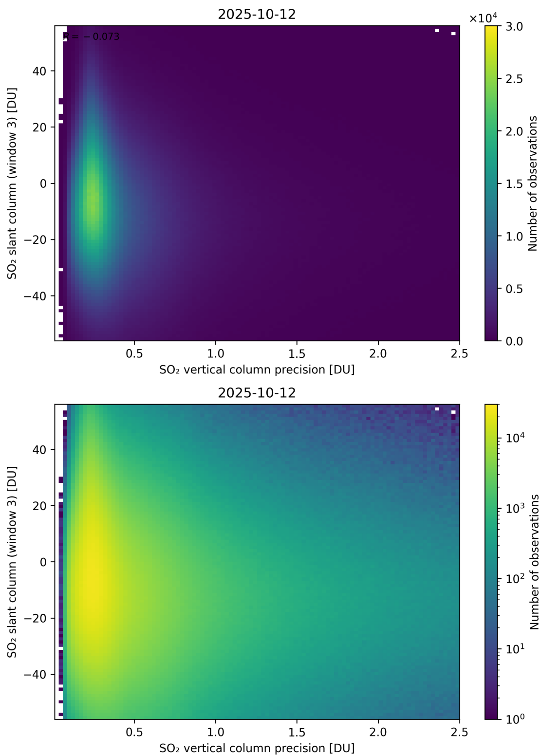
Figure 344: Scatter density plot of “SO 2 vertical column precision” against “SO 2 slant column (window 3)” for 2025-10-11 to 2025-10-13.
