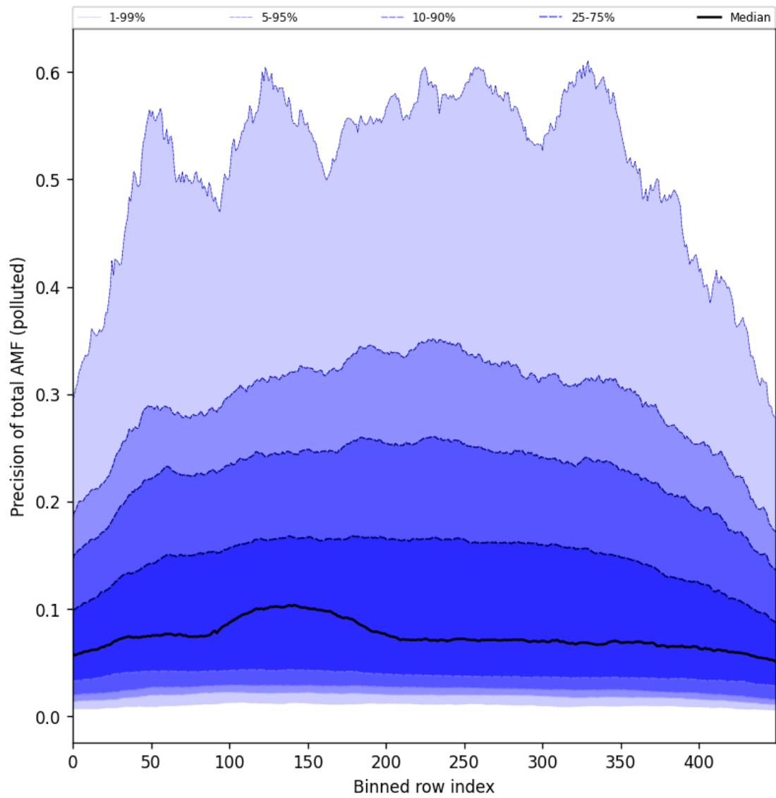
Figure 106: Along track statistics of “Precision of total AMF (polluted)” for 2025-10-11 to 2025-10-13
