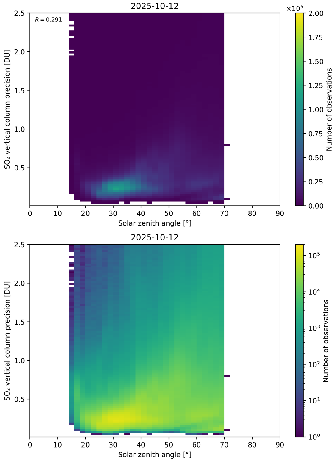
Figure 192: Scatter density plot of “Solar zenith angle” against “SO 2 vertical column precision” for 2025-10-11 to 2025-10-13.
