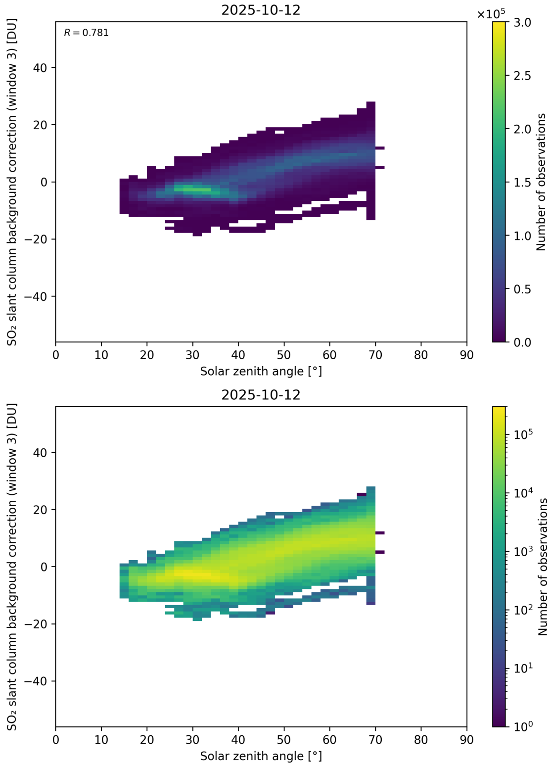
Figure 173: Scatter density plot of “Solar zenith angle” against “SO 2 slant column background correction (window 3)” for 2025-10-11 to 2025-10-13.
