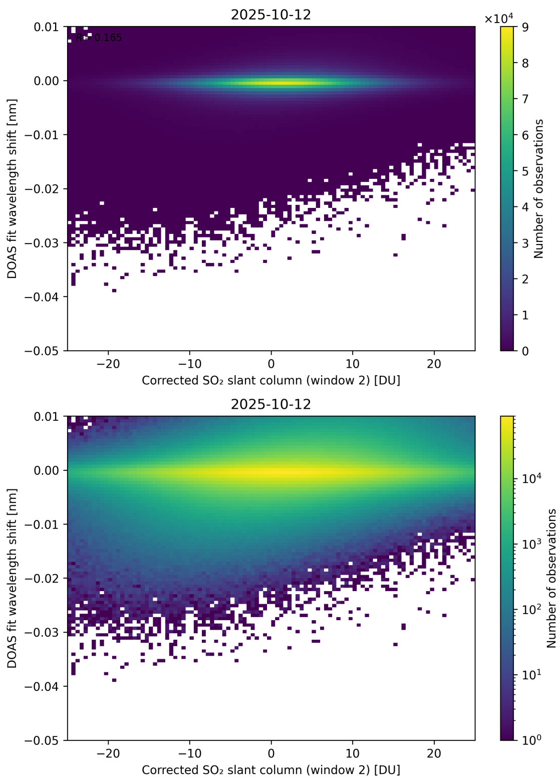
Figure 246: Scatter density plot of “Corrected SO 2 slant column (window 2)” against “DOAS fit wavelength shift” for 2025-10-11 to 2025-10-13.
