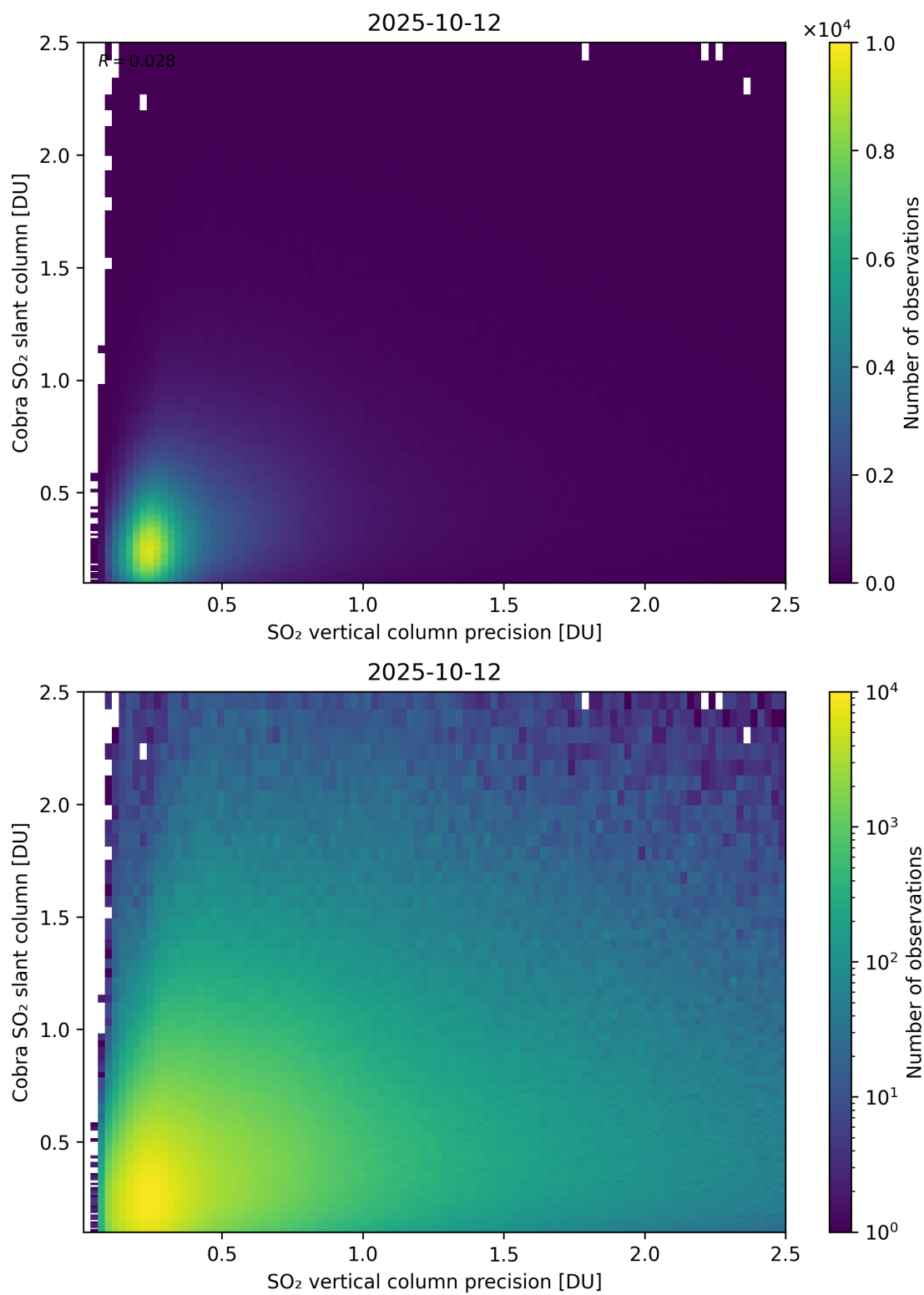
Figure 336: Scatter density plot of “SO 2 vertical column precision” against “Cobra SO 2 slant column” for 2025-10-11 to 2025-10-13.
