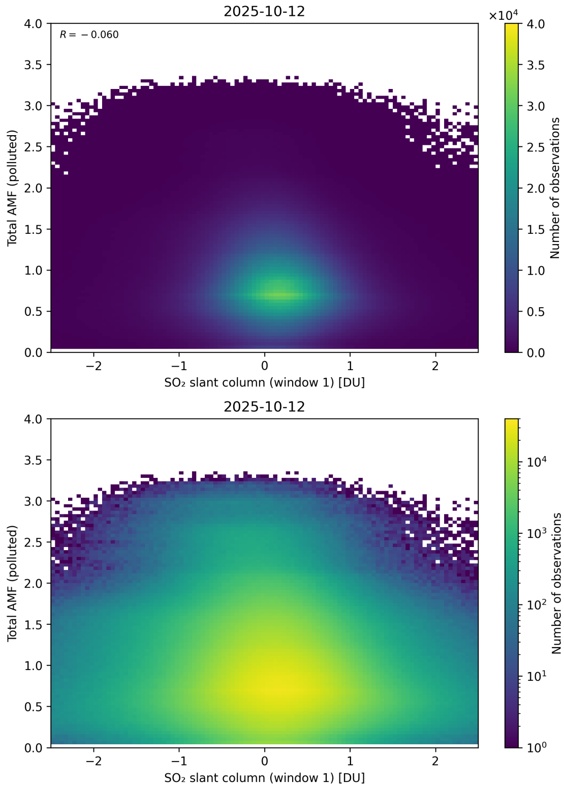
Figure 289: Scatter density plot of “SO 2 slant column (window 1)” against “Total AMF (polluted)” for 2025-10-11 to 2025-10-13.
