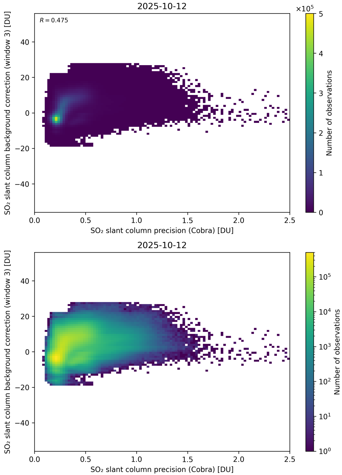
Figure 201: Scatter density plot of “SO 2 slant column precision (Cobra)” against “SO 2 slant column background correction (window 3)” for 2025-10-11 to 2025-10-13.
