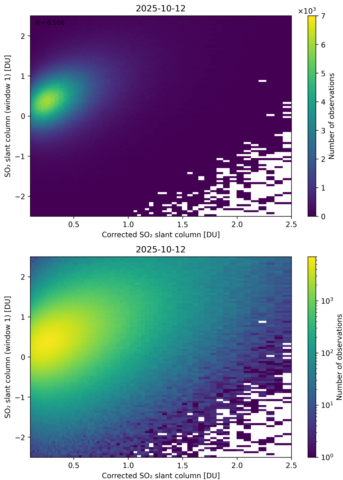
Figure 237: Scatter density plot of “Corrected SO 2 slant column” against “SO 2 slant column (window 1)” for 2025-10-11 to 2025-10-13.
