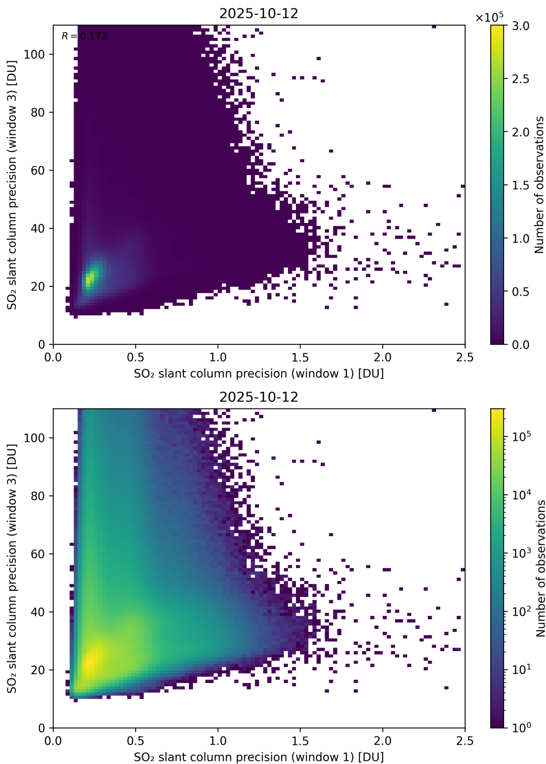
Figure 279: Scatter density plot of “SO 2 slant column precision (window 1)” against “SO 2 slant column precision (window 3)” for 2025-10-11 to 2025-10-13.
