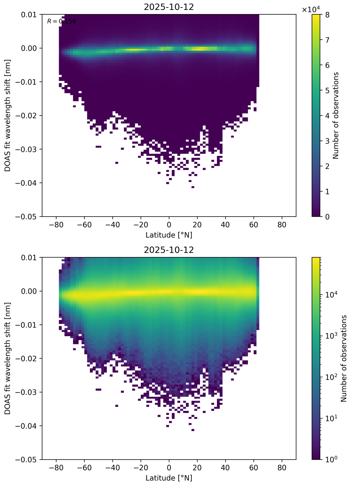
Figure 153: Scatter density plot of “Latitude” against “DOAS fit wavelength shift” for 2025-10-11 to 2025-10-13.
