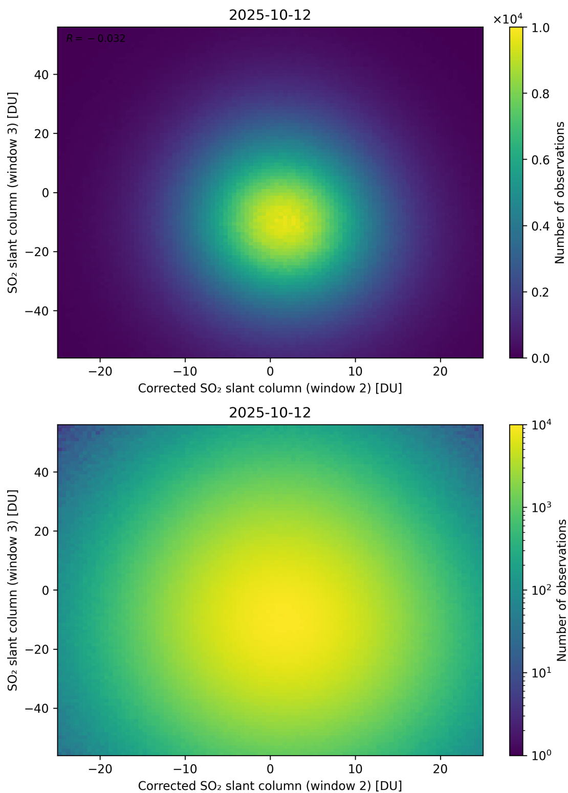
Figure 251: Scatter density plot of “Corrected SO 2 slant column (window 2)” against “SO 2 slant column (window 3)” for 2025-10-11 to 2025-10-13.
