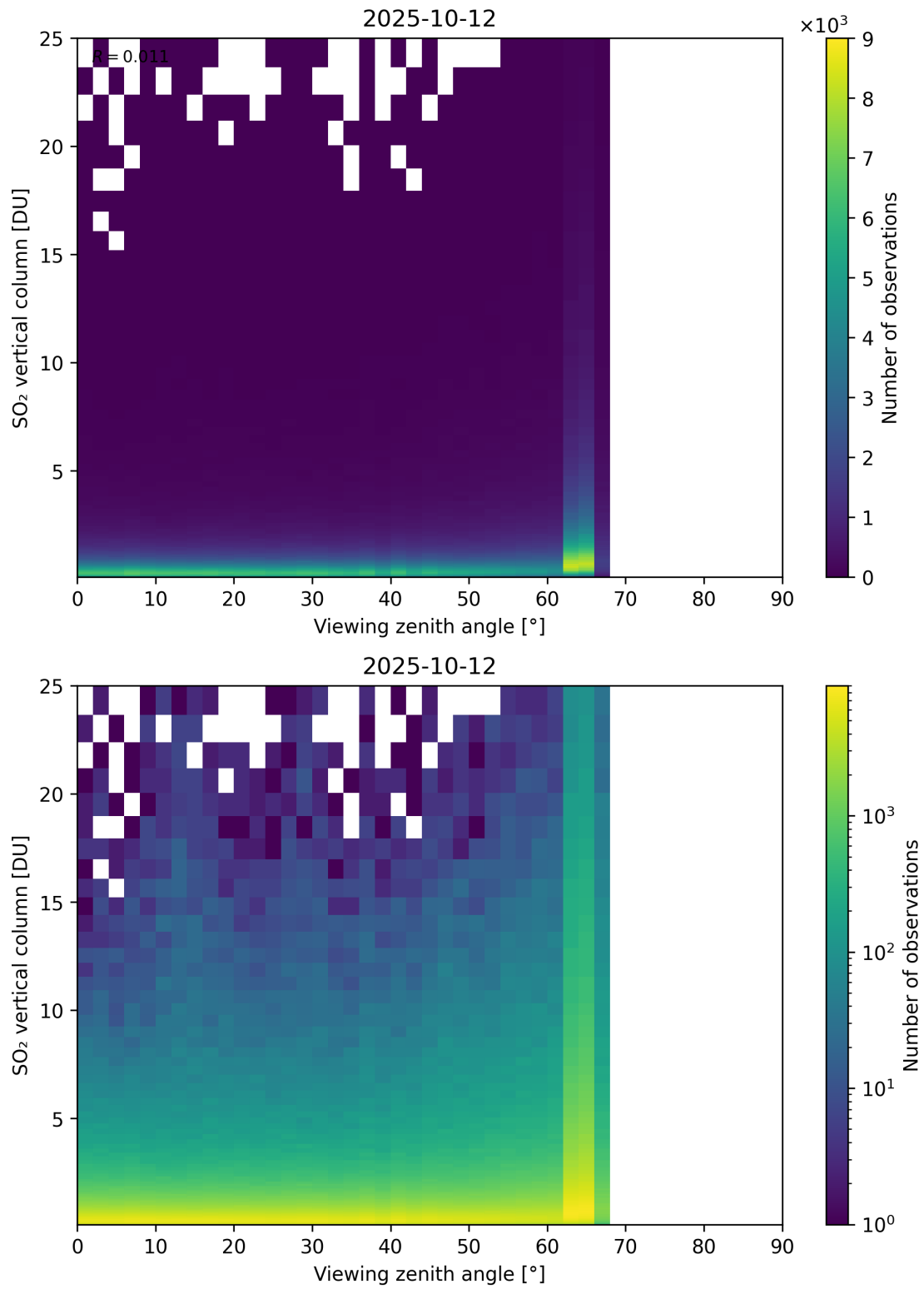
Figure 383: Scatter density plot of “Viewing zenith angle” against “SO 2 vertical column” for 2025-10-11 to 2025-10-13.
