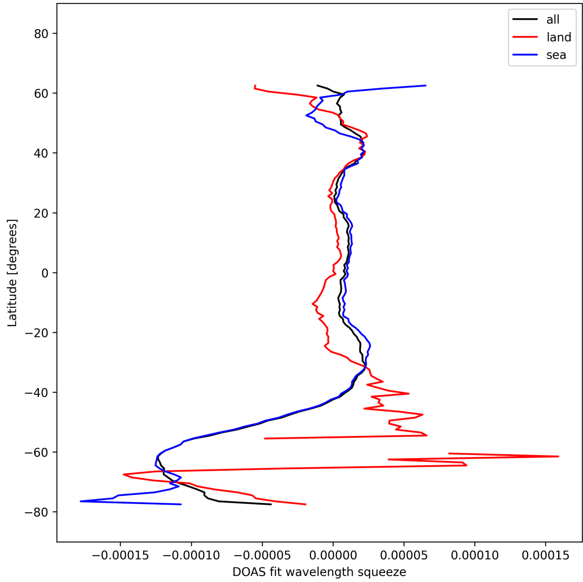
Figure 51: Zonal average of “DOAS fit wavelength squeeze” for 2025-10-11 to 2025-10-13.
