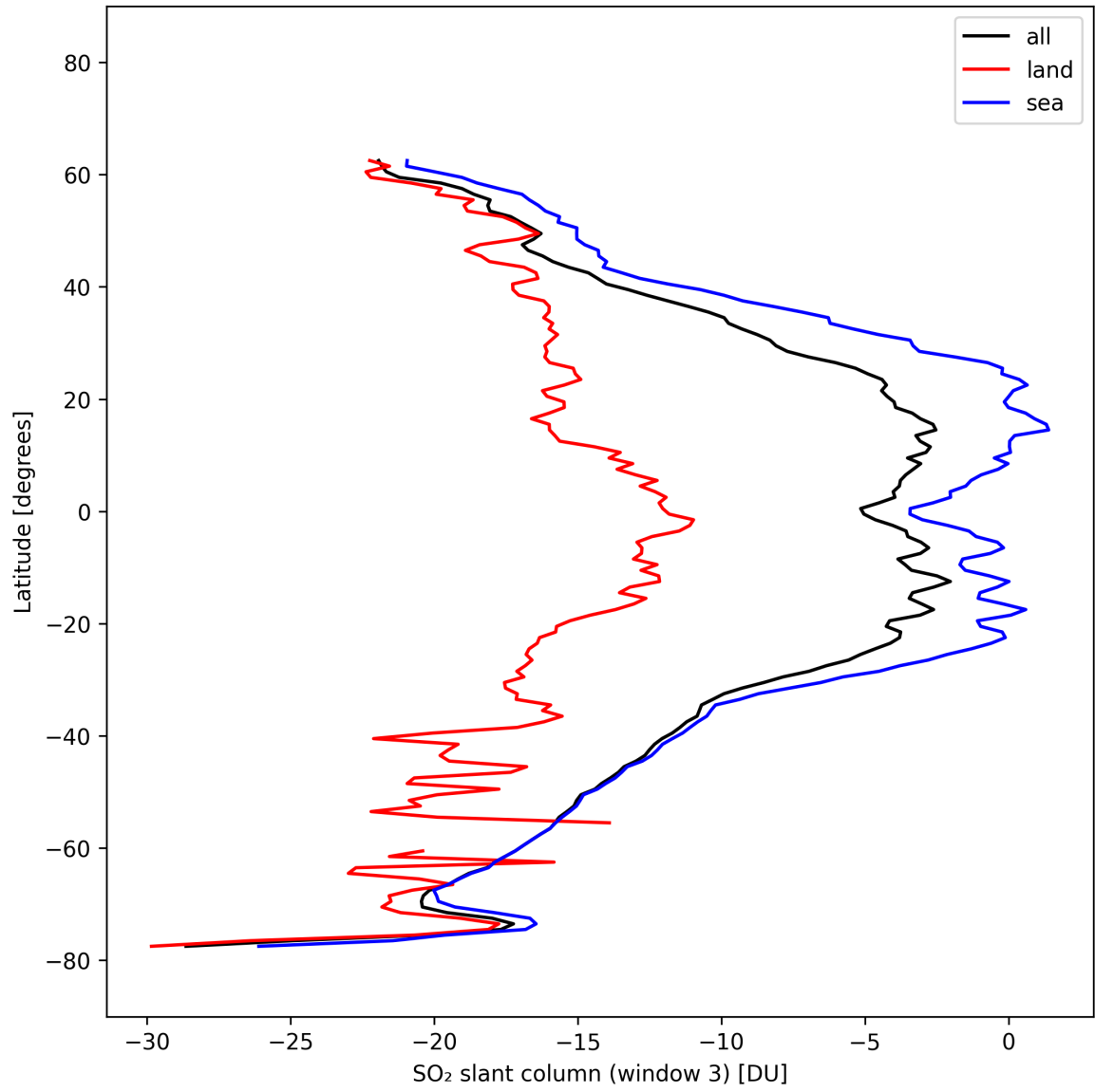
Figure 45: Zonal average of “SO 2 slant column (window 3)” for 2025-10-11 to 2025-10-13.
