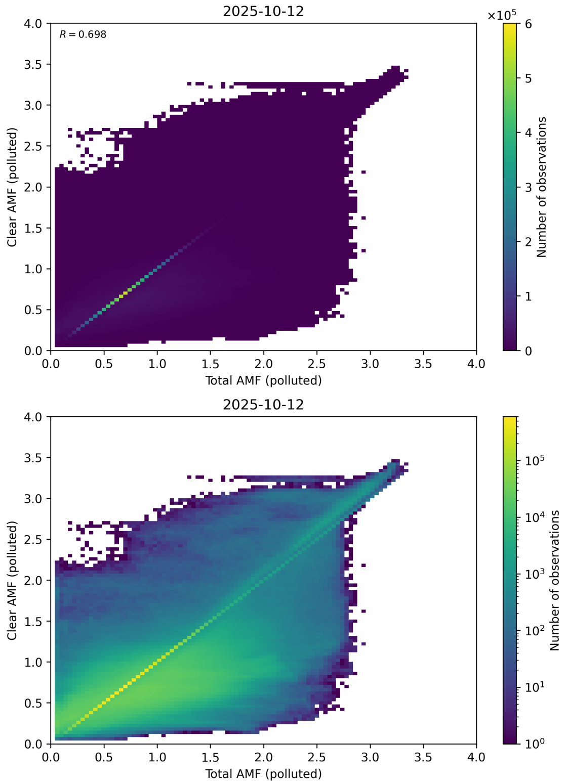
Figure 321: Scatter density plot of “Total AMF (polluted)” against “Clear AMF (polluted)” for 2025-10-11 to 2025-10-13.
