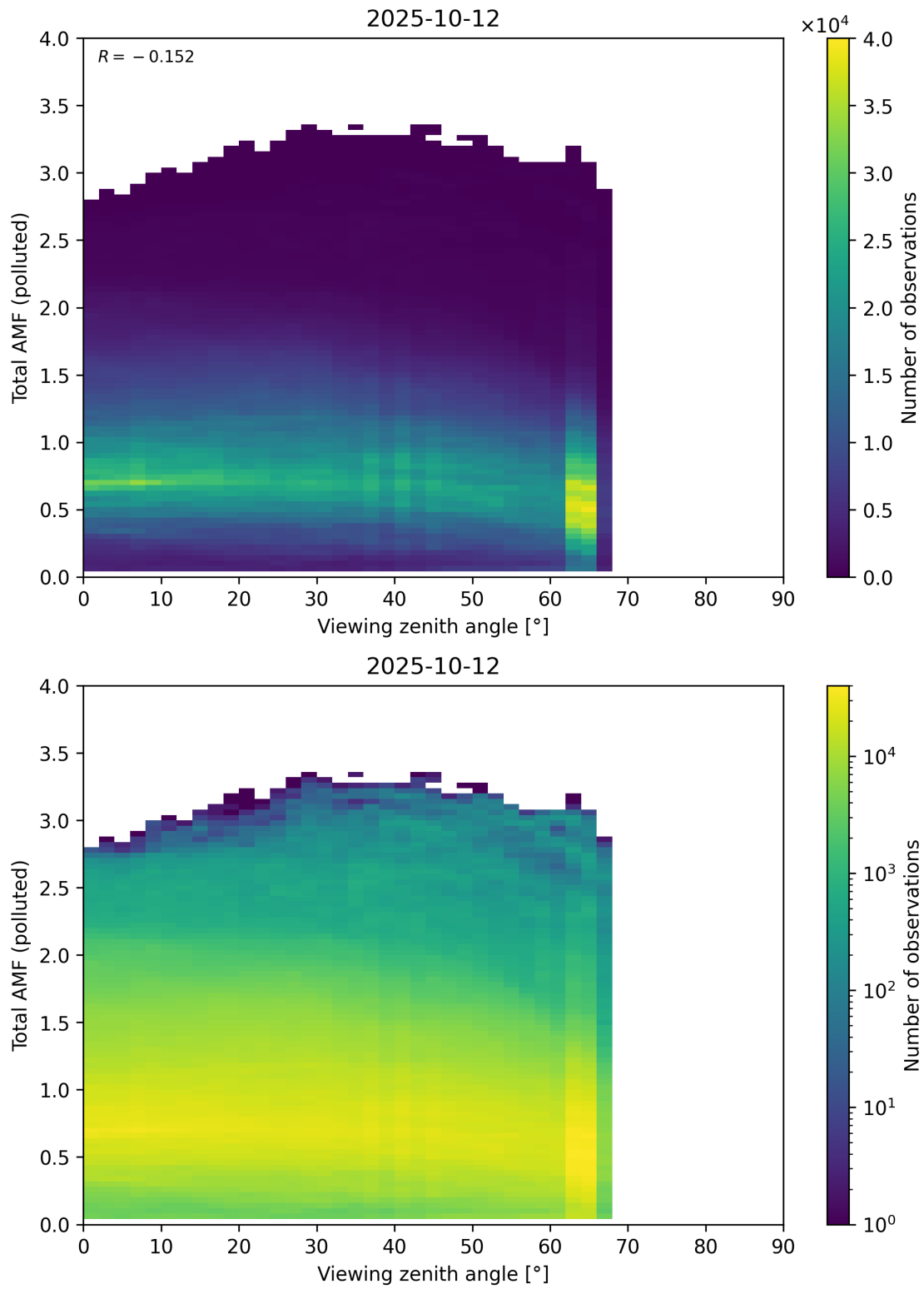
Figure 381: Scatter density plot of “Viewing zenith angle” against “Total AMF (polluted)” for 2025-10-11 to 2025-10-13.
