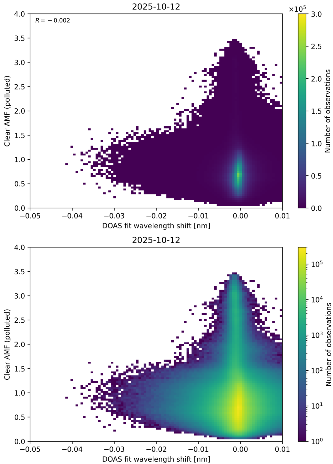
Figure 140: Scatter density plot of “DOAS fit wavelength shift” against “Clear AMF (polluted)” for 2025-10-11 to 2025-10-13.
