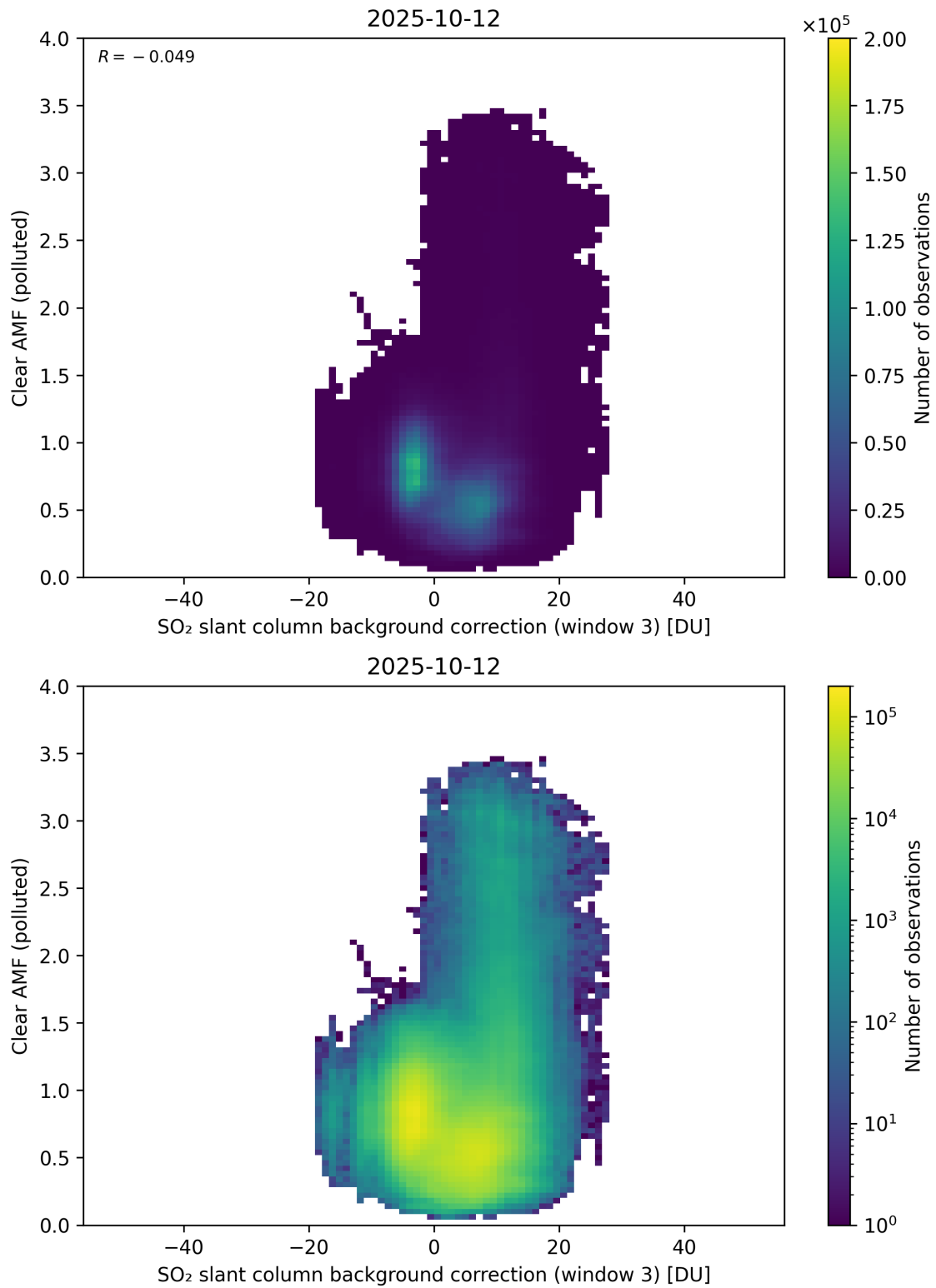
Figure 135: Scatter density plot of “SO 2 slant column background correction (window 3)” against “Clear AMF (polluted)” for 2025-10-11 to 2025-10-13.
