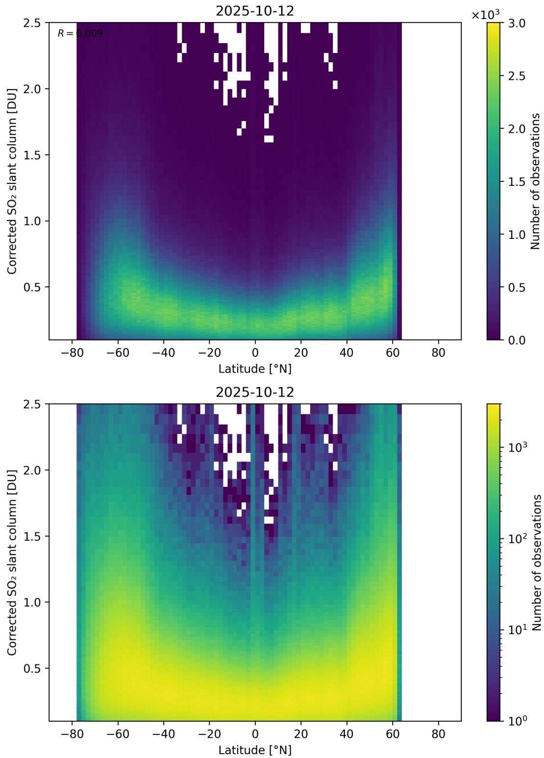
Figure 159: Scatter density plot of “Latitude” against “Corrected SO 2 slant column” for 2025-10-11 to 2025-10-13.
