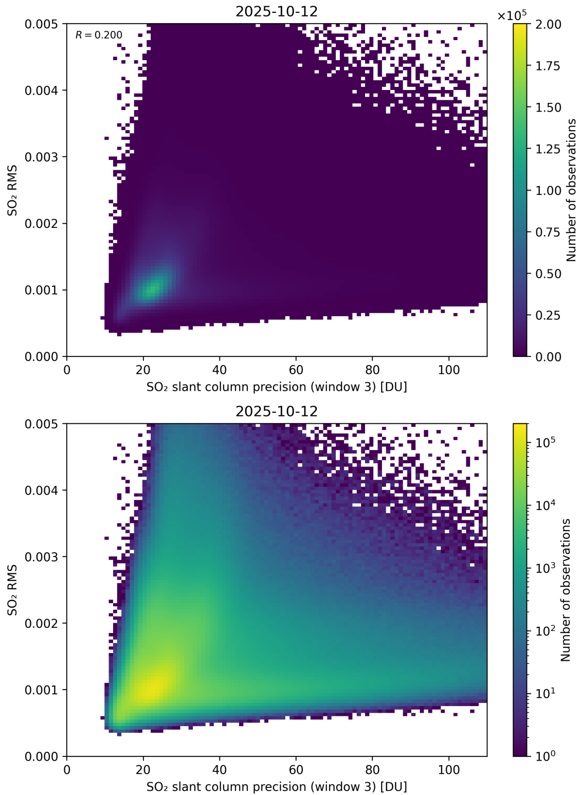
Figure 310: Scatter density plot of “SO 2 slant column precision (window 3)” against “SO 2 RMS” for 2025-10-11 to 2025-10-13.
