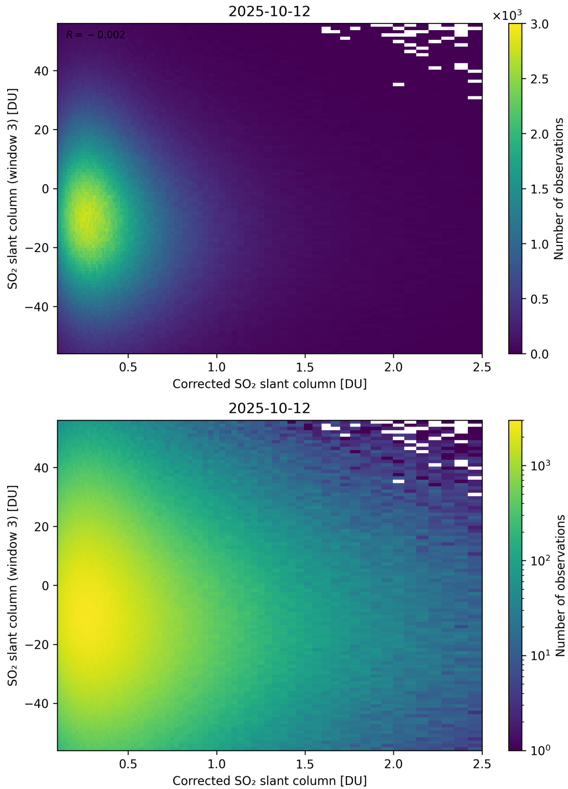
Figure 240: Scatter density plot of “Corrected SO 2 slant column” against “SO 2 slant column (window 3)” for 2025-10-11 to 2025-10-13.
