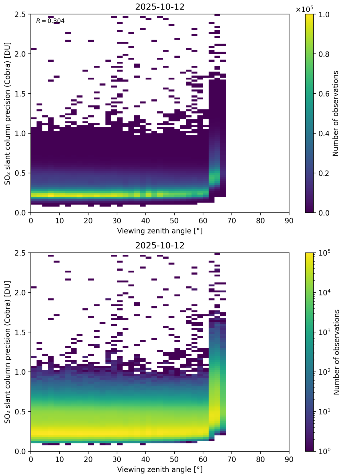
Figure 372: Scatter density plot of “Viewing zenith angle” against “SO 2 slant column precision (Cobra)” for 2025-10-11 to 2025-10-13.
