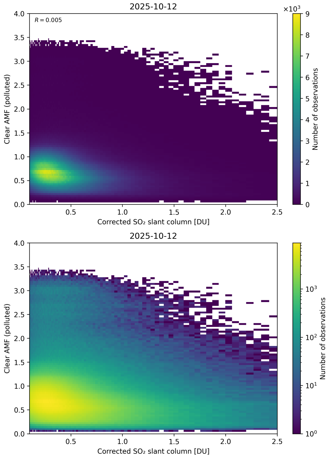
Figure 232: Scatter density plot of “Corrected SO 2 slant column” against “Clear AMF (polluted)” for 2025-10-11 to 2025-10-13.
