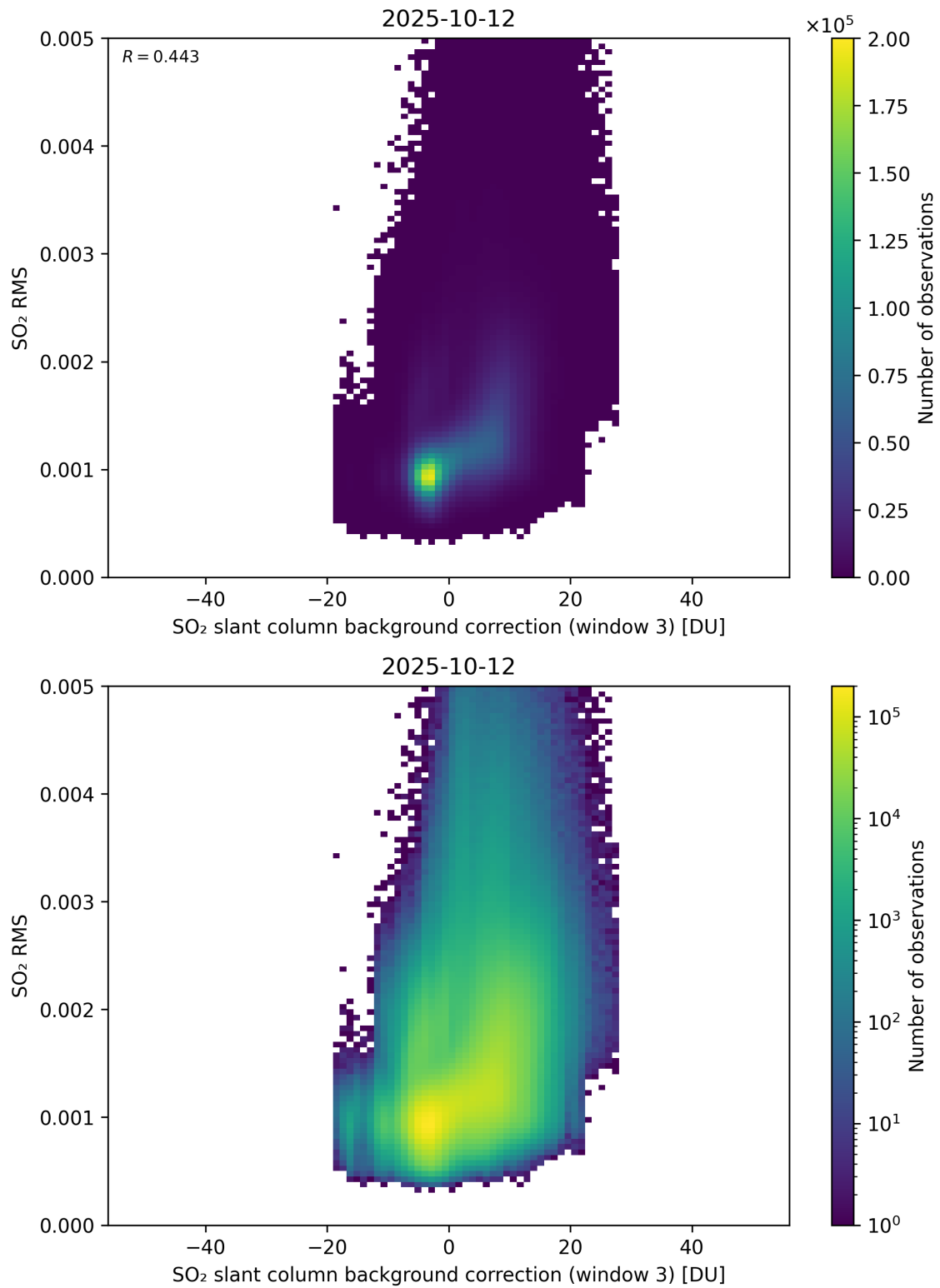
Figure 134: Scatter density plot of “SO 2 slant column background correction (window 3)” against “SO 2 RMS” for 2025-10-11 to 2025-10-13.
