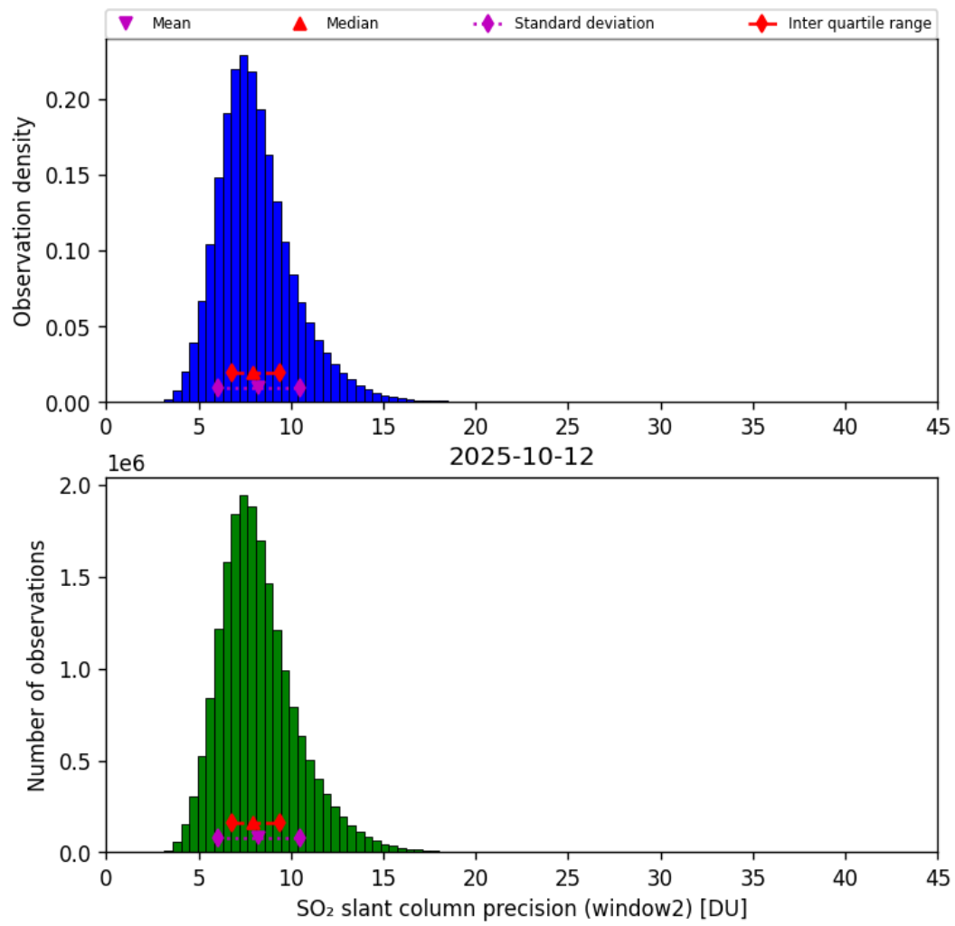
Figure 68: Histogram of “SO 2 slant column precision (window2)” for 2025-10-11 to 2025-10-13
