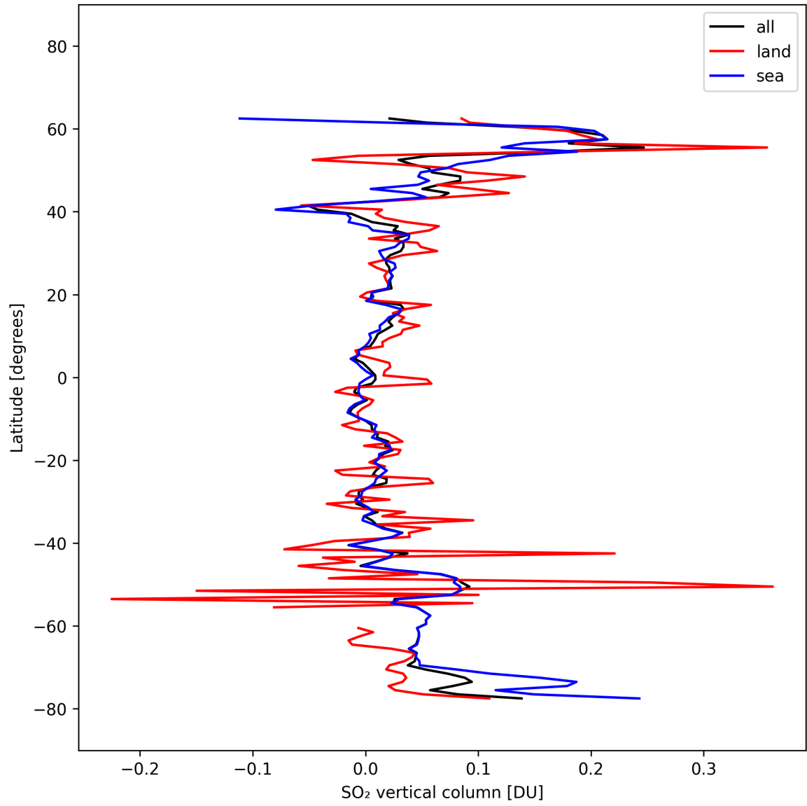
Figure 32: Zonal average of “SO 2 vertical column” for 2025-10-11 to 2025-10-13.
