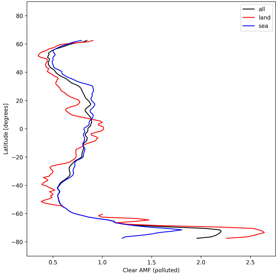
Figure 55: Zonal average of “Clear AMF (polluted)” for 2025-10-11 to 2025-10-13.
