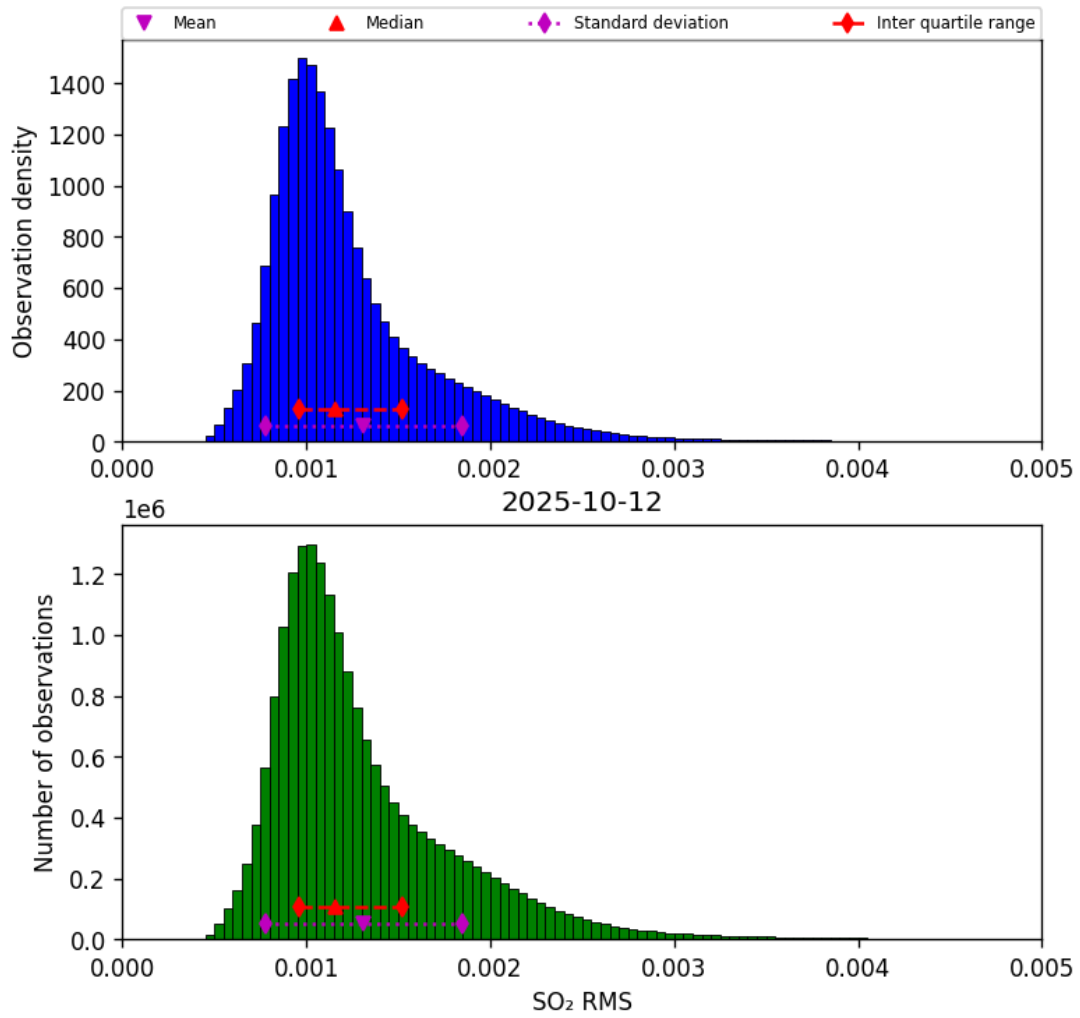
Figure 78: Histogram of “SO 2 RMS” for 2025-10-11 to 2025-10-13
