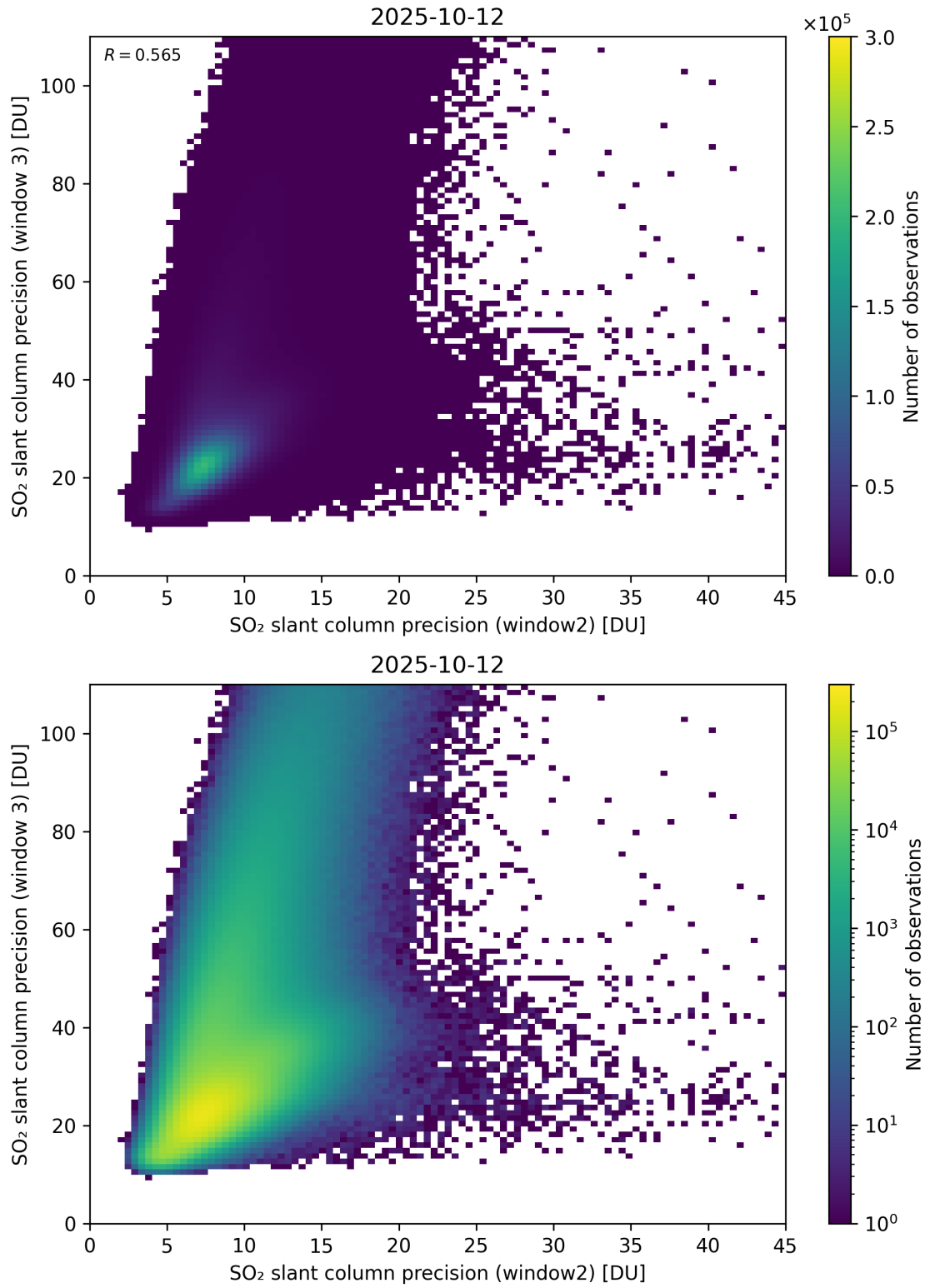
Figure 300: Scatter density plot of “SO 2 slant column precision (window2)” against “SO 2 slant column precision (window 3)” for 2025-10-11 to 2025-10-13.
