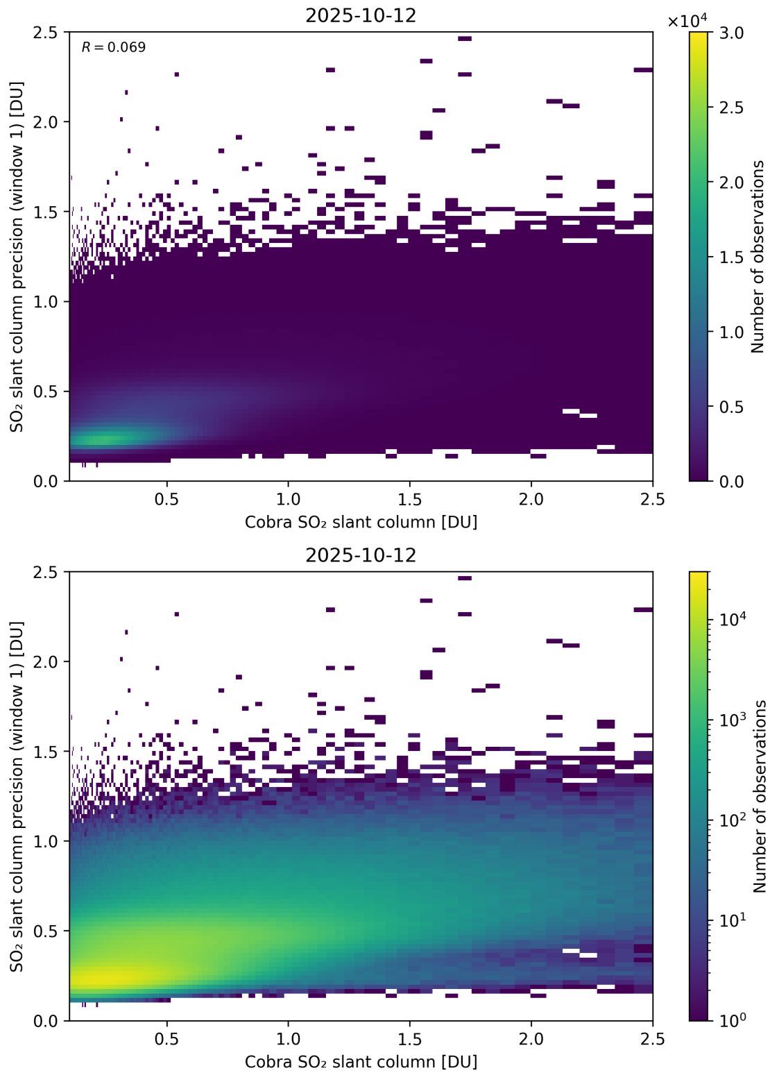
Figure 220: Scatter density plot of “Cobra SO 2 slant column” against “SO 2 slant column precision (window 1)” for 2025-10-11 to 2025-10-13.
