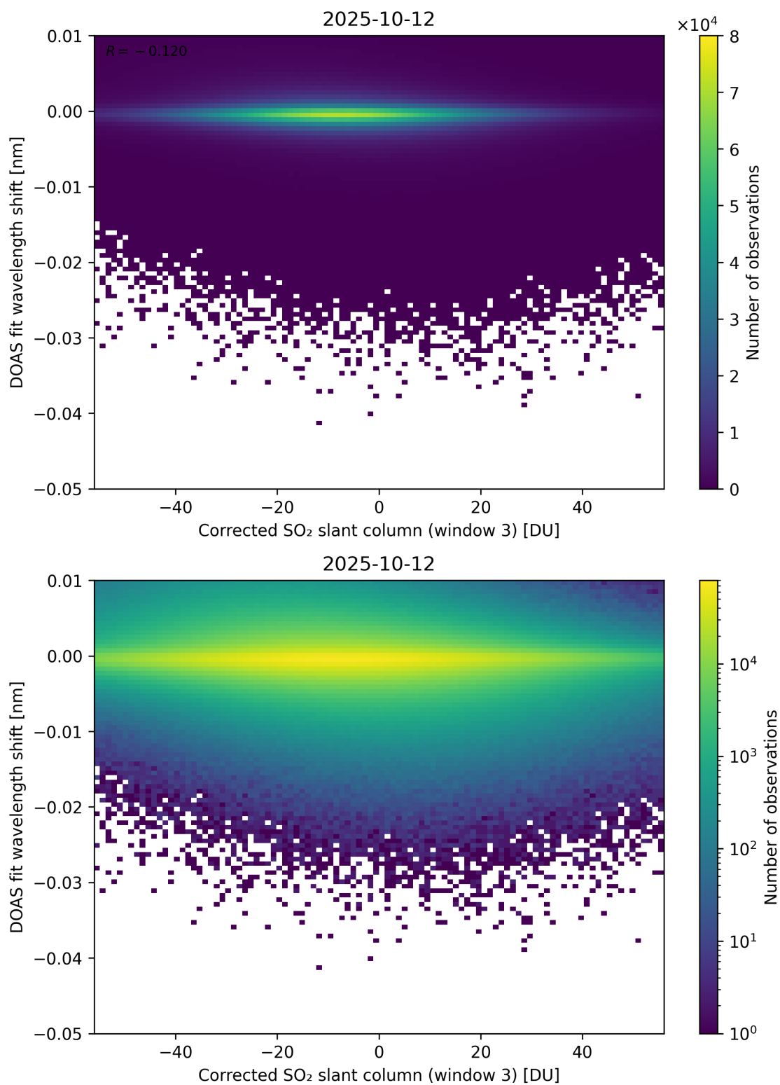
Figure 256: Scatter density plot of “Corrected SO 2 slant column (window 3)” against “DOAS fit wavelength shift” for 2025-10-11 to 2025-10-13.
