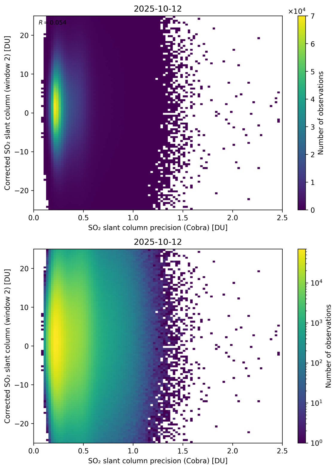
Figure 206: Scatter density plot of “SO 2 slant column precision (Cobra)” against “Corrected SO 2 slant column (window 2)” for 2025-10-11 to 2025-10-13.
