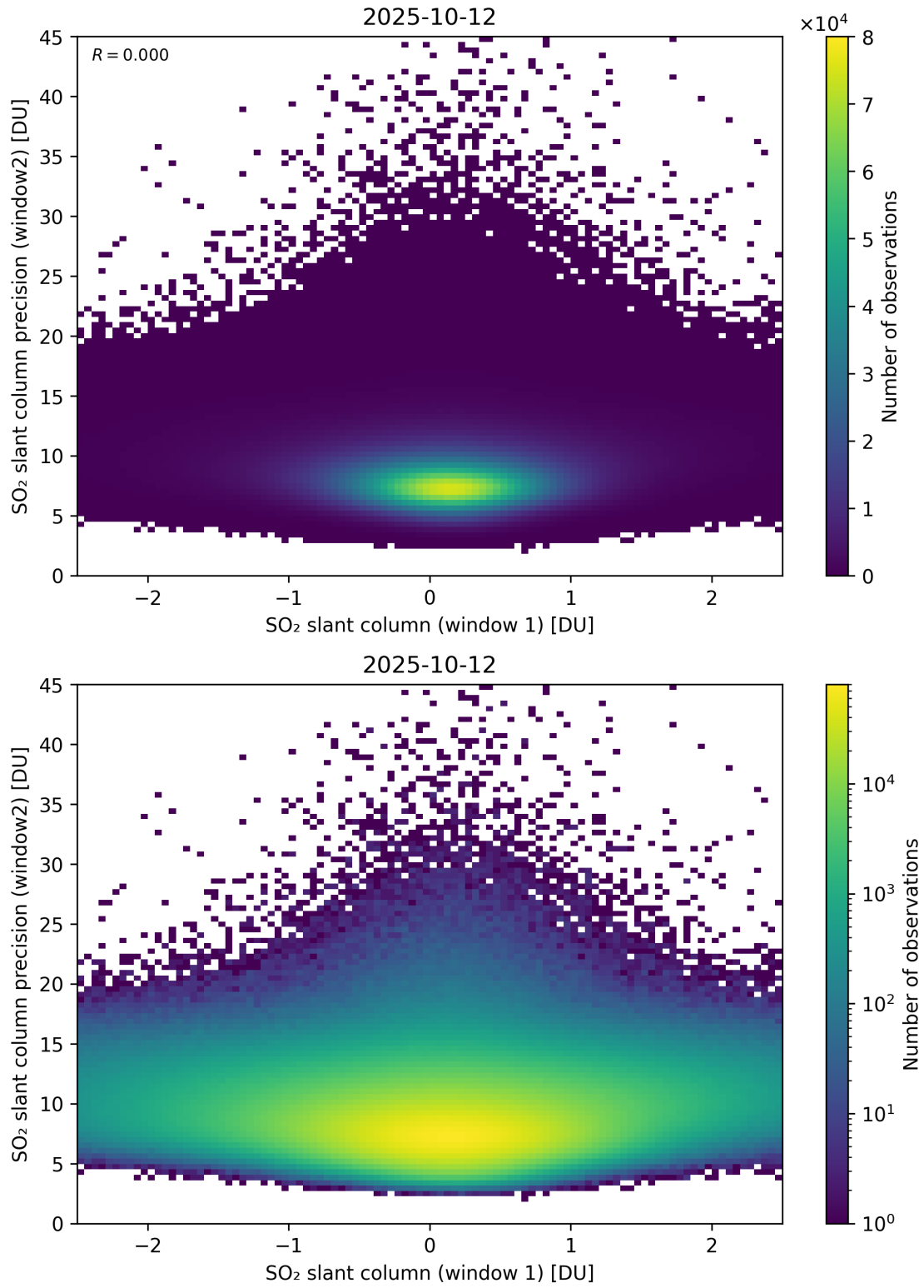
Figure 286: Scatter density plot of “SO 2 slant column (window 1)” against “SO 2 slant column precision (window2)” for 2025-10-11 to 2025-10-13.
