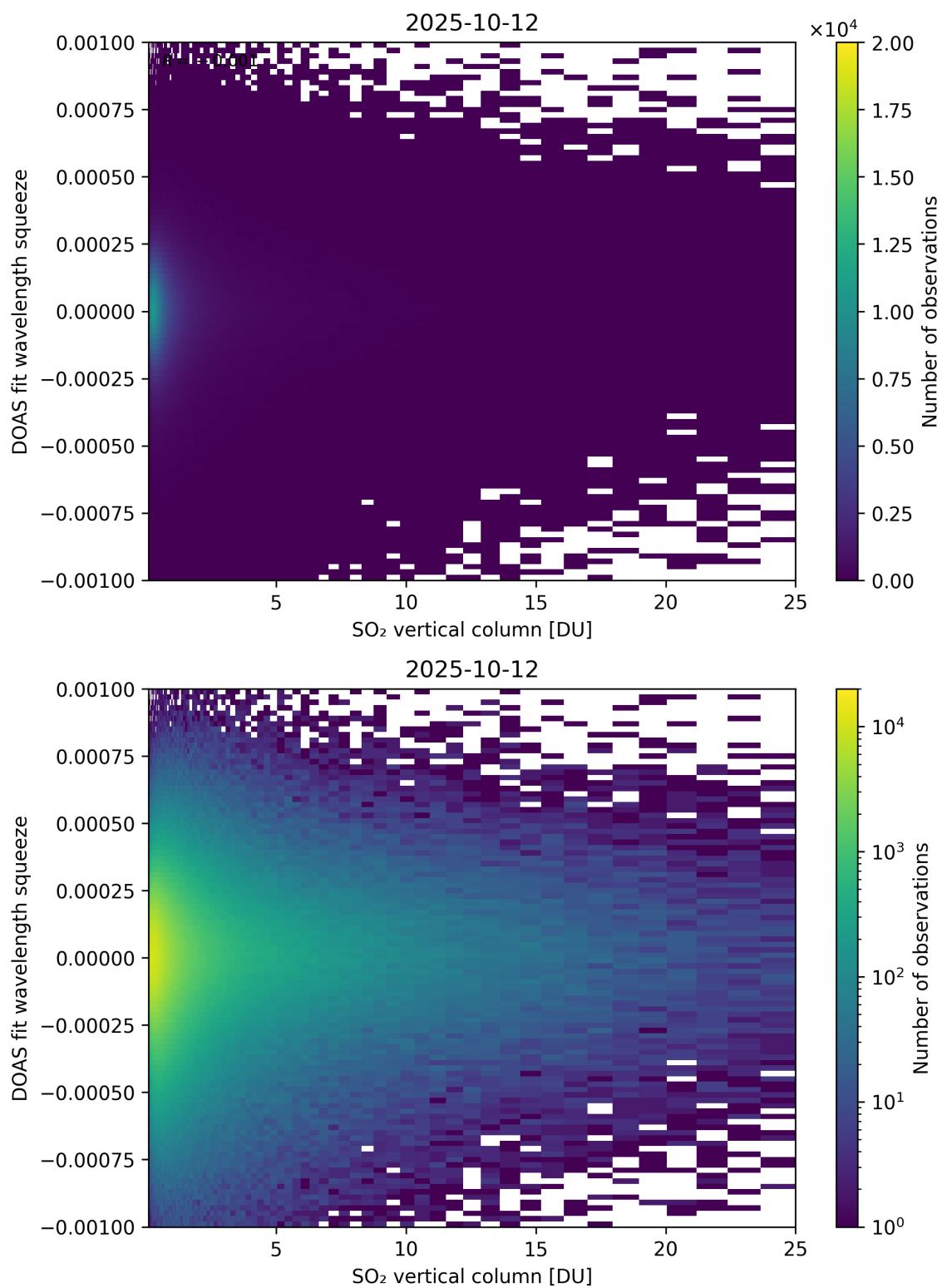
Figure 327: Scatter density plot of “SO 2 vertical column” against “DOAS fit wavelength squeeze” for 2025-10-11 to 2025-10-13.
