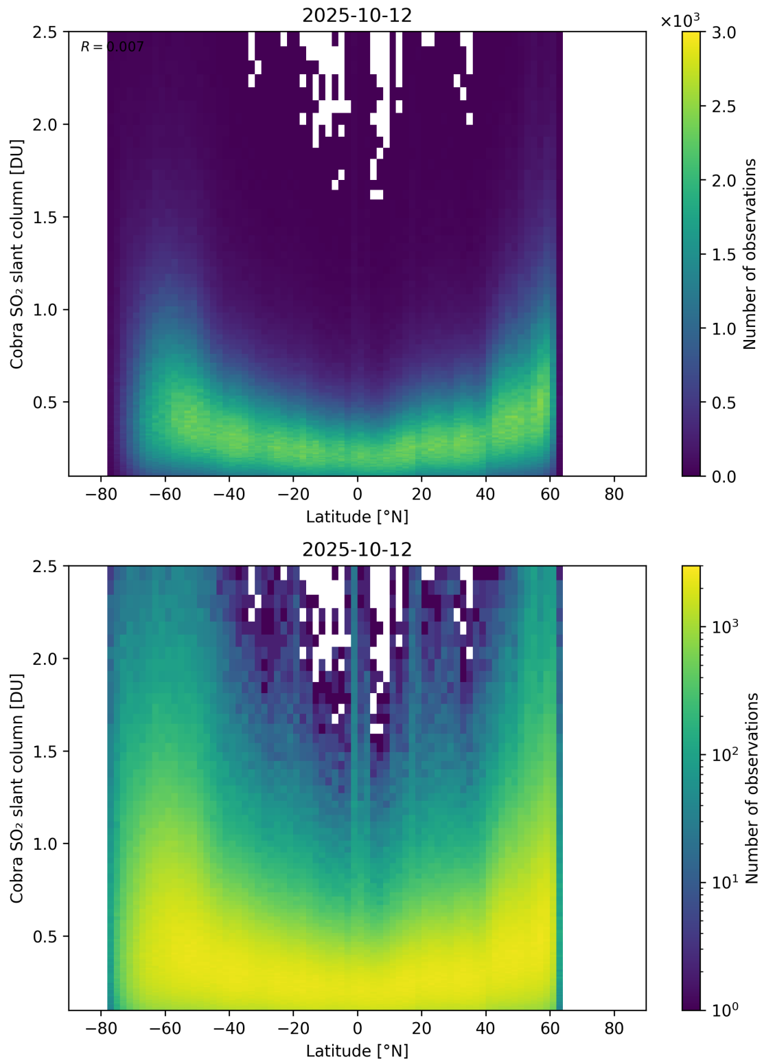
Figure 157: Scatter density plot of “Latitude” against “Cobra SO 2 slant column” for 2025-10-11 to 2025-10-13.
