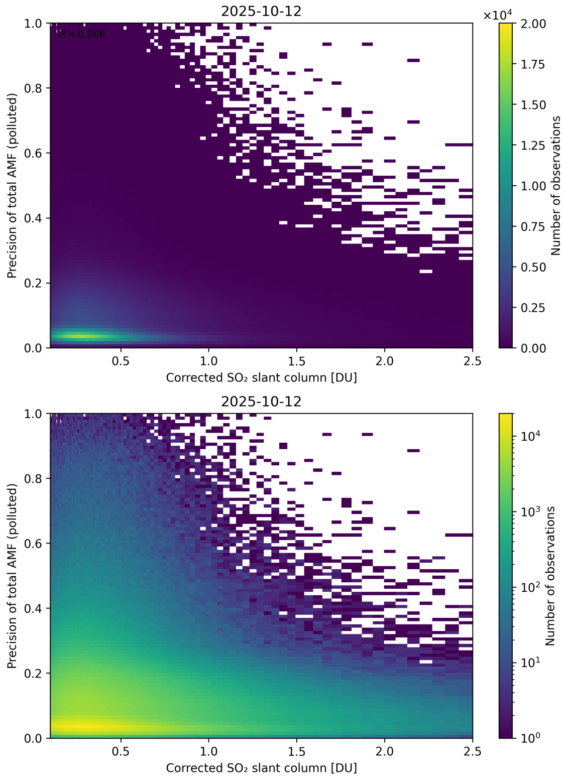
Figure 243: Scatter density plot of “Corrected SO 2 slant column” against “Precision of total AMF (polluted)” for 2025-10-11 to 2025-10-13.
