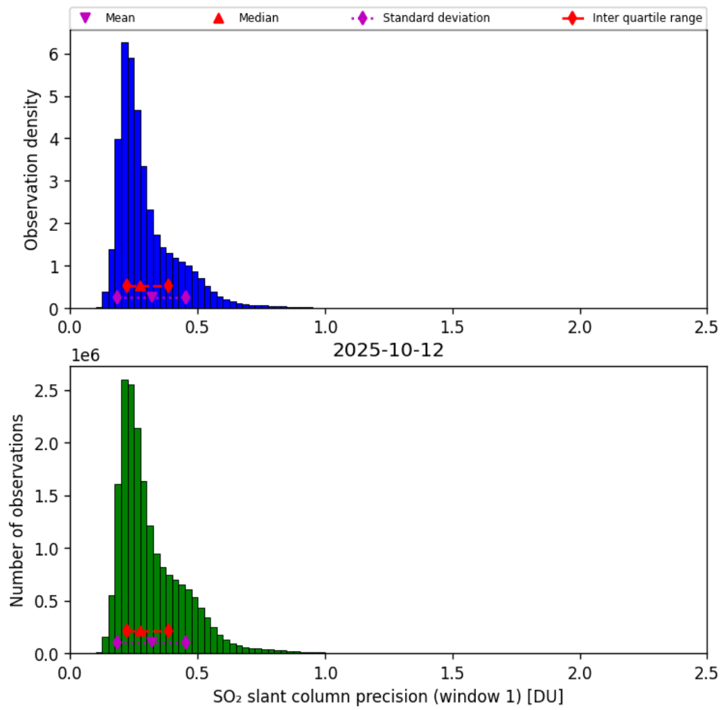
Figure 64: Histogram of “SO 2 slant column precision (window 1)” for 2025-10-11 to 2025-10-13
