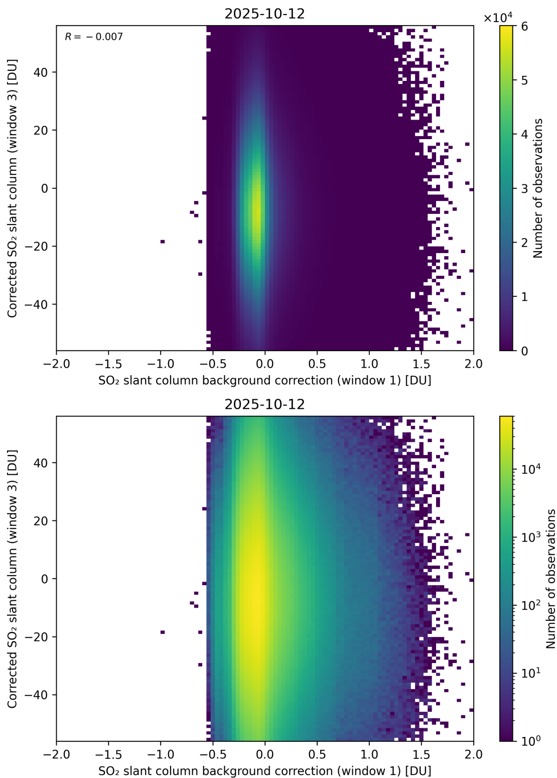
Figure 116: Scatter density plot of “SO 2 slant column background correction (window 1)” against “Corrected SO 2 slant column (window 3)” for 2025-10-11 to 2025-10-13.
