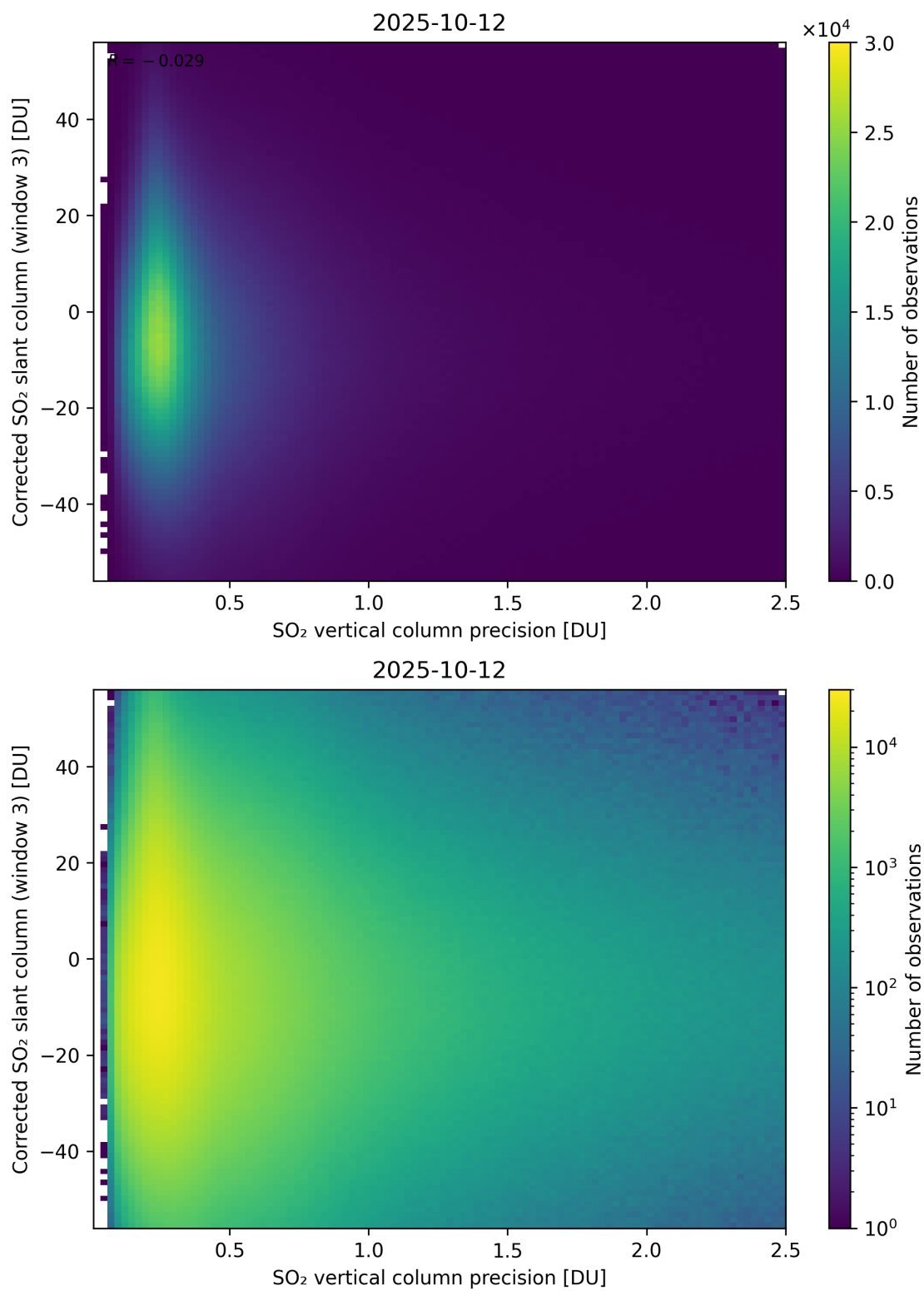
Figure 340: Scatter density plot of “SO 2 vertical column precision” against “Corrected SO 2 slant column (window 3)” for 2025-10-11 to 2025-10-13.
