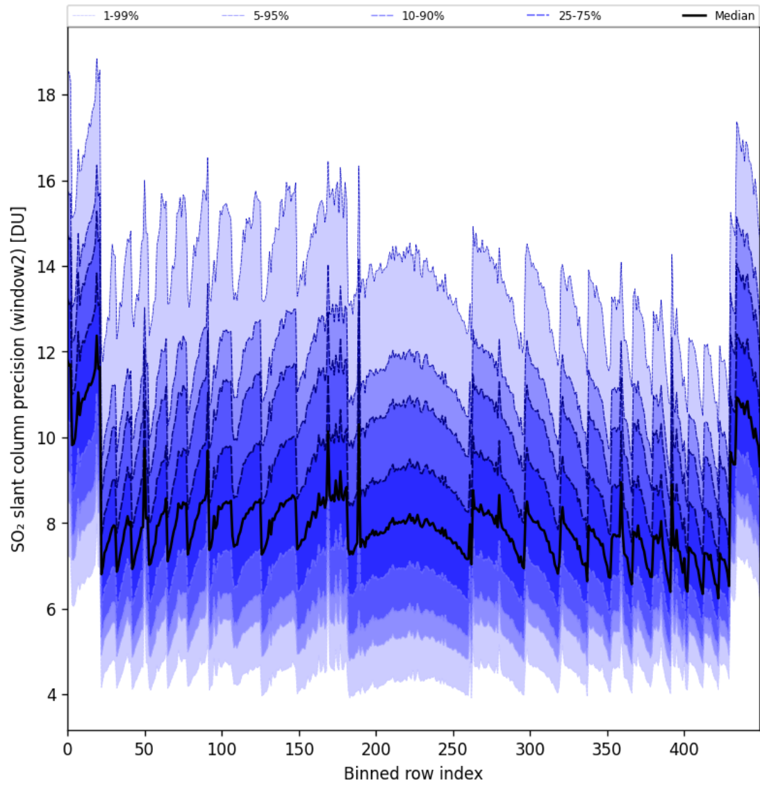
Figure 94: Along track statistics of “SO 2 slant column precision (window2)” for 2025-10-11 to 2025-10-13
