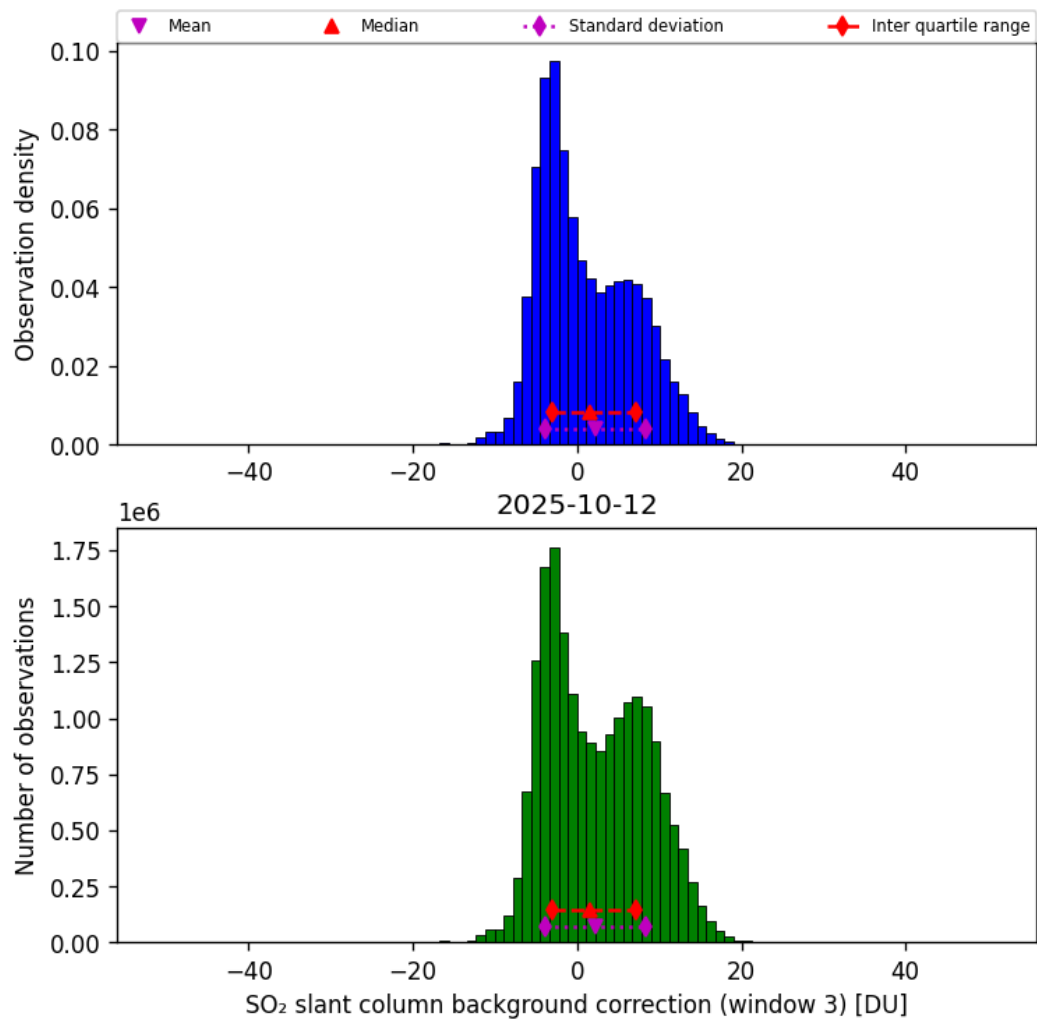
Figure 74: Histogram of “SO 2 slant column background correction (window 3)” for 2025-10-11 to 2025-10-13
