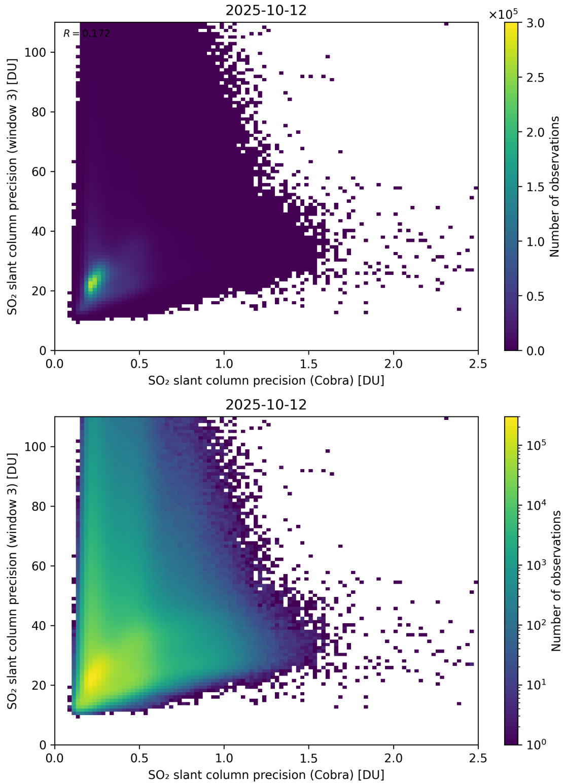
Figure 212: Scatter density plot of “SO 2 slant column precision (Cobra)” against “SO 2 slant column precision (window 3)” for 2025-10-11 to 2025-10-13.
