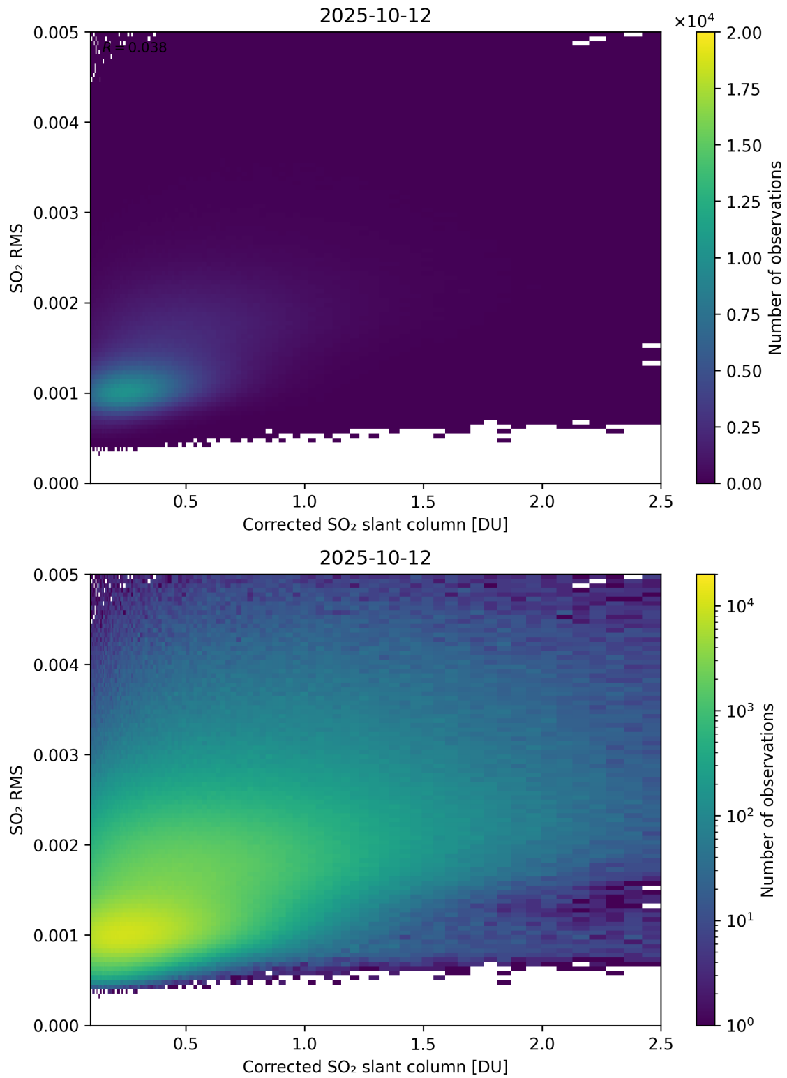
Figure 231: Scatter density plot of “Corrected SO 2 slant column” against “SO 2 RMS” for 2025-10-11 to 2025-10-13.
