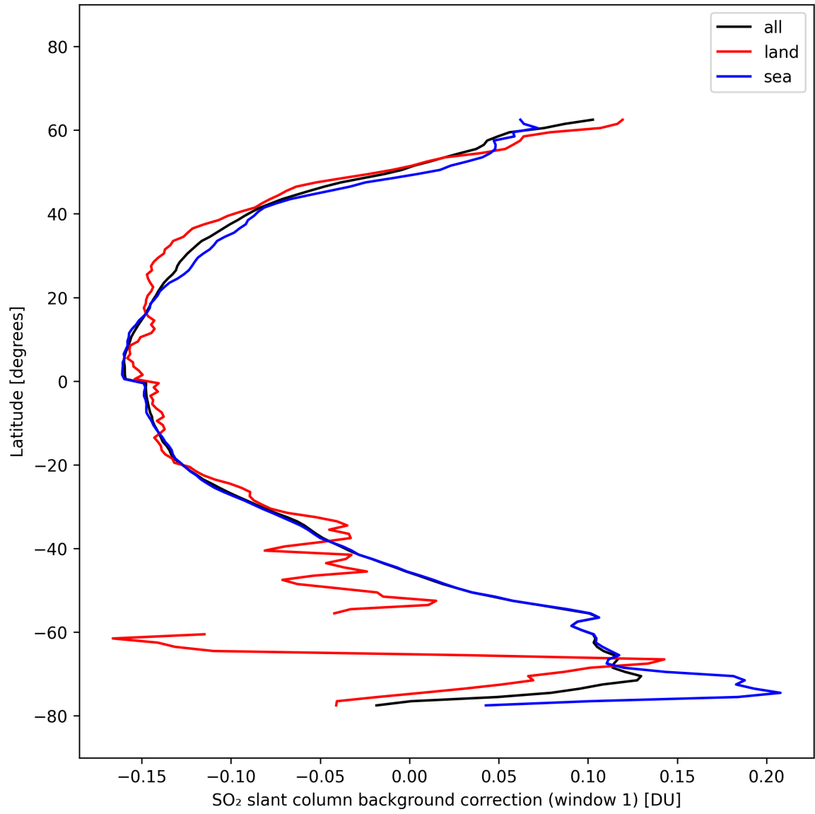
Figure 40: Zonal average of “SO 2 slant column background correction (window 1)” for 2025-10-11 to 2025-10-13.
