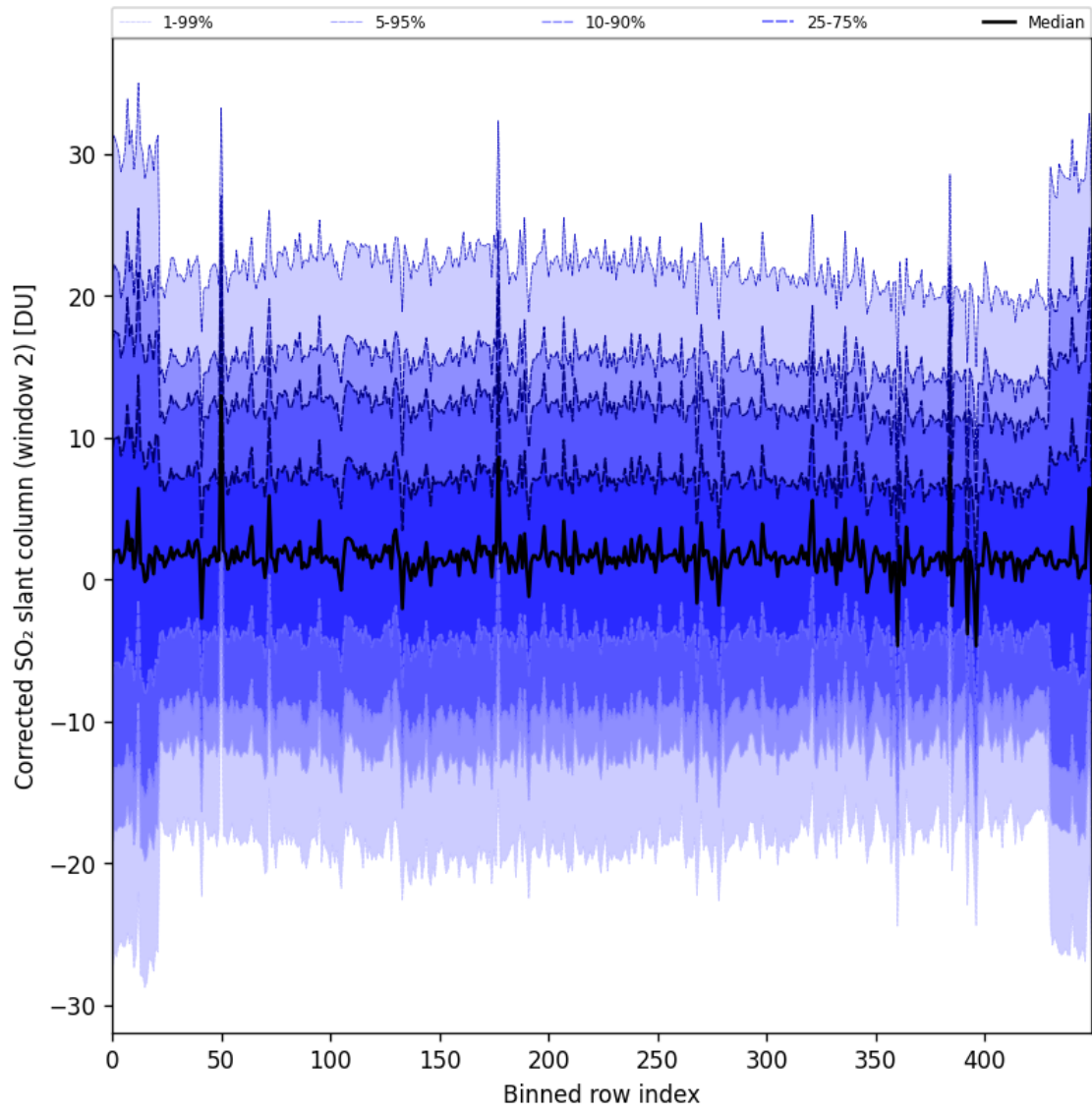
Figure 95: Along track statistics of “Corrected SO 2 slant column (window 2)” for 2025-10-11 to 2025-10-13
