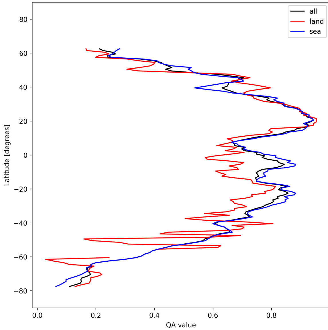
Figure 31: Zonal average of “QA value” for 2025-10-11 to 2025-10-13.
