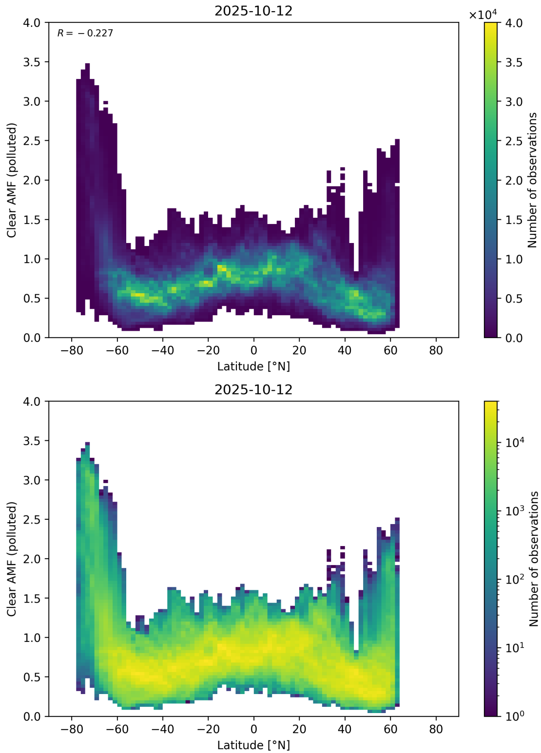
Figure 156: Scatter density plot of “Latitude” against “Clear AMF (polluted)” for 2025-10-11 to 2025-10-13.
