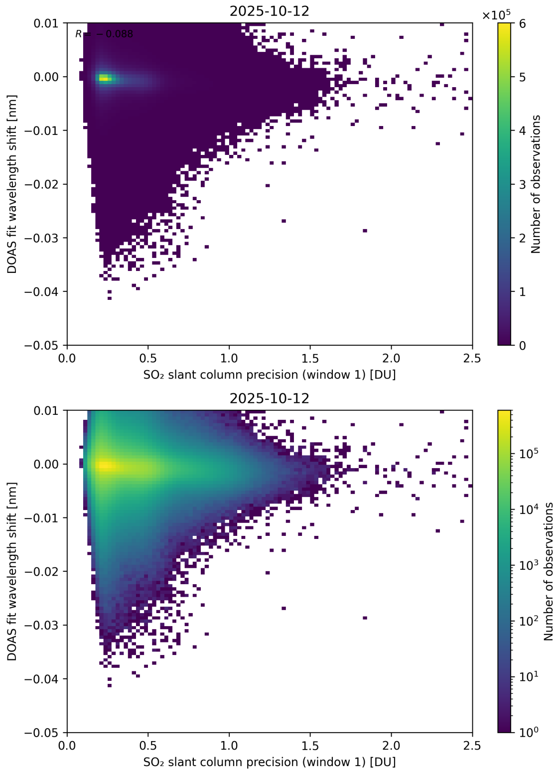
Figure 271: Scatter density plot of “SO 2 slant column precision (window 1)” against “DOAS fit wavelength shift” for 2025-10-11 to 2025-10-13.
