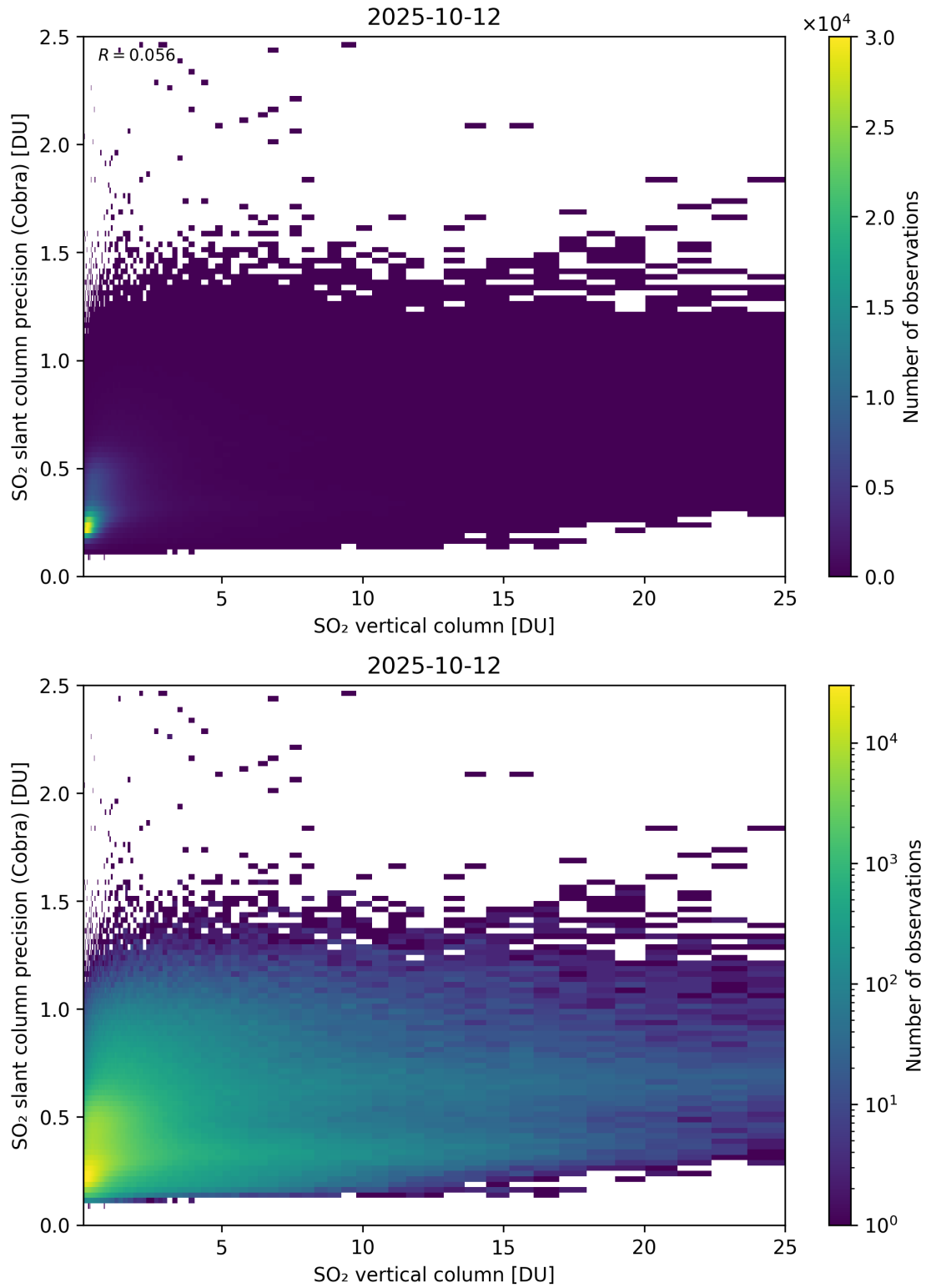
Figure 350: Scatter density plot of “SO 2 vertical column” against “SO 2 slant column precision (Cobra)” for 2025-10-11 to 2025-10-13.
