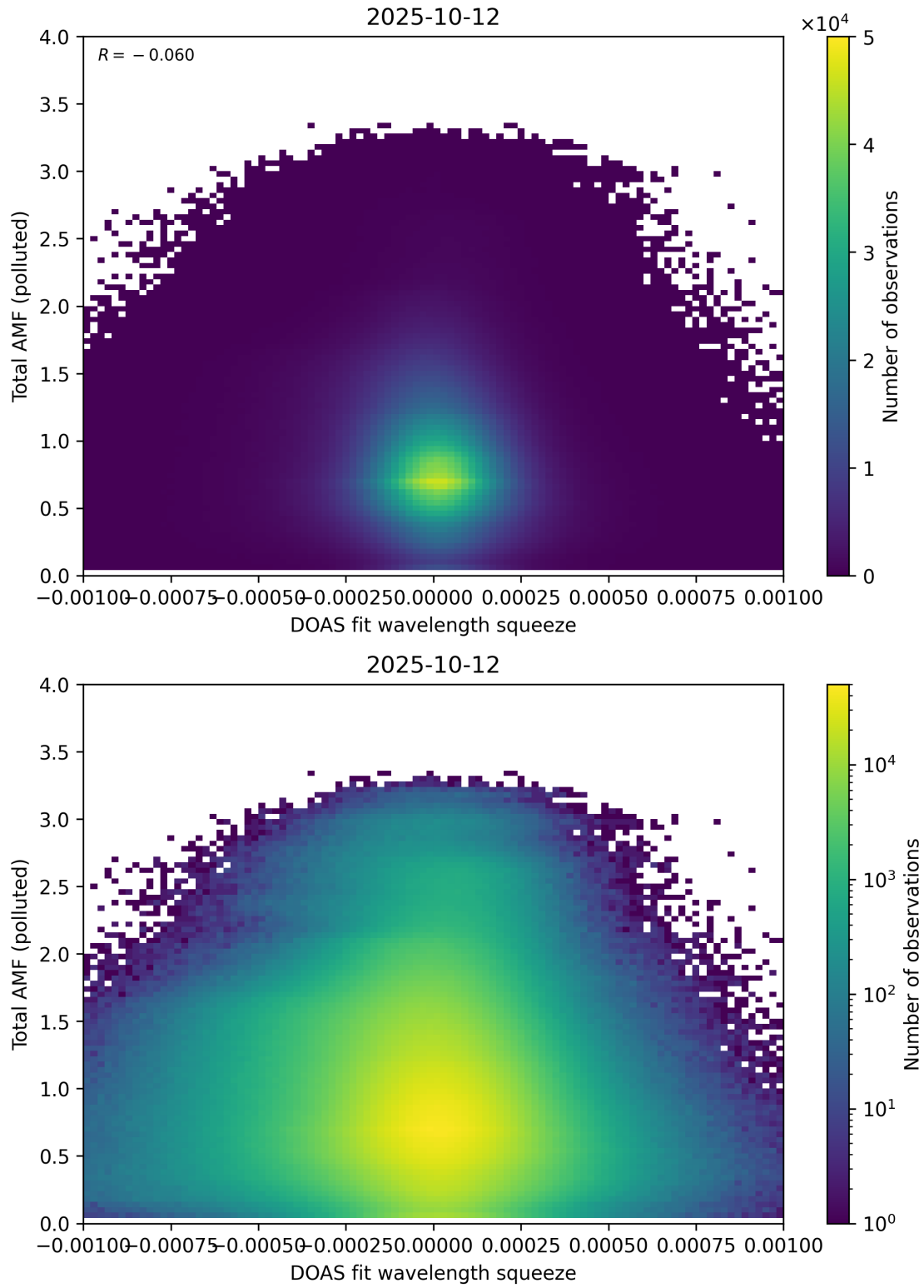
Figure 145: Scatter density plot of “DOAS fit wavelength squeeze” against “Total AMF (polluted)” for 2025-10-11 to 2025-10-13.
