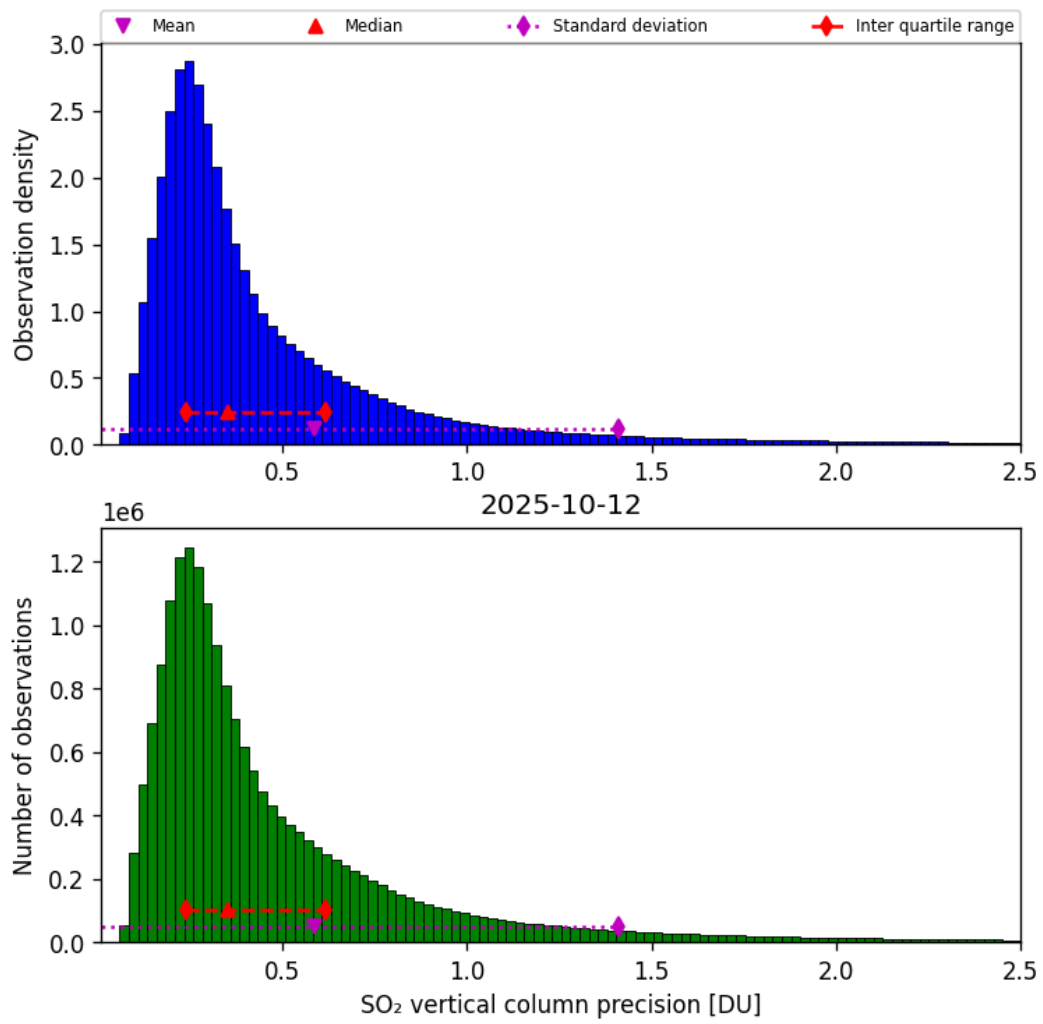
Figure 59: Histogram of “SO 2 vertical column precision” for 2025-10-11 to 2025-10-13
