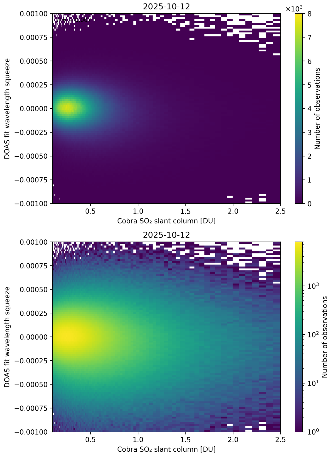
Figure 197: Scatter density plot of “Cobra SO 2 slant column” against “DOAS fit wavelength squeeze” for 2025-10-11 to 2025-10-13.
