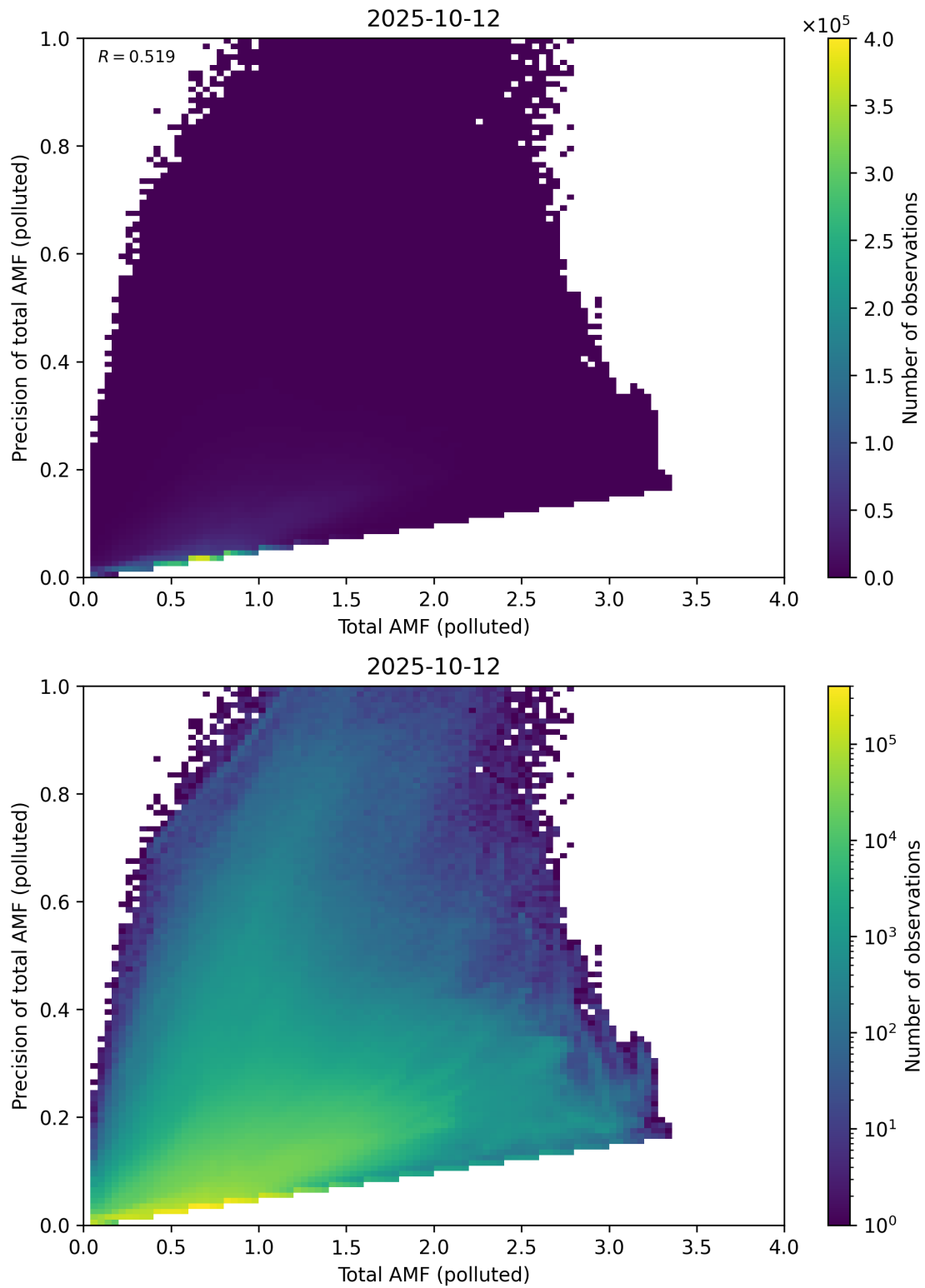
Figure 322: Scatter density plot of “Total AMF (polluted)” against “Precision of total AMF (polluted)” for 2025-10-11 to 2025-10-13.
