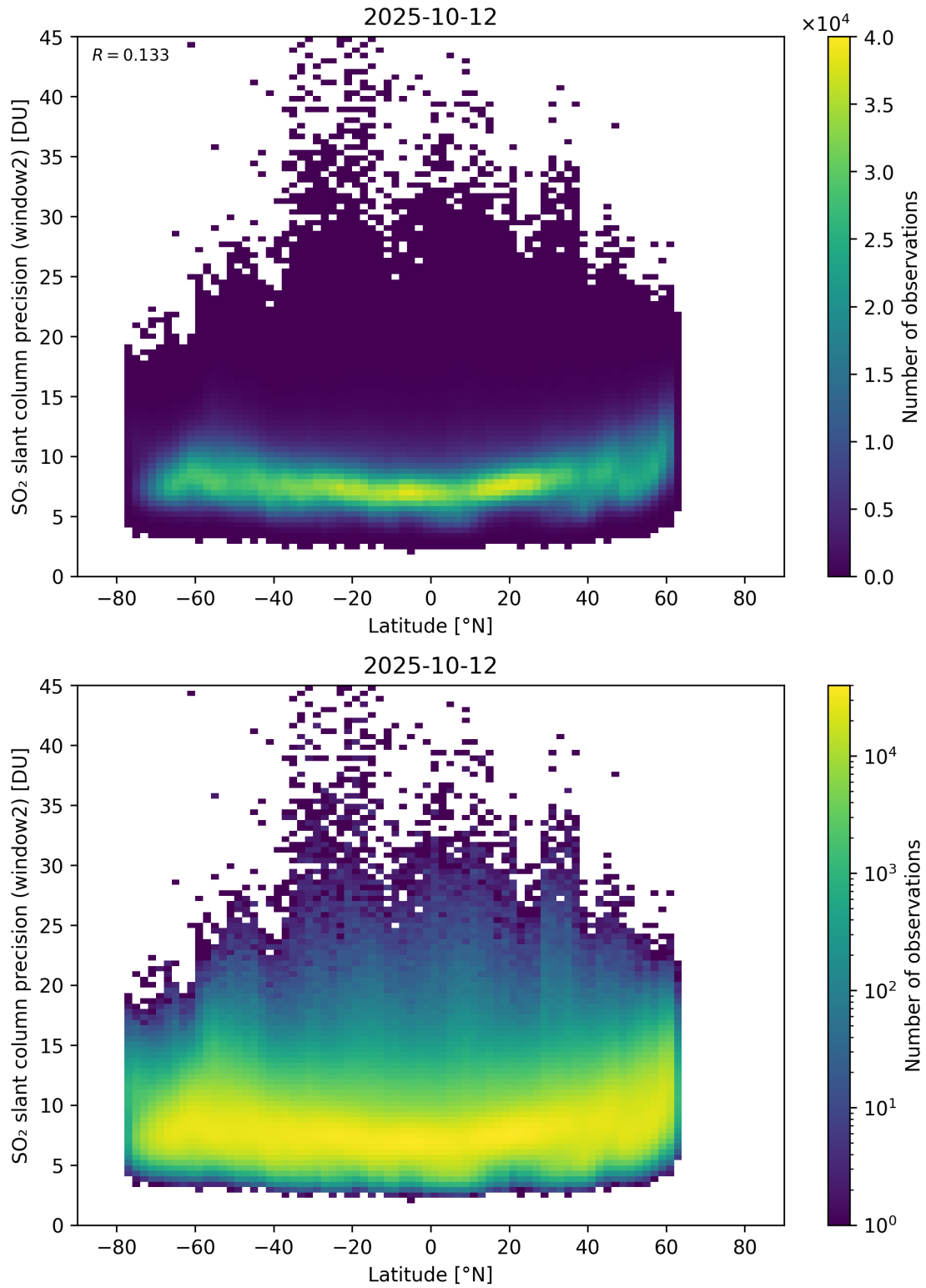
Figure 164: Scatter density plot of “Latitude” against “SO 2 slant column precision (window2)” for 2025-10-11 to 2025-10-13.
