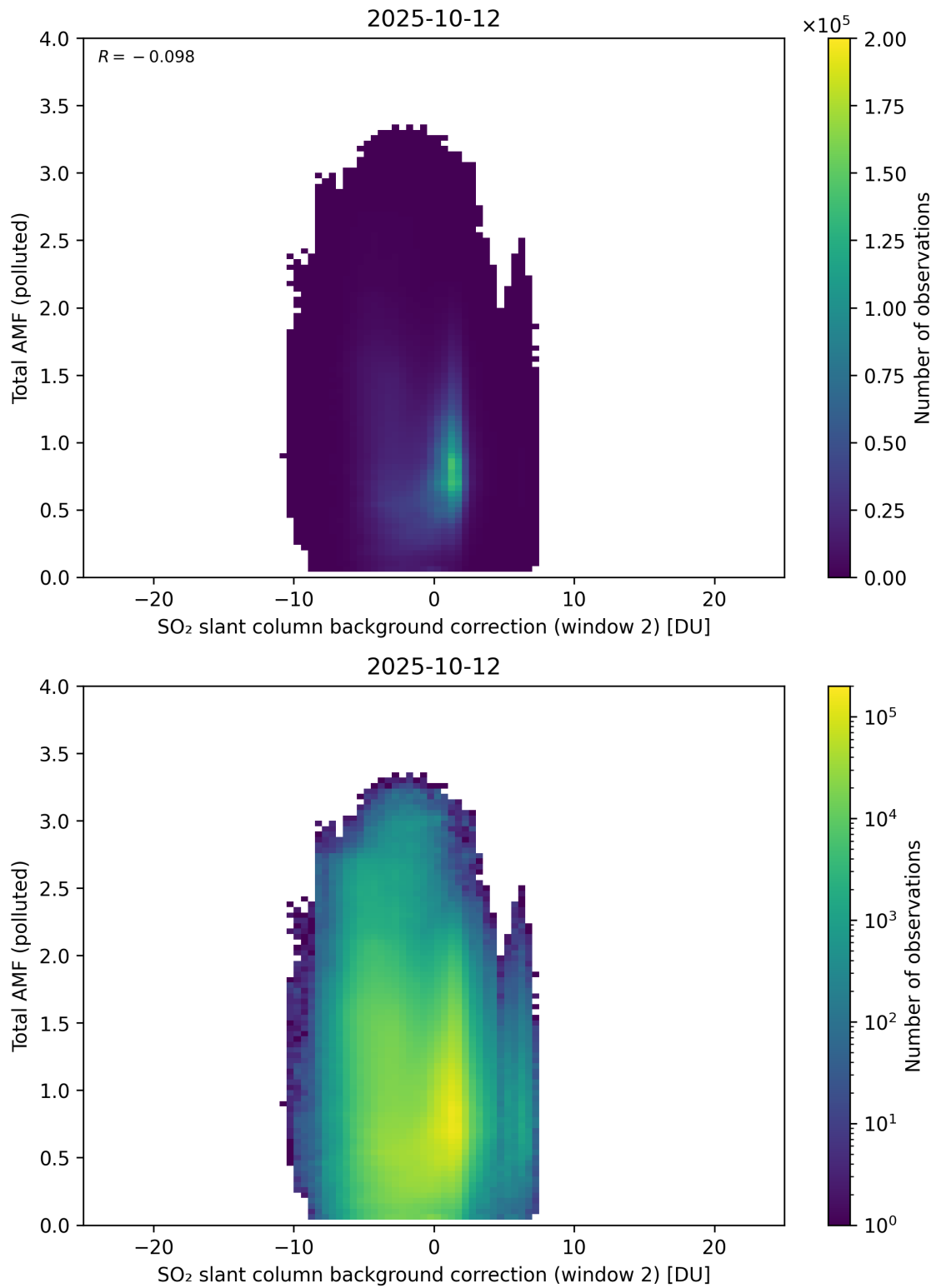
Figure 130: Scatter density plot of “SO 2 slant column background correction (window 2)” against “Total AMF (polluted)” for 2025-10-11 to 2025-10-13.
