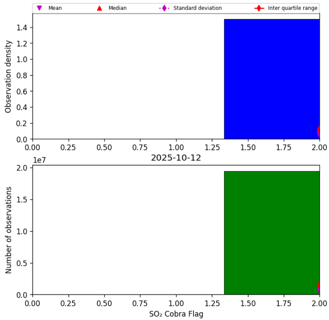
Figure 75: Histogram of “SO 2 Cobra Flag” for 2025-10-11 to 2025-10-13
