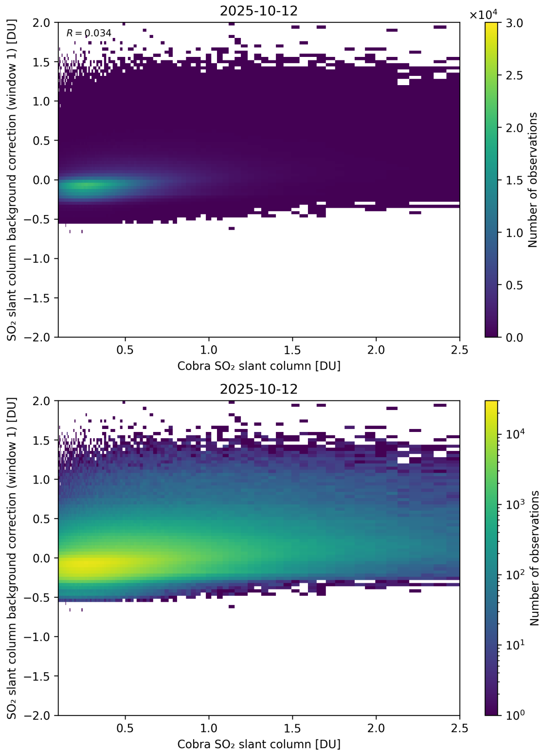
Figure 193: Scatter density plot of “Cobra SO 2 slant column” against “SO 2 slant column background correction (window 1)” for 2025-10-11 to 2025-10-13.
