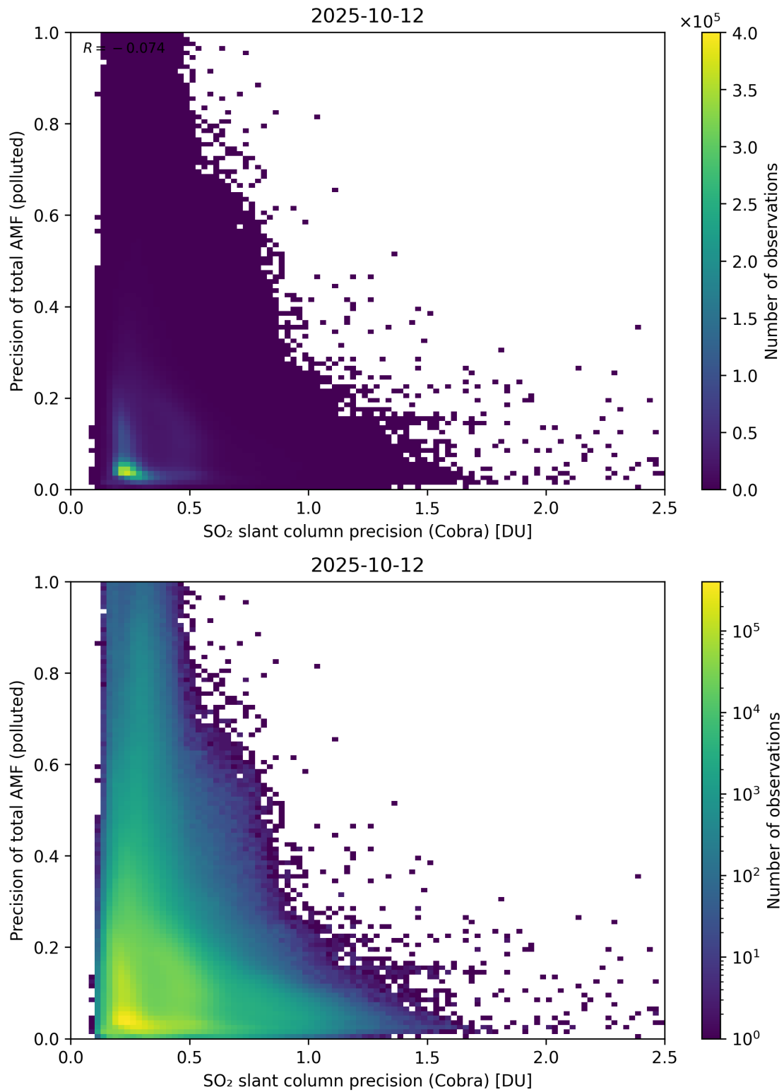
Figure 214: Scatter density plot of “SO 2 slant column precision (Cobra)” against “Precision of total AMF (polluted)” for 2025-10-11 to 2025-10-13.
