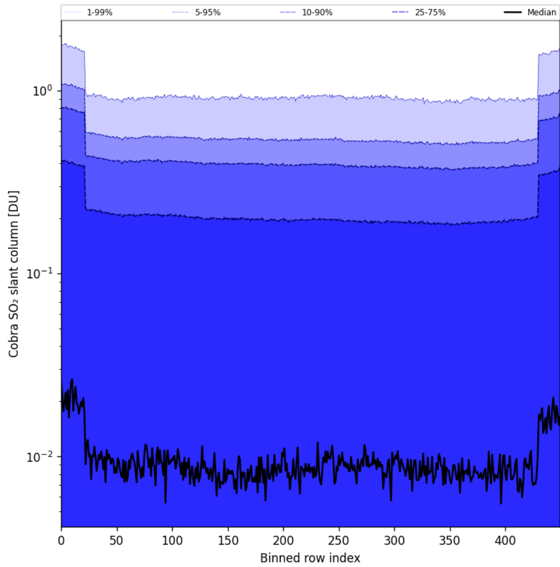
Figure 87: Along track statistics of "Cobra SO 2 slant column" for 2025-10-11 to 2025-10-13
