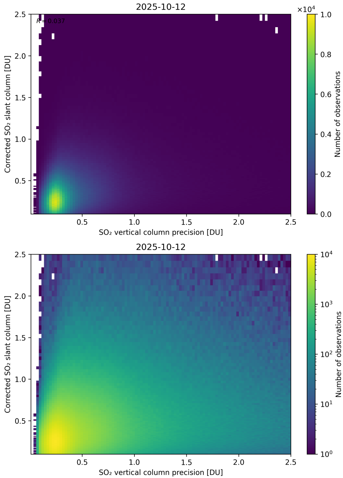
Figure 338: Scatter density plot of “SO 2 vertical column precision” against “Corrected SO 2 slant column” for 2025-10-11 to 2025-10-13.
