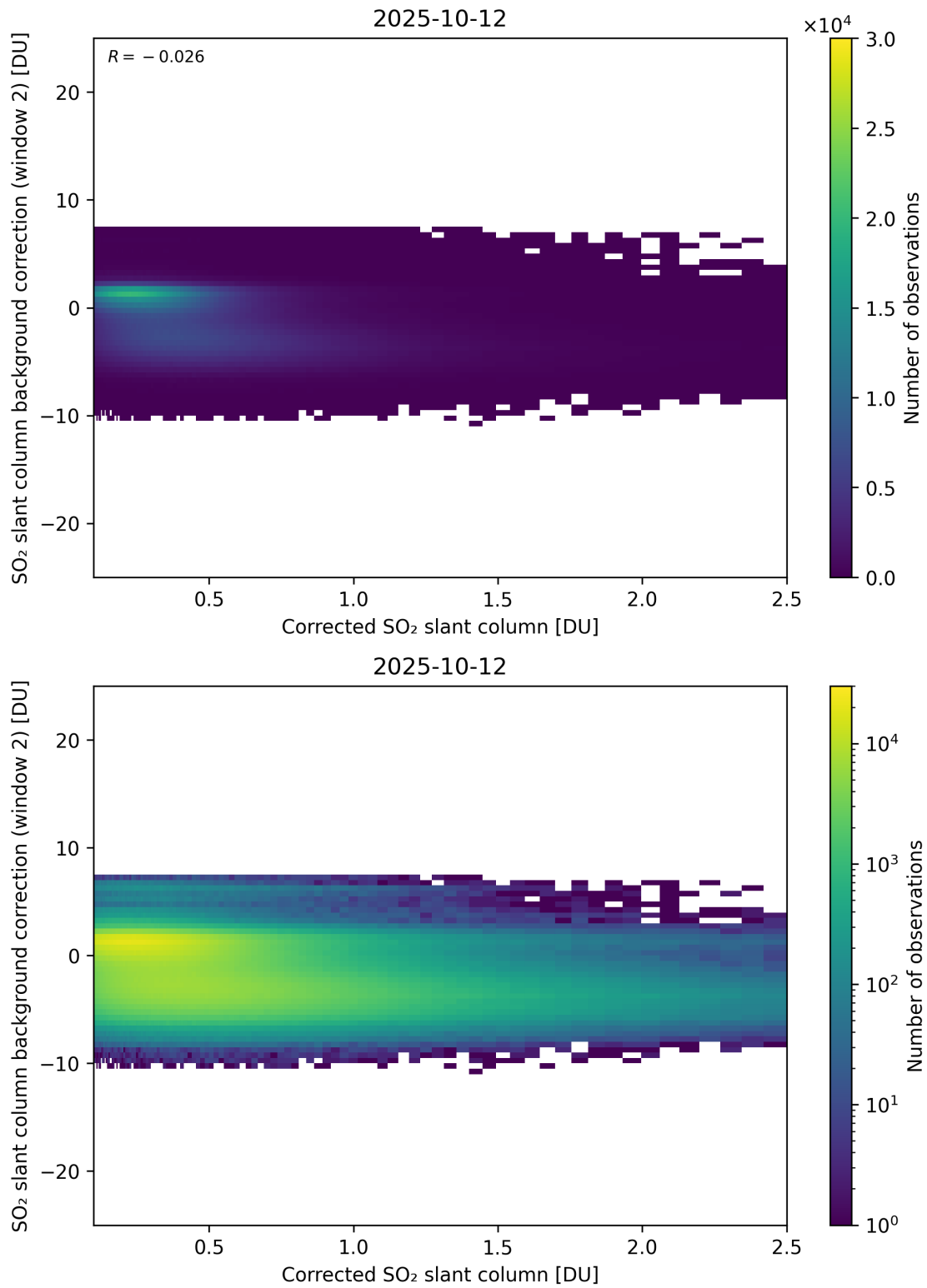
Figure 227: Scatter density plot of “Corrected SO 2 slant column” against “SO 2 slant column background correction (window 2)” for 2025-10-11 to 2025-10-13.
