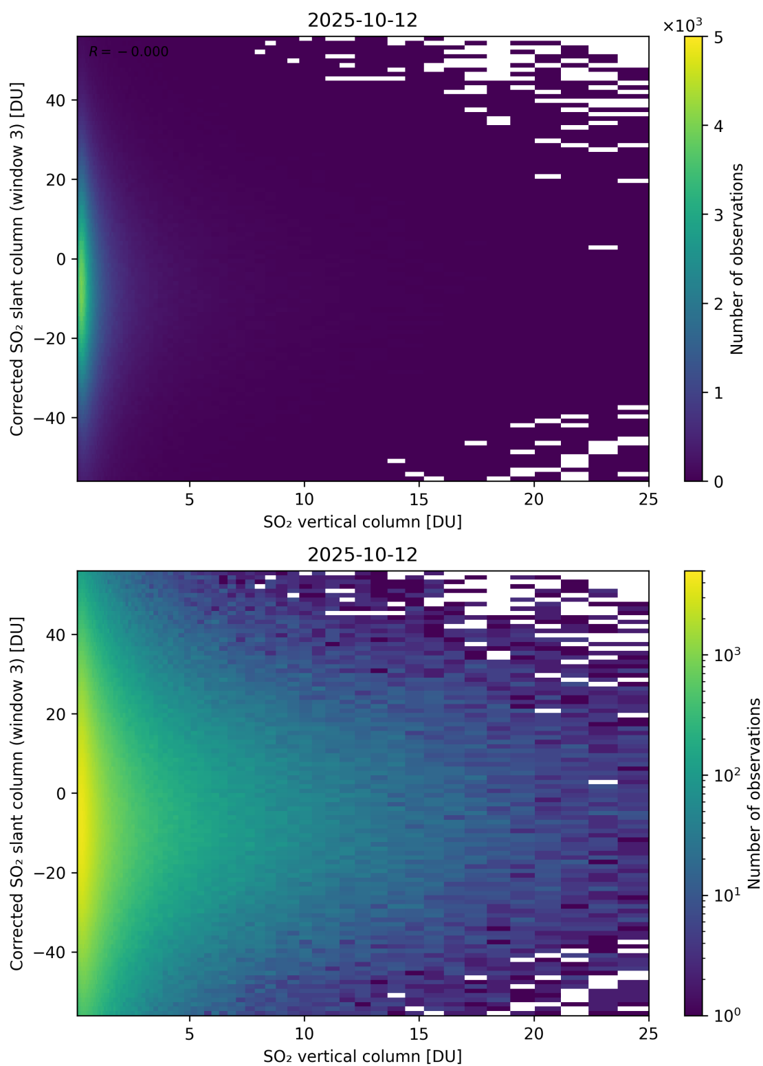
Figure 353: Scatter density plot of “SO 2 vertical column” against “Corrected SO 2 slant column (window 3)” for 2025-10-11 to 2025-10-13.
