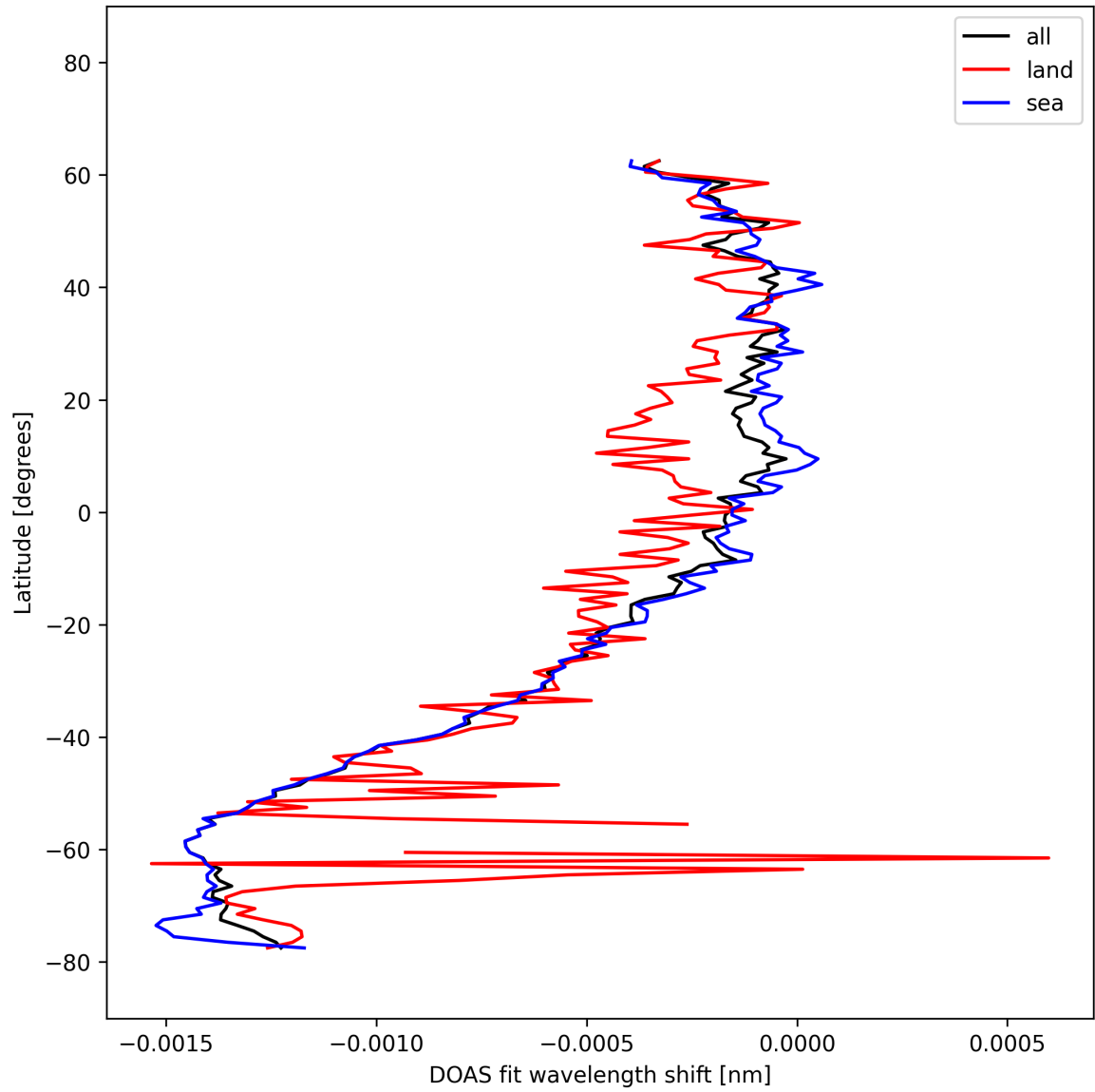
Figure 50: Zonal average of “DOAS fit wavelength shift” for 2025-10-11 to 2025-10-13.
