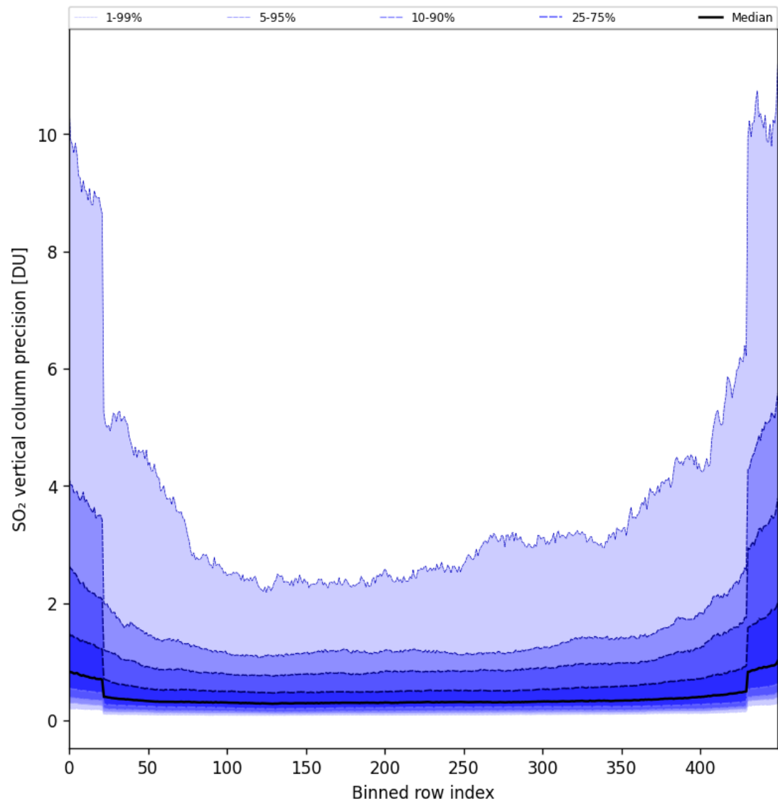
Figure 85: Along track statistics of “SO 2 vertical column precision” for 2025-10-11 to 2025-10-13
