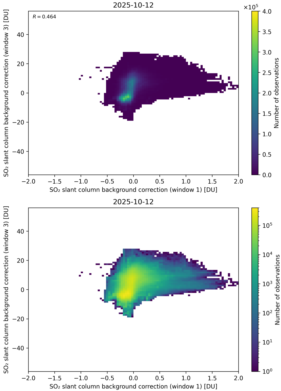
Figure 110: Scatter density plot of “SO 2 slant column background correction (window 1)” against “SO 2 slant column background correction (window 3)” for 2025-10-11 to 2025-10-13.
