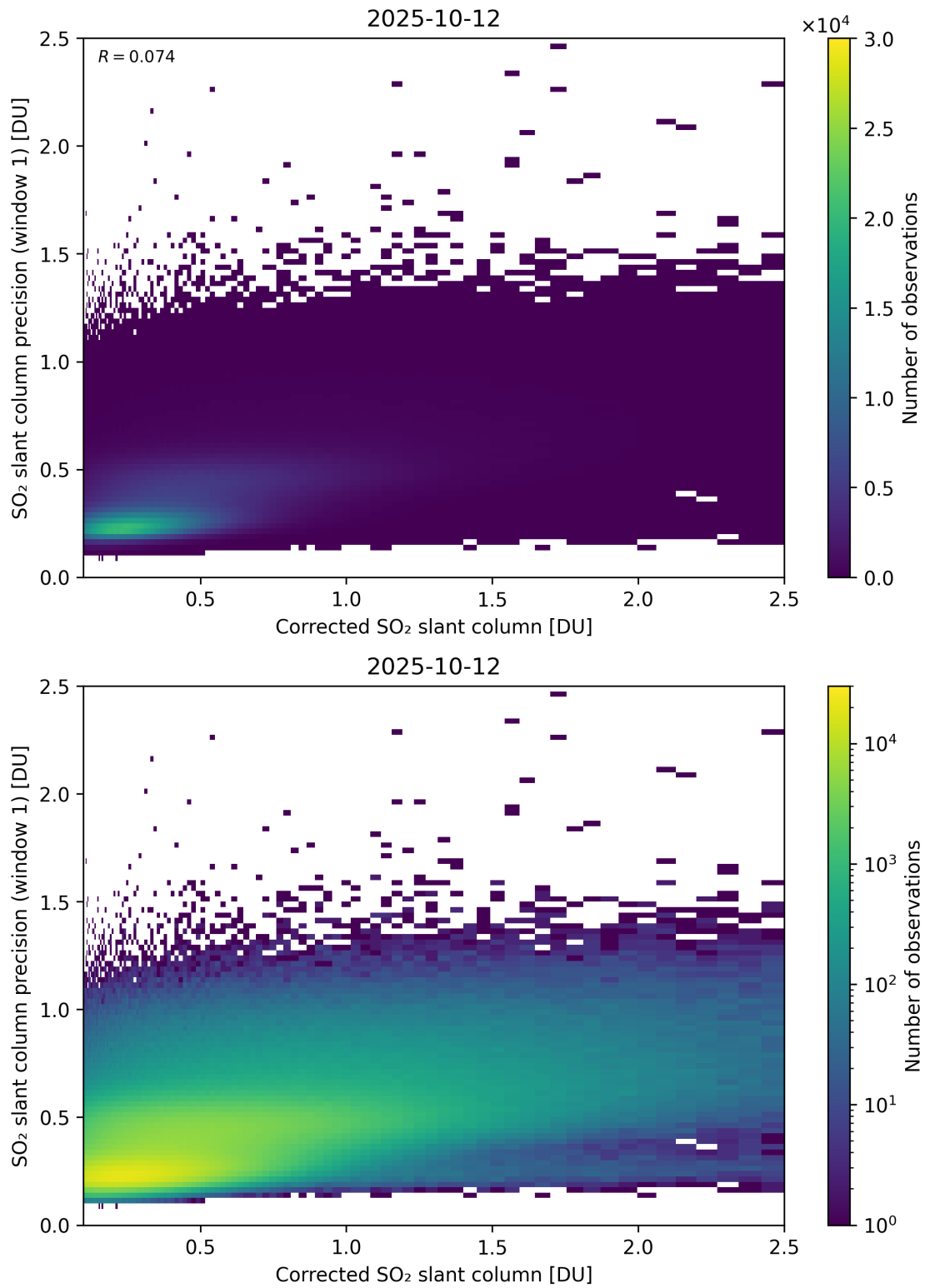
Figure 238: Scatter density plot of “Corrected SO 2 slant column” against “SO 2 slant column precision (window 1)” for 2025-10-11 to 2025-10-13.
