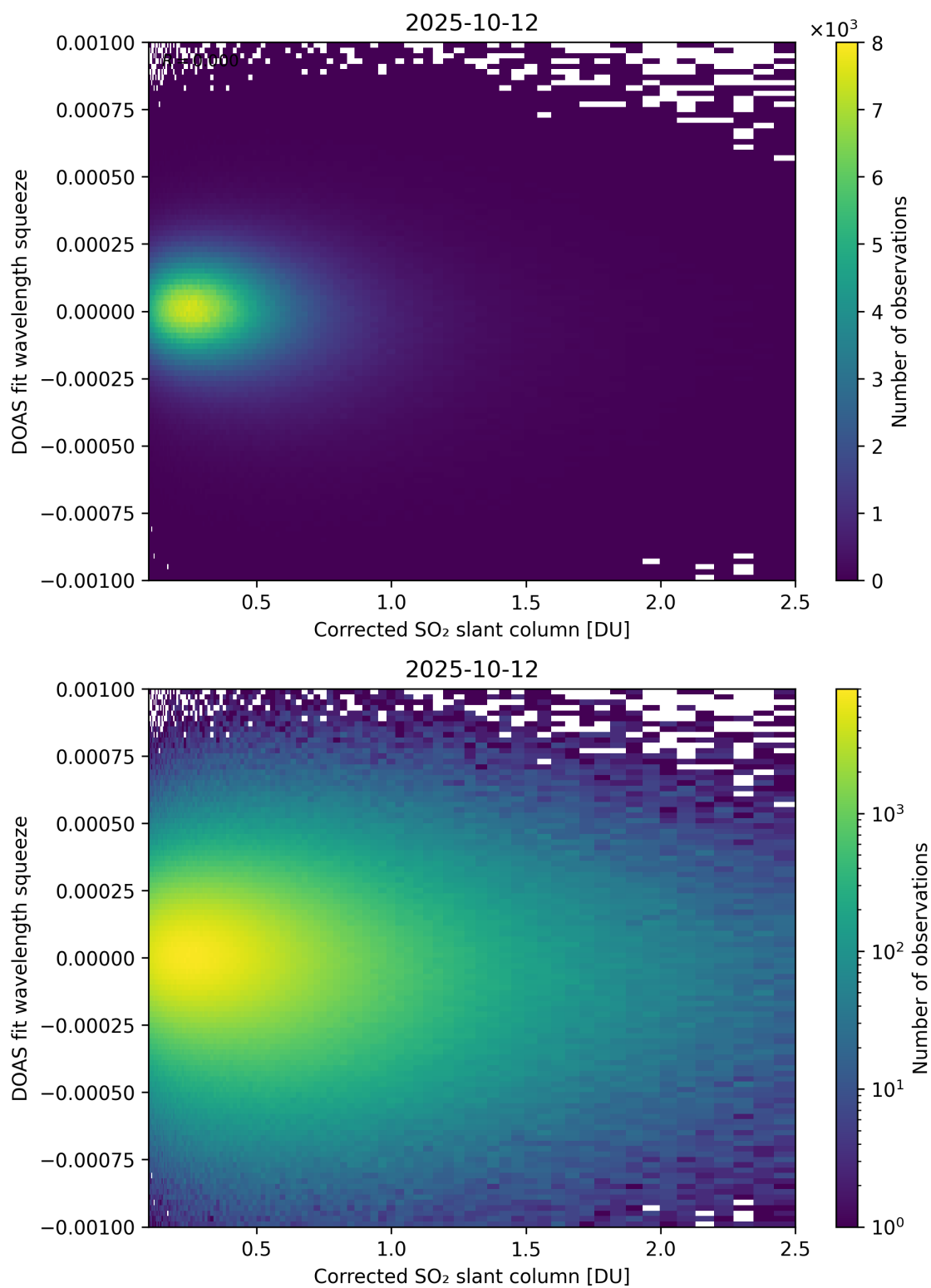
Figure 230: Scatter density plot of "Corrected SO 2 slant column" against "DOAS fit wavelength squeeze" for 2025-10-11 to 2025-10-13.
