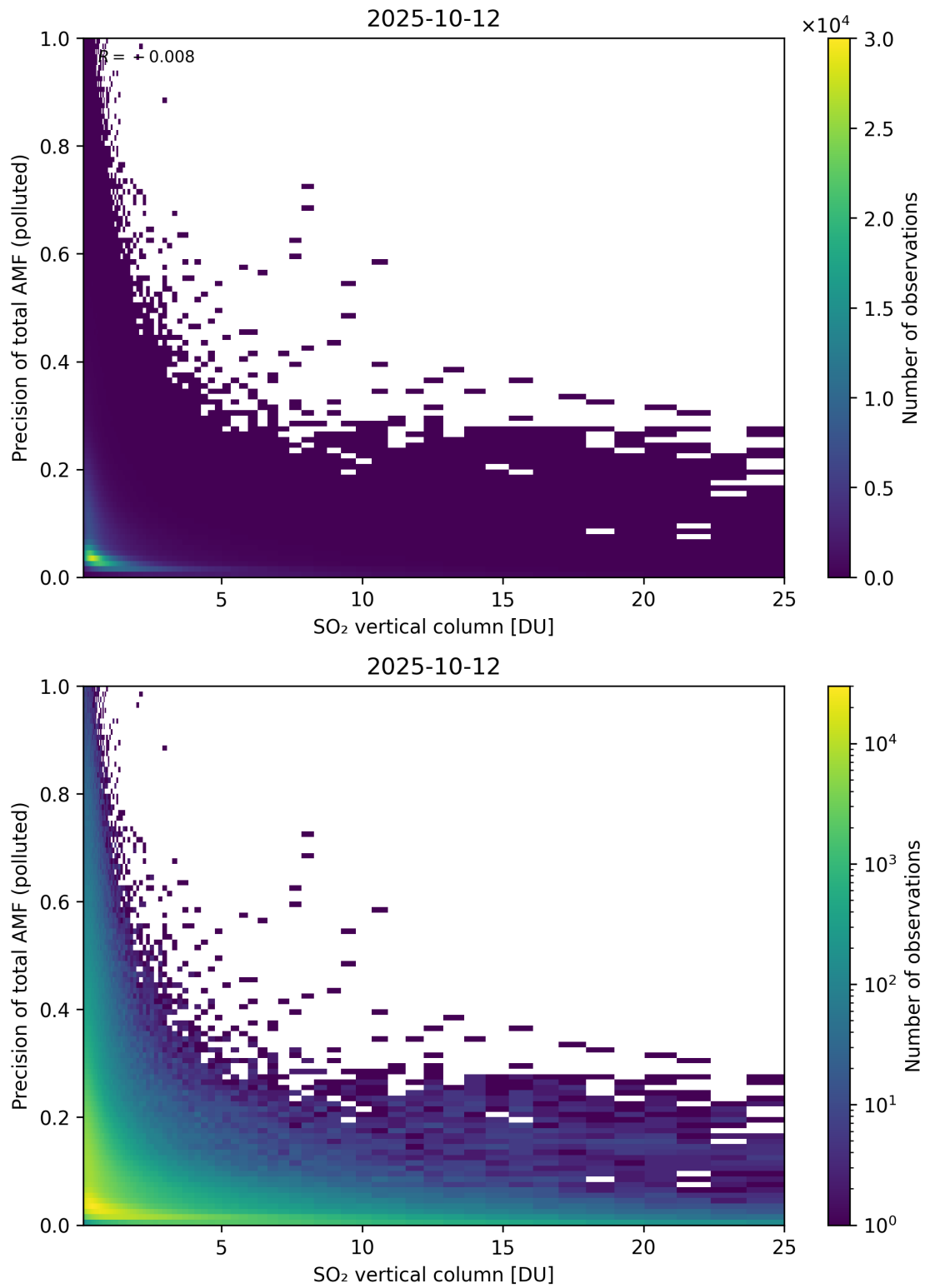
Figure 360: Scatter density plot of “SO 2 vertical column” against “Precision of total AMF (polluted)” for 2025-10-11 to 2025-10-13.
