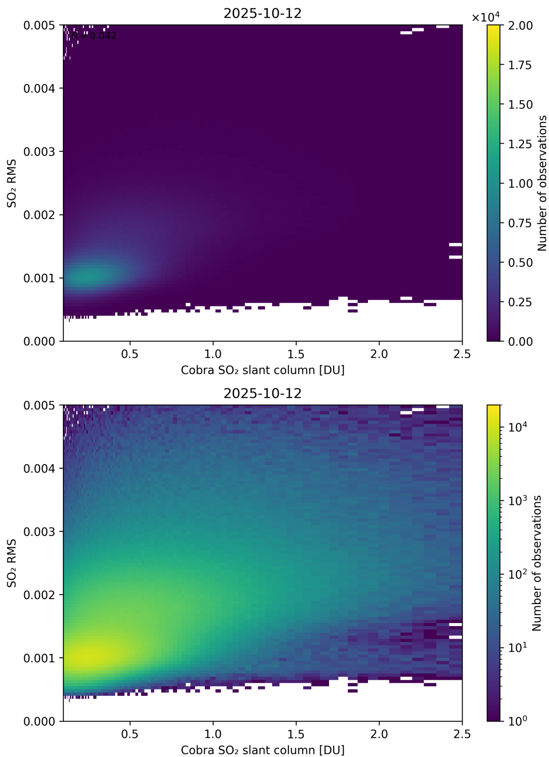
Figure 198: Scatter density plot of “Cobra SO 2 slant column” against “SO 2 RMS” for 2025-10-11 to 2025-10-13.
