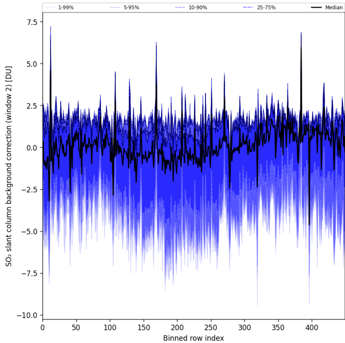
Figure 96: Along track statistics of “SO 2 slant column background correction (window 2)” for 2025-10-11 to 2025-10-13
