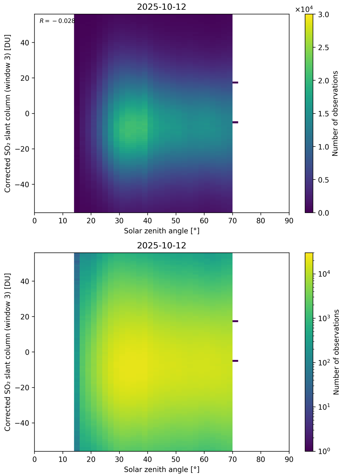
Figure 183: Scatter density plot of “Solar zenith angle” against “Corrected SO 2 slant column (window 3)” for 2025-10-11 to 2025-10-13.
