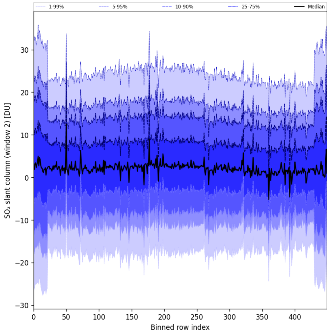
Figure 93: Along track statistics of “SO 2 slant column (window 2)” for 2025-10-11 to 2025-10-13
