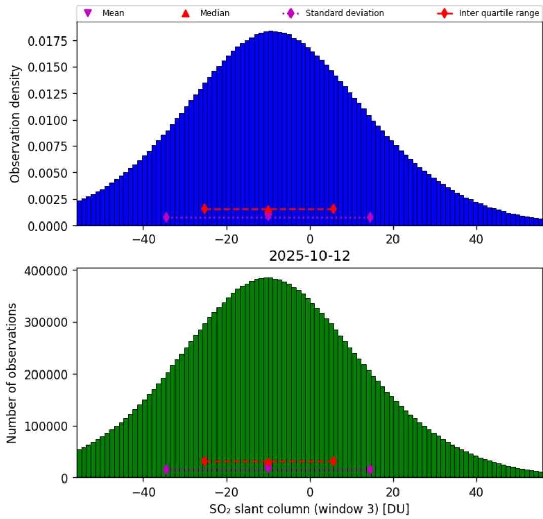
Figure 71: Histogram of “SO 2 slant column (window 3)” for 2025-10-11 to 2025-10-13
