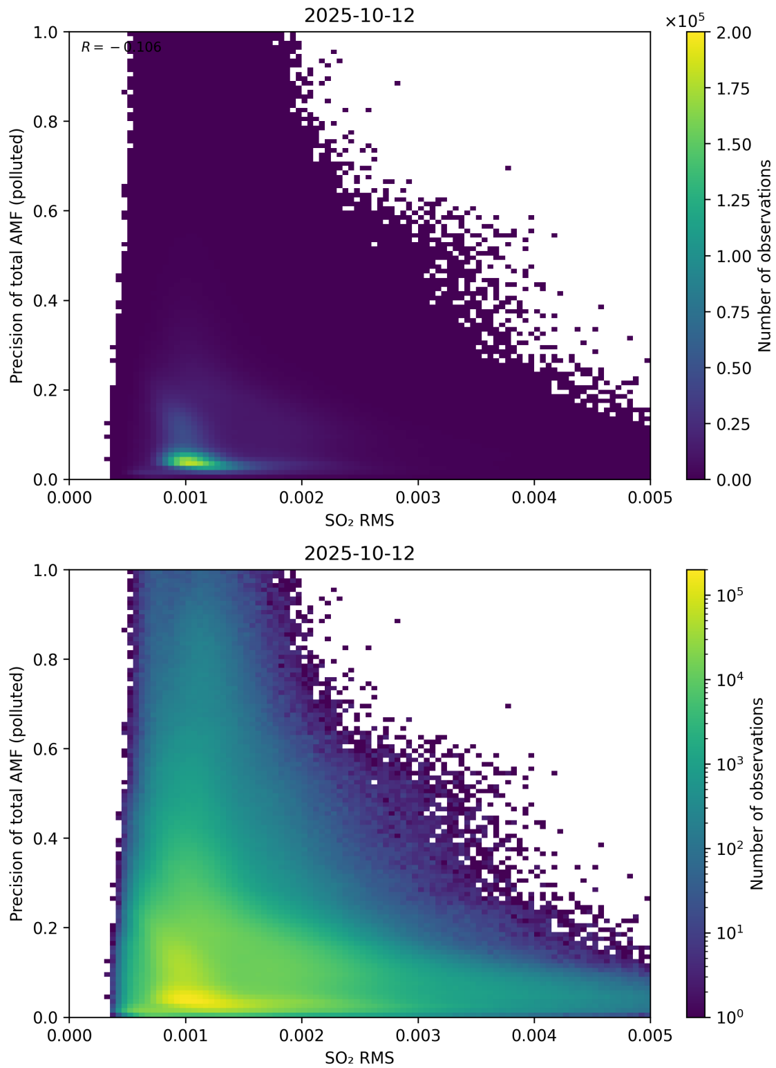
Figure 149: Scatter density plot of “SO 2 RMS” against “Precision of total AMF (polluted)” for 2025-10-11 to 2025-10-13.
