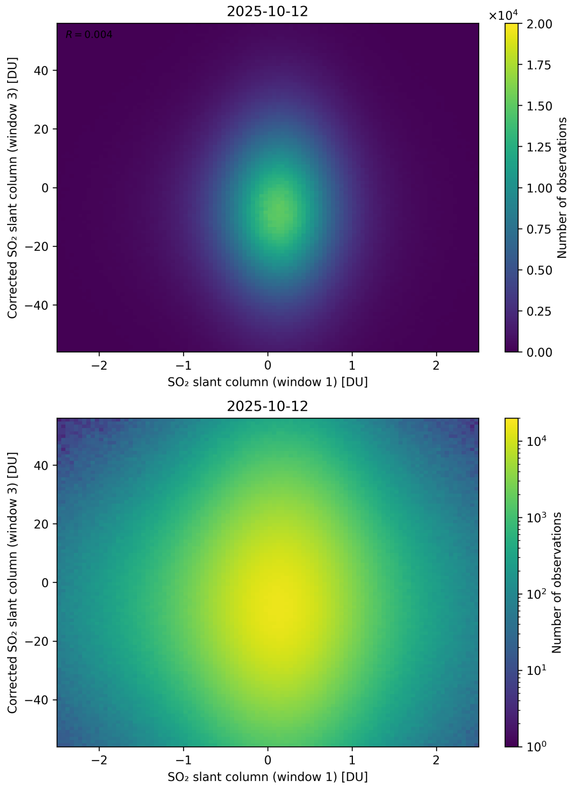
Figure 284: Scatter density plot of “SO 2 slant column (window 1)” against “Corrected SO 2 slant column (window 3)” for 2025-10-11 to 2025-10-13.
