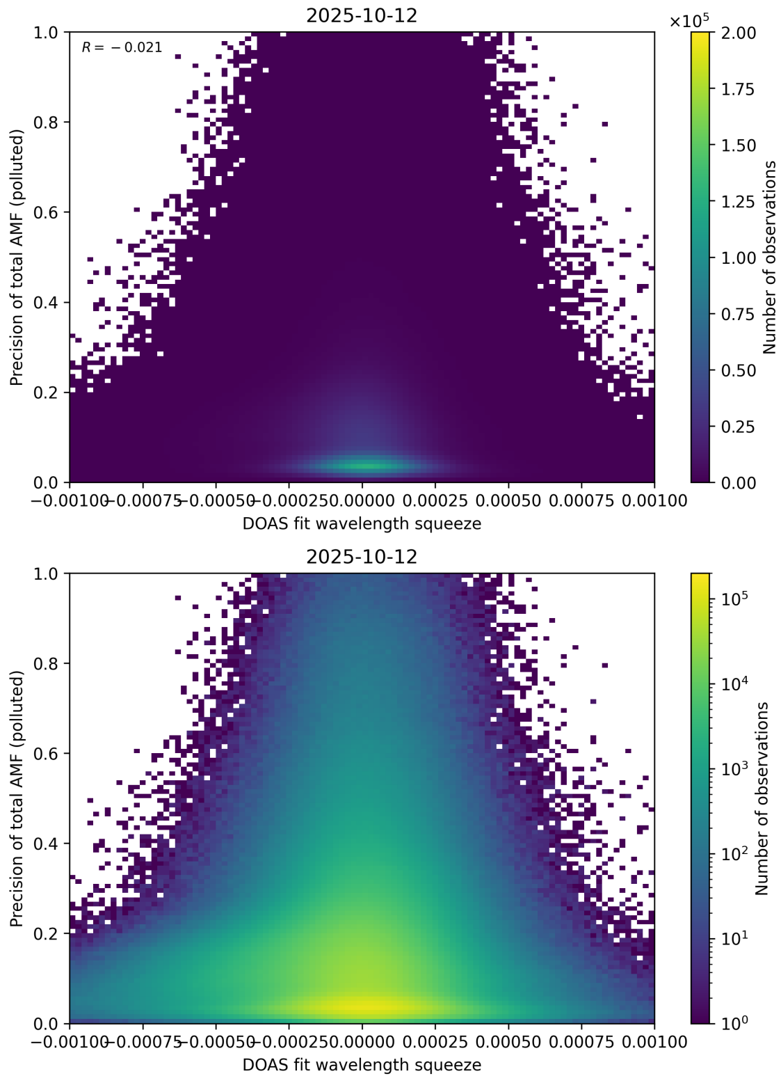
Figure 146: Scatter density plot of “DOAS fit wavelength squeeze” against “Precision of total AMF (polluted)” for 2025-10-11 to 2025-10-13.
