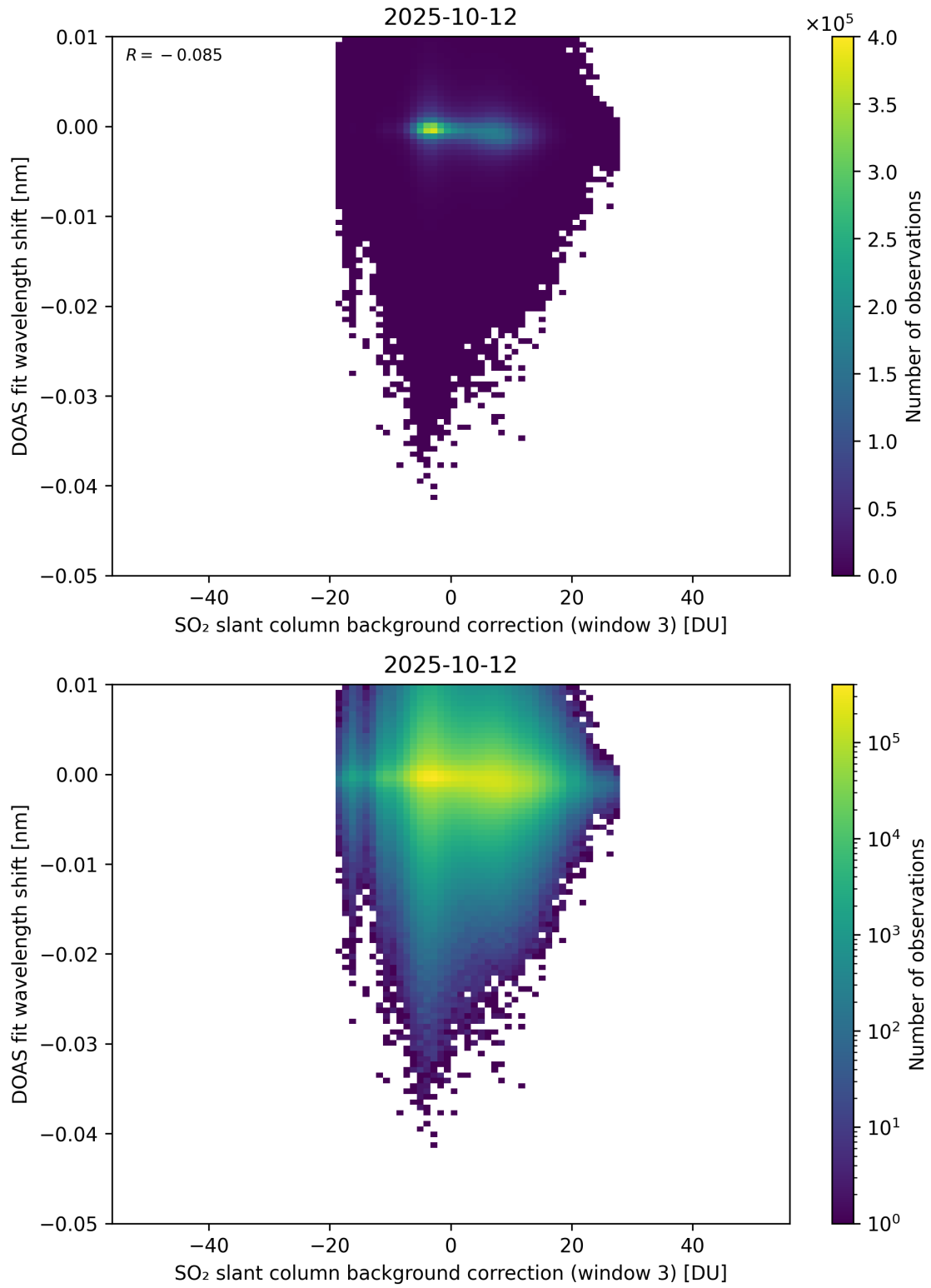
Figure 132: Scatter density plot of “SO 2 slant column background correction (window 3)” against “DOAS fit wavelength shift” for 2025-10-11 to 2025-10-13.
