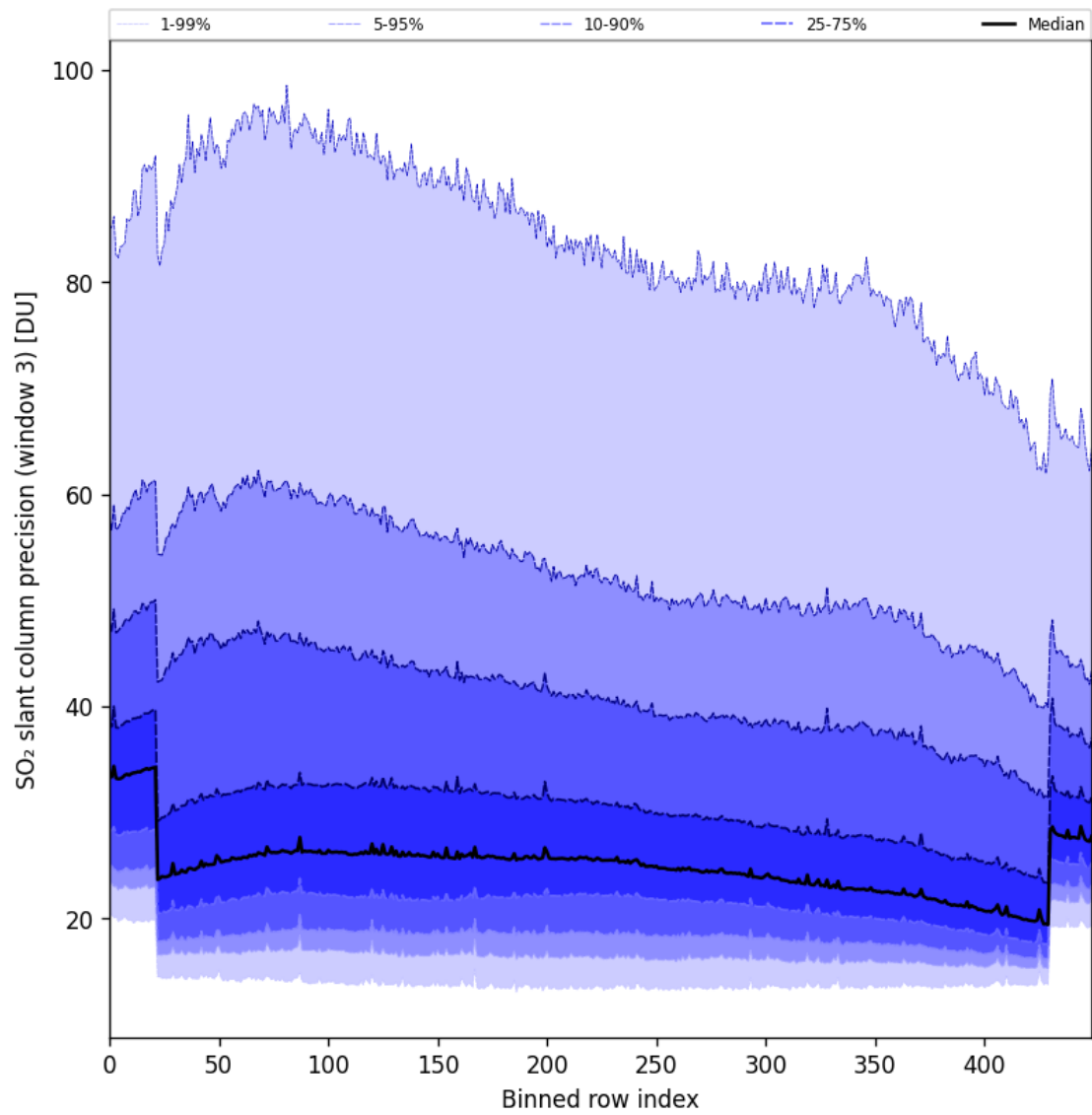
Figure 98: Along track statistics of “SO 2 slant column precision (window 3)” for 2025-10-11 to 2025-10-13
