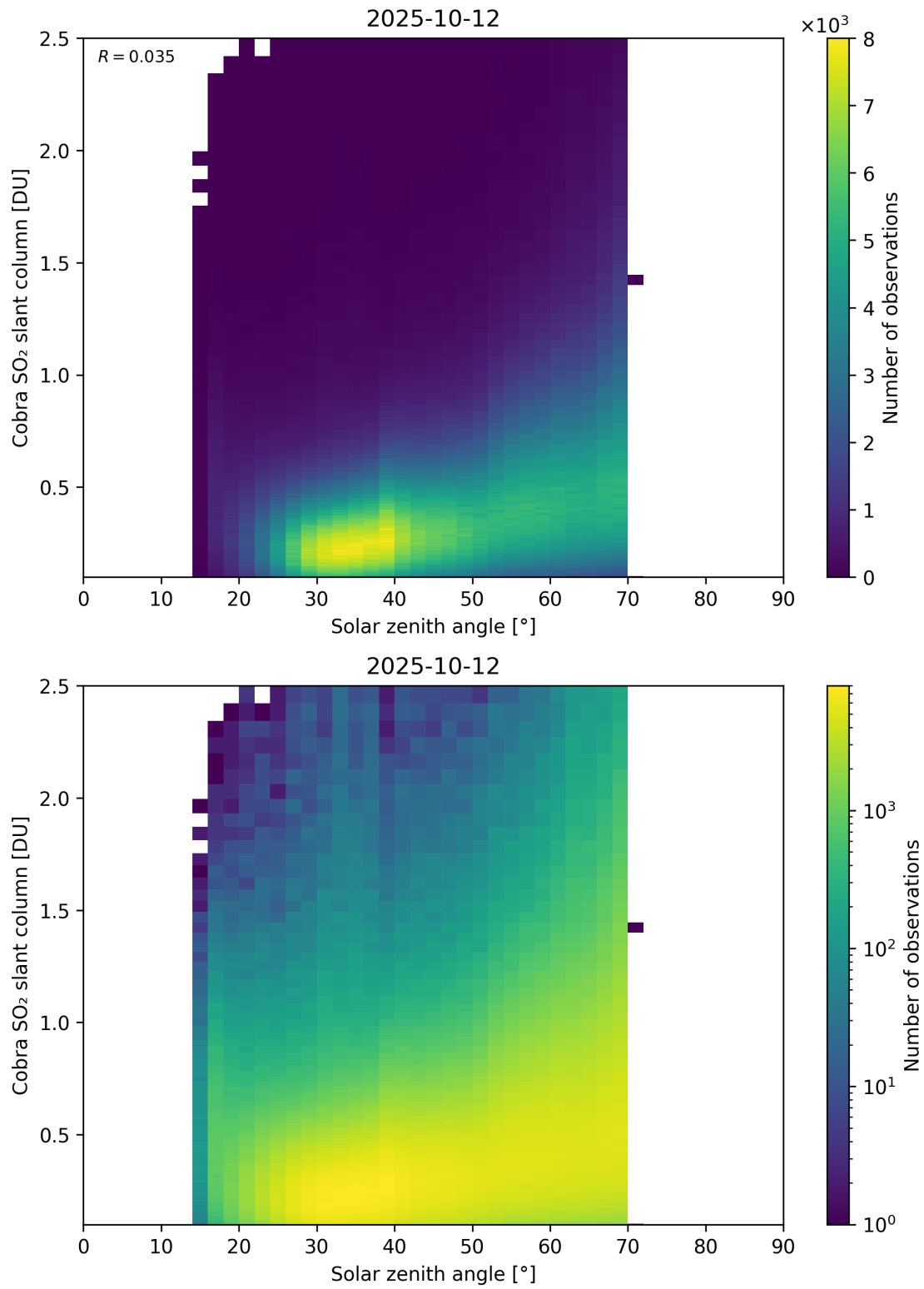
Figure 179: Scatter density plot of “Solar zenith angle” against “Cobra SO 2 slant column” for 2025-10-11 to 2025-10-13.
