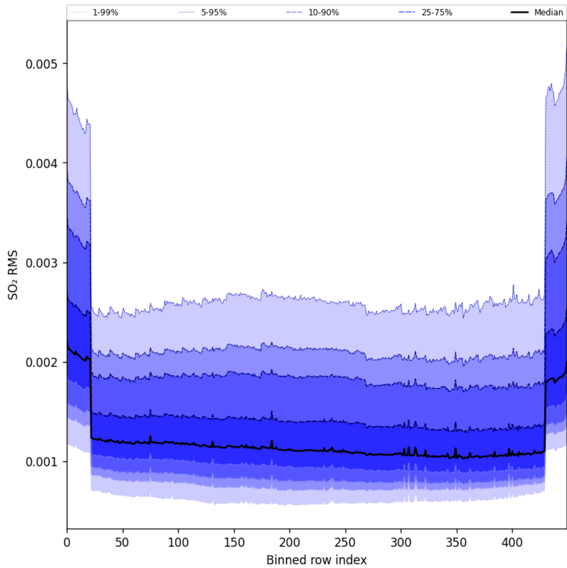
Figure 104: Along track statistics of “SO 2 RMS” for 2025-10-11 to 2025-10-13
