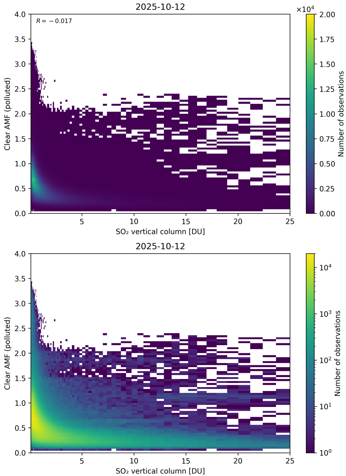
Figure 348: Scatter density plot of “SO 2 vertical column” against “Clear AMF (polluted)” for 2025-10-11 to 2025-10-13.
