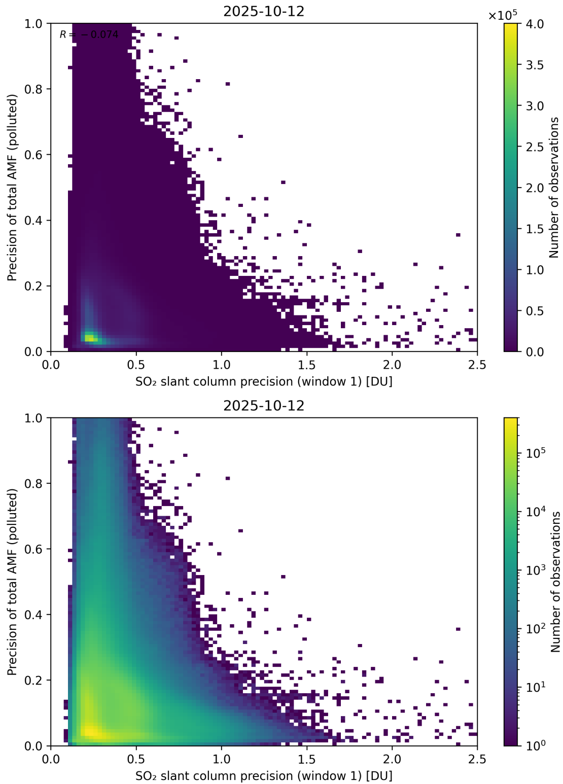
Figure 281: Scatter density plot of “SO 2 slant column precision (window 1)” against “Precision of total AMF (polluted)” for 2025-10-11 to 2025-10-13.
