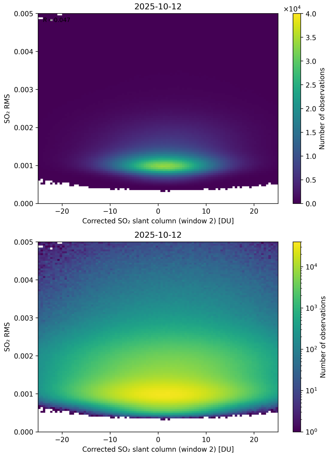
Figure 248: Scatter density plot of “Corrected SO 2 slant column (window 2)” against “SO 2 RMS” for 2025-10-11 to 2025-10-13.
