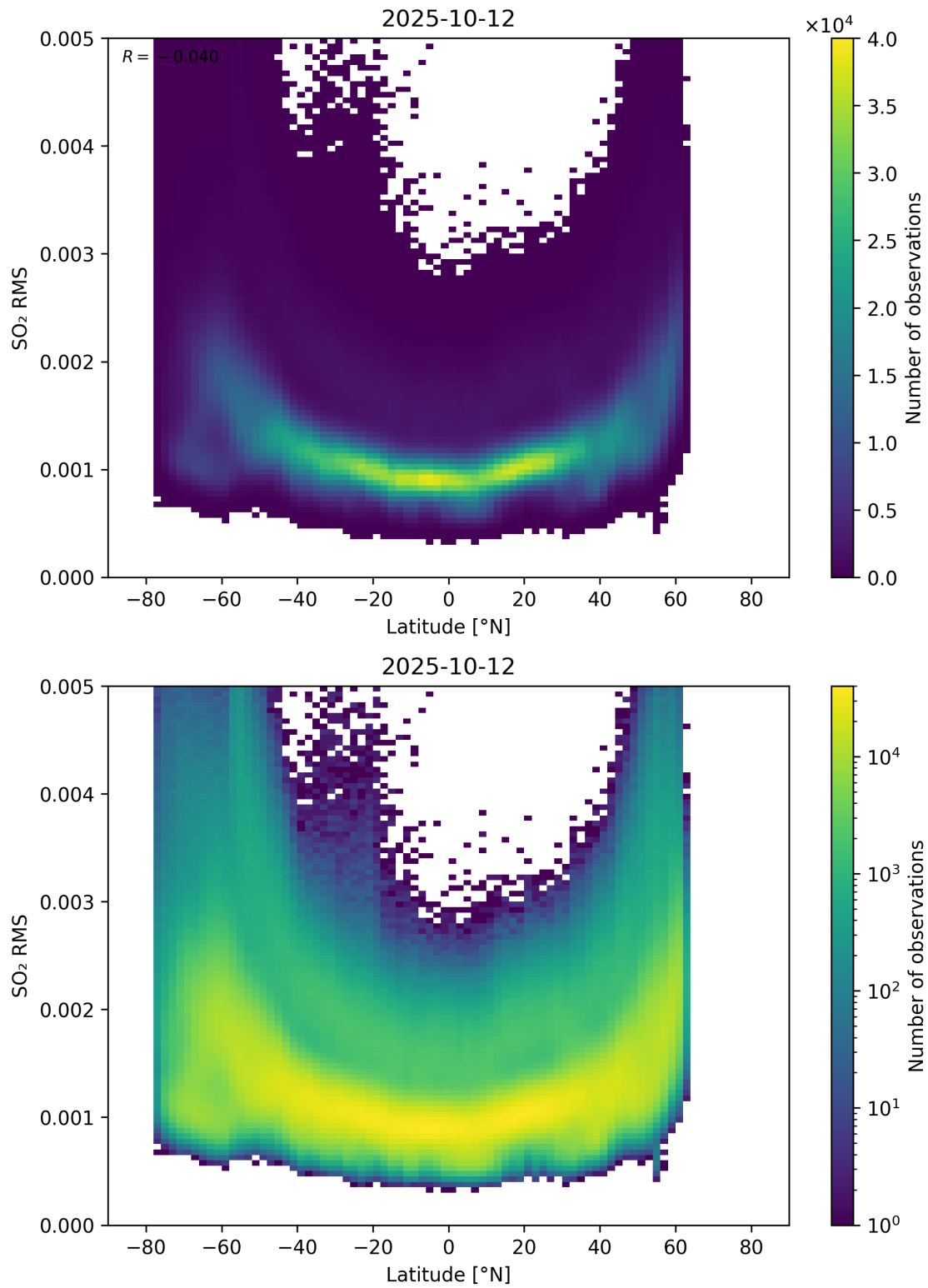
Figure 155: Scatter density plot of “Latitude” against “SO 2 RMS” for 2025-10-11 to 2025-10-13.
