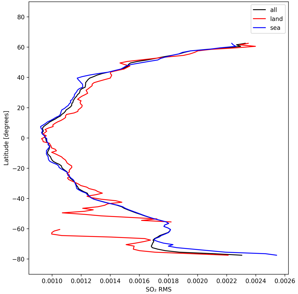
Figure 52: Zonal average of “SO 2 RMS” for 2025-10-11 to 2025-10-13.
