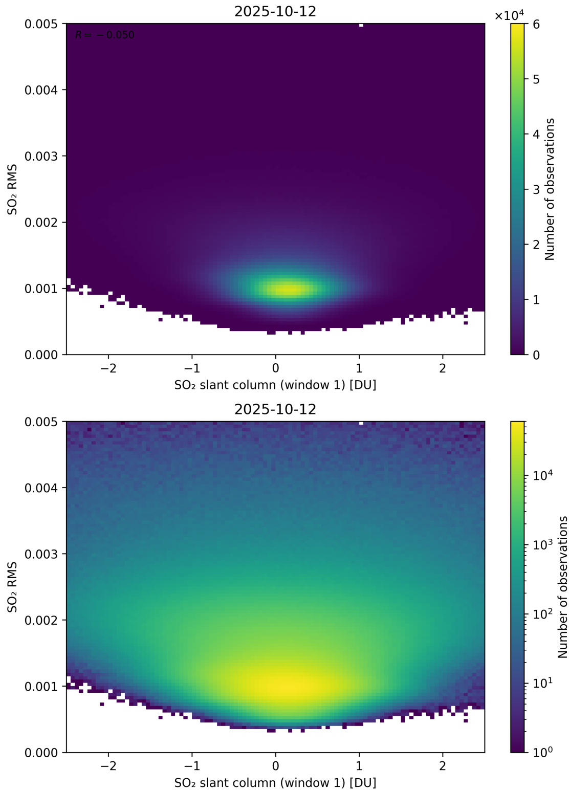
Figure 267: Scatter density plot of “SO 2 slant column (window 1)” against “SO 2 RMS” for 2025-10-11 to 2025-10-13.
