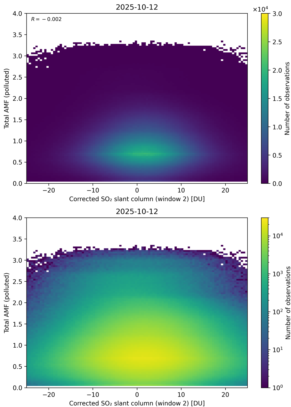
Figure 253: Scatter density plot of “Corrected SO 2 slant column (window 2)” against “Total AMF (polluted)” for 2025-10-11 to 2025-10-13.
