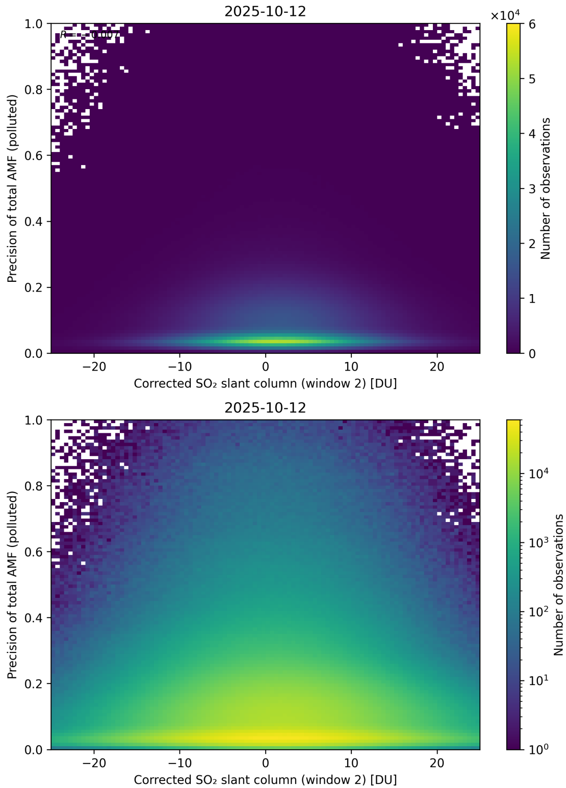
Figure 254: Scatter density plot of “Corrected SO 2 slant column (window 2)” against “Precision of total AMF (polluted)” for 2025-10-11 to 2025-10-13.
