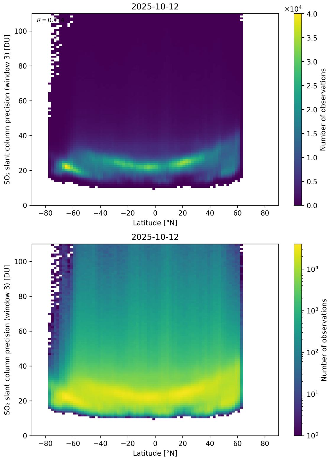
Figure 166: Scatter density plot of “Latitude” against “SO 2 slant column precision (window 3)” for 2025-10-11 to 2025-10-13.
