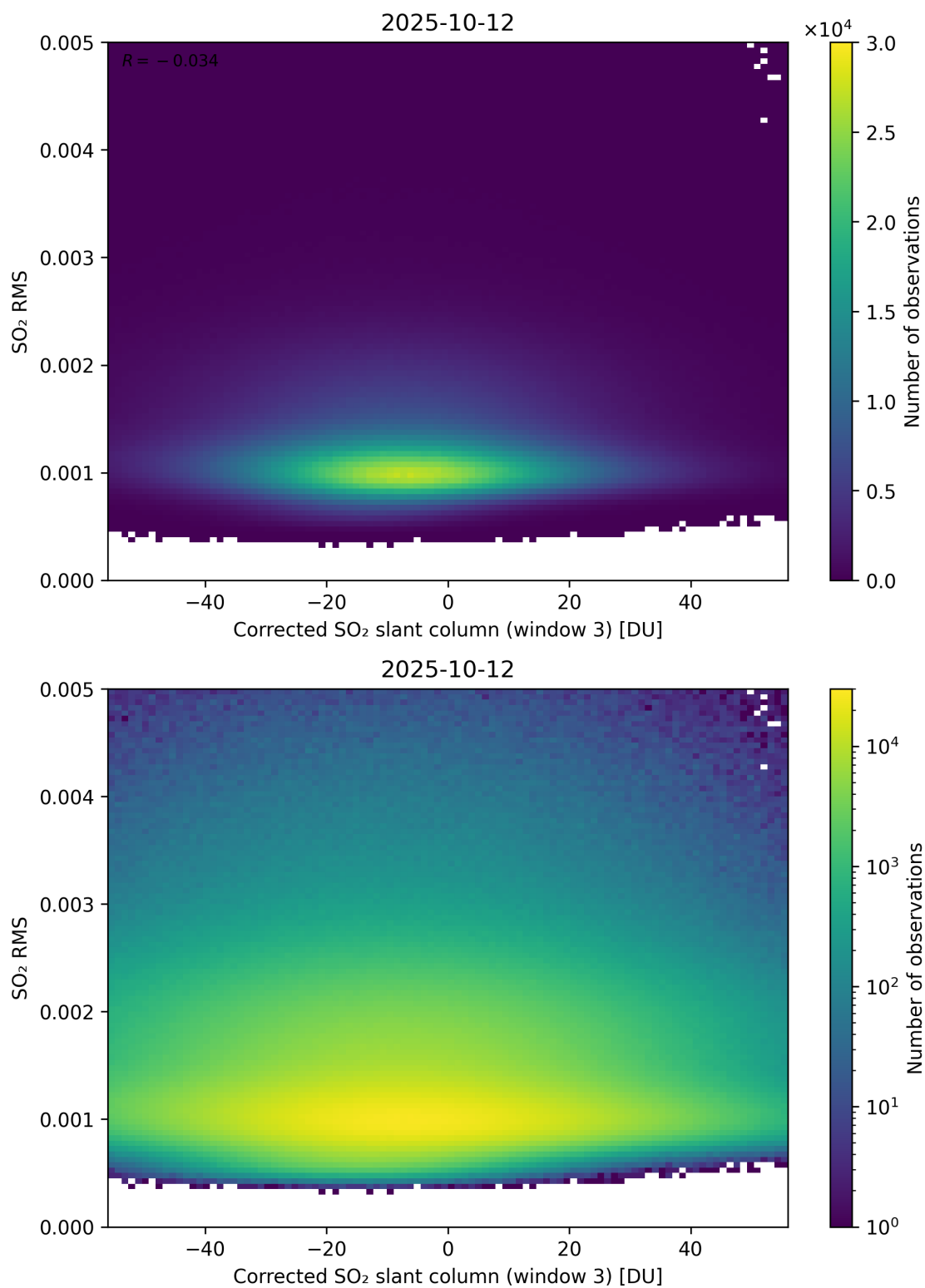
Figure 258: Scatter density plot of “Corrected SO 2 slant column (window 3)” against “SO 2 RMS” for 2025-10-11 to 2025-10-13.
