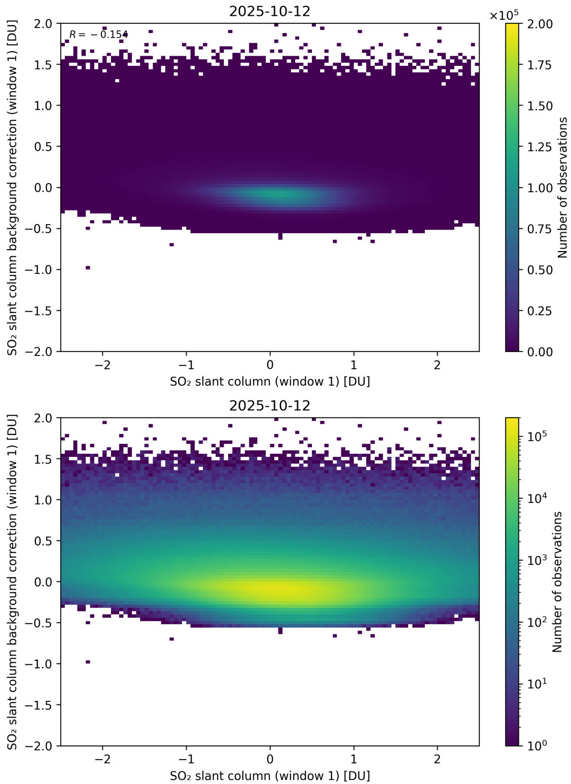
Figure 262: Scatter density plot of “SO 2 slant column (window 1)” against “SO 2 slant column background correction (window 1)” for 2025-10-11 to 2025-10-13.
