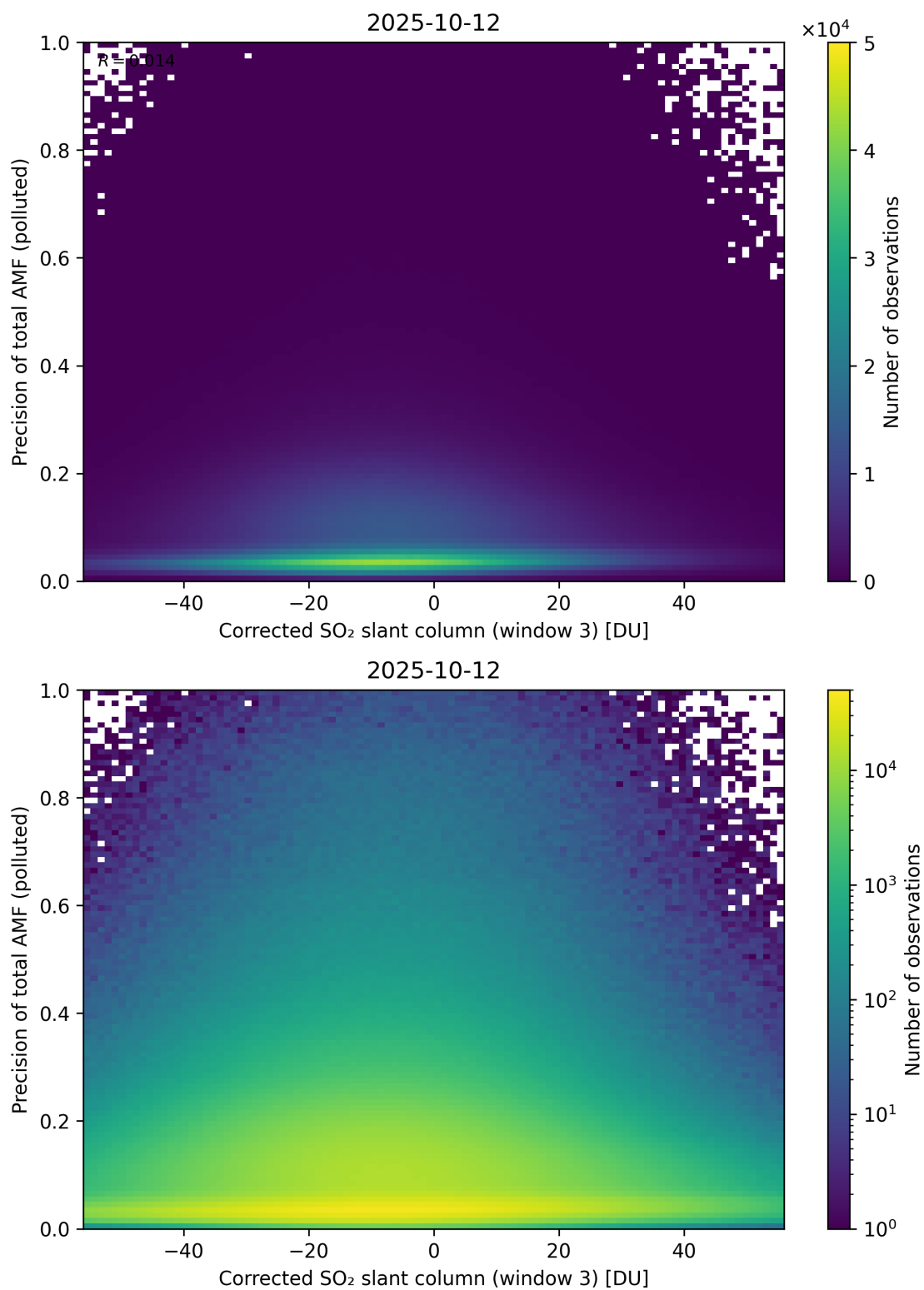
Figure 261: Scatter density plot of “Corrected SO 2 slant column (window 3)” against “Precision of total AMF (polluted)” for 2025-10-11 to 2025-10-13.
