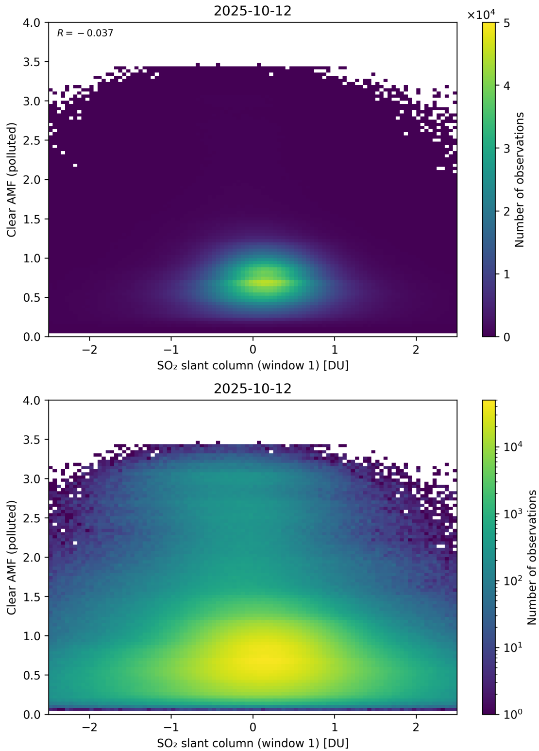
Figure 282: Scatter density plot of “SO 2 slant column (window 1)” against “Clear AMF (polluted)” for 2025-10-11 to 2025-10-13.
