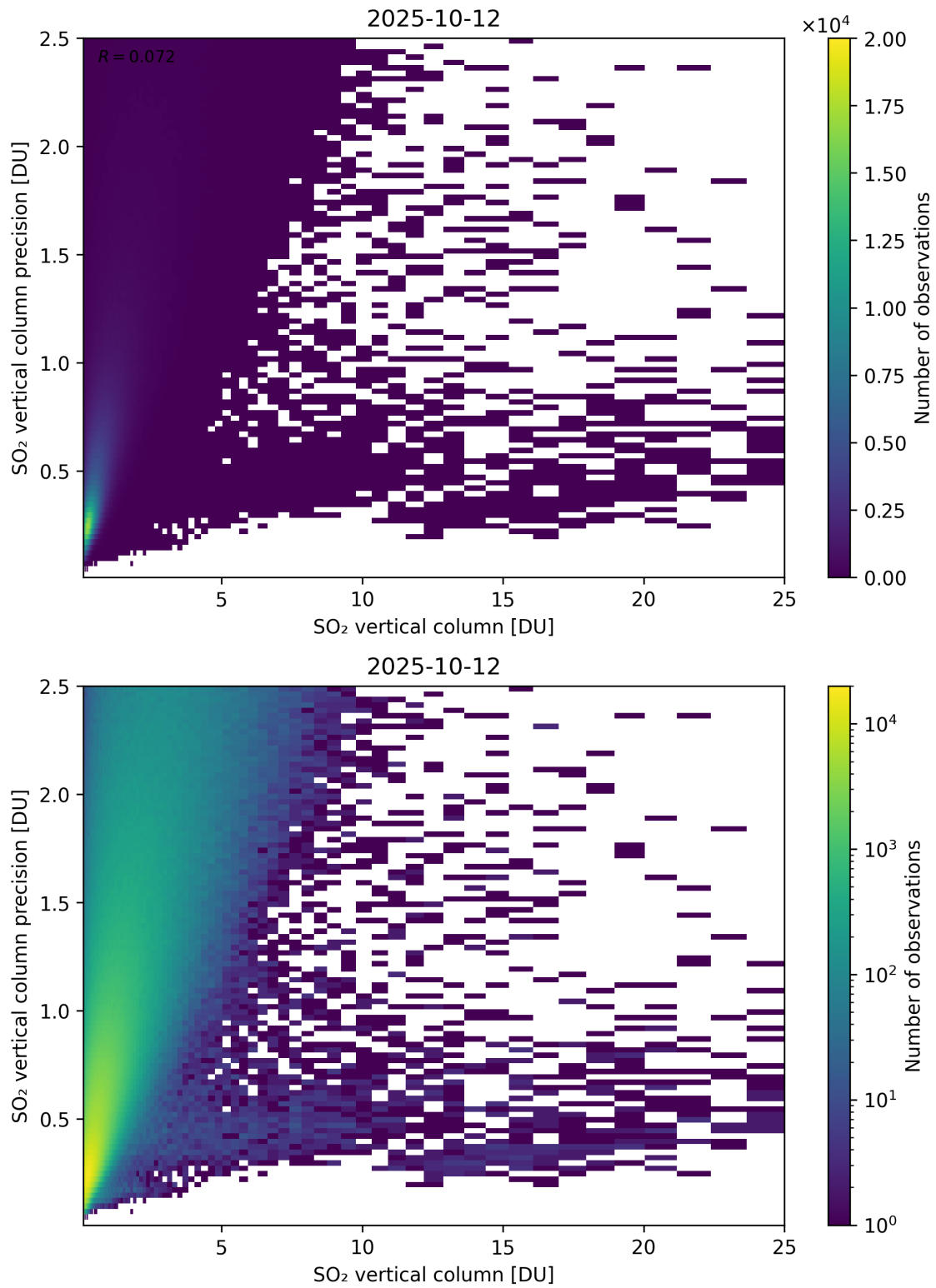
Figure 361: Scatter density plot of “SO 2 vertical column” against “SO 2 vertical column precision” for 2025-10-11 to 2025-10-13.
