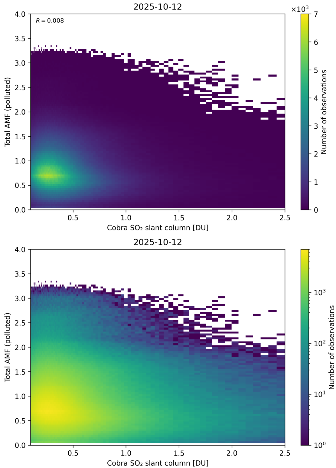
Figure 224: Scatter density plot of “Cobra SO 2 slant column” against “Total AMF (polluted)” for 2025-10-11 to 2025-10-13.
