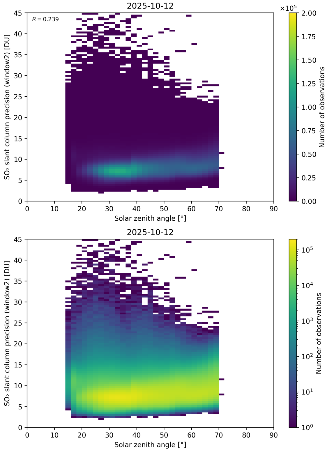
Figure 186: Scatter density plot of “Solar zenith angle” against “SO 2 slant column precision (window2)” for 2025-10-11 to 2025-10-13.
