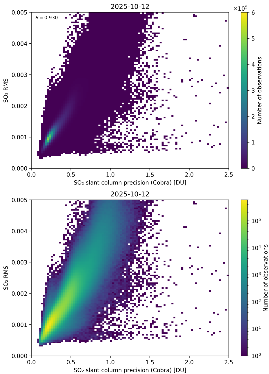
Figure 204: Scatter density plot of “SO 2 slant column precision (Cobra)” against “SO 2 RMS” for 2025-10-11 to 2025-10-13.
