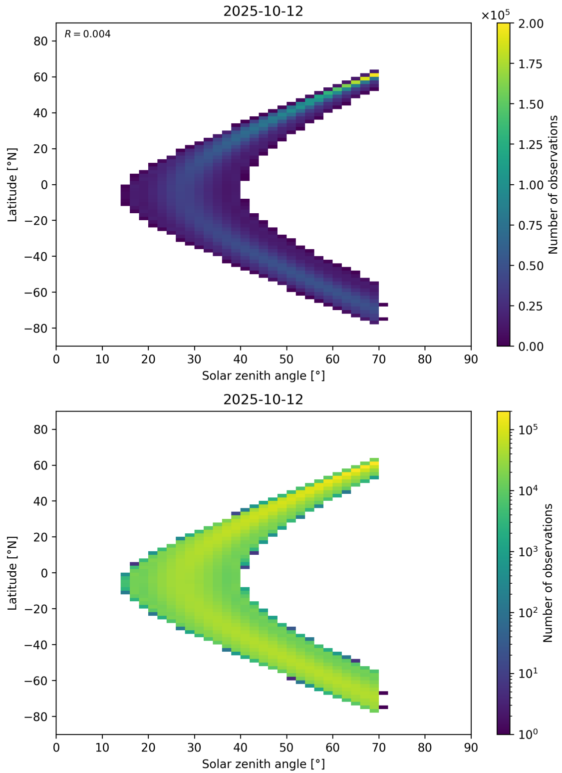
Figure 177: Scatter density plot of “Solar zenith angle” against “Latitude” for 2025-10-11 to 2025-10-13.
