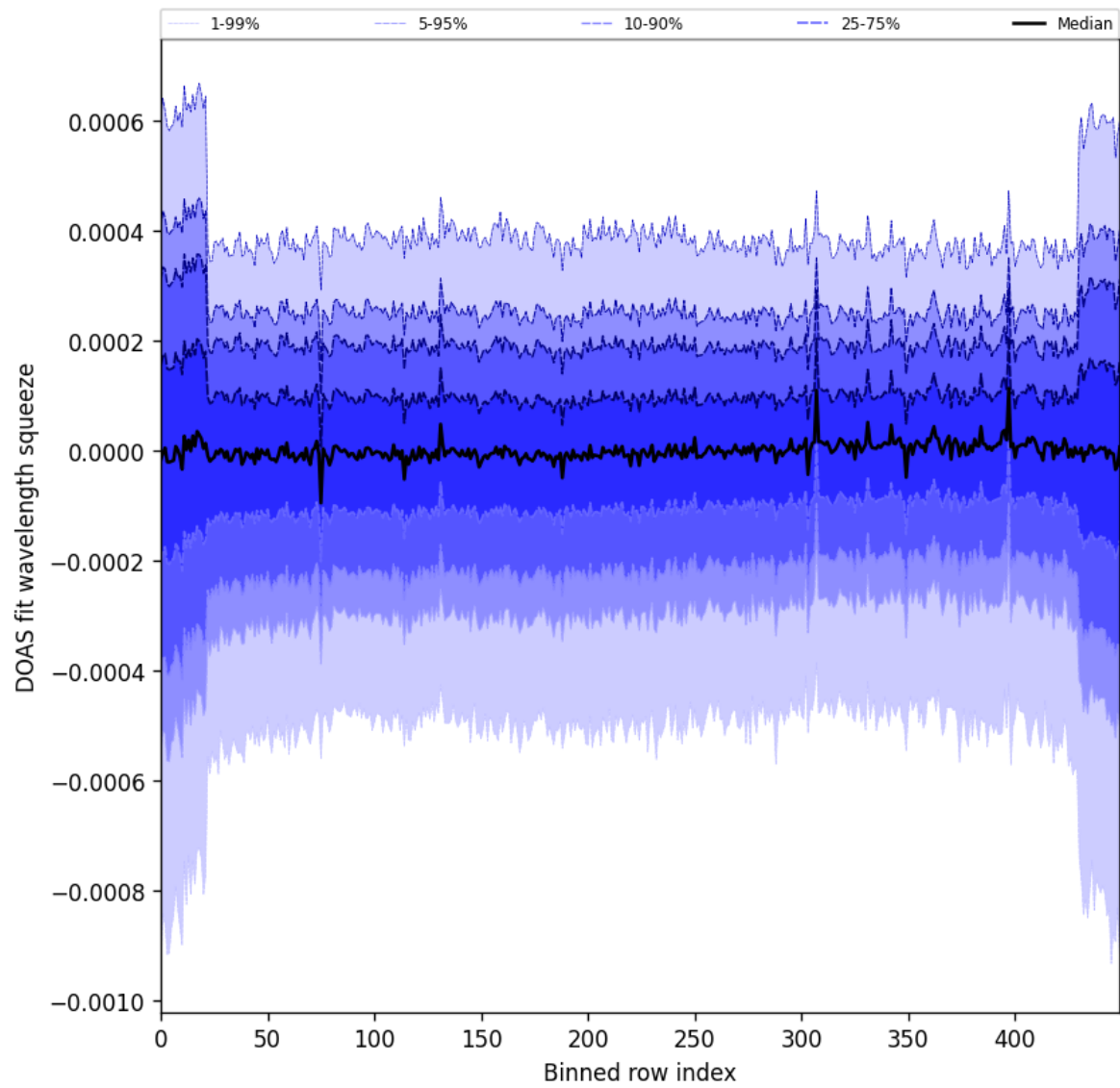
Figure 103: Along track statistics of “DOAS fit wavelength squeeze” for 2025-10-11 to 2025-10-13
