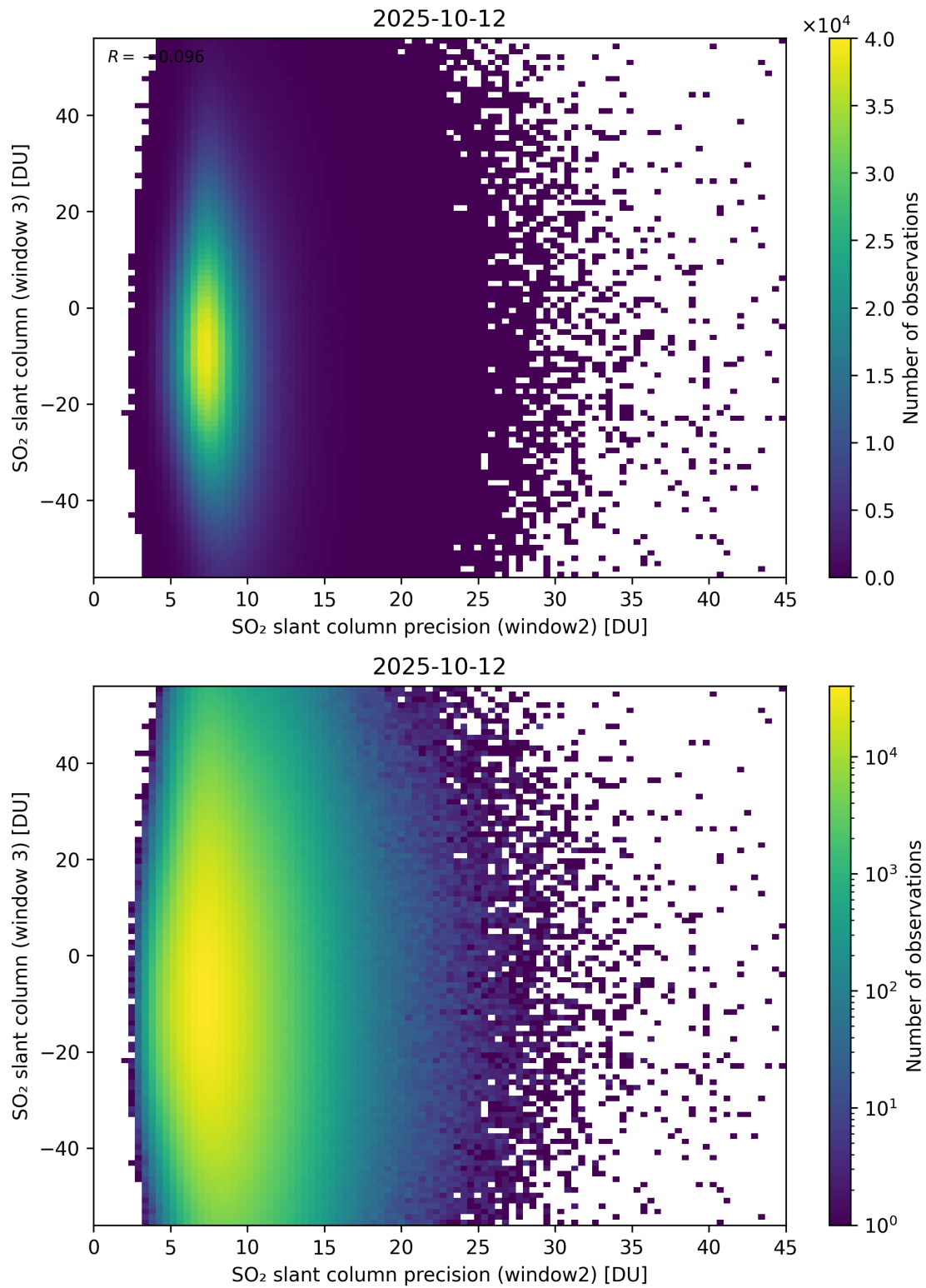
Figure 299: Scatter density plot of “SO 2 slant column precision (window2)” against “SO 2 slant column (window 3)” for 2025-10-11 to 2025-10-13.
