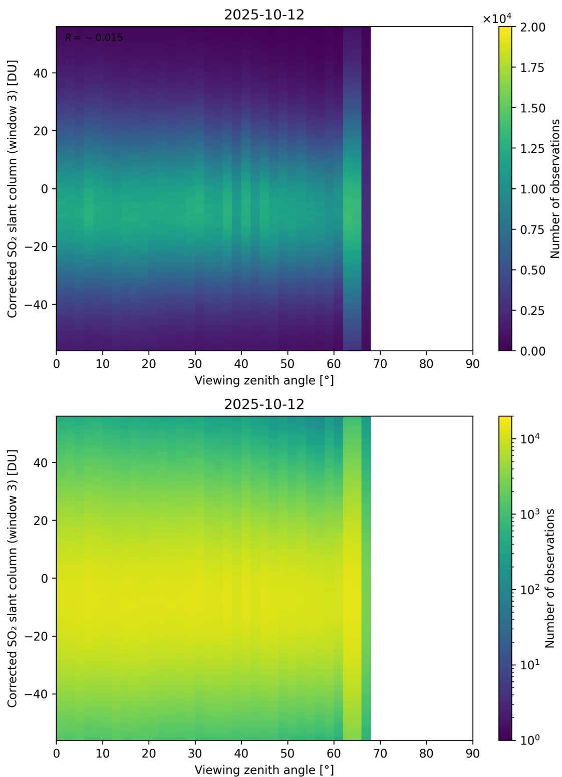
Figure 375: Scatter density plot of “Viewing zenith angle” against “Corrected SO 2 slant column (window 3)” for 2025-10-11 to 2025-10-13.
