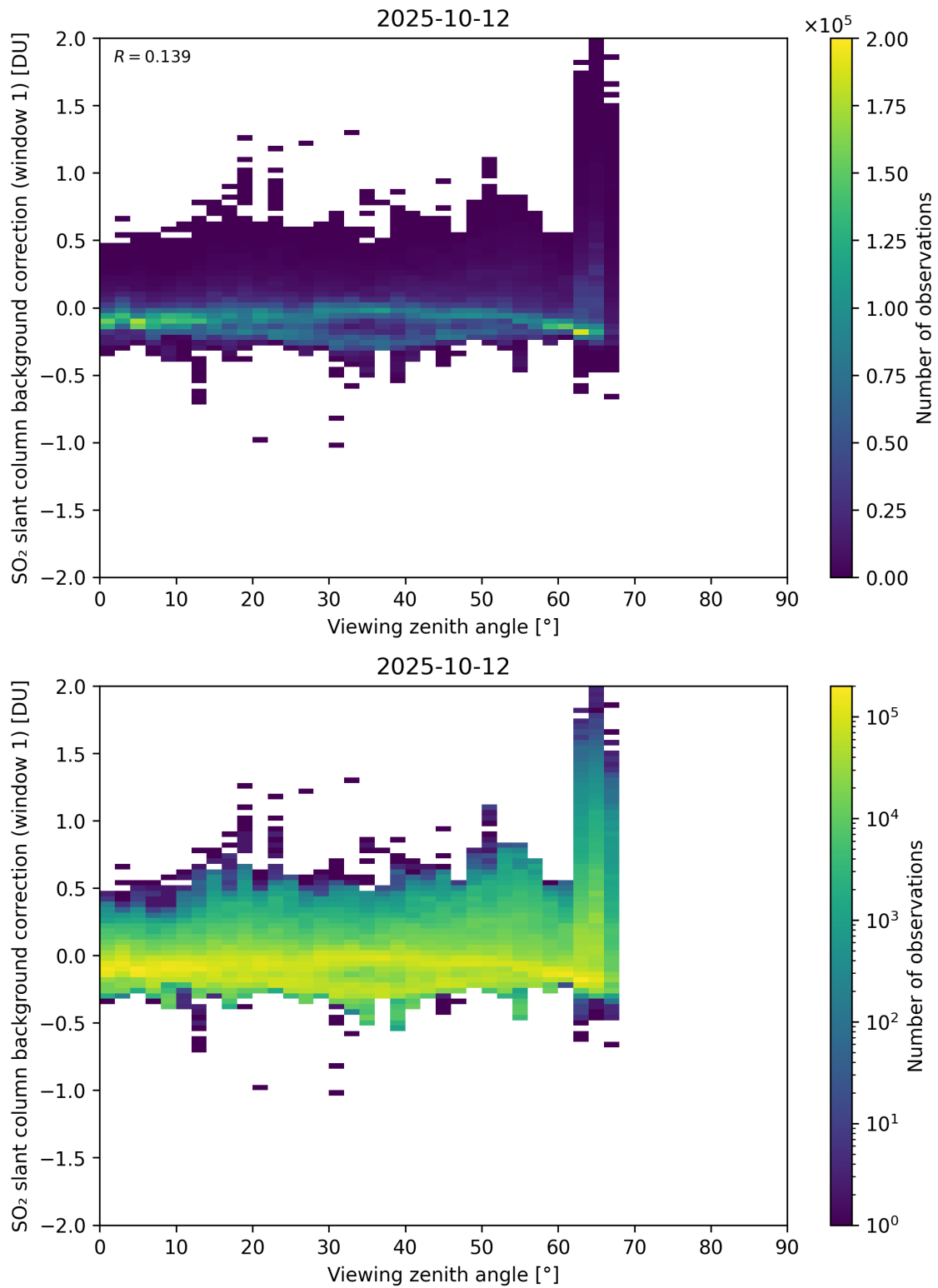
Figure 362: Scatter density plot of “Viewing zenith angle” against “SO 2 slant column background correction (window 1)” for 2025-10-11 to 2025-10-13.
