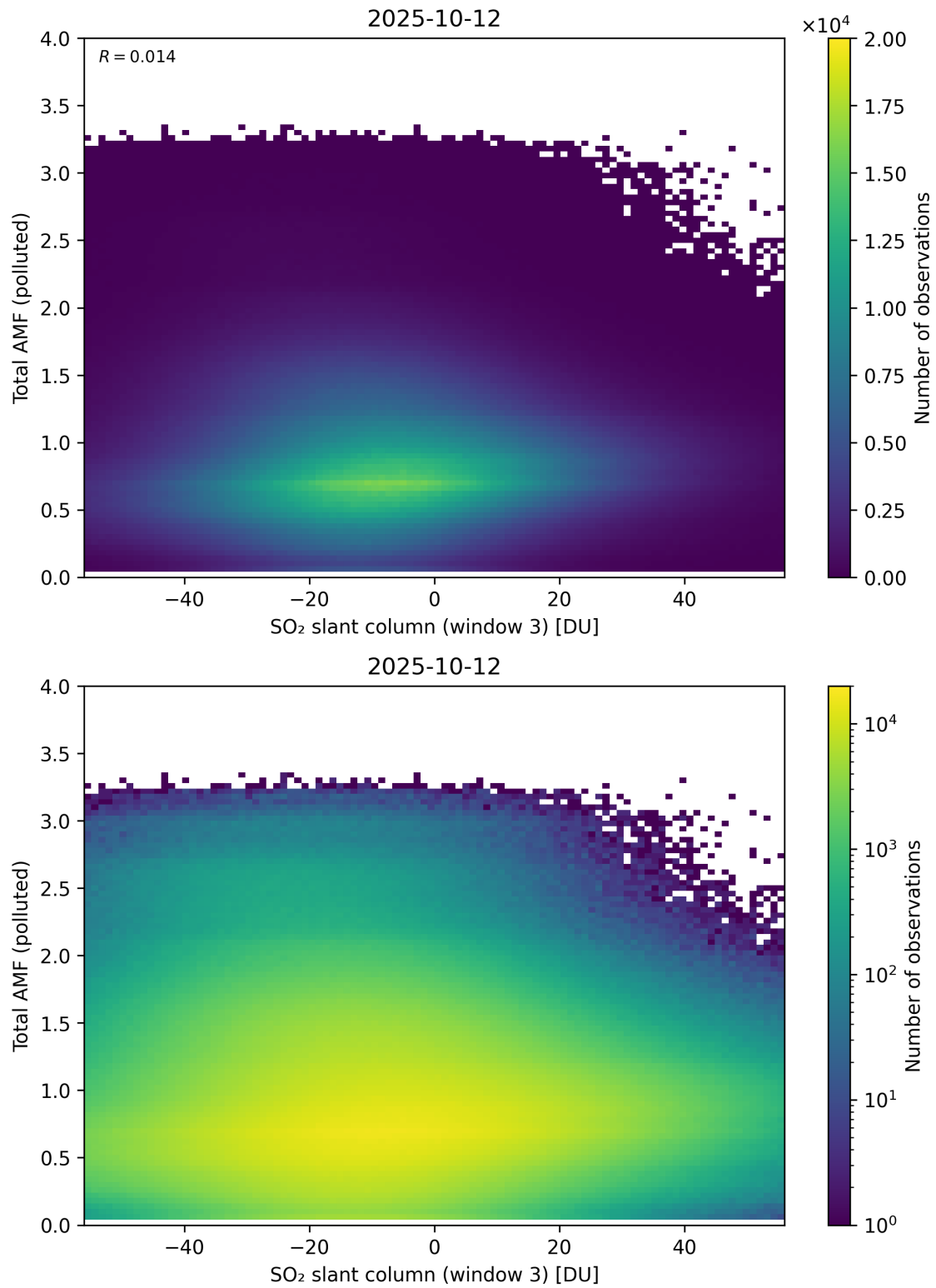
Figure 318: Scatter density plot of “SO 2 slant column (window 3)” against “Total AMF (polluted)” for 2025-10-11 to 2025-10-13.
