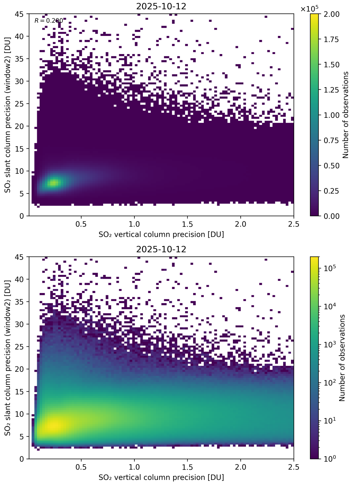
Figure 343: Scatter density plot of “SO 2 vertical column precision” against “SO 2 slant column precision (window2)” for 2025-10-11 to 2025-10-13.
