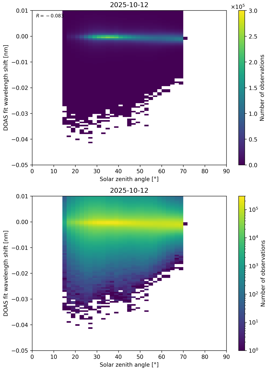
Figure 174: Scatter density plot of “Solar zenith angle” against “DOAS fit wavelength shift” for 2025-10-11 to 2025-10-13.
