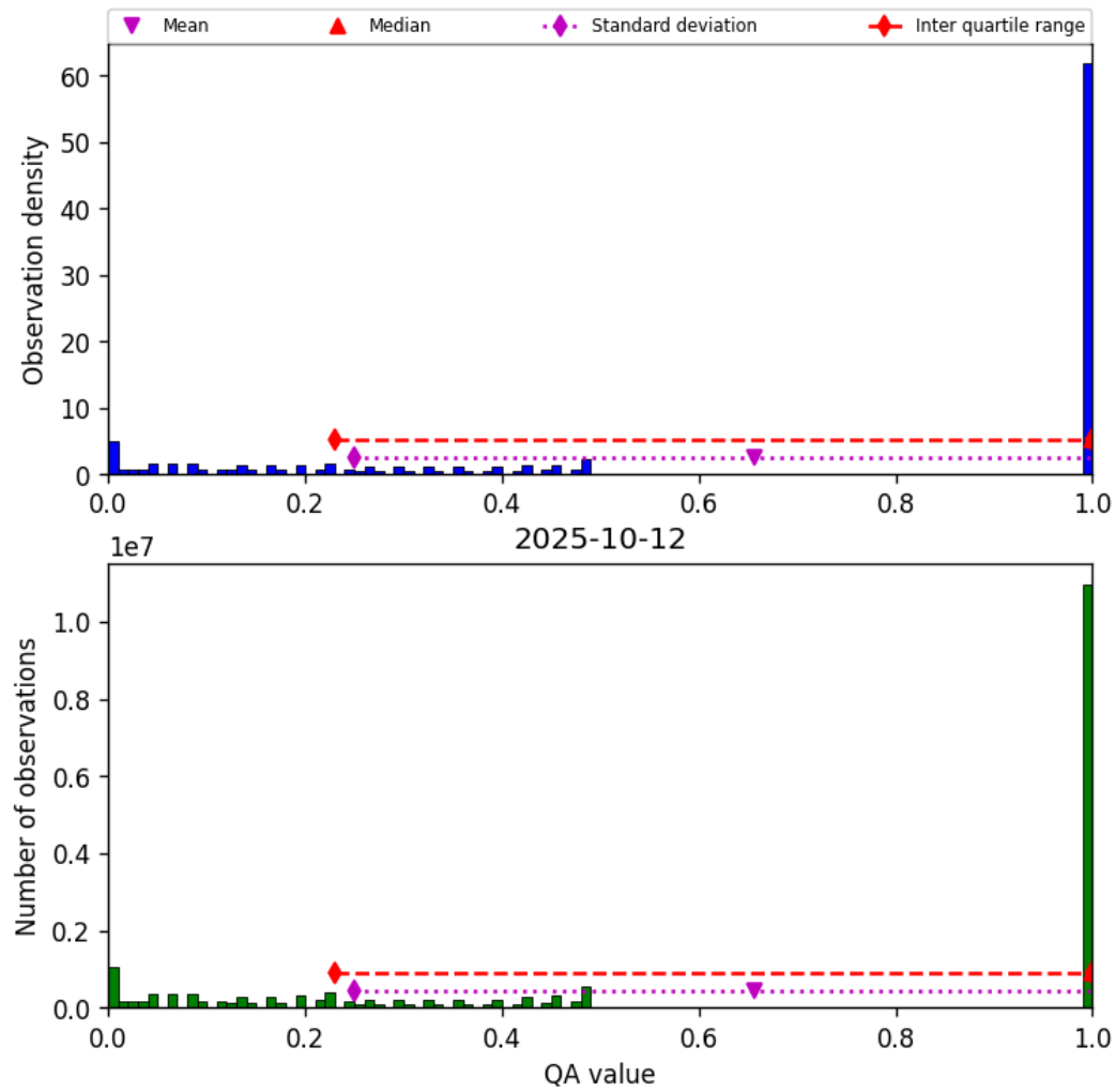
Figure 57: Histogram of “QA value” for 2025-10-11 to 2025-10-13
