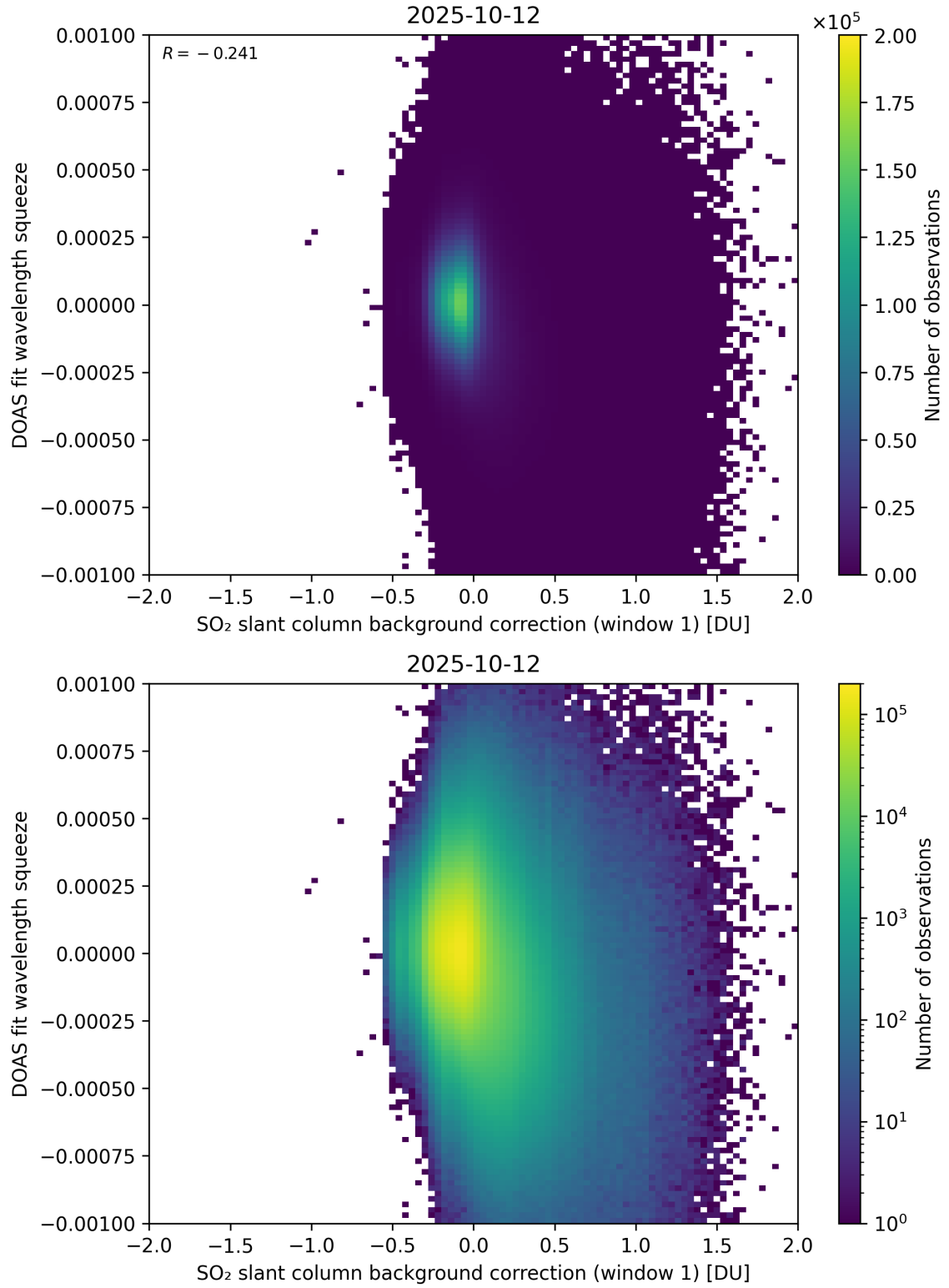
Figure 112: Scatter density plot of “SO 2 slant column background correction (window 1)” against “DOAS fit wavelength squeeze” for 2025-10-11 to 2025-10-13.
