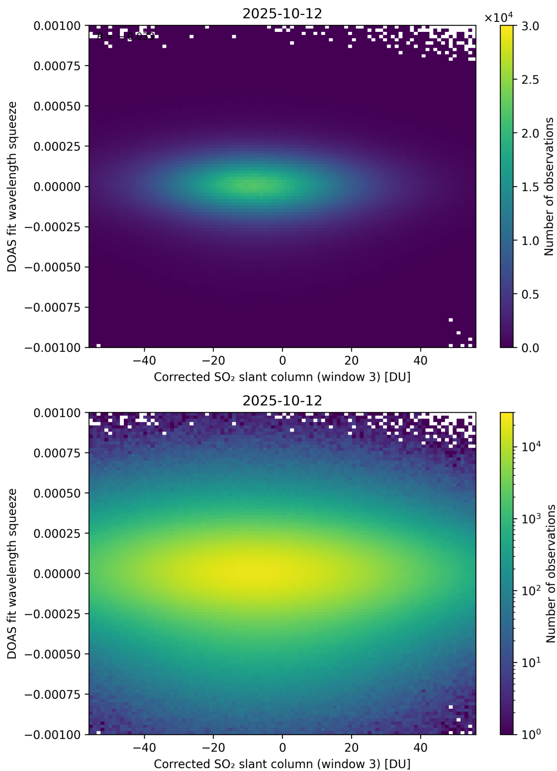
Figure 257: Scatter density plot of “Corrected SO 2 slant column (window 3)” against “DOAS fit wavelength squeeze” for 2025-10-11 to 2025-10-13.
