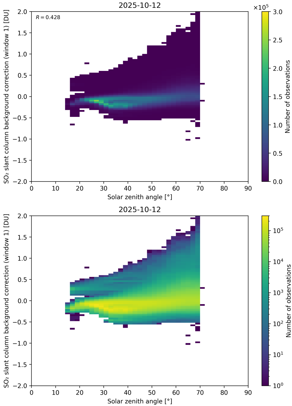
Figure 171: Scatter density plot of “Solar zenith angle” against “SO 2 slant column background correction (window 1)” for 2025-10-11 to 2025-10-13.
