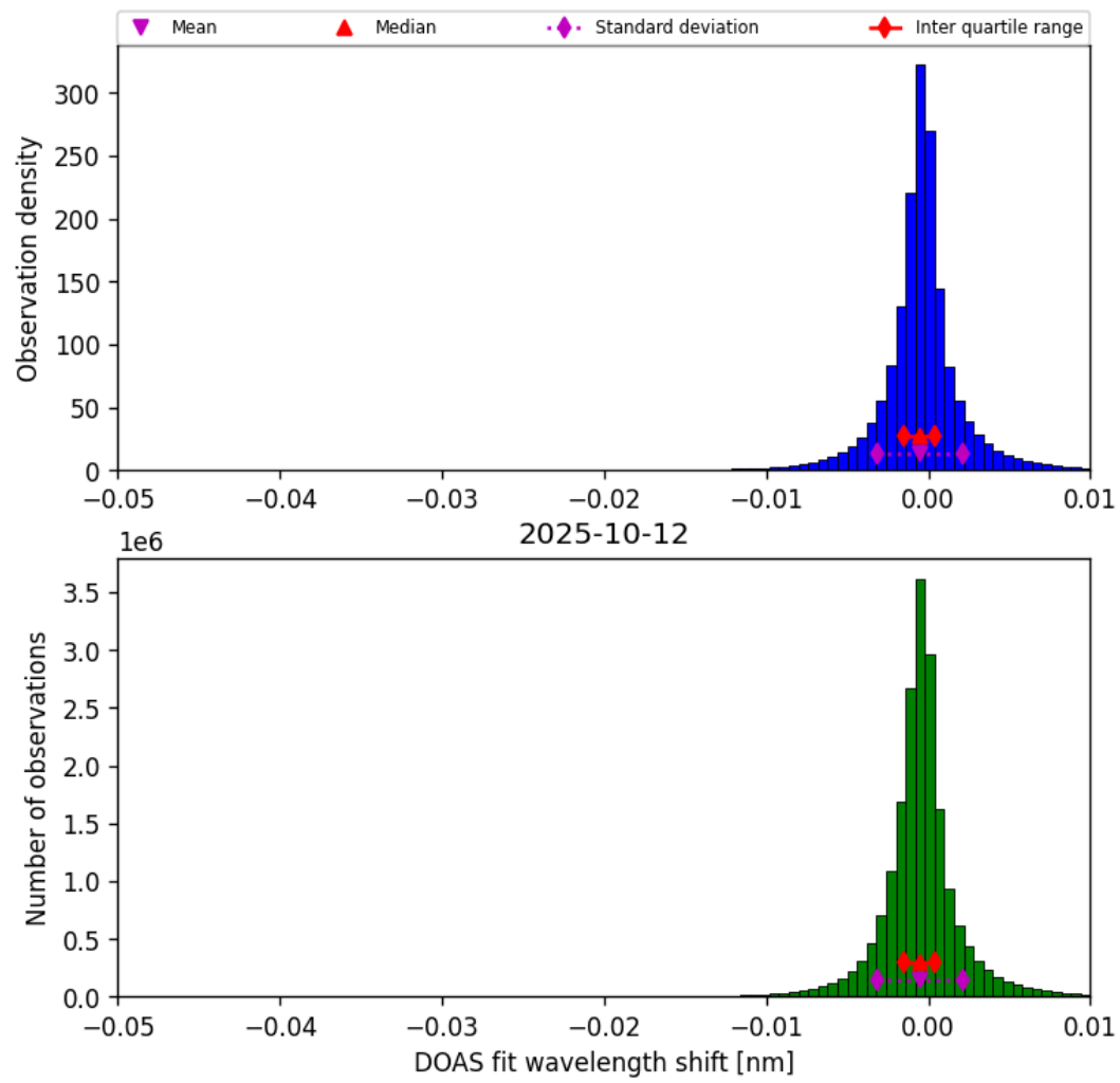
Figure 76: Histogram of “DOAS fit wavelength shift” for 2025-10-11 to 2025-10-13
