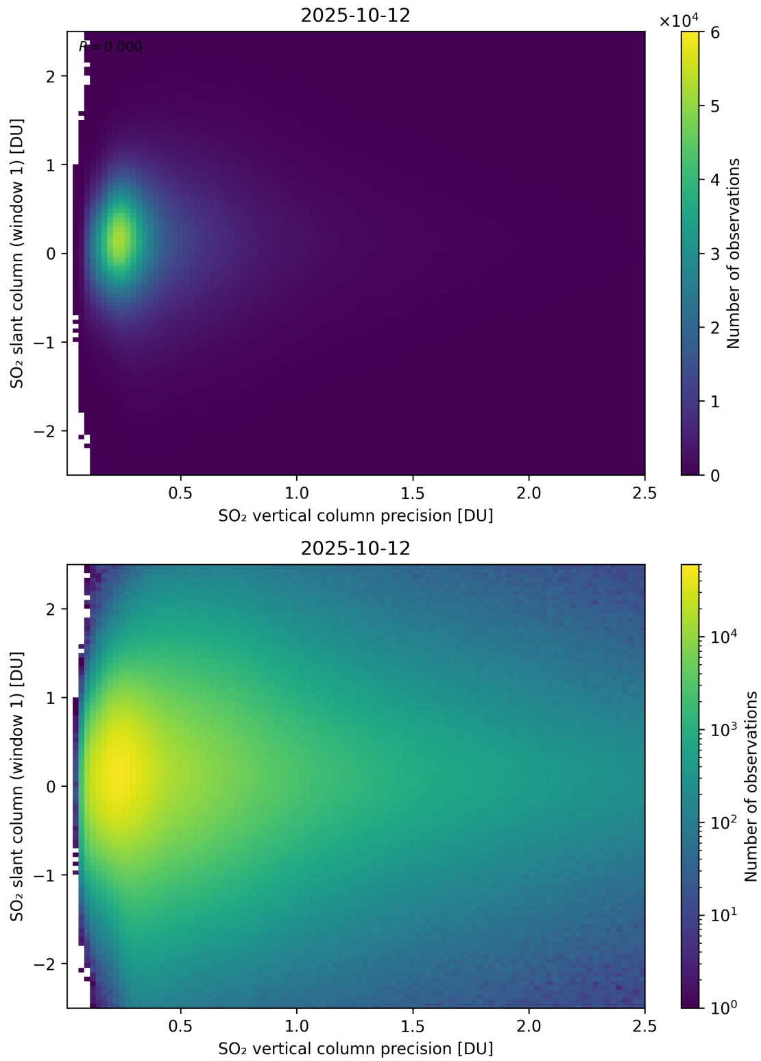
Figure 341: Scatter density plot of “SO 2 vertical column precision” against “SO 2 slant column (window 1)” for 2025-10-11 to 2025-10-13.
