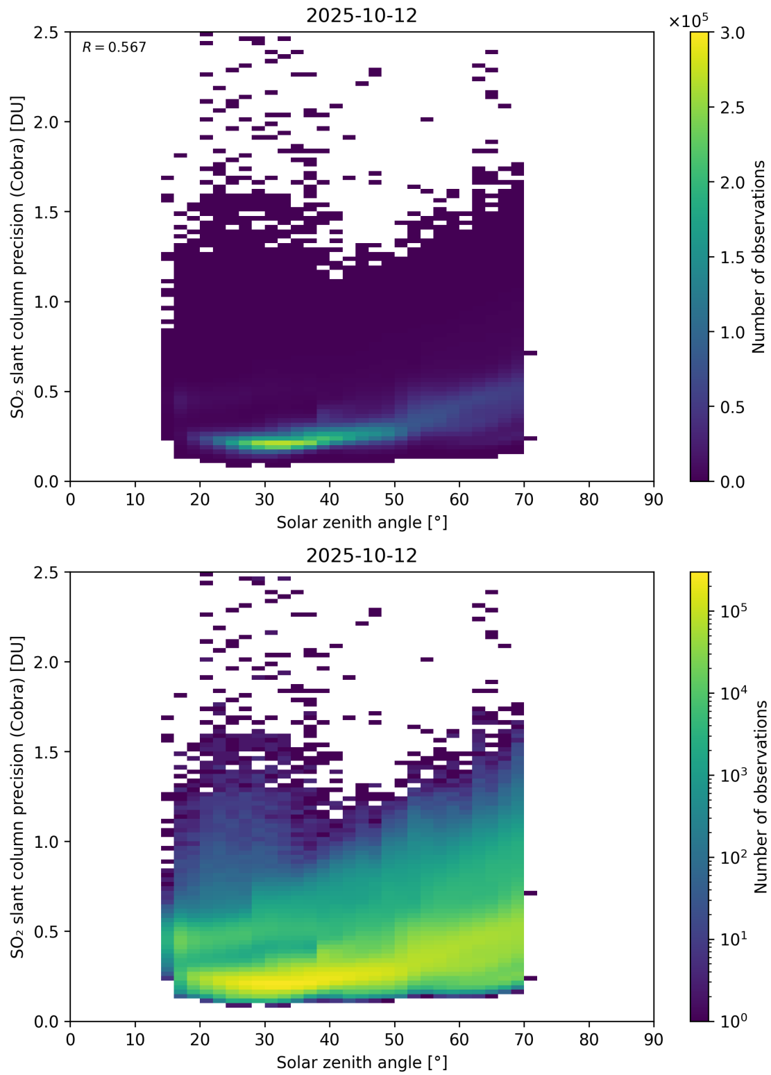
Figure 180: Scatter density plot of “Solar zenith angle” against “SO 2 slant column precision (Cobra)” for 2025-10-11 to 2025-10-13.
