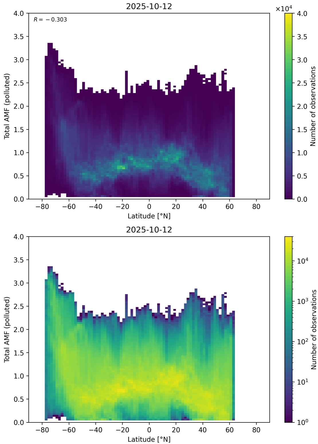
Figure 167: Scatter density plot of “Latitude” against “Total AMF (polluted)” for 2025-10-11 to 2025-10-13.
