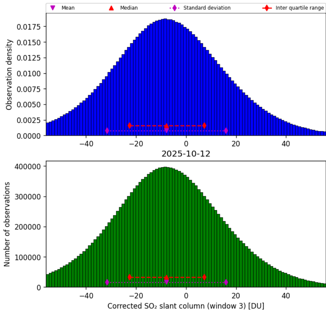
Figure 73: Histogram of “Corrected SO 2 slant column (window 3)” for 2025-10-11 to 2025-10-13
