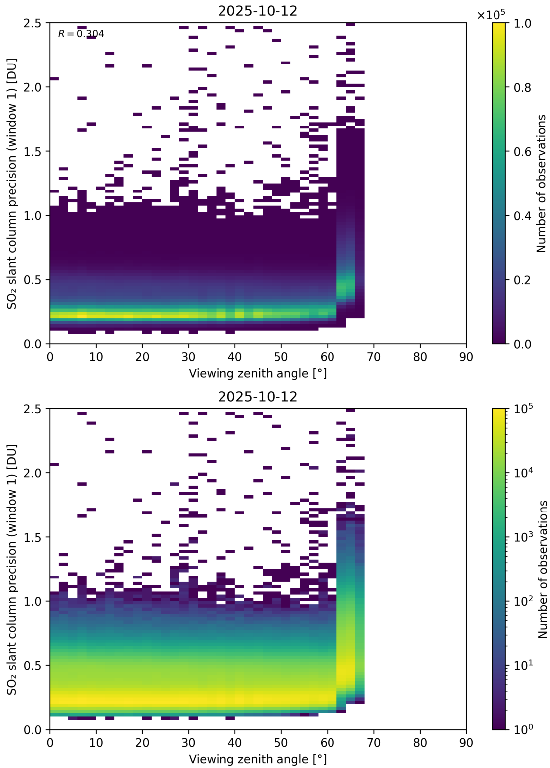
Figure 377: Scatter density plot of “Viewing zenith angle” against “SO 2 slant column precision (window 1)” for 2025-10-11 to 2025-10-13.
