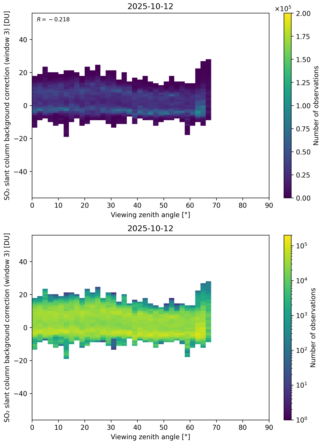
Figure 364: Scatter density plot of “Viewing zenith angle” against “SO 2 slant column background correction (window 3)” for 2025-10-11 to 2025-10-13.
