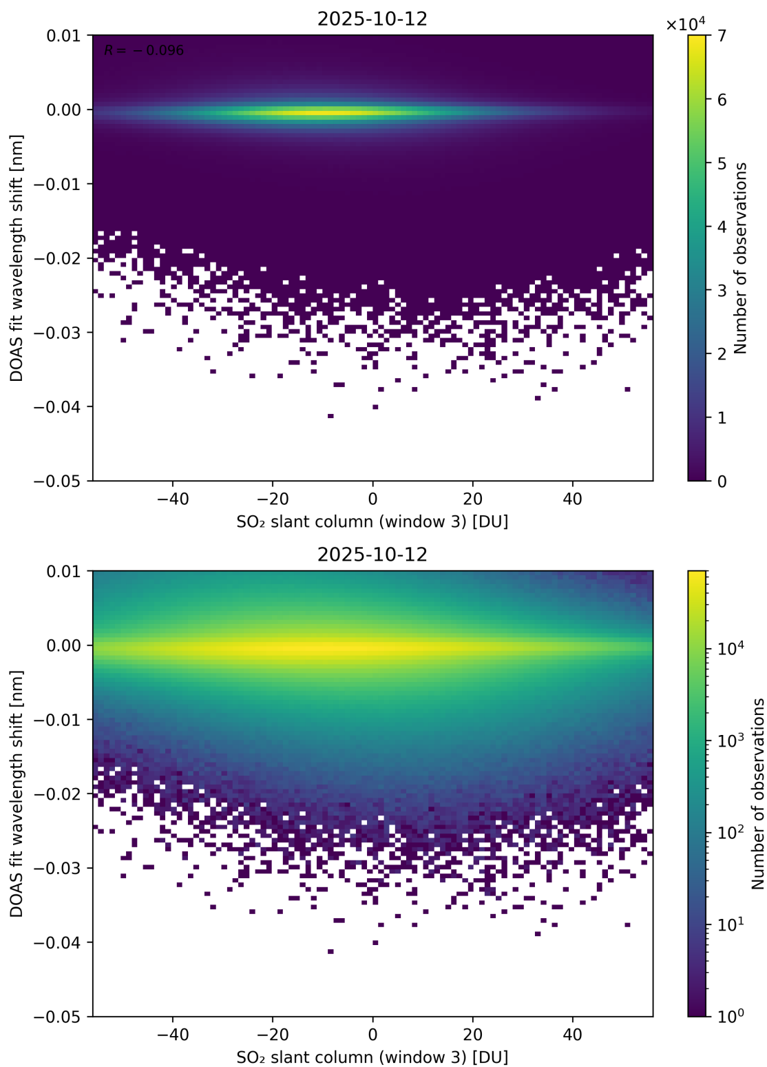
Figure 304: Scatter density plot of “SO 2 slant column (window 3)” against “DOAS fit wavelength shift” for 2025-10-11 to 2025-10-13.
