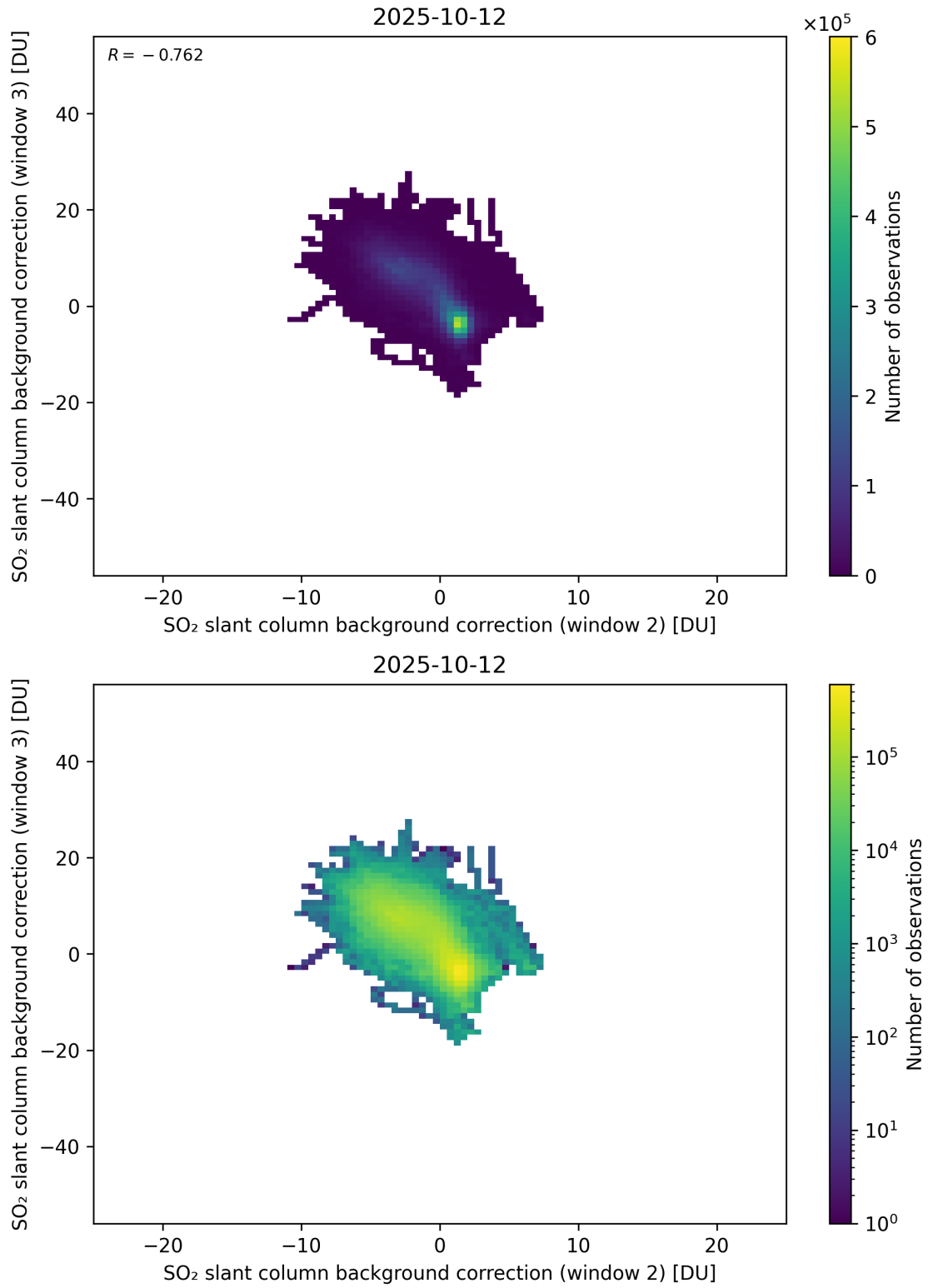
Figure 122: Scatter density plot of “SO 2 slant column background correction (window 2)” against “SO 2 slant column background correction (window 3)” for 2025-10-11 to 2025-10-13.
