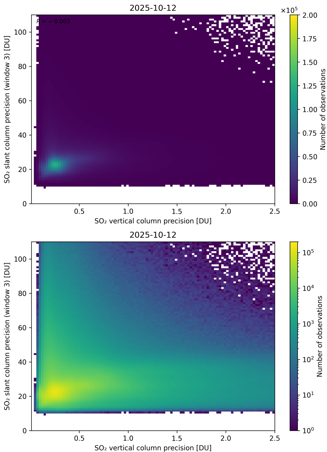
Figure 345: Scatter density plot of “SO 2 vertical column precision” against “SO 2 slant column precision (window 3)” for 2025-10-11 to 2025-10-13.
