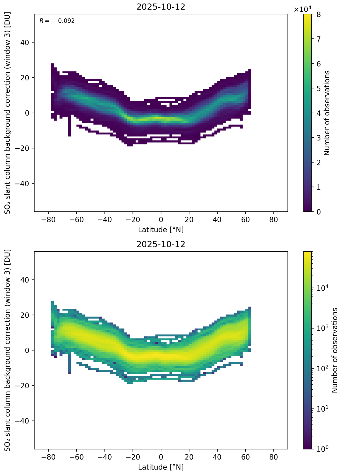
Figure 152: Scatter density plot of “Latitude” against “SO 2 slant column background correction (window 3)” for 2025-10-11 to 2025-10-13.
