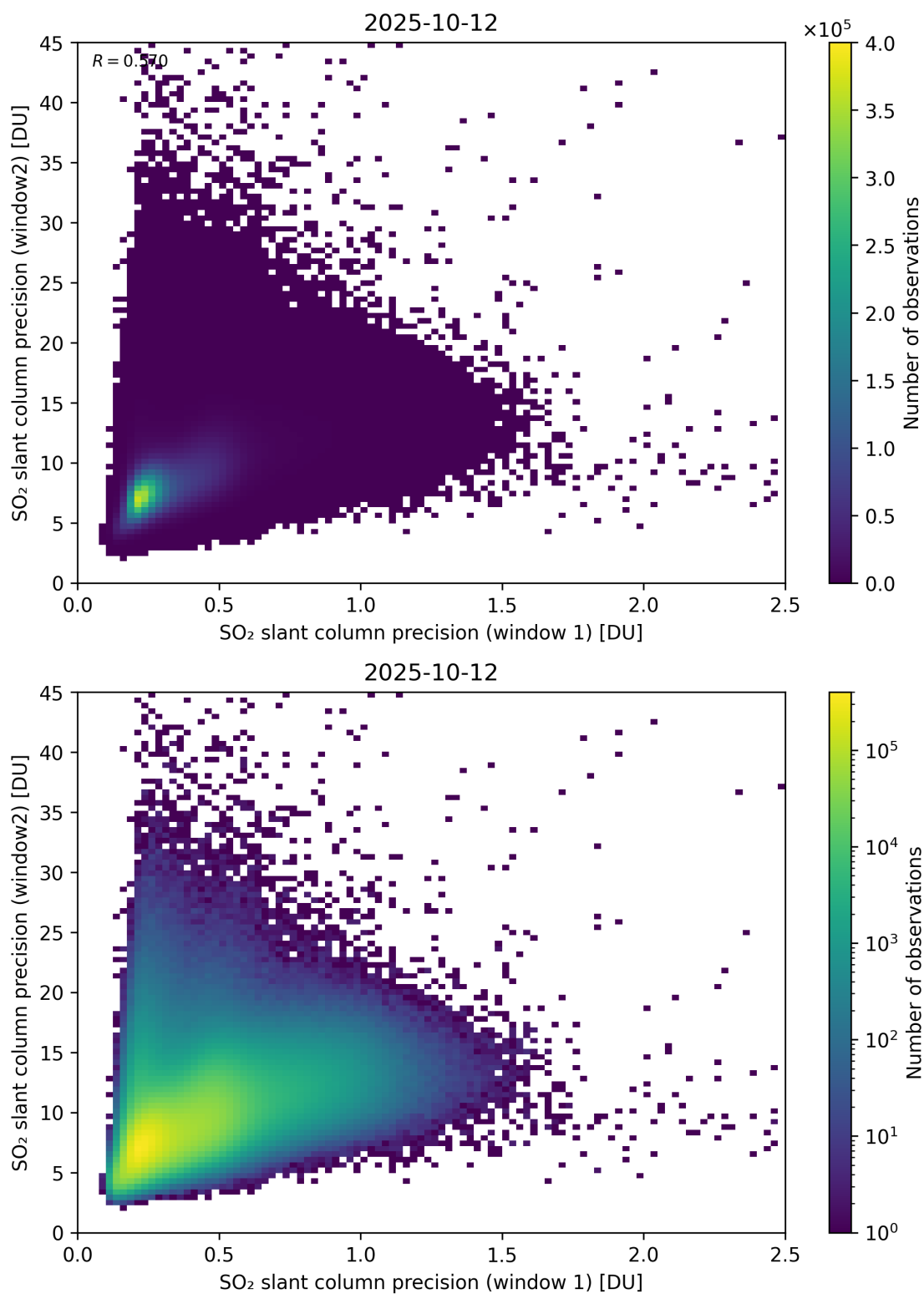
Figure 277: Scatter density plot of “SO 2 slant column precision (window 1)” against “SO 2 slant column precision (window2)” for 2025-10-11 to 2025-10-13.
