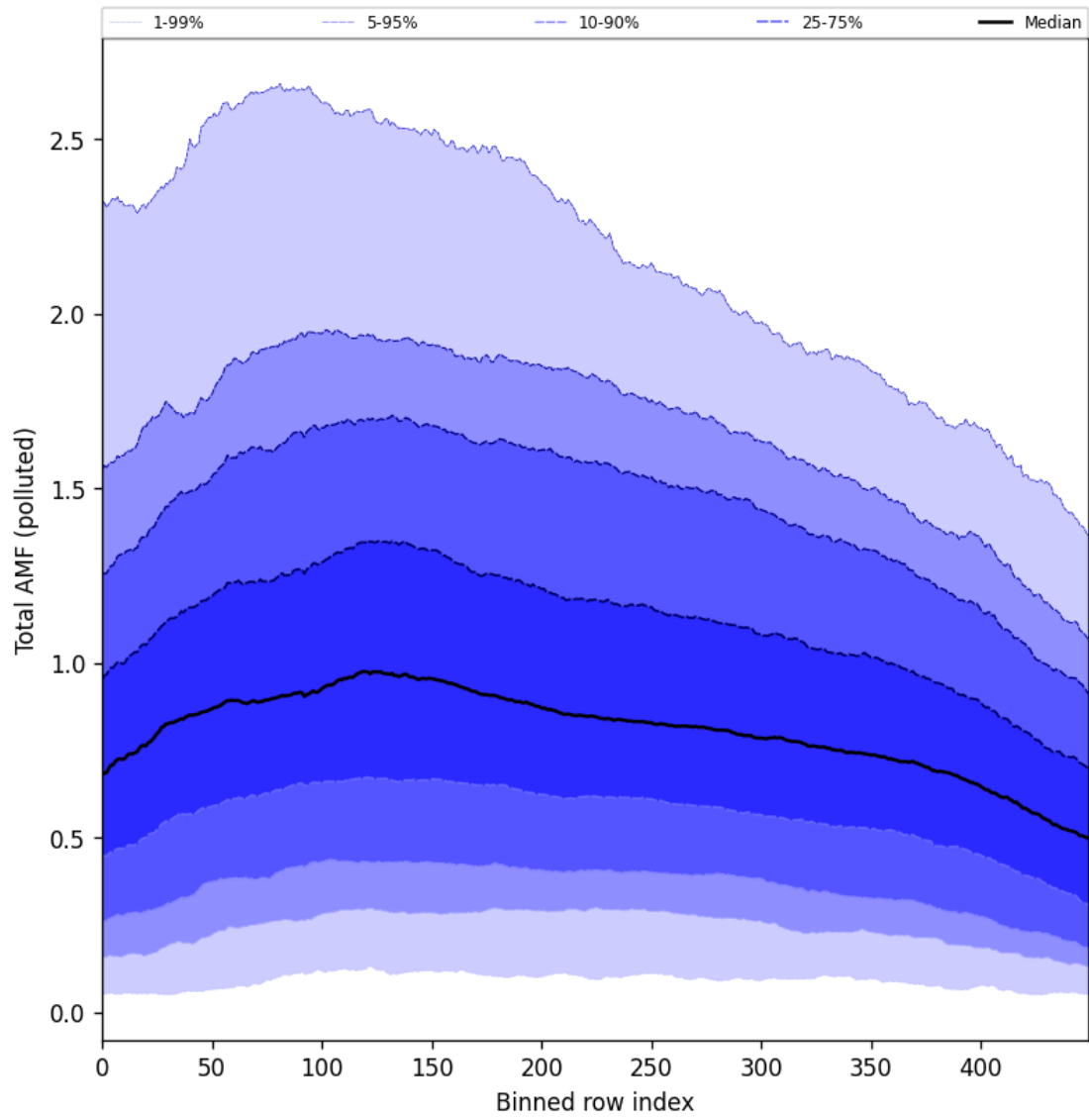
Figure 105: Along track statistics of “Total AMF (polluted)” for 2025-10-11 to 2025-10-13
