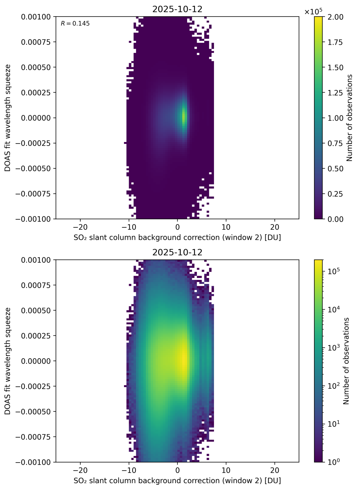
Figure 124: Scatter density plot of “SO 2 slant column background correction (window 2)” against “DOAS fit wavelength squeeze” for 2025-10-11 to 2025-10-13.
