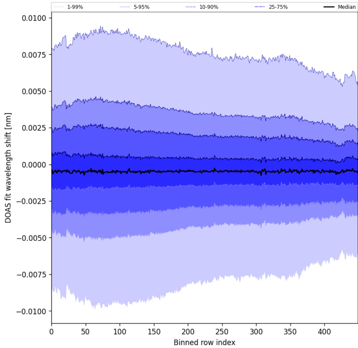
Figure 102: Along track statistics of “DOAS fit wavelength shift” for 2025-10-11 to 2025-10-13
