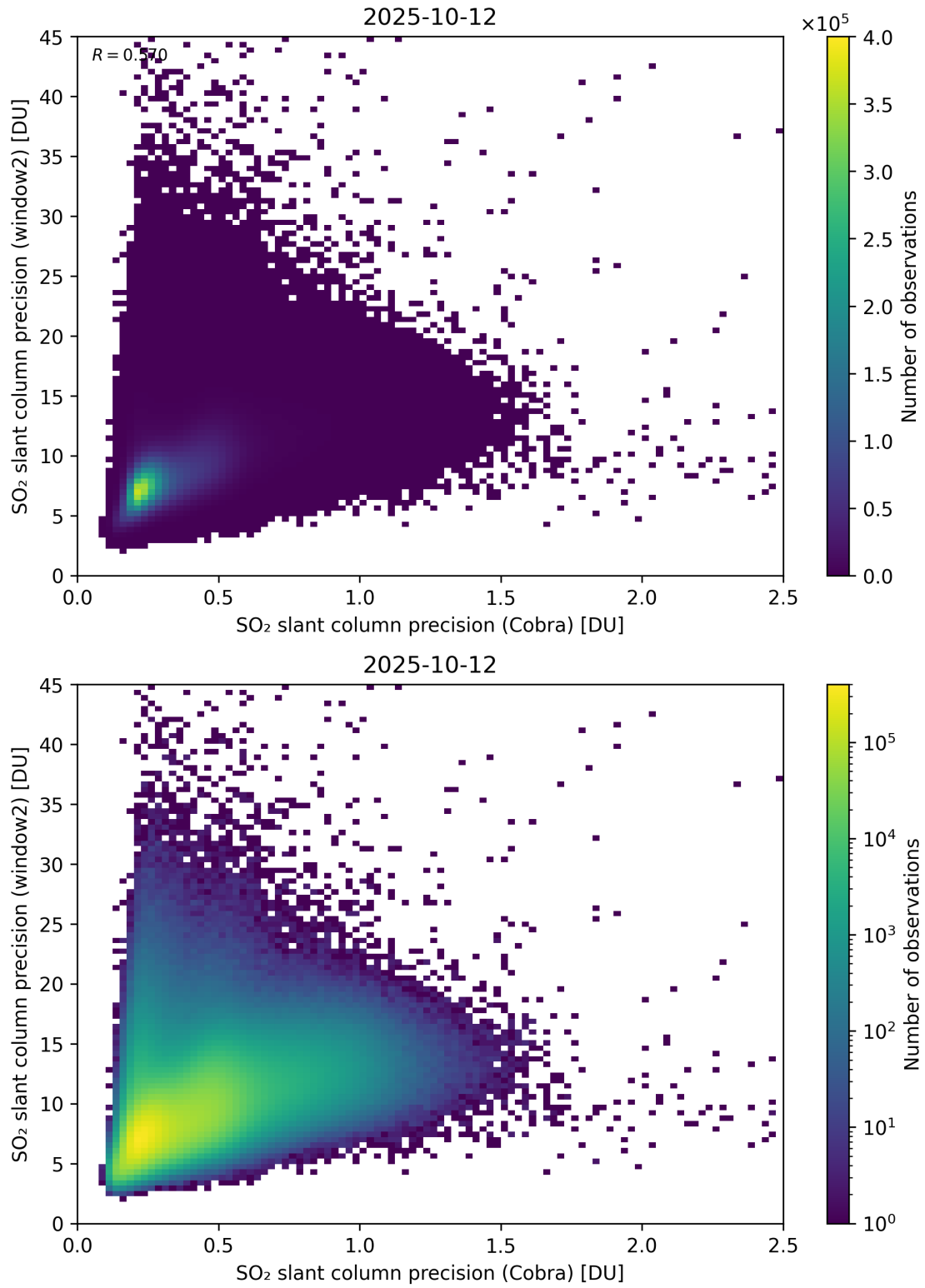
Figure 210: Scatter density plot of “SO 2 slant column precision (Cobra)” against “SO 2 slant column precision (window2)” for 2025-10-11 to 2025-10-13.
