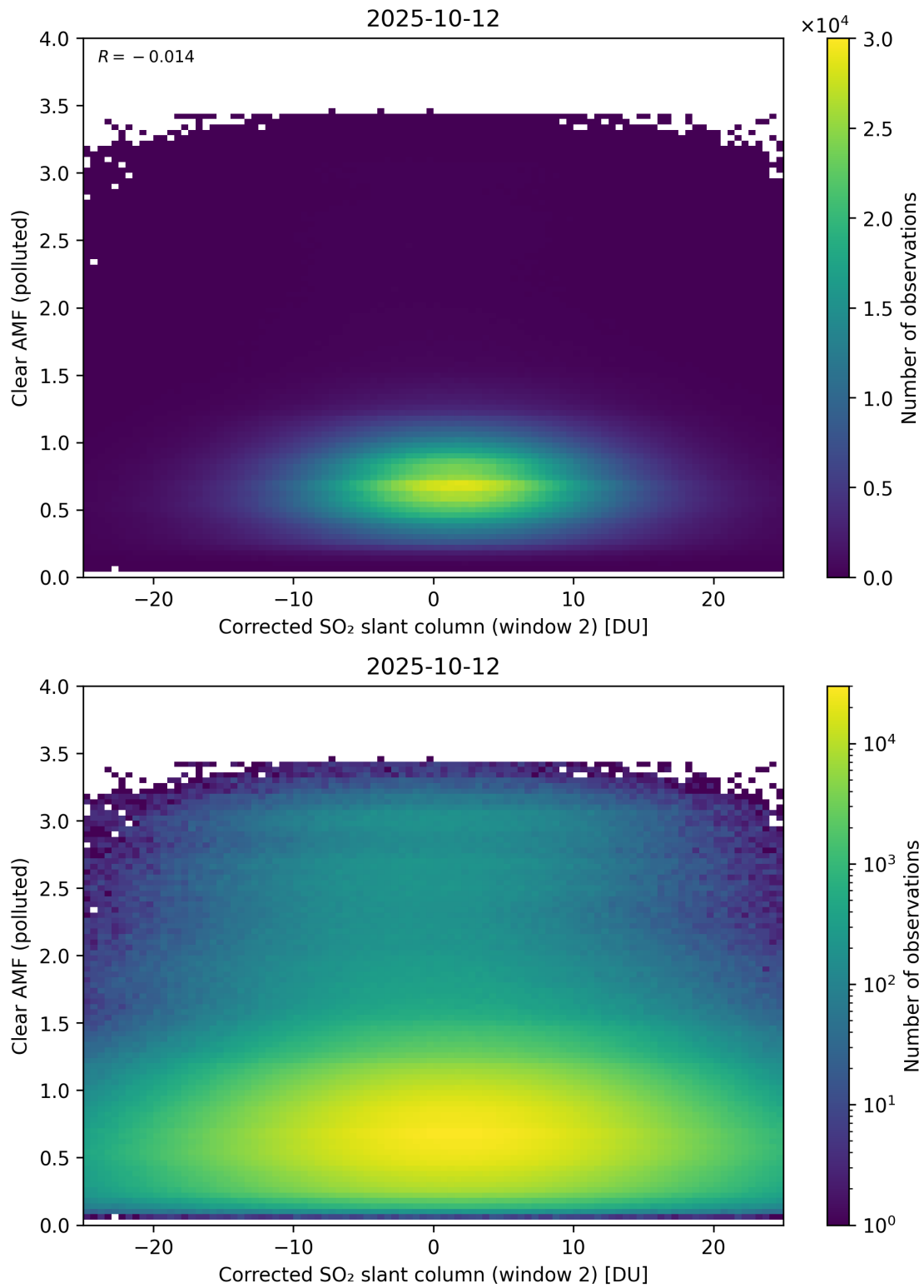
Figure 249: Scatter density plot of “Corrected SO 2 slant column (window 2)” against “Clear AMF (polluted)” for 2025-10-11 to 2025-10-13.
