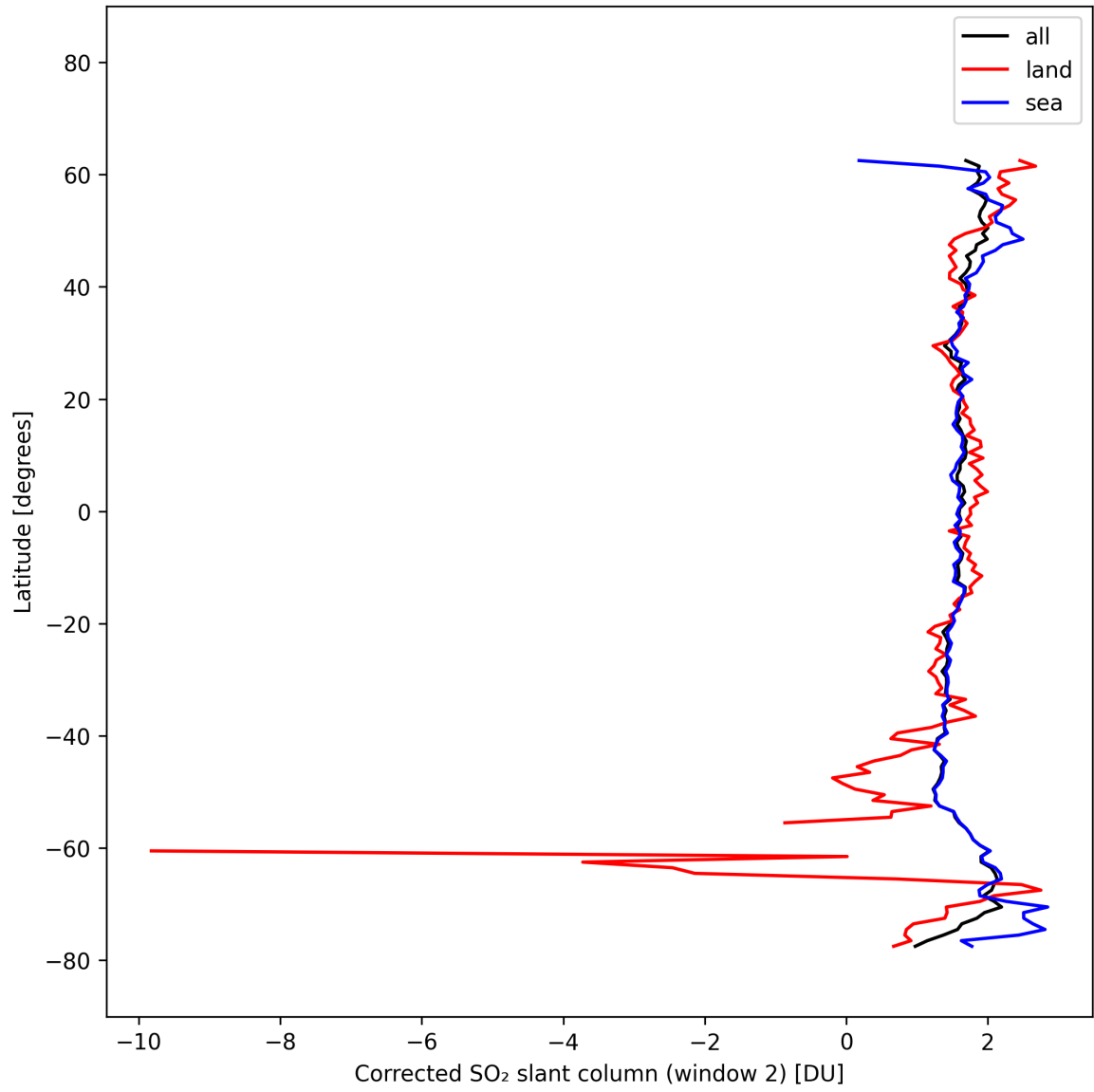
Figure 43: Zonal average of “Corrected SO 2 slant column (window 2)” for 2025-10-11 to 2025-10-13.
