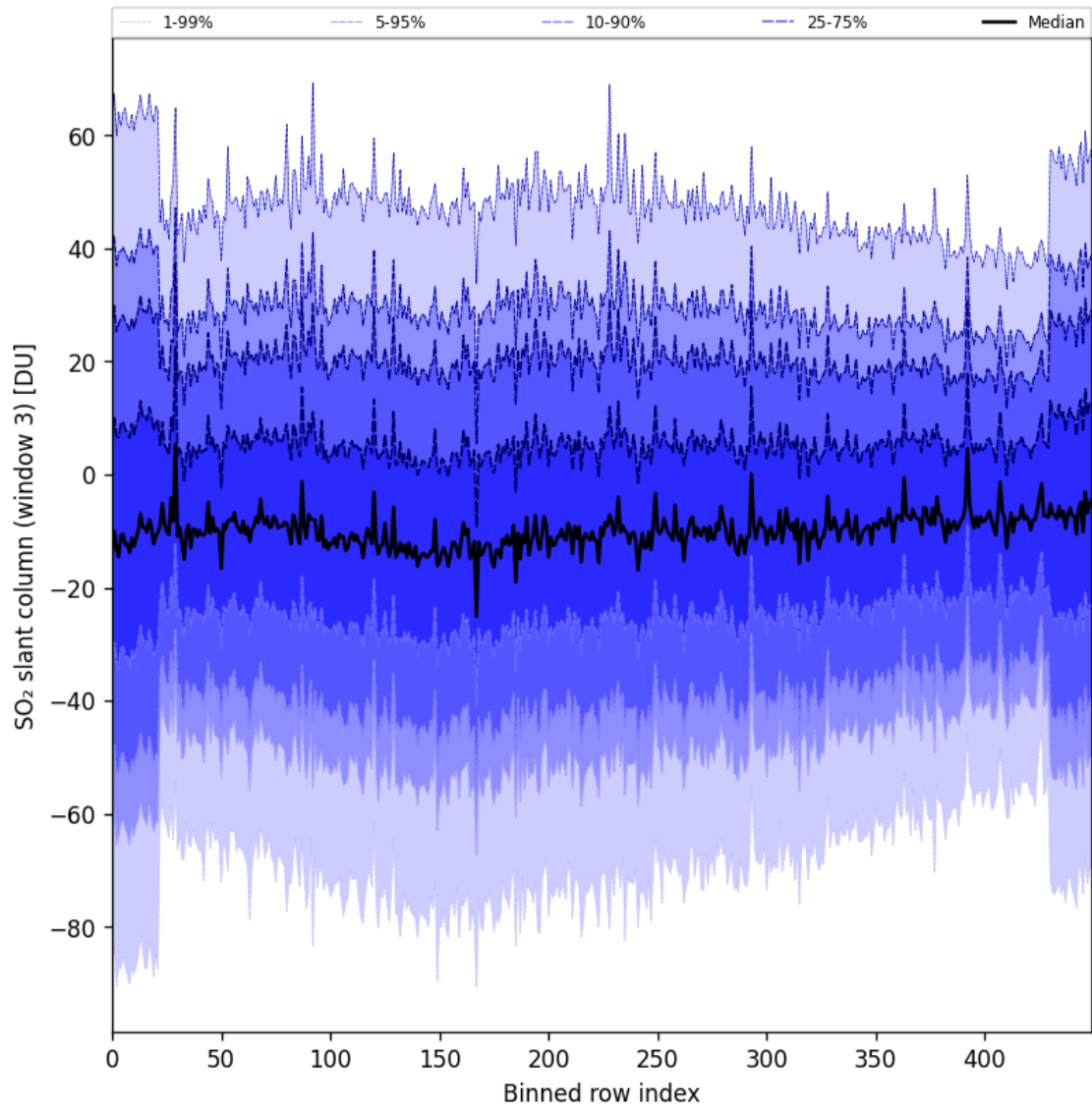
Figure 97: Along track statistics of “SO 2 slant column (window 3)” for 2025-10-11 to 2025-10-13
