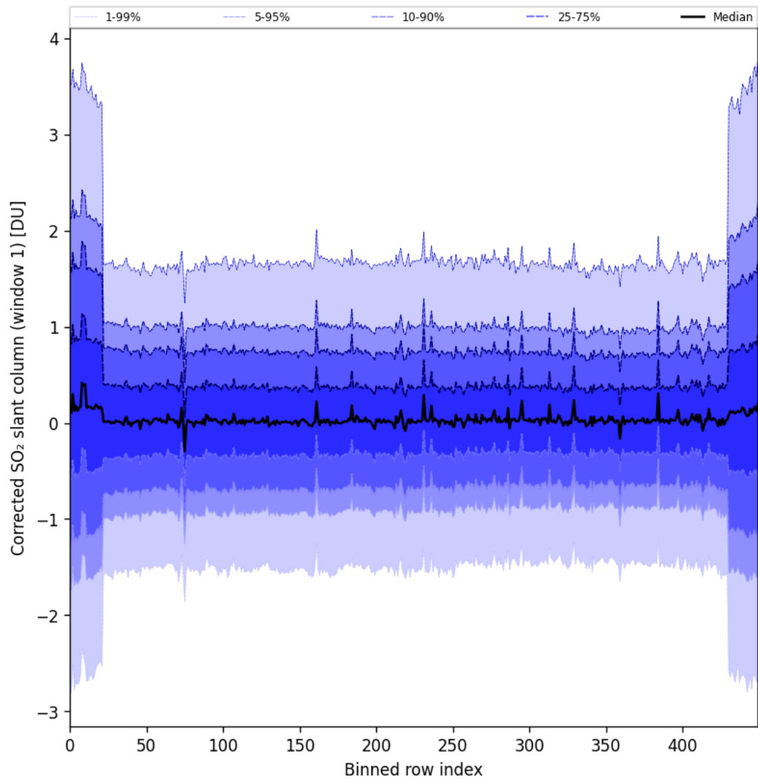
Figure 91: Along track statistics of “Corrected SO 2 slant column (window 1)” for 2025-10-11 to 2025-10-13
