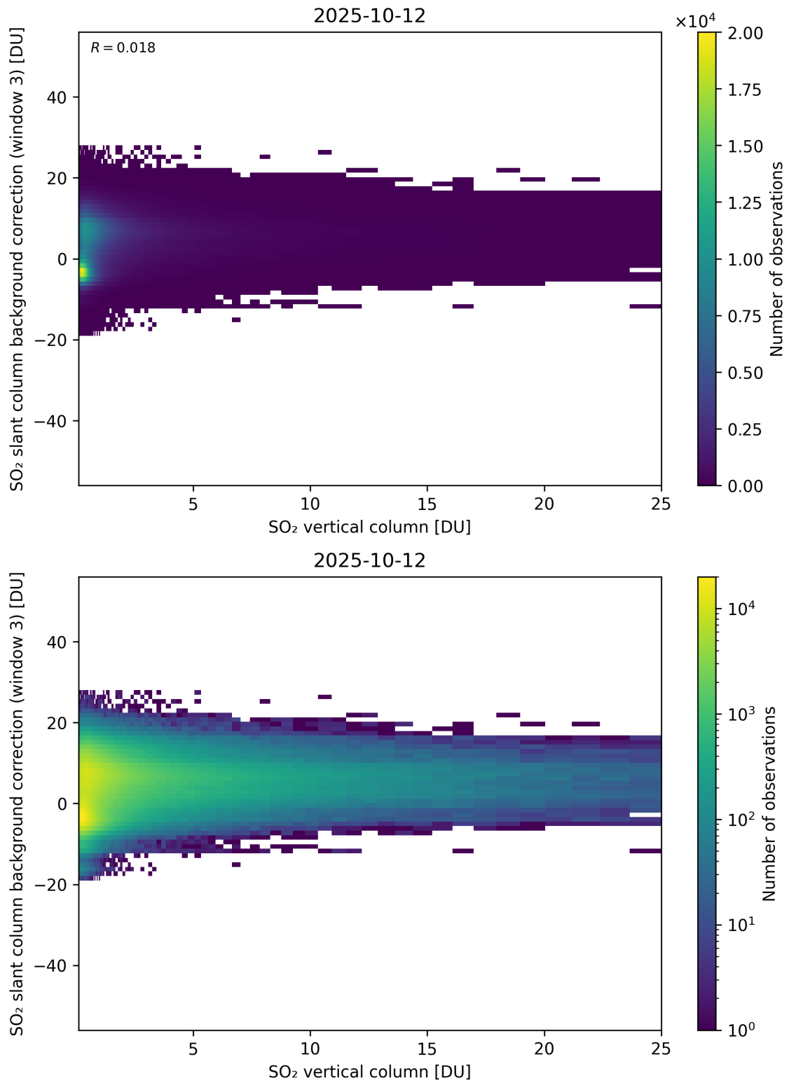
Figure 325: Scatter density plot of “SO 2 vertical column” against “SO 2 slant column background correction (window 3)” for 2025-10-11 to 2025-10-13.
