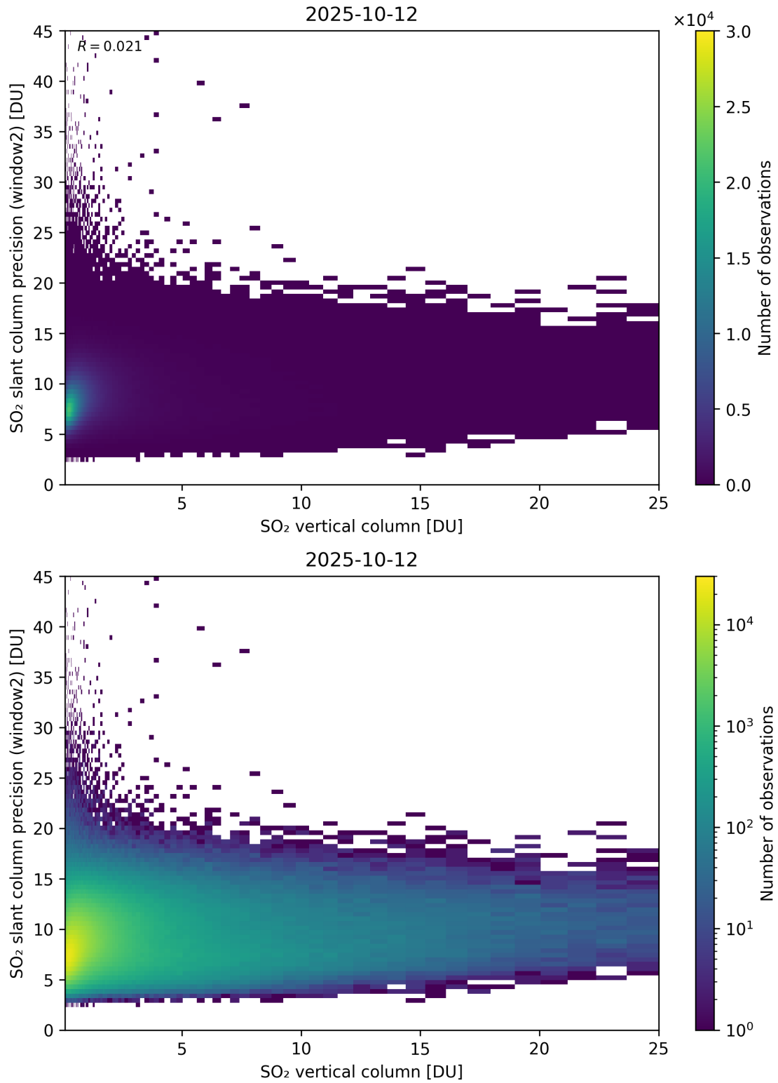
Figure 356: Scatter density plot of “SO 2 vertical column” against “SO 2 slant column precision (window2)” for 2025-10-11 to 2025-10-13.
