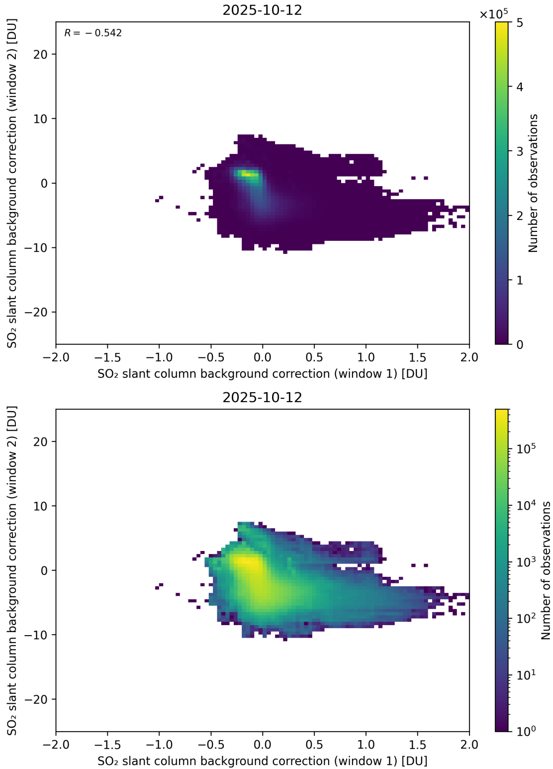
Figure 109: Scatter density plot of “SO 2 slant column background correction (window 1)” against “SO 2 slant column background correction (window 2)” for 2025-10-11 to 2025-10-13.
