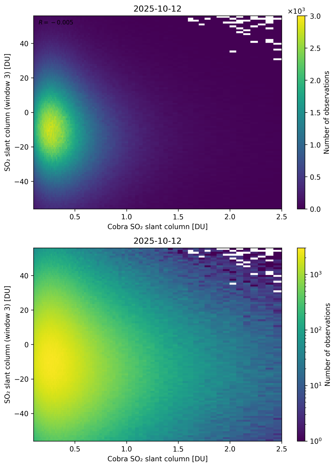
Figure 222: Scatter density plot of “Cobra SO 2 slant column” against “SO 2 slant column (window 3)” for 2025-10-11 to 2025-10-13.
