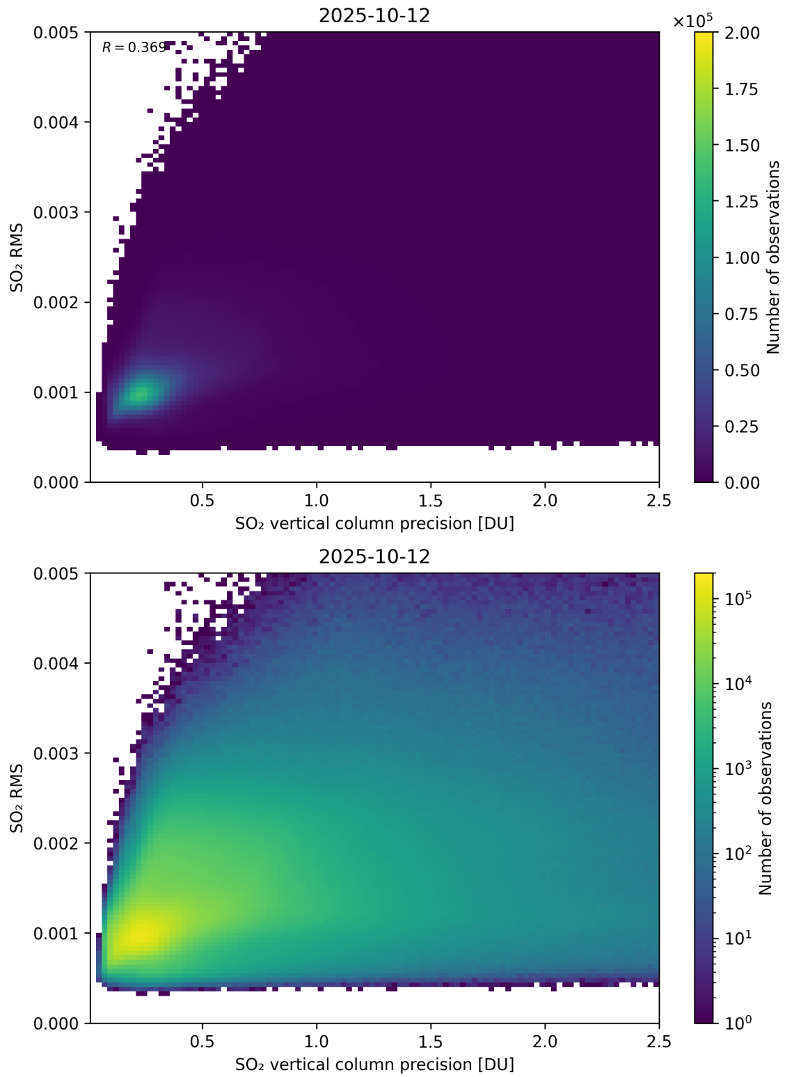
Figure 334: Scatter density plot of “SO 2 vertical column precision” against “SO 2 RMS” for 2025-10-11 to 2025-10-13.
