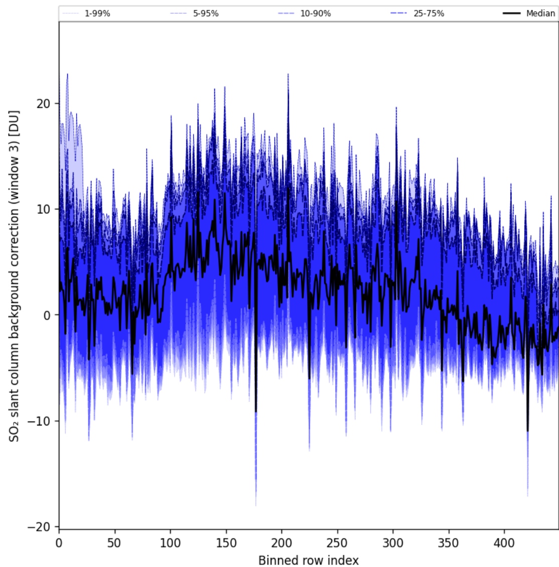
Figure 100: Along track statistics of “SO 2 slant column background correction (window 3)” for 2025-10-11 to 2025-10-13
