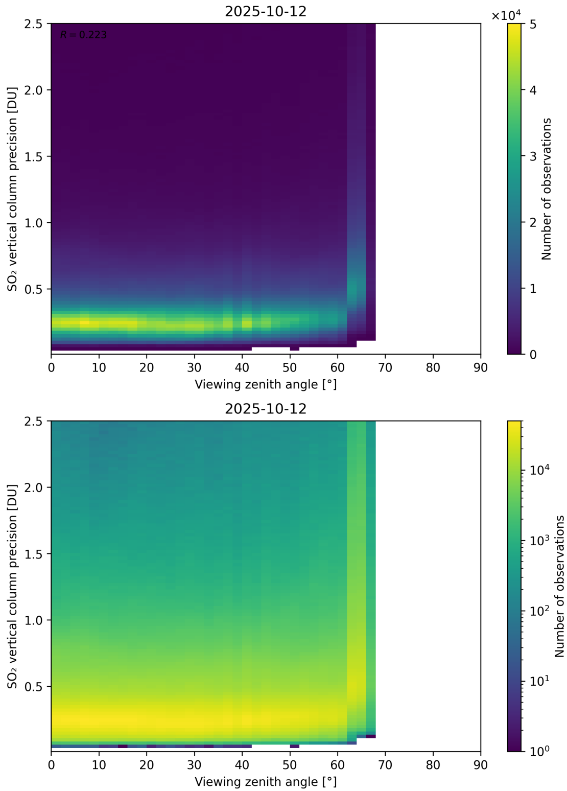
Figure 384: Scatter density plot of “Viewing zenith angle” against “SO 2 vertical column precision” for 2025-10-11 to 2025-10-13.
