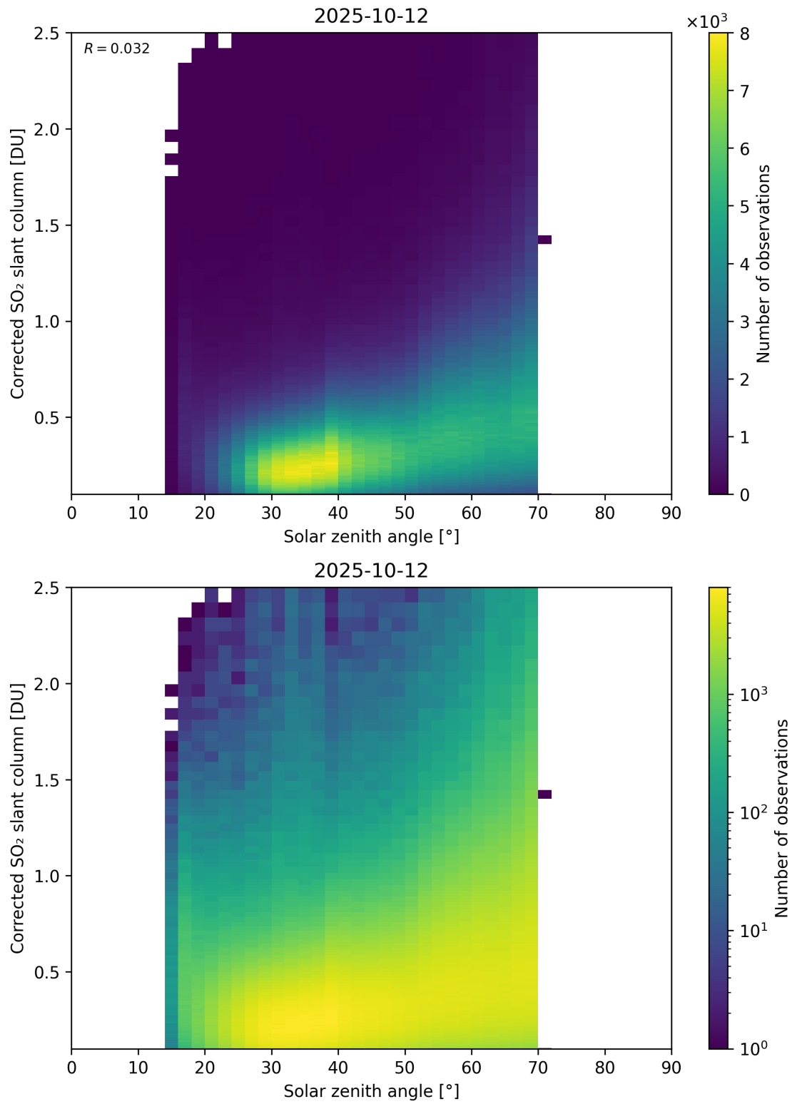
Figure 181: Scatter density plot of “Solar zenith angle” against “Corrected SO 2 slant column” for 2025-10-11 to 2025-10-13.
