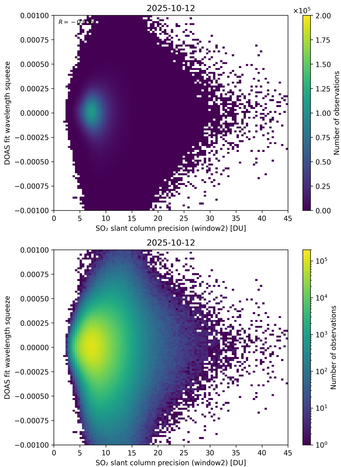
Figure 294: Scatter density plot of “SO 2 slant column precision (window2)” against “DOAS fit wavelength squeeze” for 2025-10-11 to 2025-10-13.
