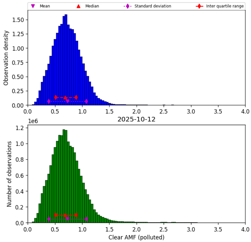
Figure 81: Histogram of “Clear AMF (polluted)” for 2025-10-11 to 2025-10-13
