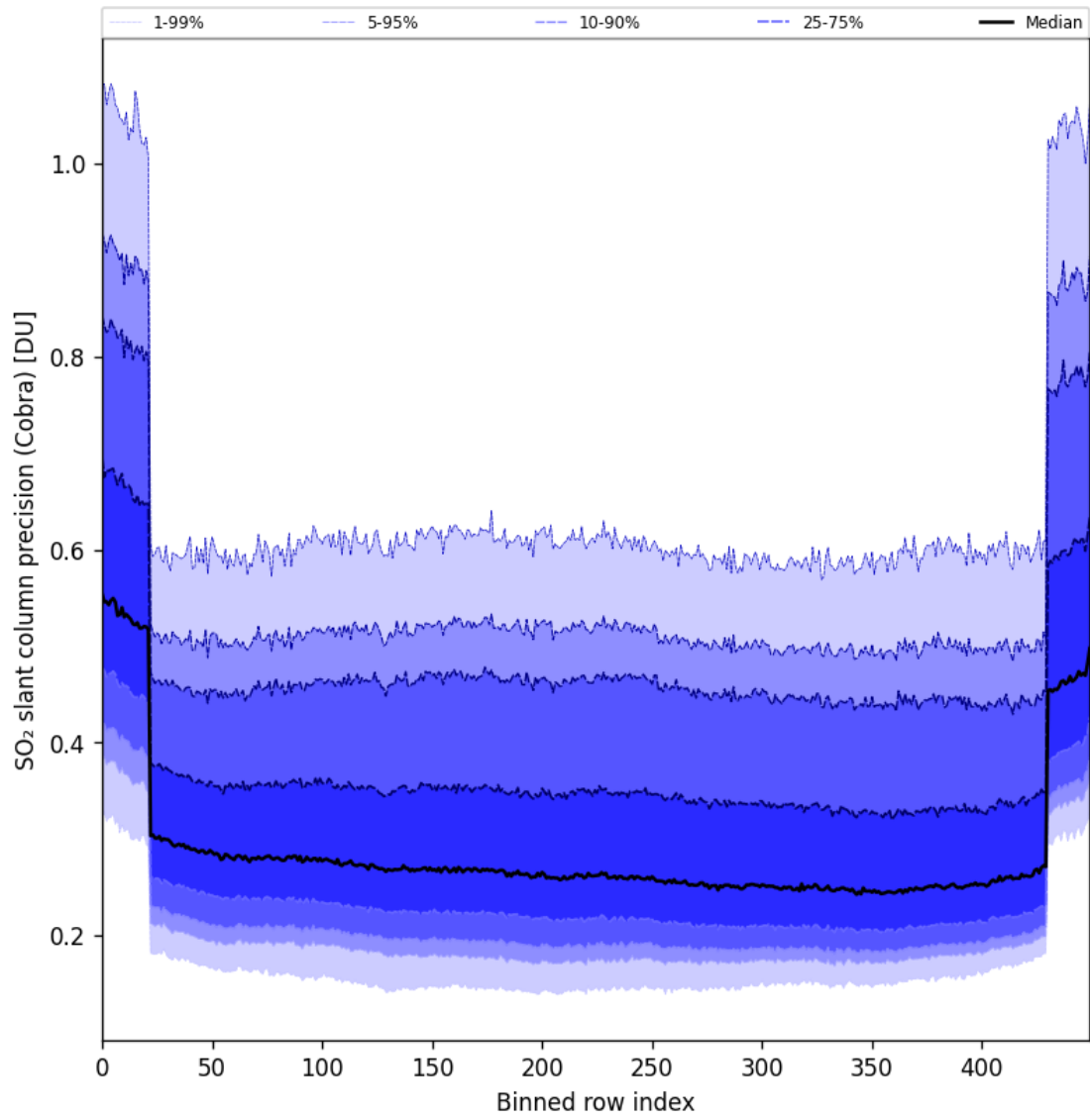
Figure 88: Along track statistics of “SO 2 slant column precision (Cobra)” for 2025-10-11 to 2025-10-13
