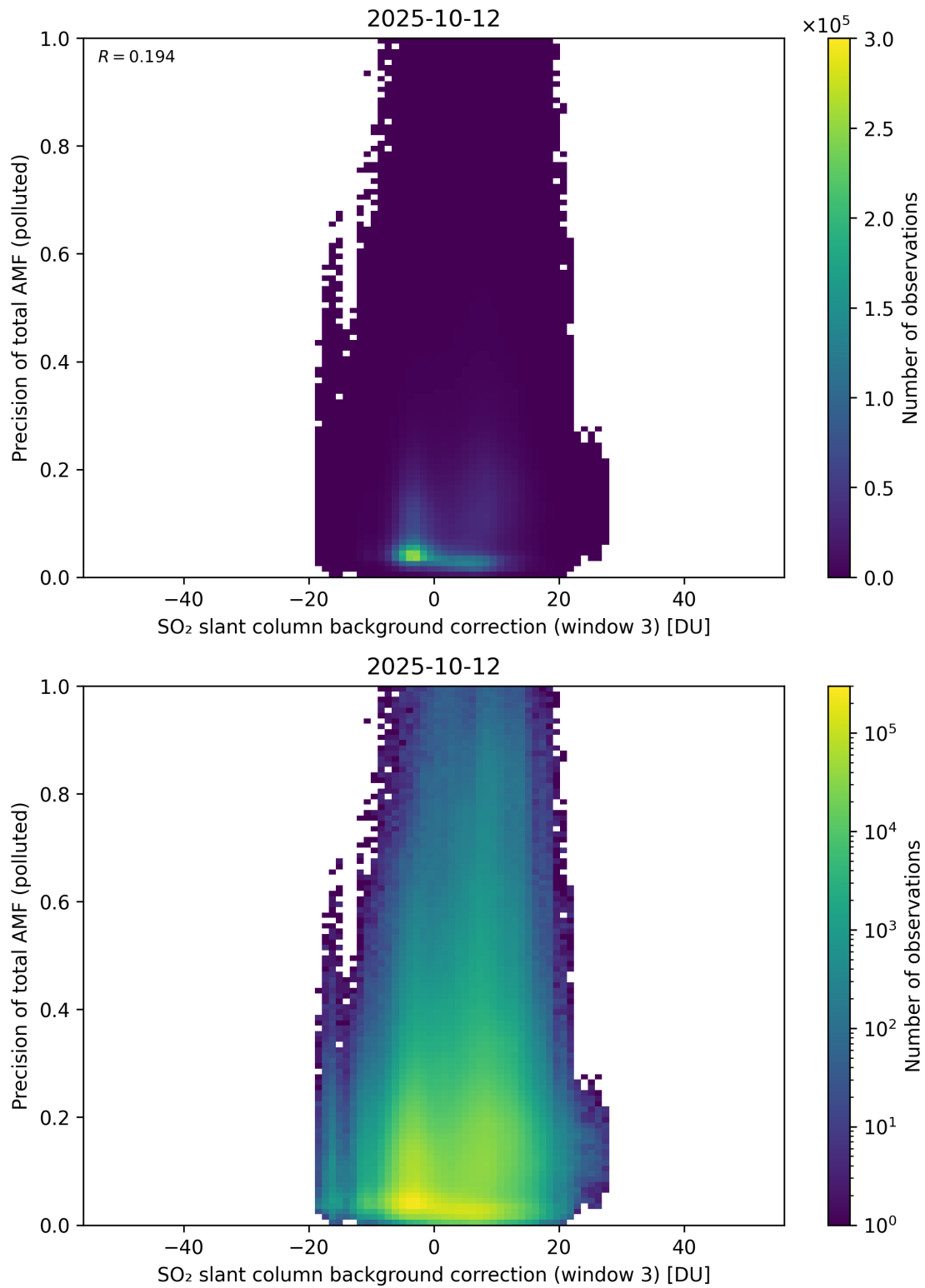
Figure 137: Scatter density plot of “SO 2 slant column background correction (window 3)” against “Precision of total AMF (polluted)” for 2025-10-11 to 2025-10-13.
