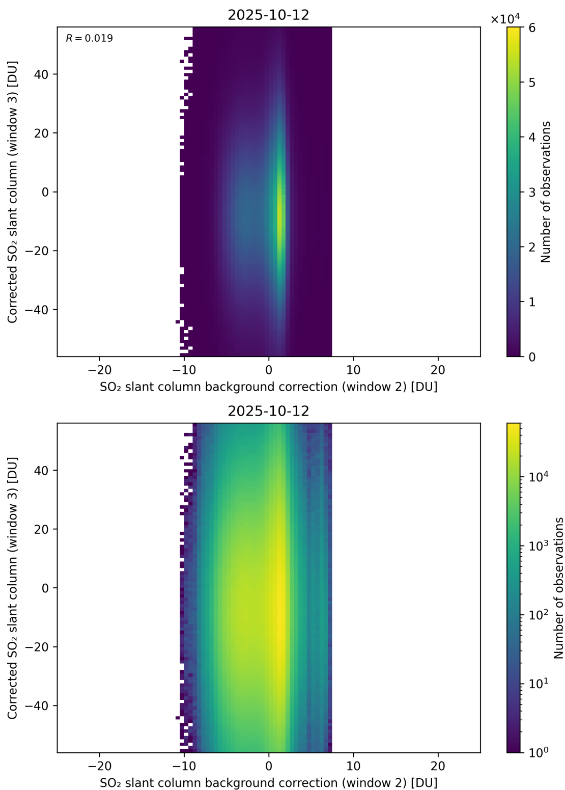
Figure 127: Scatter density plot of “SO 2 slant column background correction (window 2)” against “Corrected SO 2 slant column (window 3)” for 2025-10-11 to 2025-10-13.
