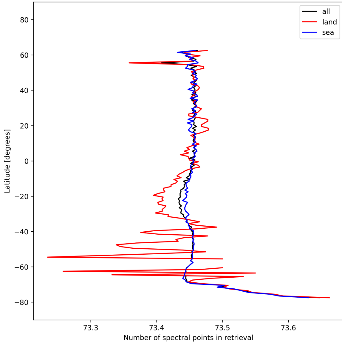
Figure 56: Zonal average of “Number of spectral points in retrieval” for 2025-10-11 to 2025-10-13.
