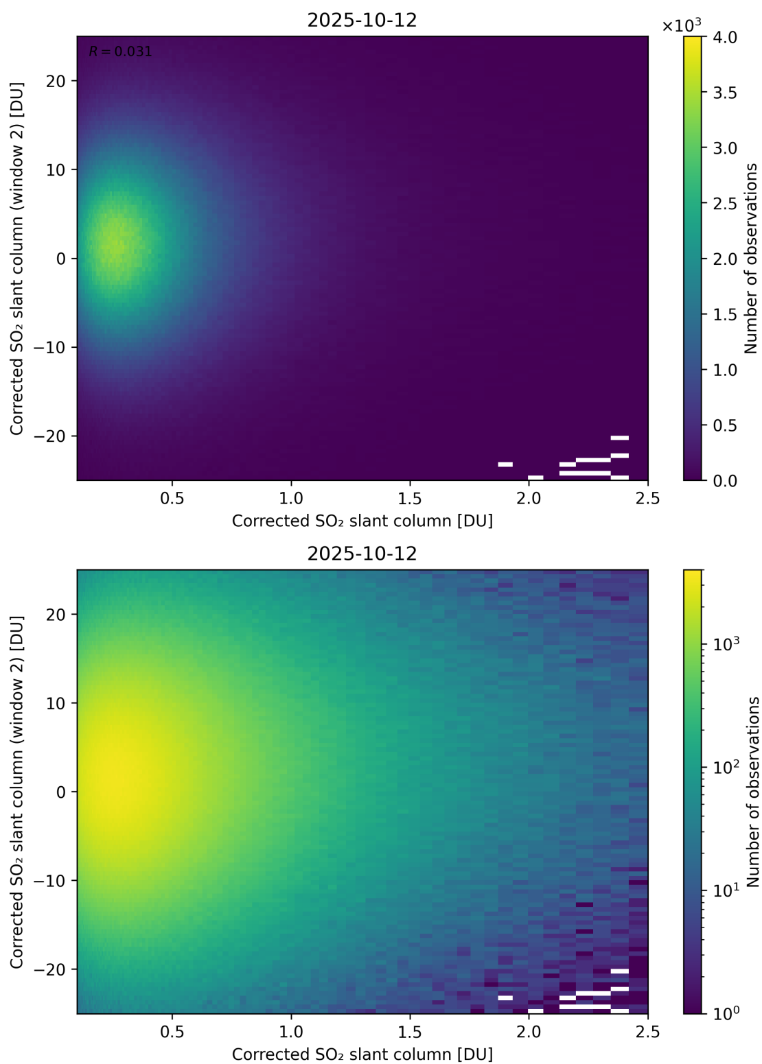
Figure 235: Scatter density plot of “Corrected SO 2 slant column” against “Corrected SO 2 slant column (window 2)” for 2025-10-11 to 2025-10-13.
