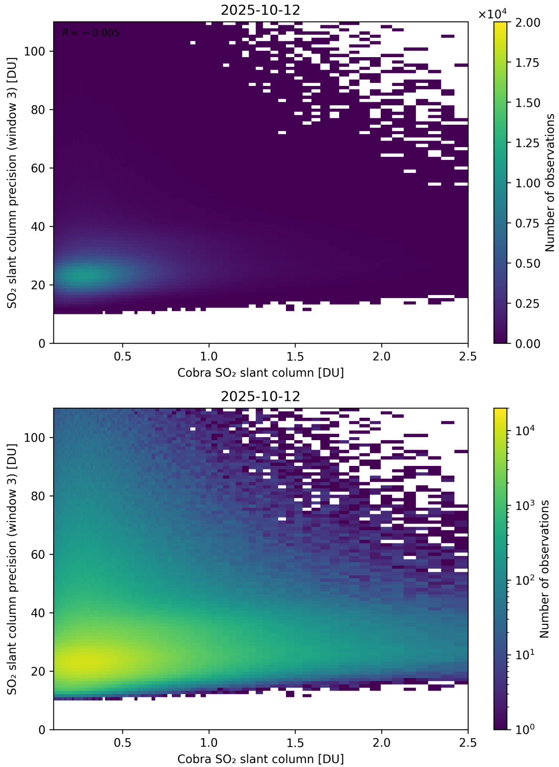
Figure 223: Scatter density plot of “Cobra SO 2 slant column” against “SO 2 slant column precision (window 3)” for 2025-10-11 to 2025-10-13.
