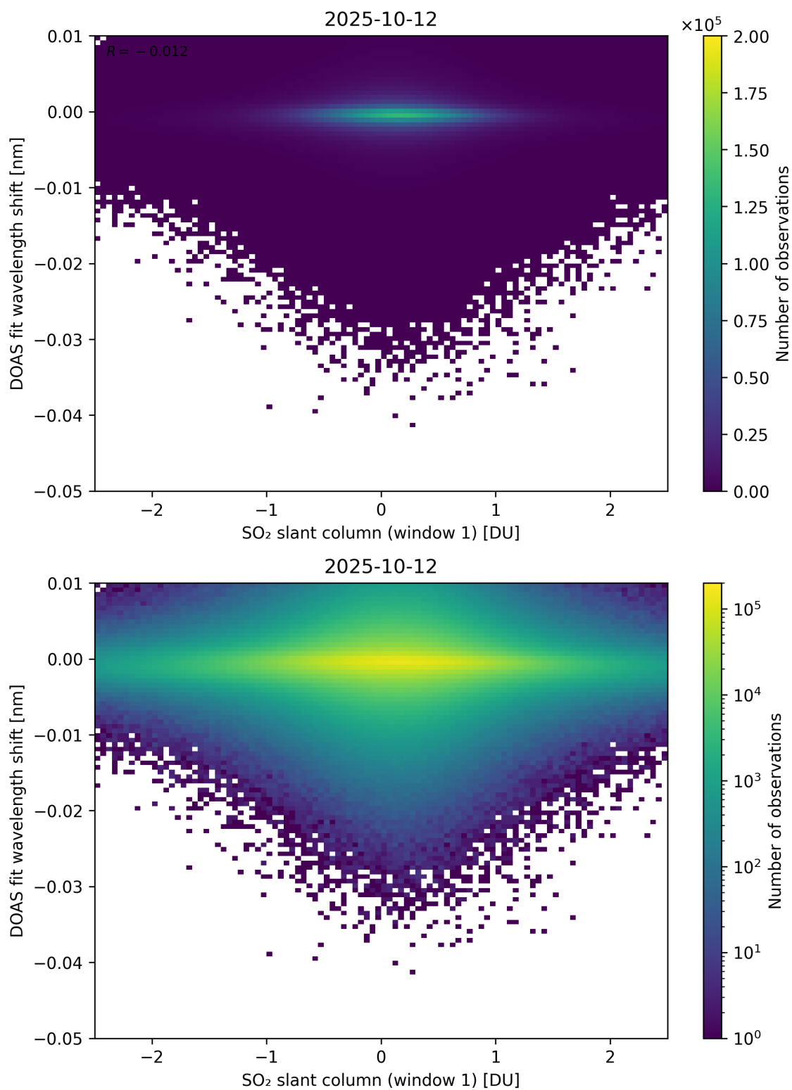
Figure 265: Scatter density plot of “SO 2 slant column (window 1)” against “DOAS fit wavelength shift” for 2025-10-11 to 2025-10-13.
