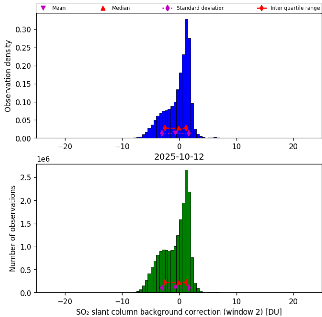
Figure 70: Histogram of “SO 2 slant column background correction (window 2)” for 2025-10-11 to 2025-10-13
