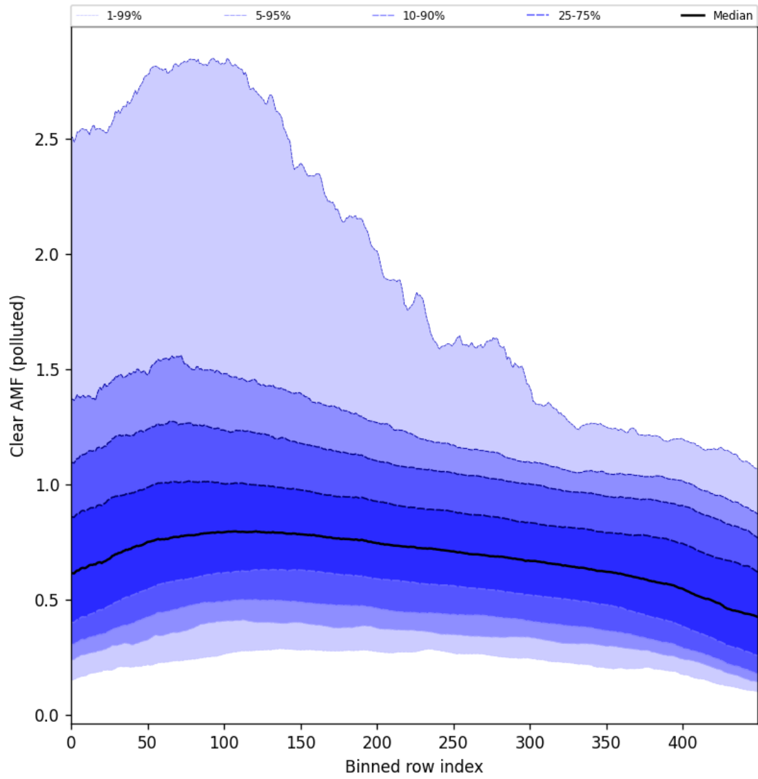
Figure 107: Along track statistics of “Clear AMF (polluted)” for 2025-10-11 to 2025-10-13
