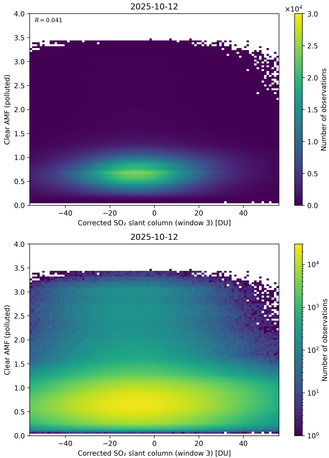
Figure 259: Scatter density plot of “Corrected SO 2 slant column (window 3)” against “Clear AMF (polluted)” for 2025-10-11 to 2025-10-13.
