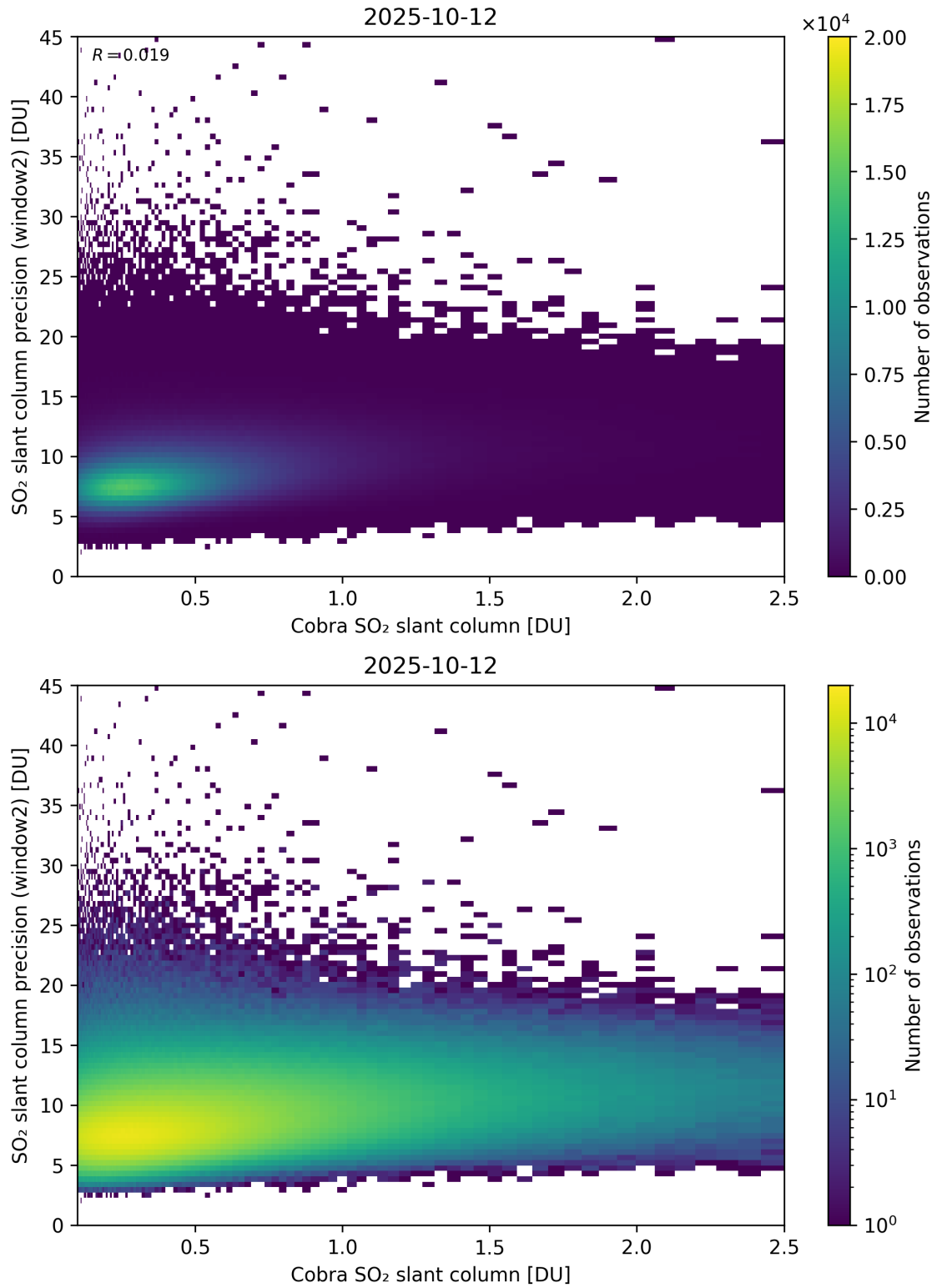
Figure 221: Scatter density plot of “Cobra SO 2 slant column” against “SO 2 slant column precision (window2)” for 2025-10-11 to 2025-10-13.
