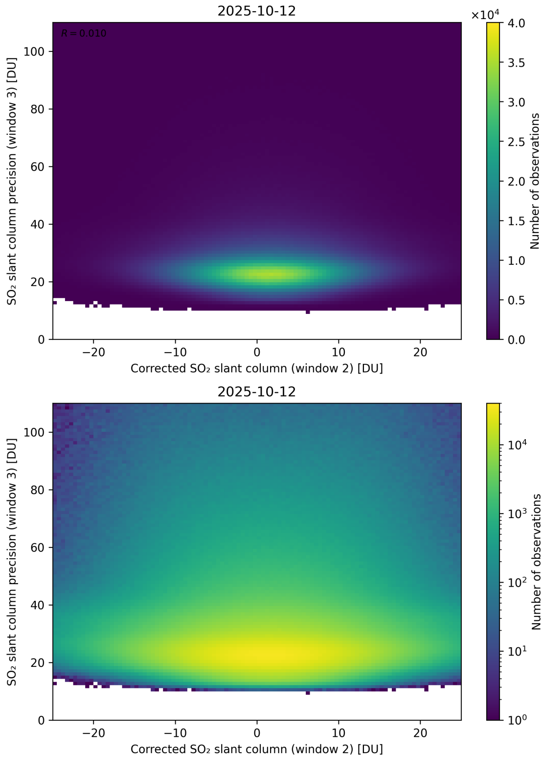
Figure 252: Scatter density plot of “Corrected SO 2 slant column (window 2)” against “SO 2 slant column precision (window 3)” for 2025-10-11 to 2025-10-13.
