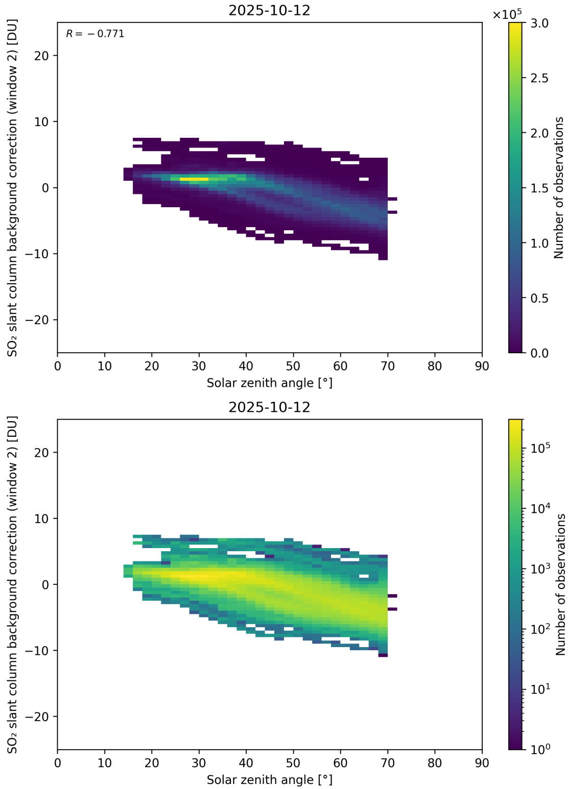
Figure 172: Scatter density plot of “Solar zenith angle” against “SO 2 slant column background correction (window 2)” for 2025-10-11 to 2025-10-13.
