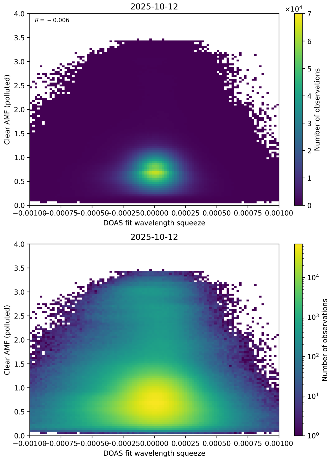
Figure 144: Scatter density plot of “DOAS fit wavelength squeeze” against “Clear AMF (polluted)” for 2025-10-11 to 2025-10-13.
