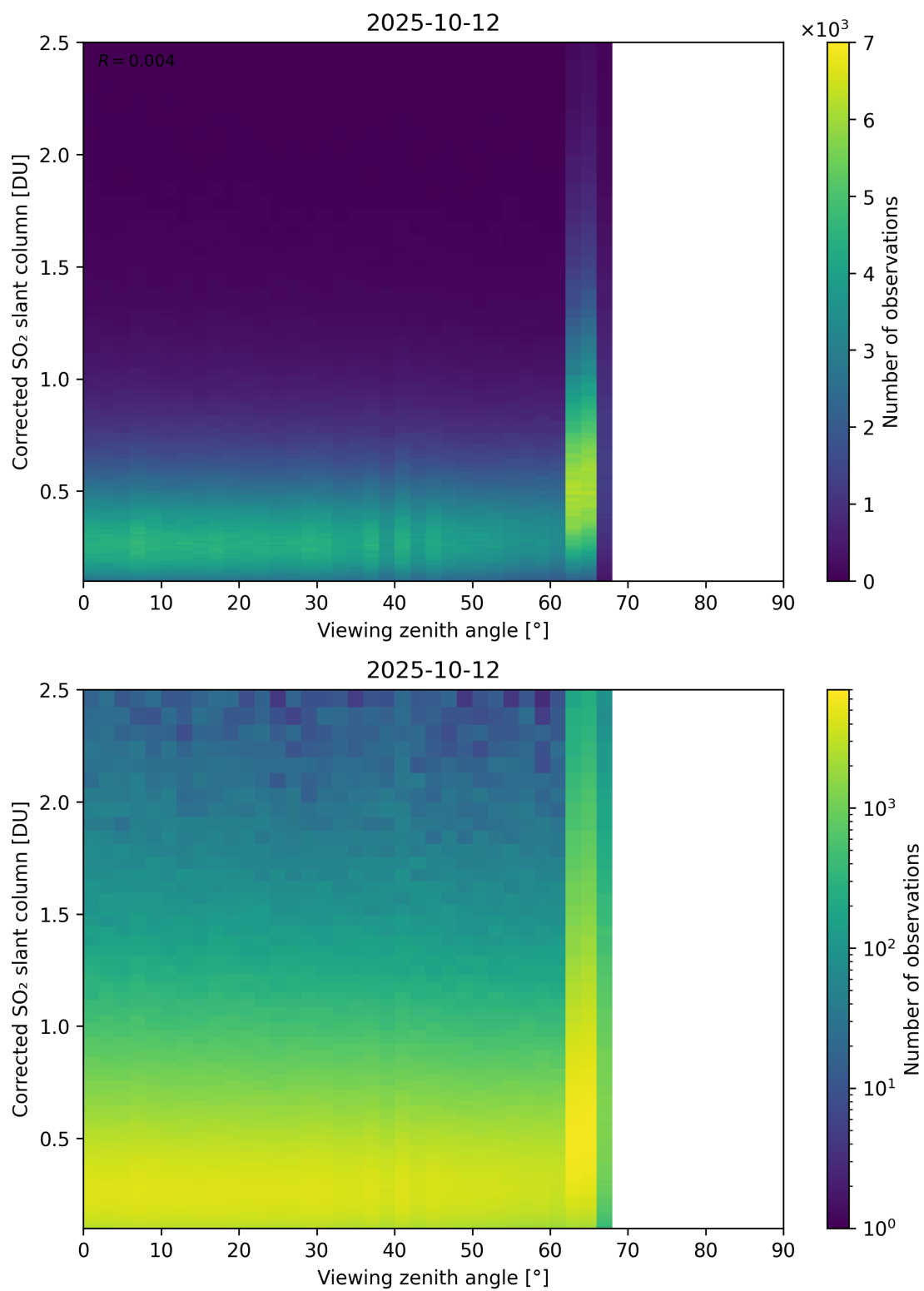
Figure 373: Scatter density plot of “Viewing zenith angle” against “Corrected SO 2 slant column” for 2025-10-11 to 2025-10-13.
