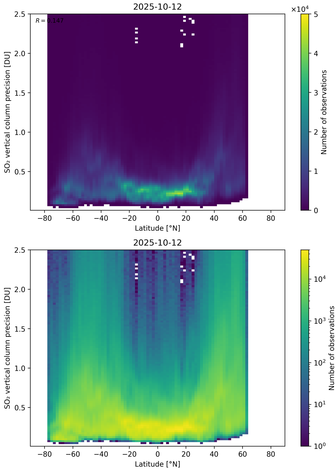
Figure 170: Scatter density plot of “Latitude” against “SO 2 vertical column precision” for 2025-10-11 to 2025-10-13.
