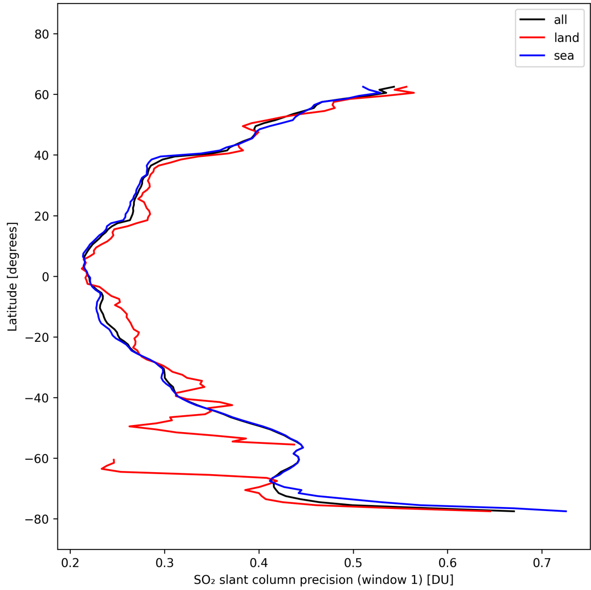
Figure 38: Zonal average of “SO 2 slant column precision (window 1)” for 2025-10-11 to 2025-10-13.
