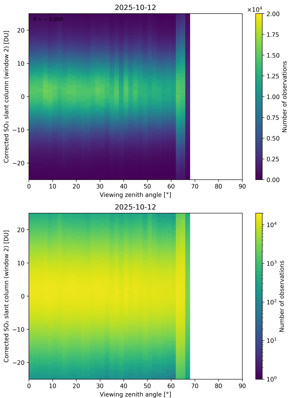
Figure 374: Scatter density plot of “Viewing zenith angle” against “Corrected SO 2 slant column (window 2)” for 2025-10-11 to 2025-10-13.
