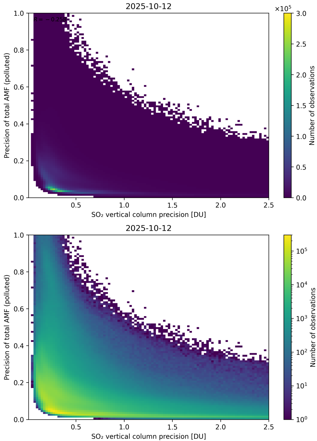
Figure 347: Scatter density plot of “SO 2 vertical column precision” against “Precision of total AMF (polluted)” for 2025-10-11 to 2025-10-13.
