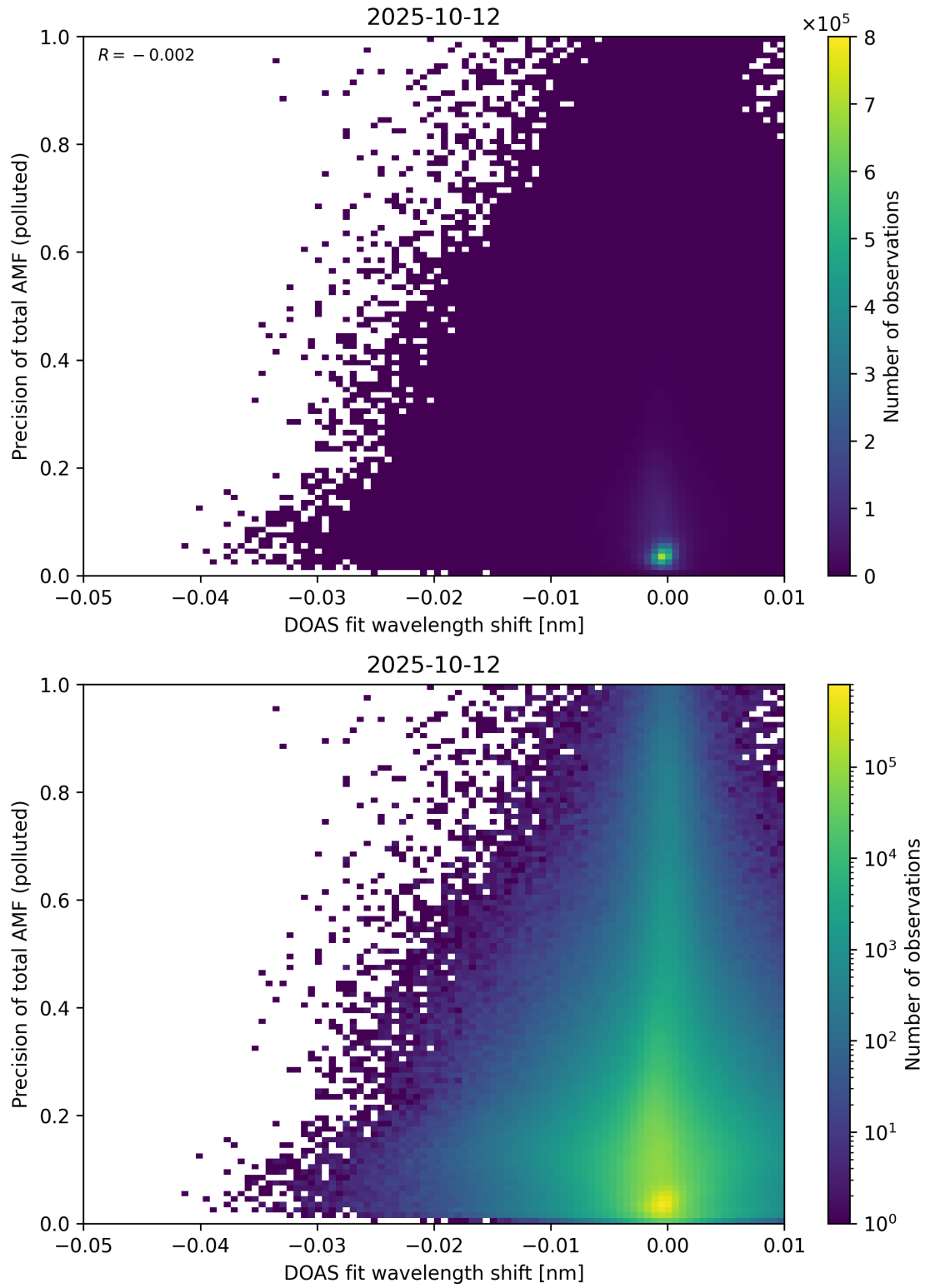
Figure 142: Scatter density plot of “DOAS fit wavelength shift” against “Precision of total AMF (polluted)” for 2025-10-11 to 2025-10-13.
