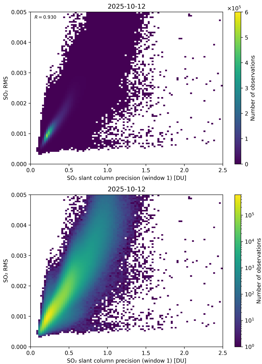
Figure 273: Scatter density plot of “SO 2 slant column precision (window 1)” against “SO 2 RMS” for 2025-10-11 to 2025-10-13.
