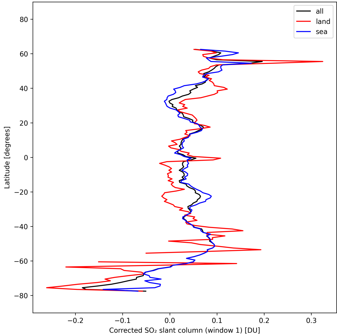
Figure 39: Zonal average of “Corrected SO 2 slant column (window 1)” for 2025-10-11 to 2025-10-13.
