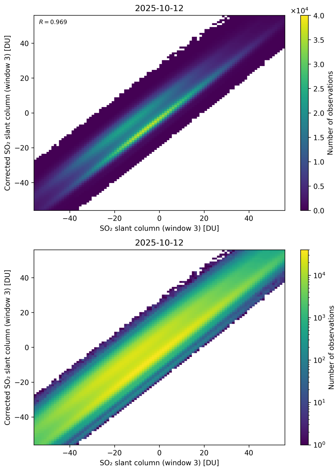
Figure 316: Scatter density plot of “SO 2 slant column (window 3)” against “Corrected SO 2 slant column (window 3)” for 2025-10-11 to 2025-10-13.
