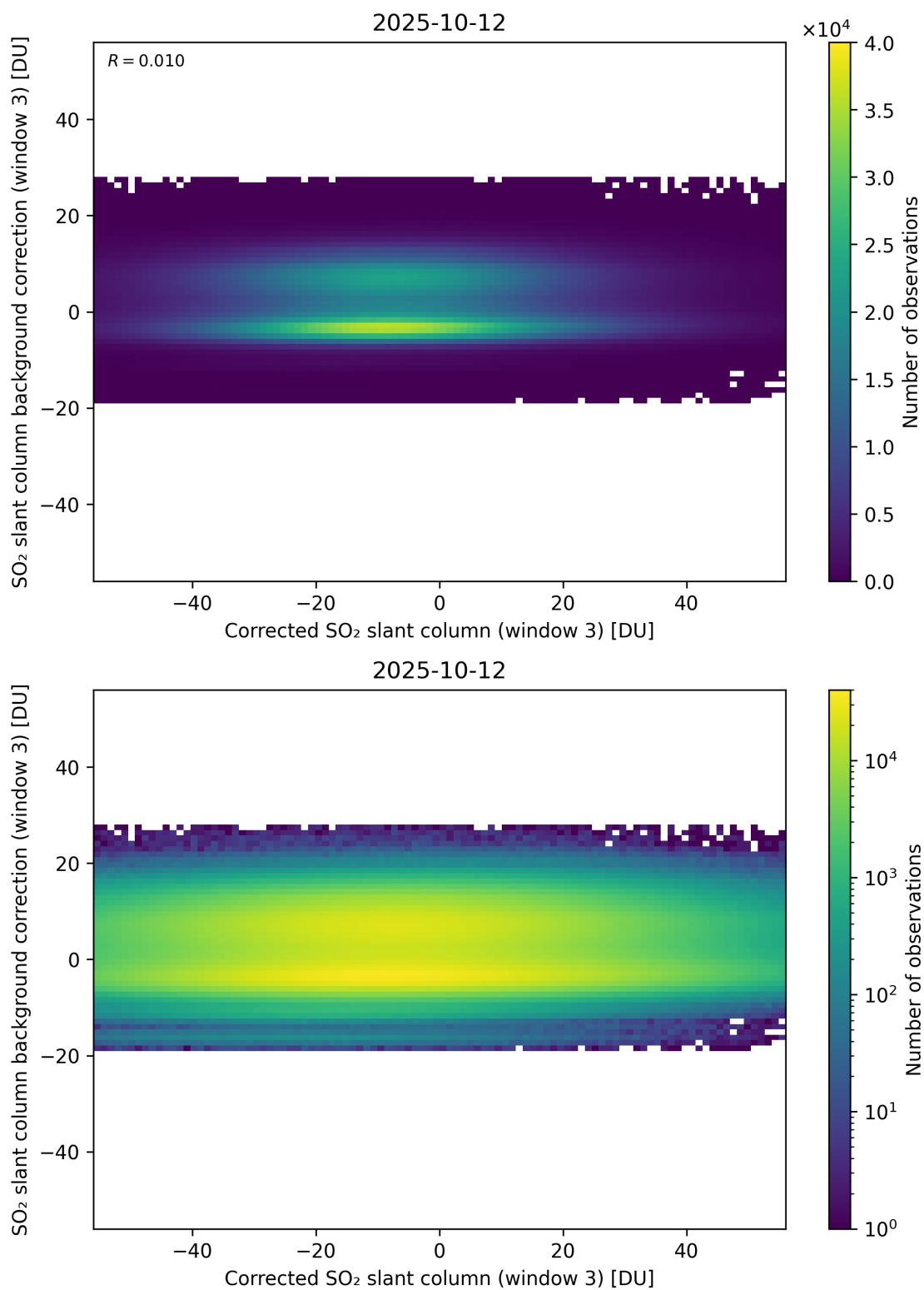
Figure 255: Scatter density plot of “Corrected SO 2 slant column (window 3)” against “SO 2 slant column background correction (window 3)” for 2025-10-11 to 2025-10-13.
