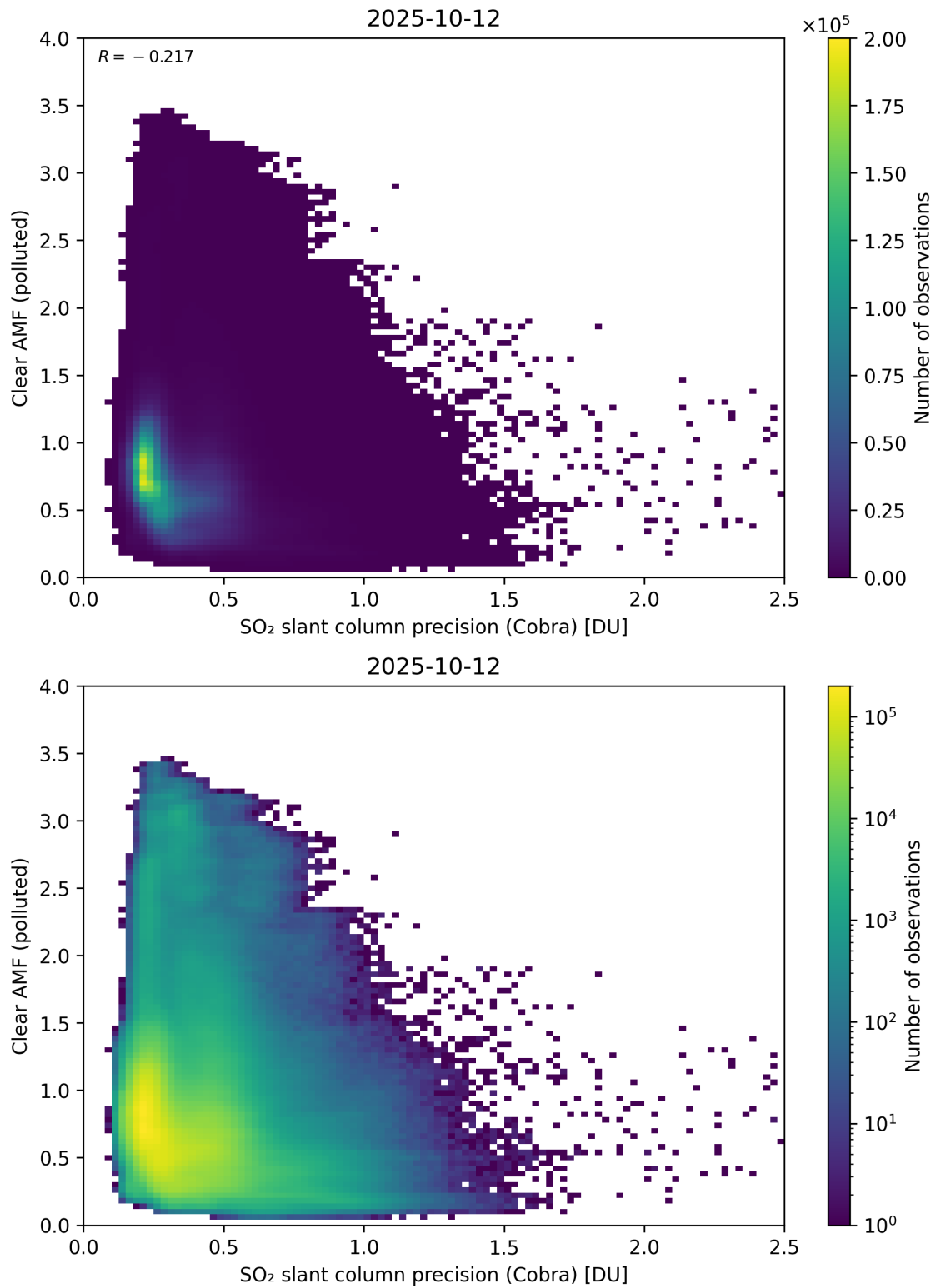
Figure 205: Scatter density plot of “SO 2 slant column precision (Cobra)” against “Clear AMF (polluted)” for 2025-10-11 to 2025-10-13.
