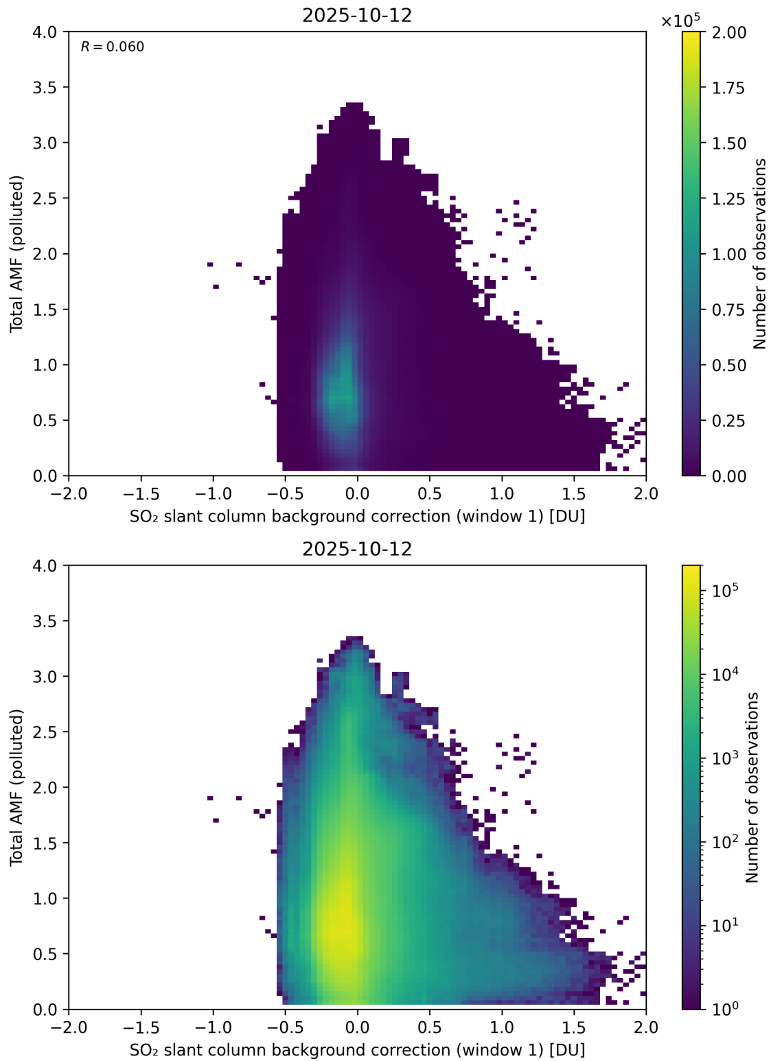
Figure 120: Scatter density plot of “SO 2 slant column background correction (window 1)” against “Total AMF (polluted)” for 2025-10-11 to 2025-10-13.
