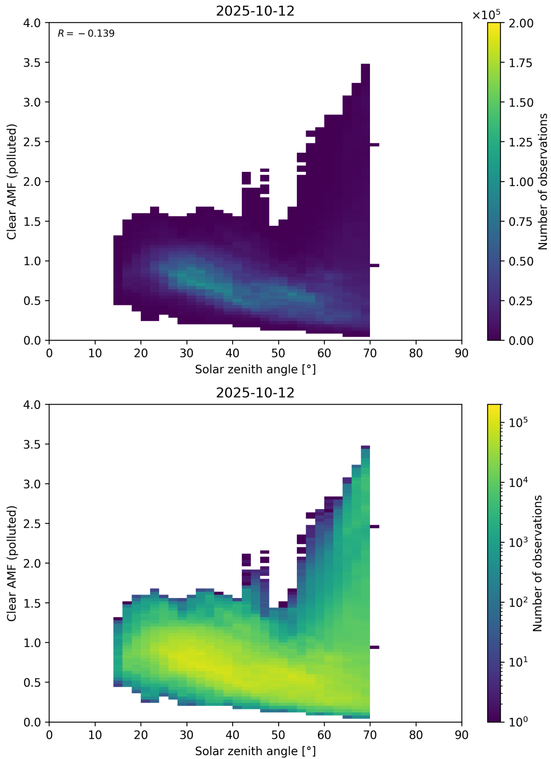
Figure 178: Scatter density plot of “Solar zenith angle” against “Clear AMF (polluted)” for 2025-10-11 to 2025-10-13.
