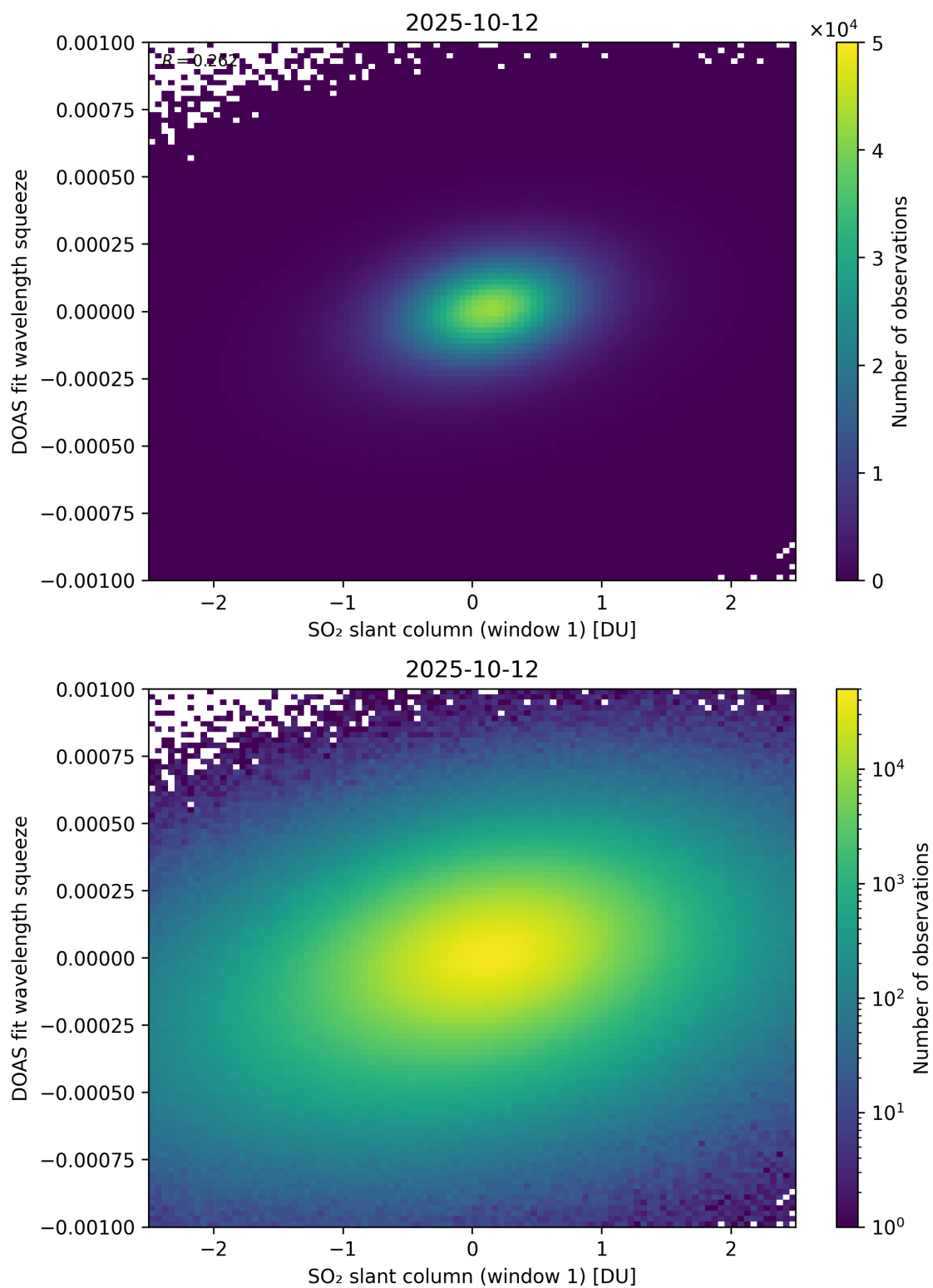
Figure 266: Scatter density plot of “SO 2 slant column (window 1)” against “DOAS fit wavelength squeeze” for 2025-10-11 to 2025-10-13.
