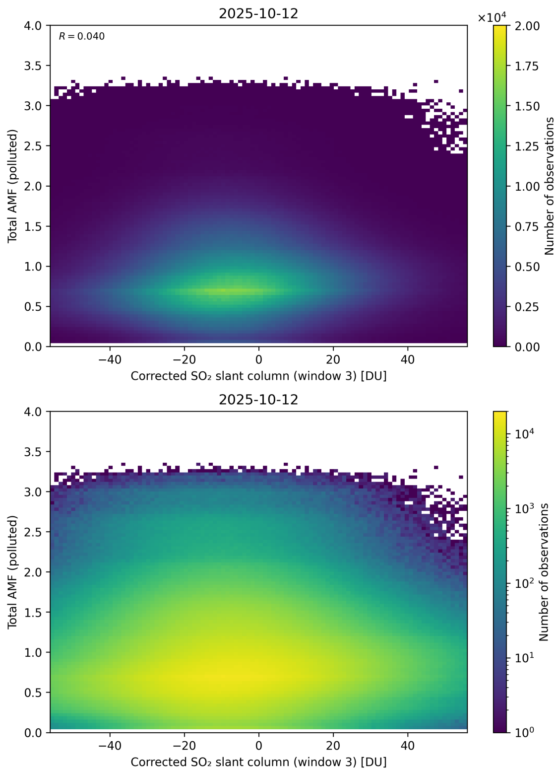
Figure 260: Scatter density plot of “Corrected SO 2 slant column (window 3)” against “Total AMF (polluted)” for 2025-10-11 to 2025-10-13.
