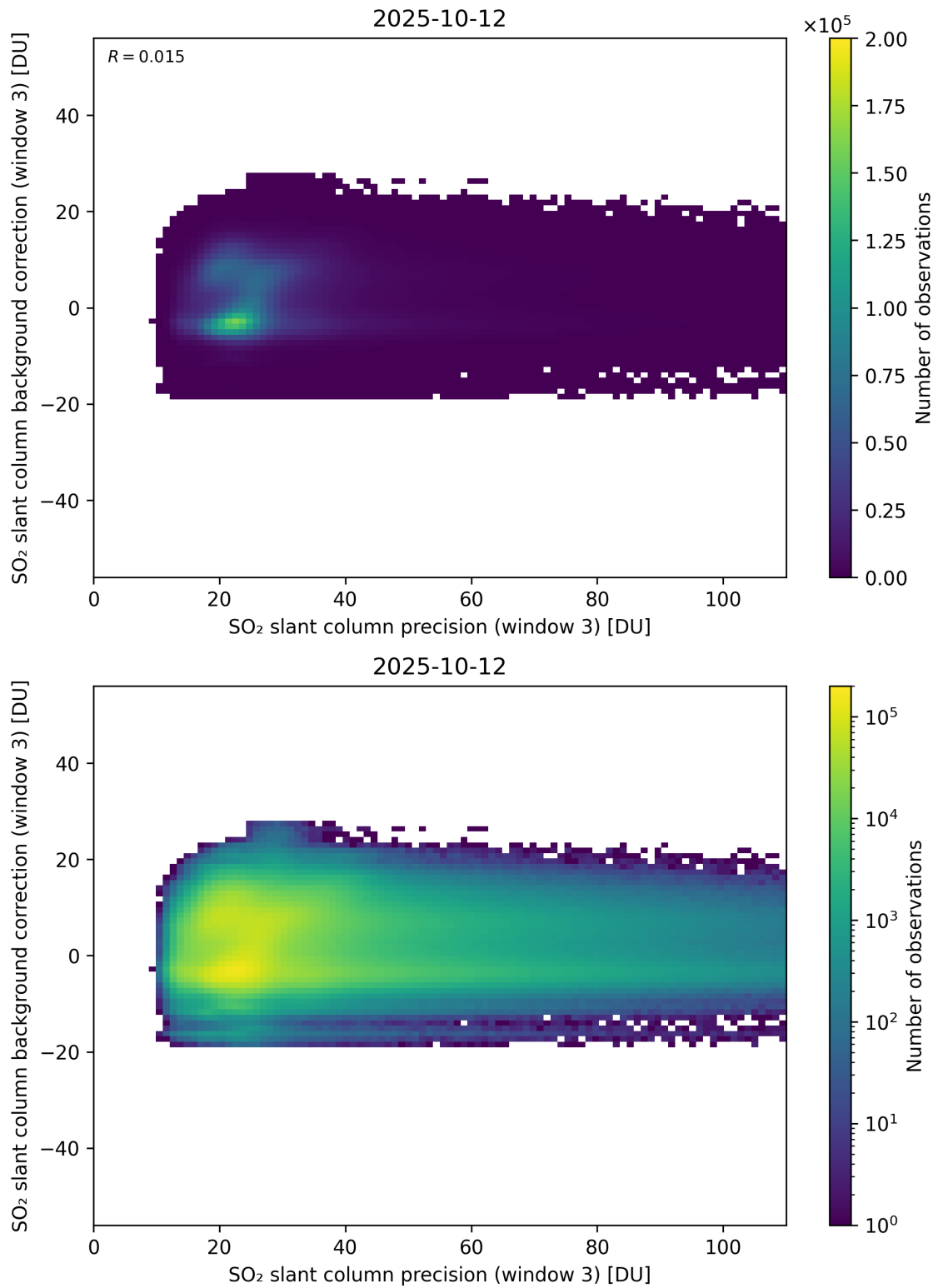
Figure 307: Scatter density plot of “SO 2 slant column precision (window 3)” against “SO 2 slant column background correction (window 3)” for 2025-10-11 to 2025-10-13.
