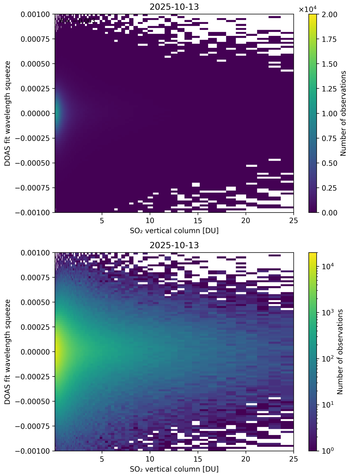
Figure 327: Scatter density plot of “SO 2 vertical column” against “DOAS fit wavelength squeeze” for 2025-10-12 to 2025-10-14.
