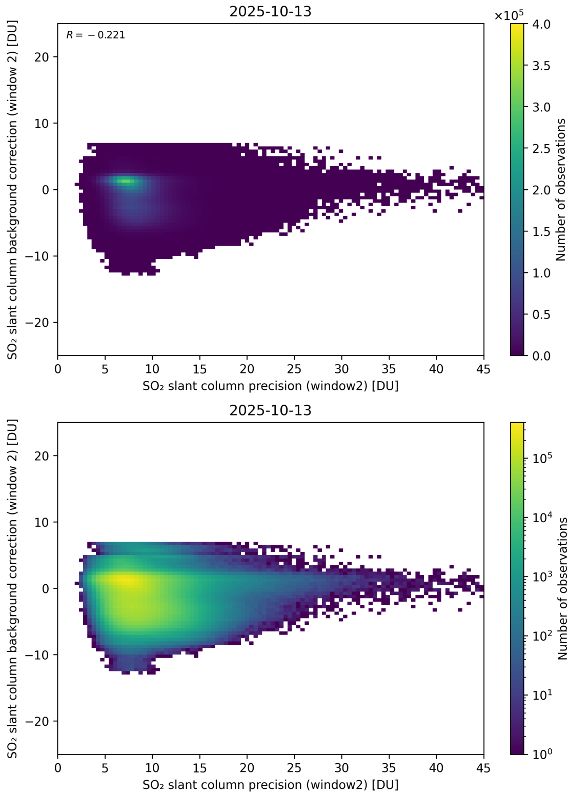
Figure 291: Scatter density plot of “SO 2 slant column precision (window2)” against “SO 2 slant column background correction (window 2)” for 2025-10-12 to 2025-10-14.
