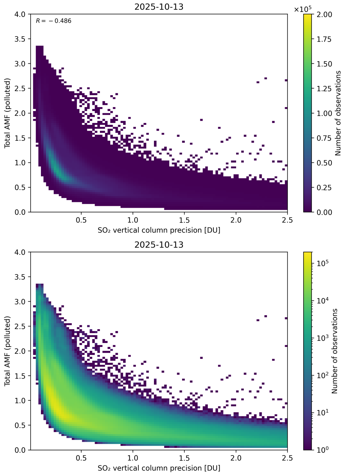
Figure 346: Scatter density plot of “SO 2 vertical column precision” against “Total AMF (polluted)” for 2025-10-12 to 2025-10-14.
