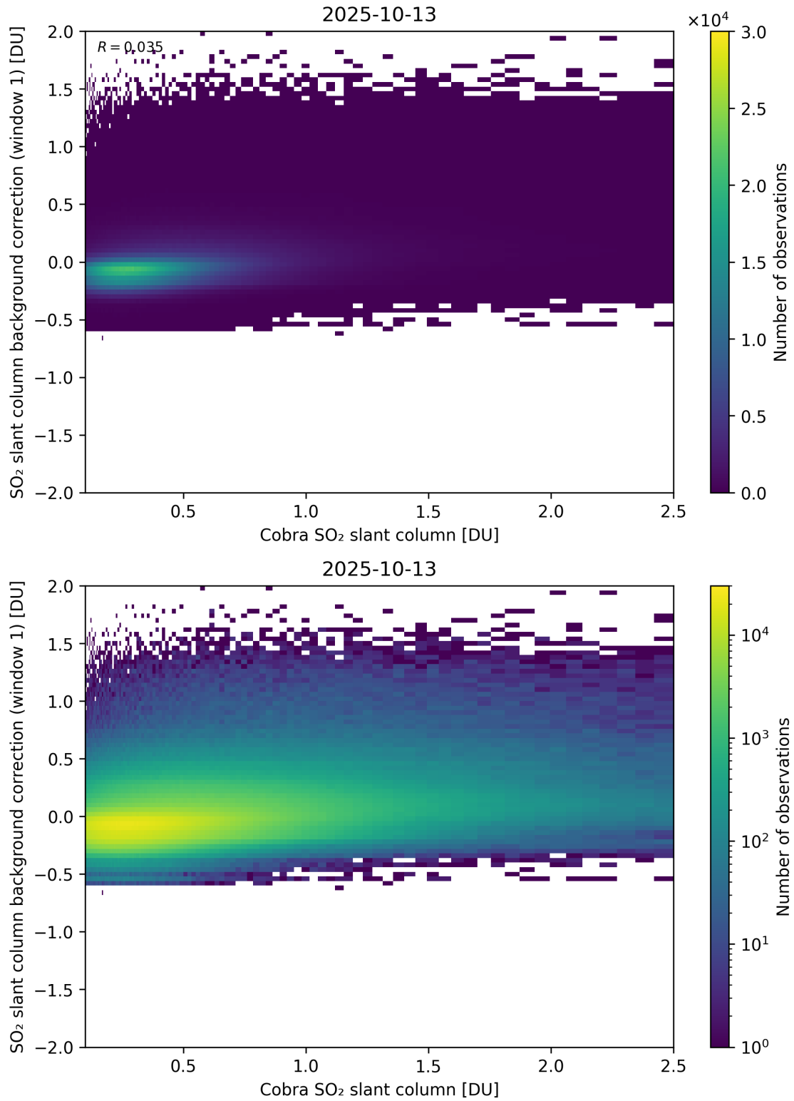
Figure 193: Scatter density plot of “Cobra SO 2 slant column” against “SO 2 slant column background correction (window 1)” for 2025-10-12 to 2025-10-14.
