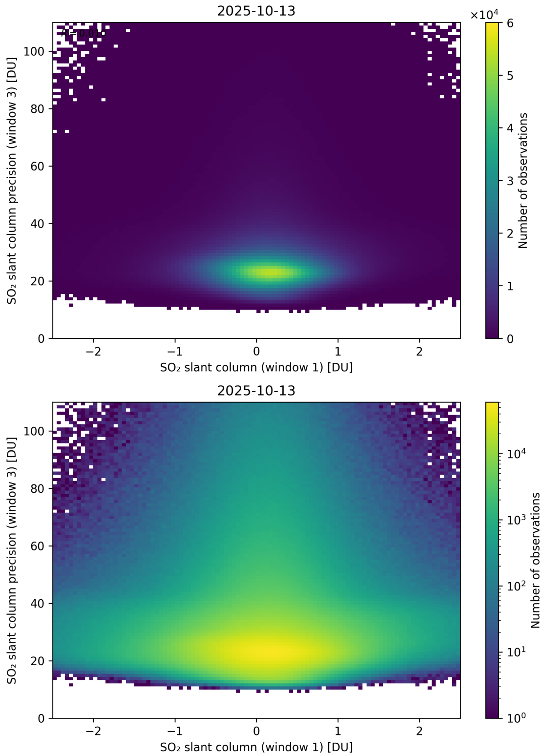
Figure 288: Scatter density plot of “SO 2 slant column (window 1)” against “SO 2 slant column precision (window 3)” for 2025-10-12 to 2025-10-14.
