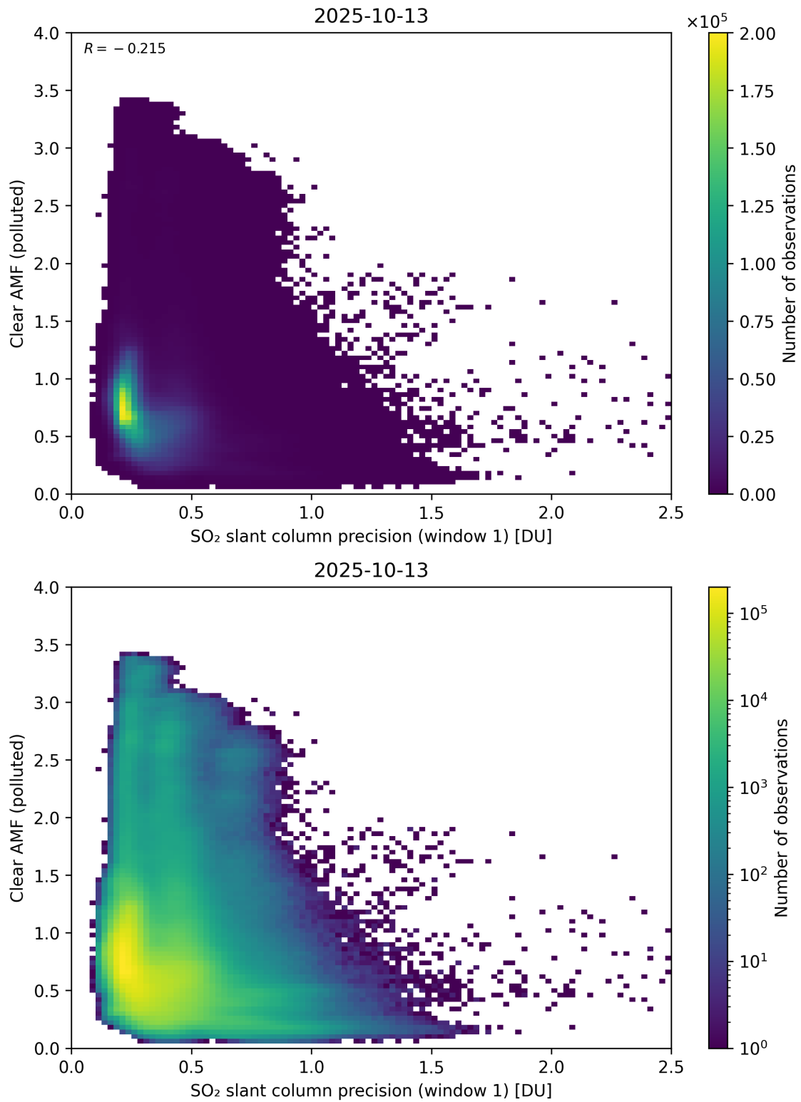
Figure 274: Scatter density plot of “SO 2 slant column precision (window 1)” against “Clear AMF (polluted)” for 2025-10-12 to 2025-10-14.
