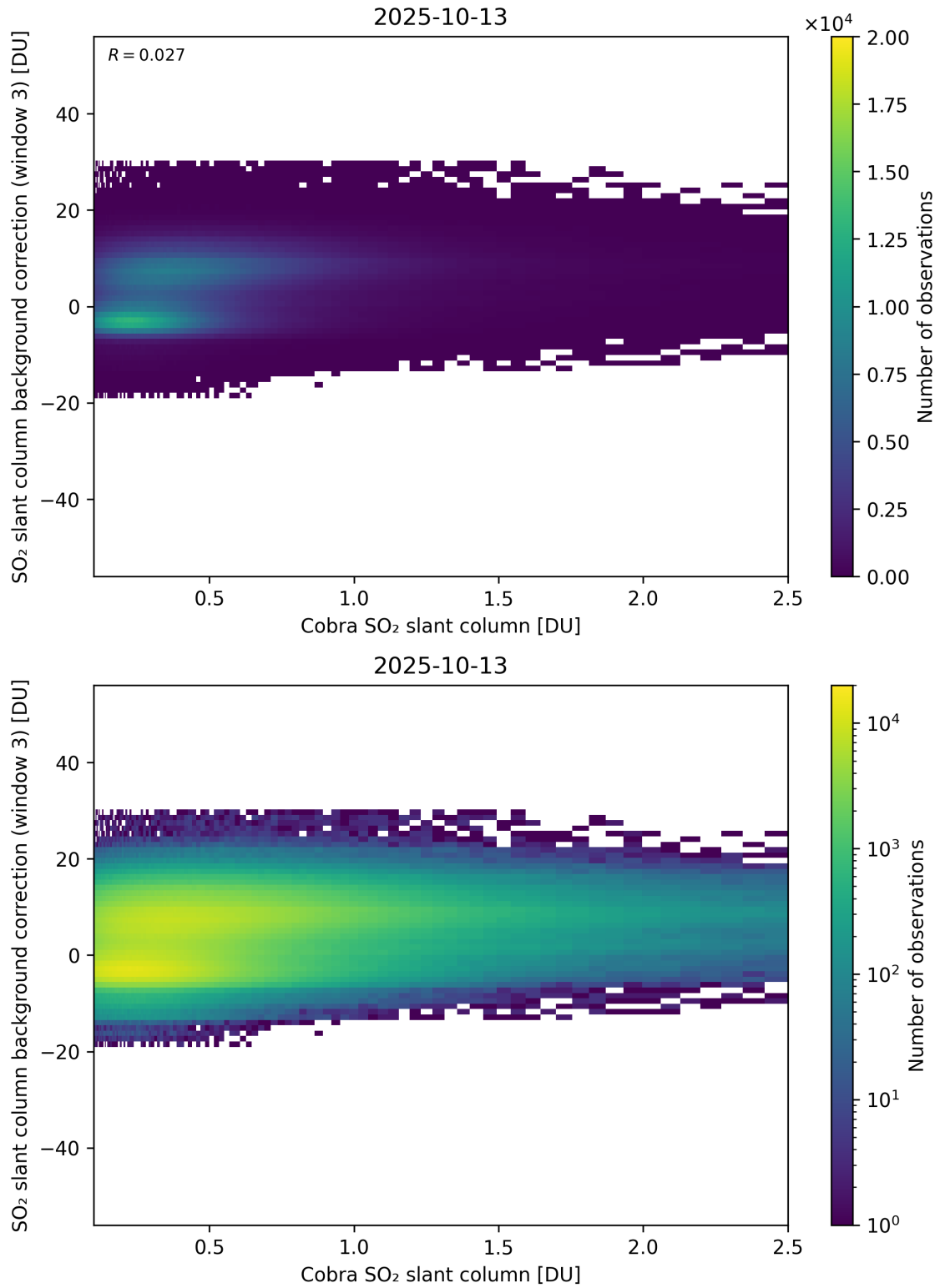
Figure 195: Scatter density plot of “Cobra SO 2 slant column” against “SO 2 slant column background correction (window 3)” for 2025-10-12 to 2025-10-14.
