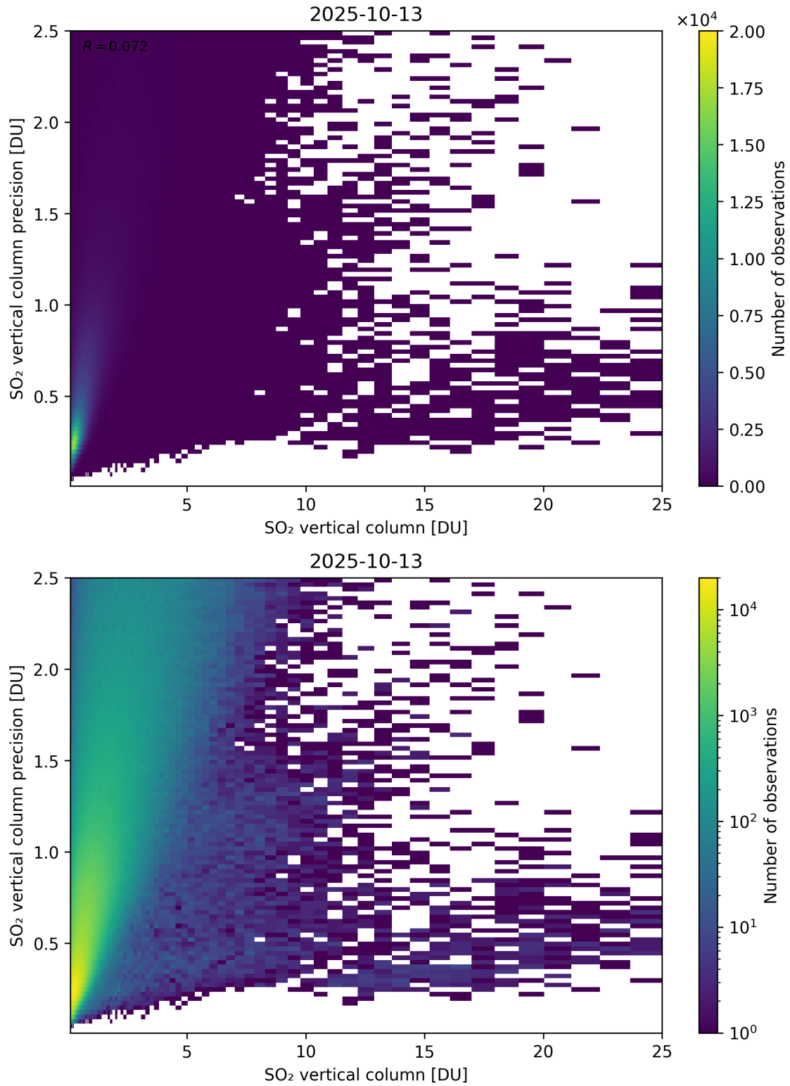
Figure 361: Scatter density plot of “SO 2 vertical column” against “SO 2 vertical column precision” for 2025-10-12 to 2025-10-14.
