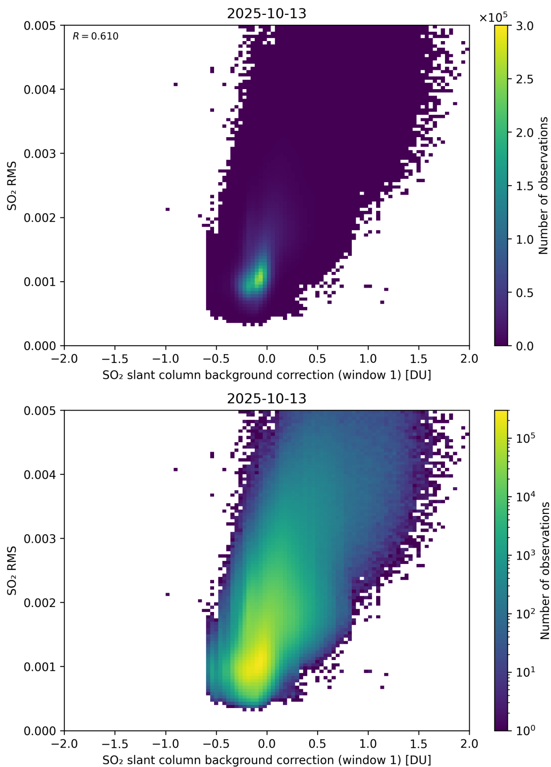
Figure 113: Scatter density plot of “SO 2 slant column background correction (window 1)” against “SO 2 RMS” for 2025-10-12 to 2025-10-14.
