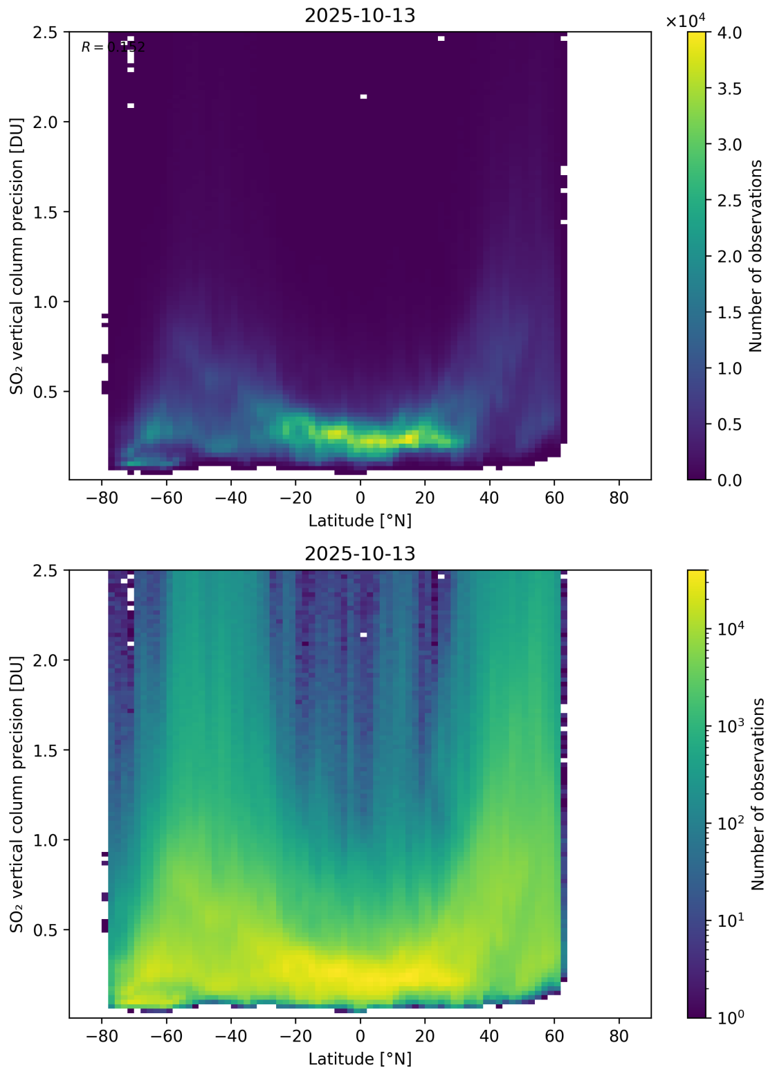
Figure 170: Scatter density plot of “Latitude” against “SO 2 vertical column precision” for 2025-10-12 to 2025-10-14.
