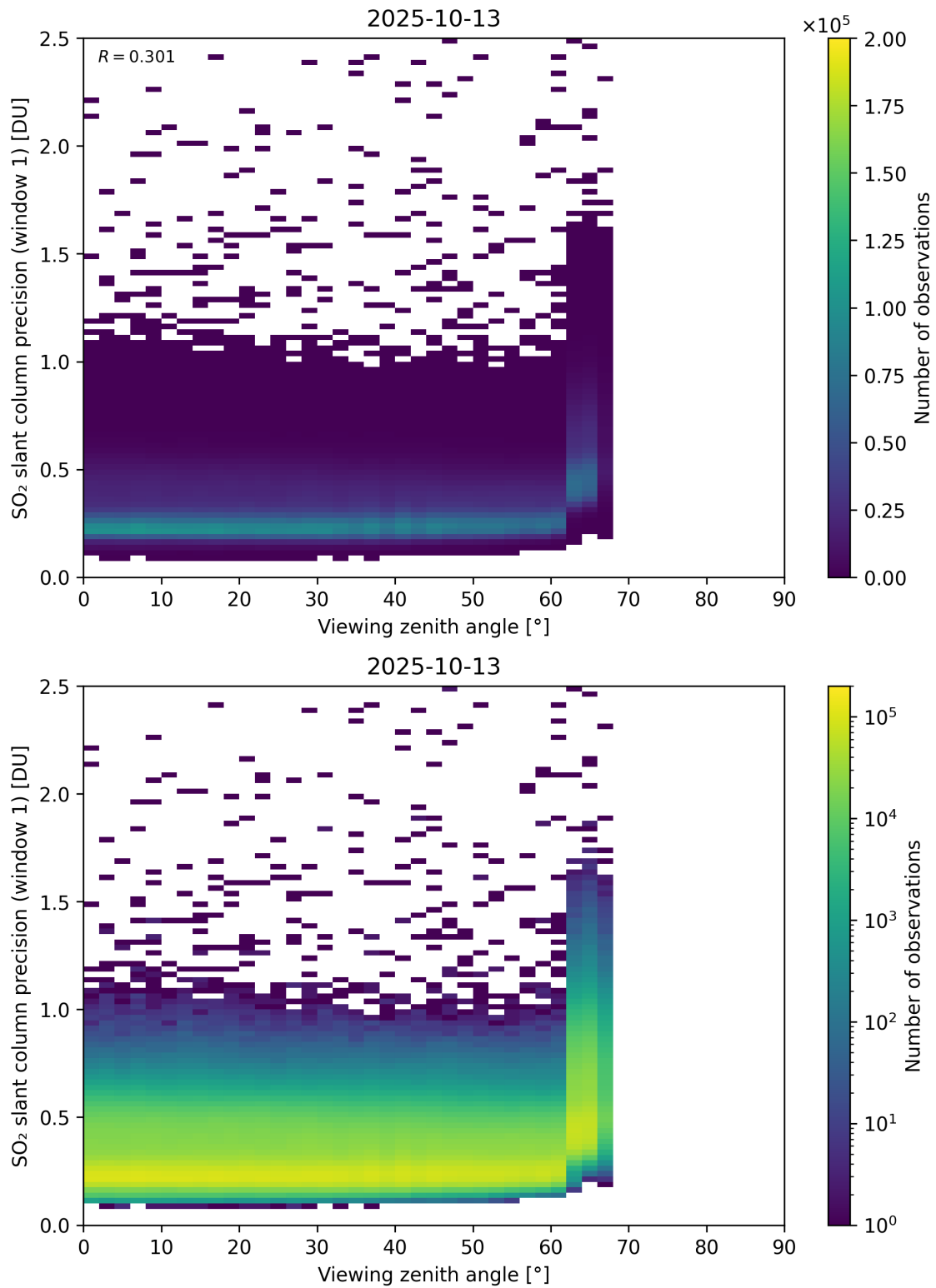
Figure 377: Scatter density plot of “Viewing zenith angle” against “SO 2 slant column precision (window 1)” for 2025-10-12 to 2025-10-14.
