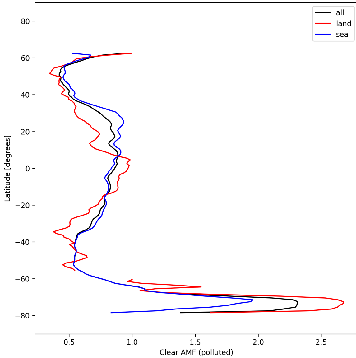
Figure 55: Zonal average of “Clear AMF (polluted)” for 2025-10-12 to 2025-10-14.
