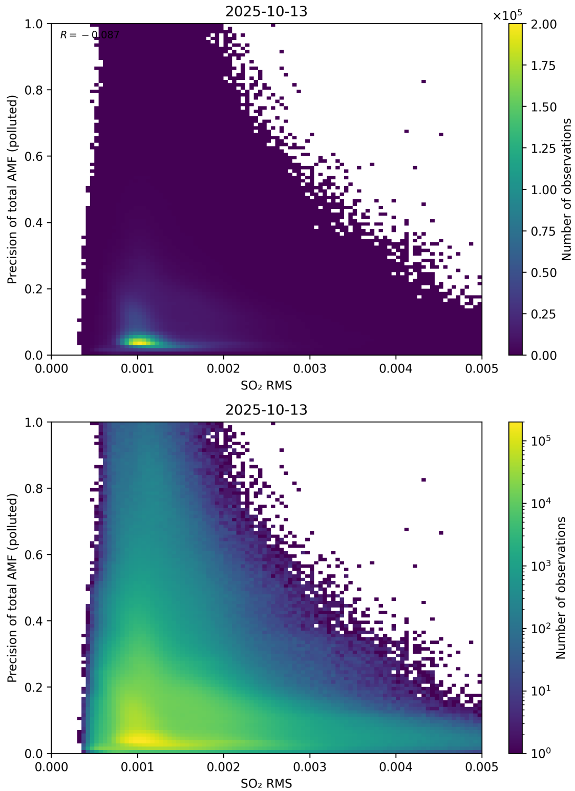
Figure 149: Scatter density plot of “SO 2 RMS” against “Precision of total AMF (polluted)” for 2025-10-12 to 2025-10-14.
