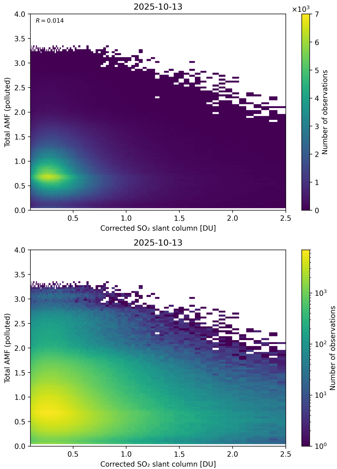
Figure 242: Scatter density plot of “Corrected SO 2 slant column” against “Total AMF (polluted)” for 2025-10-12 to 2025-10-14.
