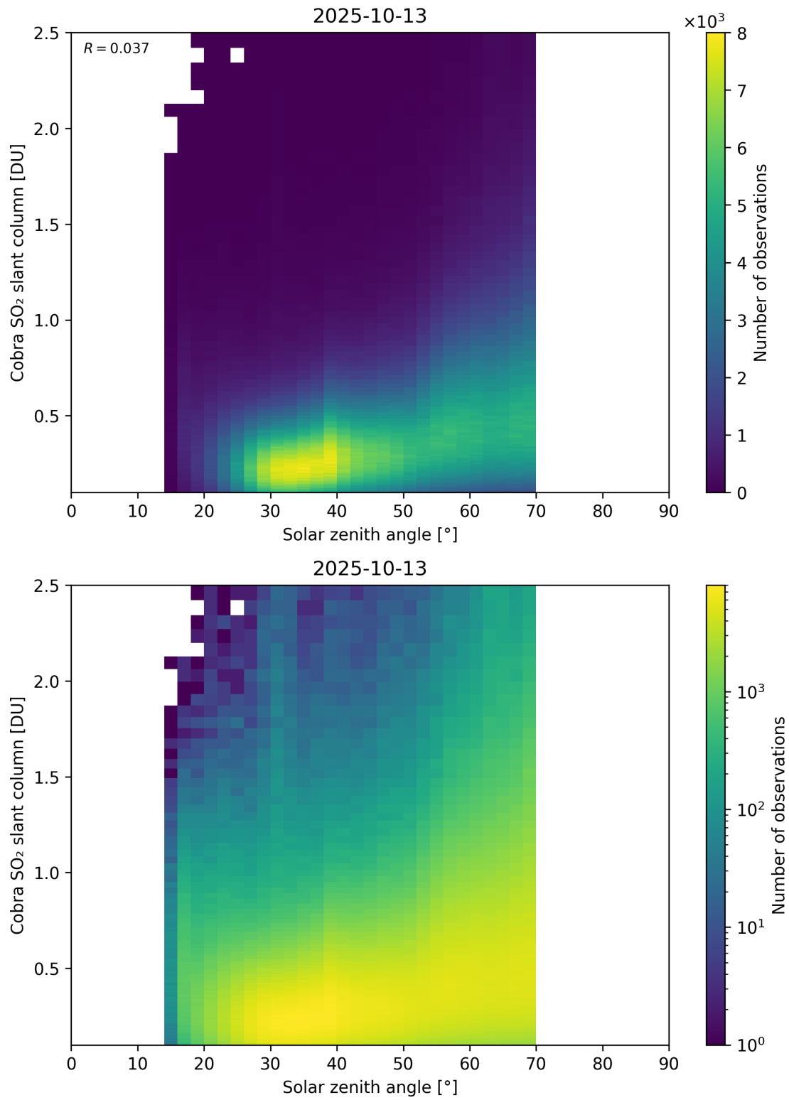
Figure 179: Scatter density plot of “Solar zenith angle” against “Cobra SO 2 slant column” for 2025-10-12 to 2025-10-14.
