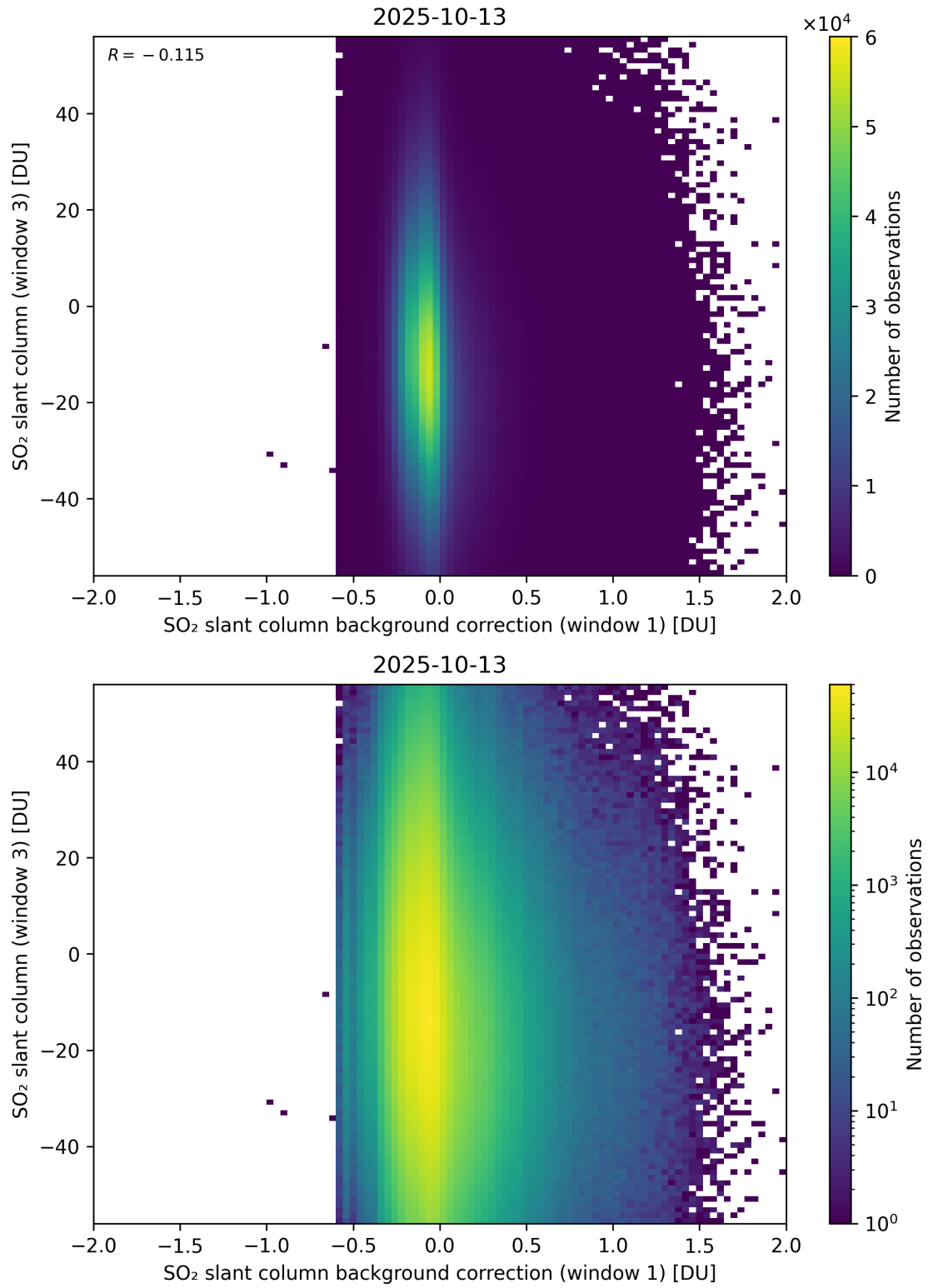
Figure 118: Scatter density plot of “SO 2 slant column background correction (window 1)” against “SO 2 slant column (window 3)” for 2025-10-12 to 2025-10-14.
