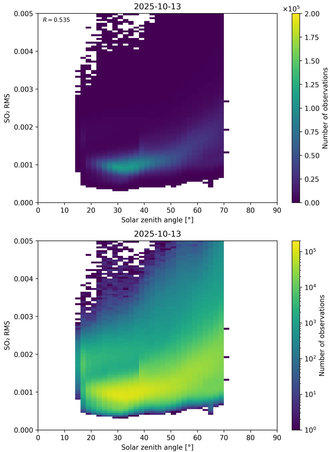
Figure 176: Scatter density plot of “Solar zenith angle” against “SO 2 RMS” for 2025-10-12 to 2025-10-14.
