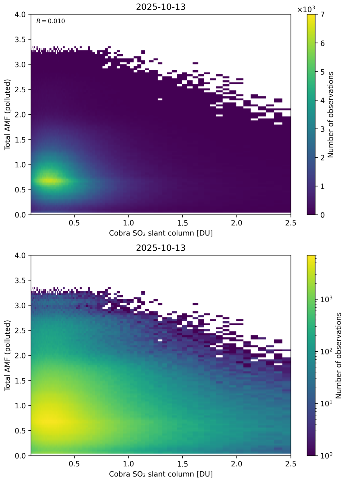
Figure 224: Scatter density plot of “Cobra SO 2 slant column” against “Total AMF (polluted)” for 2025-10-12 to 2025-10-14.
