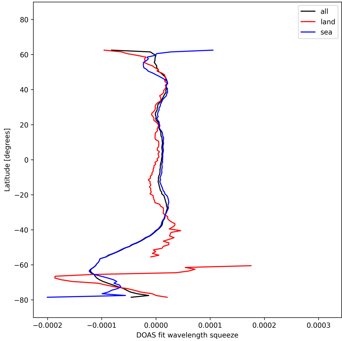
Figure 51: Zonal average of “DOAS fit wavelength squeeze” for 2025-10-12 to 2025-10-14.
