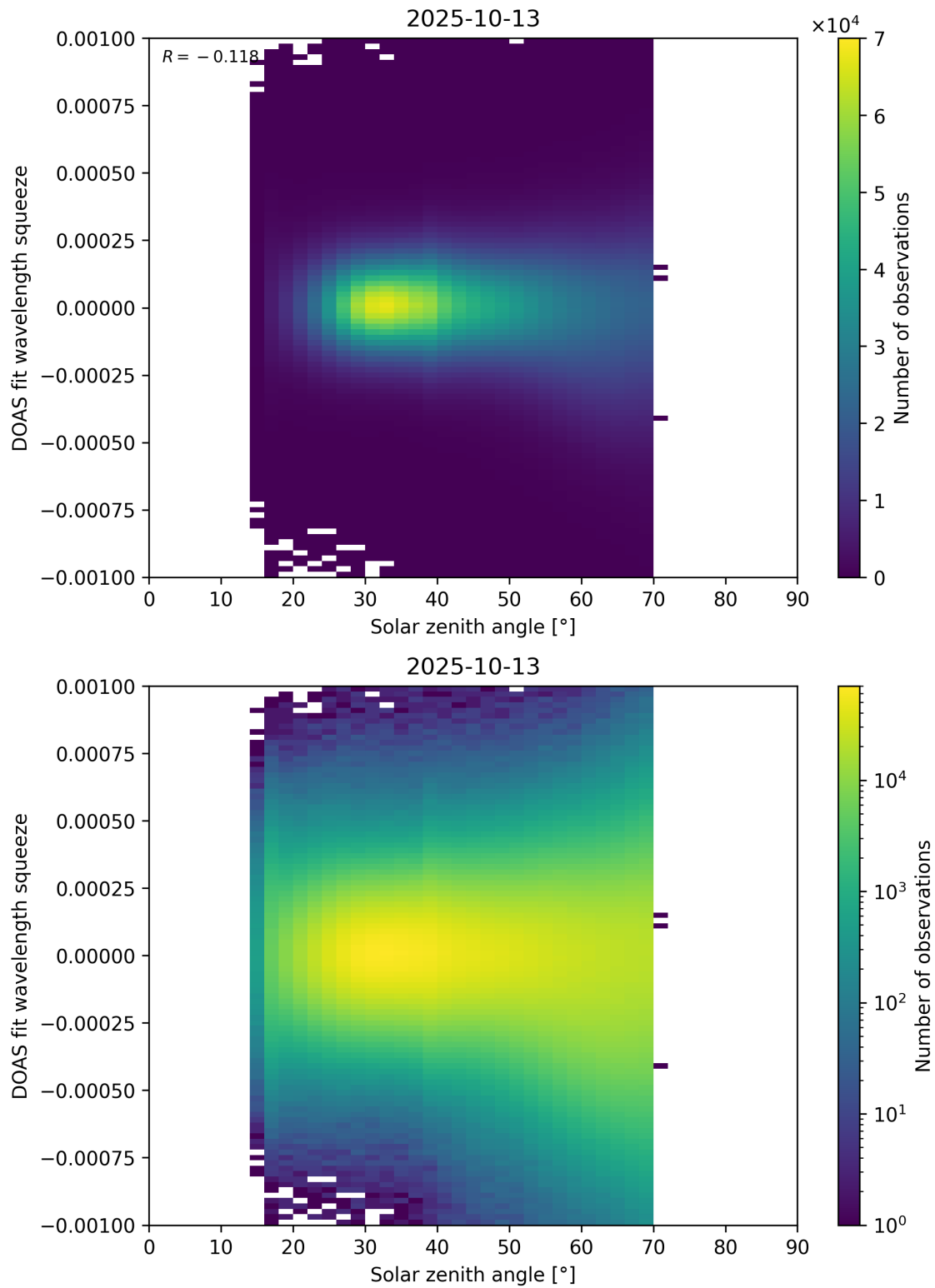
Figure 175: Scatter density plot of “Solar zenith angle” against “DOAS fit wavelength squeeze” for 2025-10-12 to 2025-10-14.
