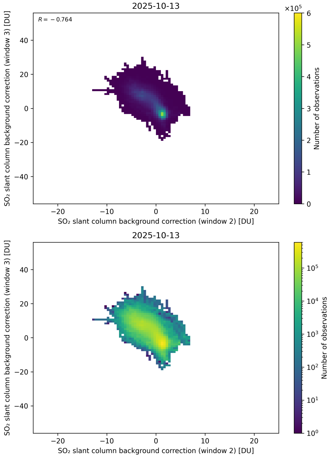
Figure 122: Scatter density plot of “SO 2 slant column background correction (window 2)” against “SO 2 slant column background correction (window 3)” for 2025-10-12 to 2025-10-14.
