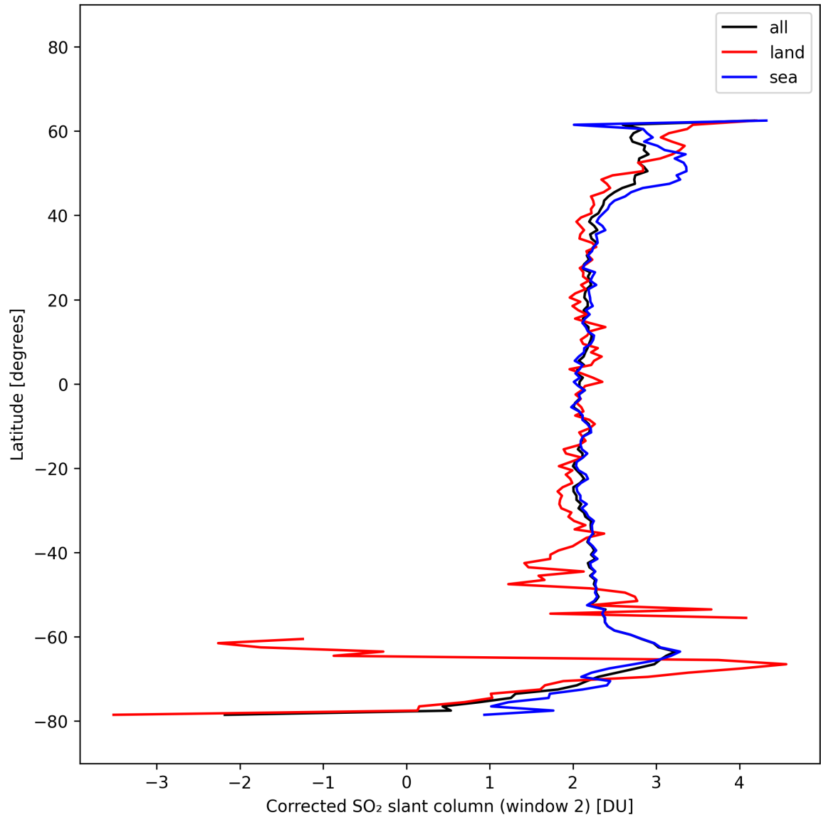
Figure 43: Zonal average of “Corrected SO 2 slant column (window 2)” for 2025-10-12 to 2025-10-14.
