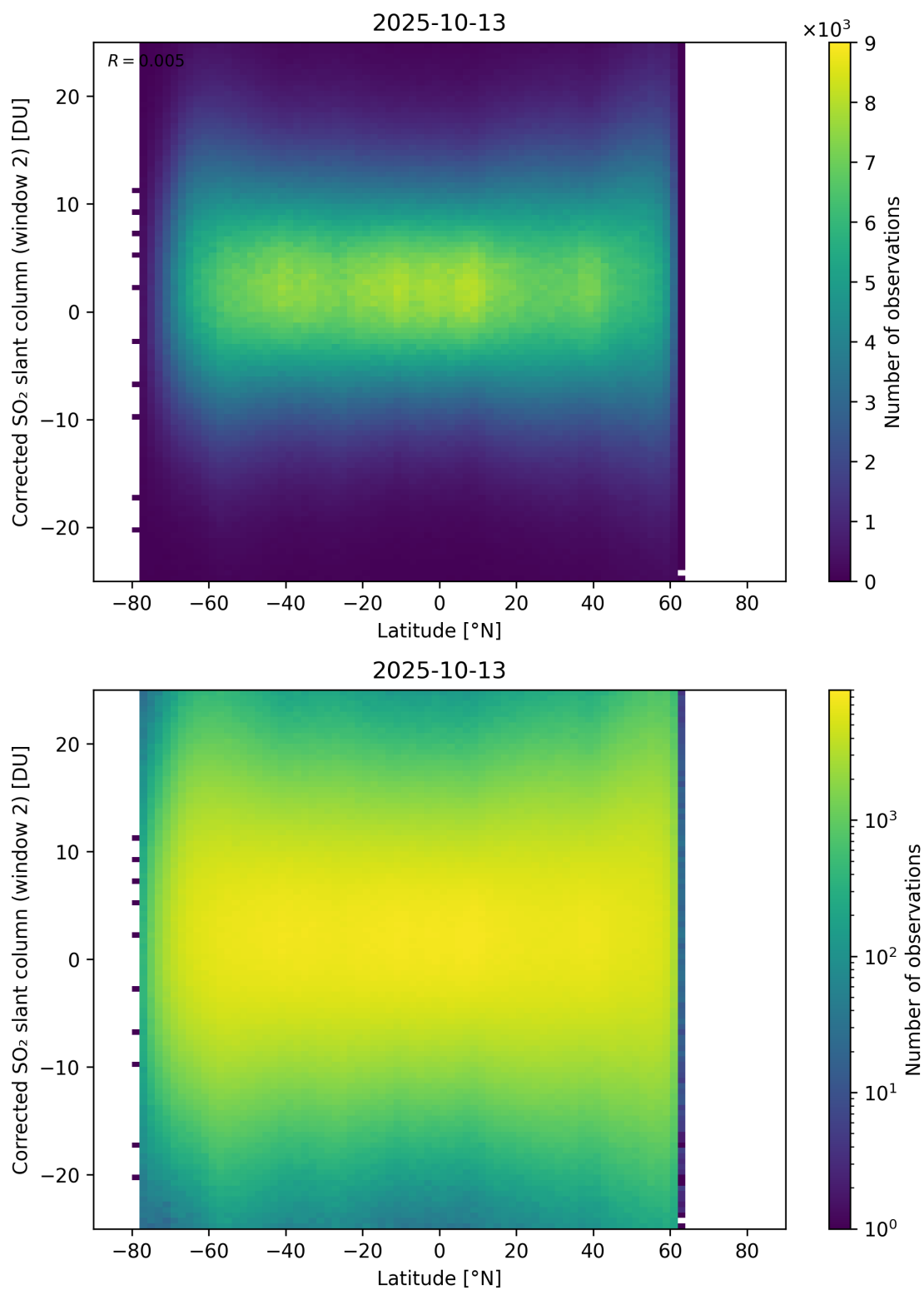
Figure 160: Scatter density plot of “Latitude” against “Corrected SO 2 slant column (window 2)” for 2025-10-12 to 2025-10-14.
