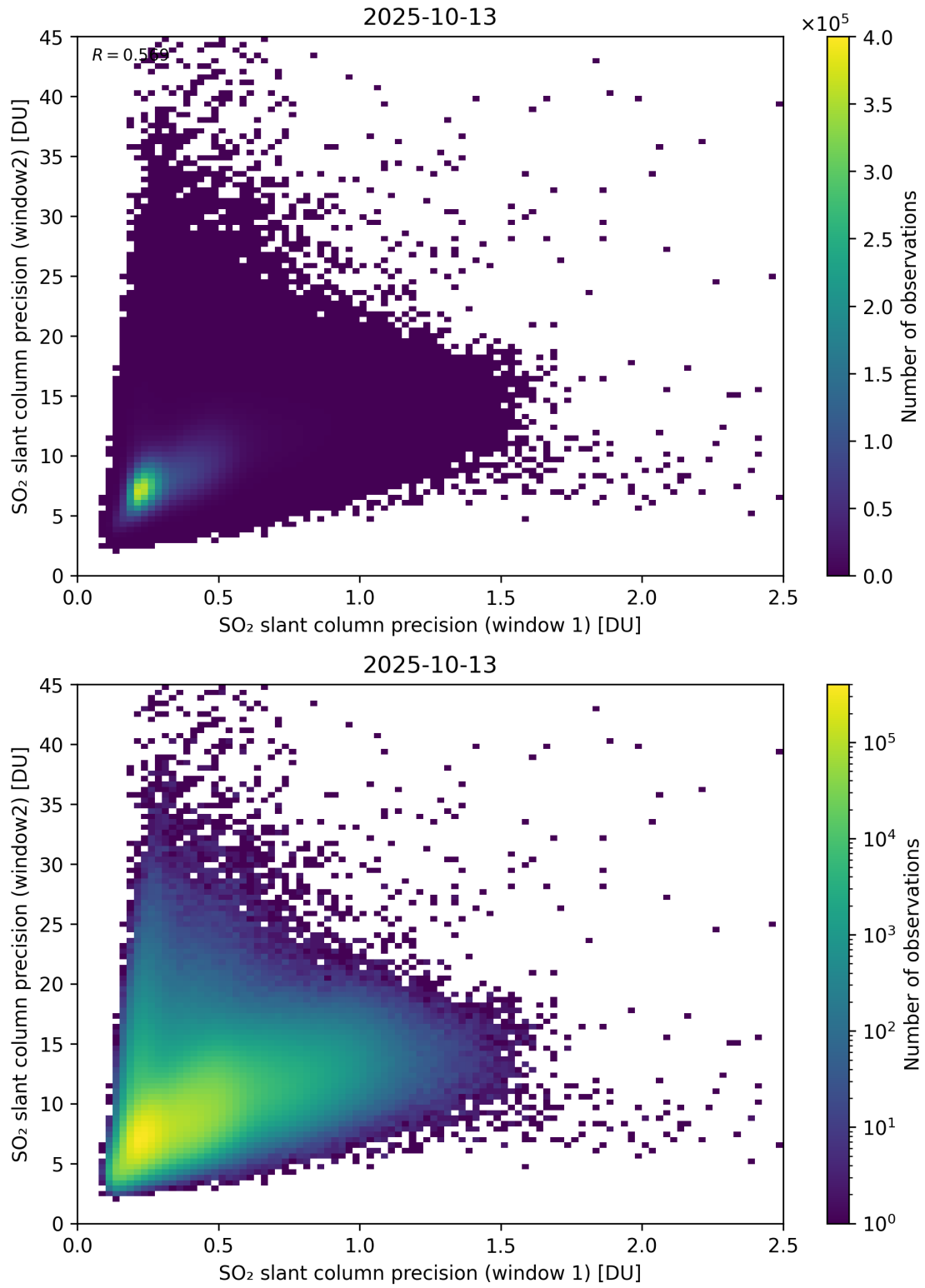
Figure 277: Scatter density plot of “SO 2 slant column precision (window 1)” against “SO 2 slant column precision (window2)” for 2025-10-12 to 2025-10-14.
