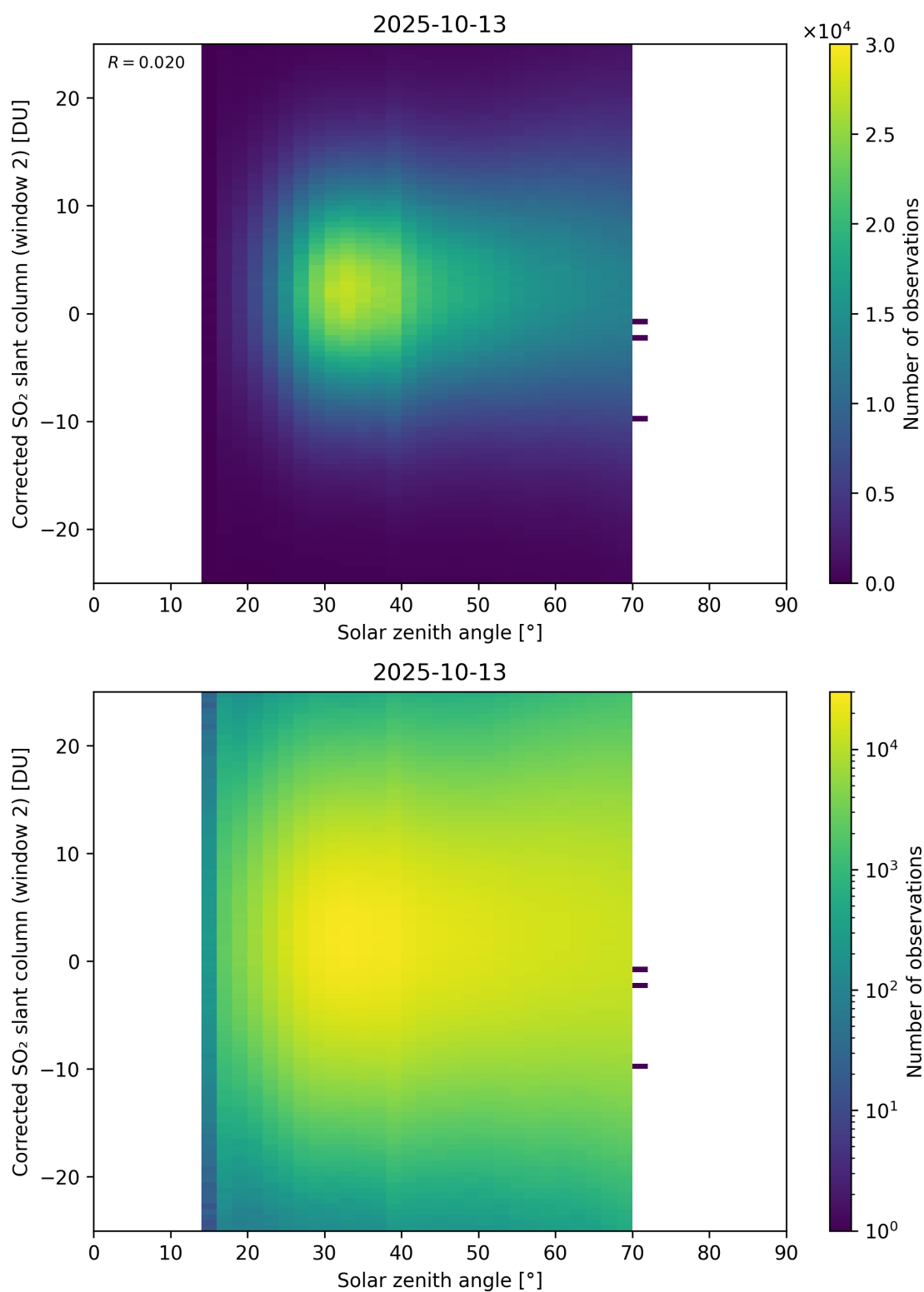
Figure 182: Scatter density plot of “Solar zenith angle” against “Corrected SO 2 slant column (window 2)” for 2025-10-12 to 2025-10-14.
