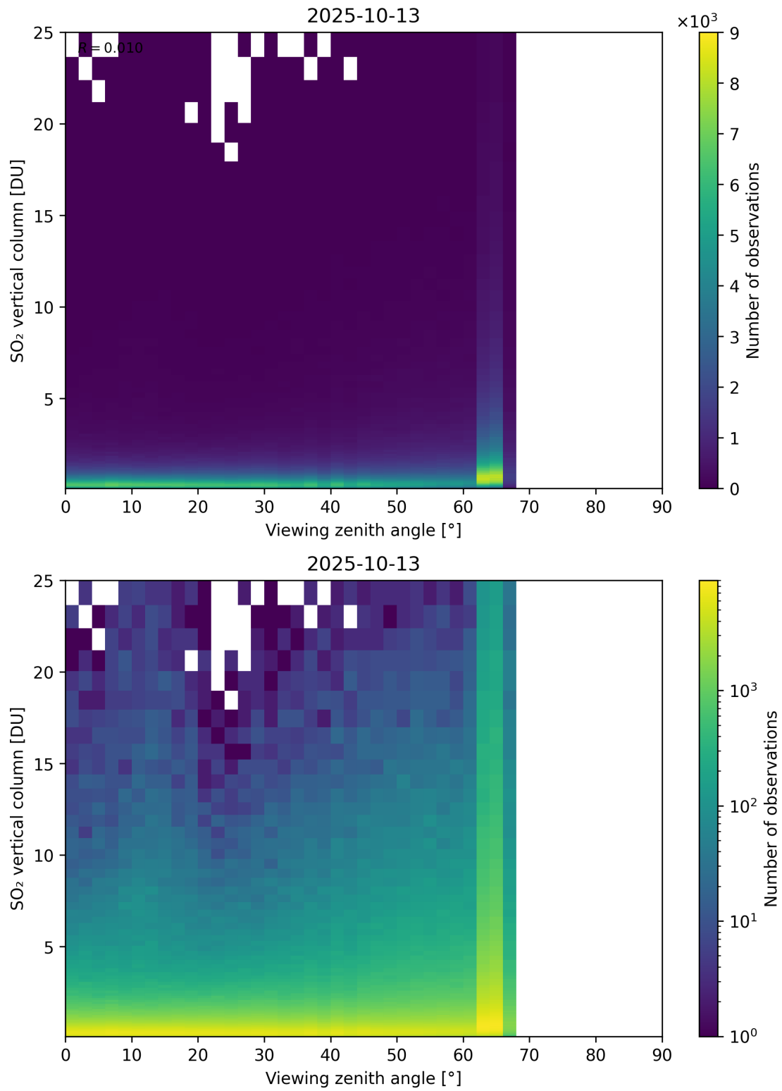
Figure 383: Scatter density plot of “Viewing zenith angle” against “SO 2 vertical column” for 2025-10-12 to 2025-10-14.
