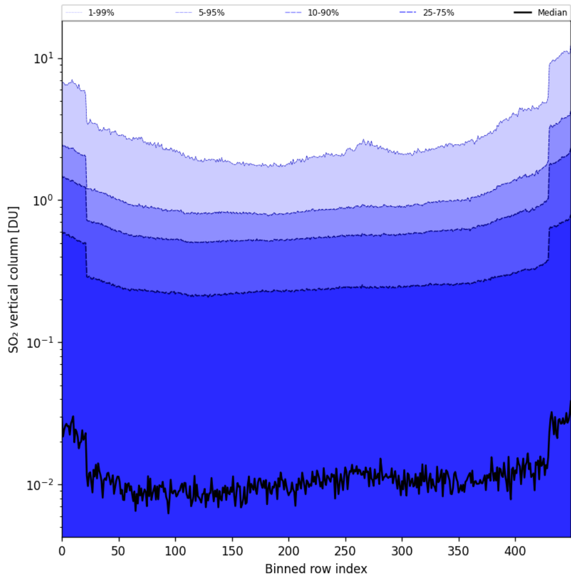
Figure 84: Along track statistics of “SO 2 vertical column” for 2025-10-12 to 2025-10-14
