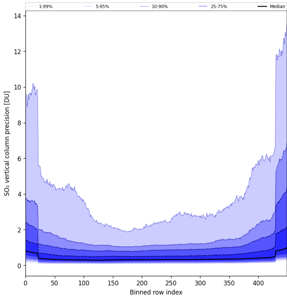
Figure 85: Along track statistics of “SO 2 vertical column precision” for 2025-10-12 to 2025-10-14
