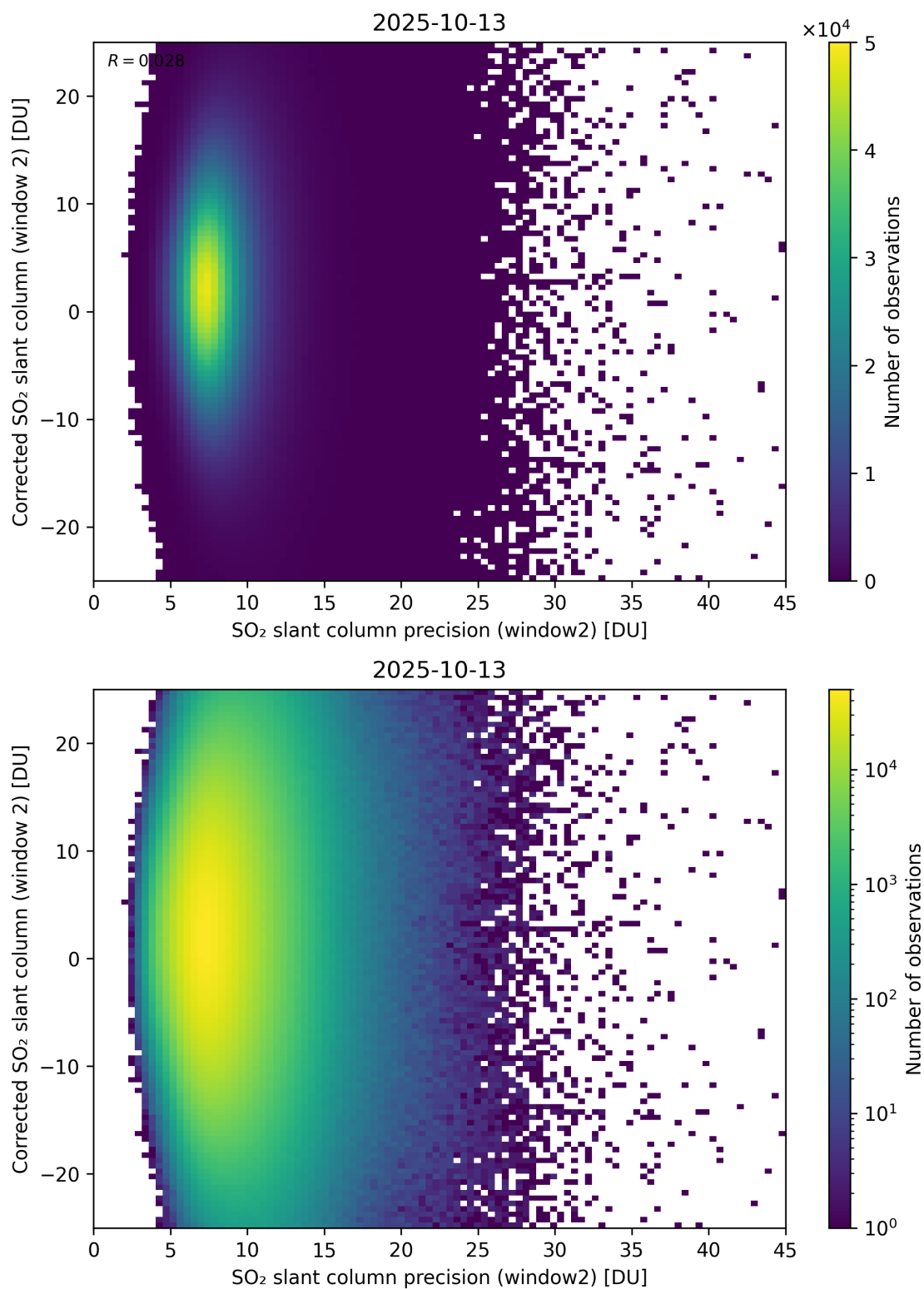
Figure 297: Scatter density plot of “SO 2 slant column precision (window2)” against “Corrected SO 2 slant column (window 2)” for 2025-10-12 to 2025-10-14.
