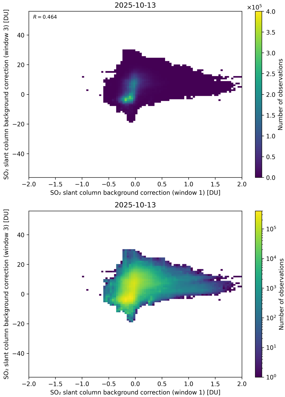
Figure 110: Scatter density plot of “SO 2 slant column background correction (window 1)” against “SO 2 slant column background correction (window 3)” for 2025-10-12 to 2025-10-14.
