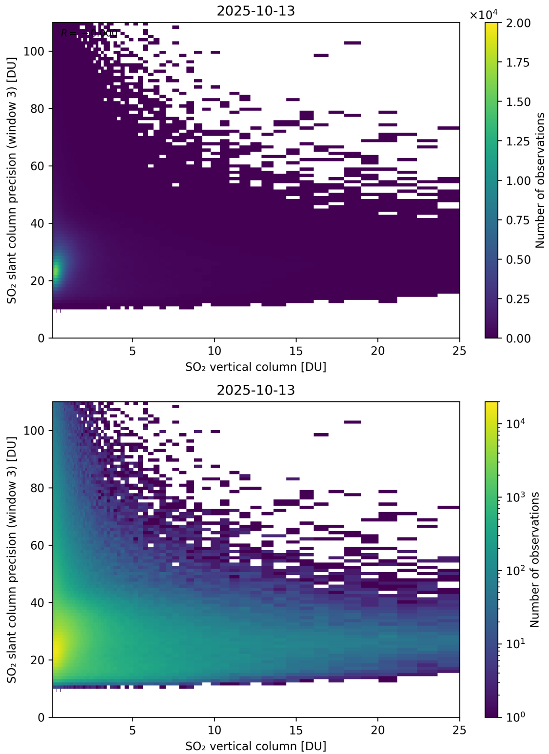
Figure 358: Scatter density plot of “SO 2 vertical column” against “SO 2 slant column precision (window 3)” for 2025-10-12 to 2025-10-14.
