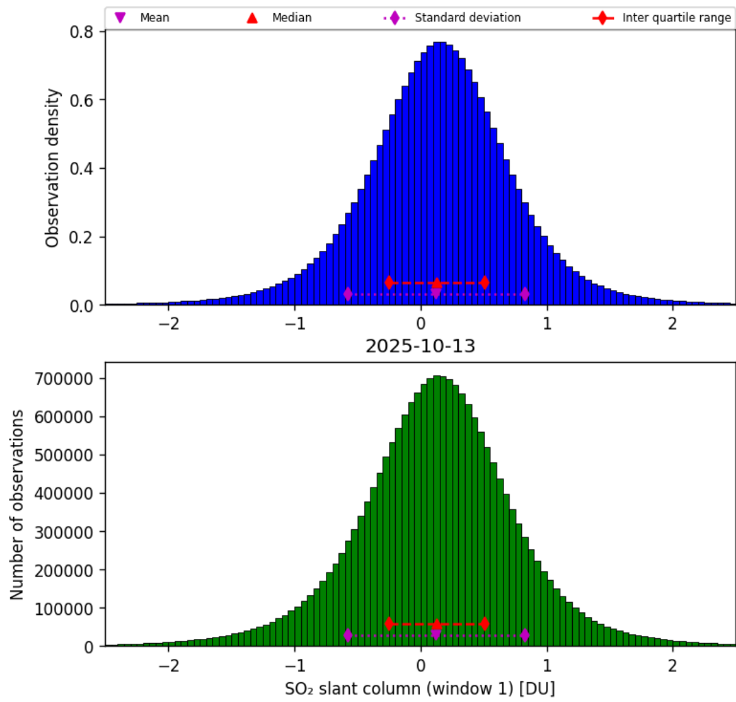
Figure 63: Histogram of “SO 2 slant column (window 1)” for 2025-10-12 to 2025-10-14
