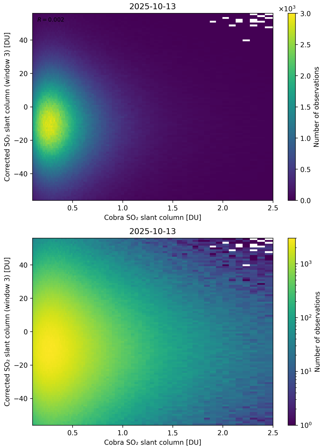
Figure 218: Scatter density plot of “Cobra SO 2 slant column” against “Corrected SO 2 slant column (window 3)” for 2025-10-12 to 2025-10-14.
