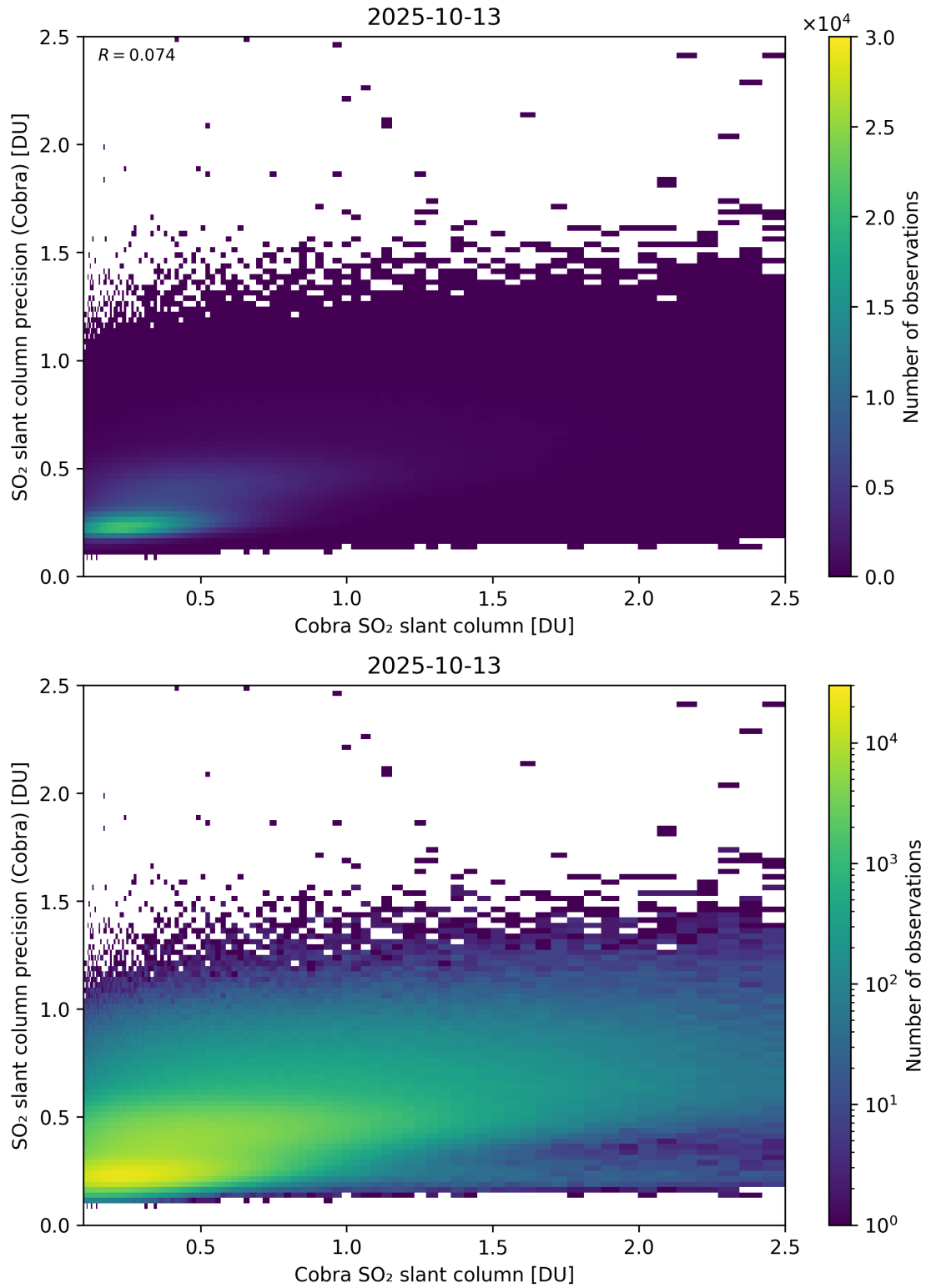
Figure 216: Scatter density plot of “Cobra SO 2 slant column” against “SO 2 slant column precision (Cobra)” for 2025-10-12 to 2025-10-14.
