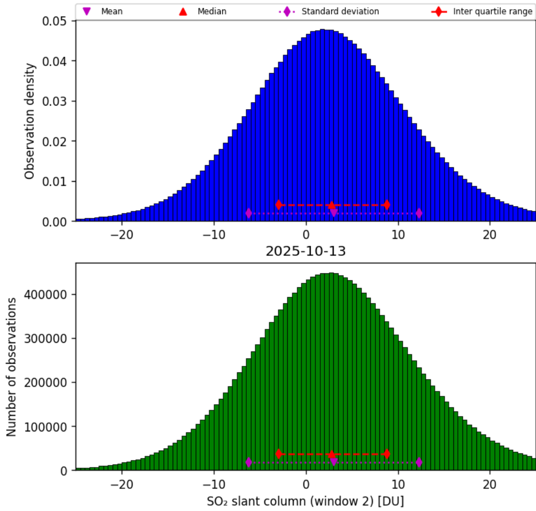
Figure 67: Histogram of “SO 2 slant column (window 2)” for 2025-10-12 to 2025-10-14
