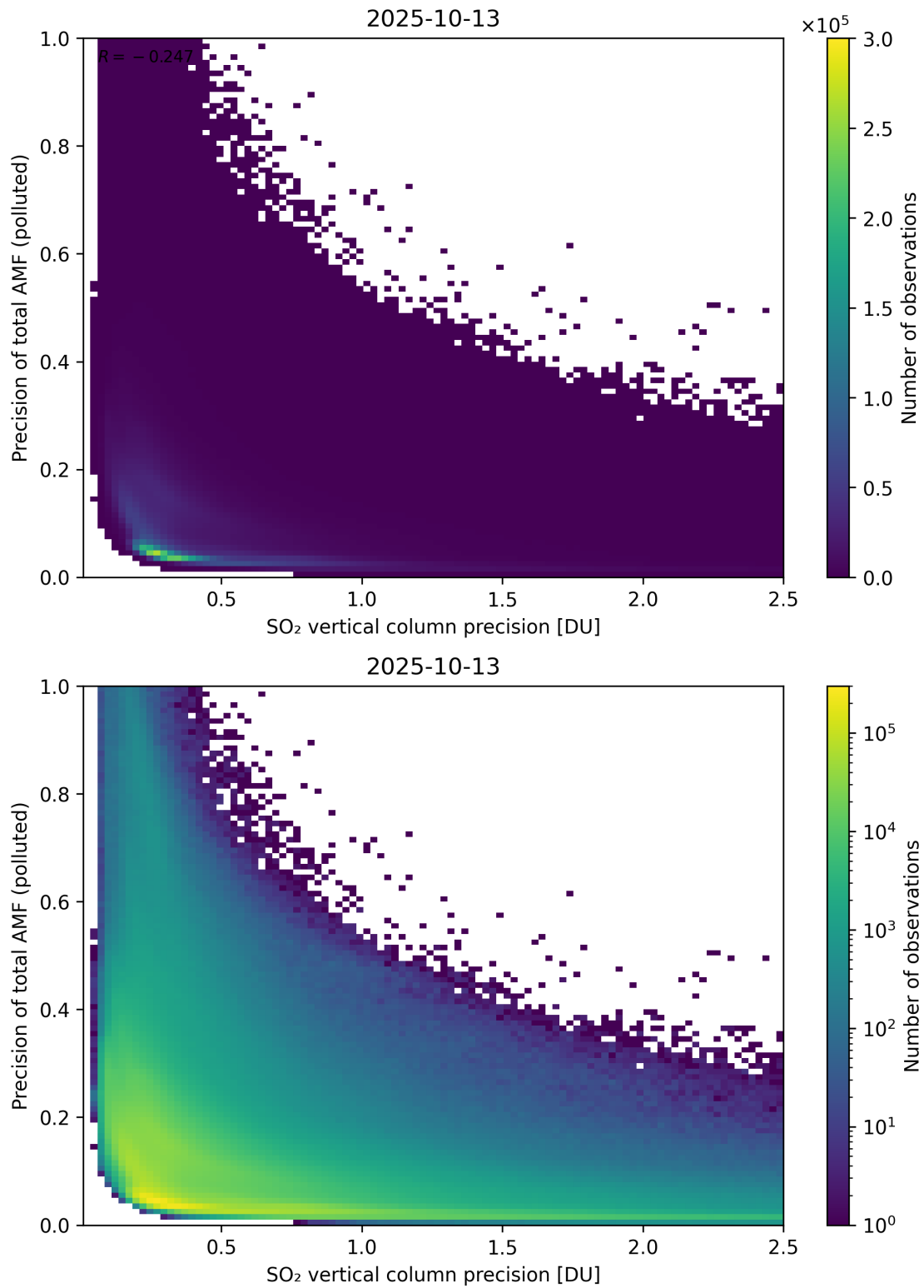
Figure 347: Scatter density plot of “SO 2 vertical column precision” against “Precision of total AMF (polluted)” for 2025-10-12 to 2025-10-14.
