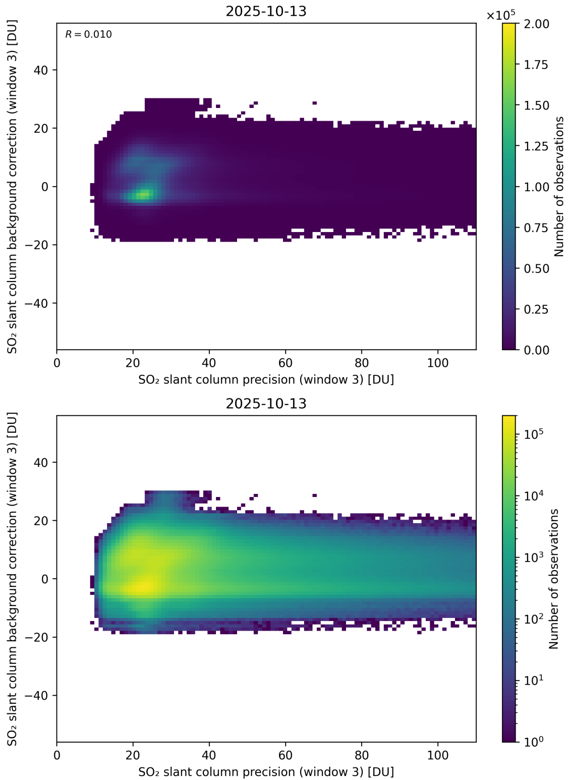
Figure 307: Scatter density plot of “SO 2 slant column precision (window 3)” against “SO 2 slant column background correction (window 3)” for 2025-10-12 to 2025-10-14.
