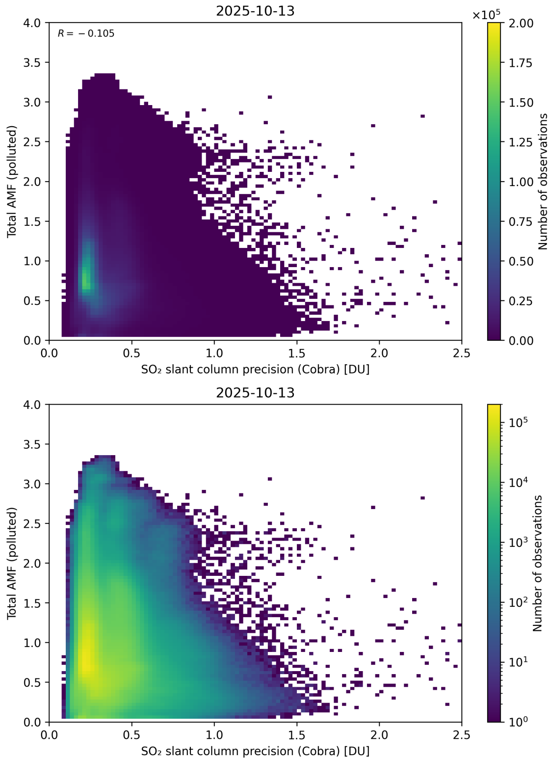
Figure 213: Scatter density plot of “SO 2 slant column precision (Cobra)” against “Total AMF (polluted)” for 2025-10-12 to 2025-10-14.
