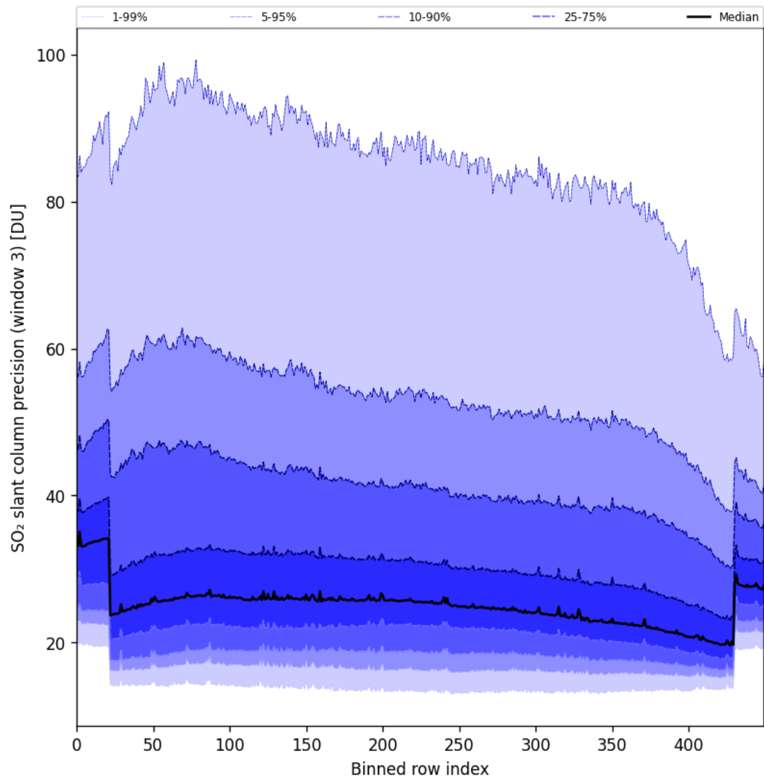
Figure 98: Along track statistics of “SO 2 slant column precision (window 3)” for 2025-10-12 to 2025-10-14
