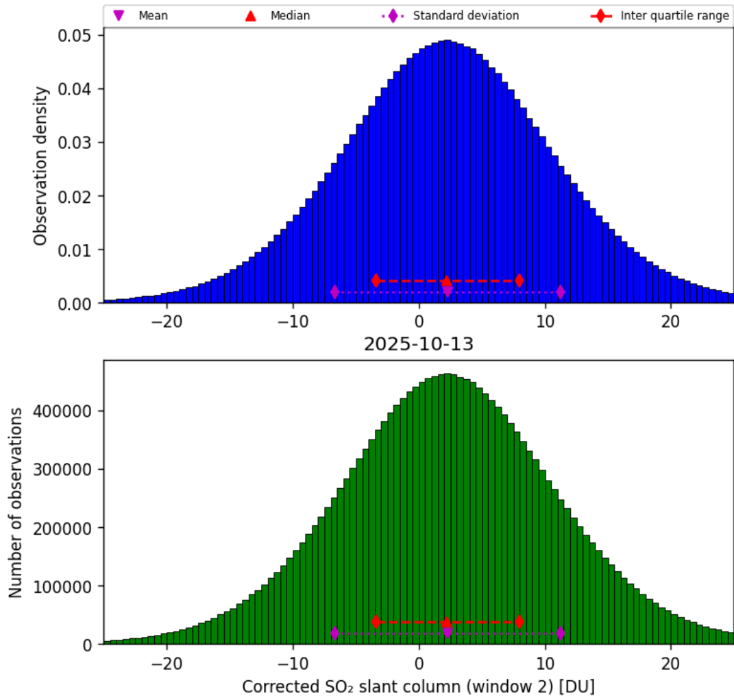
Figure 69: Histogram of “Corrected SO 2 slant column (window 2)” for 2025-10-12 to 2025-10-14
