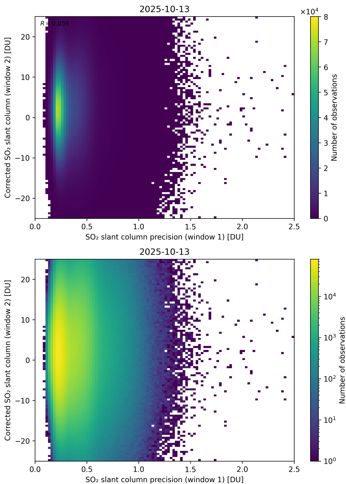
Figure 275: Scatter density plot of “SO 2 slant column precision (window 1)” against “Corrected SO 2 slant column (window 2)” for 2025-10-12 to 2025-10-14.
