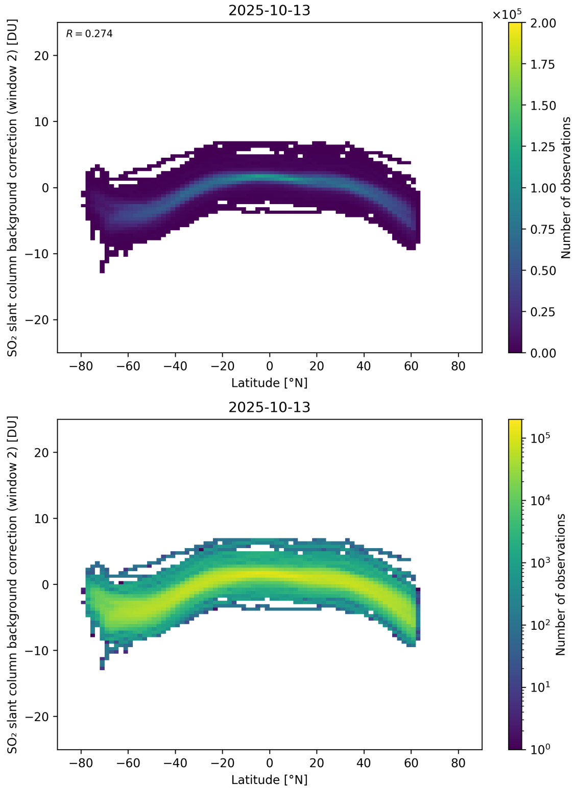
Figure 151: Scatter density plot of “Latitude” against “SO 2 slant column background correction (window 2)” for 2025-10-12 to 2025-10-14.
