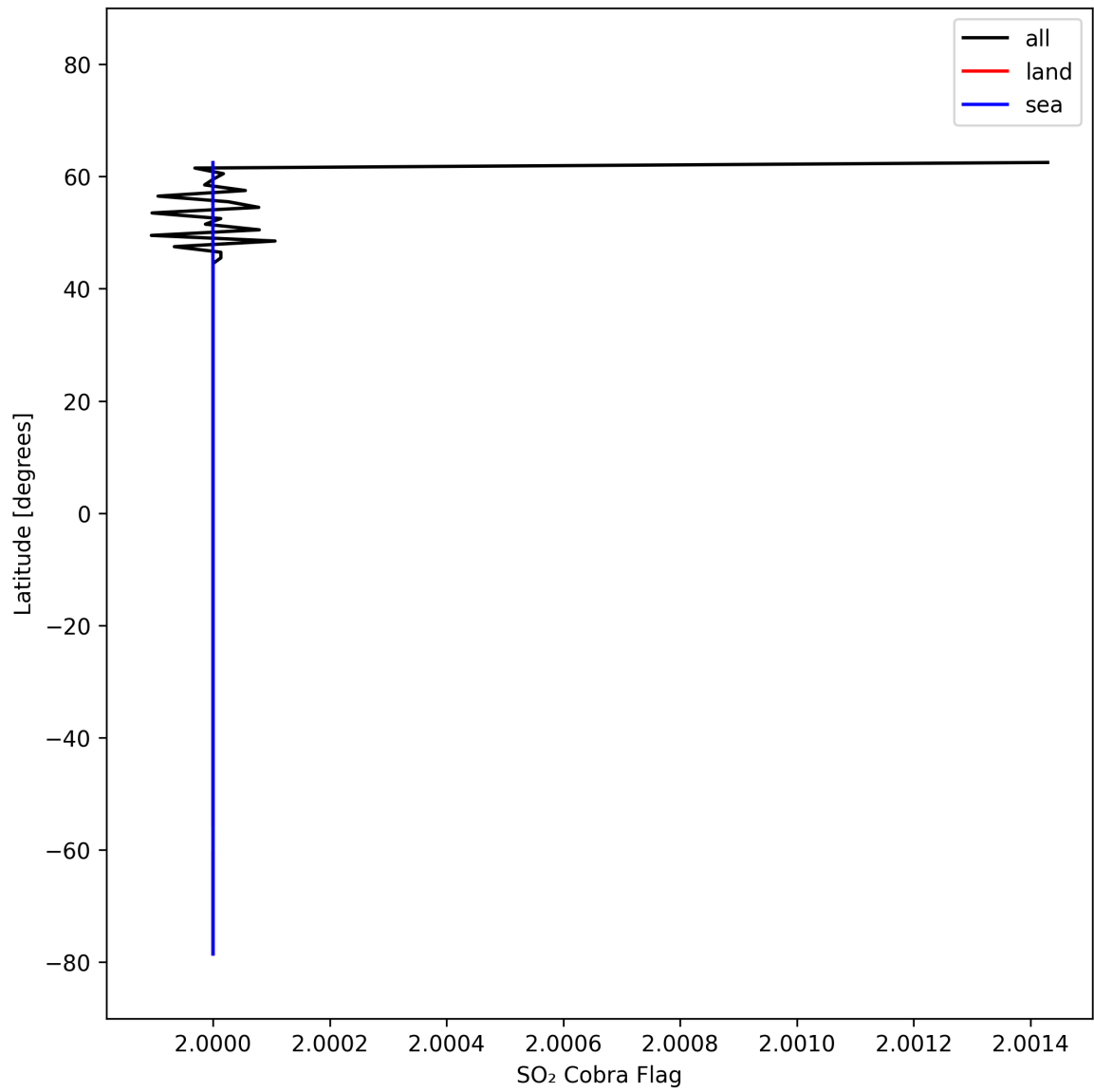
Figure 49: Zonal average of “SO 2 Cobra Flag” for 2025-10-12 to 2025-10-14.
