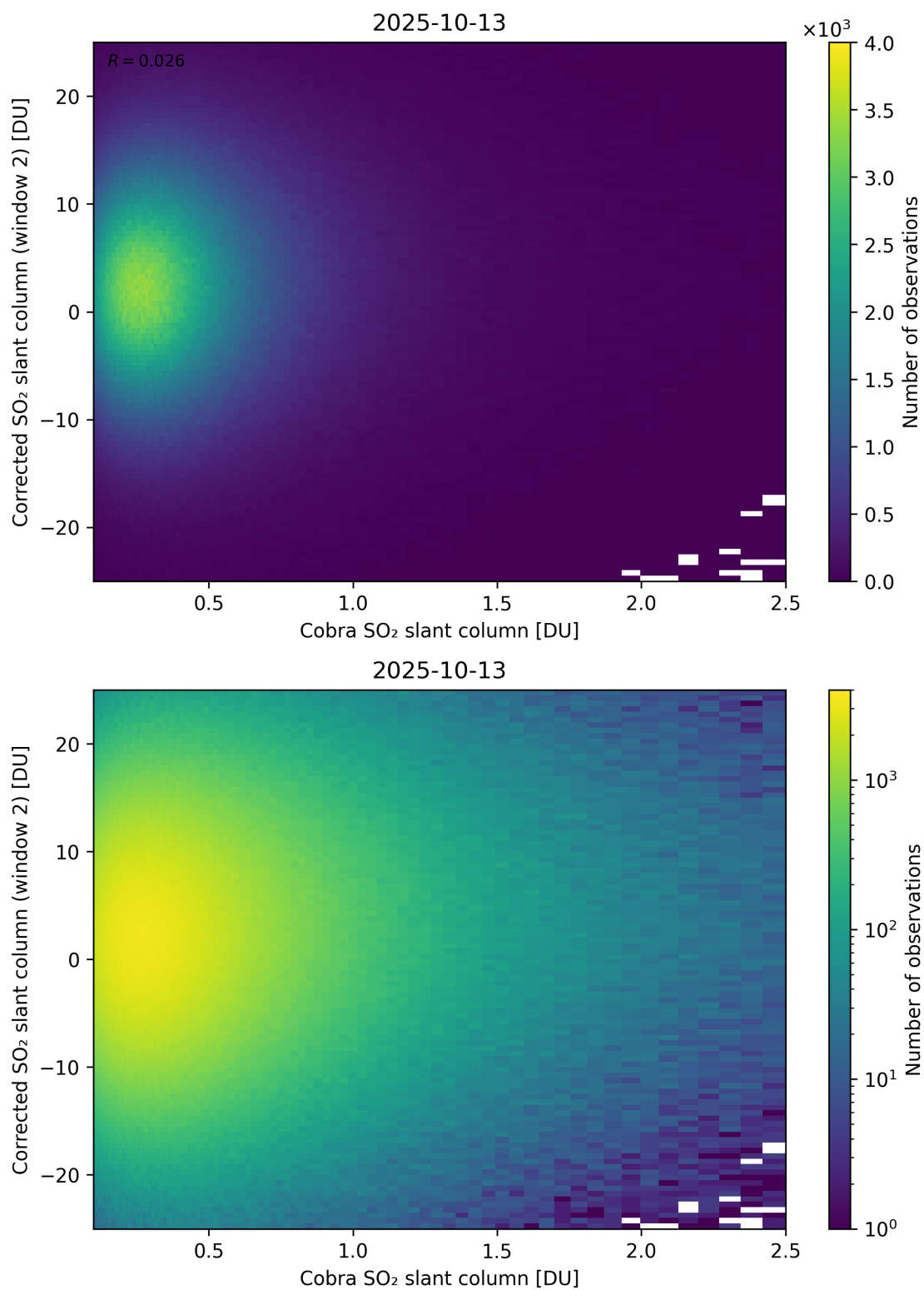
Figure 217: Scatter density plot of “Cobra SO 2 slant column” against “Corrected SO 2 slant column (window 2)” for 2025-10-12 to 2025-10-14.
