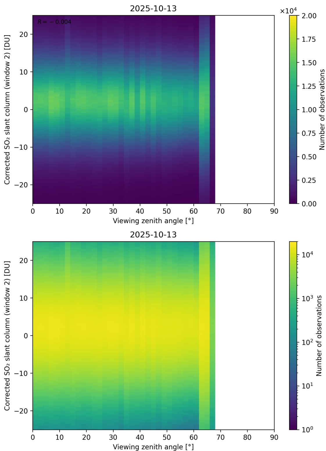
Figure 374: Scatter density plot of “Viewing zenith angle” against “Corrected SO 2 slant column (window 2)” for 2025-10-12 to 2025-10-14.
