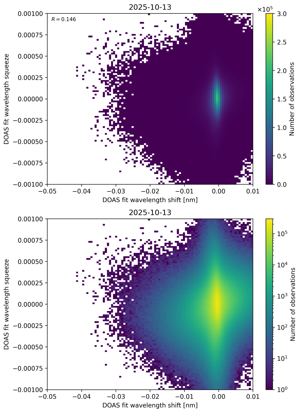
Figure 138: Scatter density plot of “DOAS fit wavelength shift” against “DOAS fit wavelength squeeze” for 2025-10-12 to 2025-10-14.
