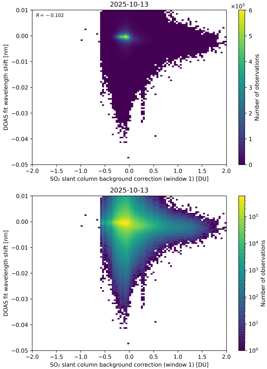
Figure 111: Scatter density plot of “SO 2 slant column background correction (window 1)” against “DOAS fit wavelength shift” for 2025-10-12 to 2025-10-14.
