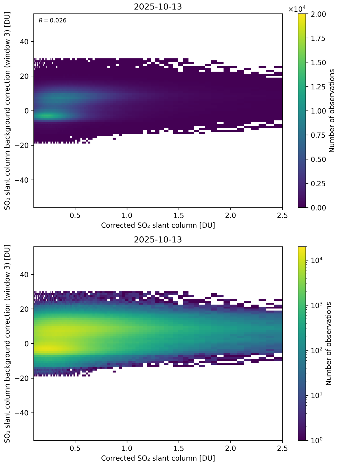
Figure 228: Scatter density plot of “Corrected SO 2 slant column” against “SO 2 slant column background correction (window 3)” for 2025-10-12 to 2025-10-14.
