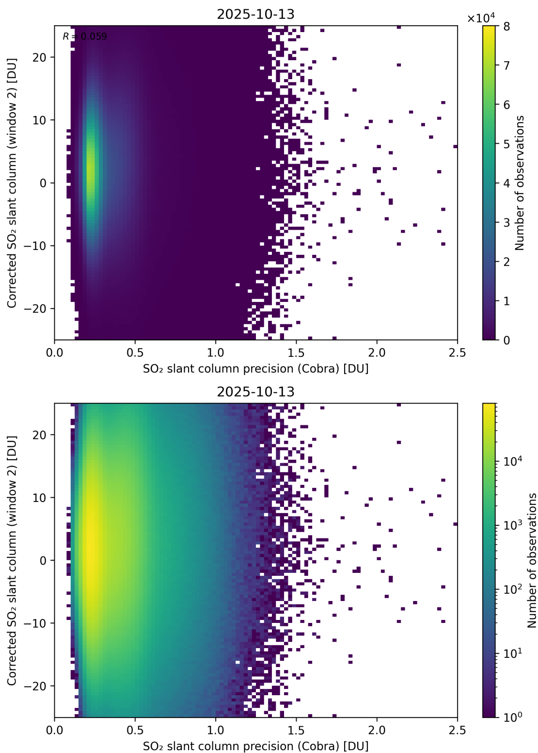
Figure 206: Scatter density plot of “SO 2 slant column precision (Cobra)” against “Corrected SO 2 slant column (window 2)” for 2025-10-12 to 2025-10-14.
