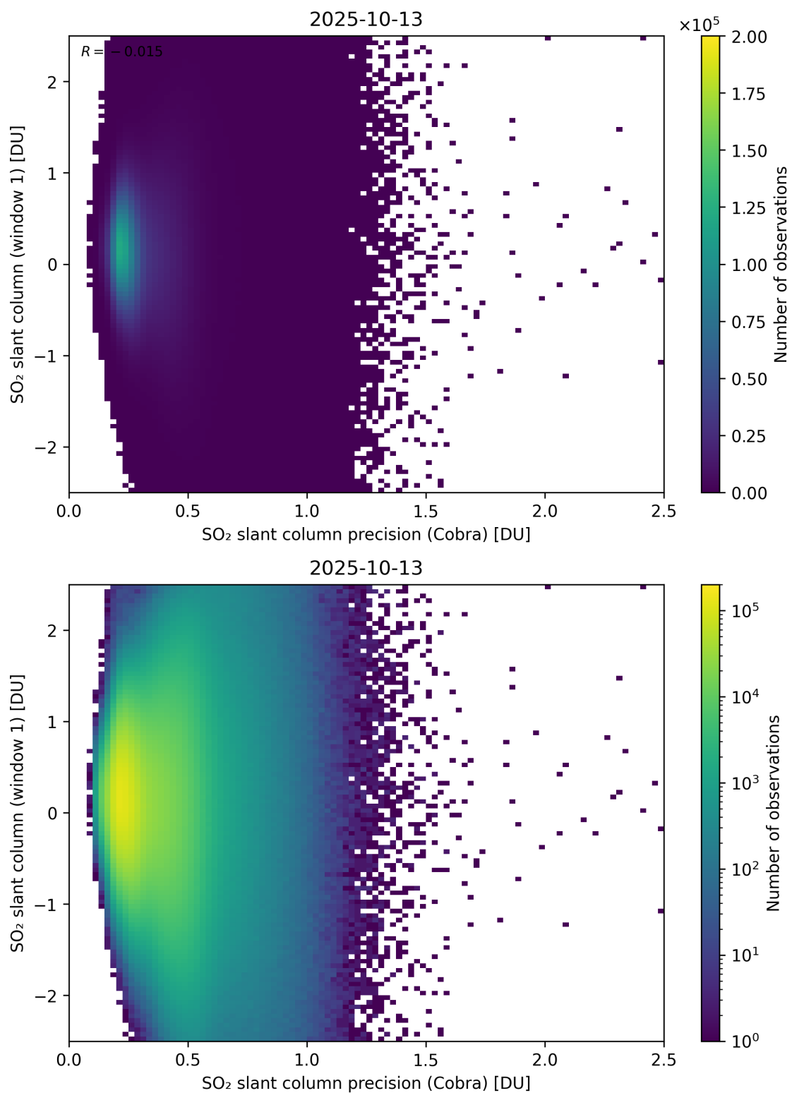
Figure 208: Scatter density plot of “SO 2 slant column precision (Cobra)” against “SO 2 slant column (window 1)” for 2025-10-12 to 2025-10-14.
