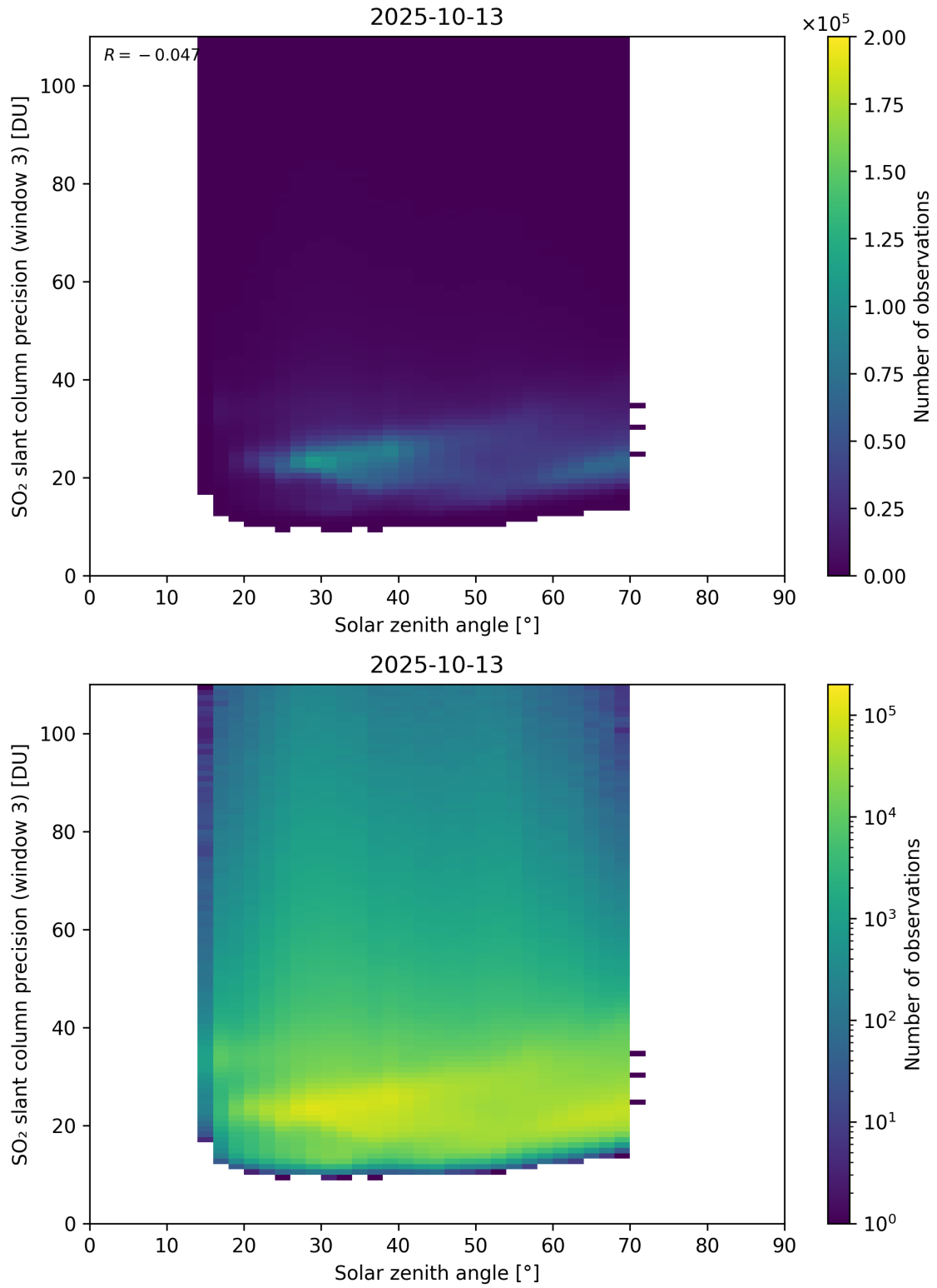
Figure 188: Scatter density plot of “Solar zenith angle” against “SO 2 slant column precision (window 3)” for 2025-10-12 to 2025-10-14.
