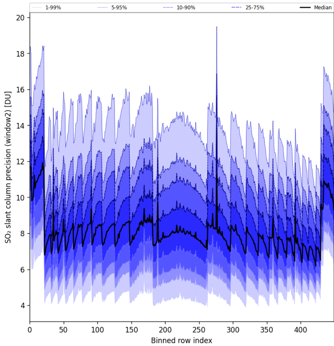
Figure 94: Along track statistics of “SO 2 slant column precision (window2)” for 2025-10-12 to 2025-10-14
