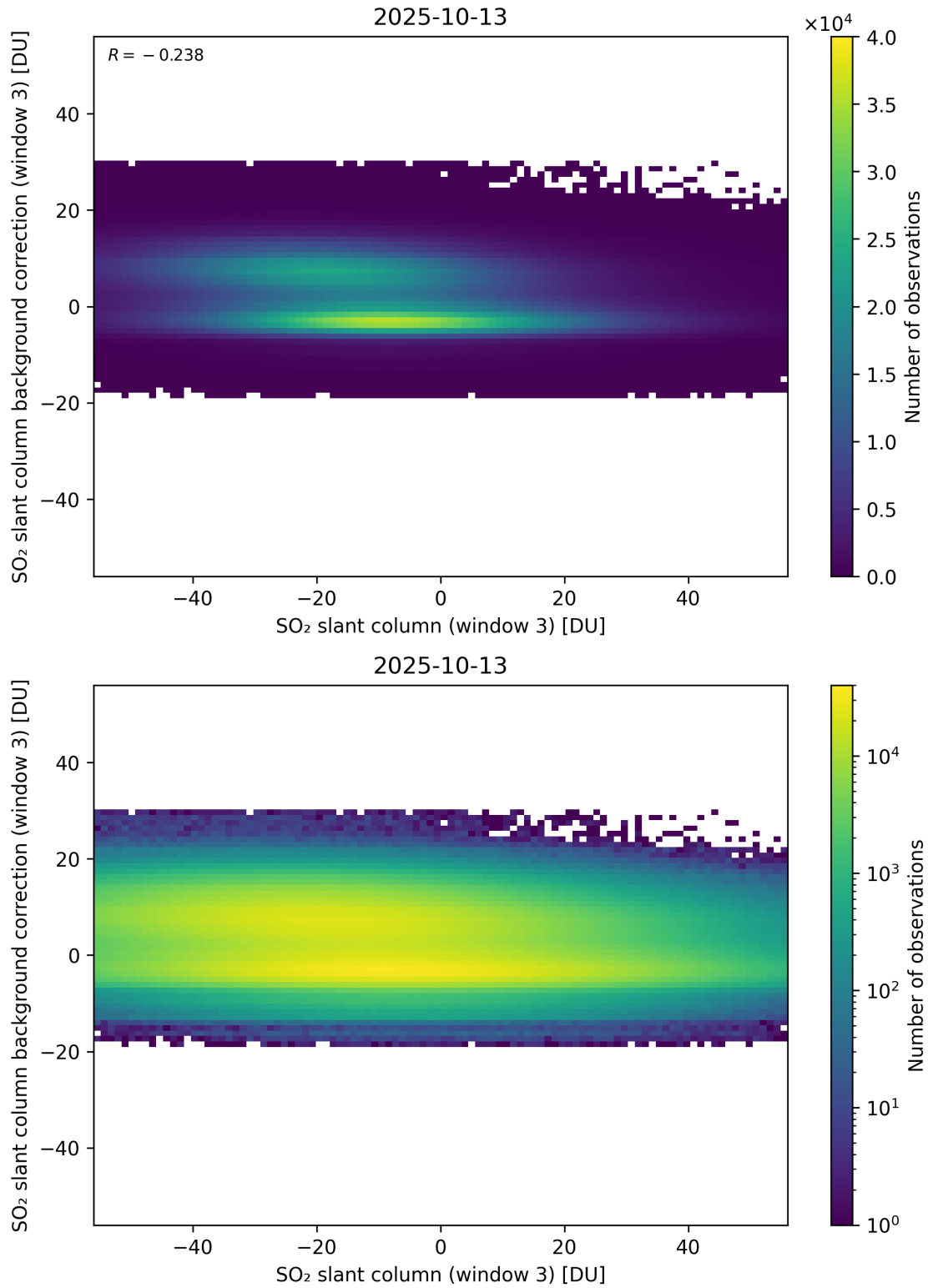
Figure 303: Scatter density plot of “SO 2 slant column (window 3)” against “SO 2 slant column background correction (window 3)” for 2025-10-12 to 2025-10-14.
