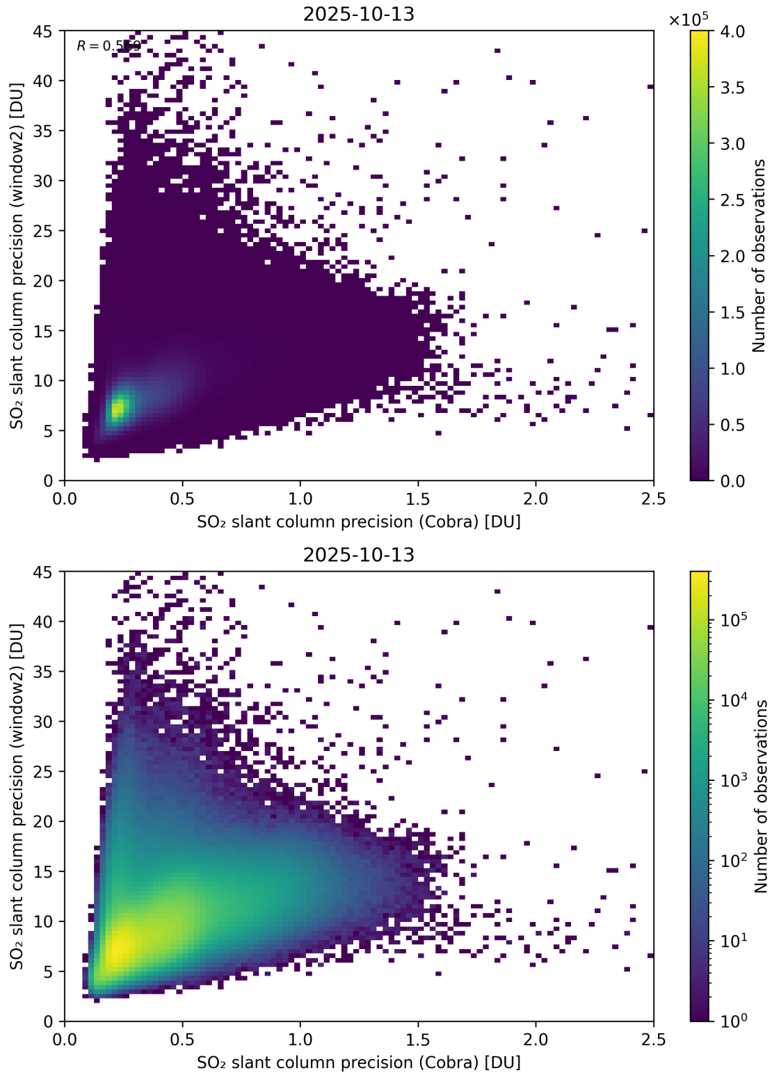
Figure 210: Scatter density plot of “SO 2 slant column precision (Cobra)” against “SO 2 slant column precision (window2)” for 2025-10-12 to 2025-10-14.
