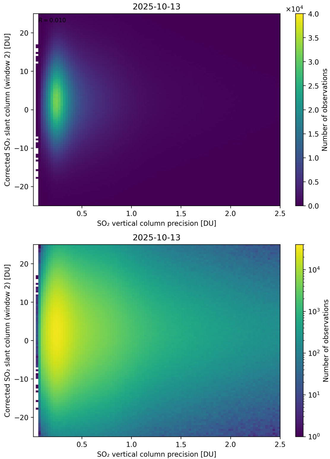
Figure 339: Scatter density plot of “SO 2 vertical column precision” against “Corrected SO 2 slant column (window 2)” for 2025-10-12 to 2025-10-14.
