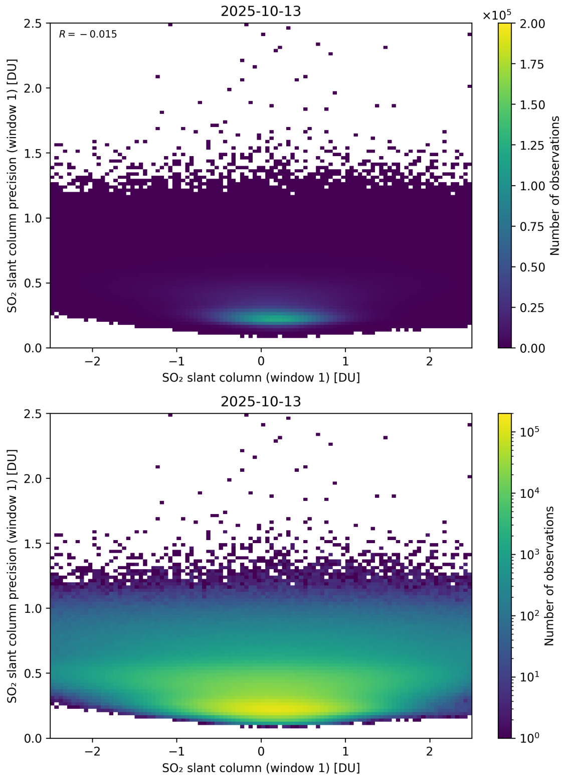
Figure 285: Scatter density plot of “SO 2 slant column (window 1)” against “SO 2 slant column precision (window 1)” for 2025-10-12 to 2025-10-14.
