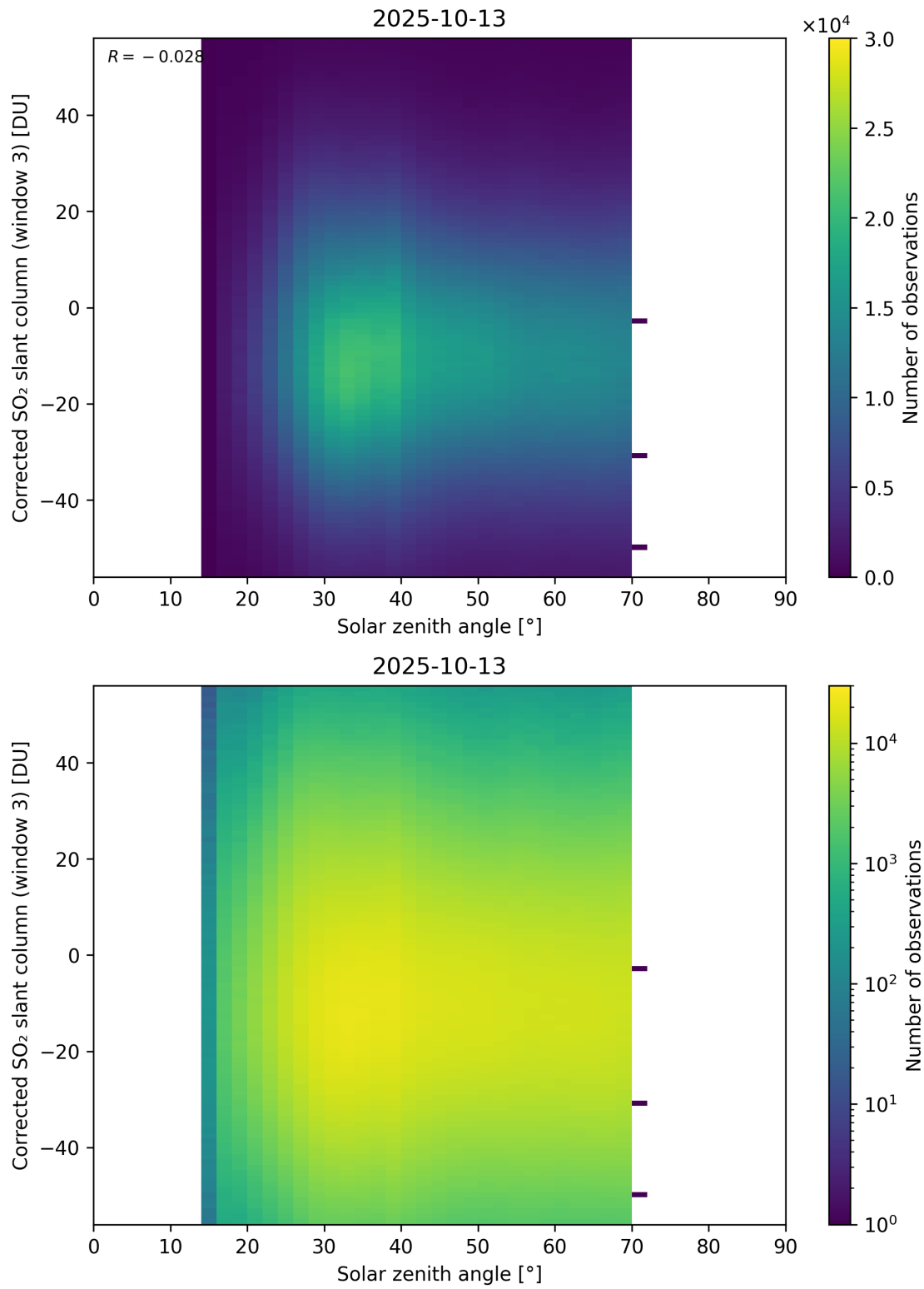
Figure 183: Scatter density plot of “Solar zenith angle” against “Corrected SO 2 slant column (window 3)” for 2025-10-12 to 2025-10-14.
