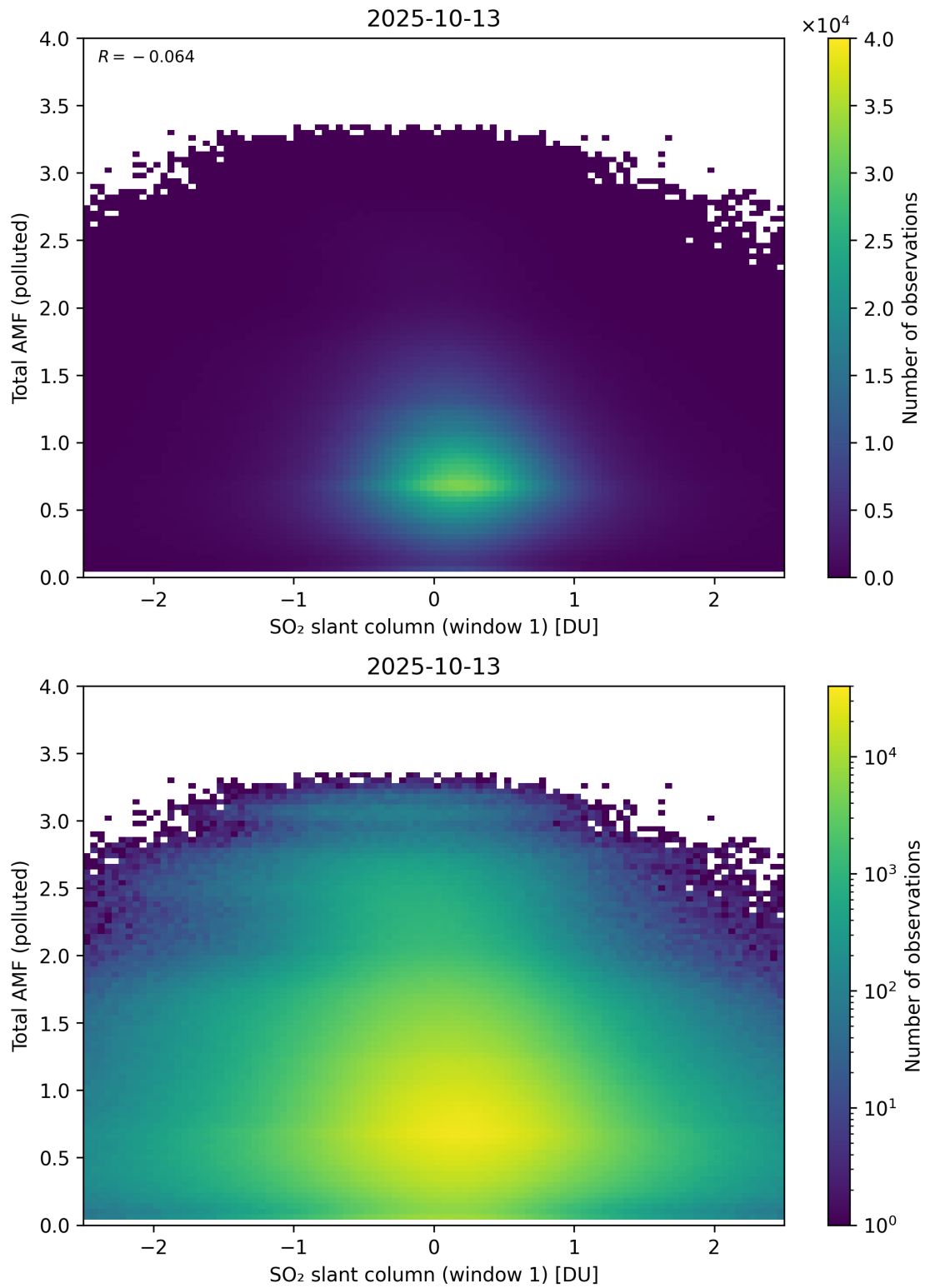
Figure 289: Scatter density plot of “SO 2 slant column (window 1)” against “Total AMF (polluted)” for 2025-10-12 to 2025-10-14.
