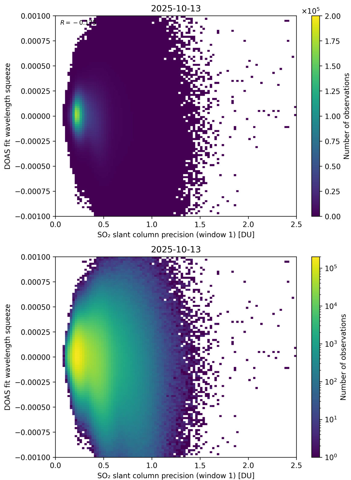
Figure 272: Scatter density plot of “SO 2 slant column precision (window 1)” against “DOAS fit wavelength squeeze” for 2025-10-12 to 2025-10-14.
