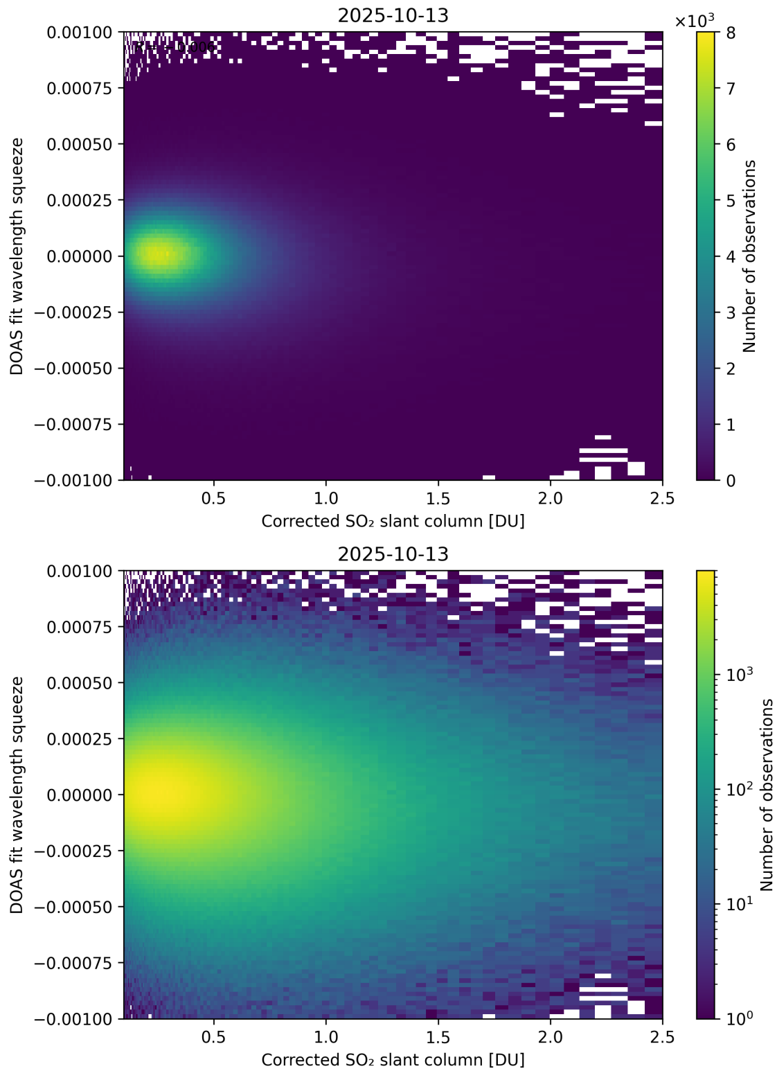
Figure 230: Scatter density plot of "Corrected SO 2 slant column" against "DOAS fit wavelength squeeze" for 2025-10-12 to 2025-10-14.
