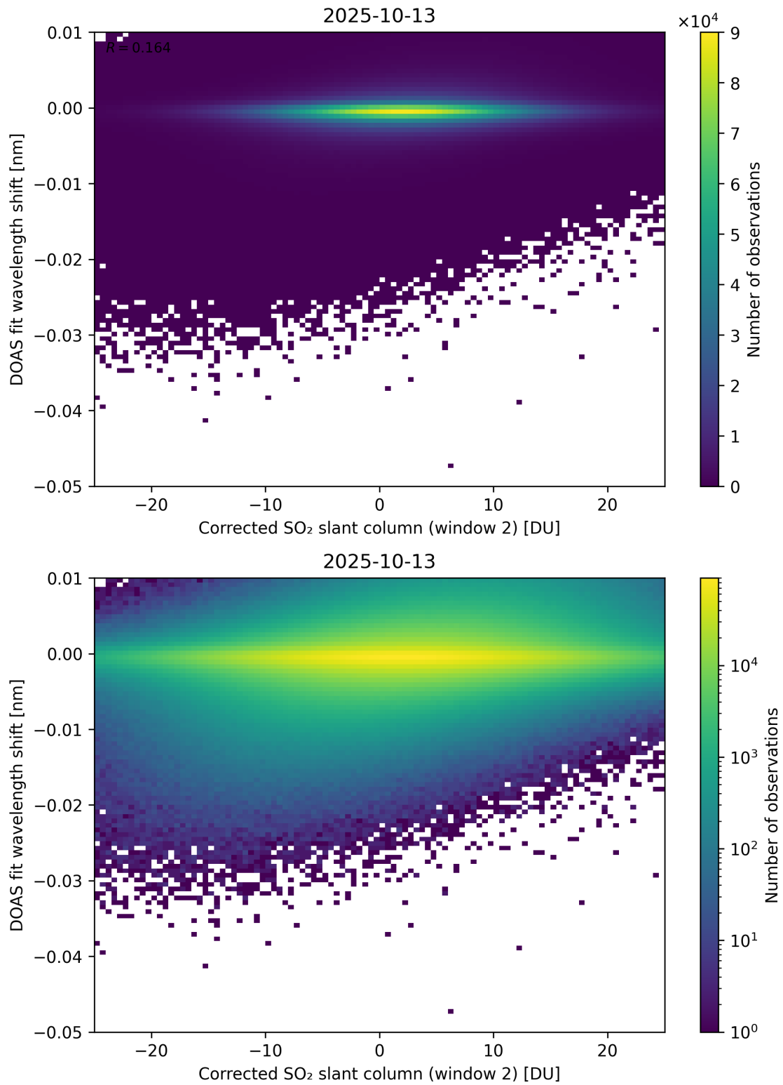
Figure 246: Scatter density plot of “Corrected SO 2 slant column (window 2)” against “DOAS fit wavelength shift” for 2025-10-12 to 2025-10-14.
