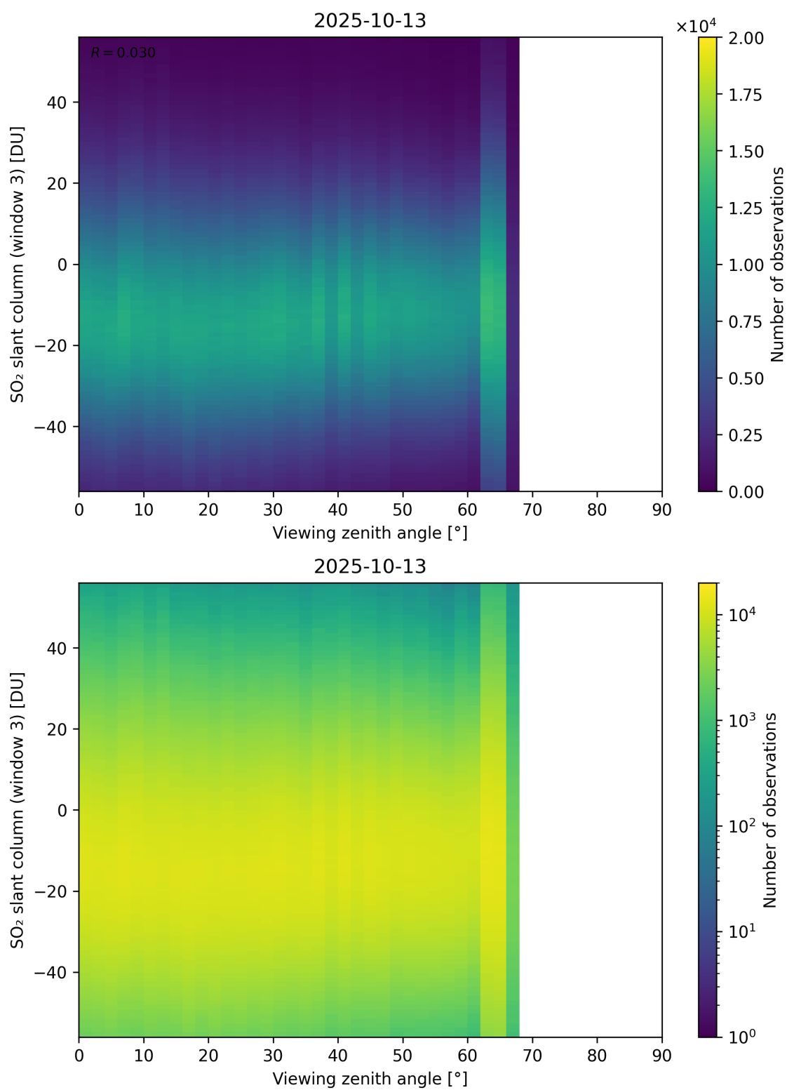
Figure 379: Scatter density plot of “Viewing zenith angle” against “SO 2 slant column (window 3)” for 2025-10-12 to 2025-10-14.
