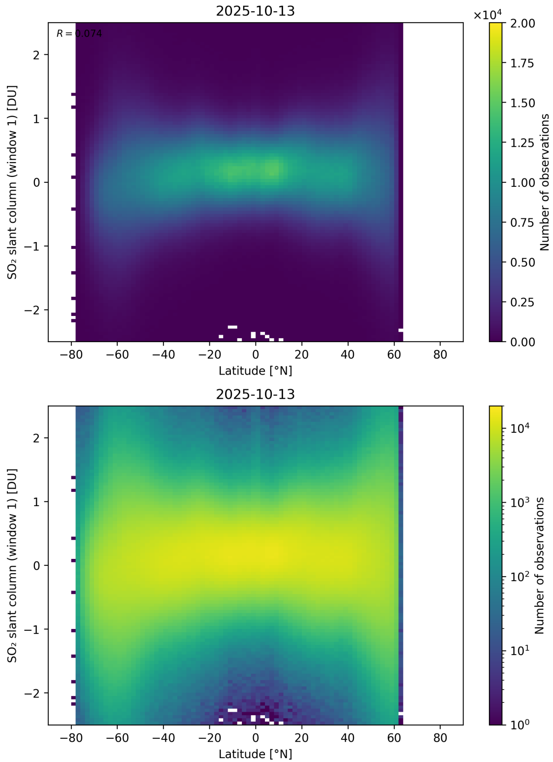
Figure 162: Scatter density plot of “Latitude” against “SO 2 slant column (window 1)” for 2025-10-12 to 2025-10-14.
