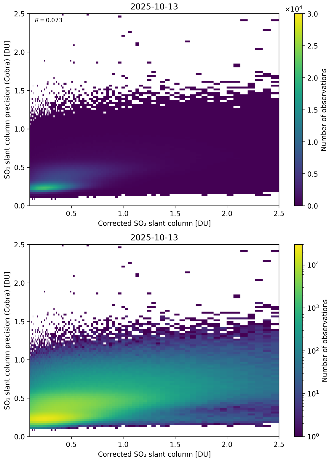
Figure 234: Scatter density plot of “Corrected SO 2 slant column” against “SO 2 slant column precision (Cobra)” for 2025-10-12 to 2025-10-14.
