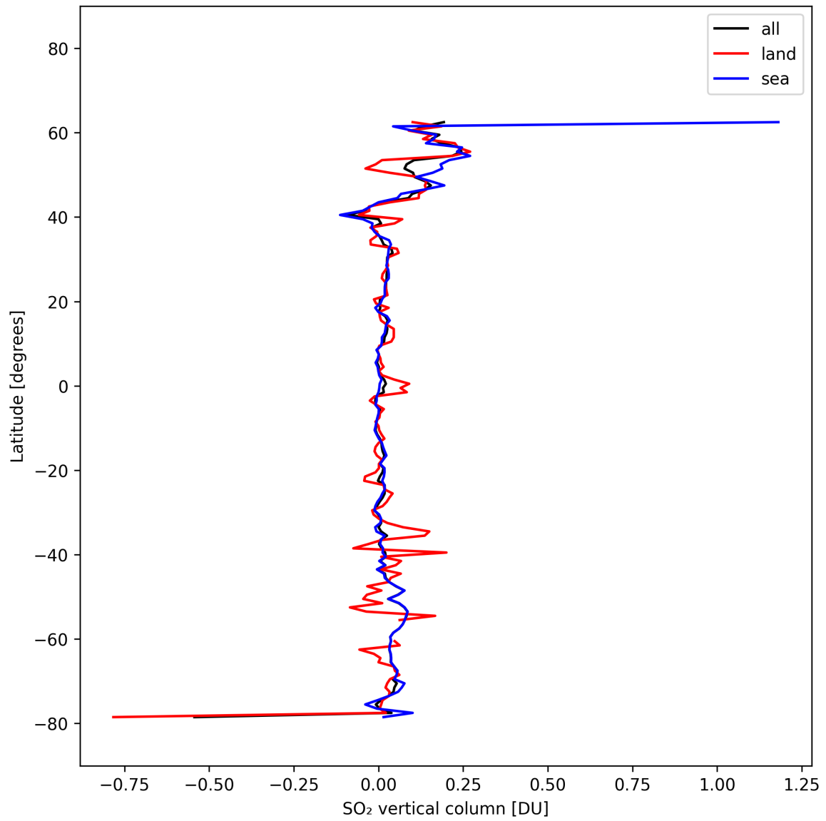
Figure 32: Zonal average of “SO 2 vertical column” for 2025-10-12 to 2025-10-14.
