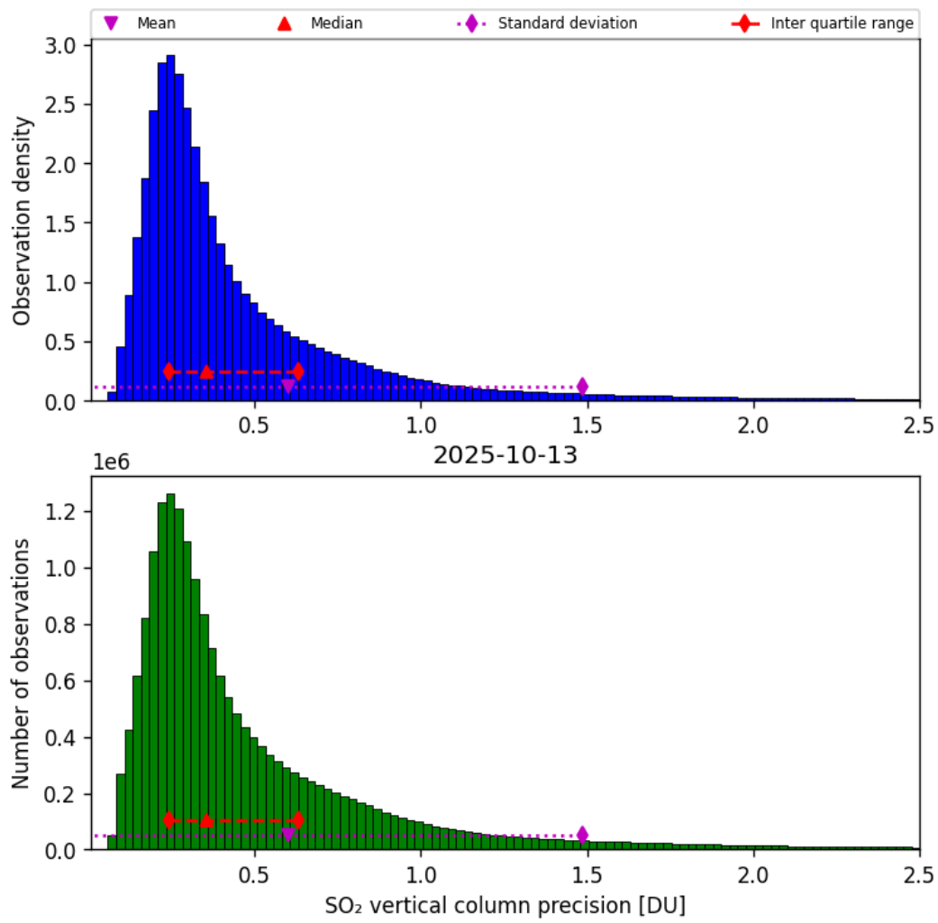
Figure 59: Histogram of “SO 2 vertical column precision” for 2025-10-12 to 2025-10-14
