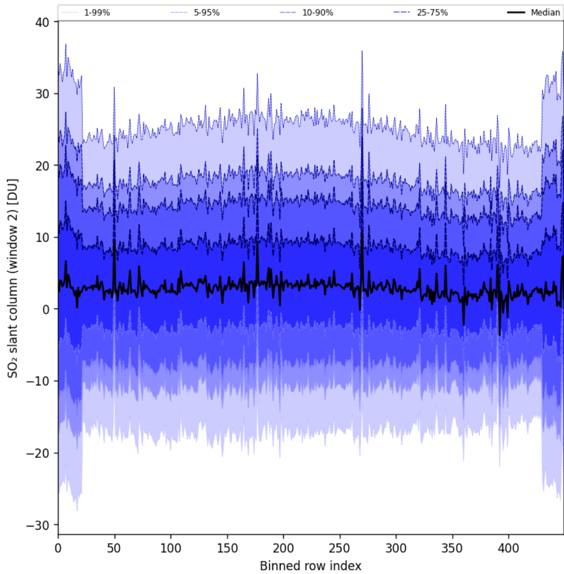
Figure 93: Along track statistics of “SO 2 slant column (window 2)” for 2025-10-12 to 2025-10-14
