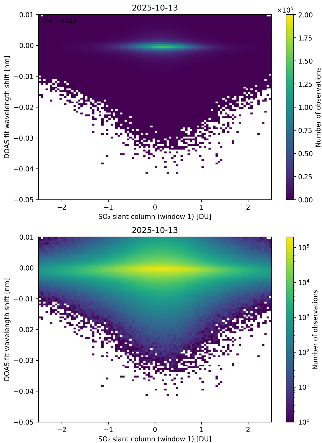
Figure 265: Scatter density plot of “SO 2 slant column (window 1)” against “DOAS fit wavelength shift” for 2025-10-12 to 2025-10-14.
