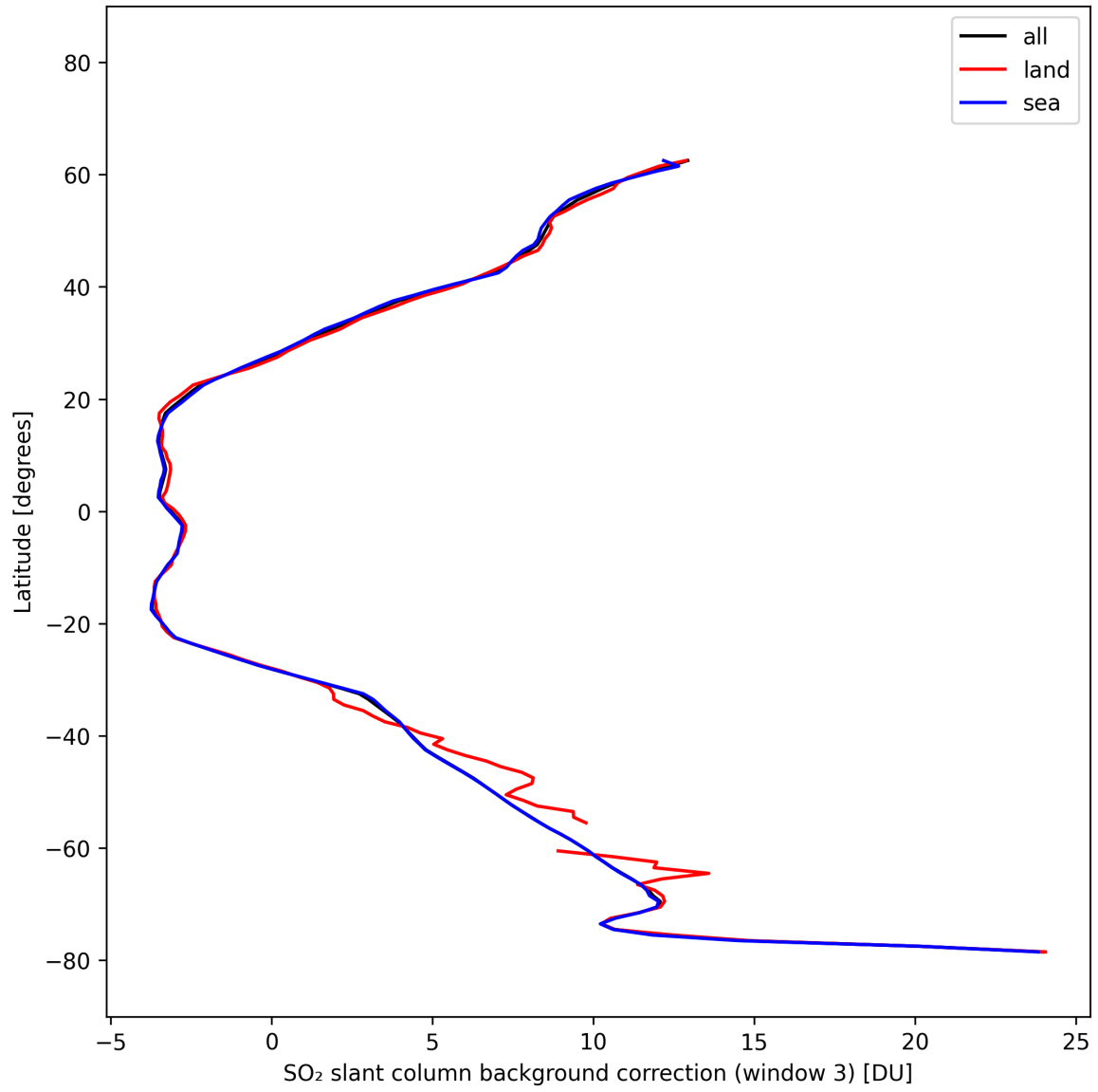
Figure 48: Zonal average of “SO 2 slant column background correction (window 3)” for 2025-10-12 to 2025-10-14.
