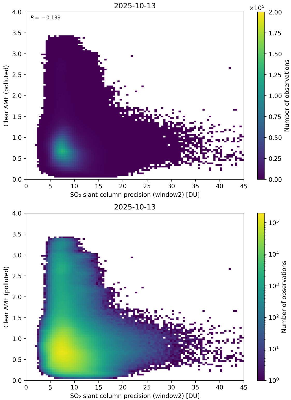
Figure 296: Scatter density plot of “SO 2 slant column precision (window2)” against “Clear AMF (polluted)” for 2025-10-12 to 2025-10-14.
