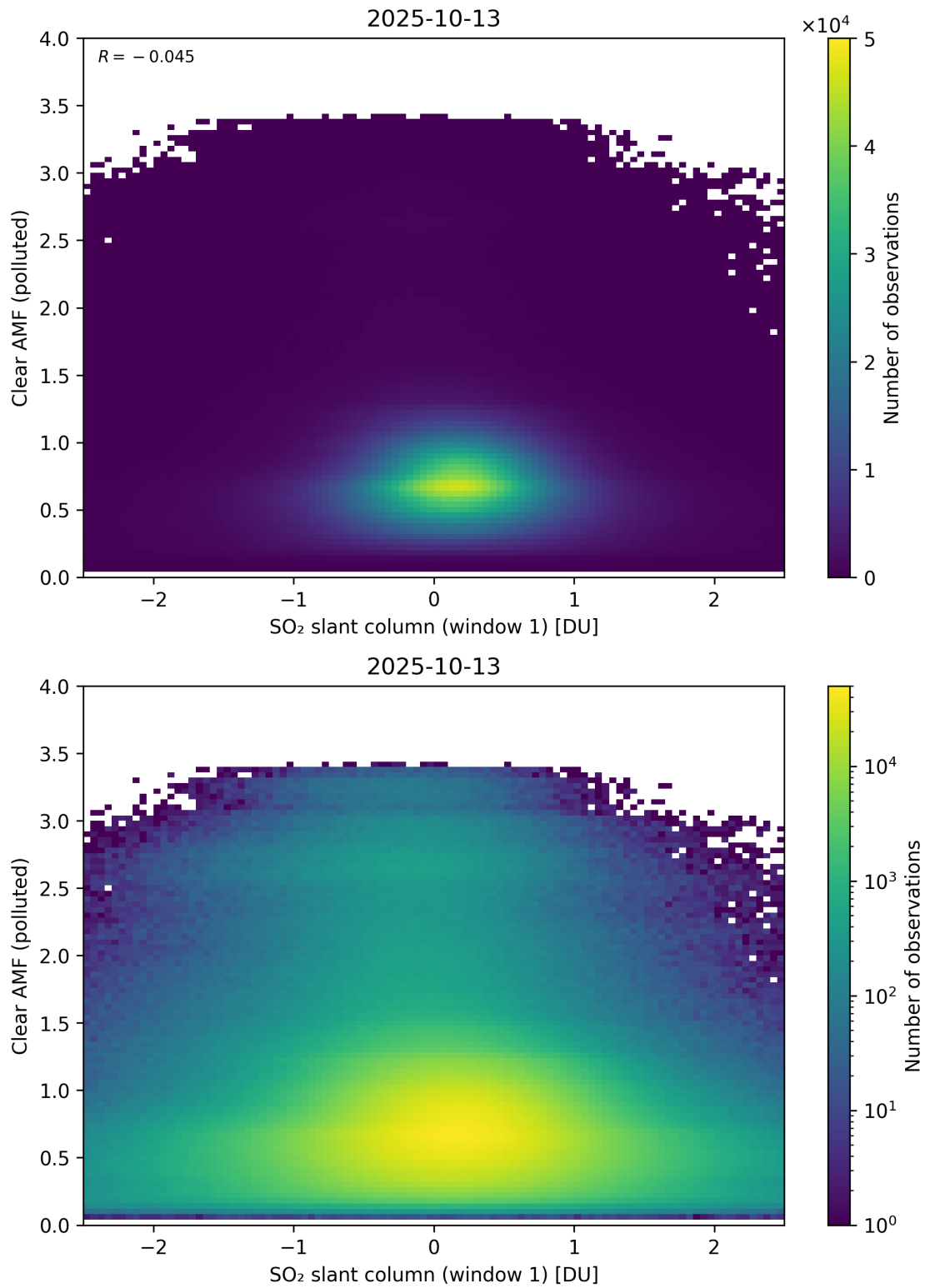
Figure 282: Scatter density plot of “SO 2 slant column (window 1)” against “Clear AMF (polluted)” for 2025-10-12 to 2025-10-14.
