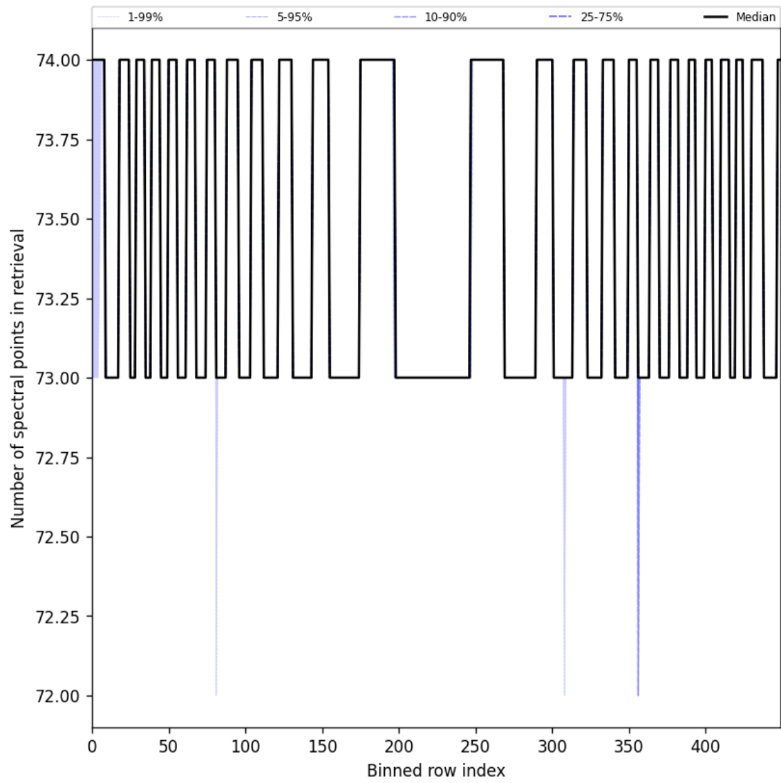
Figure 108: Along track statistics of “Number of spectral points in retrieval” for 2025-10-12 to 2025-10-14
