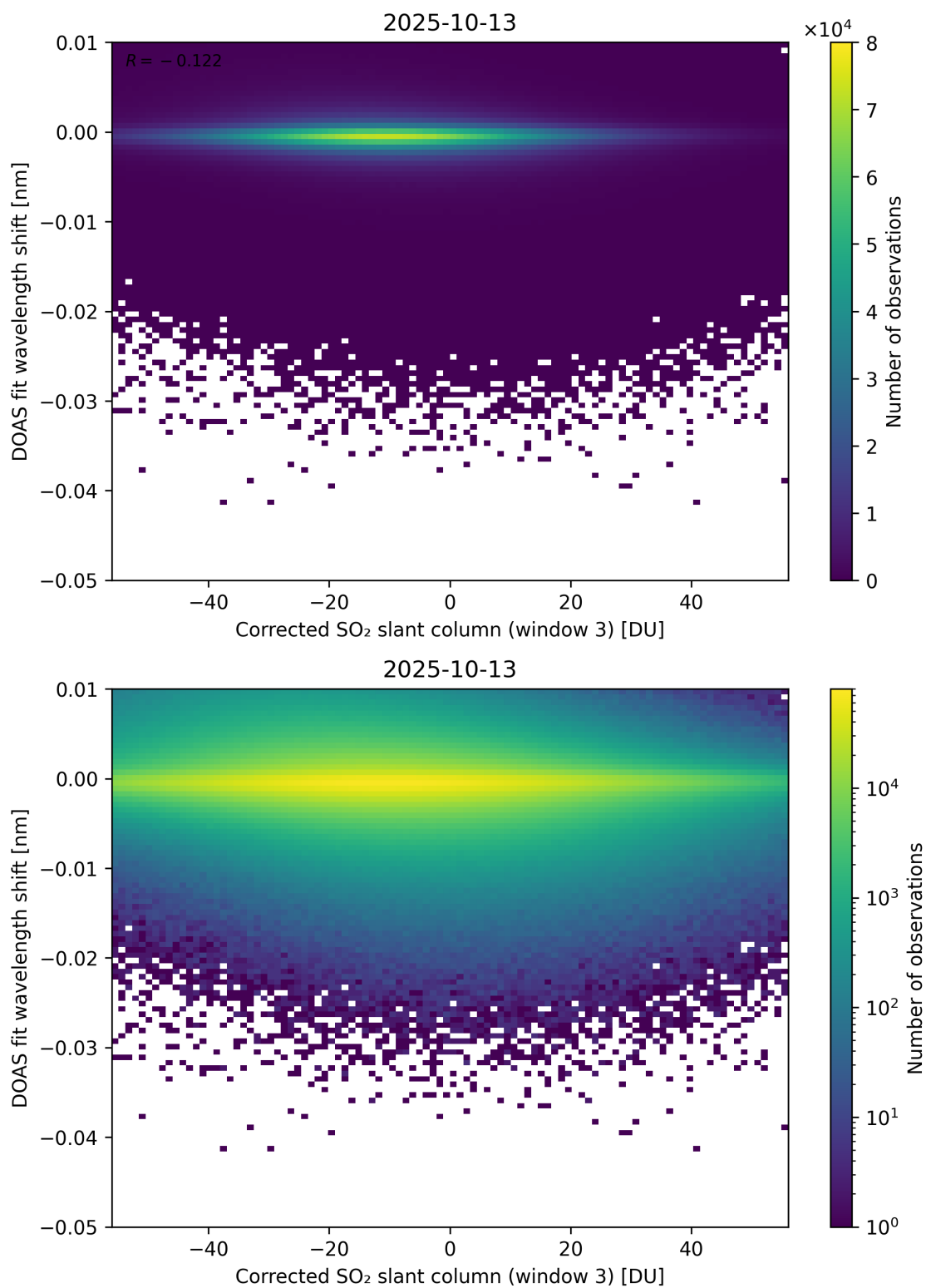
Figure 256: Scatter density plot of “Corrected SO 2 slant column (window 3)” against “DOAS fit wavelength shift” for 2025-10-12 to 2025-10-14.
