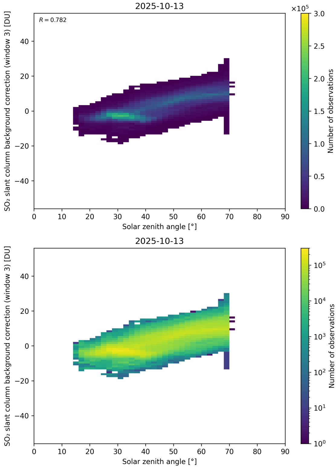
Figure 173: Scatter density plot of “Solar zenith angle” against “SO 2 slant column background correction (window 3)” for 2025-10-12 to 2025-10-14.
