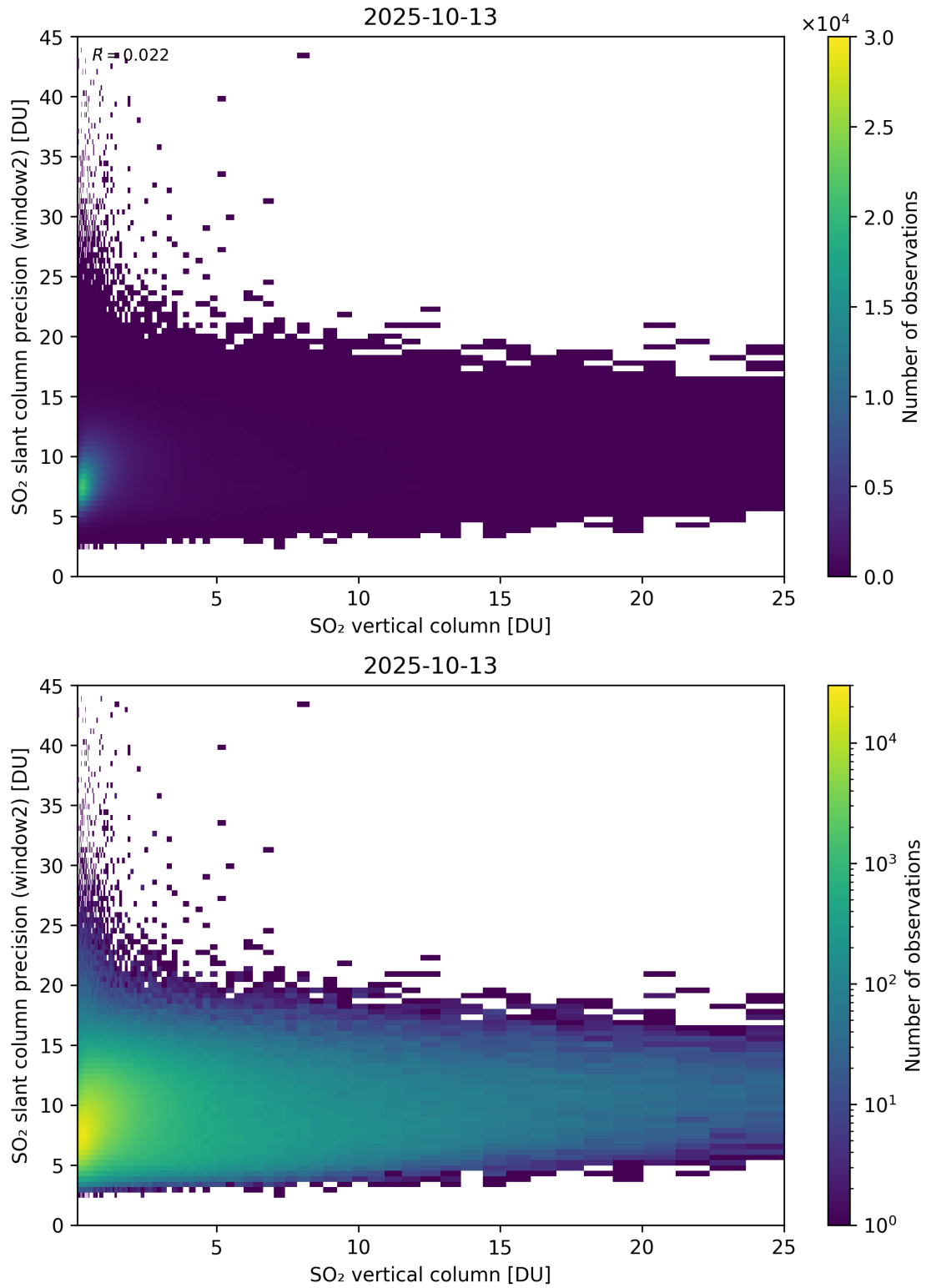
Figure 356: Scatter density plot of “SO 2 vertical column” against “SO 2 slant column precision (window2)” for 2025-10-12 to 2025-10-14.
