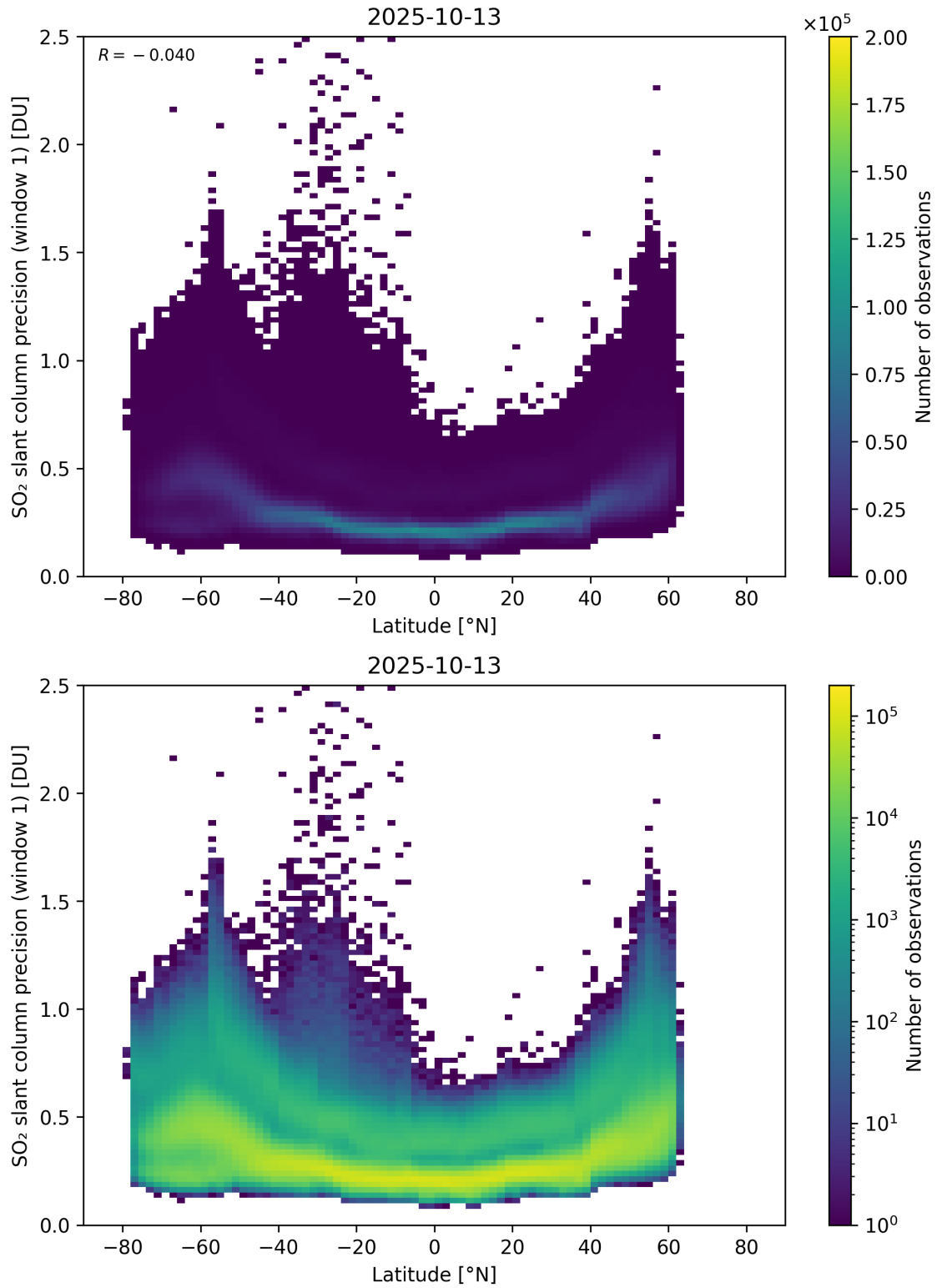
Figure 163: Scatter density plot of “Latitude” against “SO 2 slant column precision (window 1)” for 2025-10-12 to 2025-10-14.
