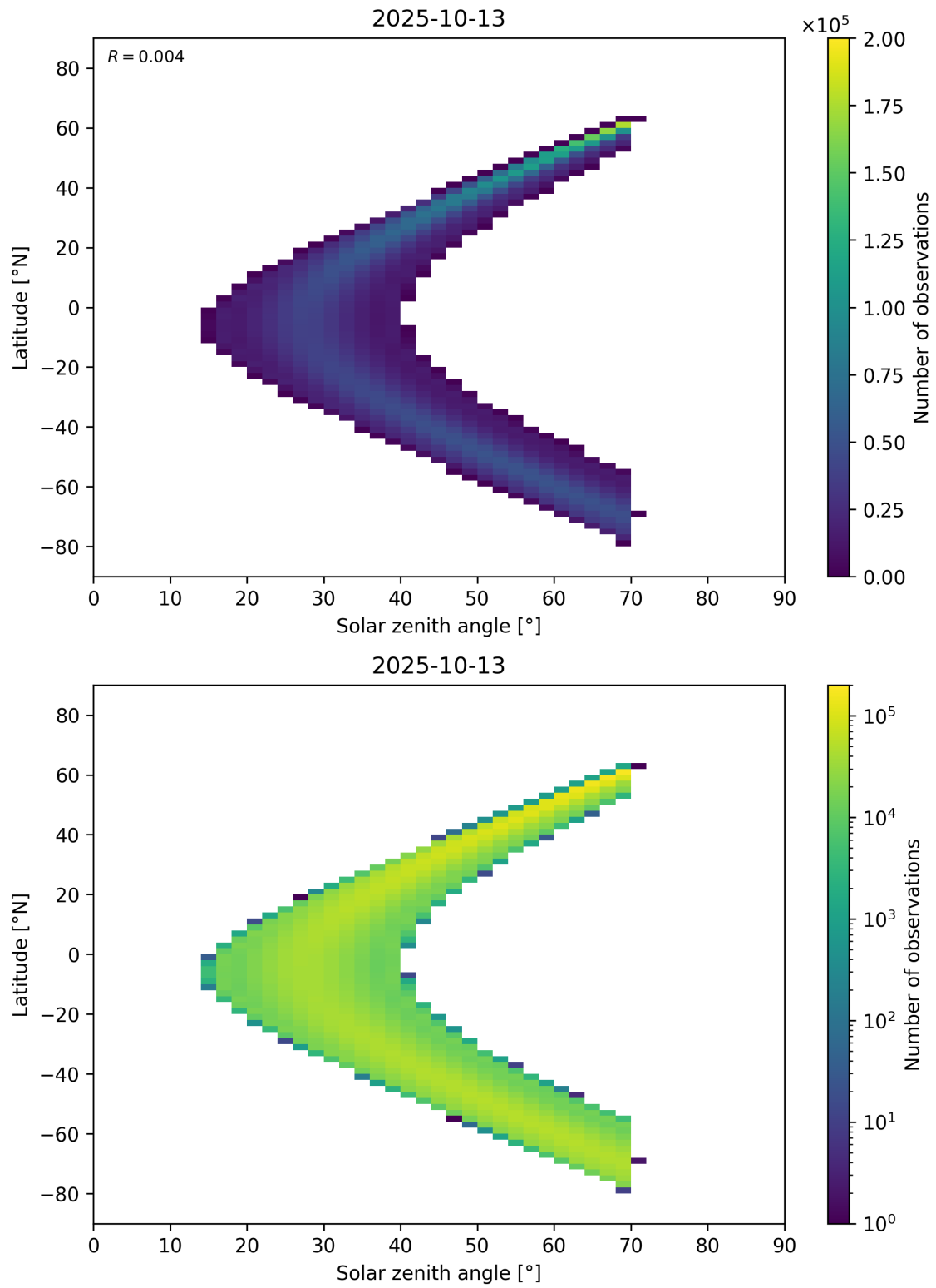
Figure 177: Scatter density plot of “Solar zenith angle” against “Latitude” for 2025-10-12 to 2025-10-14.
