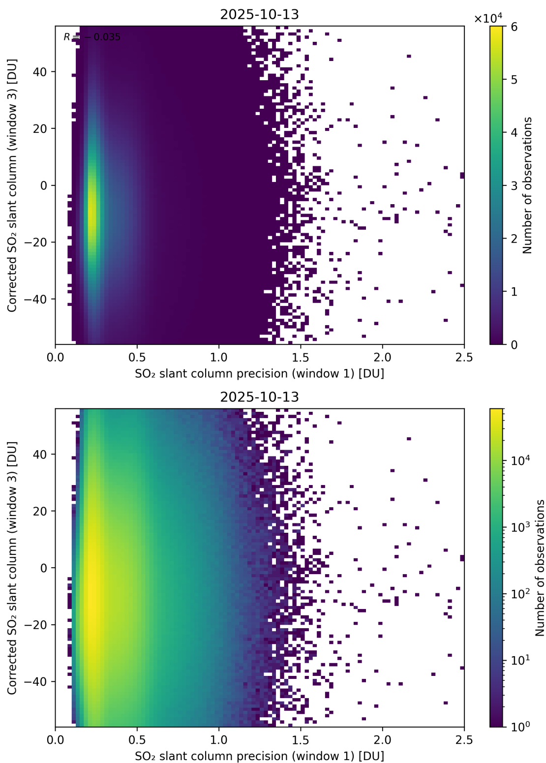
Figure 276: Scatter density plot of “SO 2 slant column precision (window 1)” against “Corrected SO 2 slant column (window 3)” for 2025-10-12 to 2025-10-14.
