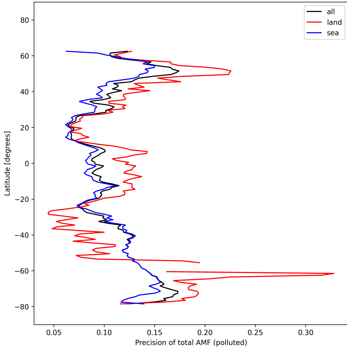
Figure 54: Zonal average of “Precision of total AMF (polluted)” for 2025-10-12 to 2025-10-14.
