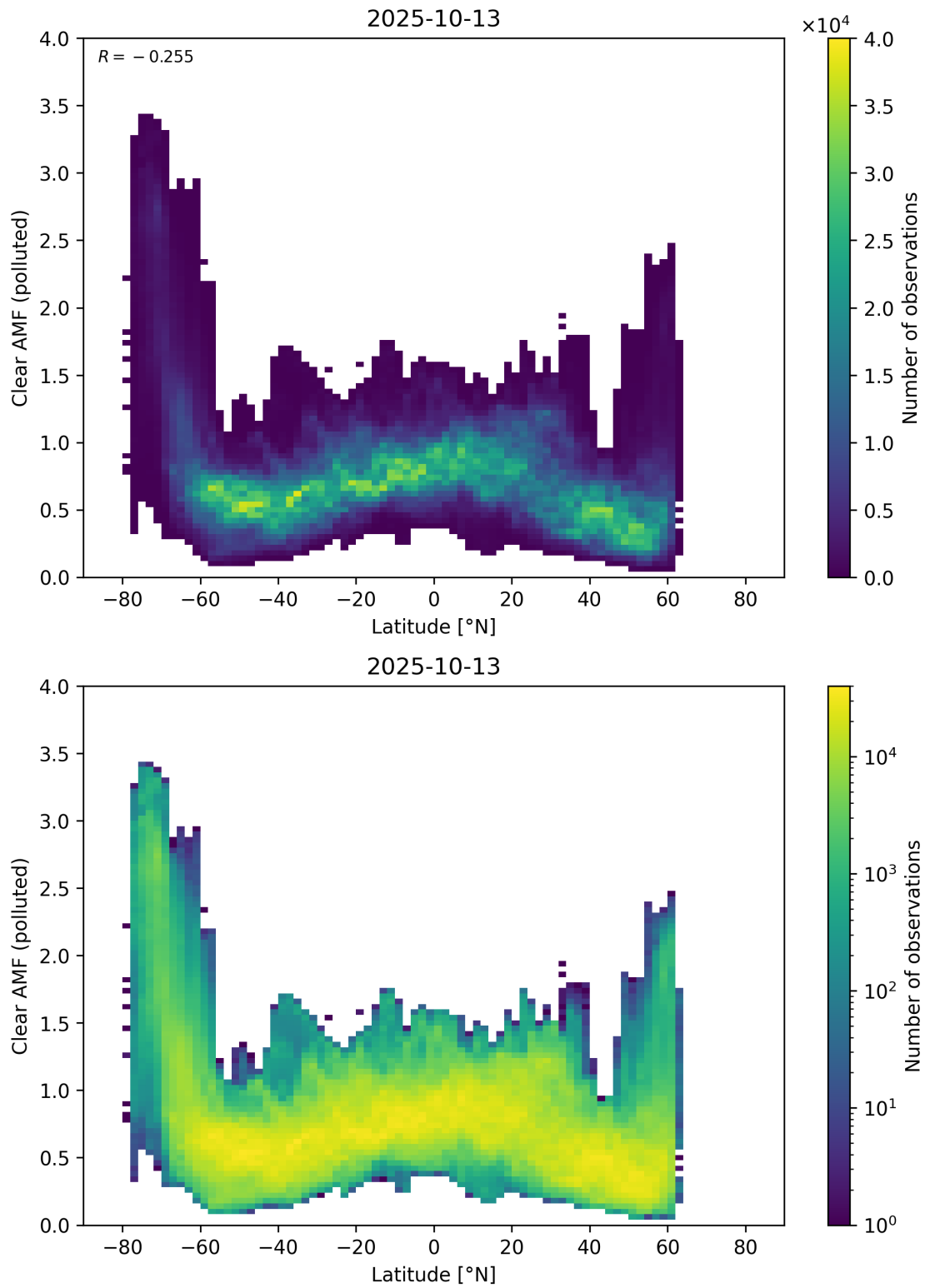
Figure 156: Scatter density plot of “Latitude” against “Clear AMF (polluted)” for 2025-10-12 to 2025-10-14.
