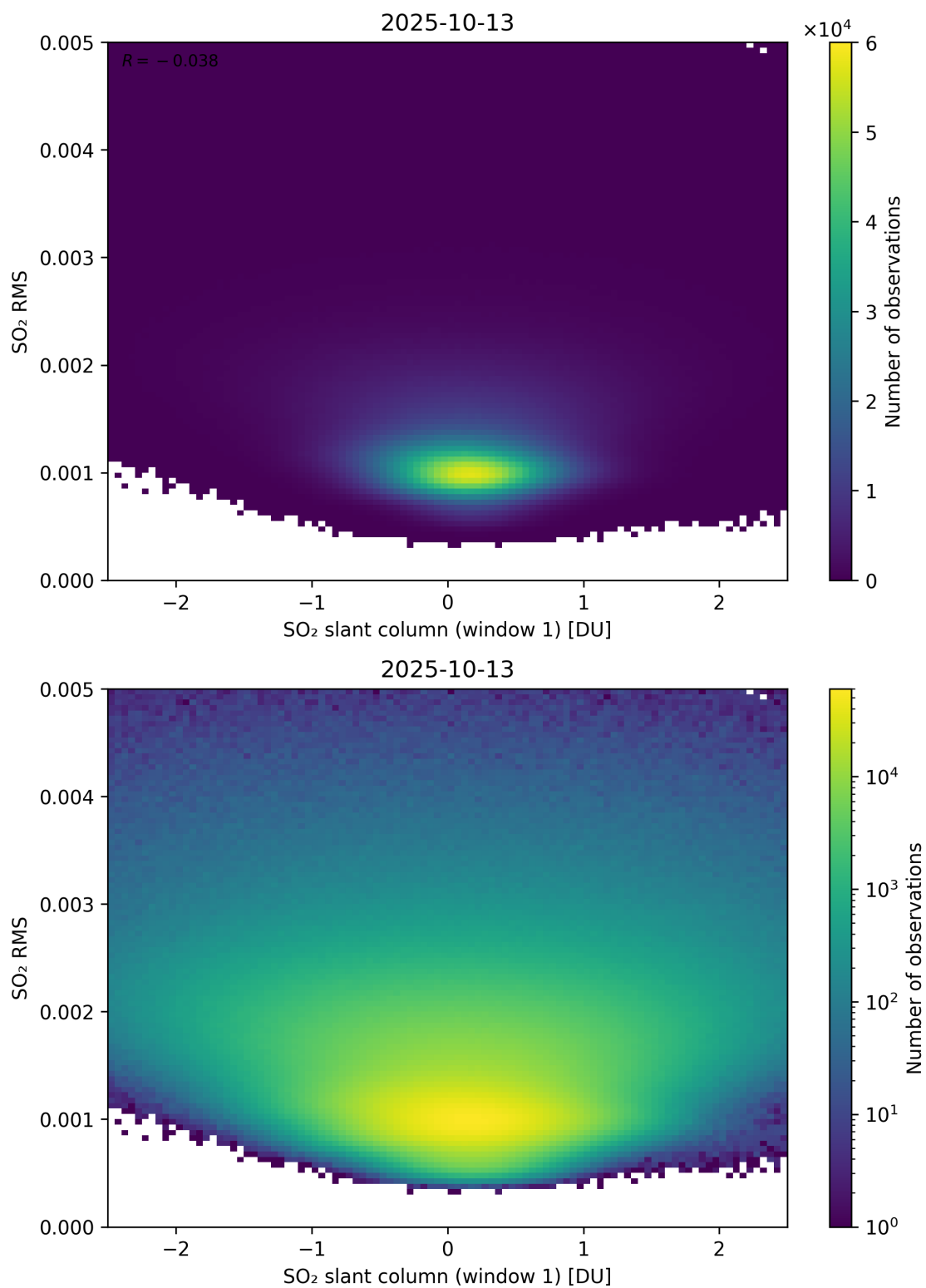
Figure 267: Scatter density plot of “SO 2 slant column (window 1)” against “SO 2 RMS” for 2025-10-12 to 2025-10-14.
