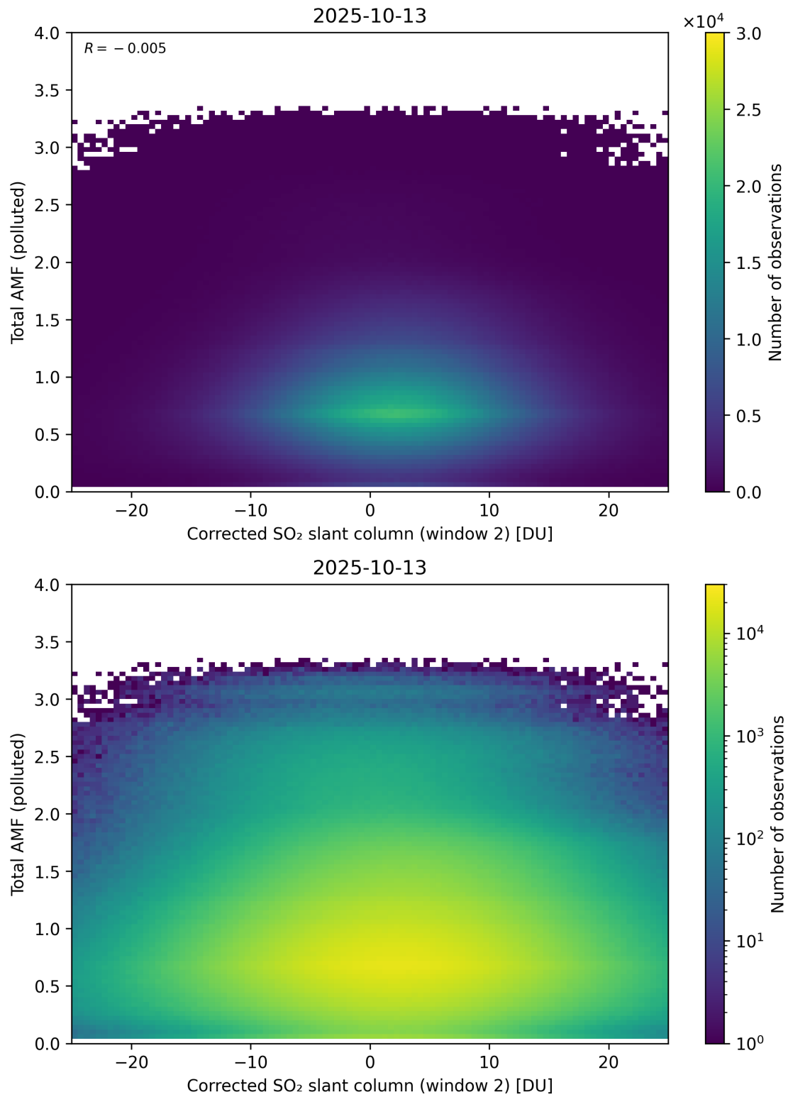
Figure 253: Scatter density plot of “Corrected SO 2 slant column (window 2)” against “Total AMF (polluted)” for 2025-10-12 to 2025-10-14.
