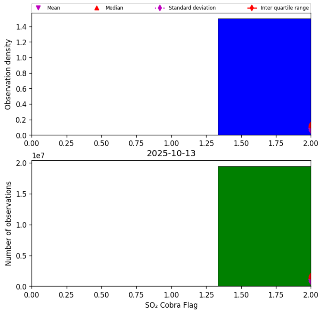
Figure 75: Histogram of “SO 2 Cobra Flag” for 2025-10-12 to 2025-10-14
