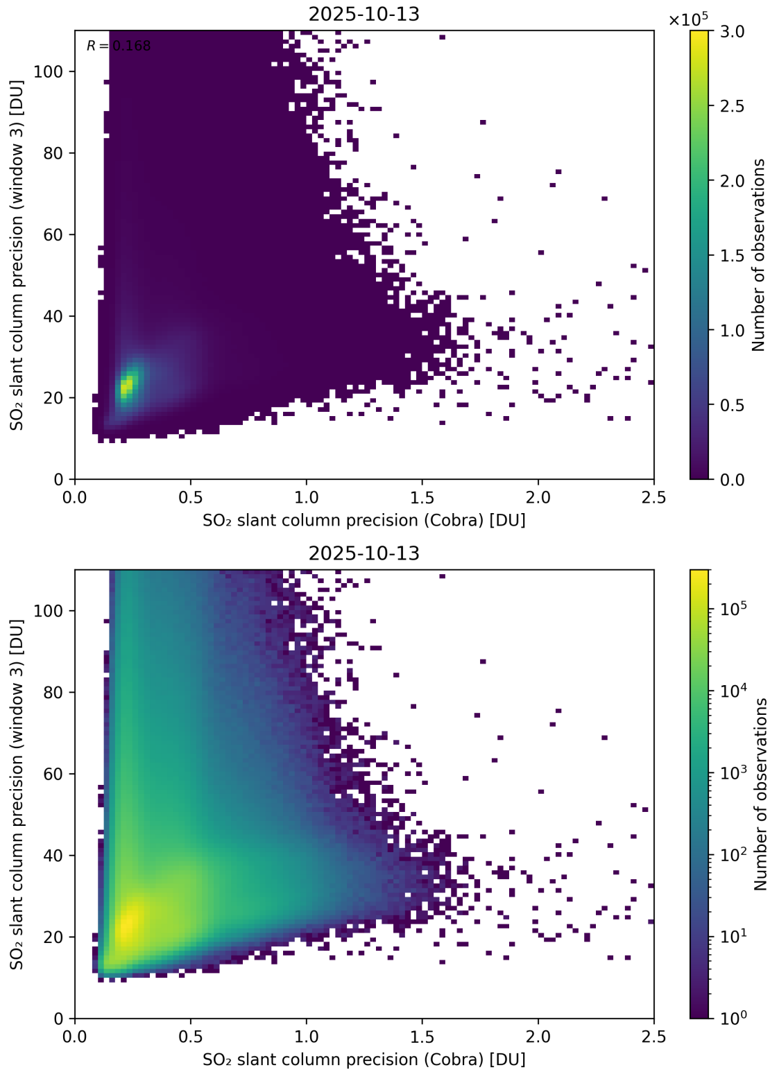
Figure 212: Scatter density plot of “SO 2 slant column precision (Cobra)” against “SO 2 slant column precision (window 3)” for 2025-10-12 to 2025-10-14.
