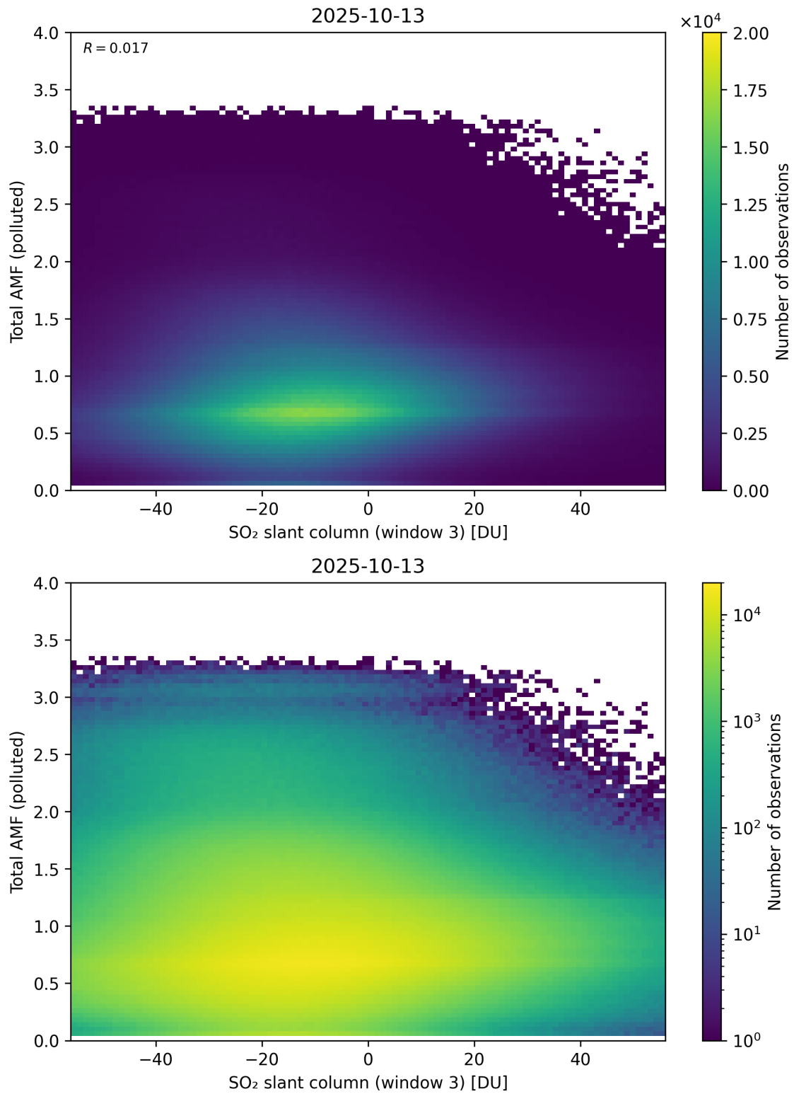
Figure 318: Scatter density plot of “SO 2 slant column (window 3)” against “Total AMF (polluted)” for 2025-10-12 to 2025-10-14.
