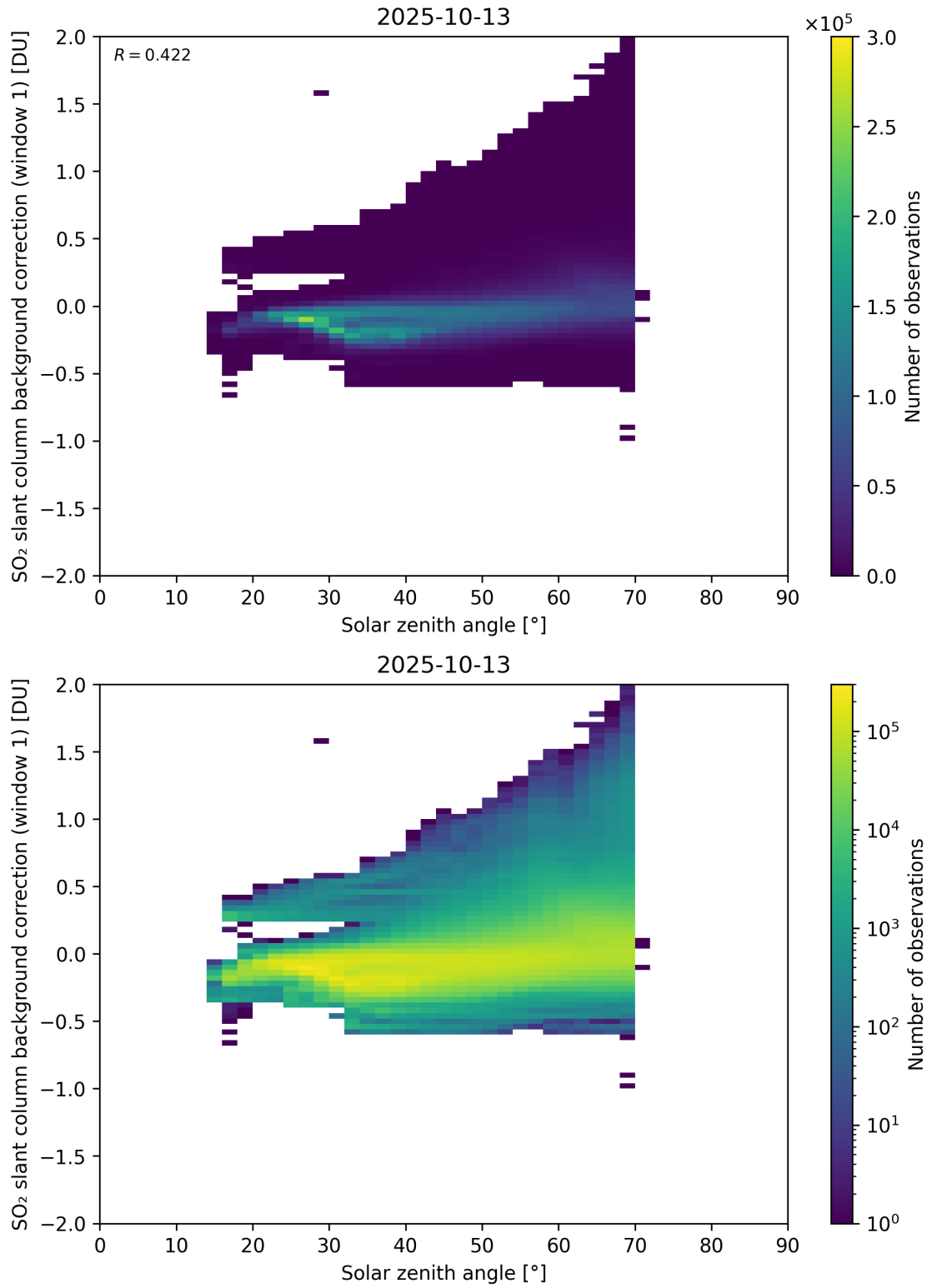
Figure 171: Scatter density plot of “Solar zenith angle” against “SO 2 slant column background correction (window 1)” for 2025-10-12 to 2025-10-14.
