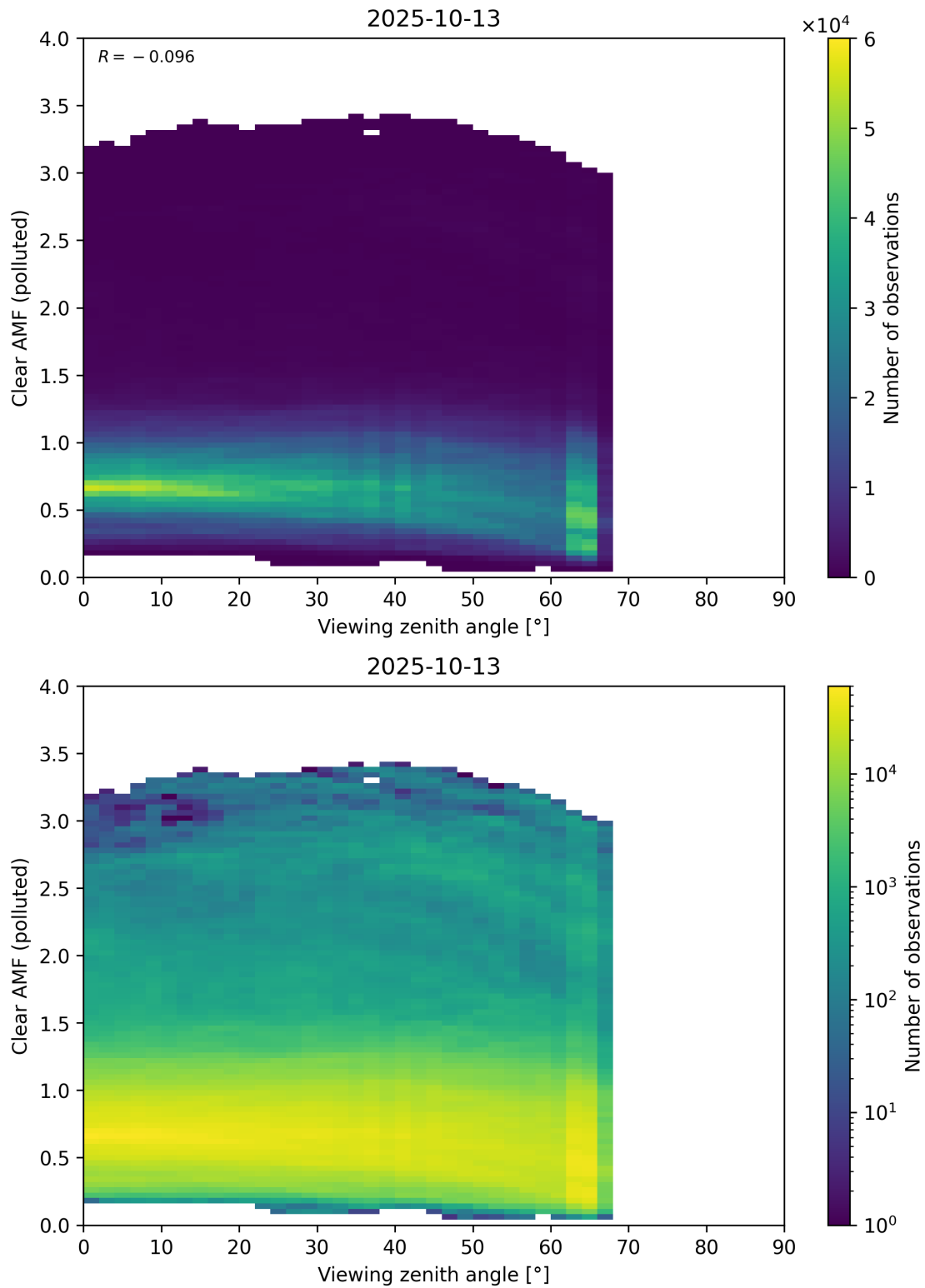
Figure 370: Scatter density plot of “Viewing zenith angle” against “Clear AMF (polluted)” for 2025-10-12 to 2025-10-14.
