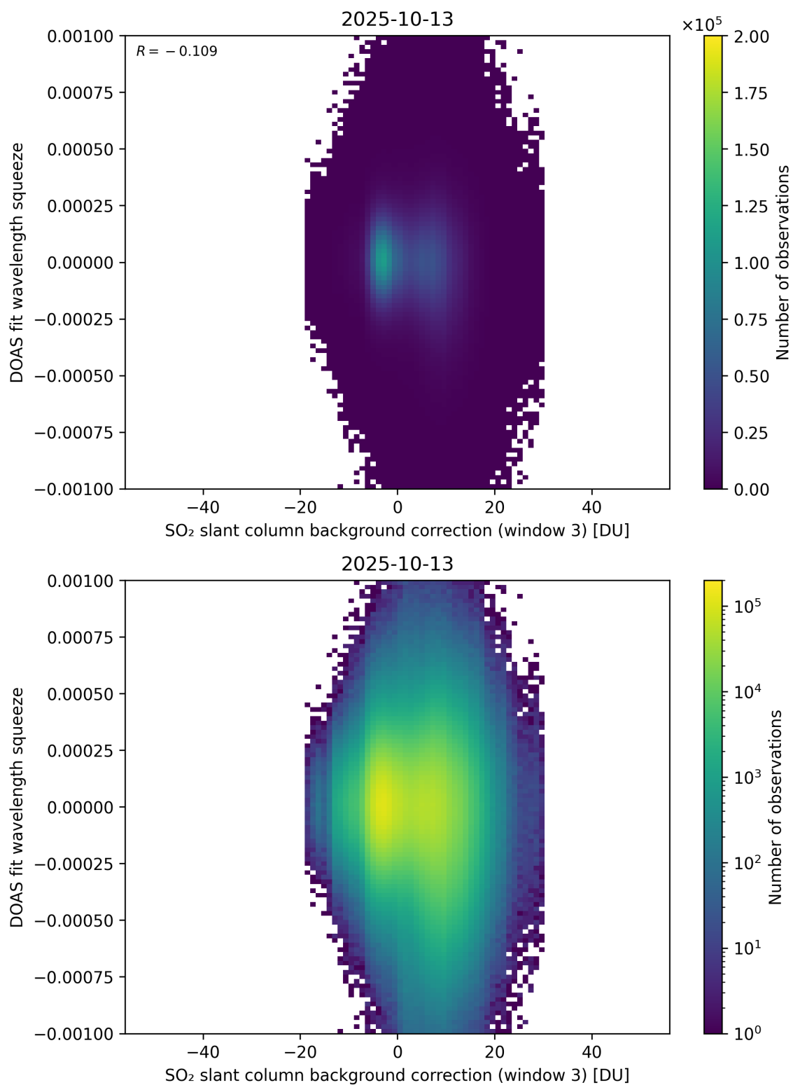
Figure 133: Scatter density plot of “SO 2 slant column background correction (window 3)” against “DOAS fit wavelength squeeze” for 2025-10-12 to 2025-10-14.
