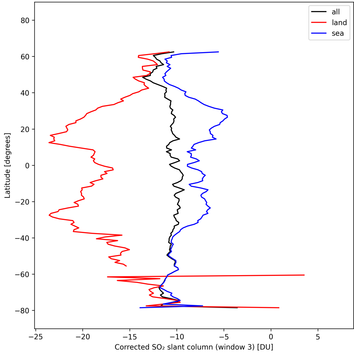
Figure 47: Zonal average of “Corrected SO 2 slant column (window 3)” for 2025-10-12 to 2025-10-14.
