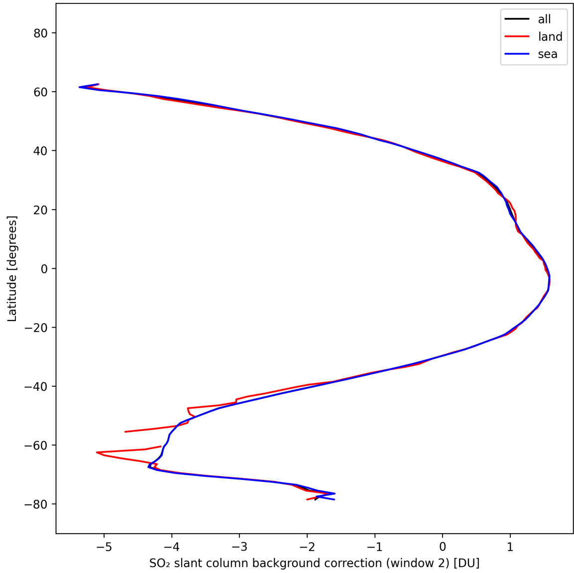
Figure 44: Zonal average of “SO 2 slant column background correction (window 2)” for 2025-10-12 to 2025-10-14.
