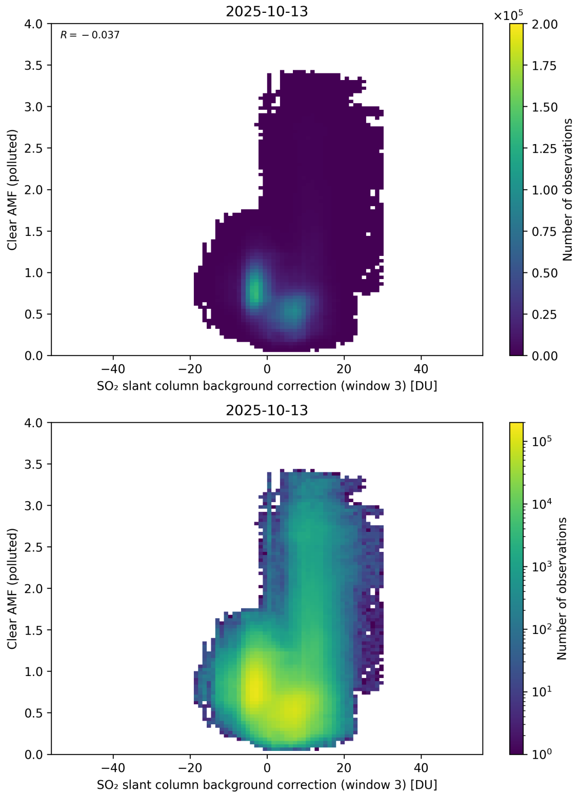
Figure 135: Scatter density plot of “SO 2 slant column background correction (window 3)” against “Clear AMF (polluted)” for 2025-10-12 to 2025-10-14.
