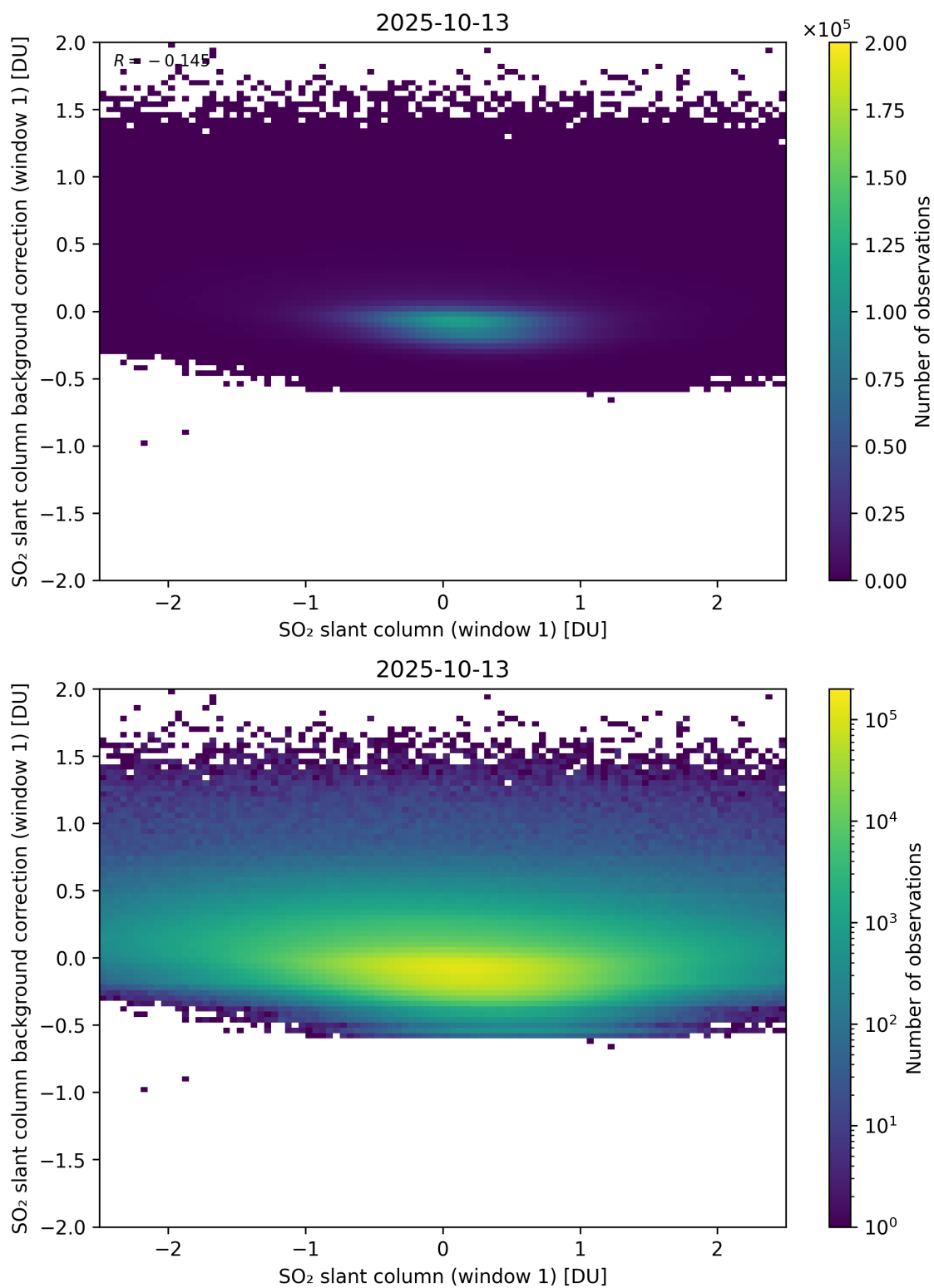
Figure 262: Scatter density plot of “SO 2 slant column (window 1)” against “SO 2 slant column background correction (window 1)” for 2025-10-12 to 2025-10-14.
