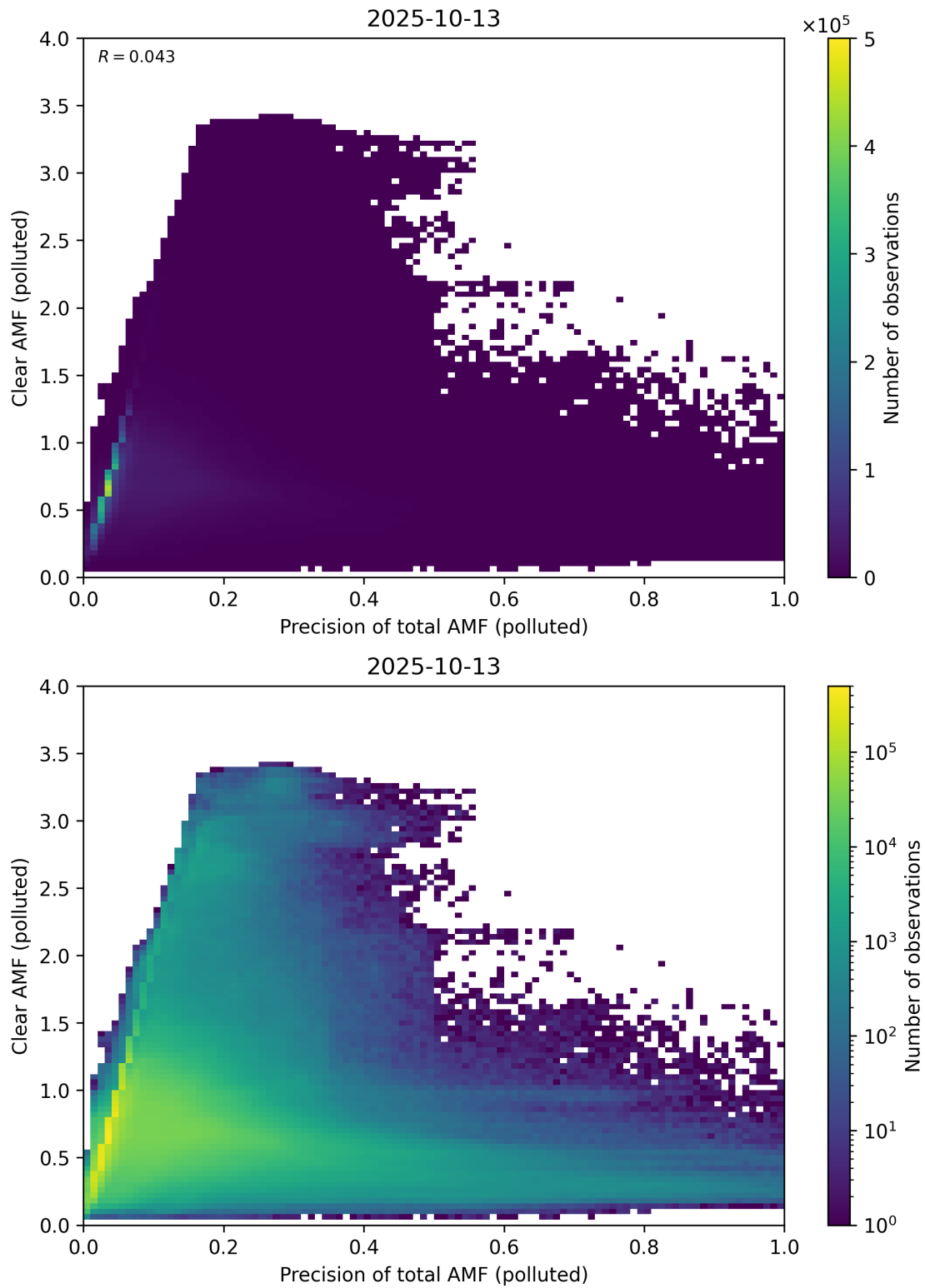
Figure 320: Scatter density plot of “Precision of total AMF (polluted)” against “Clear AMF (polluted)” for 2025-10-12 to 2025-10-14.
