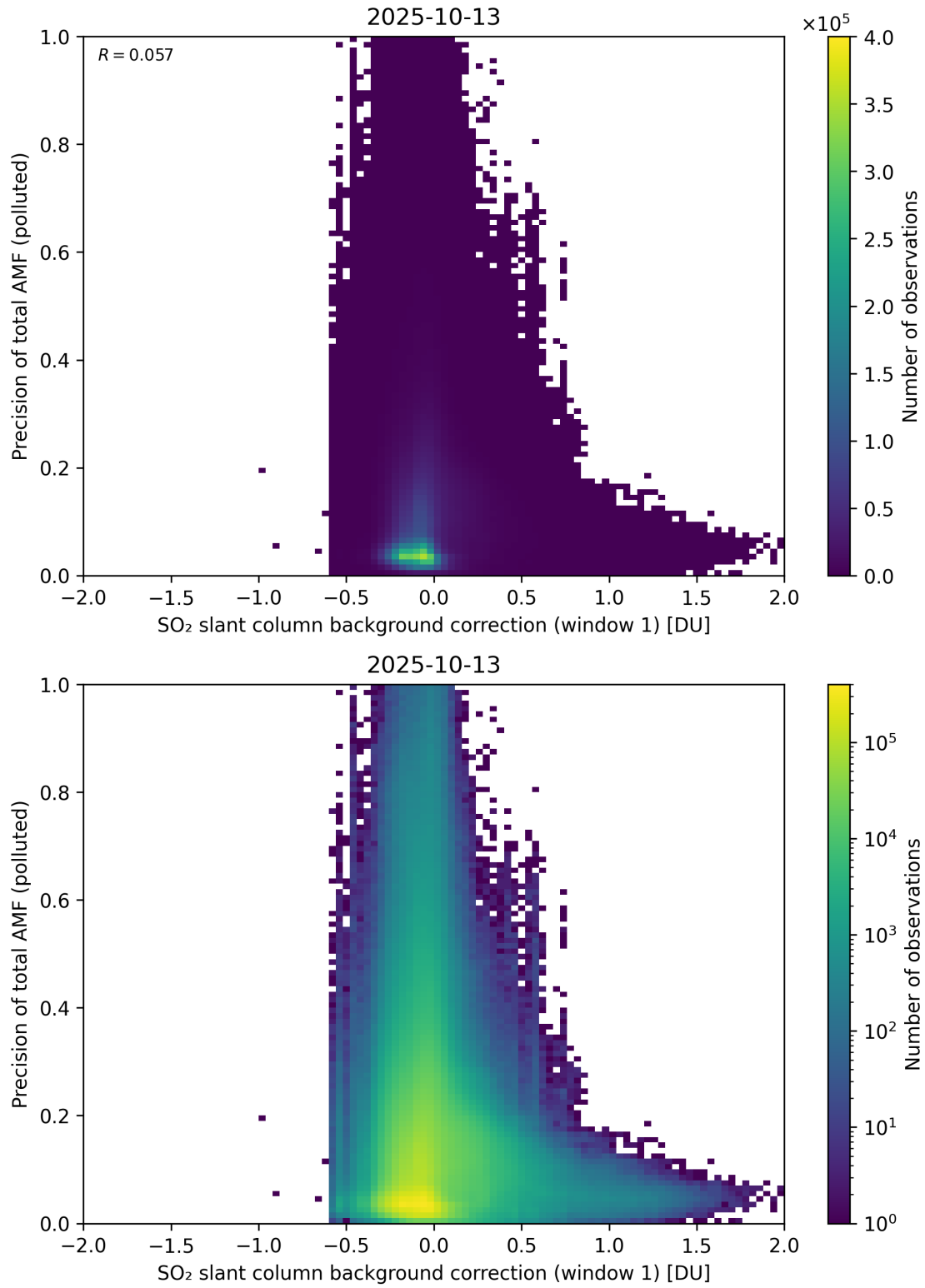
Figure 121: Scatter density plot of “SO 2 slant column background correction (window 1)” against “Precision of total AMF (polluted)” for 2025-10-12 to 2025-10-14.
