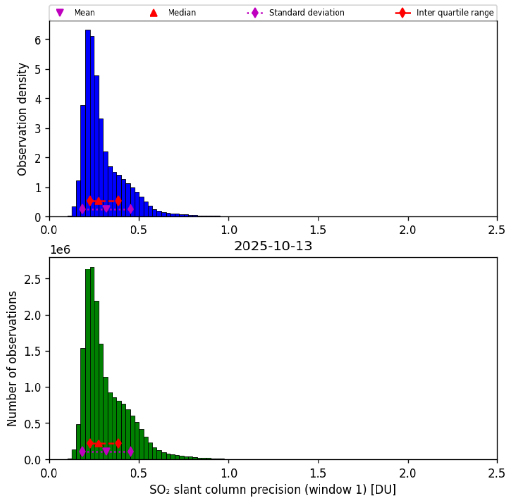
Figure 64: Histogram of “SO 2 slant column precision (window 1)” for 2025-10-12 to 2025-10-14
