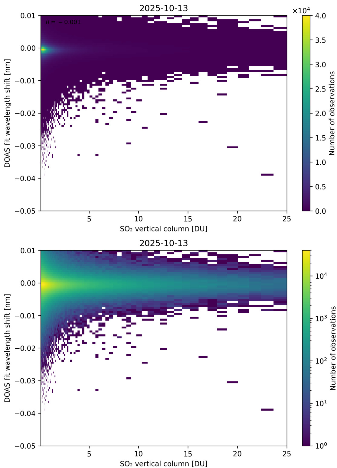
Figure 326: Scatter density plot of “SO 2 vertical column” against “DOAS fit wavelength shift” for 2025-10-12 to 2025-10-14.
