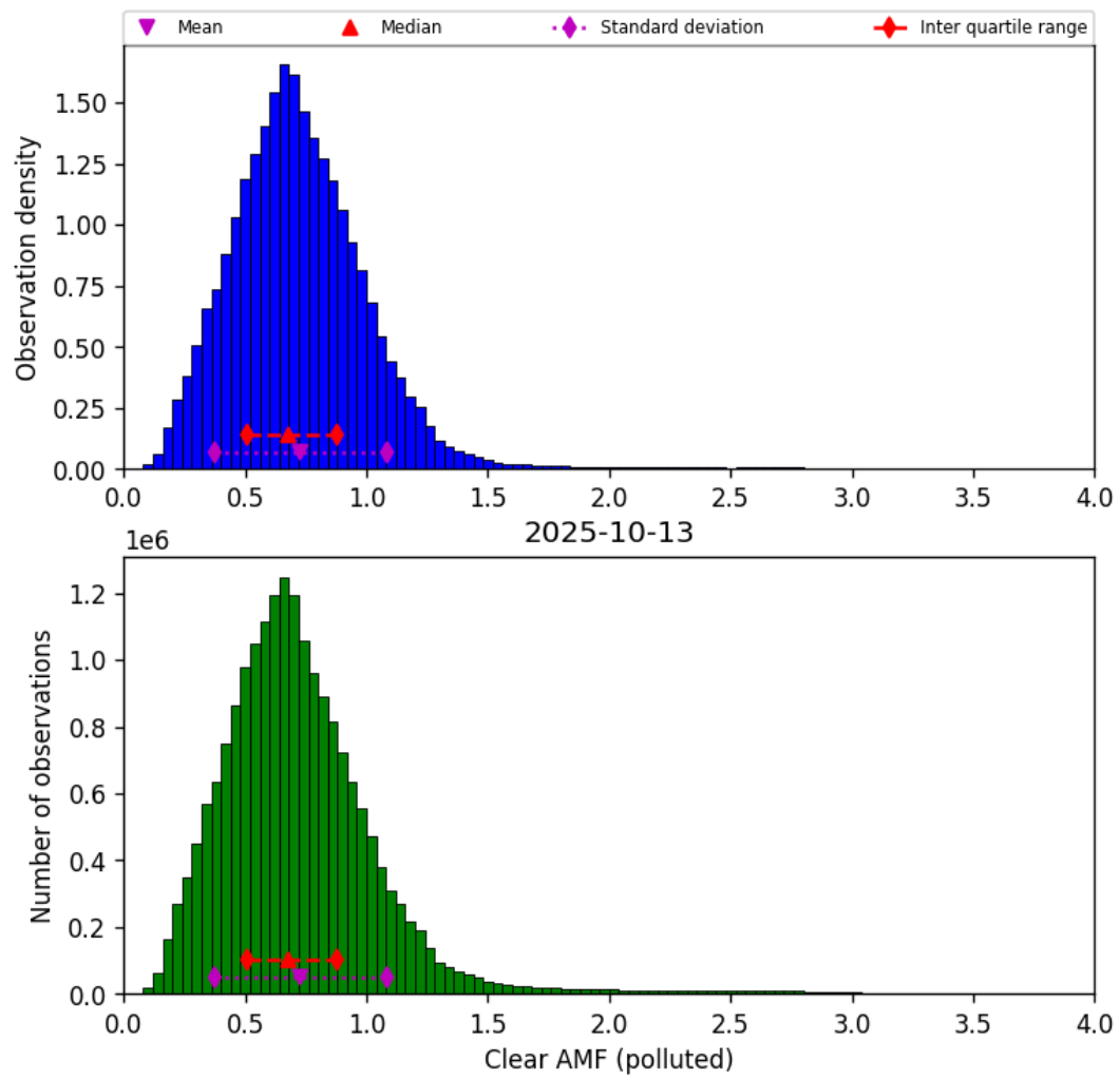
Figure 81: Histogram of “Clear AMF (polluted)” for 2025-10-12 to 2025-10-14
