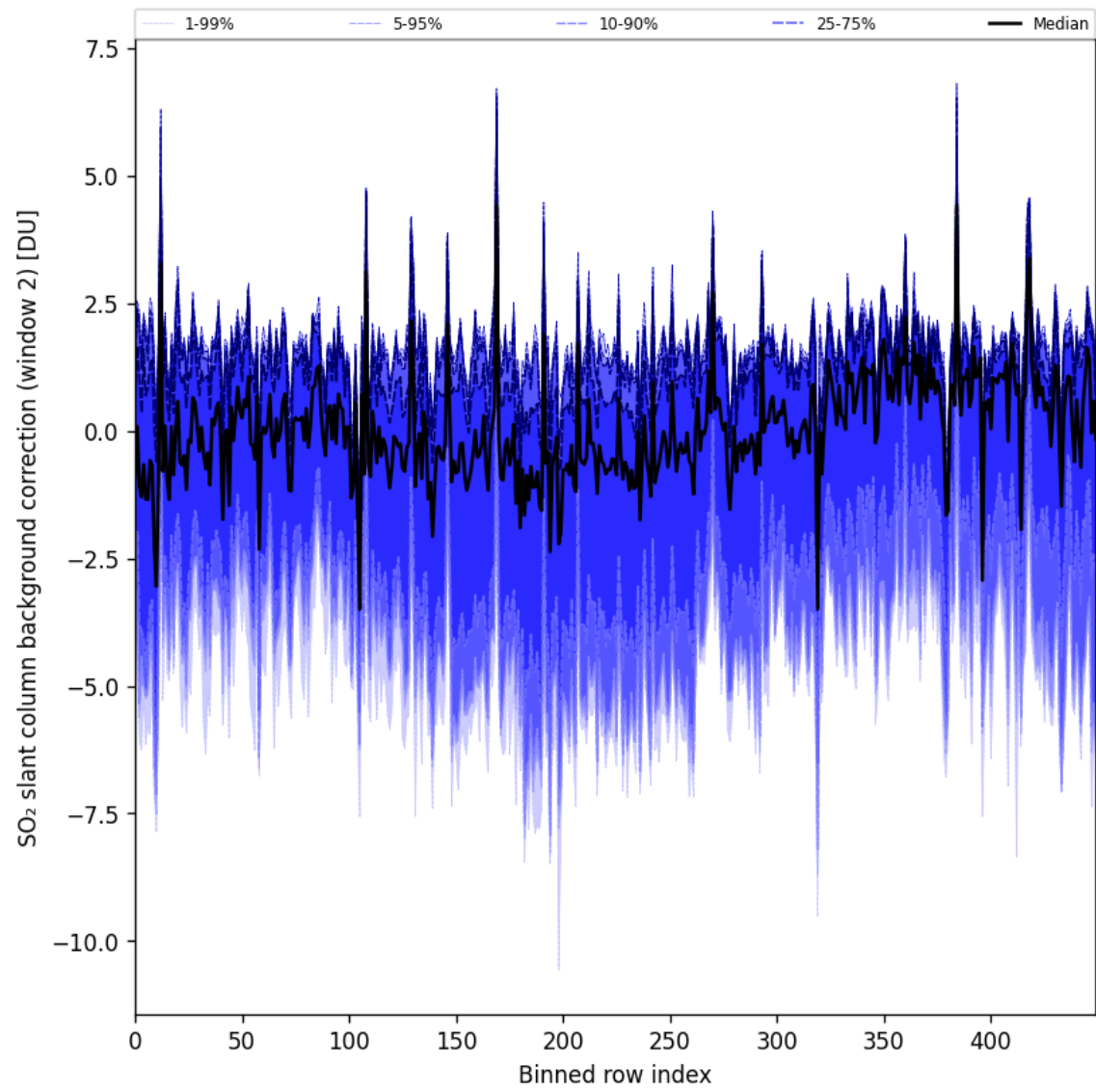
Figure 96: Along track statistics of “SO 2 slant column background correction (window 2)” for 2025-10-12 to 2025-10-14
