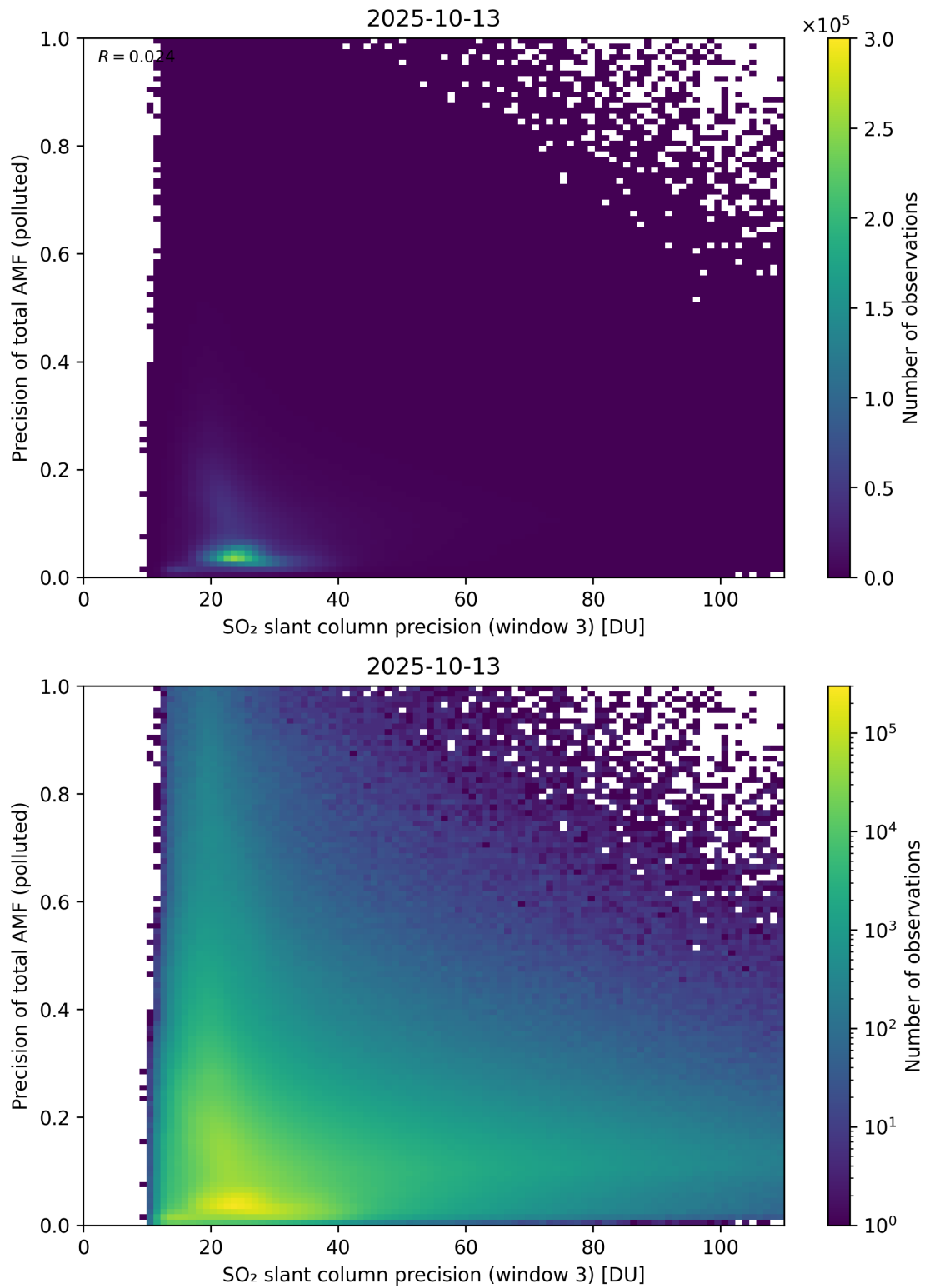
Figure 314: Scatter density plot of “SO 2 slant column precision (window 3)” against “Precision of total AMF (polluted)” for 2025-10-12 to 2025-10-14.
