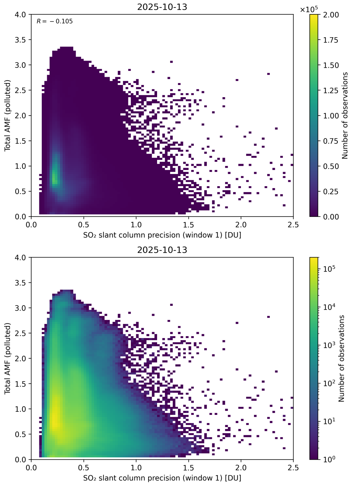
Figure 280: Scatter density plot of “SO 2 slant column precision (window 1)” against “Total AMF (polluted)” for 2025-10-12 to 2025-10-14.
