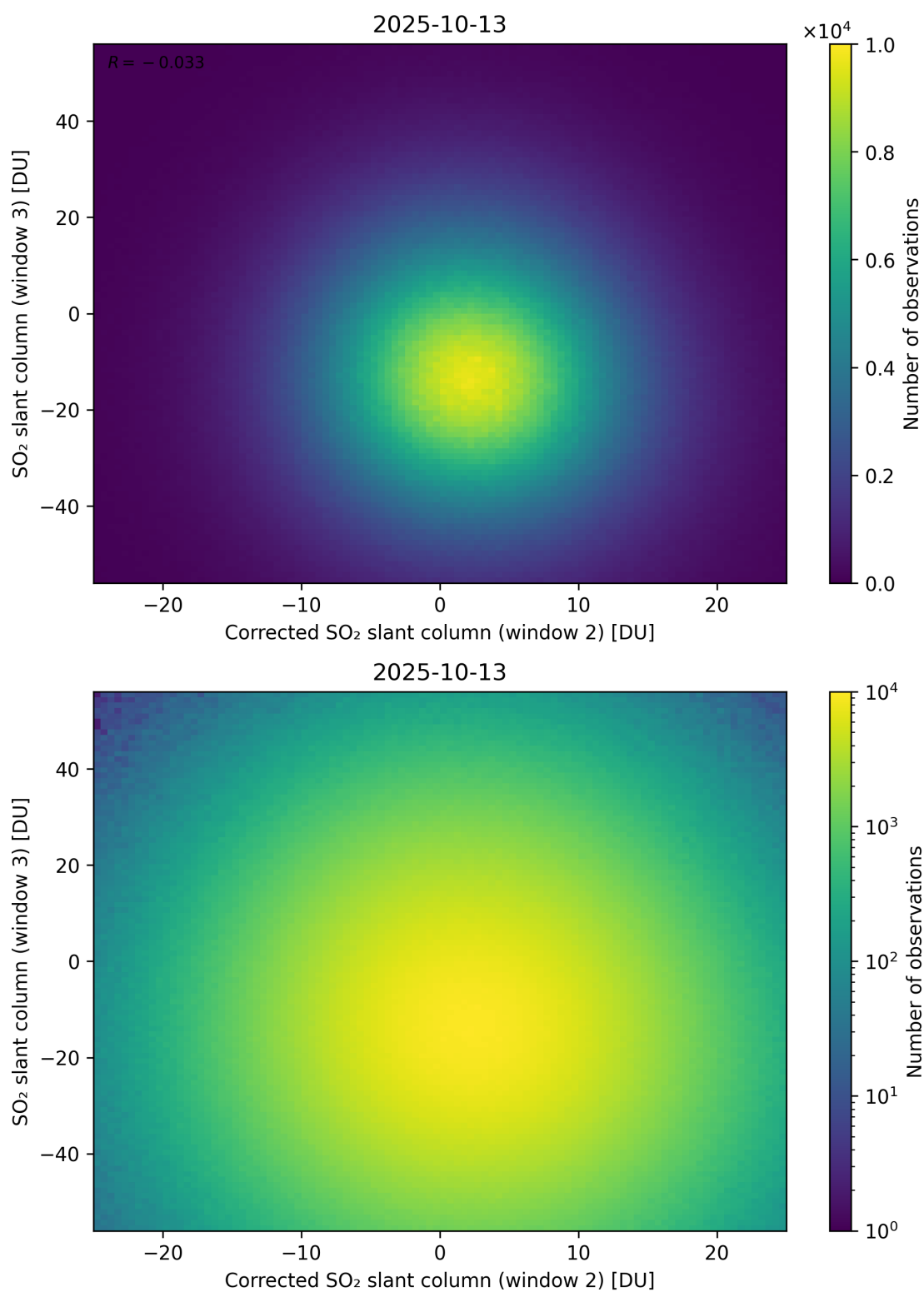
Figure 251: Scatter density plot of “Corrected SO 2 slant column (window 2)” against “SO 2 slant column (window 3)” for 2025-10-12 to 2025-10-14.
