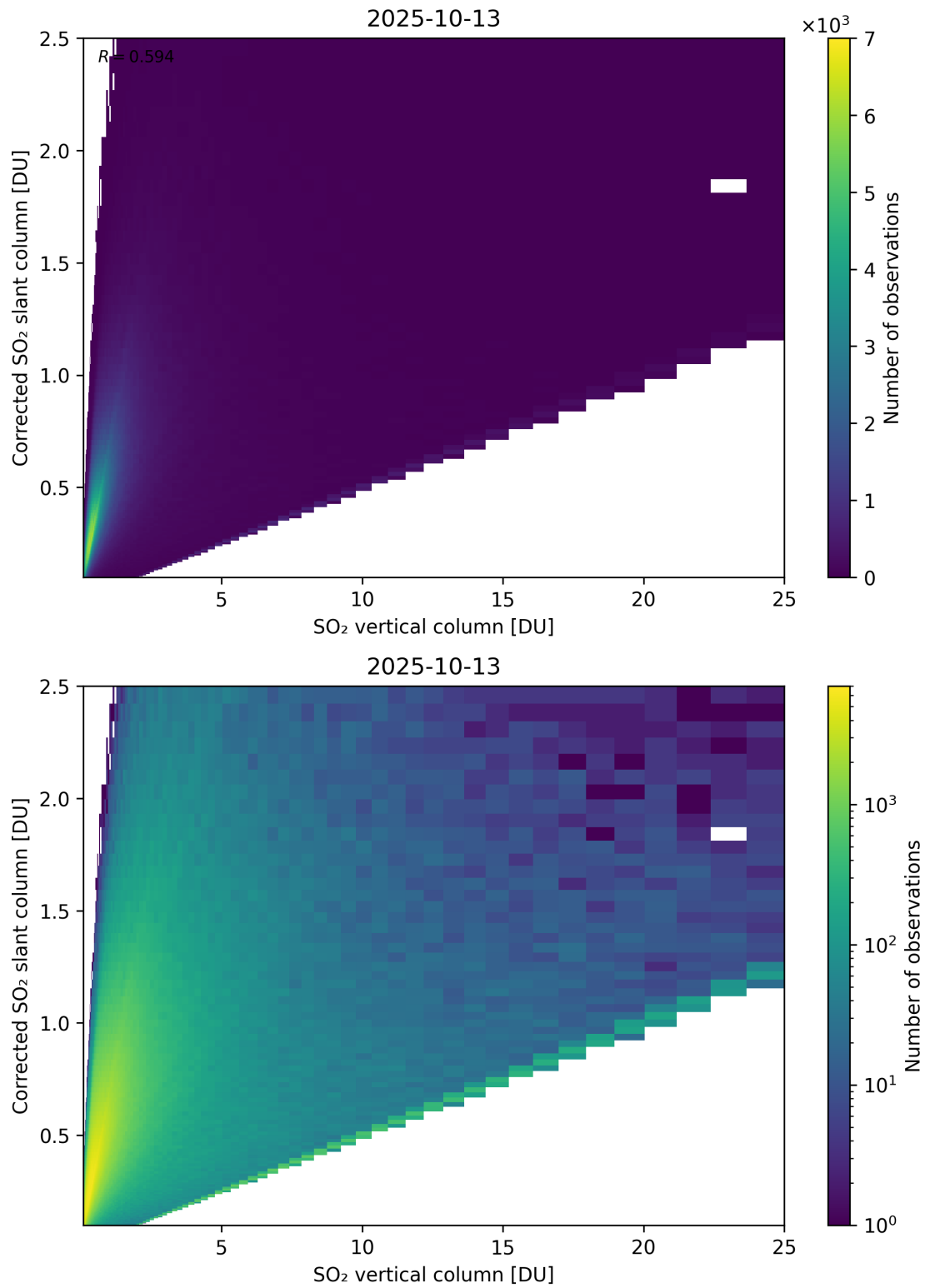
Figure 351: Scatter density plot of “SO 2 vertical column” against “Corrected SO 2 slant column” for 2025-10-12 to 2025-10-14.
