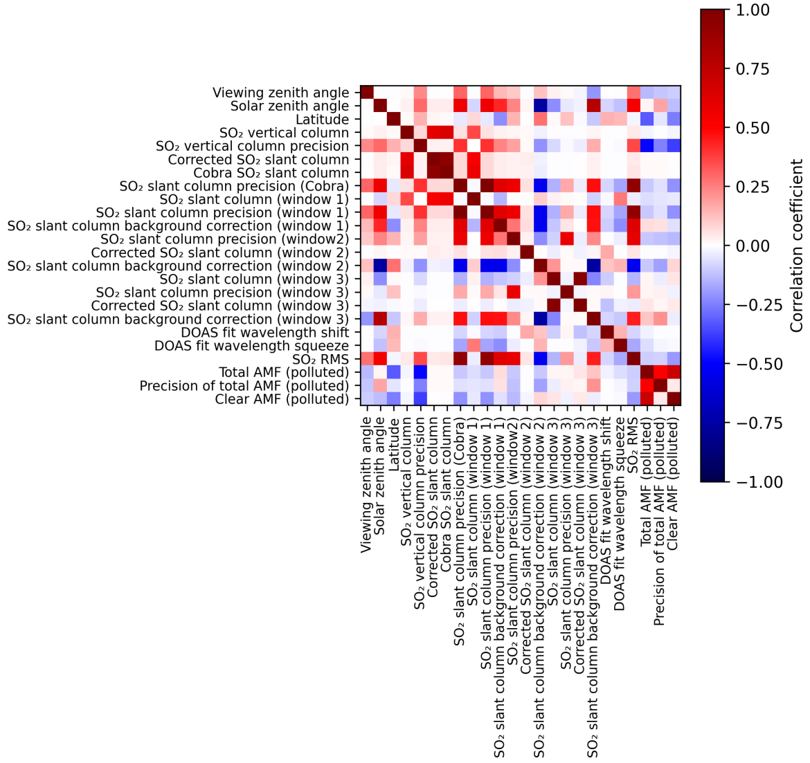
Figure 2: Map of correlation matrix for 2025-10-12 to 2025-10-14.
