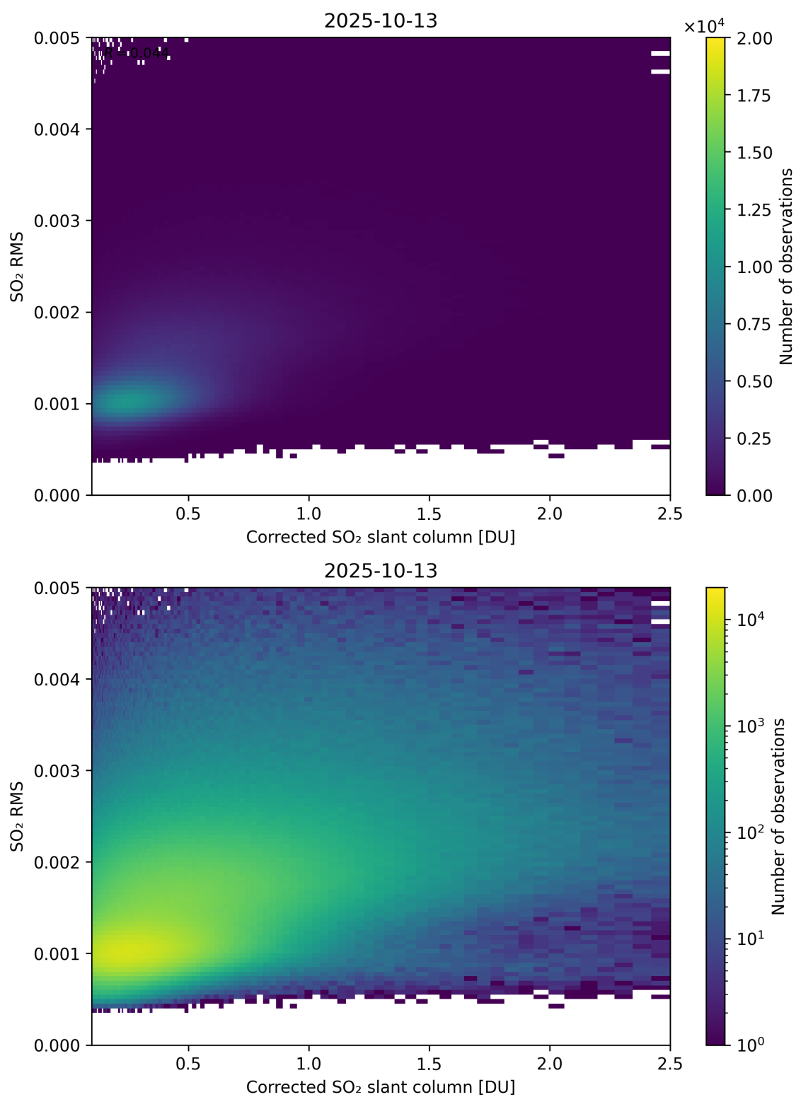
Figure 231: Scatter density plot of “Corrected SO 2 slant column” against “SO 2 RMS” for 2025-10-12 to 2025-10-14.
