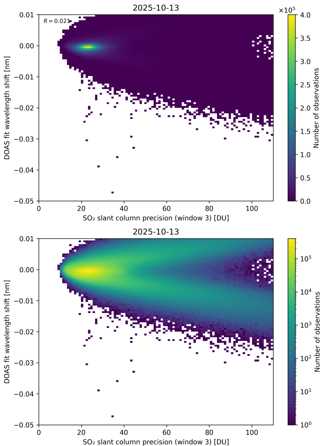
Figure 308: Scatter density plot of “SO 2 slant column precision (window 3)” against “DOAS fit wavelength shift” for 2025-10-12 to 2025-10-14.
