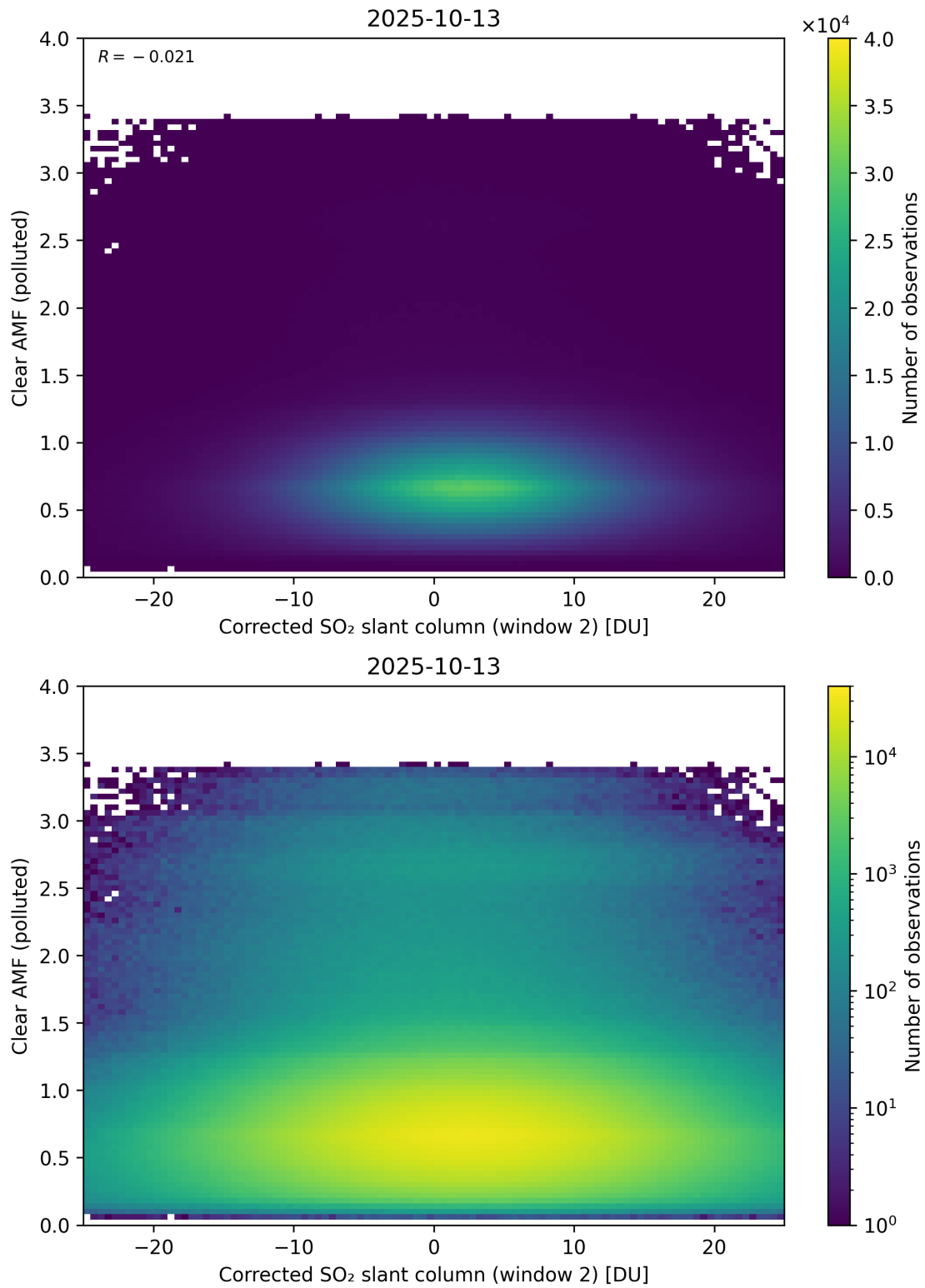
Figure 249: Scatter density plot of “Corrected SO 2 slant column (window 2)” against “Clear AMF (polluted)” for 2025-10-12 to 2025-10-14.
