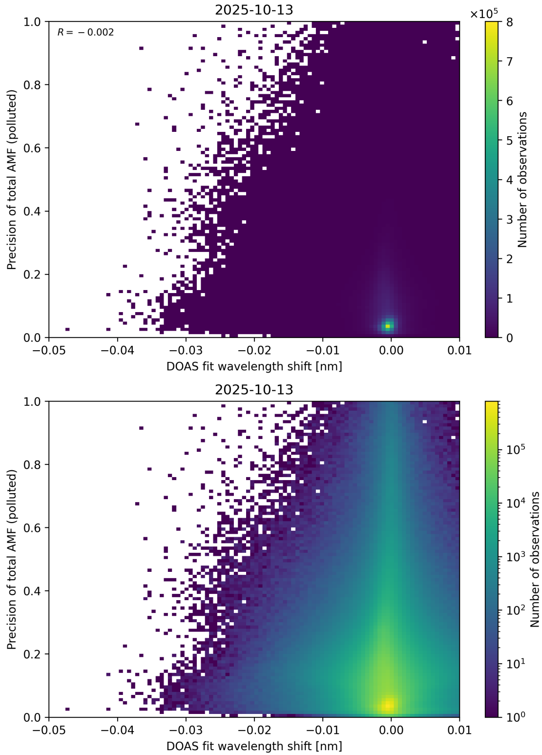
Figure 142: Scatter density plot of “DOAS fit wavelength shift” against “Precision of total AMF (polluted)” for 2025-10-12 to 2025-10-14.
