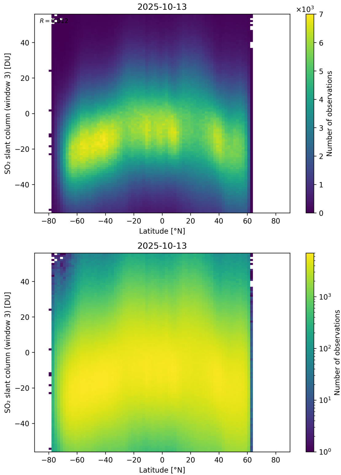
Figure 165: Scatter density plot of “Latitude” against “SO 2 slant column (window 3)” for 2025-10-12 to 2025-10-14.
