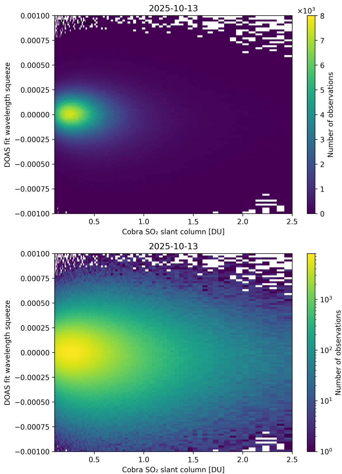
Figure 197: Scatter density plot of “Cobra SO 2 slant column” against “DOAS fit wavelength squeeze” for 2025-10-12 to 2025-10-14.
