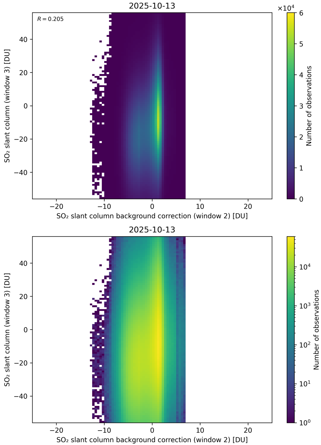
Figure 128: Scatter density plot of “SO 2 slant column background correction (window 2)” against “SO 2 slant column (window 3)” for 2025-10-12 to 2025-10-14.
