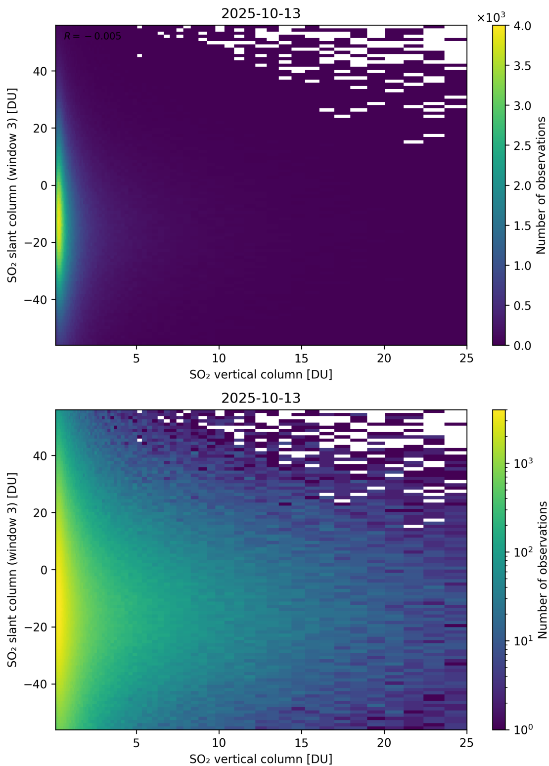
Figure 357: Scatter density plot of “SO 2 vertical column” against “SO 2 slant column (window 3)” for 2025-10-12 to 2025-10-14.
