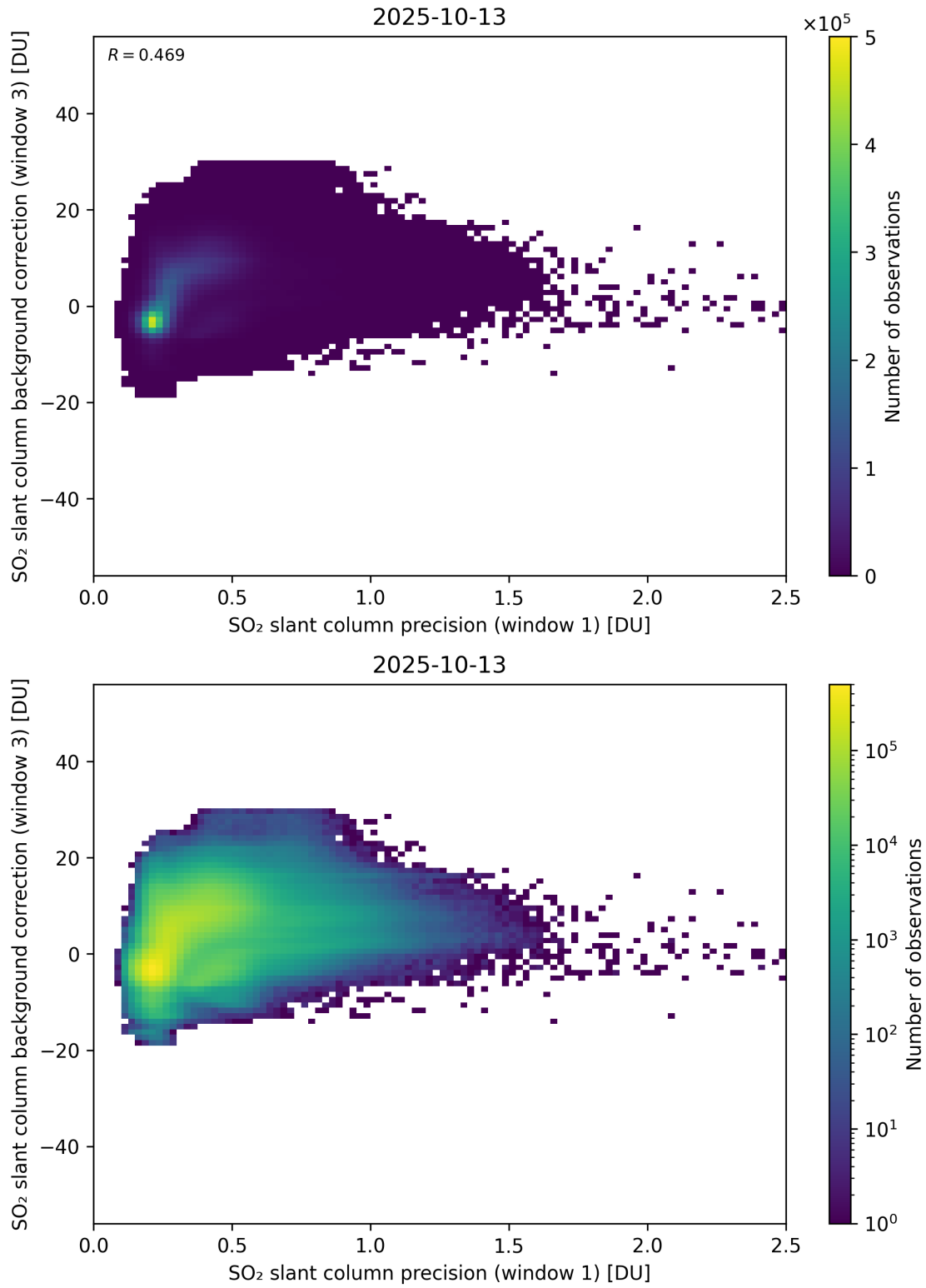
Figure 270: Scatter density plot of “SO 2 slant column precision (window 1)” against “SO 2 slant column background correction (window 3)” for 2025-10-12 to 2025-10-14.
