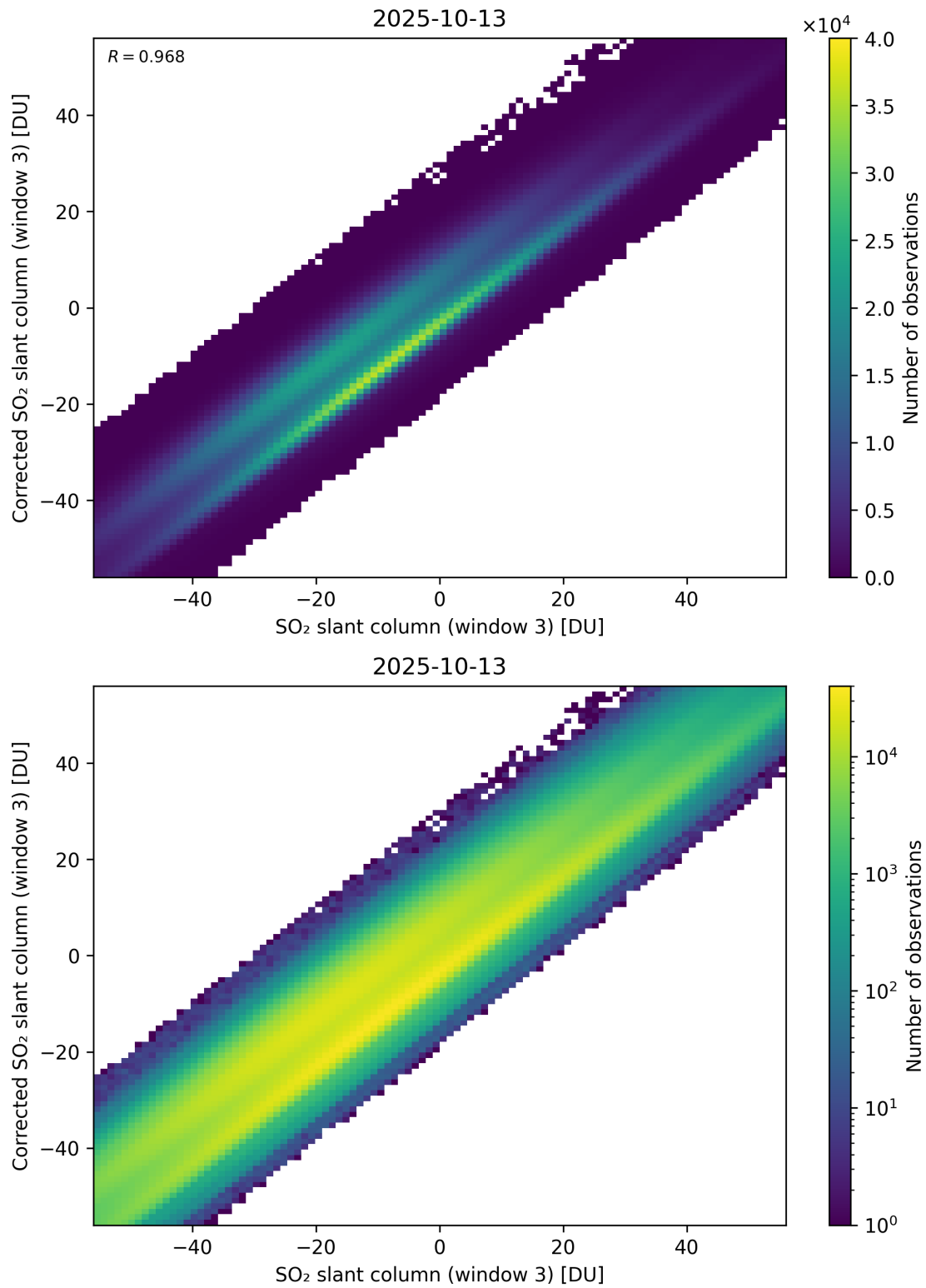
Figure 316: Scatter density plot of “SO 2 slant column (window 3)” against “Corrected SO 2 slant column (window 3)” for 2025-10-12 to 2025-10-14.
