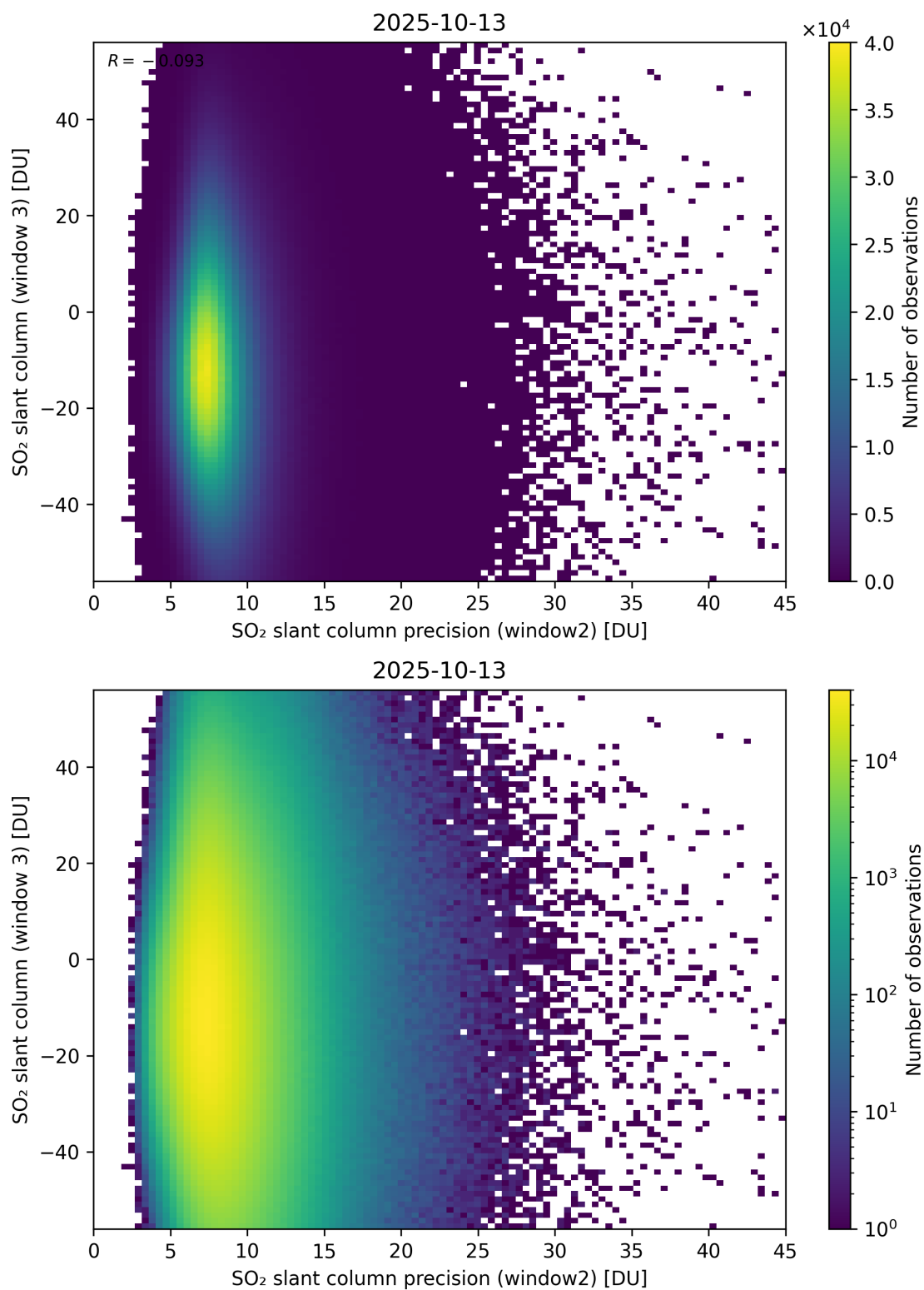
Figure 299: Scatter density plot of “SO 2 slant column precision (window2)” against “SO 2 slant column (window 3)” for 2025-10-12 to 2025-10-14.
