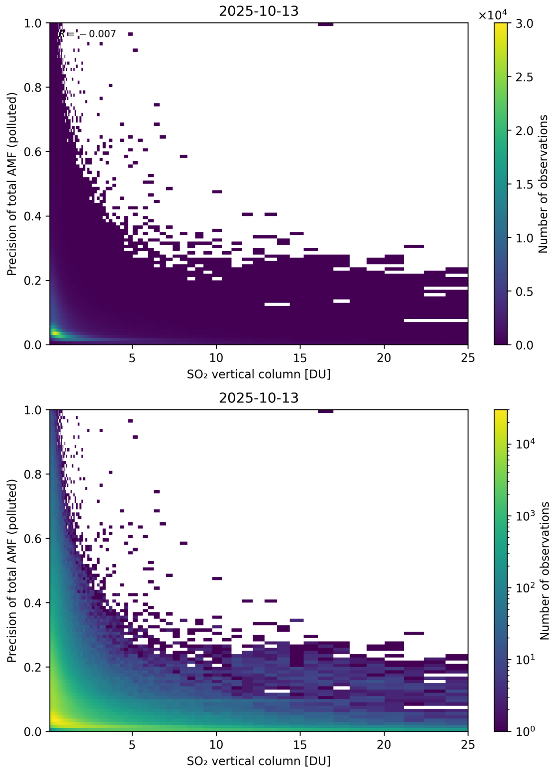
Figure 360: Scatter density plot of “SO 2 vertical column” against “Precision of total AMF (polluted)” for 2025-10-12 to 2025-10-14.
