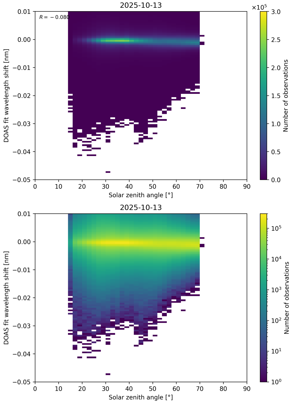
Figure 174: Scatter density plot of “Solar zenith angle” against “DOAS fit wavelength shift” for 2025-10-12 to 2025-10-14.
