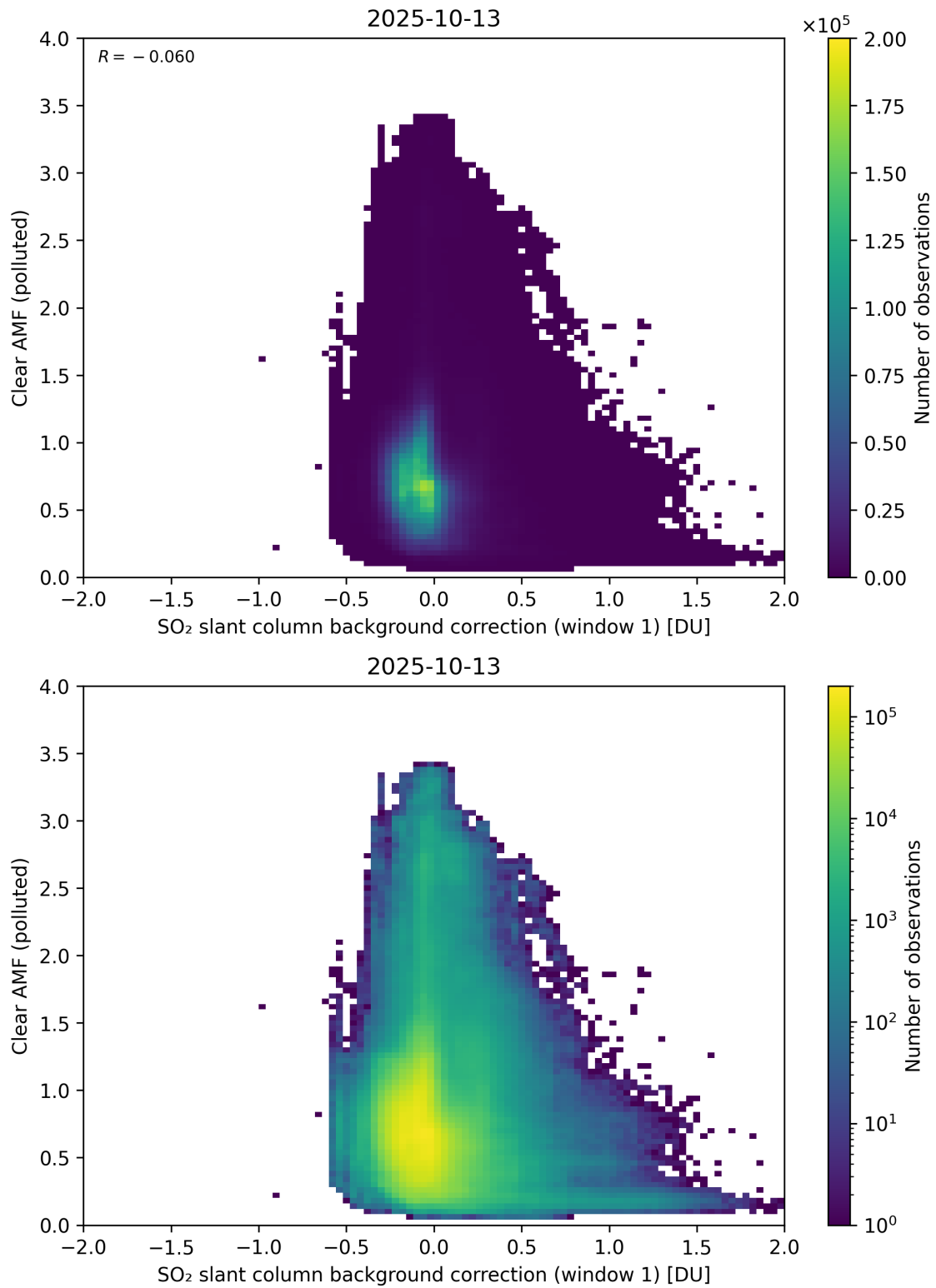
Figure 114: Scatter density plot of “SO 2 slant column background correction (window 1)” against “Clear AMF (polluted)” for 2025-10-12 to 2025-10-14.
