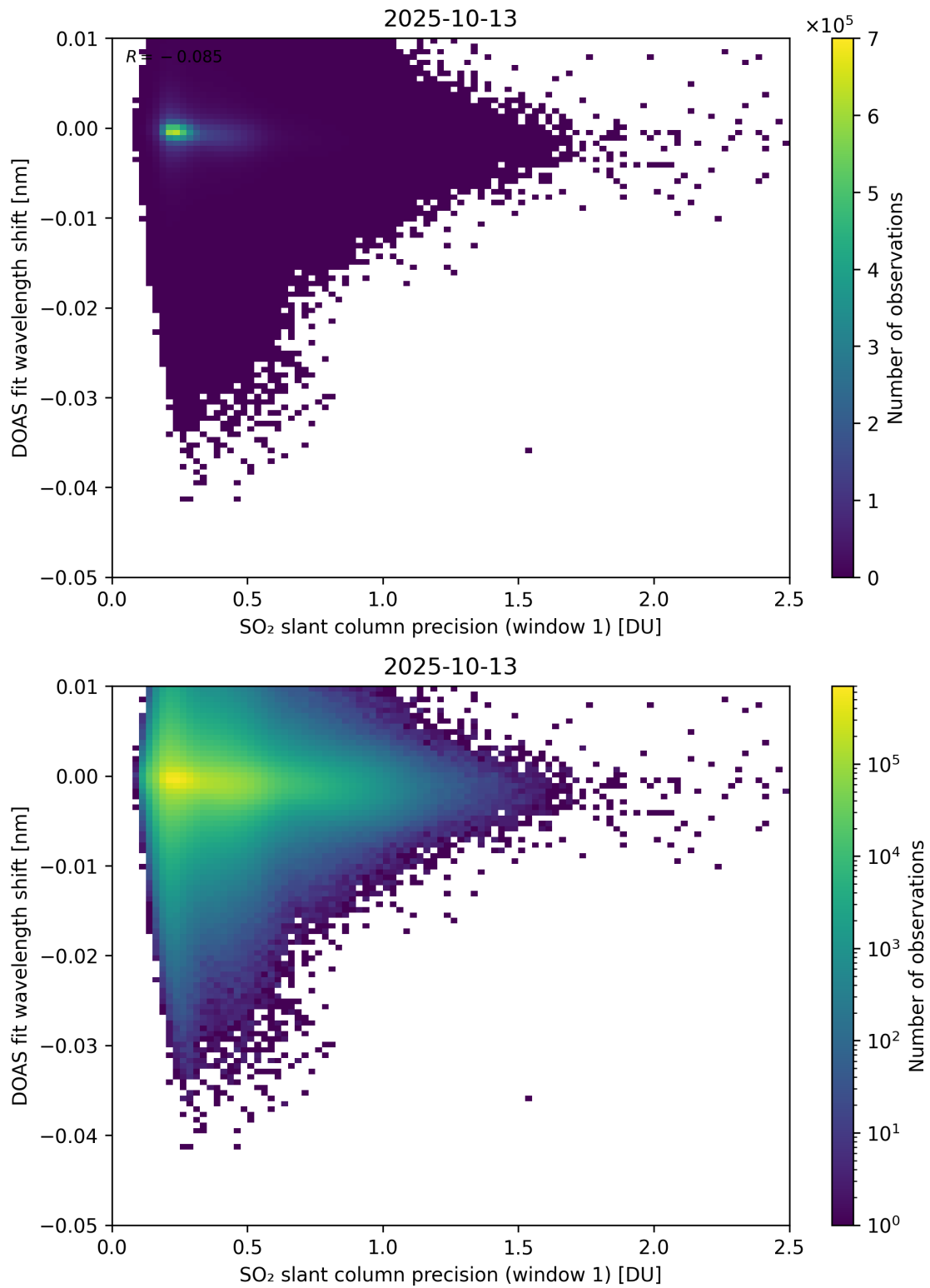
Figure 271: Scatter density plot of “SO 2 slant column precision (window 1)” against “DOAS fit wavelength shift” for 2025-10-12 to 2025-10-14.
