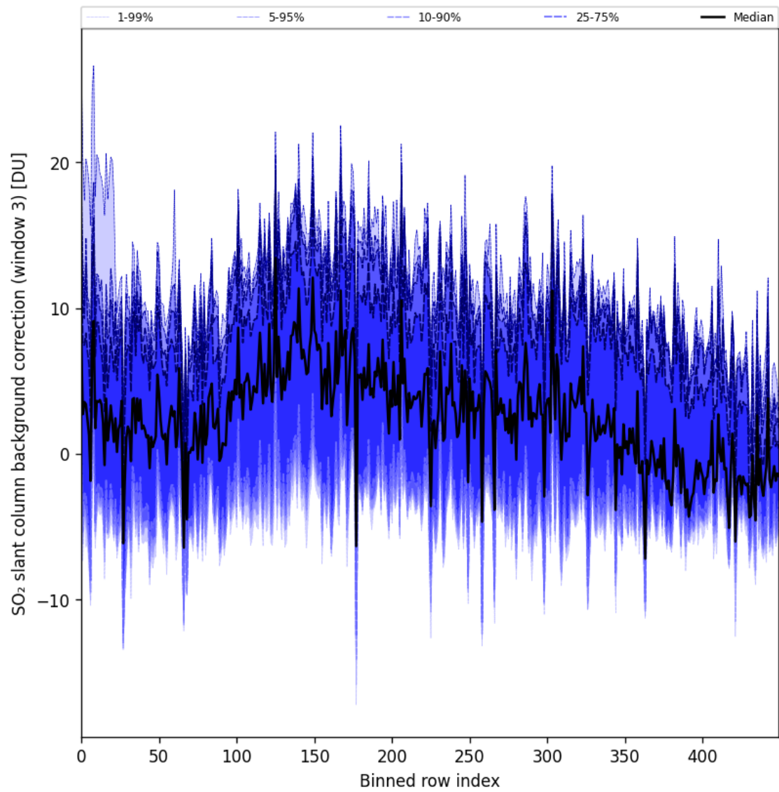
Figure 100: Along track statistics of “SO 2 slant column background correction (window 3)” for 2025-10-12 to 2025-10-14
