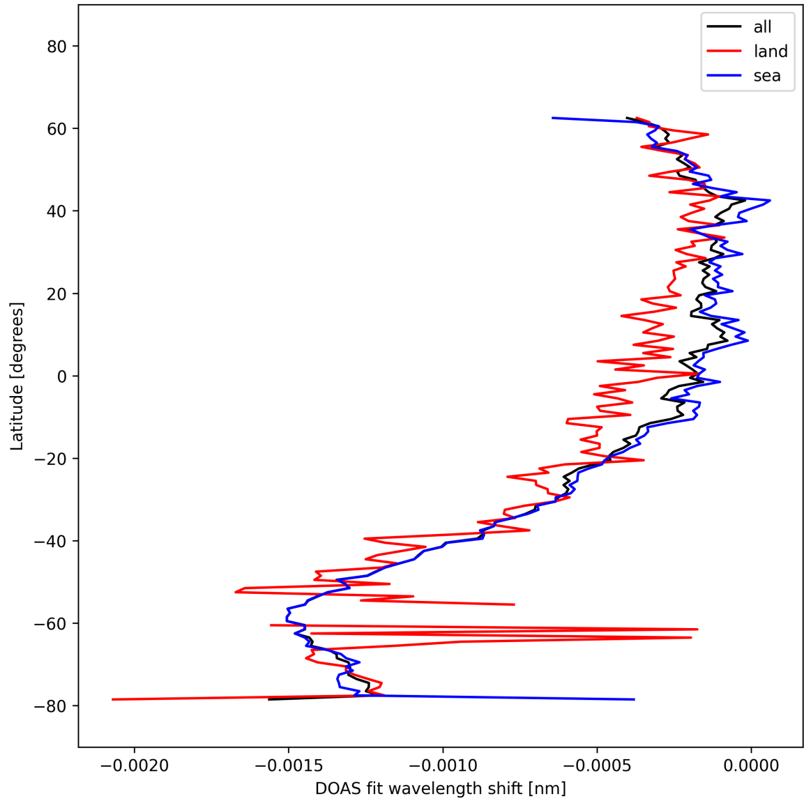
Figure 50: Zonal average of “DOAS fit wavelength shift” for 2025-10-12 to 2025-10-14.
