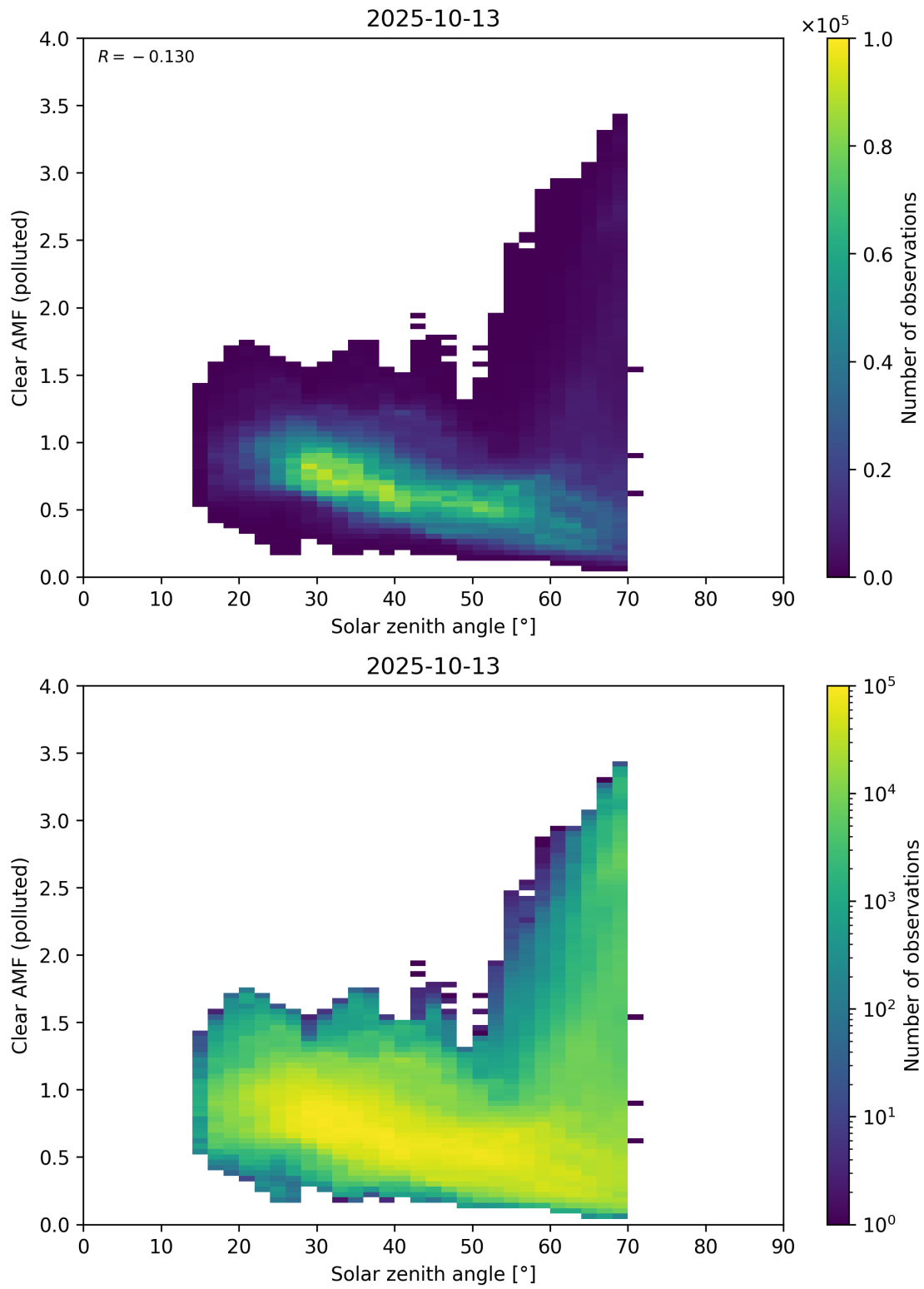
Figure 178: Scatter density plot of “Solar zenith angle” against “Clear AMF (polluted)” for 2025-10-12 to 2025-10-14.
