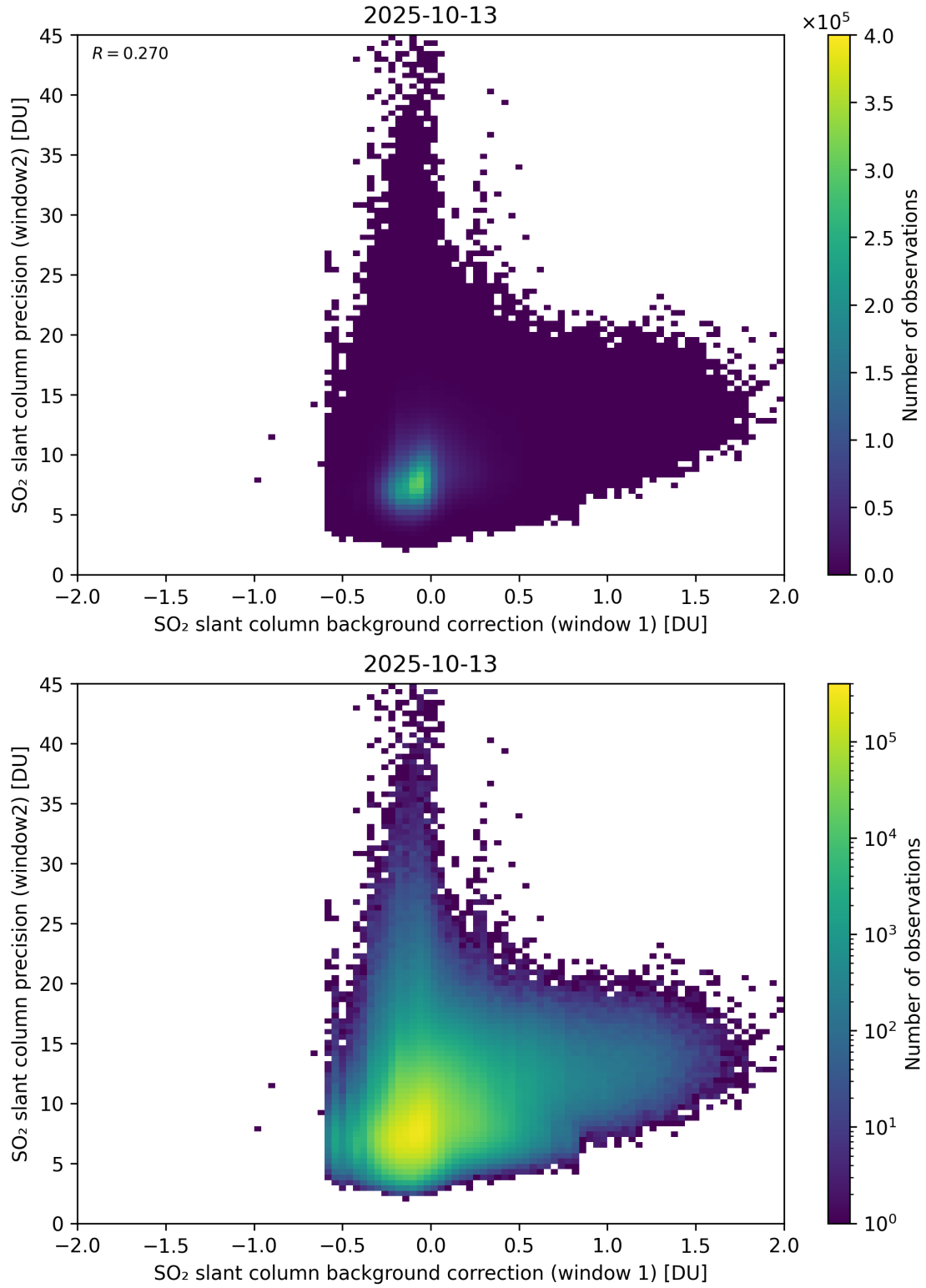
Figure 117: Scatter density plot of “SO 2 slant column background correction (window 1)” against “SO 2 slant column precision (window2)” for 2025-10-12 to 2025-10-14.
