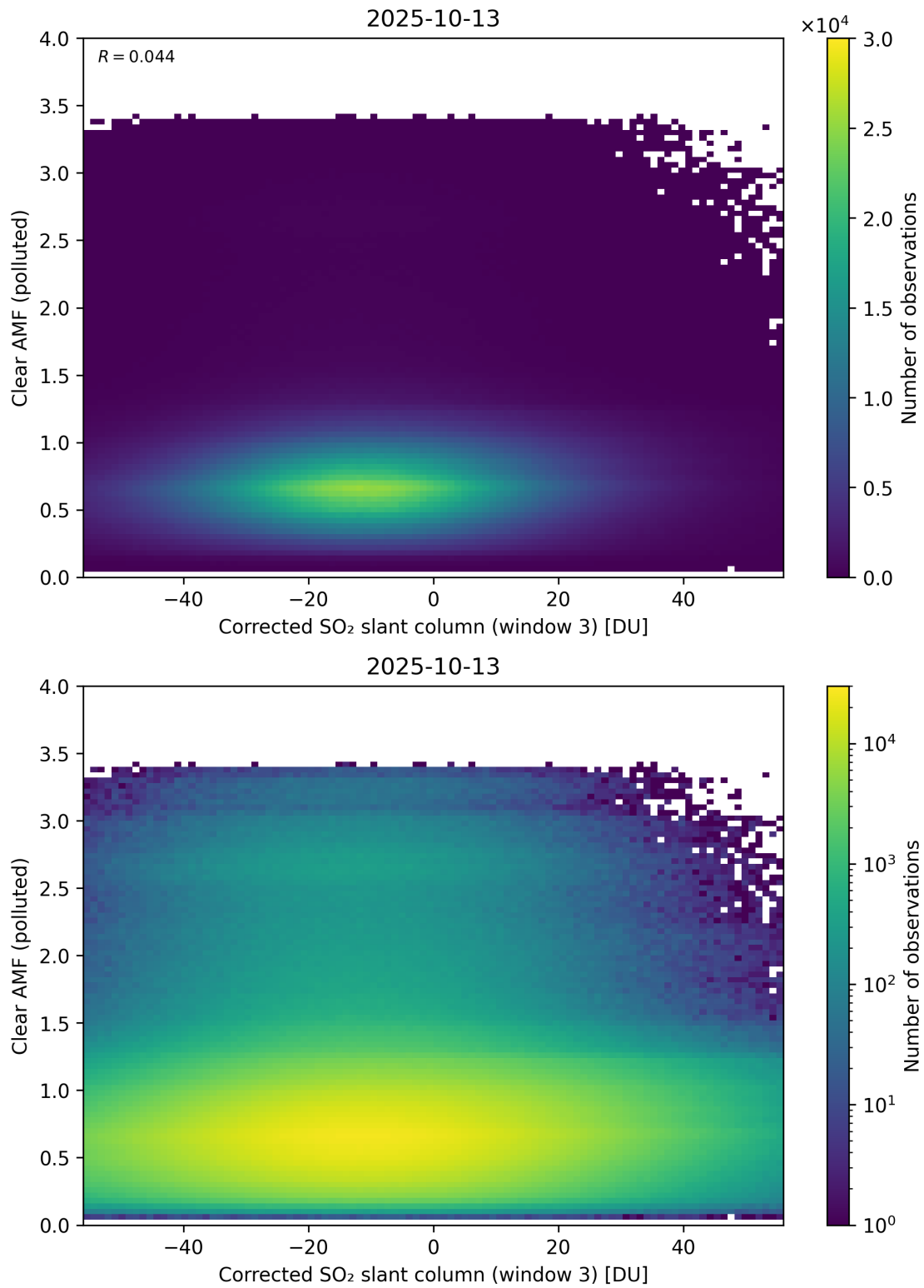
Figure 259: Scatter density plot of “Corrected SO 2 slant column (window 3)” against “Clear AMF (polluted)” for 2025-10-12 to 2025-10-14.
