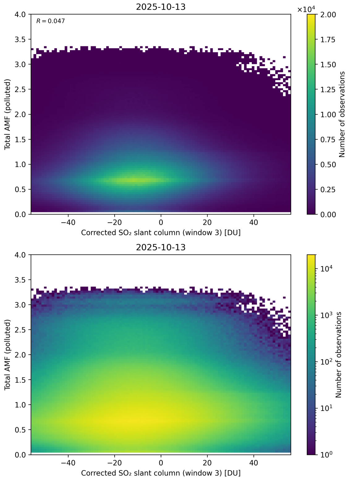
Figure 260: Scatter density plot of “Corrected SO 2 slant column (window 3)” against “Total AMF (polluted)” for 2025-10-12 to 2025-10-14.
