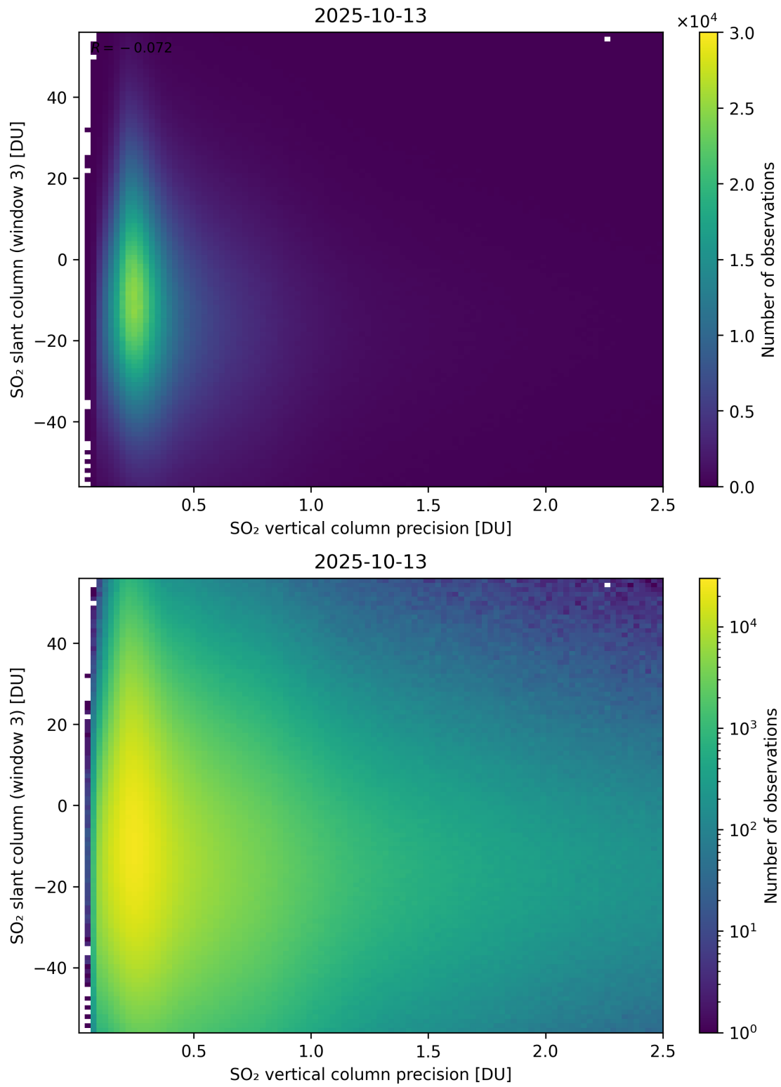
Figure 344: Scatter density plot of “SO 2 vertical column precision” against “SO 2 slant column (window 3)” for 2025-10-12 to 2025-10-14.
