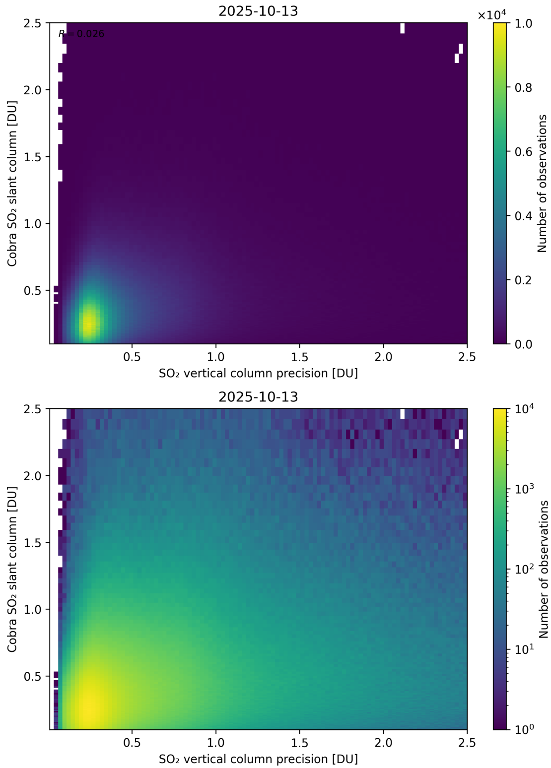
Figure 336: Scatter density plot of “SO 2 vertical column precision” against “Cobra SO 2 slant column” for 2025-10-12 to 2025-10-14.
