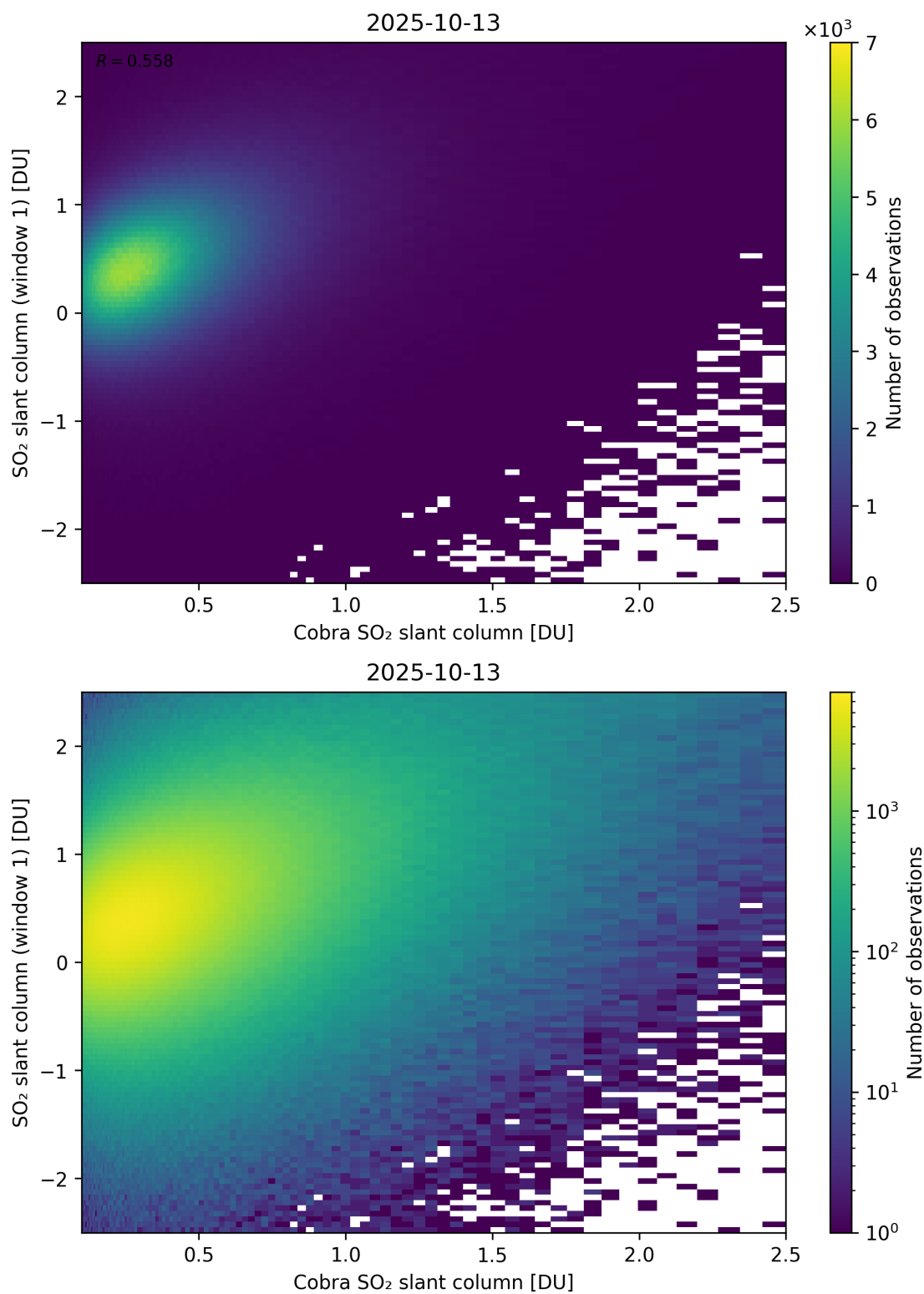
Figure 219: Scatter density plot of “Cobra SO 2 slant column” against “SO 2 slant column (window 1)” for 2025-10-12 to 2025-10-14.
