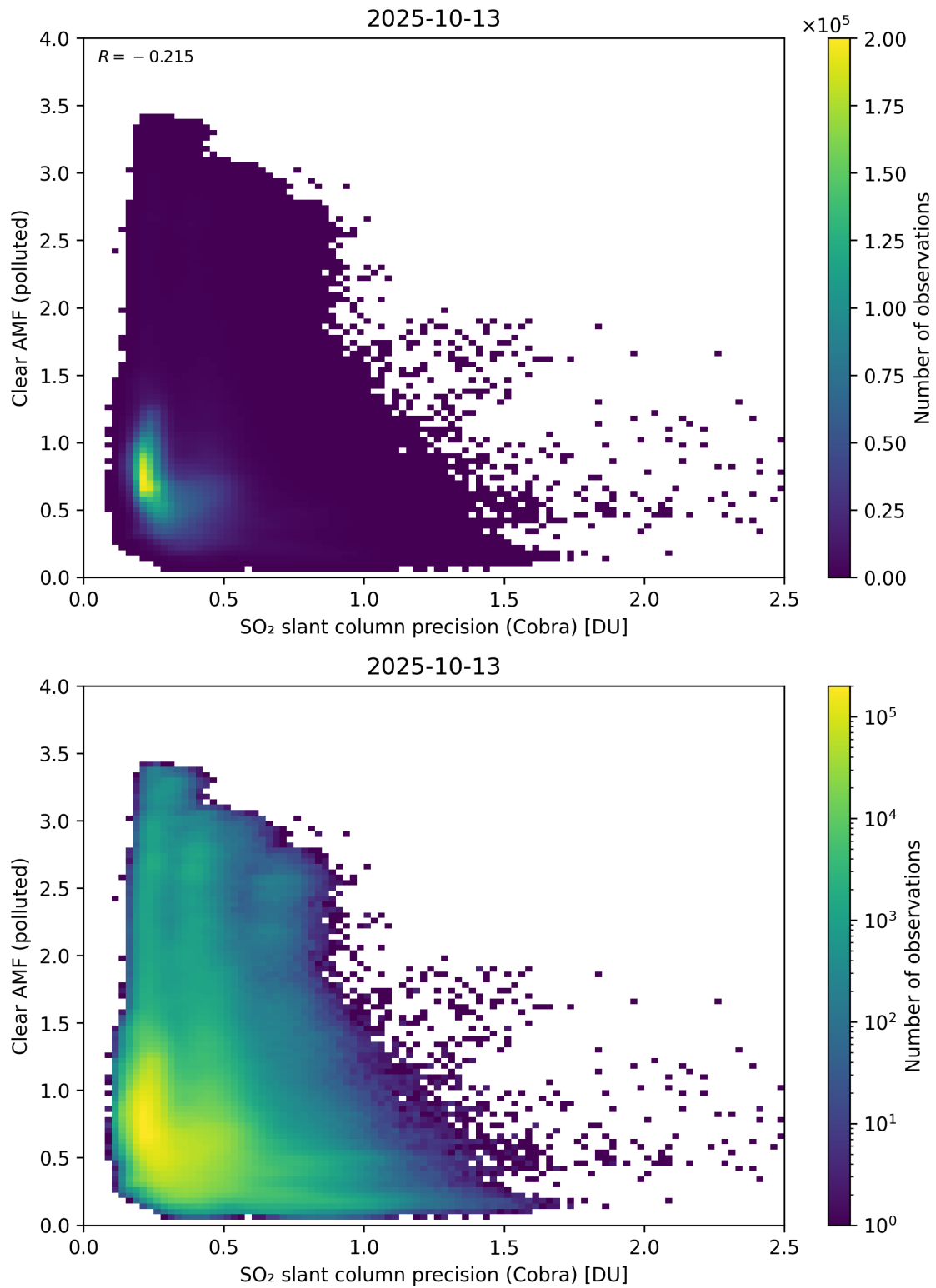
Figure 205: Scatter density plot of “SO 2 slant column precision (Cobra)” against “Clear AMF (polluted)” for 2025-10-12 to 2025-10-14.
