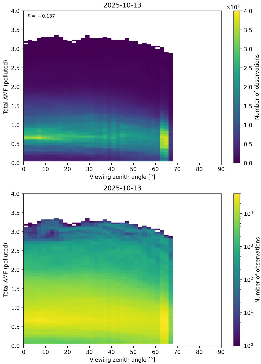
Figure 381: Scatter density plot of “Viewing zenith angle” against “Total AMF (polluted)” for 2025-10-12 to 2025-10-14.
