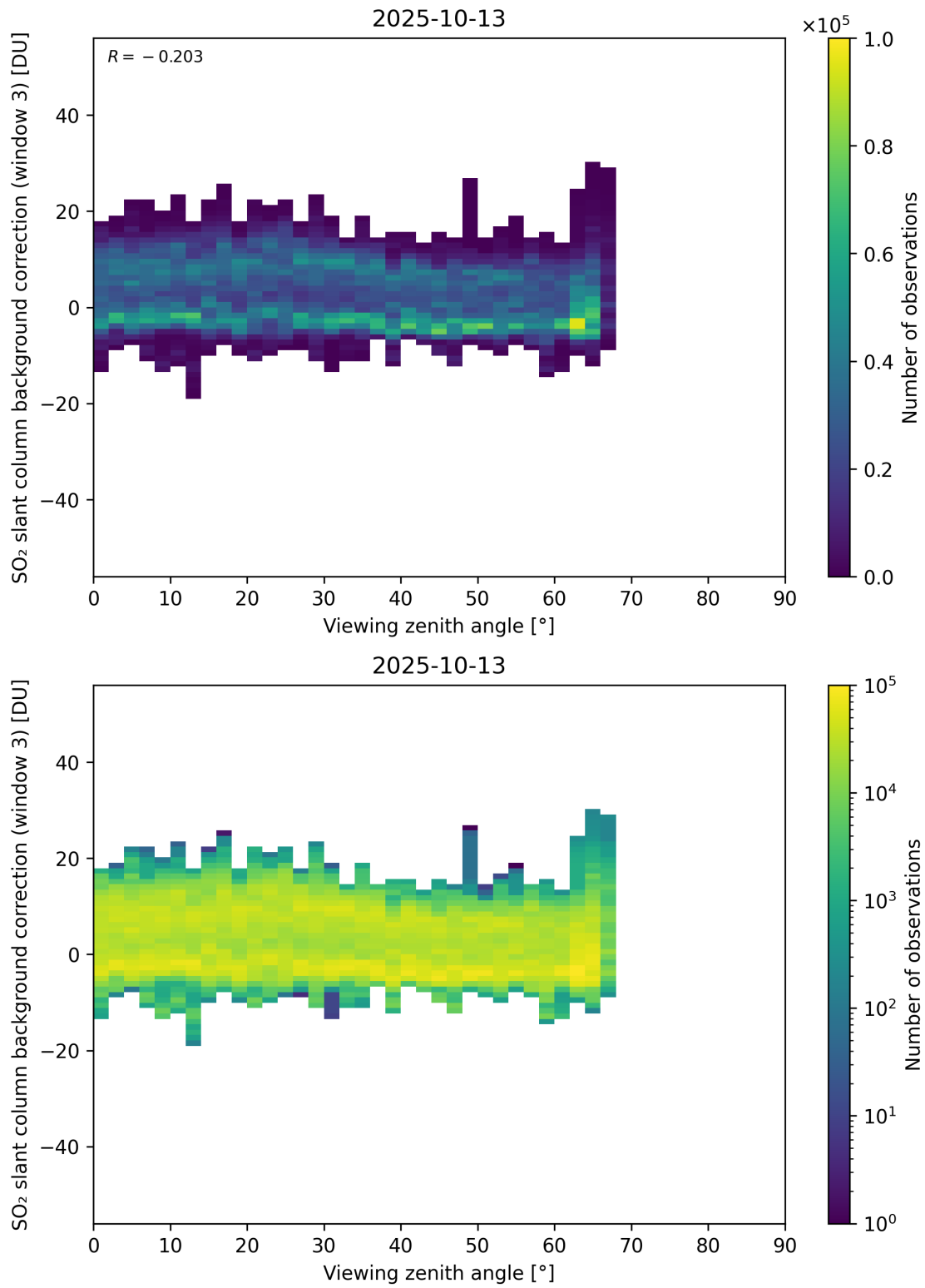
Figure 364: Scatter density plot of “Viewing zenith angle” against “SO 2 slant column background correction (window 3)” for 2025-10-12 to 2025-10-14.
