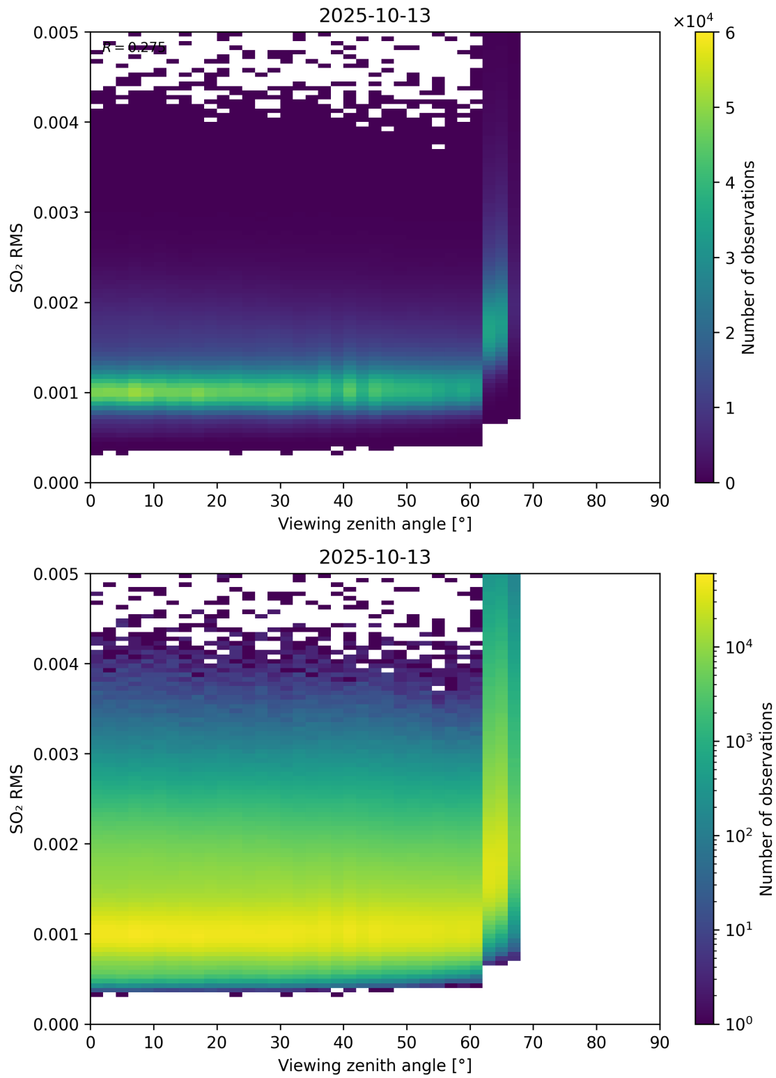
Figure 367: Scatter density plot of “Viewing zenith angle” against “SO 2 RMS” for 2025-10-12 to 2025-10-14.
