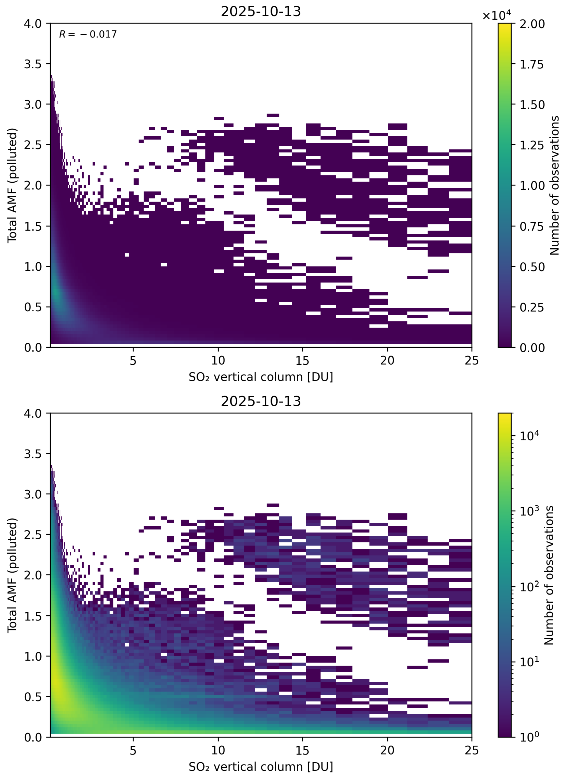
Figure 359: Scatter density plot of “SO 2 vertical column” against “Total AMF (polluted)” for 2025-10-12 to 2025-10-14.
