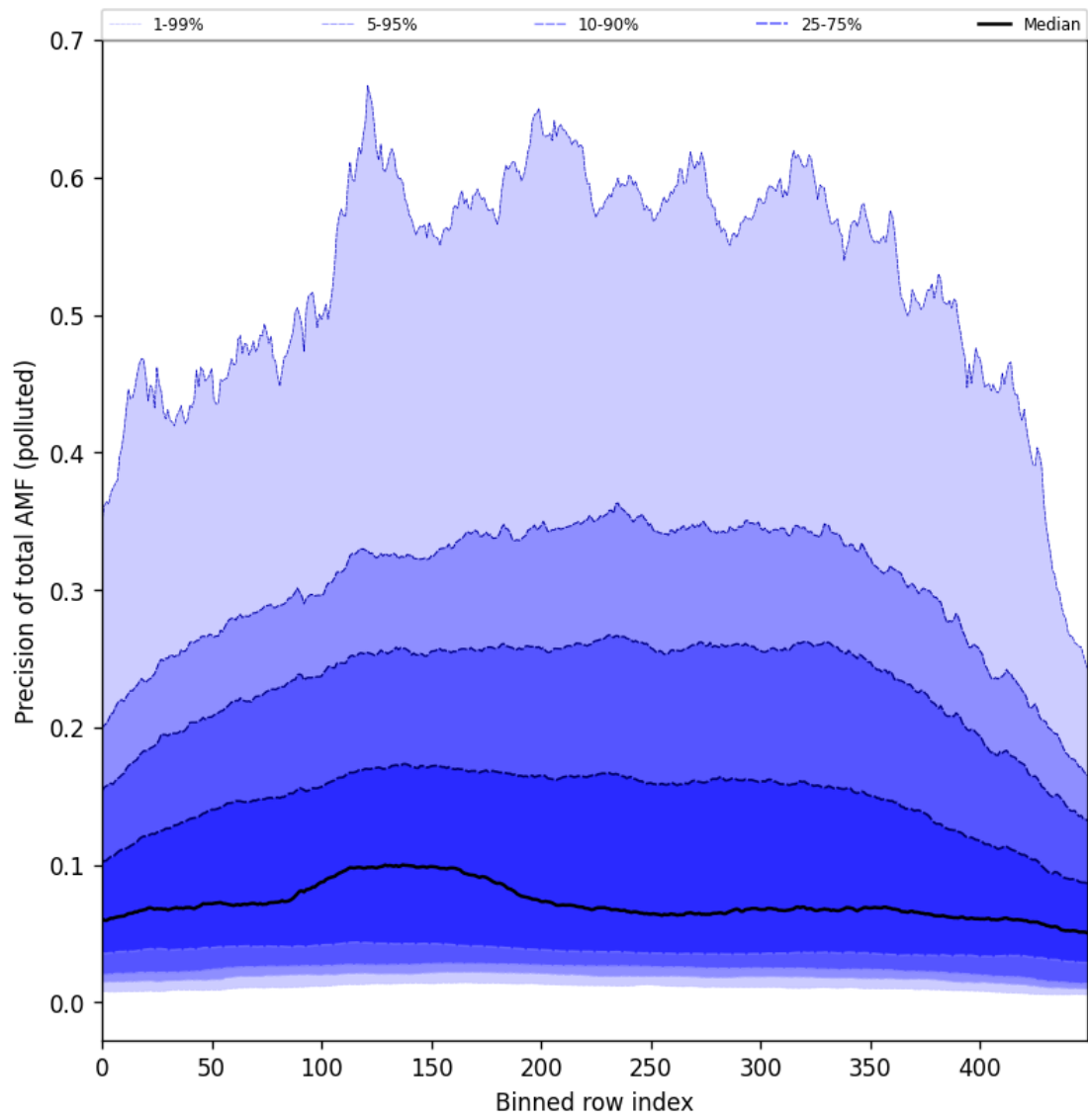
Figure 106: Along track statistics of “Precision of total AMF (polluted)” for 2025-10-12 to 2025-10-14
