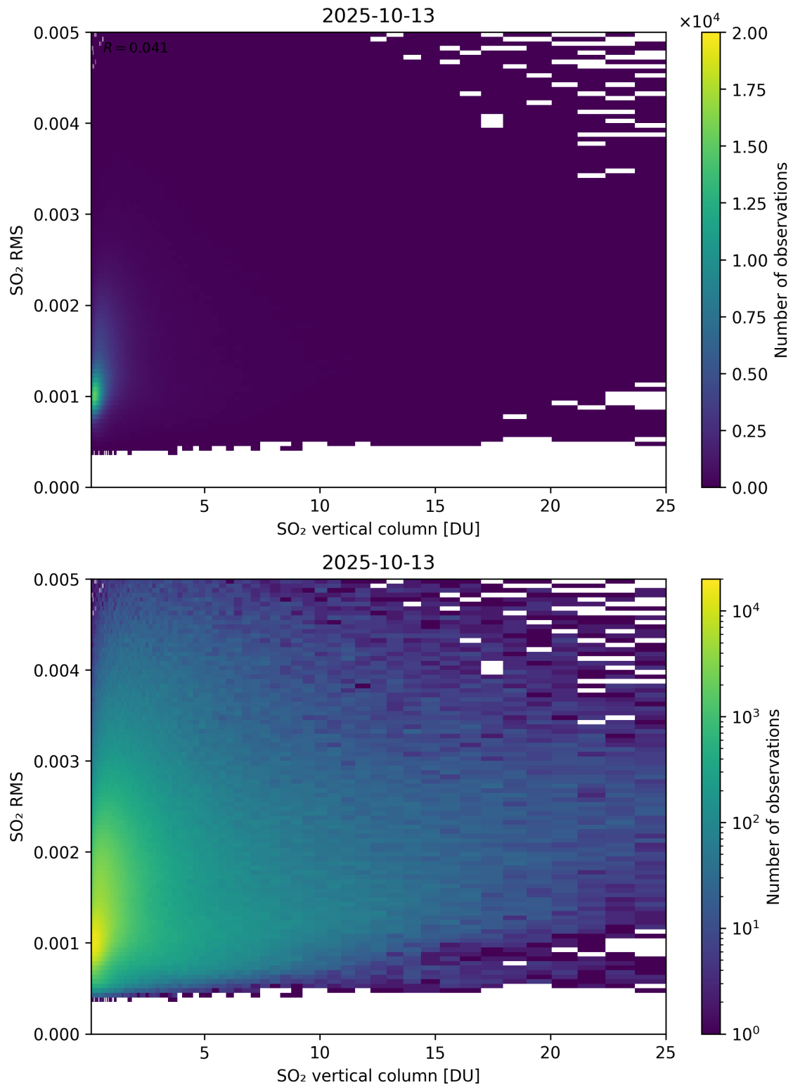
Figure 328: Scatter density plot of “SO 2 vertical column” against “SO 2 RMS” for 2025-10-12 to 2025-10-14.
