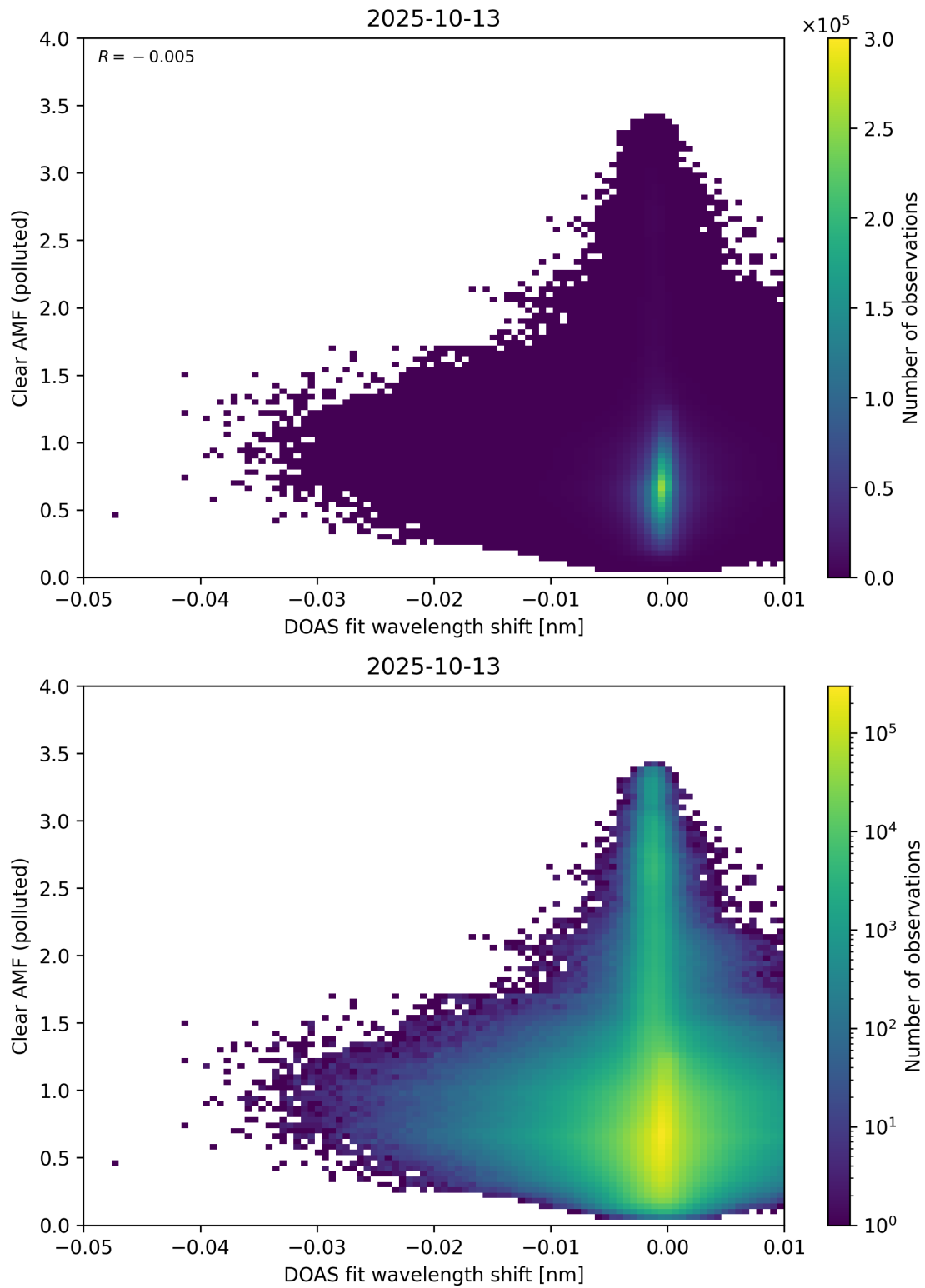
Figure 140: Scatter density plot of “DOAS fit wavelength shift” against “Clear AMF (polluted)” for 2025-10-12 to 2025-10-14.
