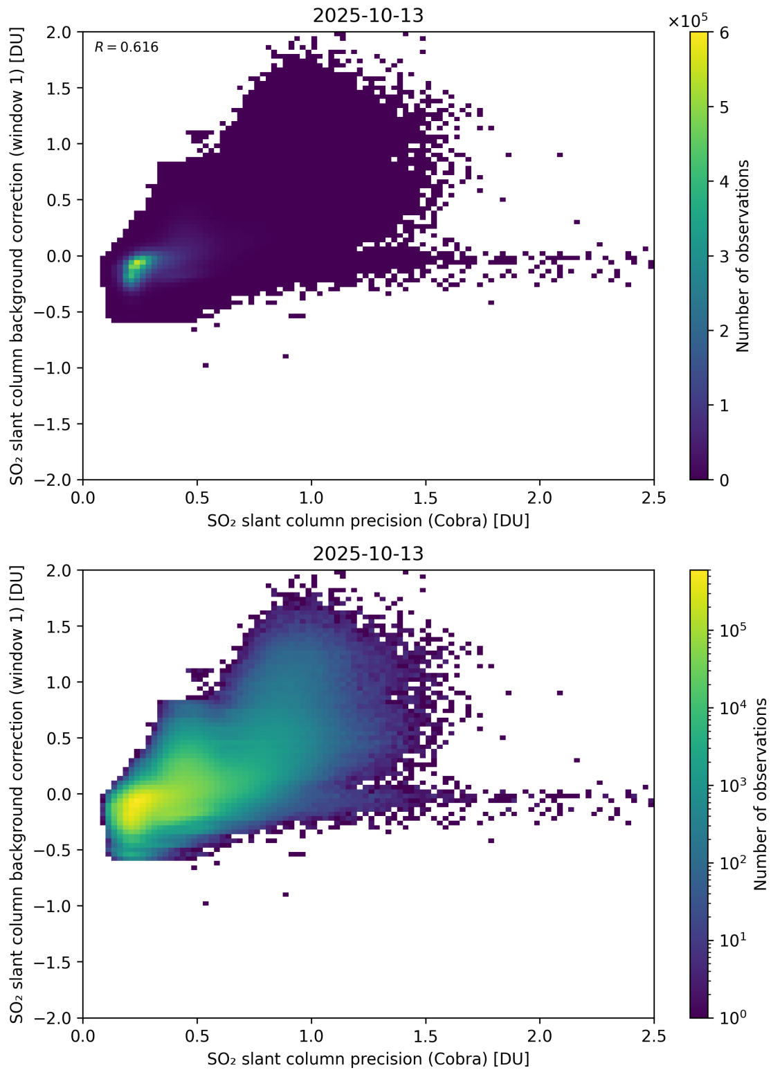
Figure 199: Scatter density plot of “SO 2 slant column precision (Cobra)” against “SO 2 slant column background correction (window 1)” for 2025-10-12 to 2025-10-14.
