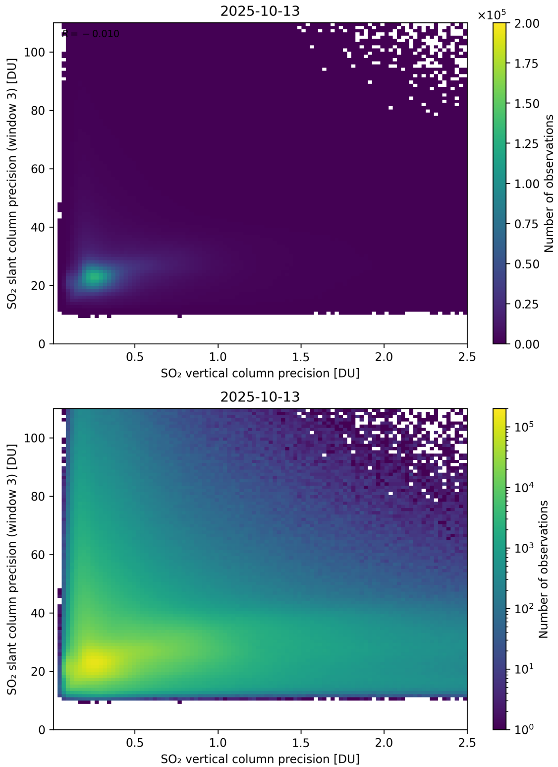
Figure 345: Scatter density plot of “SO 2 vertical column precision” against “SO 2 slant column precision (window 3)” for 2025-10-12 to 2025-10-14.
