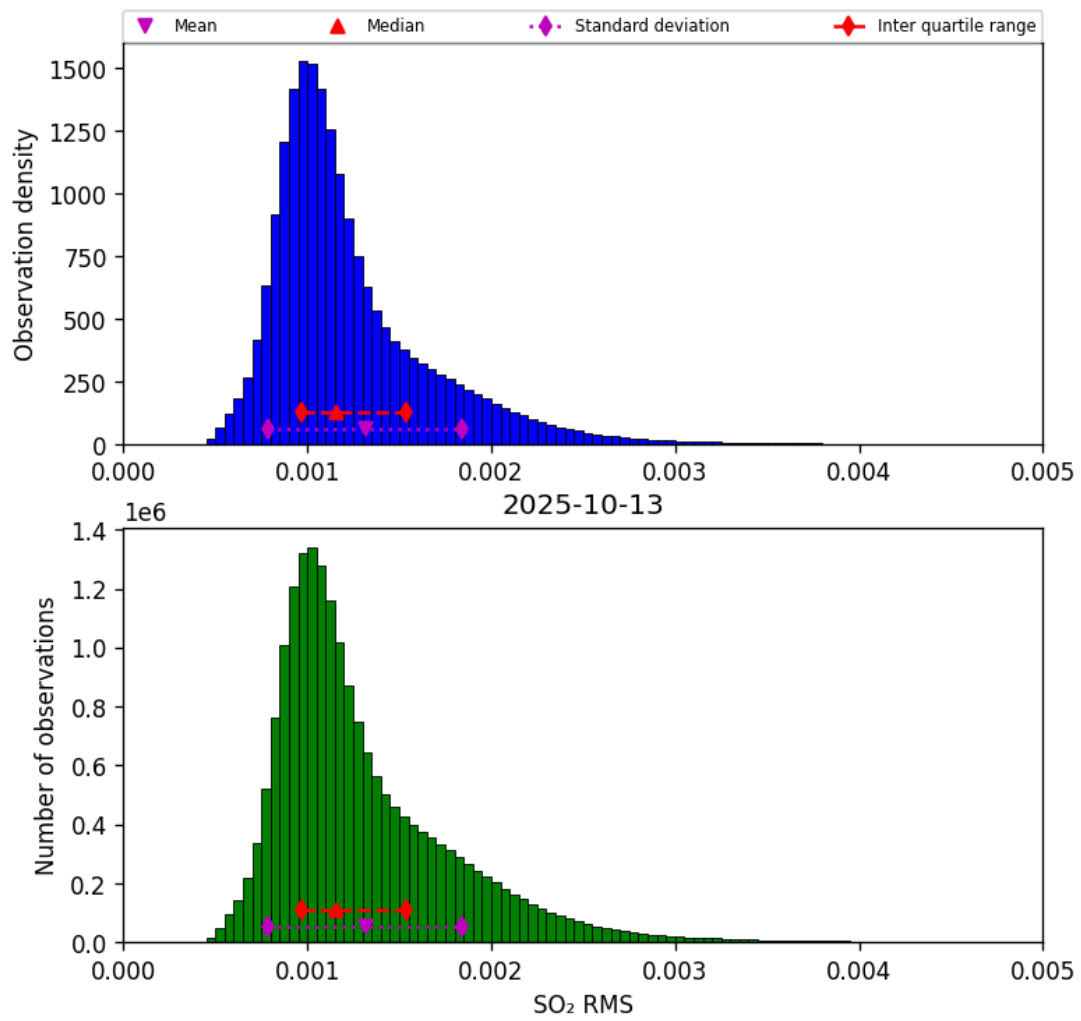
Figure 78: Histogram of “SO 2 RMS” for 2025-10-12 to 2025-10-14
