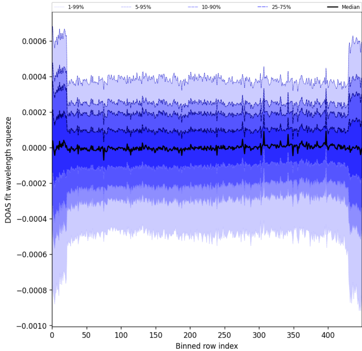
Figure 103: Along track statistics of “DOAS fit wavelength squeeze” for 2025-10-12 to 2025-10-14
