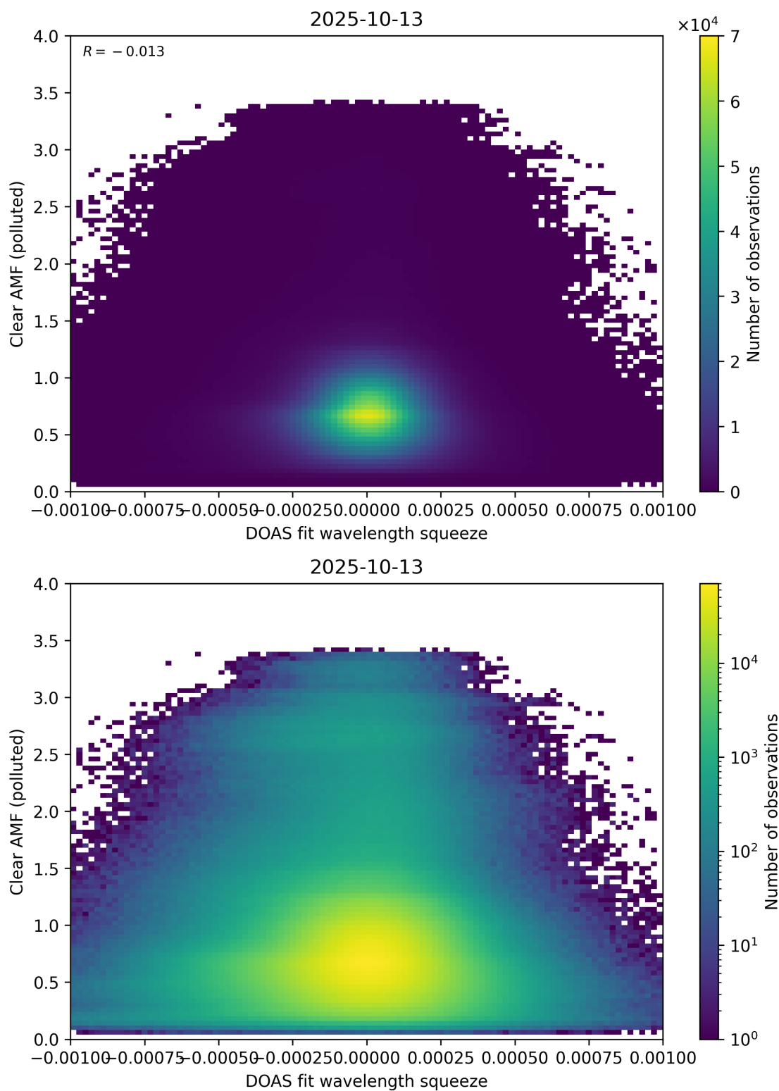
Figure 144: Scatter density plot of “DOAS fit wavelength squeeze” against “Clear AMF (polluted)” for 2025-10-12 to 2025-10-14.
