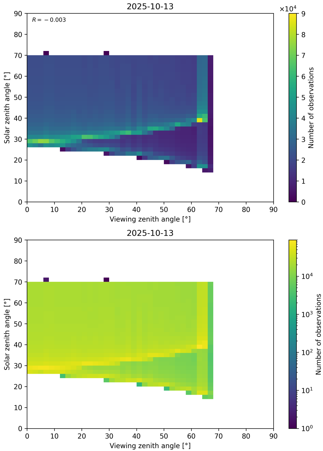
Figure 369: Scatter density plot of “Viewing zenith angle” against “Solar zenith angle” for 2025-10-12 to 2025-10-14.
