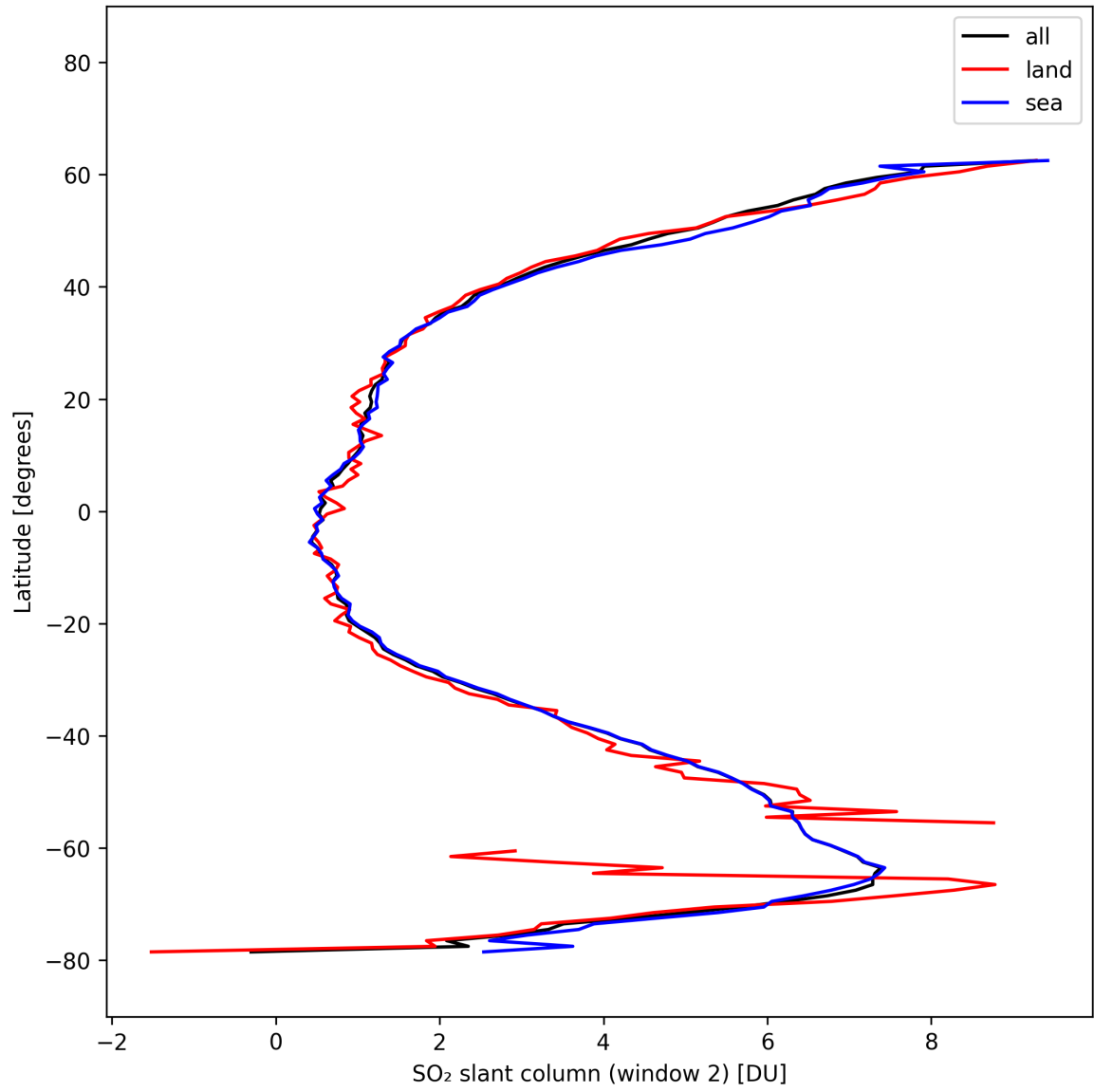
Figure 41: Zonal average of “SO 2 slant column (window 2)” for 2025-10-12 to 2025-10-14.
