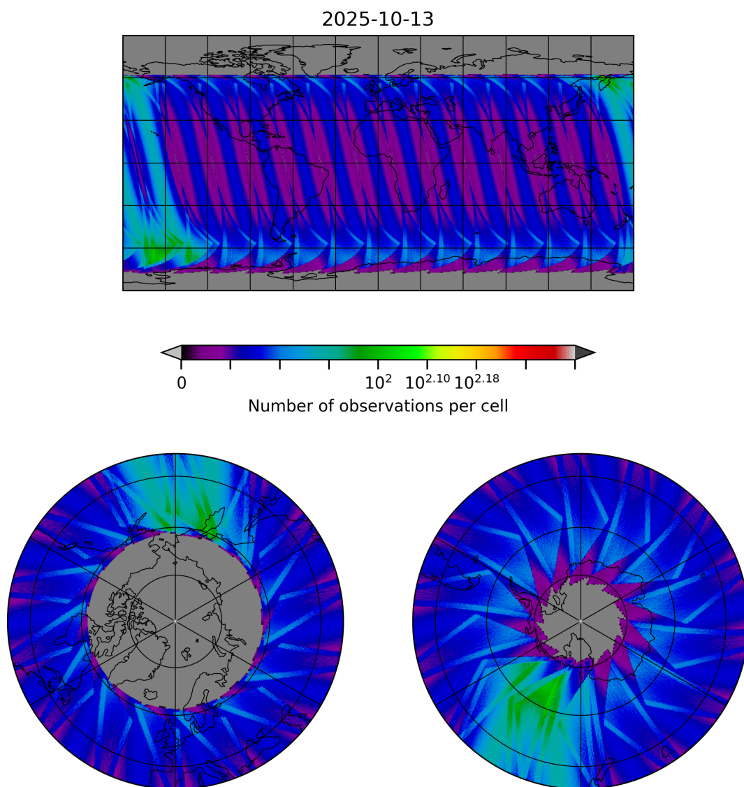
Figure 30: Map of the number of observations for 2025-10-12 to 2025-10-14
