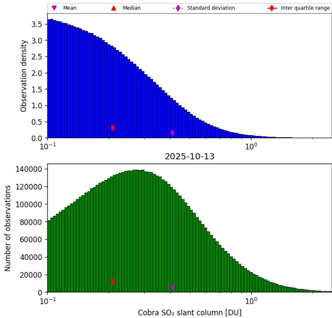
Figure 61: Histogram of “Cobra SO 2 slant column” for 2025-10-12 to 2025-10-14
