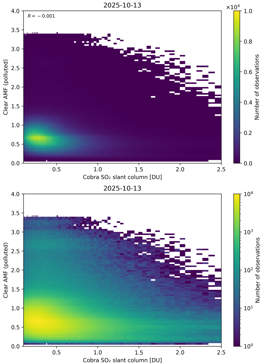
Figure 215: Scatter density plot of “Cobra SO 2 slant column” against “Clear AMF (polluted)” for 2025-10-12 to 2025-10-14.
