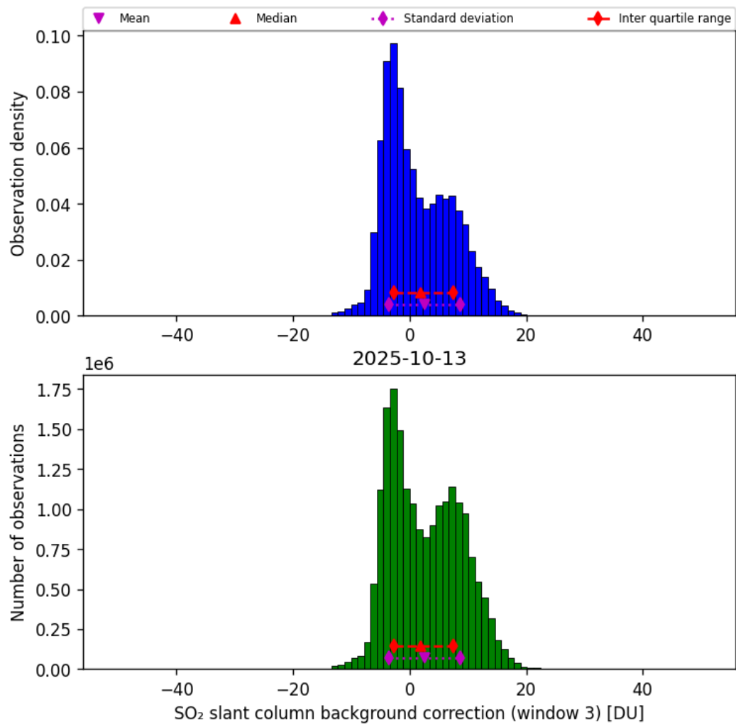
Figure 74: Histogram of “SO 2 slant column background correction (window 3)” for 2025-10-12 to 2025-10-14
