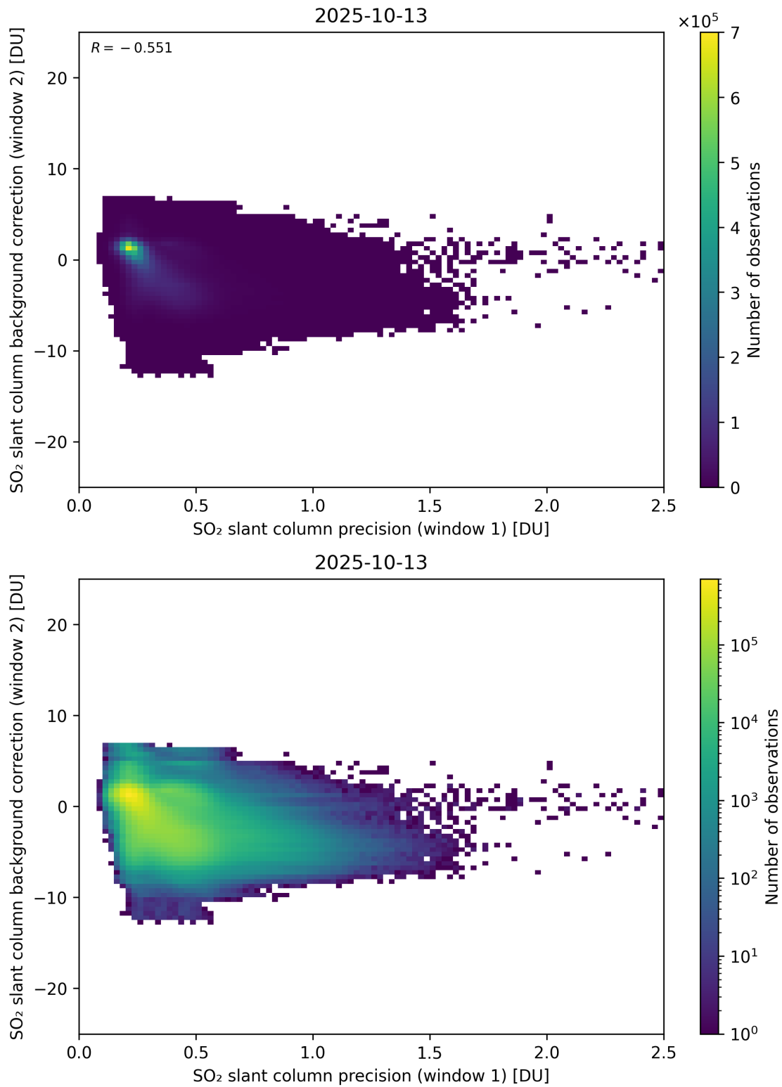
Figure 269: Scatter density plot of “SO 2 slant column precision (window 1)” against “SO 2 slant column background correction (window 2)” for 2025-10-12 to 2025-10-14.
