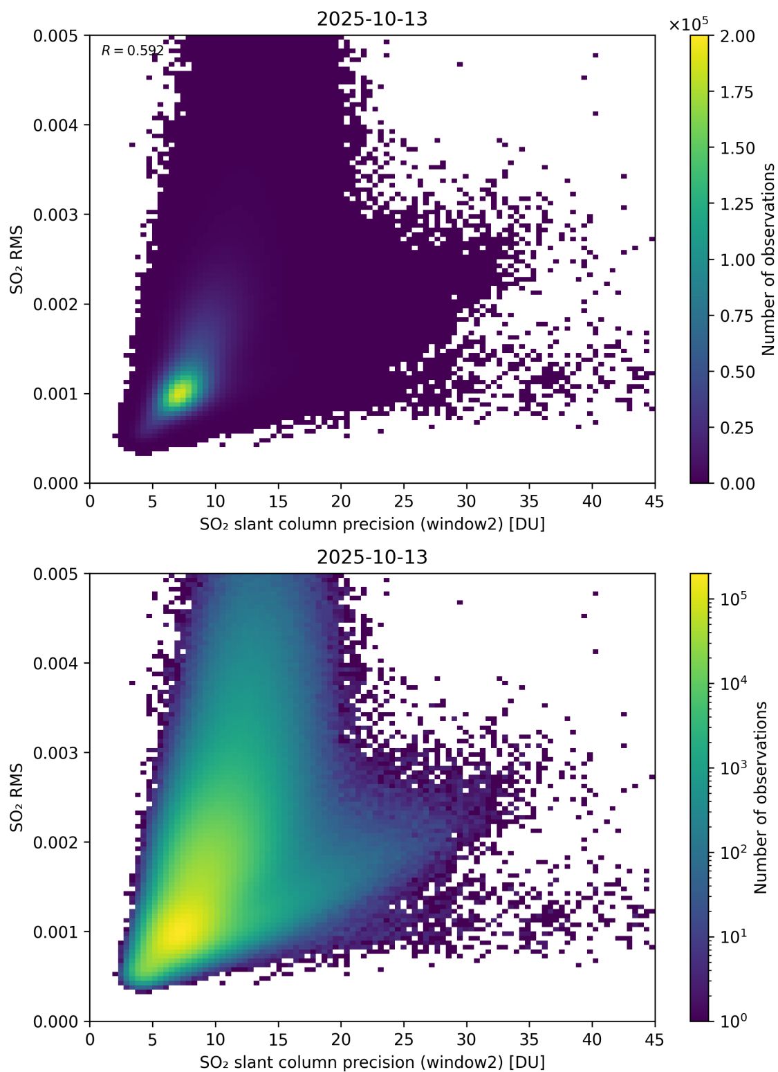
Figure 295: Scatter density plot of “SO 2 slant column precision (window2)” against “SO 2 RMS” for 2025-10-12 to 2025-10-14.
