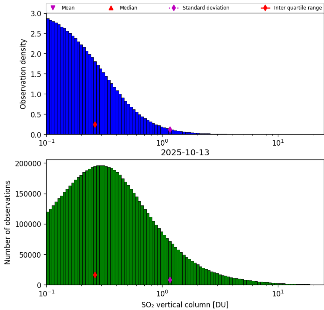
Figure 58: Histogram of “SO 2 vertical column” for 2025-10-12 to 2025-10-14
