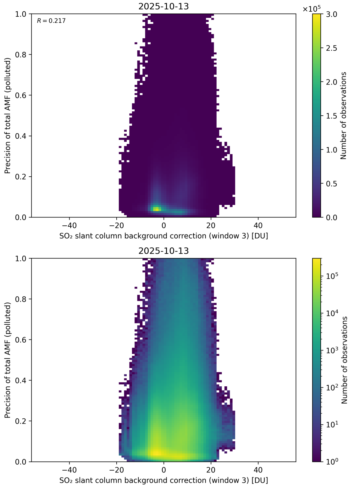
Figure 137: Scatter density plot of “SO 2 slant column background correction (window 3)” against “Precision of total AMF (polluted)” for 2025-10-12 to 2025-10-14.
