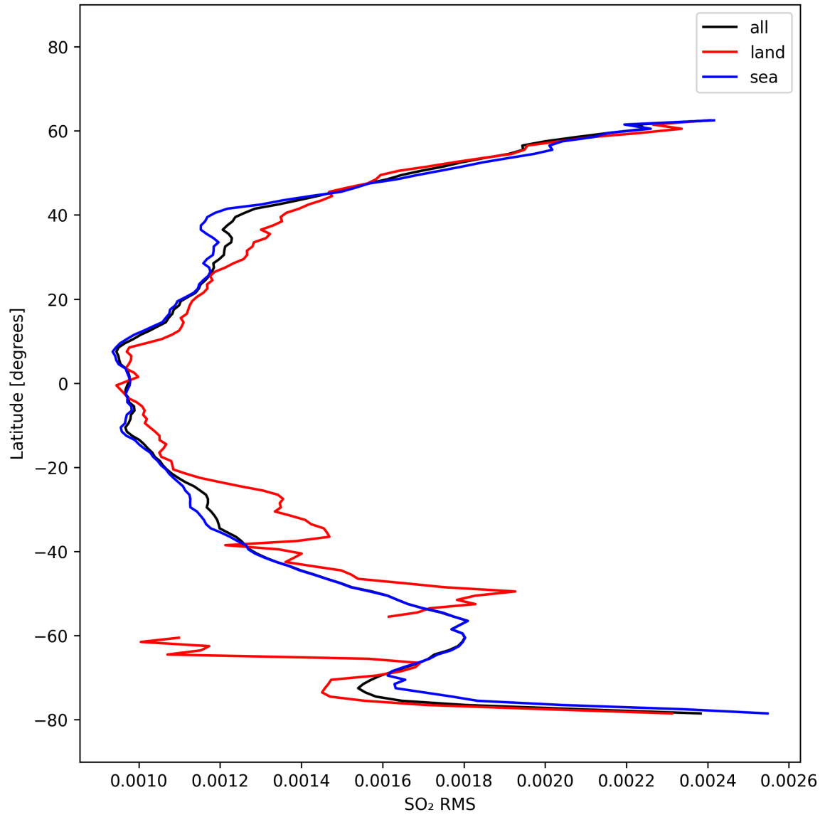
Figure 52: Zonal average of “SO 2 RMS” for 2025-10-12 to 2025-10-14.
