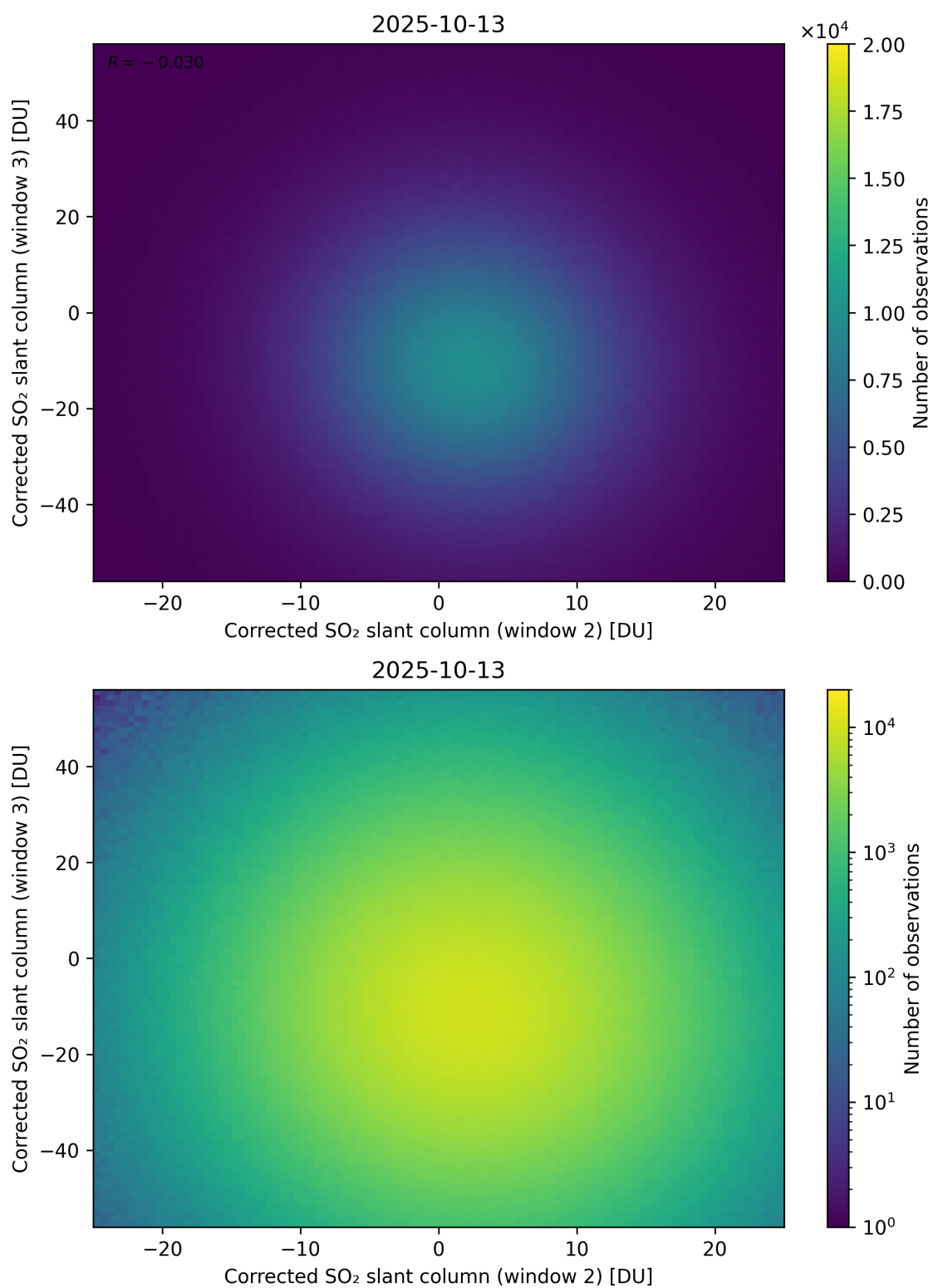
Figure 250: Scatter density plot of “Corrected SO 2 slant column (window 2)” against “Corrected SO 2 slant column (window 3)” for 2025-10-12 to 2025-10-14.
