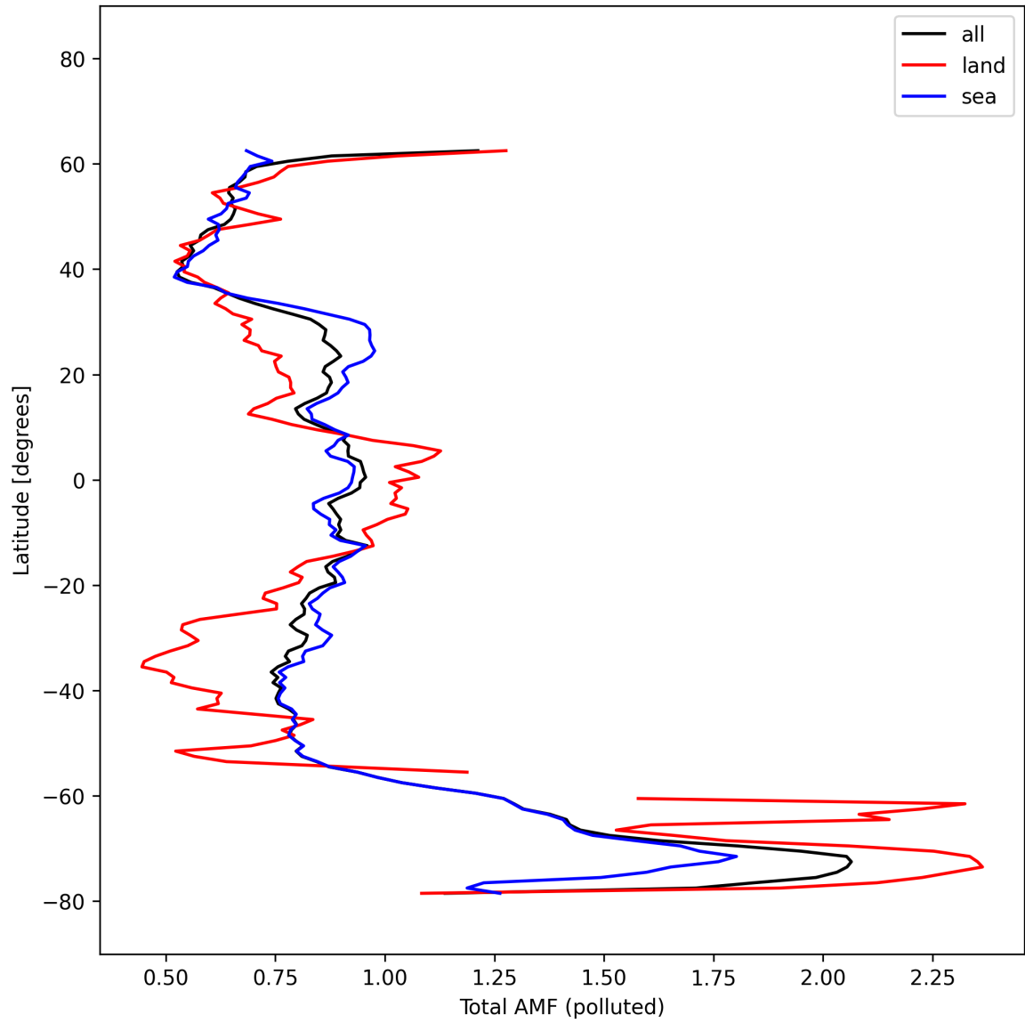
Figure 53: Zonal average of “Total AMF (polluted)” for 2025-10-12 to 2025-10-14.
