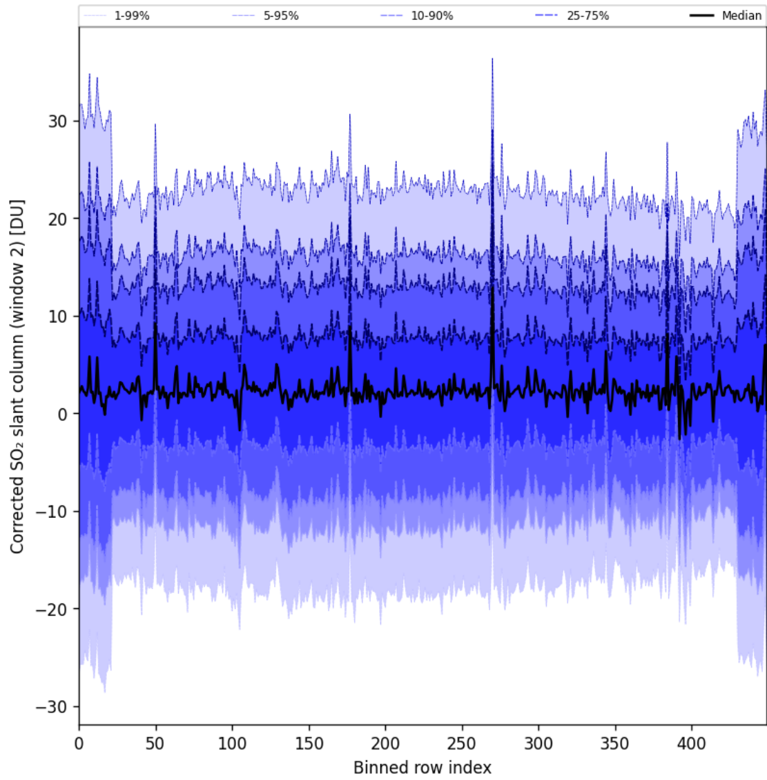
Figure 95: Along track statistics of “Corrected SO 2 slant column (window 2)” for 2025-10-12 to 2025-10-14
