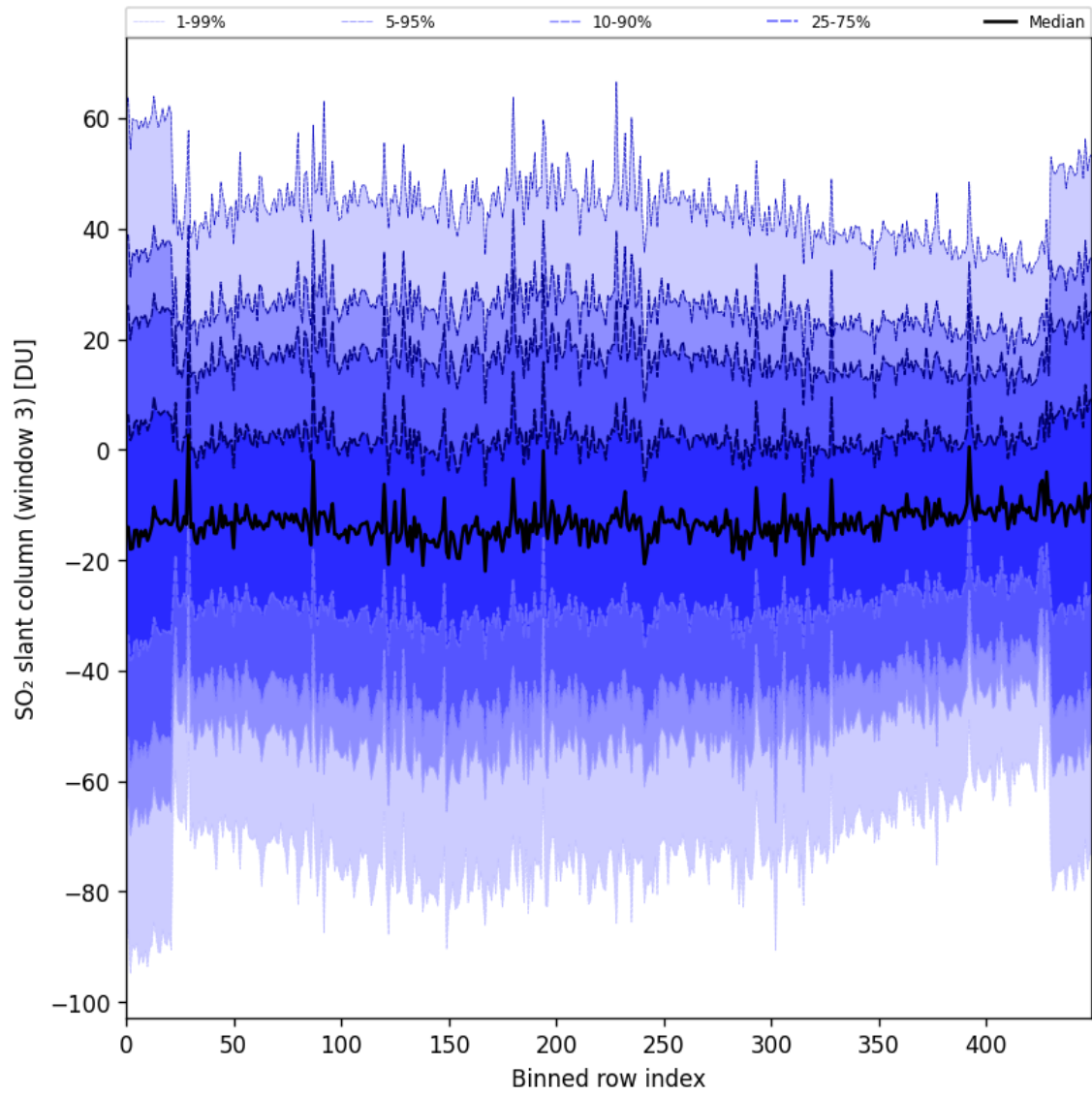
Figure 97: Along track statistics of “SO 2 slant column (window 3)” for 2025-10-12 to 2025-10-14
