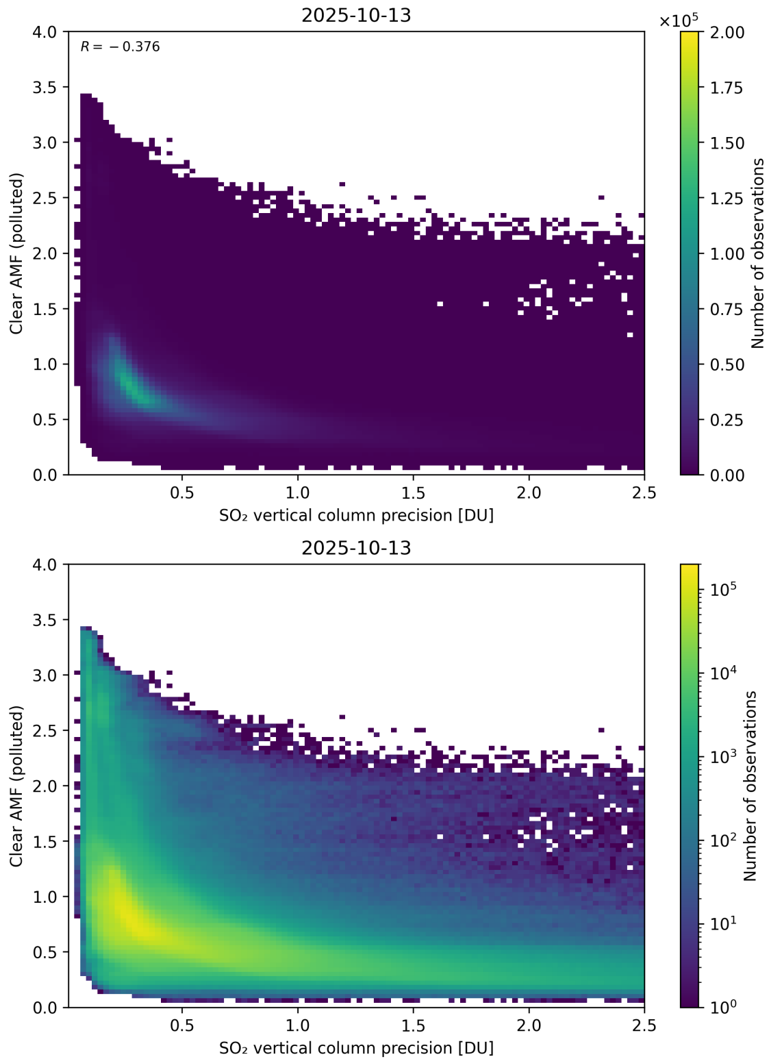
Figure 335: Scatter density plot of “SO 2 vertical column precision” against “Clear AMF (polluted)” for 2025-10-12 to 2025-10-14.
