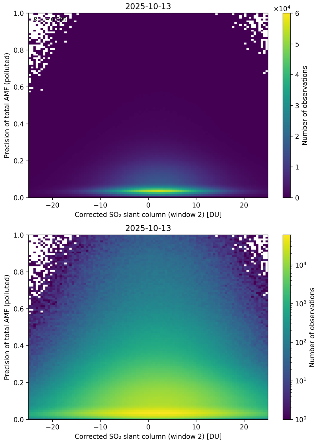
Figure 254: Scatter density plot of “Corrected SO 2 slant column (window 2)” against “Precision of total AMF (polluted)” for 2025-10-12 to 2025-10-14.
