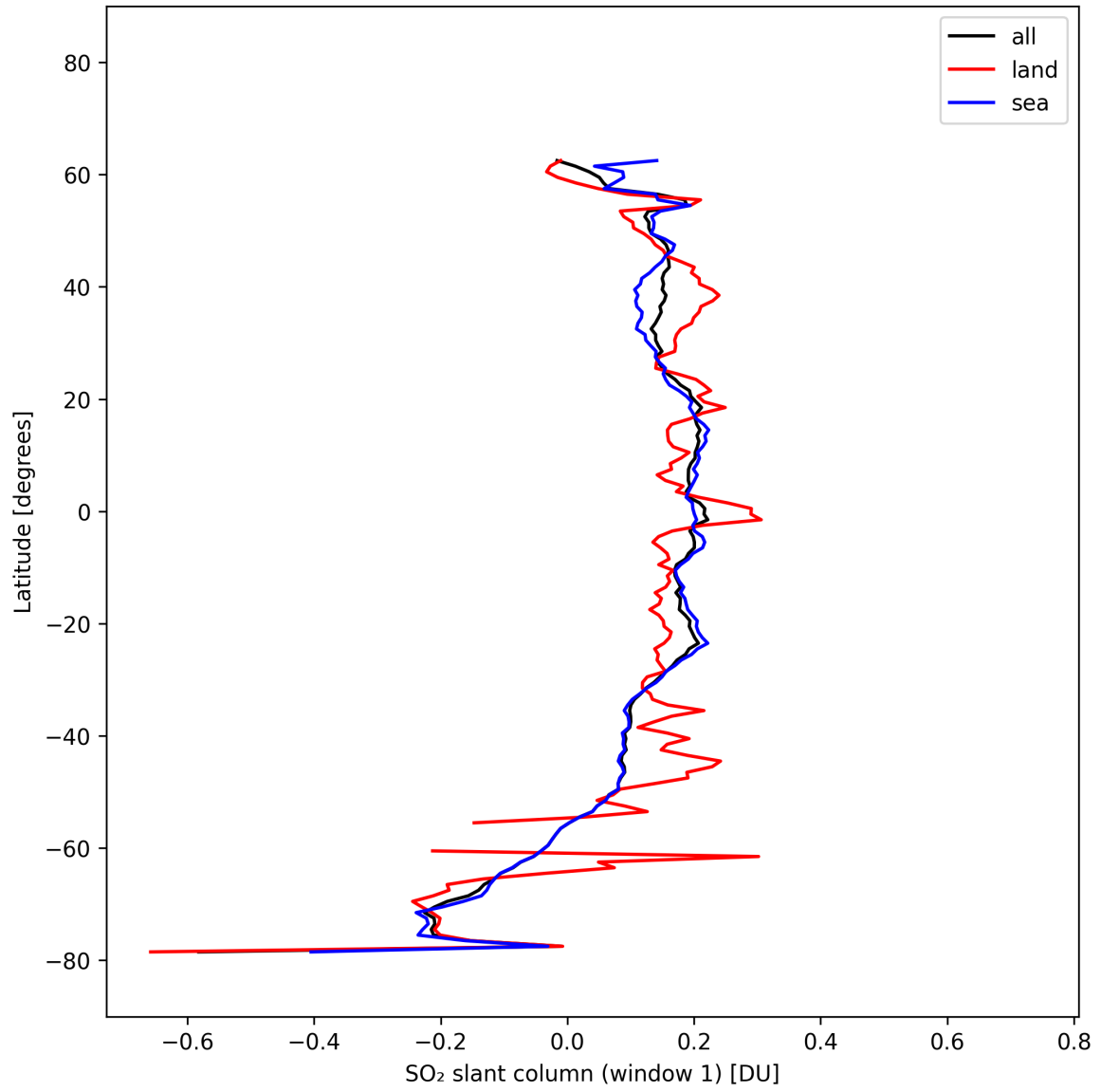
Figure 37: Zonal average of “SO 2 slant column (window 1)” for 2025-10-12 to 2025-10-14.
