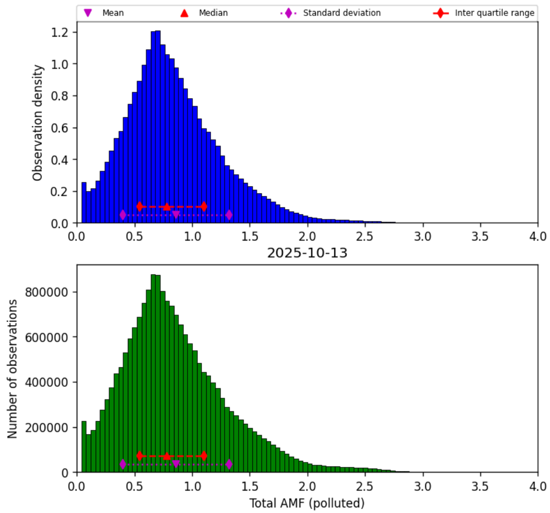
Figure 79: Histogram of “Total AMF (polluted)” for 2025-10-12 to 2025-10-14
