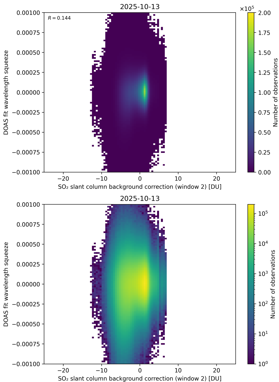
Figure 124: Scatter density plot of “SO 2 slant column background correction (window 2)” against “DOAS fit wavelength squeeze” for 2025-10-12 to 2025-10-14.
