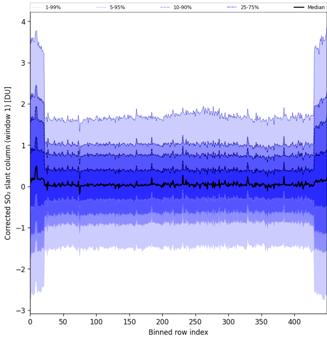
Figure 91: Along track statistics of “Corrected SO 2 slant column (window 1)” for 2025-10-12 to 2025-10-14
