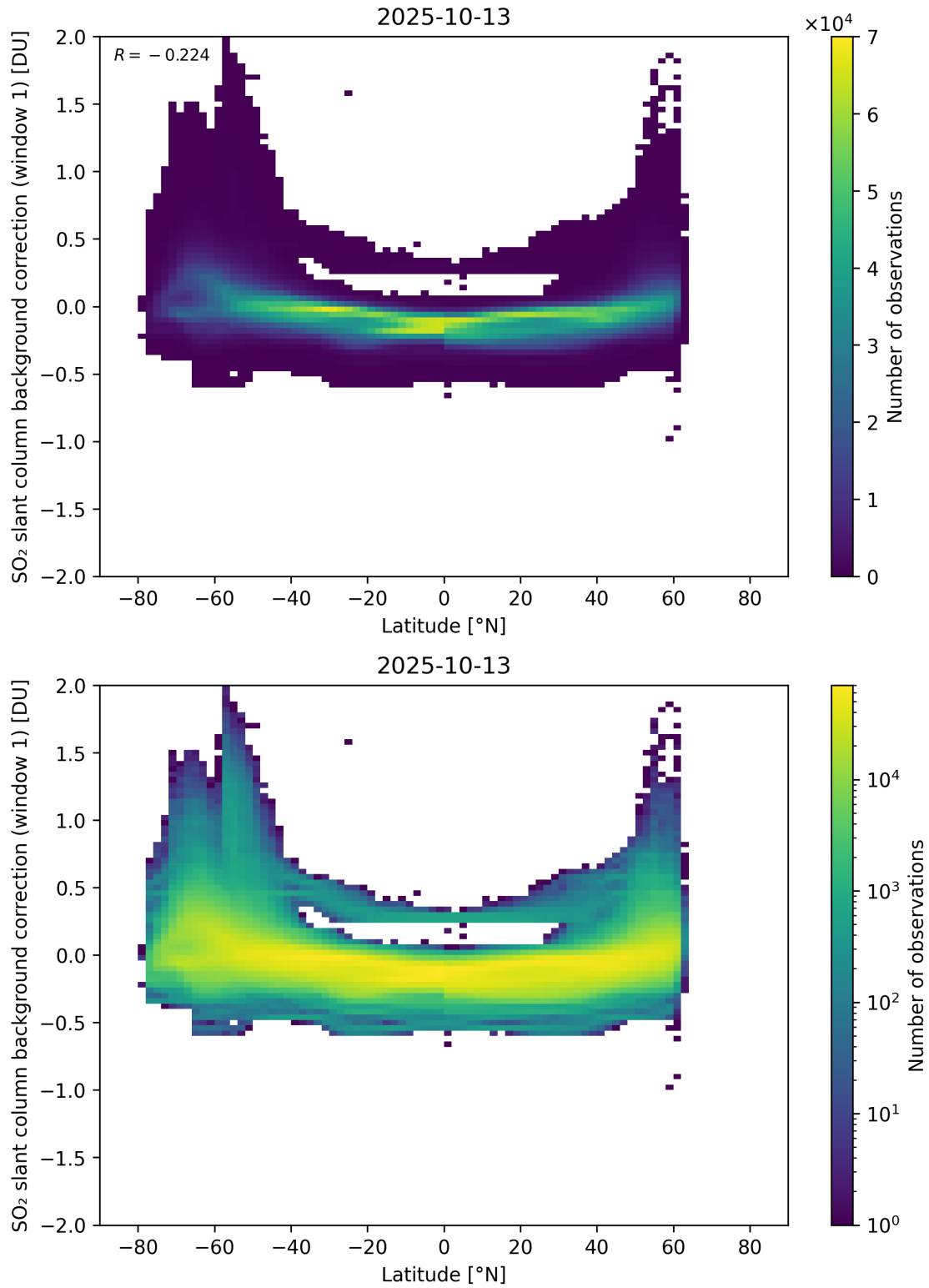
Figure 150: Scatter density plot of “Latitude” against “SO 2 slant column background correction (window 1)” for 2025-10-12 to 2025-10-14.
