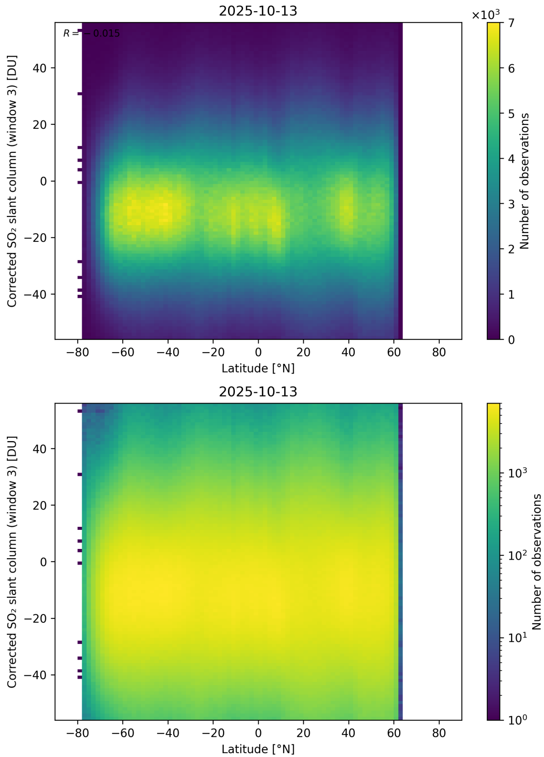
Figure 161: Scatter density plot of “Latitude” against “Corrected SO 2 slant column (window 3)” for 2025-10-12 to 2025-10-14.
