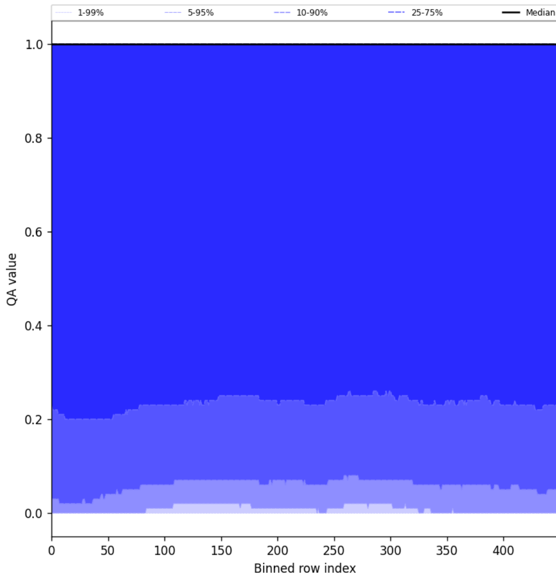
Figure 83: Along track statistics of “QA value” for 2025-10-12 to 2025-10-14
