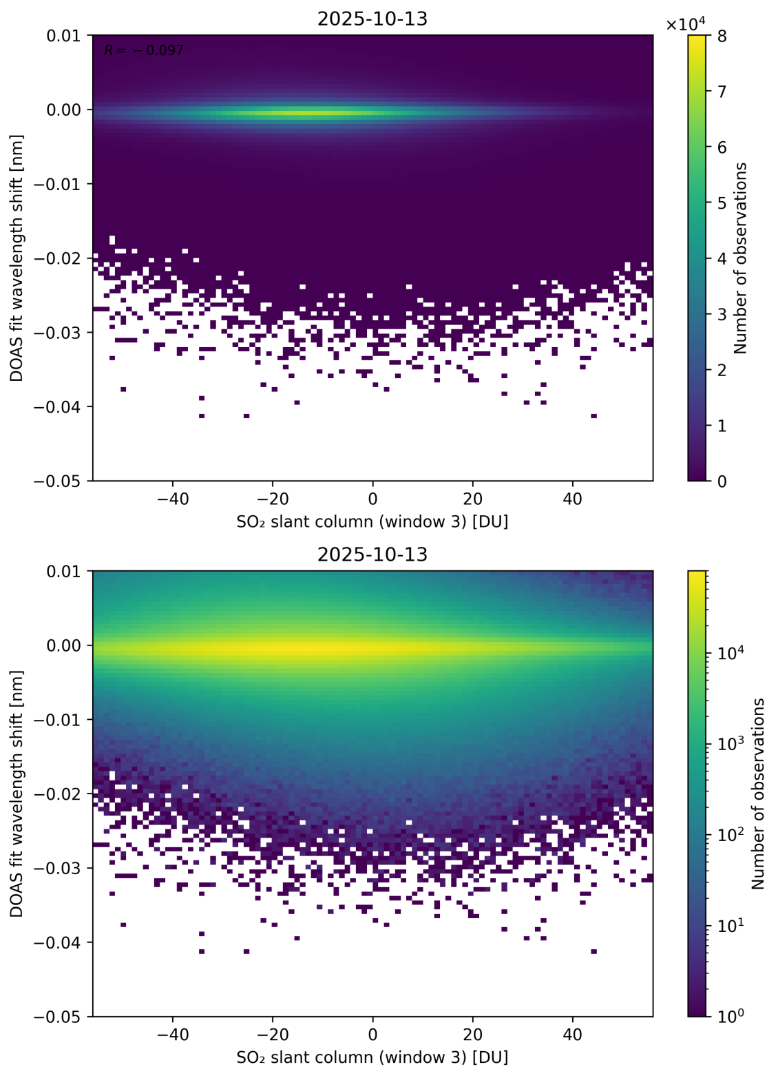
Figure 304: Scatter density plot of “SO 2 slant column (window 3)” against “DOAS fit wavelength shift” for 2025-10-12 to 2025-10-14.
