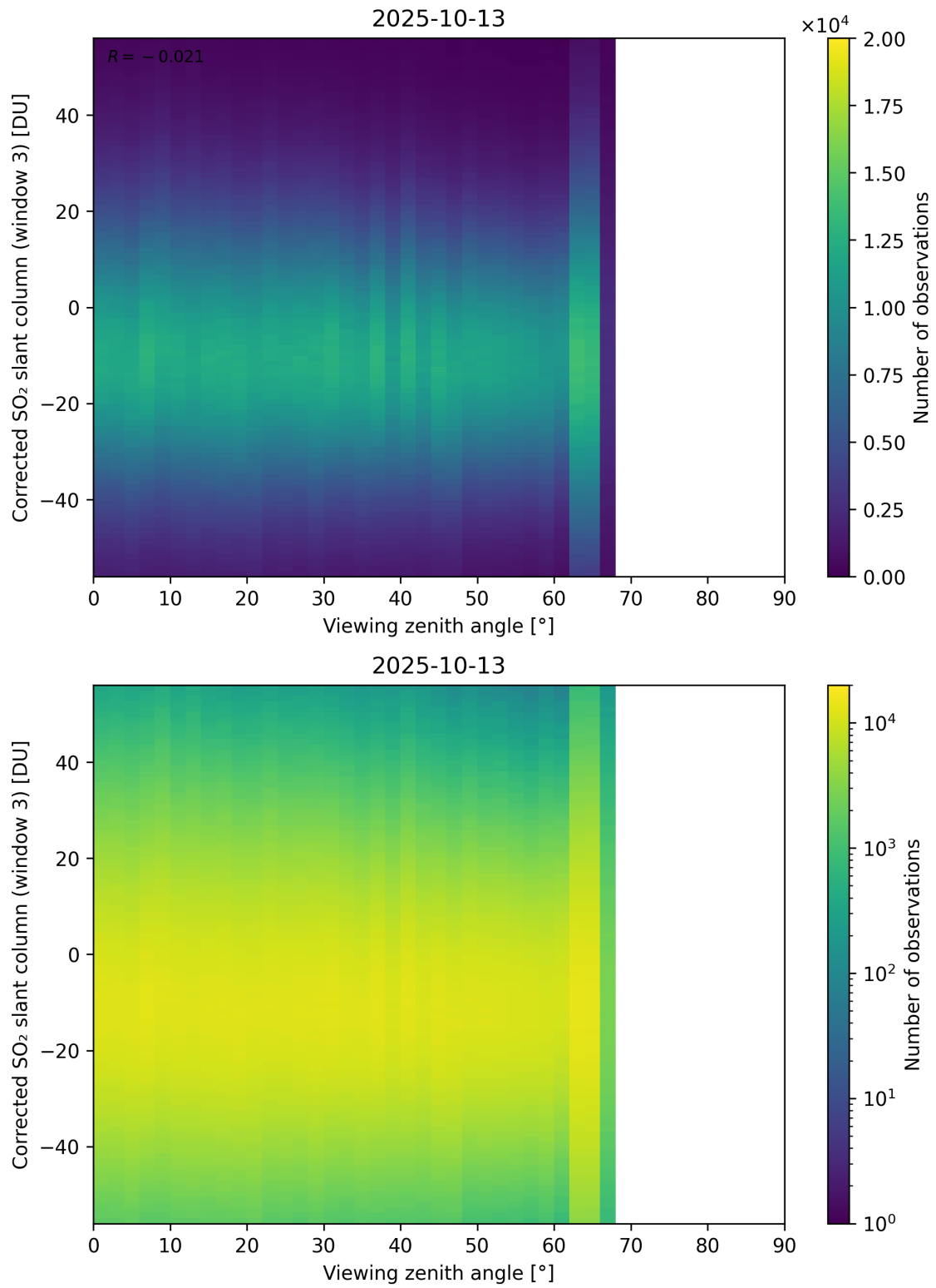
Figure 375: Scatter density plot of “Viewing zenith angle” against “Corrected SO 2 slant column (window 3)” for 2025-10-12 to 2025-10-14.
