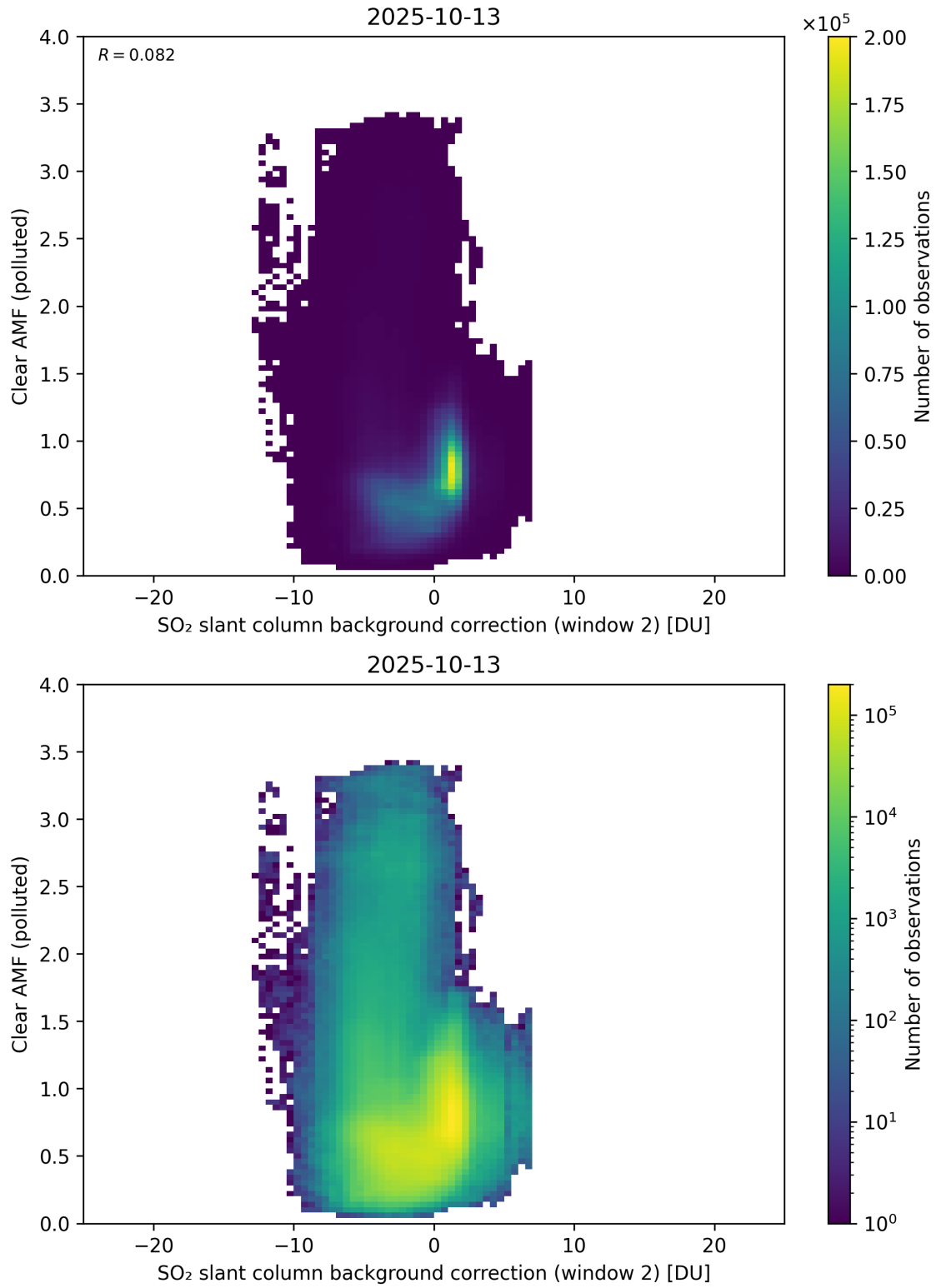
Figure 126: Scatter density plot of “SO 2 slant column background correction (window 2)” against “Clear AMF (polluted)” for 2025-10-12 to 2025-10-14.
