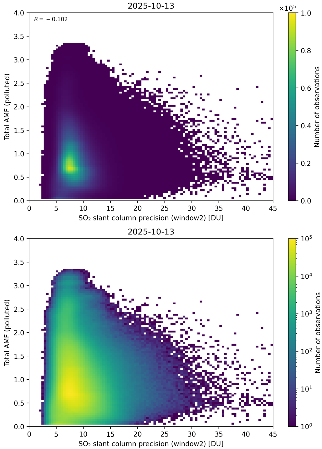
Figure 301: Scatter density plot of “SO 2 slant column precision (window2)” against “Total AMF (polluted)” for 2025-10-12 to 2025-10-14.
