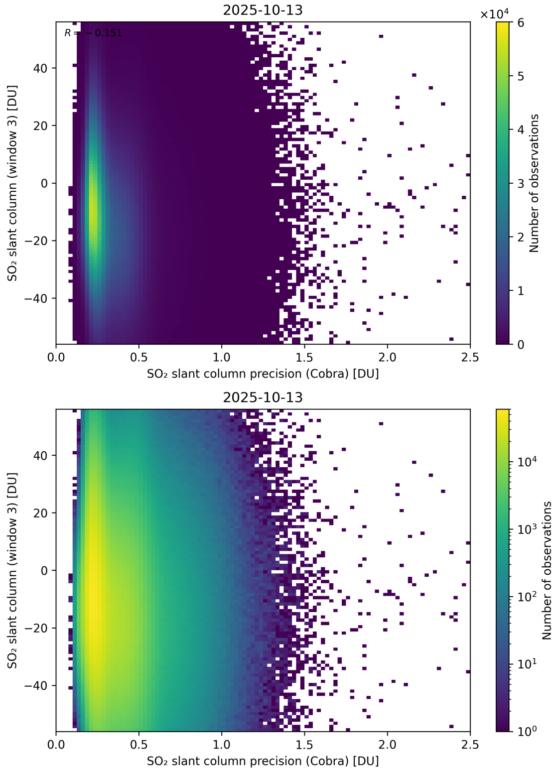
Figure 211: Scatter density plot of “SO 2 slant column precision (Cobra)” against “SO 2 slant column (window 3)” for 2025-10-12 to 2025-10-14.
