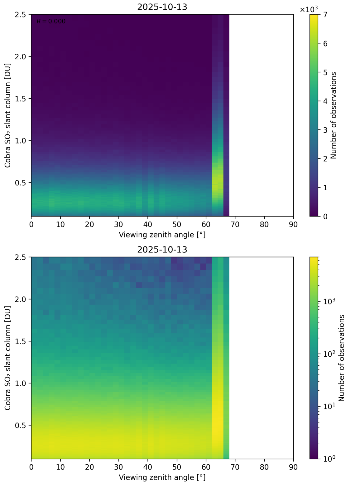
Figure 371: Scatter density plot of “Viewing zenith angle” against “Cobra SO 2 slant column” for 2025-10-12 to 2025-10-14.
