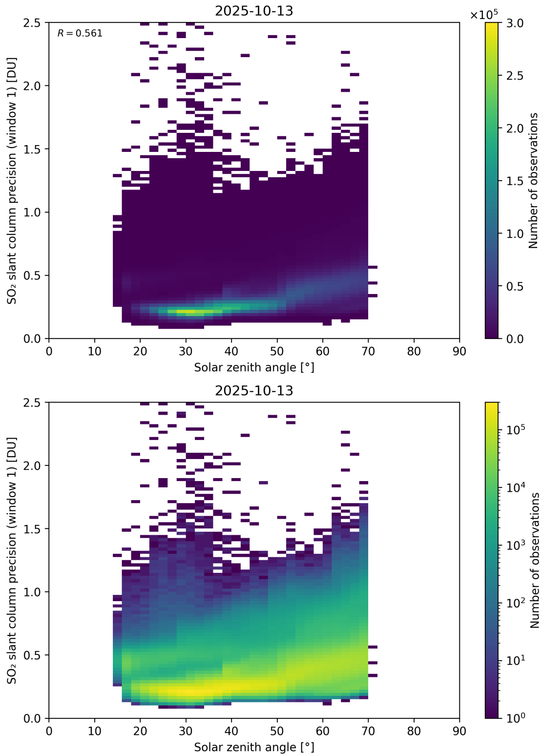
Figure 185: Scatter density plot of “Solar zenith angle” against “SO 2 slant column precision (window 1)” for 2025-10-12 to 2025-10-14.
