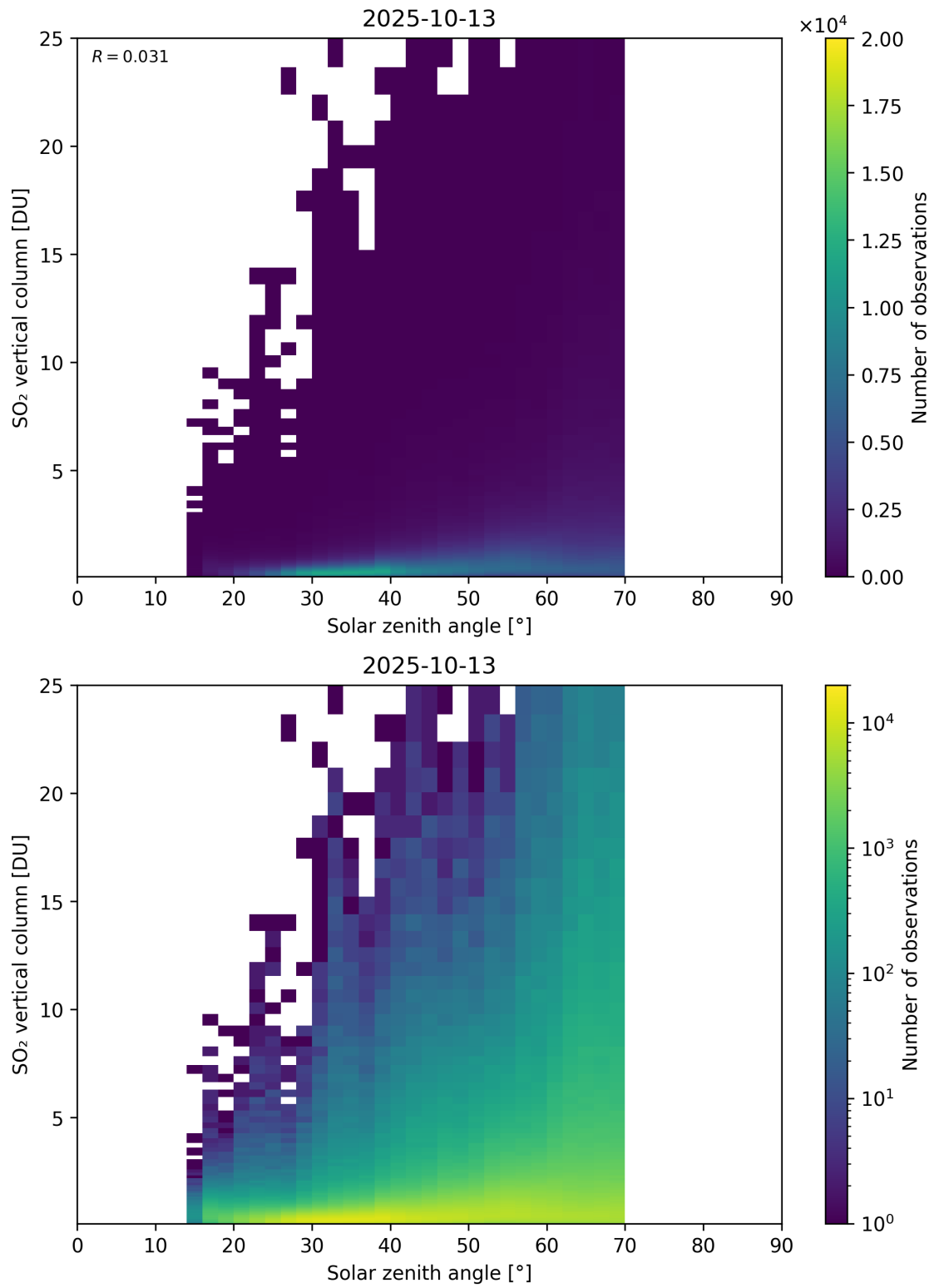
Figure 191: Scatter density plot of “Solar zenith angle” against “SO 2 vertical column” for 2025-10-12 to 2025-10-14.
