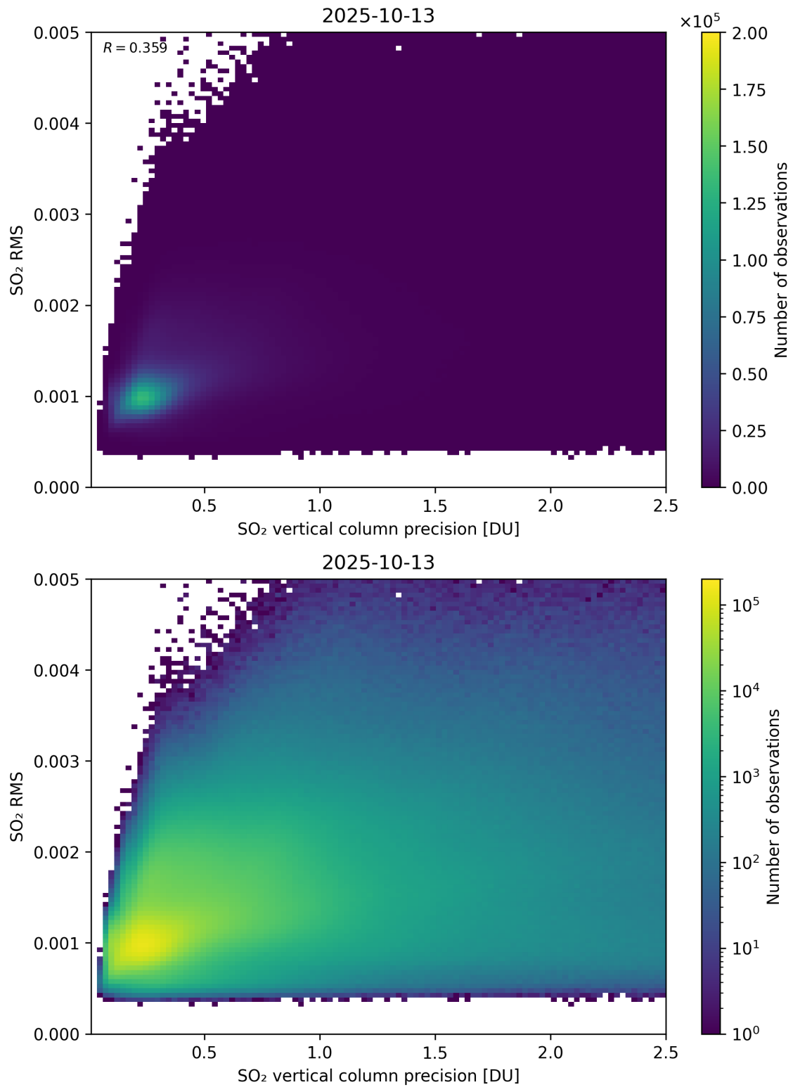
Figure 334: Scatter density plot of “SO 2 vertical column precision” against “SO 2 RMS” for 2025-10-12 to 2025-10-14.
