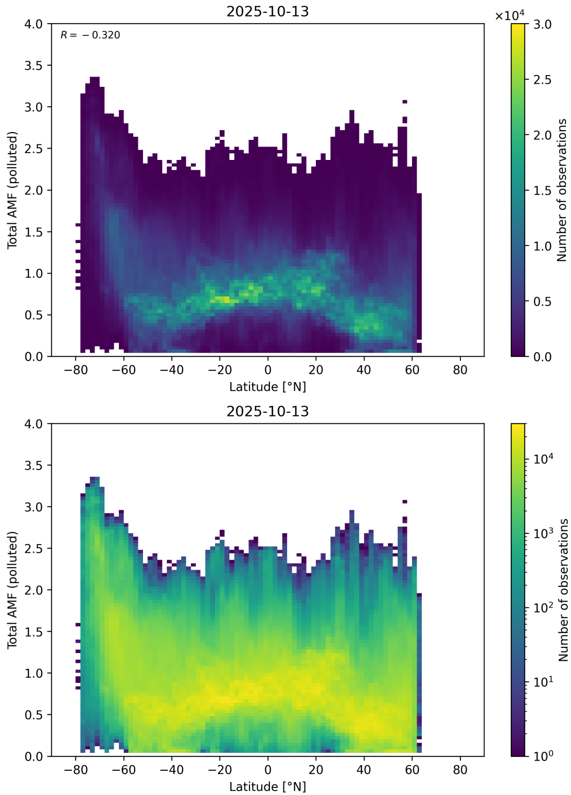
Figure 167: Scatter density plot of “Latitude” against “Total AMF (polluted)” for 2025-10-12 to 2025-10-14.
