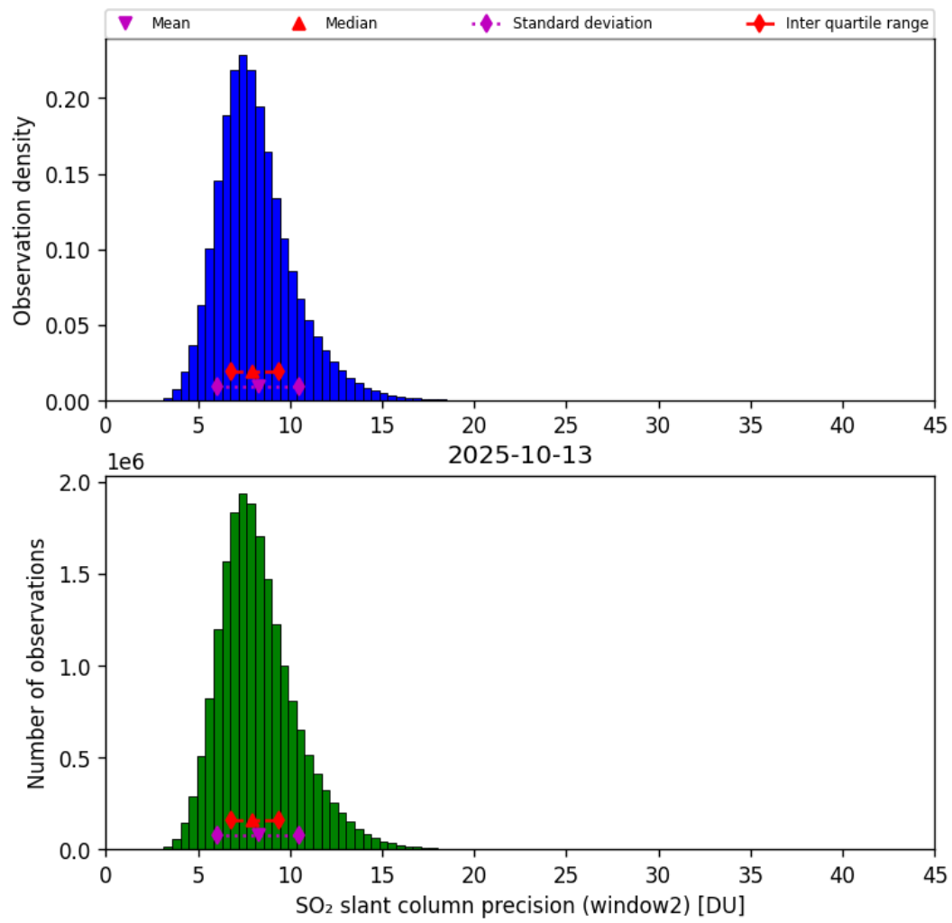
Figure 68: Histogram of “SO 2 slant column precision (window2)” for 2025-10-12 to 2025-10-14
