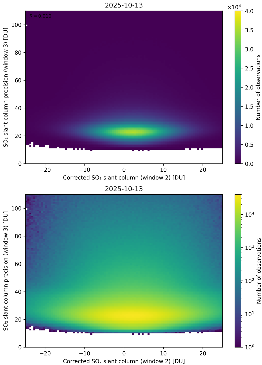
Figure 252: Scatter density plot of “Corrected SO 2 slant column (window 2)” against “SO 2 slant column precision (window 3)” for 2025-10-12 to 2025-10-14.
