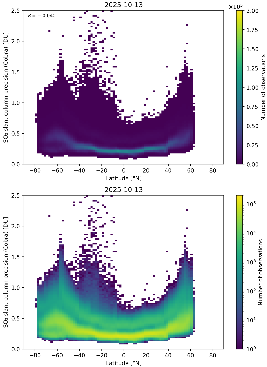
Figure 158: Scatter density plot of “Latitude” against “SO 2 slant column precision (Cobra)” for 2025-10-12 to 2025-10-14.
