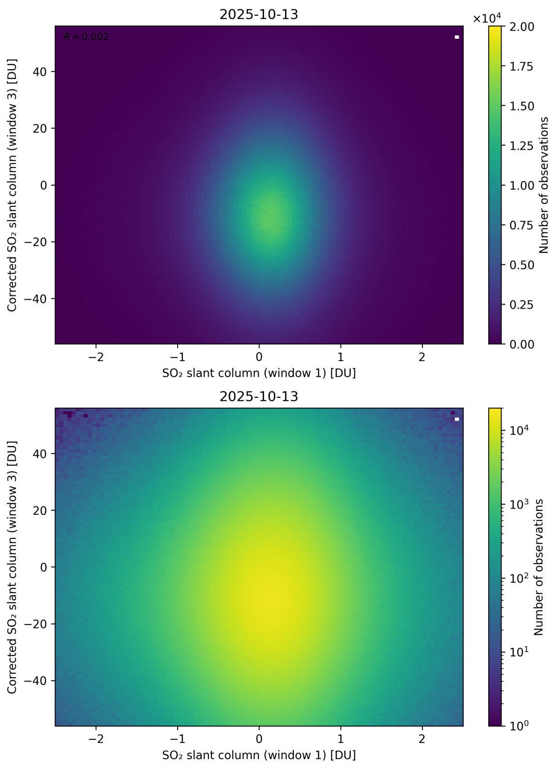
Figure 284: Scatter density plot of “SO 2 slant column (window 1)” against “Corrected SO 2 slant column (window 3)” for 2025-10-12 to 2025-10-14.
