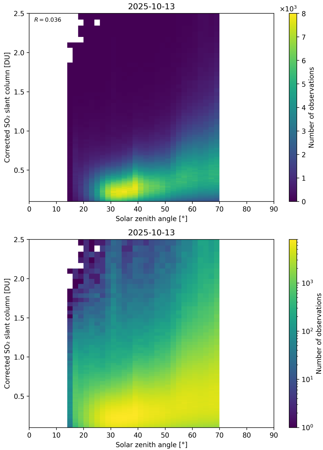
Figure 181: Scatter density plot of “Solar zenith angle” against “Corrected SO 2 slant column” for 2025-10-12 to 2025-10-14.
