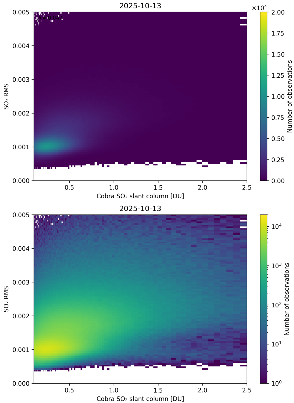
Figure 198: Scatter density plot of “Cobra SO 2 slant column” against “SO 2 RMS” for 2025-10-12 to 2025-10-14.
