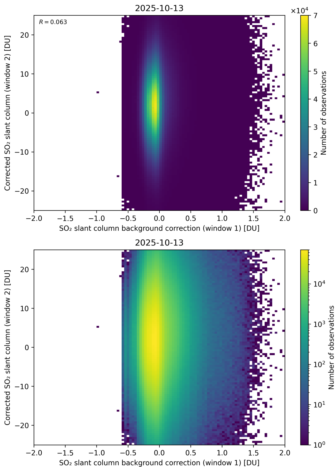
Figure 115: Scatter density plot of “SO 2 slant column background correction (window 1)” against “Corrected SO 2 slant column (window 2)” for 2025-10-12 to 2025-10-14.
