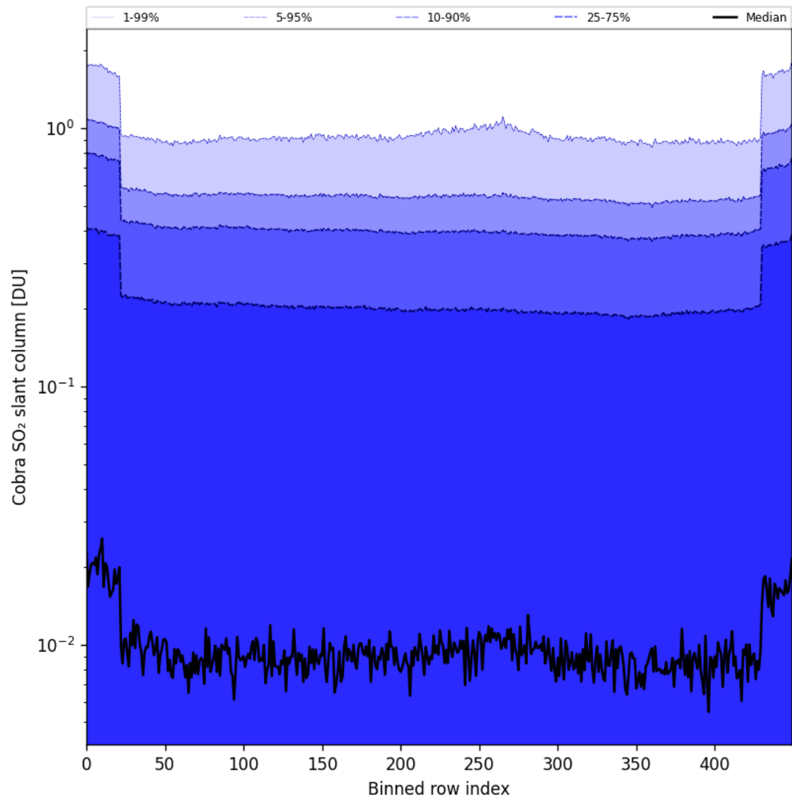
Figure 87: Along track statistics of “Cobra SO 2 slant column” for 2025-10-12 to 2025-10-14
