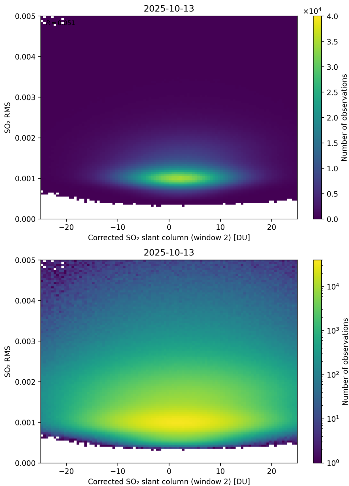
Figure 248: Scatter density plot of “Corrected SO 2 slant column (window 2)” against “SO 2 RMS” for 2025-10-12 to 2025-10-14.
