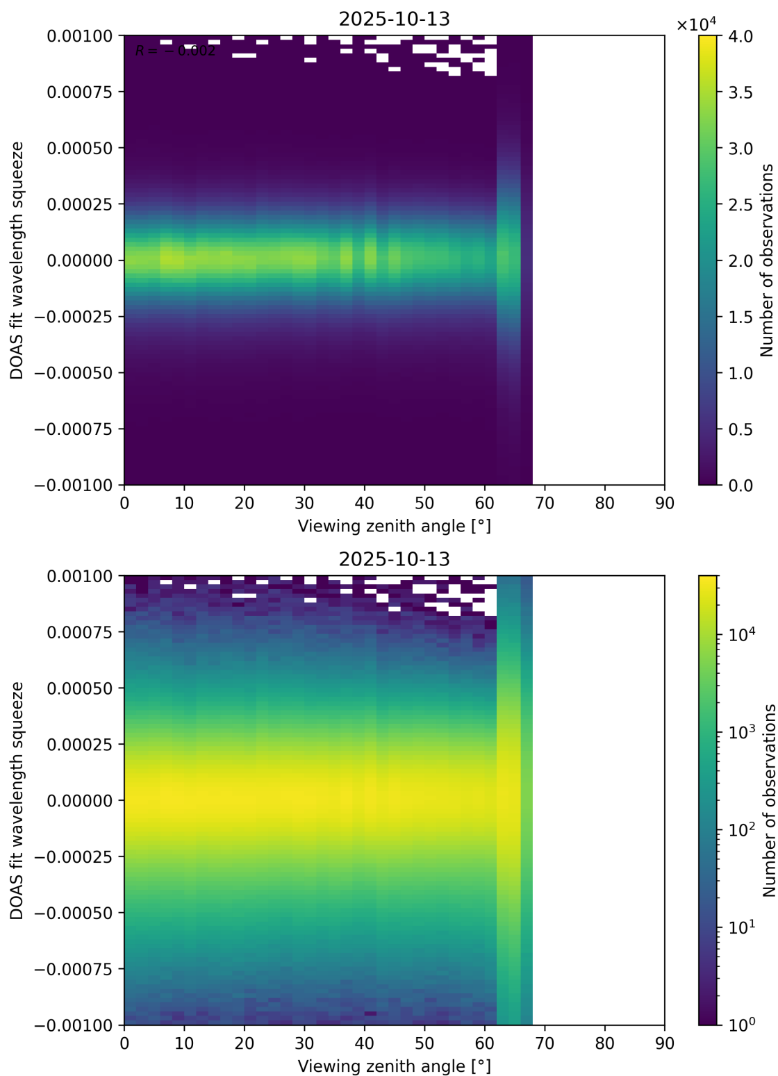
Figure 366: Scatter density plot of “Viewing zenith angle” against “DOAS fit wavelength squeeze” for 2025-10-12 to 2025-10-14.
