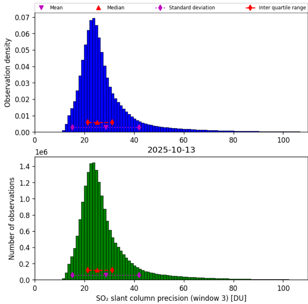
Figure 72: Histogram of “SO 2 slant column precision (window 3)” for 2025-10-12 to 2025-10-14
