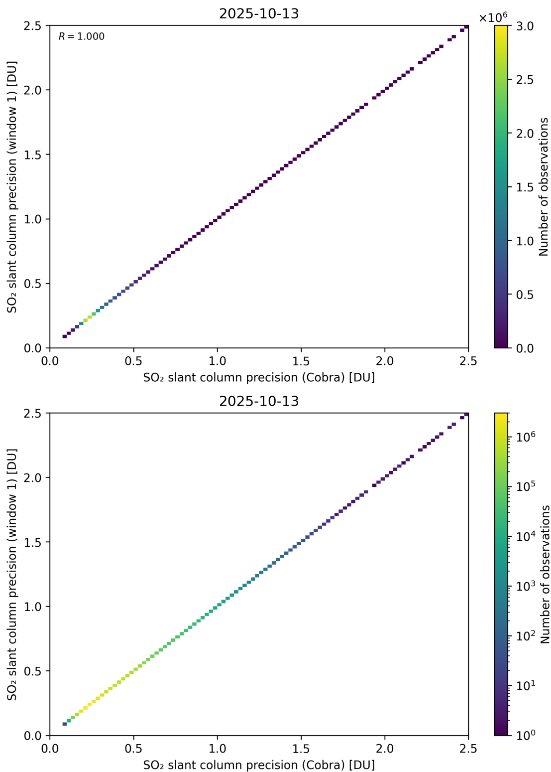
Figure 209: Scatter density plot of “SO 2 slant column precision (Cobra)” against “SO 2 slant column precision (window 1)” for 2025-10-12 to 2025-10-14.
