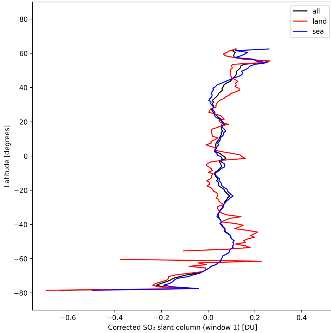
Figure 39: Zonal average of “Corrected SO 2 slant column (window 1)” for 2025-10-12 to 2025-10-14.
