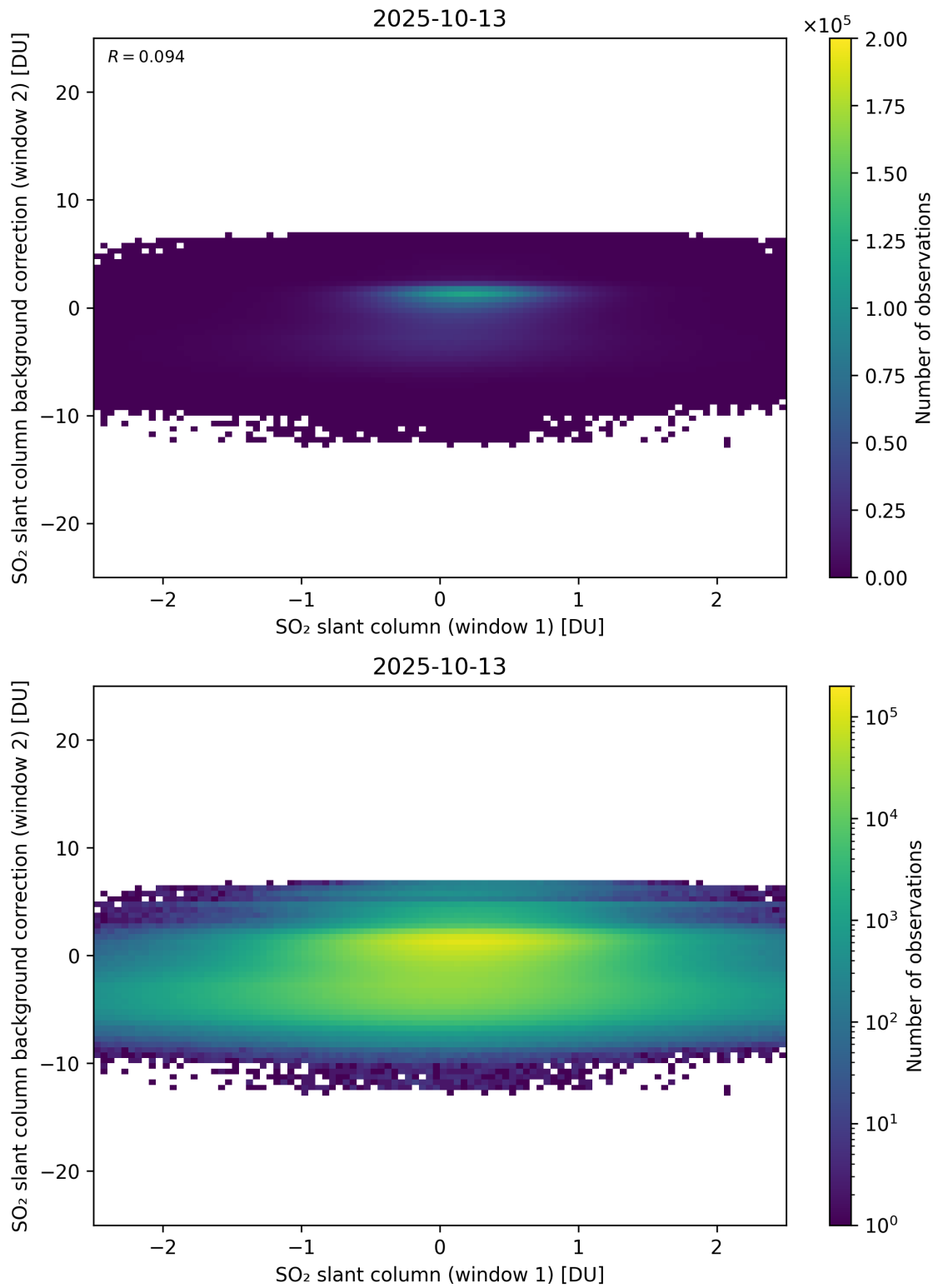
Figure 263: Scatter density plot of “SO 2 slant column (window 1)” against “SO 2 slant column background correction (window 2)” for 2025-10-12 to 2025-10-14.
