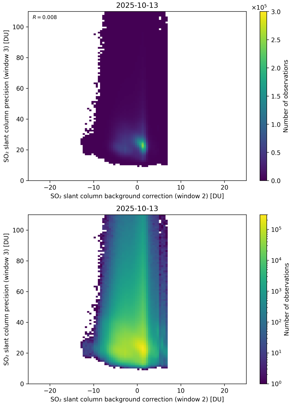
Figure 129: Scatter density plot of “SO 2 slant column background correction (window 2)” against “SO 2 slant column precision (window 3)” for 2025-10-12 to 2025-10-14.
