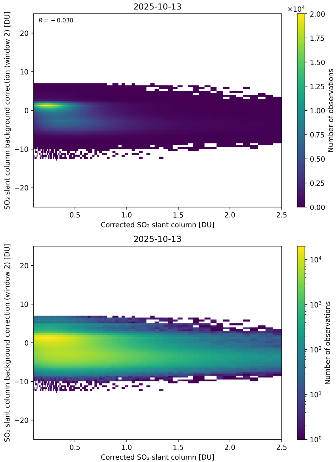
Figure 227: Scatter density plot of “Corrected SO 2 slant column” against “SO 2 slant column background correction (window 2)” for 2025-10-12 to 2025-10-14.
