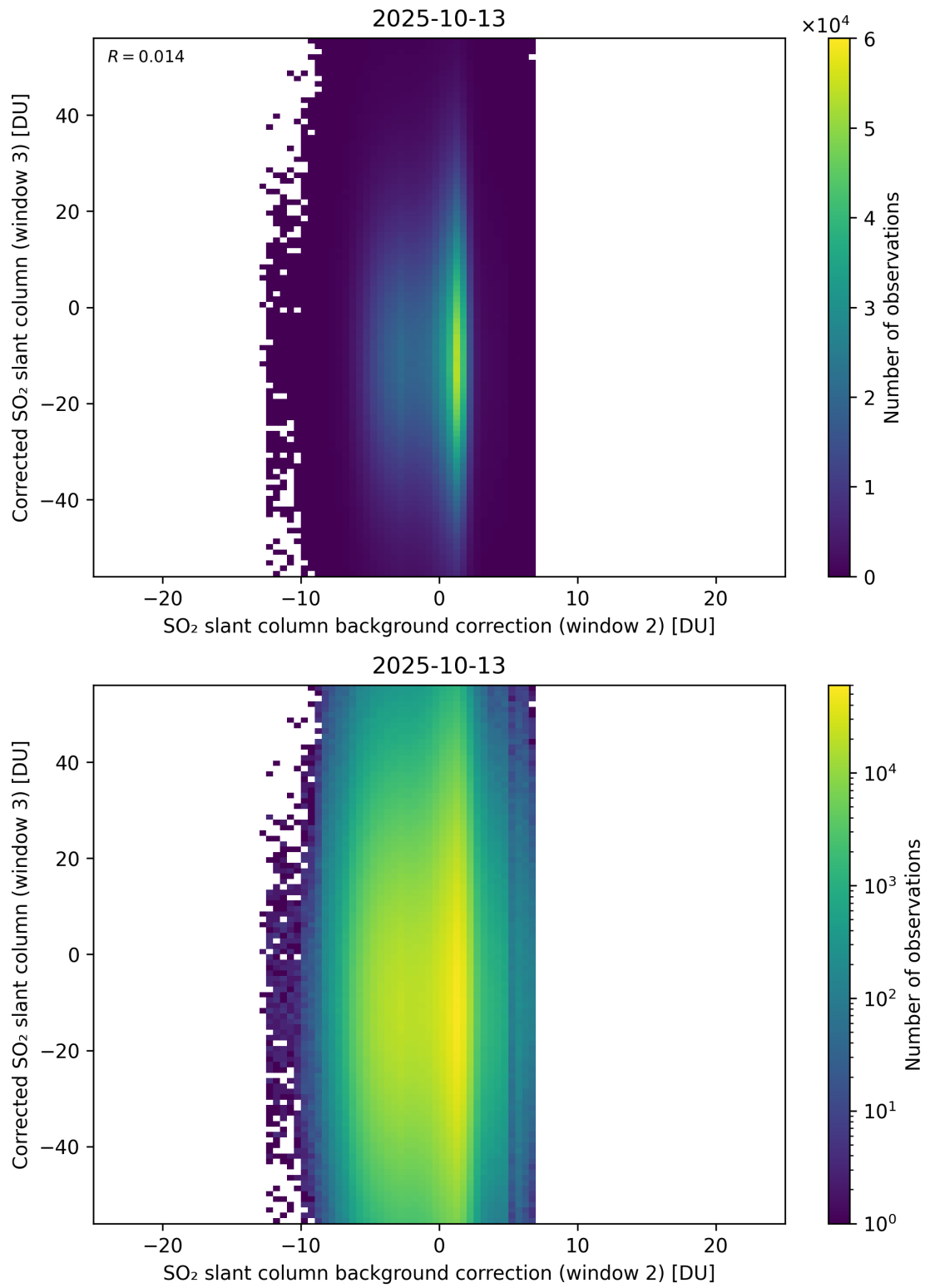
Figure 127: Scatter density plot of “SO 2 slant column background correction (window 2)” against “Corrected SO 2 slant column (window 3)” for 2025-10-12 to 2025-10-14.
