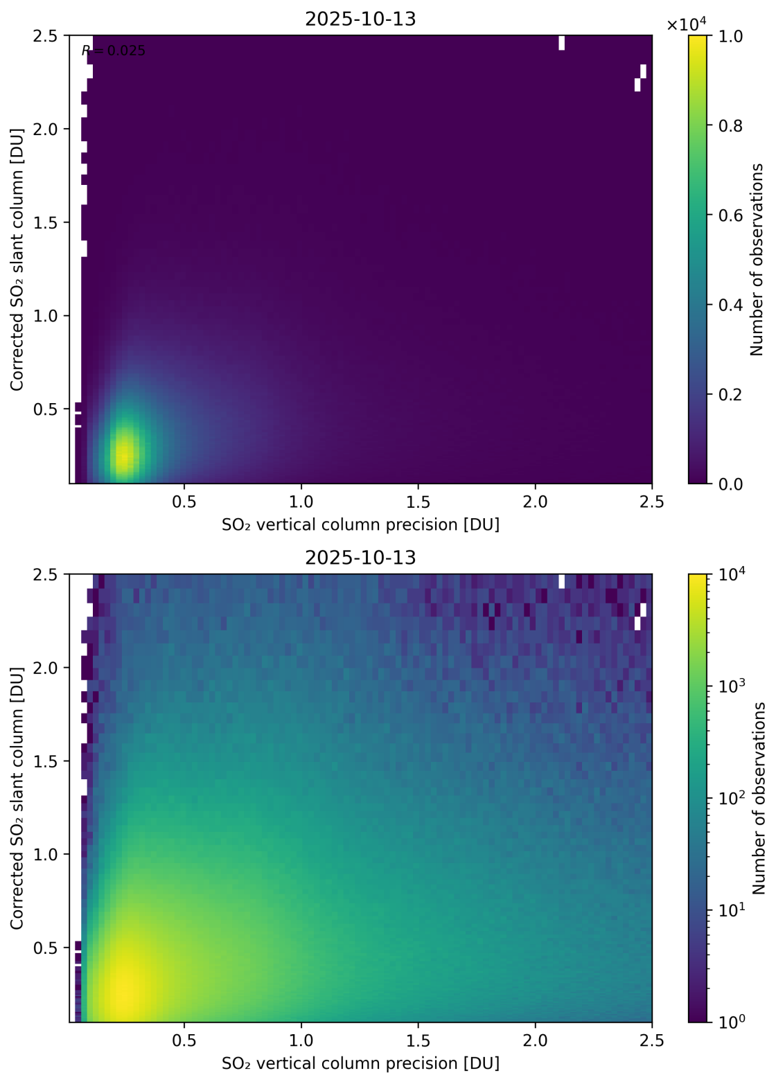
Figure 338: Scatter density plot of “SO 2 vertical column precision” against “Corrected SO 2 slant column” for 2025-10-12 to 2025-10-14.
