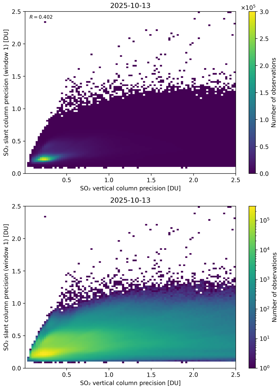
Figure 342: Scatter density plot of “SO 2 vertical column precision” against “SO 2 slant column precision (window 1)” for 2025-10-12 to 2025-10-14.
