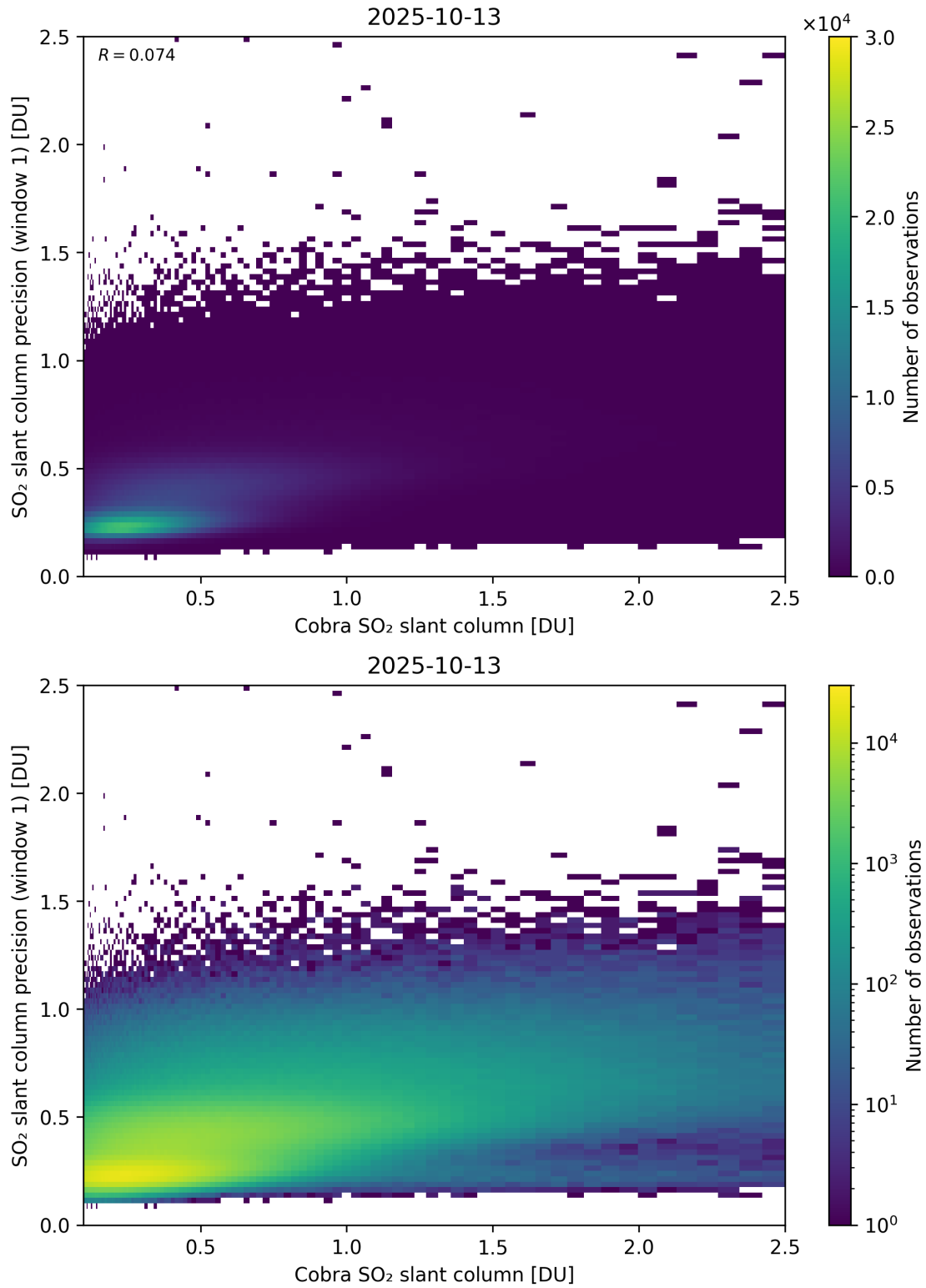
Figure 220: Scatter density plot of “Cobra SO 2 slant column” against “SO 2 slant column precision (window 1)” for 2025-10-12 to 2025-10-14.
