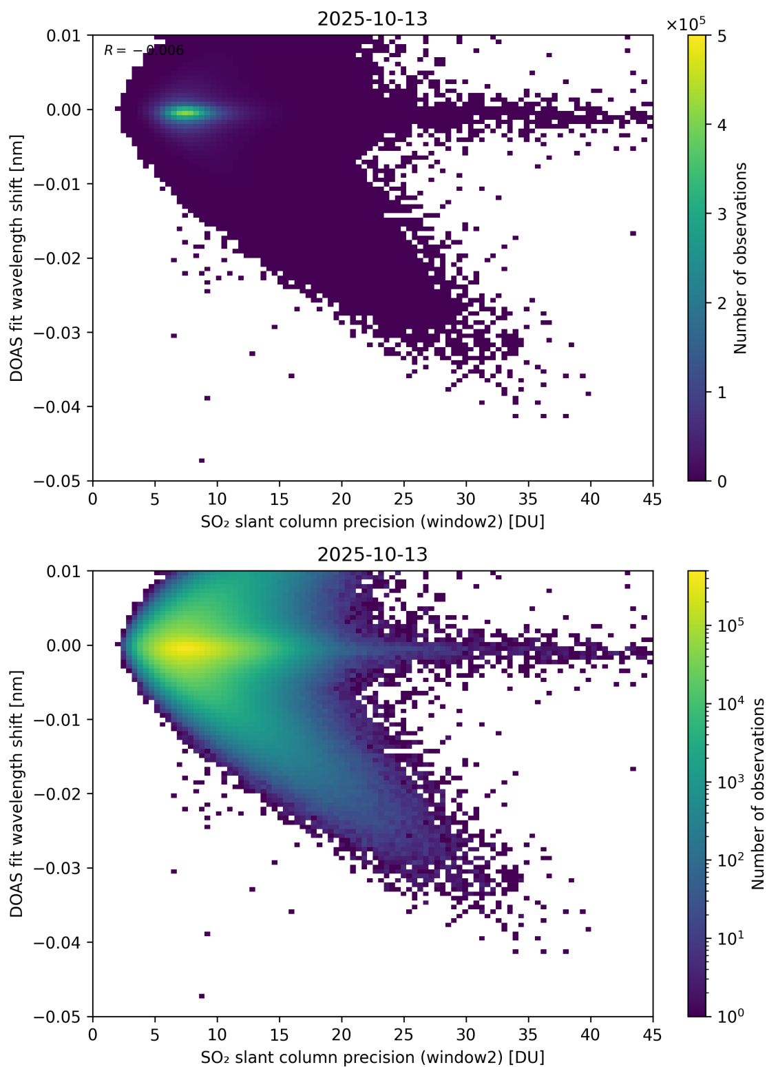
Figure 293: Scatter density plot of “SO 2 slant column precision (window2)” against “DOAS fit wavelength shift” for 2025-10-12 to 2025-10-14.
