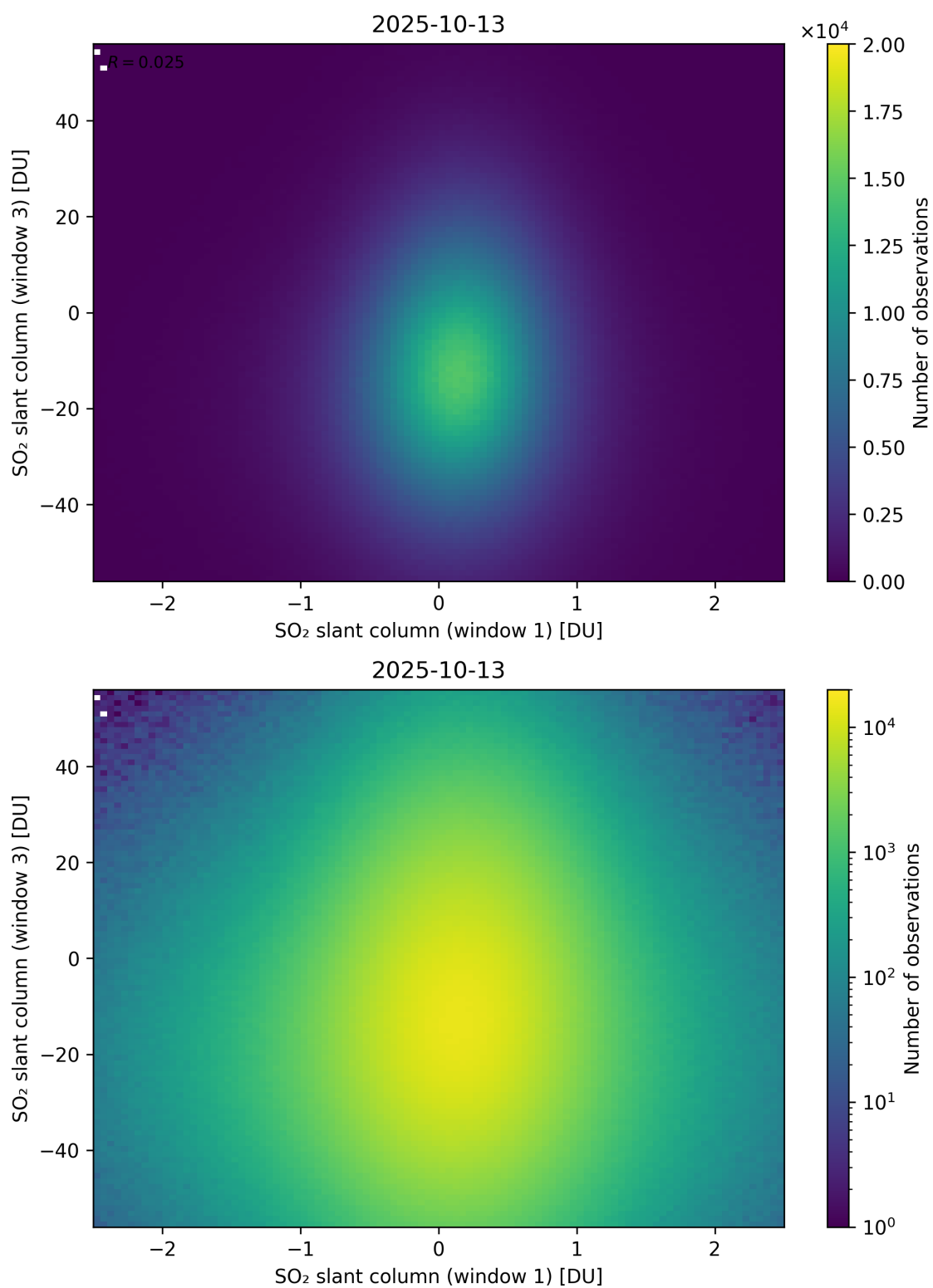
Figure 287: Scatter density plot of “SO 2 slant column (window 1)” against “SO 2 slant column (window 3)” for 2025-10-12 to 2025-10-14.
