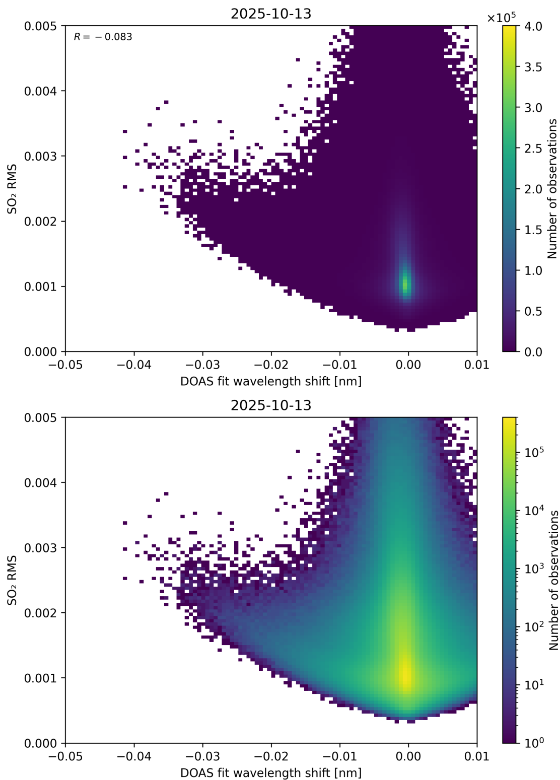
Figure 139: Scatter density plot of “DOAS fit wavelength shift” against “SO 2 RMS” for 2025-10-12 to 2025-10-14.
