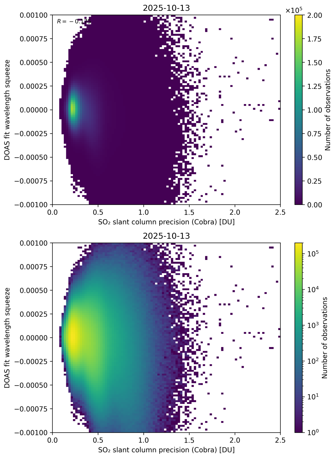
Figure 203: Scatter density plot of “SO 2 slant column precision (Cobra)” against “DOAS fit wavelength squeeze” for 2025-10-12 to 2025-10-14.
