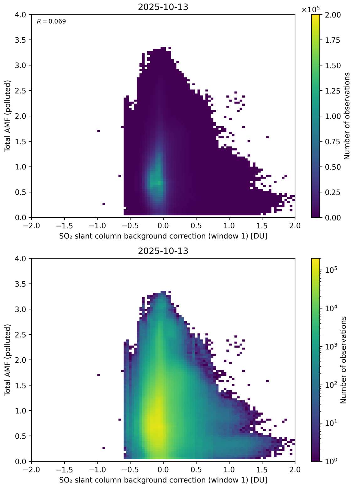
Figure 120: Scatter density plot of “SO 2 slant column background correction (window 1)” against “Total AMF (polluted)” for 2025-10-12 to 2025-10-14.
