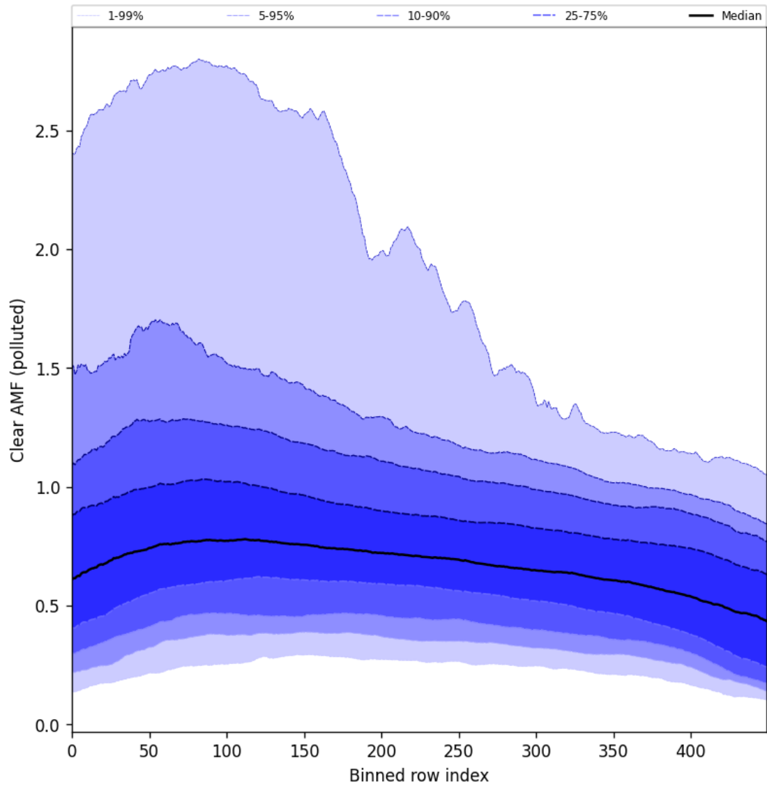
Figure 107: Along track statistics of “Clear AMF (polluted)” for 2025-10-12 to 2025-10-14
