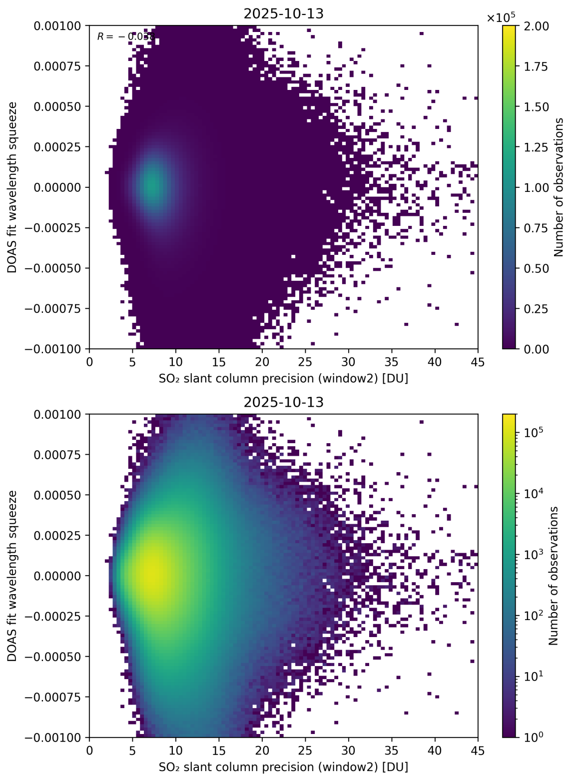
Figure 294: Scatter density plot of “SO 2 slant column precision (window2)” against “DOAS fit wavelength squeeze” for 2025-10-12 to 2025-10-14.
