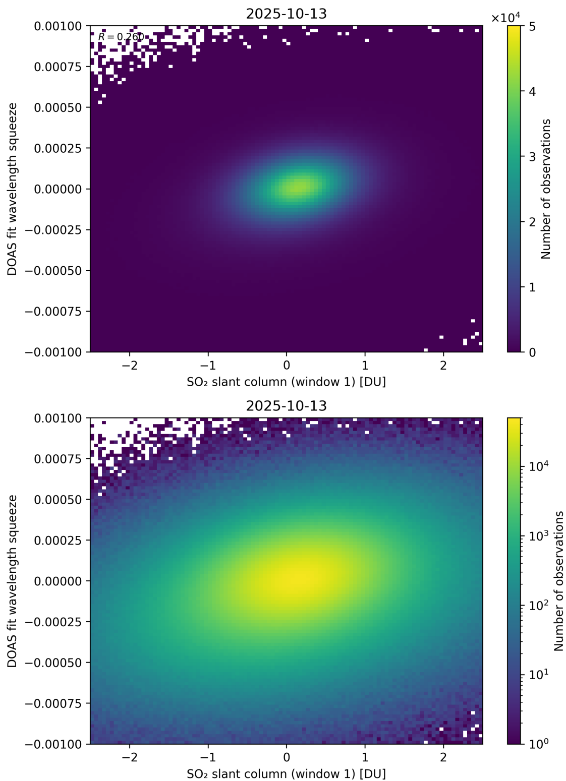
Figure 266: Scatter density plot of “SO 2 slant column (window 1)” against “DOAS fit wavelength squeeze” for 2025-10-12 to 2025-10-14.
