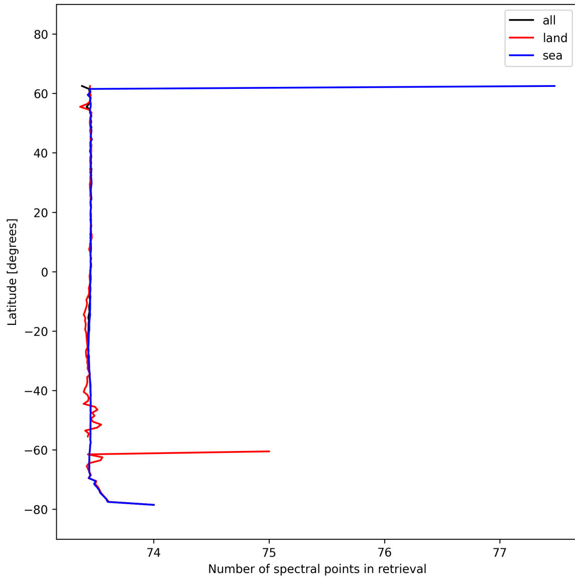
Figure 56: Zonal average of “Number of spectral points in retrieval” for 2025-10-12 to 2025-10-14.
