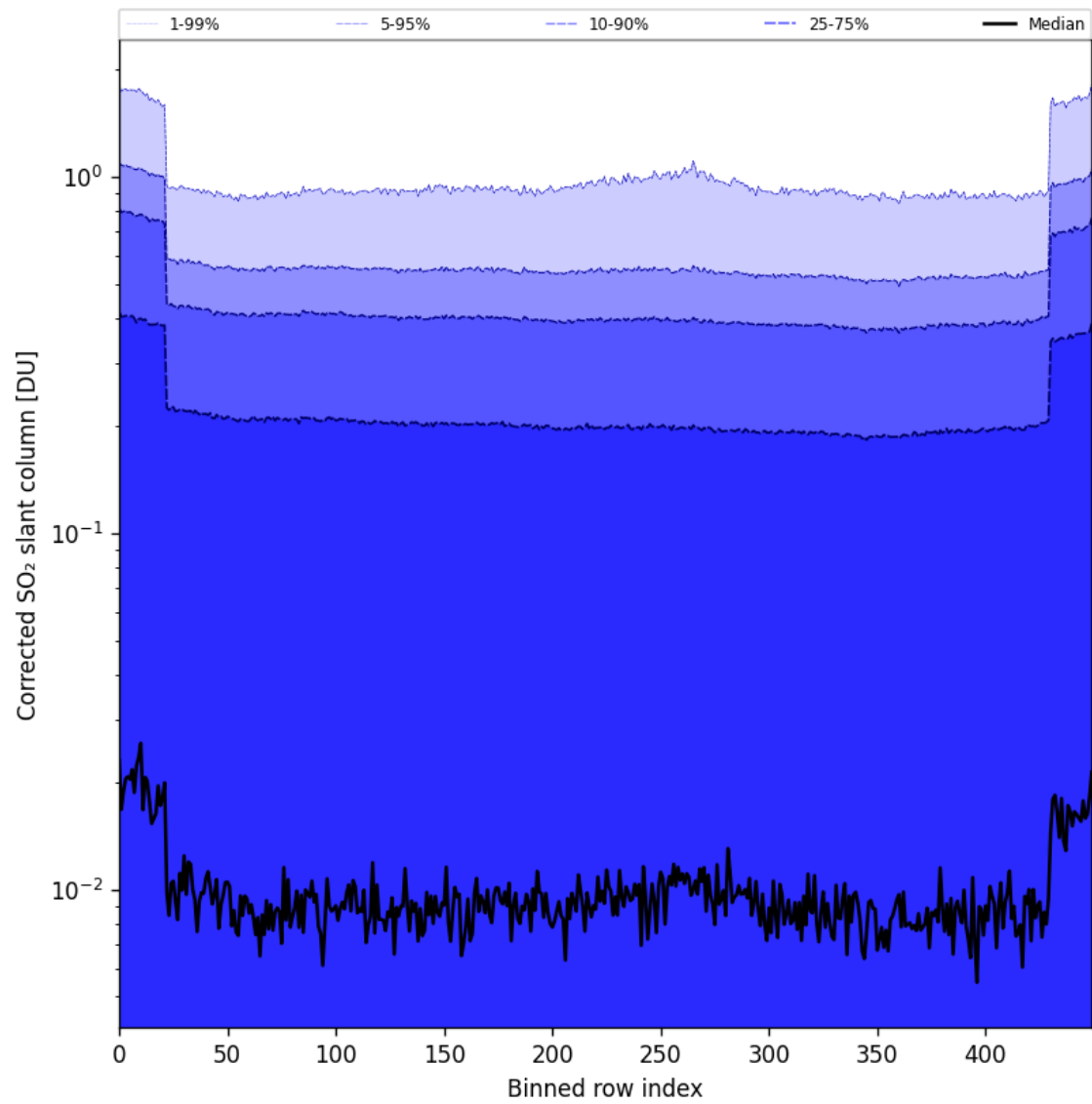
Figure 86: Along track statistics of “Corrected SO 2 slant column” for 2025-10-12 to 2025-10-14
