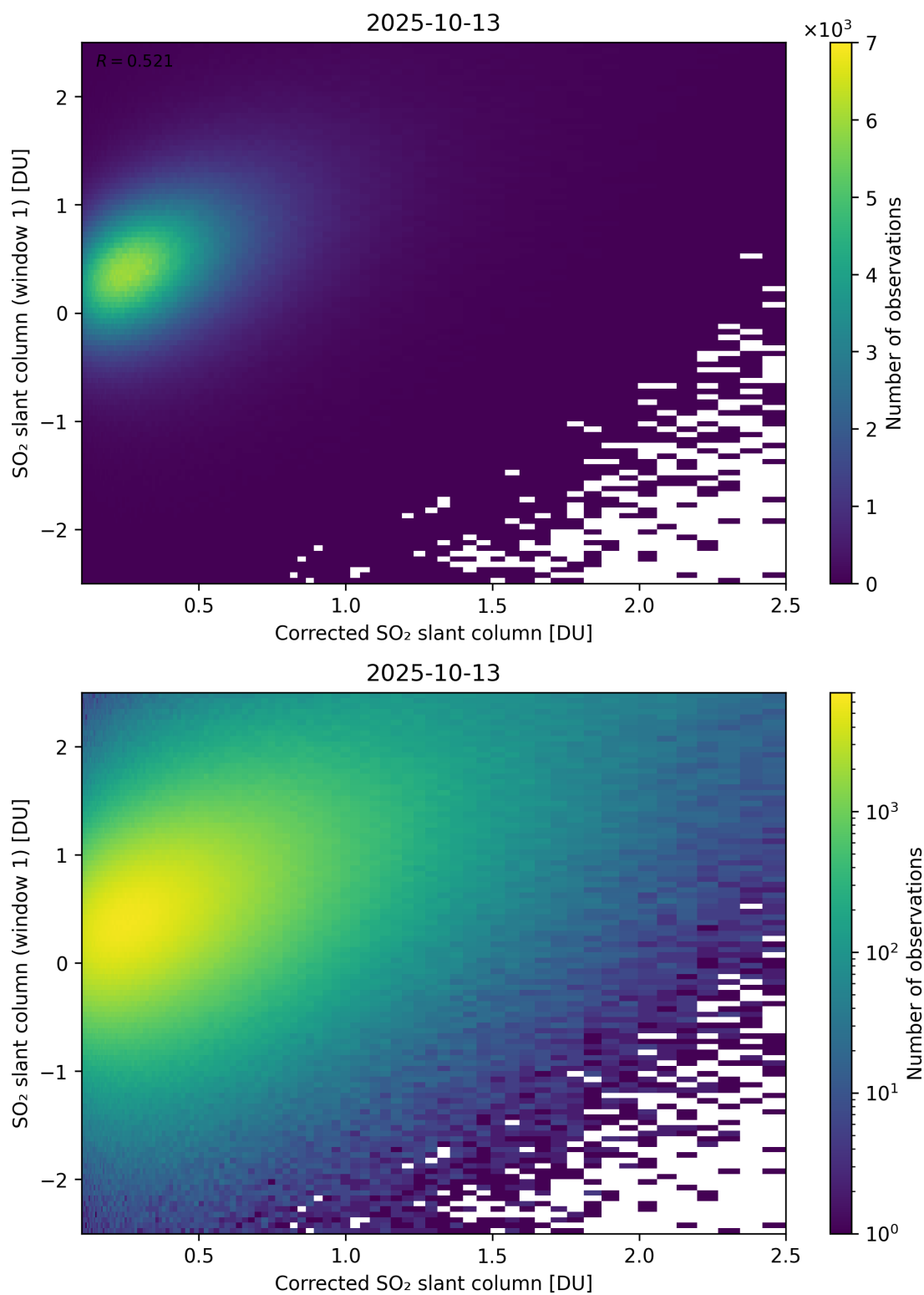
Figure 237: Scatter density plot of “Corrected SO 2 slant column” against “SO 2 slant column (window 1)” for 2025-10-12 to 2025-10-14.
