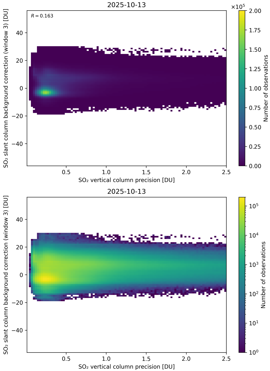
Figure 331: Scatter density plot of “SO 2 vertical column precision” against “SO 2 slant column background correction (window 3)” for 2025-10-12 to 2025-10-14.
