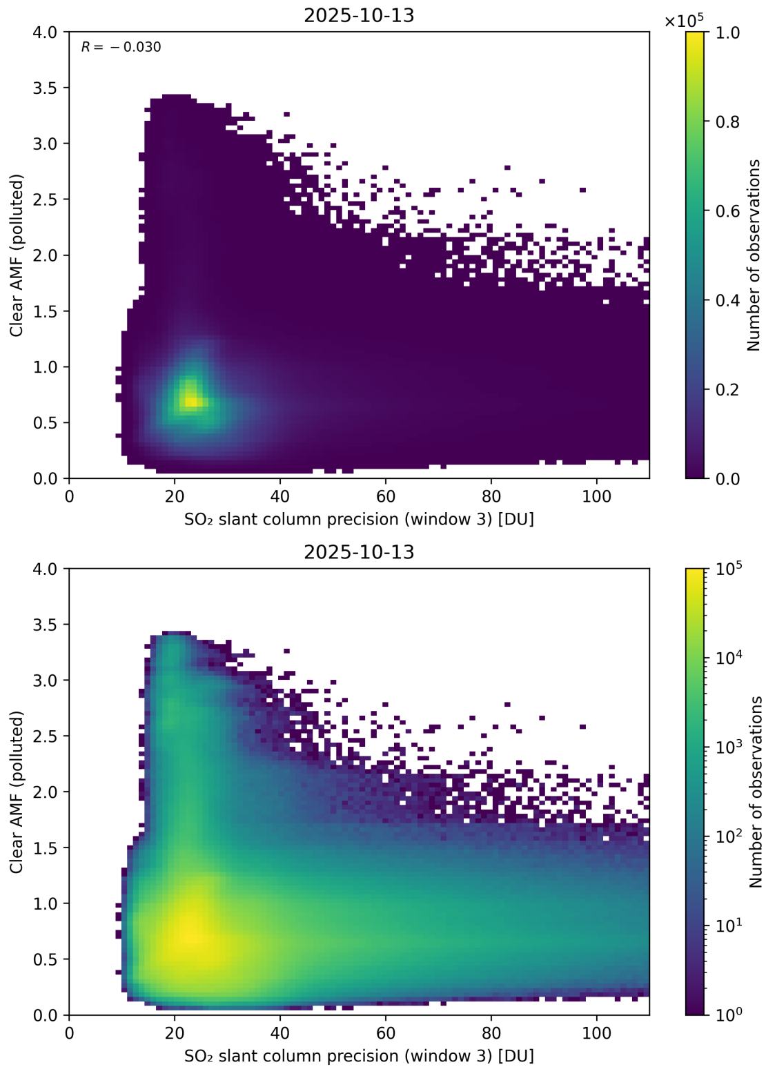
Figure 311: Scatter density plot of “SO 2 slant column precision (window 3)” against “Clear AMF (polluted)” for 2025-10-12 to 2025-10-14.
