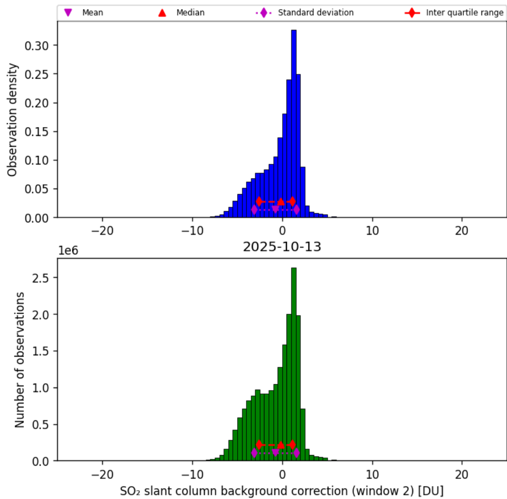
Figure 70: Histogram of “SO 2 slant column background correction (window 2)” for 2025-10-12 to 2025-10-14
