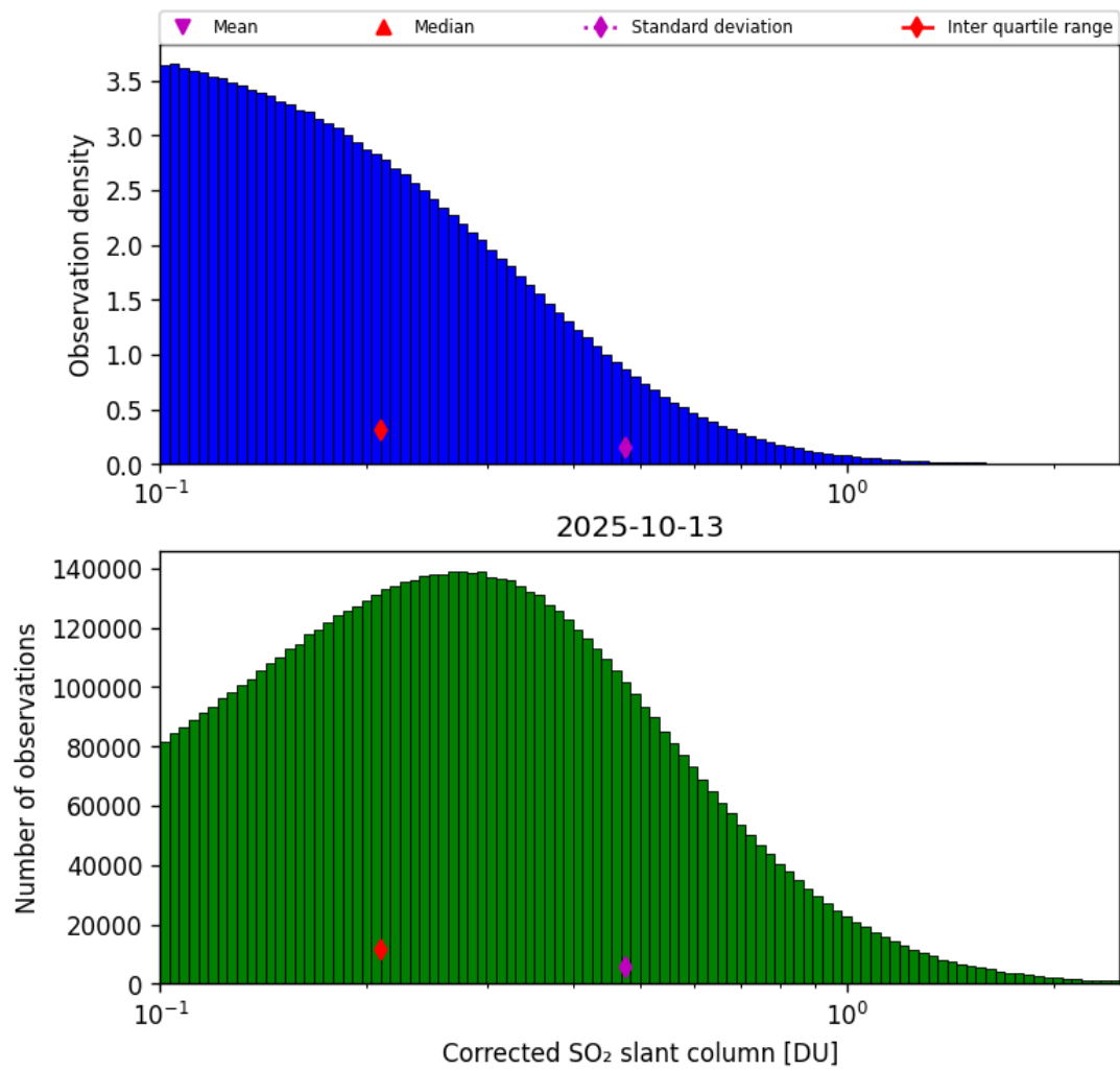
Figure 60: Histogram of “Corrected SO 2 slant column” for 2025-10-12 to 2025-10-14
