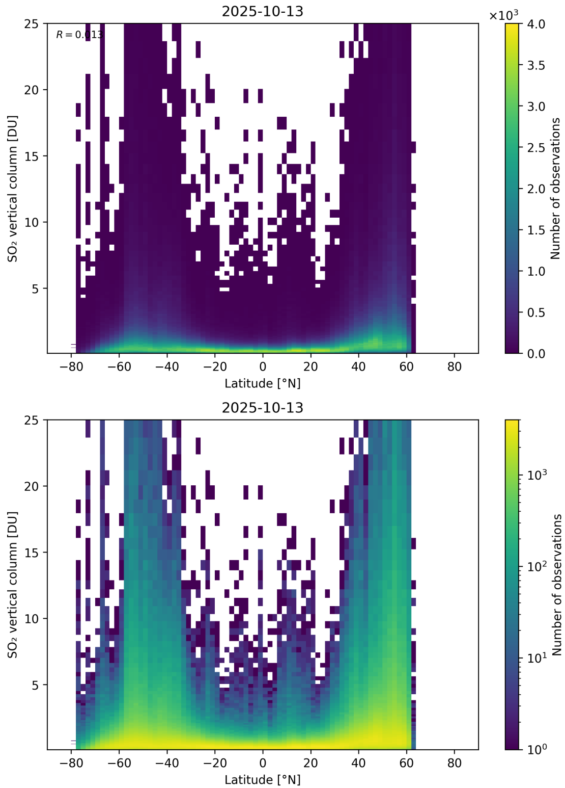
Figure 169: Scatter density plot of “Latitude” against “SO 2 vertical column” for 2025-10-12 to 2025-10-14.
