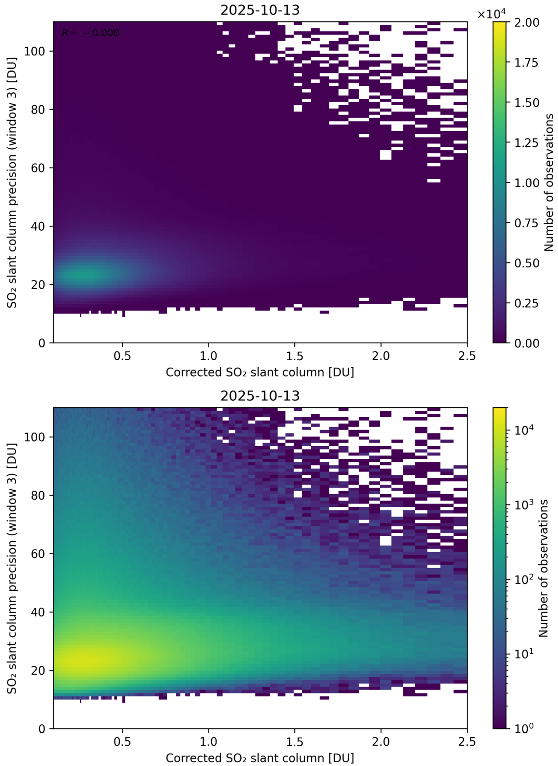
Figure 241: Scatter density plot of “Corrected SO 2 slant column” against “SO 2 slant column precision (window 3)” for 2025-10-12 to 2025-10-14.
