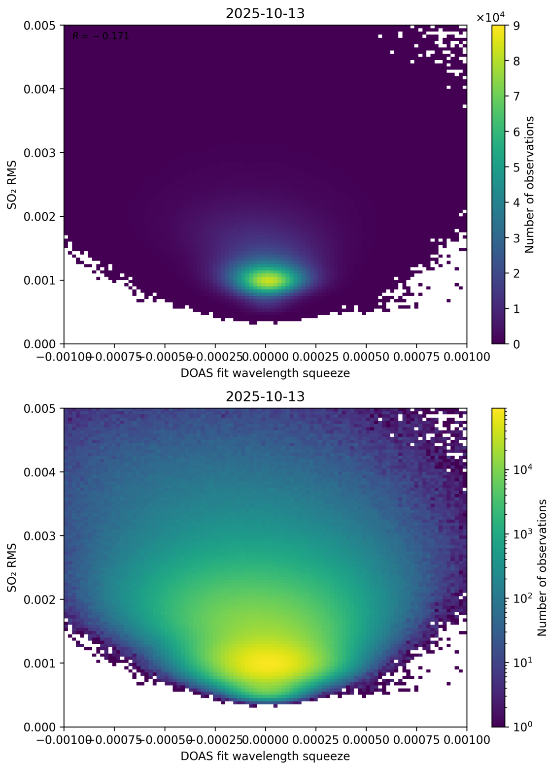
Figure 143: Scatter density plot of “DOAS fit wavelength squeeze” against “SO 2 RMS” for 2025-10-12 to 2025-10-14.
