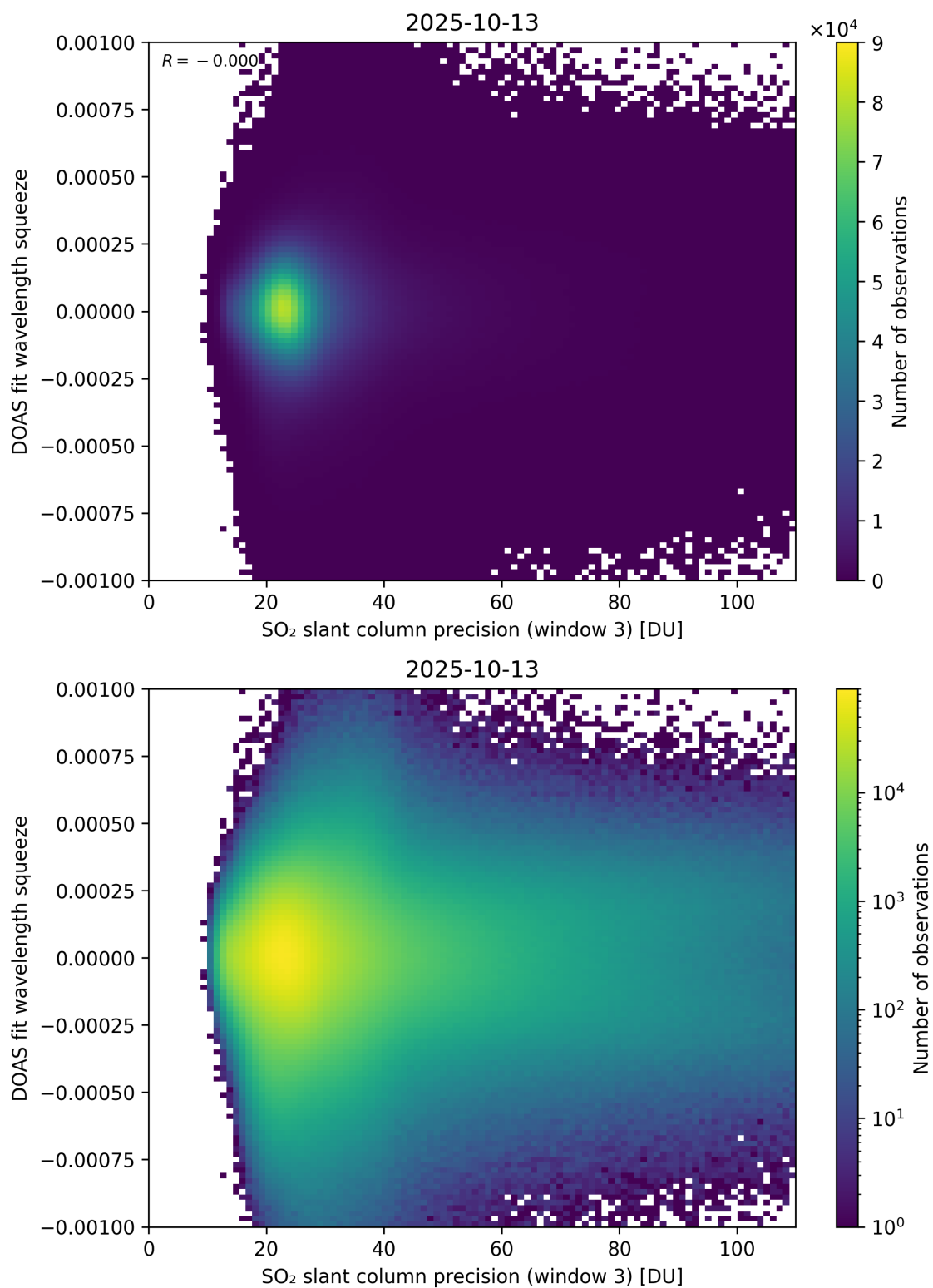
Figure 309: Scatter density plot of “SO 2 slant column precision (window 3)” against “DOAS fit wavelength squeeze” for 2025-10-12 to 2025-10-14.
