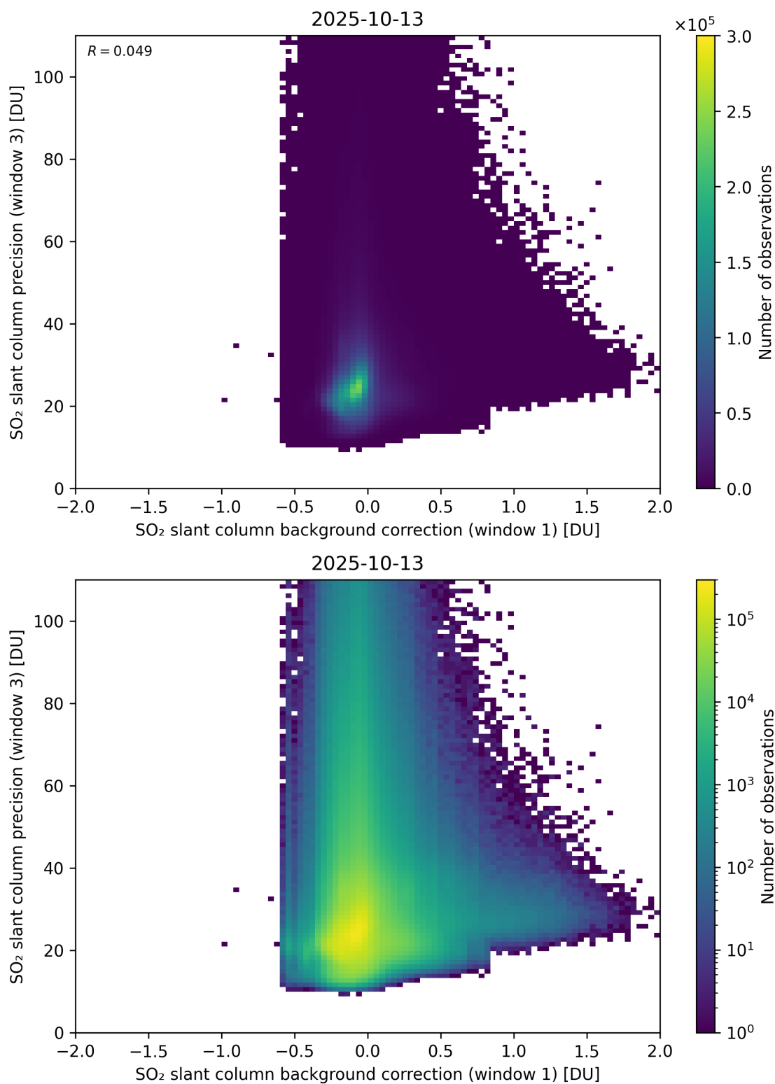
Figure 119: Scatter density plot of “SO 2 slant column background correction (window 1)” against “SO 2 slant column precision (window 3)” for 2025-10-12 to 2025-10-14.
