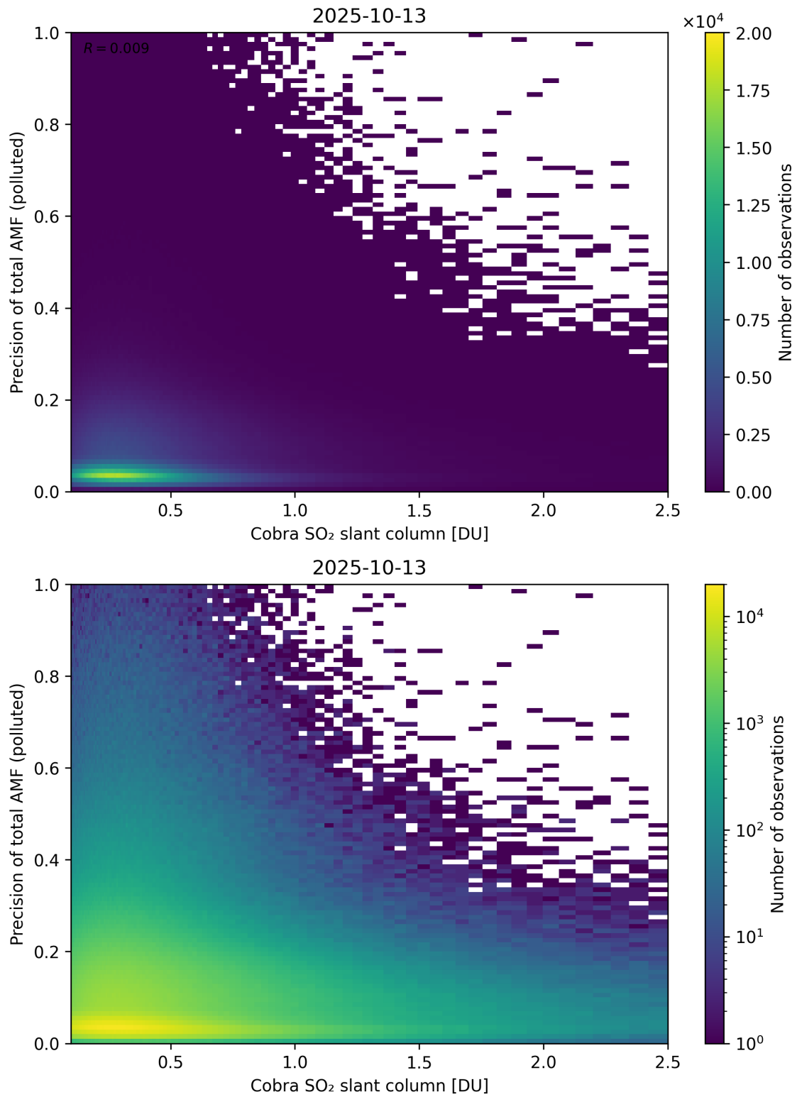
Figure 225: Scatter density plot of “Cobra SO 2 slant column” against “Precision of total AMF (polluted)” for 2025-10-12 to 2025-10-14.
