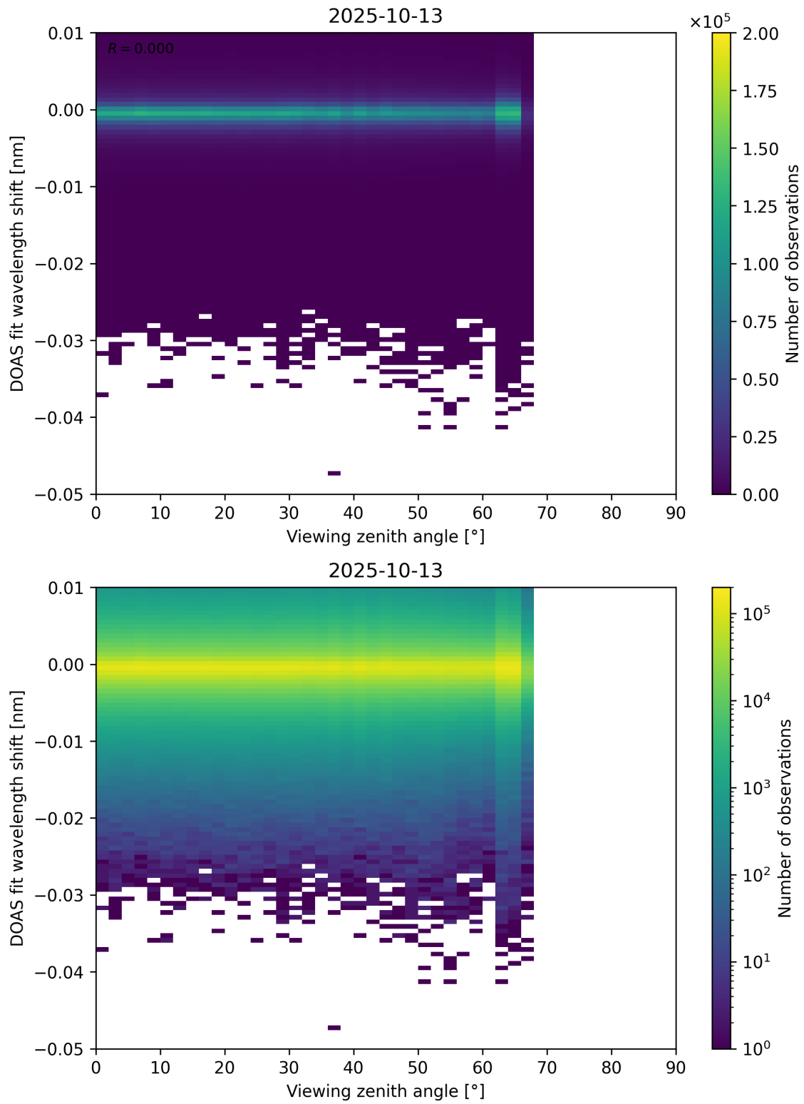
Figure 365: Scatter density plot of “Viewing zenith angle” against “DOAS fit wavelength shift” for 2025-10-12 to 2025-10-14.
