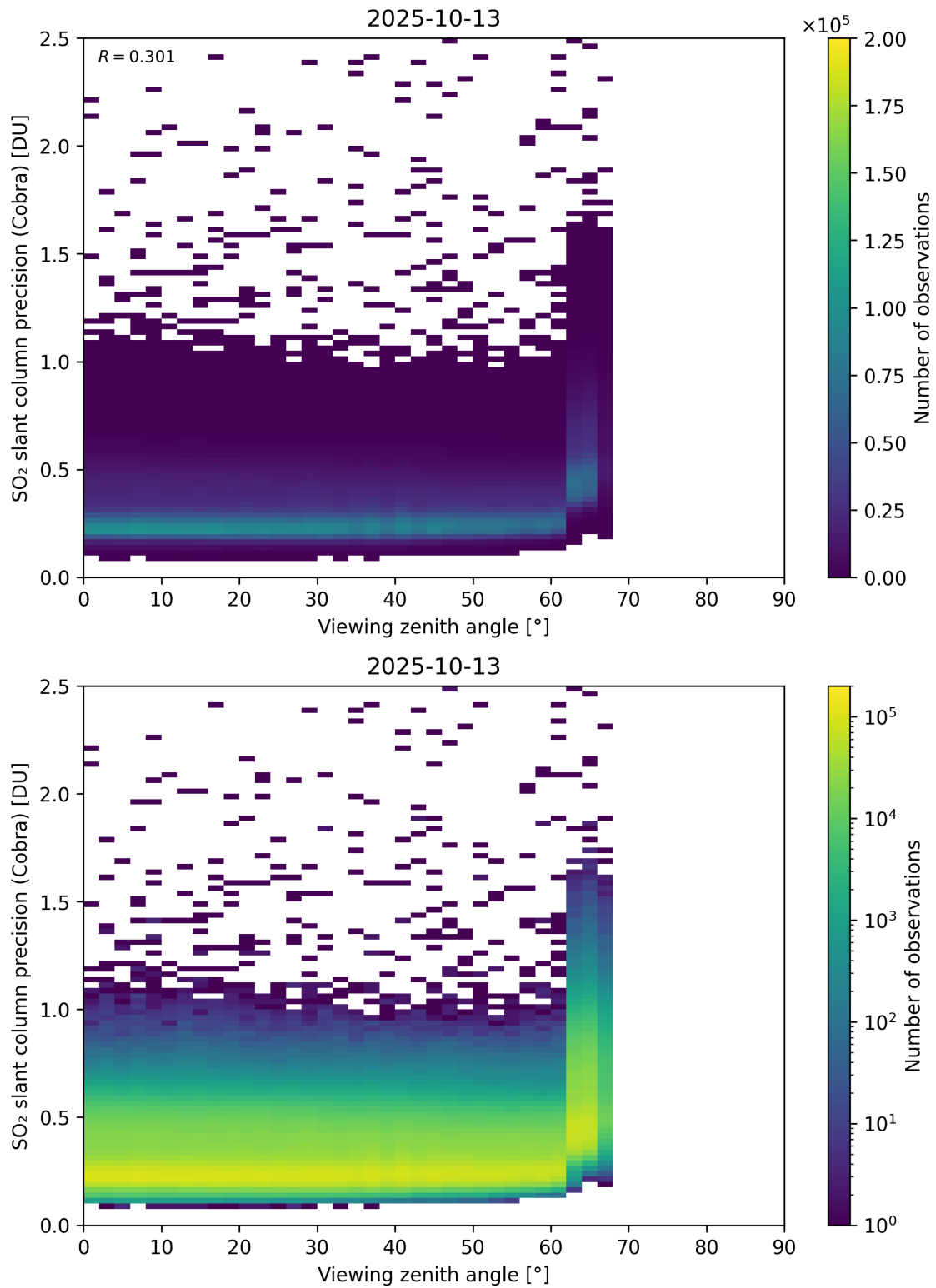
Figure 372: Scatter density plot of “Viewing zenith angle” against “SO 2 slant column precision (Cobra)” for 2025-10-12 to 2025-10-14.
