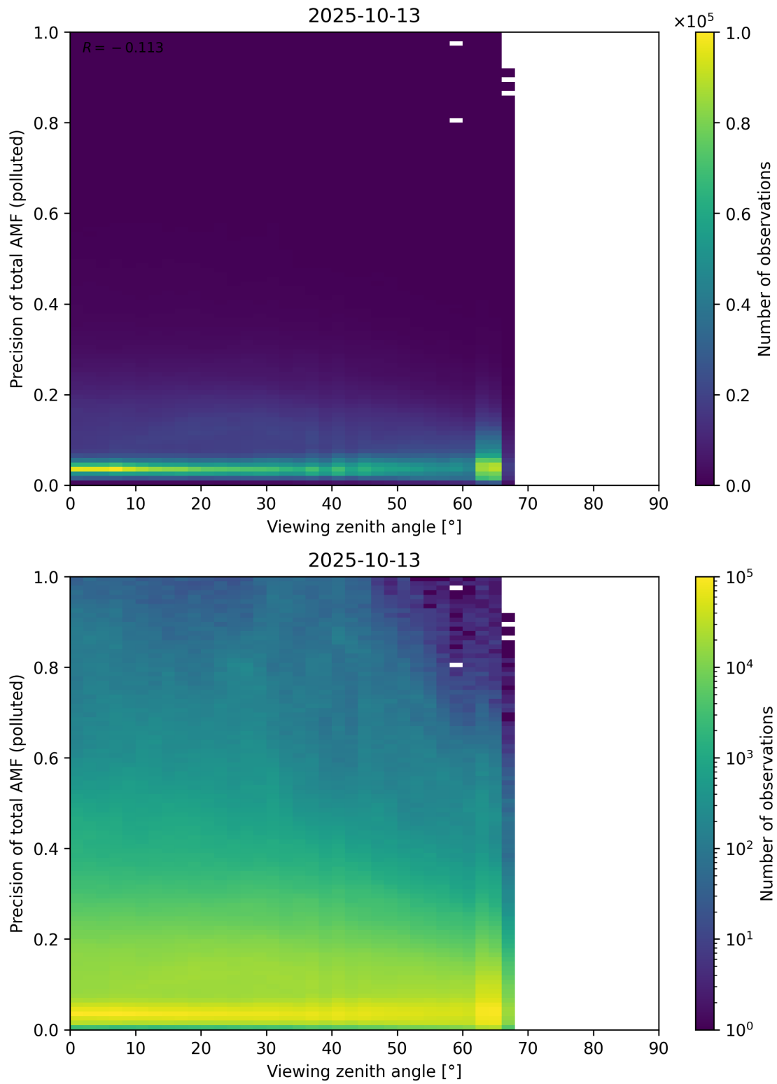
Figure 382: Scatter density plot of “Viewing zenith angle” against “Precision of total AMF (polluted)” for 2025-10-12 to 2025-10-14.
