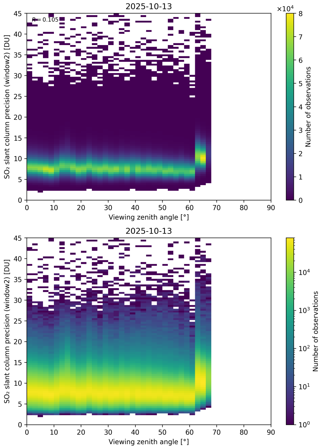
Figure 378: Scatter density plot of “Viewing zenith angle” against “SO 2 slant column precision (window2)” for 2025-10-12 to 2025-10-14.
