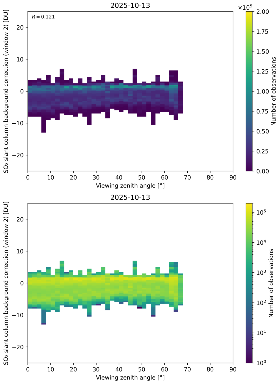
Figure 363: Scatter density plot of “Viewing zenith angle” against “SO 2 slant column background correction (window 2)” for 2025-10-12 to 2025-10-14.
