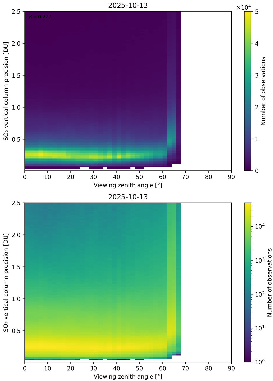
Figure 384: Scatter density plot of “Viewing zenith angle” against “SO 2 vertical column precision” for 2025-10-12 to 2025-10-14.
