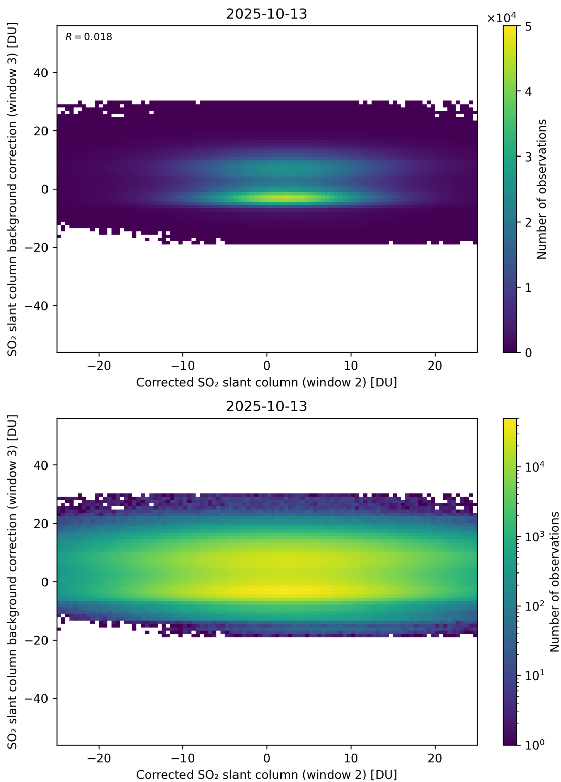
Figure 245: Scatter density plot of “Corrected SO 2 slant column (window 2)” against “SO 2 slant column background correction (window 3)” for 2025-10-12 to 2025-10-14.
