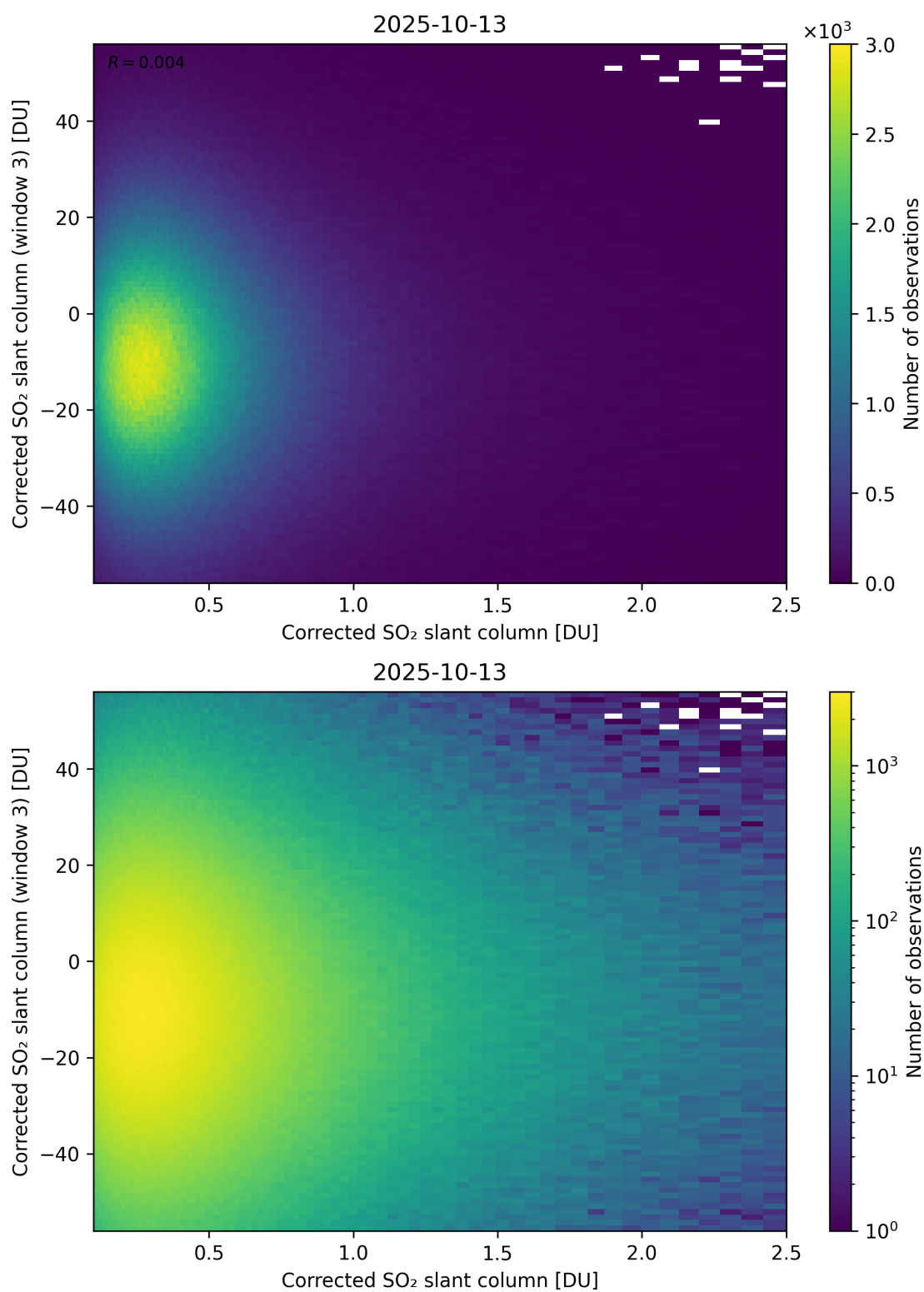
Figure 236: Scatter density plot of “Corrected SO 2 slant column” against “Corrected SO 2 slant column (window 3)” for 2025-10-12 to 2025-10-14.
