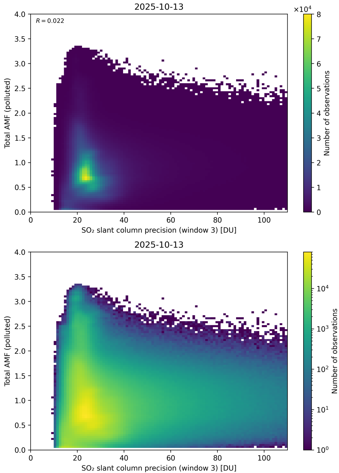
Figure 313: Scatter density plot of “SO 2 slant column precision (window 3)” against “Total AMF (polluted)” for 2025-10-12 to 2025-10-14.
