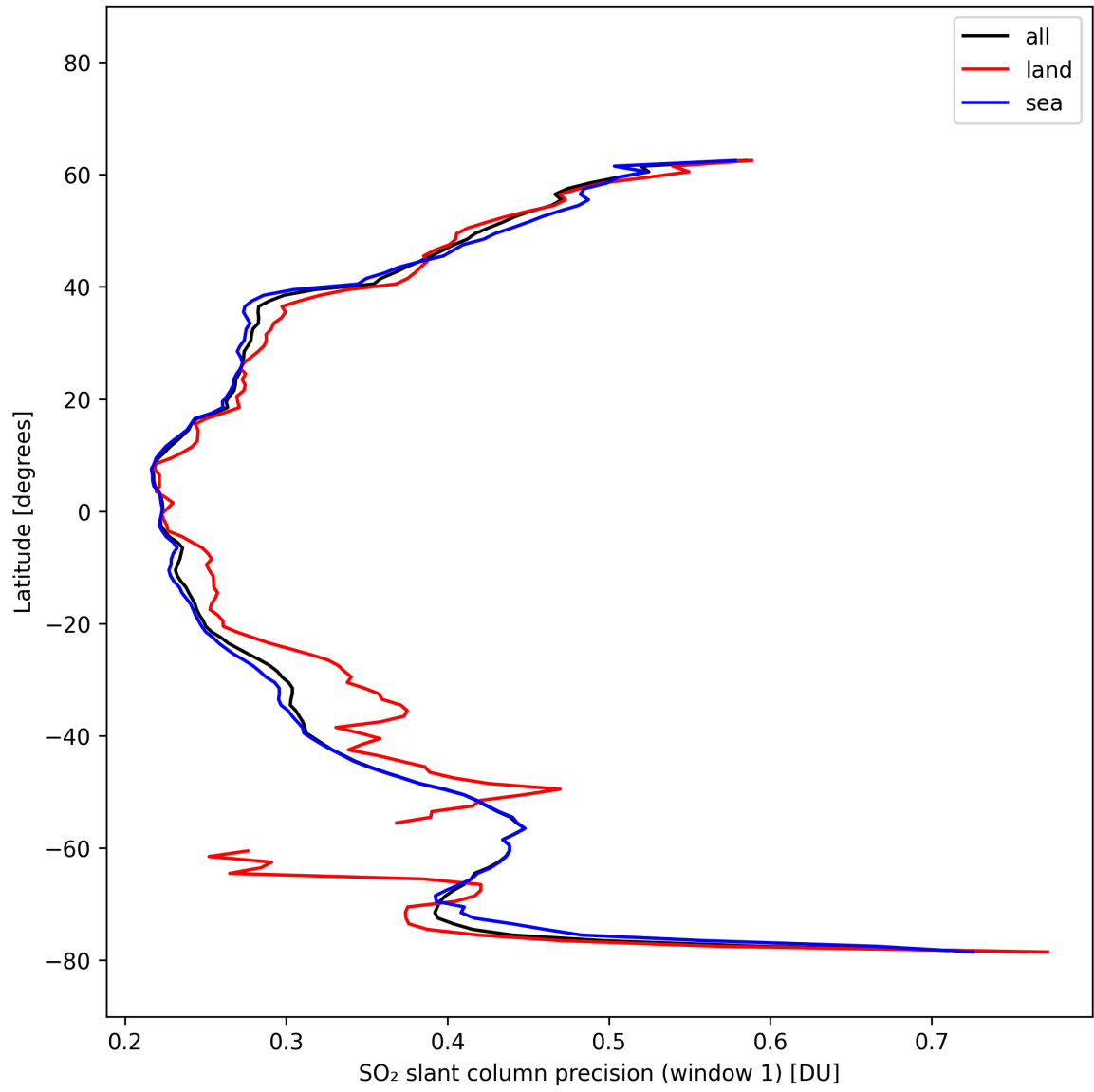
Figure 38: Zonal average of “SO 2 slant column precision (window 1)” for 2025-10-12 to 2025-10-14.
