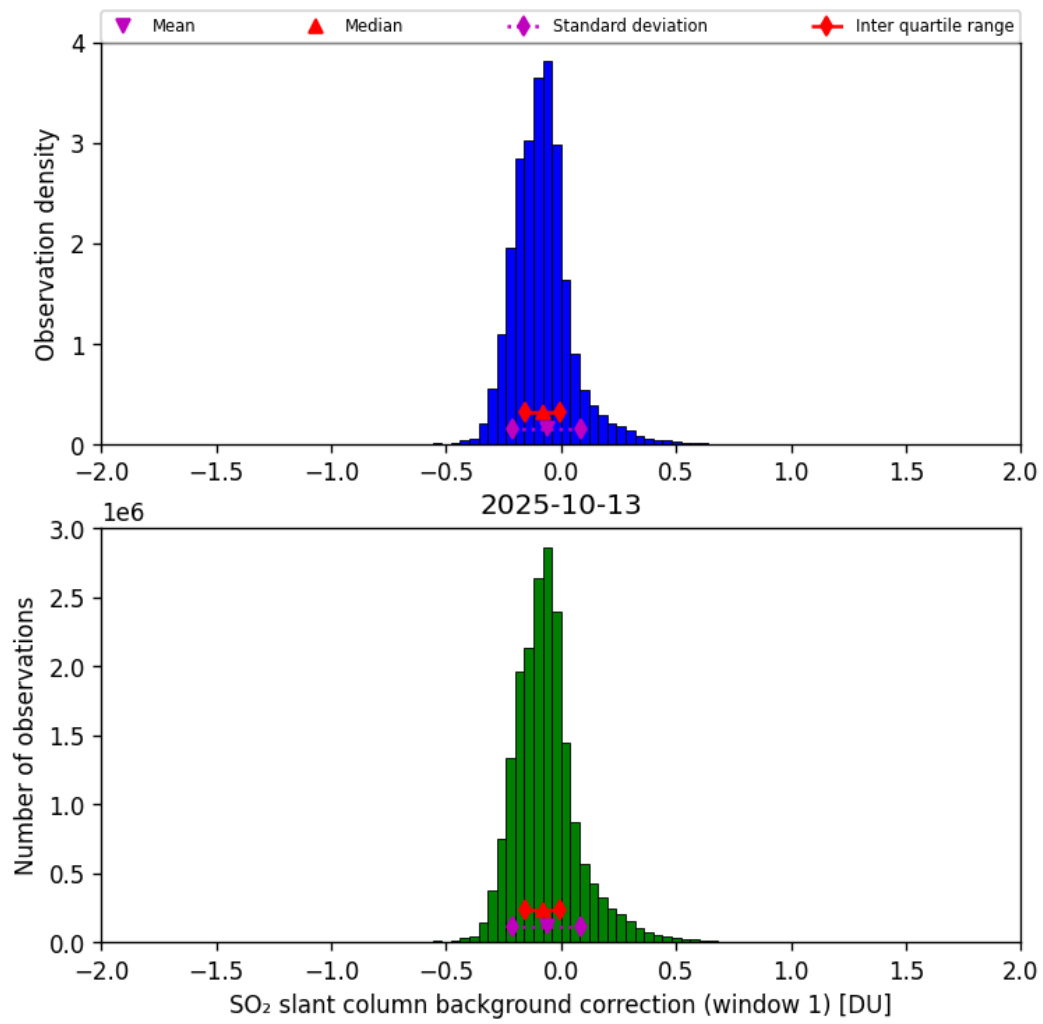
Figure 66: Histogram of “SO 2 slant column background correction (window 1)” for 2025-10-12 to 2025-10-14
