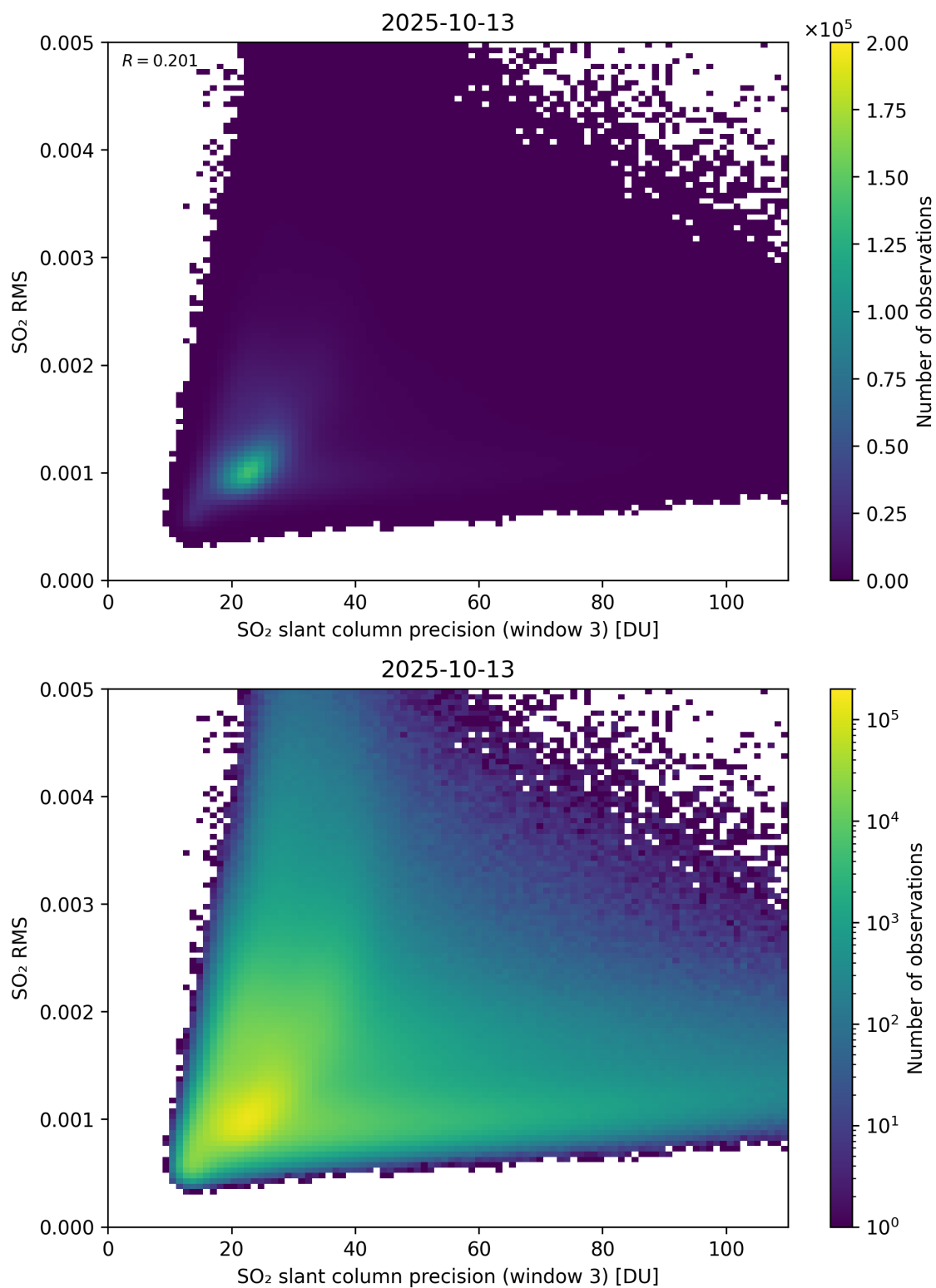
Figure 310: Scatter density plot of “SO 2 slant column precision (window 3)” against “SO 2 RMS” for 2025-10-12 to 2025-10-14.
