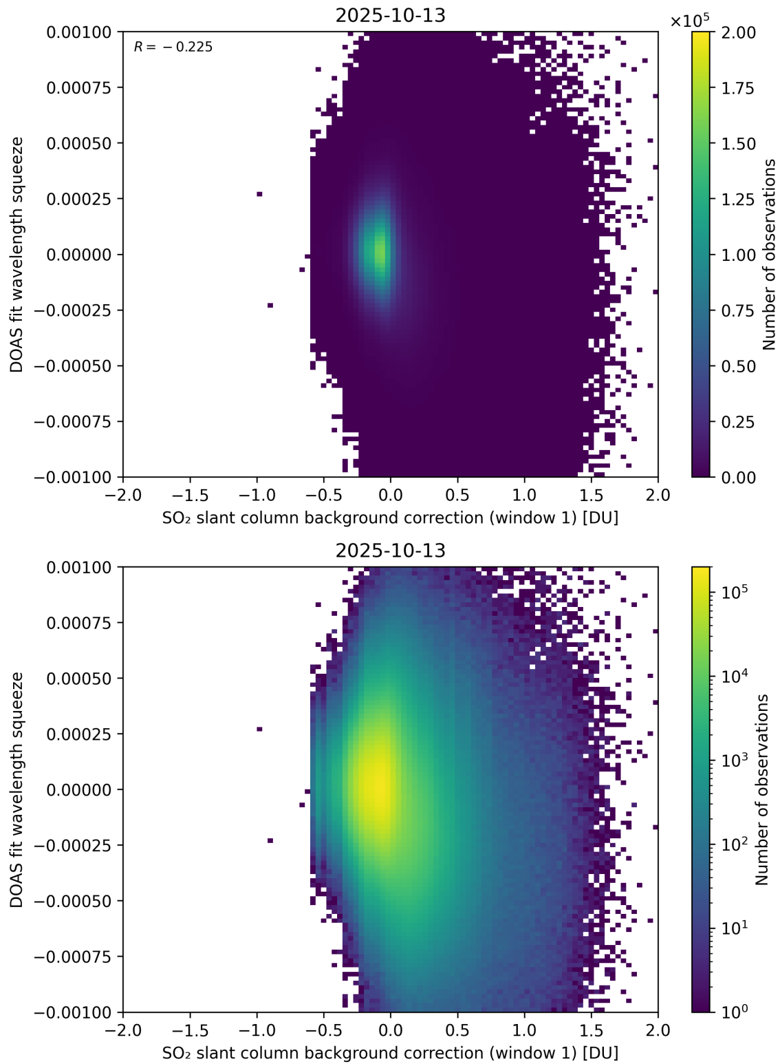
Figure 112: Scatter density plot of “SO 2 slant column background correction (window 1)” against “DOAS fit wavelength squeeze” for 2025-10-12 to 2025-10-14.
