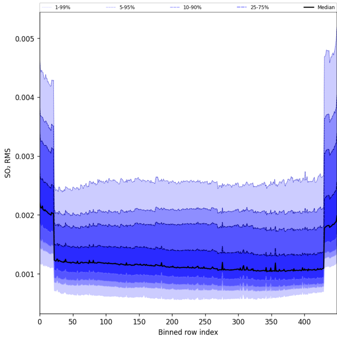
Figure 104: Along track statistics of “SO 2 RMS” for 2025-10-12 to 2025-10-14
