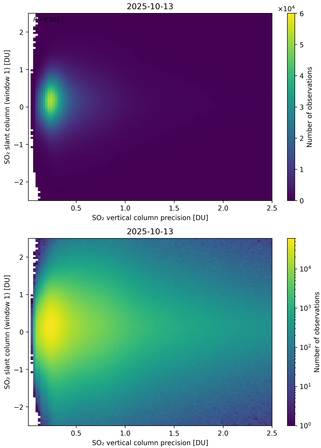
Figure 341: Scatter density plot of “SO 2 vertical column precision” against “SO 2 slant column (window 1)” for 2025-10-12 to 2025-10-14.
