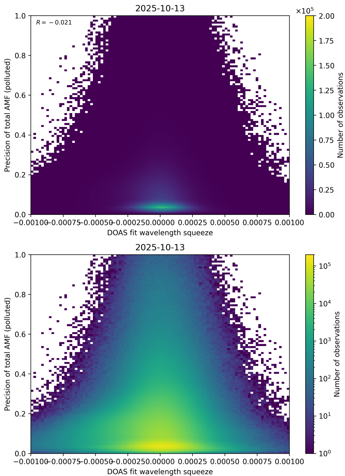
Figure 146: Scatter density plot of “DOAS fit wavelength squeeze” against “Precision of total AMF (polluted)” for 2025-10-12 to 2025-10-14.
