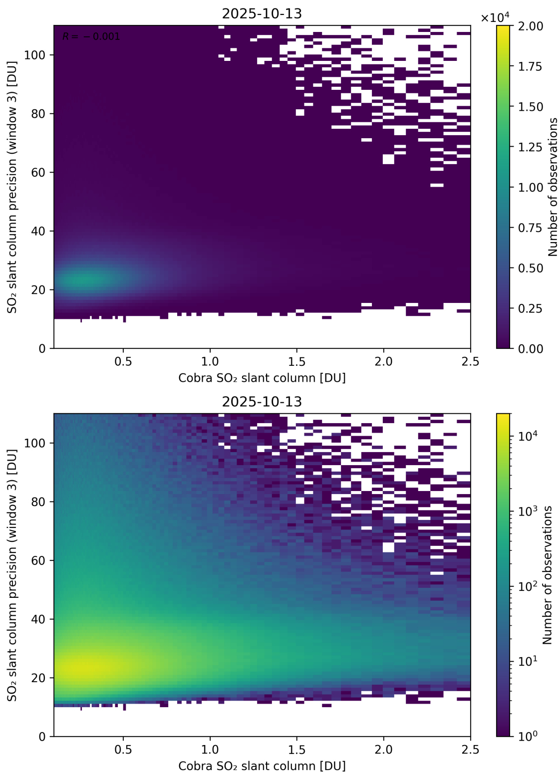
Figure 223: Scatter density plot of “Cobra SO 2 slant column” against “SO 2 slant column precision (window 3)” for 2025-10-12 to 2025-10-14.
