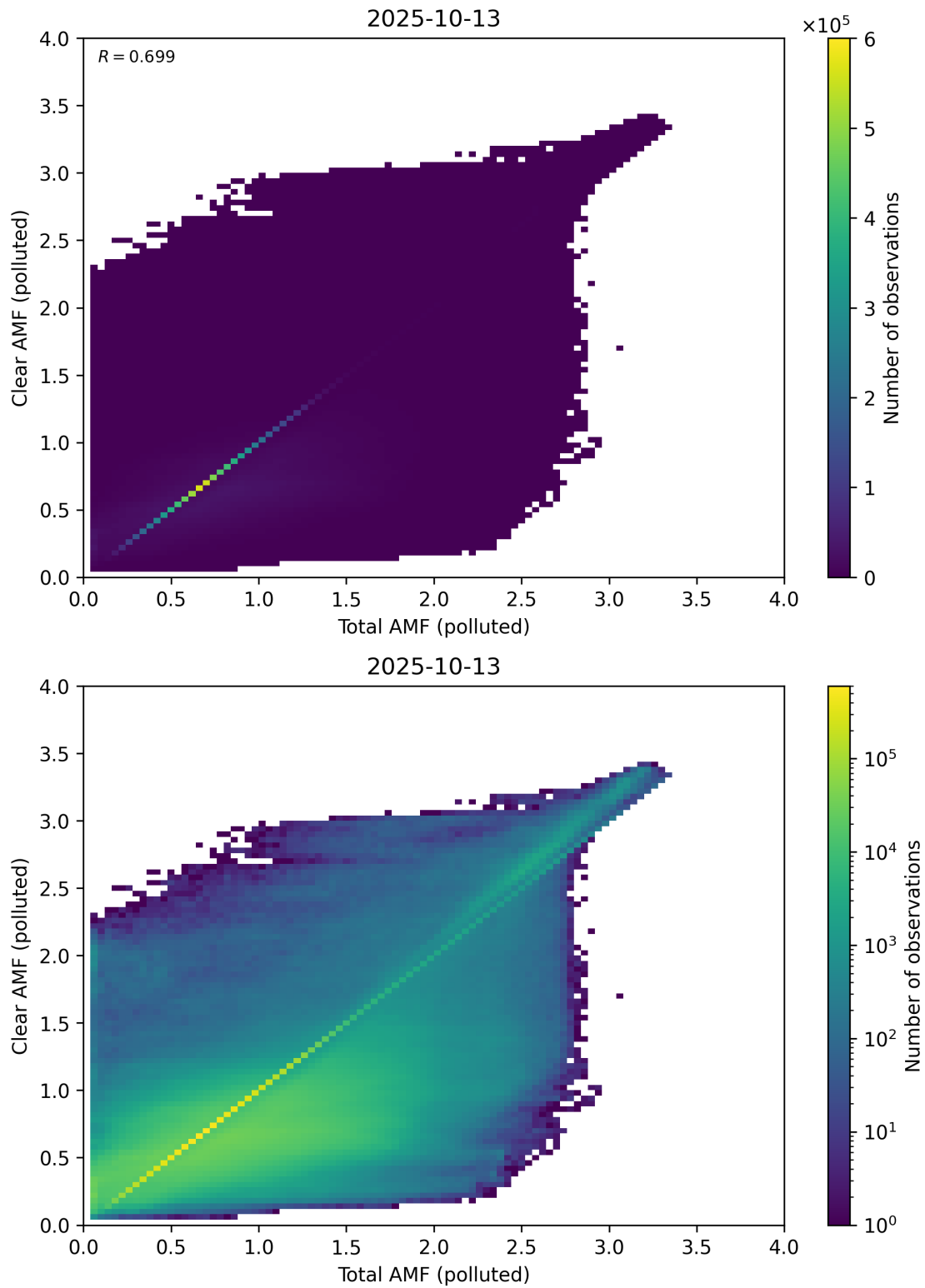
Figure 321: Scatter density plot of “Total AMF (polluted)” against “Clear AMF (polluted)” for 2025-10-12 to 2025-10-14.
