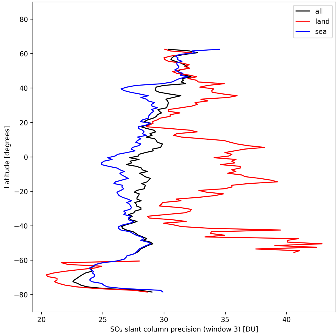
Figure 46: Zonal average of “SO 2 slant column precision (window 3)” for 2025-10-12 to 2025-10-14.
