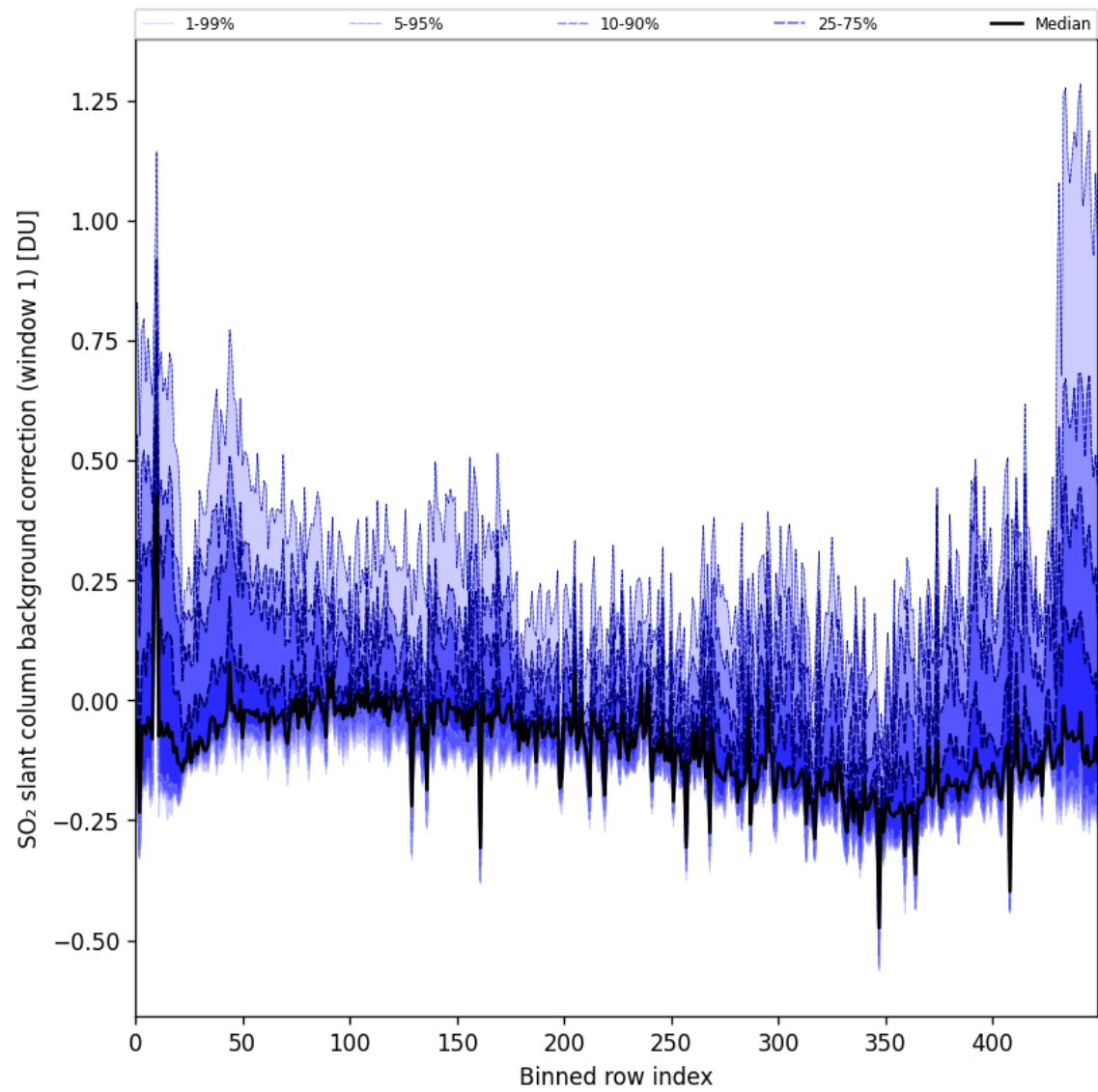
Figure 92: Along track statistics of “SO 2 slant column background correction (window 1)” for 2025-10-12 to 2025-10-14
