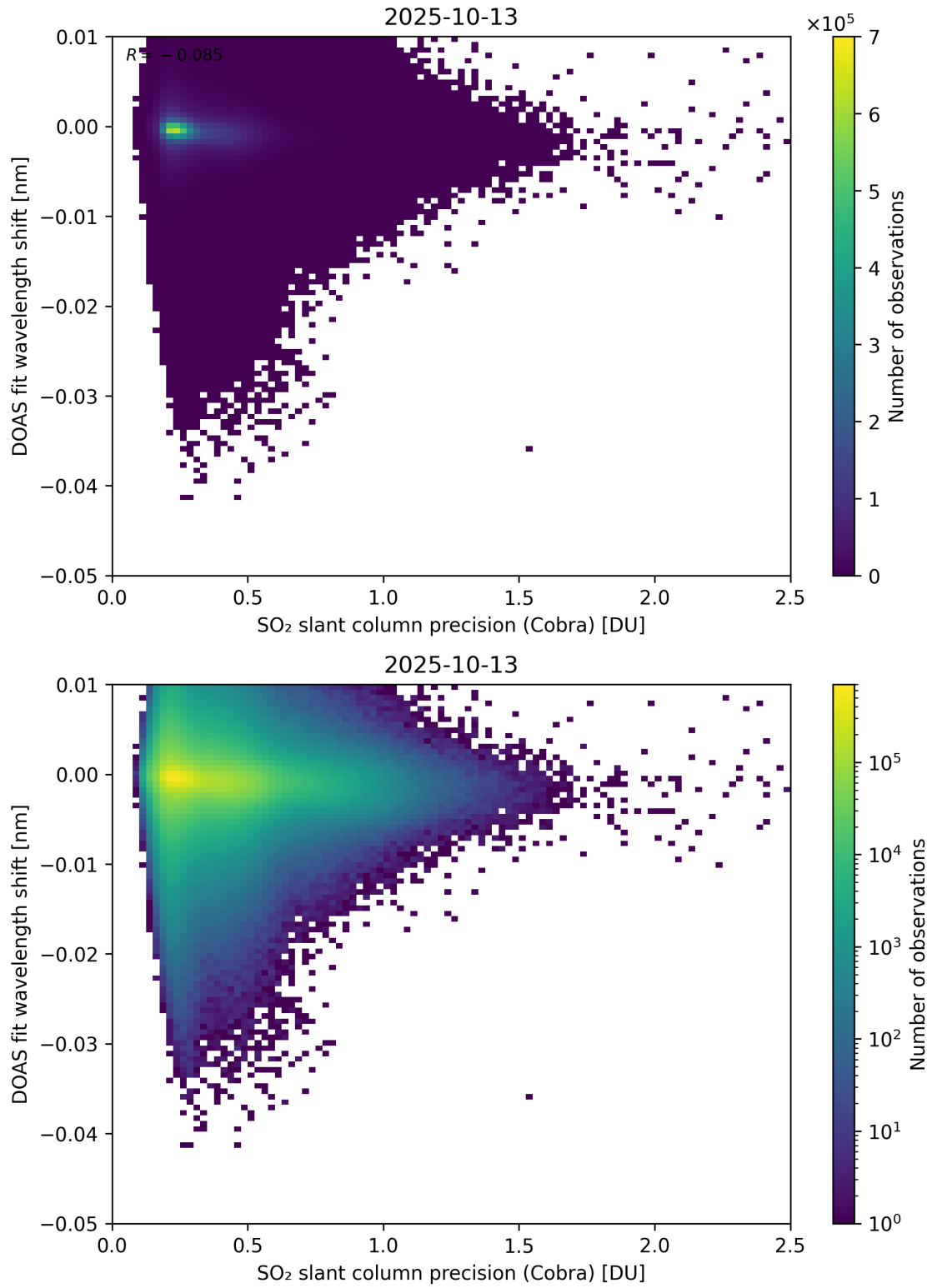
Figure 202: Scatter density plot of “SO 2 slant column precision (Cobra)” against “DOAS fit wavelength shift” for 2025-10-12 to 2025-10-14.
