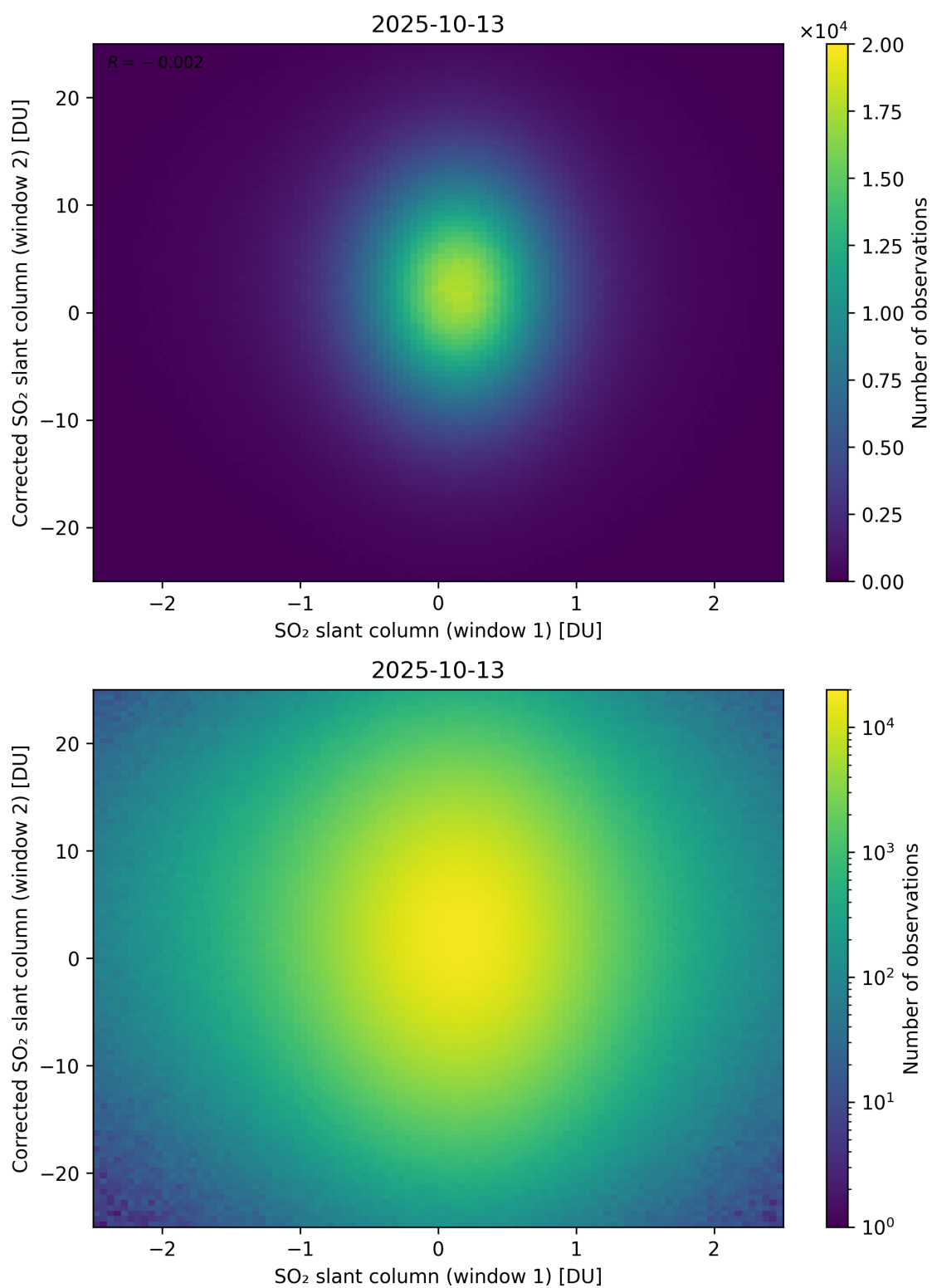
Figure 283: Scatter density plot of “SO 2 slant column (window 1)” against “Corrected SO 2 slant column (window 2)” for 2025-10-12 to 2025-10-14.
