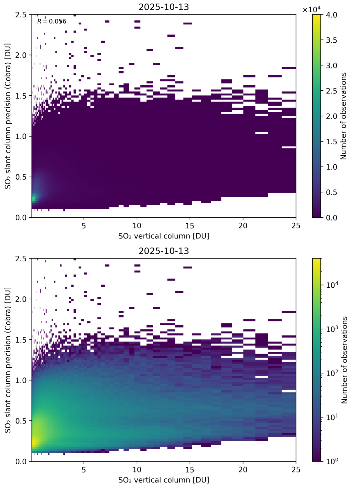
Figure 350: Scatter density plot of “SO 2 vertical column” against “SO 2 slant column precision (Cobra)” for 2025-10-12 to 2025-10-14.
