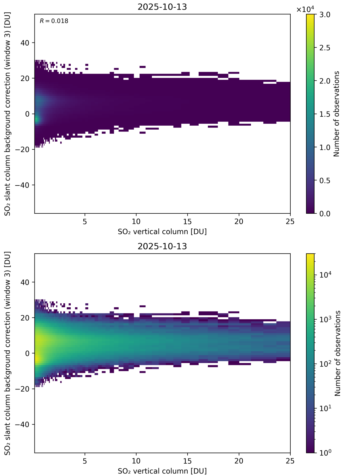
Figure 325: Scatter density plot of “SO 2 vertical column” against “SO 2 slant column background correction (window 3)” for 2025-10-12 to 2025-10-14.
