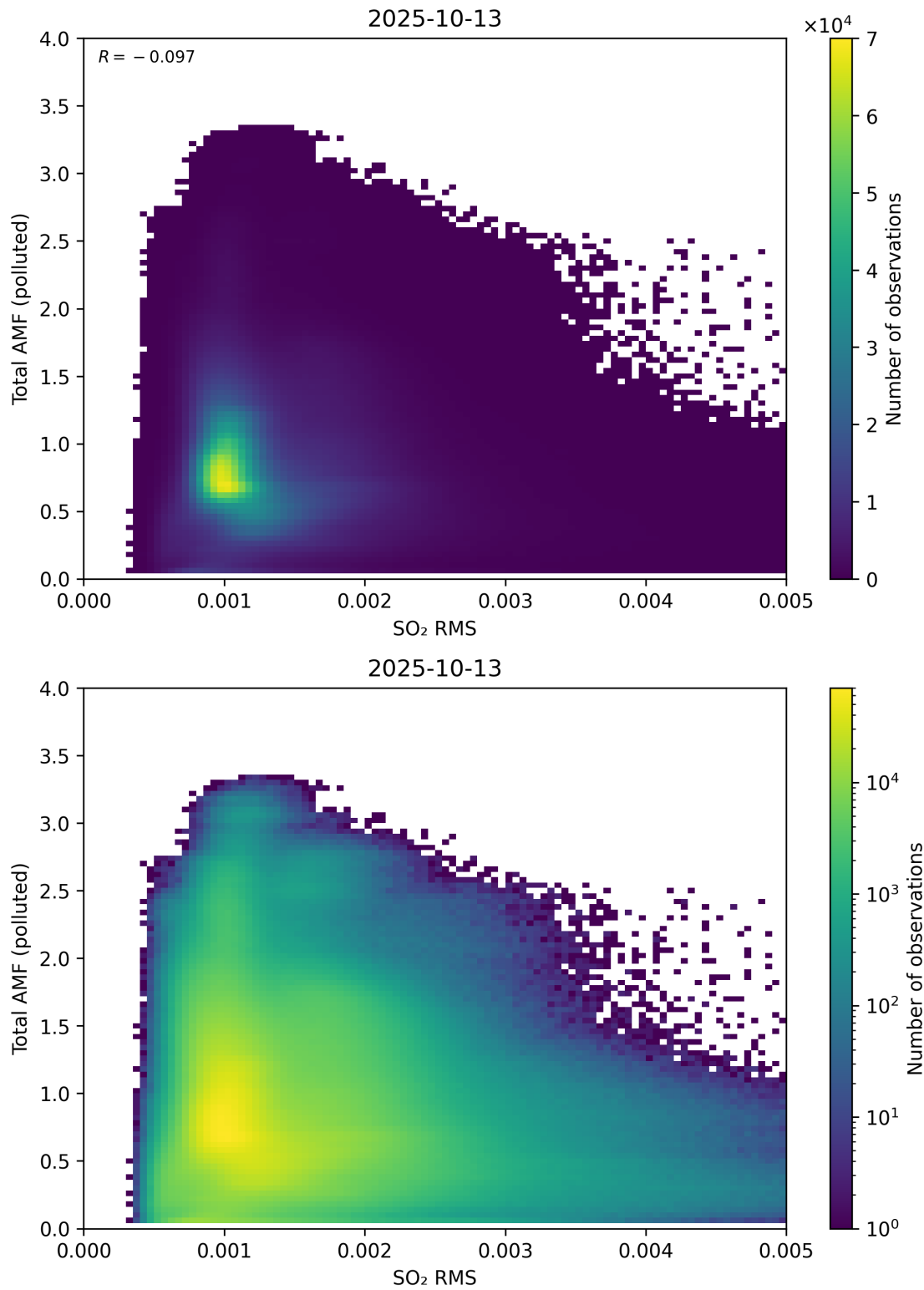
Figure 148: Scatter density plot of “SO 2 RMS” against “Total AMF (polluted)” for 2025-10-12 to 2025-10-14.
