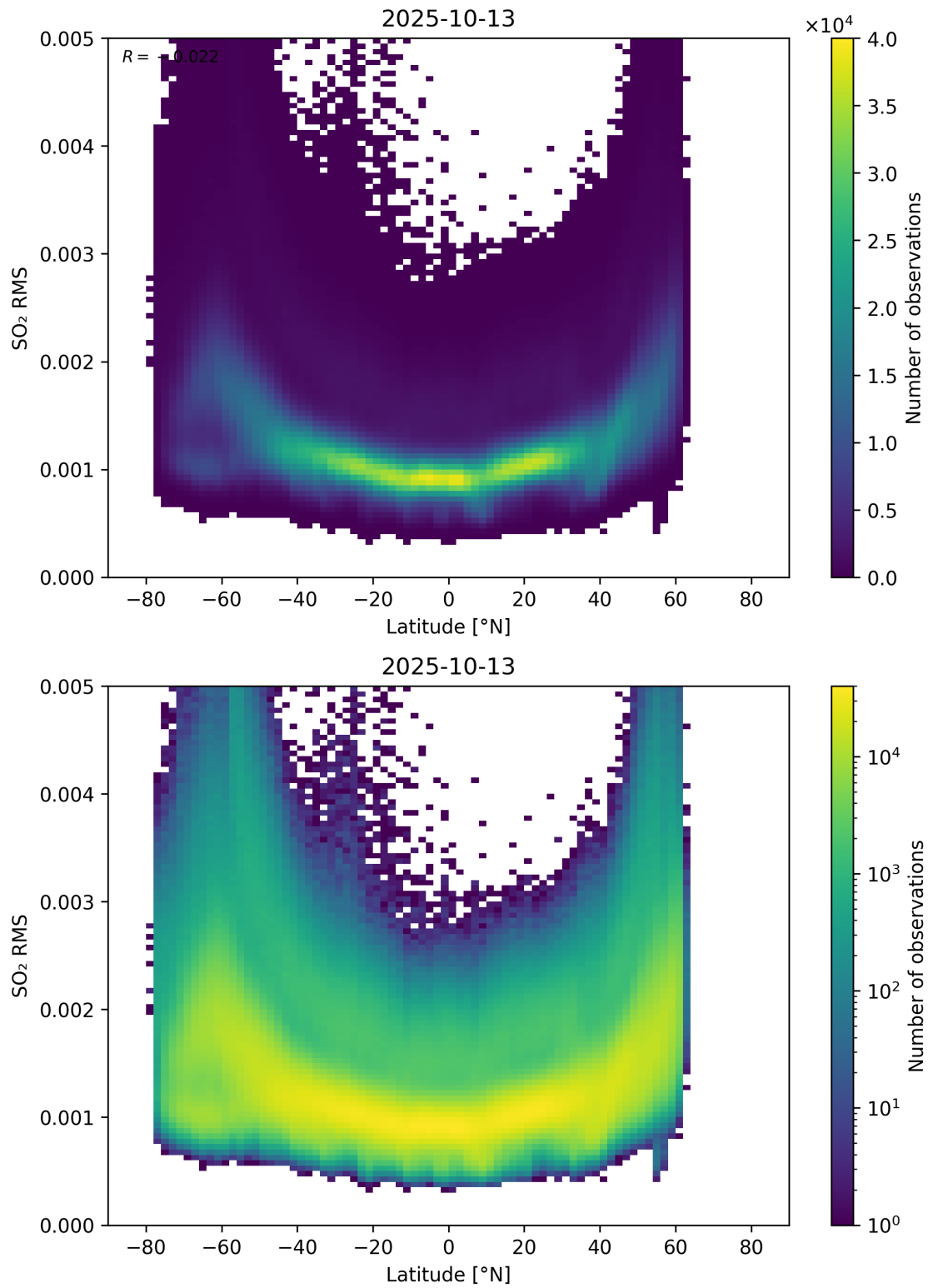
Figure 155: Scatter density plot of “Latitude” against “SO 2 RMS” for 2025-10-12 to 2025-10-14.
