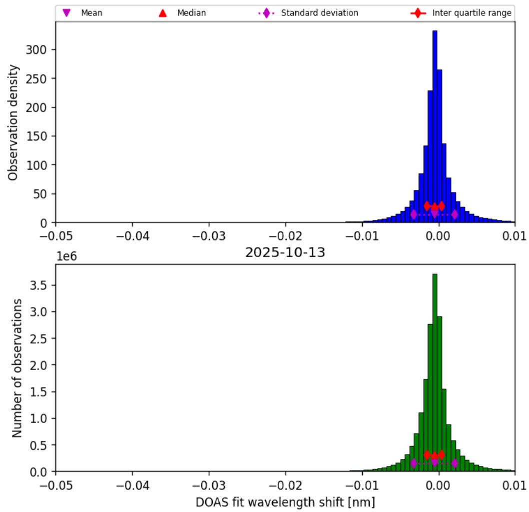
Figure 76: Histogram of “DOAS fit wavelength shift” for 2025-10-12 to 2025-10-14
