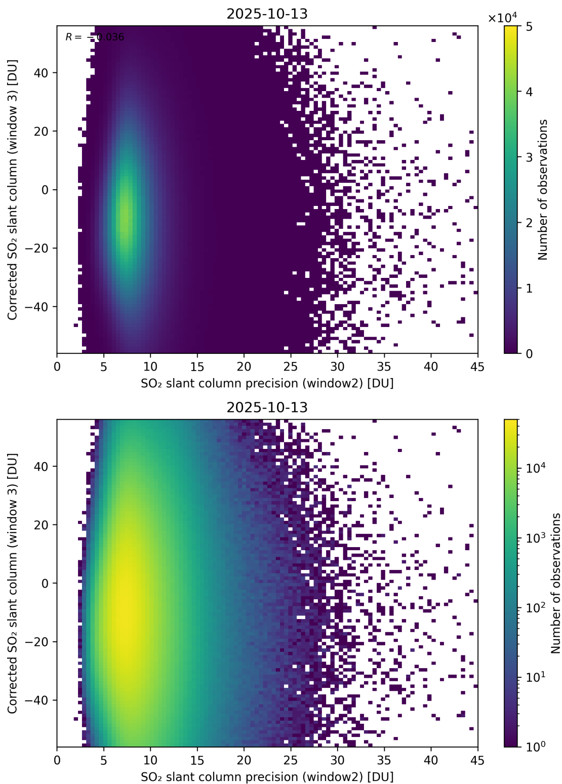
Figure 298: Scatter density plot of “SO 2 slant column precision (window2)” against “Corrected SO 2 slant column (window 3)” for 2025-10-12 to 2025-10-14.
