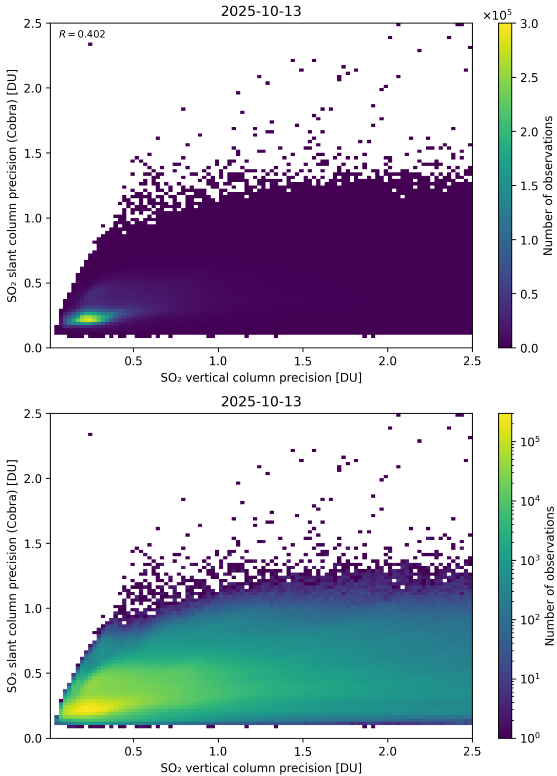
Figure 337: Scatter density plot of “SO 2 vertical column precision” against “SO 2 slant column precision (Cobra)” for 2025-10-12 to 2025-10-14.
