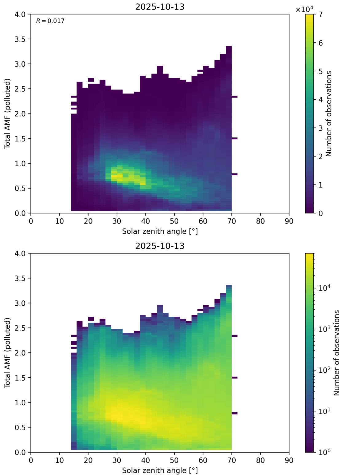
Figure 189: Scatter density plot of “Solar zenith angle” against “Total AMF (polluted)” for 2025-10-12 to 2025-10-14.
