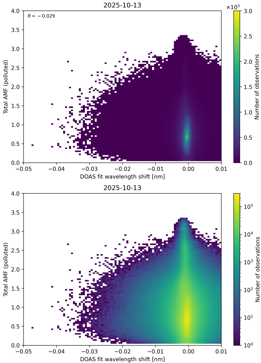
Figure 141: Scatter density plot of “DOAS fit wavelength shift” against “Total AMF (polluted)” for 2025-10-12 to 2025-10-14.
