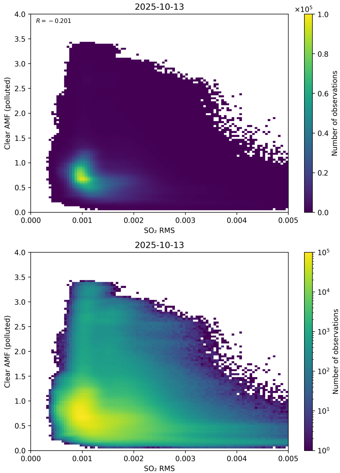
Figure 147: Scatter density plot of “SO 2 RMS” against “Clear AMF (polluted)” for 2025-10-12 to 2025-10-14.
