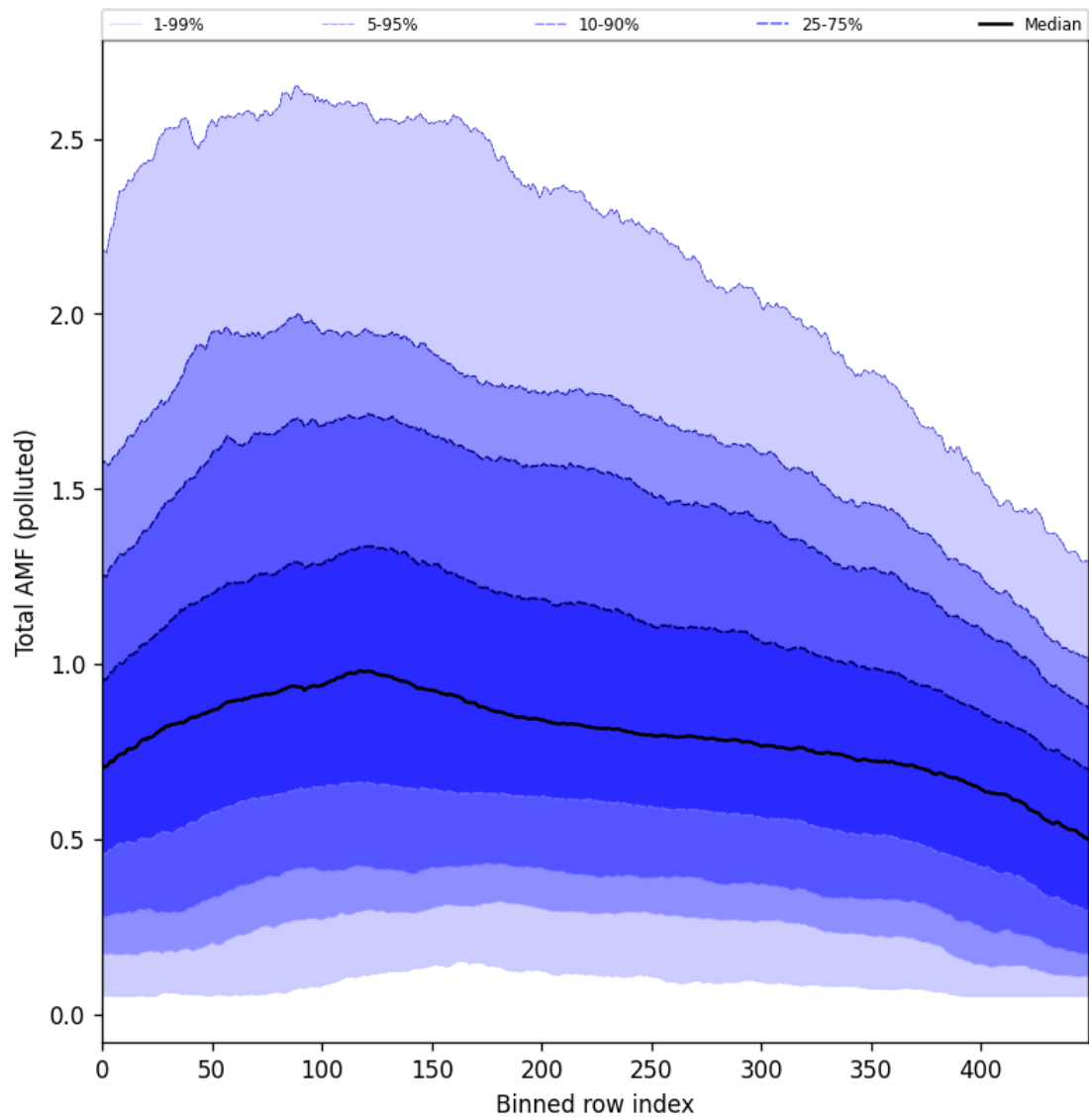
Figure 105: Along track statistics of “Total AMF (polluted)” for 2025-10-12 to 2025-10-14
