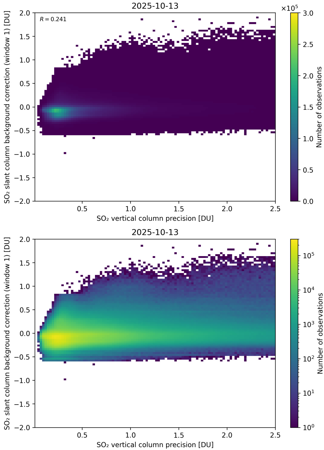
Figure 329: Scatter density plot of “SO 2 vertical column precision” against “SO 2 slant column background correction (window 1)” for 2025-10-12 to 2025-10-14.
