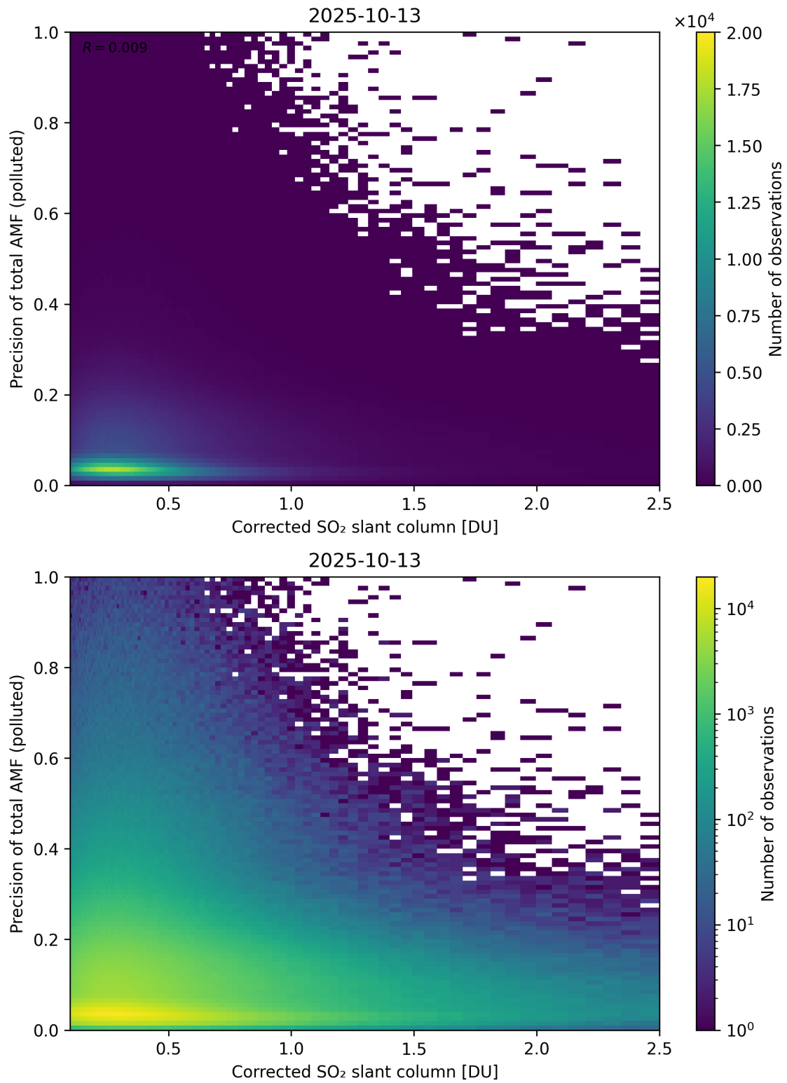
Figure 243: Scatter density plot of “Corrected SO 2 slant column” against “Precision of total AMF (polluted)” for 2025-10-12 to 2025-10-14.
