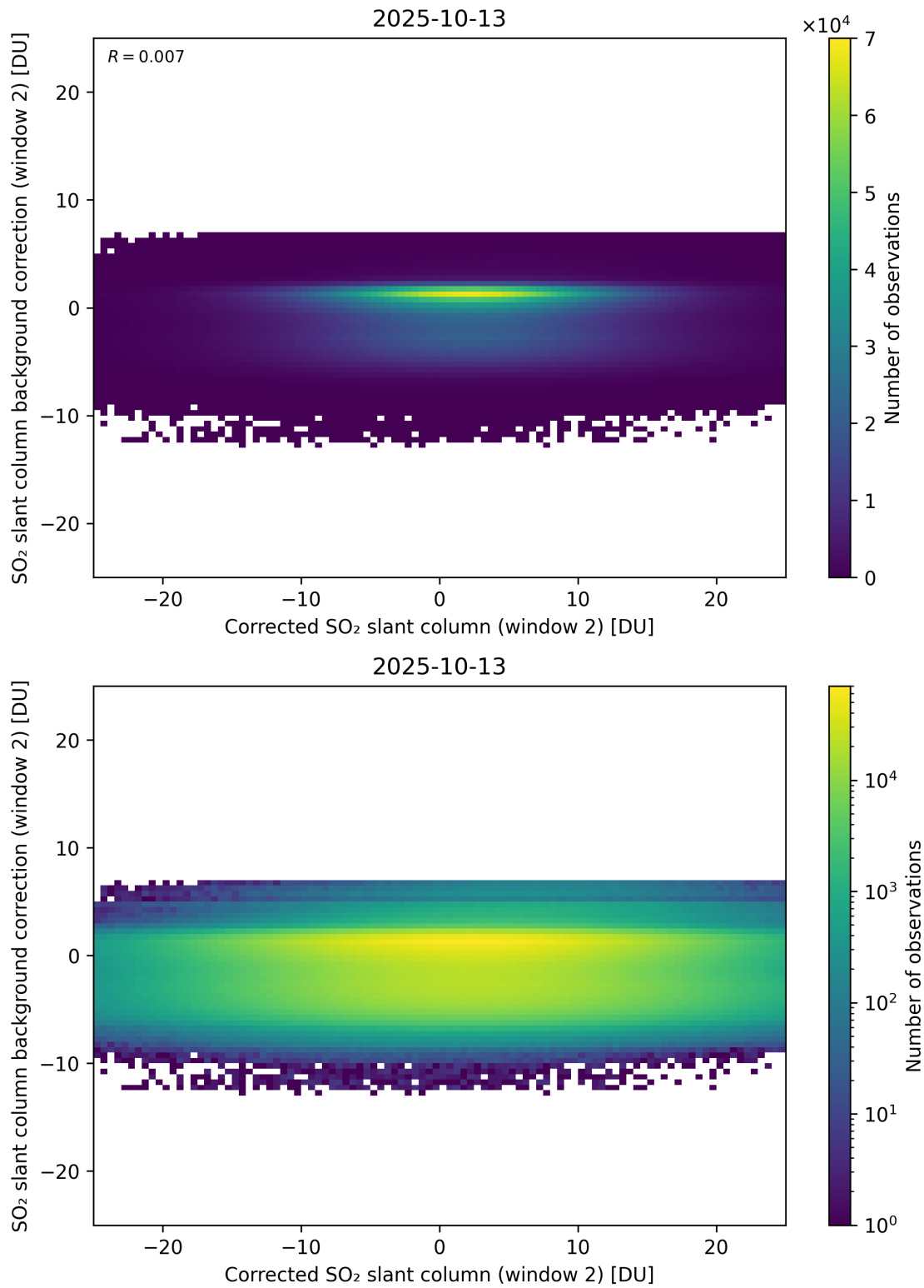
Figure 244: Scatter density plot of “Corrected SO 2 slant column (window 2)” against “SO 2 slant column background correction (window 2)” for 2025-10-12 to 2025-10-14.
