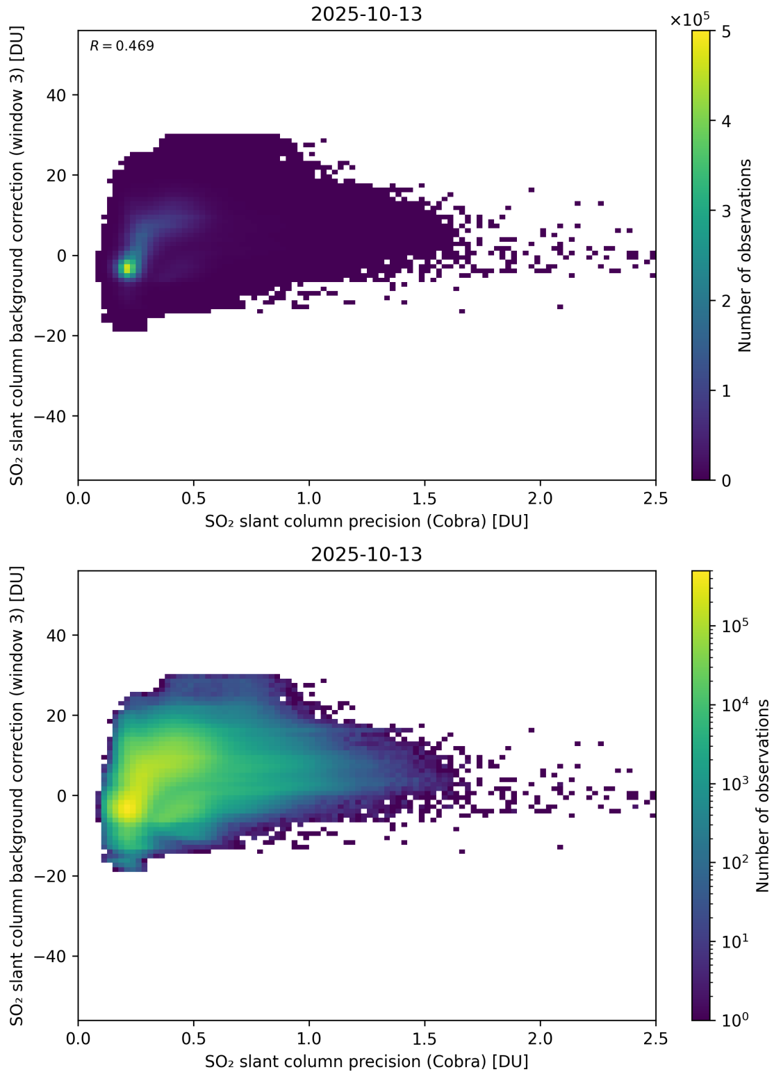
Figure 201: Scatter density plot of “SO 2 slant column precision (Cobra)” against “SO 2 slant column background correction (window 3)” for 2025-10-12 to 2025-10-14.
