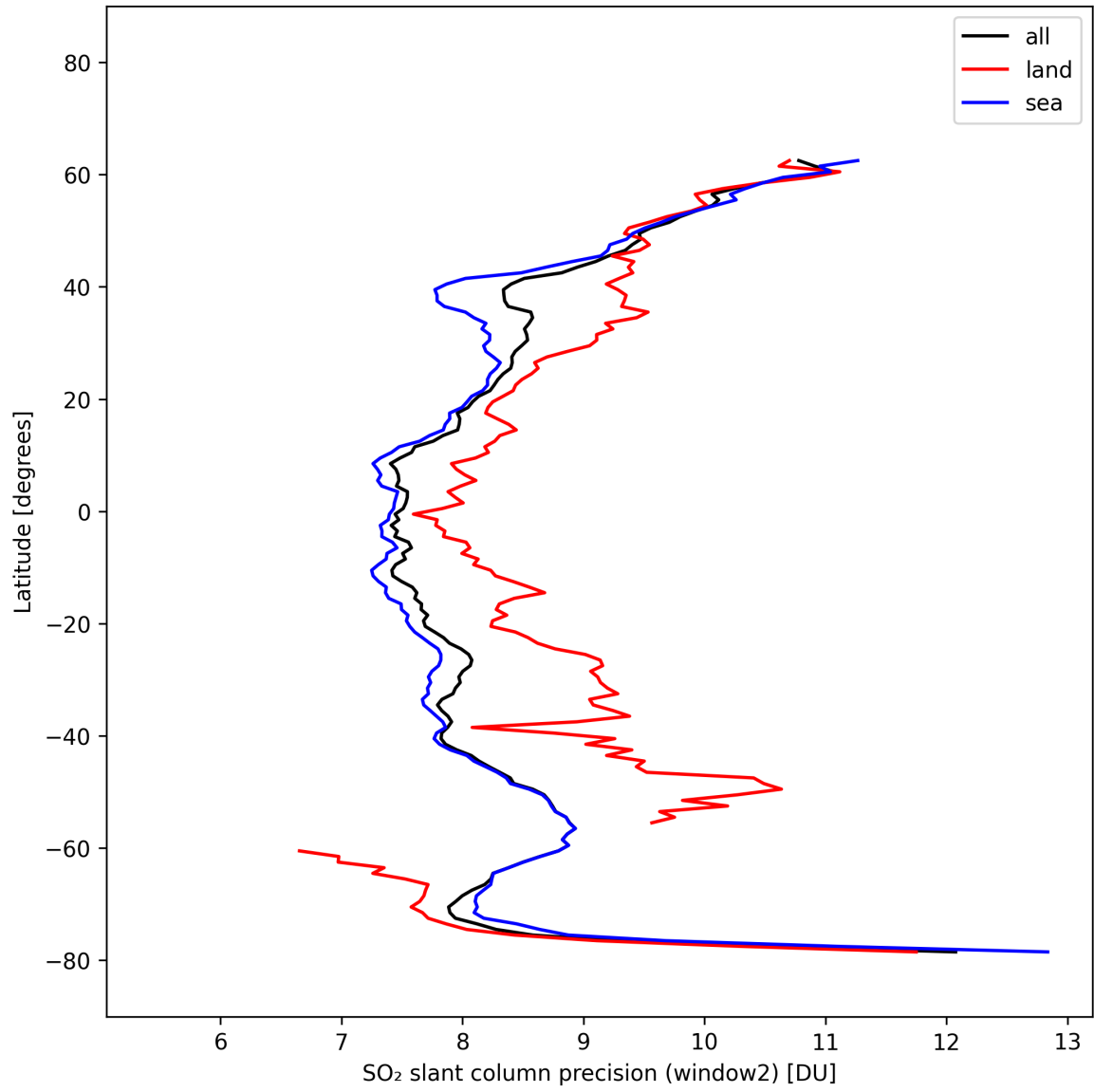
Figure 42: Zonal average of “SO 2 slant column precision (window2)” for 2025-10-12 to 2025-10-14.
