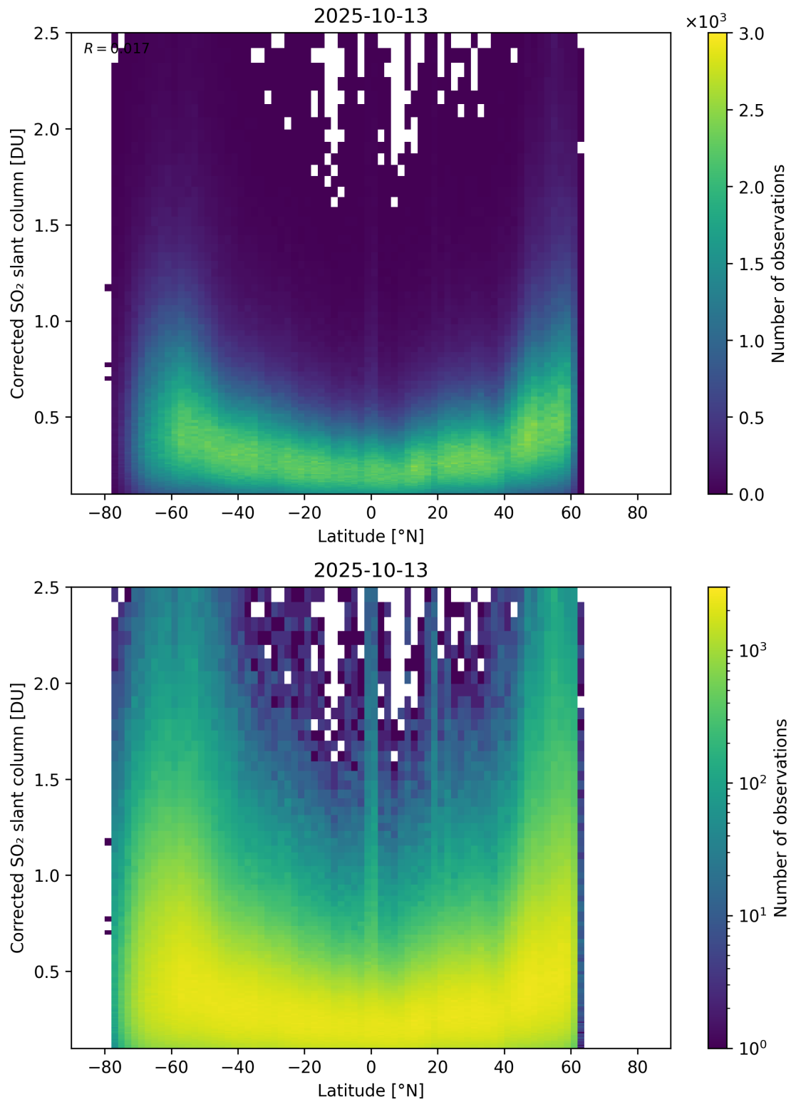
Figure 159: Scatter density plot of “Latitude” against “Corrected SO 2 slant column” for 2025-10-12 to 2025-10-14.
