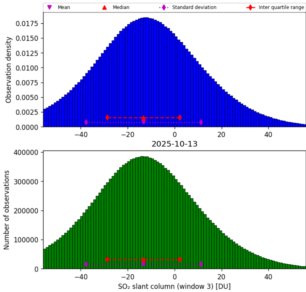
Figure 71: Histogram of “SO 2 slant column (window 3)” for 2025-10-12 to 2025-10-14
