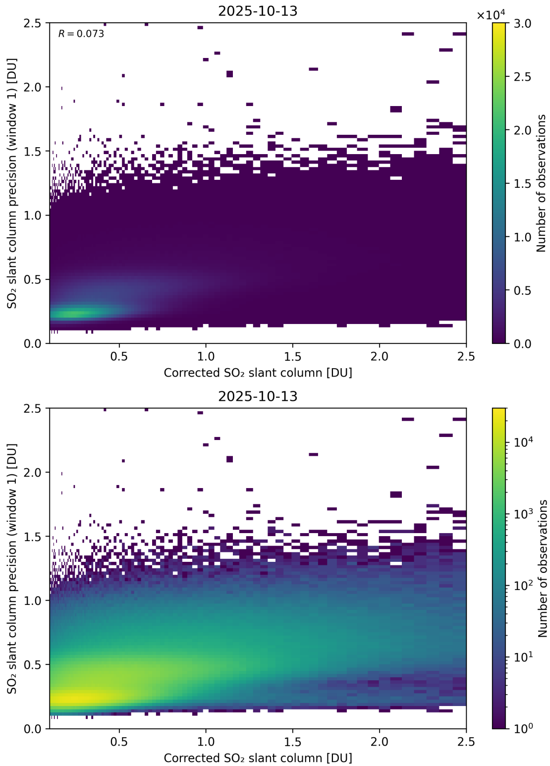
Figure 238: Scatter density plot of “Corrected SO 2 slant column” against “SO 2 slant column precision (window 1)” for 2025-10-12 to 2025-10-14.
