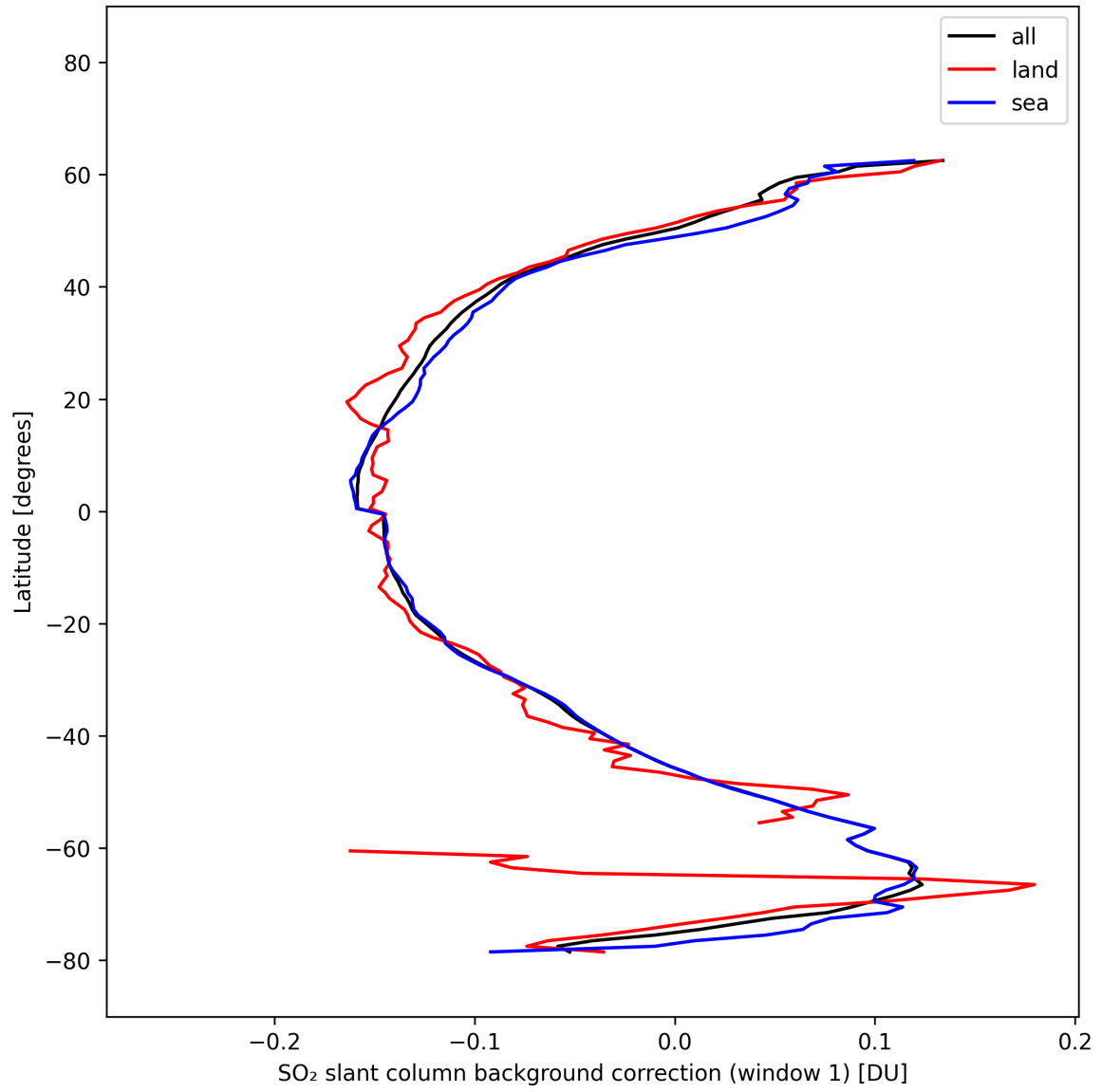
Figure 40: Zonal average of “SO 2 slant column background correction (window 1)” for 2025-10-12 to 2025-10-14.
