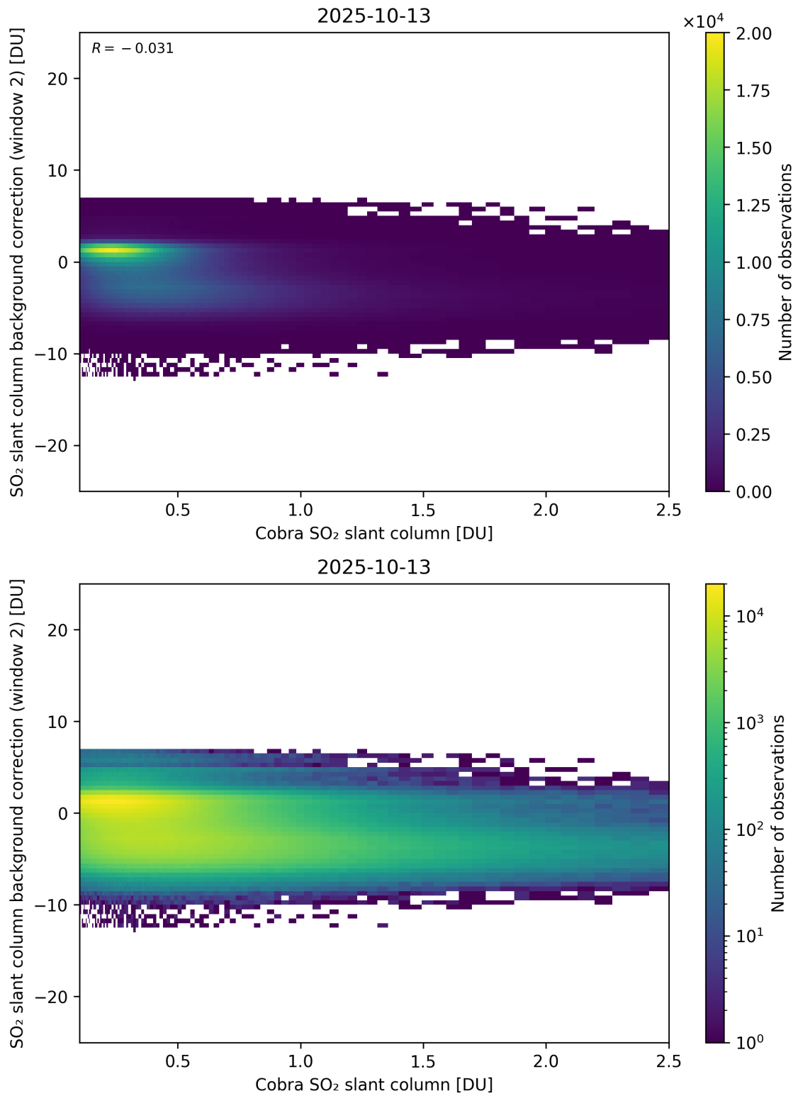
Figure 194: Scatter density plot of “Cobra SO 2 slant column” against “SO 2 slant column background correction (window 2)” for 2025-10-12 to 2025-10-14.
