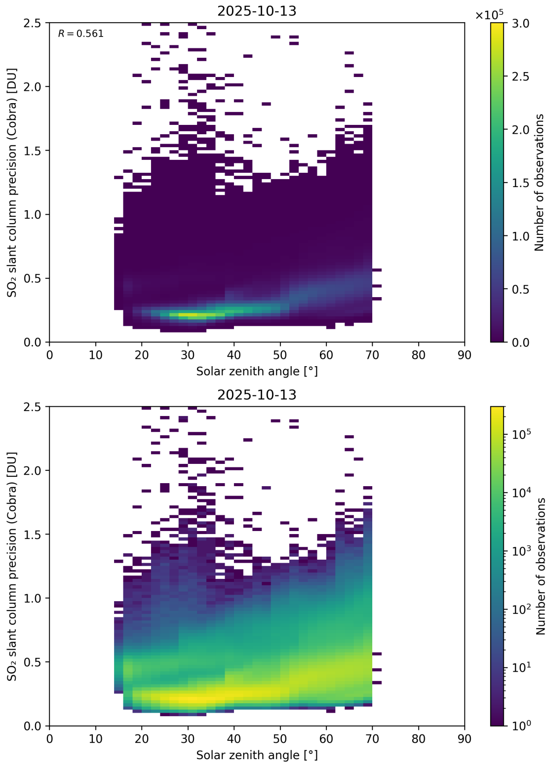
Figure 180: Scatter density plot of “Solar zenith angle” against “SO 2 slant column precision (Cobra)” for 2025-10-12 to 2025-10-14.
