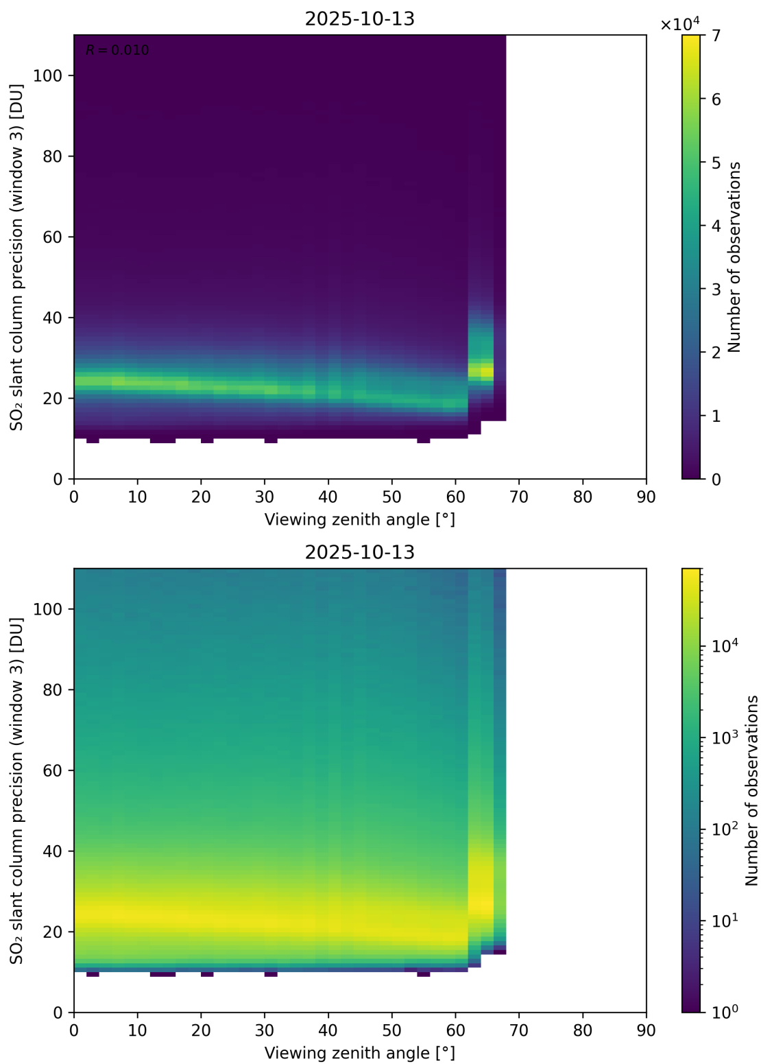
Figure 380: Scatter density plot of “Viewing zenith angle” against “SO 2 slant column precision (window 3)” for 2025-10-12 to 2025-10-14.
