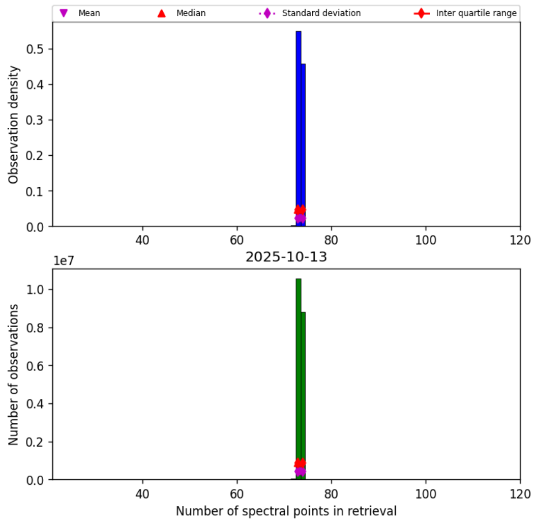
Figure 82: Histogram of “Number of spectral points in retrieval” for 2025-10-12 to 2025-10-14
