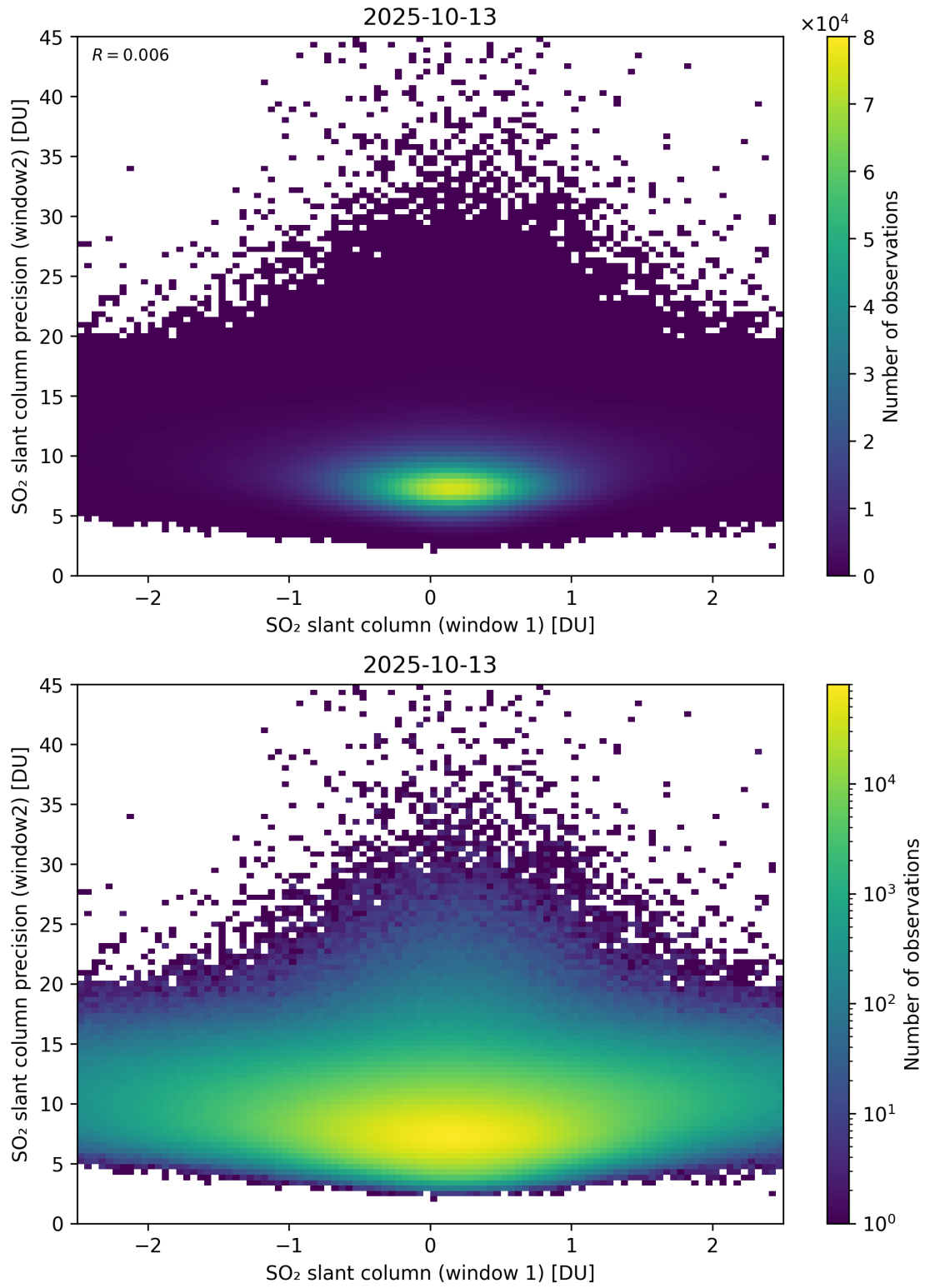
Figure 286: Scatter density plot of “SO 2 slant column (window 1)” against “SO 2 slant column precision (window2)” for 2025-10-12 to 2025-10-14.
