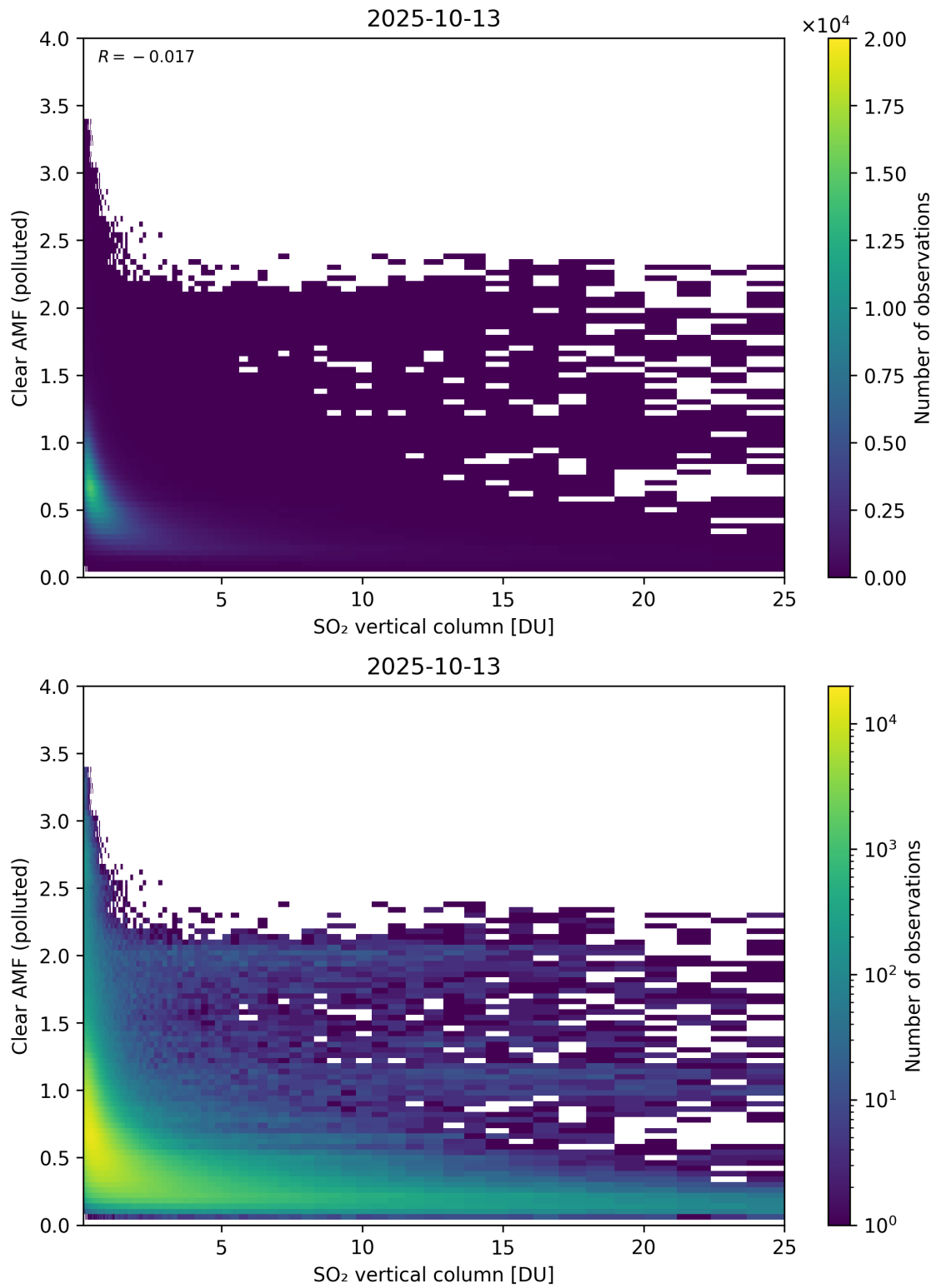
Figure 348: Scatter density plot of “SO 2 vertical column” against “Clear AMF (polluted)” for 2025-10-12 to 2025-10-14.
