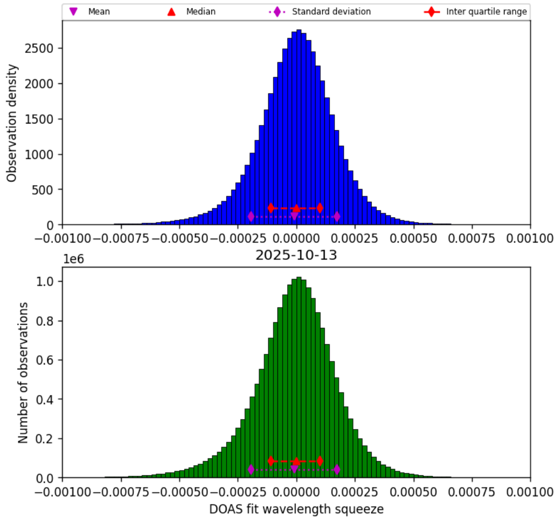
Figure 77: Histogram of “DOAS fit wavelength squeeze” for 2025-10-12 to 2025-10-14
