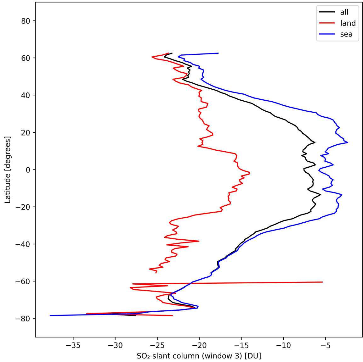
Figure 45: Zonal average of “SO 2 slant column (window 3)” for 2025-10-12 to 2025-10-14.
