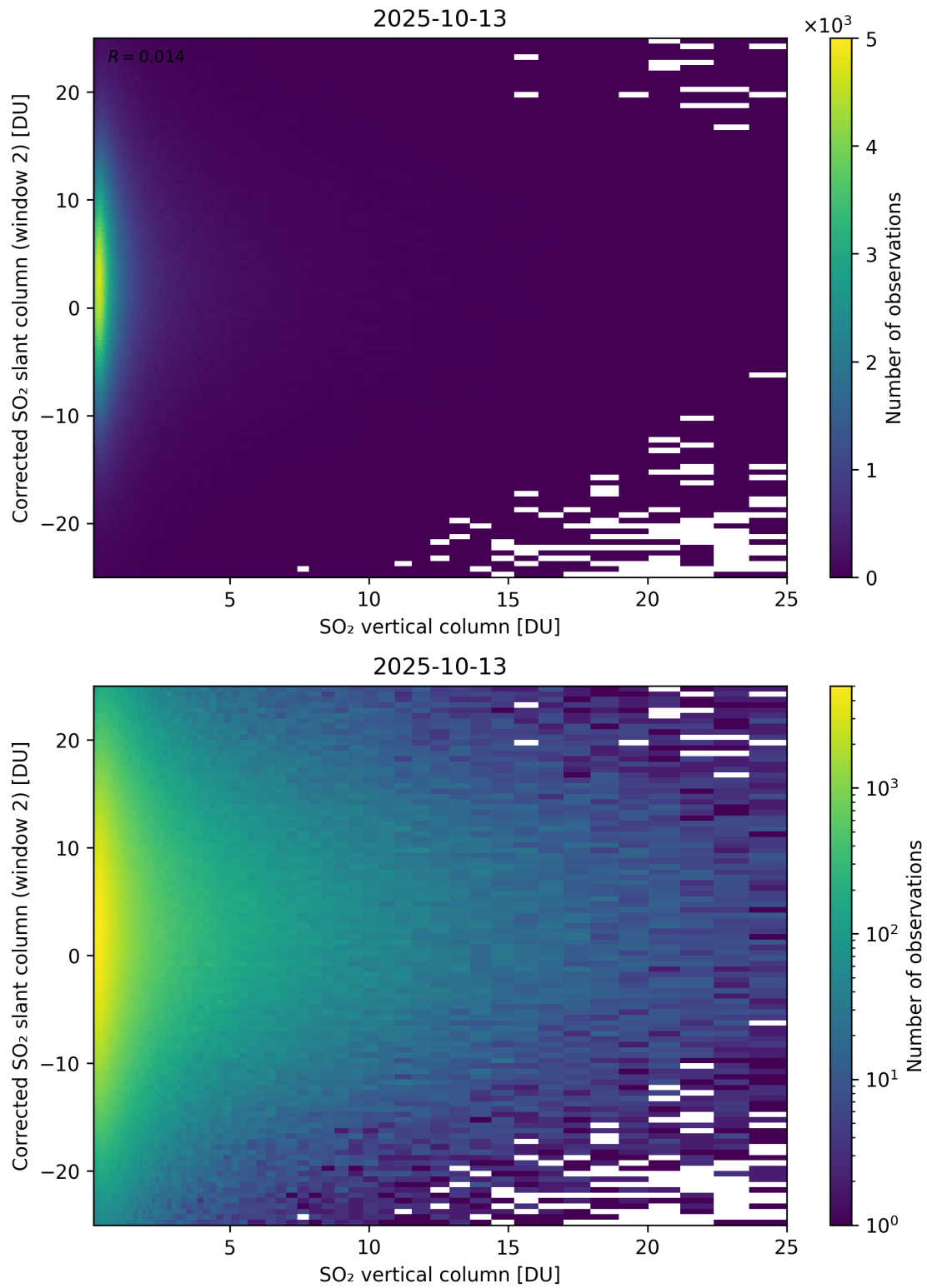
Figure 352: Scatter density plot of “SO 2 vertical column” against “Corrected SO 2 slant column (window 2)” for 2025-10-12 to 2025-10-14.
