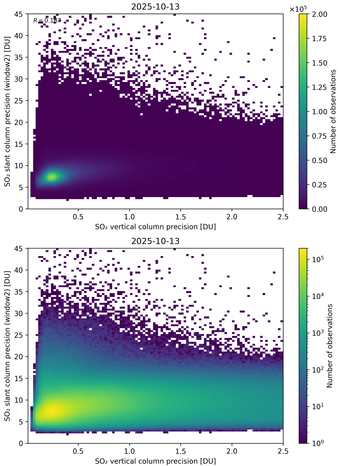
Figure 343: Scatter density plot of “SO 2 vertical column precision” against “SO 2 slant column precision (window2)” for 2025-10-12 to 2025-10-14.
