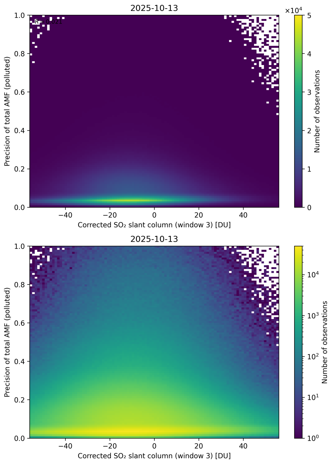
Figure 261: Scatter density plot of “Corrected SO 2 slant column (window 3)” against “Precision of total AMF (polluted)” for 2025-10-12 to 2025-10-14.
