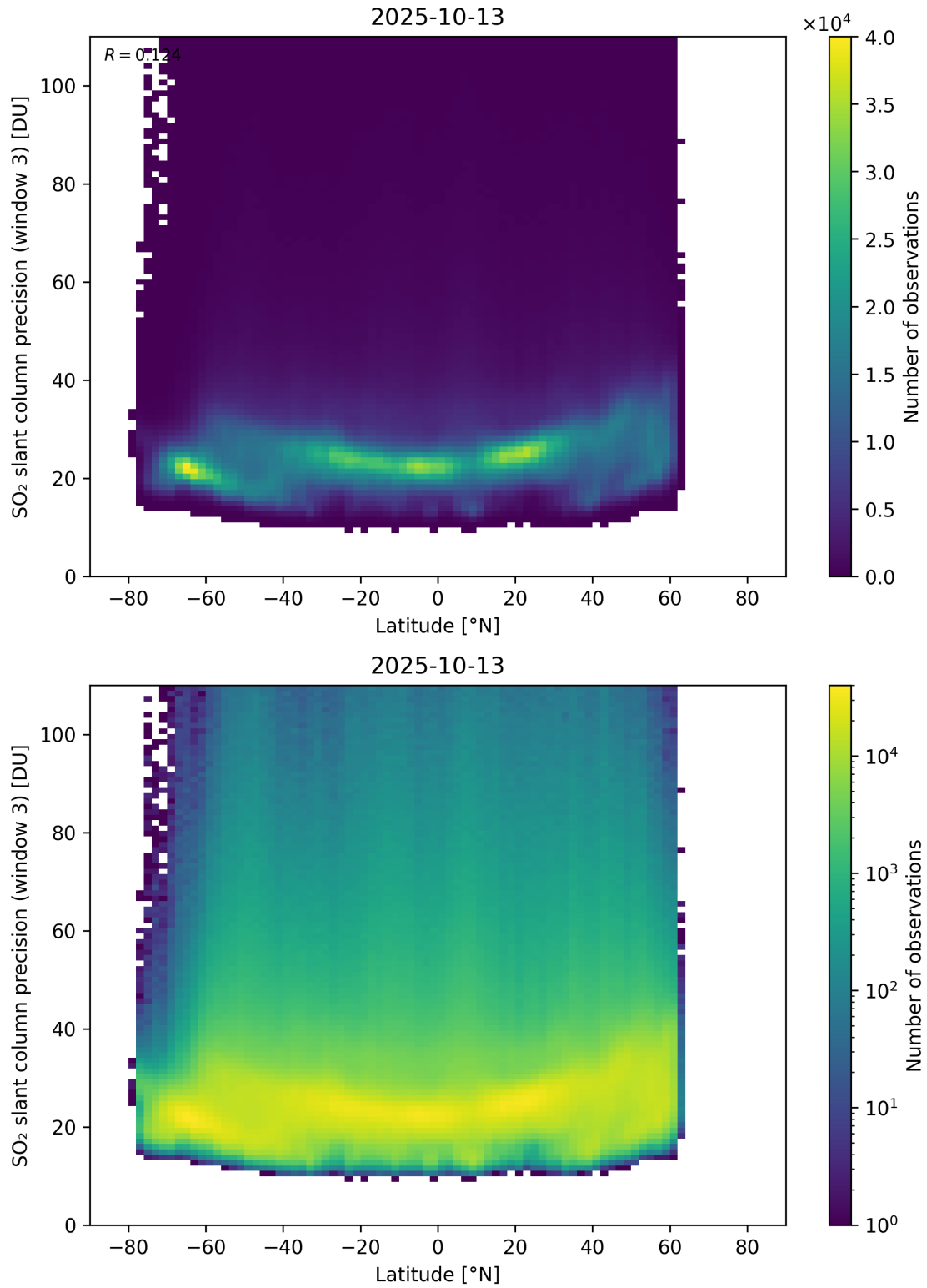
Figure 166: Scatter density plot of “Latitude” against “SO 2 slant column precision (window 3)” for 2025-10-12 to 2025-10-14.
