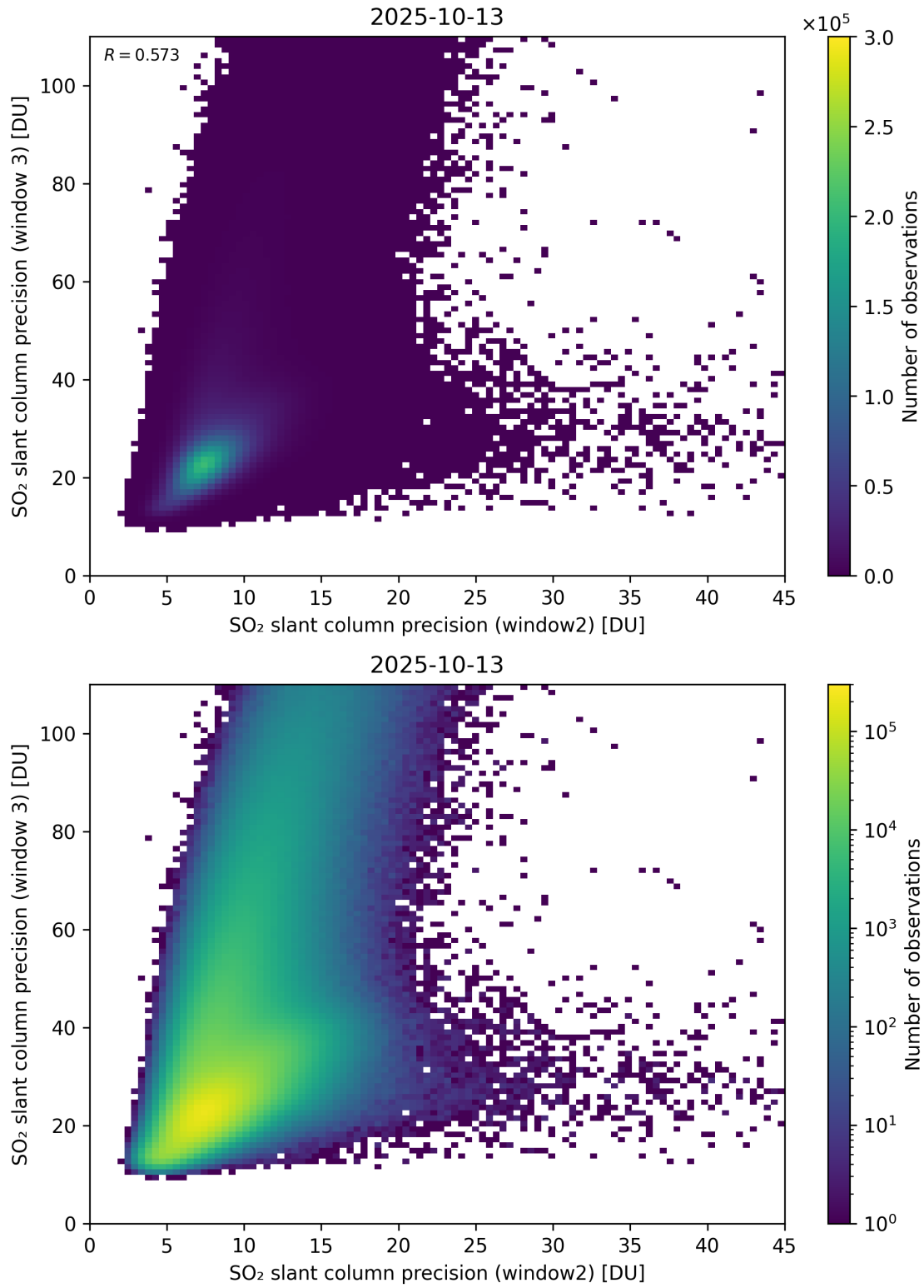
Figure 300: Scatter density plot of “SO 2 slant column precision (window2)” against “SO 2 slant column precision (window 3)” for 2025-10-12 to 2025-10-14.
