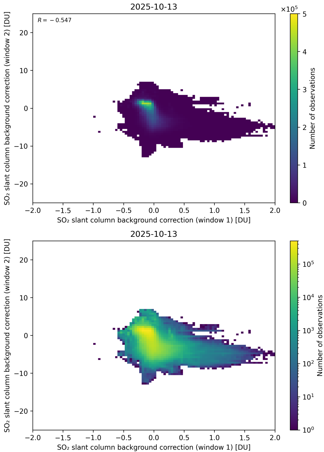
Figure 109: Scatter density plot of “SO 2 slant column background correction (window 1)” against “SO 2 slant column background correction (window 2)” for 2025-10-12 to 2025-10-14.
