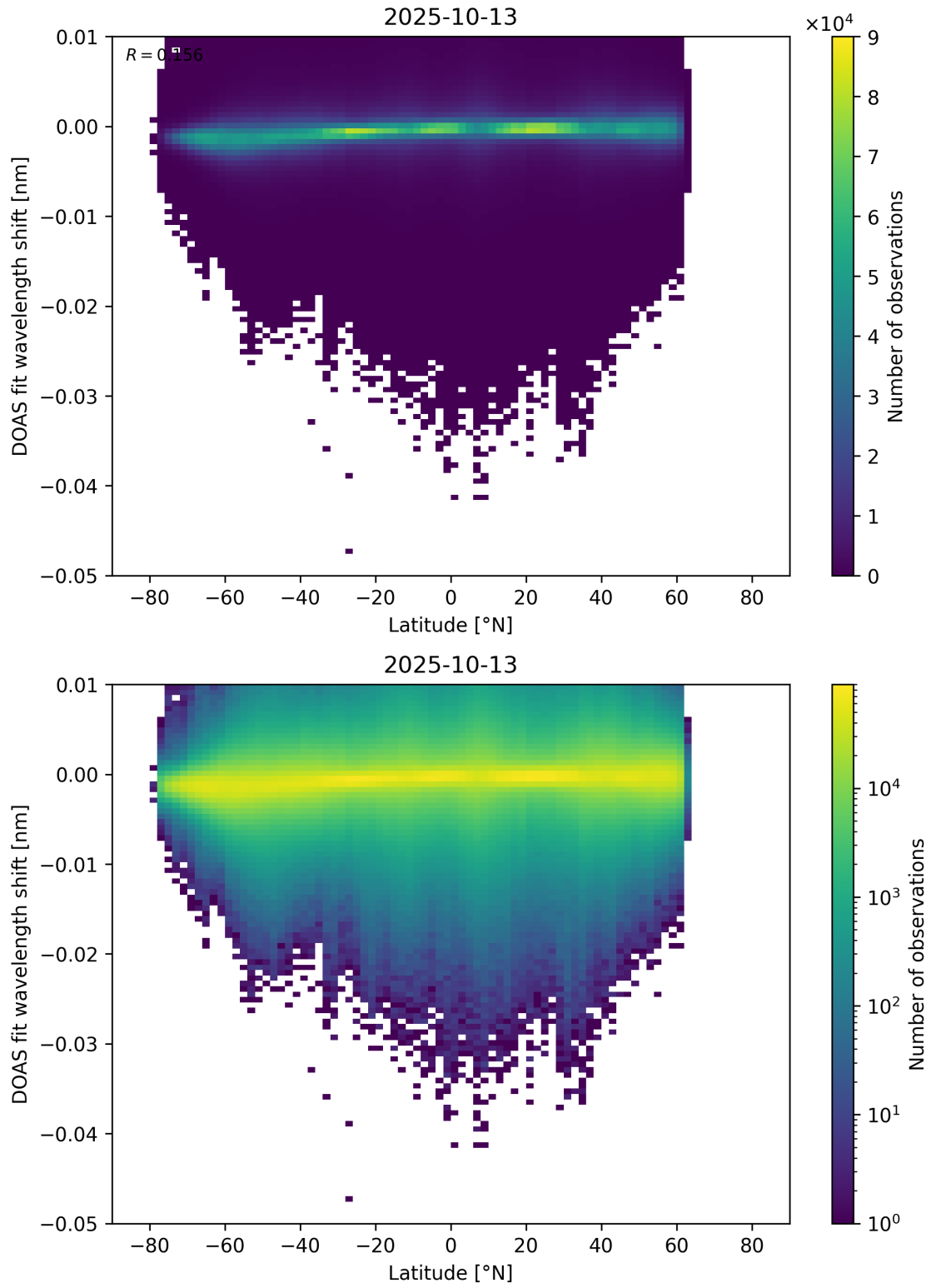
Figure 153: Scatter density plot of “Latitude” against “DOAS fit wavelength shift” for 2025-10-12 to 2025-10-14.
