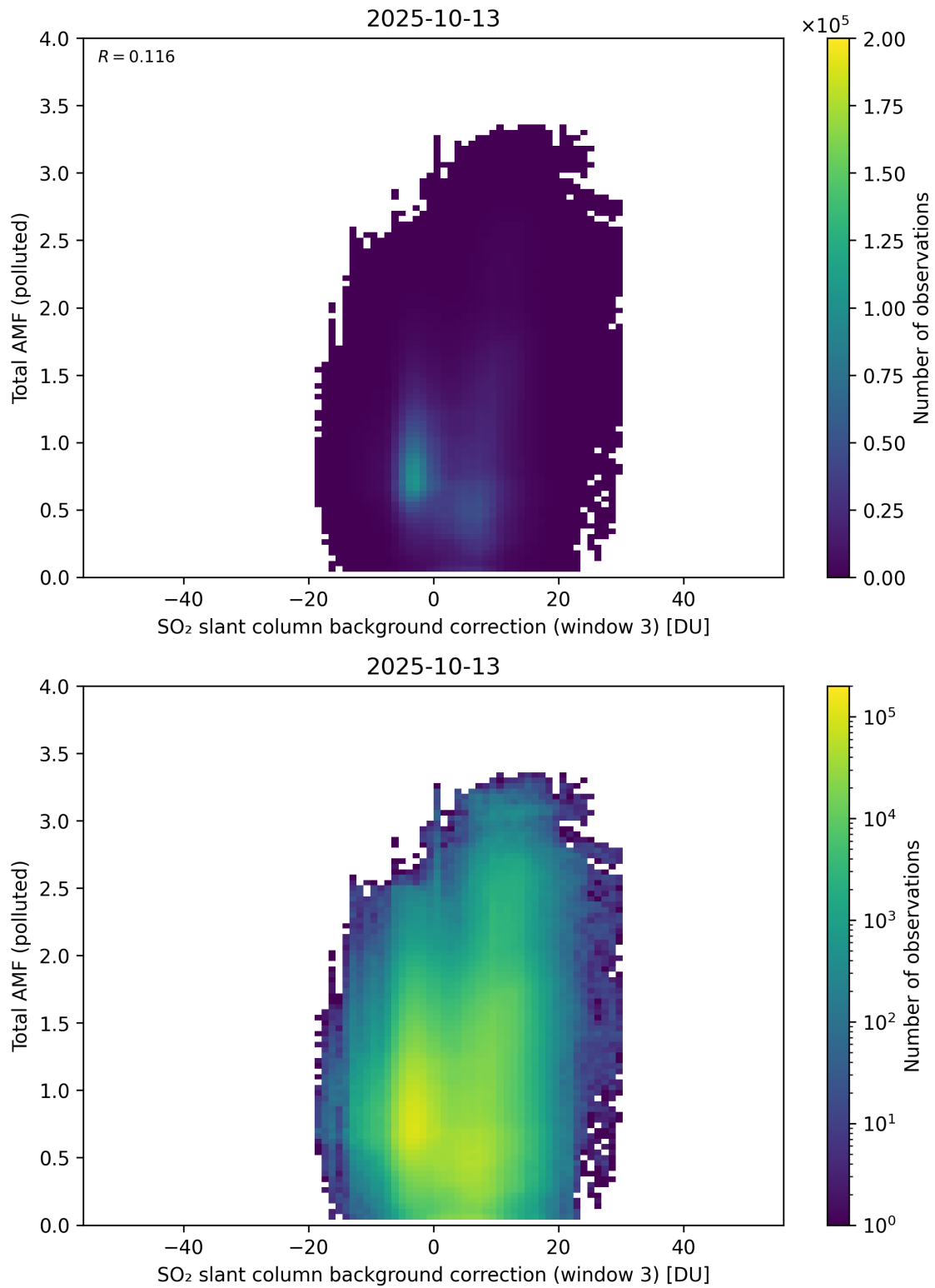
Figure 136: Scatter density plot of “SO 2 slant column background correction (window 3)” against “Total AMF (polluted)” for 2025-10-12 to 2025-10-14.
