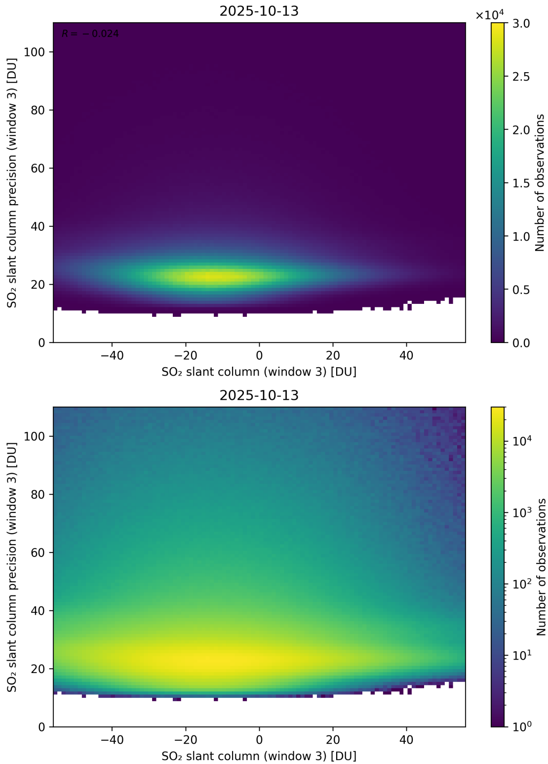
Figure 317: Scatter density plot of “SO 2 slant column (window 3)” against “SO 2 slant column precision (window 3)” for 2025-10-12 to 2025-10-14.
