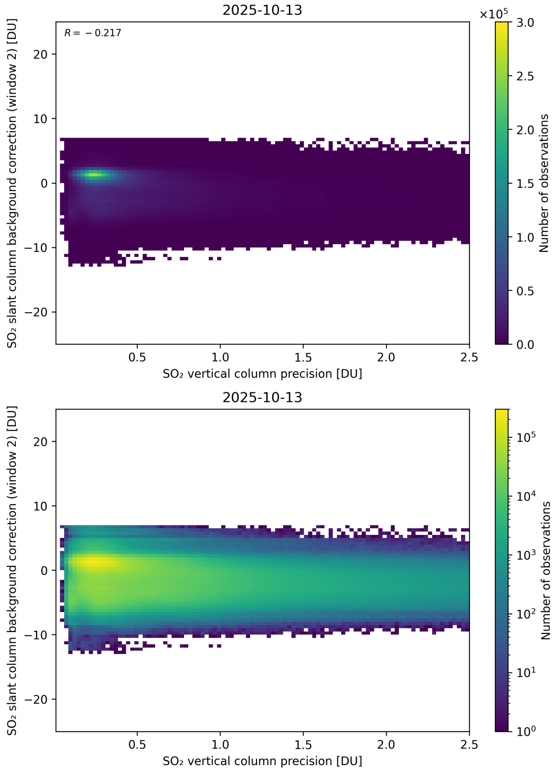
Figure 330: Scatter density plot of “SO 2 vertical column precision” against “SO 2 slant column background correction (window 2)” for 2025-10-12 to 2025-10-14.
