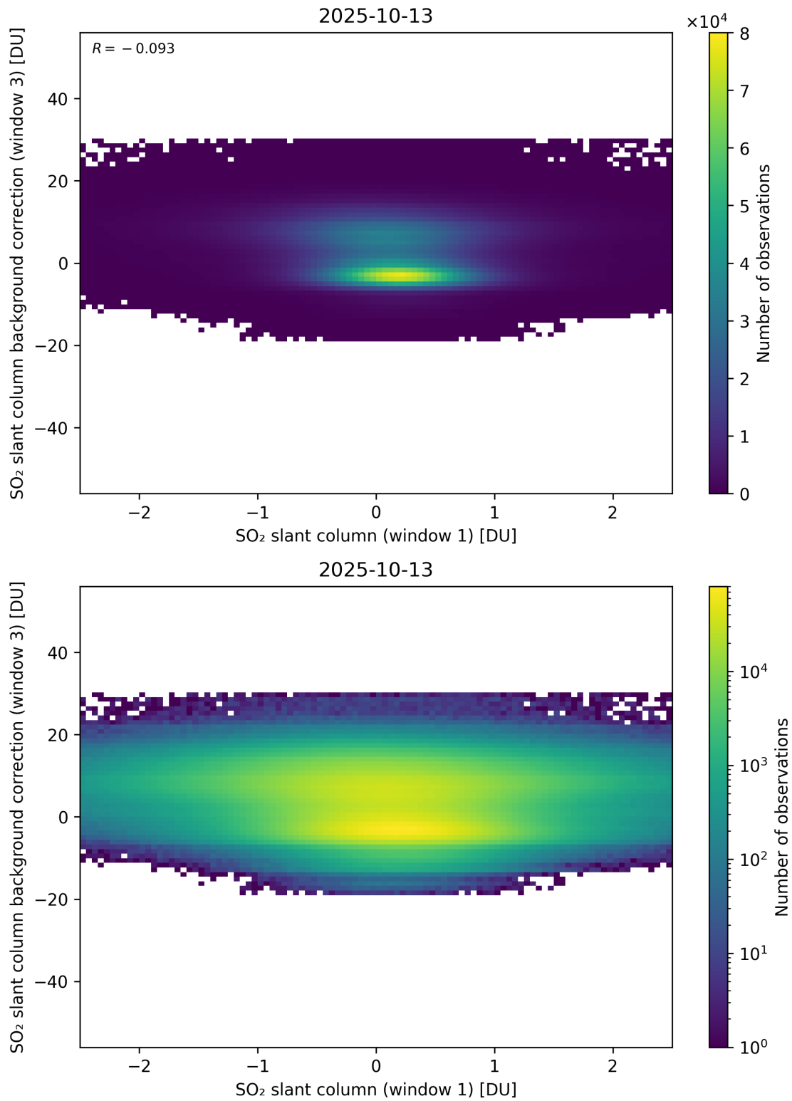
Figure 264: Scatter density plot of “SO 2 slant column (window 1)” against “SO 2 slant column background correction (window 3)” for 2025-10-12 to 2025-10-14.
