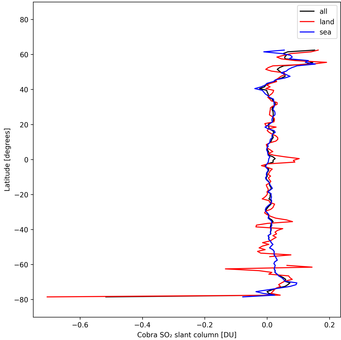
Figure 35: Zonal average of “Cobra SO 2 slant column” for 2025-10-12 to 2025-10-14.
