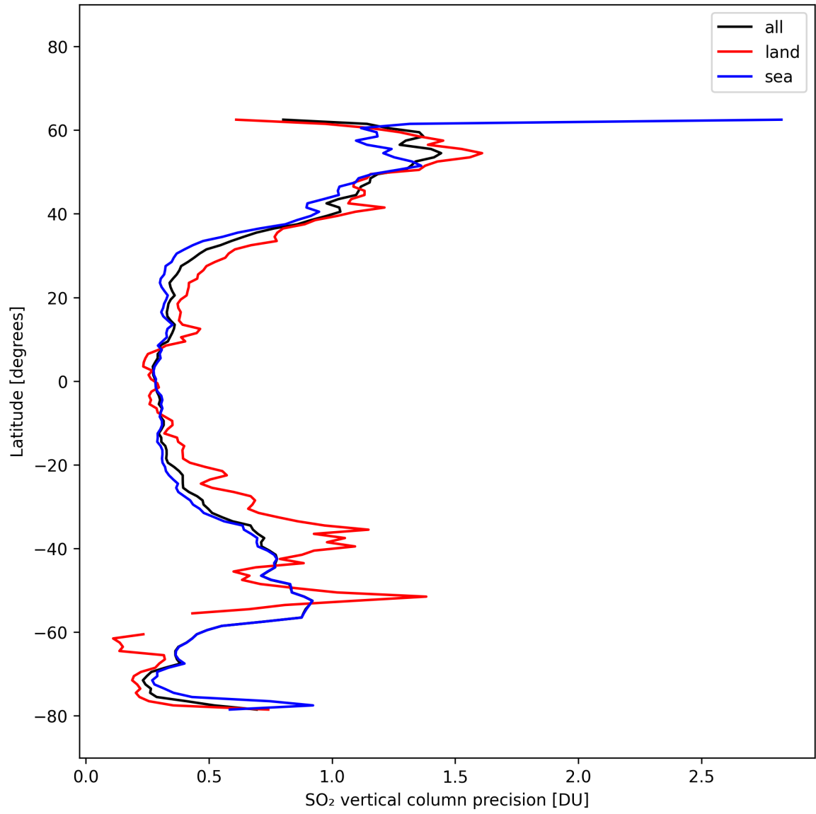
Figure 33: Zonal average of “SO 2 vertical column precision” for 2025-10-12 to 2025-10-14.
