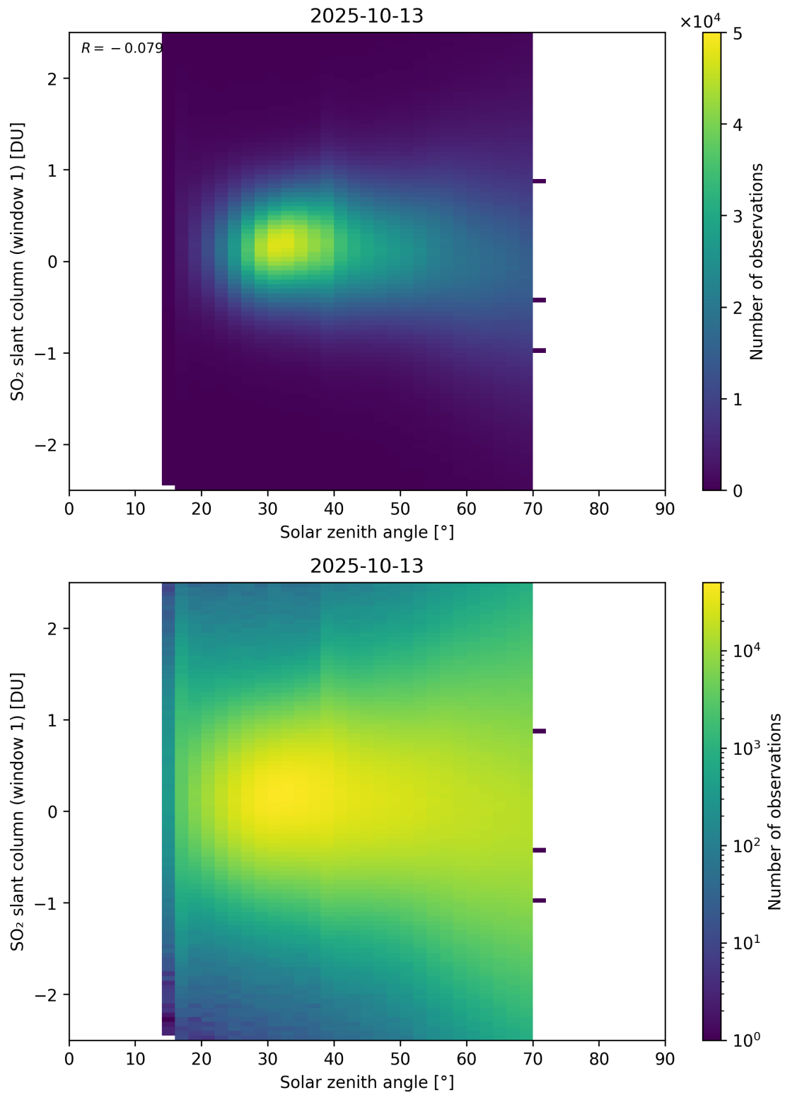
Figure 184: Scatter density plot of “Solar zenith angle” against “SO 2 slant column (window 1)” for 2025-10-12 to 2025-10-14.
