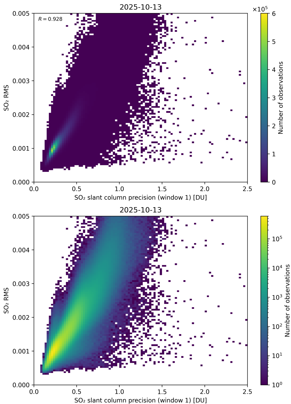
Figure 273: Scatter density plot of “SO 2 slant column precision (window 1)” against “SO 2 RMS” for 2025-10-12 to 2025-10-14.
