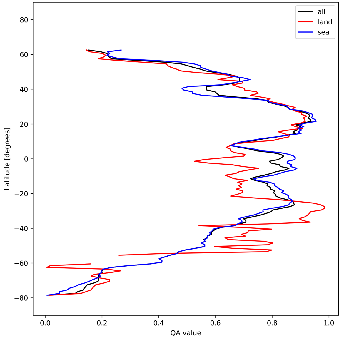
Figure 31: Zonal average of “QA value” for 2025-10-12 to 2025-10-14.
