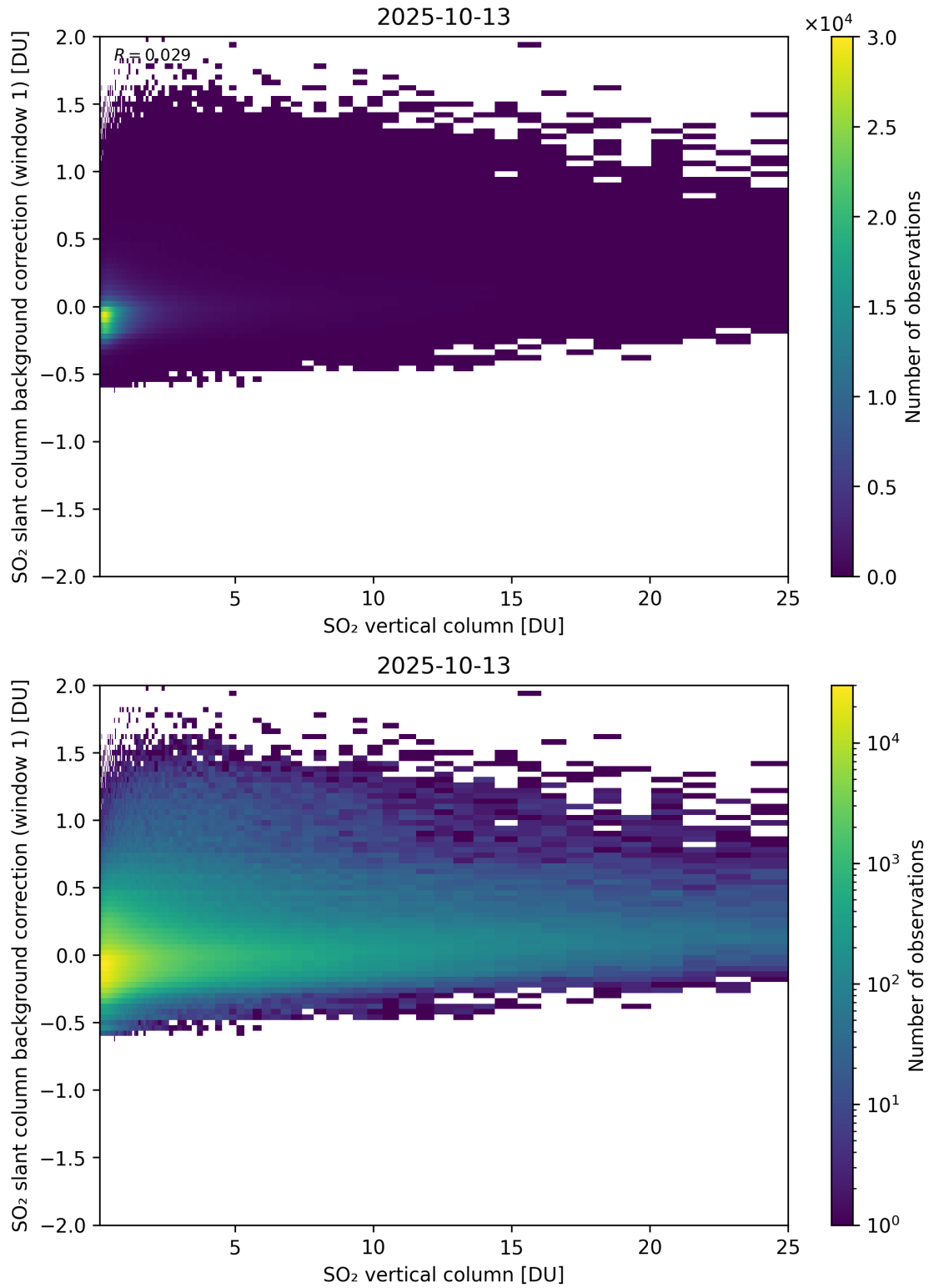
Figure 323: Scatter density plot of “SO 2 vertical column” against “SO 2 slant column background correction (window 1)” for 2025-10-12 to 2025-10-14.
