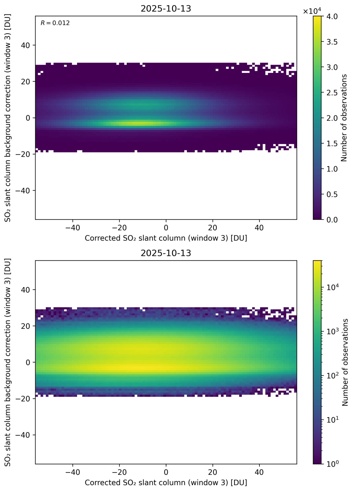
Figure 255: Scatter density plot of “Corrected SO 2 slant column (window 3)” against “SO 2 slant column background correction (window 3)” for 2025-10-12 to 2025-10-14.
