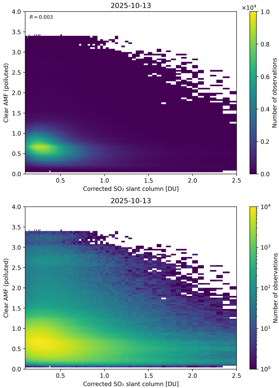
Figure 232: Scatter density plot of “Corrected SO 2 slant column” against “Clear AMF (polluted)” for 2025-10-12 to 2025-10-14.
