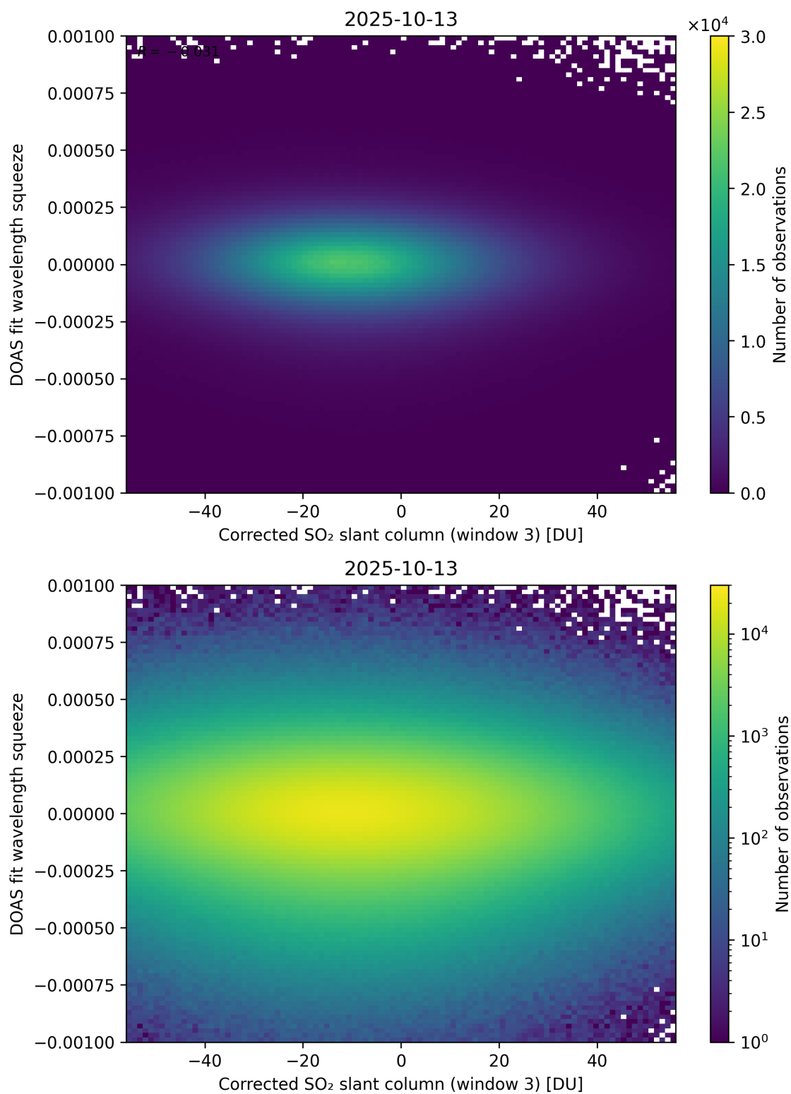
Figure 257: Scatter density plot of “Corrected SO 2 slant column (window 3)” against “DOAS fit wavelength squeeze” for 2025-10-12 to 2025-10-14.
