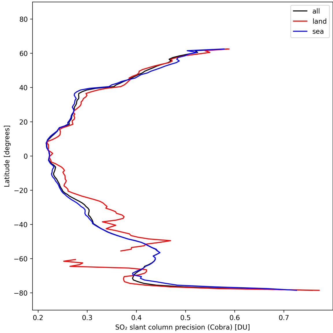
Figure 36: Zonal average of “SO 2 slant column precision (Cobra)” for 2025-10-12 to 2025-10-14.
