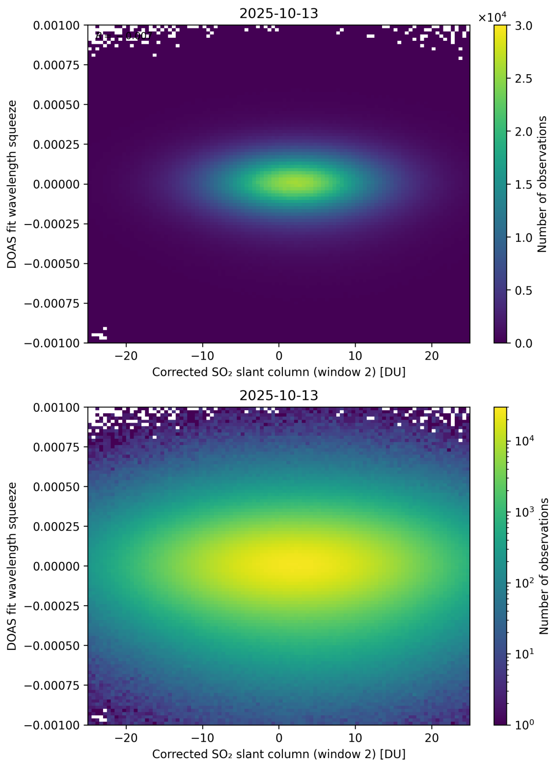
Figure 247: Scatter density plot of “Corrected SO 2 slant column (window 2)” against “DOAS fit wavelength squeeze” for 2025-10-12 to 2025-10-14.
