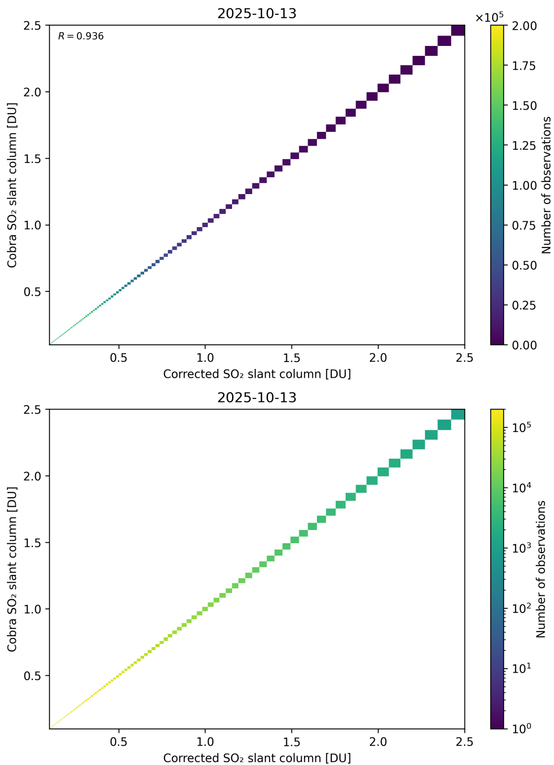
Figure 233: Scatter density plot of “Corrected SO 2 slant column” against “Cobra SO 2 slant column” for 2025-10-12 to 2025-10-14.
