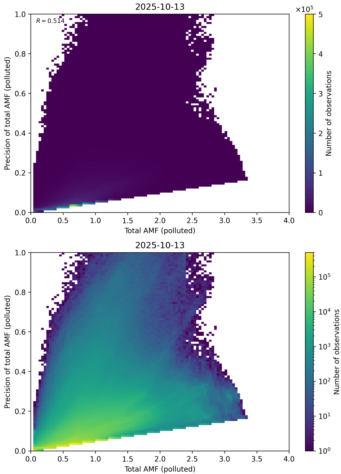
Figure 322: Scatter density plot of “Total AMF (polluted)” against “Precision of total AMF (polluted)” for 2025-10-12 to 2025-10-14.
