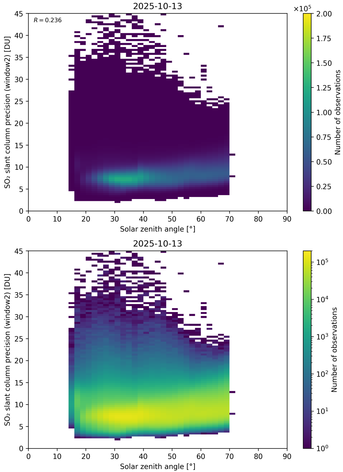
Figure 186: Scatter density plot of “Solar zenith angle” against “SO 2 slant column precision (window2)” for 2025-10-12 to 2025-10-14.
