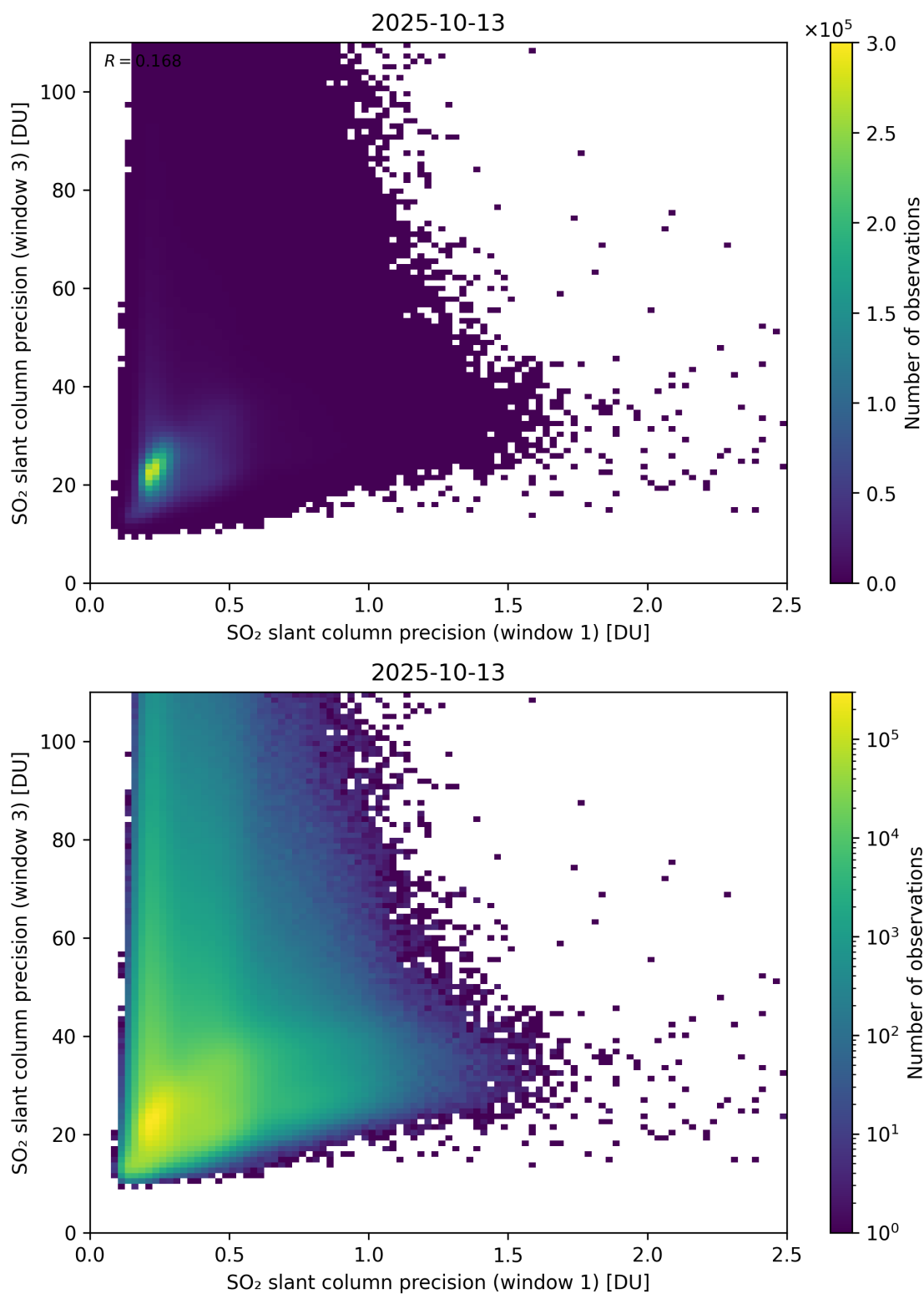
Figure 279: Scatter density plot of “SO 2 slant column precision (window 1)” against “SO 2 slant column precision (window 3)” for 2025-10-12 to 2025-10-14.
