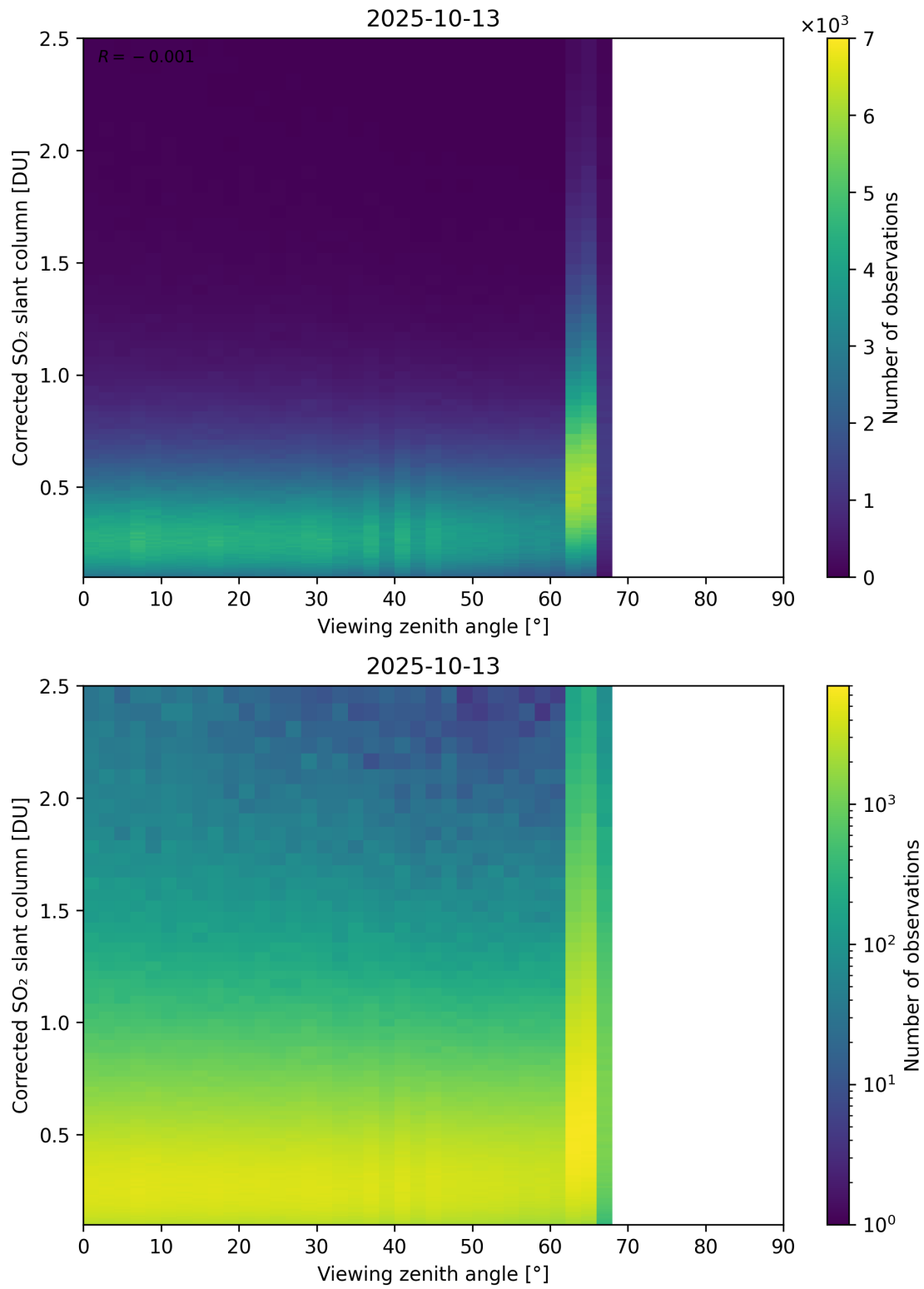
Figure 373: Scatter density plot of “Viewing zenith angle” against “Corrected SO 2 slant column” for 2025-10-12 to 2025-10-14.
