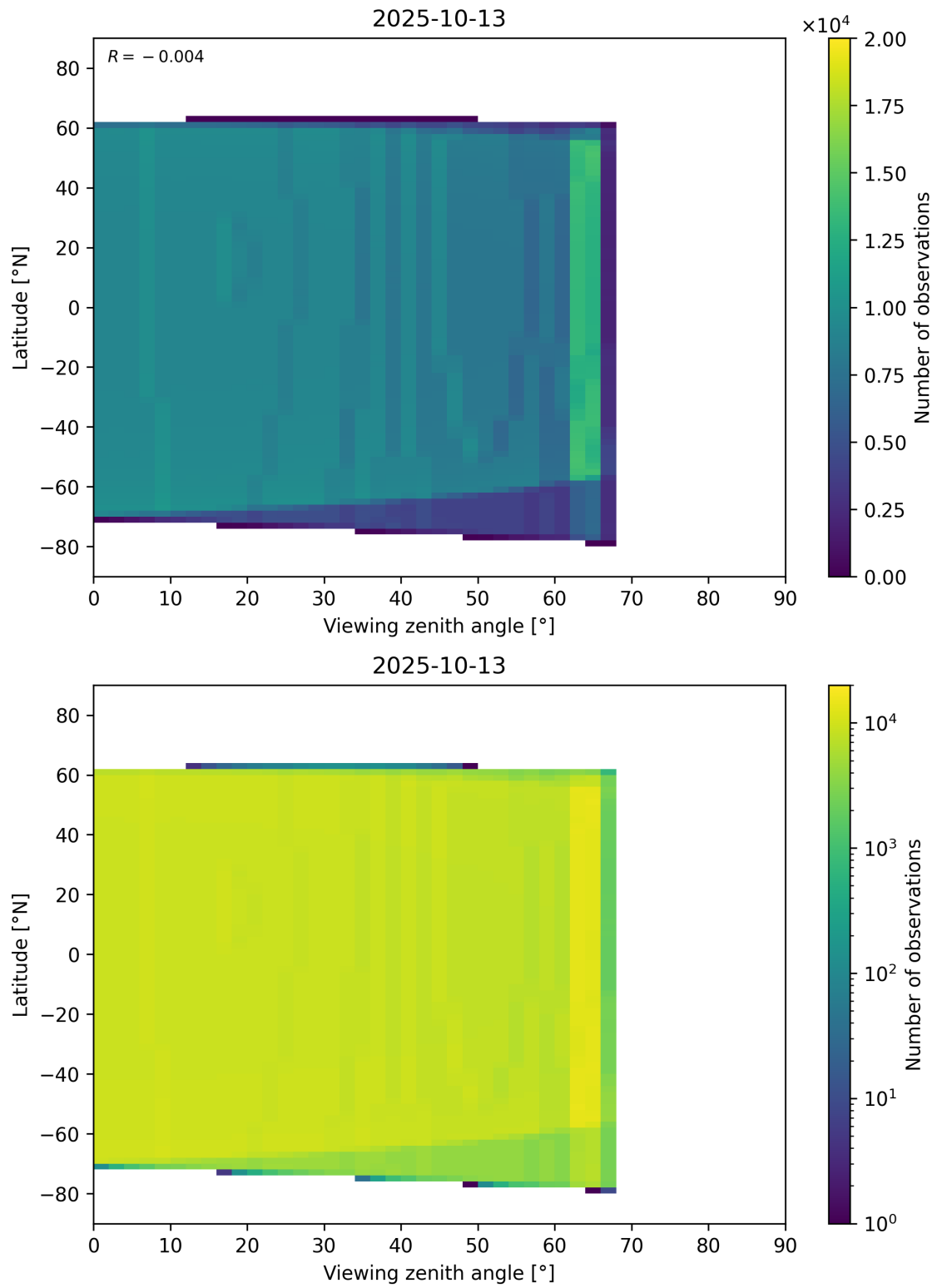
Figure 368: Scatter density plot of “Viewing zenith angle” against “Latitude” for 2025-10-12 to 2025-10-14.
