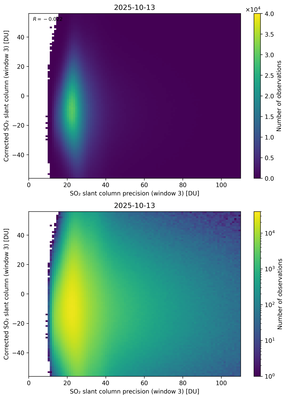
Figure 312: Scatter density plot of “SO 2 slant column precision (window 3)” against “Corrected SO 2 slant column (window 3)” for 2025-10-12 to 2025-10-14.
