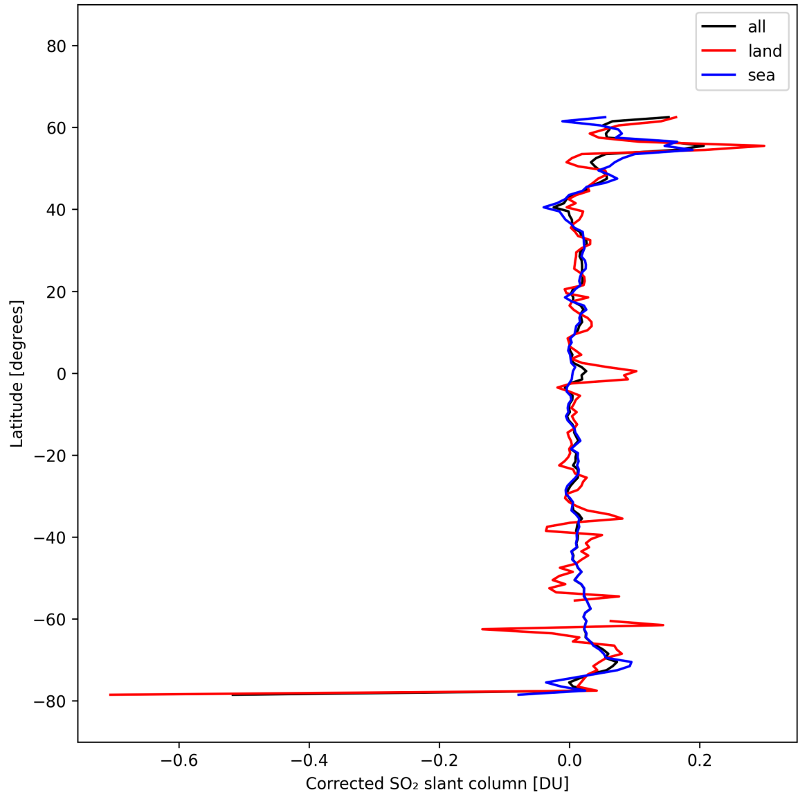
Figure 34: Zonal average of “Corrected SO 2 slant column” for 2025-10-12 to 2025-10-14.
