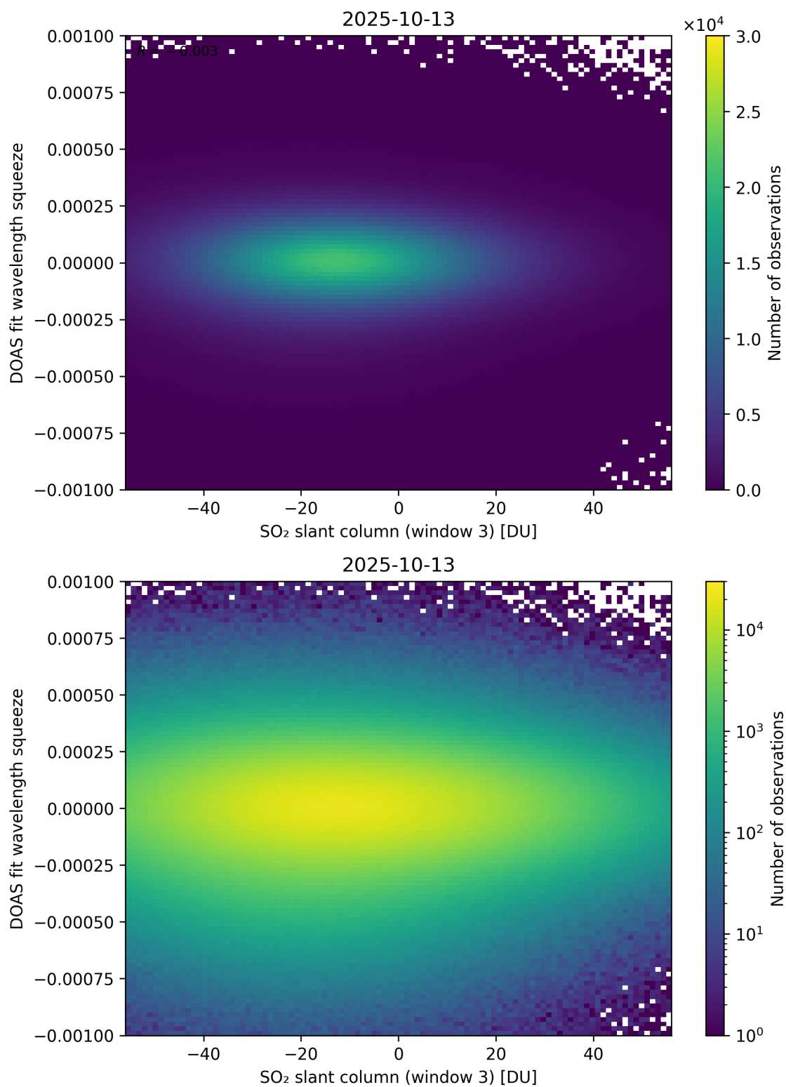
Figure 305: Scatter density plot of “SO 2 slant column (window 3)” against “DOAS fit wavelength squeeze” for 2025-10-12 to 2025-10-14.
