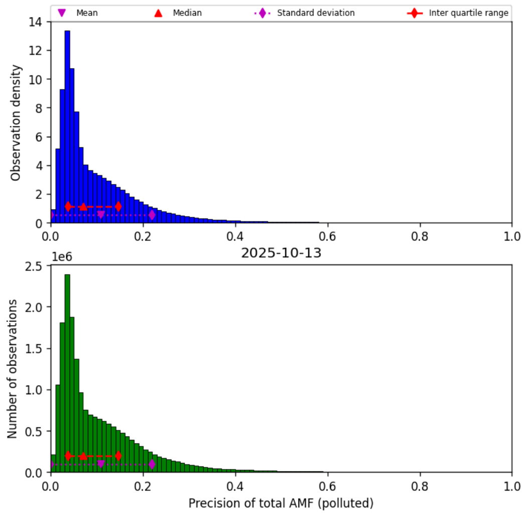
Figure 80: Histogram of “Precision of total AMF (polluted)” for 2025-10-12 to 2025-10-14
