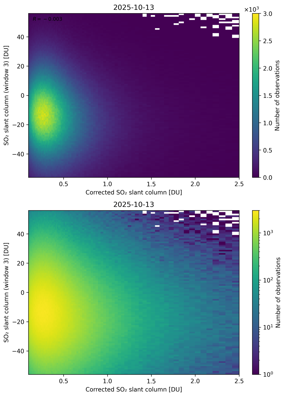
Figure 240: Scatter density plot of “Corrected SO 2 slant column” against “SO 2 slant column (window 3)” for 2025-10-12 to 2025-10-14.
