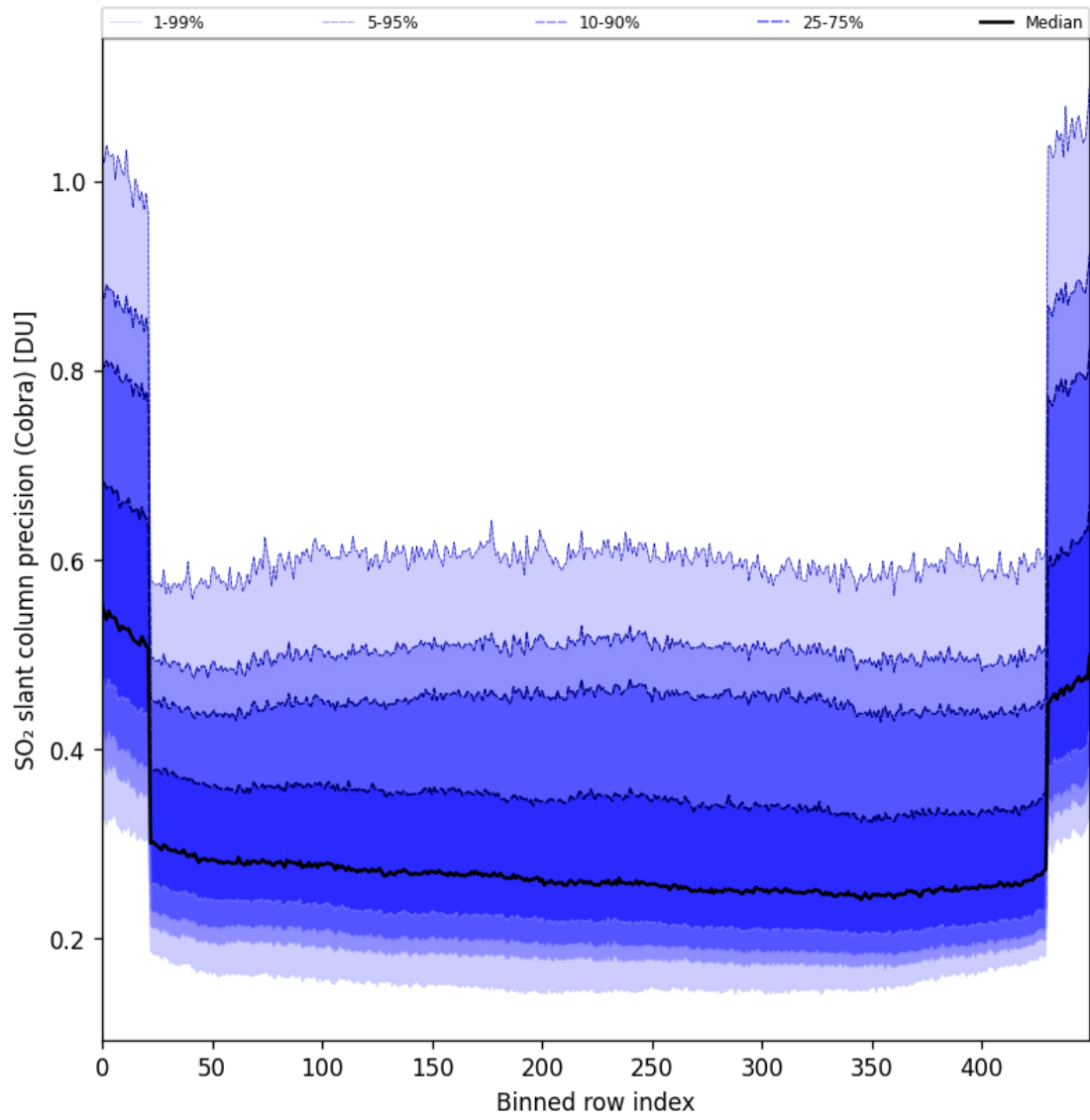
Figure 88: Along track statistics of “SO 2 slant column precision (Cobra)” for 2025-10-12 to 2025-10-14
