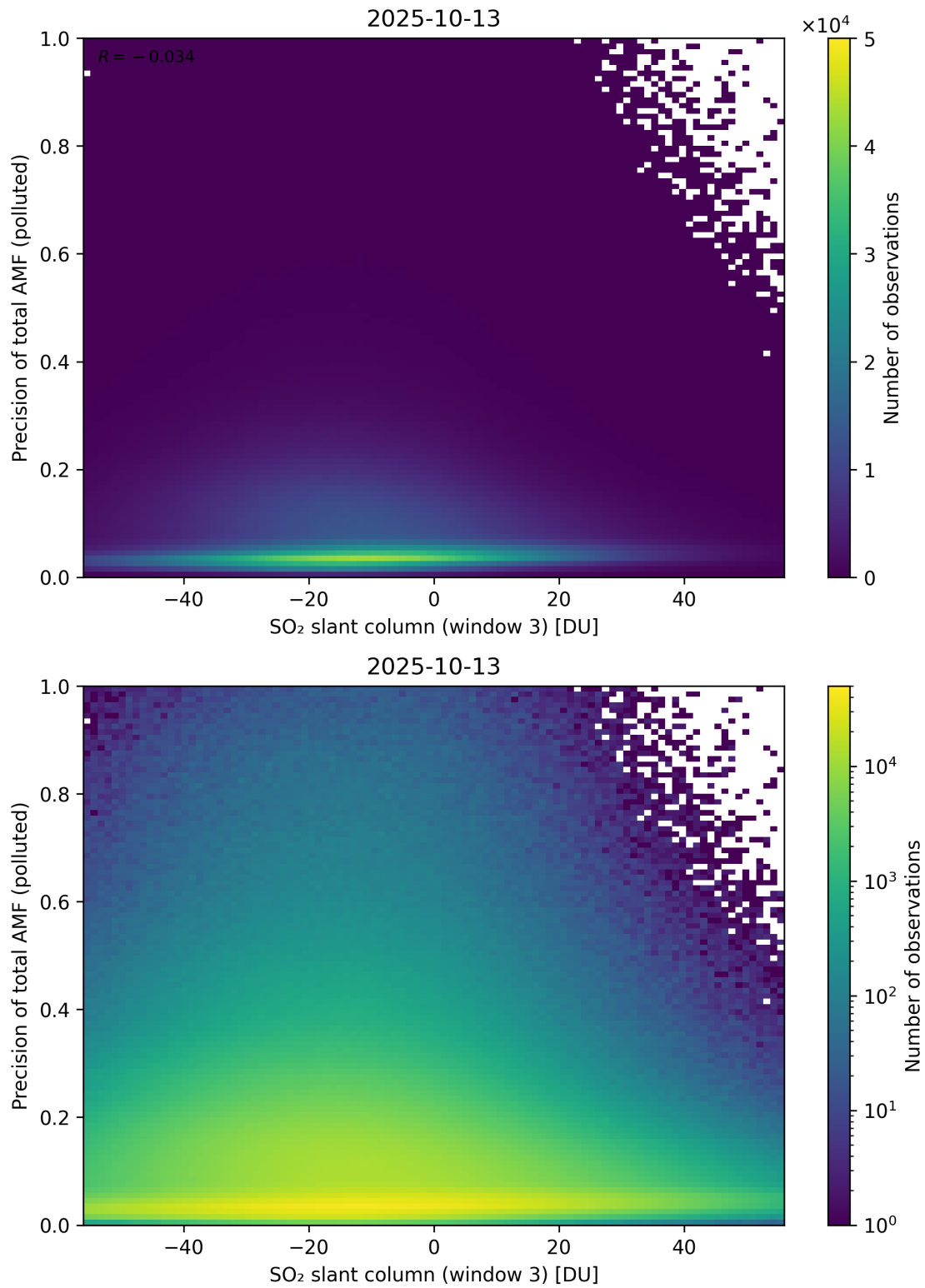
Figure 319: Scatter density plot of “SO 2 slant column (window 3)” against “Precision of total AMF (polluted)” for 2025-10-12 to 2025-10-14.
