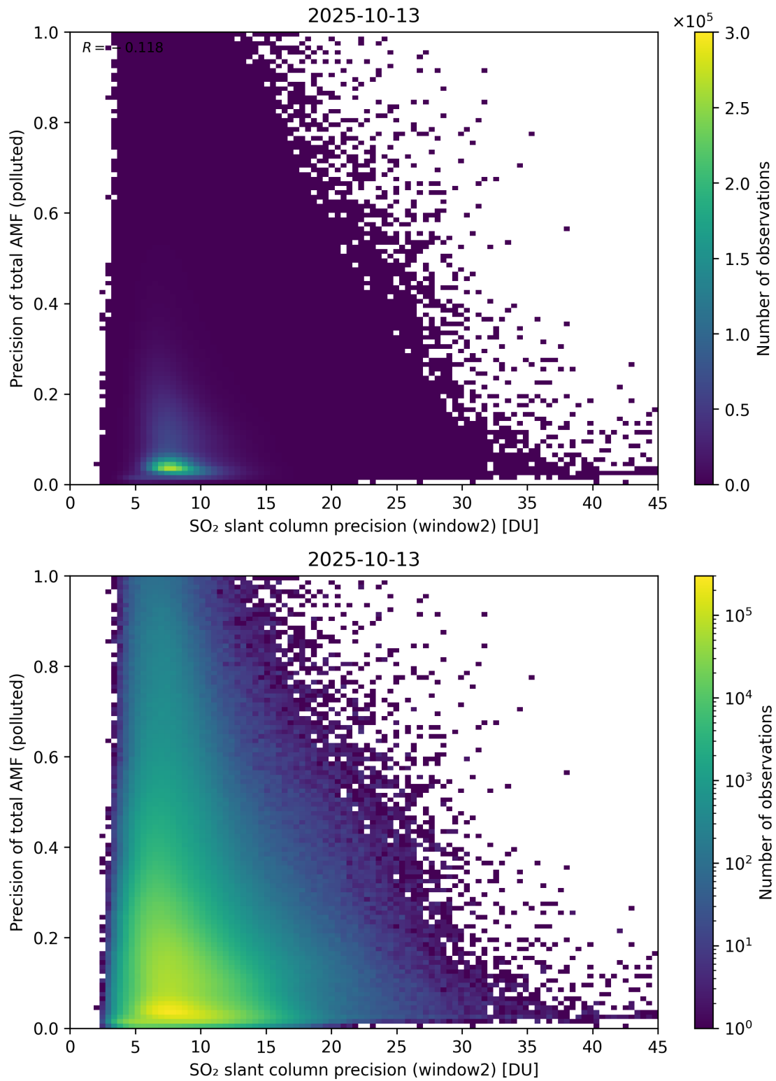
Figure 302: Scatter density plot of “SO 2 slant column precision (window2)” against “Precision of total AMF (polluted)” for 2025-10-12 to 2025-10-14.
