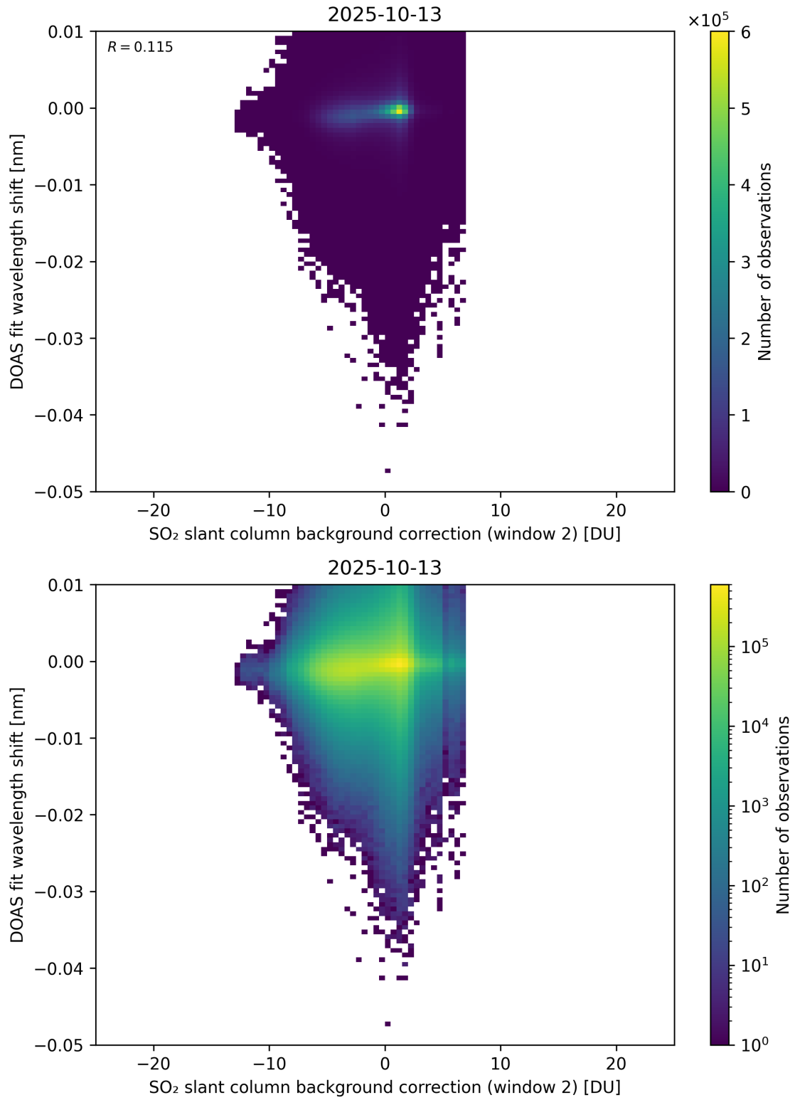
Figure 123: Scatter density plot of “SO 2 slant column background correction (window 2)” against “DOAS fit wavelength shift” for 2025-10-12 to 2025-10-14.
