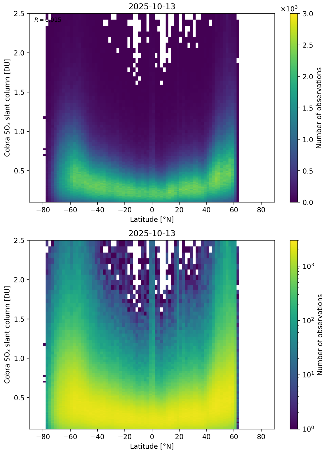
Figure 157: Scatter density plot of “Latitude” against “Cobra SO 2 slant column” for 2025-10-12 to 2025-10-14.
