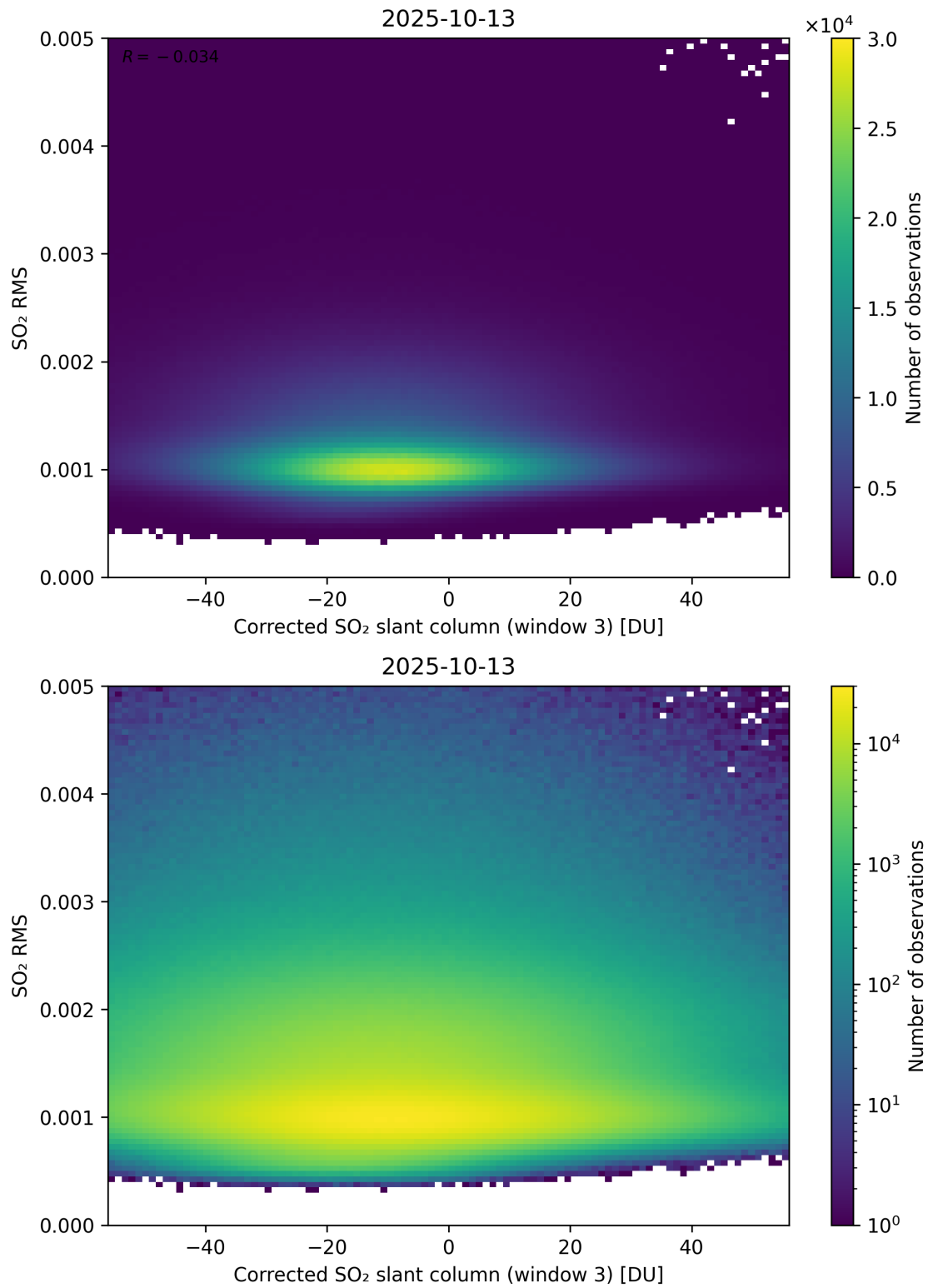
Figure 258: Scatter density plot of “Corrected SO 2 slant column (window 3)” against “SO 2 RMS” for 2025-10-12 to 2025-10-14.
