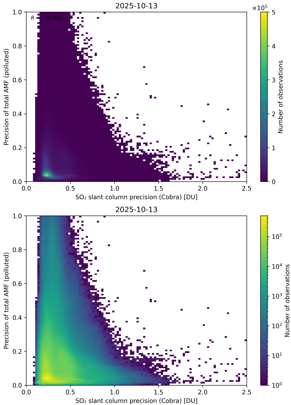
Figure 214: Scatter density plot of “SO 2 slant column precision (Cobra)” against “Precision of total AMF (polluted)” for 2025-10-12 to 2025-10-14.
