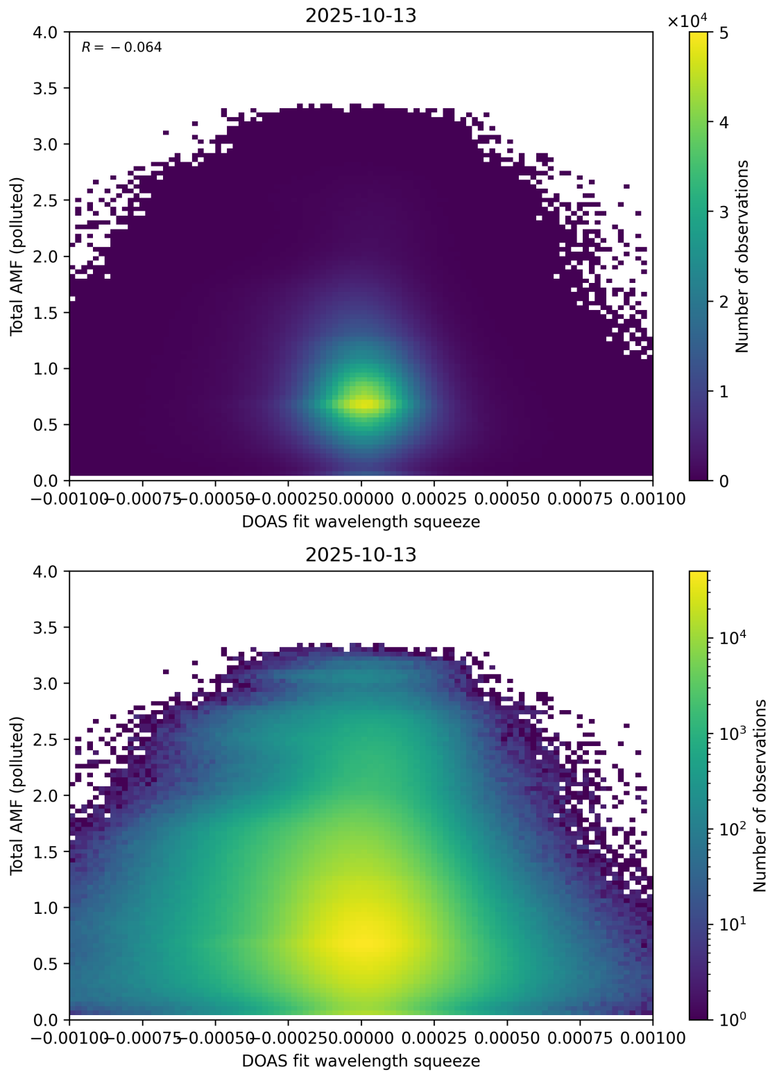
Figure 145: Scatter density plot of “DOAS fit wavelength squeeze” against “Total AMF (polluted)” for 2025-10-12 to 2025-10-14.
