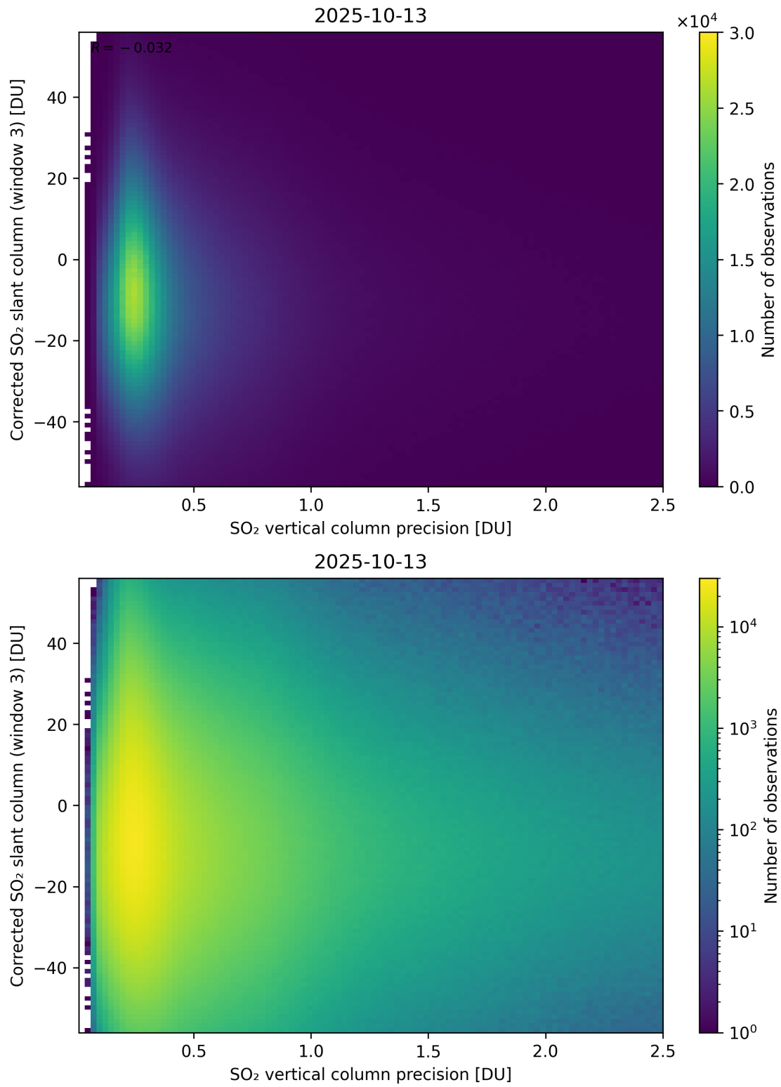
Figure 340: Scatter density plot of “SO 2 vertical column precision” against “Corrected SO 2 slant column (window 3)” for 2025-10-12 to 2025-10-14.
