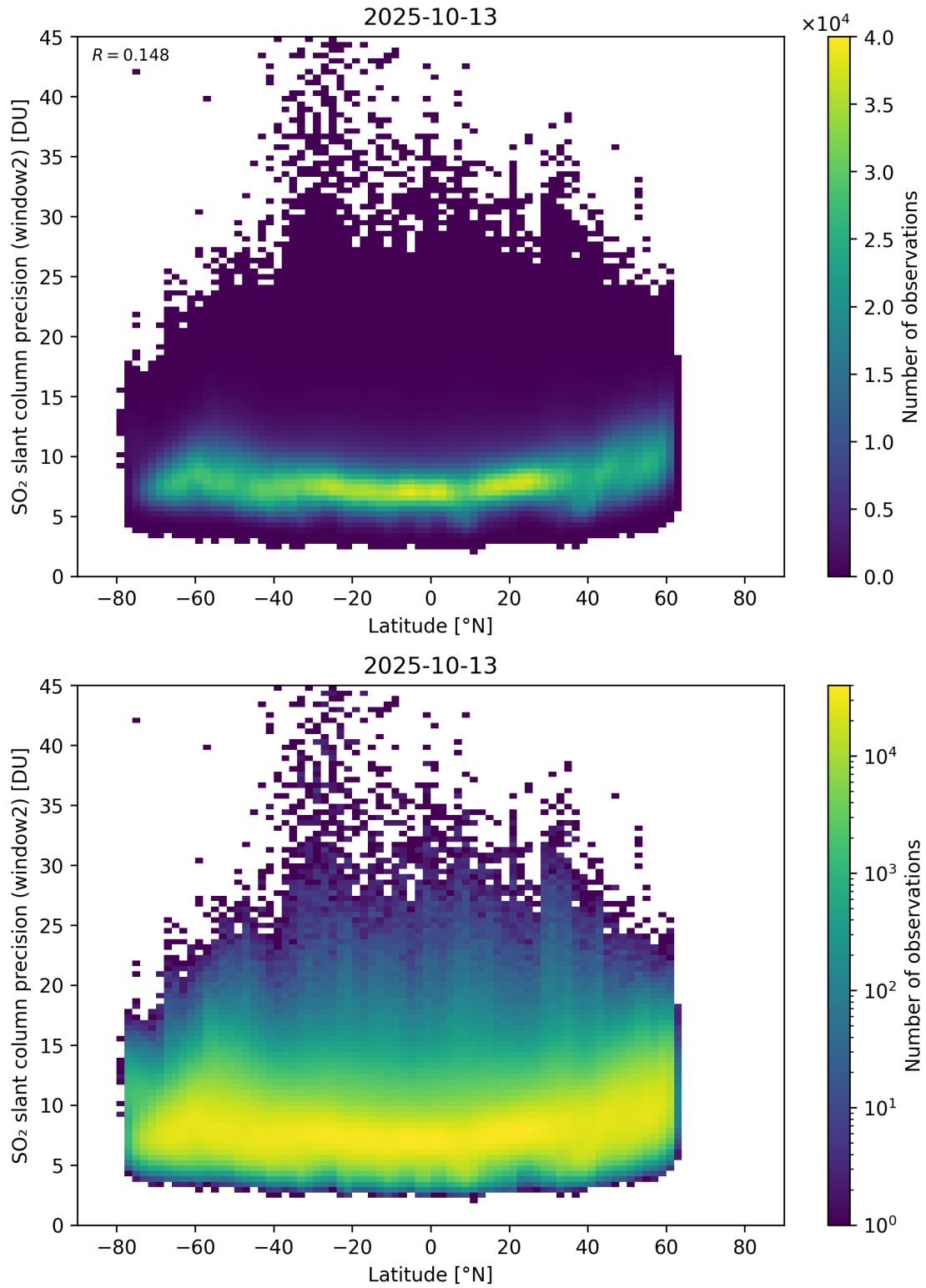
Figure 164: Scatter density plot of “Latitude” against “SO 2 slant column precision (window2)” for 2025-10-12 to 2025-10-14.
