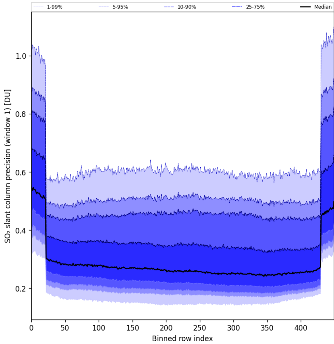
Figure 90: Along track statistics of “SO 2 slant column precision (window 1)” for 2025-10-12 to 2025-10-14
