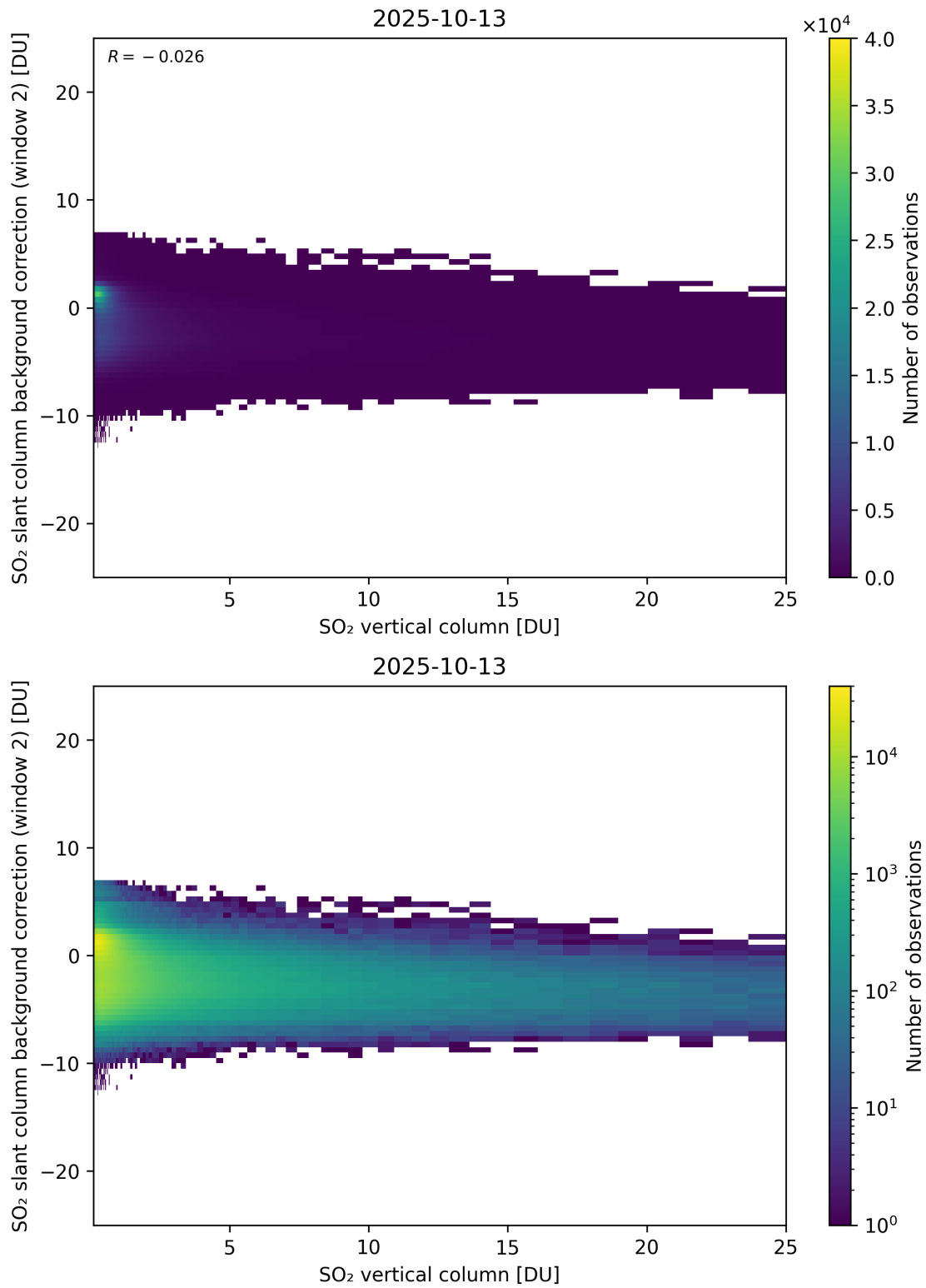
Figure 324: Scatter density plot of “SO 2 vertical column” against “SO 2 slant column background correction (window 2)” for 2025-10-12 to 2025-10-14.
