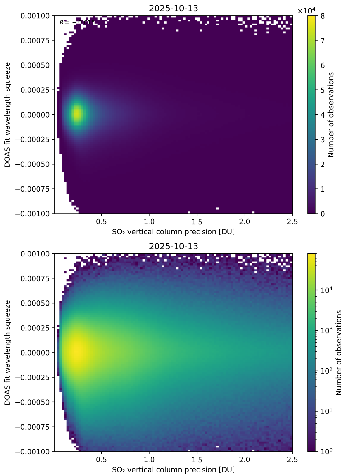
Figure 333: Scatter density plot of “SO 2 vertical column precision” against “DOAS fit wavelength squeeze” for 2025-10-12 to 2025-10-14.
