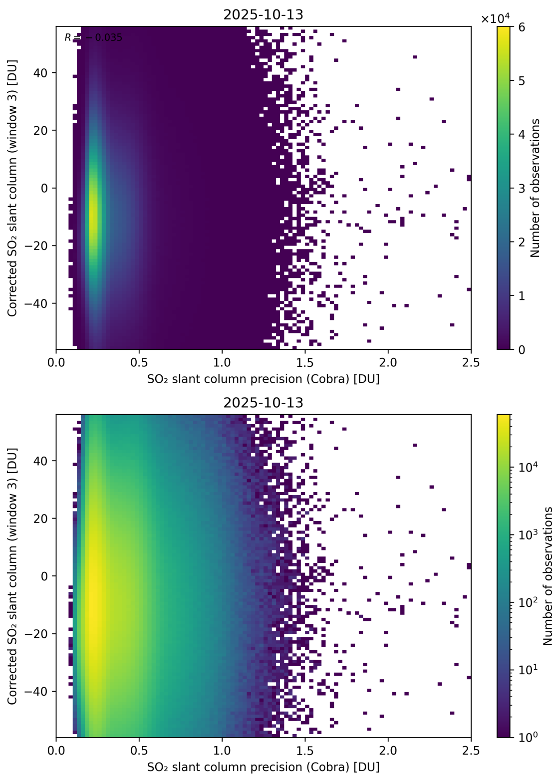
Figure 207: Scatter density plot of “SO 2 slant column precision (Cobra)” against “Corrected SO 2 slant column (window 3)” for 2025-10-12 to 2025-10-14.
