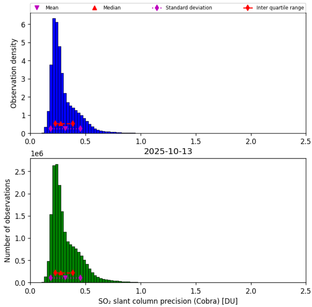
Figure 62: Histogram of “SO 2 slant column precision (Cobra)” for 2025-10-12 to 2025-10-14
