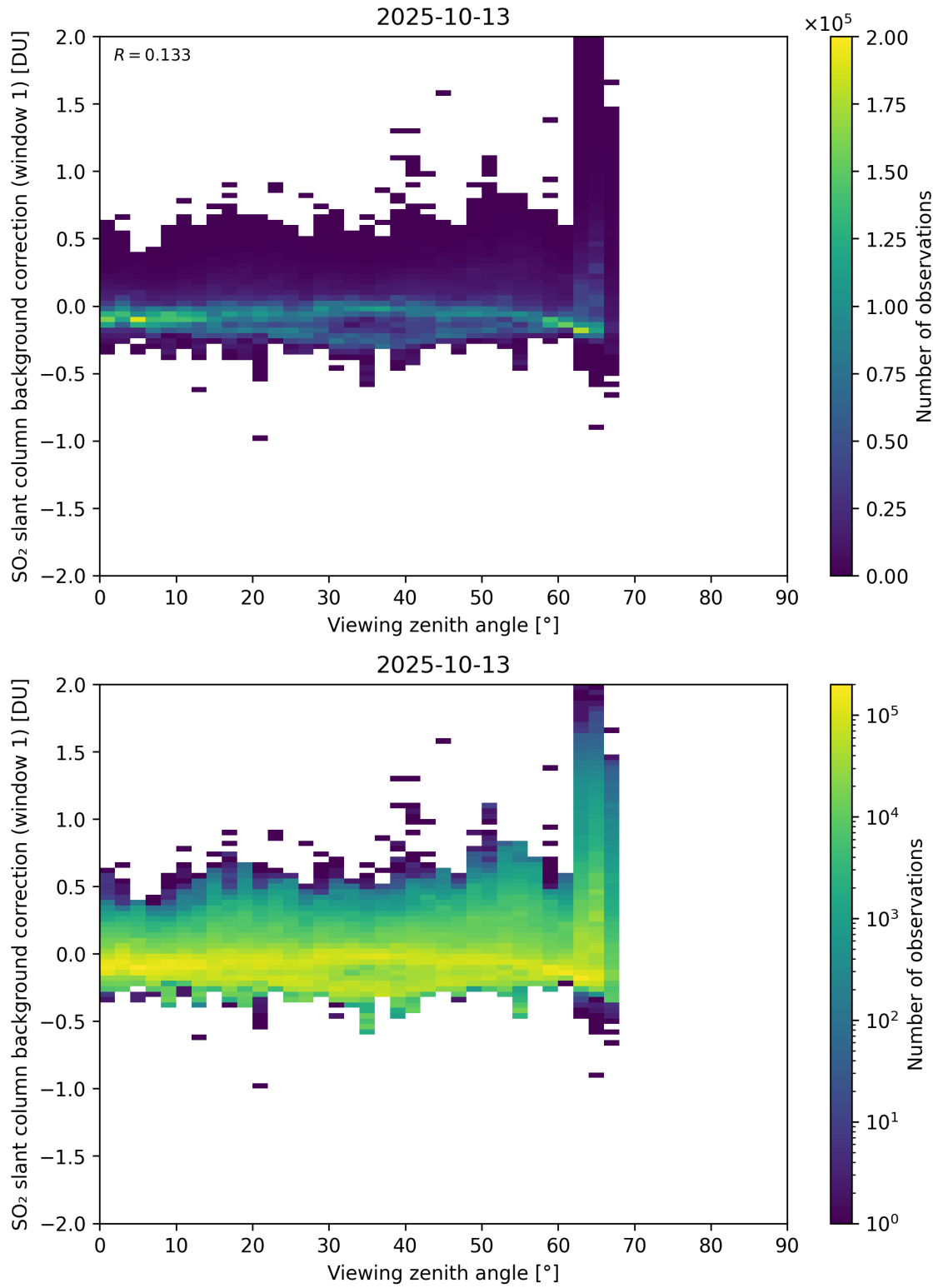
Figure 362: Scatter density plot of “Viewing zenith angle” against “SO 2 slant column background correction (window 1)” for 2025-10-12 to 2025-10-14.
