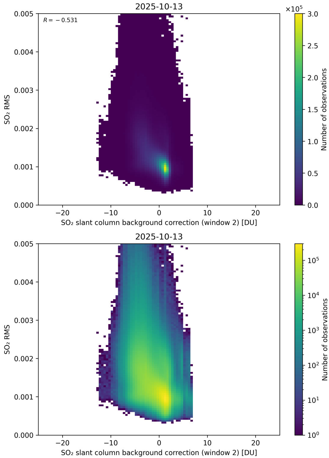
Figure 125: Scatter density plot of “SO 2 slant column background correction (window 2)” against “SO 2 RMS” for 2025-10-12 to 2025-10-14.
