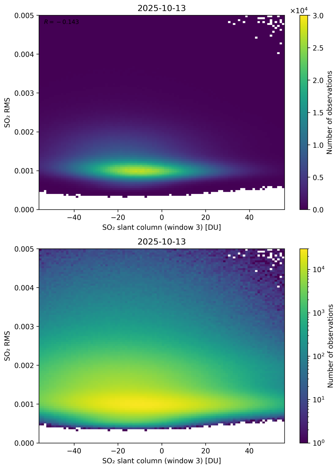
Figure 306: Scatter density plot of “SO 2 slant column (window 3)” against “SO 2 RMS” for 2025-10-12 to 2025-10-14.
