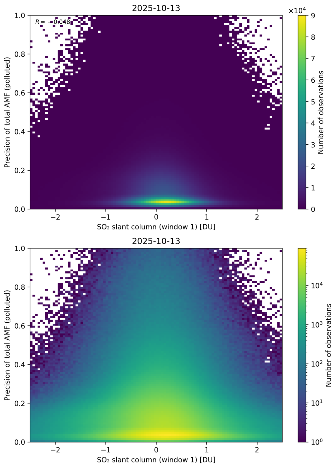
Figure 290: Scatter density plot of “SO 2 slant column (window 1)” against “Precision of total AMF (polluted)” for 2025-10-12 to 2025-10-14.
