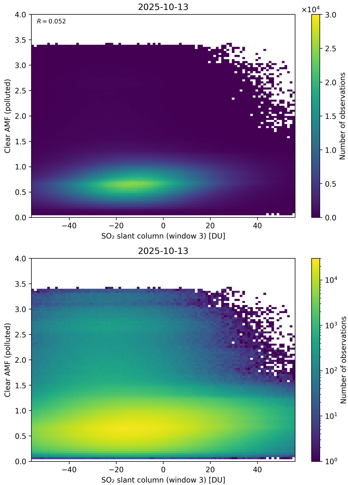
Figure 315: Scatter density plot of “SO 2 slant column (window 3)” against “Clear AMF (polluted)” for 2025-10-12 to 2025-10-14.
