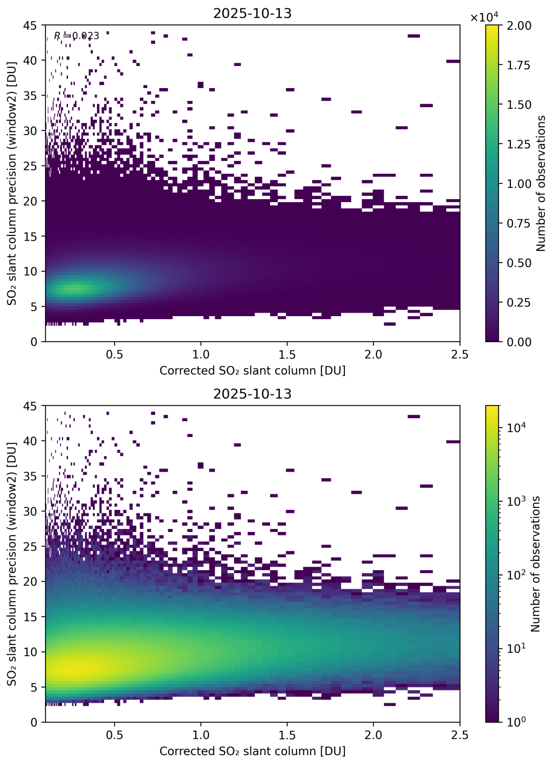
Figure 239: Scatter density plot of “Corrected SO 2 slant column” against “SO 2 slant column precision (window2)” for 2025-10-12 to 2025-10-14.
