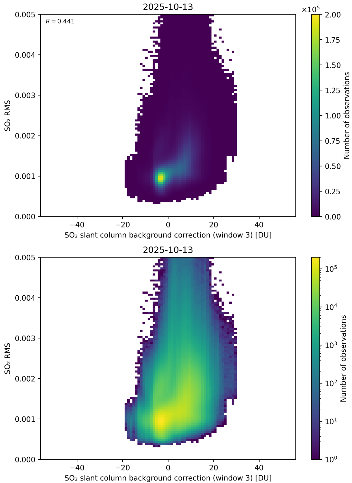
Figure 134: Scatter density plot of “SO 2 slant column background correction (window 3)” against “SO 2 RMS” for 2025-10-12 to 2025-10-14.
