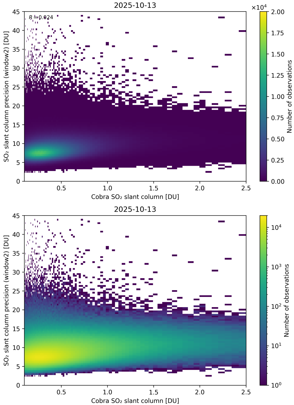
Figure 221: Scatter density plot of “Cobra SO 2 slant column” against “SO 2 slant column precision (window2)” for 2025-10-12 to 2025-10-14.
