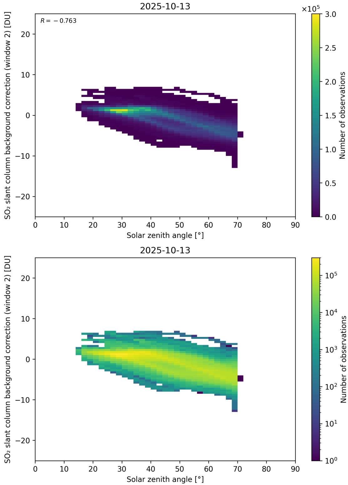
Figure 172: Scatter density plot of “Solar zenith angle” against “SO 2 slant column background correction (window 2)” for 2025-10-12 to 2025-10-14.
