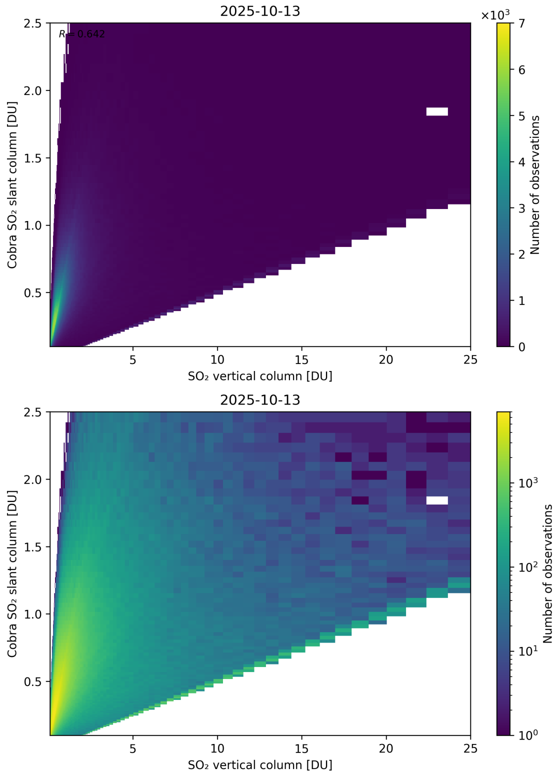
Figure 349: Scatter density plot of “SO 2 vertical column” against “Cobra SO 2 slant column” for 2025-10-12 to 2025-10-14.
