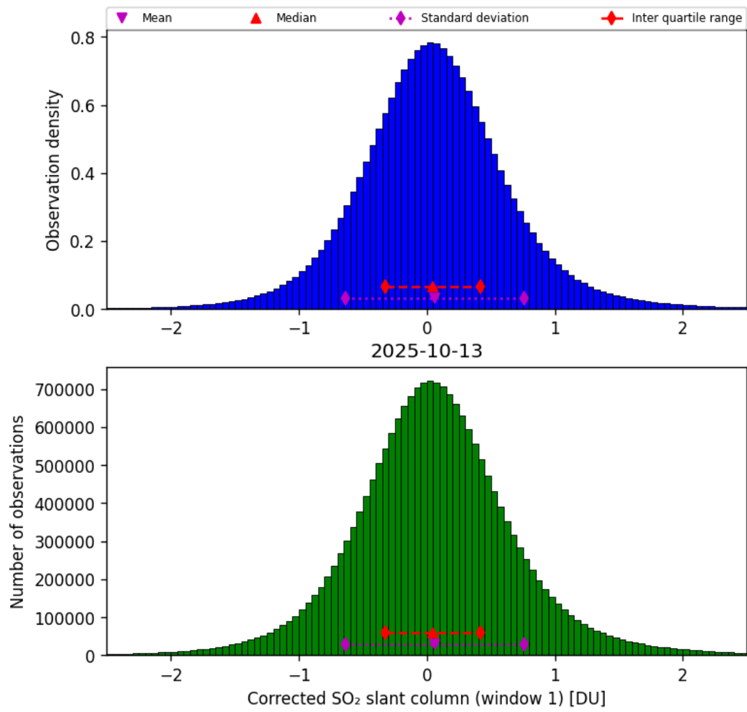
Figure 65: Histogram of “Corrected SO 2 slant column (window 1)” for 2025-10-12 to 2025-10-14
