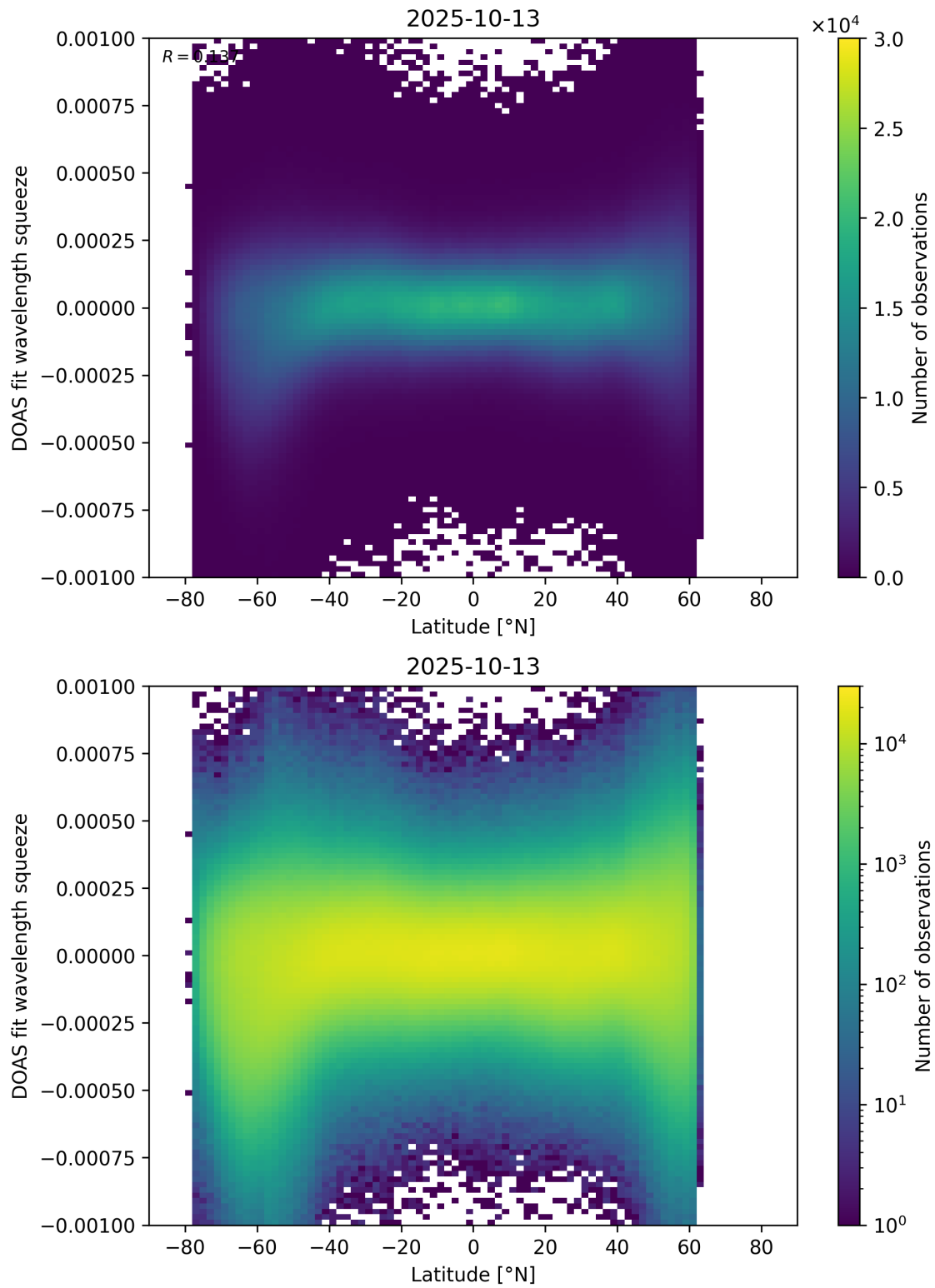
Figure 154: Scatter density plot of “Latitude” against “DOAS fit wavelength squeeze” for 2025-10-12 to 2025-10-14.
