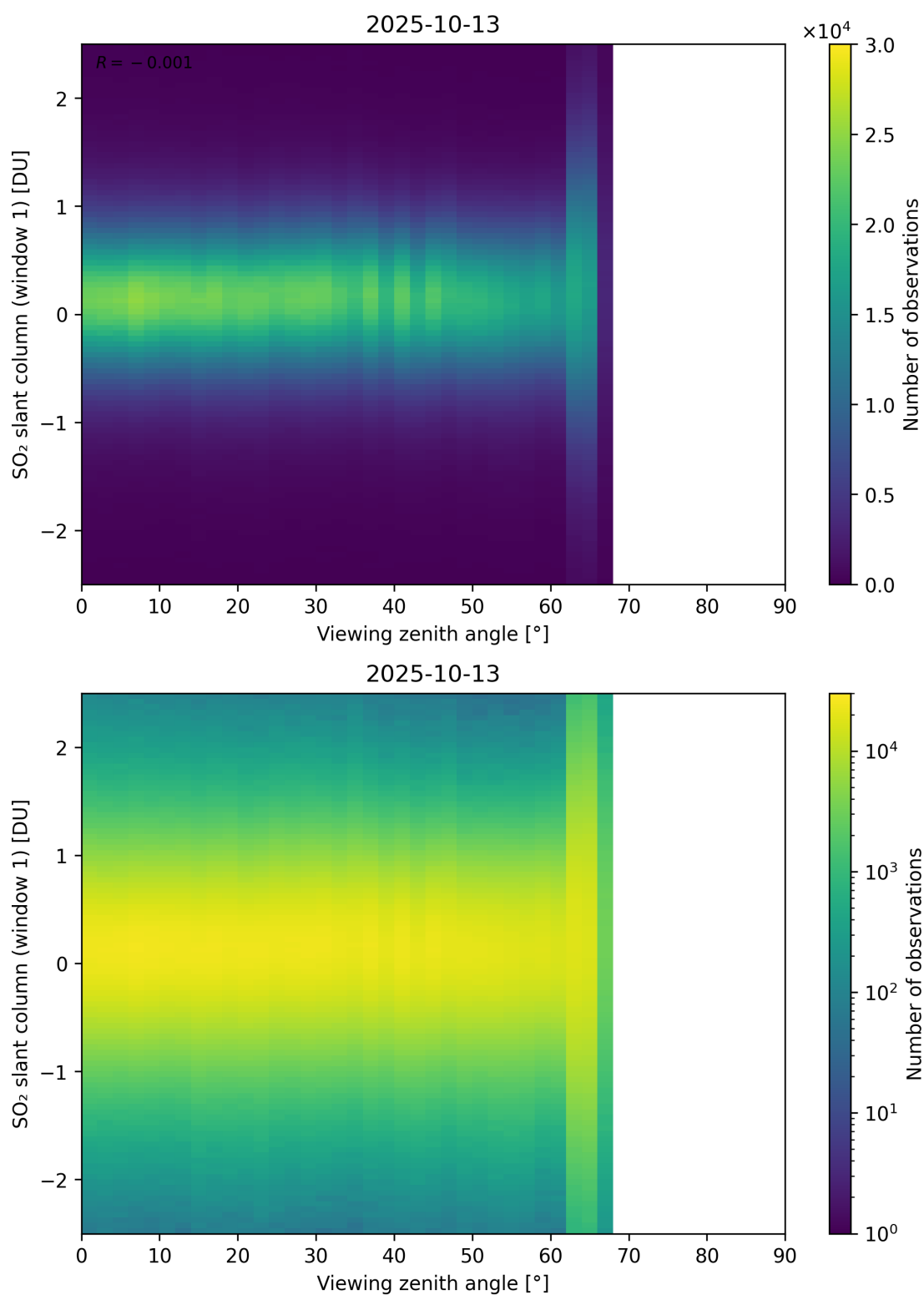
Figure 376: Scatter density plot of “Viewing zenith angle” against “SO 2 slant column (window 1)” for 2025-10-12 to 2025-10-14.
