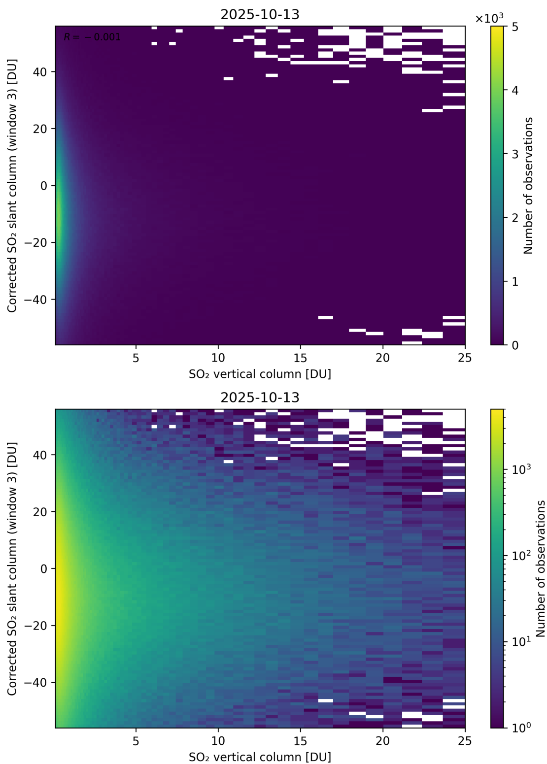
Figure 353: Scatter density plot of “SO 2 vertical column” against “Corrected SO 2 slant column (window 3)” for 2025-10-12 to 2025-10-14.
