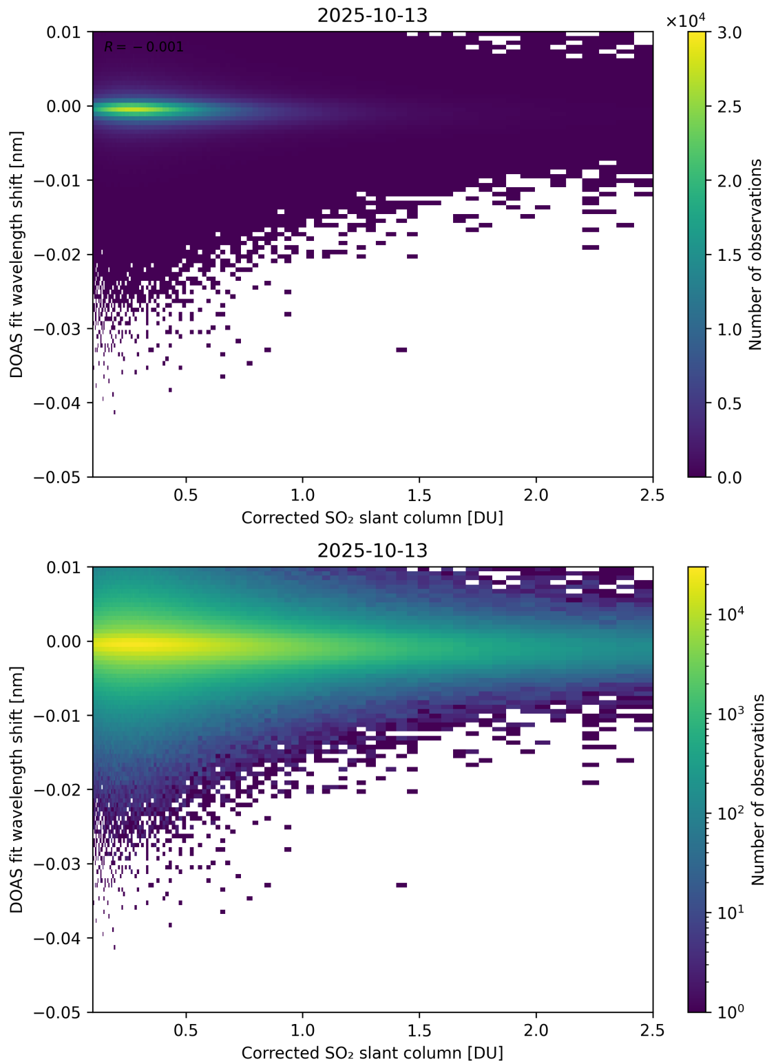
Figure 229: Scatter density plot of “Corrected SO 2 slant column” against “DOAS fit wavelength shift” for 2025-10-12 to 2025-10-14.
