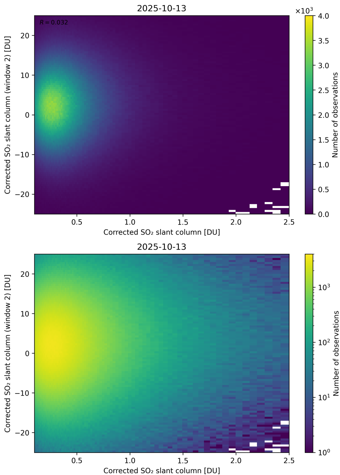
Figure 235: Scatter density plot of “Corrected SO 2 slant column” against “Corrected SO 2 slant column (window 2)” for 2025-10-12 to 2025-10-14.
