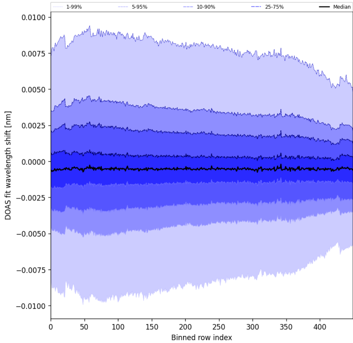
Figure 102: Along track statistics of “DOAS fit wavelength shift” for 2025-10-12 to 2025-10-14
