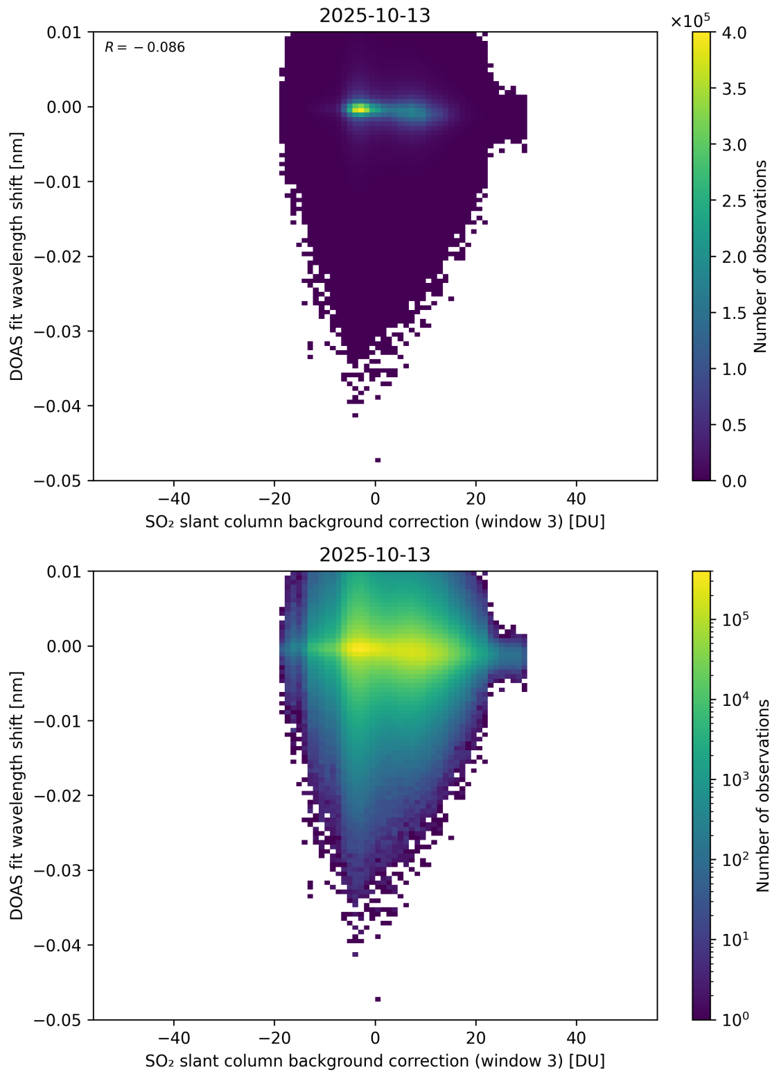
Figure 132: Scatter density plot of “SO 2 slant column background correction (window 3)” against “DOAS fit wavelength shift” for 2025-10-12 to 2025-10-14.
