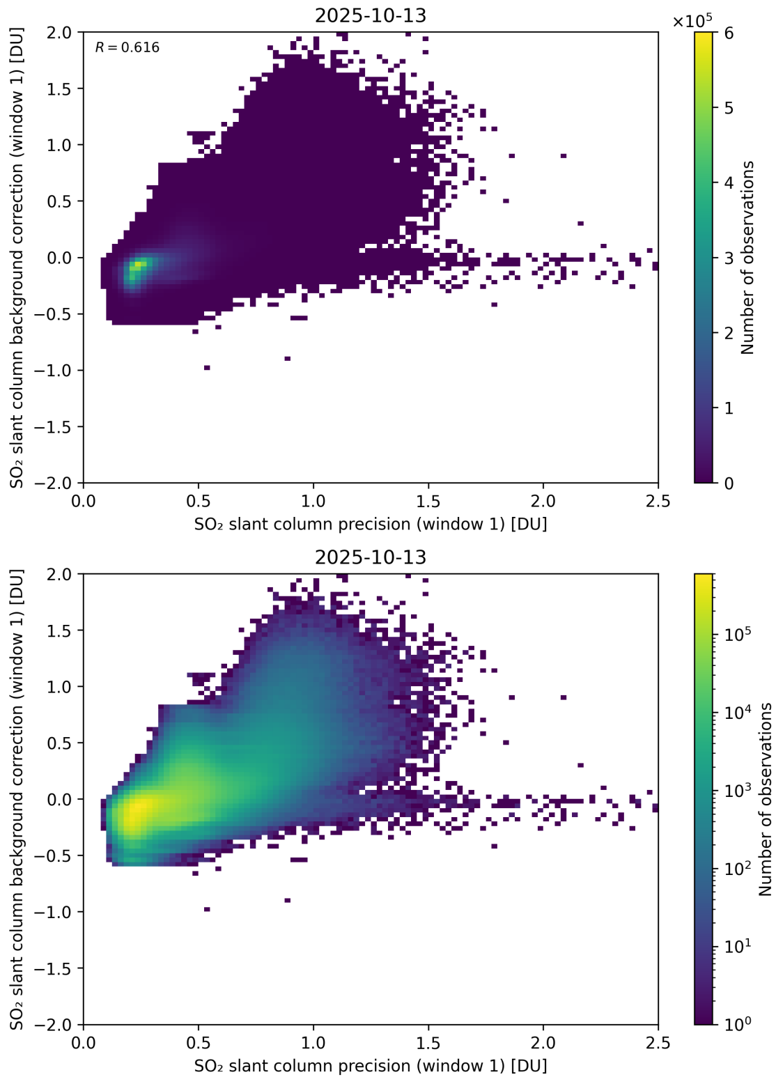
Figure 268: Scatter density plot of “SO 2 slant column precision (window 1)” against “SO 2 slant column background correction (window 1)” for 2025-10-12 to 2025-10-14.
