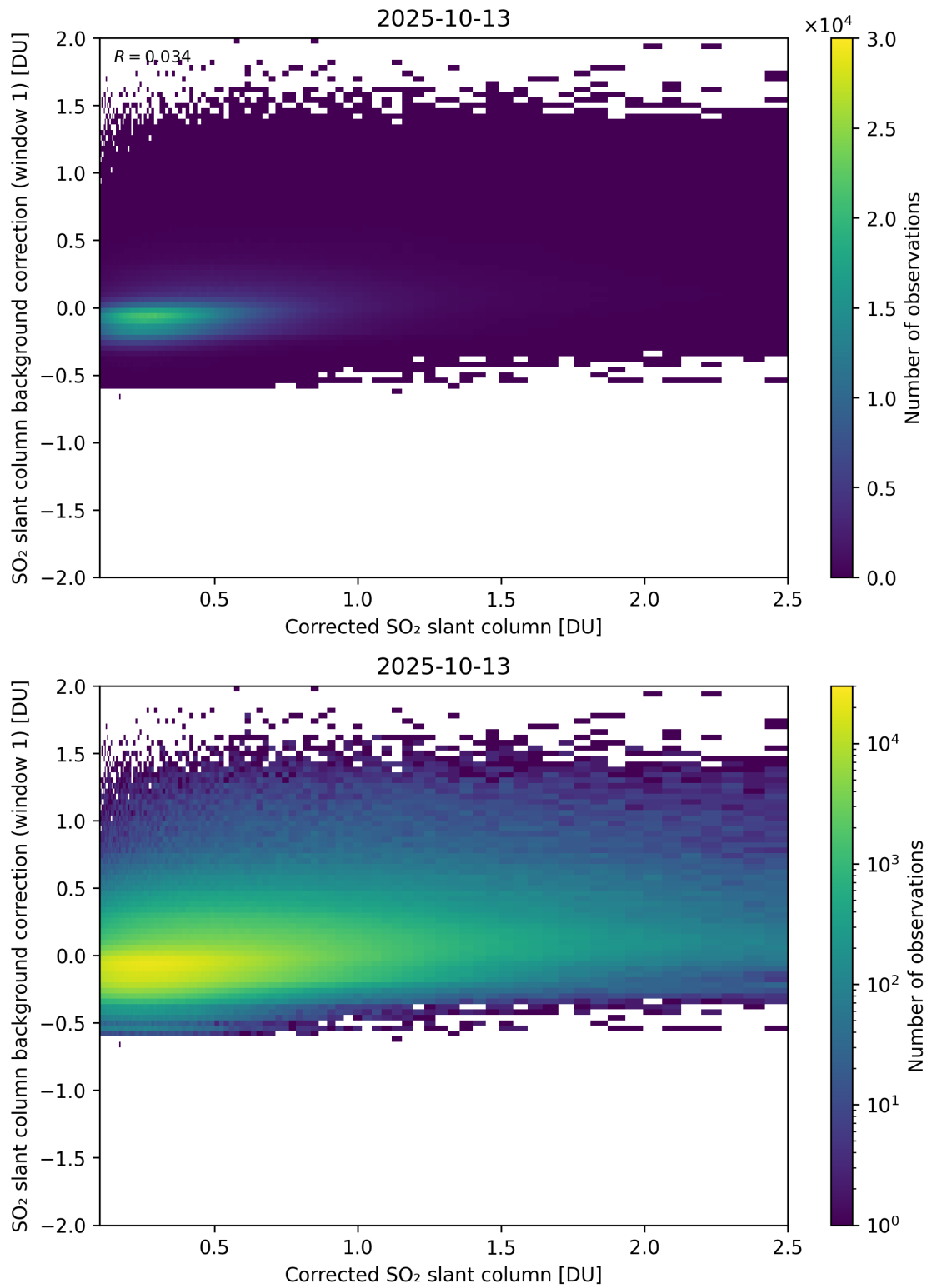
Figure 226: Scatter density plot of “Corrected SO 2 slant column” against “SO 2 slant column background correction (window 1)” for 2025-10-12 to 2025-10-14.
