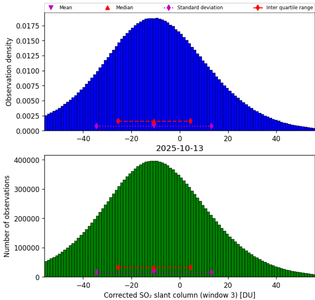
Figure 73: Histogram of “Corrected SO 2 slant column (window 3)” for 2025-10-12 to 2025-10-14
