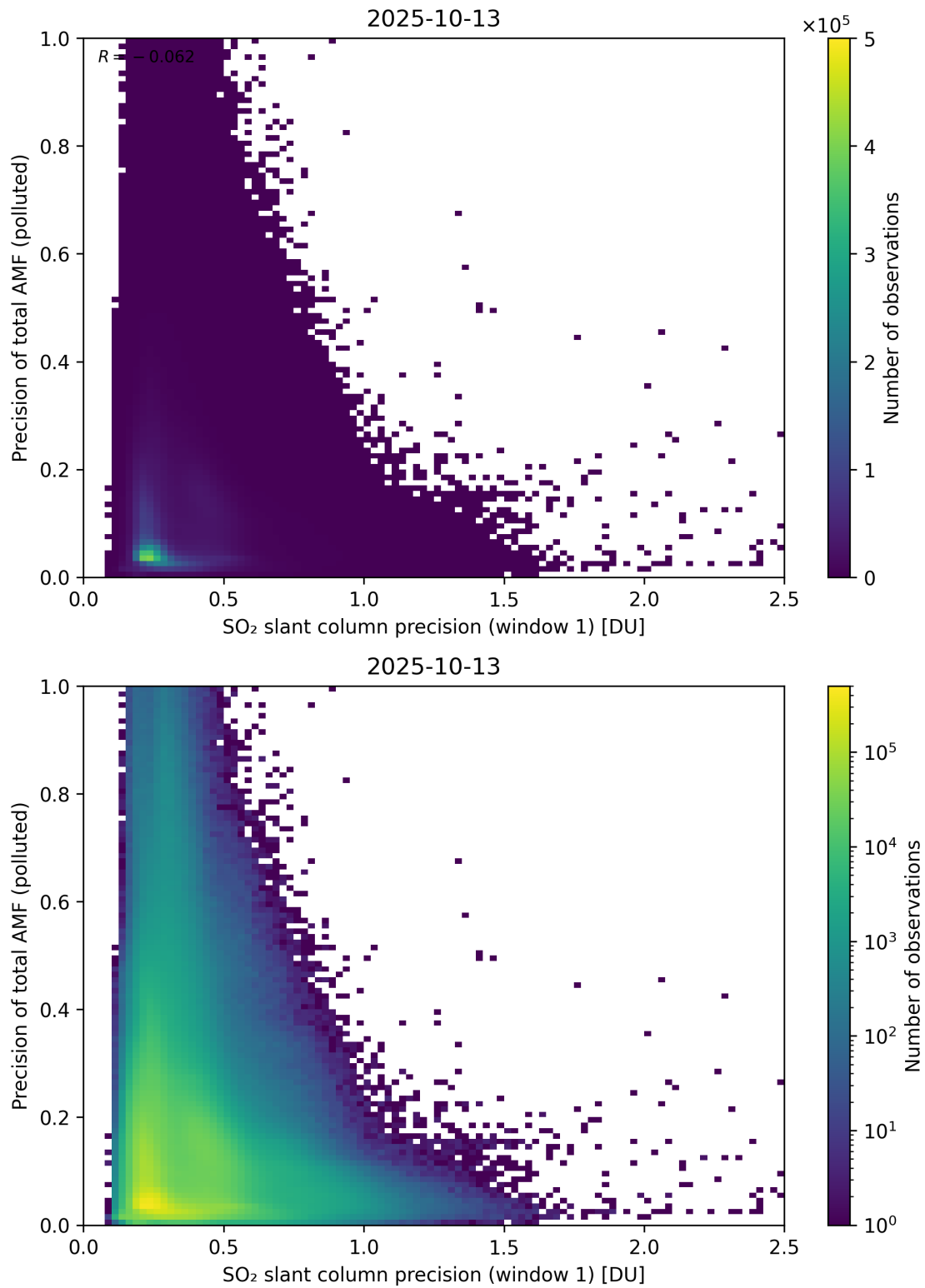
Figure 281: Scatter density plot of “SO 2 slant column precision (window 1)” against “Precision of total AMF (polluted)” for 2025-10-12 to 2025-10-14.
