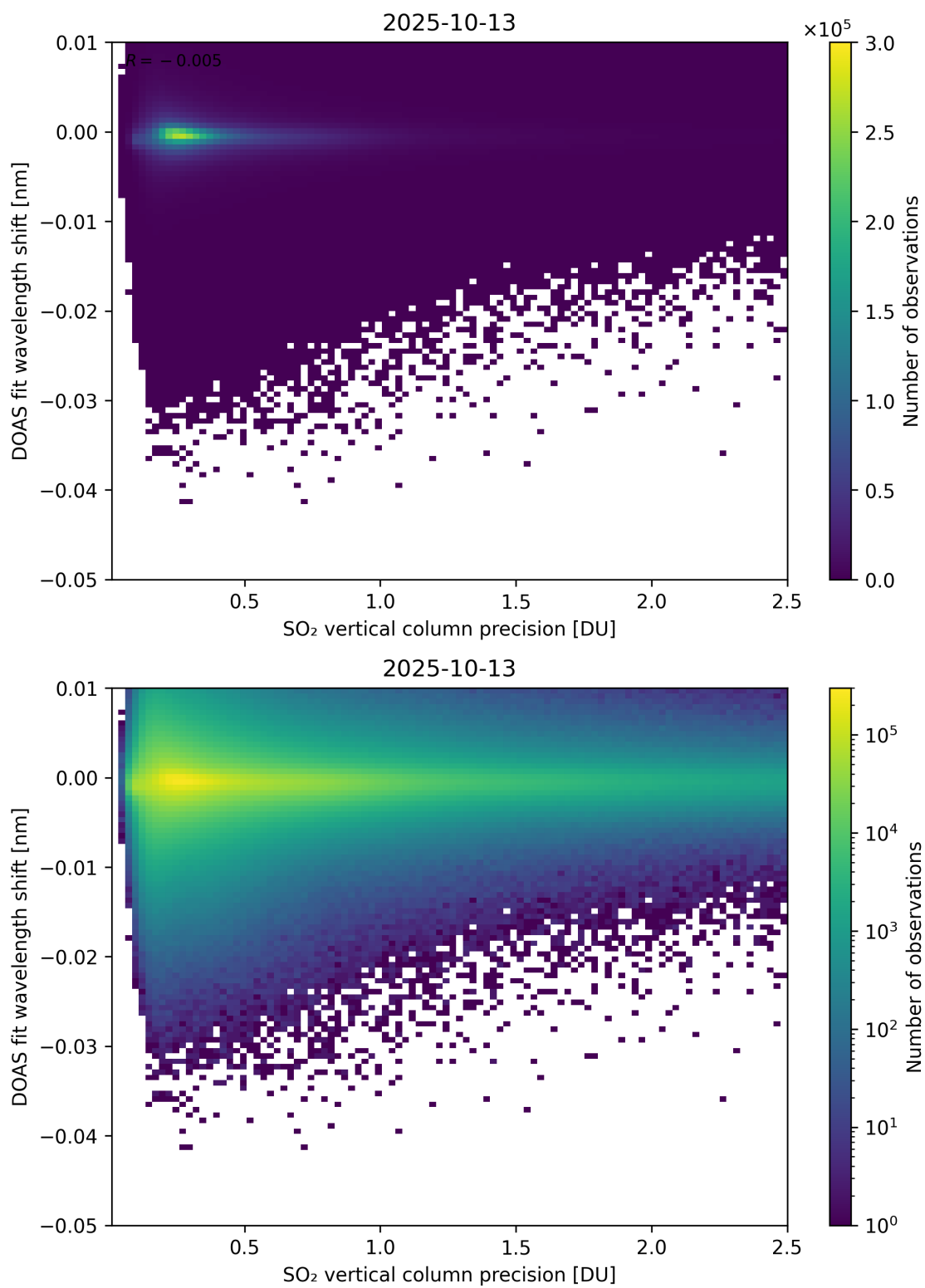
Figure 332: Scatter density plot of “SO 2 vertical column precision” against “DOAS fit wavelength shift” for 2025-10-12 to 2025-10-14.
