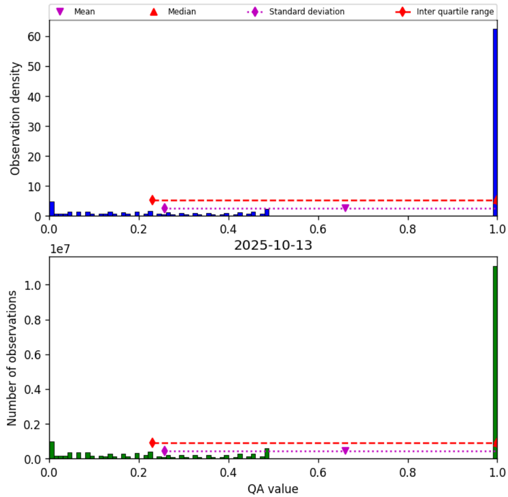
Figure 57: Histogram of “QA value” for 2025-10-12 to 2025-10-14
