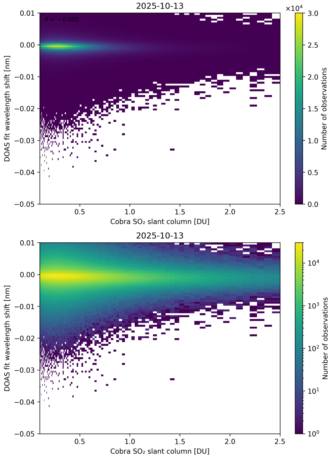
Figure 196: Scatter density plot of “Cobra SO 2 slant column” against “DOAS fit wavelength shift” for 2025-10-12 to 2025-10-14.
