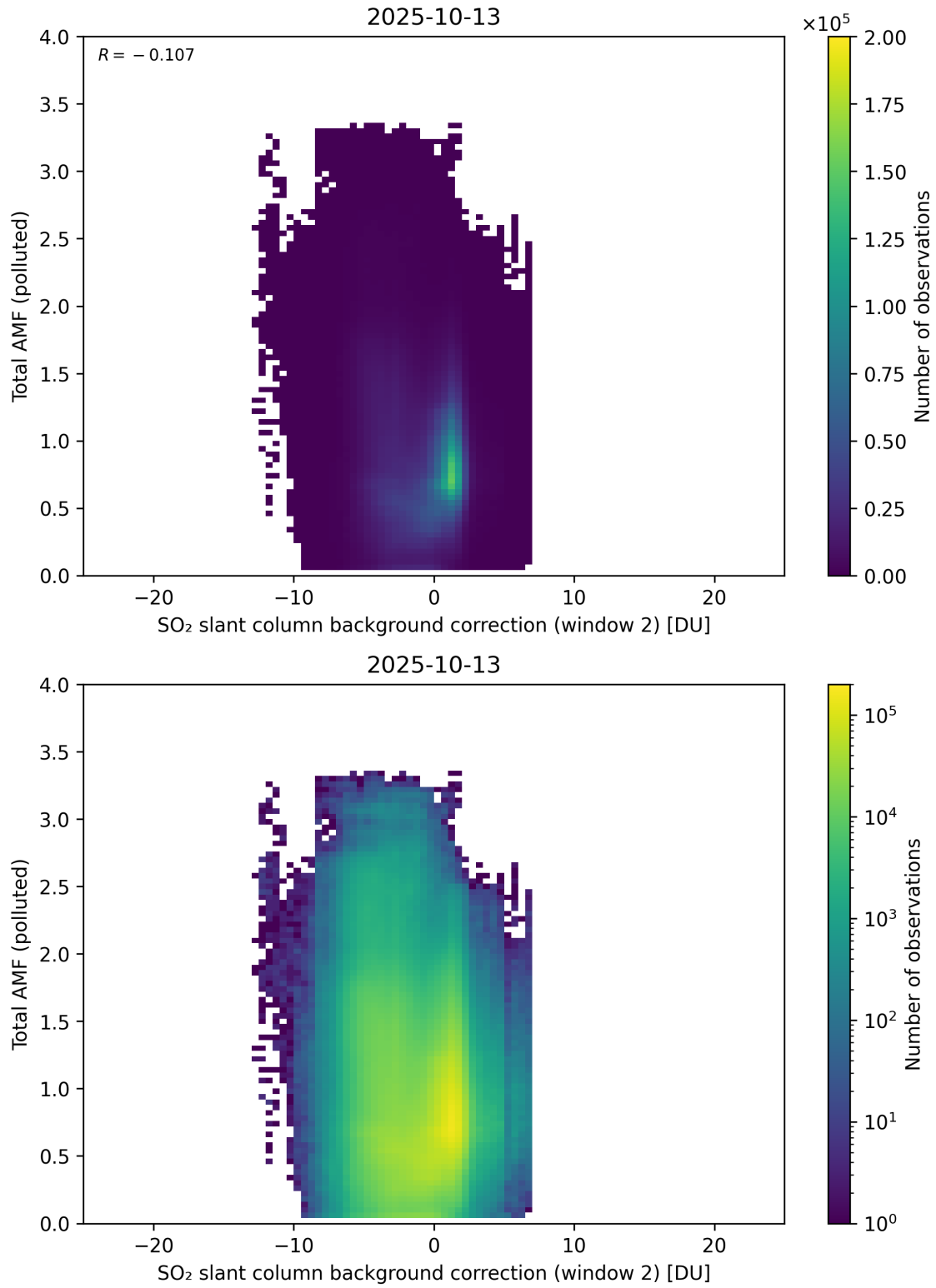
Figure 130: Scatter density plot of “SO 2 slant column background correction (window 2)” against “Total AMF (polluted)” for 2025-10-12 to 2025-10-14.
