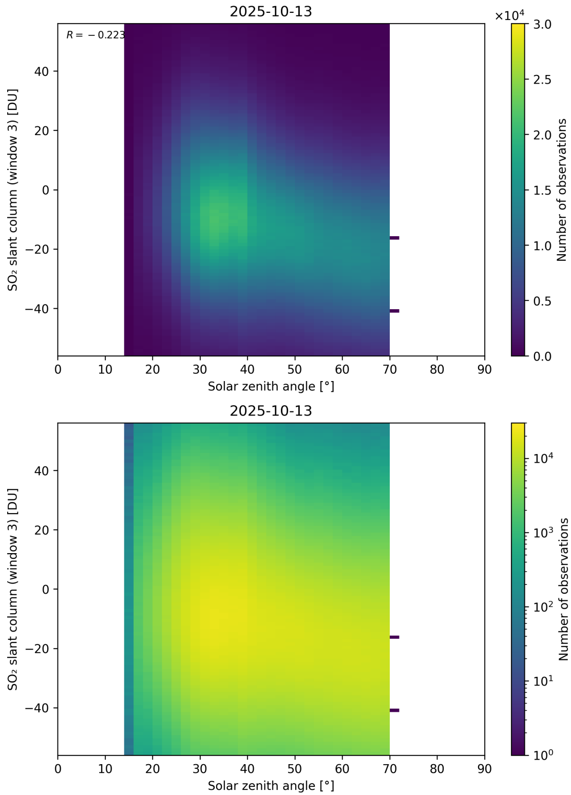
Figure 187: Scatter density plot of “Solar zenith angle” against “SO 2 slant column (window 3)” for 2025-10-12 to 2025-10-14.
