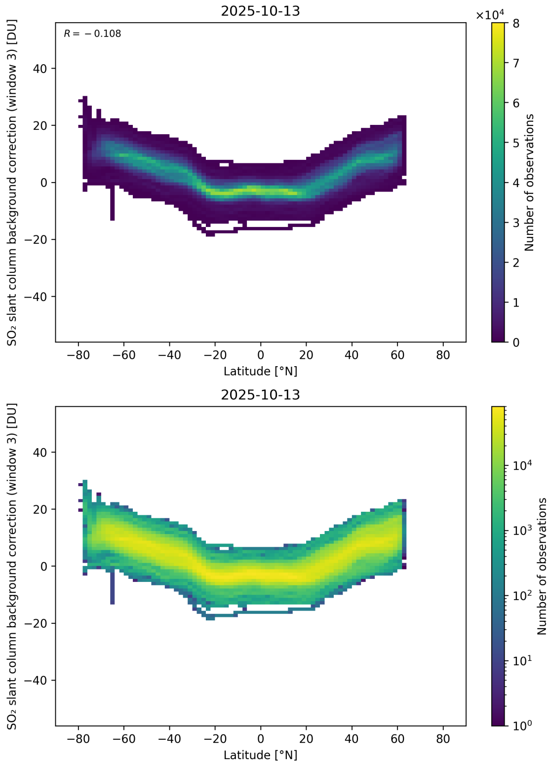
Figure 152: Scatter density plot of “Latitude” against “SO 2 slant column background correction (window 3)” for 2025-10-12 to 2025-10-14.
