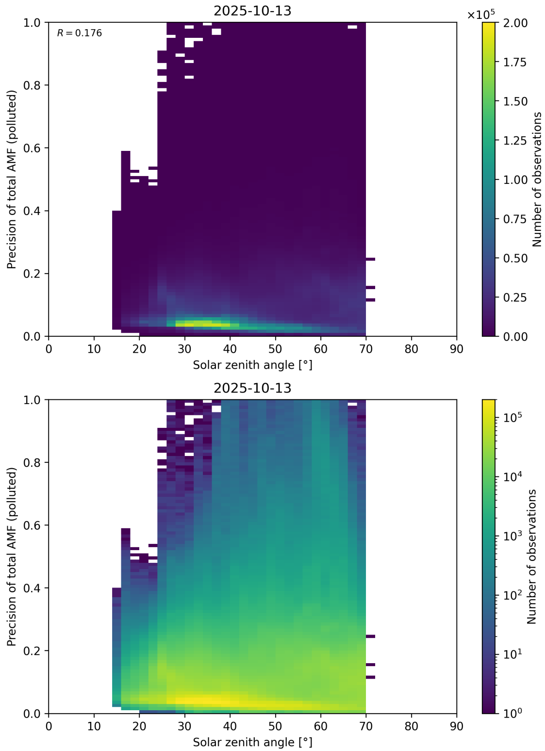
Figure 190: Scatter density plot of “Solar zenith angle” against “Precision of total AMF (polluted)” for 2025-10-12 to 2025-10-14.
