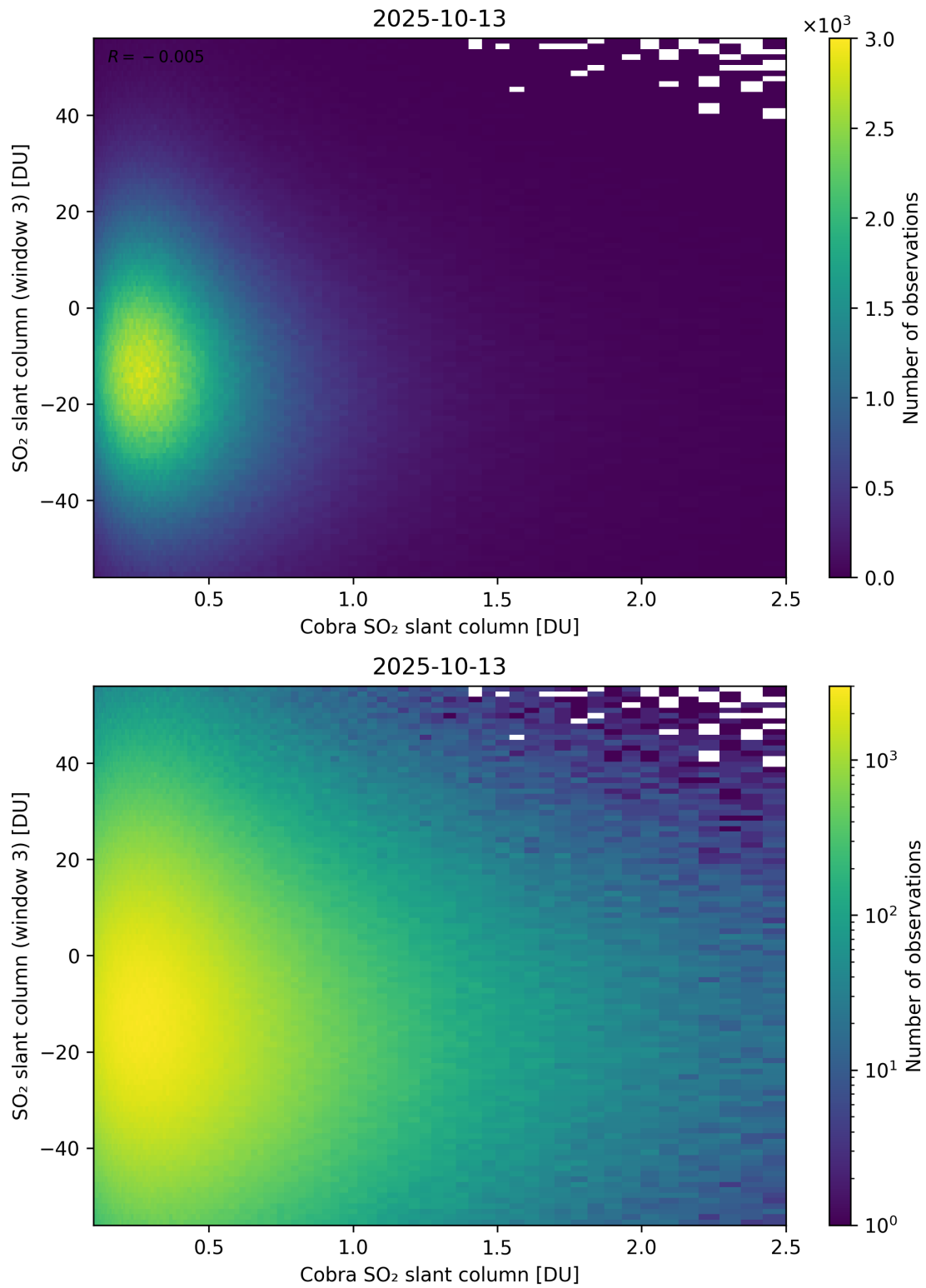
Figure 222: Scatter density plot of “Cobra SO 2 slant column” against “SO 2 slant column (window 3)” for 2025-10-12 to 2025-10-14.
