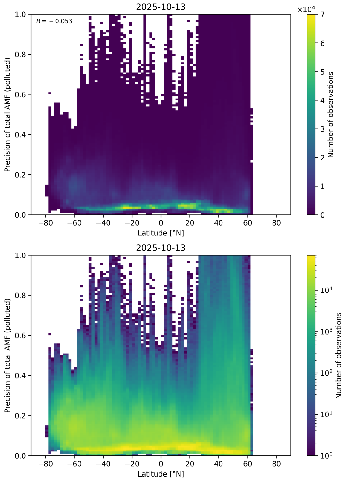
Figure 168: Scatter density plot of “Latitude” against “Precision of total AMF (polluted)” for 2025-10-12 to 2025-10-14.
