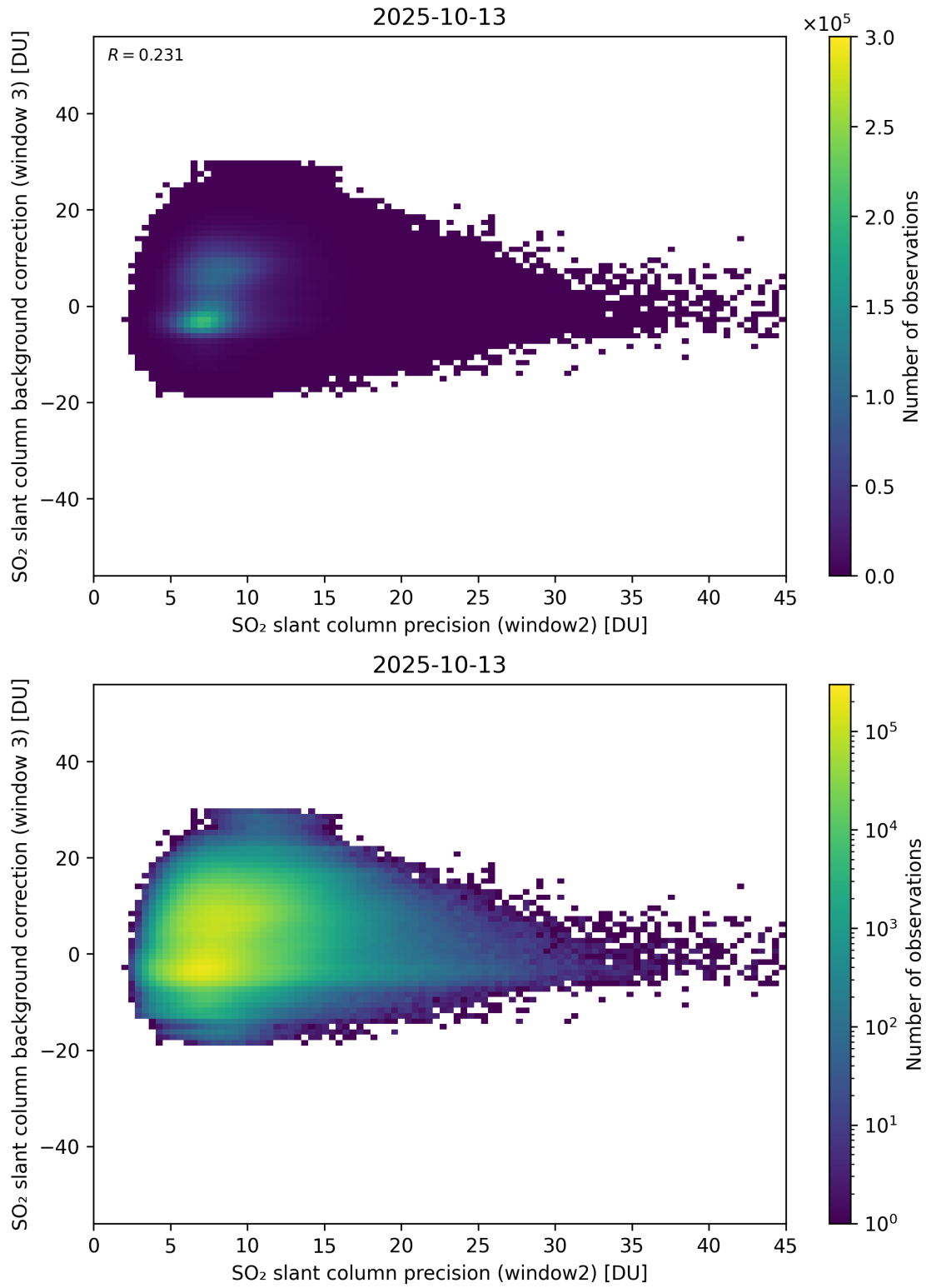
Figure 292: Scatter density plot of “SO 2 slant column precision (window2)” against “SO 2 slant column background correction (window 3)” for 2025-10-12 to 2025-10-14.
