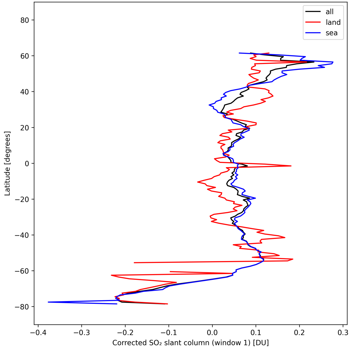
Figure 39: Zonal average of “Corrected SO 2 slant column (window 1)” for 2025-10-14 to 2025-10-16.
