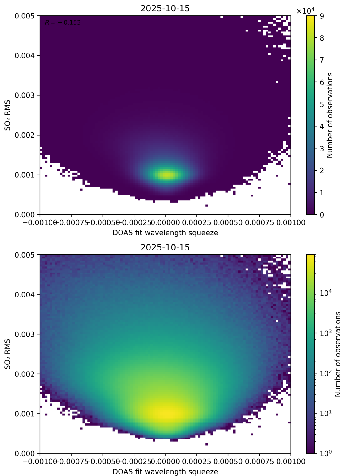
Figure 143: Scatter density plot of “DOAS fit wavelength squeeze” against “SO 2 RMS” for 2025-10-14 to 2025-10-16.
