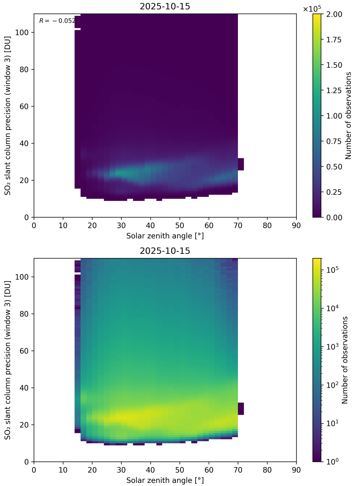
Figure 188: Scatter density plot of “Solar zenith angle” against “SO 2 slant column precision (window 3)” for 2025-10-14 to 2025-10-16.
