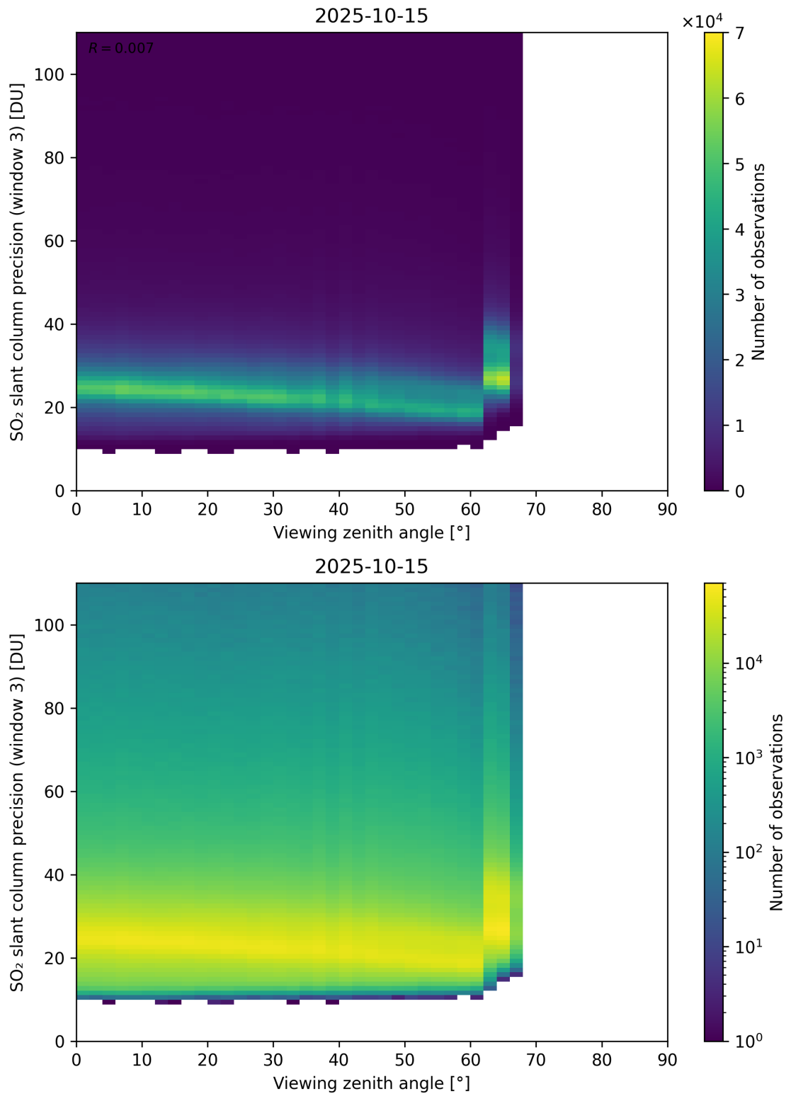
Figure 380: Scatter density plot of “Viewing zenith angle” against “SO 2 slant column precision (window 3)” for 2025-10-14 to 2025-10-16.
