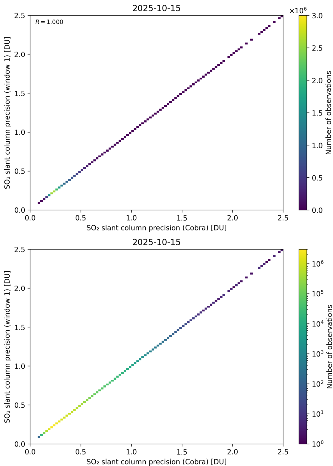
Figure 209: Scatter density plot of “SO 2 slant column precision (Cobra)” against “SO 2 slant column precision (window 1)” for 2025-10-14 to 2025-10-16.
