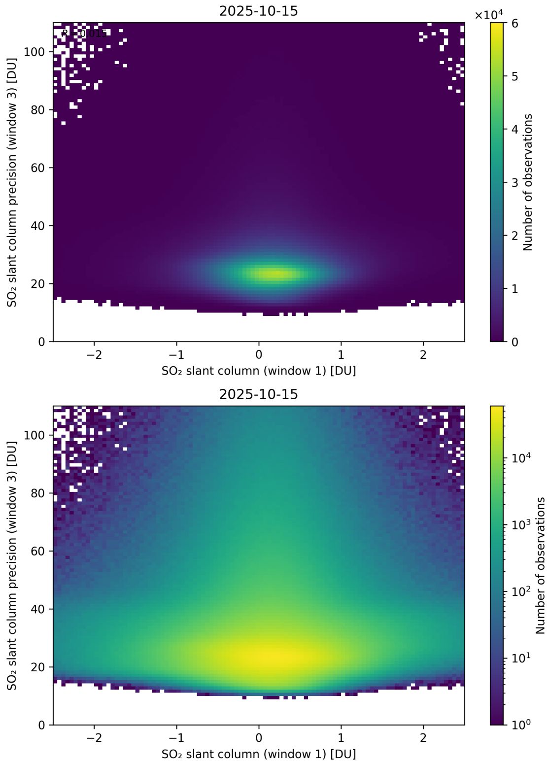
Figure 288: Scatter density plot of “SO 2 slant column (window 1)” against “SO 2 slant column precision (window 3)” for 2025-10-14 to 2025-10-16.
