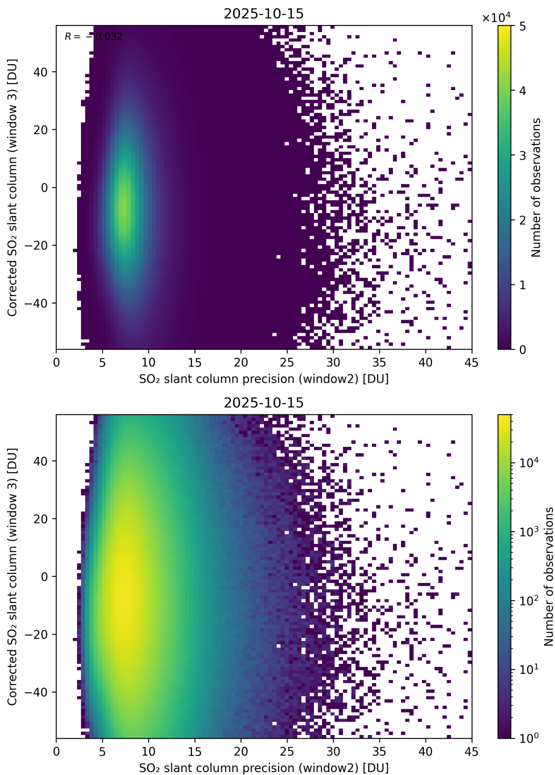
Figure 298: Scatter density plot of “SO 2 slant column precision (window2)” against “Corrected SO 2 slant column (window 3)” for 2025-10-14 to 2025-10-16.
