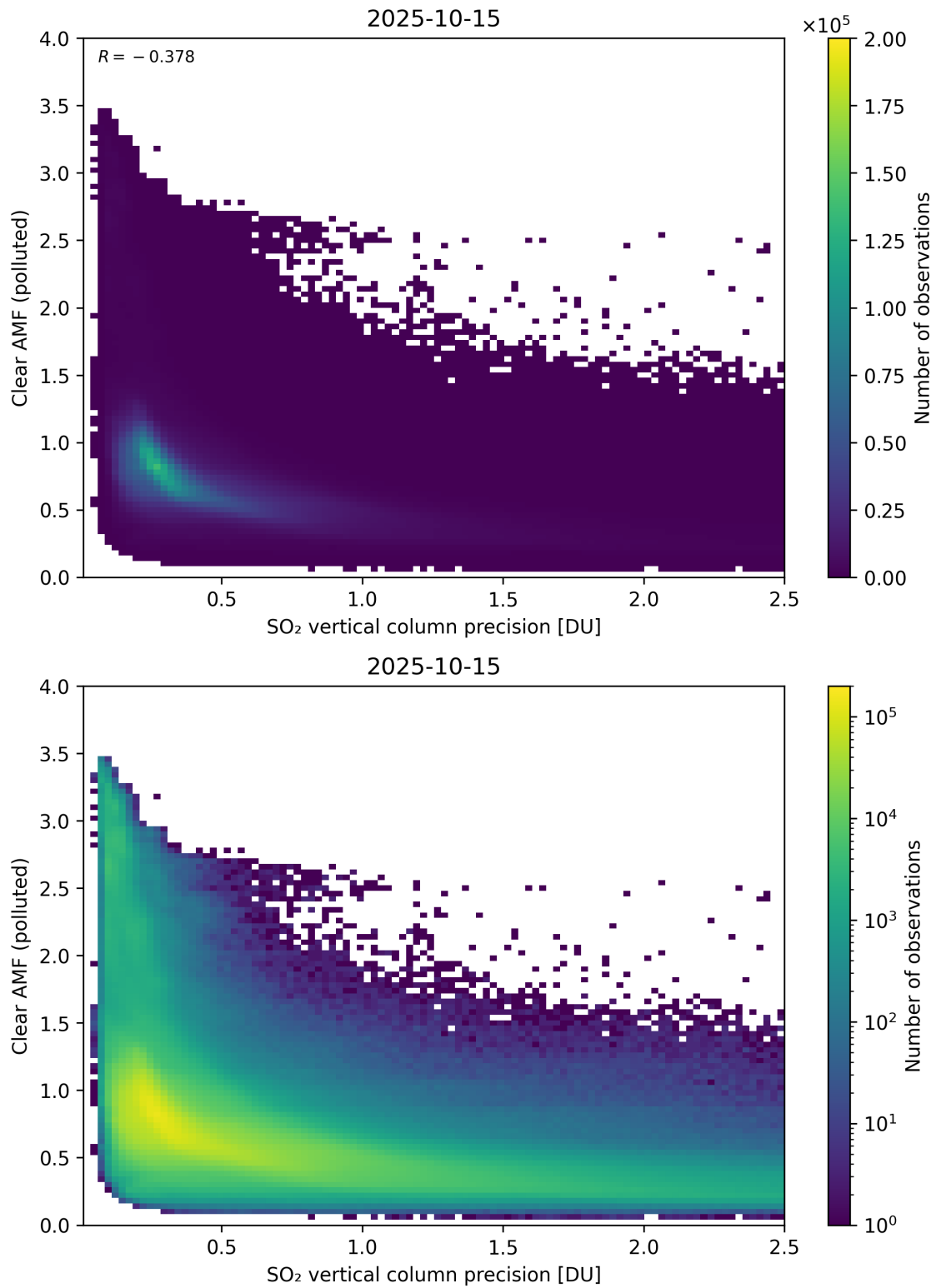
Figure 335: Scatter density plot of “SO 2 vertical column precision” against “Clear AMF (polluted)” for 2025-10-14 to 2025-10-16.
