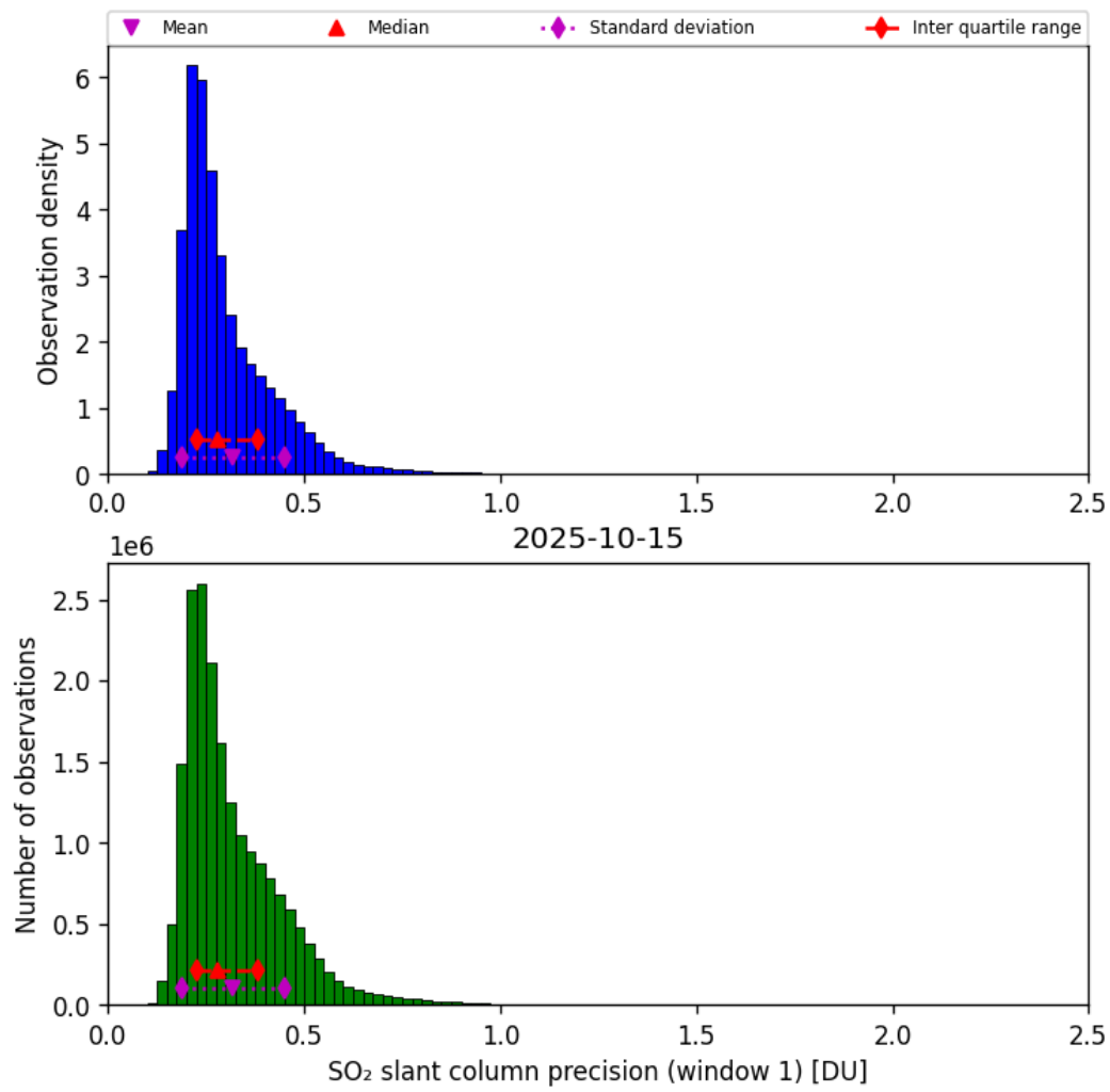
Figure 64: Histogram of “SO 2 slant column precision (window 1)” for 2025-10-14 to 2025-10-16
