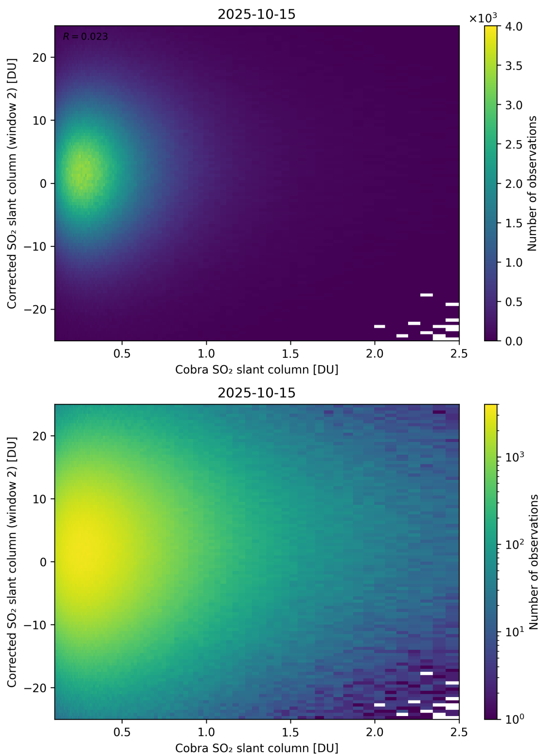
Figure 217: Scatter density plot of “Cobra SO 2 slant column” against “Corrected SO 2 slant column (window 2)” for 2025-10-14 to 2025-10-16.
