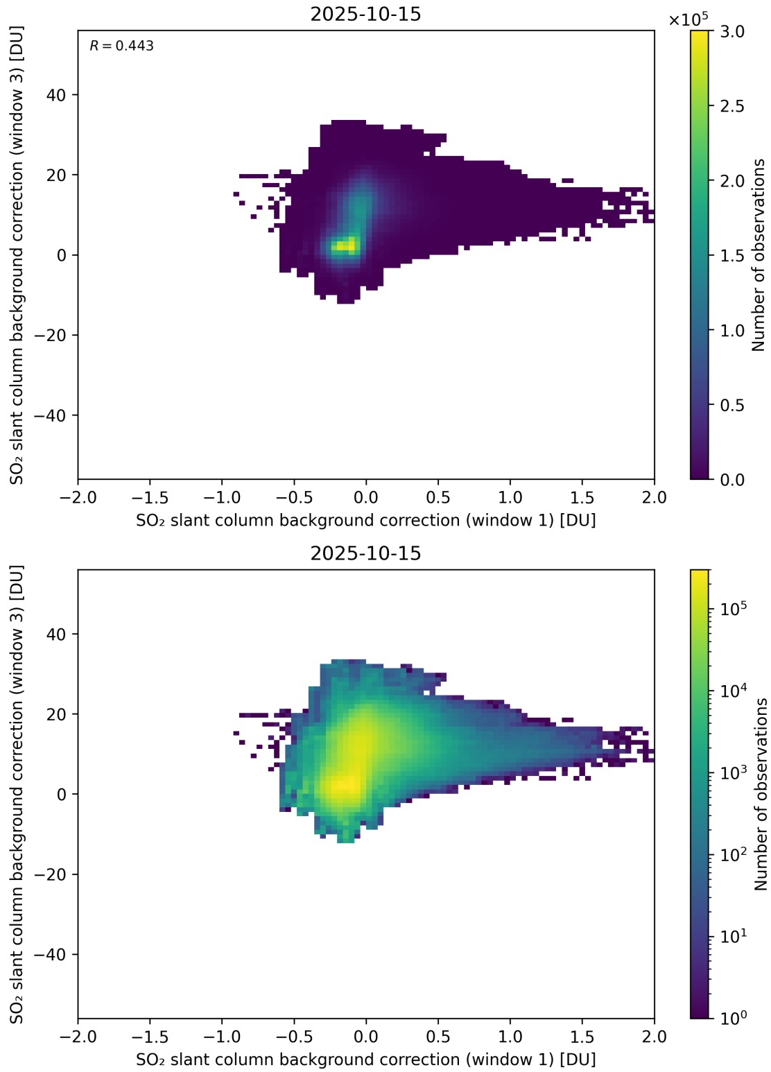
Figure 110: Scatter density plot of “SO 2 slant column background correction (window 1)” against “SO 2 slant column background correction (window 3)” for 2025-10-14 to 2025-10-16.
