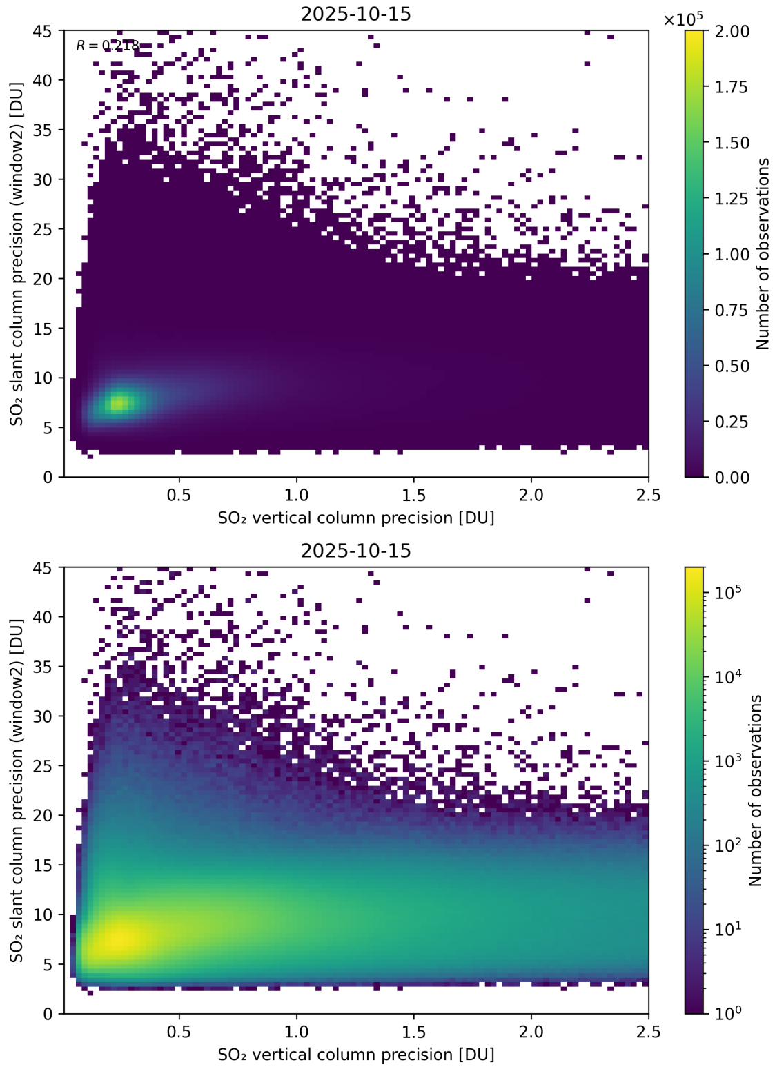
Figure 343: Scatter density plot of “SO 2 vertical column precision” against “SO 2 slant column precision (window2)” for 2025-10-14 to 2025-10-16.
