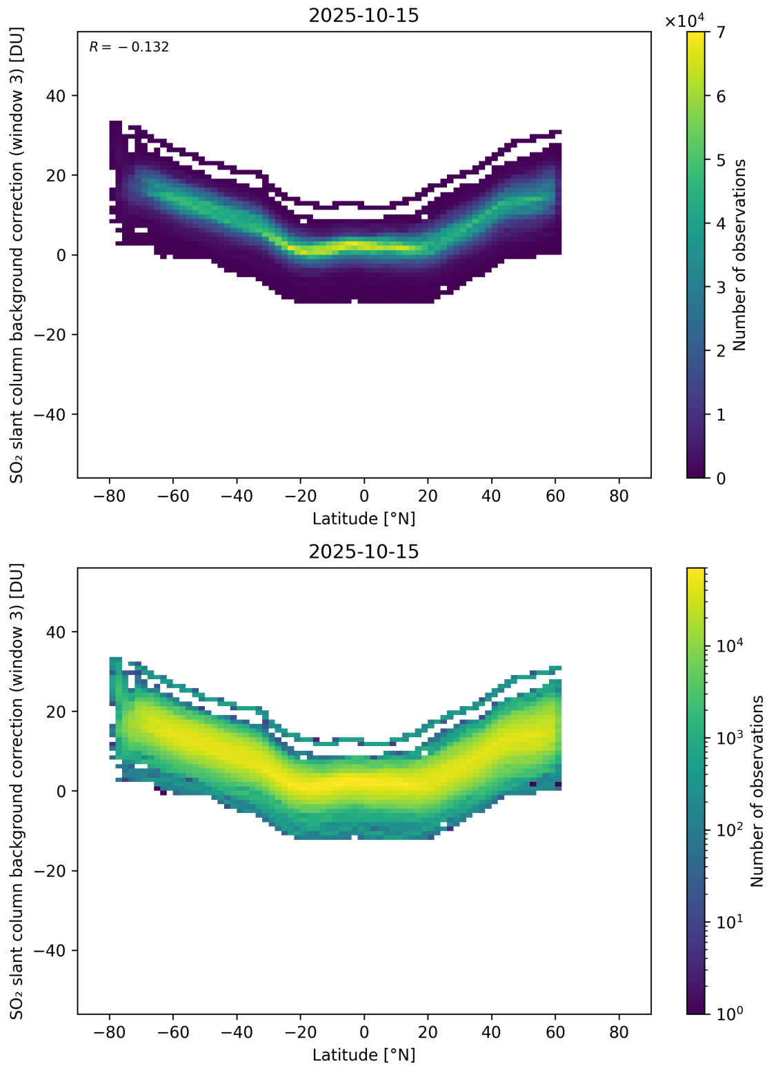
Figure 152: Scatter density plot of “Latitude” against “SO 2 slant column background correction (window 3)” for 2025-10-14 to 2025-10-16.
