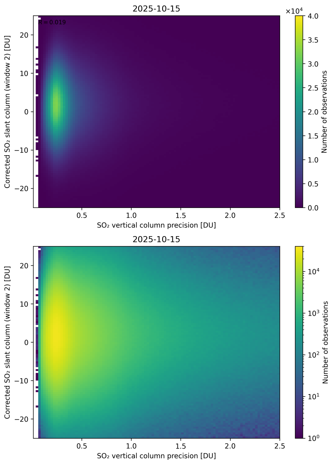
Figure 339: Scatter density plot of “SO 2 vertical column precision” against “Corrected SO 2 slant column (window 2)” for 2025-10-14 to 2025-10-16.
