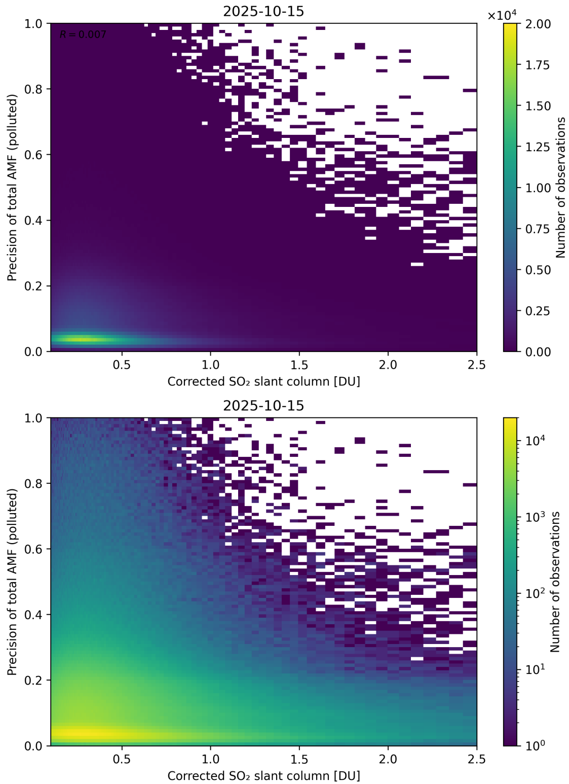
Figure 243: Scatter density plot of “Corrected SO 2 slant column” against “Precision of total AMF (polluted)” for 2025-10-14 to 2025-10-16.
