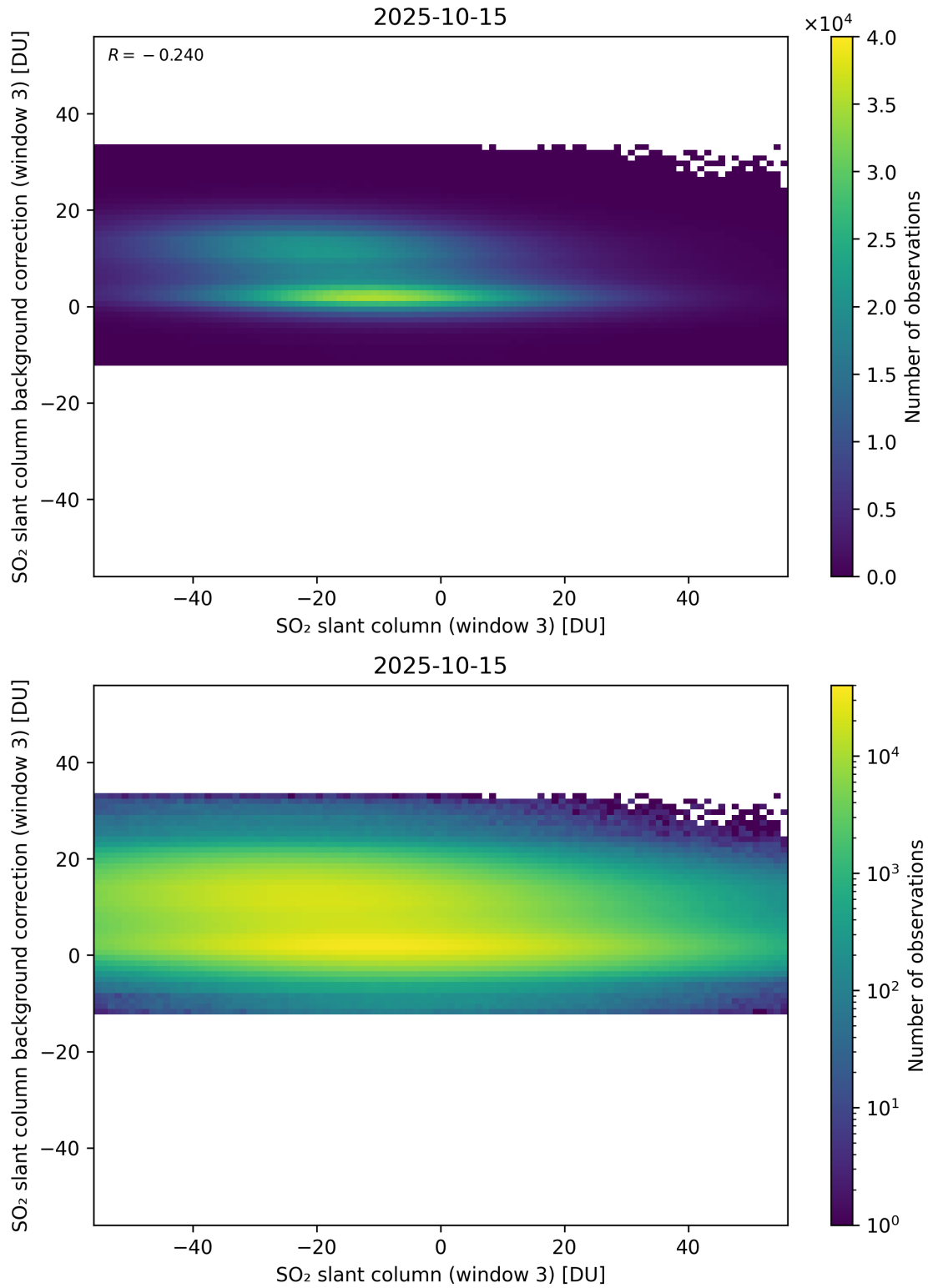
Figure 303: Scatter density plot of “SO 2 slant column (window 3)” against “SO 2 slant column background correction (window 3)” for 2025-10-14 to 2025-10-16.
