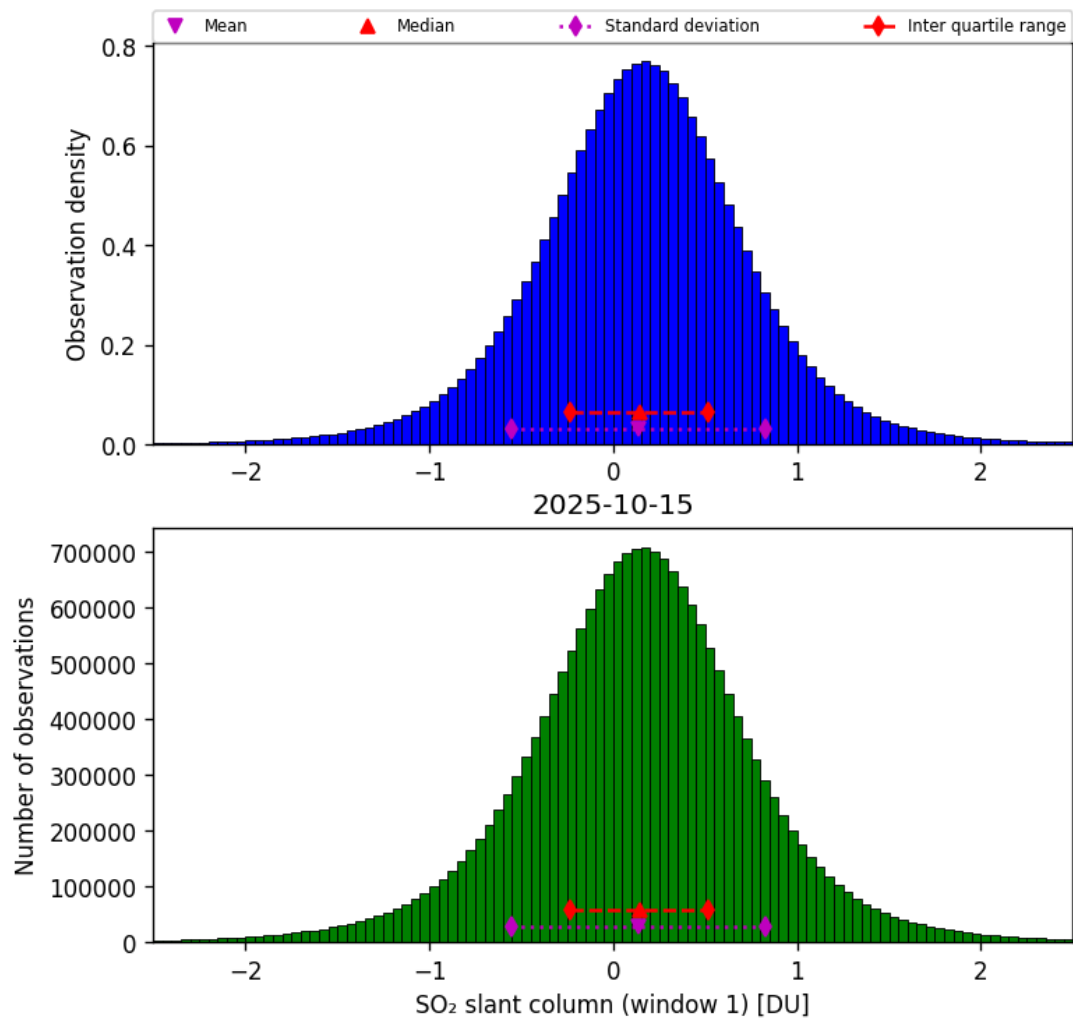
Figure 63: Histogram of “SO 2 slant column (window 1)” for 2025-10-14 to 2025-10-16
