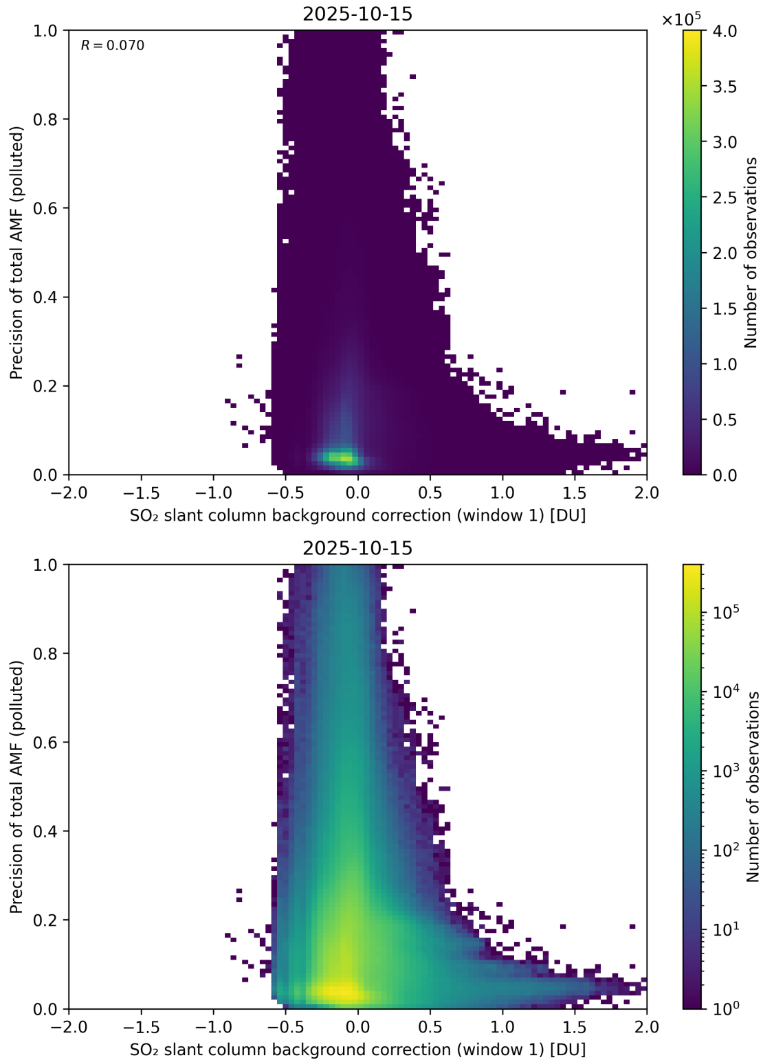
Figure 121: Scatter density plot of “SO 2 slant column background correction (window 1)” against “Precision of total AMF (polluted)” for 2025-10-14 to 2025-10-16.
