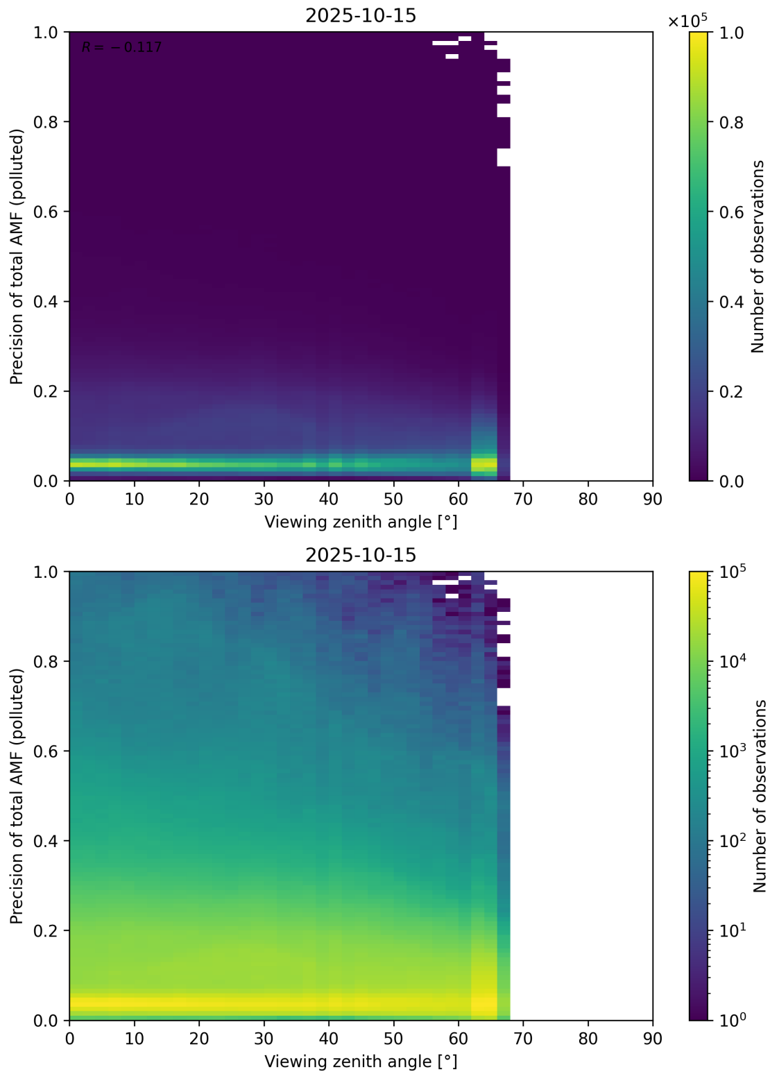
Figure 382: Scatter density plot of “Viewing zenith angle” against “Precision of total AMF (polluted)” for 2025-10-14 to 2025-10-16.
