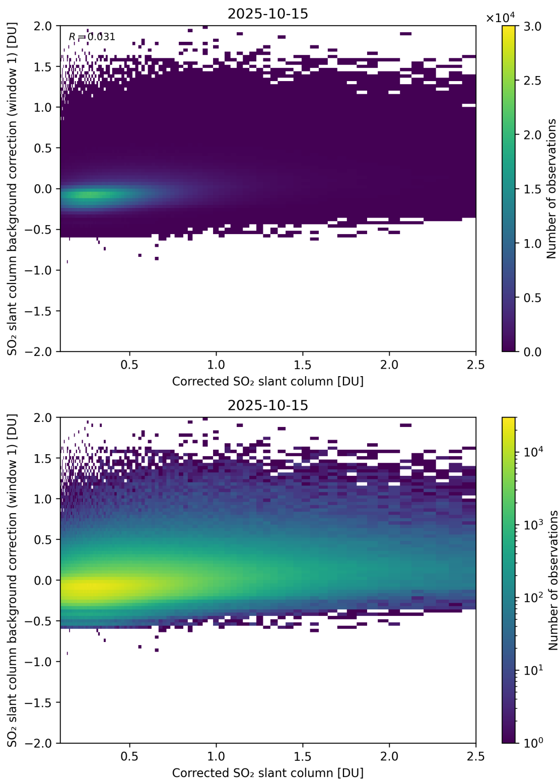
Figure 226: Scatter density plot of “Corrected SO 2 slant column” against “SO 2 slant column background correction (window 1)” for 2025-10-14 to 2025-10-16.
