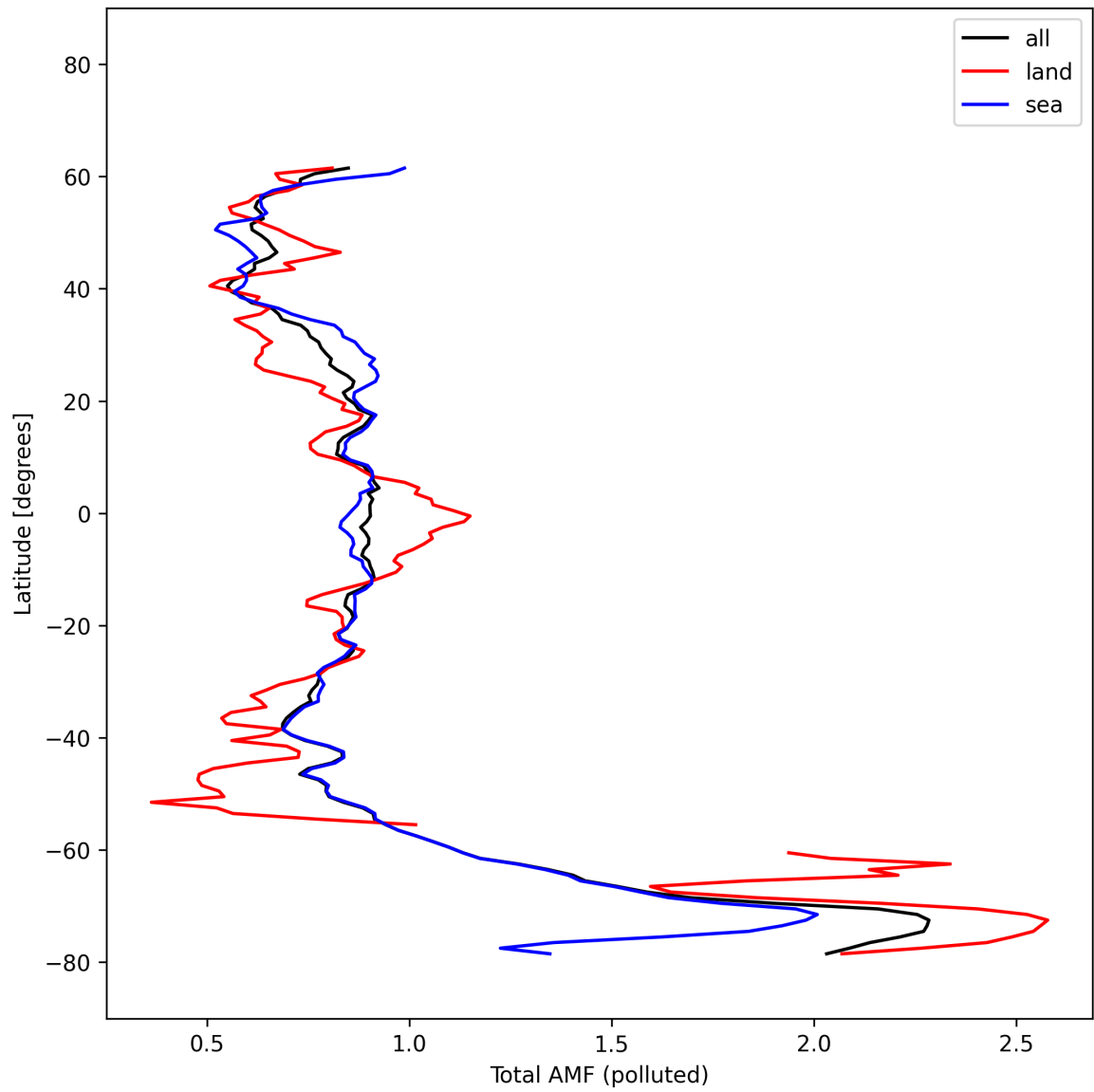
Figure 53: Zonal average of “Total AMF (polluted)” for 2025-10-14 to 2025-10-16.
