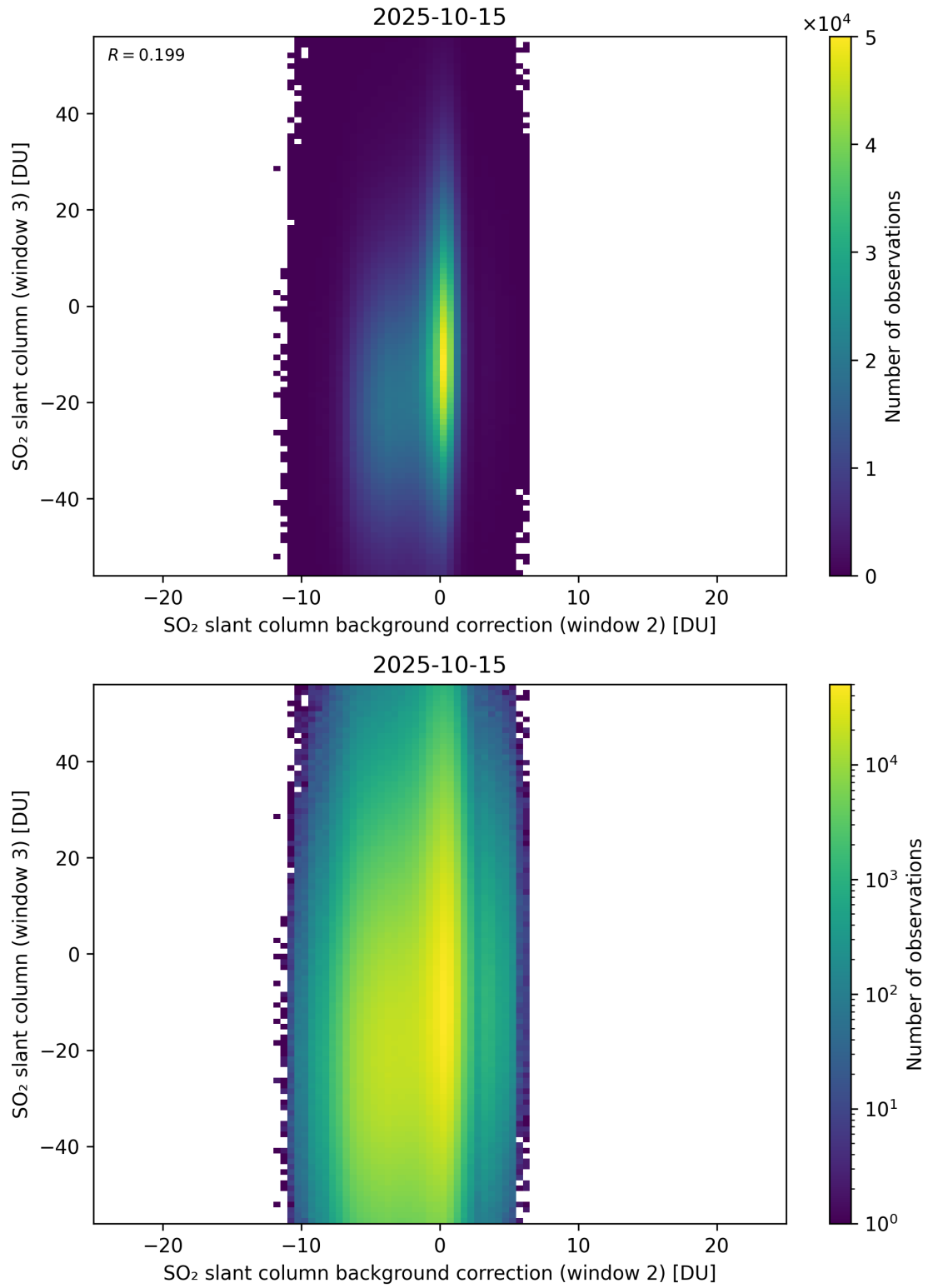
Figure 128: Scatter density plot of “SO 2 slant column background correction (window 2)” against “SO 2 slant column (window 3)” for 2025-10-14 to 2025-10-16.
