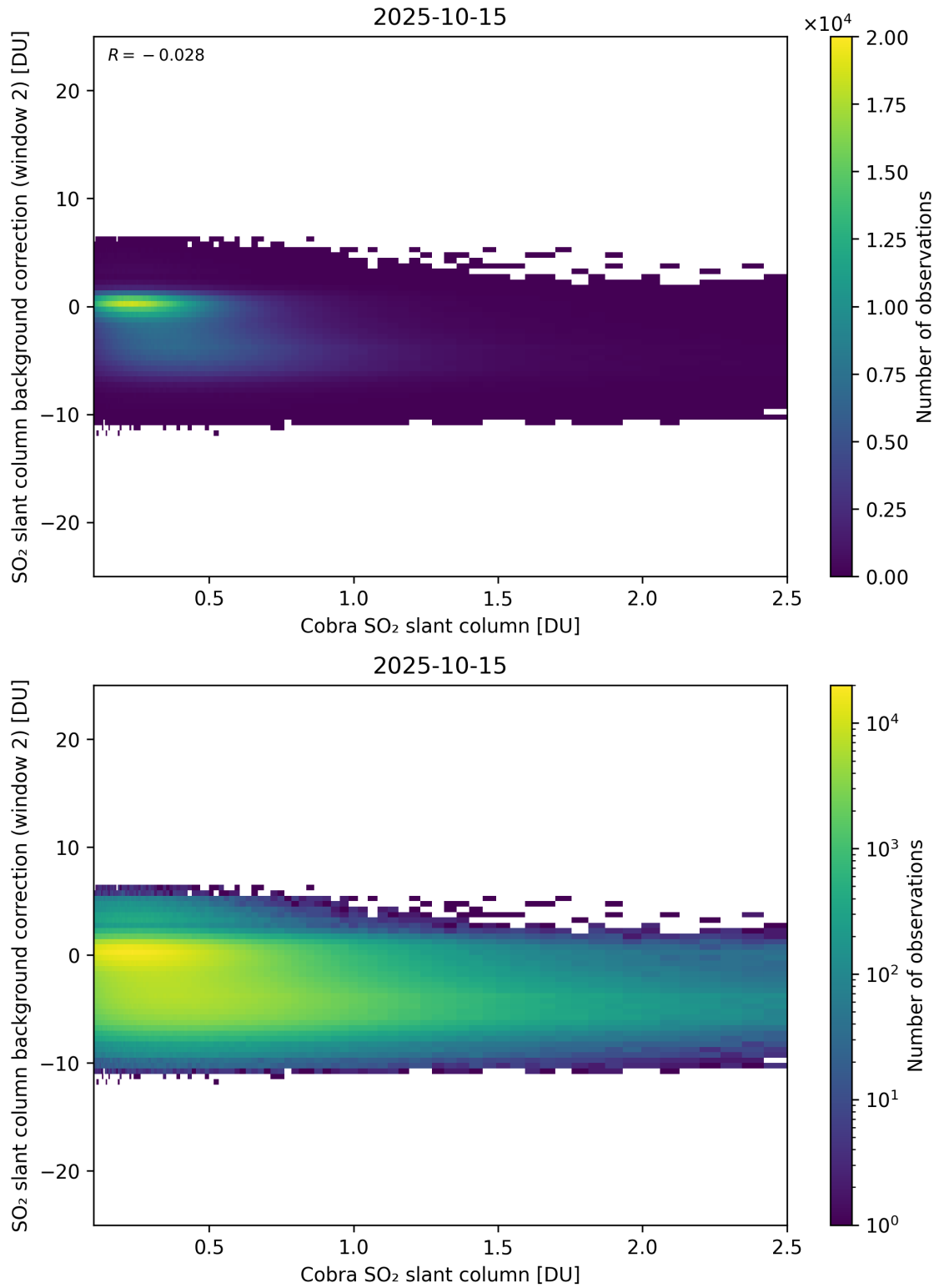
Figure 194: Scatter density plot of “Cobra SO 2 slant column” against “SO 2 slant column background correction (window 2)” for 2025-10-14 to 2025-10-16.
