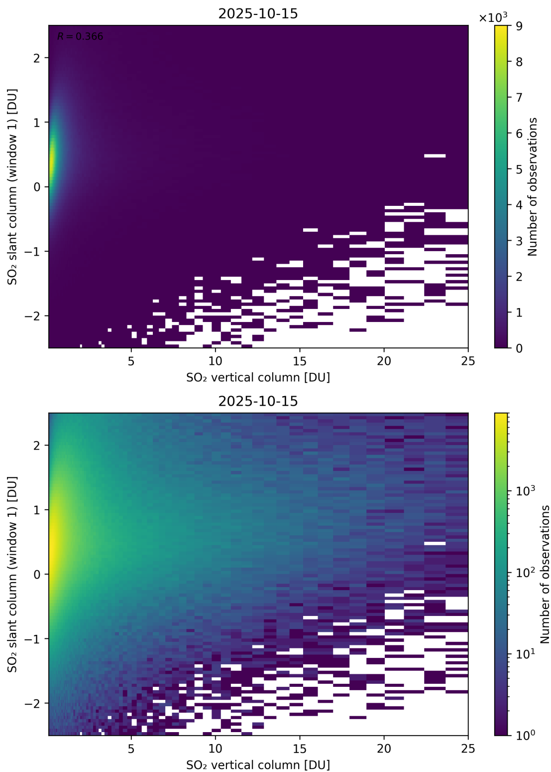
Figure 354: Scatter density plot of “SO 2 vertical column” against “SO 2 slant column (window 1)” for 2025-10-14 to 2025-10-16.
