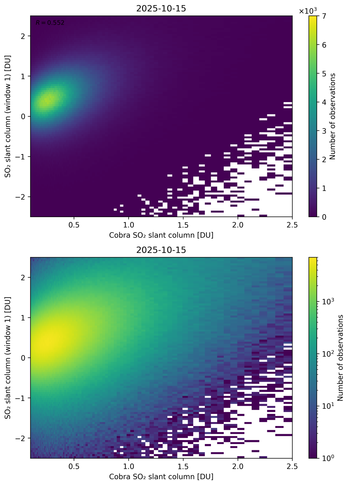
Figure 219: Scatter density plot of “Cobra SO 2 slant column” against “SO 2 slant column (window 1)” for 2025-10-14 to 2025-10-16.
