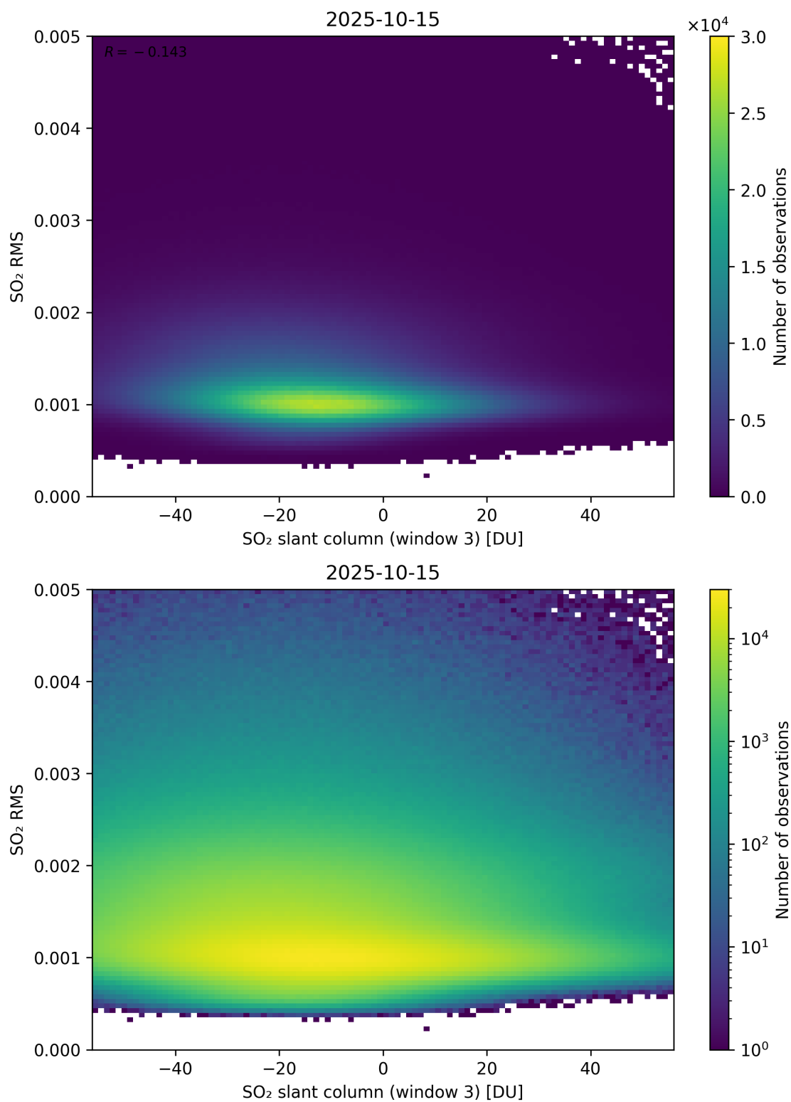
Figure 306: Scatter density plot of “SO 2 slant column (window 3)” against “SO 2 RMS” for 2025-10-14 to 2025-10-16.
