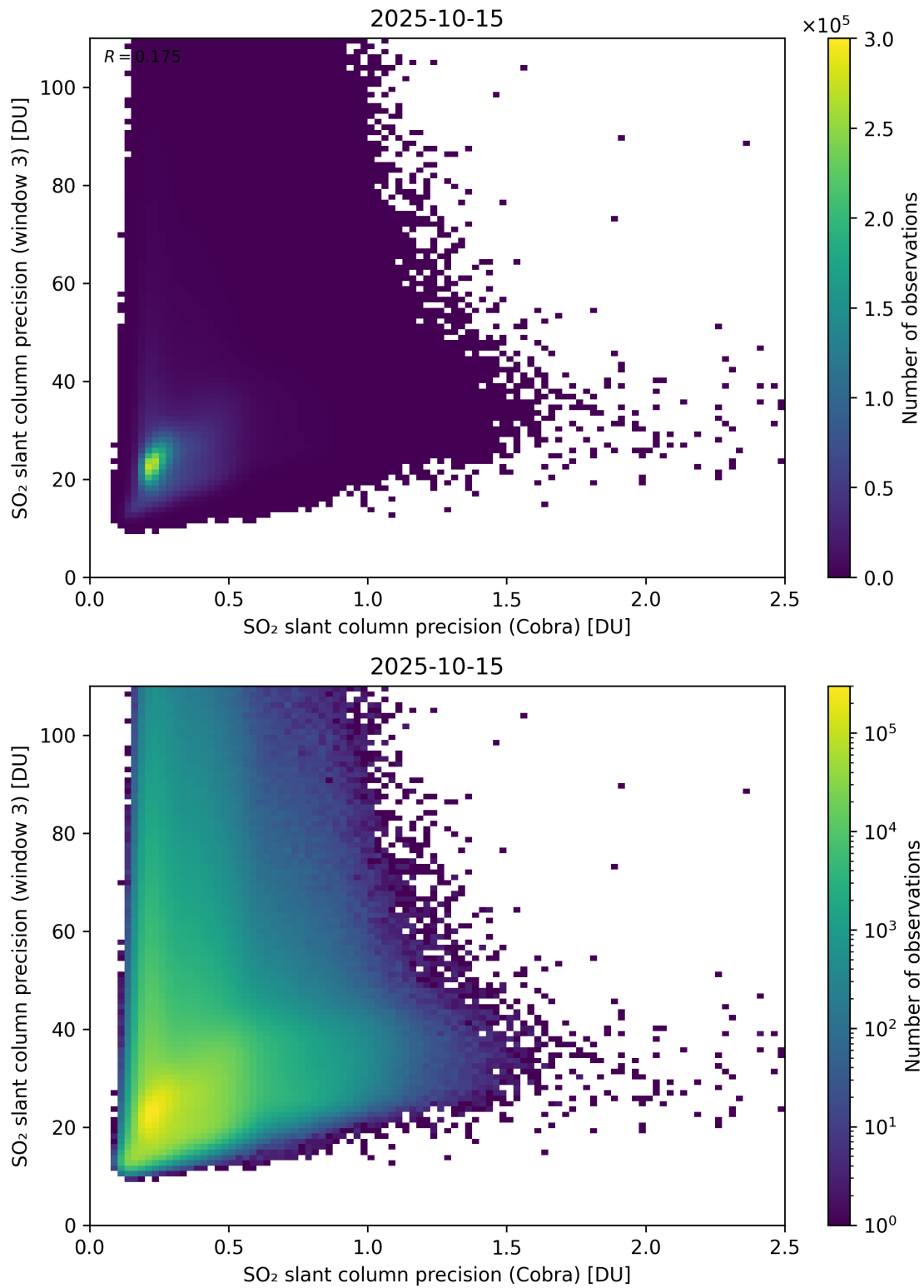
Figure 212: Scatter density plot of “SO 2 slant column precision (Cobra)” against “SO 2 slant column precision (window 3)” for 2025-10-14 to 2025-10-16.
