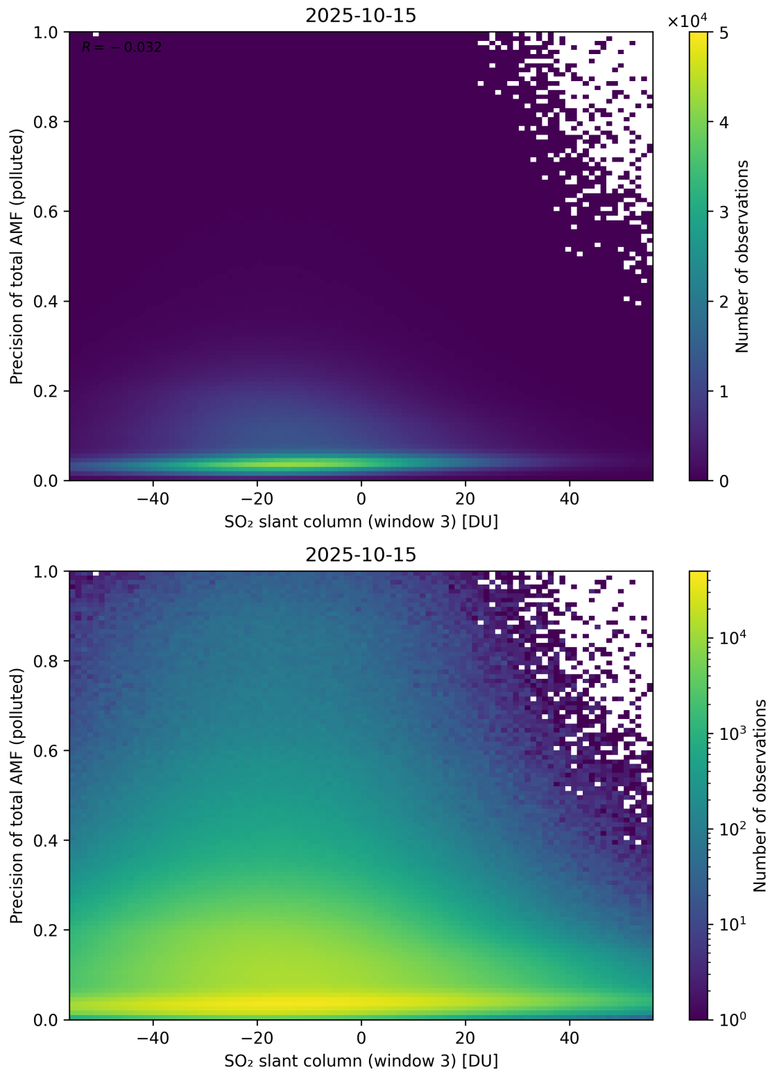
Figure 319: Scatter density plot of “SO 2 slant column (window 3)” against “Precision of total AMF (polluted)” for 2025-10-14 to 2025-10-16.
