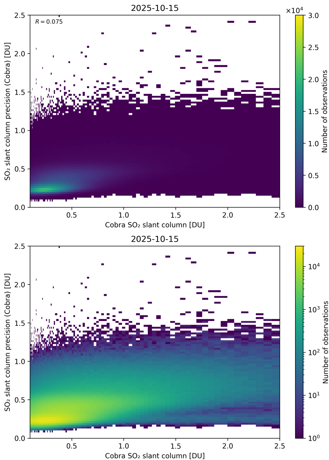
Figure 216: Scatter density plot of “Cobra SO 2 slant column” against “SO 2 slant column precision (Cobra)” for 2025-10-14 to 2025-10-16.
