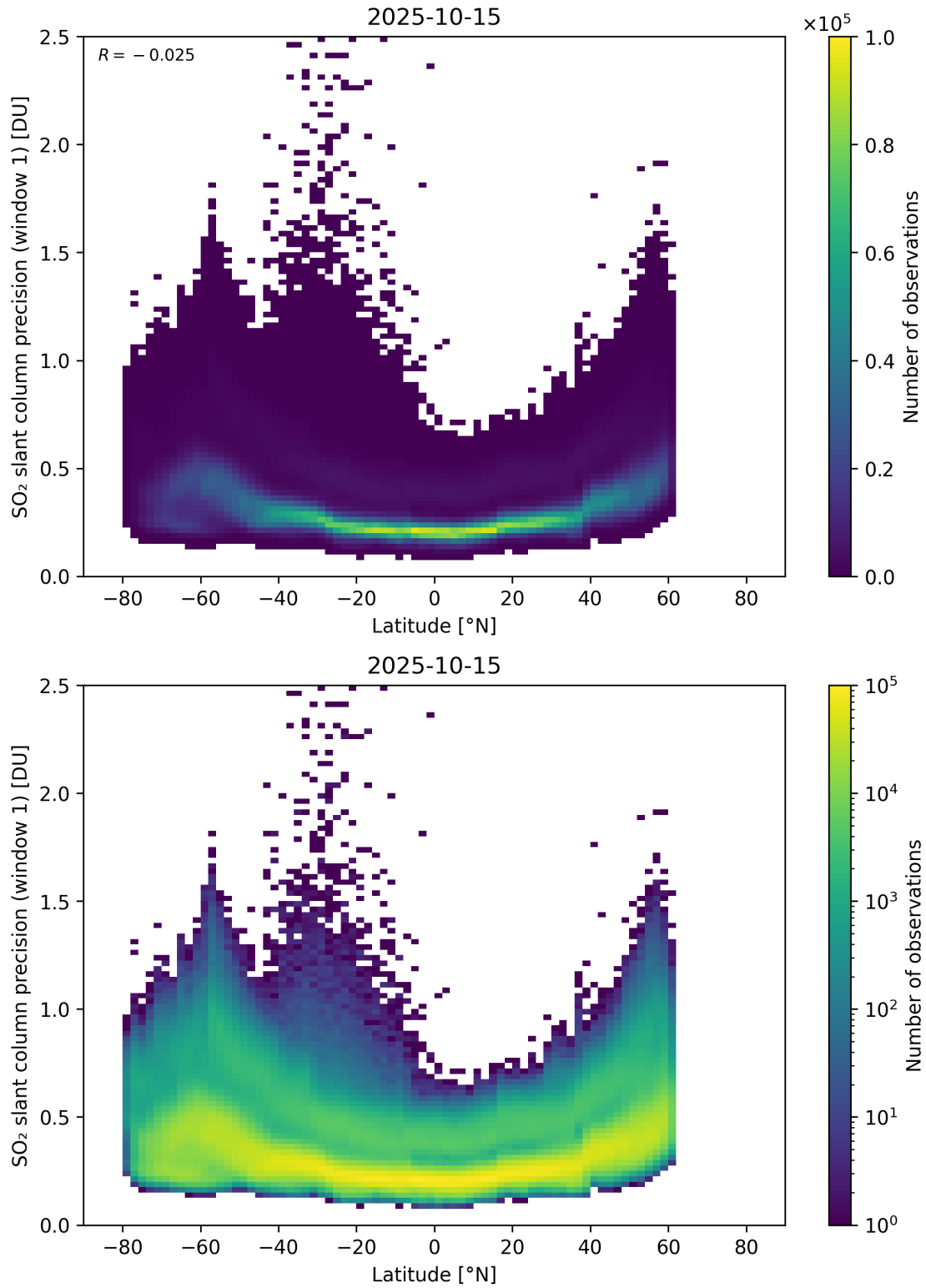
Figure 163: Scatter density plot of “Latitude” against “SO 2 slant column precision (window 1)” for 2025-10-14 to 2025-10-16.
