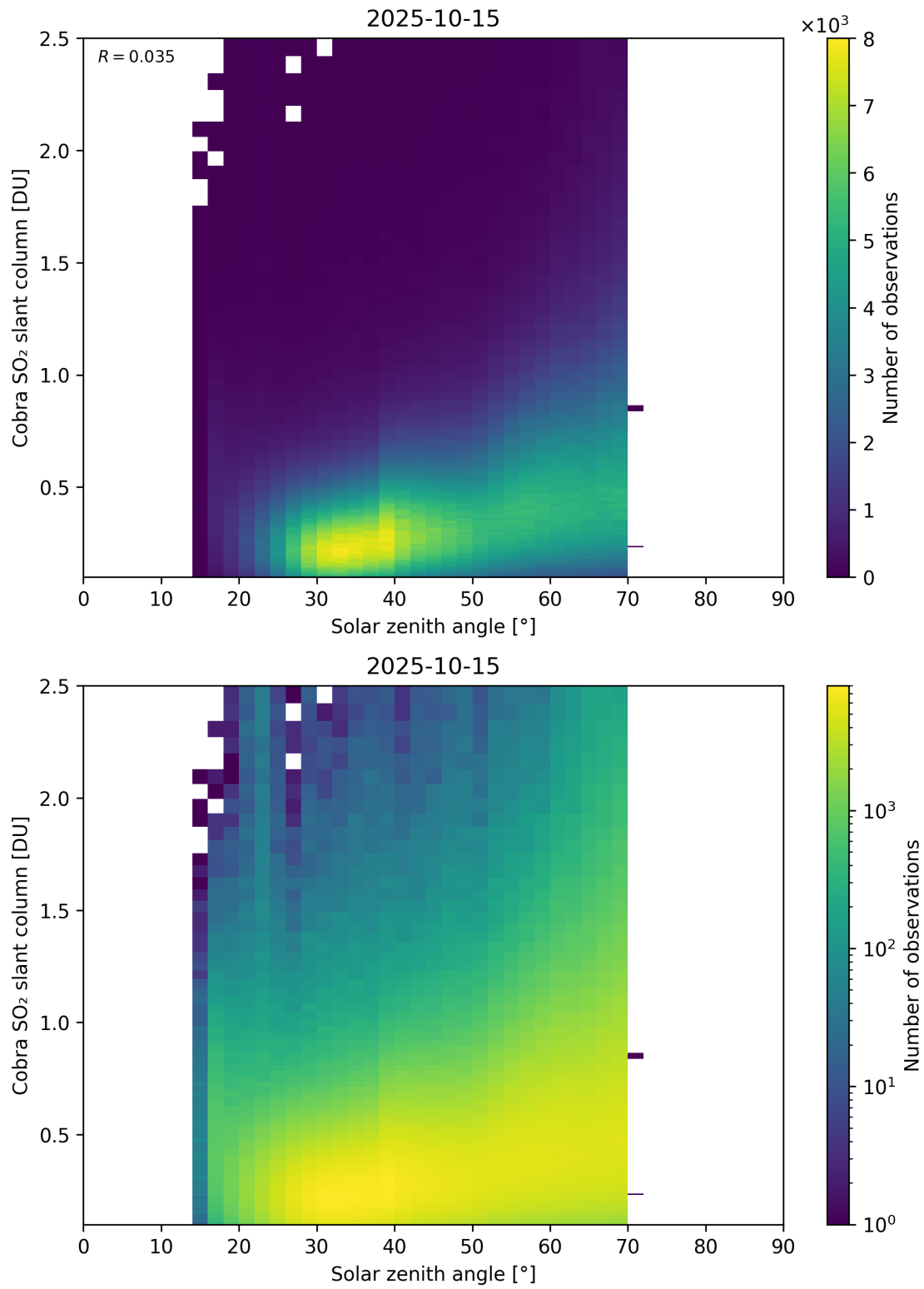
Figure 179: Scatter density plot of “Solar zenith angle” against “Cobra SO 2 slant column” for 2025-10-14 to 2025-10-16.
