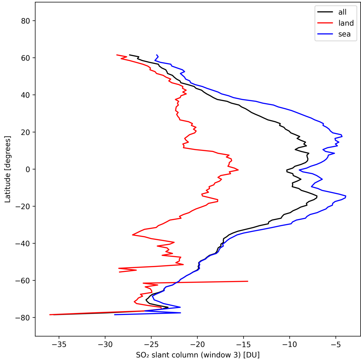
Figure 45: Zonal average of “SO 2 slant column (window 3)” for 2025-10-14 to 2025-10-16.
