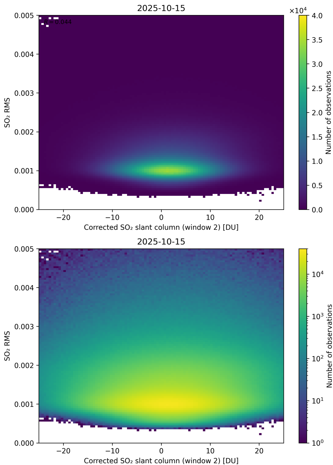
Figure 248: Scatter density plot of “Corrected SO 2 slant column (window 2)” against “SO 2 RMS” for 2025-10-14 to 2025-10-16.
