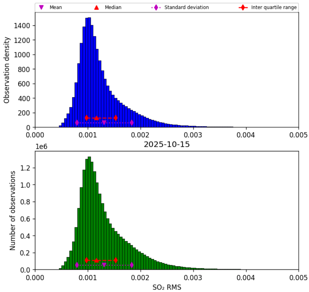
Figure 78: Histogram of “SO 2 RMS” for 2025-10-14 to 2025-10-16
