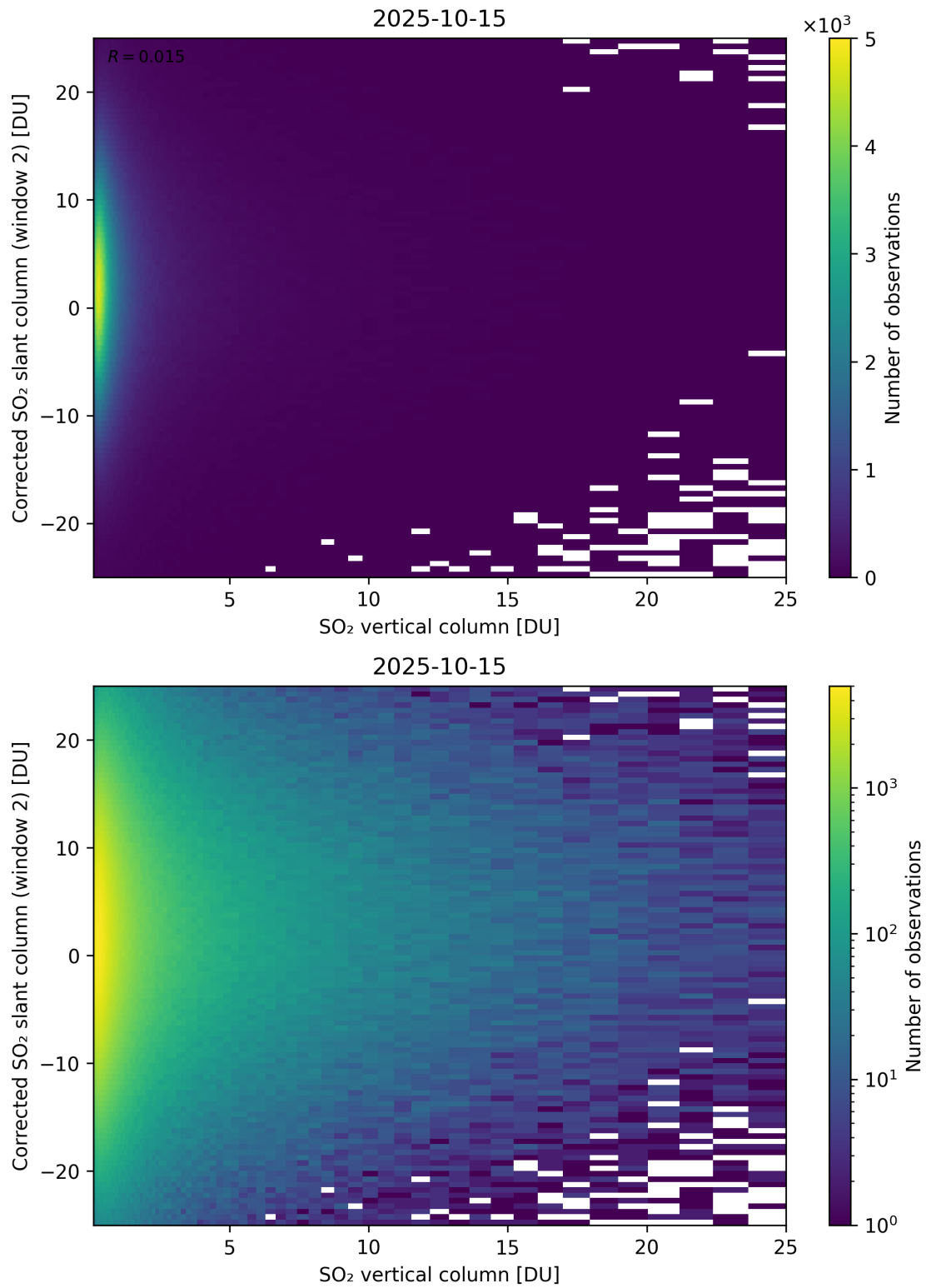
Figure 352: Scatter density plot of “SO 2 vertical column” against “Corrected SO 2 slant column (window 2)” for 2025-10-14 to 2025-10-16.
