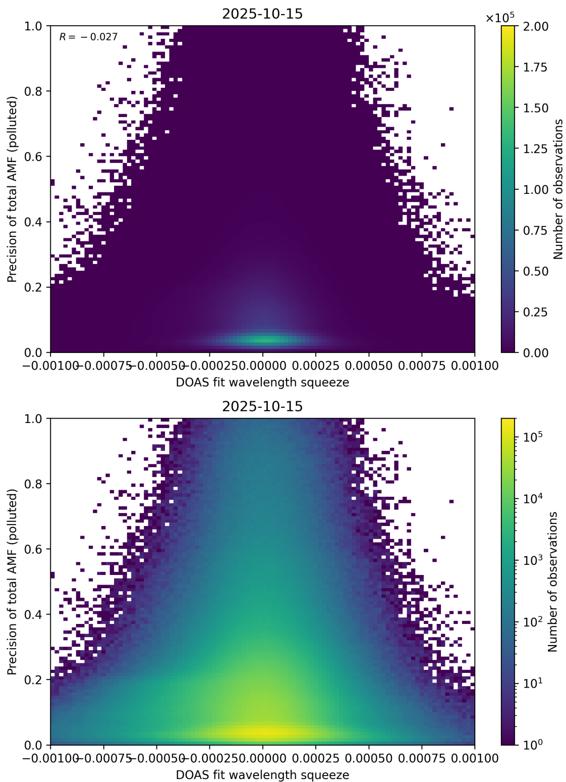
Figure 146: Scatter density plot of “DOAS fit wavelength squeeze” against “Precision of total AMF (polluted)” for 2025-10-14 to 2025-10-16.
