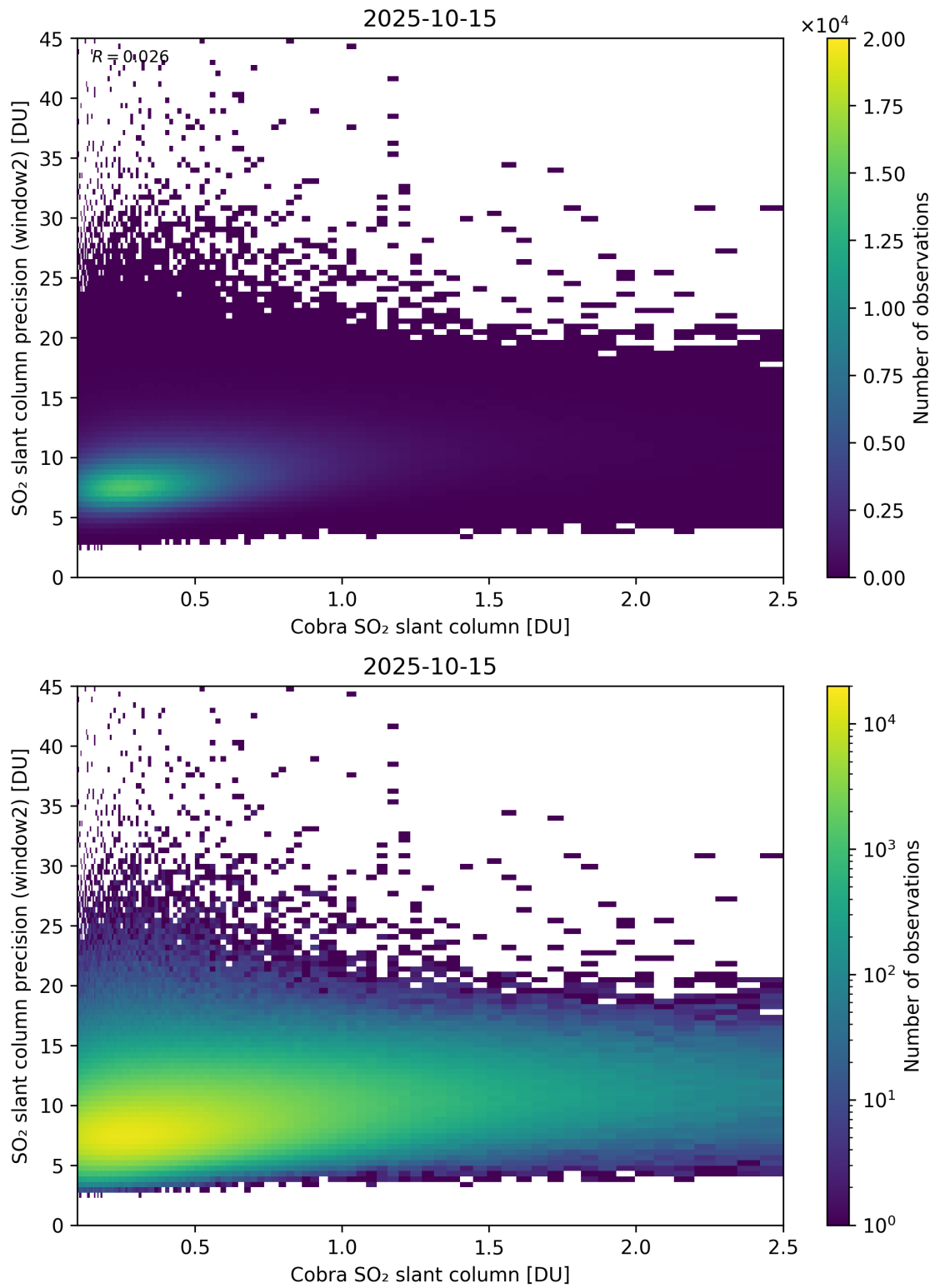
Figure 221: Scatter density plot of “Cobra SO 2 slant column” against “SO 2 slant column precision (window2)” for 2025-10-14 to 2025-10-16.
