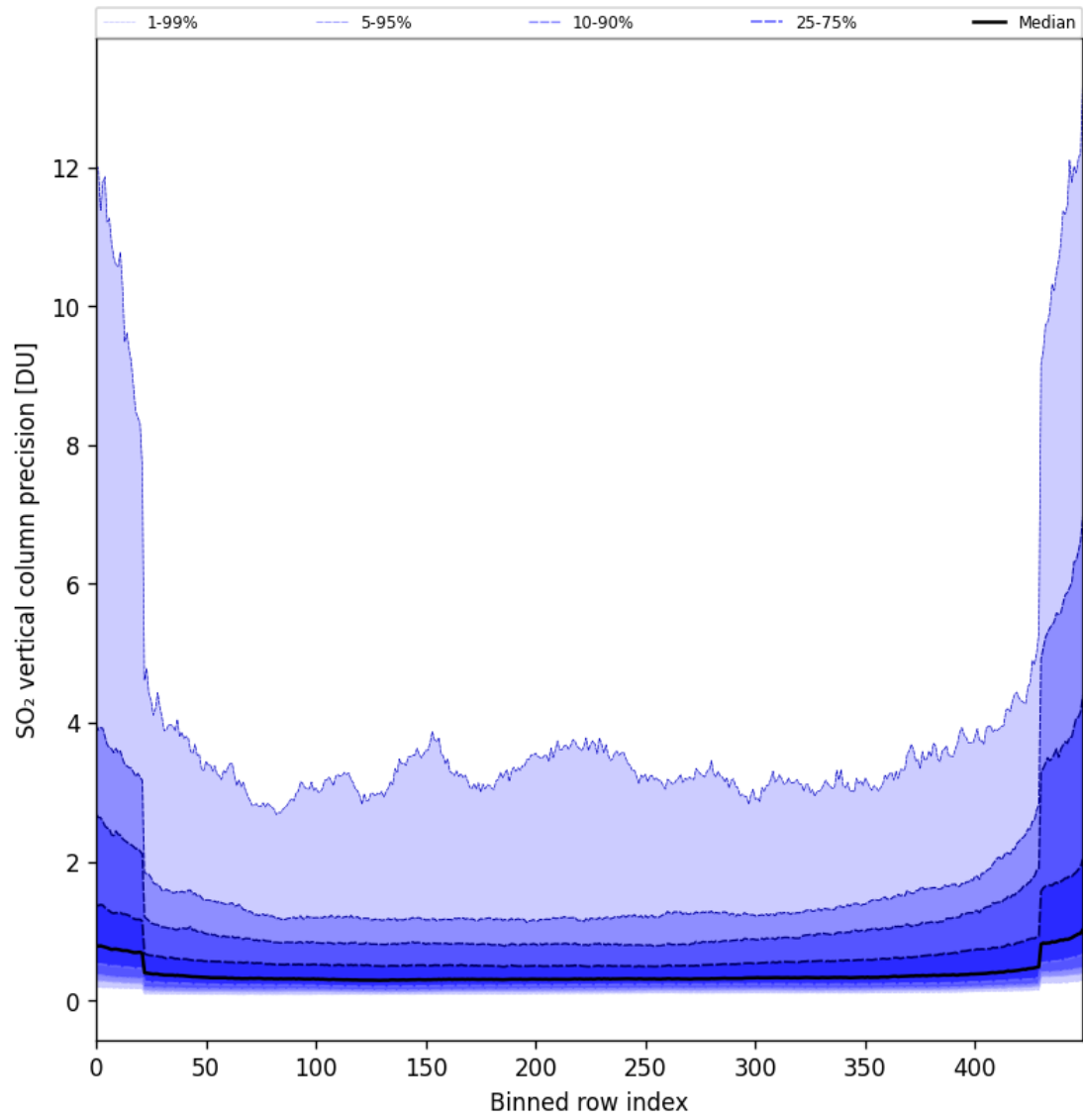
Figure 85: Along track statistics of “SO 2 vertical column precision” for 2025-10-14 to 2025-10-16
