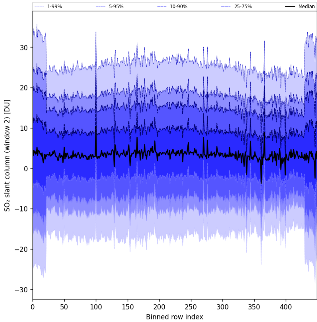
Figure 93: Along track statistics of “SO 2 slant column (window 2)” for 2025-10-14 to 2025-10-16
