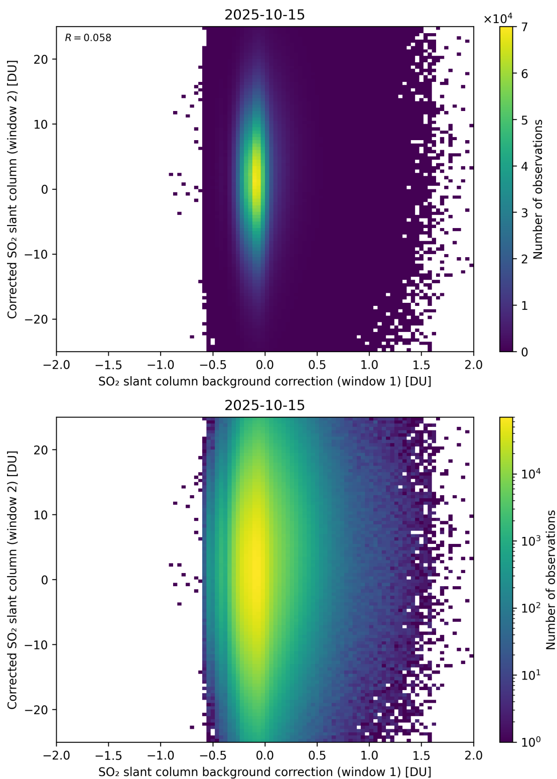
Figure 115: Scatter density plot of “SO 2 slant column background correction (window 1)” against “Corrected SO 2 slant column (window 2)” for 2025-10-14 to 2025-10-16.
