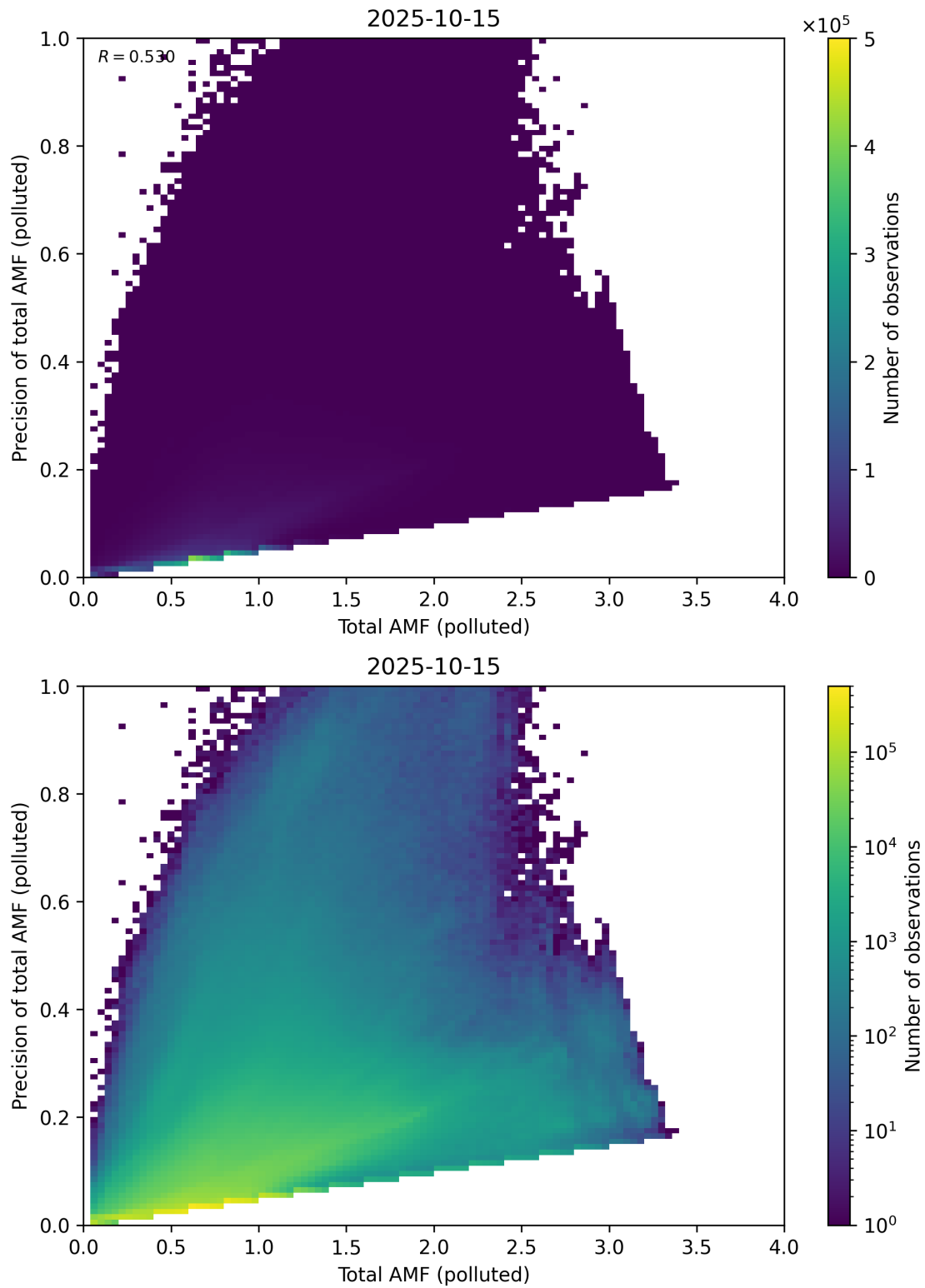
Figure 322: Scatter density plot of “Total AMF (polluted)” against “Precision of total AMF (polluted)” for 2025-10-14 to 2025-10-16.
