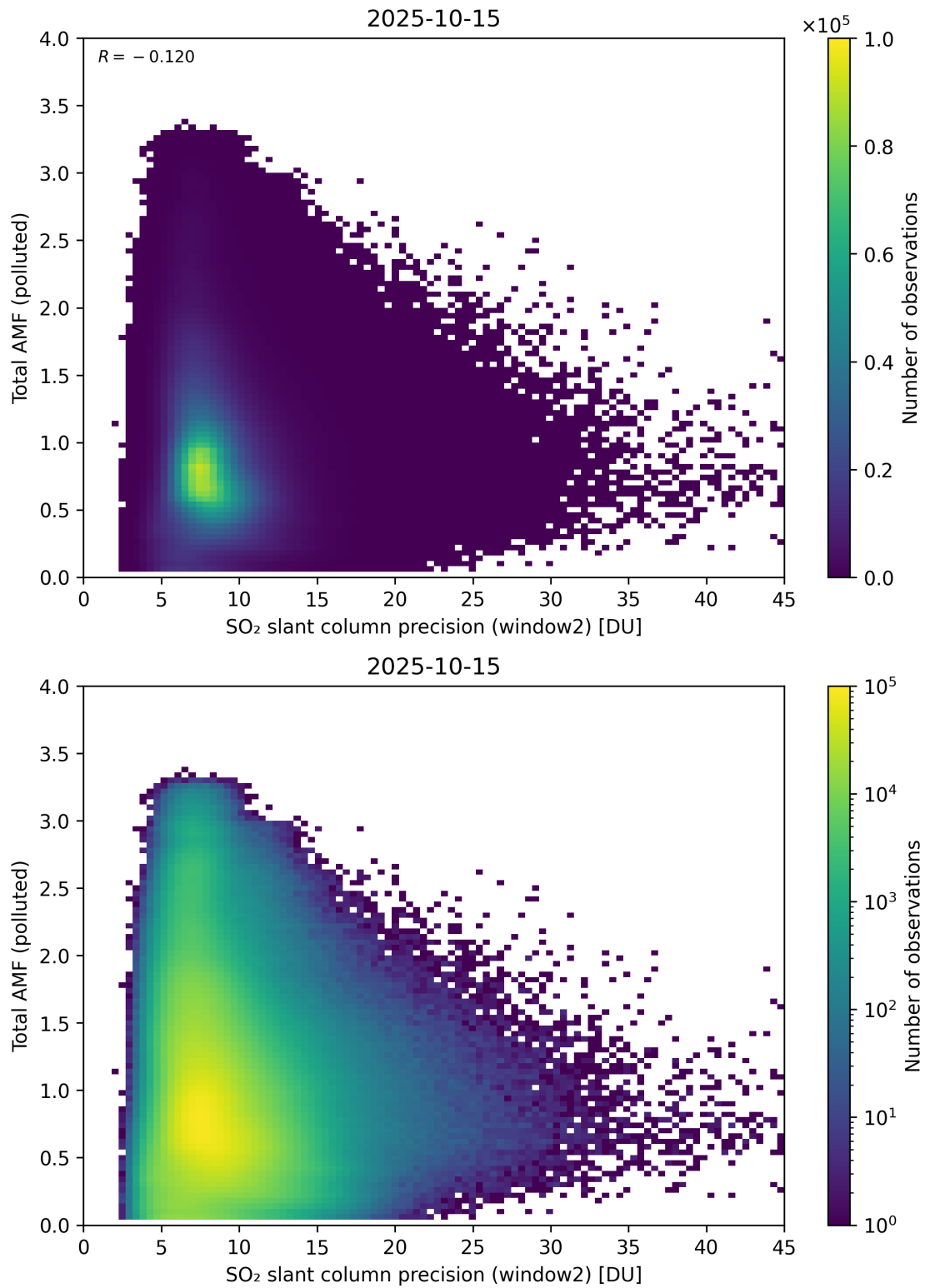
Figure 301: Scatter density plot of “SO 2 slant column precision (window2)” against “Total AMF (polluted)” for 2025-10-14 to 2025-10-16.
