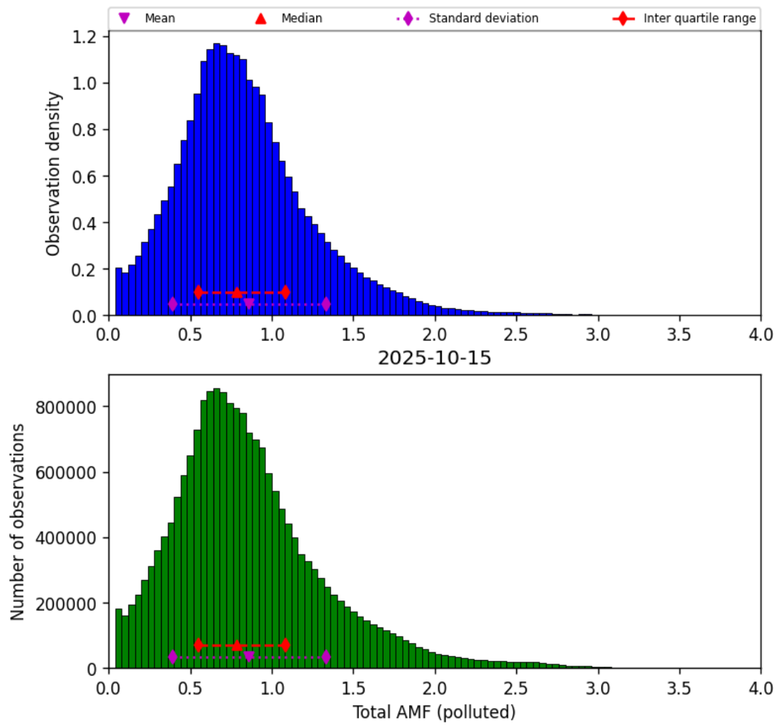
Figure 79: Histogram of “Total AMF (polluted)” for 2025-10-14 to 2025-10-16
