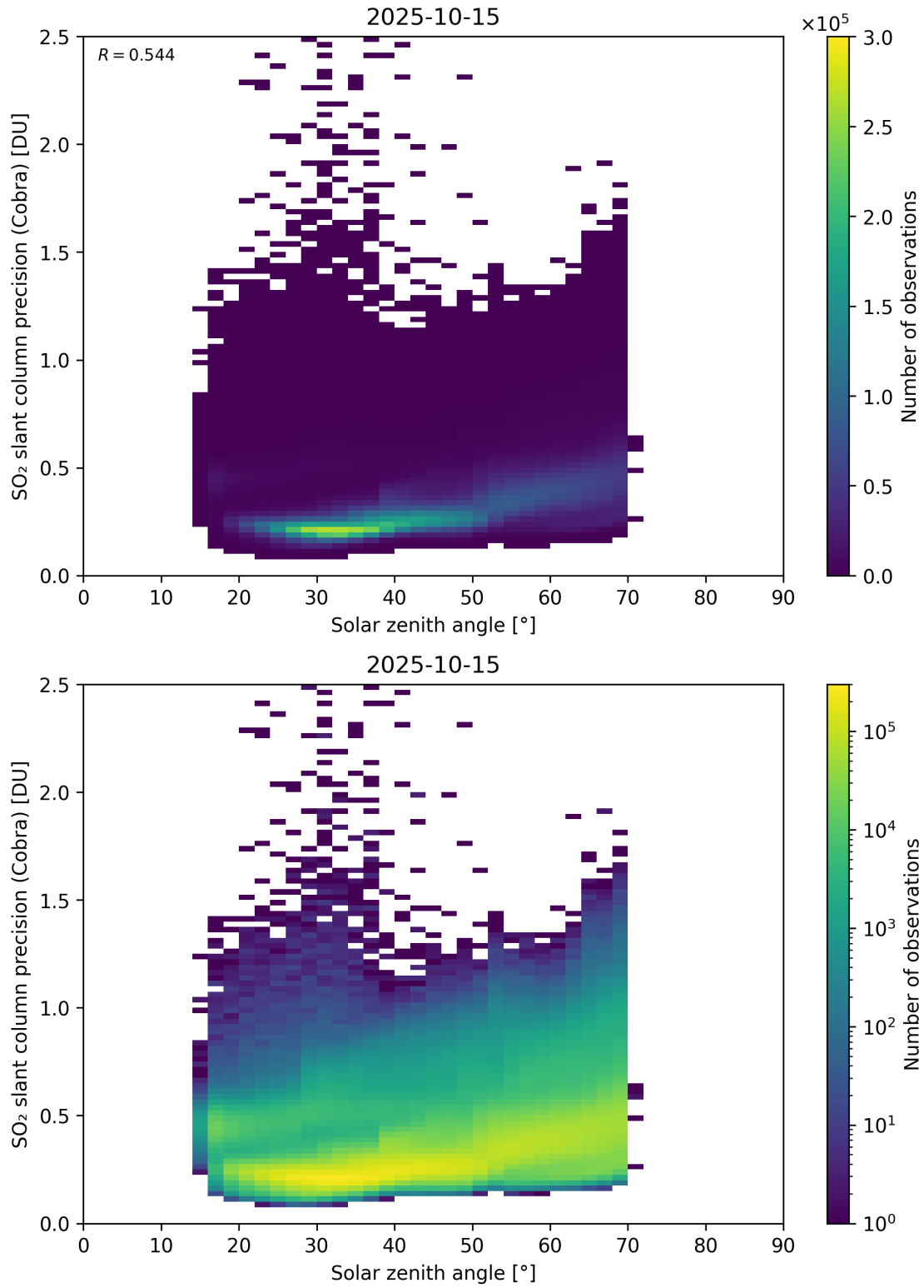
Figure 180: Scatter density plot of “Solar zenith angle” against “SO 2 slant column precision (Cobra)” for 2025-10-14 to 2025-10-16.
