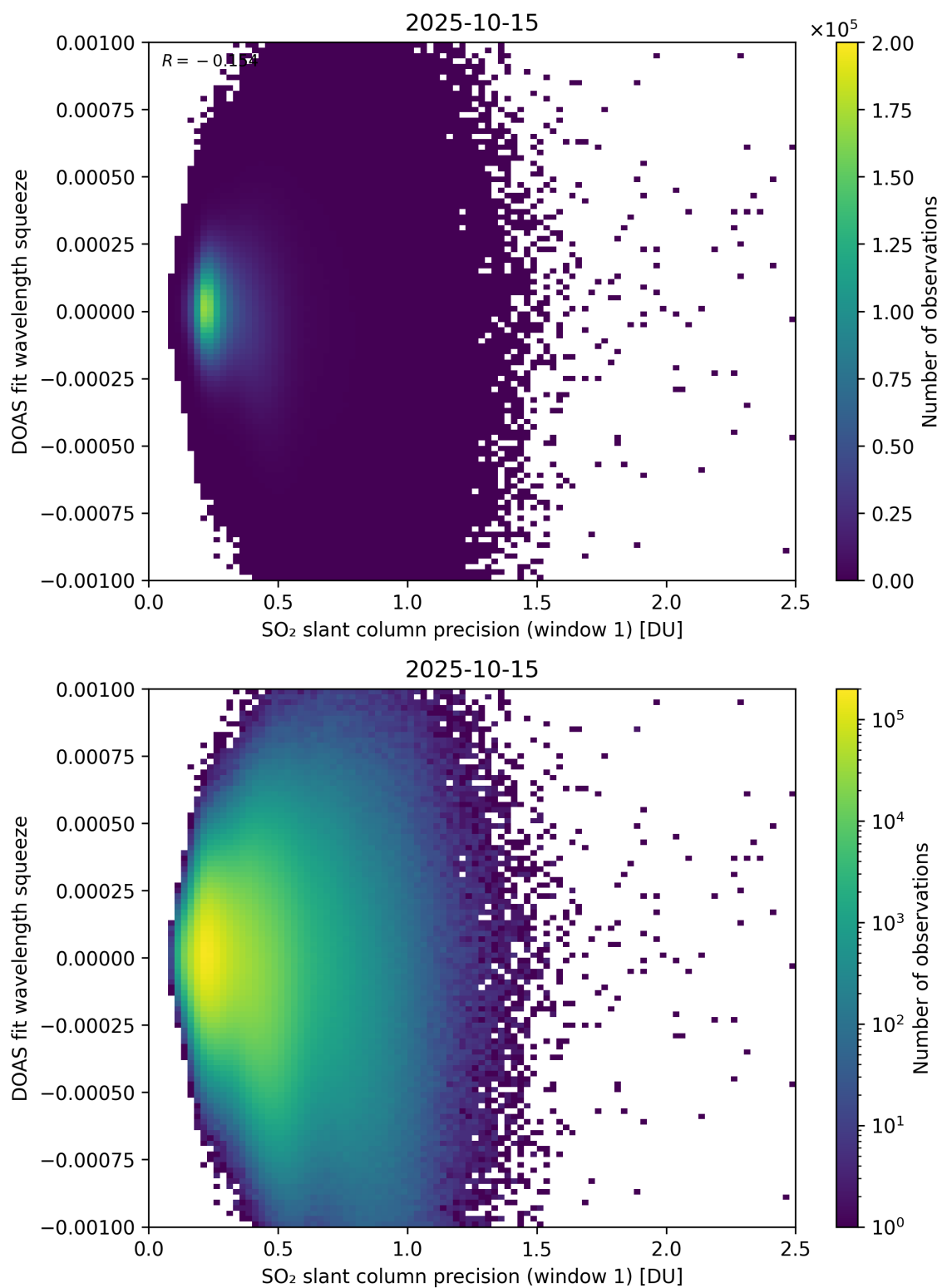
Figure 272: Scatter density plot of “SO 2 slant column precision (window 1)” against “DOAS fit wavelength squeeze” for 2025-10-14 to 2025-10-16.
