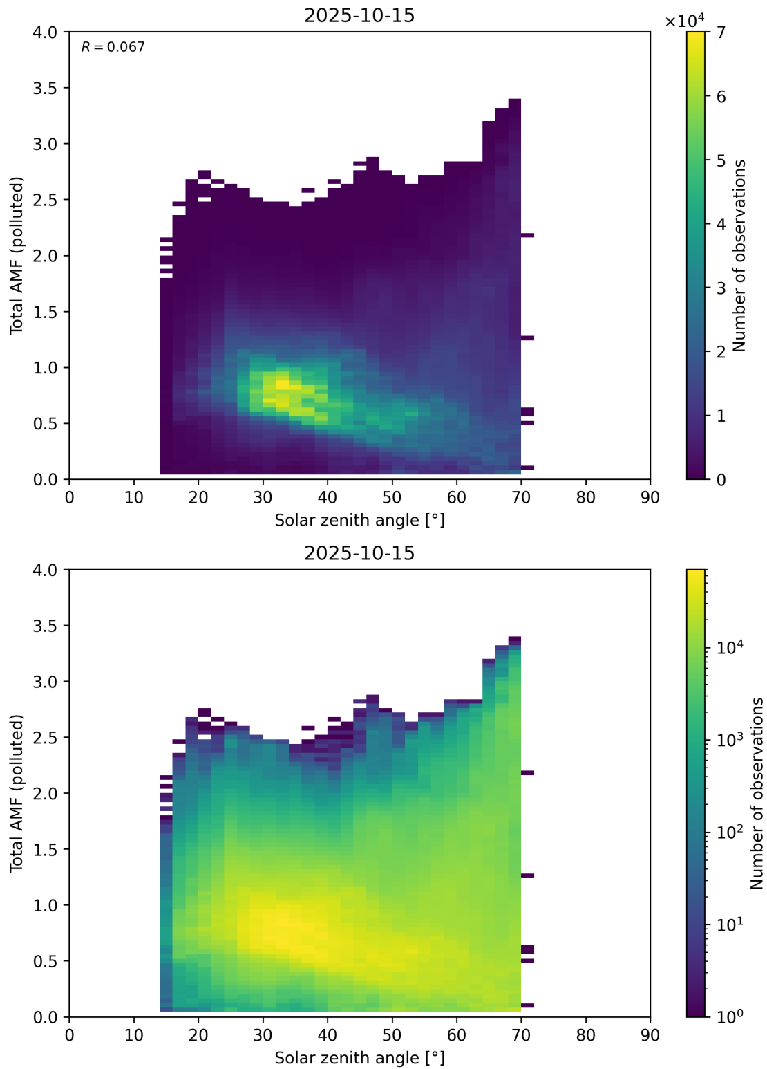
Figure 189: Scatter density plot of “Solar zenith angle” against “Total AMF (polluted)” for 2025-10-14 to 2025-10-16.
