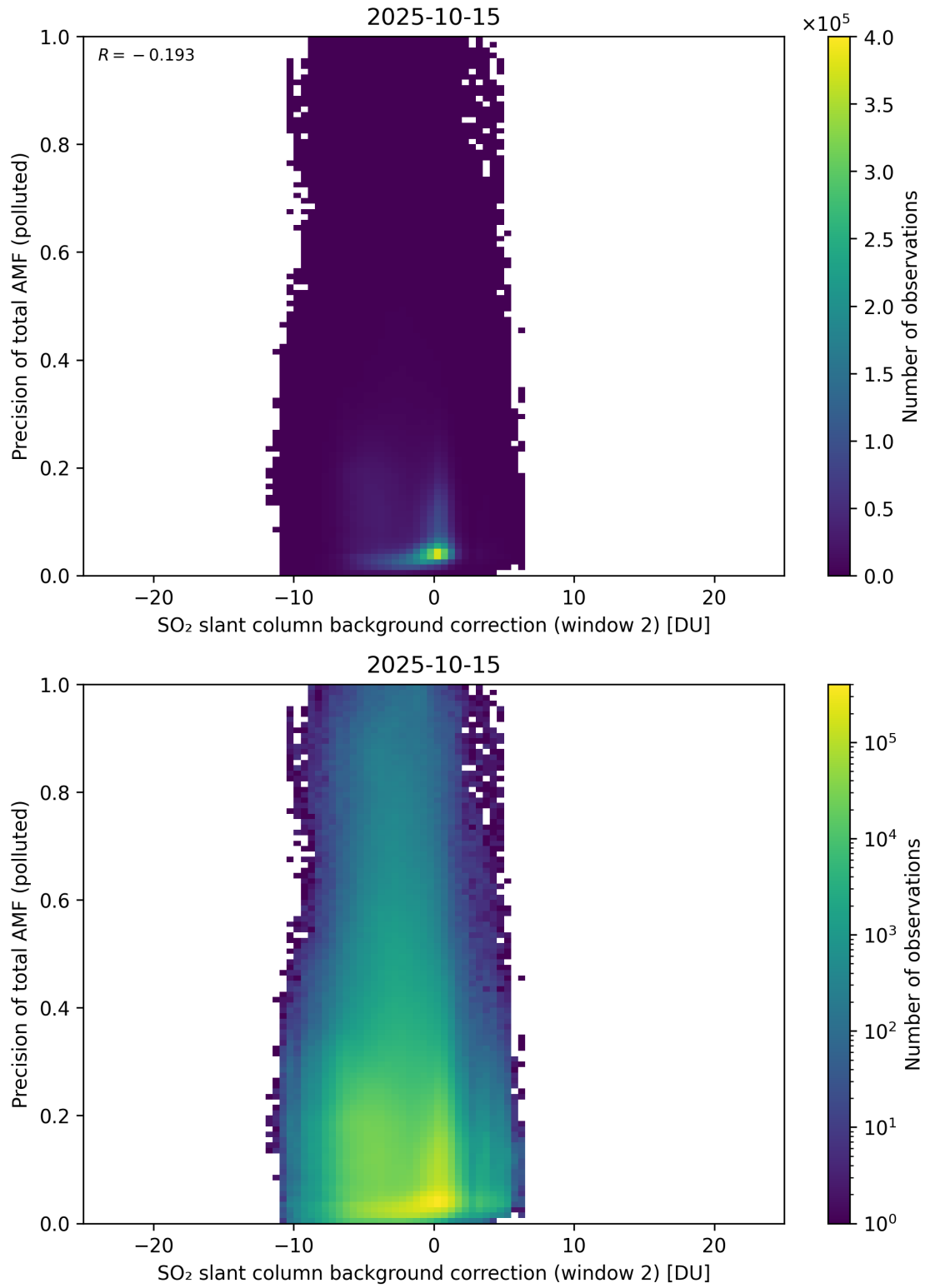
Figure 131: Scatter density plot of “SO 2 slant column background correction (window 2)” against “Precision of total AMF (polluted)” for 2025-10-14 to 2025-10-16.
