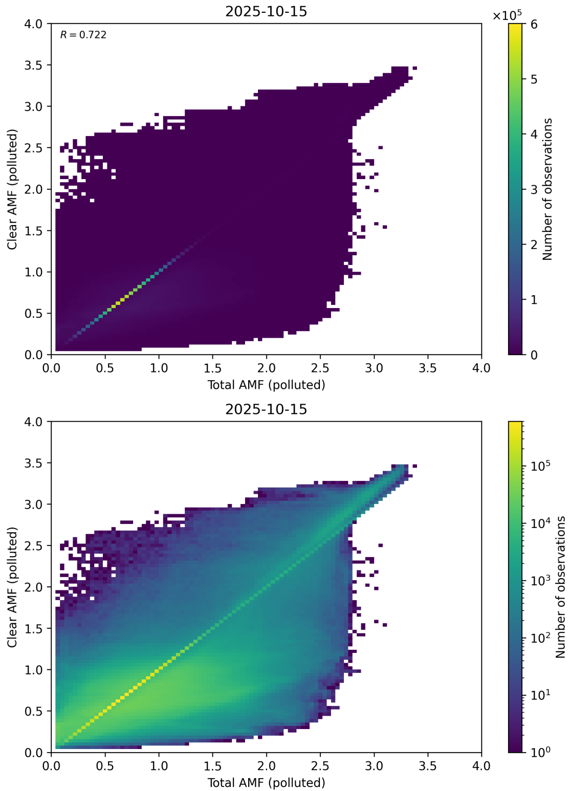
Figure 321: Scatter density plot of “Total AMF (polluted)” against “Clear AMF (polluted)” for 2025-10-14 to 2025-10-16.
