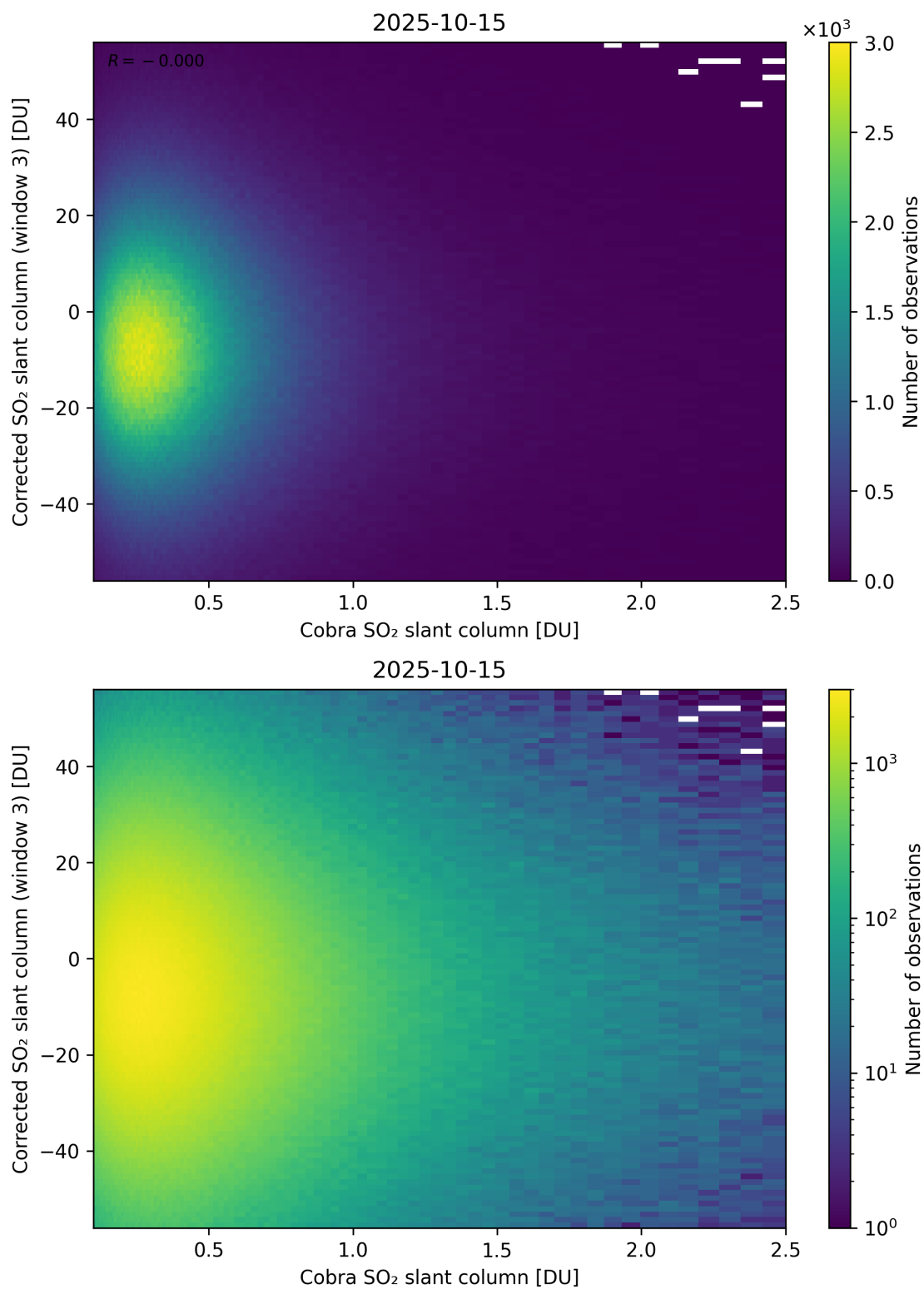
Figure 218: Scatter density plot of “Cobra SO 2 slant column” against “Corrected SO 2 slant column (window 3)” for 2025-10-14 to 2025-10-16.
