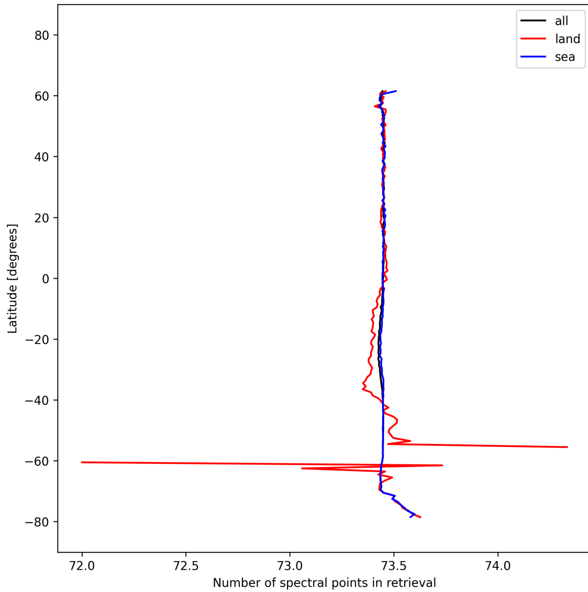
Figure 56: Zonal average of “Number of spectral points in retrieval” for 2025-10-14 to 2025-10-16.
