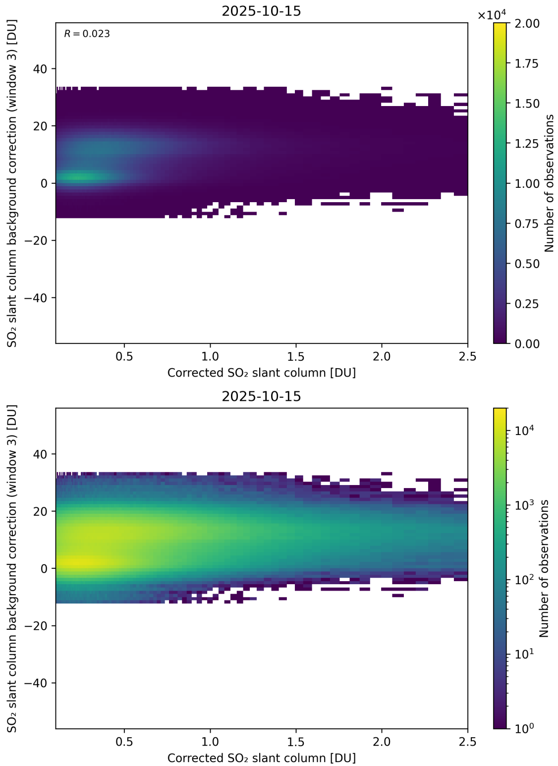
Figure 228: Scatter density plot of “Corrected SO 2 slant column” against “SO 2 slant column background correction (window 3)” for 2025-10-14 to 2025-10-16.
