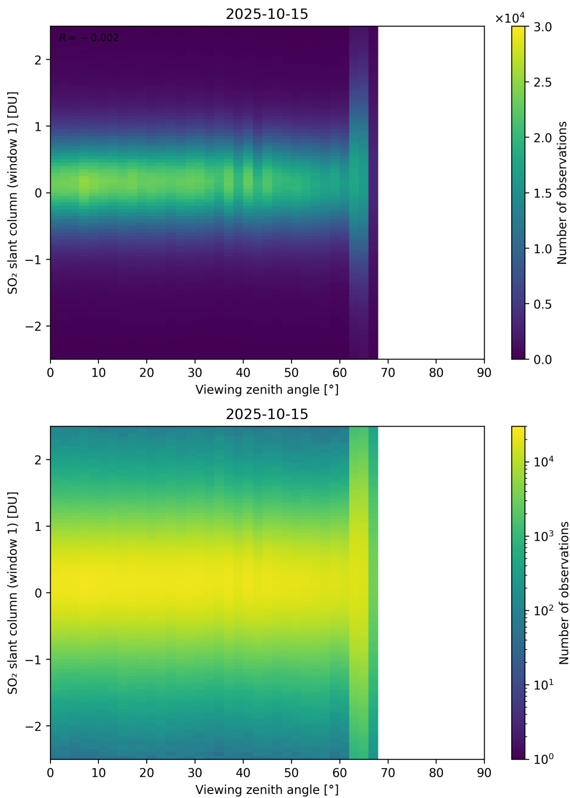
Figure 376: Scatter density plot of “Viewing zenith angle” against “SO 2 slant column (window 1)” for 2025-10-14 to 2025-10-16.
