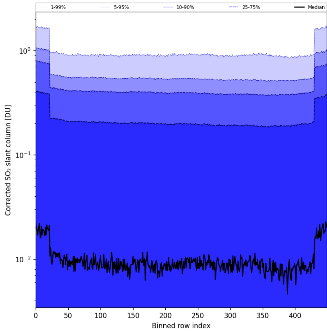
Figure 86: Along track statistics of “Corrected SO 2 slant column” for 2025-10-14 to 2025-10-16
