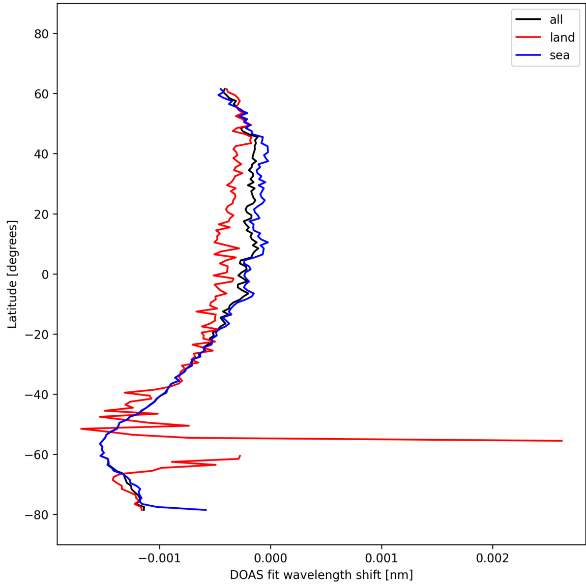
Figure 50: Zonal average of "DOAS fit wavelength shift" for 2025-10-14 to 2025-10-16.
