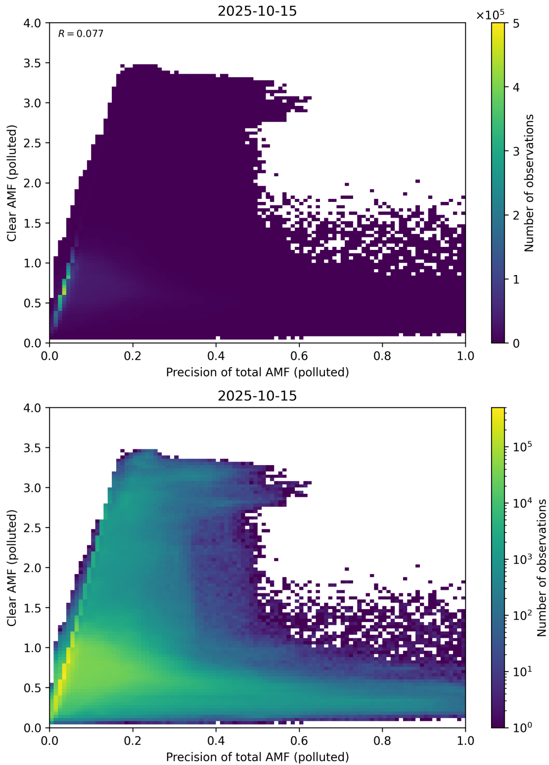
Figure 320: Scatter density plot of “Precision of total AMF (polluted)” against “Clear AMF (polluted)” for 2025-10-14 to 2025-10-16.
