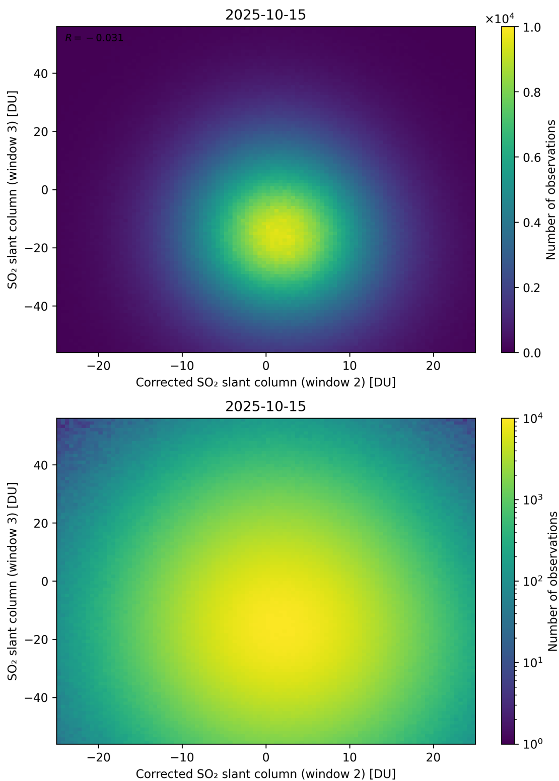
Figure 251: Scatter density plot of “Corrected SO 2 slant column (window 2)” against “SO 2 slant column (window 3)” for 2025-10-14 to 2025-10-16.
