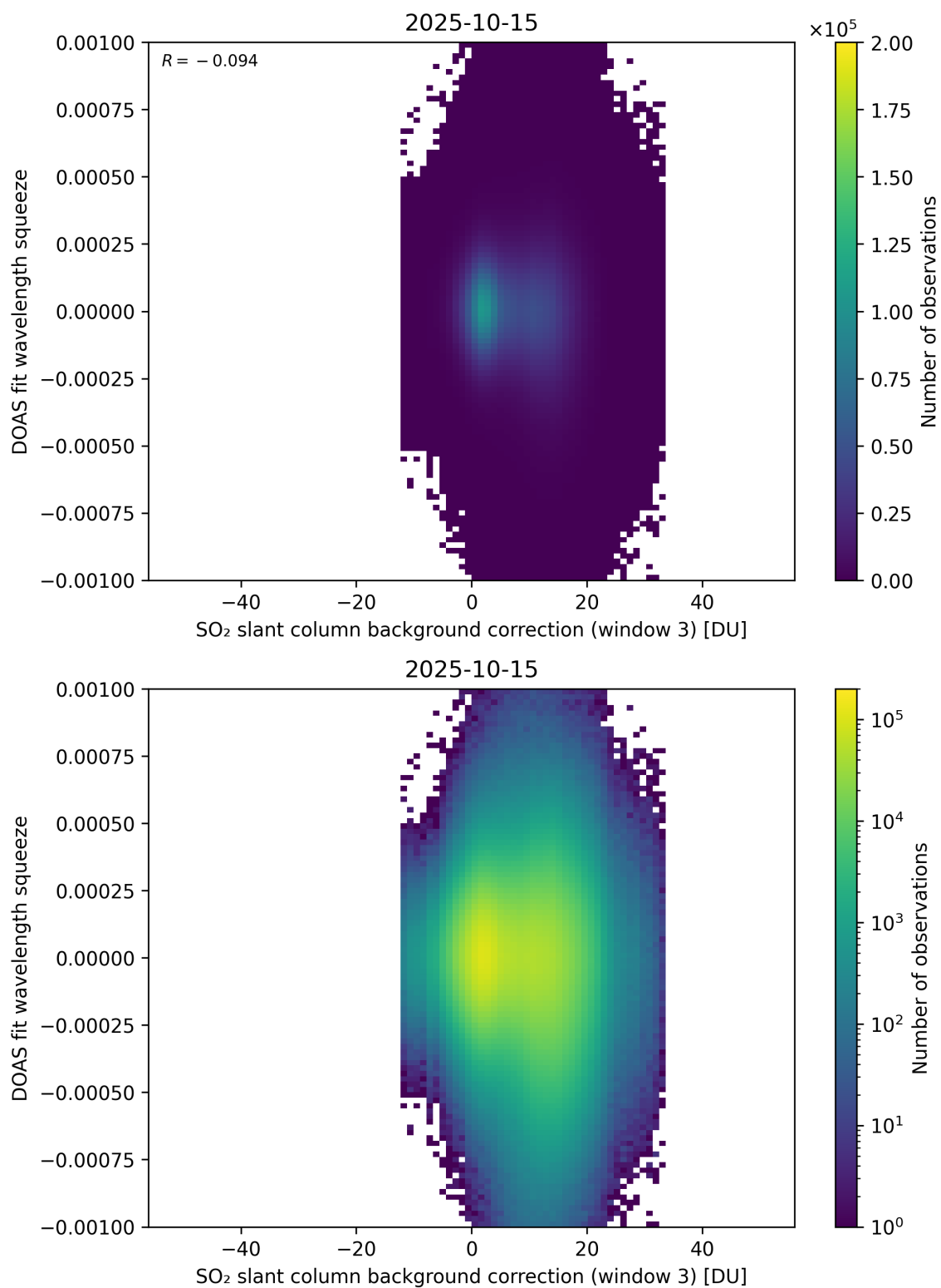
Figure 133: Scatter density plot of “SO 2 slant column background correction (window 3)” against “DOAS fit wavelength squeeze” for 2025-10-14 to 2025-10-16.
