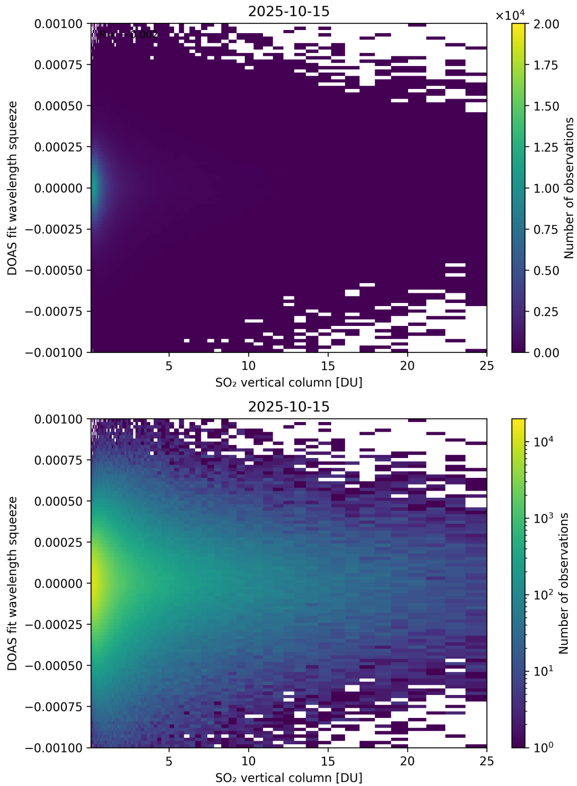
Figure 327: Scatter density plot of “SO 2 vertical column” against “DOAS fit wavelength squeeze” for 2025-10-14 to 2025-10-16.
