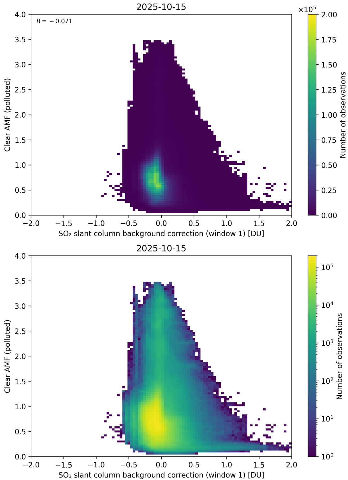
Figure 114: Scatter density plot of “SO 2 slant column background correction (window 1)” against “Clear AMF (polluted)” for 2025-10-14 to 2025-10-16.
