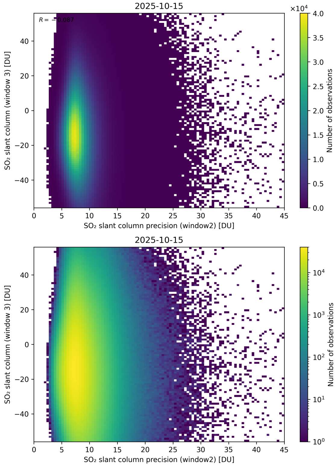
Figure 299: Scatter density plot of “SO 2 slant column precision (window2)” against “SO 2 slant column (window 3)” for 2025-10-14 to 2025-10-16.
