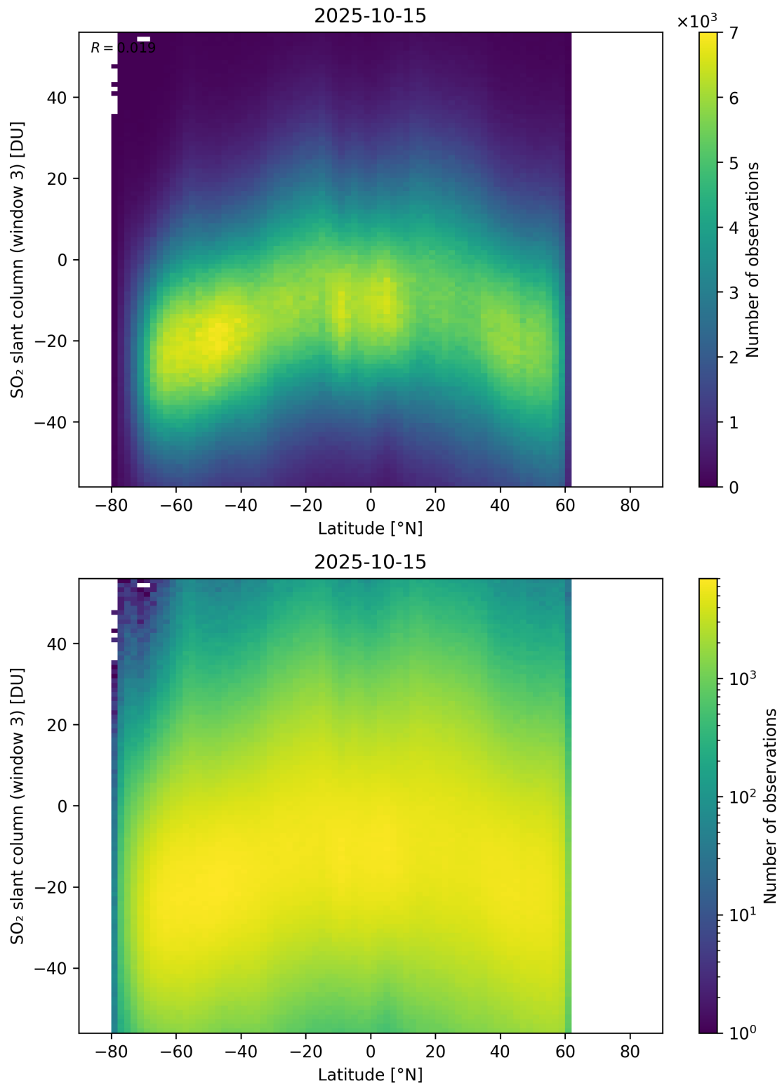
Figure 165: Scatter density plot of “Latitude” against “SO 2 slant column (window 3)” for 2025-10-14 to 2025-10-16.
