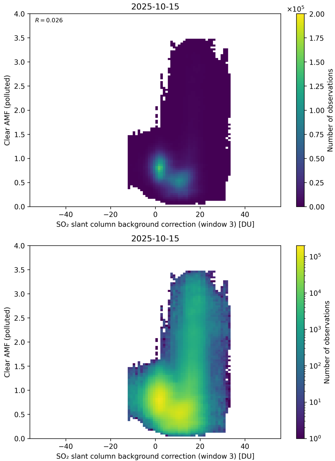
Figure 135: Scatter density plot of “SO 2 slant column background correction (window 3)” against “Clear AMF (polluted)” for 2025-10-14 to 2025-10-16.
