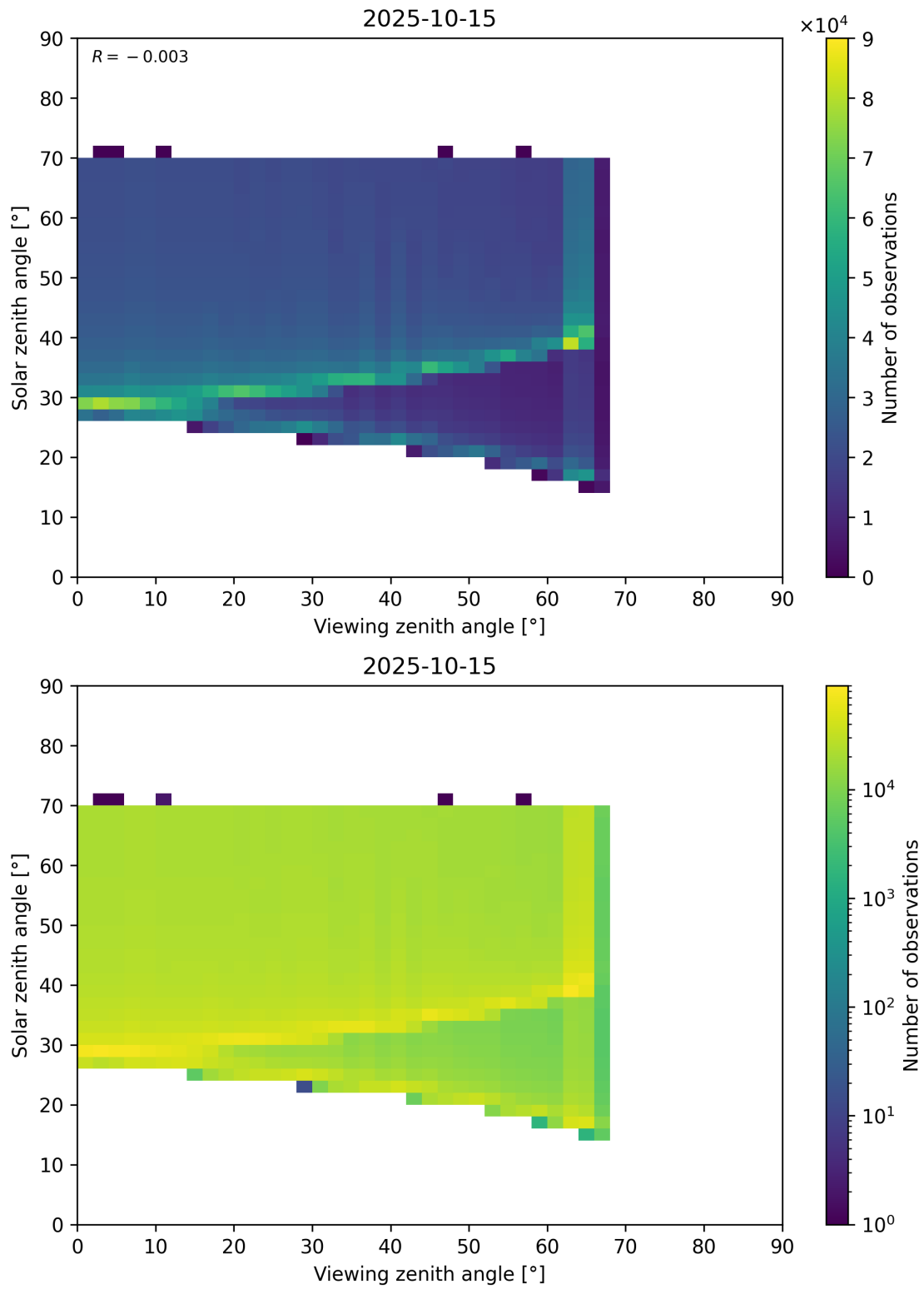
Figure 369: Scatter density plot of “Viewing zenith angle” against “Solar zenith angle” for 2025-10-14 to 2025-10-16.
