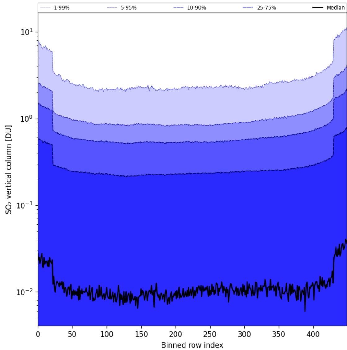
Figure 84: Along track statistics of “SO 2 vertical column” for 2025-10-14 to 2025-10-16
