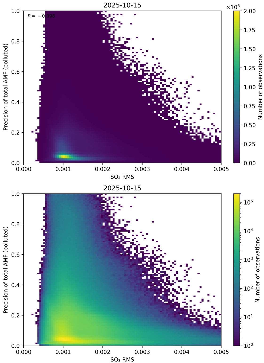
Figure 149: Scatter density plot of “SO 2 RMS” against “Precision of total AMF (polluted)” for 2025-10-14 to 2025-10-16.
