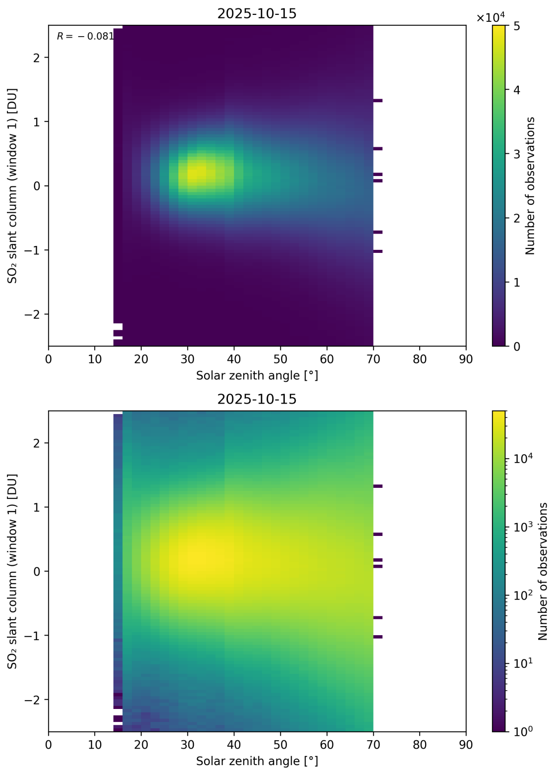
Figure 184: Scatter density plot of “Solar zenith angle” against “SO 2 slant column (window 1)” for 2025-10-14 to 2025-10-16.
