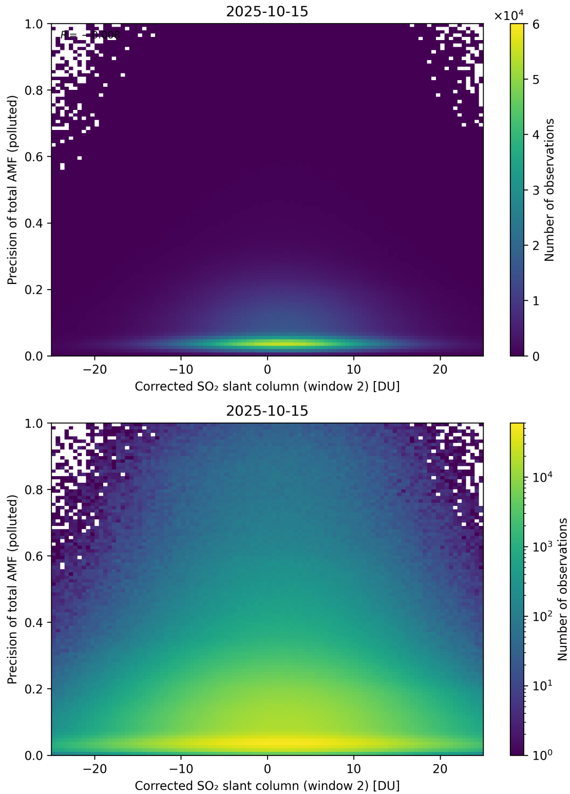
Figure 254: Scatter density plot of “Corrected SO 2 slant column (window 2)” against “Precision of total AMF (polluted)” for 2025-10-14 to 2025-10-16.
