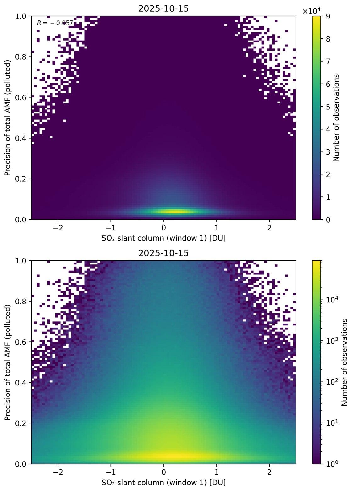
Figure 290: Scatter density plot of “SO 2 slant column (window 1)” against “Precision of total AMF (polluted)” for 2025-10-14 to 2025-10-16.
