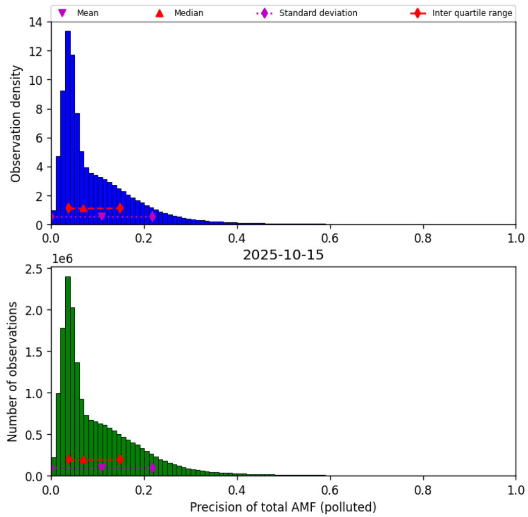
Figure 80: Histogram of “Precision of total AMF (polluted)” for 2025-10-14 to 2025-10-16
