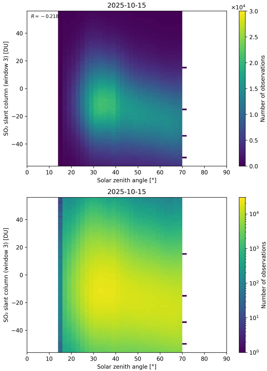
Figure 187: Scatter density plot of “Solar zenith angle” against “SO 2 slant column (window 3)” for 2025-10-14 to 2025-10-16.
