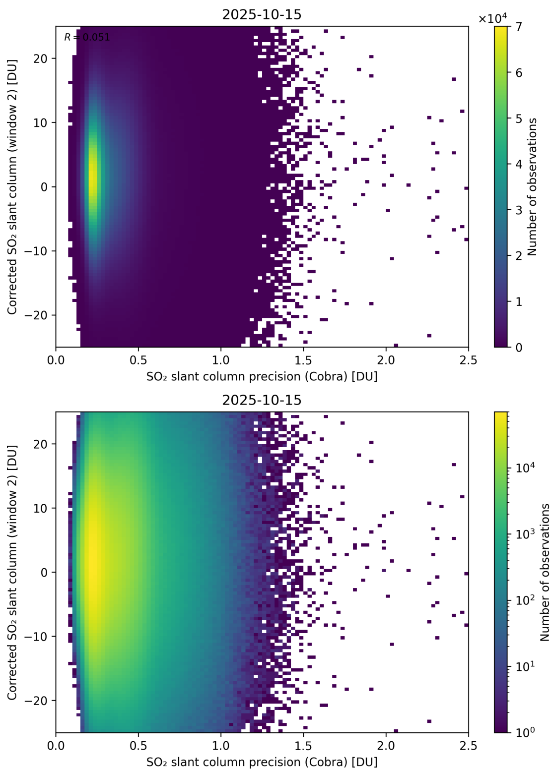
Figure 206: Scatter density plot of “SO 2 slant column precision (Cobra)” against “Corrected SO 2 slant column (window 2)” for 2025-10-14 to 2025-10-16.
