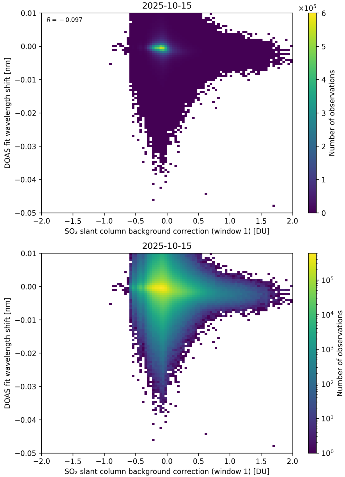
Figure 111: Scatter density plot of “SO 2 slant column background correction (window 1)” against “DOAS fit wavelength shift” for 2025-10-14 to 2025-10-16.
