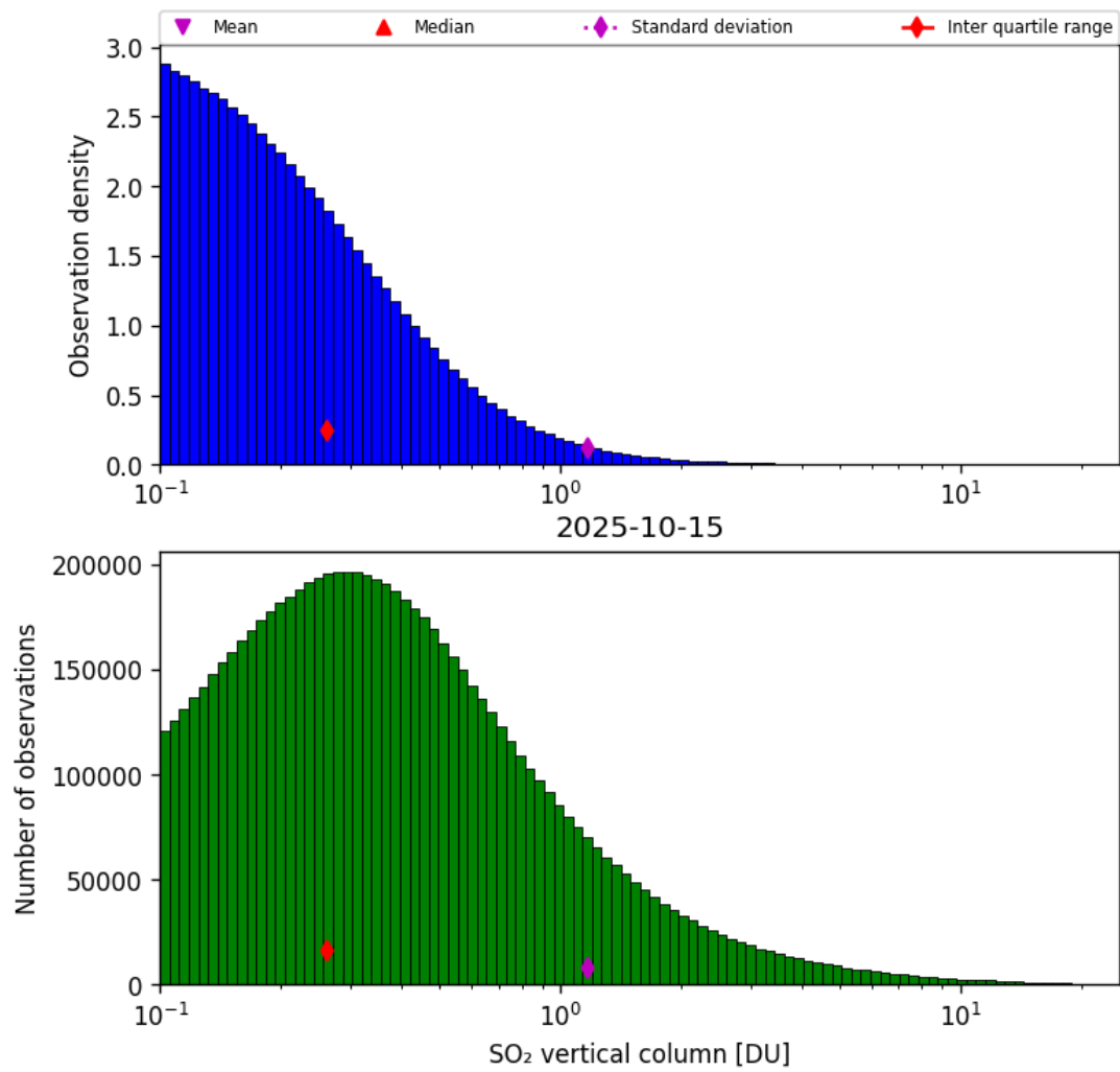
Figure 58: Histogram of “SO 2 vertical column” for 2025-10-14 to 2025-10-16
