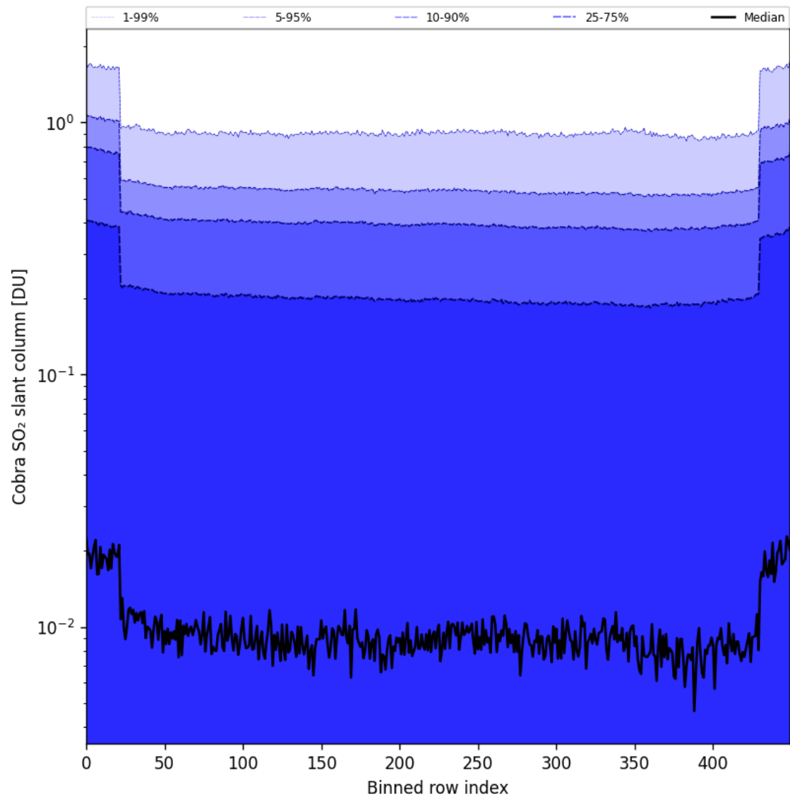
Figure 87: Along track statistics of "Cobra SO 2 slant column" for 2025-10-14 to 2025-10-16
