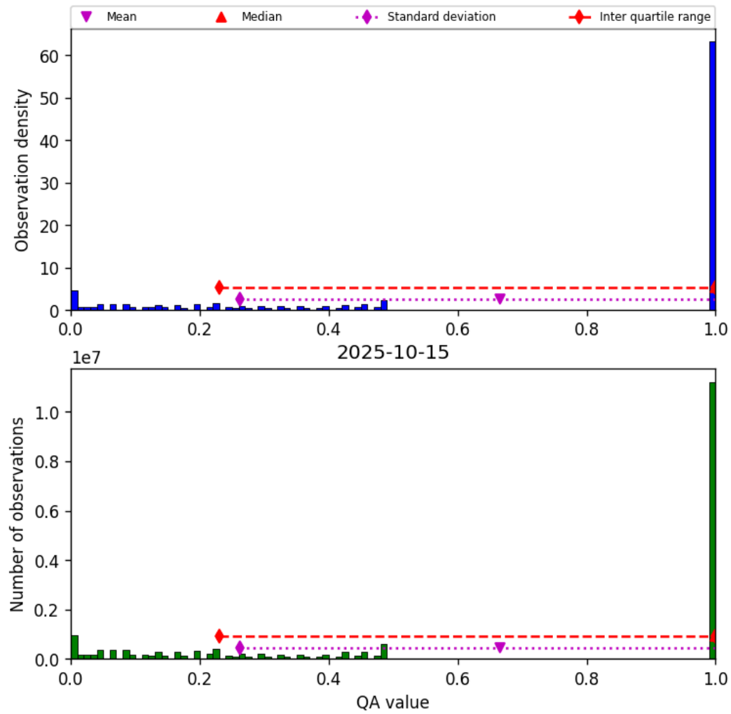
Figure 57: Histogram of “QA value” for 2025-10-14 to 2025-10-16
