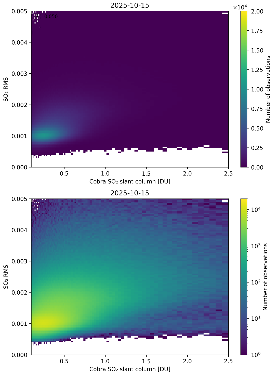
Figure 198: Scatter density plot of “Cobra SO 2 slant column” against “SO 2 RMS” for 2025-10-14 to 2025-10-16.
