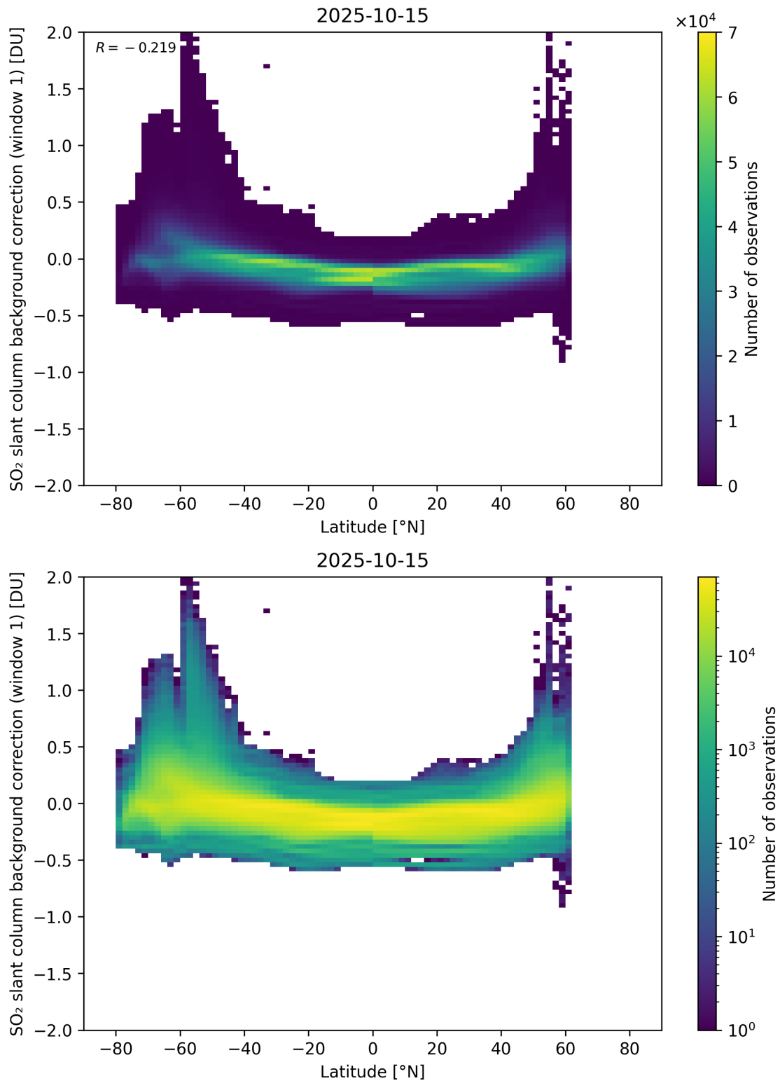
Figure 150: Scatter density plot of “Latitude” against “SO 2 slant column background correction (window 1)” for 2025-10-14 to 2025-10-16.
