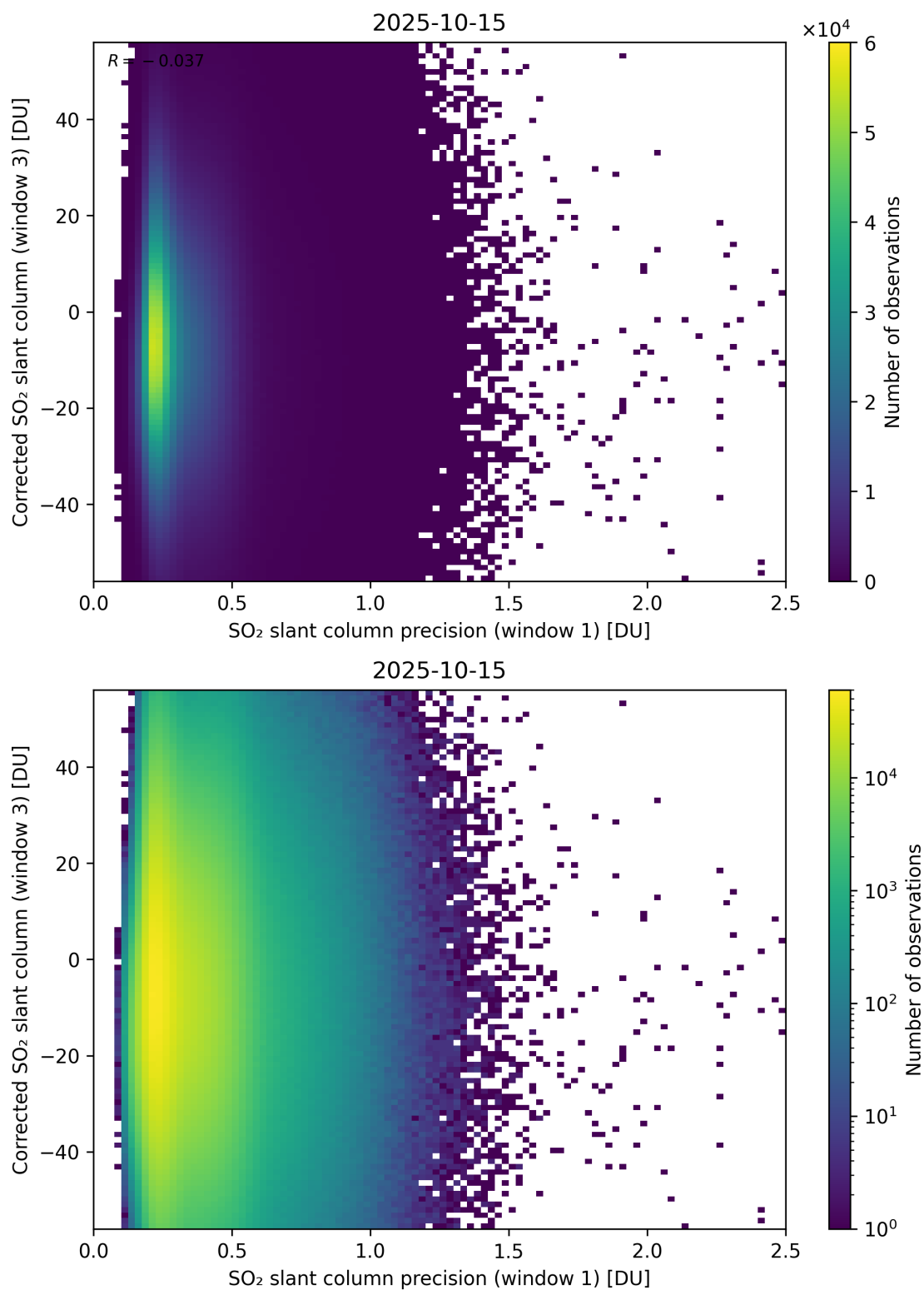
Figure 276: Scatter density plot of “SO 2 slant column precision (window 1)” against “Corrected SO 2 slant column (window 3)” for 2025-10-14 to 2025-10-16.
