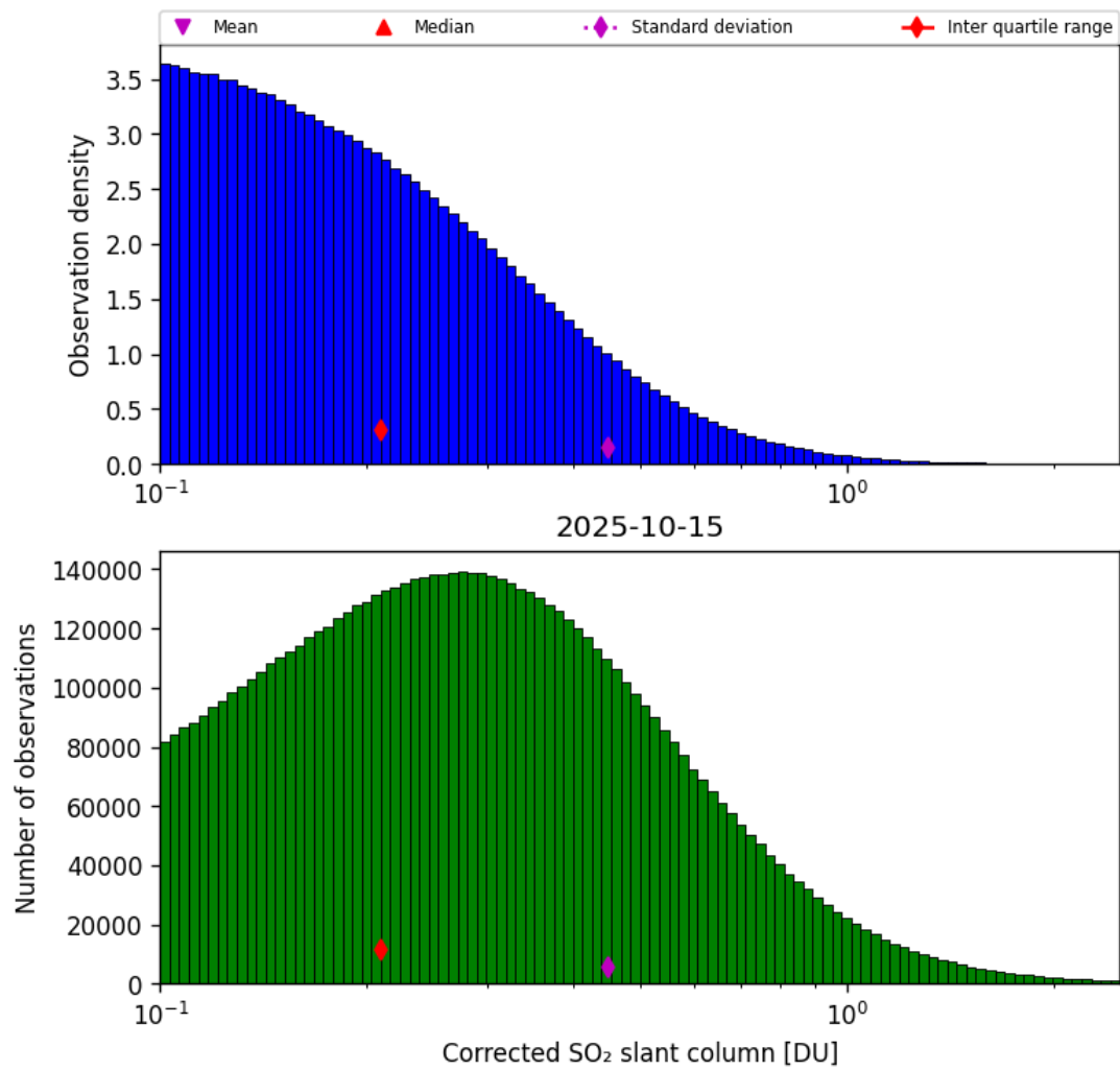
Figure 60: Histogram of “Corrected SO 2 slant column” for 2025-10-14 to 2025-10-16
