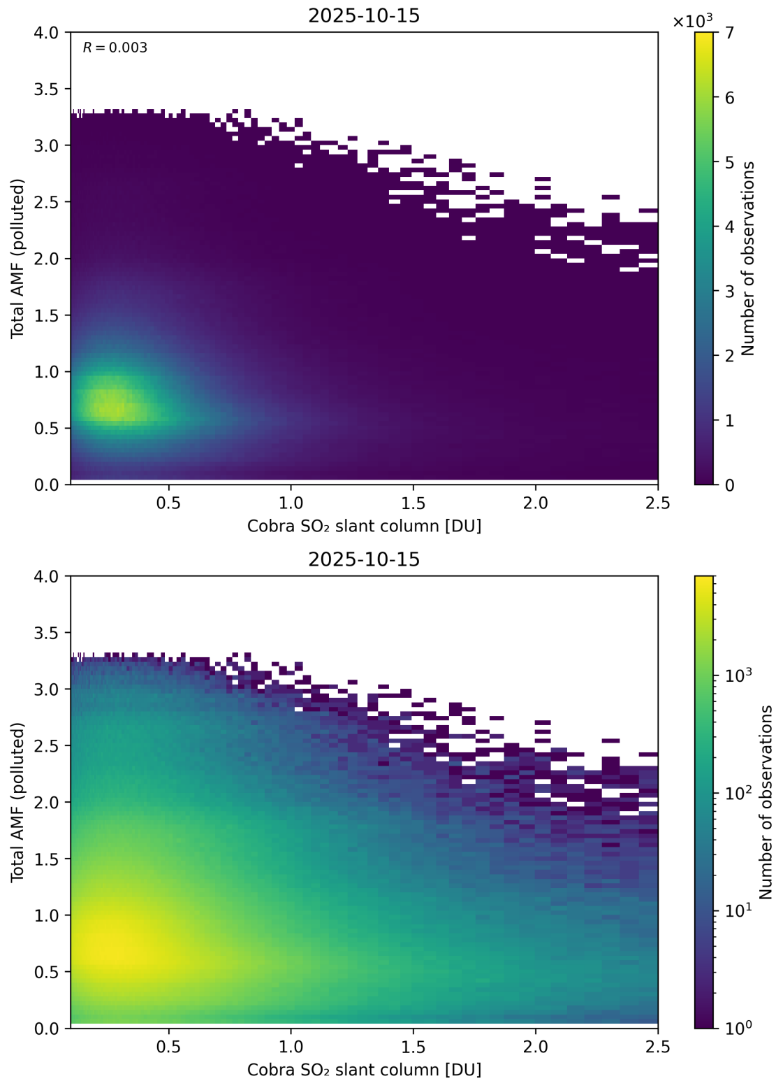
Figure 224: Scatter density plot of “Cobra SO 2 slant column” against “Total AMF (polluted)” for 2025-10-14 to 2025-10-16.
