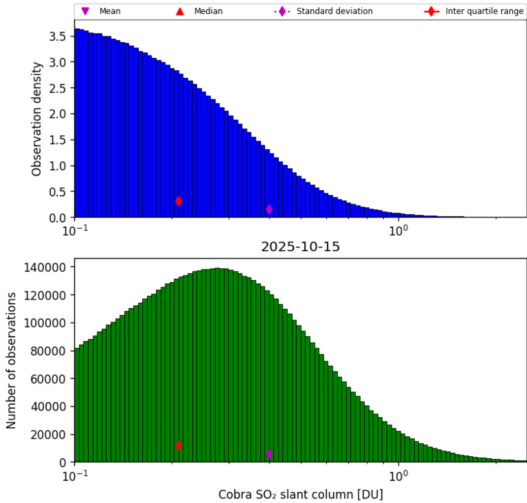
Figure 61: Histogram of “Cobra SO 2 slant column” for 2025-10-14 to 2025-10-16
