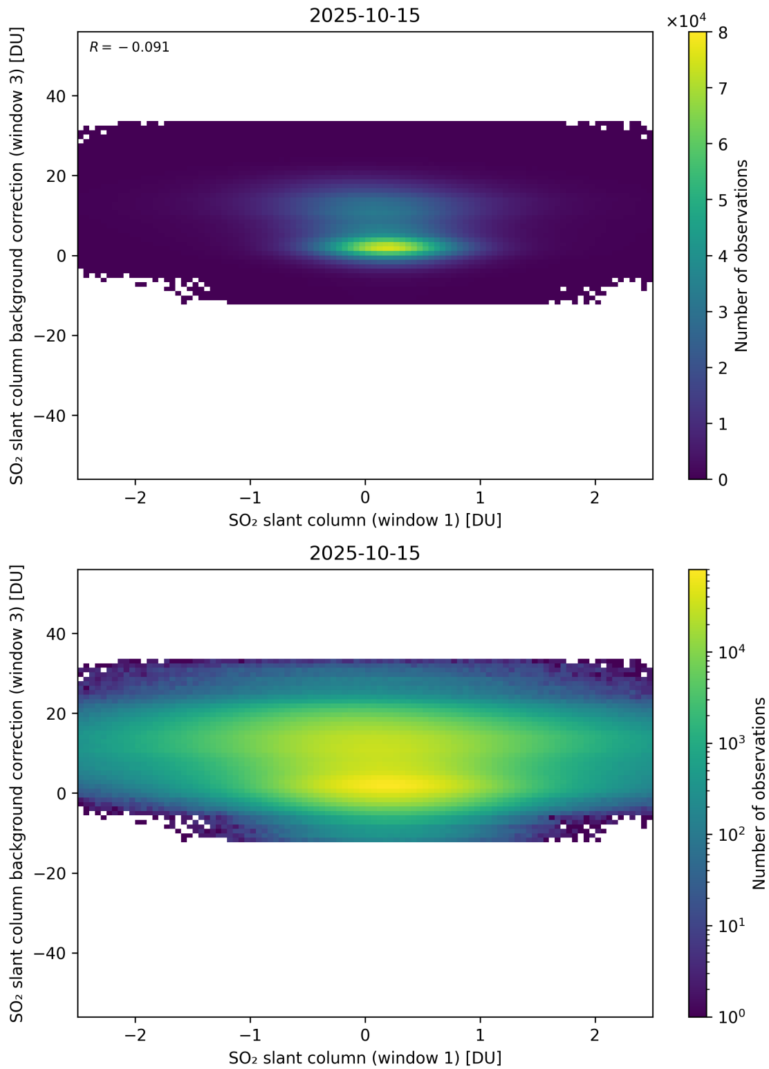
Figure 264: Scatter density plot of “SO 2 slant column (window 1)” against “SO 2 slant column background correction (window 3)” for 2025-10-14 to 2025-10-16.
