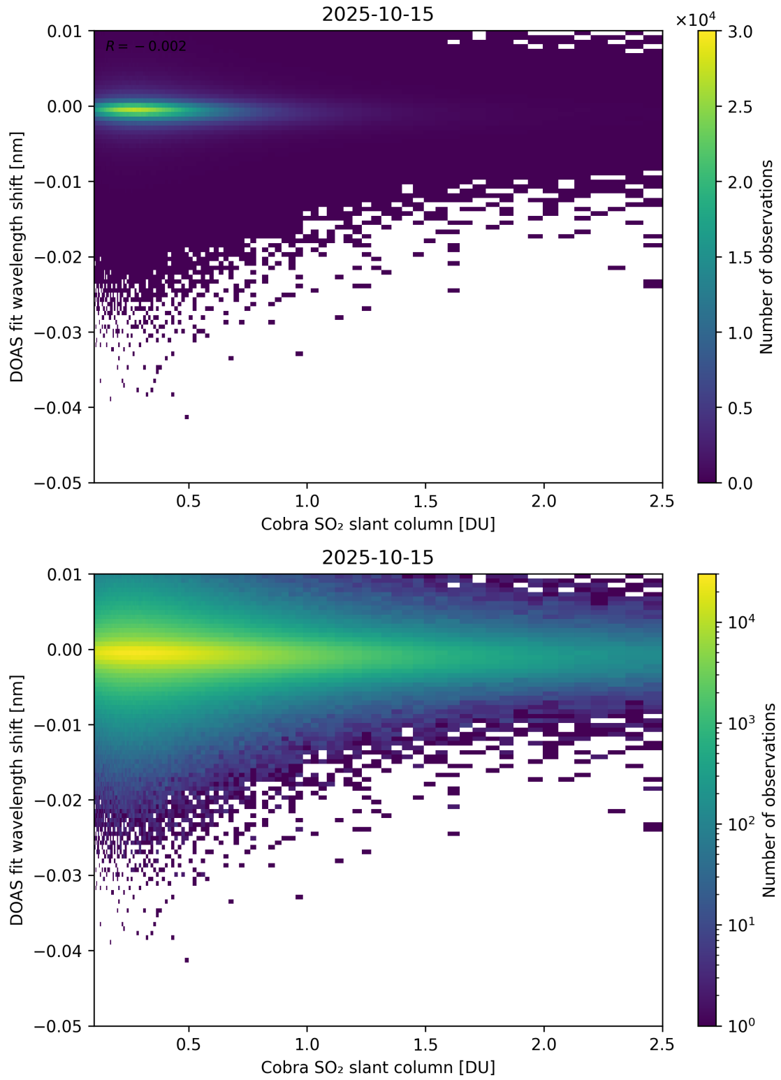
Figure 196: Scatter density plot of “Cobra SO 2 slant column” against “DOAS fit wavelength shift” for 2025-10-14 to 2025-10-16.
