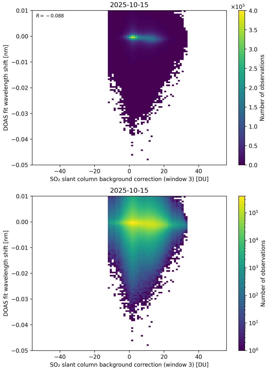
Figure 132: Scatter density plot of “SO 2 slant column background correction (window 3)” against “DOAS fit wavelength shift” for 2025-10-14 to 2025-10-16.
