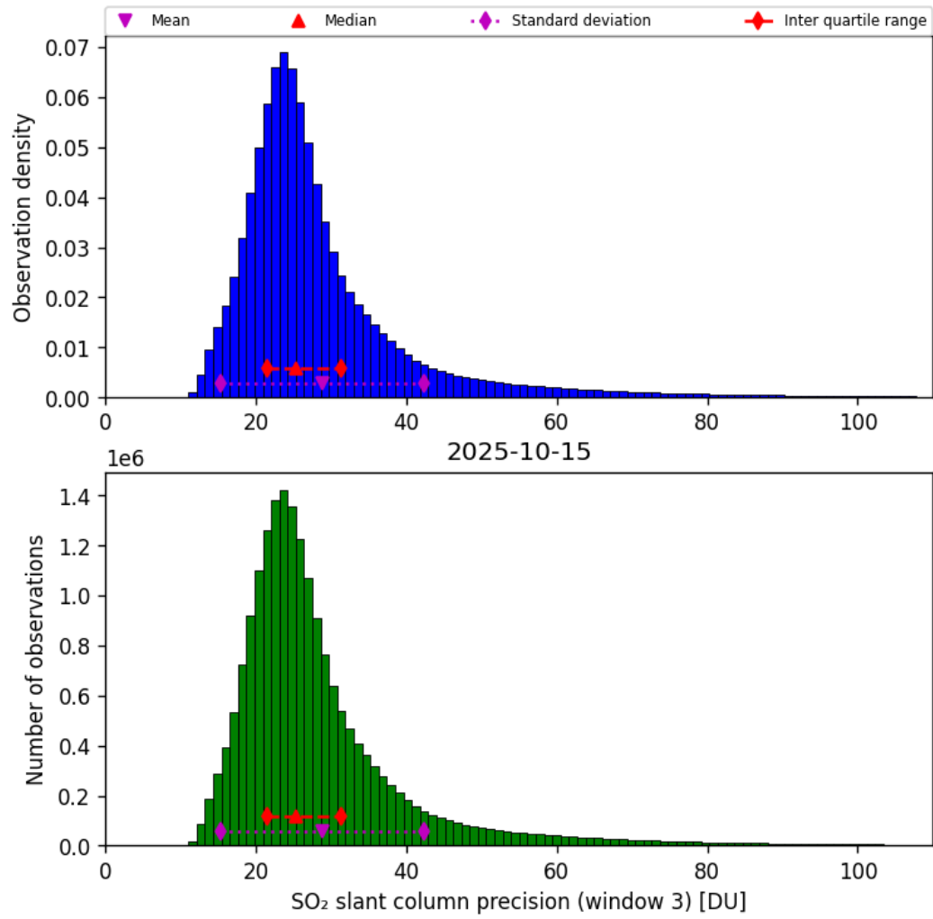
Figure 72: Histogram of “SO 2 slant column precision (window 3)” for 2025-10-14 to 2025-10-16
