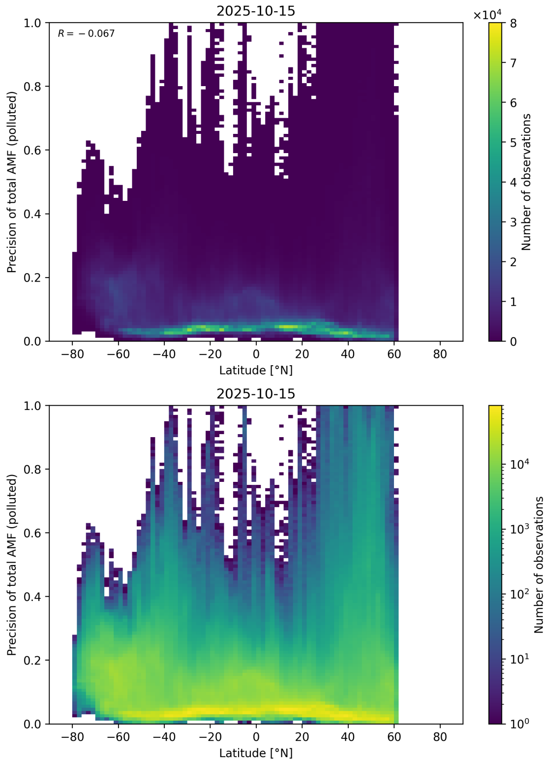
Figure 168: Scatter density plot of “Latitude” against “Precision of total AMF (polluted)” for 2025-10-14 to 2025-10-16.
