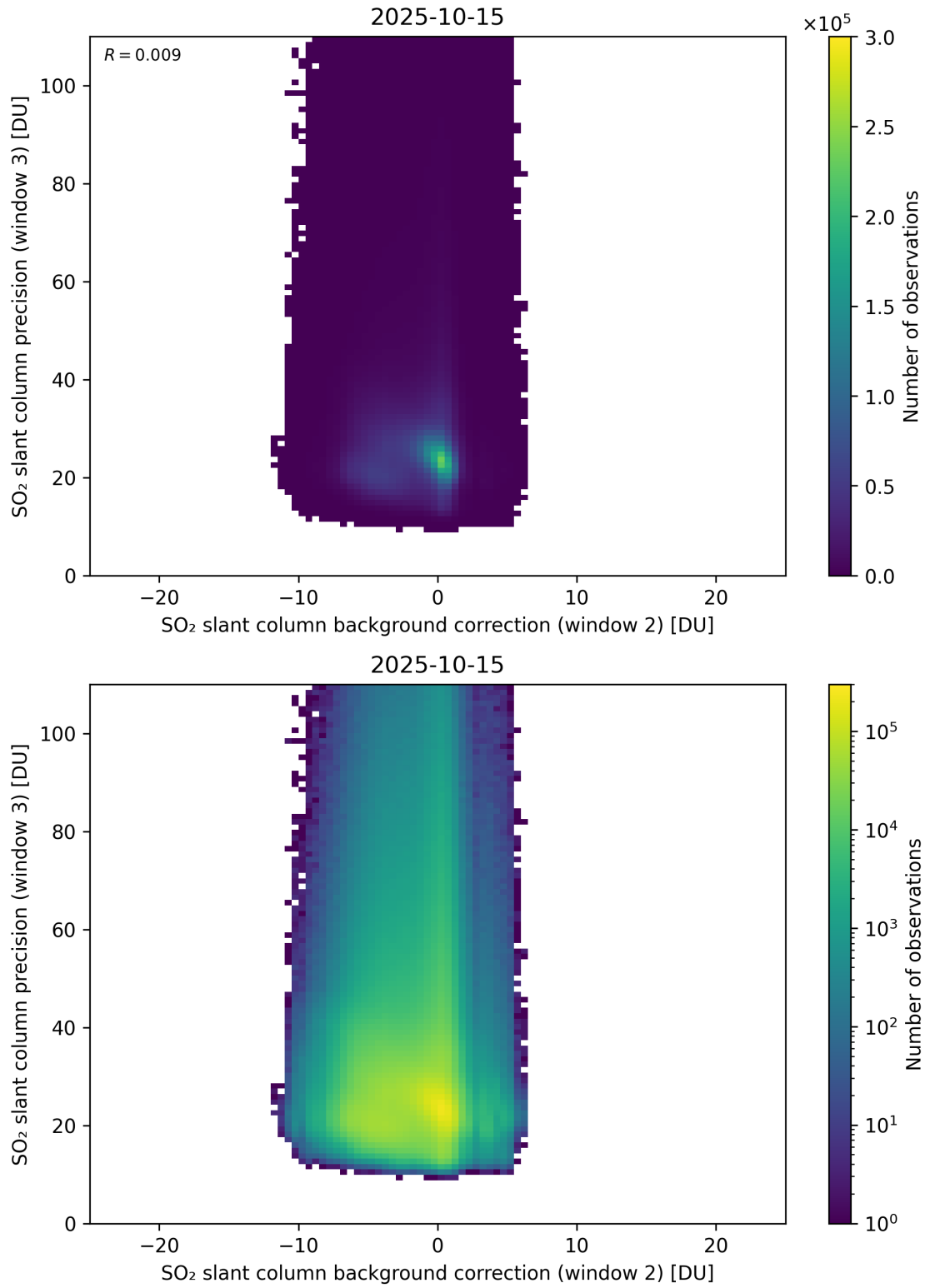
Figure 129: Scatter density plot of “SO 2 slant column background correction (window 2)” against “SO 2 slant column precision (window 3)” for 2025-10-14 to 2025-10-16.
