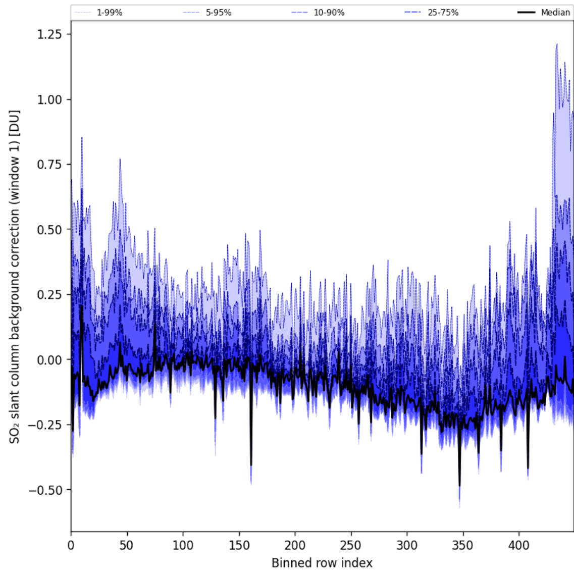
Figure 92: Along track statistics of “SO 2 slant column background correction (window 1)” for 2025-10-14 to 2025-10-16
