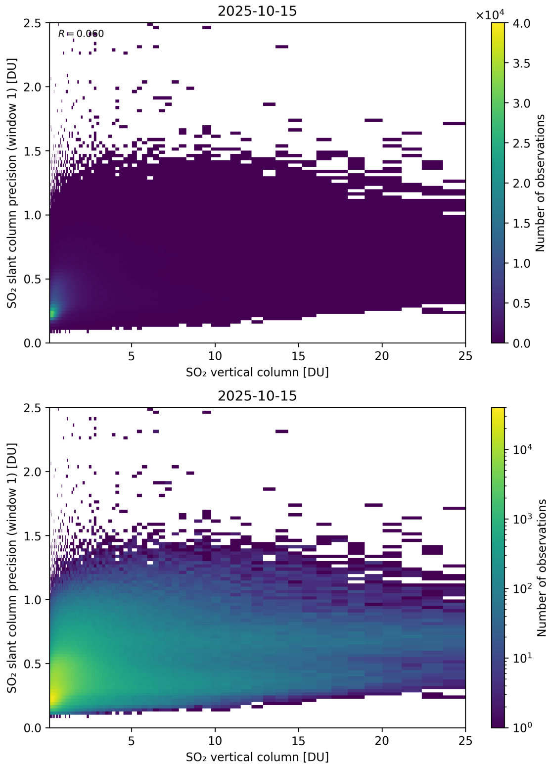
Figure 355: Scatter density plot of “SO 2 vertical column” against “SO 2 slant column precision (window 1)” for 2025-10-14 to 2025-10-16.
