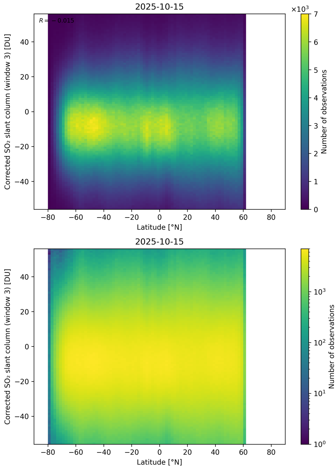
Figure 161: Scatter density plot of “Latitude” against “Corrected SO 2 slant column (window 3)” for 2025-10-14 to 2025-10-16.
