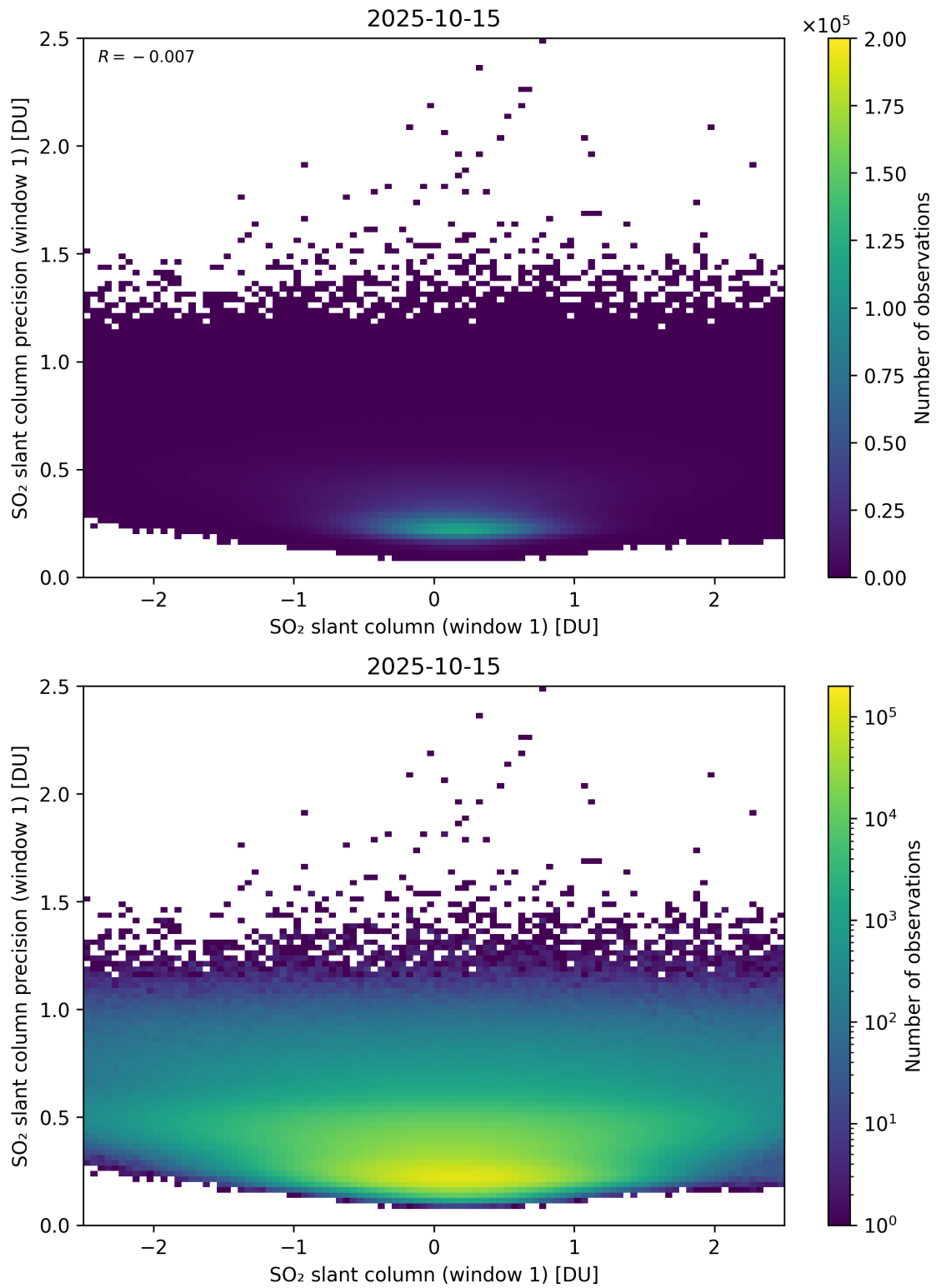
Figure 285: Scatter density plot of “SO 2 slant column (window 1)” against “SO 2 slant column precision (window 1)” for 2025-10-14 to 2025-10-16.
