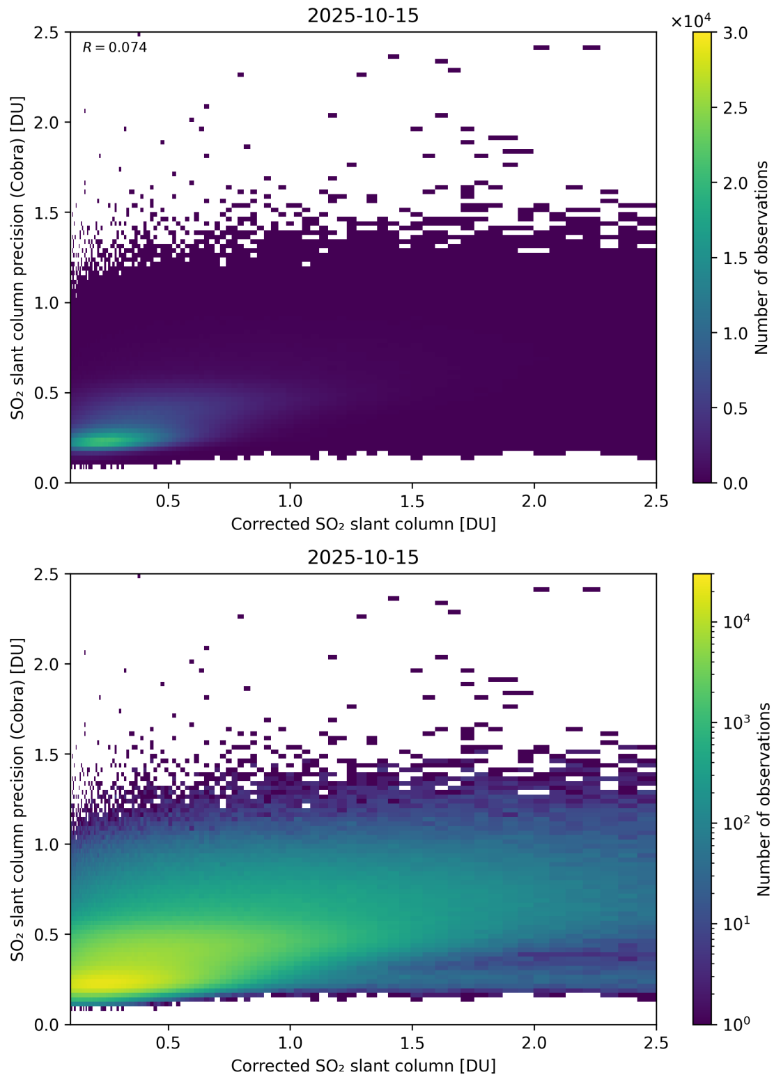
Figure 234: Scatter density plot of “Corrected SO 2 slant column” against “SO 2 slant column precision (Cobra)” for 2025-10-14 to 2025-10-16.
