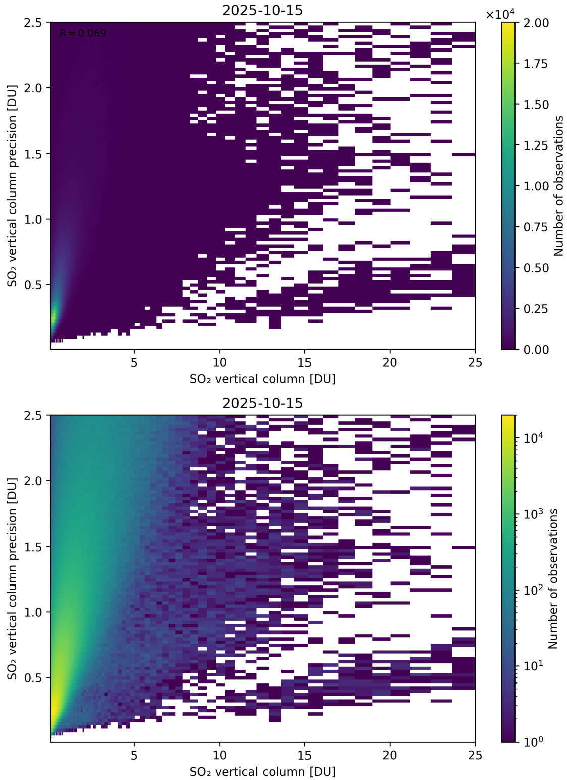
Figure 361: Scatter density plot of “SO 2 vertical column” against “SO 2 vertical column precision” for 2025-10-14 to 2025-10-16.
