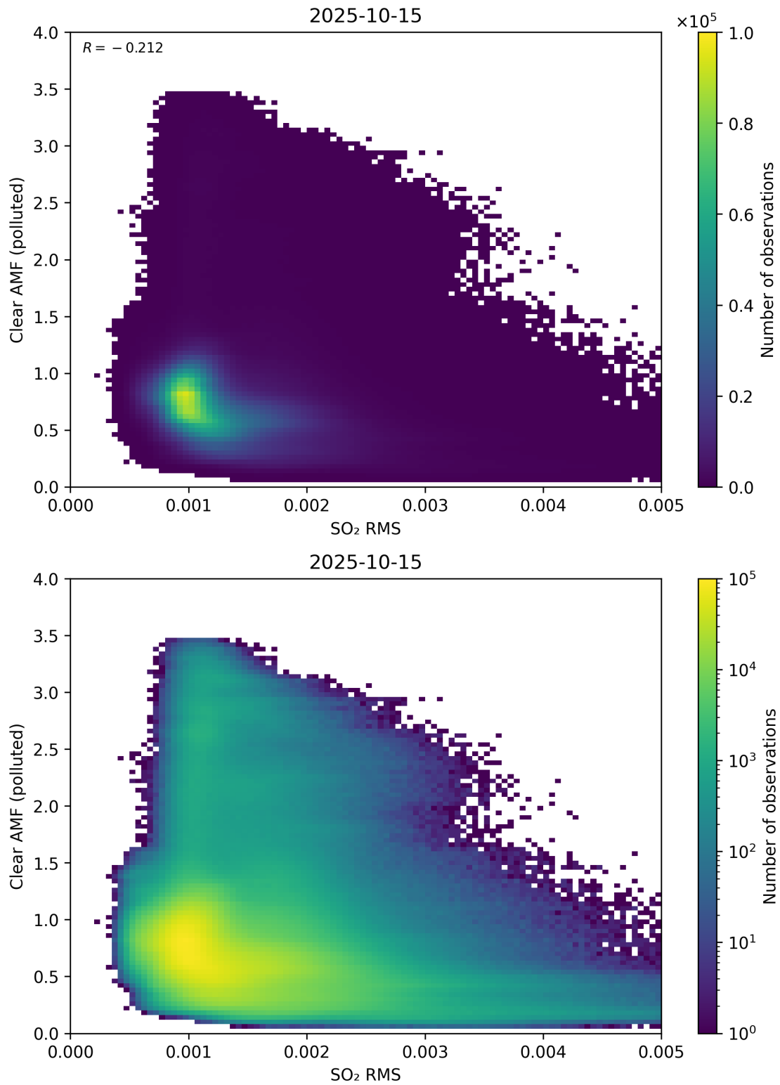
Figure 147: Scatter density plot of “SO 2 RMS” against “Clear AMF (polluted)” for 2025-10-14 to 2025-10-16.
