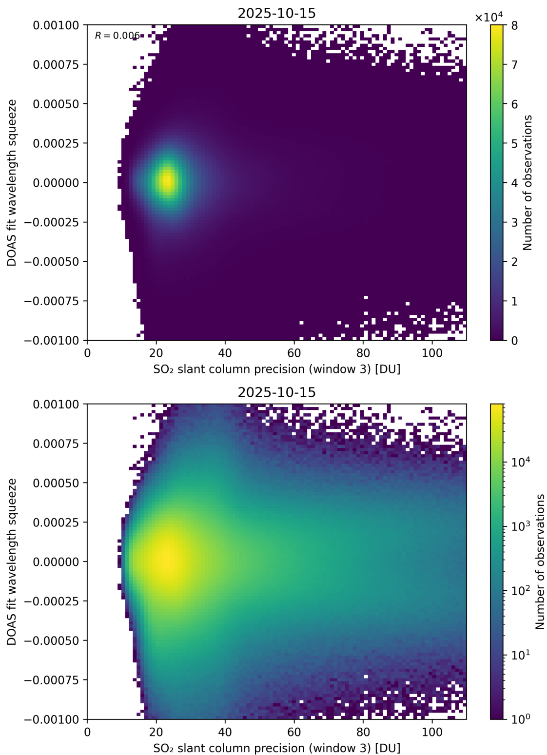
Figure 309: Scatter density plot of “SO 2 slant column precision (window 3)” against “DOAS fit wavelength squeeze” for 2025-10-14 to 2025-10-16.
