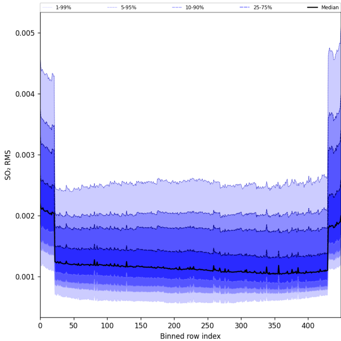
Figure 104: Along track statistics of “SO 2 RMS” for 2025-10-14 to 2025-10-16
