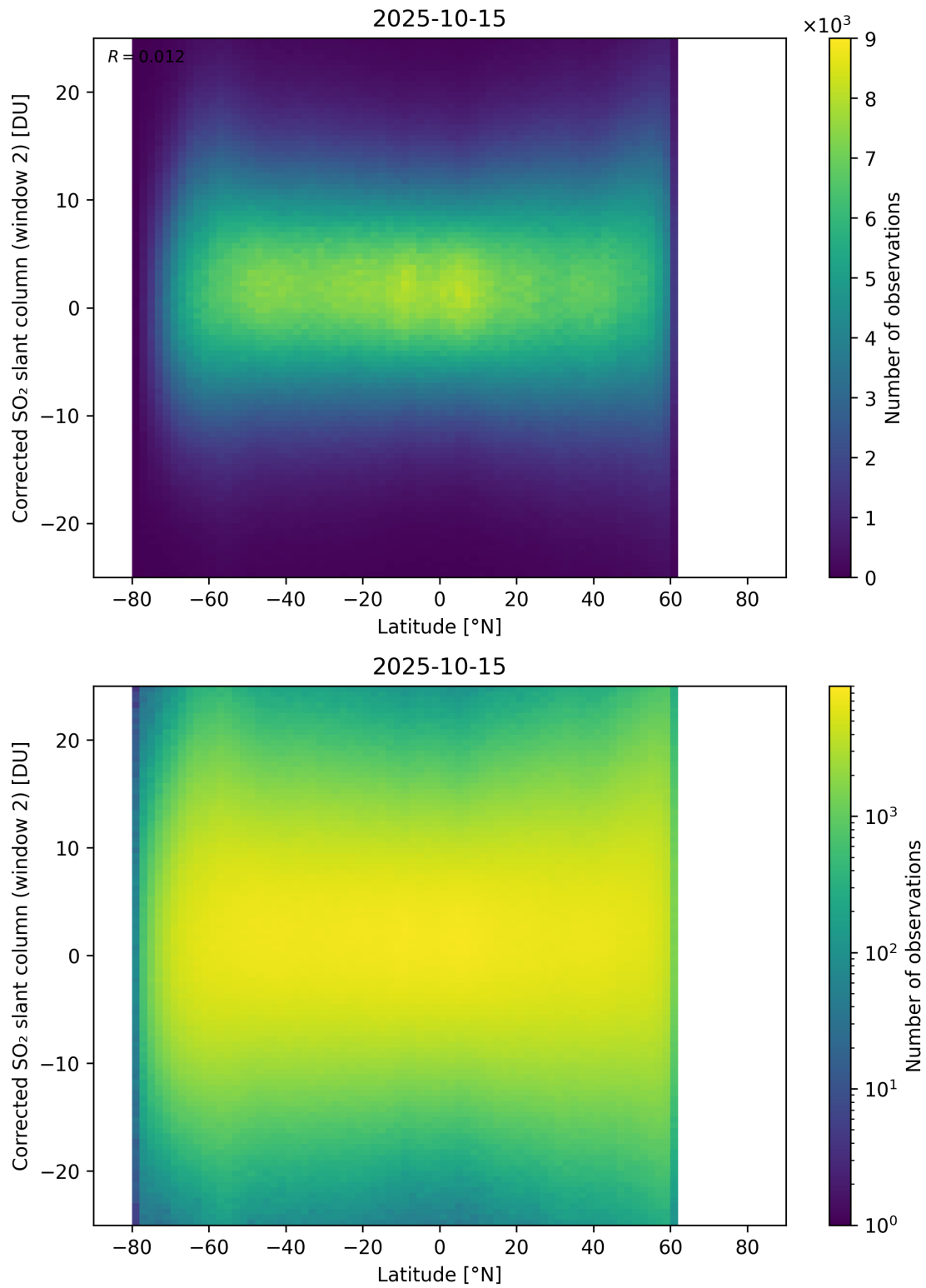
Figure 160: Scatter density plot of “Latitude” against “Corrected SO 2 slant column (window 2)” for 2025-10-14 to 2025-10-16.
