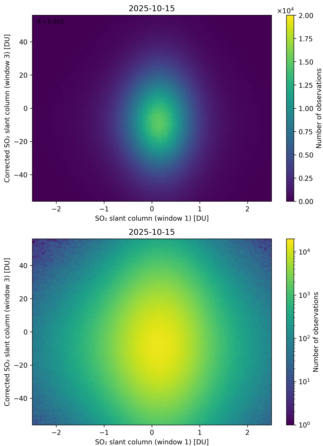
Figure 284: Scatter density plot of “SO 2 slant column (window 1)” against “Corrected SO 2 slant column (window 3)” for 2025-10-14 to 2025-10-16.
