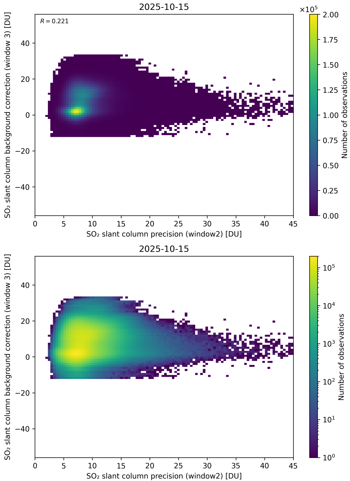
Figure 292: Scatter density plot of “SO 2 slant column precision (window2)” against “SO 2 slant column background correction (window 3)” for 2025-10-14 to 2025-10-16.
