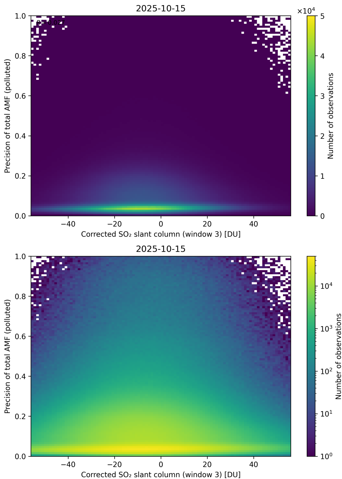
Figure 261: Scatter density plot of “Corrected SO 2 slant column (window 3)” against “Precision of total AMF (polluted)” for 2025-10-14 to 2025-10-16.
