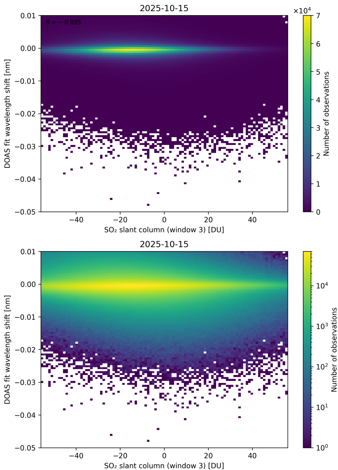
Figure 304: Scatter density plot of “SO 2 slant column (window 3)” against “DOAS fit wavelength shift” for 2025-10-14 to 2025-10-16.
