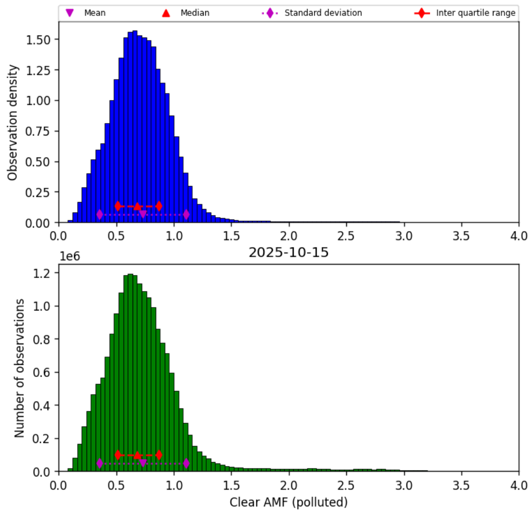
Figure 81: Histogram of “Clear AMF (polluted)” for 2025-10-14 to 2025-10-16
