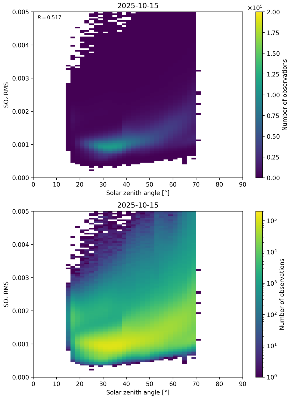
Figure 176: Scatter density plot of “Solar zenith angle” against “SO 2 RMS” for 2025-10-14 to 2025-10-16.
