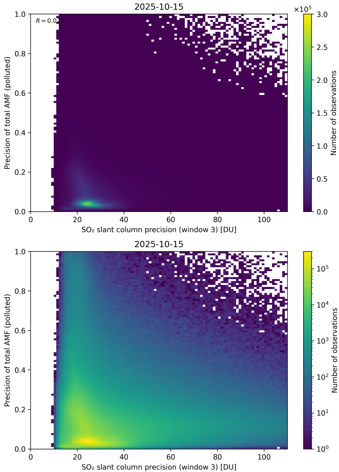
Figure 314: Scatter density plot of “SO 2 slant column precision (window 3)” against “Precision of total AMF (polluted)” for 2025-10-14 to 2025-10-16.
