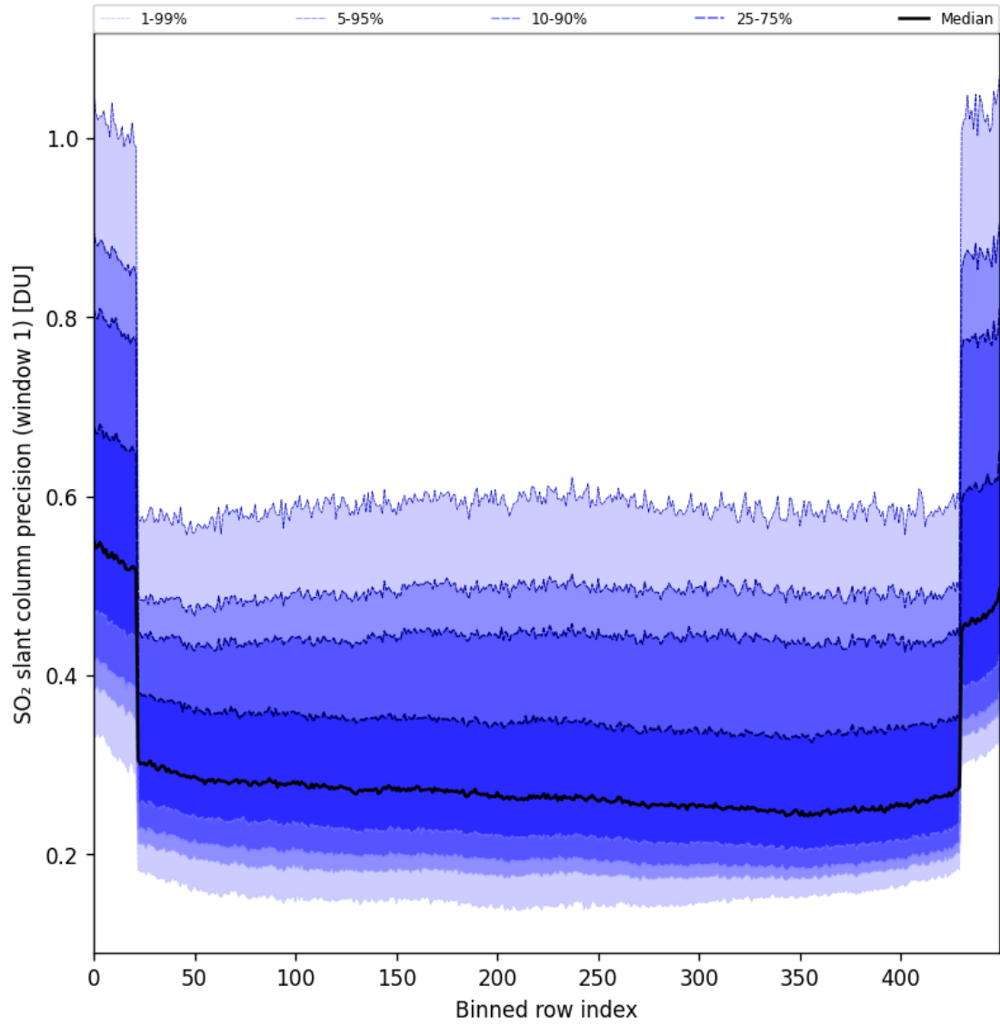
Figure 90: Along track statistics of “SO 2 slant column precision (window 1)” for 2025-10-14 to 2025-10-16
