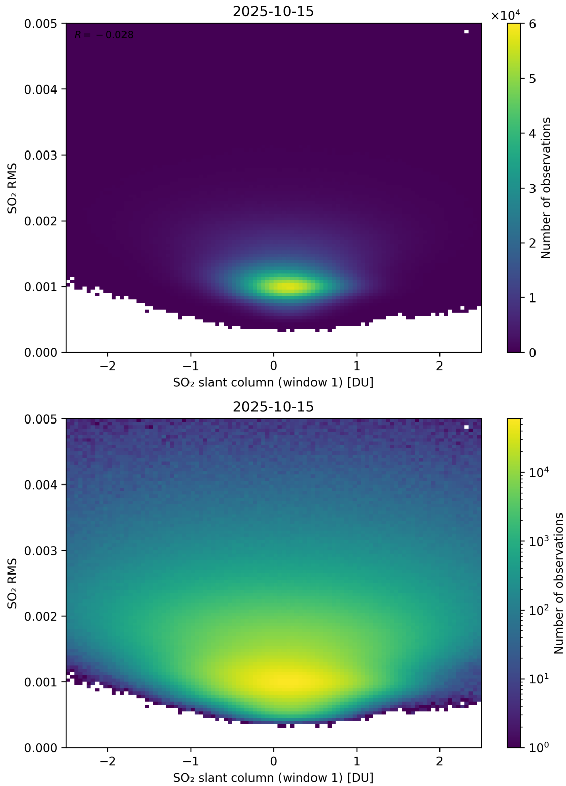
Figure 267: Scatter density plot of “SO 2 slant column (window 1)” against “SO 2 RMS” for 2025-10-14 to 2025-10-16.
