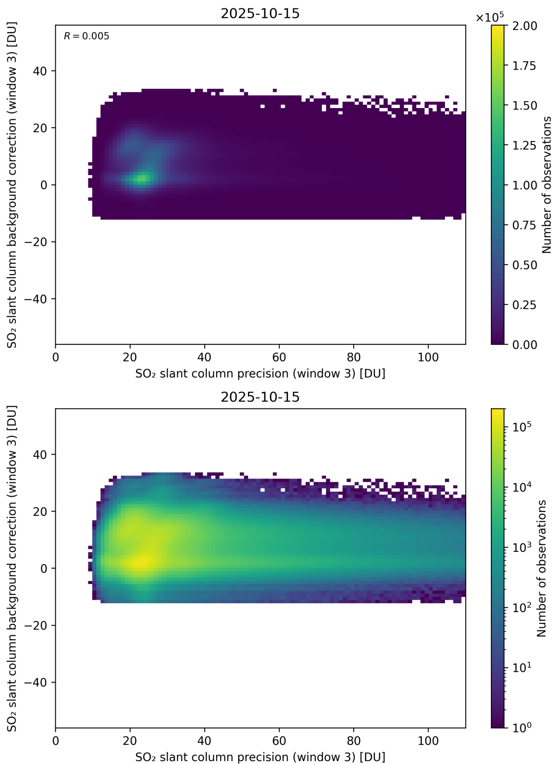
Figure 307: Scatter density plot of “SO 2 slant column precision (window 3)” against “SO 2 slant column background correction (window 3)” for 2025-10-14 to 2025-10-16.
