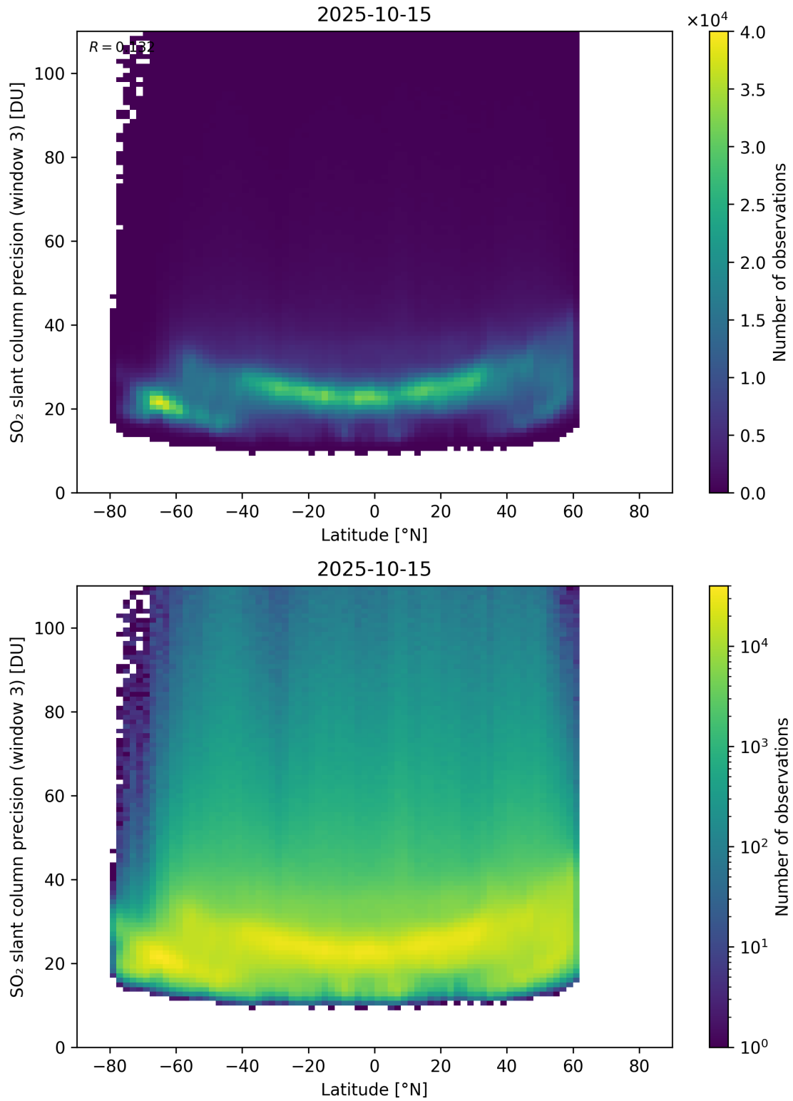
Figure 166: Scatter density plot of “Latitude” against “SO 2 slant column precision (window 3)” for 2025-10-14 to 2025-10-16.
