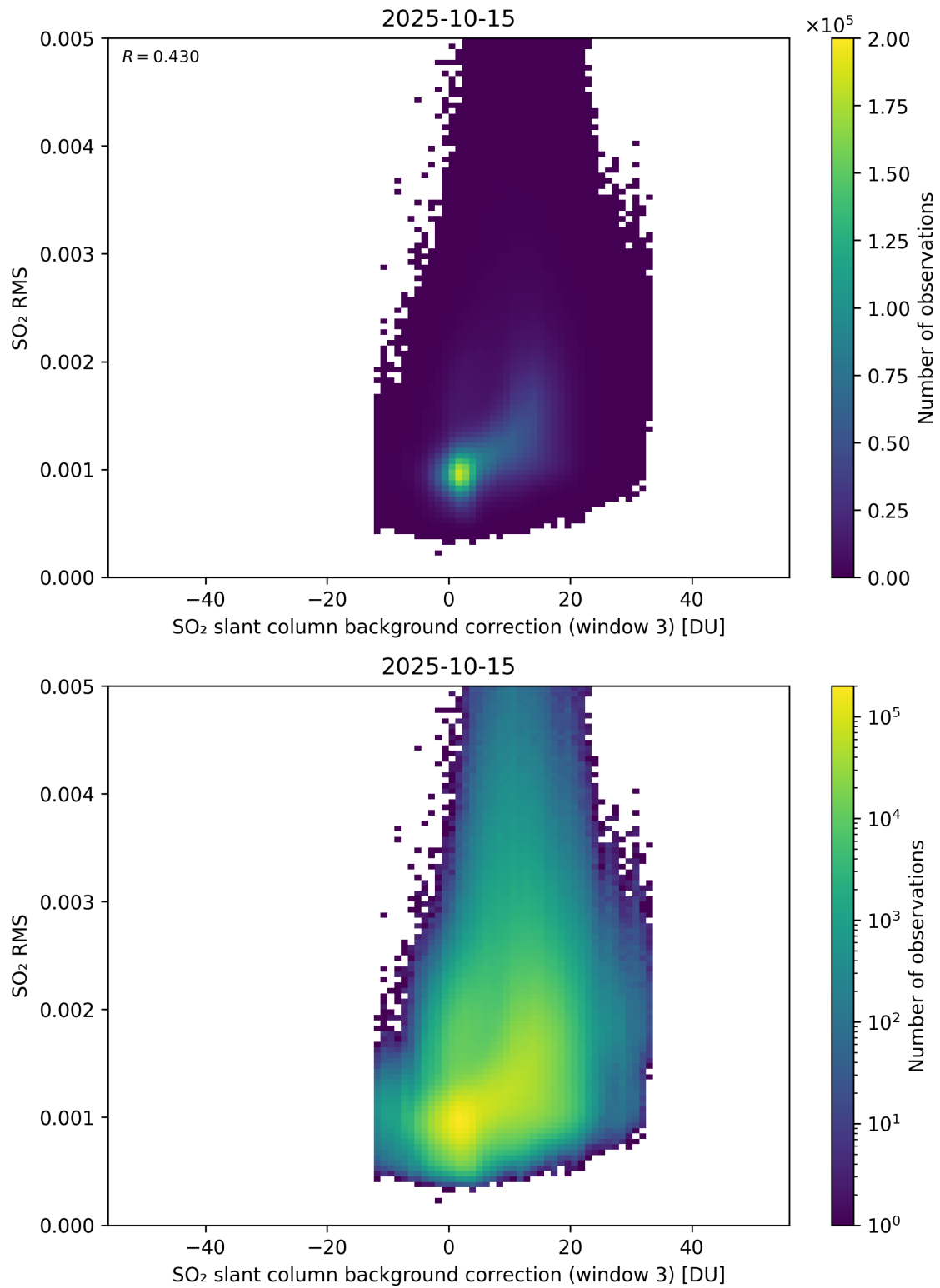
Figure 134: Scatter density plot of “SO 2 slant column background correction (window 3)” against “SO 2 RMS” for 2025-10-14 to 2025-10-16.
