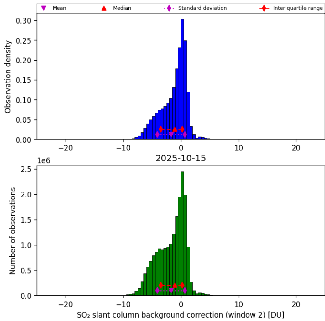
Figure 70: Histogram of “SO 2 slant column background correction (window 2)” for 2025-10-14 to 2025-10-16
