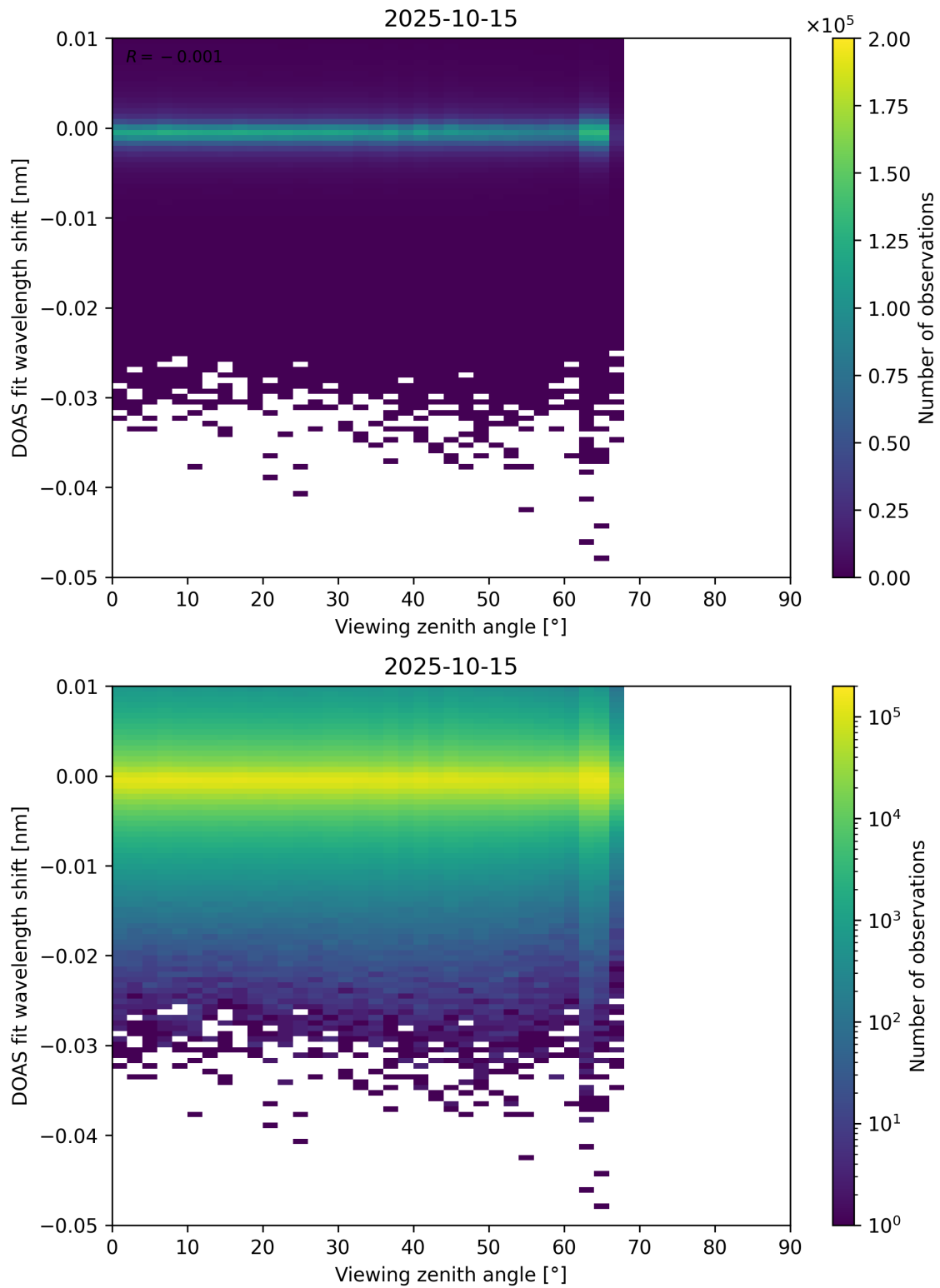
Figure 365: Scatter density plot of “Viewing zenith angle” against “DOAS fit wavelength shift” for 2025-10-14 to 2025-10-16.
