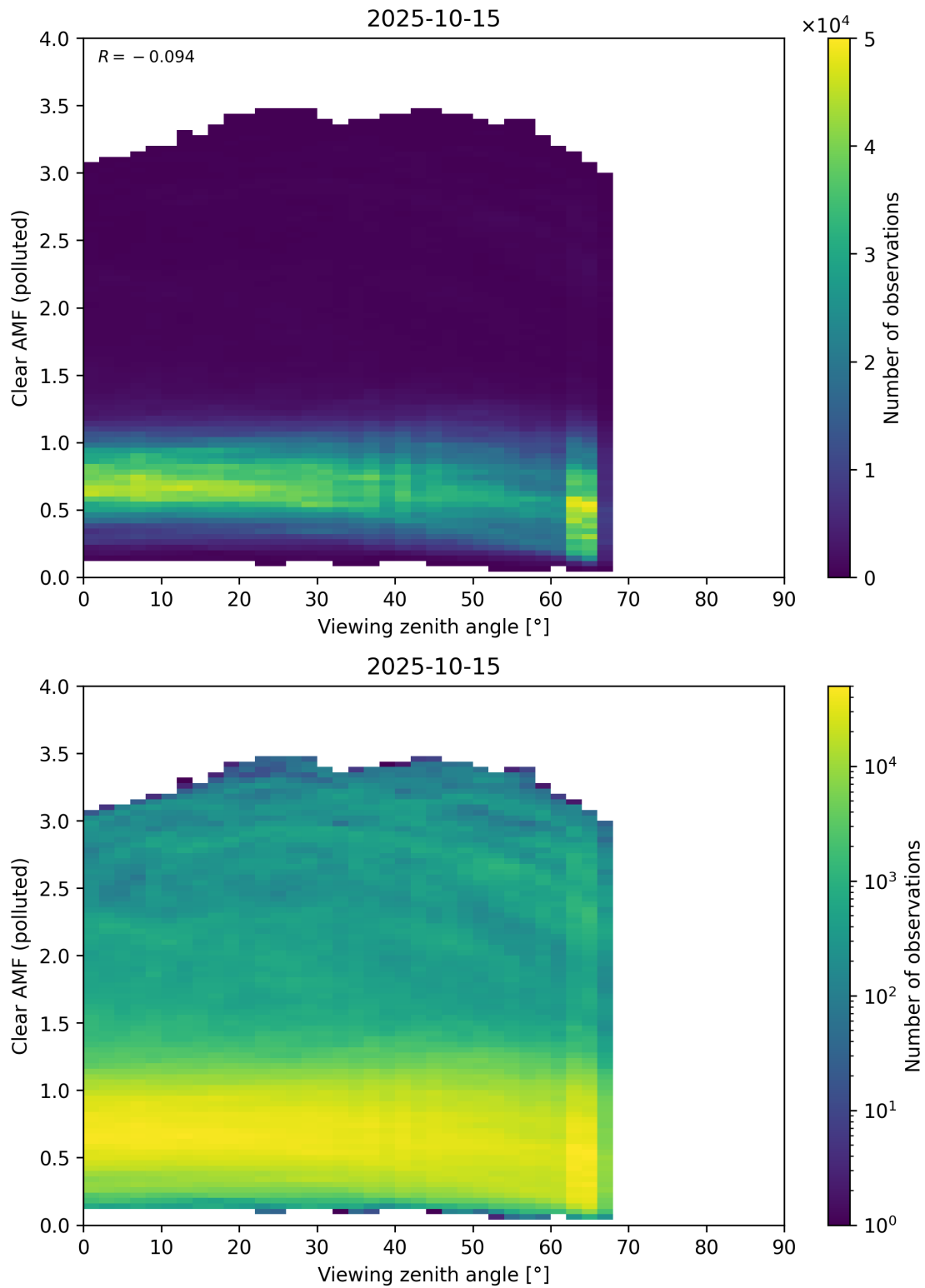
Figure 370: Scatter density plot of “Viewing zenith angle” against “Clear AMF (polluted)” for 2025-10-14 to 2025-10-16.
