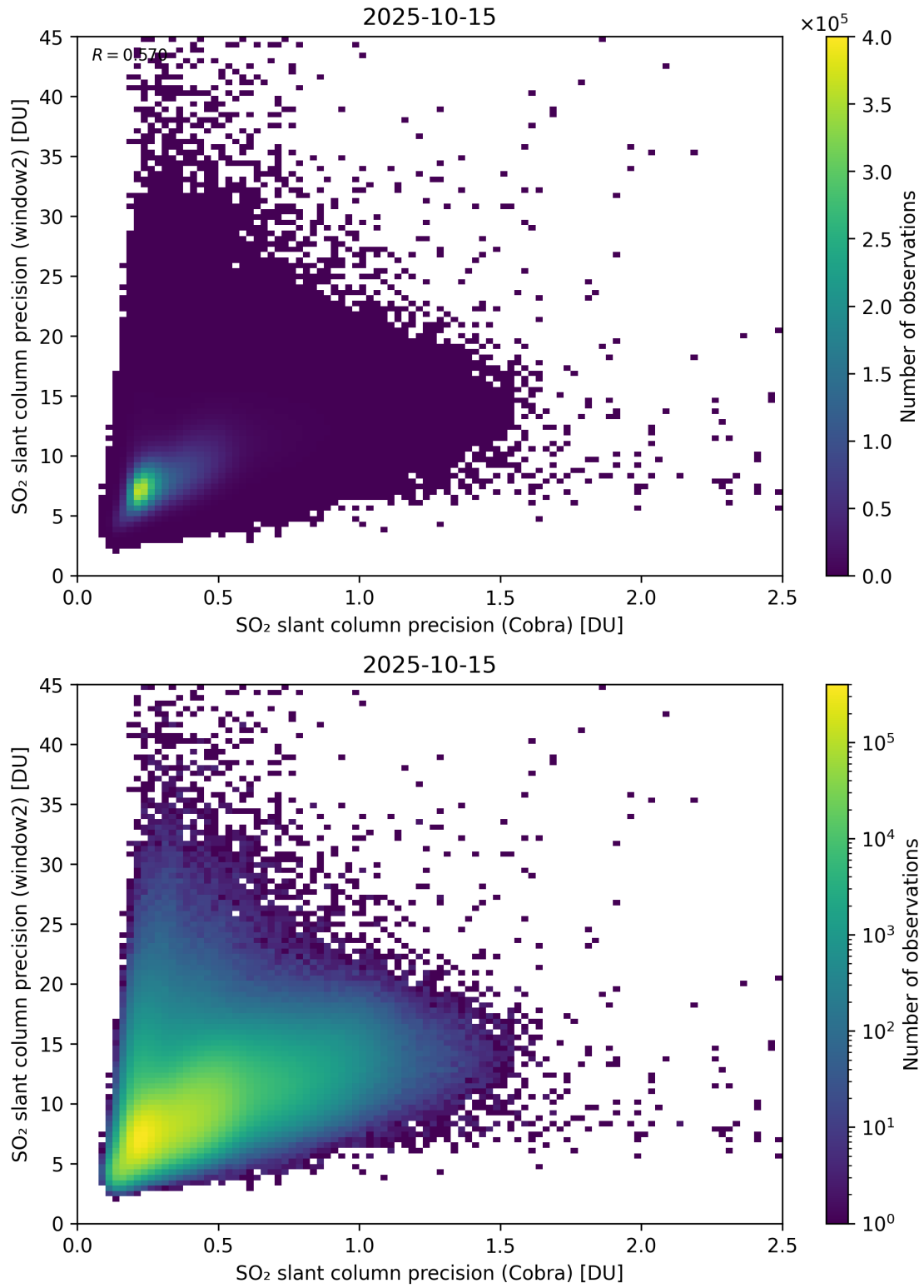
Figure 210: Scatter density plot of “SO 2 slant column precision (Cobra)” against “SO 2 slant column precision (window2)” for 2025-10-14 to 2025-10-16.
