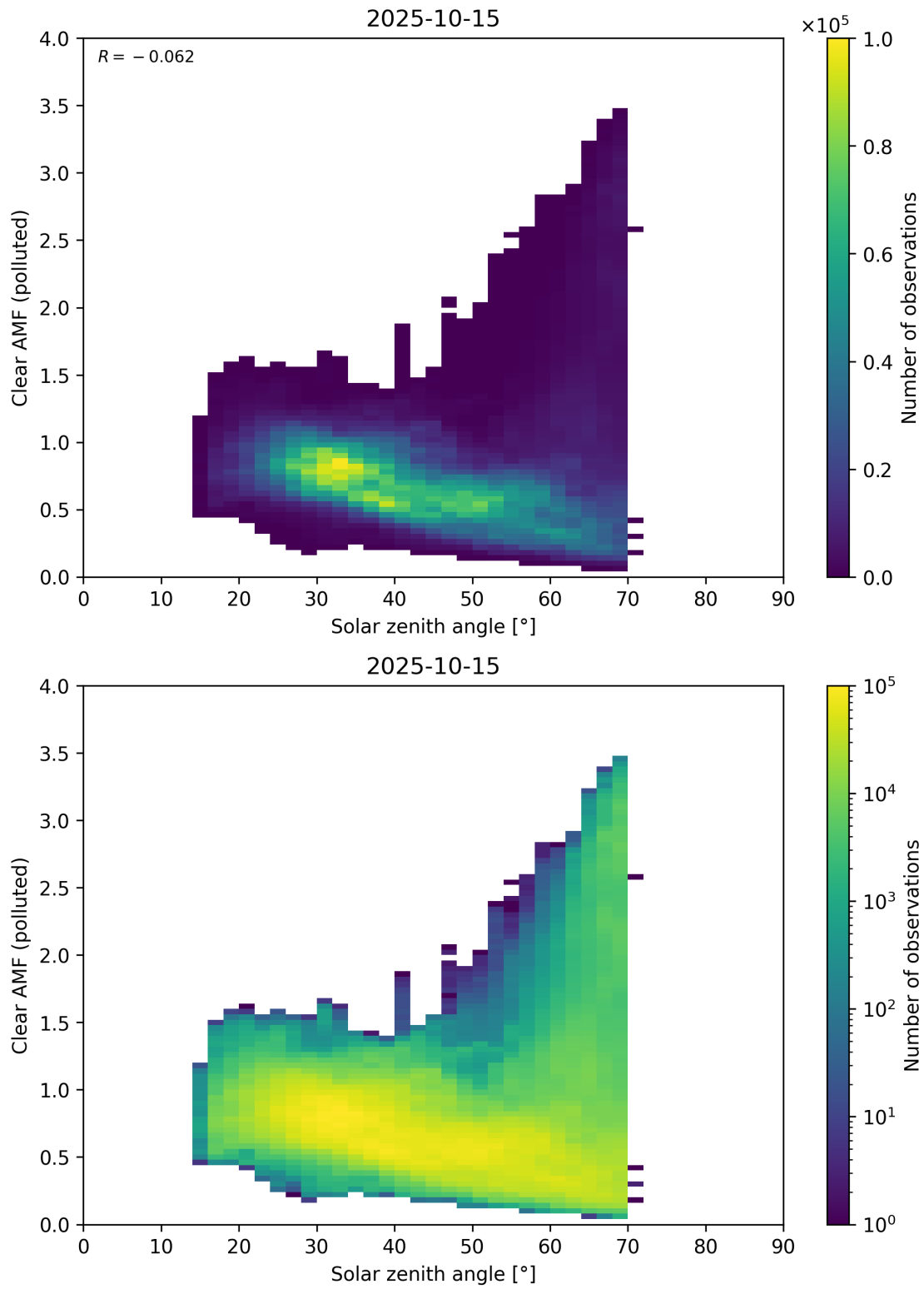
Figure 178: Scatter density plot of “Solar zenith angle” against “Clear AMF (polluted)” for 2025-10-14 to 2025-10-16.
