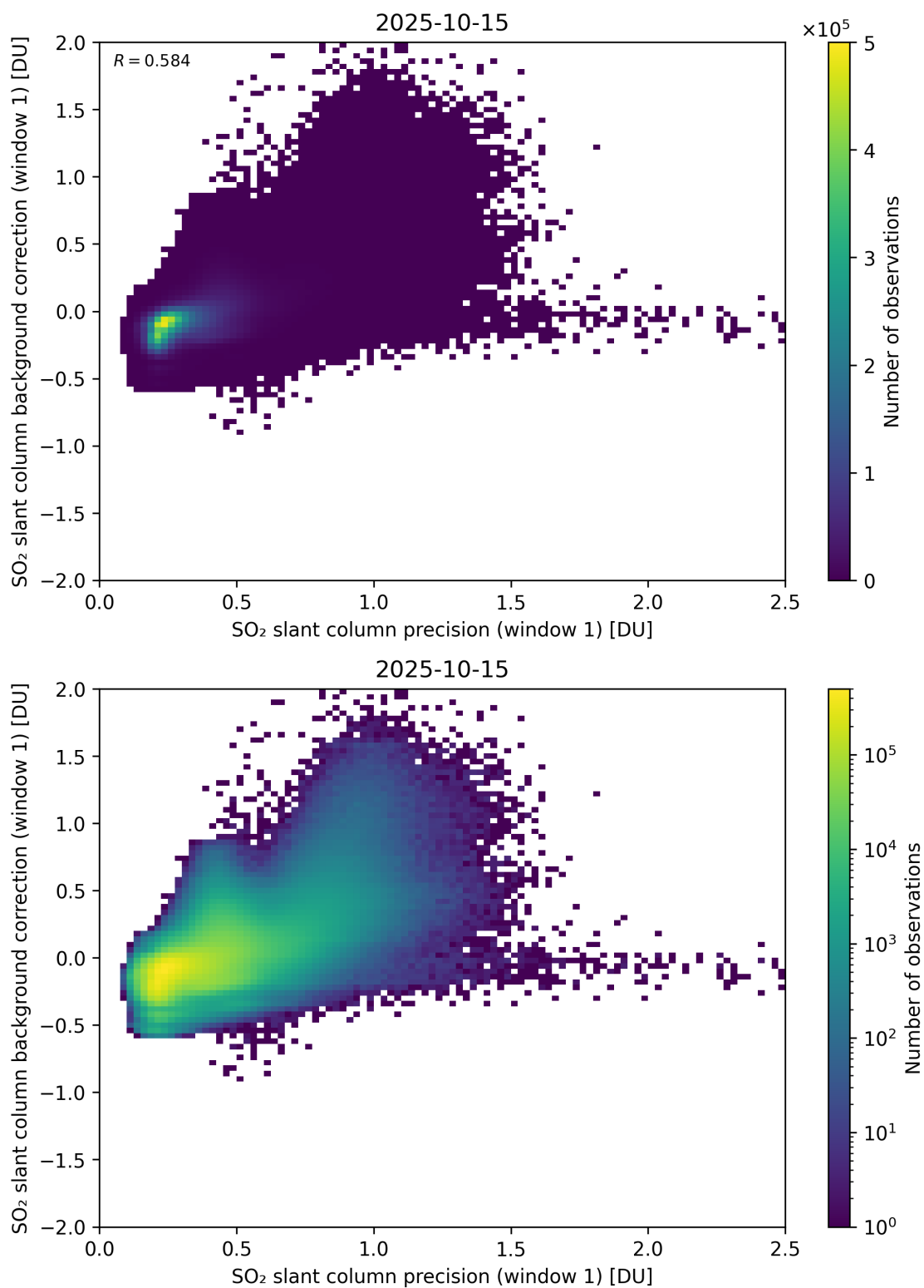
Figure 268: Scatter density plot of “SO 2 slant column precision (window 1)” against “SO 2 slant column background correction (window 1)” for 2025-10-14 to 2025-10-16.
