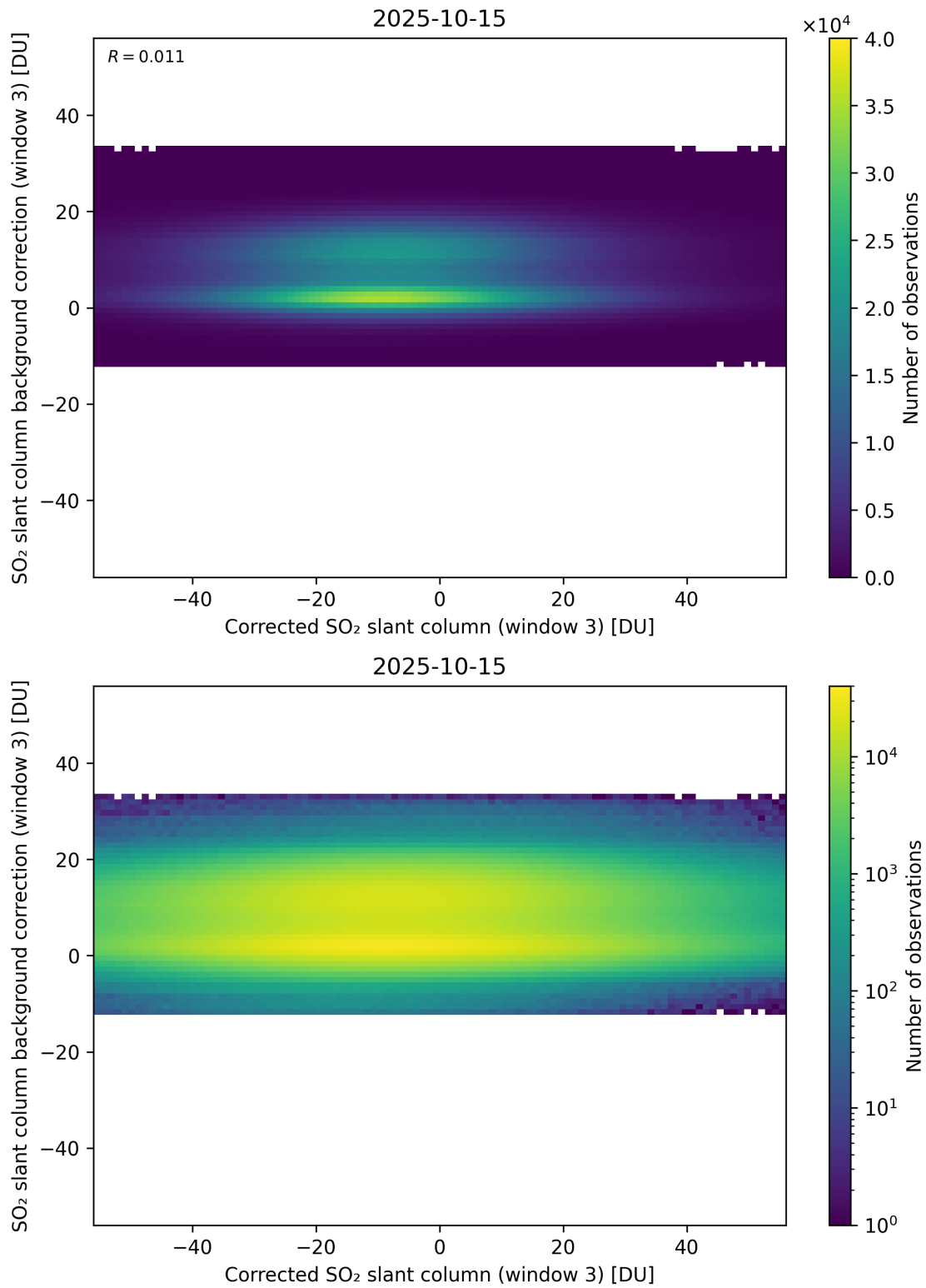
Figure 255: Scatter density plot of “Corrected SO 2 slant column (window 3)” against “SO 2 slant column background correction (window 3)” for 2025-10-14 to 2025-10-16.
