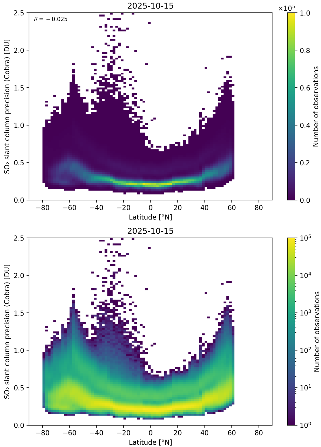
Figure 158: Scatter density plot of “Latitude” against “SO 2 slant column precision (Cobra)” for 2025-10-14 to 2025-10-16.
