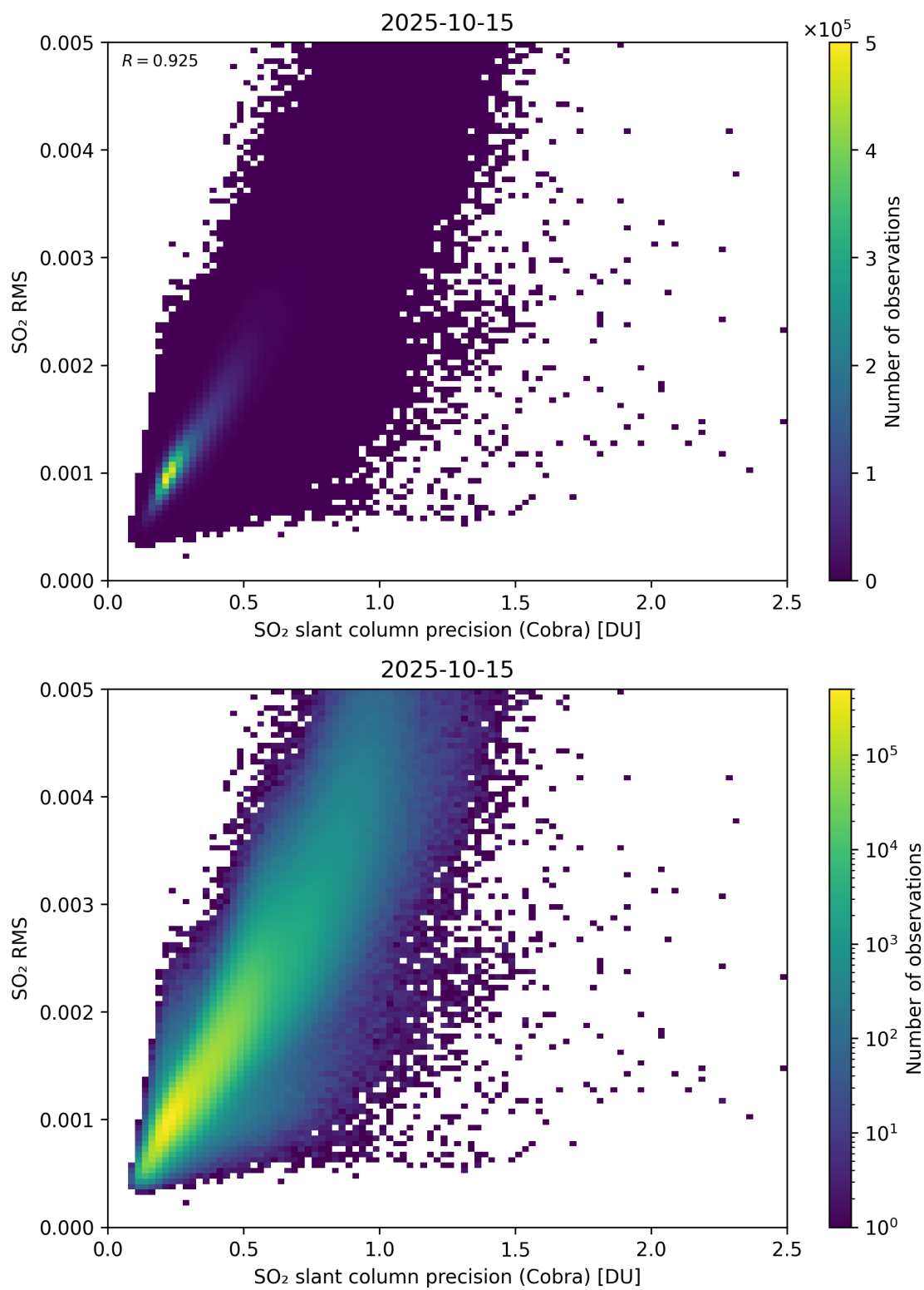
Figure 204: Scatter density plot of “SO 2 slant column precision (Cobra)” against “SO 2 RMS” for 2025-10-14 to 2025-10-16.
