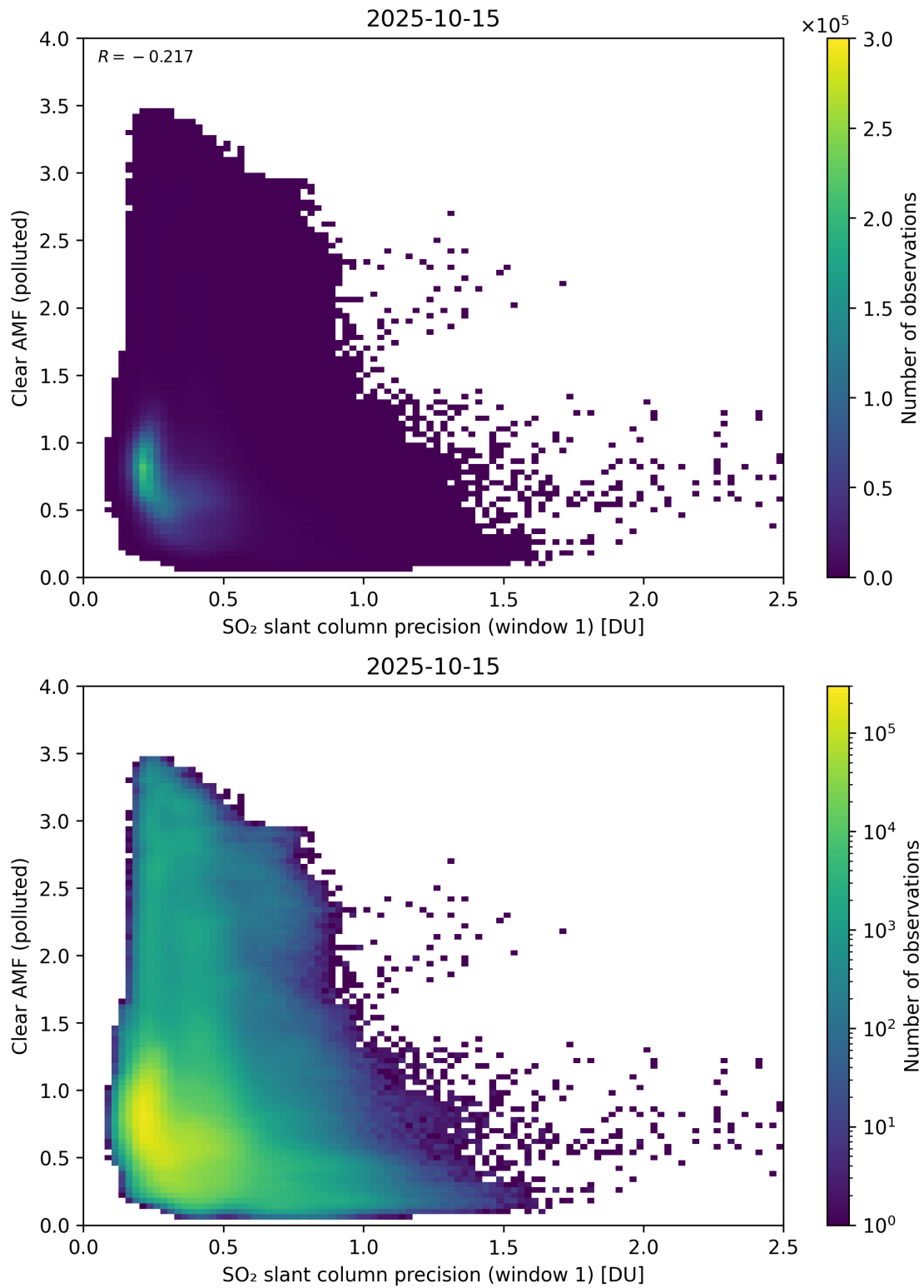
Figure 274: Scatter density plot of “SO 2 slant column precision (window 1)” against “Clear AMF (polluted)” for 2025-10-14 to 2025-10-16.
