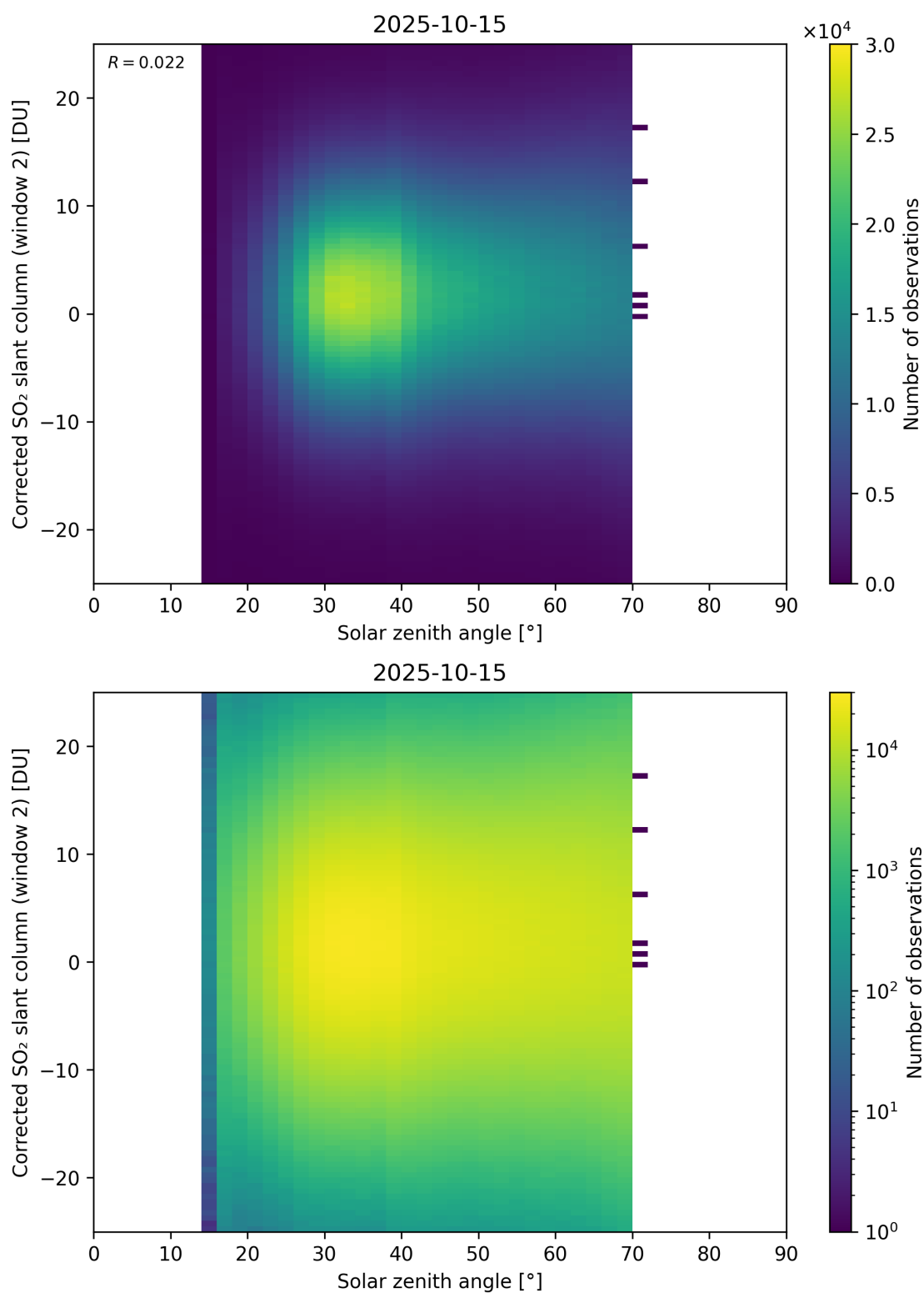
Figure 182: Scatter density plot of “Solar zenith angle” against “Corrected SO 2 slant column (window 2)” for 2025-10-14 to 2025-10-16.
