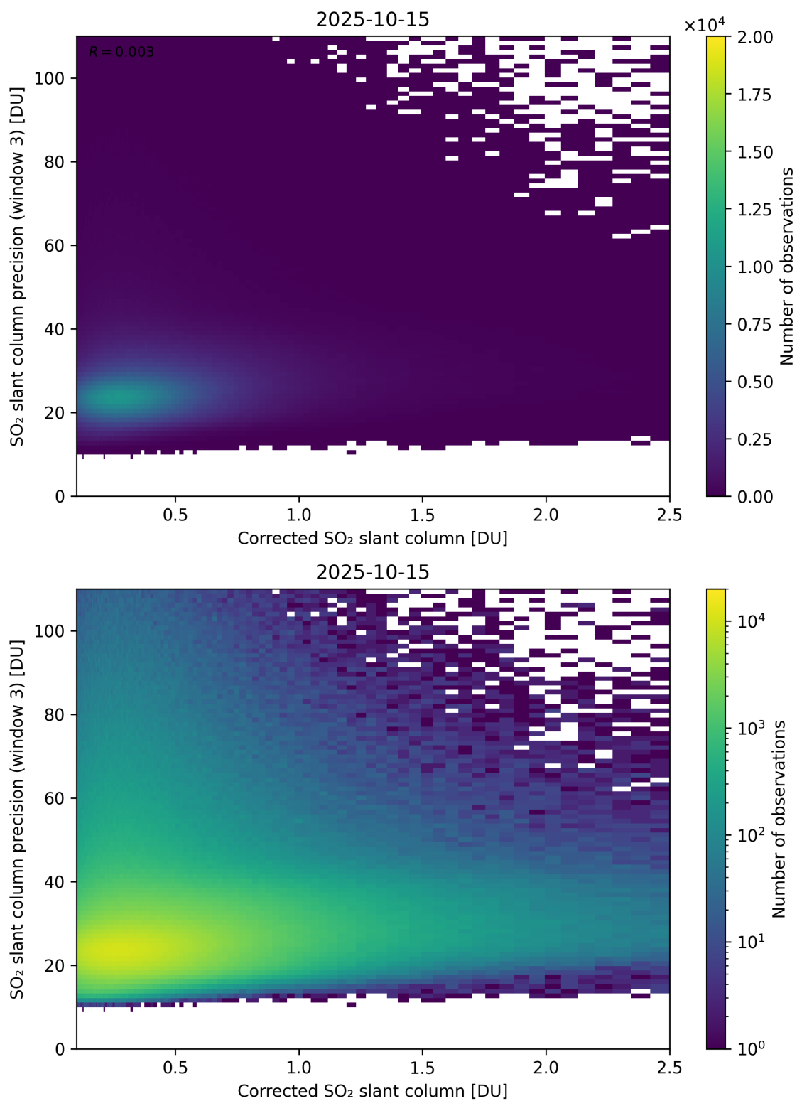
Figure 241: Scatter density plot of “Corrected SO 2 slant column” against “SO 2 slant column precision (window 3)” for 2025-10-14 to 2025-10-16.
