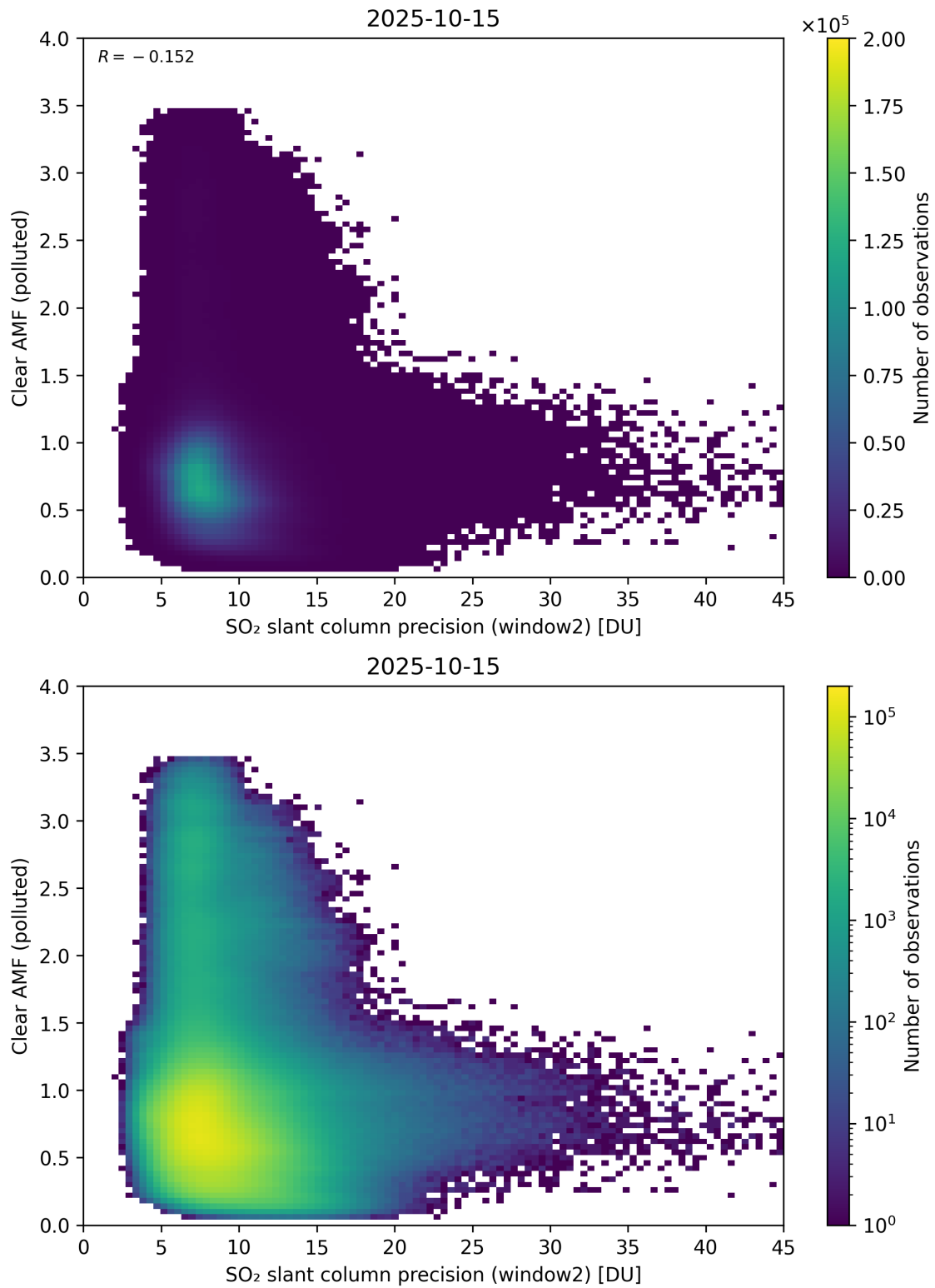
Figure 296: Scatter density plot of “SO 2 slant column precision (window2)” against “Clear AMF (polluted)” for 2025-10-14 to 2025-10-16.
