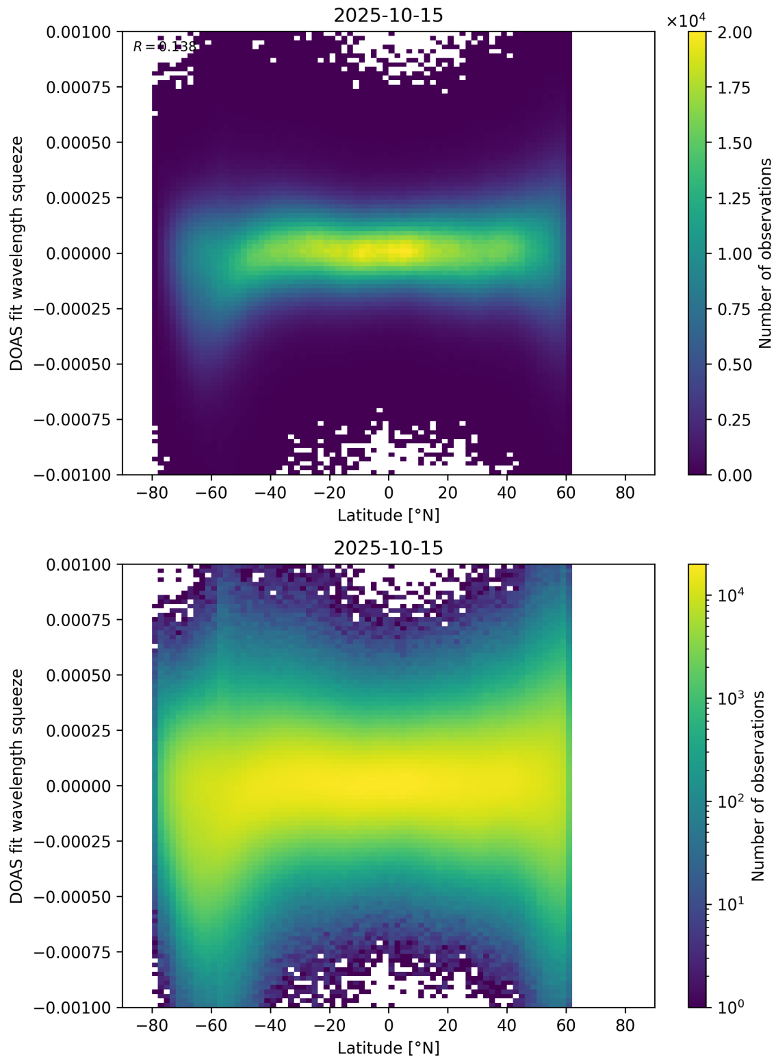
Figure 154: Scatter density plot of “Latitude” against “DOAS fit wavelength squeeze” for 2025-10-14 to 2025-10-16.
