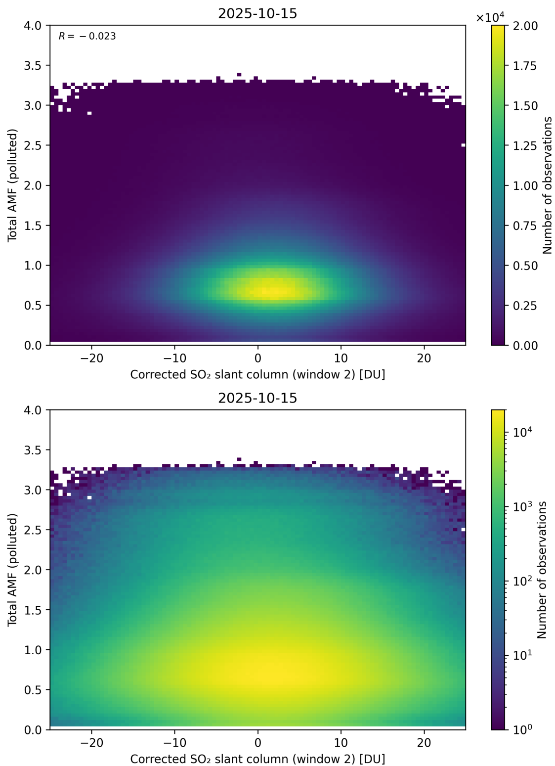
Figure 253: Scatter density plot of “Corrected SO 2 slant column (window 2)” against “Total AMF (polluted)” for 2025-10-14 to 2025-10-16.
