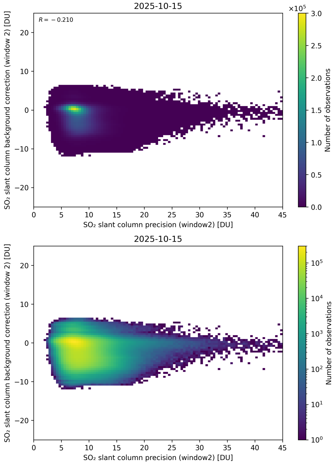
Figure 291: Scatter density plot of “SO 2 slant column precision (window2)” against “SO 2 slant column background correction (window 2)” for 2025-10-14 to 2025-10-16.
