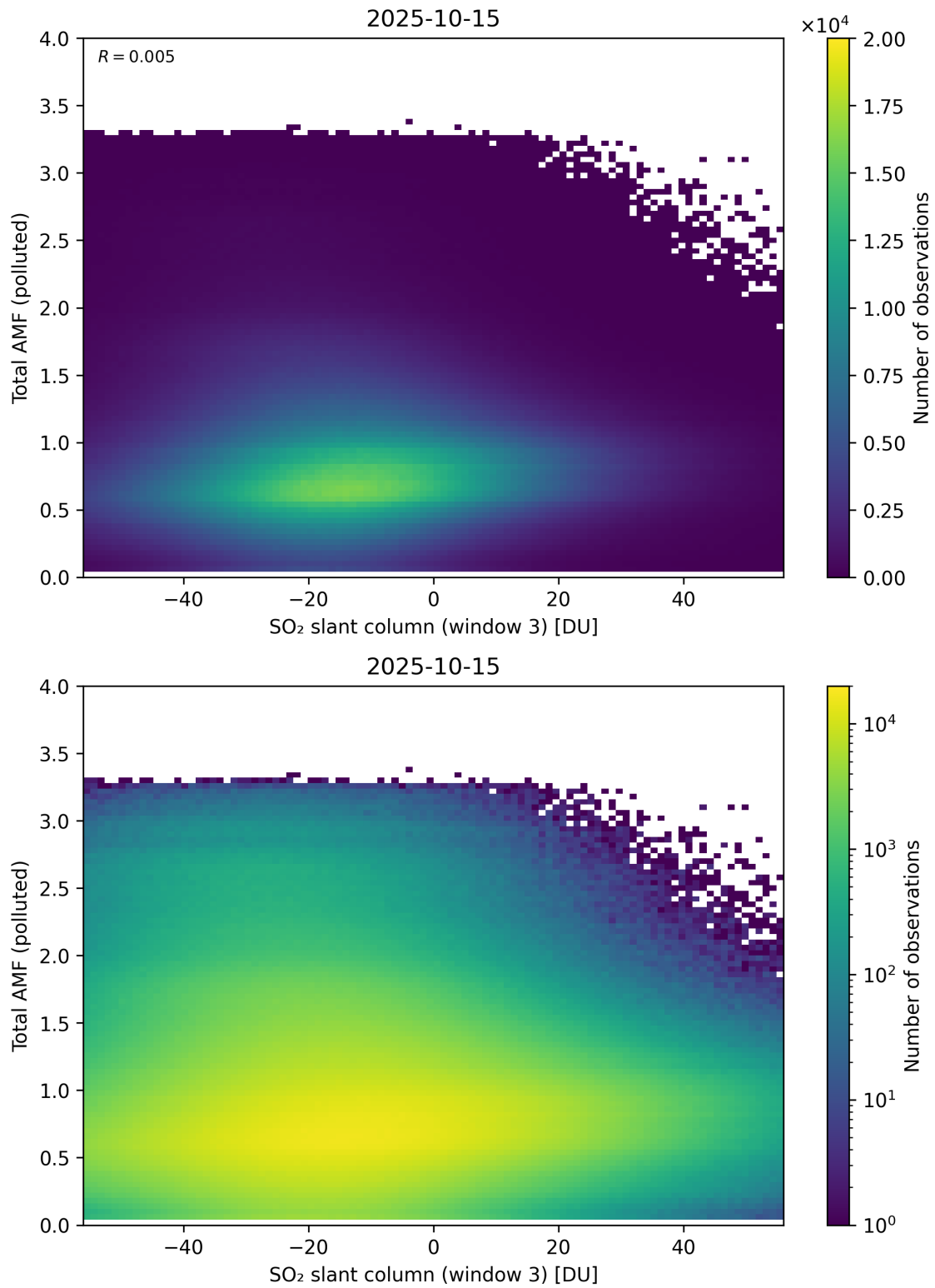
Figure 318: Scatter density plot of “SO 2 slant column (window 3)” against “Total AMF (polluted)” for 2025-10-14 to 2025-10-16.
