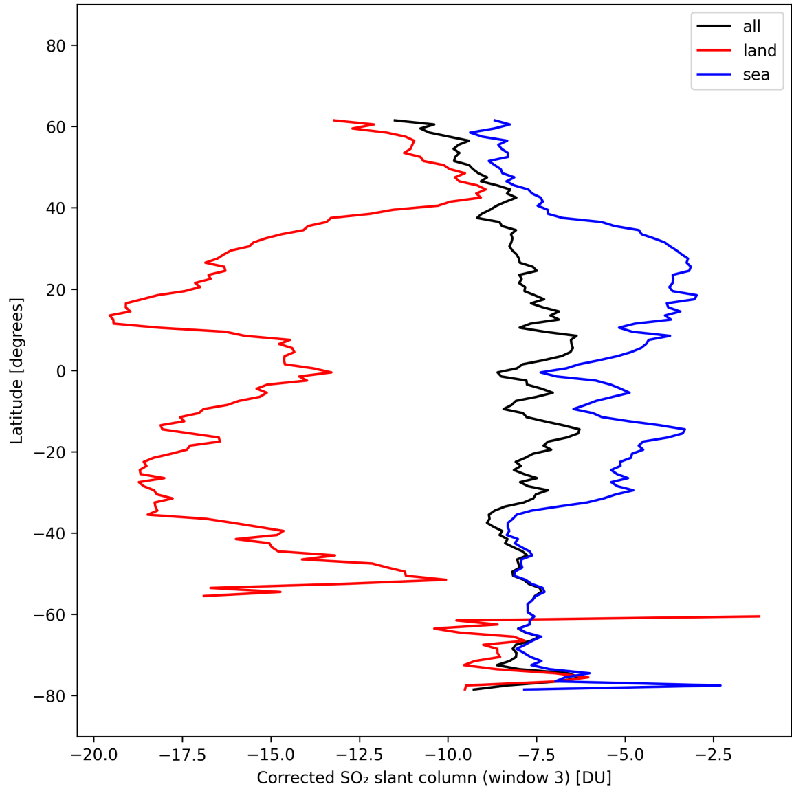
Figure 47: Zonal average of “Corrected SO 2 slant column (window 3)” for 2025-10-14 to 2025-10-16.
