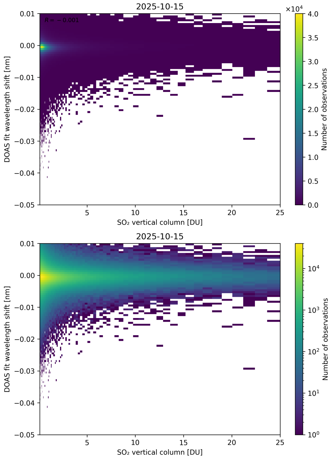
Figure 326: Scatter density plot of “SO 2 vertical column” against “DOAS fit wavelength shift” for 2025-10-14 to 2025-10-16.
