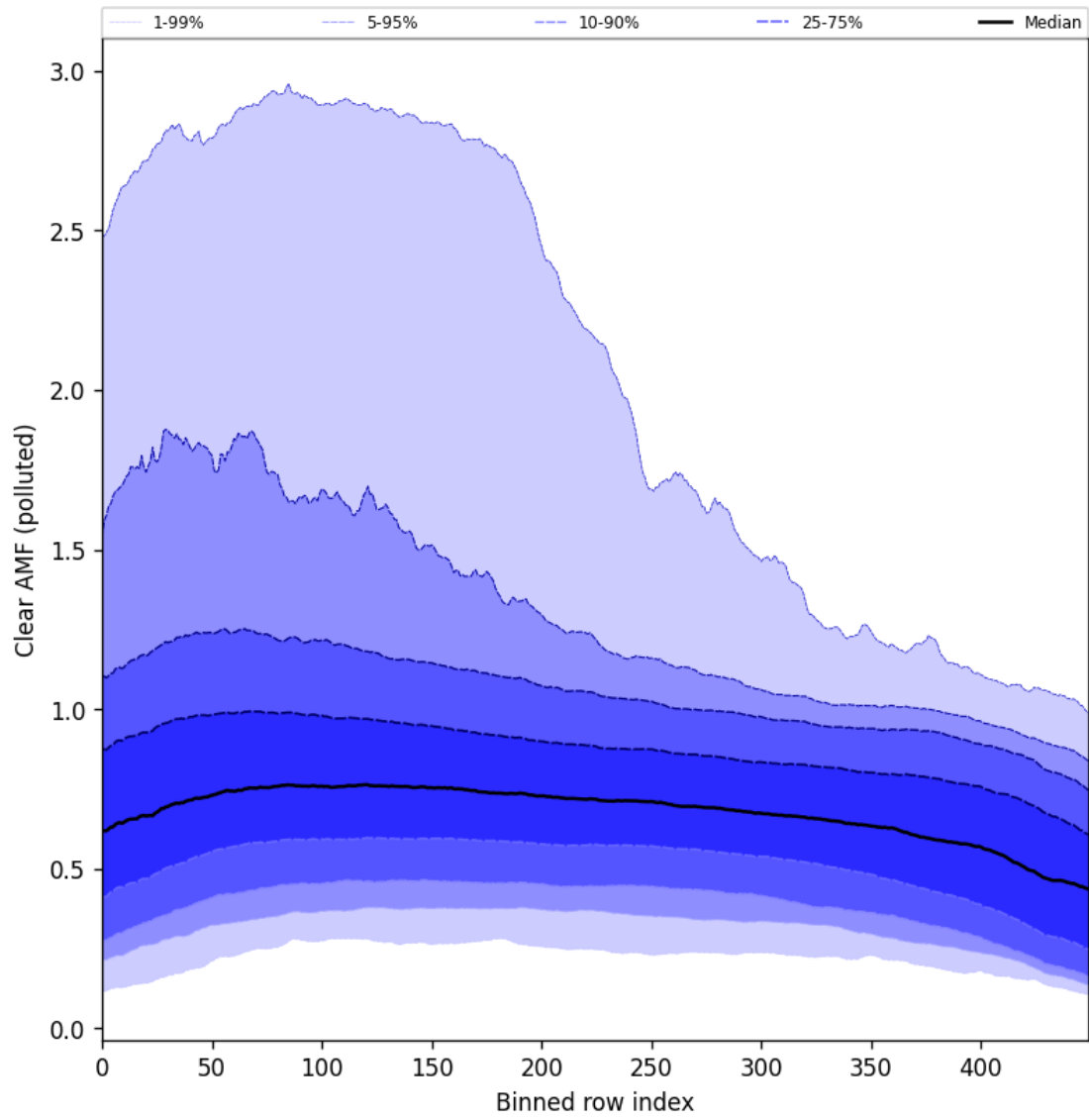
Figure 107: Along track statistics of “Clear AMF (polluted)” for 2025-10-14 to 2025-10-16
