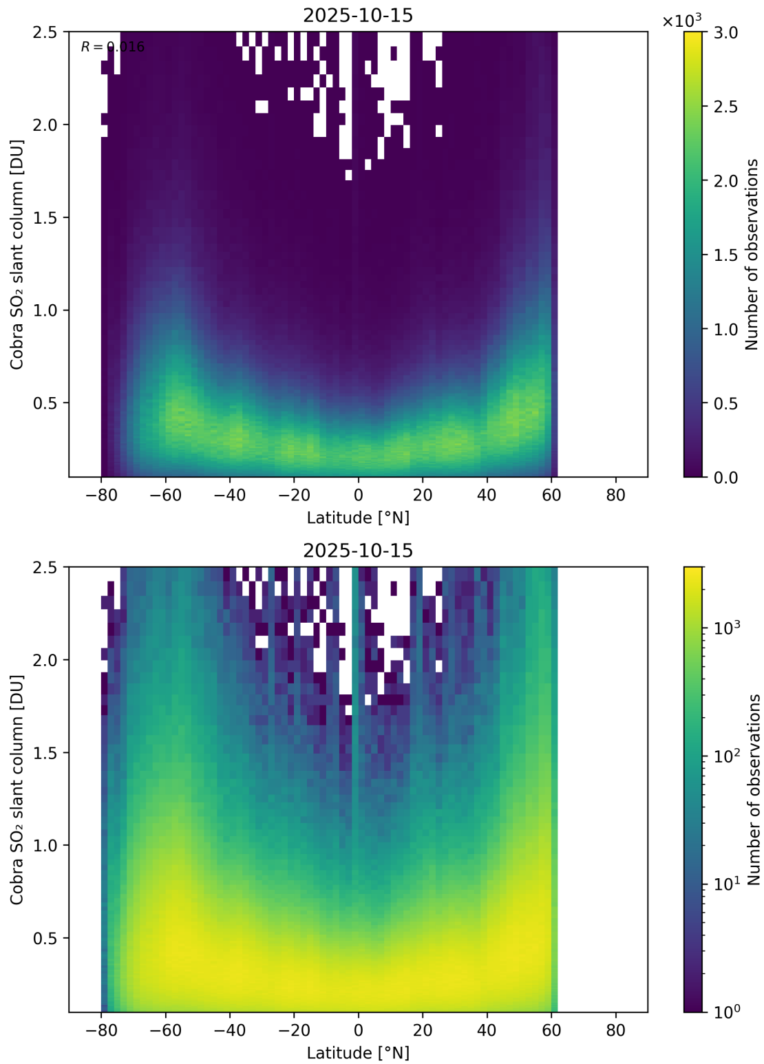
Figure 157: Scatter density plot of “Latitude” against “Cobra SO 2 slant column” for 2025-10-14 to 2025-10-16.
