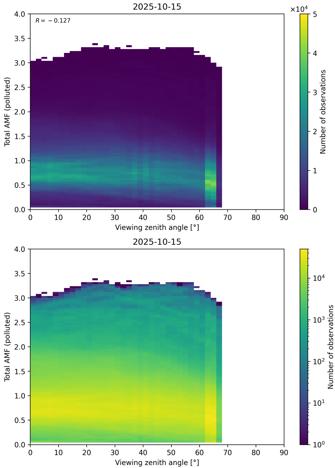
Figure 381: Scatter density plot of “Viewing zenith angle” against “Total AMF (polluted)” for 2025-10-14 to 2025-10-16.
