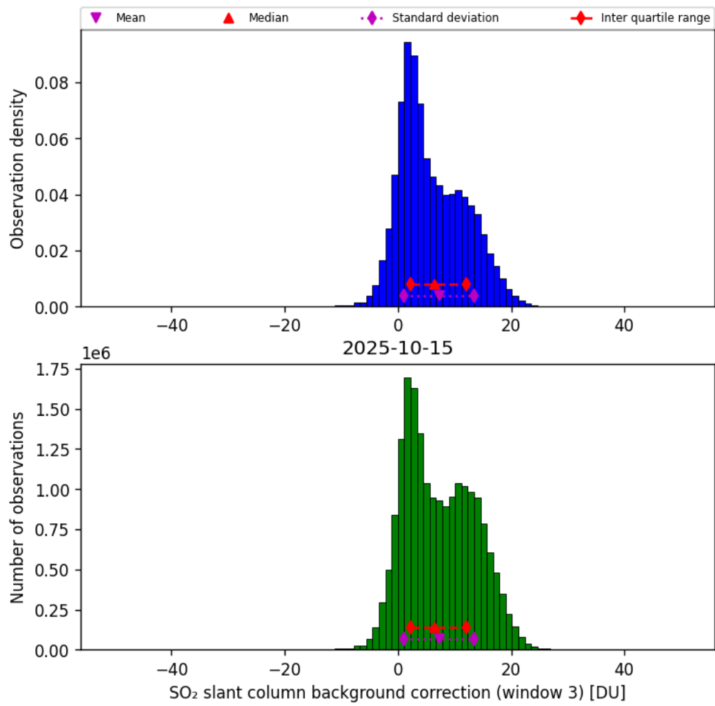
Figure 74: Histogram of “SO 2 slant column background correction (window 3)” for 2025-10-14 to 2025-10-16
