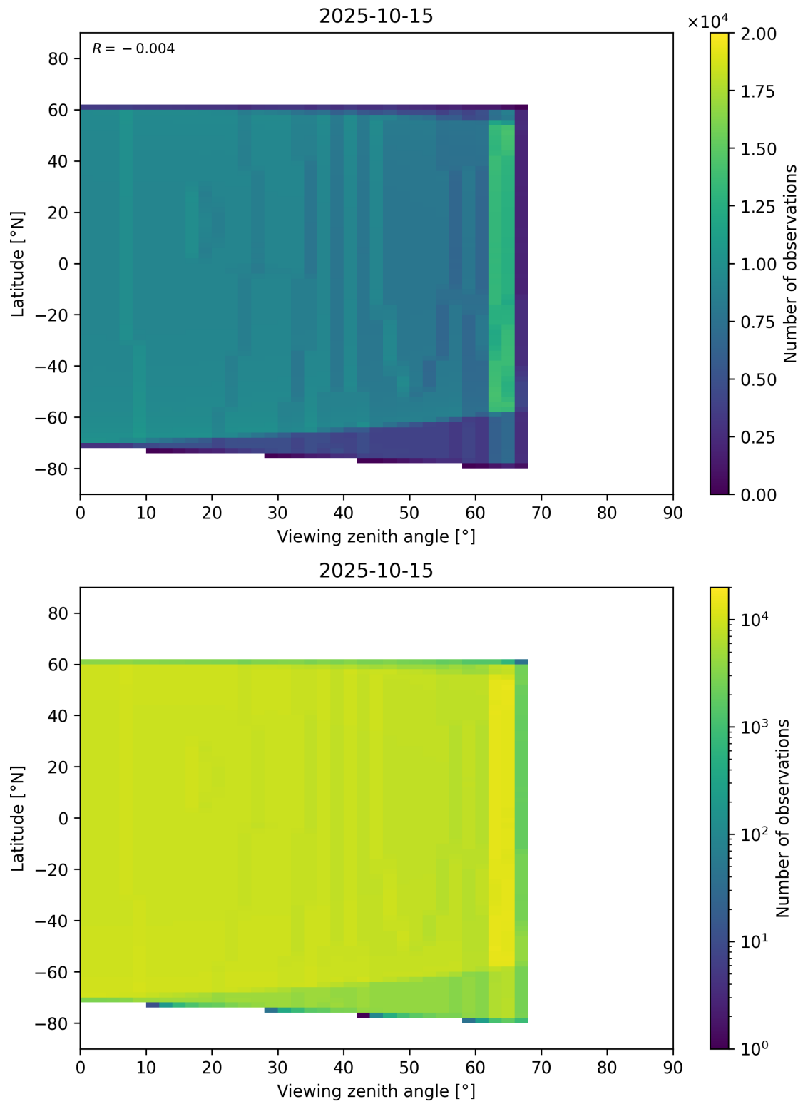
Figure 368: Scatter density plot of “Viewing zenith angle” against “Latitude” for 2025-10-14 to 2025-10-16.
