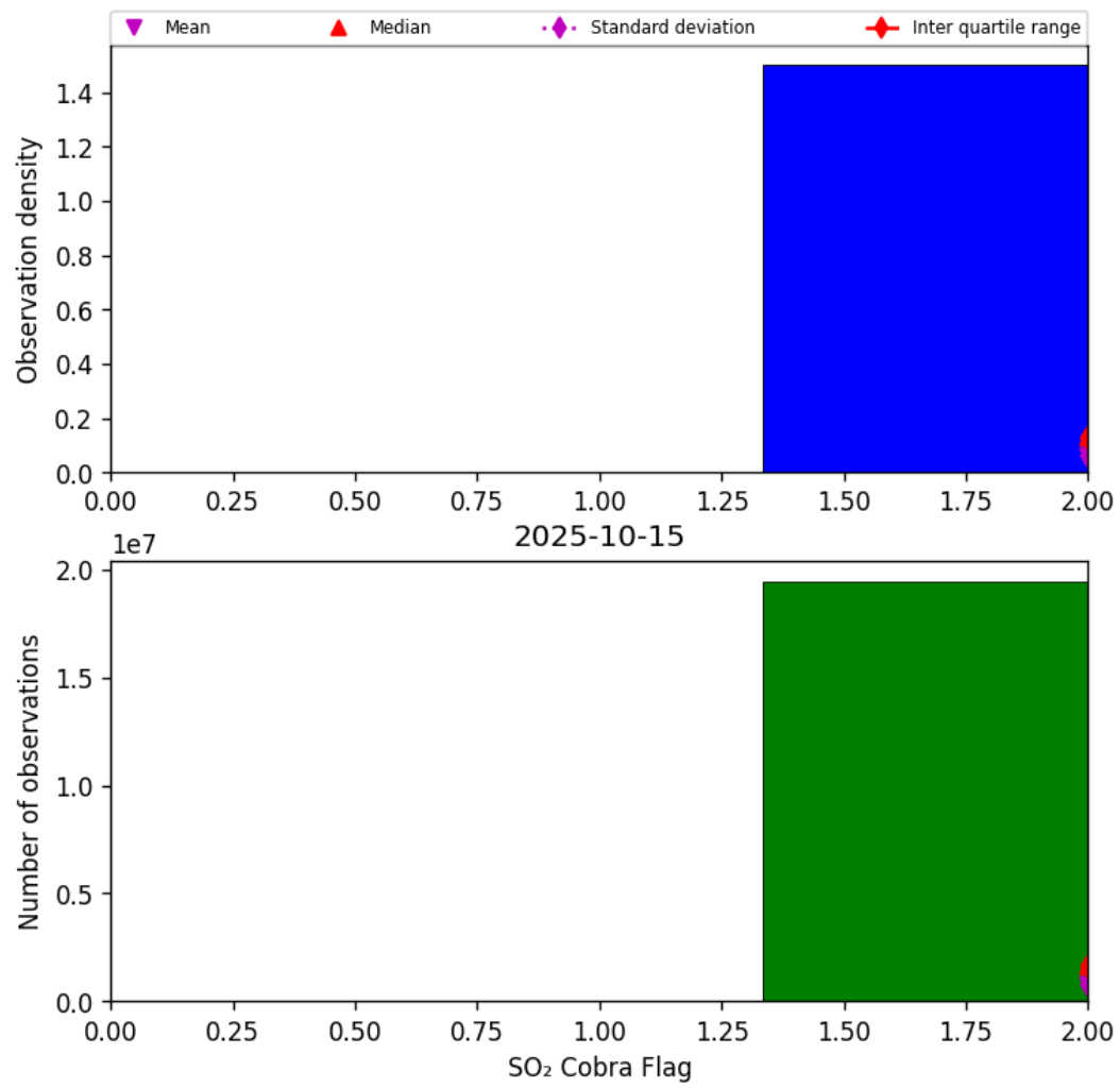
Figure 75: Histogram of “SO 2 Cobra Flag” for 2025-10-14 to 2025-10-16
