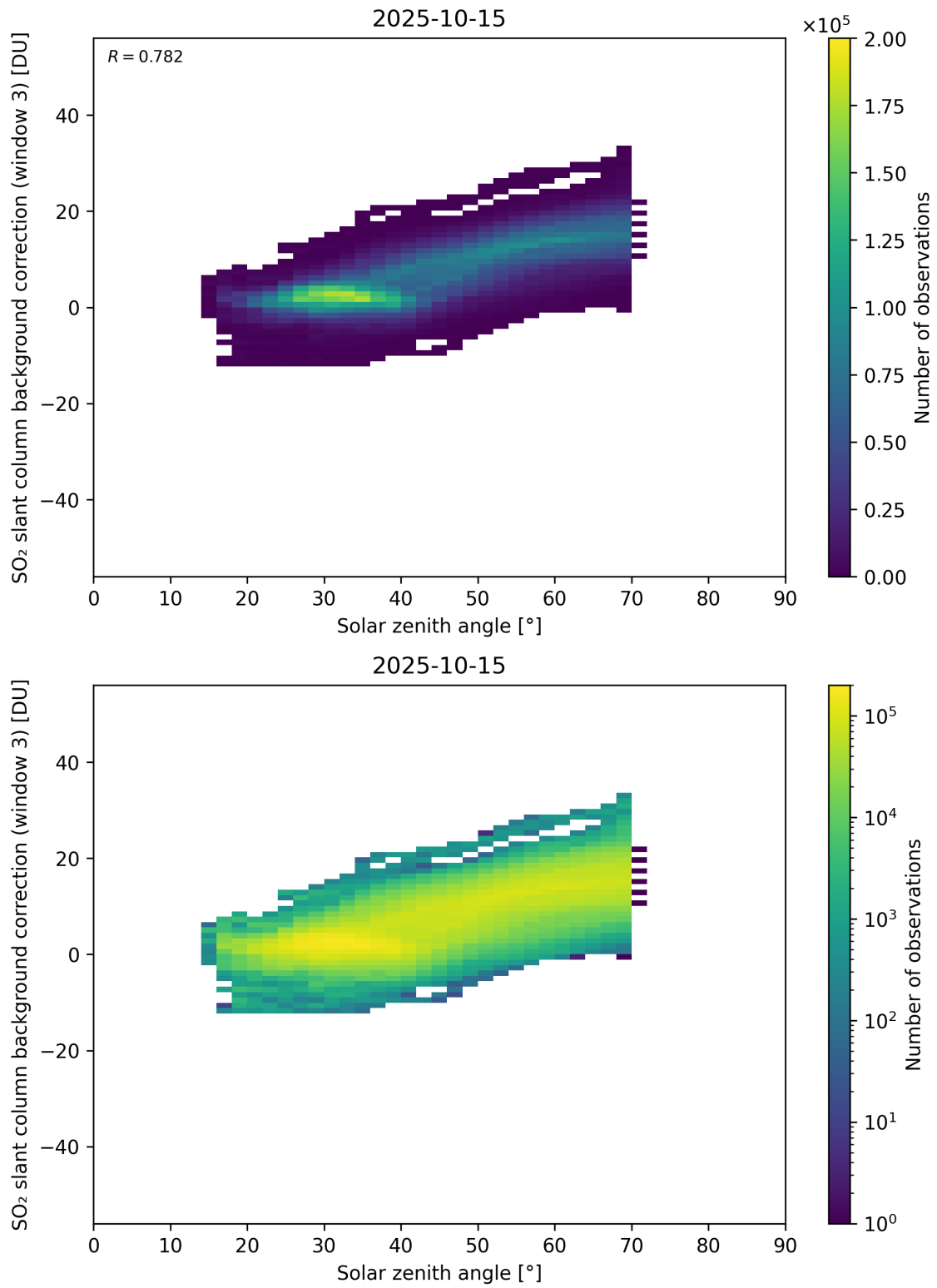
Figure 173: Scatter density plot of “Solar zenith angle” against “SO 2 slant column background correction (window 3)” for 2025-10-14 to 2025-10-16.
