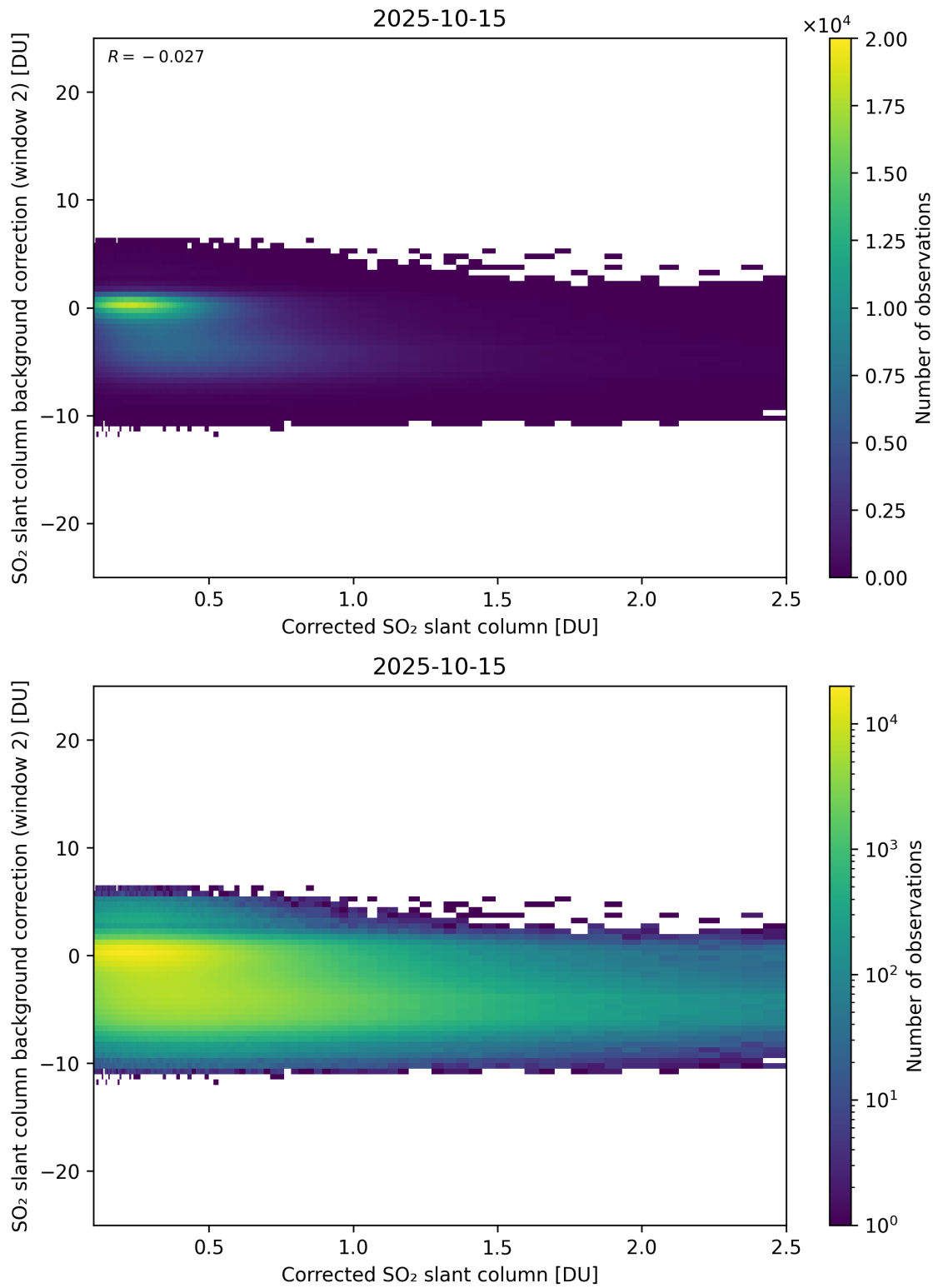
Figure 227: Scatter density plot of “Corrected SO 2 slant column” against “SO 2 slant column background correction (window 2)” for 2025-10-14 to 2025-10-16.
