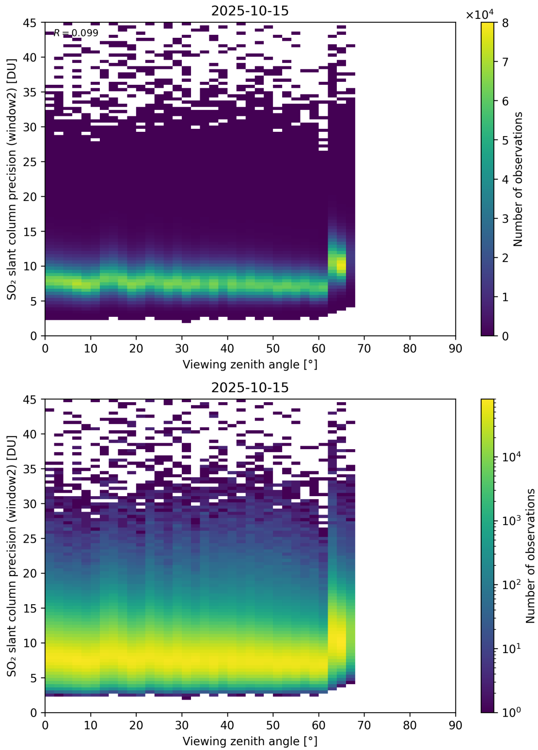
Figure 378: Scatter density plot of “Viewing zenith angle” against “SO 2 slant column precision (window2)” for 2025-10-14 to 2025-10-16.
