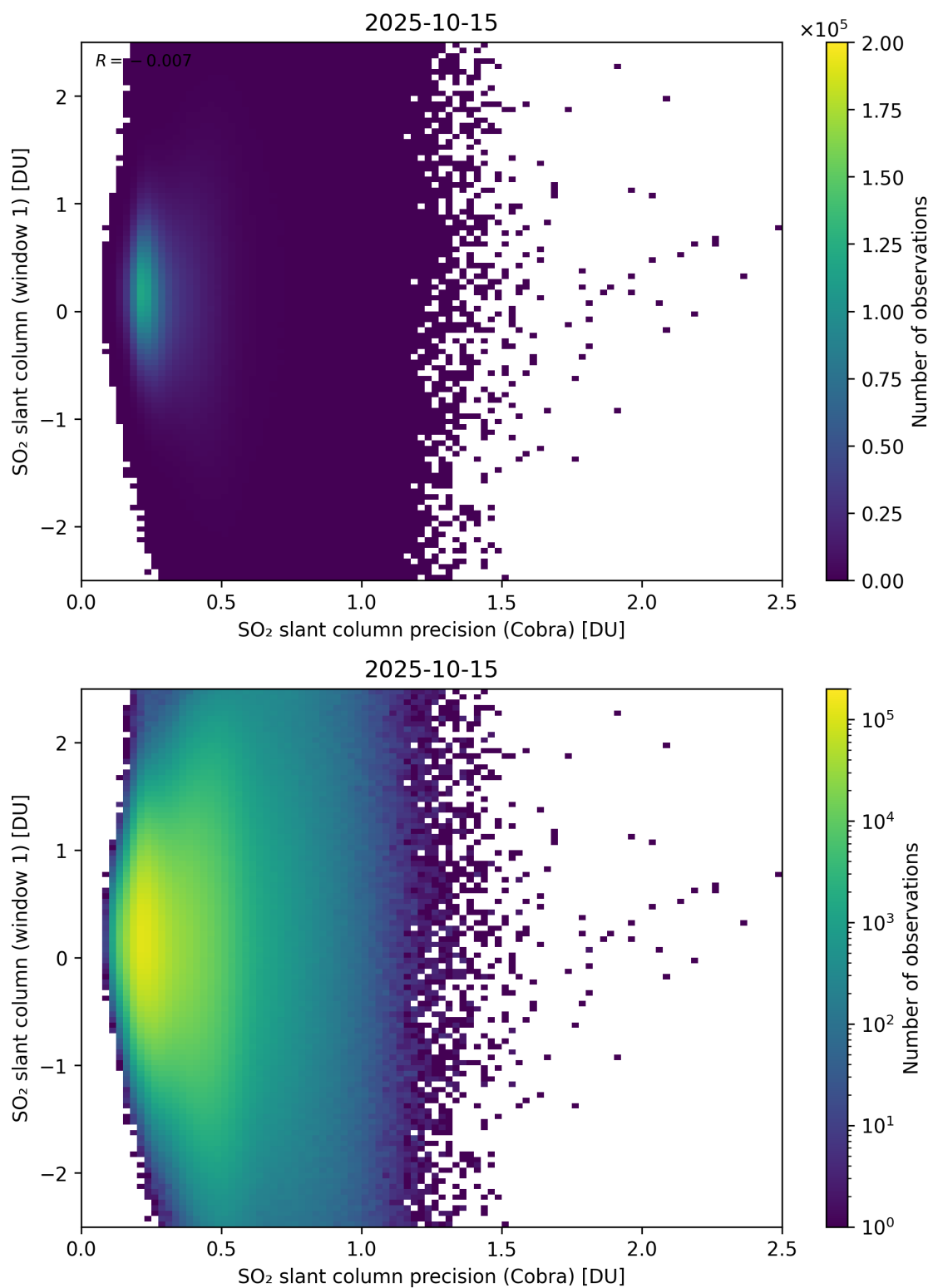
Figure 208: Scatter density plot of “SO 2 slant column precision (Cobra)” against “SO 2 slant column (window 1)” for 2025-10-14 to 2025-10-16.
