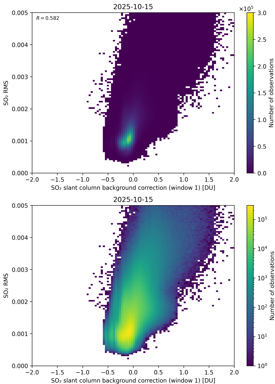
Figure 113: Scatter density plot of “SO 2 slant column background correction (window 1)” against “SO 2 RMS” for 2025-10-14 to 2025-10-16.
