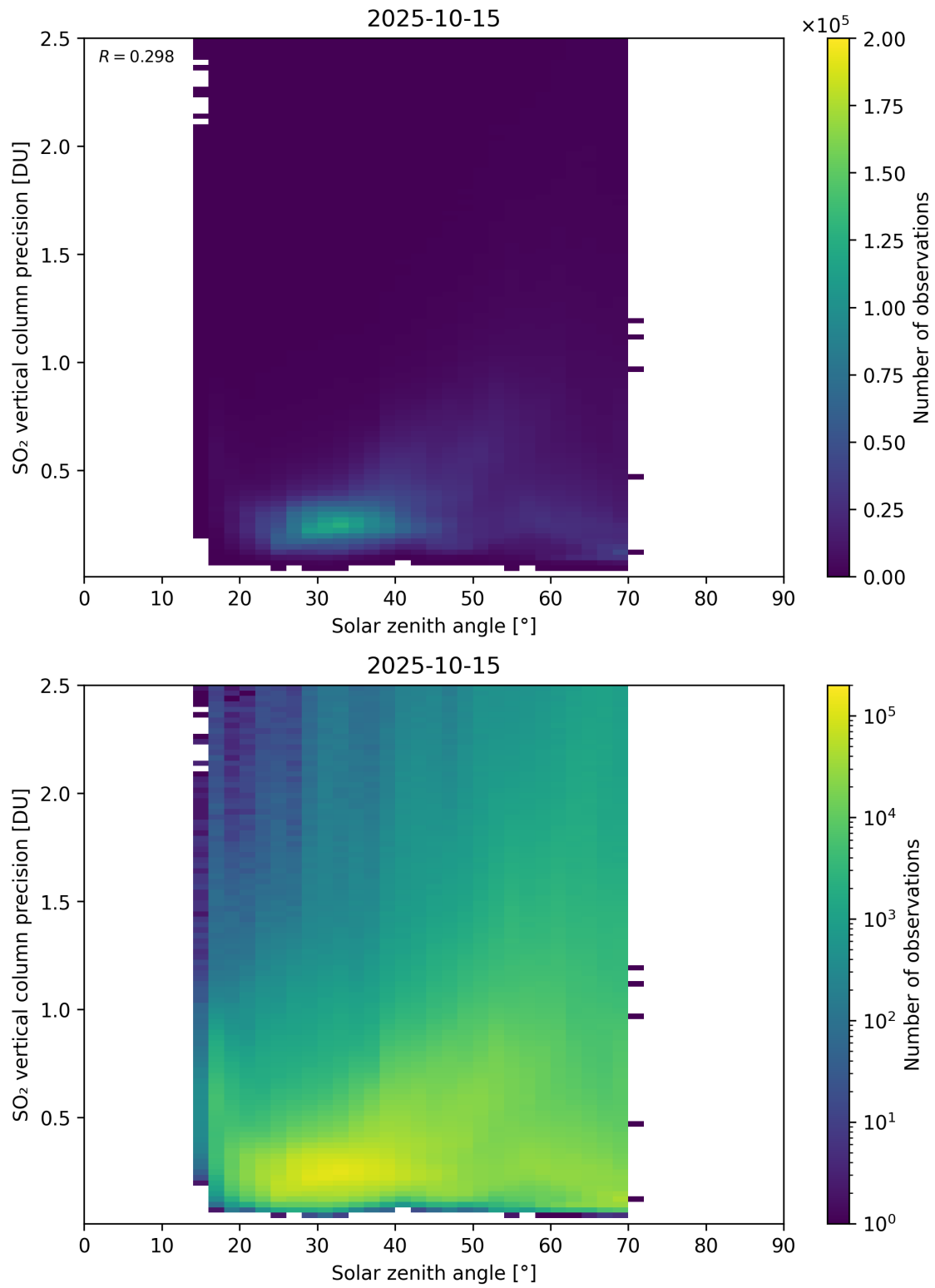
Figure 192: Scatter density plot of “Solar zenith angle” against “SO 2 vertical column precision” for 2025-10-14 to 2025-10-16.
