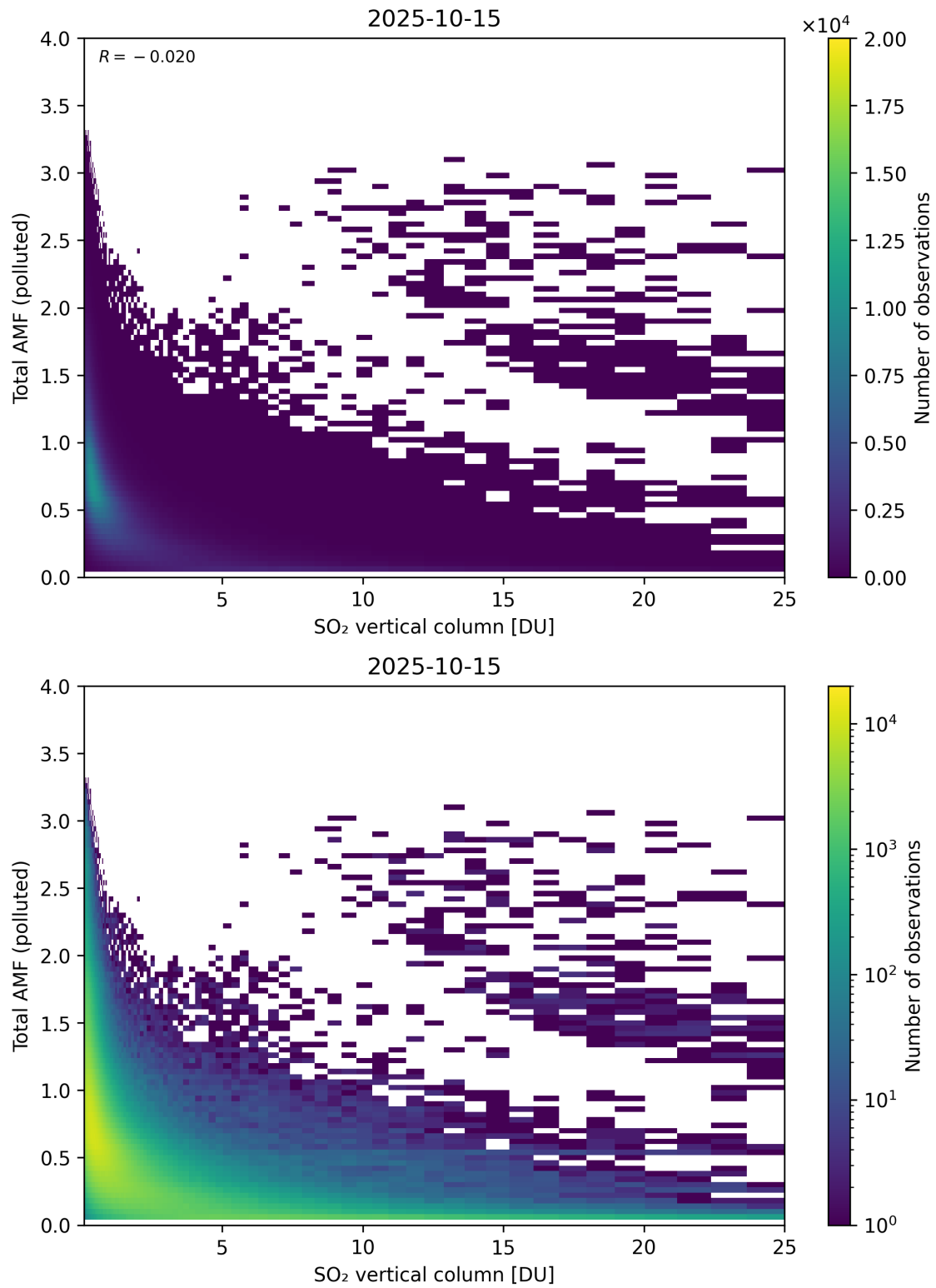
Figure 359: Scatter density plot of “SO 2 vertical column” against “Total AMF (polluted)” for 2025-10-14 to 2025-10-16.
