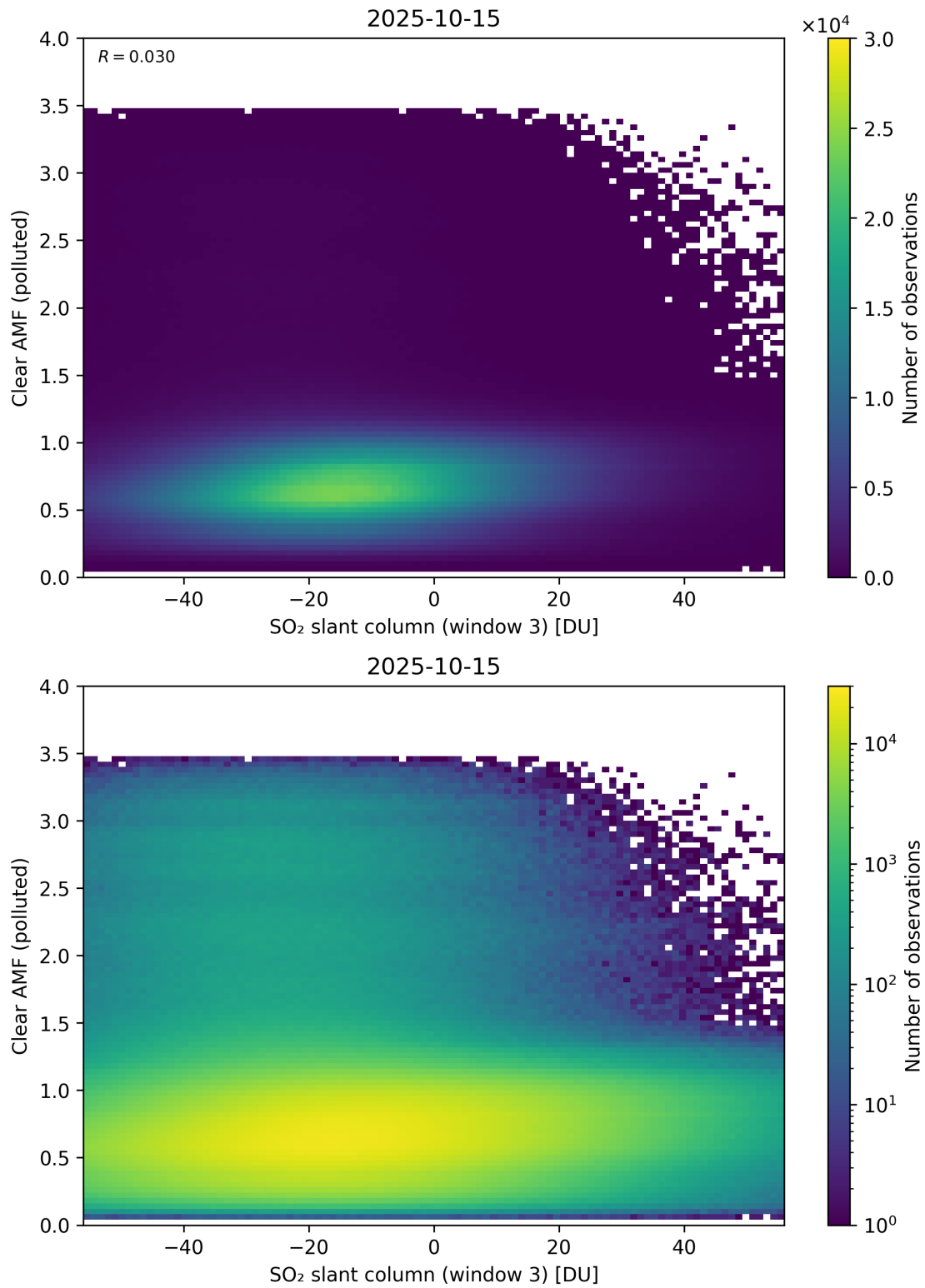
Figure 315: Scatter density plot of “SO 2 slant column (window 3)” against “Clear AMF (polluted)” for 2025-10-14 to 2025-10-16.
