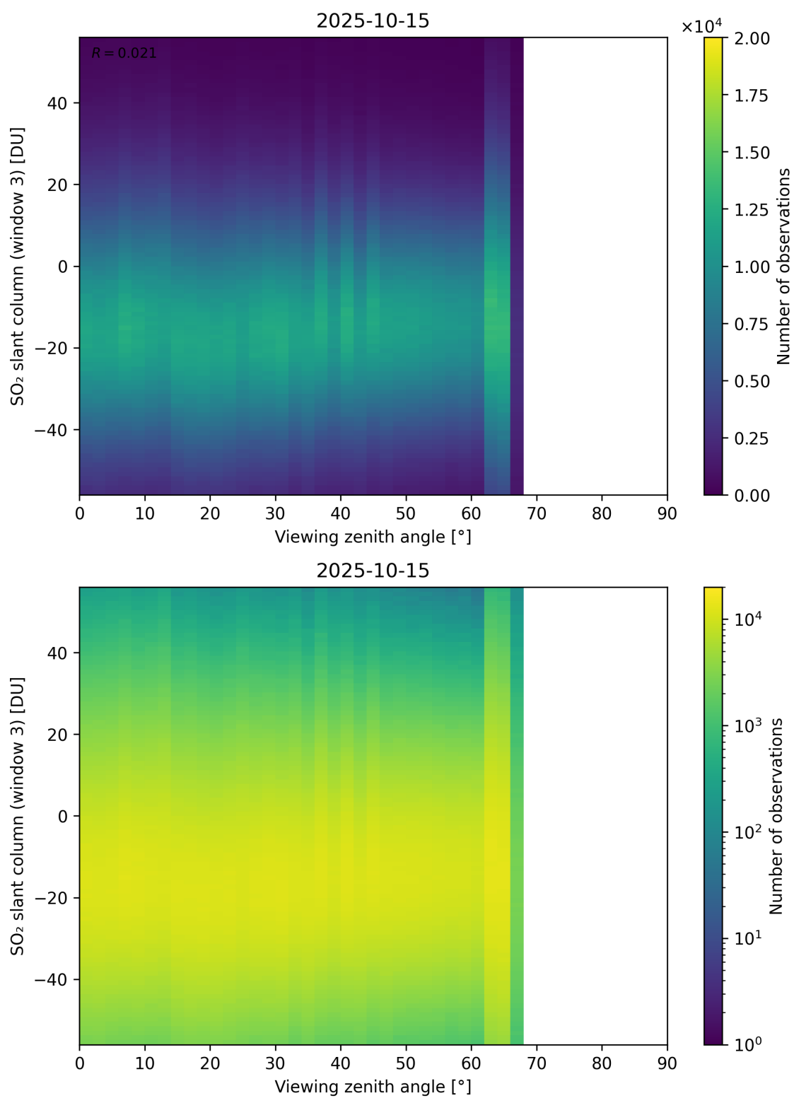
Figure 379: Scatter density plot of “Viewing zenith angle” against “SO 2 slant column (window 3)” for 2025-10-14 to 2025-10-16.
