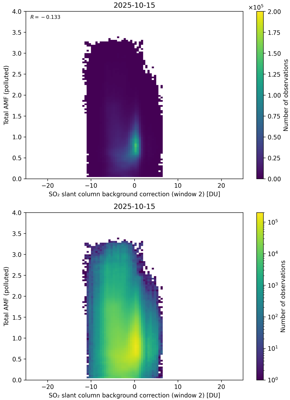
Figure 130: Scatter density plot of “SO 2 slant column background correction (window 2)” against “Total AMF (polluted)” for 2025-10-14 to 2025-10-16.
