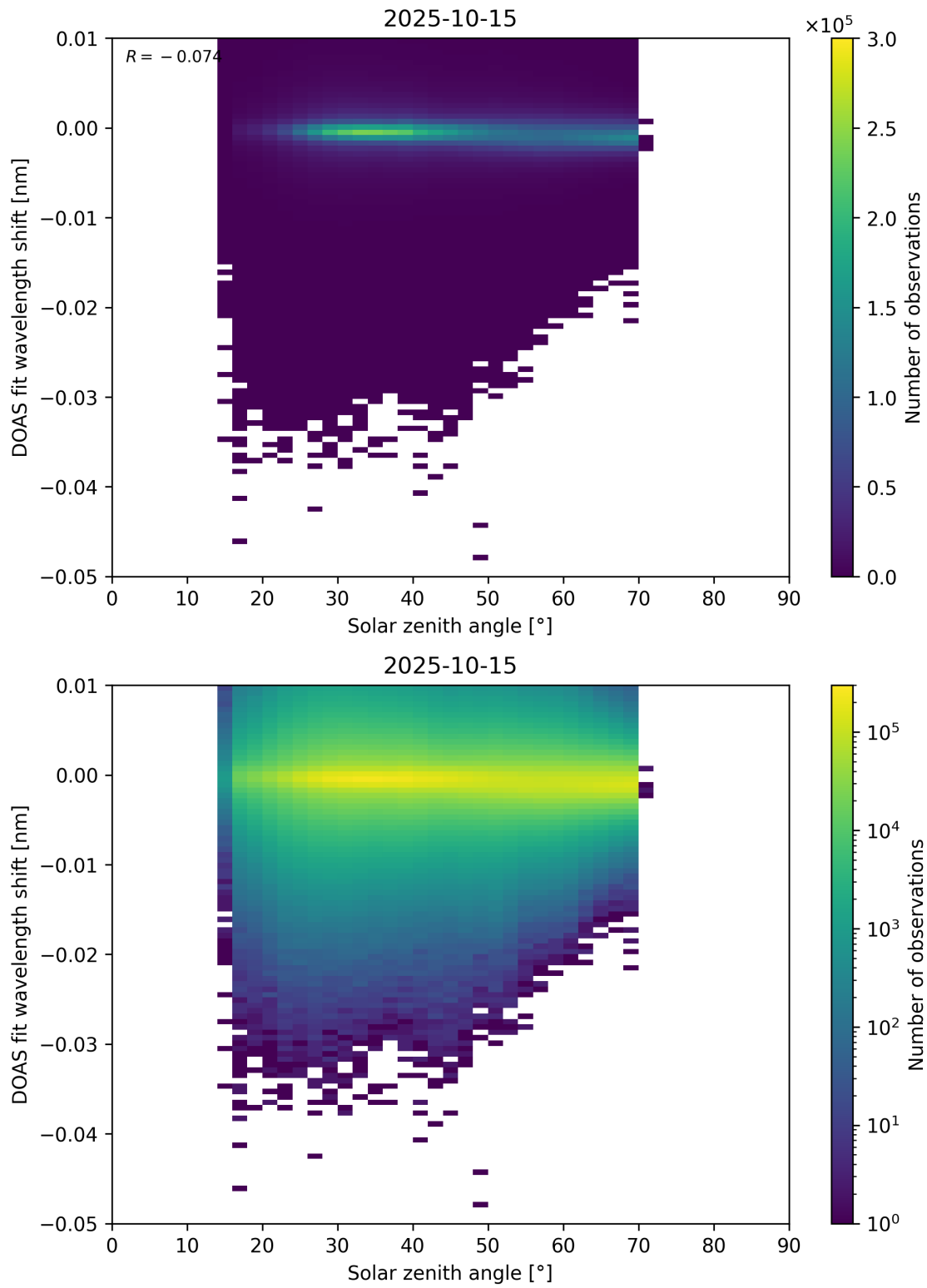
Figure 174: Scatter density plot of “Solar zenith angle” against “DOAS fit wavelength shift” for 2025-10-14 to 2025-10-16.
