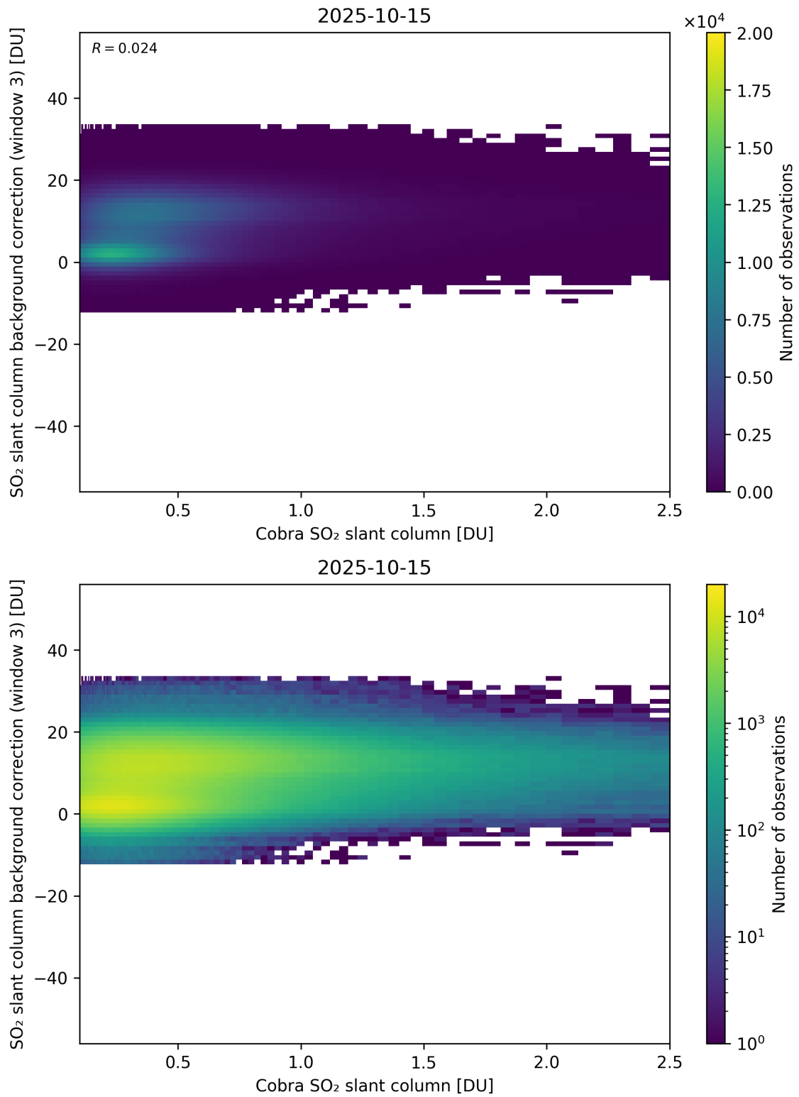
Figure 195: Scatter density plot of “Cobra SO 2 slant column” against “SO 2 slant column background correction (window 3)” for 2025-10-14 to 2025-10-16.
