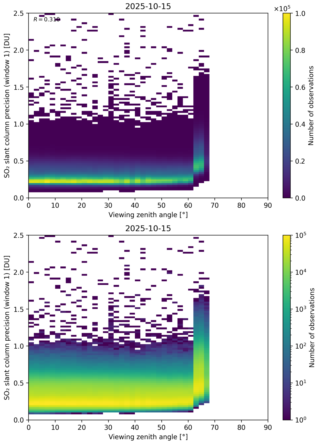
Figure 377: Scatter density plot of “Viewing zenith angle” against “SO 2 slant column precision (window 1)” for 2025-10-14 to 2025-10-16.
