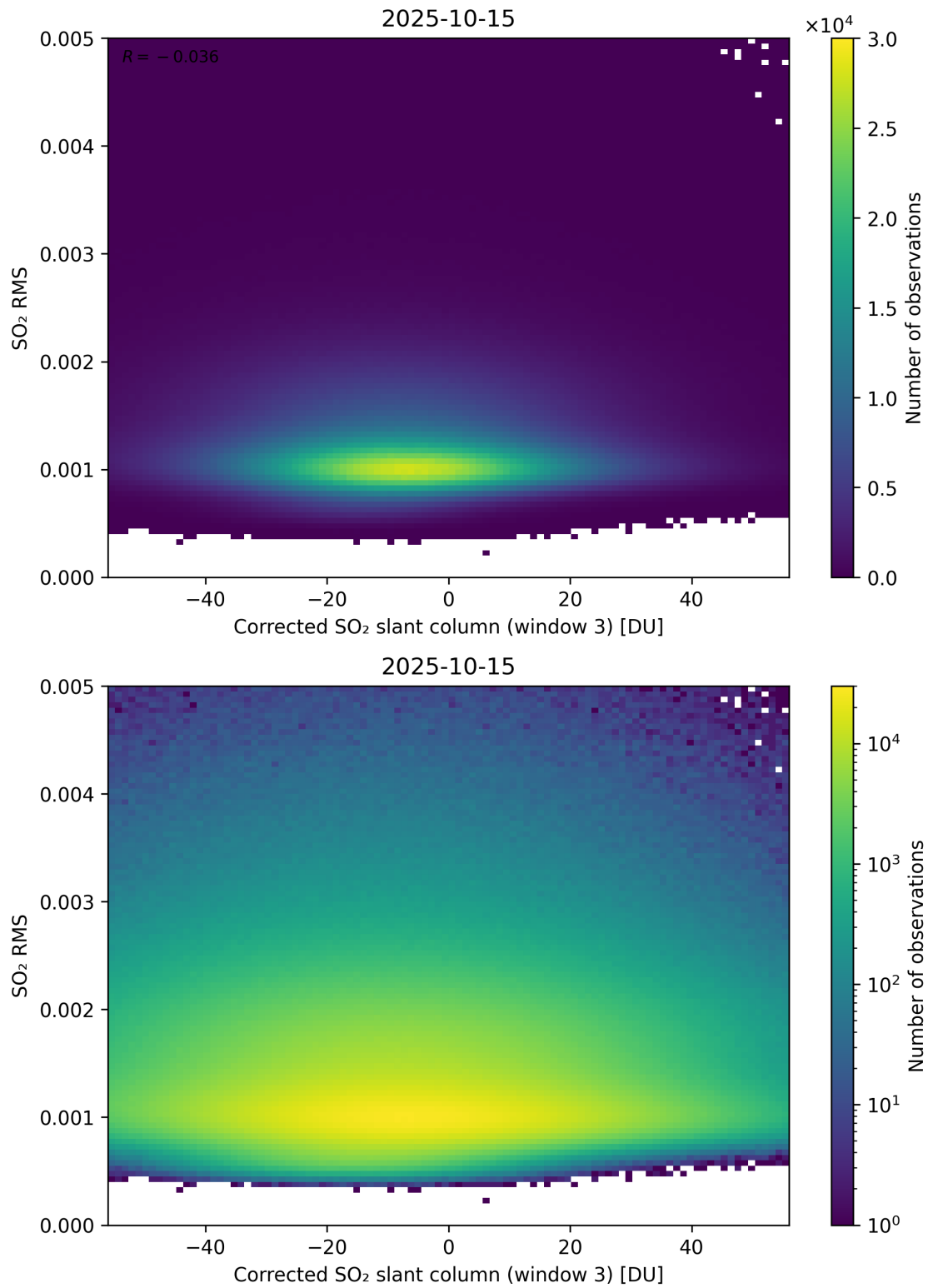
Figure 258: Scatter density plot of “Corrected SO 2 slant column (window 3)” against “SO 2 RMS” for 2025-10-14 to 2025-10-16.
