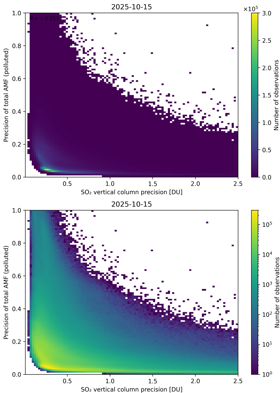
Figure 347: Scatter density plot of “SO 2 vertical column precision” against “Precision of total AMF (polluted)” for 2025-10-14 to 2025-10-16.
