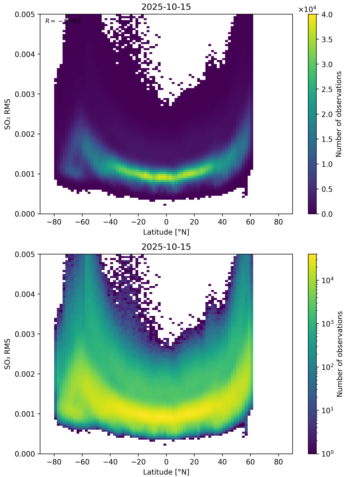
Figure 155: Scatter density plot of “Latitude” against “SO 2 RMS” for 2025-10-14 to 2025-10-16.
