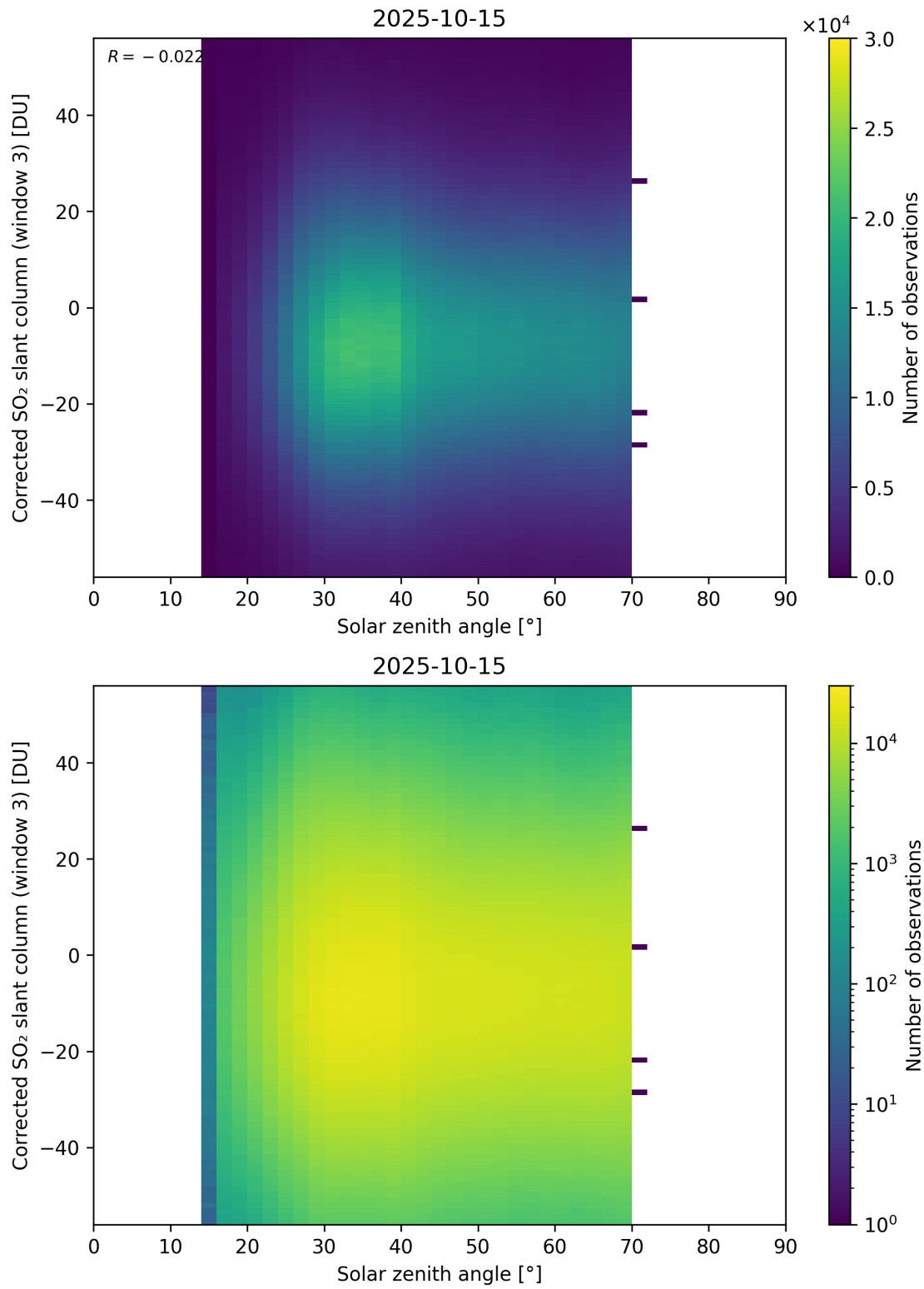
Figure 183: Scatter density plot of “Solar zenith angle” against “Corrected SO 2 slant column (window 3)” for 2025-10-14 to 2025-10-16.
