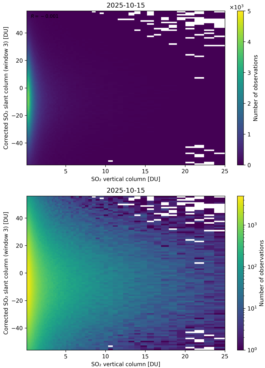
Figure 353: Scatter density plot of “SO 2 vertical column” against “Corrected SO 2 slant column (window 3)” for 2025-10-14 to 2025-10-16.
