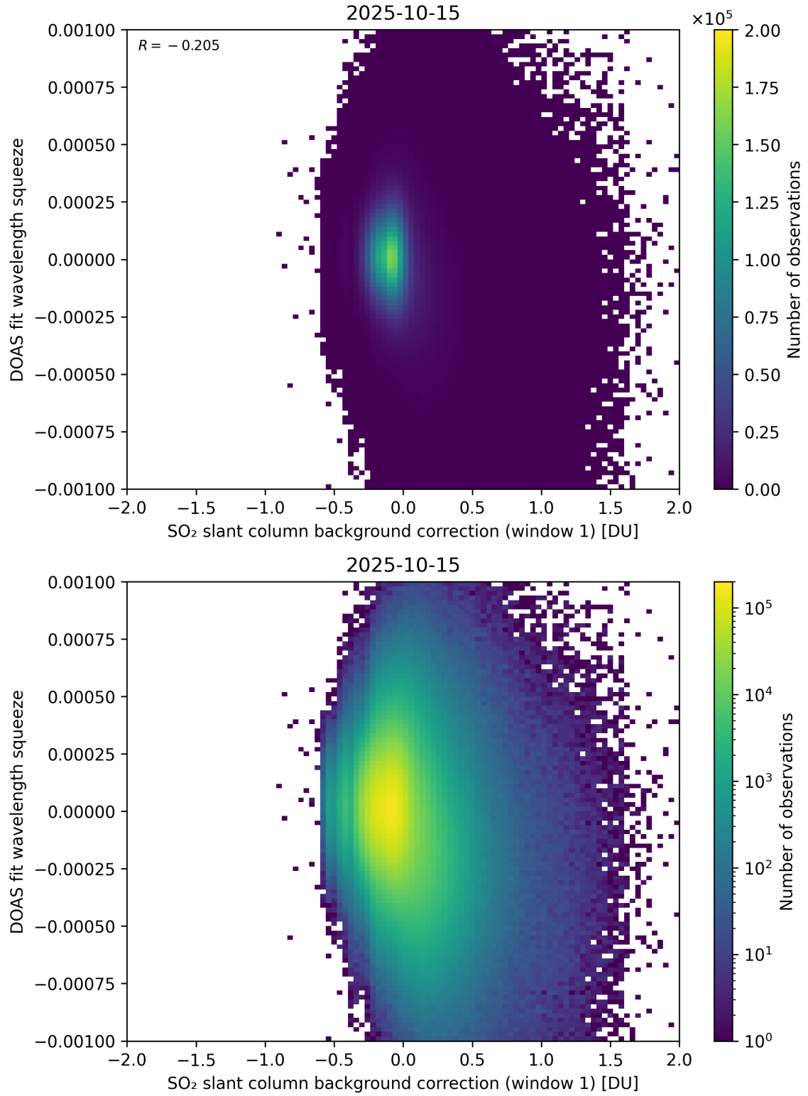
Figure 112: Scatter density plot of “SO 2 slant column background correction (window 1)” against “DOAS fit wavelength squeeze” for 2025-10-14 to 2025-10-16.
