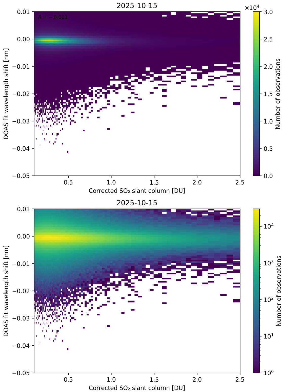
Figure 229: Scatter density plot of “Corrected SO 2 slant column” against “DOAS fit wavelength shift” for 2025-10-14 to 2025-10-16.
