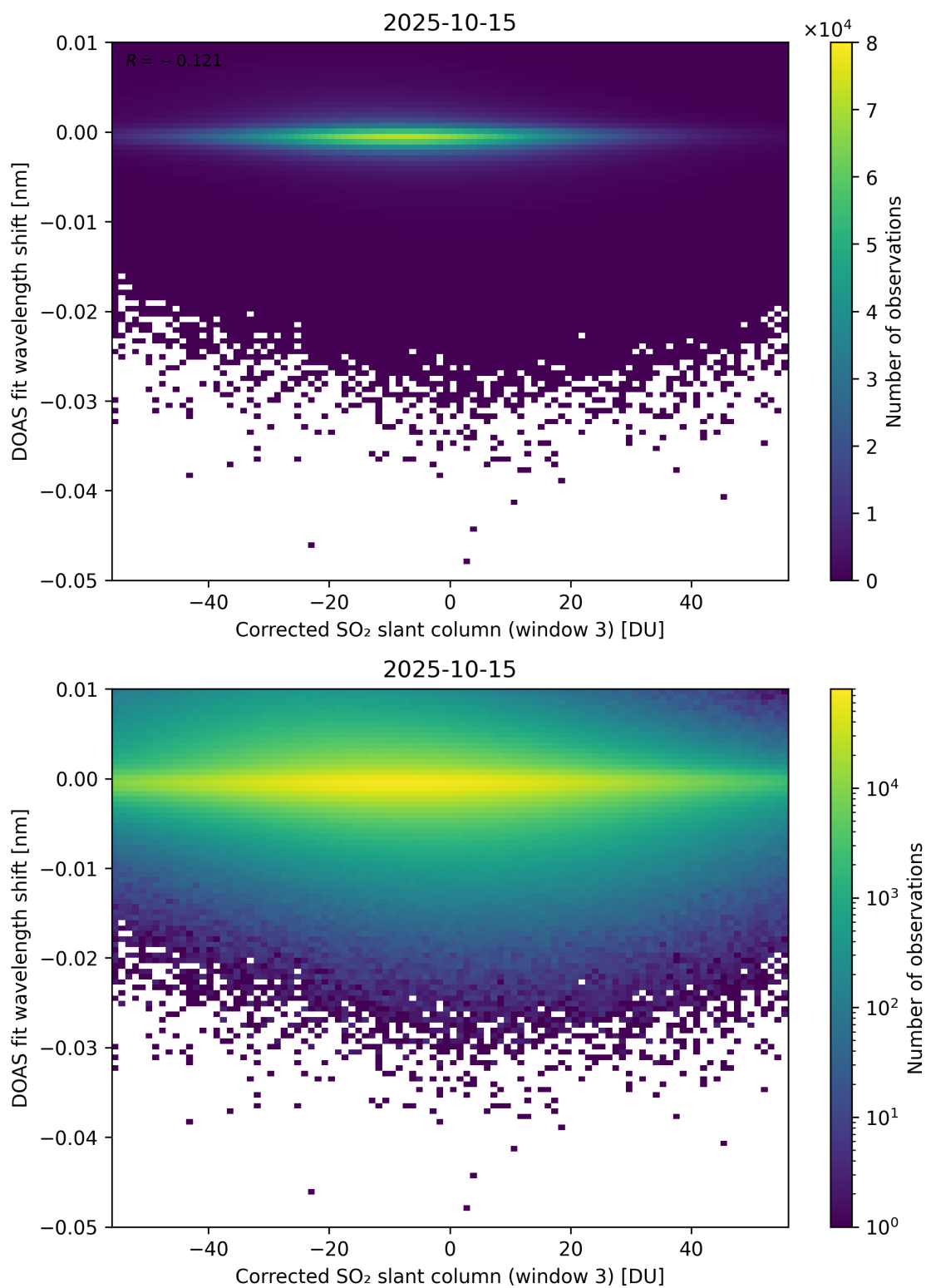
Figure 256: Scatter density plot of “Corrected SO 2 slant column (window 3)” against “DOAS fit wavelength shift” for 2025-10-14 to 2025-10-16.
