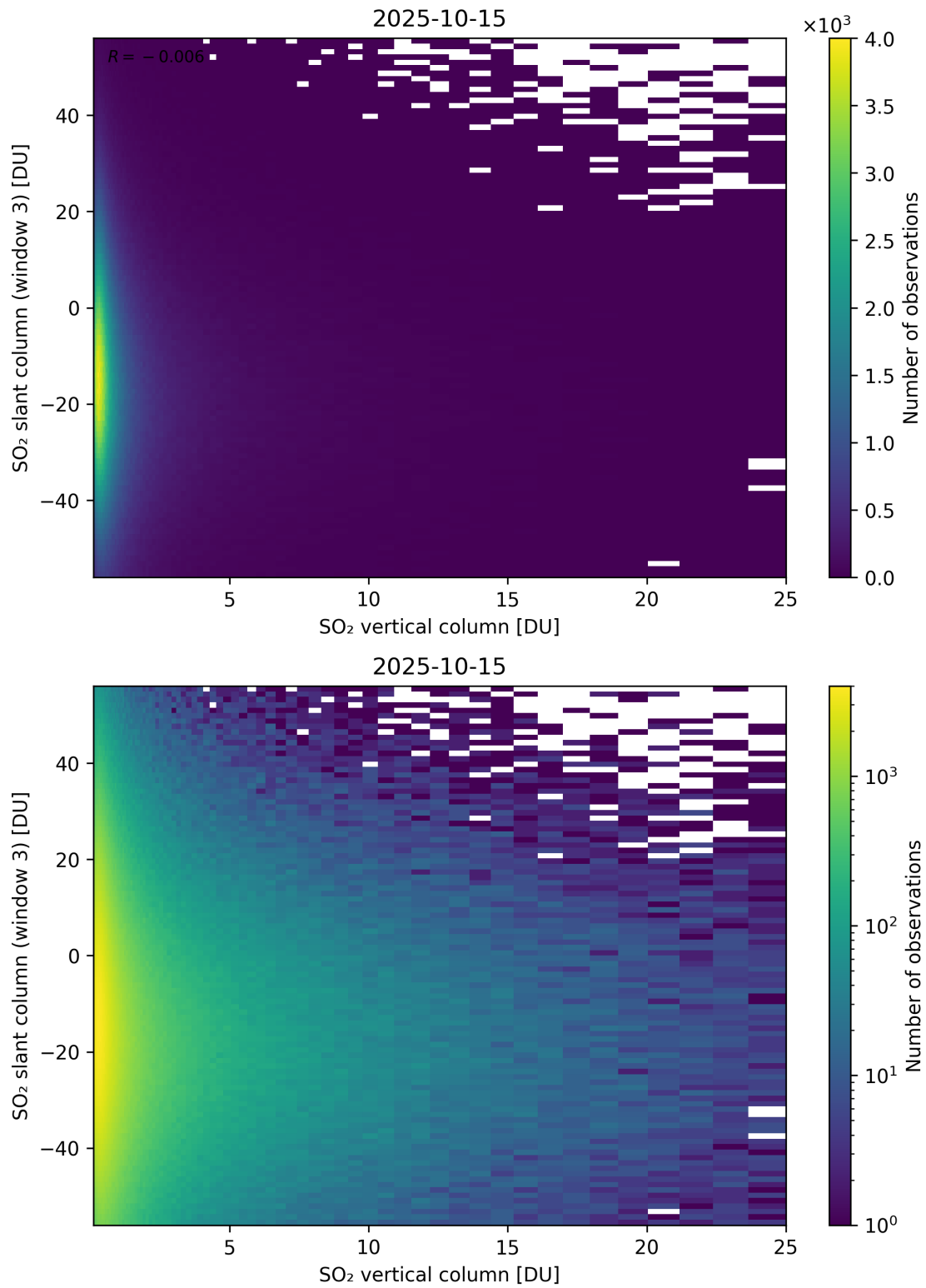
Figure 357: Scatter density plot of “SO 2 vertical column” against “SO 2 slant column (window 3)” for 2025-10-14 to 2025-10-16.
