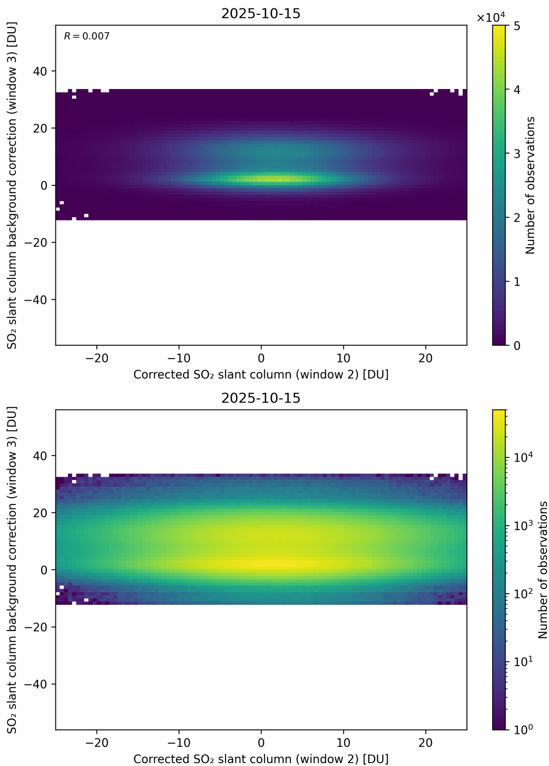
Figure 245: Scatter density plot of “Corrected SO 2 slant column (window 2)” against “SO 2 slant column background correction (window 3)” for 2025-10-14 to 2025-10-16.
