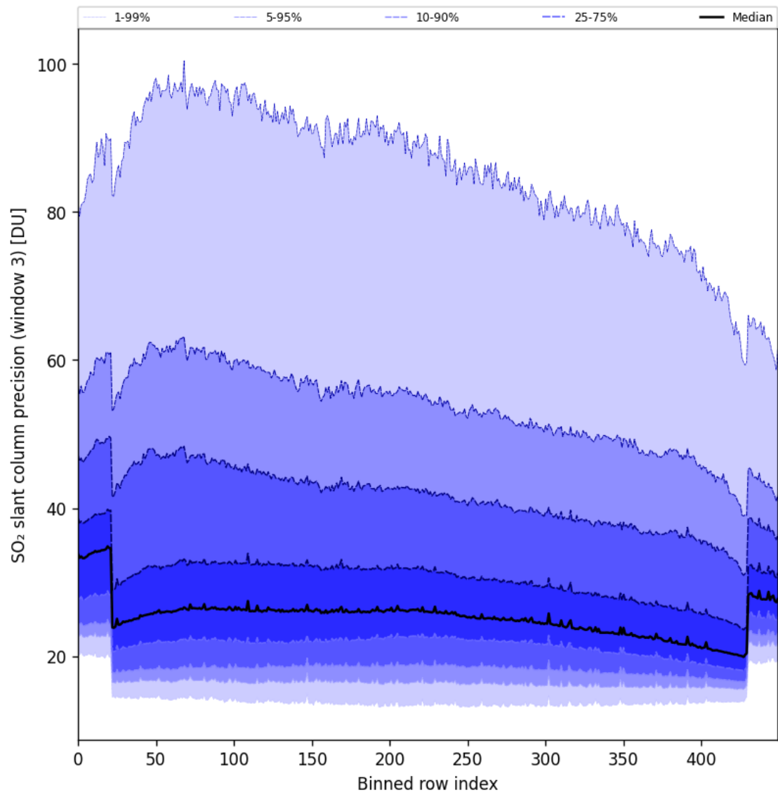
Figure 98: Along track statistics of “SO 2 slant column precision (window 3)” for 2025-10-14 to 2025-10-16
