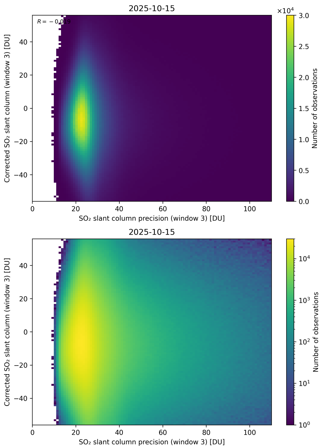
Figure 312: Scatter density plot of “SO 2 slant column precision (window 3)” against “Corrected SO 2 slant column (window 3)” for 2025-10-14 to 2025-10-16.
