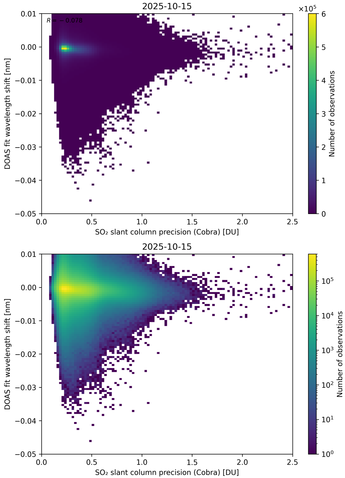
Figure 202: Scatter density plot of “SO 2 slant column precision (Cobra)” against “DOAS fit wavelength shift” for 2025-10-14 to 2025-10-16.
