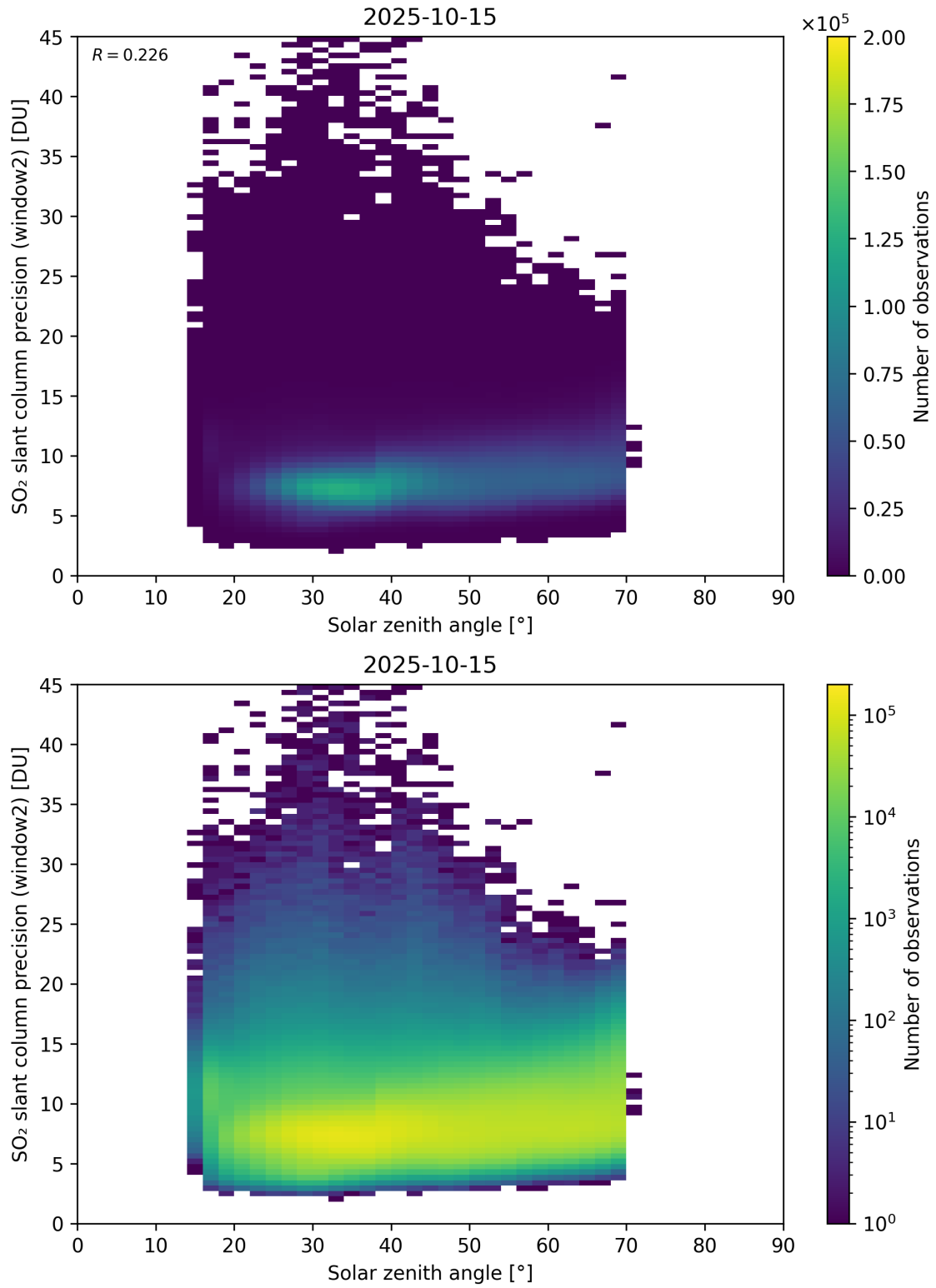
Figure 186: Scatter density plot of “Solar zenith angle” against “SO 2 slant column precision (window2)” for 2025-10-14 to 2025-10-16.
