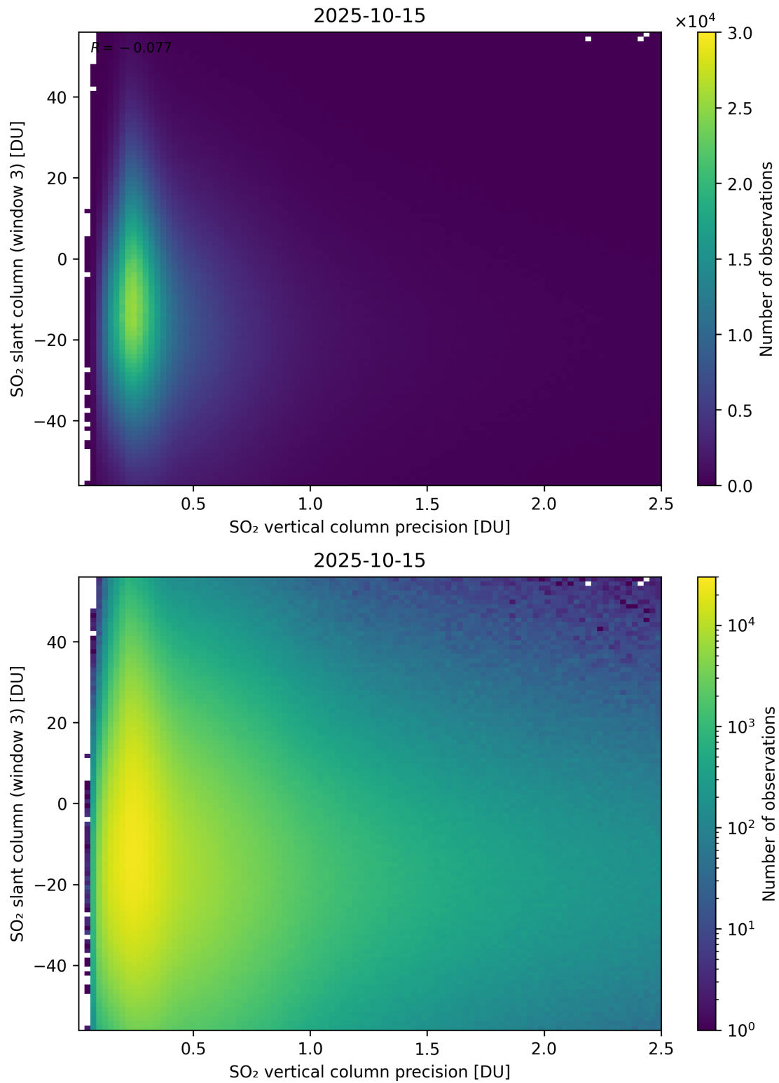
Figure 344: Scatter density plot of “SO 2 vertical column precision” against “SO 2 slant column (window 3)” for 2025-10-14 to 2025-10-16.
