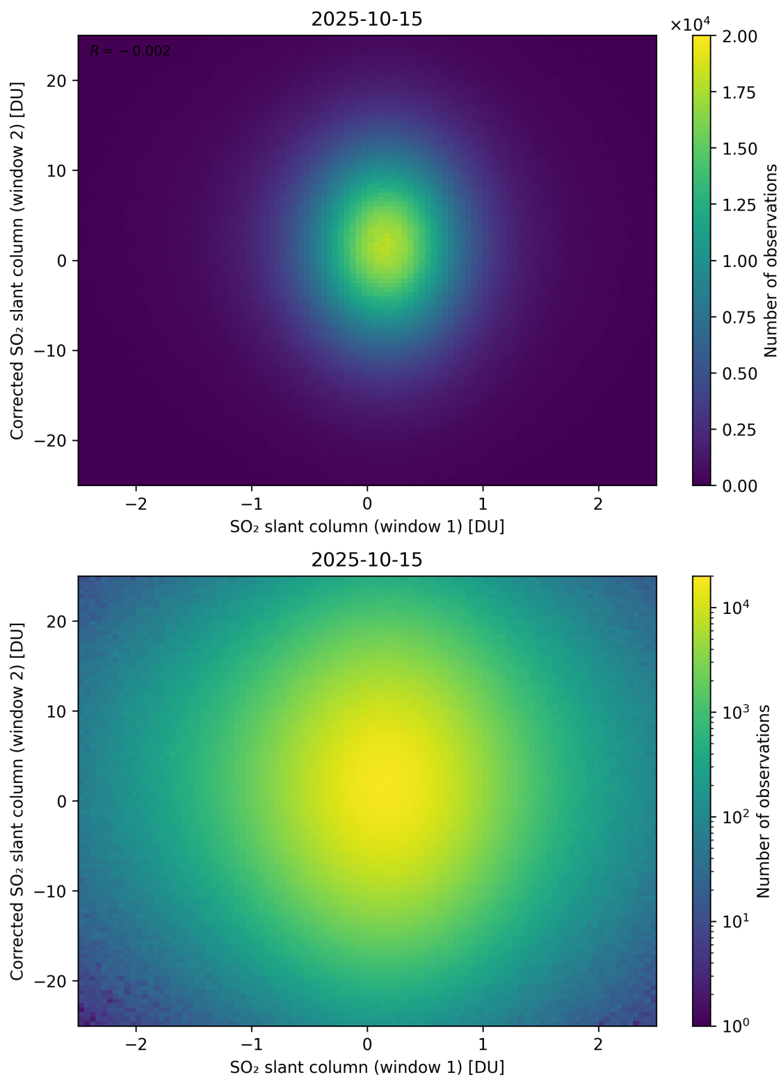
Figure 283: Scatter density plot of “SO 2 slant column (window 1)” against “Corrected SO 2 slant column (window 2)” for 2025-10-14 to 2025-10-16.
