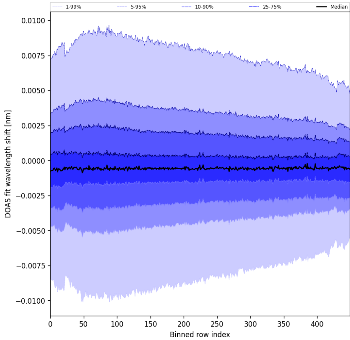
Figure 102: Along track statistics of “DOAS fit wavelength shift” for 2025-10-14 to 2025-10-16
