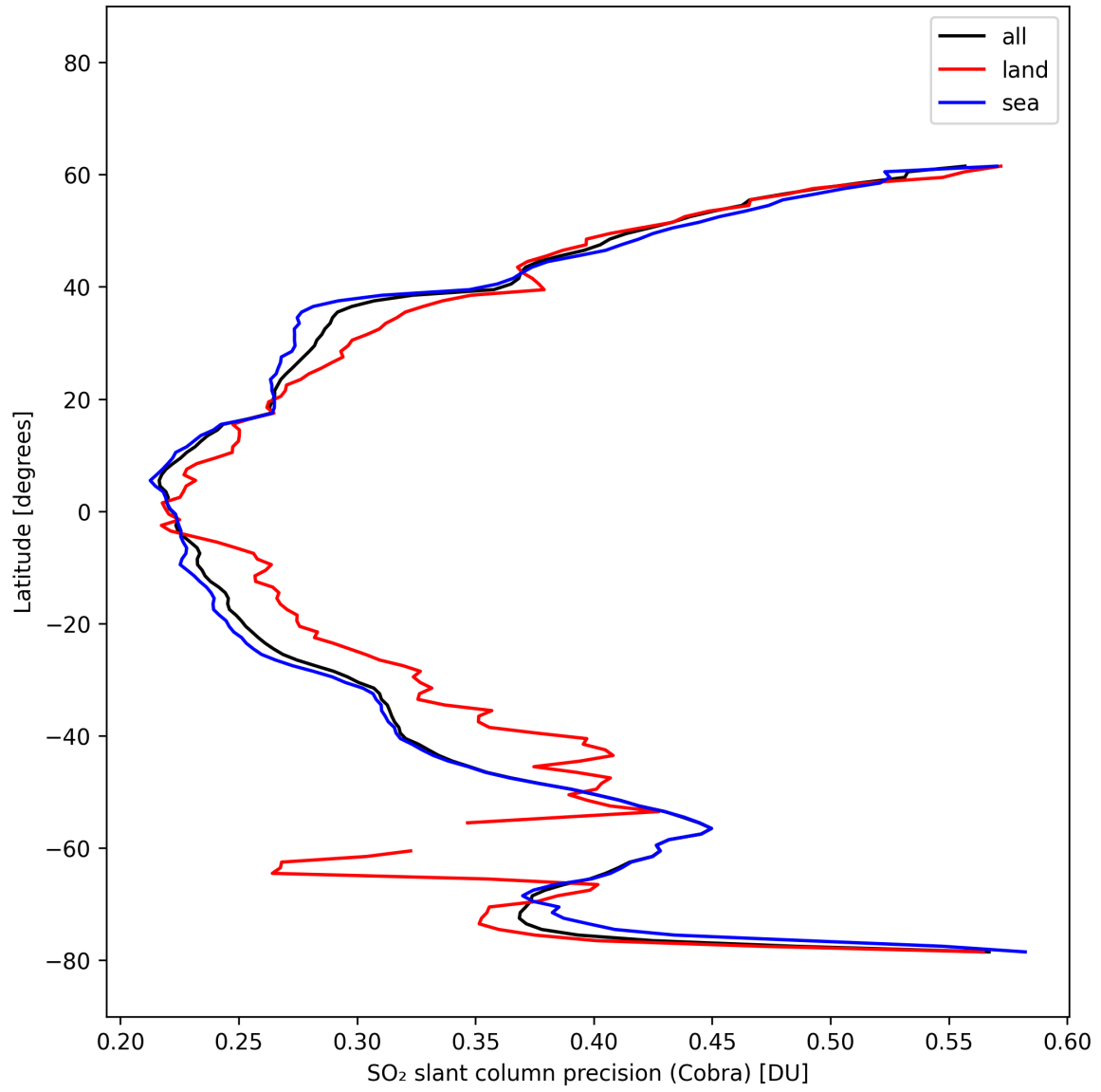
Figure 36: Zonal average of "SO 2 slant column precision (Cobra)" for 2025-10-14 to 2025-10-16.
