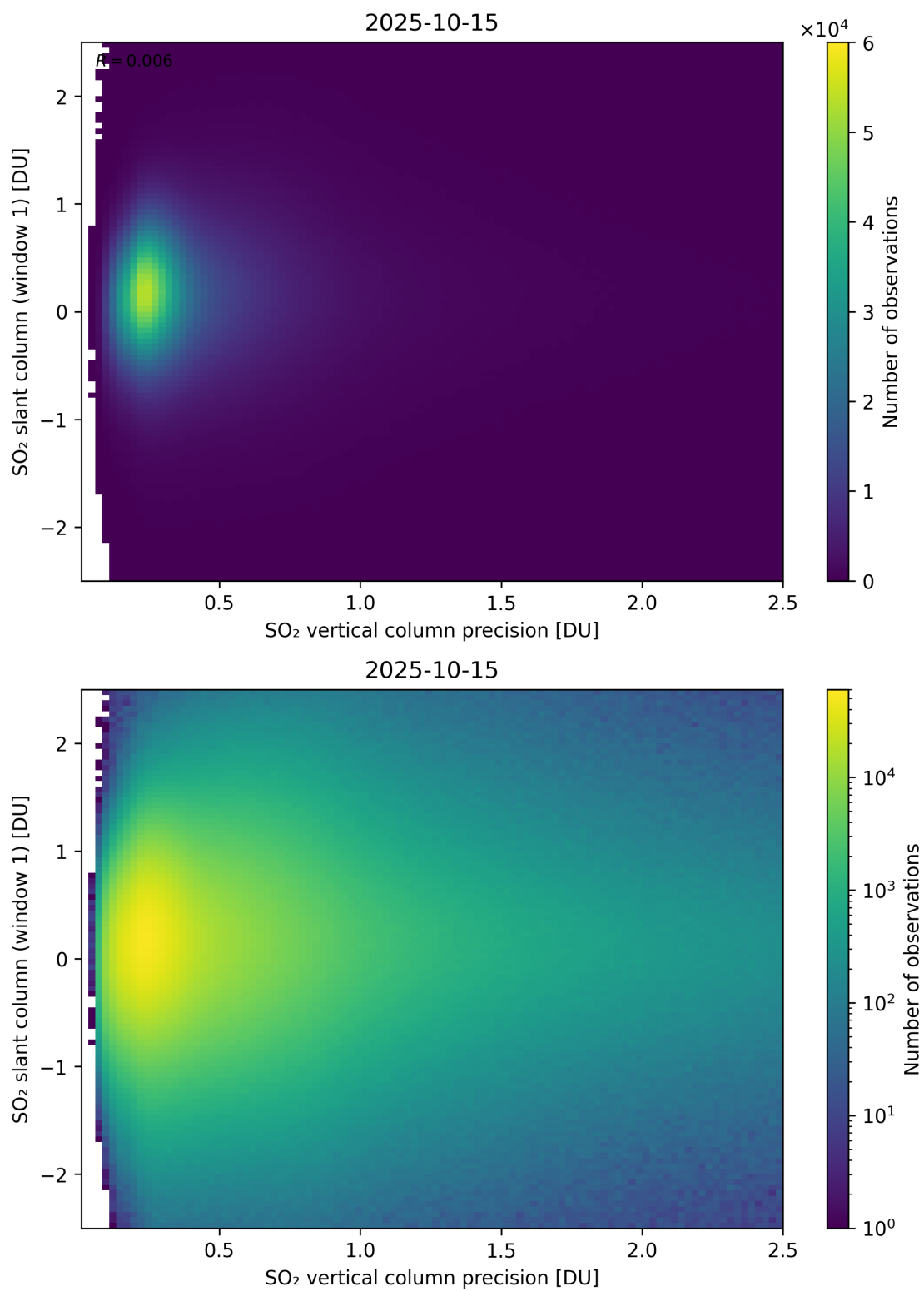
Figure 341: Scatter density plot of “SO 2 vertical column precision” against “SO 2 slant column (window 1)” for 2025-10-14 to 2025-10-16.
