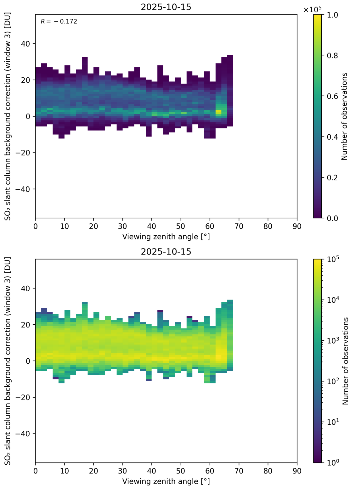
Figure 364: Scatter density plot of “Viewing zenith angle” against “SO 2 slant column background correction (window 3)” for 2025-10-14 to 2025-10-16.
