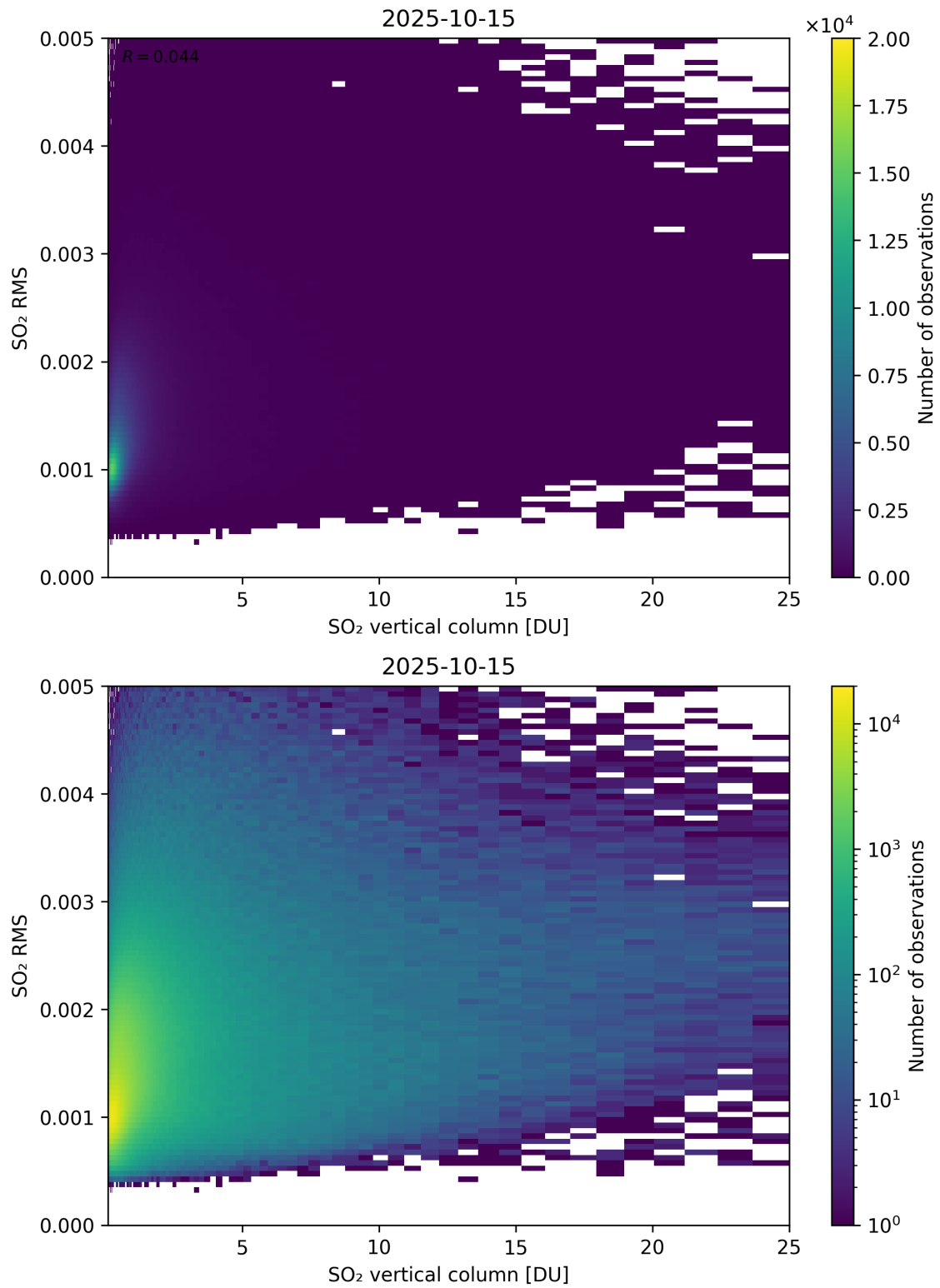
Figure 328: Scatter density plot of “SO 2 vertical column” against “SO 2 RMS” for 2025-10-14 to 2025-10-16.
