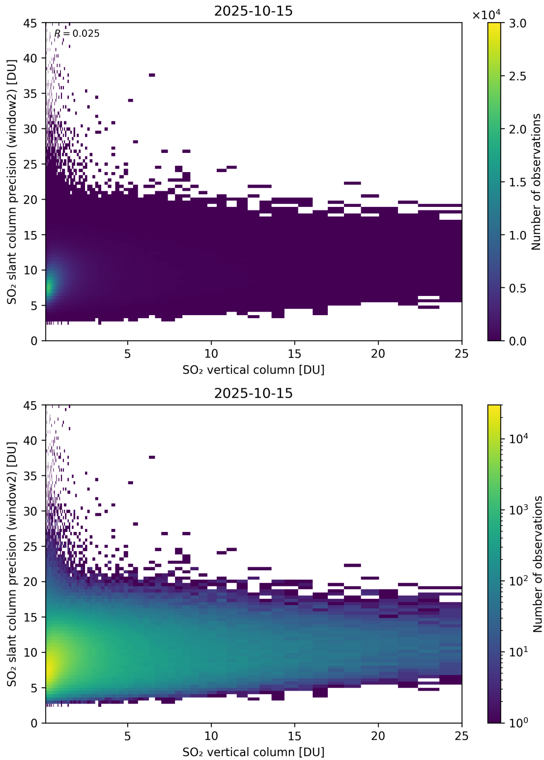
Figure 356: Scatter density plot of “SO 2 vertical column” against “SO 2 slant column precision (window2)” for 2025-10-14 to 2025-10-16.
