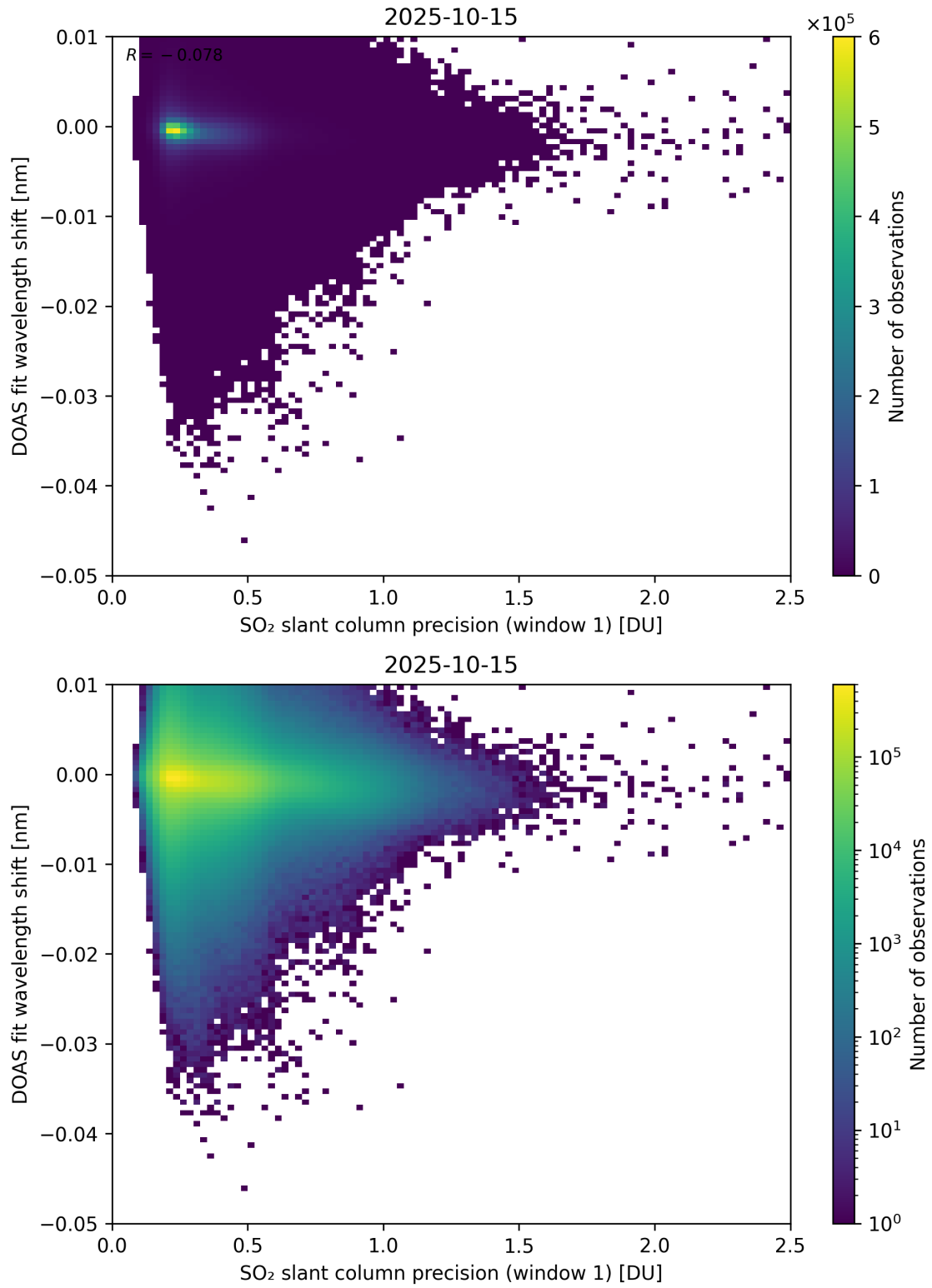
Figure 271: Scatter density plot of “SO 2 slant column precision (window 1)” against “DOAS fit wavelength shift” for 2025-10-14 to 2025-10-16.
