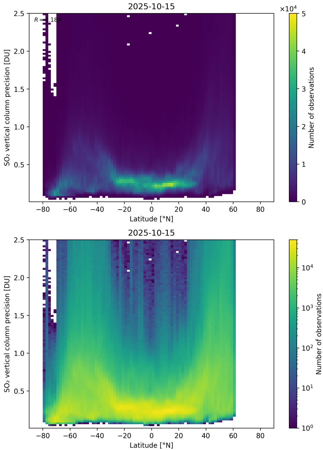
Figure 170: Scatter density plot of “Latitude” against “SO 2 vertical column precision” for 2025-10-14 to 2025-10-16.
