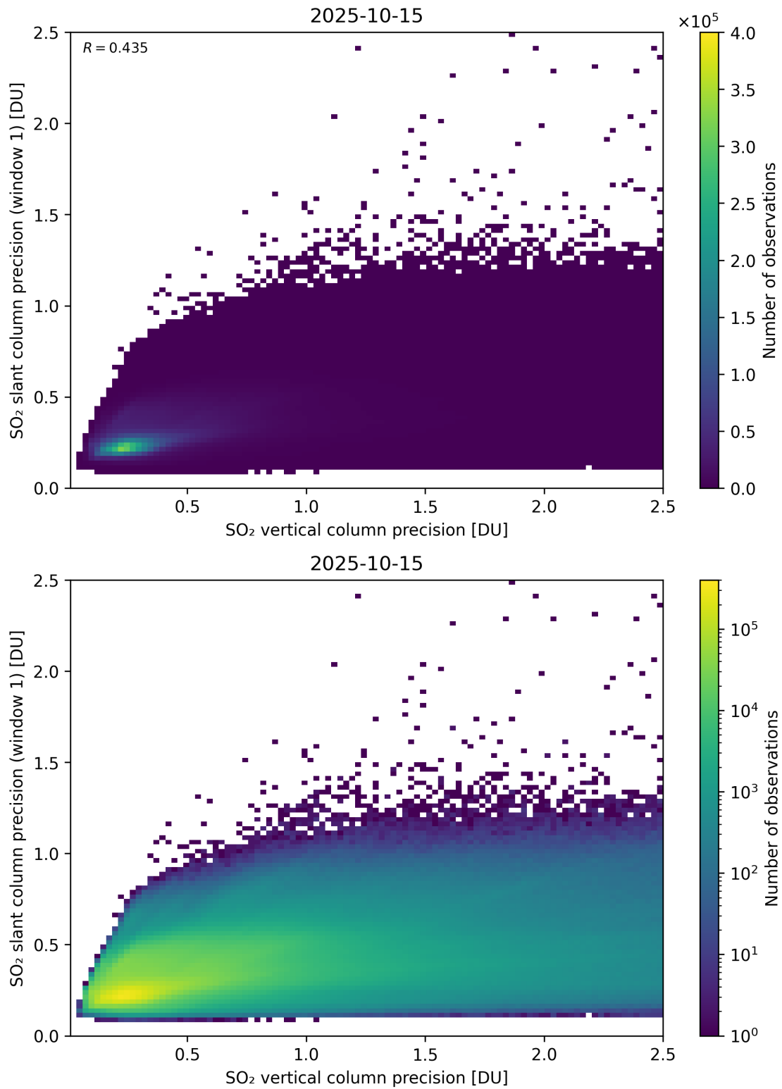
Figure 342: Scatter density plot of “SO 2 vertical column precision” against “SO 2 slant column precision (window 1)” for 2025-10-14 to 2025-10-16.
