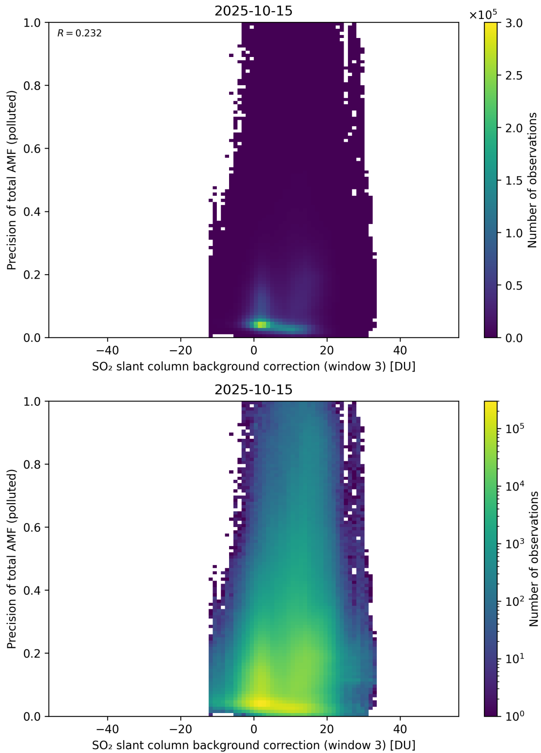
Figure 137: Scatter density plot of “SO 2 slant column background correction (window 3)” against “Precision of total AMF (polluted)” for 2025-10-14 to 2025-10-16.
