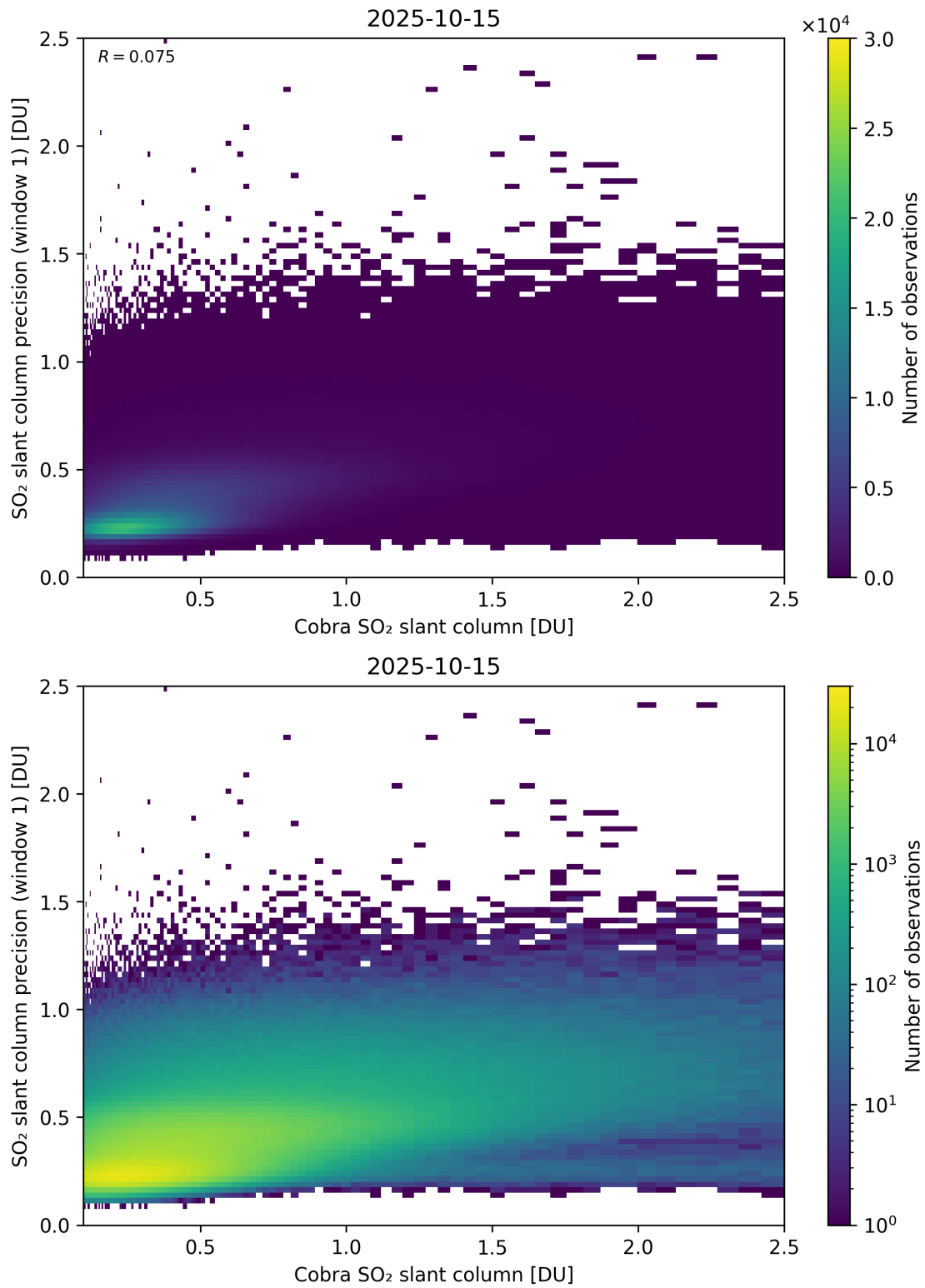
Figure 220: Scatter density plot of “Cobra SO 2 slant column” against “SO 2 slant column precision (window 1)” for 2025-10-14 to 2025-10-16.
