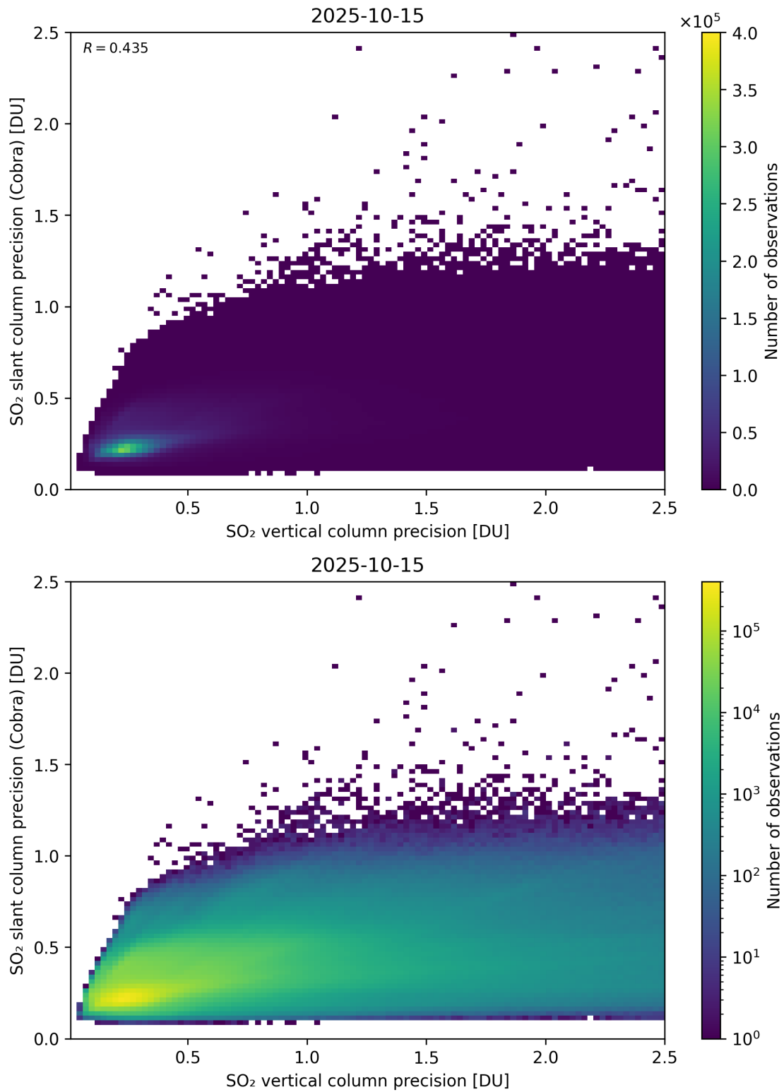
Figure 337: Scatter density plot of “SO 2 vertical column precision” against “SO 2 slant column precision (Cobra)” for 2025-10-14 to 2025-10-16.
