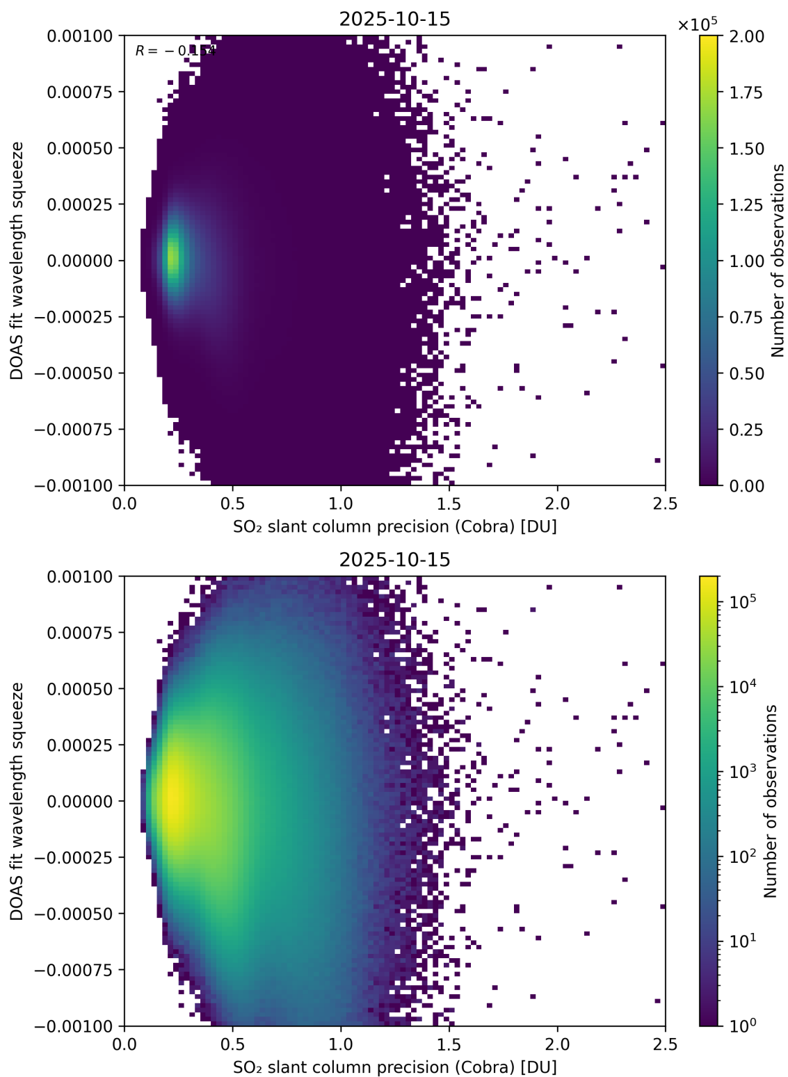
Figure 203: Scatter density plot of “SO 2 slant column precision (Cobra)” against “DOAS fit wavelength squeeze” for 2025-10-14 to 2025-10-16.
