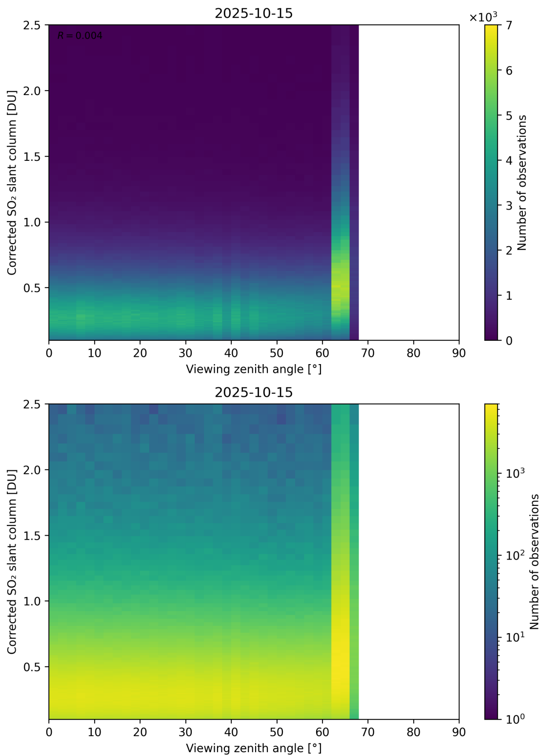
Figure 373: Scatter density plot of “Viewing zenith angle” against “Corrected SO 2 slant column” for 2025-10-14 to 2025-10-16.
