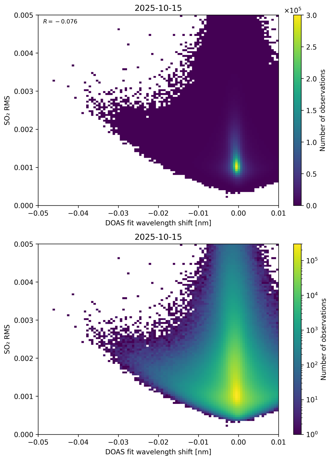
Figure 139: Scatter density plot of “DOAS fit wavelength shift” against “SO 2 RMS” for 2025-10-14 to 2025-10-16.
