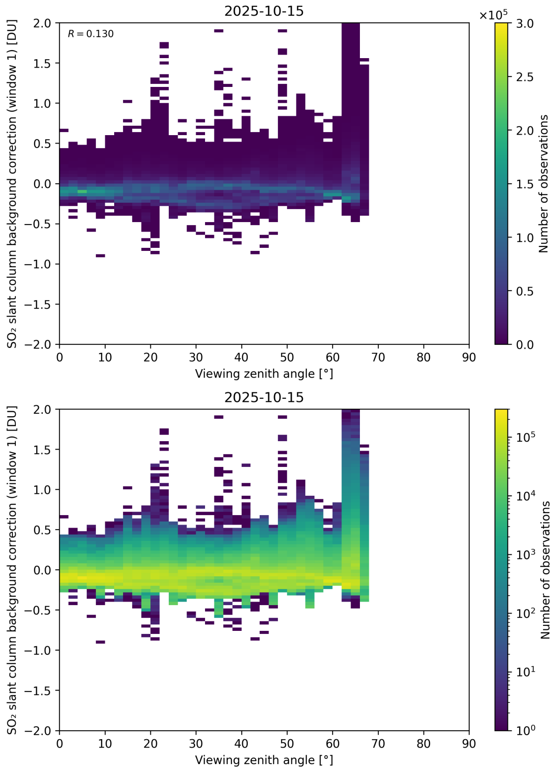
Figure 362: Scatter density plot of “Viewing zenith angle” against “SO 2 slant column background correction (window 1)” for 2025-10-14 to 2025-10-16.
