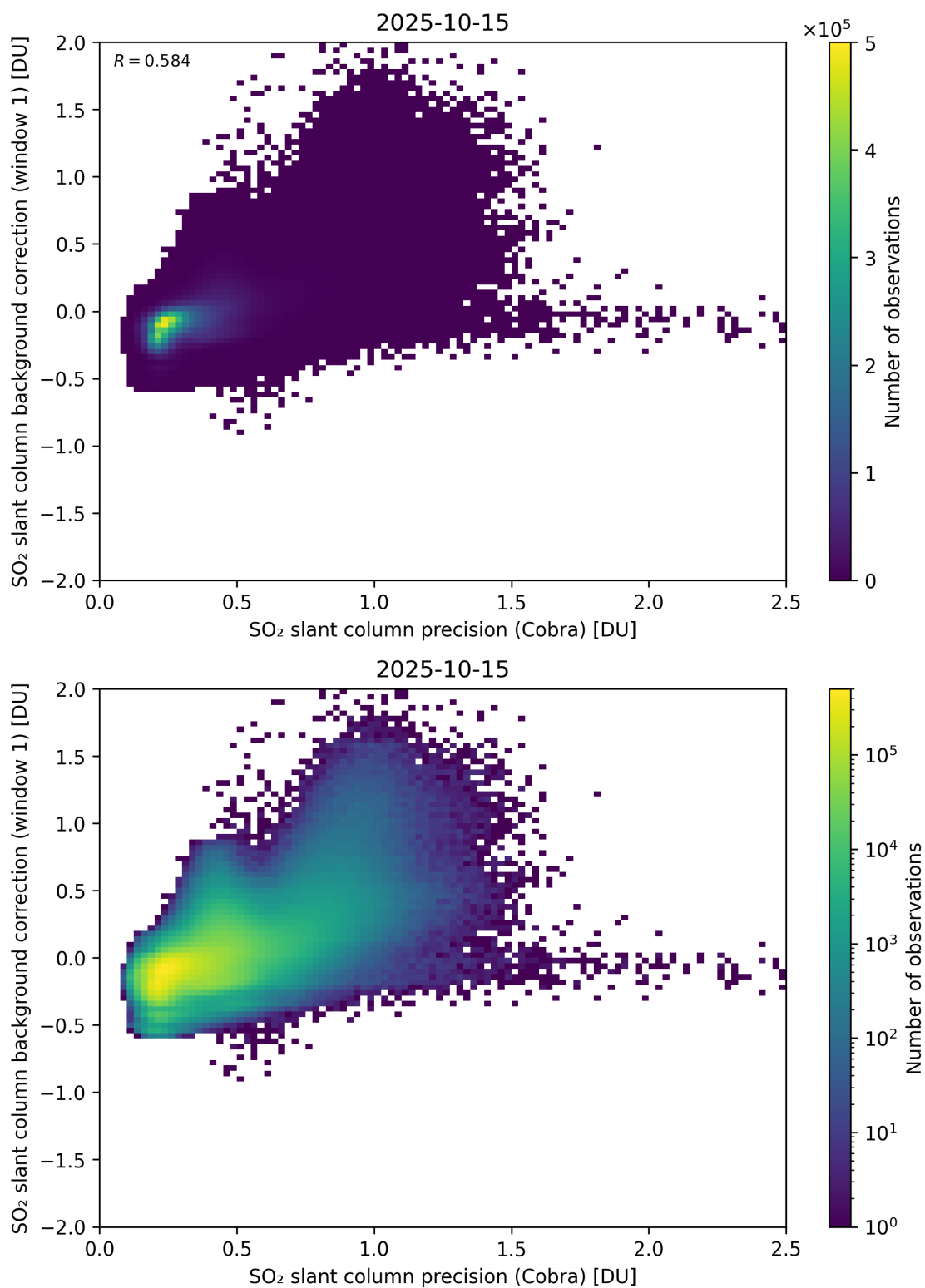
Figure 199: Scatter density plot of “SO 2 slant column precision (Cobra)” against “SO 2 slant column background correction (window 1)” for 2025-10-14 to 2025-10-16.
