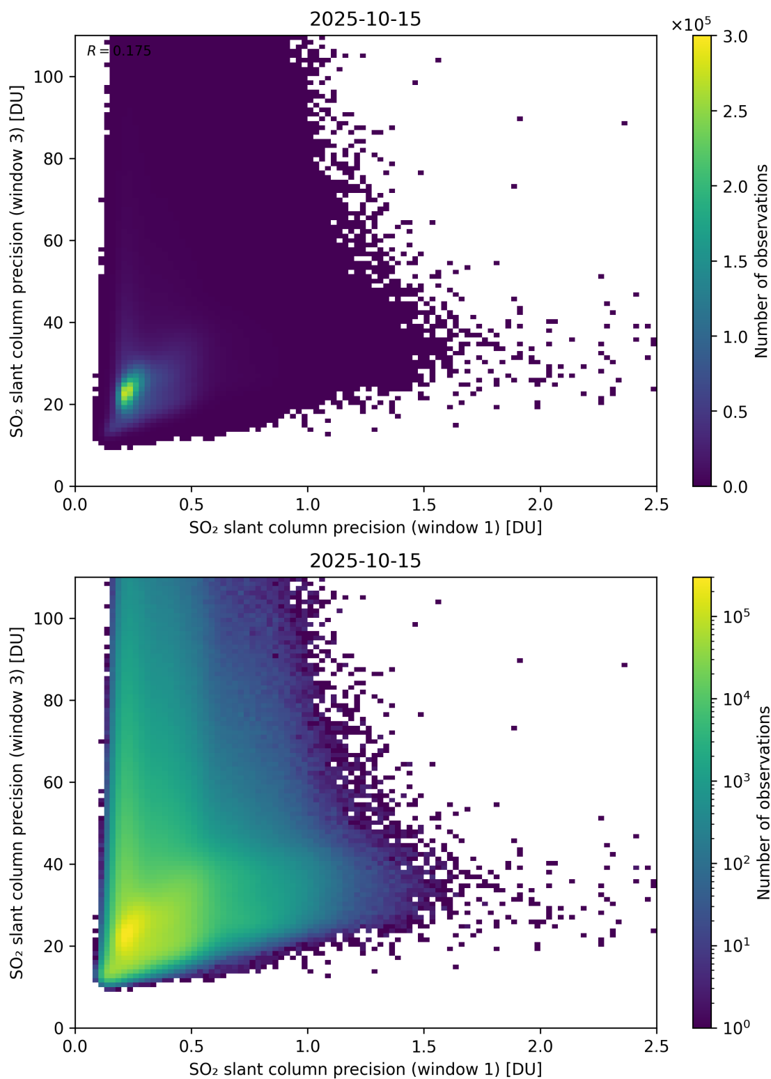
Figure 279: Scatter density plot of “SO 2 slant column precision (window 1)” against “SO 2 slant column precision (window 3)” for 2025-10-14 to 2025-10-16.
