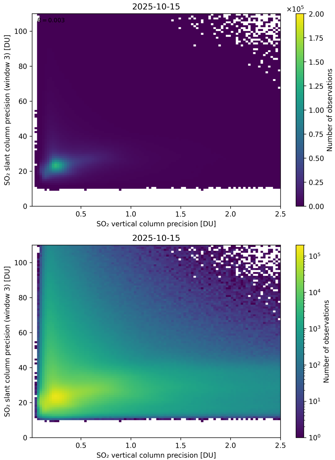
Figure 345: Scatter density plot of “SO 2 vertical column precision” against “SO 2 slant column precision (window 3)” for 2025-10-14 to 2025-10-16.
