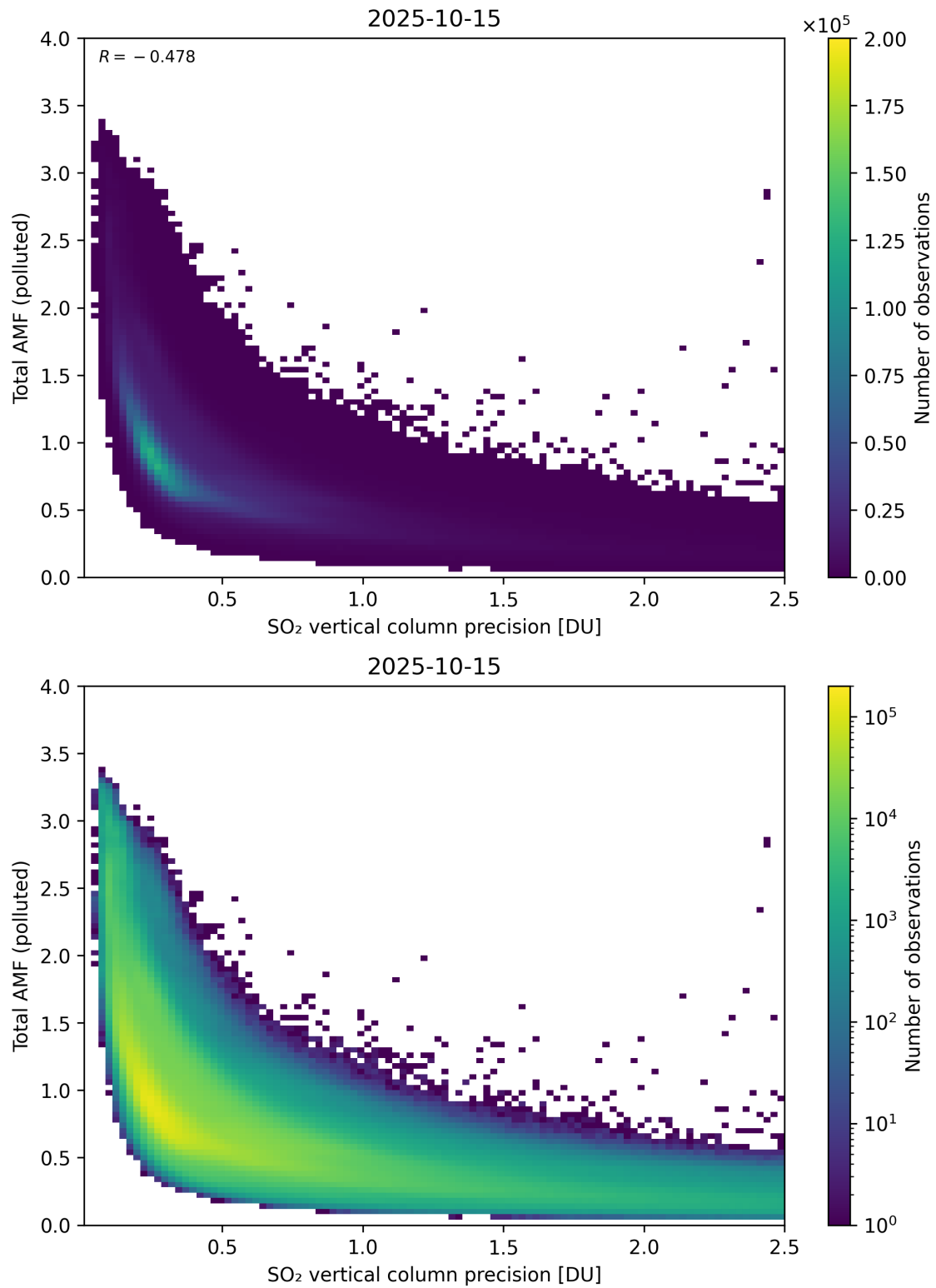
Figure 346: Scatter density plot of “SO 2 vertical column precision” against “Total AMF (polluted)” for 2025-10-14 to 2025-10-16.
