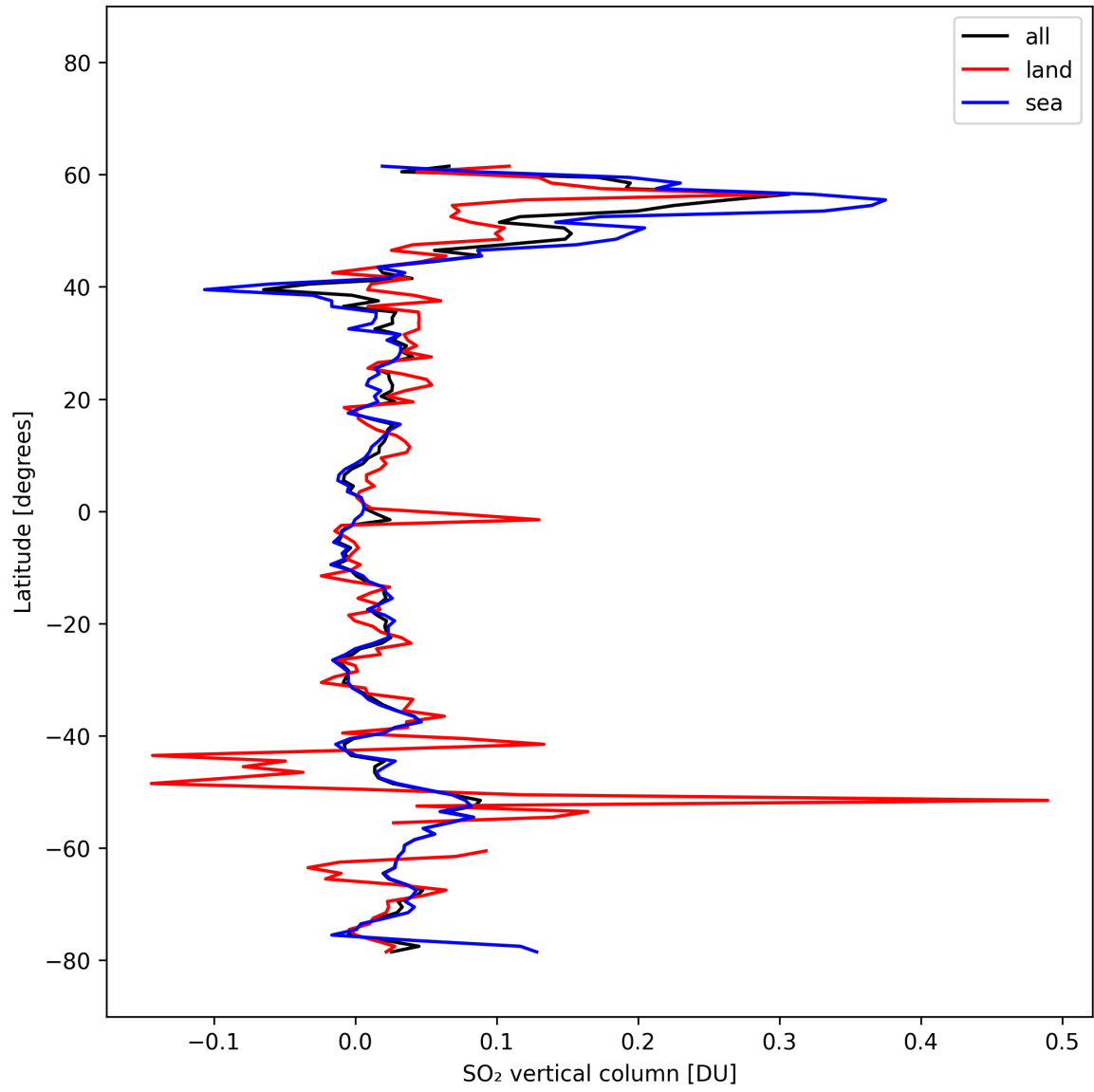
Figure 32: Zonal average of “SO 2 vertical column” for 2025-10-14 to 2025-10-16.
