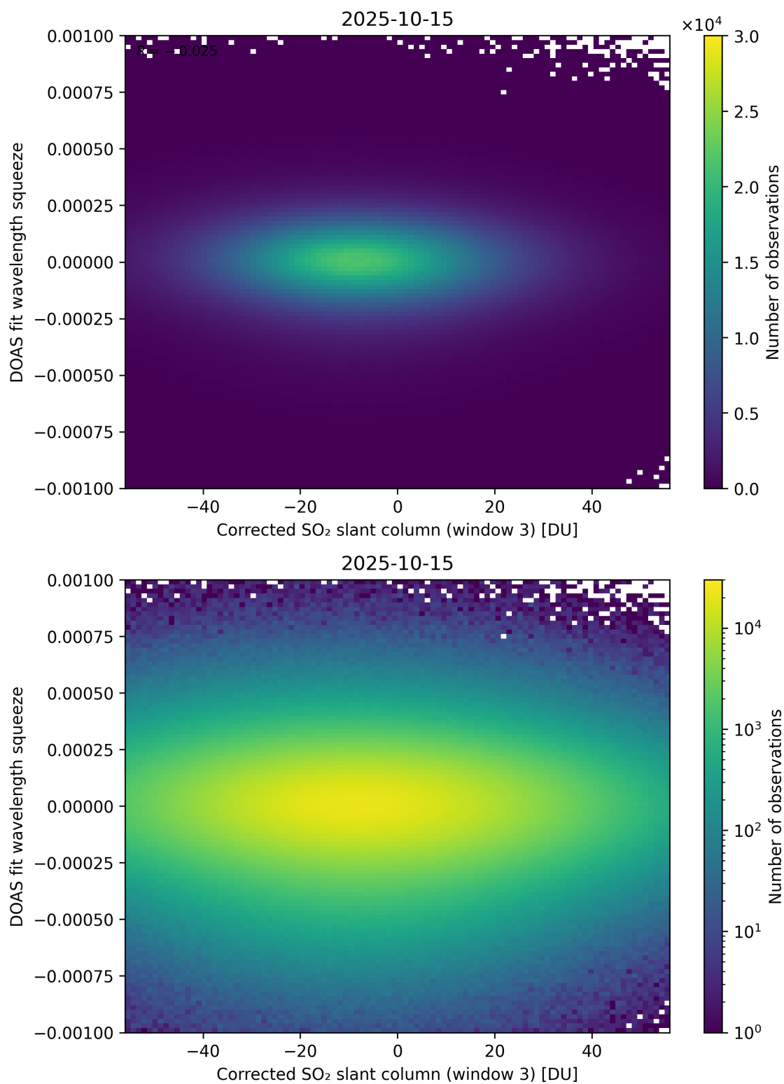
Figure 257: Scatter density plot of “Corrected SO 2 slant column (window 3)” against “DOAS fit wavelength squeeze” for 2025-10-14 to 2025-10-16.
