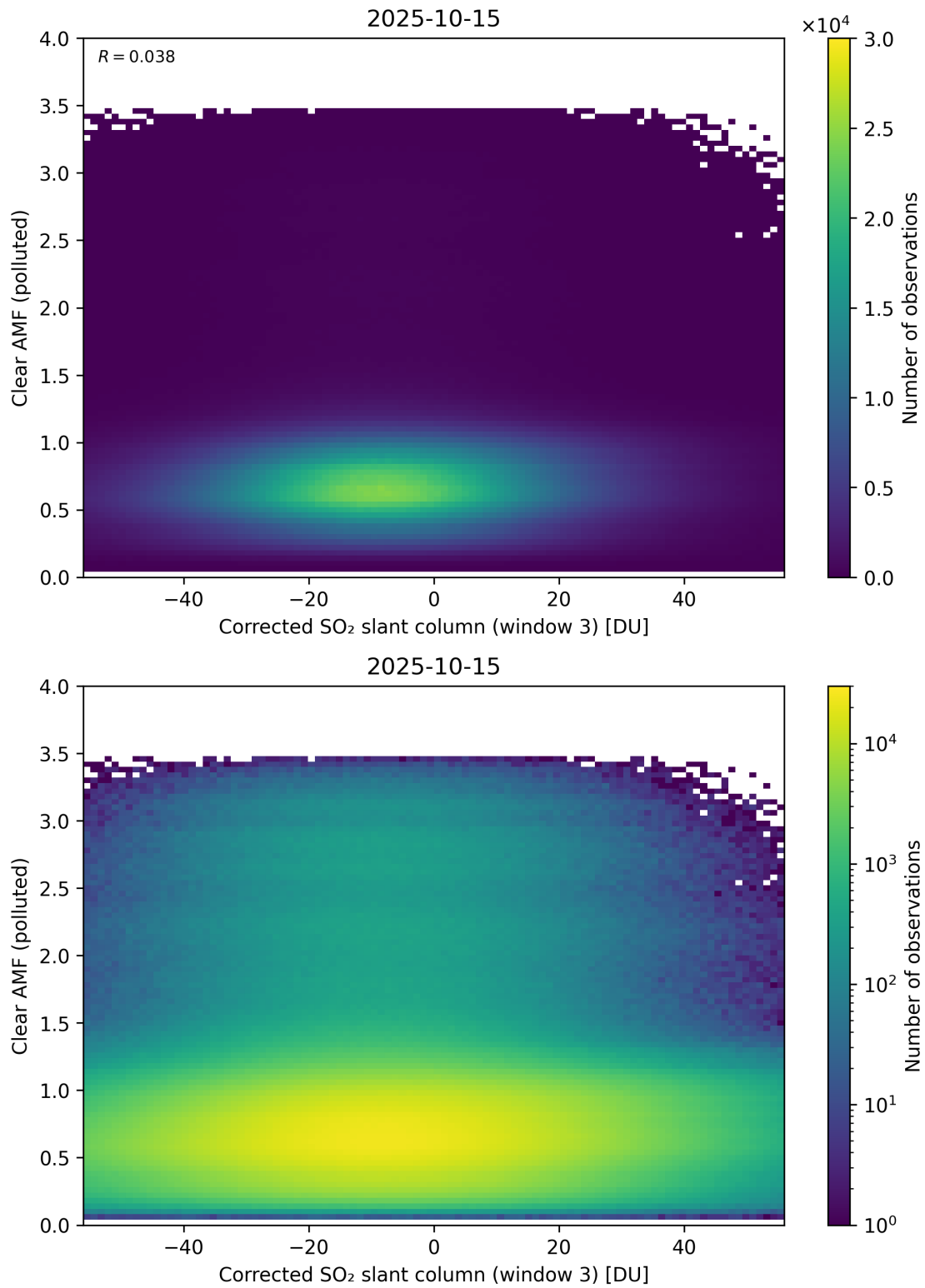
Figure 259: Scatter density plot of “Corrected SO 2 slant column (window 3)” against “Clear AMF (polluted)” for 2025-10-14 to 2025-10-16.
