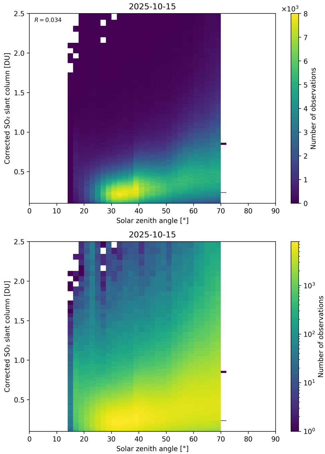
Figure 181: Scatter density plot of “Solar zenith angle” against “Corrected SO 2 slant column” for 2025-10-14 to 2025-10-16.
