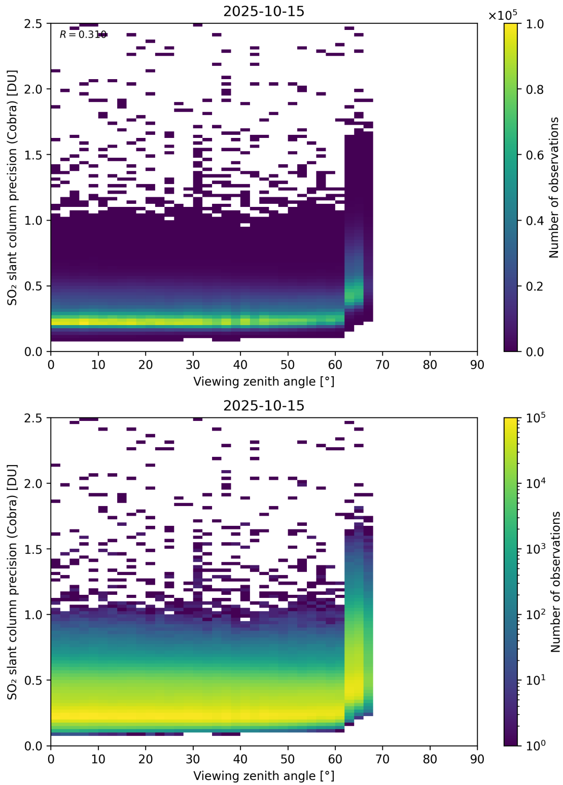
Figure 372: Scatter density plot of “Viewing zenith angle” against “SO 2 slant column precision (Cobra)” for 2025-10-14 to 2025-10-16.
