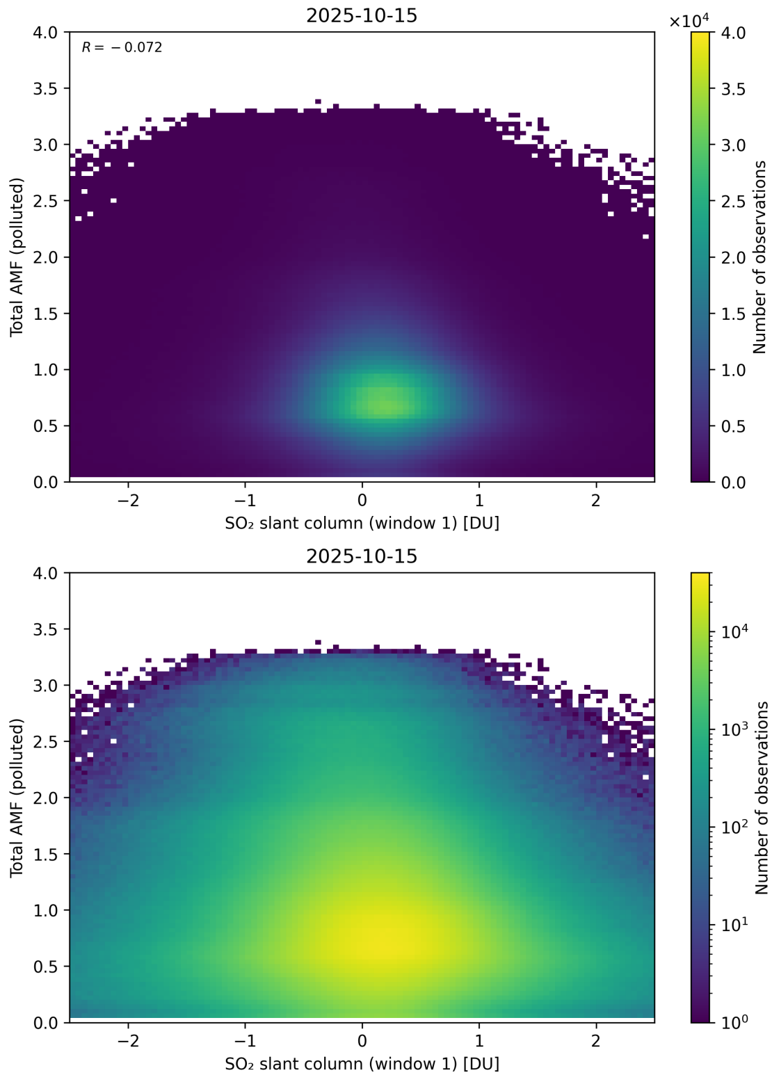
Figure 289: Scatter density plot of “SO 2 slant column (window 1)” against “Total AMF (polluted)” for 2025-10-14 to 2025-10-16.
