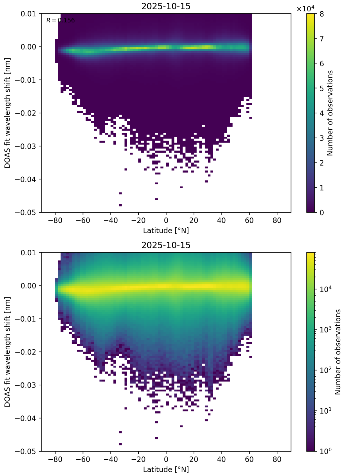
Figure 153: Scatter density plot of “Latitude” against “DOAS fit wavelength shift” for 2025-10-14 to 2025-10-16.
