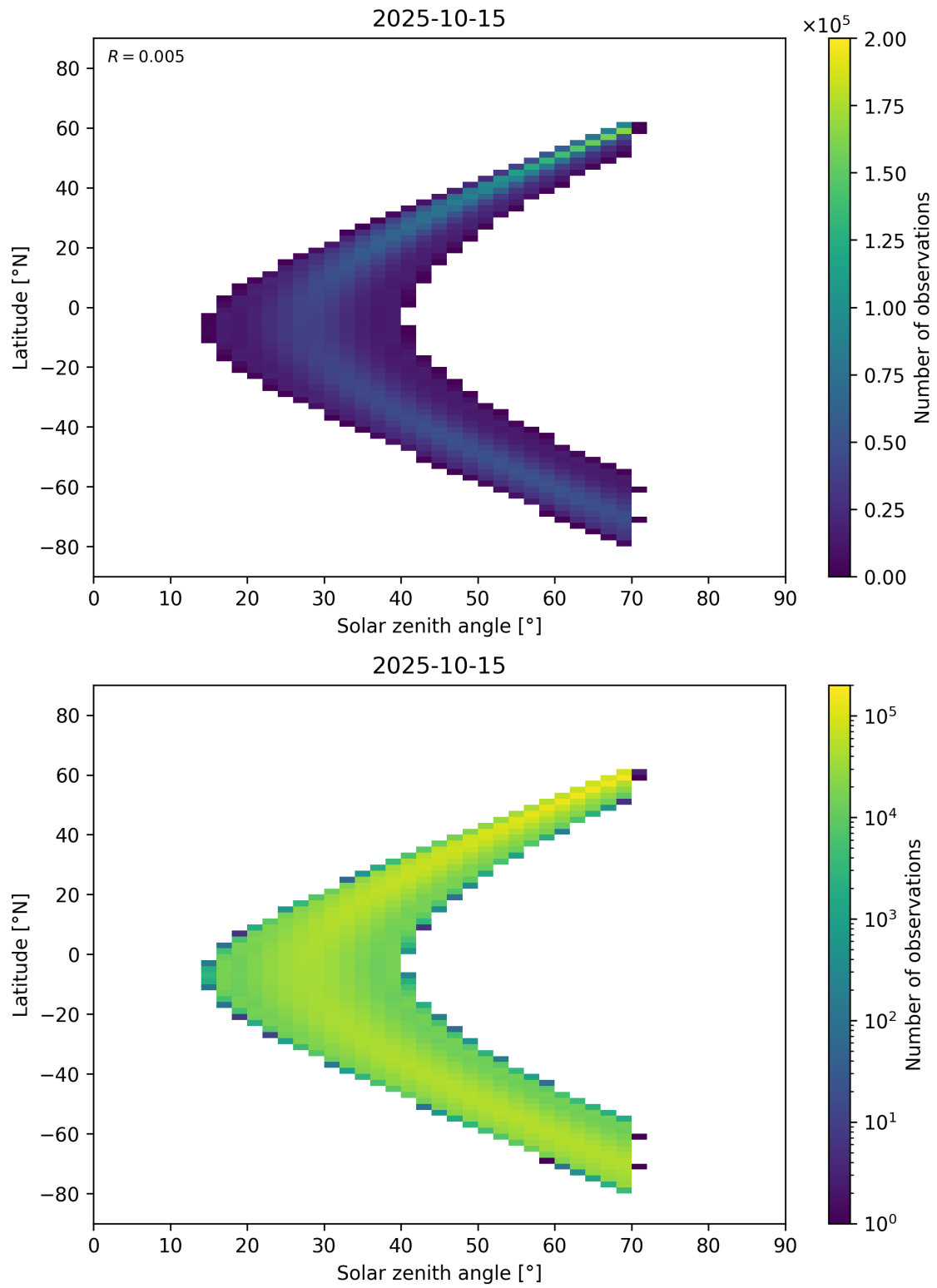
Figure 177: Scatter density plot of “Solar zenith angle” against “Latitude” for 2025-10-14 to 2025-10-16.
