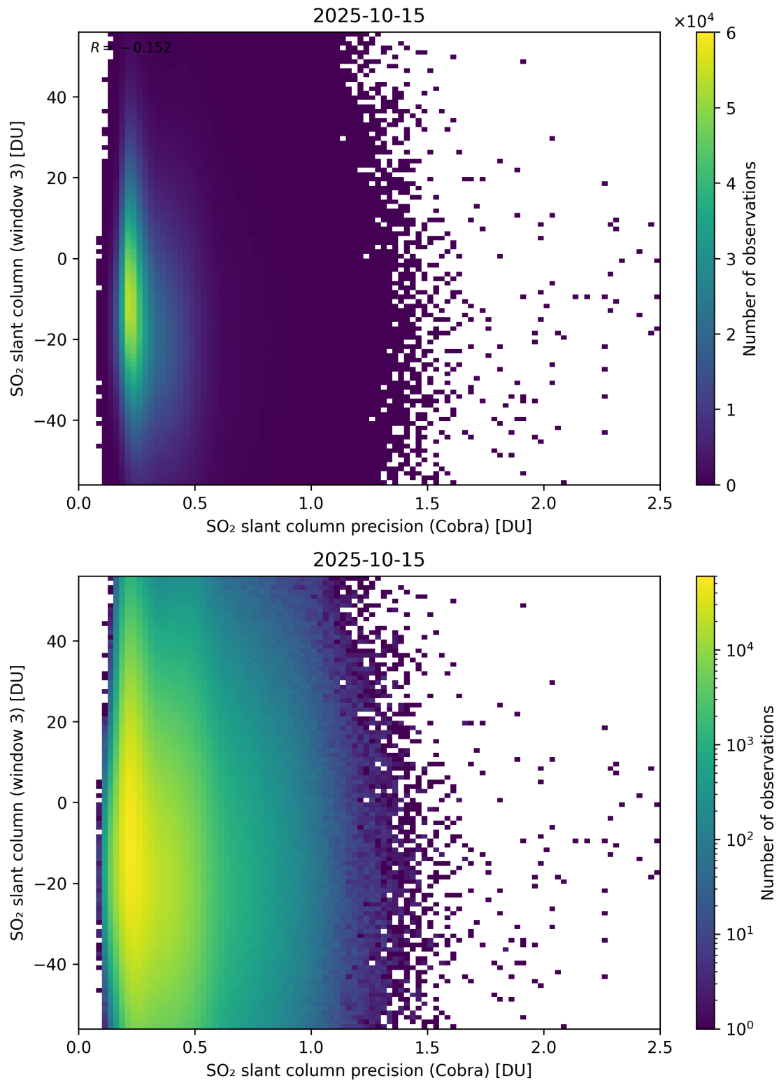
Figure 211: Scatter density plot of “SO 2 slant column precision (Cobra)” against “SO 2 slant column (window 3)” for 2025-10-14 to 2025-10-16.
