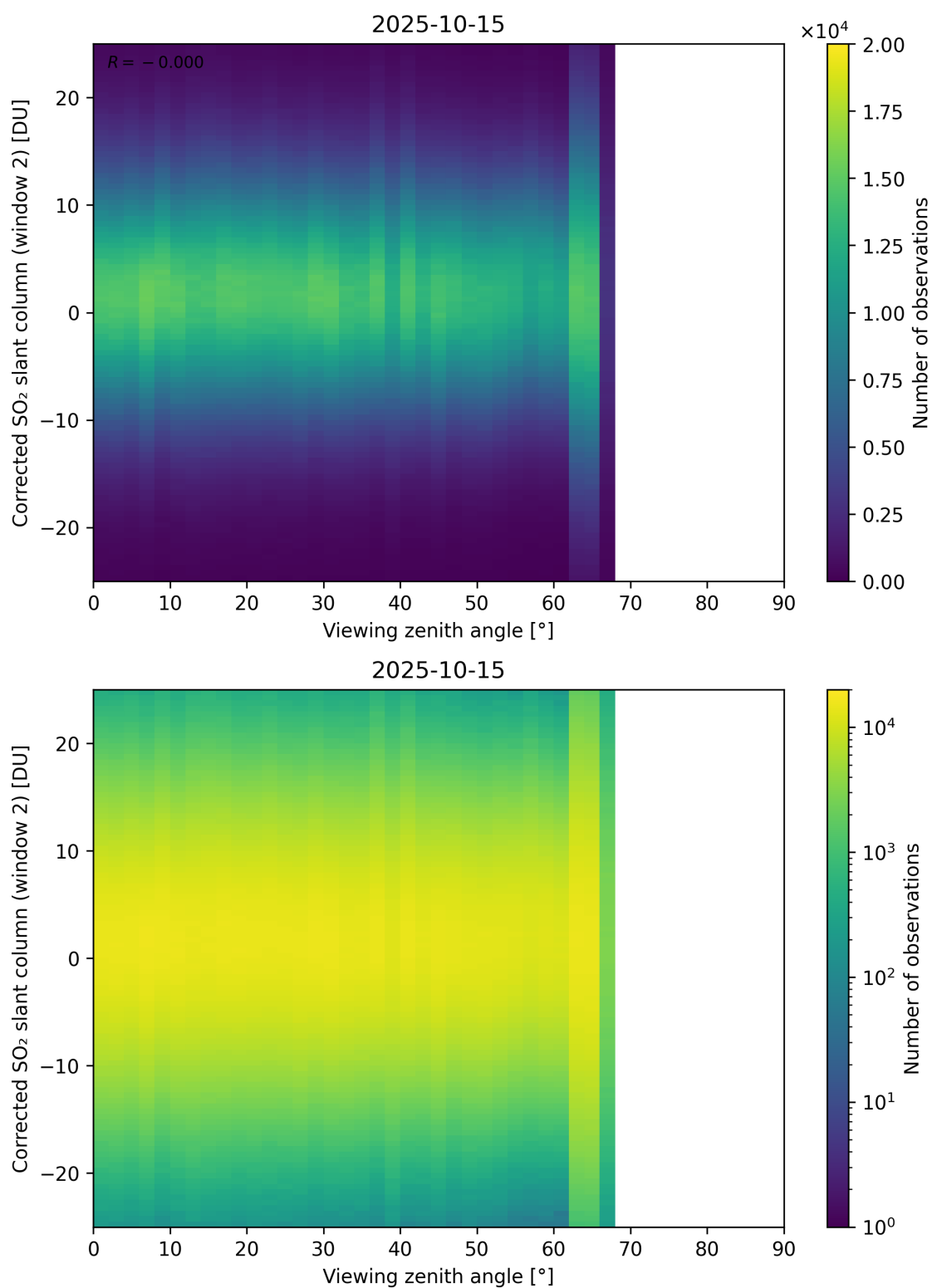
Figure 374: Scatter density plot of “Viewing zenith angle” against “Corrected SO 2 slant column (window 2)” for 2025-10-14 to 2025-10-16.
