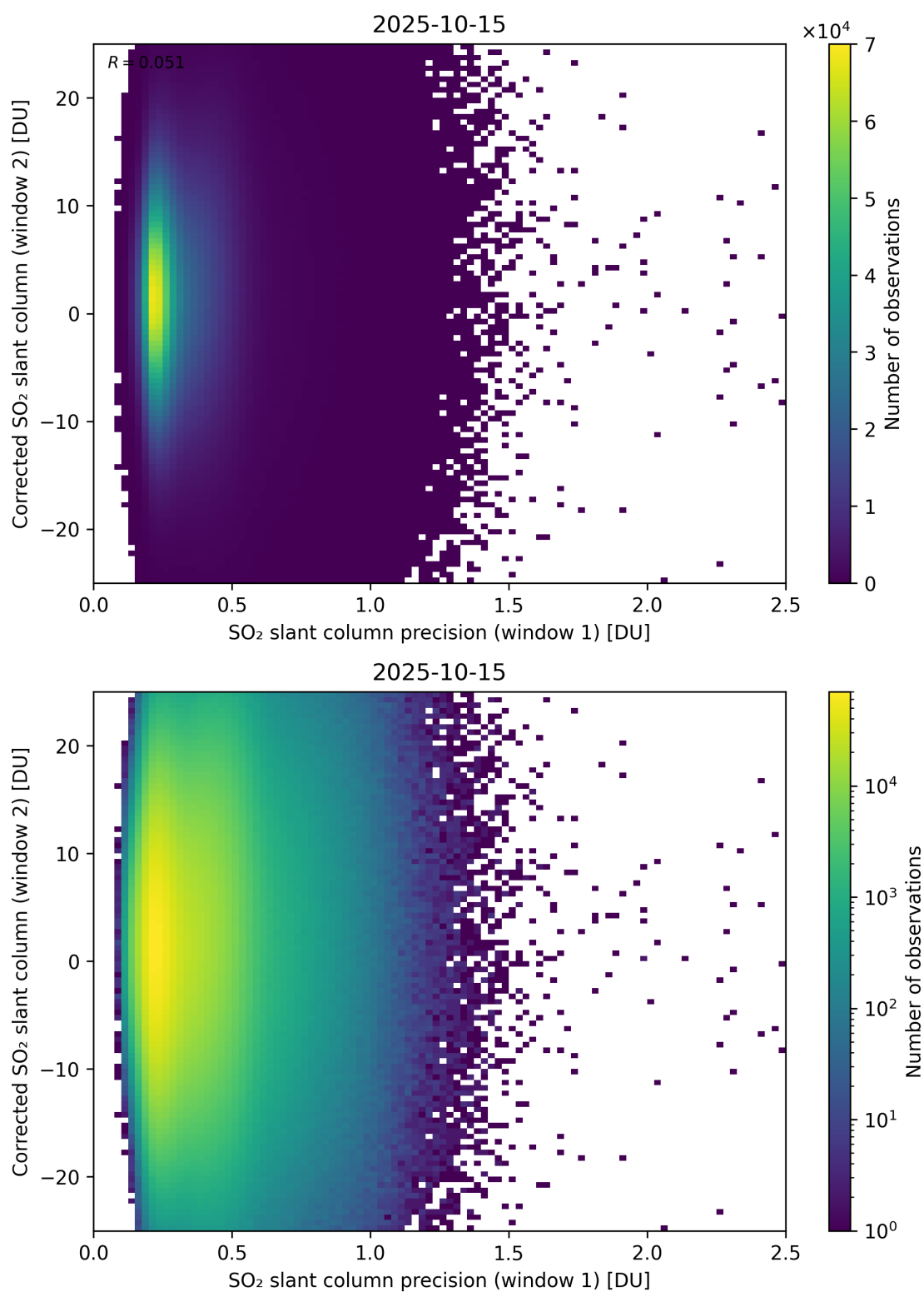
Figure 275: Scatter density plot of “SO 2 slant column precision (window 1)” against “Corrected SO 2 slant column (window 2)” for 2025-10-14 to 2025-10-16.
