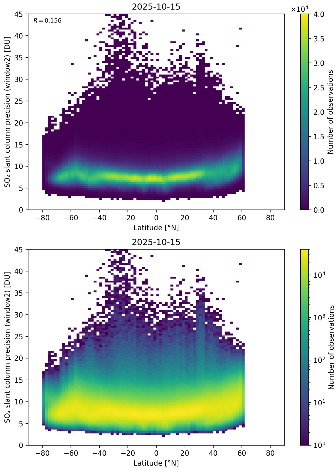
Figure 164: Scatter density plot of “Latitude” against “SO 2 slant column precision (window2)” for 2025-10-14 to 2025-10-16.
