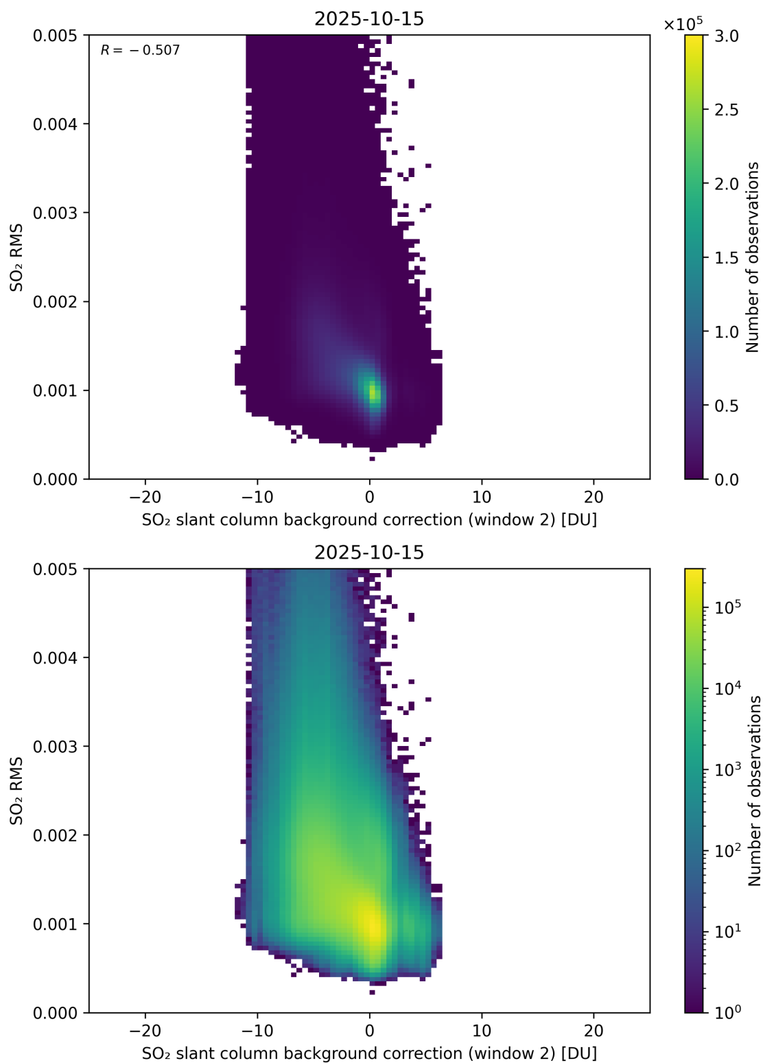
Figure 125: Scatter density plot of “SO 2 slant column background correction (window 2)” against “SO 2 RMS” for 2025-10-14 to 2025-10-16.
