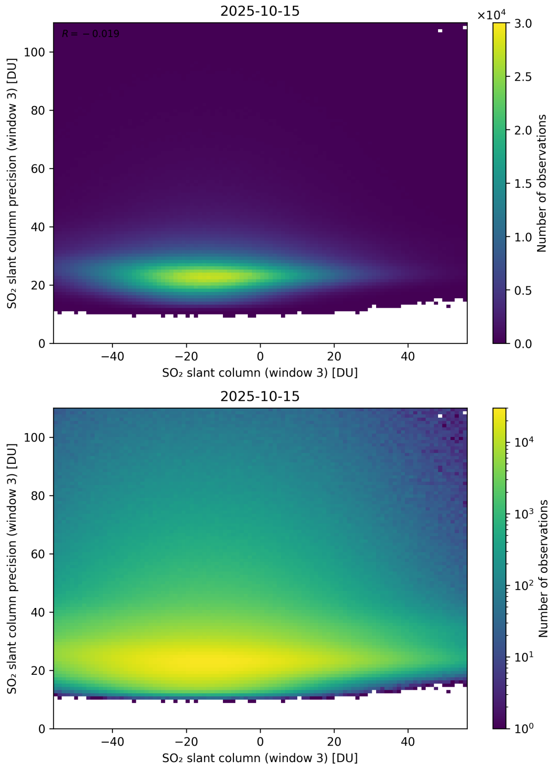
Figure 317: Scatter density plot of “SO 2 slant column (window 3)” against “SO 2 slant column precision (window 3)” for 2025-10-14 to 2025-10-16.
