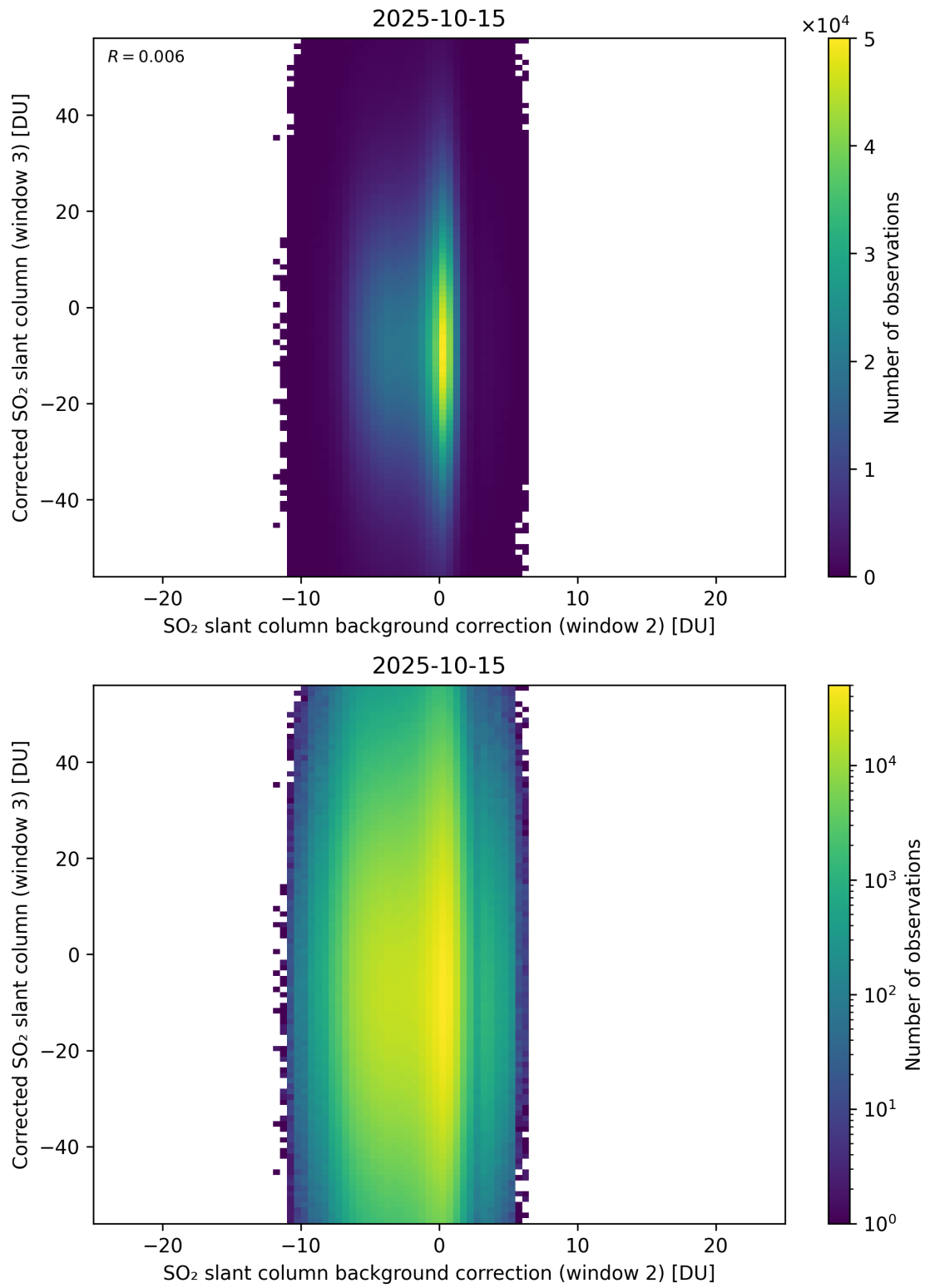
Figure 127: Scatter density plot of “SO 2 slant column background correction (window 2)” against “Corrected SO 2 slant column (window 3)” for 2025-10-14 to 2025-10-16.
