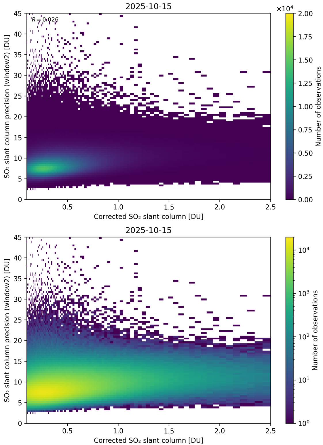
Figure 239: Scatter density plot of “Corrected SO 2 slant column” against “SO 2 slant column precision (window2)” for 2025-10-14 to 2025-10-16.
