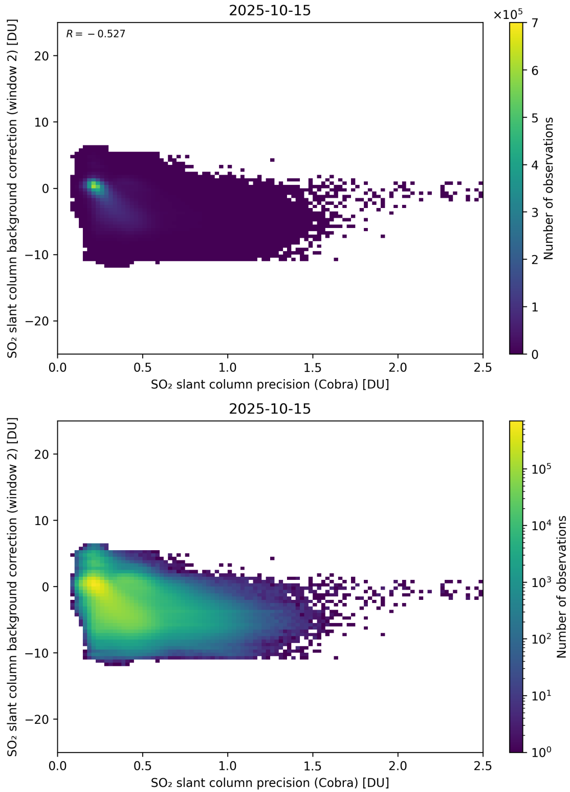
Figure 200: Scatter density plot of “SO 2 slant column precision (Cobra)” against “SO 2 slant column background correction (window 2)” for 2025-10-14 to 2025-10-16.
