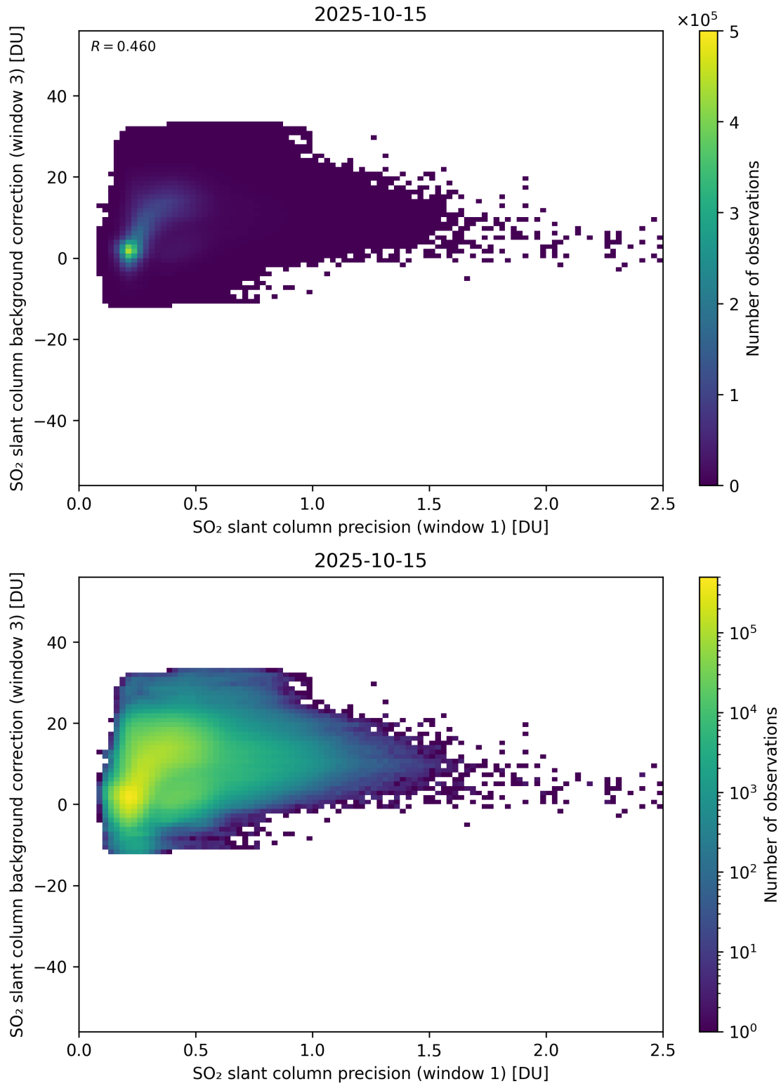
Figure 270: Scatter density plot of “SO 2 slant column precision (window 1)” against “SO 2 slant column background correction (window 3)” for 2025-10-14 to 2025-10-16.
