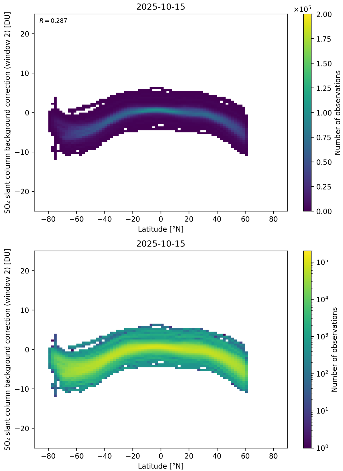
Figure 151: Scatter density plot of “Latitude” against “SO 2 slant column background correction (window 2)” for 2025-10-14 to 2025-10-16.
