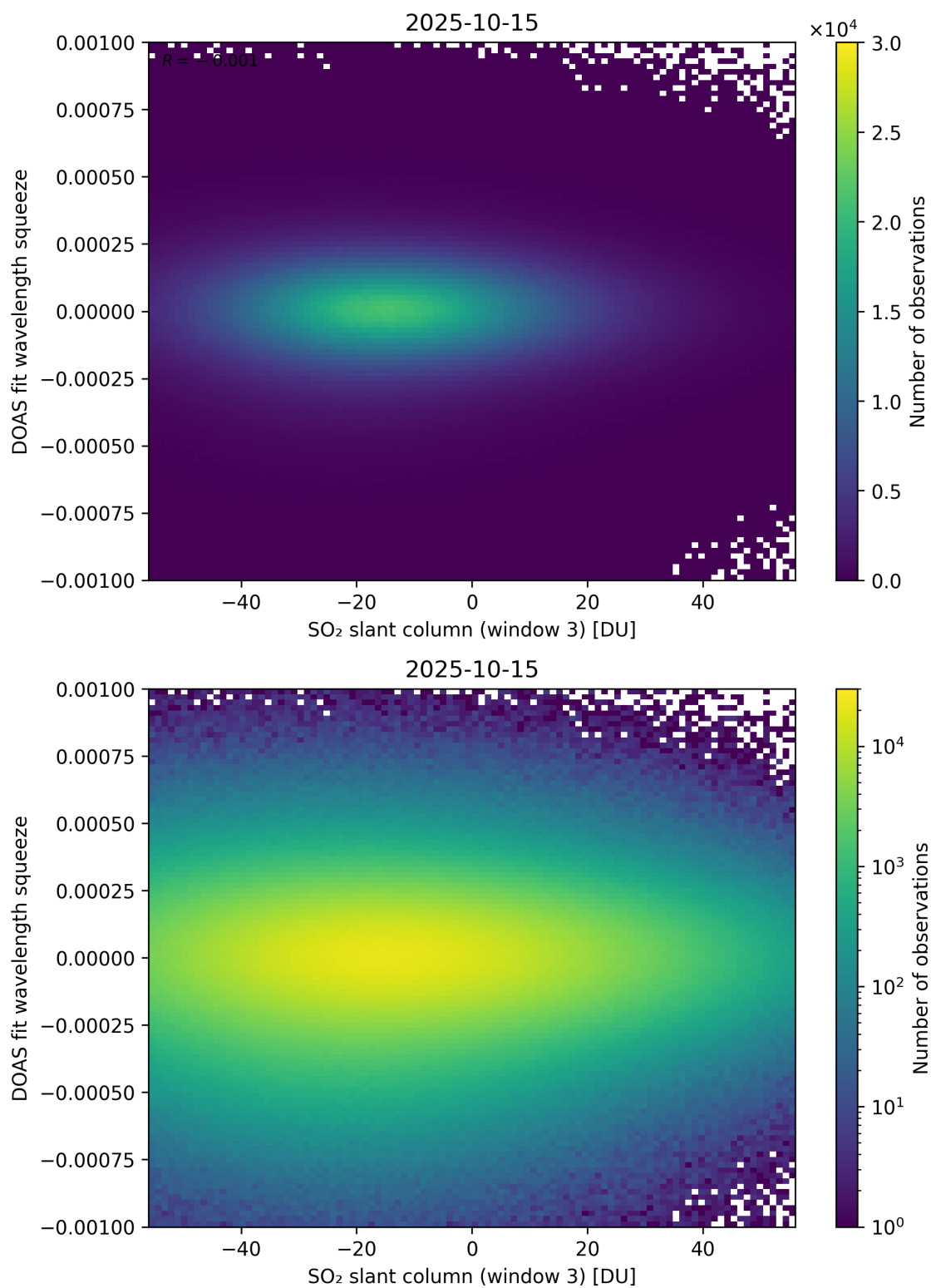
Figure 305: Scatter density plot of “SO 2 slant column (window 3)” against “DOAS fit wavelength squeeze” for 2025-10-14 to 2025-10-16.
