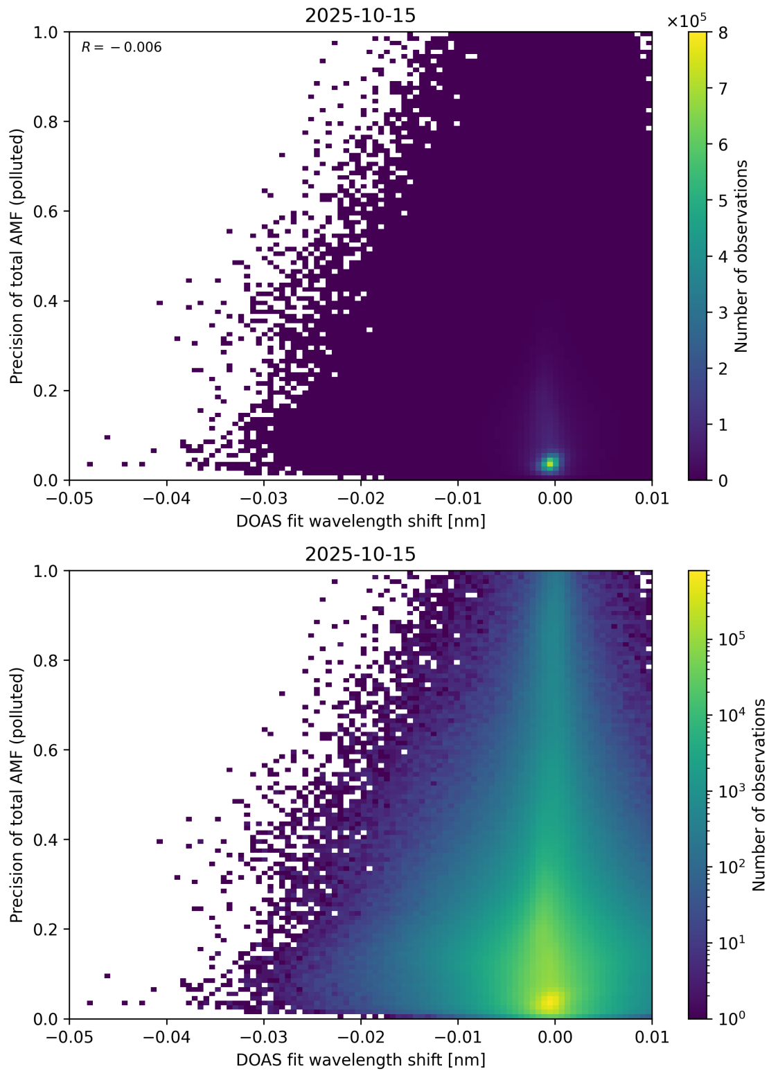
Figure 142: Scatter density plot of “DOAS fit wavelength shift” against “Precision of total AMF (polluted)” for 2025-10-14 to 2025-10-16.
