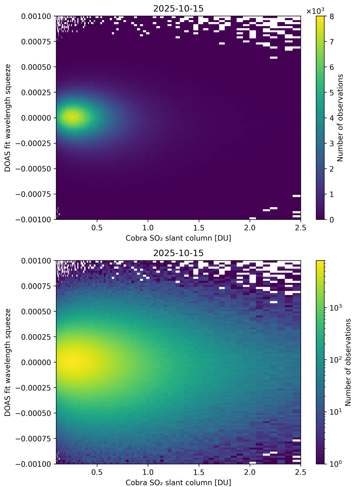
Figure 197: Scatter density plot of “Cobra SO 2 slant column” against “DOAS fit wavelength squeeze” for 2025-10-14 to 2025-10-16.
