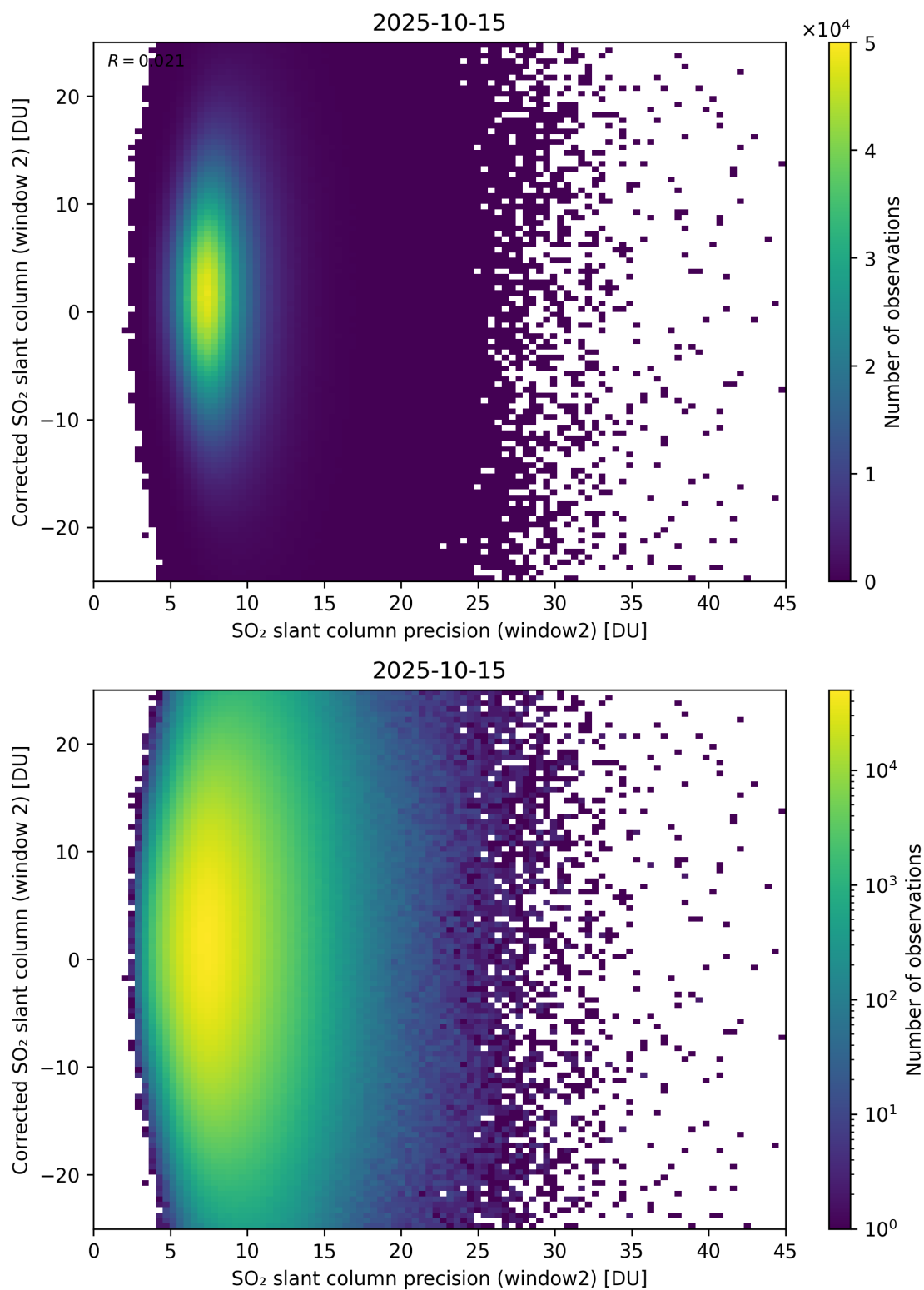
Figure 297: Scatter density plot of “SO 2 slant column precision (window2)” against “Corrected SO 2 slant column (window 2)” for 2025-10-14 to 2025-10-16.
