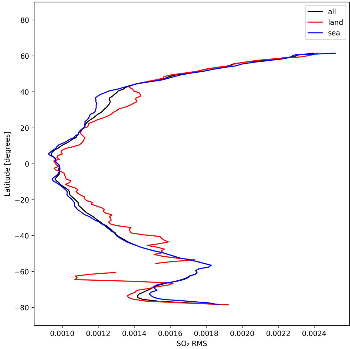
Figure 52: Zonal average of “SO 2 RMS” for 2025-10-14 to 2025-10-16.
