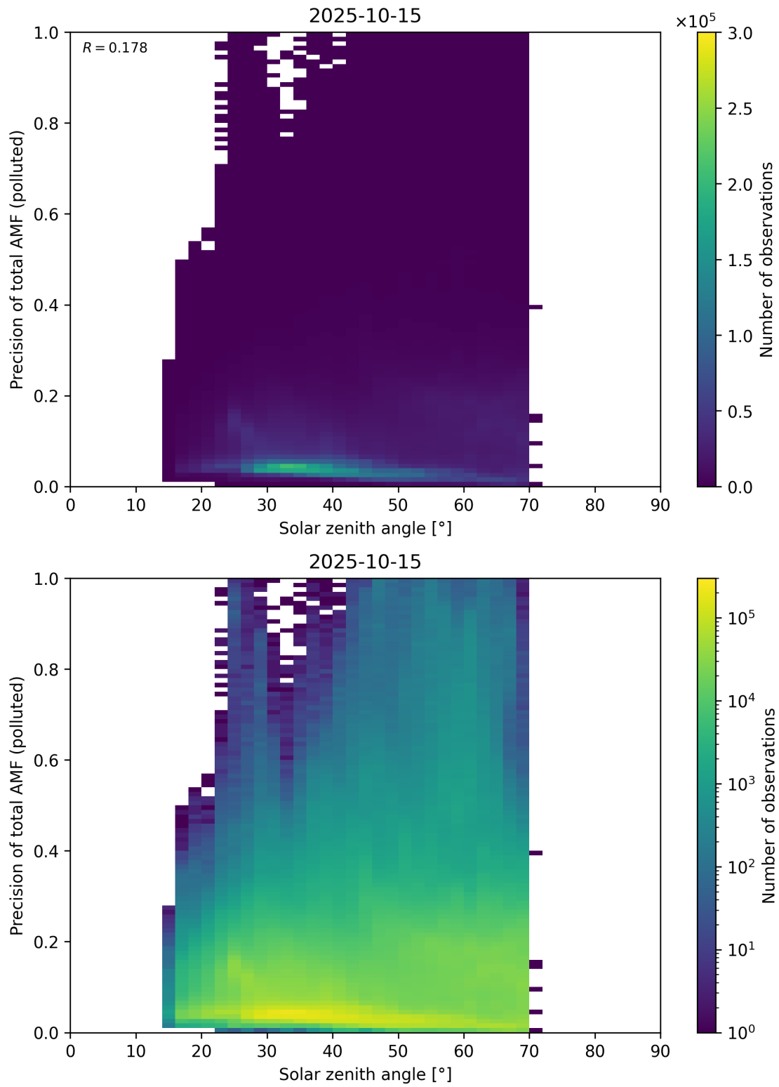
Figure 190: Scatter density plot of “Solar zenith angle” against “Precision of total AMF (polluted)” for 2025-10-14 to 2025-10-16.
