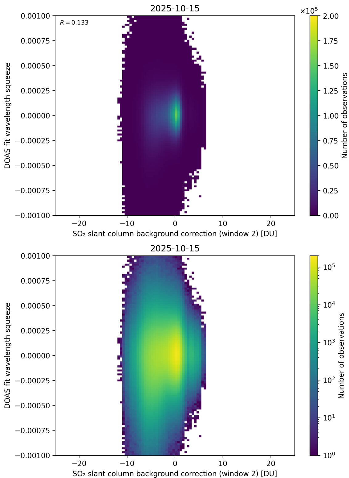
Figure 124: Scatter density plot of “SO 2 slant column background correction (window 2)” against “DOAS fit wavelength squeeze” for 2025-10-14 to 2025-10-16.
