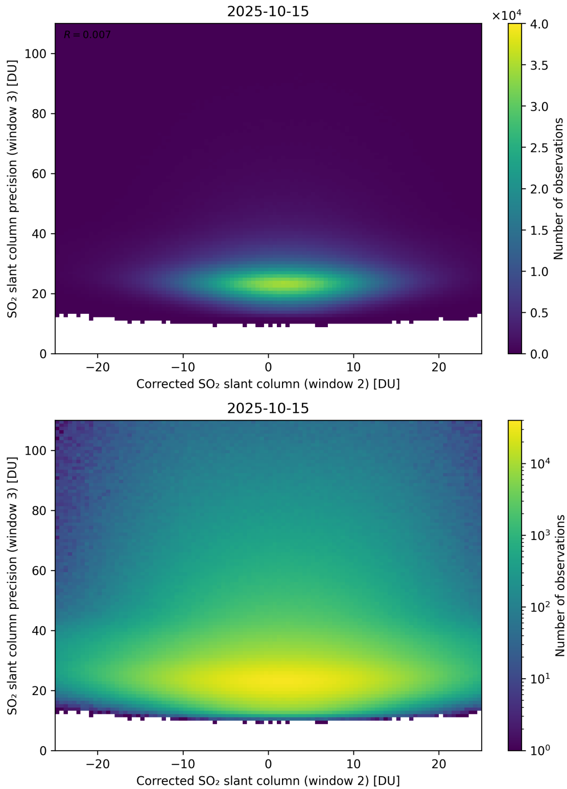
Figure 252: Scatter density plot of “Corrected SO 2 slant column (window 2)” against “SO 2 slant column precision (window 3)” for 2025-10-14 to 2025-10-16.
