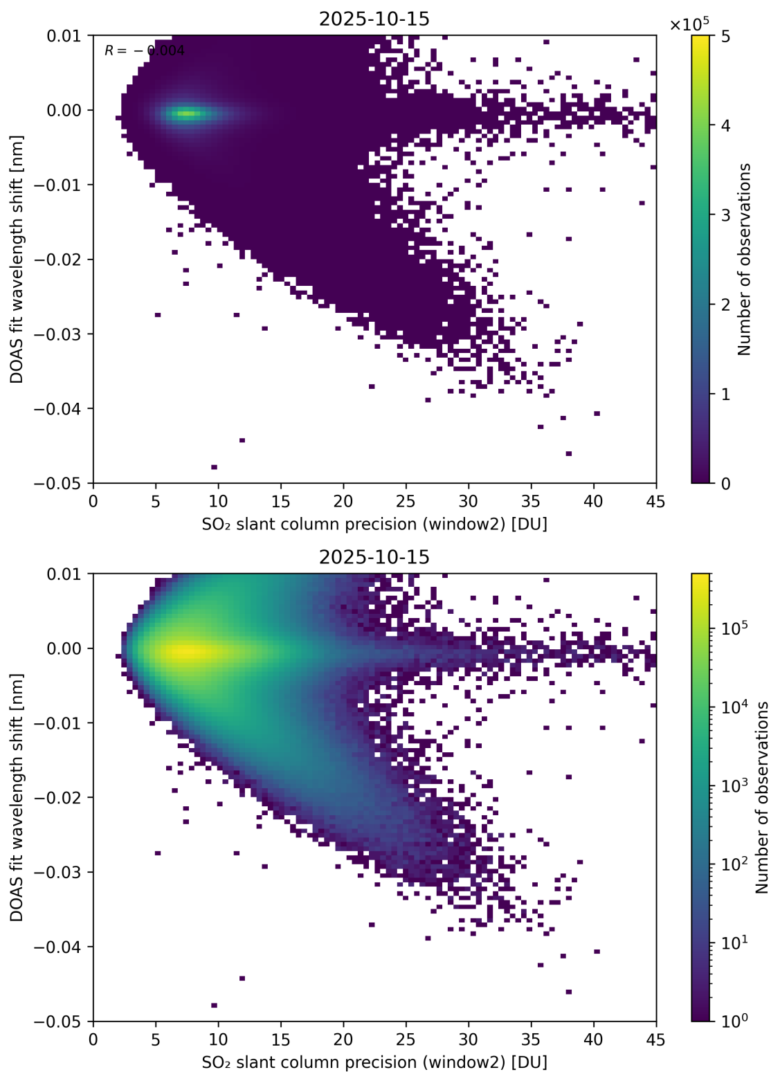
Figure 293: Scatter density plot of “SO 2 slant column precision (window2)” against “DOAS fit wavelength shift” for 2025-10-14 to 2025-10-16.
