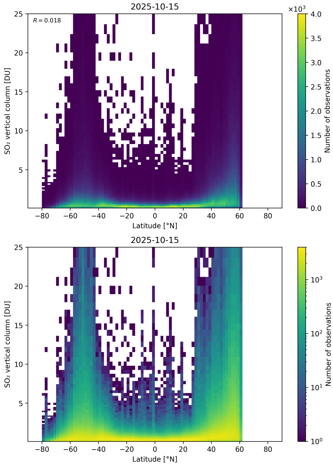
Figure 169: Scatter density plot of “Latitude” against “SO 2 vertical column” for 2025-10-14 to 2025-10-16.
