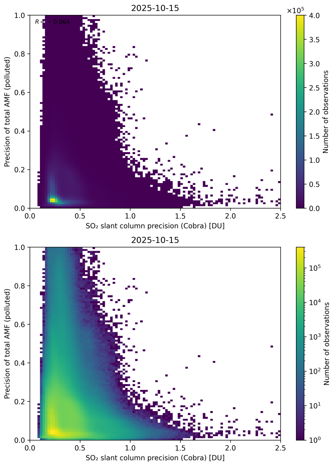
Figure 214: Scatter density plot of “SO 2 slant column precision (Cobra)” against “Precision of total AMF (polluted)” for 2025-10-14 to 2025-10-16.
