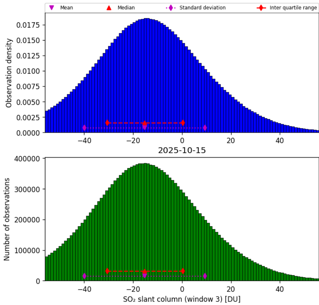
Figure 71: Histogram of “SO 2 slant column (window 3)” for 2025-10-14 to 2025-10-16
