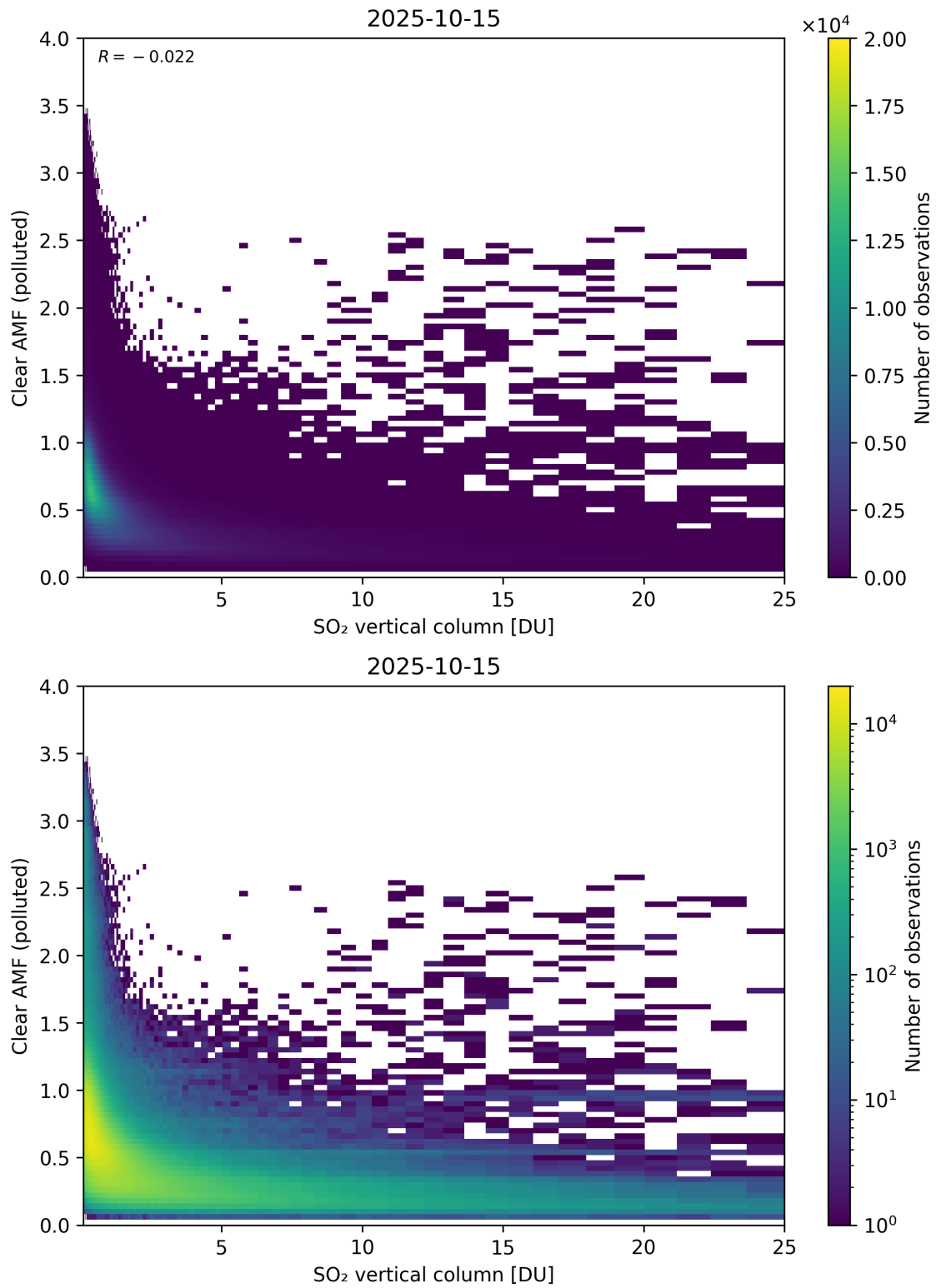
Figure 348: Scatter density plot of “SO 2 vertical column” against “Clear AMF (polluted)” for 2025-10-14 to 2025-10-16.
