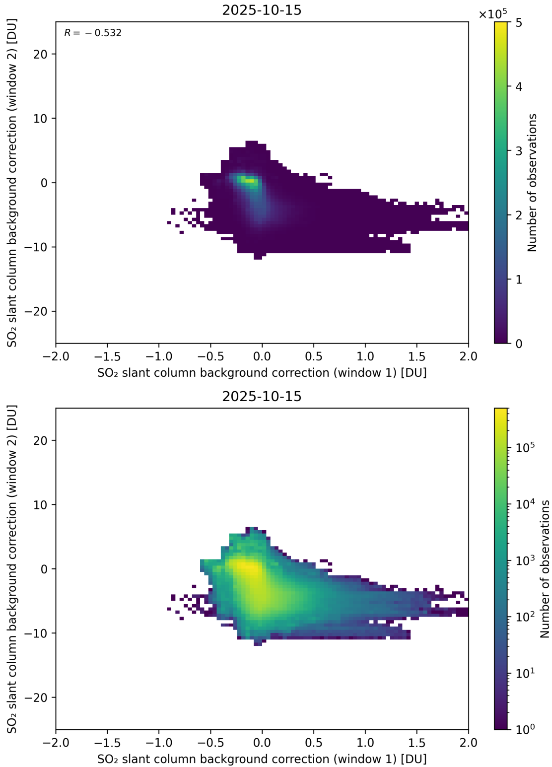
Figure 109: Scatter density plot of “SO 2 slant column background correction (window 1)” against “SO 2 slant column background correction (window 2)” for 2025-10-14 to 2025-10-16.
