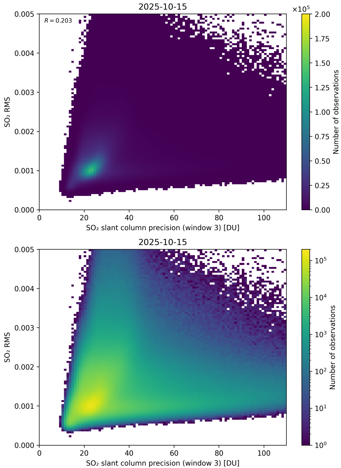
Figure 310: Scatter density plot of “SO 2 slant column precision (window 3)” against “SO 2 RMS” for 2025-10-14 to 2025-10-16.
