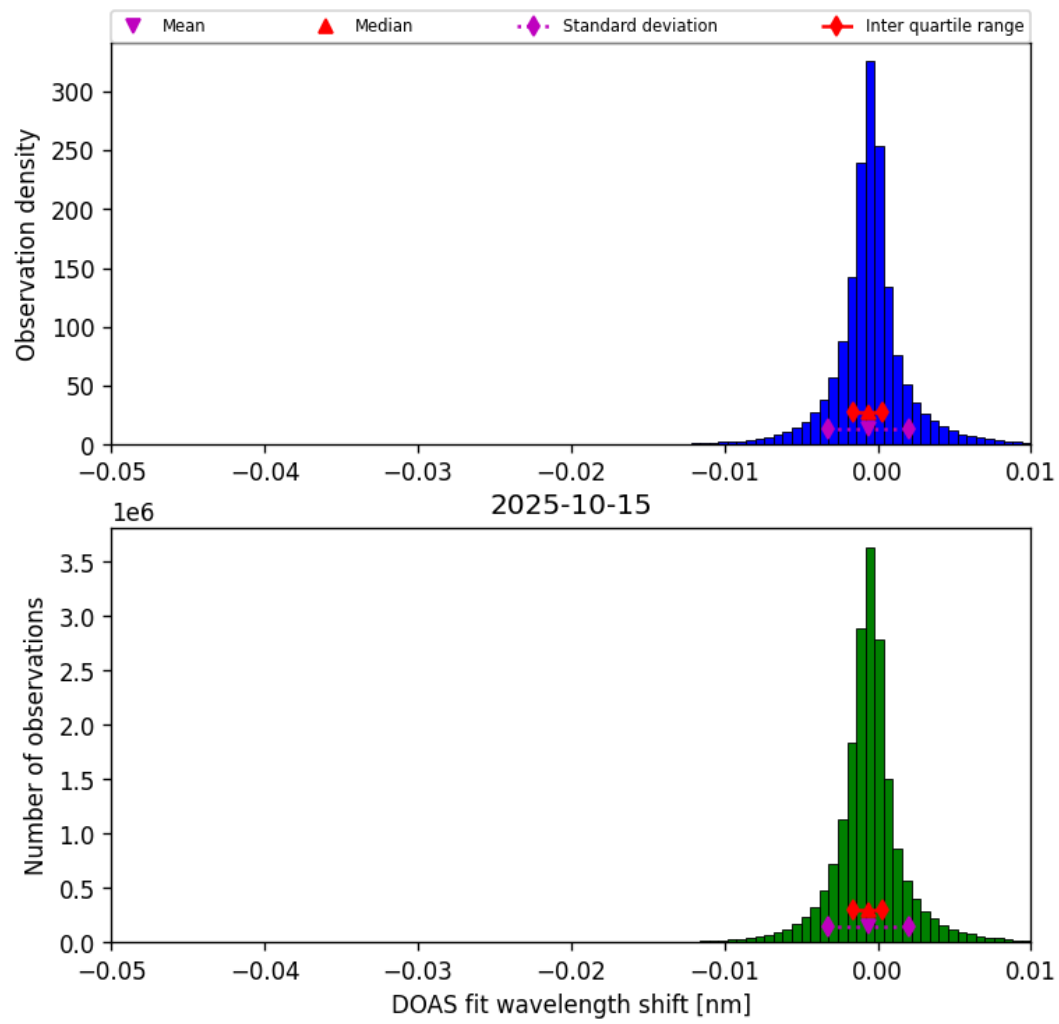
Figure 76: Histogram of “DOAS fit wavelength shift” for 2025-10-14 to 2025-10-16
