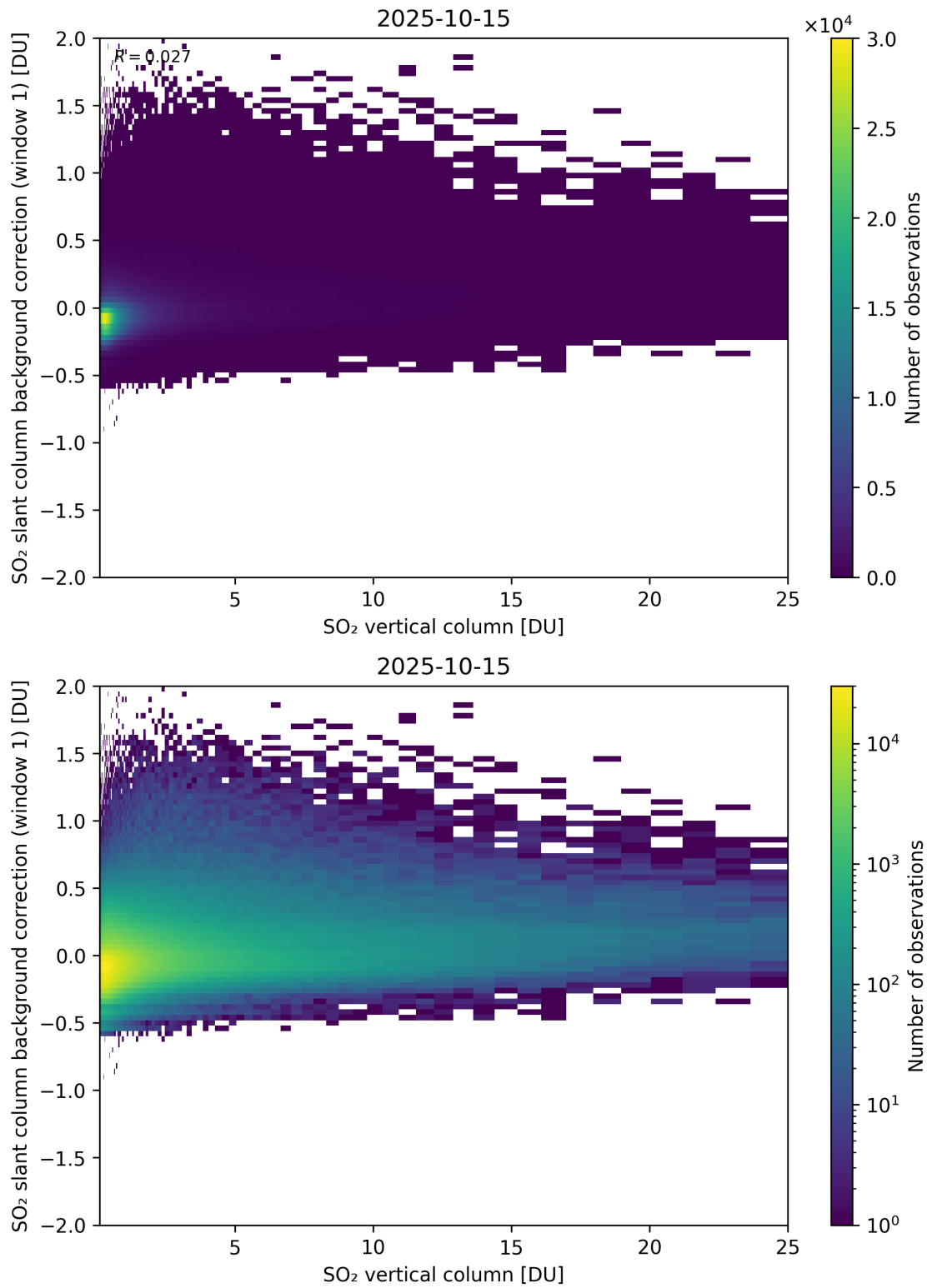
Figure 323: Scatter density plot of “SO 2 vertical column” against “SO 2 slant column background correction (window 1)” for 2025-10-14 to 2025-10-16.
