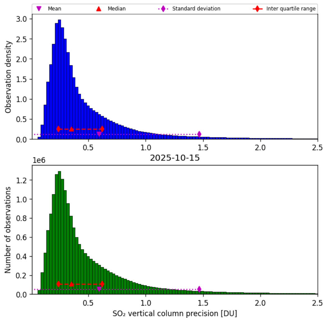
Figure 59: Histogram of “SO 2 vertical column precision” for 2025-10-14 to 2025-10-16
