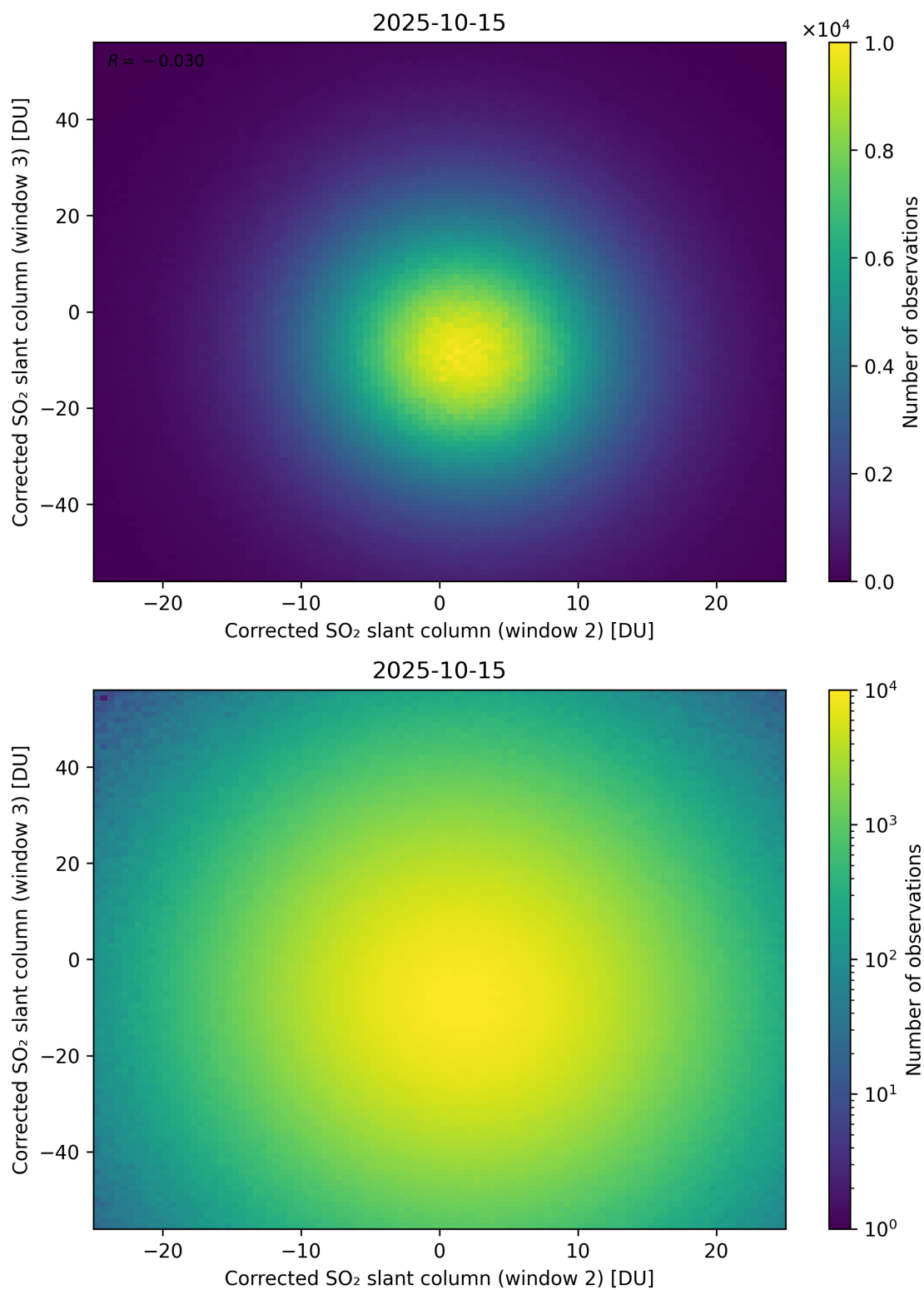
Figure 250: Scatter density plot of “Corrected SO 2 slant column (window 2)” against “Corrected SO 2 slant column (window 3)” for 2025-10-14 to 2025-10-16.
