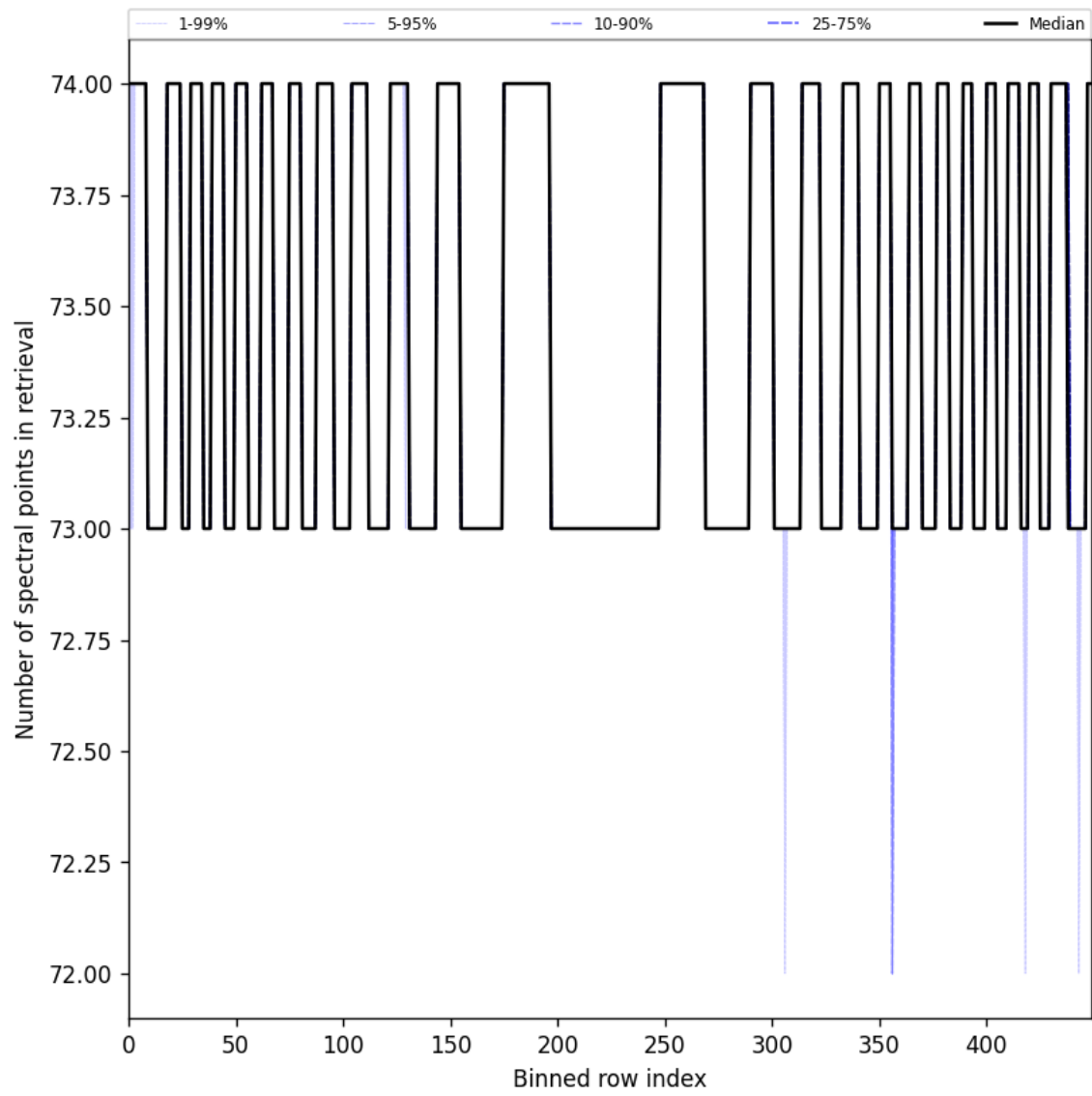
Figure 108: Along track statistics of “Number of spectral points in retrieval” for 2025-10-14 to 2025-10-16
