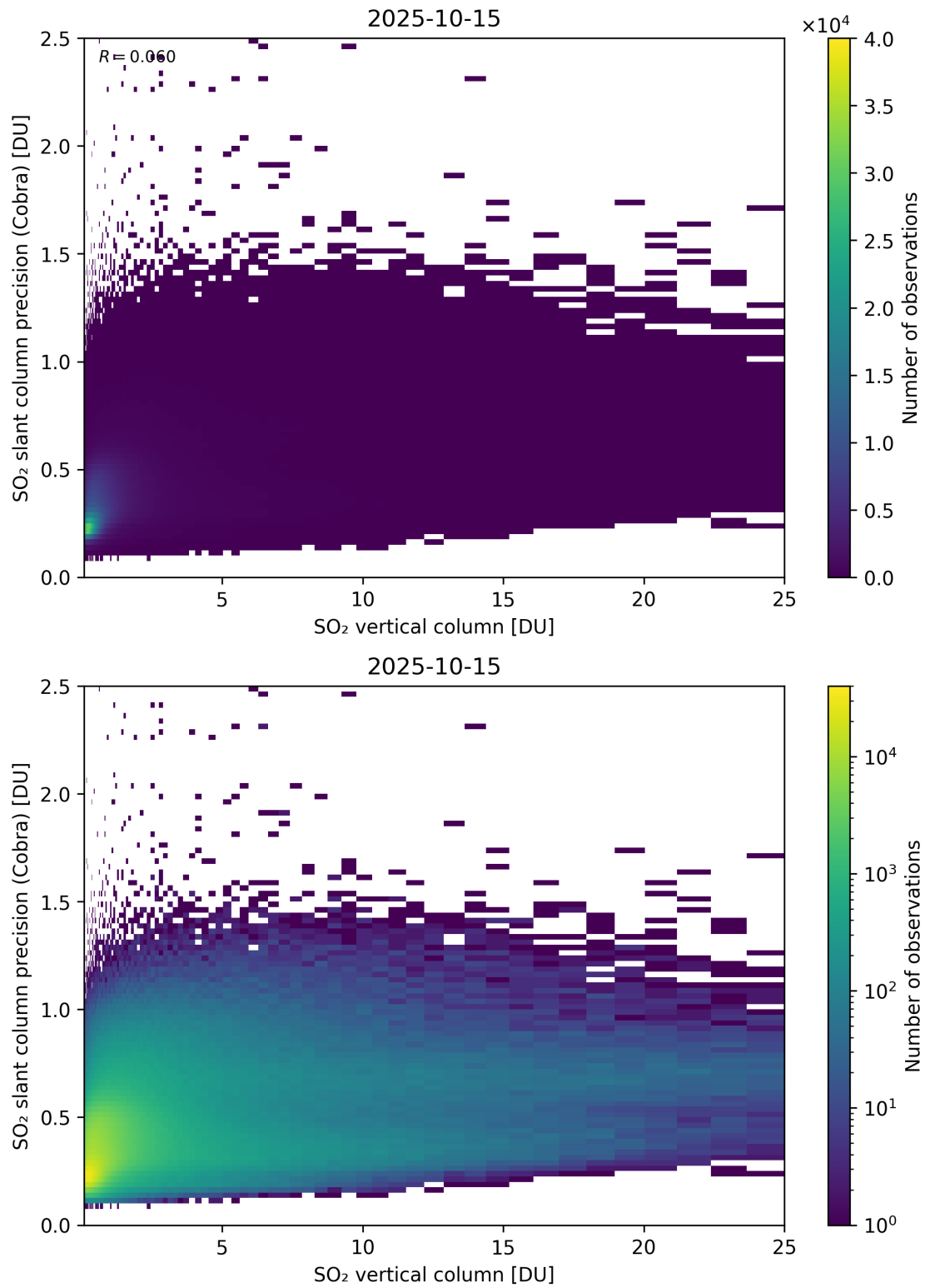
Figure 350: Scatter density plot of “SO 2 vertical column” against “SO 2 slant column precision (Cobra)” for 2025-10-14 to 2025-10-16.
