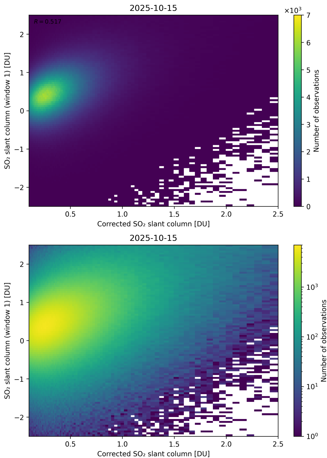
Figure 237: Scatter density plot of “Corrected SO 2 slant column” against “SO 2 slant column (window 1)” for 2025-10-14 to 2025-10-16.
