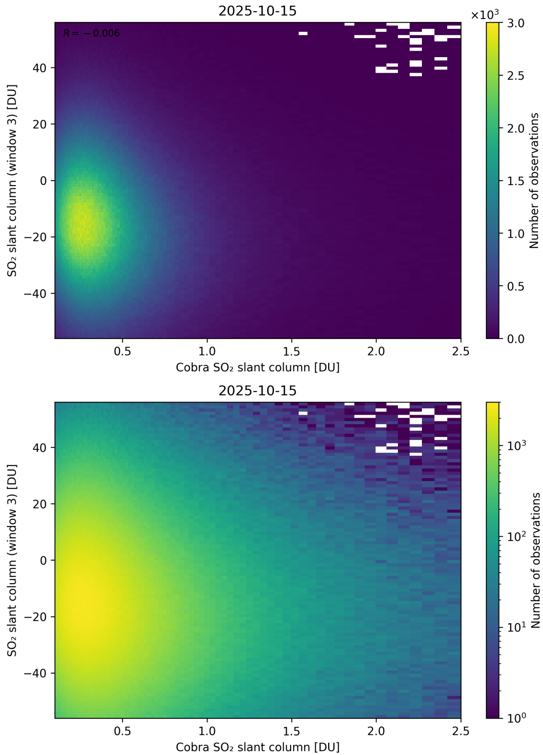
Figure 222: Scatter density plot of “Cobra SO 2 slant column” against “SO 2 slant column (window 3)” for 2025-10-14 to 2025-10-16.
