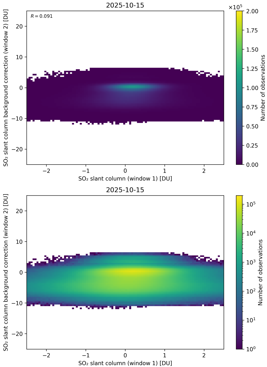
Figure 263: Scatter density plot of “SO 2 slant column (window 1)” against “SO 2 slant column background correction (window 2)” for 2025-10-14 to 2025-10-16.
