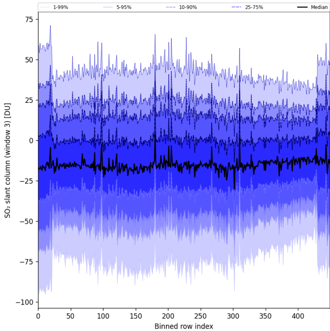
Figure 97: Along track statistics of “SO 2 slant column (window 3)” for 2025-10-14 to 2025-10-16
