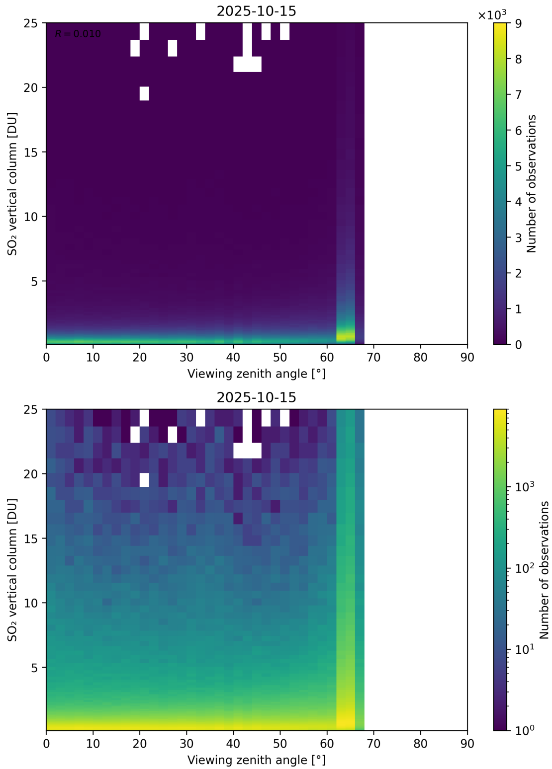
Figure 383: Scatter density plot of “Viewing zenith angle” against “SO 2 vertical column” for 2025-10-14 to 2025-10-16.
