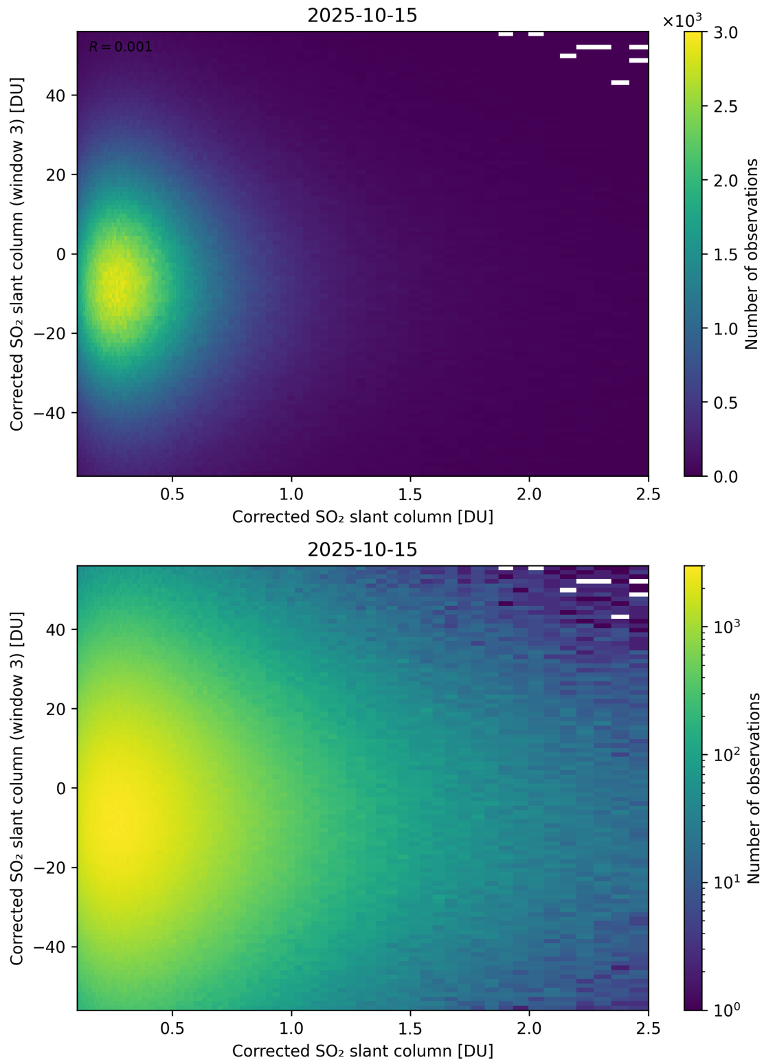
Figure 236: Scatter density plot of “Corrected SO 2 slant column” against “Corrected SO 2 slant column (window 3)” for 2025-10-14 to 2025-10-16.
