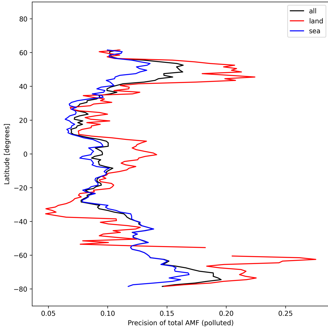
Figure 54: Zonal average of “Precision of total AMF (polluted)” for 2025-10-14 to 2025-10-16.
