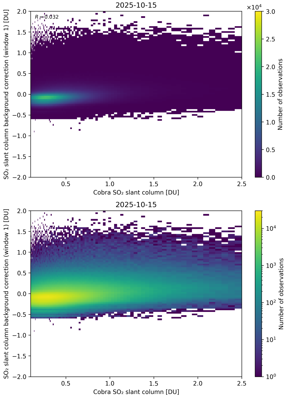
Figure 193: Scatter density plot of “Cobra SO 2 slant column” against “SO 2 slant column background correction (window 1)” for 2025-10-14 to 2025-10-16.
