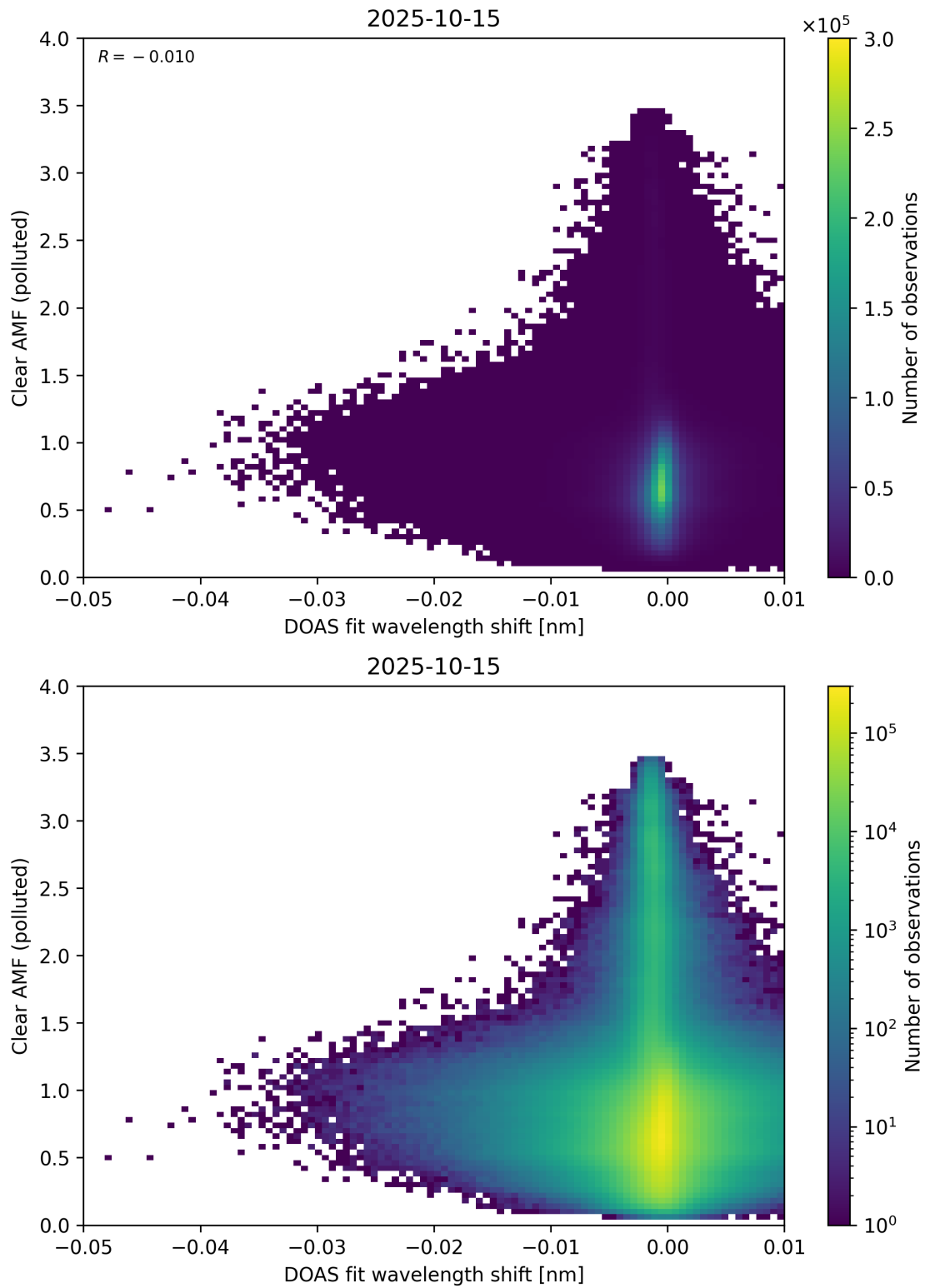
Figure 140: Scatter density plot of “DOAS fit wavelength shift” against “Clear AMF (polluted)” for 2025-10-14 to 2025-10-16.
