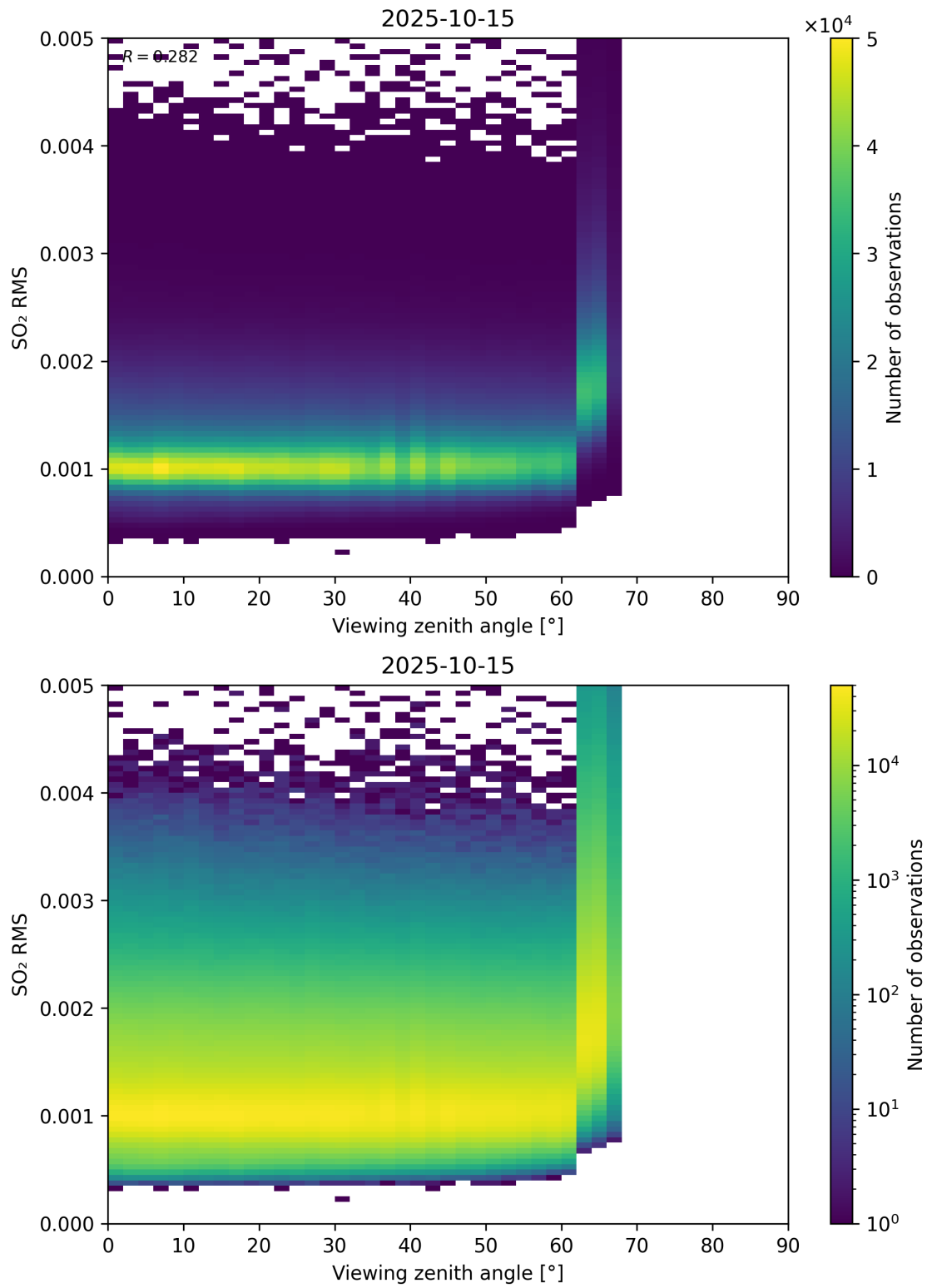
Figure 367: Scatter density plot of “Viewing zenith angle” against “SO 2 RMS” for 2025-10-14 to 2025-10-16.
