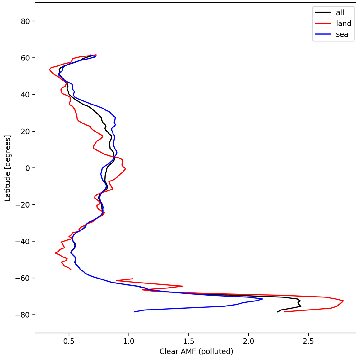
Figure 55: Zonal average of “Clear AMF (polluted)” for 2025-10-14 to 2025-10-16.
