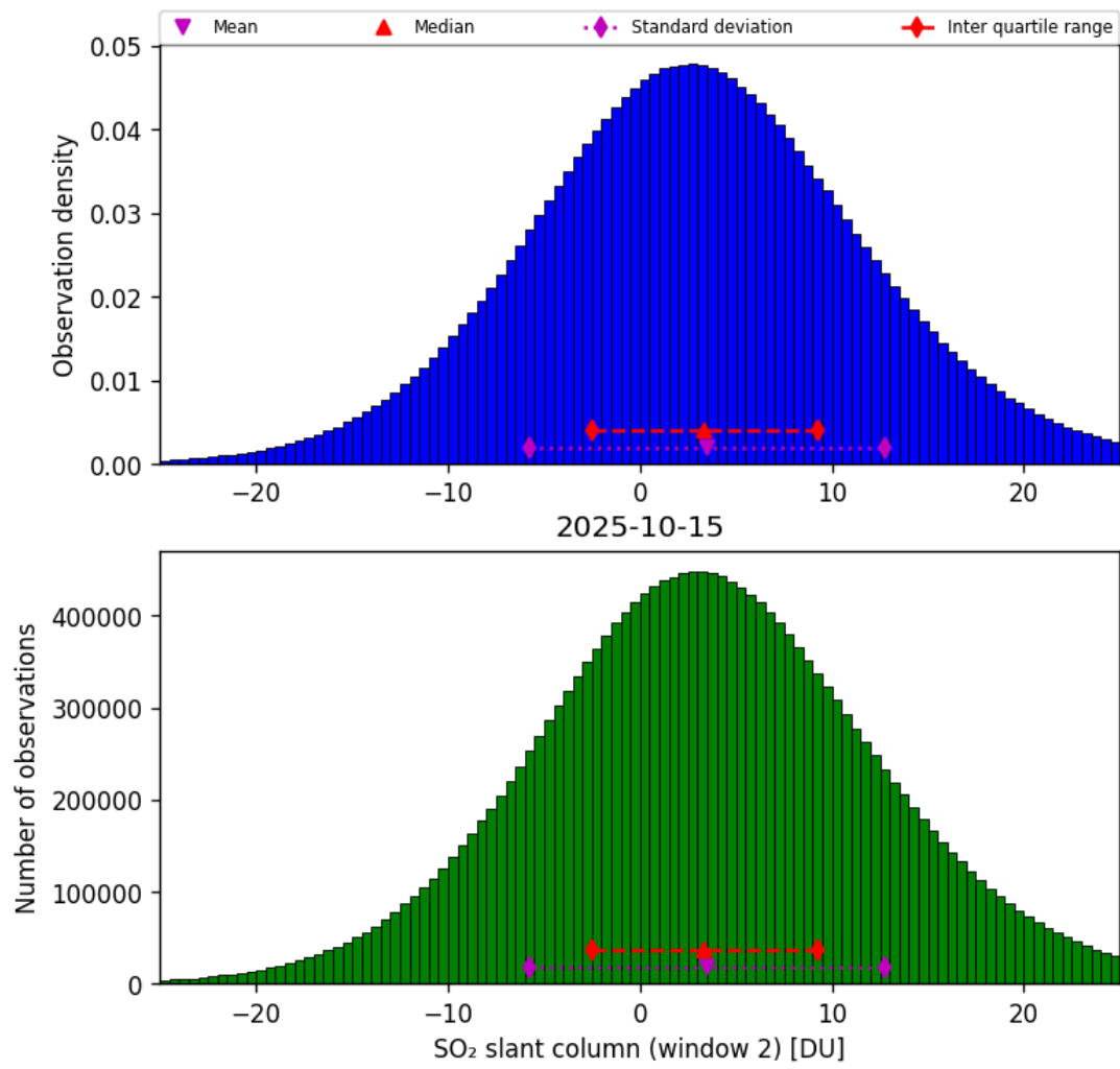
Figure 67: Histogram of “SO 2 slant column (window 2)” for 2025-10-14 to 2025-10-16
