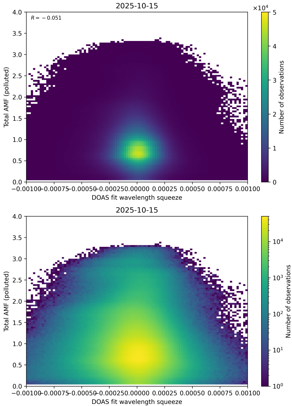
Figure 145: Scatter density plot of “DOAS fit wavelength squeeze” against “Total AMF (polluted)” for 2025-10-14 to 2025-10-16.
