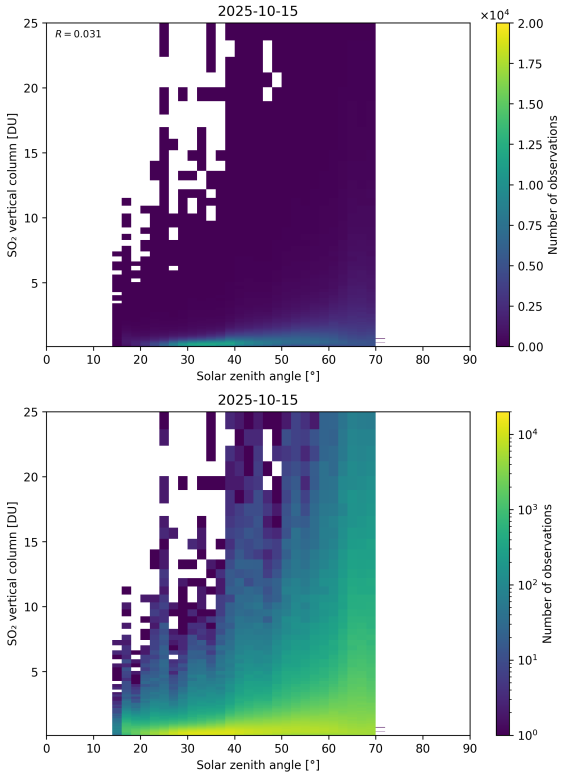
Figure 191: Scatter density plot of “Solar zenith angle” against “SO 2 vertical column” for 2025-10-14 to 2025-10-16.
