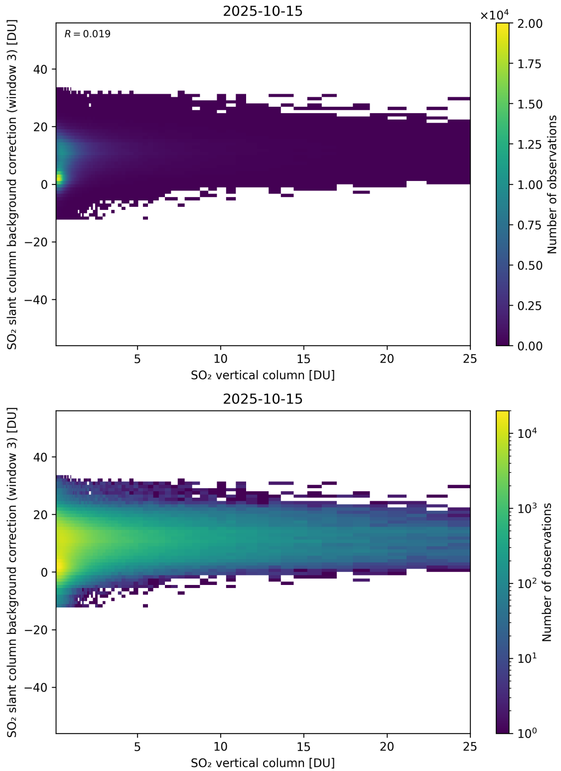
Figure 325: Scatter density plot of “SO 2 vertical column” against “SO 2 slant column background correction (window 3)” for 2025-10-14 to 2025-10-16.
