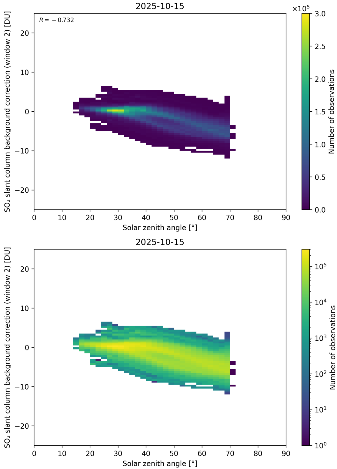
Figure 172: Scatter density plot of “Solar zenith angle” against “SO 2 slant column background correction (window 2)” for 2025-10-14 to 2025-10-16.
