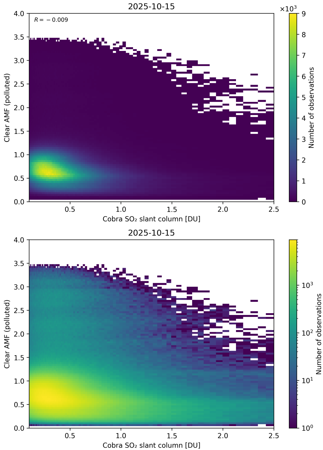
Figure 215: Scatter density plot of “Cobra SO 2 slant column” against “Clear AMF (polluted)” for 2025-10-14 to 2025-10-16.
