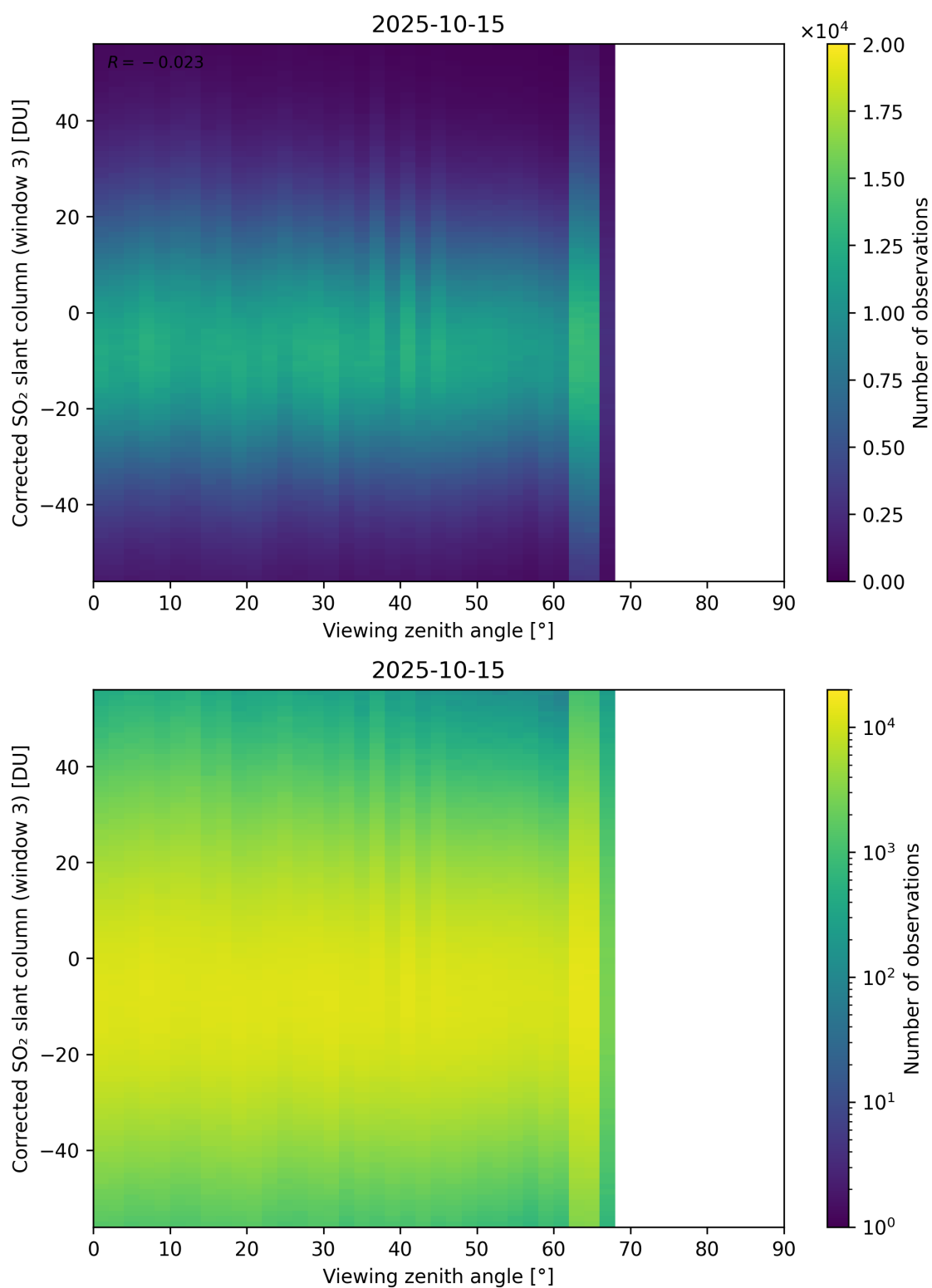
Figure 375: Scatter density plot of “Viewing zenith angle” against “Corrected SO 2 slant column (window 3)” for 2025-10-14 to 2025-10-16.
