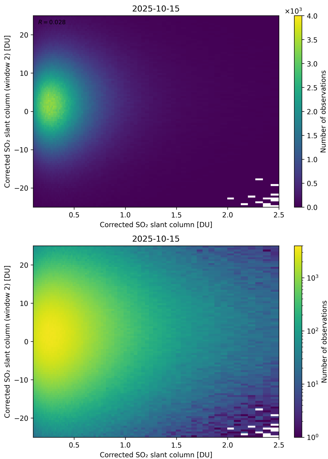
Figure 235: Scatter density plot of “Corrected SO 2 slant column” against “Corrected SO 2 slant column (window 2)” for 2025-10-14 to 2025-10-16.
