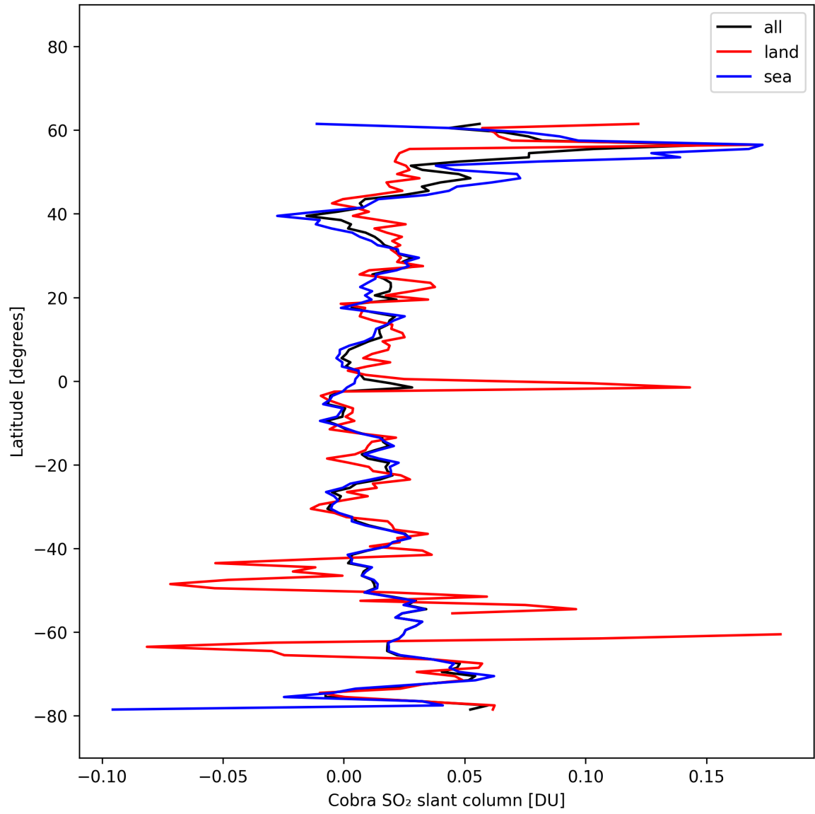
Figure 35: Zonal average of “Cobra SO 2 slant column” for 2025-10-14 to 2025-10-16.
