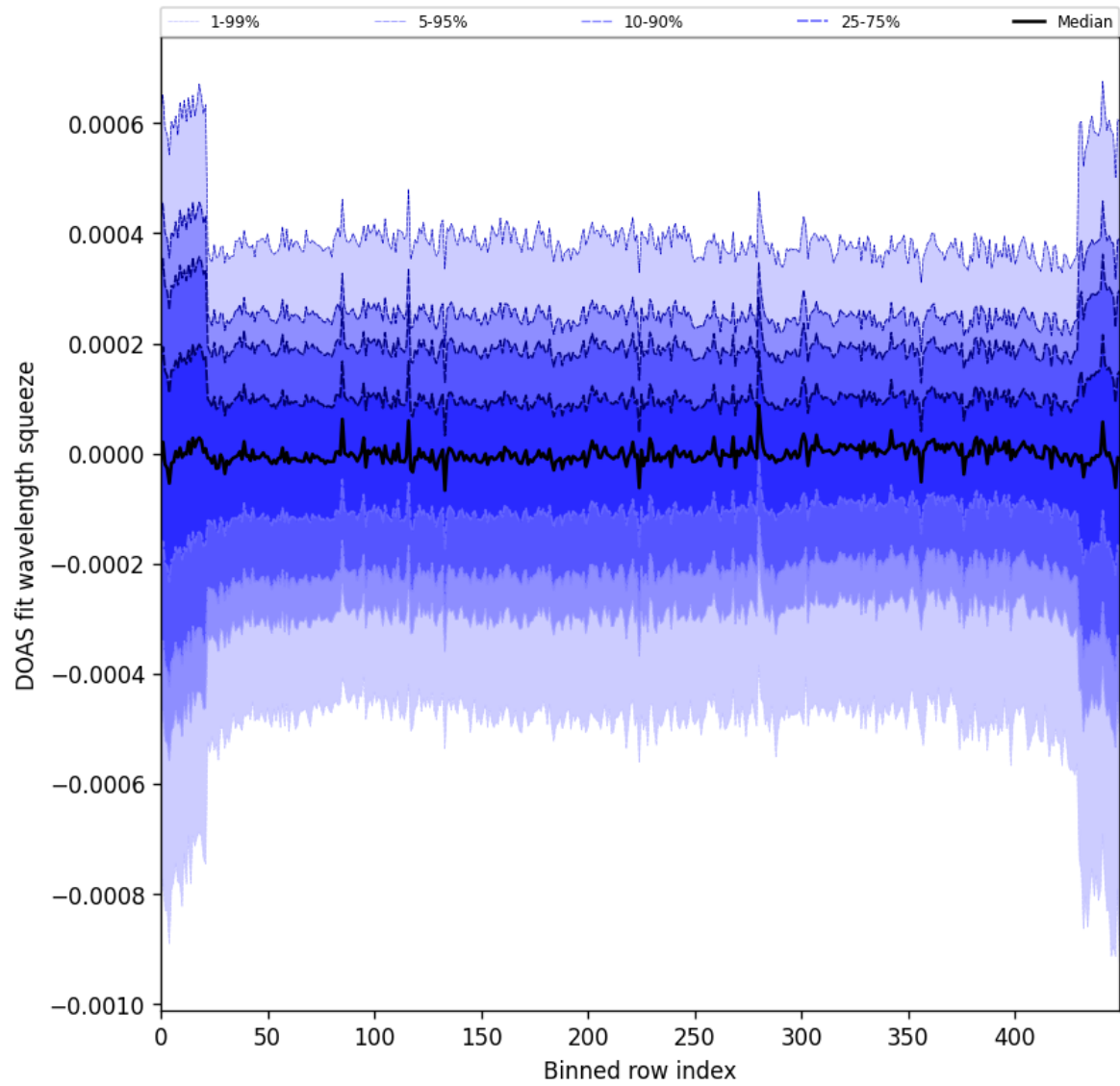
Figure 103: Along track statistics of “DOAS fit wavelength squeeze” for 2025-10-14 to 2025-10-16
