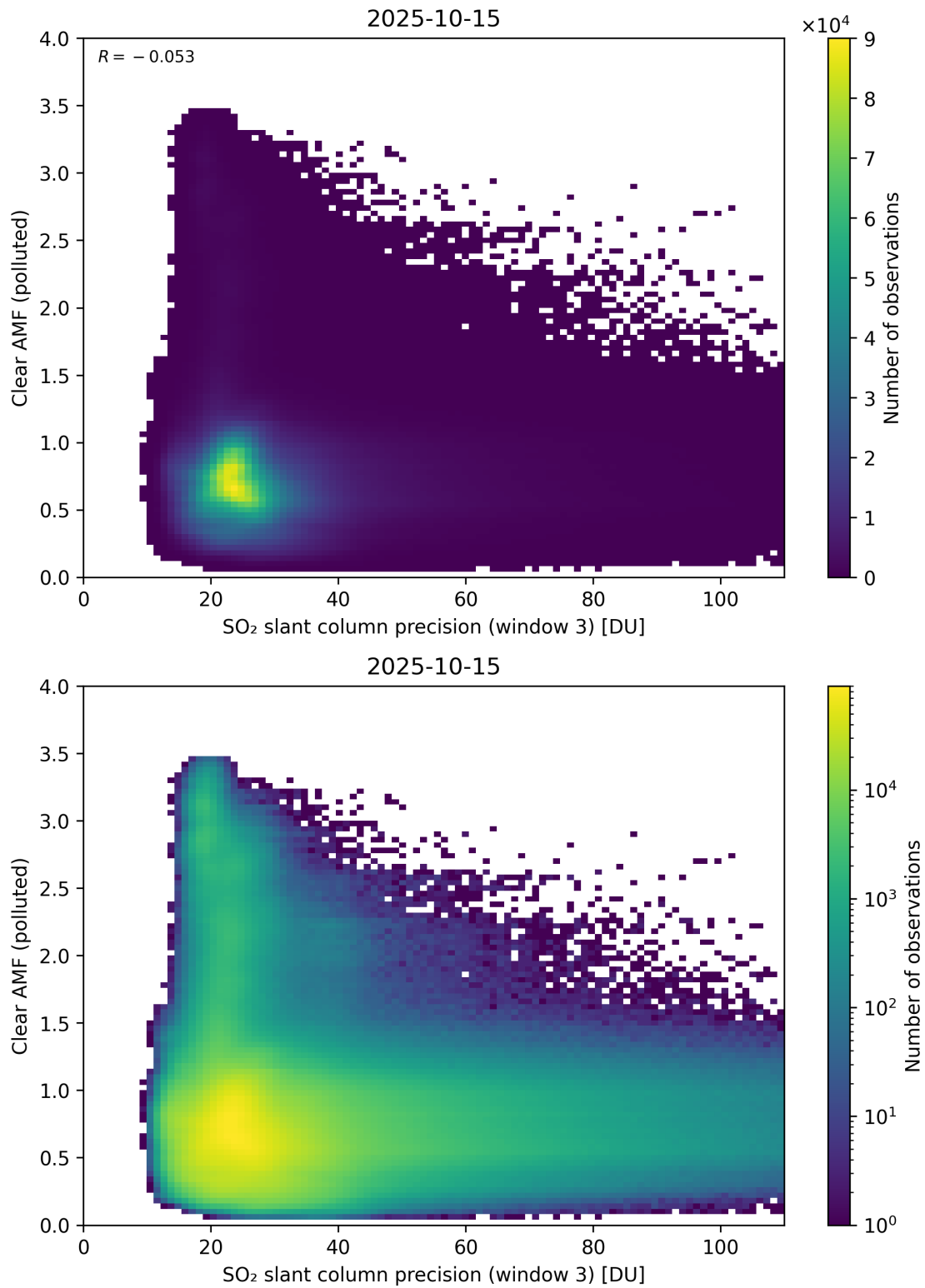
Figure 311: Scatter density plot of “SO 2 slant column precision (window 3)” against “Clear AMF (polluted)” for 2025-10-14 to 2025-10-16.
