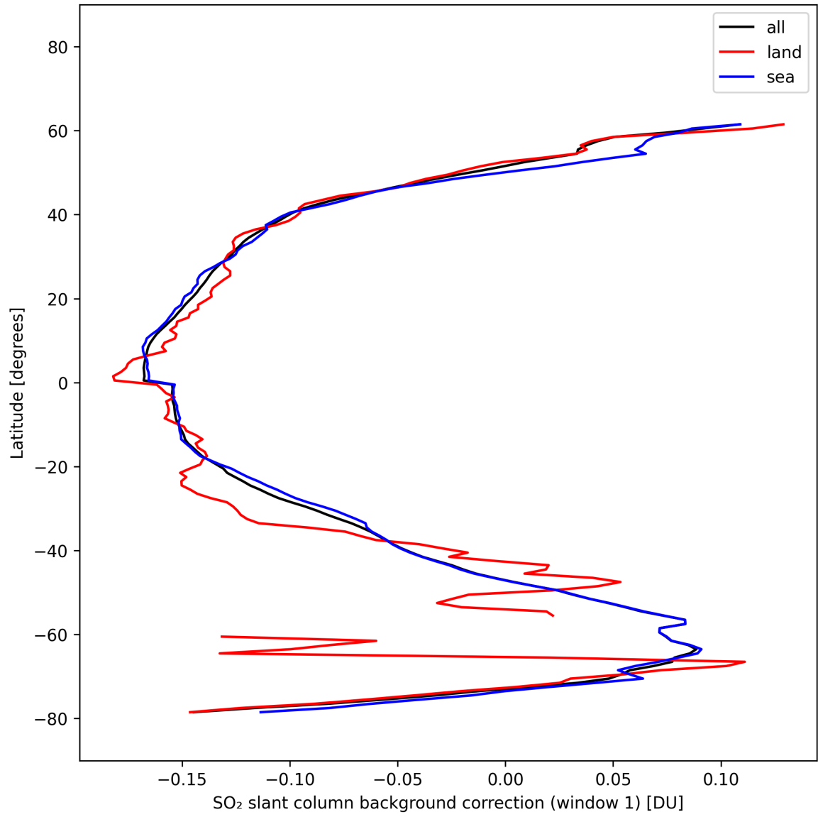
Figure 40: Zonal average of “SO 2 slant column background correction (window 1)” for 2025-10-14 to 2025-10-16.
