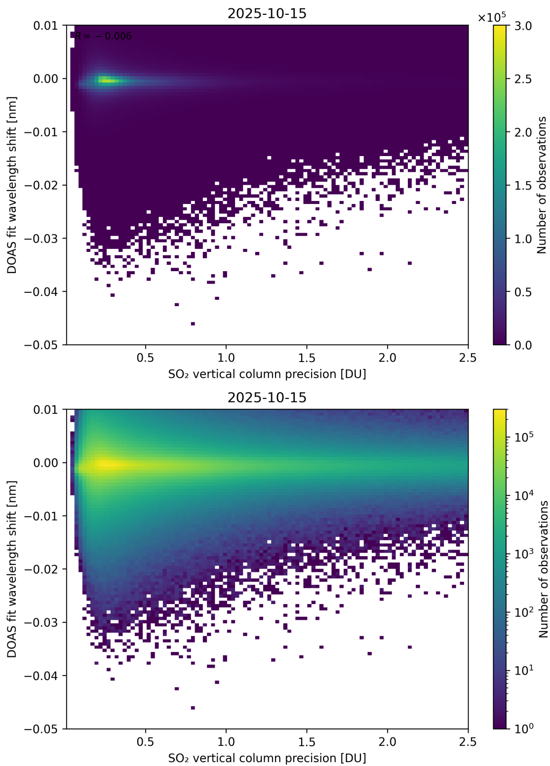
Figure 332: Scatter density plot of “SO 2 vertical column precision” against “DOAS fit wavelength shift” for 2025-10-14 to 2025-10-16.
