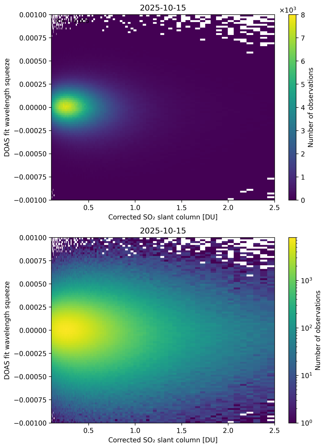
Figure 230: Scatter density plot of "Corrected SO 2 slant column" against "DOAS fit wavelength squeeze" for 2025-10-14 to 2025-10-16.
