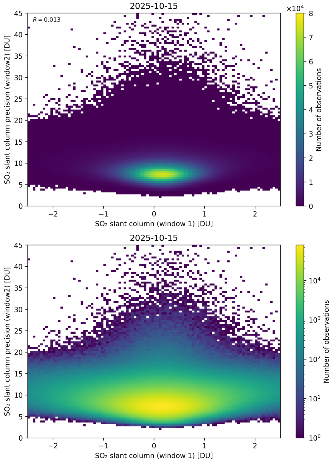
Figure 286: Scatter density plot of “SO 2 slant column (window 1)” against “SO 2 slant column precision (window2)” for 2025-10-14 to 2025-10-16.
