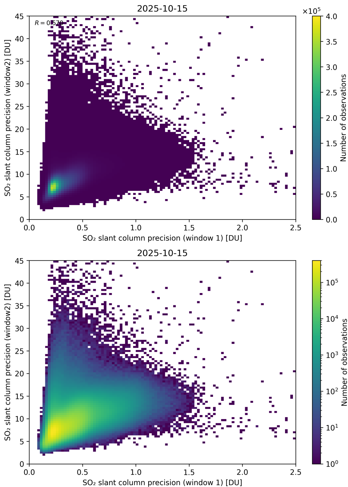
Figure 277: Scatter density plot of “SO 2 slant column precision (window 1)” against “SO 2 slant column precision (window2)” for 2025-10-14 to 2025-10-16.
