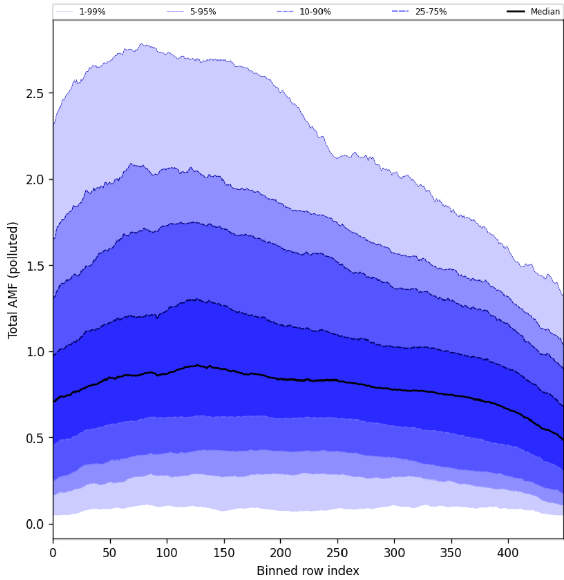
Figure 105: Along track statistics of “Total AMF (polluted)” for 2025-10-14 to 2025-10-16
