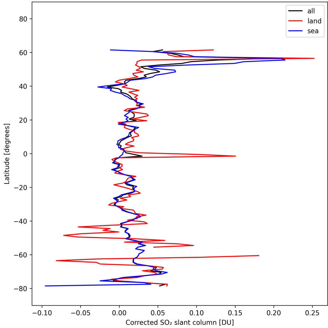
Figure 34: Zonal average of “Corrected SO 2 slant column” for 2025-10-14 to 2025-10-16.
