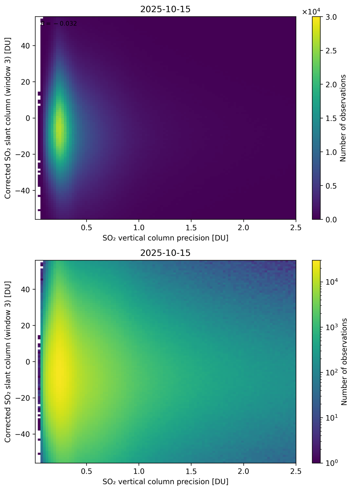
Figure 340: Scatter density plot of “SO 2 vertical column precision” against “Corrected SO 2 slant column (window 3)” for 2025-10-14 to 2025-10-16.
