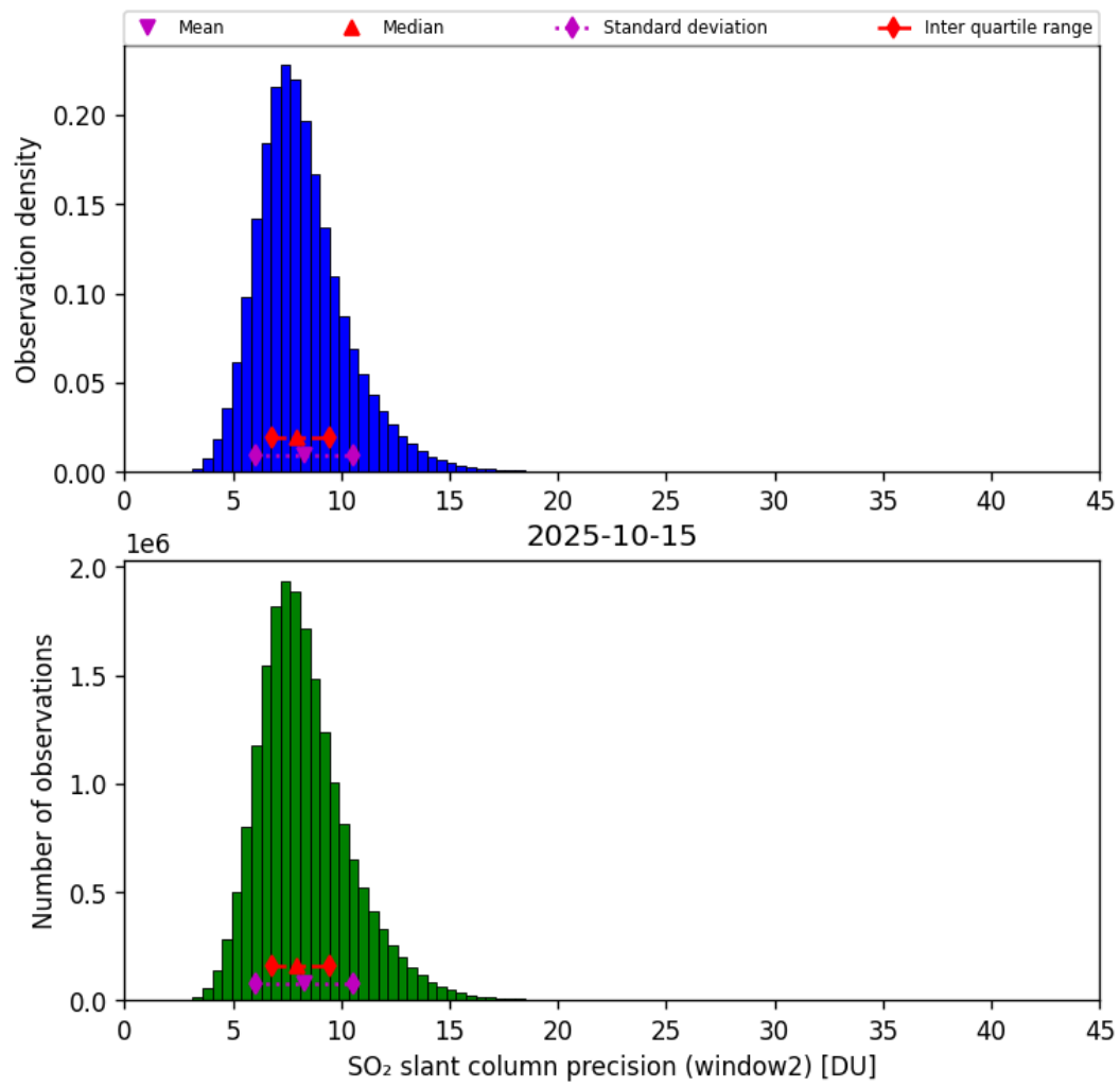
Figure 68: Histogram of “SO 2 slant column precision (window2)” for 2025-10-14 to 2025-10-16
