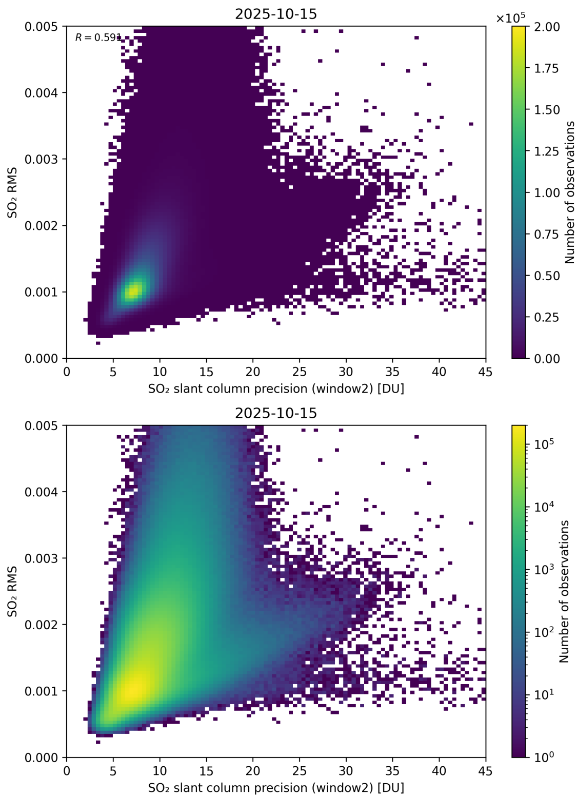
Figure 295: Scatter density plot of “SO 2 slant column precision (window2)” against “SO 2 RMS” for 2025-10-14 to 2025-10-16.
