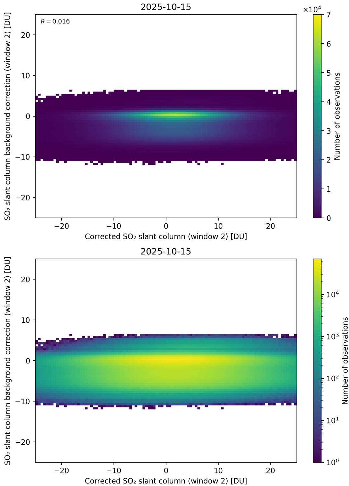
Figure 244: Scatter density plot of “Corrected SO 2 slant column (window 2)” against “SO 2 slant column background correction (window 2)” for 2025-10-14 to 2025-10-16.
