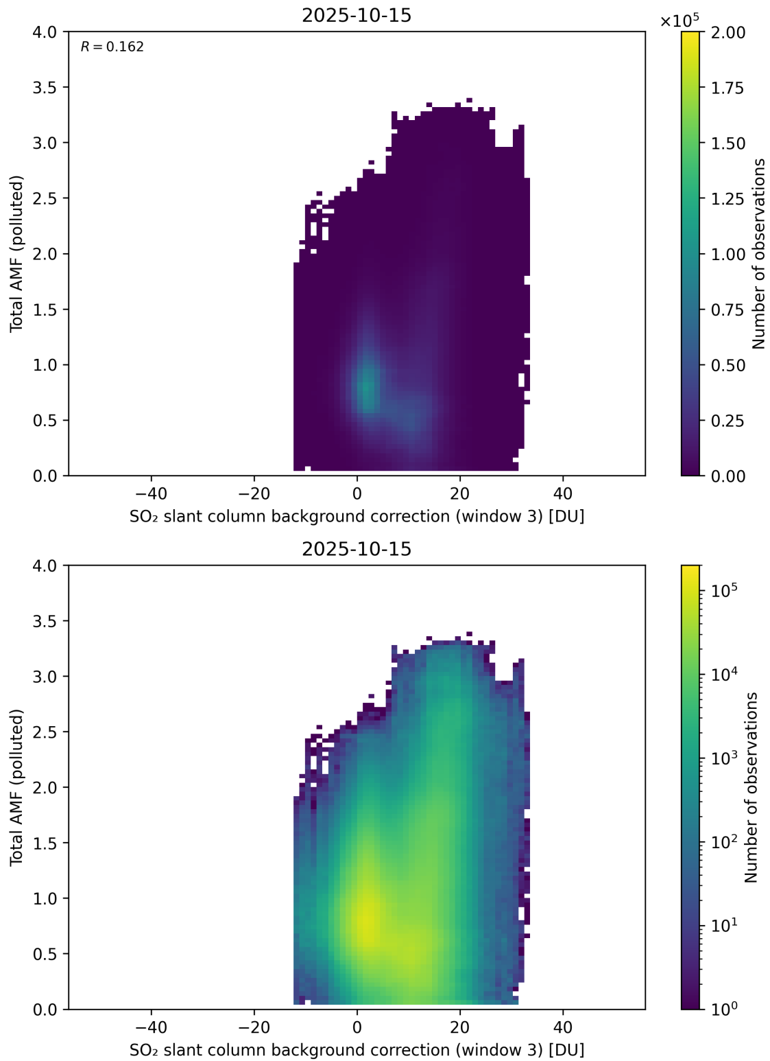
Figure 136: Scatter density plot of “SO 2 slant column background correction (window 3)” against “Total AMF (polluted)” for 2025-10-14 to 2025-10-16.
