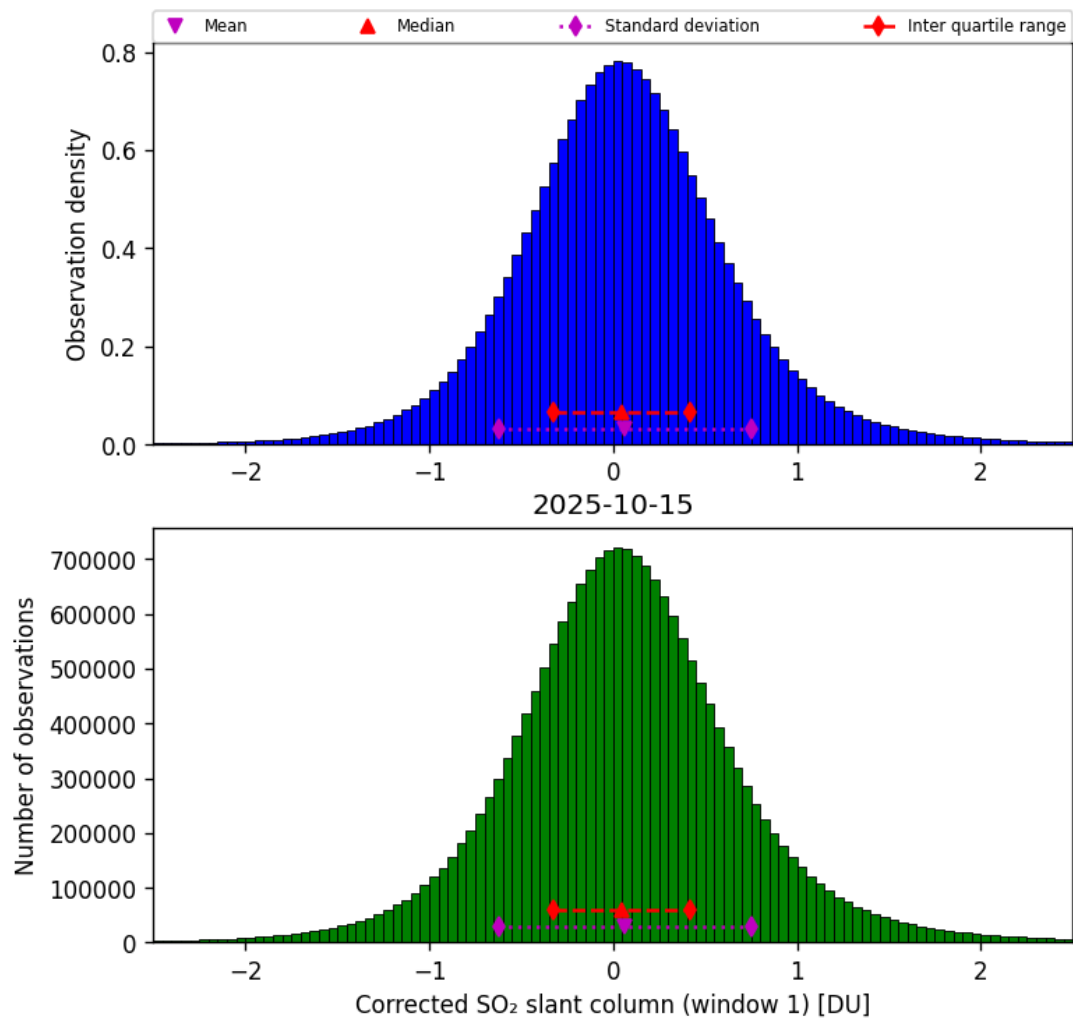
Figure 65: Histogram of “Corrected SO 2 slant column (window 1)” for 2025-10-14 to 2025-10-16
