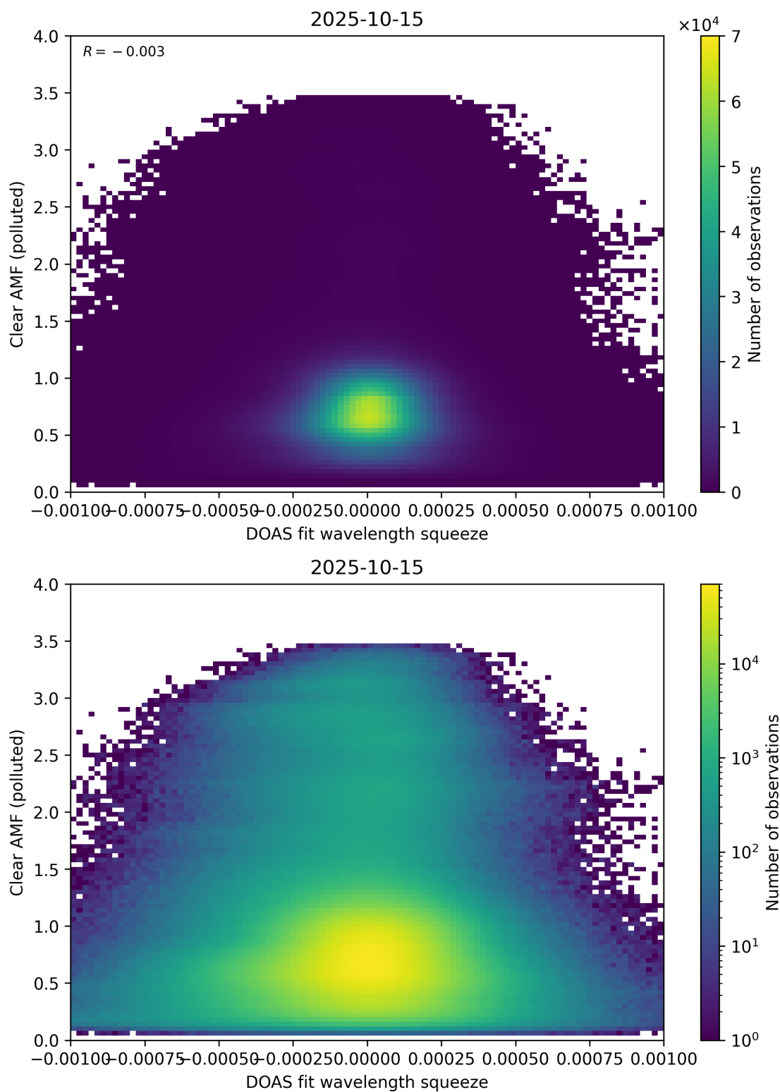
Figure 144: Scatter density plot of “DOAS fit wavelength squeeze” against “Clear AMF (polluted)” for 2025-10-14 to 2025-10-16.
