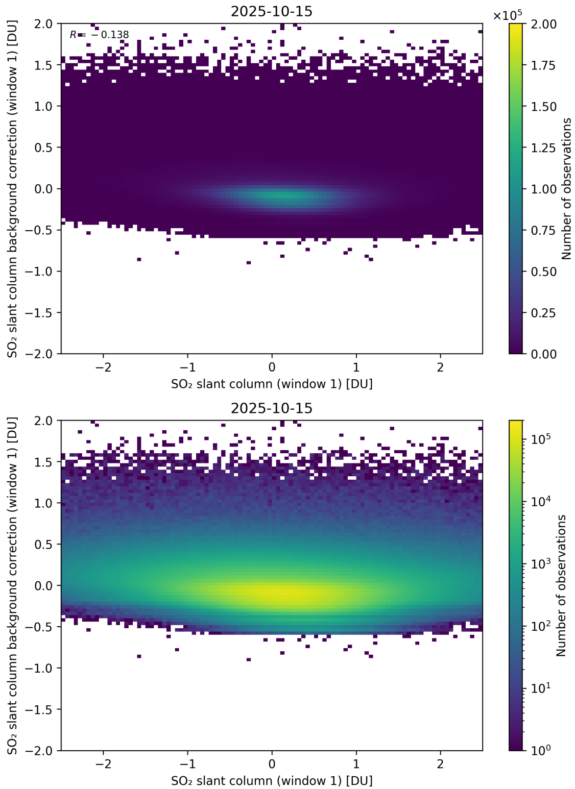
Figure 262: Scatter density plot of “SO 2 slant column (window 1)” against “SO 2 slant column background correction (window 1)” for 2025-10-14 to 2025-10-16.
