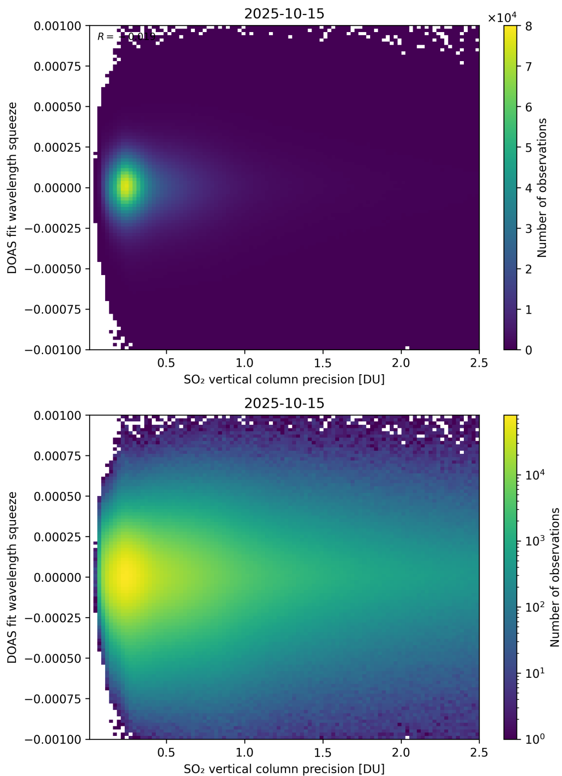
Figure 333: Scatter density plot of “SO 2 vertical column precision” against “DOAS fit wavelength squeeze” for 2025-10-14 to 2025-10-16.
