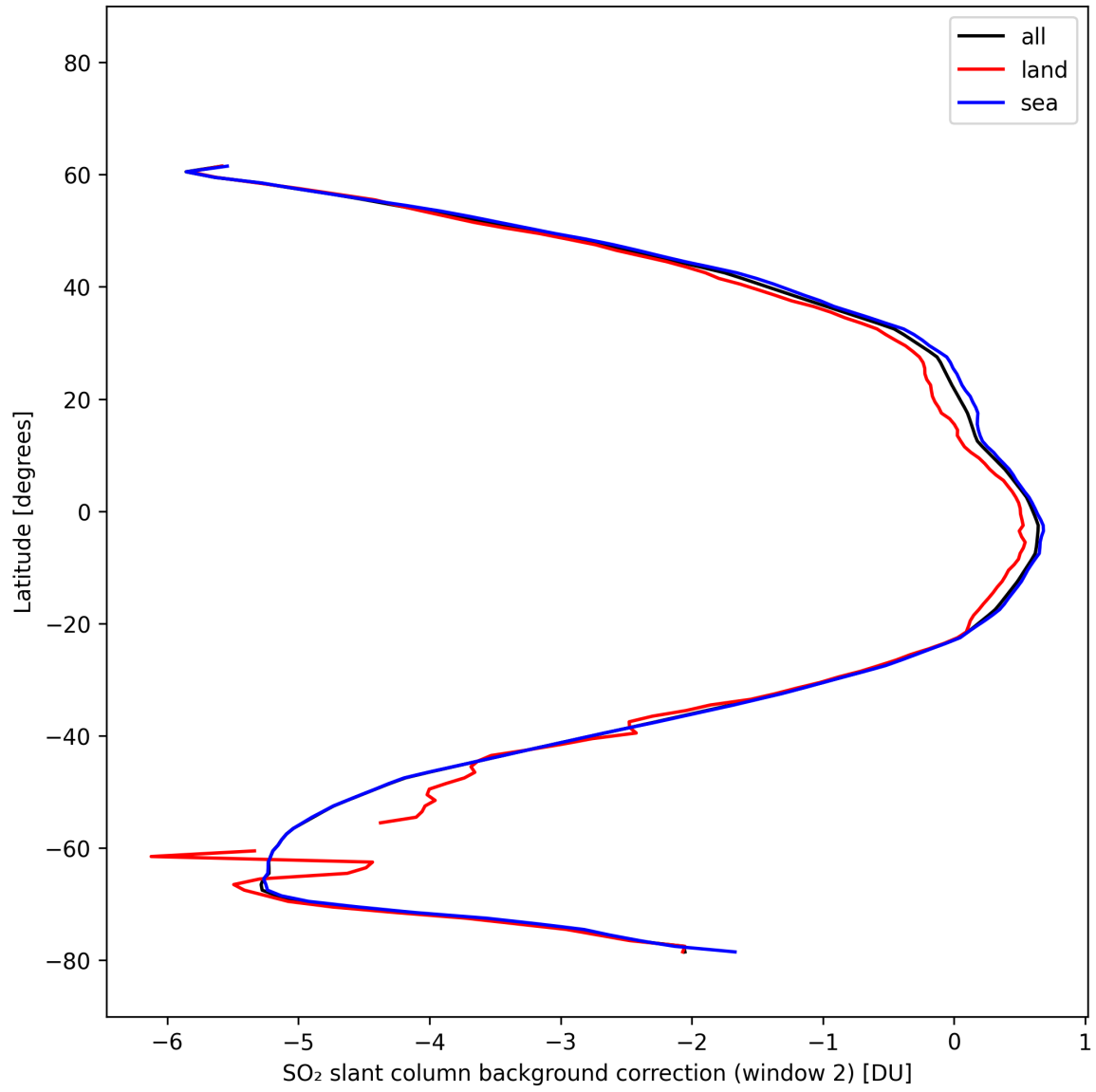
Figure 44: Zonal average of “SO 2 slant column background correction (window 2)” for 2025-10-14 to 2025-10-16.
