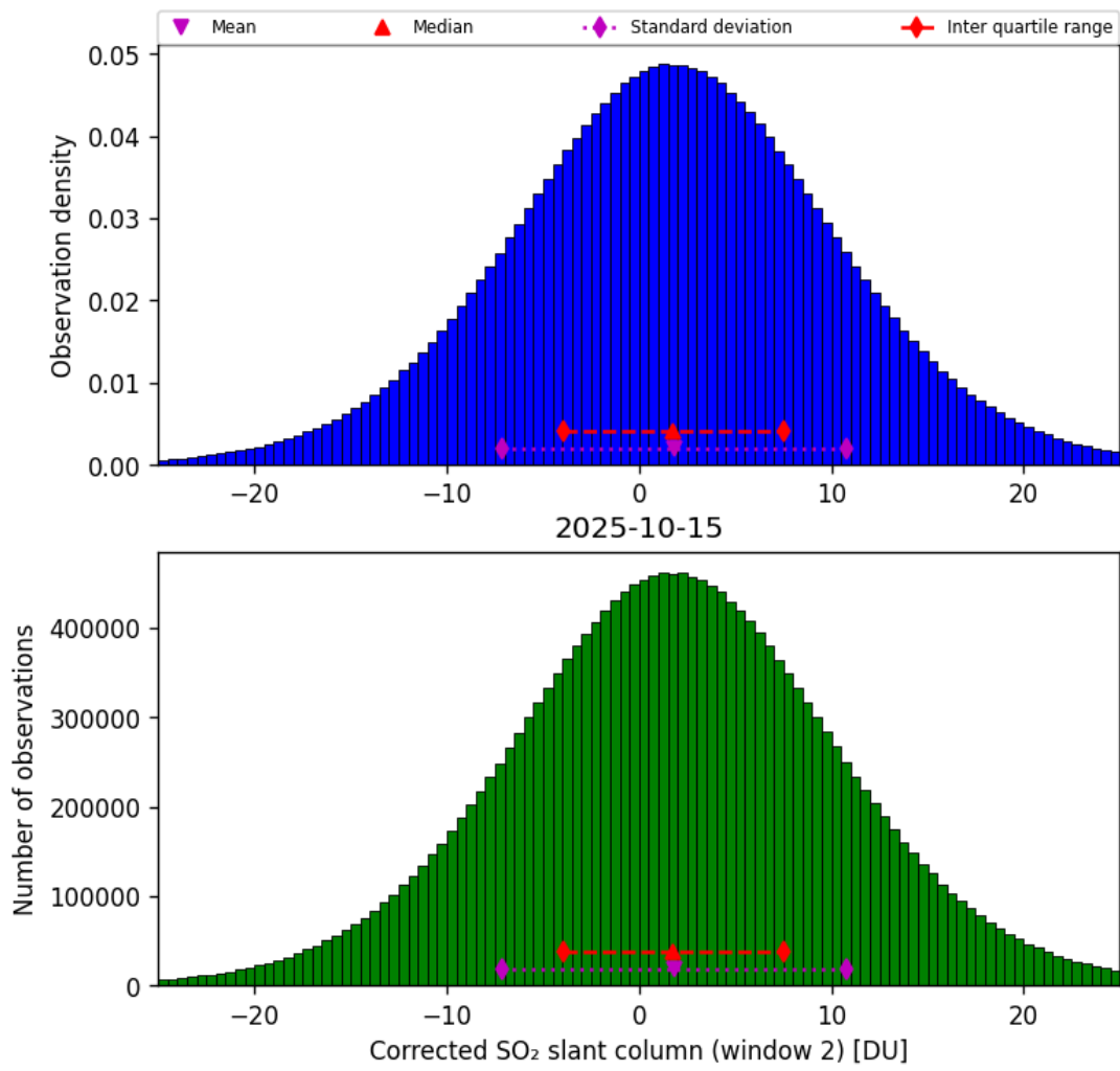
Figure 69: Histogram of “Corrected SO 2 slant column (window 2)” for 2025-10-14 to 2025-10-16
