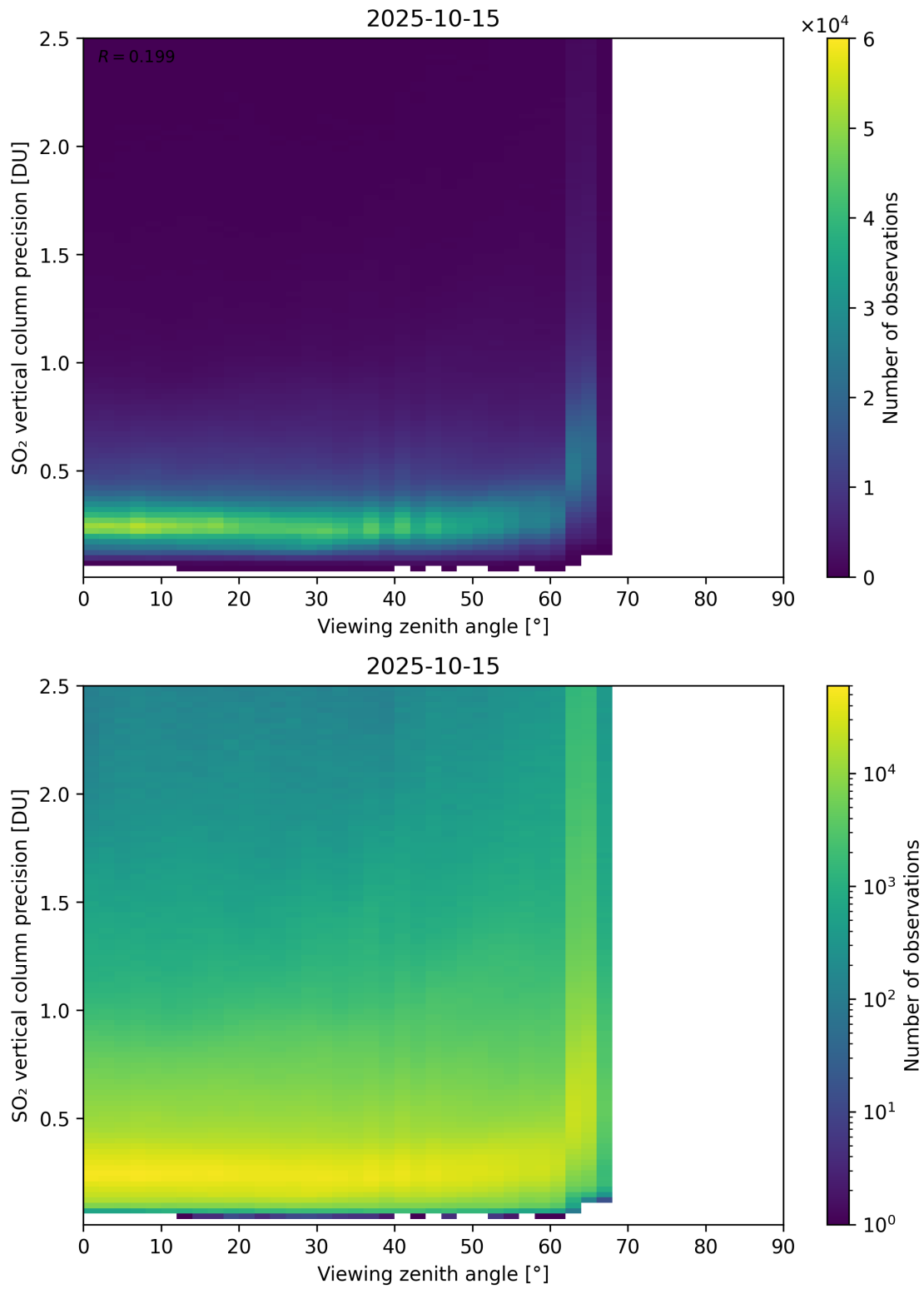
Figure 384: Scatter density plot of “Viewing zenith angle” against “SO 2 vertical column precision” for 2025-10-14 to 2025-10-16.
