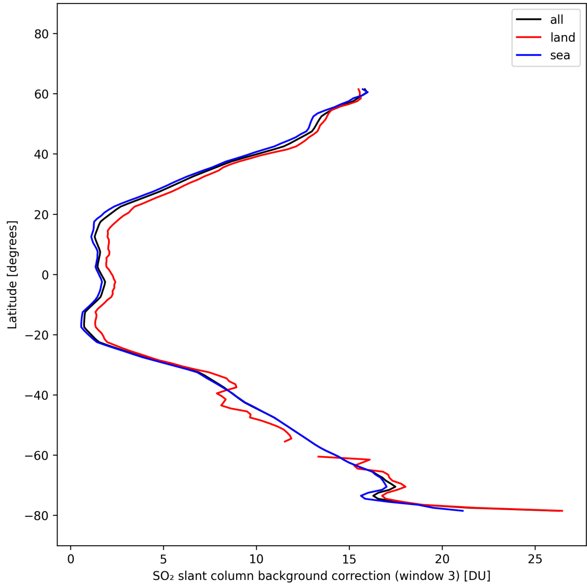
Figure 48: Zonal average of "SO 2 slant column background correction (window 3)" for 2025-10-14 to 2025-10-16.
