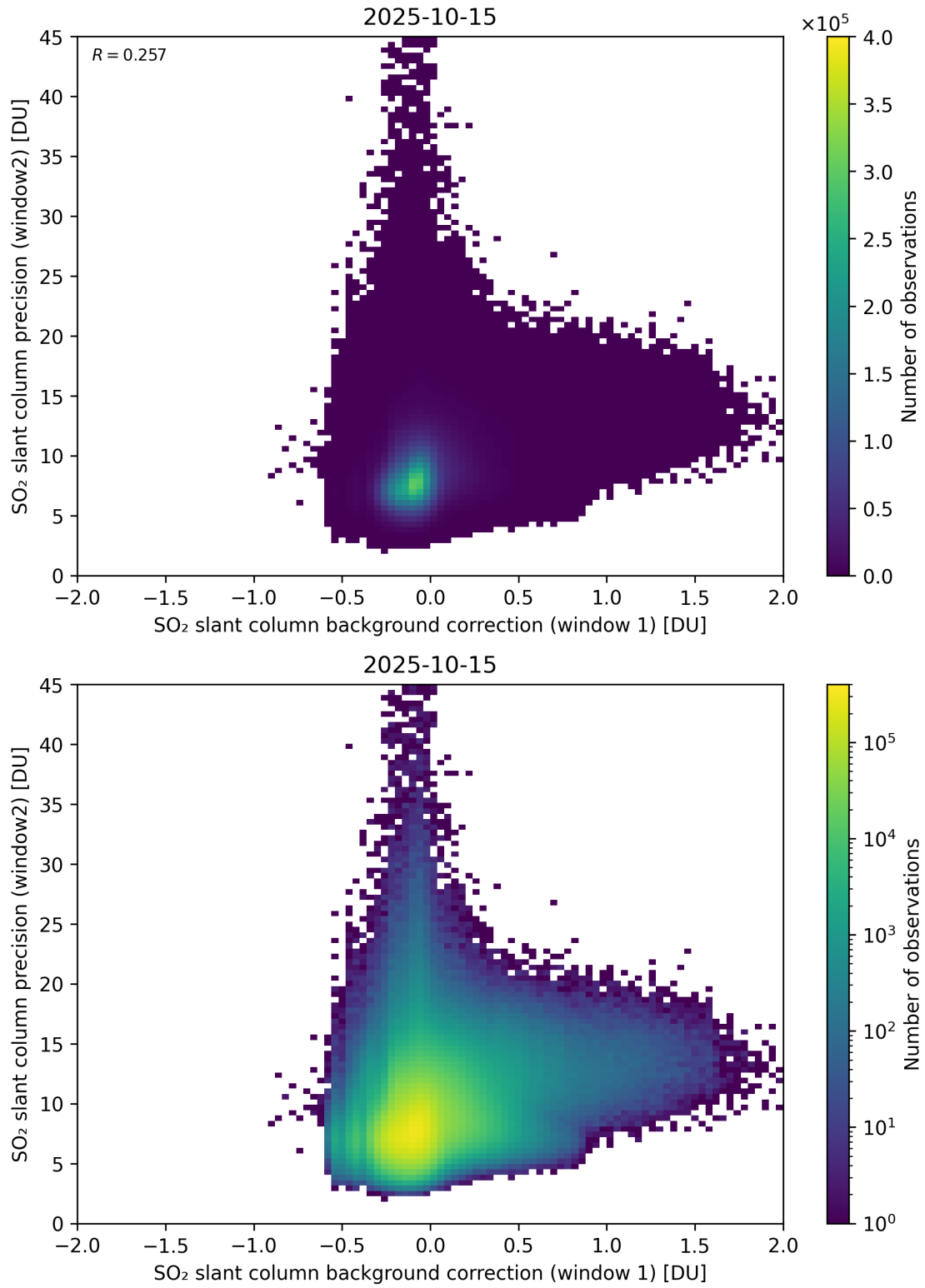
Figure 117: Scatter density plot of “SO 2 slant column background correction (window 1)” against “SO 2 slant column precision (window2)” for 2025-10-14 to 2025-10-16.
