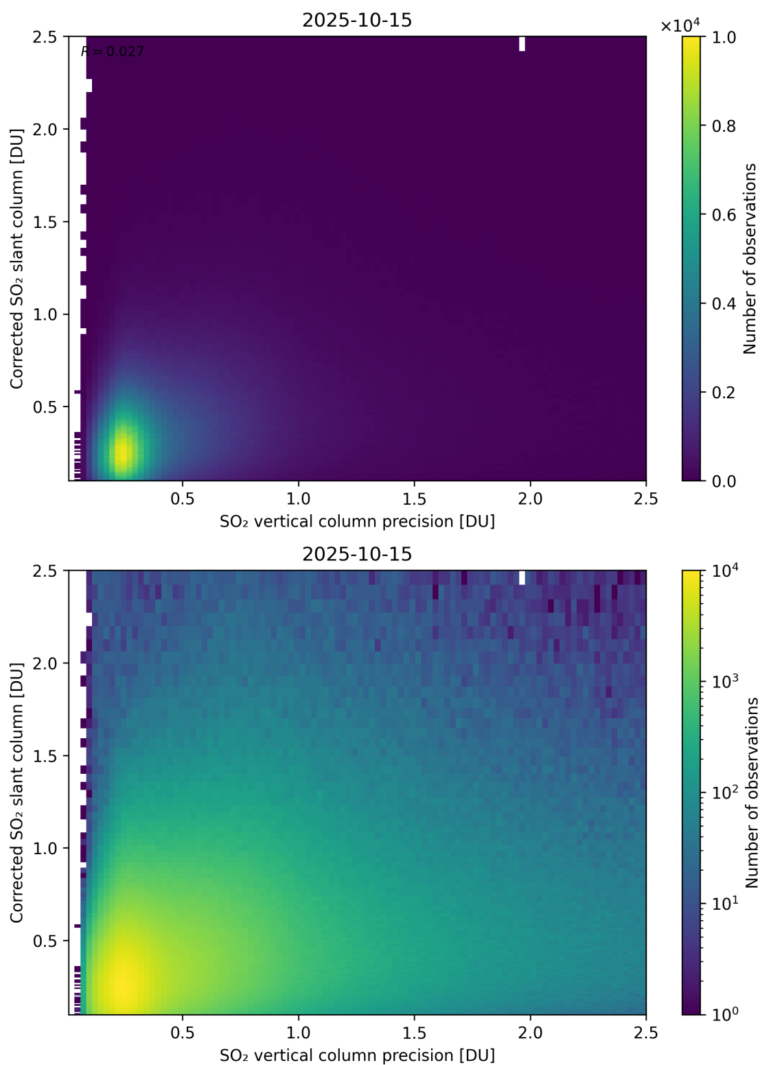
Figure 338: Scatter density plot of “SO 2 vertical column precision” against “Corrected SO 2 slant column” for 2025-10-14 to 2025-10-16.
