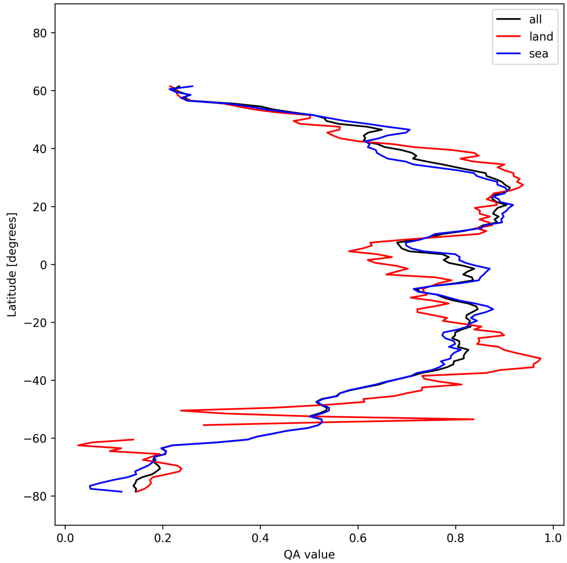
Figure 31: Zonal average of “QA value” for 2025-10-14 to 2025-10-16.
