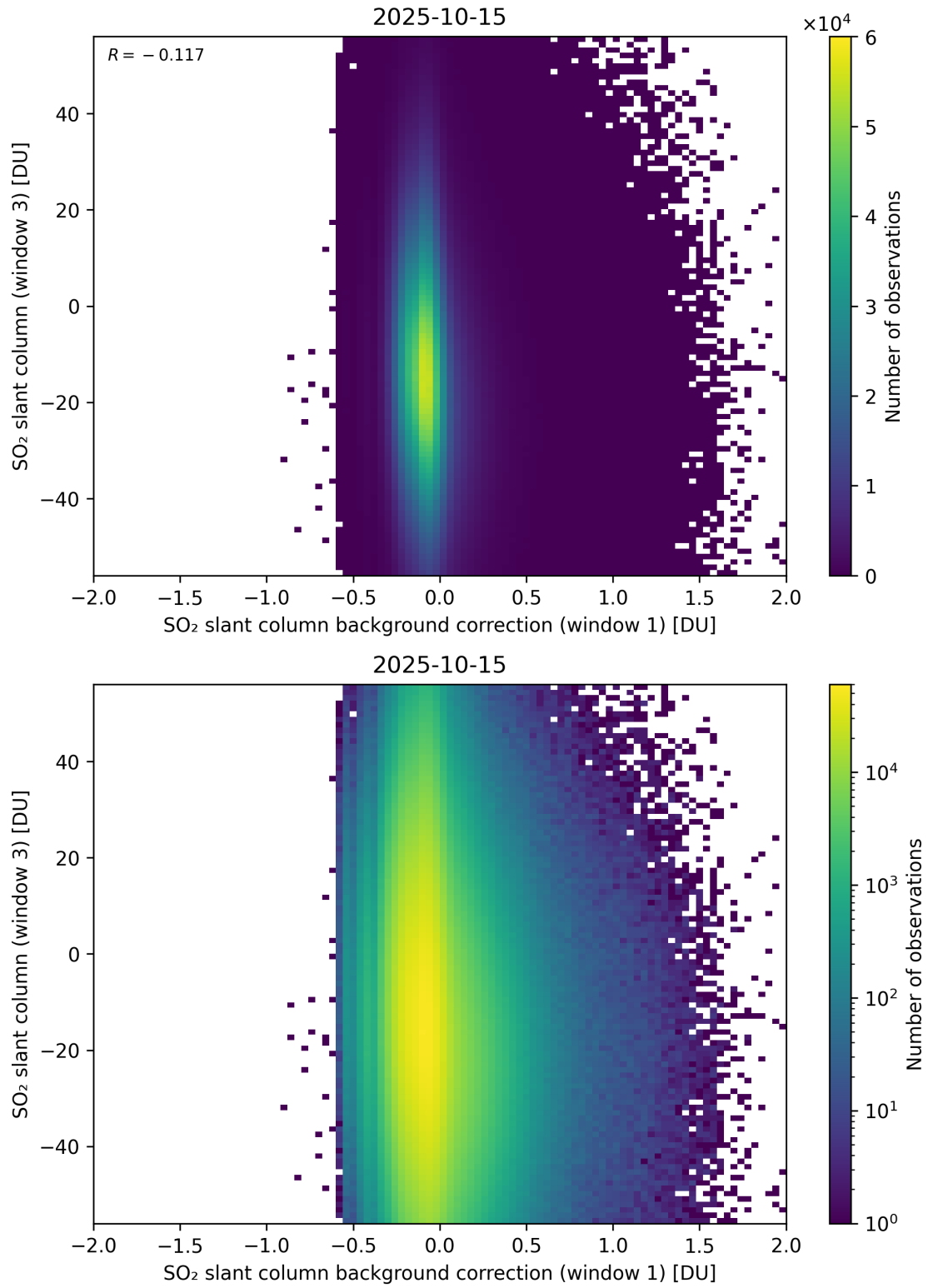
Figure 118: Scatter density plot of “SO 2 slant column background correction (window 1)” against “SO 2 slant column (window 3)” for 2025-10-14 to 2025-10-16.
