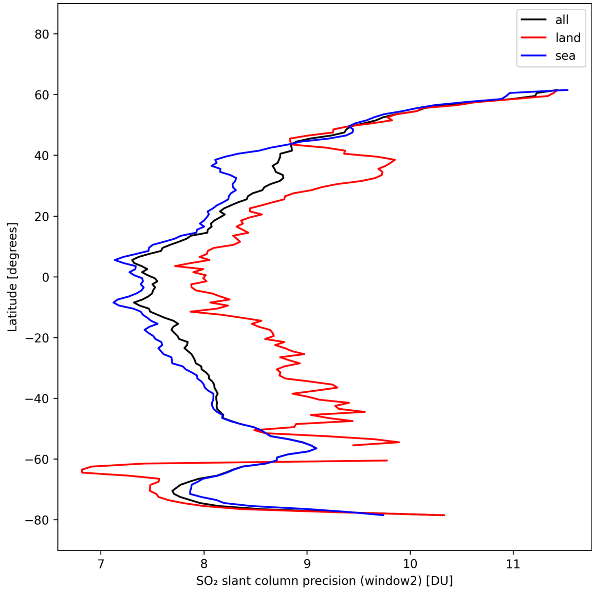
Figure 42: Zonal average of “SO 2 slant column precision (window2)” for 2025-10-14 to 2025-10-16.
