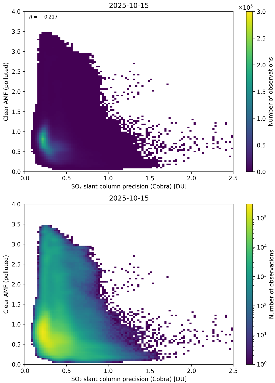
Figure 205: Scatter density plot of “SO 2 slant column precision (Cobra)” against “Clear AMF (polluted)” for 2025-10-14 to 2025-10-16.
