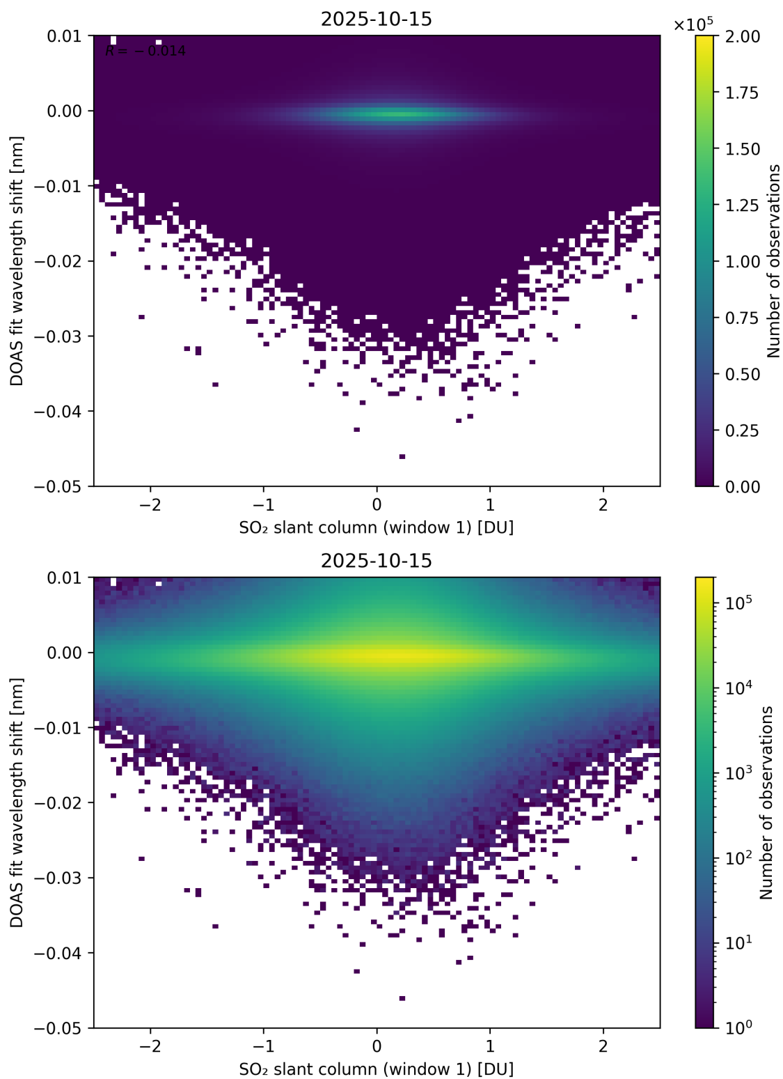
Figure 265: Scatter density plot of “SO 2 slant column (window 1)” against “DOAS fit wavelength shift” for 2025-10-14 to 2025-10-16.
