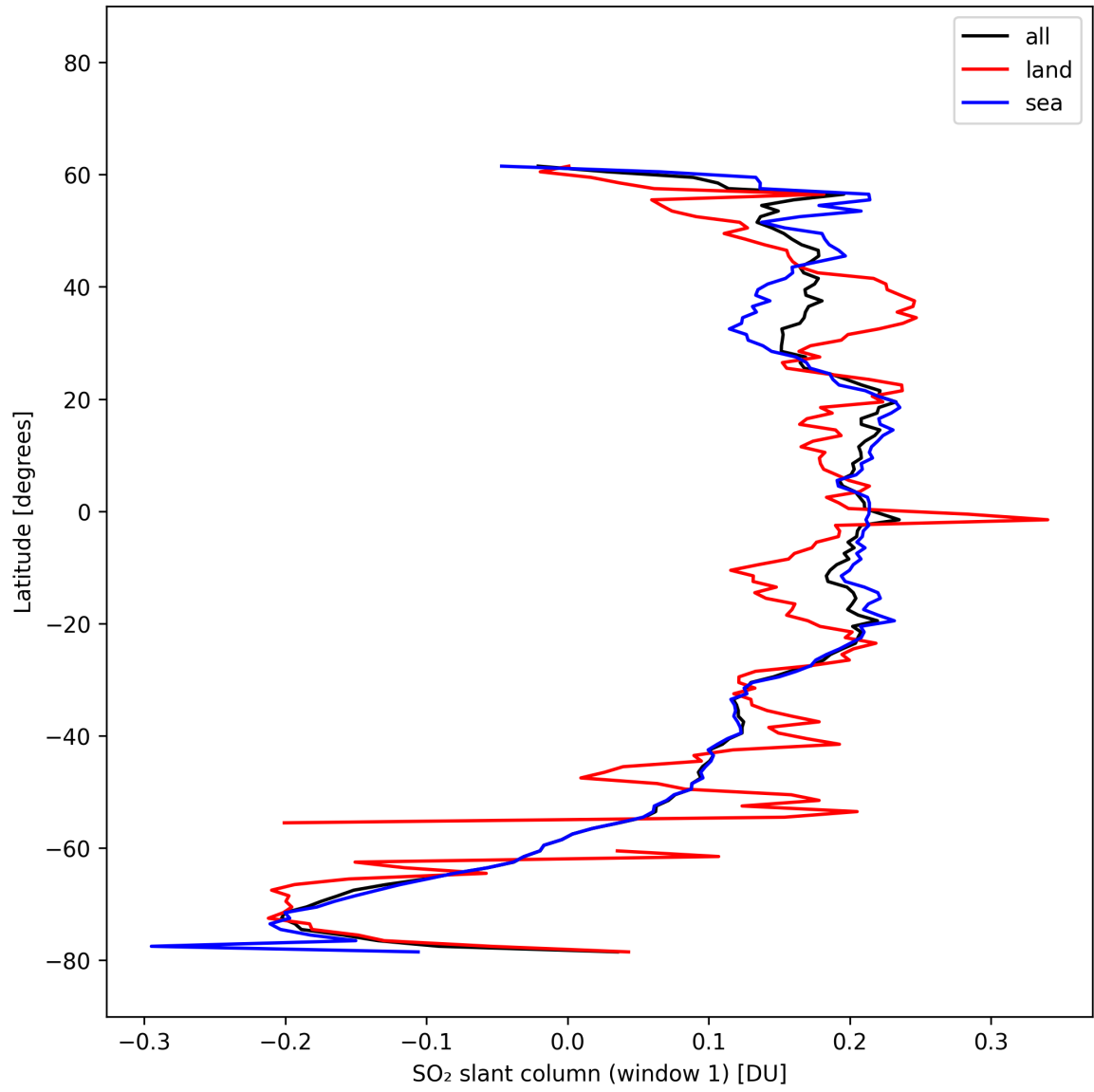
Figure 37: Zonal average of “SO 2 slant column (window 1)” for 2025-10-14 to 2025-10-16.
