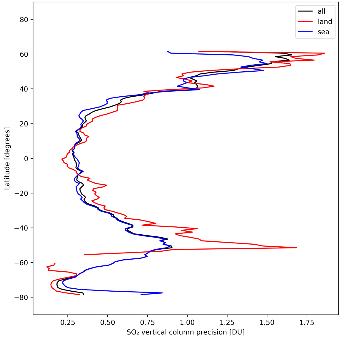
Figure 33: Zonal average of “SO 2 vertical column precision” for 2025-10-14 to 2025-10-16.
