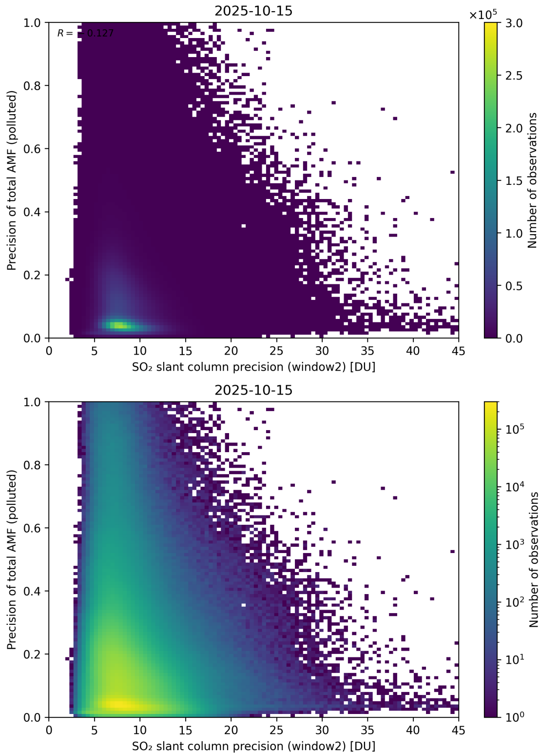
Figure 302: Scatter density plot of “SO 2 slant column precision (window2)” against “Precision of total AMF (polluted)” for 2025-10-14 to 2025-10-16.
