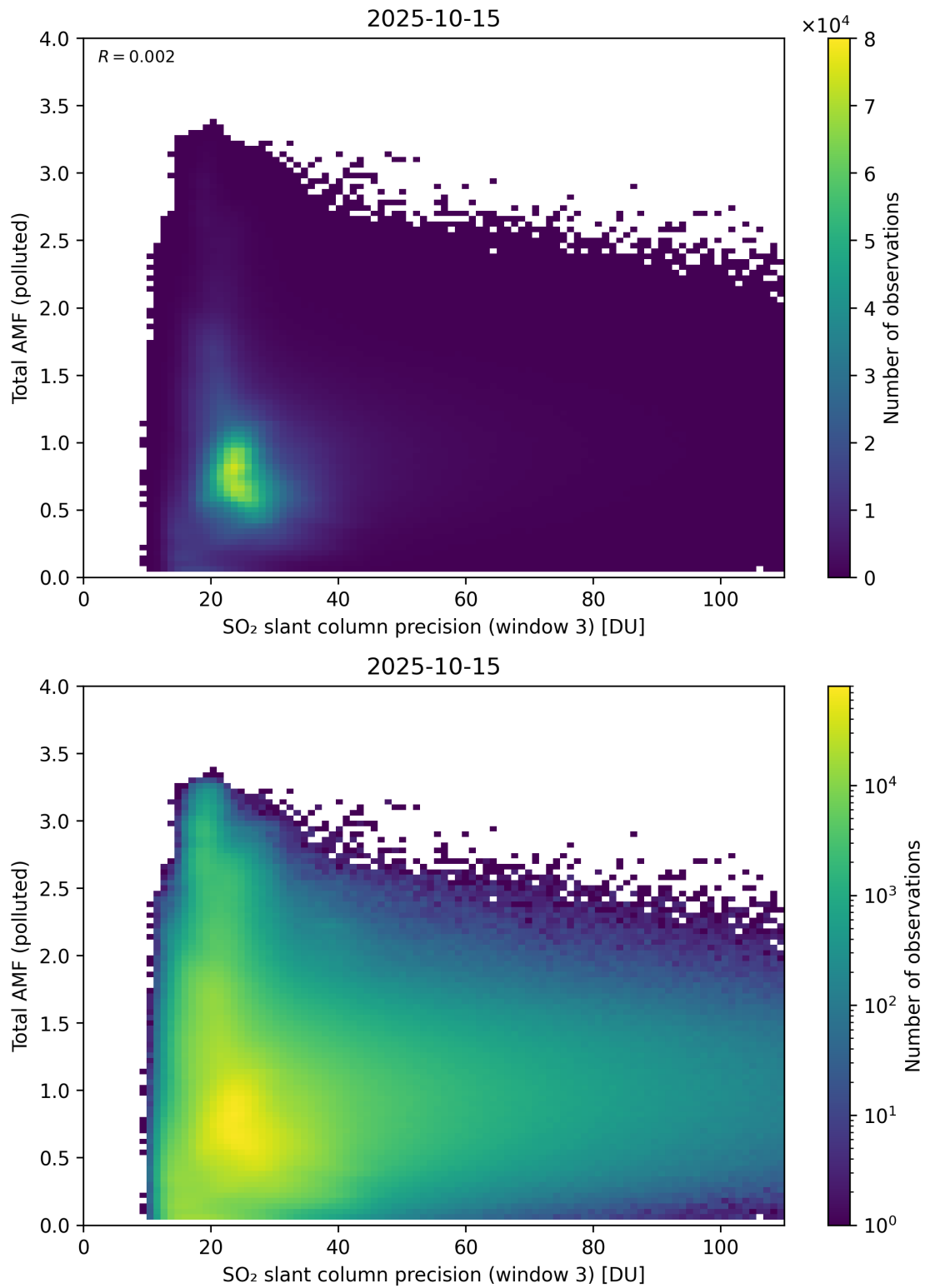
Figure 313: Scatter density plot of “SO 2 slant column precision (window 3)” against “Total AMF (polluted)” for 2025-10-14 to 2025-10-16.
