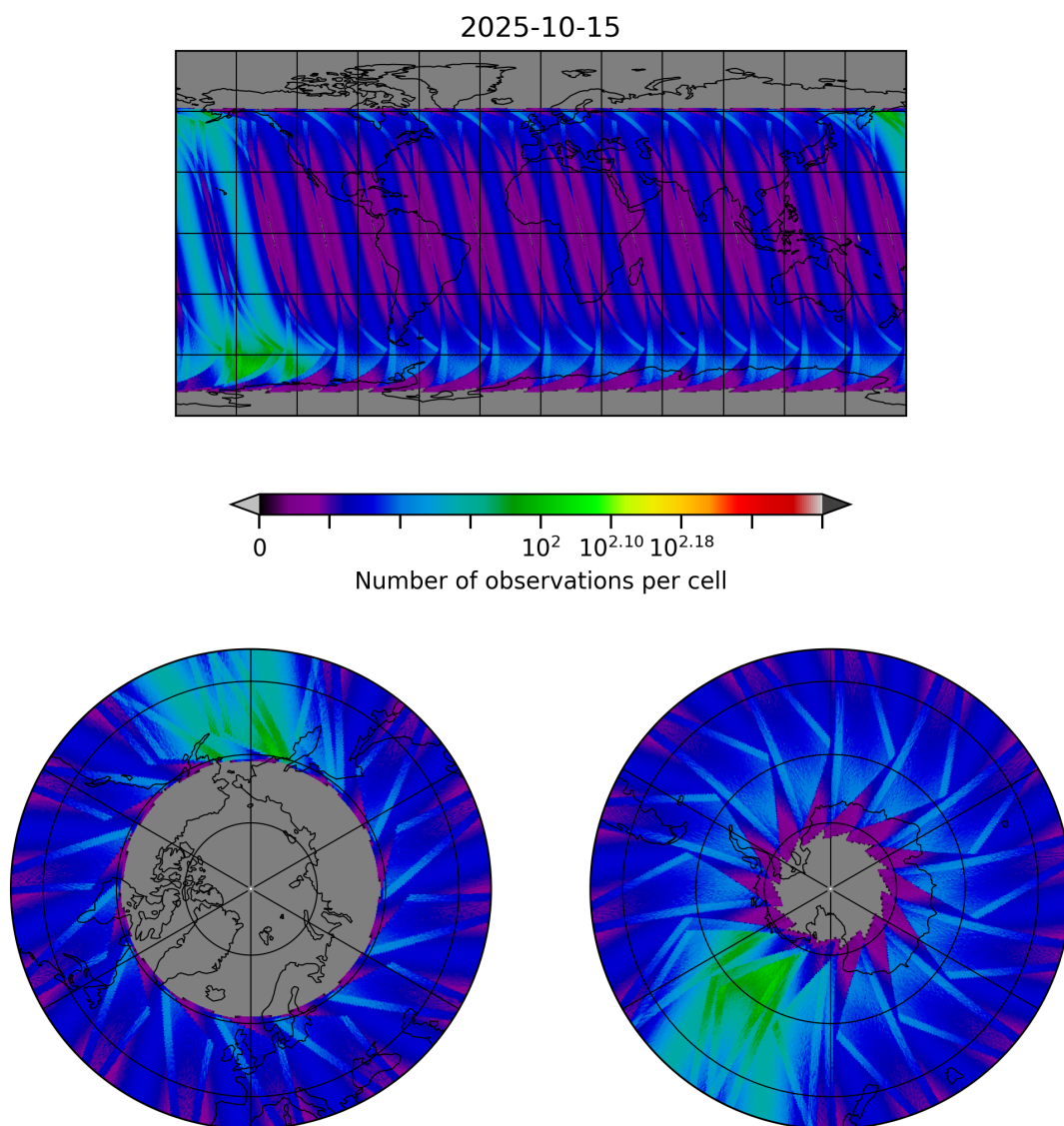
Figure 30: Map of the number of observations for 2025-10-14 to 2025-10-16
