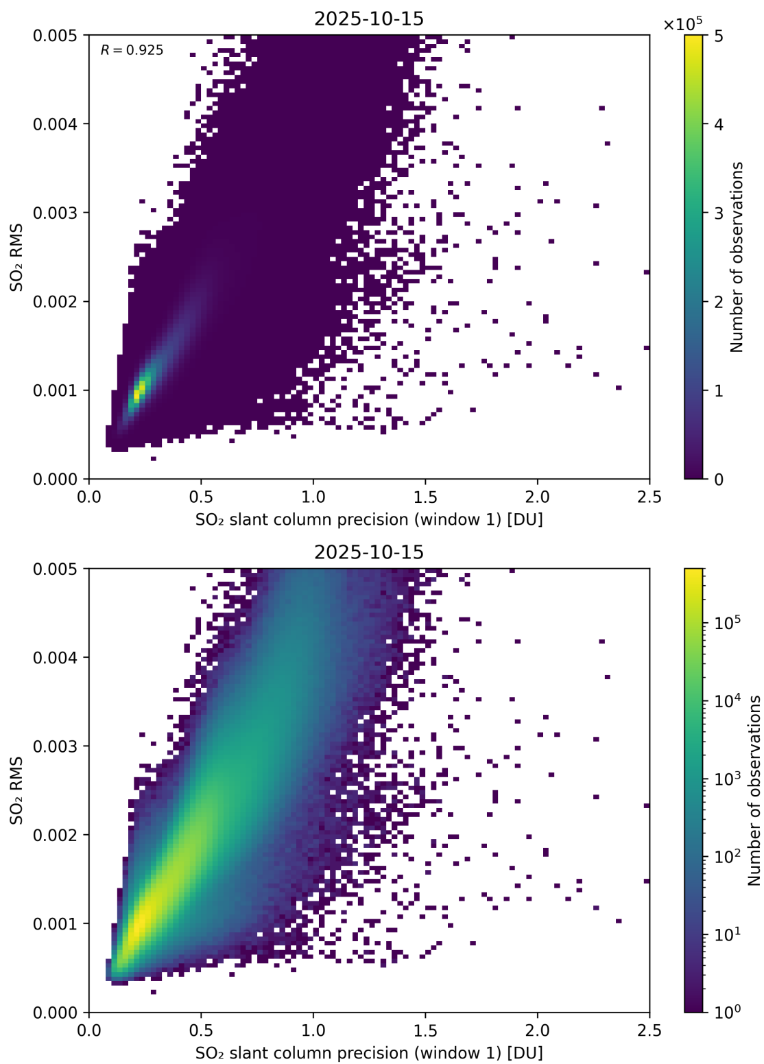
Figure 273: Scatter density plot of “SO 2 slant column precision (window 1)” against “SO 2 RMS” for 2025-10-14 to 2025-10-16.
