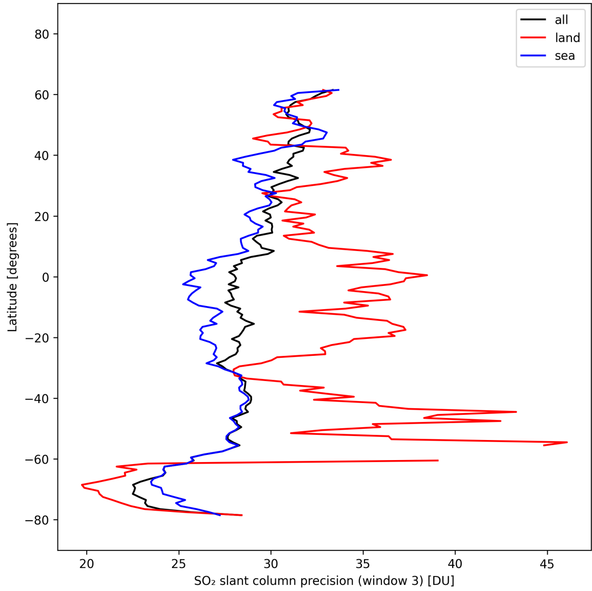
Figure 46: Zonal average of “SO 2 slant column precision (window 3)” for 2025-10-14 to 2025-10-16.
