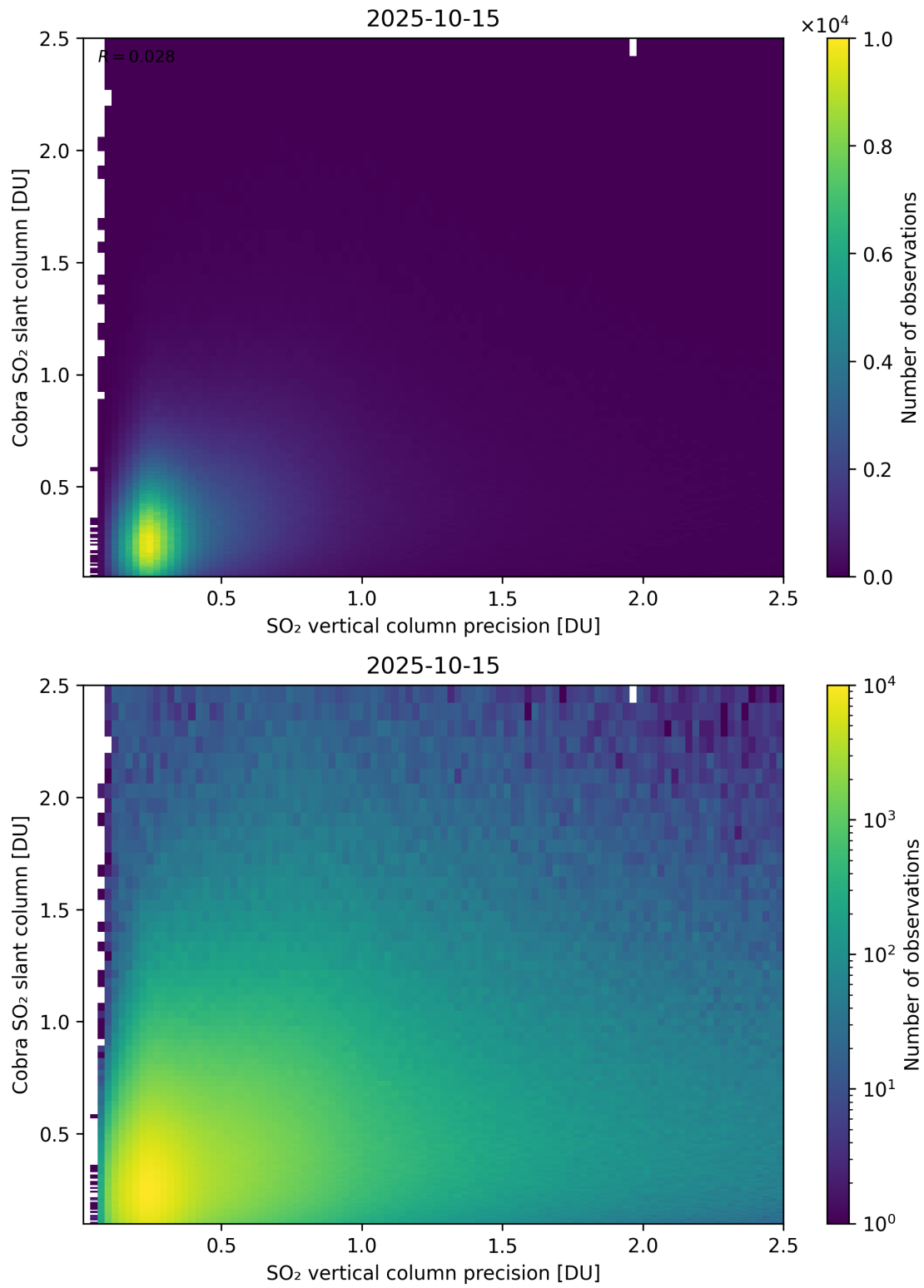
Figure 336: Scatter density plot of “SO 2 vertical column precision” against “Cobra SO 2 slant column” for 2025-10-14 to 2025-10-16.
