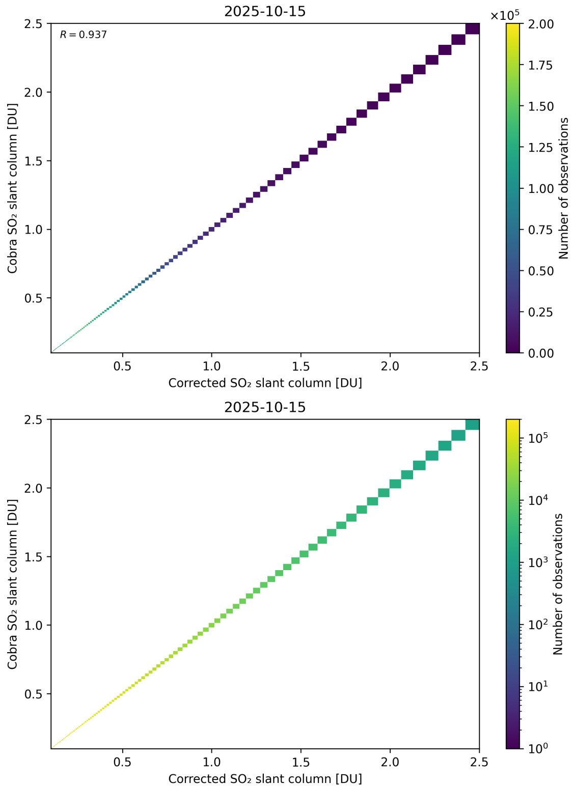
Figure 233: Scatter density plot of “Corrected SO 2 slant column” against “Cobra SO 2 slant column” for 2025-10-14 to 2025-10-16.
