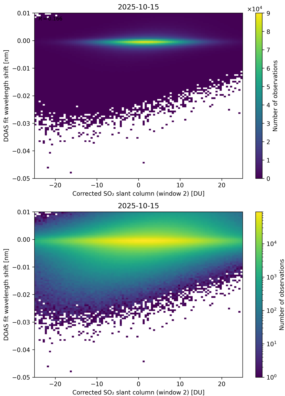
Figure 246: Scatter density plot of “Corrected SO 2 slant column (window 2)” against “DOAS fit wavelength shift” for 2025-10-14 to 2025-10-16.
