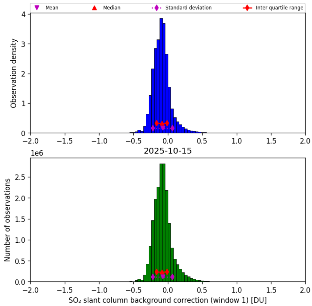
Figure 66: Histogram of “SO 2 slant column background correction (window 1)” for 2025-10-14 to 2025-10-16
