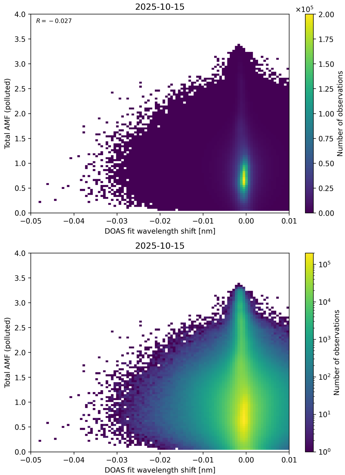
Figure 141: Scatter density plot of “DOAS fit wavelength shift” against “Total AMF (polluted)” for 2025-10-14 to 2025-10-16.
