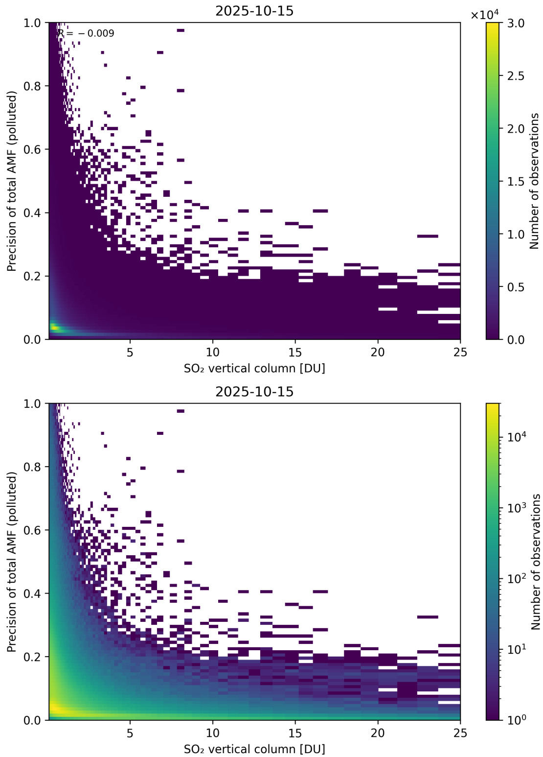
Figure 360: Scatter density plot of “SO 2 vertical column” against “Precision of total AMF (polluted)” for 2025-10-14 to 2025-10-16.
