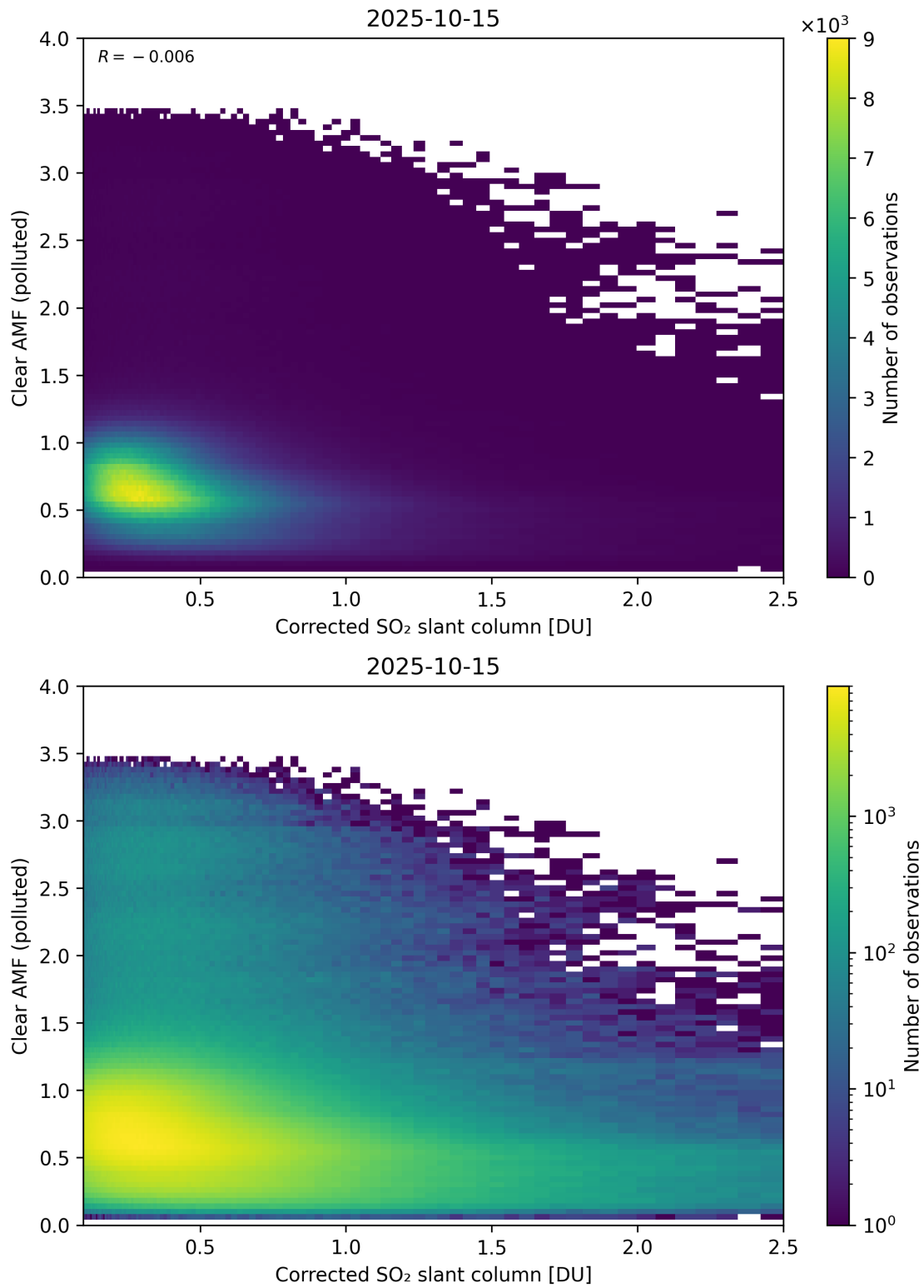
Figure 232: Scatter density plot of “Corrected SO 2 slant column” against “Clear AMF (polluted)” for 2025-10-14 to 2025-10-16.
