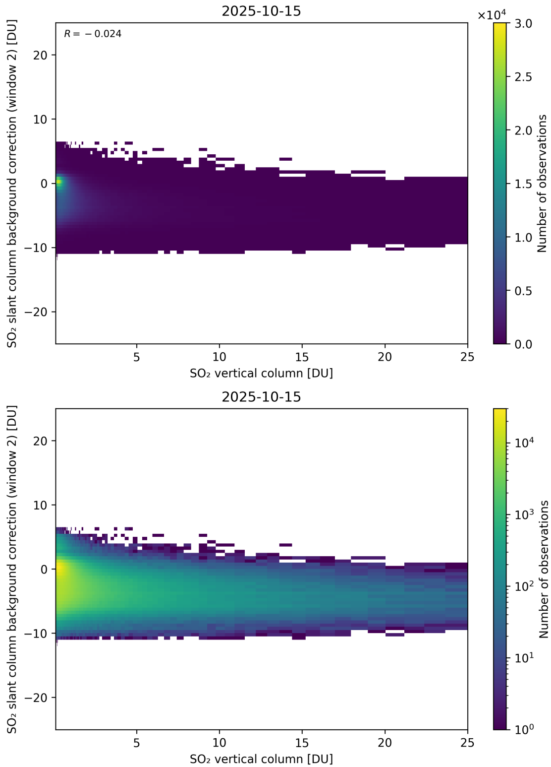
Figure 324: Scatter density plot of “SO 2 vertical column” against “SO 2 slant column background correction (window 2)” for 2025-10-14 to 2025-10-16.
