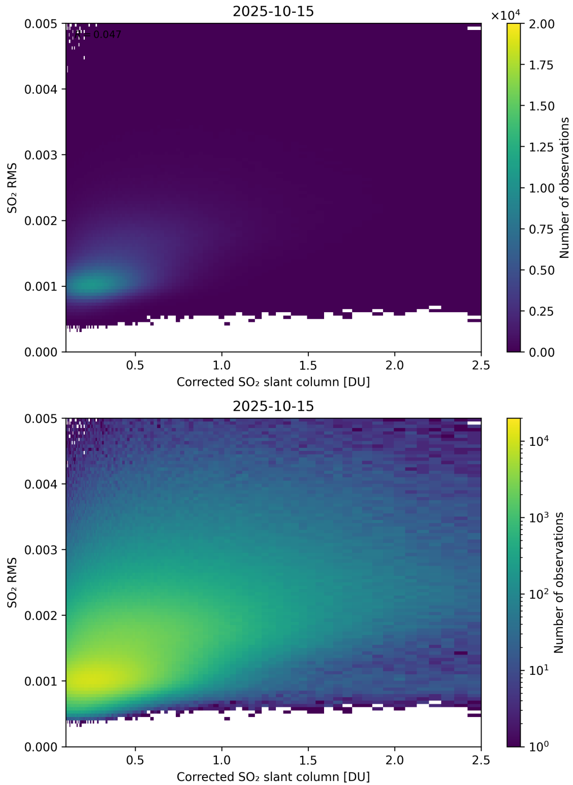
Figure 231: Scatter density plot of “Corrected SO 2 slant column” against “SO 2 RMS” for 2025-10-14 to 2025-10-16.
