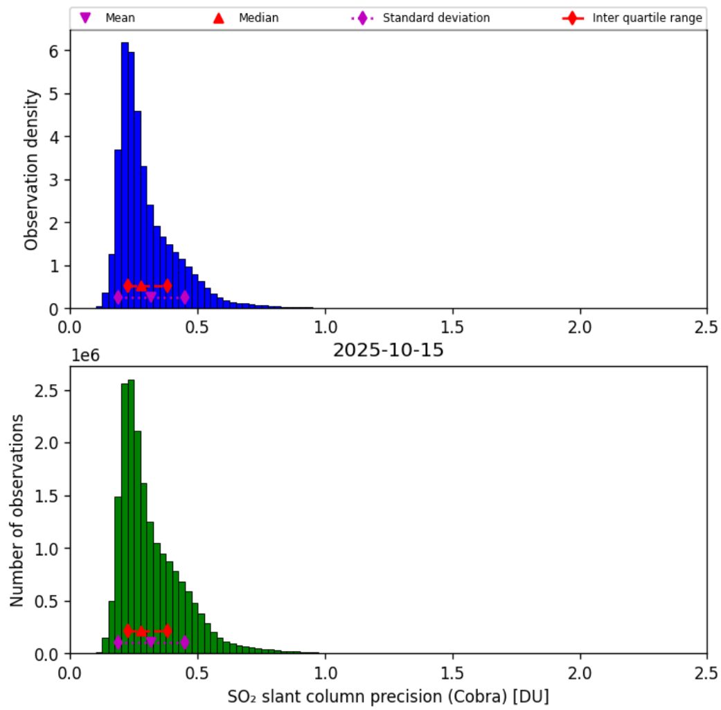
Figure 62: Histogram of “SO 2 slant column precision (Cobra)” for 2025-10-14 to 2025-10-16
