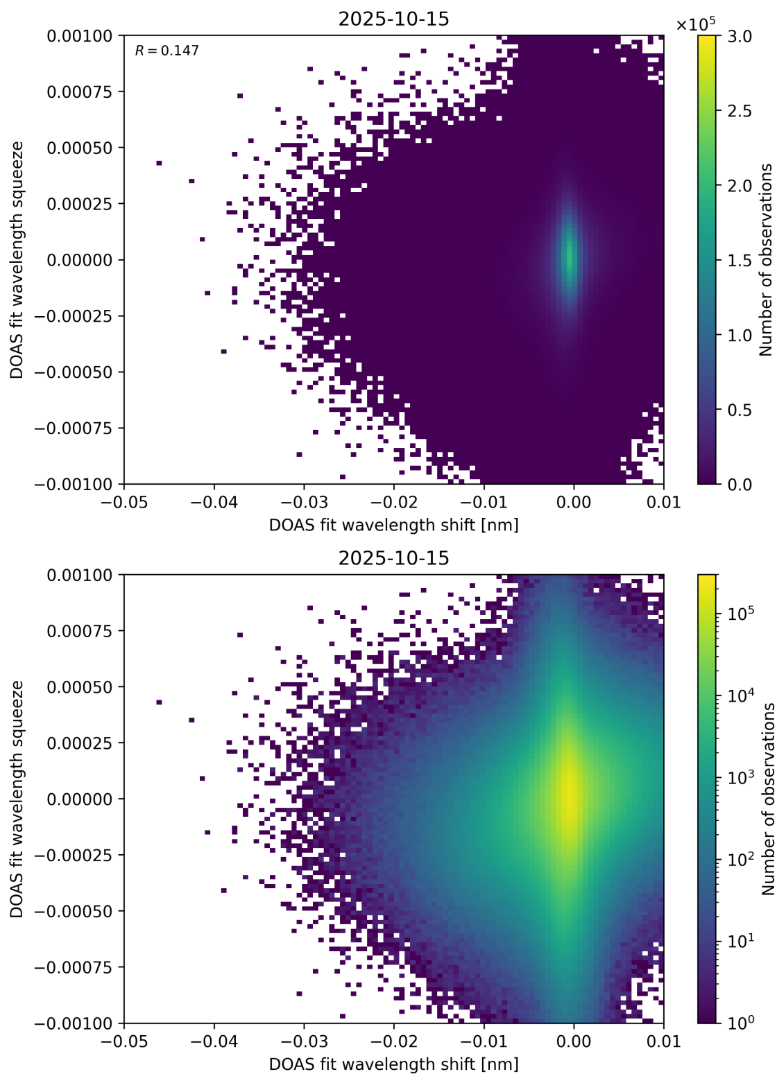
Figure 138: Scatter density plot of “DOAS fit wavelength shift” against “DOAS fit wavelength squeeze” for 2025-10-14 to 2025-10-16.
