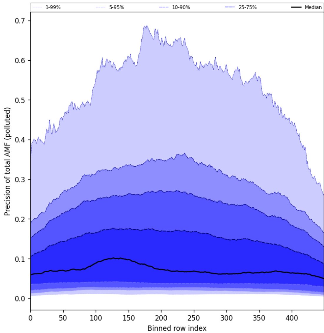
Figure 106: Along track statistics of “Precision of total AMF (polluted)” for 2025-10-14 to 2025-10-16
