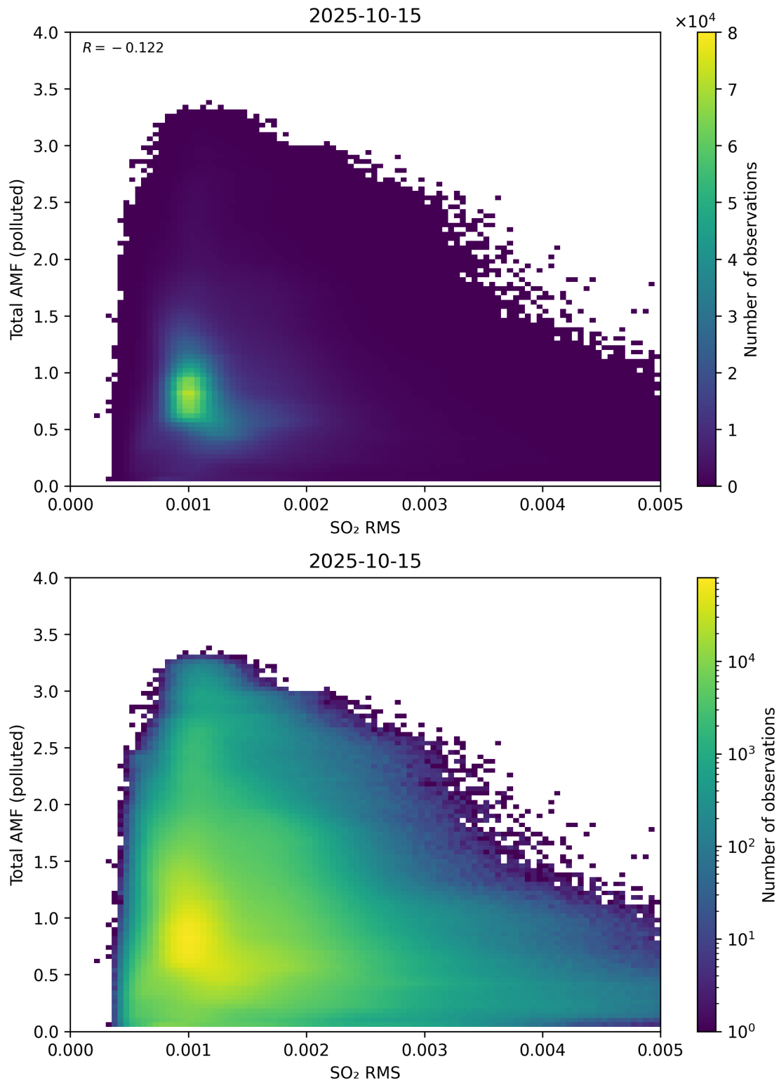
Figure 148: Scatter density plot of “SO 2 RMS” against “Total AMF (polluted)” for 2025-10-14 to 2025-10-16.
