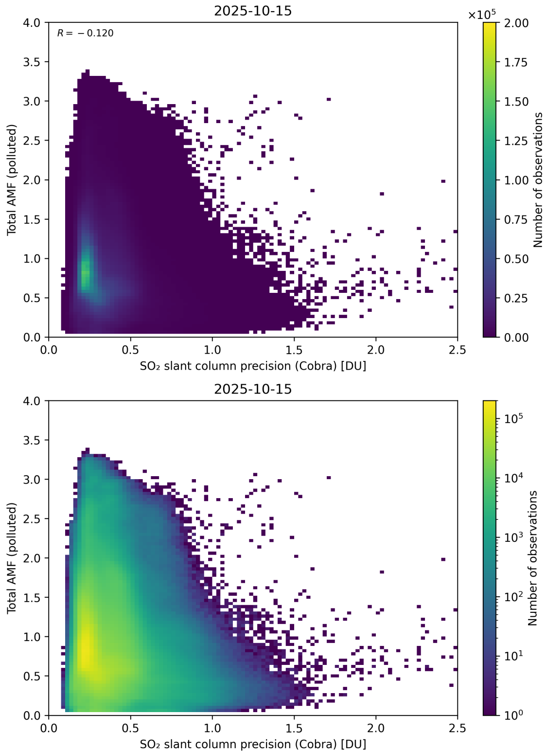
Figure 213: Scatter density plot of “SO 2 slant column precision (Cobra)” against “Total AMF (polluted)” for 2025-10-14 to 2025-10-16.
