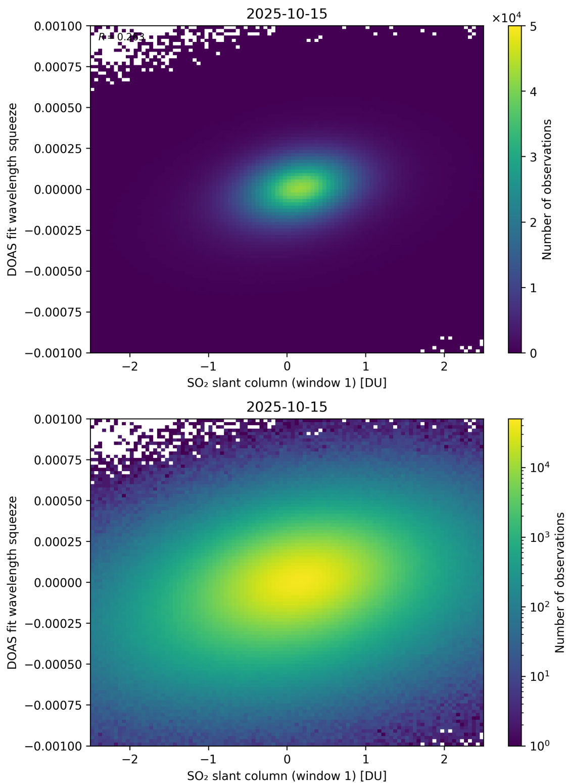
Figure 266: Scatter density plot of “SO 2 slant column (window 1)” against “DOAS fit wavelength squeeze” for 2025-10-14 to 2025-10-16.
