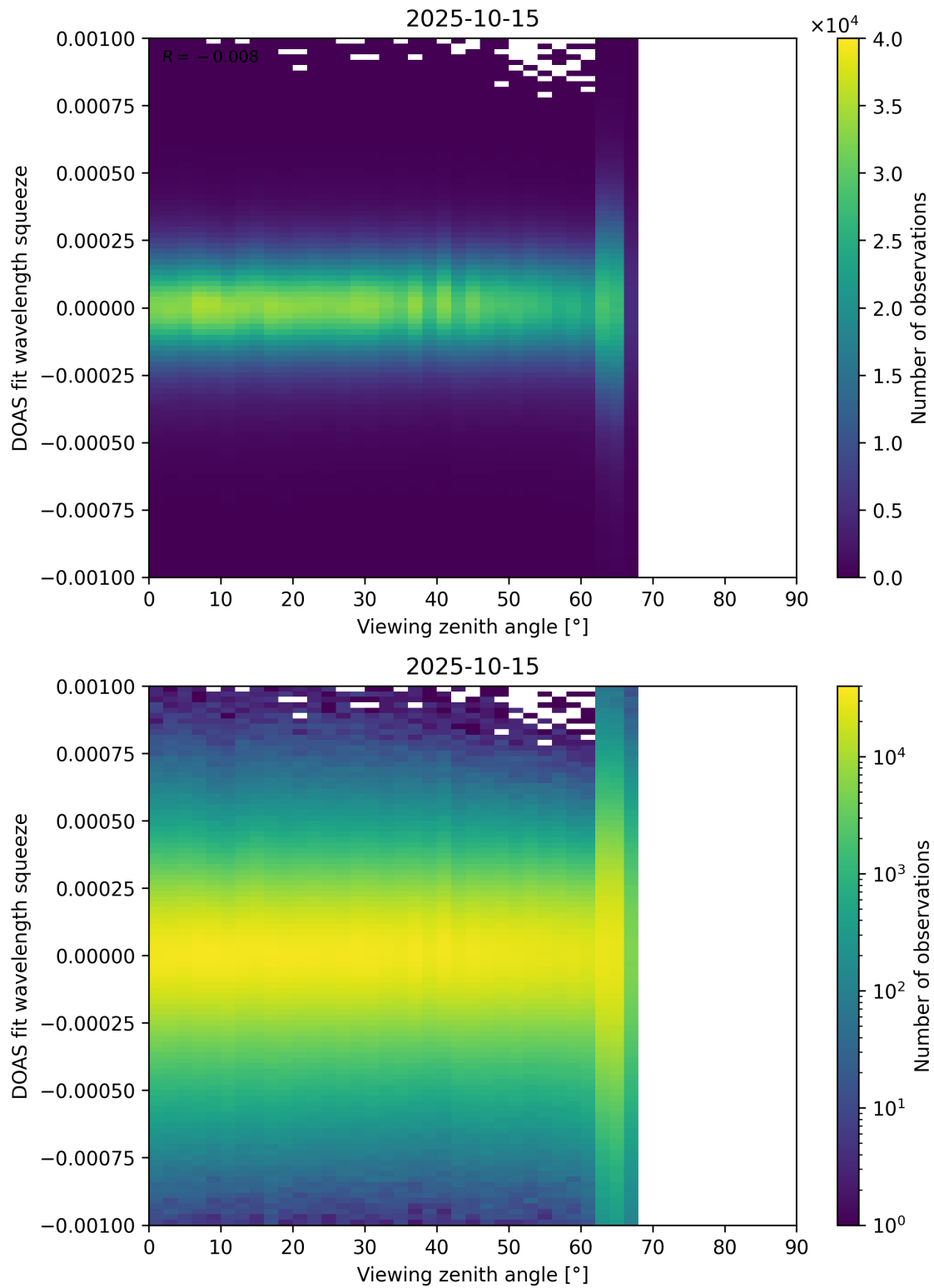
Figure 366: Scatter density plot of “Viewing zenith angle” against “DOAS fit wavelength squeeze” for 2025-10-14 to 2025-10-16.
