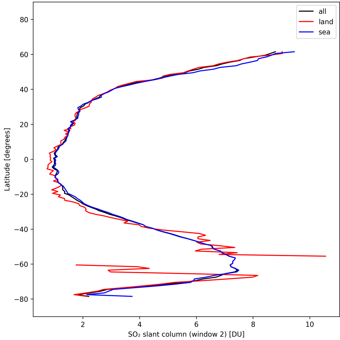
Figure 41: Zonal average of “SO 2 slant column (window 2)” for 2025-10-14 to 2025-10-16.
