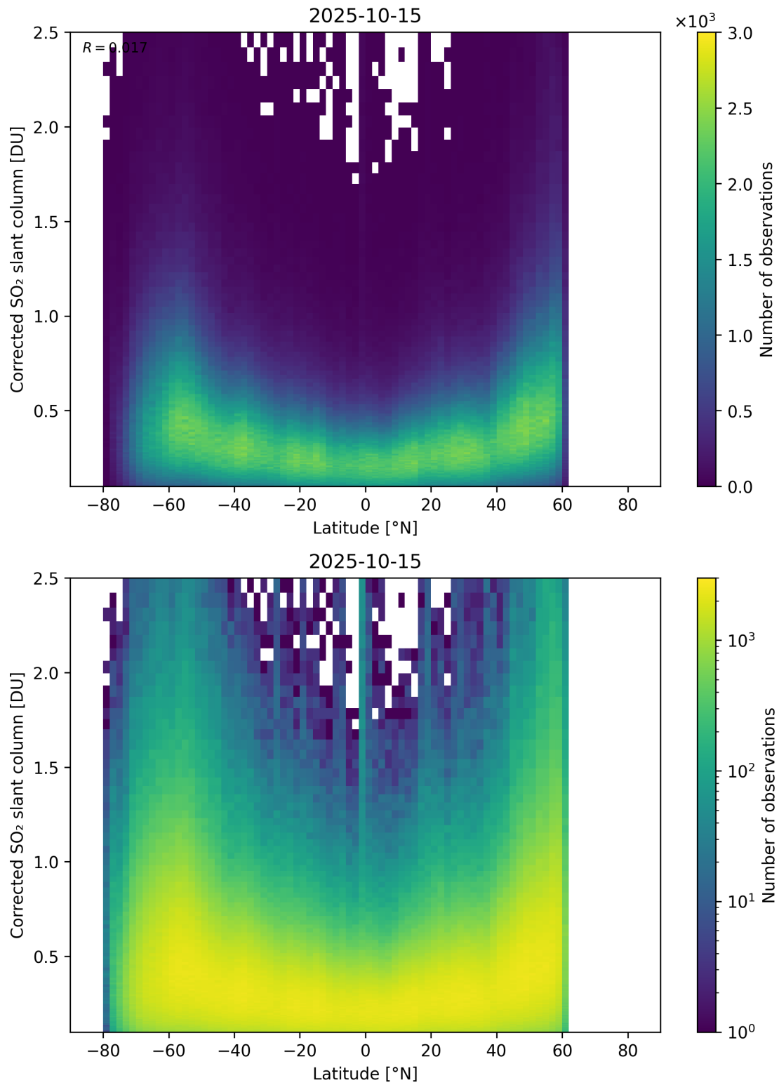
Figure 159: Scatter density plot of “Latitude” against “Corrected SO 2 slant column” for 2025-10-14 to 2025-10-16.
