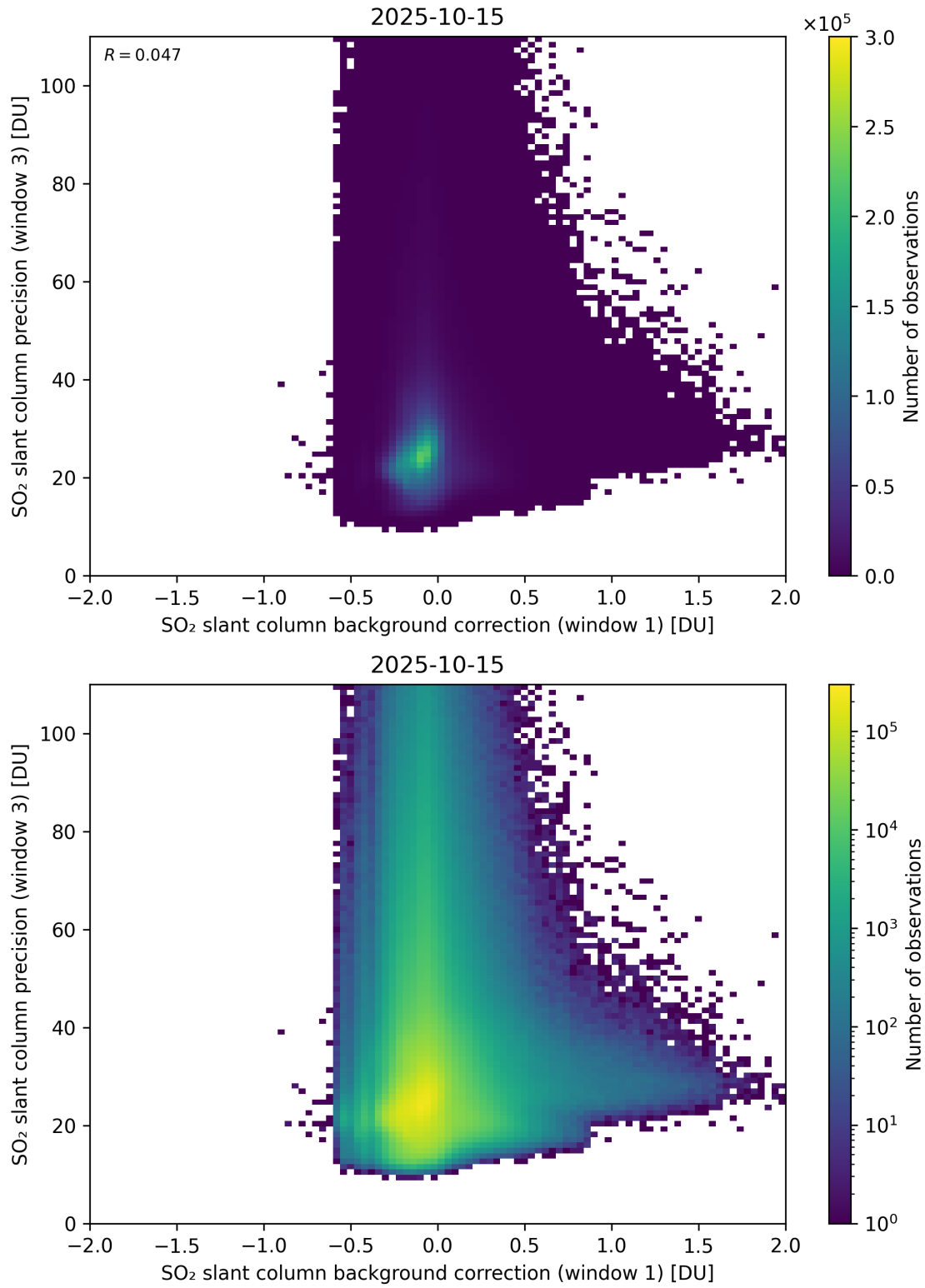
Figure 119: Scatter density plot of “SO 2 slant column background correction (window 1)” against “SO 2 slant column precision (window 3)” for 2025-10-14 to 2025-10-16.
