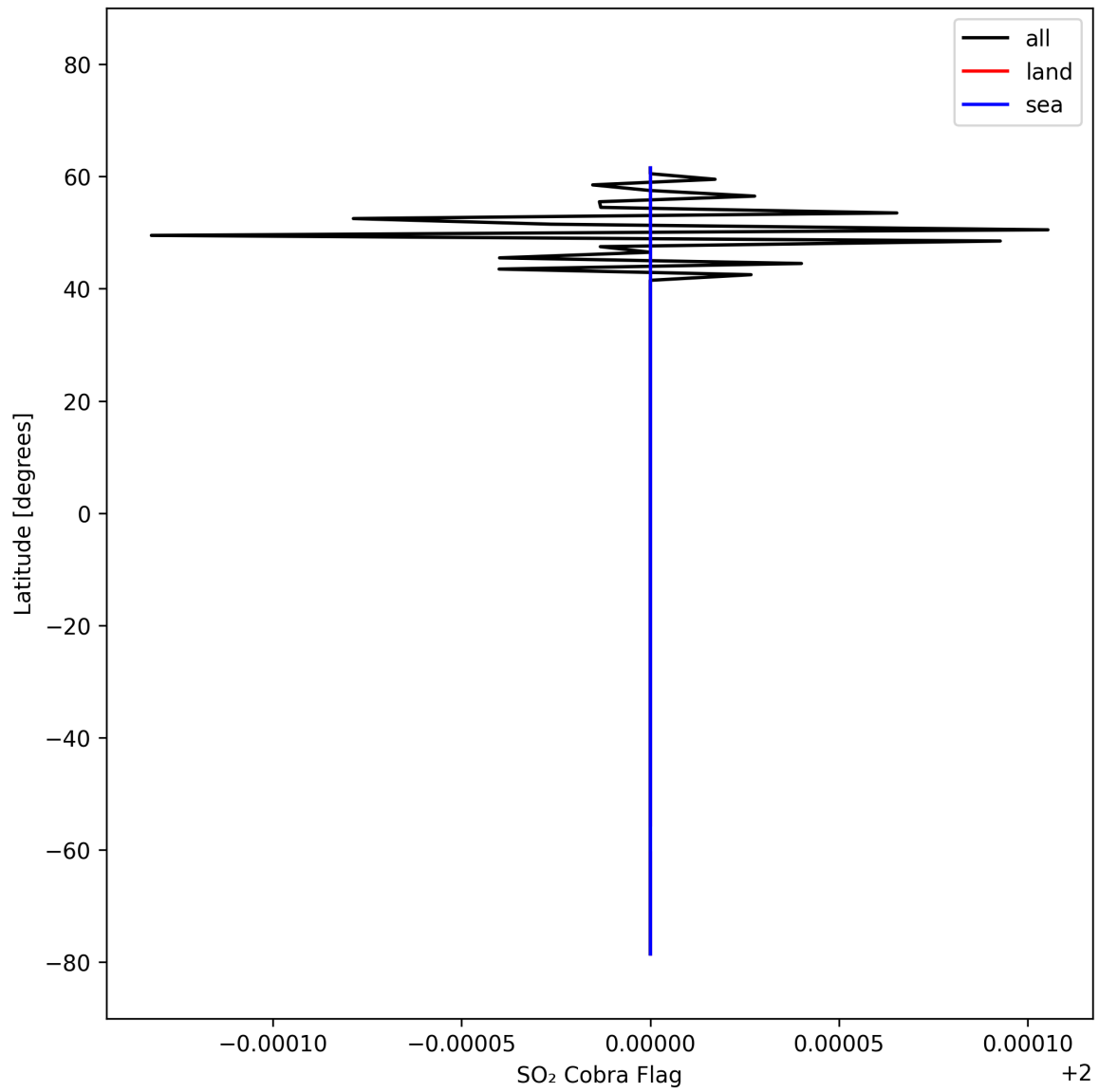
Figure 49: Zonal average of "SO 2 Cobra Flag" for 2025-10-14 to 2025-10-16.
