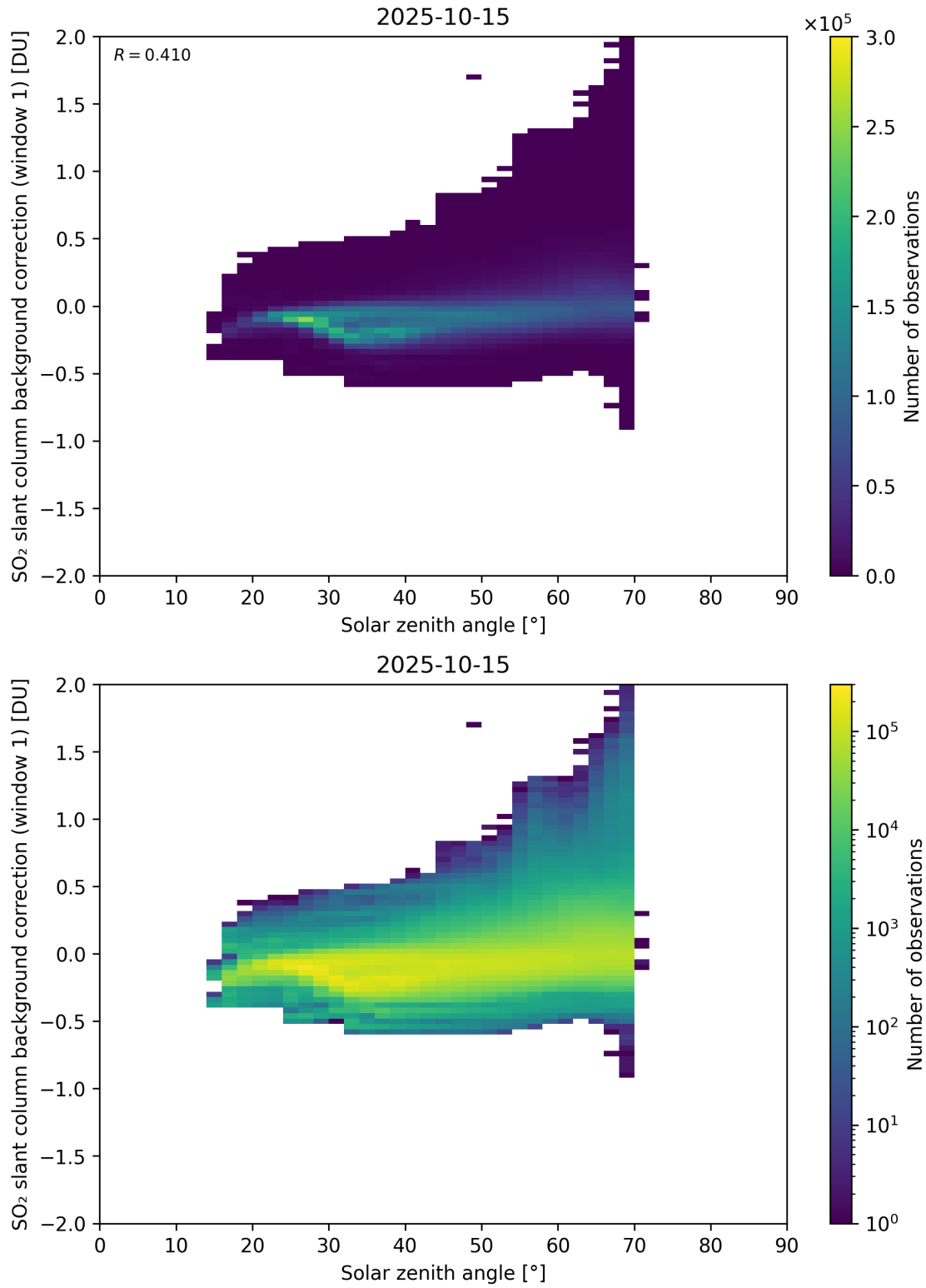
Figure 171: Scatter density plot of “Solar zenith angle” against “SO 2 slant column background correction (window 1)” for 2025-10-14 to 2025-10-16.
