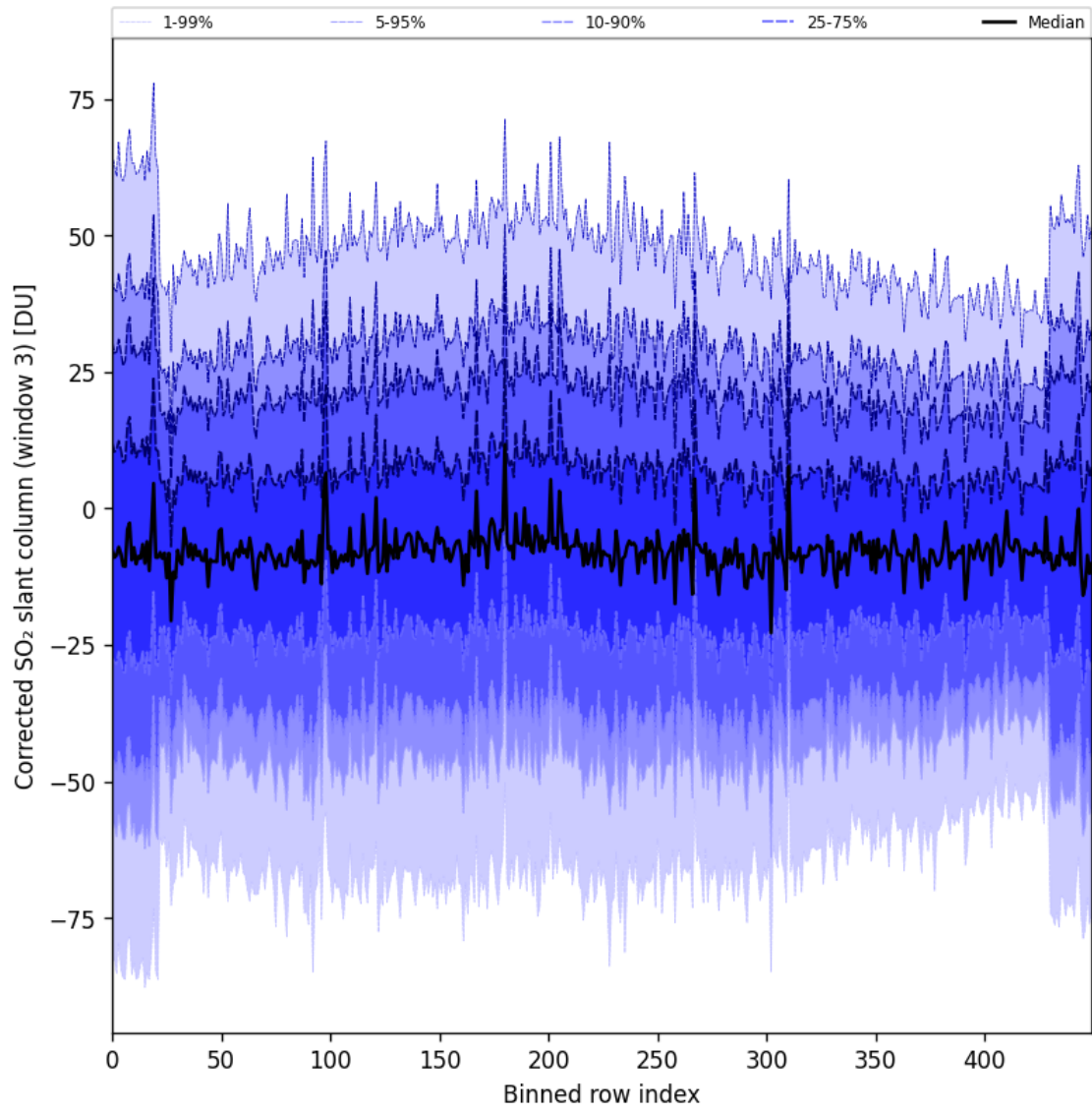
Figure 99: Along track statistics of “Corrected SO 2 slant column (window 3)” for 2025-10-14 to 2025-10-16
