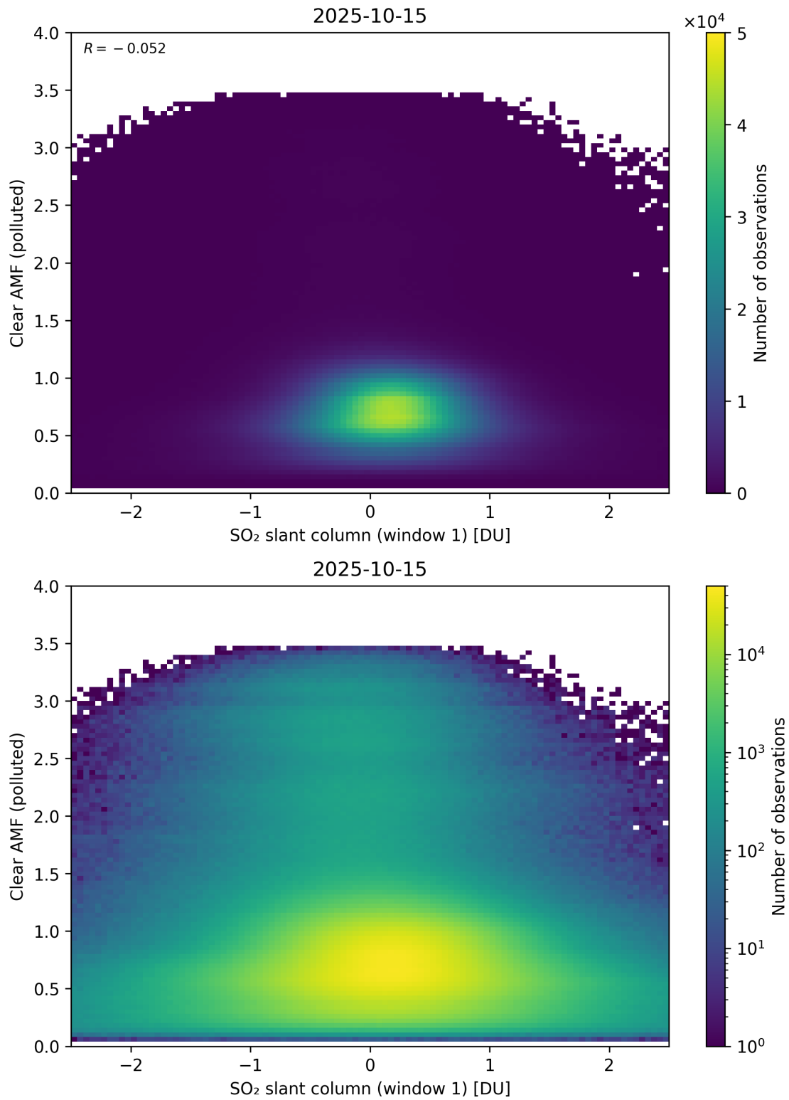
Figure 282: Scatter density plot of “SO 2 slant column (window 1)” against “Clear AMF (polluted)” for 2025-10-14 to 2025-10-16.
