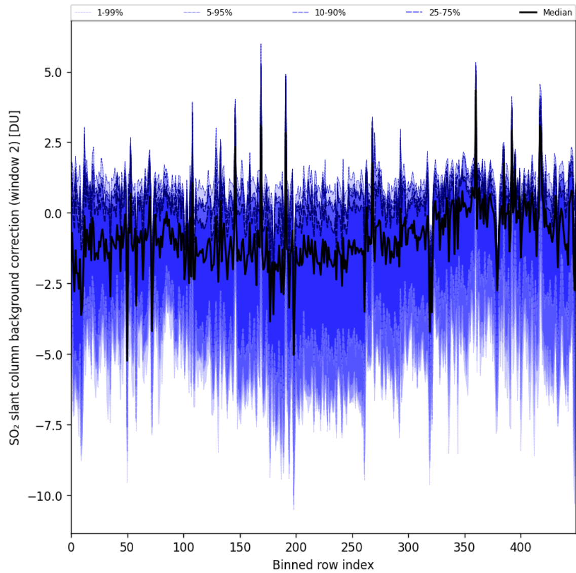
Figure 96: Along track statistics of “SO 2 slant column background correction (window 2)” for 2025-10-14 to 2025-10-16
