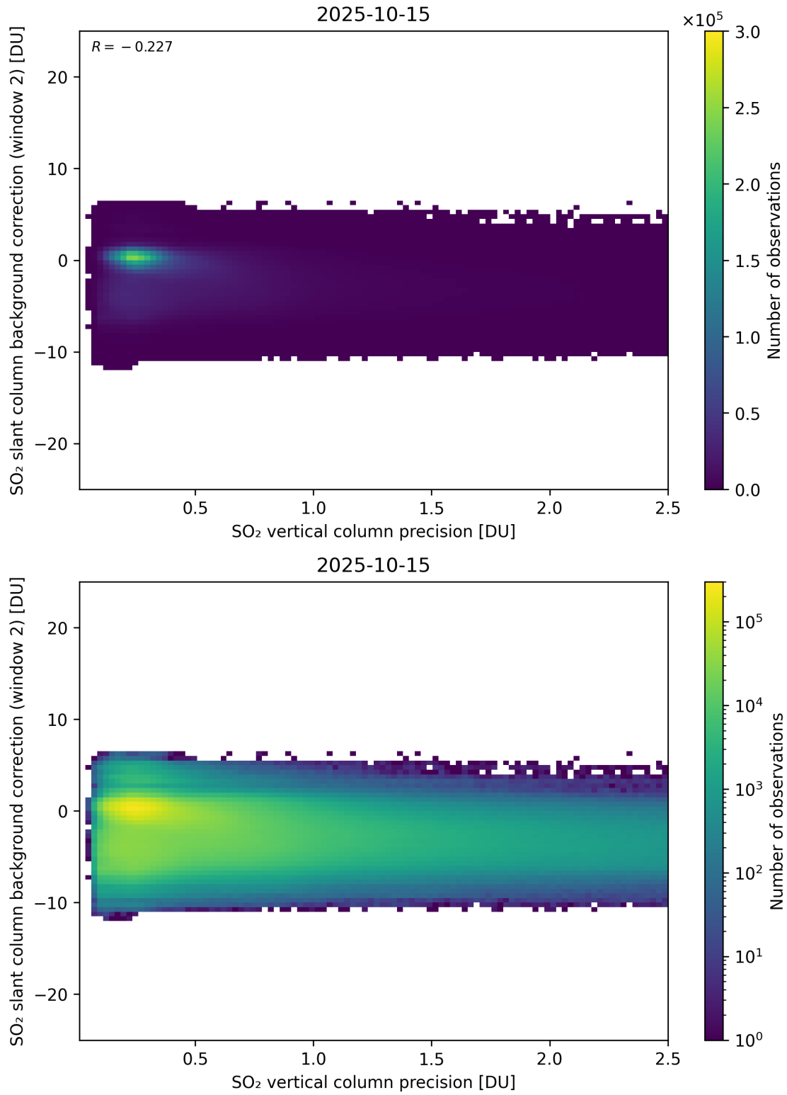
Figure 330: Scatter density plot of “SO 2 vertical column precision” against “SO 2 slant column background correction (window 2)” for 2025-10-14 to 2025-10-16.
