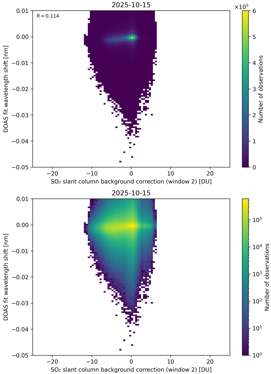
Figure 123: Scatter density plot of “SO 2 slant column background correction (window 2)” against “DOAS fit wavelength shift” for 2025-10-14 to 2025-10-16.
