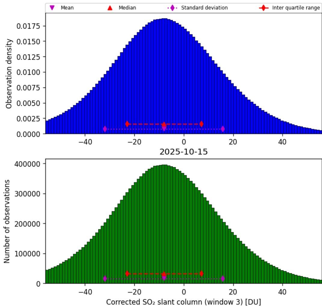
Figure 73: Histogram of “Corrected SO 2 slant column (window 3)” for 2025-10-14 to 2025-10-16
