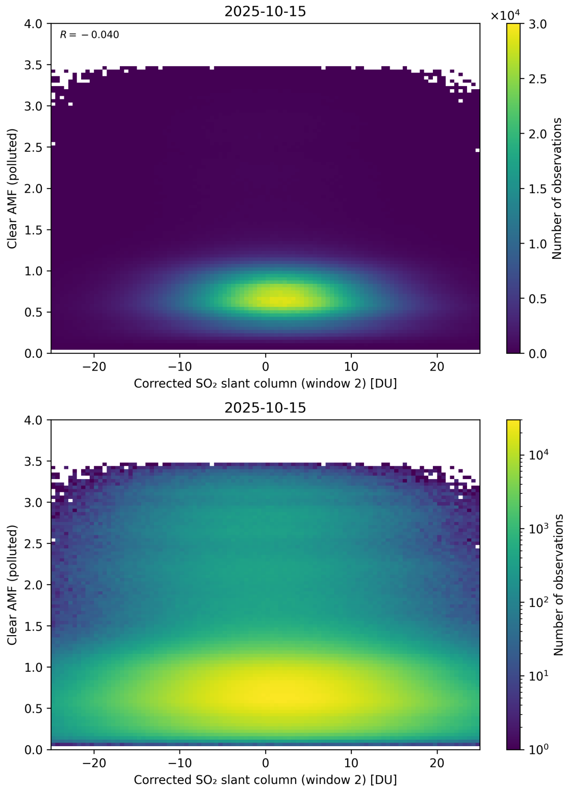
Figure 249: Scatter density plot of “Corrected SO 2 slant column (window 2)” against “Clear AMF (polluted)” for 2025-10-14 to 2025-10-16.
