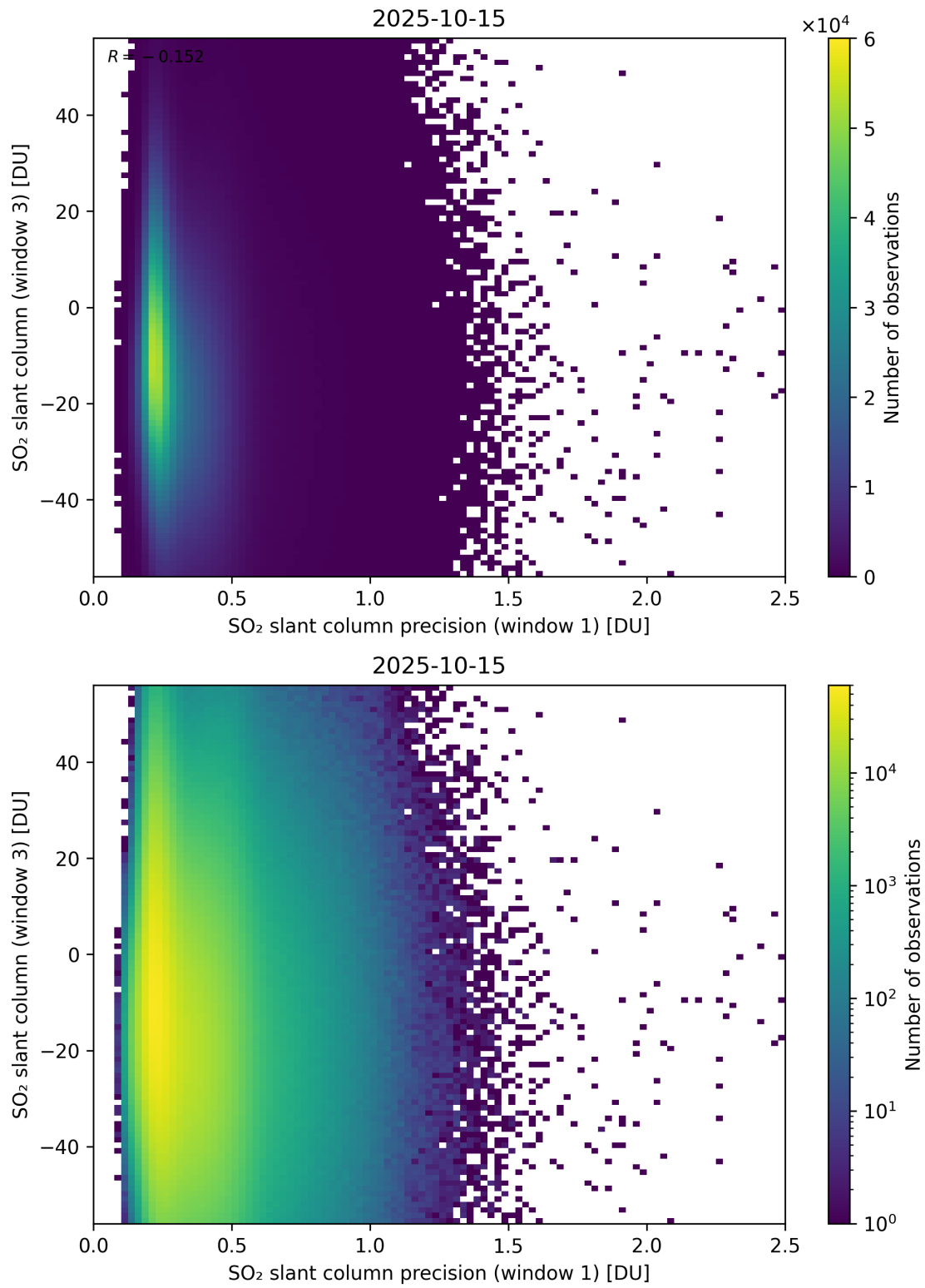
Figure 278: Scatter density plot of “SO 2 slant column precision (window 1)” against “SO 2 slant column (window 3)” for 2025-10-14 to 2025-10-16.
