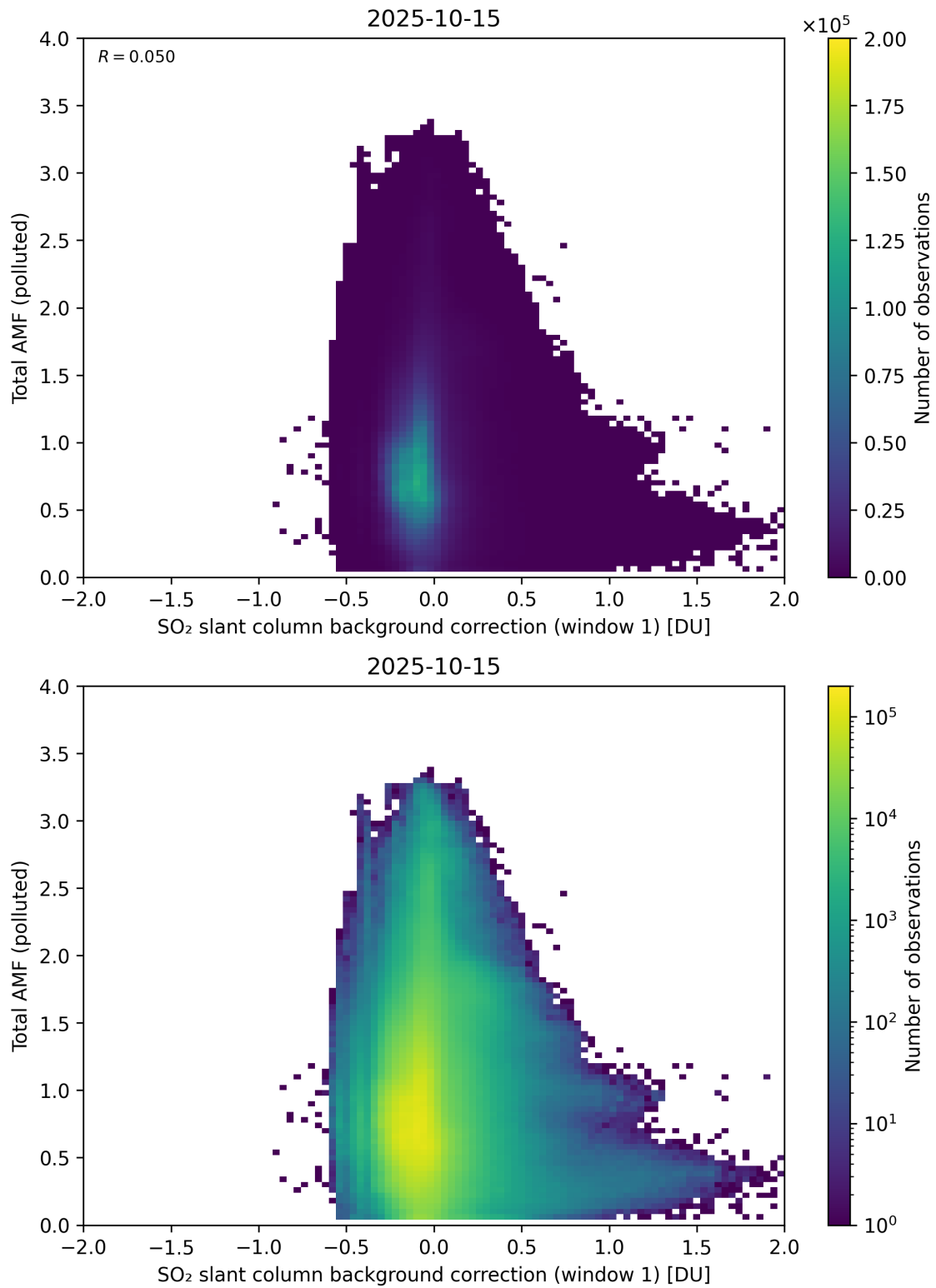
Figure 120: Scatter density plot of “SO 2 slant column background correction (window 1)” against “Total AMF (polluted)” for 2025-10-14 to 2025-10-16.
