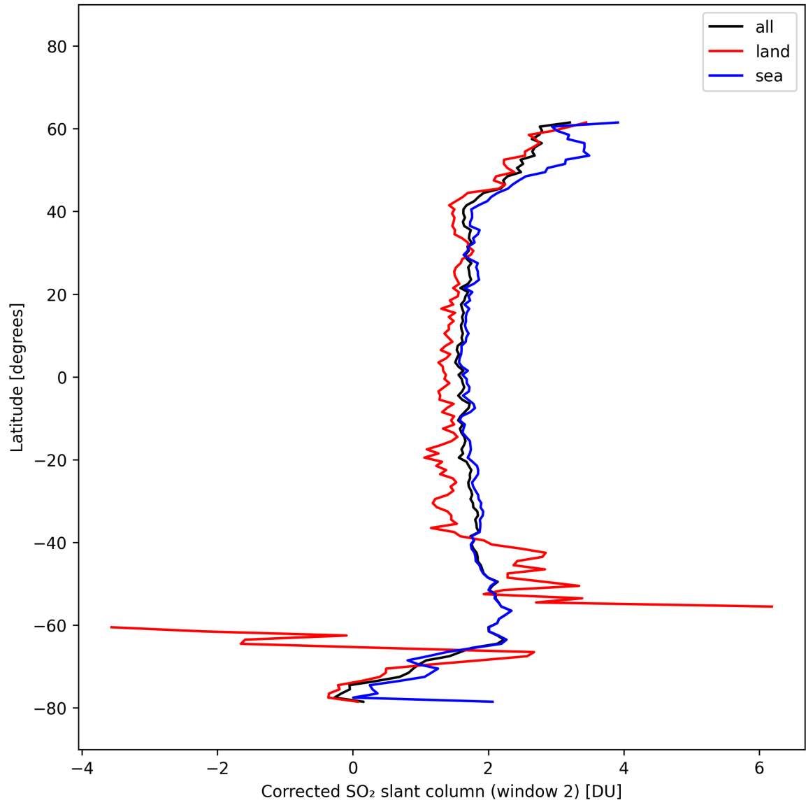
Figure 43: Zonal average of “Corrected SO 2 slant column (window 2)” for 2025-10-14 to 2025-10-16.
