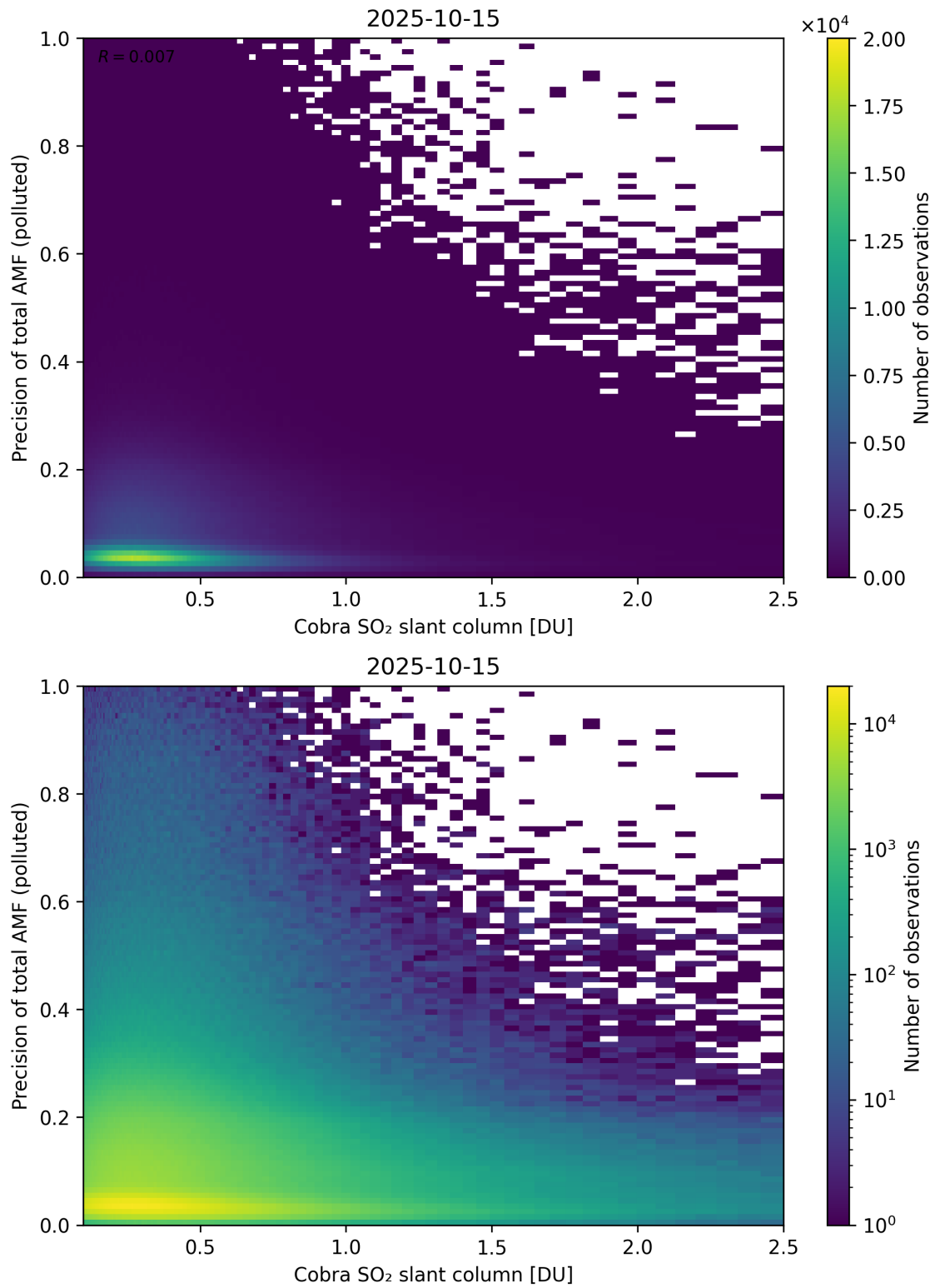
Figure 225: Scatter density plot of “Cobra SO 2 slant column” against “Precision of total AMF (polluted)” for 2025-10-14 to 2025-10-16.
