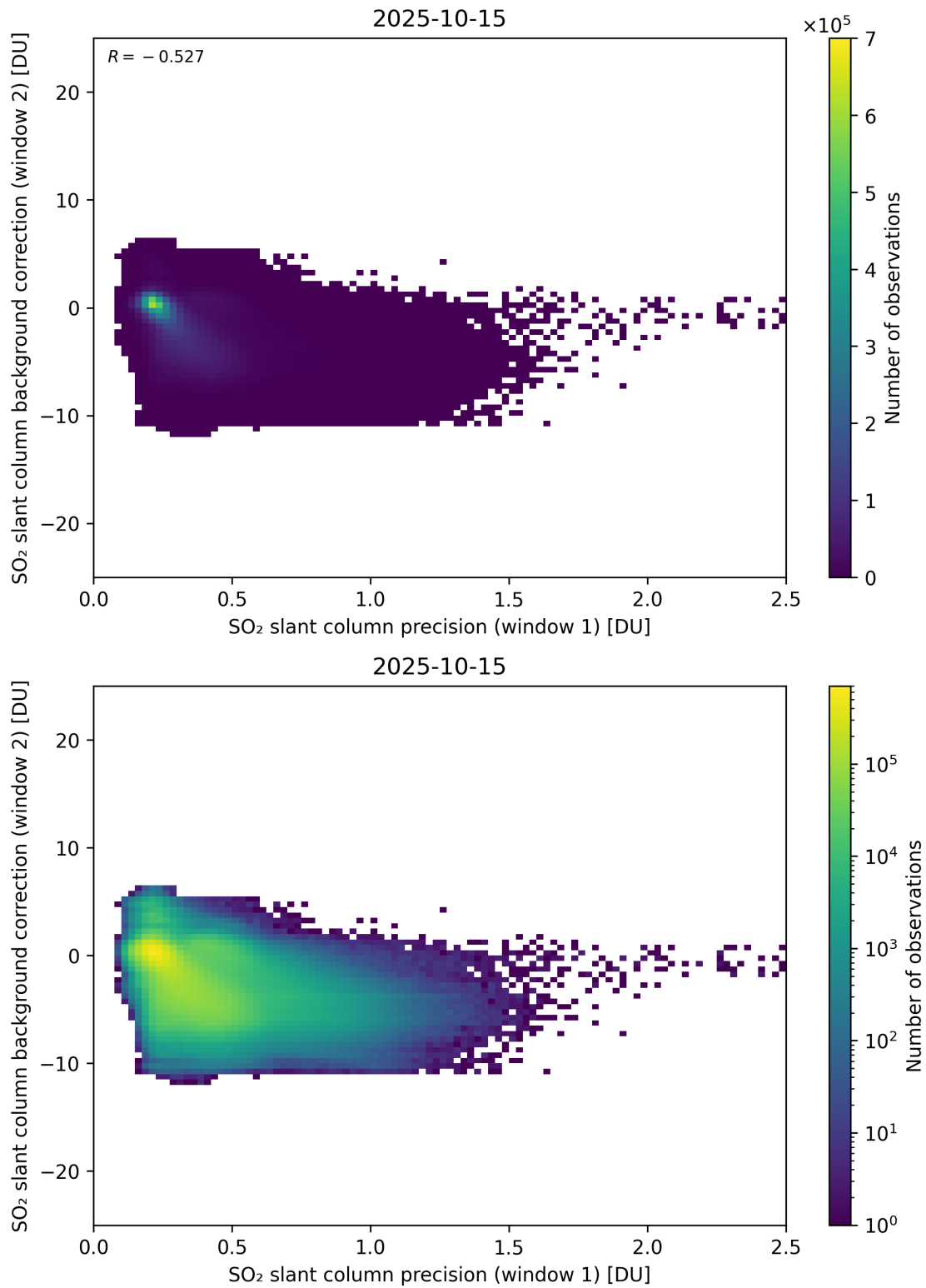
Figure 269: Scatter density plot of “SO 2 slant column precision (window 1)” against “SO 2 slant column background correction (window 2)” for 2025-10-14 to 2025-10-16.
