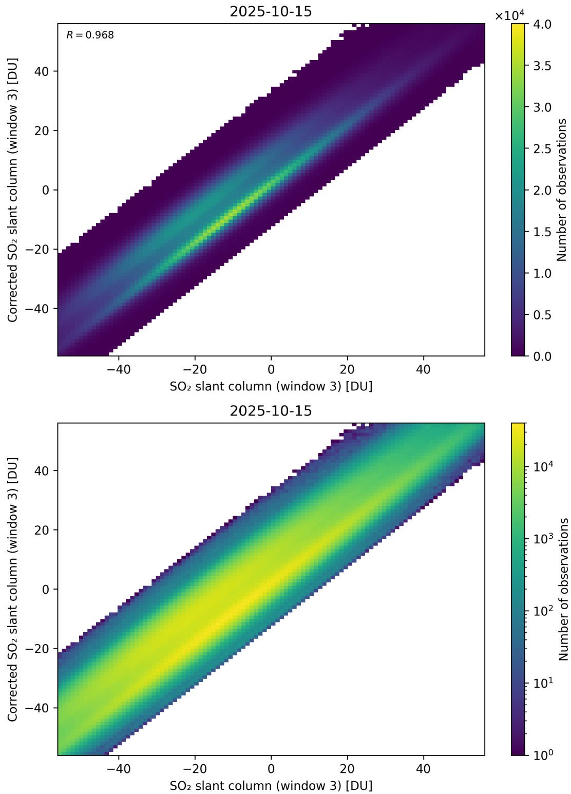
Figure 316: Scatter density plot of “SO 2 slant column (window 3)” against “Corrected SO 2 slant column (window 3)” for 2025-10-14 to 2025-10-16.
