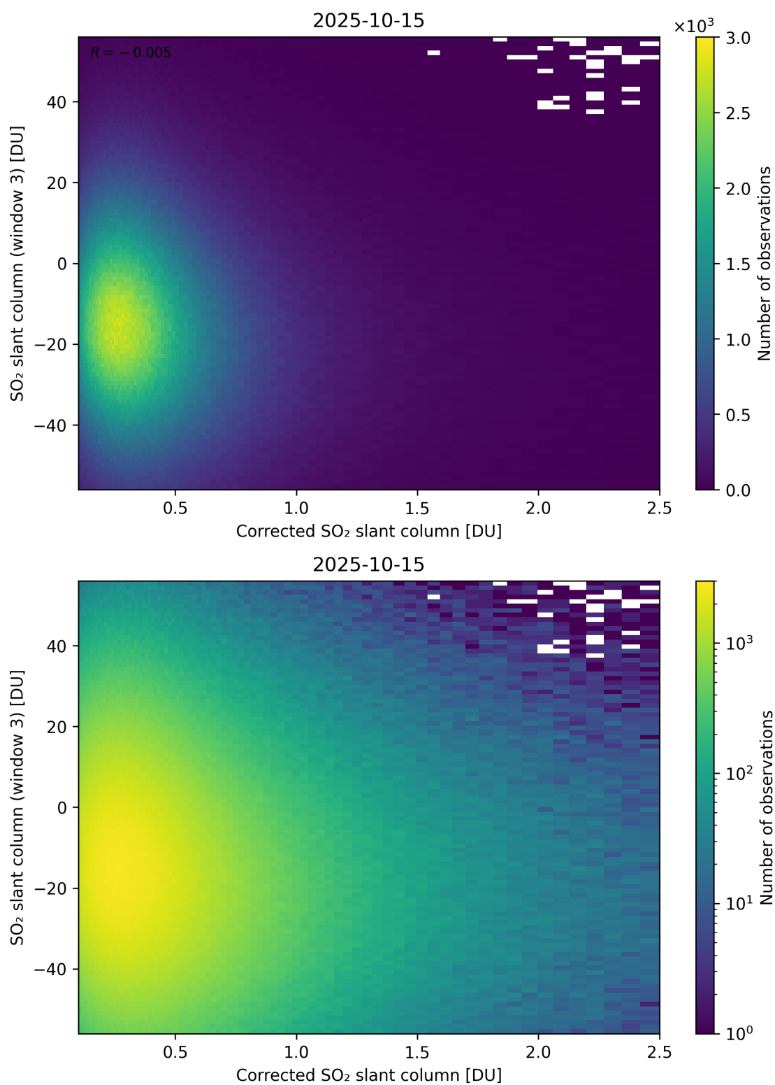
Figure 240: Scatter density plot of “Corrected SO 2 slant column” against “SO 2 slant column (window 3)” for 2025-10-14 to 2025-10-16.
