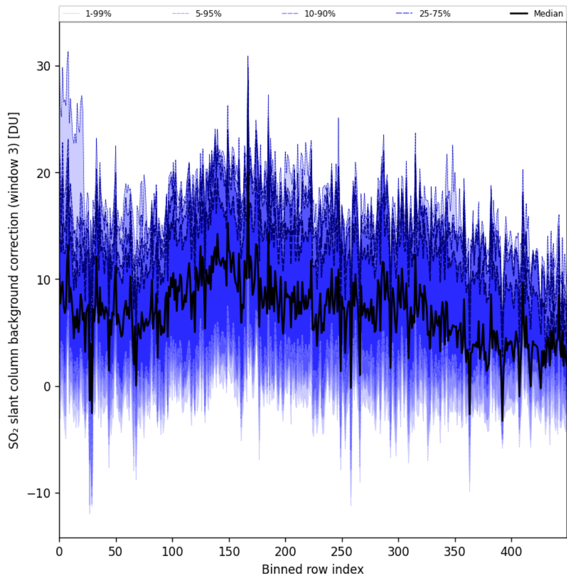
Figure 100: Along track statistics of “SO 2 slant column background correction (window 3)” for 2025-10-14 to 2025-10-16
