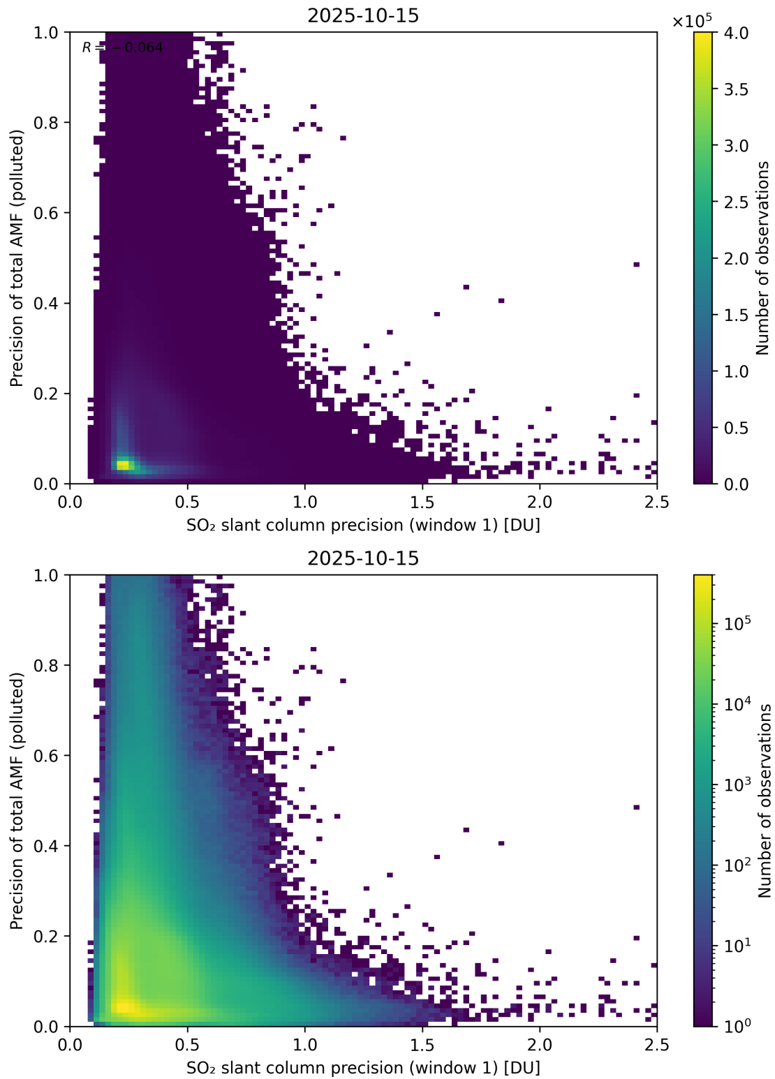
Figure 281: Scatter density plot of “SO 2 slant column precision (window 1)” against “Precision of total AMF (polluted)” for 2025-10-14 to 2025-10-16.
