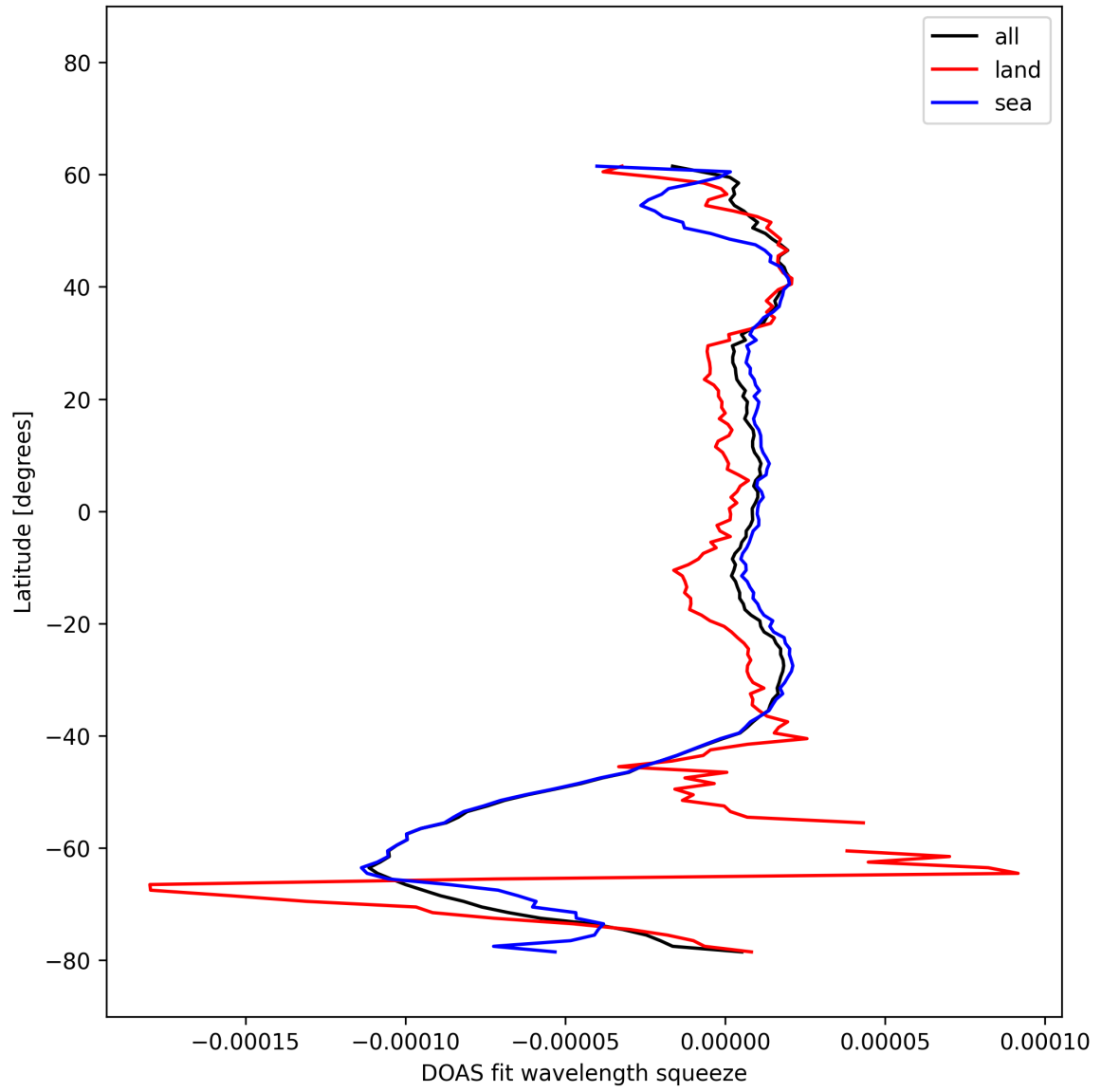
Figure 51: Zonal average of “DOAS fit wavelength squeeze” for 2025-10-14 to 2025-10-16.
