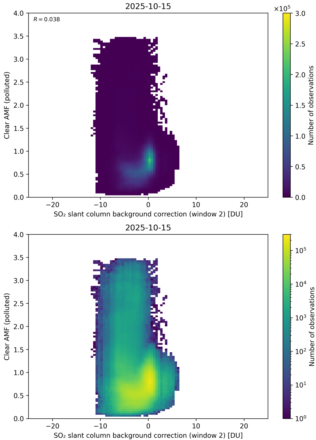
Figure 126: Scatter density plot of “SO 2 slant column background correction (window 2)” against “Clear AMF (polluted)” for 2025-10-14 to 2025-10-16.
