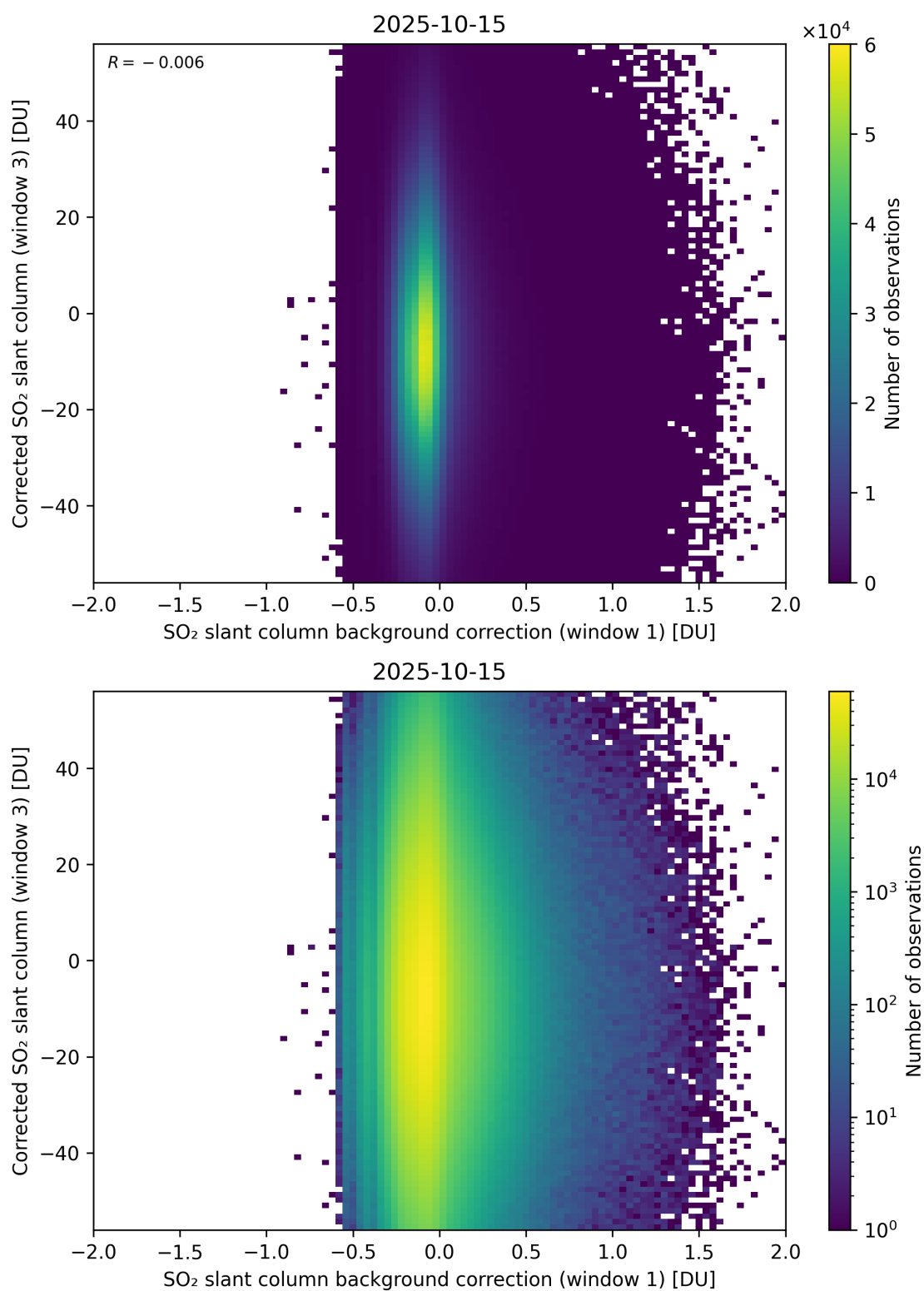
Figure 116: Scatter density plot of “SO 2 slant column background correction (window 1)” against “Corrected SO 2 slant column (window 3)” for 2025-10-14 to 2025-10-16.
