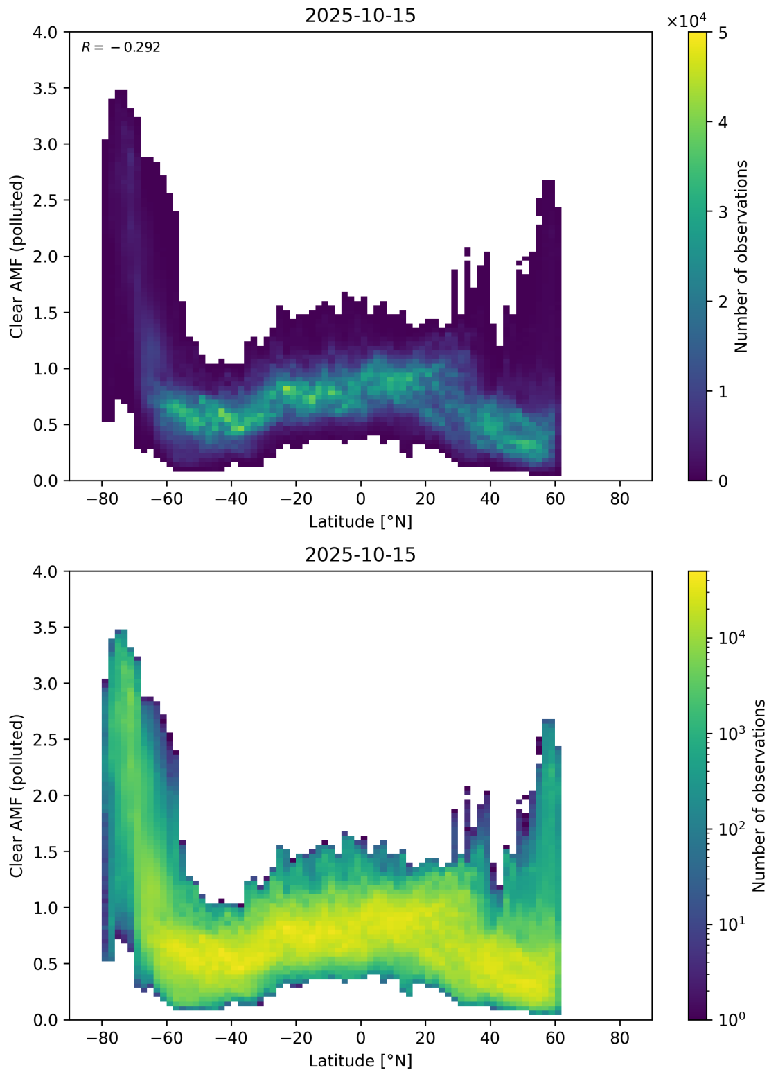
Figure 156: Scatter density plot of “Latitude” against “Clear AMF (polluted)” for 2025-10-14 to 2025-10-16.
