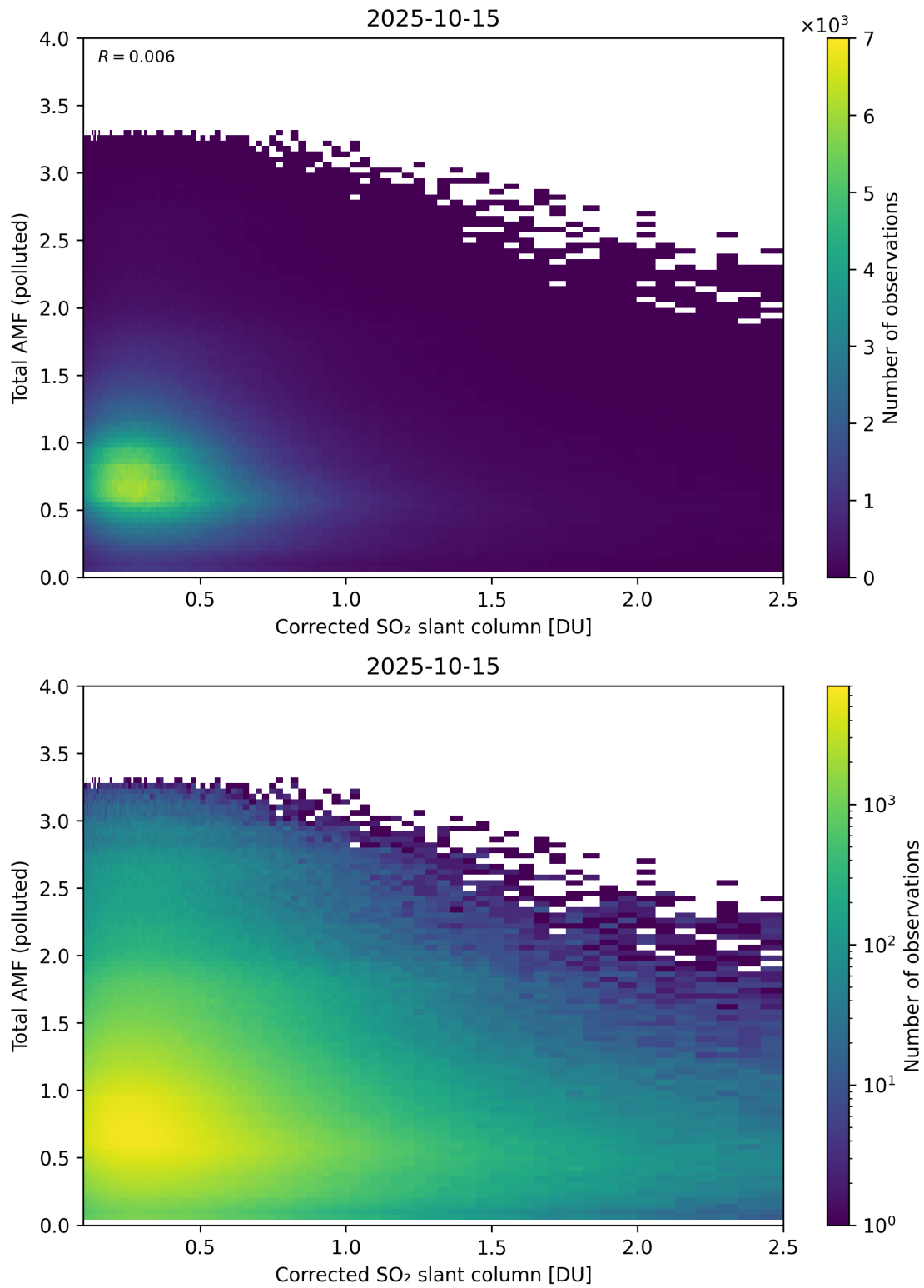
Figure 242: Scatter density plot of “Corrected SO 2 slant column” against “Total AMF (polluted)” for 2025-10-14 to 2025-10-16.
