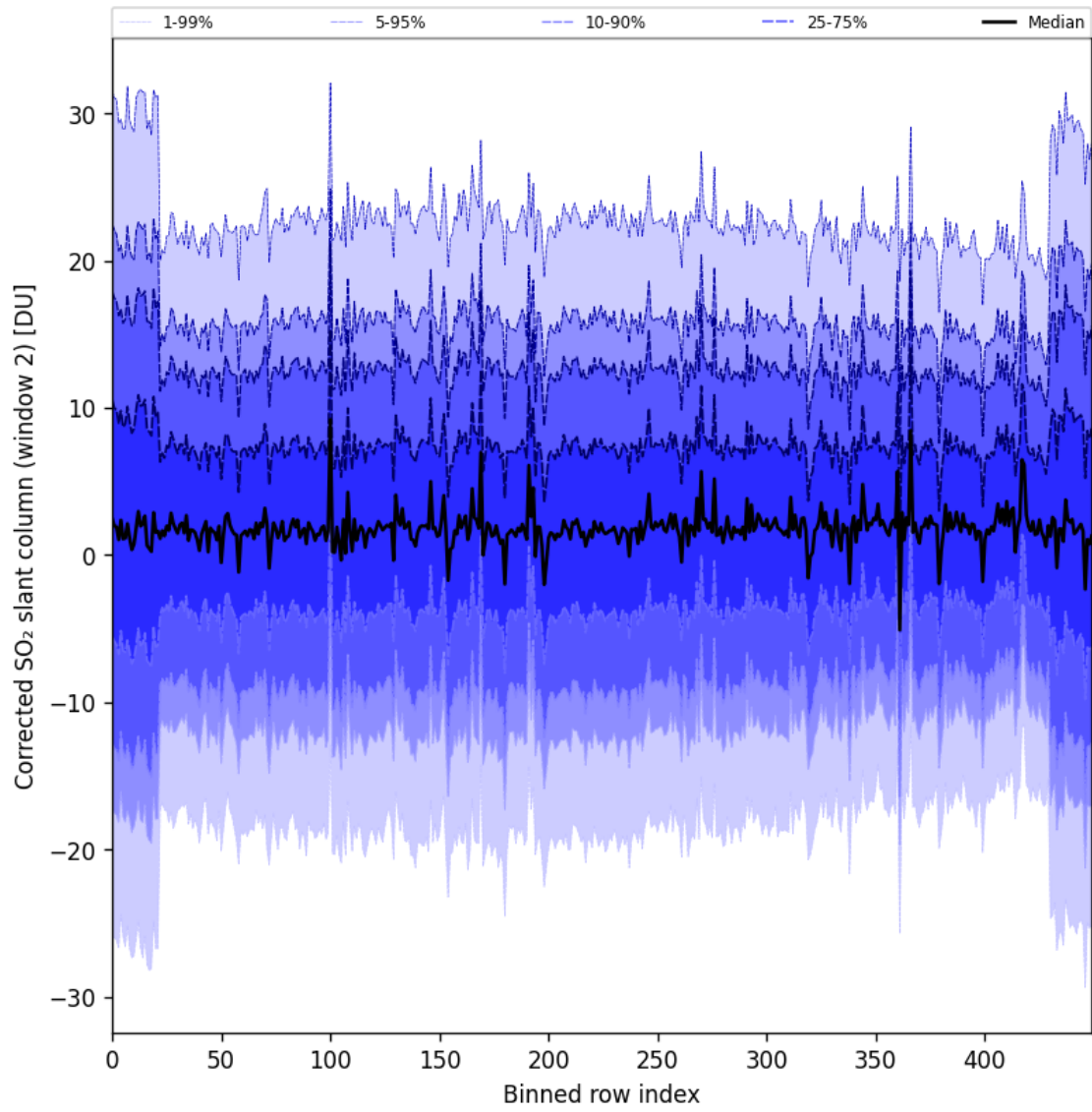
Figure 95: Along track statistics of “Corrected SO 2 slant column (window 2)” for 2025-10-14 to 2025-10-16
