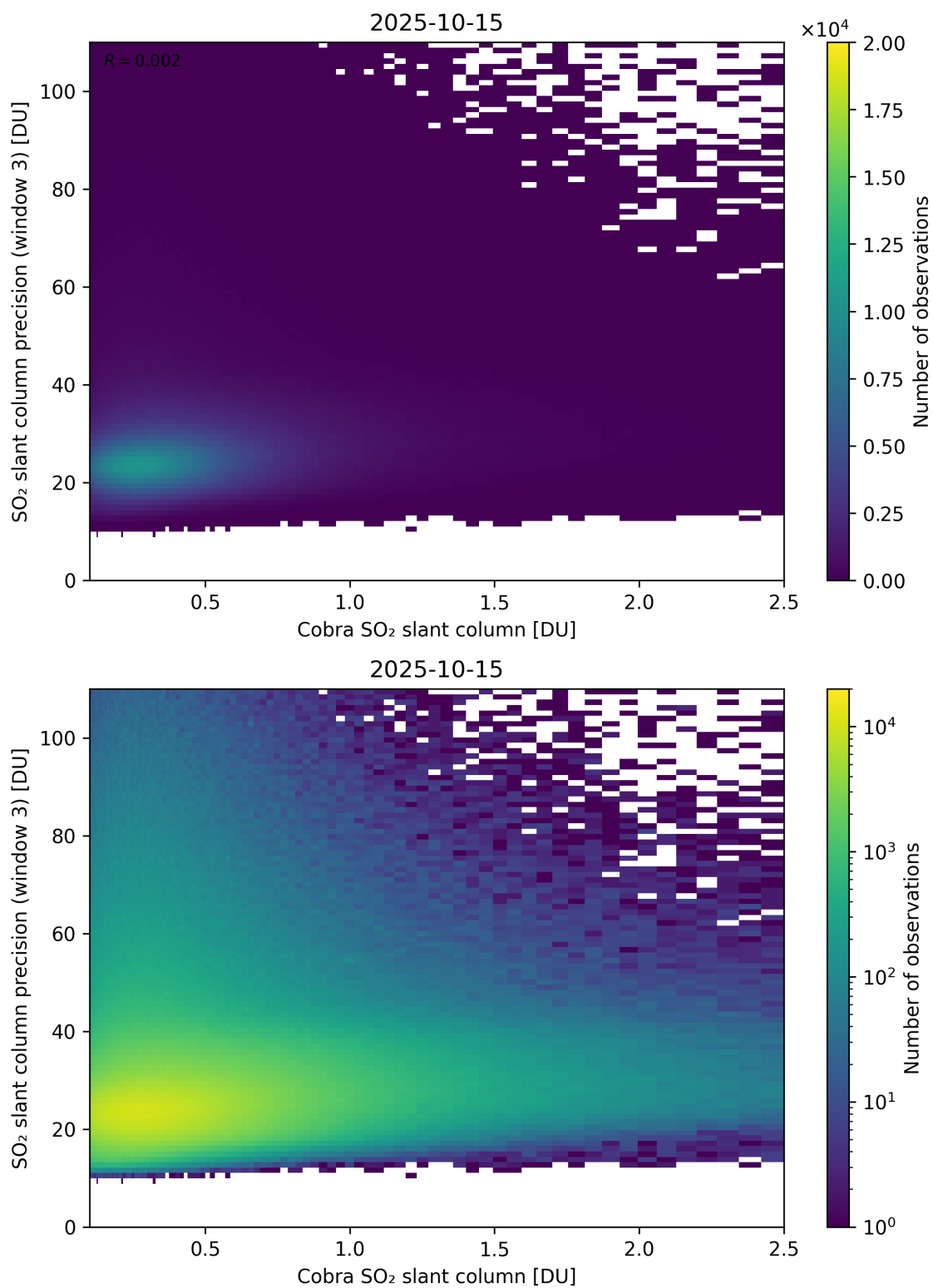
Figure 223: Scatter density plot of “Cobra SO 2 slant column” against “SO 2 slant column precision (window 3)” for 2025-10-14 to 2025-10-16.
