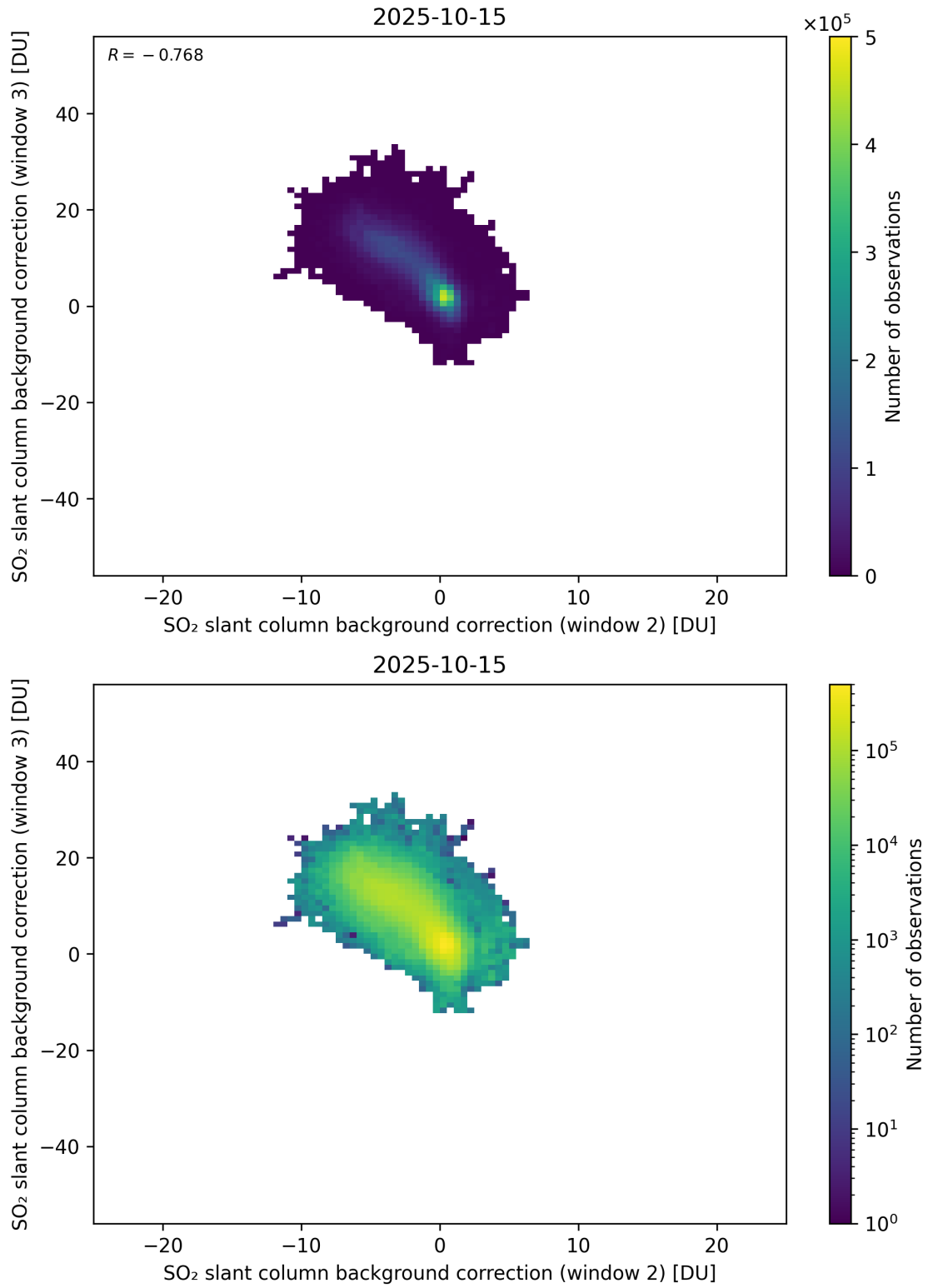
Figure 122: Scatter density plot of “SO 2 slant column background correction (window 2)” against “SO 2 slant column background correction (window 3)” for 2025-10-14 to 2025-10-16.
