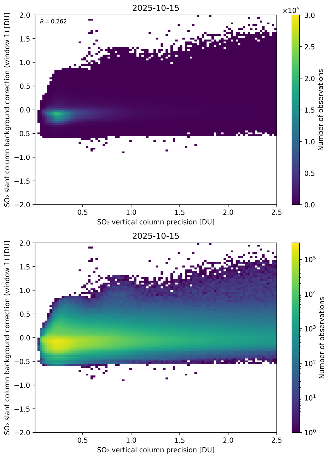
Figure 329: Scatter density plot of “SO 2 vertical column precision” against “SO 2 slant column background correction (window 1)” for 2025-10-14 to 2025-10-16.
