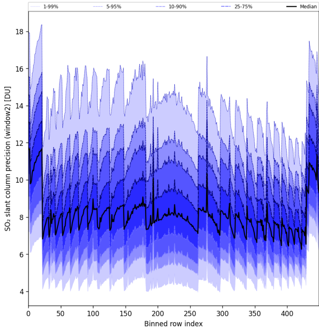
Figure 94: Along track statistics of “SO 2 slant column precision (window2)” for 2025-10-14 to 2025-10-16
