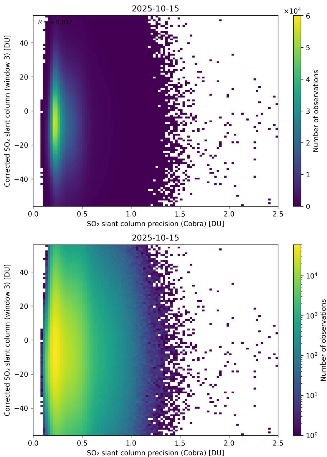
Figure 207: Scatter density plot of “SO 2 slant column precision (Cobra)” against “Corrected SO 2 slant column (window 3)” for 2025-10-14 to 2025-10-16.
