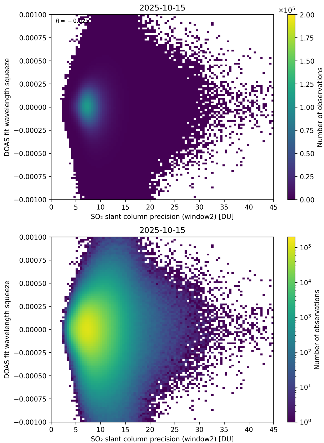
Figure 294: Scatter density plot of “SO 2 slant column precision (window2)” against “DOAS fit wavelength squeeze” for 2025-10-14 to 2025-10-16.
