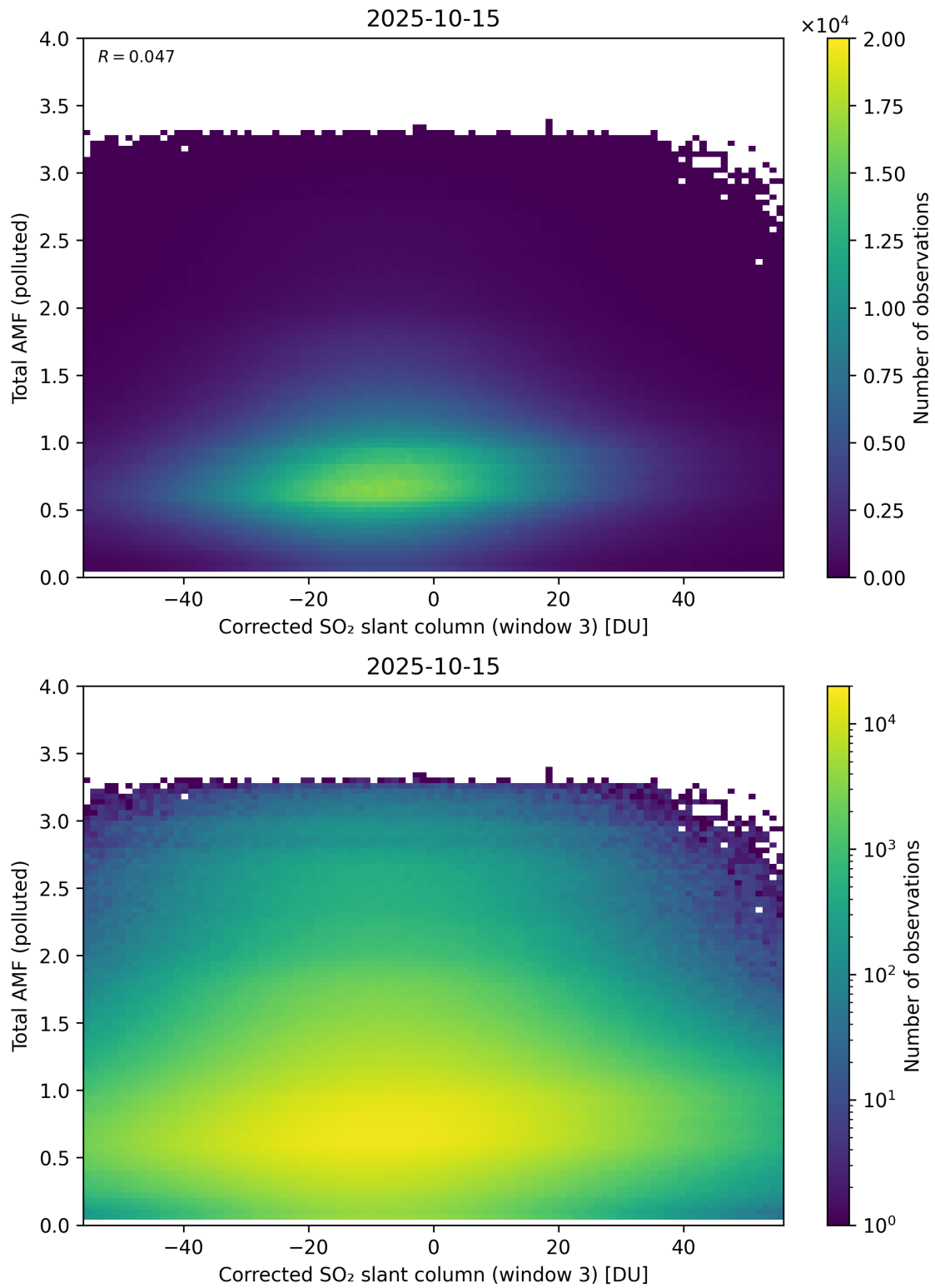
Figure 260: Scatter density plot of “Corrected SO 2 slant column (window 3)” against “Total AMF (polluted)” for 2025-10-14 to 2025-10-16.
