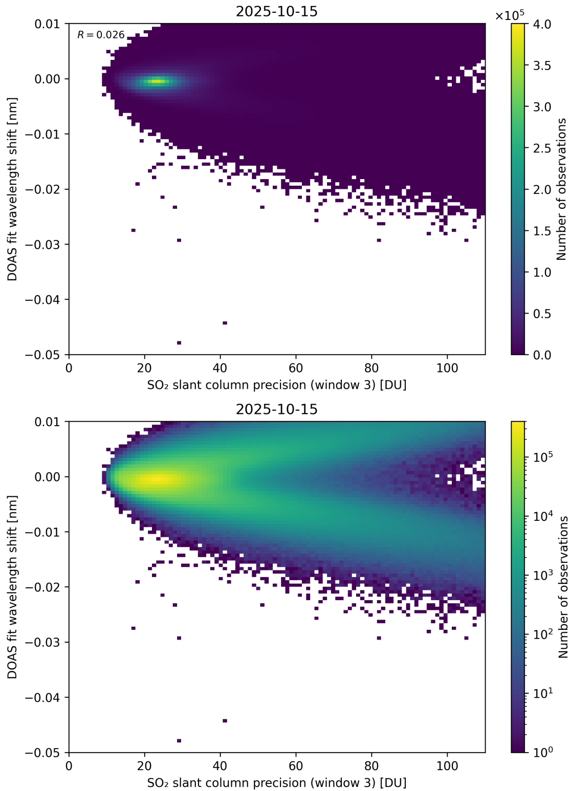
Figure 308: Scatter density plot of “SO 2 slant column precision (window 3)” against “DOAS fit wavelength shift” for 2025-10-14 to 2025-10-16.
