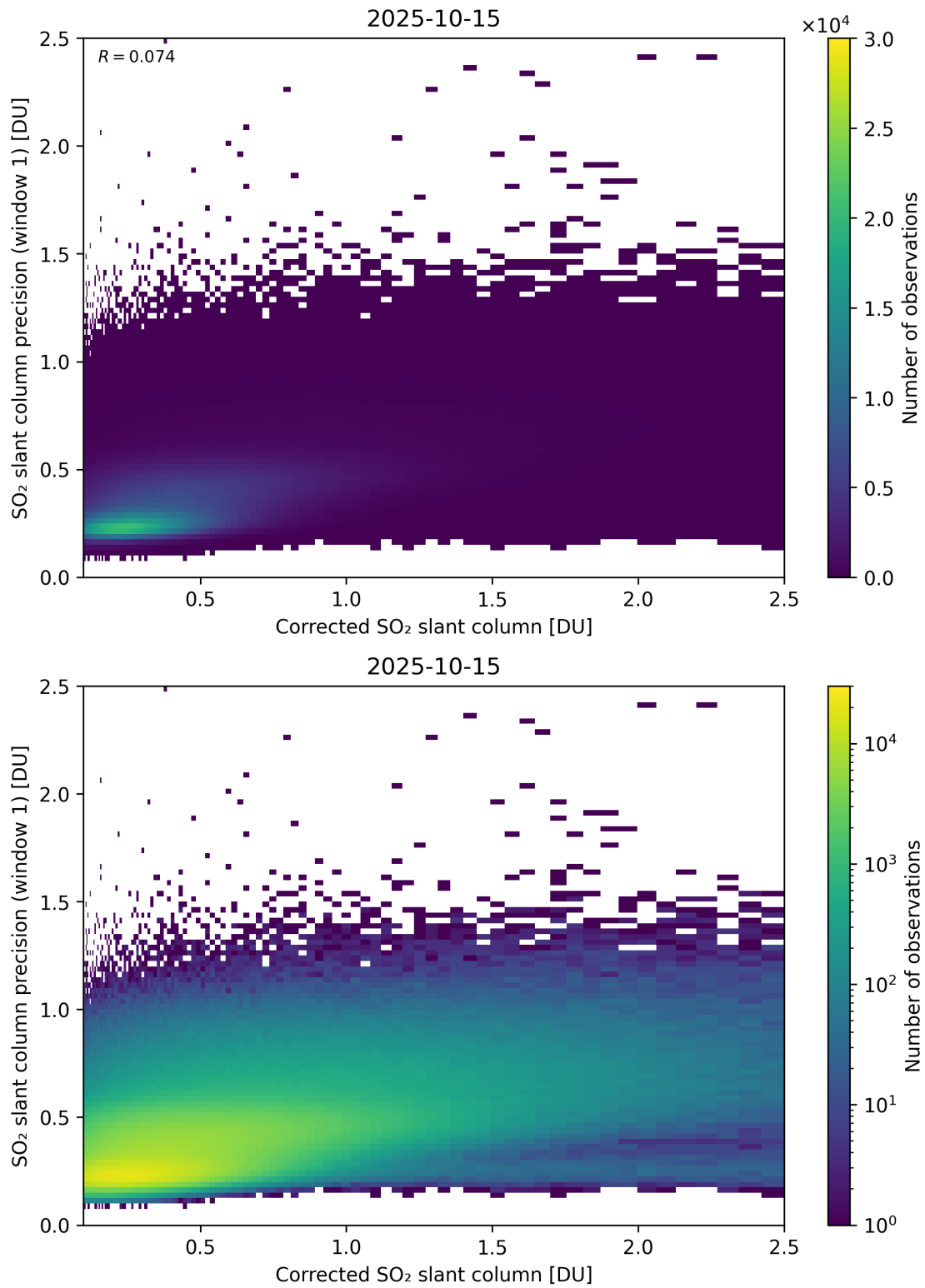
Figure 238: Scatter density plot of “Corrected SO 2 slant column” against “SO 2 slant column precision (window 1)” for 2025-10-14 to 2025-10-16.
