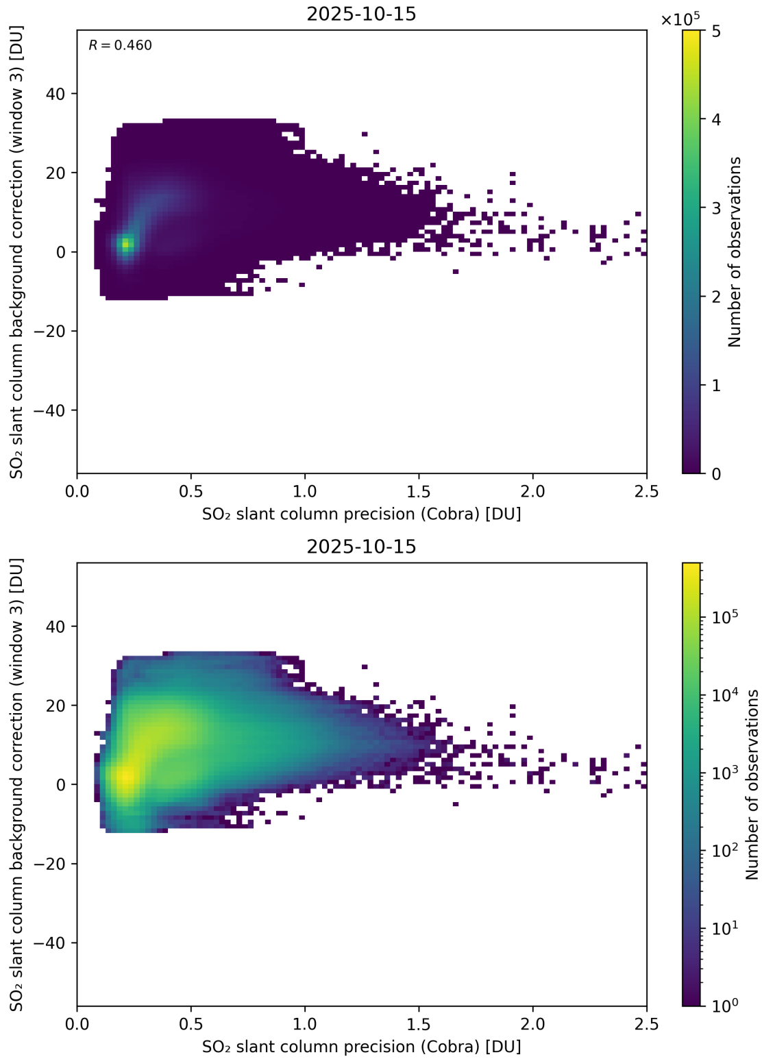
Figure 201: Scatter density plot of “SO 2 slant column precision (Cobra)” against “SO 2 slant column background correction (window 3)” for 2025-10-14 to 2025-10-16.
