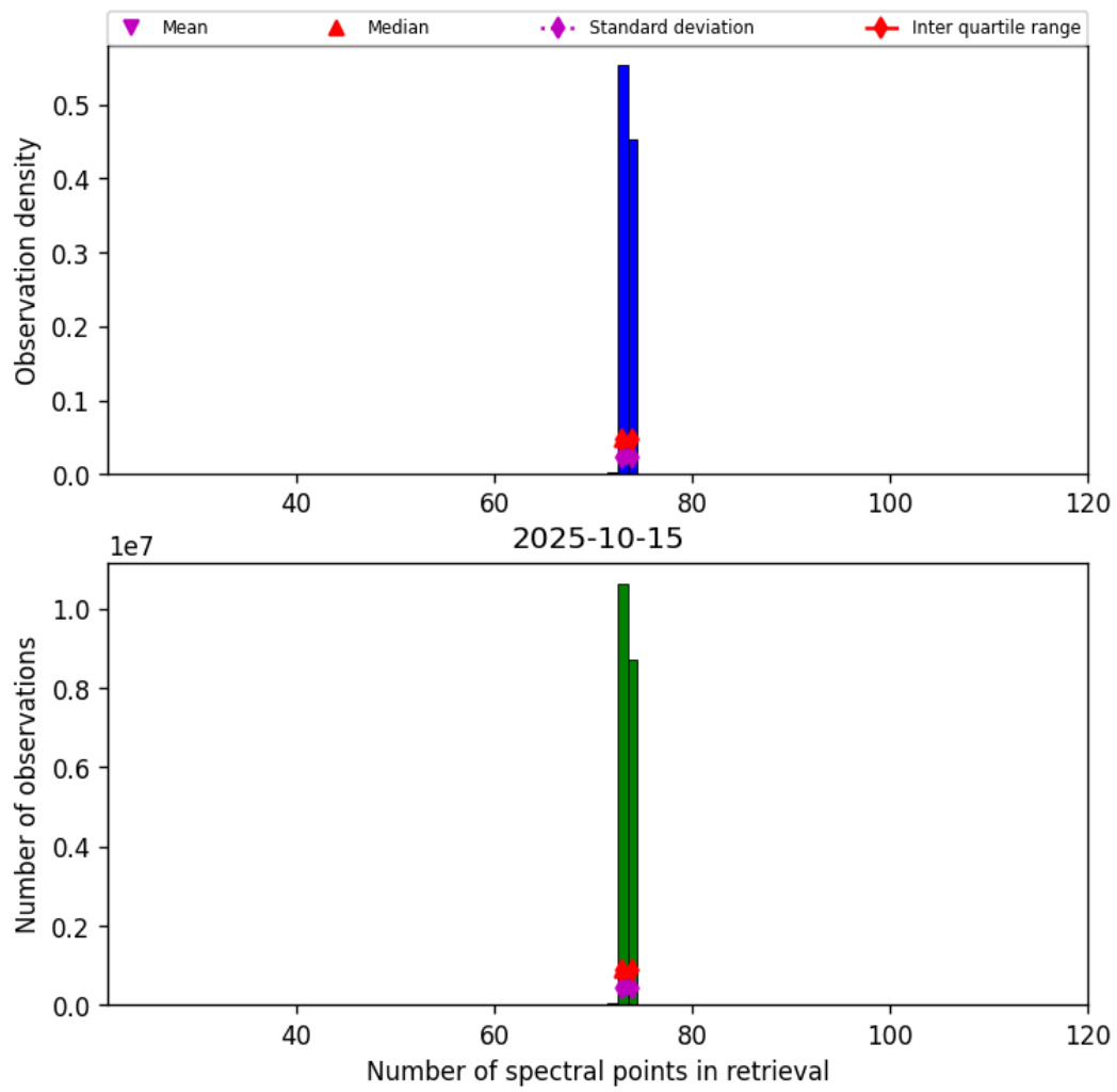
Figure 82: Histogram of “Number of spectral points in retrieval” for 2025-10-14 to 2025-10-16
