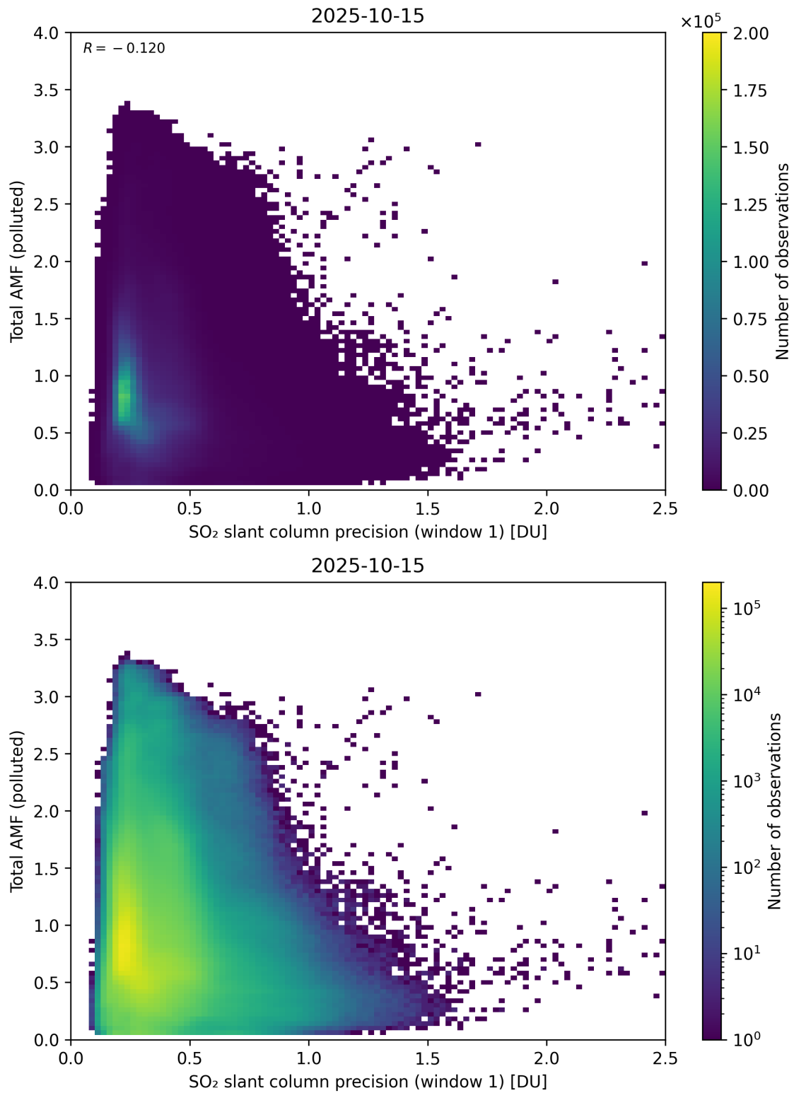
Figure 280: Scatter density plot of “SO 2 slant column precision (window 1)” against “Total AMF (polluted)” for 2025-10-14 to 2025-10-16.
