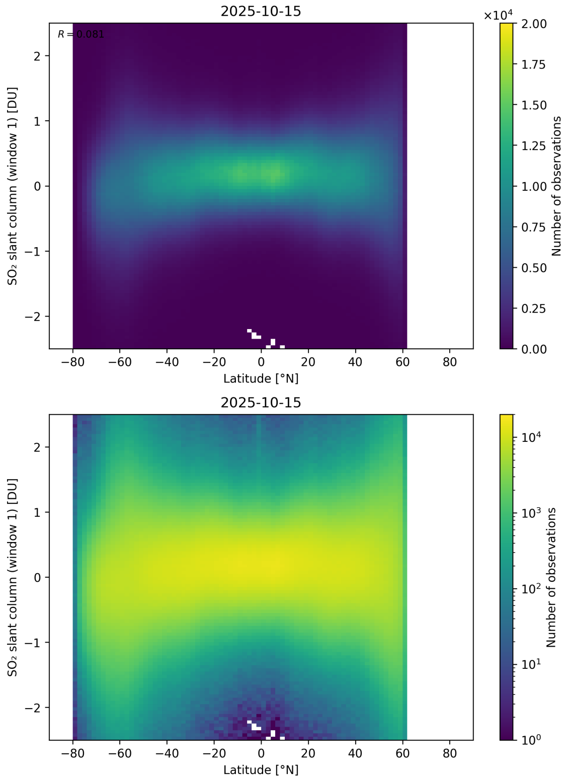
Figure 162: Scatter density plot of “Latitude” against “SO 2 slant column (window 1)” for 2025-10-14 to 2025-10-16.
