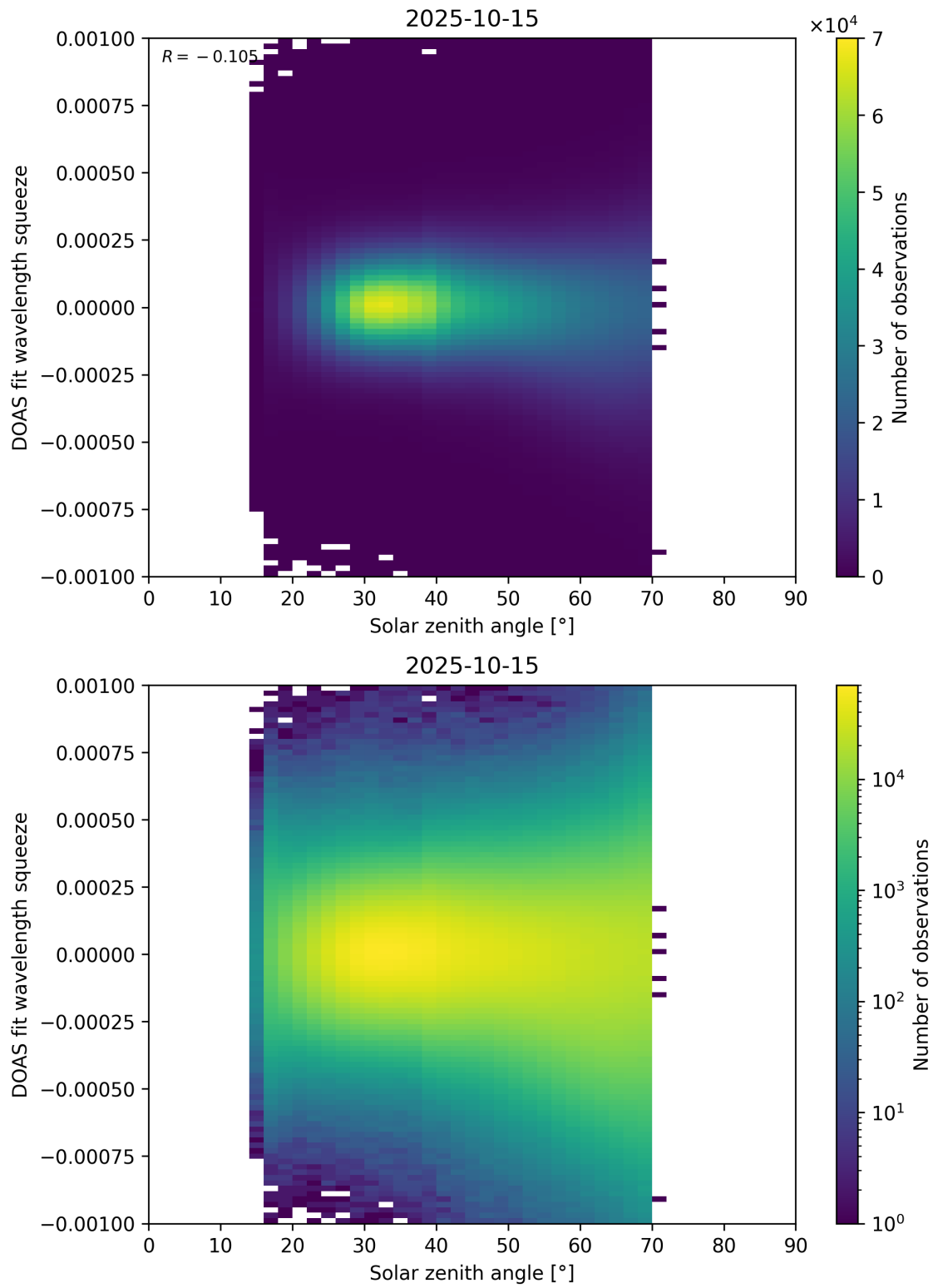
Figure 175: Scatter density plot of “Solar zenith angle” against “DOAS fit wavelength squeeze” for 2025-10-14 to 2025-10-16.
