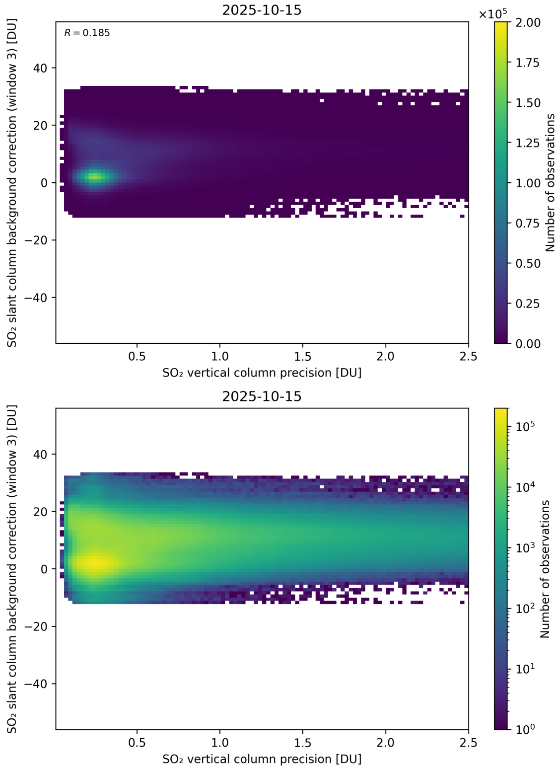
Figure 331: Scatter density plot of “SO 2 vertical column precision” against “SO 2 slant column background correction (window 3)” for 2025-10-14 to 2025-10-16.
