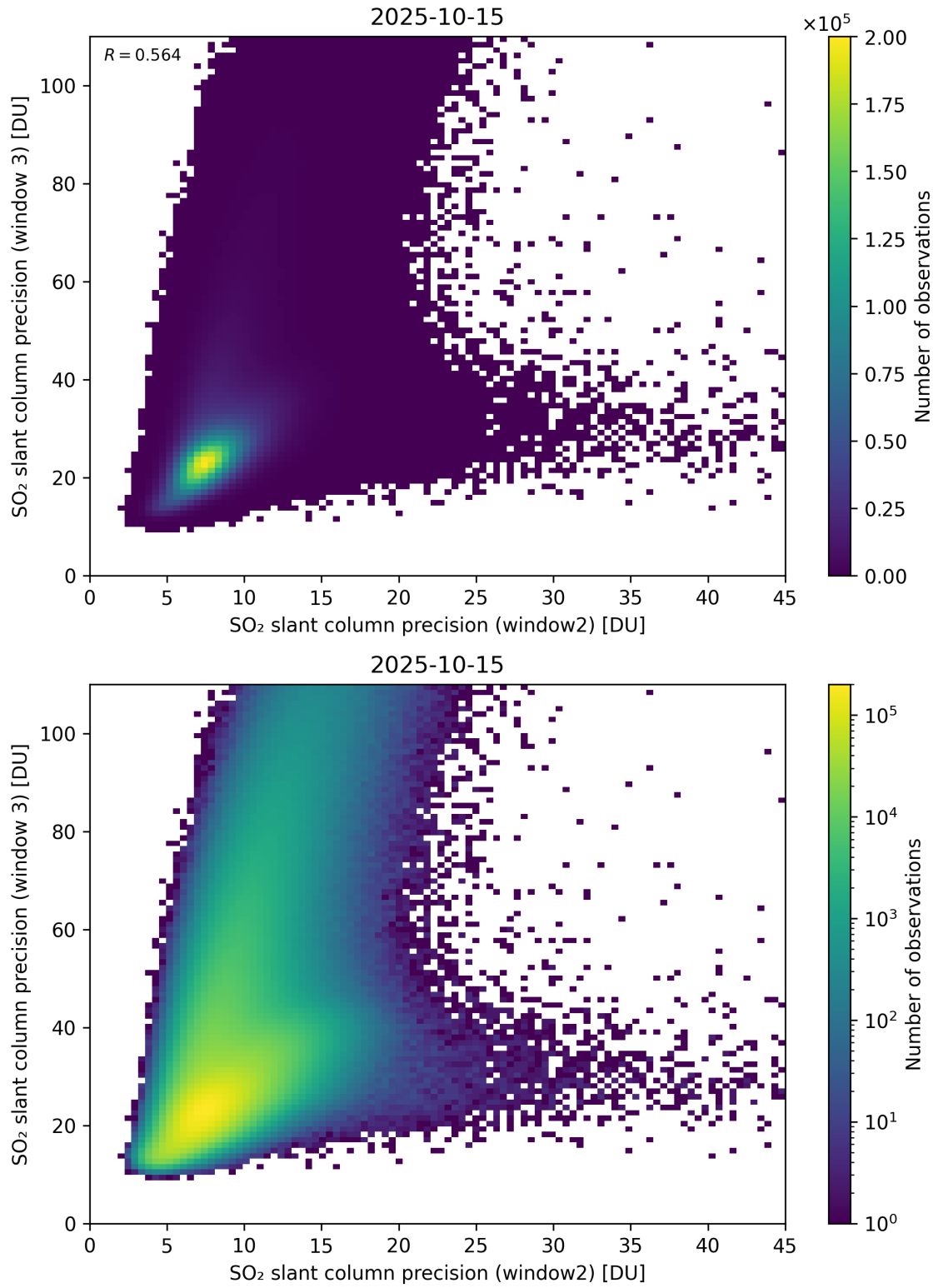
Figure 300: Scatter density plot of “SO 2 slant column precision (window2)” against “SO 2 slant column precision (window 3)” for 2025-10-14 to 2025-10-16.
