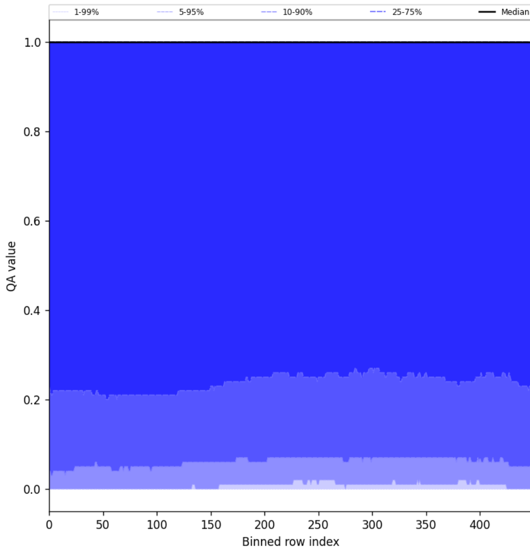
Figure 83: Along track statistics of “QA value” for 2025-10-14 to 2025-10-16
