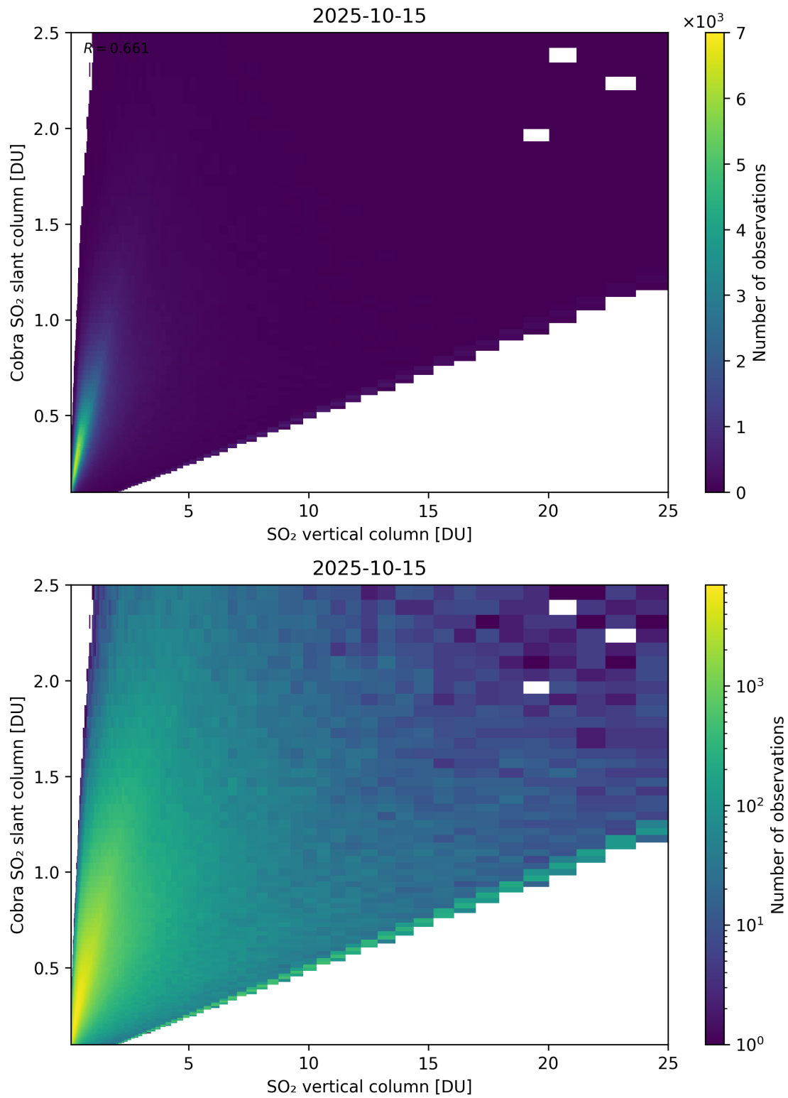
Figure 349: Scatter density plot of “SO 2 vertical column” against “Cobra SO 2 slant column” for 2025-10-14 to 2025-10-16.
