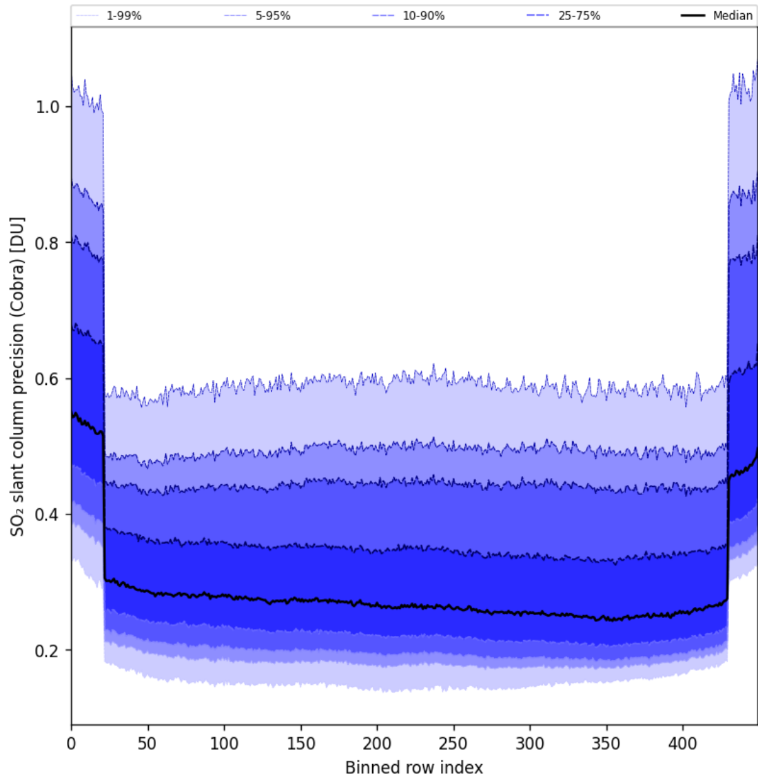
Figure 88: Along track statistics of “SO 2 slant column precision (Cobra)” for 2025-10-14 to 2025-10-16
