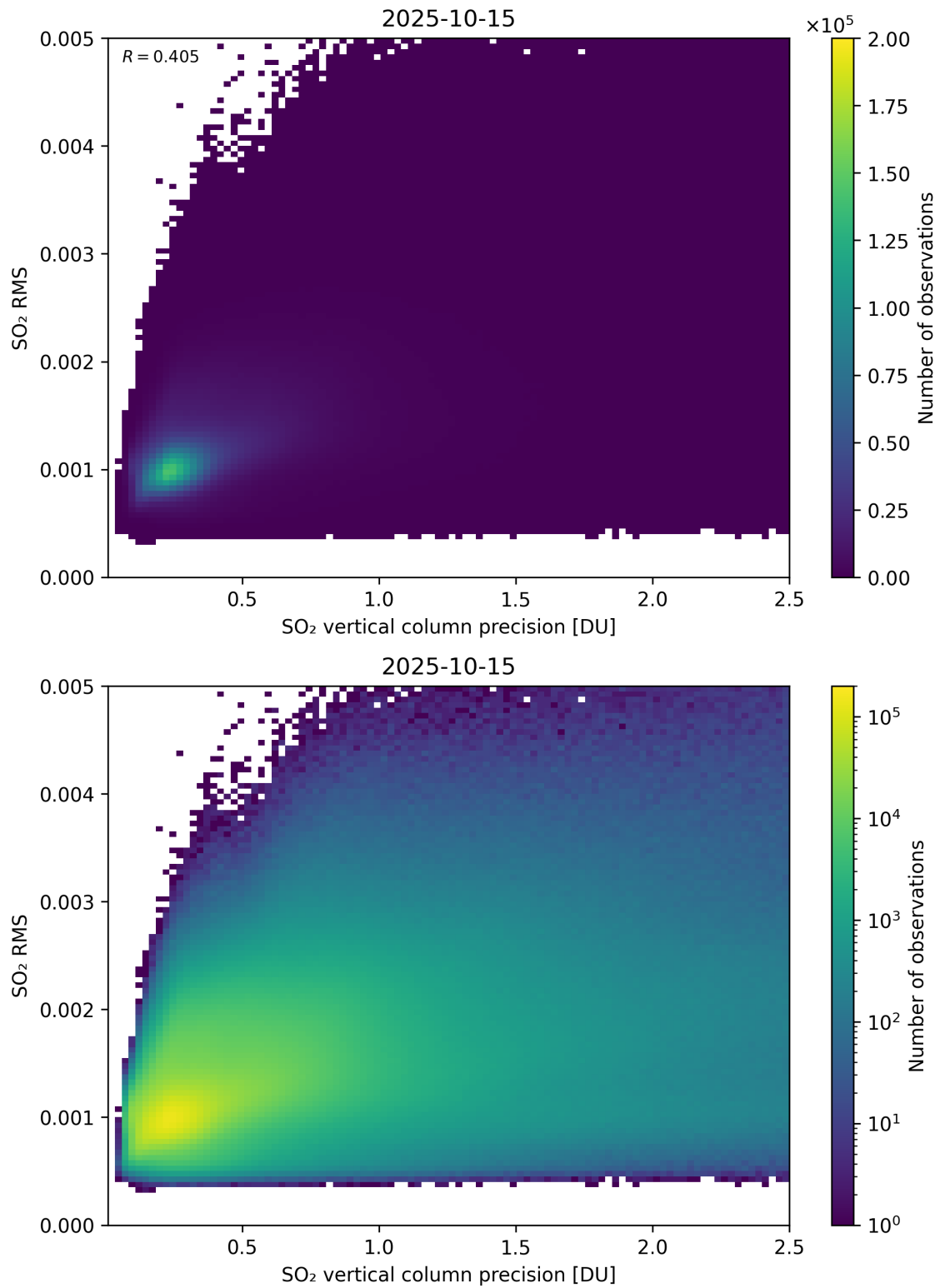
Figure 334: Scatter density plot of “SO 2 vertical column precision” against “SO 2 RMS” for 2025-10-14 to 2025-10-16.
