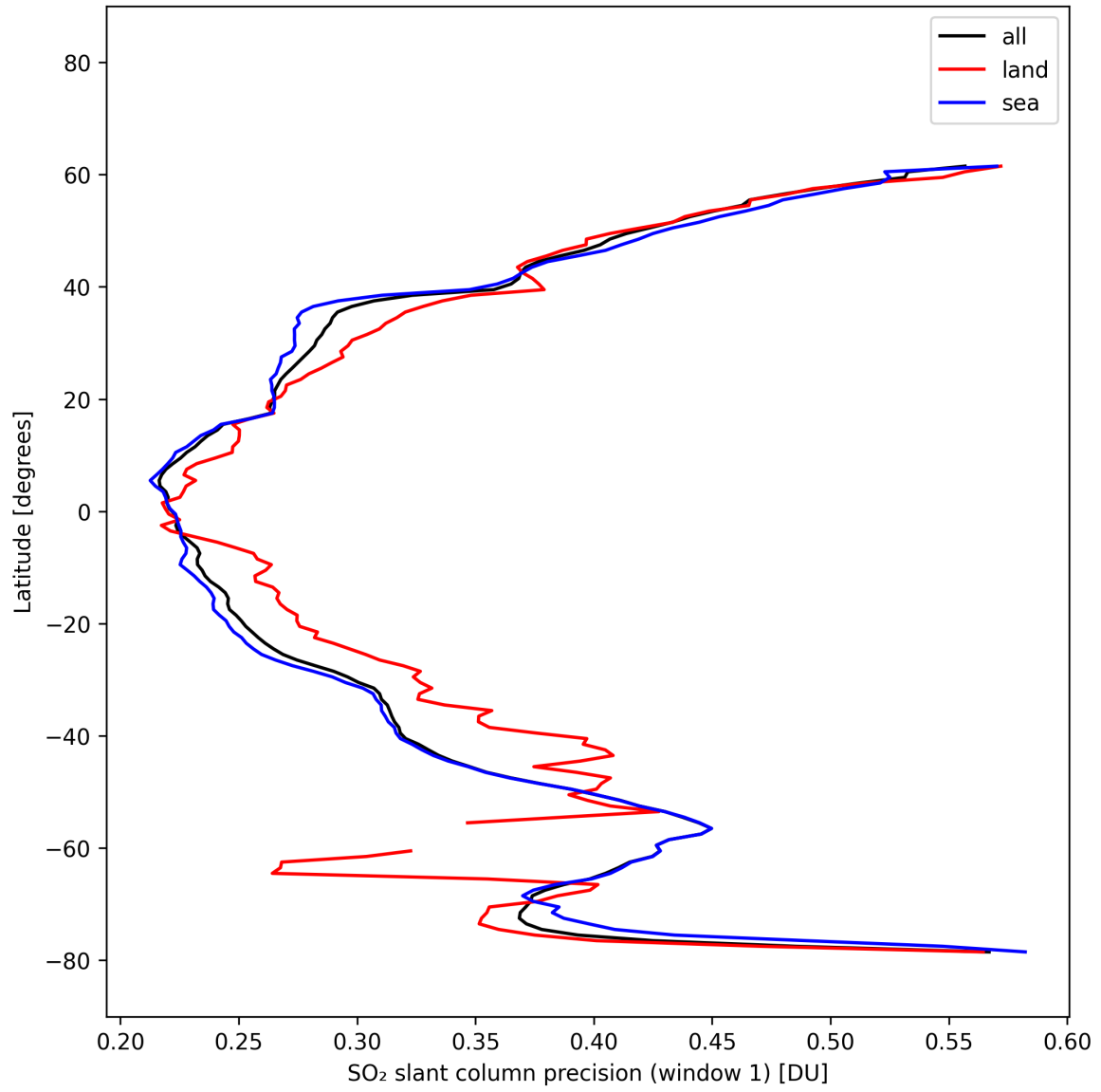
Figure 38: Zonal average of “SO 2 slant column precision (window 1)” for 2025-10-14 to 2025-10-16.
