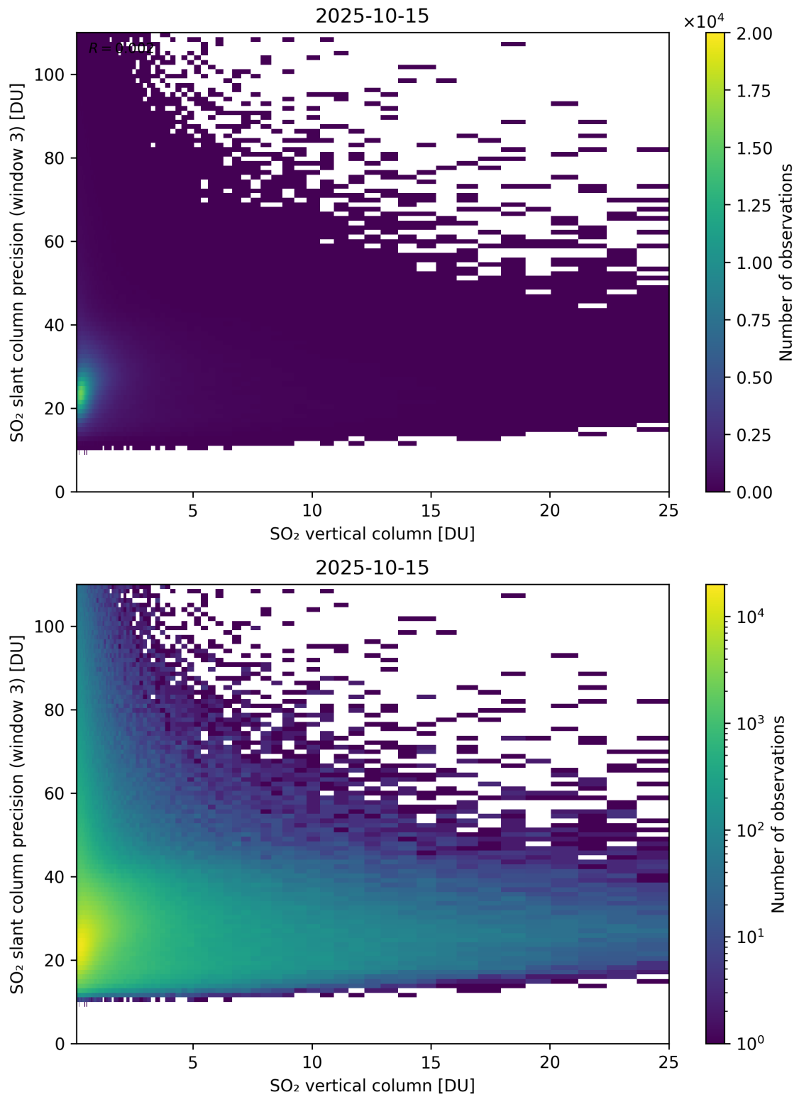
Figure 358: Scatter density plot of “SO 2 vertical column” against “SO 2 slant column precision (window 3)” for 2025-10-14 to 2025-10-16.
