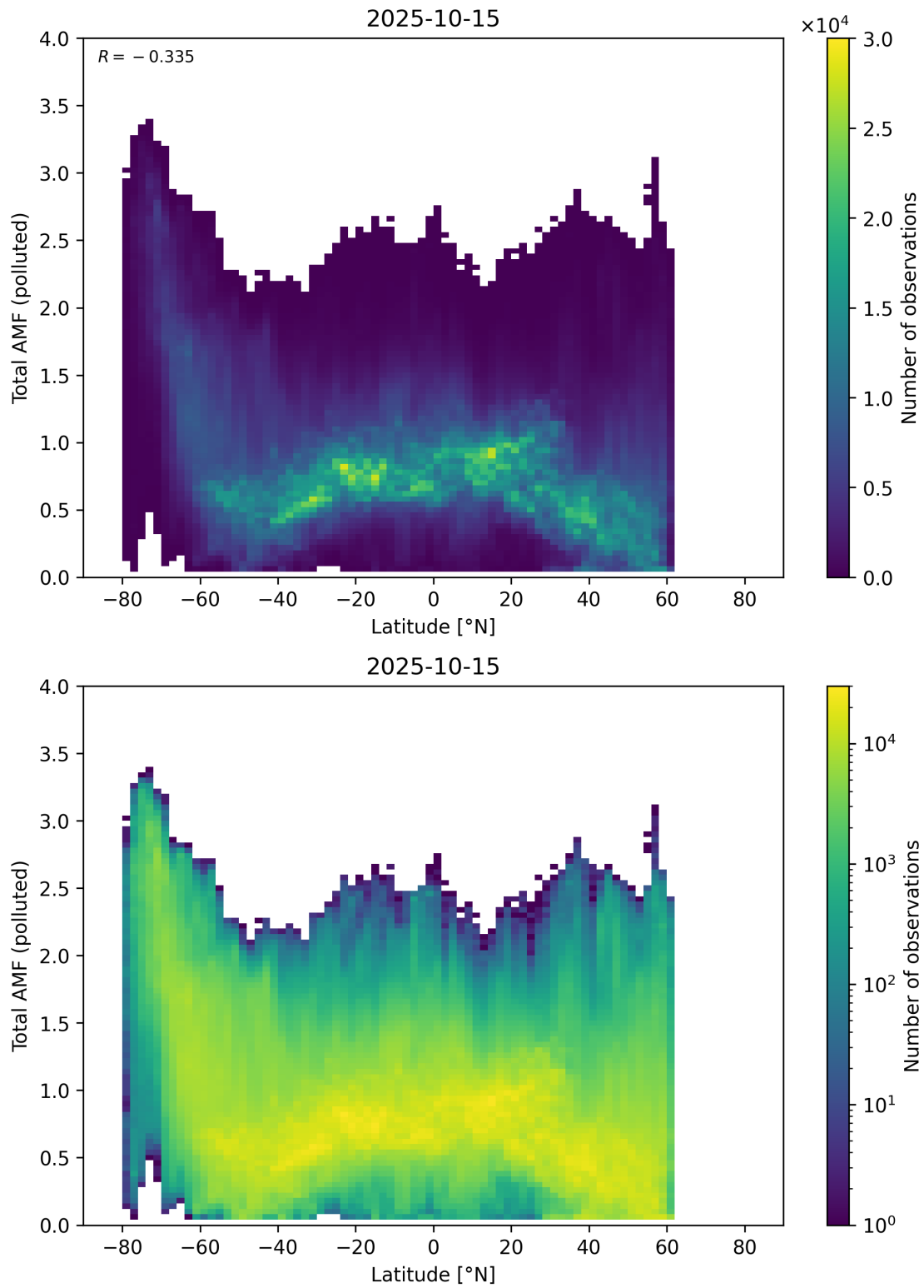
Figure 167: Scatter density plot of “Latitude” against “Total AMF (polluted)” for 2025-10-14 to 2025-10-16.
