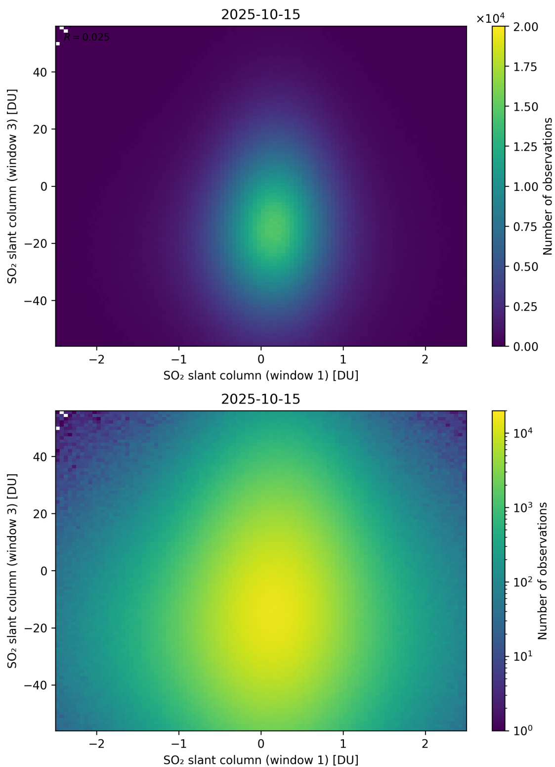
Figure 287: Scatter density plot of “SO 2 slant column (window 1)” against “SO 2 slant column (window 3)” for 2025-10-14 to 2025-10-16.
