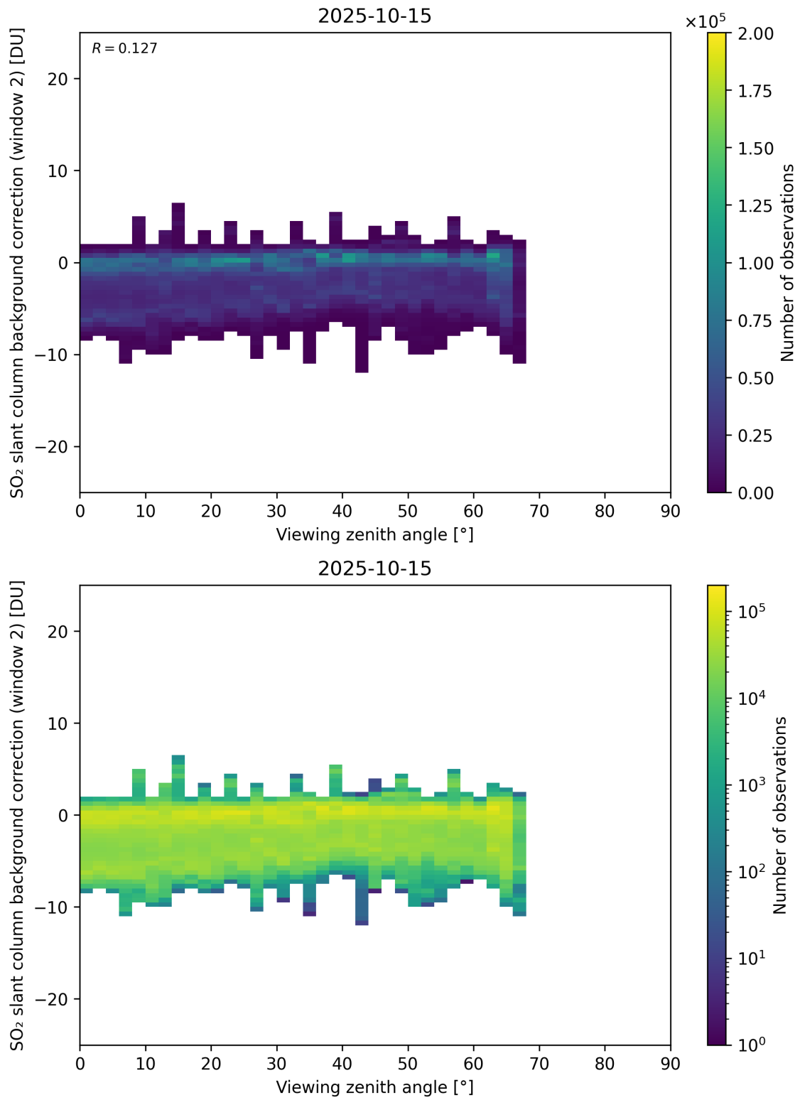
Figure 363: Scatter density plot of “Viewing zenith angle” against “SO 2 slant column background correction (window 2)” for 2025-10-14 to 2025-10-16.
