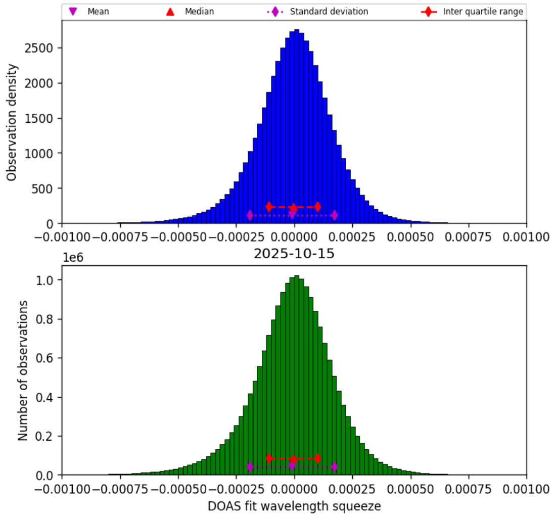
Figure 77: Histogram of “DOAS fit wavelength squeeze” for 2025-10-14 to 2025-10-16
