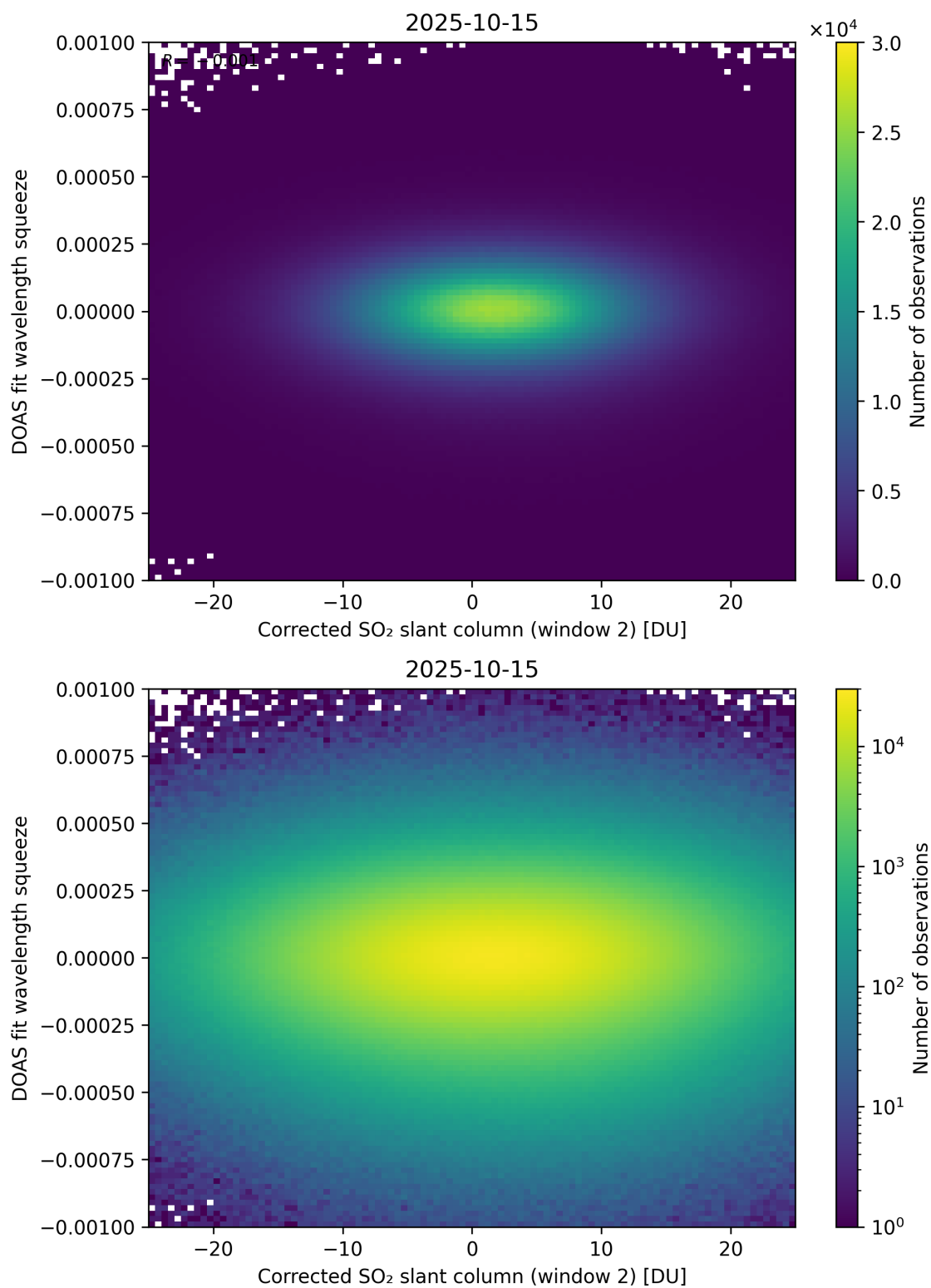
Figure 247: Scatter density plot of “Corrected SO 2 slant column (window 2)” against “DOAS fit wavelength squeeze” for 2025-10-14 to 2025-10-16.
