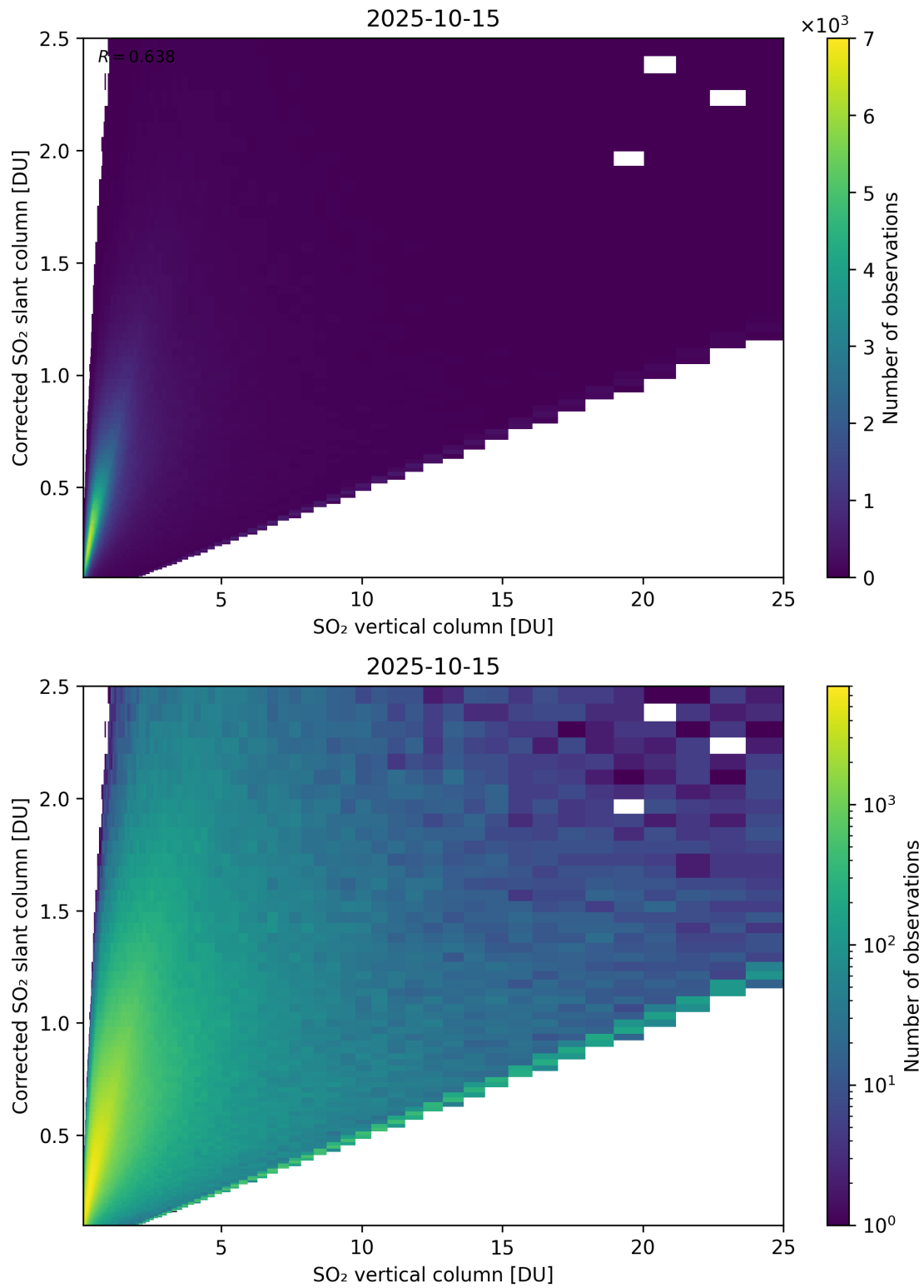
Figure 351: Scatter density plot of “SO 2 vertical column” against “Corrected SO 2 slant column” for 2025-10-14 to 2025-10-16.
