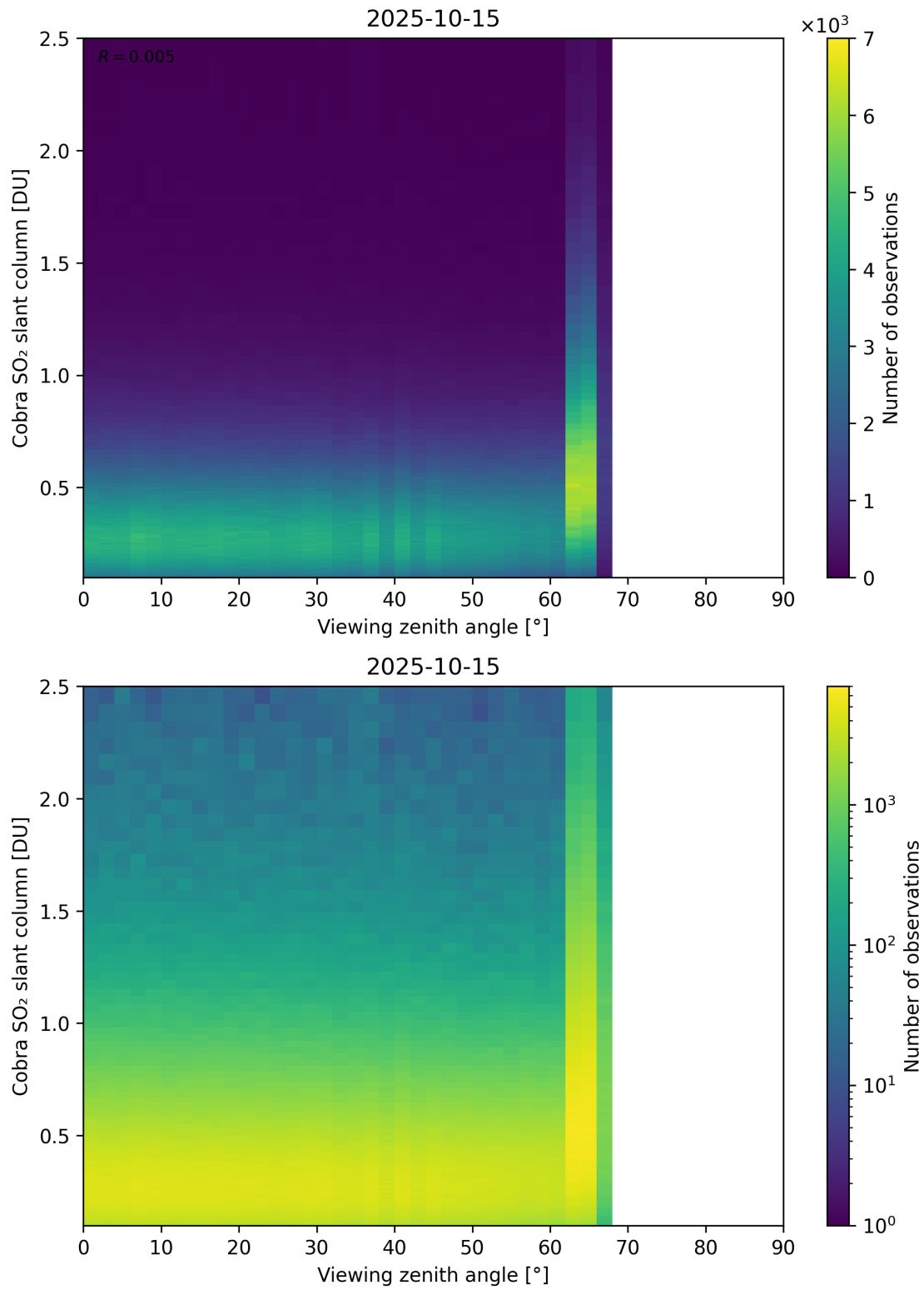
Figure 371: Scatter density plot of “Viewing zenith angle” against “Cobra SO 2 slant column” for 2025-10-14 to 2025-10-16.
