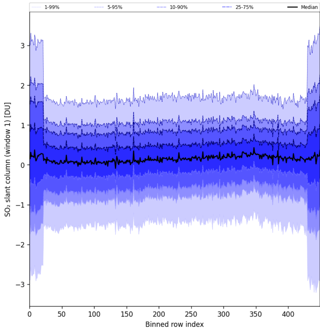
Figure 89: Along track statistics of “SO 2 slant column (window 1)” for 2025-10-14 to 2025-10-16
