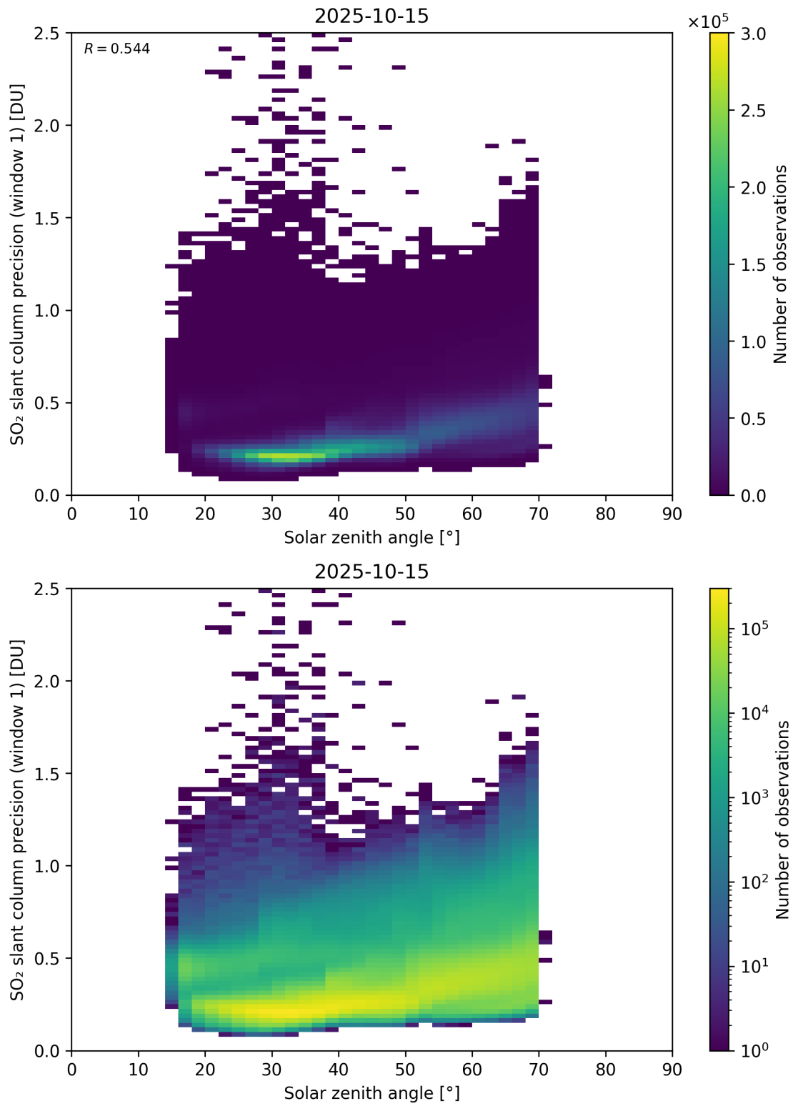
Figure 185: Scatter density plot of “Solar zenith angle” against “SO 2 slant column precision (window 1)” for 2025-10-14 to 2025-10-16.
