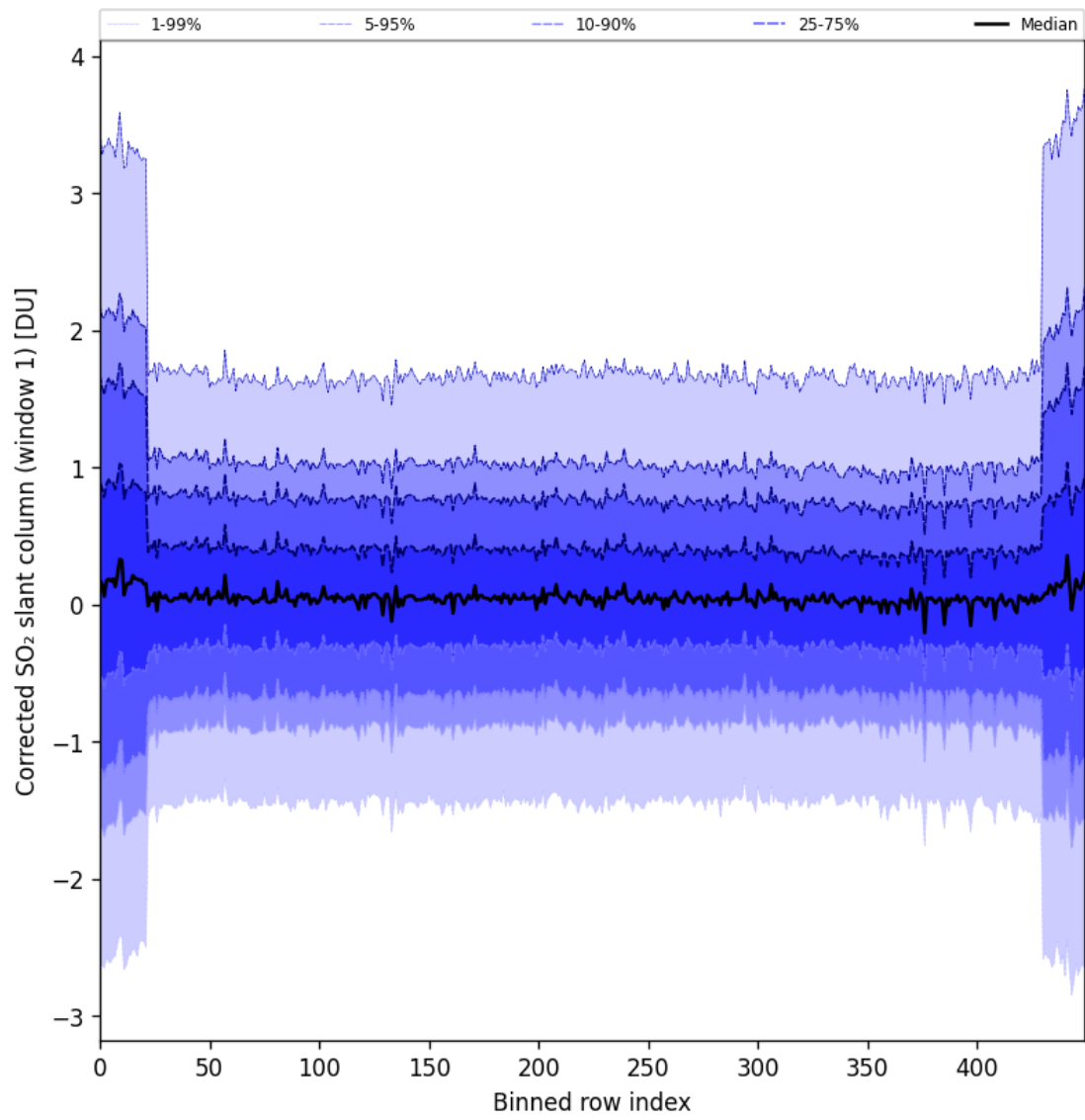
Figure 91: Along track statistics of “Corrected SO 2 slant column (window 1)” for 2025-10-14 to 2025-10-16
