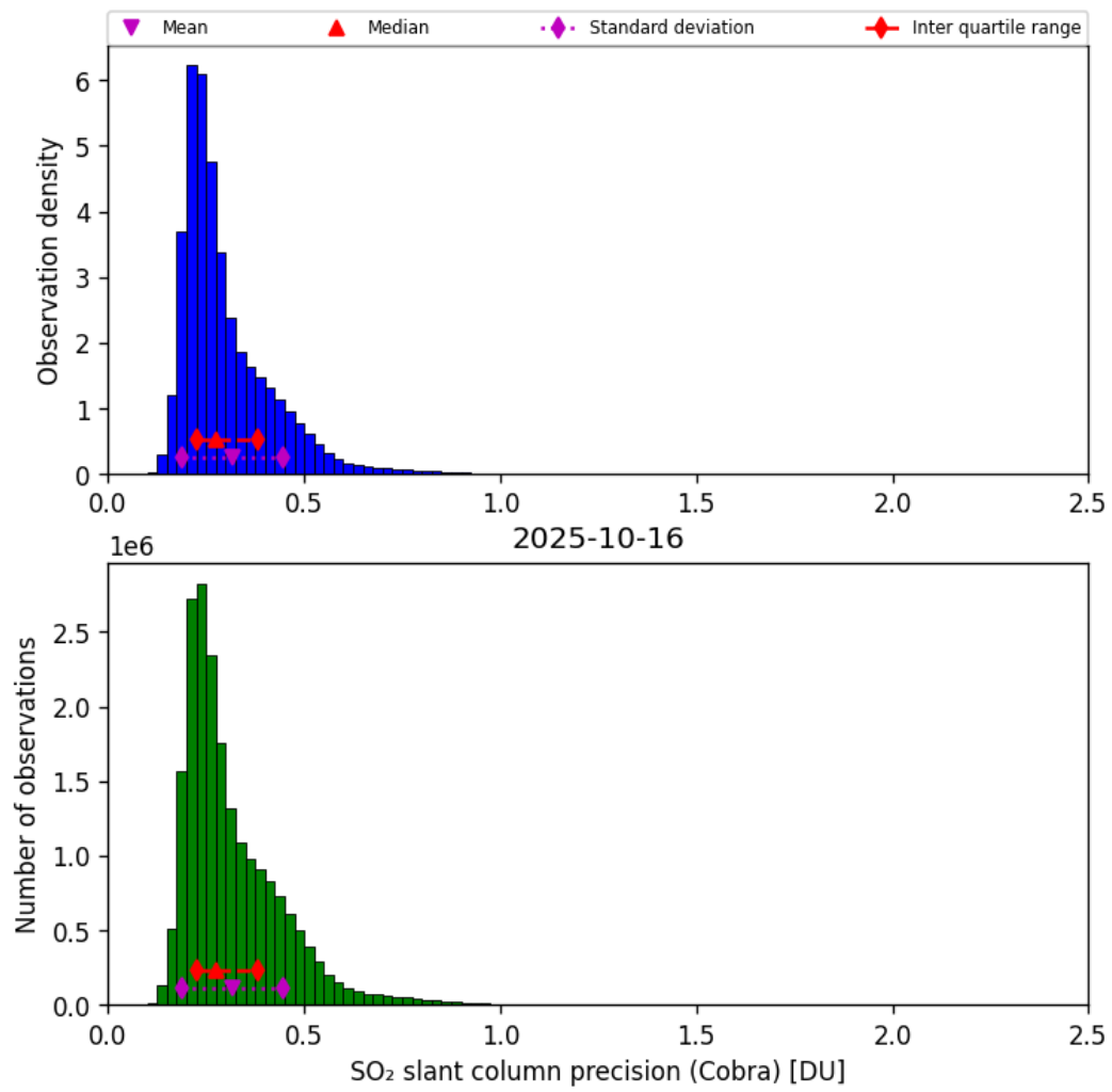
Figure 62: Histogram of “SO 2 slant column precision (Cobra)” for 2025-10-15 to 2025-10-17
