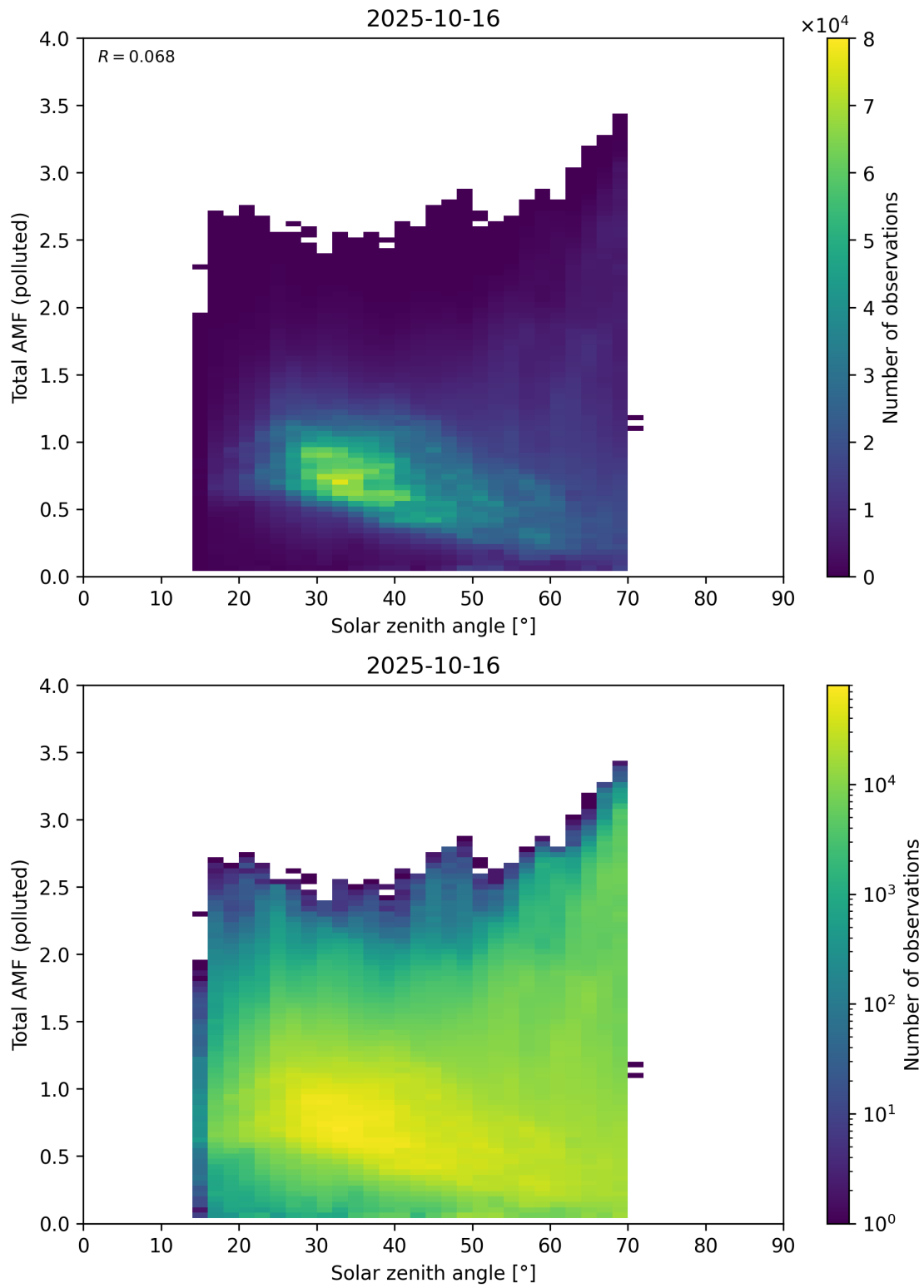
Figure 189: Scatter density plot of “Solar zenith angle” against “Total AMF (polluted)” for 2025-10-15 to 2025-10-17.
