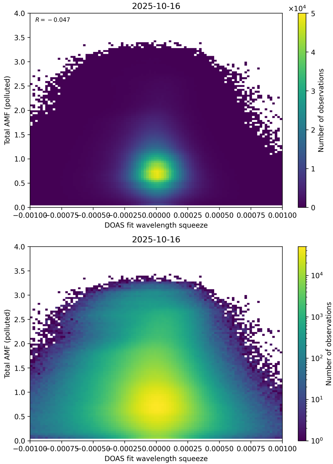
Figure 145: Scatter density plot of “DOAS fit wavelength squeeze” against “Total AMF (polluted)” for 2025-10-15 to 2025-10-17.
