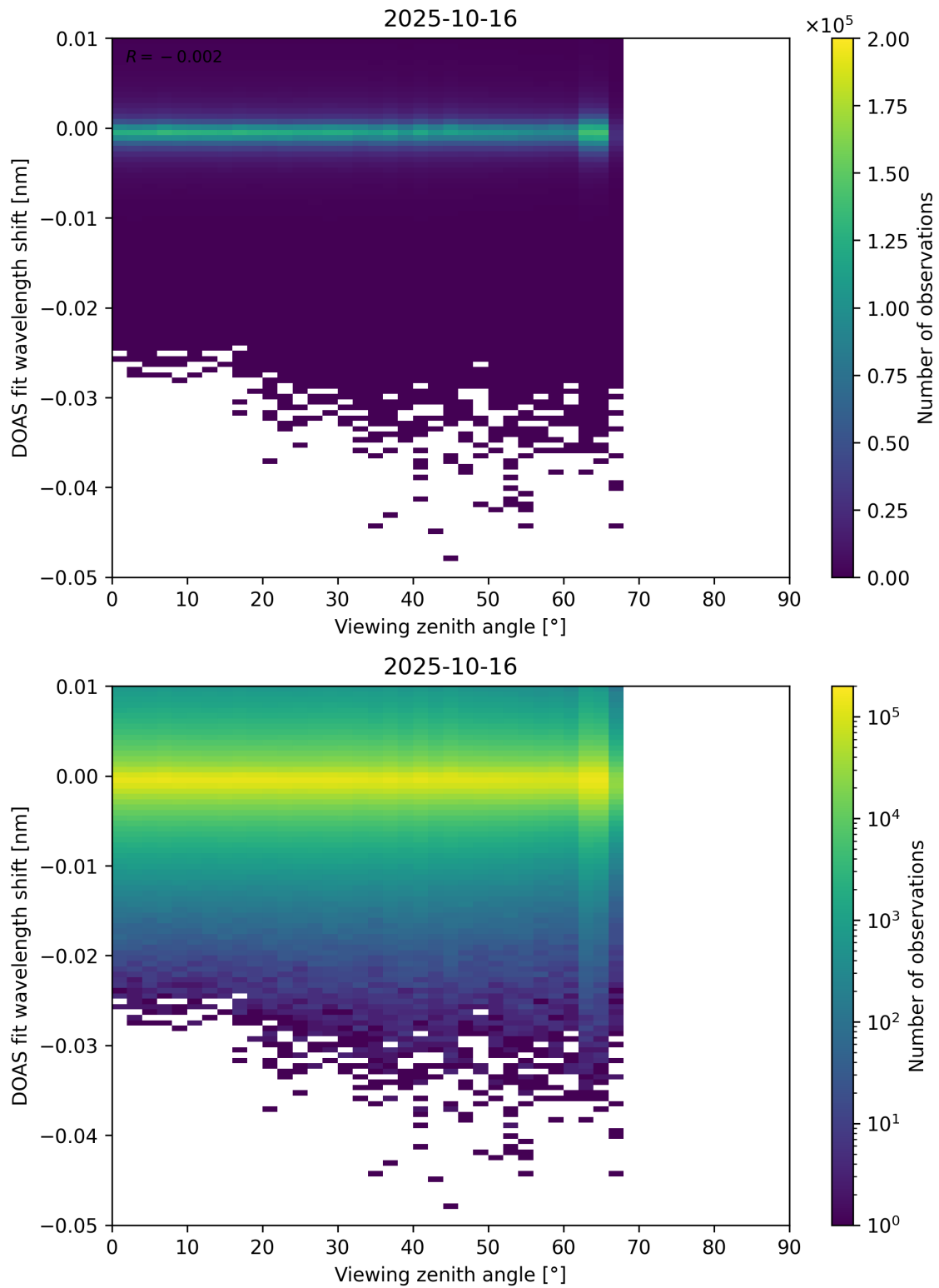
Figure 365: Scatter density plot of “Viewing zenith angle” against “DOAS fit wavelength shift” for 2025-10-15 to 2025-10-17.
