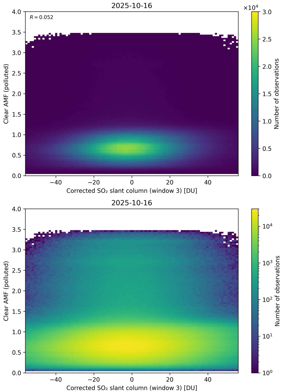
Figure 259: Scatter density plot of “Corrected SO 2 slant column (window 3)” against “Clear AMF (polluted)” for 2025-10-15 to 2025-10-17.
