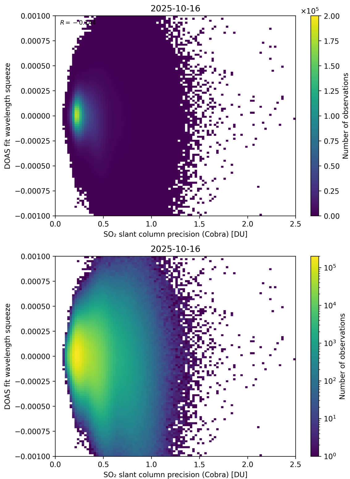
Figure 203: Scatter density plot of “SO 2 slant column precision (Cobra)” against “DOAS fit wavelength squeeze” for 2025-10-15 to 2025-10-17.
