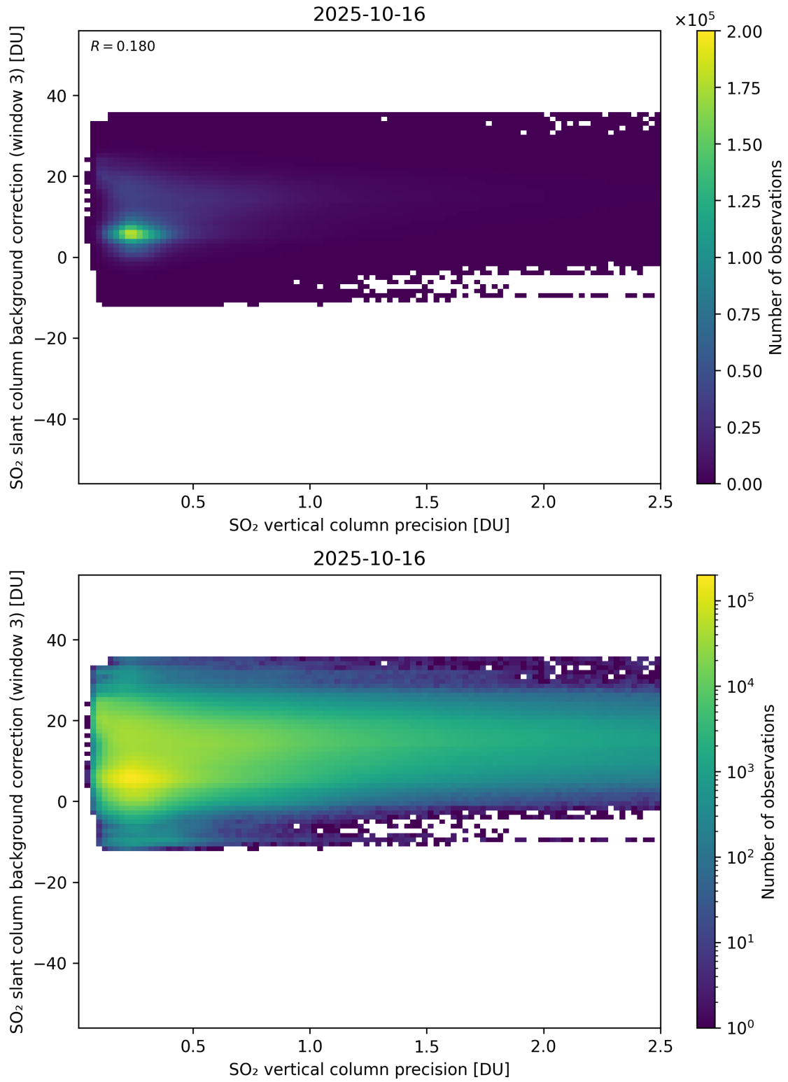
Figure 331: Scatter density plot of “SO 2 vertical column precision” against “SO 2 slant column background correction (window 3)” for 2025-10-15 to 2025-10-17.
