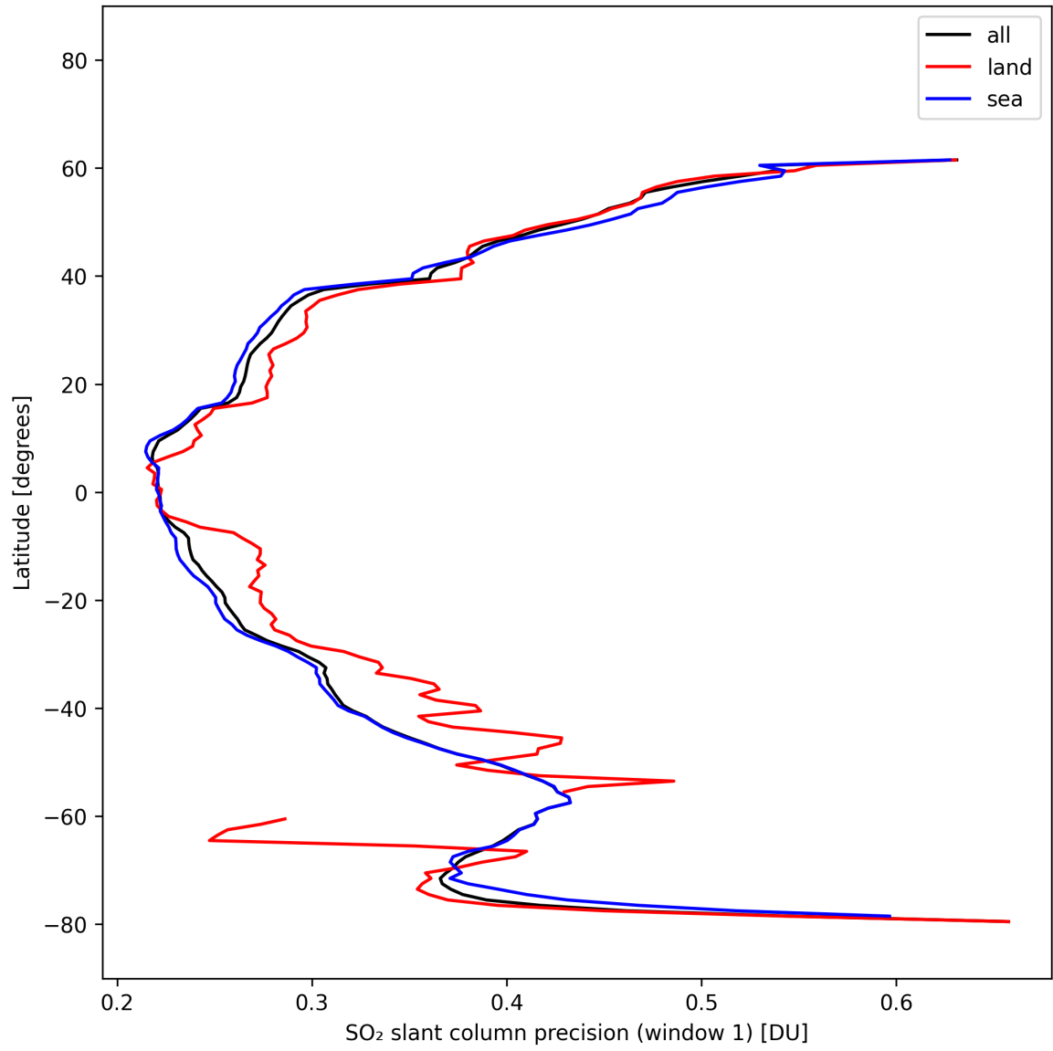
Figure 38: Zonal average of “SO 2 slant column precision (window 1)” for 2025-10-15 to 2025-10-17.
