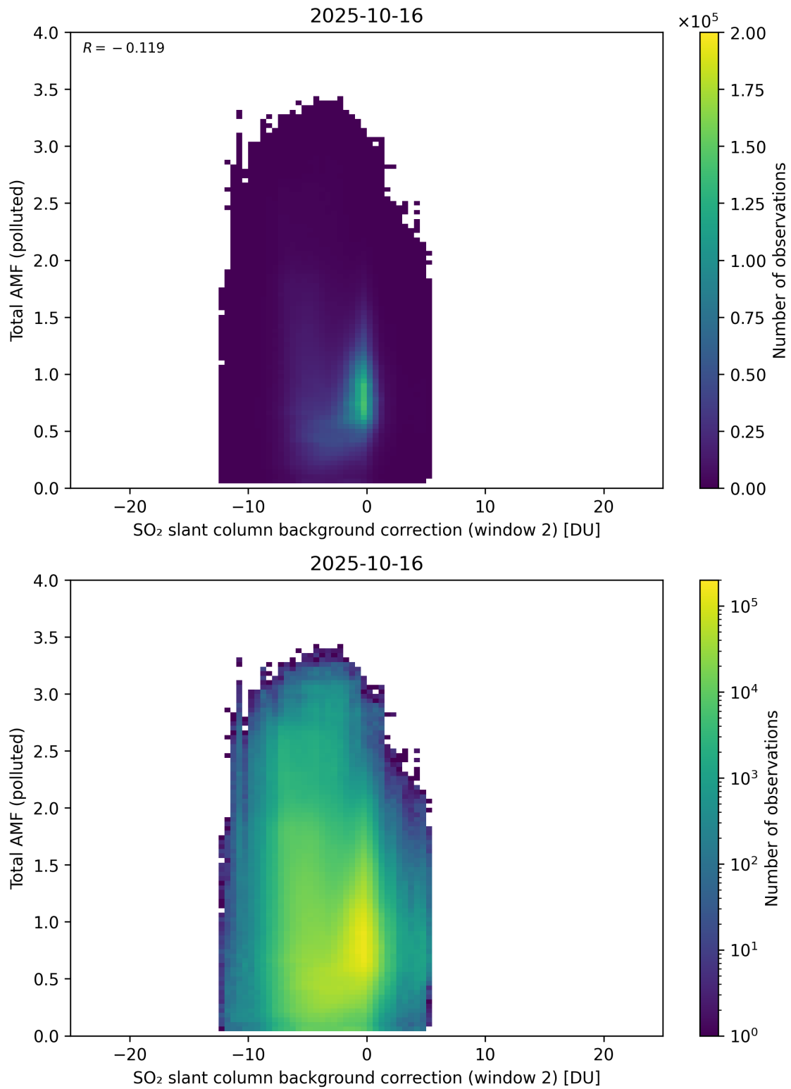
Figure 130: Scatter density plot of “SO 2 slant column background correction (window 2)” against “Total AMF (polluted)” for 2025-10-15 to 2025-10-17.
