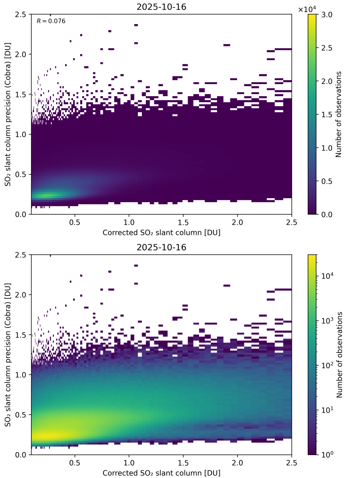
Figure 234: Scatter density plot of “Corrected SO 2 slant column” against “SO 2 slant column precision (Cobra)” for 2025-10-15 to 2025-10-17.
