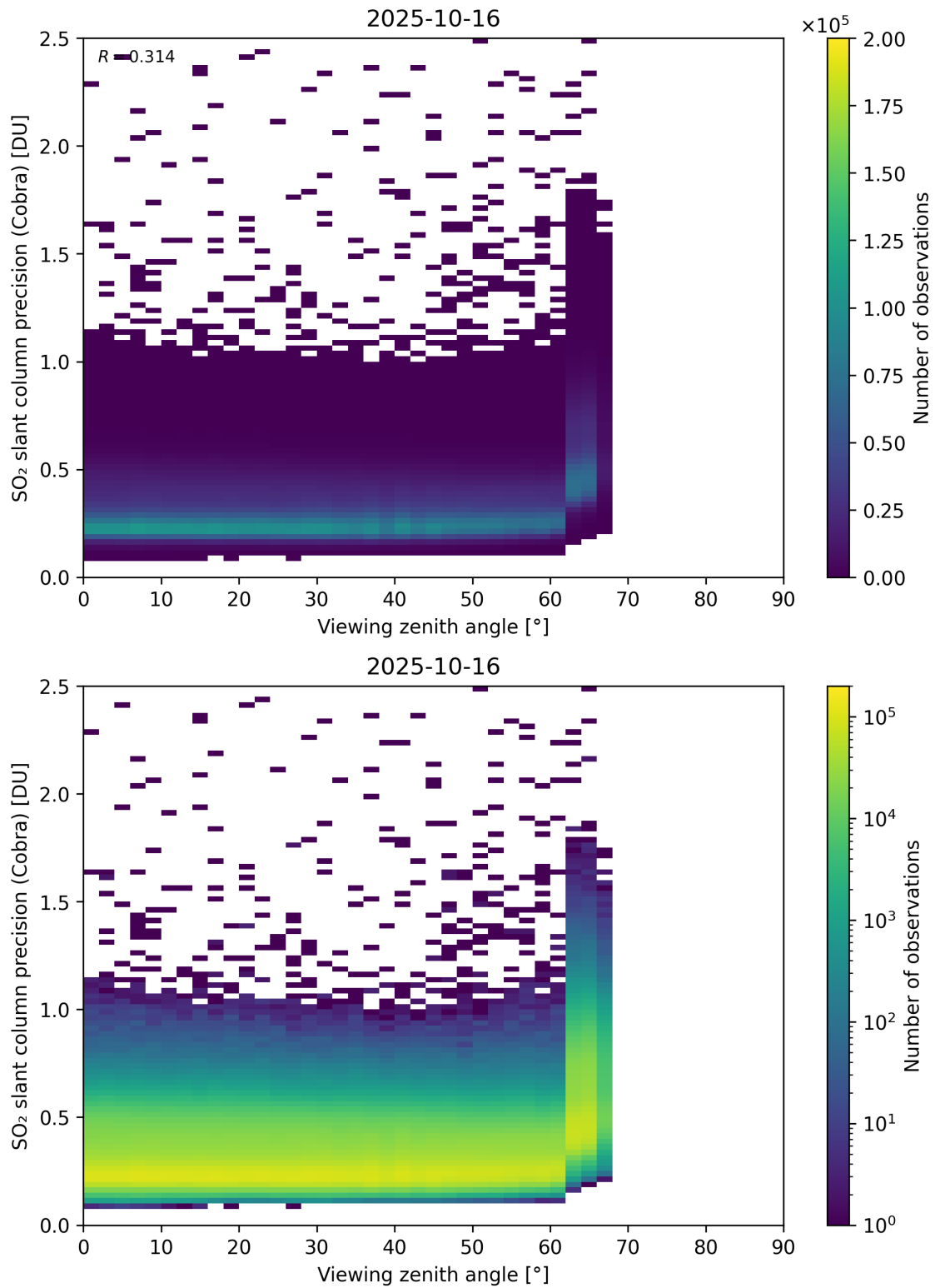
Figure 372: Scatter density plot of “Viewing zenith angle” against “SO 2 slant column precision (Cobra)” for 2025-10-15 to 2025-10-17.
