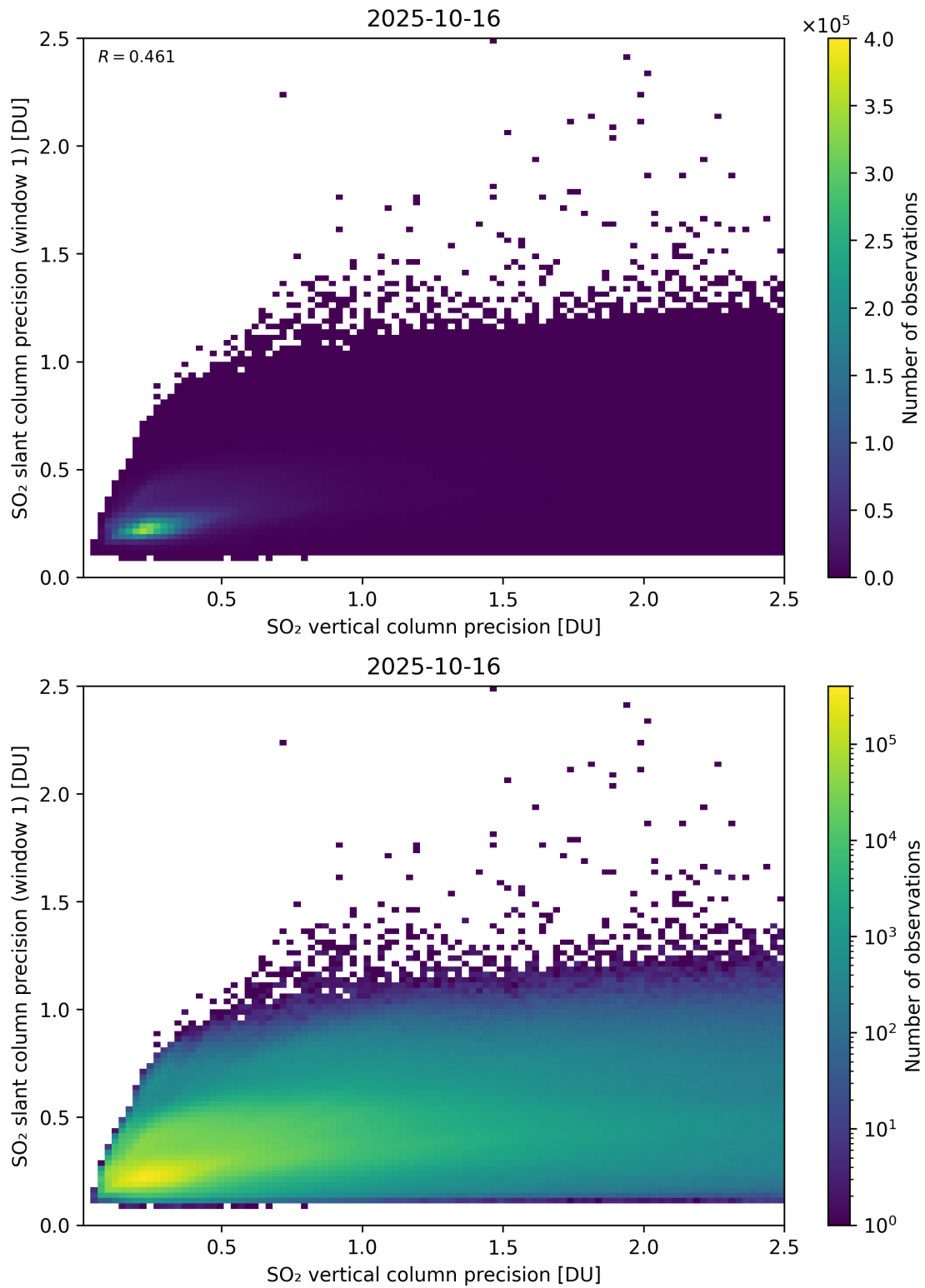
Figure 342: Scatter density plot of “SO 2 vertical column precision” against “SO 2 slant column precision (window 1)” for 2025-10-15 to 2025-10-17.
