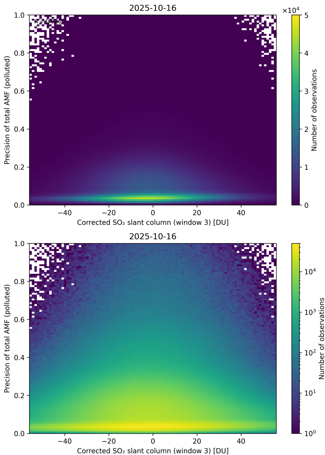
Figure 261: Scatter density plot of “Corrected SO 2 slant column (window 3)” against “Precision of total AMF (polluted)” for 2025-10-15 to 2025-10-17.
