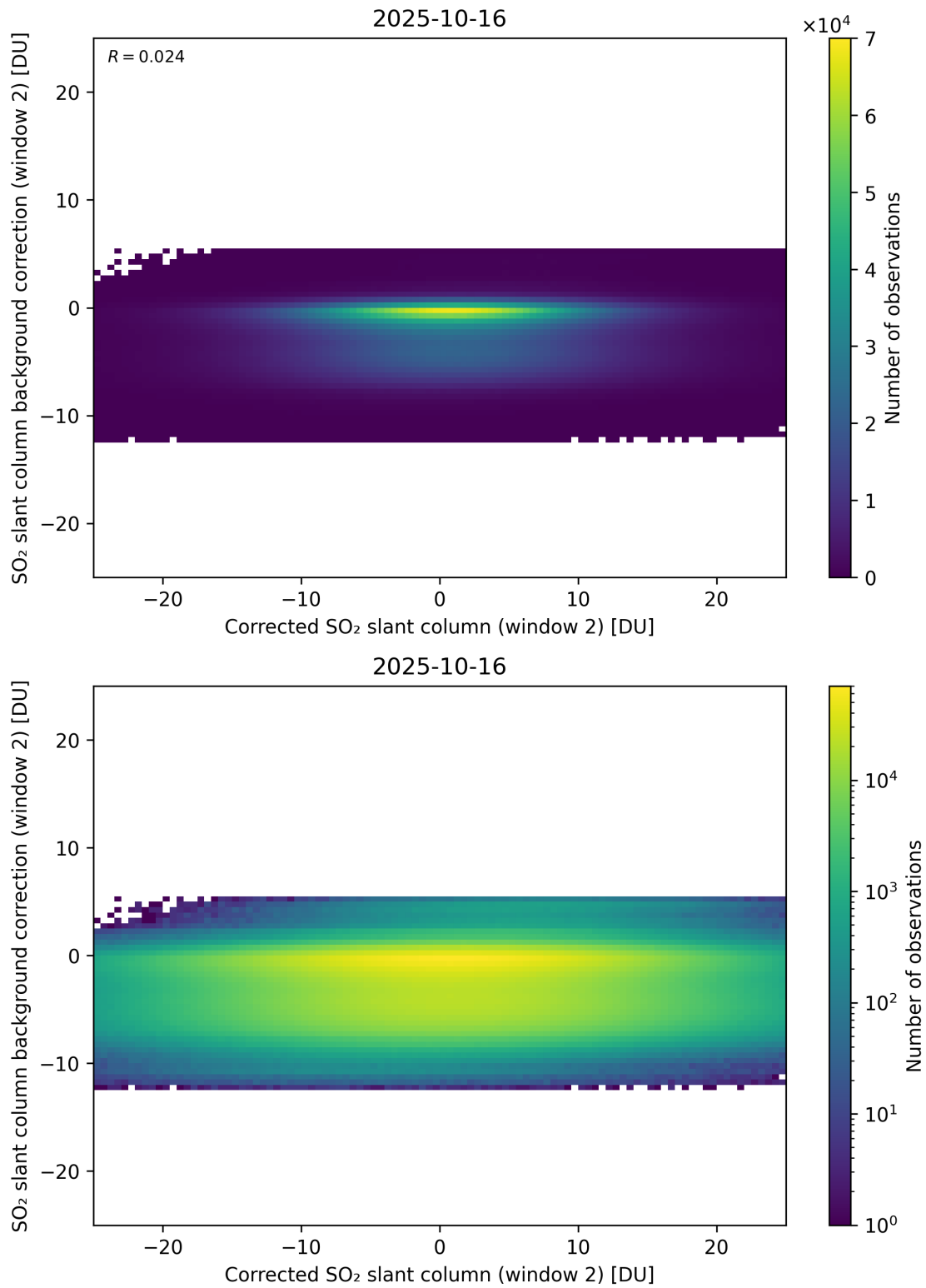
Figure 244: Scatter density plot of “Corrected SO 2 slant column (window 2)” against “SO 2 slant column background correction (window 2)” for 2025-10-15 to 2025-10-17.
