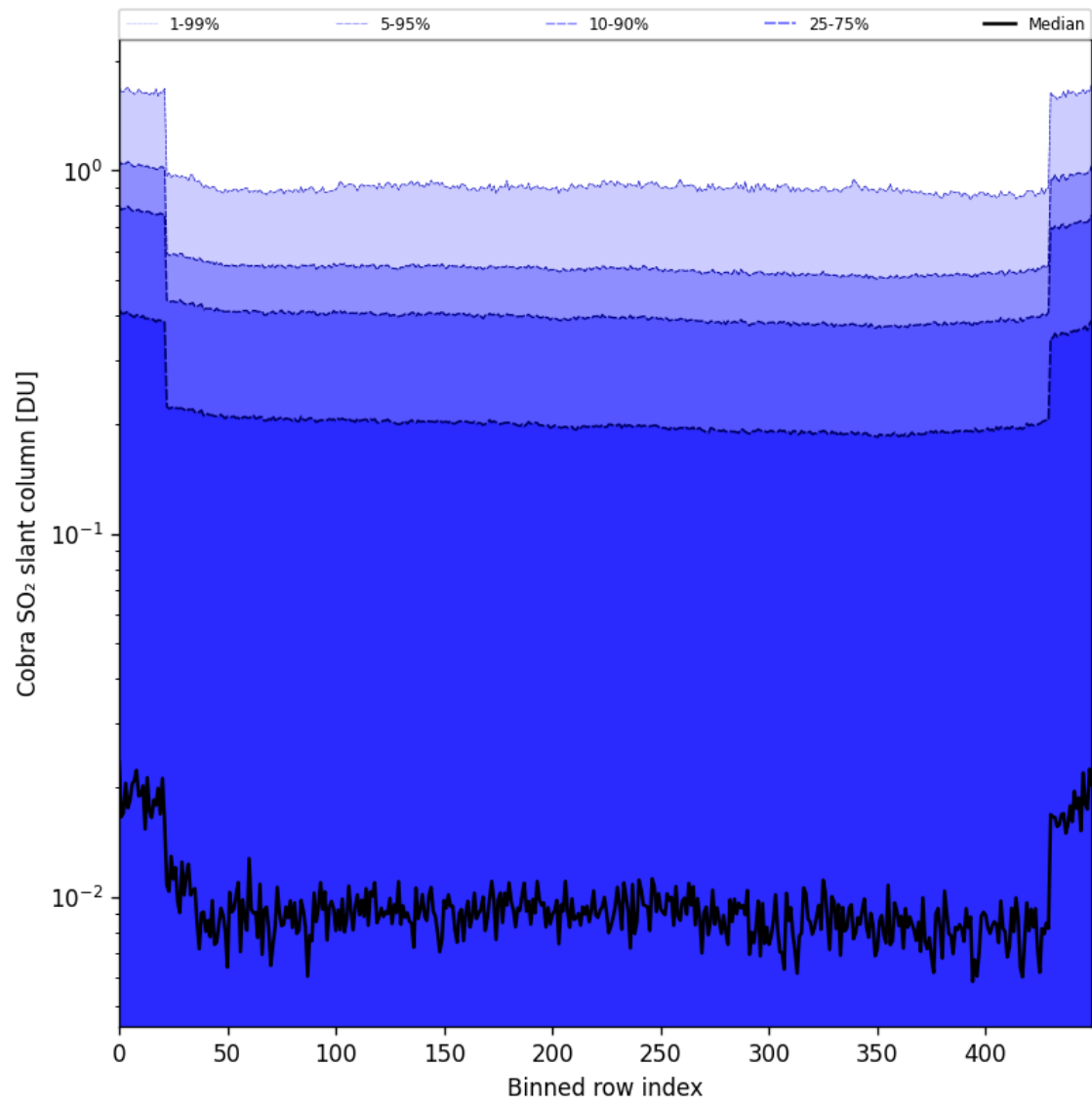
Figure 87: Along track statistics of “Cobra SO 2 slant column” for 2025-10-15 to 2025-10-17
