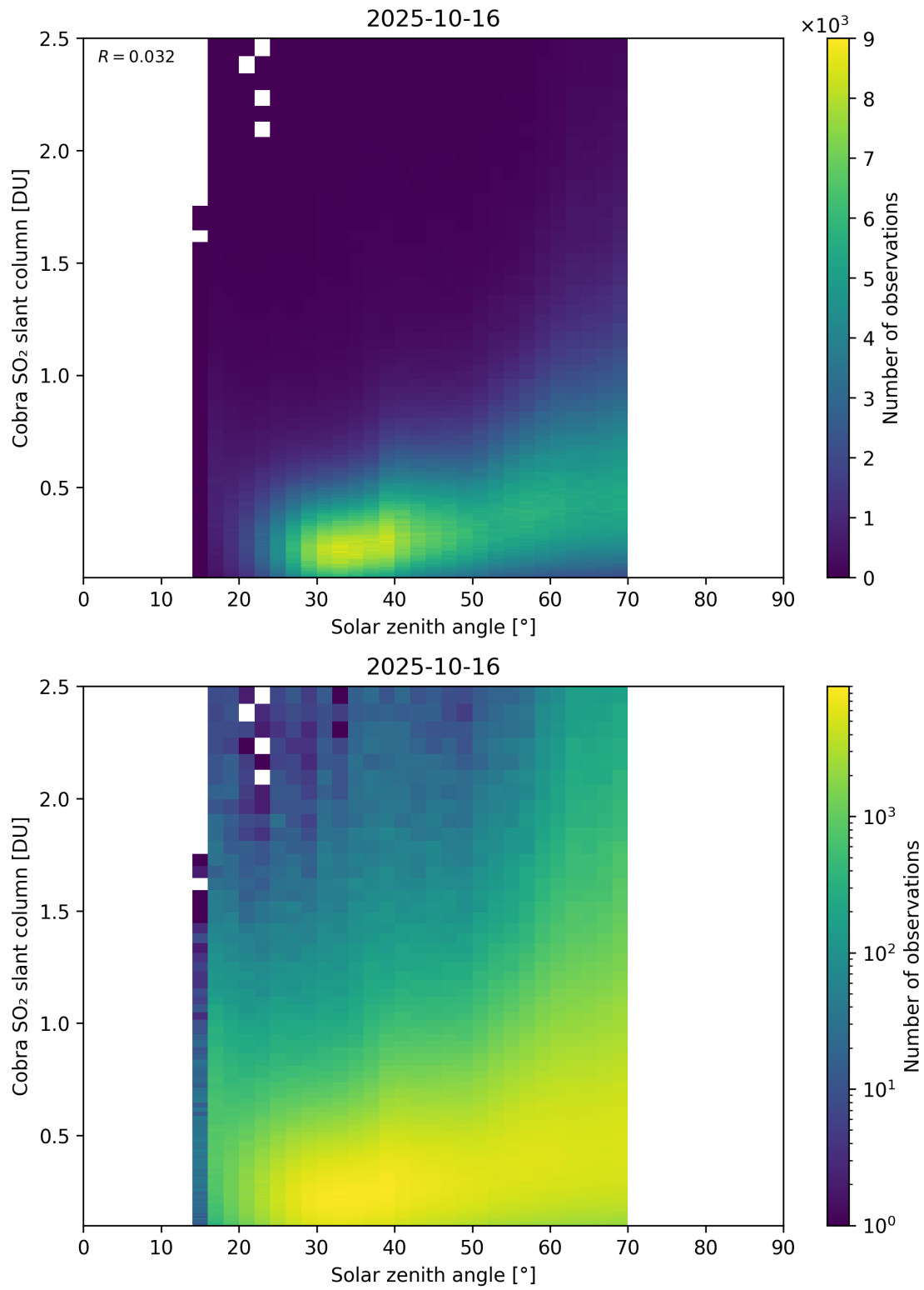
Figure 179: Scatter density plot of “Solar zenith angle” against “Cobra SO 2 slant column” for 2025-10-15 to 2025-10-17.
