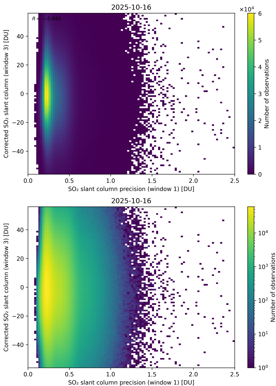
Figure 276: Scatter density plot of “SO 2 slant column precision (window 1)” against “Corrected SO 2 slant column (window 3)” for 2025-10-15 to 2025-10-17.
