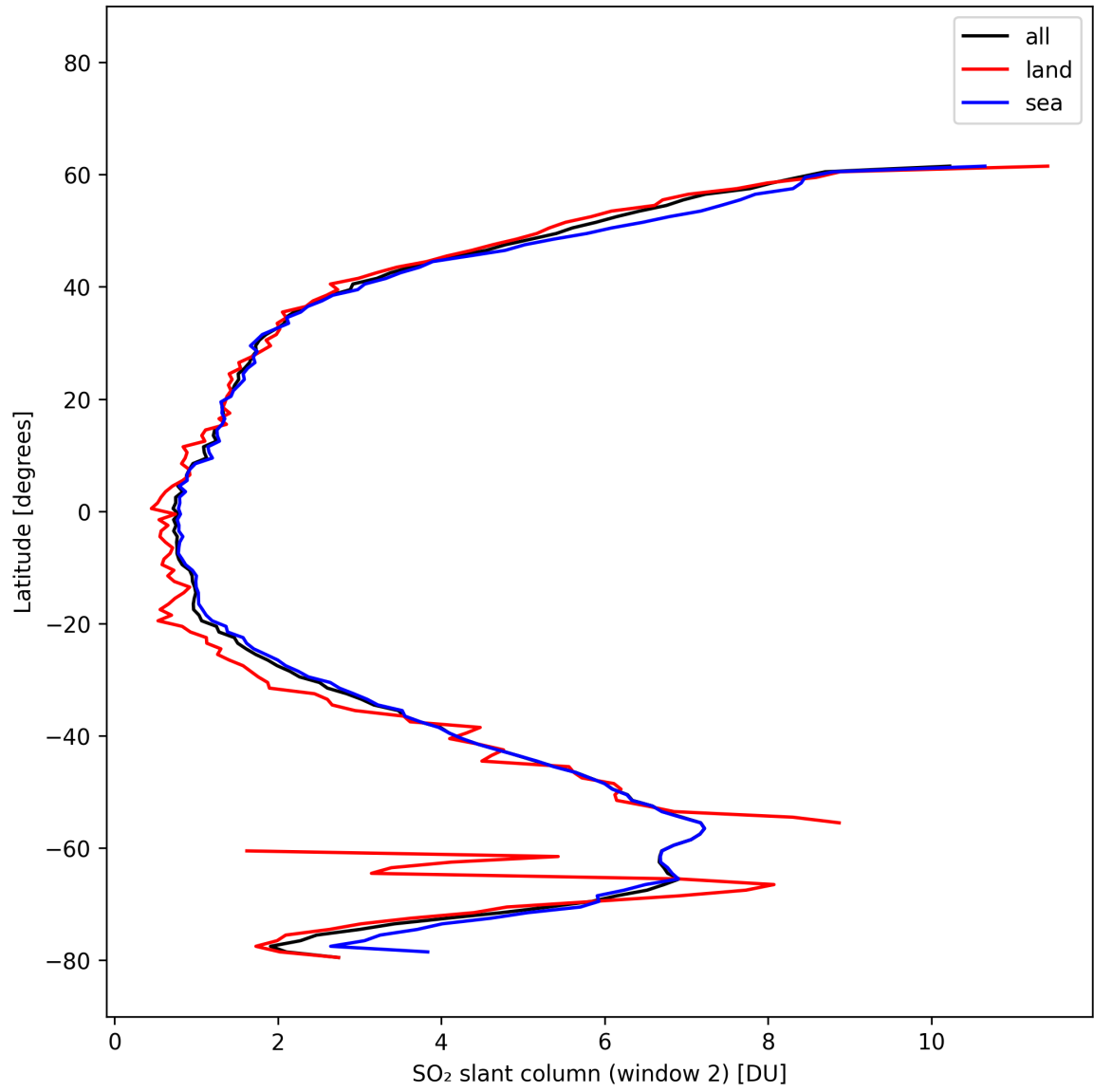
Figure 41: Zonal average of “SO 2 slant column (window 2)” for 2025-10-15 to 2025-10-17.
