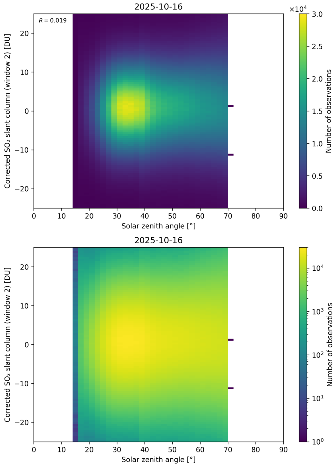
Figure 182: Scatter density plot of “Solar zenith angle” against “Corrected SO 2 slant column (window 2)” for 2025-10-15 to 2025-10-17.
