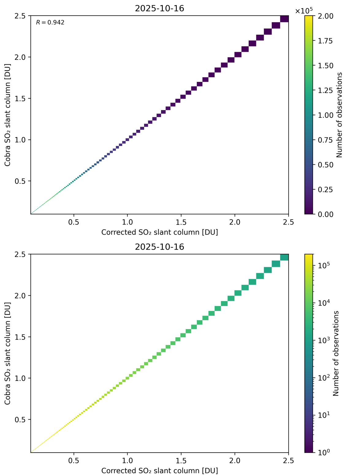
Figure 233: Scatter density plot of “Corrected SO 2 slant column” against “Cobra SO 2 slant column” for 2025-10-15 to 2025-10-17.
