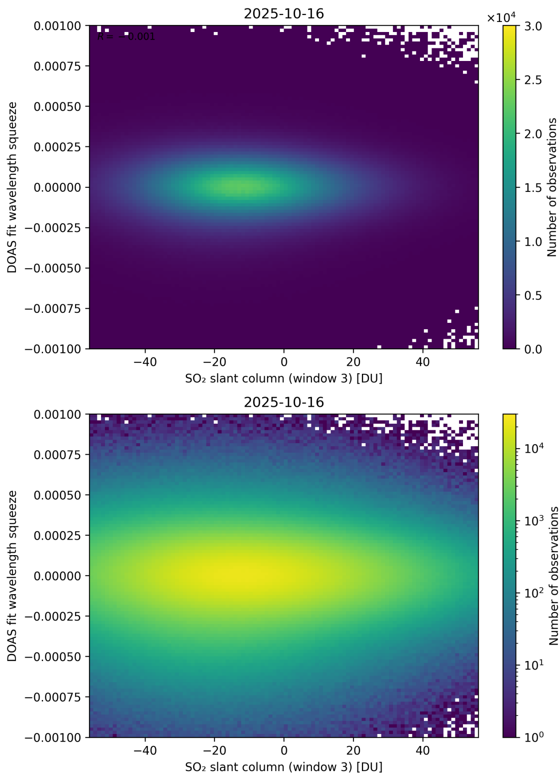
Figure 305: Scatter density plot of “SO 2 slant column (window 3)” against “DOAS fit wavelength squeeze” for 2025-10-15 to 2025-10-17.
