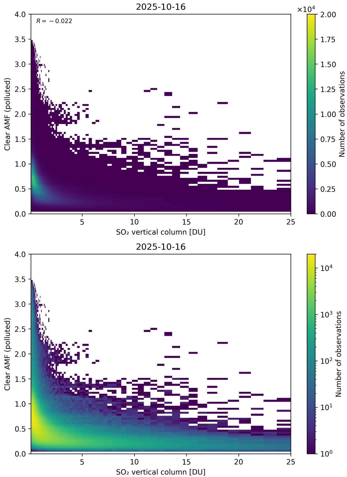
Figure 348: Scatter density plot of “SO 2 vertical column” against “Clear AMF (polluted)” for 2025-10-15 to 2025-10-17.
