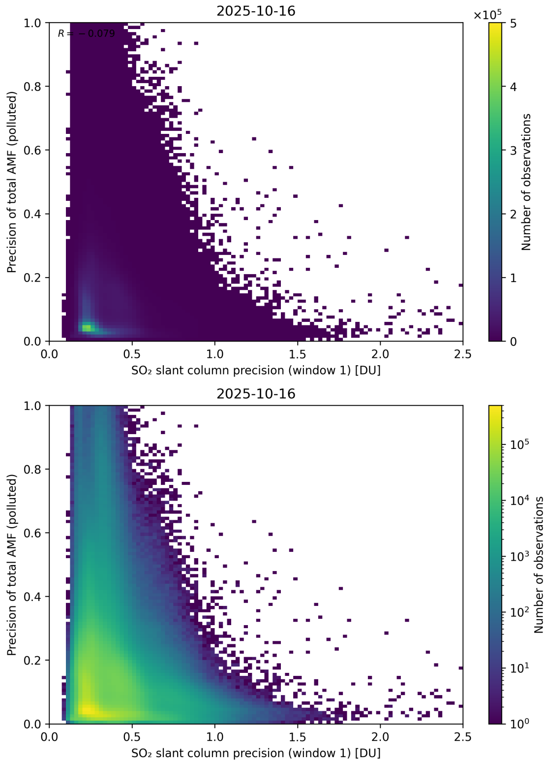
Figure 281: Scatter density plot of “SO 2 slant column precision (window 1)” against “Precision of total AMF (polluted)” for 2025-10-15 to 2025-10-17.
