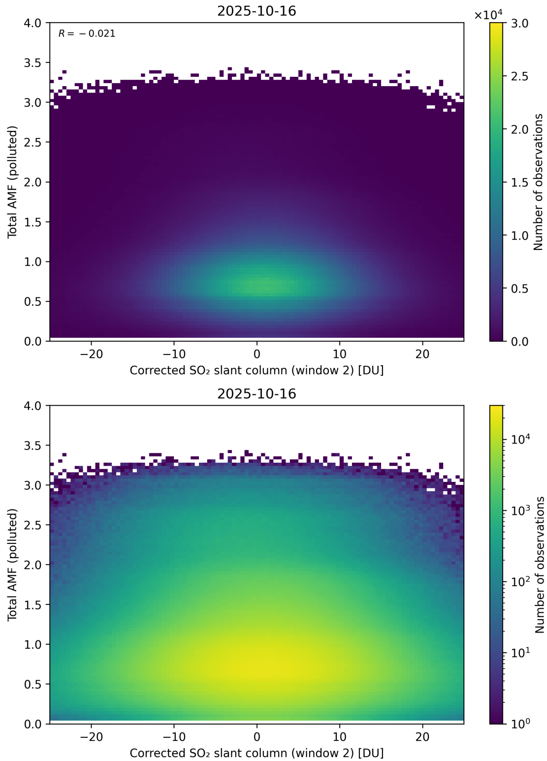
Figure 253: Scatter density plot of “Corrected SO 2 slant column (window 2)” against “Total AMF (polluted)” for 2025-10-15 to 2025-10-17.
