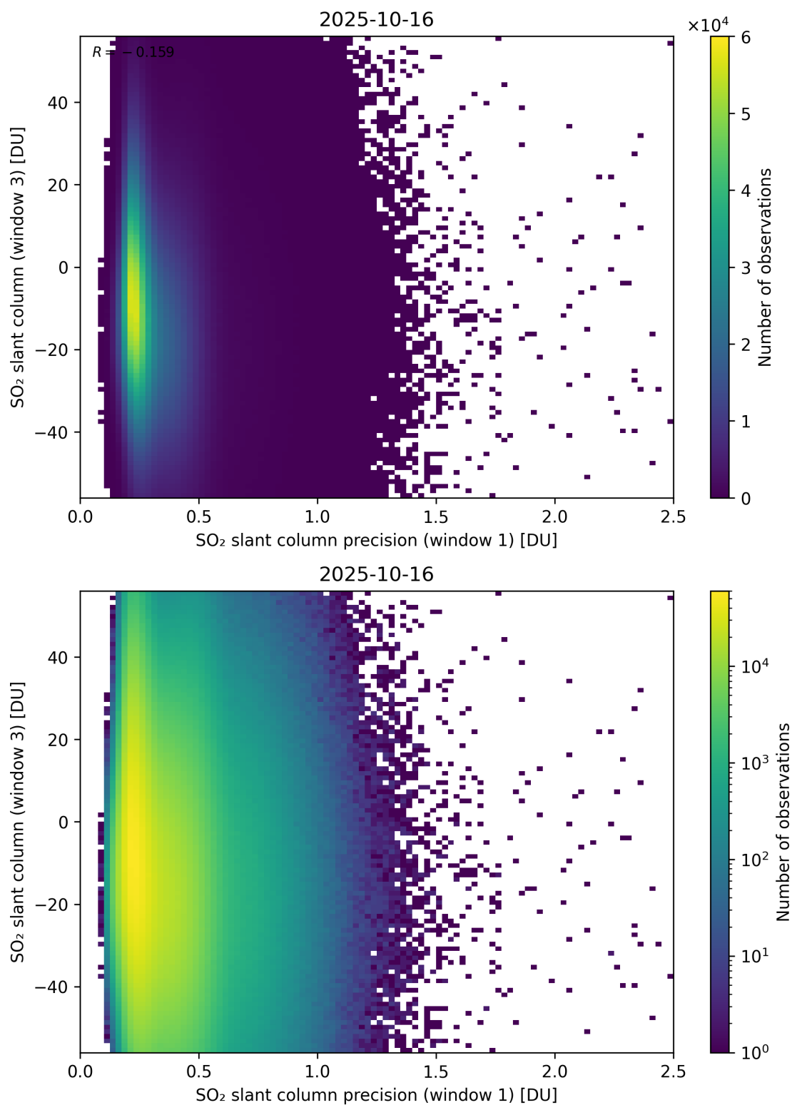
Figure 278: Scatter density plot of “SO 2 slant column precision (window 1)” against “SO 2 slant column (window 3)” for 2025-10-15 to 2025-10-17.
