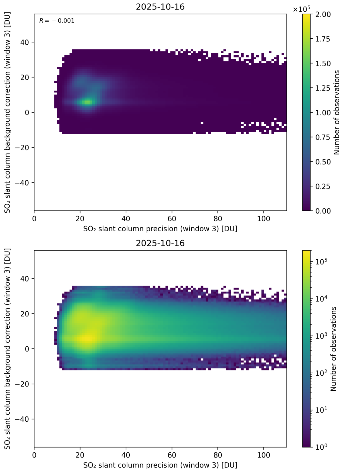
Figure 307: Scatter density plot of “SO 2 slant column precision (window 3)” against “SO 2 slant column background correction (window 3)” for 2025-10-15 to 2025-10-17.
