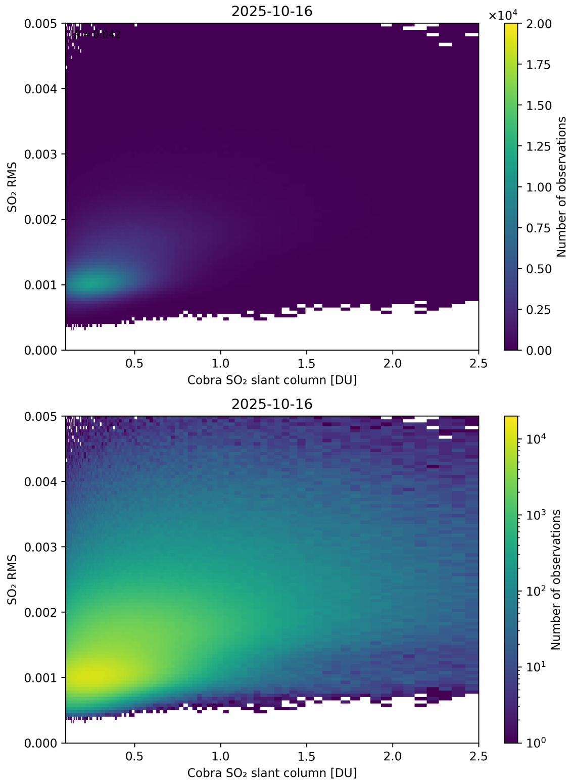
Figure 198: Scatter density plot of “Cobra SO 2 slant column” against “SO 2 RMS” for 2025-10-15 to 2025-10-17.
