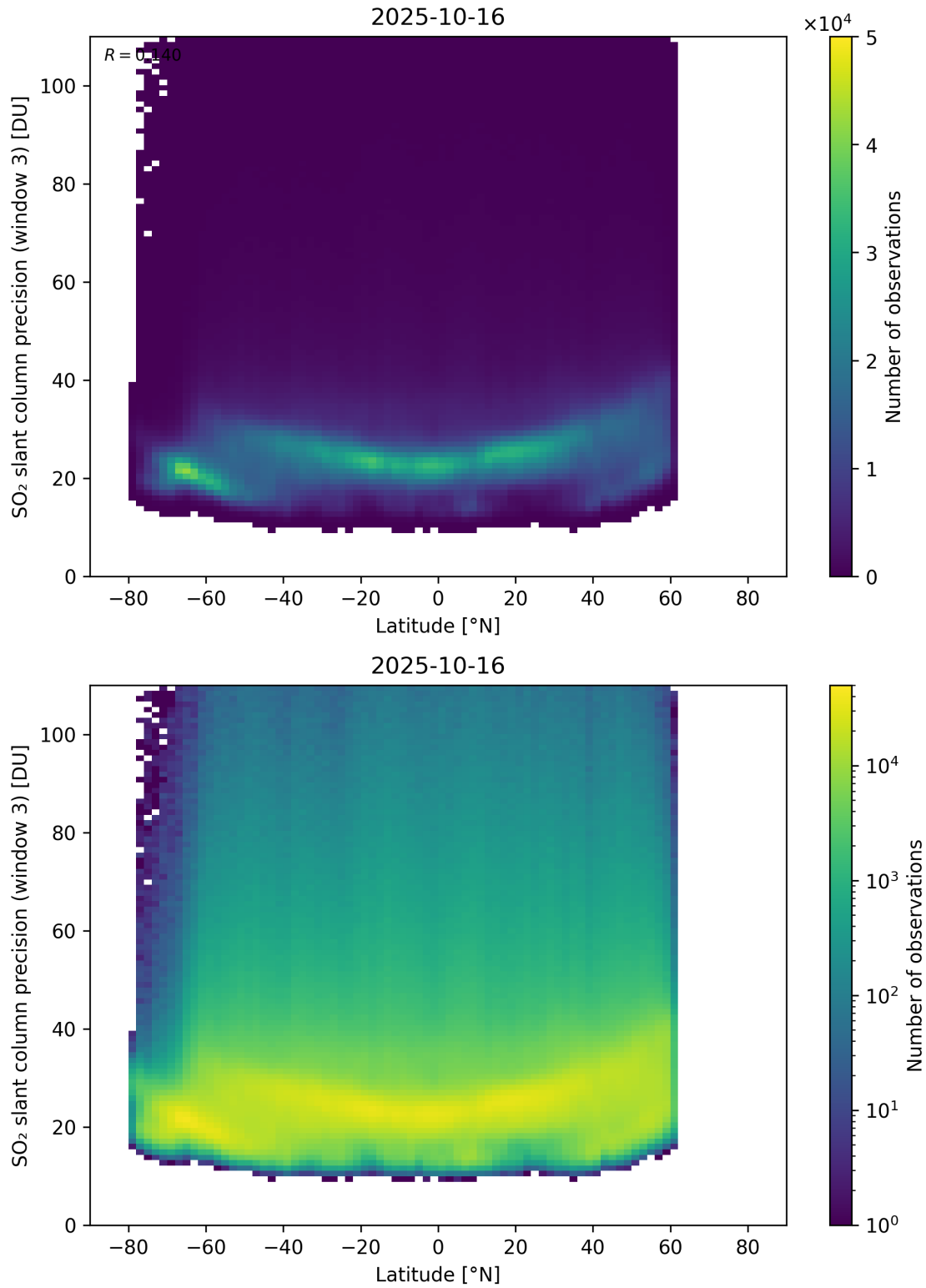
Figure 166: Scatter density plot of “Latitude” against “SO 2 slant column precision (window 3)” for 2025-10-15 to 2025-10-17.
