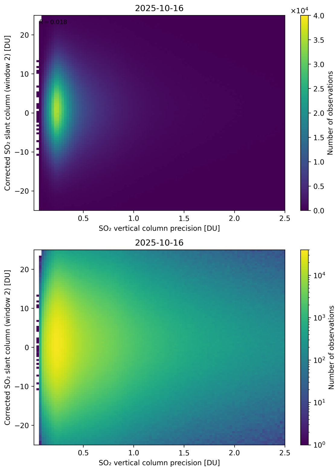
Figure 339: Scatter density plot of “SO 2 vertical column precision” against “Corrected SO 2 slant column (window 2)” for 2025-10-15 to 2025-10-17.
