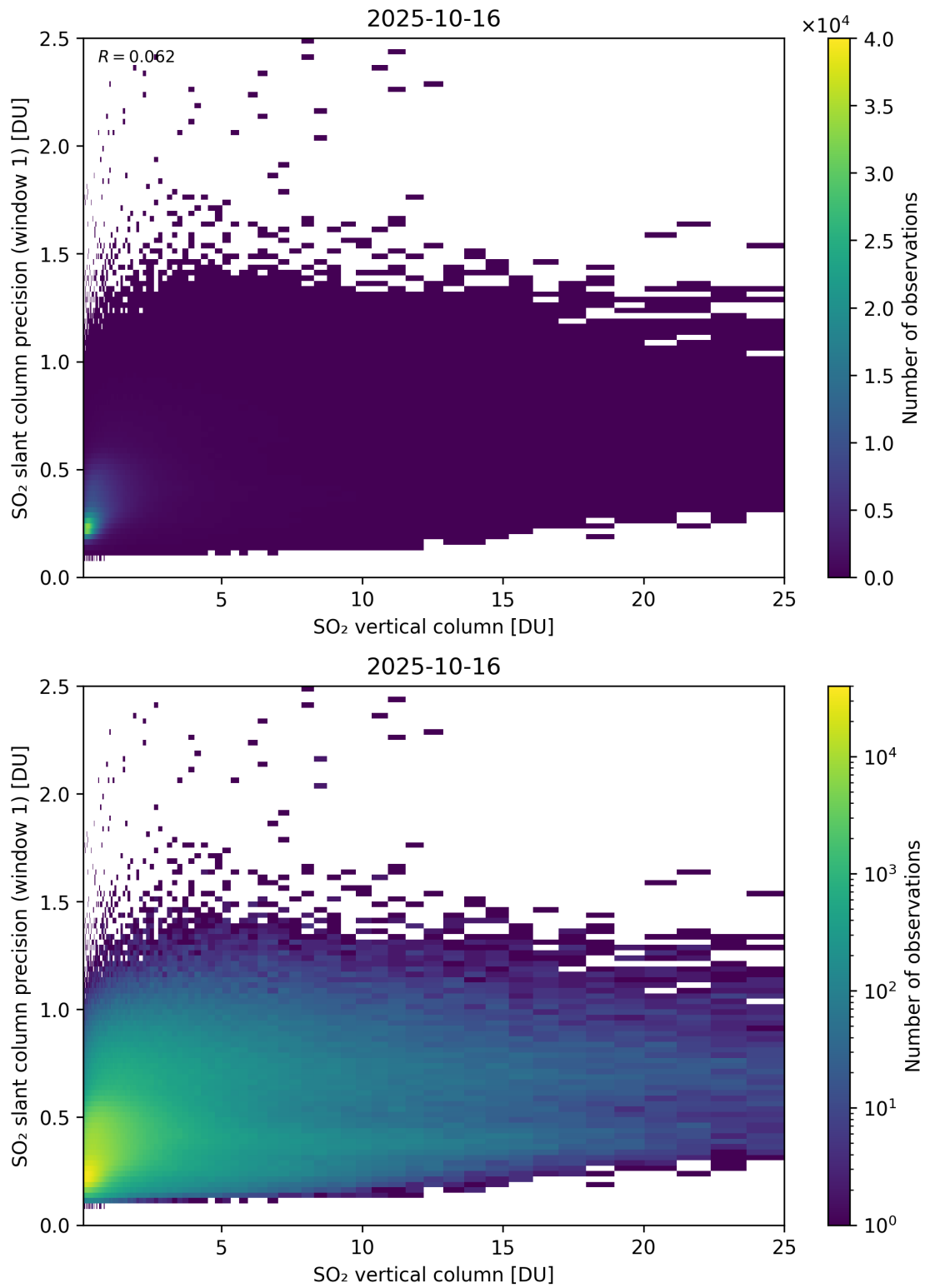
Figure 355: Scatter density plot of “SO 2 vertical column” against “SO 2 slant column precision (window 1)” for 2025-10-15 to 2025-10-17.
