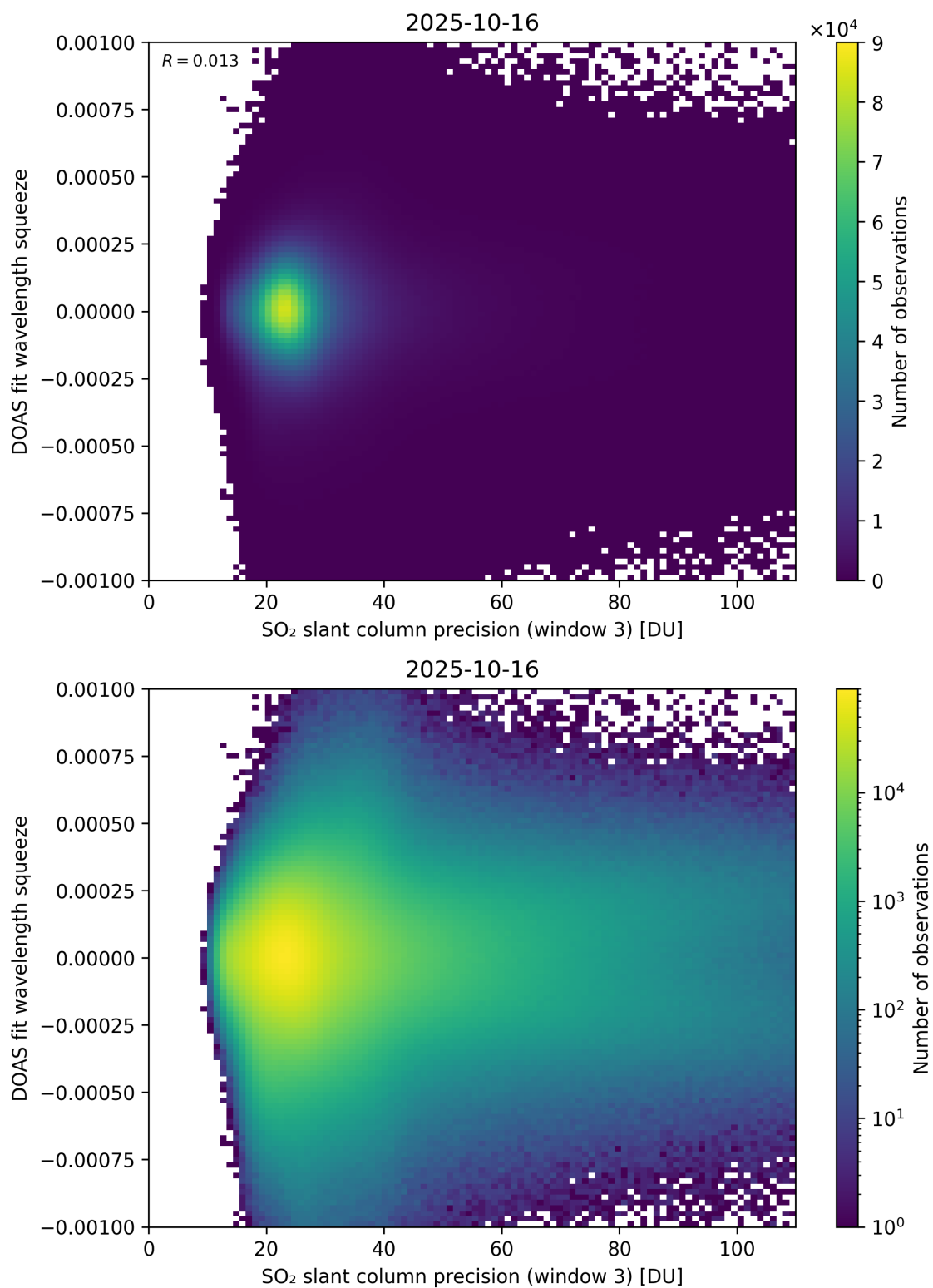
Figure 309: Scatter density plot of “SO 2 slant column precision (window 3)” against “DOAS fit wavelength squeeze” for 2025-10-15 to 2025-10-17.
