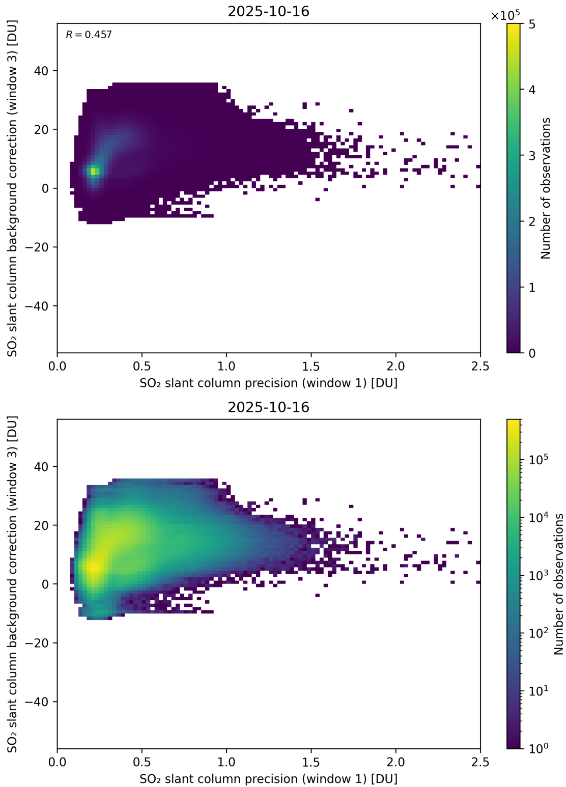
Figure 270: Scatter density plot of “SO 2 slant column precision (window 1)” against “SO 2 slant column background correction (window 3)” for 2025-10-15 to 2025-10-17.
