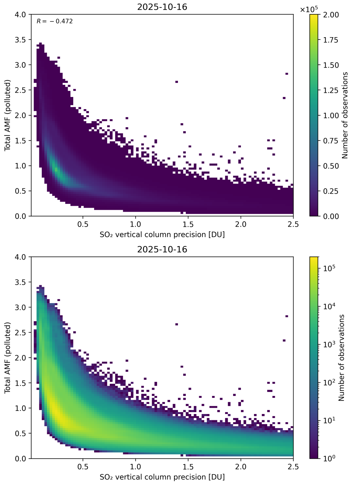
Figure 346: Scatter density plot of “SO 2 vertical column precision” against “Total AMF (polluted)” for 2025-10-15 to 2025-10-17.
