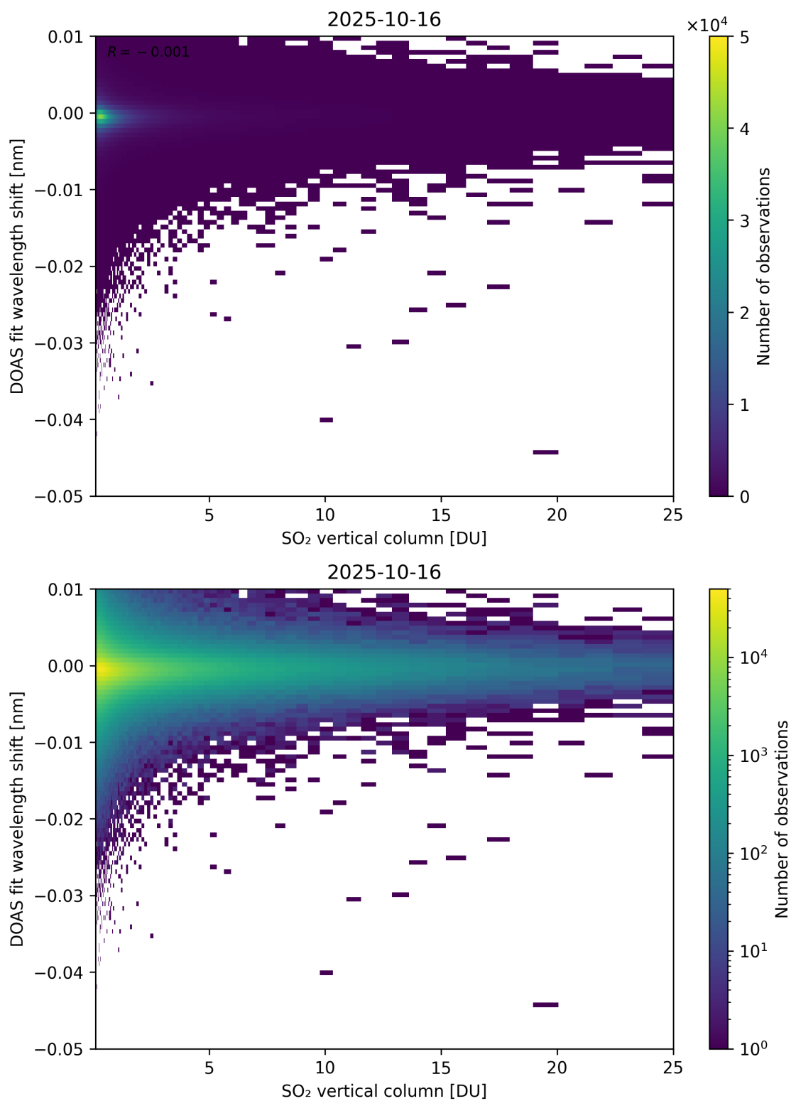
Figure 326: Scatter density plot of “SO 2 vertical column” against “DOAS fit wavelength shift” for 2025-10-15 to 2025-10-17.
