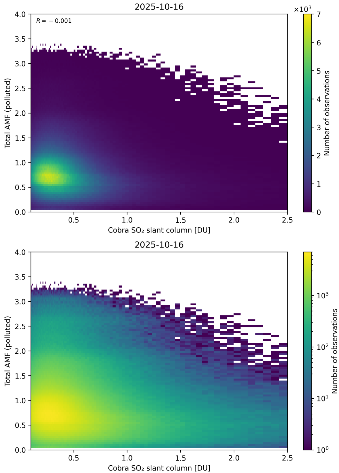
Figure 224: Scatter density plot of “Cobra SO 2 slant column” against “Total AMF (polluted)” for 2025-10-15 to 2025-10-17.
