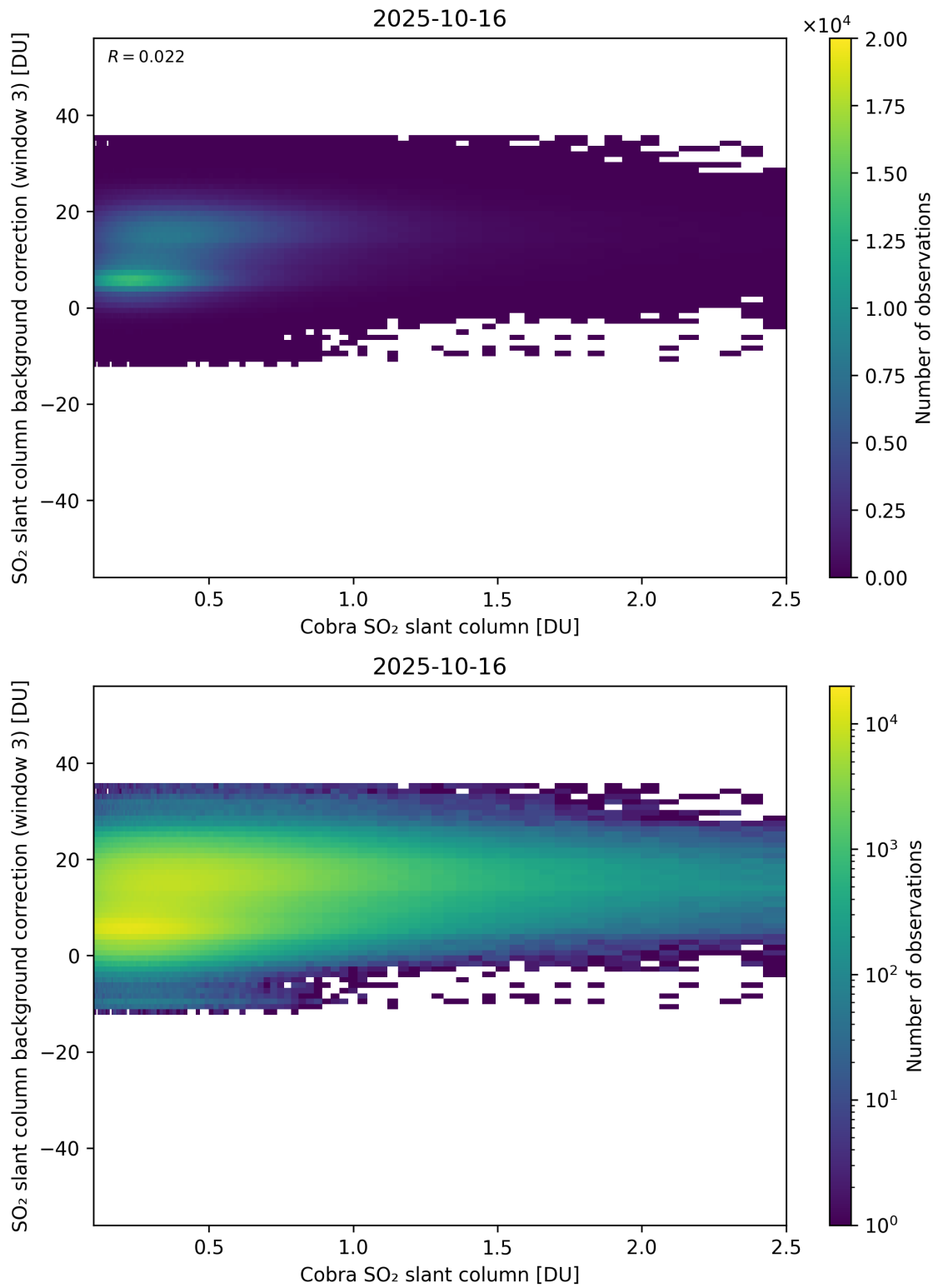
Figure 195: Scatter density plot of “Cobra SO 2 slant column” against “SO 2 slant column background correction (window 3)” for 2025-10-15 to 2025-10-17.
