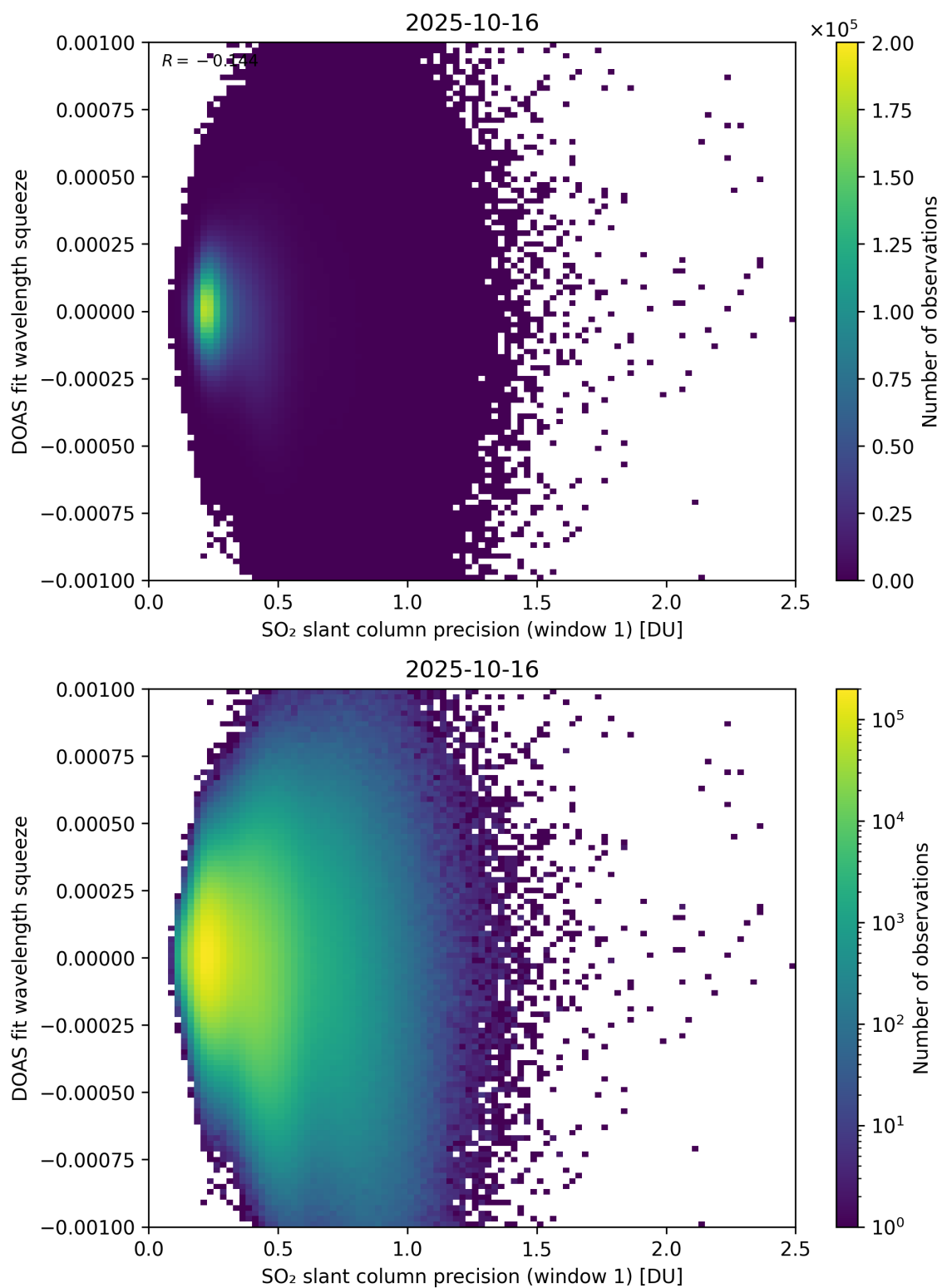
Figure 272: Scatter density plot of “SO 2 slant column precision (window 1)” against “DOAS fit wavelength squeeze” for 2025-10-15 to 2025-10-17.
