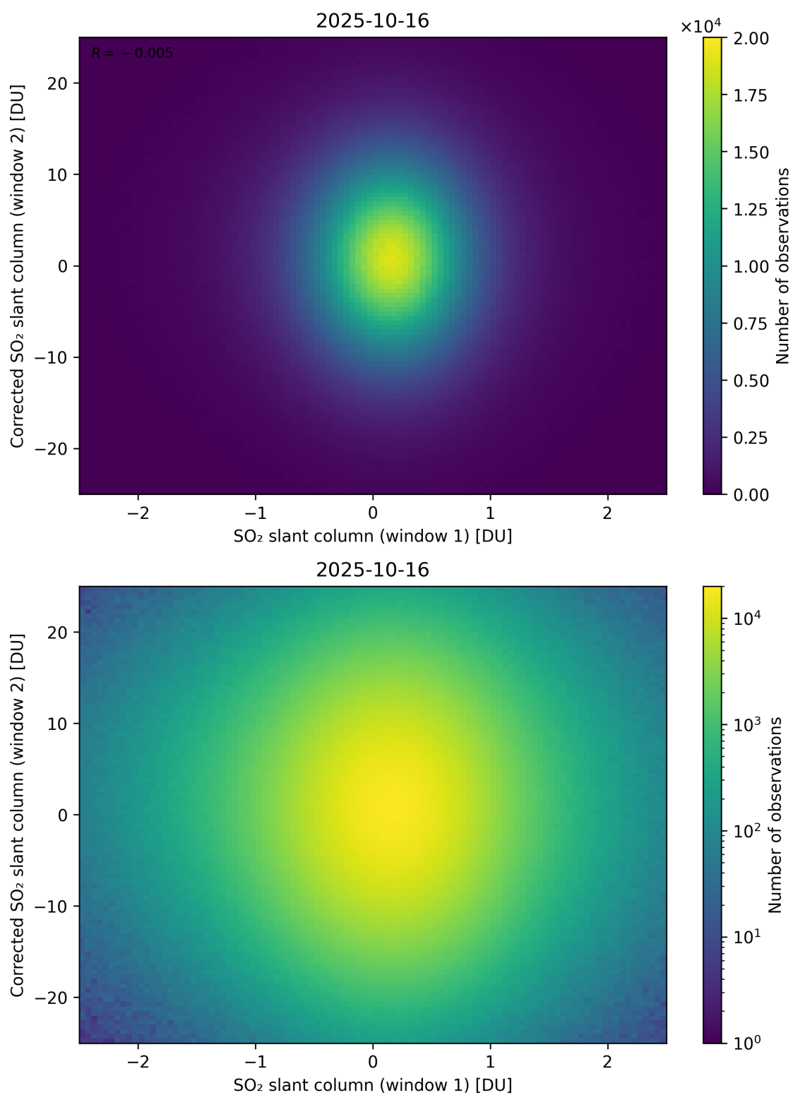
Figure 283: Scatter density plot of “SO 2 slant column (window 1)” against “Corrected SO 2 slant column (window 2)” for 2025-10-15 to 2025-10-17.
