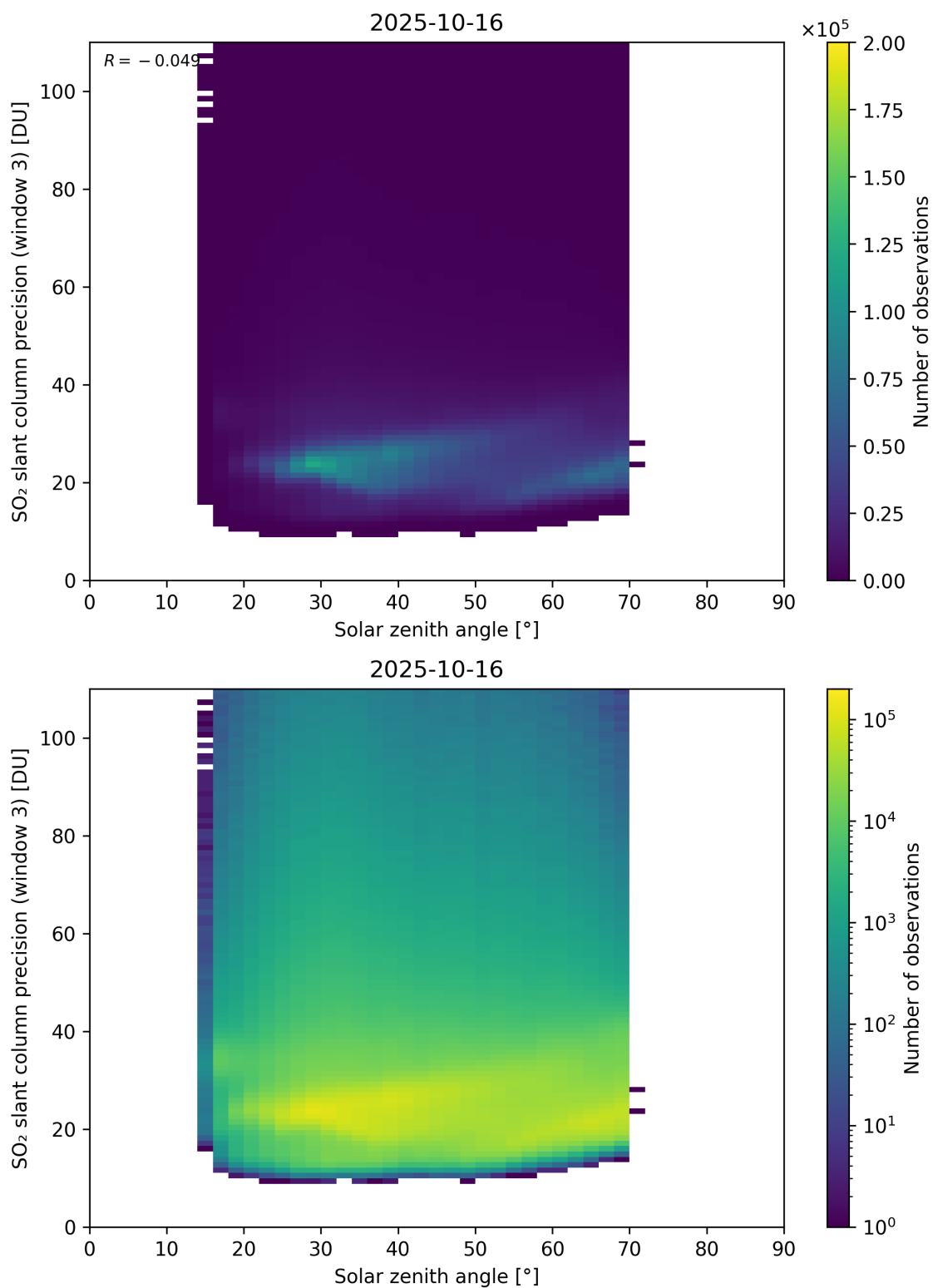
Figure 188: Scatter density plot of “Solar zenith angle” against “SO 2 slant column precision (window 3)” for 2025-10-15 to 2025-10-17.
