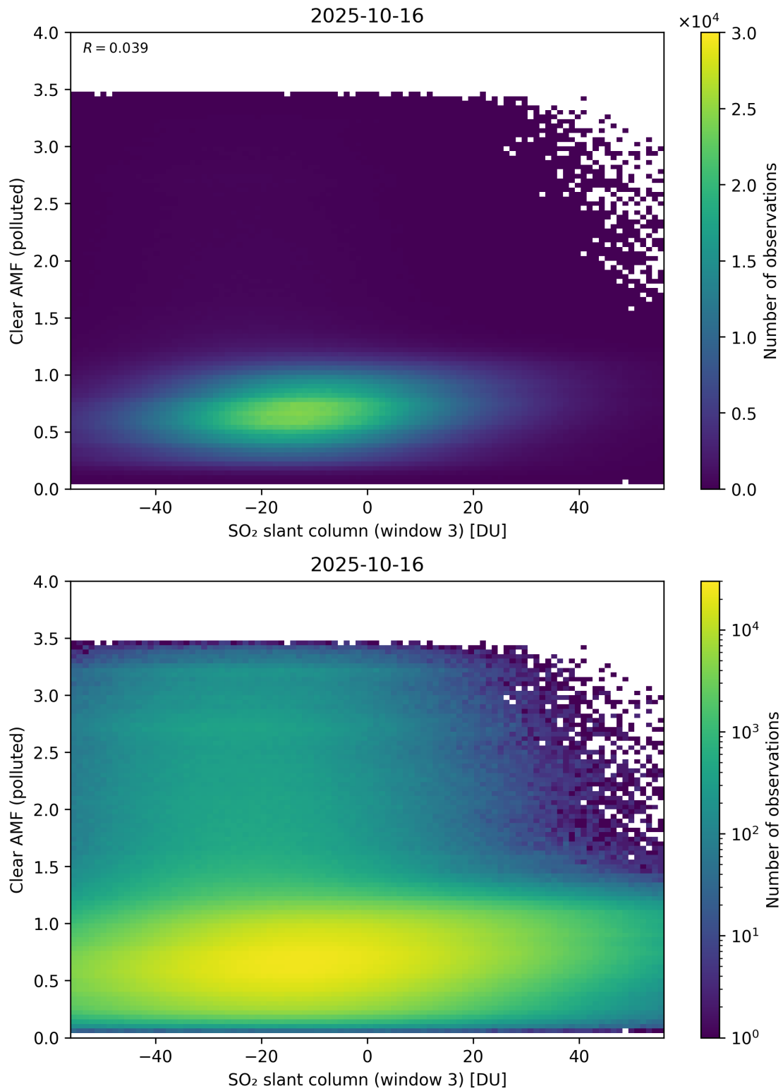
Figure 315: Scatter density plot of “SO 2 slant column (window 3)” against “Clear AMF (polluted)” for 2025-10-15 to 2025-10-17.
