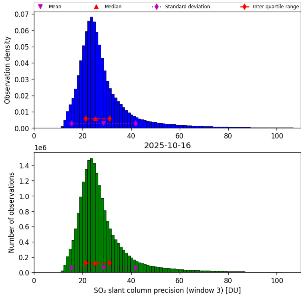
Figure 72: Histogram of “SO 2 slant column precision (window 3)” for 2025-10-15 to 2025-10-17
