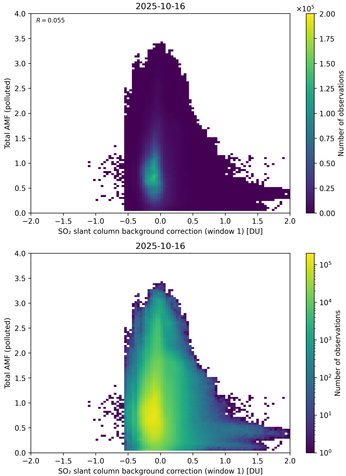
Figure 120: Scatter density plot of “SO 2 slant column background correction (window 1)” against “Total AMF (polluted)” for 2025-10-15 to 2025-10-17.
