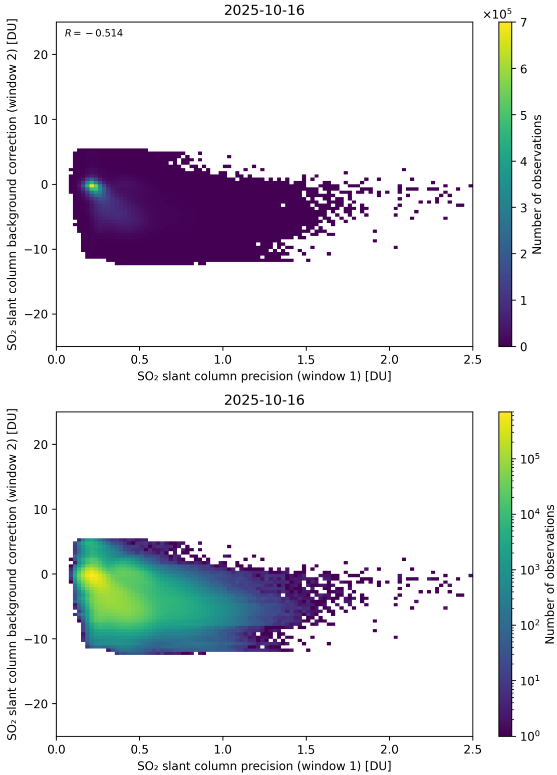
Figure 269: Scatter density plot of “SO 2 slant column precision (window 1)” against “SO 2 slant column background correction (window 2)” for 2025-10-15 to 2025-10-17.
