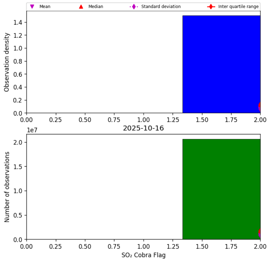
Figure 75: Histogram of “SO 2 Cobra Flag” for 2025-10-15 to 2025-10-17
