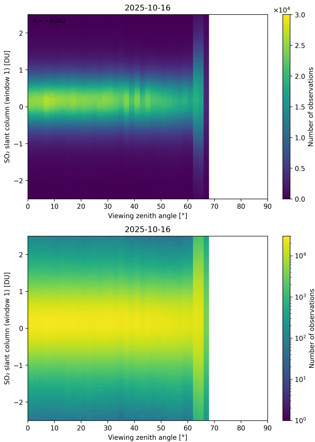
Figure 376: Scatter density plot of “Viewing zenith angle” against “SO 2 slant column (window 1)” for 2025-10-15 to 2025-10-17.
