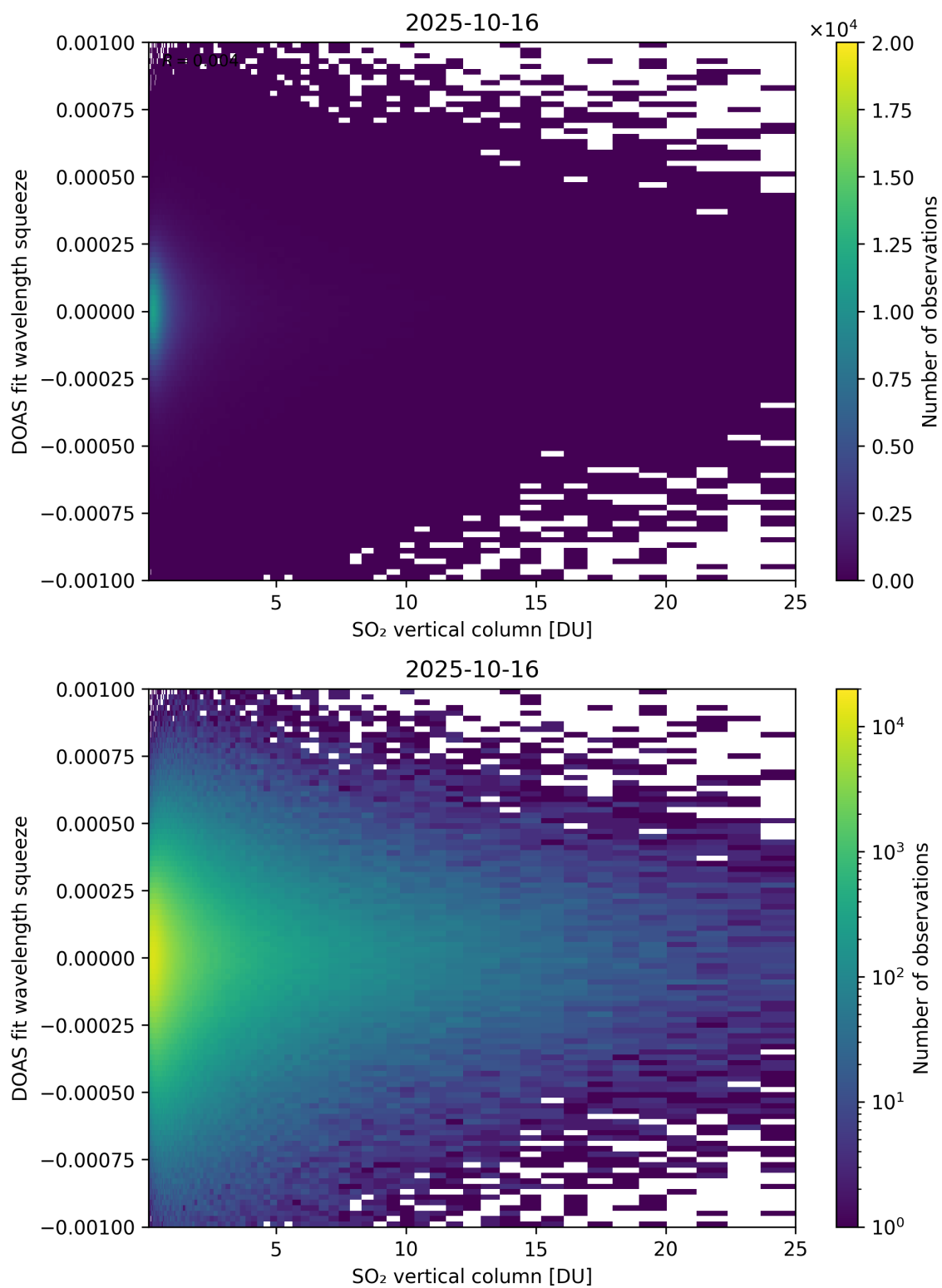
Figure 327: Scatter density plot of “SO 2 vertical column” against “DOAS fit wavelength squeeze” for 2025-10-15 to 2025-10-17.
