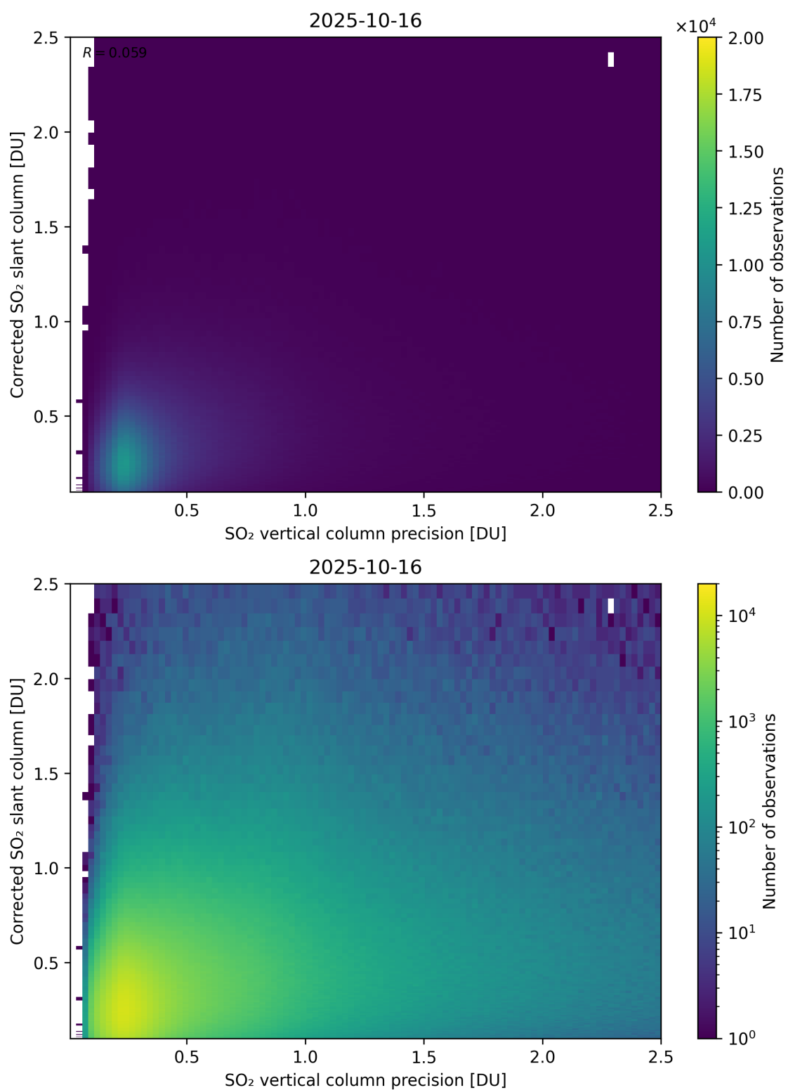
Figure 338: Scatter density plot of “SO 2 vertical column precision” against “Corrected SO 2 slant column” for 2025-10-15 to 2025-10-17.
