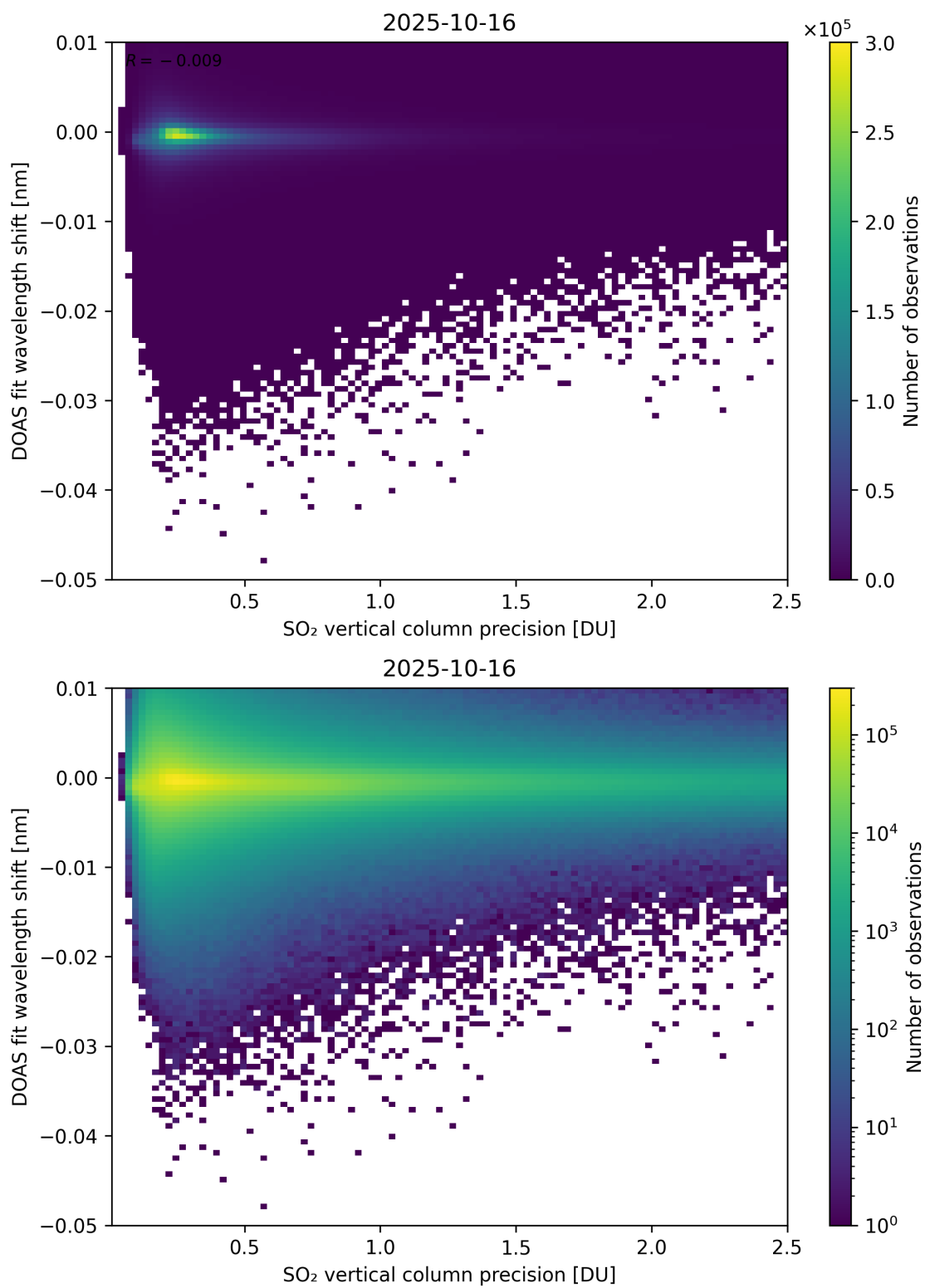
Figure 332: Scatter density plot of “SO 2 vertical column precision” against “DOAS fit wavelength shift” for 2025-10-15 to 2025-10-17.
