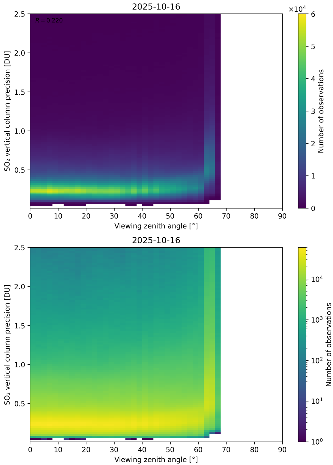
Figure 384: Scatter density plot of “Viewing zenith angle” against “SO 2 vertical column precision” for 2025-10-15 to 2025-10-17.
