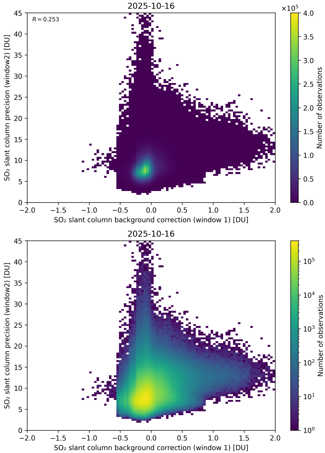
Figure 117: Scatter density plot of “SO 2 slant column background correction (window 1)” against “SO 2 slant column precision (window2)” for 2025-10-15 to 2025-10-17.
