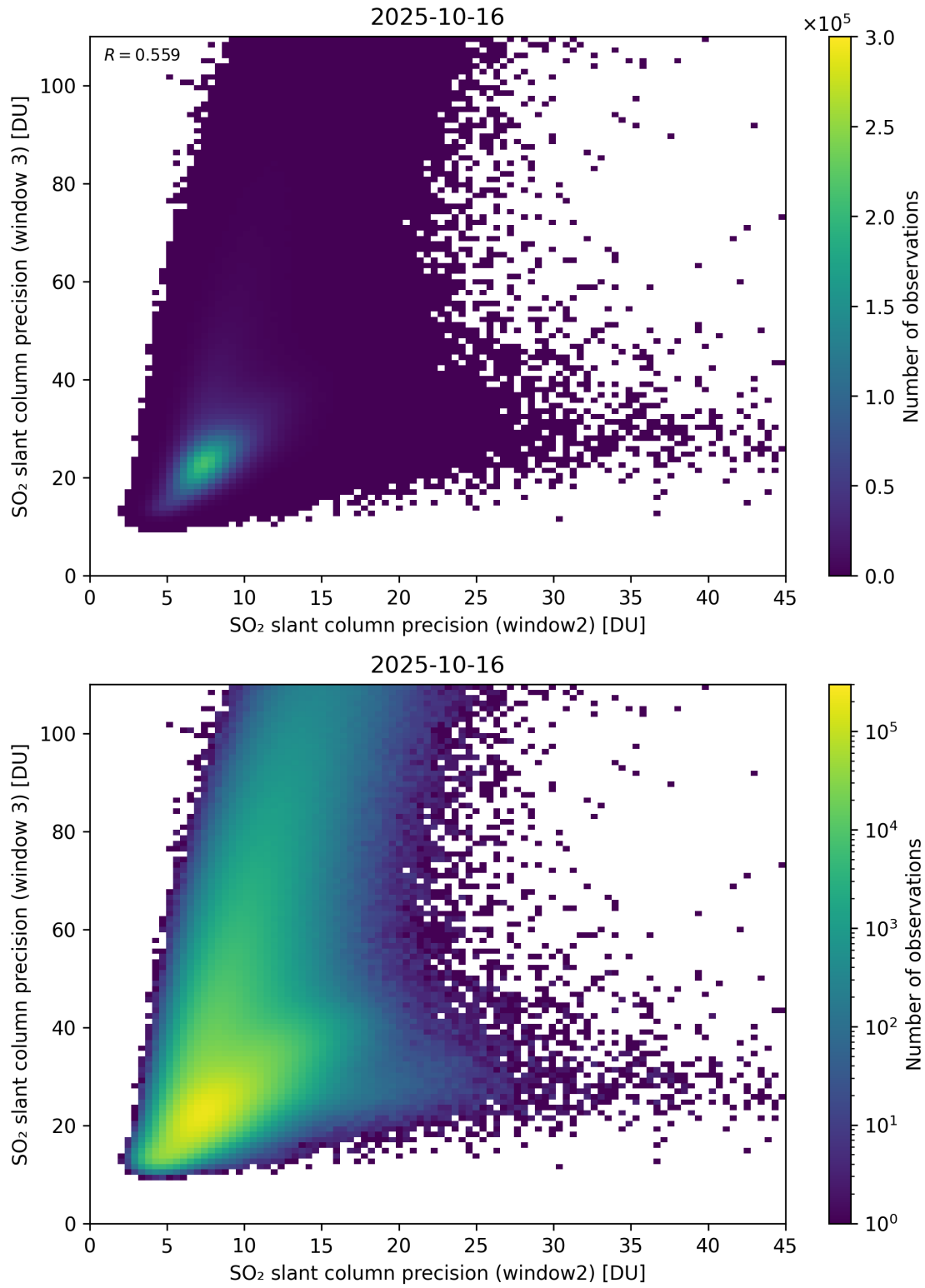
Figure 300: Scatter density plot of “SO 2 slant column precision (window2)” against “SO 2 slant column precision (window 3)” for 2025-10-15 to 2025-10-17.
