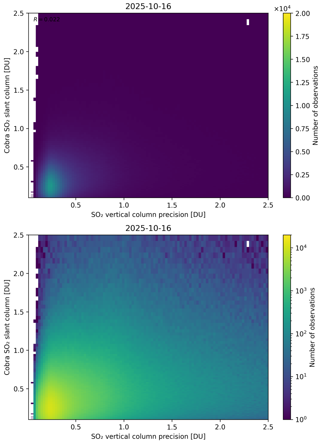
Figure 336: Scatter density plot of “SO 2 vertical column precision” against “Cobra SO 2 slant column” for 2025-10-15 to 2025-10-17.
