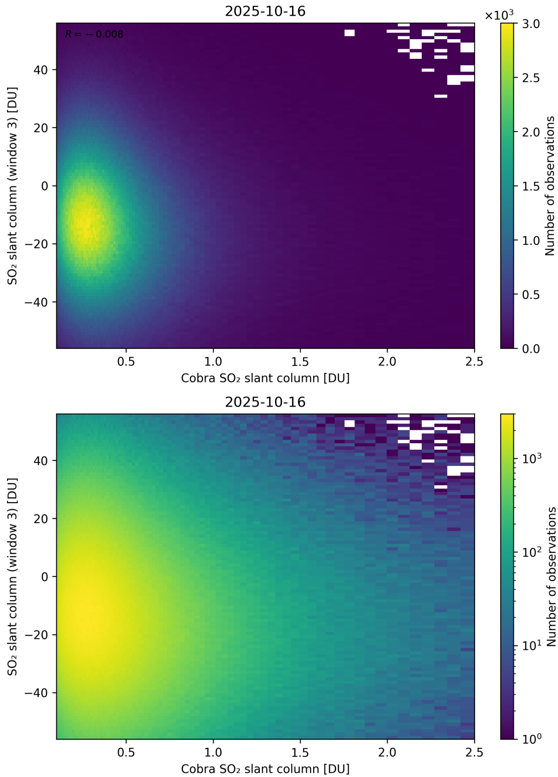
Figure 222: Scatter density plot of “Cobra SO 2 slant column” against “SO 2 slant column (window 3)” for 2025-10-15 to 2025-10-17.
