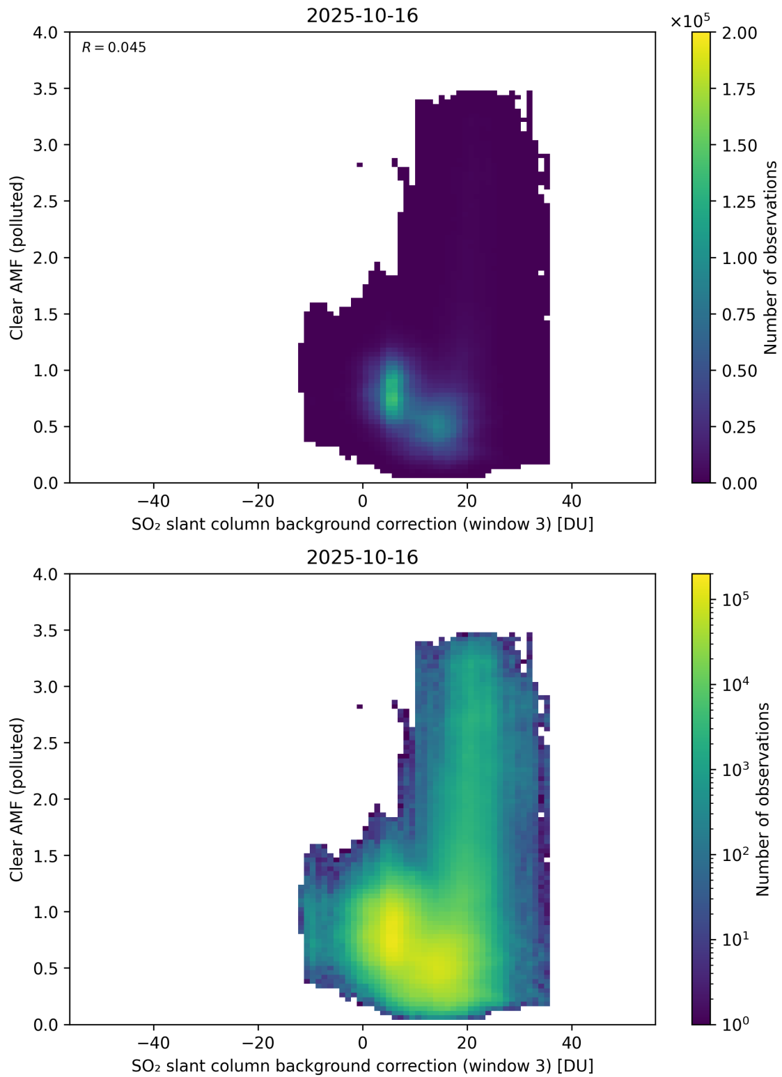
Figure 135: Scatter density plot of “SO 2 slant column background correction (window 3)” against “Clear AMF (polluted)” for 2025-10-15 to 2025-10-17.
