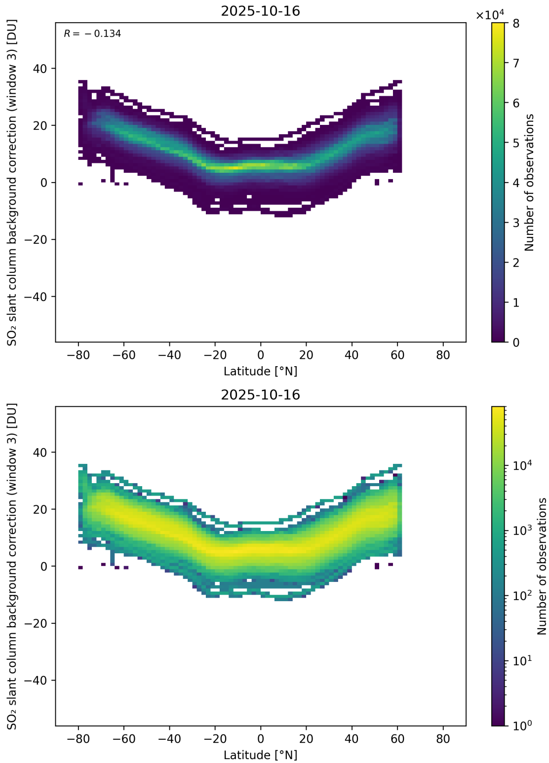
Figure 152: Scatter density plot of “Latitude” against “SO 2 slant column background correction (window 3)” for 2025-10-15 to 2025-10-17.
