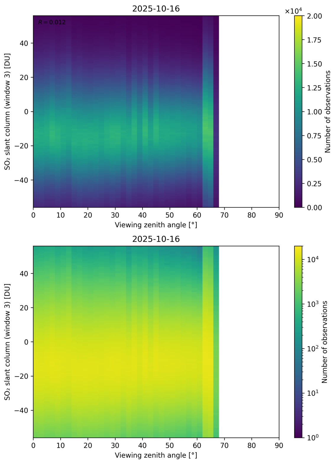
Figure 379: Scatter density plot of “Viewing zenith angle” against “SO 2 slant column (window 3)” for 2025-10-15 to 2025-10-17.
