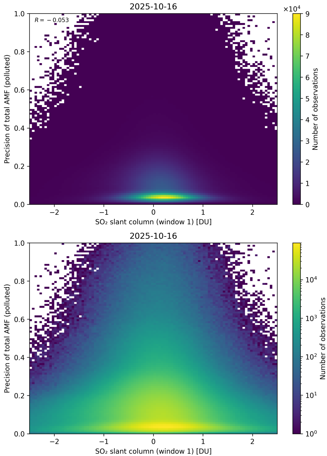
Figure 290: Scatter density plot of “SO 2 slant column (window 1)” against “Precision of total AMF (polluted)” for 2025-10-15 to 2025-10-17.
