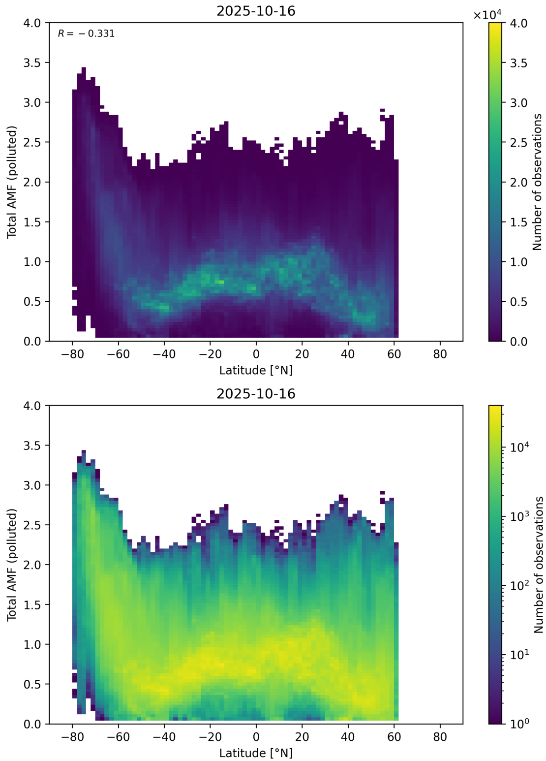
Figure 167: Scatter density plot of “Latitude” against “Total AMF (polluted)” for 2025-10-15 to 2025-10-17.
