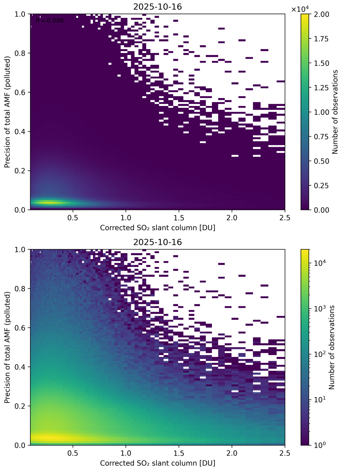
Figure 243: Scatter density plot of “Corrected SO 2 slant column” against “Precision of total AMF (polluted)” for 2025-10-15 to 2025-10-17.
