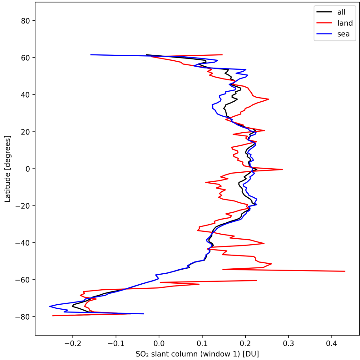
Figure 37: Zonal average of “SO 2 slant column (window 1)” for 2025-10-15 to 2025-10-17.
