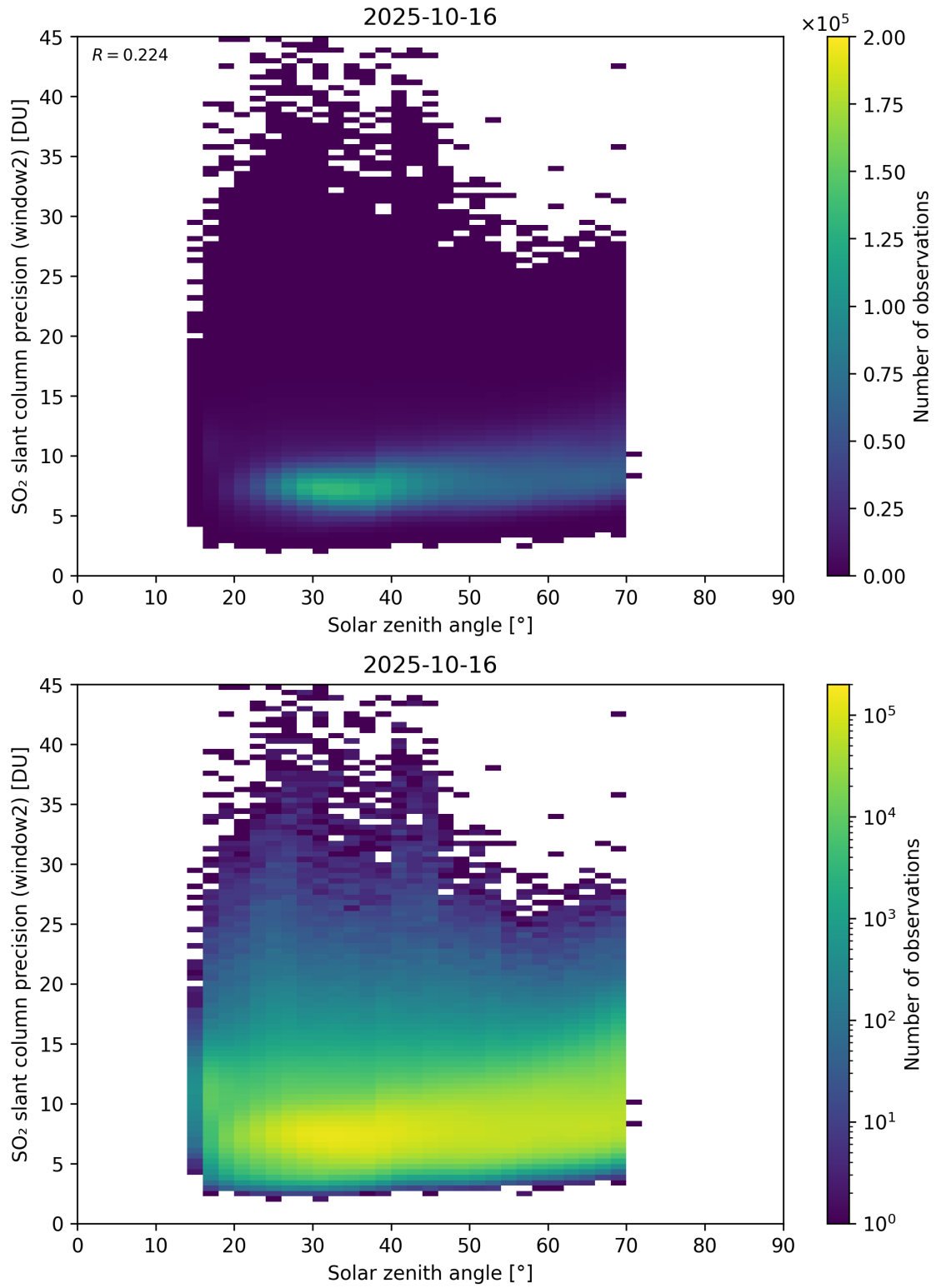
Figure 186: Scatter density plot of “Solar zenith angle” against “SO 2 slant column precision (window2)” for 2025-10-15 to 2025-10-17.
