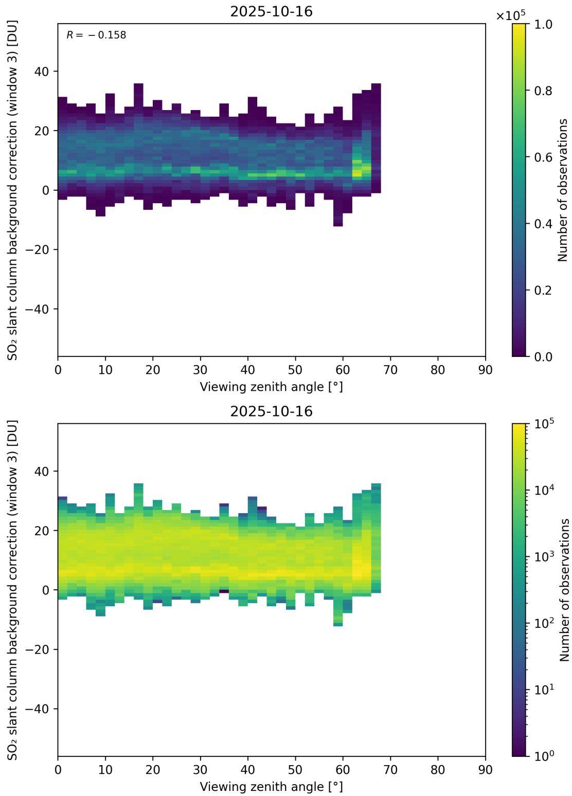
Figure 364: Scatter density plot of “Viewing zenith angle” against “SO 2 slant column background correction (window 3)” for 2025-10-15 to 2025-10-17.
