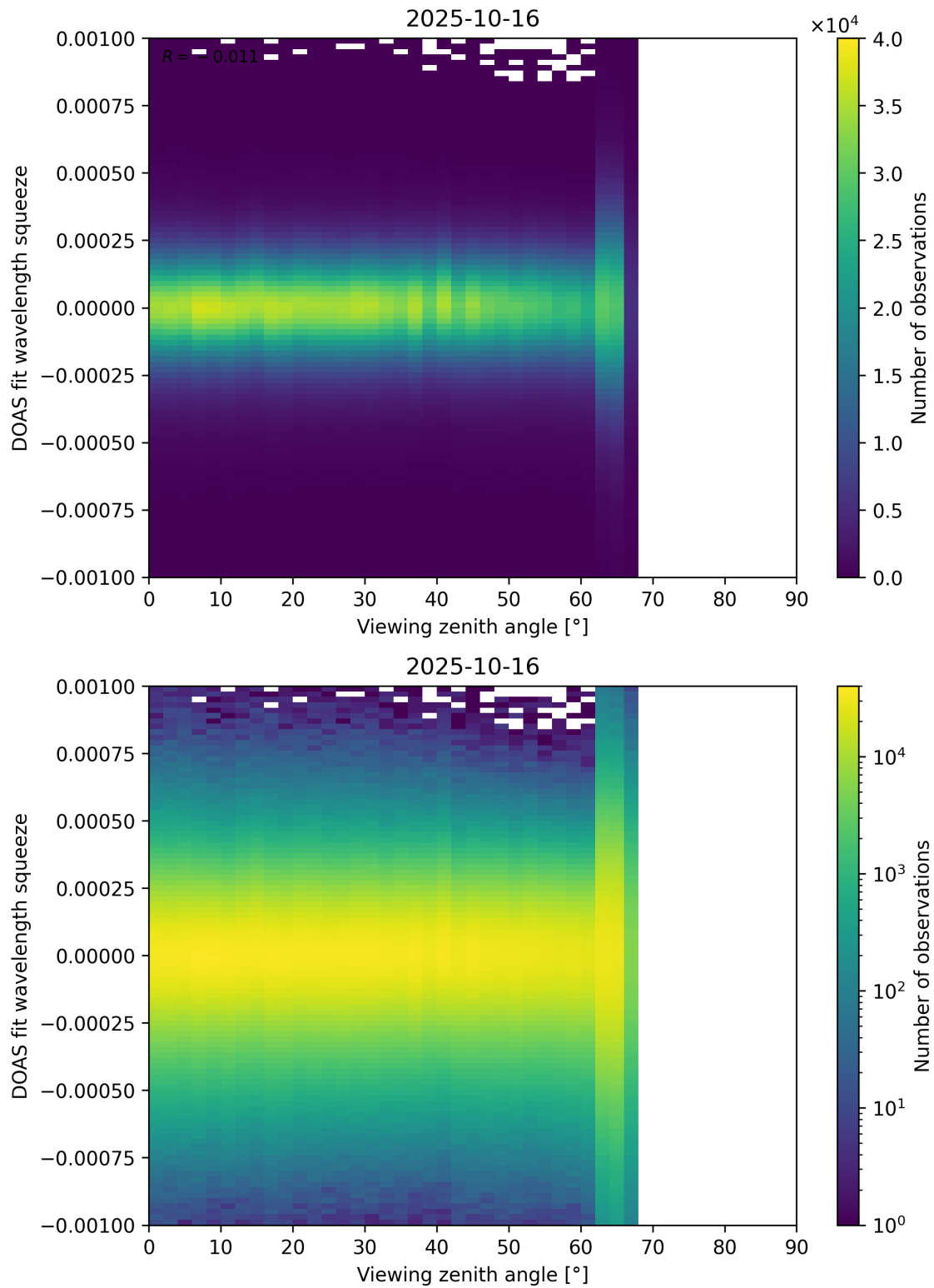
Figure 366: Scatter density plot of “Viewing zenith angle” against “DOAS fit wavelength squeeze” for 2025-10-15 to 2025-10-17.
