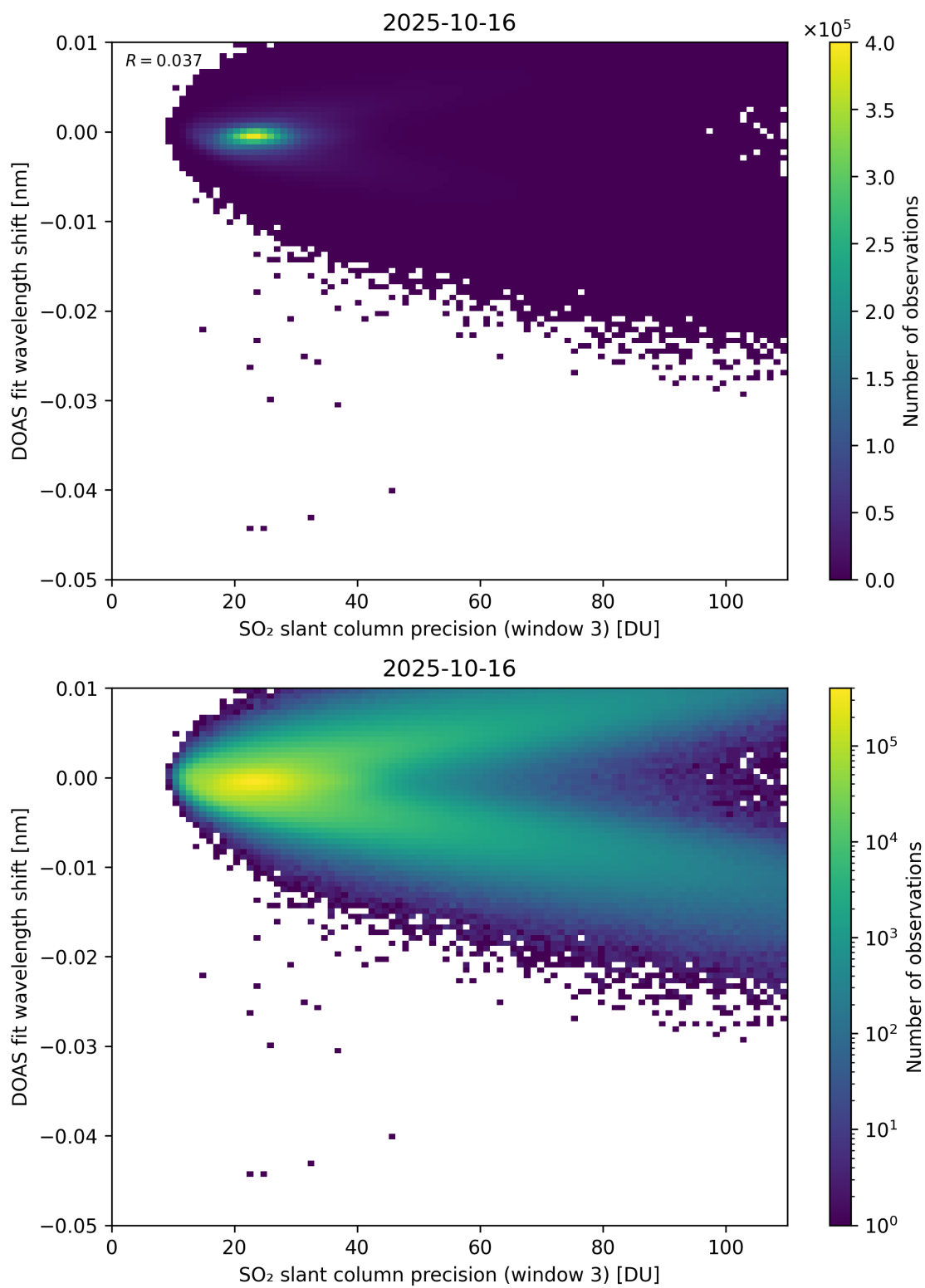
Figure 308: Scatter density plot of “SO 2 slant column precision (window 3)” against “DOAS fit wavelength shift” for 2025-10-15 to 2025-10-17.
