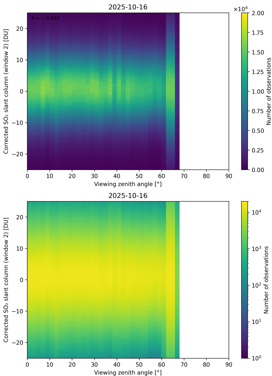
Figure 374: Scatter density plot of “Viewing zenith angle” against “Corrected SO 2 slant column (window 2)” for 2025-10-15 to 2025-10-17.
