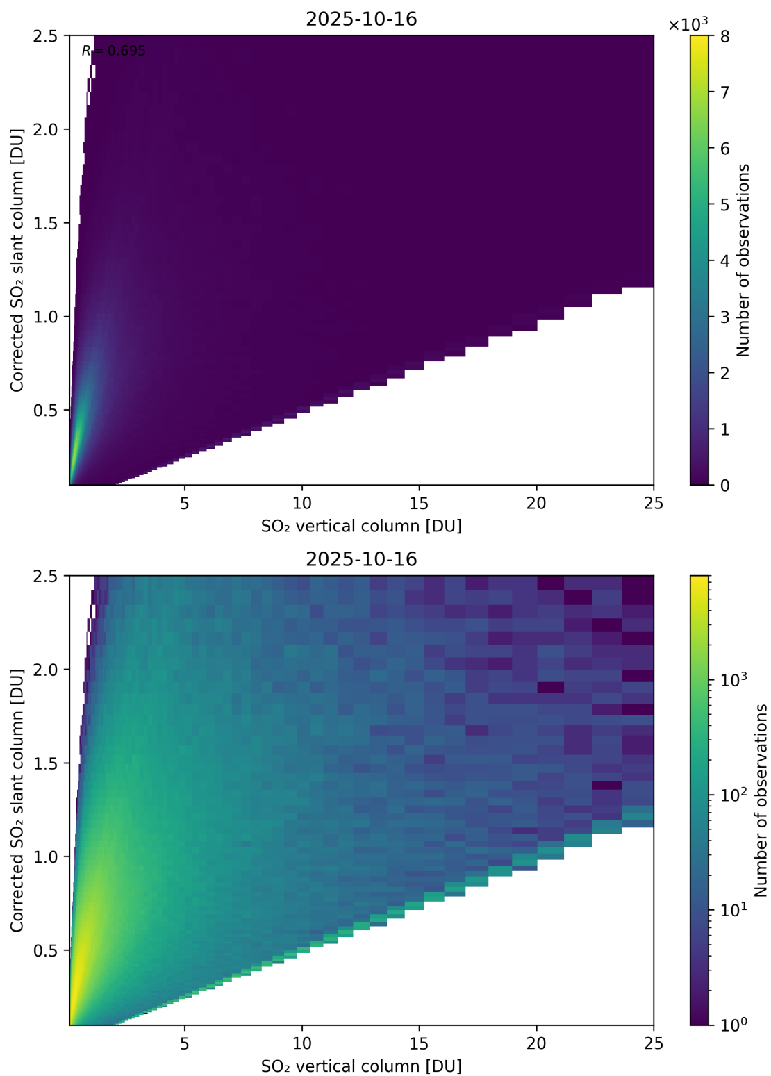
Figure 351: Scatter density plot of “SO 2 vertical column” against “Corrected SO 2 slant column” for 2025-10-15 to 2025-10-17.
