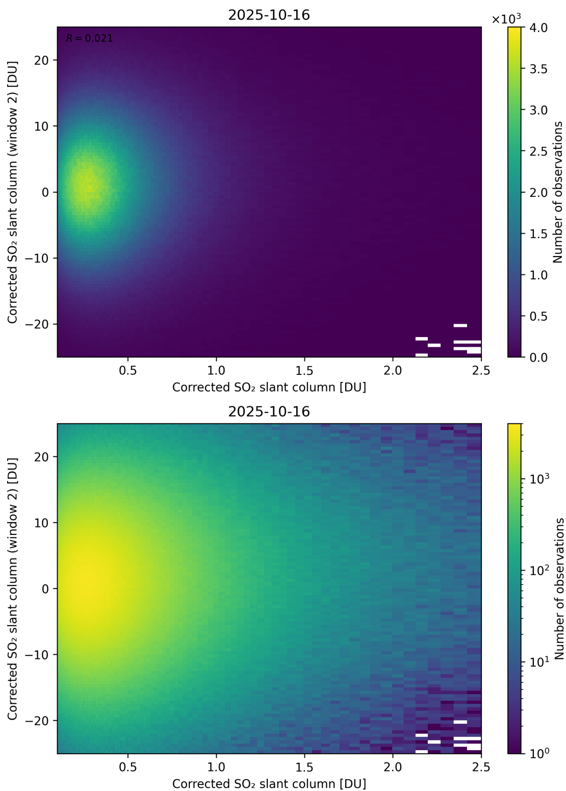
Figure 235: Scatter density plot of “Corrected SO 2 slant column” against “Corrected SO 2 slant column (window 2)” for 2025-10-15 to 2025-10-17.
