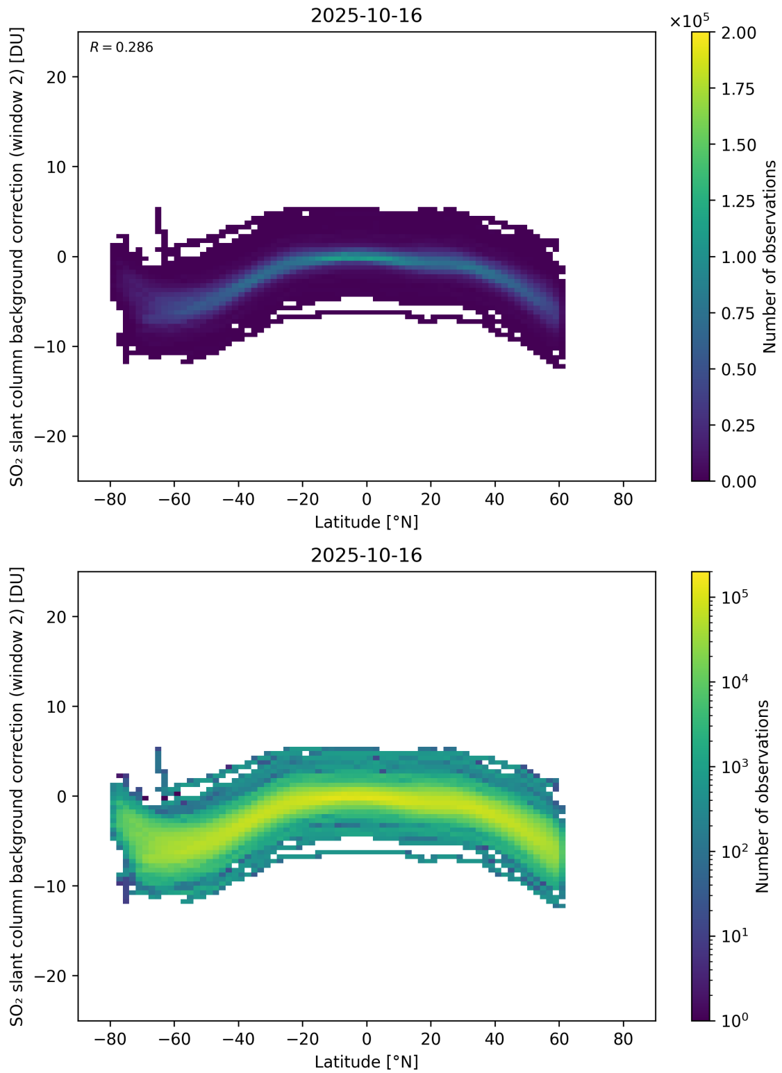
Figure 151: Scatter density plot of “Latitude” against “SO 2 slant column background correction (window 2)” for 2025-10-15 to 2025-10-17.
