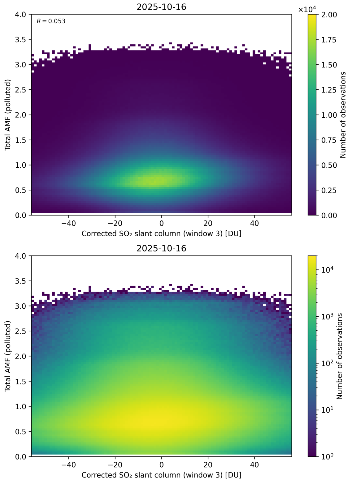
Figure 260: Scatter density plot of “Corrected SO 2 slant column (window 3)” against “Total AMF (polluted)” for 2025-10-15 to 2025-10-17.
