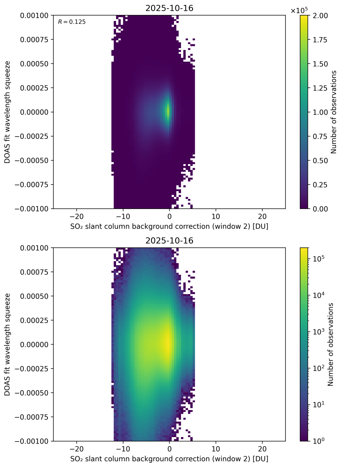
Figure 124: Scatter density plot of “SO 2 slant column background correction (window 2)” against “DOAS fit wavelength squeeze” for 2025-10-15 to 2025-10-17.
