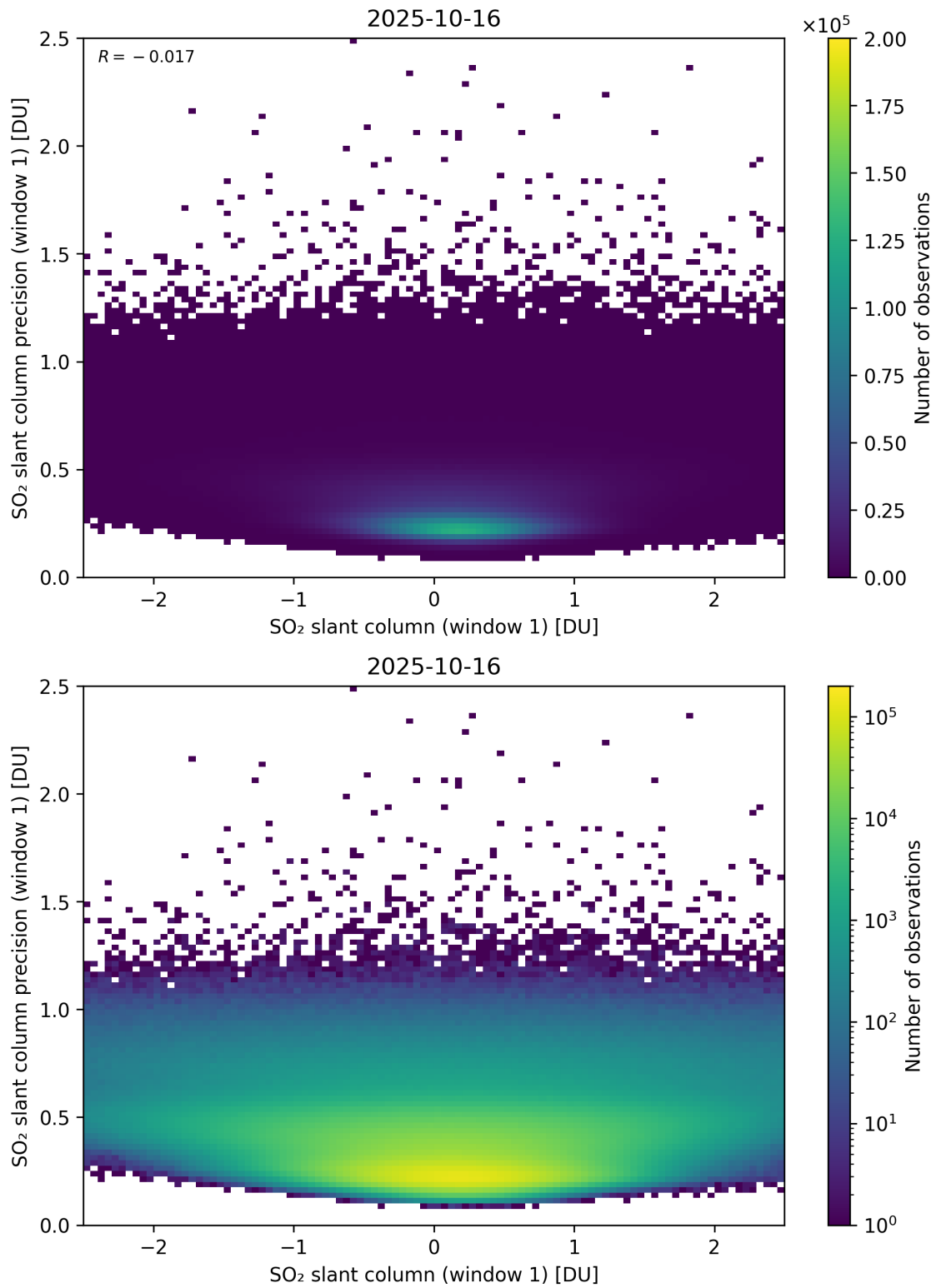
Figure 285: Scatter density plot of “SO 2 slant column (window 1)” against “SO 2 slant column precision (window 1)” for 2025-10-15 to 2025-10-17.
