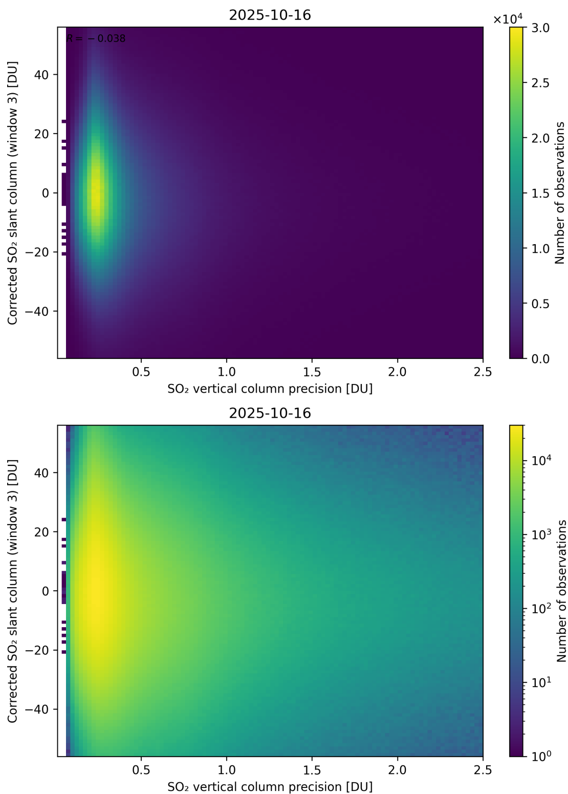
Figure 340: Scatter density plot of “SO 2 vertical column precision” against “Corrected SO 2 slant column (window 3)” for 2025-10-15 to 2025-10-17.
