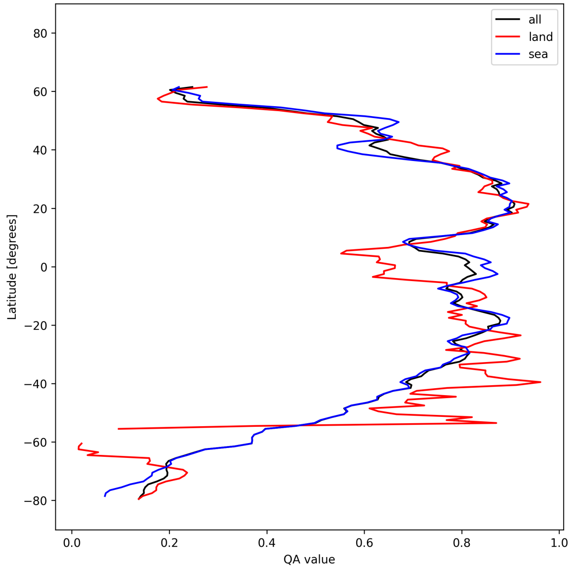
Figure 31: Zonal average of “QA value” for 2025-10-15 to 2025-10-17.
