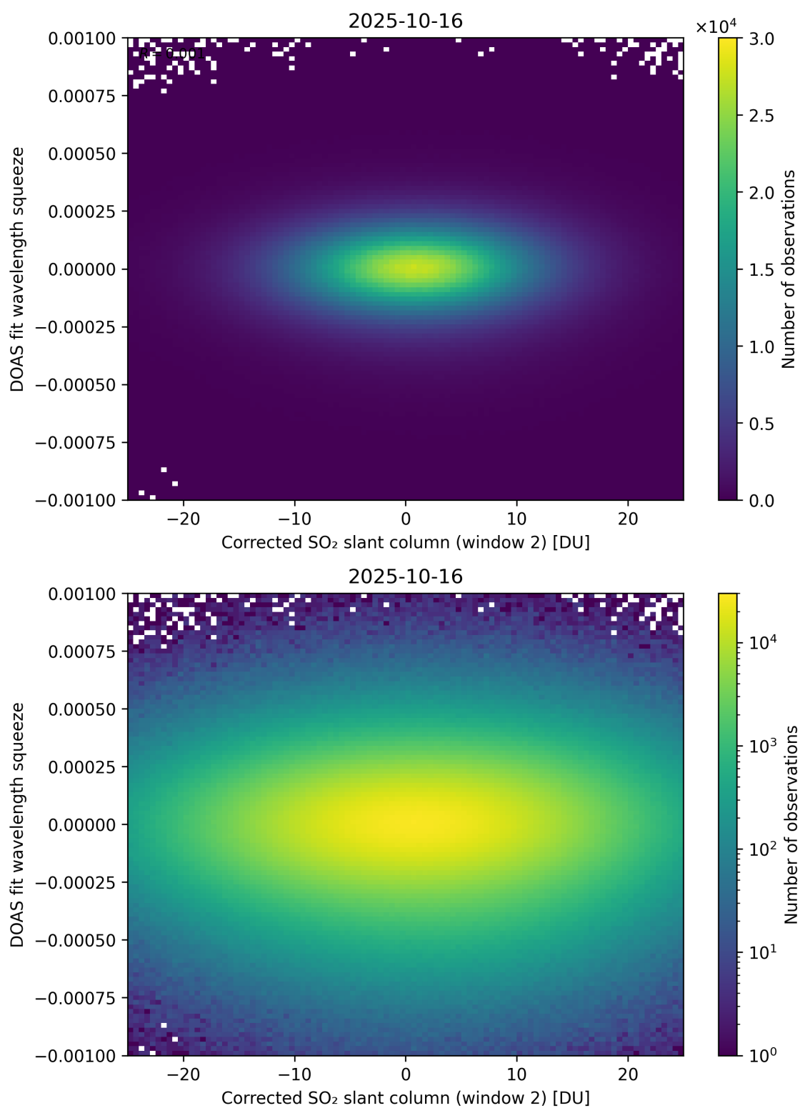
Figure 247: Scatter density plot of “Corrected SO 2 slant column (window 2)” against “DOAS fit wavelength squeeze” for 2025-10-15 to 2025-10-17.
