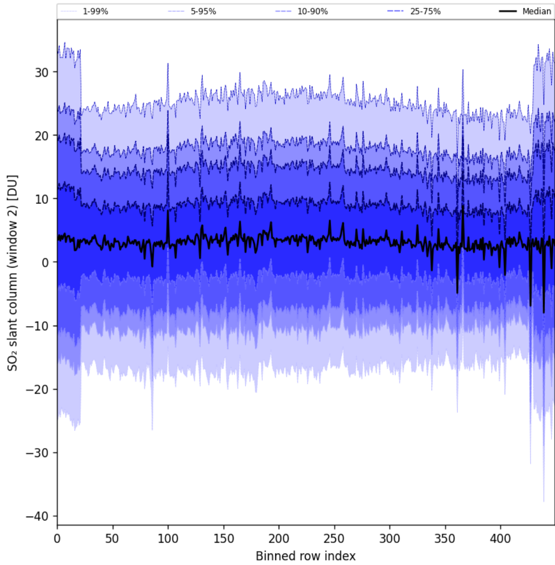
Figure 93: Along track statistics of “SO 2 slant column (window 2)” for 2025-10-15 to 2025-10-17
