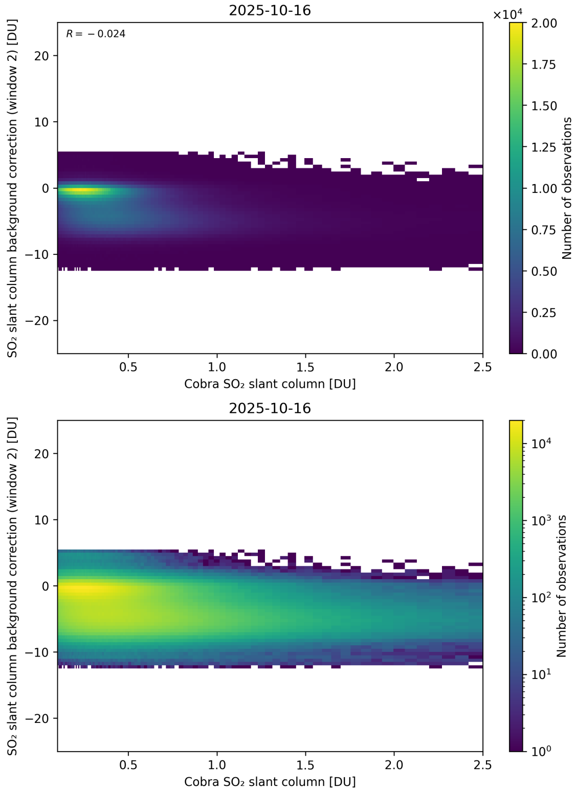
Figure 194: Scatter density plot of “Cobra SO 2 slant column” against “SO 2 slant column background correction (window 2)” for 2025-10-15 to 2025-10-17.
