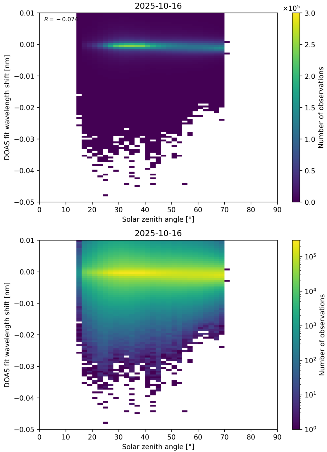
Figure 174: Scatter density plot of “Solar zenith angle” against “DOAS fit wavelength shift” for 2025-10-15 to 2025-10-17.
