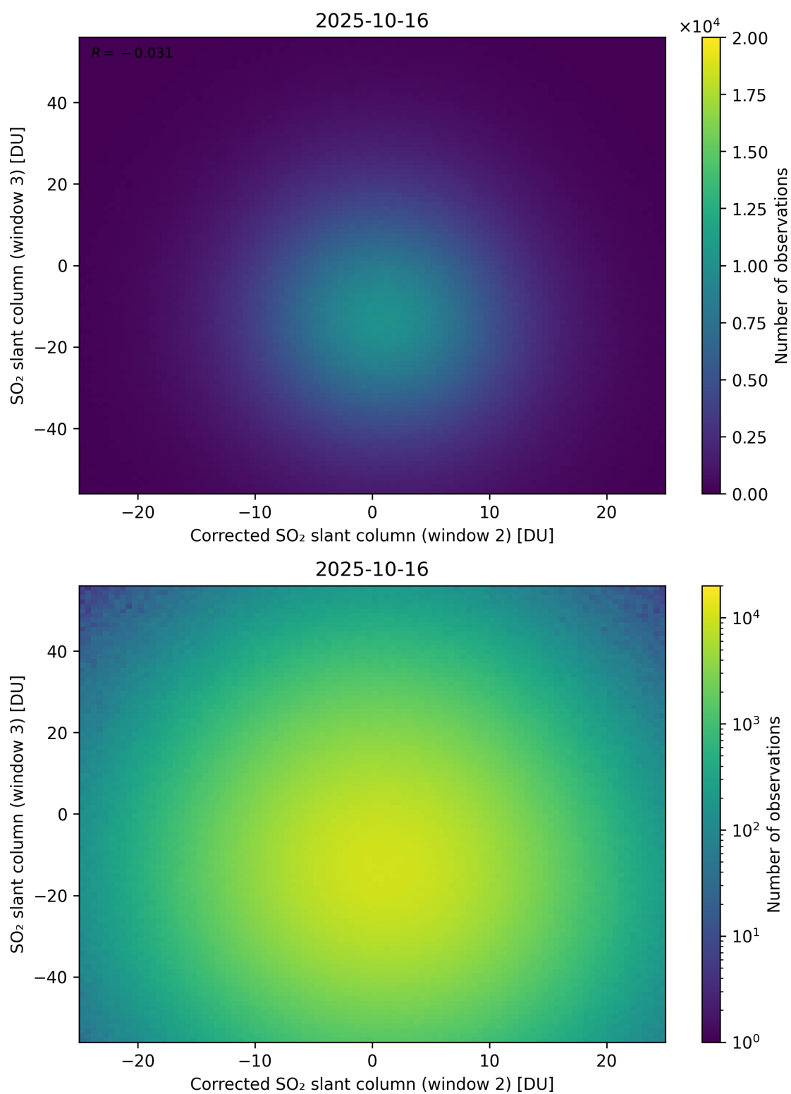
Figure 251: Scatter density plot of “Corrected SO 2 slant column (window 2)” against “SO 2 slant column (window 3)” for 2025-10-15 to 2025-10-17.
