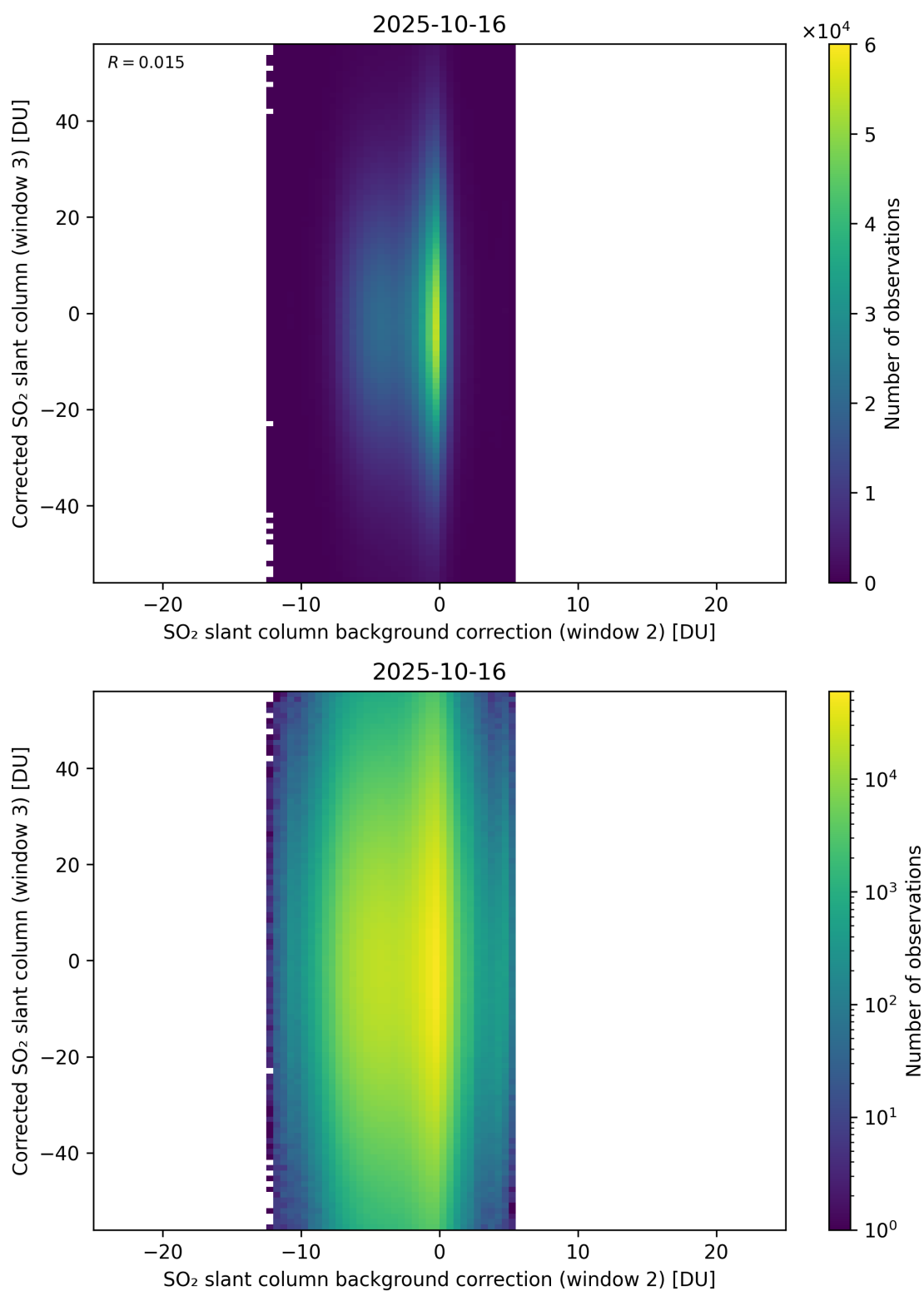
Figure 127: Scatter density plot of “SO 2 slant column background correction (window 2)” against “Corrected SO 2 slant column (window 3)” for 2025-10-15 to 2025-10-17.
