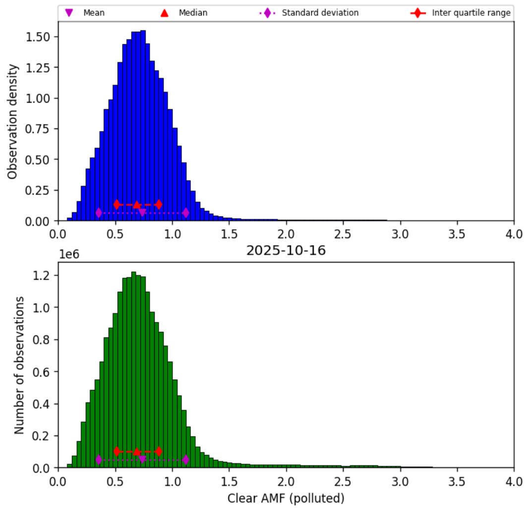
Figure 81: Histogram of “Clear AMF (polluted)” for 2025-10-15 to 2025-10-17
