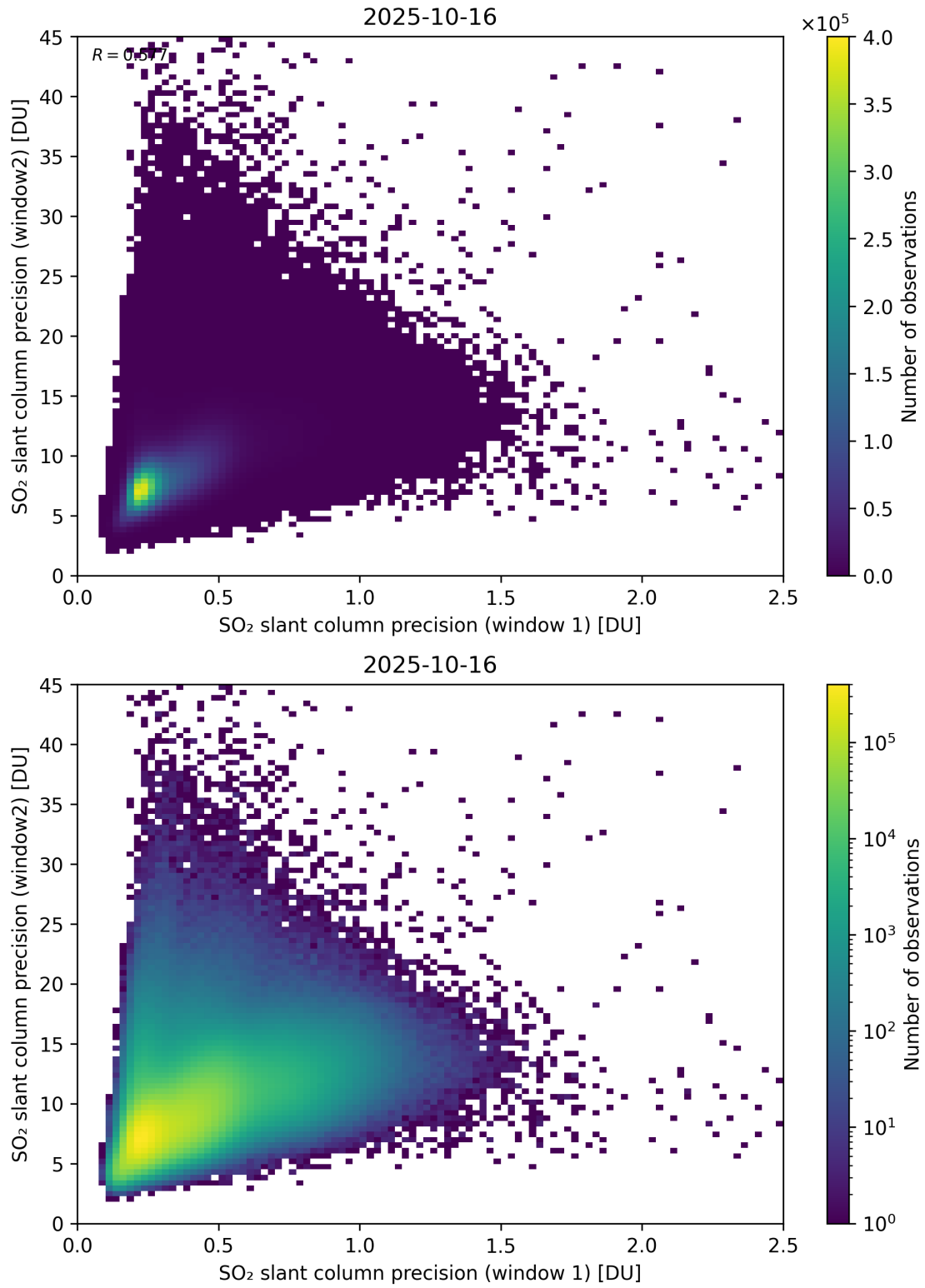
Figure 277: Scatter density plot of “SO 2 slant column precision (window 1)” against “SO 2 slant column precision (window2)” for 2025-10-15 to 2025-10-17.
