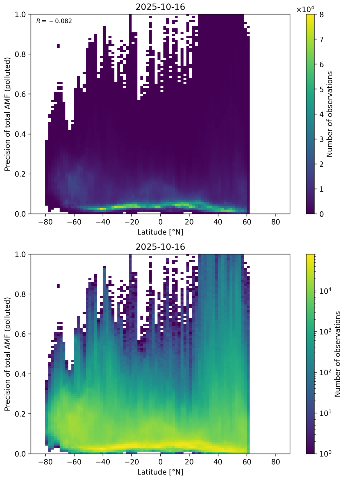
Figure 168: Scatter density plot of “Latitude” against “Precision of total AMF (polluted)” for 2025-10-15 to 2025-10-17.
