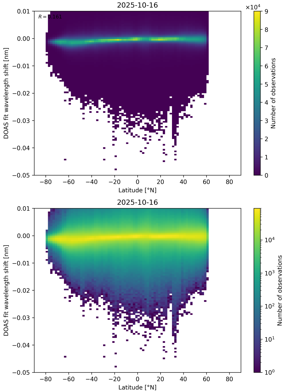
Figure 153: Scatter density plot of “Latitude” against “DOAS fit wavelength shift” for 2025-10-15 to 2025-10-17.
