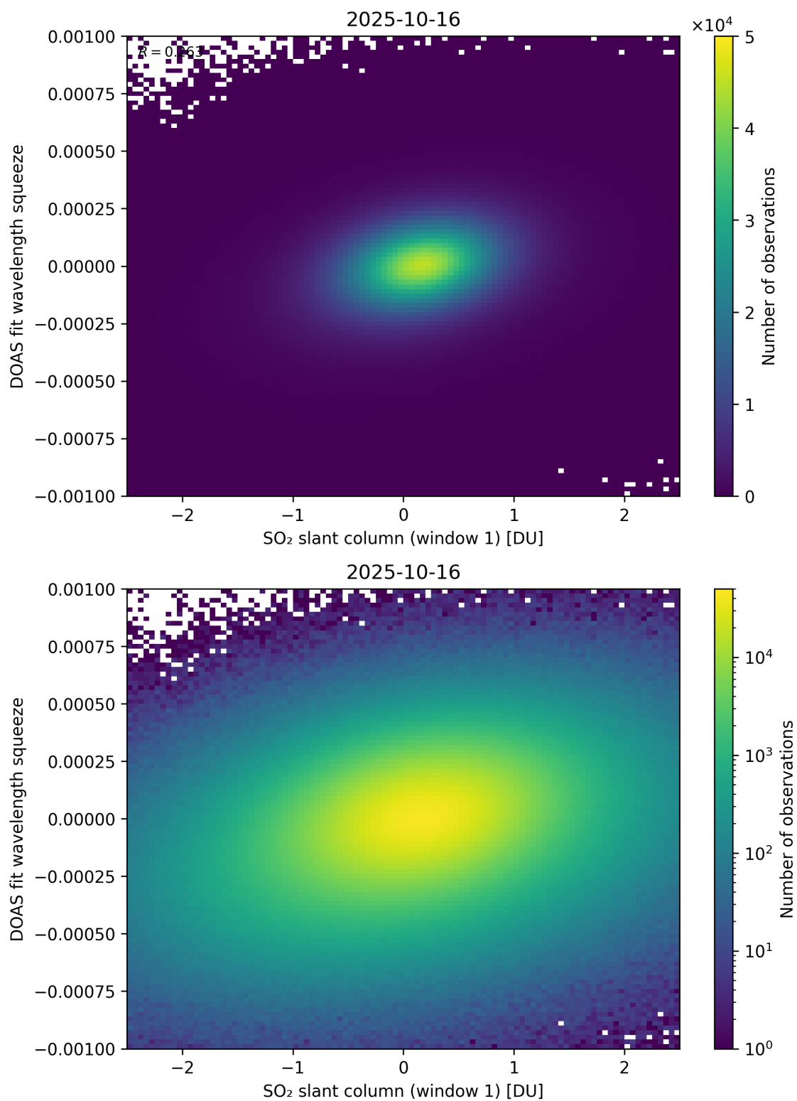
Figure 266: Scatter density plot of “SO 2 slant column (window 1)” against “DOAS fit wavelength squeeze” for 2025-10-15 to 2025-10-17.
