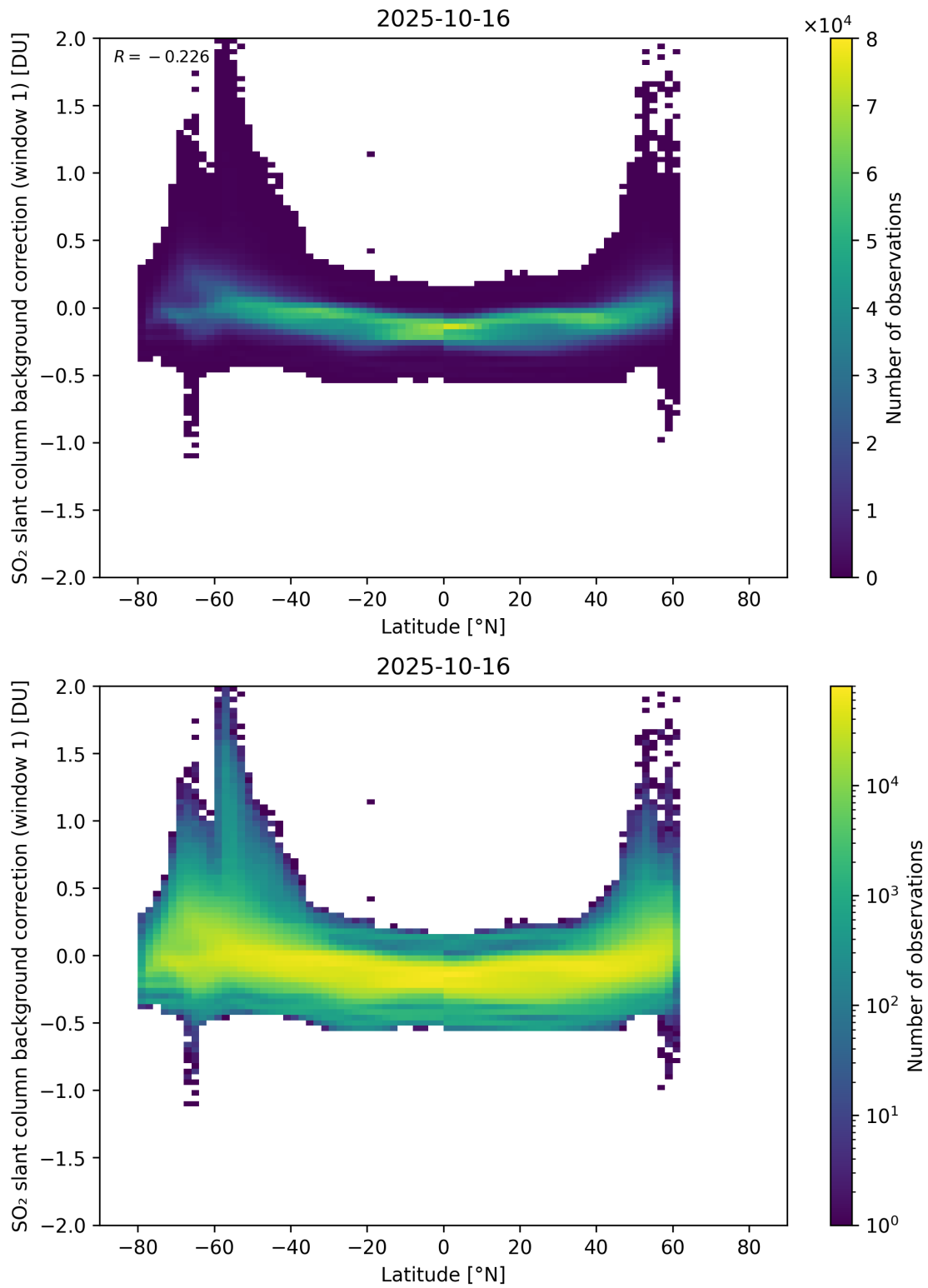
Figure 150: Scatter density plot of “Latitude” against “SO 2 slant column background correction (window 1)” for 2025-10-15 to 2025-10-17.
