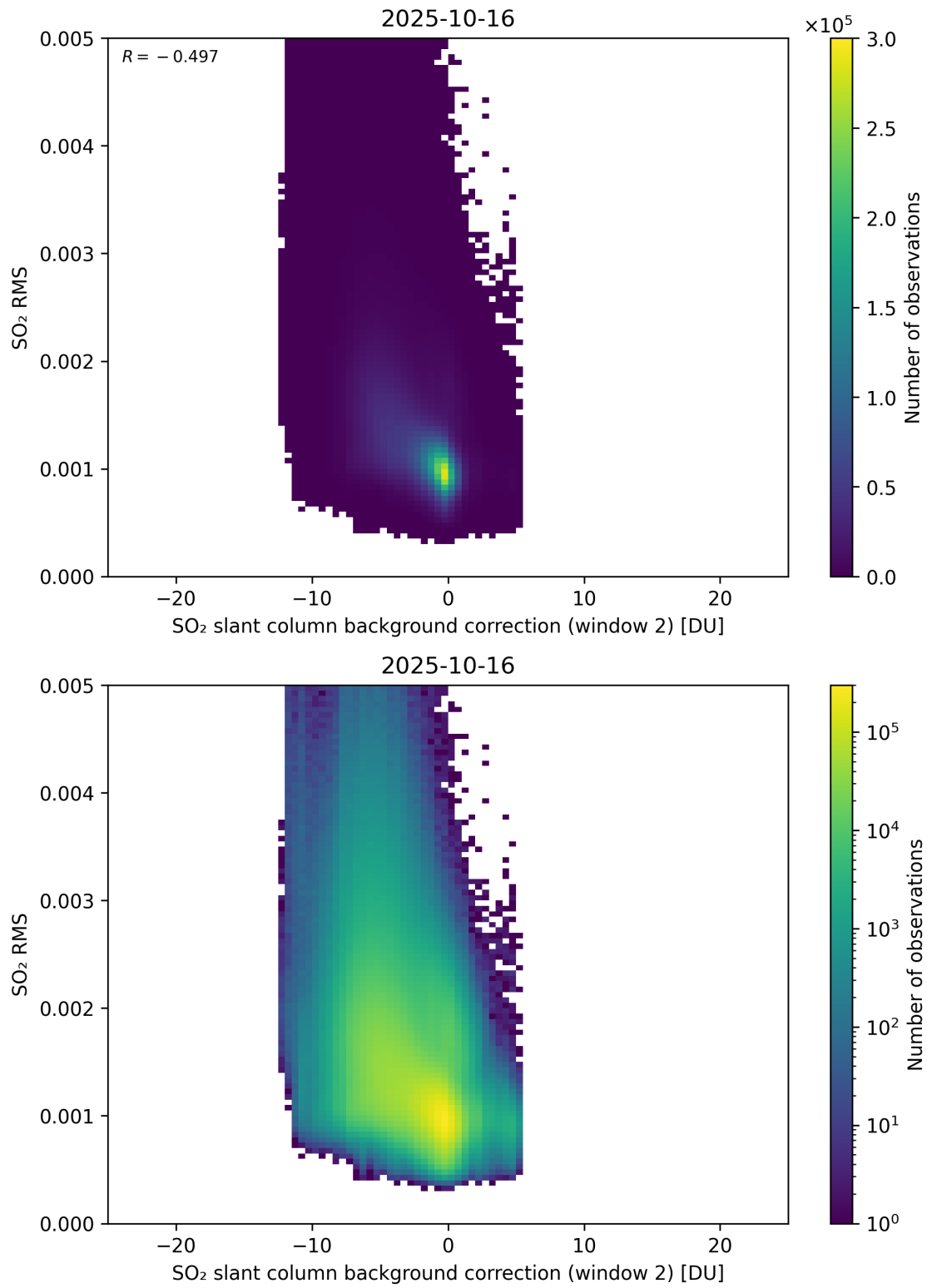
Figure 125: Scatter density plot of “SO 2 slant column background correction (window 2)” against “SO 2 RMS” for 2025-10-15 to 2025-10-17.
