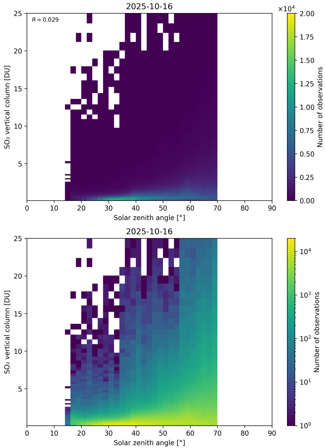
Figure 191: Scatter density plot of “Solar zenith angle” against “SO 2 vertical column” for 2025-10-15 to 2025-10-17.
