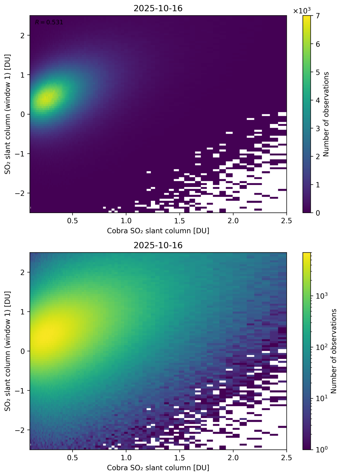
Figure 219: Scatter density plot of “Cobra SO 2 slant column” against “SO 2 slant column (window 1)” for 2025-10-15 to 2025-10-17.
