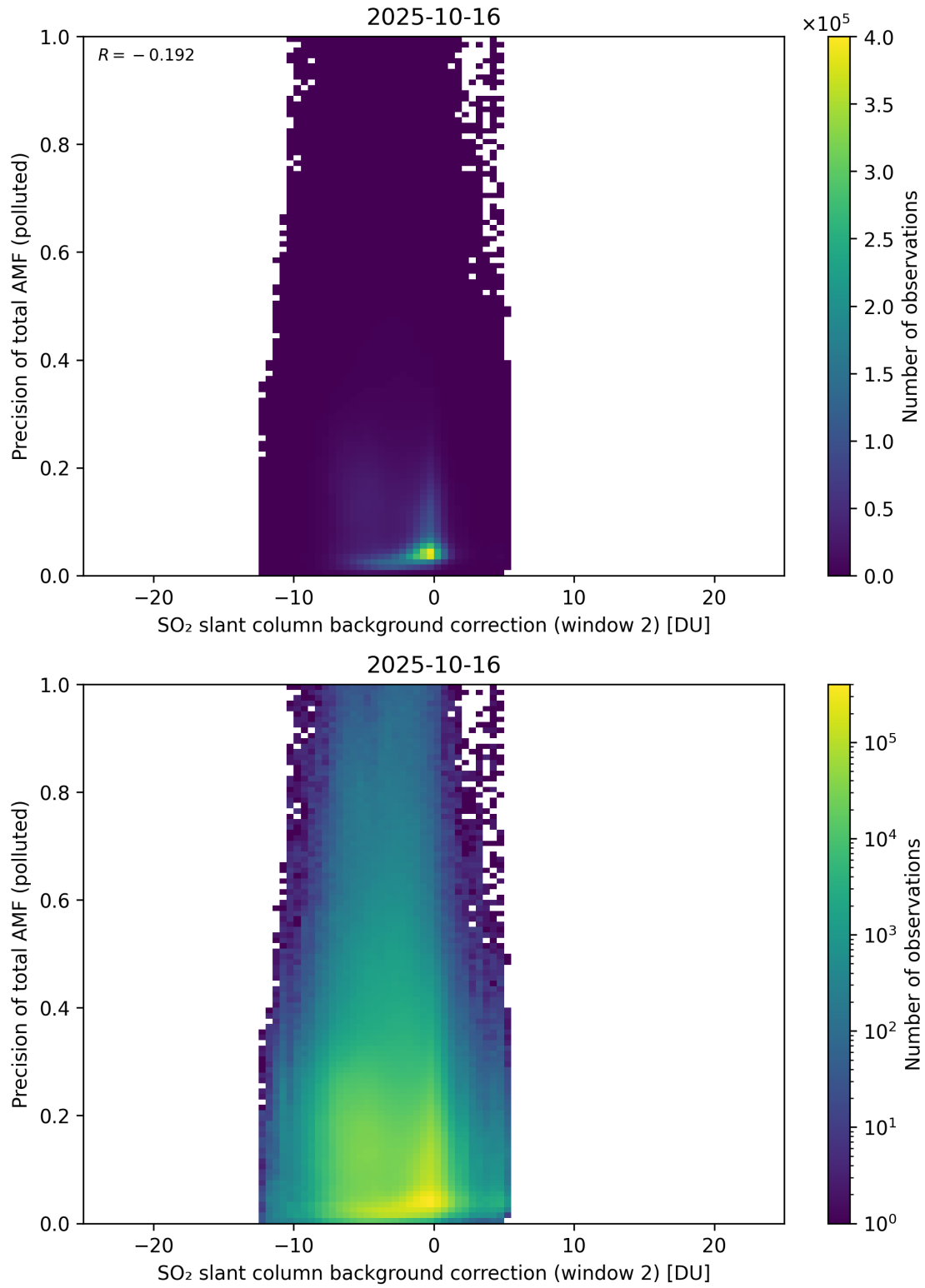
Figure 131: Scatter density plot of “SO 2 slant column background correction (window 2)” against “Precision of total AMF (polluted)” for 2025-10-15 to 2025-10-17.
