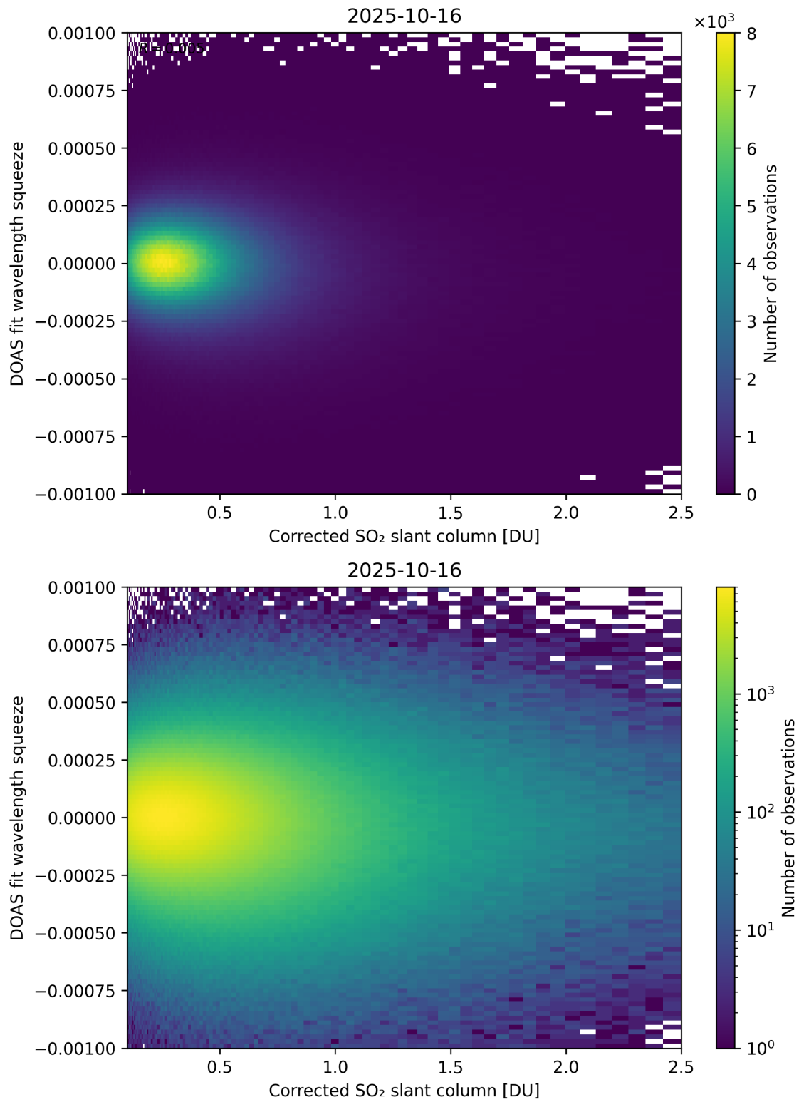
Figure 230: Scatter density plot of “Corrected SO 2 slant column” against “DOAS fit wavelength squeeze” for 2025-10-15 to 2025-10-17.
