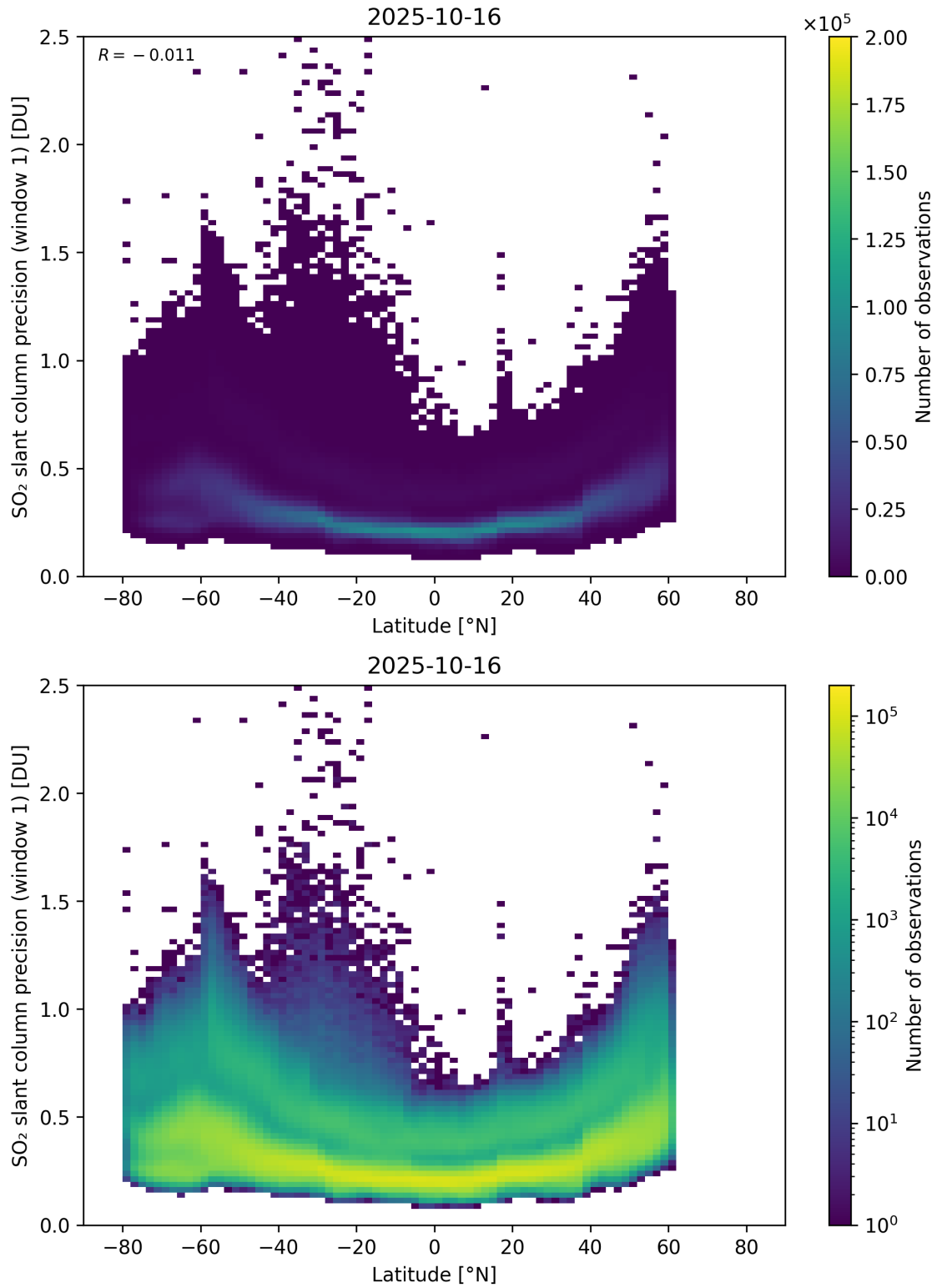
Figure 163: Scatter density plot of “Latitude” against “SO 2 slant column precision (window 1)” for 2025-10-15 to 2025-10-17.
