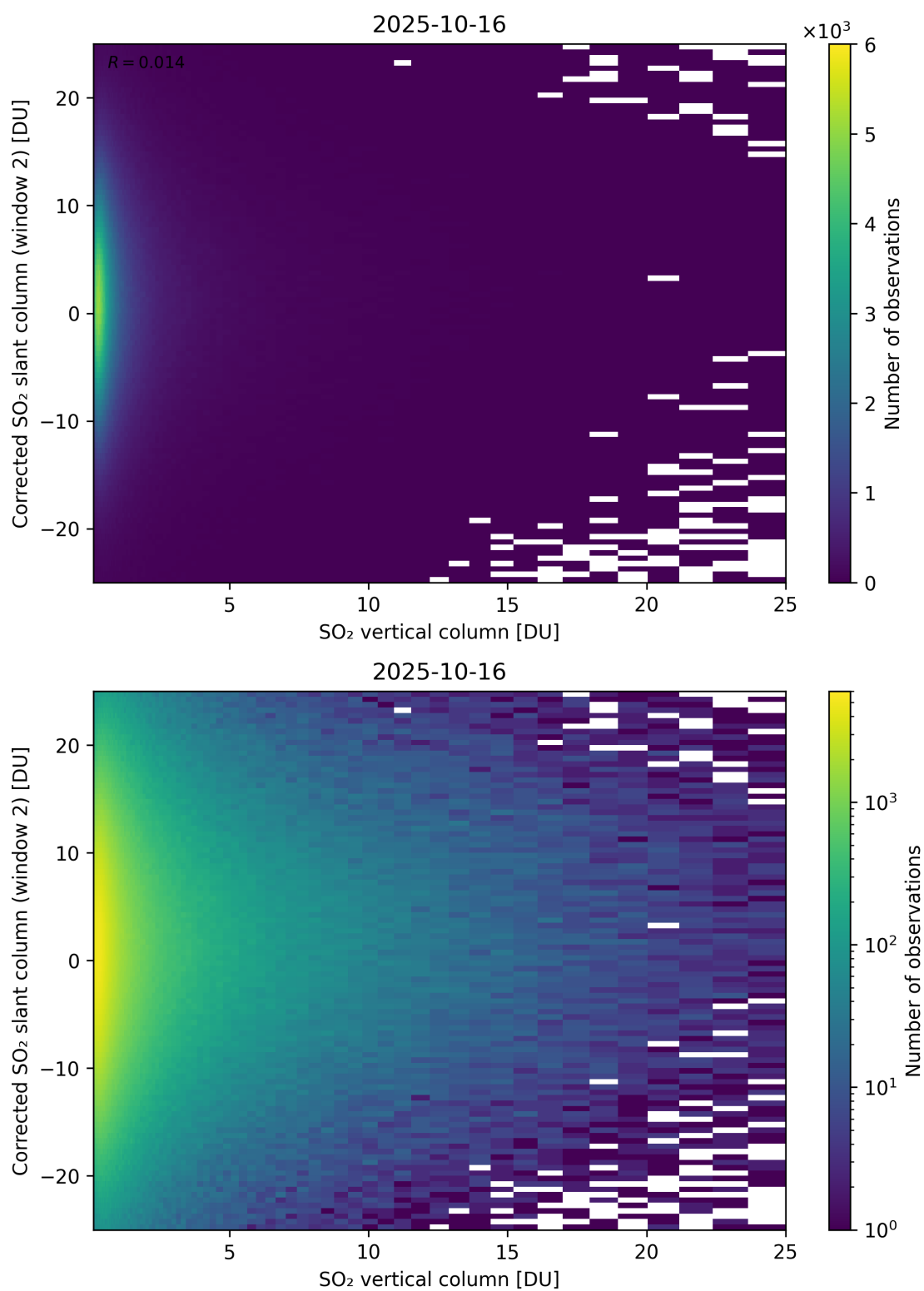
Figure 352: Scatter density plot of “SO 2 vertical column” against “Corrected SO 2 slant column (window 2)” for 2025-10-15 to 2025-10-17.
