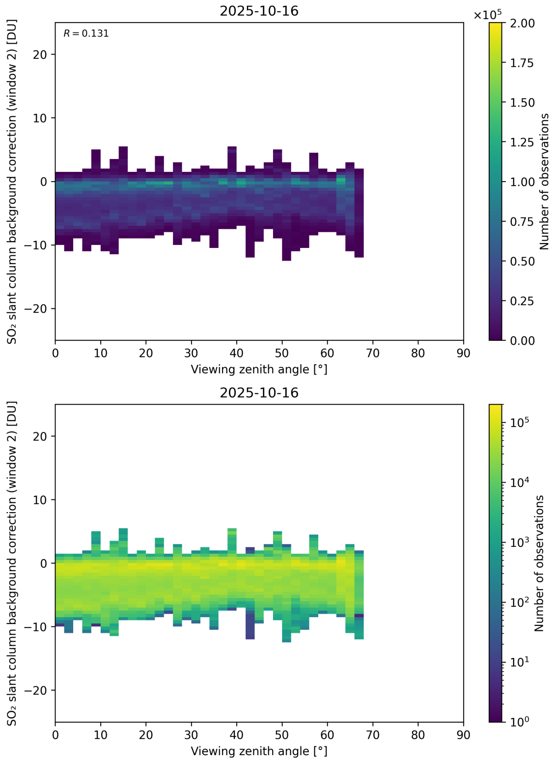
Figure 363: Scatter density plot of “Viewing zenith angle” against “SO 2 slant column background correction (window 2)” for 2025-10-15 to 2025-10-17.
