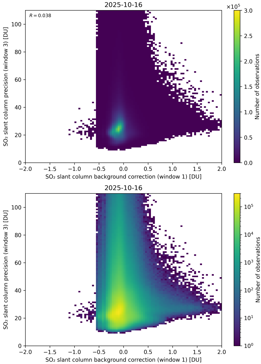
Figure 119: Scatter density plot of “SO 2 slant column background correction (window 1)” against “SO 2 slant column precision (window 3)” for 2025-10-15 to 2025-10-17.
