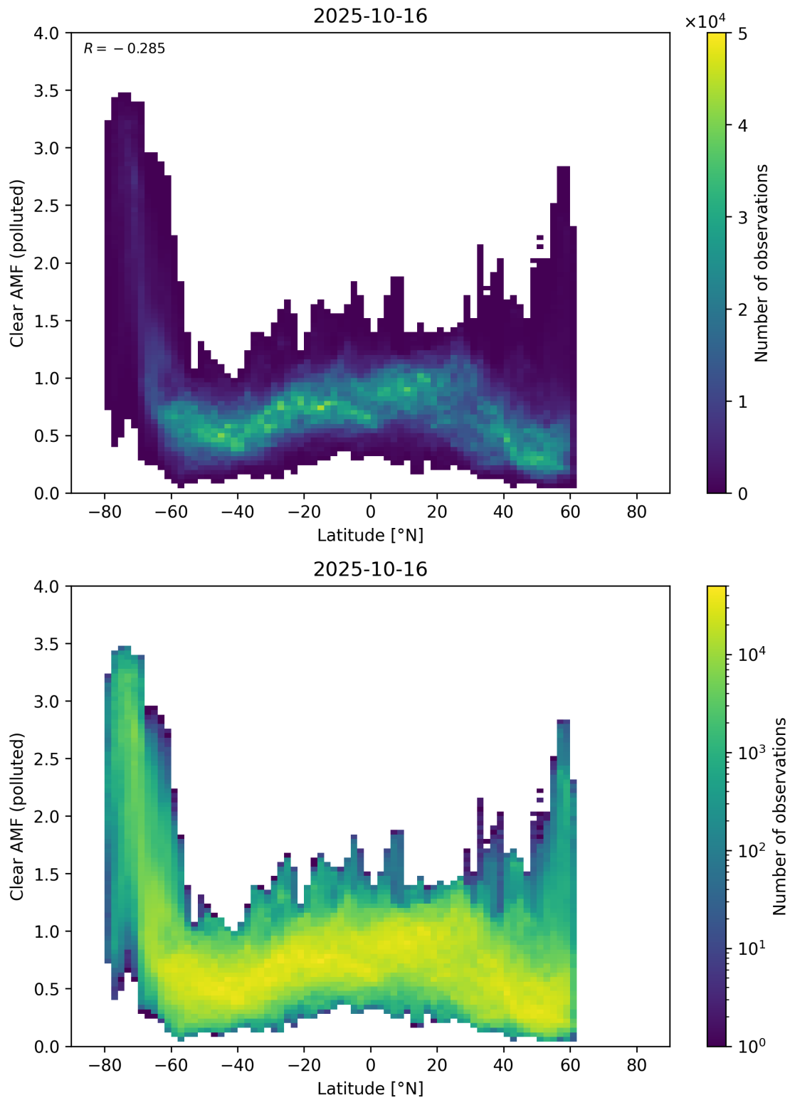
Figure 156: Scatter density plot of “Latitude” against “Clear AMF (polluted)” for 2025-10-15 to 2025-10-17.
