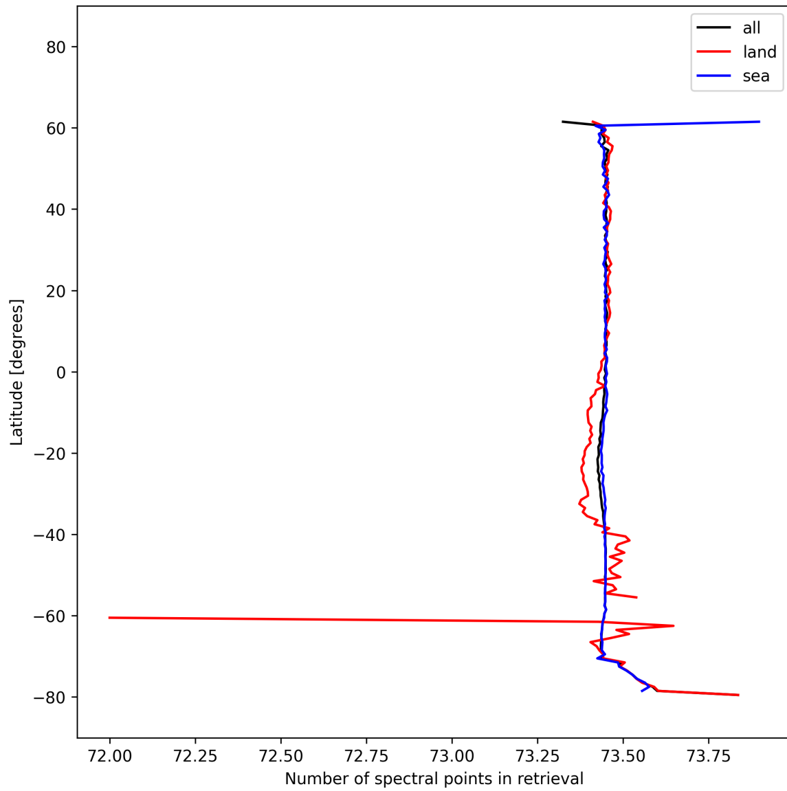
Figure 56: Zonal average of “Number of spectral points in retrieval” for 2025-10-15 to 2025-10-17.
