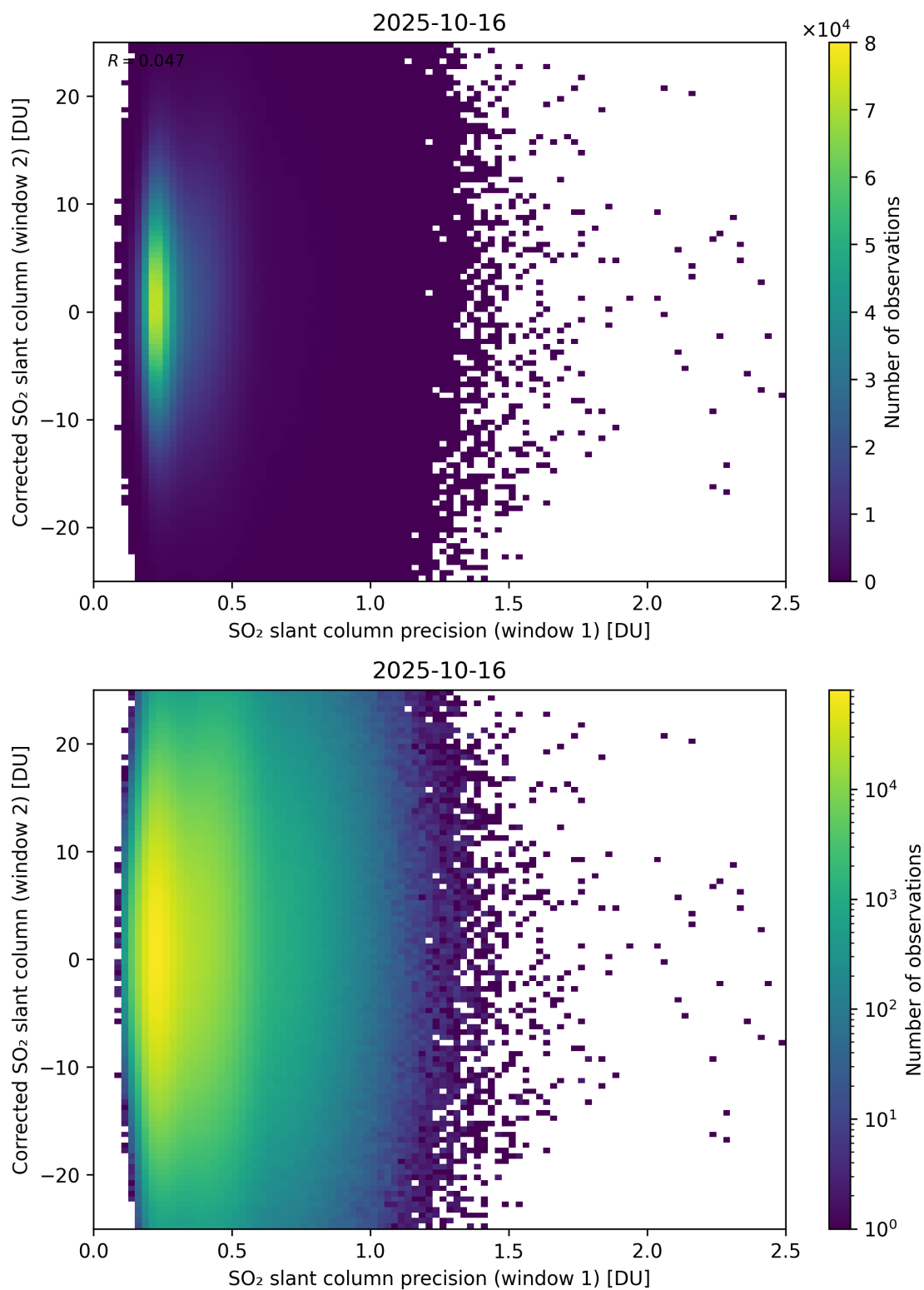
Figure 275: Scatter density plot of “SO 2 slant column precision (window 1)” against “Corrected SO 2 slant column (window 2)” for 2025-10-15 to 2025-10-17.
