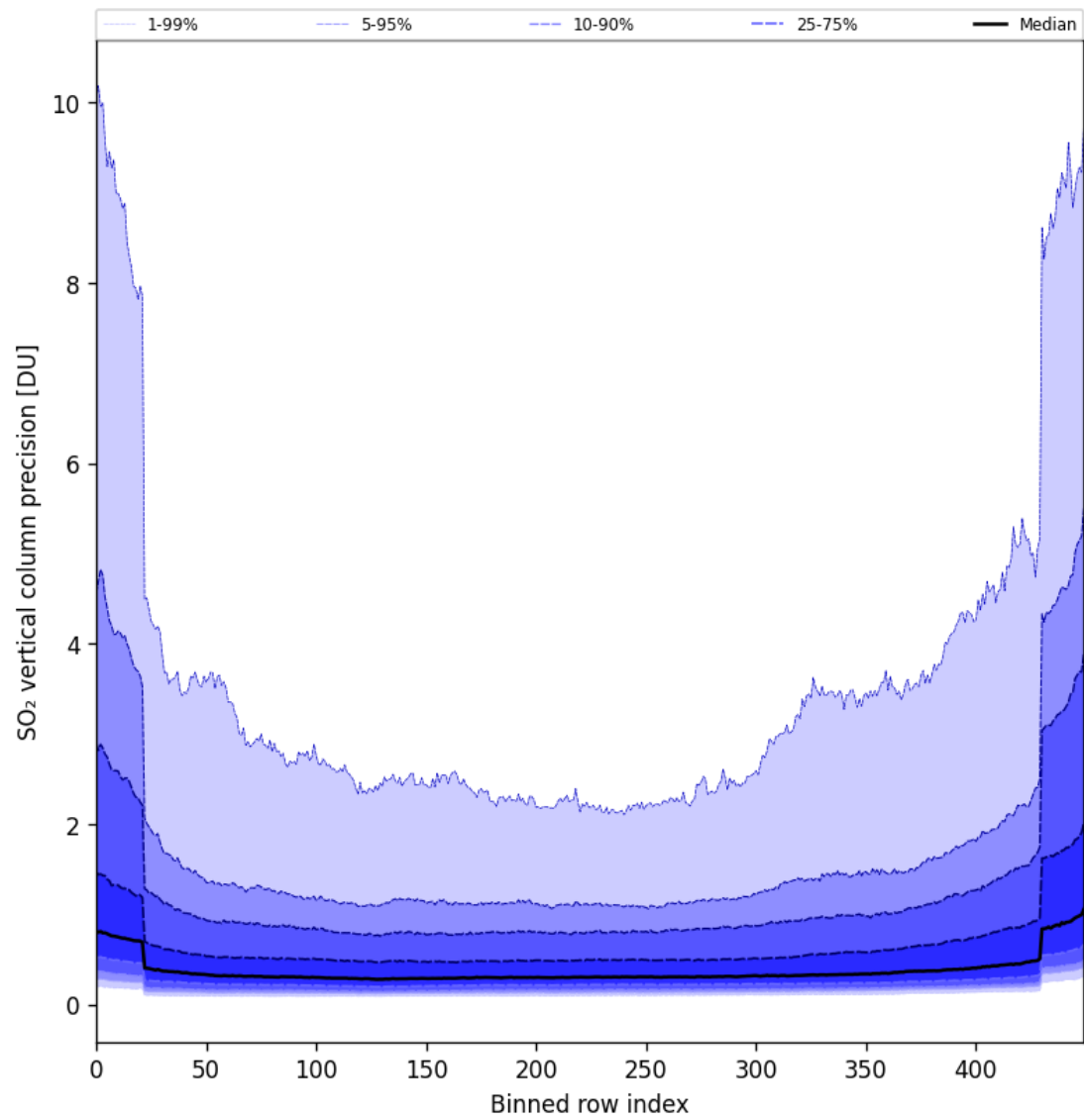
Figure 85: Along track statistics of “SO 2 vertical column precision” for 2025-10-15 to 2025-10-17
