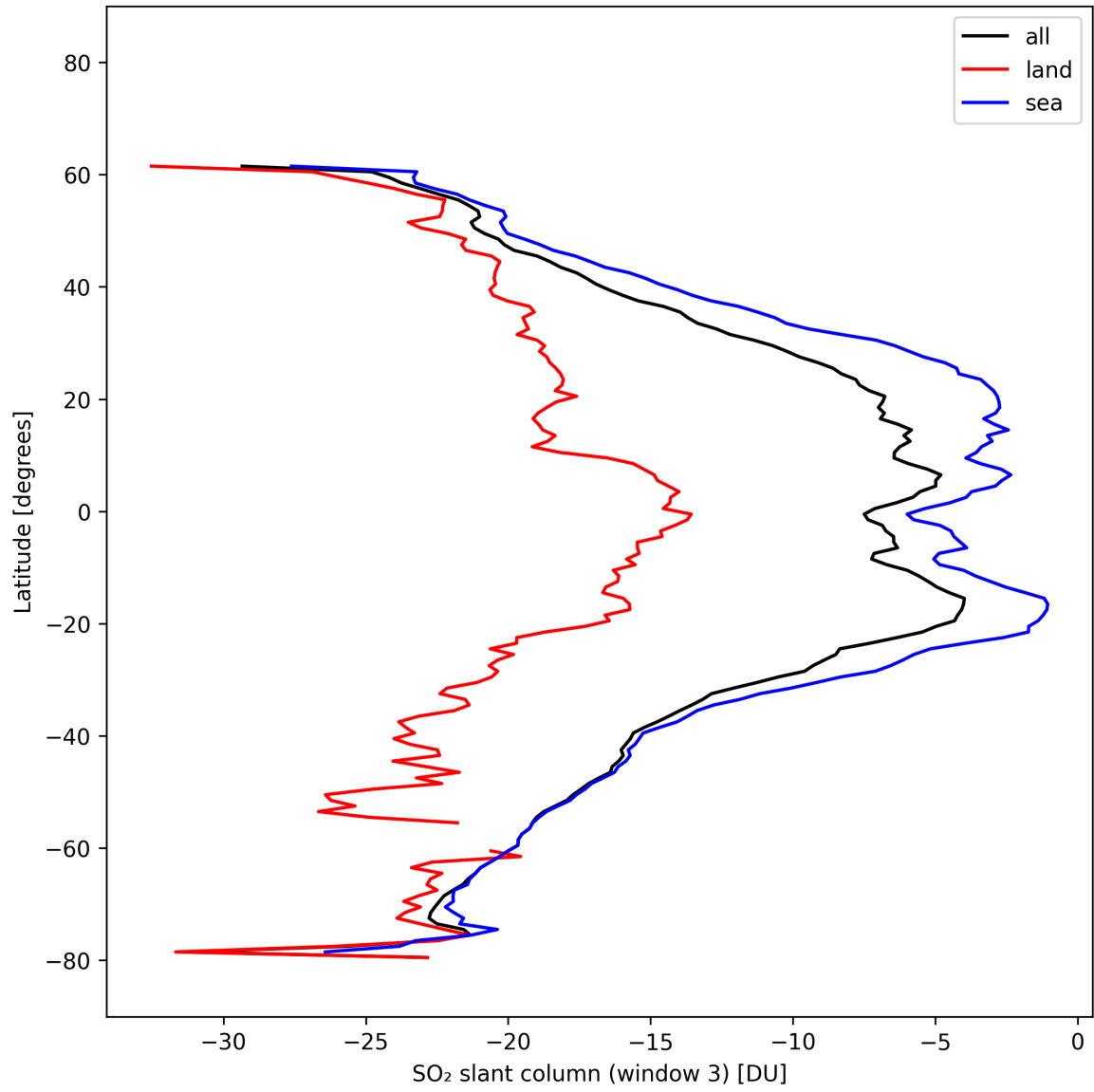
Figure 45: Zonal average of “SO 2 slant column (window 3)” for 2025-10-15 to 2025-10-17.
