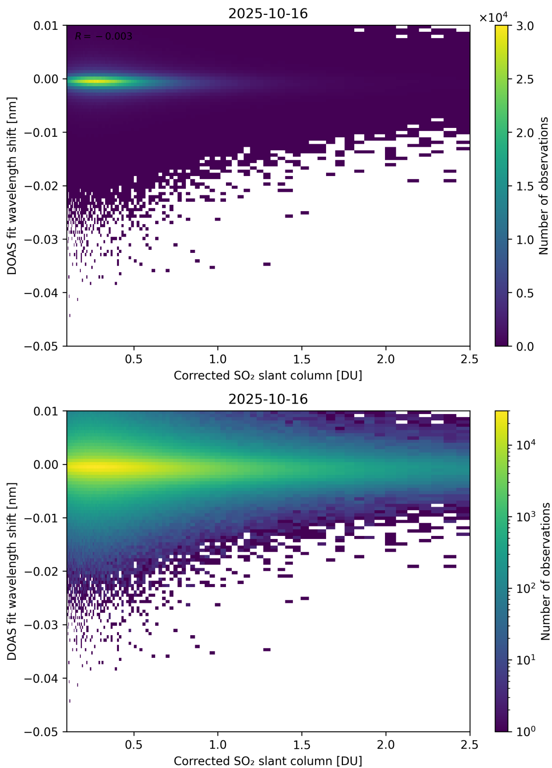
Figure 229: Scatter density plot of “Corrected SO 2 slant column” against “DOAS fit wavelength shift” for 2025-10-15 to 2025-10-17.
