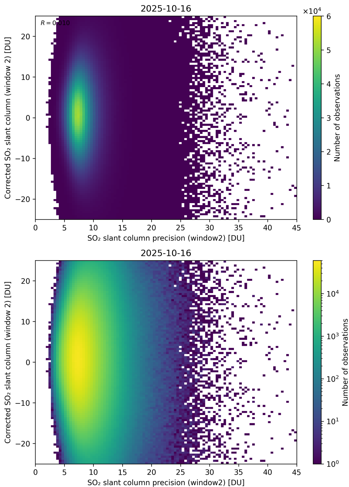
Figure 297: Scatter density plot of “SO 2 slant column precision (window2)” against “Corrected SO 2 slant column (window 2)” for 2025-10-15 to 2025-10-17.
