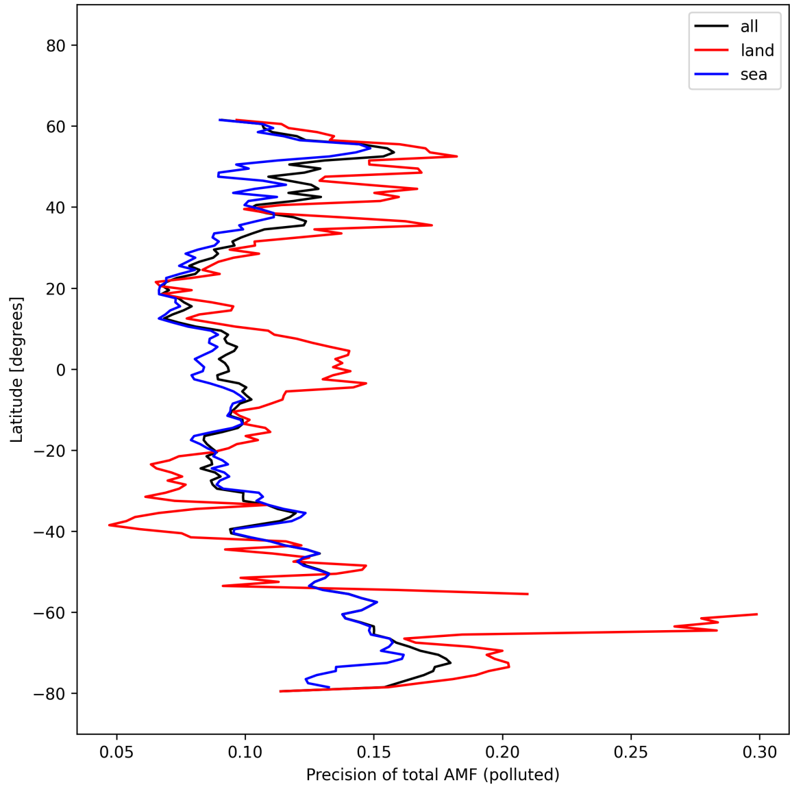
Figure 54: Zonal average of “Precision of total AMF (polluted)” for 2025-10-15 to 2025-10-17.
