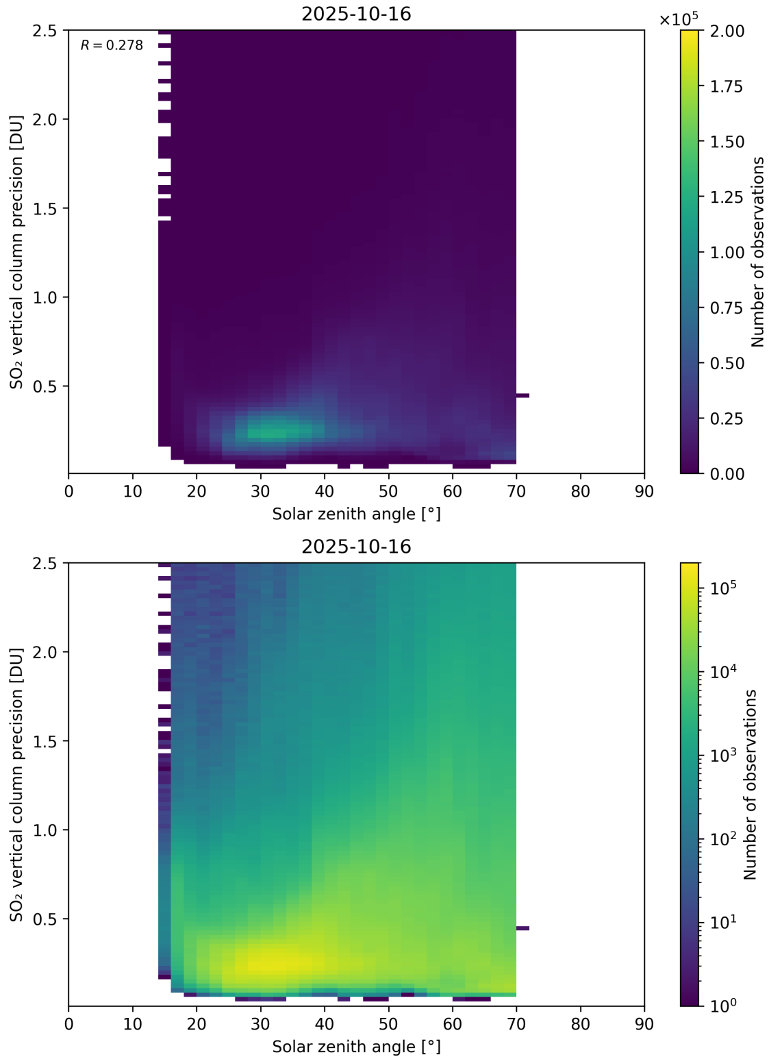
Figure 192: Scatter density plot of “Solar zenith angle” against “SO 2 vertical column precision” for 2025-10-15 to 2025-10-17.
