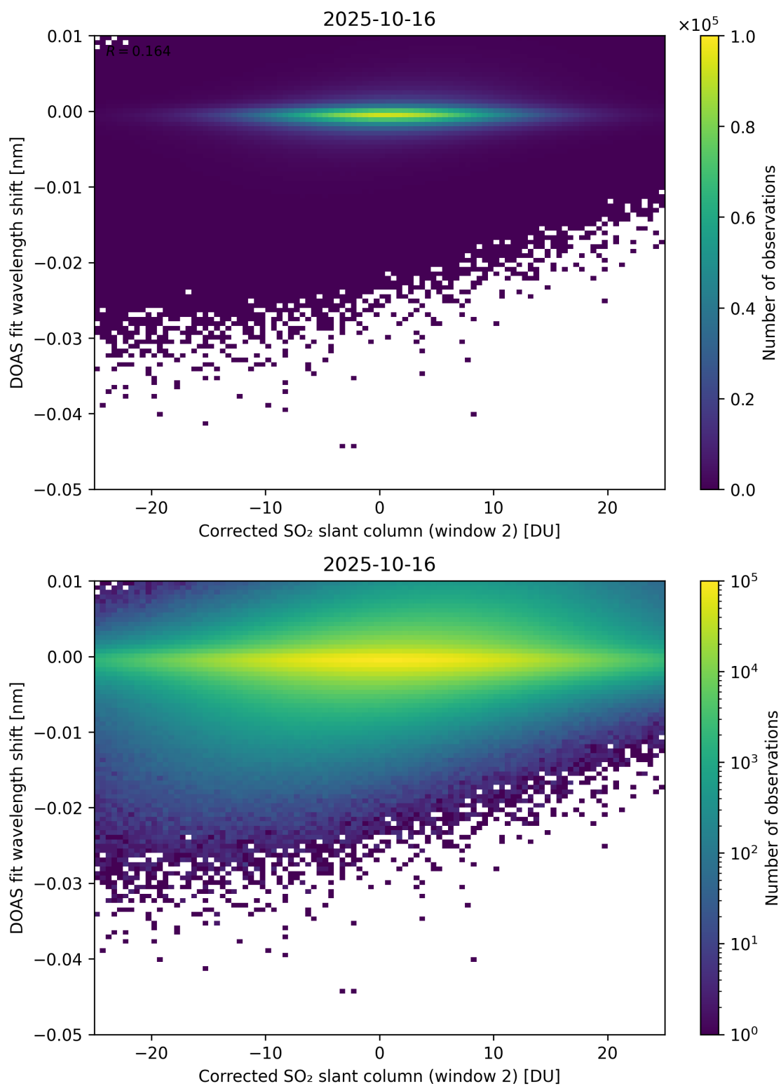
Figure 246: Scatter density plot of “Corrected SO 2 slant column (window 2)” against “DOAS fit wavelength shift” for 2025-10-15 to 2025-10-17.
