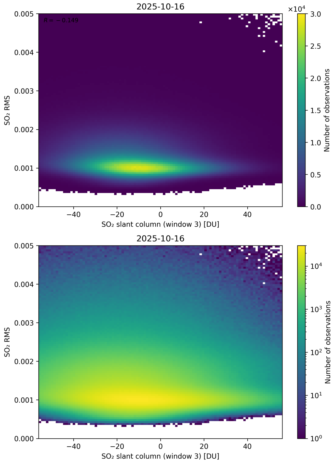
Figure 306: Scatter density plot of “SO 2 slant column (window 3)” against “SO 2 RMS” for 2025-10-15 to 2025-10-17.
