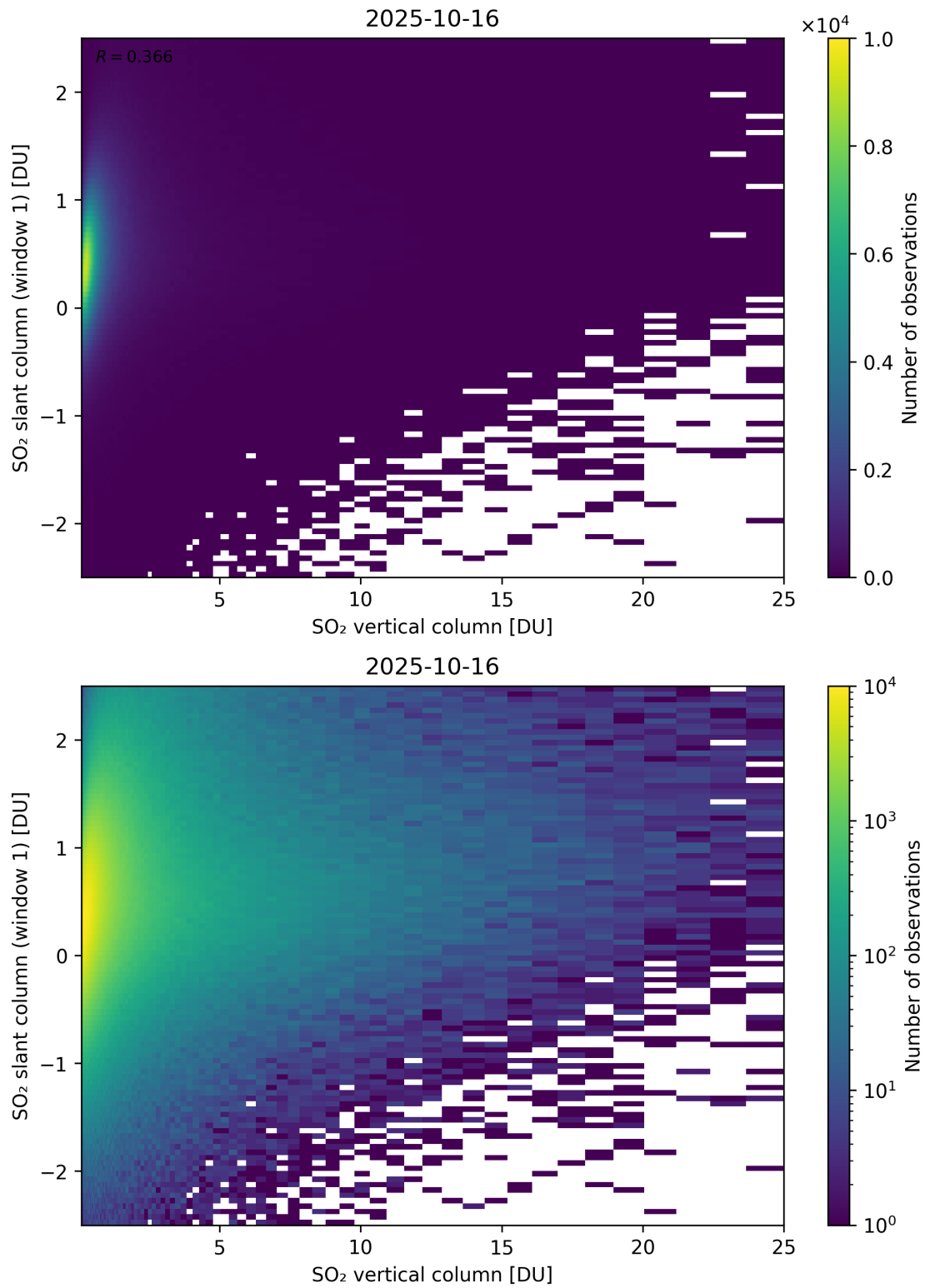
Figure 354: Scatter density plot of “SO 2 vertical column” against “SO 2 slant column (window 1)” for 2025-10-15 to 2025-10-17.
