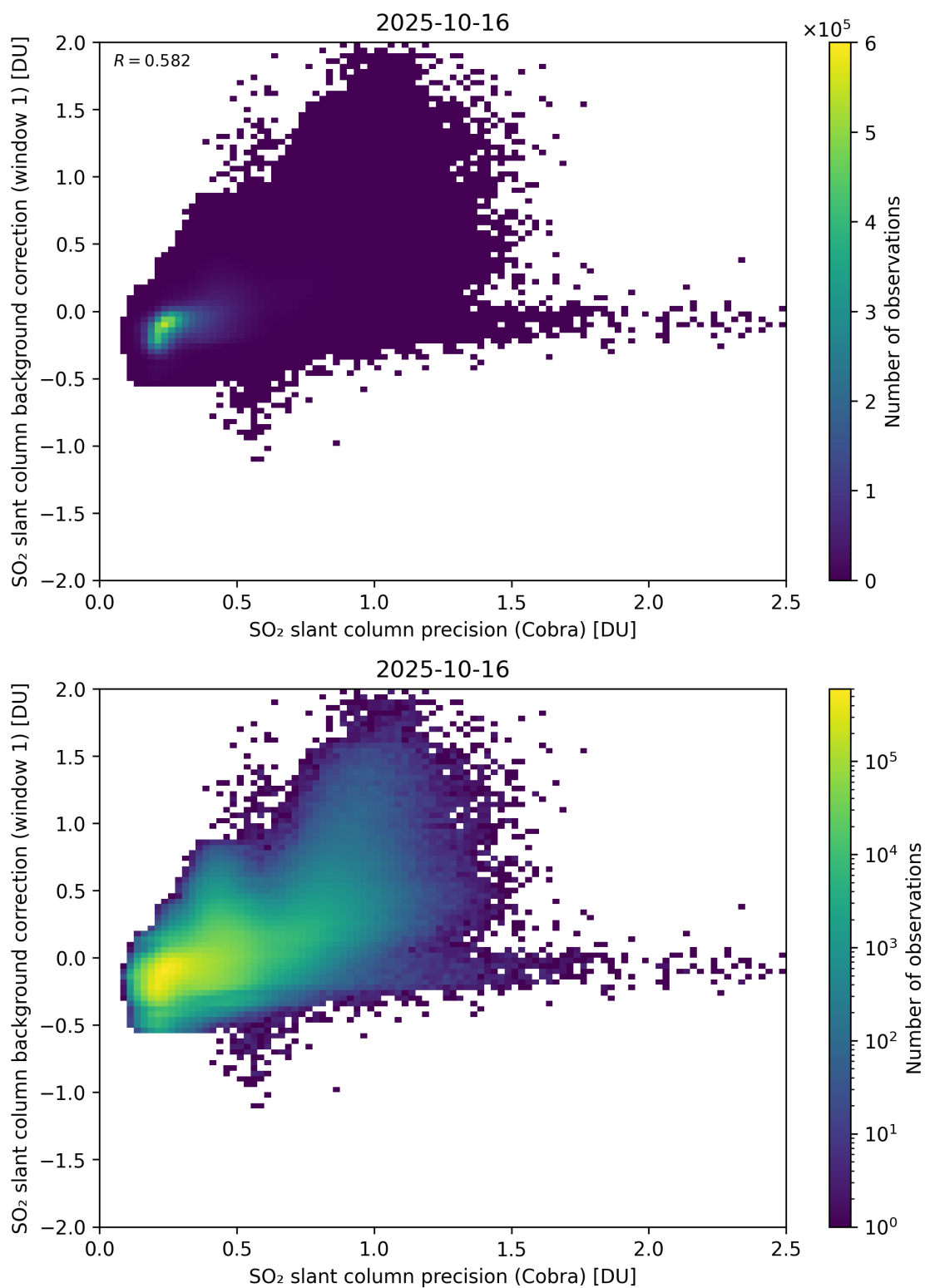
Figure 199: Scatter density plot of “SO 2 slant column precision (Cobra)” against “SO 2 slant column background correction (window 1)” for 2025-10-15 to 2025-10-17.
