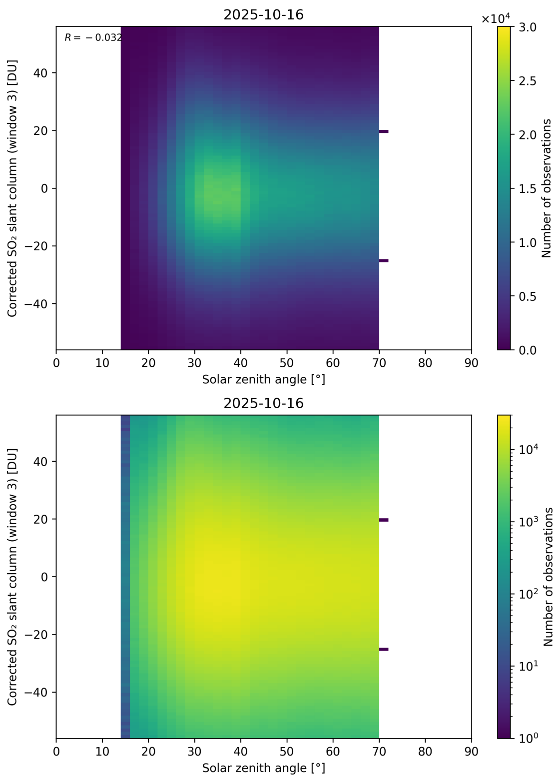
Figure 183: Scatter density plot of “Solar zenith angle” against “Corrected SO 2 slant column (window 3)” for 2025-10-15 to 2025-10-17.
