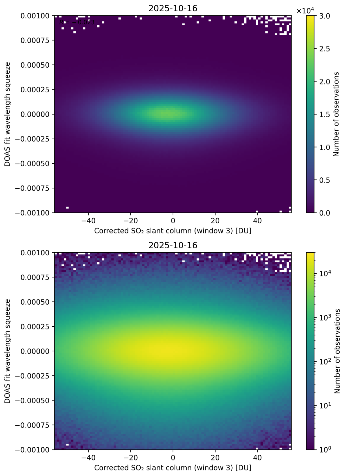
Figure 257: Scatter density plot of “Corrected SO 2 slant column (window 3)” against “DOAS fit wavelength squeeze” for 2025-10-15 to 2025-10-17.
