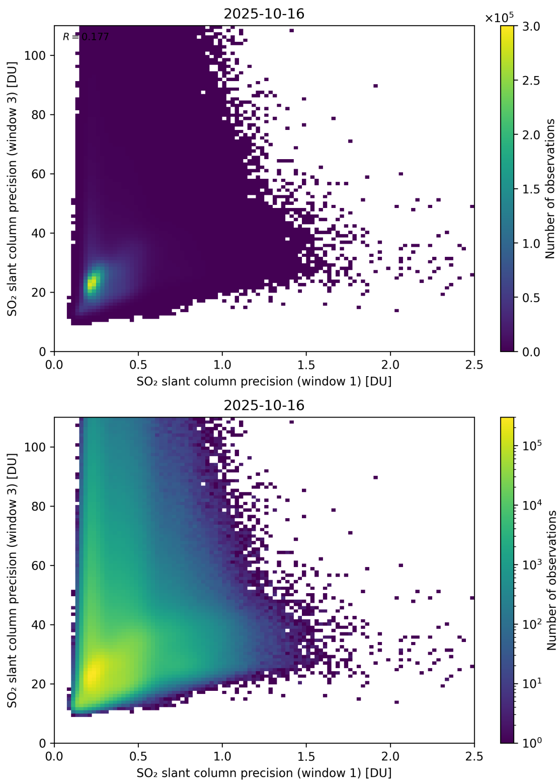
Figure 279: Scatter density plot of “SO 2 slant column precision (window 1)” against “SO 2 slant column precision (window 3)” for 2025-10-15 to 2025-10-17.
