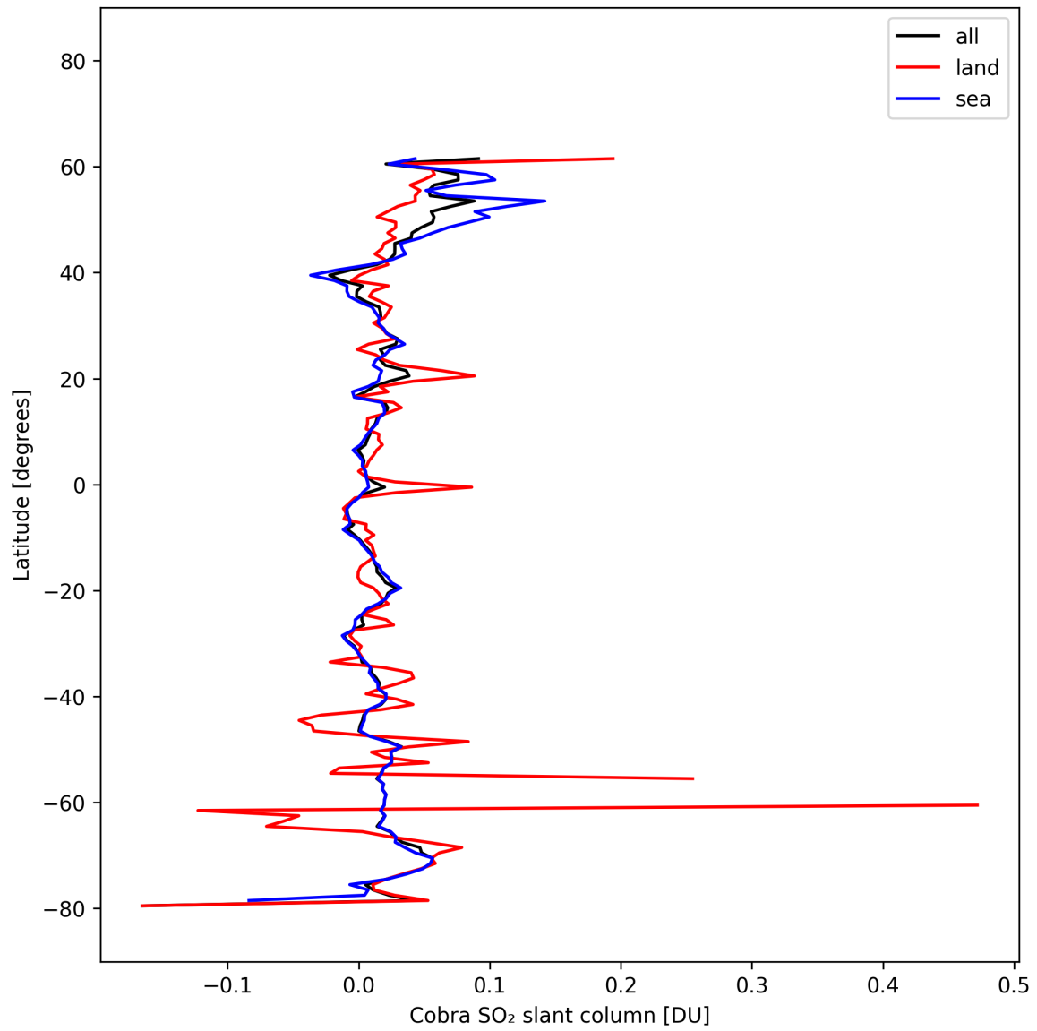
Figure 35: Zonal average of “Cobra SO 2 slant column” for 2025-10-15 to 2025-10-17.
