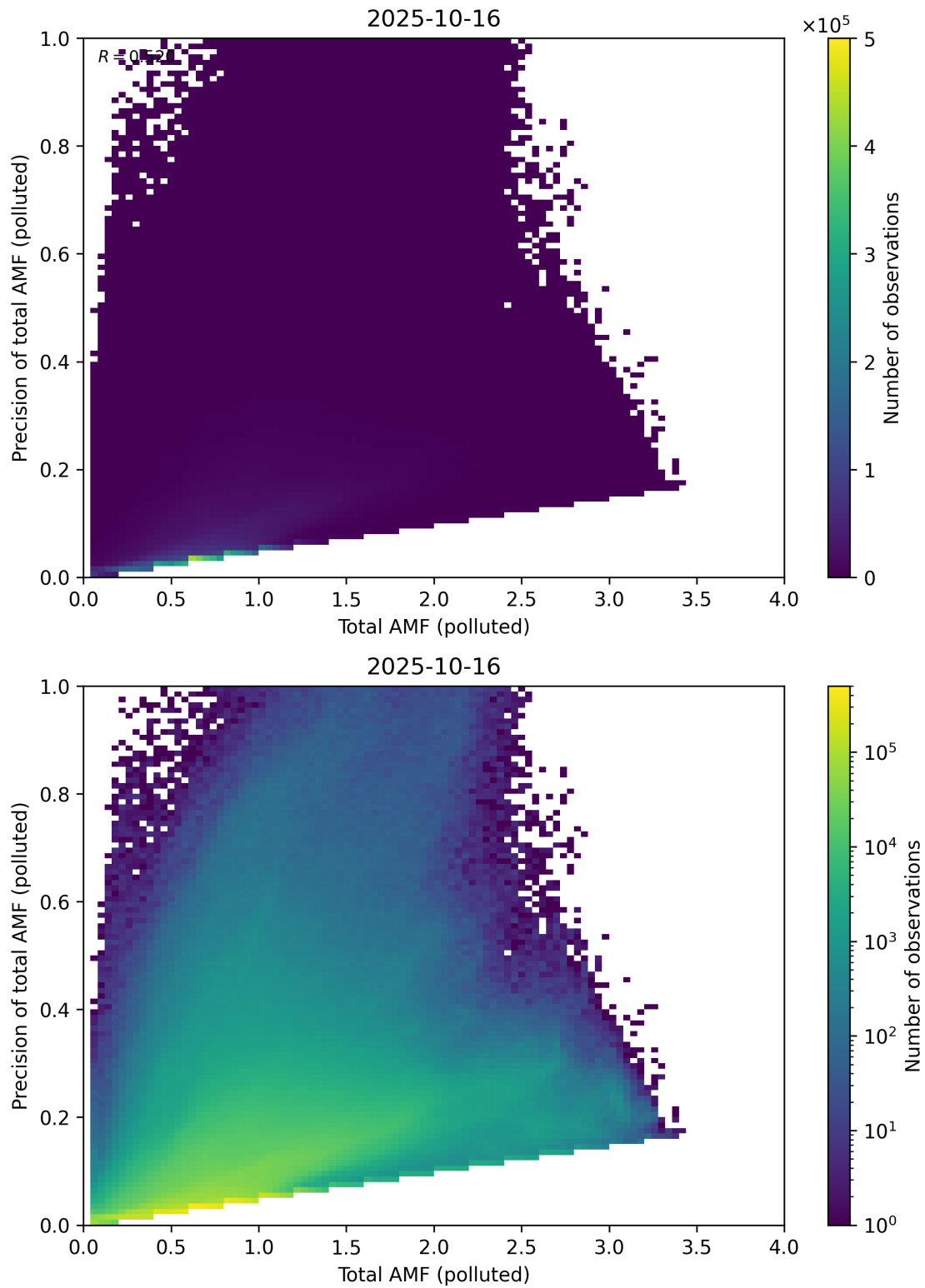
Figure 322: Scatter density plot of “Total AMF (polluted)” against “Precision of total AMF (polluted)” for 2025-10-15 to 2025-10-17.
