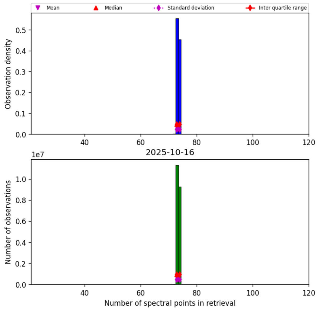
Figure 82: Histogram of “Number of spectral points in retrieval” for 2025-10-15 to 2025-10-17
