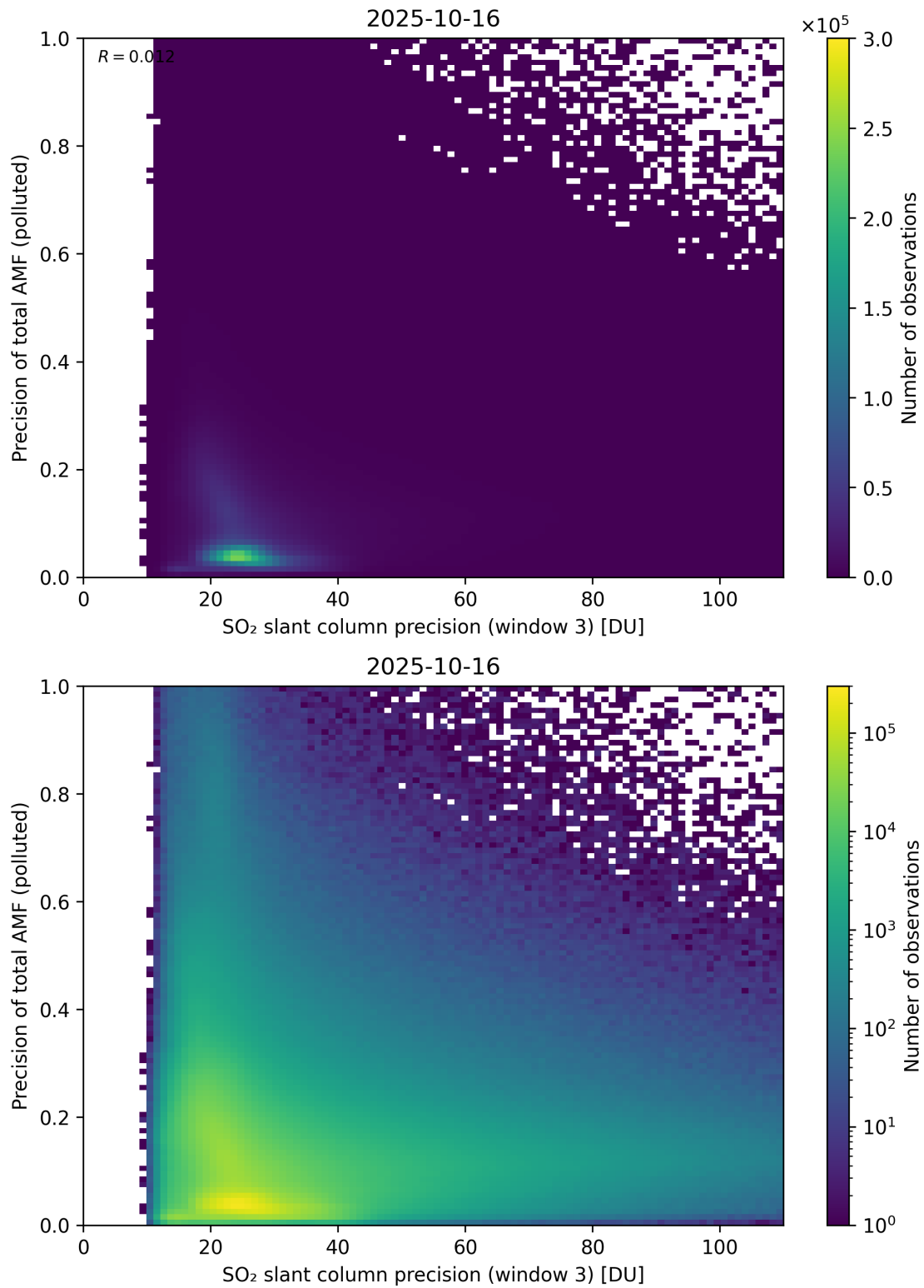
Figure 314: Scatter density plot of “SO 2 slant column precision (window 3)” against “Precision of total AMF (polluted)” for 2025-10-15 to 2025-10-17.
