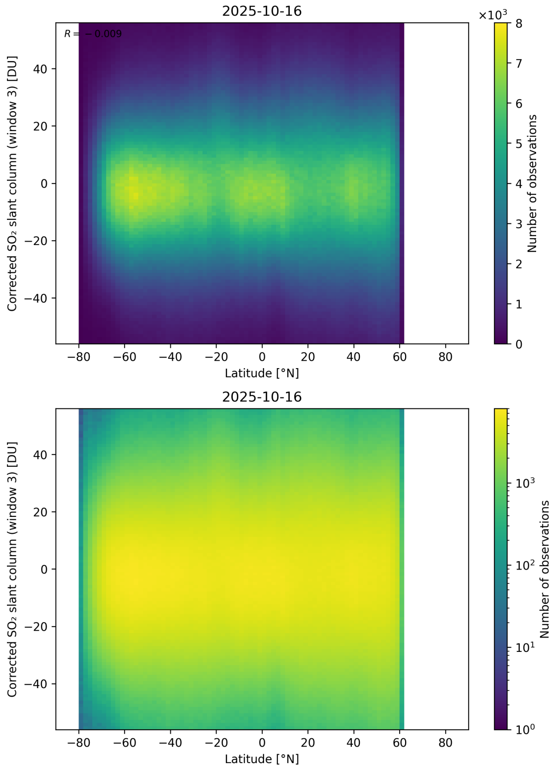
Figure 161: Scatter density plot of “Latitude” against “Corrected SO 2 slant column (window 3)” for 2025-10-15 to 2025-10-17.
