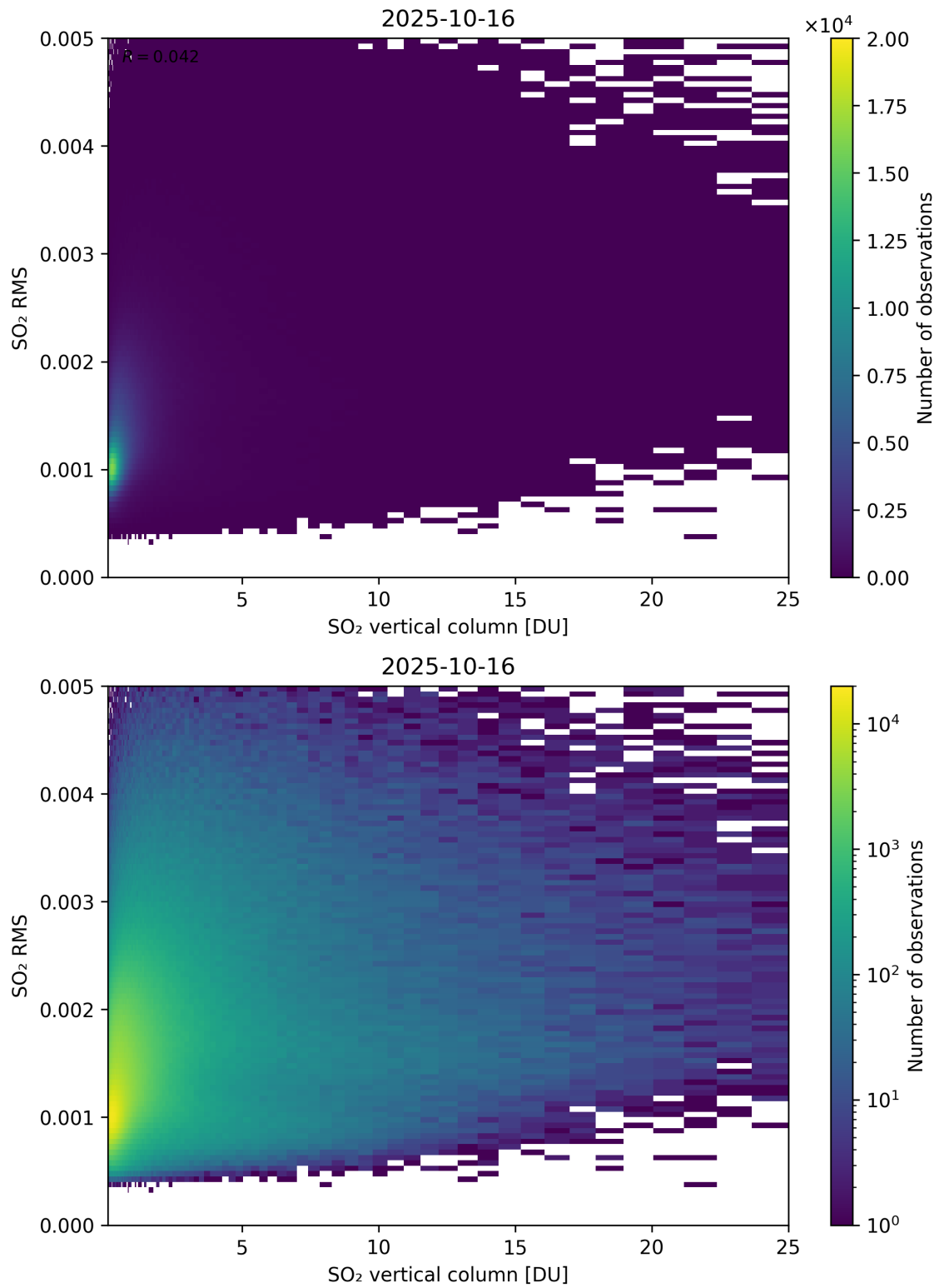
Figure 328: Scatter density plot of “SO 2 vertical column” against “SO 2 RMS” for 2025-10-15 to 2025-10-17.
