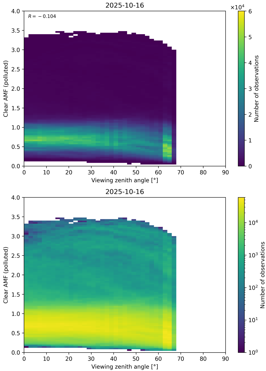
Figure 370: Scatter density plot of “Viewing zenith angle” against “Clear AMF (polluted)” for 2025-10-15 to 2025-10-17.
