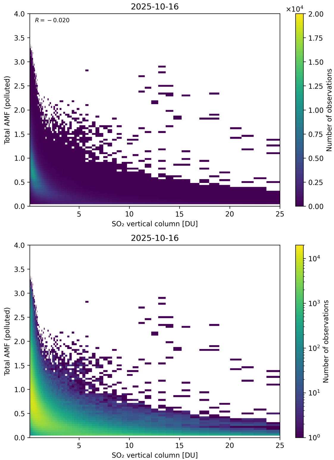
Figure 359: Scatter density plot of “SO 2 vertical column” against “Total AMF (polluted)” for 2025-10-15 to 2025-10-17.
