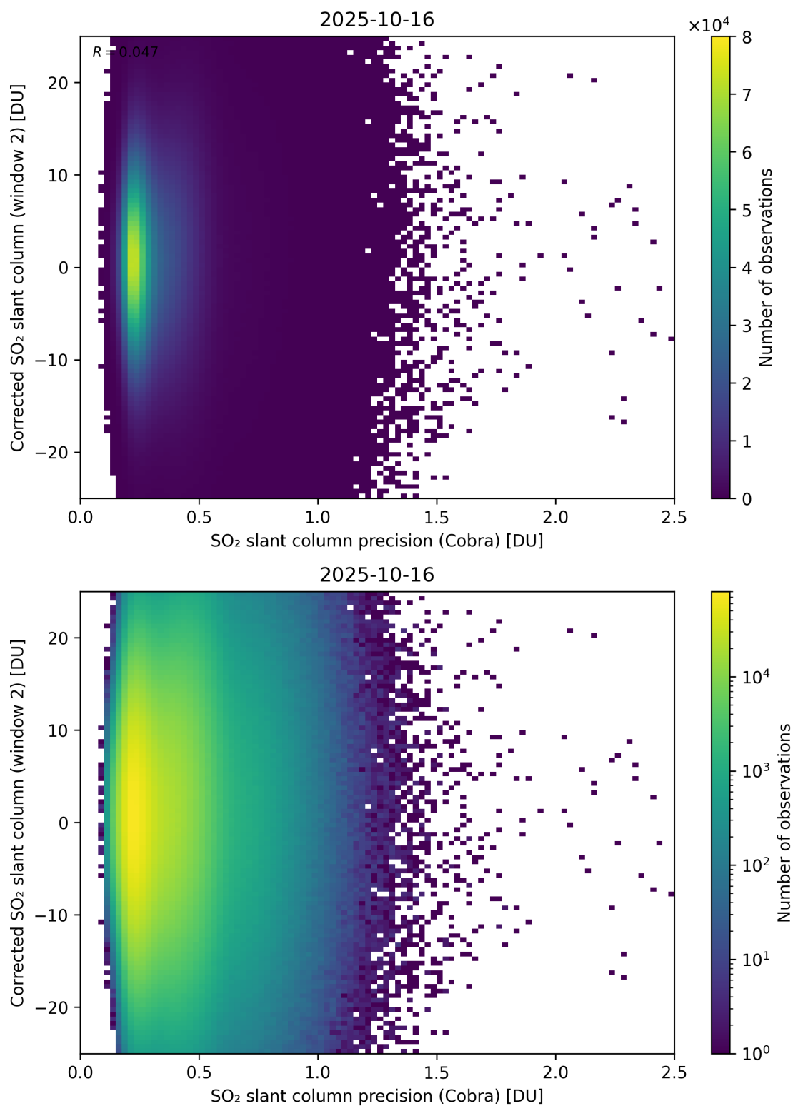
Figure 206: Scatter density plot of “SO 2 slant column precision (Cobra)” against “Corrected SO 2 slant column (window 2)” for 2025-10-15 to 2025-10-17.
