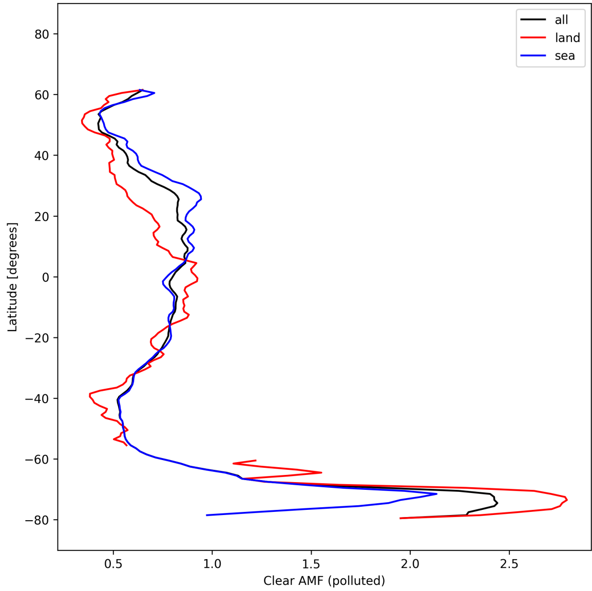
Figure 55: Zonal average of “Clear AMF (polluted)” for 2025-10-15 to 2025-10-17.
