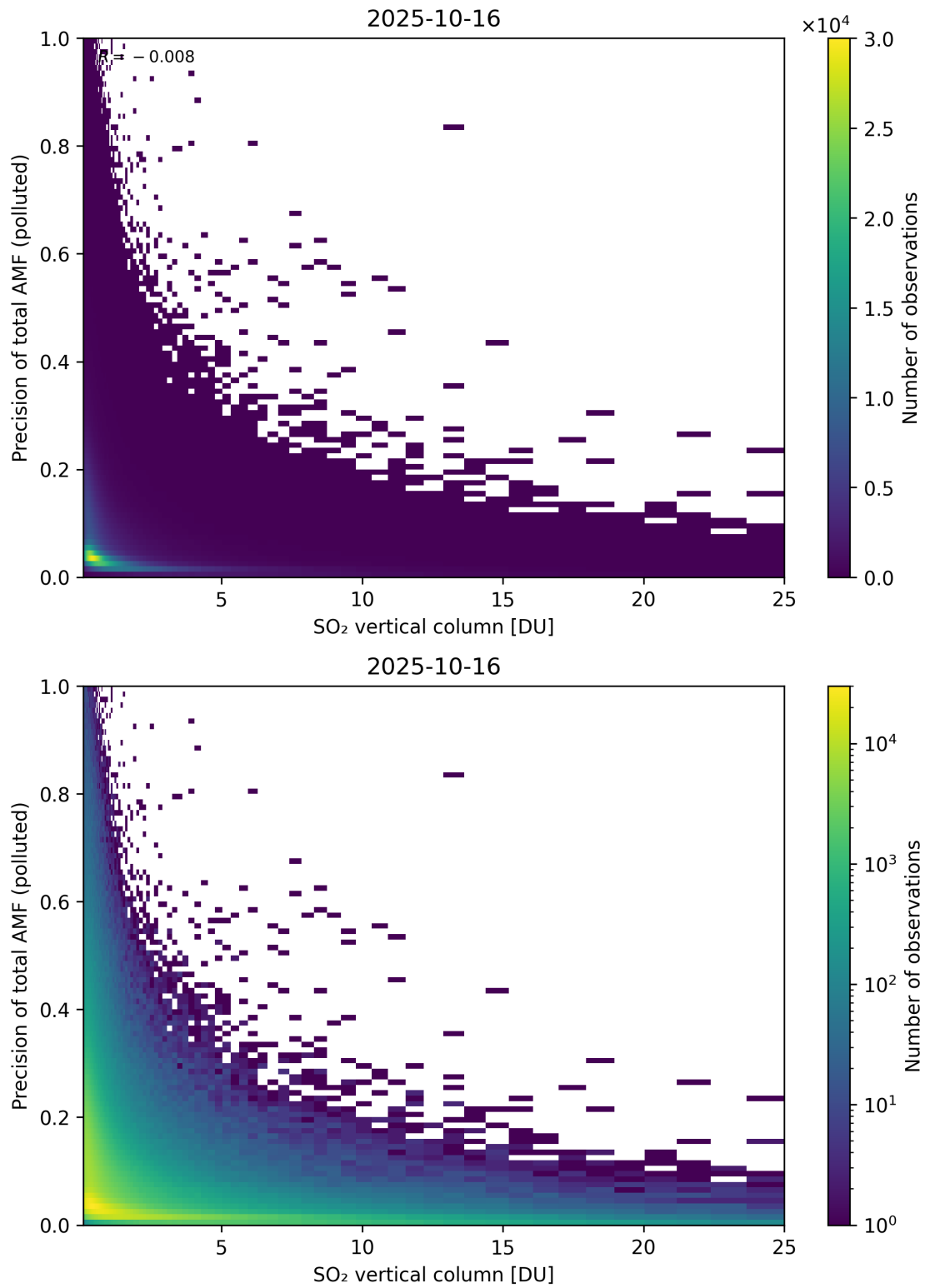
Figure 360: Scatter density plot of “SO 2 vertical column” against “Precision of total AMF (polluted)” for 2025-10-15 to 2025-10-17.
