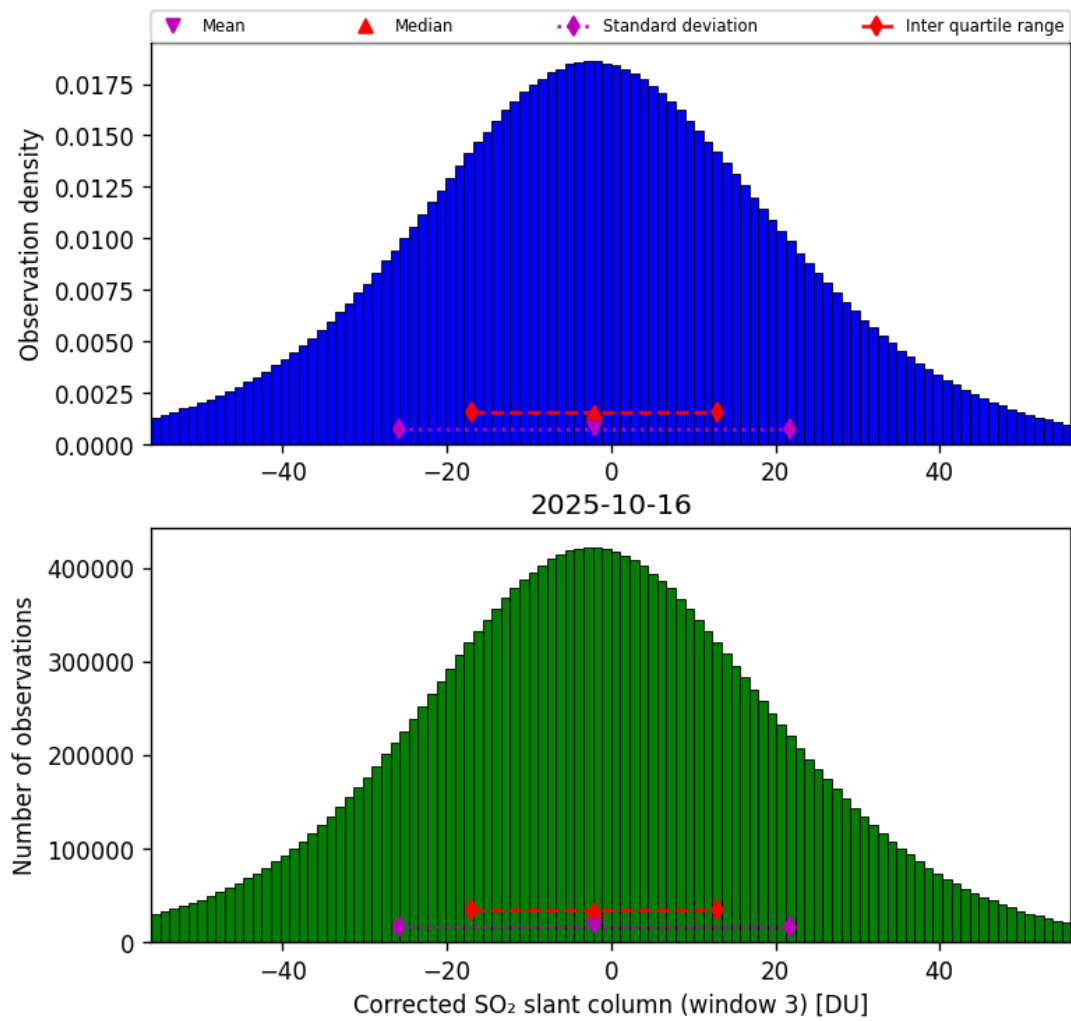
Figure 73: Histogram of “Corrected SO 2 slant column (window 3)” for 2025-10-15 to 2025-10-17
