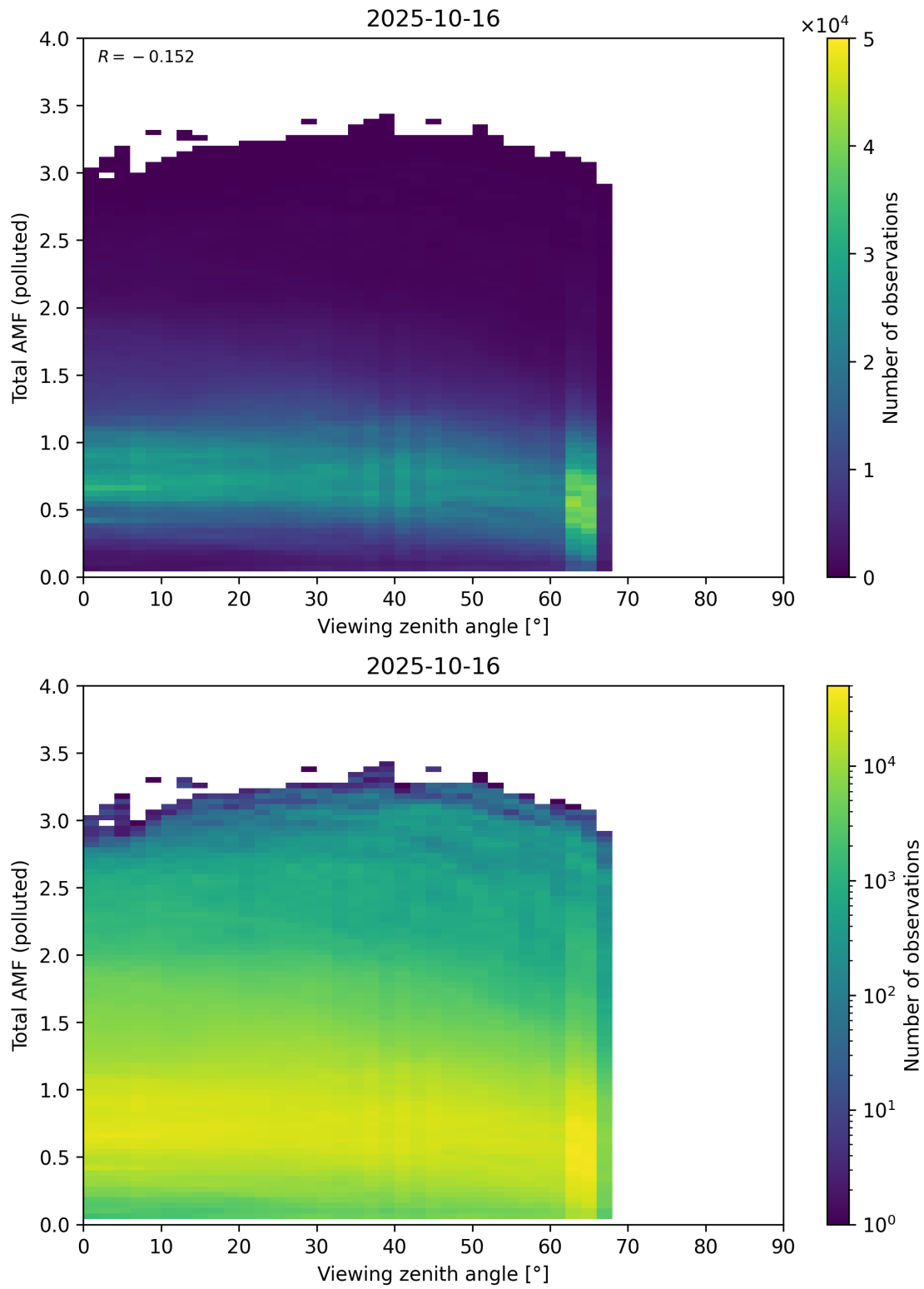
Figure 381: Scatter density plot of “Viewing zenith angle” against “Total AMF (polluted)” for 2025-10-15 to 2025-10-17.
