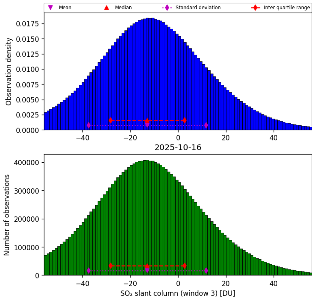
Figure 71: Histogram of “SO 2 slant column (window 3)” for 2025-10-15 to 2025-10-17
