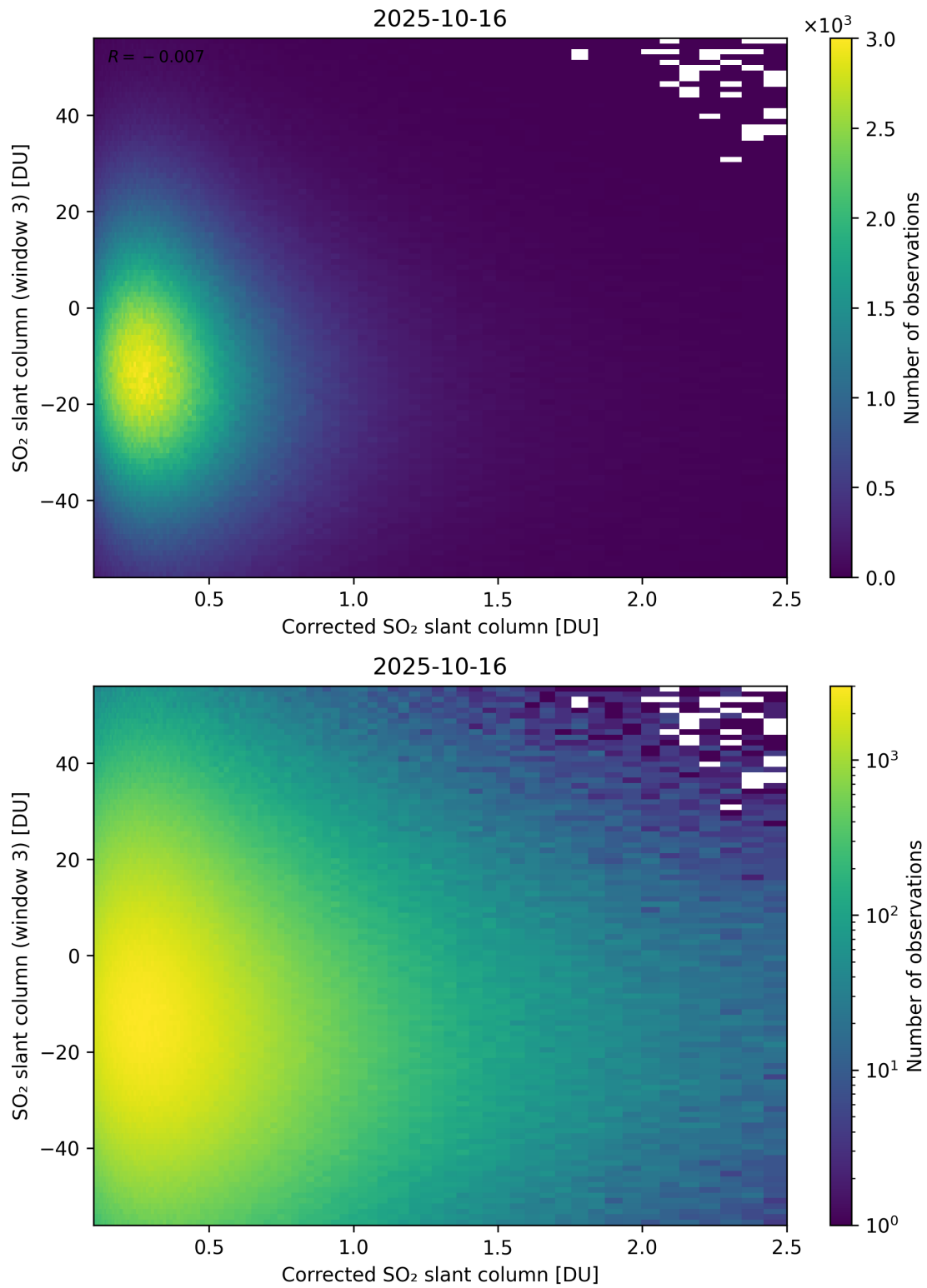
Figure 240: Scatter density plot of “Corrected SO 2 slant column” against “SO 2 slant column (window 3)” for 2025-10-15 to 2025-10-17.
