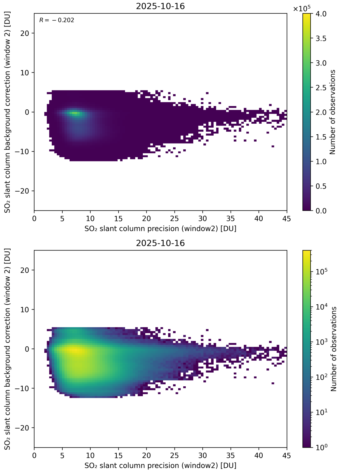
Figure 291: Scatter density plot of “SO 2 slant column precision (window2)” against “SO 2 slant column background correction (window 2)” for 2025-10-15 to 2025-10-17.
