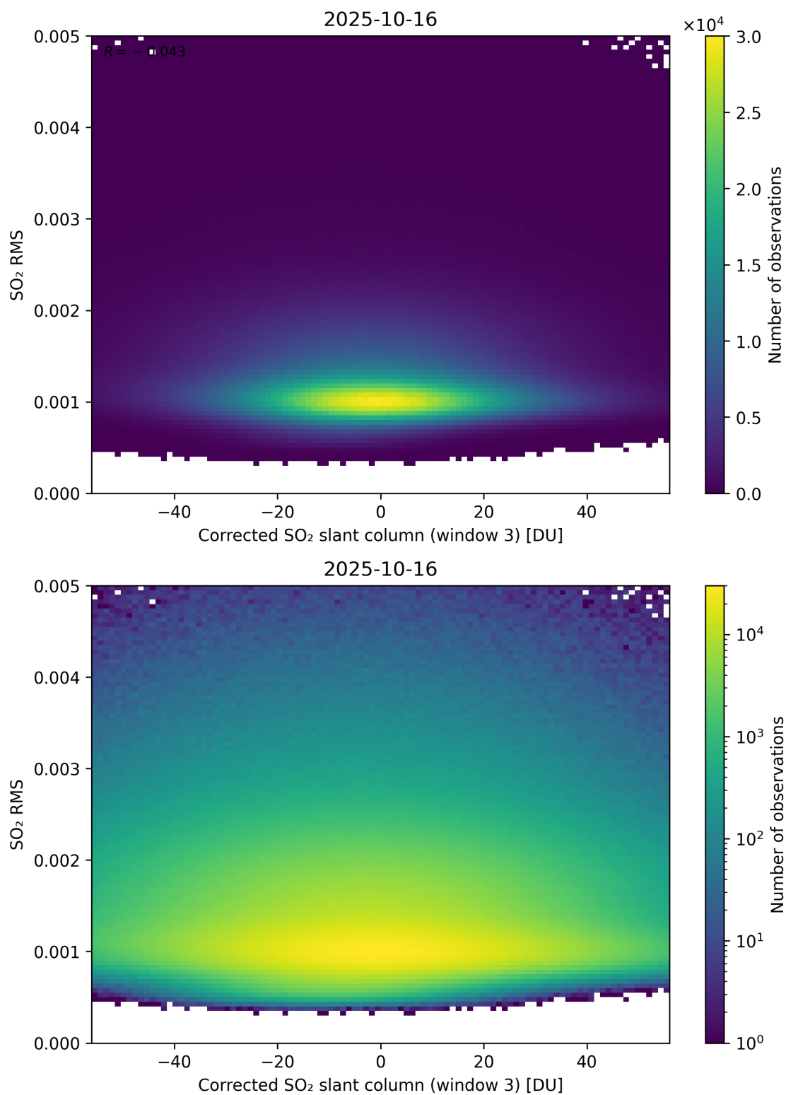
Figure 258: Scatter density plot of “Corrected SO 2 slant column (window 3)” against “SO 2 RMS” for 2025-10-15 to 2025-10-17.
