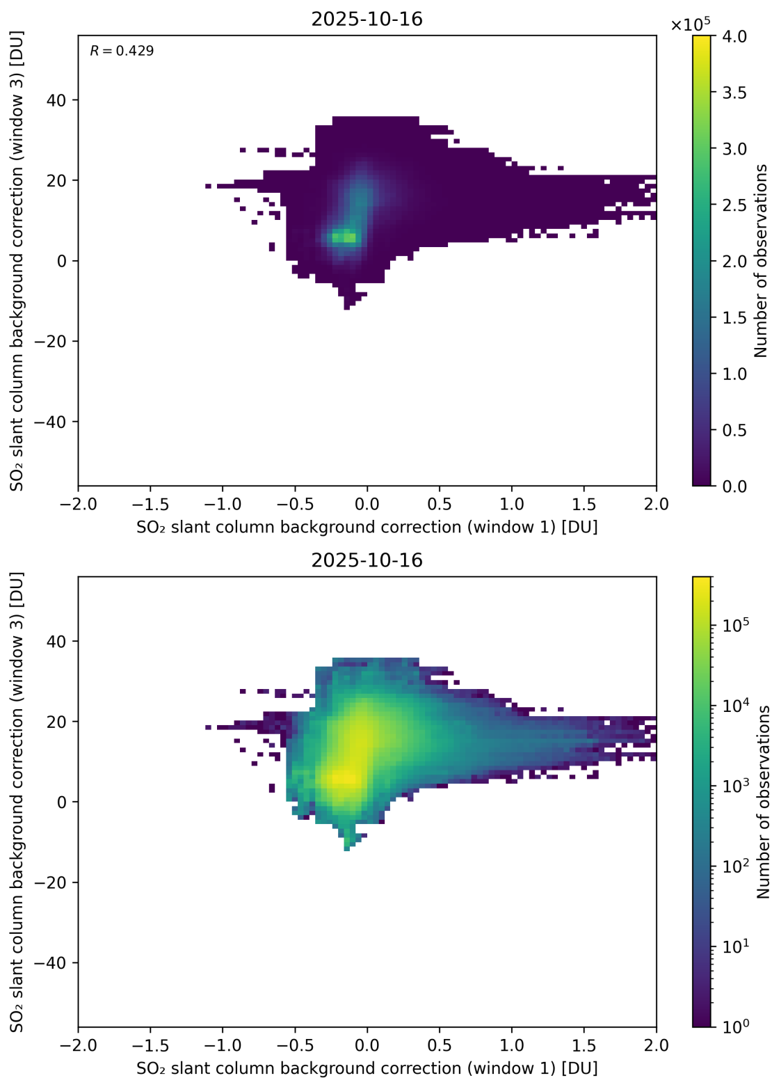
Figure 110: Scatter density plot of “SO 2 slant column background correction (window 1)” against “SO 2 slant column background correction (window 3)” for 2025-10-15 to 2025-10-17.
