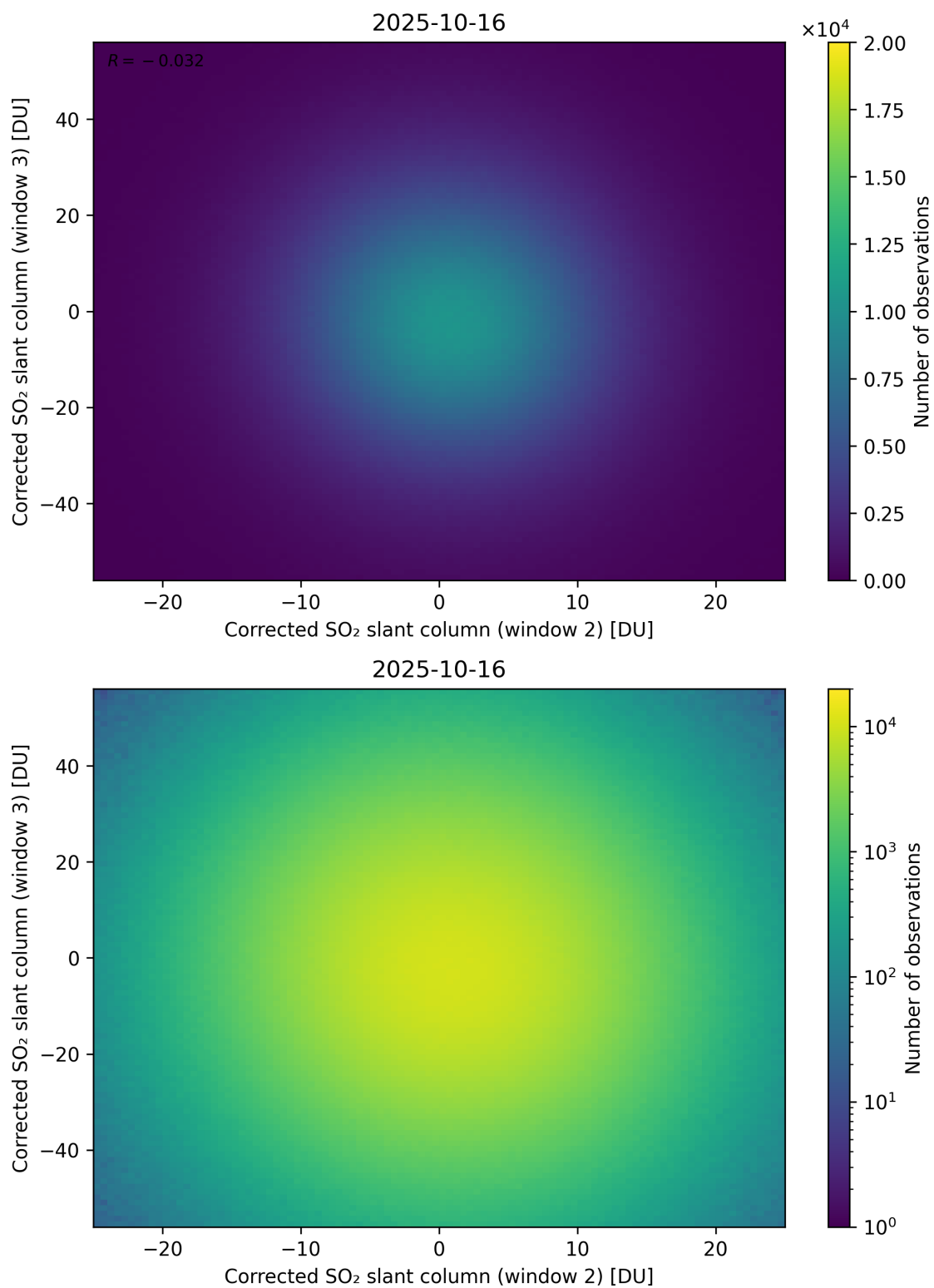
Figure 250: Scatter density plot of “Corrected SO 2 slant column (window 2)” against “Corrected SO 2 slant column (window 3)” for 2025-10-15 to 2025-10-17.
