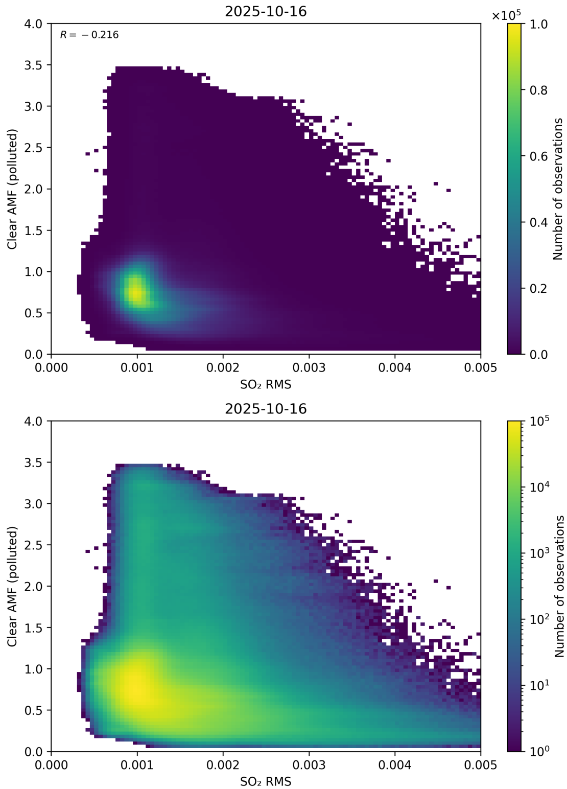
Figure 147: Scatter density plot of “SO 2 RMS” against “Clear AMF (polluted)” for 2025-10-15 to 2025-10-17.
