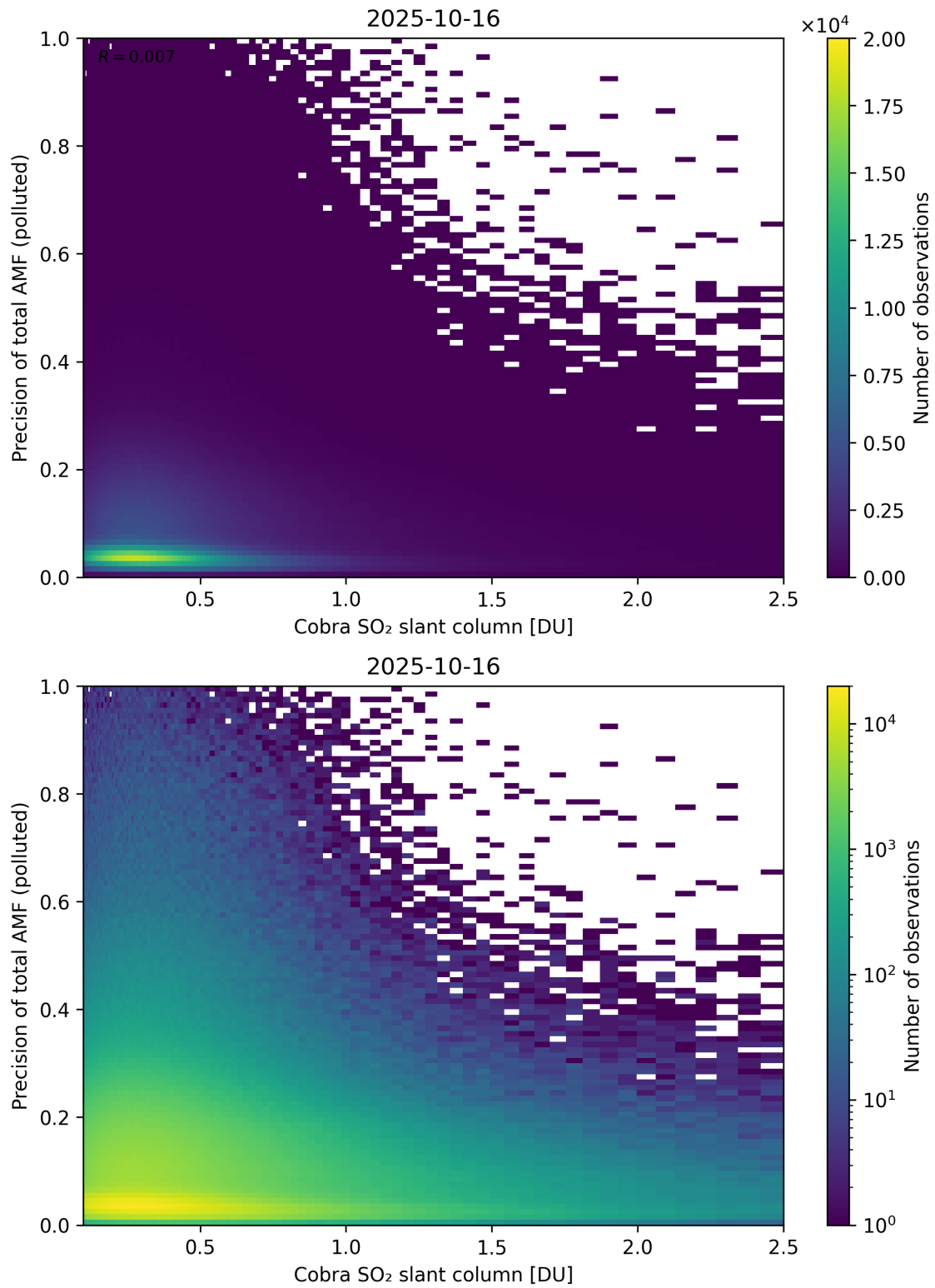
Figure 225: Scatter density plot of “Cobra SO 2 slant column” against “Precision of total AMF (polluted)” for 2025-10-15 to 2025-10-17.
