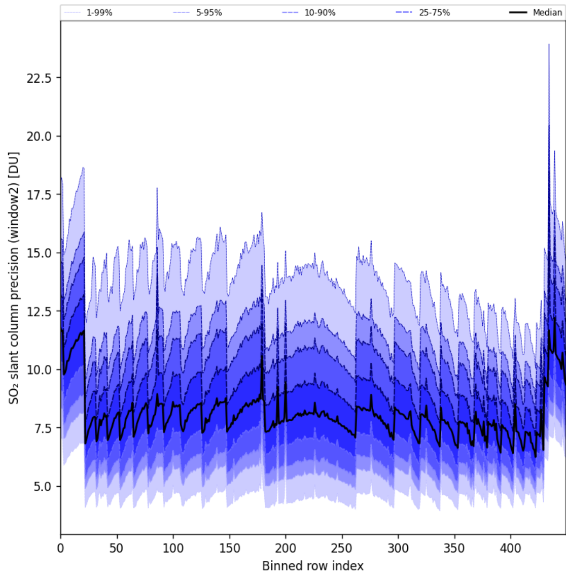
Figure 94: Along track statistics of “SO 2 slant column precision (window2)” for 2025-10-15 to 2025-10-17
