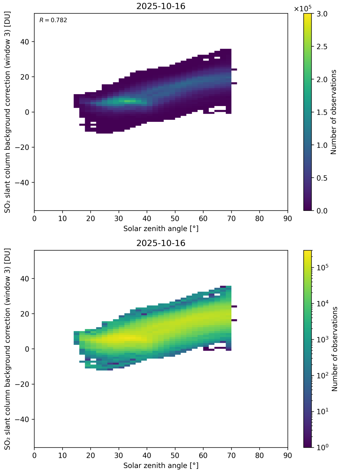
Figure 173: Scatter density plot of “Solar zenith angle” against “SO 2 slant column background correction (window 3)” for 2025-10-15 to 2025-10-17.
