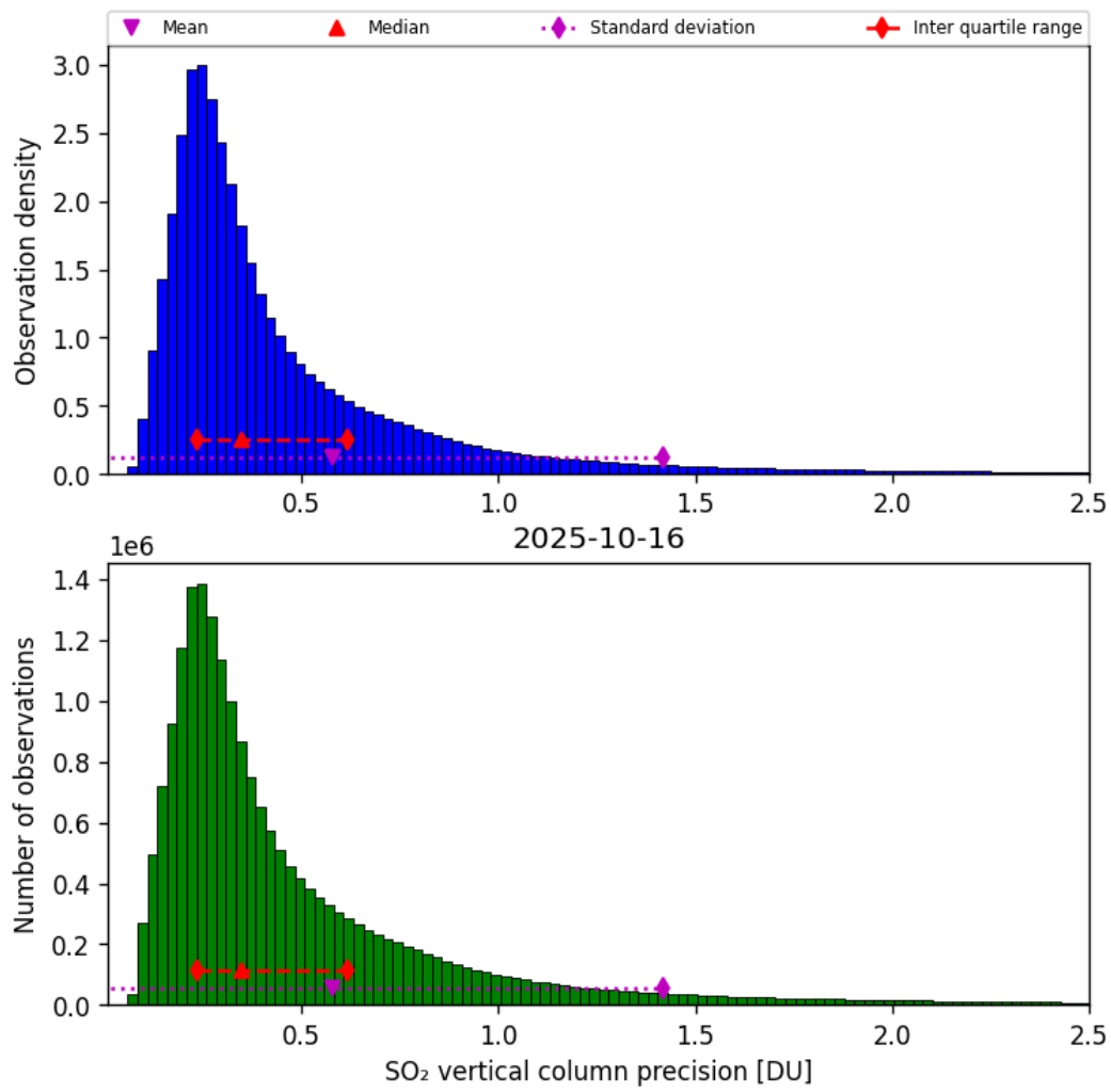
Figure 59: Histogram of “SO 2 vertical column precision” for 2025-10-15 to 2025-10-17
