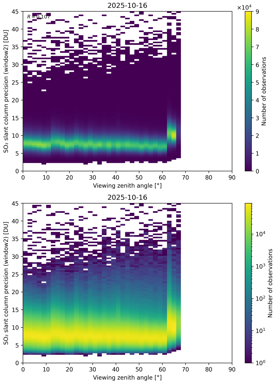
Figure 378: Scatter density plot of “Viewing zenith angle” against “SO 2 slant column precision (window2)” for 2025-10-15 to 2025-10-17.
