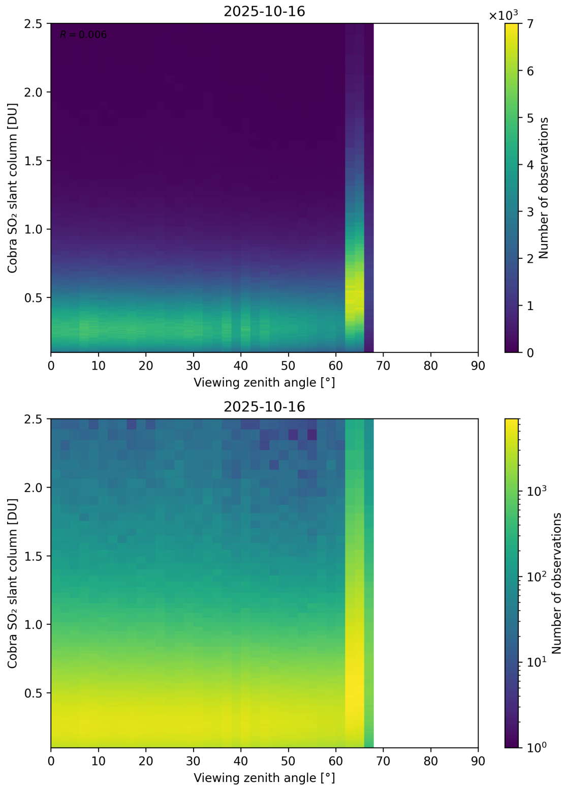
Figure 371: Scatter density plot of “Viewing zenith angle” against “Cobra SO 2 slant column” for 2025-10-15 to 2025-10-17.
