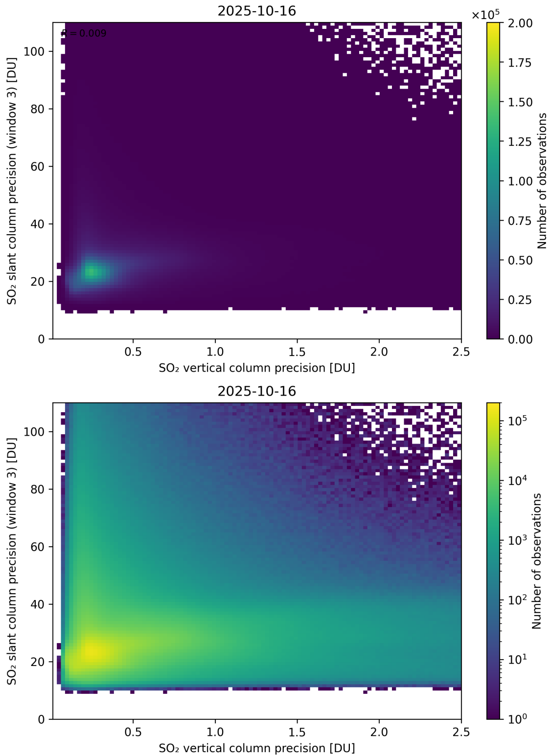
Figure 345: Scatter density plot of “SO 2 vertical column precision” against “SO 2 slant column precision (window 3)” for 2025-10-15 to 2025-10-17.
