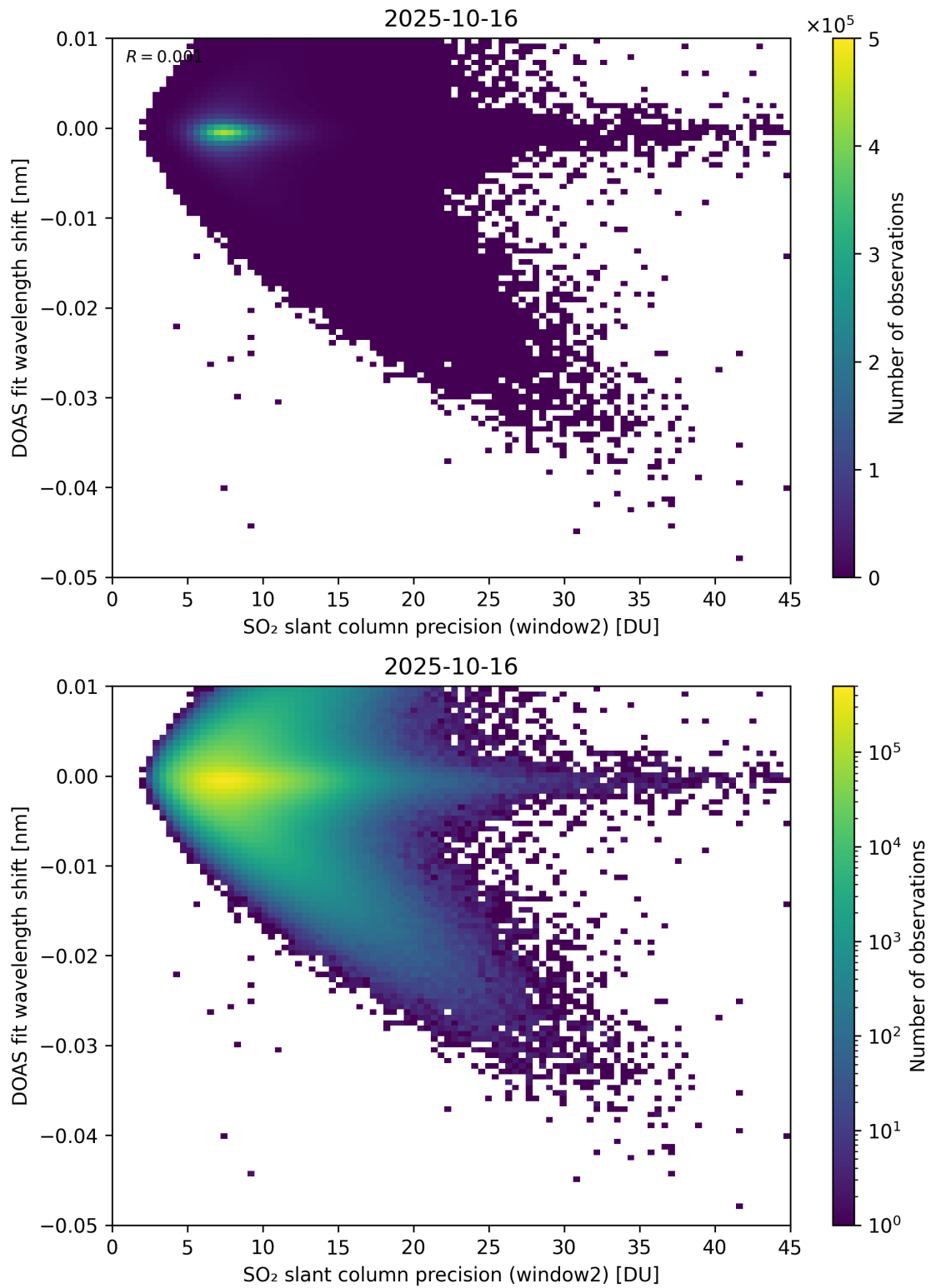
Figure 293: Scatter density plot of “SO 2 slant column precision (window2)” against “DOAS fit wavelength shift” for 2025-10-15 to 2025-10-17.
