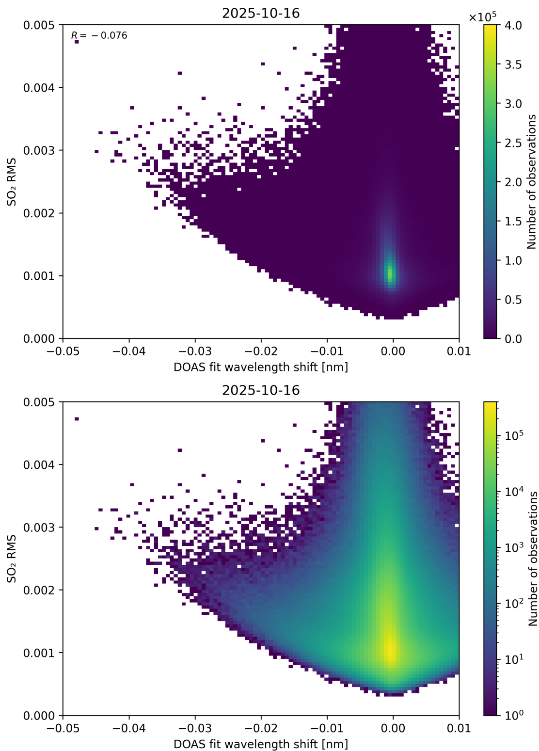
Figure 139: Scatter density plot of “DOAS fit wavelength shift” against “SO 2 RMS” for 2025-10-15 to 2025-10-17.
