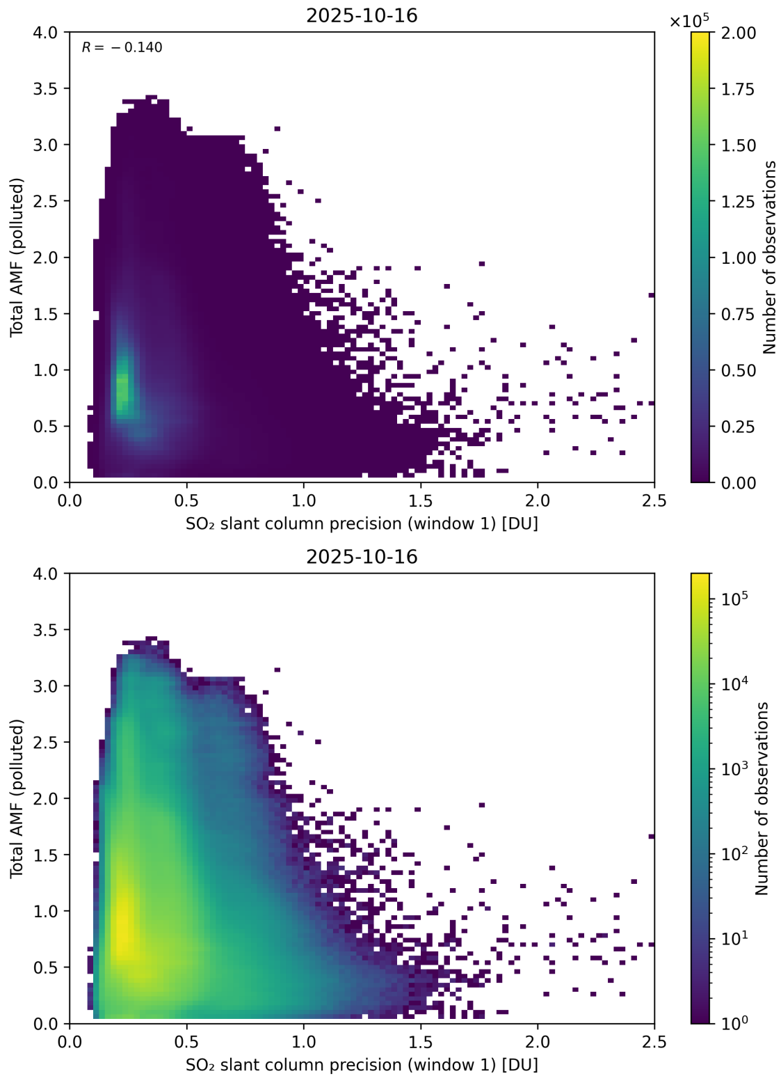
Figure 280: Scatter density plot of “SO 2 slant column precision (window 1)” against “Total AMF (polluted)” for 2025-10-15 to 2025-10-17.
