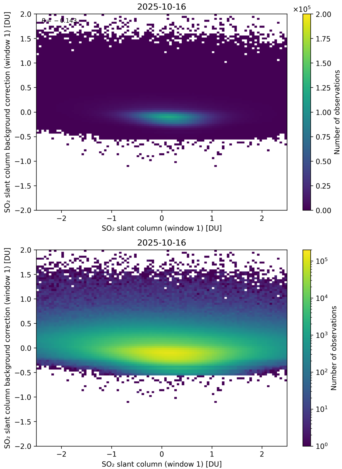
Figure 262: Scatter density plot of “SO 2 slant column (window 1)” against “SO 2 slant column background correction (window 1)” for 2025-10-15 to 2025-10-17.
