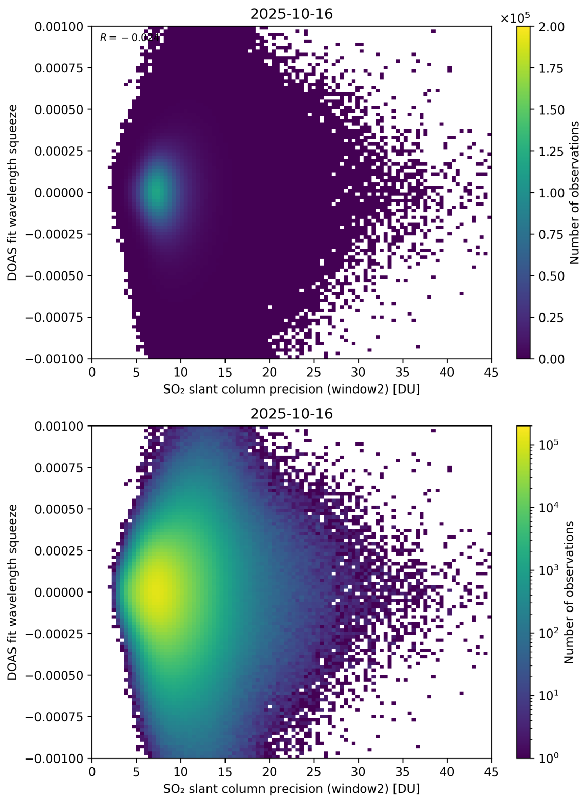
Figure 294: Scatter density plot of “SO 2 slant column precision (window2)” against “DOAS fit wavelength squeeze” for 2025-10-15 to 2025-10-17.
