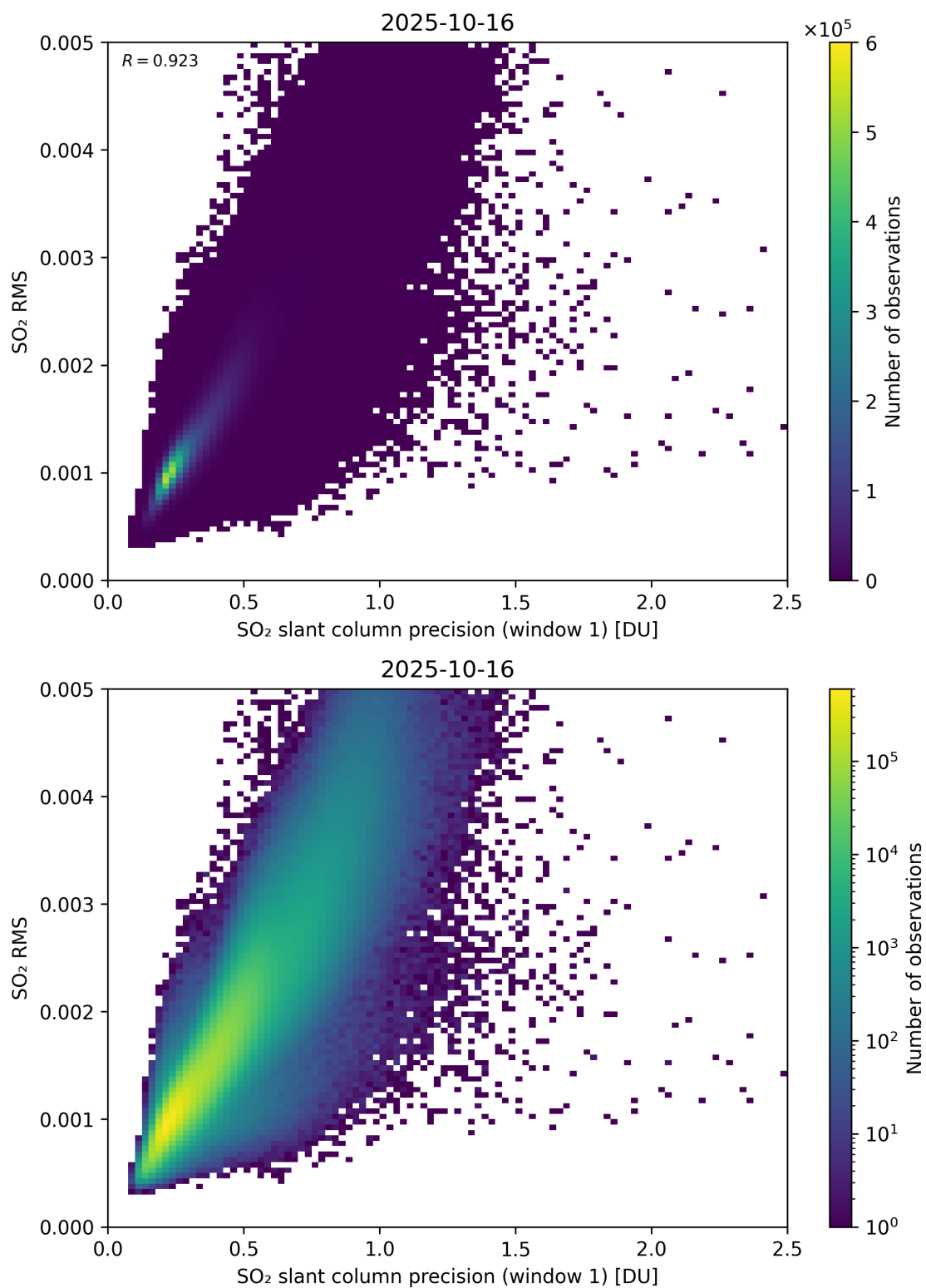
Figure 273: Scatter density plot of “SO 2 slant column precision (window 1)” against “SO 2 RMS” for 2025-10-15 to 2025-10-17.
