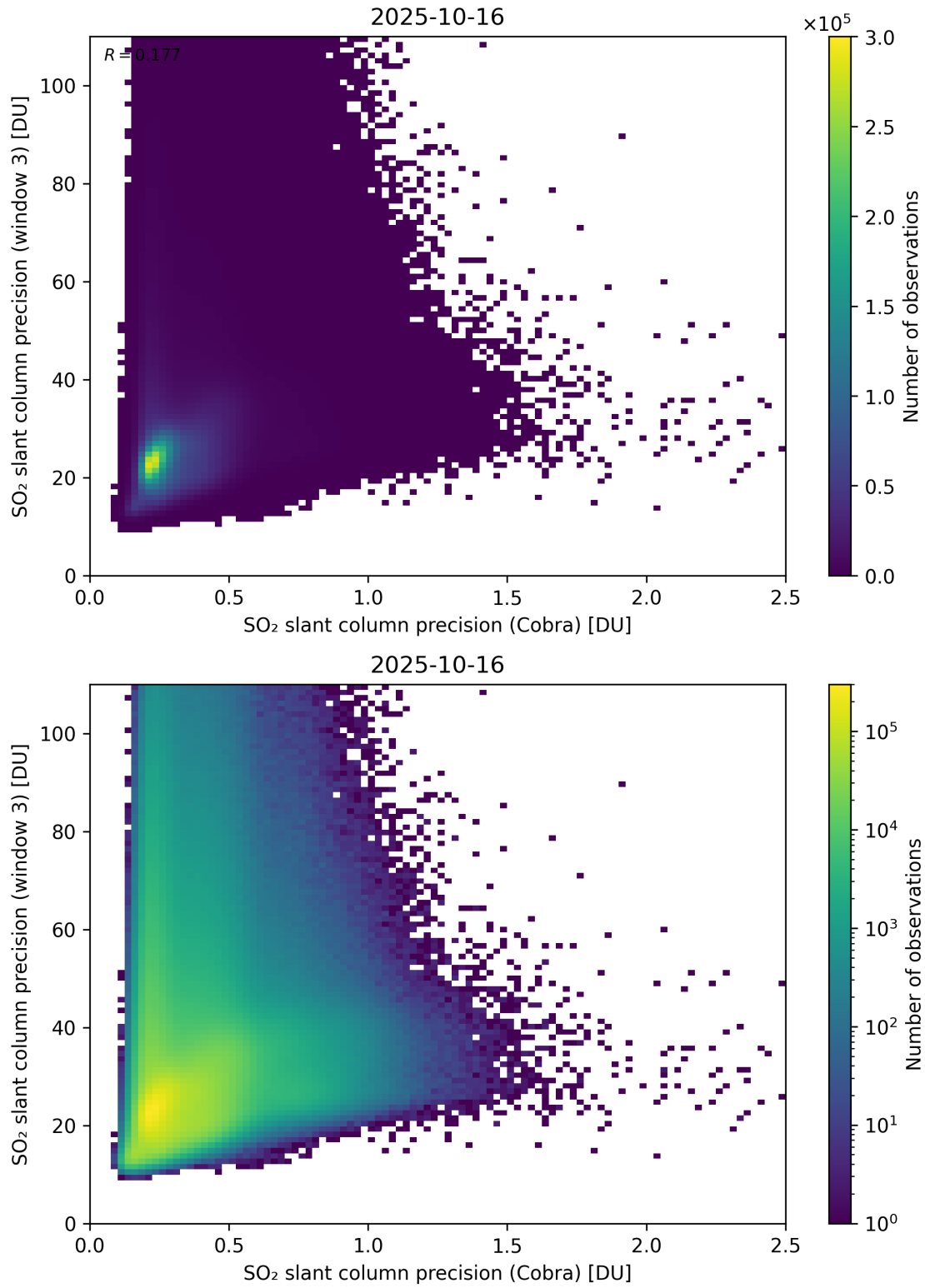
Figure 212: Scatter density plot of “SO 2 slant column precision (Cobra)” against “SO 2 slant column precision (window 3)” for 2025-10-15 to 2025-10-17.
