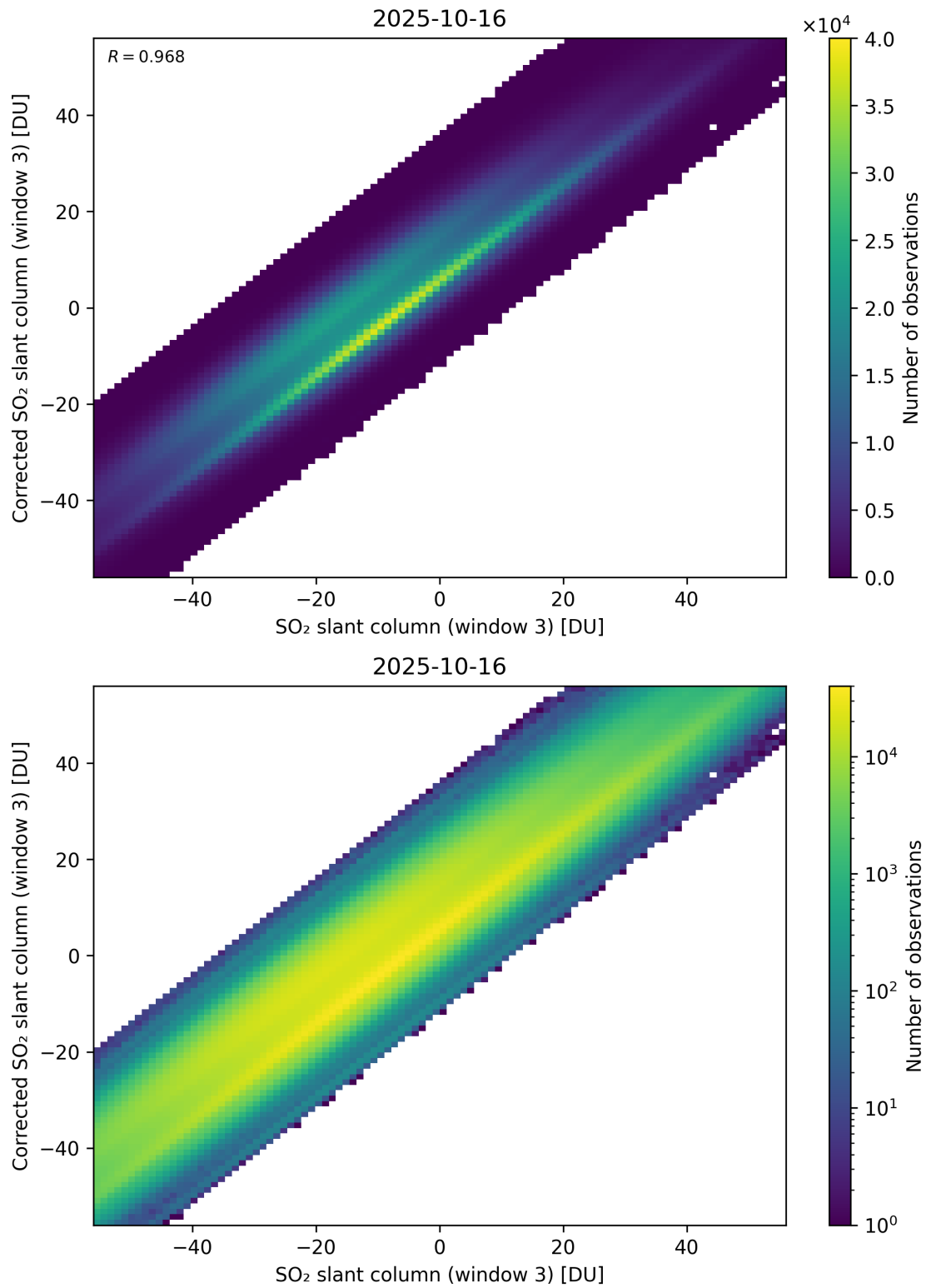
Figure 316: Scatter density plot of “SO 2 slant column (window 3)” against “Corrected SO 2 slant column (window 3)” for 2025-10-15 to 2025-10-17.
