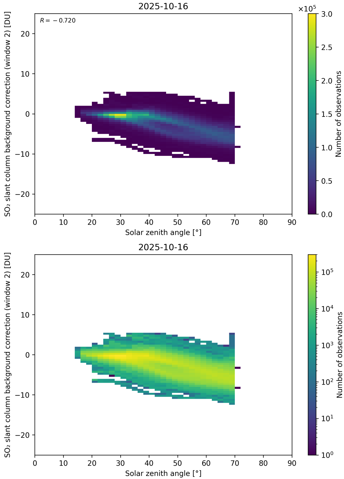
Figure 172: Scatter density plot of “Solar zenith angle” against “SO 2 slant column background correction (window 2)” for 2025-10-15 to 2025-10-17.
