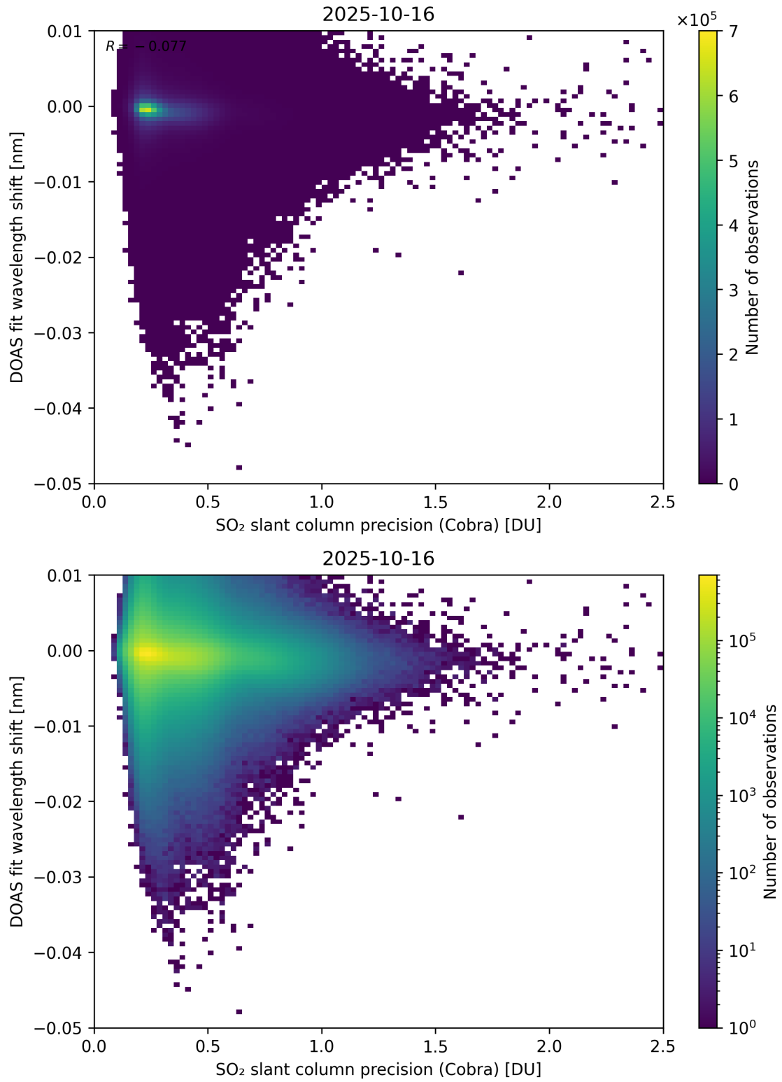
Figure 202: Scatter density plot of “SO 2 slant column precision (Cobra)” against “DOAS fit wavelength shift” for 2025-10-15 to 2025-10-17.
