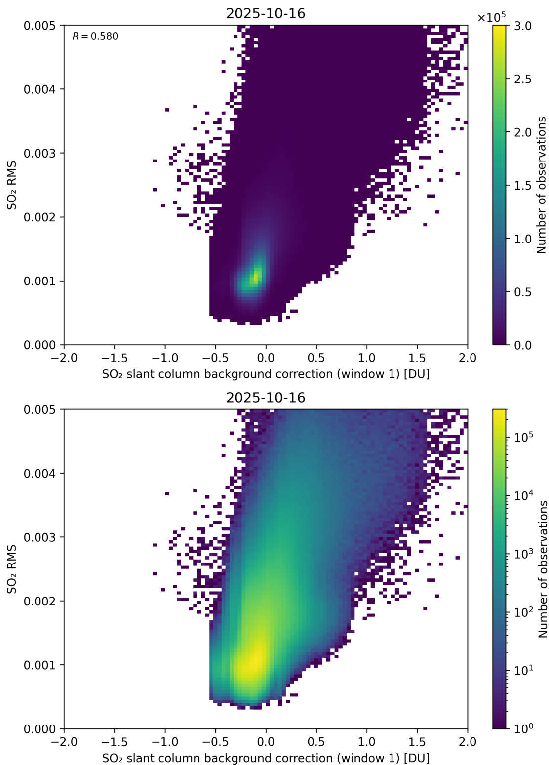
Figure 113: Scatter density plot of “SO 2 slant column background correction (window 1)” against “SO 2 RMS” for 2025-10-15 to 2025-10-17.
