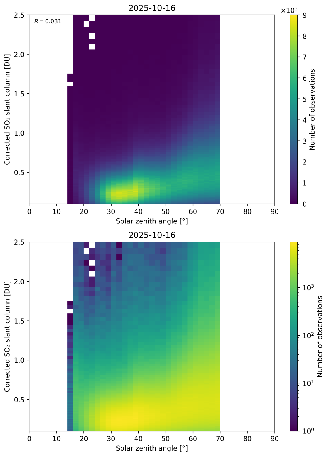
Figure 181: Scatter density plot of “Solar zenith angle” against “Corrected SO 2 slant column” for 2025-10-15 to 2025-10-17.
