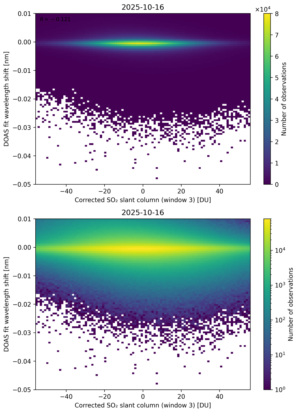
Figure 256: Scatter density plot of “Corrected SO 2 slant column (window 3)” against “DOAS fit wavelength shift” for 2025-10-15 to 2025-10-17.
