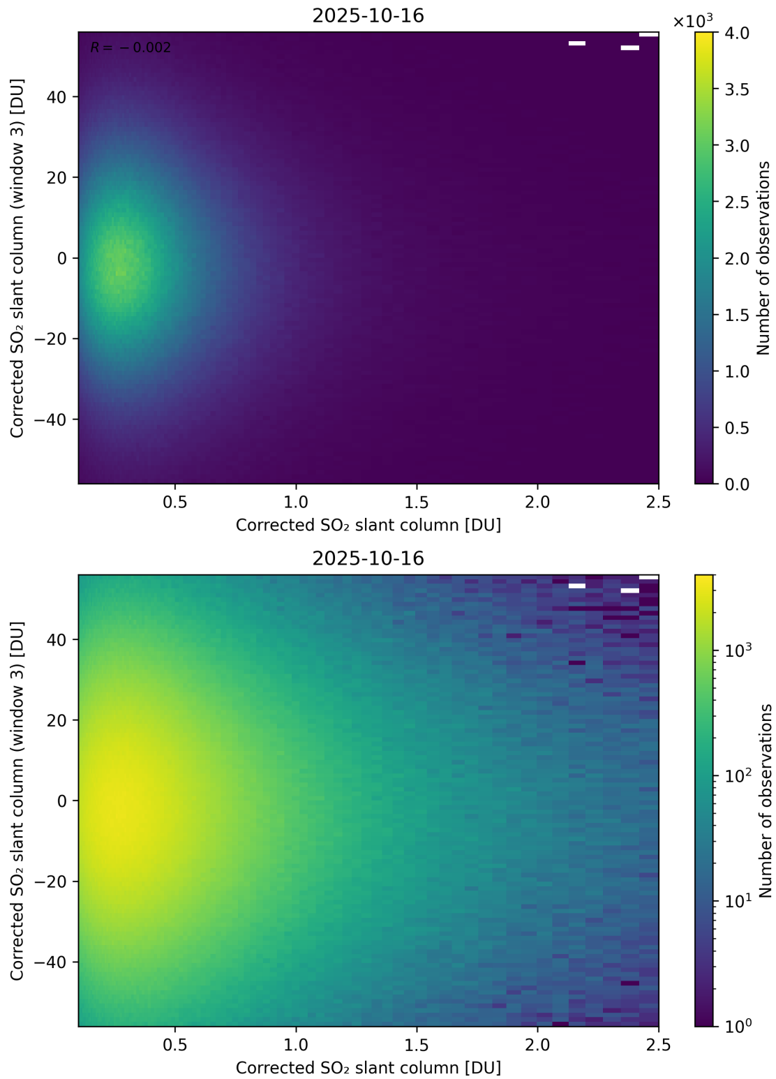
Figure 236: Scatter density plot of “Corrected SO 2 slant column” against “Corrected SO 2 slant column (window 3)” for 2025-10-15 to 2025-10-17.
