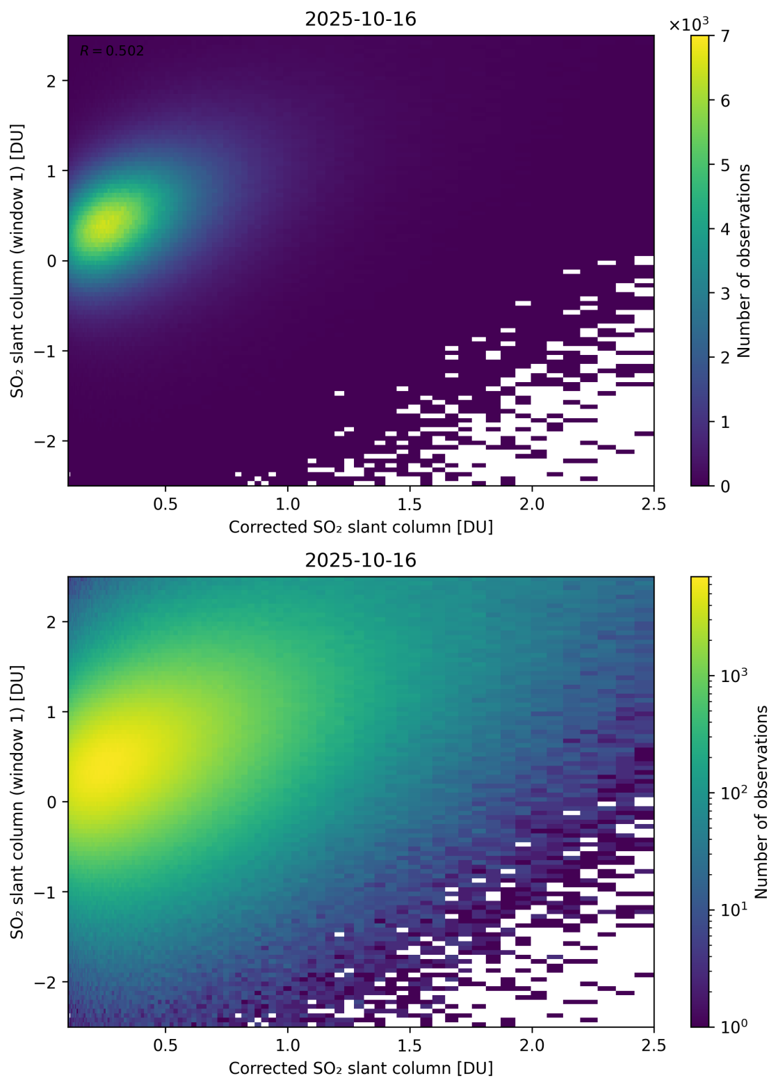
Figure 237: Scatter density plot of “Corrected SO 2 slant column” against “SO 2 slant column (window 1)” for 2025-10-15 to 2025-10-17.
