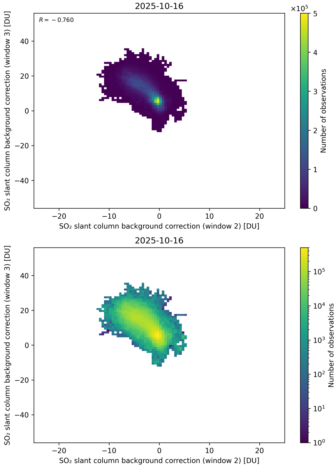
Figure 122: Scatter density plot of “SO 2 slant column background correction (window 2)” against “SO 2 slant column background correction (window 3)” for 2025-10-15 to 2025-10-17.
