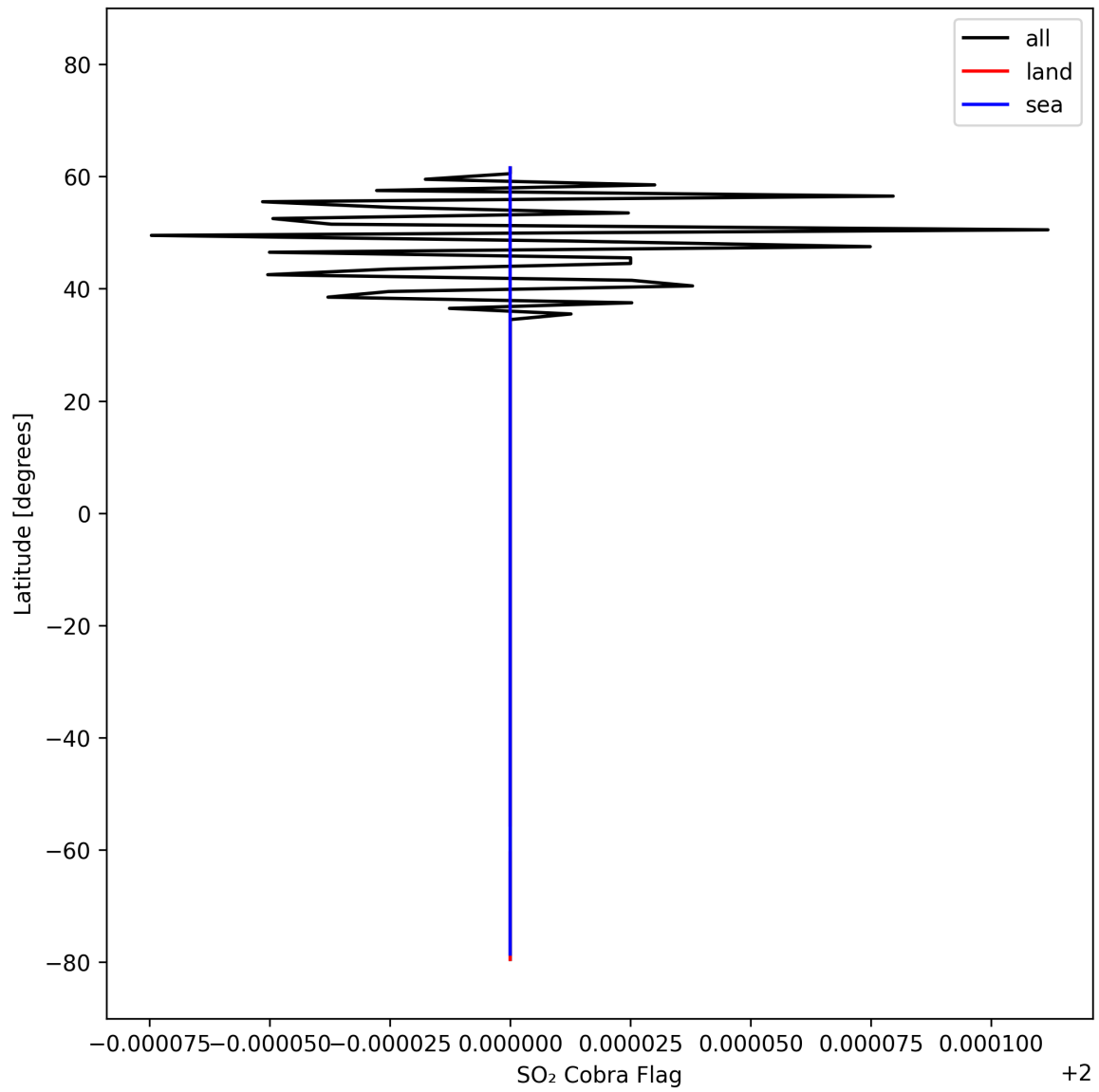
Figure 49: Zonal average of "SO 2 Cobra Flag" for 2025-10-15 to 2025-10-17.
