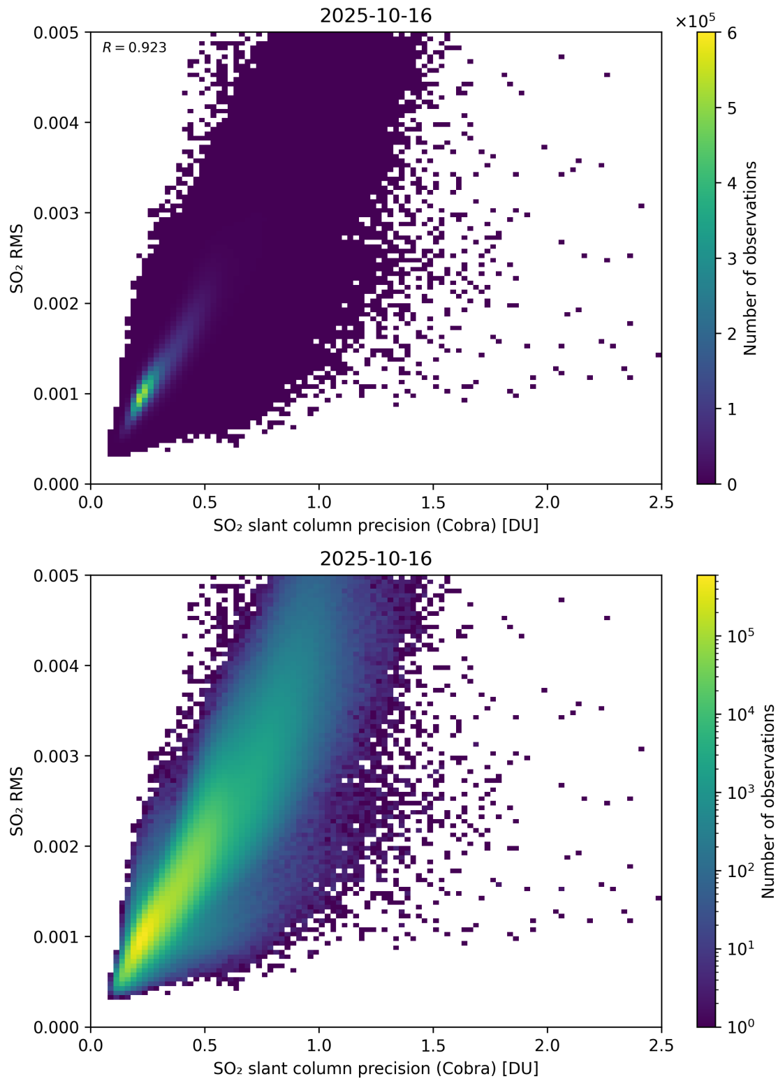
Figure 204: Scatter density plot of “SO 2 slant column precision (Cobra)” against “SO 2 RMS” for 2025-10-15 to 2025-10-17.
