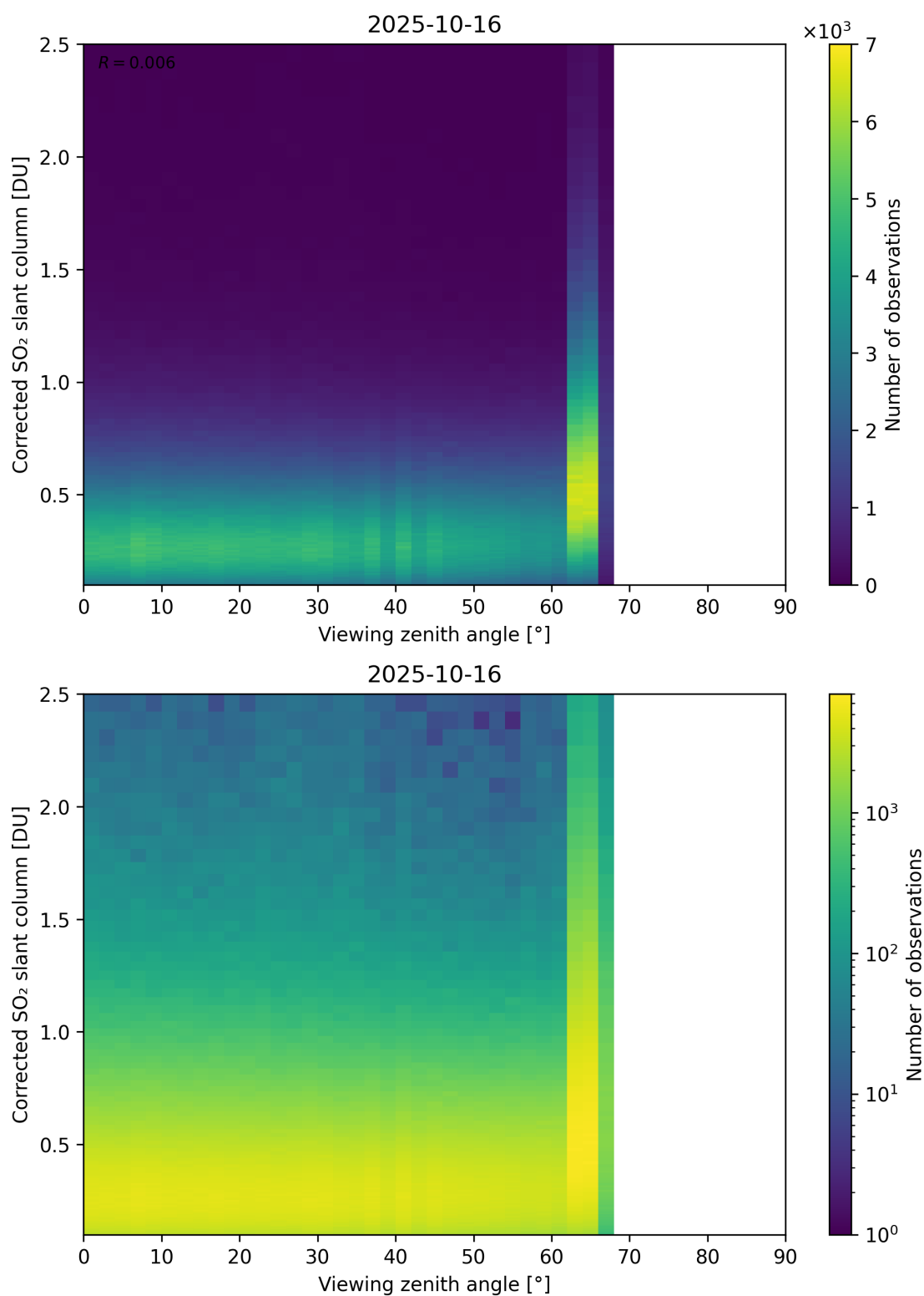
Figure 373: Scatter density plot of “Viewing zenith angle” against “Corrected SO 2 slant column” for 2025-10-15 to 2025-10-17.
