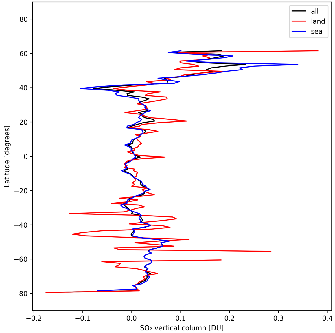
Figure 32: Zonal average of “SO 2 vertical column” for 2025-10-15 to 2025-10-17.
