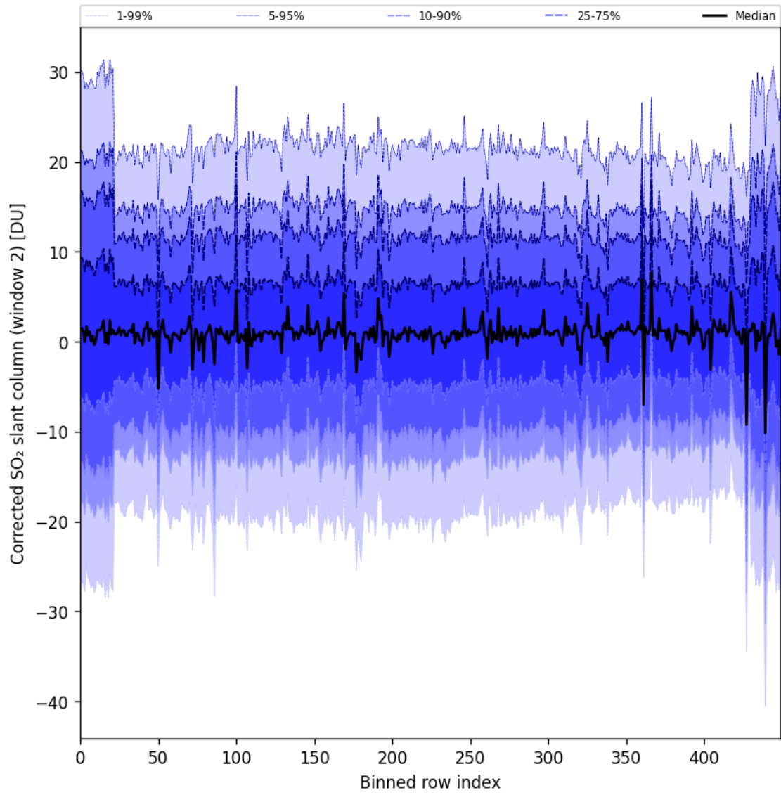
Figure 95: Along track statistics of “Corrected SO 2 slant column (window 2)” for 2025-10-15 to 2025-10-17
