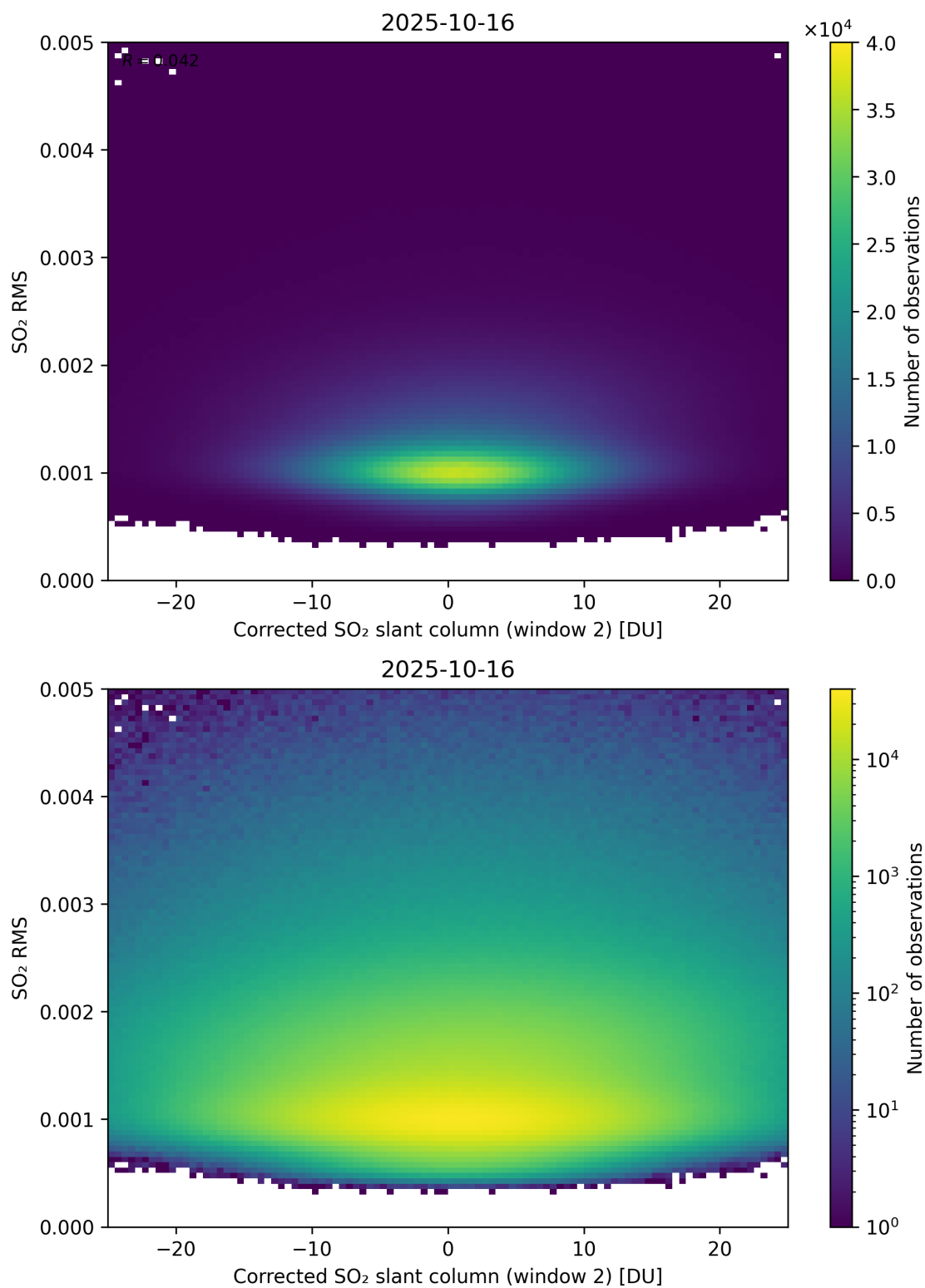
Figure 248: Scatter density plot of “Corrected SO 2 slant column (window 2)” against “SO 2 RMS” for 2025-10-15 to 2025-10-17.
