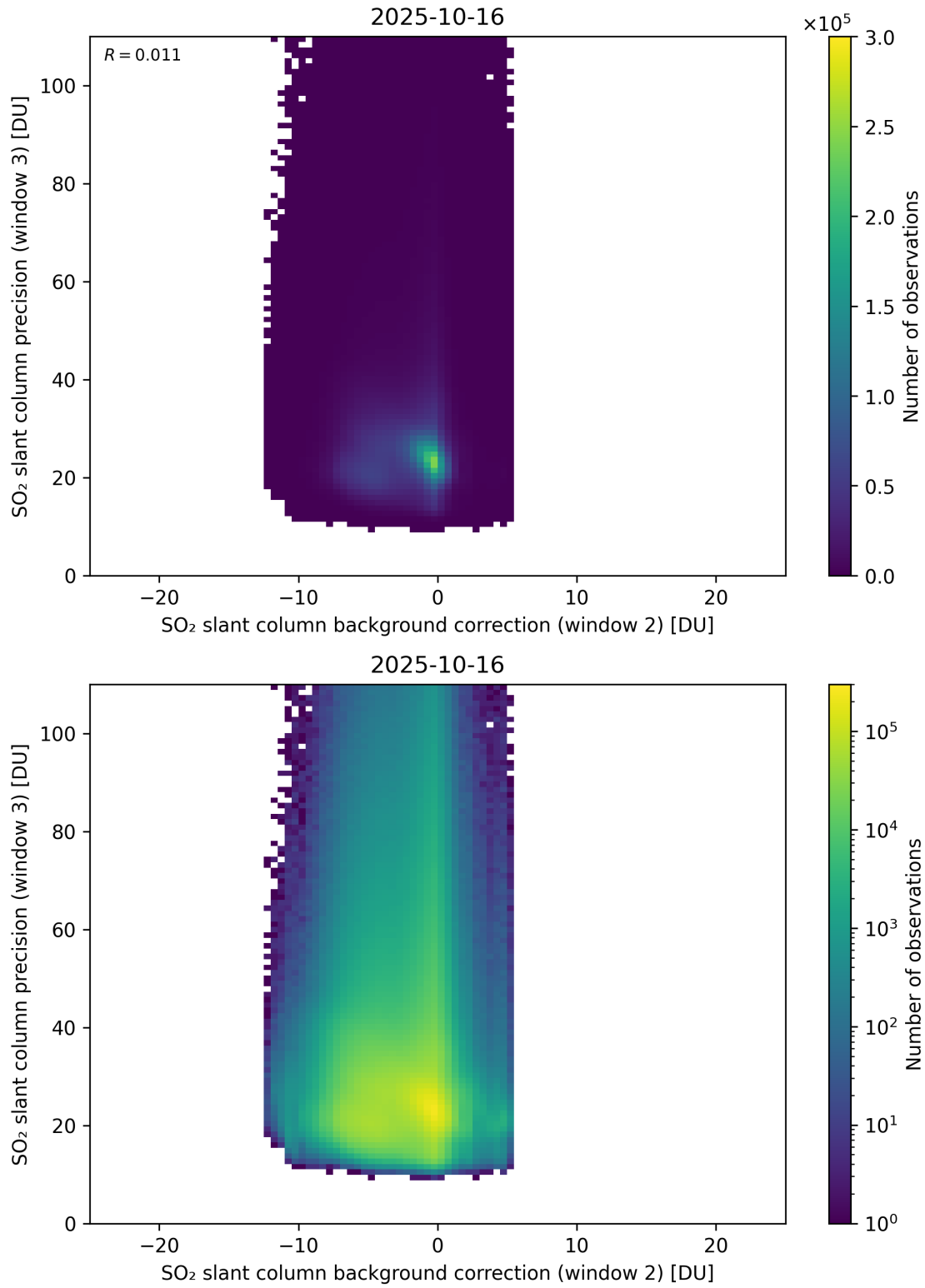
Figure 129: Scatter density plot of “SO 2 slant column background correction (window 2)” against “SO 2 slant column precision (window 3)” for 2025-10-15 to 2025-10-17.
