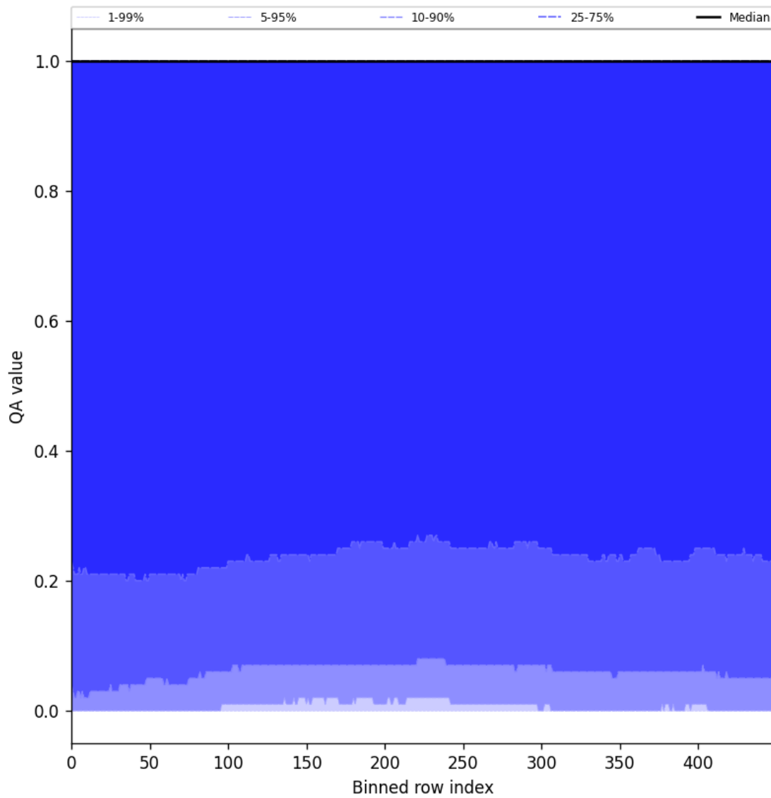
Figure 83: Along track statistics of “QA value” for 2025-10-15 to 2025-10-17
