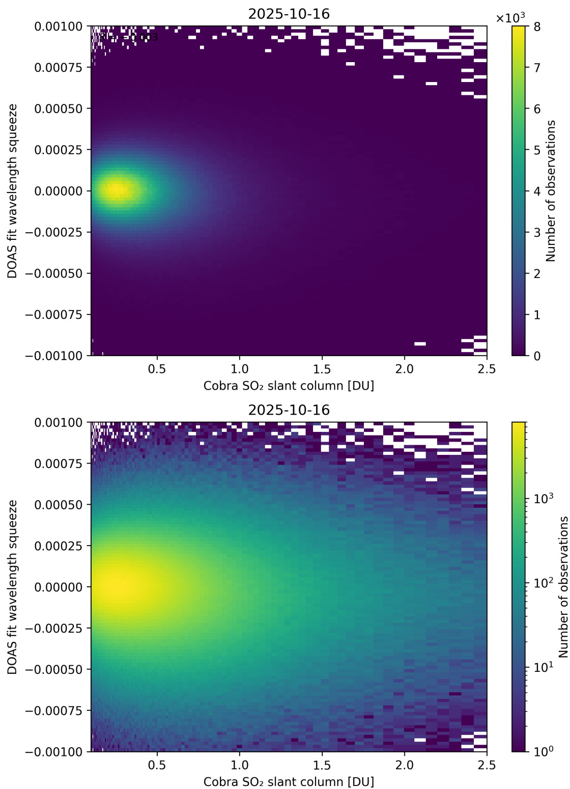
Figure 197: Scatter density plot of “Cobra SO 2 slant column” against “DOAS fit wavelength squeeze” for 2025-10-15 to 2025-10-17.
