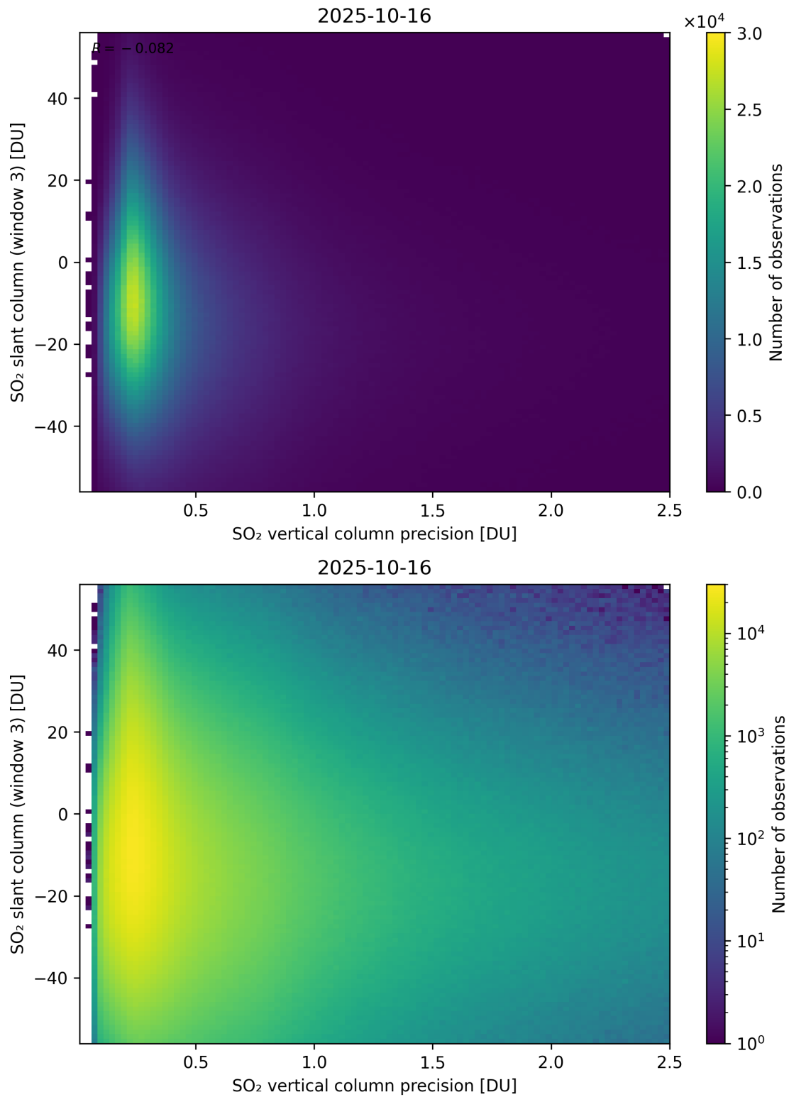
Figure 344: Scatter density plot of “SO 2 vertical column precision” against “SO 2 slant column (window 3)” for 2025-10-15 to 2025-10-17.
