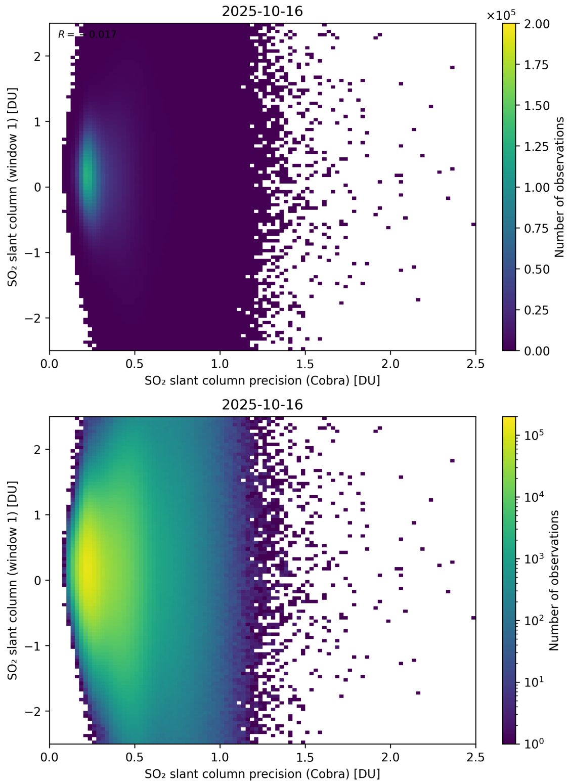
Figure 208: Scatter density plot of “SO 2 slant column precision (Cobra)” against “SO 2 slant column (window 1)” for 2025-10-15 to 2025-10-17.
