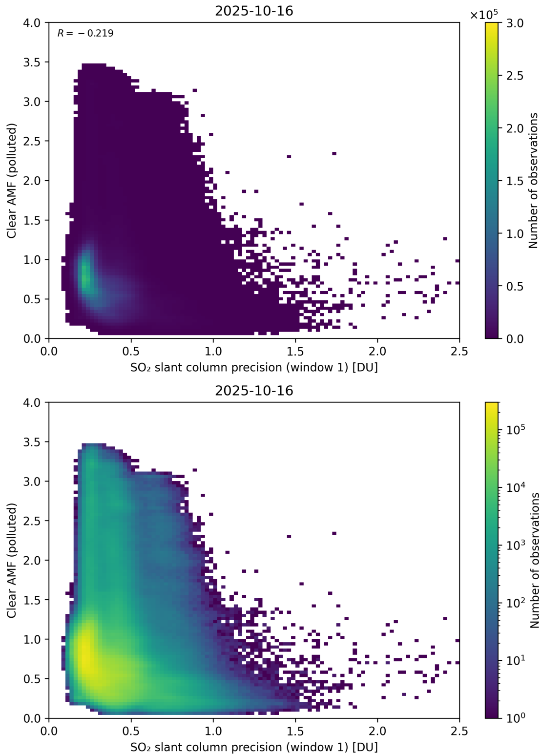
Figure 274: Scatter density plot of “SO 2 slant column precision (window 1)” against “Clear AMF (polluted)” for 2025-10-15 to 2025-10-17.
