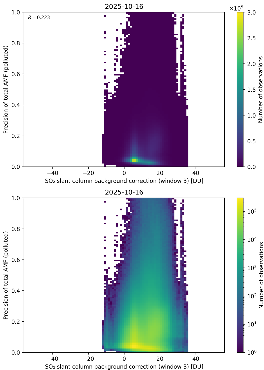
Figure 137: Scatter density plot of “SO 2 slant column background correction (window 3)” against “Precision of total AMF (polluted)” for 2025-10-15 to 2025-10-17.
