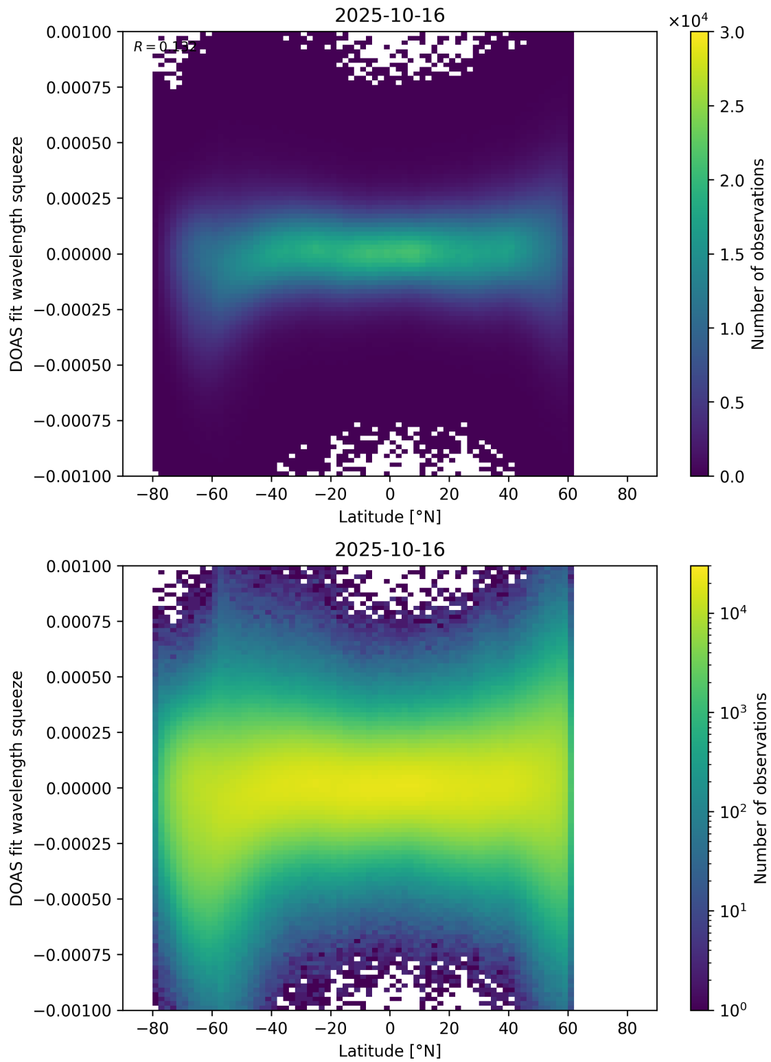
Figure 154: Scatter density plot of “Latitude” against “DOAS fit wavelength squeeze” for 2025-10-15 to 2025-10-17.
