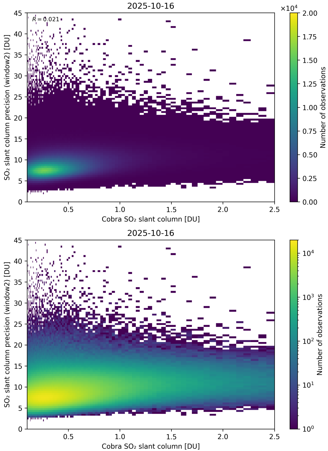
Figure 221: Scatter density plot of “Cobra SO 2 slant column” against “SO 2 slant column precision (window2)” for 2025-10-15 to 2025-10-17.
