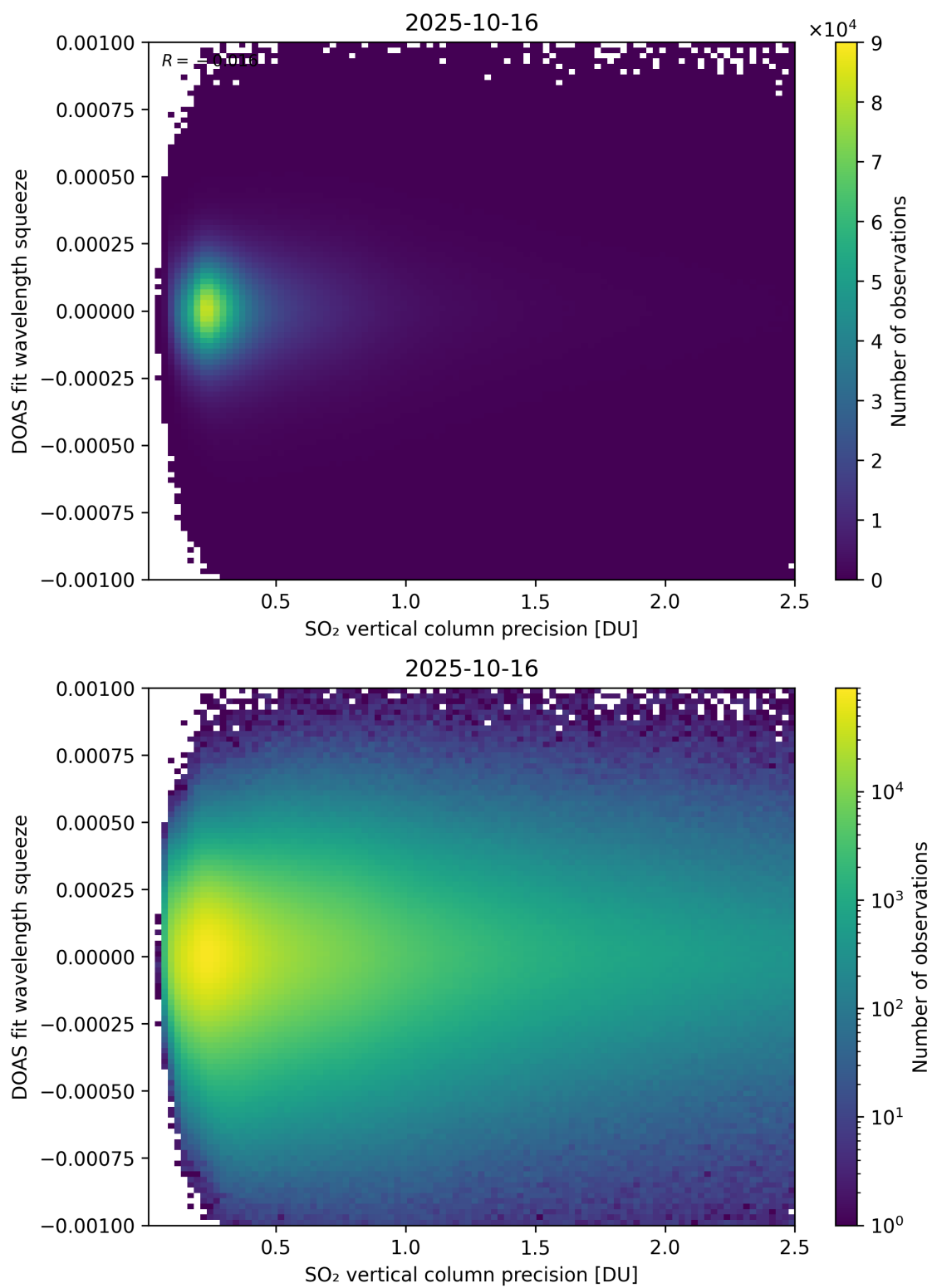
Figure 333: Scatter density plot of “SO 2 vertical column precision” against “DOAS fit wavelength squeeze” for 2025-10-15 to 2025-10-17.
