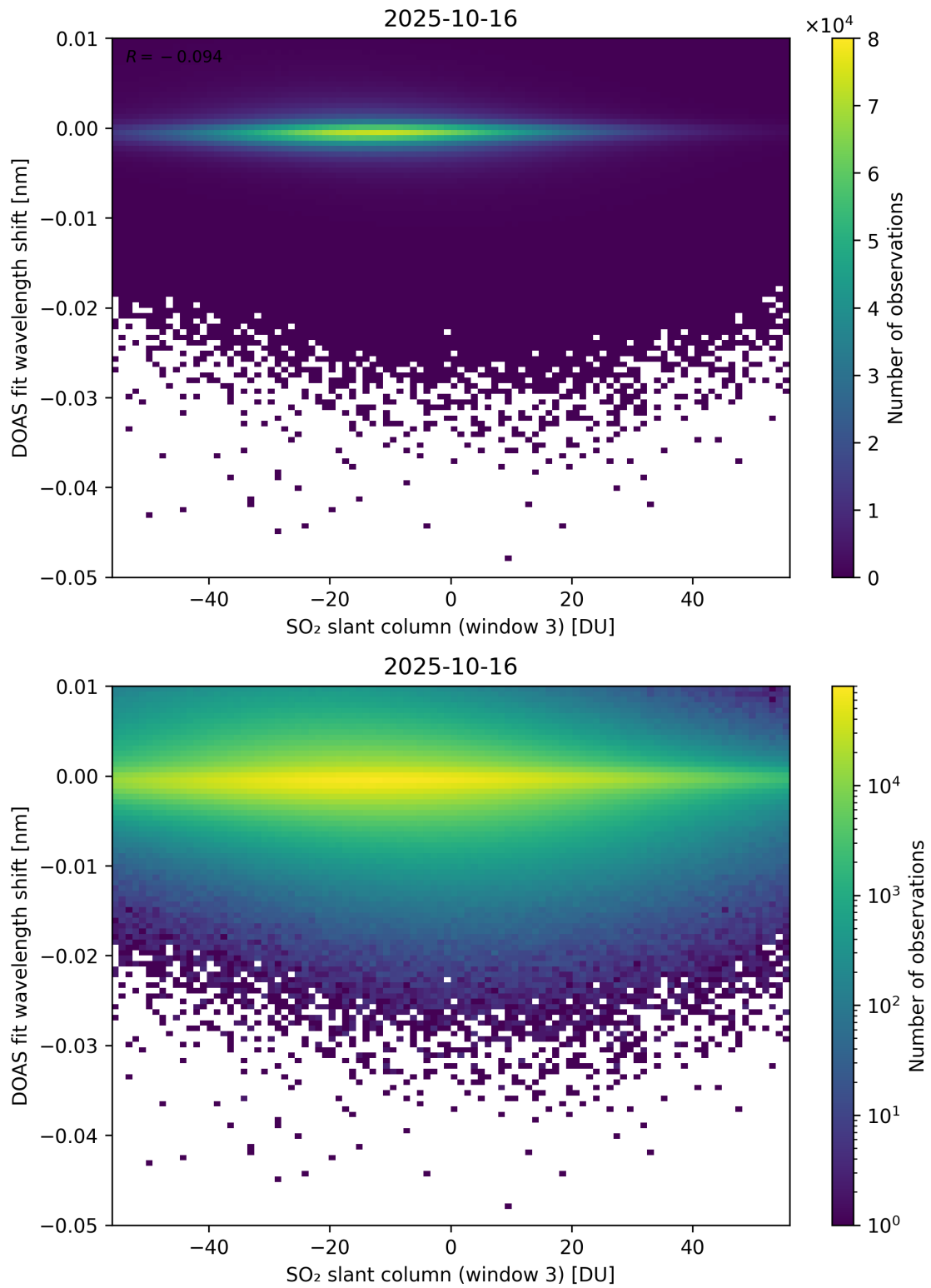
Figure 304: Scatter density plot of “SO 2 slant column (window 3)” against “DOAS fit wavelength shift” for 2025-10-15 to 2025-10-17.
