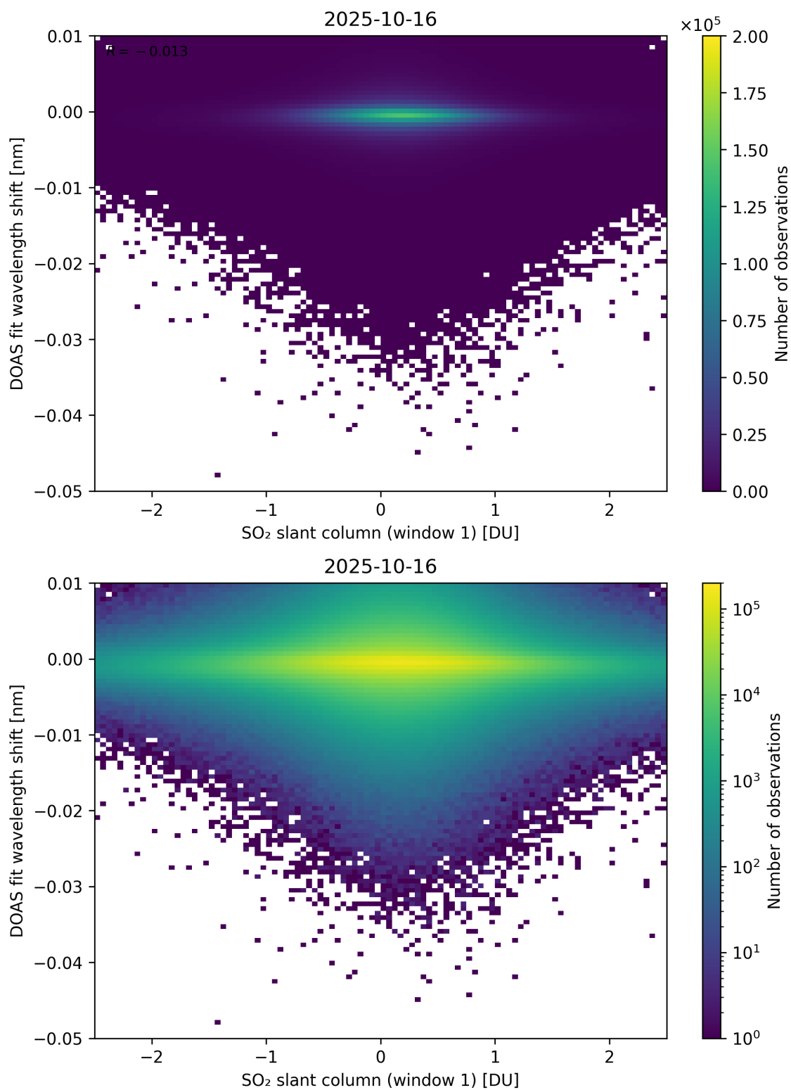
Figure 265: Scatter density plot of “SO 2 slant column (window 1)” against “DOAS fit wavelength shift” for 2025-10-15 to 2025-10-17.
