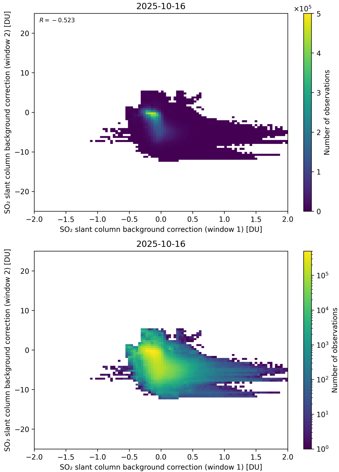
Figure 109: Scatter density plot of “SO 2 slant column background correction (window 1)” against “SO 2 slant column background correction (window 2)” for 2025-10-15 to 2025-10-17.
