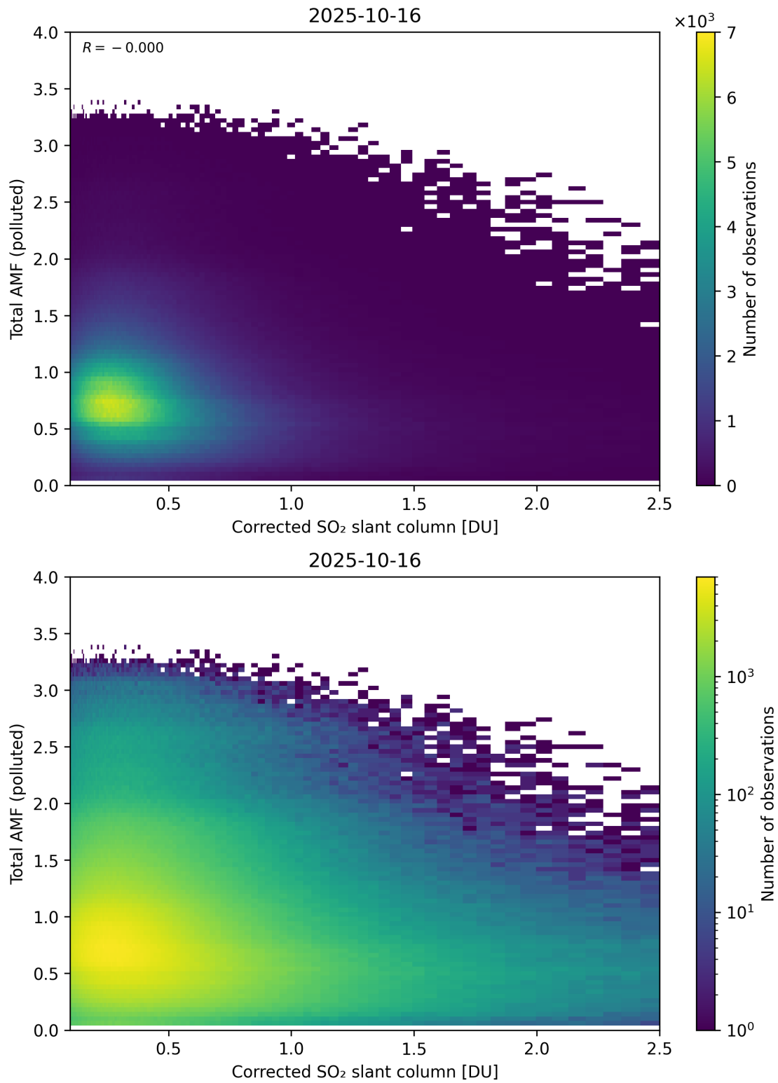
Figure 242: Scatter density plot of “Corrected SO 2 slant column” against “Total AMF (polluted)” for 2025-10-15 to 2025-10-17.
