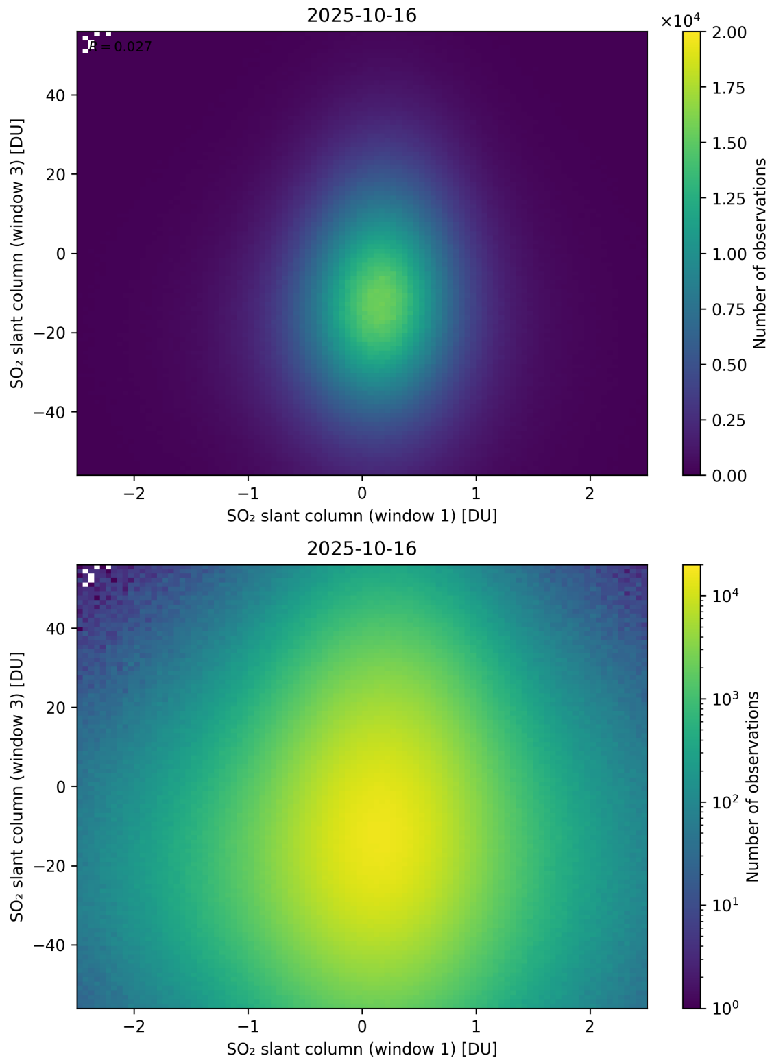
Figure 287: Scatter density plot of “SO 2 slant column (window 1)” against “SO 2 slant column (window 3)” for 2025-10-15 to 2025-10-17.
