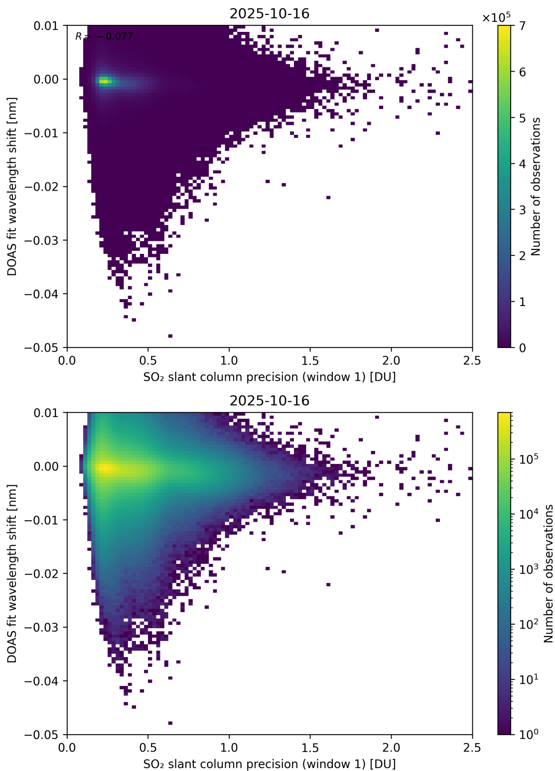
Figure 271: Scatter density plot of “SO 2 slant column precision (window 1)” against “DOAS fit wavelength shift” for 2025-10-15 to 2025-10-17.
