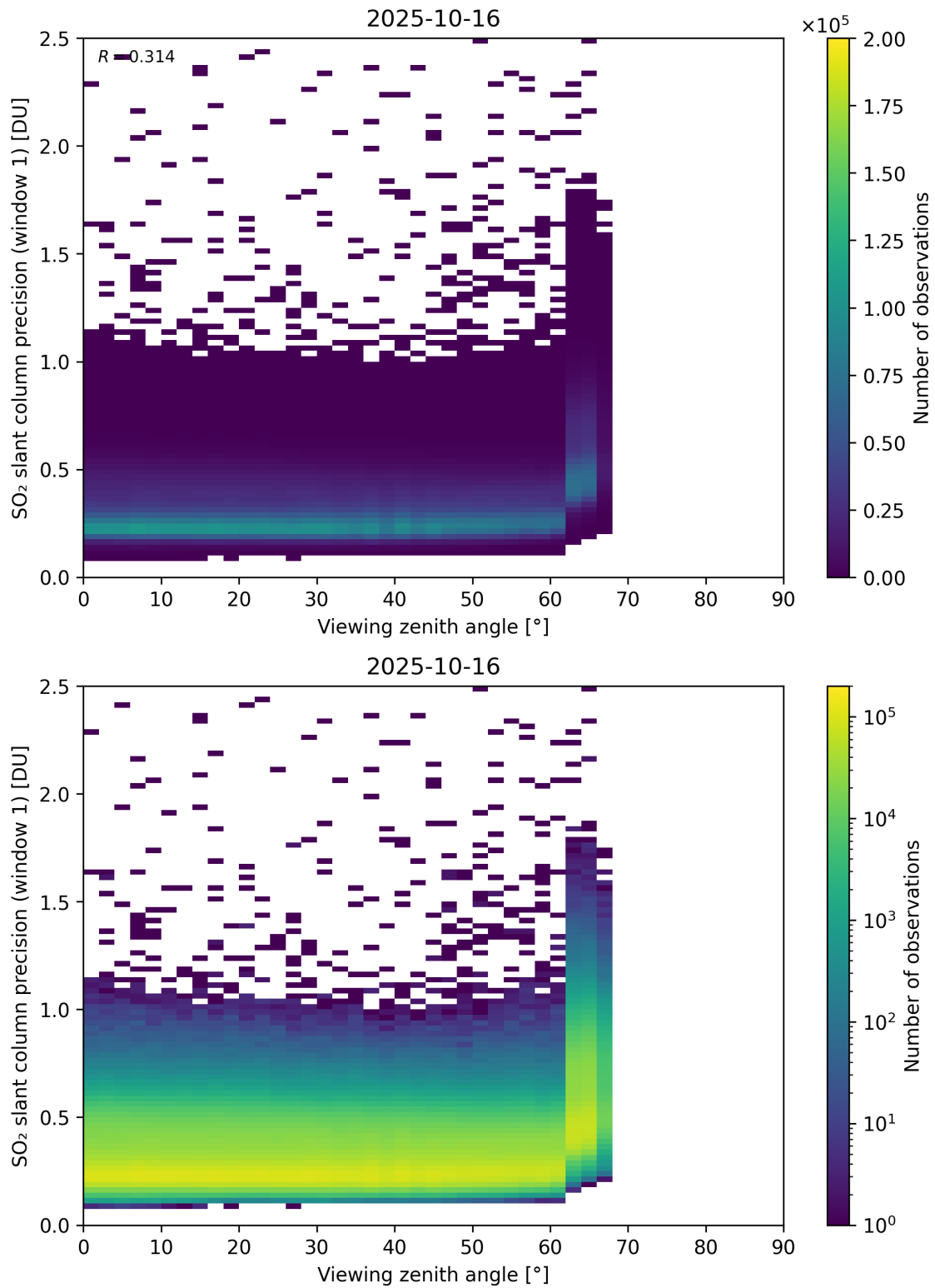
Figure 377: Scatter density plot of “Viewing zenith angle” against “SO 2 slant column precision (window 1)” for 2025-10-15 to 2025-10-17.
