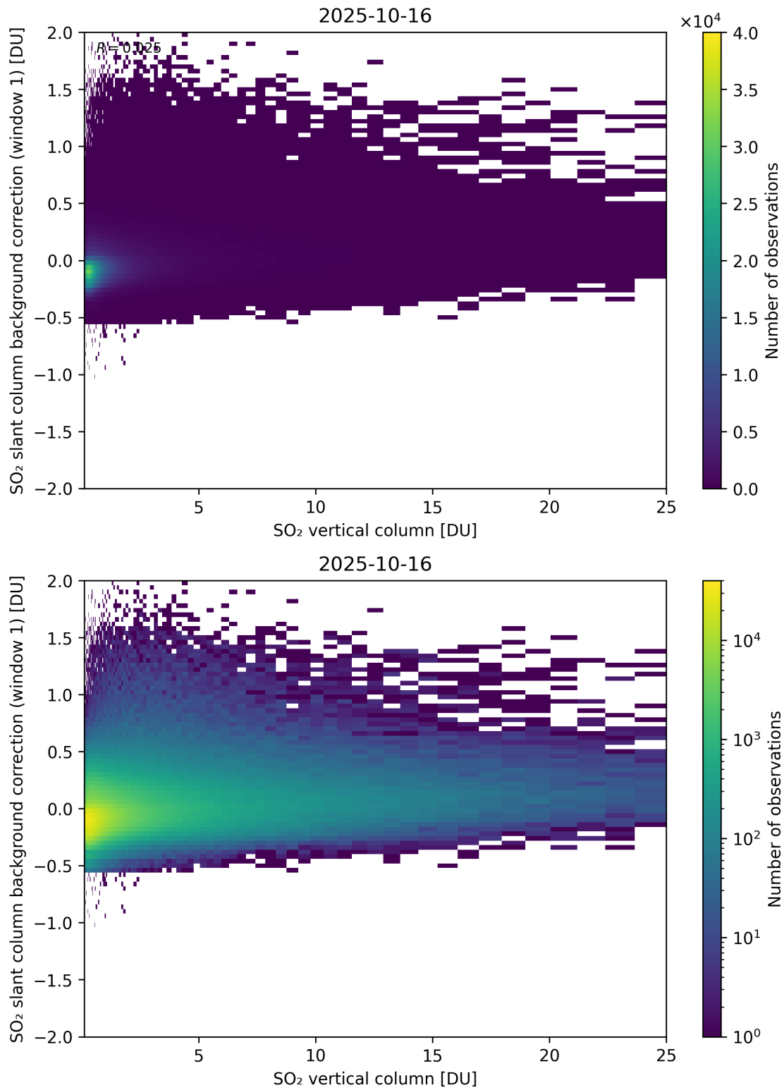
Figure 323: Scatter density plot of “SO 2 vertical column” against “SO 2 slant column background correction (window 1)” for 2025-10-15 to 2025-10-17.
