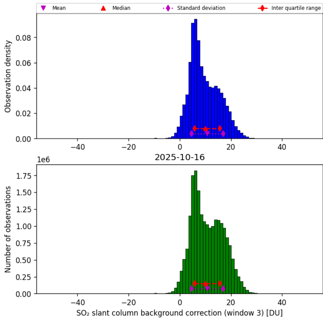
Figure 74: Histogram of “SO 2 slant column background correction (window 3)” for 2025-10-15 to 2025-10-17
