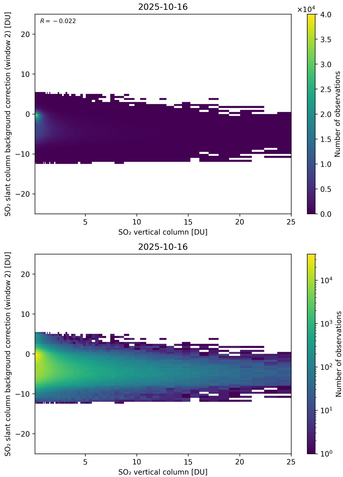
Figure 324: Scatter density plot of “SO 2 vertical column” against “SO 2 slant column background correction (window 2)” for 2025-10-15 to 2025-10-17.
