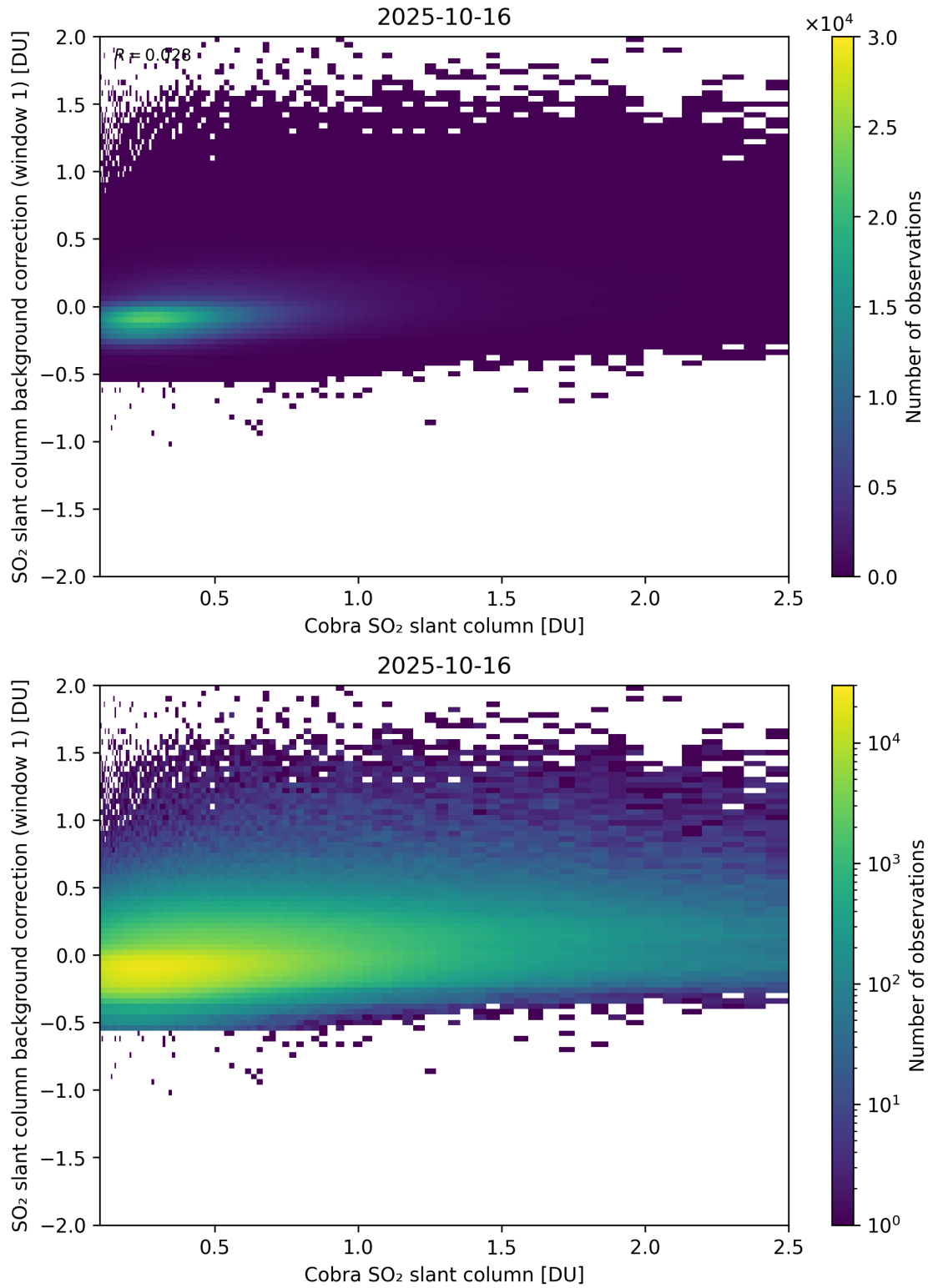
Figure 193: Scatter density plot of “Cobra SO 2 slant column” against “SO 2 slant column background correction (window 1)” for 2025-10-15 to 2025-10-17.
