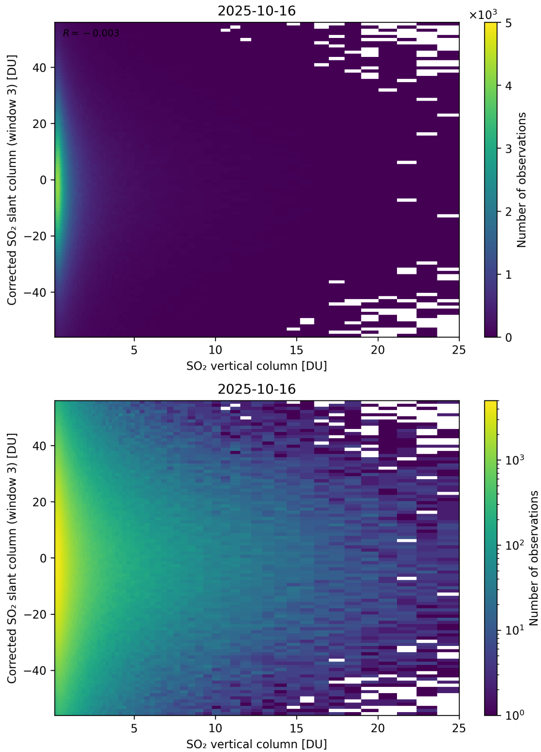
Figure 353: Scatter density plot of “SO 2 vertical column” against “Corrected SO 2 slant column (window 3)” for 2025-10-15 to 2025-10-17.
