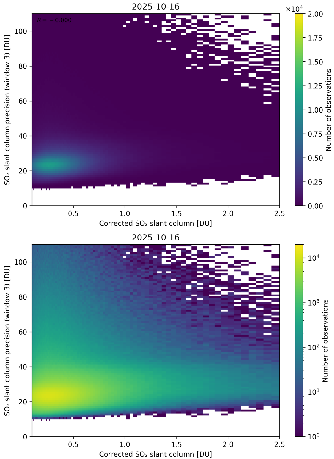
Figure 241: Scatter density plot of “Corrected SO 2 slant column” against “SO 2 slant column precision (window 3)” for 2025-10-15 to 2025-10-17.
