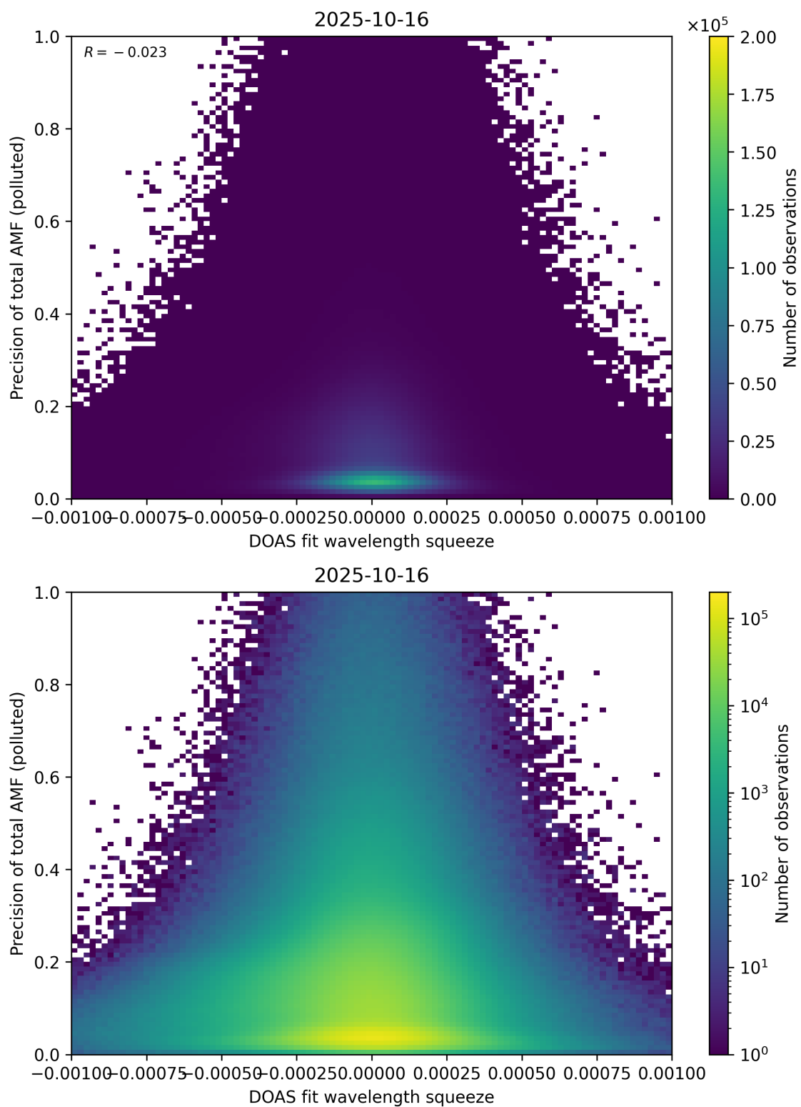
Figure 146: Scatter density plot of “DOAS fit wavelength squeeze” against “Precision of total AMF (polluted)” for 2025-10-15 to 2025-10-17.
