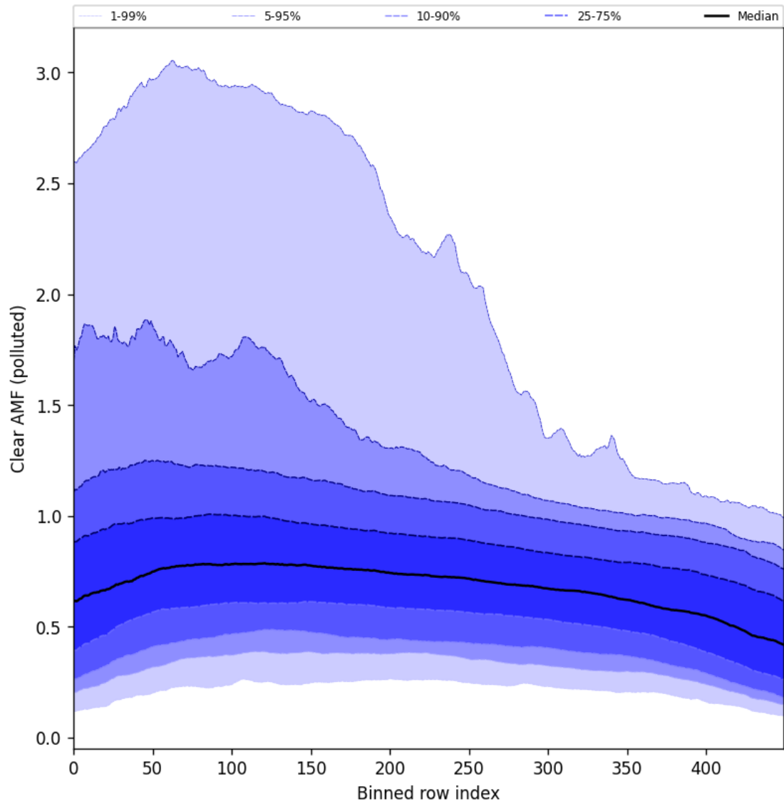
Figure 107: Along track statistics of “Clear AMF (polluted)” for 2025-10-15 to 2025-10-17
