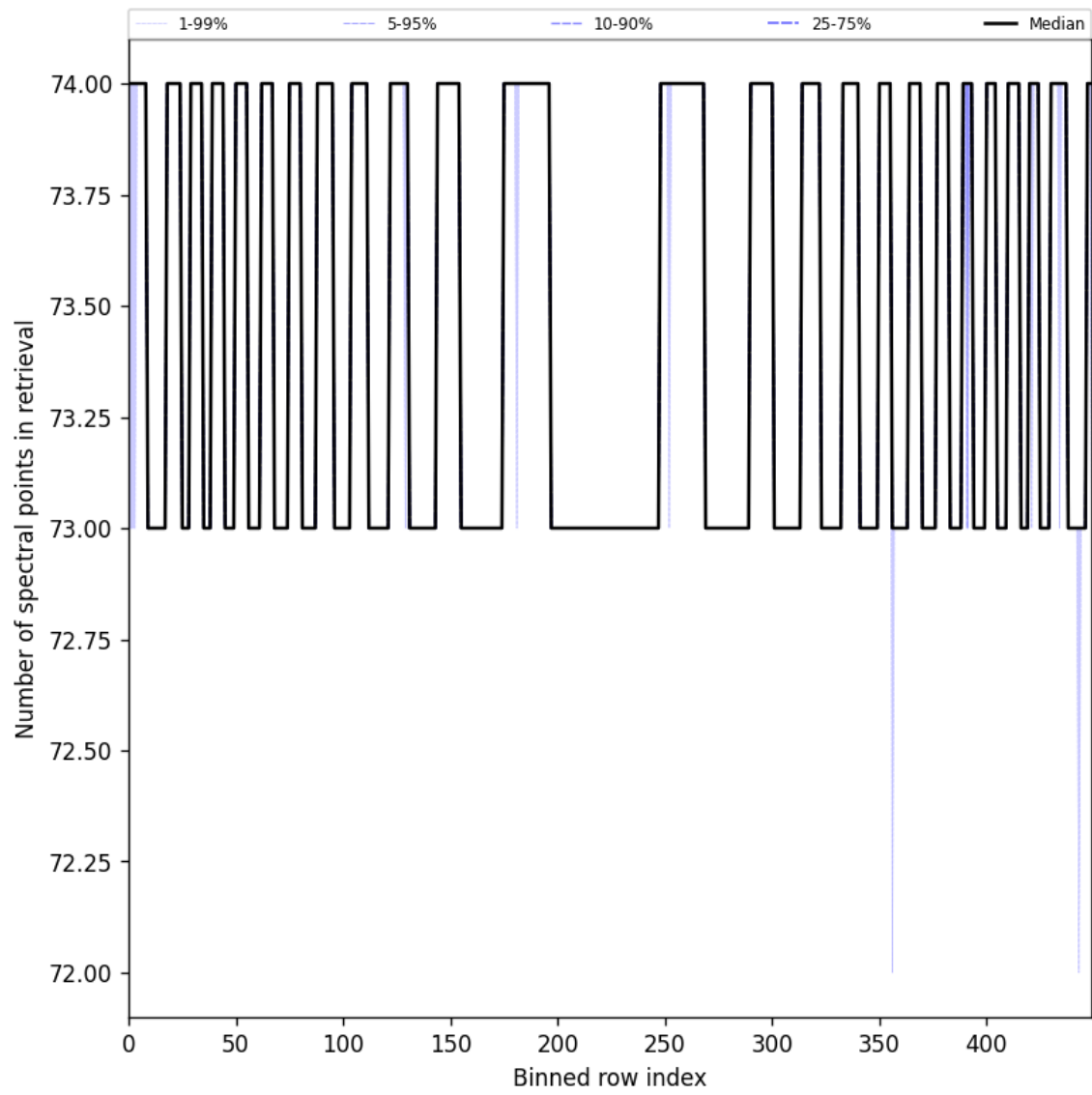
Figure 108: Along track statistics of “Number of spectral points in retrieval” for 2025-10-15 to 2025-10-17
