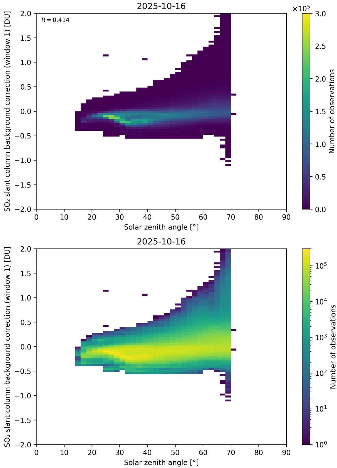
Figure 171: Scatter density plot of “Solar zenith angle” against “SO 2 slant column background correction (window 1)” for 2025-10-15 to 2025-10-17.
