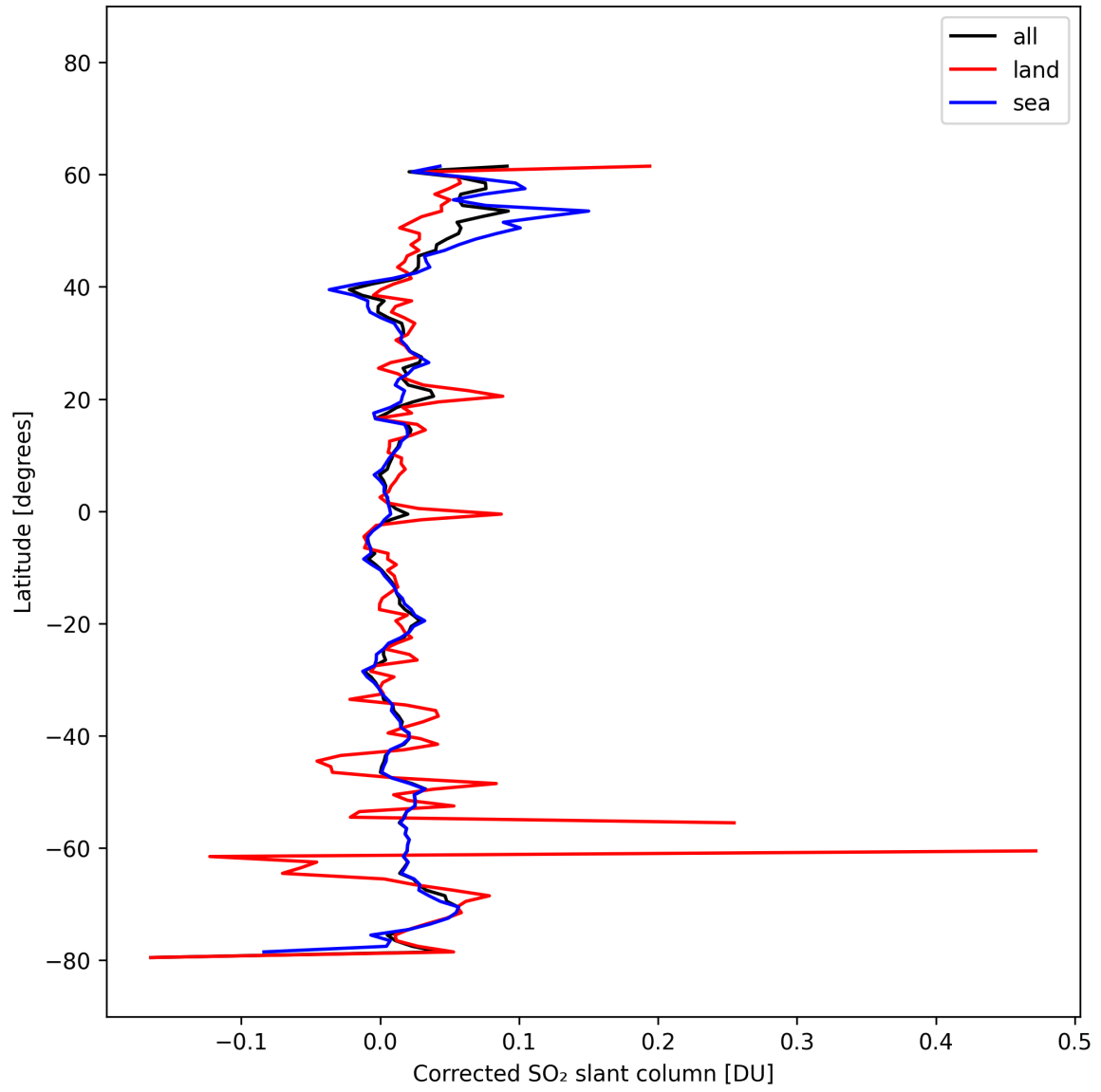
Figure 34: Zonal average of “Corrected SO 2 slant column” for 2025-10-15 to 2025-10-17.
