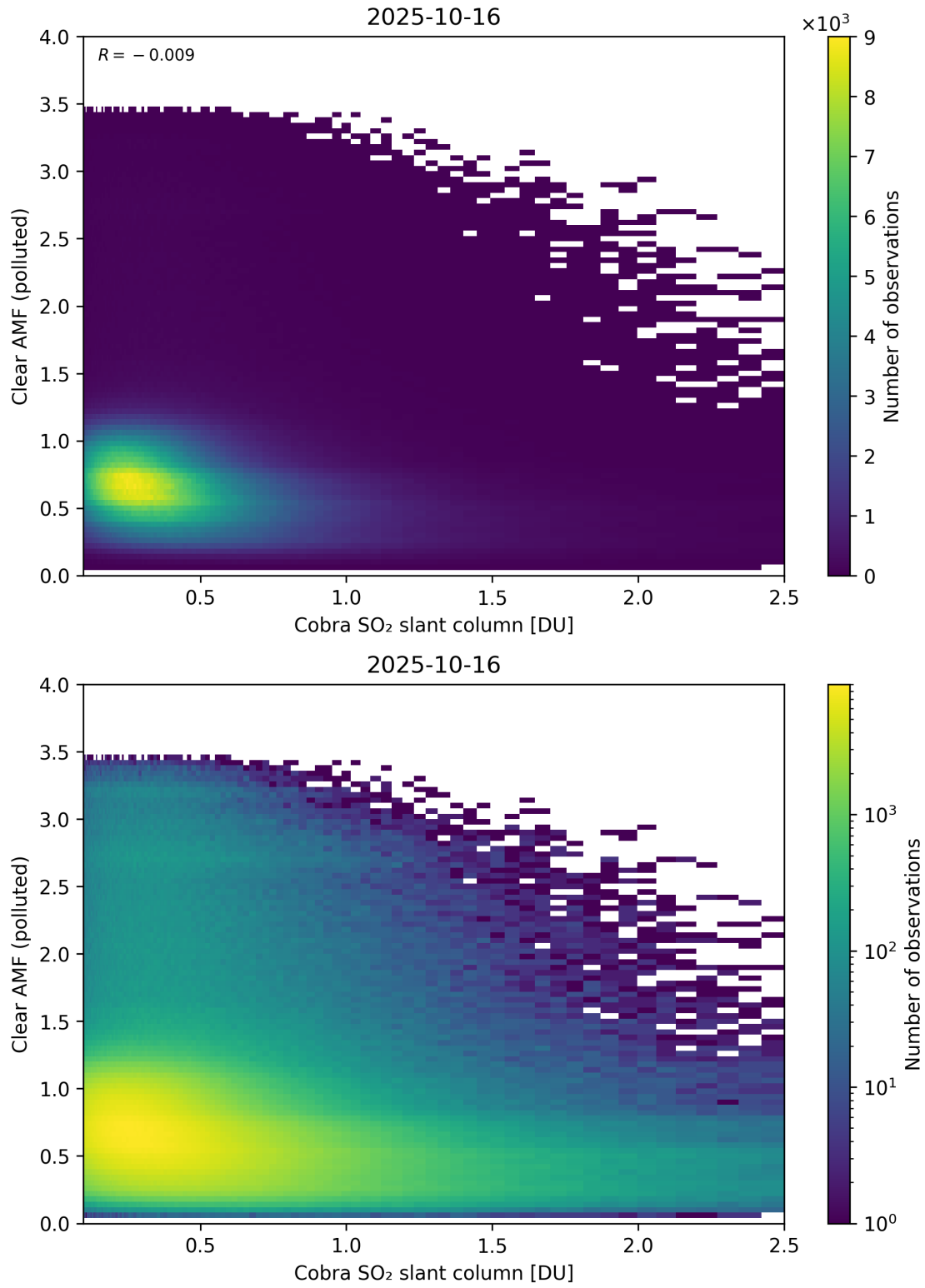
Figure 215: Scatter density plot of “Cobra SO 2 slant column” against “Clear AMF (polluted)” for 2025-10-15 to 2025-10-17.
