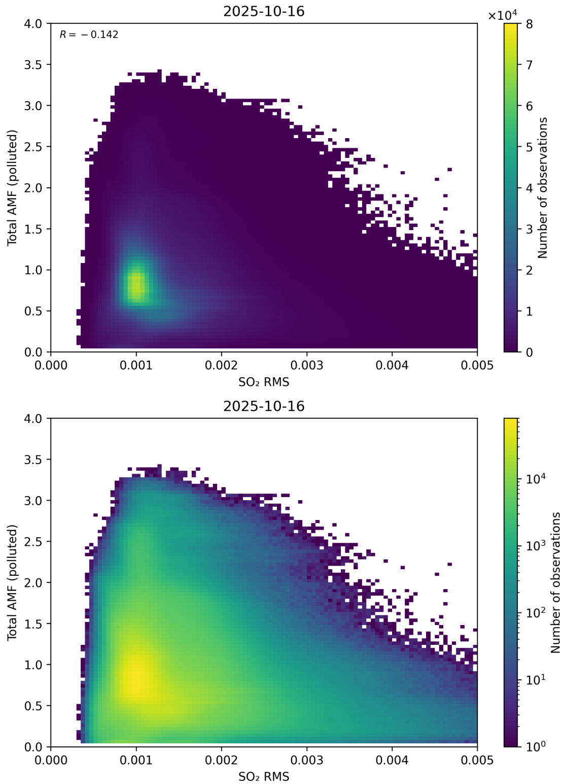
Figure 148: Scatter density plot of “SO 2 RMS” against “Total AMF (polluted)” for 2025-10-15 to 2025-10-17.
