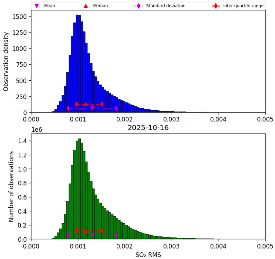
Figure 78: Histogram of “SO 2 RMS” for 2025-10-15 to 2025-10-17
