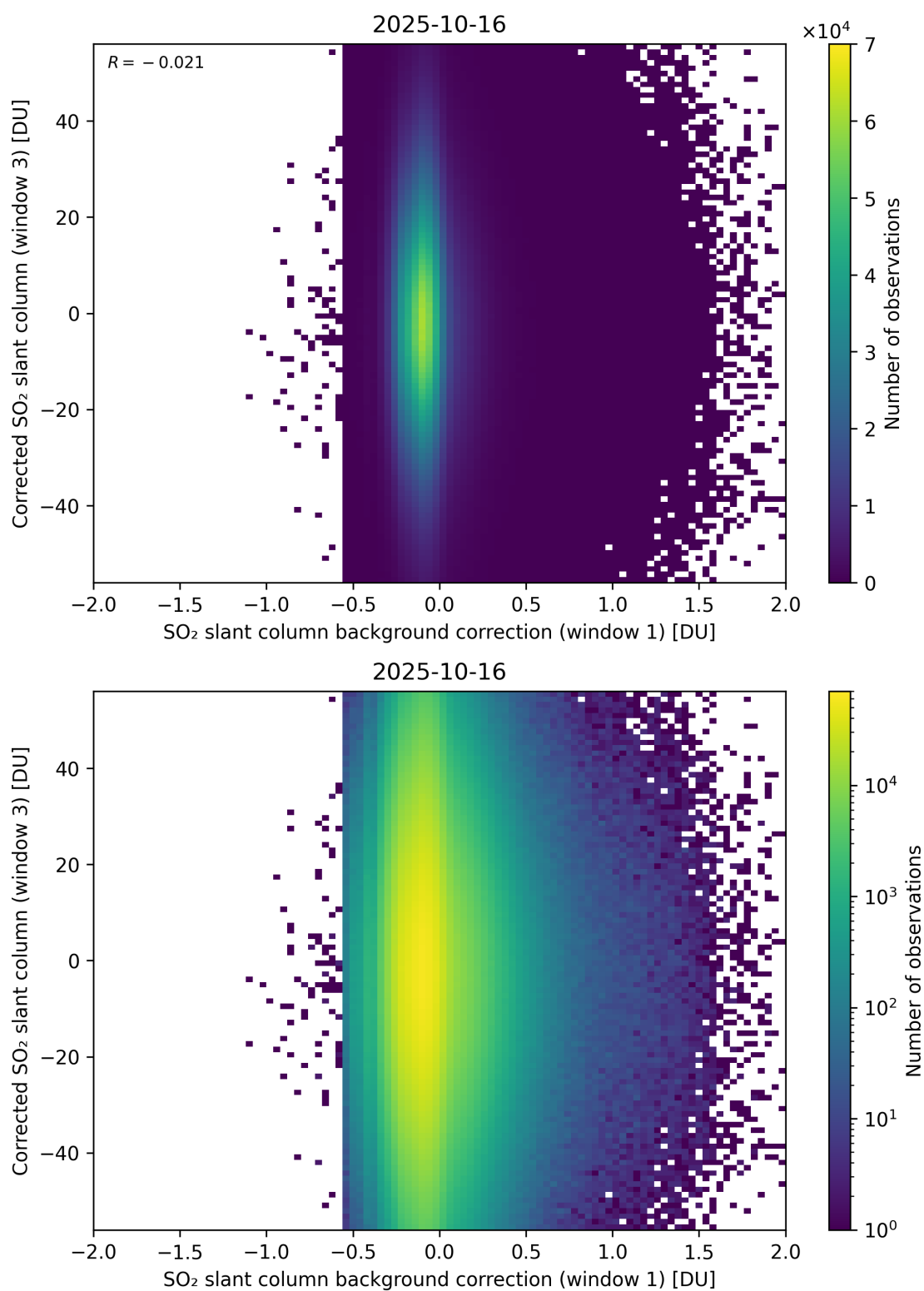
Figure 116: Scatter density plot of “SO 2 slant column background correction (window 1)” against “Corrected SO 2 slant column (window 3)” for 2025-10-15 to 2025-10-17.
