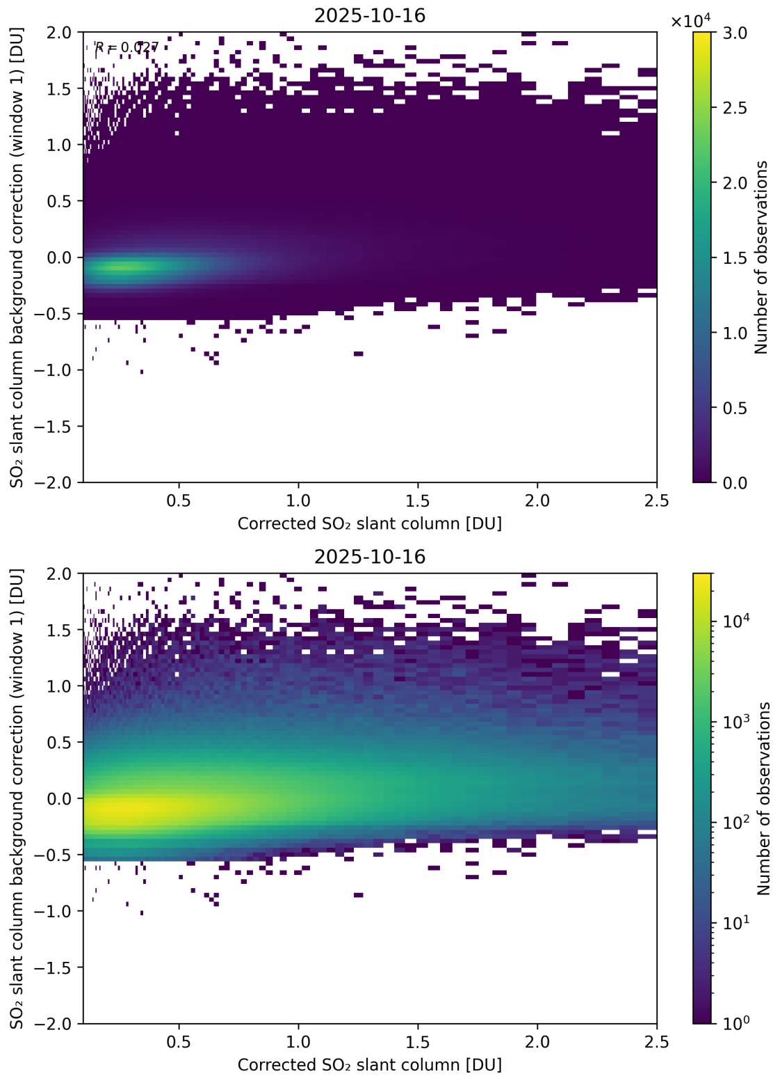
Figure 226: Scatter density plot of “Corrected SO 2 slant column” against “SO 2 slant column background correction (window 1)” for 2025-10-15 to 2025-10-17.
