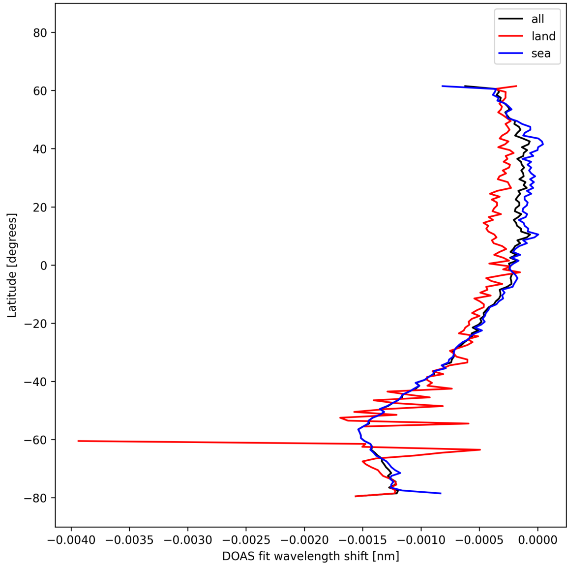
Figure 50: Zonal average of “DOAS fit wavelength shift” for 2025-10-15 to 2025-10-17.
