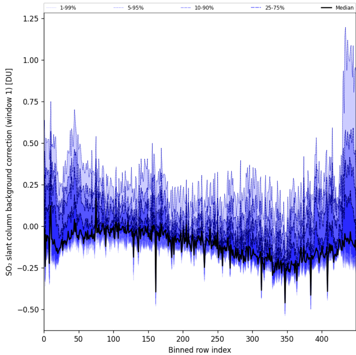
Figure 92: Along track statistics of “SO 2 slant column background correction (window 1)” for 2025-10-15 to 2025-10-17
