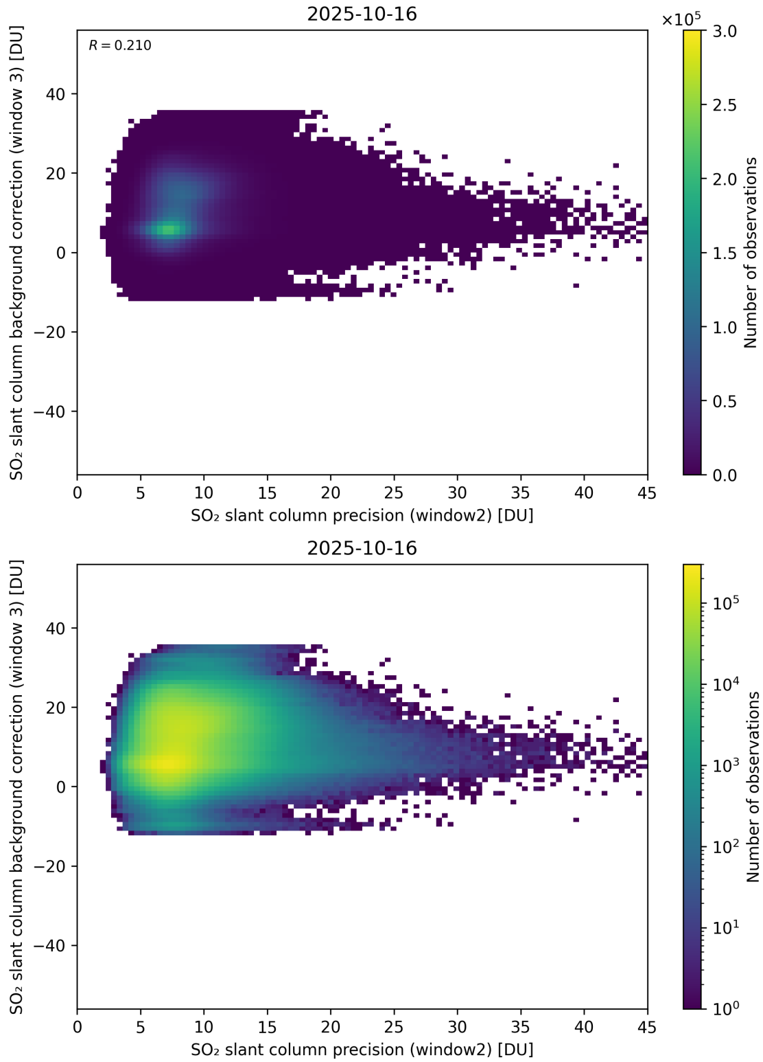
Figure 292: Scatter density plot of “SO 2 slant column precision (window2)” against “SO 2 slant column background correction (window 3)” for 2025-10-15 to 2025-10-17.
