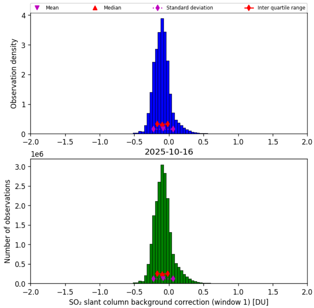
Figure 66: Histogram of “SO 2 slant column background correction (window 1)” for 2025-10-15 to 2025-10-17
