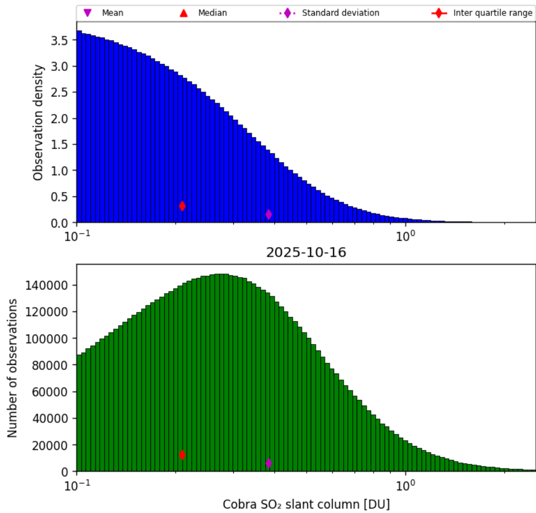
Figure 61: Histogram of “Cobra SO 2 slant column” for 2025-10-15 to 2025-10-17
