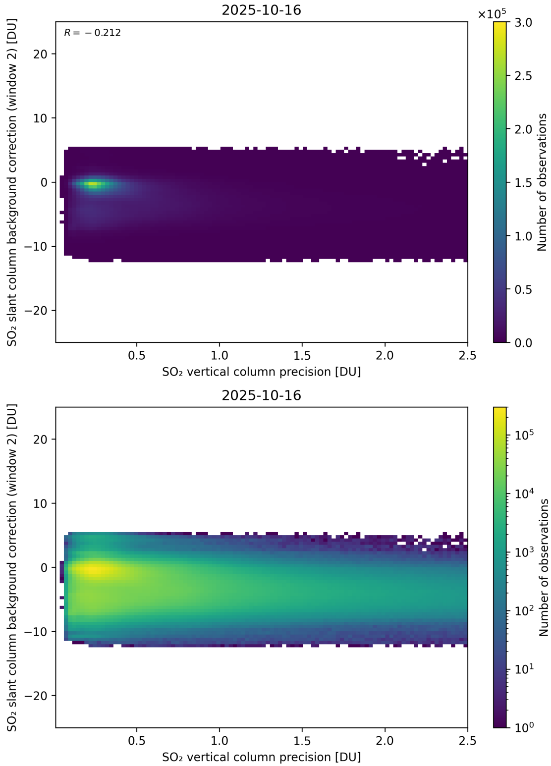
Figure 330: Scatter density plot of “SO 2 vertical column precision” against “SO 2 slant column background correction (window 2)” for 2025-10-15 to 2025-10-17.
