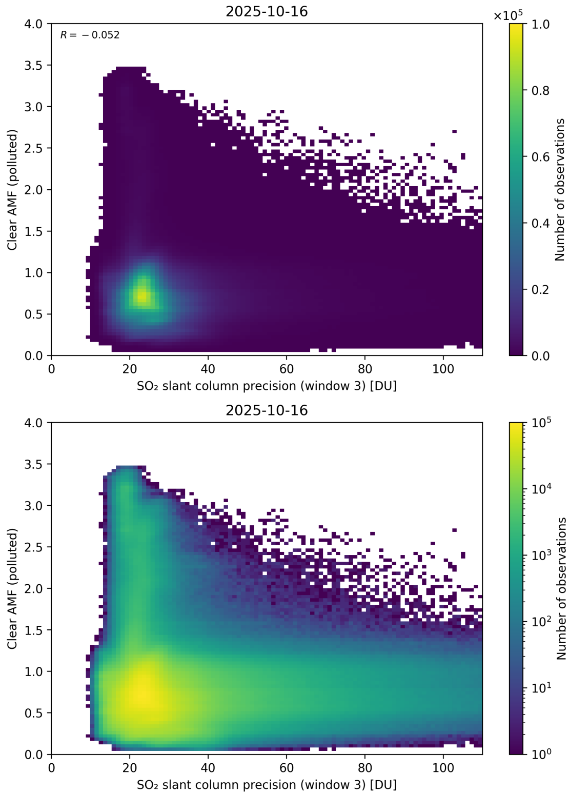
Figure 311: Scatter density plot of “SO 2 slant column precision (window 3)” against “Clear AMF (polluted)” for 2025-10-15 to 2025-10-17.
