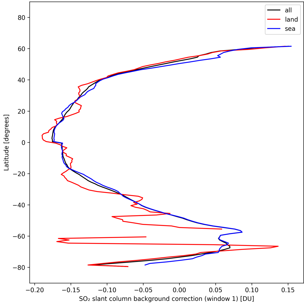
Figure 40: Zonal average of “SO 2 slant column background correction (window 1)” for 2025-10-15 to 2025-10-17.
