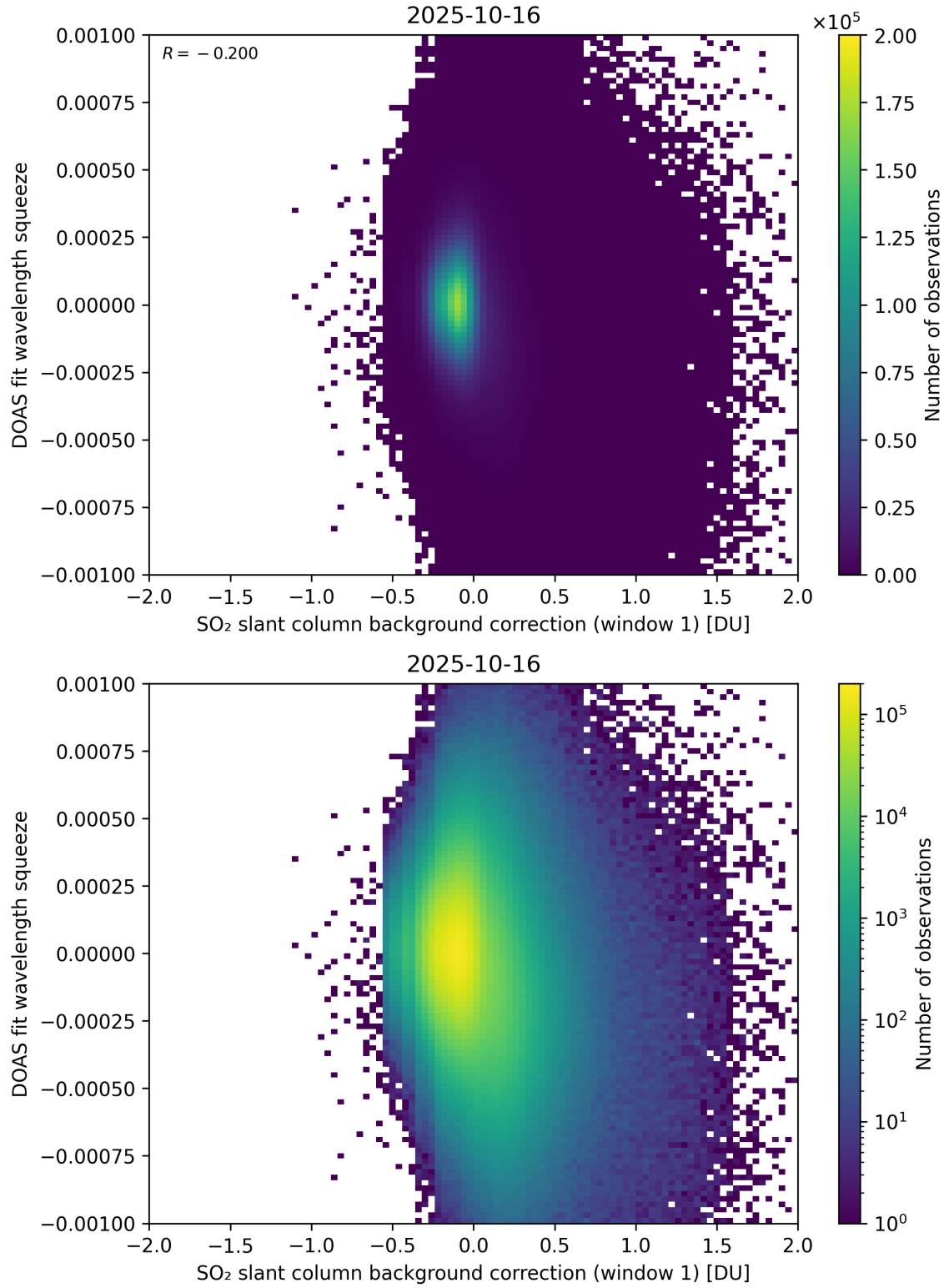
Figure 112: Scatter density plot of “SO 2 slant column background correction (window 1)” against “DOAS fit wavelength squeeze” for 2025-10-15 to 2025-10-17.
