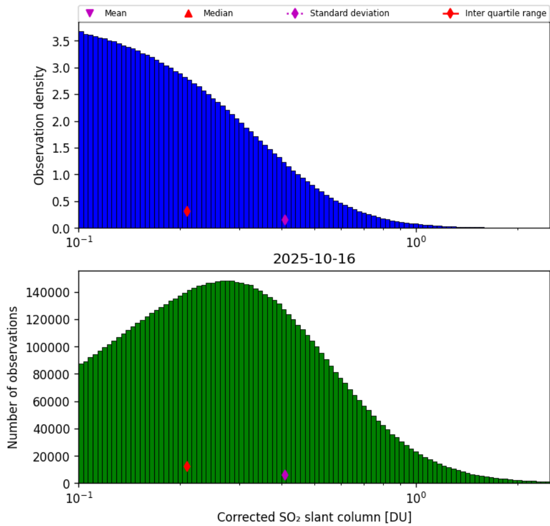
Figure 60: Histogram of "Corrected SO 2 slant column" for 2025-10-15 to 2025-10-17
