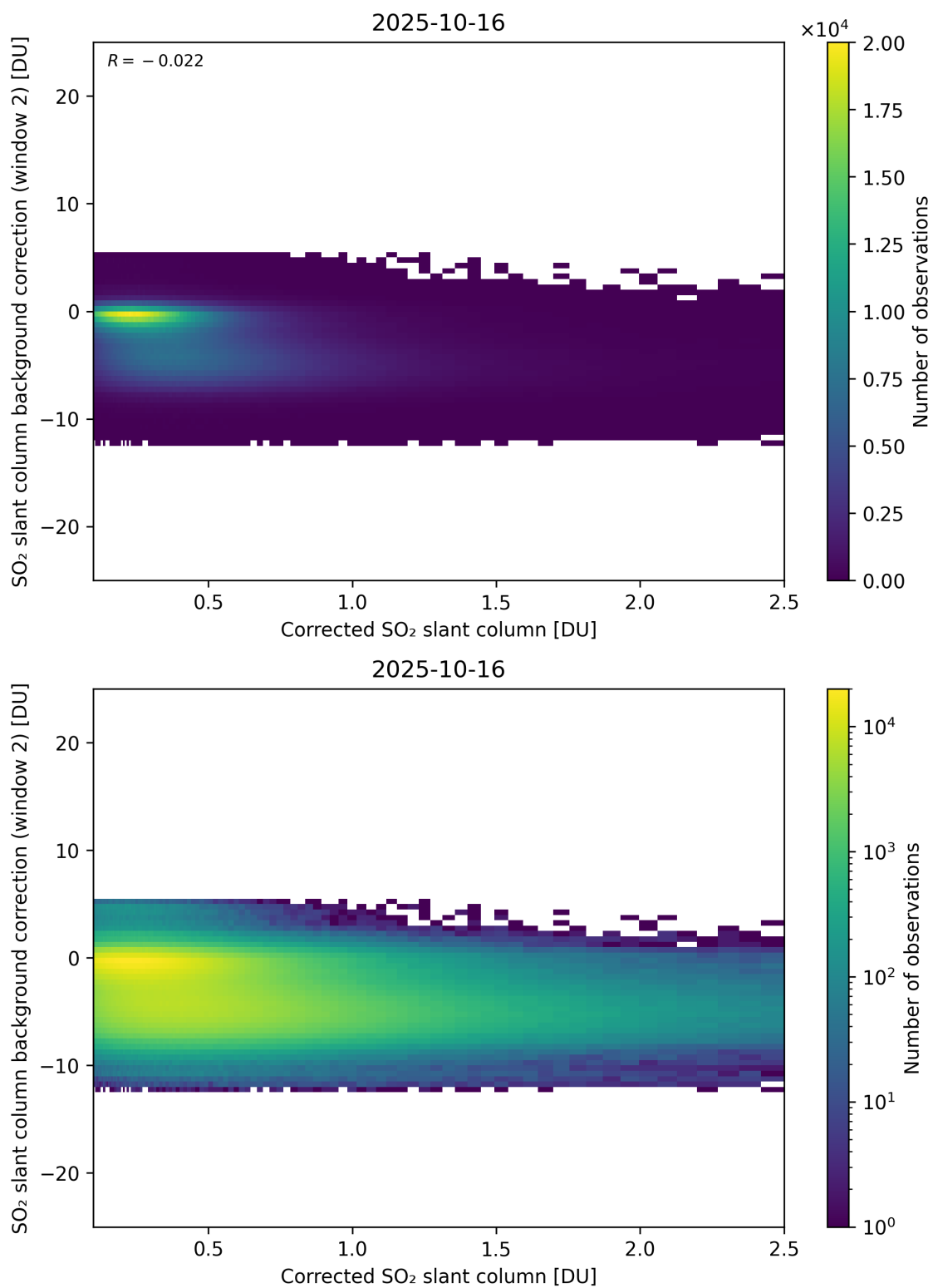
Figure 227: Scatter density plot of “Corrected SO 2 slant column” against “SO 2 slant column background correction (window 2)” for 2025-10-15 to 2025-10-17.
