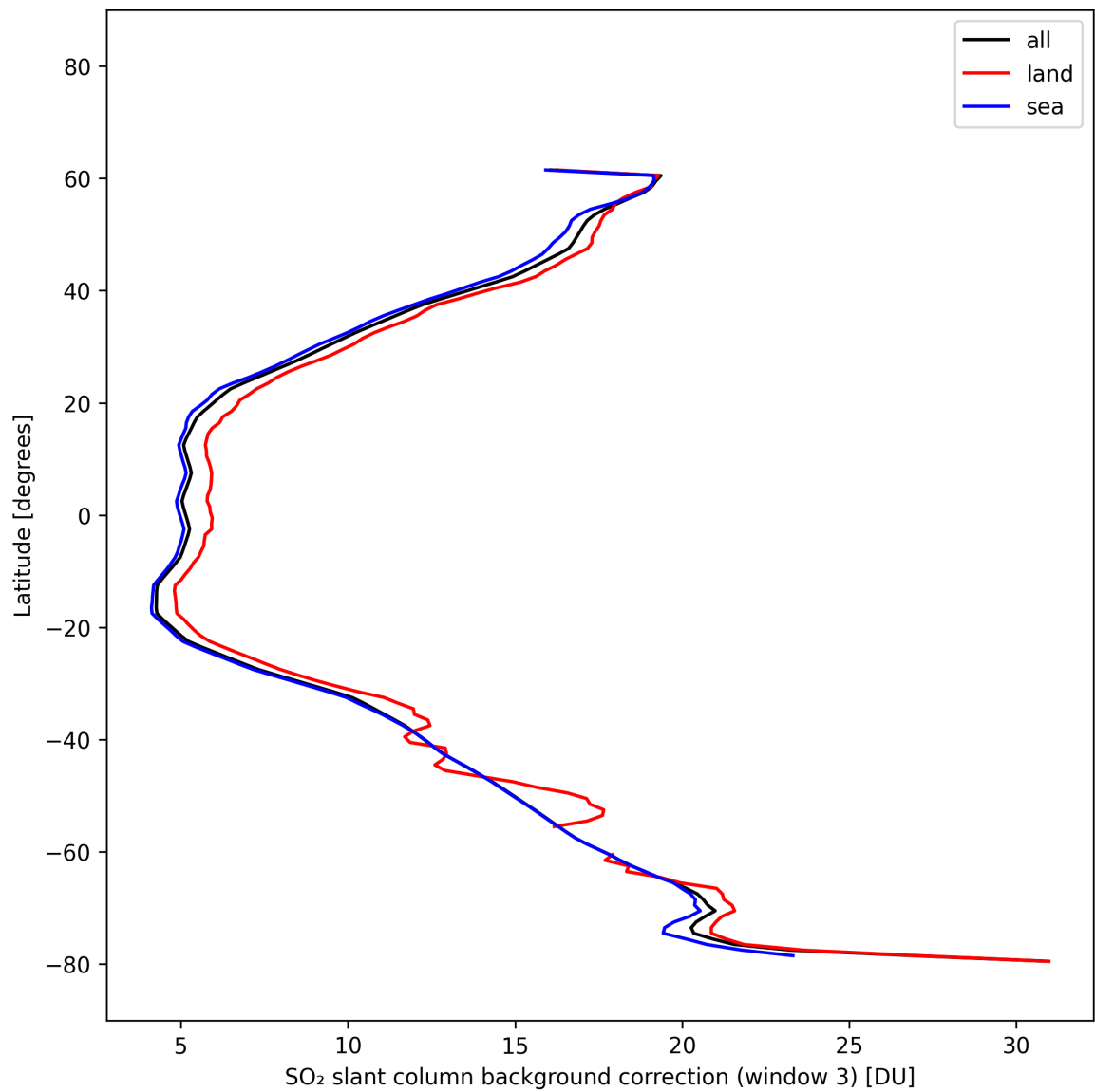
Figure 48: Zonal average of “SO 2 slant column background correction (window 3)” for 2025-10-15 to 2025-10-17.
