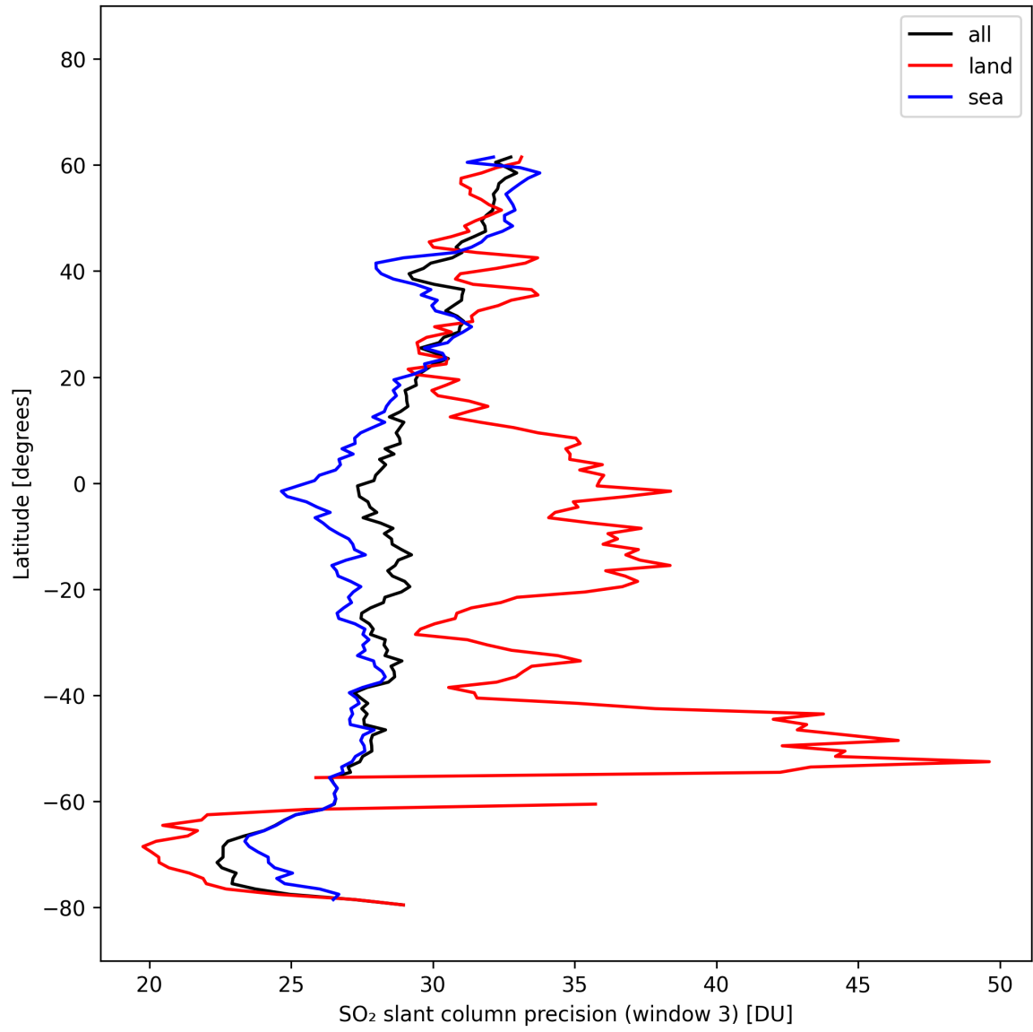
Figure 46: Zonal average of “SO 2 slant column precision (window 3)” for 2025-10-15 to 2025-10-17.
