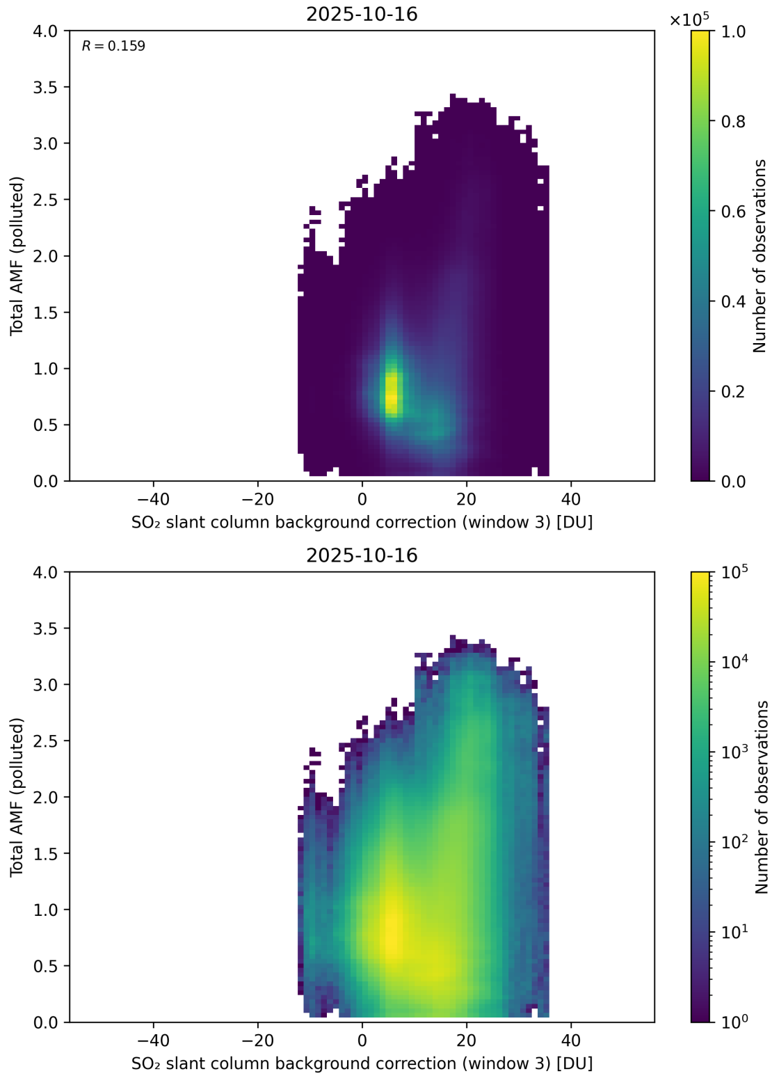
Figure 136: Scatter density plot of “SO 2 slant column background correction (window 3)” against “Total AMF (polluted)” for 2025-10-15 to 2025-10-17.
