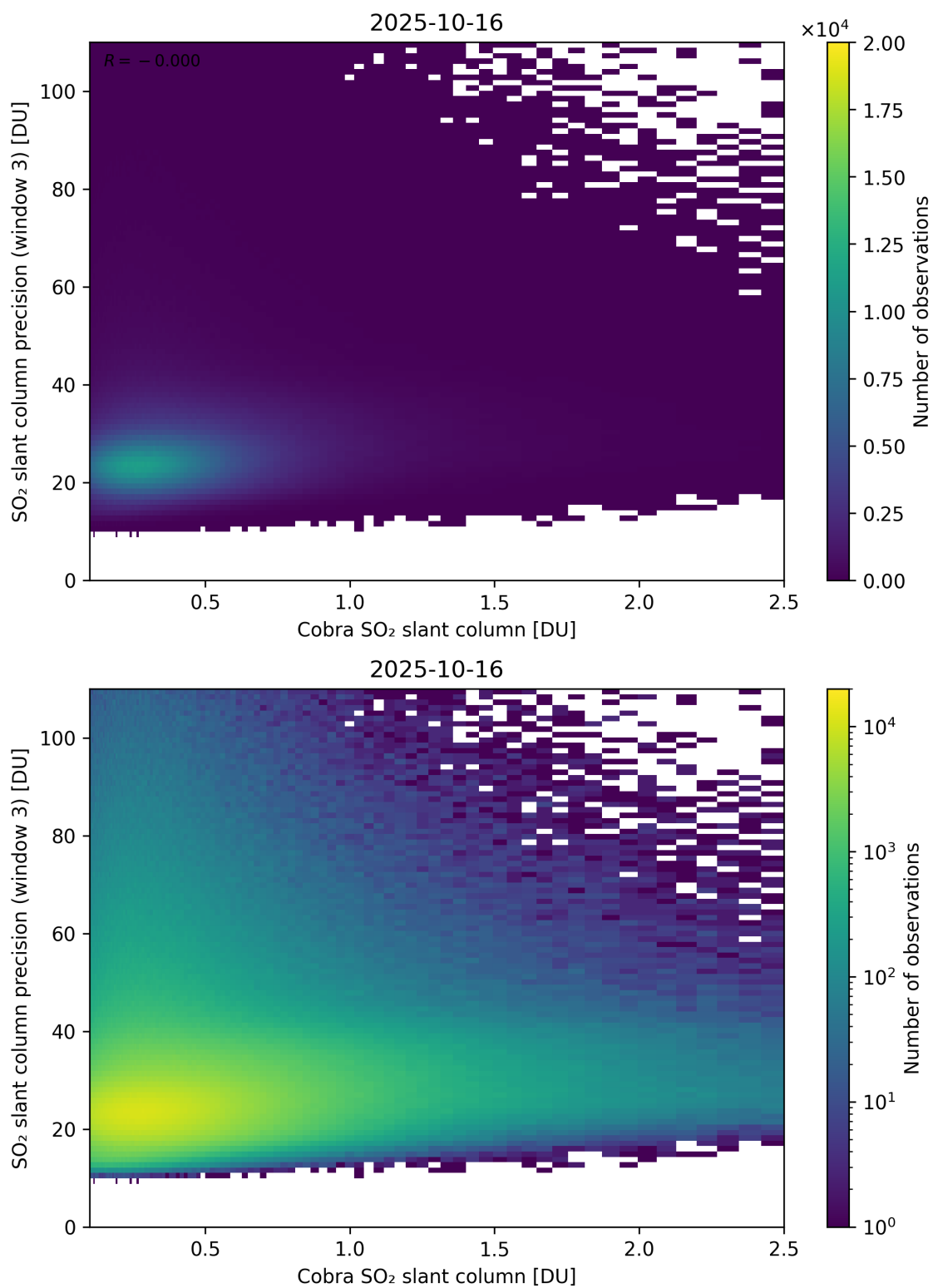
Figure 223: Scatter density plot of “Cobra SO 2 slant column” against “SO 2 slant column precision (window 3)” for 2025-10-15 to 2025-10-17.
