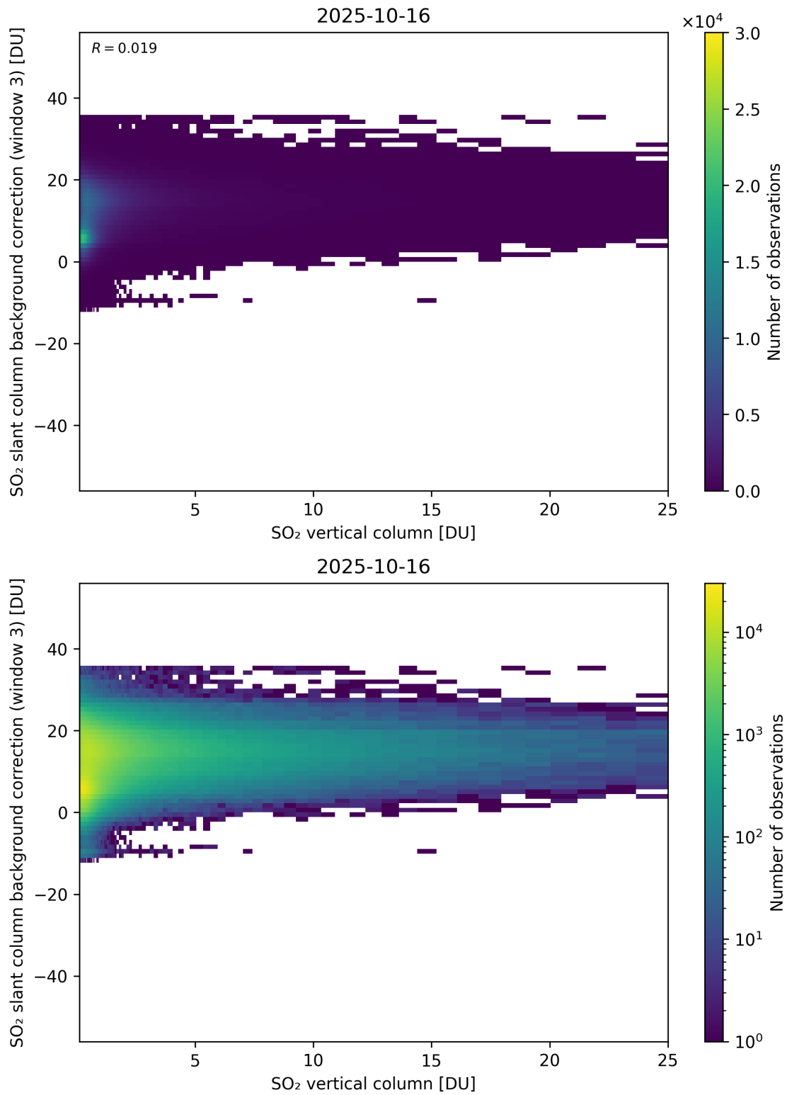
Figure 325: Scatter density plot of “SO 2 vertical column” against “SO 2 slant column background correction (window 3)” for 2025-10-15 to 2025-10-17.
