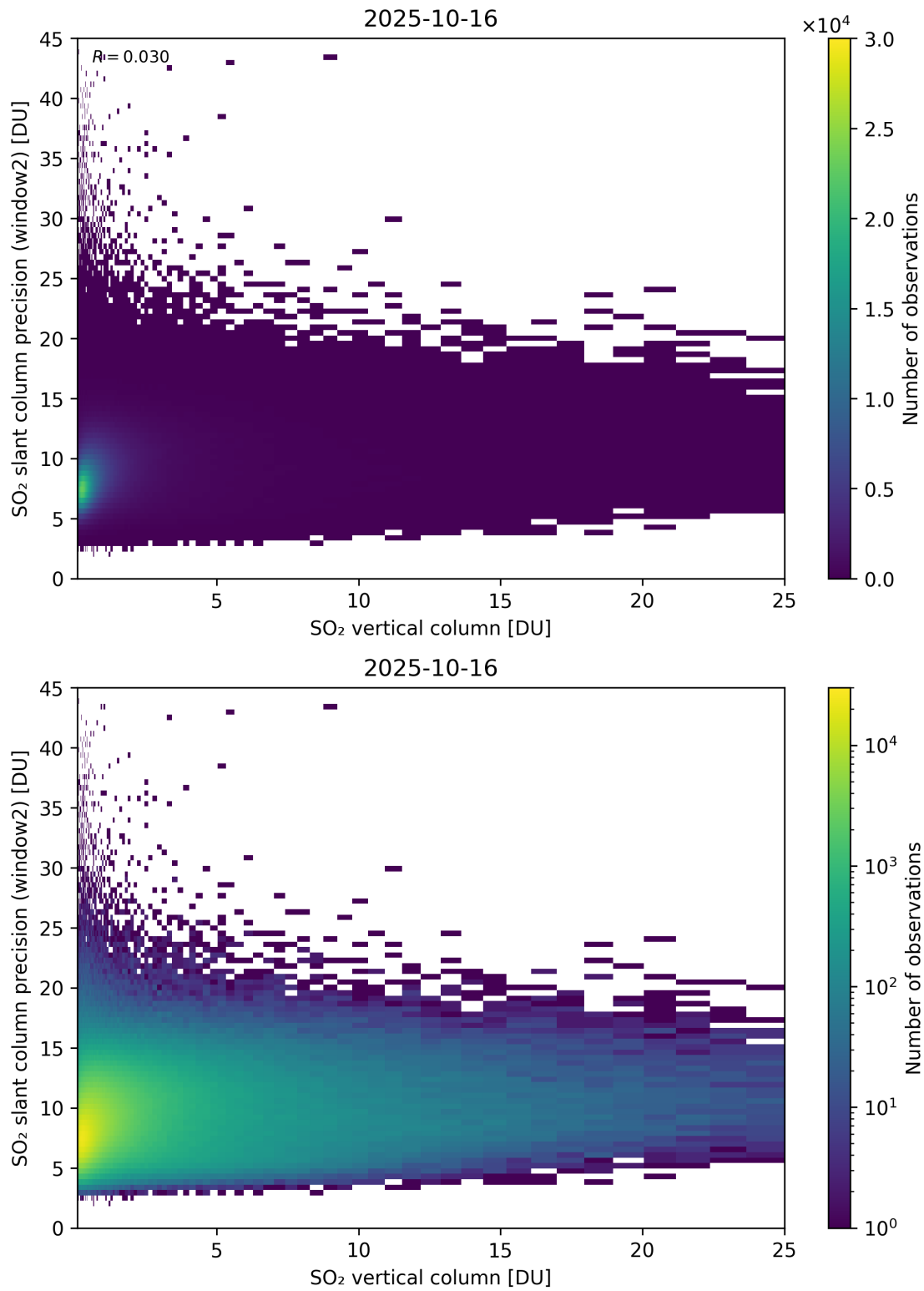
Figure 356: Scatter density plot of “SO 2 vertical column” against “SO 2 slant column precision (window2)” for 2025-10-15 to 2025-10-17.
