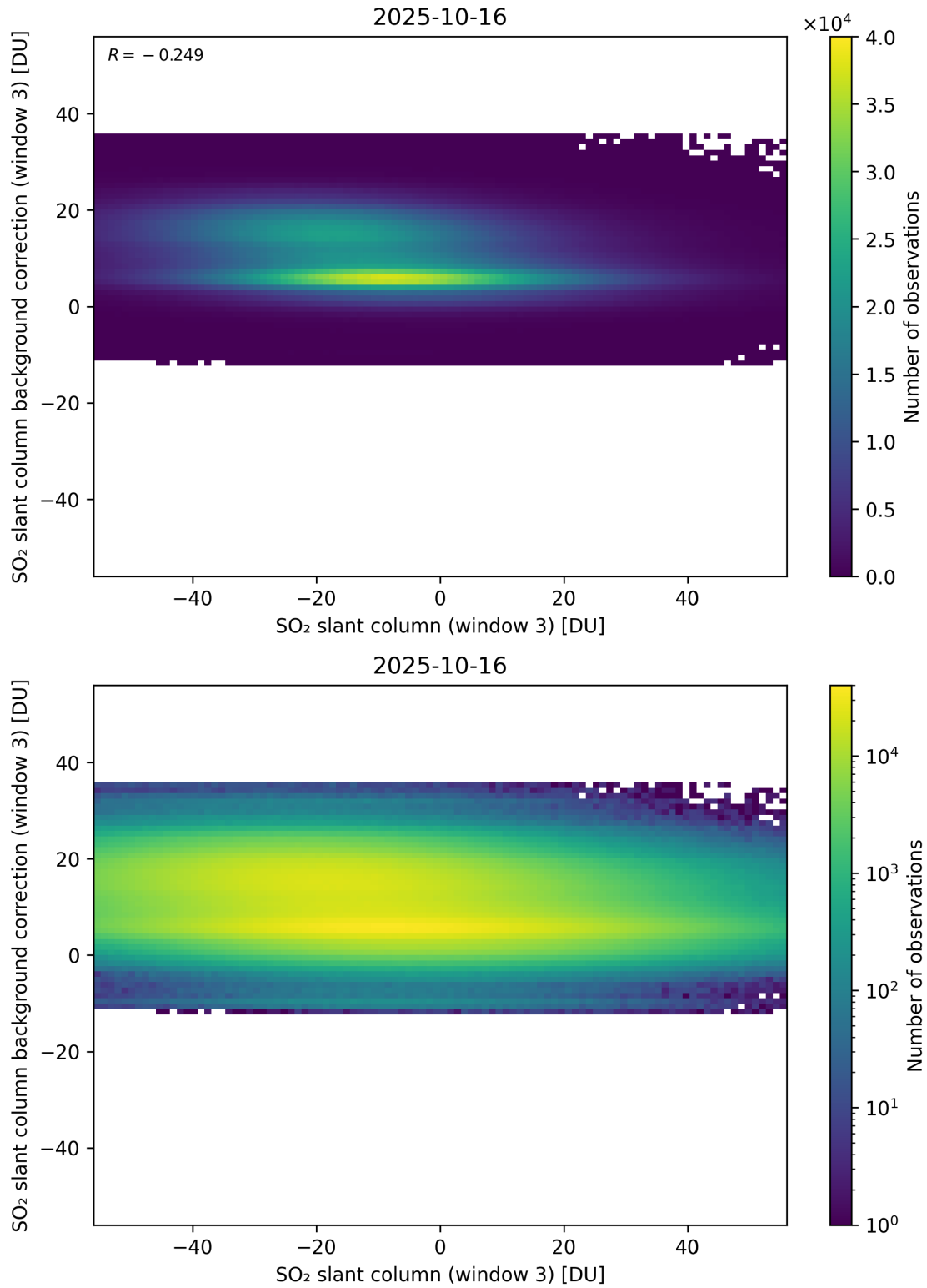
Figure 303: Scatter density plot of “SO 2 slant column (window 3)” against “SO 2 slant column background correction (window 3)” for 2025-10-15 to 2025-10-17.
