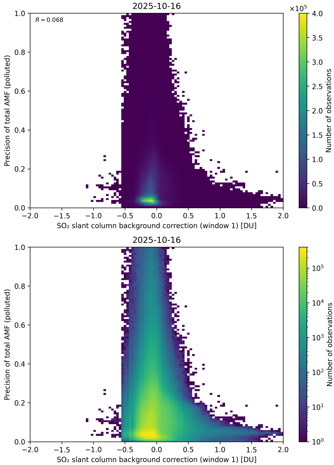
Figure 121: Scatter density plot of “SO 2 slant column background correction (window 1)” against “Precision of total AMF (polluted)” for 2025-10-15 to 2025-10-17.
