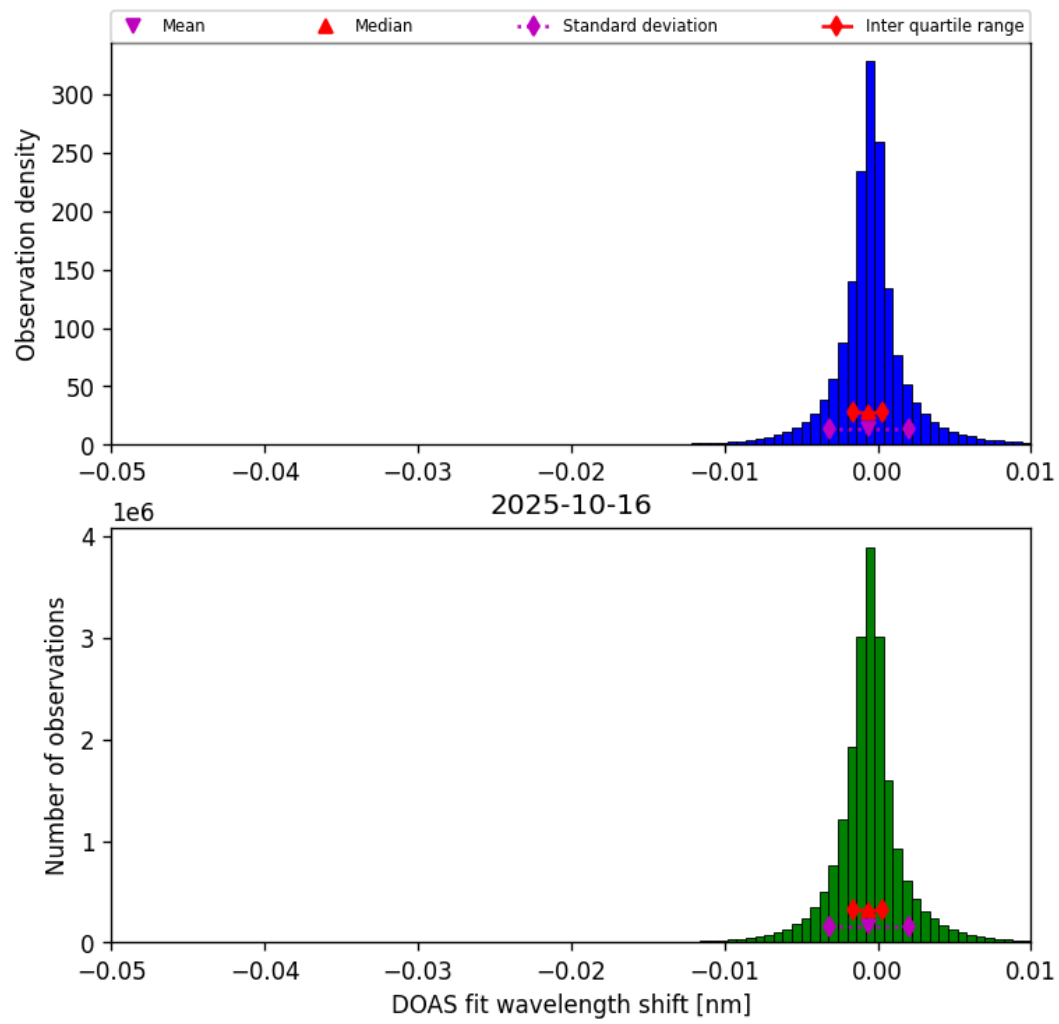
Figure 76: Histogram of “DOAS fit wavelength shift” for 2025-10-15 to 2025-10-17
