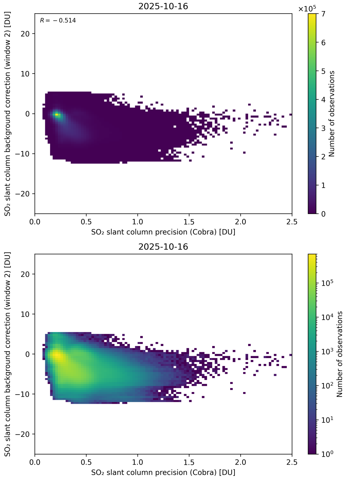
Figure 200: Scatter density plot of “SO 2 slant column precision (Cobra)” against “SO 2 slant column background correction (window 2)” for 2025-10-15 to 2025-10-17.
