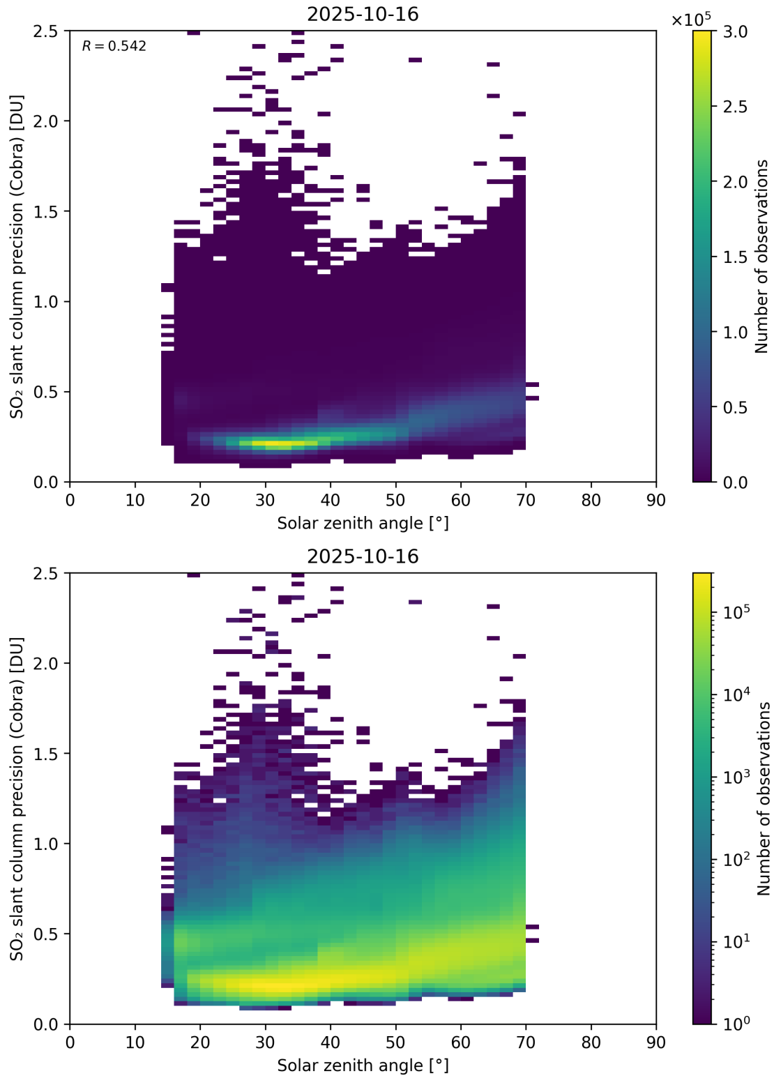
Figure 180: Scatter density plot of “Solar zenith angle” against “SO 2 slant column precision (Cobra)” for 2025-10-15 to 2025-10-17.
