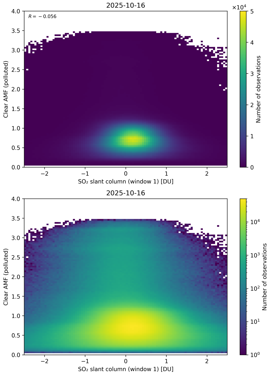
Figure 282: Scatter density plot of “SO 2 slant column (window 1)” against “Clear AMF (polluted)” for 2025-10-15 to 2025-10-17.
