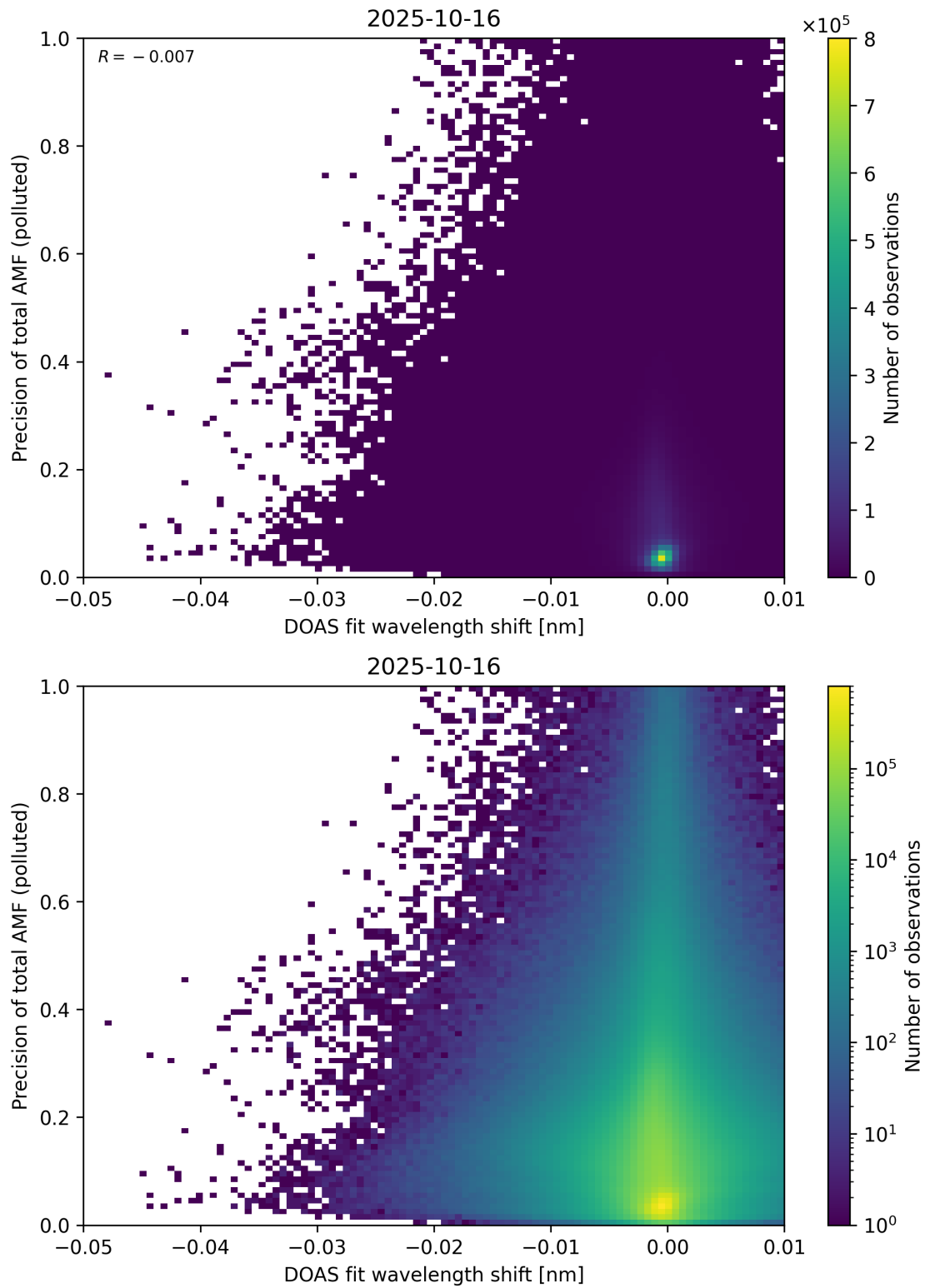
Figure 142: Scatter density plot of “DOAS fit wavelength shift” against “Precision of total AMF (polluted)” for 2025-10-15 to 2025-10-17.
