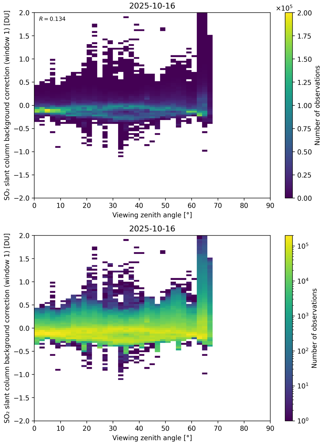
Figure 362: Scatter density plot of “Viewing zenith angle” against “SO 2 slant column background correction (window 1)” for 2025-10-15 to 2025-10-17.
