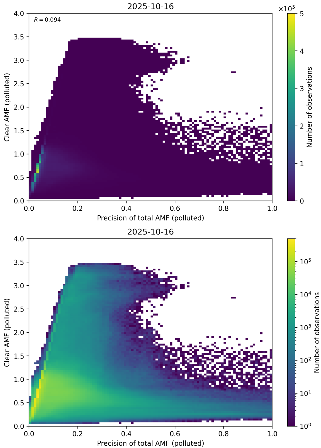
Figure 320: Scatter density plot of “Precision of total AMF (polluted)” against “Clear AMF (polluted)” for 2025-10-15 to 2025-10-17.
