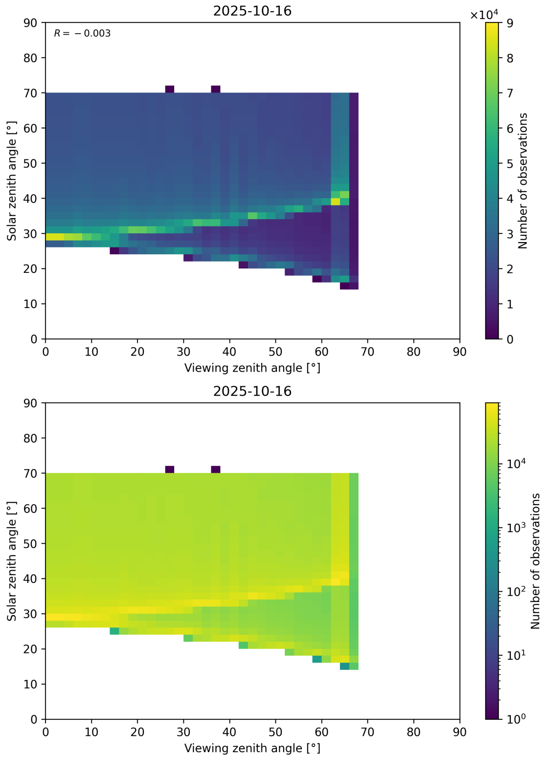
Figure 369: Scatter density plot of “Viewing zenith angle” against “Solar zenith angle” for 2025-10-15 to 2025-10-17.
