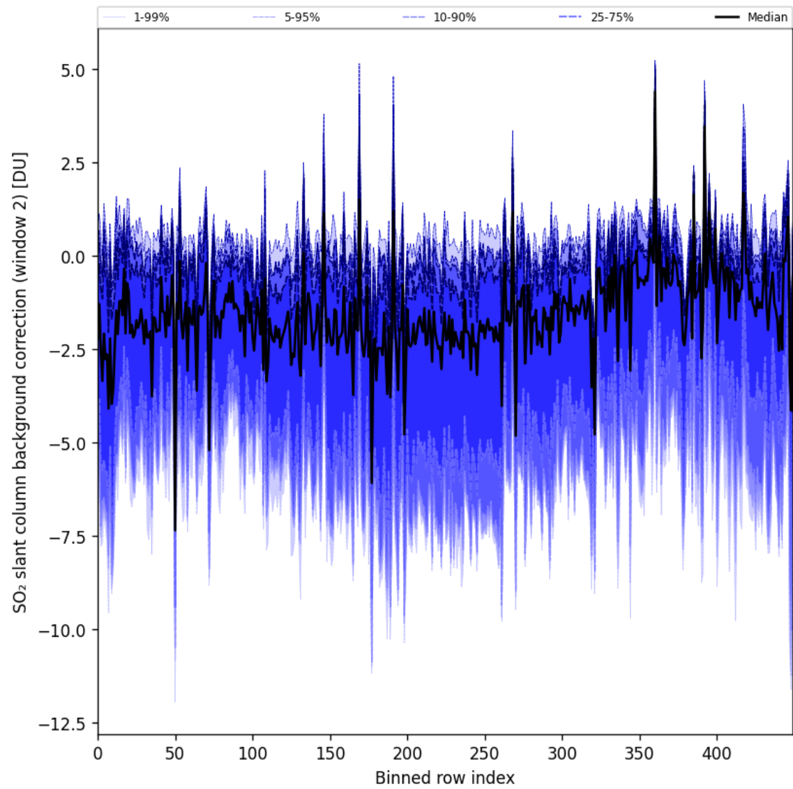
Figure 96: Along track statistics of “SO 2 slant column background correction (window 2)” for 2025-10-15 to 2025-10-17
