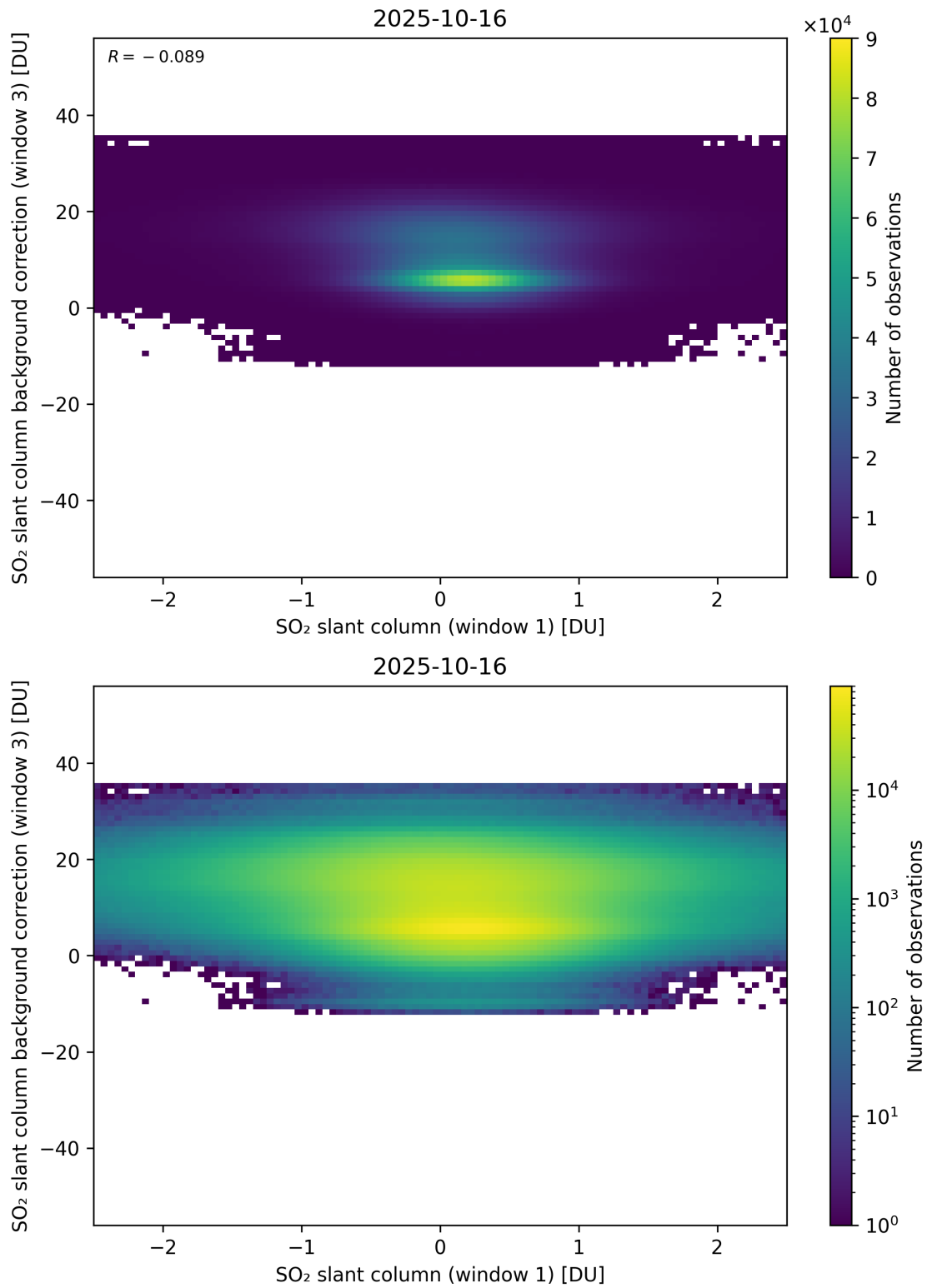
Figure 264: Scatter density plot of “SO 2 slant column (window 1)” against “SO 2 slant column background correction (window 3)” for 2025-10-15 to 2025-10-17.
