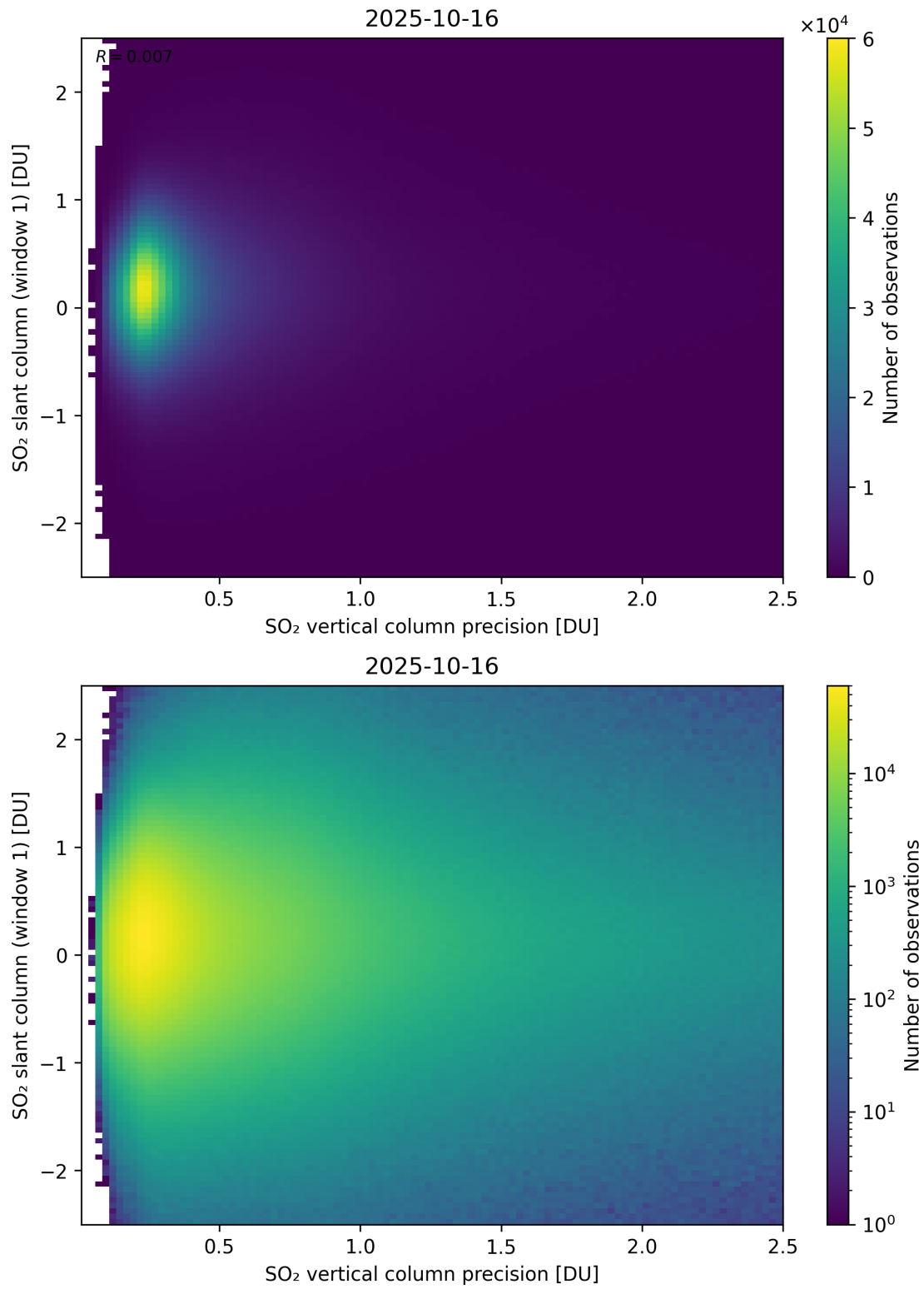
Figure 341: Scatter density plot of “SO 2 vertical column precision” against “SO 2 slant column (window 1)” for 2025-10-15 to 2025-10-17.
