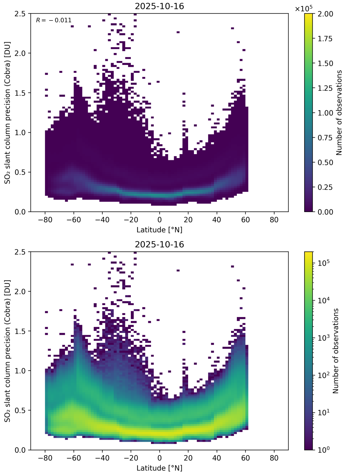
Figure 158: Scatter density plot of “Latitude” against “SO 2 slant column precision (Cobra)” for 2025-10-15 to 2025-10-17.
