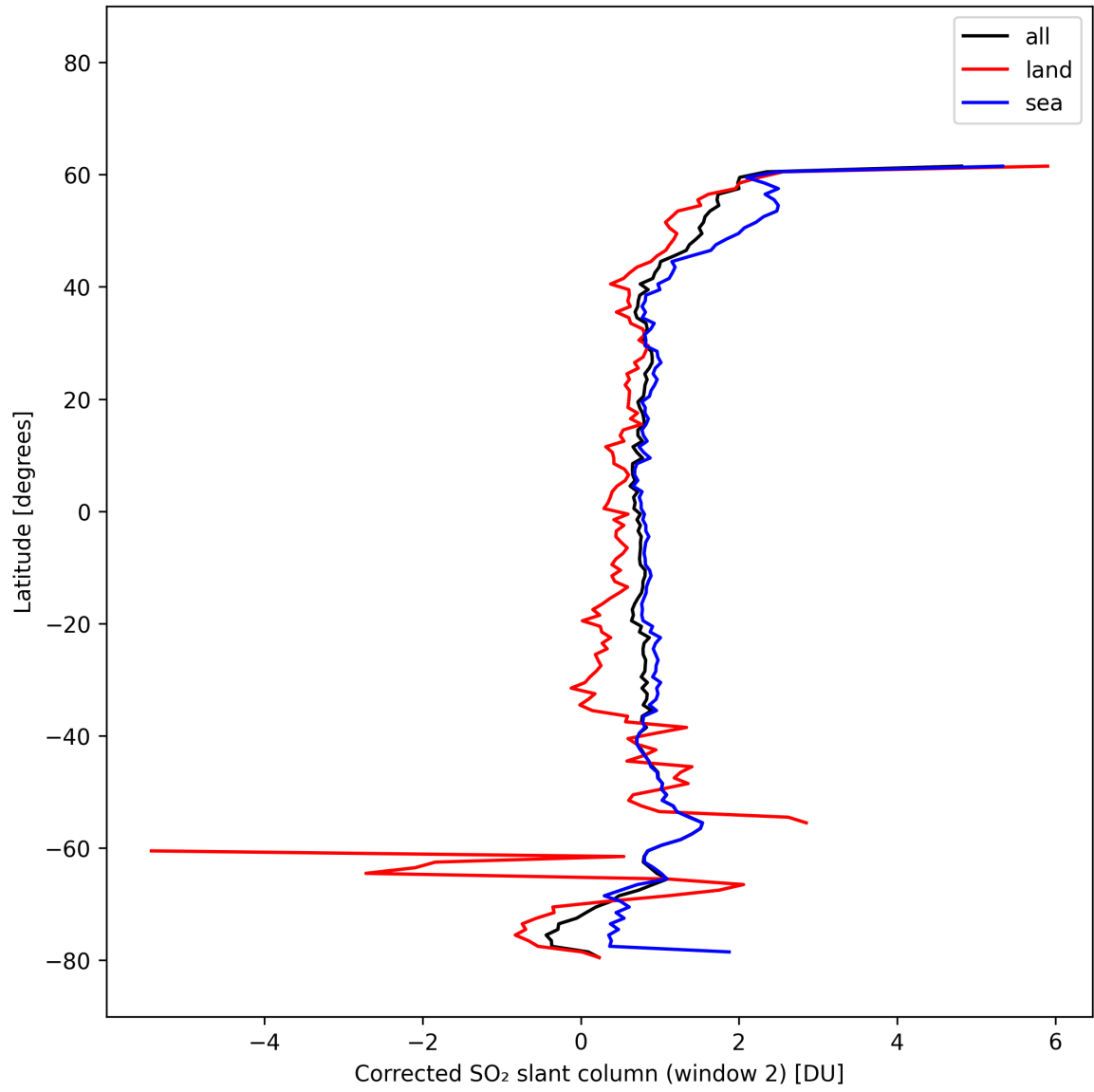
Figure 43: Zonal average of “Corrected SO 2 slant column (window 2)” for 2025-10-15 to 2025-10-17.
