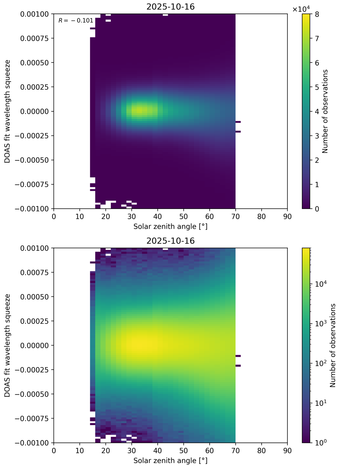
Figure 175: Scatter density plot of “Solar zenith angle” against “DOAS fit wavelength squeeze” for 2025-10-15 to 2025-10-17.
