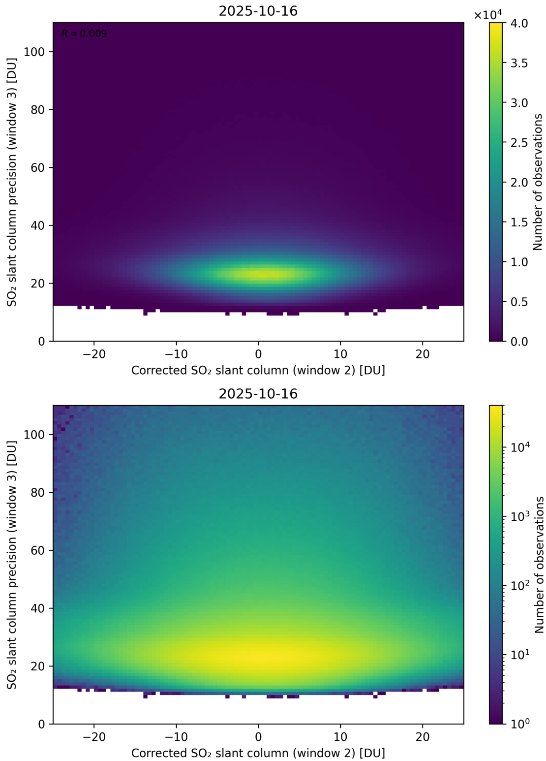
Figure 252: Scatter density plot of “Corrected SO 2 slant column (window 2)” against “SO 2 slant column precision (window 3)” for 2025-10-15 to 2025-10-17.
