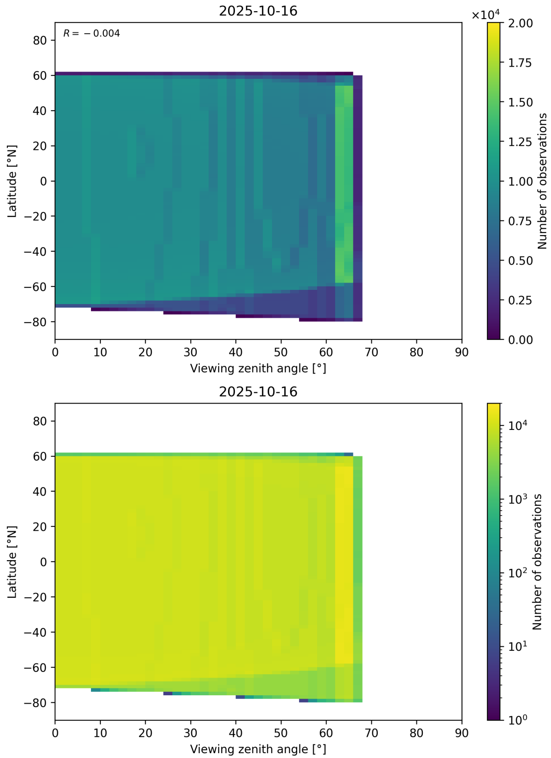
Figure 368: Scatter density plot of “Viewing zenith angle” against “Latitude” for 2025-10-15 to 2025-10-17.
