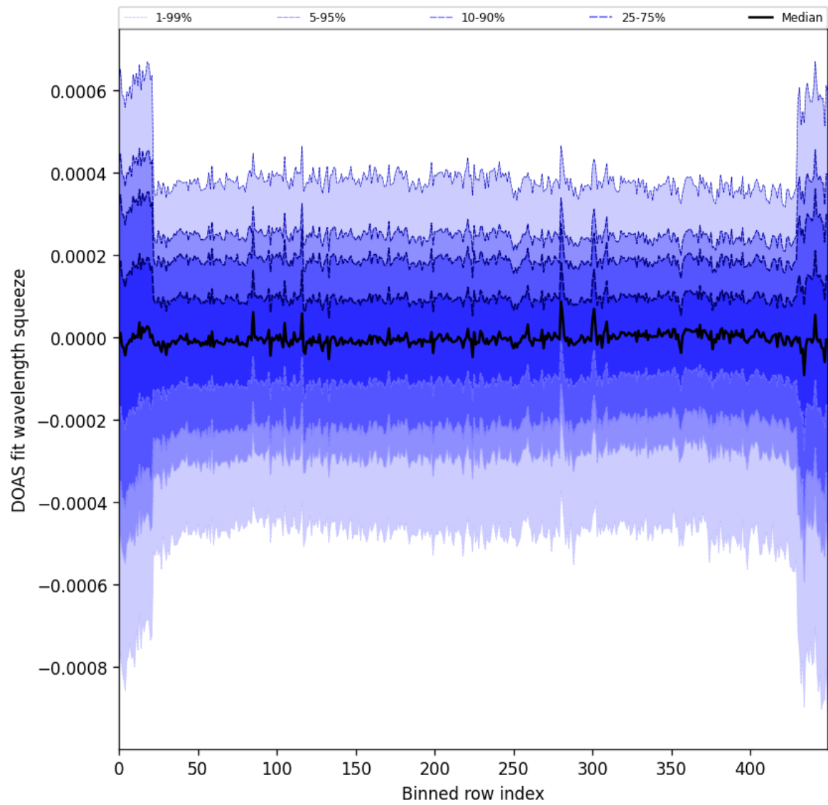
Figure 103: Along track statistics of “DOAS fit wavelength squeeze” for 2025-10-15 to 2025-10-17
