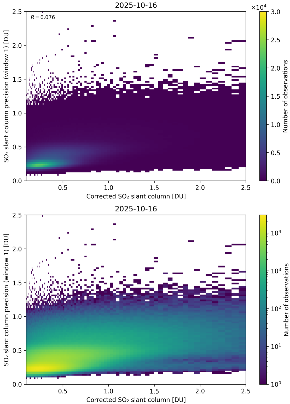
Figure 238: Scatter density plot of “Corrected SO 2 slant column” against “SO 2 slant column precision (window 1)” for 2025-10-15 to 2025-10-17.
