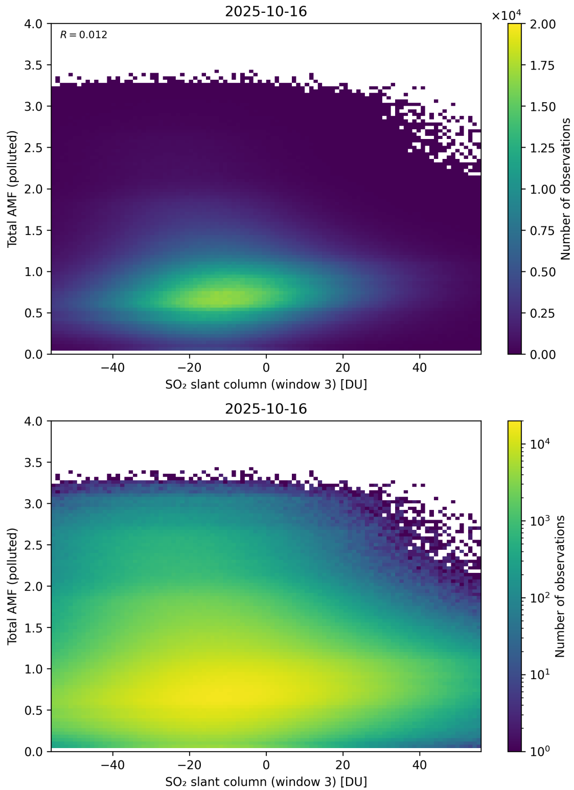
Figure 318: Scatter density plot of “SO 2 slant column (window 3)” against “Total AMF (polluted)” for 2025-10-15 to 2025-10-17.
