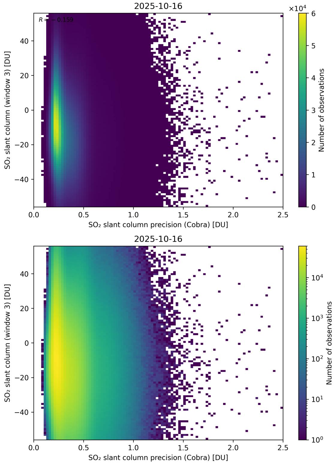
Figure 211: Scatter density plot of “SO 2 slant column precision (Cobra)” against “SO 2 slant column (window 3)” for 2025-10-15 to 2025-10-17.
