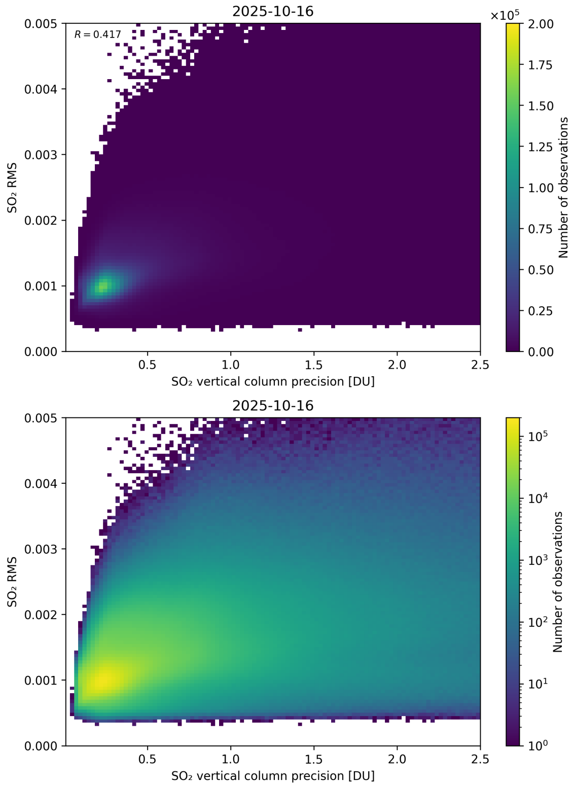
Figure 334: Scatter density plot of “SO 2 vertical column precision” against “SO 2 RMS” for 2025-10-15 to 2025-10-17.
