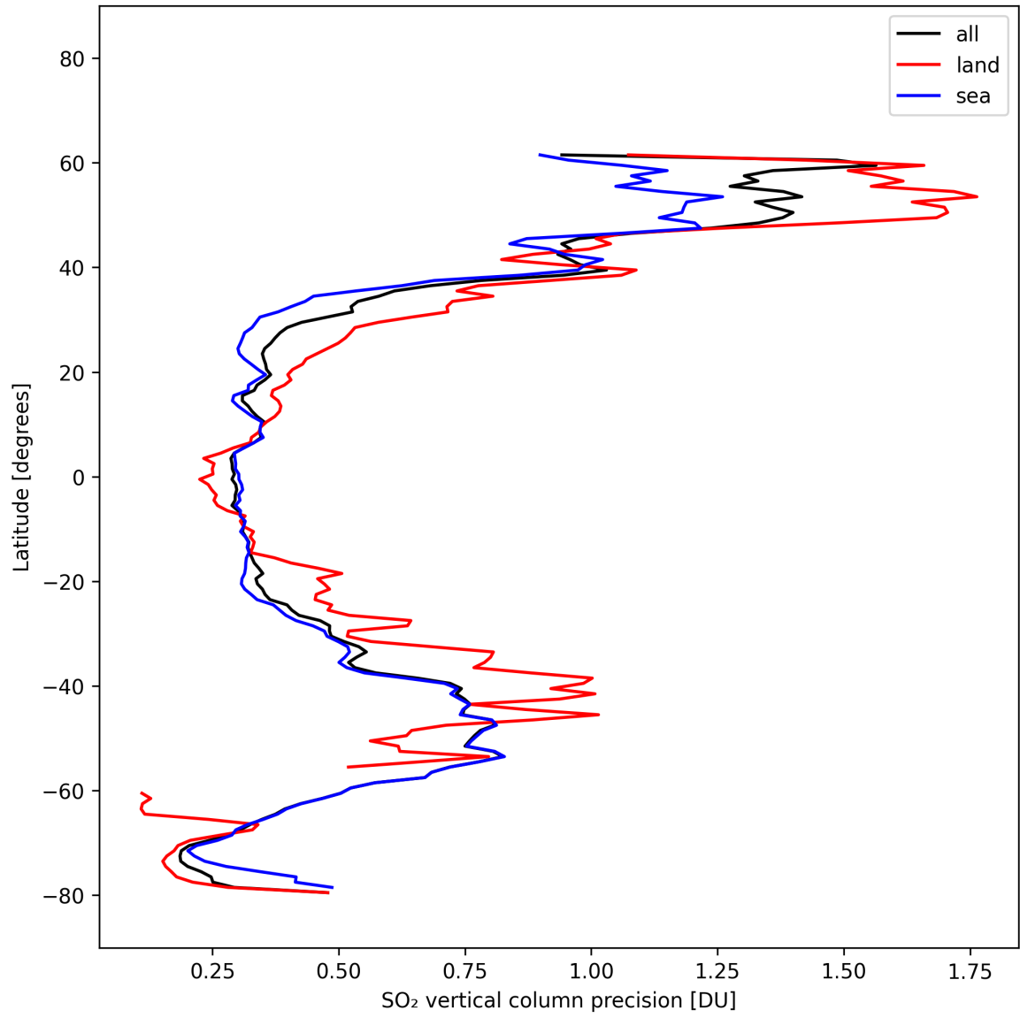
Figure 33: Zonal average of “SO 2 vertical column precision” for 2025-10-15 to 2025-10-17.
