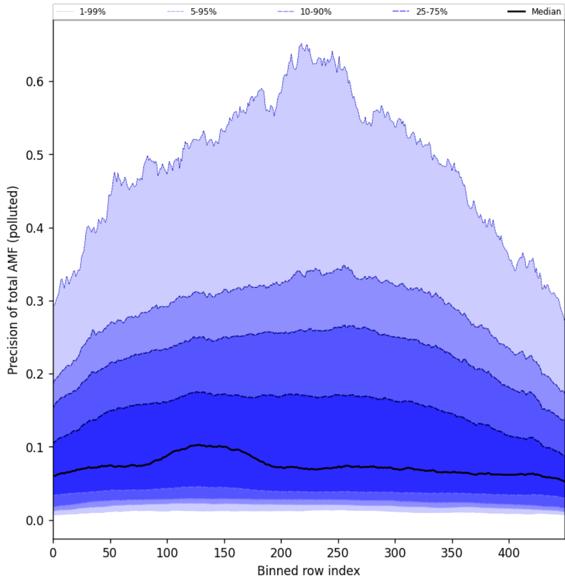
Figure 106: Along track statistics of “Precision of total AMF (polluted)” for 2025-10-15 to 2025-10-17
