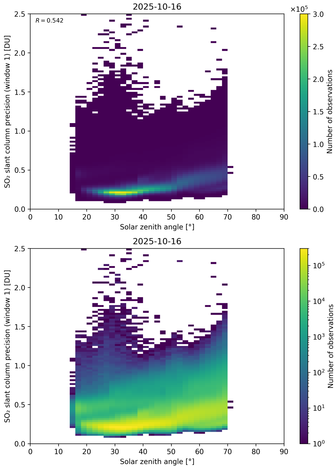
Figure 185: Scatter density plot of “Solar zenith angle” against “SO 2 slant column precision (window 1)” for 2025-10-15 to 2025-10-17.
