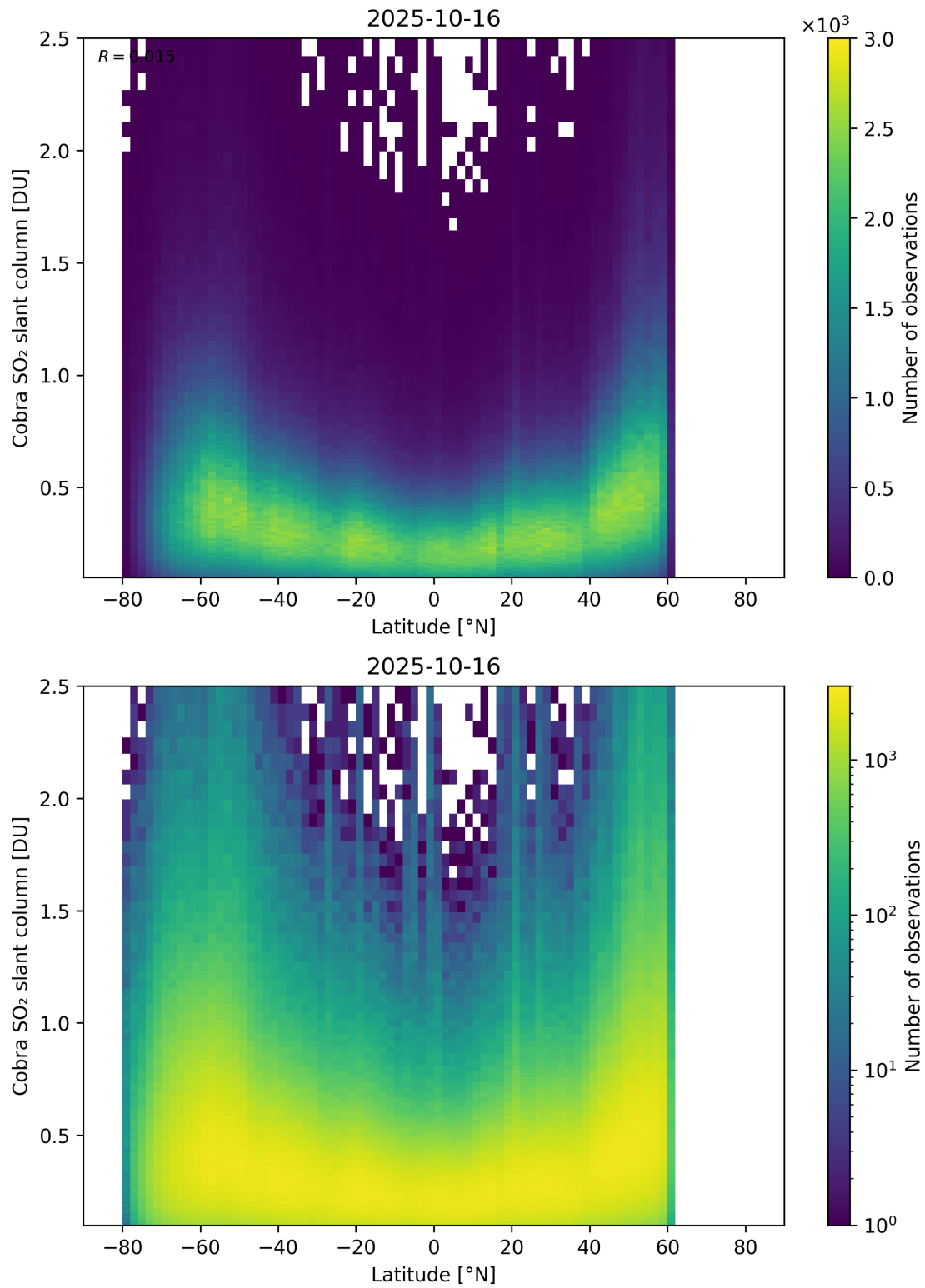
Figure 157: Scatter density plot of “Latitude” against “Cobra SO 2 slant column” for 2025-10-15 to 2025-10-17.
