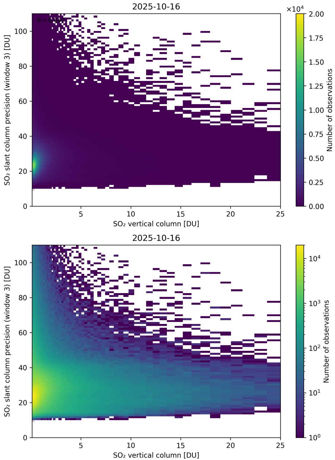
Figure 358: Scatter density plot of “SO 2 vertical column” against “SO 2 slant column precision (window 3)” for 2025-10-15 to 2025-10-17.
