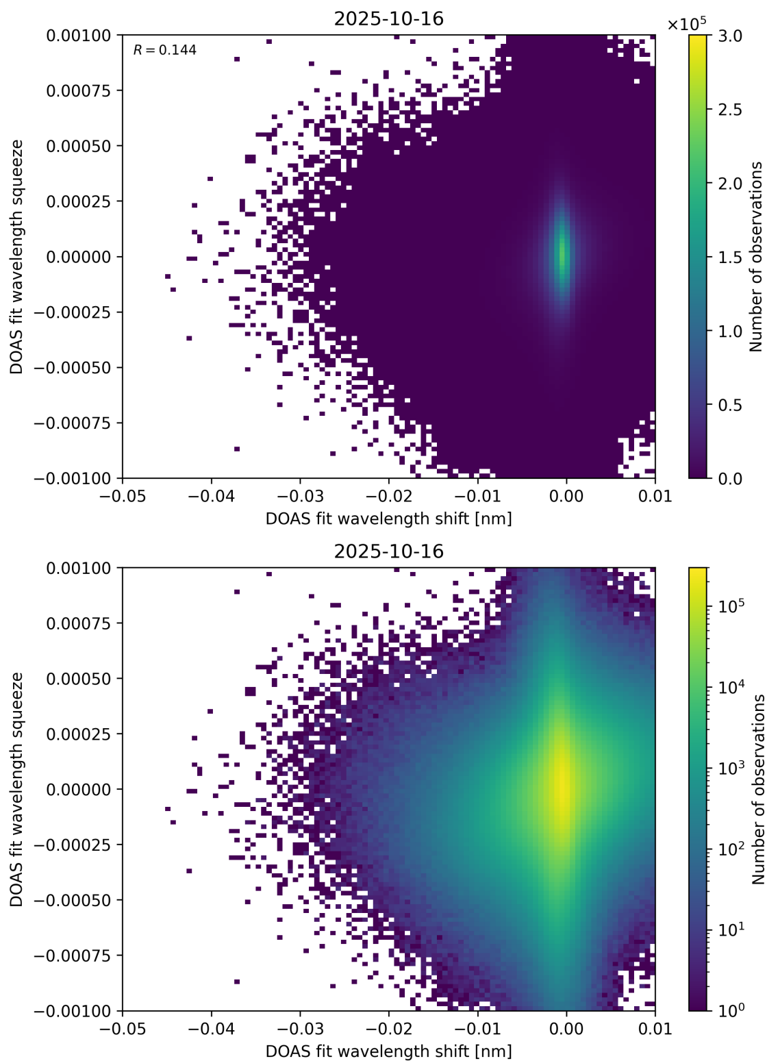
Figure 138: Scatter density plot of “DOAS fit wavelength shift” against “DOAS fit wavelength squeeze” for 2025-10-15 to 2025-10-17.
