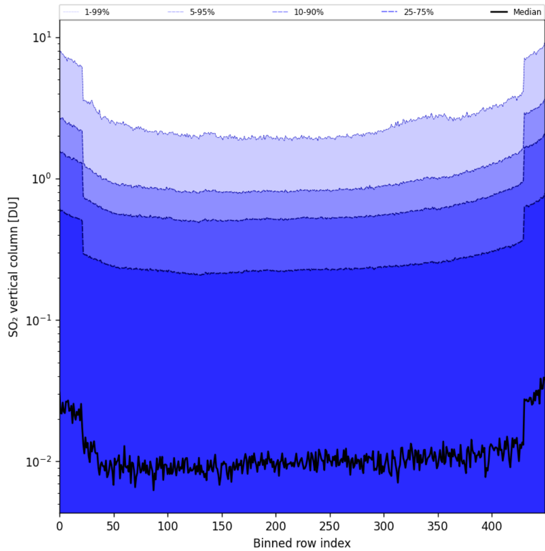
Figure 84: Along track statistics of “SO 2 vertical column” for 2025-10-15 to 2025-10-17
