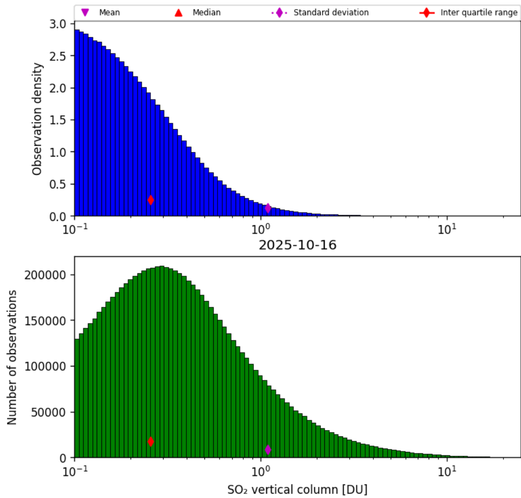
Figure 58: Histogram of “SO 2 vertical column” for 2025-10-15 to 2025-10-17
