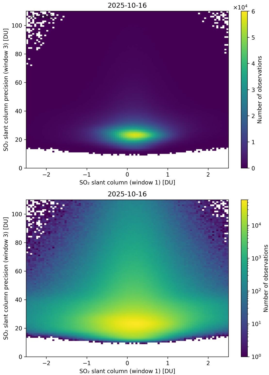
Figure 288: Scatter density plot of “SO 2 slant column (window 1)” against “SO 2 slant column precision (window 3)” for 2025-10-15 to 2025-10-17.
