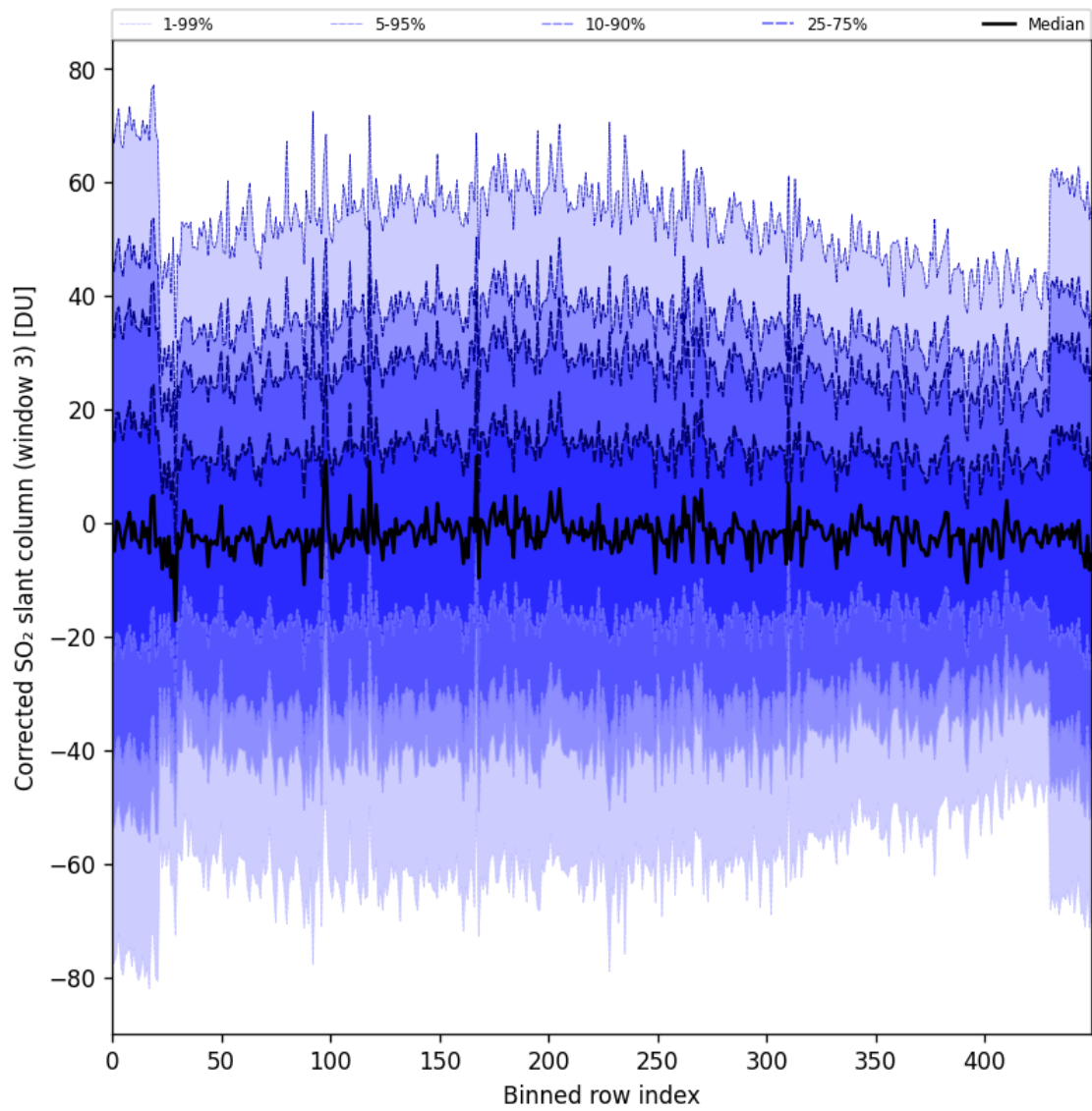
Figure 99: Along track statistics of “Corrected SO 2 slant column (window 3)” for 2025-10-15 to 2025-10-17
