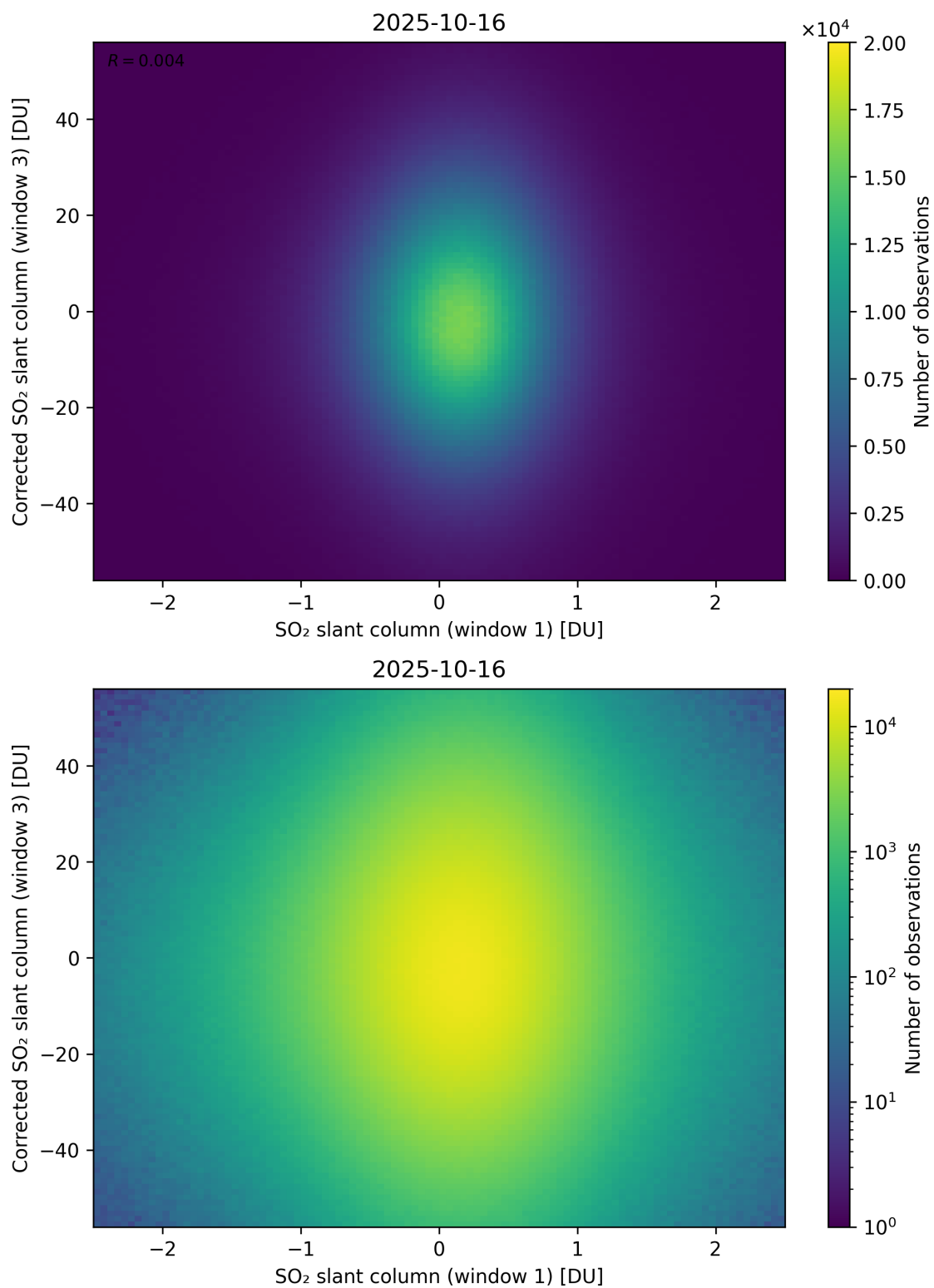
Figure 284: Scatter density plot of “SO 2 slant column (window 1)” against “Corrected SO 2 slant column (window 3)” for 2025-10-15 to 2025-10-17.
