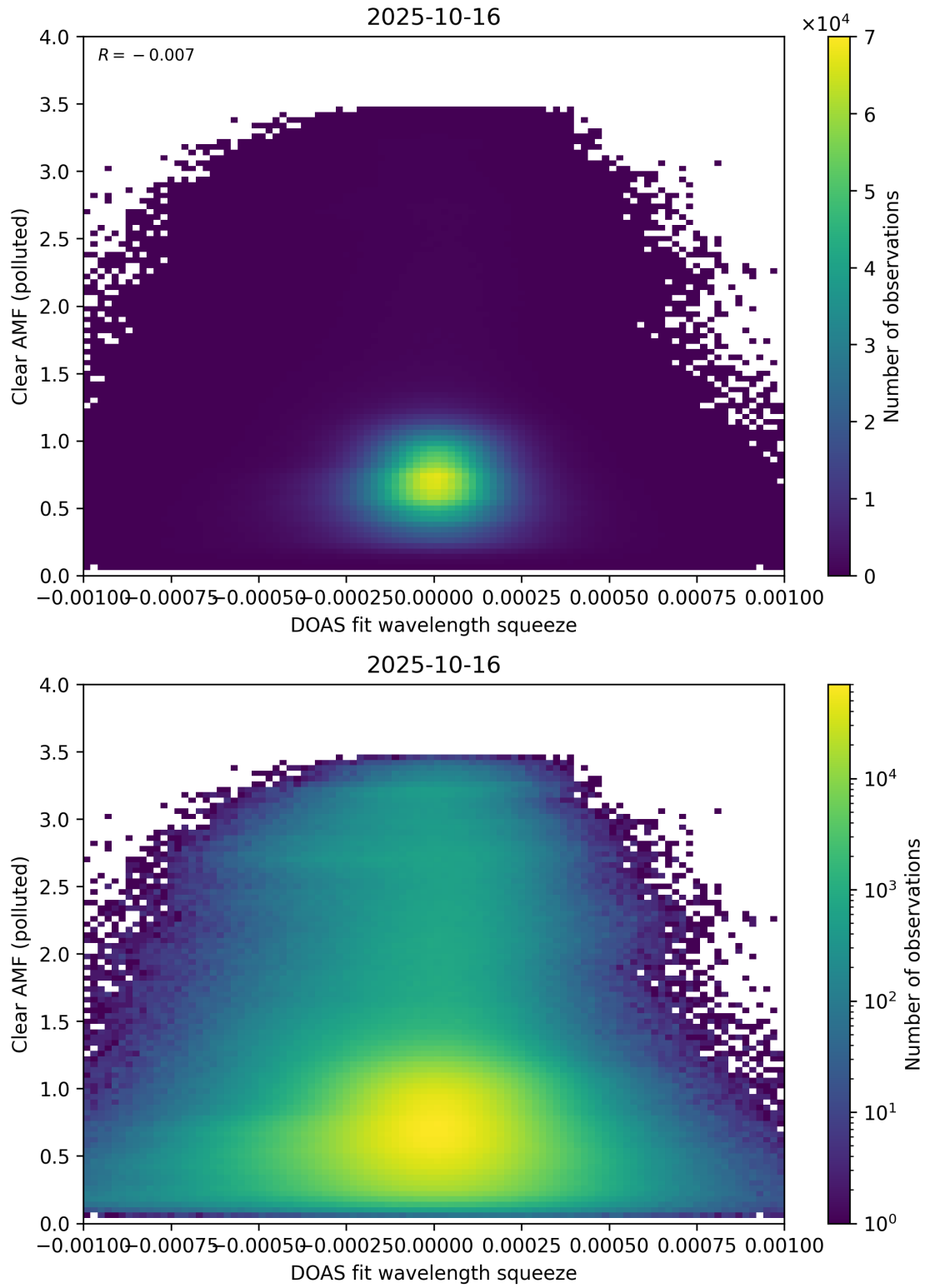
Figure 144: Scatter density plot of “DOAS fit wavelength squeeze” against “Clear AMF (polluted)” for 2025-10-15 to 2025-10-17.
