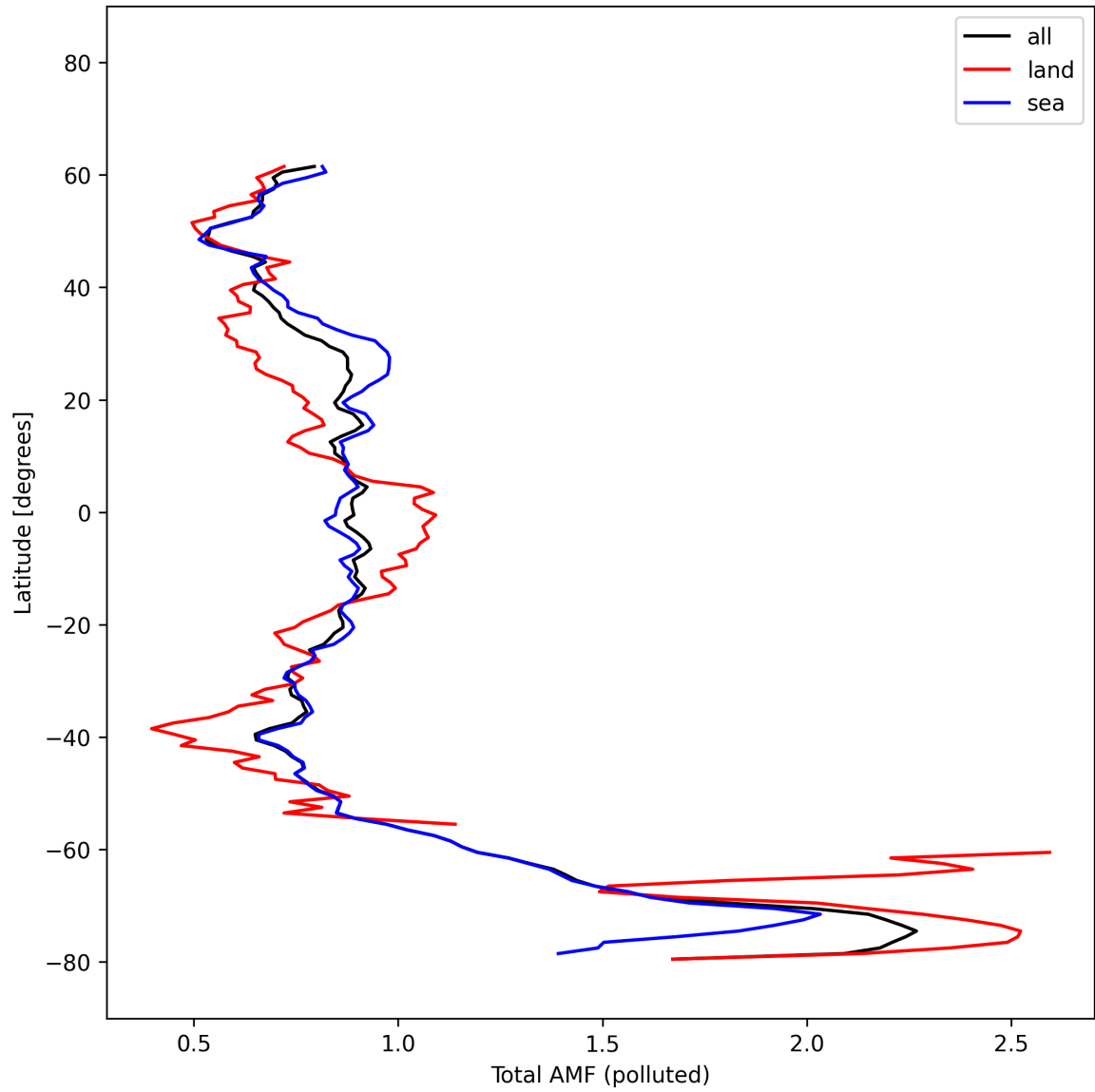
Figure 53: Zonal average of “Total AMF (polluted)” for 2025-10-15 to 2025-10-17.
