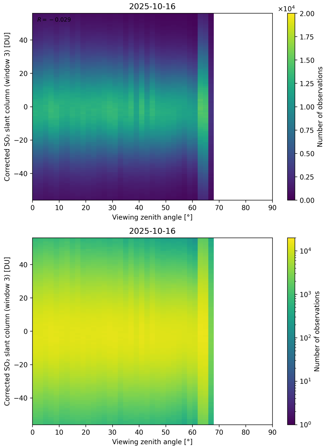
Figure 375: Scatter density plot of “Viewing zenith angle” against “Corrected SO 2 slant column (window 3)” for 2025-10-15 to 2025-10-17.
