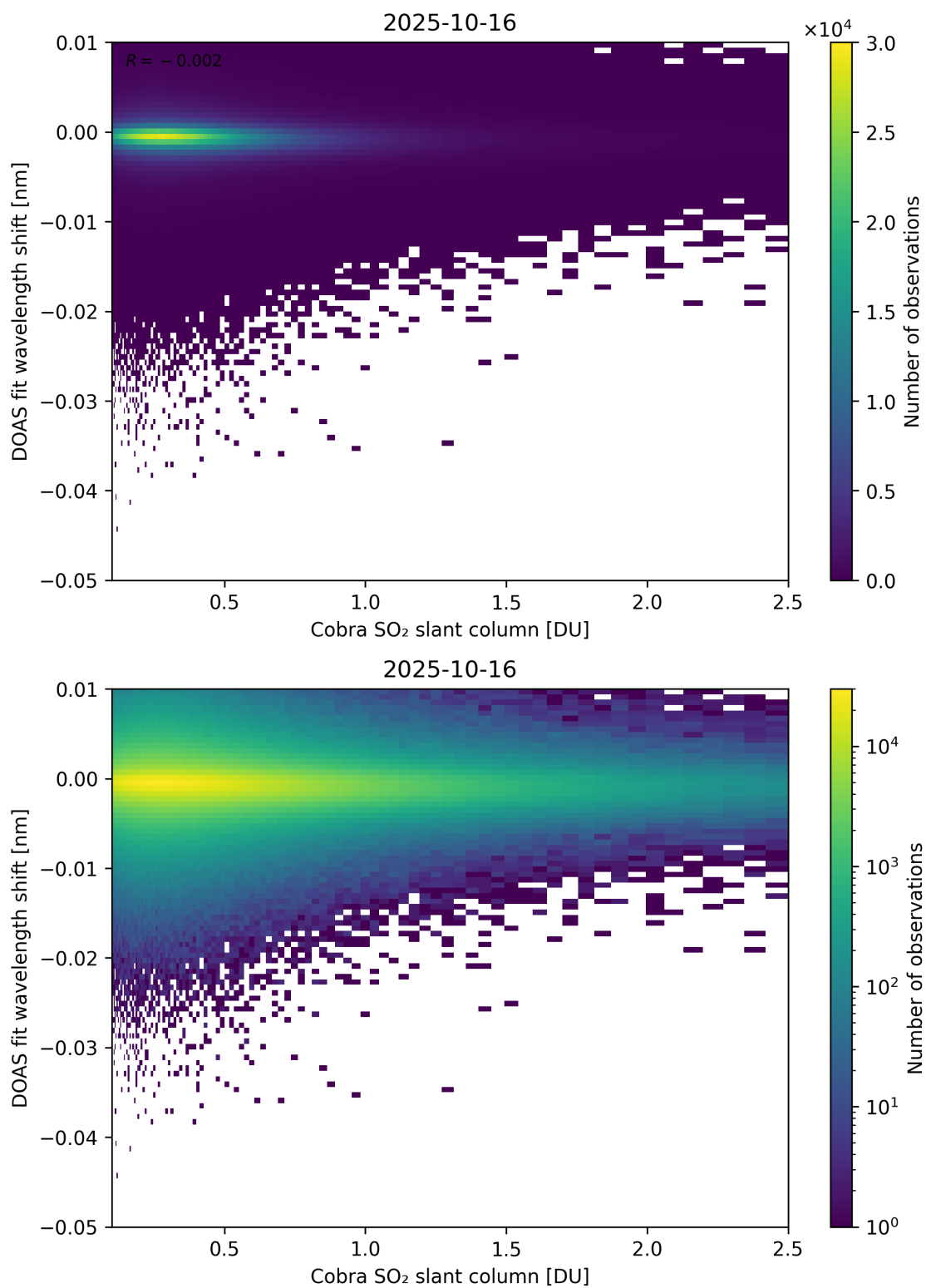
Figure 196: Scatter density plot of “Cobra SO 2 slant column” against “DOAS fit wavelength shift” for 2025-10-15 to 2025-10-17.
