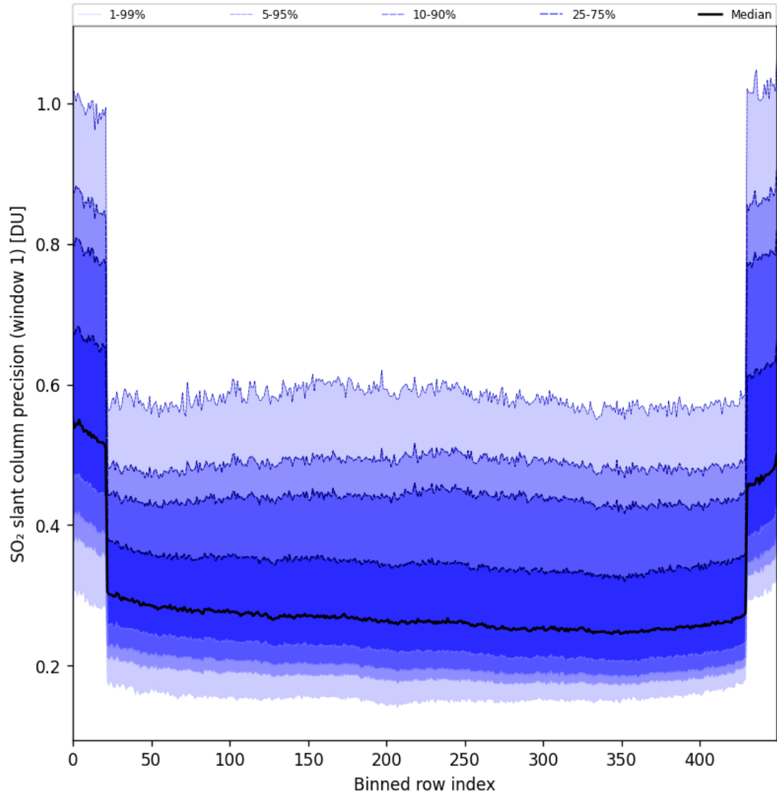
Figure 90: Along track statistics of “SO 2 slant column precision (window 1)” for 2025-10-15 to 2025-10-17
