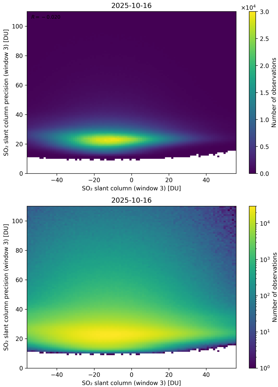
Figure 317: Scatter density plot of “SO 2 slant column (window 3)” against “SO 2 slant column precision (window 3)” for 2025-10-15 to 2025-10-17.
