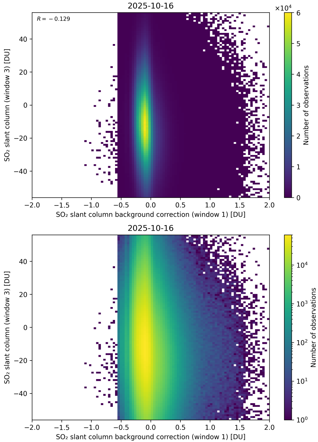
Figure 118: Scatter density plot of “SO 2 slant column background correction (window 1)” against “SO 2 slant column (window 3)” for 2025-10-15 to 2025-10-17.
