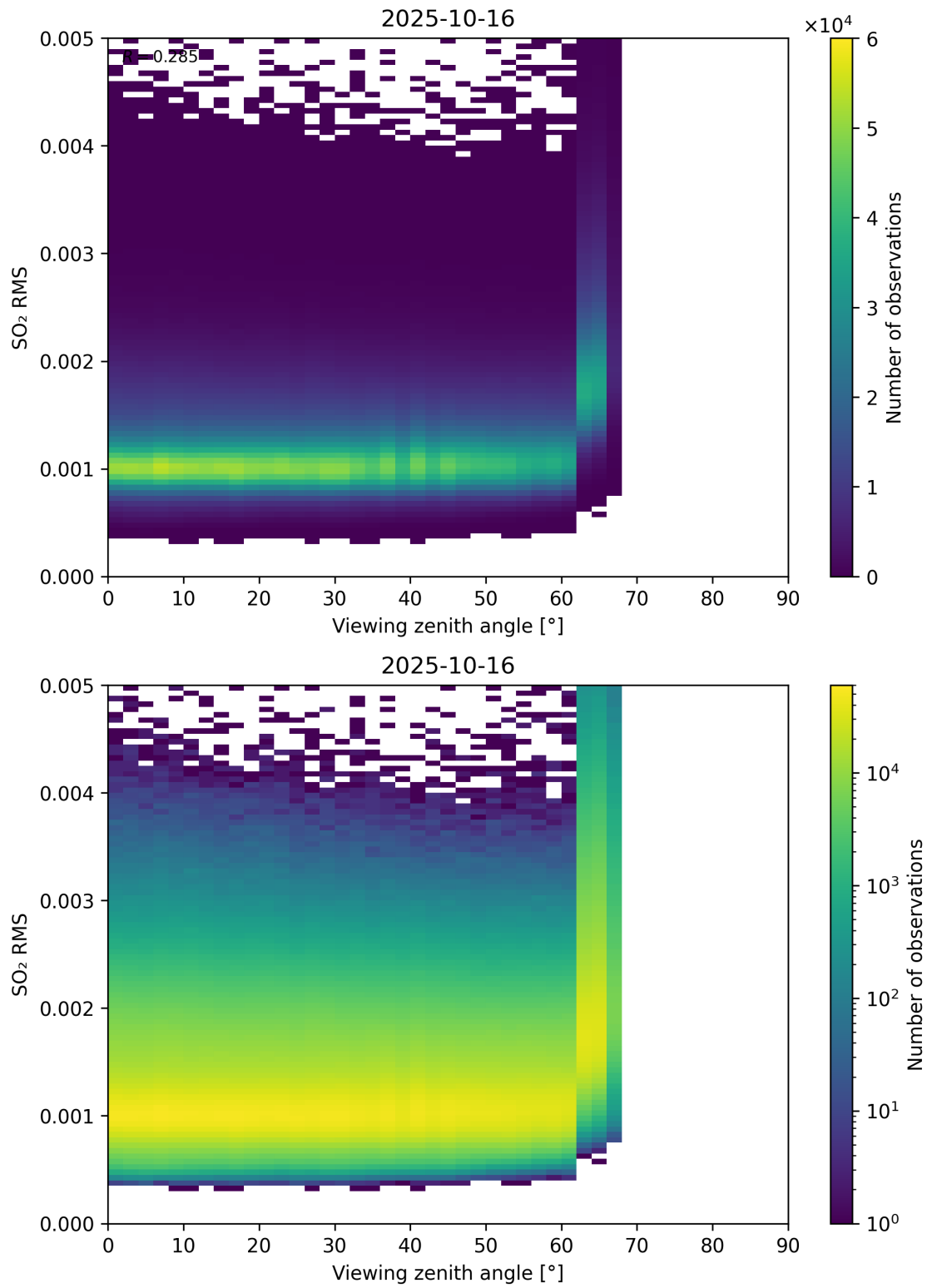
Figure 367: Scatter density plot of “Viewing zenith angle” against “SO 2 RMS” for 2025-10-15 to 2025-10-17.
