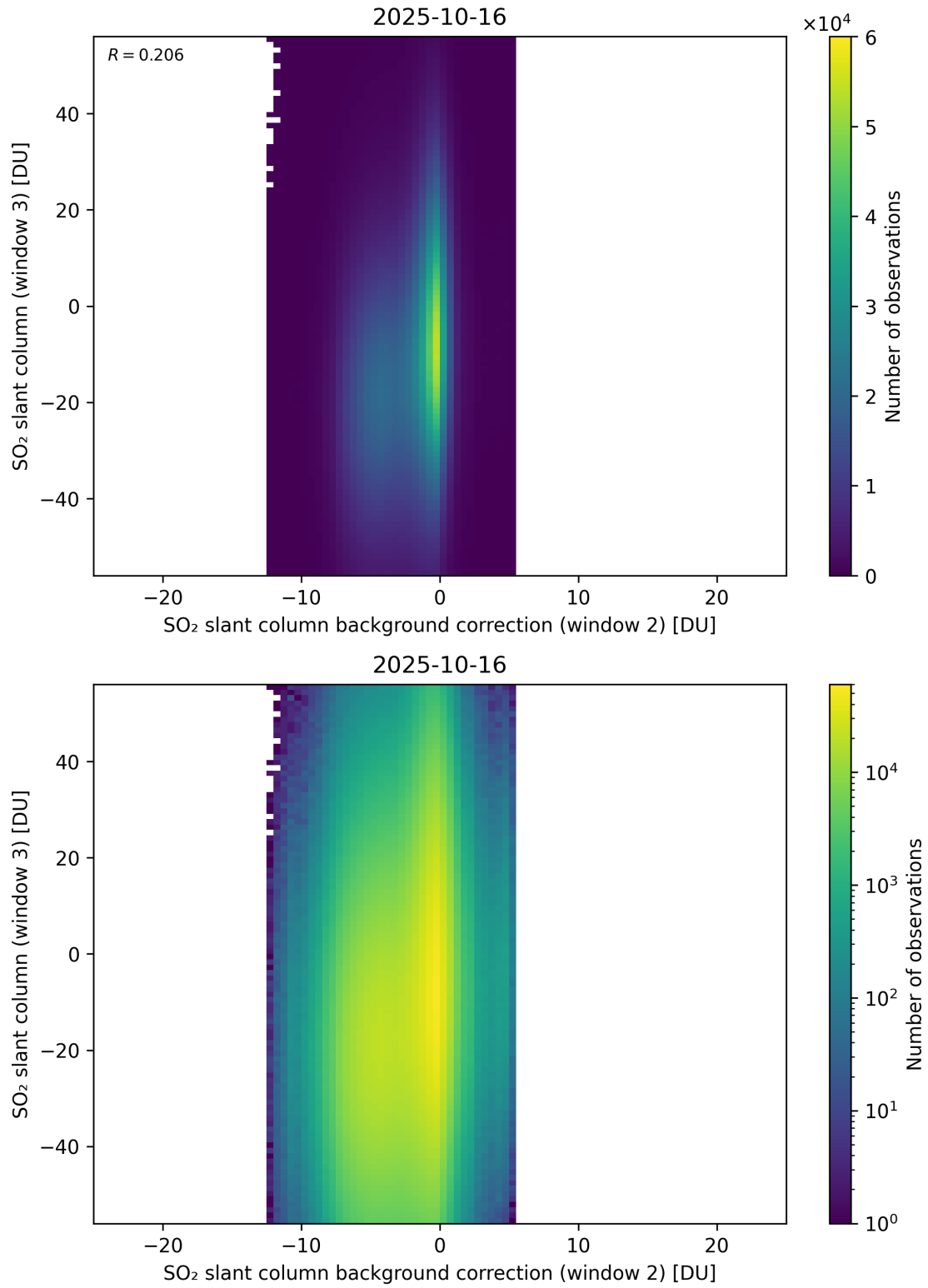
Figure 128: Scatter density plot of “SO 2 slant column background correction (window 2)” against “SO 2 slant column (window 3)” for 2025-10-15 to 2025-10-17.
