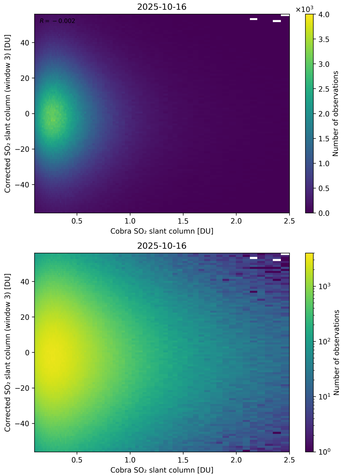
Figure 218: Scatter density plot of “Cobra SO 2 slant column” against “Corrected SO 2 slant column (window 3)” for 2025-10-15 to 2025-10-17.
