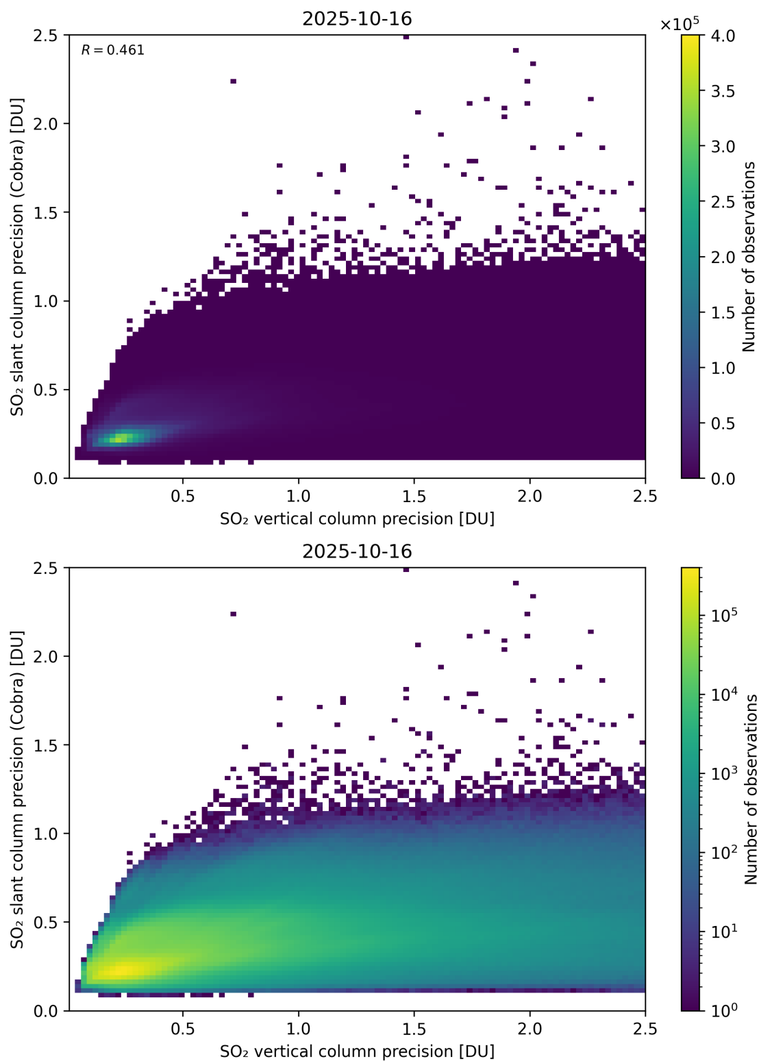
Figure 337: Scatter density plot of “SO 2 vertical column precision” against “SO 2 slant column precision (Cobra)” for 2025-10-15 to 2025-10-17.
