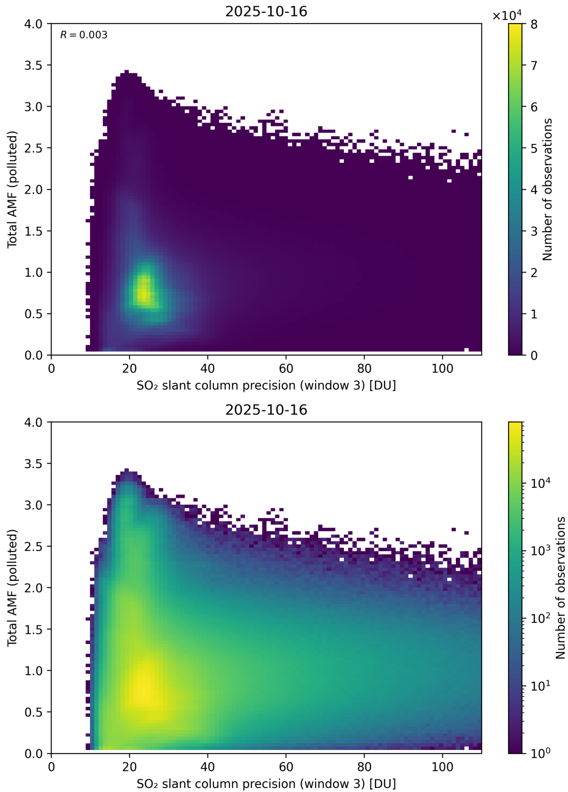
Figure 313: Scatter density plot of “SO 2 slant column precision (window 3)” against “Total AMF (polluted)” for 2025-10-15 to 2025-10-17.
