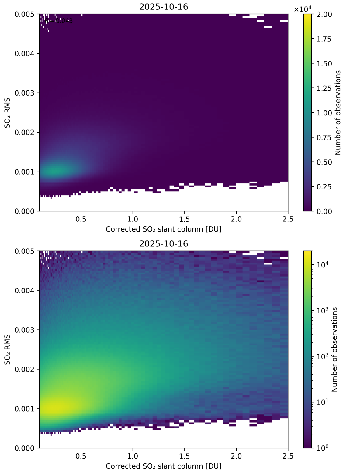
Figure 231: Scatter density plot of “Corrected SO 2 slant column” against “SO 2 RMS” for 2025-10-15 to 2025-10-17.
