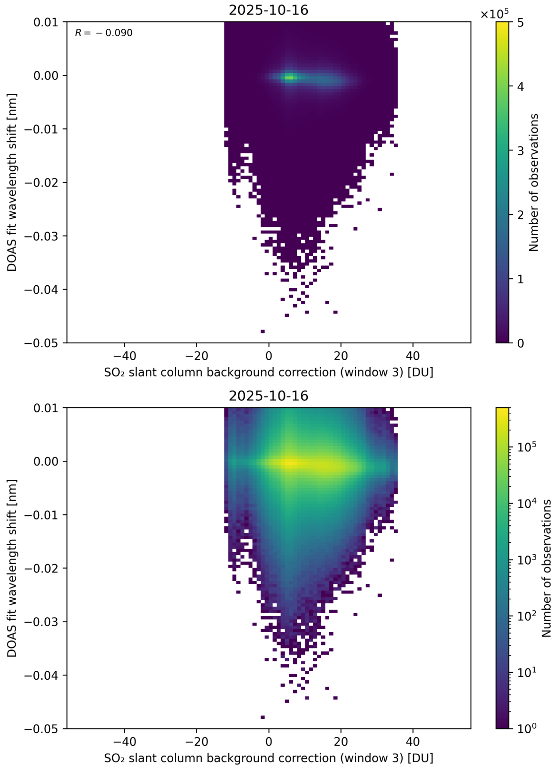
Figure 132: Scatter density plot of “SO 2 slant column background correction (window 3)” against “DOAS fit wavelength shift” for 2025-10-15 to 2025-10-17.
