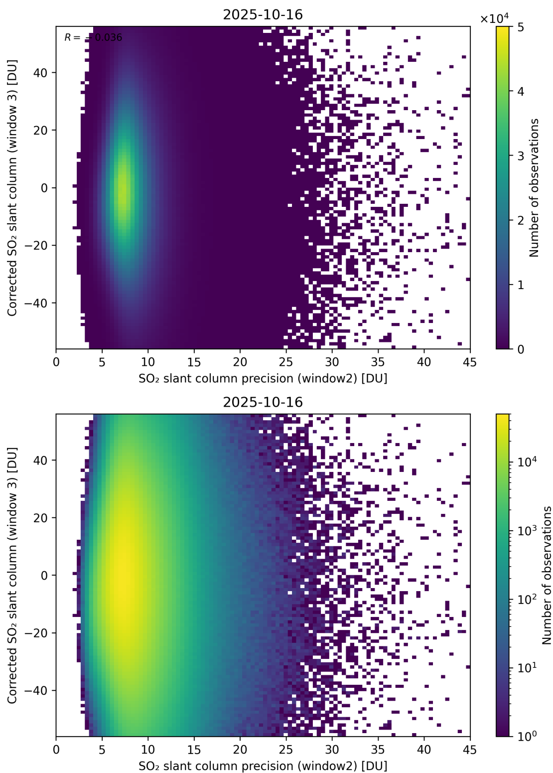
Figure 298: Scatter density plot of “SO 2 slant column precision (window2)” against “Corrected SO 2 slant column (window 3)” for 2025-10-15 to 2025-10-17.
