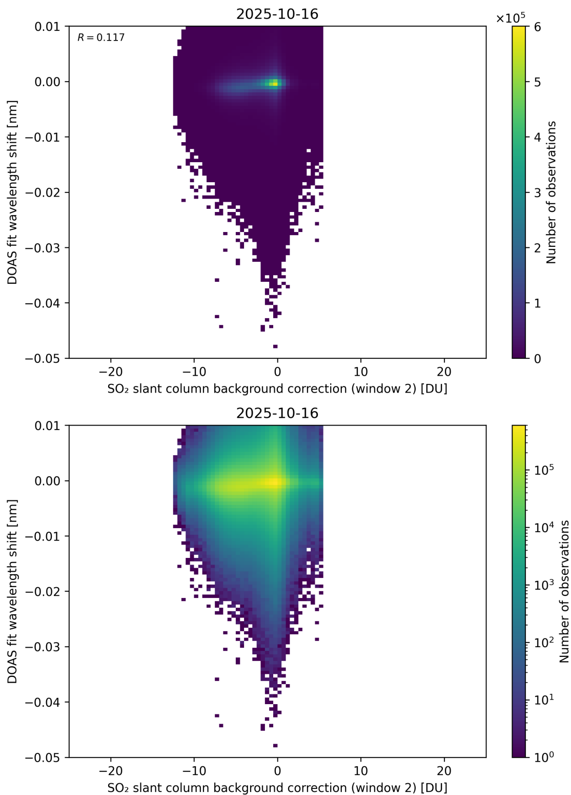
Figure 123: Scatter density plot of “SO 2 slant column background correction (window 2)” against “DOAS fit wavelength shift” for 2025-10-15 to 2025-10-17.
