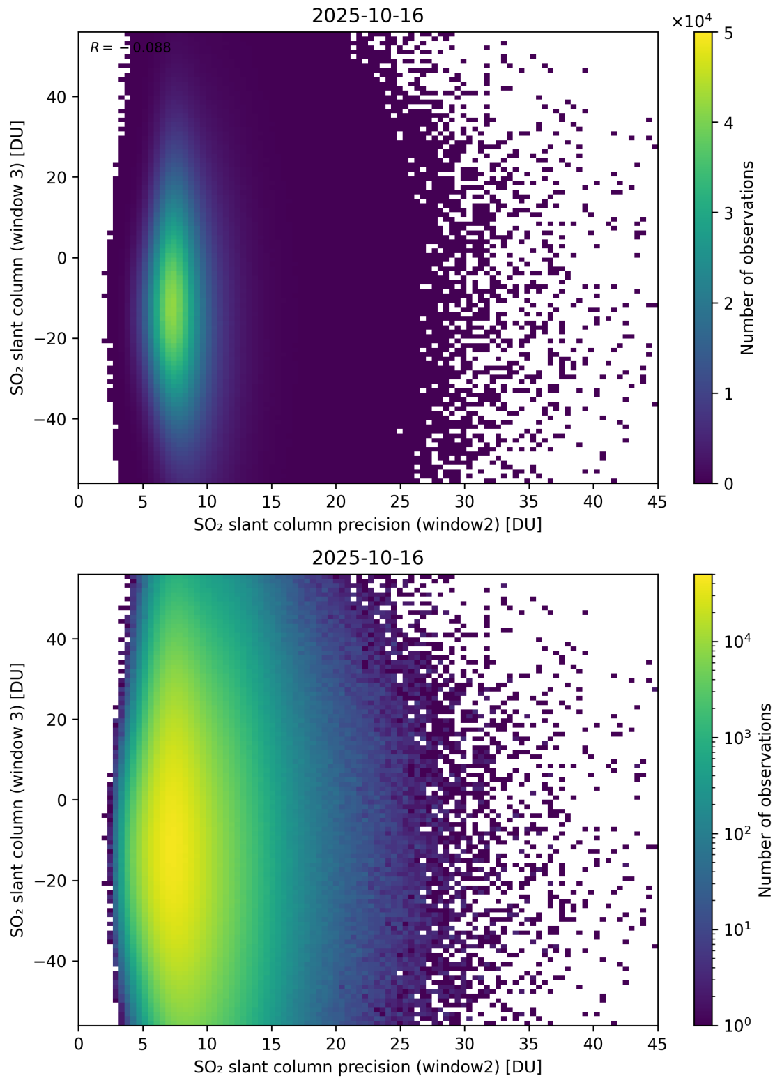
Figure 299: Scatter density plot of “SO 2 slant column precision (window2)” against “SO 2 slant column (window 3)” for 2025-10-15 to 2025-10-17.
