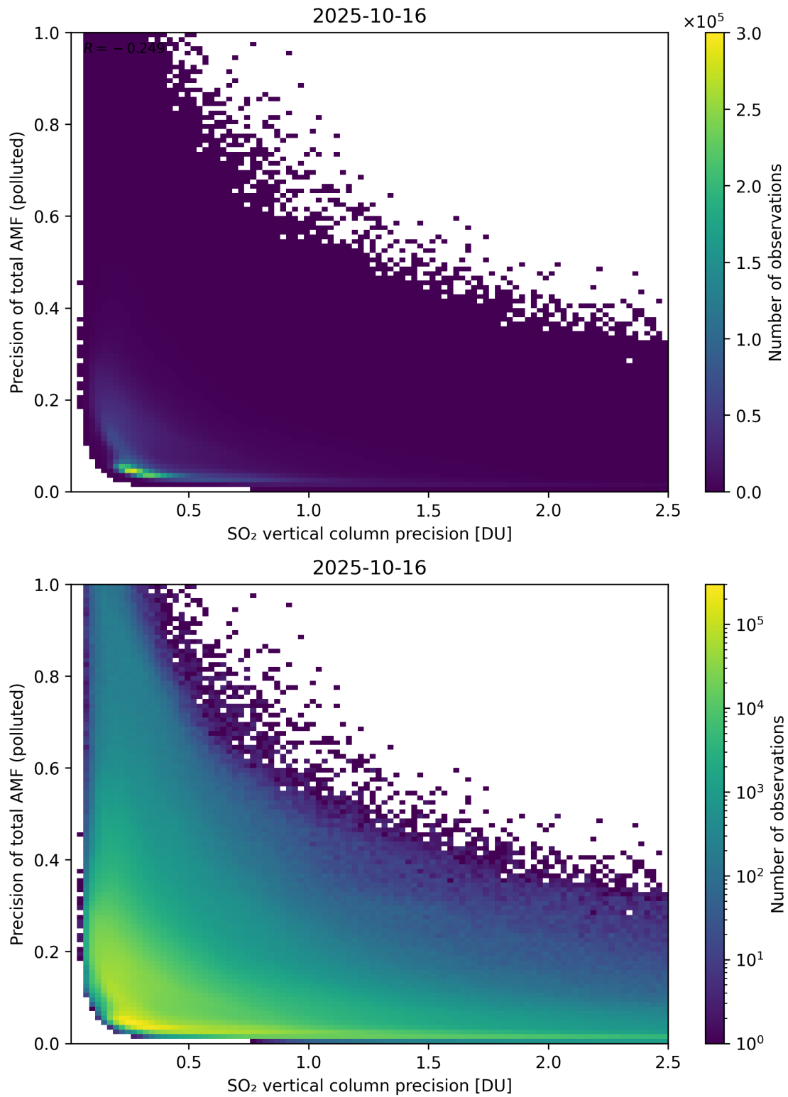
Figure 347: Scatter density plot of “SO 2 vertical column precision” against “Precision of total AMF (polluted)” for 2025-10-15 to 2025-10-17.
