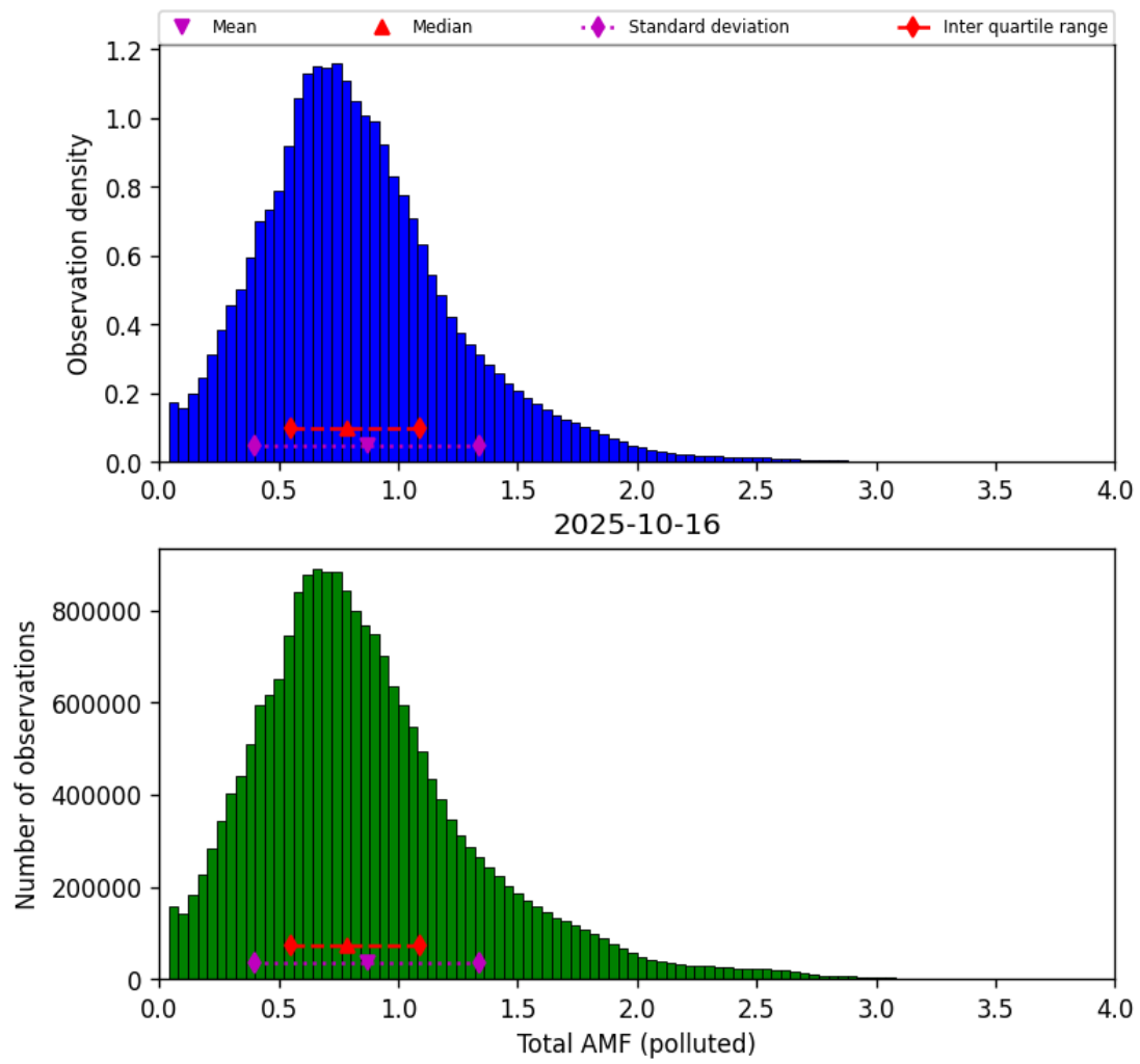
Figure 79: Histogram of “Total AMF (polluted)” for 2025-10-15 to 2025-10-17
