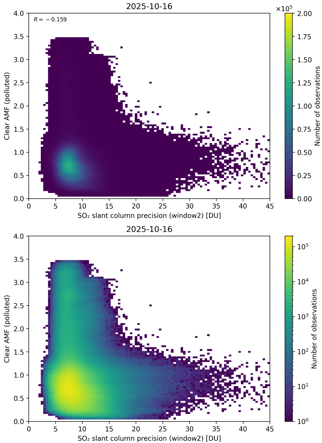
Figure 296: Scatter density plot of “SO 2 slant column precision (window2)” against “Clear AMF (polluted)” for 2025-10-15 to 2025-10-17.
