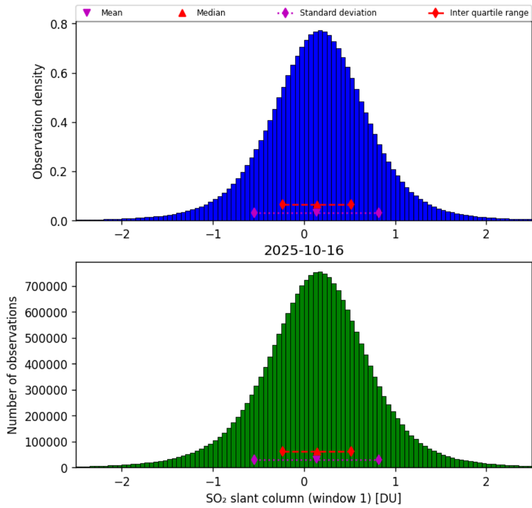
Figure 63: Histogram of “SO 2 slant column (window 1)” for 2025-10-15 to 2025-10-17
