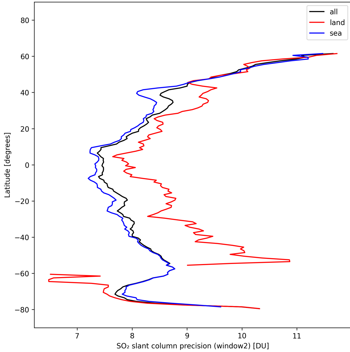
Figure 42: Zonal average of “SO 2 slant column precision (window2)” for 2025-10-15 to 2025-10-17.
