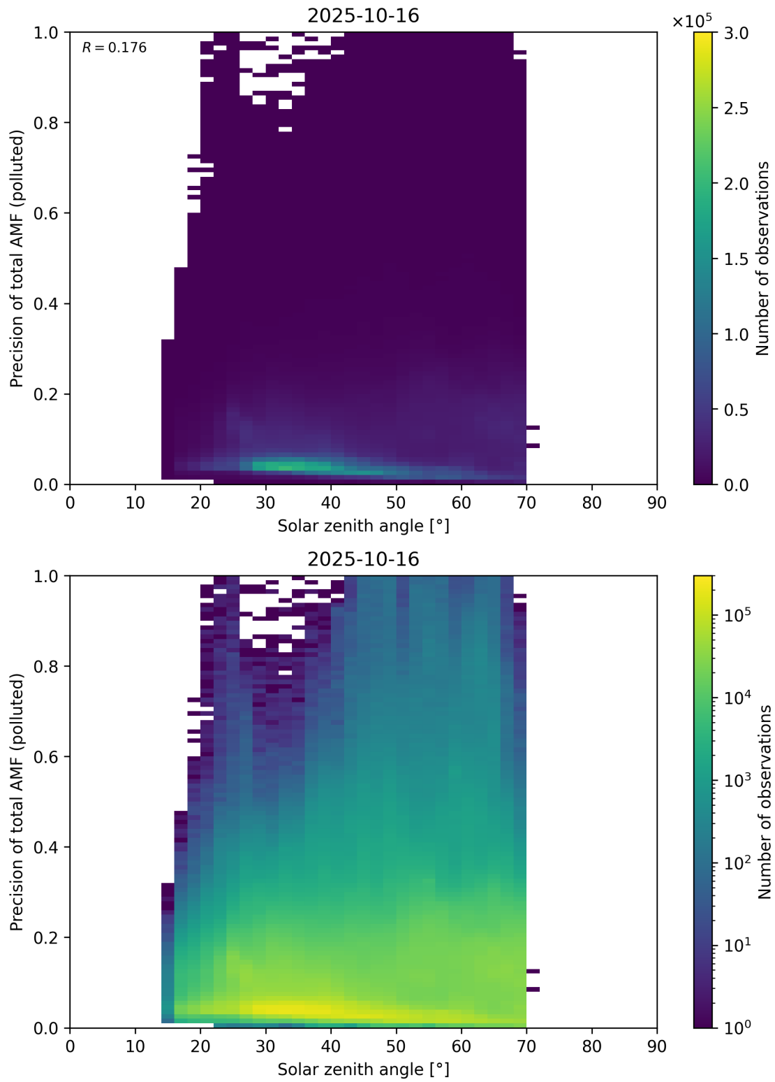
Figure 190: Scatter density plot of “Solar zenith angle” against “Precision of total AMF (polluted)” for 2025-10-15 to 2025-10-17.
