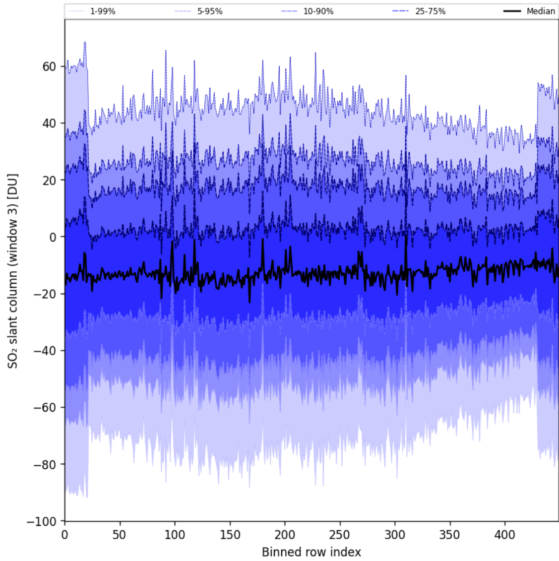
Figure 97: Along track statistics of “SO 2 slant column (window 3)” for 2025-10-15 to 2025-10-17
