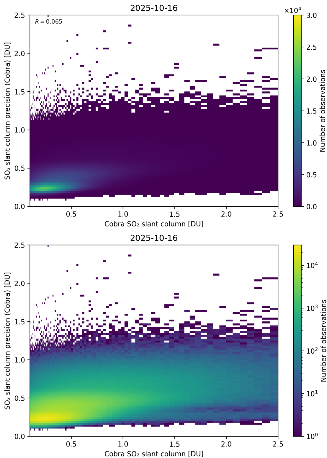
Figure 216: Scatter density plot of “Cobra SO 2 slant column” against “SO 2 slant column precision (Cobra)” for 2025-10-15 to 2025-10-17.
