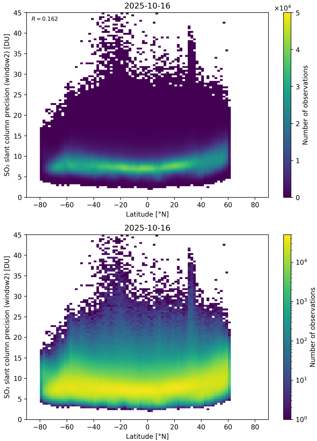
Figure 164: Scatter density plot of “Latitude” against “SO 2 slant column precision (window2)” for 2025-10-15 to 2025-10-17.
