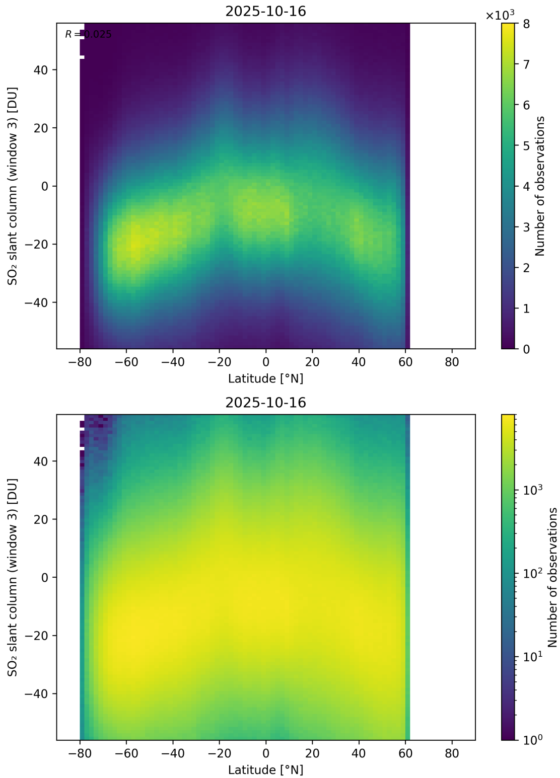
Figure 165: Scatter density plot of “Latitude” against “SO 2 slant column (window 3)” for 2025-10-15 to 2025-10-17.
