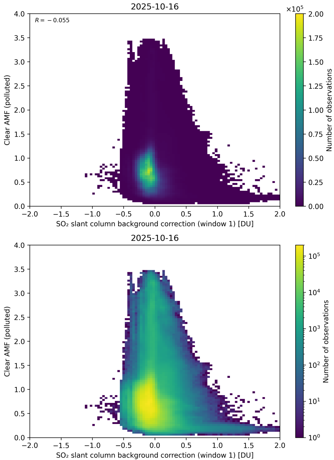
Figure 114: Scatter density plot of “SO 2 slant column background correction (window 1)” against “Clear AMF (polluted)” for 2025-10-15 to 2025-10-17.
