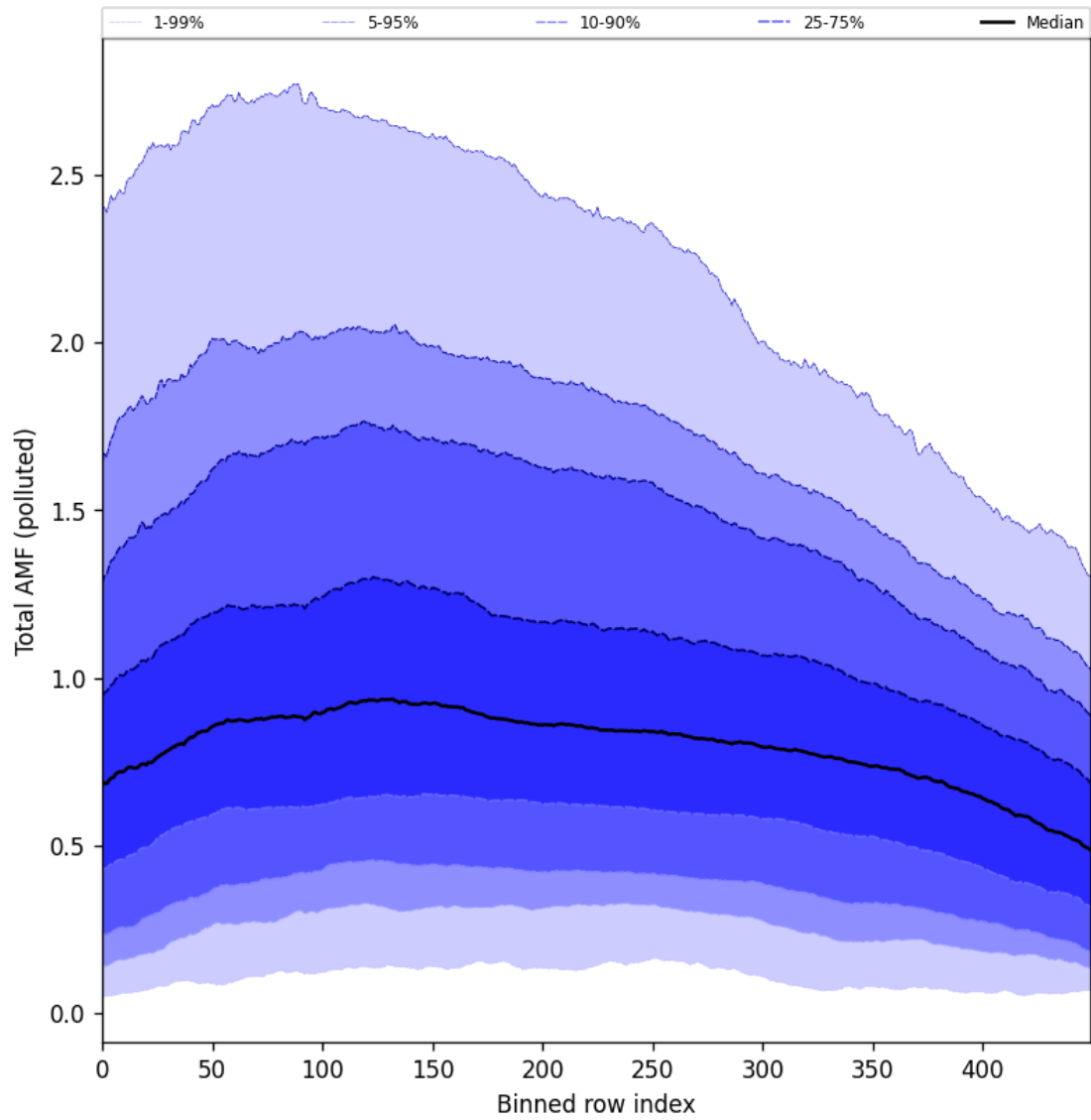
Figure 105: Along track statistics of “Total AMF (polluted)” for 2025-10-15 to 2025-10-17
