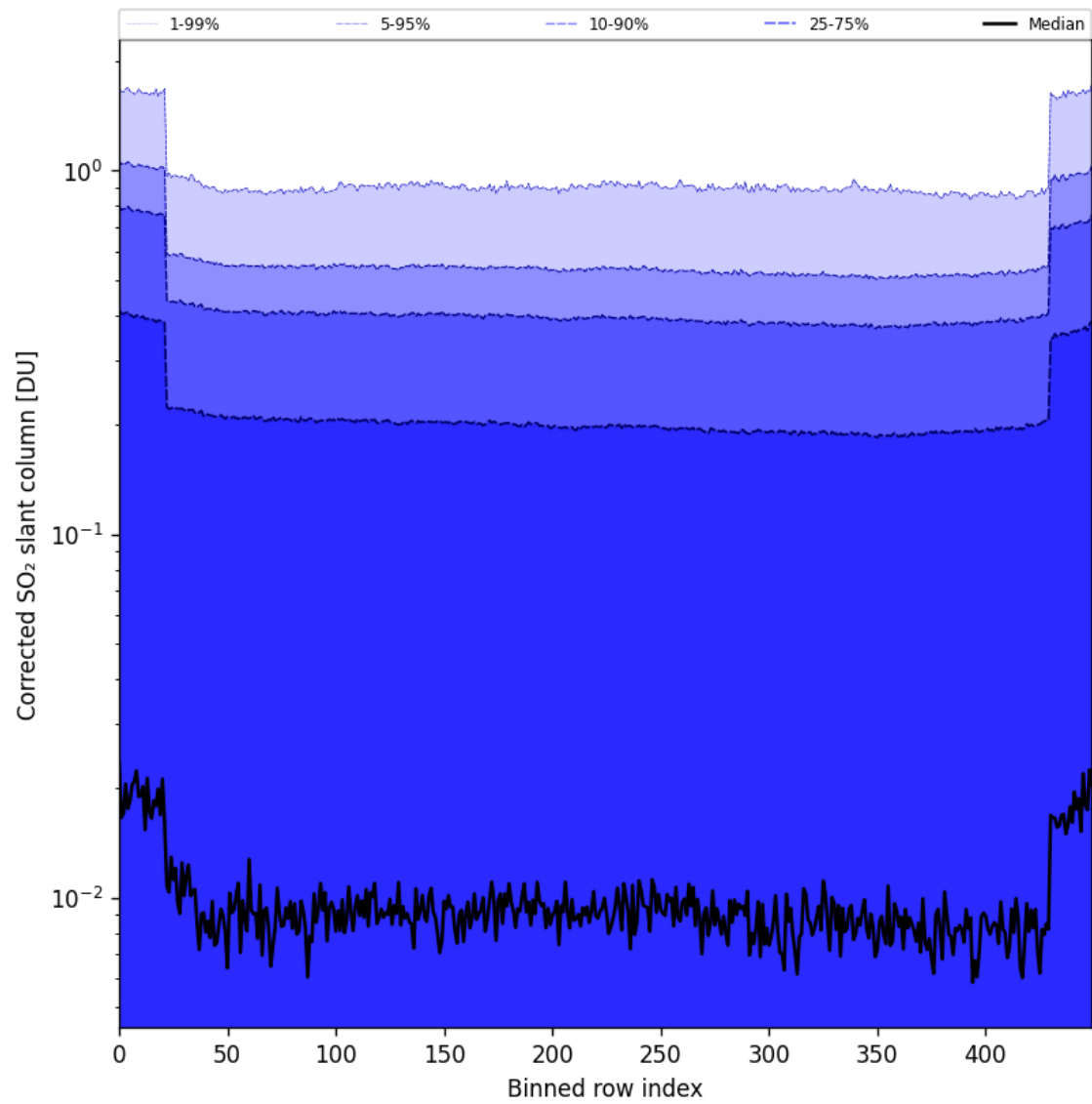
Figure 86: Along track statistics of “Corrected SO 2 slant column” for 2025-10-15 to 2025-10-17
