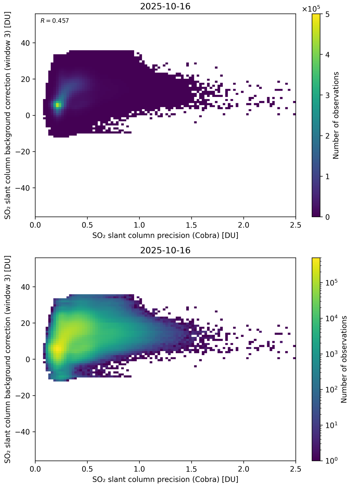
Figure 201: Scatter density plot of “SO 2 slant column precision (Cobra)” against “SO 2 slant column background correction (window 3)” for 2025-10-15 to 2025-10-17.
