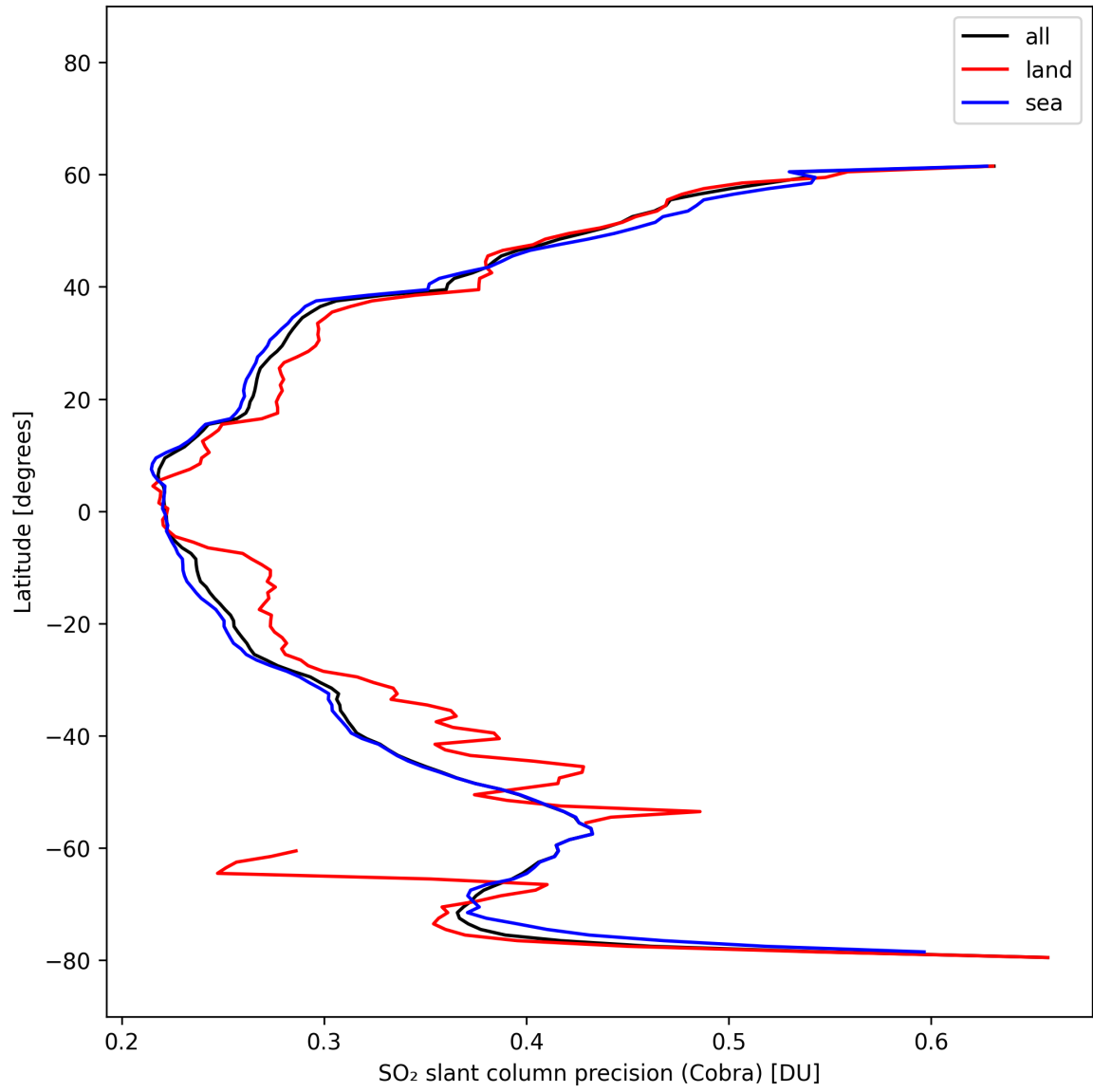
Figure 36: Zonal average of “SO 2 slant column precision (Cobra)” for 2025-10-15 to 2025-10-17.
