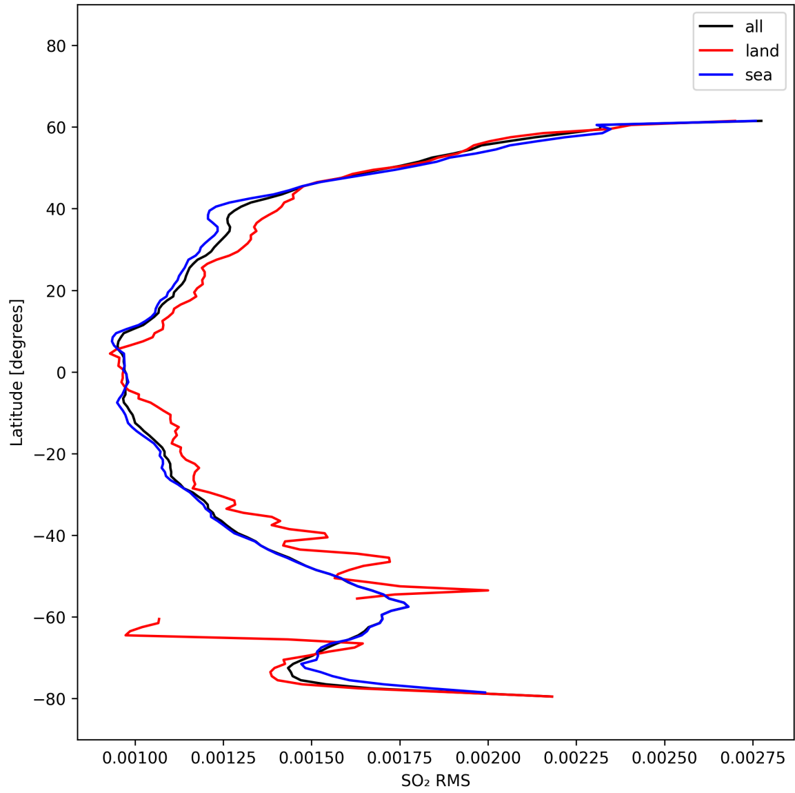
Figure 52: Zonal average of “SO 2 RMS” for 2025-10-15 to 2025-10-17.
