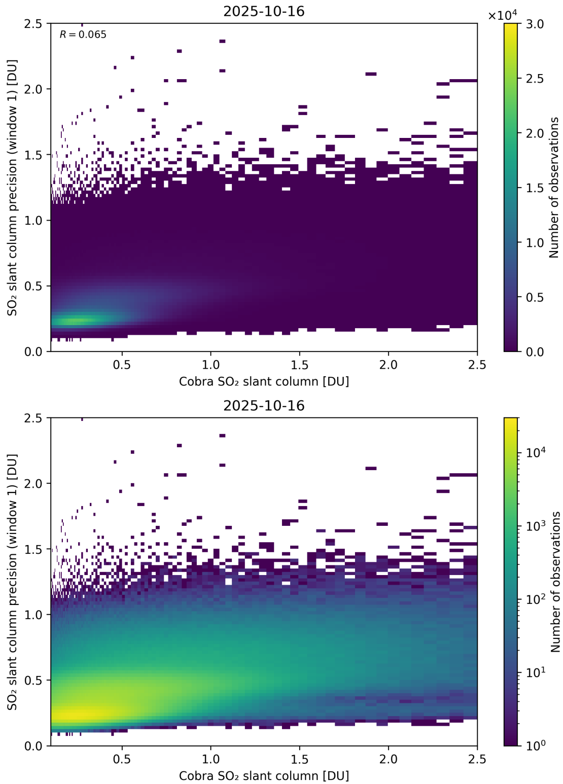
Figure 220: Scatter density plot of “Cobra SO 2 slant column” against “SO 2 slant column precision (window 1)” for 2025-10-15 to 2025-10-17.
