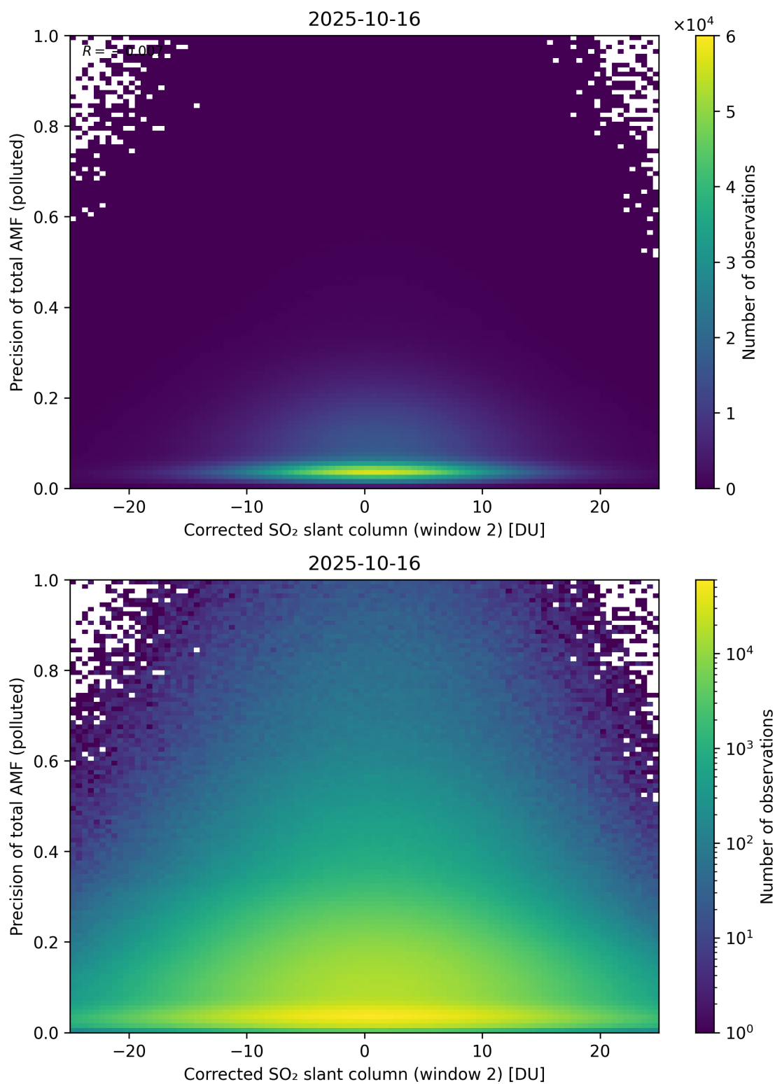
Figure 254: Scatter density plot of “Corrected SO 2 slant column (window 2)” against “Precision of total AMF (polluted)” for 2025-10-15 to 2025-10-17.
