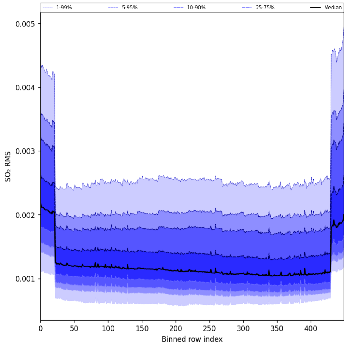
Figure 104: Along track statistics of “SO 2 RMS” for 2025-10-15 to 2025-10-17
