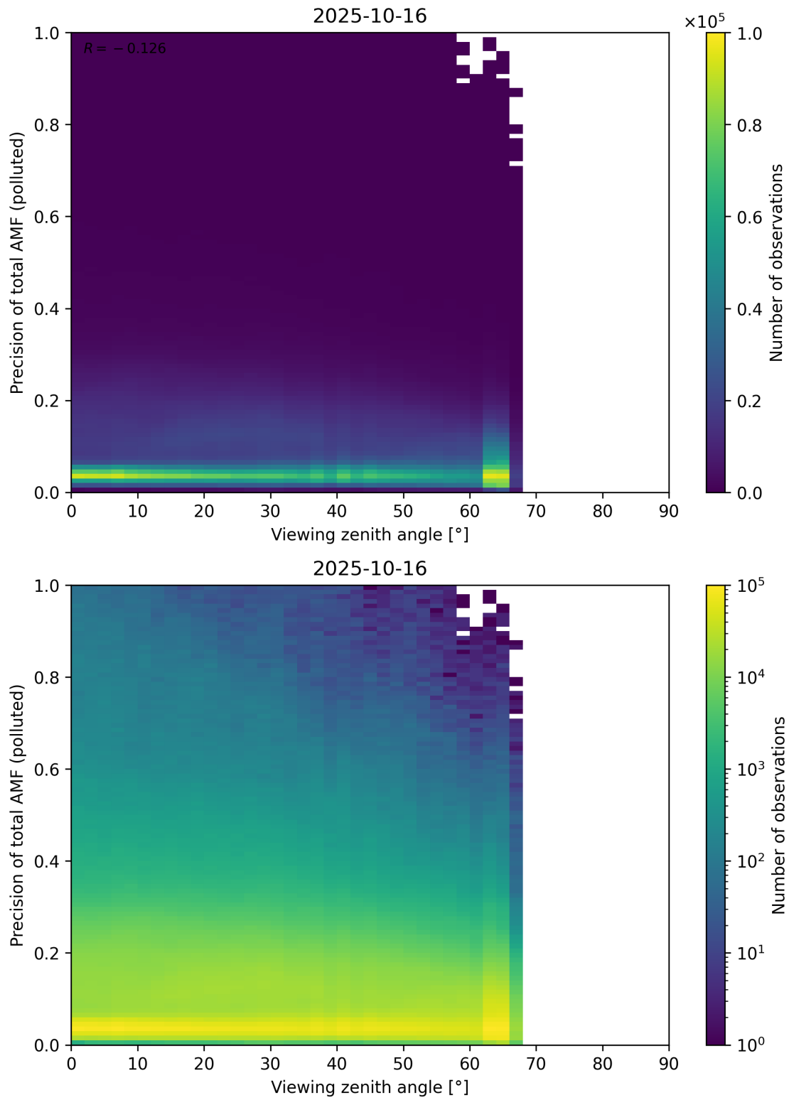
Figure 382: Scatter density plot of “Viewing zenith angle” against “Precision of total AMF (polluted)” for 2025-10-15 to 2025-10-17.
