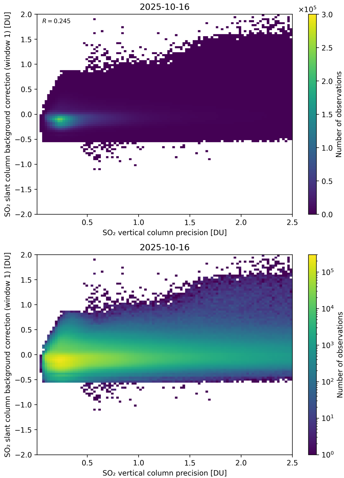
Figure 329: Scatter density plot of “SO 2 vertical column precision” against “SO 2 slant column background correction (window 1)” for 2025-10-15 to 2025-10-17.
