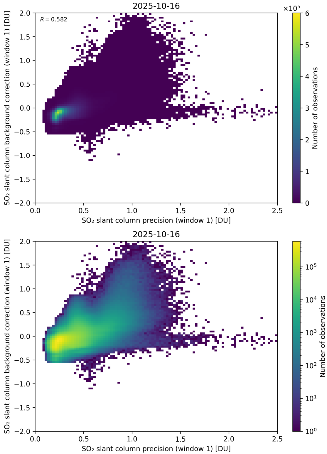
Figure 268: Scatter density plot of “SO 2 slant column precision (window 1)” against “SO 2 slant column background correction (window 1)” for 2025-10-15 to 2025-10-17.
