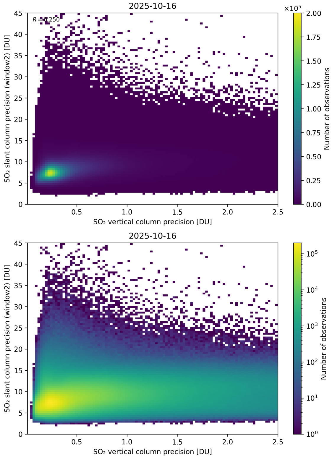
Figure 343: Scatter density plot of “SO 2 vertical column precision” against “SO 2 slant column precision (window2)” for 2025-10-15 to 2025-10-17.
