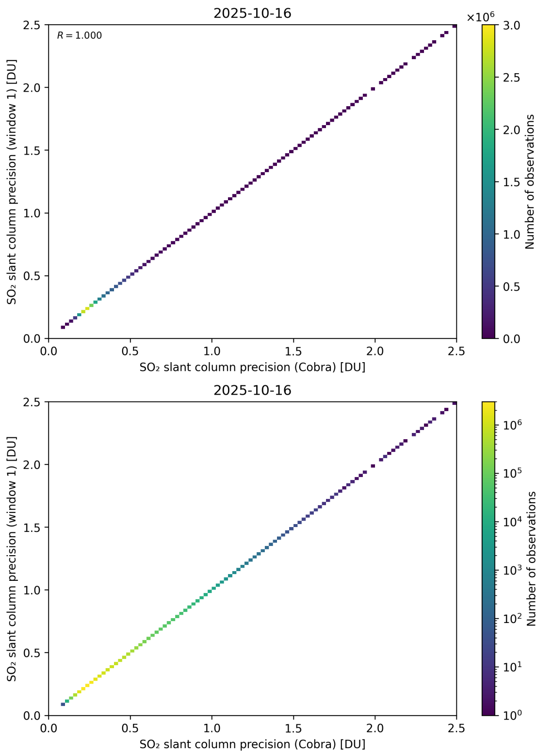
Figure 209: Scatter density plot of “SO 2 slant column precision (Cobra)” against “SO 2 slant column precision (window 1)” for 2025-10-15 to 2025-10-17.
