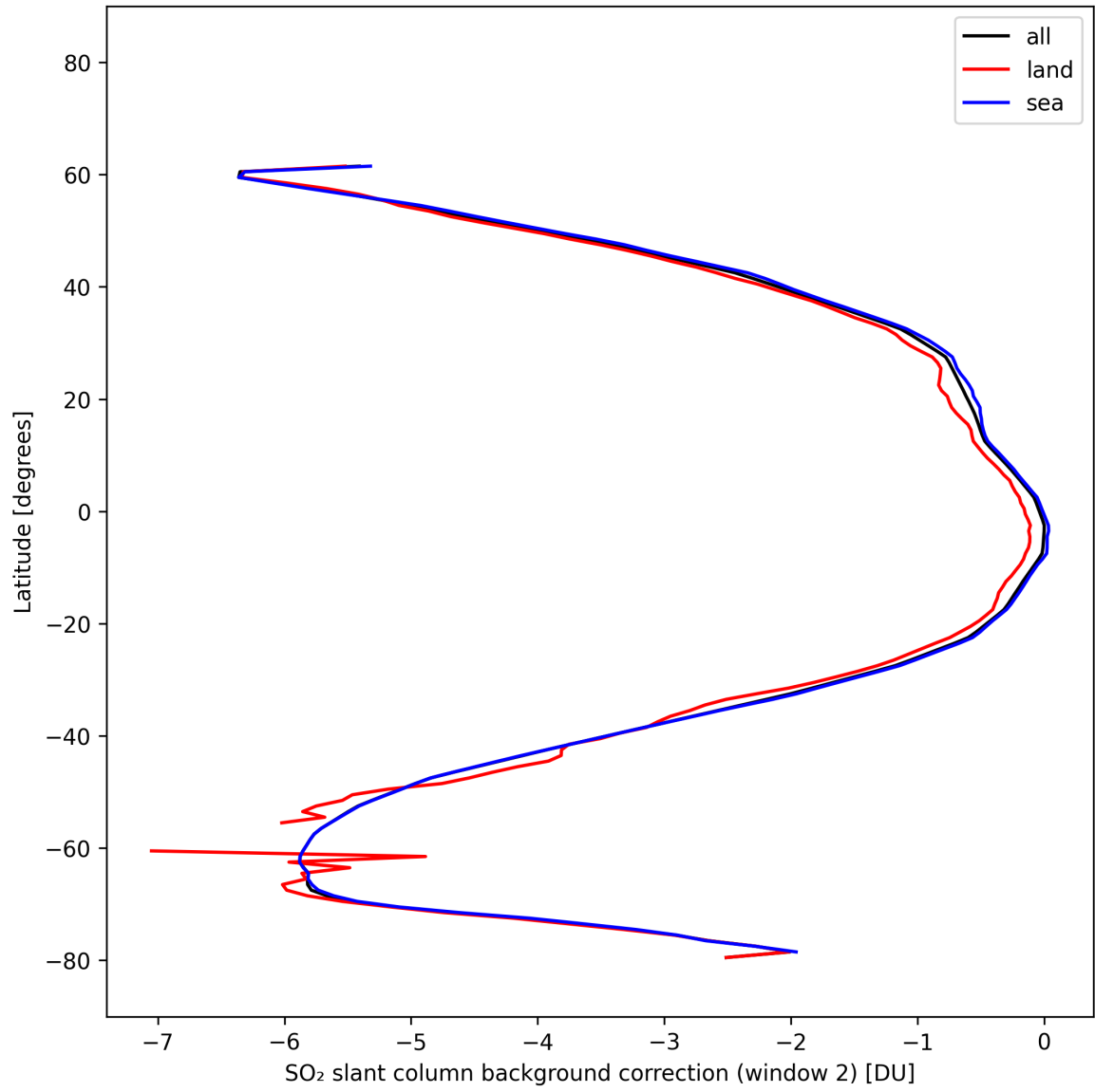
Figure 44: Zonal average of “SO 2 slant column background correction (window 2)” for 2025-10-15 to 2025-10-17.
