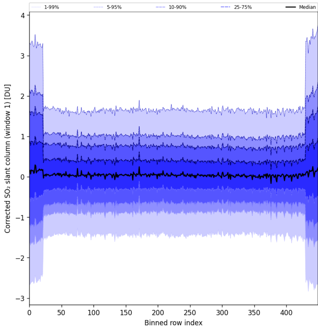
Figure 91: Along track statistics of “Corrected SO 2 slant column (window 1)” for 2025-10-15 to 2025-10-17
