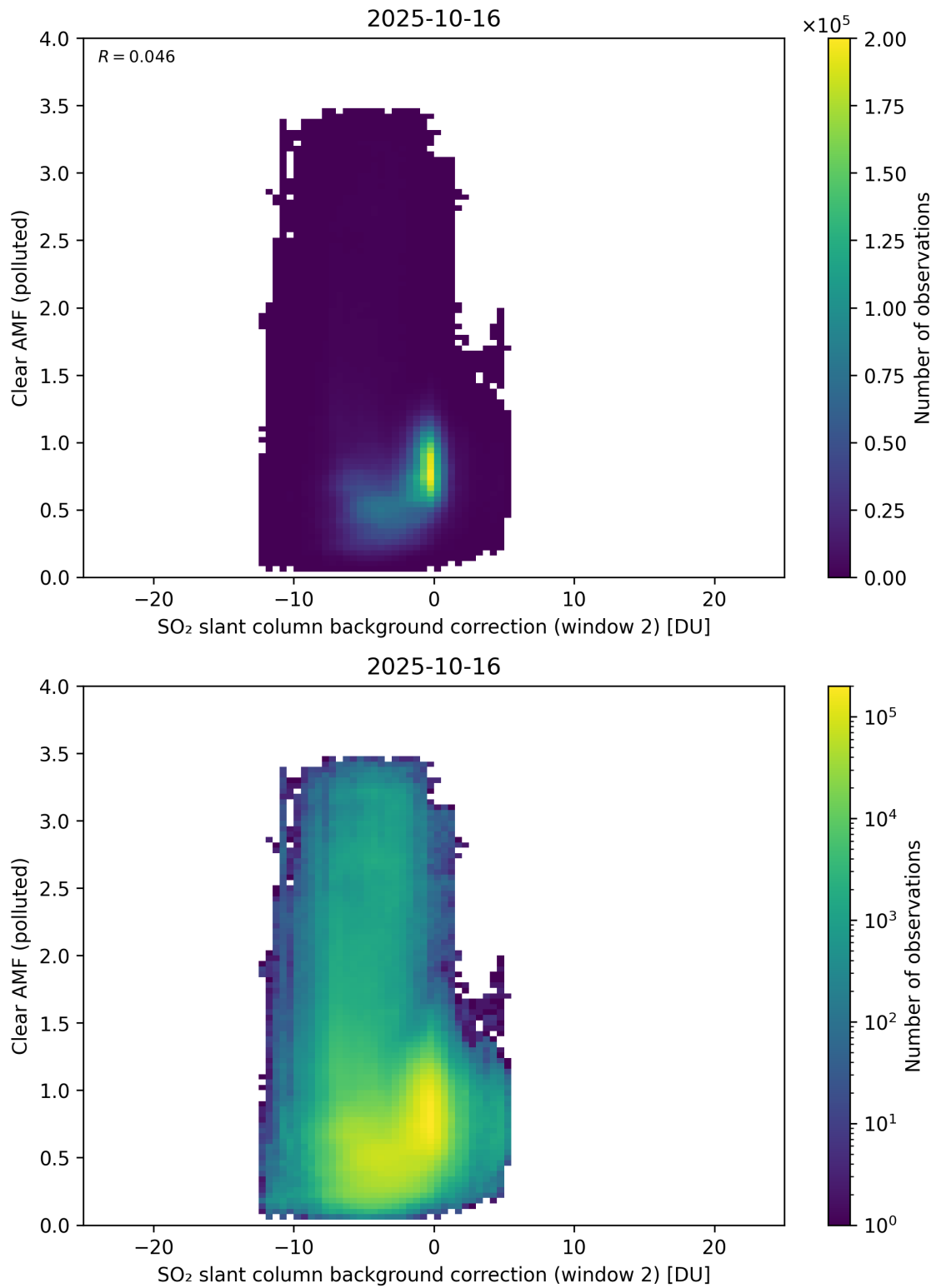
Figure 126: Scatter density plot of “SO 2 slant column background correction (window 2)” against “Clear AMF (polluted)” for 2025-10-15 to 2025-10-17.
