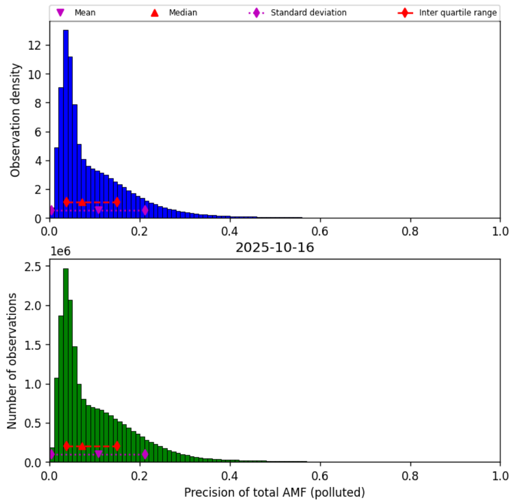
Figure 80: Histogram of “Precision of total AMF (polluted)” for 2025-10-15 to 2025-10-17
