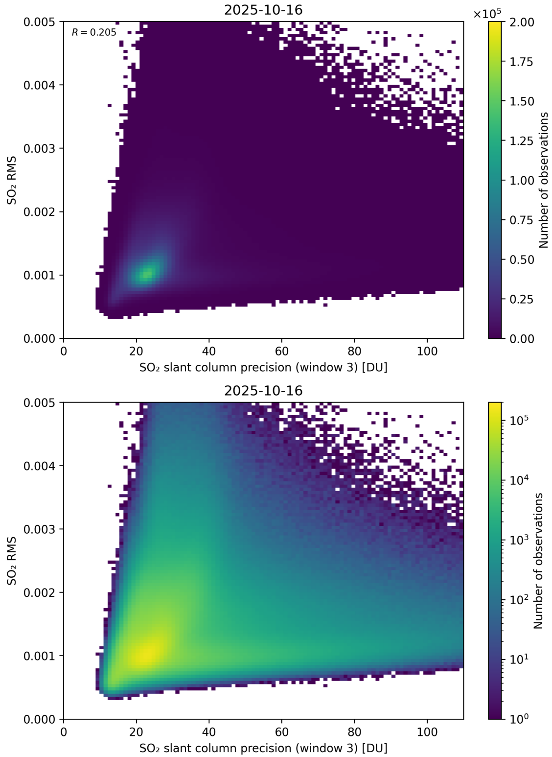
Figure 310: Scatter density plot of “SO 2 slant column precision (window 3)” against “SO 2 RMS” for 2025-10-15 to 2025-10-17.
