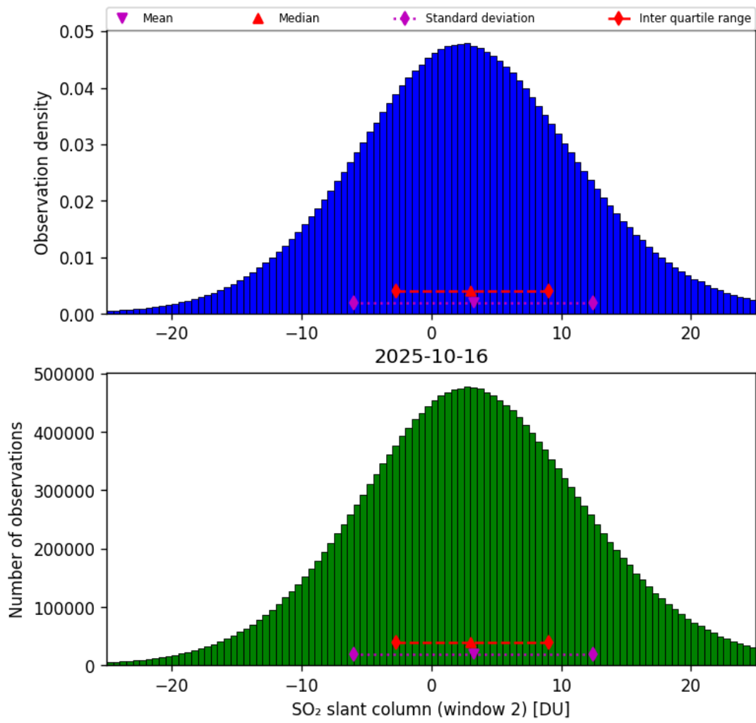
Figure 67: Histogram of “SO 2 slant column (window 2)” for 2025-10-15 to 2025-10-17
