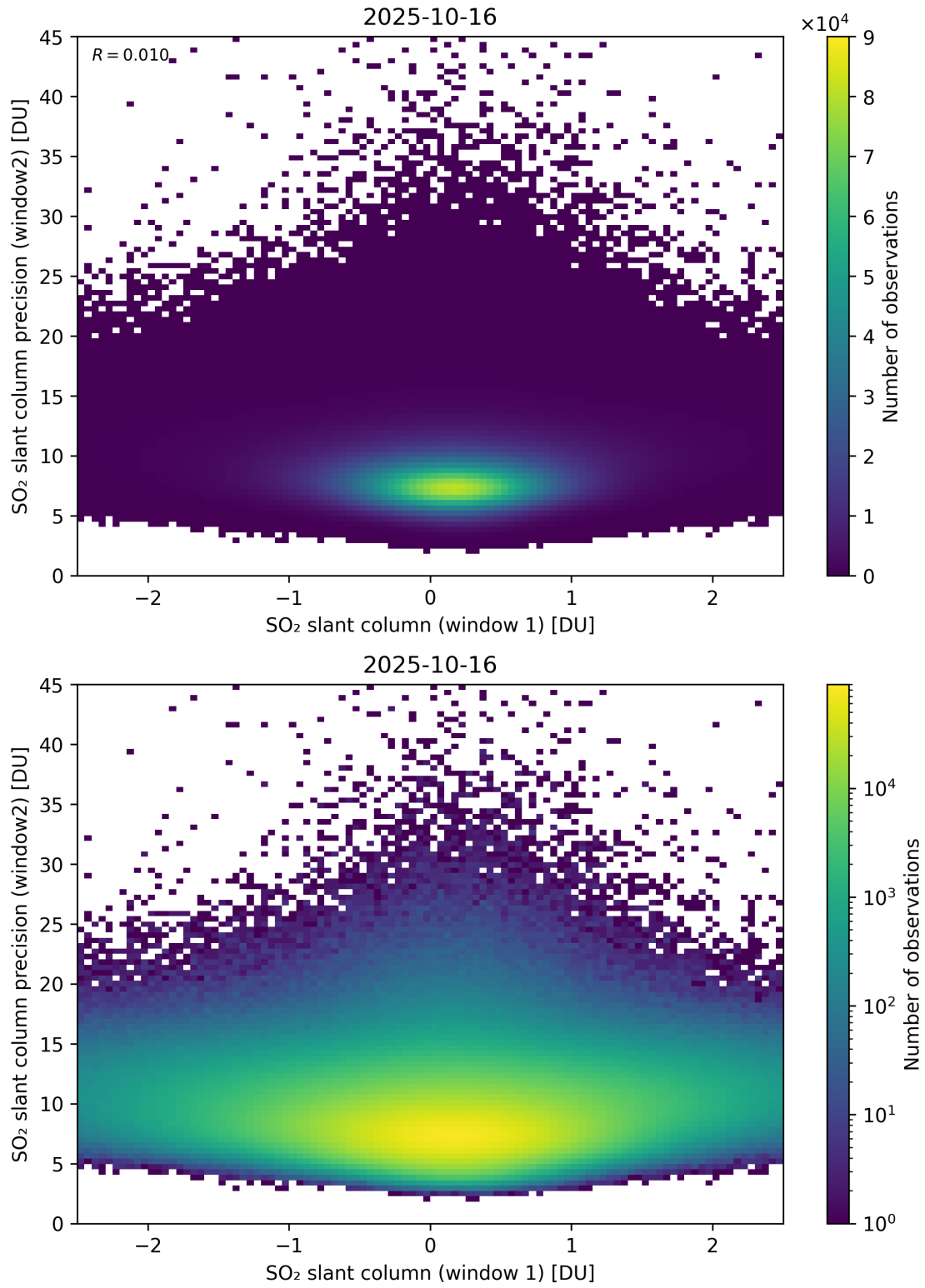
Figure 286: Scatter density plot of “SO 2 slant column (window 1)” against “SO 2 slant column precision (window2)” for 2025-10-15 to 2025-10-17.
