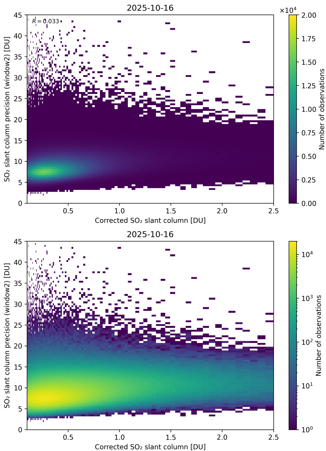
Figure 239: Scatter density plot of “Corrected SO 2 slant column” against “SO 2 slant column precision (window2)” for 2025-10-15 to 2025-10-17.
