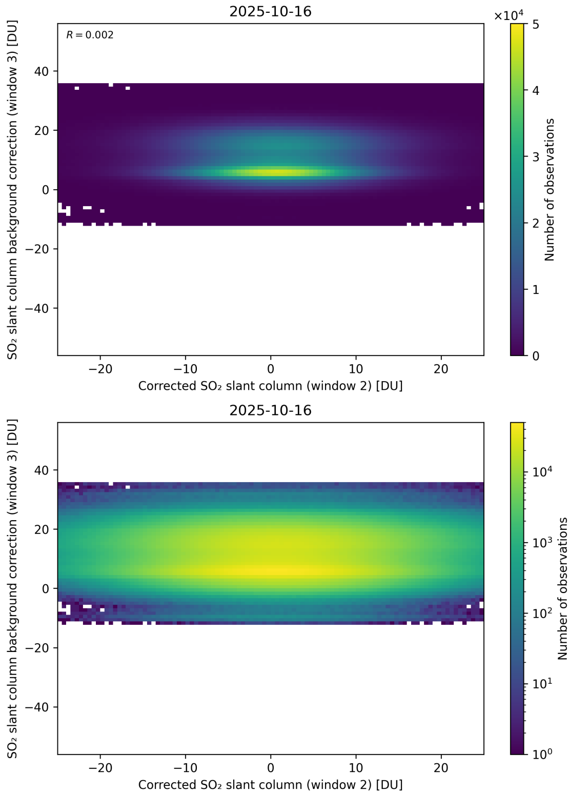
Figure 245: Scatter density plot of “Corrected SO 2 slant column (window 2)” against “SO 2 slant column background correction (window 3)” for 2025-10-15 to 2025-10-17.
