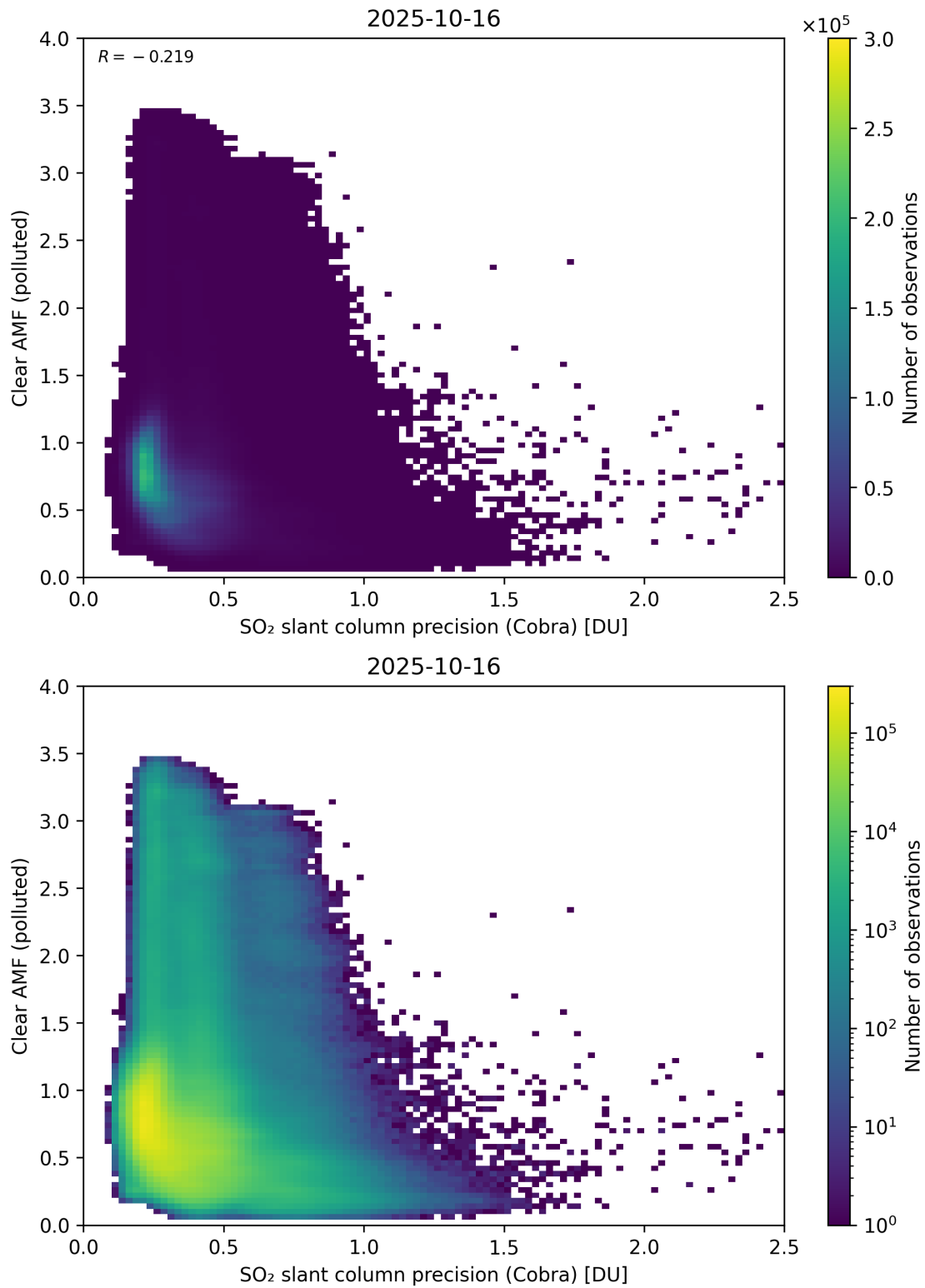
Figure 205: Scatter density plot of “SO 2 slant column precision (Cobra)” against “Clear AMF (polluted)” for 2025-10-15 to 2025-10-17.
