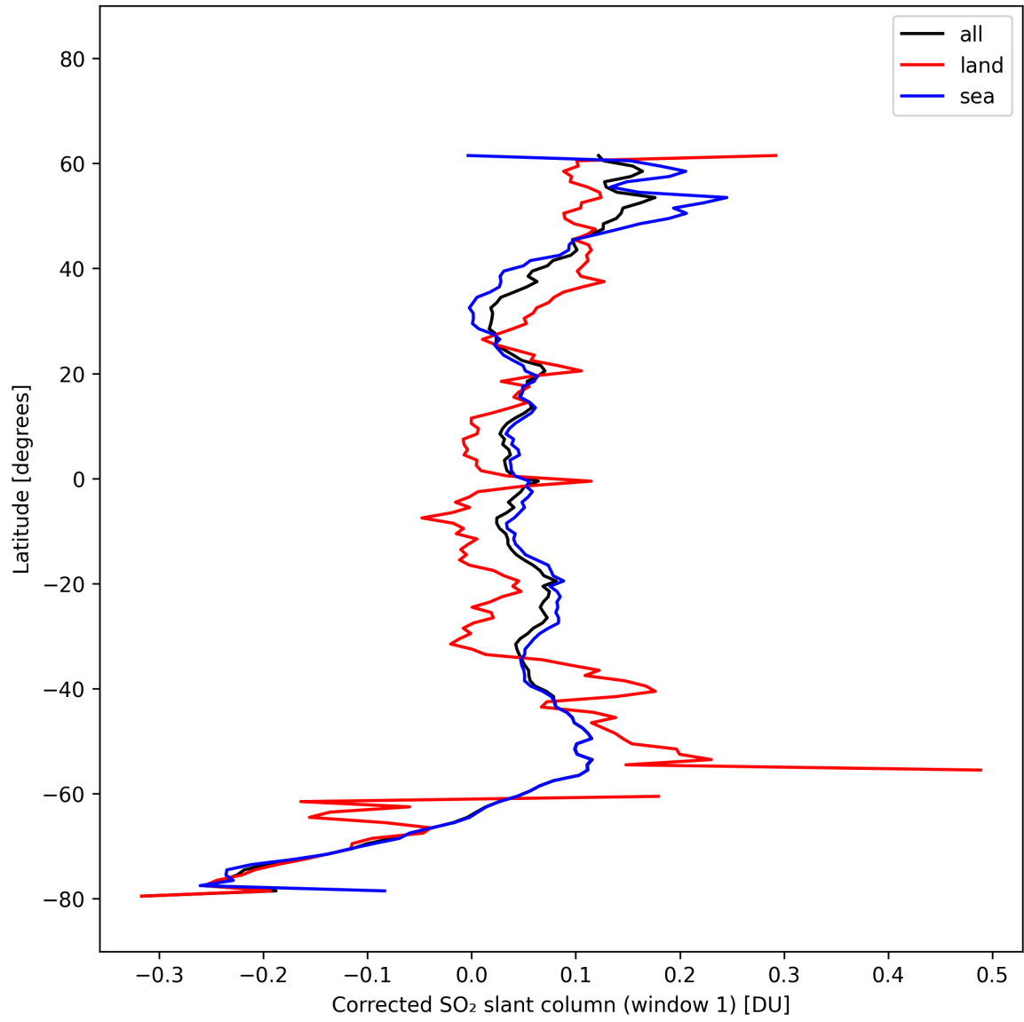
Figure 39: Zonal average of “Corrected SO 2 slant column (window 1)” for 2025-10-15 to 2025-10-17.
