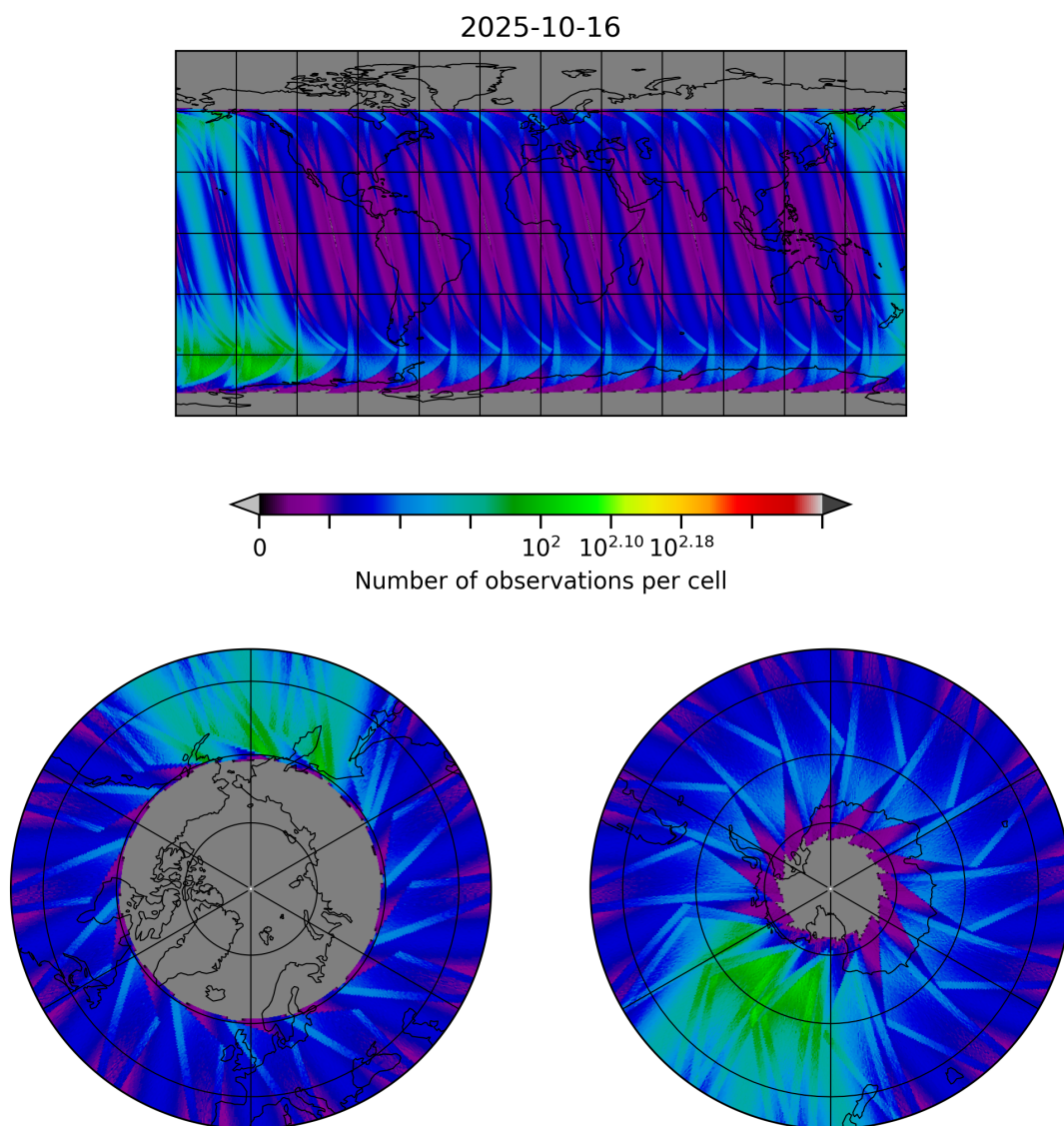
Figure 30: Map of the number of observations for 2025-10-15 to 2025-10-17
