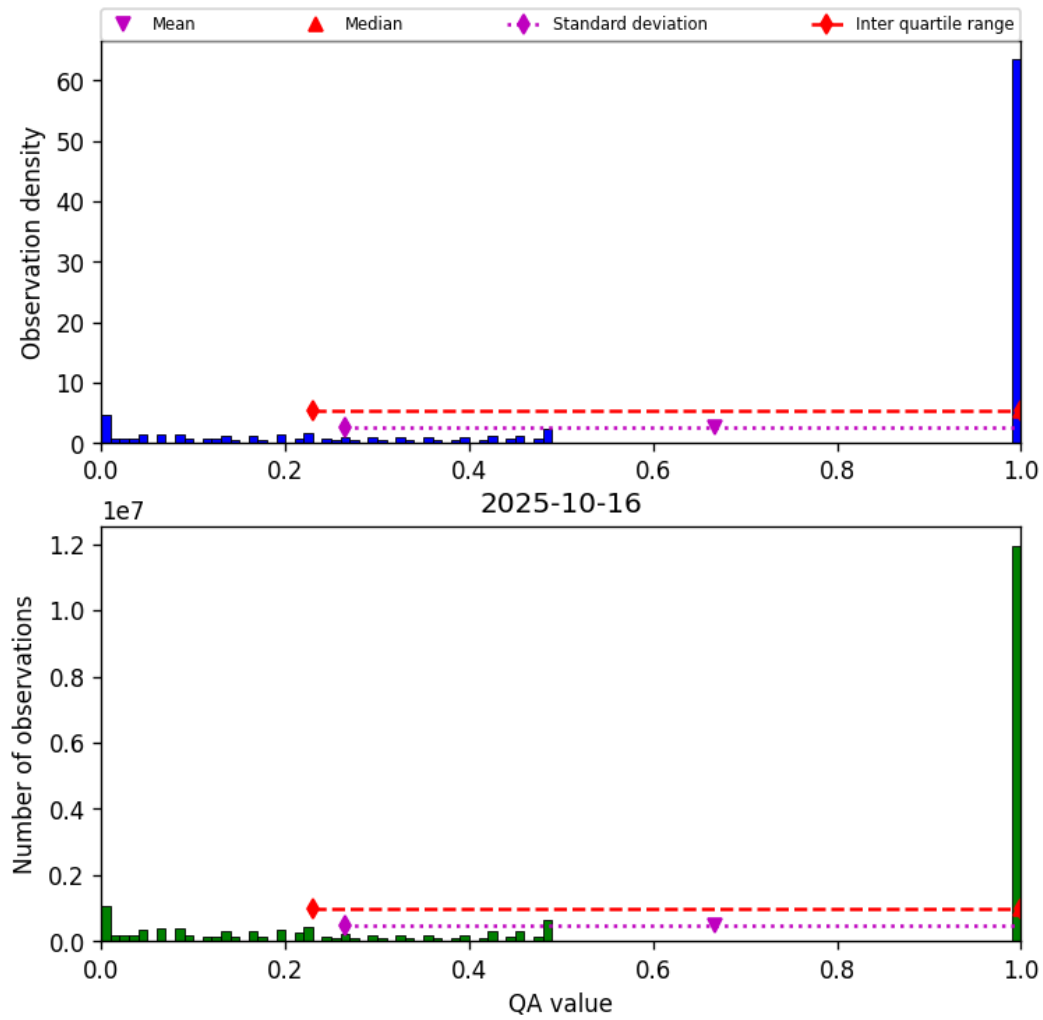
Figure 57: Histogram of “QA value” for 2025-10-15 to 2025-10-17
