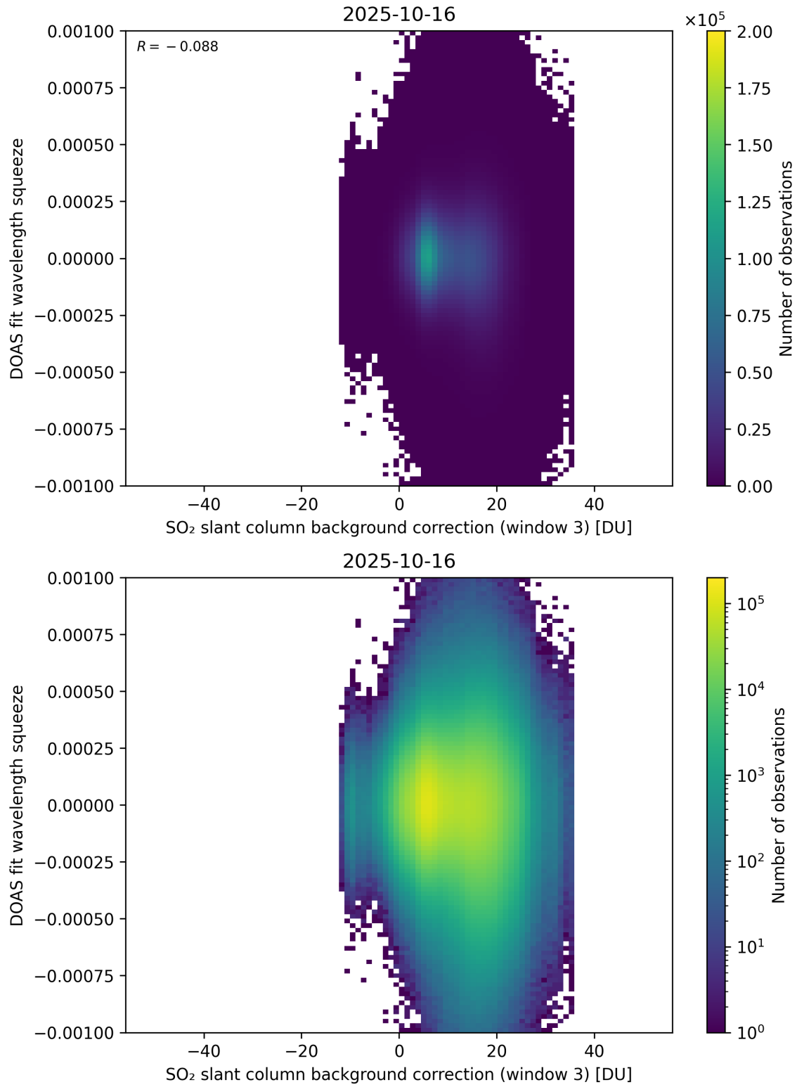
Figure 133: Scatter density plot of “SO 2 slant column background correction (window 3)” against “DOAS fit wavelength squeeze” for 2025-10-15 to 2025-10-17.
