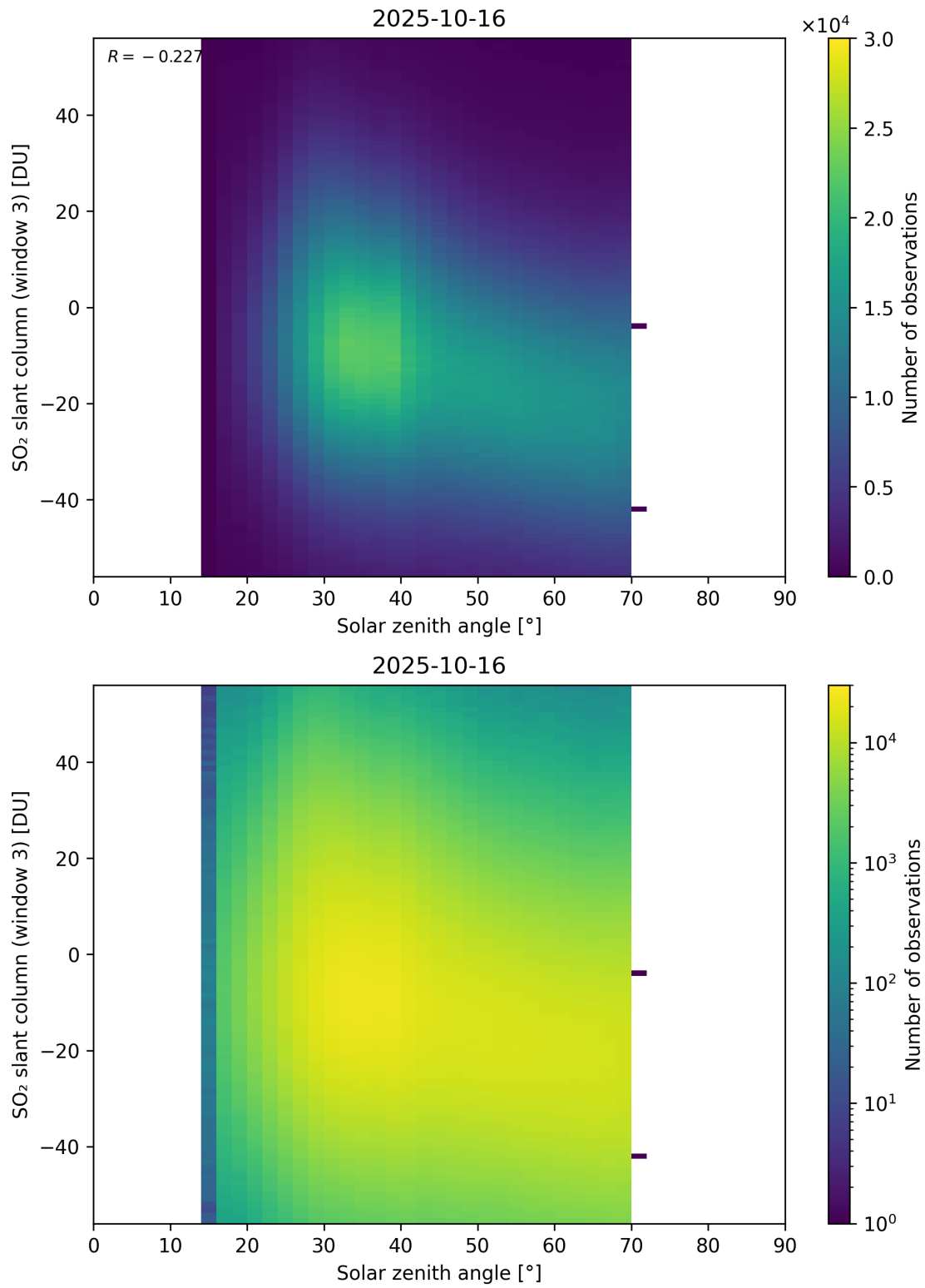
Figure 187: Scatter density plot of “Solar zenith angle” against “SO 2 slant column (window 3)” for 2025-10-15 to 2025-10-17.
