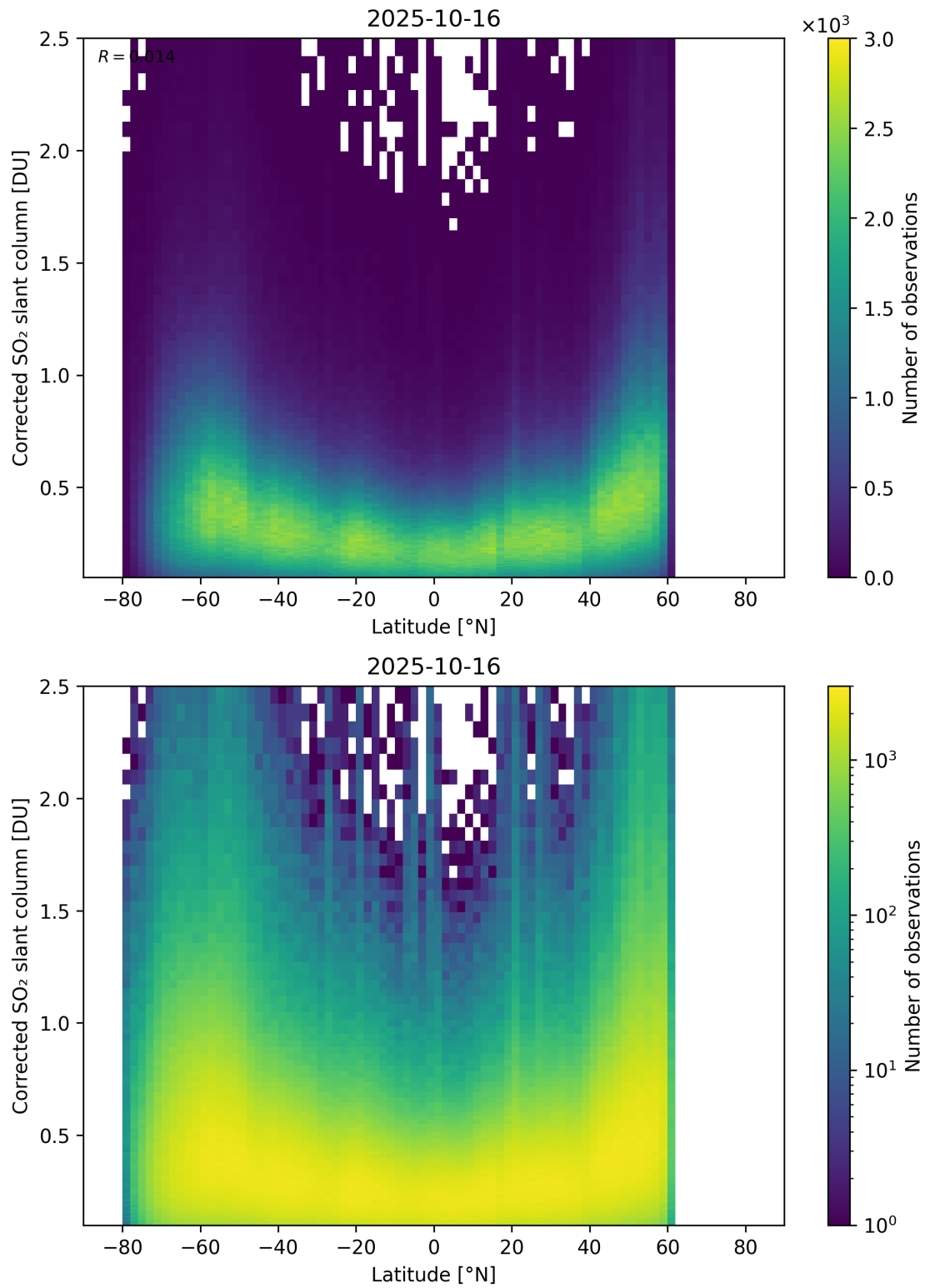
Figure 159: Scatter density plot of “Latitude” against “Corrected SO 2 slant column” for 2025-10-15 to 2025-10-17.
