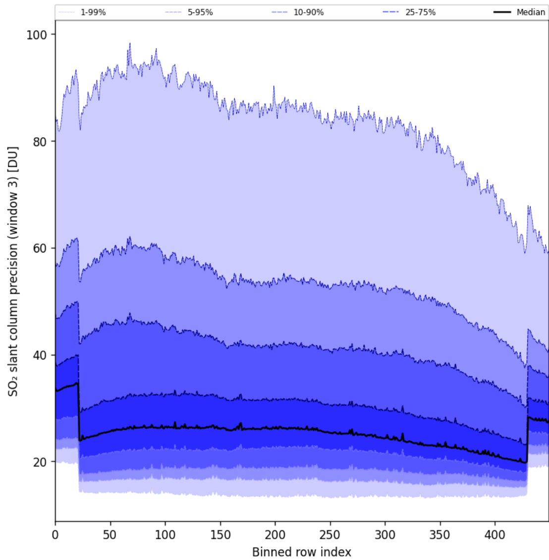
Figure 98: Along track statistics of “SO 2 slant column precision (window 3)” for 2025-10-15 to 2025-10-17
