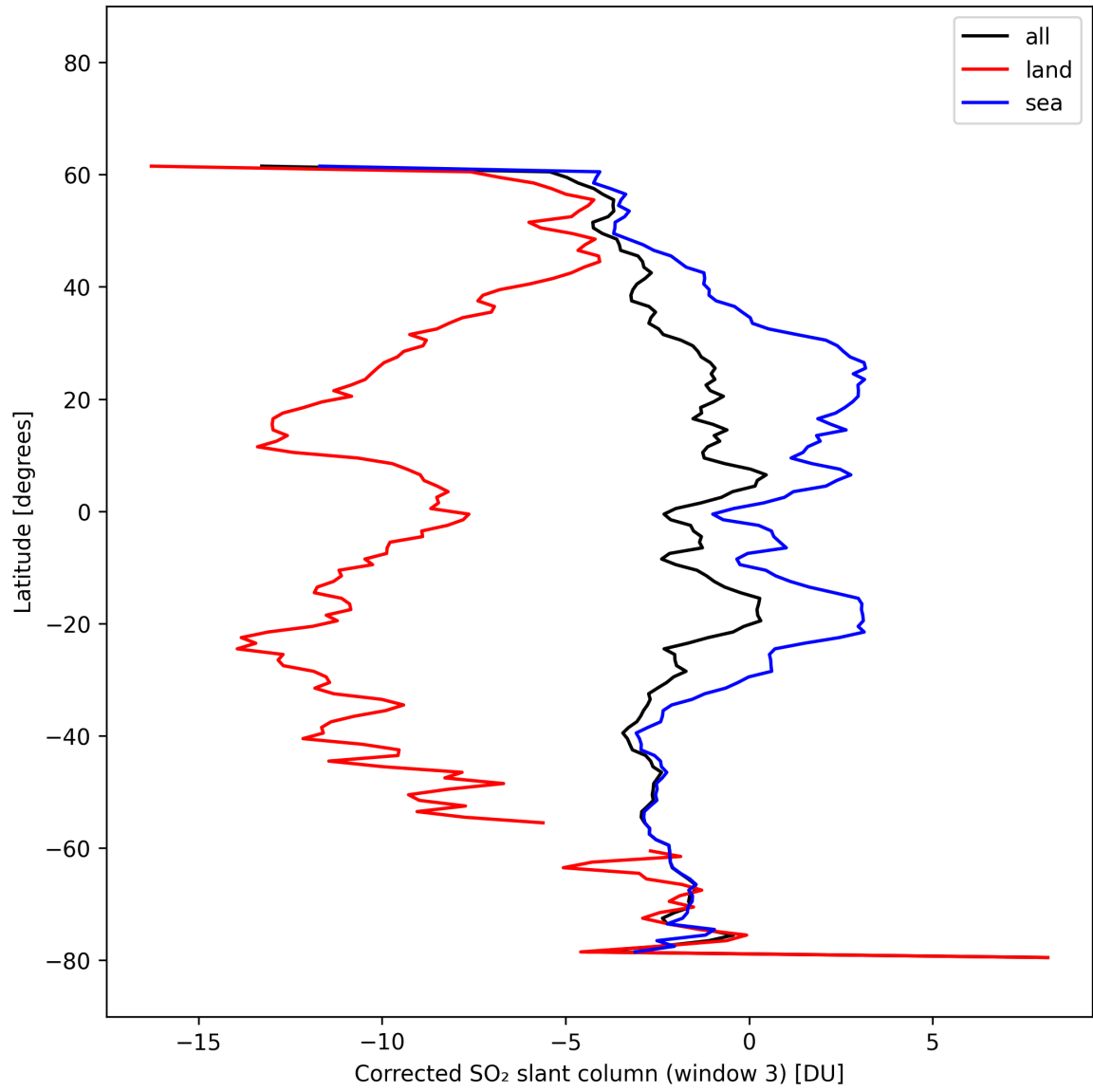
Figure 47: Zonal average of “Corrected SO 2 slant column (window 3)” for 2025-10-15 to 2025-10-17.
