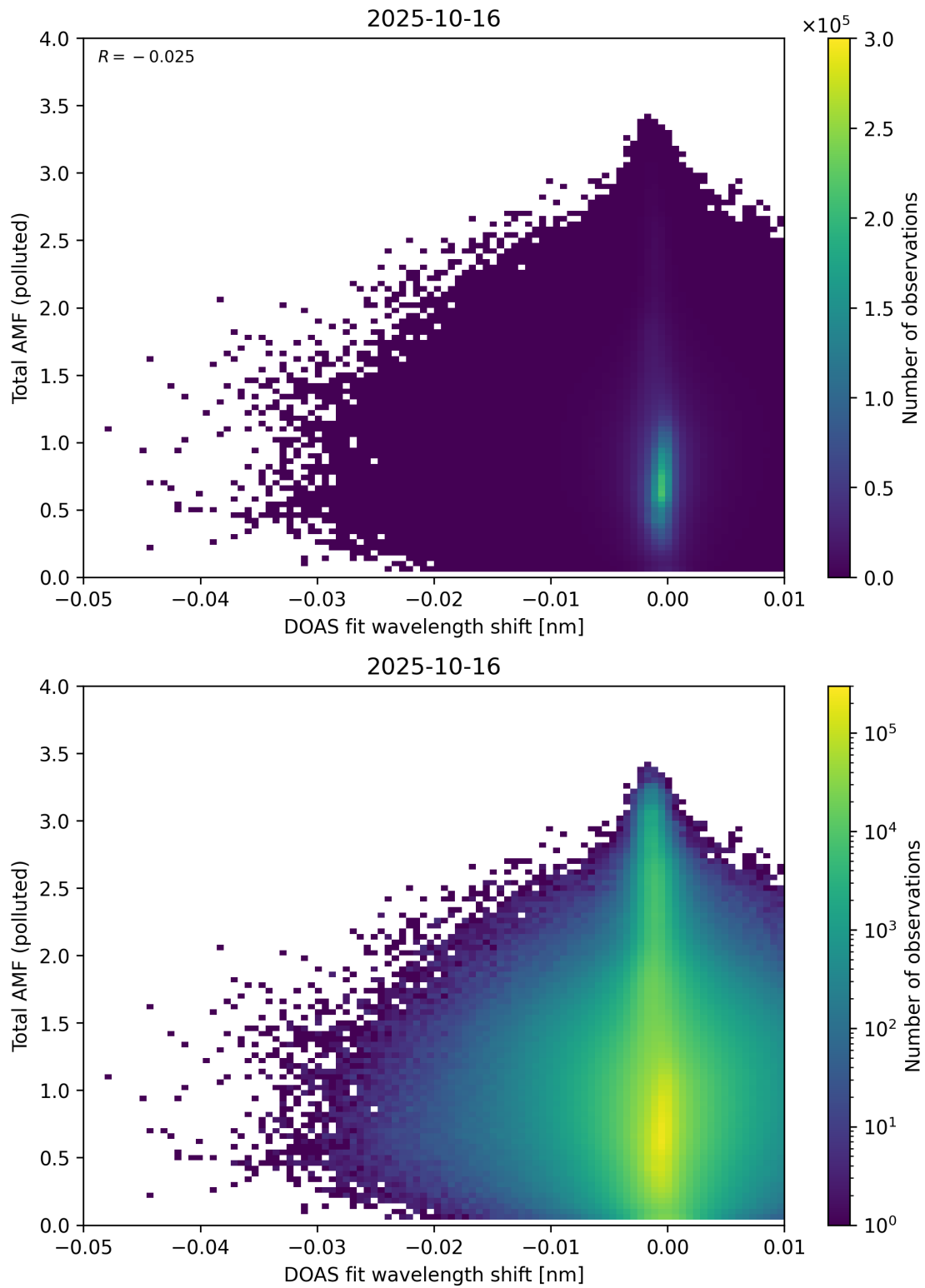
Figure 141: Scatter density plot of “DOAS fit wavelength shift” against “Total AMF (polluted)” for 2025-10-15 to 2025-10-17.
