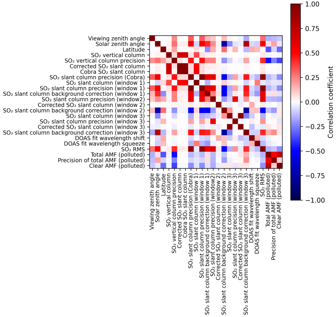
Figure 2: Map of correlation matrix for 2025-10-15 to 2025-10-17.
