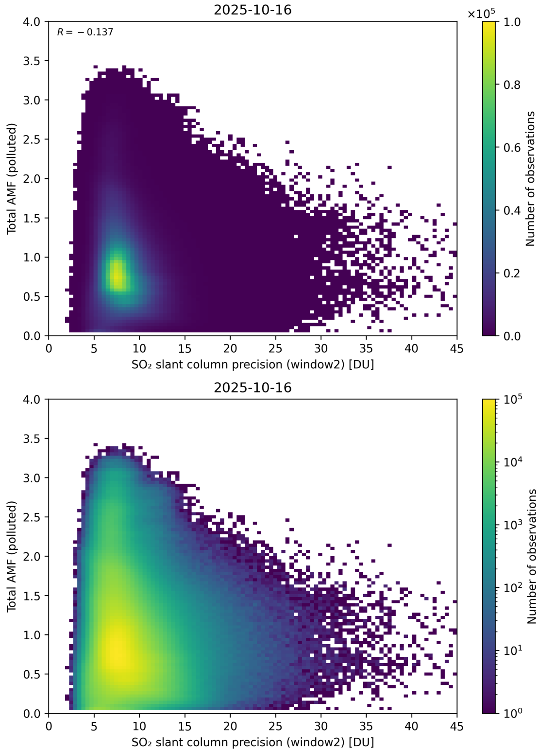
Figure 301: Scatter density plot of “SO 2 slant column precision (window2)” against “Total AMF (polluted)” for 2025-10-15 to 2025-10-17.
