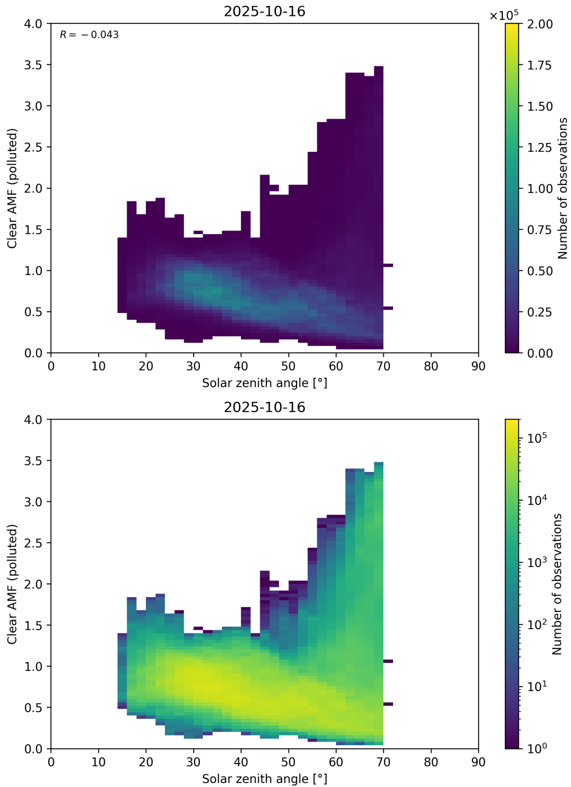
Figure 178: Scatter density plot of “Solar zenith angle” against “Clear AMF (polluted)” for 2025-10-15 to 2025-10-17.
