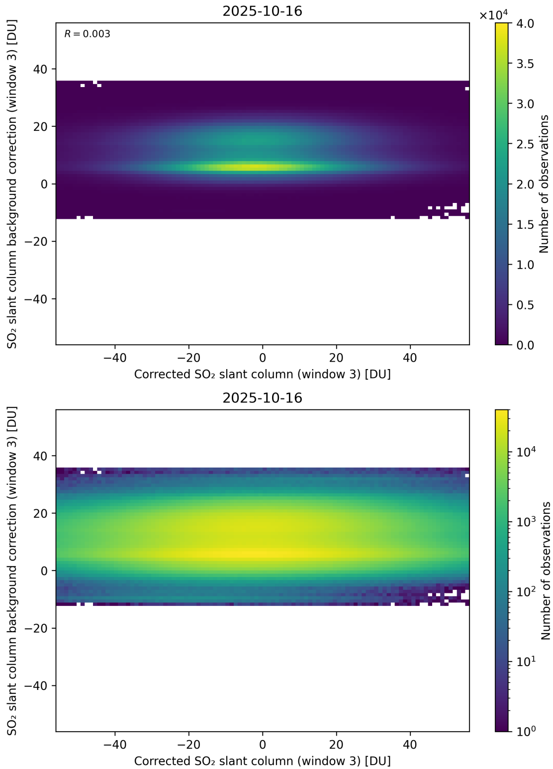
Figure 255: Scatter density plot of “Corrected SO 2 slant column (window 3)” against “SO 2 slant column background correction (window 3)” for 2025-10-15 to 2025-10-17.
