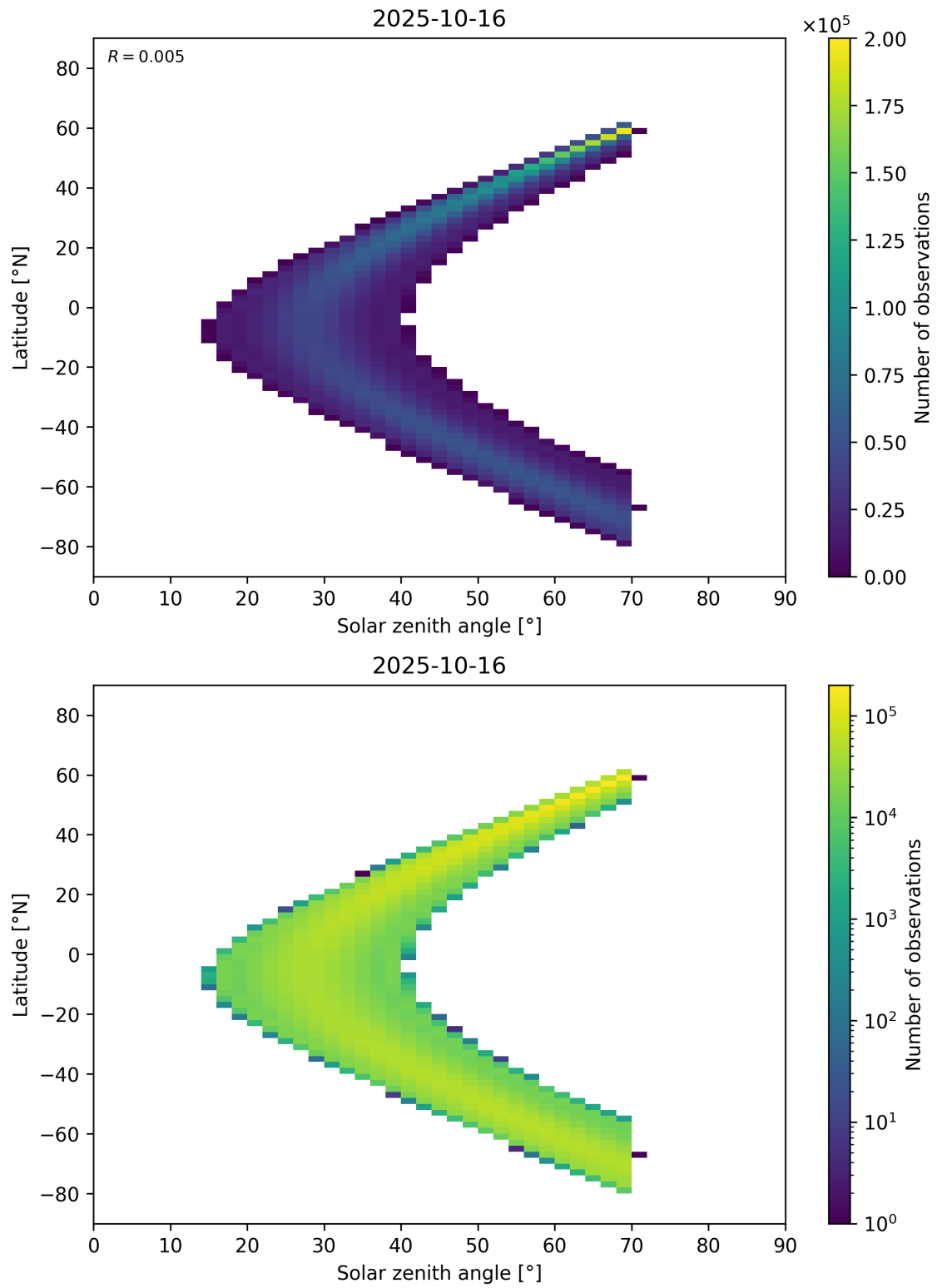
Figure 177: Scatter density plot of “Solar zenith angle” against “Latitude” for 2025-10-15 to 2025-10-17.
