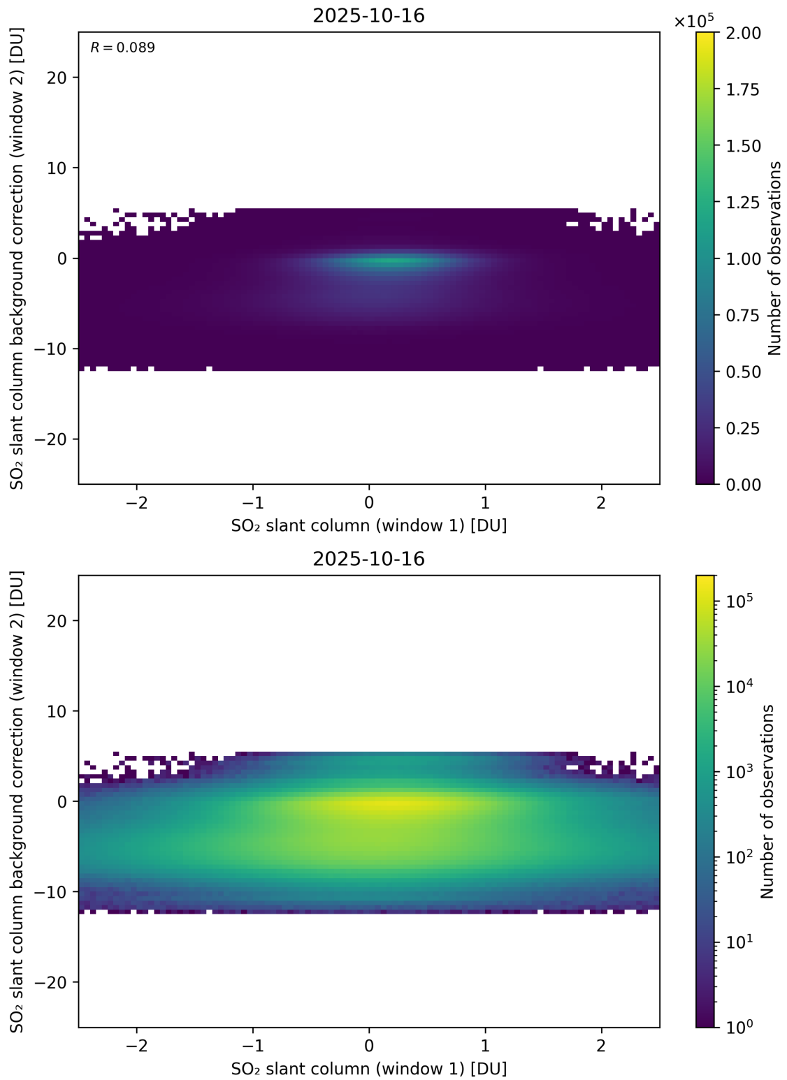
Figure 263: Scatter density plot of “SO 2 slant column (window 1)” against “SO 2 slant column background correction (window 2)” for 2025-10-15 to 2025-10-17.
