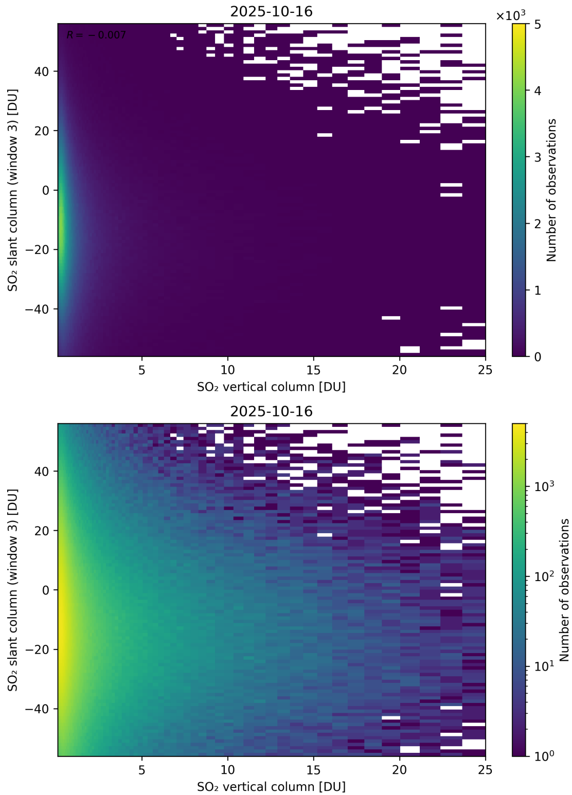
Figure 357: Scatter density plot of “SO 2 vertical column” against “SO 2 slant column (window 3)” for 2025-10-15 to 2025-10-17.
