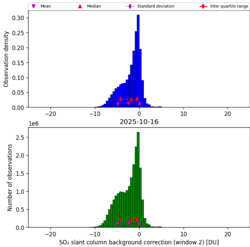
Figure 70: Histogram of “SO 2 slant column background correction (window 2)” for 2025-10-15 to 2025-10-17
