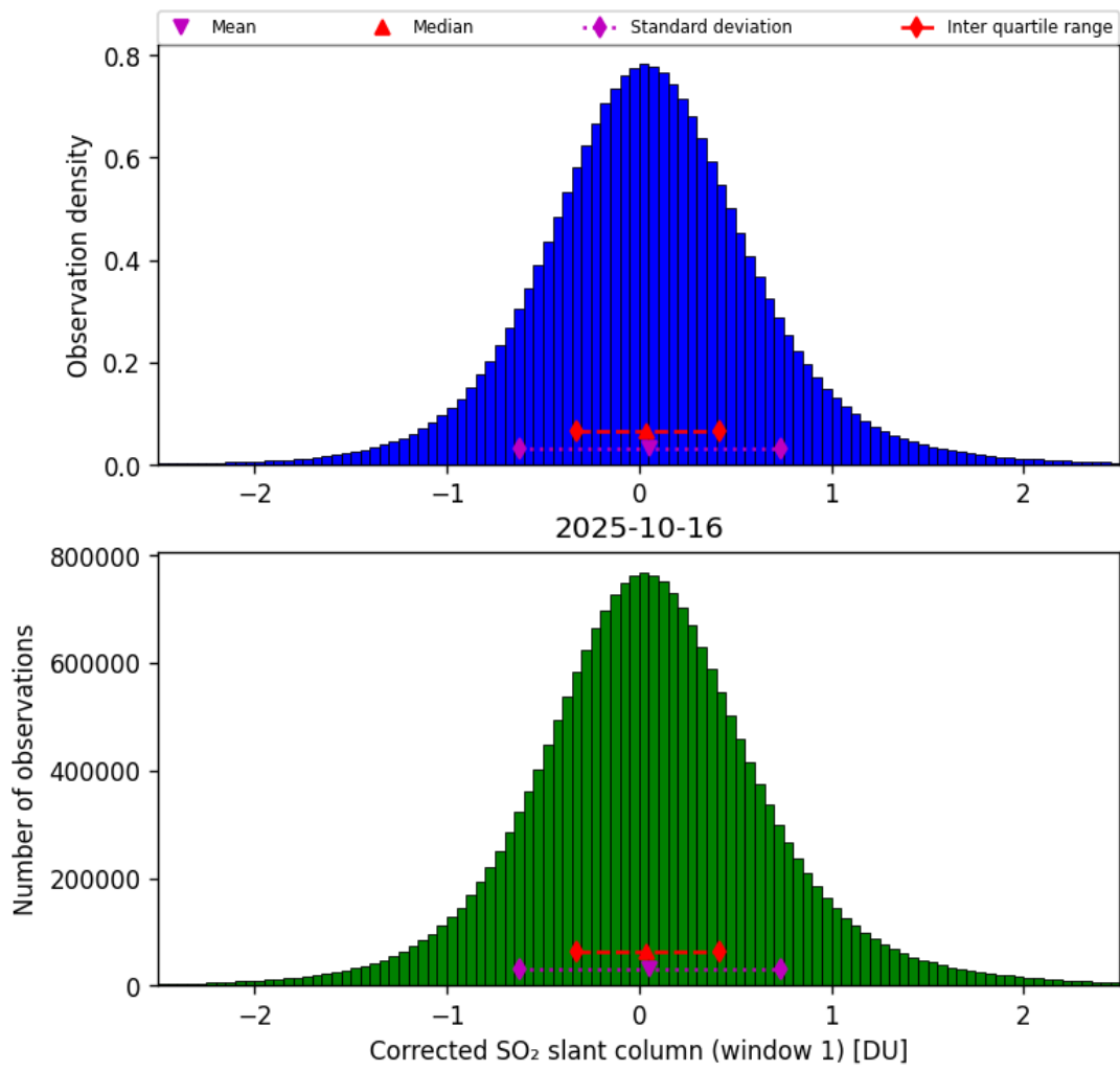
Figure 65: Histogram of “Corrected SO 2 slant column (window 1)” for 2025-10-15 to 2025-10-17
