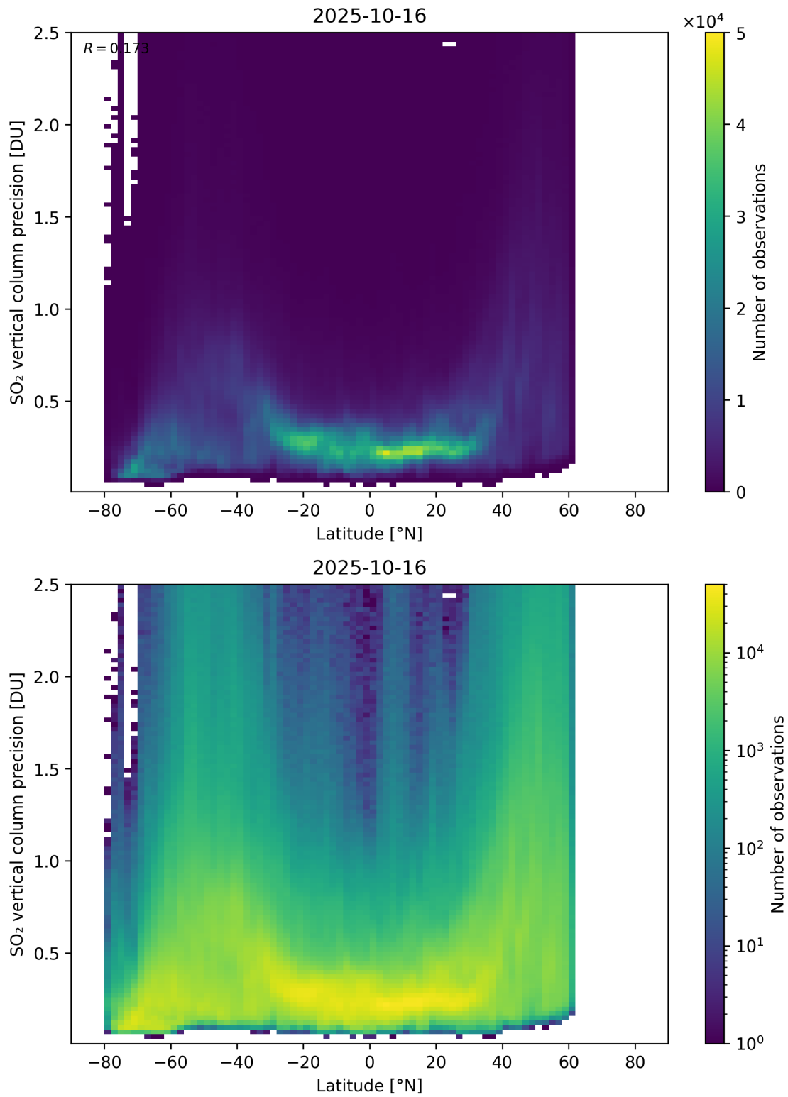
Figure 170: Scatter density plot of “Latitude” against “SO 2 vertical column precision” for 2025-10-15 to 2025-10-17.
