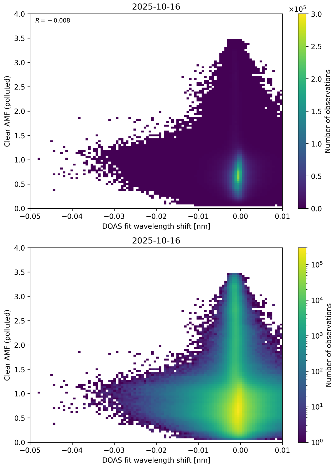
Figure 140: Scatter density plot of “DOAS fit wavelength shift” against “Clear AMF (polluted)” for 2025-10-15 to 2025-10-17.
