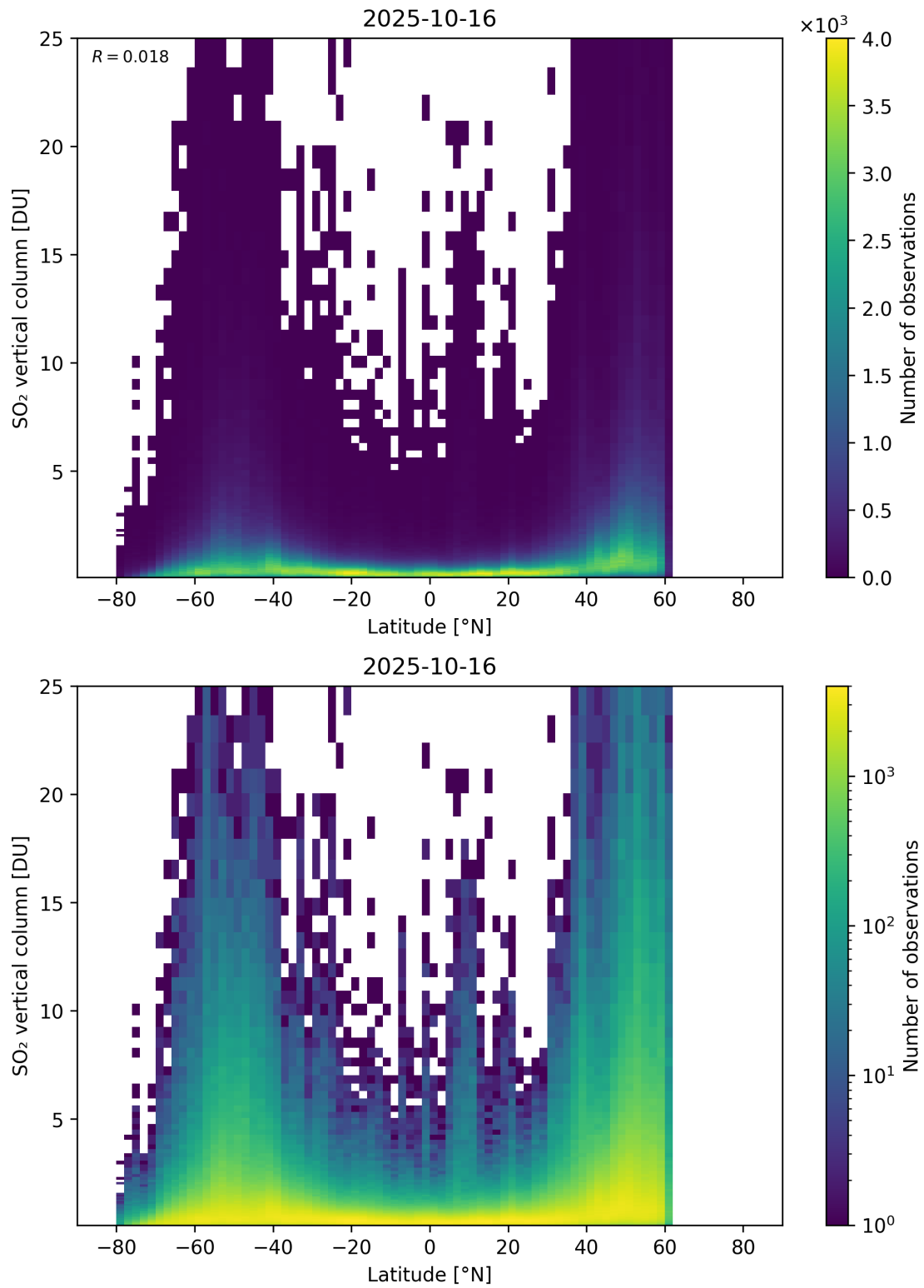
Figure 169: Scatter density plot of “Latitude” against “SO 2 vertical column” for 2025-10-15 to 2025-10-17.
