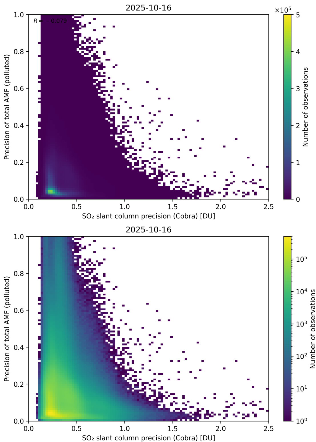
Figure 214: Scatter density plot of “SO 2 slant column precision (Cobra)” against “Precision of total AMF (polluted)” for 2025-10-15 to 2025-10-17.
