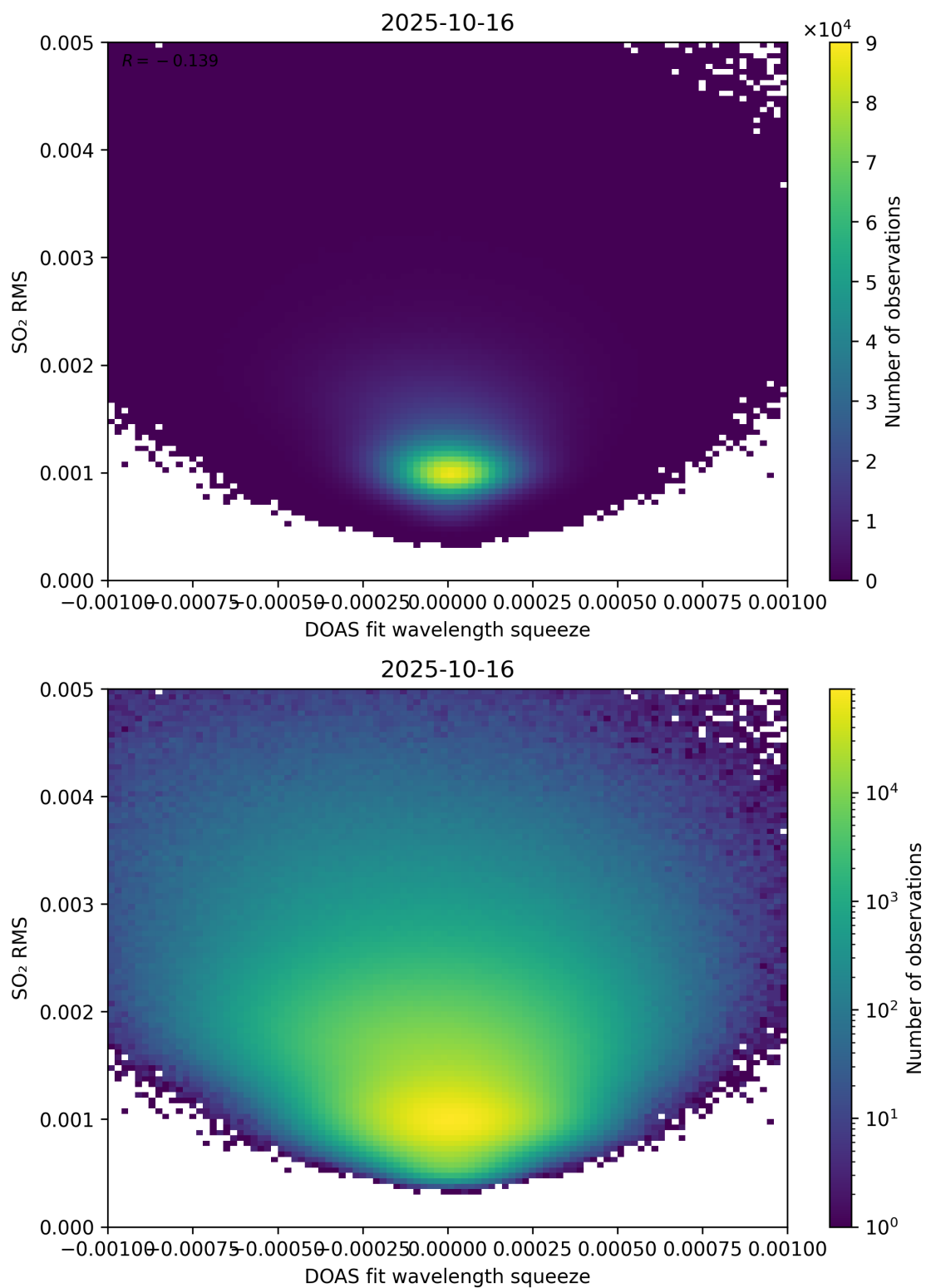
Figure 143: Scatter density plot of “DOAS fit wavelength squeeze” against “SO 2 RMS” for 2025-10-15 to 2025-10-17.
