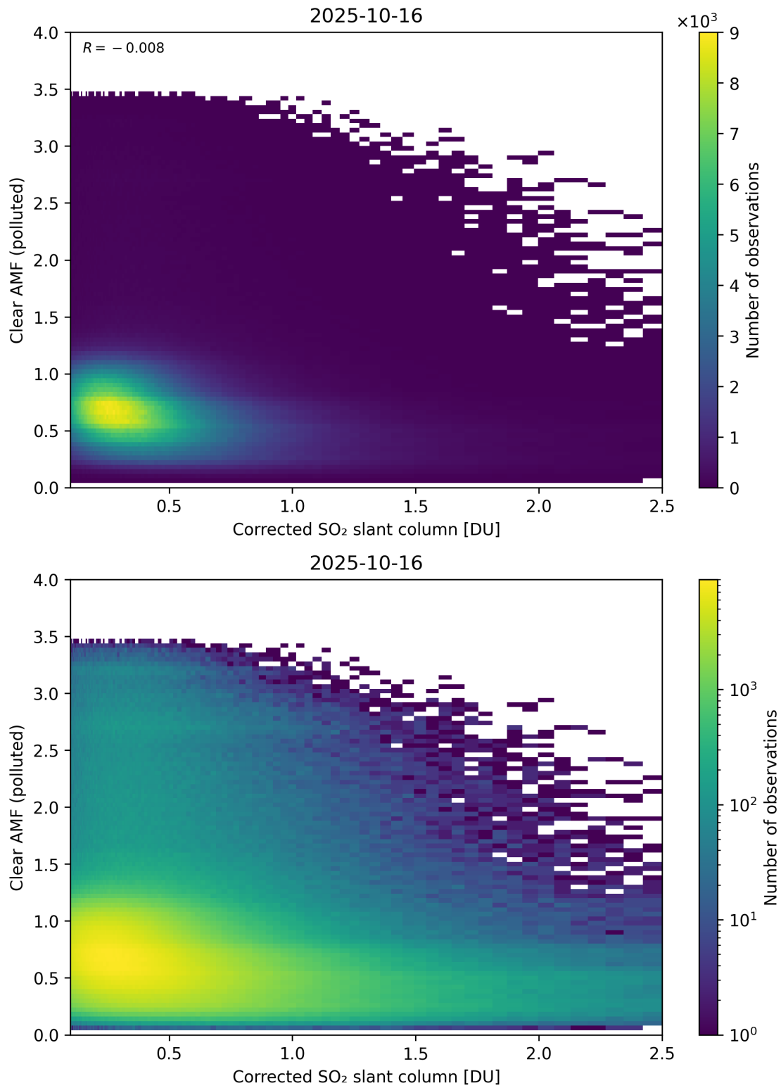
Figure 232: Scatter density plot of “Corrected SO 2 slant column” against “Clear AMF (polluted)” for 2025-10-15 to 2025-10-17.
