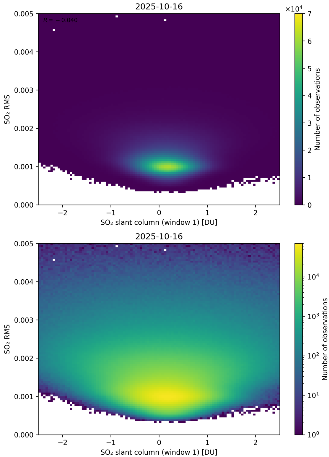
Figure 267: Scatter density plot of “SO 2 slant column (window 1)” against “SO 2 RMS” for 2025-10-15 to 2025-10-17.
