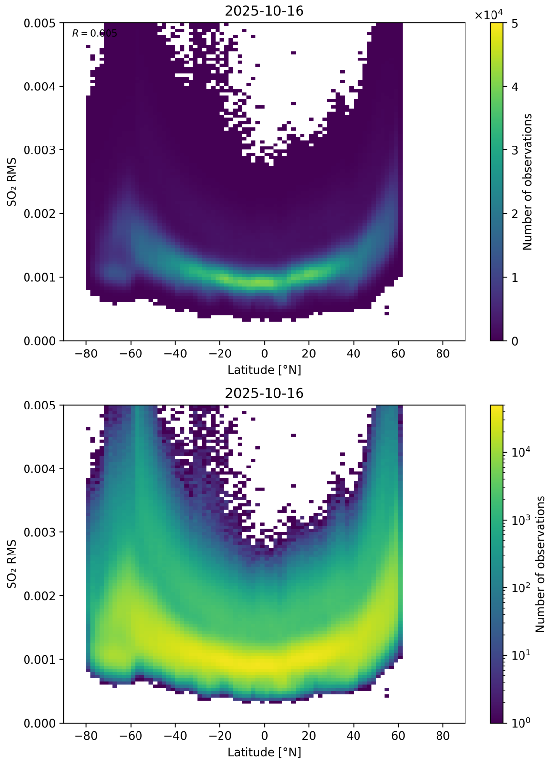
Figure 155: Scatter density plot of “Latitude” against “SO 2 RMS” for 2025-10-15 to 2025-10-17.
