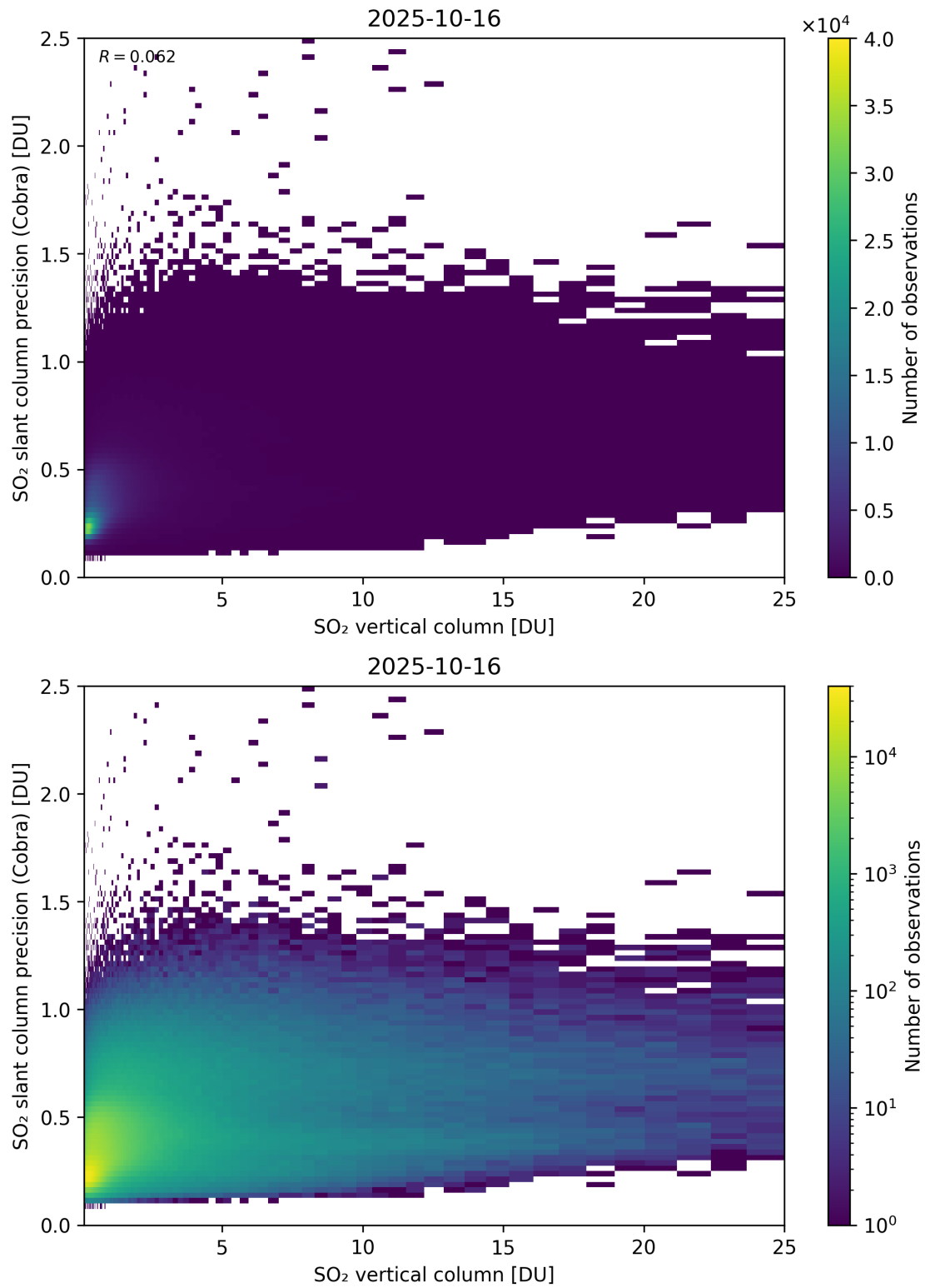
Figure 350: Scatter density plot of “SO 2 vertical column” against “SO 2 slant column precision (Cobra)” for 2025-10-15 to 2025-10-17.
