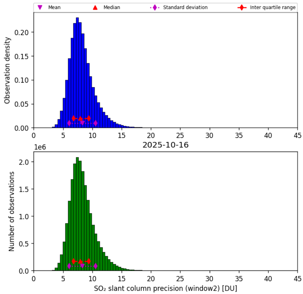
Figure 68: Histogram of “SO 2 slant column precision (window2)” for 2025-10-15 to 2025-10-17
