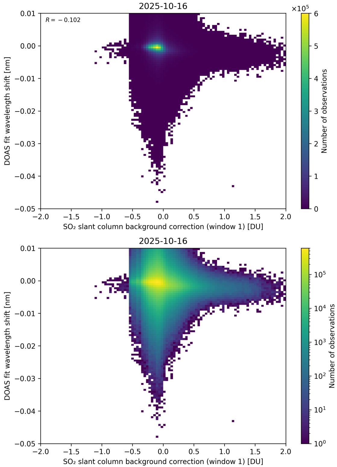
Figure 111: Scatter density plot of “SO 2 slant column background correction (window 1)” against “DOAS fit wavelength shift” for 2025-10-15 to 2025-10-17.
