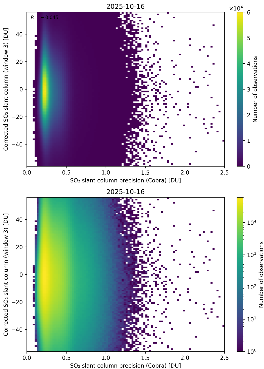
Figure 207: Scatter density plot of “SO 2 slant column precision (Cobra)” against “Corrected SO 2 slant column (window 3)” for 2025-10-15 to 2025-10-17.
