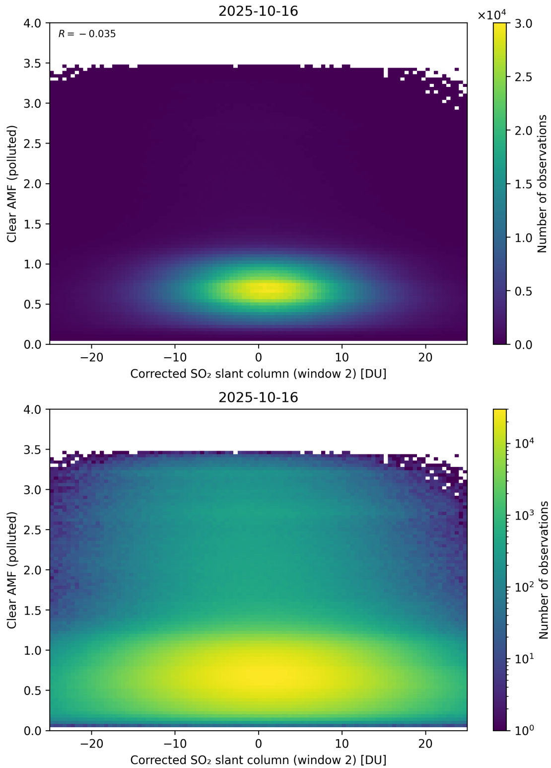
Figure 249: Scatter density plot of “Corrected SO 2 slant column (window 2)” against “Clear AMF (polluted)” for 2025-10-15 to 2025-10-17.
