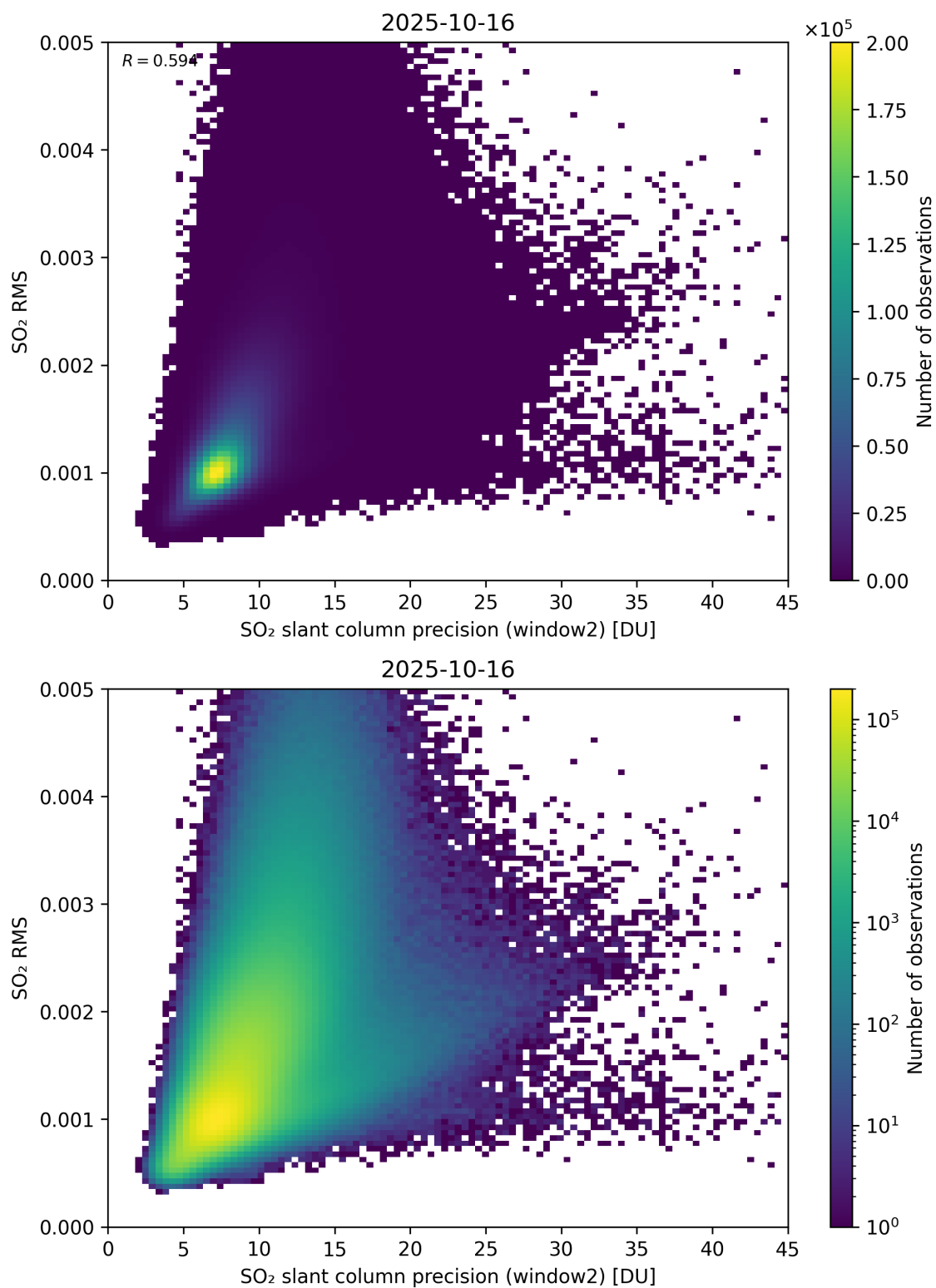
Figure 295: Scatter density plot of “SO 2 slant column precision (window2)” against “SO 2 RMS” for 2025-10-15 to 2025-10-17.
