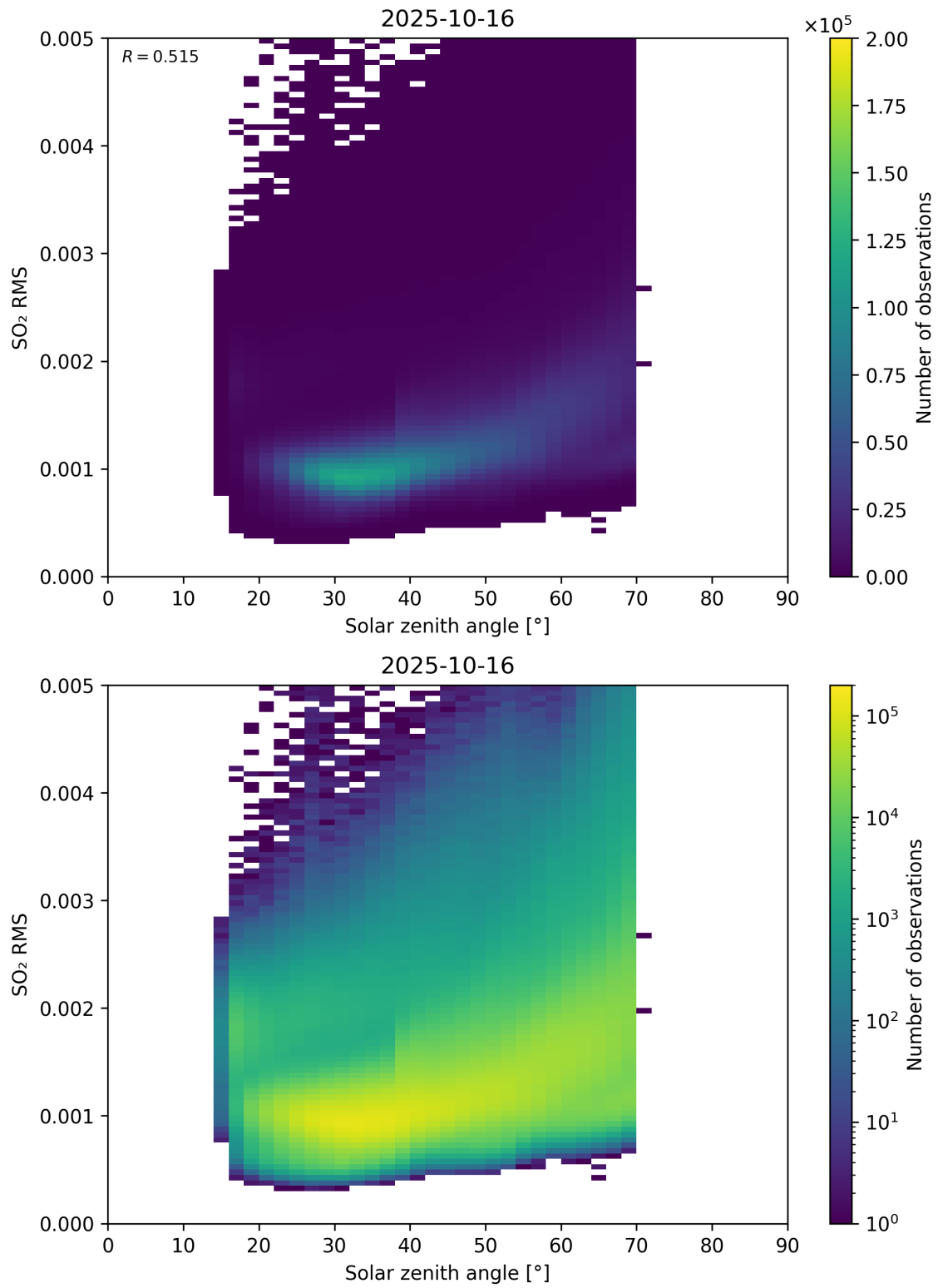
Figure 176: Scatter density plot of “Solar zenith angle” against “SO 2 RMS” for 2025-10-15 to 2025-10-17.
