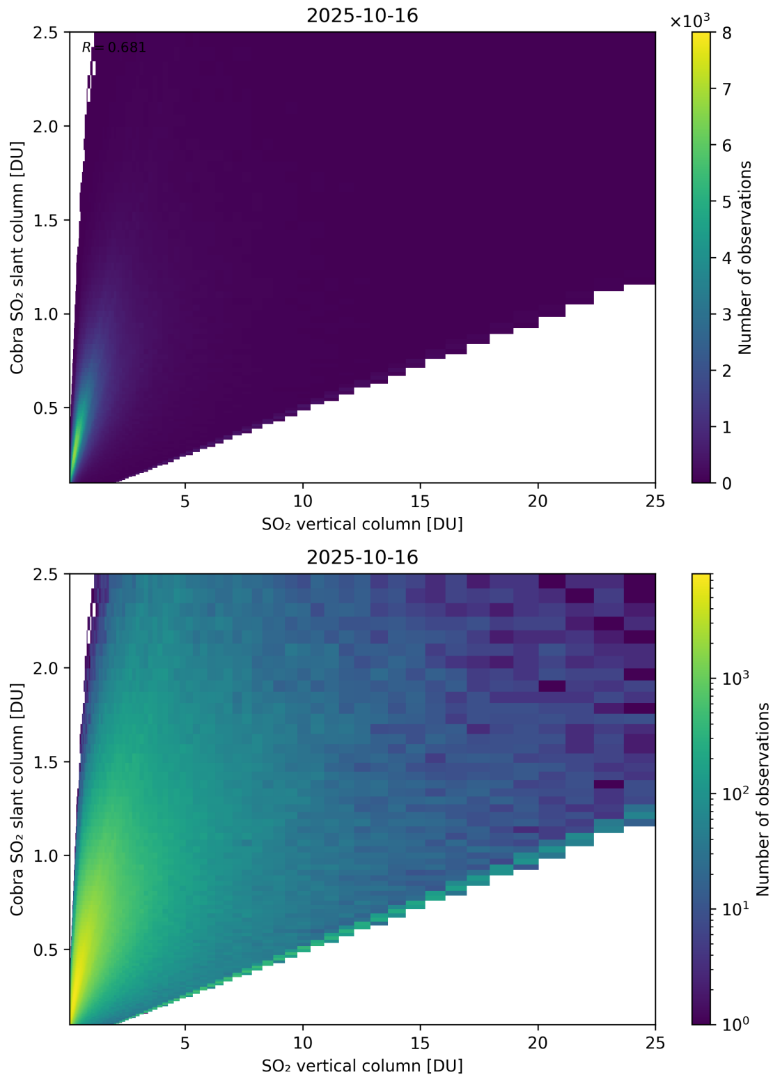
Figure 349: Scatter density plot of “SO 2 vertical column” against “Cobra SO 2 slant column” for 2025-10-15 to 2025-10-17.
