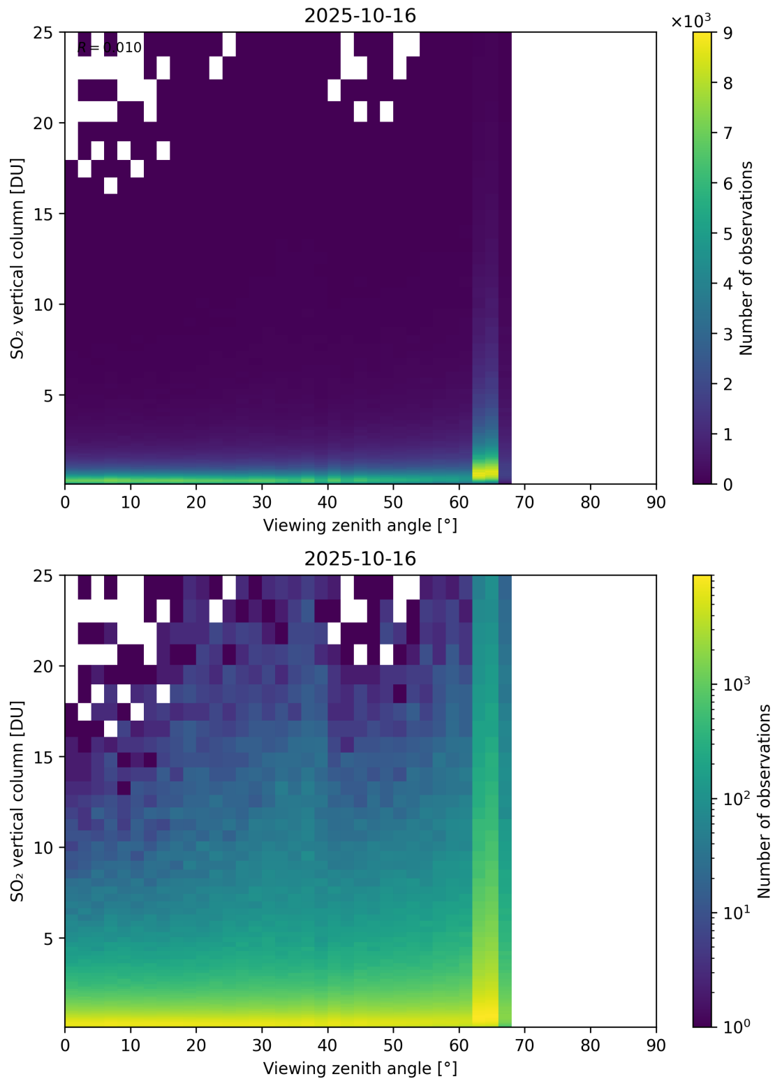
Figure 383: Scatter density plot of “Viewing zenith angle” against “SO 2 vertical column” for 2025-10-15 to 2025-10-17.
