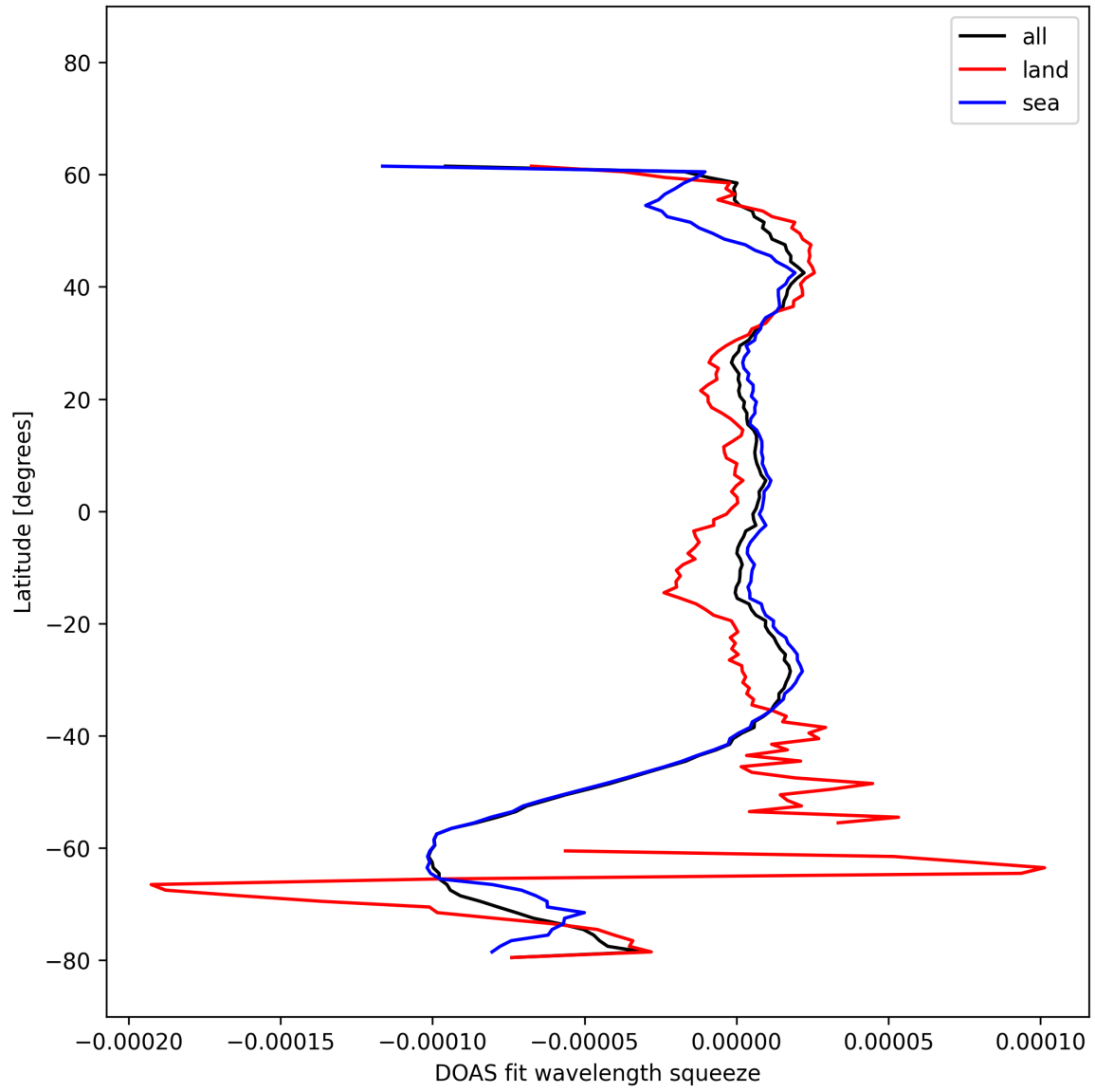
Figure 51: Zonal average of “DOAS fit wavelength squeeze” for 2025-10-15 to 2025-10-17.
