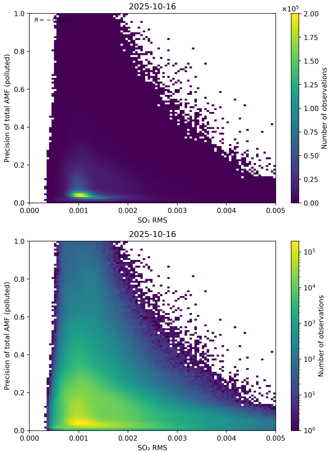
Figure 149: Scatter density plot of “SO 2 RMS” against “Precision of total AMF (polluted)” for 2025-10-15 to 2025-10-17.
