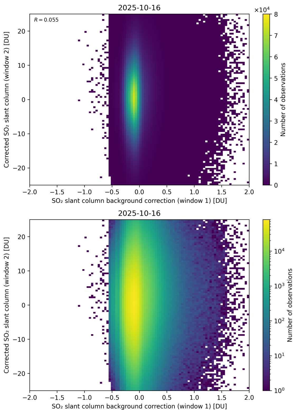
Figure 115: Scatter density plot of “SO 2 slant column background correction (window 1)” against “Corrected SO 2 slant column (window 2)” for 2025-10-15 to 2025-10-17.
