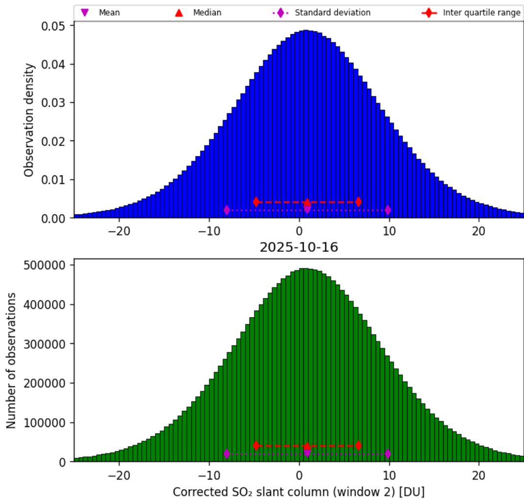
Figure 69: Histogram of “Corrected SO 2 slant column (window 2)” for 2025-10-15 to 2025-10-17
