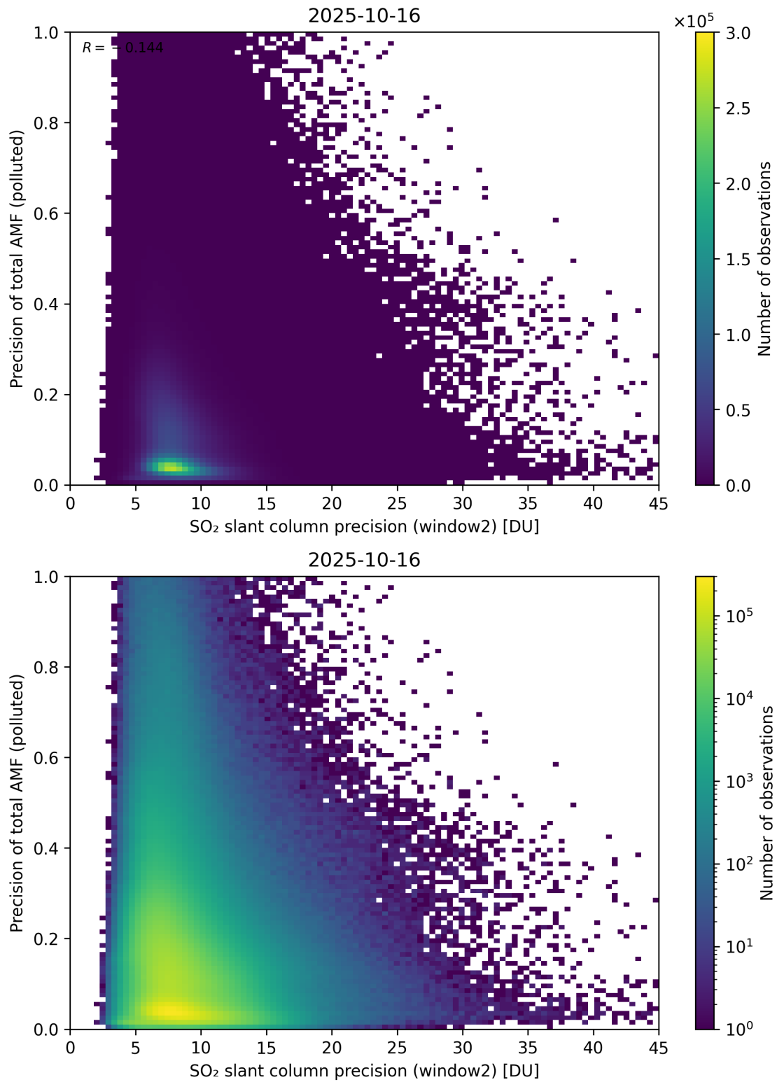
Figure 302: Scatter density plot of “SO 2 slant column precision (window2)” against “Precision of total AMF (polluted)” for 2025-10-15 to 2025-10-17.
