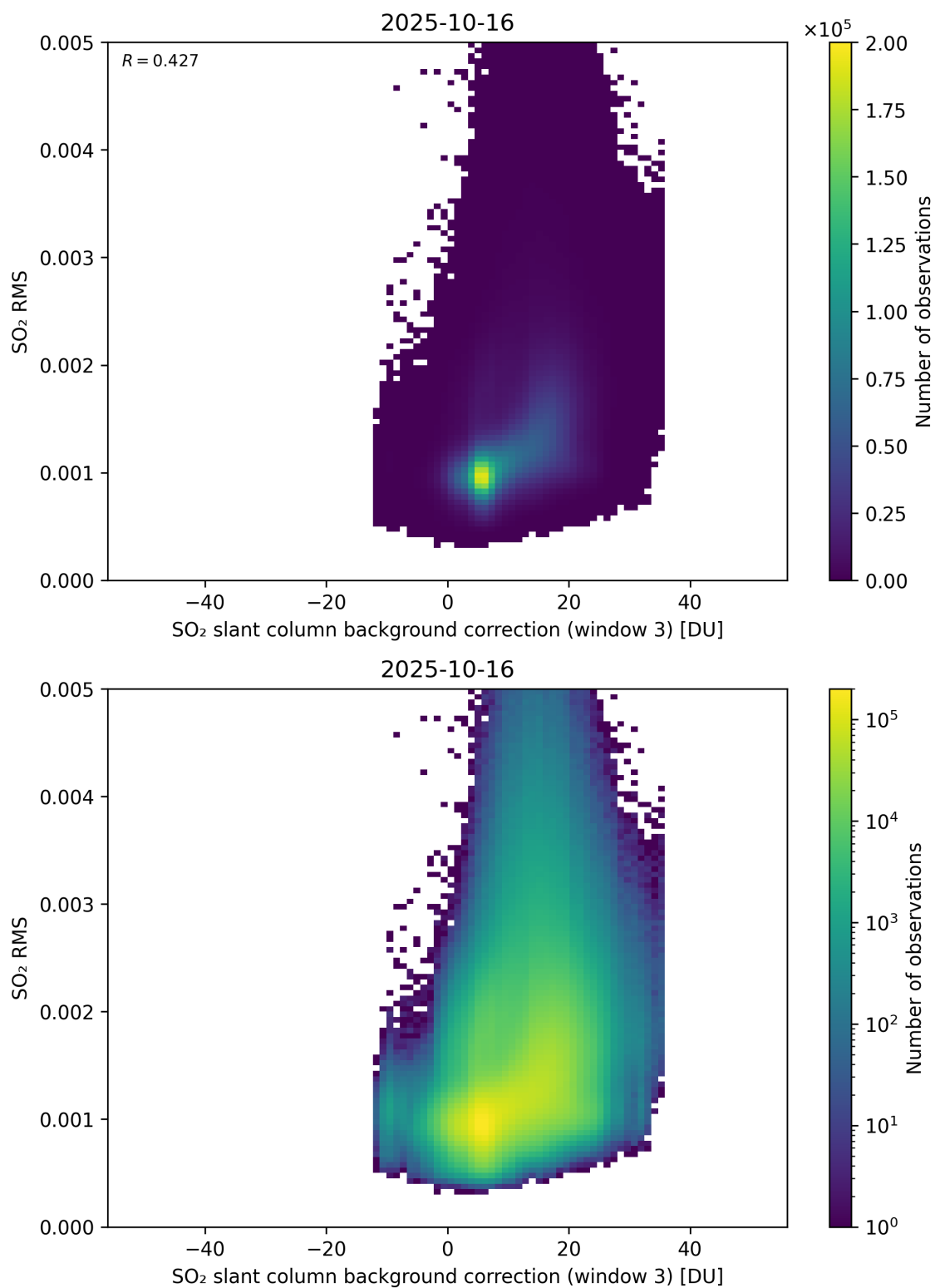
Figure 134: Scatter density plot of “SO 2 slant column background correction (window 3)” against “SO 2 RMS” for 2025-10-15 to 2025-10-17.
