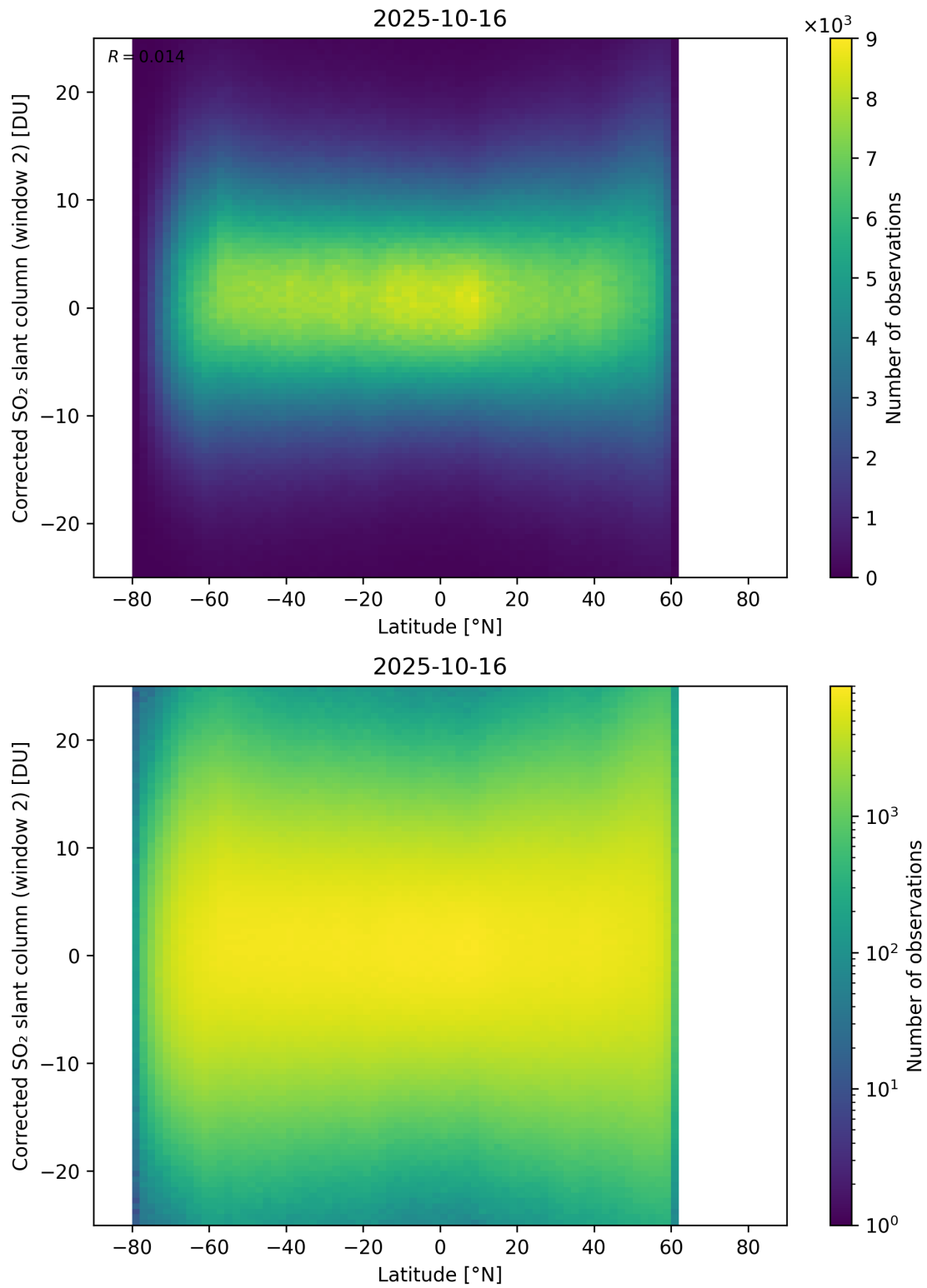
Figure 160: Scatter density plot of “Latitude” against “Corrected SO 2 slant column (window 2)” for 2025-10-15 to 2025-10-17.
