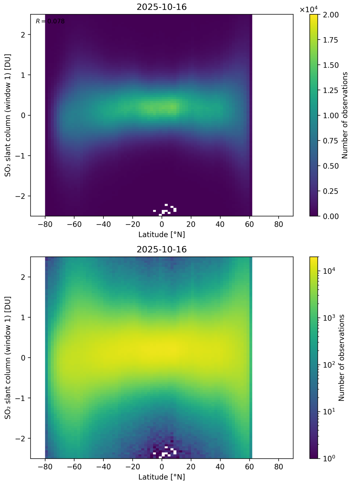
Figure 162: Scatter density plot of “Latitude” against “SO 2 slant column (window 1)” for 2025-10-15 to 2025-10-17.
