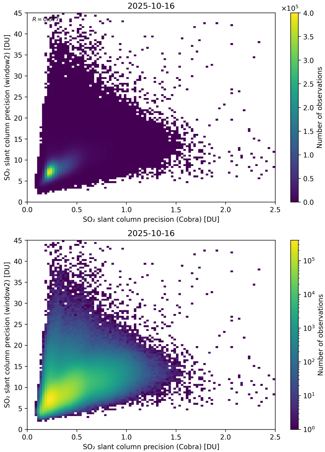
Figure 210: Scatter density plot of “SO 2 slant column precision (Cobra)” against “SO 2 slant column precision (window2)” for 2025-10-15 to 2025-10-17.
