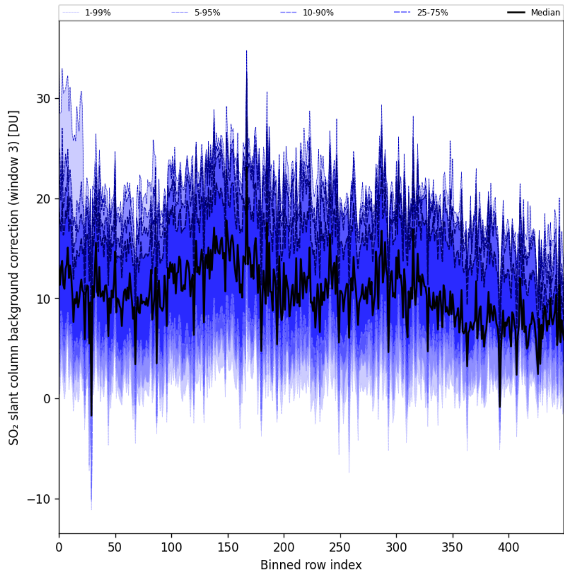
Figure 100: Along track statistics of “SO 2 slant column background correction (window 3)” for 2025-10-15 to 2025-10-17
