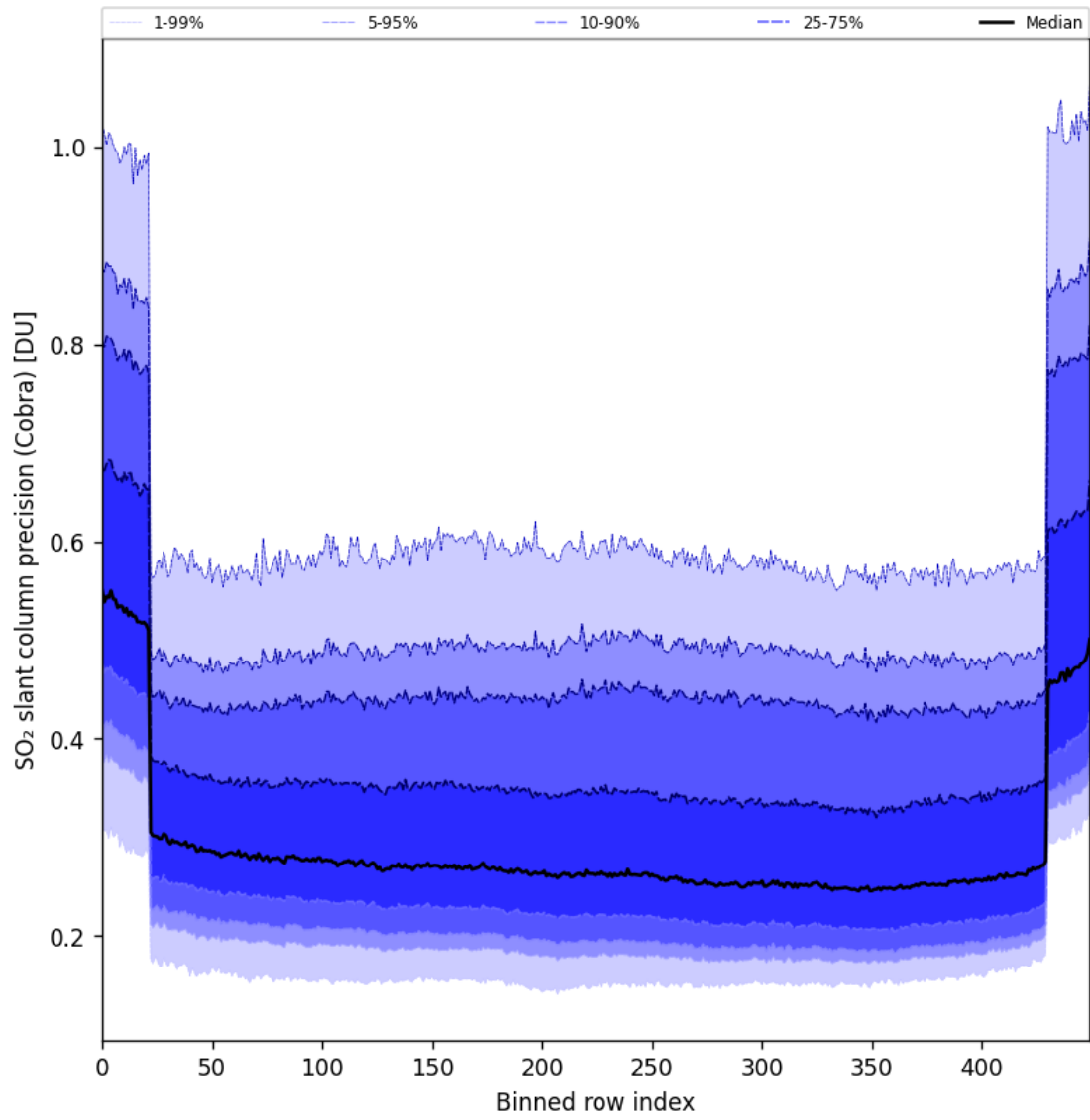
Figure 88: Along track statistics of “SO 2 slant column precision (Cobra)” for 2025-10-15 to 2025-10-17
