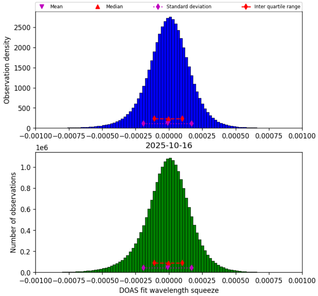
Figure 77: Histogram of “DOAS fit wavelength squeeze” for 2025-10-15 to 2025-10-17
