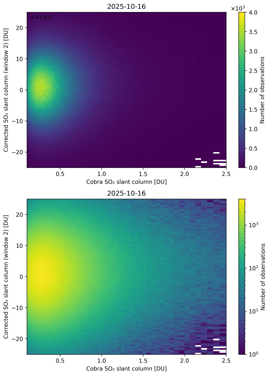
Figure 217: Scatter density plot of “Cobra SO 2 slant column” against “Corrected SO 2 slant column (window 2)” for 2025-10-15 to 2025-10-17.
