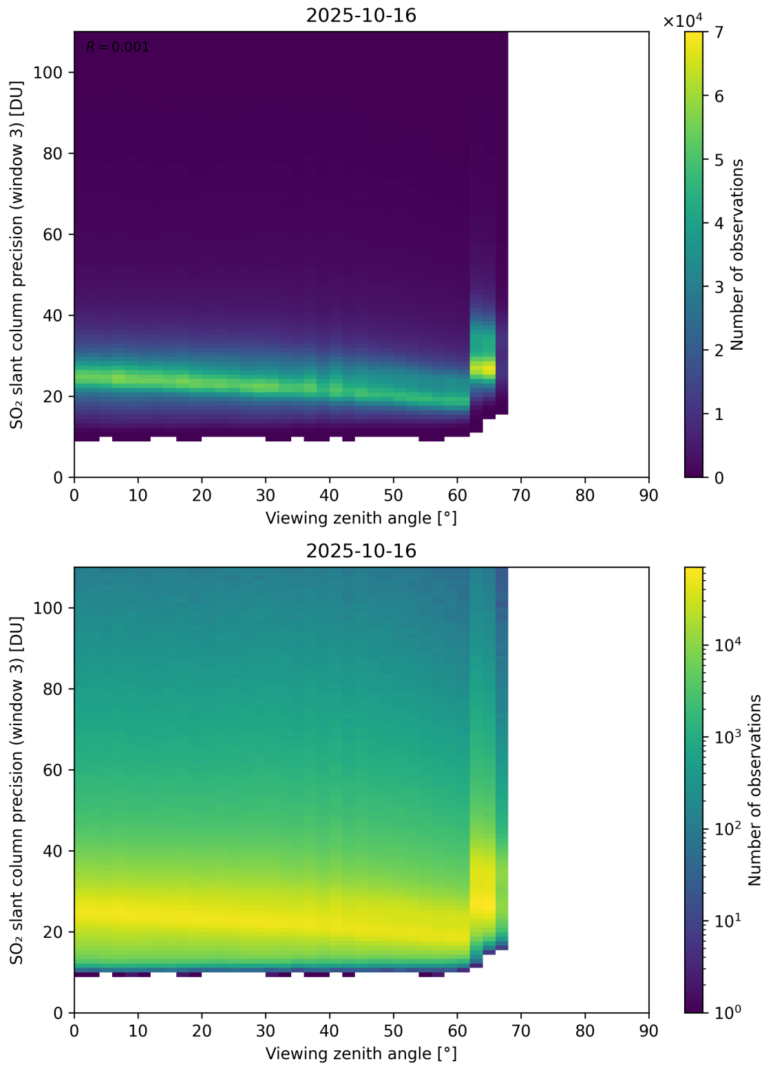
Figure 380: Scatter density plot of “Viewing zenith angle” against “SO 2 slant column precision (window 3)” for 2025-10-15 to 2025-10-17.
