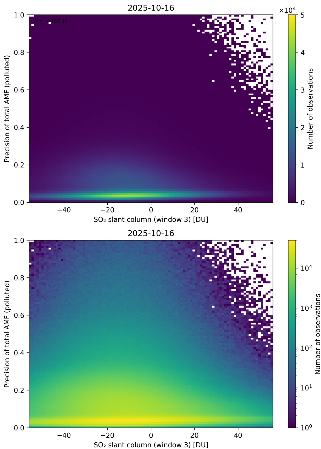
Figure 319: Scatter density plot of “SO 2 slant column (window 3)” against “Precision of total AMF (polluted)” for 2025-10-15 to 2025-10-17.
