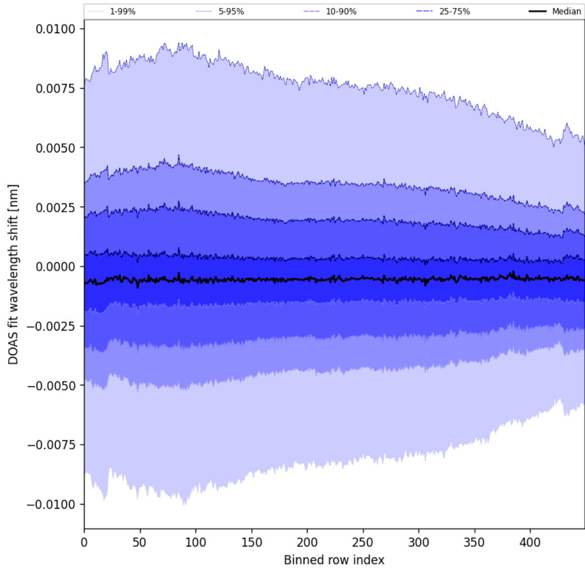
Figure 102: Along track statistics of “DOAS fit wavelength shift” for 2025-10-15 to 2025-10-17
