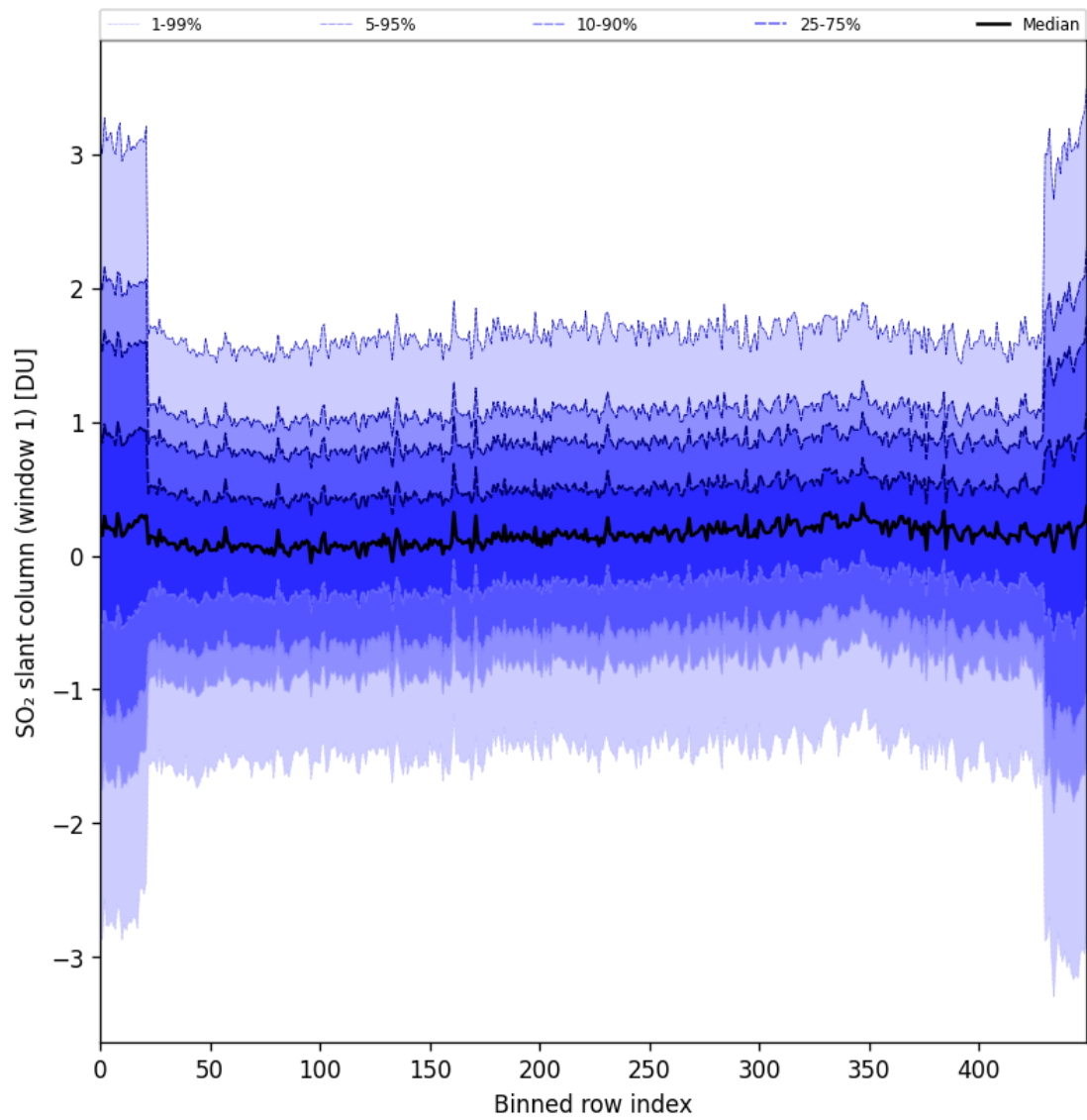
Figure 89: Along track statistics of “SO 2 slant column (window 1)” for 2025-10-15 to 2025-10-17
