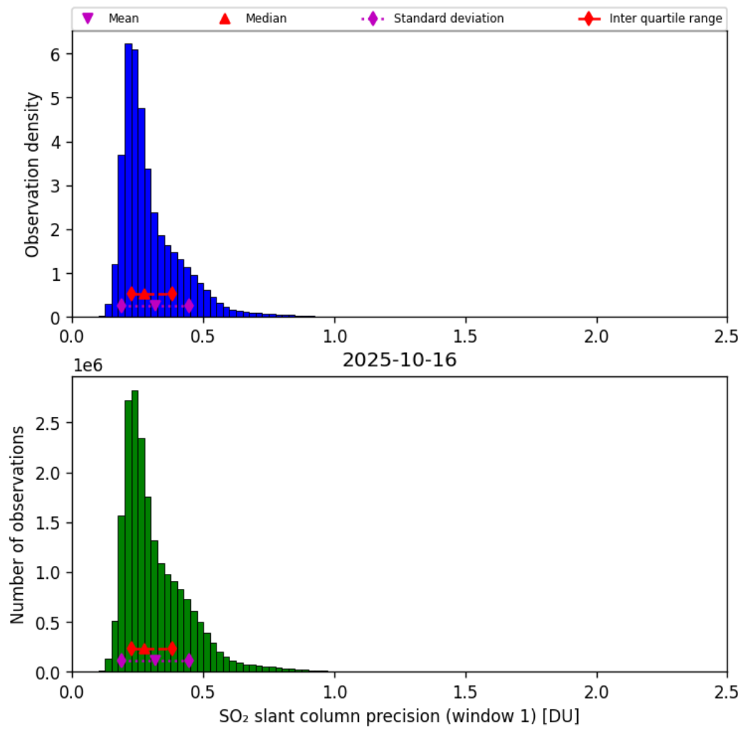
Figure 64: Histogram of “SO 2 slant column precision (window 1)” for 2025-10-15 to 2025-10-17
