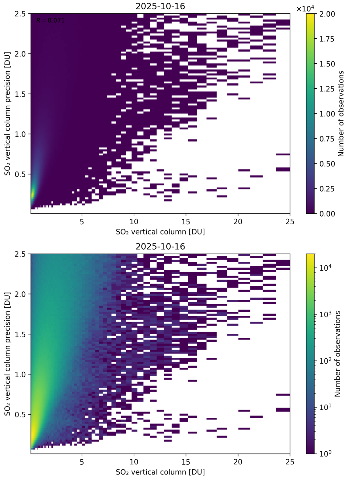
Figure 361: Scatter density plot of “SO 2 vertical column” against “SO 2 vertical column precision” for 2025-10-15 to 2025-10-17.
