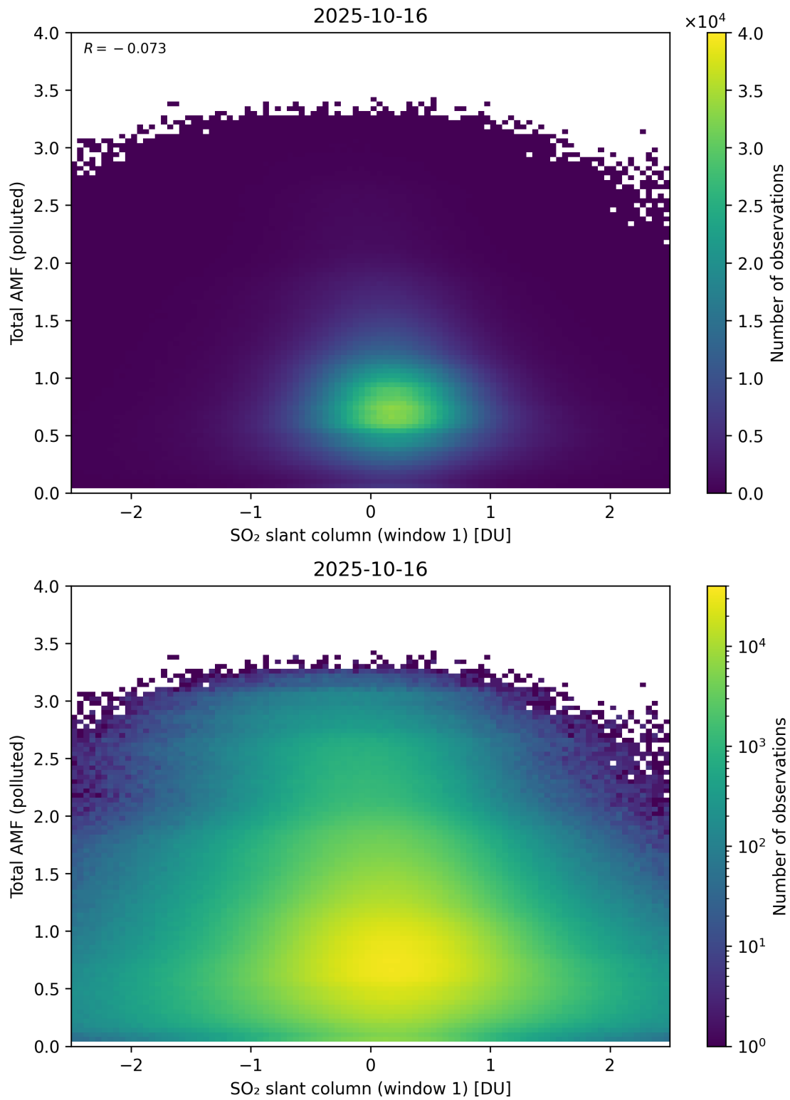
Figure 289: Scatter density plot of “SO 2 slant column (window 1)” against “Total AMF (polluted)” for 2025-10-15 to 2025-10-17.
