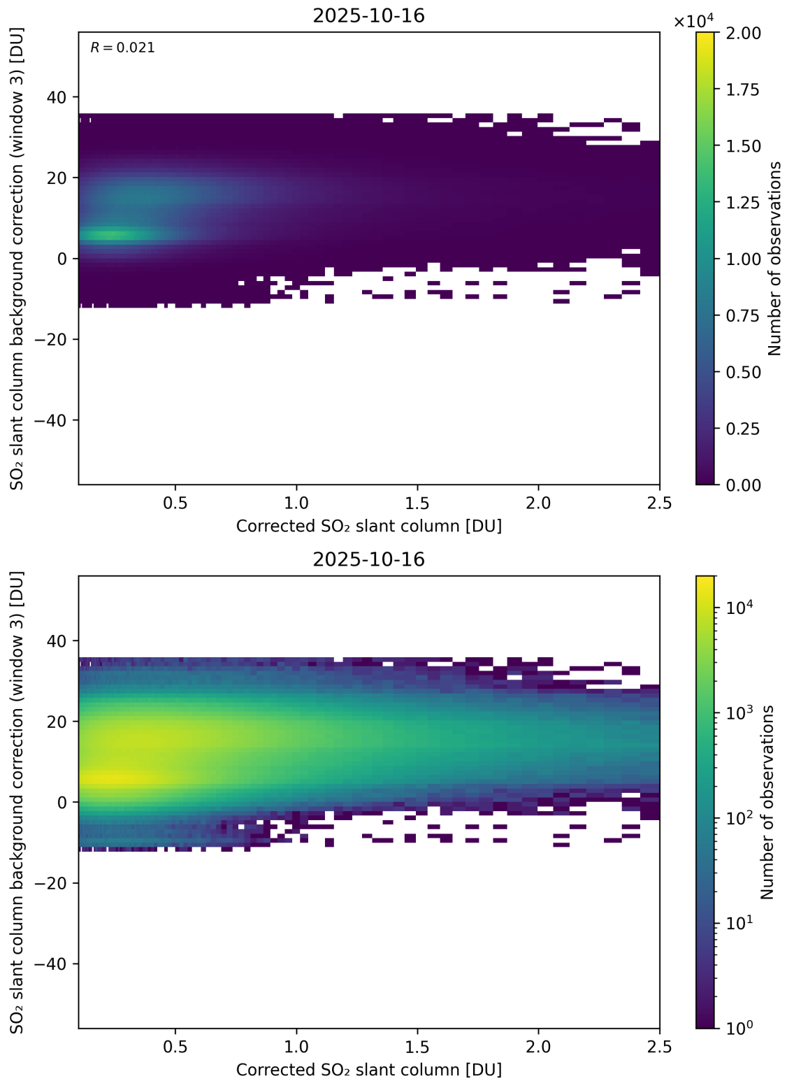
Figure 228: Scatter density plot of “Corrected SO 2 slant column” against “SO 2 slant column background correction (window 3)” for 2025-10-15 to 2025-10-17.
