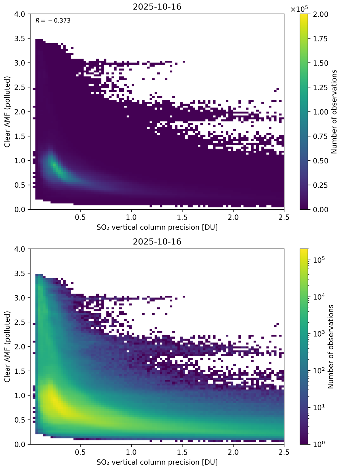
Figure 335: Scatter density plot of “SO 2 vertical column precision” against “Clear AMF (polluted)” for 2025-10-15 to 2025-10-17.
