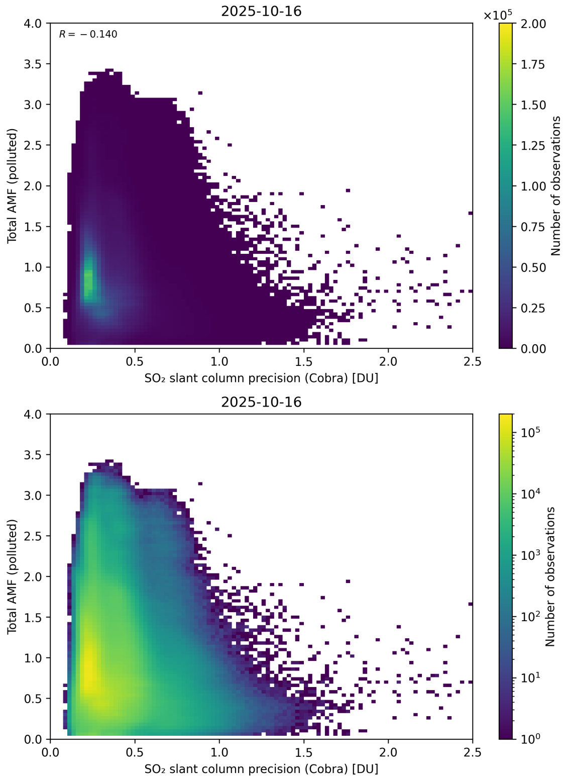
Figure 213: Scatter density plot of “SO 2 slant column precision (Cobra)” against “Total AMF (polluted)” for 2025-10-15 to 2025-10-17.
