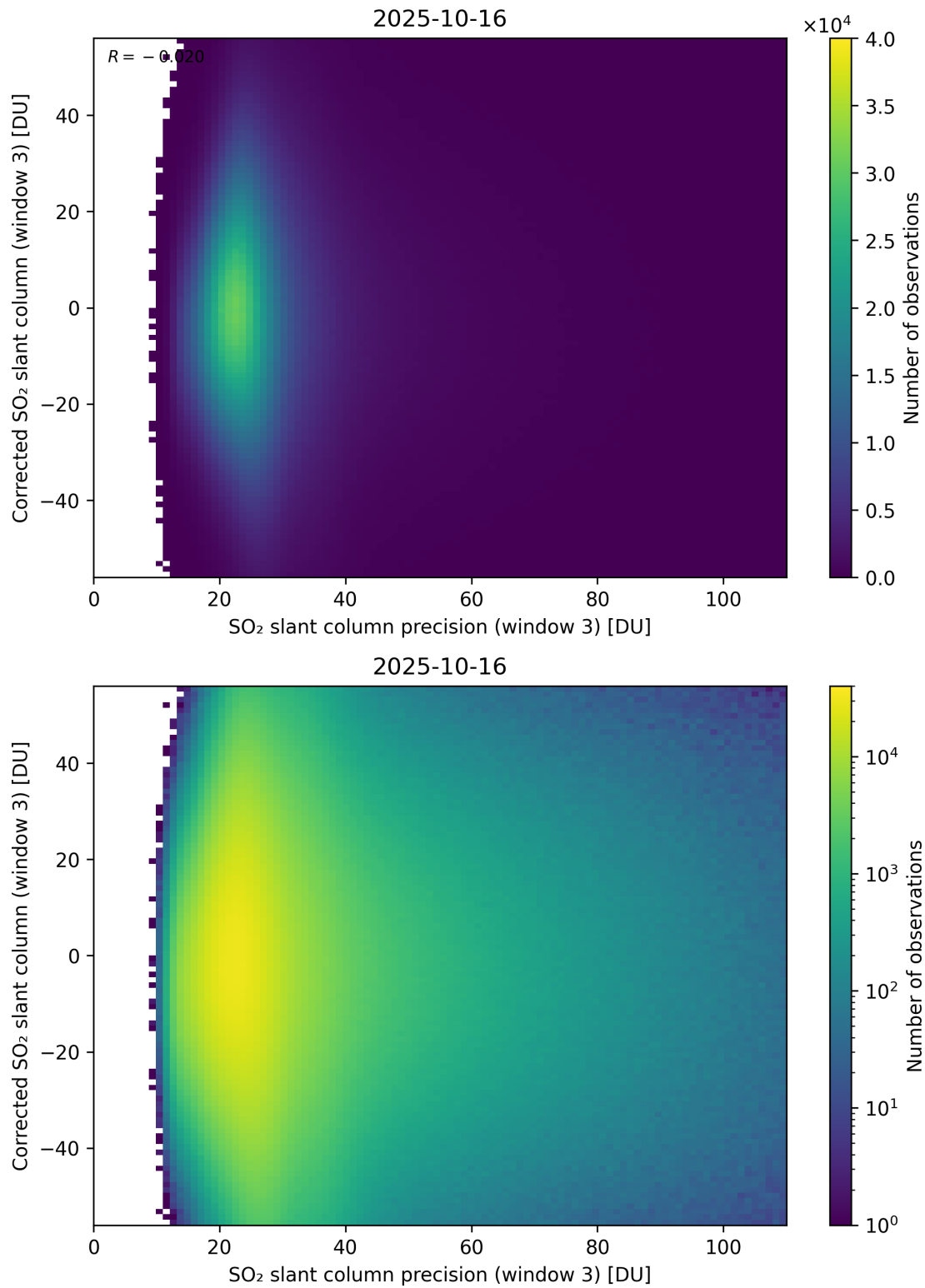
Figure 312: Scatter density plot of “SO 2 slant column precision (window 3)” against “Corrected SO 2 slant column (window 3)” for 2025-10-15 to 2025-10-17.
