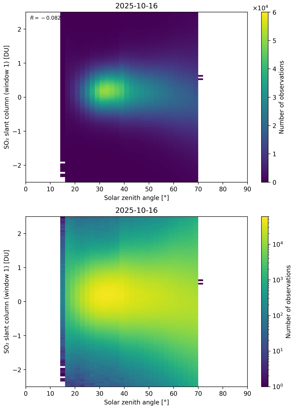
Figure 184: Scatter density plot of “Solar zenith angle” against “SO 2 slant column (window 1)” for 2025-10-15 to 2025-10-17.
