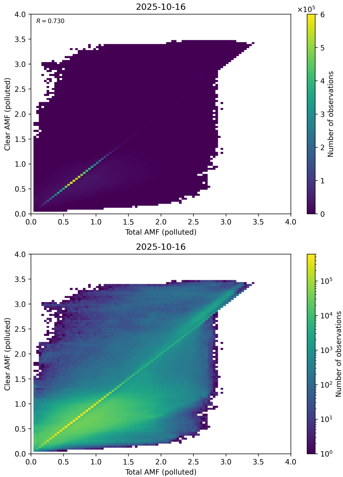
Figure 321: Scatter density plot of “Total AMF (polluted)” against “Clear AMF (polluted)” for 2025-10-15 to 2025-10-17.
