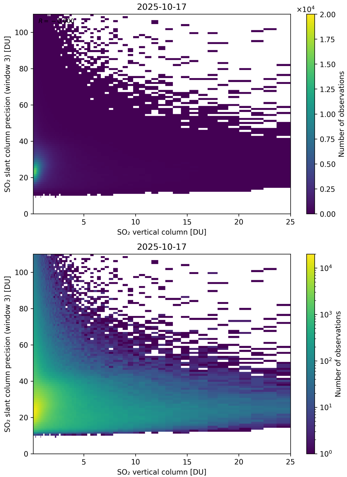
Figure 358: Scatter density plot of “SO 2 vertical column” against “SO 2 slant column precision (window 3)” for 2025-10-17 to 2025-10-18.
