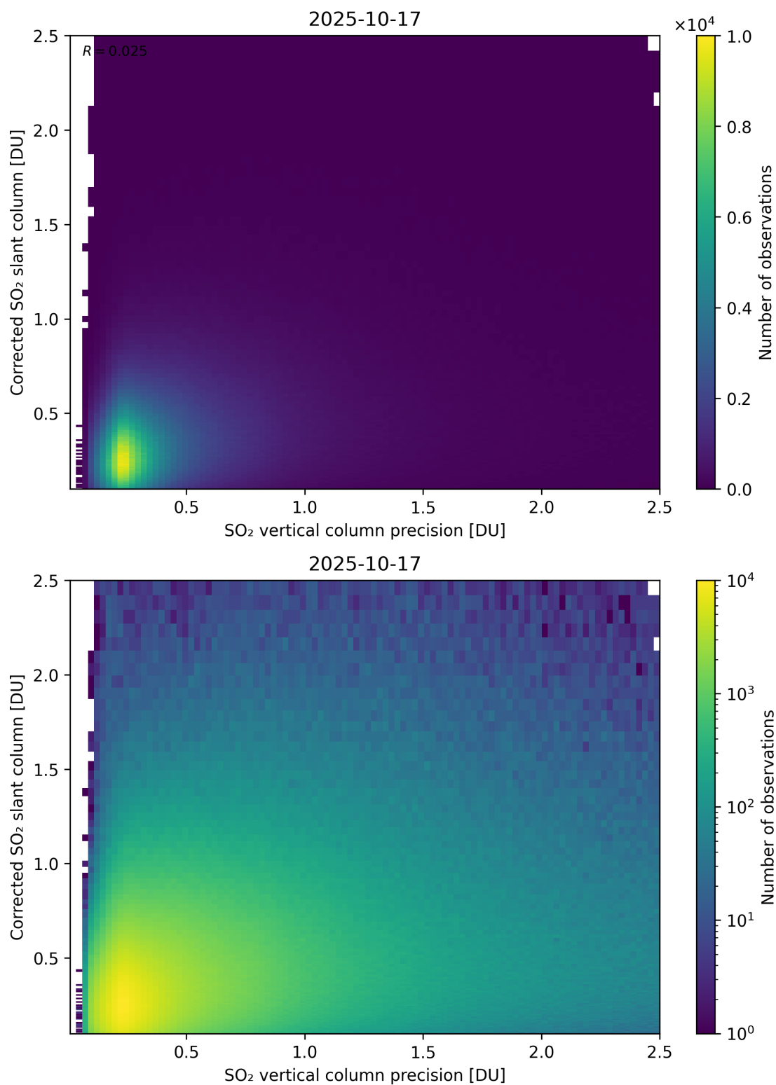
Figure 338: Scatter density plot of “SO 2 vertical column precision” against “Corrected SO 2 slant column” for 2025-10-17 to 2025-10-18.
