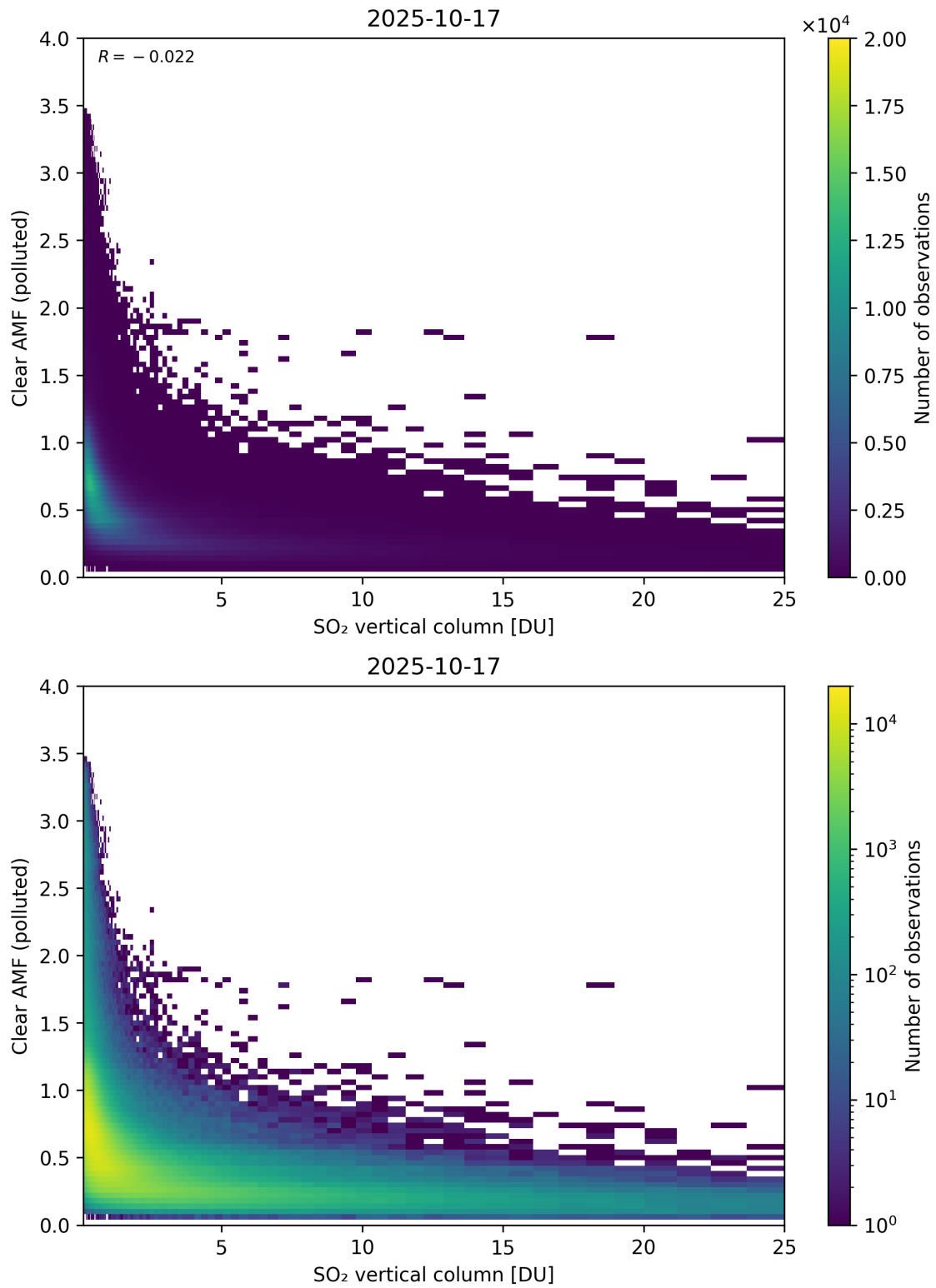
Figure 348: Scatter density plot of “SO 2 vertical column” against “Clear AMF (polluted)” for 2025-10-17 to 2025-10-18.
