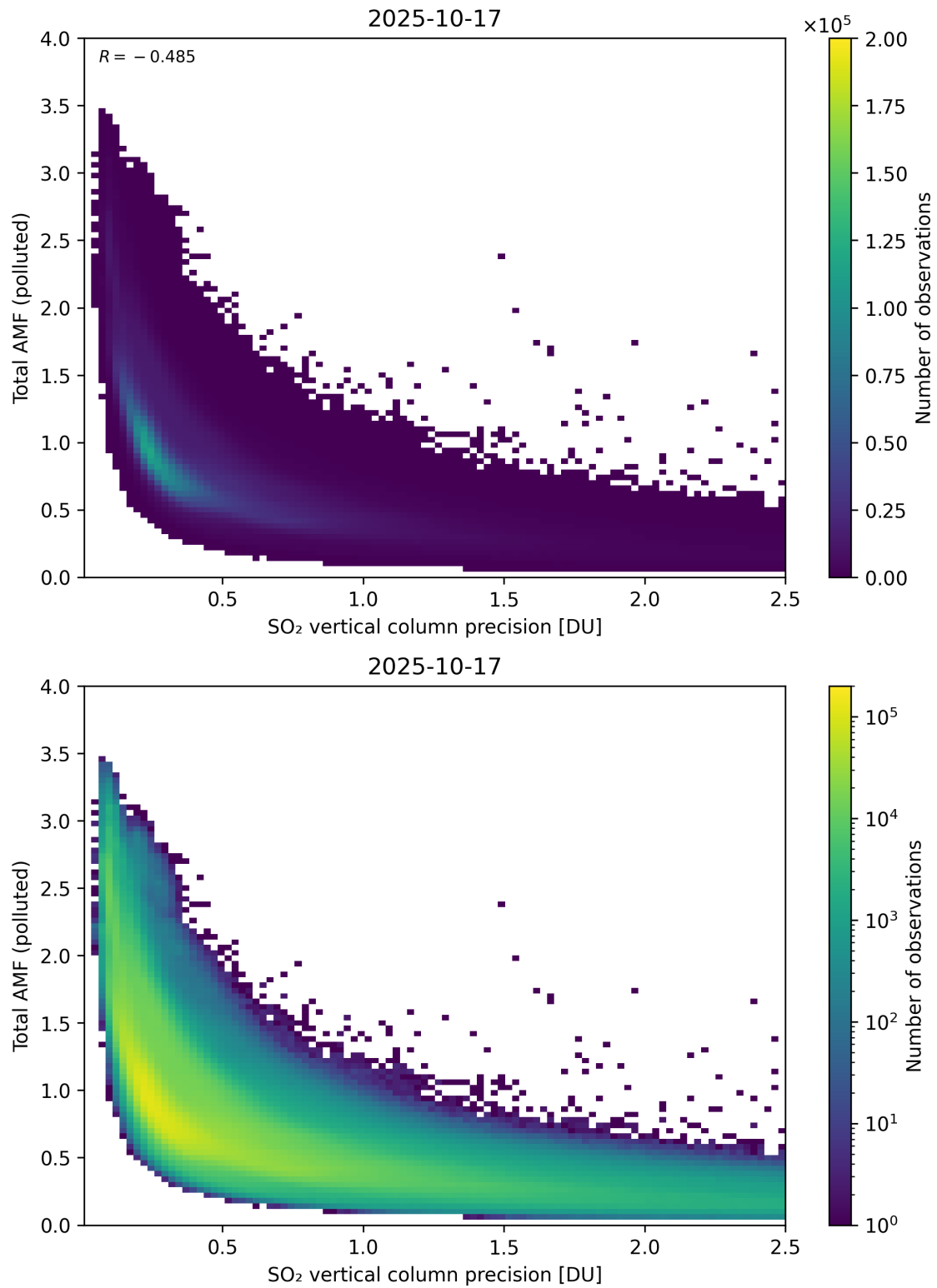
Figure 346: Scatter density plot of “SO 2 vertical column precision” against “Total AMF (polluted)” for 2025-10-17 to 2025-10-18.
