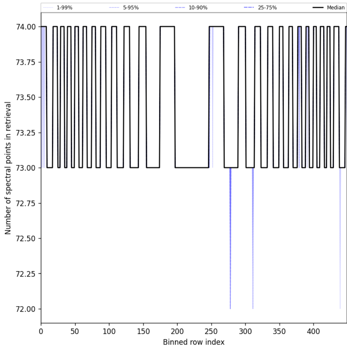
Figure 108: Along track statistics of “Number of spectral points in retrieval” for 2025-10-17 to 2025-10-18
