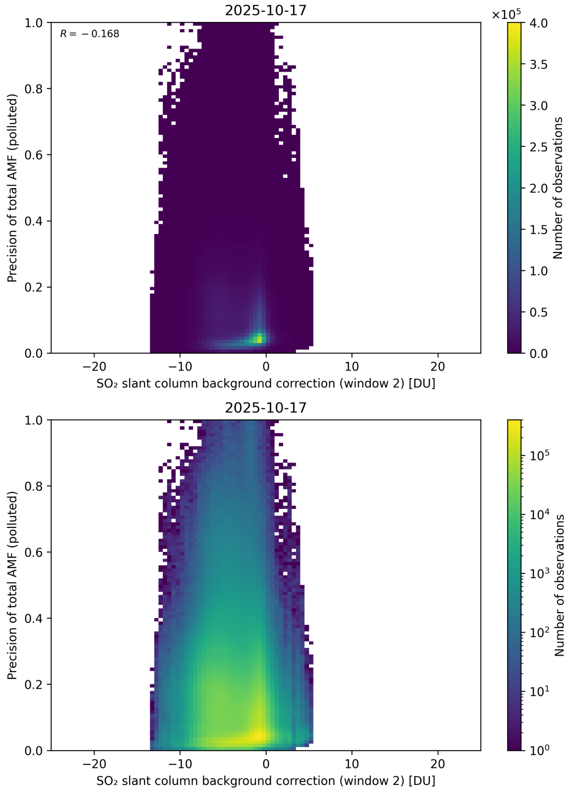
Figure 131: Scatter density plot of “SO 2 slant column background correction (window 2)” against “Precision of total AMF (polluted)” for 2025-10-17 to 2025-10-18.
