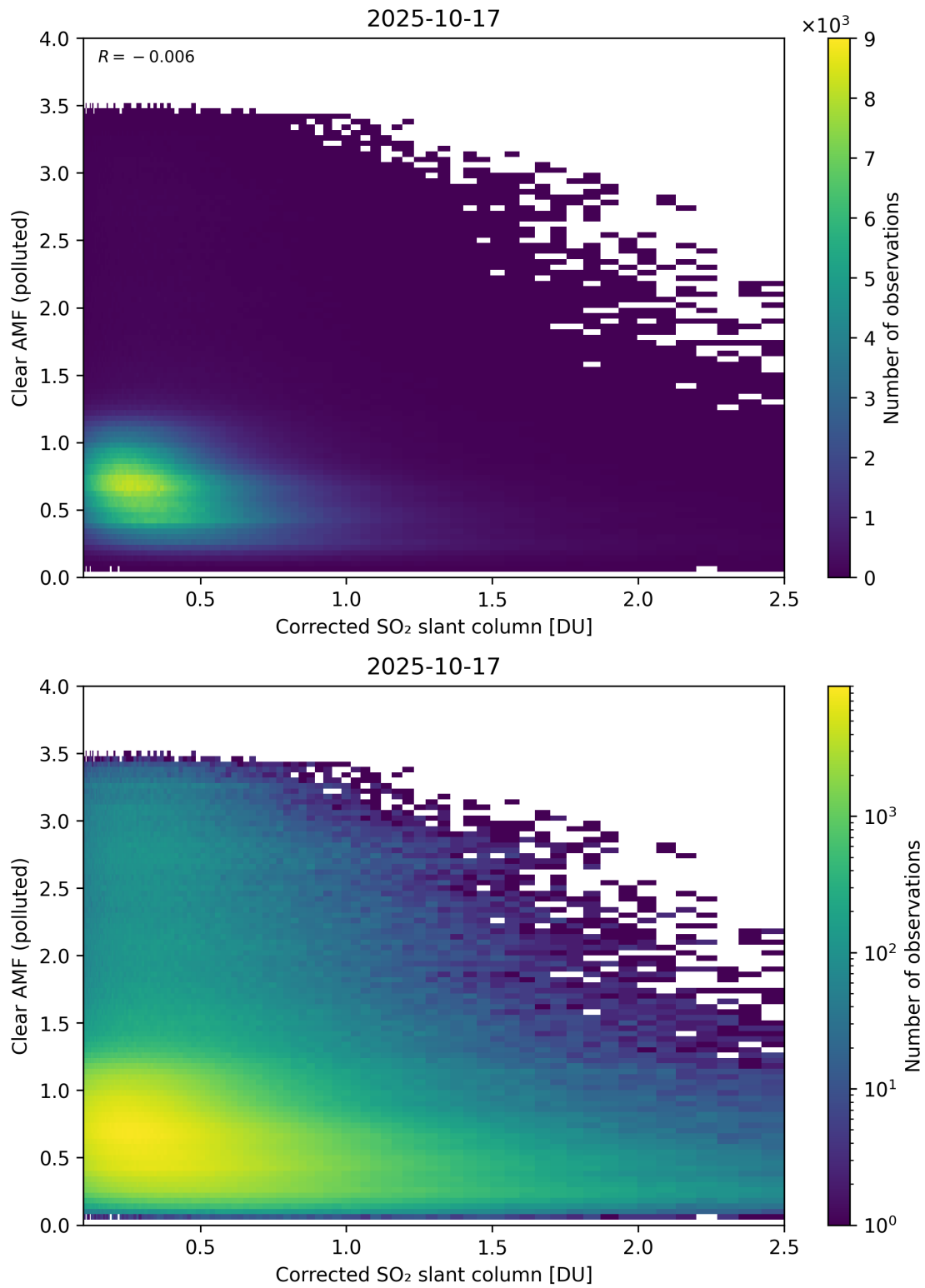
Figure 232: Scatter density plot of “Corrected SO 2 slant column” against “Clear AMF (polluted)” for 2025-10-17 to 2025-10-18.
