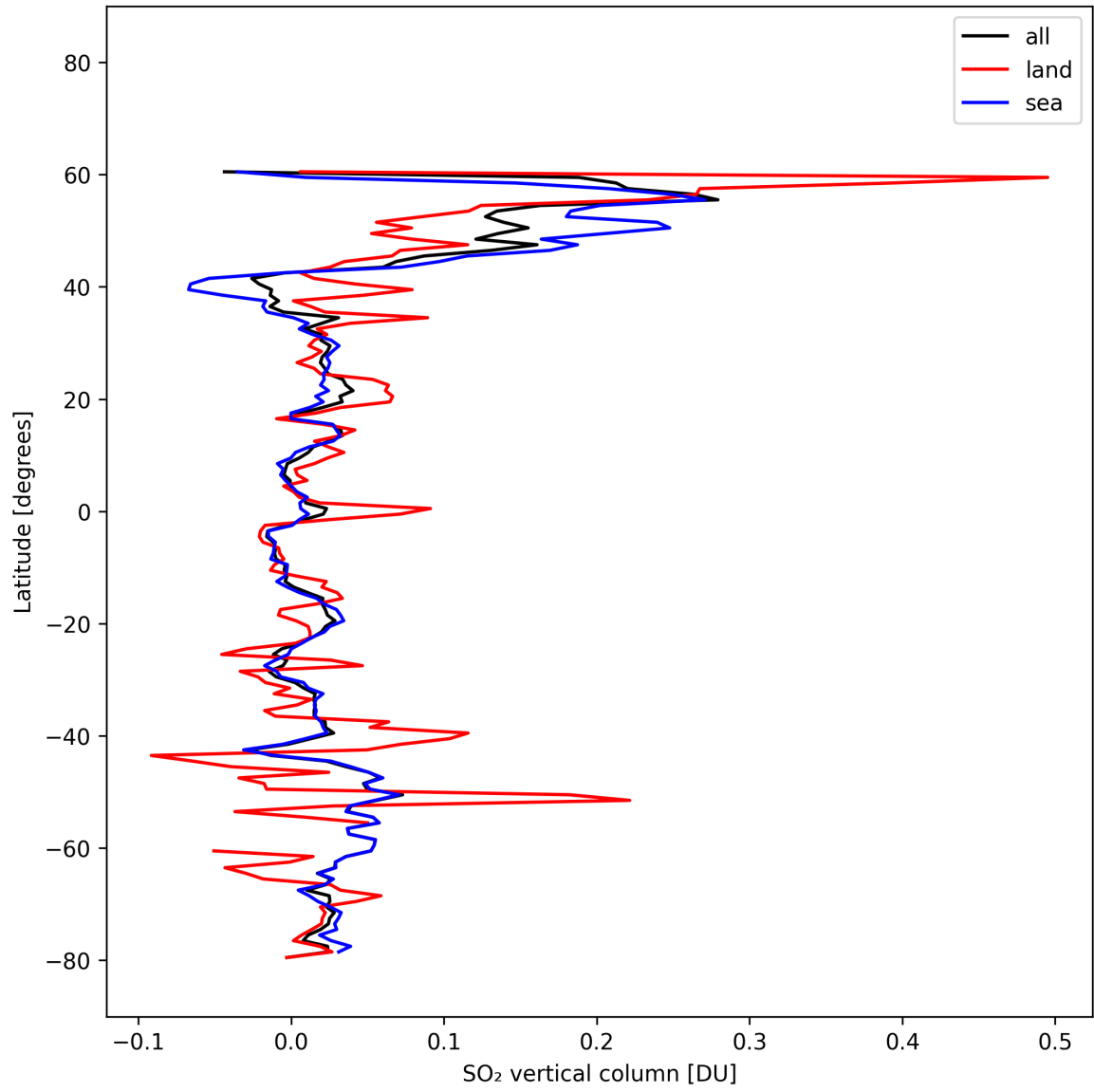
Figure 32: Zonal average of “SO 2 vertical column” for 2025-10-17 to 2025-10-18.
