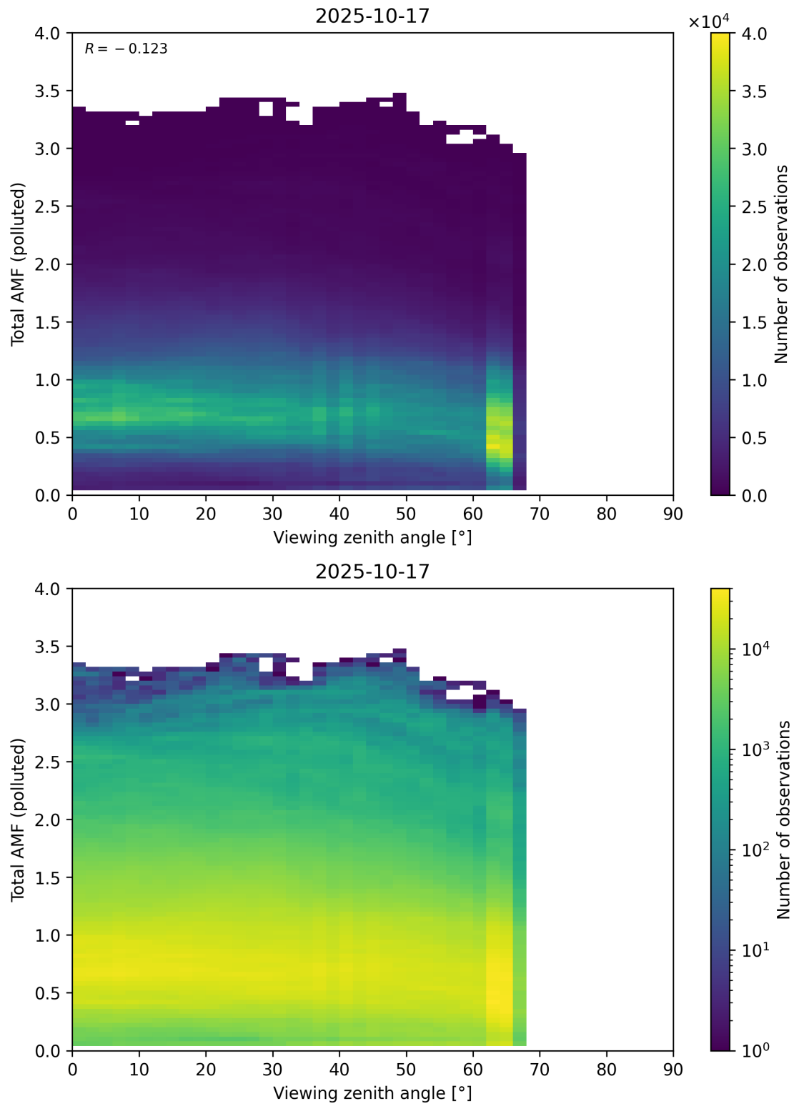
Figure 381: Scatter density plot of “Viewing zenith angle” against “Total AMF (polluted)” for 2025-10-17 to 2025-10-18.
