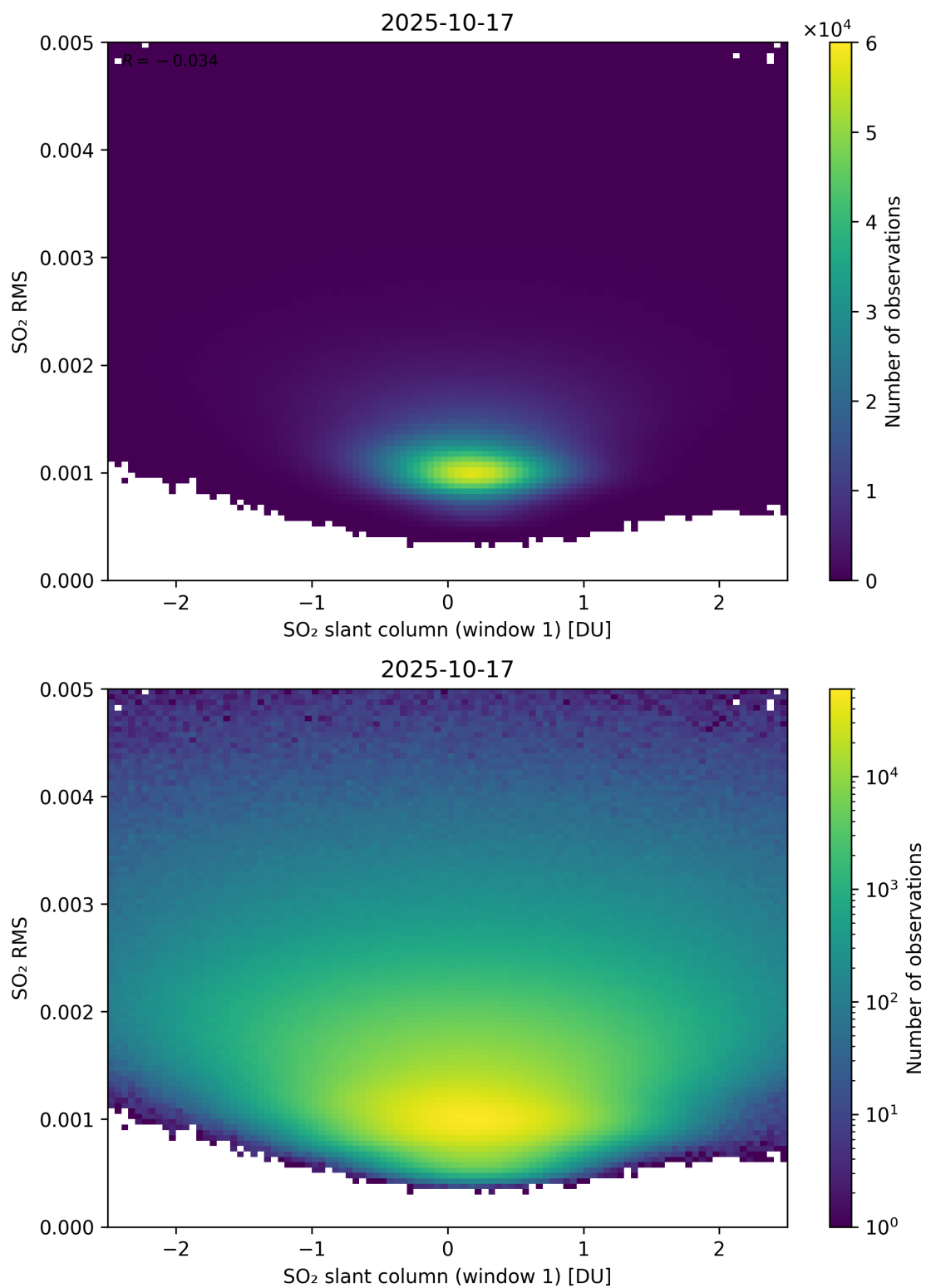
Figure 267: Scatter density plot of “SO 2 slant column (window 1)” against “SO 2 RMS” for 2025-10-17 to 2025-10-18.
