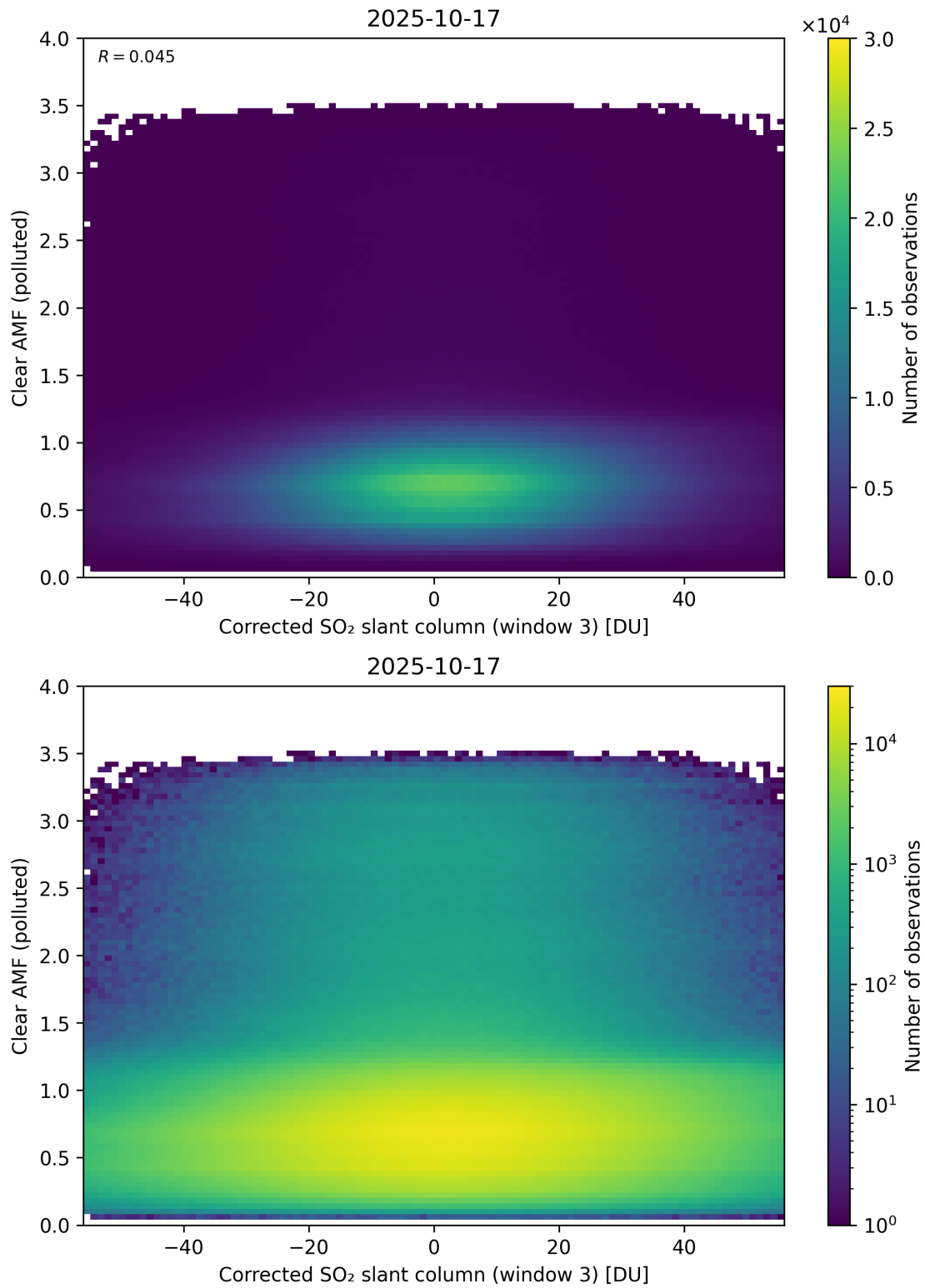
Figure 259: Scatter density plot of “Corrected SO 2 slant column (window 3)” against “Clear AMF (polluted)” for 2025-10-17 to 2025-10-18.
