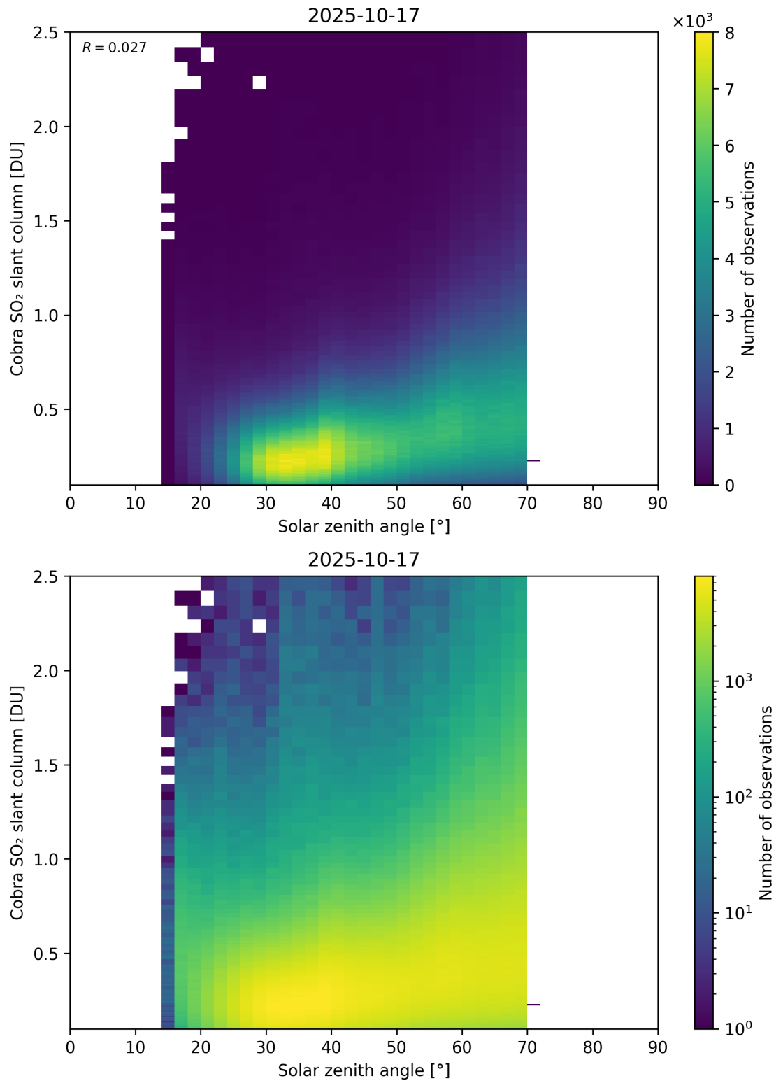
Figure 179: Scatter density plot of “Solar zenith angle” against “Cobra SO 2 slant column” for 2025-10-17 to 2025-10-18.
