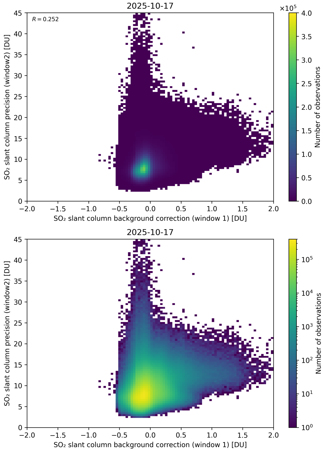
Figure 117: Scatter density plot of “SO 2 slant column background correction (window 1)” against “SO 2 slant column precision (window2)” for 2025-10-17 to 2025-10-18.
