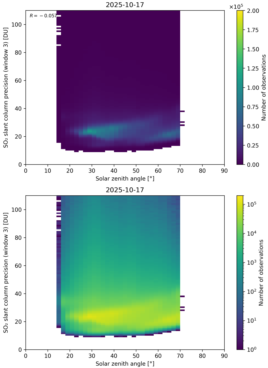
Figure 188: Scatter density plot of “Solar zenith angle” against “SO 2 slant column precision (window 3)” for 2025-10-17 to 2025-10-18.
