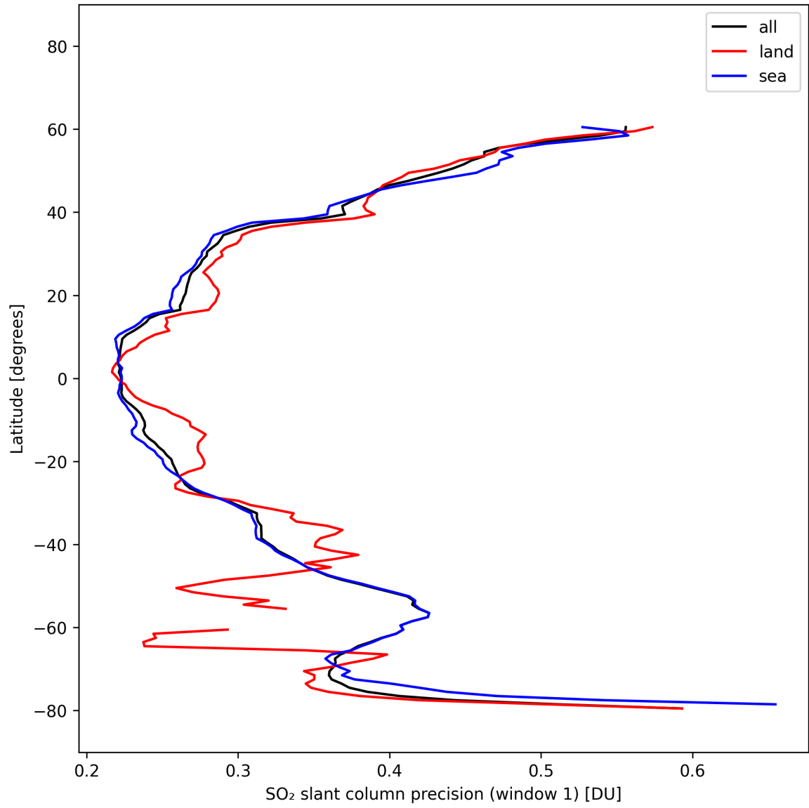
Figure 38: Zonal average of “SO 2 slant column precision (window 1)” for 2025-10-17 to 2025-10-18.
