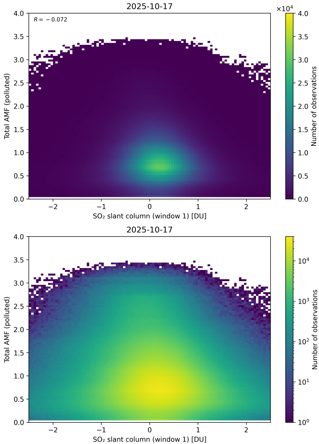
Figure 289: Scatter density plot of “SO 2 slant column (window 1)” against “Total AMF (polluted)” for 2025-10-17 to 2025-10-18.
