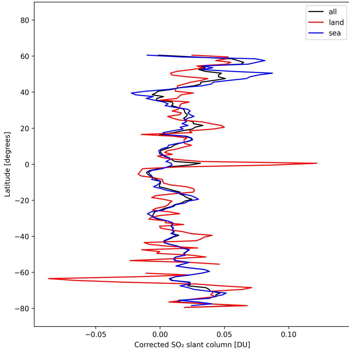
Figure 34: Zonal average of “Corrected SO 2 slant column” for 2025-10-17 to 2025-10-18.
