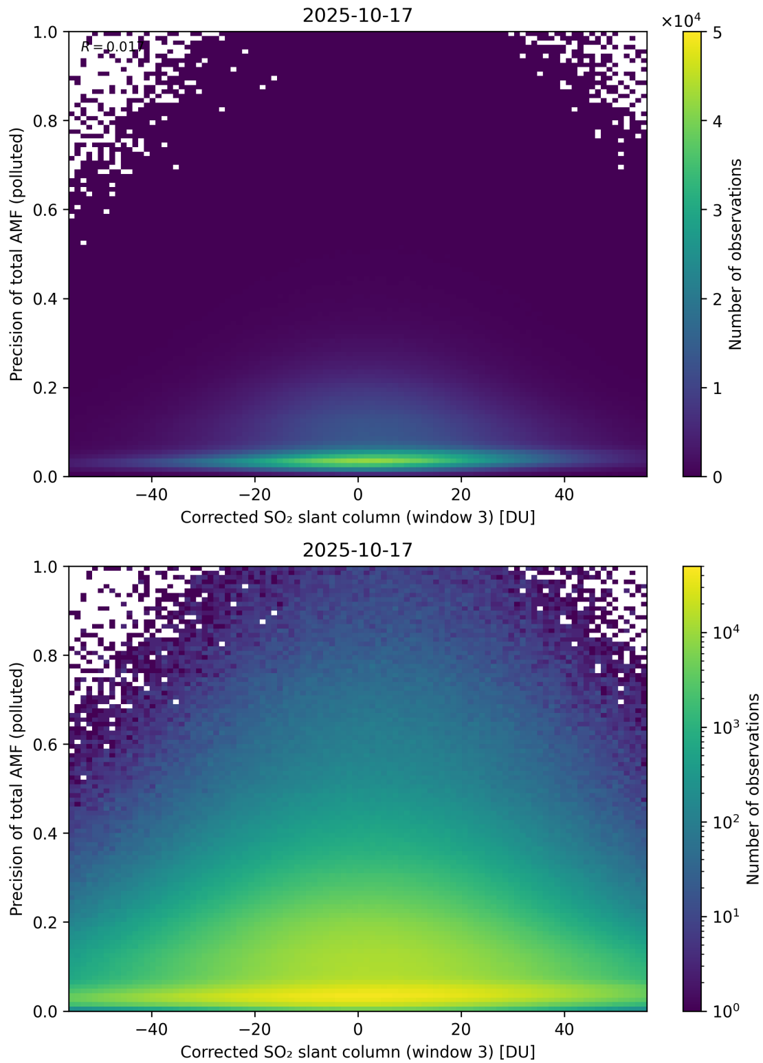
Figure 261: Scatter density plot of “Corrected SO 2 slant column (window 3)” against “Precision of total AMF (polluted)” for 2025-10-17 to 2025-10-18.
