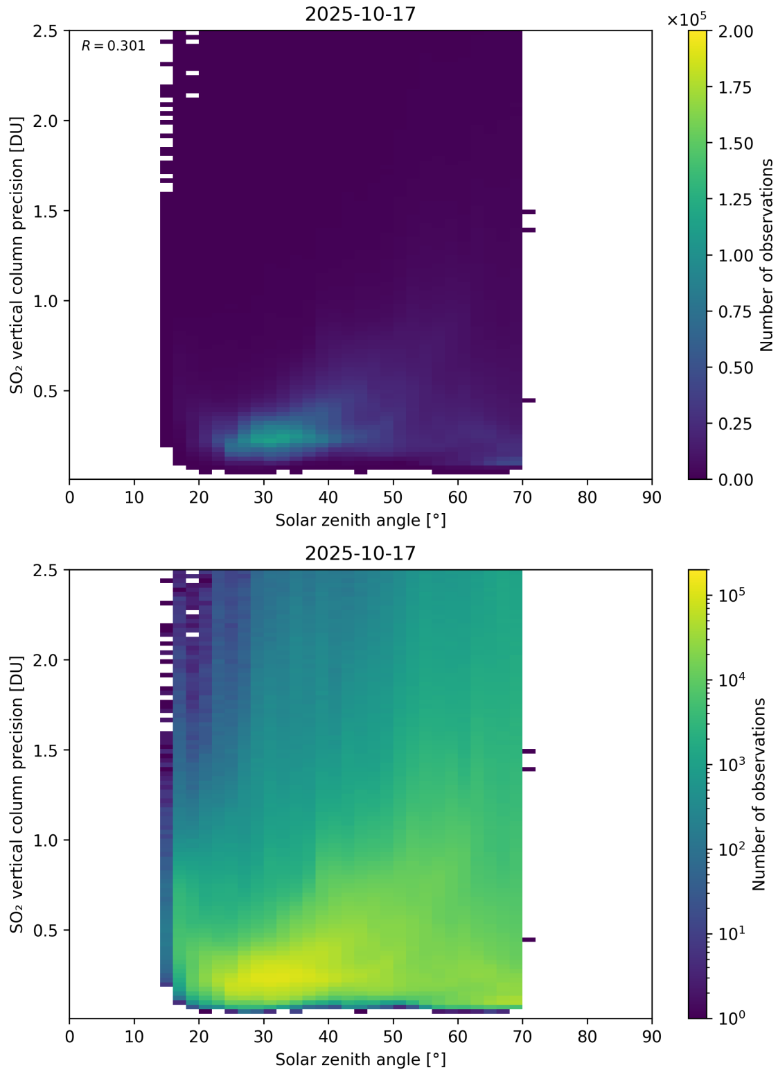
Figure 192: Scatter density plot of “Solar zenith angle” against “SO 2 vertical column precision” for 2025-10-17 to 2025-10-18.
