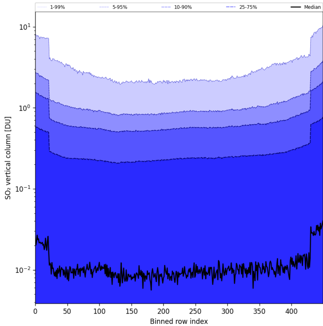
Figure 84: Along track statistics of “SO 2 vertical column” for 2025-10-17 to 2025-10-18
