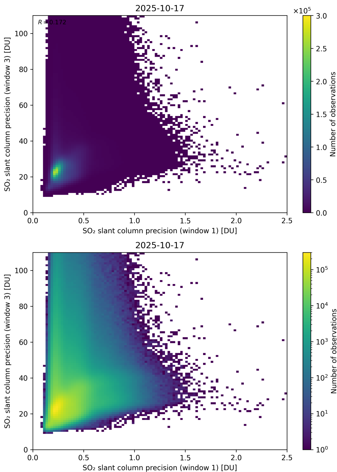
Figure 279: Scatter density plot of “SO 2 slant column precision (window 1)” against “SO 2 slant column precision (window 3)” for 2025-10-17 to 2025-10-18.
