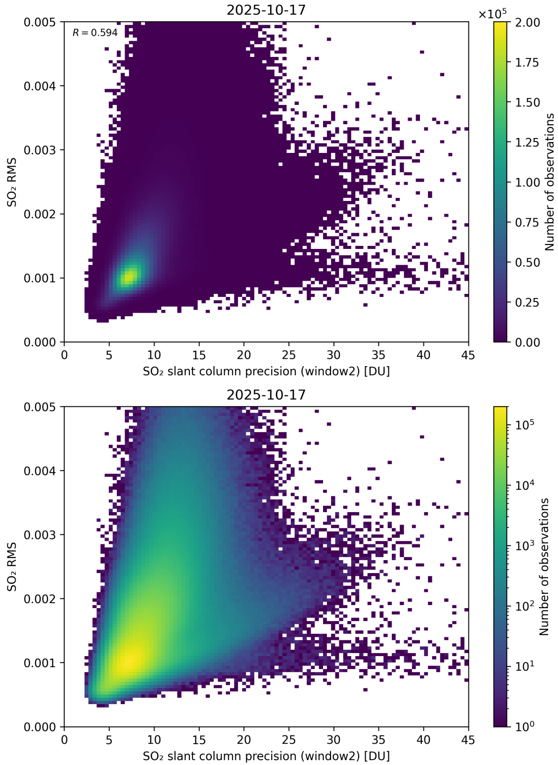
Figure 295: Scatter density plot of “SO 2 slant column precision (window2)” against “SO 2 RMS” for 2025-10-17 to 2025-10-18.
