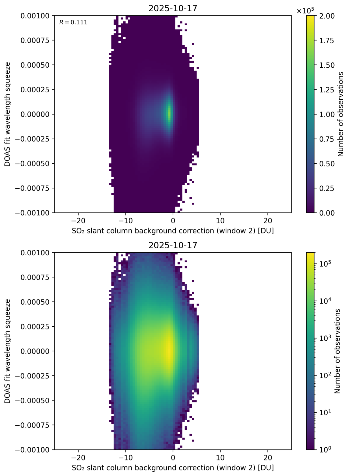
Figure 124: Scatter density plot of “SO 2 slant column background correction (window 2)” against “DOAS fit wavelength squeeze” for 2025-10-17 to 2025-10-18.
