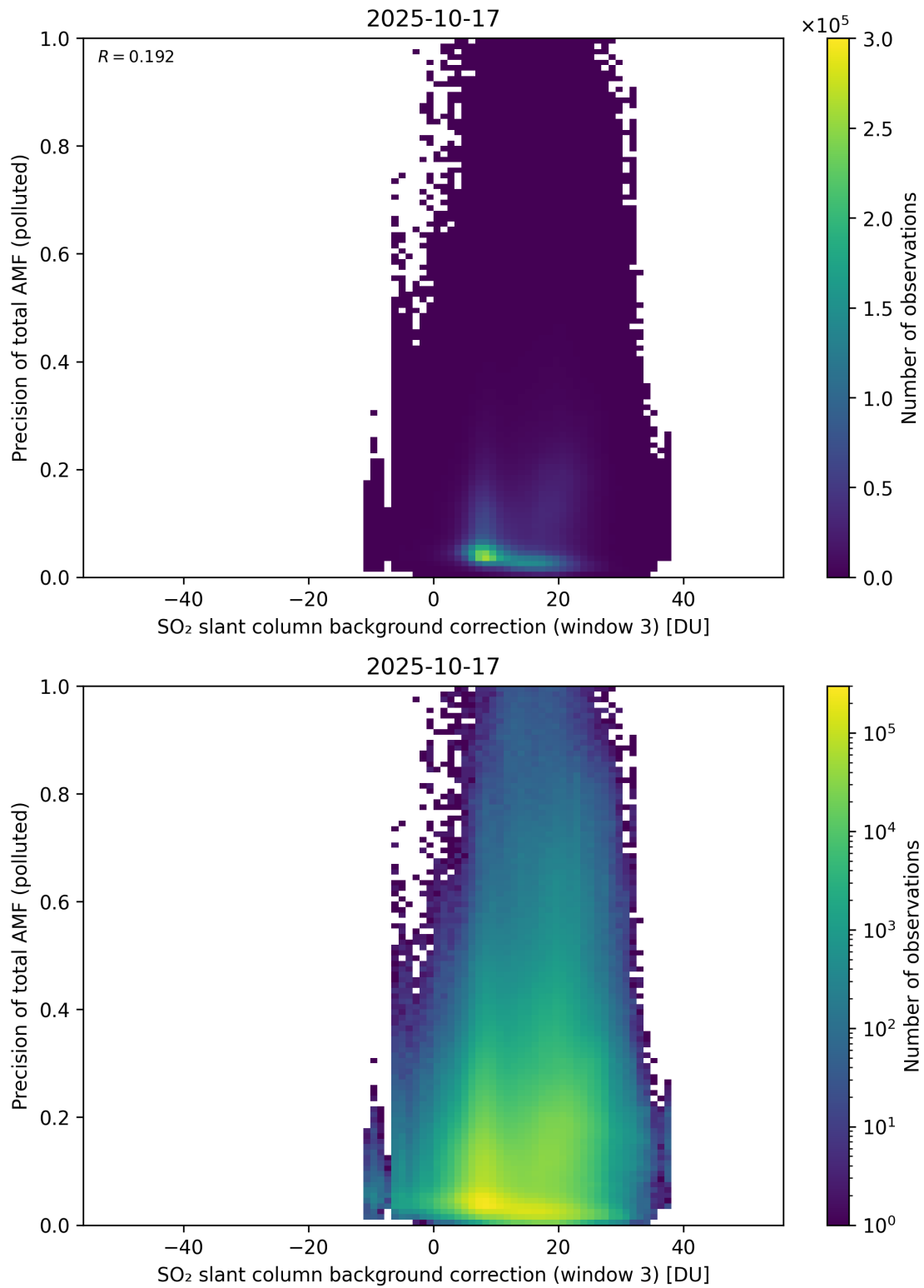
Figure 137: Scatter density plot of “SO 2 slant column background correction (window 3)” against “Precision of total AMF (polluted)” for 2025-10-17 to 2025-10-18.
