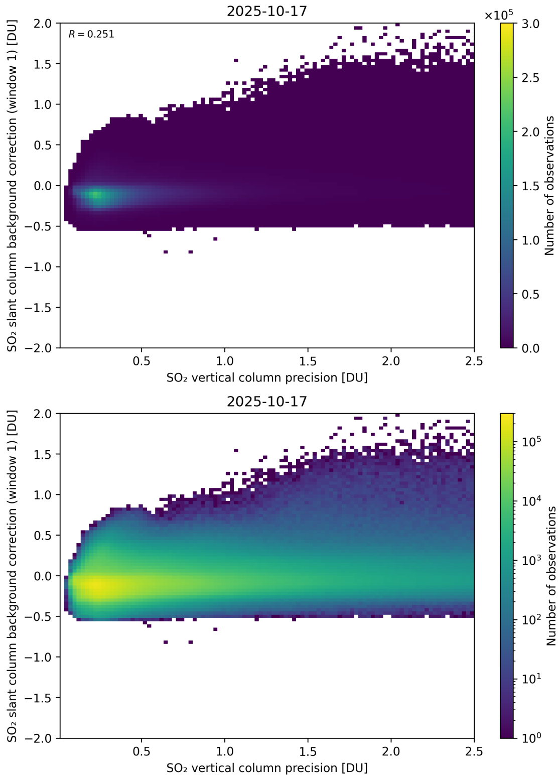
Figure 329: Scatter density plot of “SO 2 vertical column precision” against “SO 2 slant column background correction (window 1)” for 2025-10-17 to 2025-10-18.
