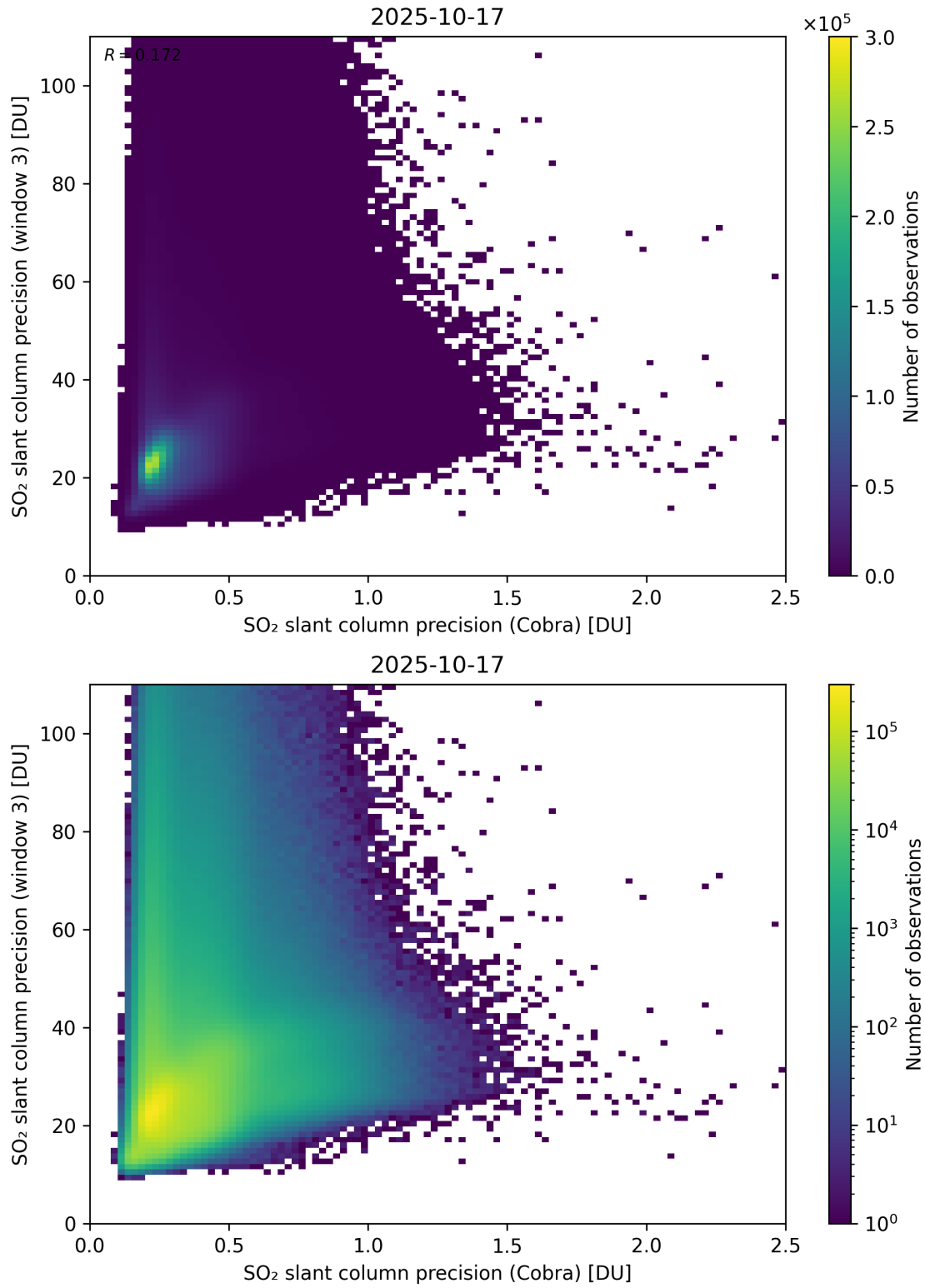
Figure 212: Scatter density plot of “SO 2 slant column precision (Cobra)” against “SO 2 slant column precision (window 3)” for 2025-10-17 to 2025-10-18.
