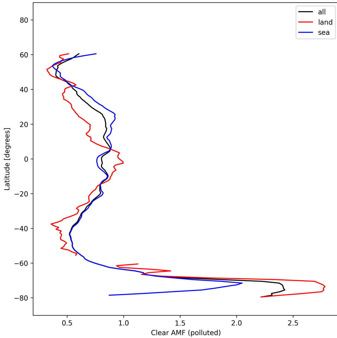
Figure 55: Zonal average of “Clear AMF (polluted)” for 2025-10-17 to 2025-10-18.
