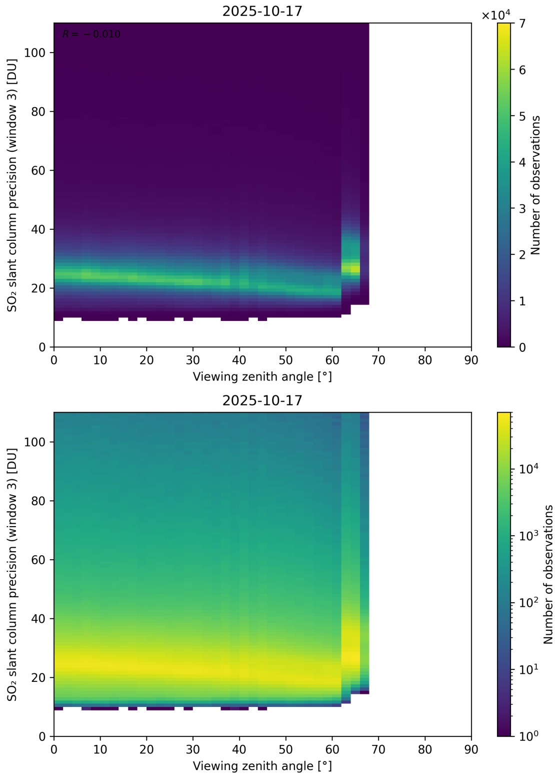
Figure 380: Scatter density plot of “Viewing zenith angle” against “SO 2 slant column precision (window 3)” for 2025-10-17 to 2025-10-18.
