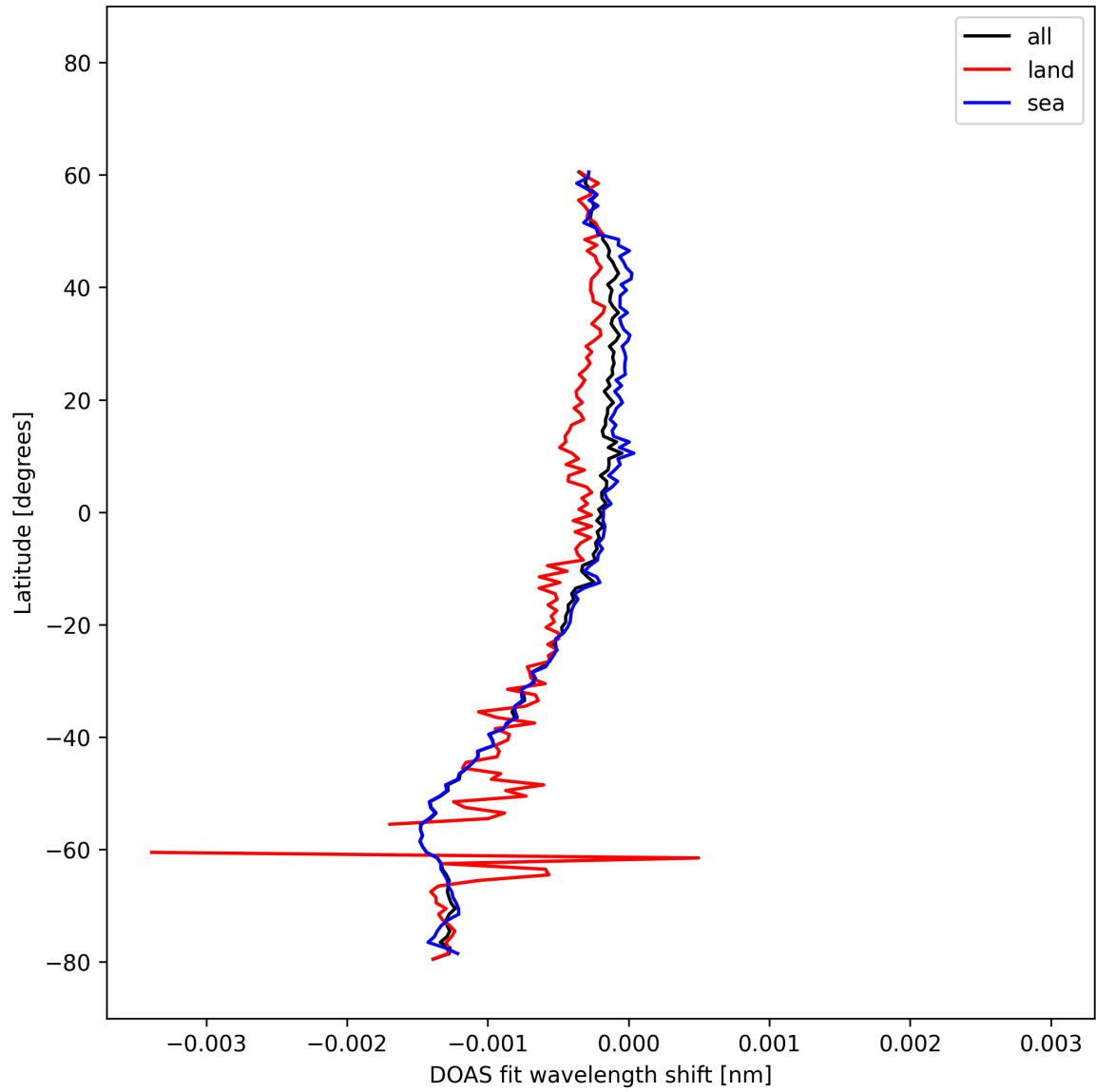
Figure 50: Zonal average of “DOAS fit wavelength shift” for 2025-10-17 to 2025-10-18.
