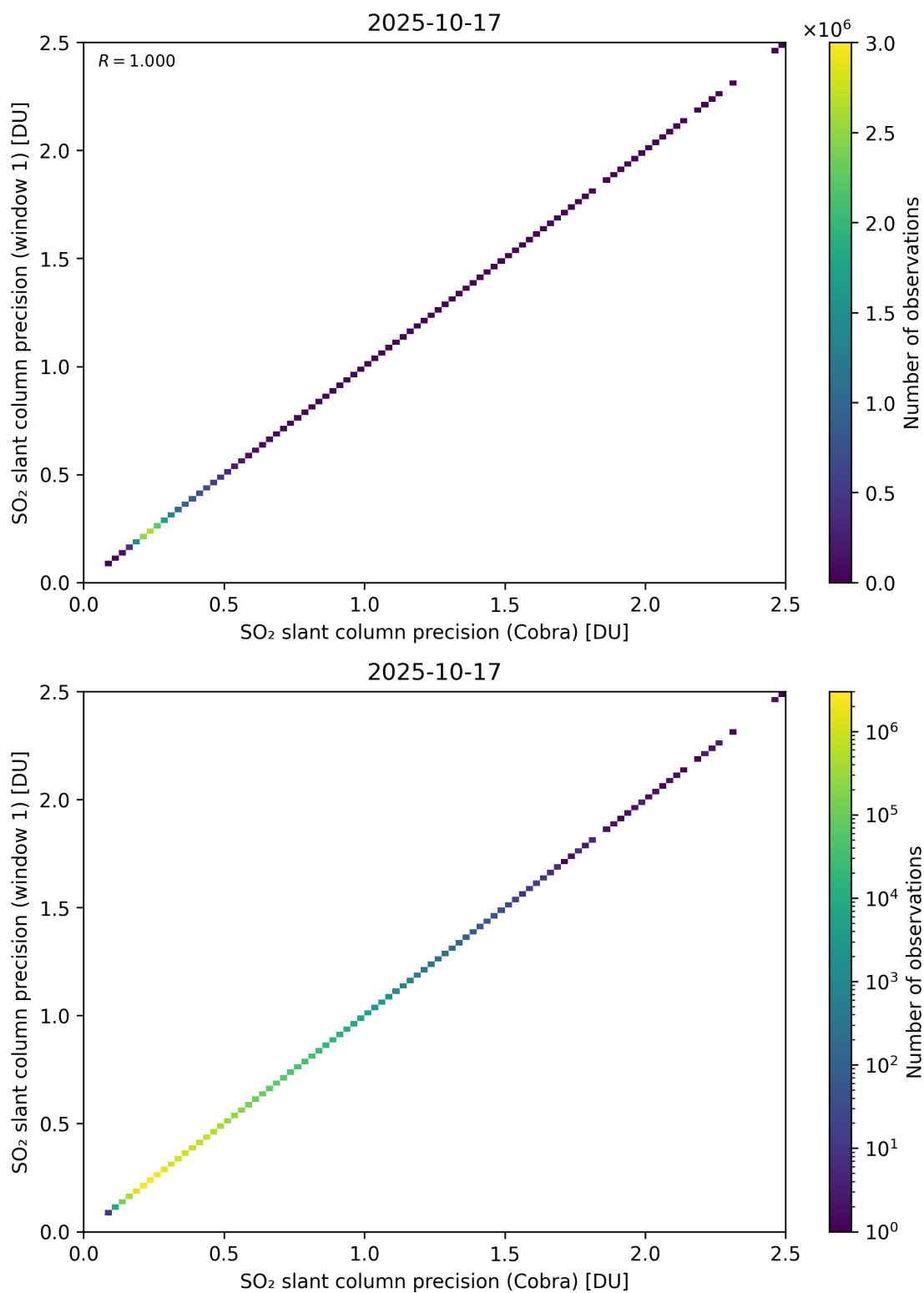
Figure 209: Scatter density plot of “SO 2 slant column precision (Cobra)” against “SO 2 slant column precision (window 1)” for 2025-10-17 to 2025-10-18.
