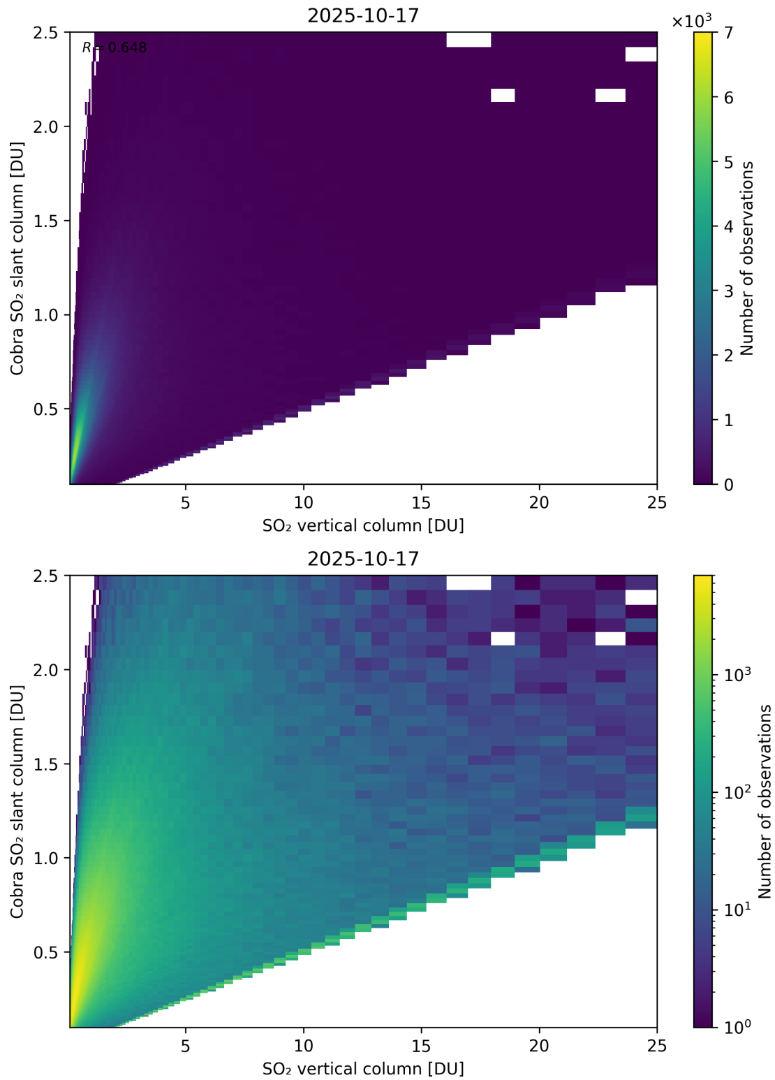
Figure 349: Scatter density plot of “SO 2 vertical column” against “Cobra SO 2 slant column” for 2025-10-17 to 2025-10-18.
