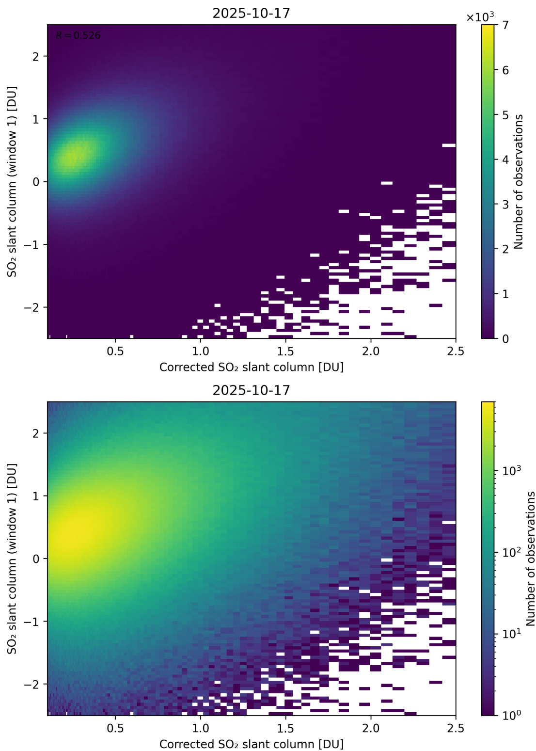
Figure 237: Scatter density plot of “Corrected SO 2 slant column” against “SO 2 slant column (window 1)” for 2025-10-17 to 2025-10-18.
