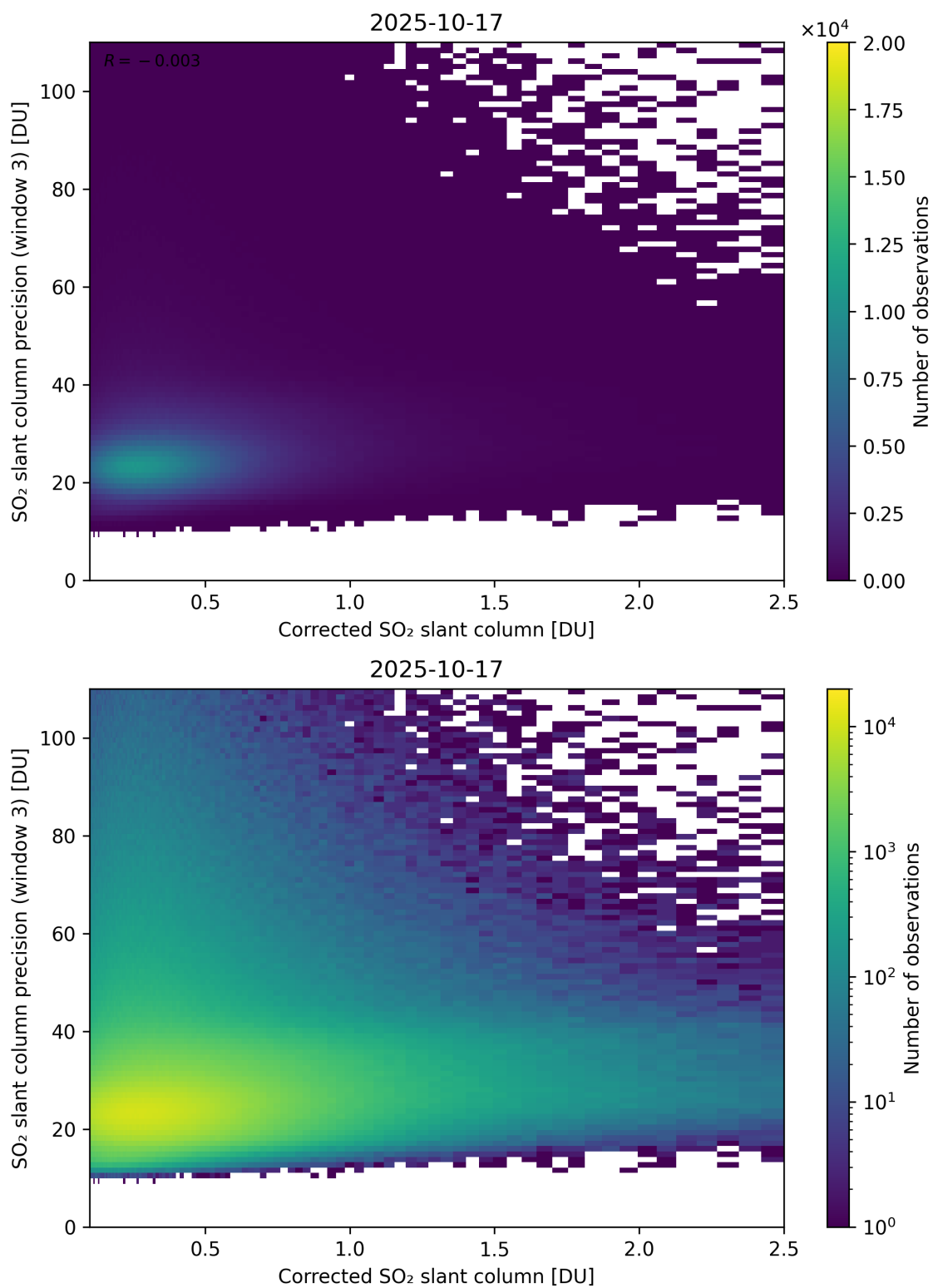
Figure 241: Scatter density plot of “Corrected SO 2 slant column” against “SO 2 slant column precision (window 3)” for 2025-10-17 to 2025-10-18.
