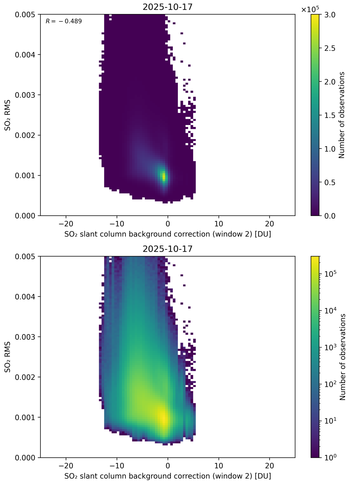
Figure 125: Scatter density plot of “SO 2 slant column background correction (window 2)” against “SO 2 RMS” for 2025-10-17 to 2025-10-18.
