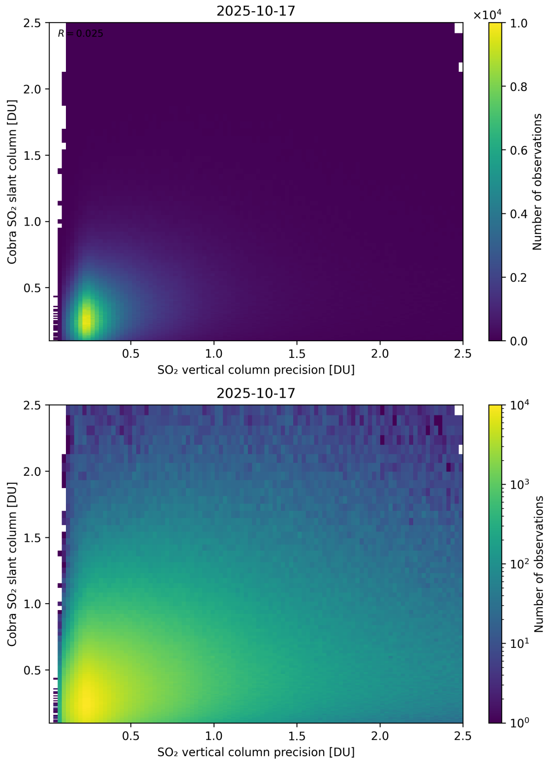
Figure 336: Scatter density plot of “SO 2 vertical column precision” against “Cobra SO 2 slant column” for 2025-10-17 to 2025-10-18.
