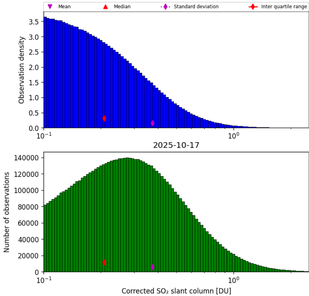
Figure 60: Histogram of “Corrected SO 2 slant column” for 2025-10-17 to 2025-10-18
