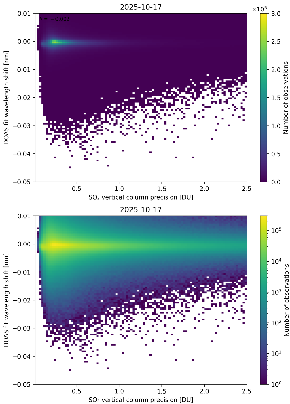
Figure 332: Scatter density plot of “SO 2 vertical column precision” against “DOAS fit wavelength shift” for 2025-10-17 to 2025-10-18.
