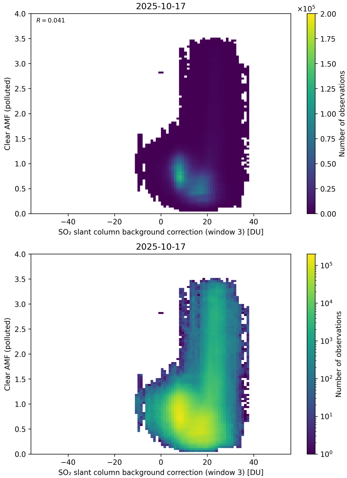
Figure 135: Scatter density plot of “SO 2 slant column background correction (window 3)” against “Clear AMF (polluted)” for 2025-10-17 to 2025-10-18.
