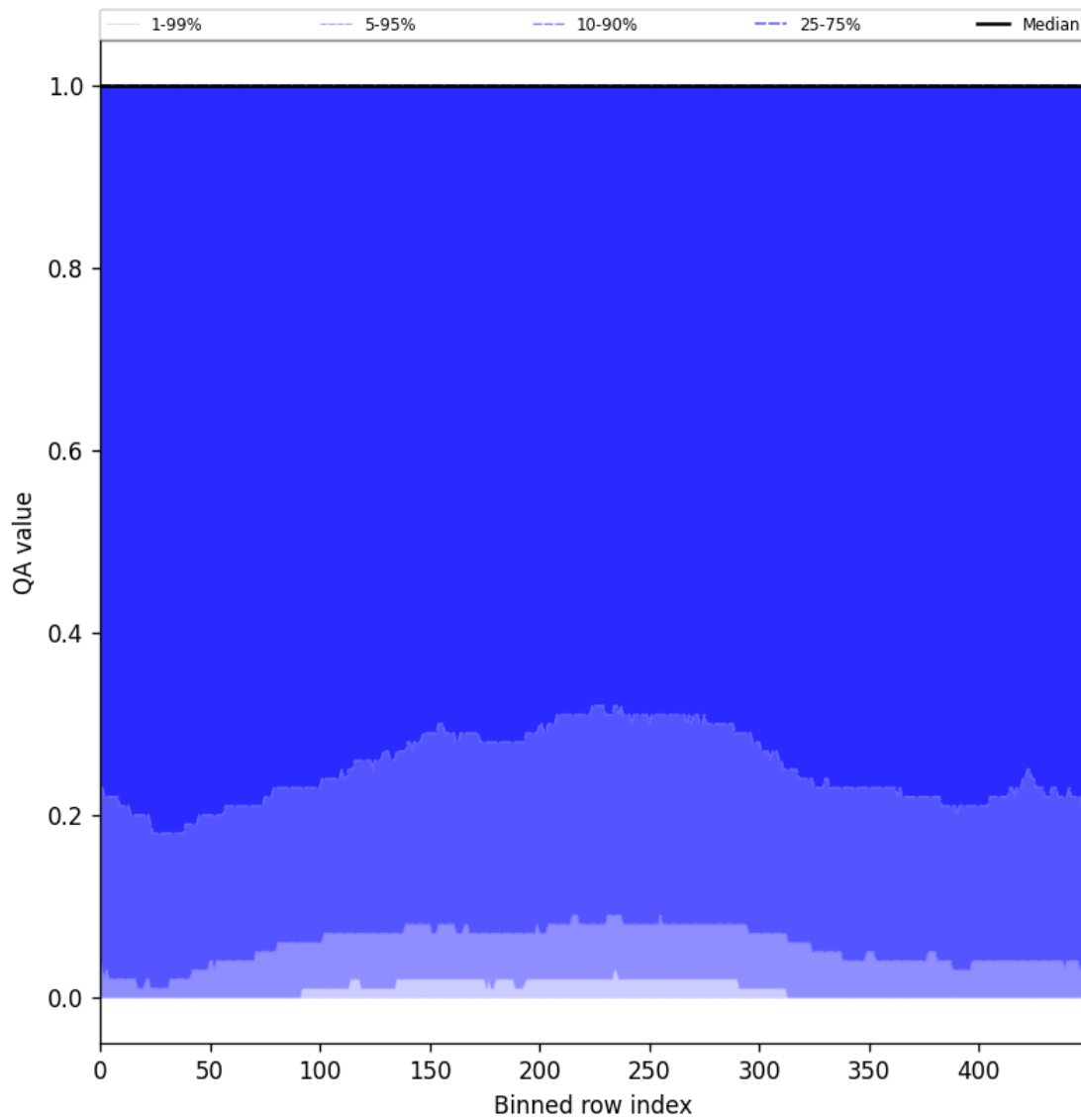
Figure 83: Along track statistics of “QA value” for 2025-10-17 to 2025-10-18
