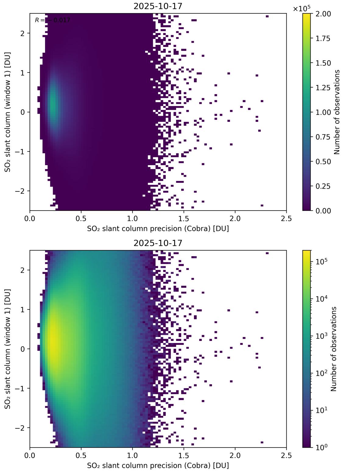
Figure 208: Scatter density plot of “SO 2 slant column precision (Cobra)” against “SO 2 slant column (window 1)” for 2025-10-17 to 2025-10-18.
