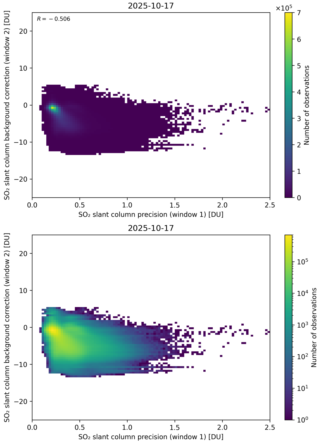
Figure 269: Scatter density plot of “SO 2 slant column precision (window 1)” against “SO 2 slant column background correction (window 2)” for 2025-10-17 to 2025-10-18.
