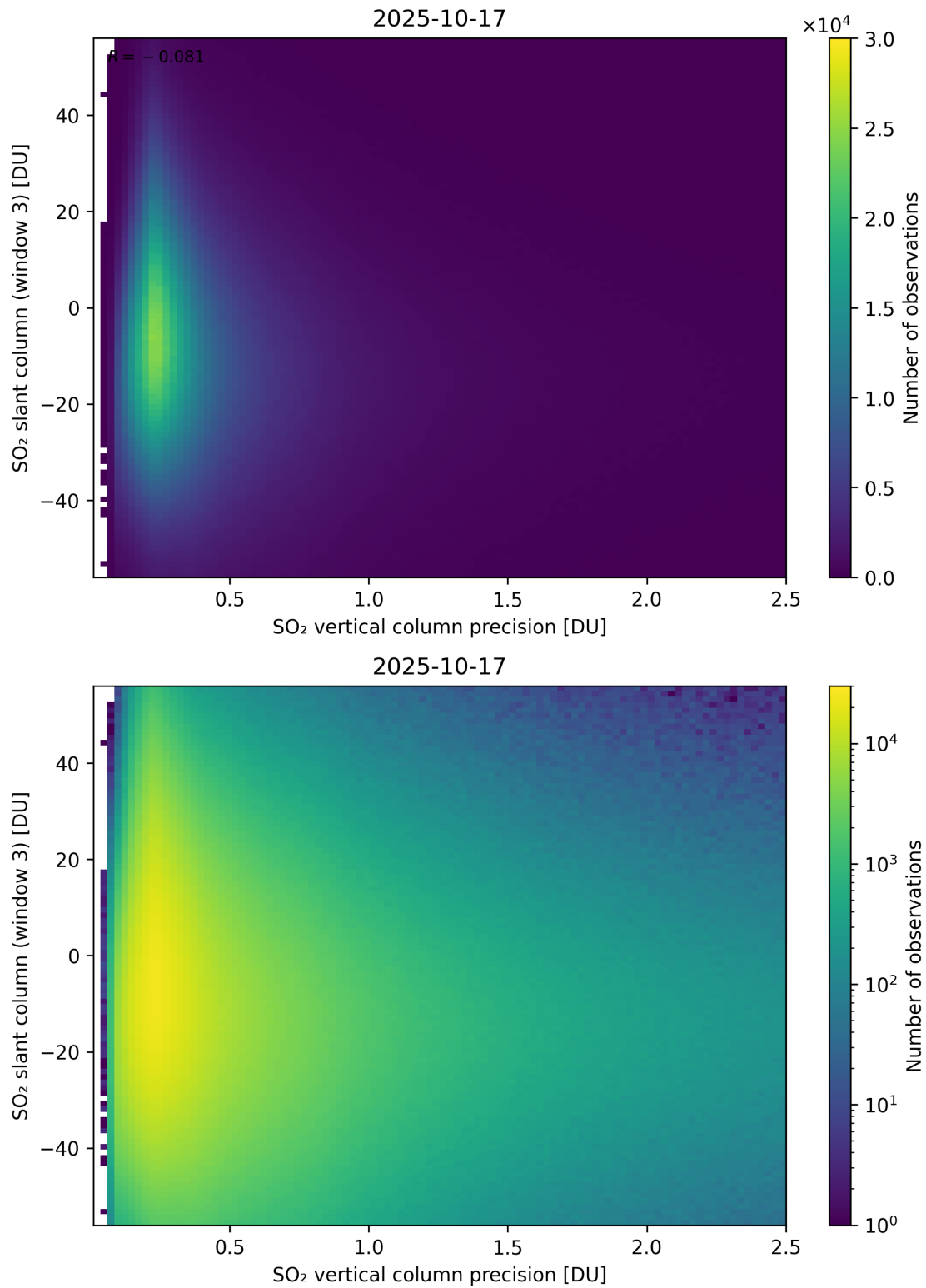
Figure 344: Scatter density plot of “SO 2 vertical column precision” against “SO 2 slant column (window 3)” for 2025-10-17 to 2025-10-18.
