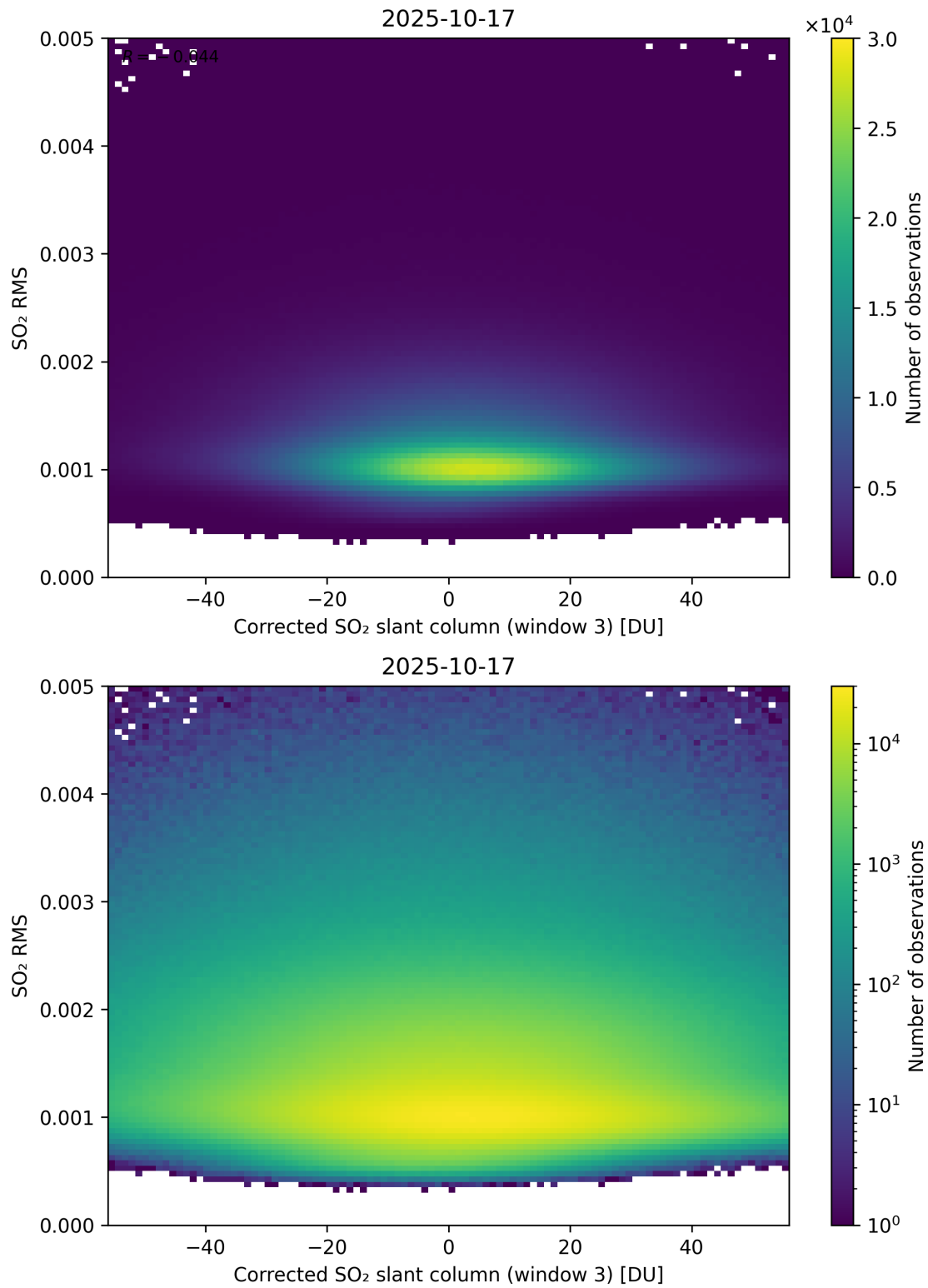
Figure 258: Scatter density plot of “Corrected SO 2 slant column (window 3)” against “SO 2 RMS” for 2025-10-17 to 2025-10-18.
