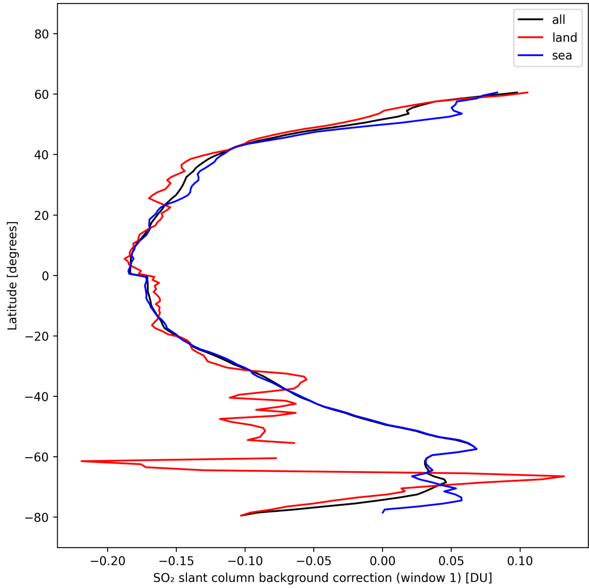
Figure 40: Zonal average of “SO 2 slant column background correction (window 1)” for 2025-10-17 to 2025-10-18.
