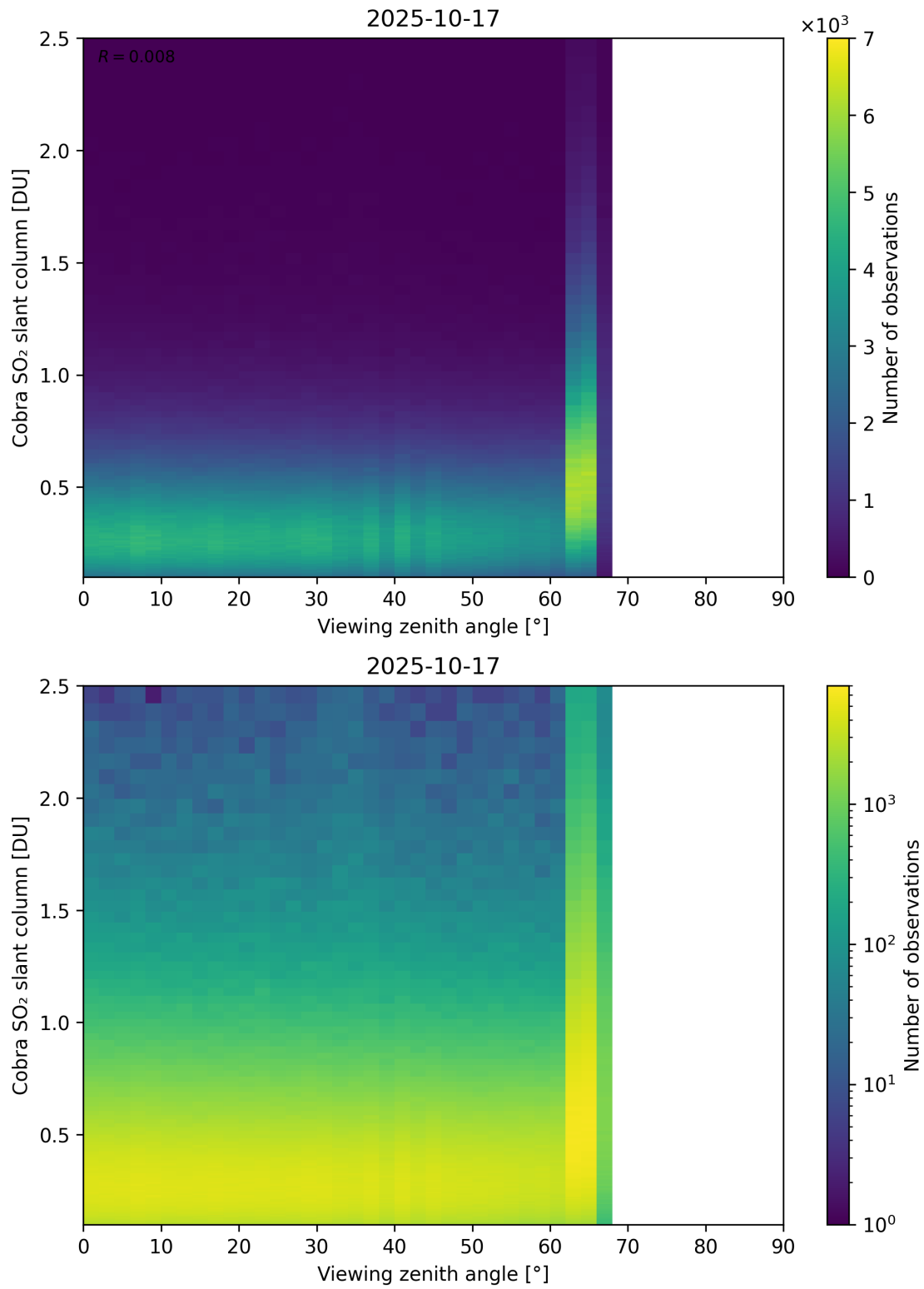
Figure 371: Scatter density plot of “Viewing zenith angle” against “Cobra SO 2 slant column” for 2025-10-17 to 2025-10-18.
