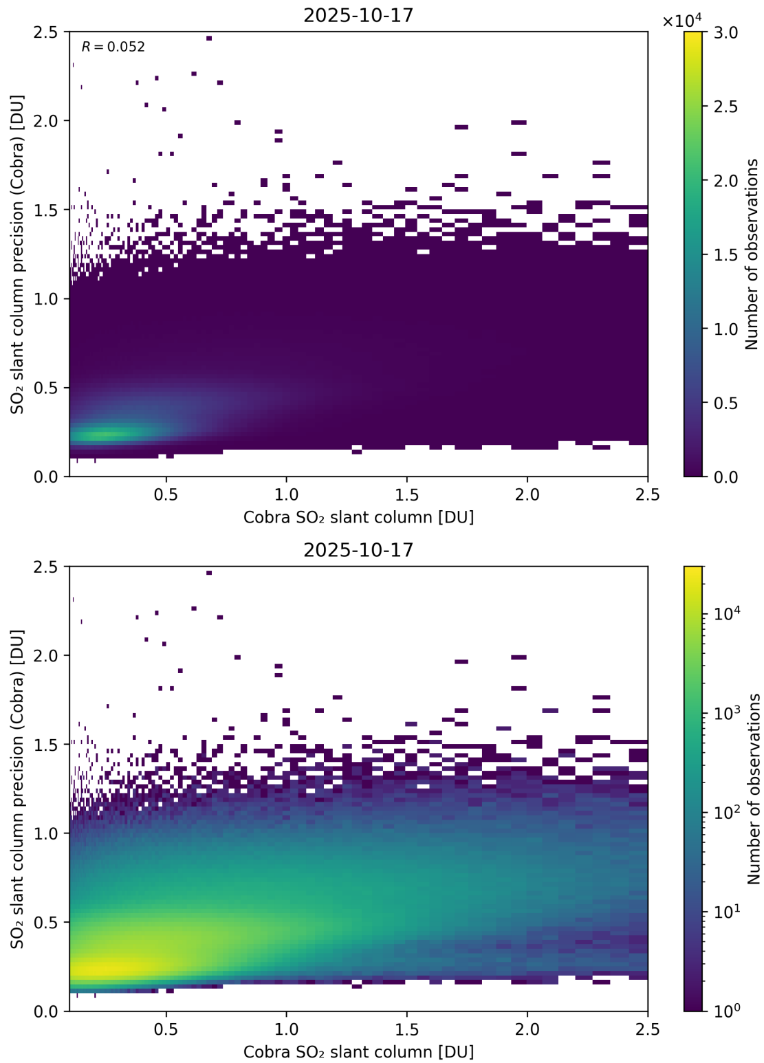
Figure 216: Scatter density plot of “Cobra SO 2 slant column” against “SO 2 slant column precision (Cobra)” for 2025-10-17 to 2025-10-18.
