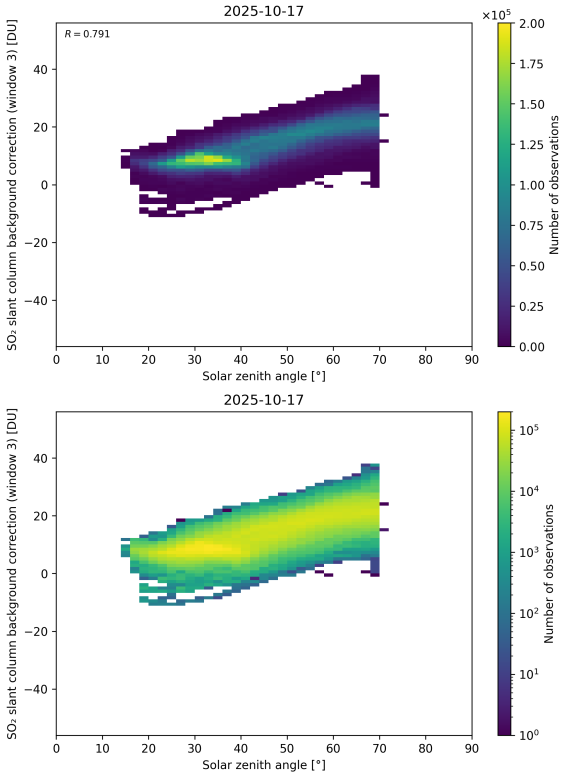
Figure 173: Scatter density plot of “Solar zenith angle” against “SO 2 slant column background correction (window 3)” for 2025-10-17 to 2025-10-18.
