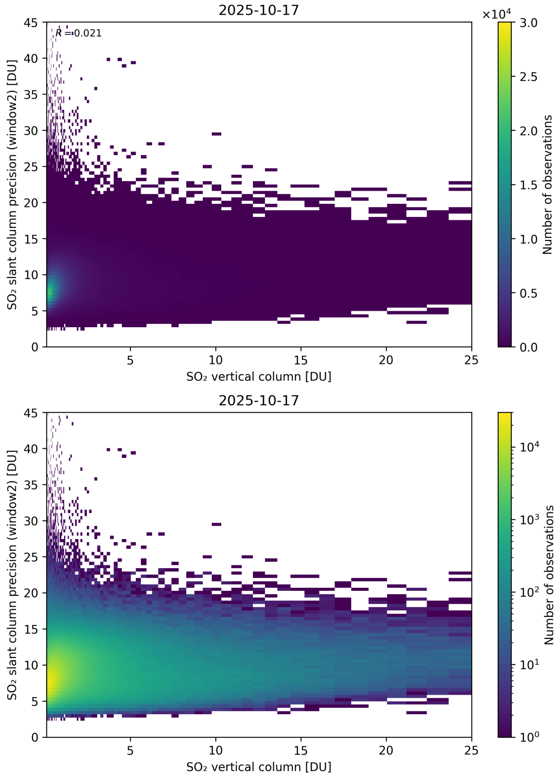
Figure 356: Scatter density plot of “SO 2 vertical column” against “SO 2 slant column precision (window2)” for 2025-10-17 to 2025-10-18.
