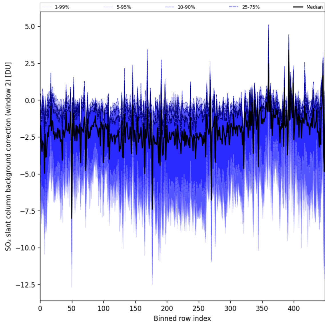
Figure 96: Along track statistics of “SO 2 slant column background correction (window 2)” for 2025-10-17 to 2025-10-18
