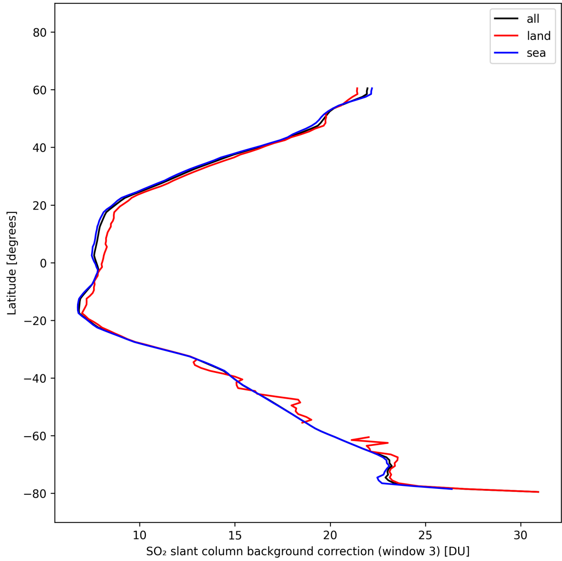
Figure 48: Zonal average of “SO 2 slant column background correction (window 3)” for 2025-10-17 to 2025-10-18.
