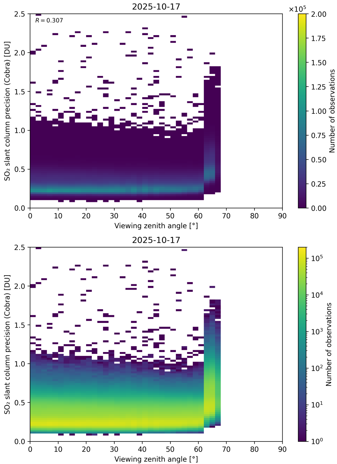
Figure 372: Scatter density plot of “Viewing zenith angle” against “SO 2 slant column precision (Cobra)” for 2025-10-17 to 2025-10-18.
