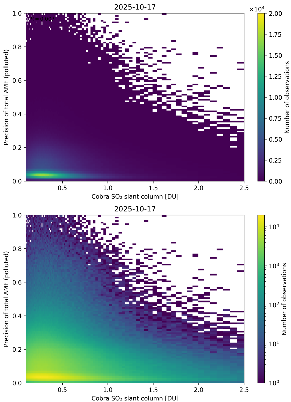
Figure 225: Scatter density plot of “Cobra SO 2 slant column” against “Precision of total AMF (polluted)” for 2025-10-17 to 2025-10-18.
