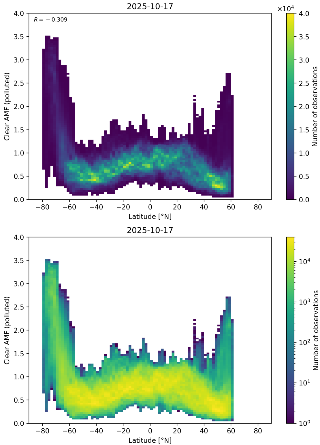
Figure 156: Scatter density plot of “Latitude” against “Clear AMF (polluted)” for 2025-10-17 to 2025-10-18.
