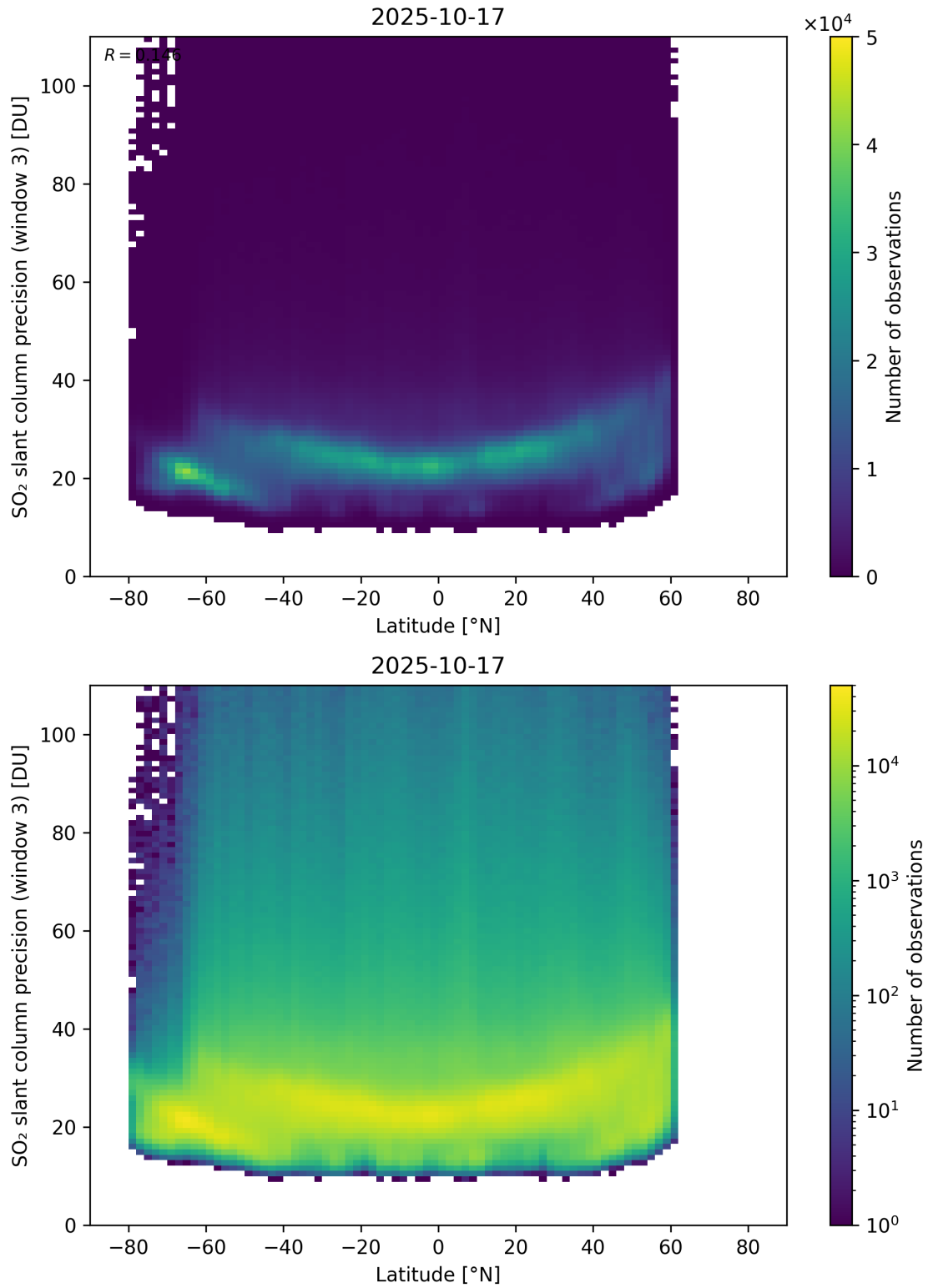
Figure 166: Scatter density plot of “Latitude” against “SO 2 slant column precision (window 3)” for 2025-10-17 to 2025-10-18.
