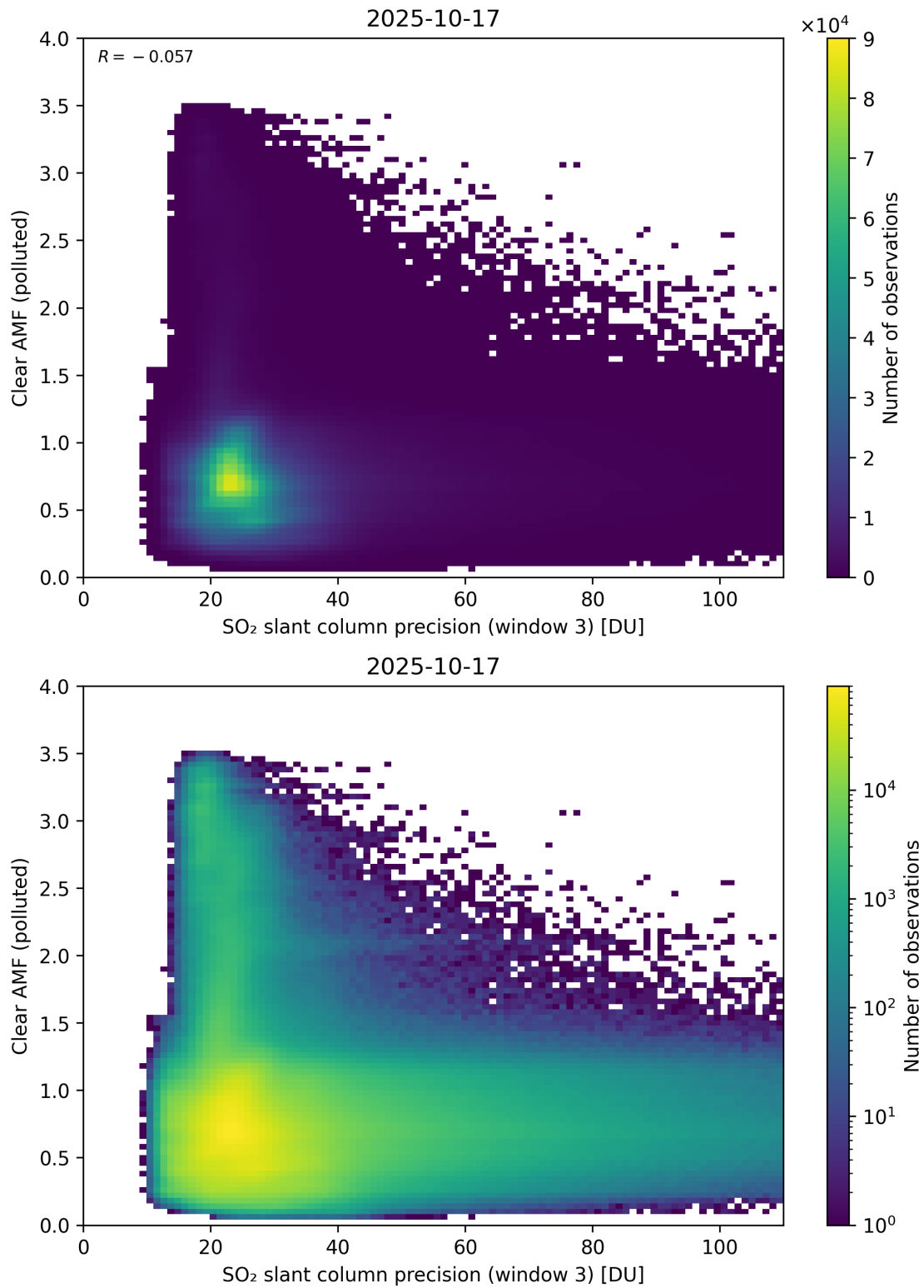
Figure 311: Scatter density plot of “SO 2 slant column precision (window 3)” against “Clear AMF (polluted)” for 2025-10-17 to 2025-10-18.
