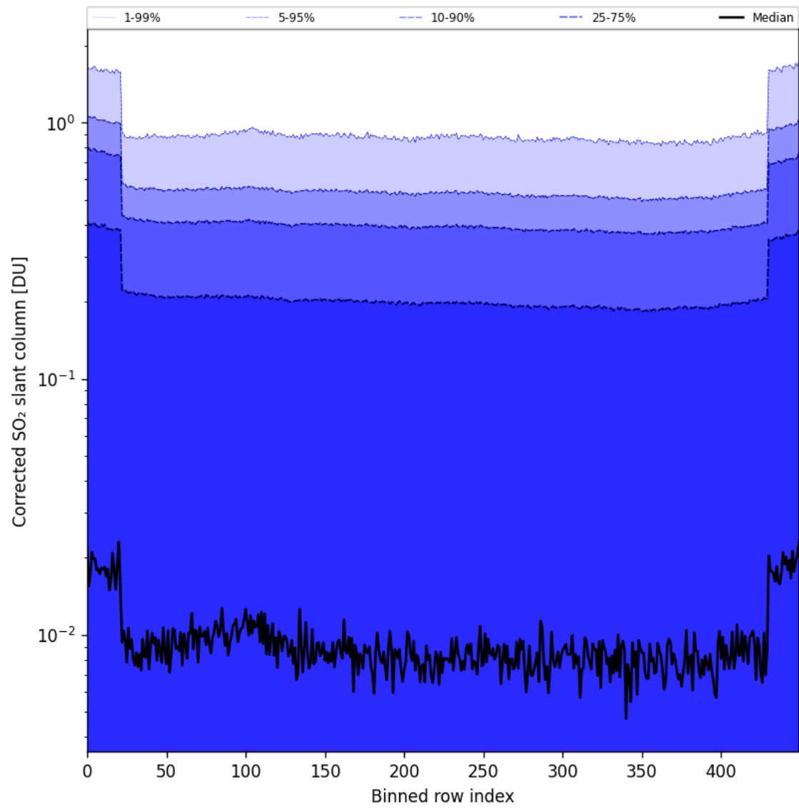
Figure 86: Along track statistics of “Corrected SO 2 slant column” for 2025-10-17 to 2025-10-18
