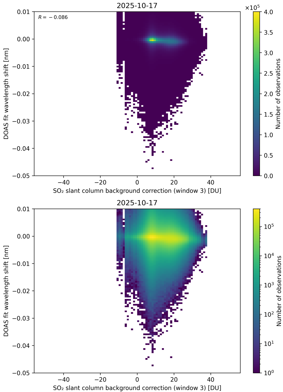
Figure 132: Scatter density plot of “SO 2 slant column background correction (window 3)” against “DOAS fit wavelength shift” for 2025-10-17 to 2025-10-18.
