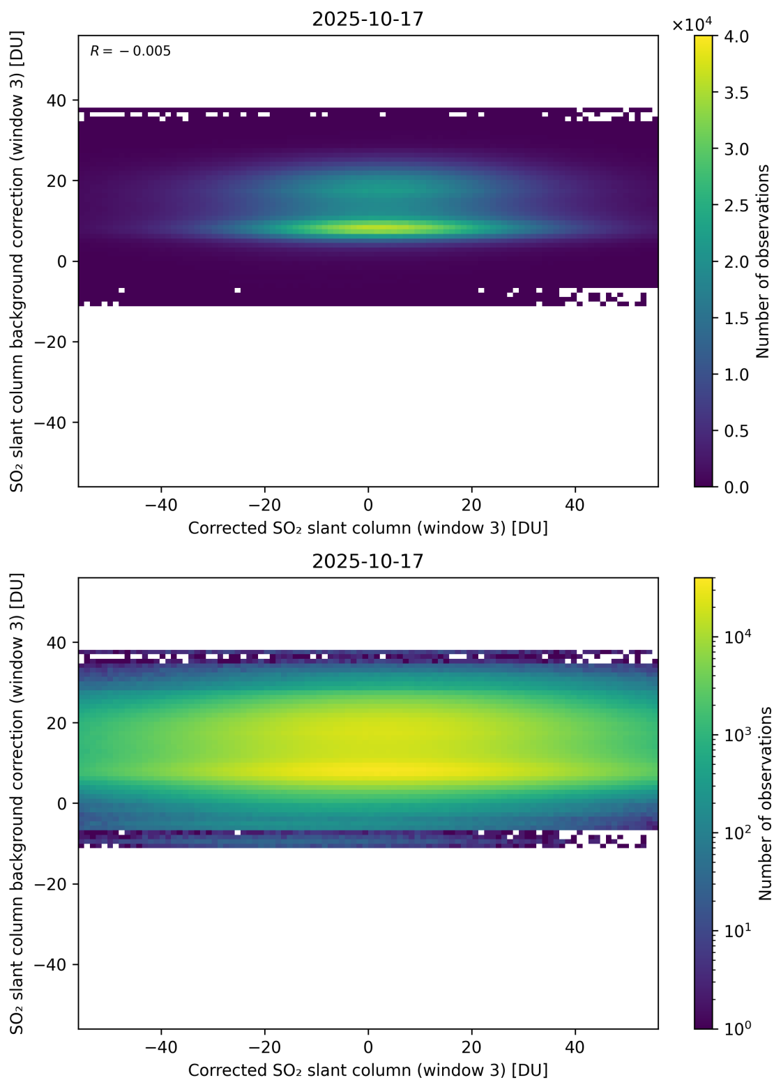
Figure 255: Scatter density plot of “Corrected SO 2 slant column (window 3)” against “SO 2 slant column background correction (window 3)” for 2025-10-17 to 2025-10-18.
