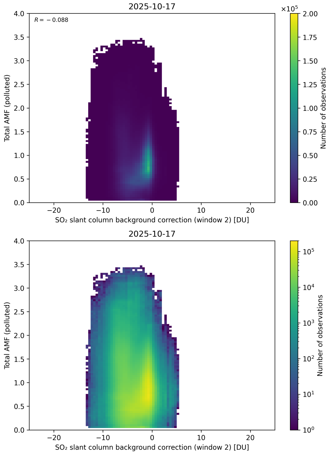
Figure 130: Scatter density plot of “SO 2 slant column background correction (window 2)” against “Total AMF (polluted)” for 2025-10-17 to 2025-10-18.
