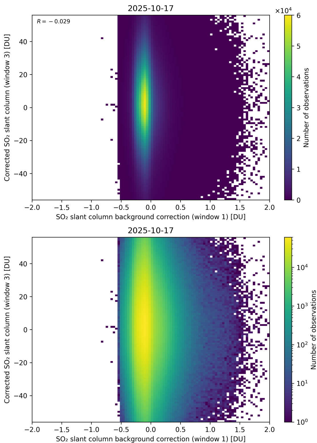
Figure 116: Scatter density plot of “SO 2 slant column background correction (window 1)” against “Corrected SO 2 slant column (window 3)” for 2025-10-17 to 2025-10-18.
