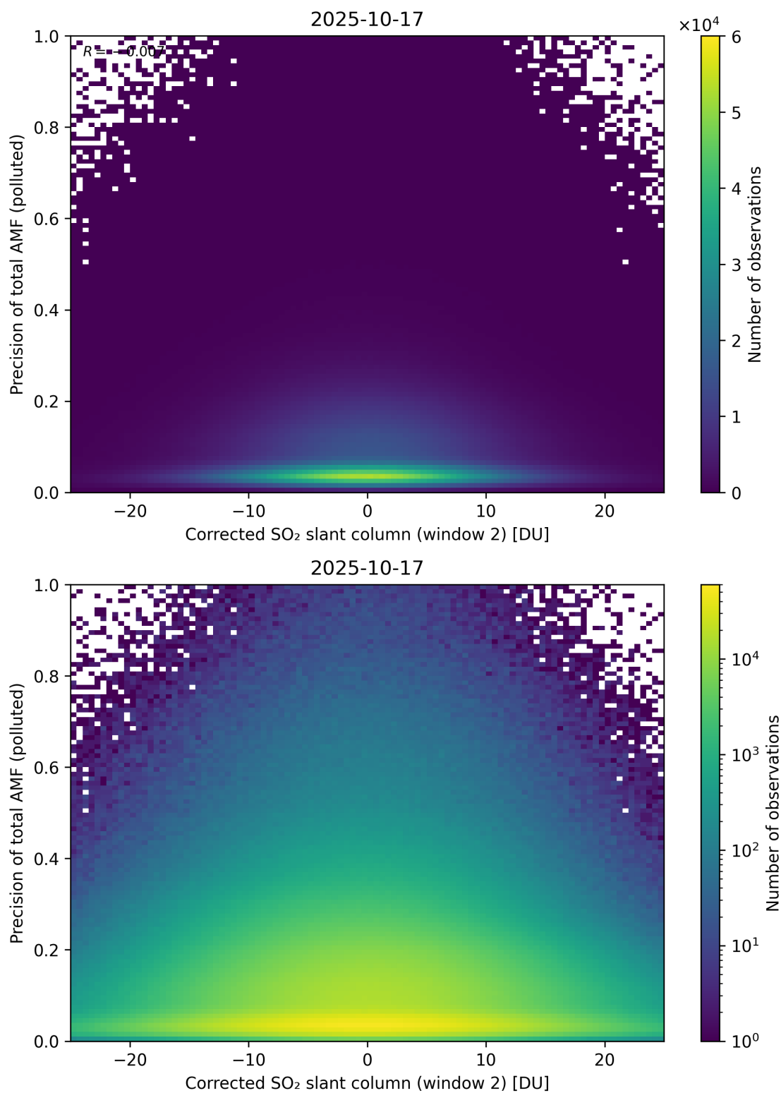
Figure 254: Scatter density plot of “Corrected SO 2 slant column (window 2)” against “Precision of total AMF (polluted)” for 2025-10-17 to 2025-10-18.
