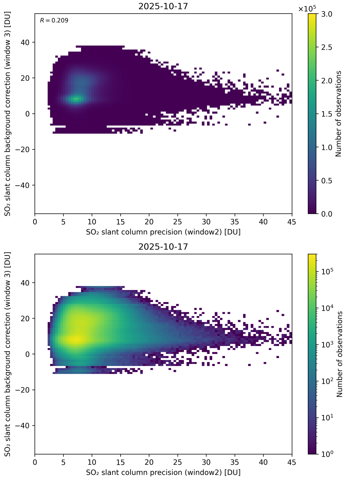
Figure 292: Scatter density plot of “SO 2 slant column precision (window2)” against “SO 2 slant column background correction (window 3)” for 2025-10-17 to 2025-10-18.
