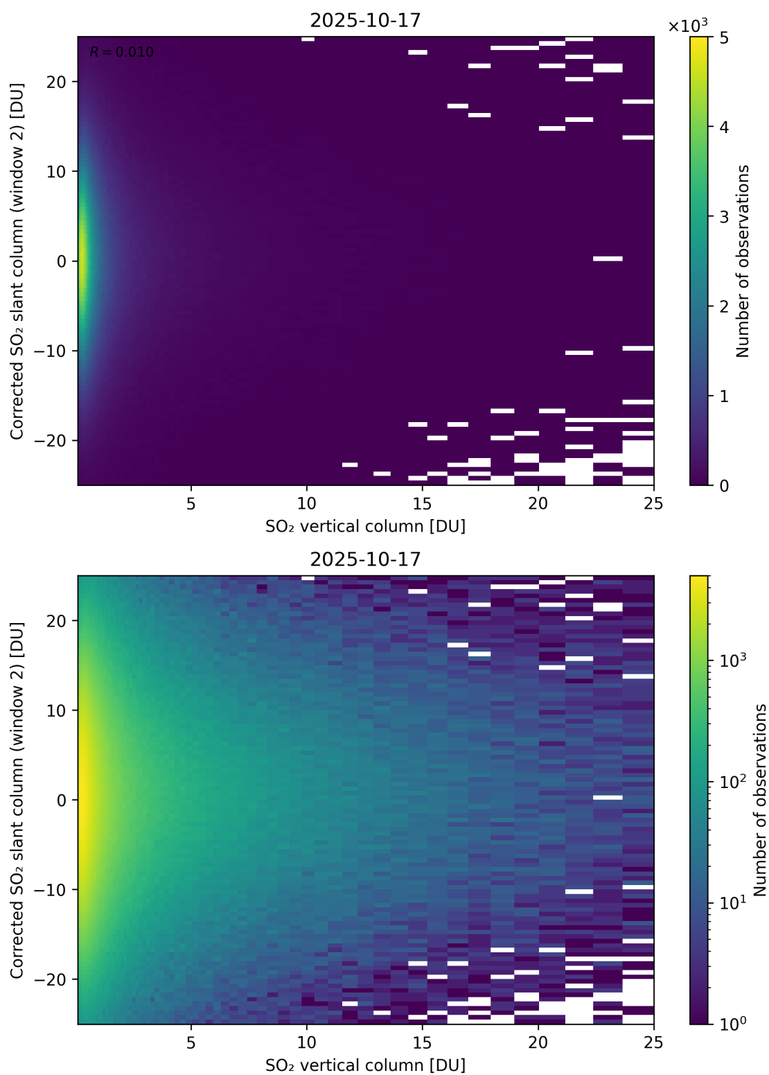
Figure 352: Scatter density plot of “SO 2 vertical column” against “Corrected SO 2 slant column (window 2)” for 2025-10-17 to 2025-10-18.
