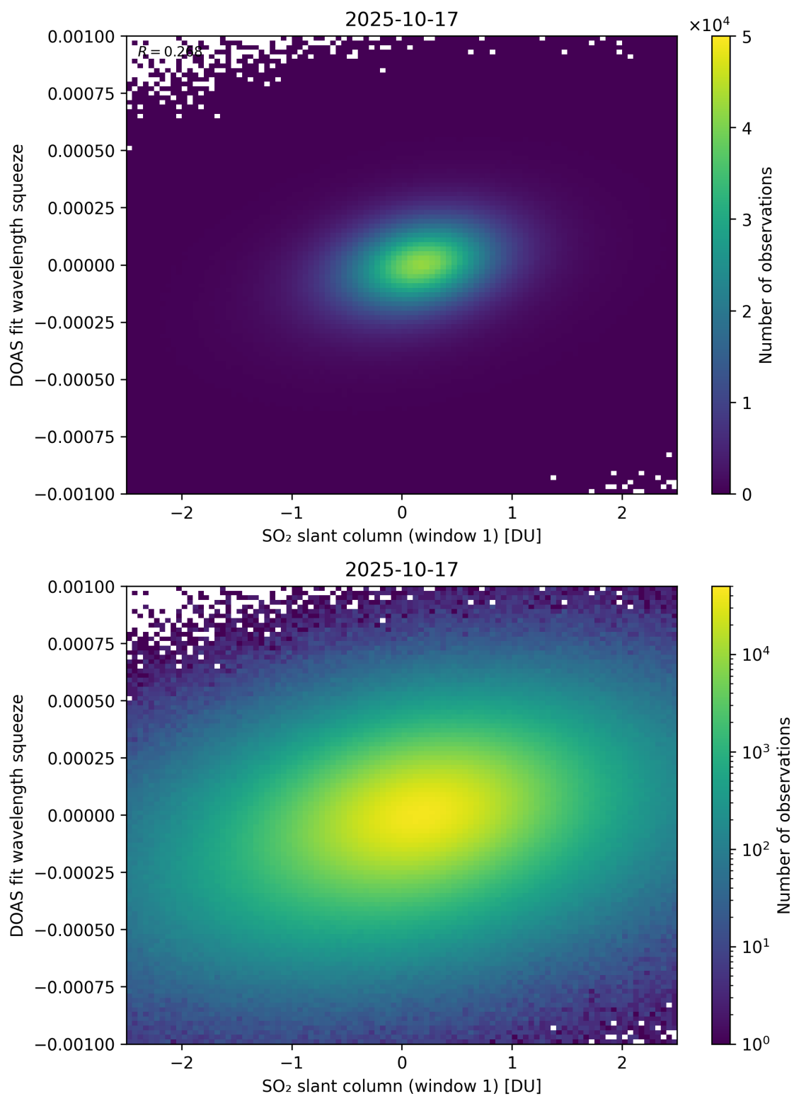
Figure 266: Scatter density plot of “SO 2 slant column (window 1)” against “DOAS fit wavelength squeeze” for 2025-10-17 to 2025-10-18.
