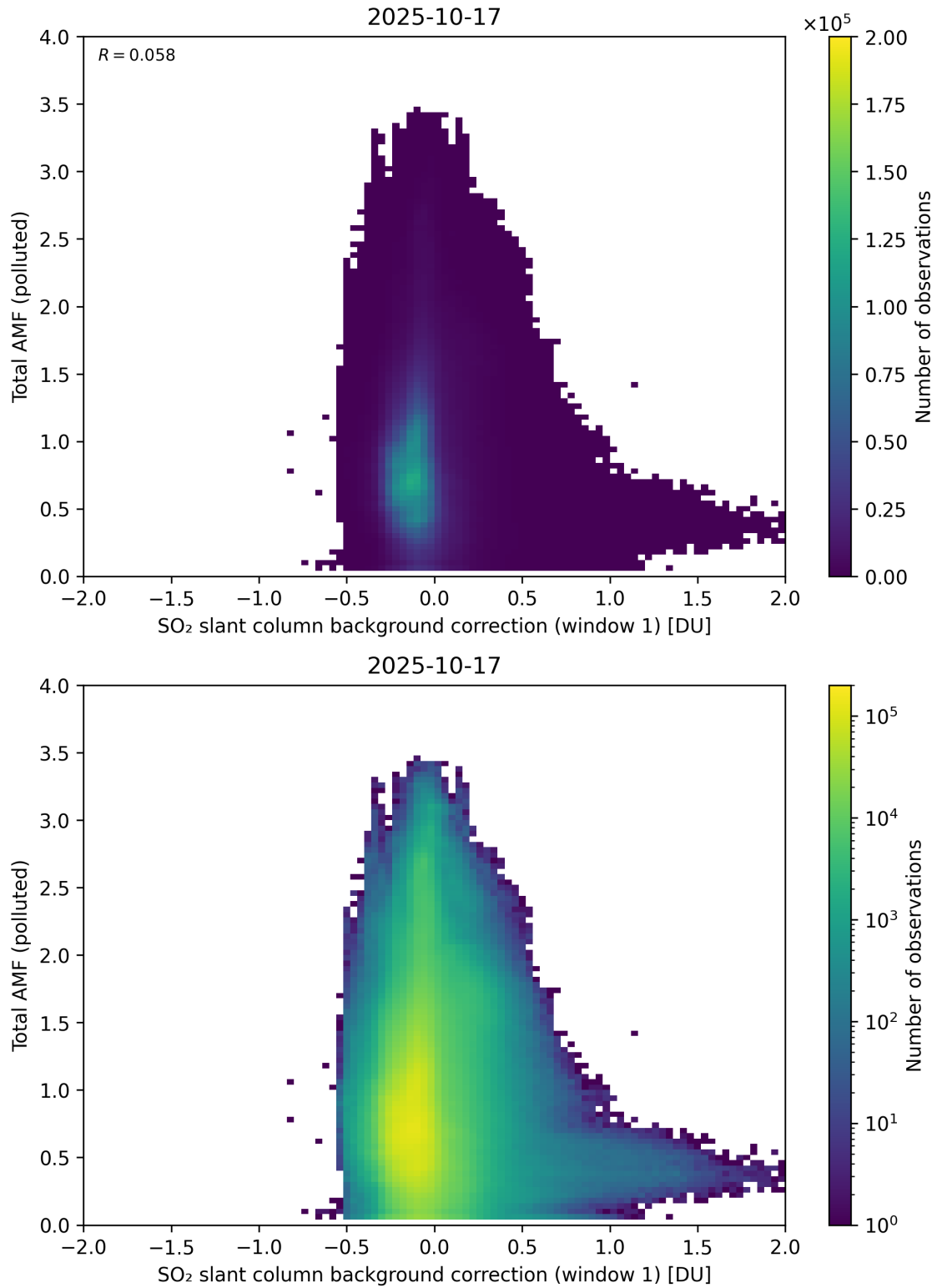
Figure 120: Scatter density plot of “SO 2 slant column background correction (window 1)” against “Total AMF (polluted)” for 2025-10-17 to 2025-10-18.
