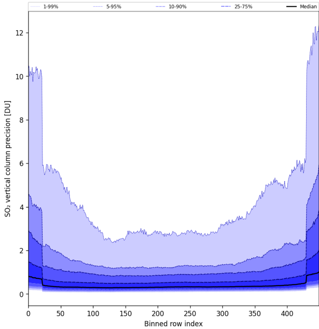
Figure 85: Along track statistics of “SO 2 vertical column precision” for 2025-10-17 to 2025-10-18
