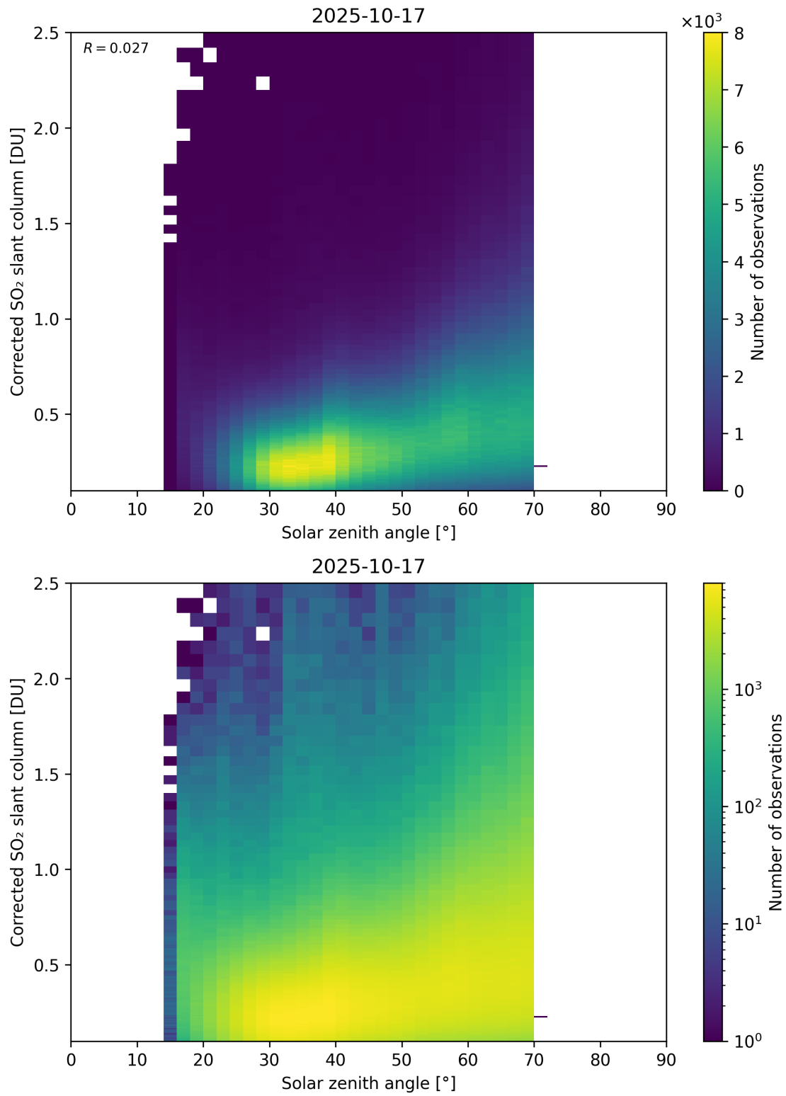
Figure 181: Scatter density plot of “Solar zenith angle” against “Corrected SO 2 slant column” for 2025-10-17 to 2025-10-18.
