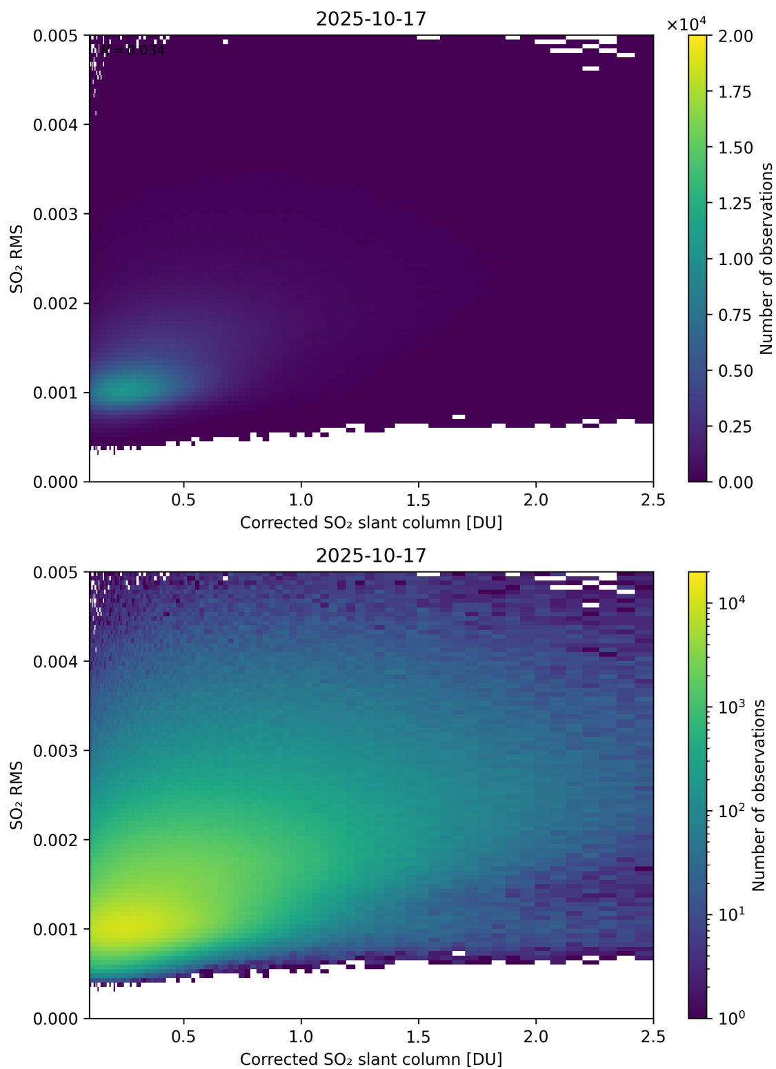
Figure 231: Scatter density plot of “Corrected SO 2 slant column” against “SO 2 RMS” for 2025-10-17 to 2025-10-18.
