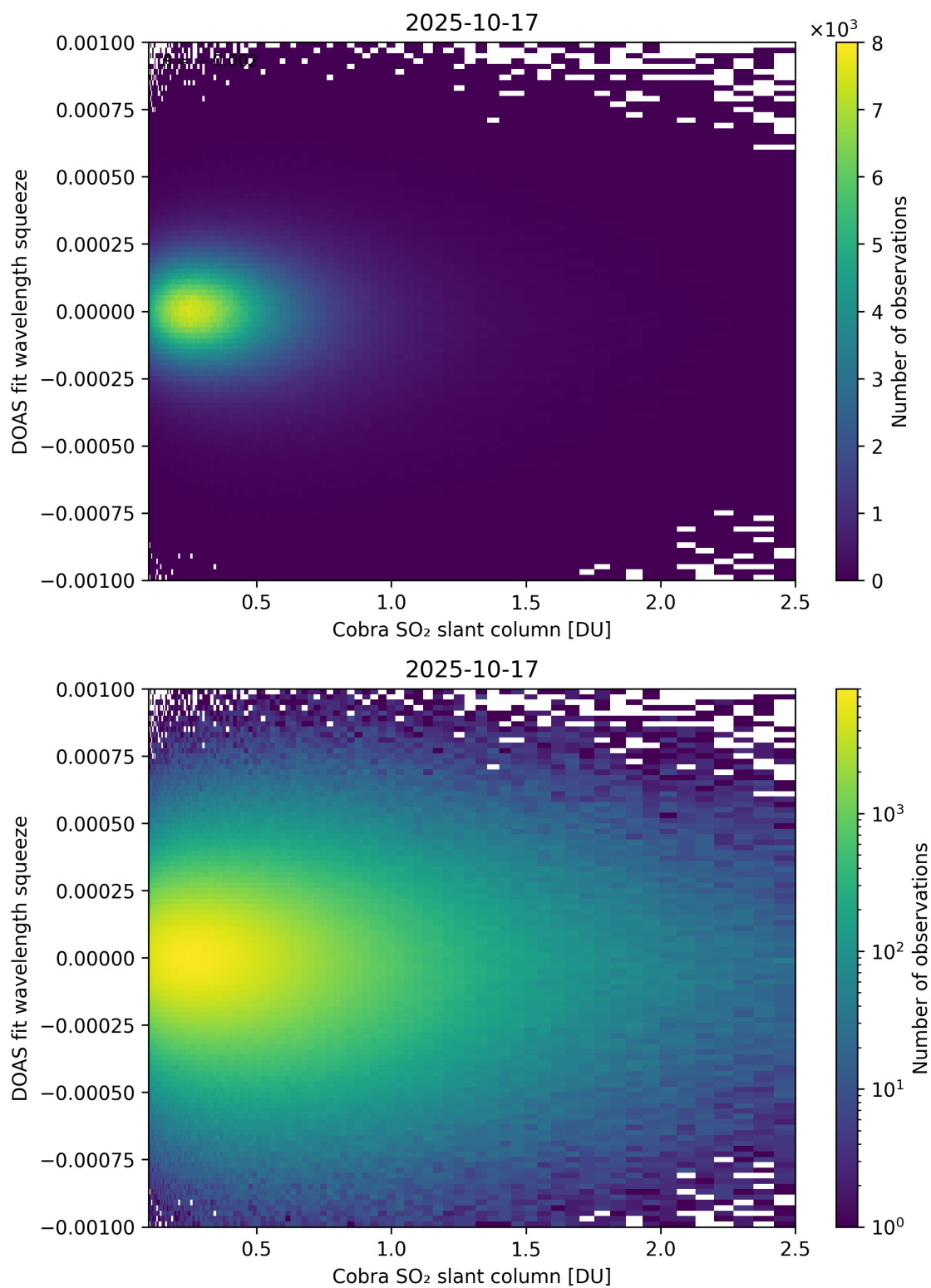
Figure 197: Scatter density plot of “Cobra SO 2 slant column” against “DOAS fit wavelength squeeze” for 2025-10-17 to 2025-10-18.
