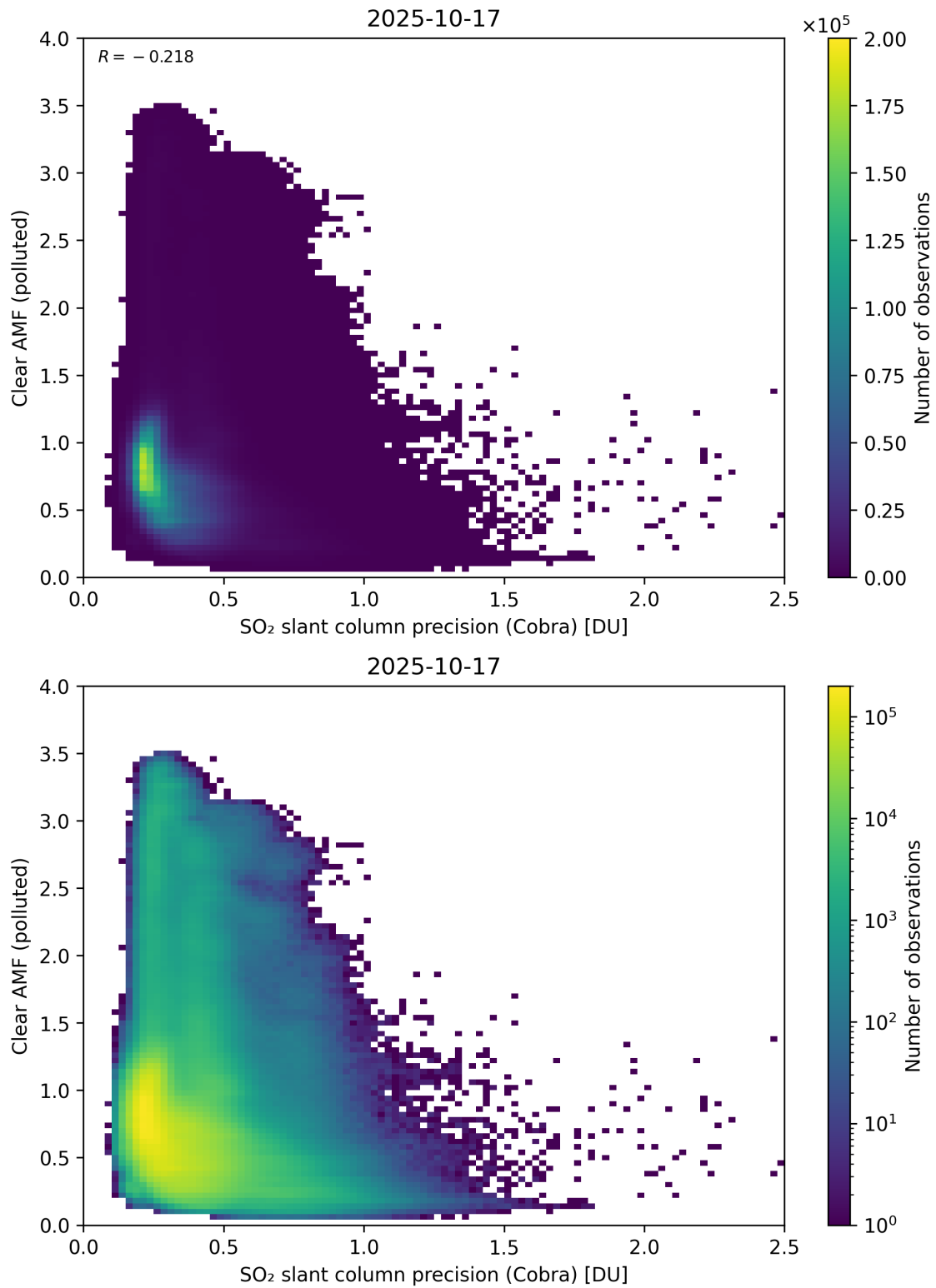
Figure 205: Scatter density plot of “SO 2 slant column precision (Cobra)” against “Clear AMF (polluted)” for 2025-10-17 to 2025-10-18.
