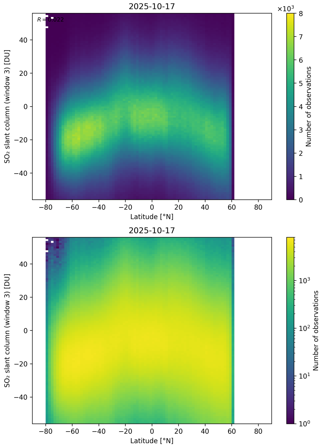
Figure 165: Scatter density plot of “Latitude” against “SO 2 slant column (window 3)” for 2025-10-17 to 2025-10-18.
