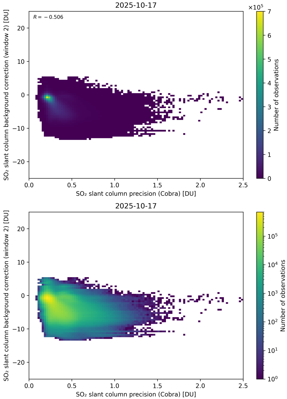
Figure 200: Scatter density plot of “SO 2 slant column precision (Cobra)” against “SO 2 slant column background correction (window 2)” for 2025-10-17 to 2025-10-18.
