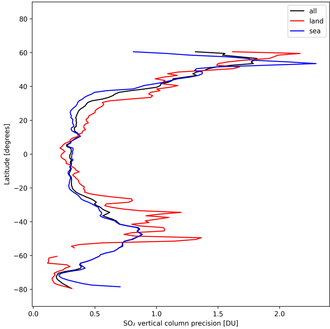
Figure 33: Zonal average of “SO 2 vertical column precision” for 2025-10-17 to 2025-10-18.
