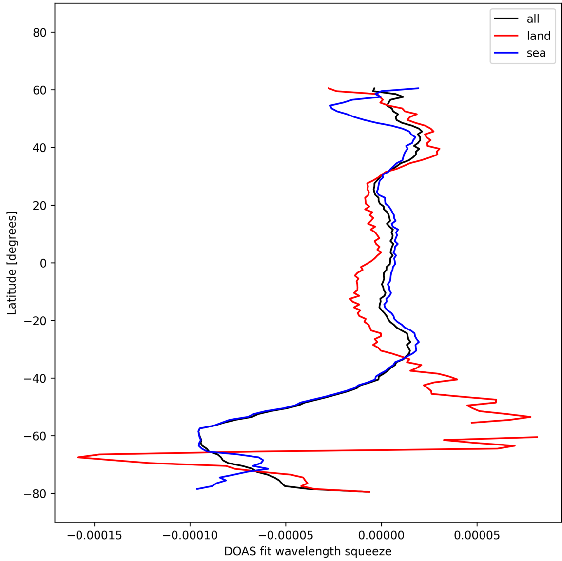
Figure 51: Zonal average of “DOAS fit wavelength squeeze” for 2025-10-17 to 2025-10-18.
