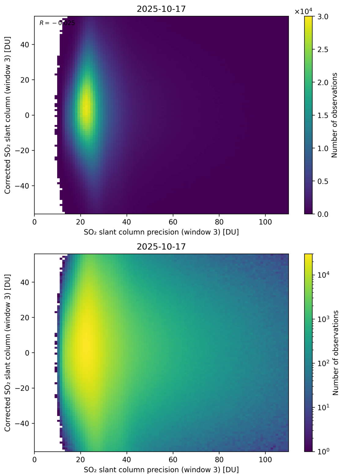
Figure 312: Scatter density plot of “SO 2 slant column precision (window 3)” against “Corrected SO 2 slant column (window 3)” for 2025-10-17 to 2025-10-18.
