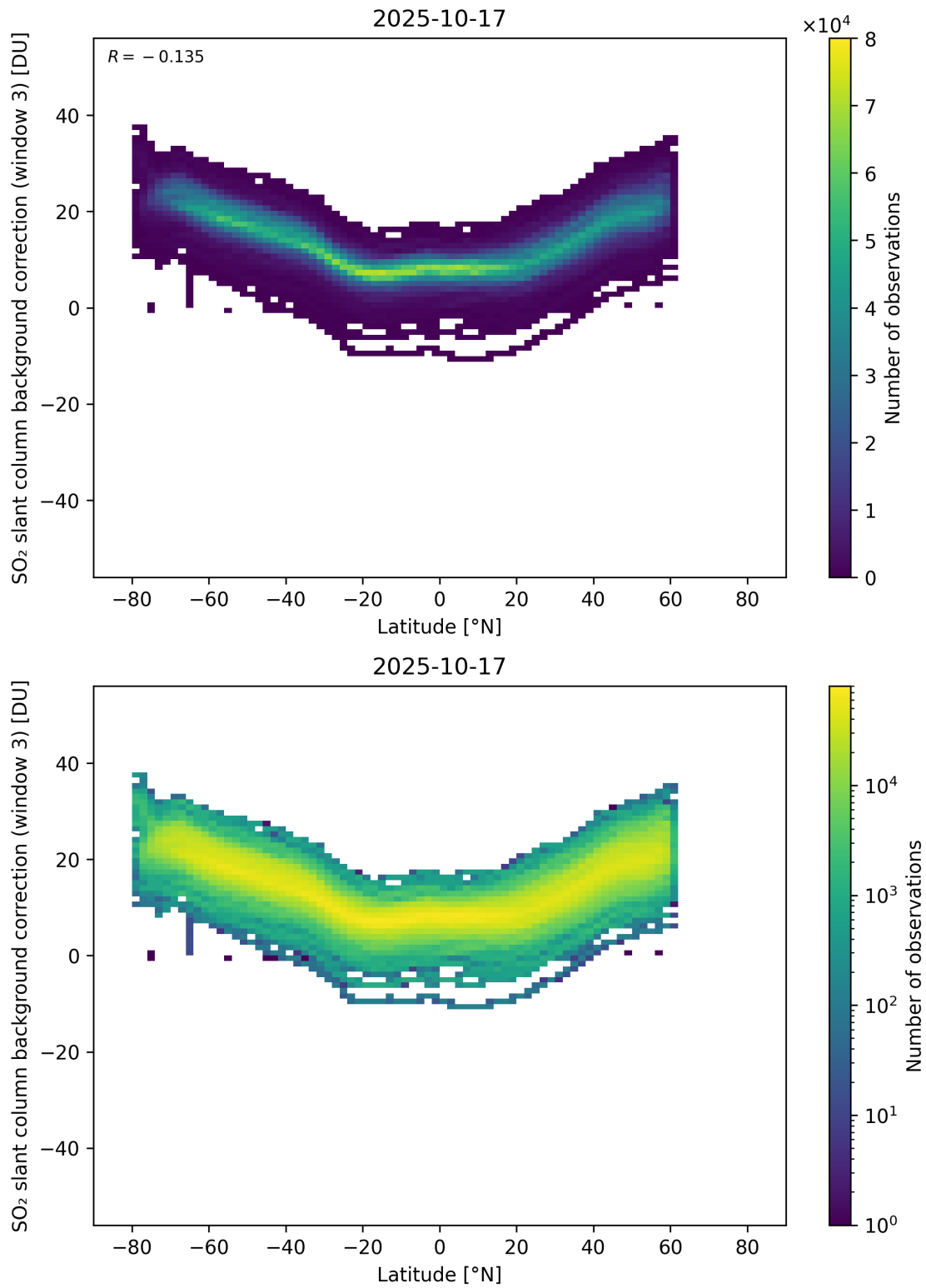
Figure 152: Scatter density plot of “Latitude” against “SO 2 slant column background correction (window 3)” for 2025-10-17 to 2025-10-18.
