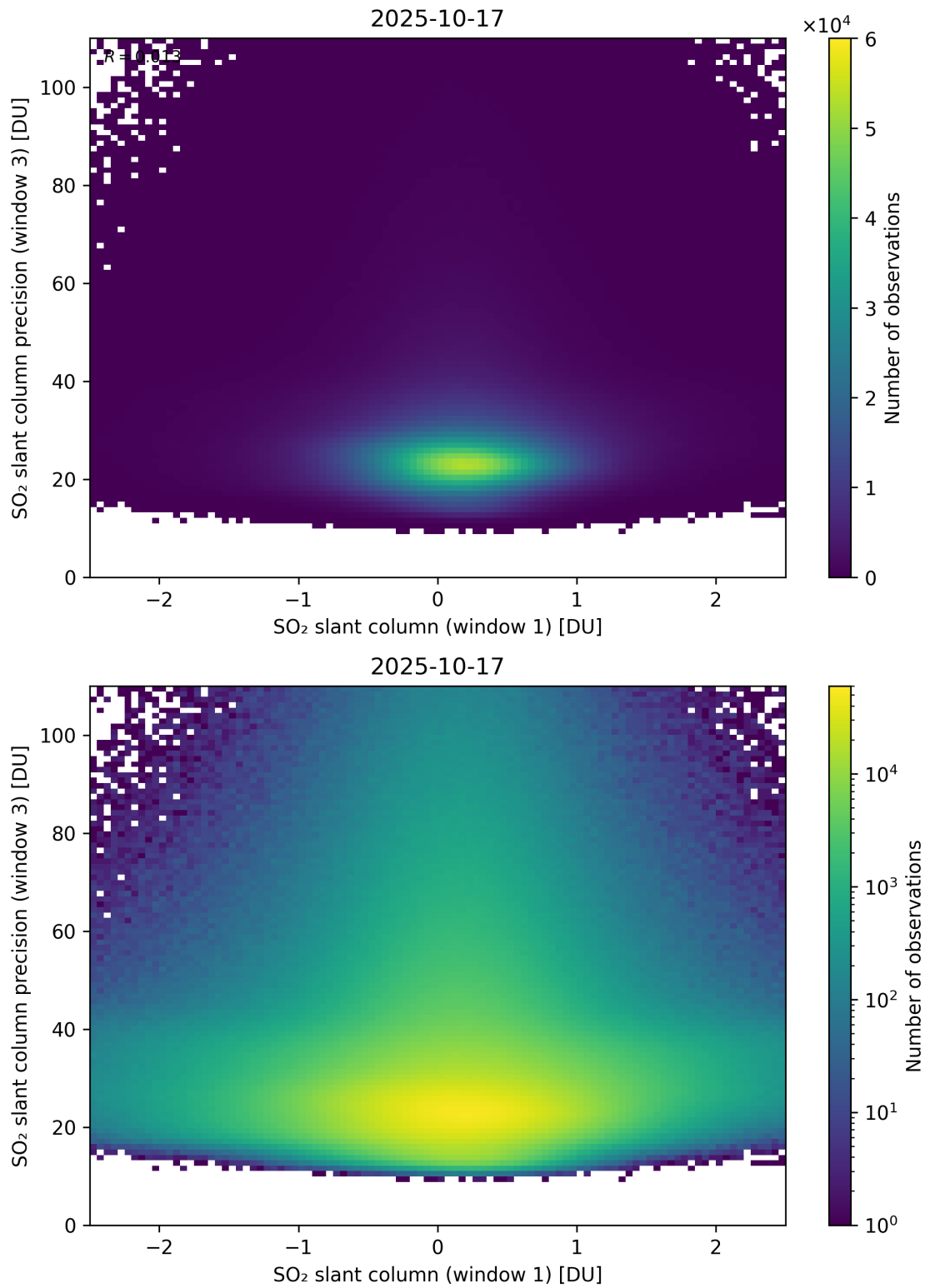
Figure 288: Scatter density plot of “SO 2 slant column (window 1)” against “SO 2 slant column precision (window 3)” for 2025-10-17 to 2025-10-18.
