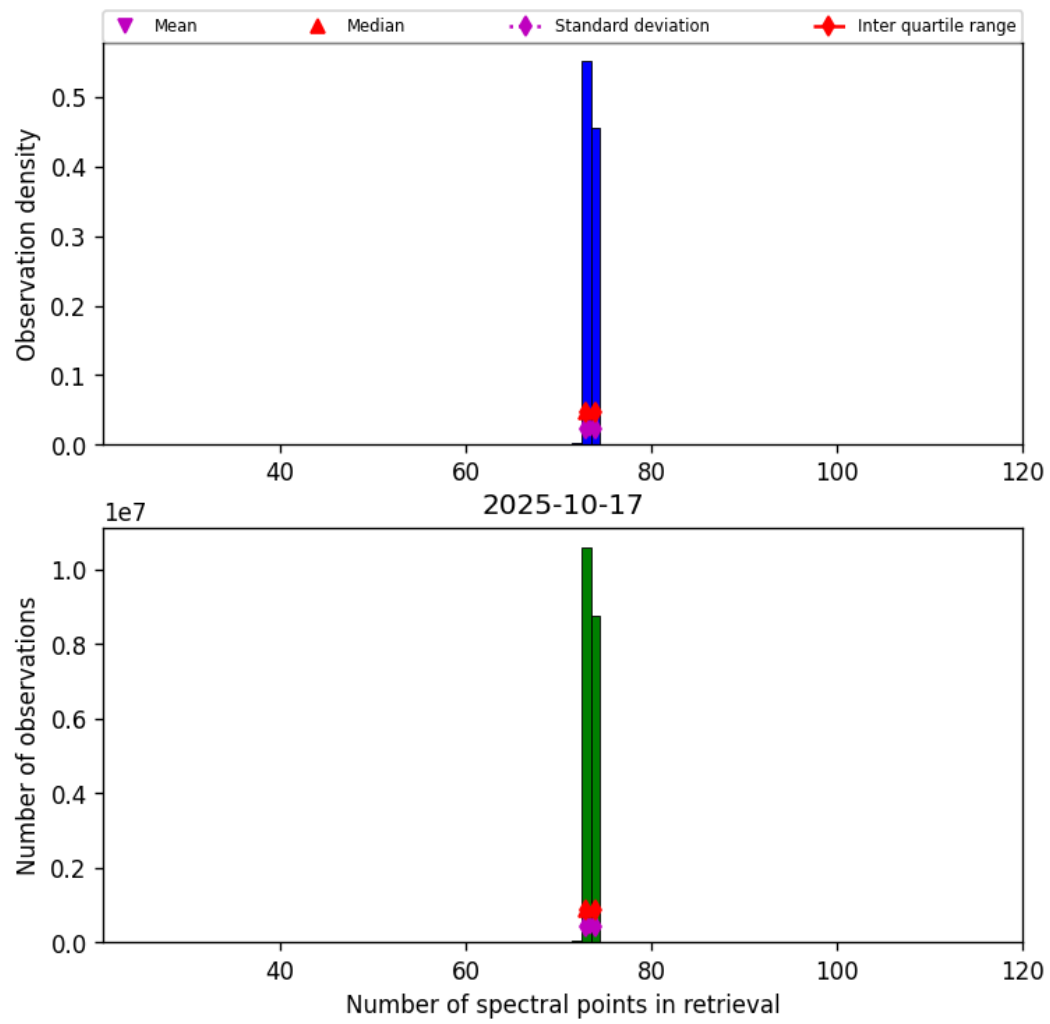
Figure 82: Histogram of “Number of spectral points in retrieval” for 2025-10-17 to 2025-10-18
