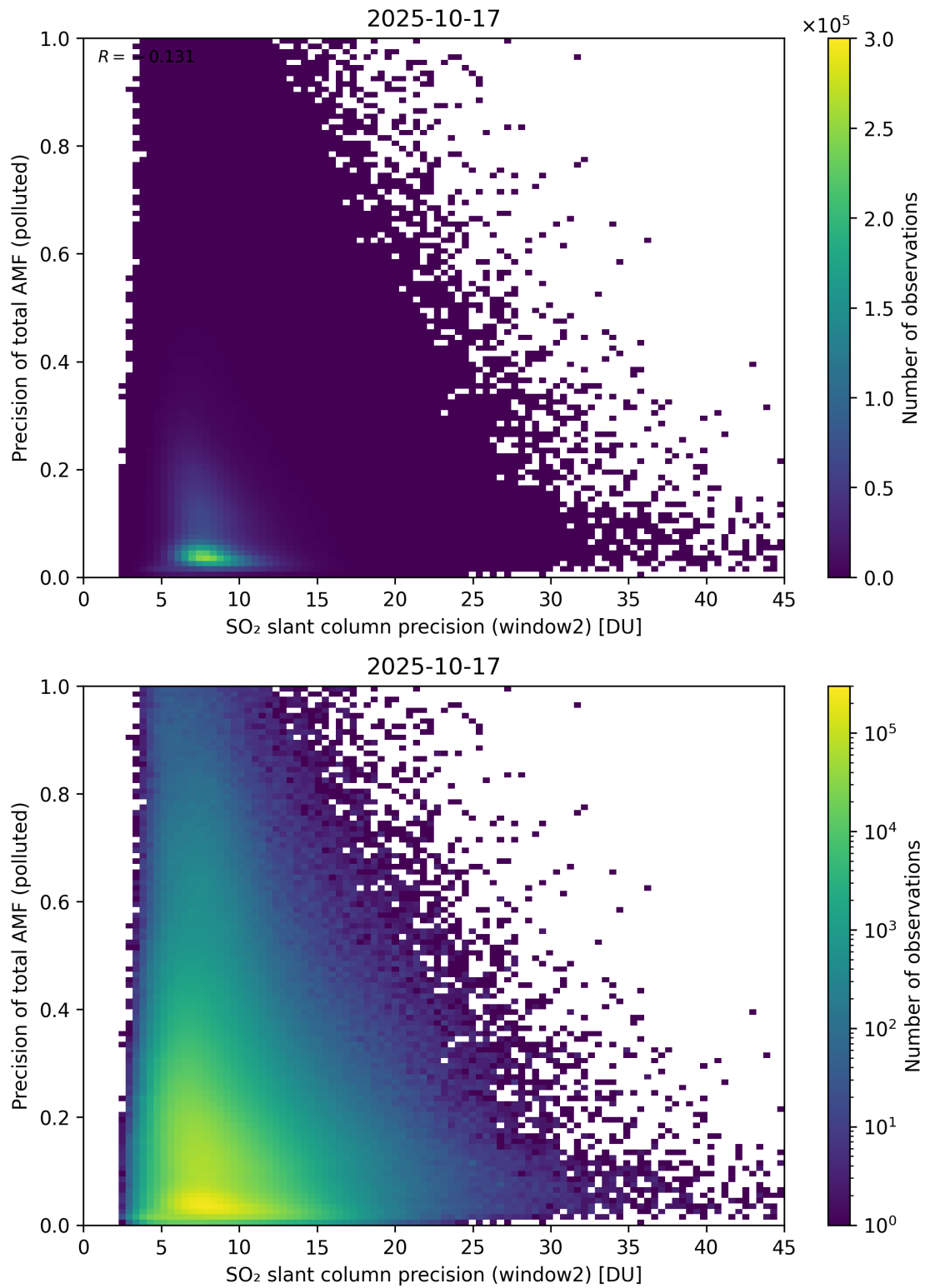
Figure 302: Scatter density plot of “SO 2 slant column precision (window2)” against “Precision of total AMF (polluted)” for 2025-10-17 to 2025-10-18.
