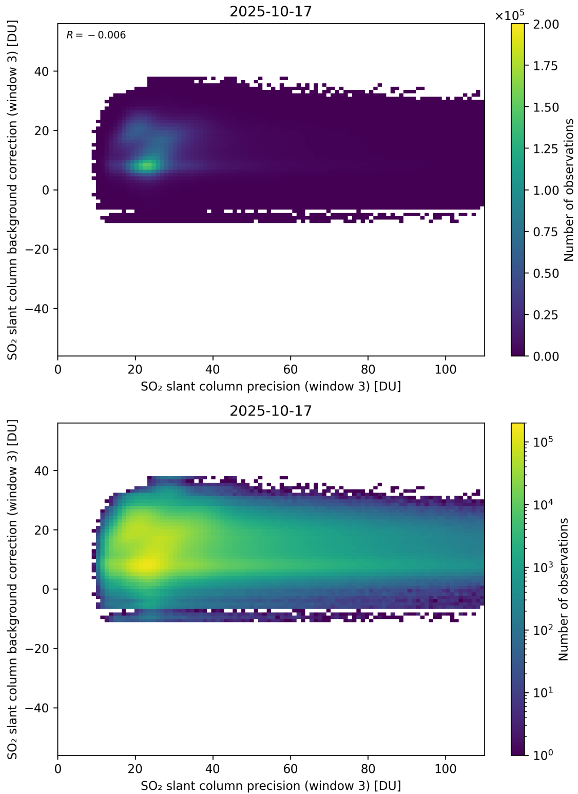
Figure 307: Scatter density plot of “SO 2 slant column precision (window 3)” against “SO 2 slant column background correction (window 3)” for 2025-10-17 to 2025-10-18.
