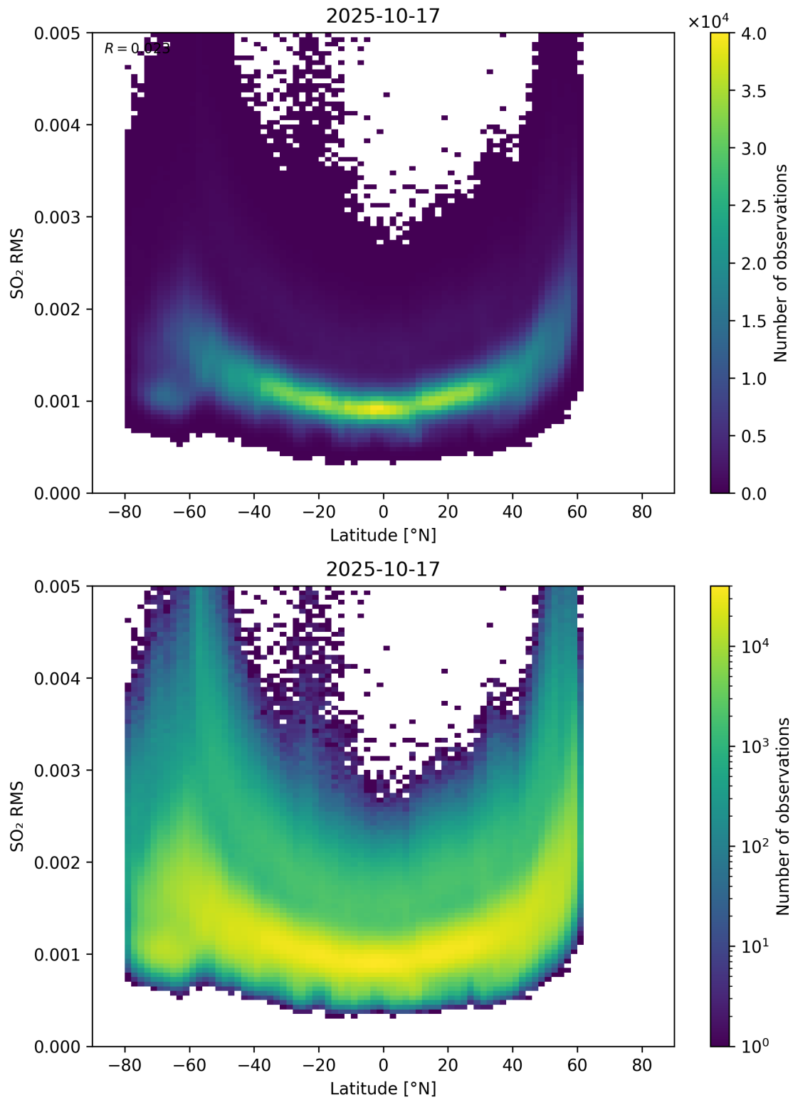
Figure 155: Scatter density plot of “Latitude” against “SO 2 RMS” for 2025-10-17 to 2025-10-18.
