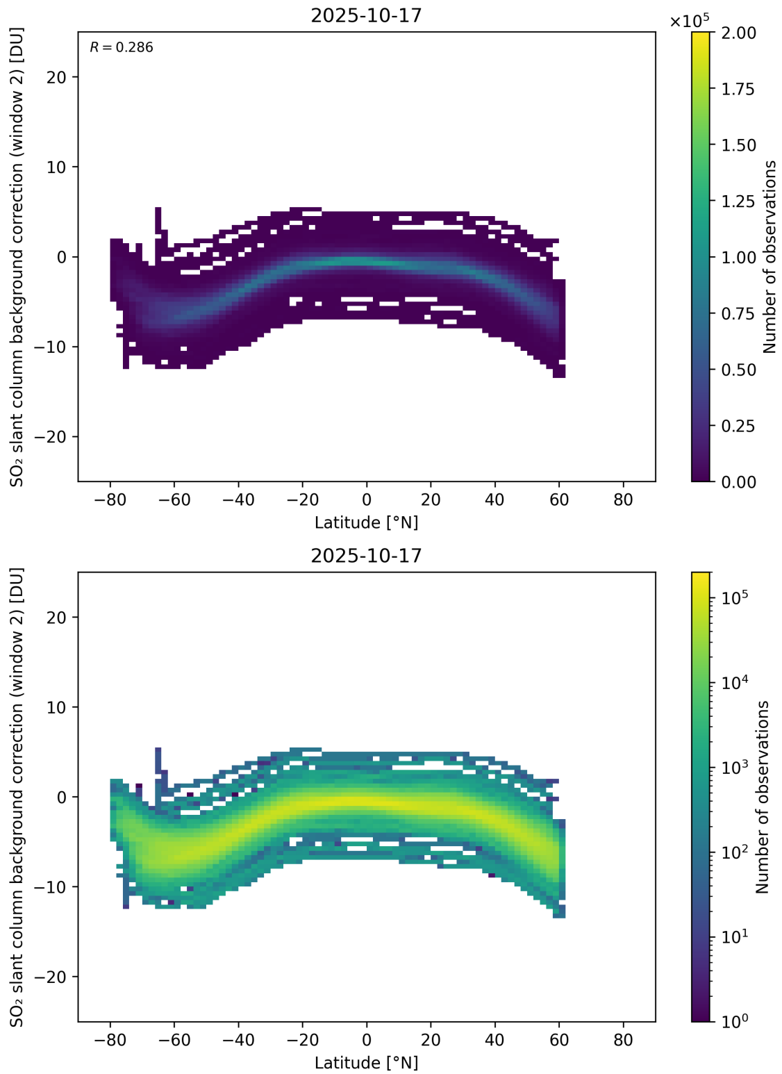
Figure 151: Scatter density plot of “Latitude” against “SO 2 slant column background correction (window 2)” for 2025-10-17 to 2025-10-18.
