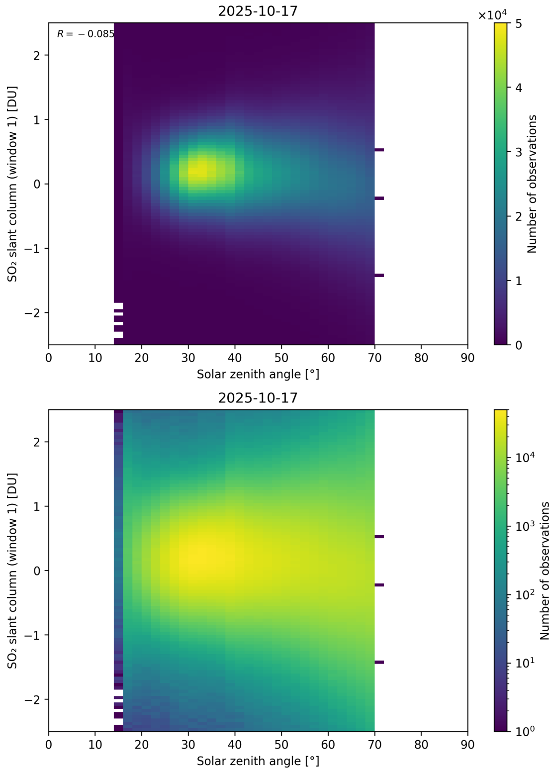
Figure 184: Scatter density plot of “Solar zenith angle” against “SO 2 slant column (window 1)” for 2025-10-17 to 2025-10-18.
