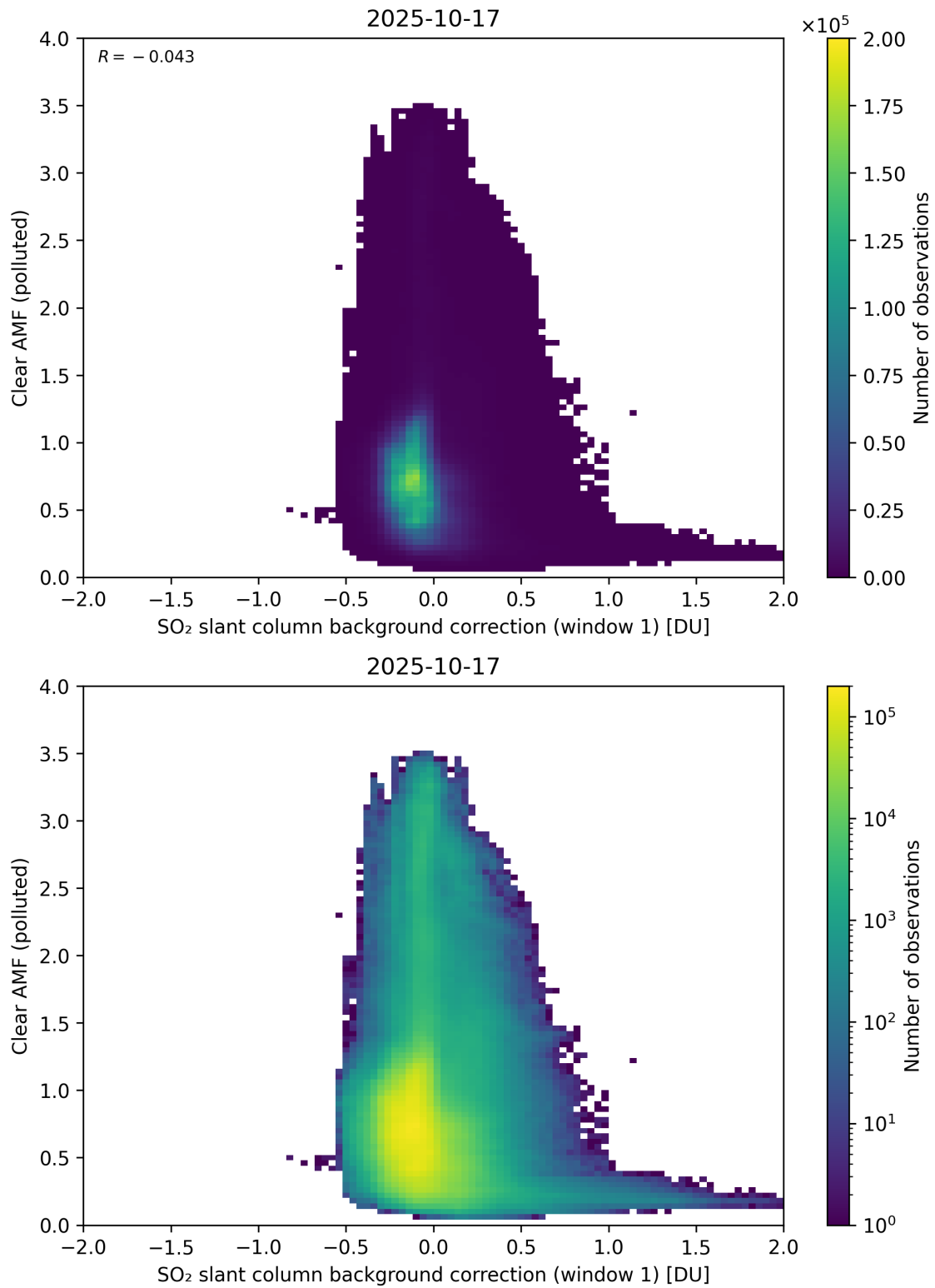
Figure 114: Scatter density plot of “SO 2 slant column background correction (window 1)” against “Clear AMF (polluted)” for 2025-10-17 to 2025-10-18.
