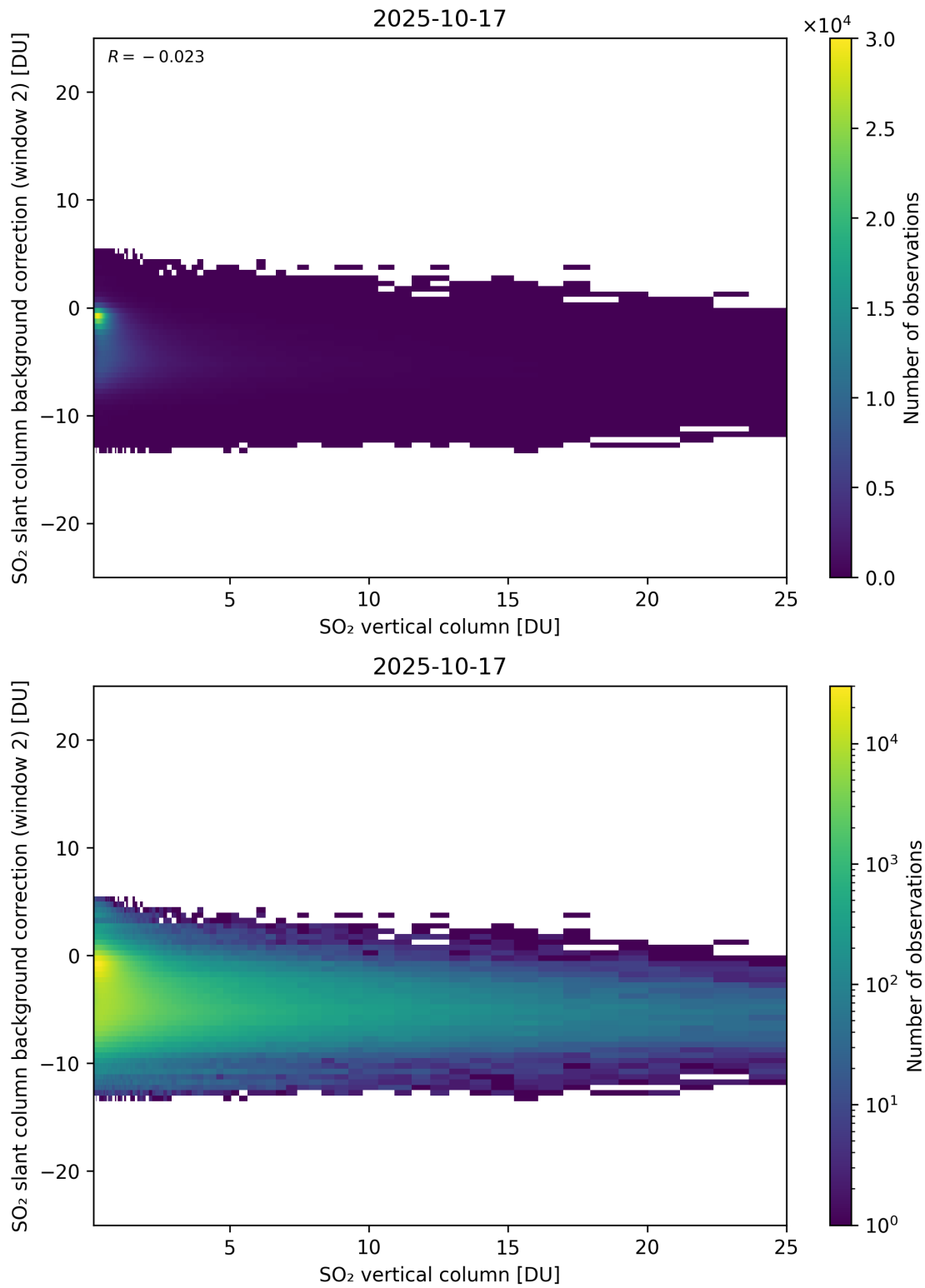
Figure 324: Scatter density plot of “SO 2 vertical column” against “SO 2 slant column background correction (window 2)” for 2025-10-17 to 2025-10-18.
