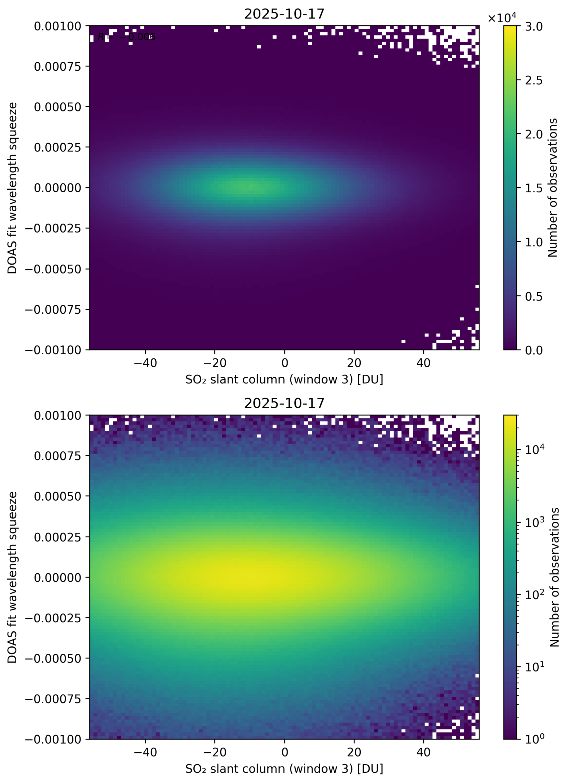
Figure 305: Scatter density plot of “SO 2 slant column (window 3)” against “DOAS fit wavelength squeeze” for 2025-10-17 to 2025-10-18.
