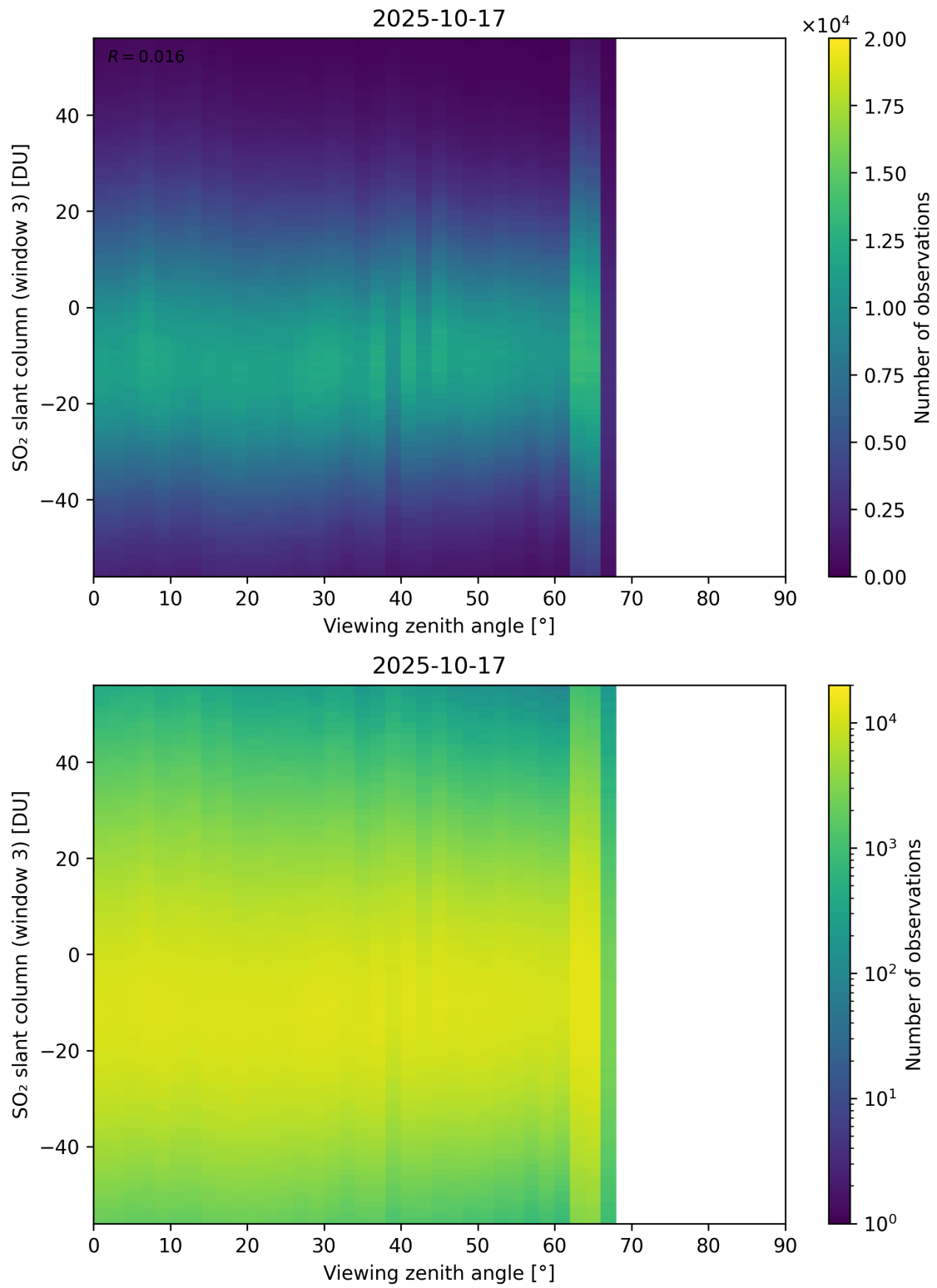
Figure 379: Scatter density plot of “Viewing zenith angle” against “SO 2 slant column (window 3)” for 2025-10-17 to 2025-10-18.
