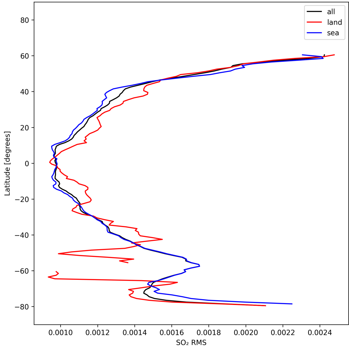
Figure 52: Zonal average of “SO 2 RMS” for 2025-10-17 to 2025-10-18.
