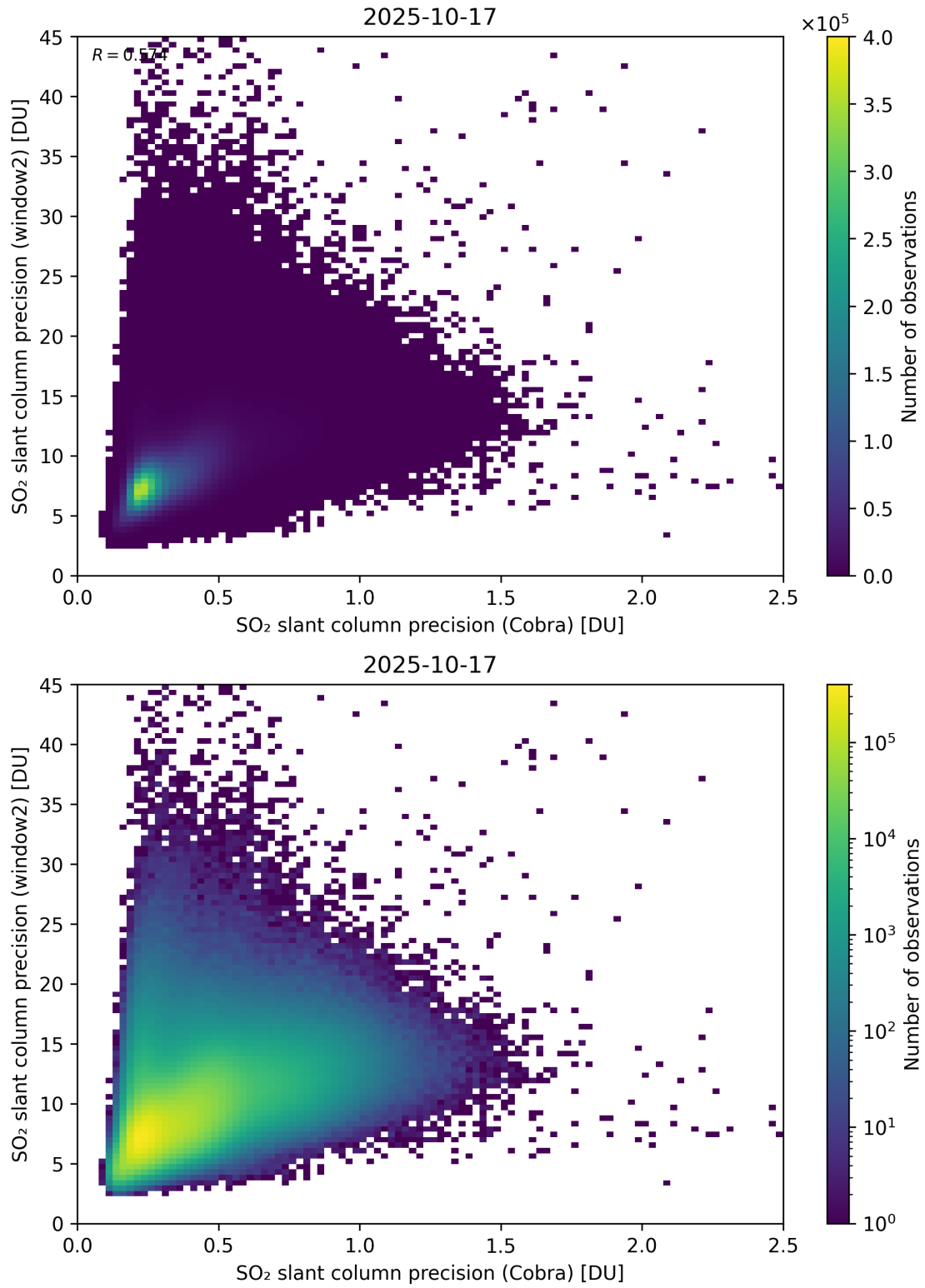
Figure 210: Scatter density plot of “SO 2 slant column precision (Cobra)” against “SO 2 slant column precision (window2)” for 2025-10-17 to 2025-10-18.
