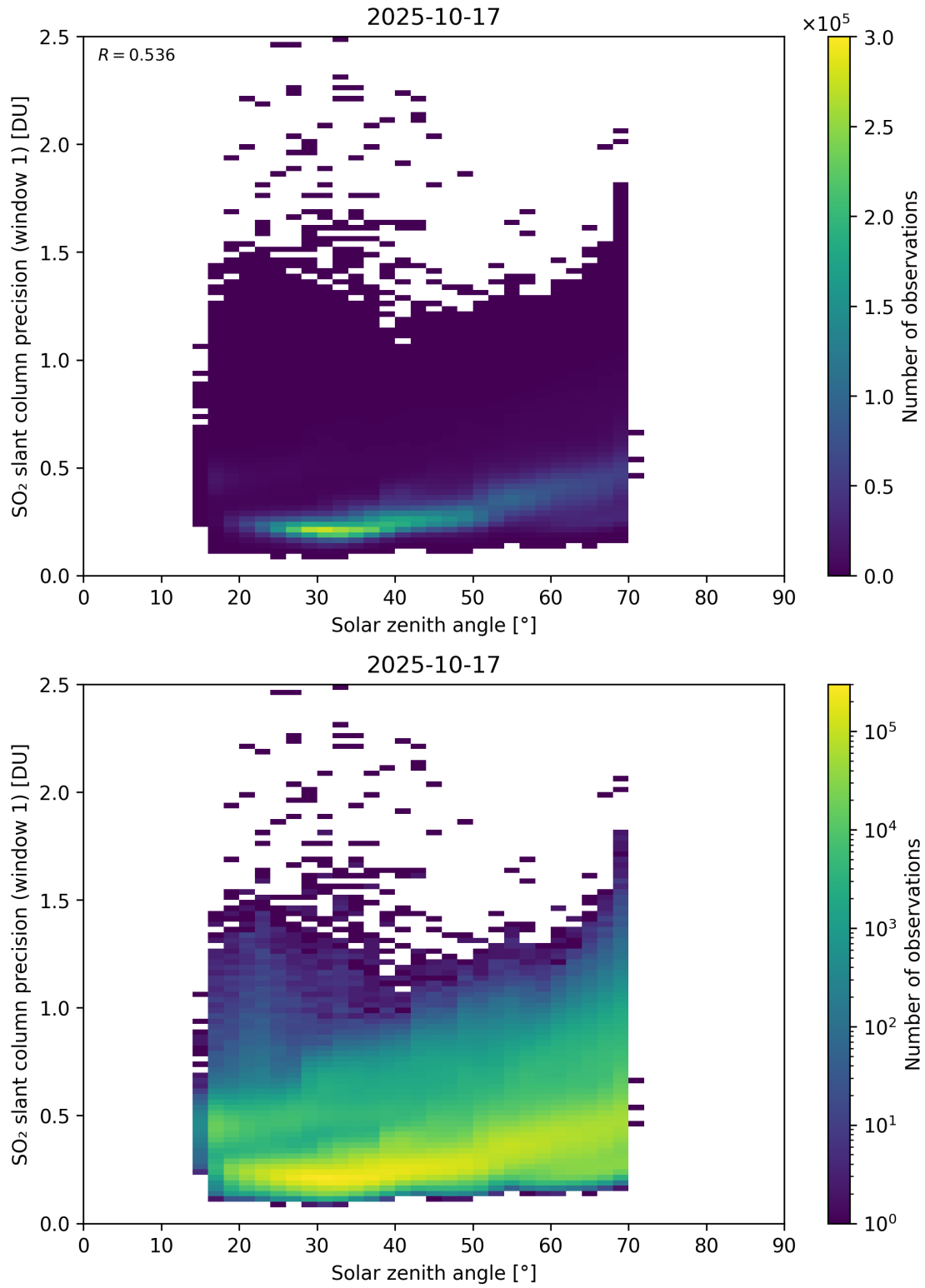
Figure 185: Scatter density plot of “Solar zenith angle” against “SO 2 slant column precision (window 1)” for 2025-10-17 to 2025-10-18.
