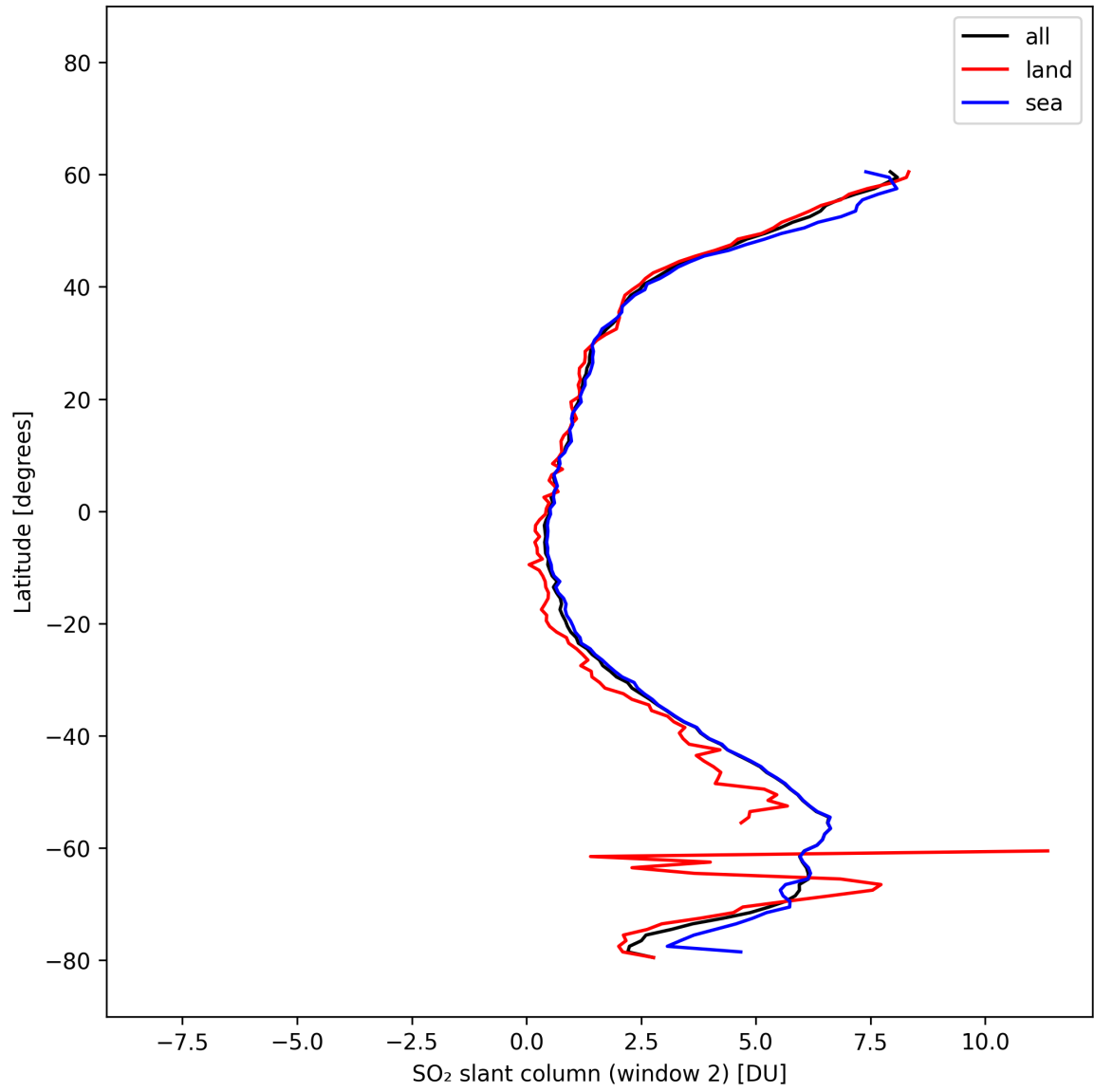
Figure 41: Zonal average of “SO 2 slant column (window 2)” for 2025-10-17 to 2025-10-18.
