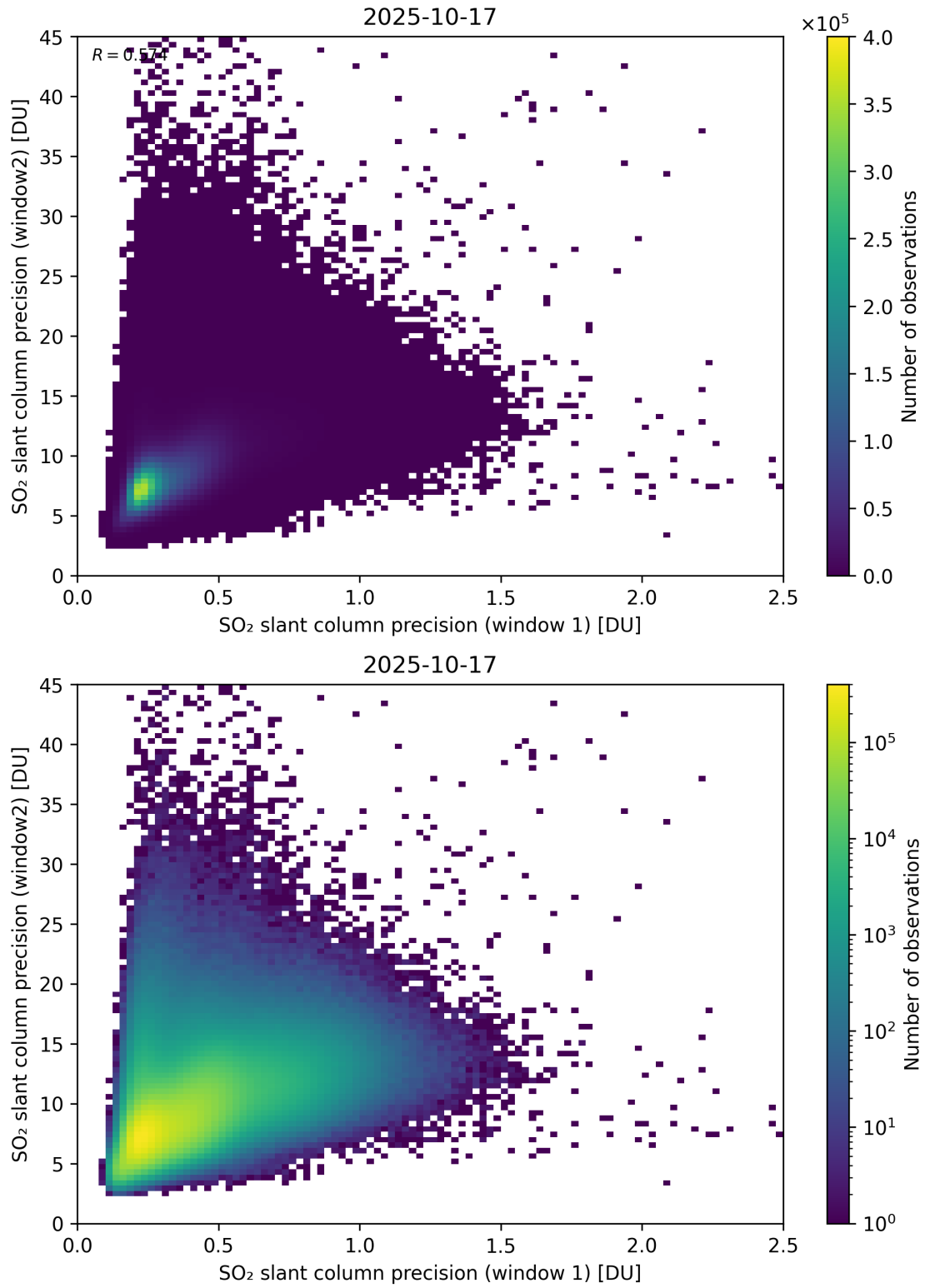
Figure 277: Scatter density plot of “SO 2 slant column precision (window 1)” against “SO 2 slant column precision (window2)” for 2025-10-17 to 2025-10-18.
