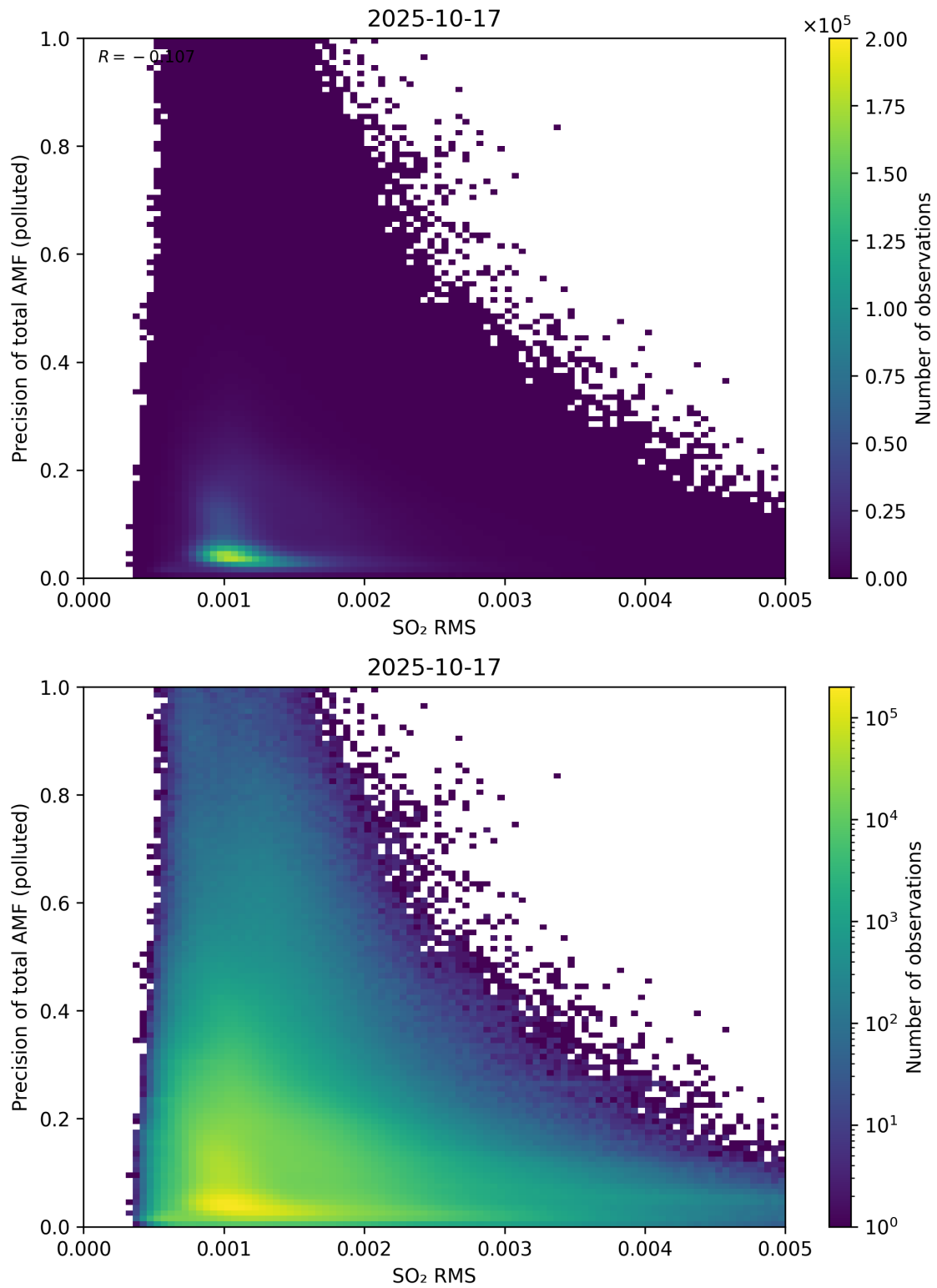
Figure 149: Scatter density plot of “SO 2 RMS” against “Precision of total AMF (polluted)” for 2025-10-17 to 2025-10-18.
