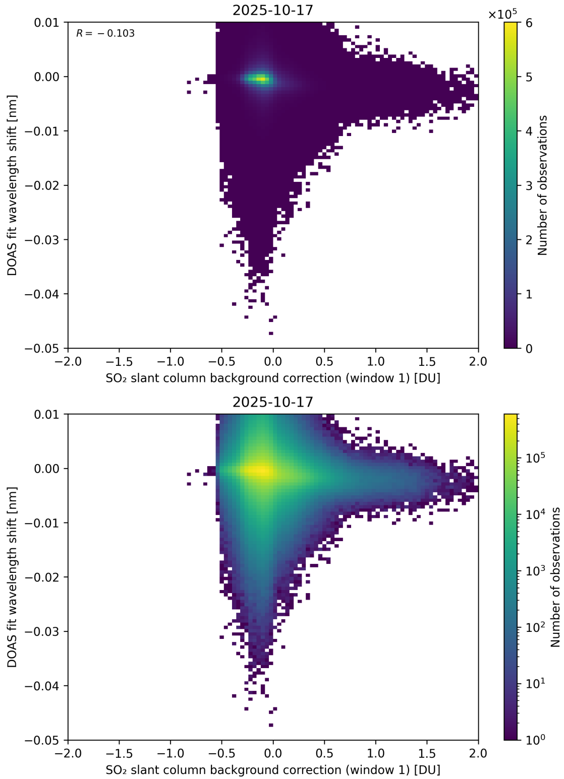
Figure 111: Scatter density plot of “SO 2 slant column background correction (window 1)” against “DOAS fit wavelength shift” for 2025-10-17 to 2025-10-18.
