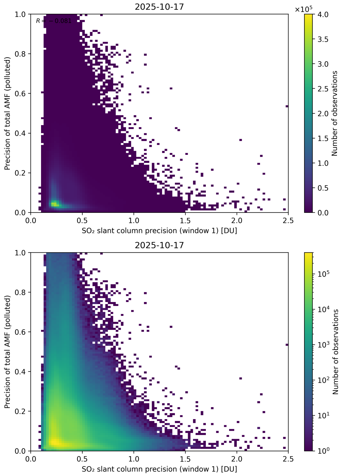
Figure 281: Scatter density plot of “SO 2 slant column precision (window 1)” against “Precision of total AMF (polluted)” for 2025-10-17 to 2025-10-18.
