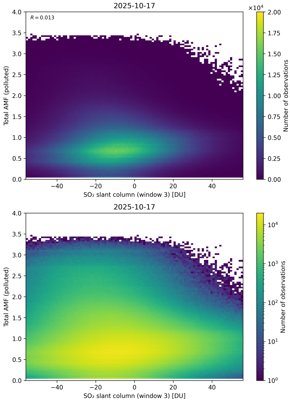
Figure 318: Scatter density plot of “SO 2 slant column (window 3)” against “Total AMF (polluted)” for 2025-10-17 to 2025-10-18.
