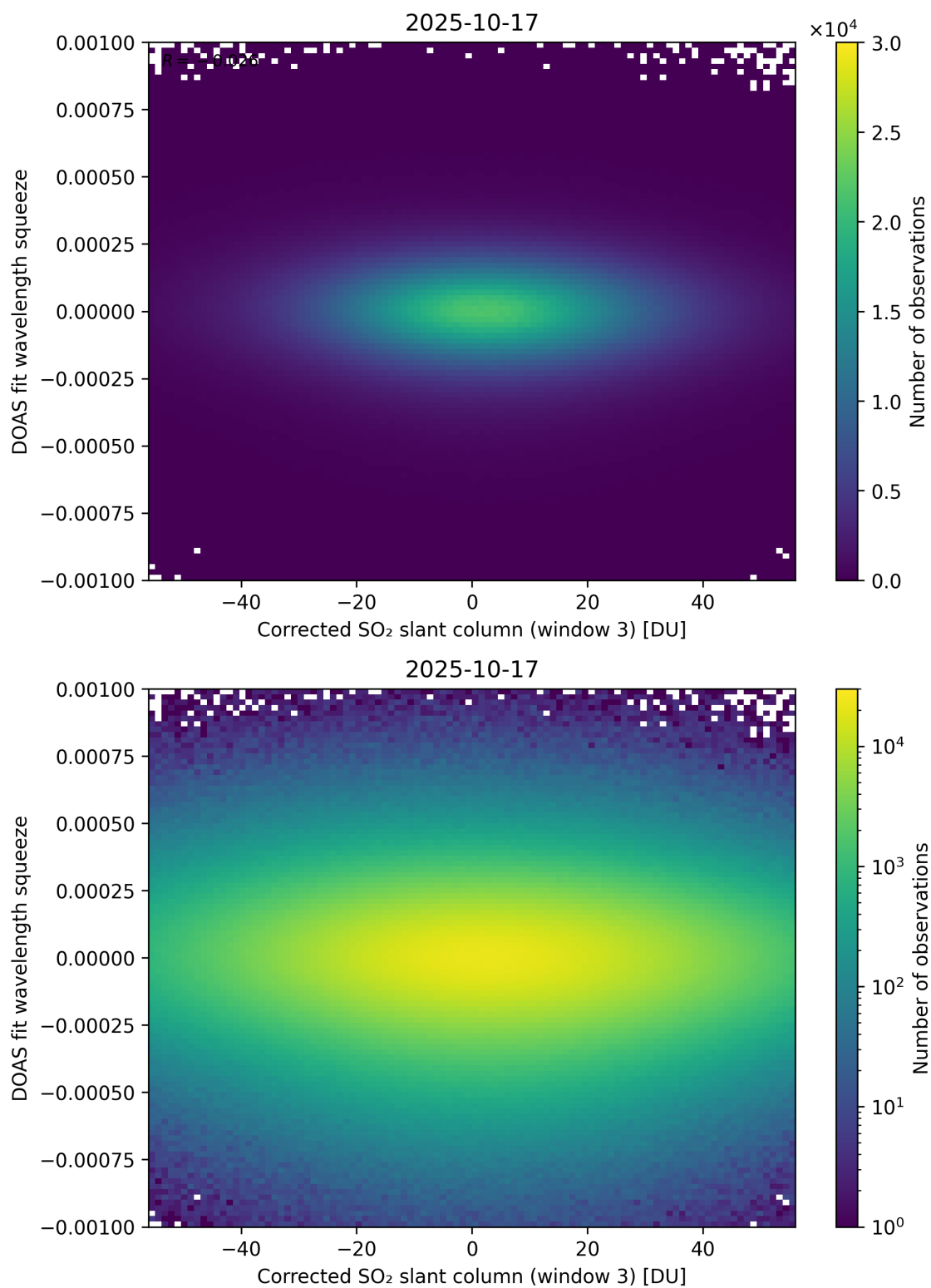
Figure 257: Scatter density plot of “Corrected SO 2 slant column (window 3)” against “DOAS fit wavelength squeeze” for 2025-10-17 to 2025-10-18.
