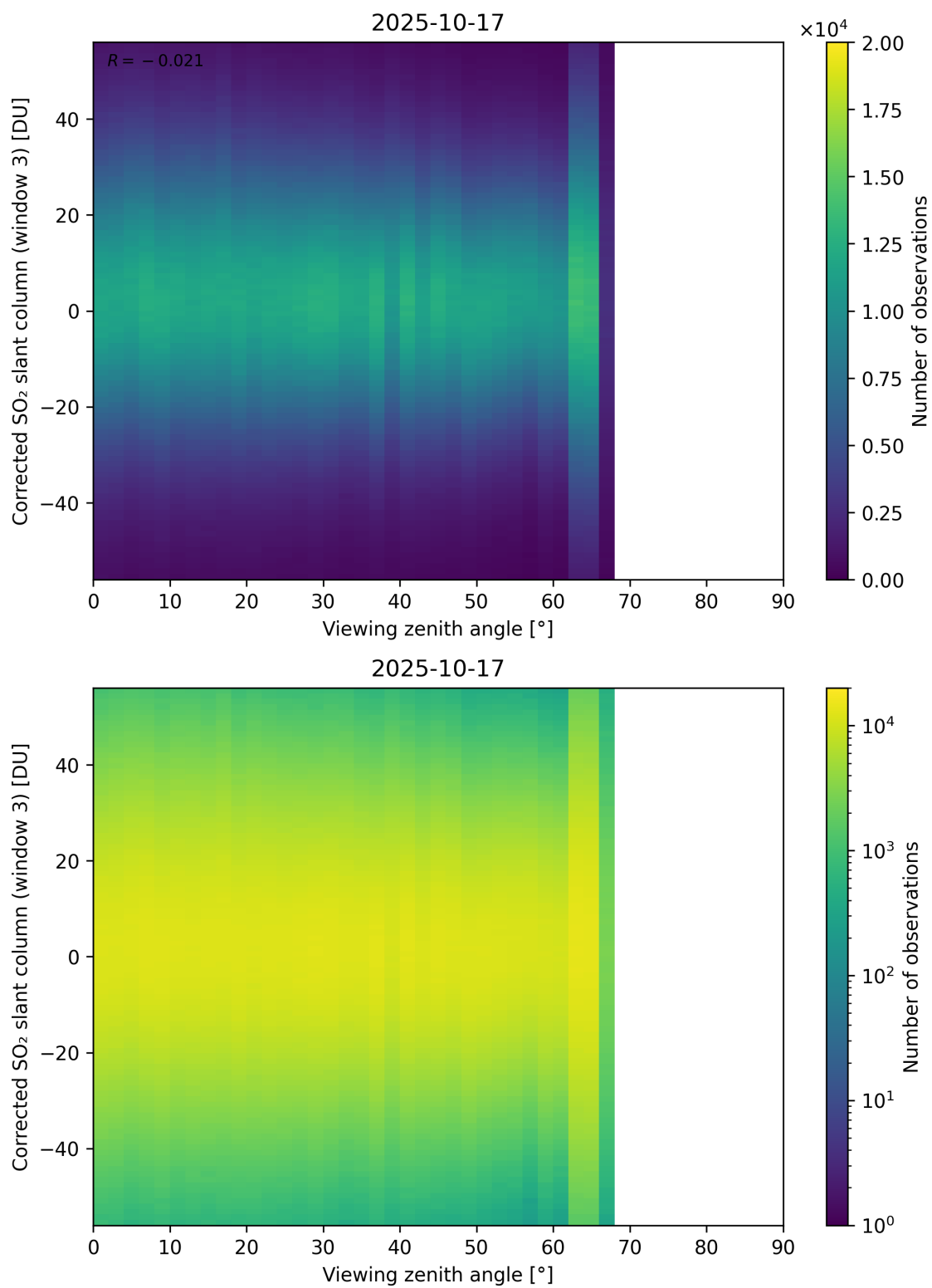
Figure 375: Scatter density plot of “Viewing zenith angle” against “Corrected SO 2 slant column (window 3)” for 2025-10-17 to 2025-10-18.
