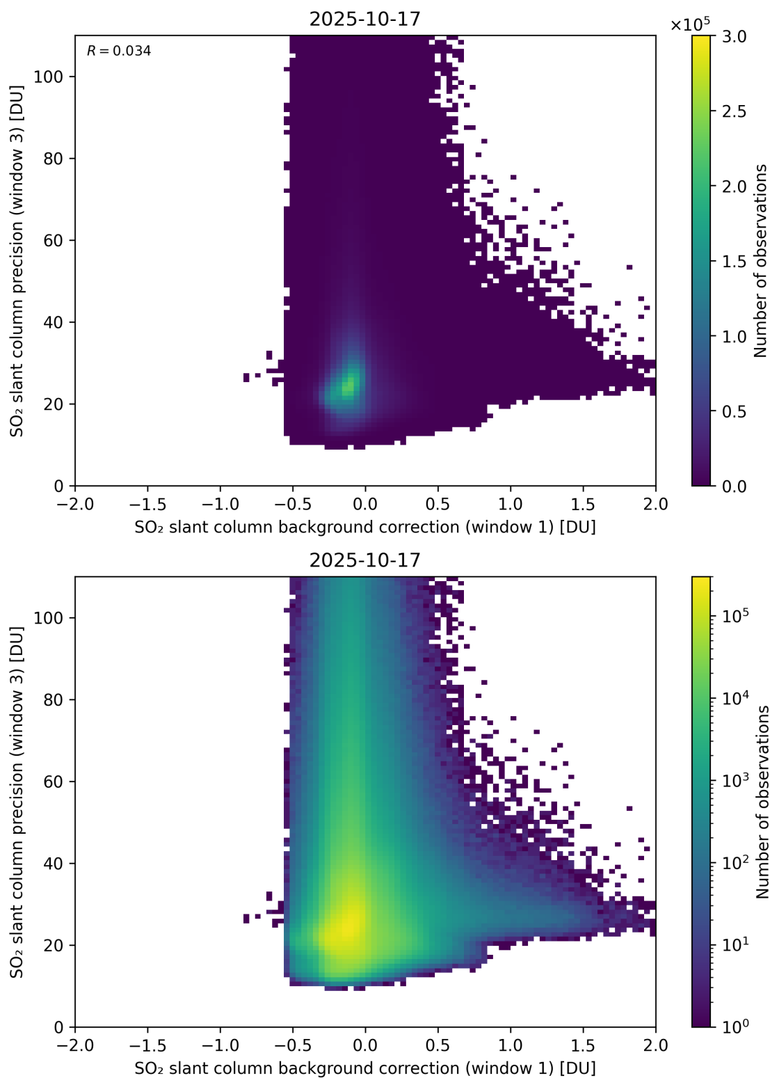
Figure 119: Scatter density plot of “SO 2 slant column background correction (window 1)” against “SO 2 slant column precision (window 3)” for 2025-10-17 to 2025-10-18.
