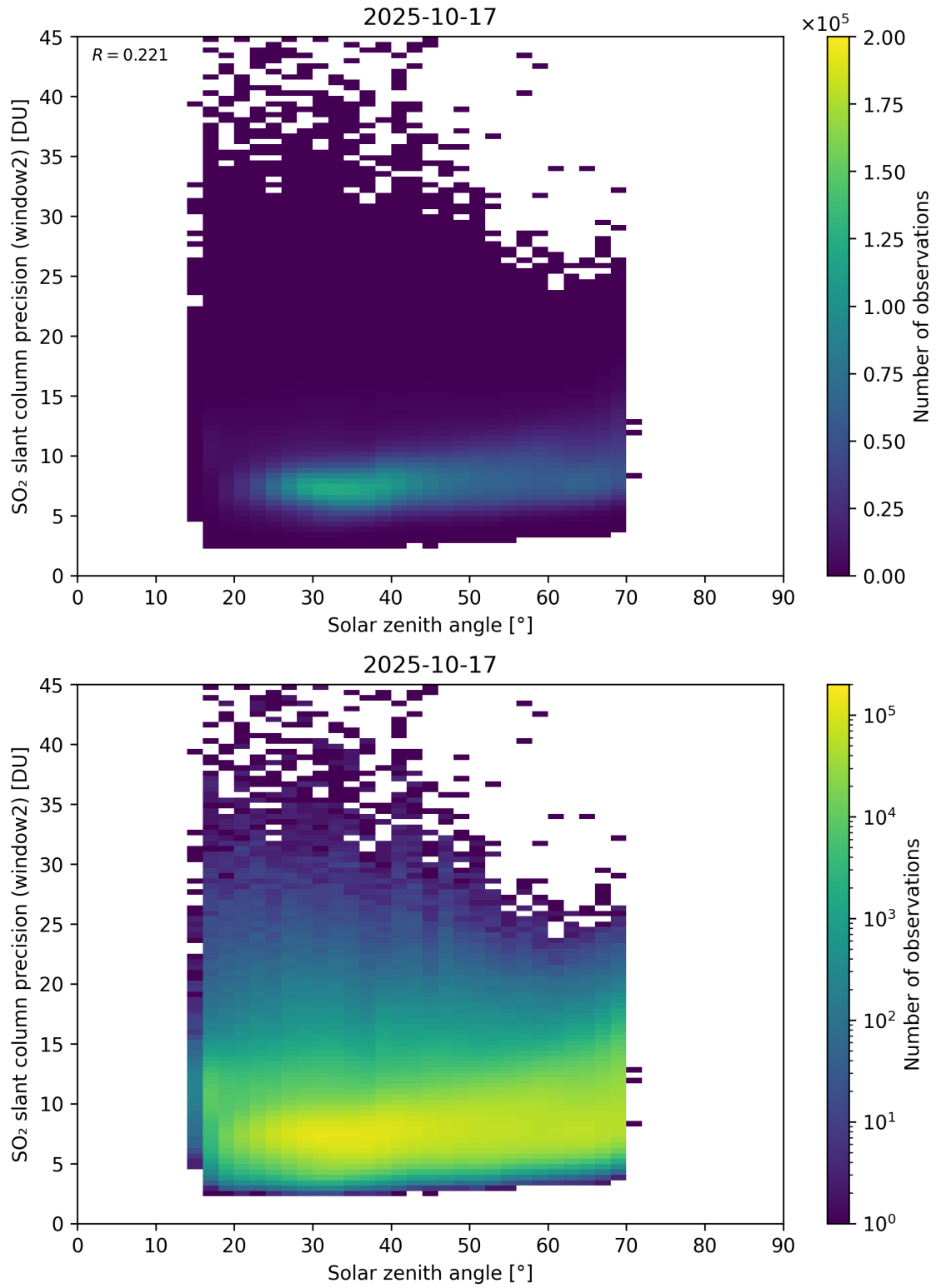
Figure 186: Scatter density plot of “Solar zenith angle” against “SO 2 slant column precision (window2)” for 2025-10-17 to 2025-10-18.
