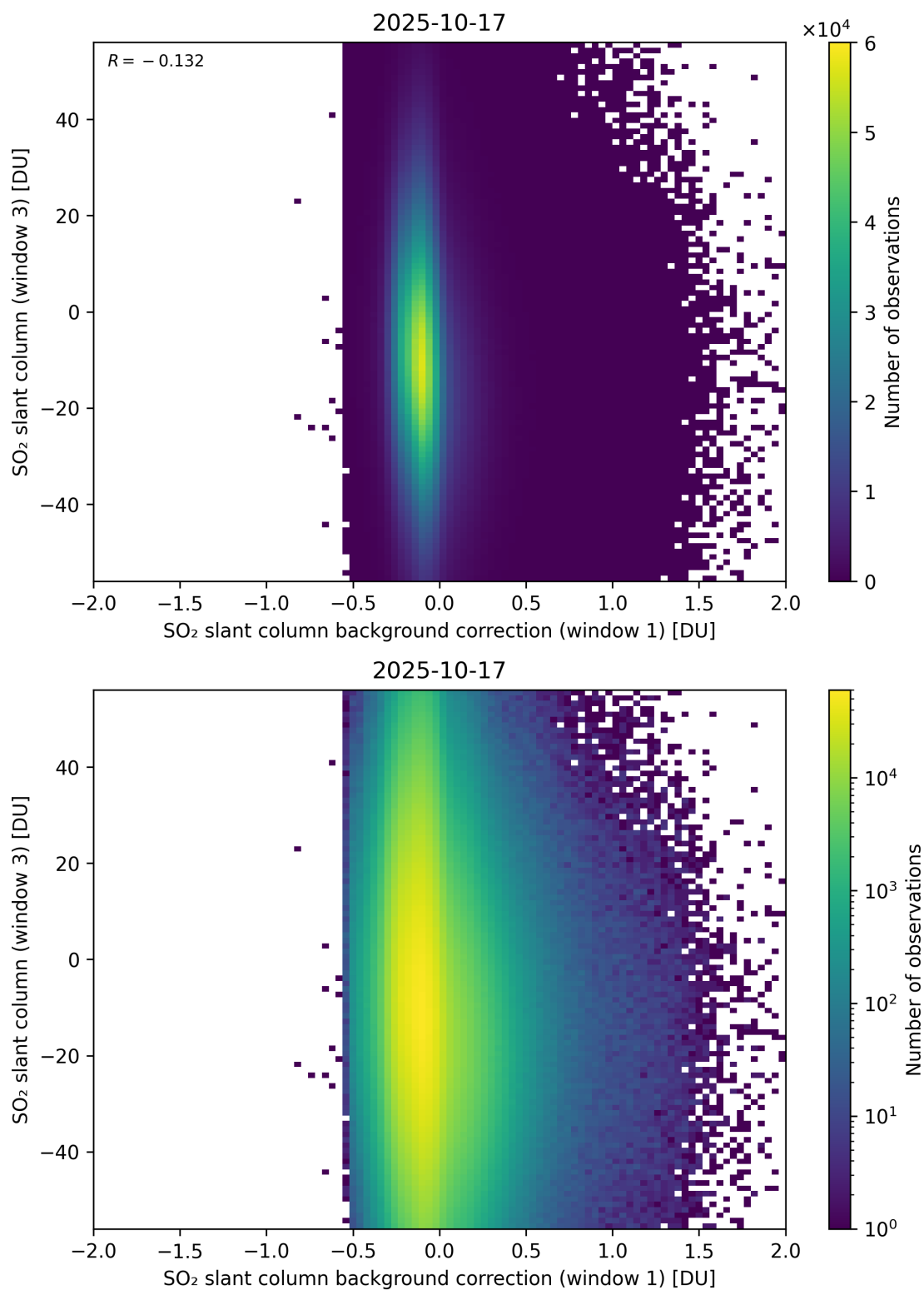
Figure 118: Scatter density plot of “SO 2 slant column background correction (window 1)” against “SO 2 slant column (window 3)” for 2025-10-17 to 2025-10-18.
