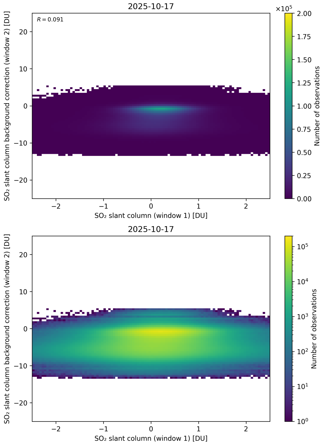
Figure 263: Scatter density plot of “SO 2 slant column (window 1)” against “SO 2 slant column background correction (window 2)” for 2025-10-17 to 2025-10-18.
