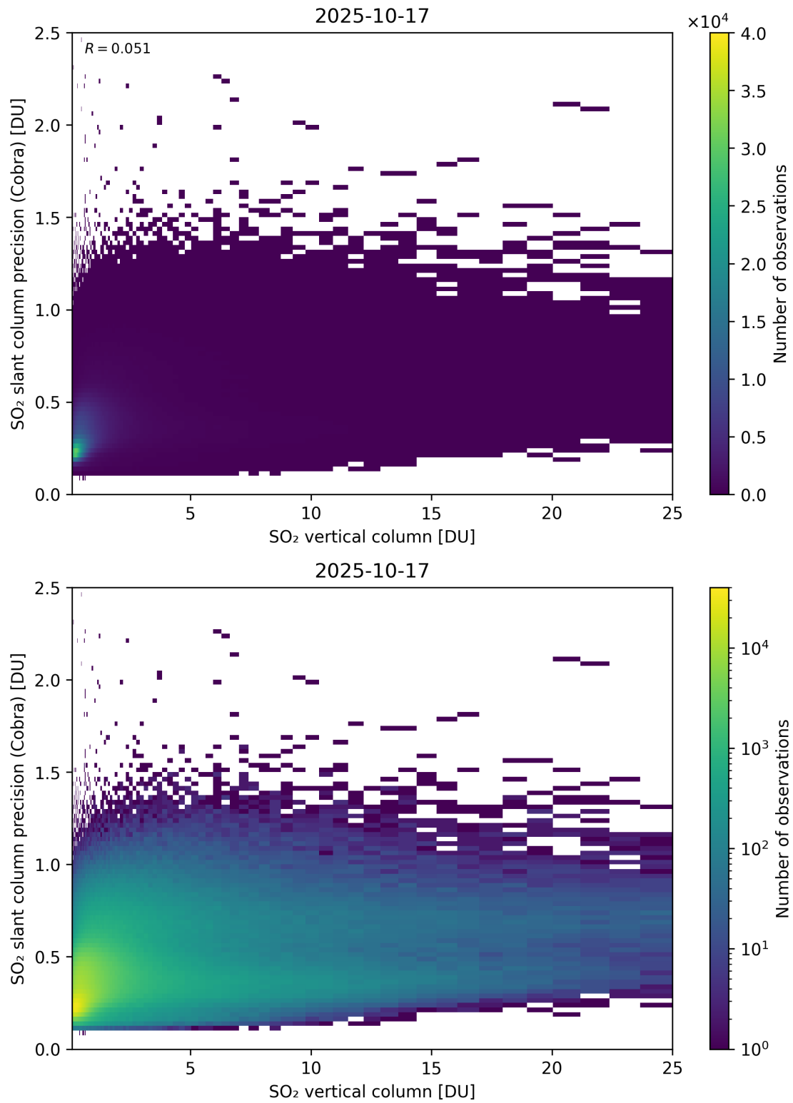
Figure 350: Scatter density plot of “SO 2 vertical column” against “SO 2 slant column precision (Cobra)” for 2025-10-17 to 2025-10-18.
