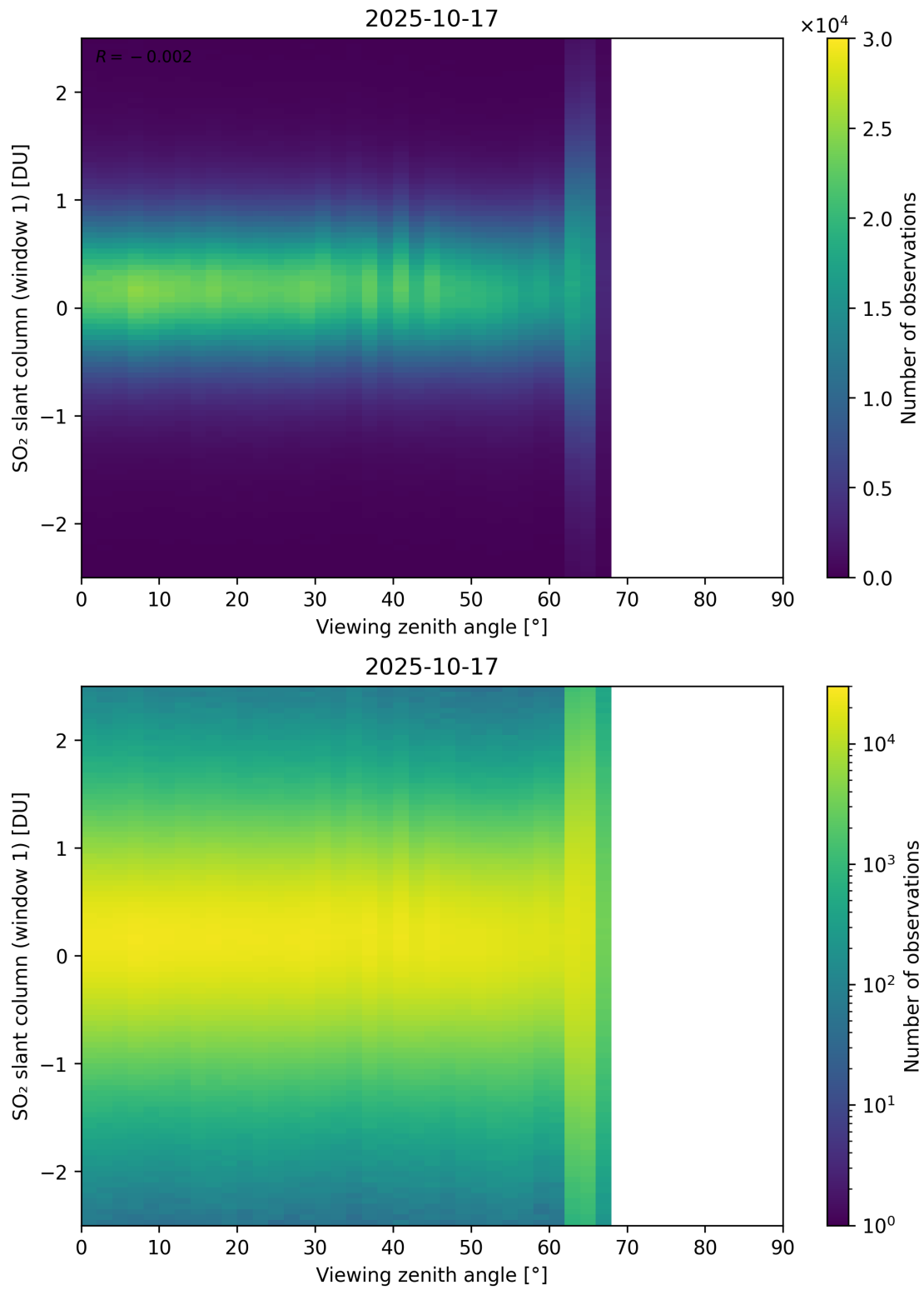
Figure 376: Scatter density plot of “Viewing zenith angle” against “SO 2 slant column (window 1)” for 2025-10-17 to 2025-10-18.
