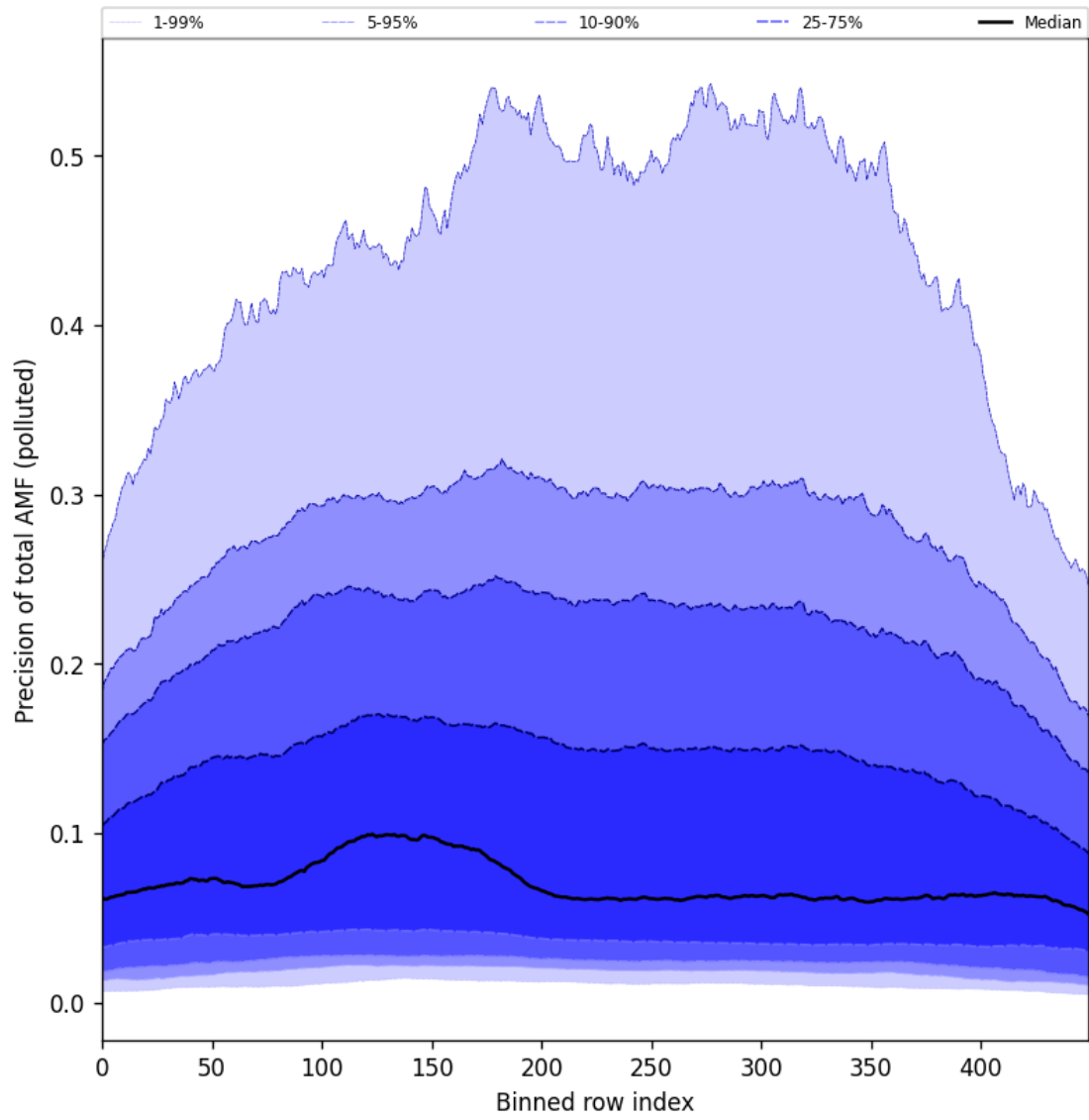
Figure 106: Along track statistics of “Precision of total AMF (polluted)” for 2025-10-17 to 2025-10-18
