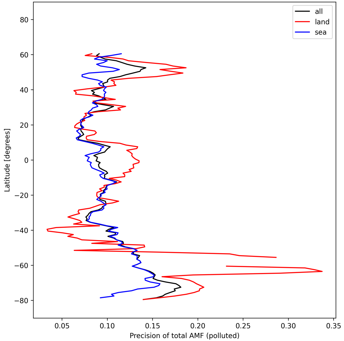
Figure 54: Zonal average of “Precision of total AMF (polluted)” for 2025-10-17 to 2025-10-18.
