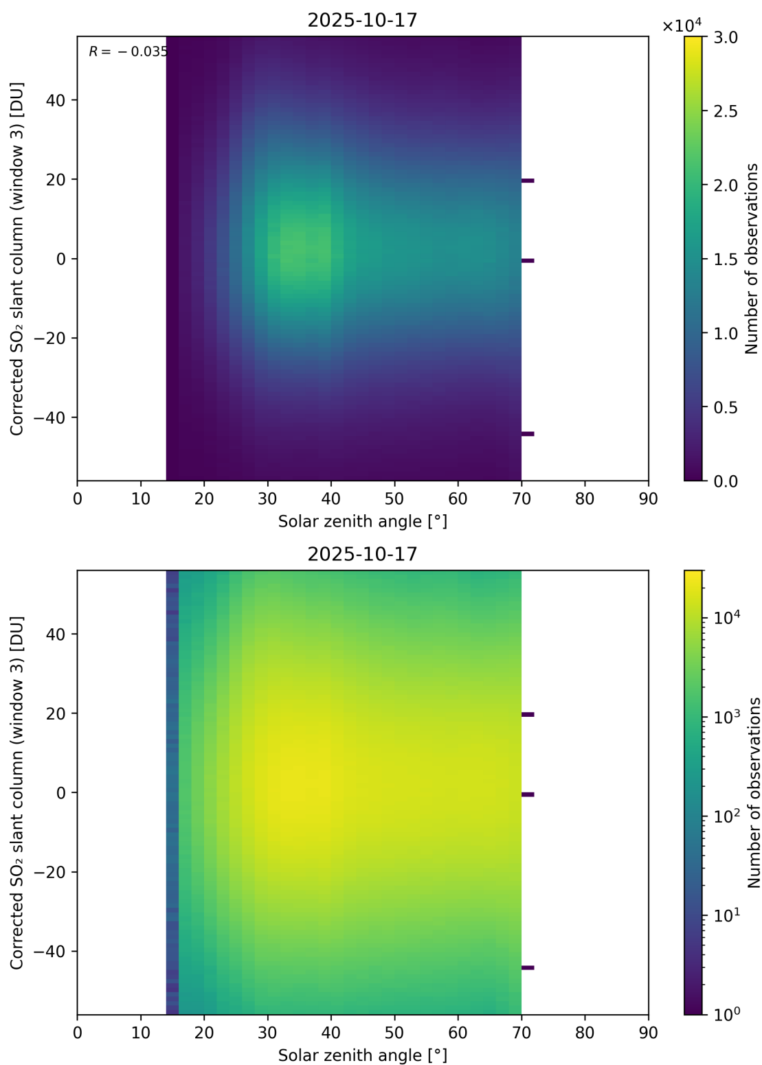
Figure 183: Scatter density plot of “Solar zenith angle” against “Corrected SO 2 slant column (window 3)” for 2025-10-17 to 2025-10-18.
