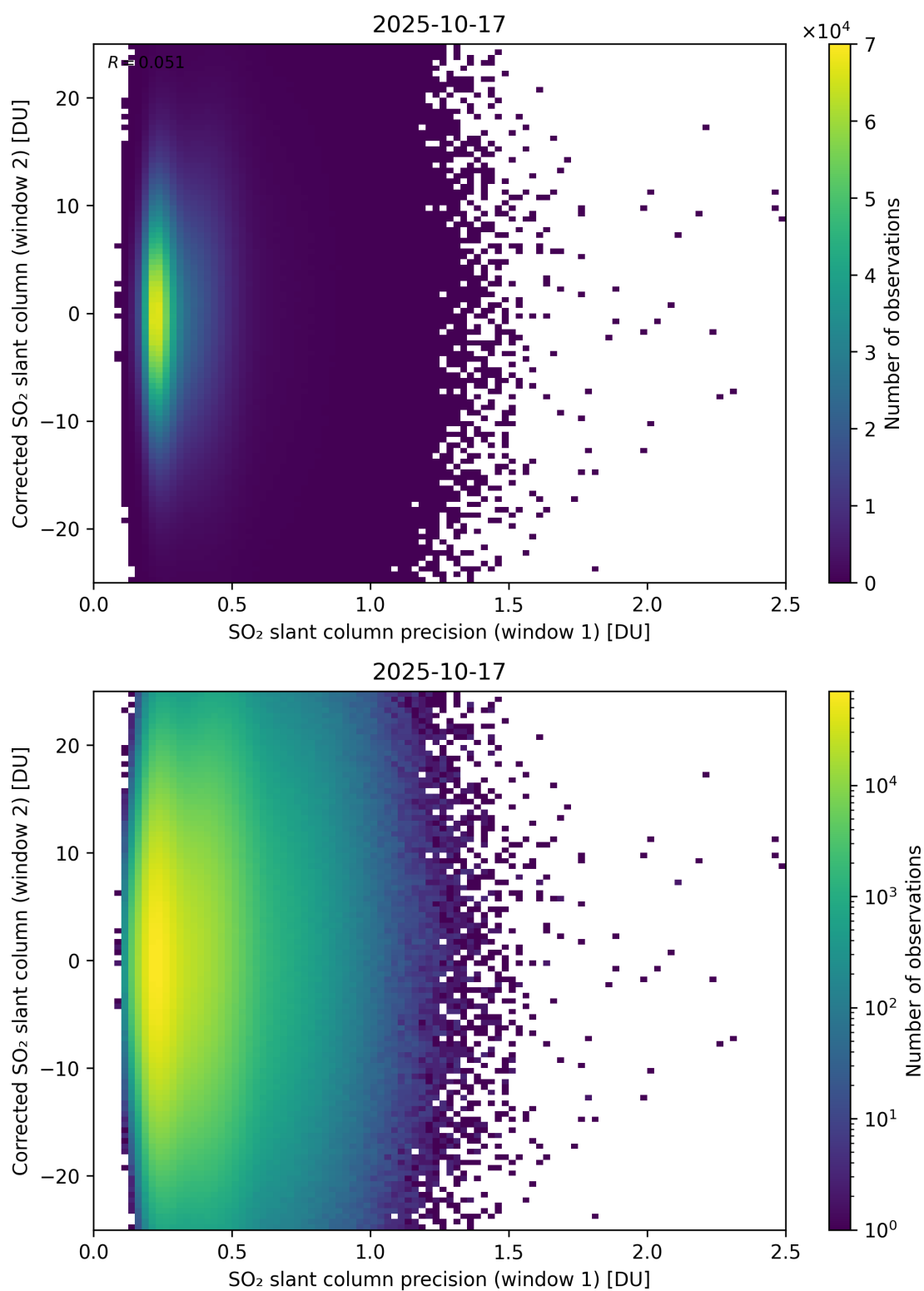
Figure 275: Scatter density plot of “SO 2 slant column precision (window 1)” against “Corrected SO 2 slant column (window 2)” for 2025-10-17 to 2025-10-18.
