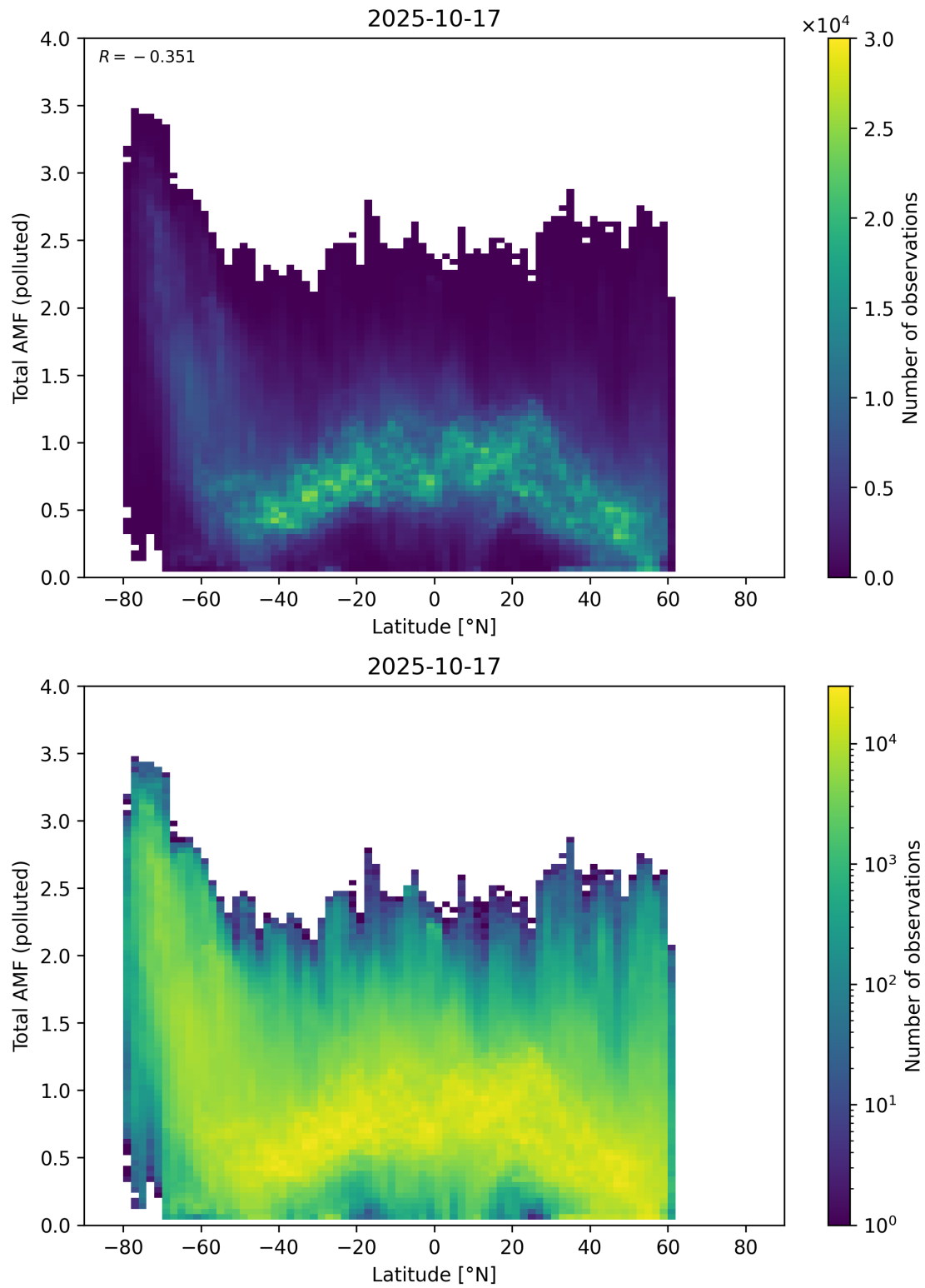
Figure 167: Scatter density plot of “Latitude” against “Total AMF (polluted)” for 2025-10-17 to 2025-10-18.
