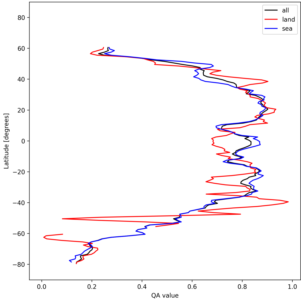
Figure 31: Zonal average of “QA value” for 2025-10-17 to 2025-10-18.
