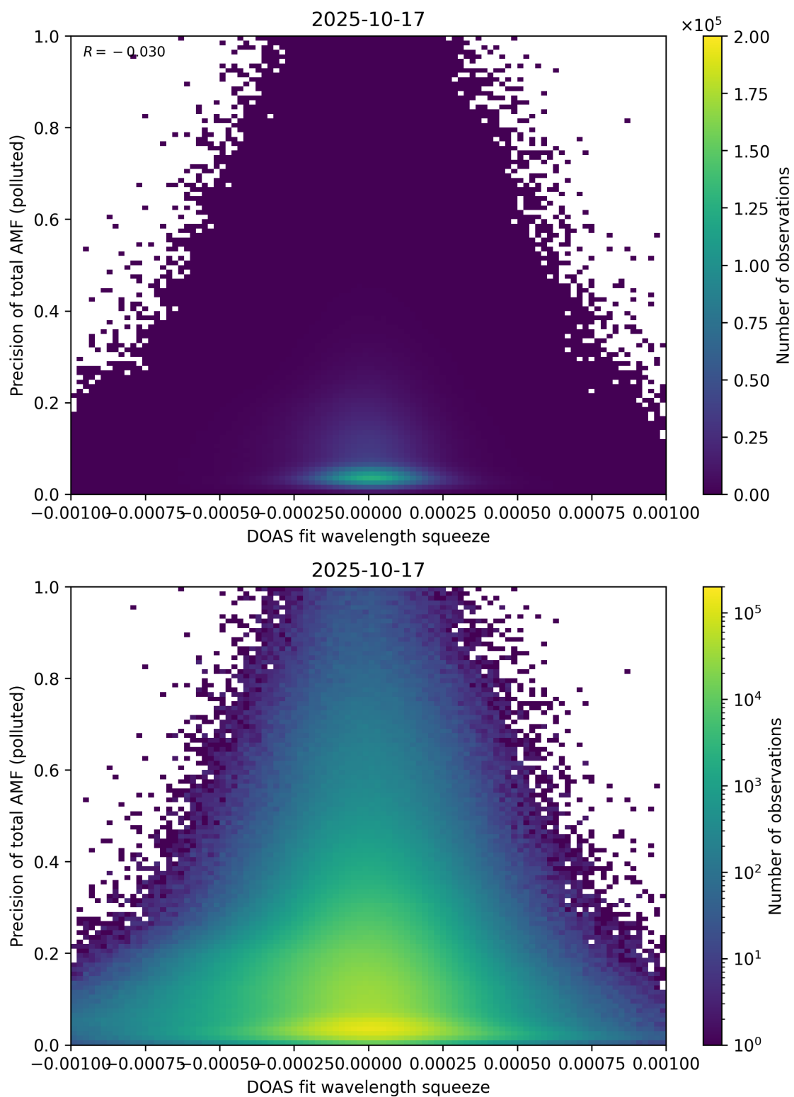
Figure 146: Scatter density plot of “DOAS fit wavelength squeeze” against “Precision of total AMF (polluted)” for 2025-10-17 to 2025-10-18.
