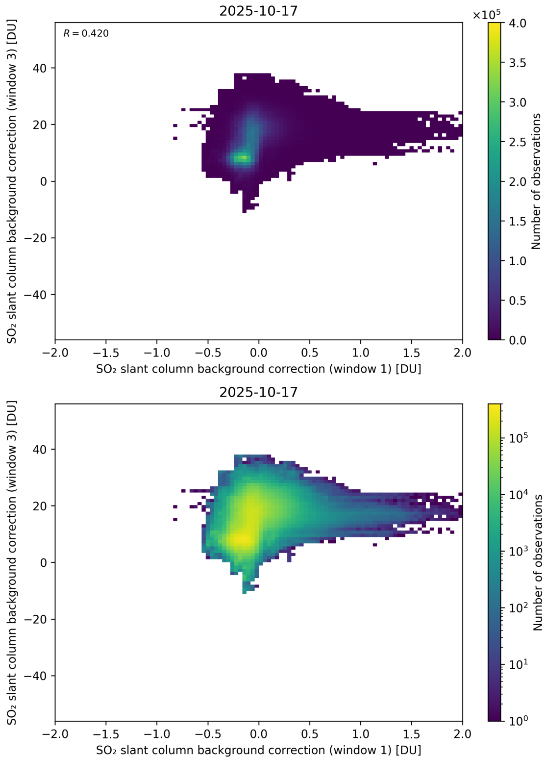
Figure 110: Scatter density plot of “SO 2 slant column background correction (window 1)” against “SO 2 slant column background correction (window 3)” for 2025-10-17 to 2025-10-18.
