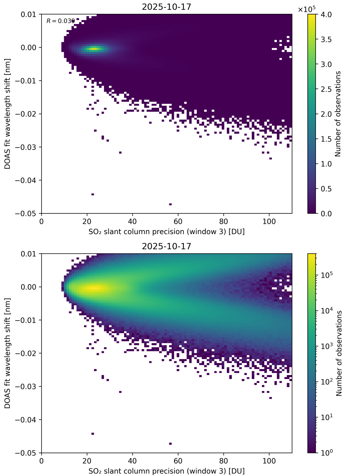
Figure 308: Scatter density plot of “SO 2 slant column precision (window 3)” against “DOAS fit wavelength shift” for 2025-10-17 to 2025-10-18.
