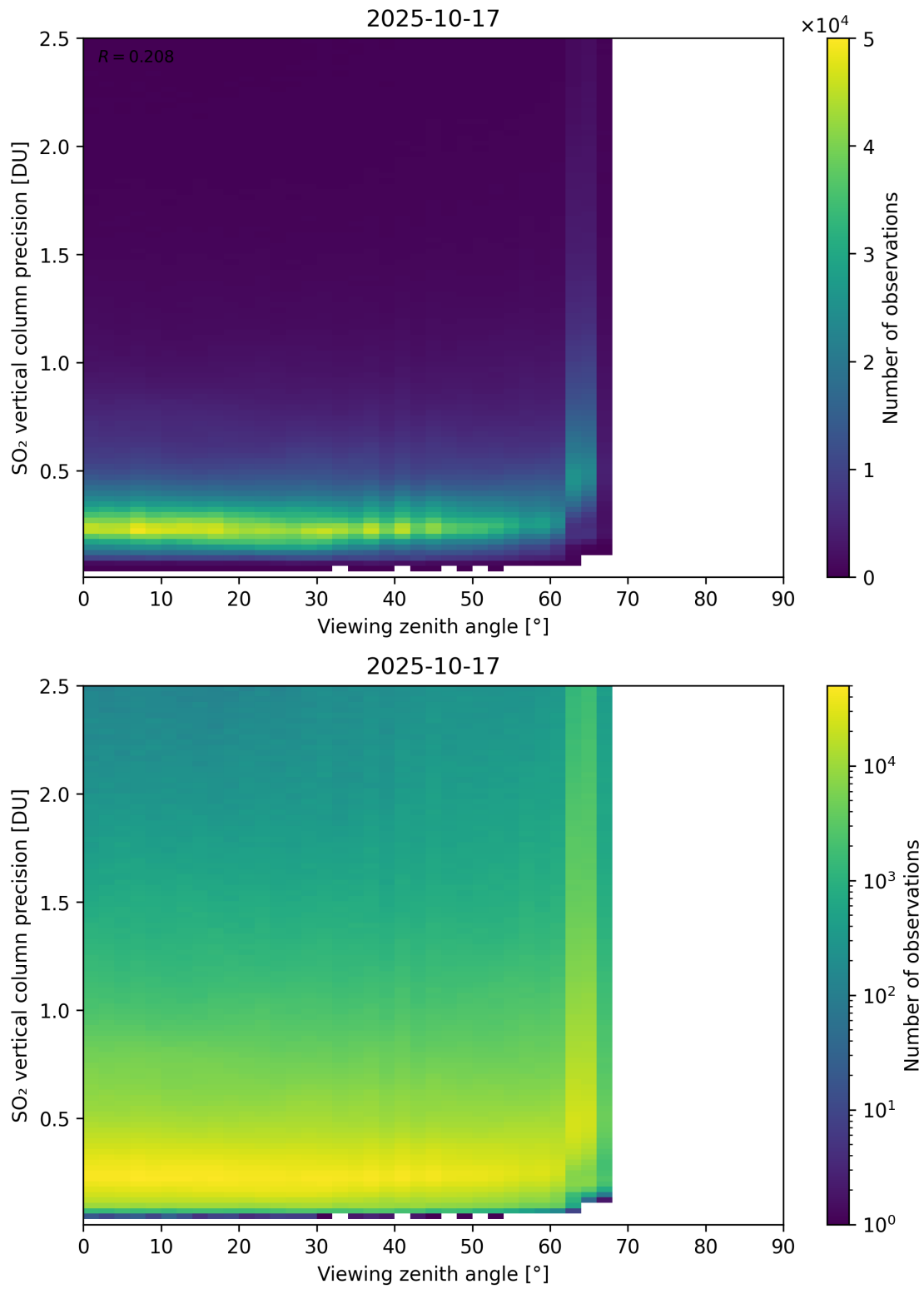
Figure 384: Scatter density plot of “Viewing zenith angle” against “SO 2 vertical column precision” for 2025-10-17 to 2025-10-18.
