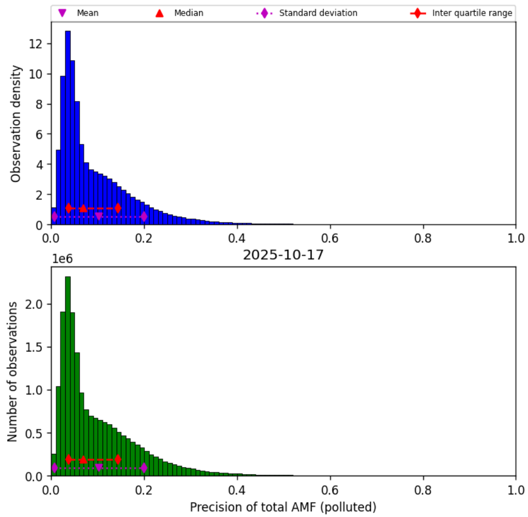
Figure 80: Histogram of “Precision of total AMF (polluted)” for 2025-10-17 to 2025-10-18
