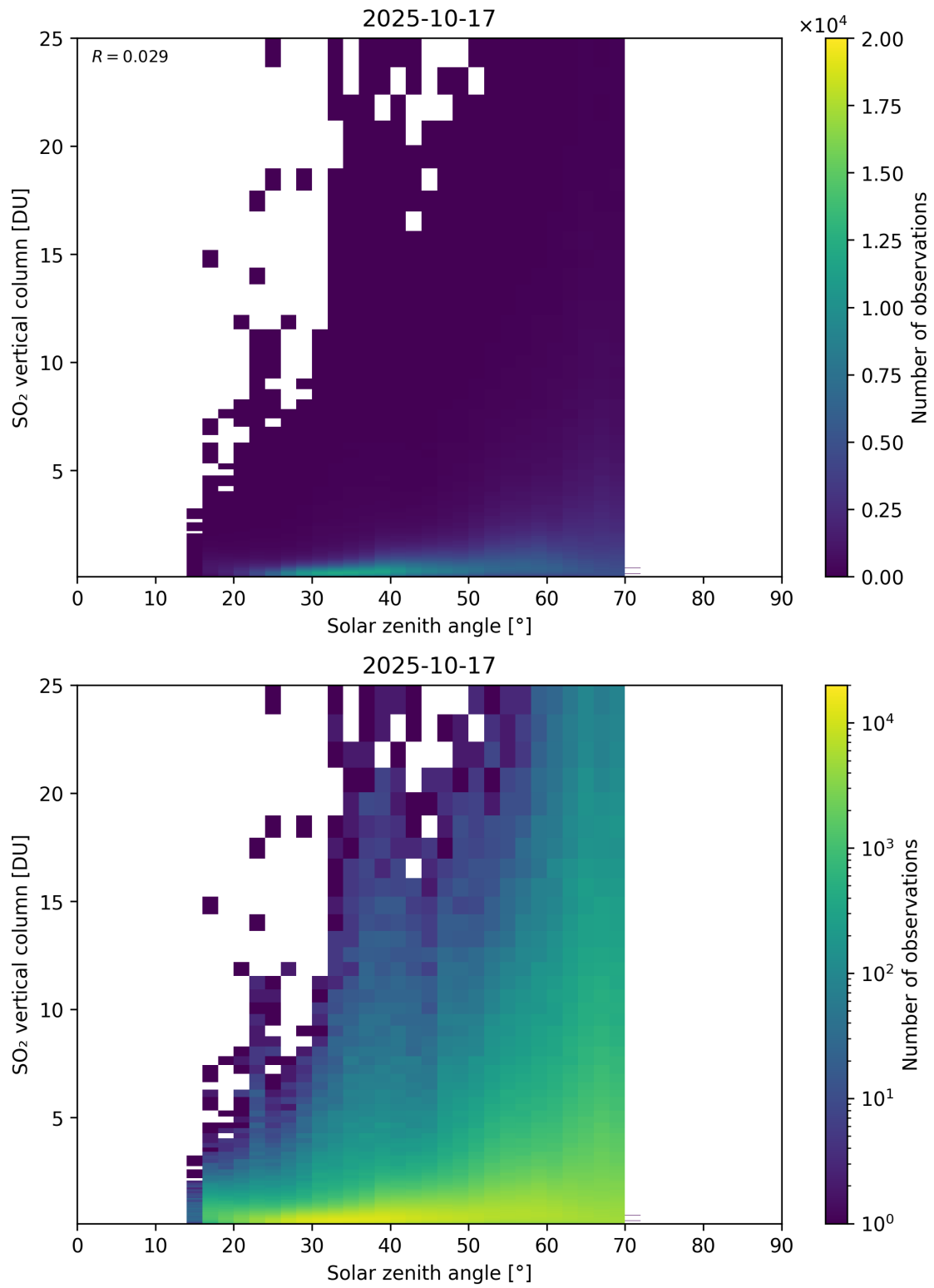
Figure 191: Scatter density plot of “Solar zenith angle” against “SO 2 vertical column” for 2025-10-17 to 2025-10-18.
