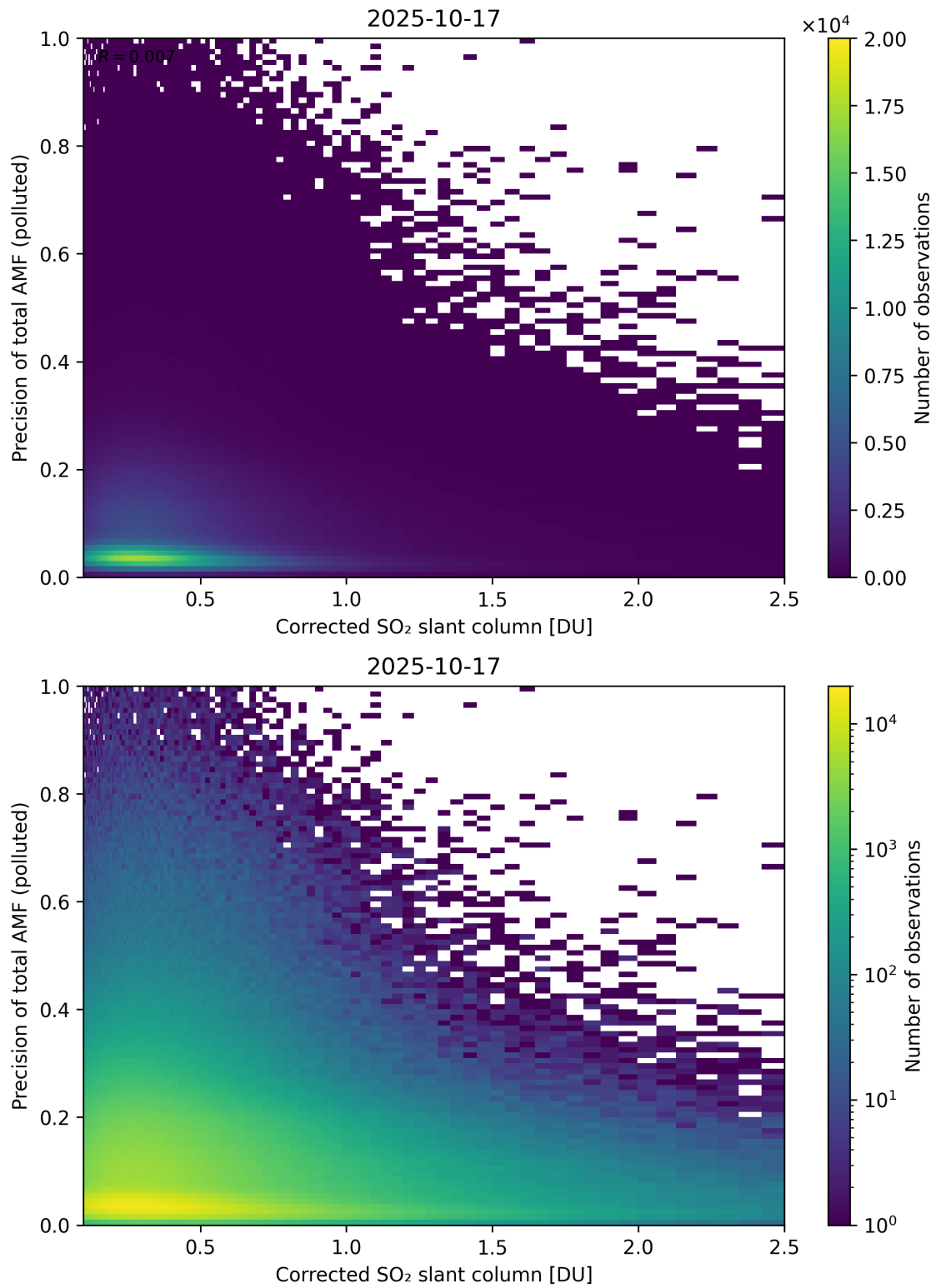
Figure 243: Scatter density plot of “Corrected SO 2 slant column” against “Precision of total AMF (polluted)” for 2025-10-17 to 2025-10-18.
