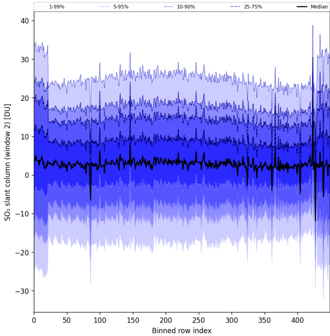
Figure 93: Along track statistics of “SO 2 slant column (window 2)” for 2025-10-17 to 2025-10-18
