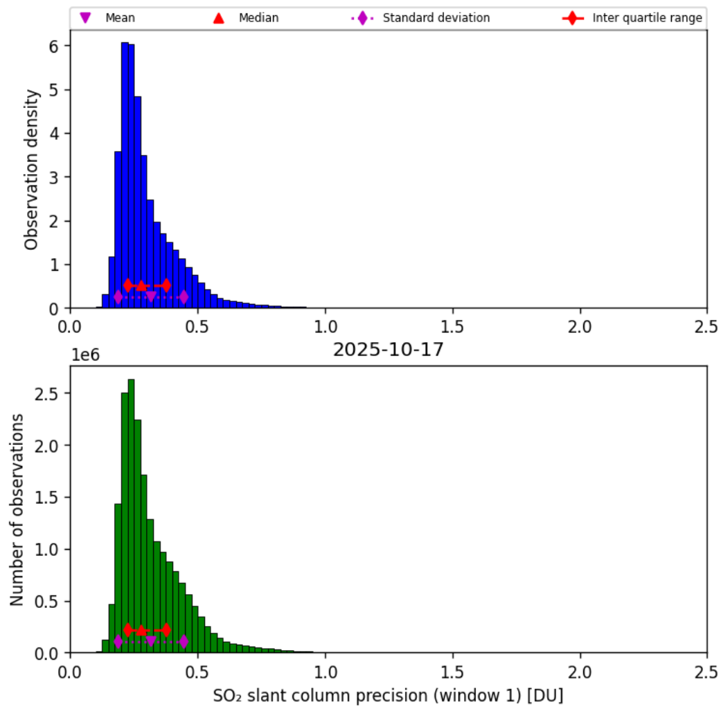
Figure 64: Histogram of “SO 2 slant column precision (window 1)” for 2025-10-17 to 2025-10-18
