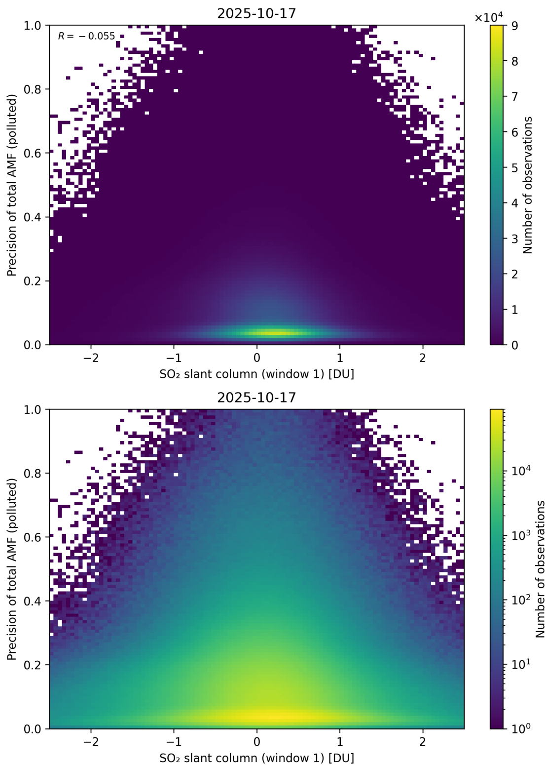
Figure 290: Scatter density plot of “SO 2 slant column (window 1)” against “Precision of total AMF (polluted)” for 2025-10-17 to 2025-10-18.
