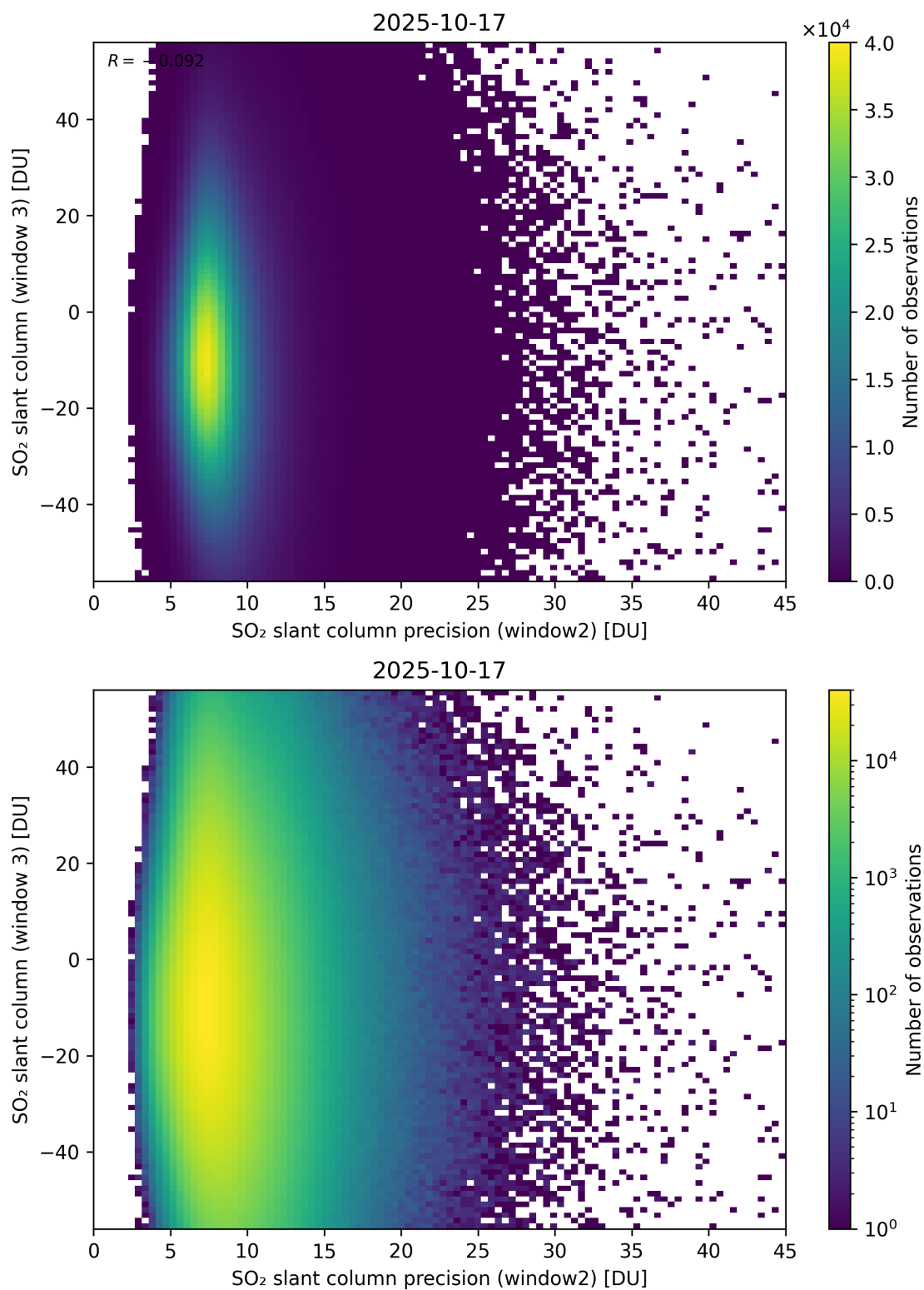
Figure 299: Scatter density plot of “SO 2 slant column precision (window2)” against “SO 2 slant column (window 3)” for 2025-10-17 to 2025-10-18.
