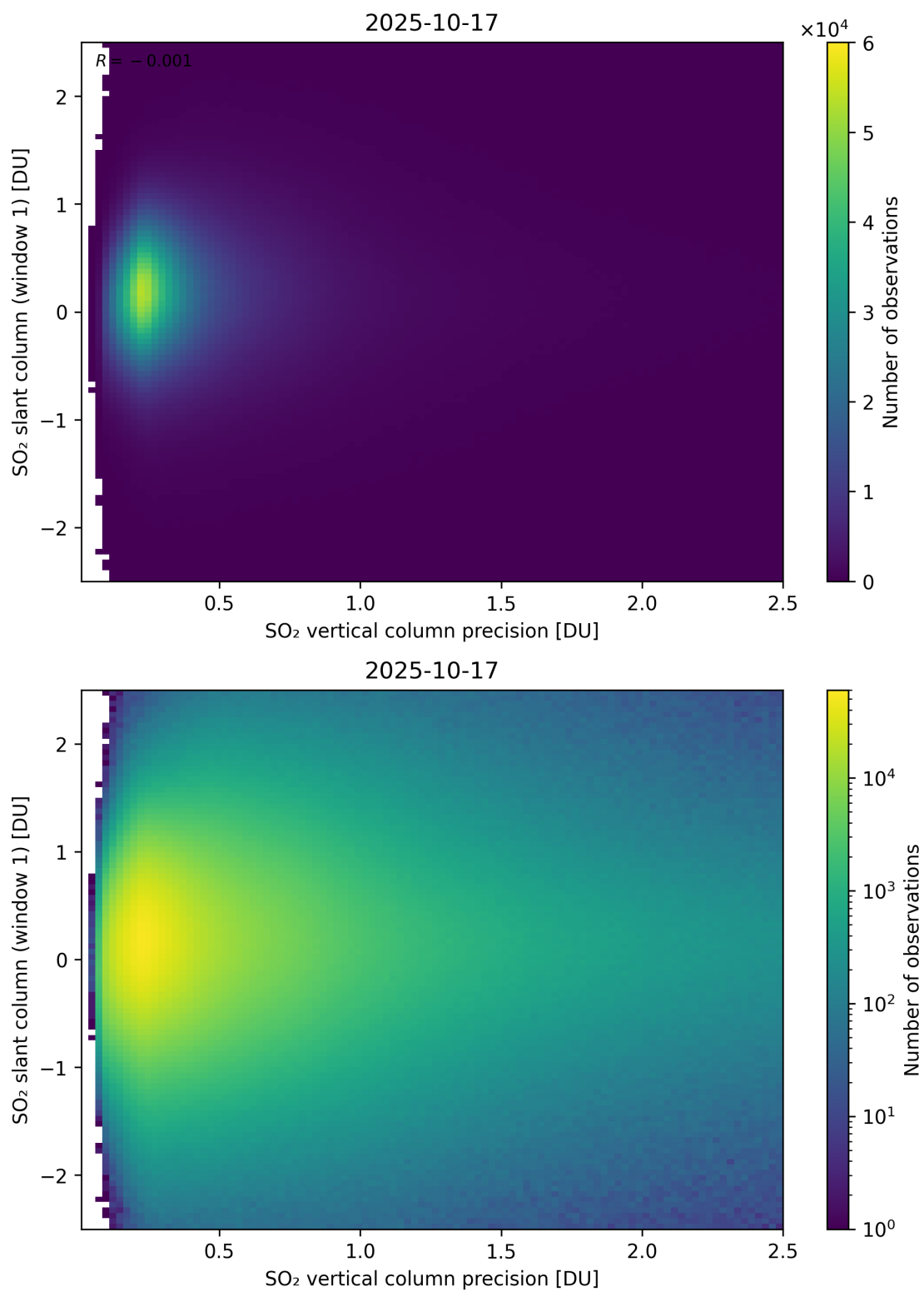
Figure 341: Scatter density plot of “SO 2 vertical column precision” against “SO 2 slant column (window 1)” for 2025-10-17 to 2025-10-18.
