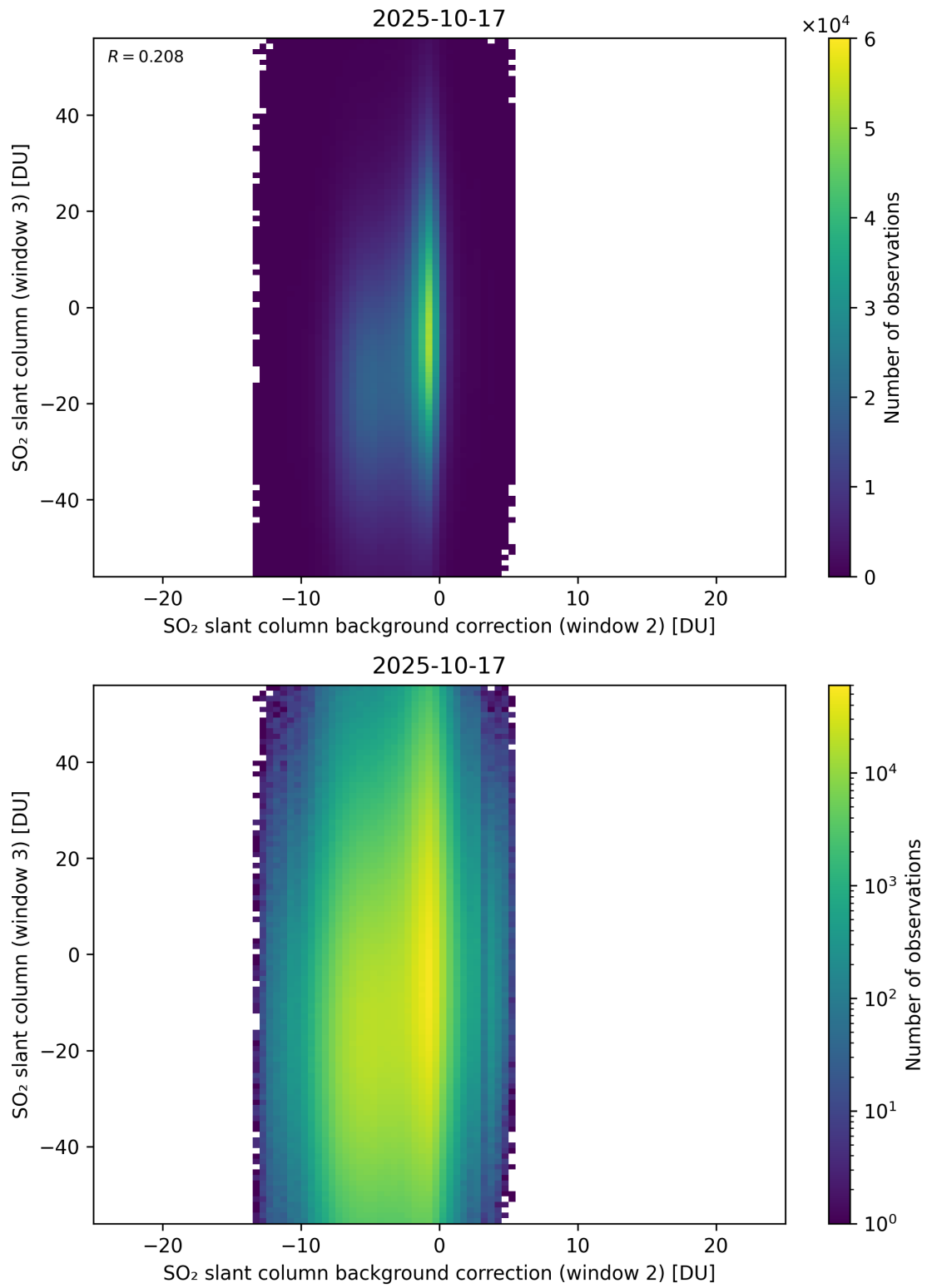
Figure 128: Scatter density plot of “SO 2 slant column background correction (window 2)” against “SO 2 slant column (window 3)” for 2025-10-17 to 2025-10-18.
