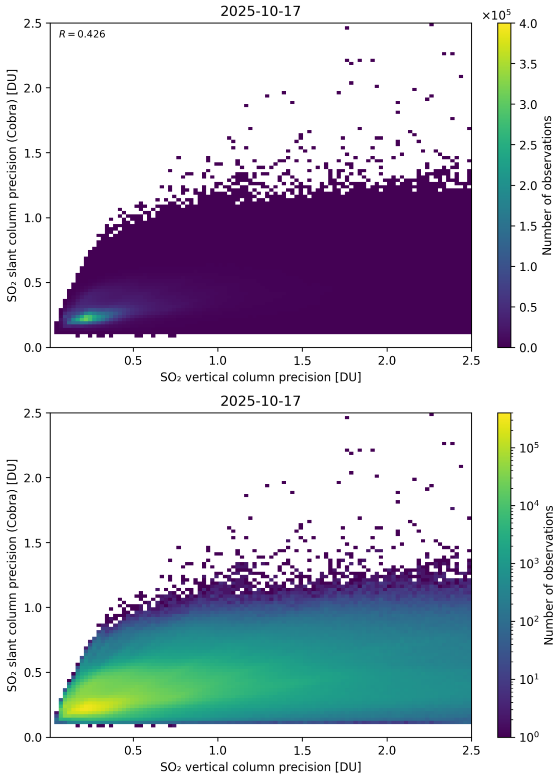
Figure 337: Scatter density plot of “SO 2 vertical column precision” against “SO 2 slant column precision (Cobra)” for 2025-10-17 to 2025-10-18.
