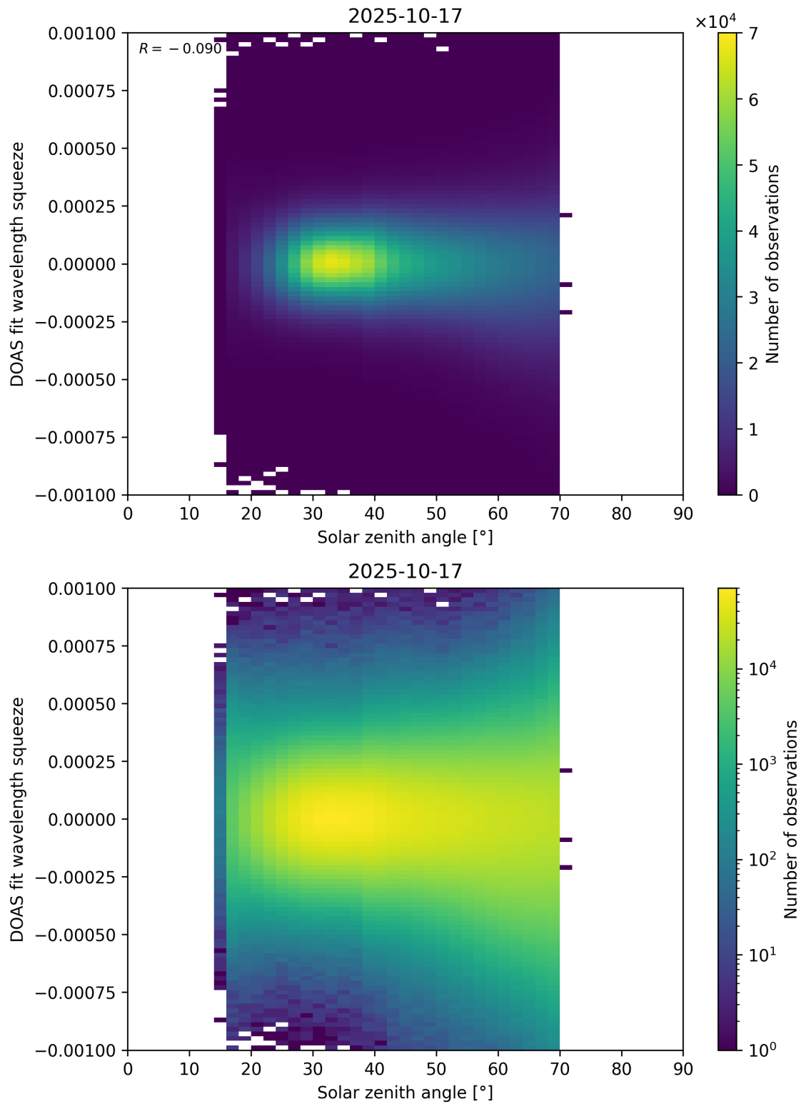
Figure 175: Scatter density plot of “Solar zenith angle” against “DOAS fit wavelength squeeze” for 2025-10-17 to 2025-10-18.
