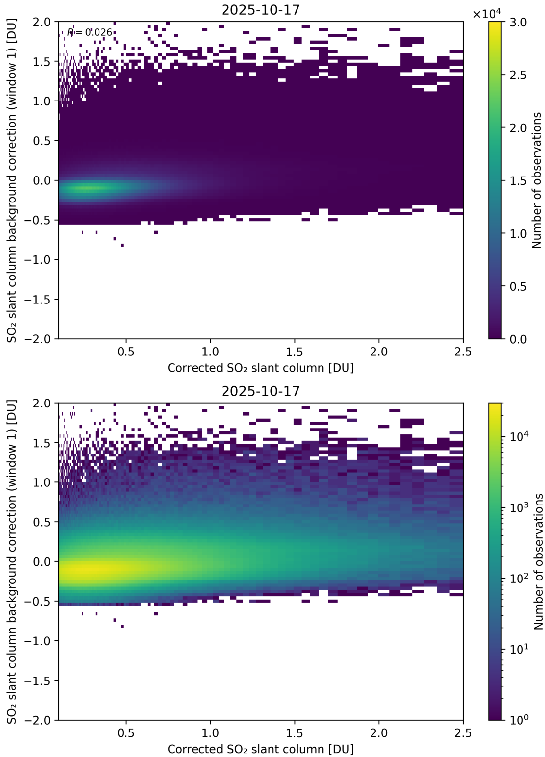
Figure 226: Scatter density plot of “Corrected SO 2 slant column” against “SO 2 slant column background correction (window 1)” for 2025-10-17 to 2025-10-18.
