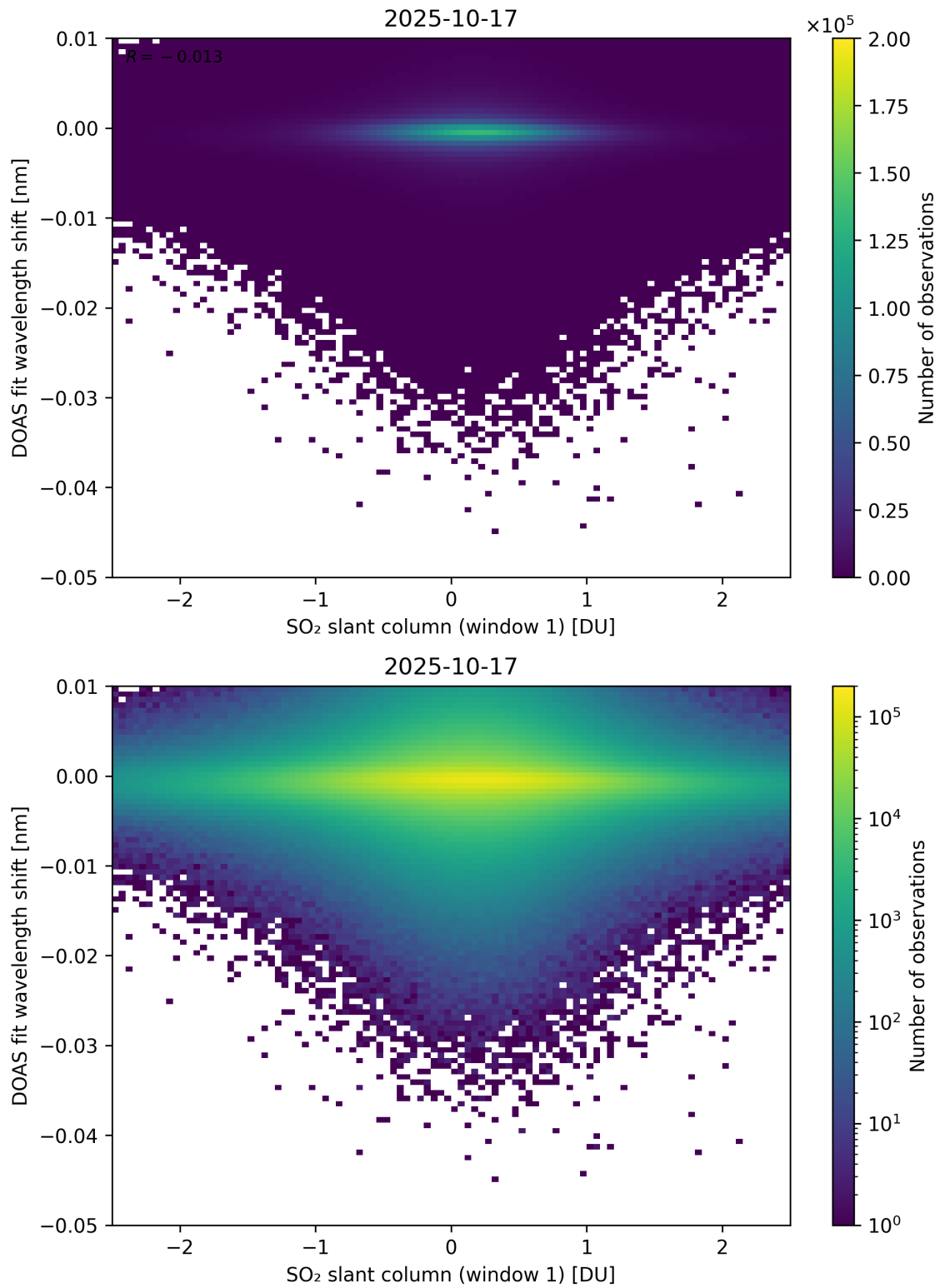
Figure 265: Scatter density plot of “SO 2 slant column (window 1)” against “DOAS fit wavelength shift” for 2025-10-17 to 2025-10-18.
