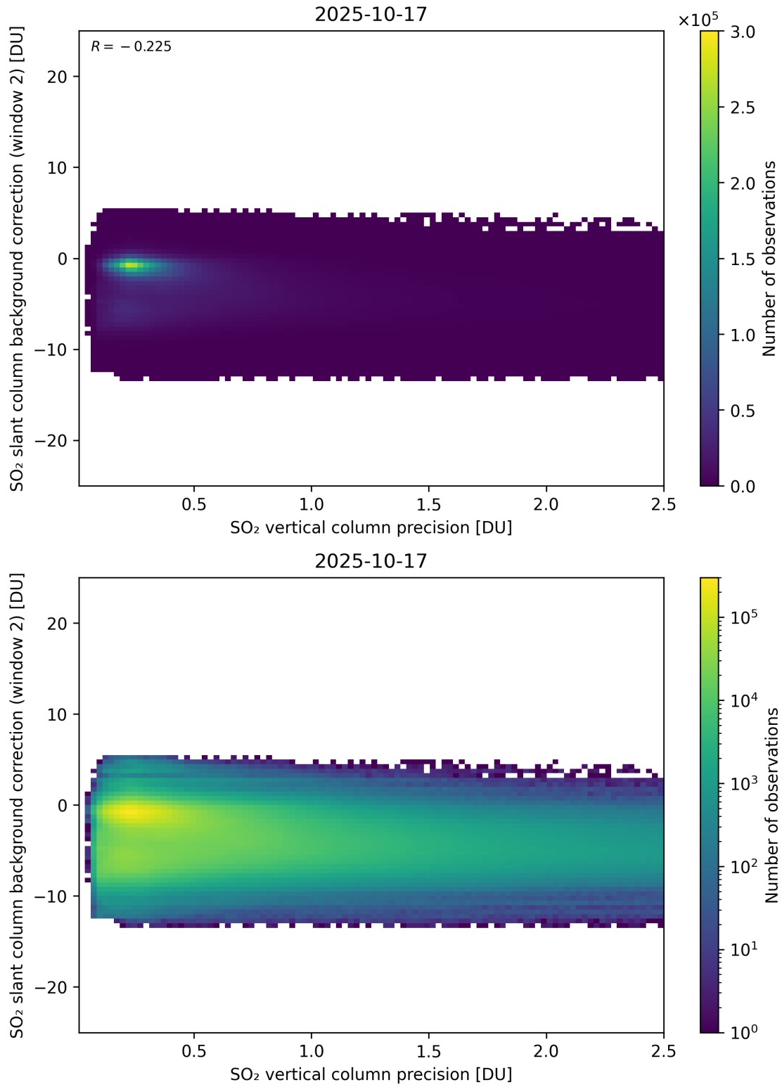
Figure 330: Scatter density plot of “SO 2 vertical column precision” against “SO 2 slant column background correction (window 2)” for 2025-10-17 to 2025-10-18.
