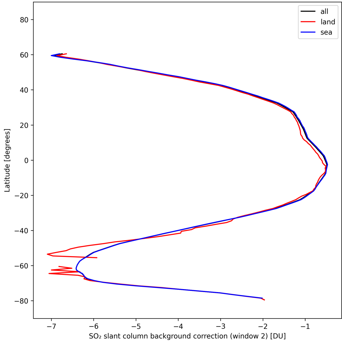
Figure 44: Zonal average of “SO 2 slant column background correction (window 2)” for 2025-10-17 to 2025-10-18.
