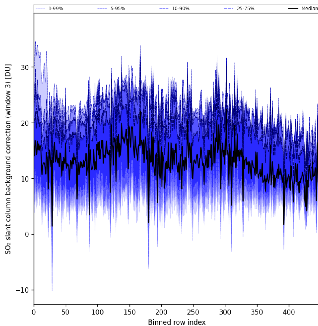
Figure 100: Along track statistics of “SO 2 slant column background correction (window 3)” for 2025-10-17 to 2025-10-18
