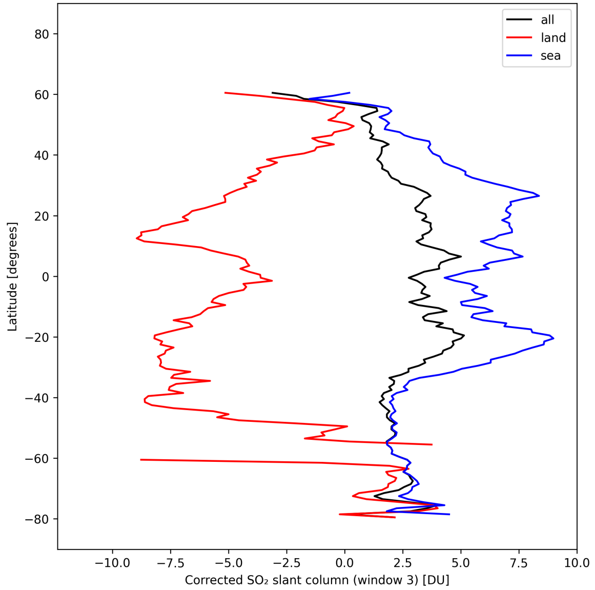
Figure 47: Zonal average of “Corrected SO 2 slant column (window 3)” for 2025-10-17 to 2025-10-18.
