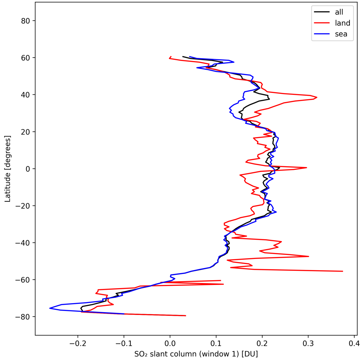
Figure 37: Zonal average of “SO 2 slant column (window 1)” for 2025-10-17 to 2025-10-18.
