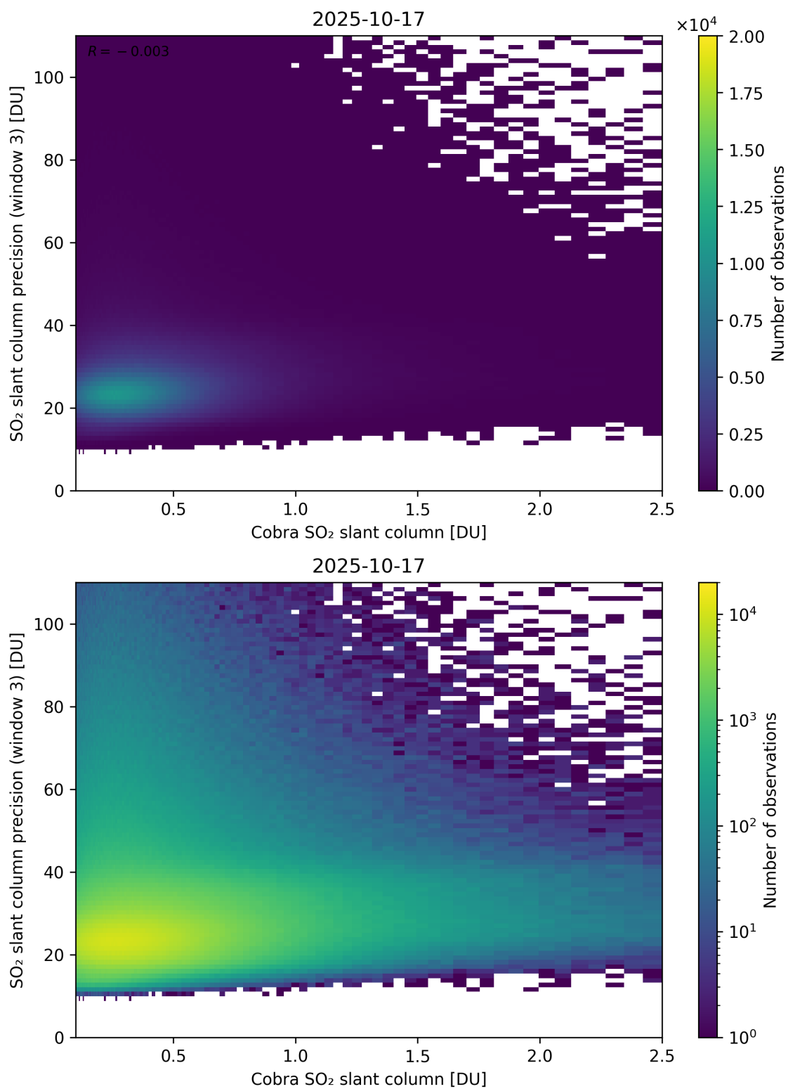
Figure 223: Scatter density plot of “Cobra SO 2 slant column” against “SO 2 slant column precision (window 3)” for 2025-10-17 to 2025-10-18.
