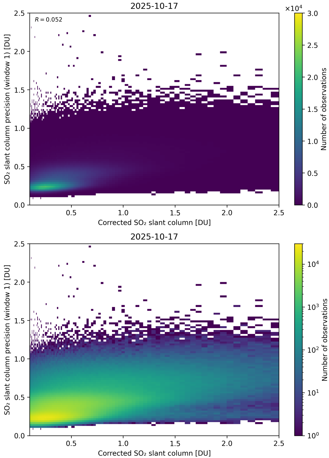
Figure 238: Scatter density plot of “Corrected SO 2 slant column” against “SO 2 slant column precision (window 1)” for 2025-10-17 to 2025-10-18.
