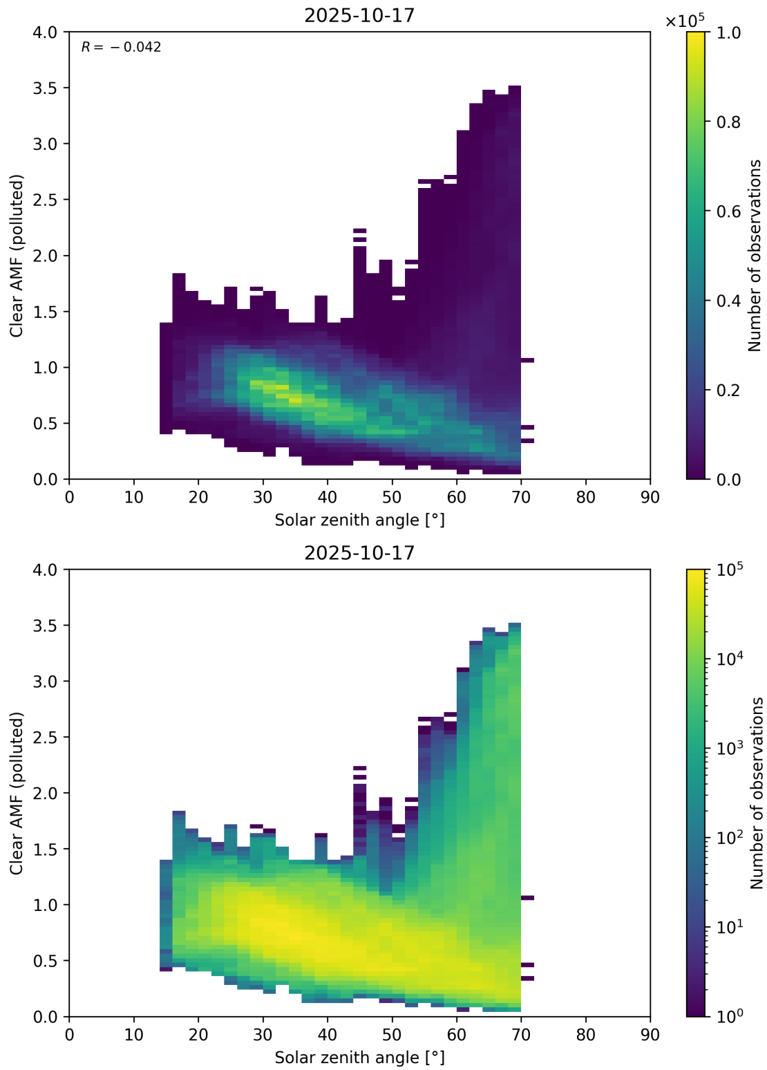
Figure 178: Scatter density plot of “Solar zenith angle” against “Clear AMF (polluted)” for 2025-10-17 to 2025-10-18.
