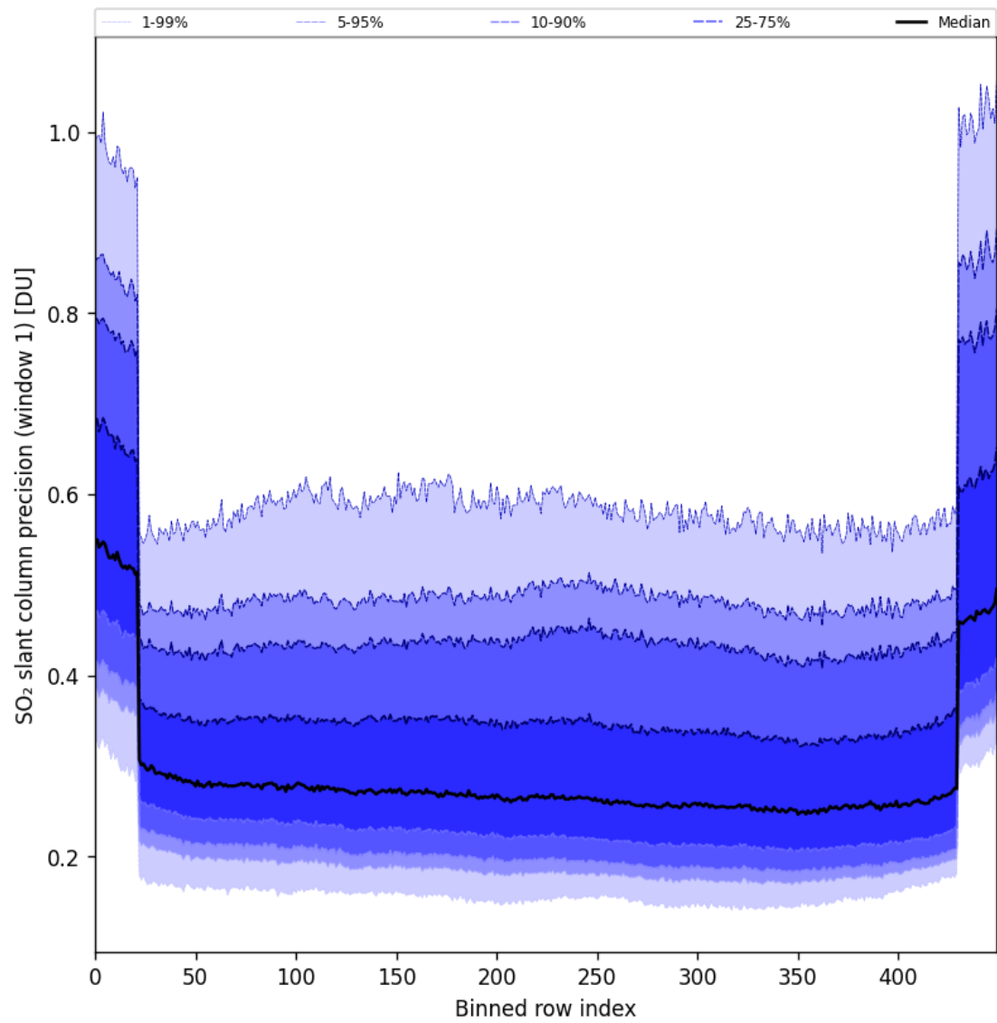
Figure 90: Along track statistics of "SO 2 slant column precision (window 1)" for 2025-10-17 to 2025-10-18
