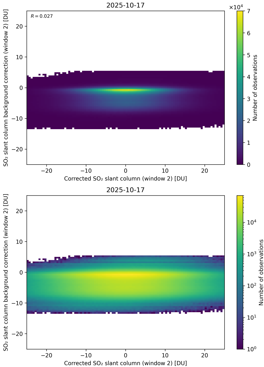
Figure 244: Scatter density plot of “Corrected SO 2 slant column (window 2)” against “SO 2 slant column background correction (window 2)” for 2025-10-17 to 2025-10-18.
