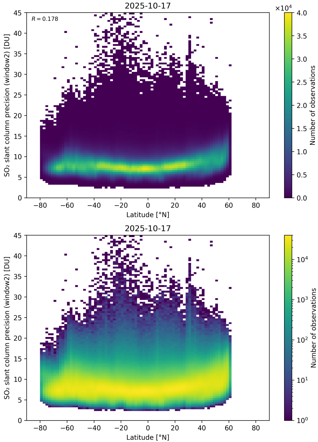
Figure 164: Scatter density plot of “Latitude” against “SO 2 slant column precision (window2)” for 2025-10-17 to 2025-10-18.
