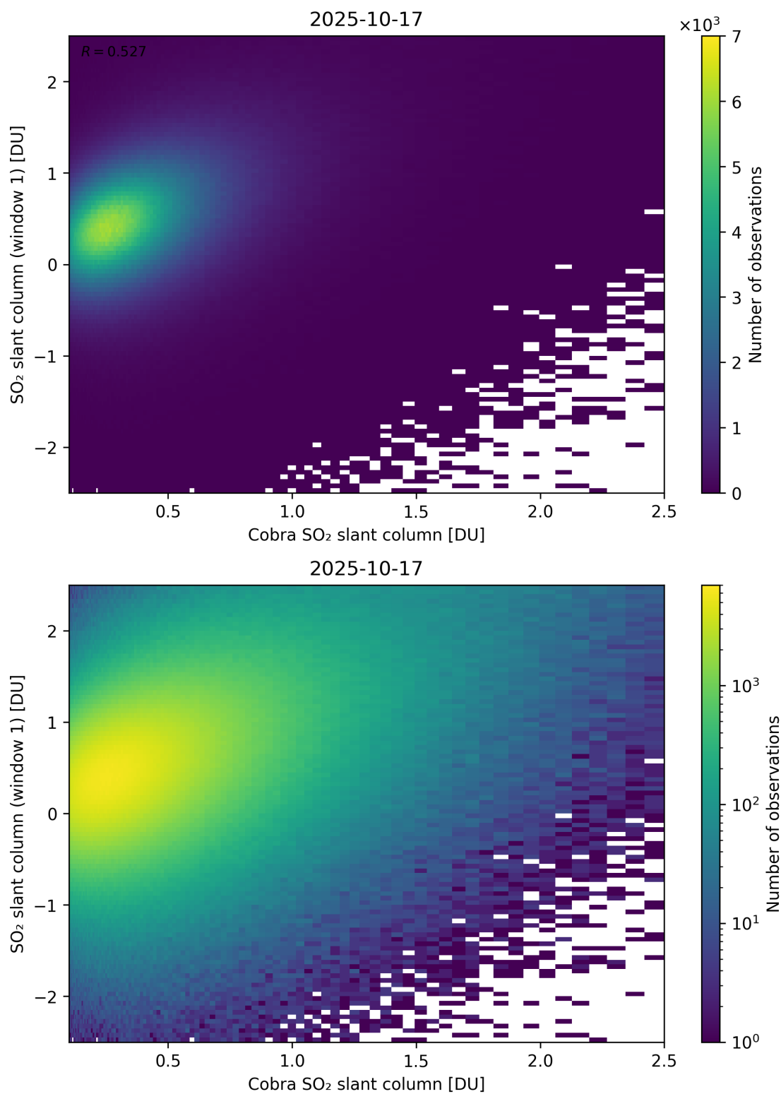
Figure 219: Scatter density plot of “Cobra SO 2 slant column” against “SO 2 slant column (window 1)” for 2025-10-17 to 2025-10-18.
