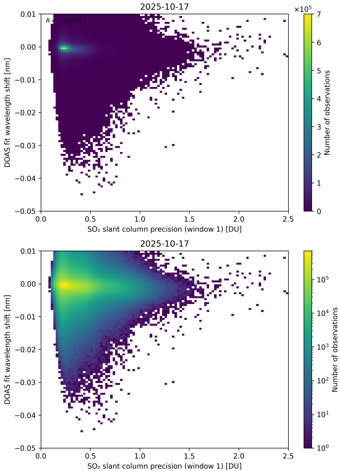
Figure 271: Scatter density plot of “SO 2 slant column precision (window 1)” against “DOAS fit wavelength shift” for 2025-10-17 to 2025-10-18.
