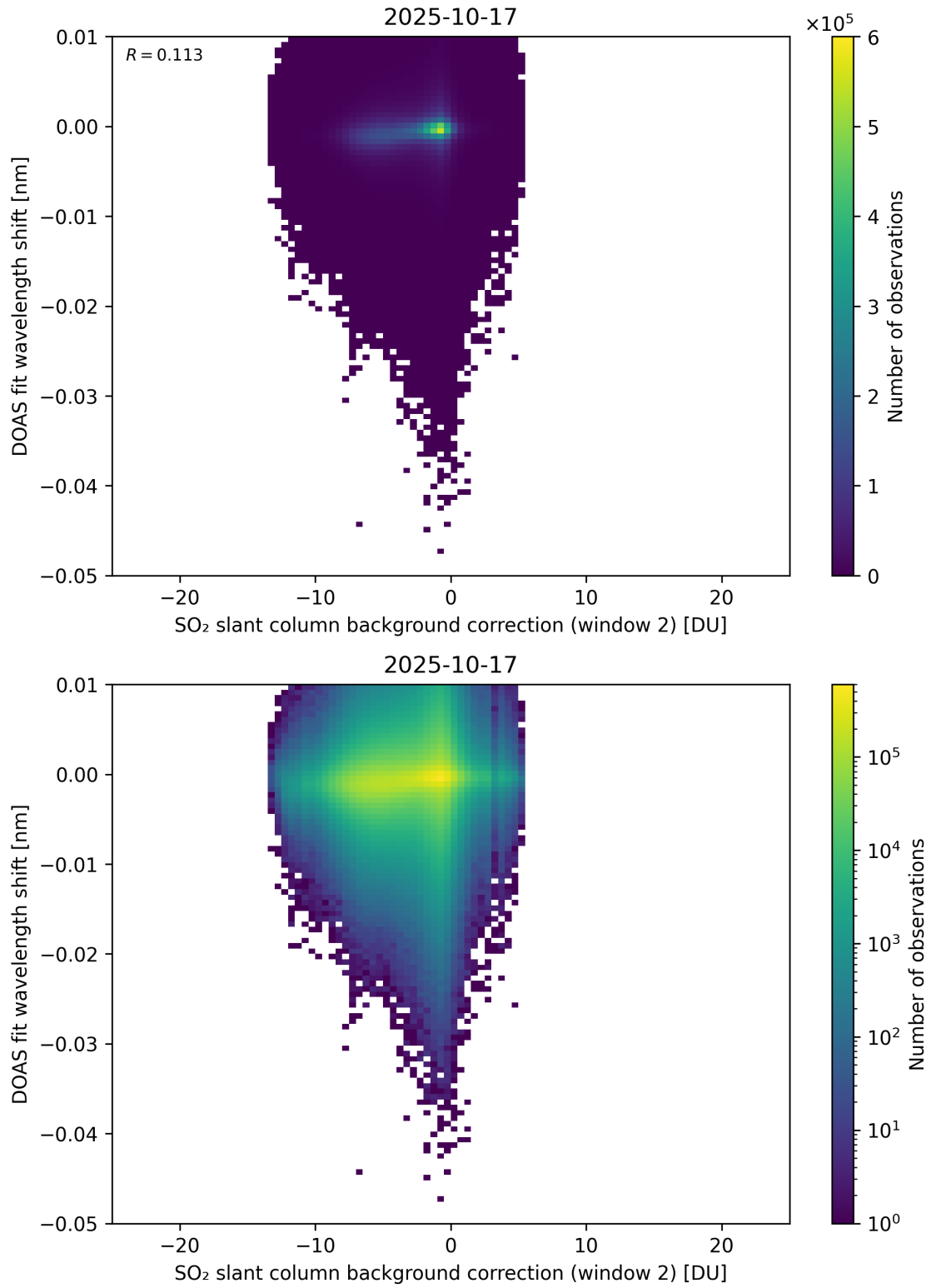
Figure 123: Scatter density plot of “SO 2 slant column background correction (window 2)” against “DOAS fit wavelength shift” for 2025-10-17 to 2025-10-18.
