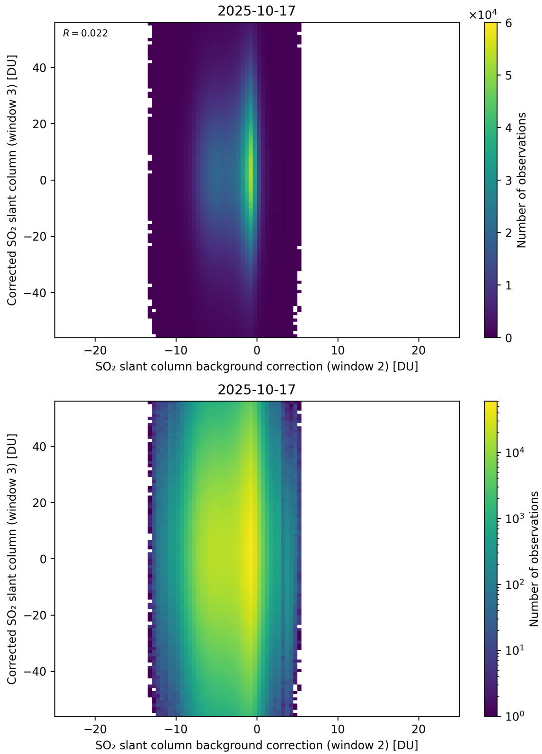
Figure 127: Scatter density plot of “SO 2 slant column background correction (window 2)” against “Corrected SO 2 slant column (window 3)” for 2025-10-17 to 2025-10-18.
