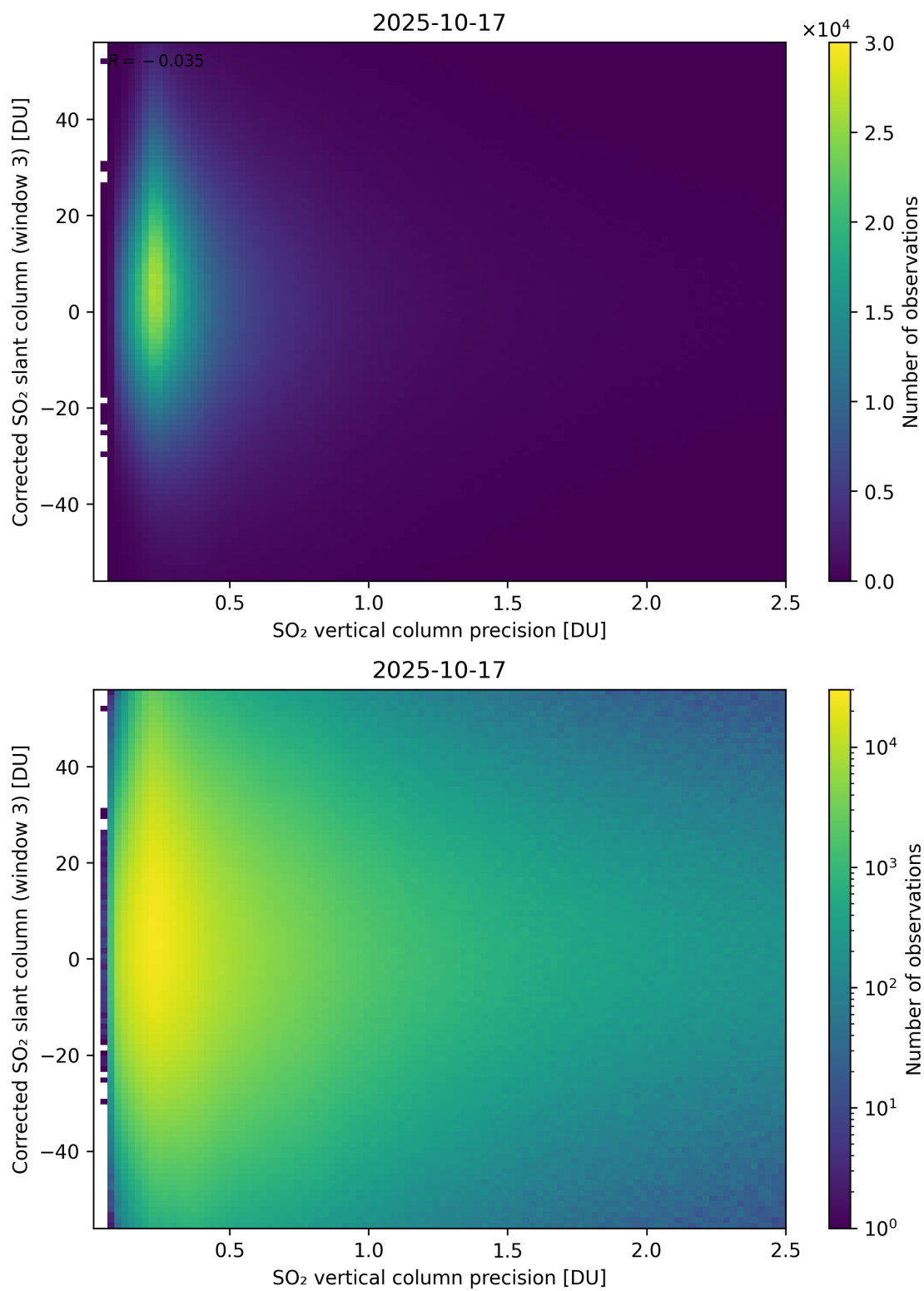
Figure 340: Scatter density plot of “SO 2 vertical column precision” against “Corrected SO 2 slant column (window 3)” for 2025-10-17 to 2025-10-18.
