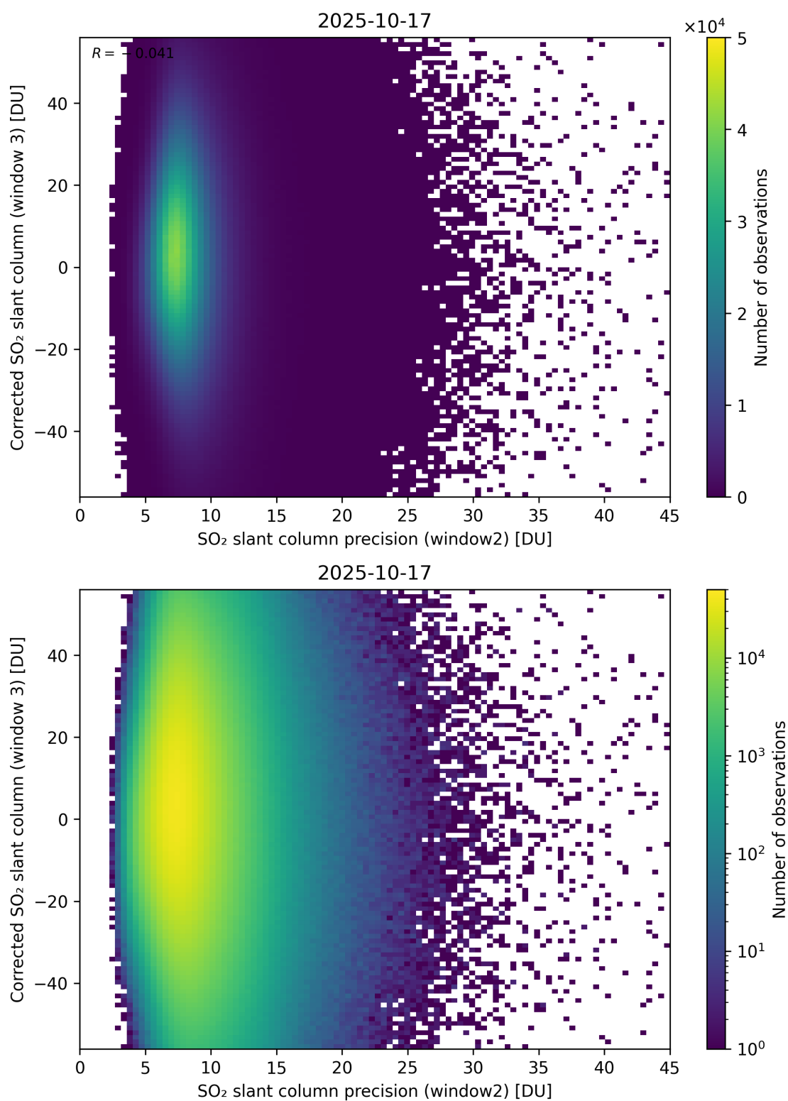
Figure 298: Scatter density plot of “SO 2 slant column precision (window2)” against “Corrected SO 2 slant column (window 3)” for 2025-10-17 to 2025-10-18.
