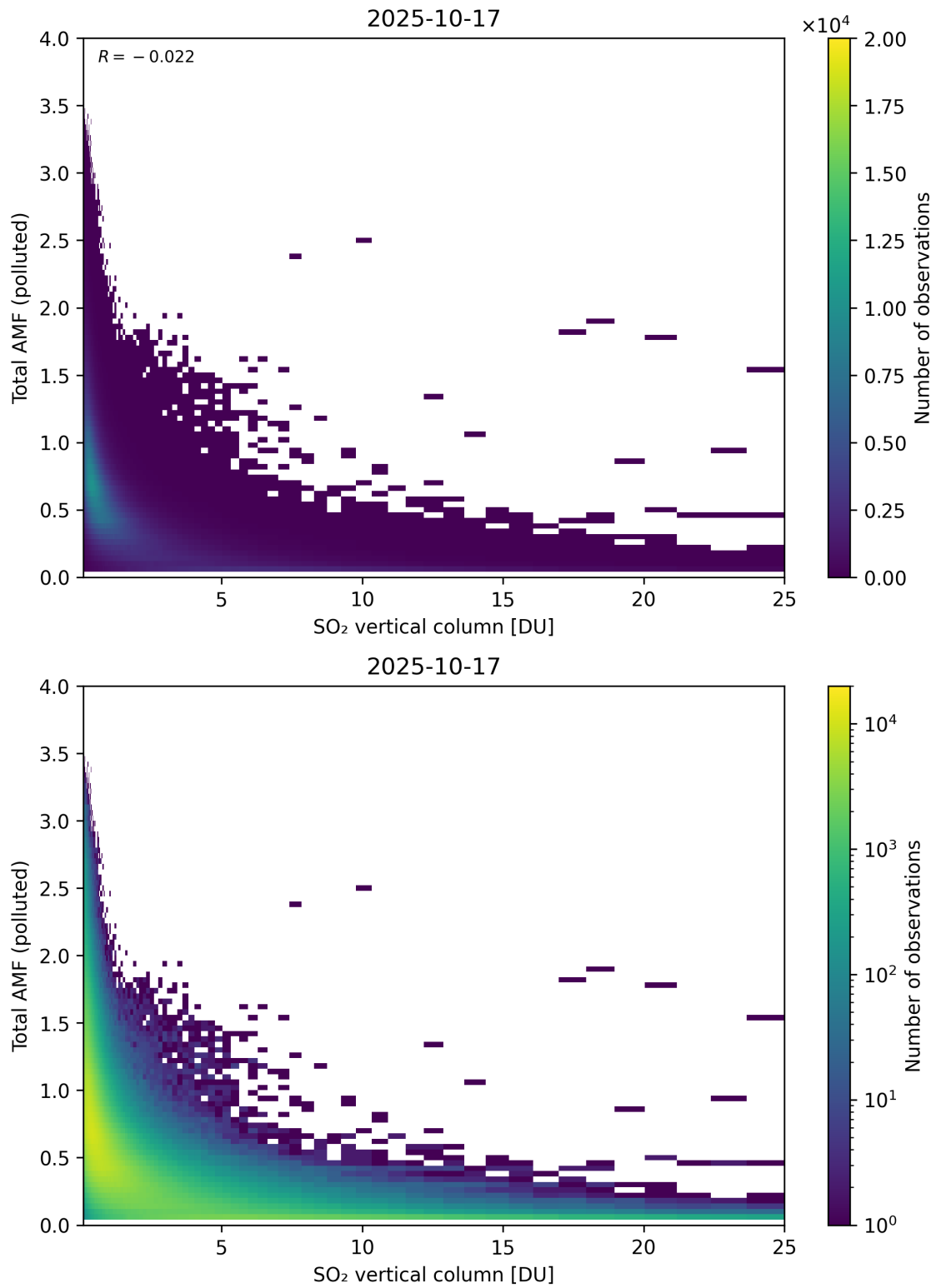
Figure 359: Scatter density plot of “SO 2 vertical column” against “Total AMF (polluted)” for 2025-10-17 to 2025-10-18.
