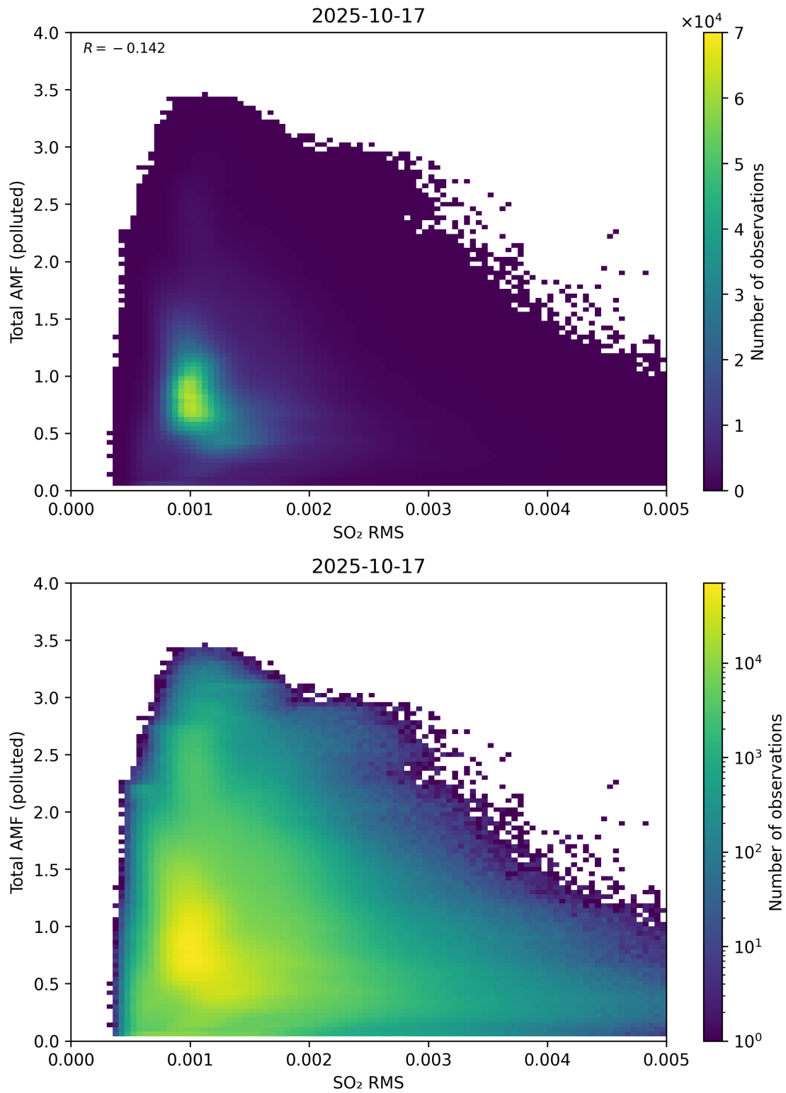
Figure 148: Scatter density plot of “SO 2 RMS” against “Total AMF (polluted)” for 2025-10-17 to 2025-10-18.
