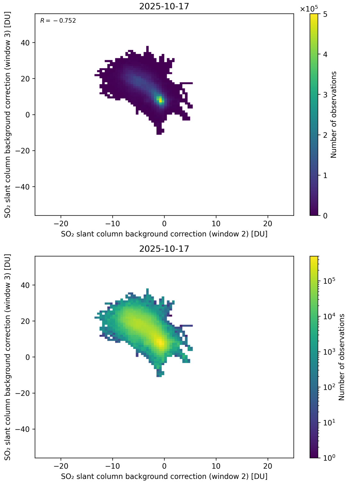
Figure 122: Scatter density plot of “SO 2 slant column background correction (window 2)” against “SO 2 slant column background correction (window 3)” for 2025-10-17 to 2025-10-18.
