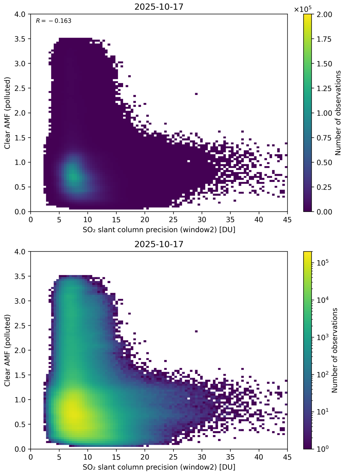
Figure 296: Scatter density plot of “SO 2 slant column precision (window2)” against “Clear AMF (polluted)” for 2025-10-17 to 2025-10-18.
