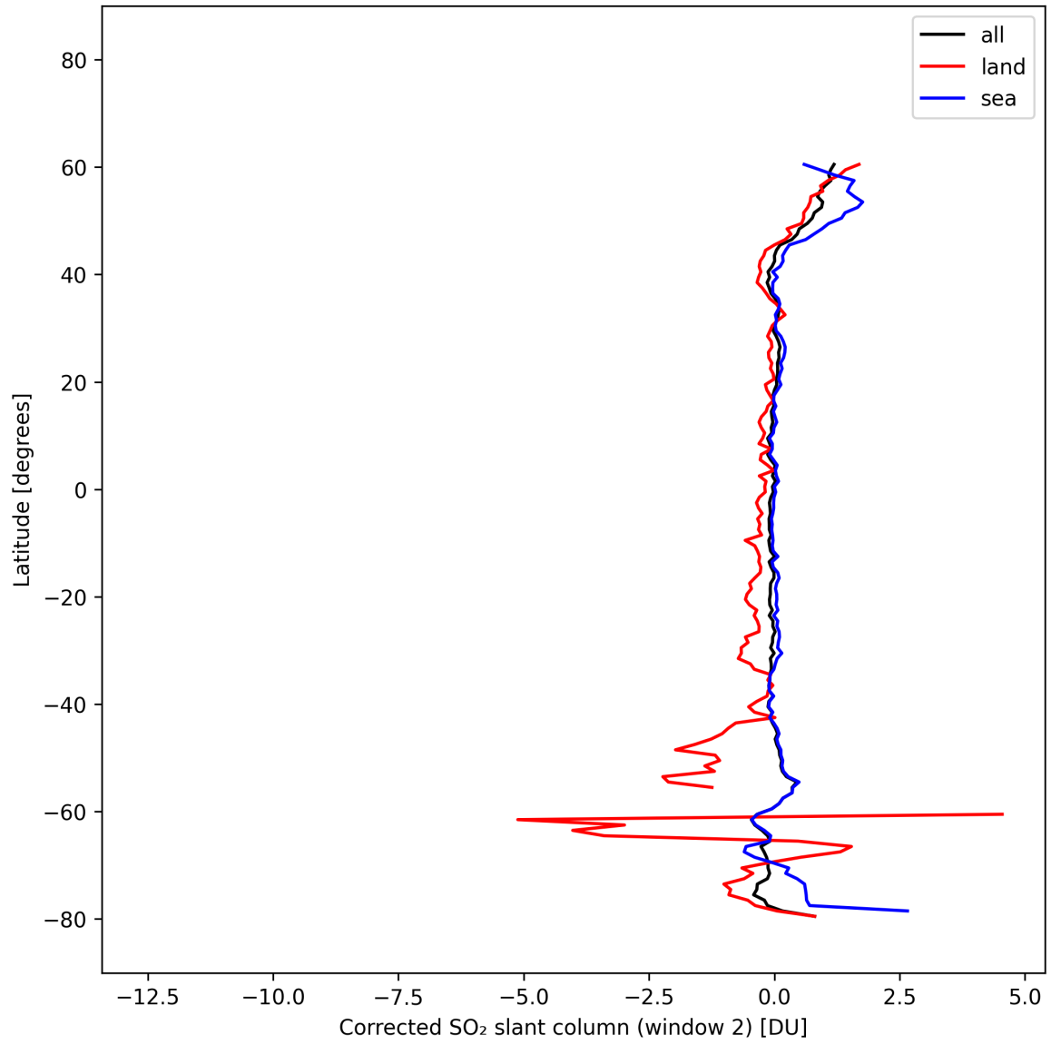
Figure 43: Zonal average of “Corrected SO 2 slant column (window 2)” for 2025-10-17 to 2025-10-18.
