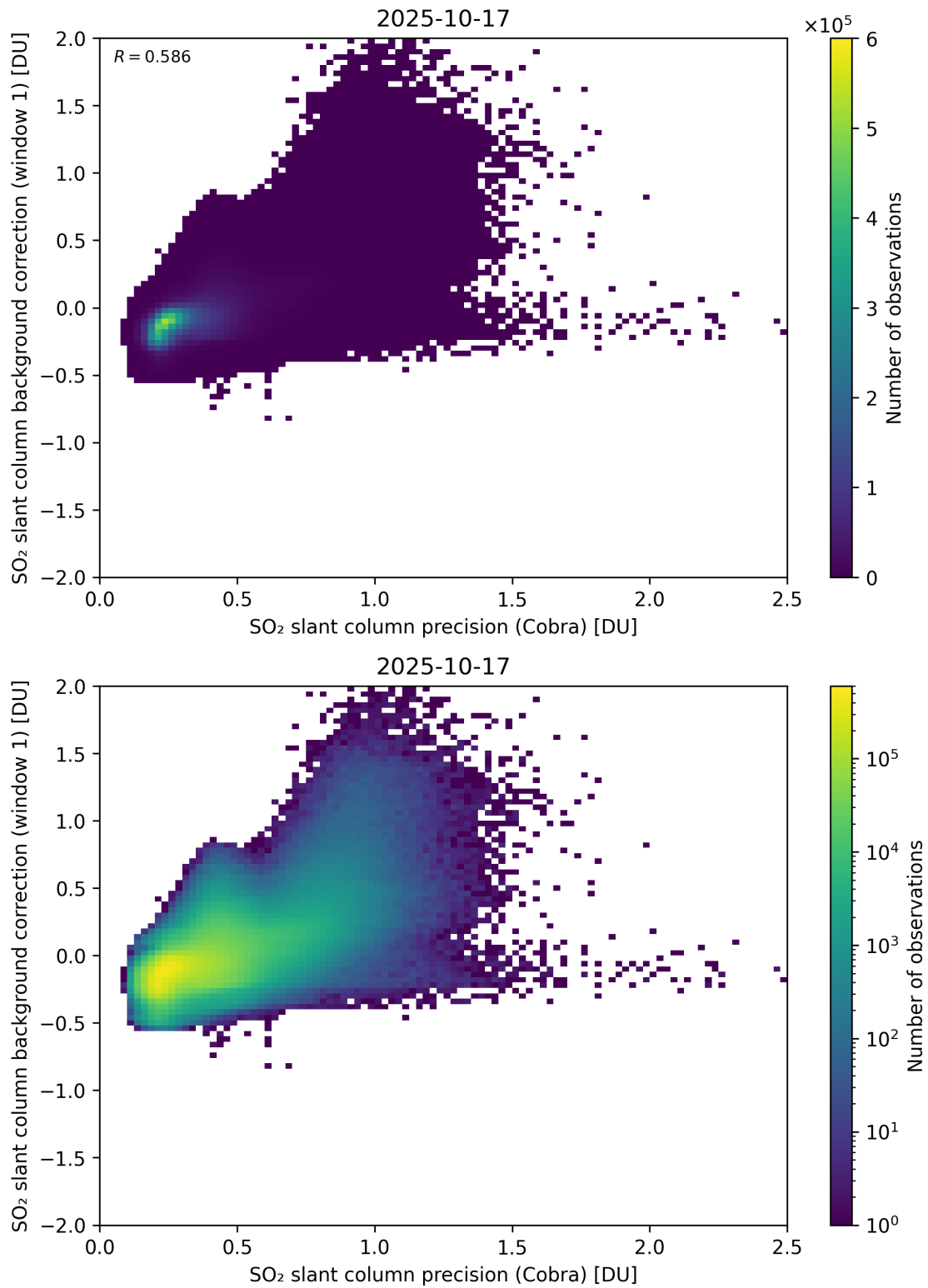
Figure 199: Scatter density plot of “SO 2 slant column precision (Cobra)” against “SO 2 slant column background correction (window 1)” for 2025-10-17 to 2025-10-18.
