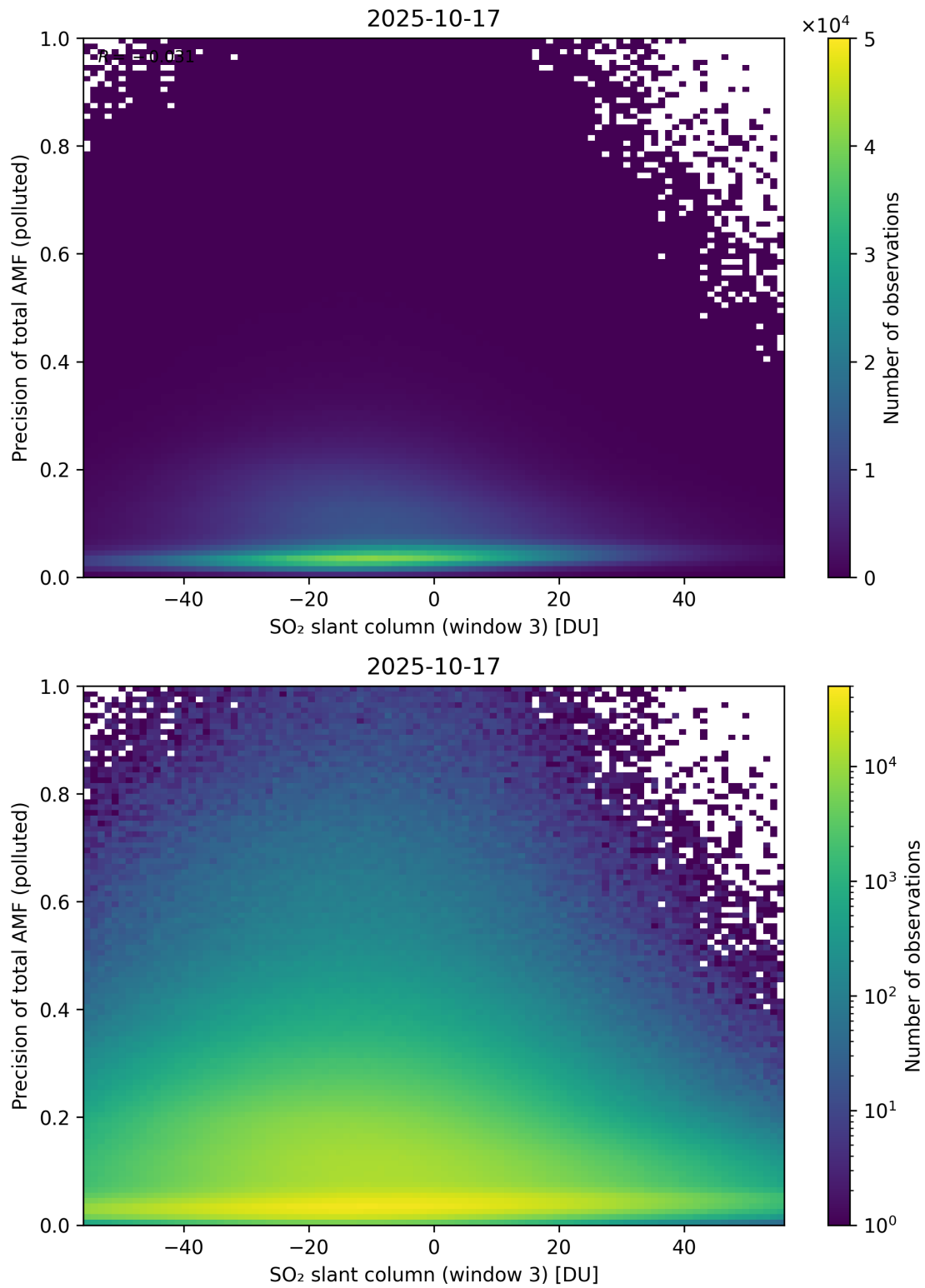
Figure 319: Scatter density plot of “SO 2 slant column (window 3)” against “Precision of total AMF (polluted)” for 2025-10-17 to 2025-10-18.
