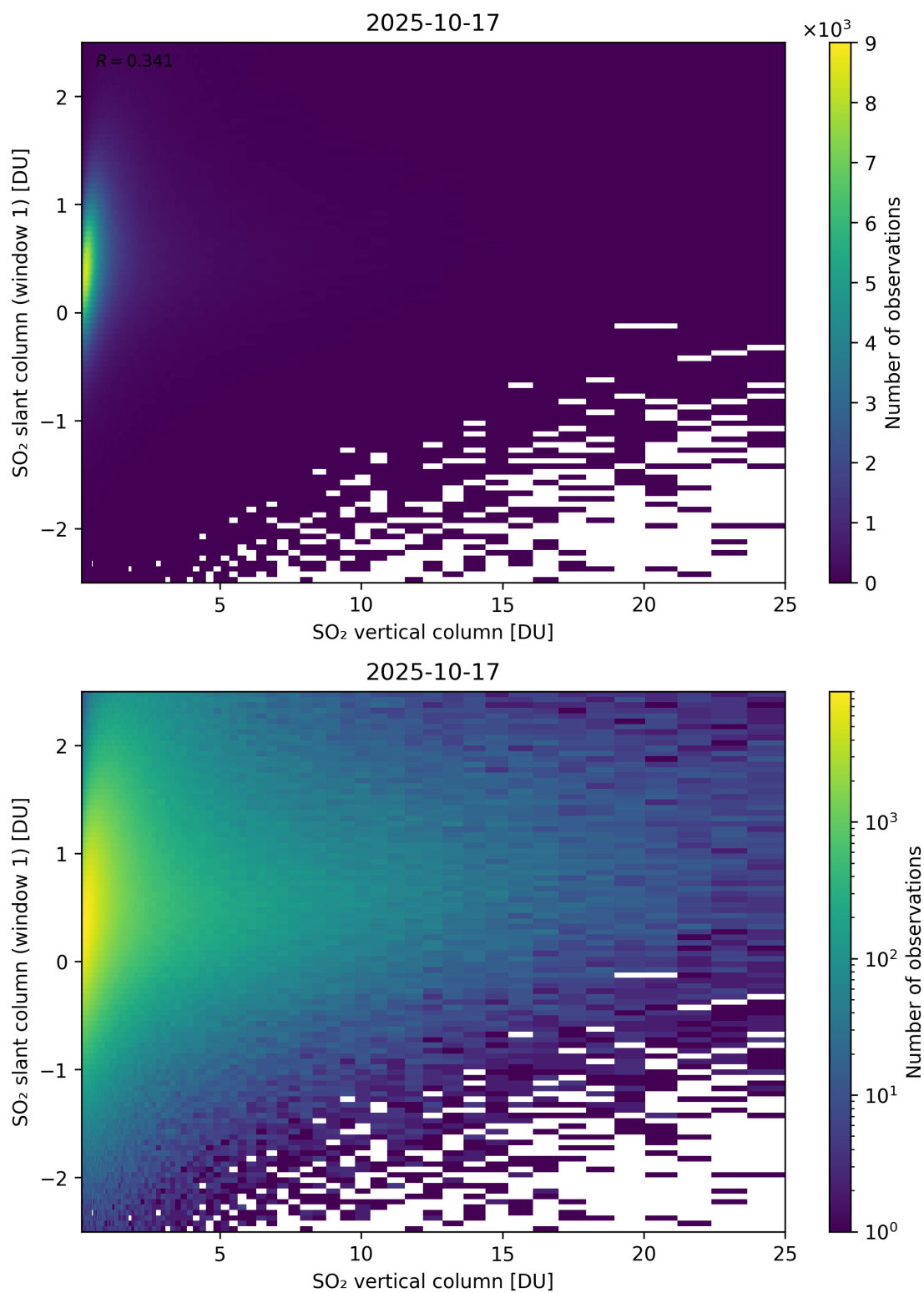
Figure 354: Scatter density plot of “SO 2 vertical column” against “SO 2 slant column (window 1)” for 2025-10-17 to 2025-10-18.
