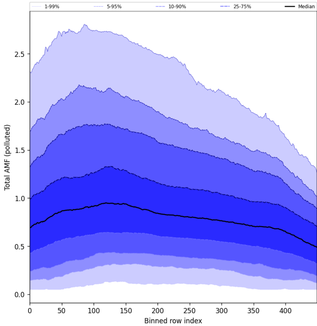
Figure 105: Along track statistics of “Total AMF (polluted)” for 2025-10-17 to 2025-10-18
