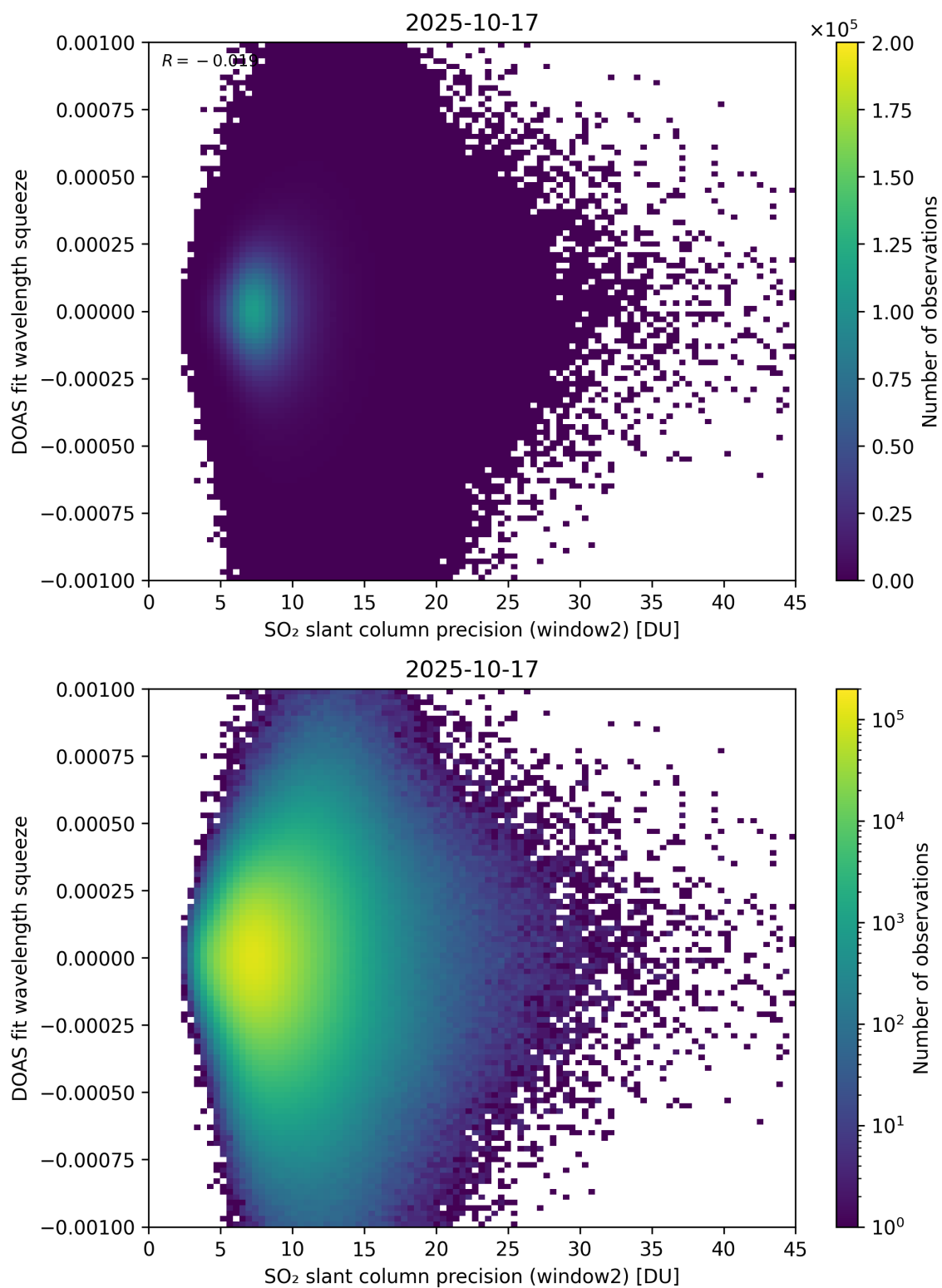
Figure 294: Scatter density plot of “SO 2 slant column precision (window2)” against “DOAS fit wavelength squeeze” for 2025-10-17 to 2025-10-18.
