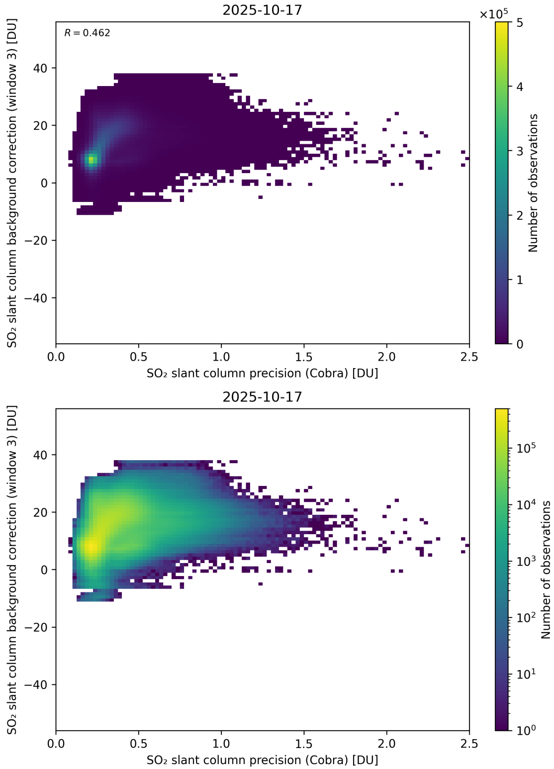
Figure 201: Scatter density plot of “SO 2 slant column precision (Cobra)” against “SO 2 slant column background correction (window 3)” for 2025-10-17 to 2025-10-18.
