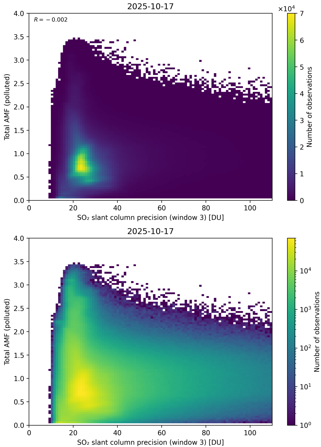
Figure 313: Scatter density plot of “SO 2 slant column precision (window 3)” against “Total AMF (polluted)” for 2025-10-17 to 2025-10-18.
