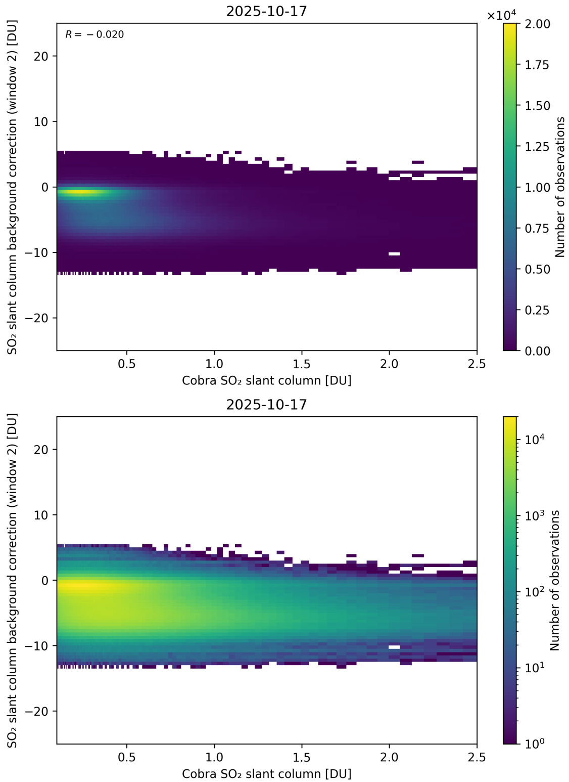
Figure 194: Scatter density plot of “Cobra SO 2 slant column” against “SO 2 slant column background correction (window 2)” for 2025-10-17 to 2025-10-18.
