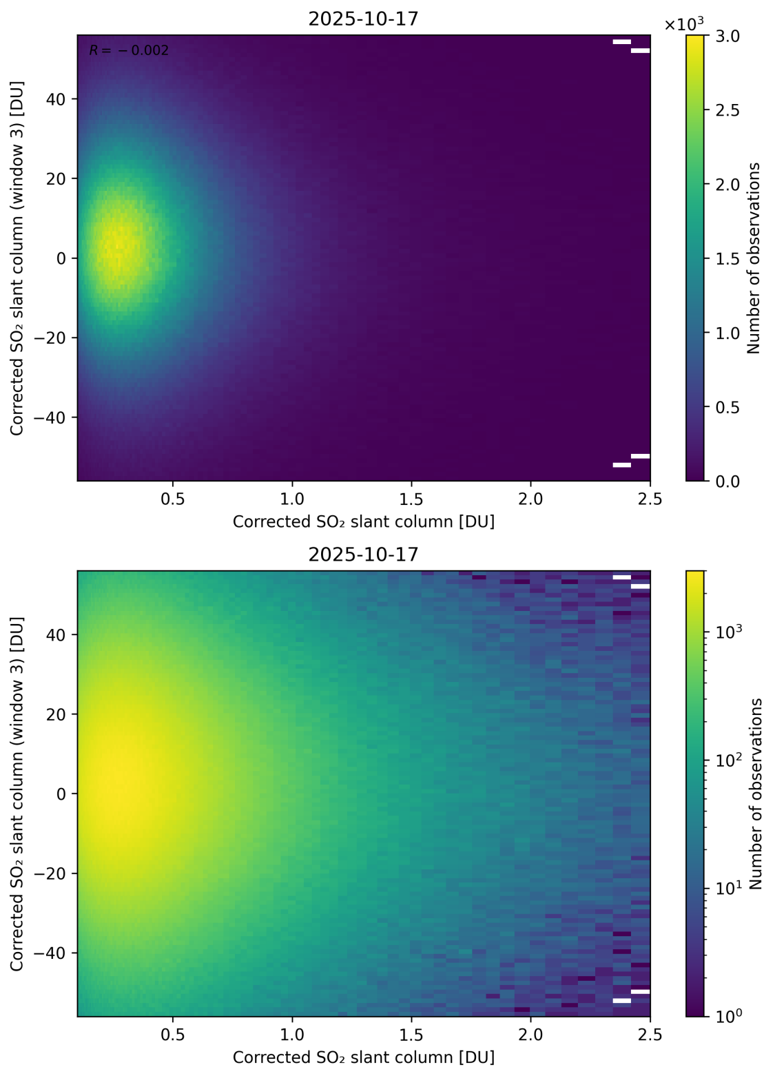
Figure 236: Scatter density plot of “Corrected SO 2 slant column” against “Corrected SO 2 slant column (window 3)” for 2025-10-17 to 2025-10-18.
