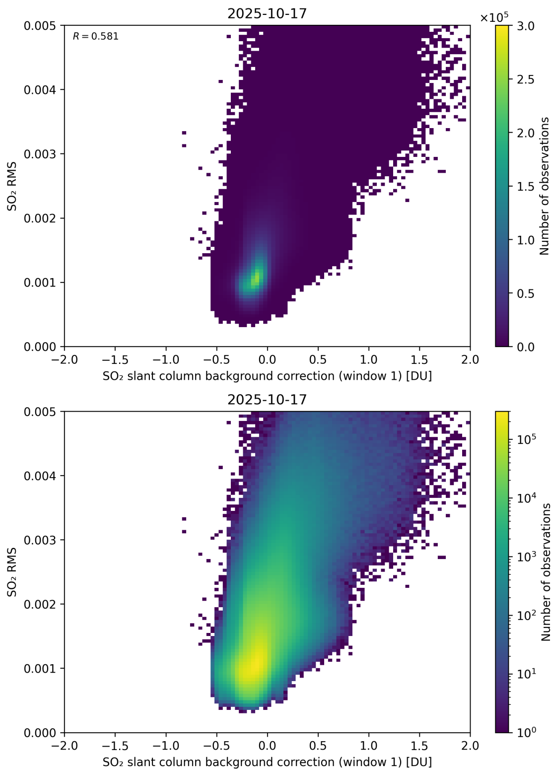
Figure 113: Scatter density plot of “SO 2 slant column background correction (window 1)” against “SO 2 RMS” for 2025-10-17 to 2025-10-18.
