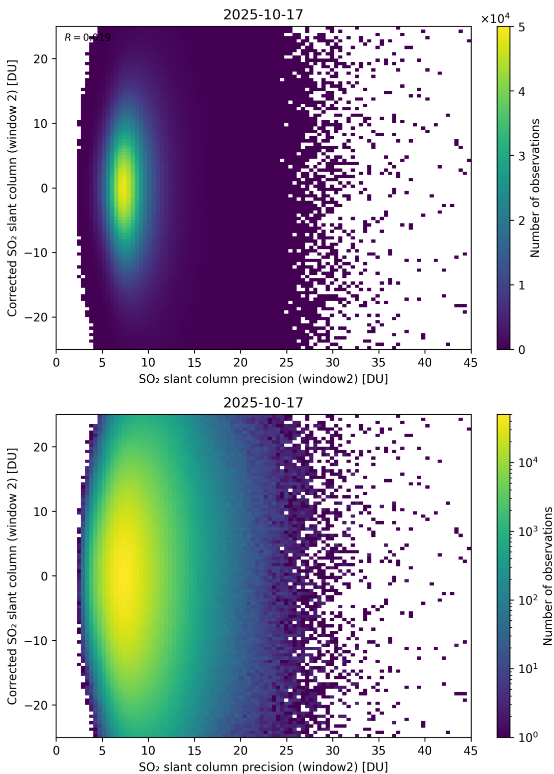
Figure 297: Scatter density plot of “SO 2 slant column precision (window2)” against “Corrected SO 2 slant column (window 2)” for 2025-10-17 to 2025-10-18.
