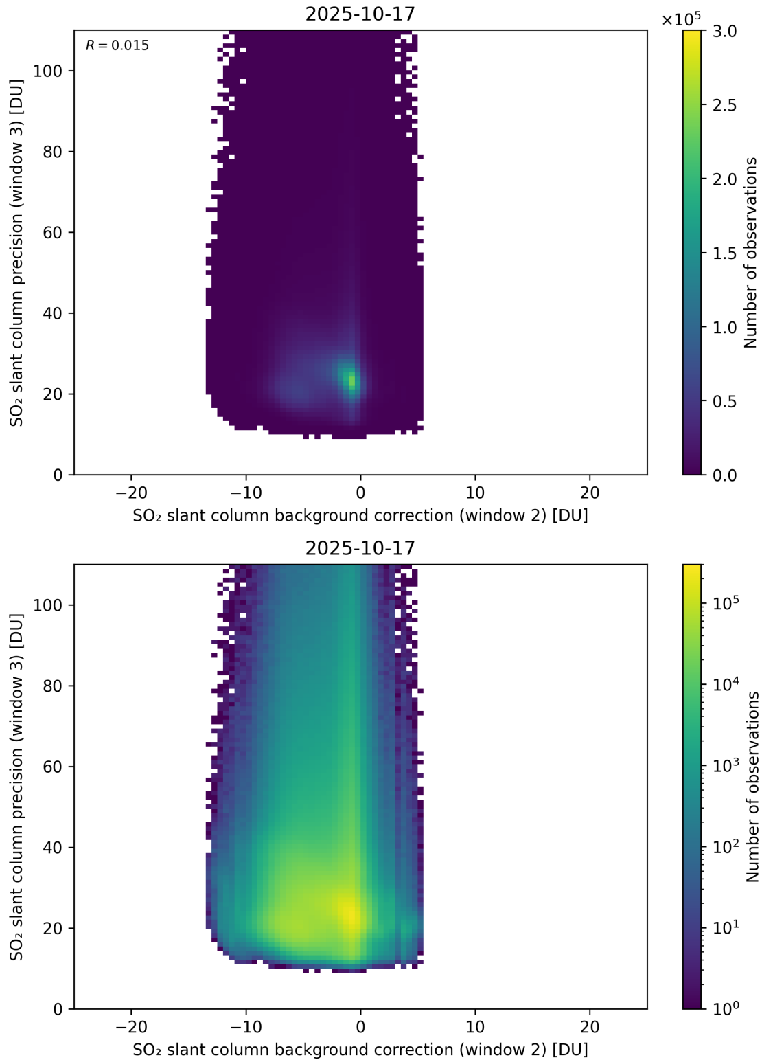
Figure 129: Scatter density plot of “SO 2 slant column background correction (window 2)” against “SO 2 slant column precision (window 3)” for 2025-10-17 to 2025-10-18.
