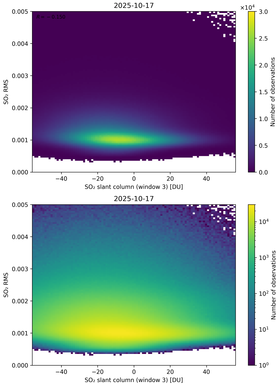
Figure 306: Scatter density plot of “SO 2 slant column (window 3)” against “SO 2 RMS” for 2025-10-17 to 2025-10-18.
