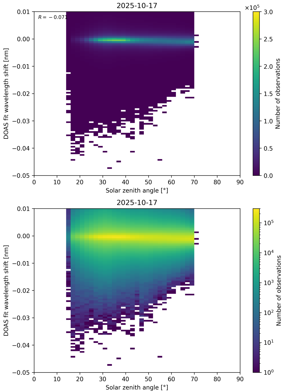
Figure 174: Scatter density plot of “Solar zenith angle” against “DOAS fit wavelength shift” for 2025-10-17 to 2025-10-18.
