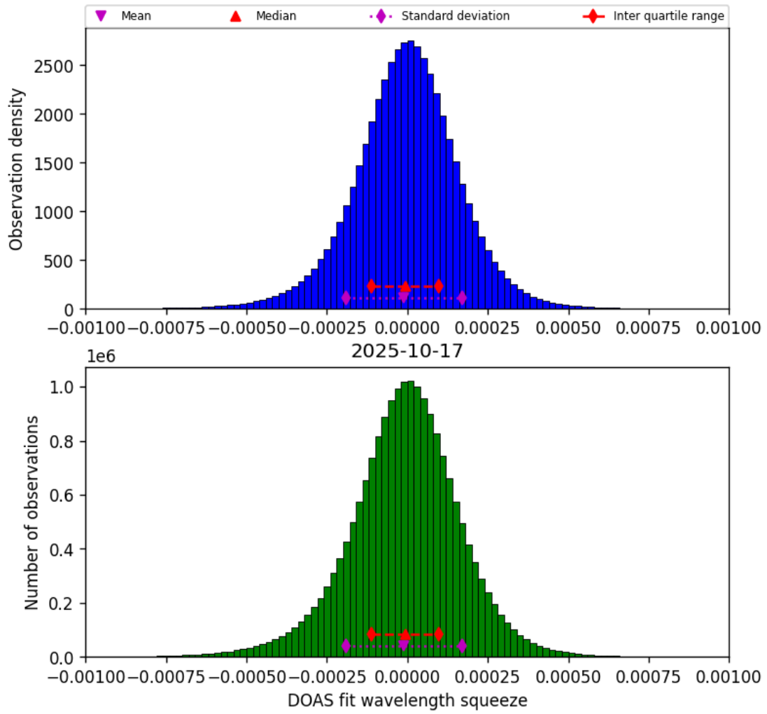
Figure 77: Histogram of “DOAS fit wavelength squeeze” for 2025-10-17 to 2025-10-18
