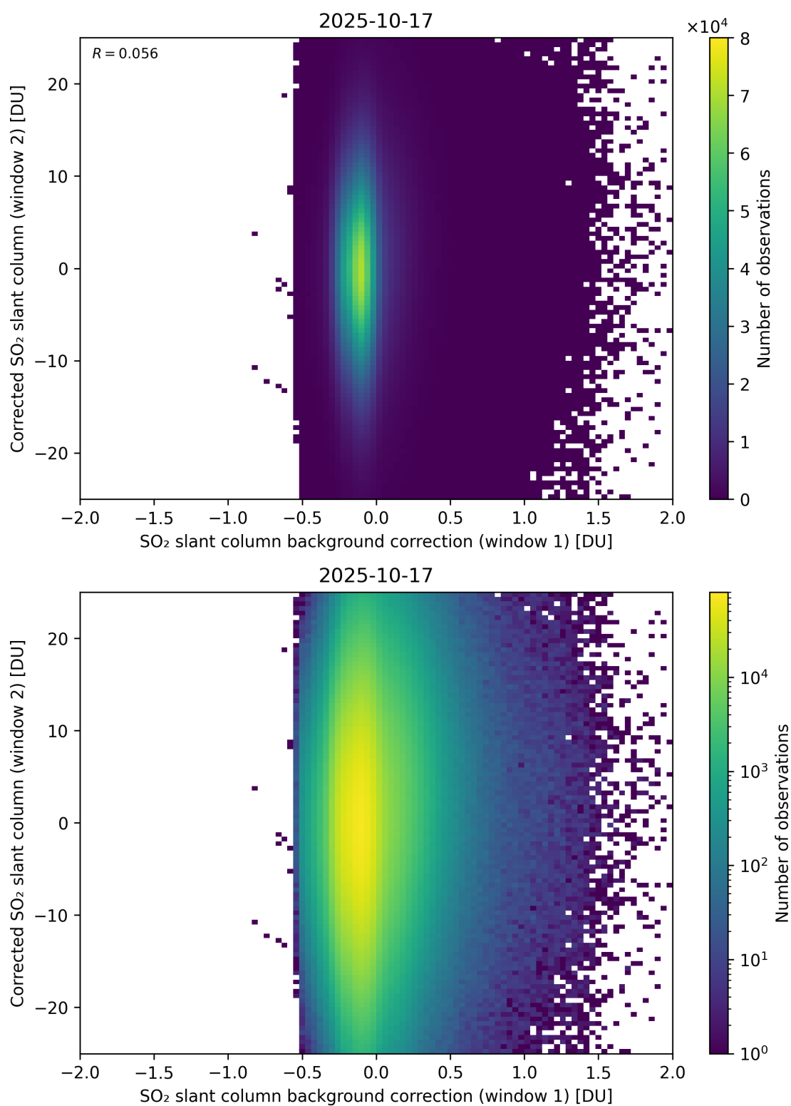
Figure 115: Scatter density plot of “SO 2 slant column background correction (window 1)” against “Corrected SO 2 slant column (window 2)” for 2025-10-17 to 2025-10-18.
