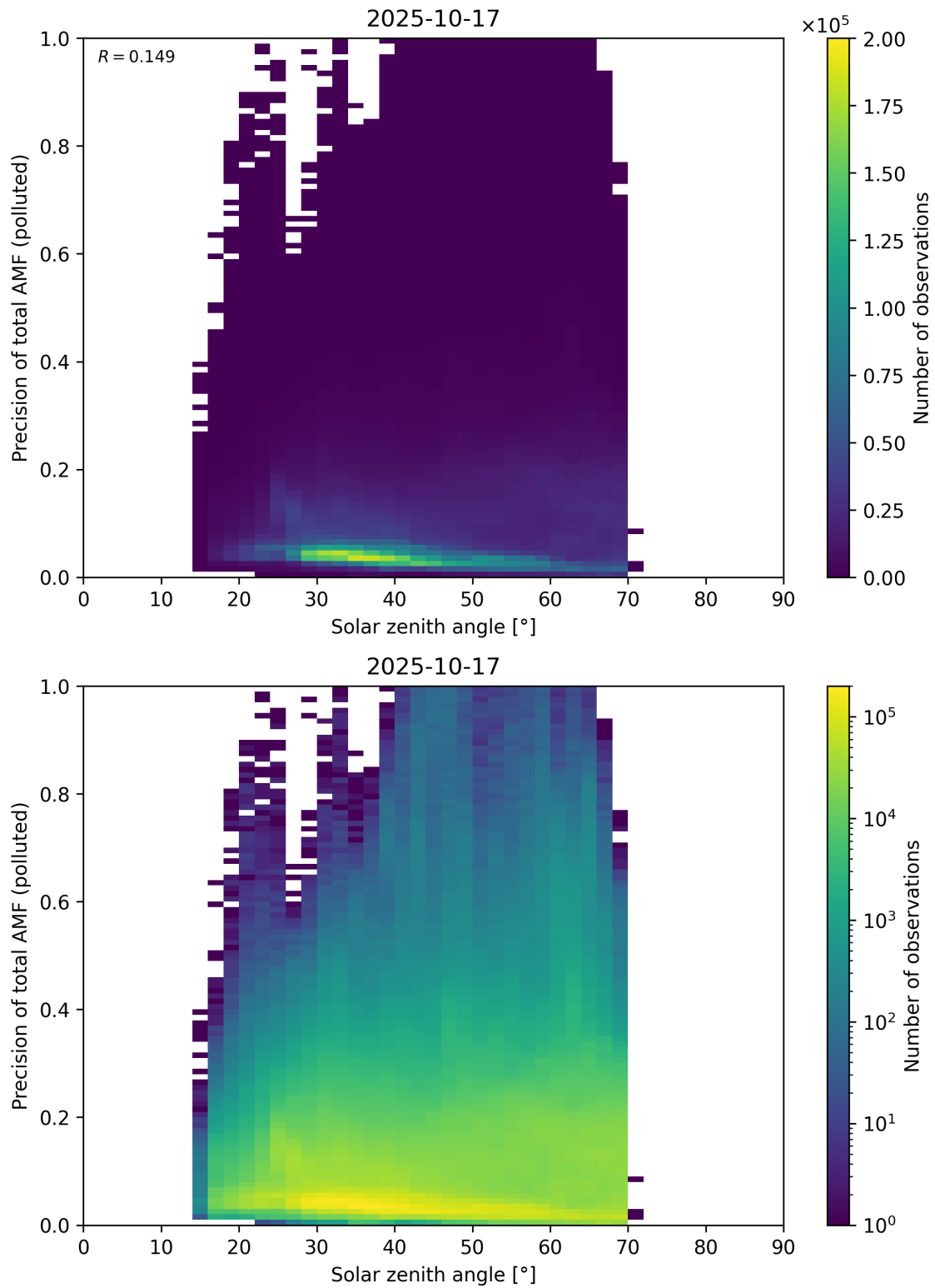
Figure 190: Scatter density plot of “Solar zenith angle” against “Precision of total AMF (polluted)” for 2025-10-17 to 2025-10-18.
