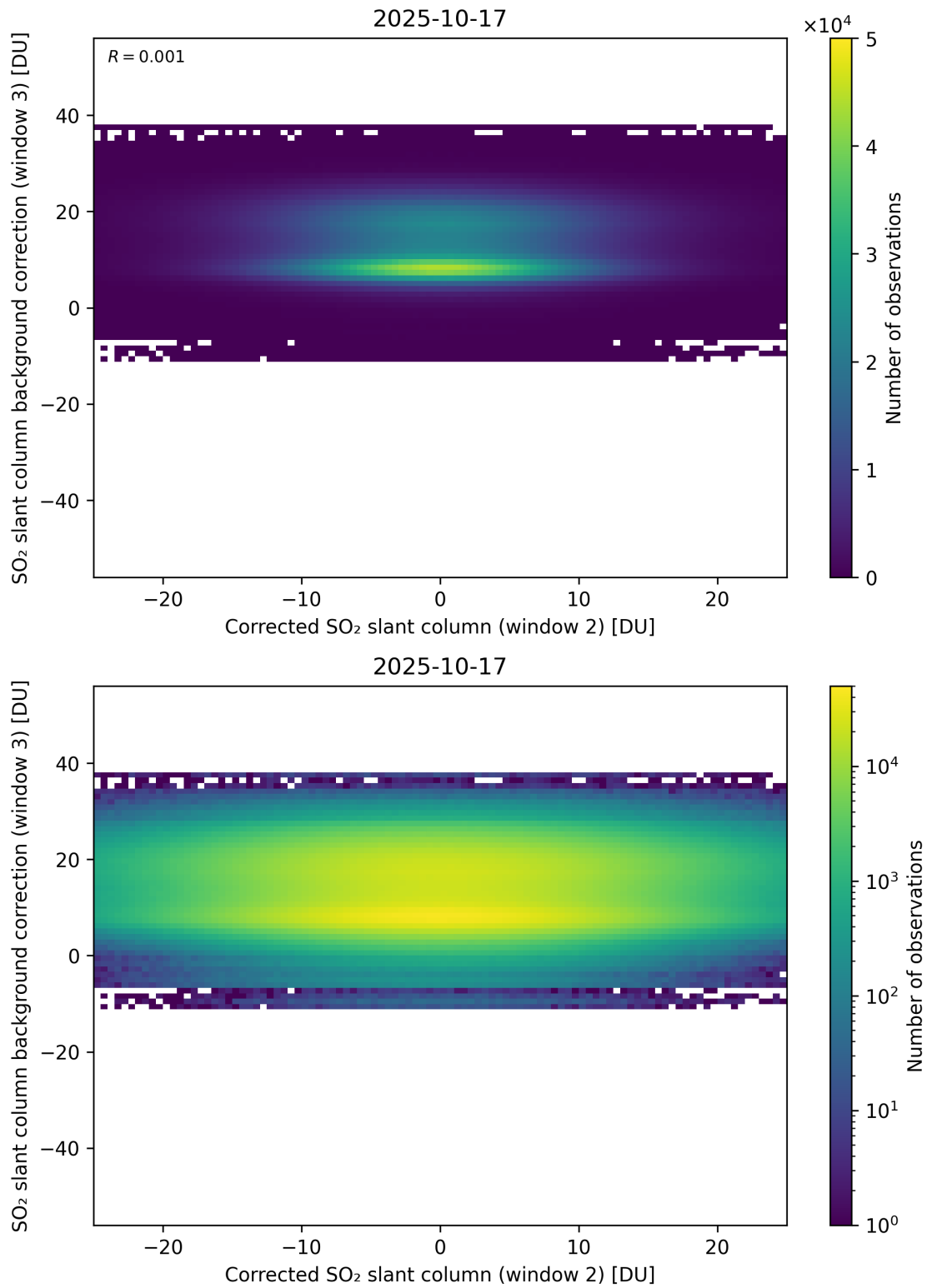
Figure 245: Scatter density plot of “Corrected SO 2 slant column (window 2)” against “SO 2 slant column background correction (window 3)” for 2025-10-17 to 2025-10-18.
