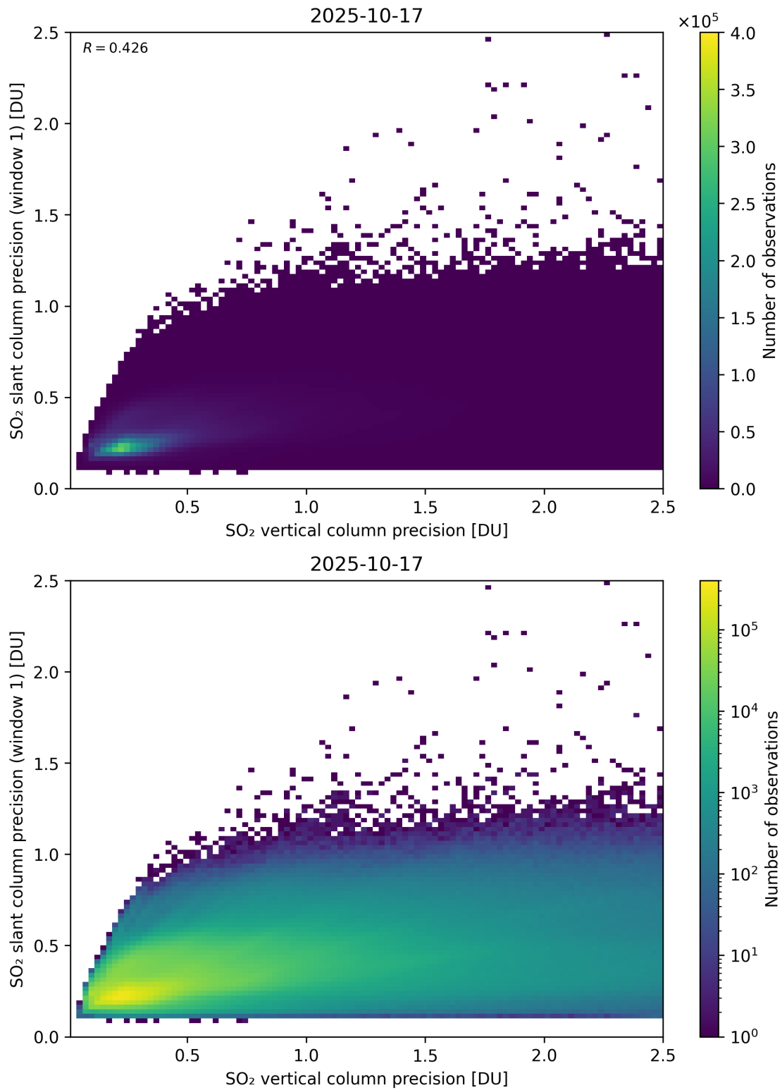
Figure 342: Scatter density plot of “SO 2 vertical column precision” against “SO 2 slant column precision (window 1)” for 2025-10-17 to 2025-10-18.
