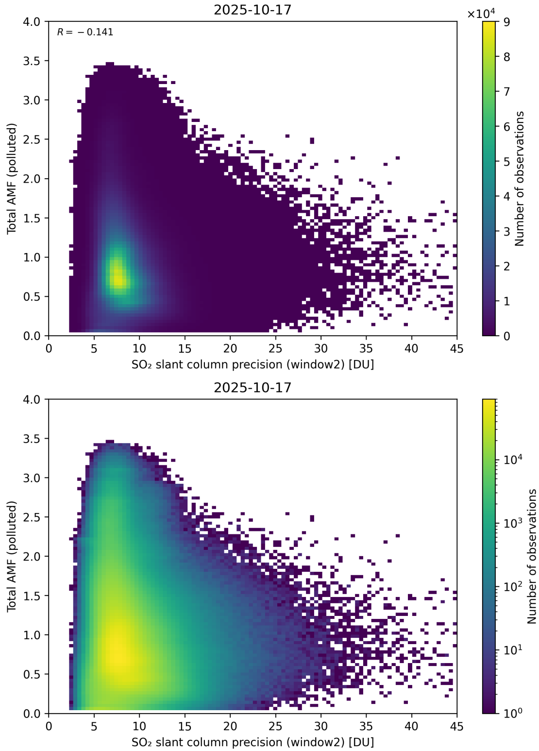
Figure 301: Scatter density plot of “SO 2 slant column precision (window2)” against “Total AMF (polluted)” for 2025-10-17 to 2025-10-18.
