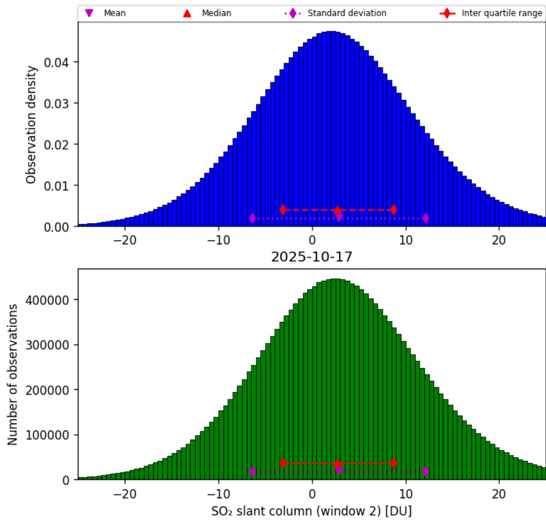
Figure 67: Histogram of “SO 2 slant column (window 2)” for 2025-10-17 to 2025-10-18
