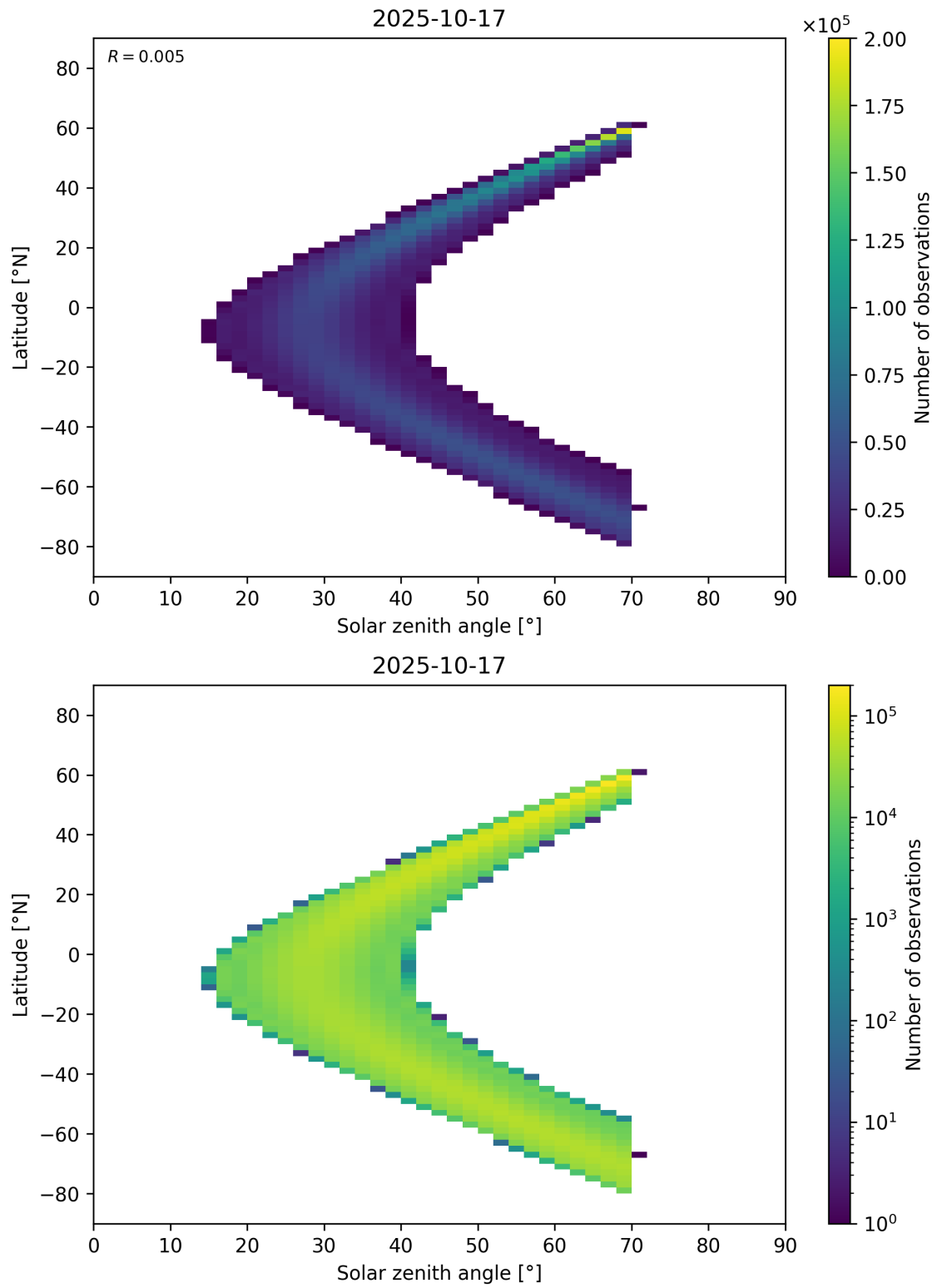
Figure 177: Scatter density plot of “Solar zenith angle” against “Latitude” for 2025-10-17 to 2025-10-18.
