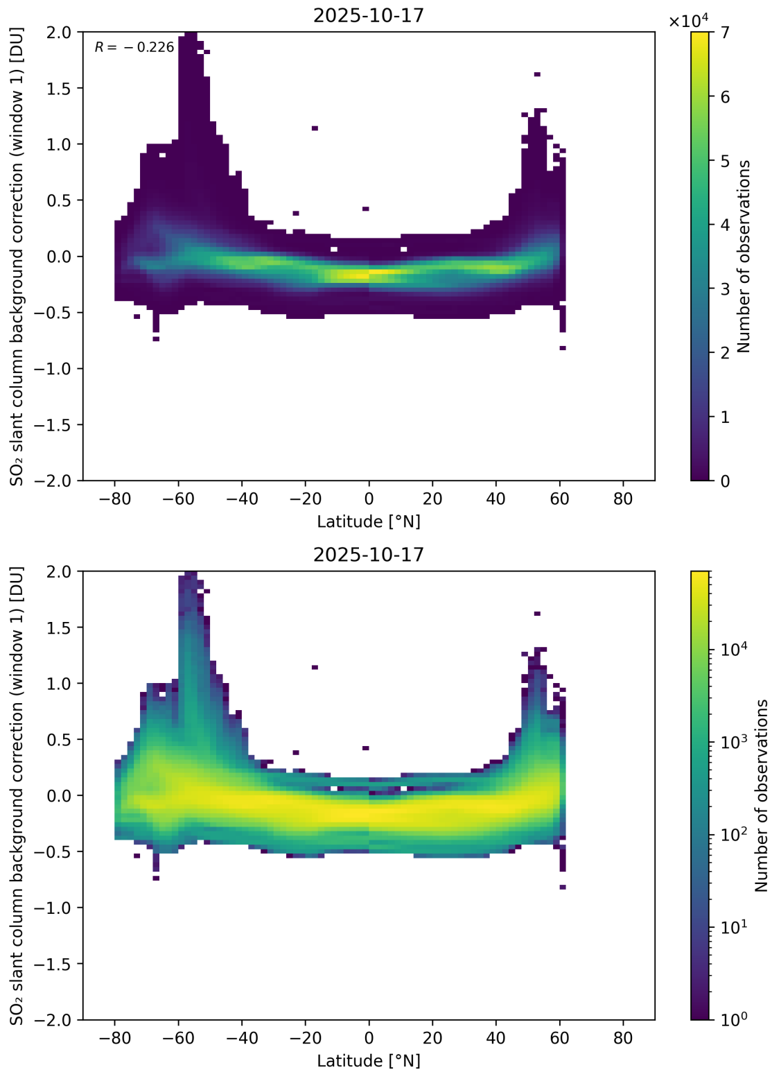
Figure 150: Scatter density plot of “Latitude” against “SO 2 slant column background correction (window 1)” for 2025-10-17 to 2025-10-18.
