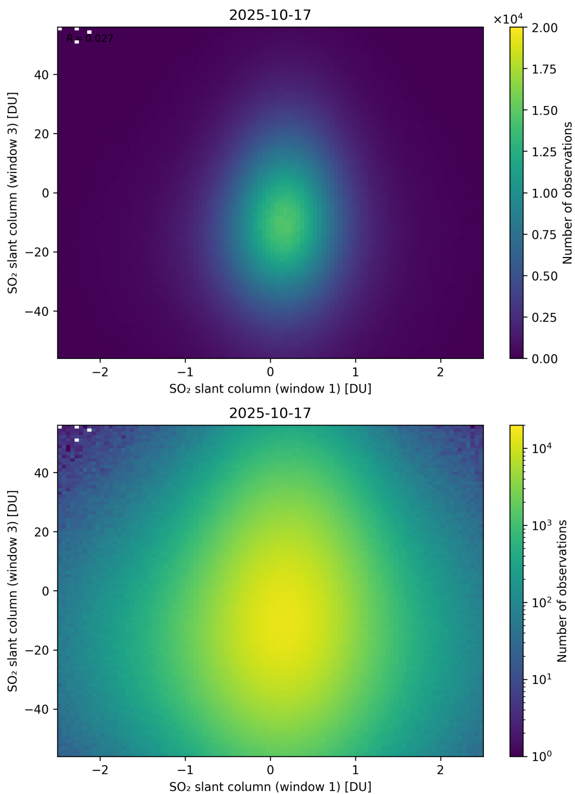
Figure 287: Scatter density plot of “SO 2 slant column (window 1)” against “SO 2 slant column (window 3)” for 2025-10-17 to 2025-10-18.
