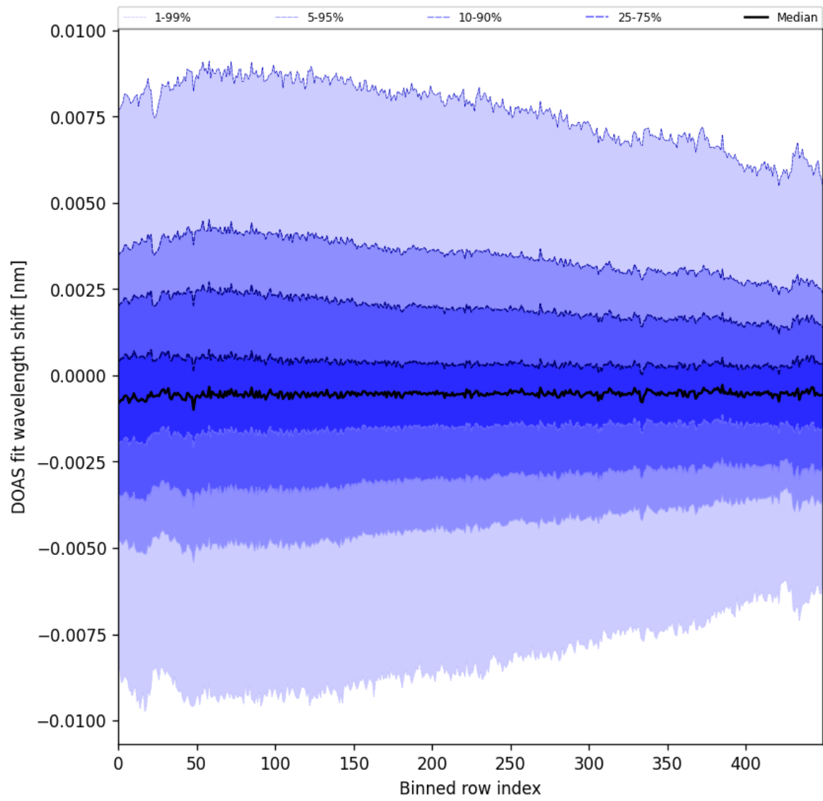
Figure 102: Along track statistics of “DOAS fit wavelength shift” for 2025-10-17 to 2025-10-18
