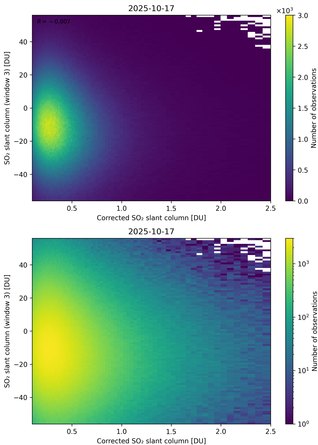
Figure 240: Scatter density plot of “Corrected SO 2 slant column” against “SO 2 slant column (window 3)” for 2025-10-17 to 2025-10-18.
