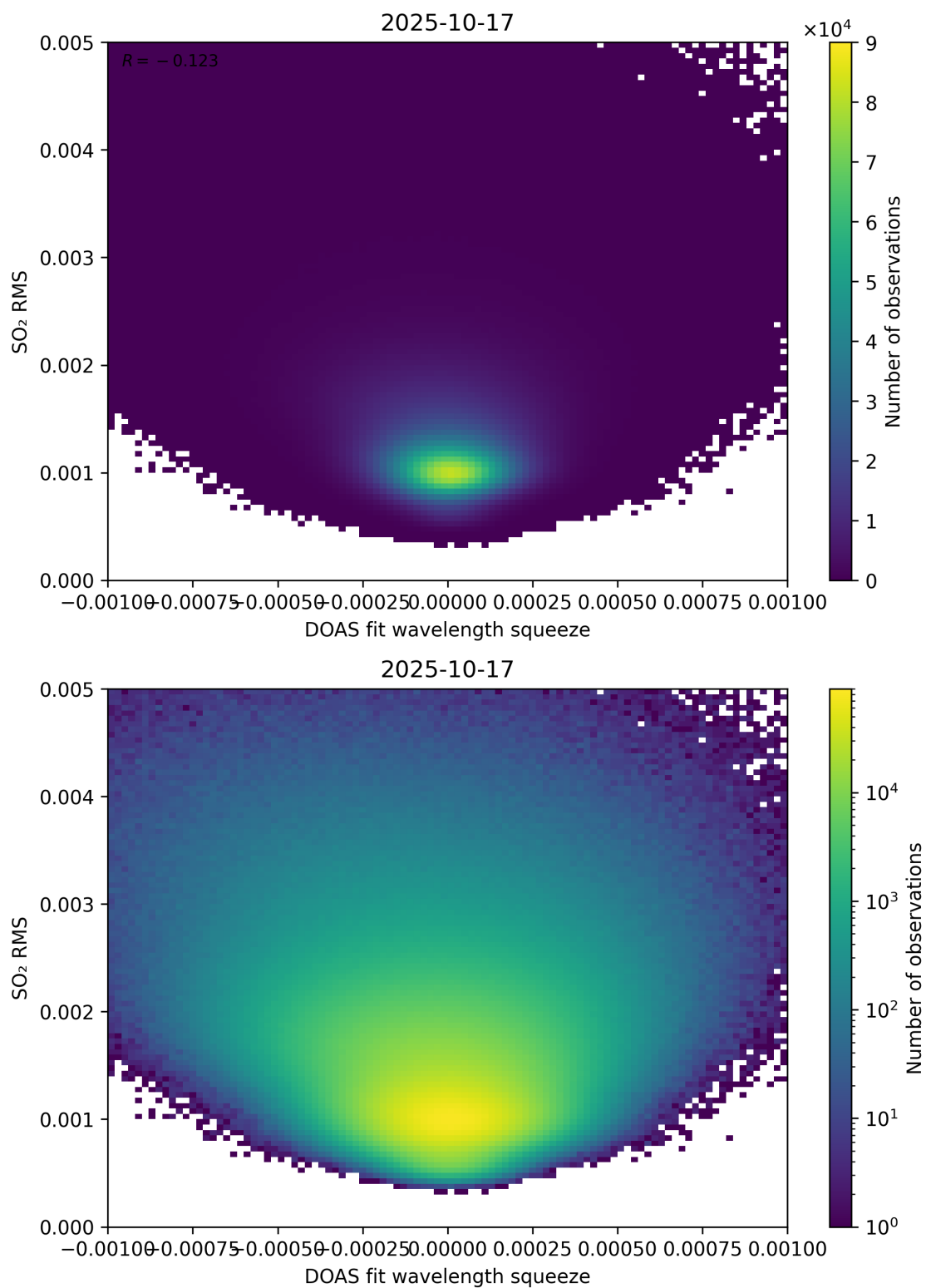
Figure 143: Scatter density plot of “DOAS fit wavelength squeeze” against “SO 2 RMS” for 2025-10-17 to 2025-10-18.
