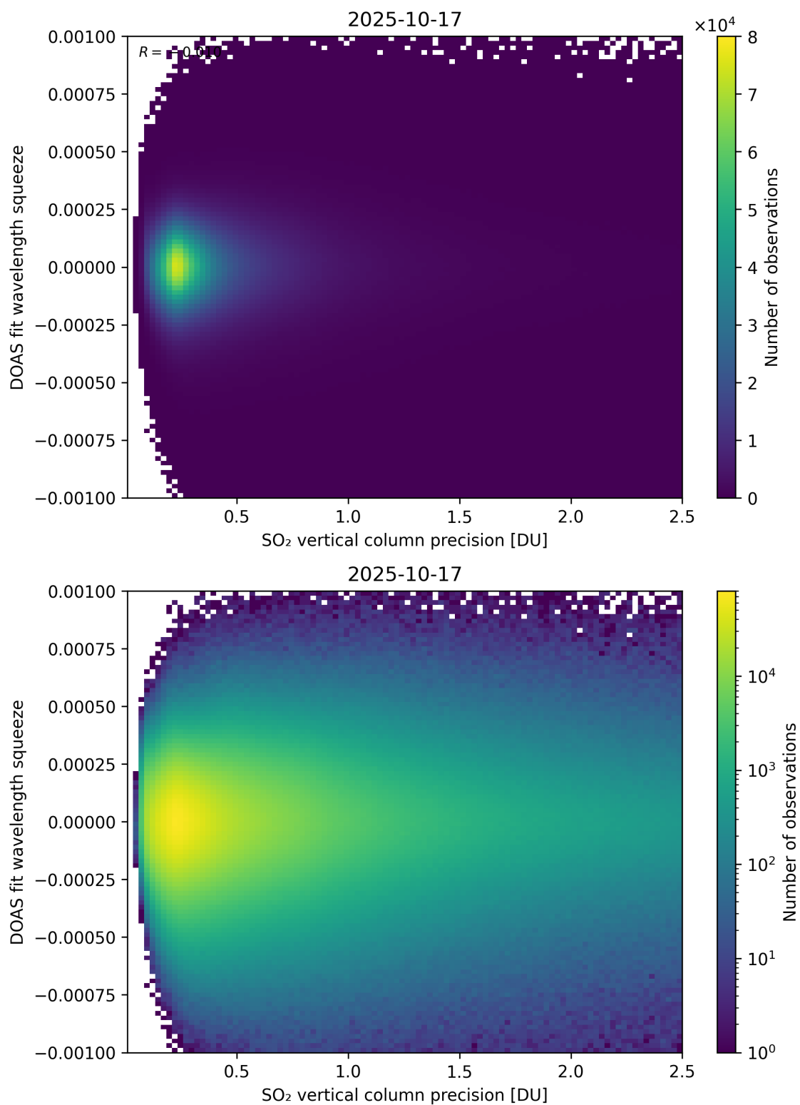
Figure 333: Scatter density plot of “SO 2 vertical column precision” against “DOAS fit wavelength squeeze” for 2025-10-17 to 2025-10-18.
