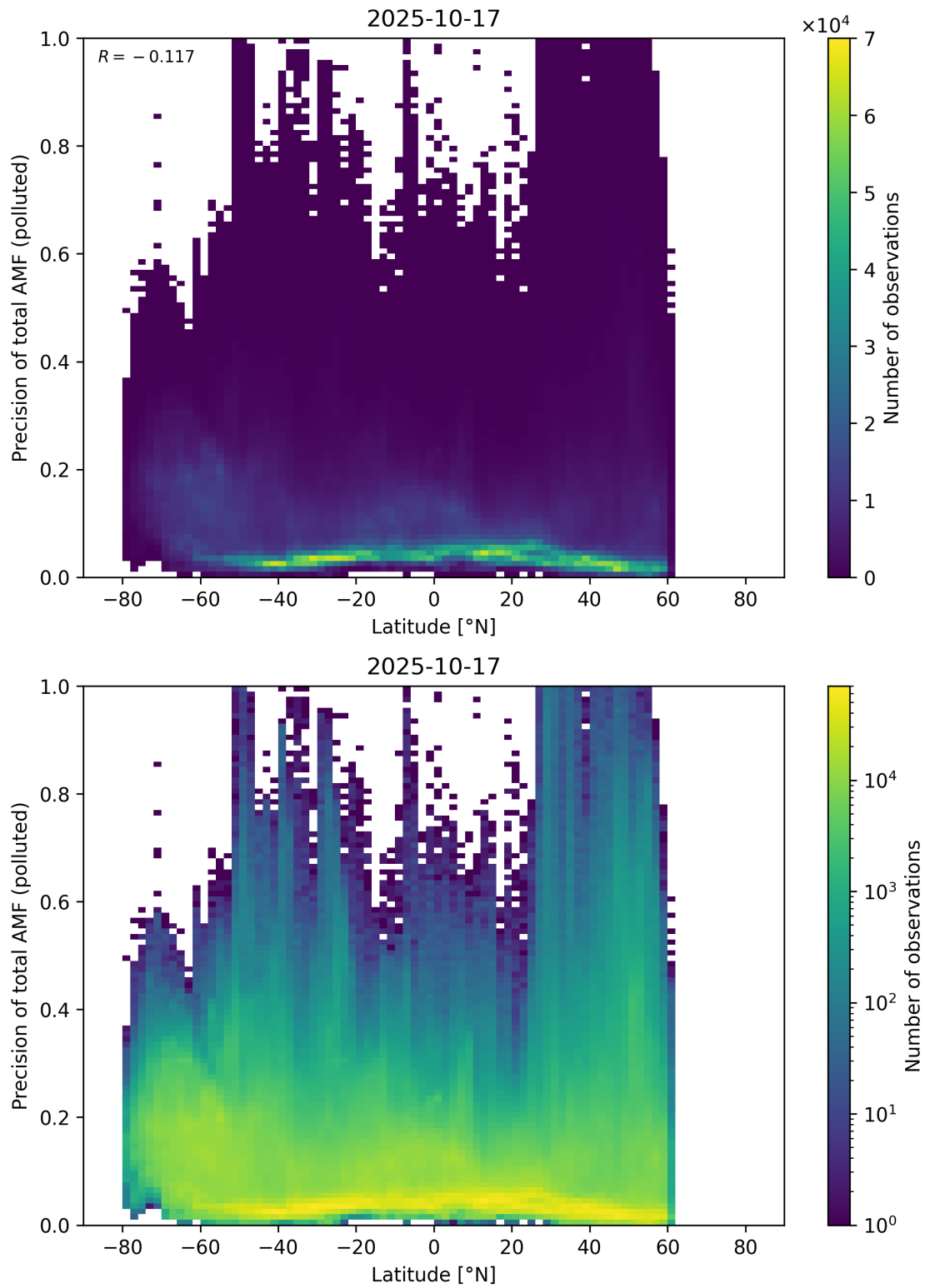
Figure 168: Scatter density plot of “Latitude” against “Precision of total AMF (polluted)” for 2025-10-17 to 2025-10-18.
