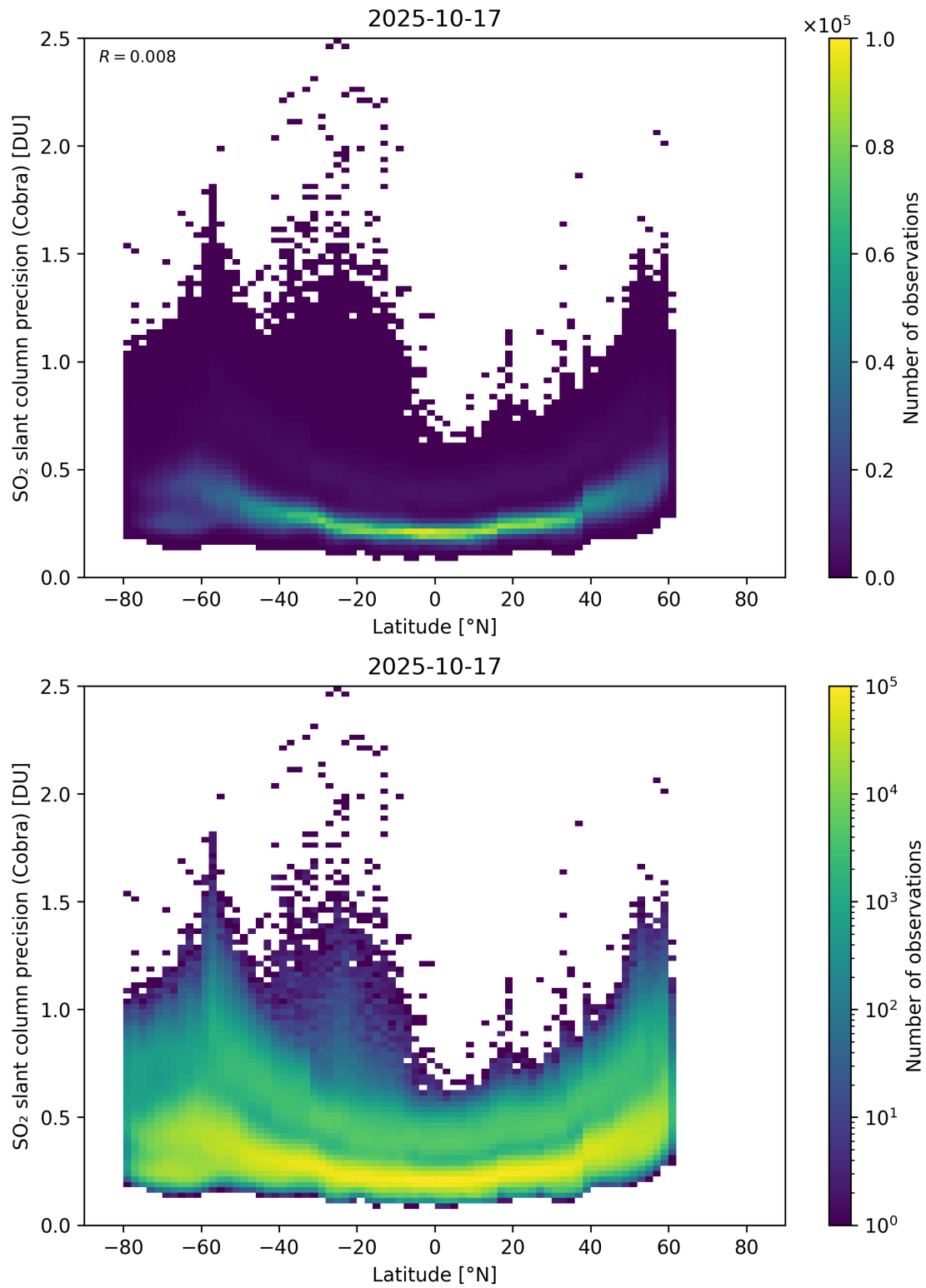
Figure 158: Scatter density plot of “Latitude” against “SO 2 slant column precision (Cobra)” for 2025-10-17 to 2025-10-18.
