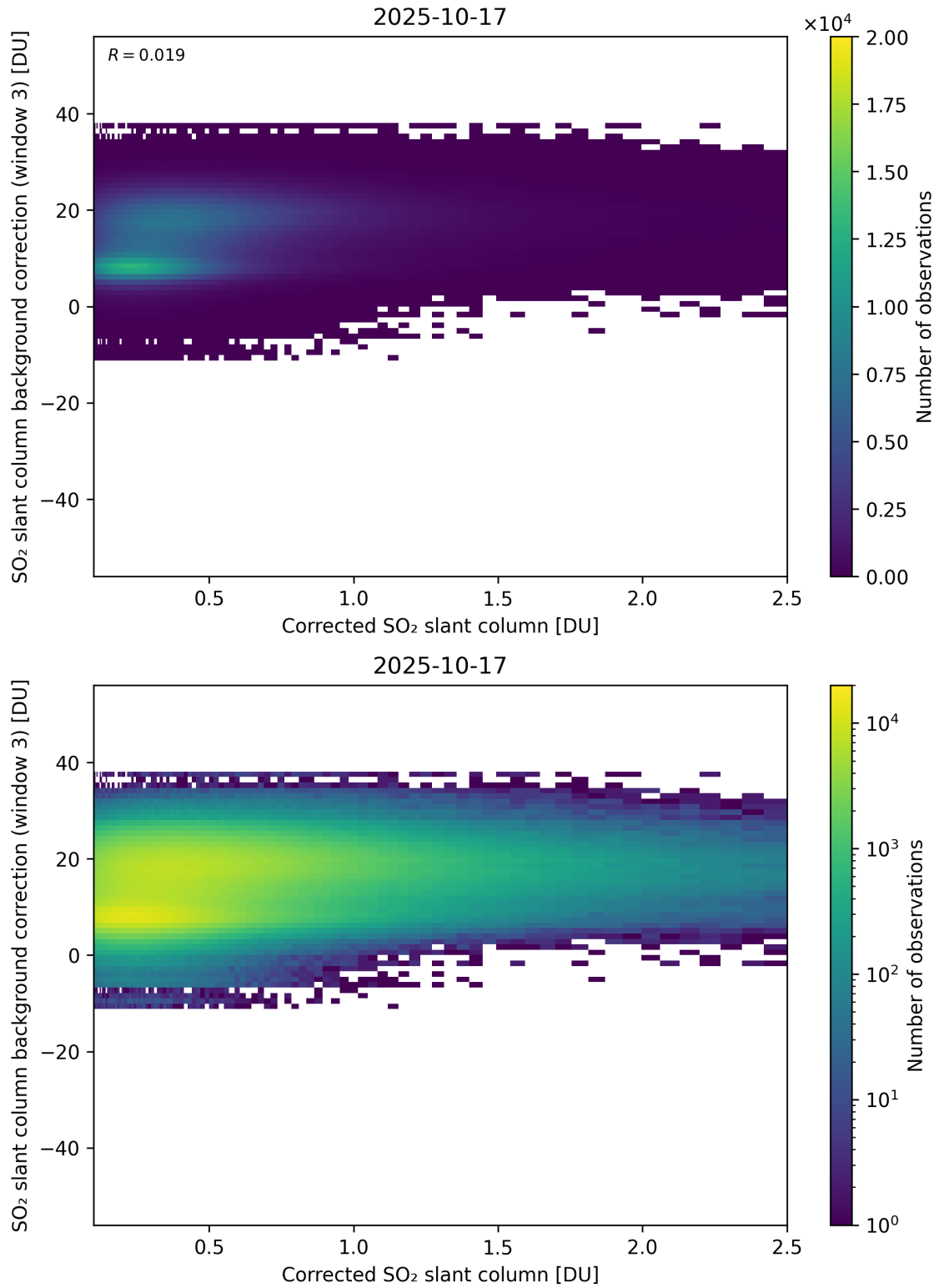
Figure 228: Scatter density plot of “Corrected SO 2 slant column” against “SO 2 slant column background correction (window 3)” for 2025-10-17 to 2025-10-18.
