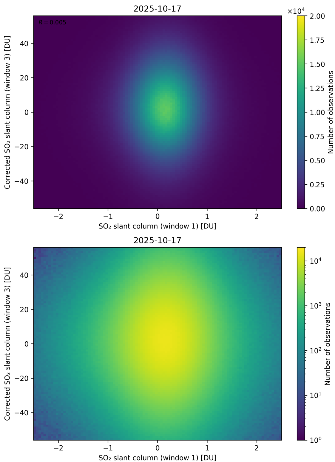
Figure 284: Scatter density plot of “SO 2 slant column (window 1)” against “Corrected SO 2 slant column (window 3)” for 2025-10-17 to 2025-10-18.
