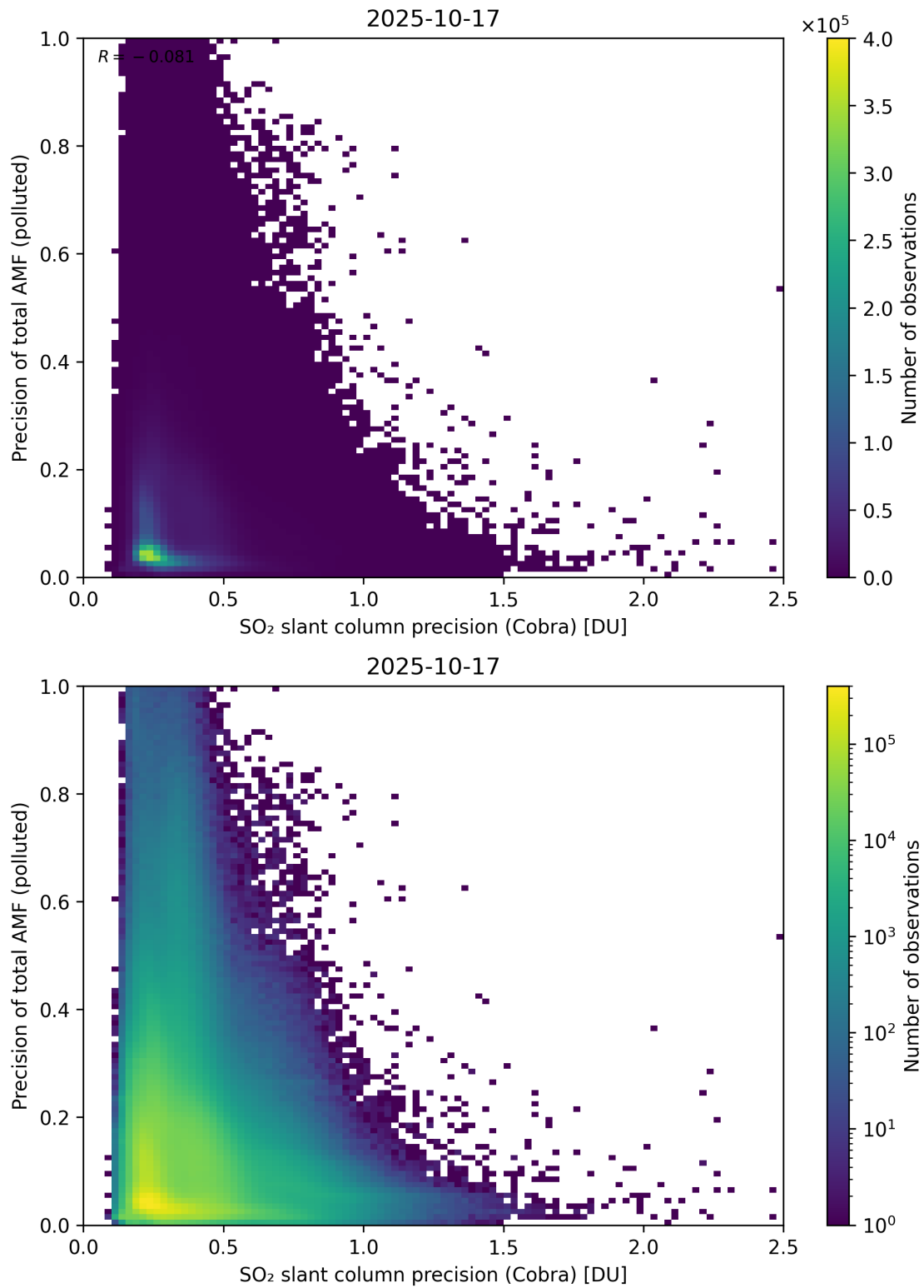
Figure 214: Scatter density plot of “SO 2 slant column precision (Cobra)” against “Precision of total AMF (polluted)” for 2025-10-17 to 2025-10-18.
