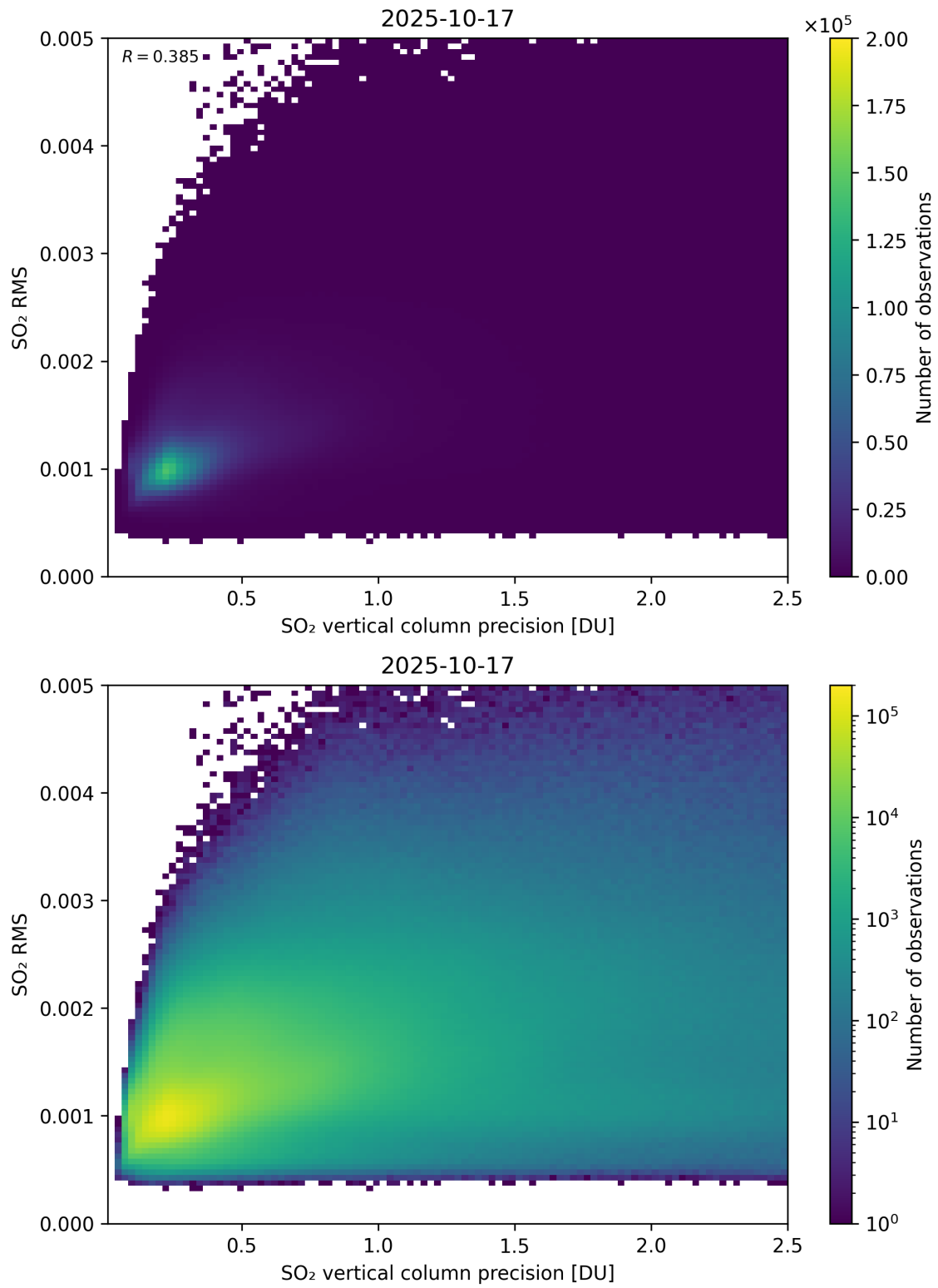
Figure 334: Scatter density plot of “SO 2 vertical column precision” against “SO 2 RMS” for 2025-10-17 to 2025-10-18.
