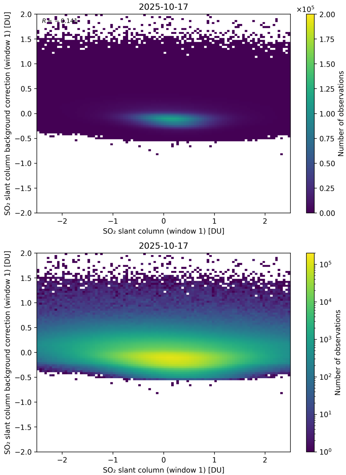
Figure 262: Scatter density plot of “SO 2 slant column (window 1)” against “SO 2 slant column background correction (window 1)” for 2025-10-17 to 2025-10-18.
