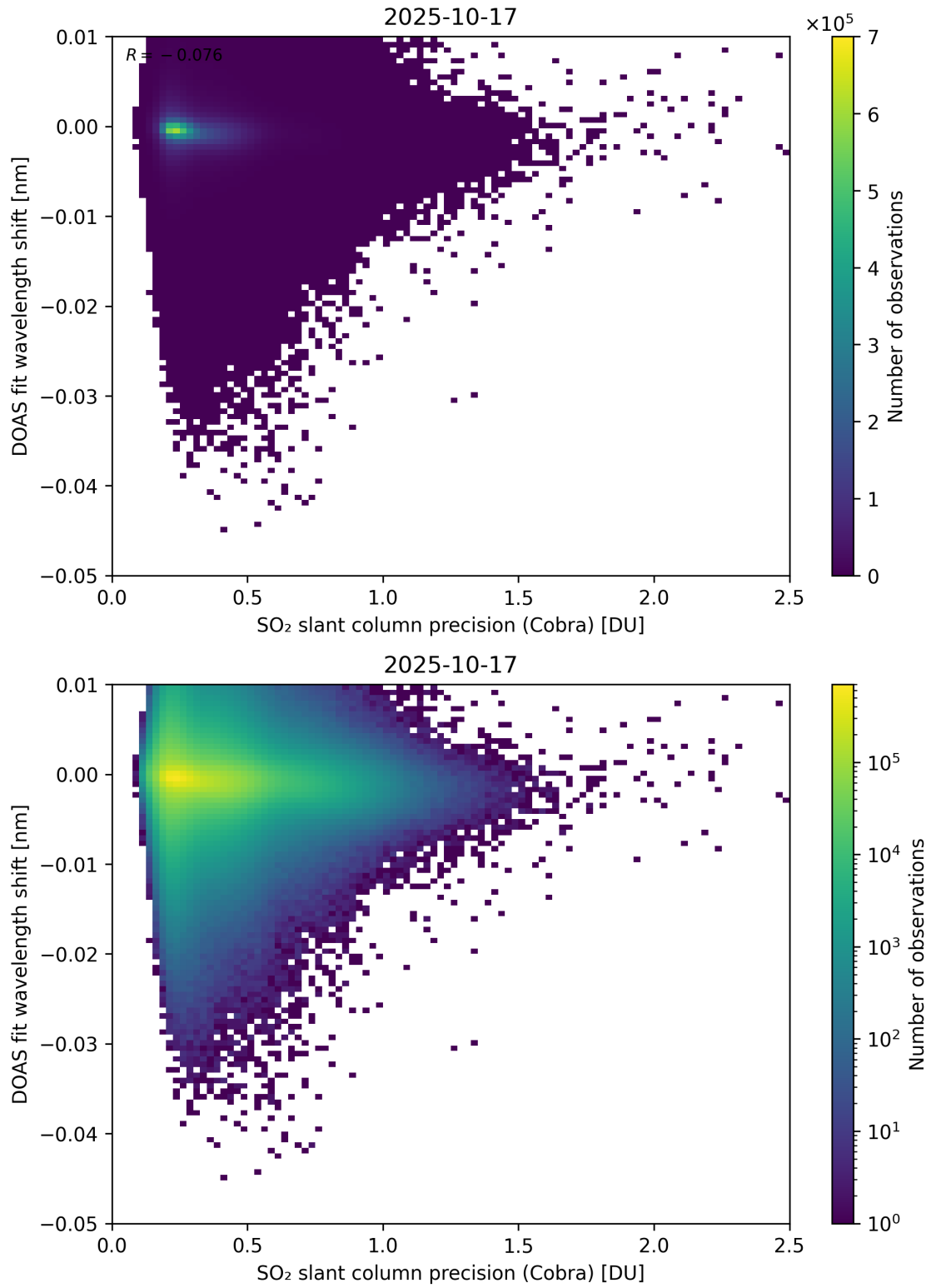
Figure 202: Scatter density plot of “SO 2 slant column precision (Cobra)” against “DOAS fit wavelength shift” for 2025-10-17 to 2025-10-18.
