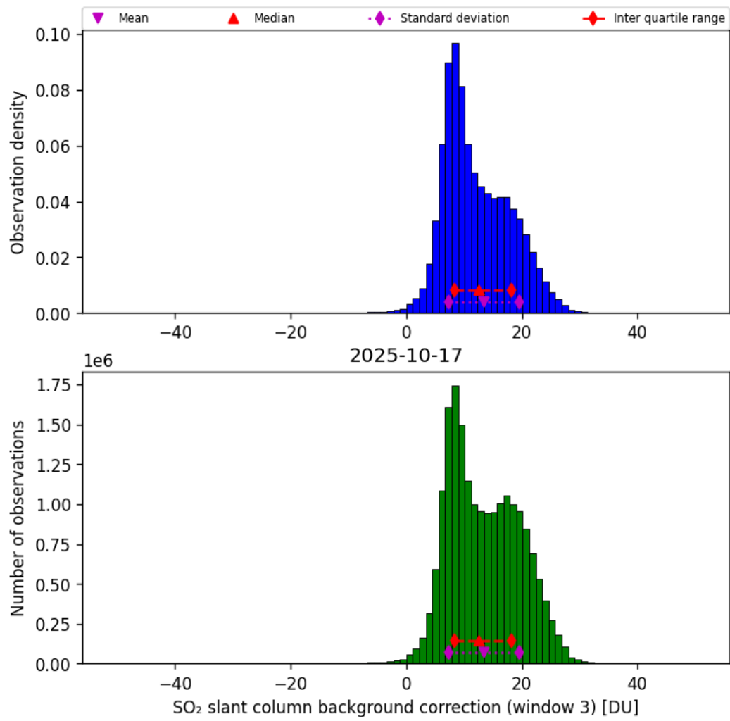
Figure 74: Histogram of “SO 2 slant column background correction (window 3)” for 2025-10-17 to 2025-10-18
