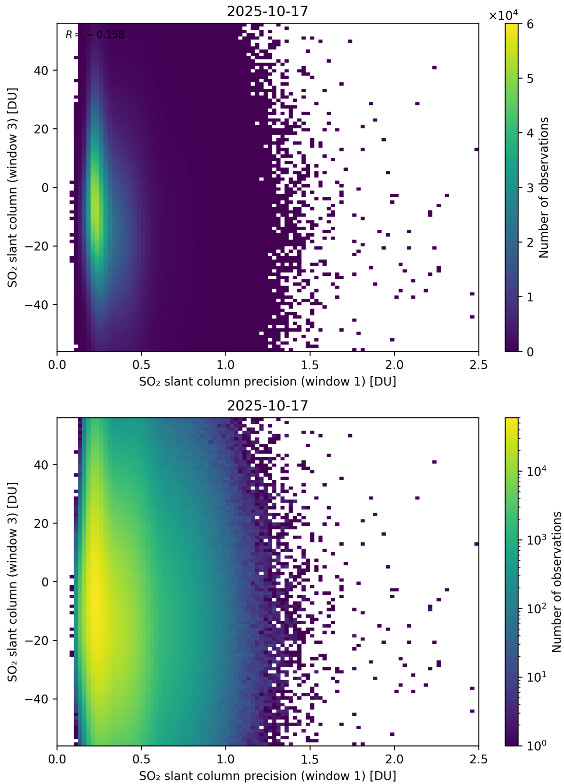
Figure 278: Scatter density plot of “SO 2 slant column precision (window 1)” against “SO 2 slant column (window 3)” for 2025-10-17 to 2025-10-18.
