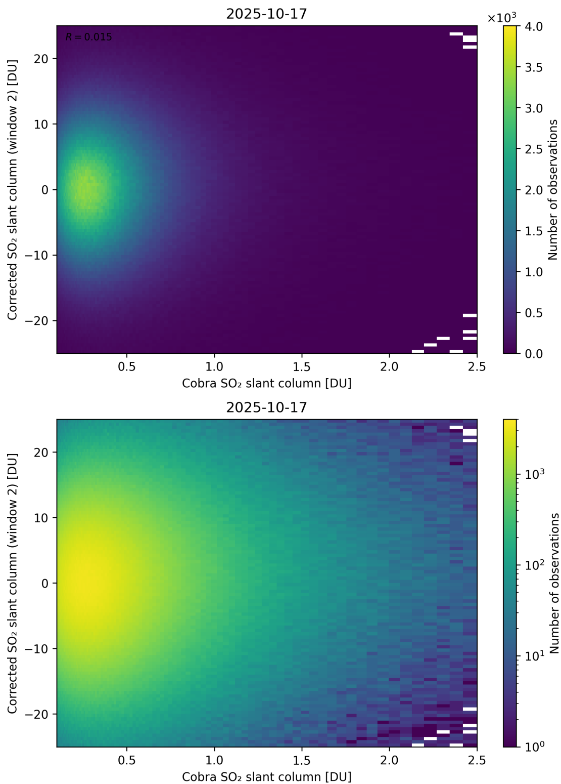
Figure 217: Scatter density plot of “Cobra SO 2 slant column” against “Corrected SO 2 slant column (window 2)” for 2025-10-17 to 2025-10-18.
