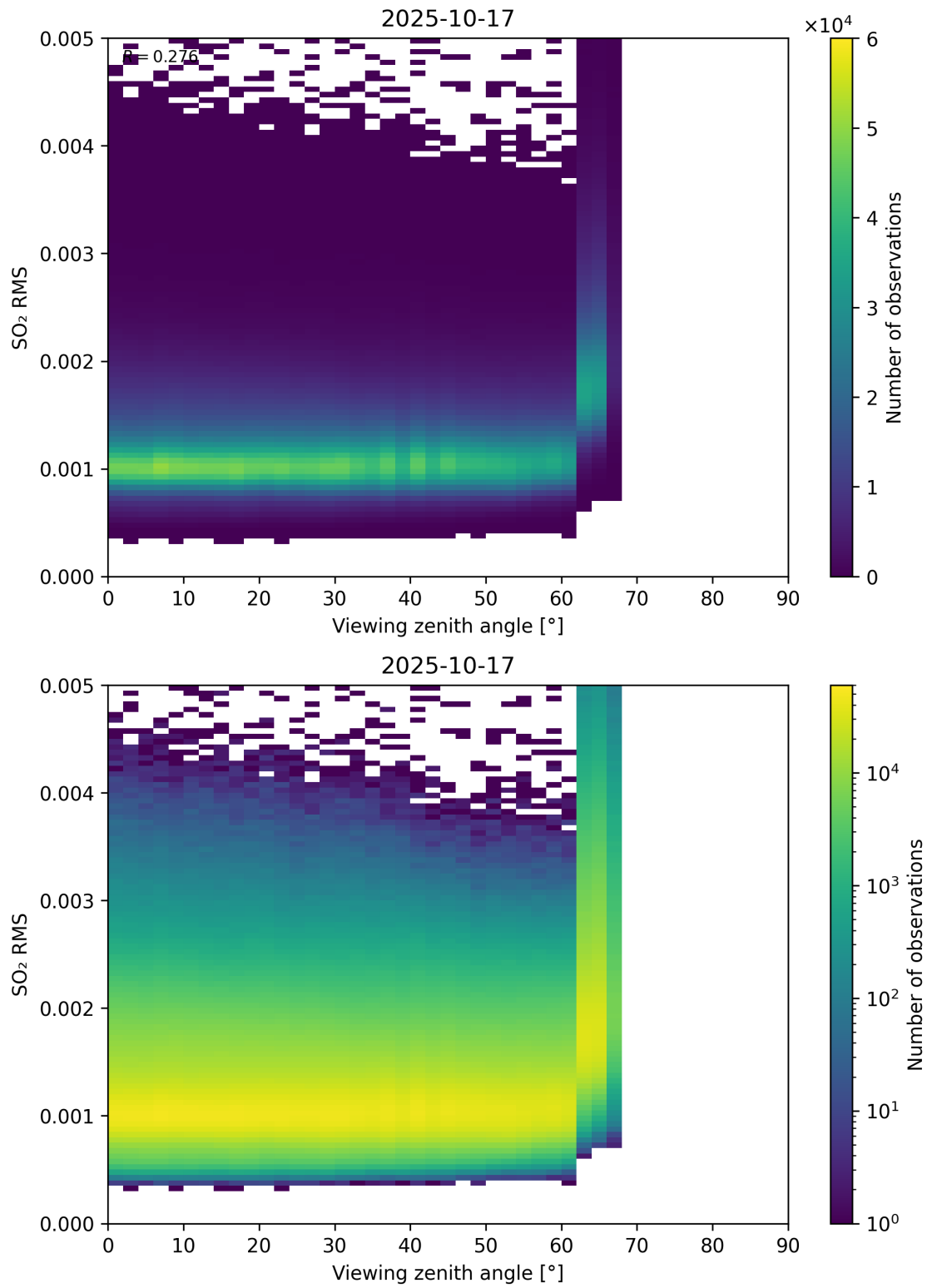
Figure 367: Scatter density plot of “Viewing zenith angle” against “SO 2 RMS” for 2025-10-17 to 2025-10-18.
