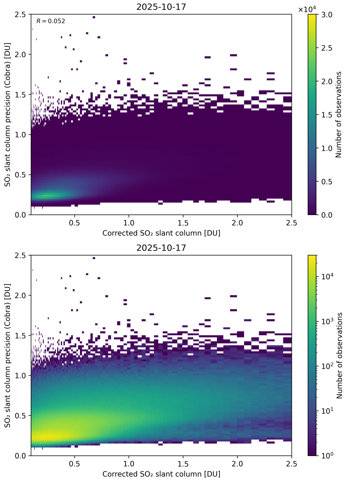
Figure 234: Scatter density plot of “Corrected SO 2 slant column” against “SO 2 slant column precision (Cobra)” for 2025-10-17 to 2025-10-18.
