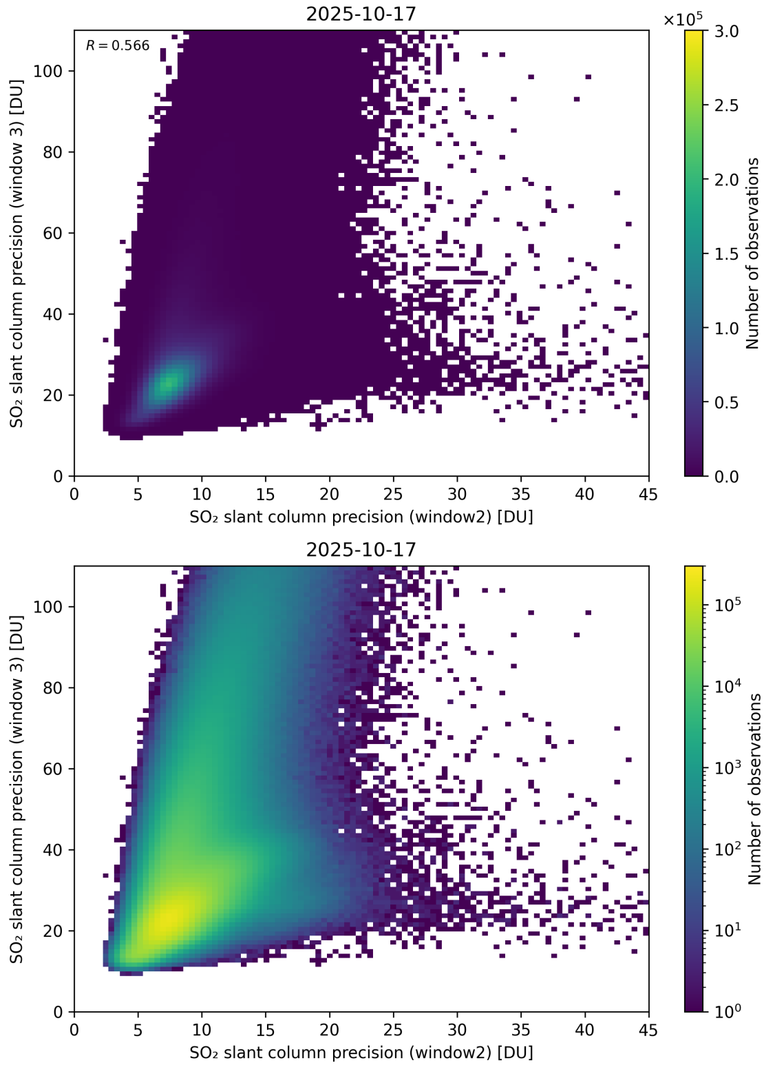
Figure 300: Scatter density plot of “SO 2 slant column precision (window2)” against “SO 2 slant column precision (window 3)” for 2025-10-17 to 2025-10-18.
