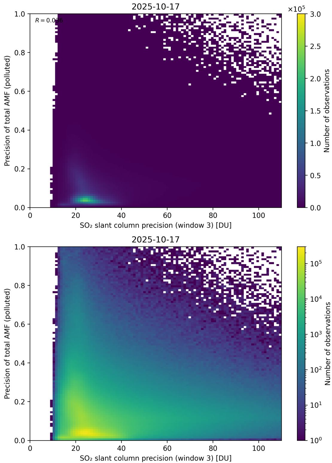
Figure 314: Scatter density plot of “SO 2 slant column precision (window 3)” against “Precision of total AMF (polluted)” for 2025-10-17 to 2025-10-18.
