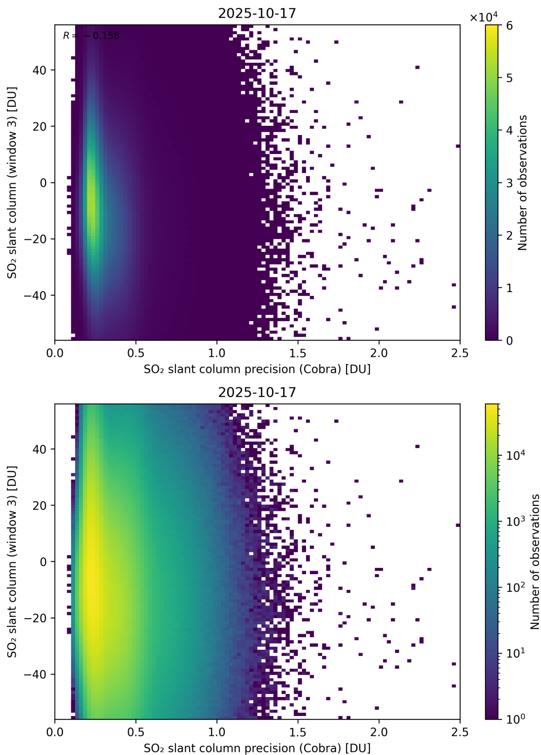
Figure 211: Scatter density plot of “SO 2 slant column precision (Cobra)” against “SO 2 slant column (window 3)” for 2025-10-17 to 2025-10-18.
