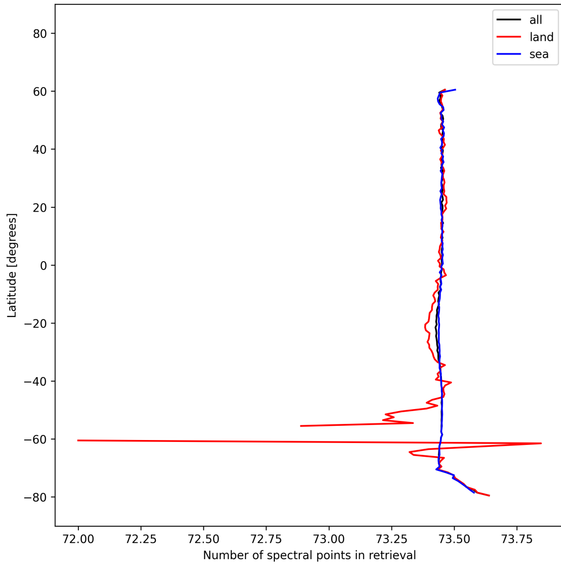
Figure 56: Zonal average of “Number of spectral points in retrieval” for 2025-10-17 to 2025-10-18.
