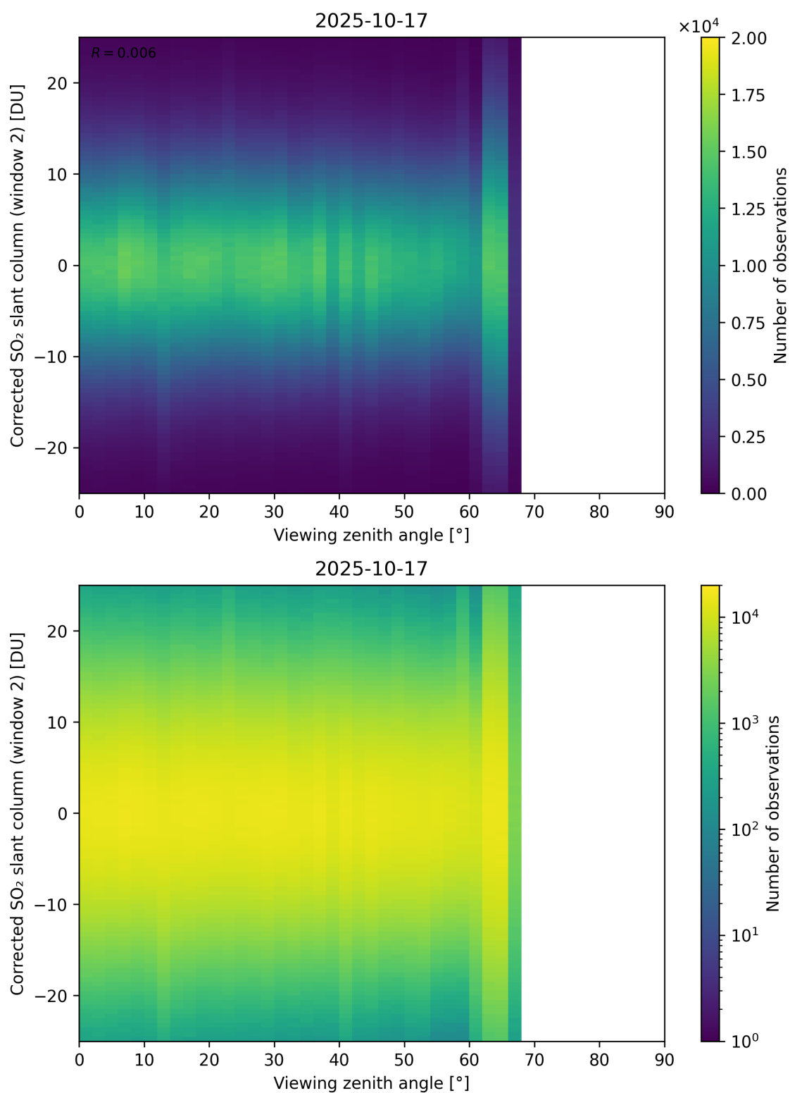
Figure 374: Scatter density plot of “Viewing zenith angle” against “Corrected SO 2 slant column (window 2)” for 2025-10-17 to 2025-10-18.
