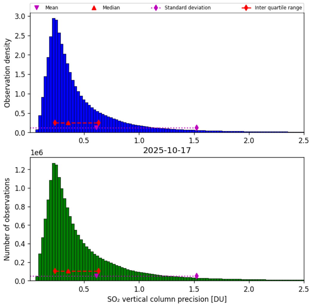
Figure 59: Histogram of “SO 2 vertical column precision” for 2025-10-17 to 2025-10-18
