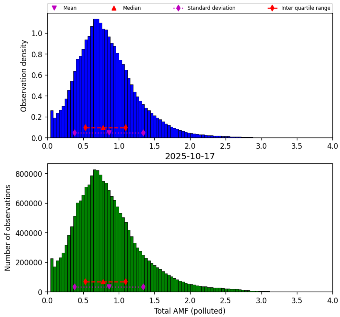
Figure 79: Histogram of “Total AMF (polluted)” for 2025-10-17 to 2025-10-18
