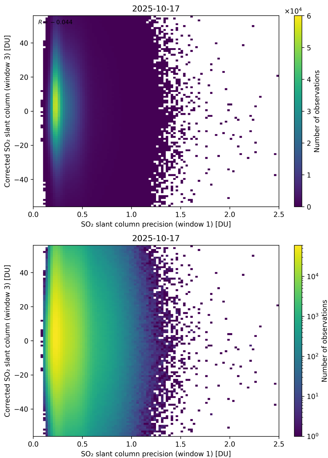
Figure 276: Scatter density plot of “SO 2 slant column precision (window 1)” against “Corrected SO 2 slant column (window 3)” for 2025-10-17 to 2025-10-18.
