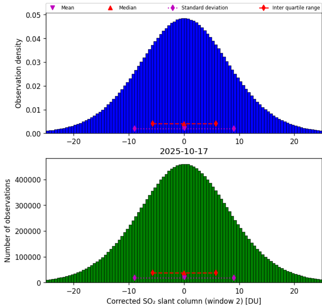
Figure 69: Histogram of “Corrected SO 2 slant column (window 2)” for 2025-10-17 to 2025-10-18
