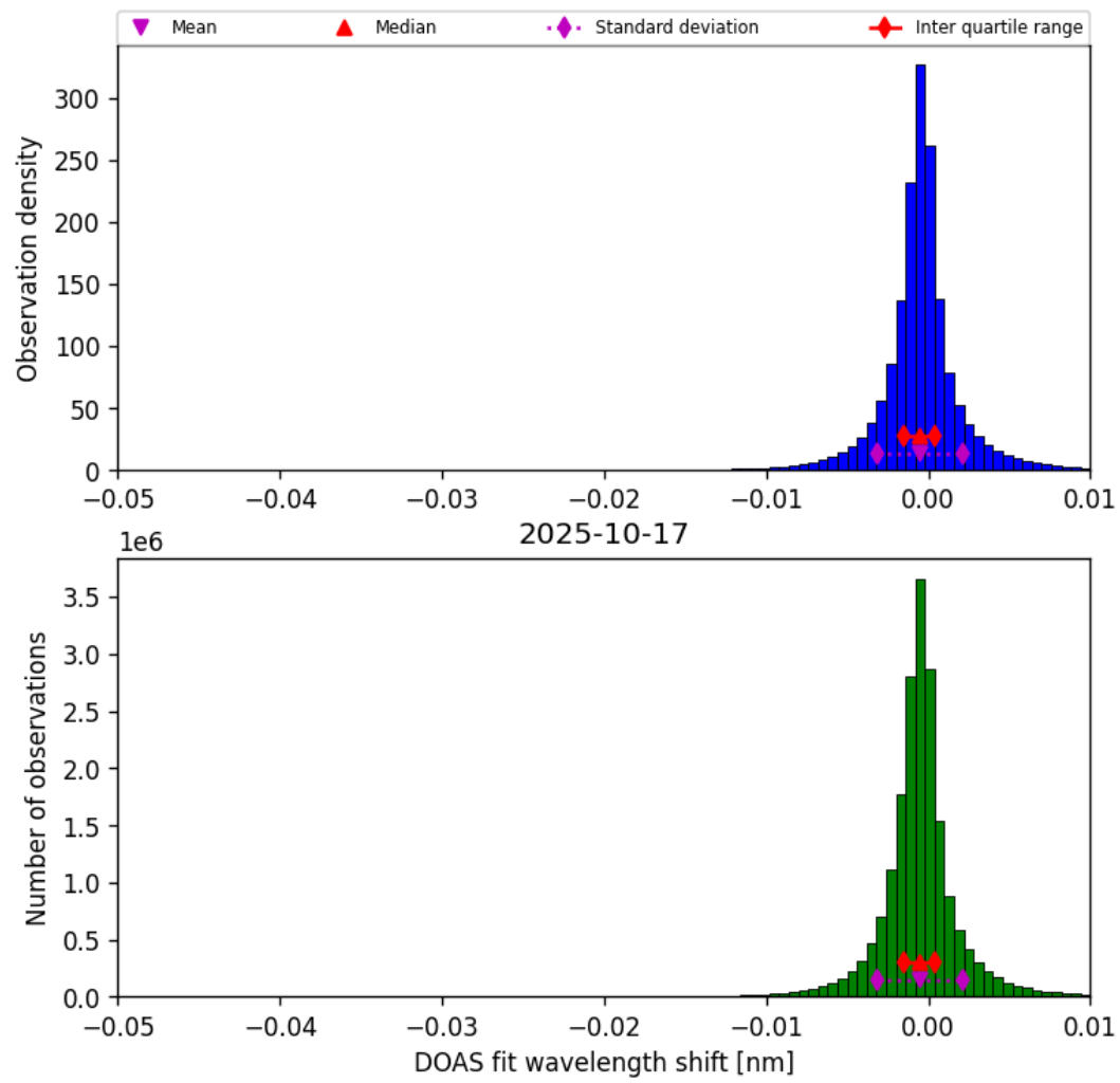
Figure 76: Histogram of “DOAS fit wavelength shift” for 2025-10-17 to 2025-10-18
