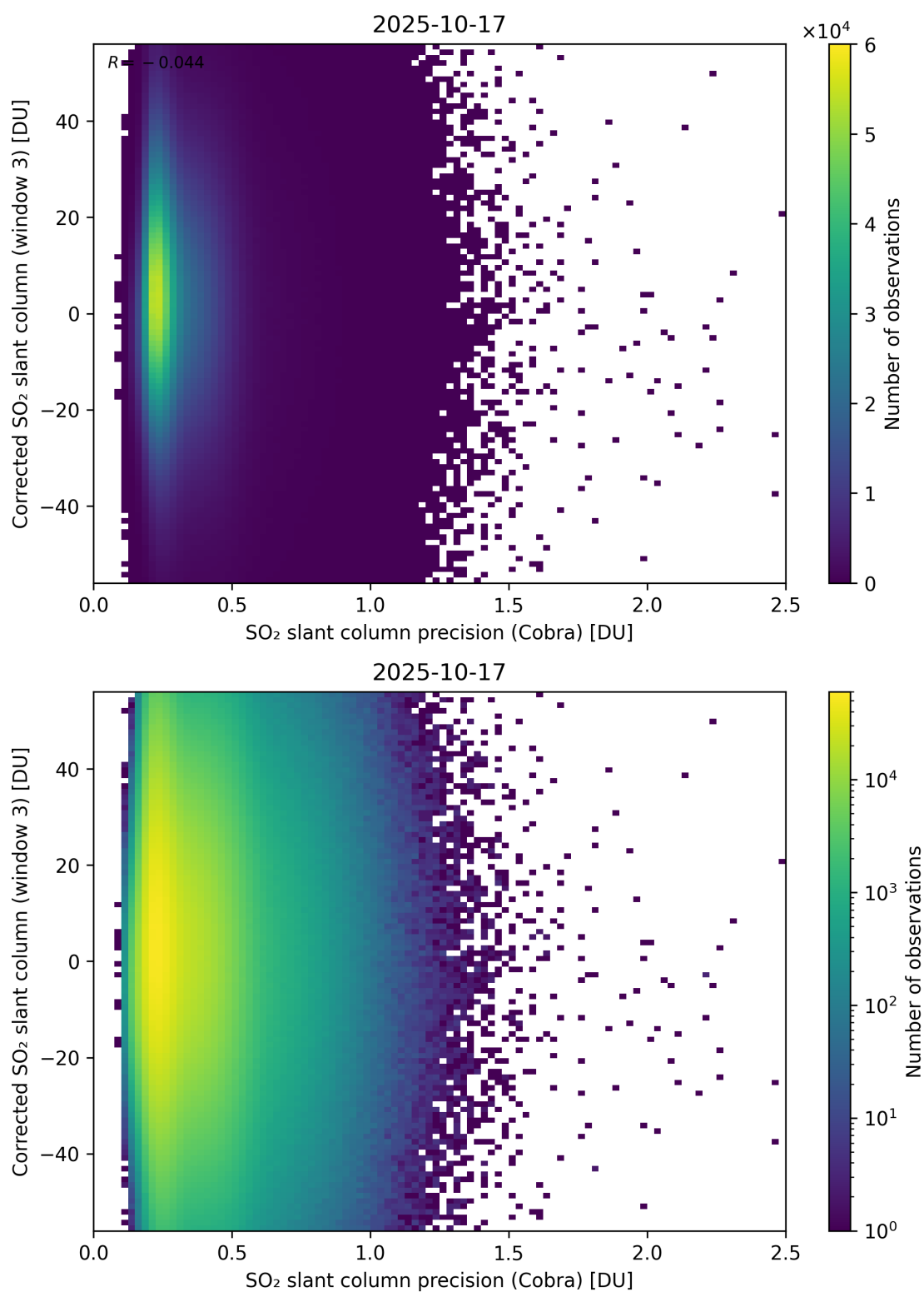
Figure 207: Scatter density plot of “SO 2 slant column precision (Cobra)” against “Corrected SO 2 slant column (window 3)” for 2025-10-17 to 2025-10-18.
