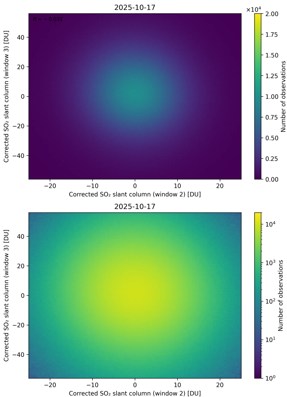
Figure 250: Scatter density plot of “Corrected SO 2 slant column (window 2)” against “Corrected SO 2 slant column (window 3)” for 2025-10-17 to 2025-10-18.
