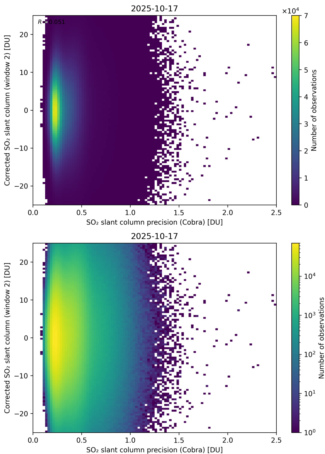
Figure 206: Scatter density plot of “SO 2 slant column precision (Cobra)” against “Corrected SO 2 slant column (window 2)” for 2025-10-17 to 2025-10-18.
