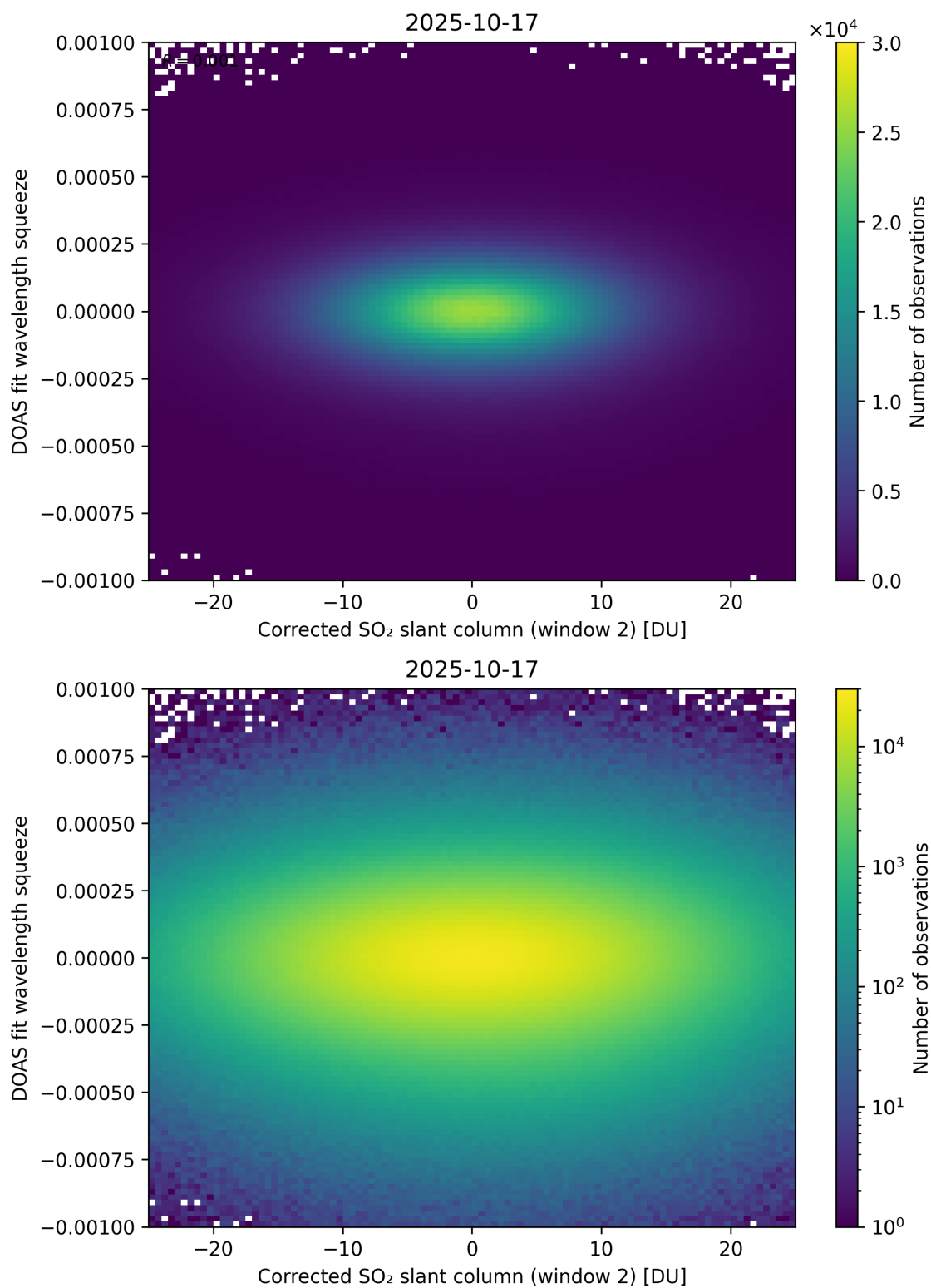
Figure 247: Scatter density plot of “Corrected SO 2 slant column (window 2)” against “DOAS fit wavelength squeeze” for 2025-10-17 to 2025-10-18.
