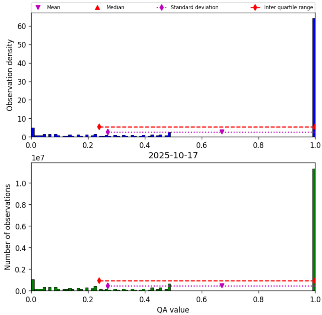
Figure 57: Histogram of “QA value” for 2025-10-17 to 2025-10-18
