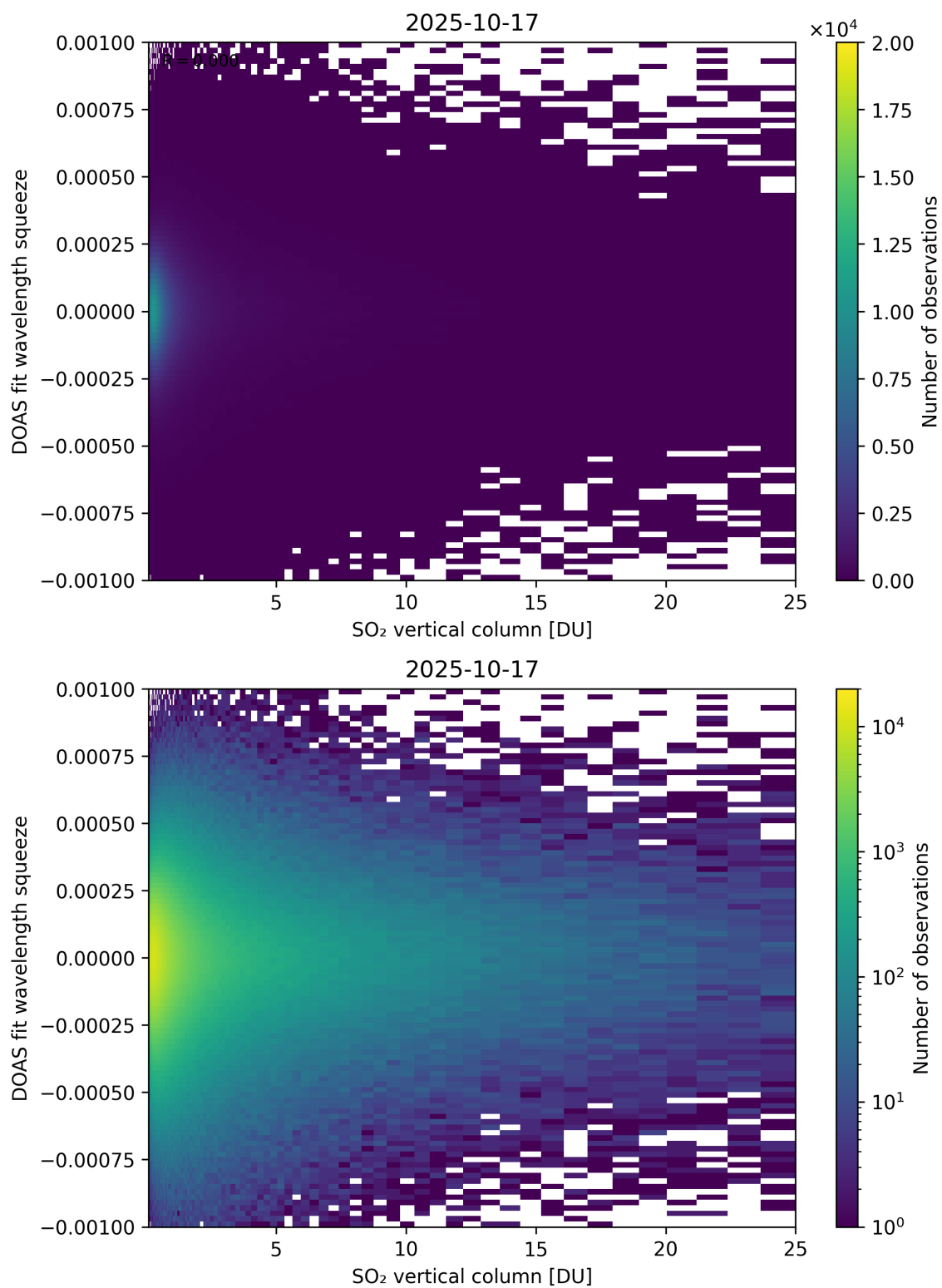
Figure 327: Scatter density plot of “SO 2 vertical column” against “DOAS fit wavelength squeeze” for 2025-10-17 to 2025-10-18.
