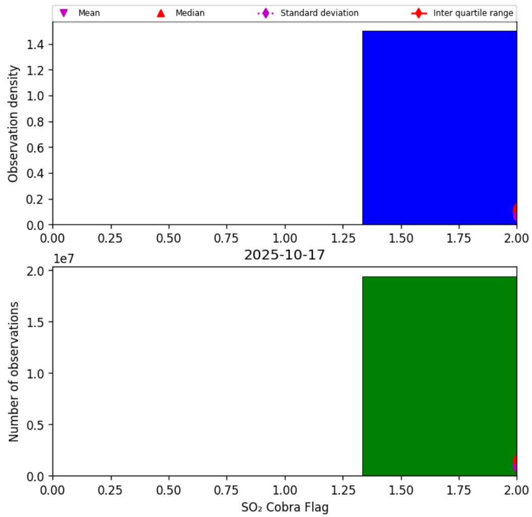
Figure 75: Histogram of “SO 2 Cobra Flag” for 2025-10-17 to 2025-10-18
