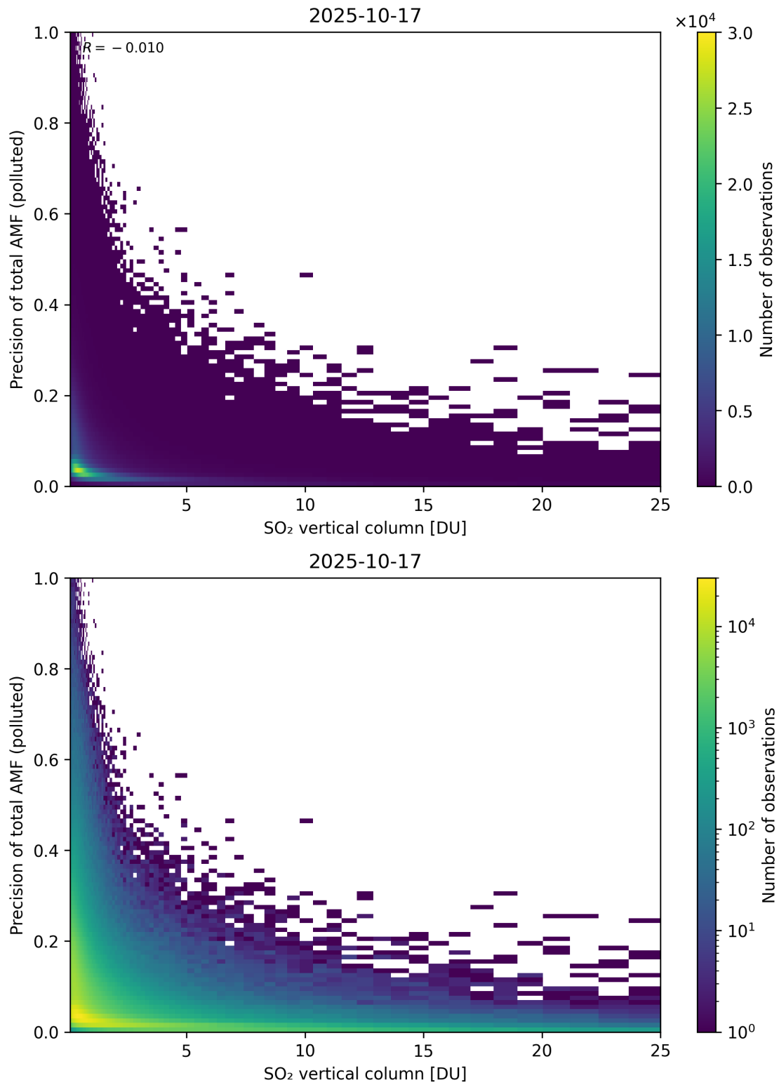
Figure 360: Scatter density plot of “SO 2 vertical column” against “Precision of total AMF (polluted)” for 2025-10-17 to 2025-10-18.
