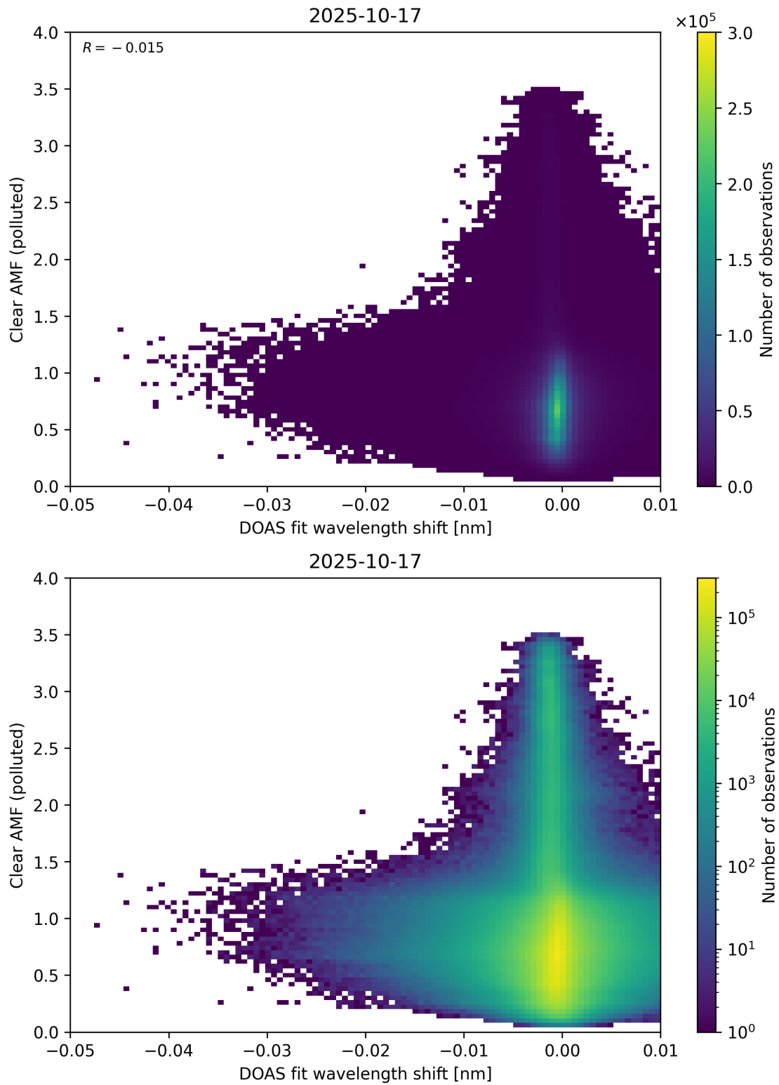
Figure 140: Scatter density plot of “DOAS fit wavelength shift” against “Clear AMF (polluted)” for 2025-10-17 to 2025-10-18.
