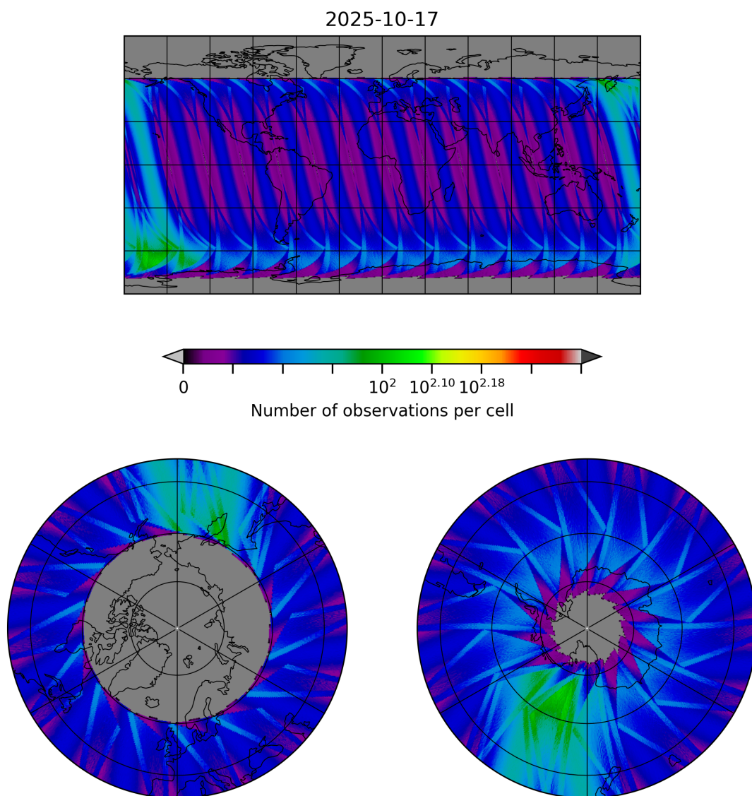
Figure 30: Map of the number of observations for 2025-10-17 to 2025-10-18
