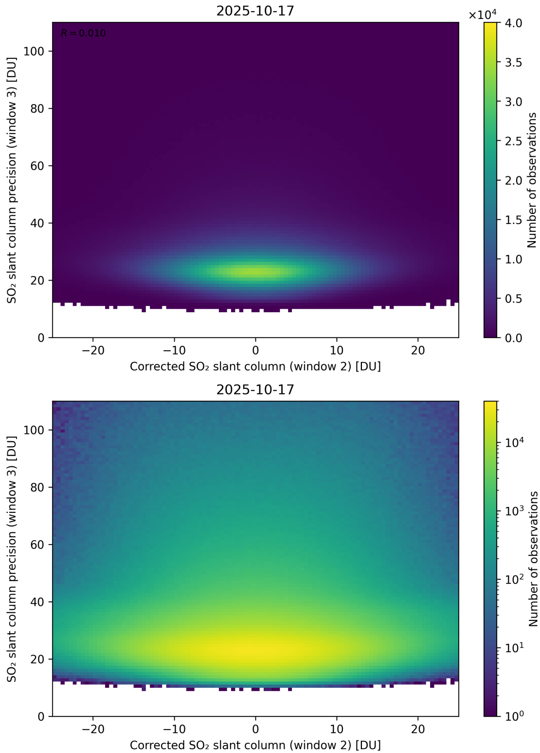
Figure 252: Scatter density plot of “Corrected SO 2 slant column (window 2)” against “SO 2 slant column precision (window 3)” for 2025-10-17 to 2025-10-18.
