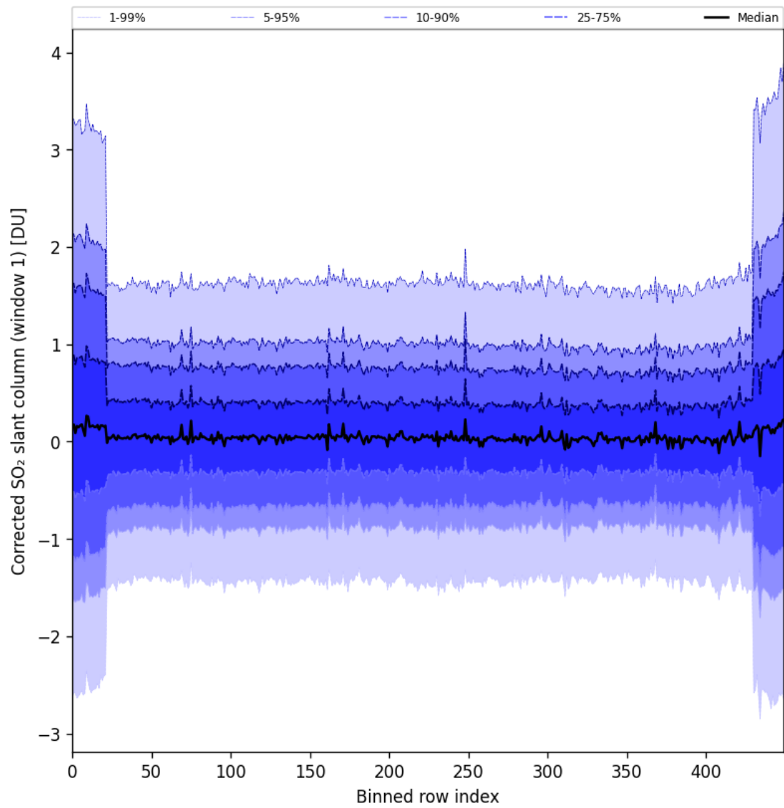
Figure 91: Along track statistics of “Corrected SO 2 slant column (window 1)” for 2025-10-17 to 2025-10-18
