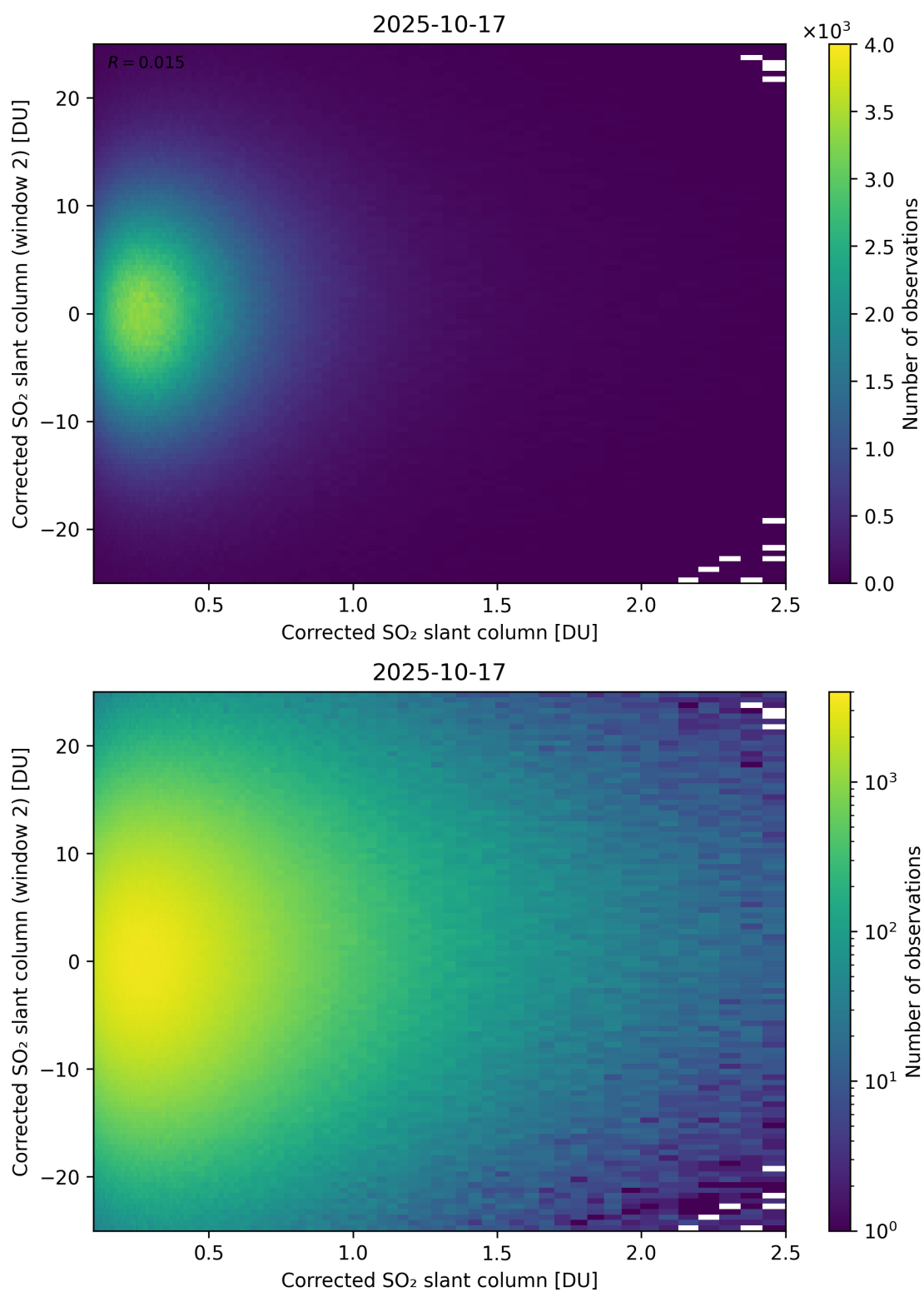
Figure 235: Scatter density plot of “Corrected SO 2 slant column” against “Corrected SO 2 slant column (window 2)” for 2025-10-17 to 2025-10-18.
