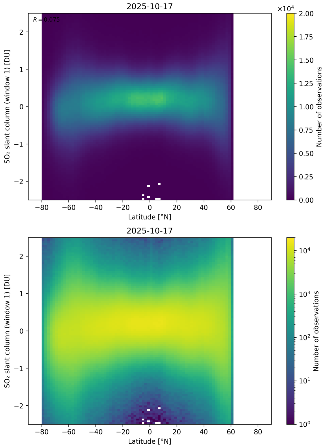
Figure 162: Scatter density plot of “Latitude” against “SO 2 slant column (window 1)” for 2025-10-17 to 2025-10-18.
