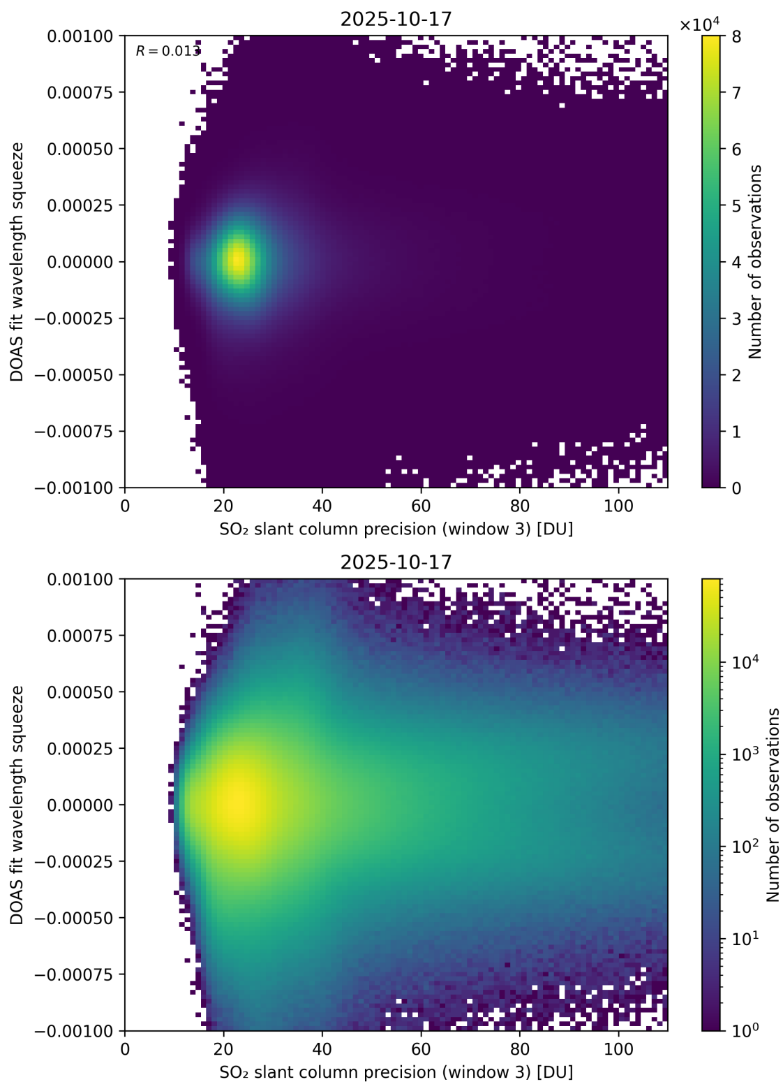
Figure 309: Scatter density plot of “SO 2 slant column precision (window 3)” against “DOAS fit wavelength squeeze” for 2025-10-17 to 2025-10-18.
