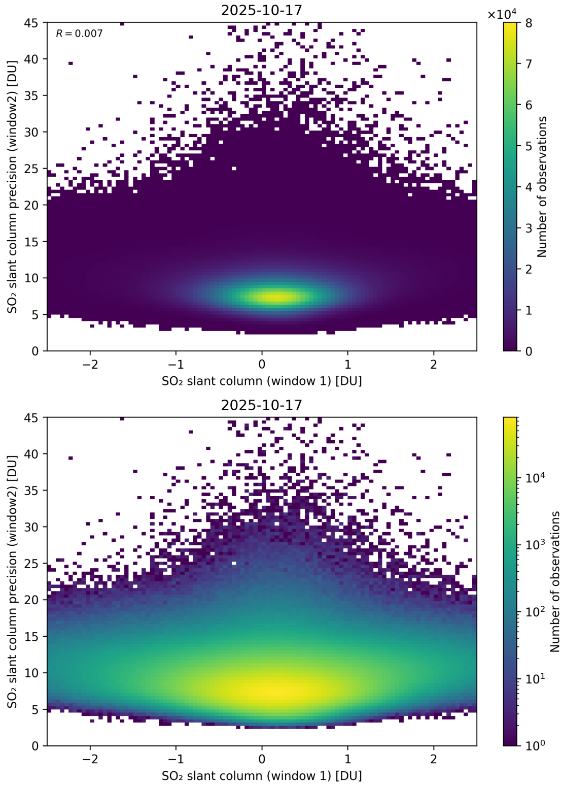
Figure 286: Scatter density plot of “SO 2 slant column (window 1)” against “SO 2 slant column precision (window2)” for 2025-10-17 to 2025-10-18.
