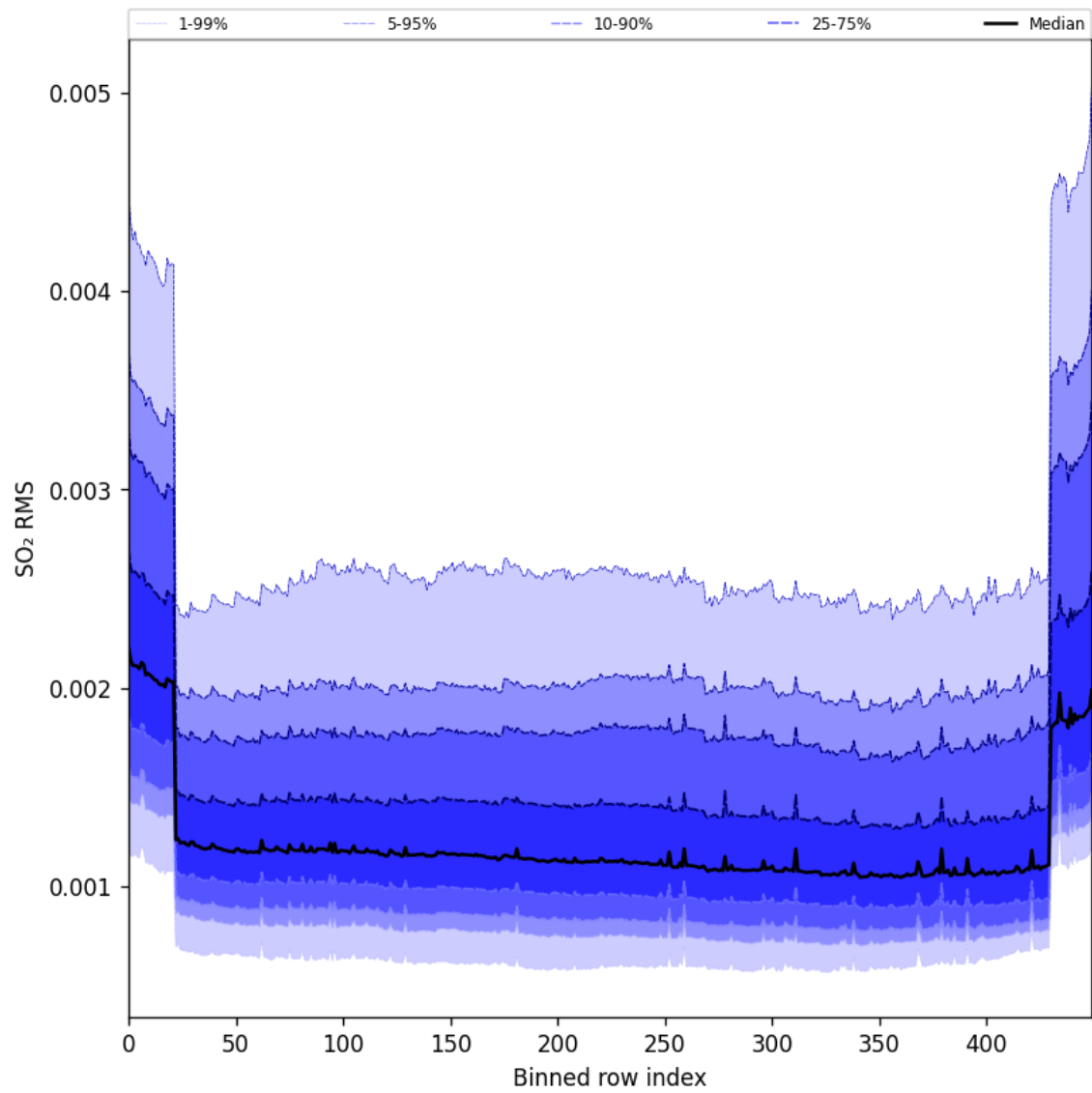
Figure 104: Along track statistics of “SO 2 RMS” for 2025-10-17 to 2025-10-18
