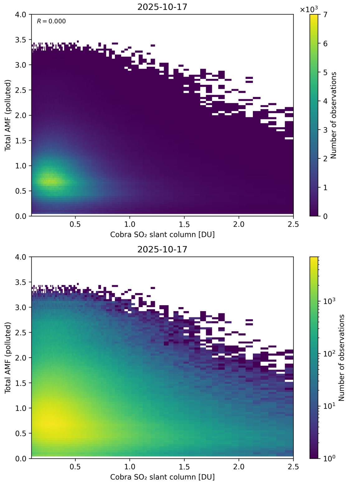
Figure 224: Scatter density plot of “Cobra SO 2 slant column” against “Total AMF (polluted)” for 2025-10-17 to 2025-10-18.
