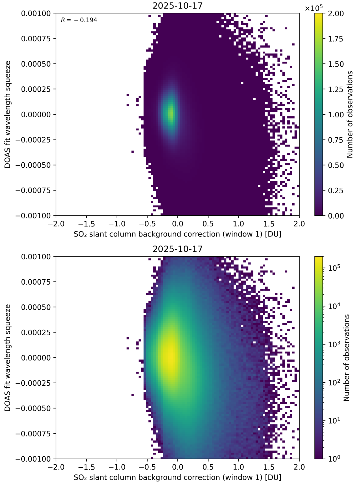
Figure 112: Scatter density plot of “SO 2 slant column background correction (window 1)” against “DOAS fit wavelength squeeze” for 2025-10-17 to 2025-10-18.
