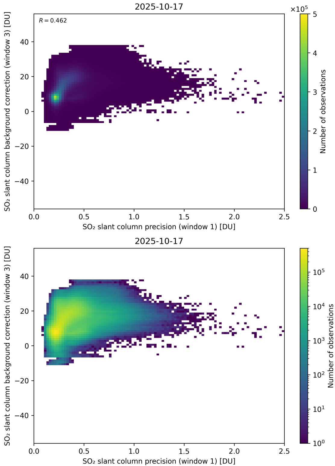
Figure 270: Scatter density plot of “SO 2 slant column precision (window 1)” against “SO 2 slant column background correction (window 3)” for 2025-10-17 to 2025-10-18.
