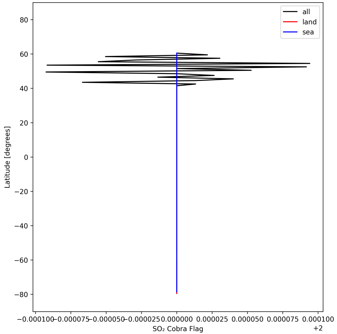
Figure 49: Zonal average of “SO 2 Cobra Flag” for 2025-10-17 to 2025-10-18.
