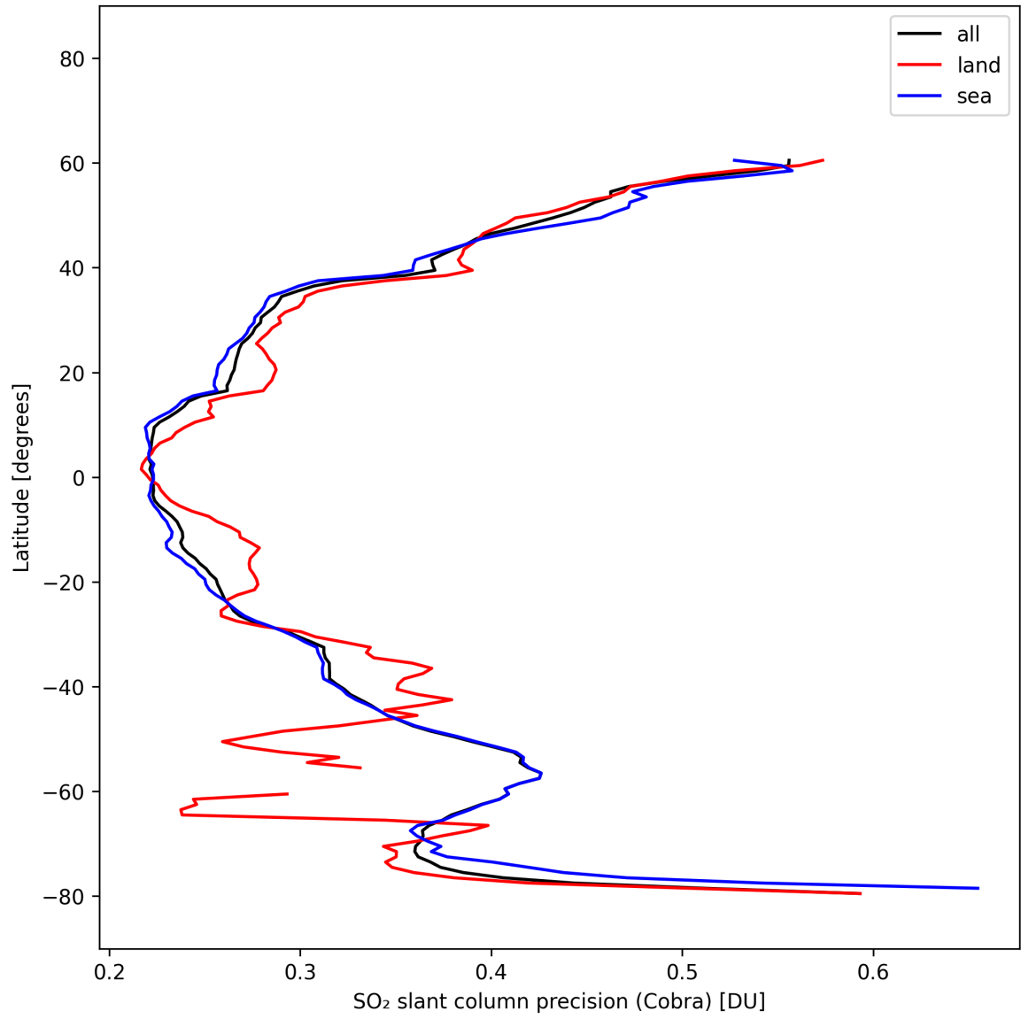
Figure 36: Zonal average of "SO 2 slant column precision (Cobra)" for 2025-10-17 to 2025-10-18.
