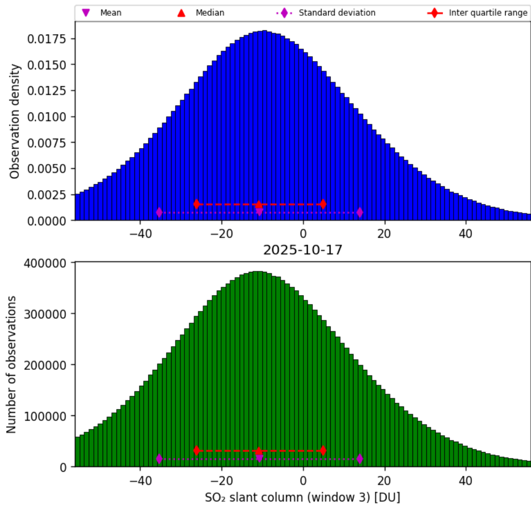
Figure 71: Histogram of “SO 2 slant column (window 3)” for 2025-10-17 to 2025-10-18
