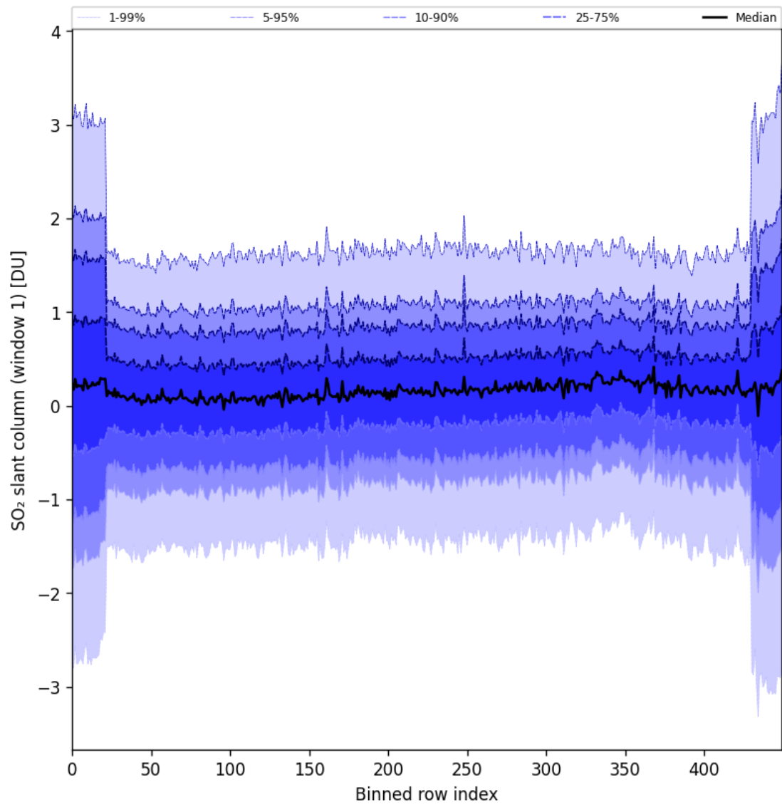
Figure 89: Along track statistics of “SO 2 slant column (window 1)” for 2025-10-17 to 2025-10-18
