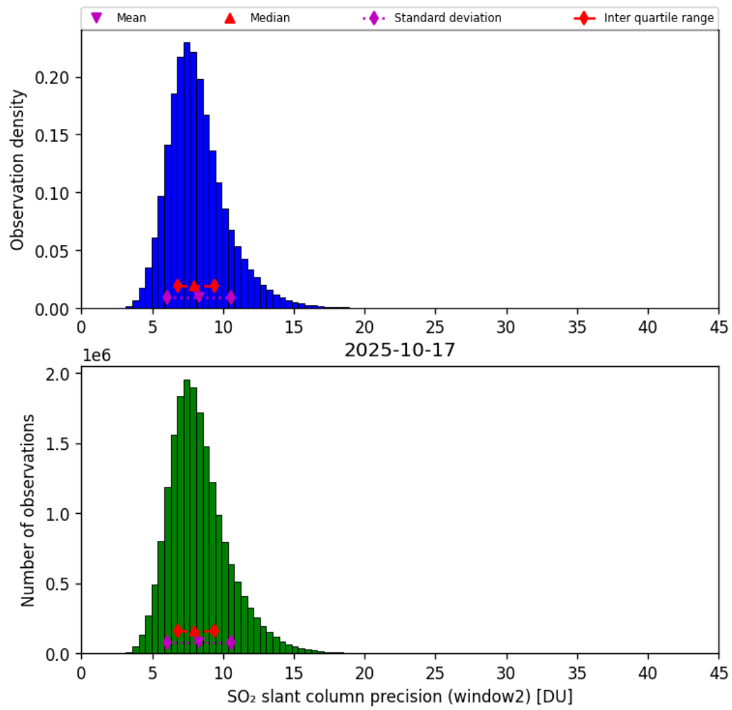
Figure 68: Histogram of “SO 2 slant column precision (window2)” for 2025-10-17 to 2025-10-18
