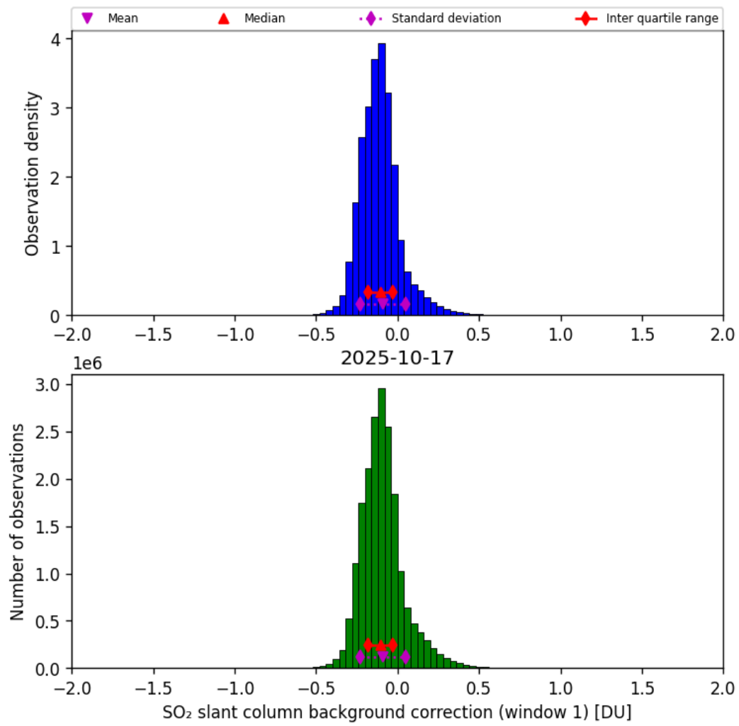
Figure 66: Histogram of “SO 2 slant column background correction (window 1)” for 2025-10-17 to 2025-10-18
