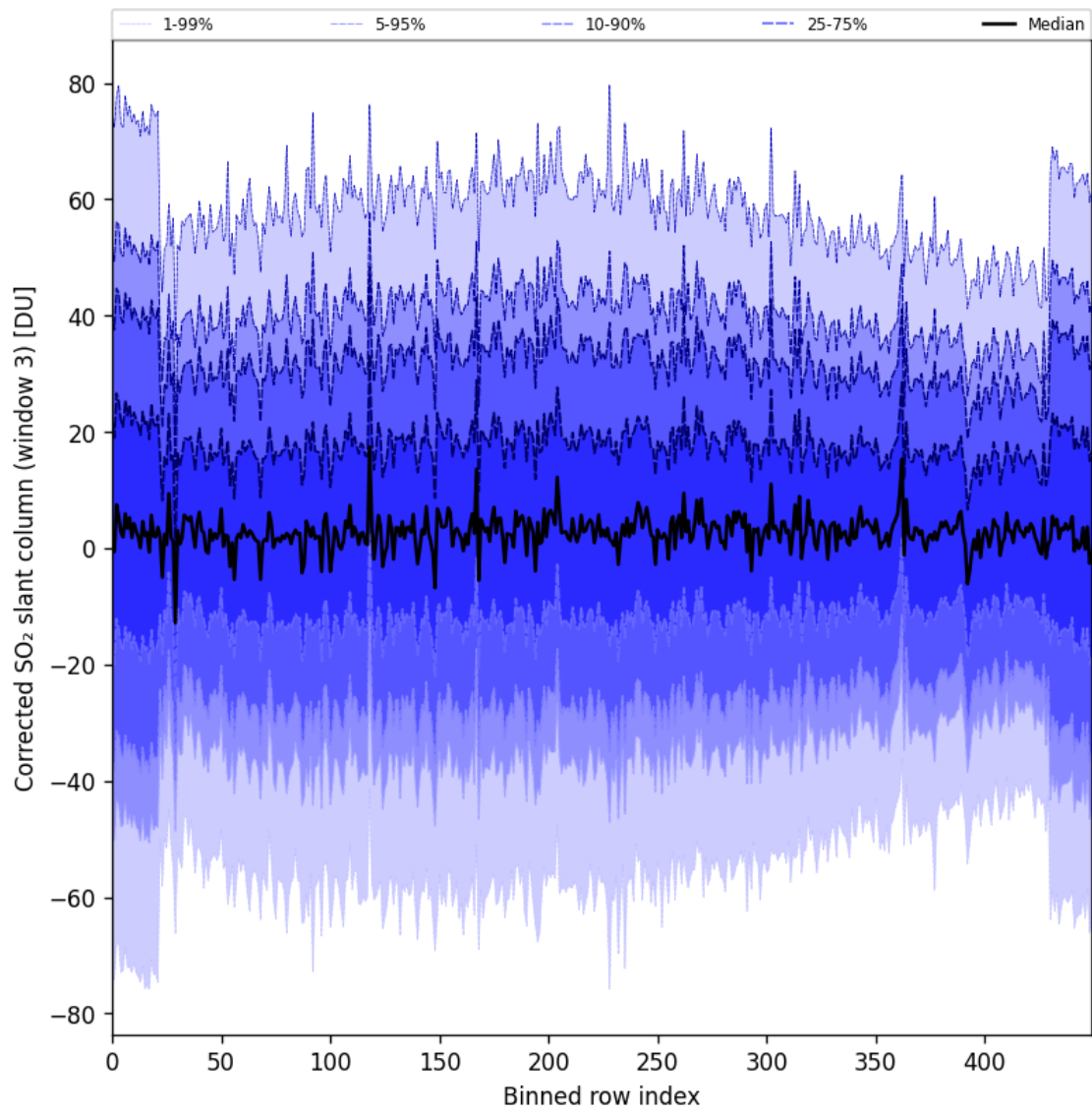
Figure 99: Along track statistics of “Corrected SO 2 slant column (window 3)” for 2025-10-17 to 2025-10-18
