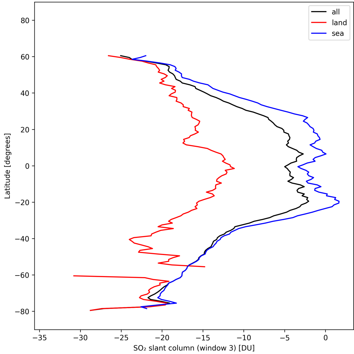
Figure 45: Zonal average of “SO 2 slant column (window 3)” for 2025-10-17 to 2025-10-18.
