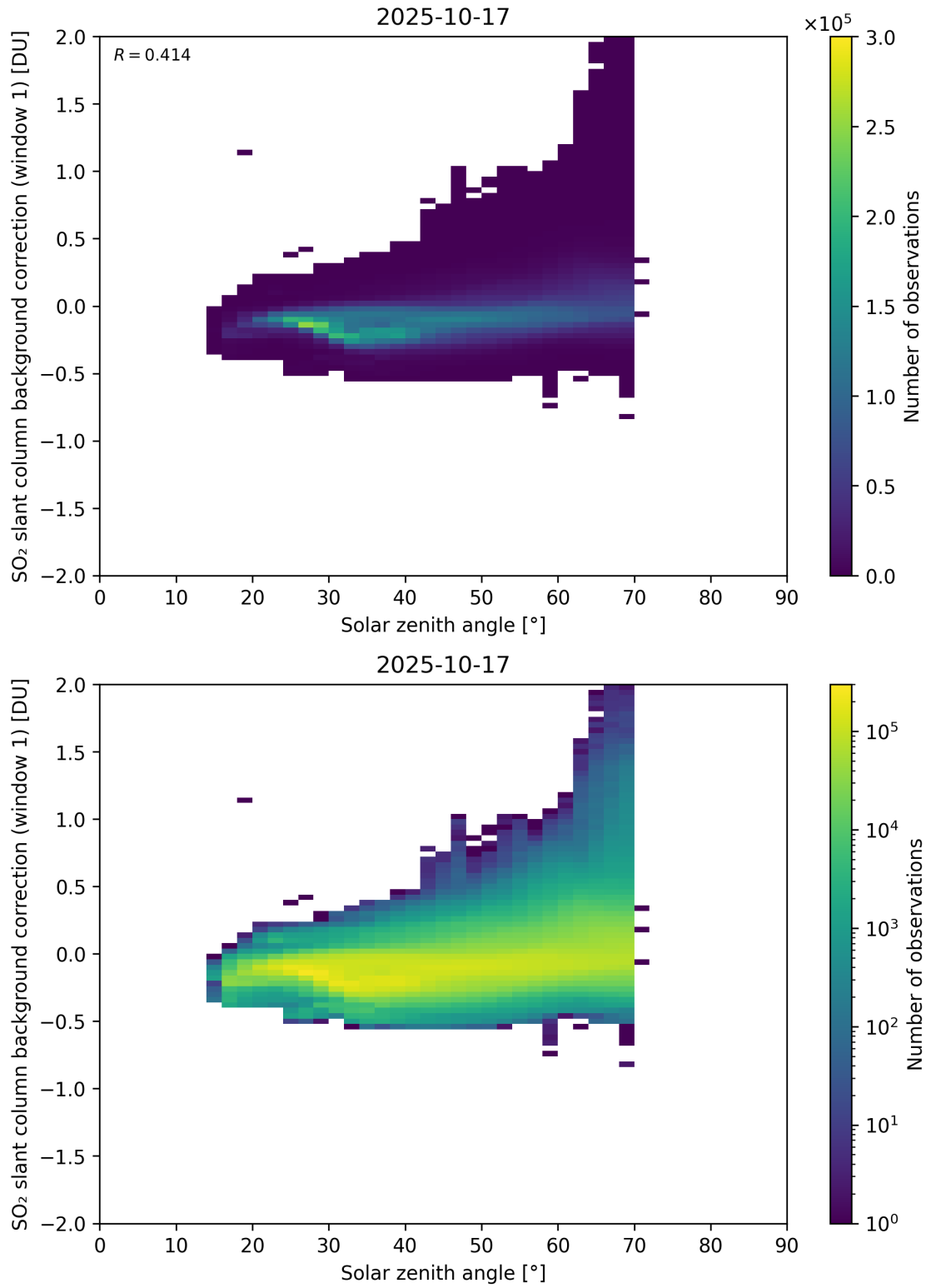
Figure 171: Scatter density plot of “Solar zenith angle” against “SO 2 slant column background correction (window 1)” for 2025-10-17 to 2025-10-18.
