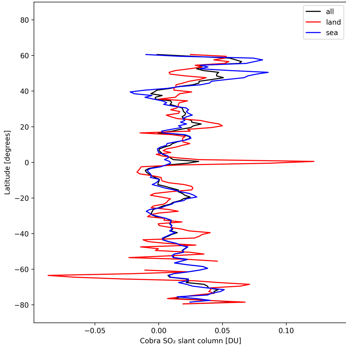
Figure 35: Zonal average of “Cobra SO 2 slant column” for 2025-10-17 to 2025-10-18.
