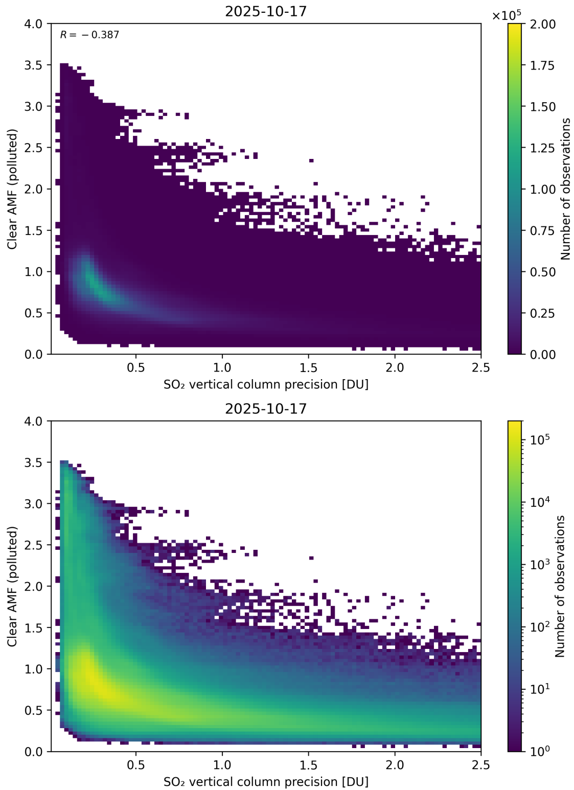
Figure 335: Scatter density plot of “SO 2 vertical column precision” against “Clear AMF (polluted)” for 2025-10-17 to 2025-10-18.
