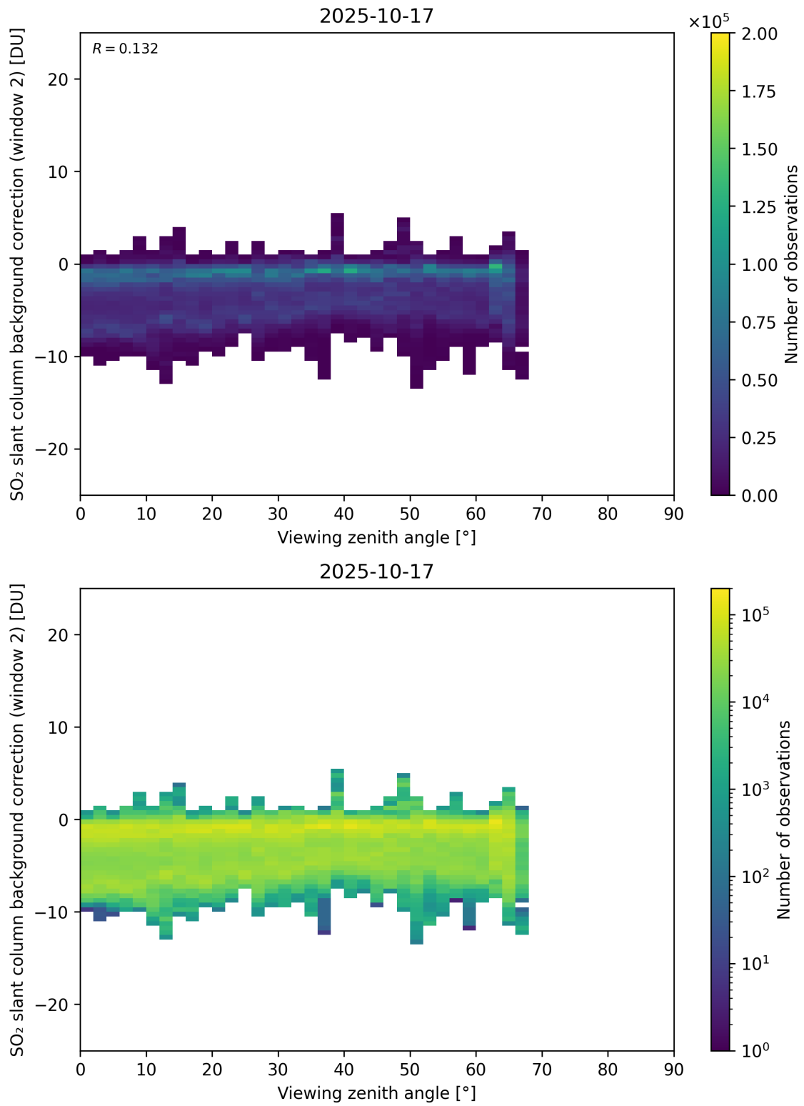
Figure 363: Scatter density plot of “Viewing zenith angle” against “SO 2 slant column background correction (window 2)” for 2025-10-17 to 2025-10-18.
