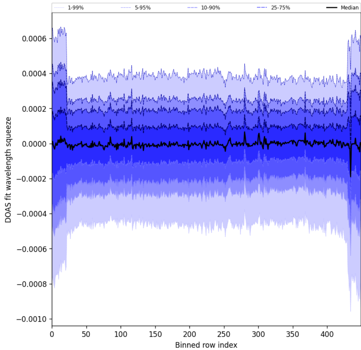
Figure 103: Along track statistics of “DOAS fit wavelength squeeze” for 2025-10-17 to 2025-10-18
