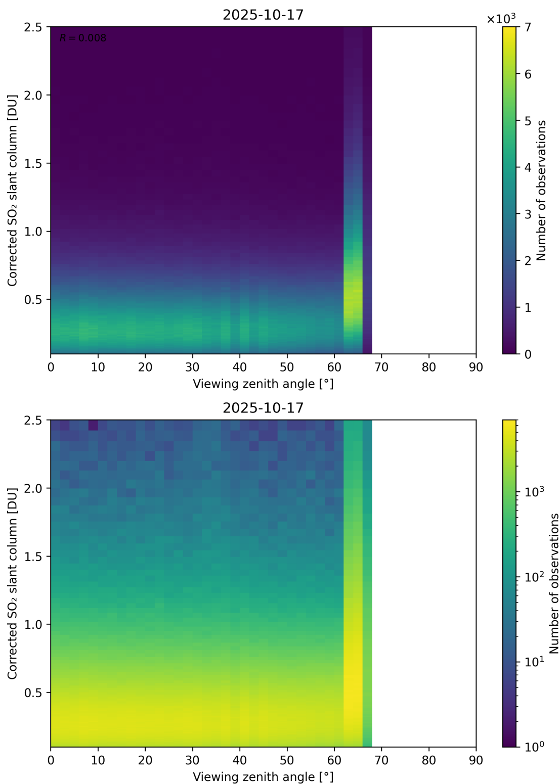
Figure 373: Scatter density plot of “Viewing zenith angle” against “Corrected SO 2 slant column” for 2025-10-17 to 2025-10-18.
