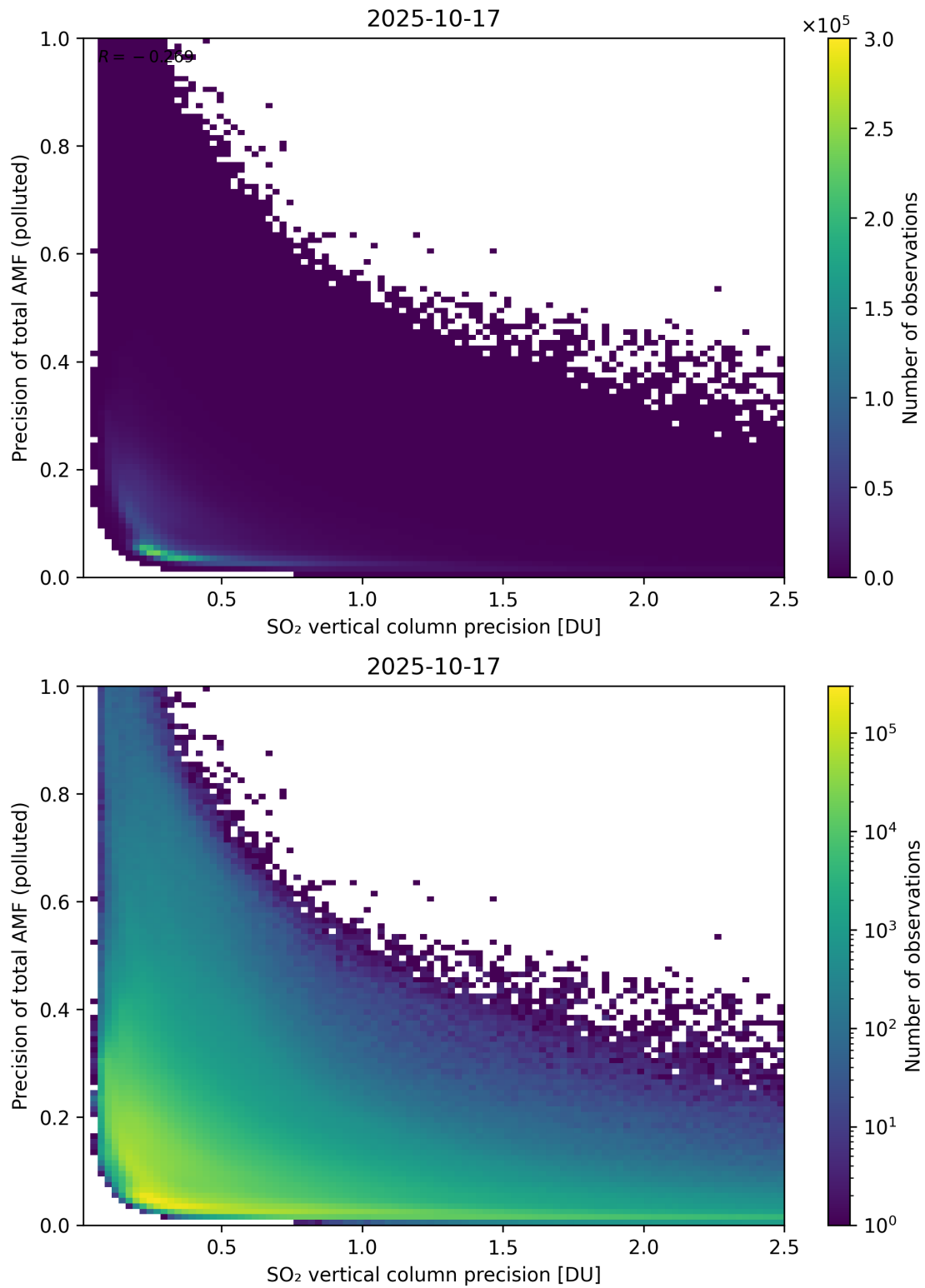
Figure 347: Scatter density plot of “SO 2 vertical column precision” against “Precision of total AMF (polluted)” for 2025-10-17 to 2025-10-18.
