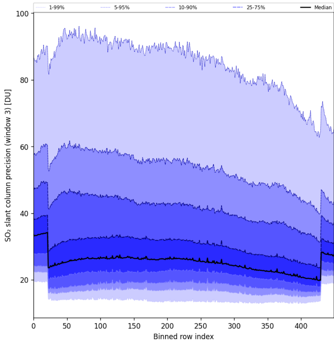
Figure 98: Along track statistics of “SO 2 slant column precision (window 3)” for 2025-10-17 to 2025-10-18
