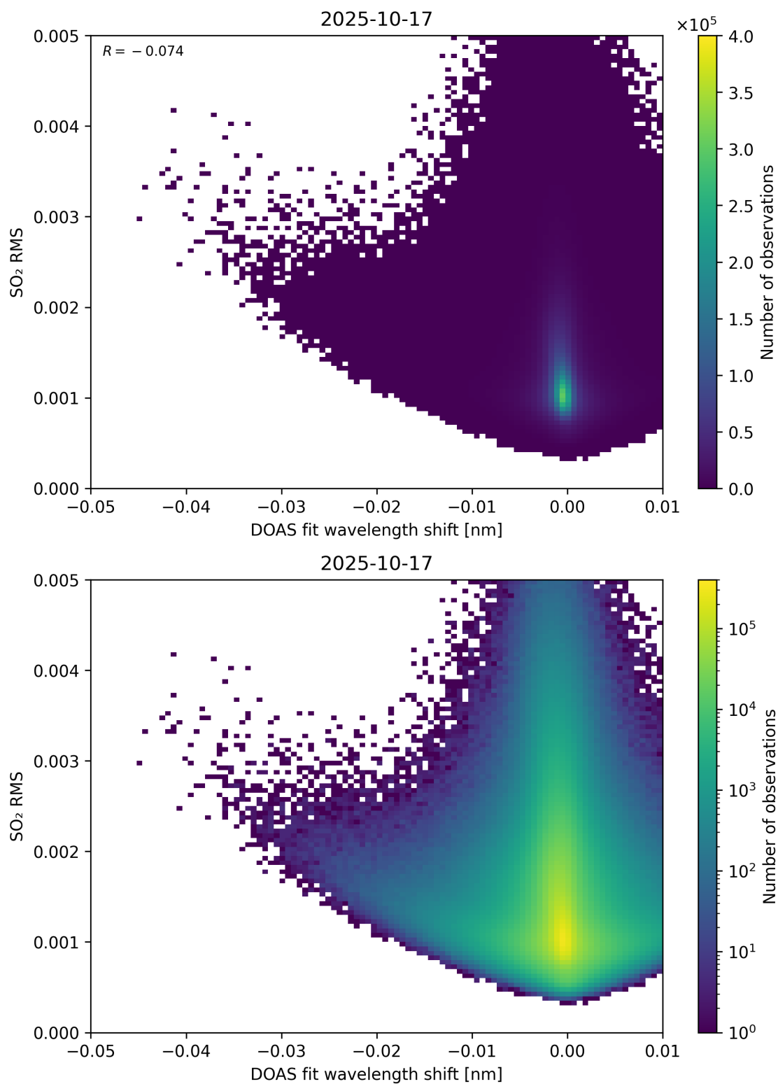
Figure 139: Scatter density plot of “DOAS fit wavelength shift” against “SO 2 RMS” for 2025-10-17 to 2025-10-18.
