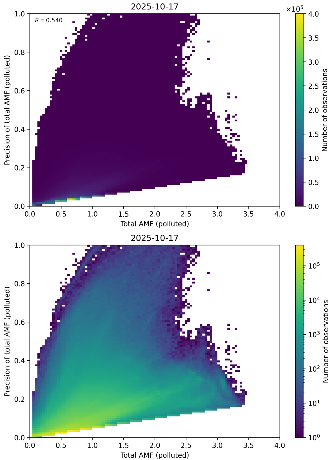
Figure 322: Scatter density plot of “Total AMF (polluted)” against “Precision of total AMF (polluted)” for 2025-10-17 to 2025-10-18.
