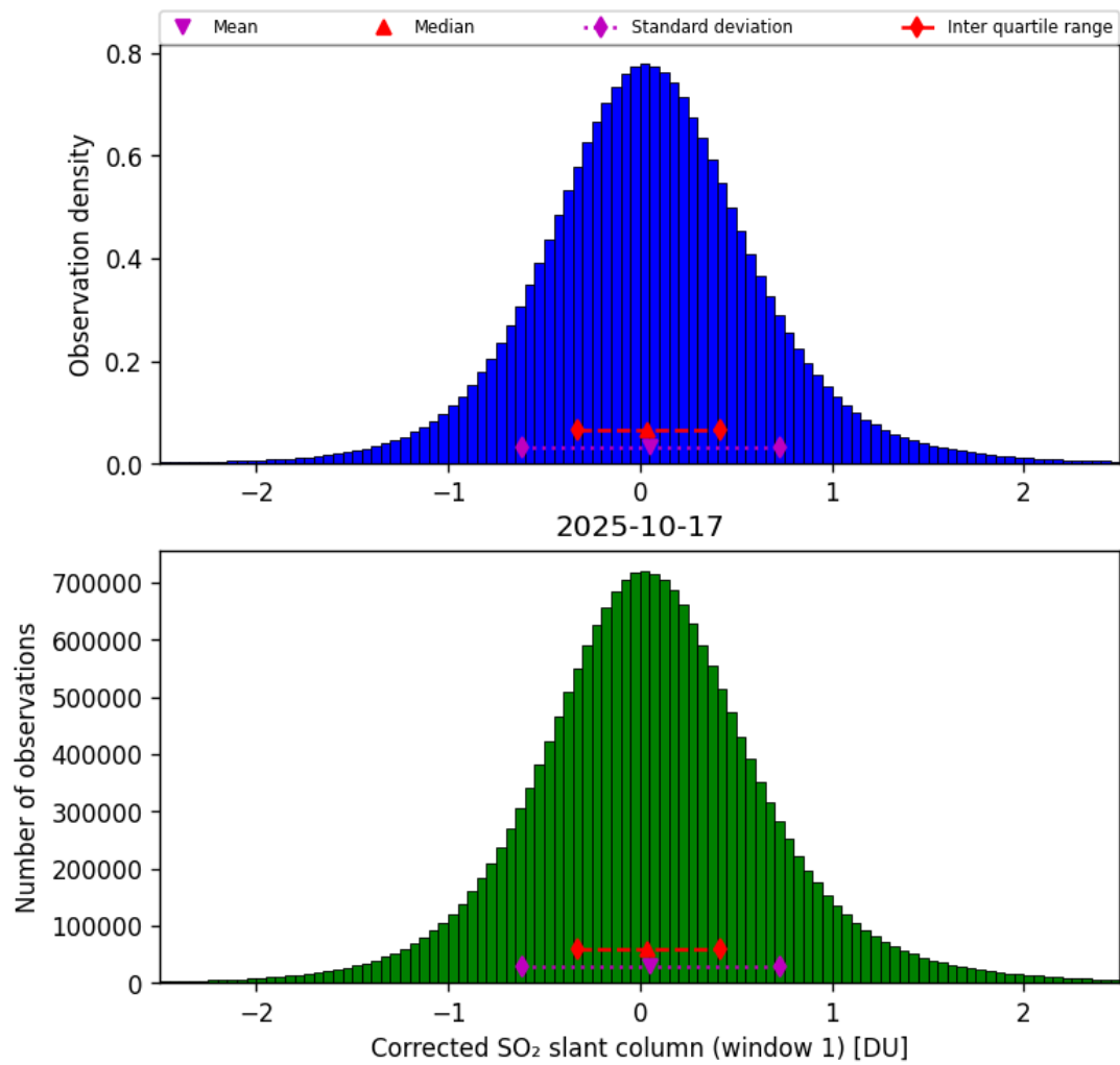
Figure 65: Histogram of “Corrected SO 2 slant column (window 1)” for 2025-10-17 to 2025-10-18
