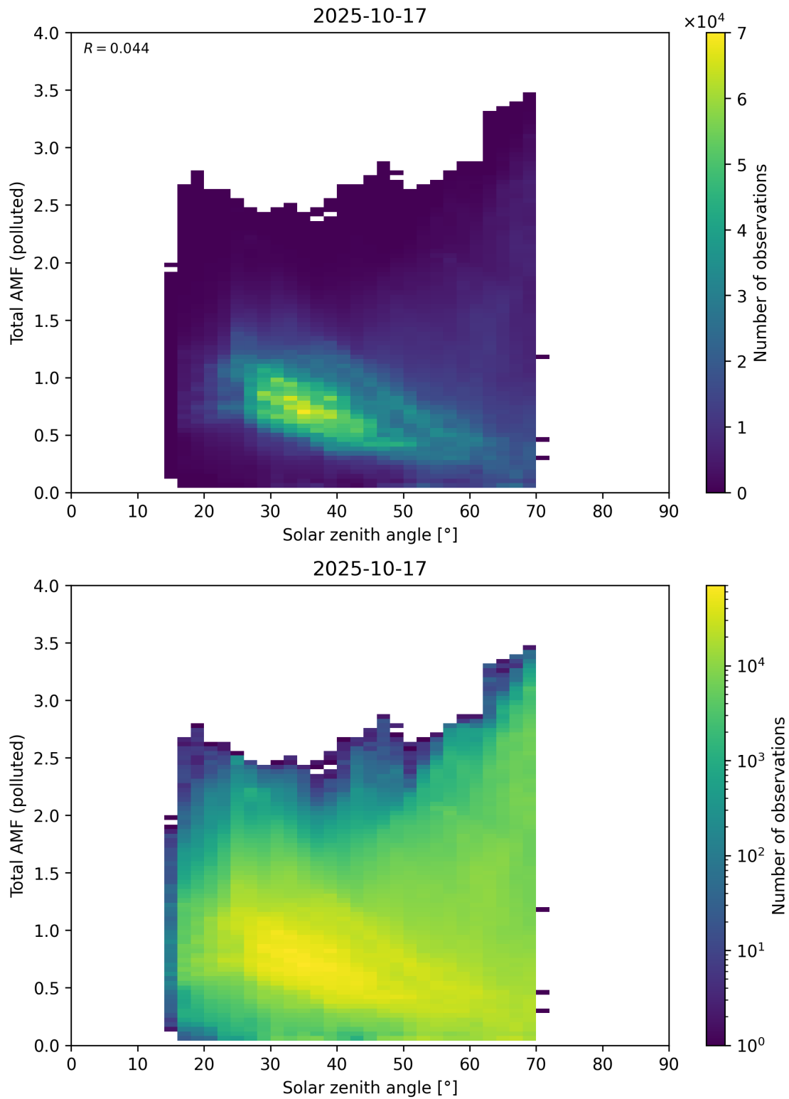
Figure 189: Scatter density plot of “Solar zenith angle” against “Total AMF (polluted)” for 2025-10-17 to 2025-10-18.
