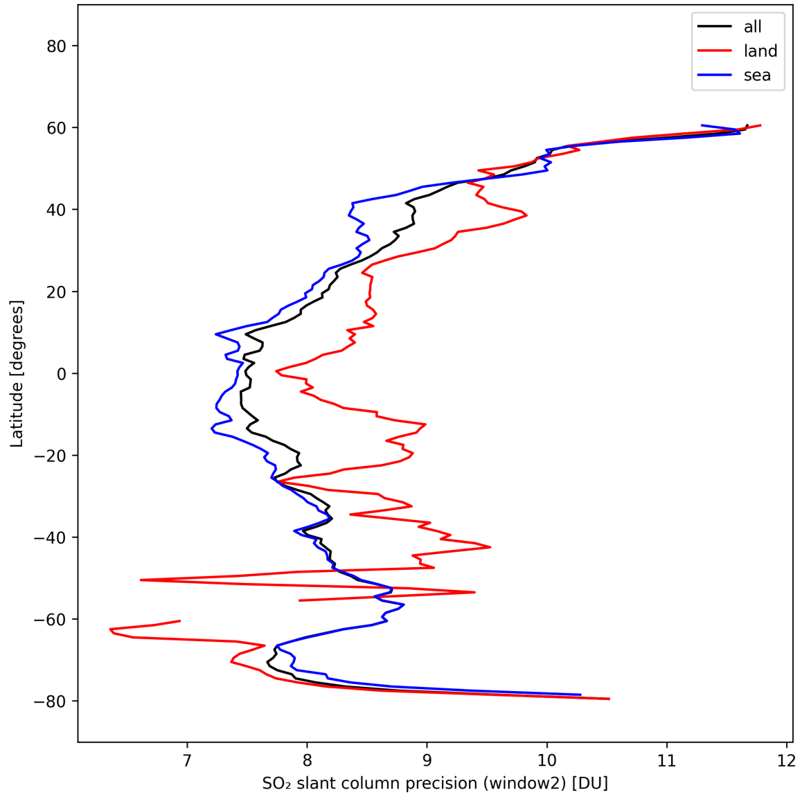
Figure 42: Zonal average of “SO 2 slant column precision (window2)” for 2025-10-17 to 2025-10-18.
