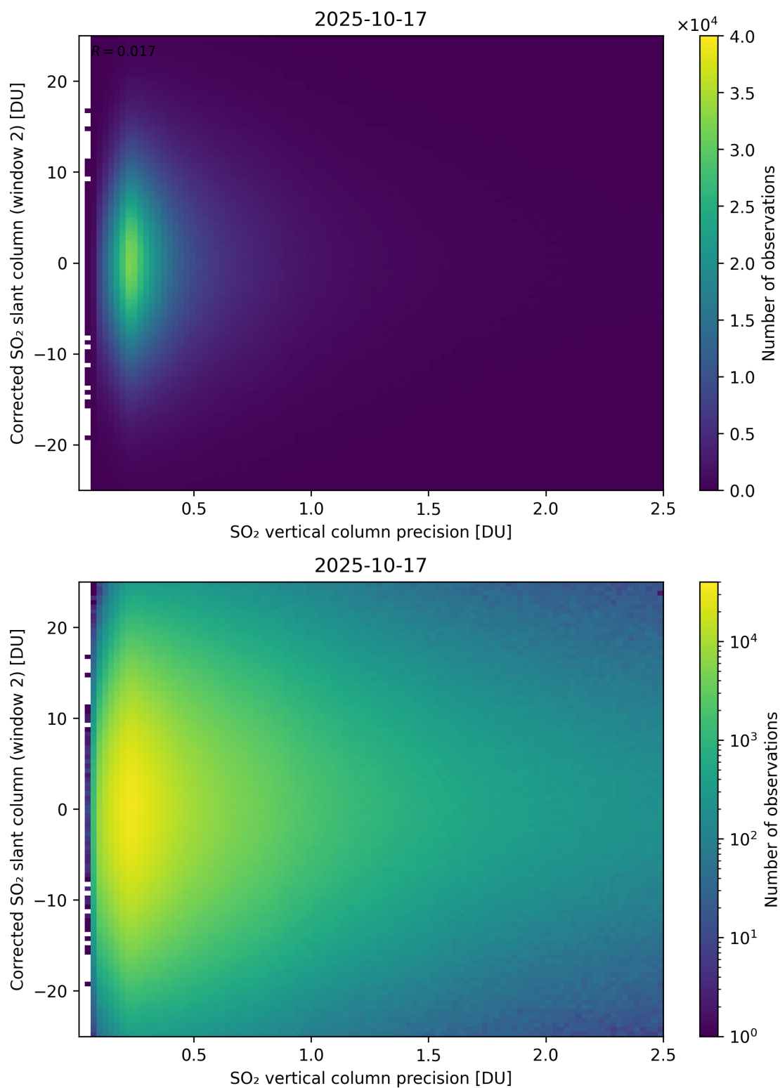
Figure 339: Scatter density plot of “SO 2 vertical column precision” against “Corrected SO 2 slant column (window 2)” for 2025-10-17 to 2025-10-18.
