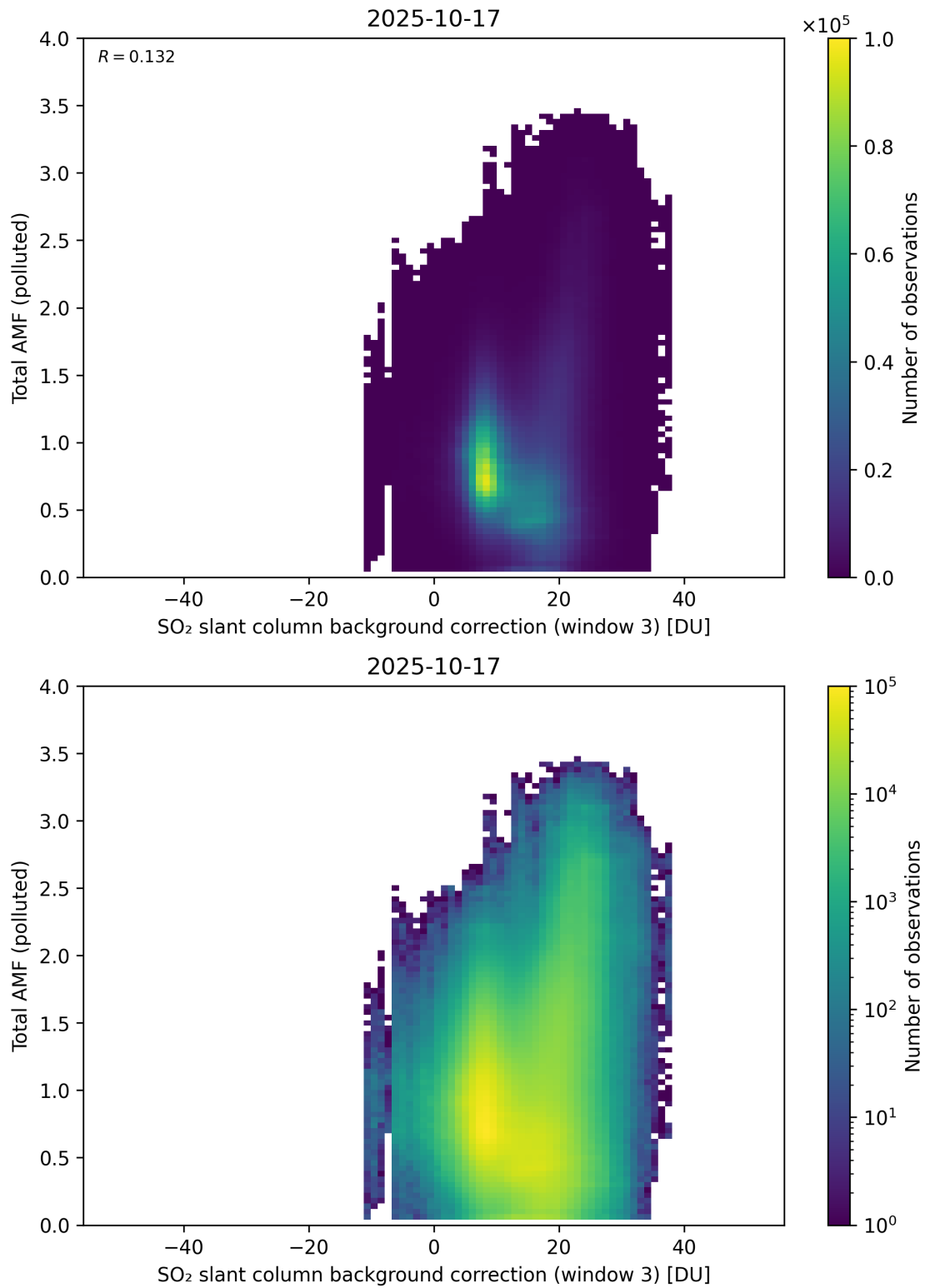
Figure 136: Scatter density plot of “SO 2 slant column background correction (window 3)” against “Total AMF (polluted)” for 2025-10-17 to 2025-10-18.
