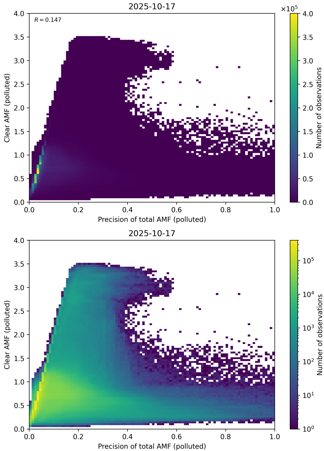
Figure 320: Scatter density plot of “Precision of total AMF (polluted)” against “Clear AMF (polluted)” for 2025-10-17 to 2025-10-18.
