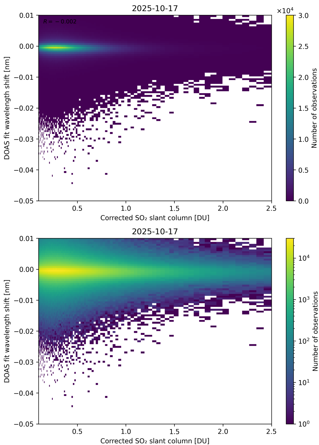
Figure 229: Scatter density plot of “Corrected SO 2 slant column” against “DOAS fit wavelength shift” for 2025-10-17 to 2025-10-18.
