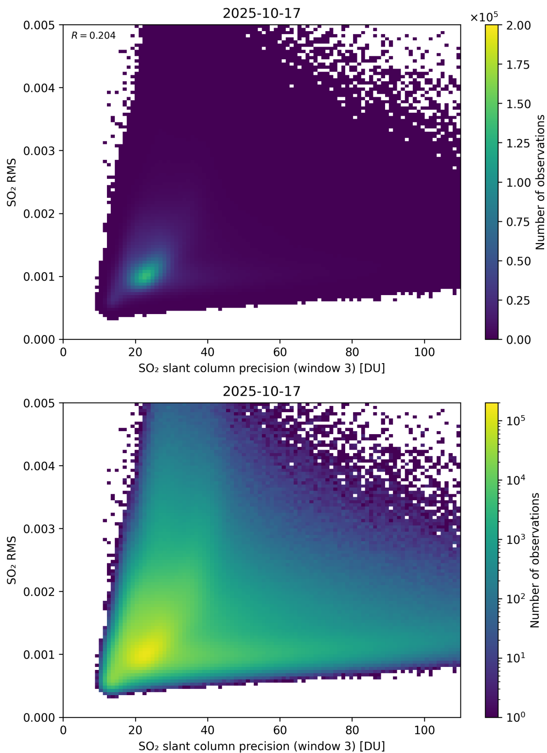
Figure 310: Scatter density plot of “SO 2 slant column precision (window 3)” against “SO 2 RMS” for 2025-10-17 to 2025-10-18.
