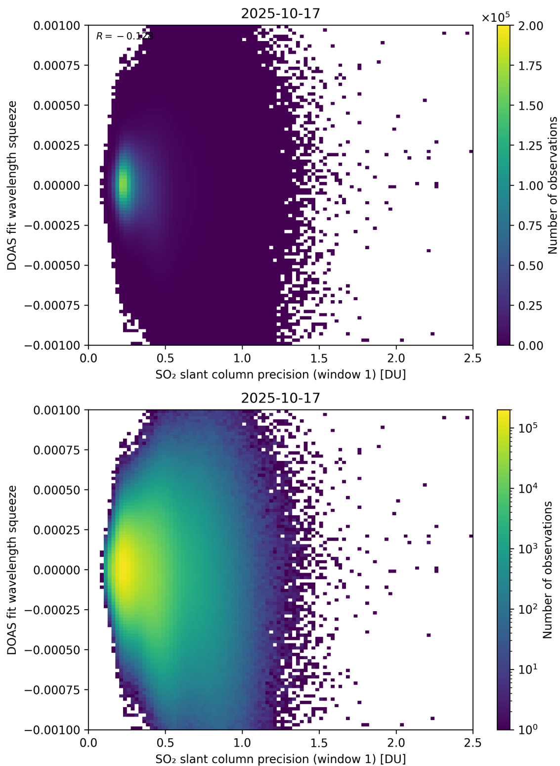
Figure 272: Scatter density plot of “SO 2 slant column precision (window 1)” against “DOAS fit wavelength squeeze” for 2025-10-17 to 2025-10-18.
