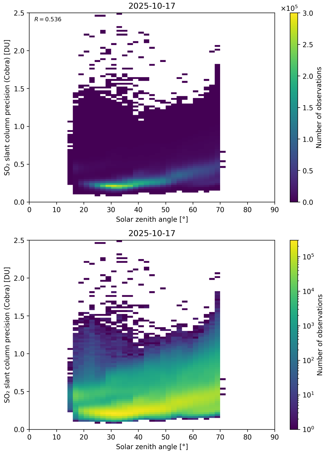
Figure 180: Scatter density plot of “Solar zenith angle” against “SO 2 slant column precision (Cobra)” for 2025-10-17 to 2025-10-18.
