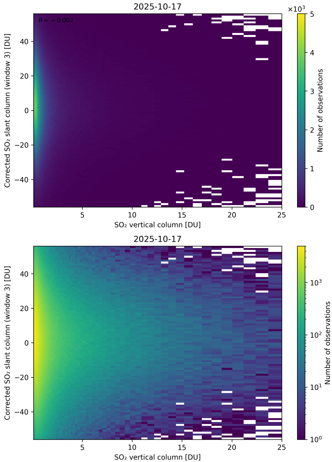
Figure 353: Scatter density plot of “SO 2 vertical column” against “Corrected SO 2 slant column (window 3)” for 2025-10-17 to 2025-10-18.
