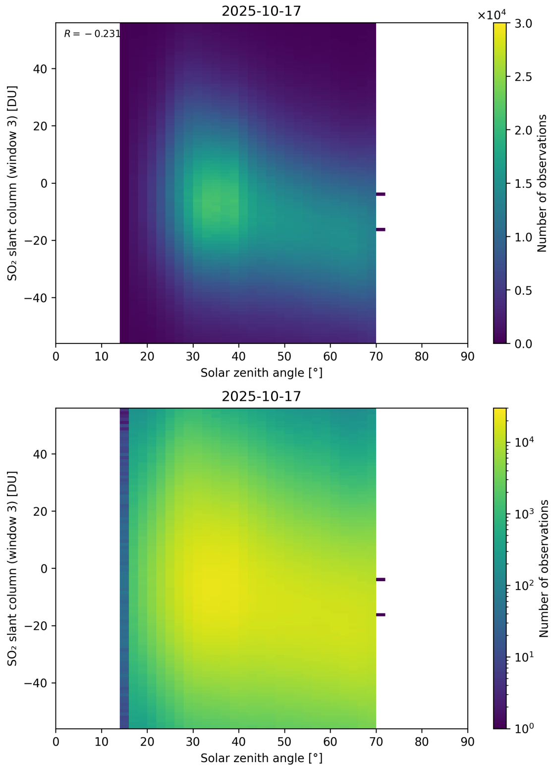
Figure 187: Scatter density plot of “Solar zenith angle” against “SO 2 slant column (window 3)” for 2025-10-17 to 2025-10-18.
