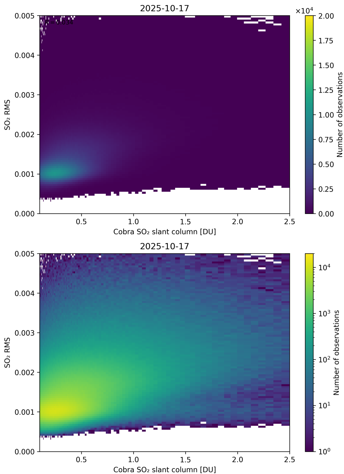
Figure 198: Scatter density plot of “Cobra SO 2 slant column” against “SO 2 RMS” for 2025-10-17 to 2025-10-18.
