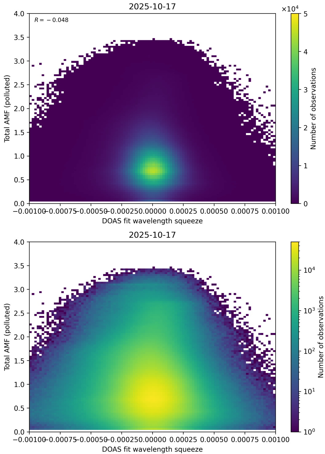
Figure 145: Scatter density plot of “DOAS fit wavelength squeeze” against “Total AMF (polluted)” for 2025-10-17 to 2025-10-18.
