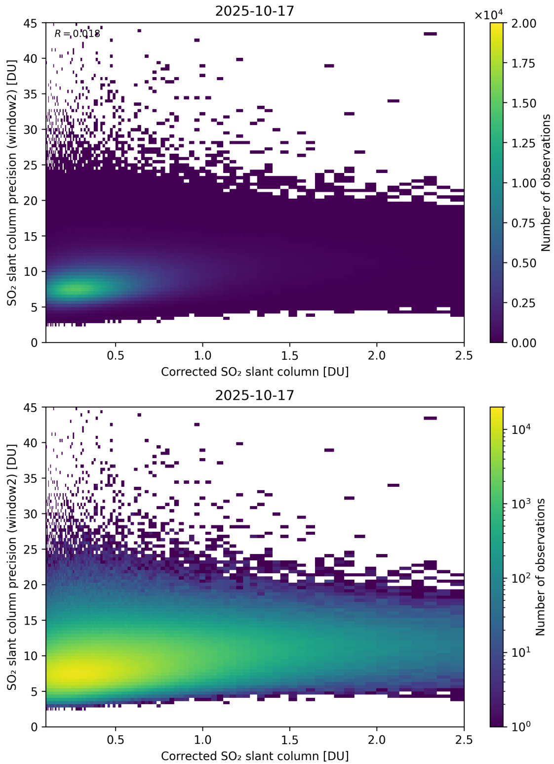
Figure 239: Scatter density plot of “Corrected SO 2 slant column” against “SO 2 slant column precision (window2)” for 2025-10-17 to 2025-10-18.
