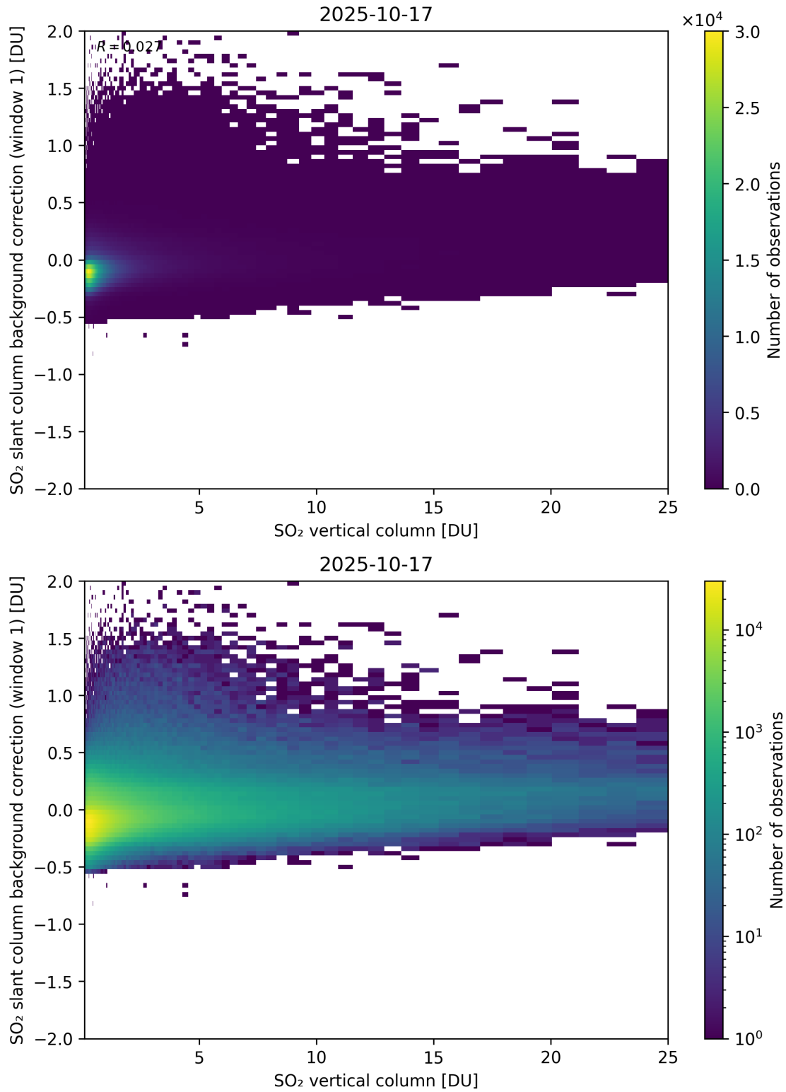
Figure 323: Scatter density plot of “SO 2 vertical column” against “SO 2 slant column background correction (window 1)” for 2025-10-17 to 2025-10-18.
