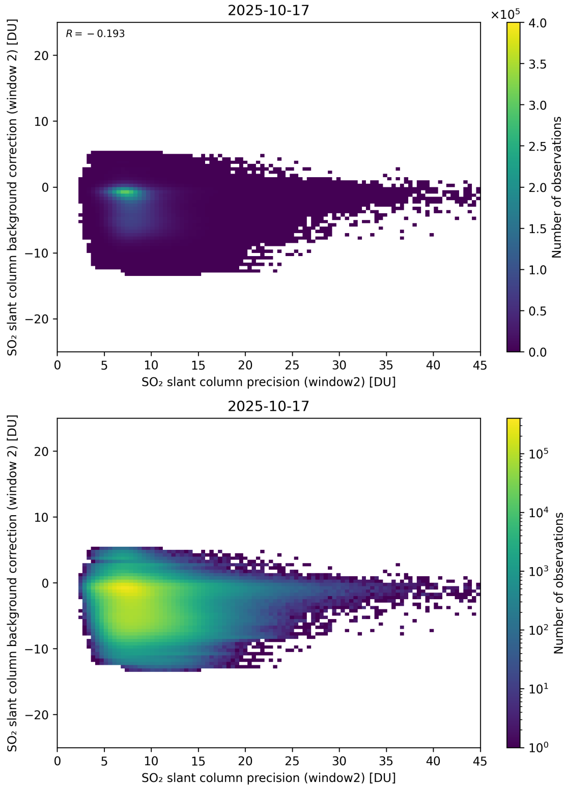
Figure 291: Scatter density plot of “SO 2 slant column precision (window2)” against “SO 2 slant column background correction (window 2)” for 2025-10-17 to 2025-10-18.
