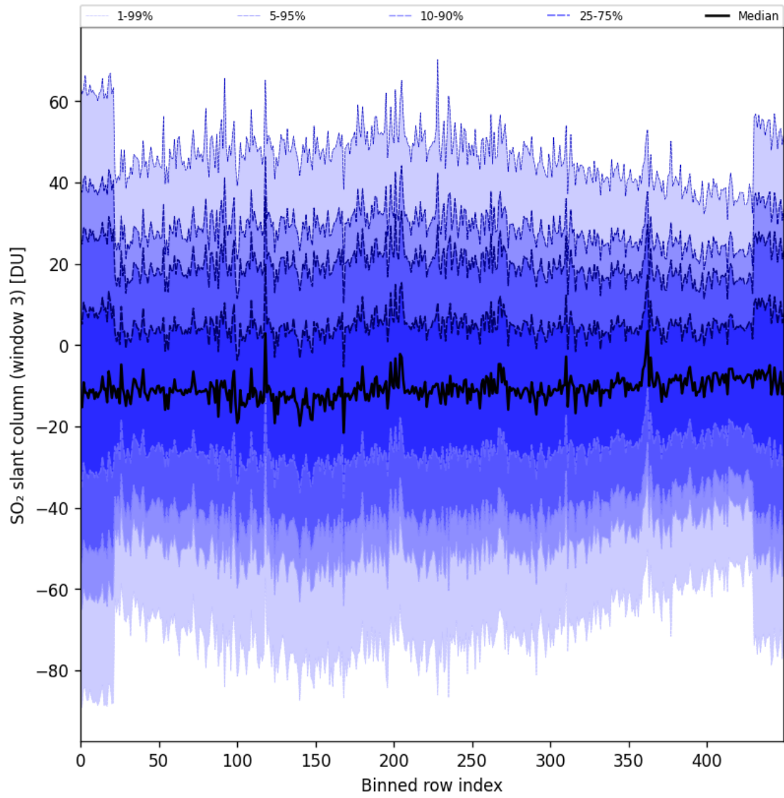
Figure 97: Along track statistics of “SO 2 slant column (window 3)” for 2025-10-17 to 2025-10-18
