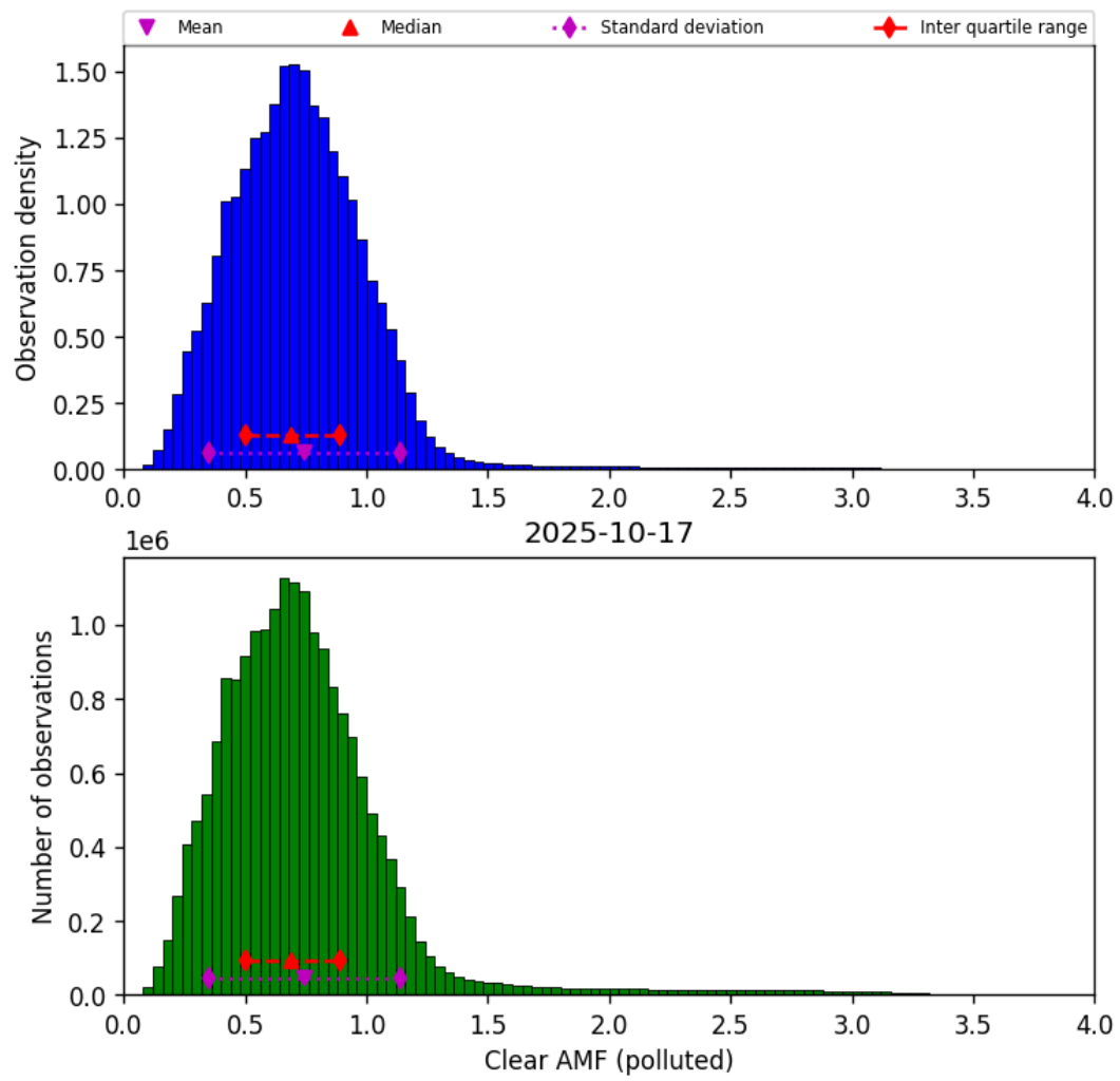
Figure 81: Histogram of “Clear AMF (polluted)” for 2025-10-17 to 2025-10-18
