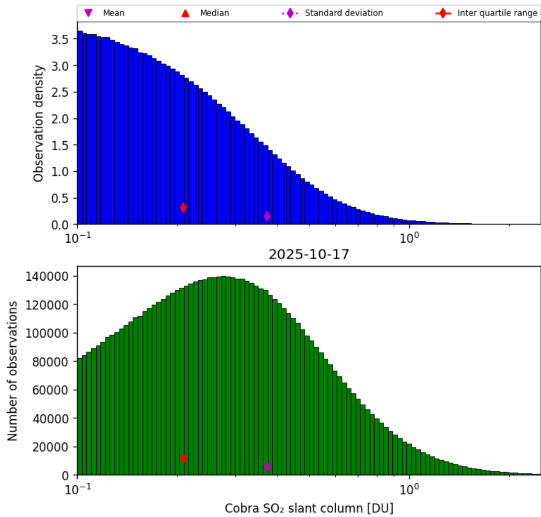
Figure 61: Histogram of “Cobra SO 2 slant column” for 2025-10-17 to 2025-10-18
