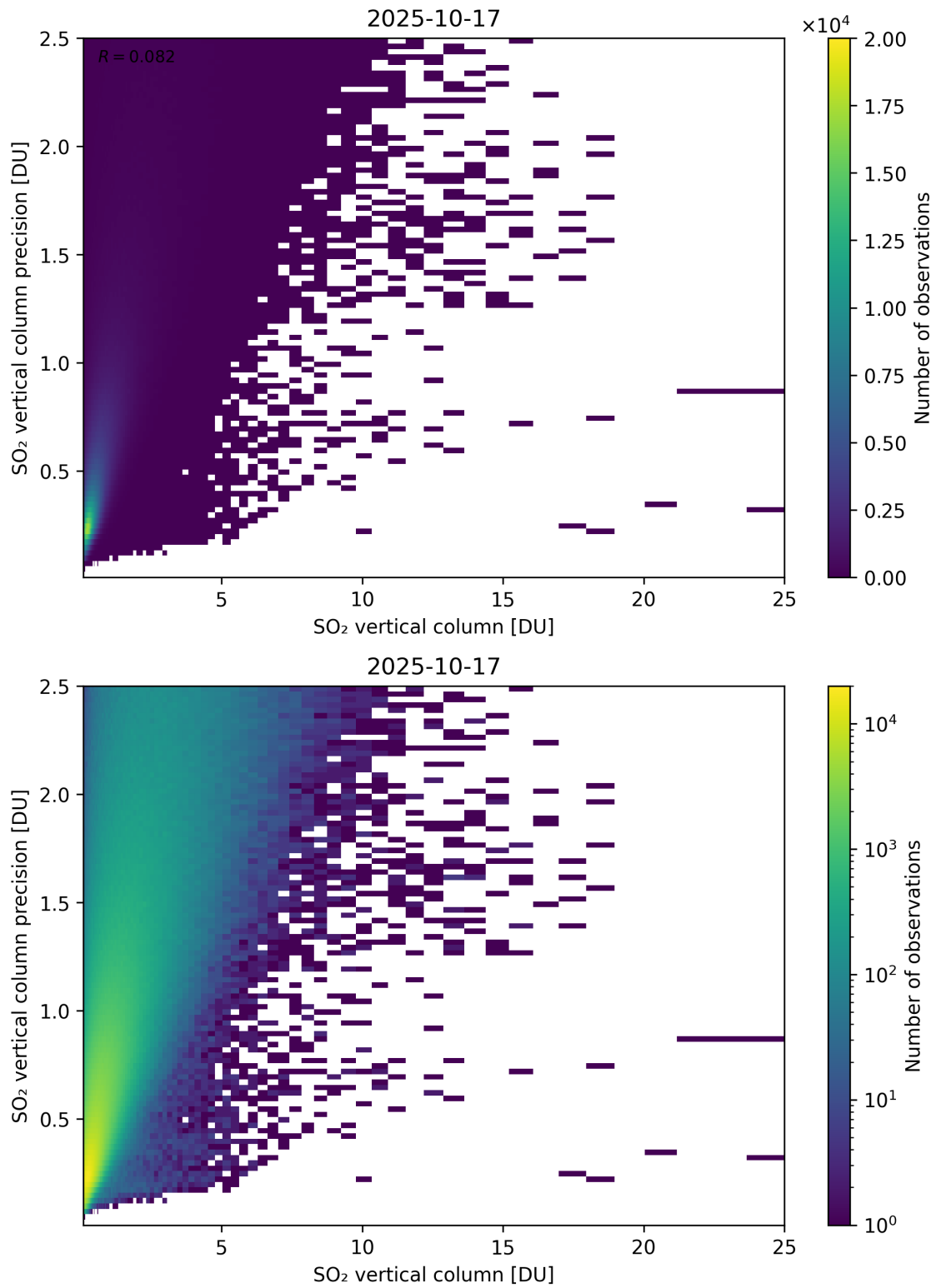
Figure 361: Scatter density plot of “SO 2 vertical column” against “SO 2 vertical column precision” for 2025-10-17 to 2025-10-18.
