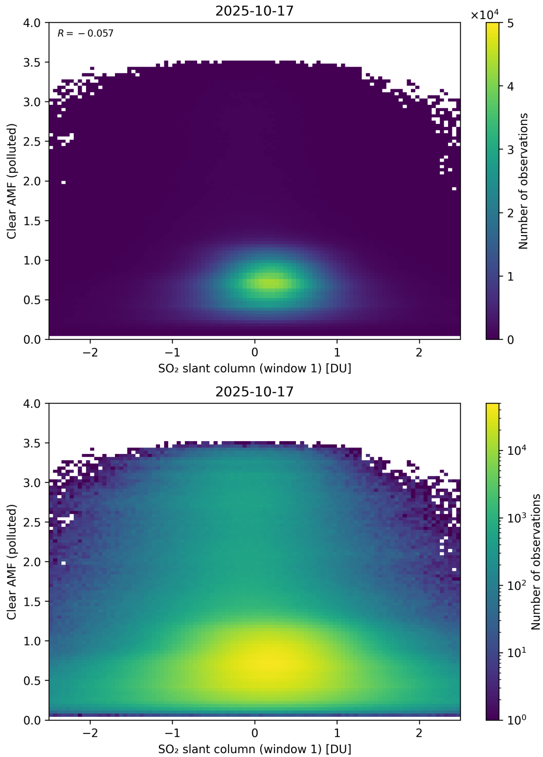
Figure 282: Scatter density plot of “SO 2 slant column (window 1)” against “Clear AMF (polluted)” for 2025-10-17 to 2025-10-18.
