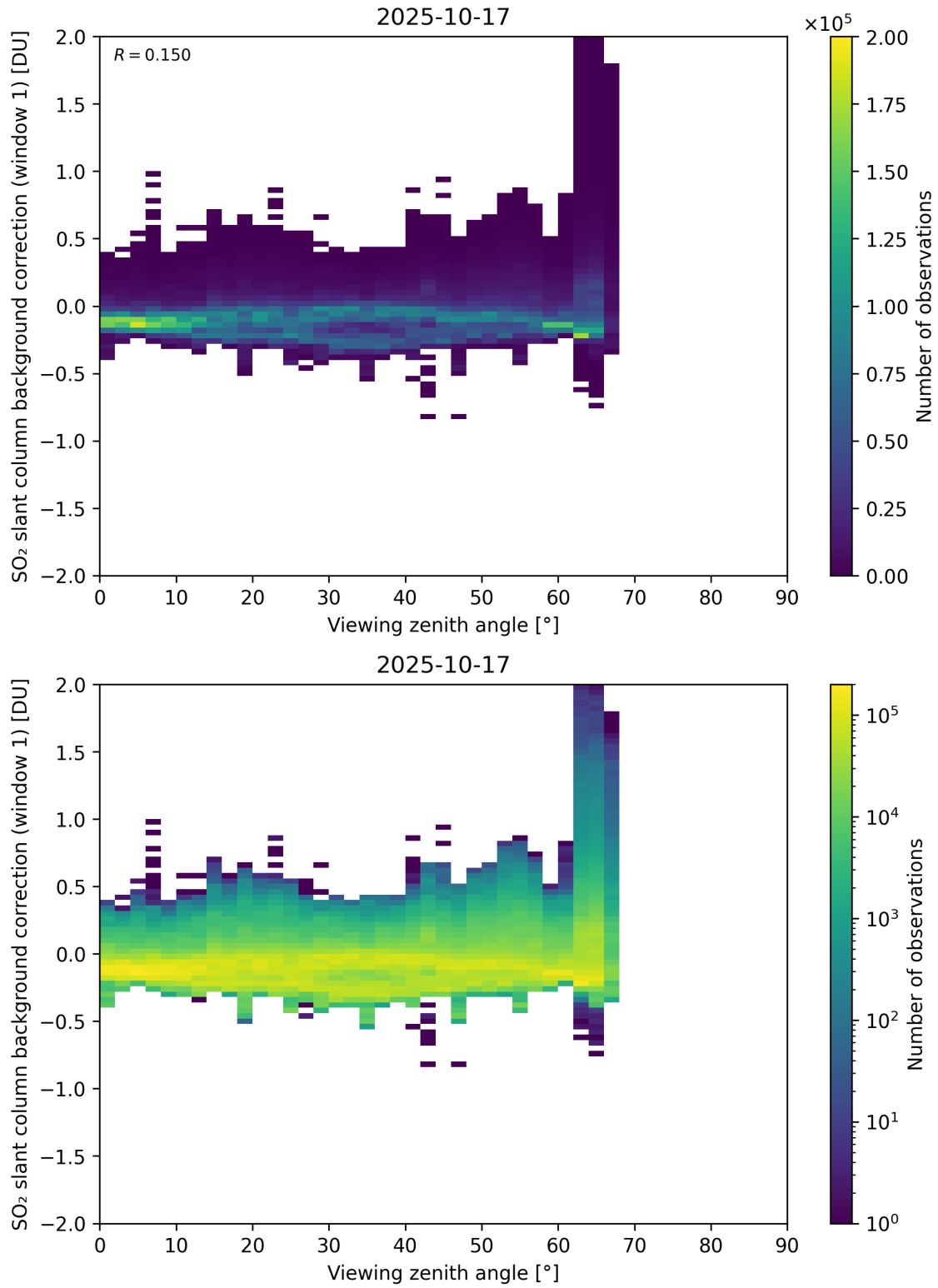
Figure 362: Scatter density plot of “Viewing zenith angle” against “SO 2 slant column background correction (window 1)” for 2025-10-17 to 2025-10-18.
