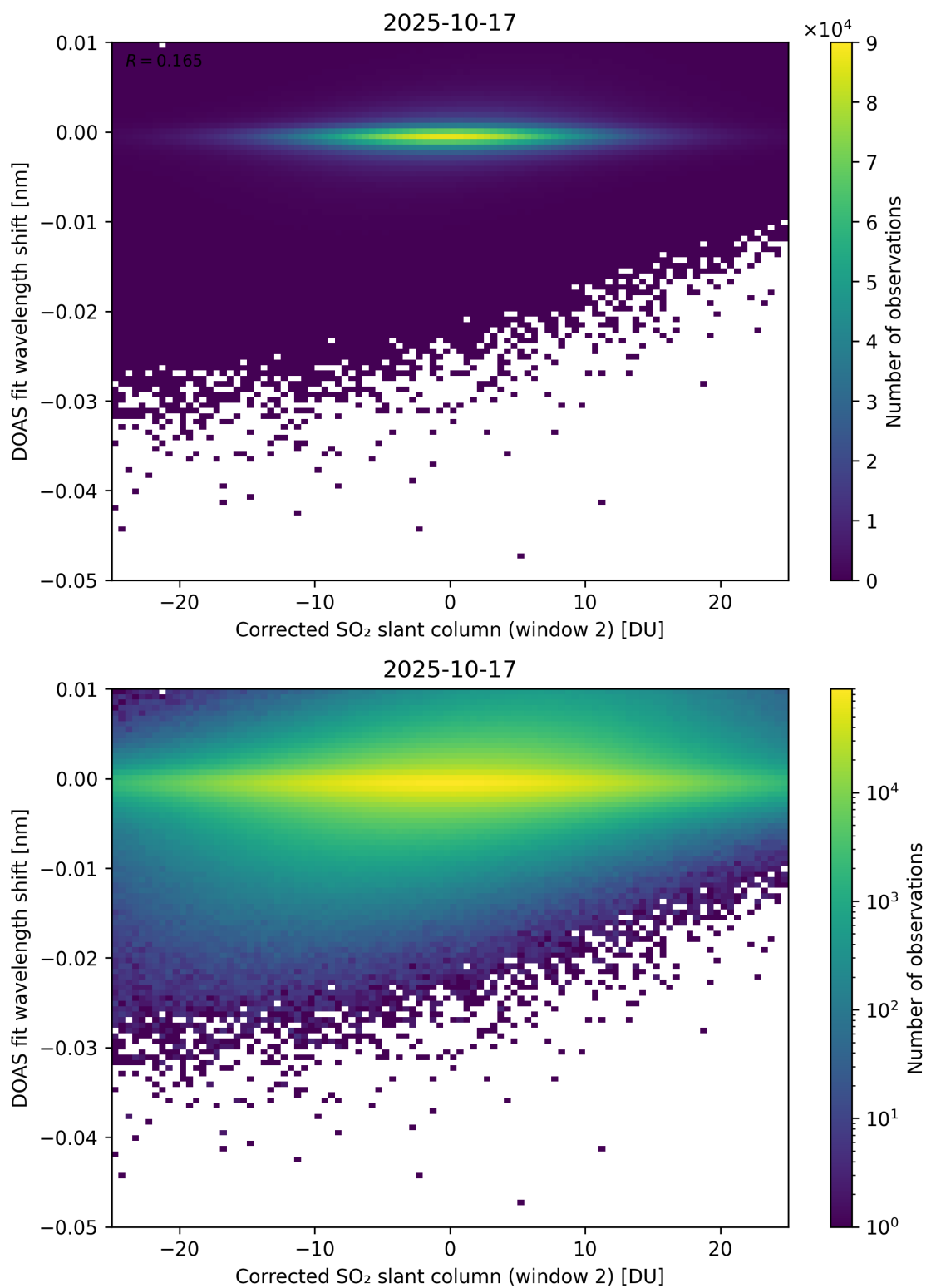
Figure 246: Scatter density plot of “Corrected SO 2 slant column (window 2)” against “DOAS fit wavelength shift” for 2025-10-17 to 2025-10-18.
