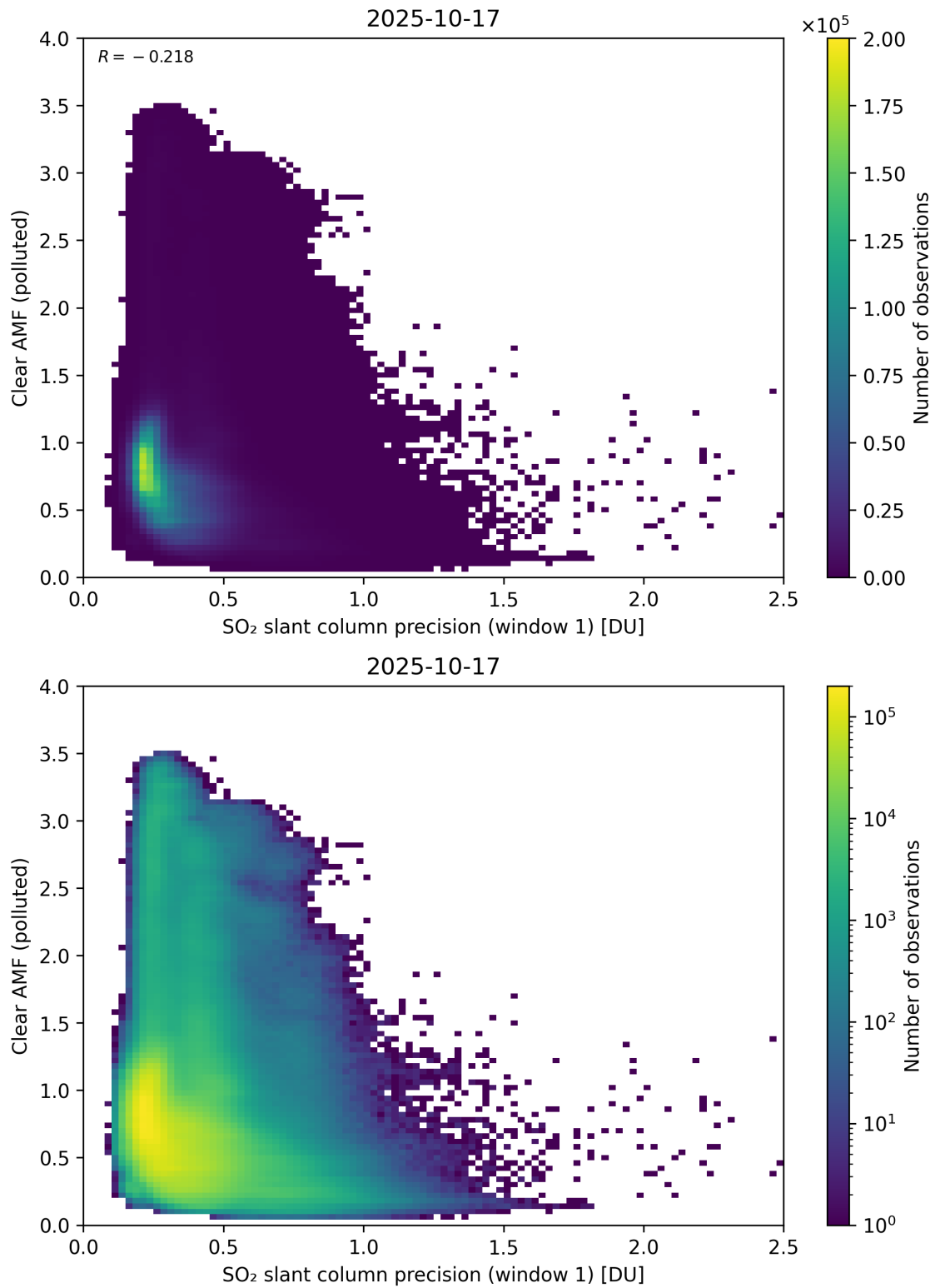
Figure 274: Scatter density plot of “SO 2 slant column precision (window 1)” against “Clear AMF (polluted)” for 2025-10-17 to 2025-10-18.
