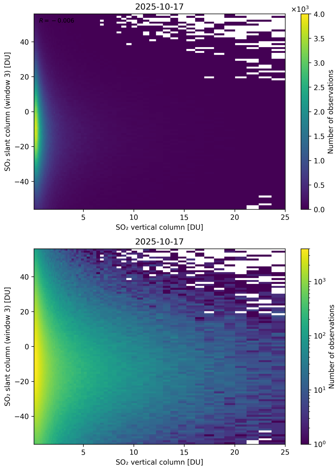
Figure 357: Scatter density plot of “SO 2 vertical column” against “SO 2 slant column (window 3)” for 2025-10-17 to 2025-10-18.
