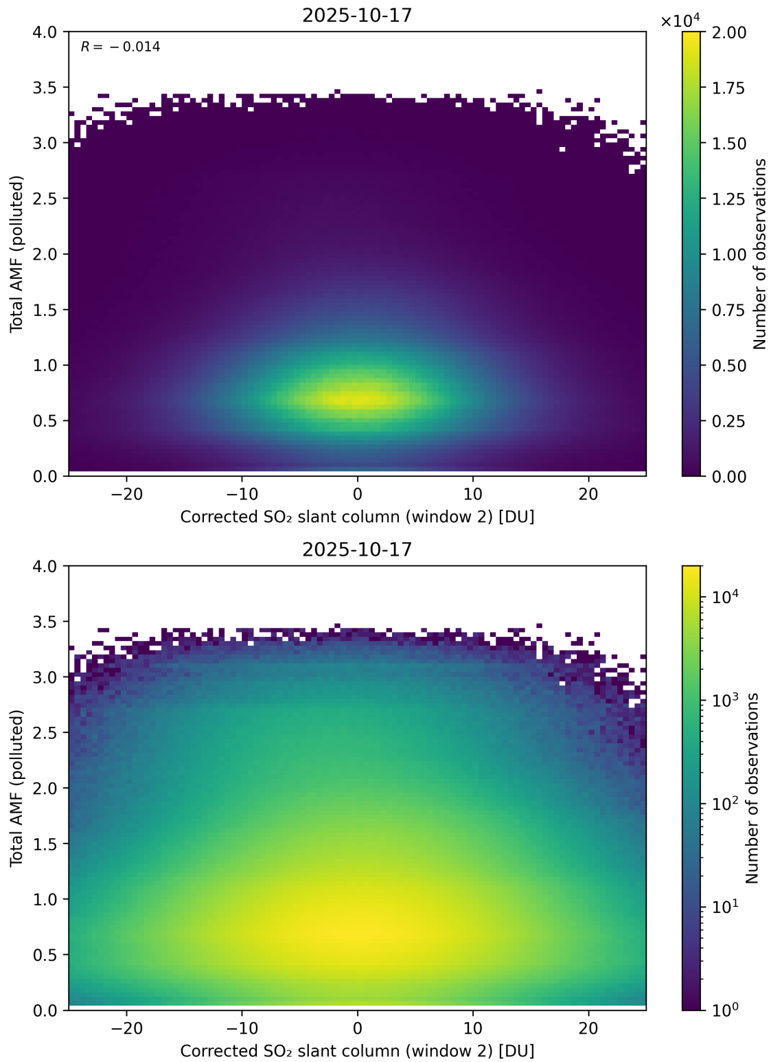
Figure 253: Scatter density plot of “Corrected SO 2 slant column (window 2)” against “Total AMF (polluted)” for 2025-10-17 to 2025-10-18.
