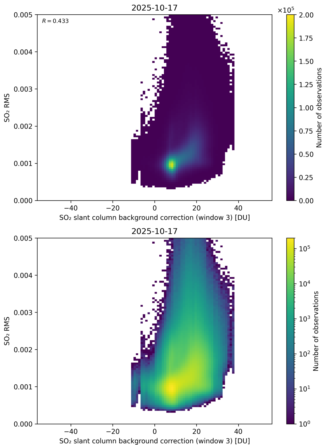
Figure 134: Scatter density plot of “SO 2 slant column background correction (window 3)” against “SO 2 RMS” for 2025-10-17 to 2025-10-18.
