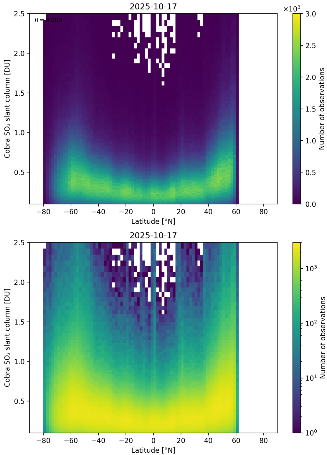
Figure 157: Scatter density plot of “Latitude” against “Cobra SO 2 slant column” for 2025-10-17 to 2025-10-18.
