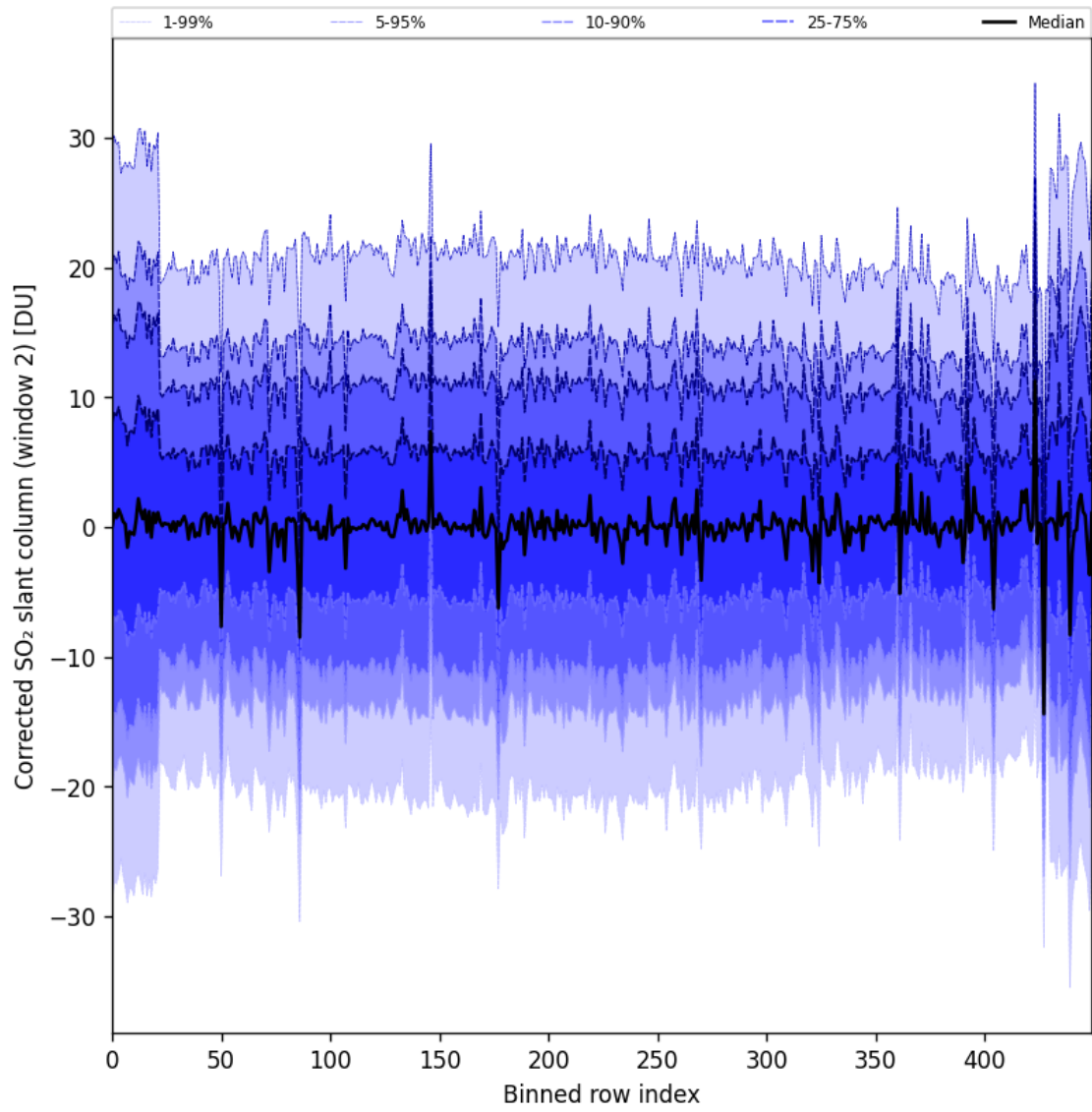
Figure 95: Along track statistics of “Corrected SO 2 slant column (window 2)” for 2025-10-17 to 2025-10-18
