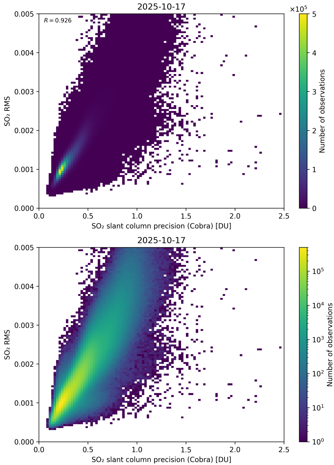
Figure 204: Scatter density plot of “SO 2 slant column precision (Cobra)” against “SO 2 RMS” for 2025-10-17 to 2025-10-18.
