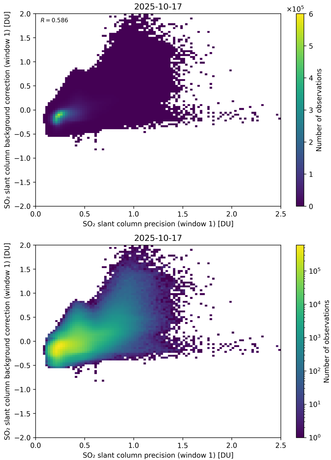
Figure 268: Scatter density plot of “SO 2 slant column precision (window 1)” against “SO 2 slant column background correction (window 1)” for 2025-10-17 to 2025-10-18.
