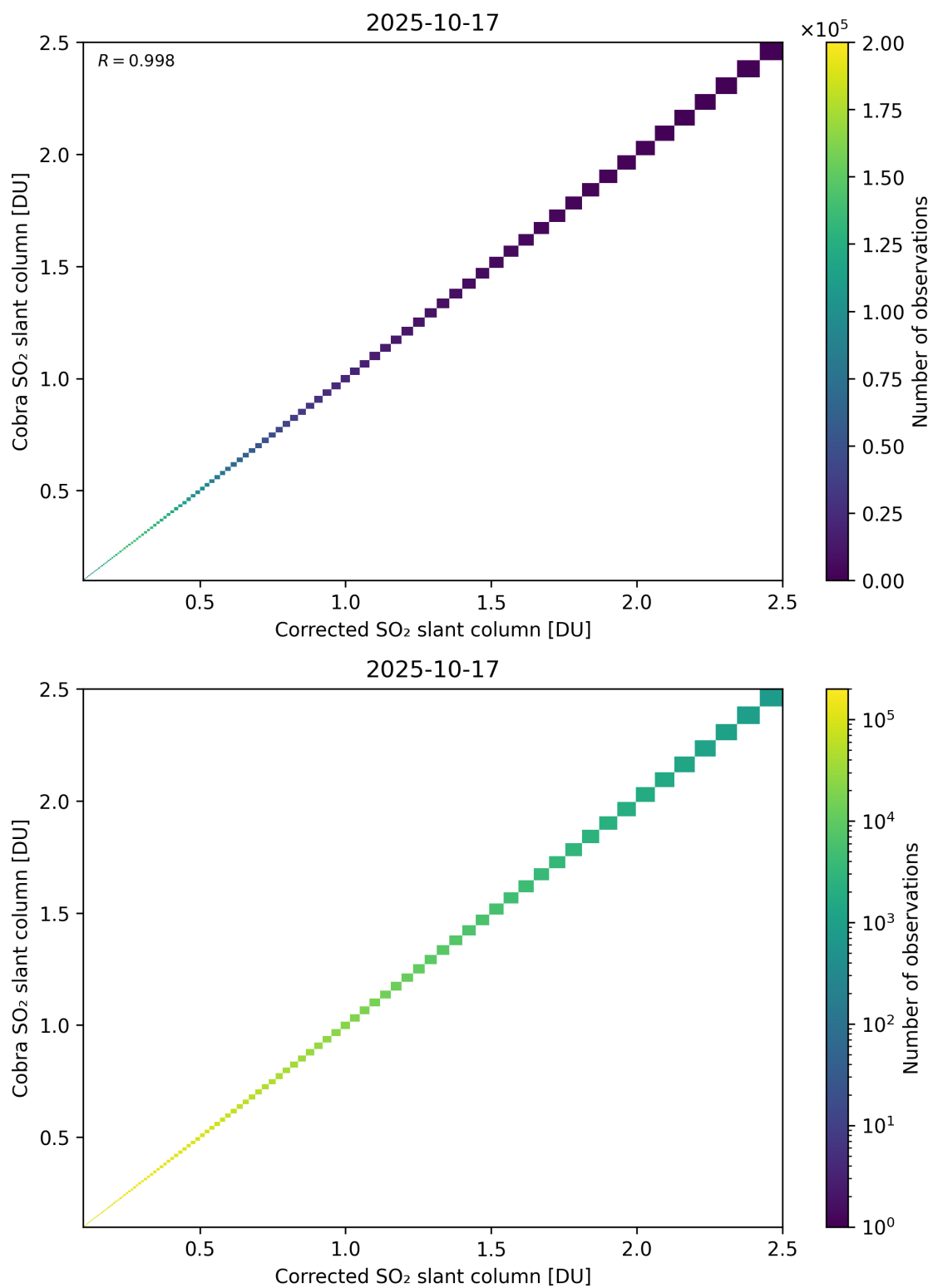
Figure 233: Scatter density plot of “Corrected SO 2 slant column” against “Cobra SO 2 slant column” for 2025-10-17 to 2025-10-18.
