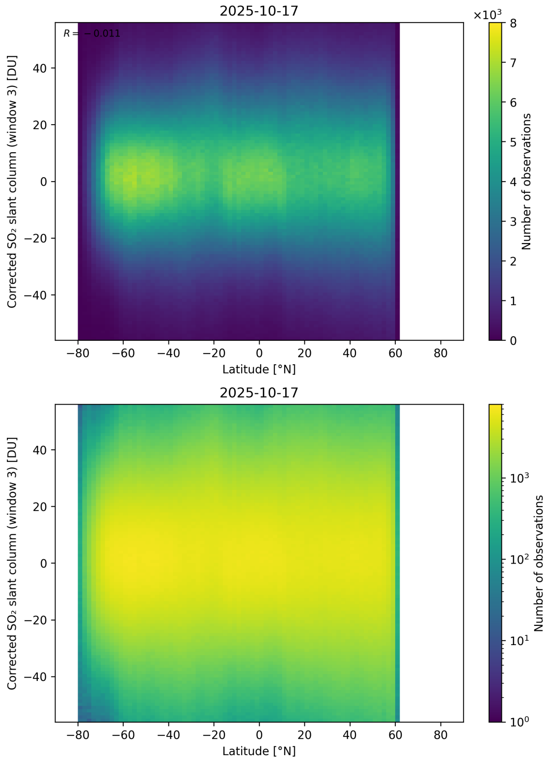
Figure 161: Scatter density plot of “Latitude” against “Corrected SO 2 slant column (window 3)” for 2025-10-17 to 2025-10-18.
