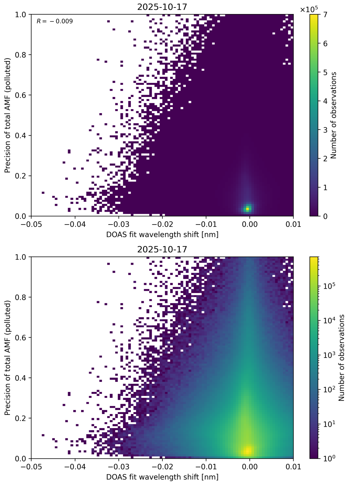
Figure 142: Scatter density plot of “DOAS fit wavelength shift” against “Precision of total AMF (polluted)” for 2025-10-17 to 2025-10-18.
