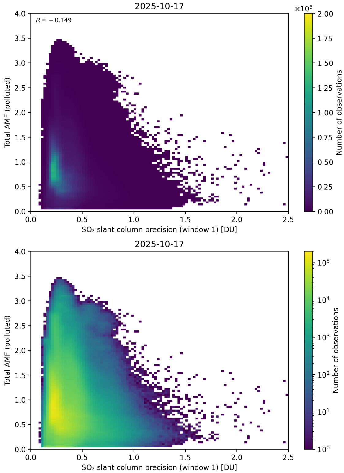
Figure 280: Scatter density plot of “SO 2 slant column precision (window 1)” against “Total AMF (polluted)” for 2025-10-17 to 2025-10-18.
