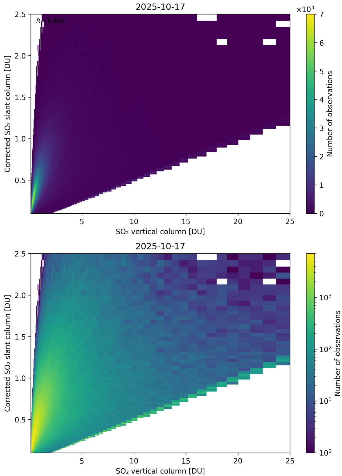
Figure 351: Scatter density plot of “SO 2 vertical column” against “Corrected SO 2 slant column” for 2025-10-17 to 2025-10-18.
