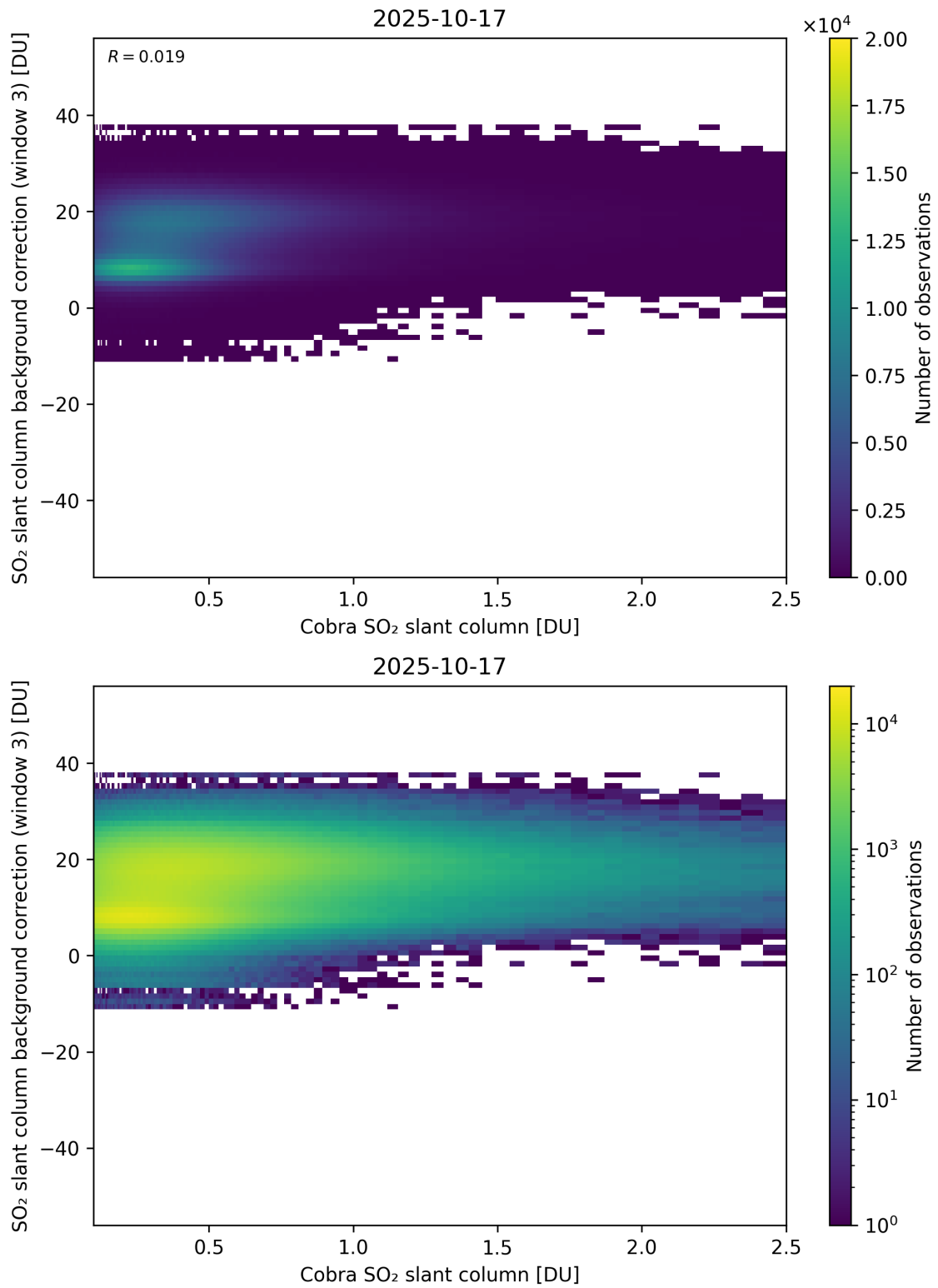
Figure 195: Scatter density plot of “Cobra SO 2 slant column” against “SO 2 slant column background correction (window 3)” for 2025-10-17 to 2025-10-18.
