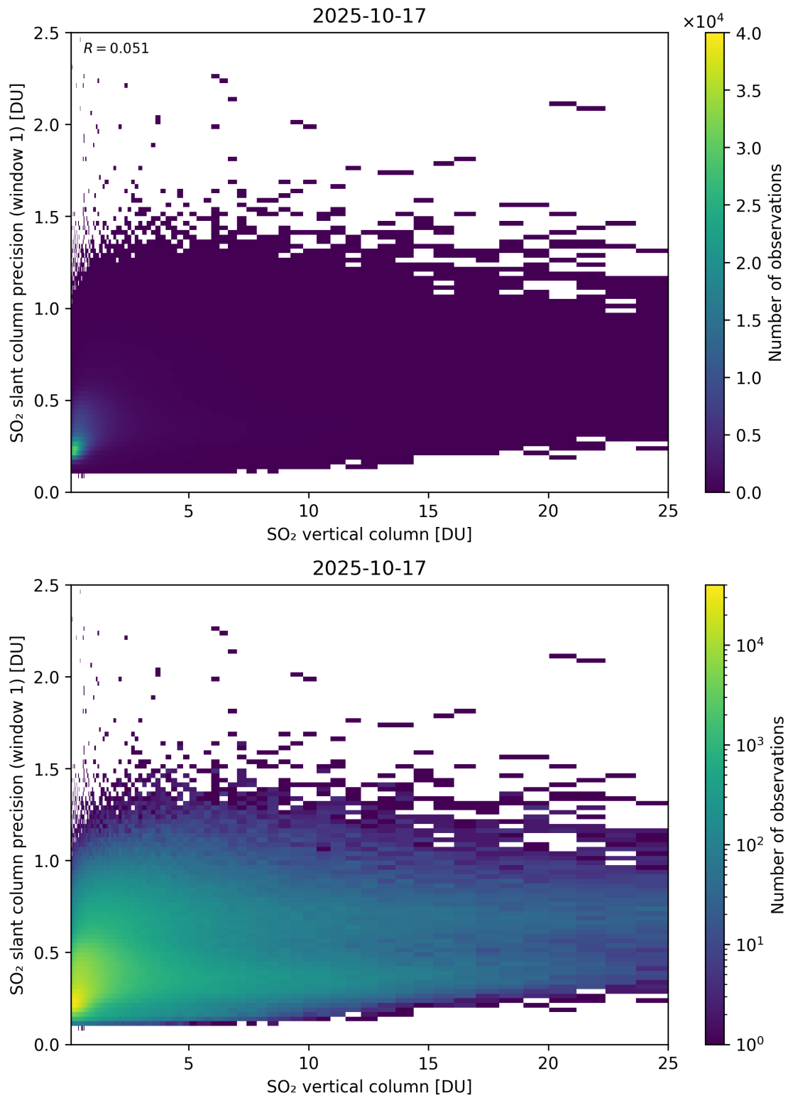
Figure 355: Scatter density plot of “SO 2 vertical column” against “SO 2 slant column precision (window 1)” for 2025-10-17 to 2025-10-18.
