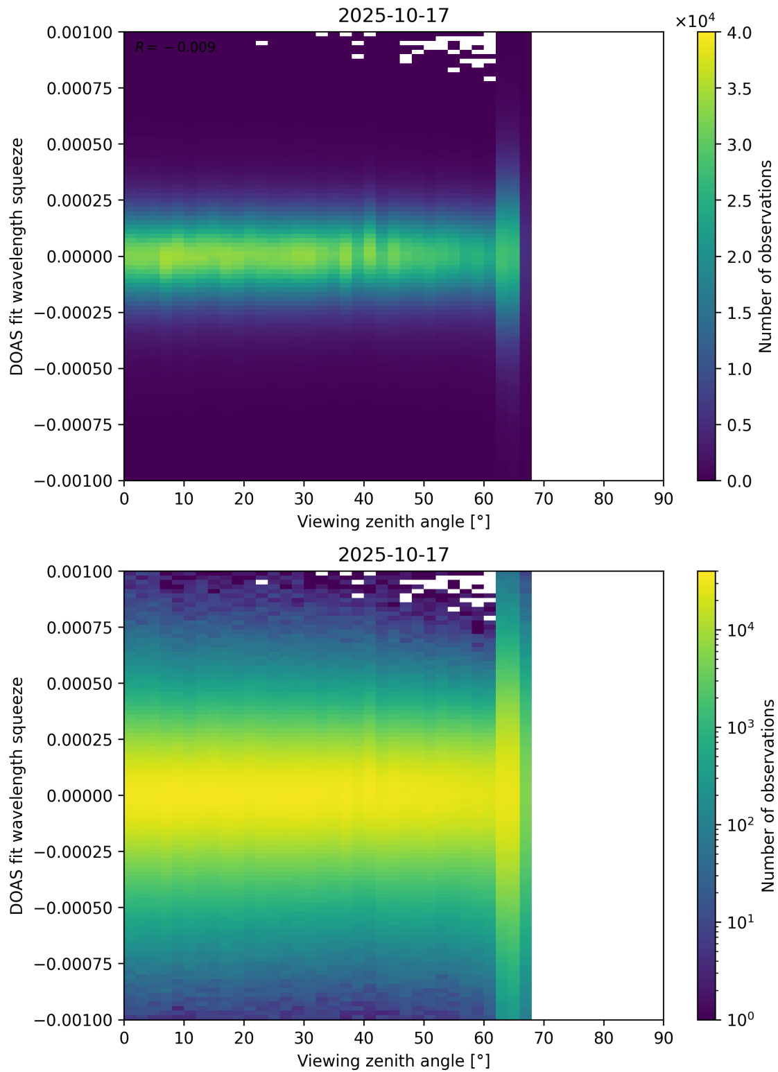
Figure 366: Scatter density plot of “Viewing zenith angle” against “DOAS fit wavelength squeeze” for 2025-10-17 to 2025-10-18.
