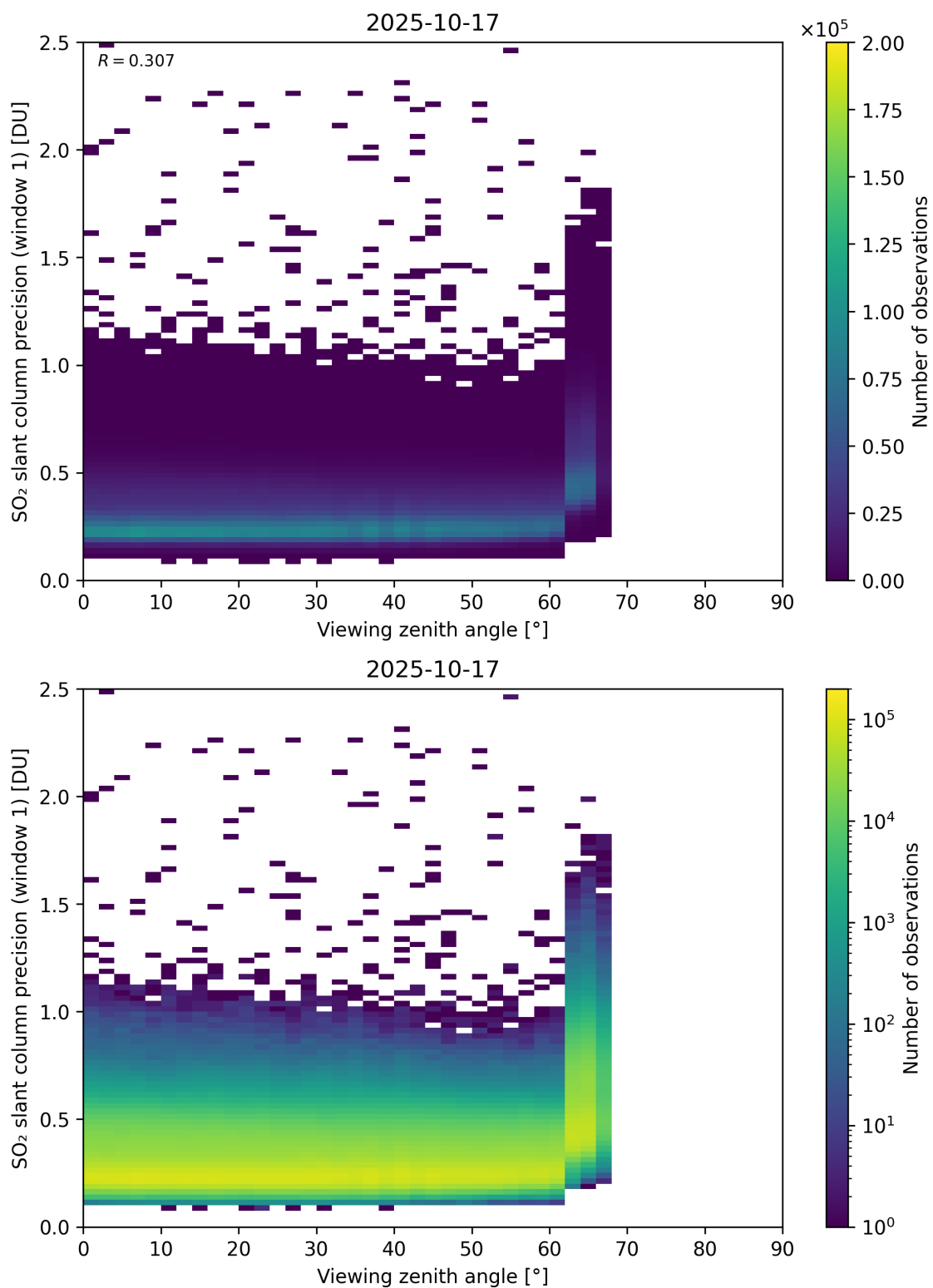
Figure 377: Scatter density plot of “Viewing zenith angle” against “SO 2 slant column precision (window 1)” for 2025-10-17 to 2025-10-18.
