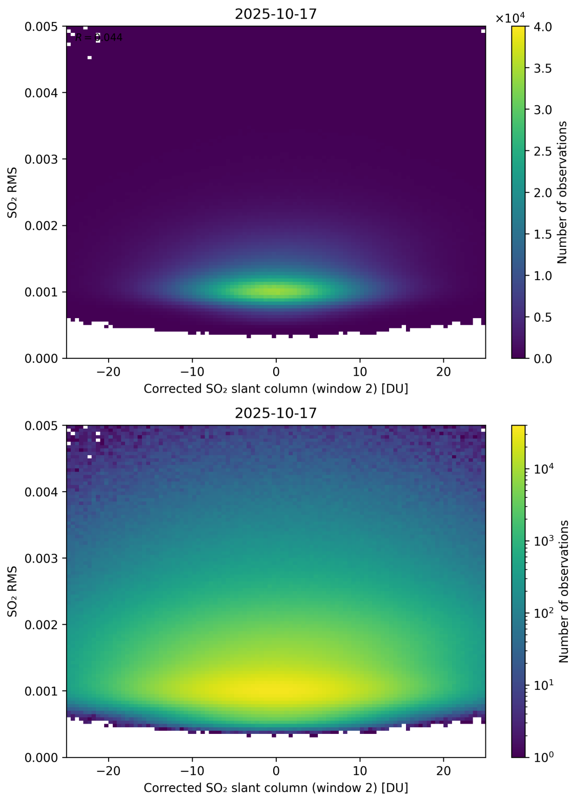
Figure 248: Scatter density plot of “Corrected SO 2 slant column (window 2)” against “SO 2 RMS” for 2025-10-17 to 2025-10-18.
