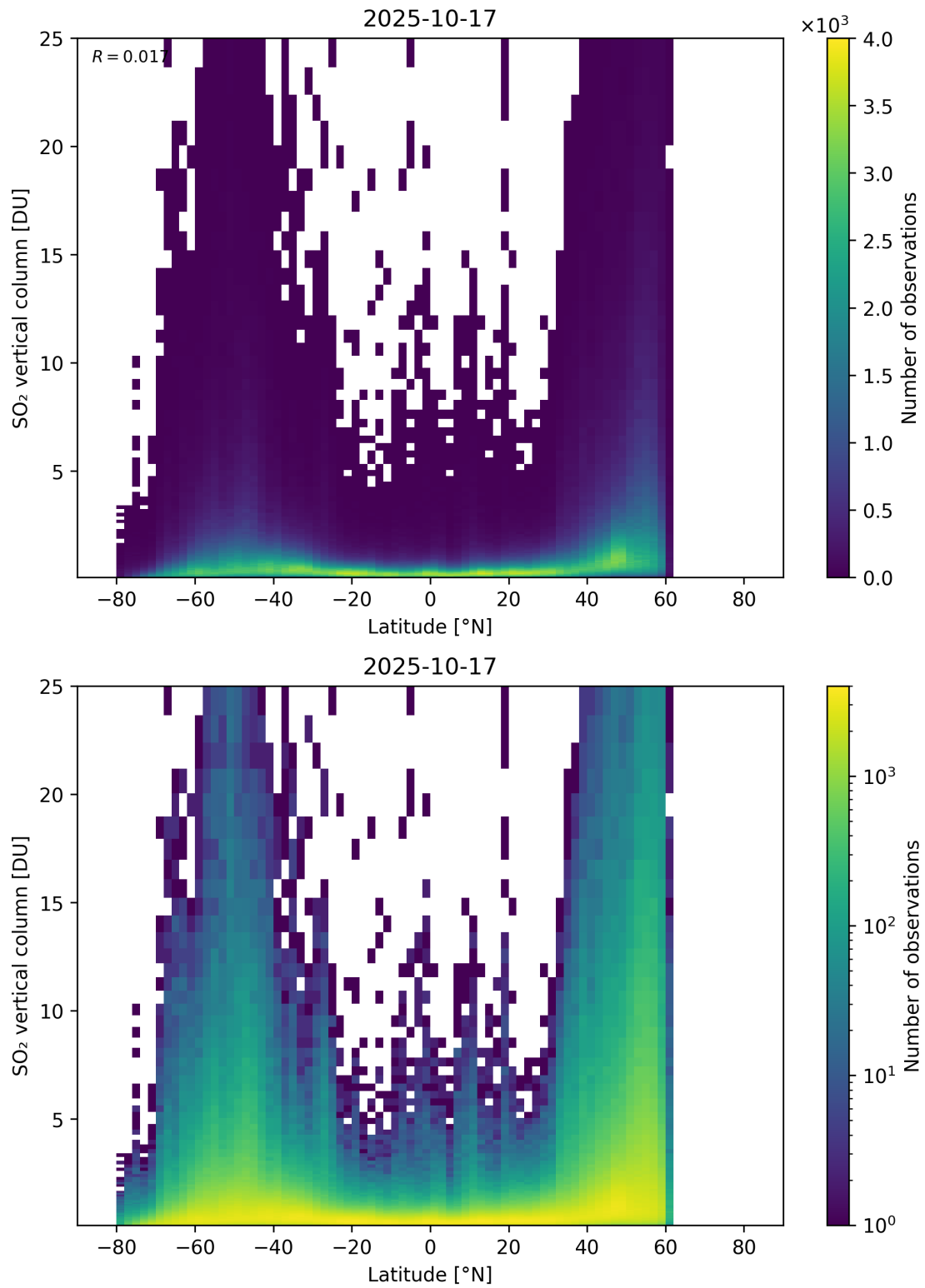
Figure 169: Scatter density plot of “Latitude” against “SO 2 vertical column” for 2025-10-17 to 2025-10-18.
