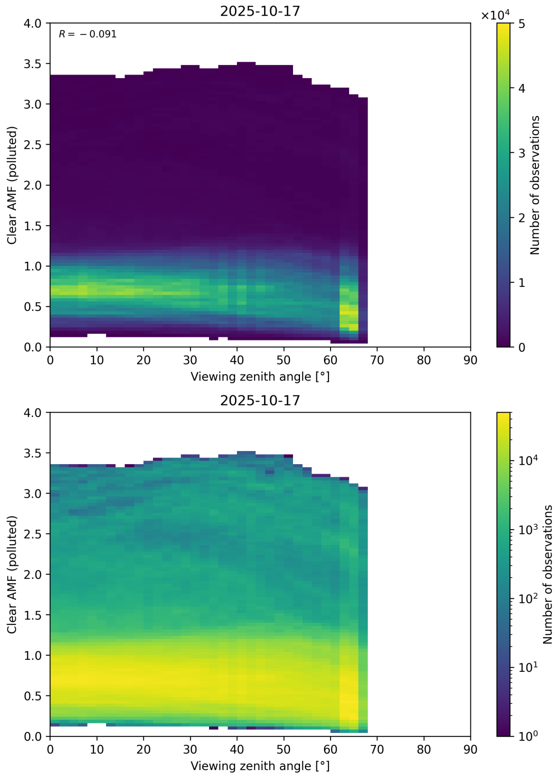
Figure 370: Scatter density plot of “Viewing zenith angle” against “Clear AMF (polluted)” for 2025-10-17 to 2025-10-18.
