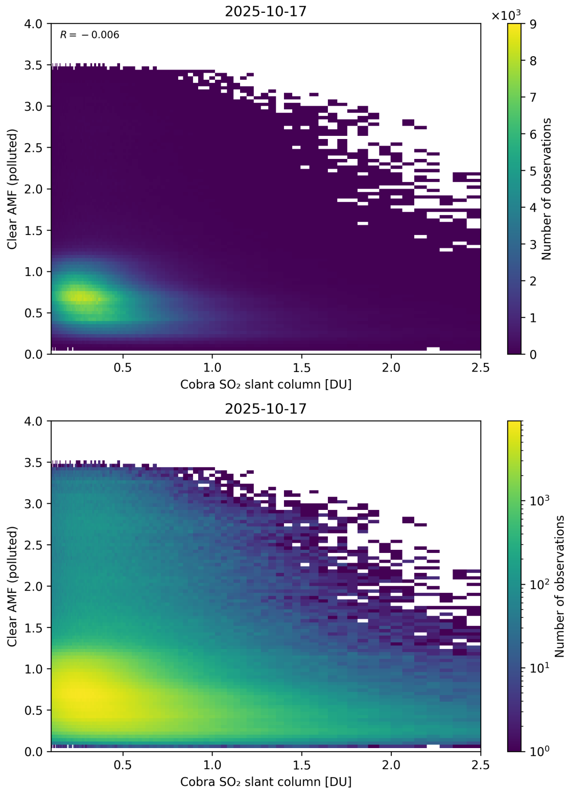
Figure 215: Scatter density plot of “Cobra SO 2 slant column” against “Clear AMF (polluted)” for 2025-10-17 to 2025-10-18.
