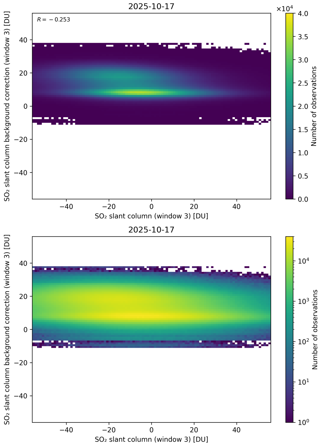
Figure 303: Scatter density plot of “SO 2 slant column (window 3)” against “SO 2 slant column background correction (window 3)” for 2025-10-17 to 2025-10-18.
