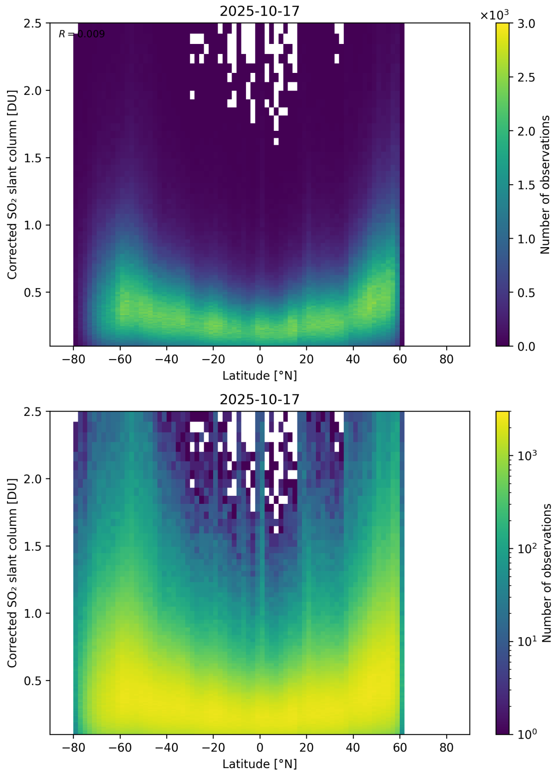
Figure 159: Scatter density plot of “Latitude” against “Corrected SO 2 slant column” for 2025-10-17 to 2025-10-18.
