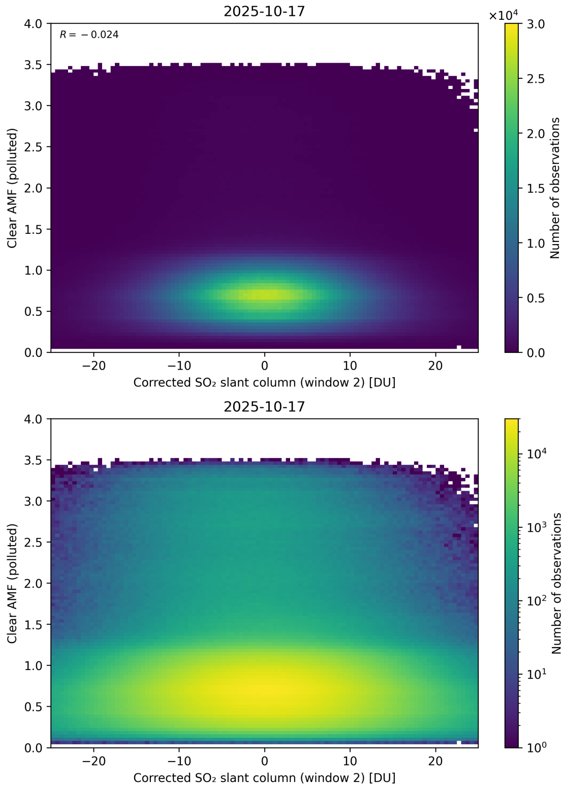
Figure 249: Scatter density plot of “Corrected SO 2 slant column (window 2)” against “Clear AMF (polluted)” for 2025-10-17 to 2025-10-18.
