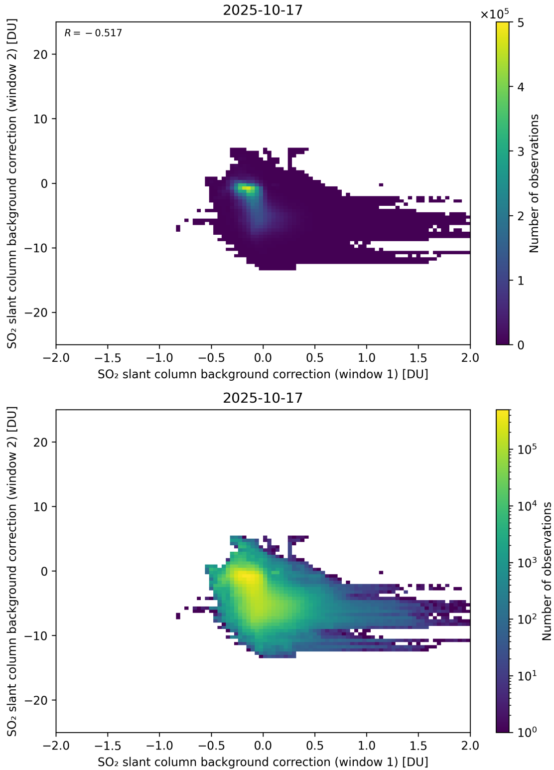
Figure 109: Scatter density plot of “SO 2 slant column background correction (window 1)” against “SO 2 slant column background correction (window 2)” for 2025-10-17 to 2025-10-18.
