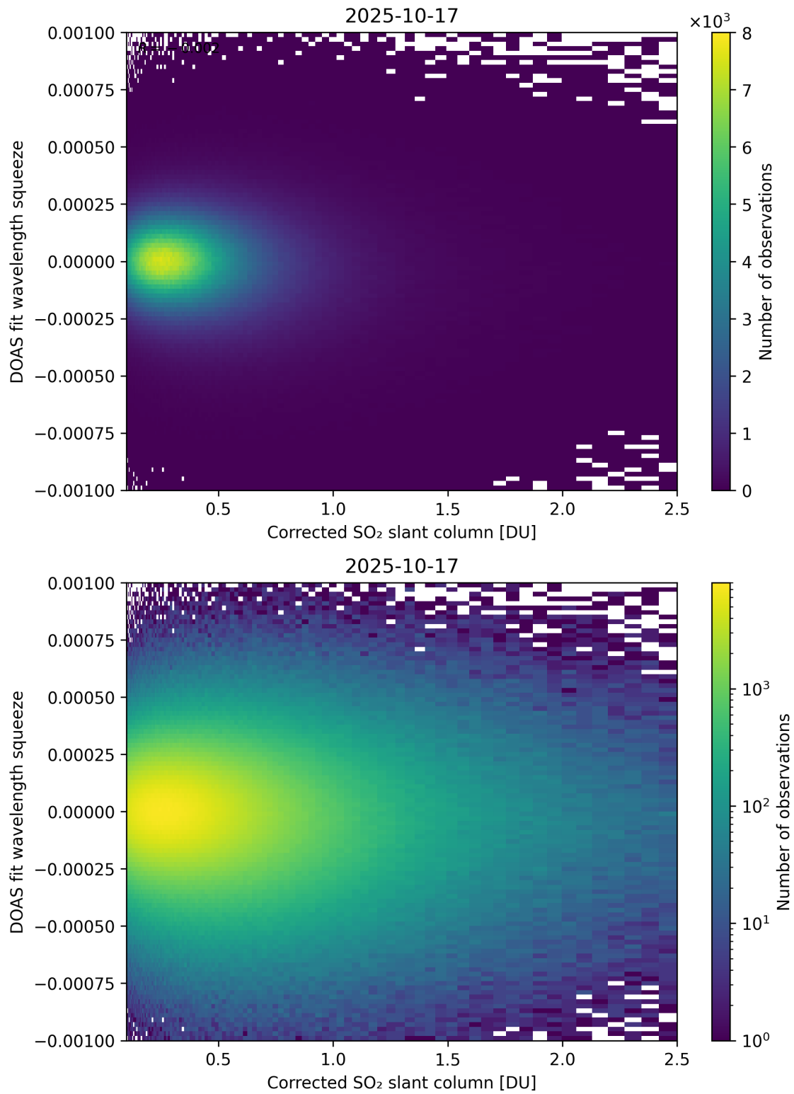
Figure 230: Scatter density plot of “Corrected SO 2 slant column” against “DOAS fit wavelength squeeze” for 2025-10-17 to 2025-10-18.
