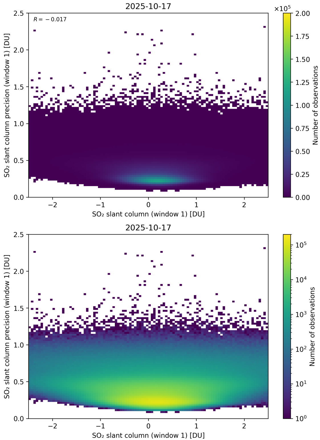
Figure 285: Scatter density plot of “SO 2 slant column (window 1)” against “SO 2 slant column precision (window 1)” for 2025-10-17 to 2025-10-18.
