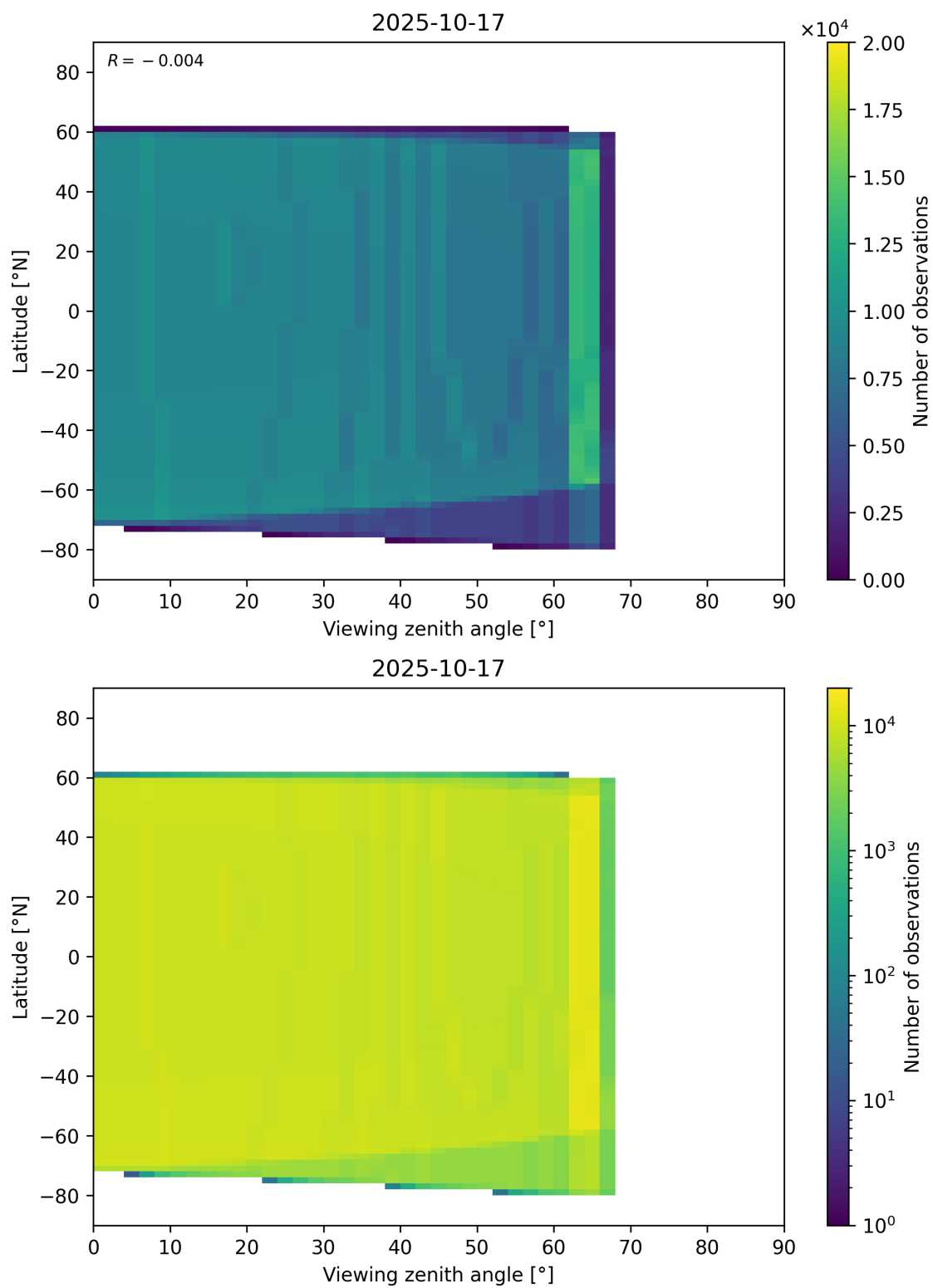
Figure 368: Scatter density plot of “Viewing zenith angle” against “Latitude” for 2025-10-17 to 2025-10-18.
