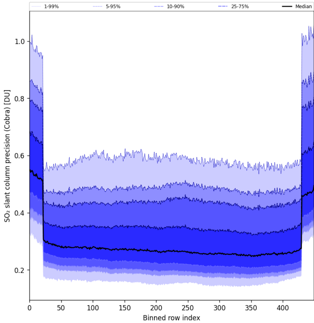
Figure 88: Along track statistics of “SO 2 slant column precision (Cobra)” for 2025-10-17 to 2025-10-18
