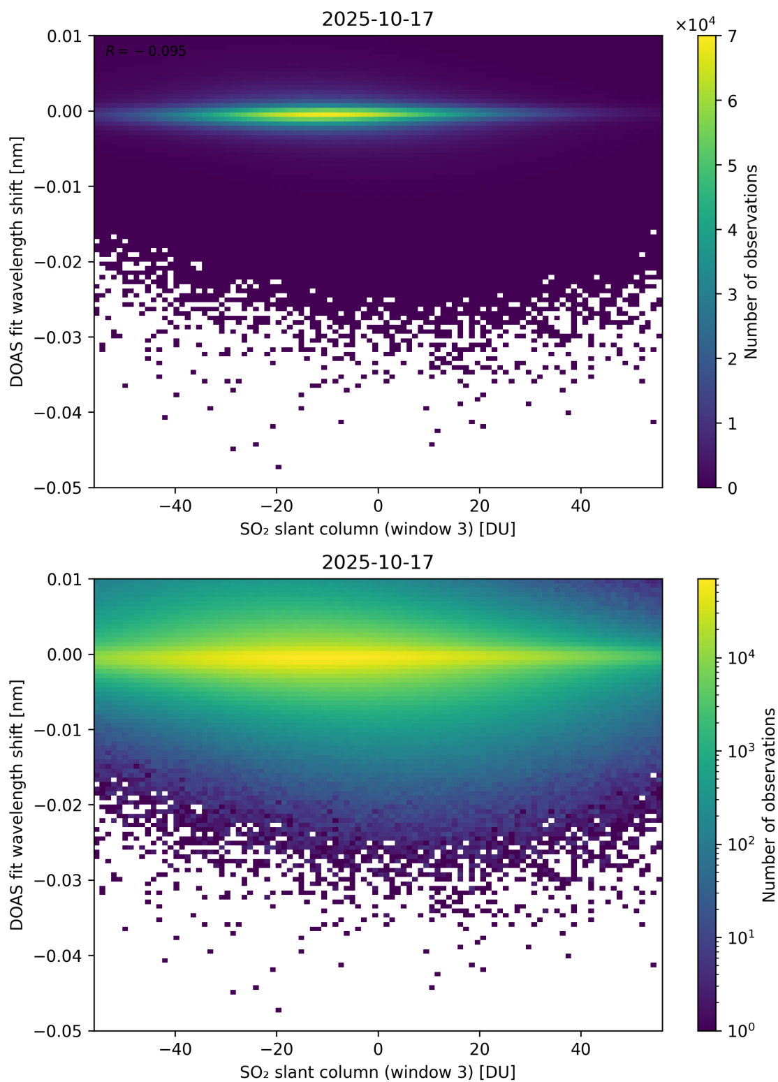
Figure 304: Scatter density plot of “SO 2 slant column (window 3)” against “DOAS fit wavelength shift” for 2025-10-17 to 2025-10-18.
