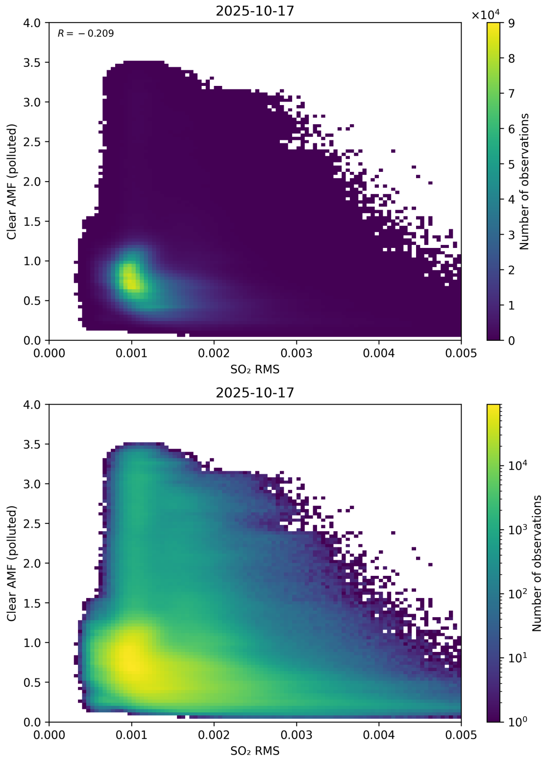
Figure 147: Scatter density plot of “SO 2 RMS” against “Clear AMF (polluted)” for 2025-10-17 to 2025-10-18.
