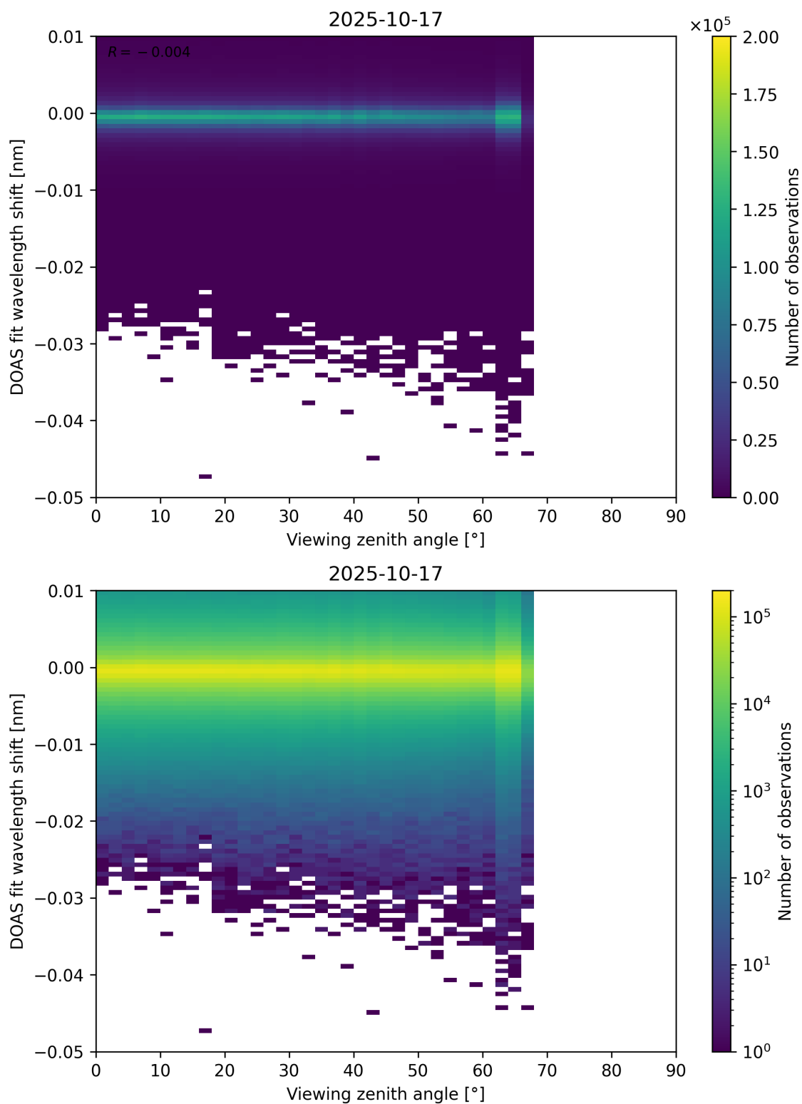
Figure 365: Scatter density plot of “Viewing zenith angle” against “DOAS fit wavelength shift” for 2025-10-17 to 2025-10-18.
