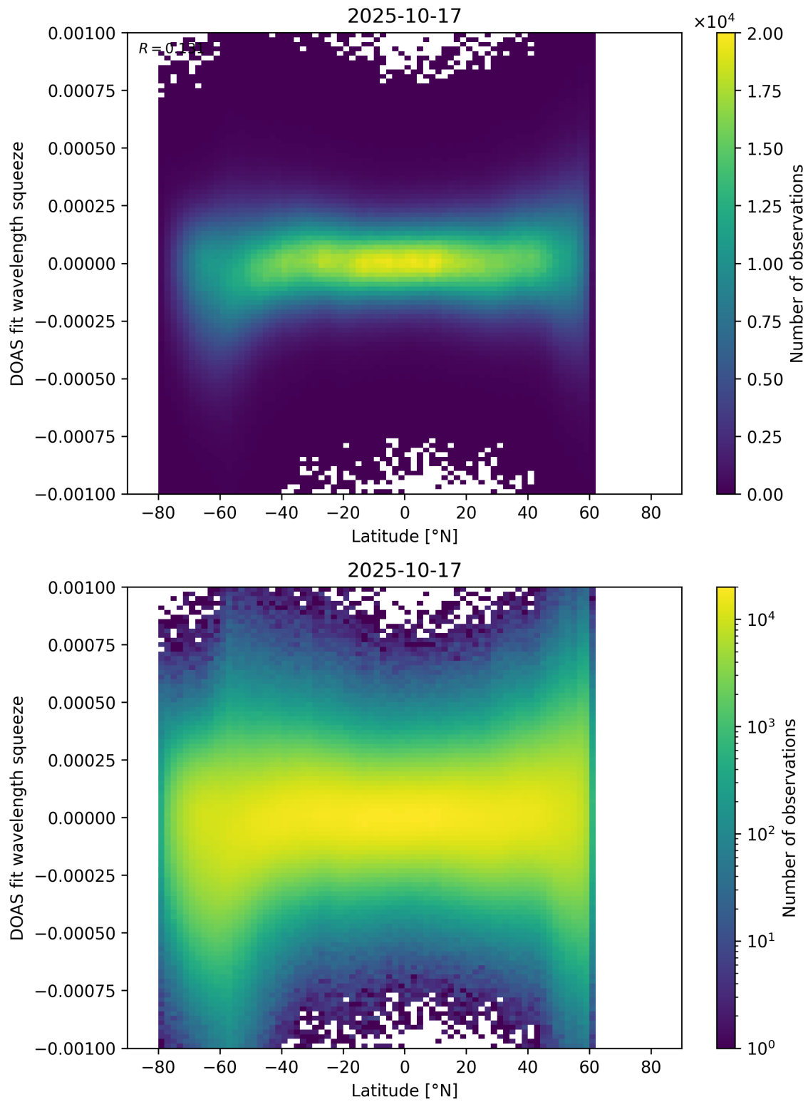
Figure 154: Scatter density plot of “Latitude” against “DOAS fit wavelength squeeze” for 2025-10-17 to 2025-10-18.
