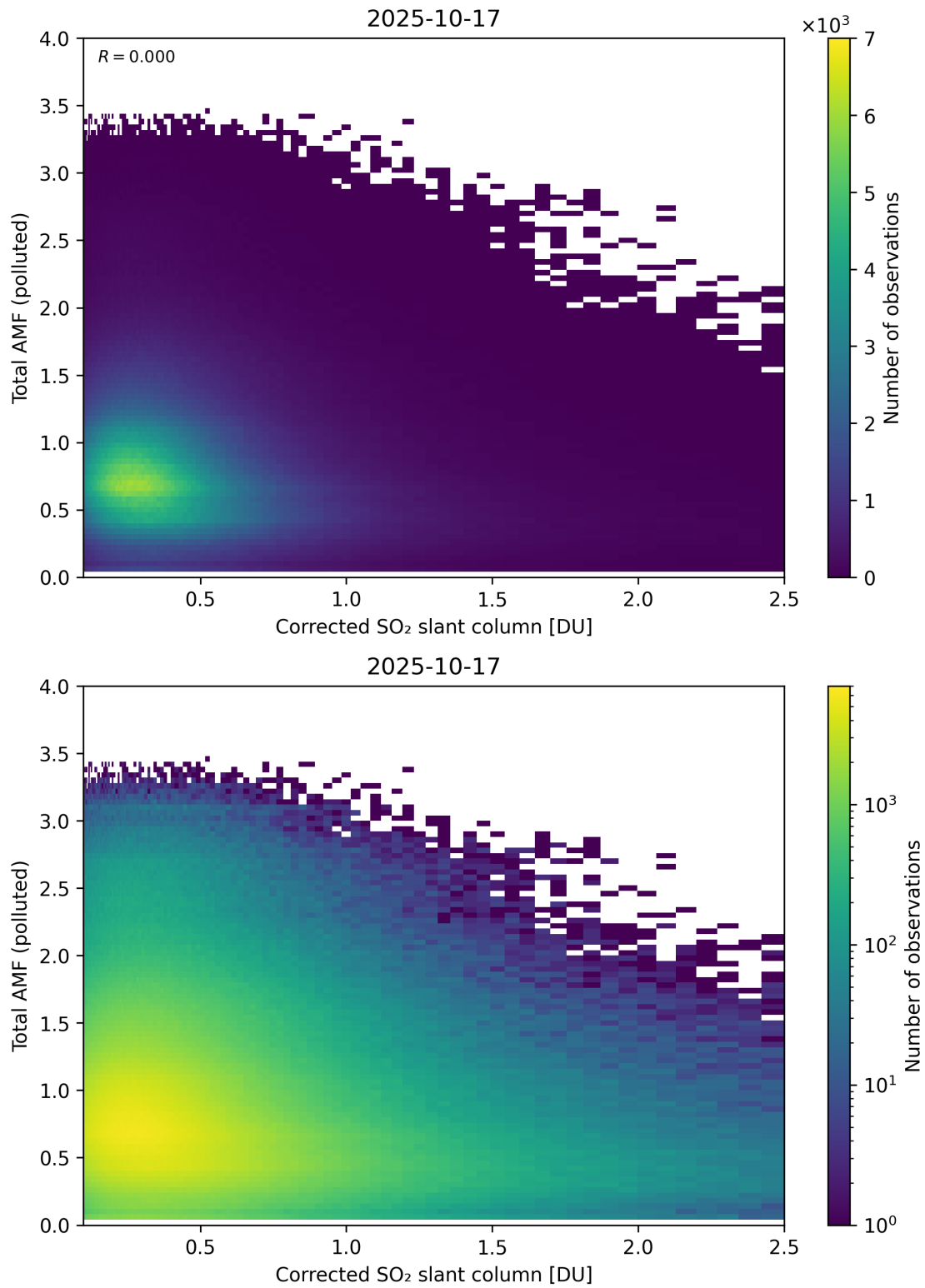
Figure 242: Scatter density plot of “Corrected SO 2 slant column” against “Total AMF (polluted)” for 2025-10-17 to 2025-10-18.
