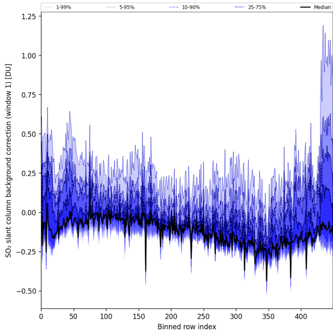
Figure 92: Along track statistics of “SO 2 slant column background correction (window 1)” for 2025-10-17 to 2025-10-18
