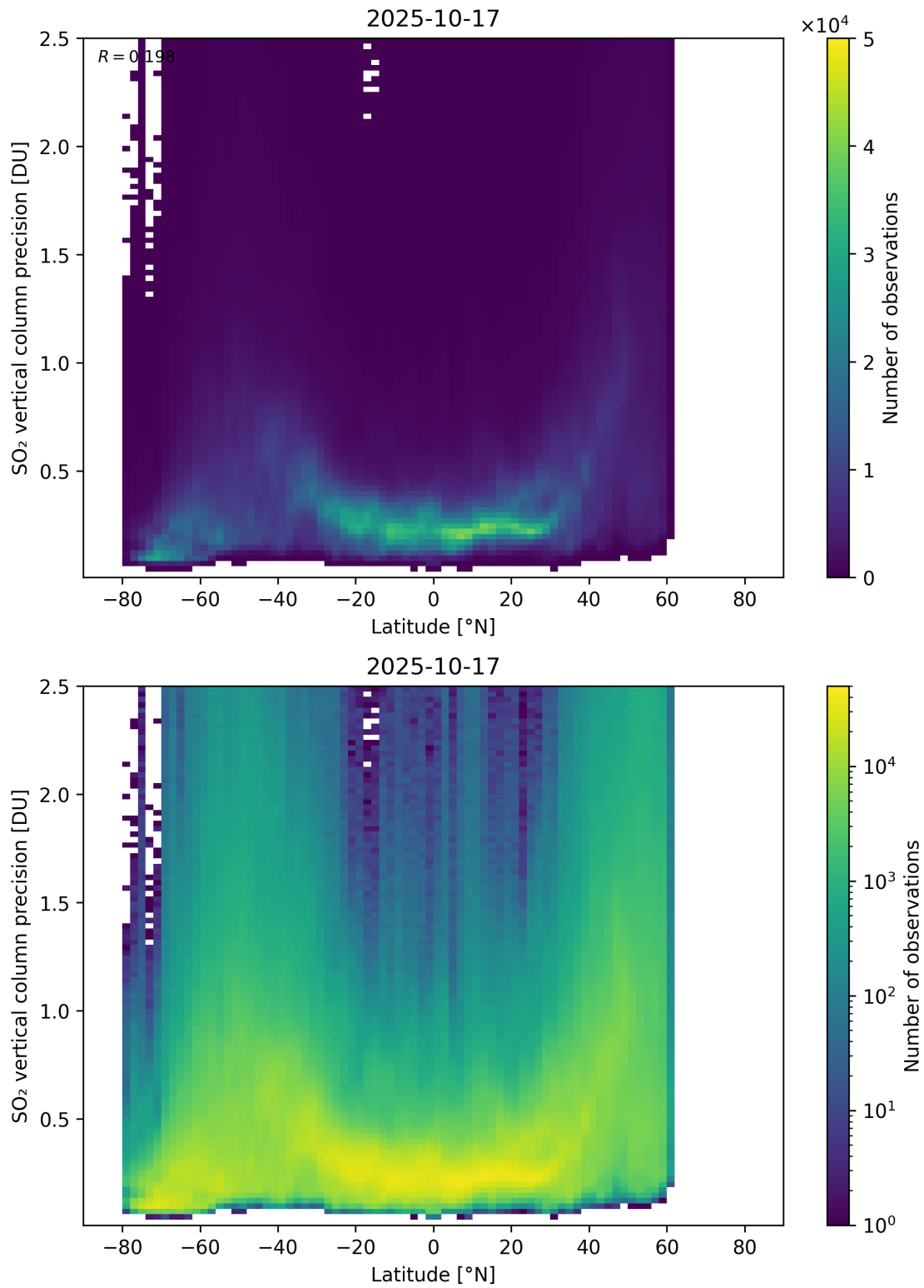
Figure 170: Scatter density plot of “Latitude” against “SO 2 vertical column precision” for 2025-10-17 to 2025-10-18.
