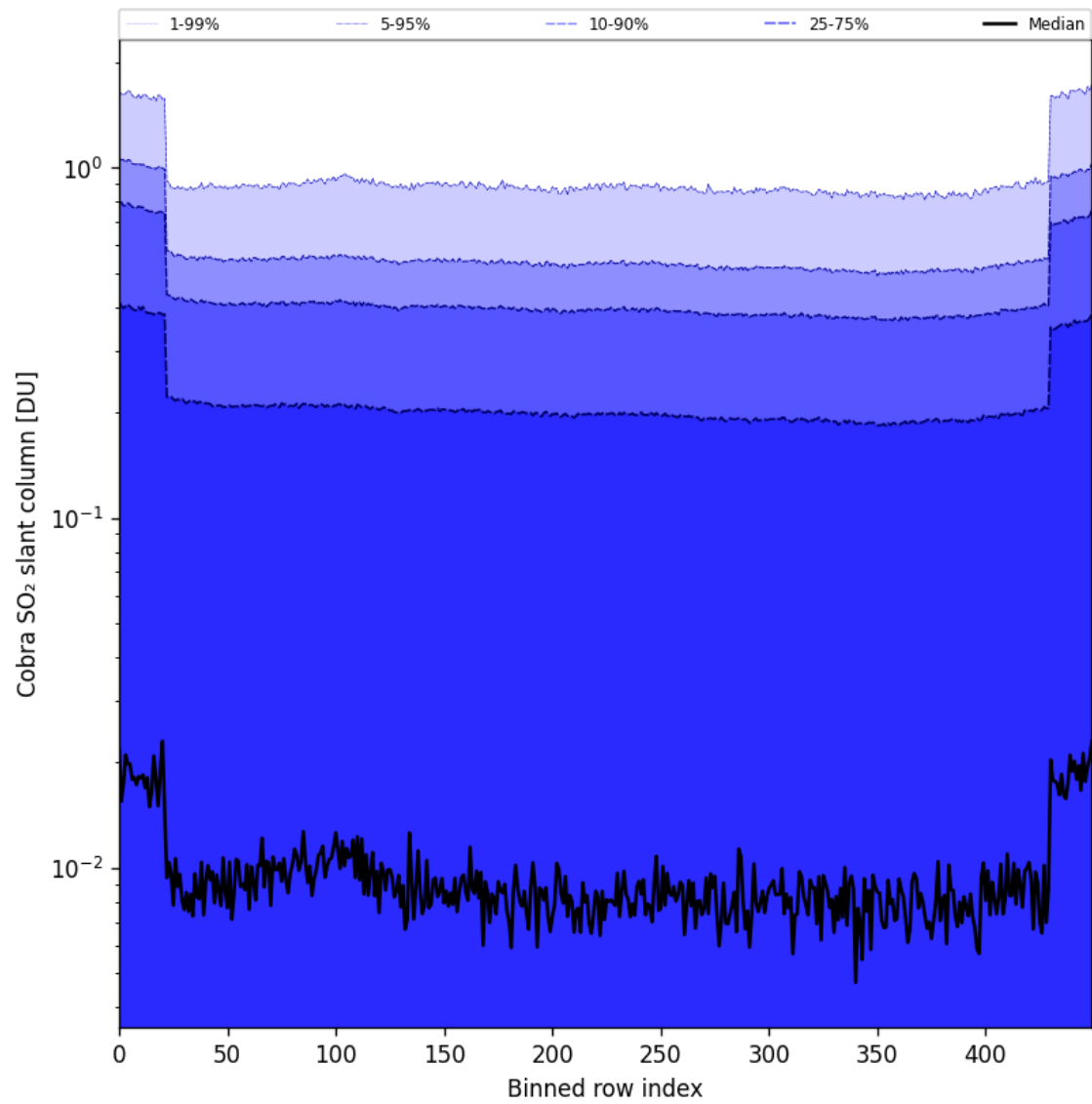
Figure 87: Along track statistics of “Cobra SO 2 slant column” for 2025-10-17 to 2025-10-18
