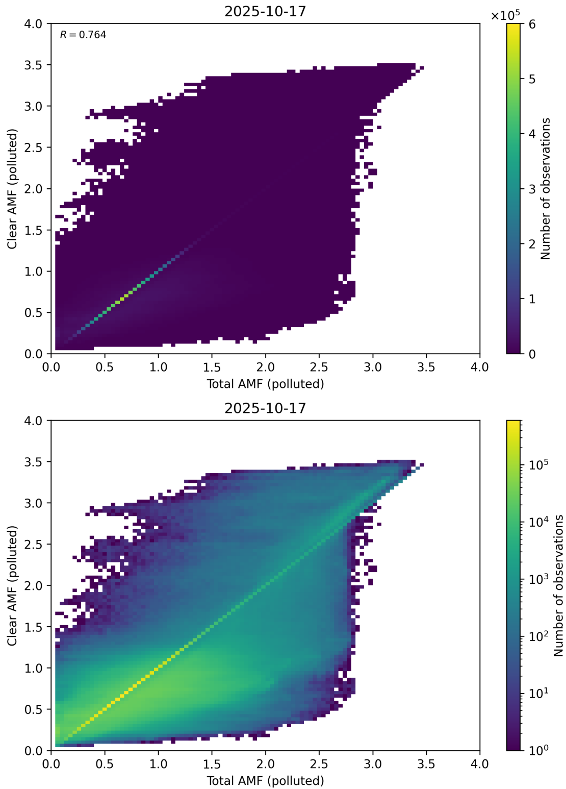
Figure 321: Scatter density plot of “Total AMF (polluted)” against “Clear AMF (polluted)” for 2025-10-17 to 2025-10-18.
