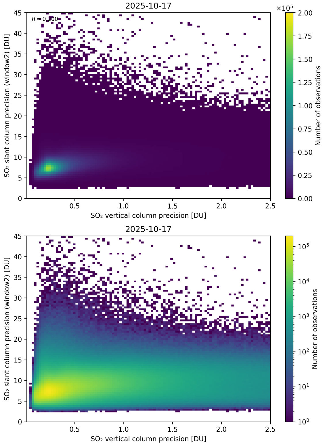
Figure 343: Scatter density plot of “SO 2 vertical column precision” against “SO 2 slant column precision (window2)” for 2025-10-17 to 2025-10-18.
