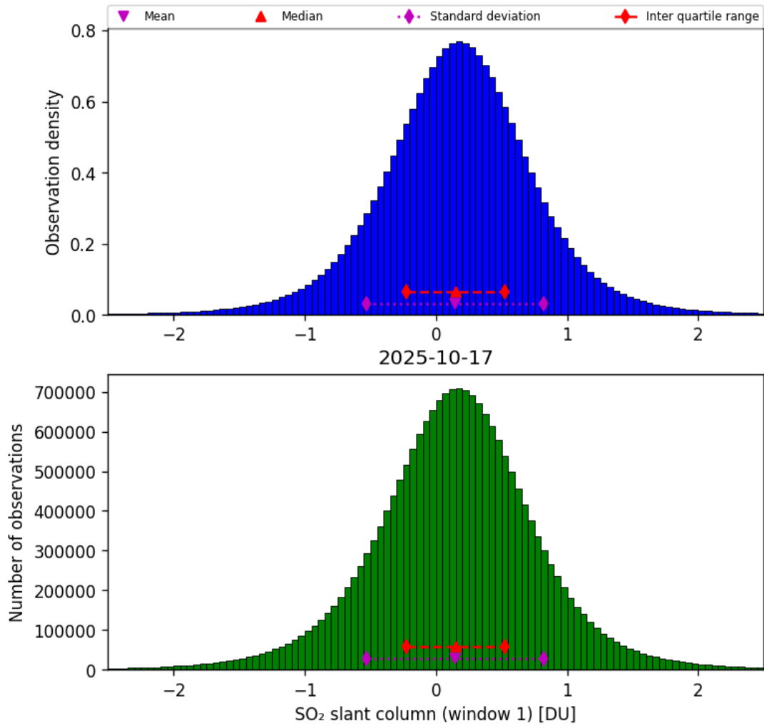
Figure 63: Histogram of “SO 2 slant column (window 1)” for 2025-10-17 to 2025-10-18
