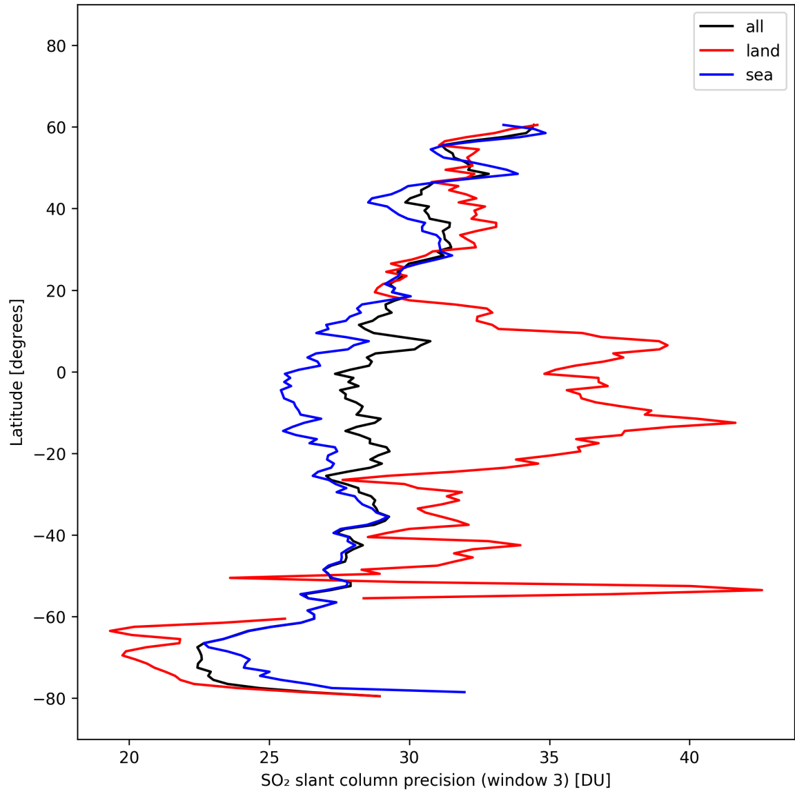
Figure 46: Zonal average of “SO 2 slant column precision (window 3)” for 2025-10-17 to 2025-10-18.
