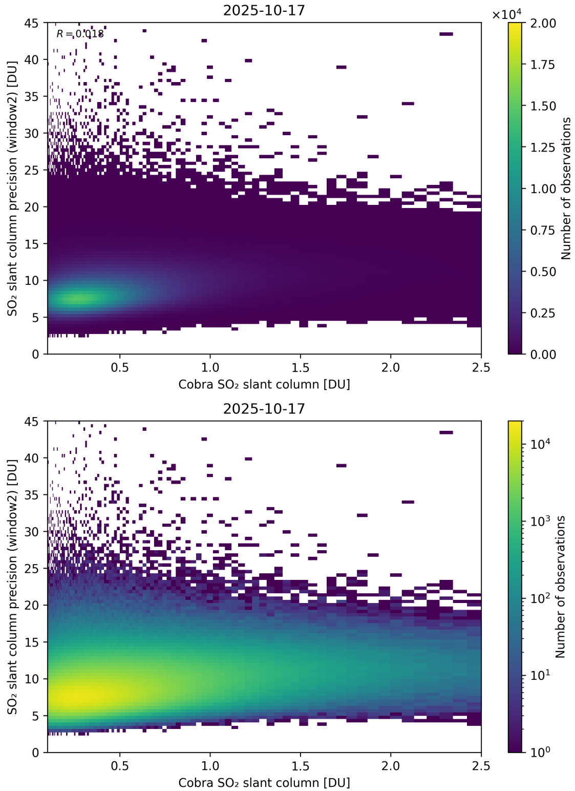
Figure 221: Scatter density plot of “Cobra SO 2 slant column” against “SO 2 slant column precision (window2)” for 2025-10-17 to 2025-10-18.
