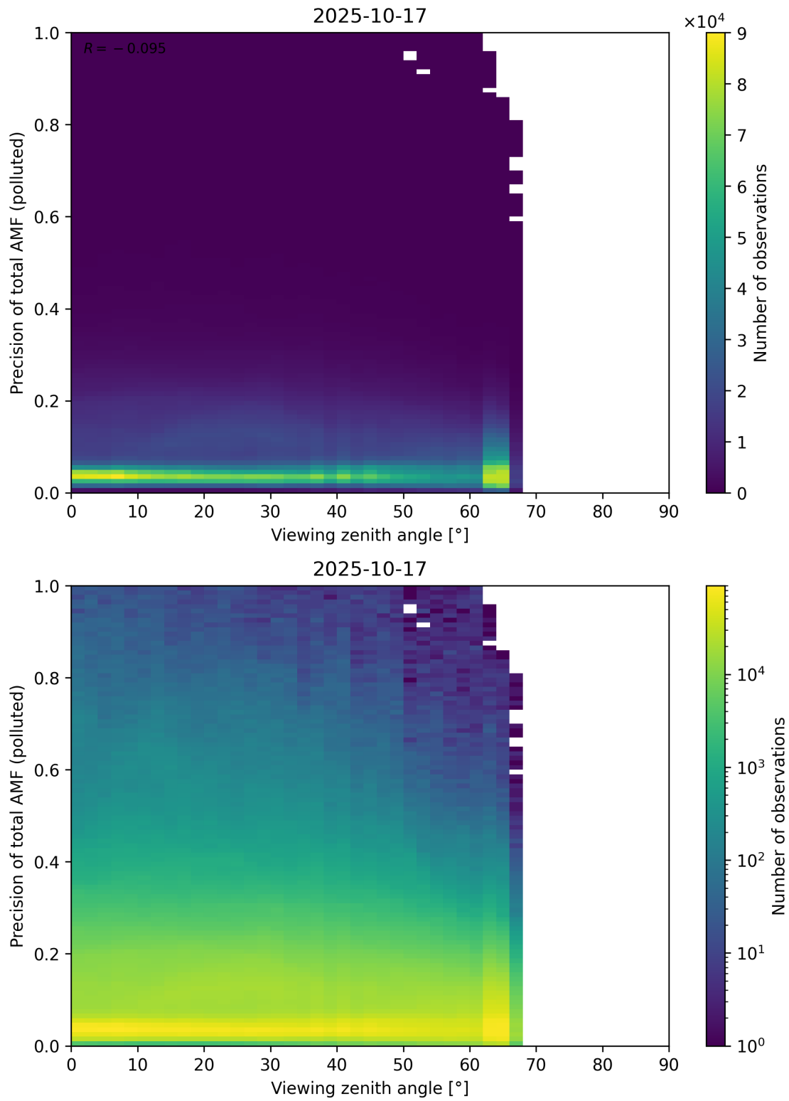
Figure 382: Scatter density plot of “Viewing zenith angle” against “Precision of total AMF (polluted)” for 2025-10-17 to 2025-10-18.
