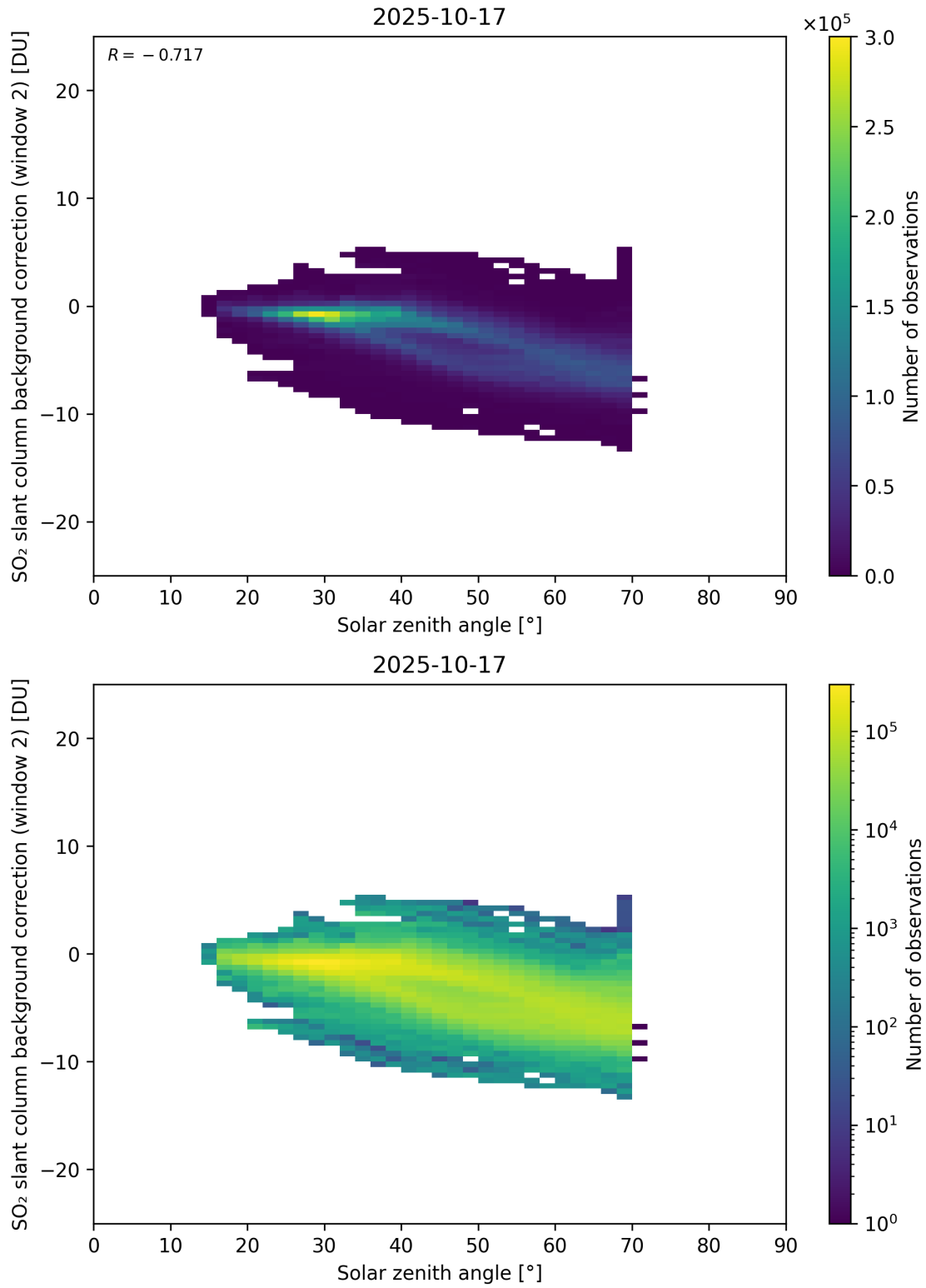
Figure 172: Scatter density plot of “Solar zenith angle” against “SO 2 slant column background correction (window 2)” for 2025-10-17 to 2025-10-18.
