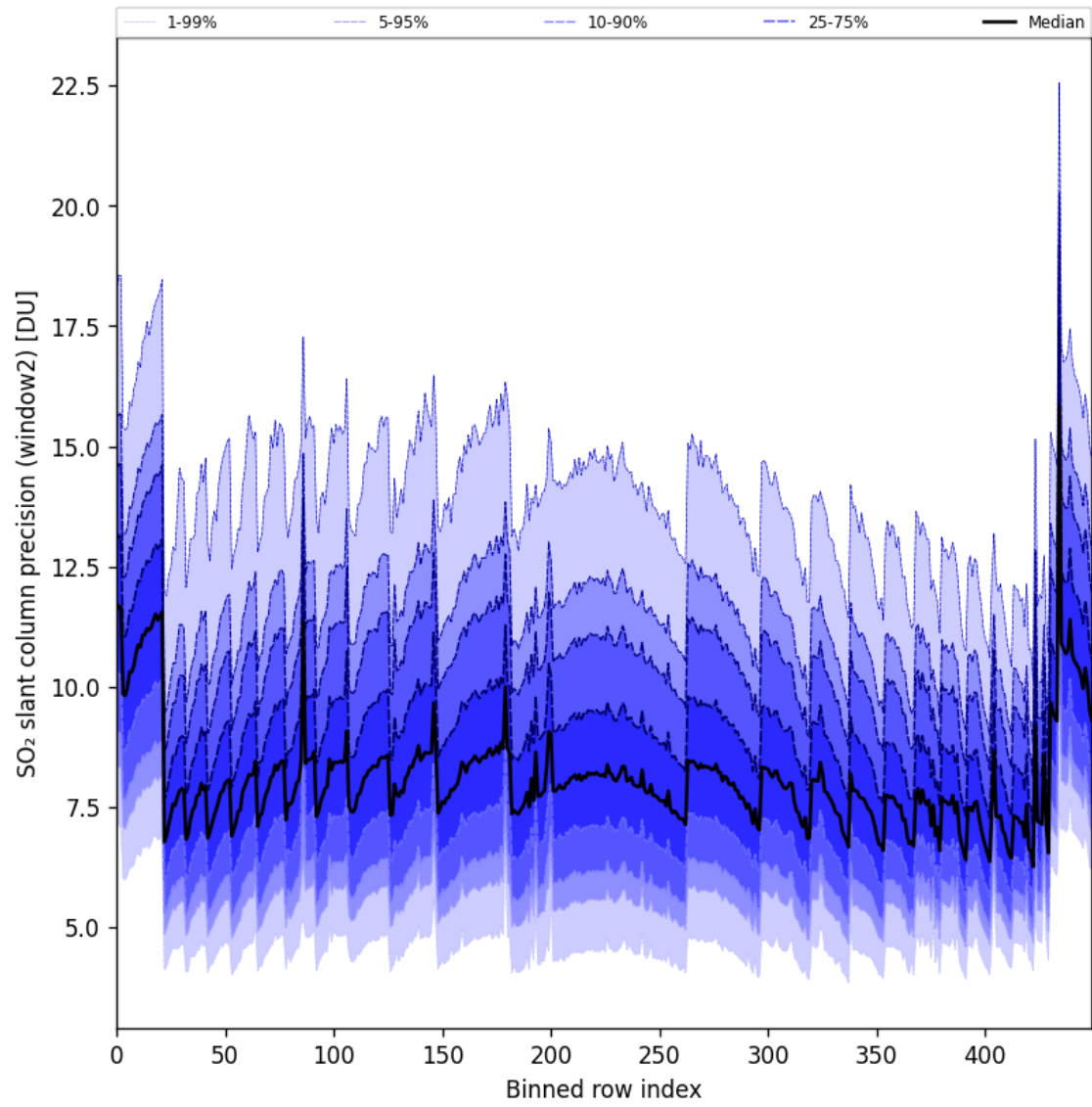
Figure 94: Along track statistics of “SO 2 slant column precision (window2)” for 2025-10-17 to 2025-10-18
