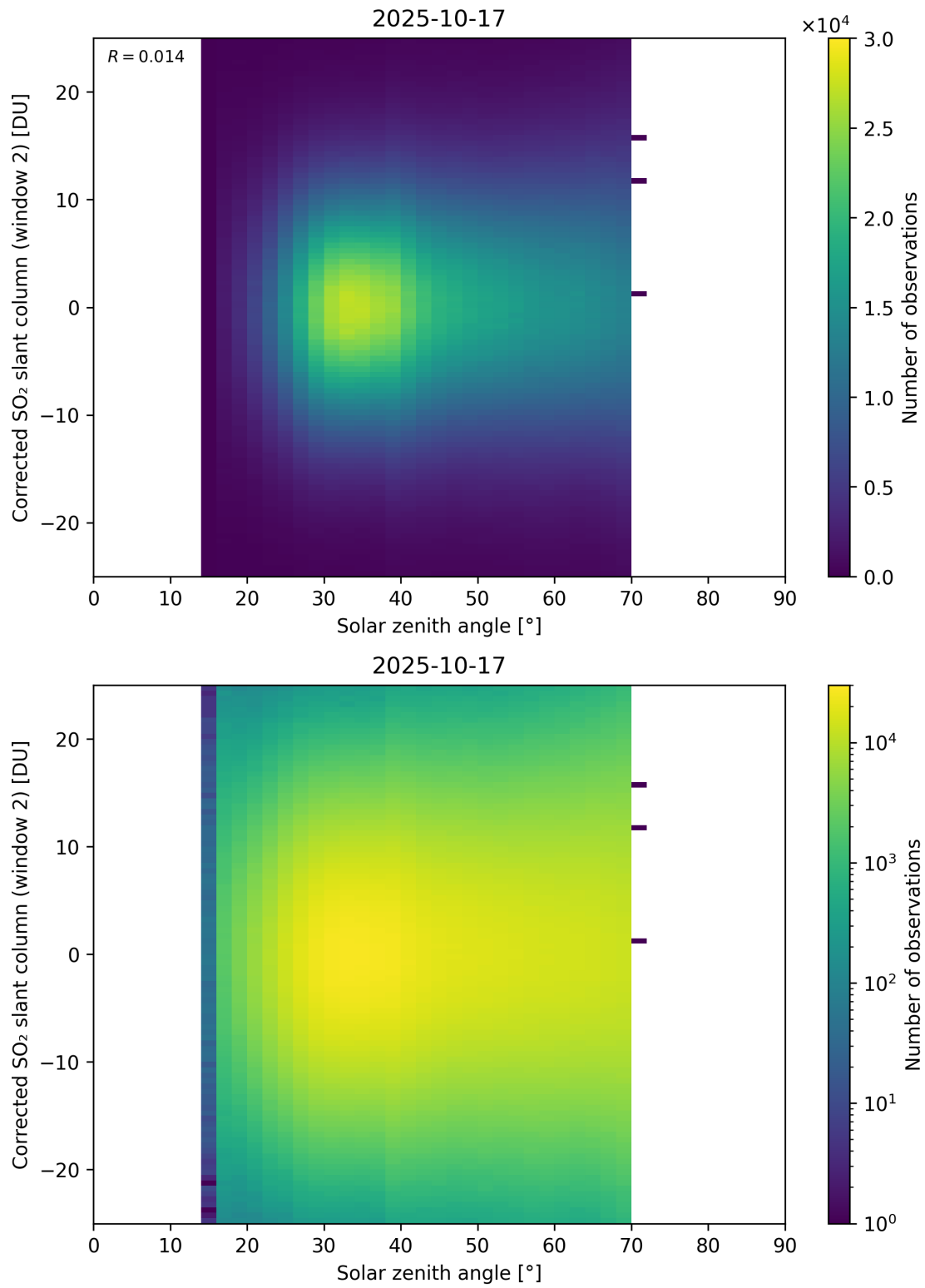
Figure 182: Scatter density plot of “Solar zenith angle” against “Corrected SO 2 slant column (window 2)” for 2025-10-17 to 2025-10-18.
