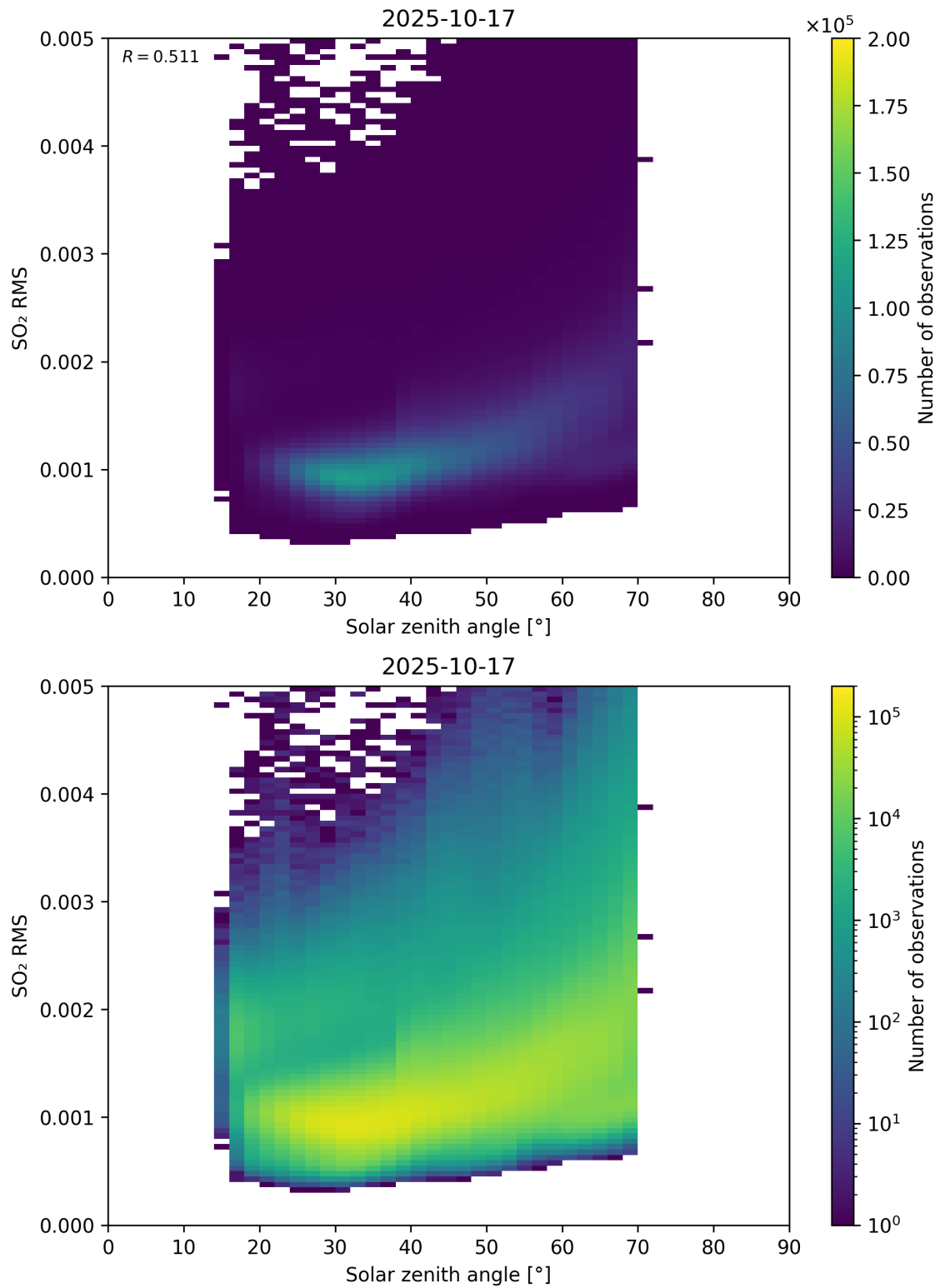
Figure 176: Scatter density plot of “Solar zenith angle” against “SO 2 RMS” for 2025-10-17 to 2025-10-18.
