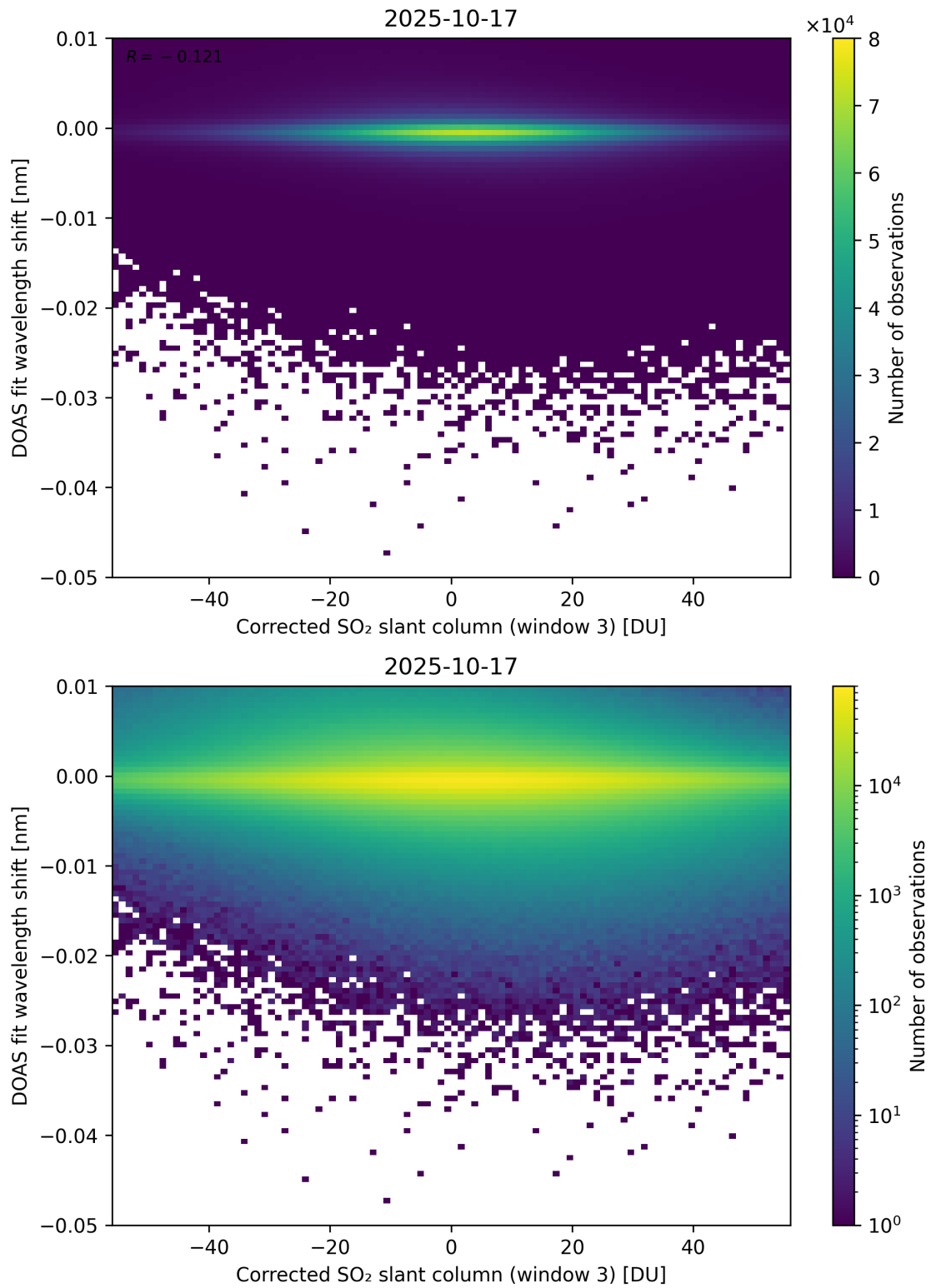
Figure 256: Scatter density plot of “Corrected SO 2 slant column (window 3)” against “DOAS fit wavelength shift” for 2025-10-17 to 2025-10-18.
