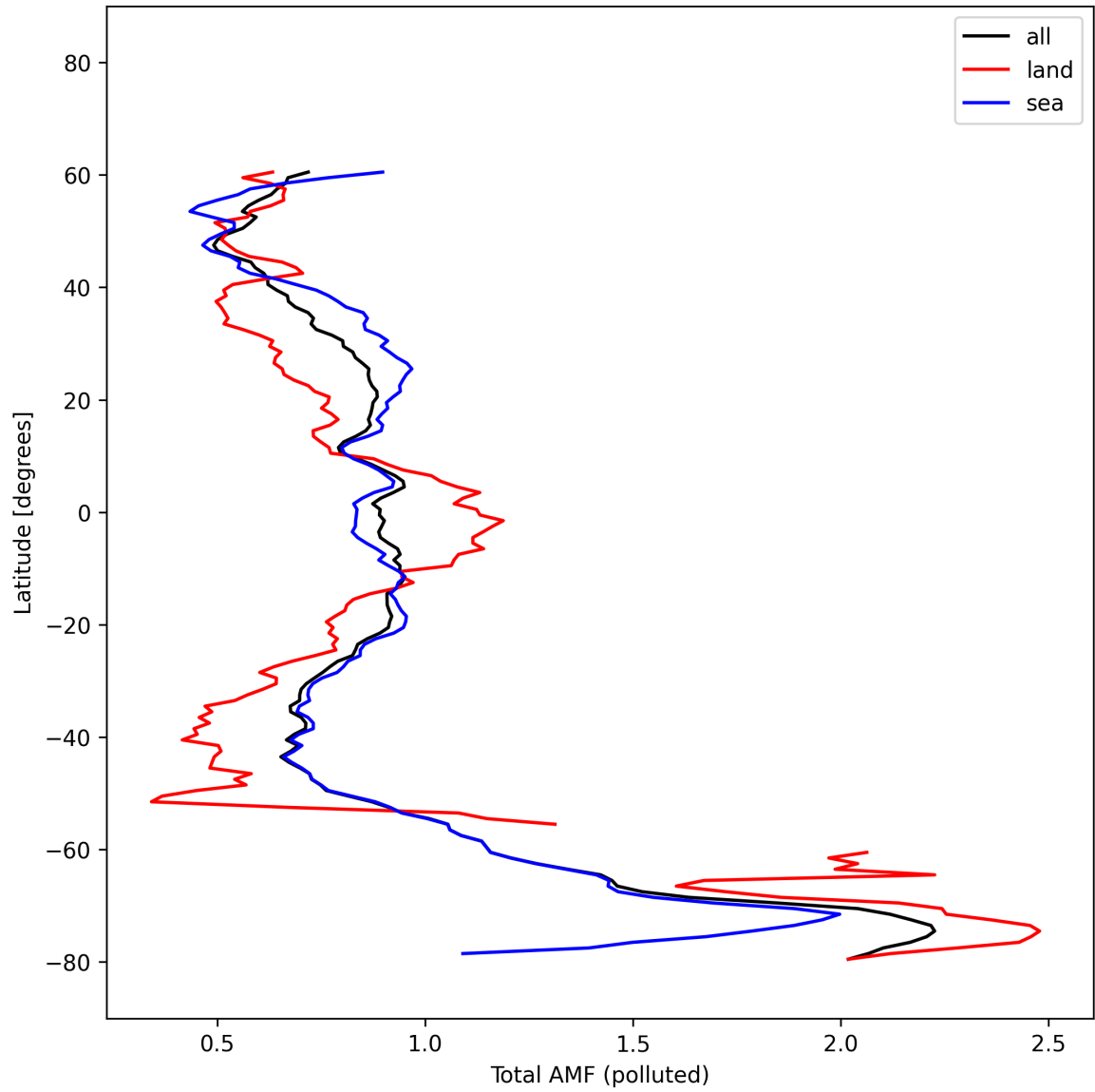
Figure 53: Zonal average of “Total AMF (polluted)” for 2025-10-17 to 2025-10-18.
