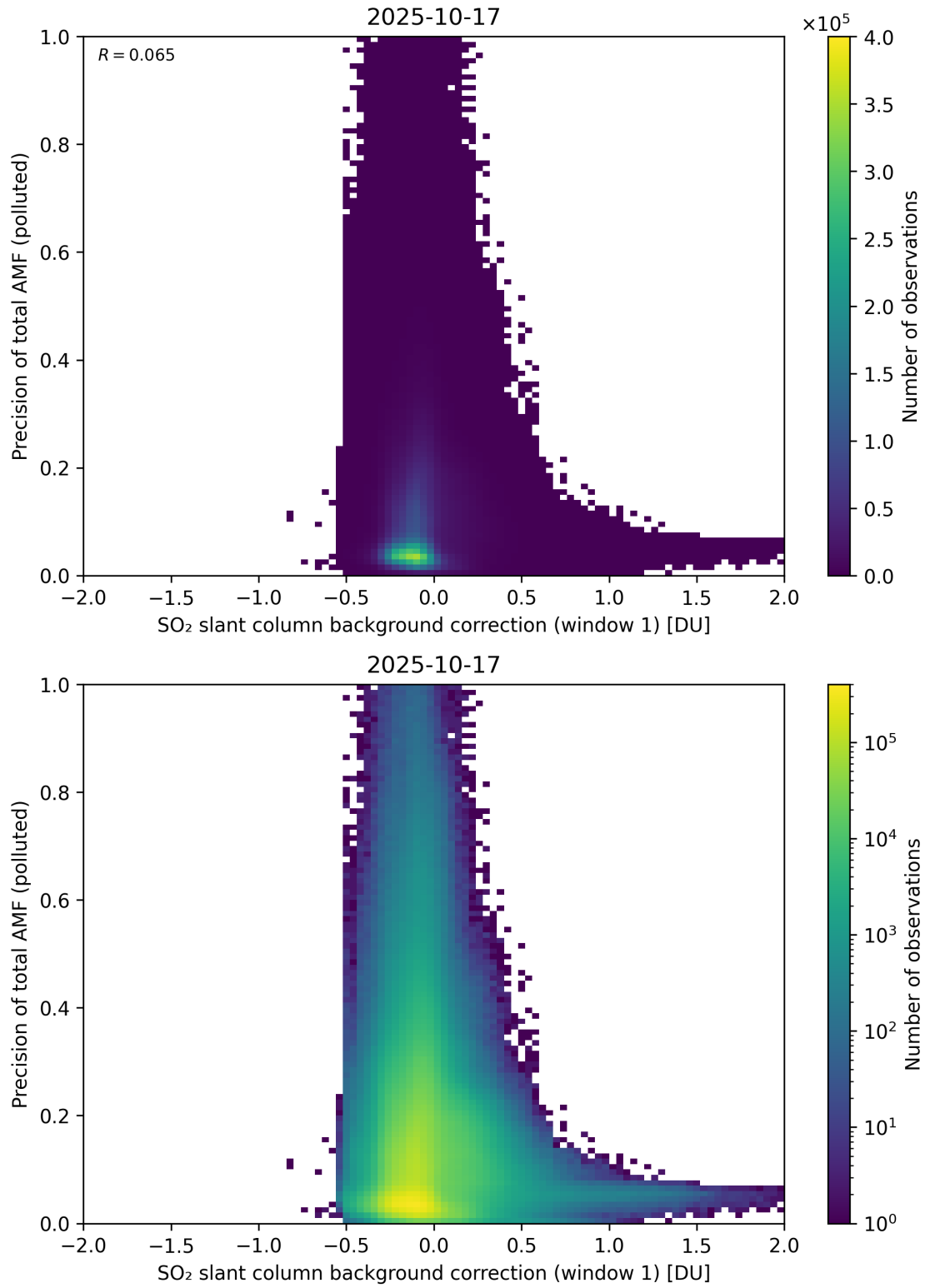
Figure 121: Scatter density plot of “SO 2 slant column background correction (window 1)” against “Precision of total AMF (polluted)” for 2025-10-17 to 2025-10-18.
