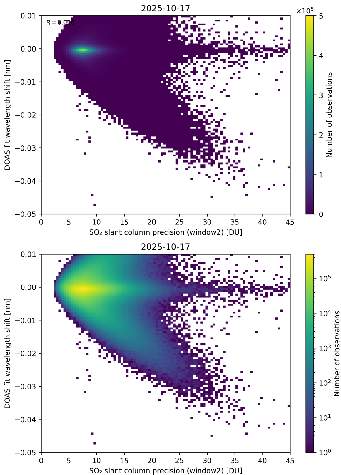
Figure 293: Scatter density plot of “SO 2 slant column precision (window2)” against “DOAS fit wavelength shift” for 2025-10-17 to 2025-10-18.
