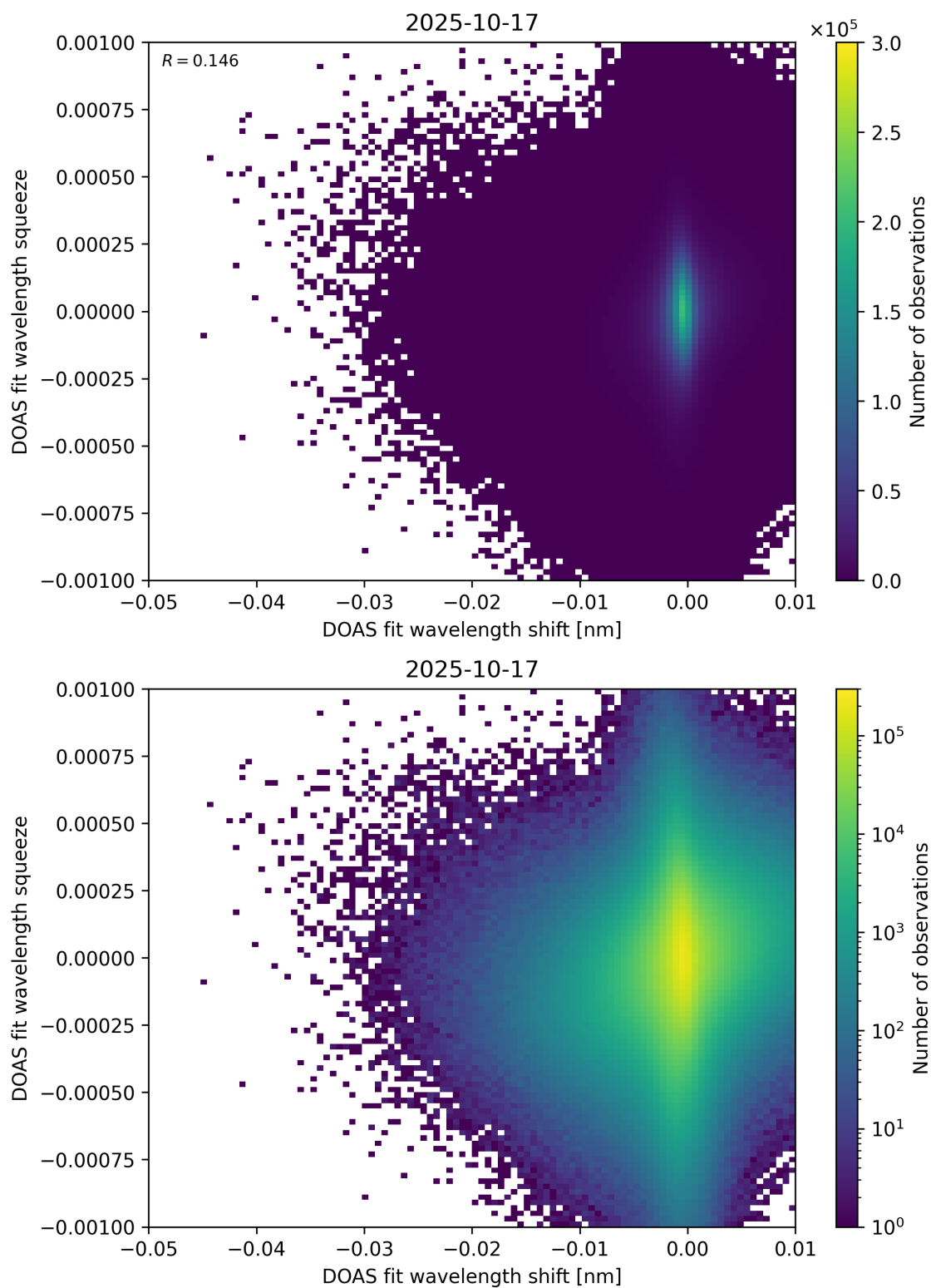
Figure 138: Scatter density plot of “DOAS fit wavelength shift” against “DOAS fit wavelength squeeze” for 2025-10-17 to 2025-10-18.
