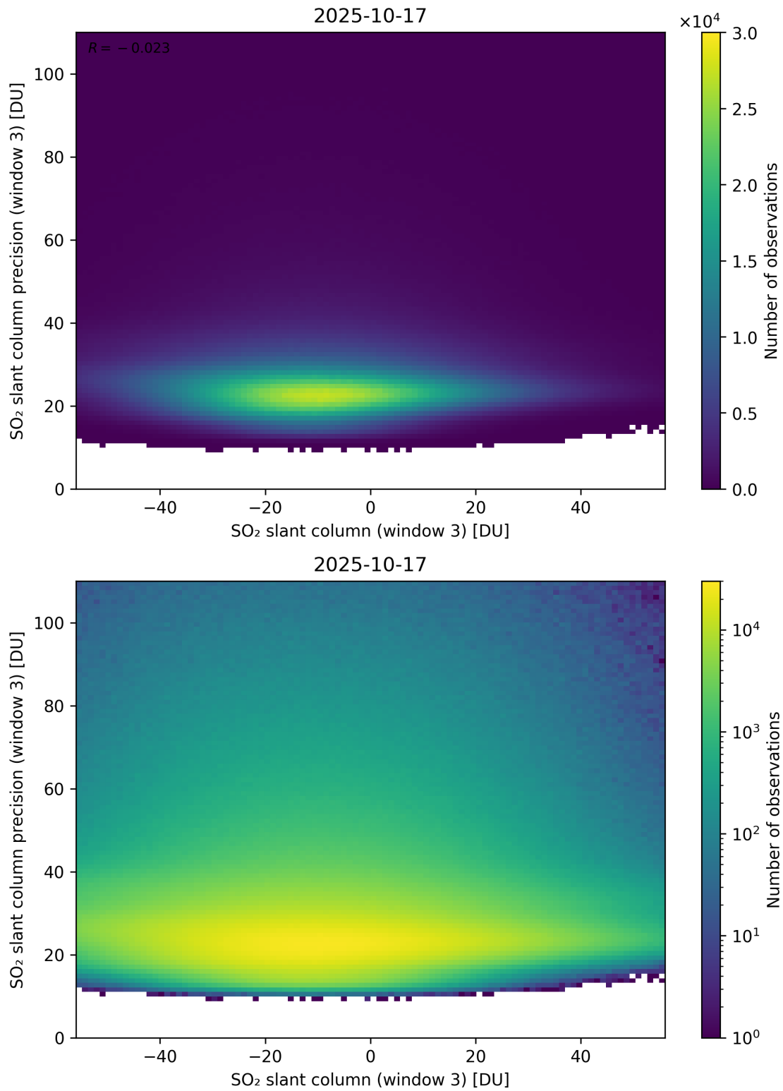
Figure 317: Scatter density plot of “SO 2 slant column (window 3)” against “SO 2 slant column precision (window 3)” for 2025-10-17 to 2025-10-18.
