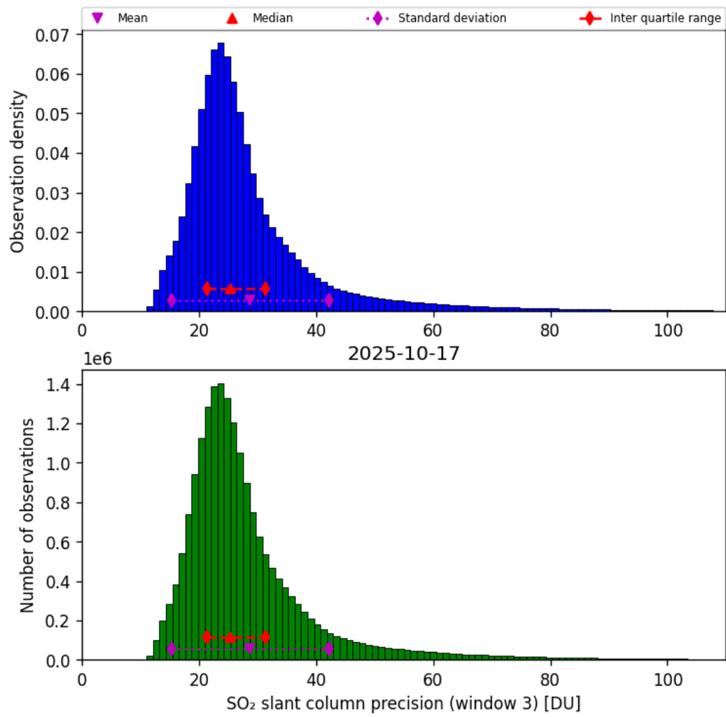
Figure 72: Histogram of “SO 2 slant column precision (window 3)” for 2025-10-17 to 2025-10-18
