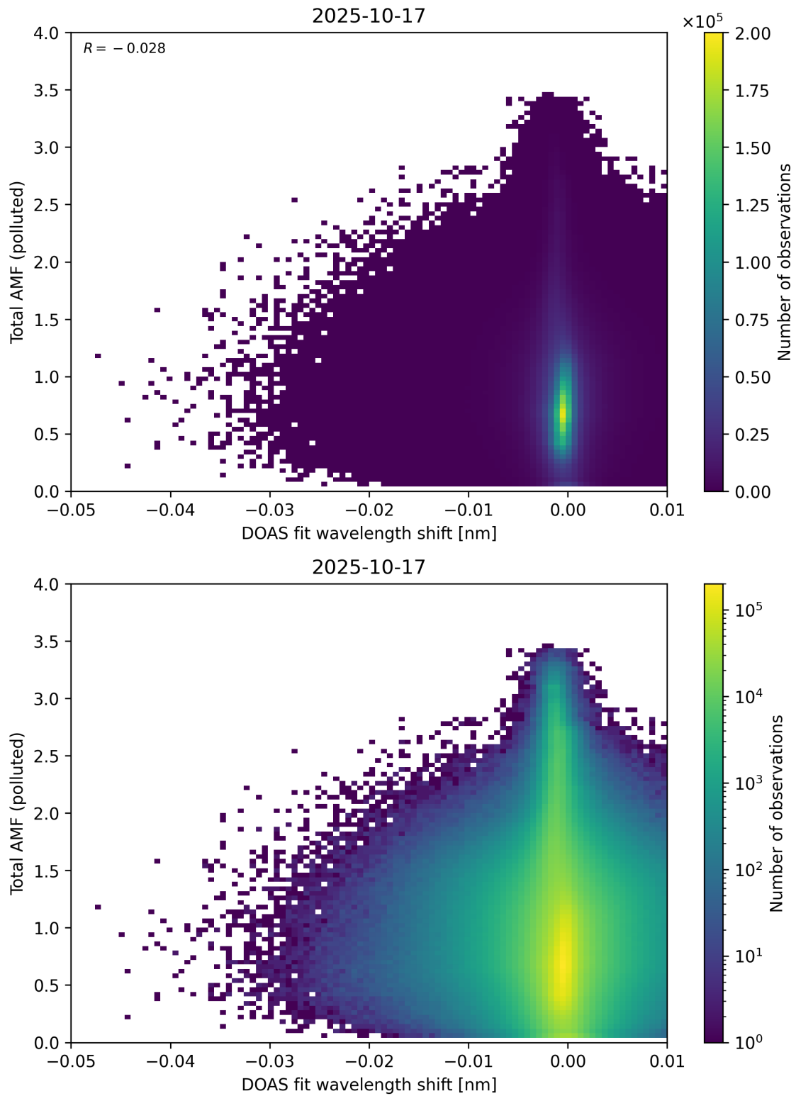
Figure 141: Scatter density plot of “DOAS fit wavelength shift” against “Total AMF (polluted)” for 2025-10-17 to 2025-10-18.
