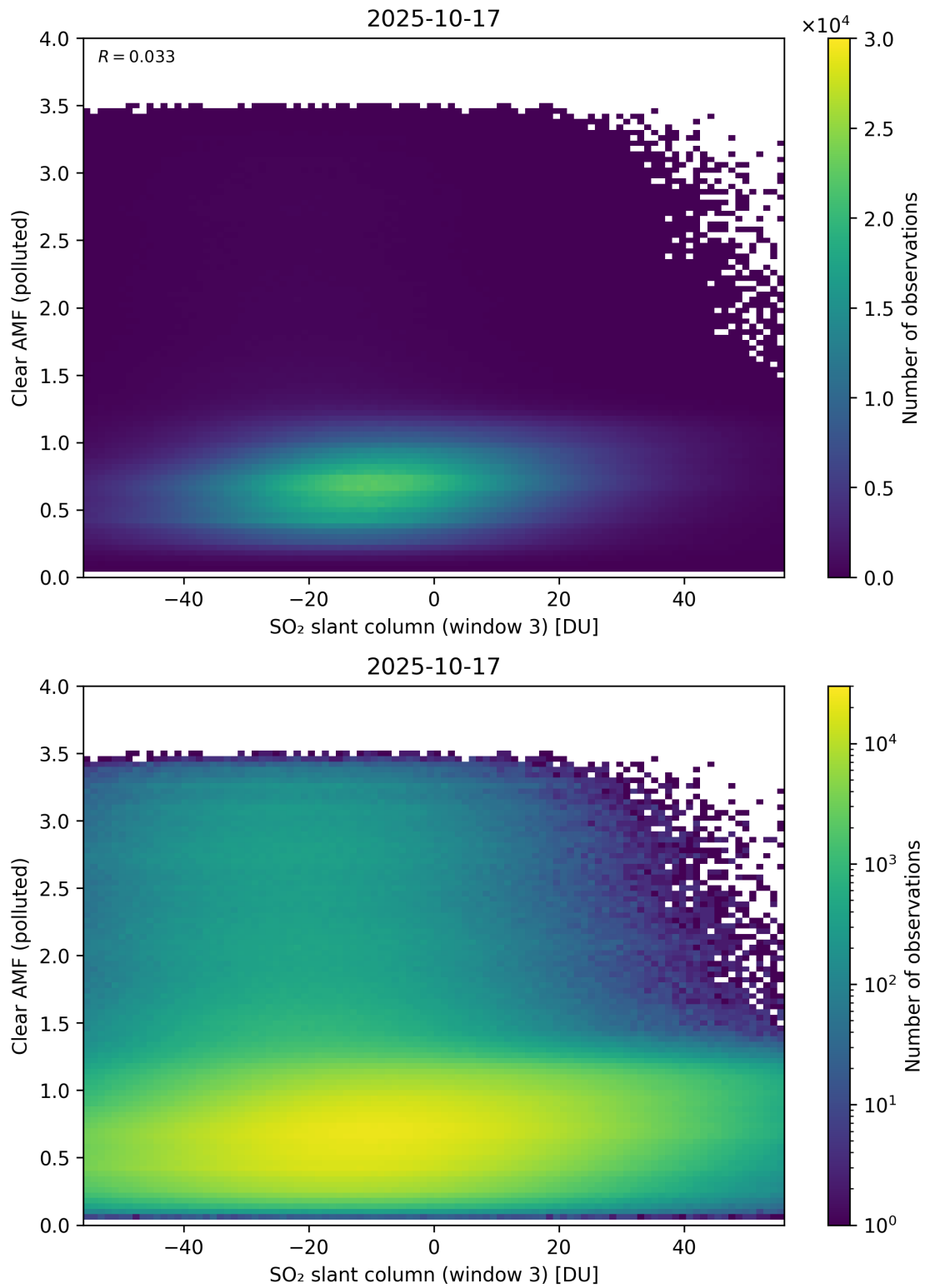
Figure 315: Scatter density plot of “SO 2 slant column (window 3)” against “Clear AMF (polluted)” for 2025-10-17 to 2025-10-18.
