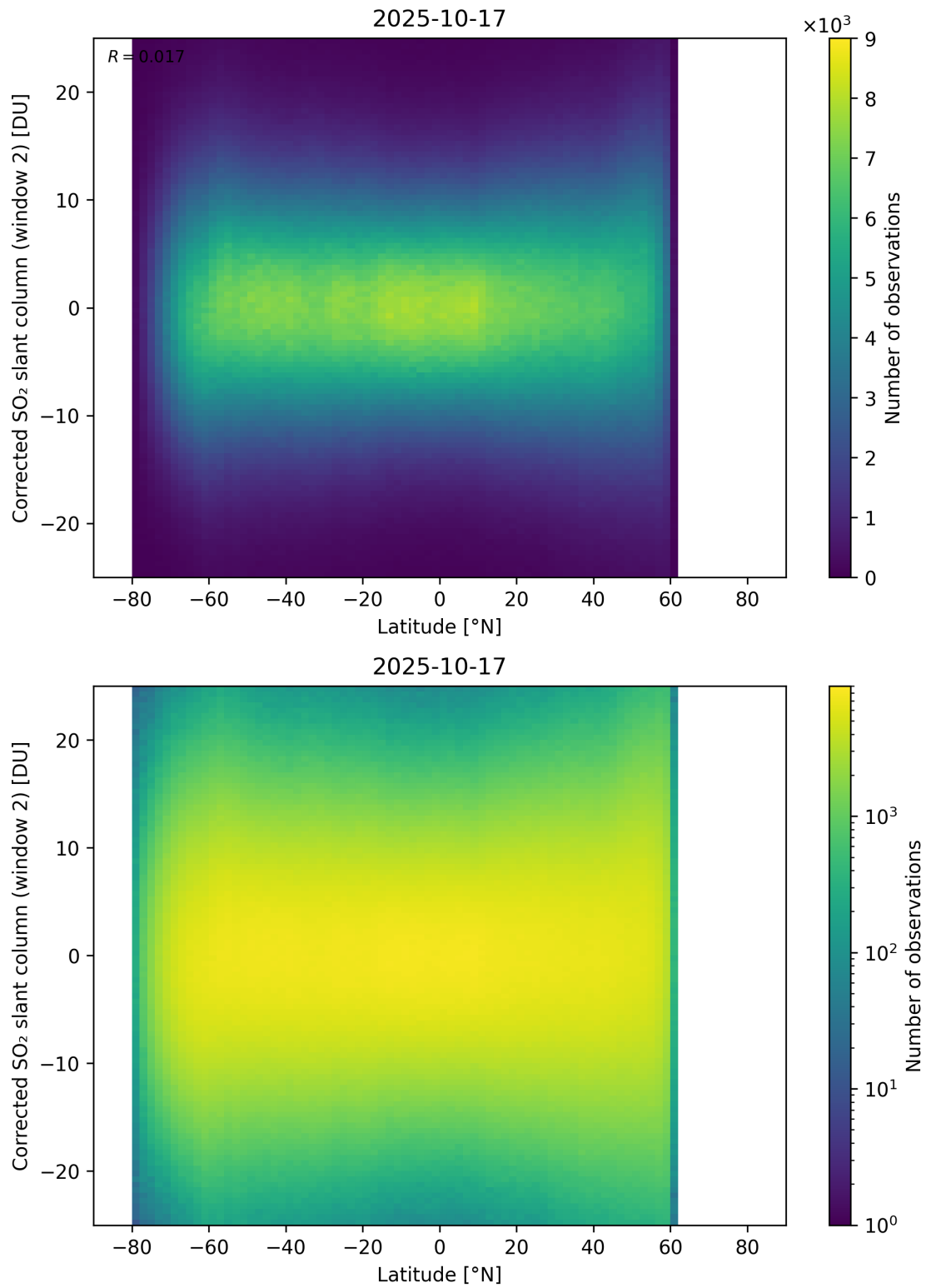
Figure 160: Scatter density plot of “Latitude” against “Corrected SO 2 slant column (window 2)” for 2025-10-17 to 2025-10-18.
