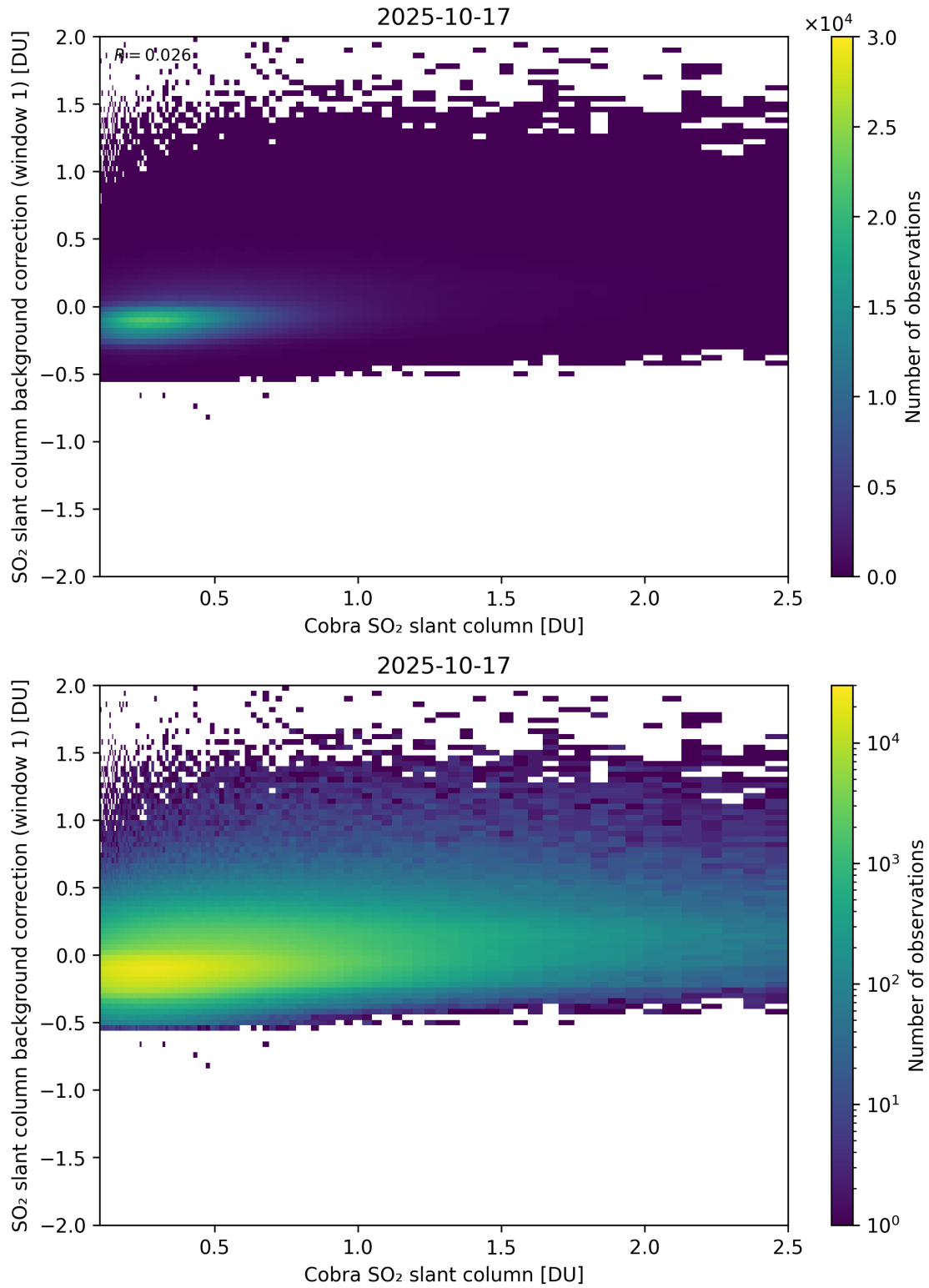
Figure 193: Scatter density plot of “Cobra SO 2 slant column” against “SO 2 slant column background correction (window 1)” for 2025-10-17 to 2025-10-18.
