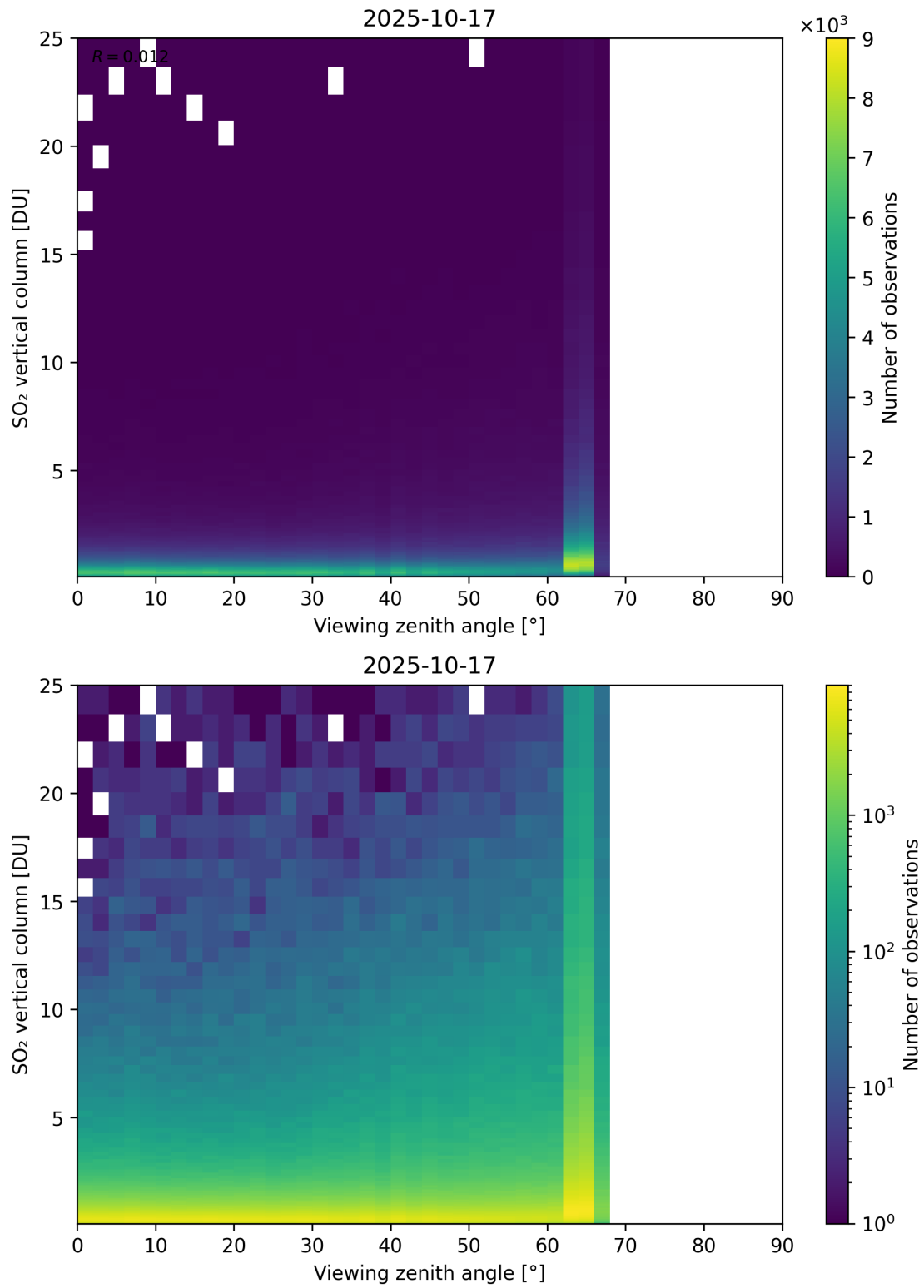
Figure 383: Scatter density plot of “Viewing zenith angle” against “SO 2 vertical column” for 2025-10-17 to 2025-10-18.
