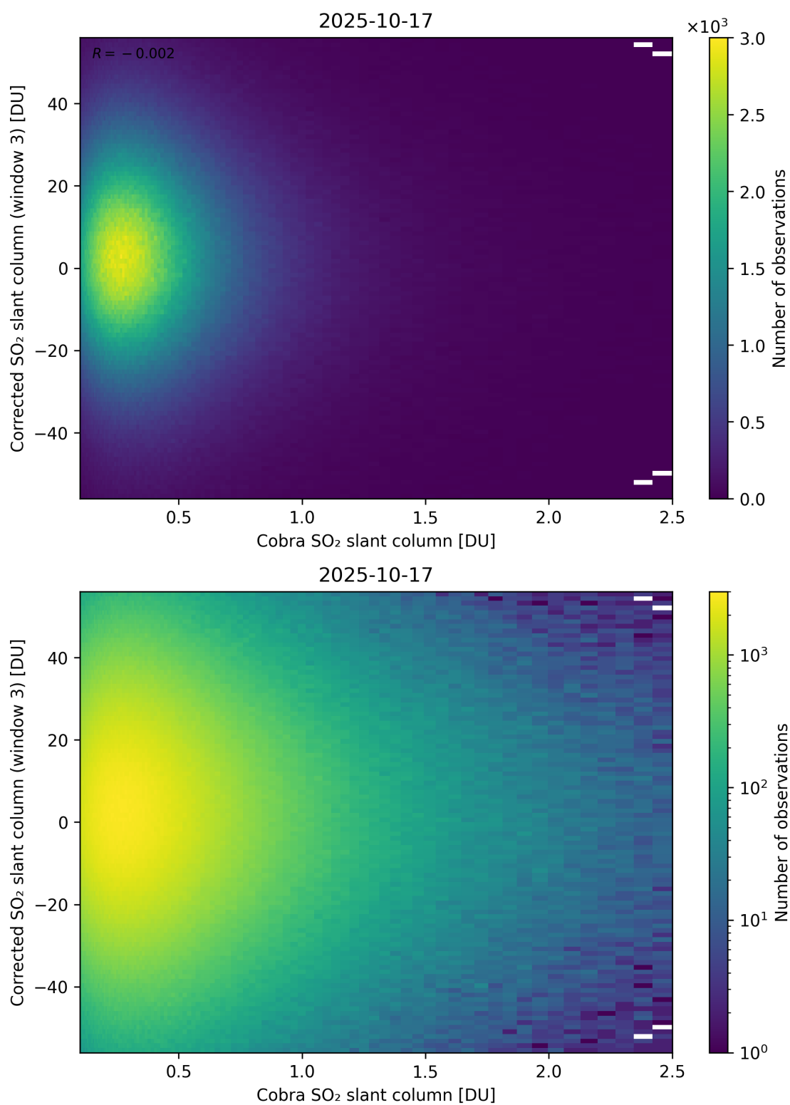
Figure 218: Scatter density plot of “Cobra SO 2 slant column” against “Corrected SO 2 slant column (window 3)” for 2025-10-17 to 2025-10-18.
