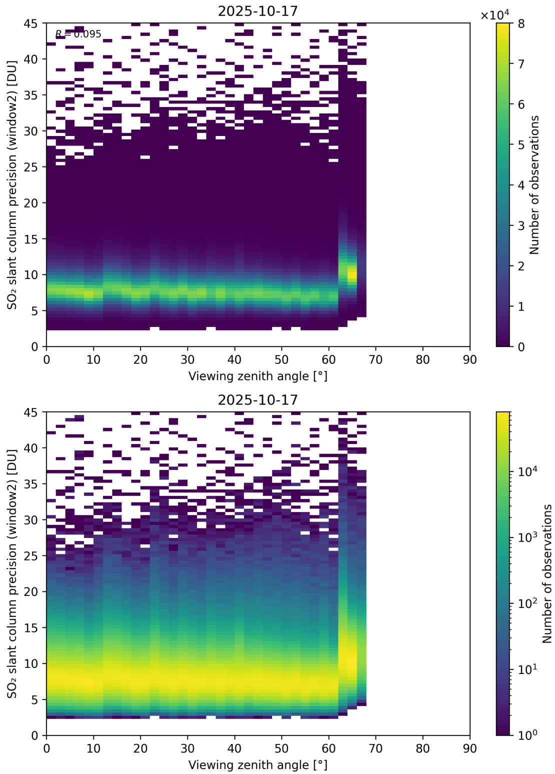
Figure 378: Scatter density plot of “Viewing zenith angle” against “SO 2 slant column precision (window2)” for 2025-10-17 to 2025-10-18.
