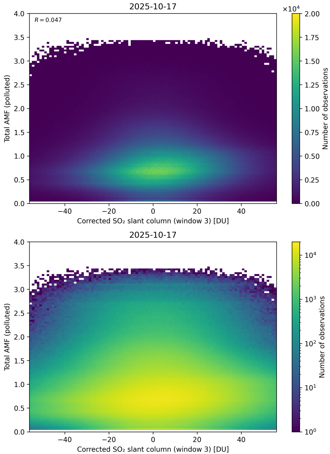
Figure 260: Scatter density plot of “Corrected SO 2 slant column (window 3)” against “Total AMF (polluted)” for 2025-10-17 to 2025-10-18.
