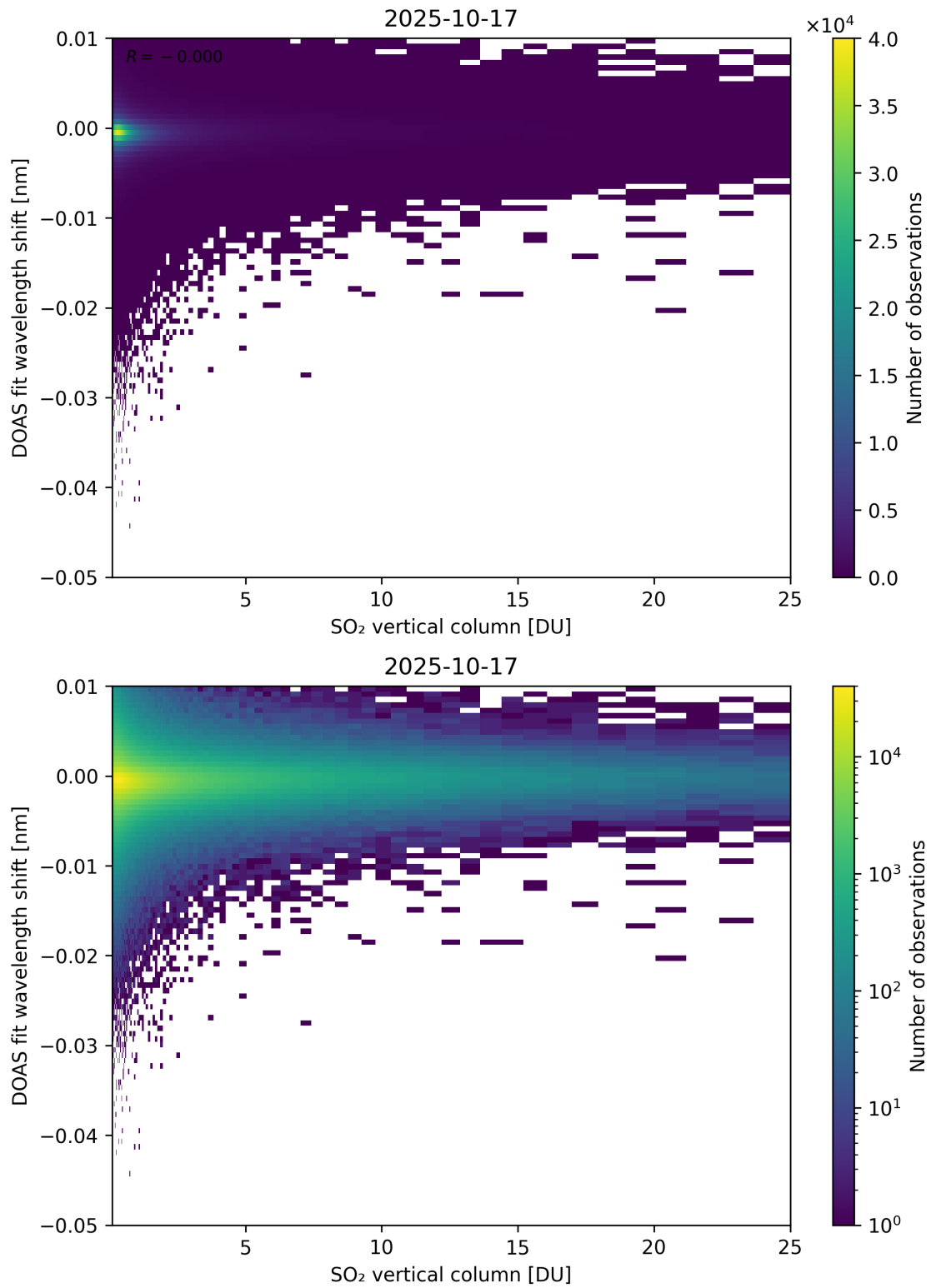
Figure 326: Scatter density plot of “SO 2 vertical column” against “DOAS fit wavelength shift” for 2025-10-17 to 2025-10-18.
