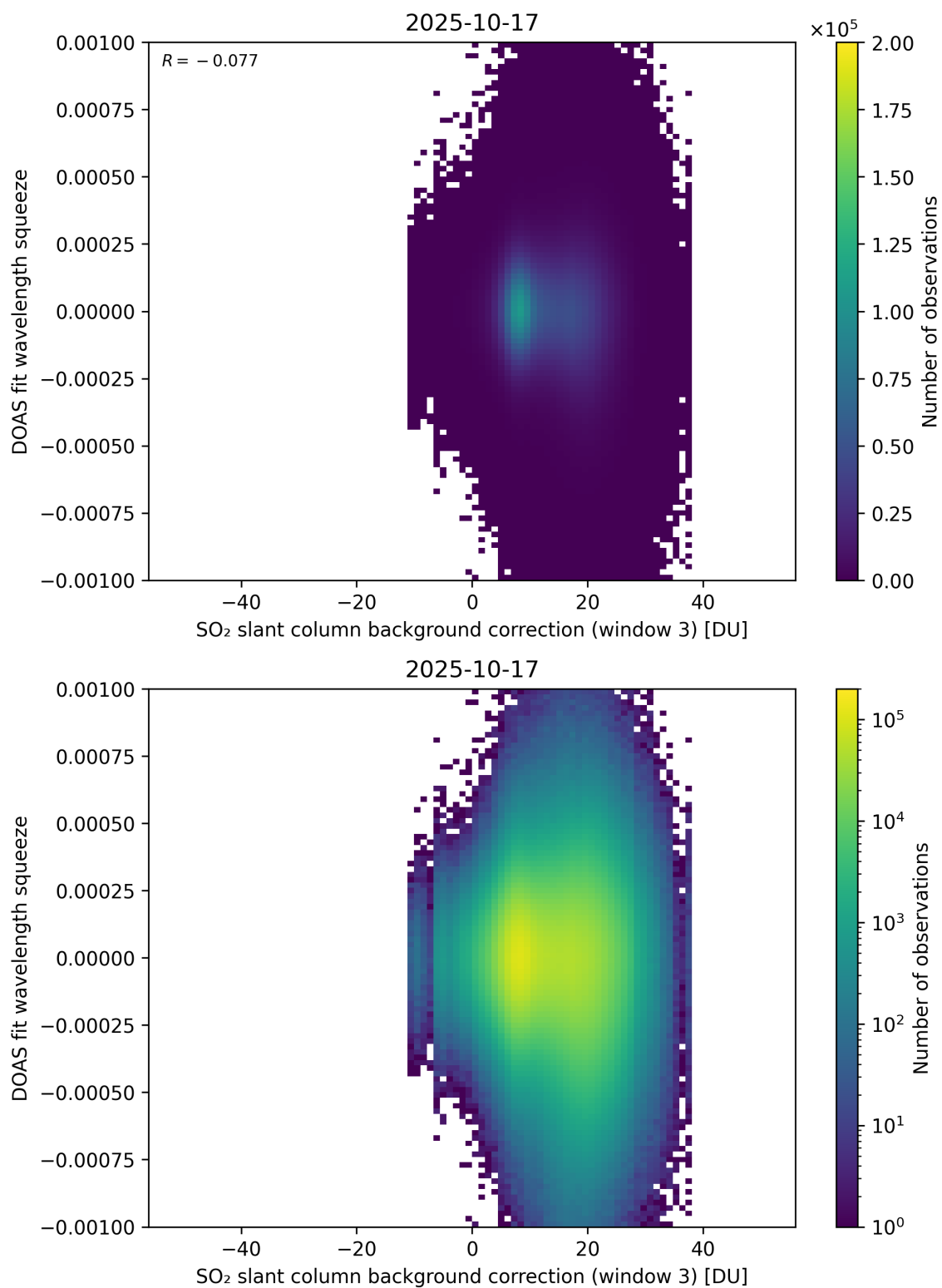
Figure 133: Scatter density plot of “SO 2 slant column background correction (window 3)” against “DOAS fit wavelength squeeze” for 2025-10-17 to 2025-10-18.
