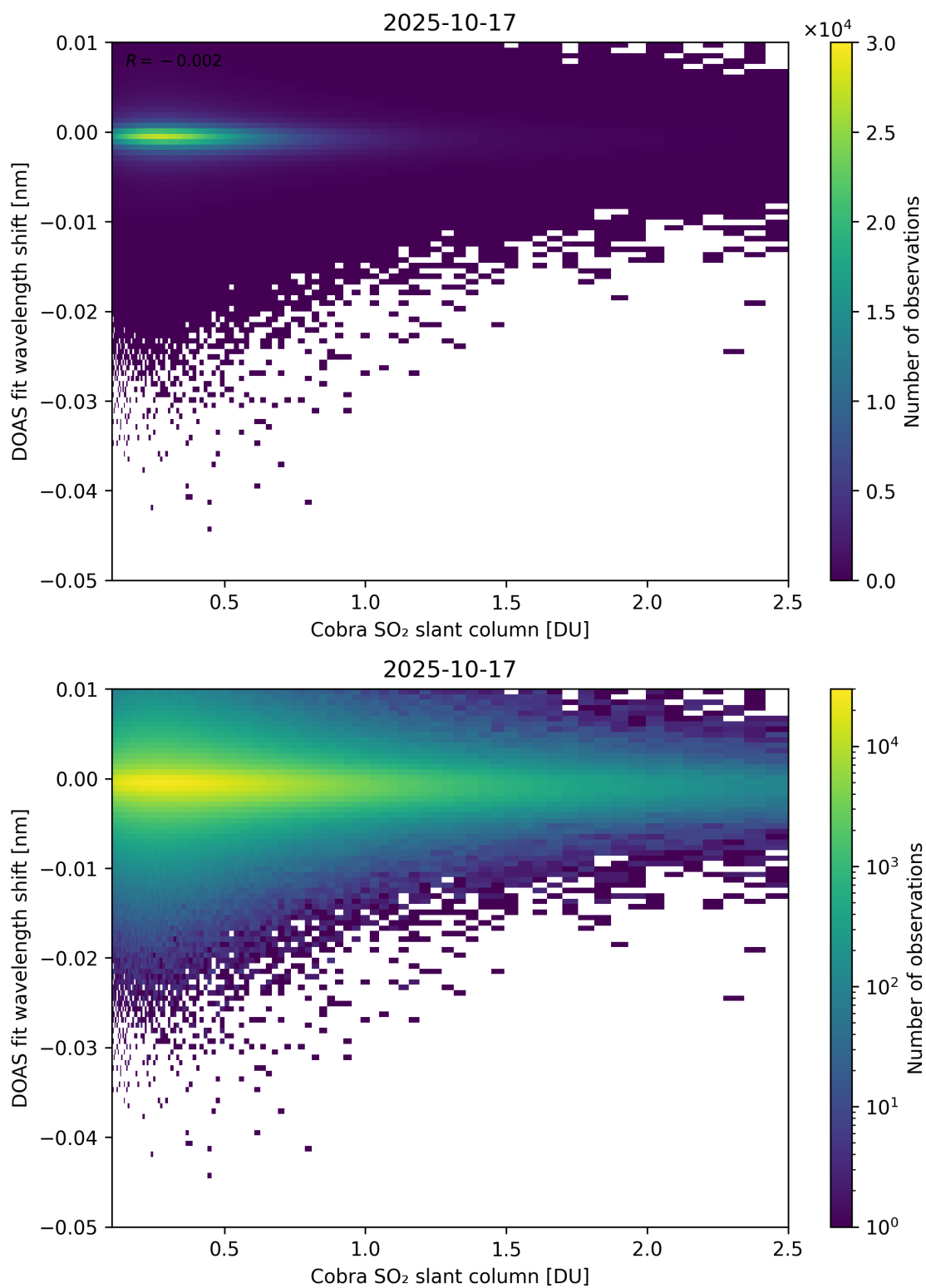
Figure 196: Scatter density plot of “Cobra SO 2 slant column” against “DOAS fit wavelength shift” for 2025-10-17 to 2025-10-18.
