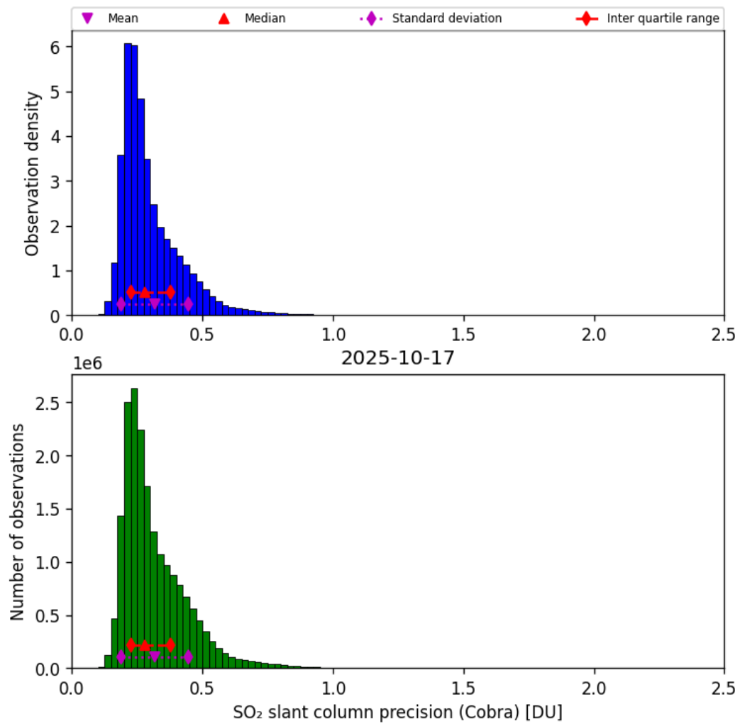
Figure 62: Histogram of “SO 2 slant column precision (Cobra)” for 2025-10-17 to 2025-10-18
