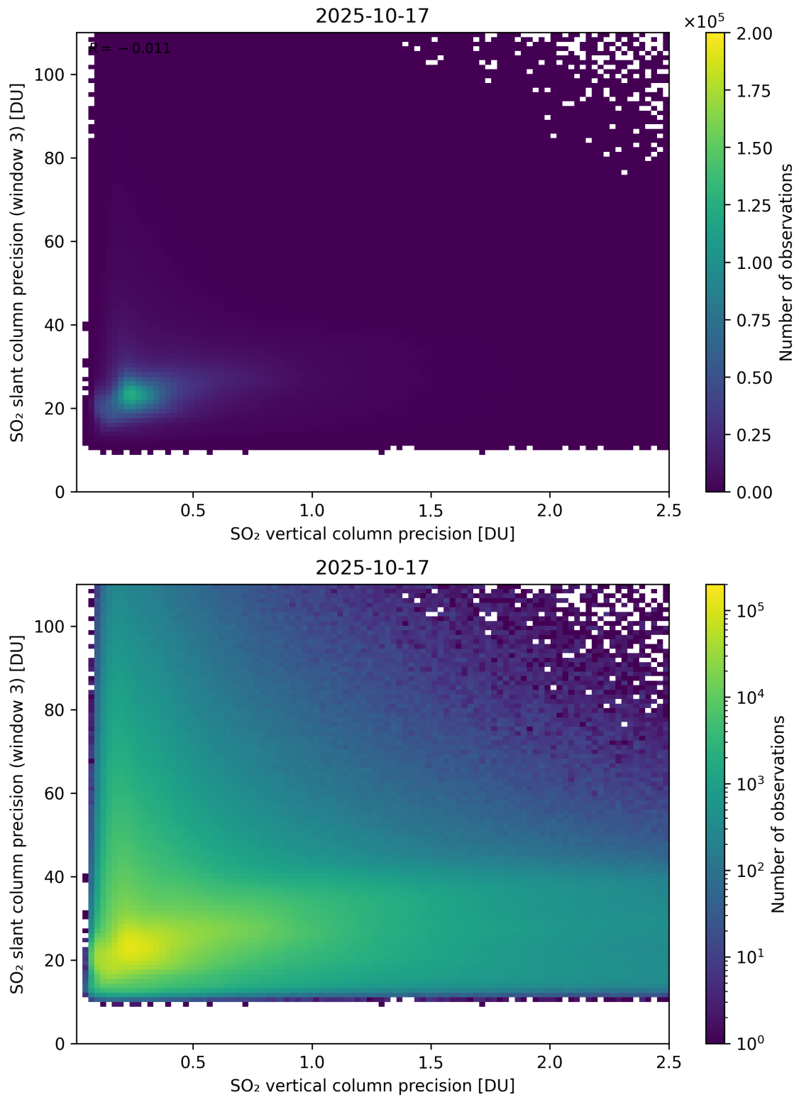
Figure 345: Scatter density plot of “SO 2 vertical column precision” against “SO 2 slant column precision (window 3)” for 2025-10-17 to 2025-10-18.
