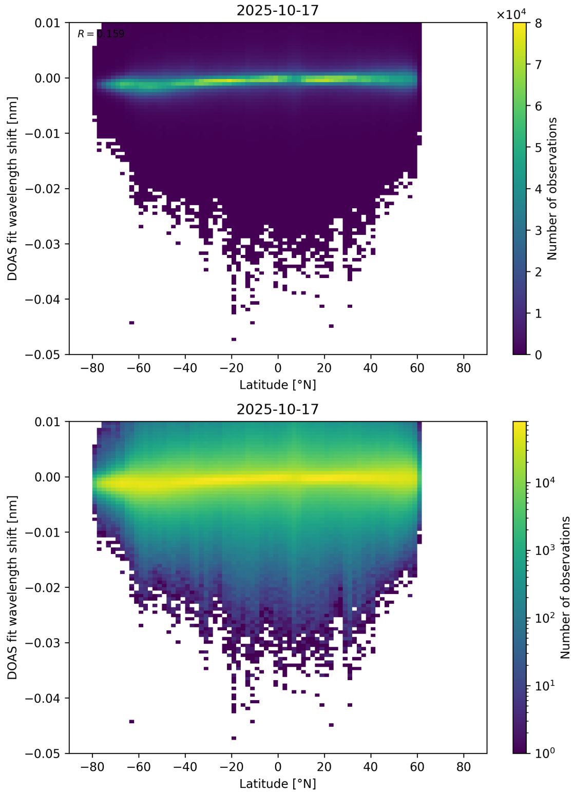
Figure 153: Scatter density plot of “Latitude” against “DOAS fit wavelength shift” for 2025-10-17 to 2025-10-18.
