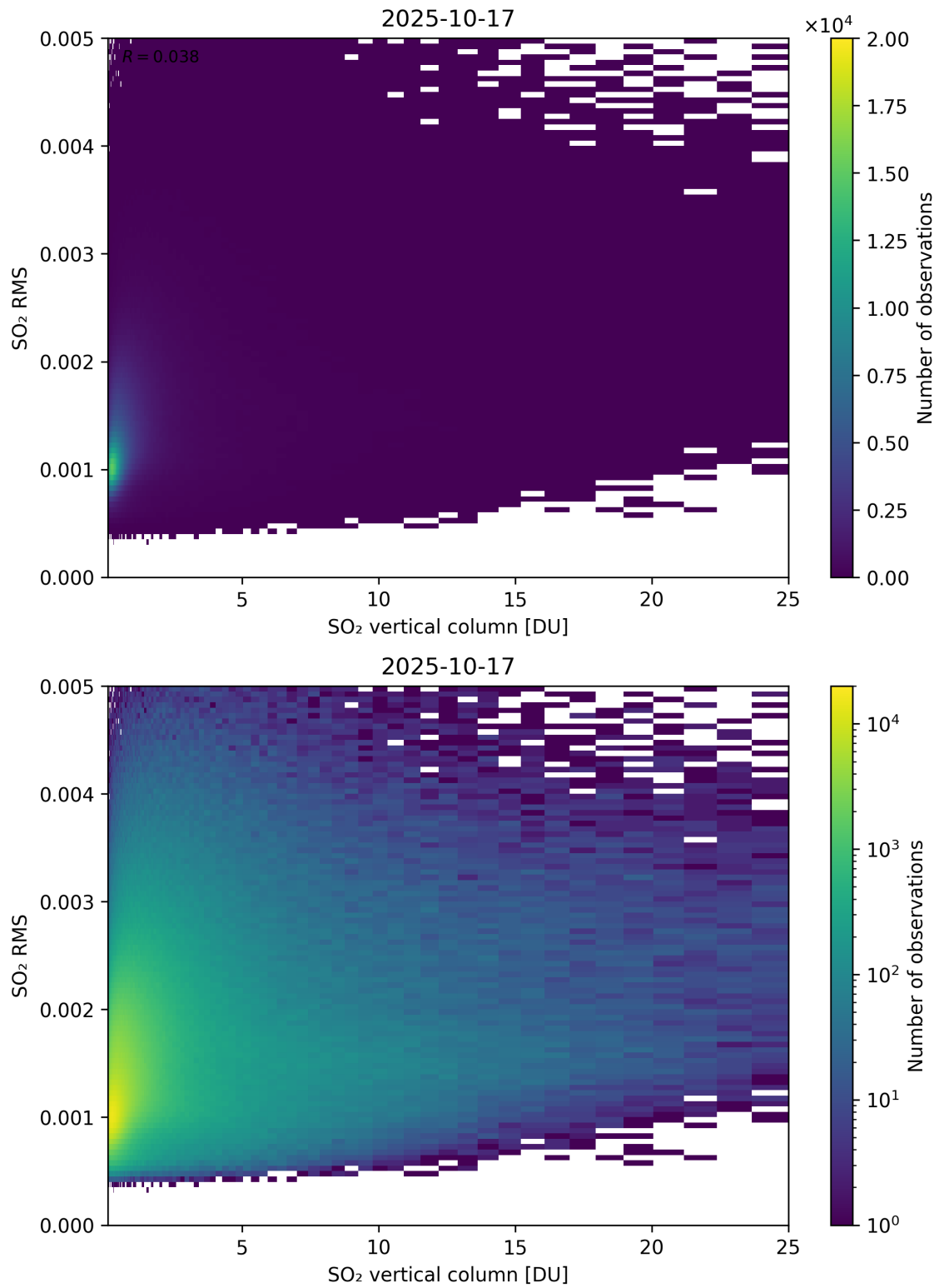
Figure 328: Scatter density plot of “SO 2 vertical column” against “SO 2 RMS” for 2025-10-17 to 2025-10-18.
