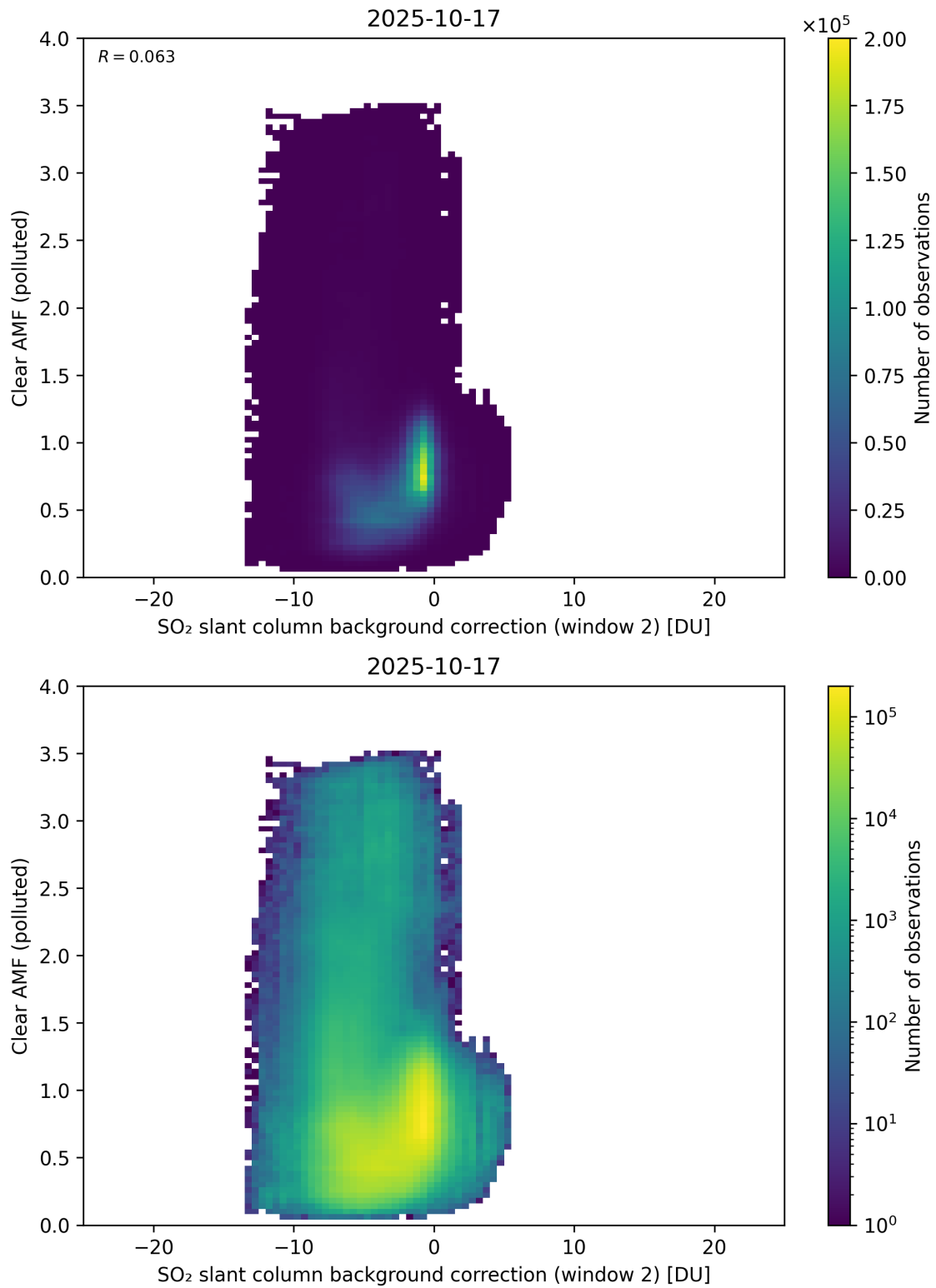
Figure 126: Scatter density plot of “SO 2 slant column background correction (window 2)” against “Clear AMF (polluted)” for 2025-10-17 to 2025-10-18.
