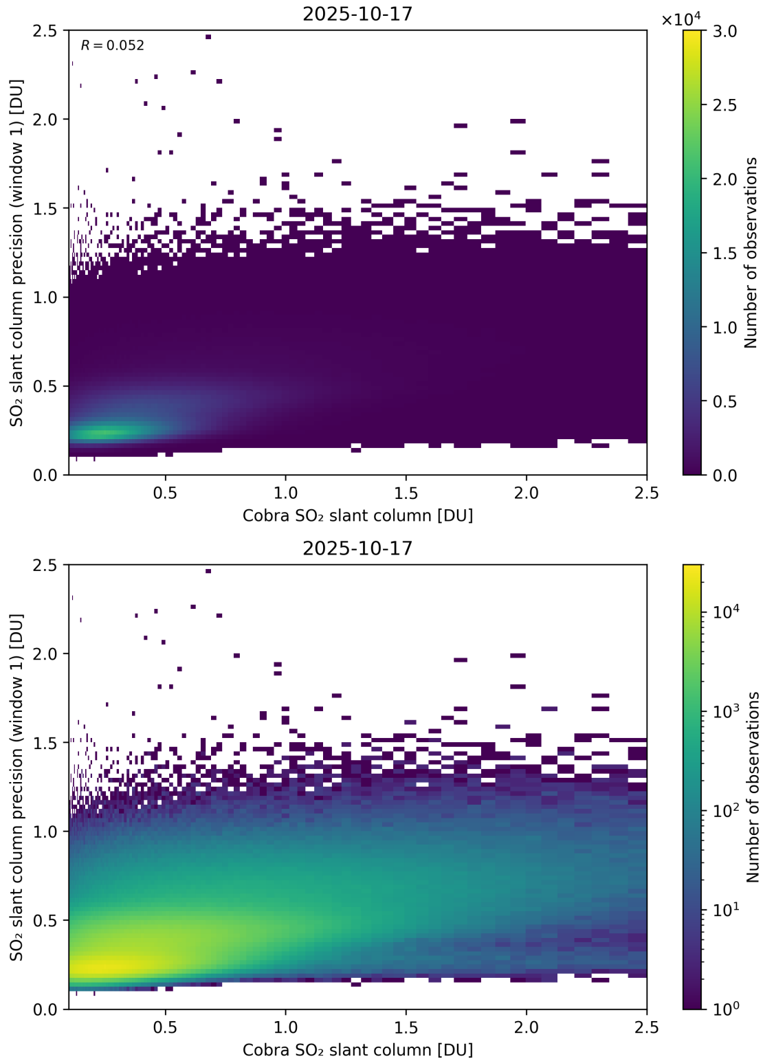
Figure 220: Scatter density plot of “Cobra SO 2 slant column” against “SO 2 slant column precision (window 1)” for 2025-10-17 to 2025-10-18.
