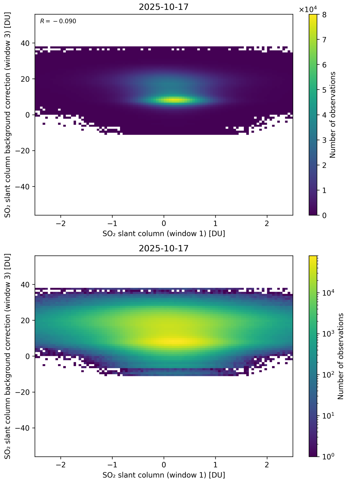
Figure 264: Scatter density plot of “SO 2 slant column (window 1)” against “SO 2 slant column background correction (window 3)” for 2025-10-17 to 2025-10-18.
