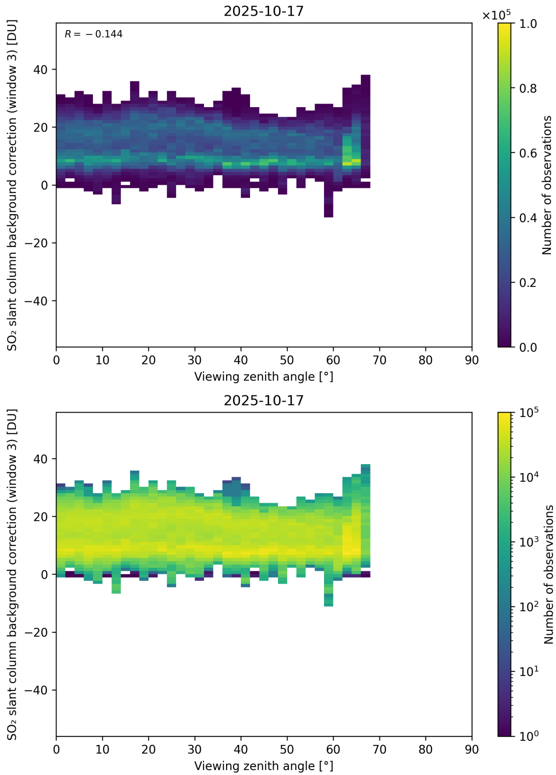
Figure 364: Scatter density plot of “Viewing zenith angle” against “SO 2 slant column background correction (window 3)” for 2025-10-17 to 2025-10-18.
