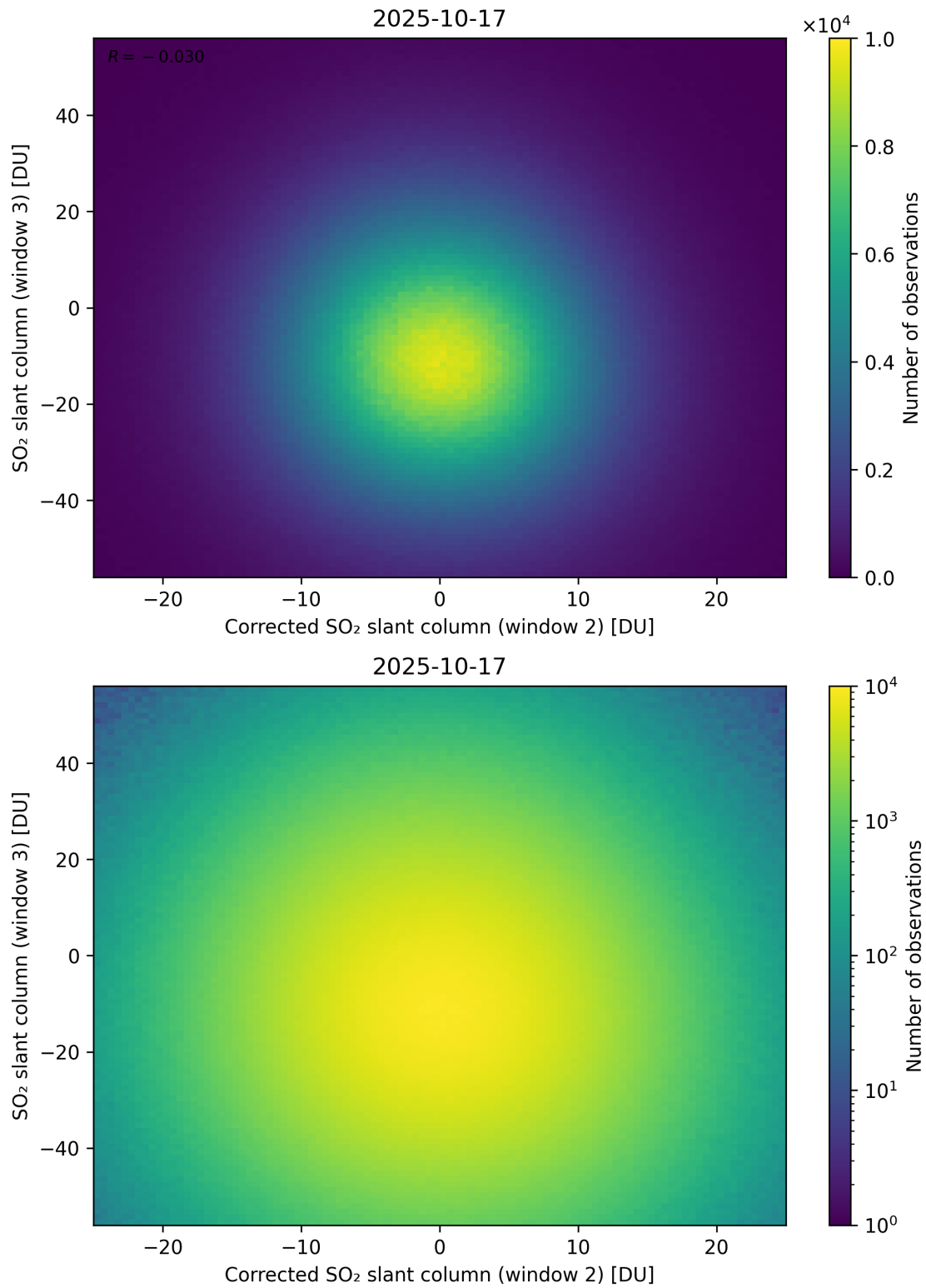
Figure 251: Scatter density plot of “Corrected SO 2 slant column (window 2)” against “SO 2 slant column (window 3)” for 2025-10-17 to 2025-10-18.
