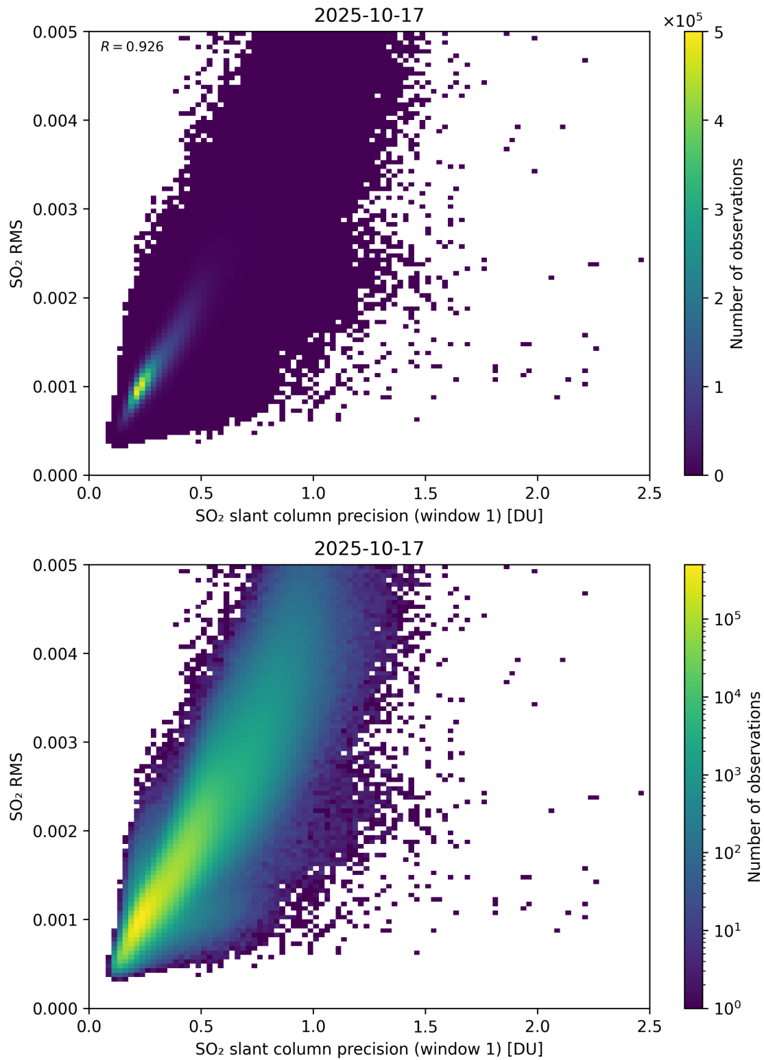
Figure 273: Scatter density plot of “SO 2 slant column precision (window 1)” against “SO 2 RMS” for 2025-10-17 to 2025-10-18.
