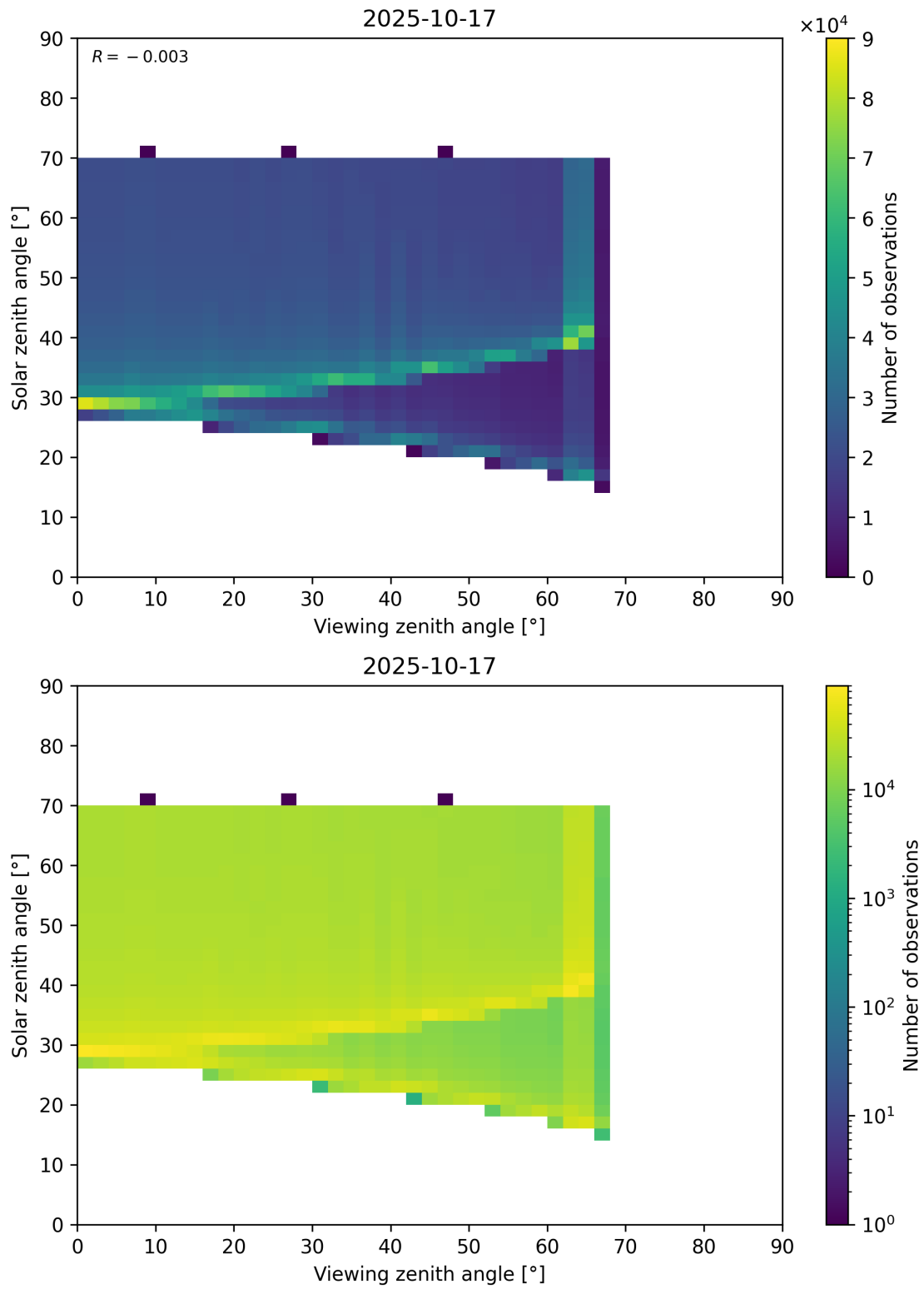
Figure 369: Scatter density plot of “Viewing zenith angle” against “Solar zenith angle” for 2025-10-17 to 2025-10-18.
