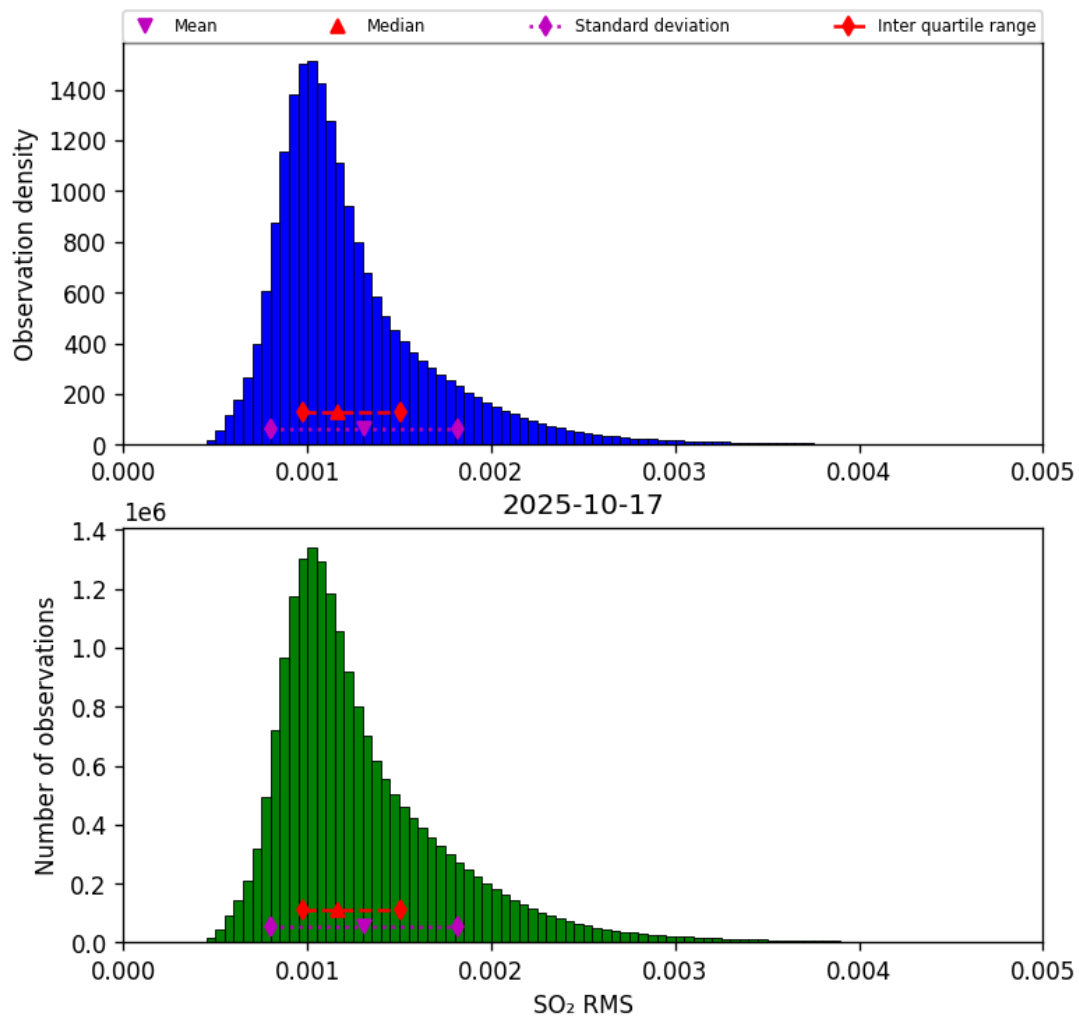
Figure 78: Histogram of “SO 2 RMS” for 2025-10-17 to 2025-10-18
