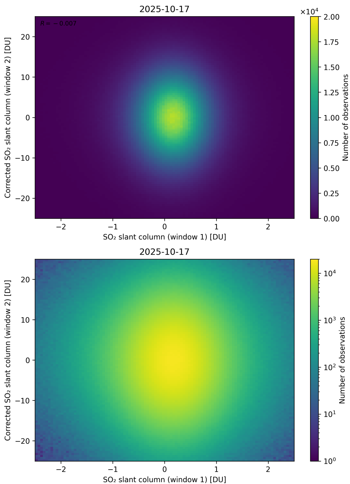
Figure 283: Scatter density plot of “SO 2 slant column (window 1)” against “Corrected SO 2 slant column (window 2)” for 2025-10-17 to 2025-10-18.
