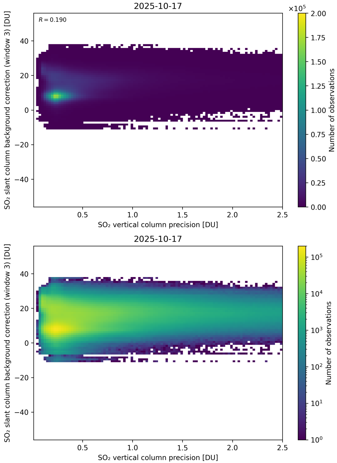
Figure 331: Scatter density plot of “SO 2 vertical column precision” against “SO 2 slant column background correction (window 3)” for 2025-10-17 to 2025-10-18.
