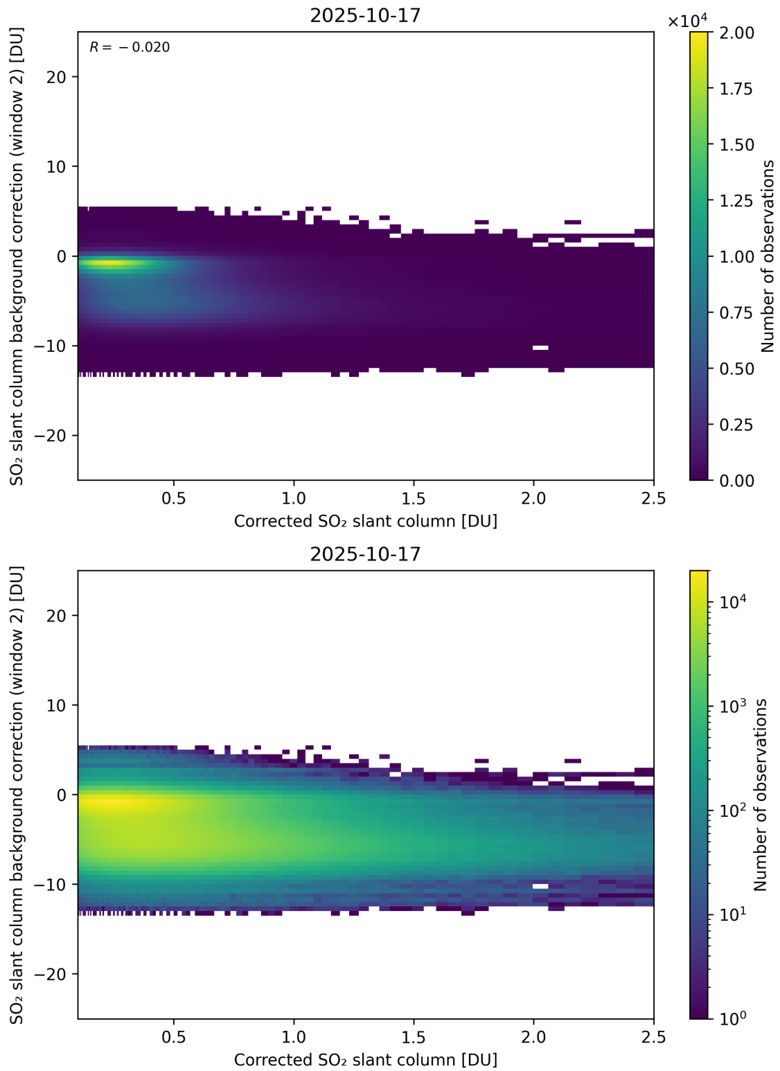
Figure 227: Scatter density plot of “Corrected SO 2 slant column” against “SO 2 slant column background correction (window 2)” for 2025-10-17 to 2025-10-18.
