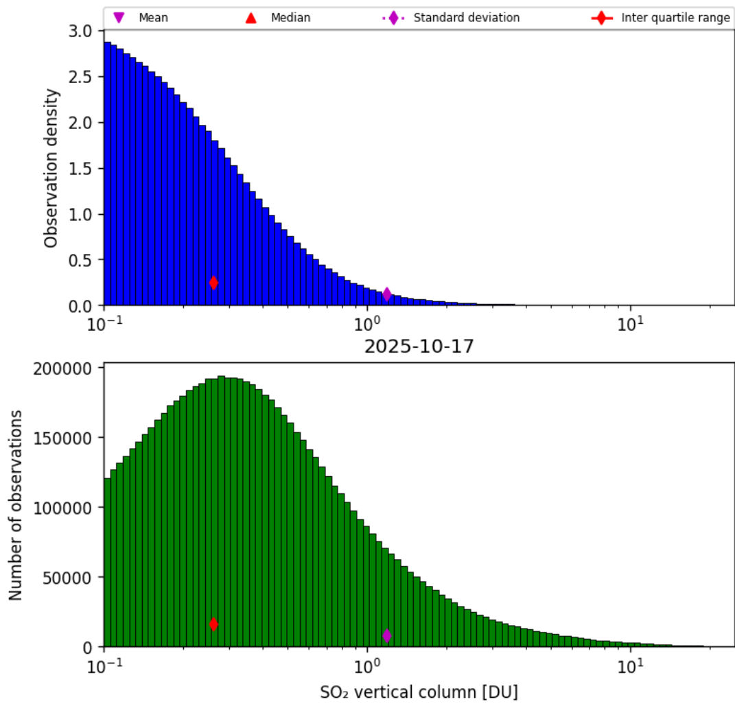
Figure 58: Histogram of “SO 2 vertical column” for 2025-10-17 to 2025-10-18
