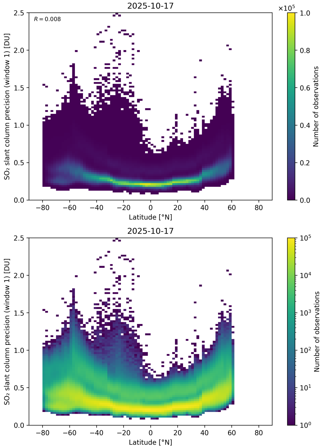
Figure 163: Scatter density plot of “Latitude” against “SO 2 slant column precision (window 1)” for 2025-10-17 to 2025-10-18.
