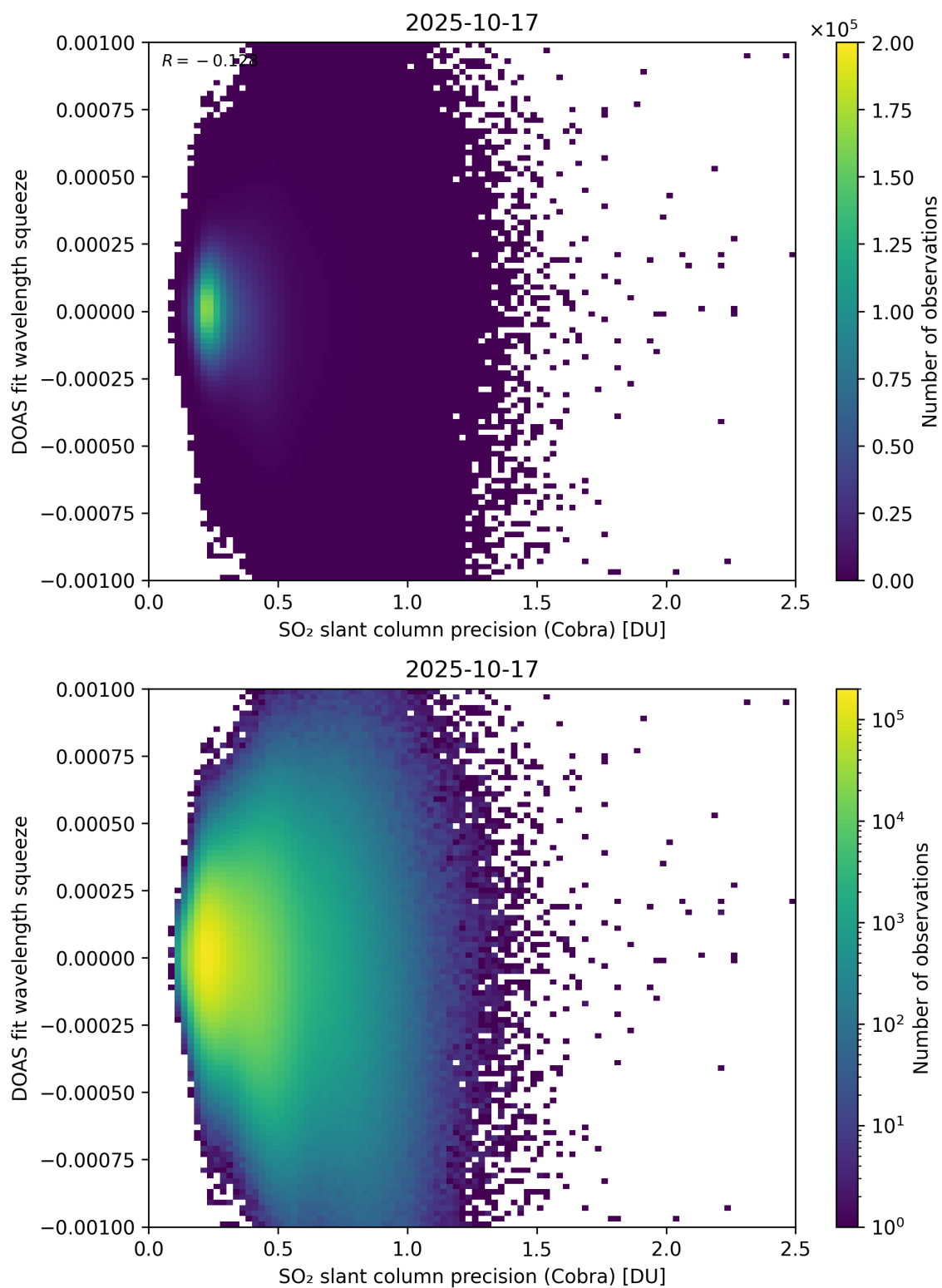
Figure 203: Scatter density plot of “SO 2 slant column precision (Cobra)” against “DOAS fit wavelength squeeze” for 2025-10-17 to 2025-10-18.
