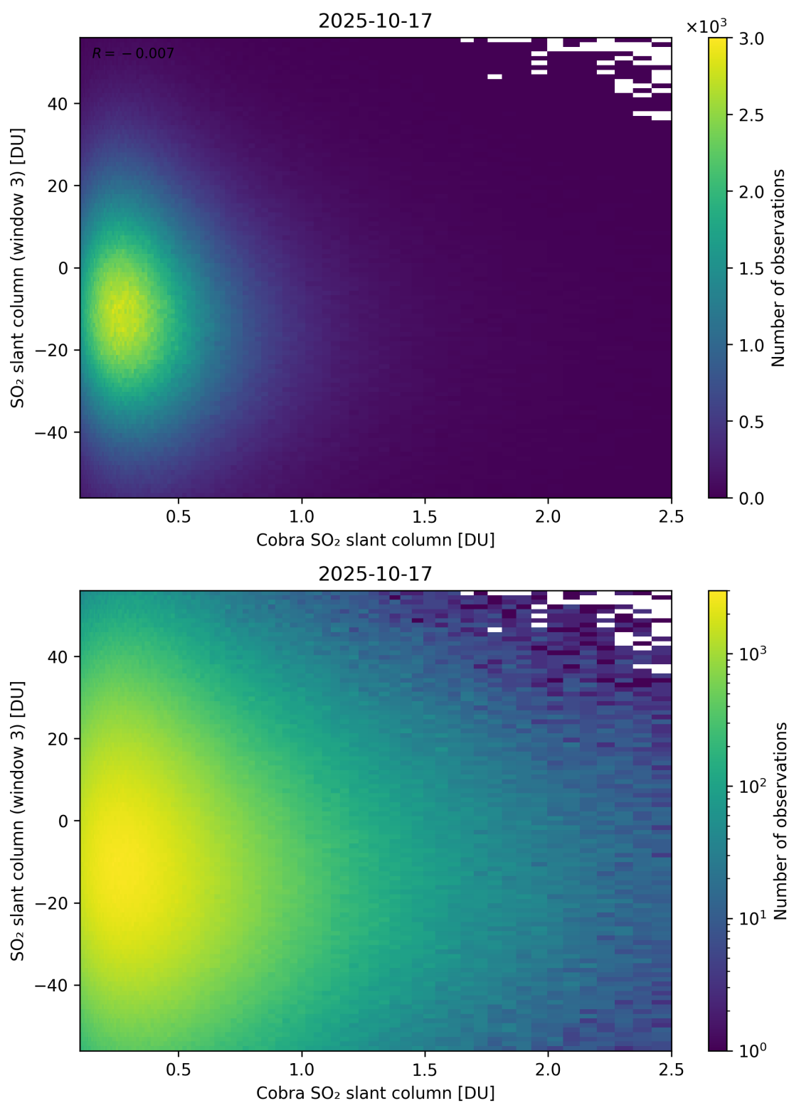
Figure 222: Scatter density plot of “Cobra SO 2 slant column” against “SO 2 slant column (window 3)” for 2025-10-17 to 2025-10-18.
