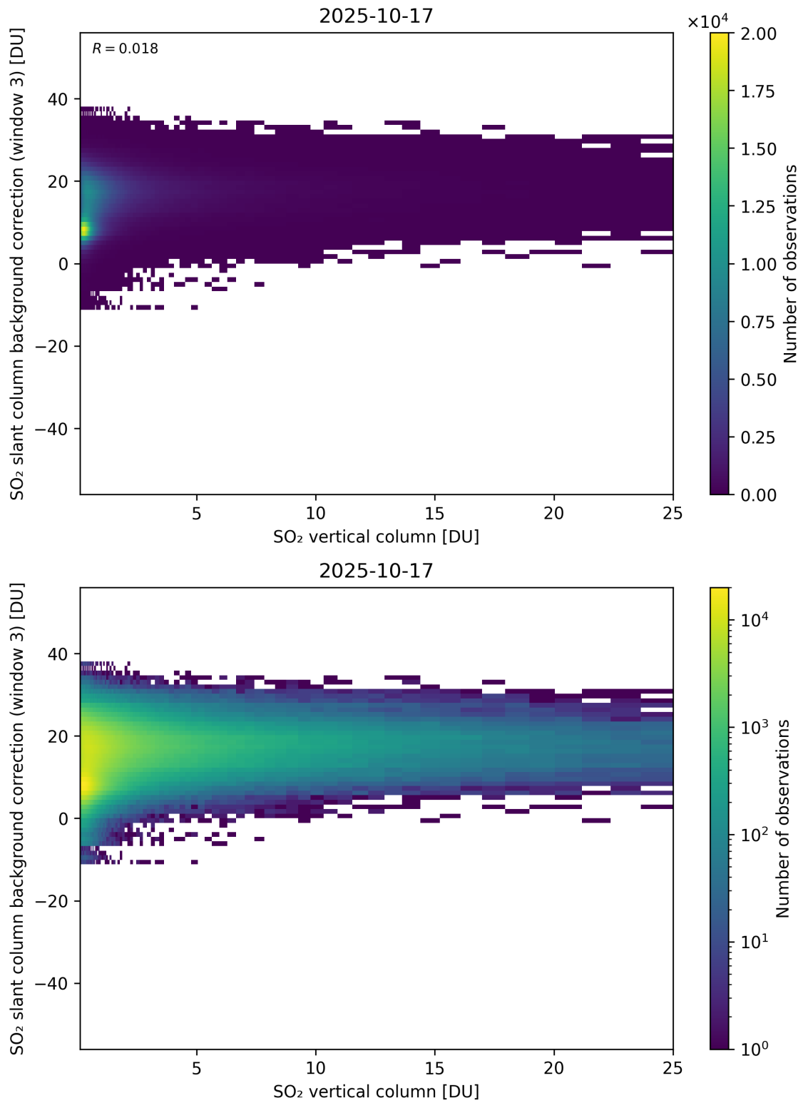
Figure 325: Scatter density plot of “SO 2 vertical column” against “SO 2 slant column background correction (window 3)” for 2025-10-17 to 2025-10-18.
