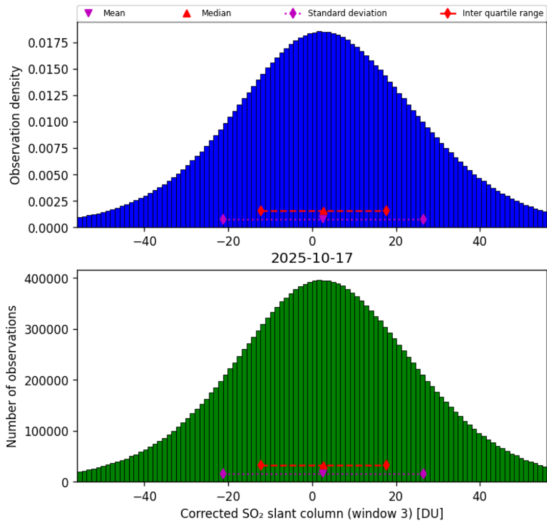
Figure 73: Histogram of “Corrected SO 2 slant column (window 3)” for 2025-10-17 to 2025-10-18
