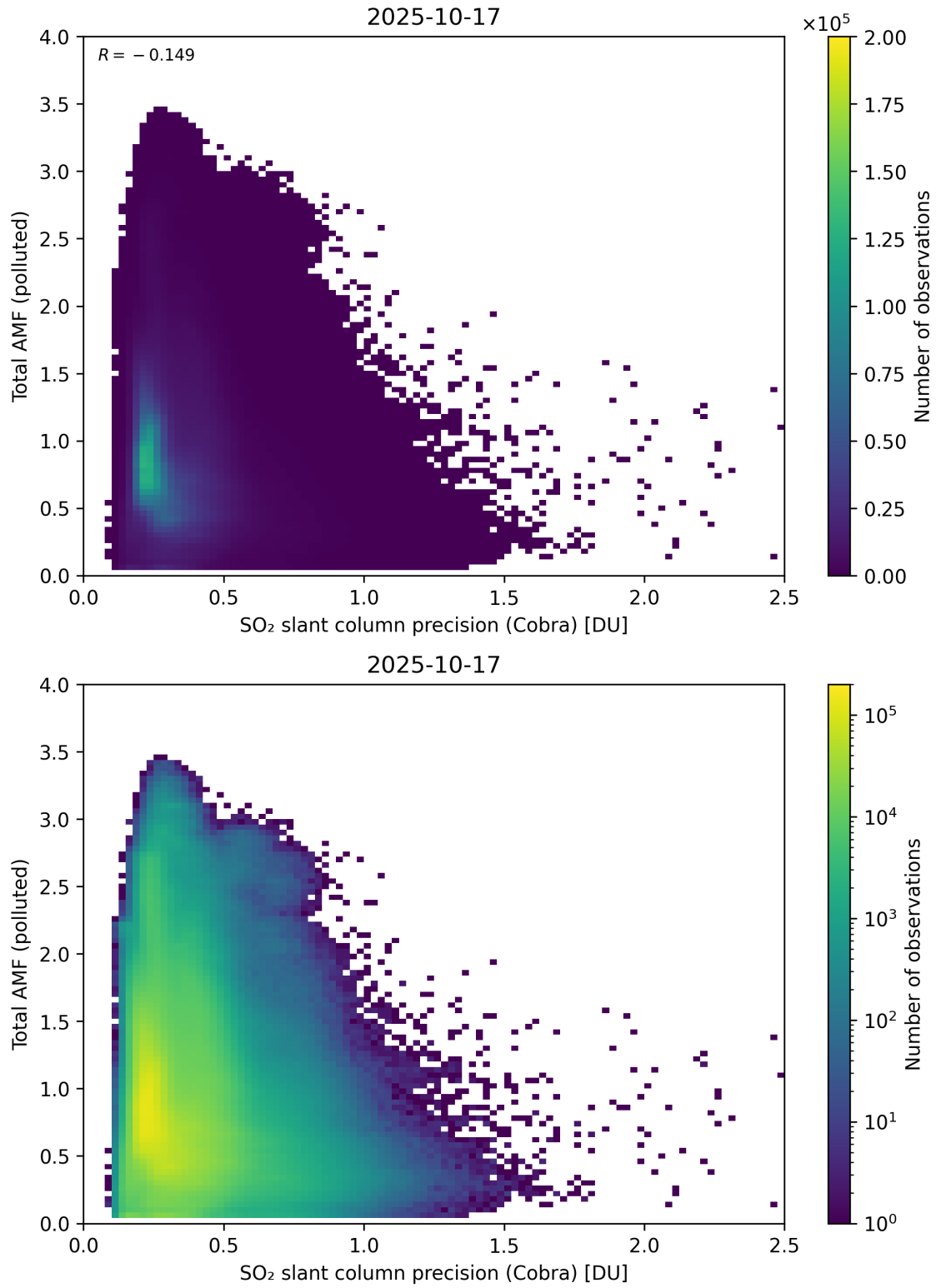
Figure 213: Scatter density plot of “SO 2 slant column precision (Cobra)” against “Total AMF (polluted)” for 2025-10-17 to 2025-10-18.
