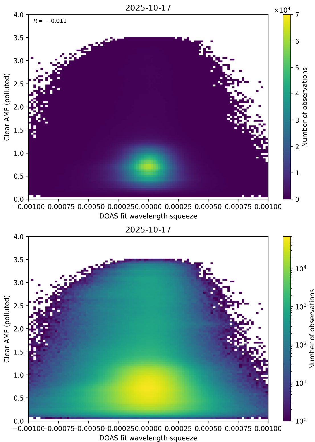
Figure 144: Scatter density plot of “DOAS fit wavelength squeeze” against “Clear AMF (polluted)” for 2025-10-17 to 2025-10-18.
