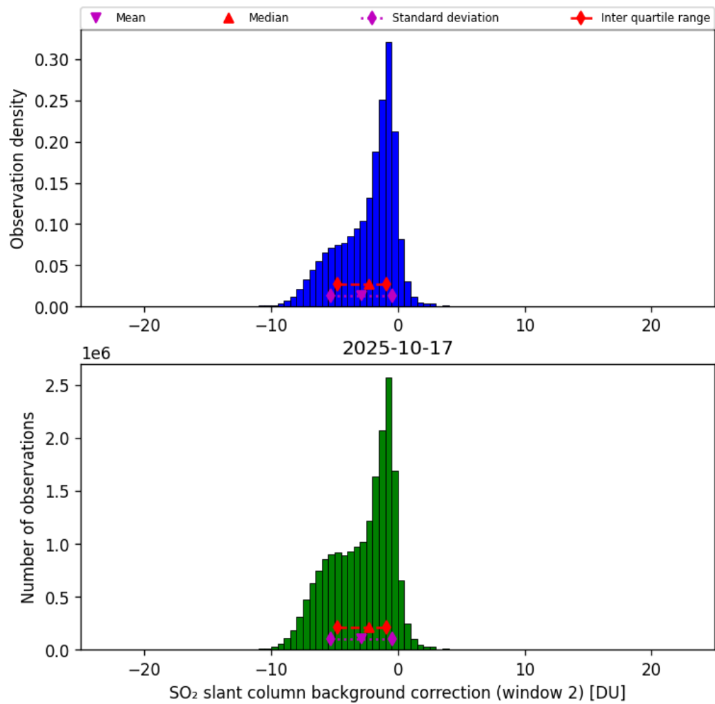
Figure 70: Histogram of “SO 2 slant column background correction (window 2)” for 2025-10-17 to 2025-10-18
