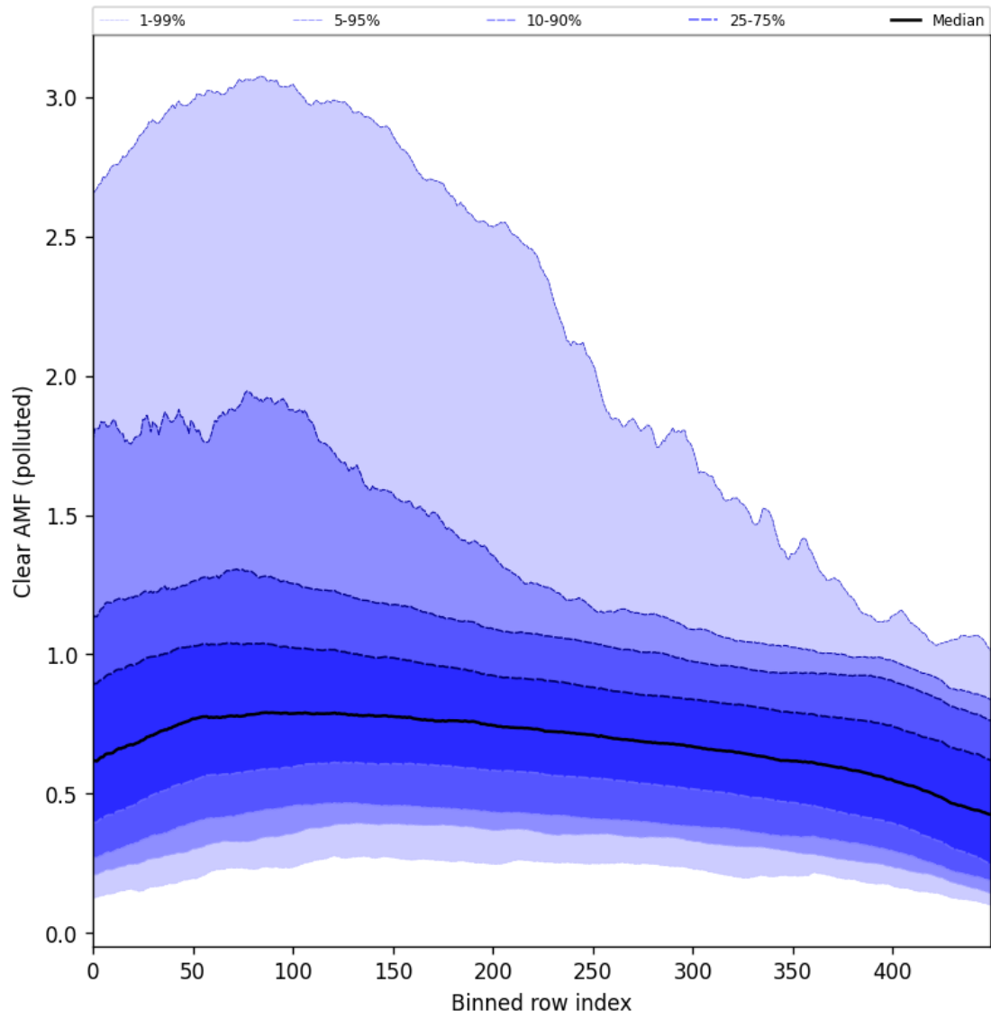
Figure 107: Along track statistics of “Clear AMF (polluted)” for 2025-10-17 to 2025-10-18
