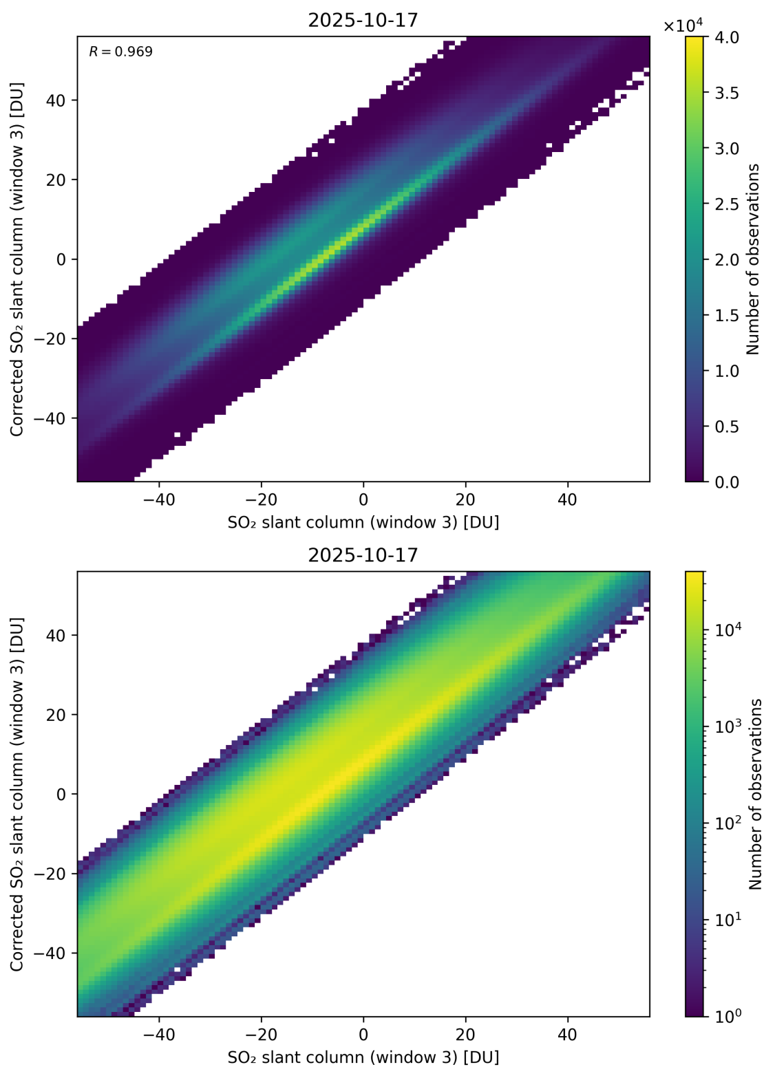
Figure 316: Scatter density plot of “SO 2 slant column (window 3)” against “Corrected SO 2 slant column (window 3)” for 2025-10-17 to 2025-10-18.
