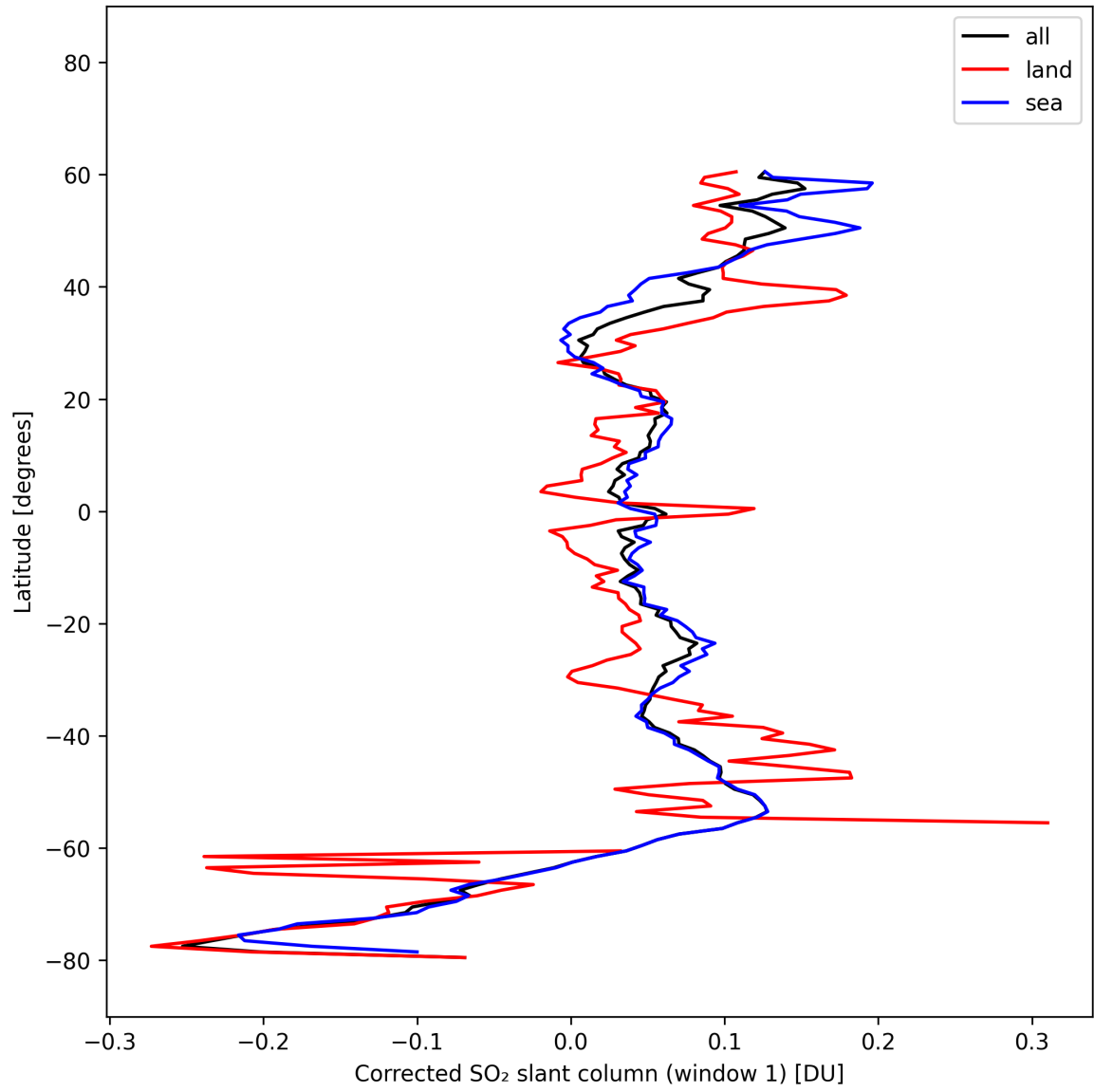
Figure 39: Zonal average of “Corrected SO 2 slant column (window 1)” for 2025-10-17 to 2025-10-18.
