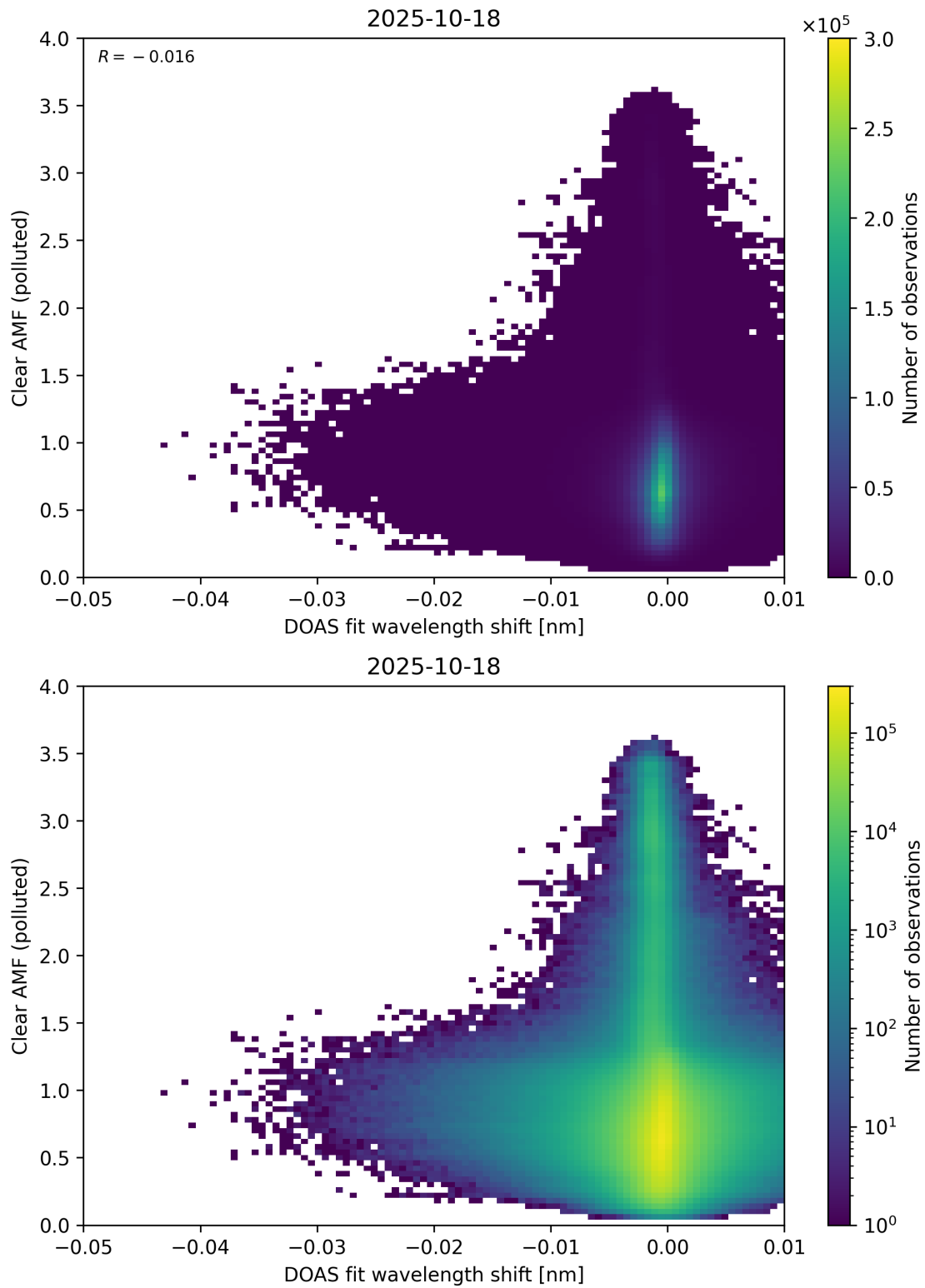
Figure 140: Scatter density plot of “DOAS fit wavelength shift” against “Clear AMF (polluted)” for 2025-10-17 to 2025-10-19.
