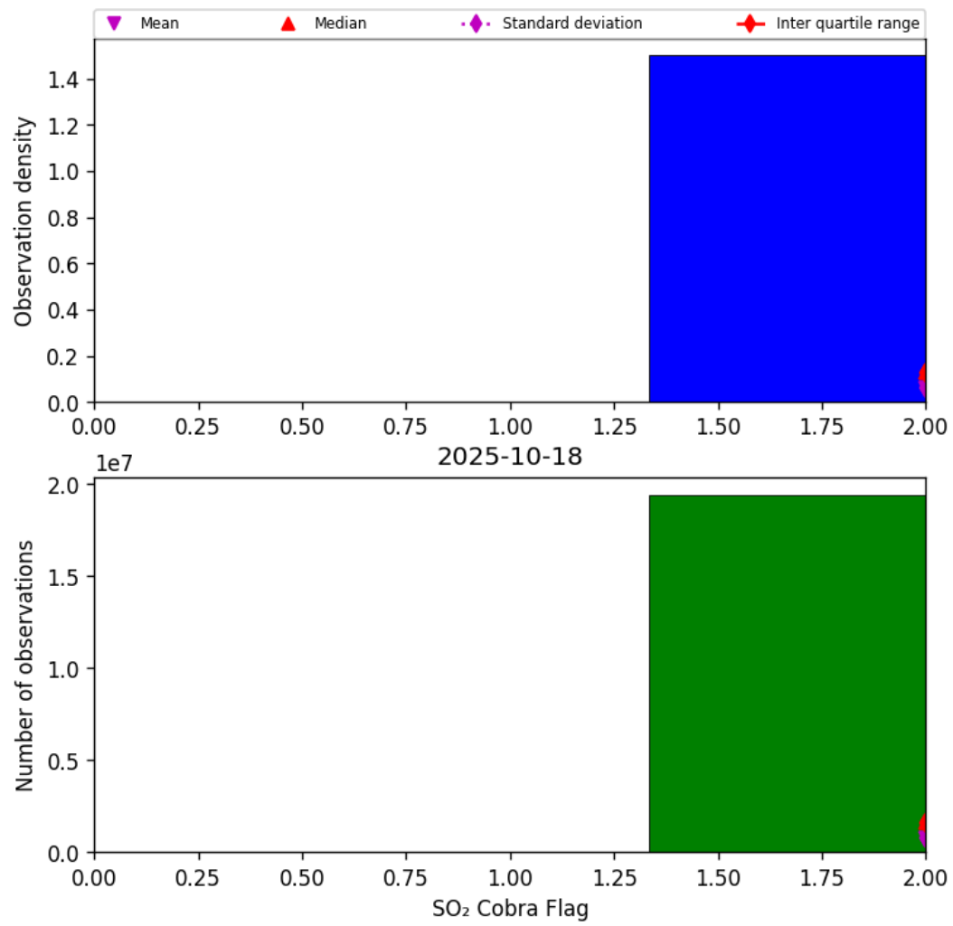
Figure 75: Histogram of "SO 2 Cobra Flag" for 2025-10-17 to 2025-10-19
