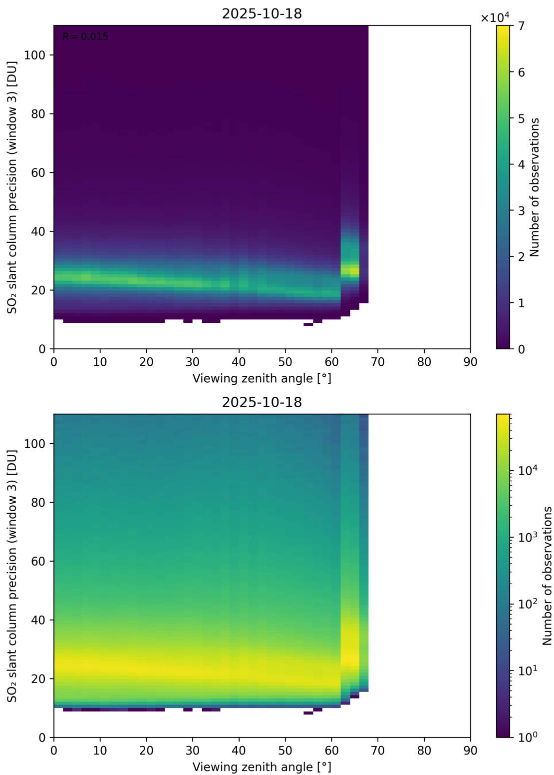
Figure 380: Scatter density plot of “Viewing zenith angle” against “SO 2 slant column precision (window 3)” for 2025-10-17 to 2025-10-19.
