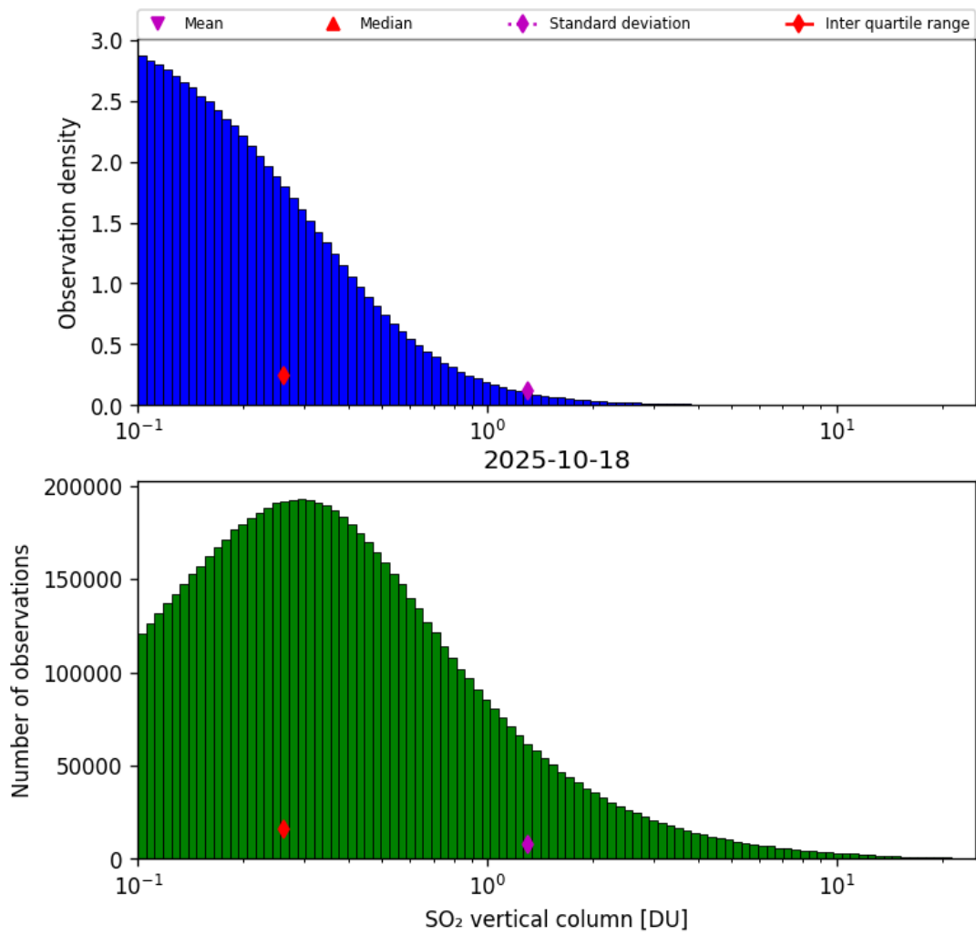
Figure 58: Histogram of “SO 2 vertical column” for 2025-10-17 to 2025-10-19
