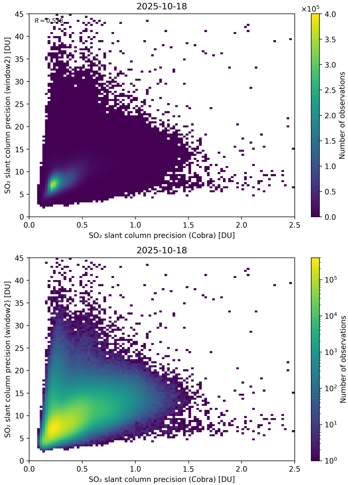
Figure 210: Scatter density plot of “SO 2 slant column precision (Cobra)” against “SO 2 slant column precision (window2)” for 2025-10-17 to 2025-10-19.
