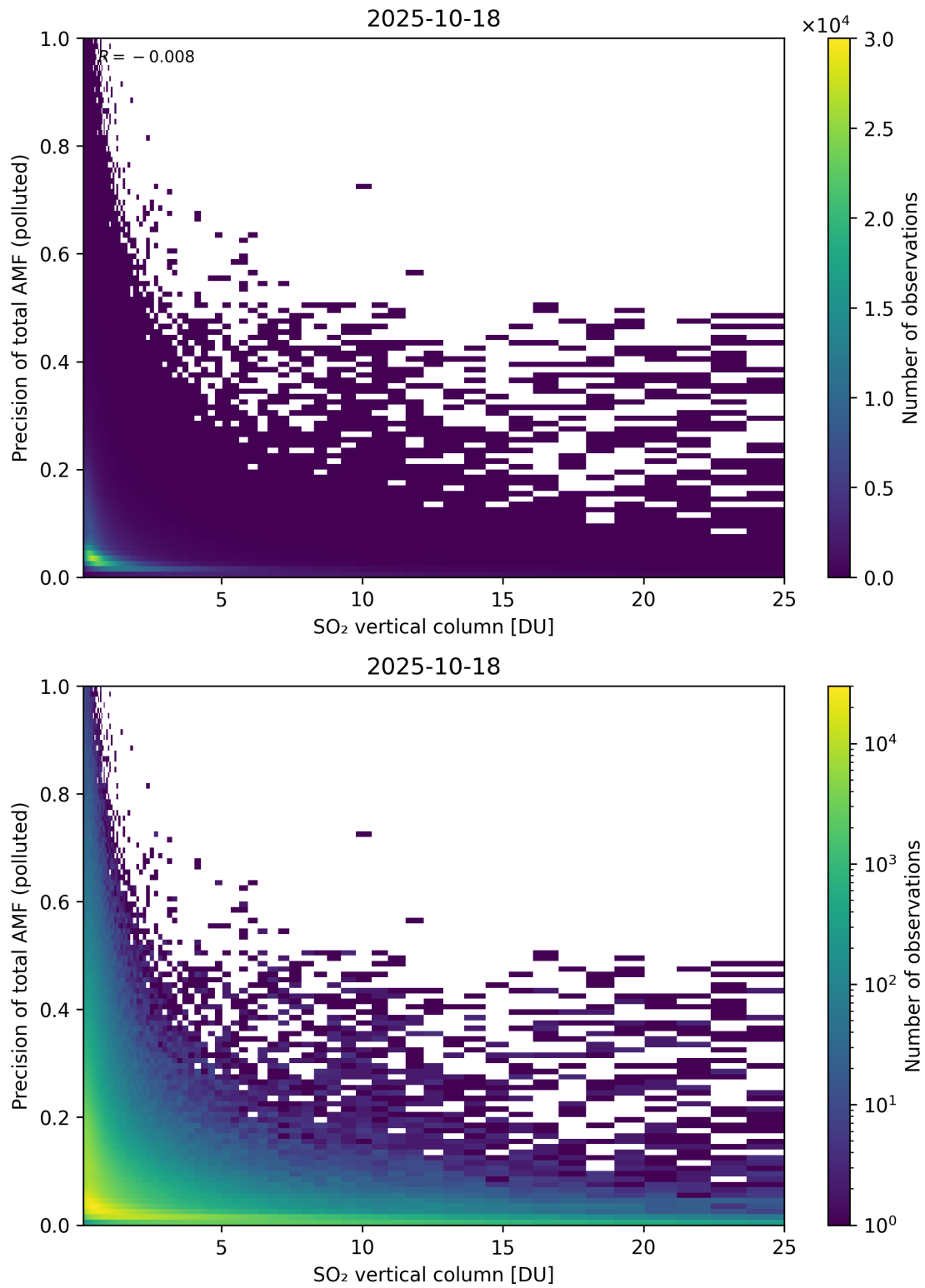
Figure 360: Scatter density plot of “SO 2 vertical column” against “Precision of total AMF (polluted)” for 2025-10-17 to 2025-10-19.
