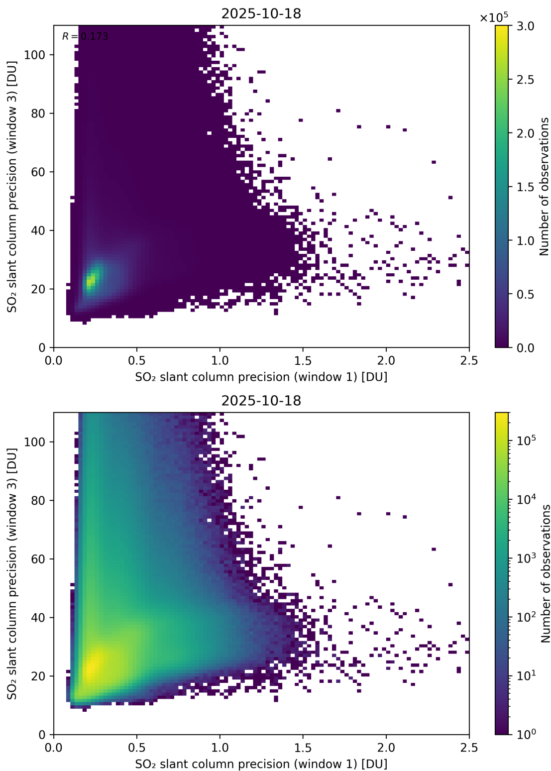
Figure 279: Scatter density plot of “SO 2 slant column precision (window 1)” against “SO 2 slant column precision (window 3)” for 2025-10-17 to 2025-10-19.
