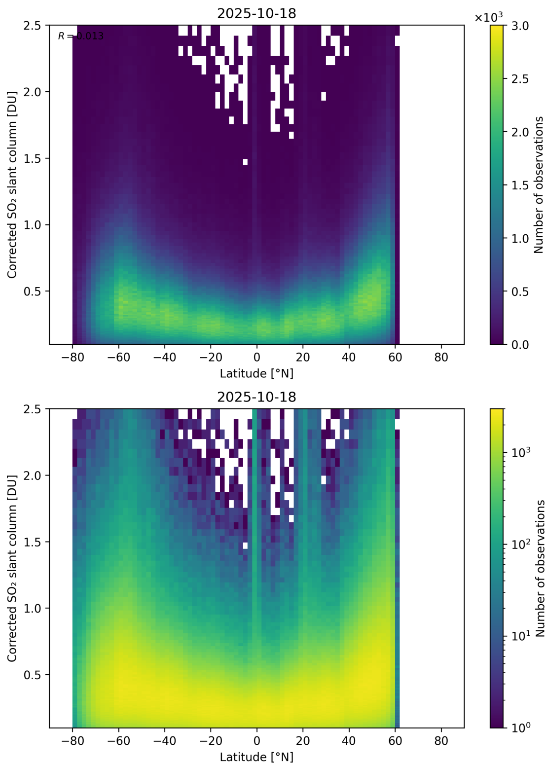
Figure 159: Scatter density plot of “Latitude” against “Corrected SO 2 slant column” for 2025-10-17 to 2025-10-19.
