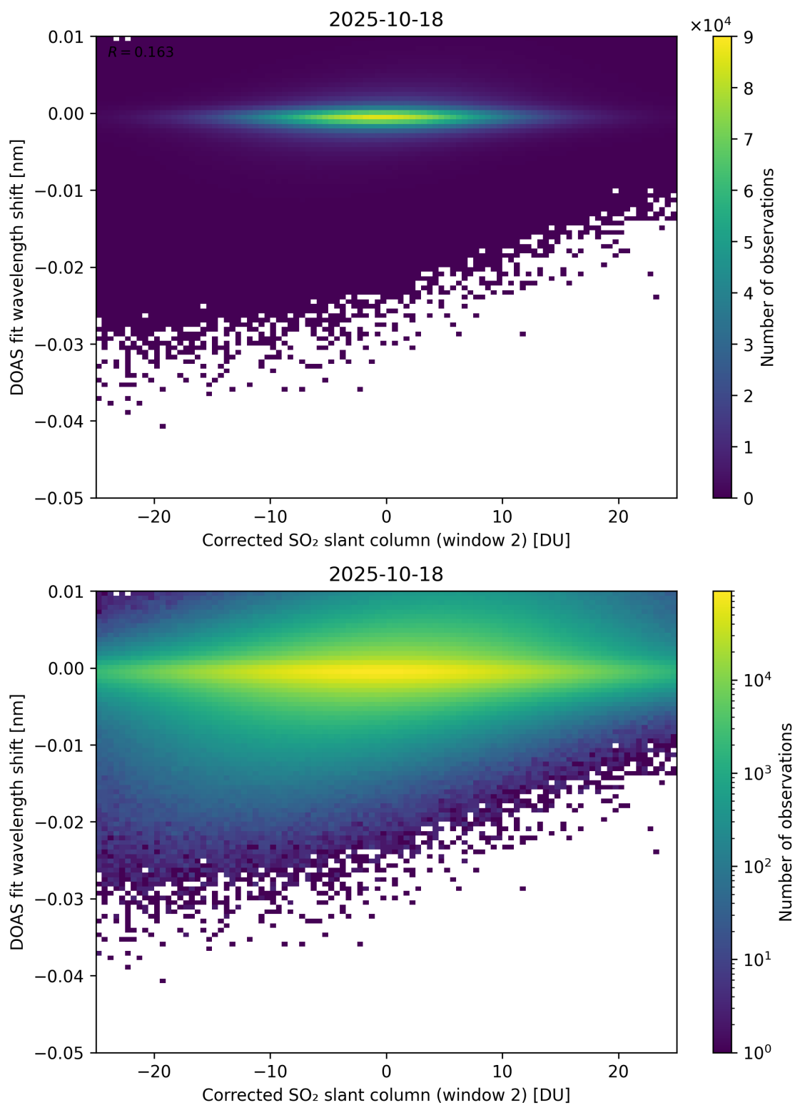
Figure 246: Scatter density plot of “Corrected SO 2 slant column (window 2)” against “DOAS fit wavelength shift” for 2025-10-17 to 2025-10-19.
