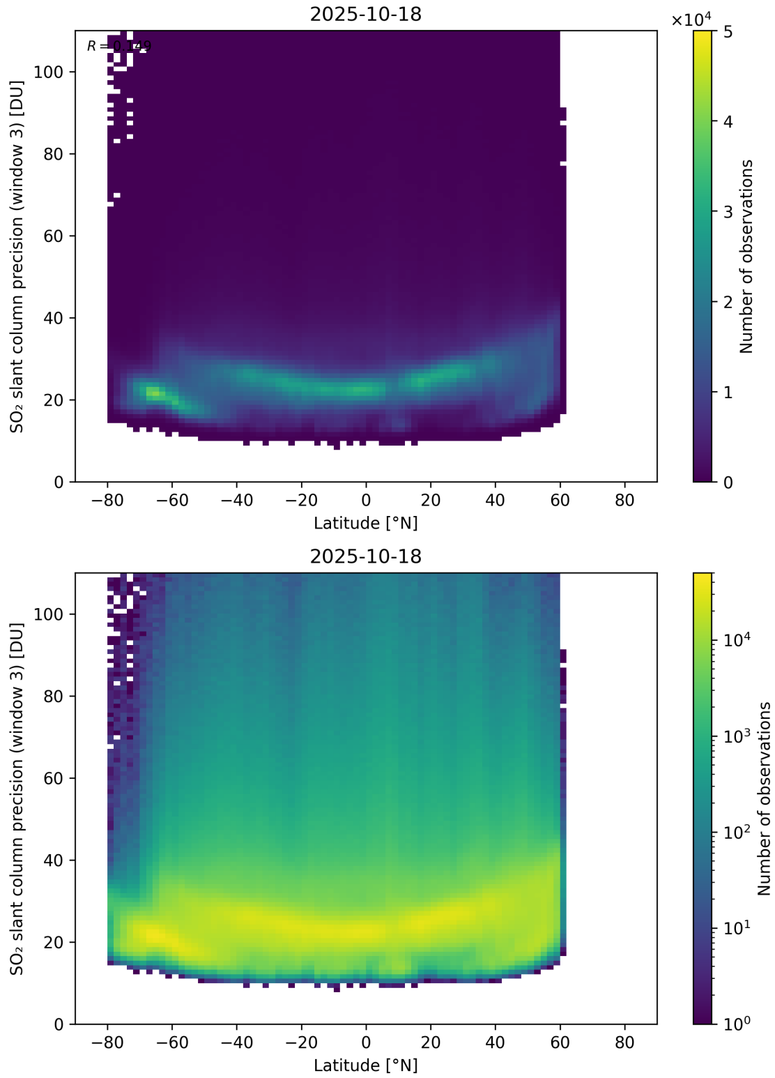
Figure 166: Scatter density plot of “Latitude” against “SO 2 slant column precision (window 3)” for 2025-10-17 to 2025-10-19.
