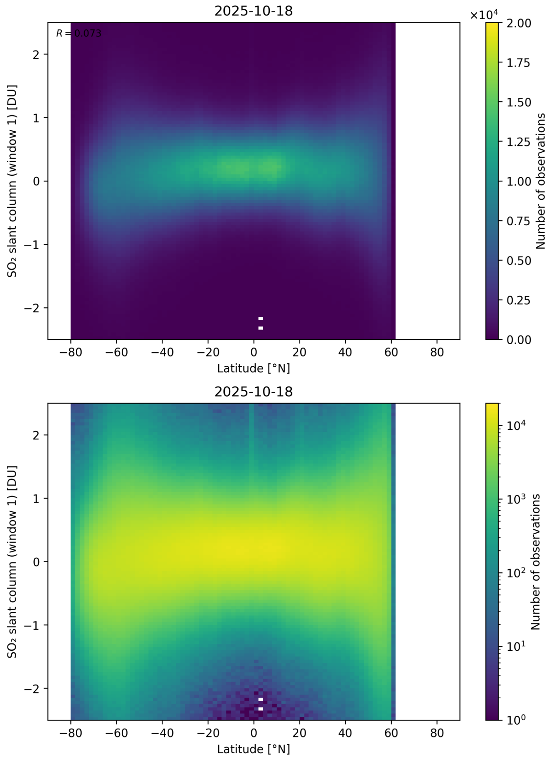
Figure 162: Scatter density plot of “Latitude” against “SO 2 slant column (window 1)” for 2025-10-17 to 2025-10-19.
