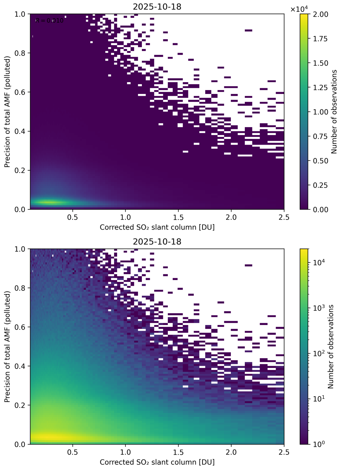
Figure 243: Scatter density plot of “Corrected SO 2 slant column” against “Precision of total AMF (polluted)” for 2025-10-17 to 2025-10-19.
