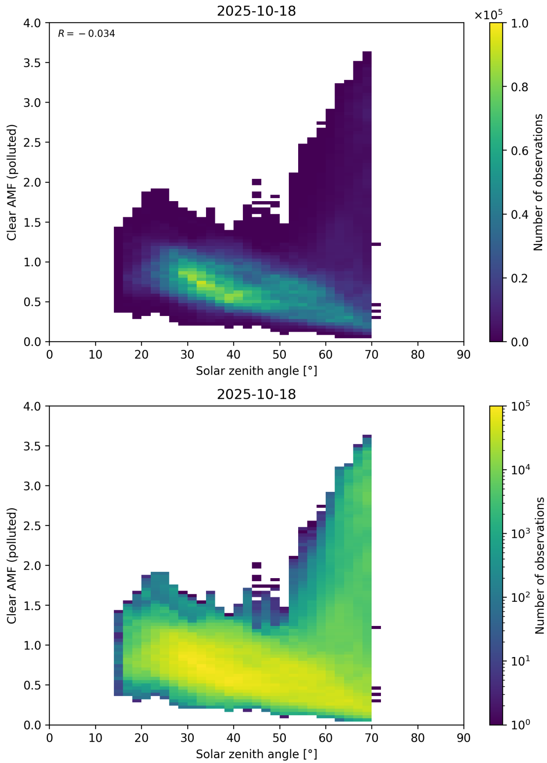
Figure 178: Scatter density plot of “Solar zenith angle” against “Clear AMF (polluted)” for 2025-10-17 to 2025-10-19.
