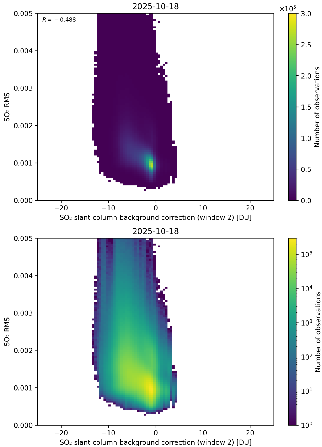
Figure 125: Scatter density plot of “SO 2 slant column background correction (window 2)” against “SO 2 RMS” for 2025-10-17 to 2025-10-19.
