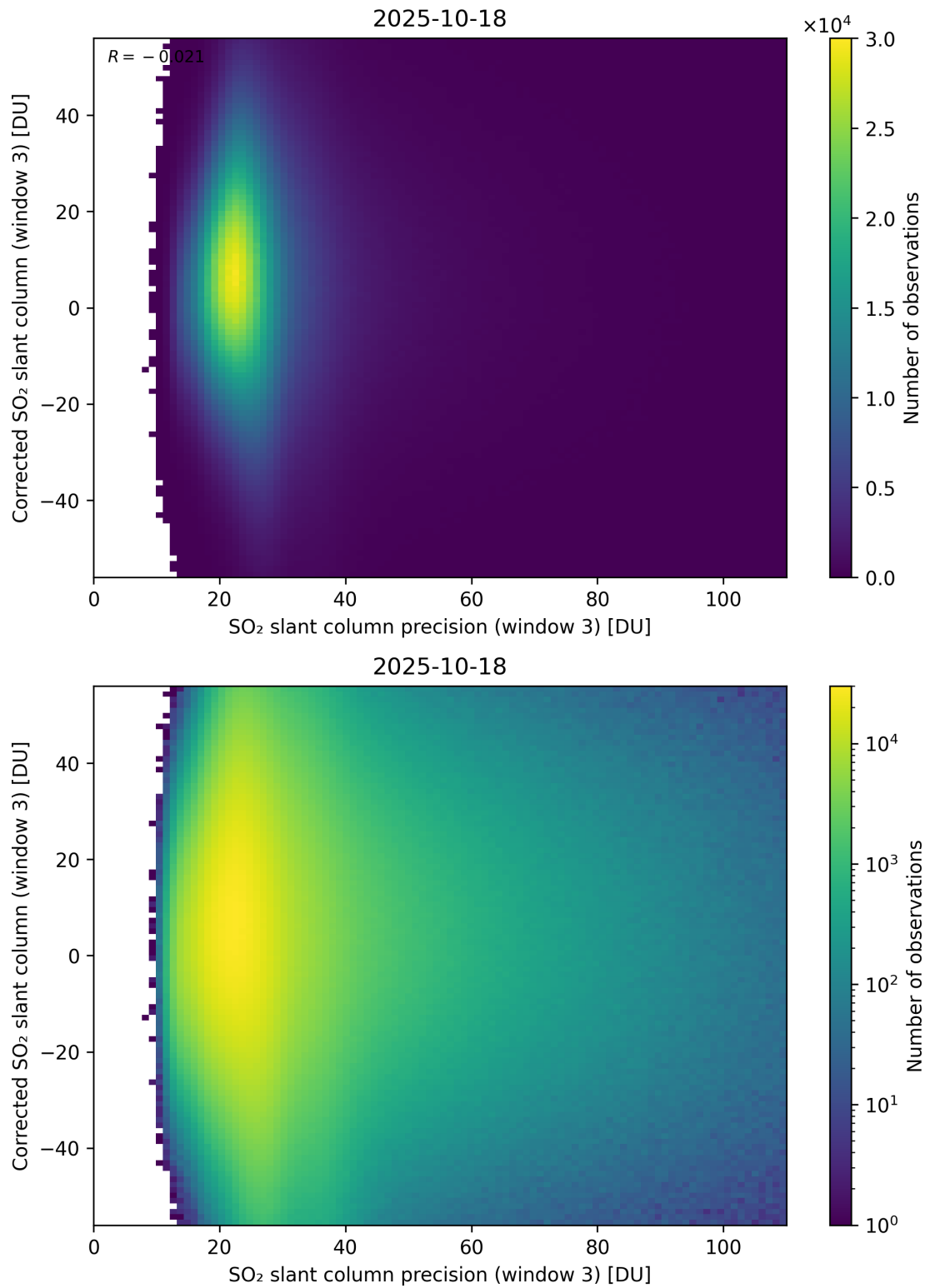
Figure 312: Scatter density plot of “SO 2 slant column precision (window 3)” against “Corrected SO 2 slant column (window 3)” for 2025-10-17 to 2025-10-19.
