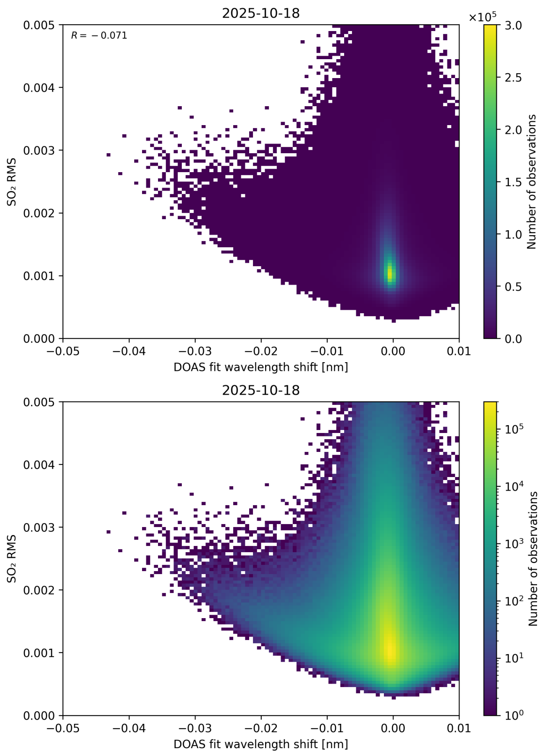
Figure 139: Scatter density plot of “DOAS fit wavelength shift” against “SO 2 RMS” for 2025-10-17 to 2025-10-19.
