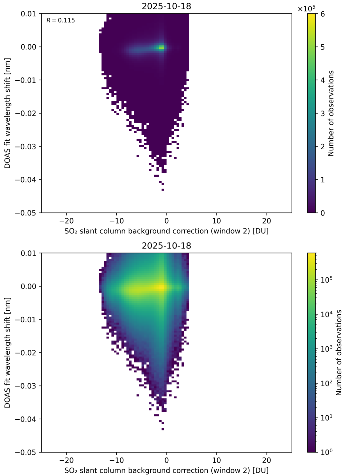
Figure 123: Scatter density plot of “SO 2 slant column background correction (window 2)” against “DOAS fit wavelength shift” for 2025-10-17 to 2025-10-19.
