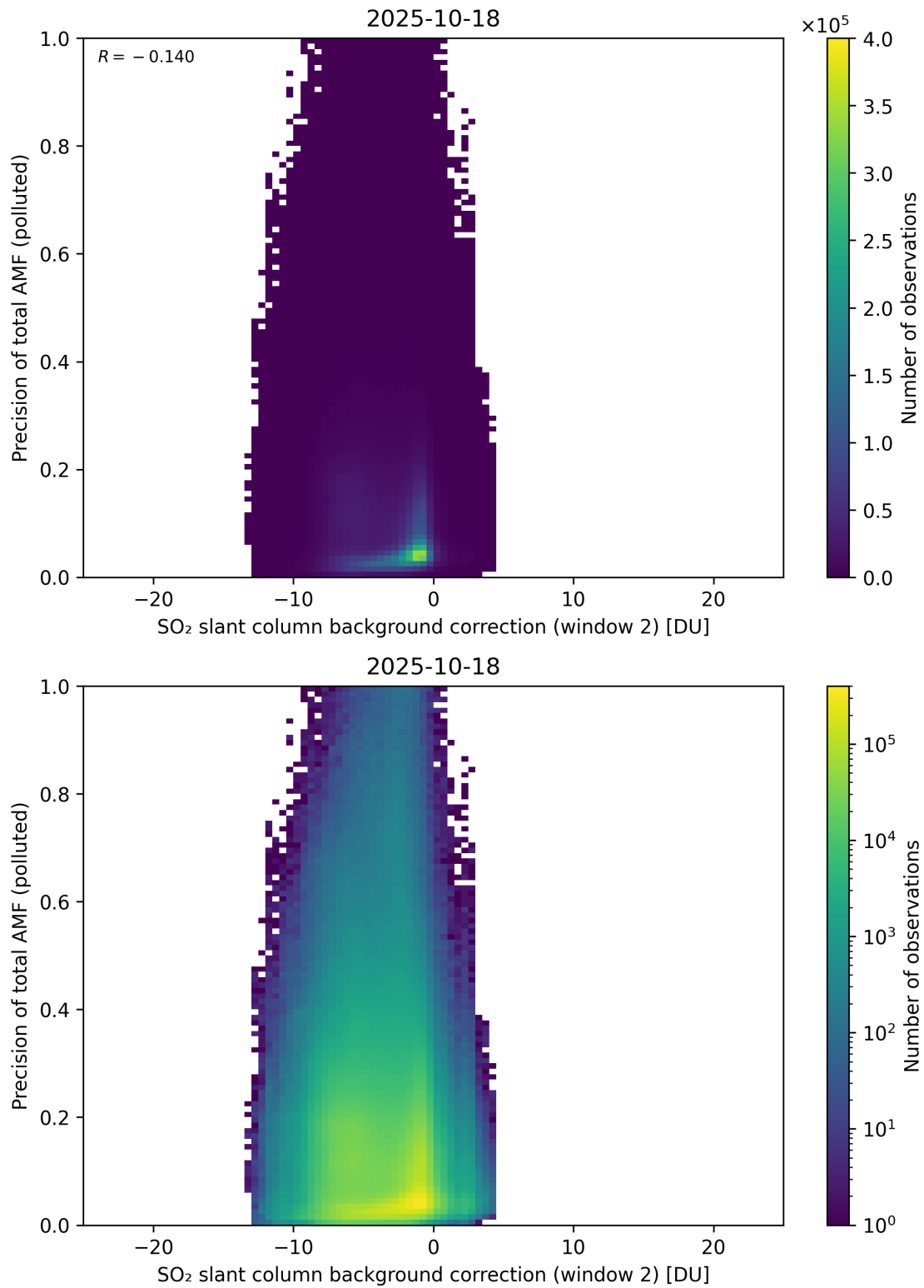
Figure 131: Scatter density plot of “SO 2 slant column background correction (window 2)” against “Precision of total AMF (polluted)” for 2025-10-17 to 2025-10-19.
