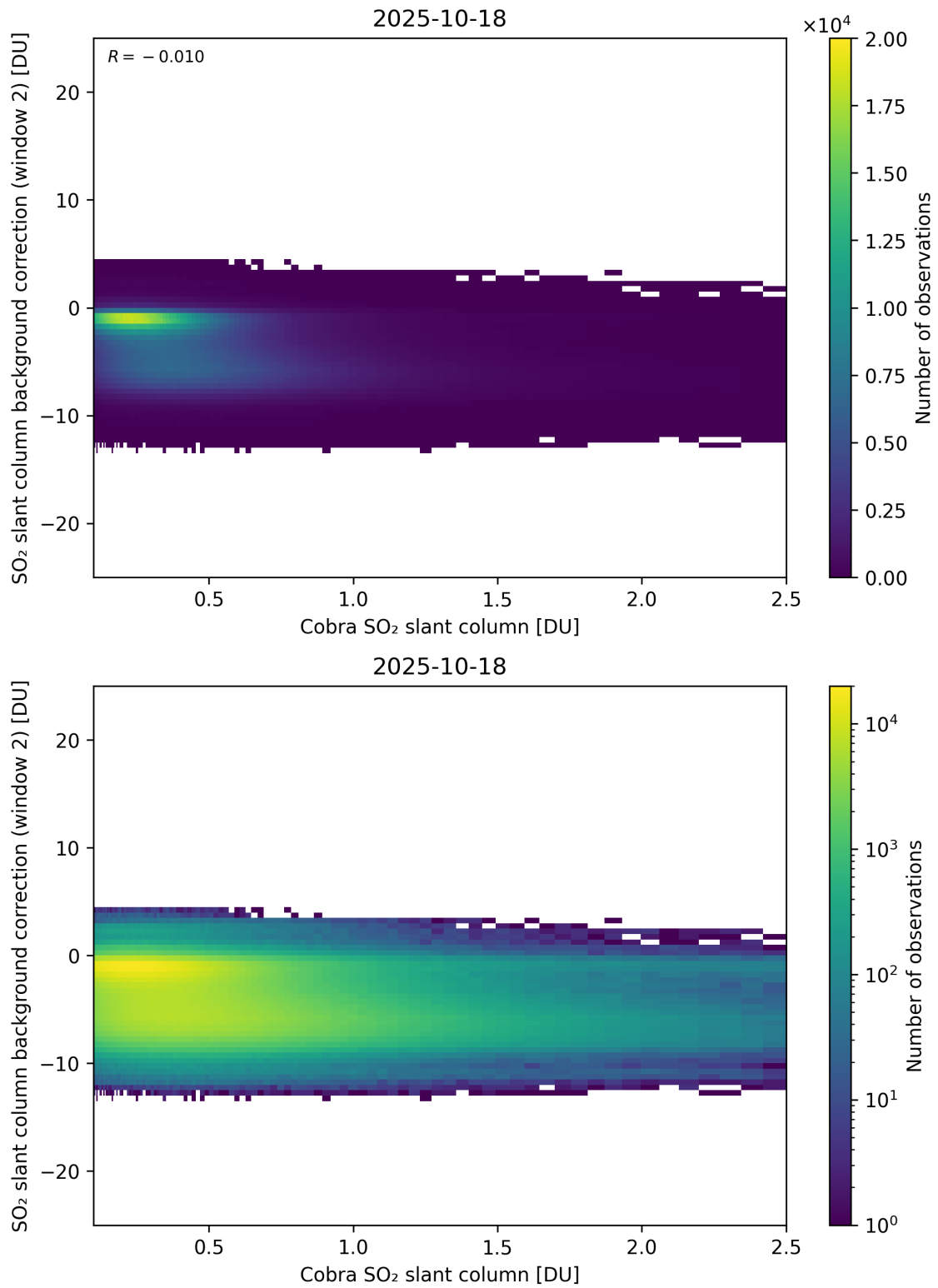
Figure 194: Scatter density plot of “Cobra SO 2 slant column” against “SO 2 slant column background correction (window 2)” for 2025-10-17 to 2025-10-19.
