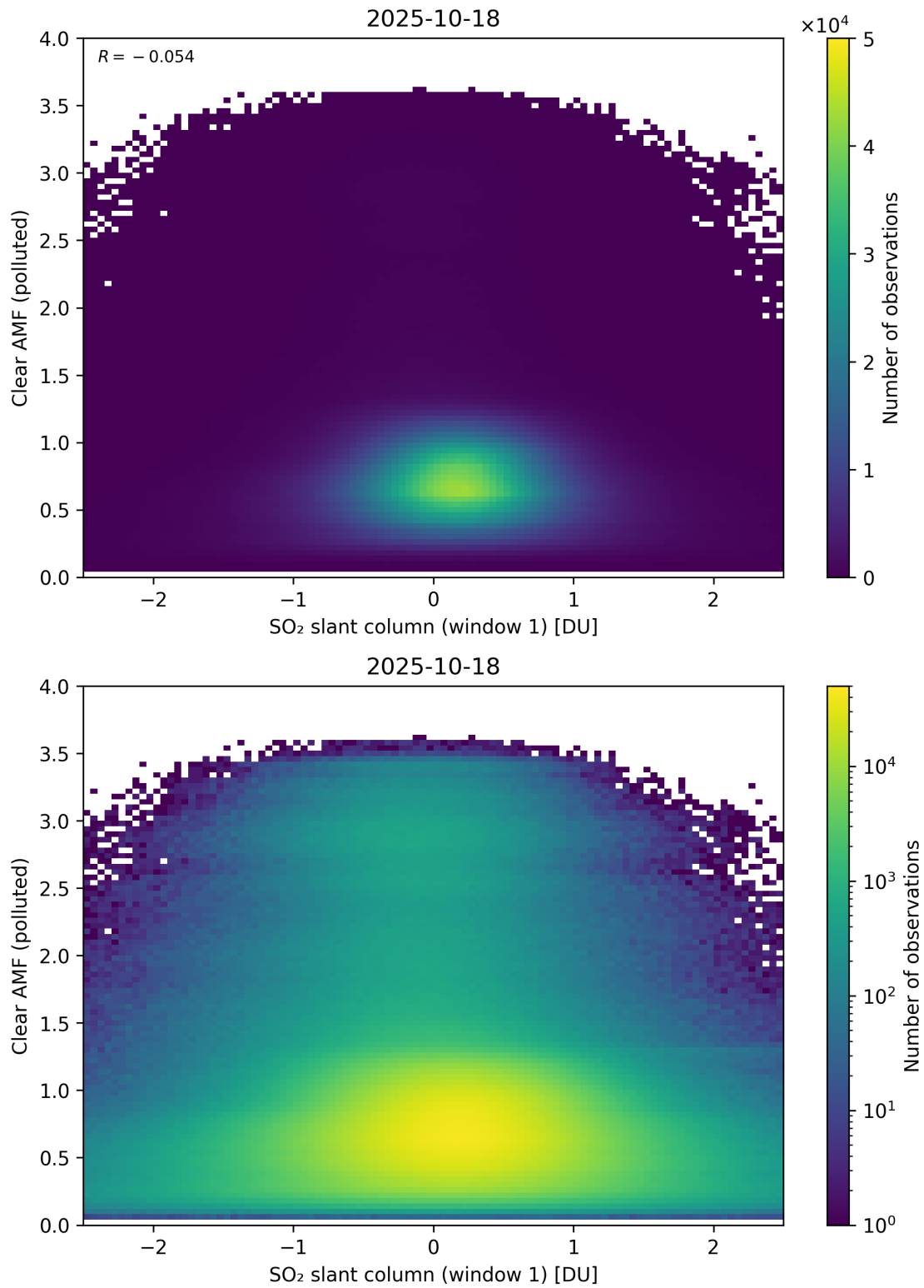
Figure 282: Scatter density plot of “SO 2 slant column (window 1)” against “Clear AMF (polluted)” for 2025-10-17 to 2025-10-19.
