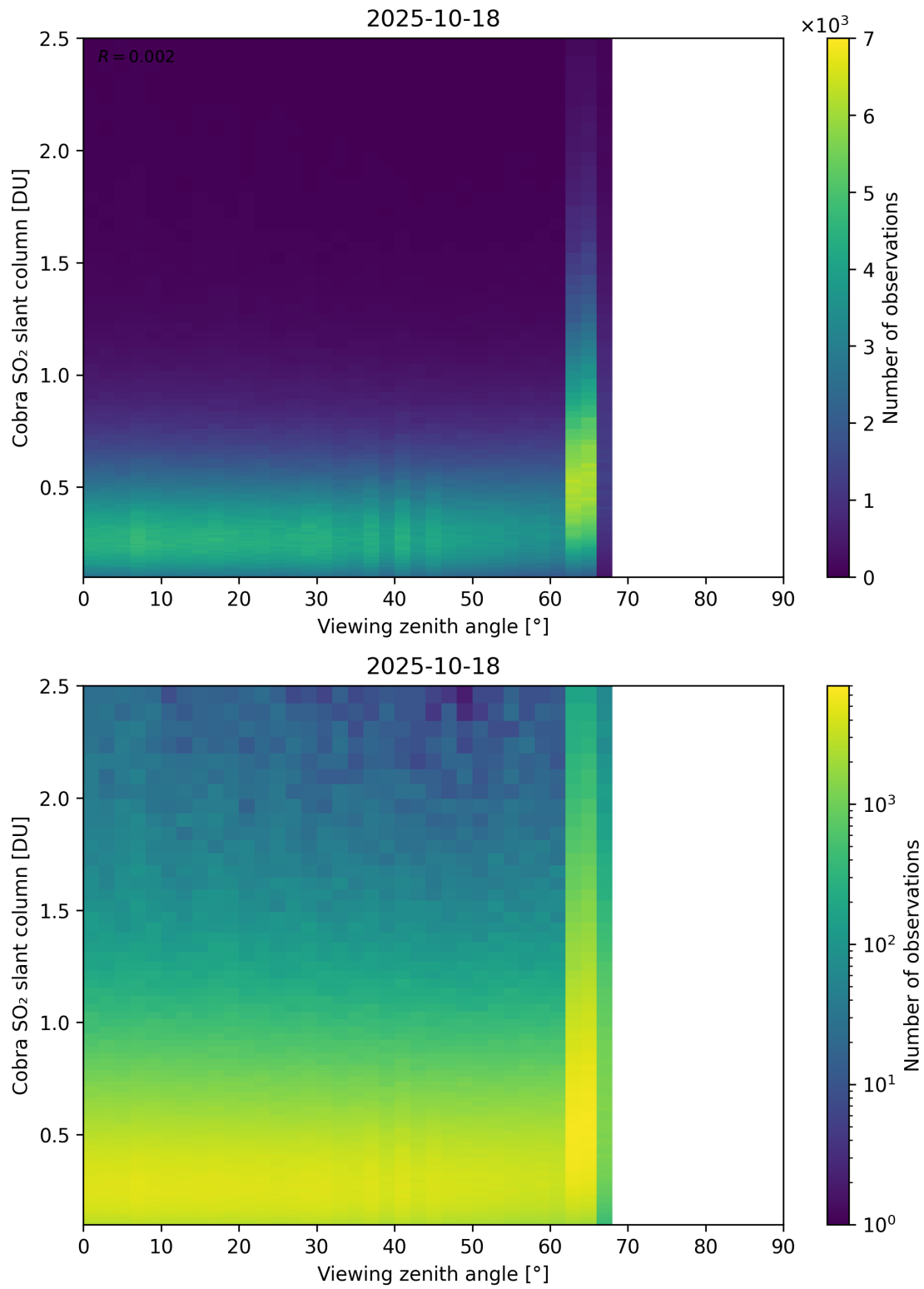
Figure 371: Scatter density plot of “Viewing zenith angle” against “Cobra SO 2 slant column” for 2025-10-17 to 2025-10-19.
