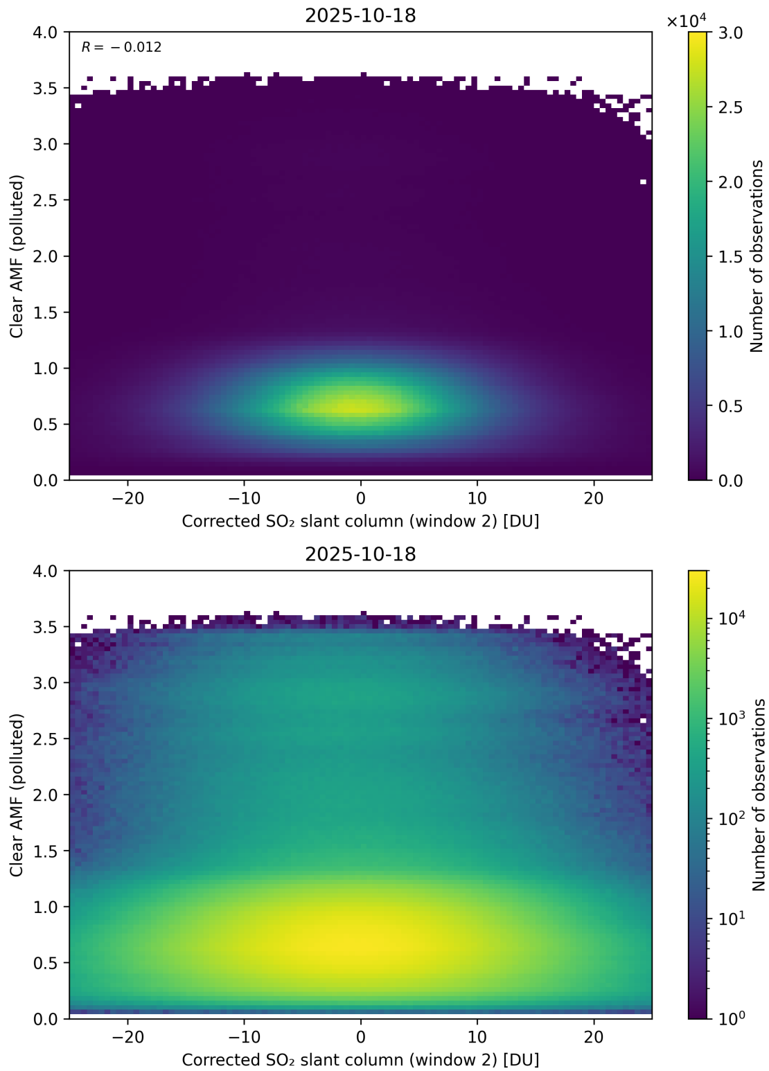
Figure 249: Scatter density plot of “Corrected SO 2 slant column (window 2)” against “Clear AMF (polluted)” for 2025-10-17 to 2025-10-19.
