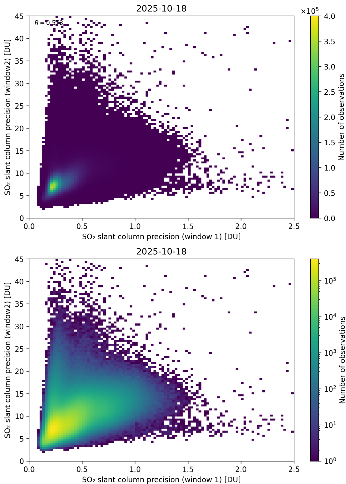
Figure 277: Scatter density plot of “SO 2 slant column precision (window 1)” against “SO 2 slant column precision (window2)” for 2025-10-17 to 2025-10-19.
