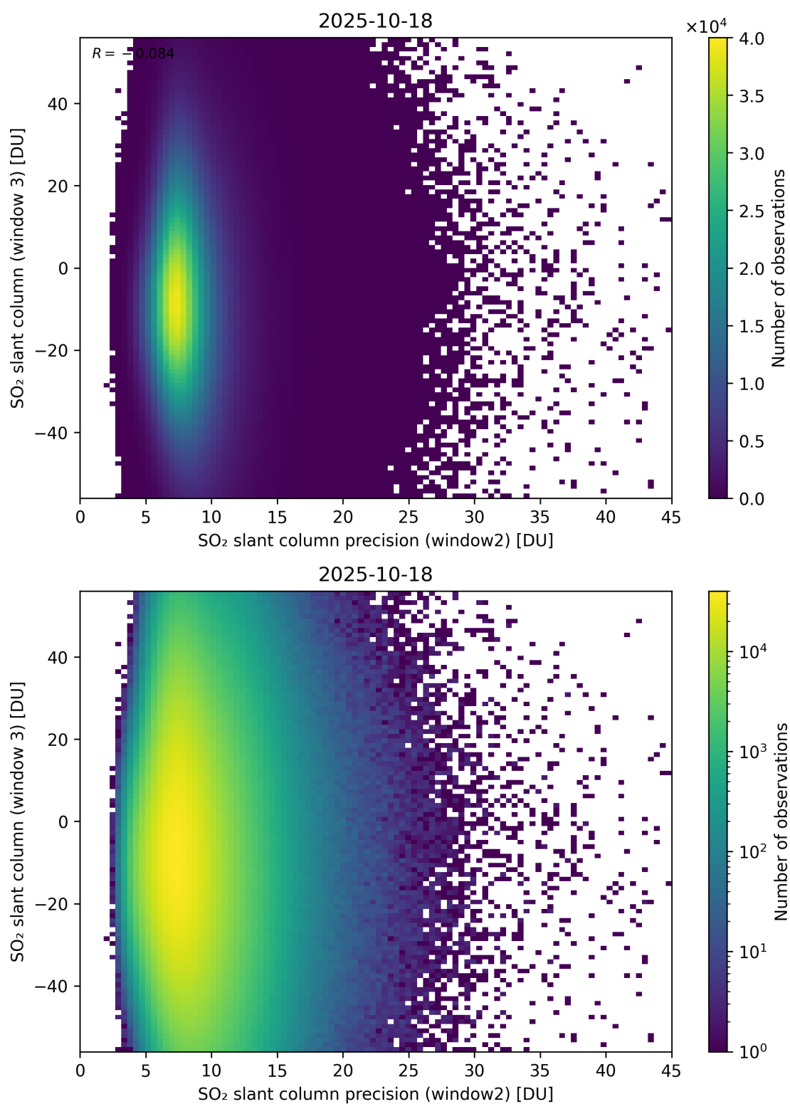
Figure 299: Scatter density plot of “SO 2 slant column precision (window2)” against “SO 2 slant column (window 3)” for 2025-10-17 to 2025-10-19.
