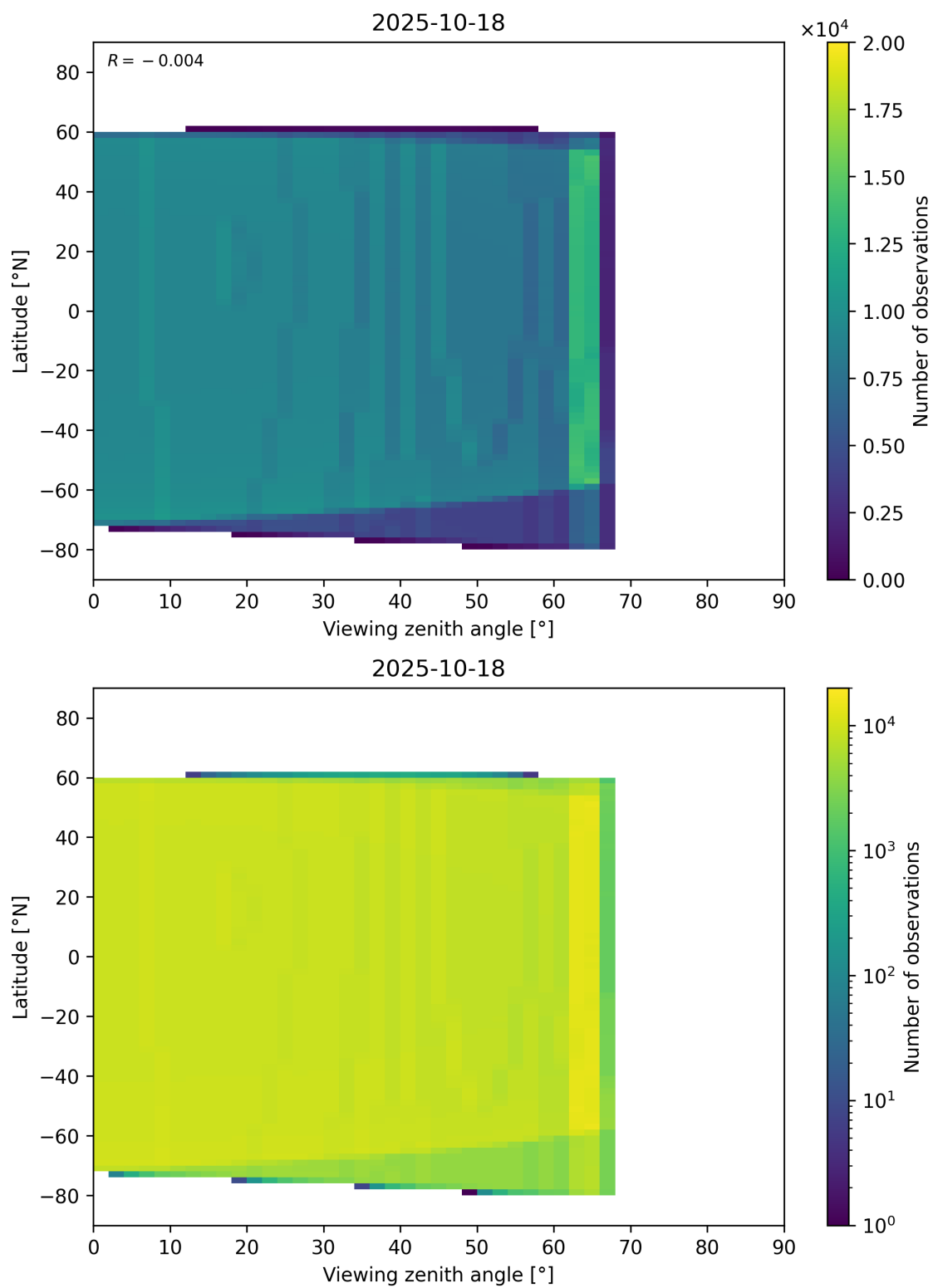
Figure 368: Scatter density plot of “Viewing zenith angle” against “Latitude” for 2025-10-17 to 2025-10-19.
