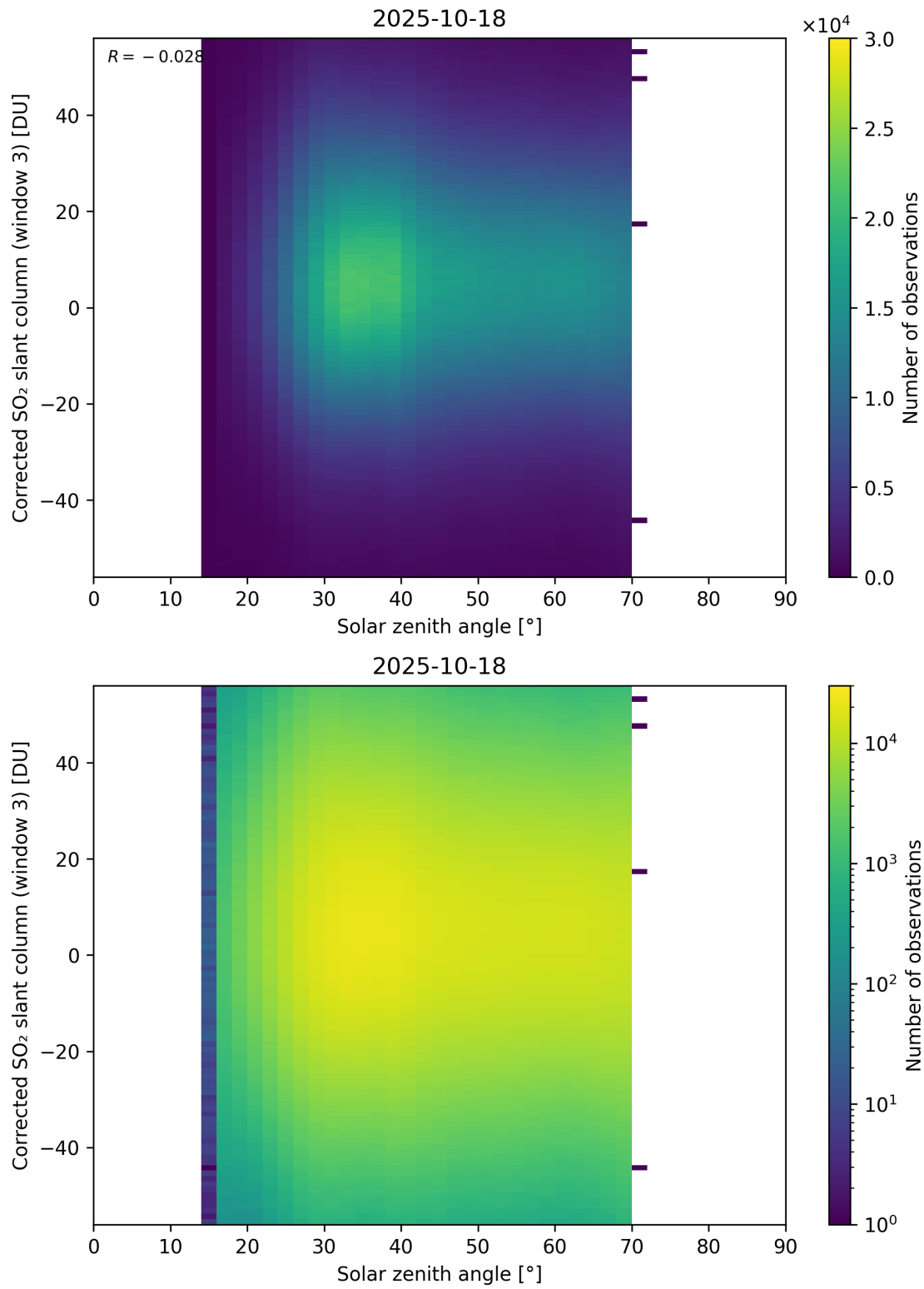
Figure 183: Scatter density plot of “Solar zenith angle” against “Corrected SO 2 slant column (window 3)” for 2025-10-17 to 2025-10-19.
