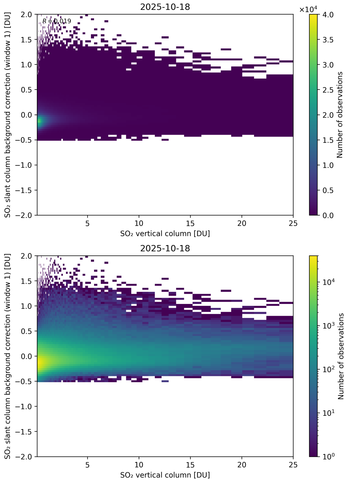
Figure 323: Scatter density plot of “SO 2 vertical column” against “SO 2 slant column background correction (window 1)” for 2025-10-17 to 2025-10-19.
