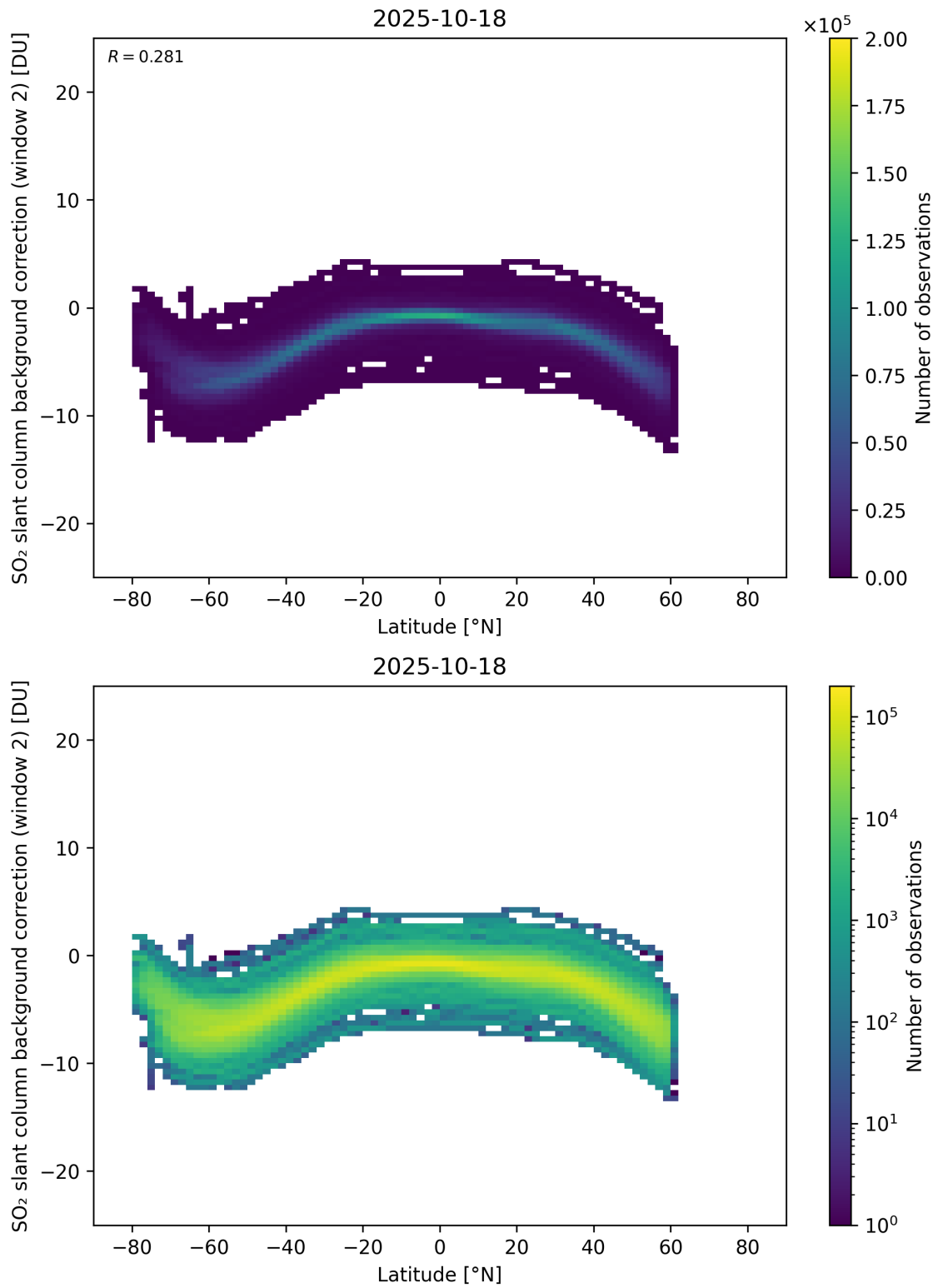
Figure 151: Scatter density plot of “Latitude” against “SO 2 slant column background correction (window 2)” for 2025-10-17 to 2025-10-19.
