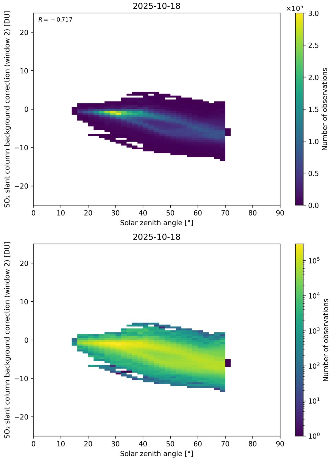
Figure 172: Scatter density plot of “Solar zenith angle” against “SO 2 slant column background correction (window 2)” for 2025-10-17 to 2025-10-19.
