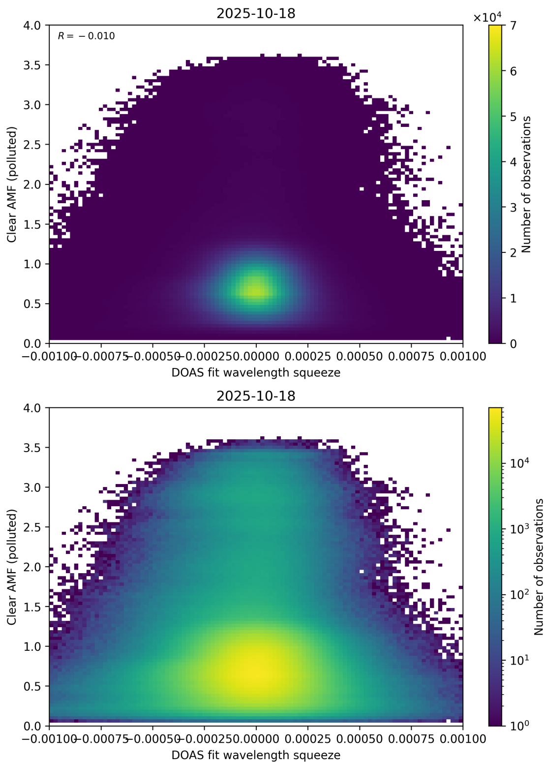
Figure 144: Scatter density plot of “DOAS fit wavelength squeeze” against “Clear AMF (polluted)” for 2025-10-17 to 2025-10-19.
