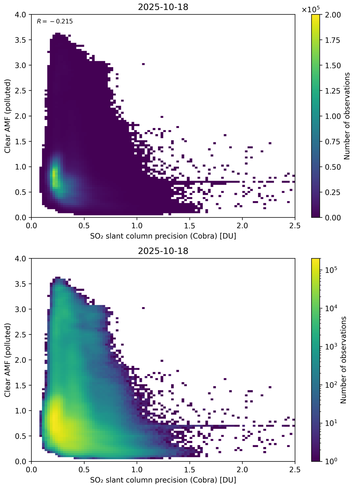
Figure 205: Scatter density plot of “SO 2 slant column precision (Cobra)” against “Clear AMF (polluted)” for 2025-10-17 to 2025-10-19.
