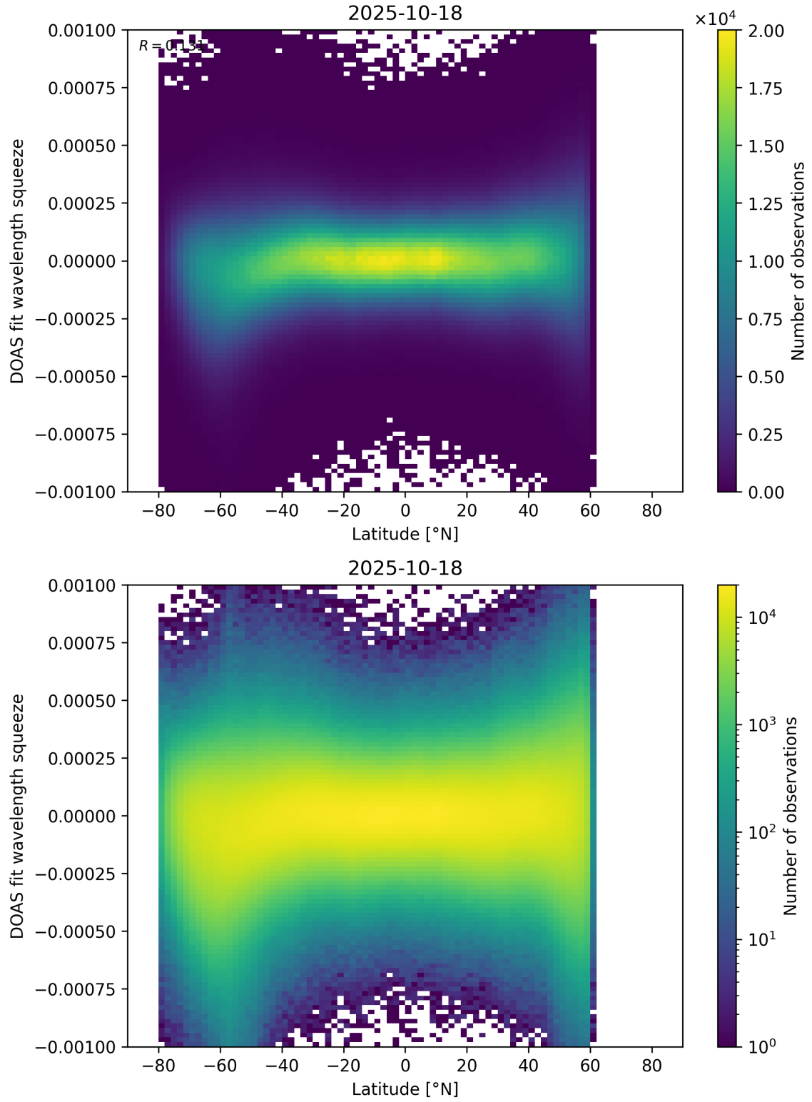
Figure 154: Scatter density plot of “Latitude” against “DOAS fit wavelength squeeze” for 2025-10-17 to 2025-10-19.
