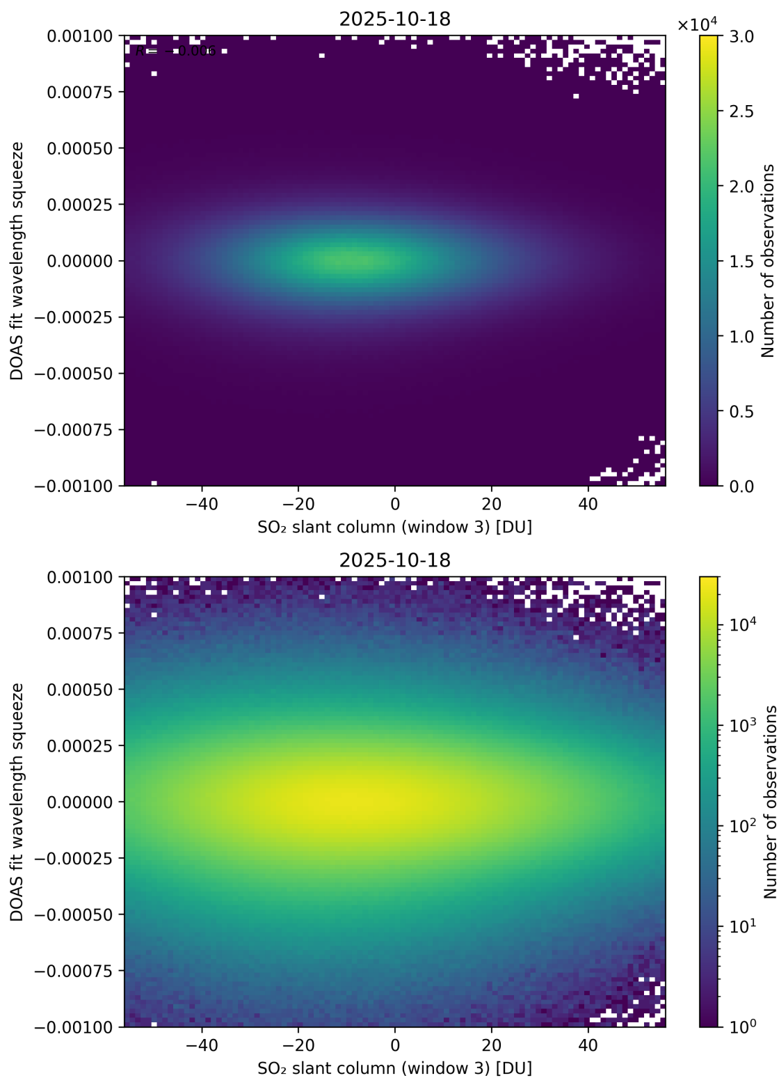
Figure 305: Scatter density plot of “SO 2 slant column (window 3)” against “DOAS fit wavelength squeeze” for 2025-10-17 to 2025-10-19.
