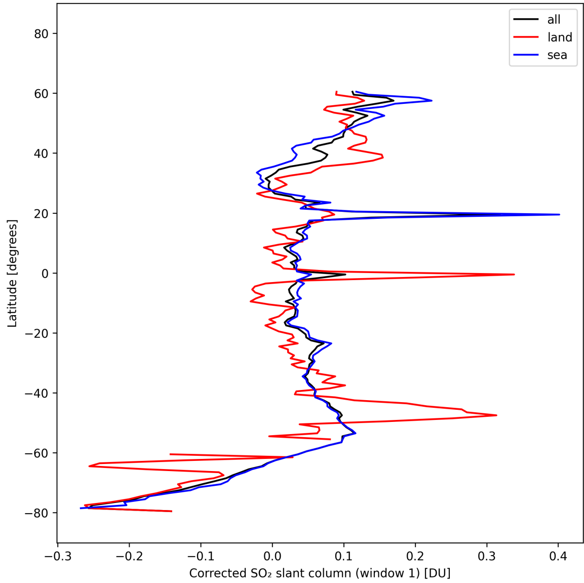
Figure 39: Zonal average of “Corrected SO 2 slant column (window 1)” for 2025-10-17 to 2025-10-19.
