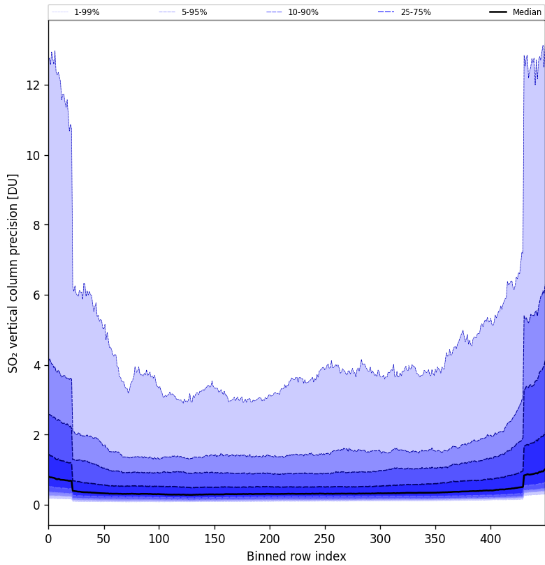
Figure 85: Along track statistics of “SO 2 vertical column precision” for 2025-10-17 to 2025-10-19
