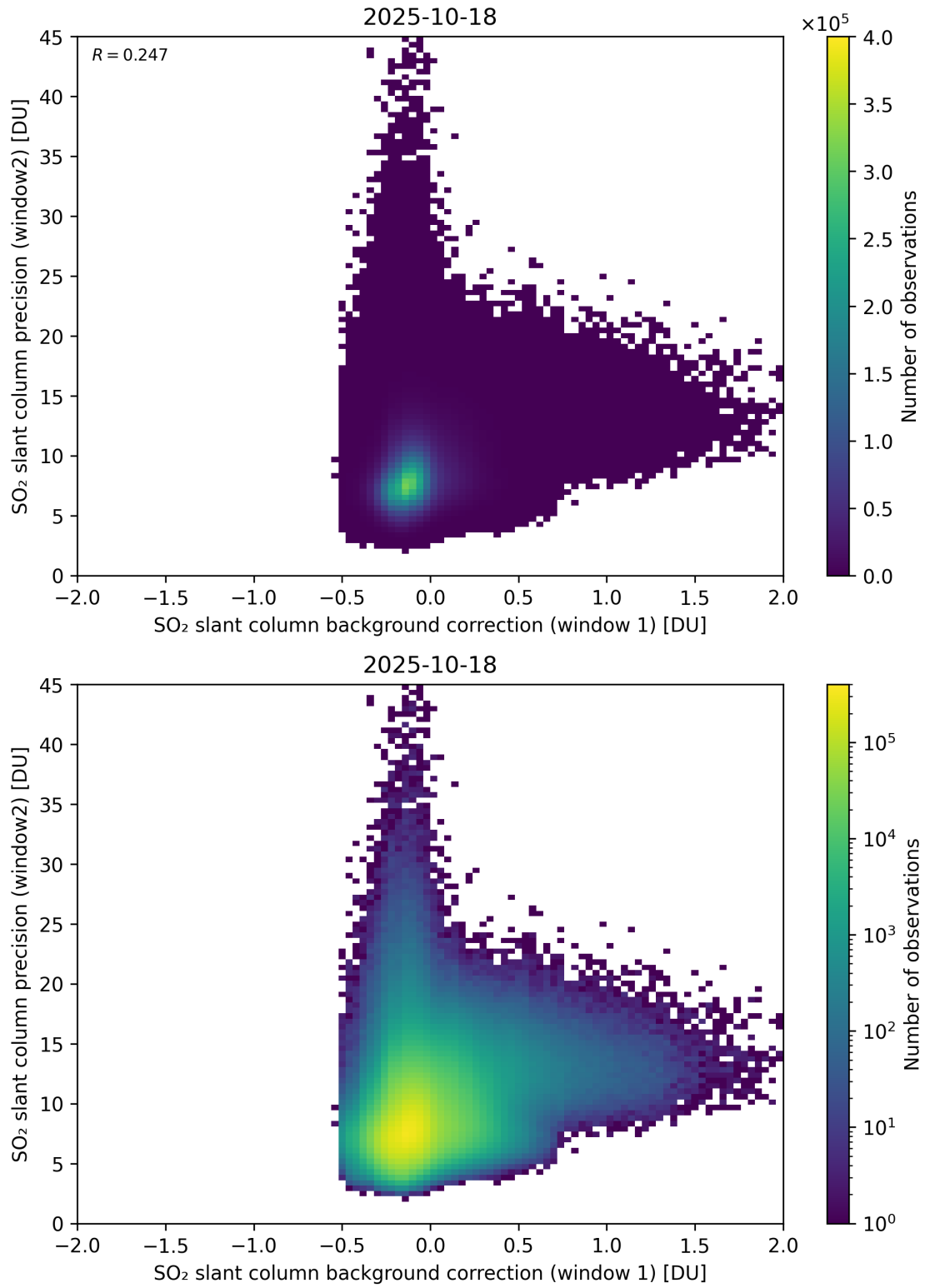
Figure 117: Scatter density plot of “SO 2 slant column background correction (window 1)” against “SO 2 slant column precision (window2)” for 2025-10-17 to 2025-10-19.
