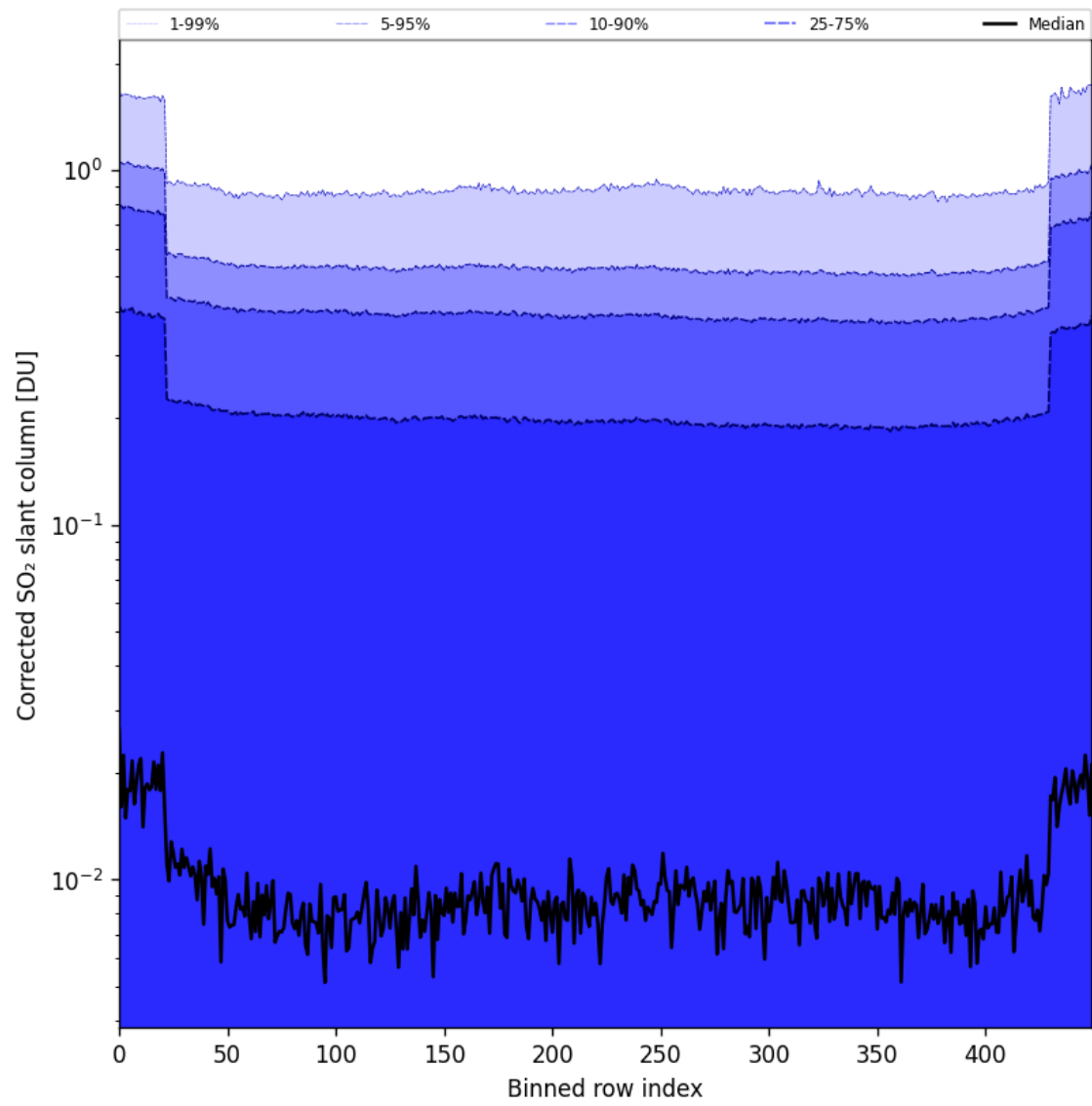
Figure 86: Along track statistics of "Corrected SO 2 slant column" for 2025-10-17 to 2025-10-19
