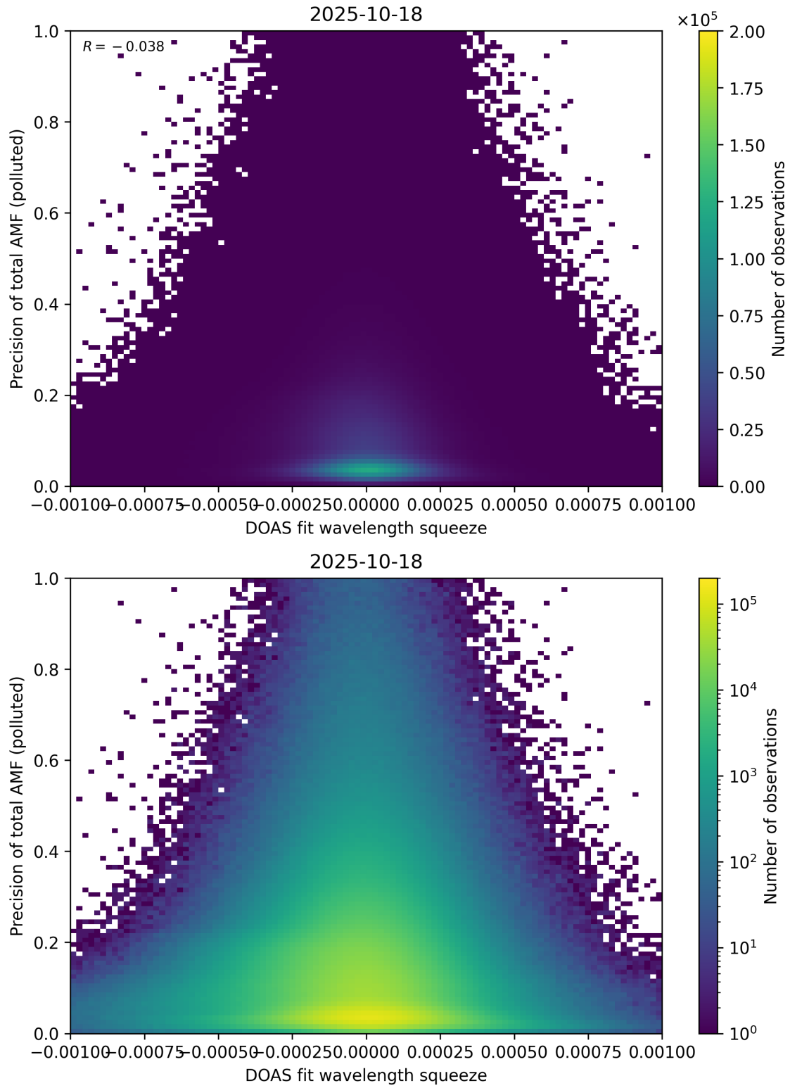
Figure 146: Scatter density plot of “DOAS fit wavelength squeeze” against “Precision of total AMF (polluted)” for 2025-10-17 to 2025-10-19.
