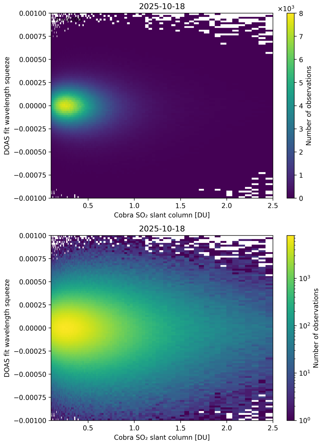
Figure 197: Scatter density plot of “Cobra SO 2 slant column” against “DOAS fit wavelength squeeze” for 2025-10-17 to 2025-10-19.
