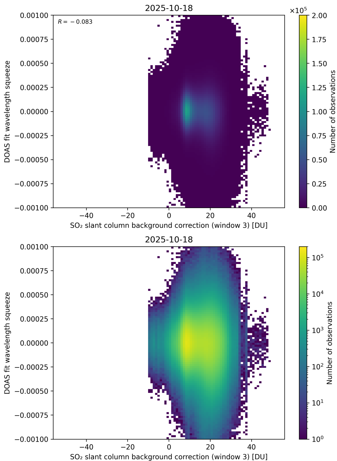
Figure 133: Scatter density plot of “SO 2 slant column background correction (window 3)” against “DOAS fit wavelength squeeze” for 2025-10-17 to 2025-10-19.
