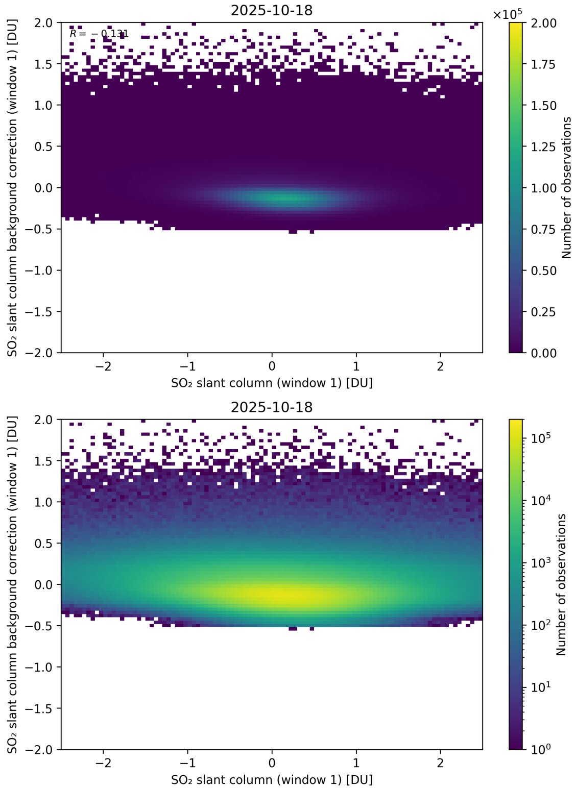
Figure 262: Scatter density plot of “SO 2 slant column (window 1)” against “SO 2 slant column background correction (window 1)” for 2025-10-17 to 2025-10-19.
