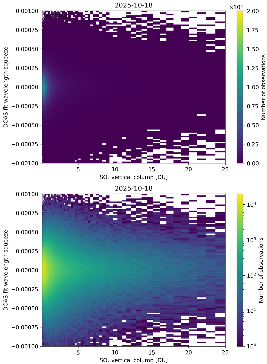
Figure 327: Scatter density plot of “SO 2 vertical column” against “DOAS fit wavelength squeeze” for 2025-10-17 to 2025-10-19.
