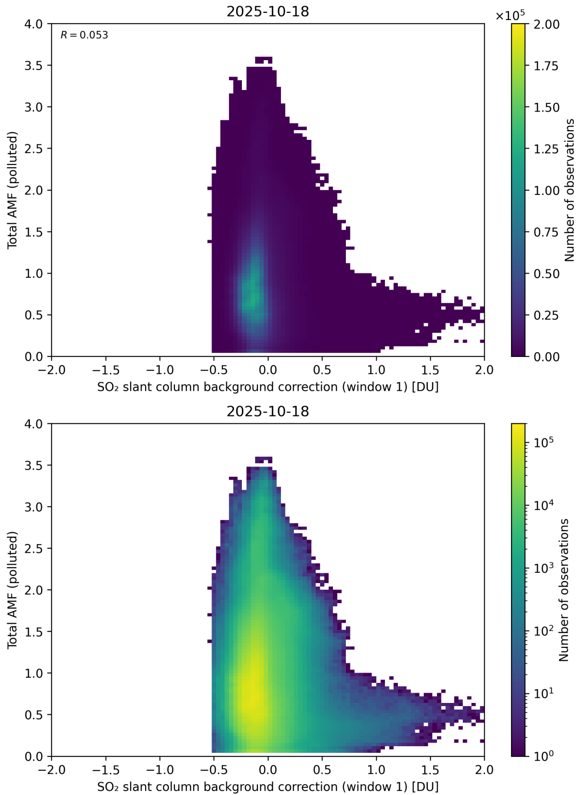
Figure 120: Scatter density plot of “SO 2 slant column background correction (window 1)” against “Total AMF (polluted)” for 2025-10-17 to 2025-10-19.
