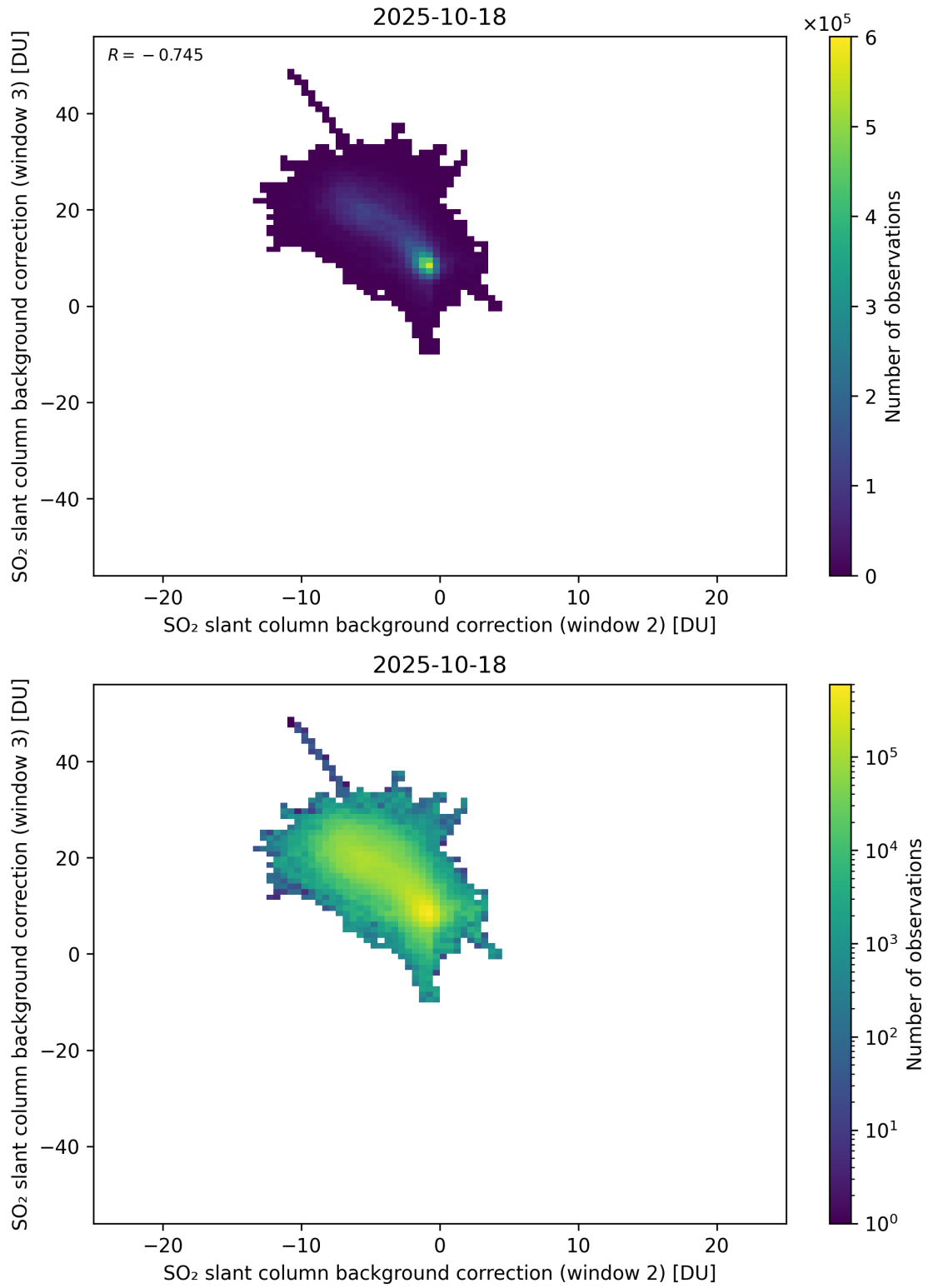
Figure 122: Scatter density plot of “SO 2 slant column background correction (window 2)” against “SO 2 slant column background correction (window 3)” for 2025-10-17 to 2025-10-19.
