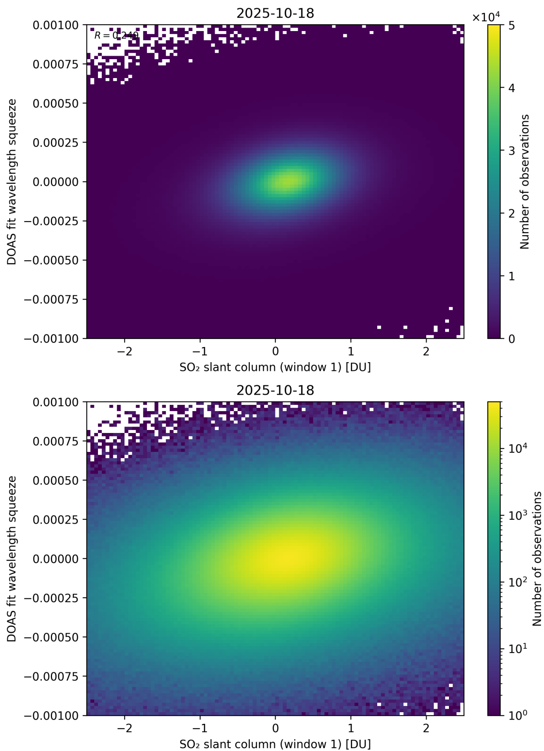
Figure 266: Scatter density plot of “SO 2 slant column (window 1)” against “DOAS fit wavelength squeeze” for 2025-10-17 to 2025-10-19.
