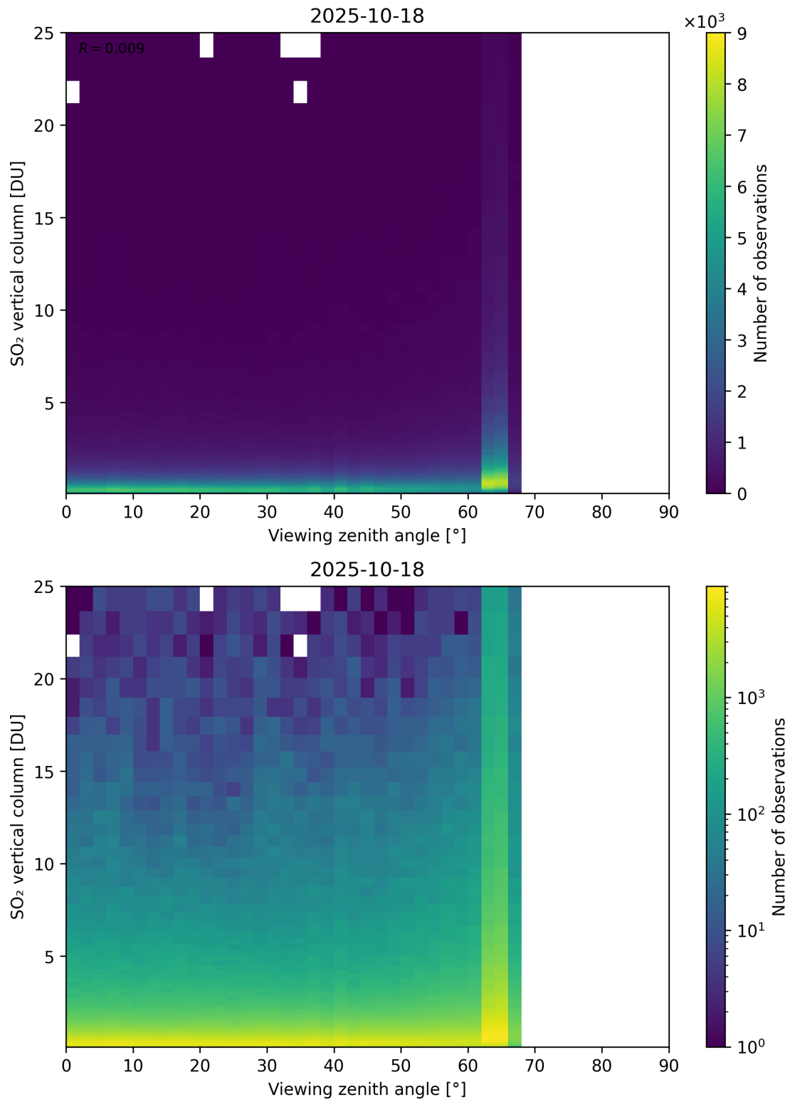
Figure 383: Scatter density plot of “Viewing zenith angle” against “SO 2 vertical column” for 2025-10-17 to 2025-10-19.
