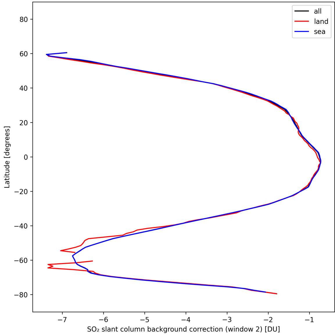
Figure 44: Zonal average of “SO 2 slant column background correction (window 2)” for 2025-10-17 to 2025-10-19.
