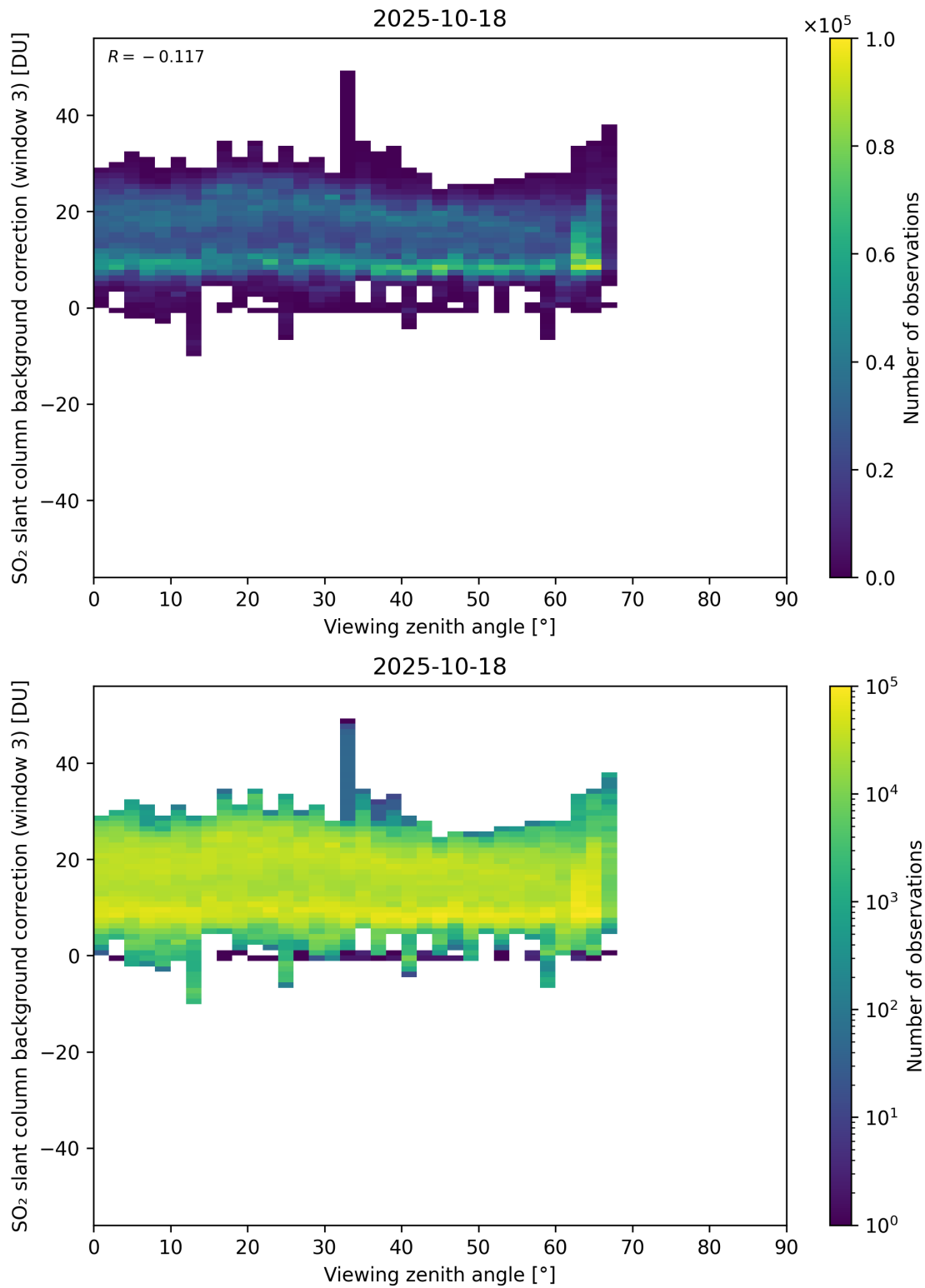
Figure 364: Scatter density plot of “Viewing zenith angle” against “SO 2 slant column background correction (window 3)” for 2025-10-17 to 2025-10-19.
