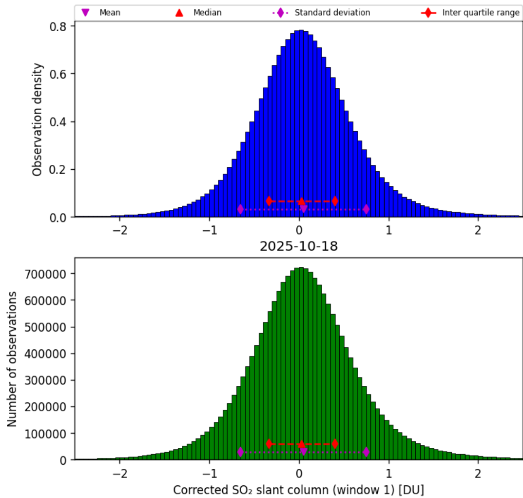
Figure 65: Histogram of “Corrected SO 2 slant column (window 1)” for 2025-10-17 to 2025-10-19
