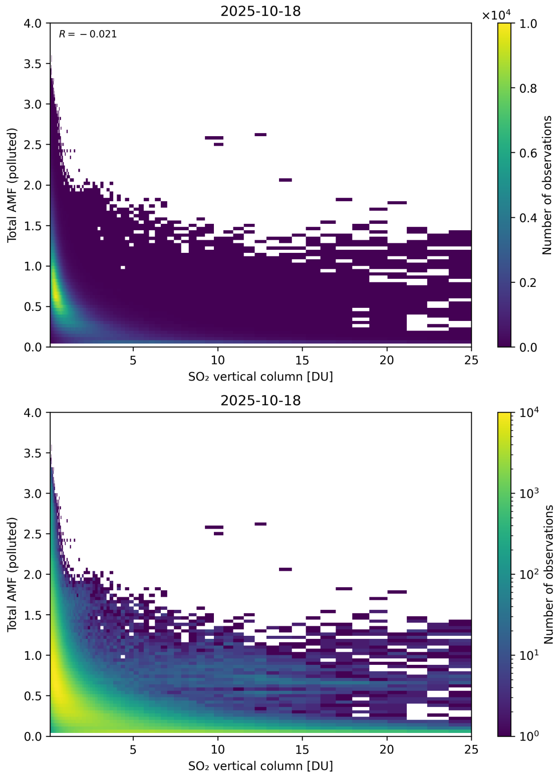
Figure 359: Scatter density plot of “SO 2 vertical column” against “Total AMF (polluted)” for 2025-10-17 to 2025-10-19.
