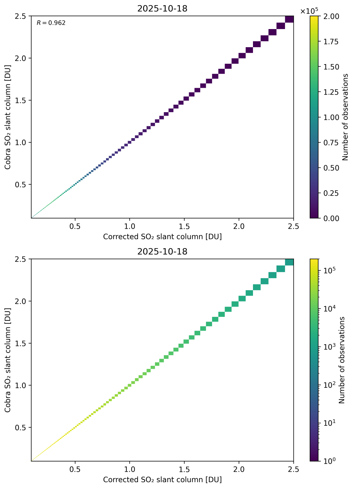
Figure 233: Scatter density plot of “Corrected SO 2 slant column” against “Cobra SO 2 slant column” for 2025-10-17 to 2025-10-19.
