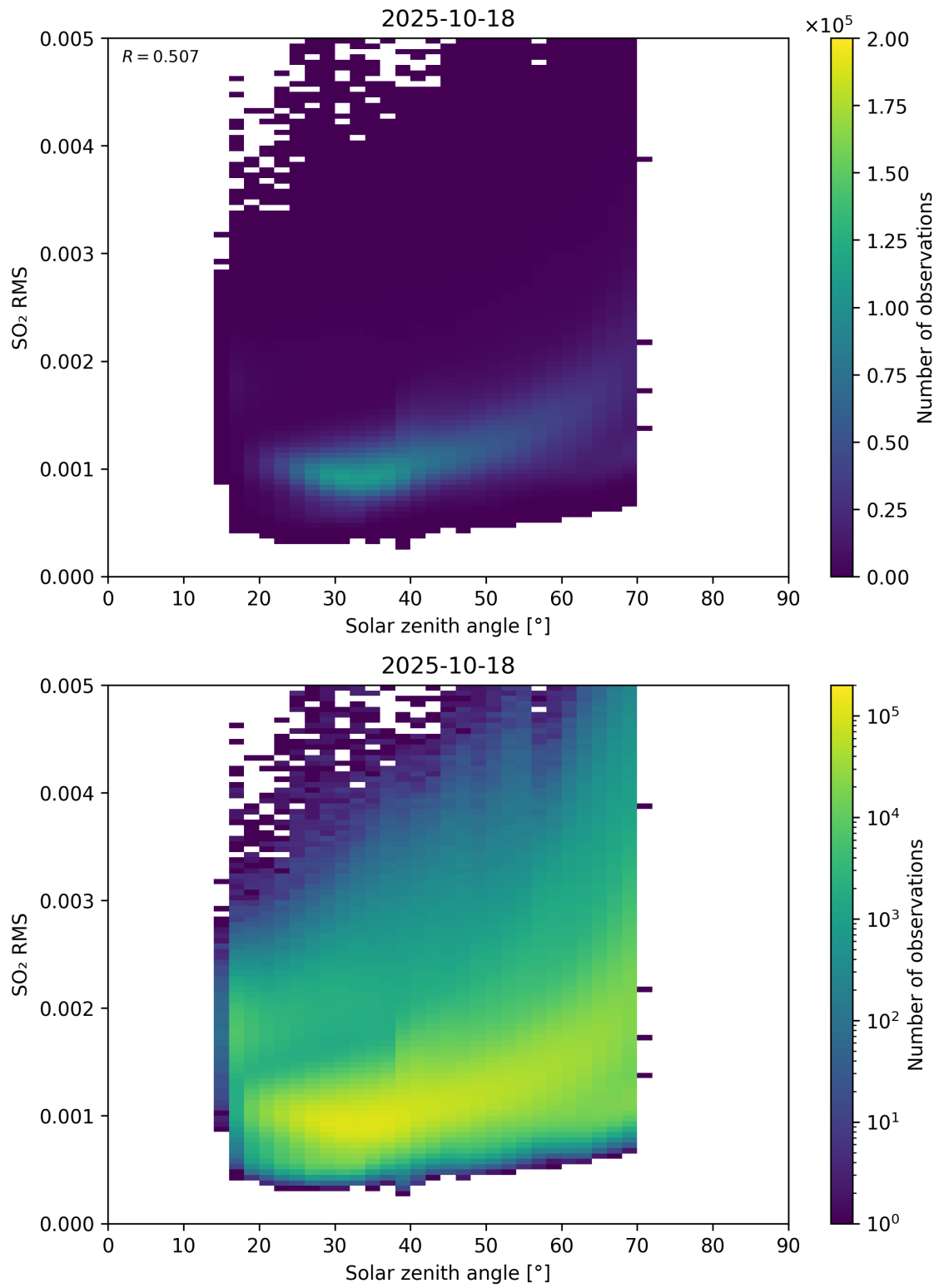
Figure 176: Scatter density plot of “Solar zenith angle” against “SO 2 RMS” for 2025-10-17 to 2025-10-19.
