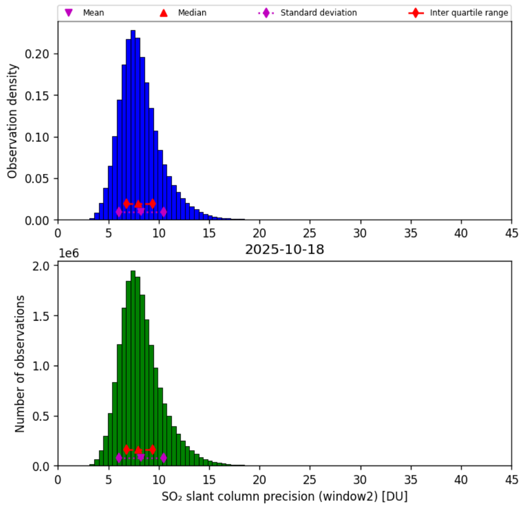
Figure 68: Histogram of “SO 2 slant column precision (window2)” for 2025-10-17 to 2025-10-19
