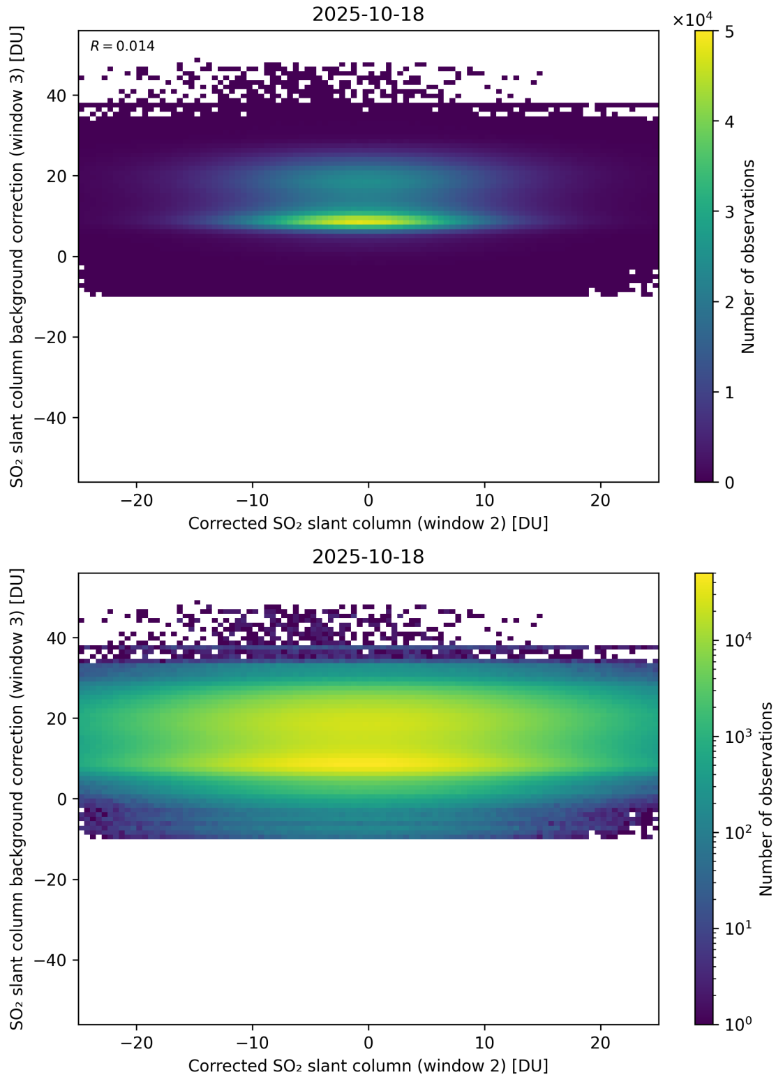
Figure 245: Scatter density plot of “Corrected SO 2 slant column (window 2)” against “SO 2 slant column background correction (window 3)” for 2025-10-17 to 2025-10-19.
