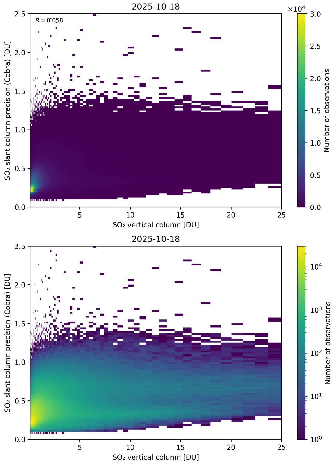
Figure 350: Scatter density plot of “SO 2 vertical column” against “SO 2 slant column precision (Cobra)” for 2025-10-17 to 2025-10-19.
