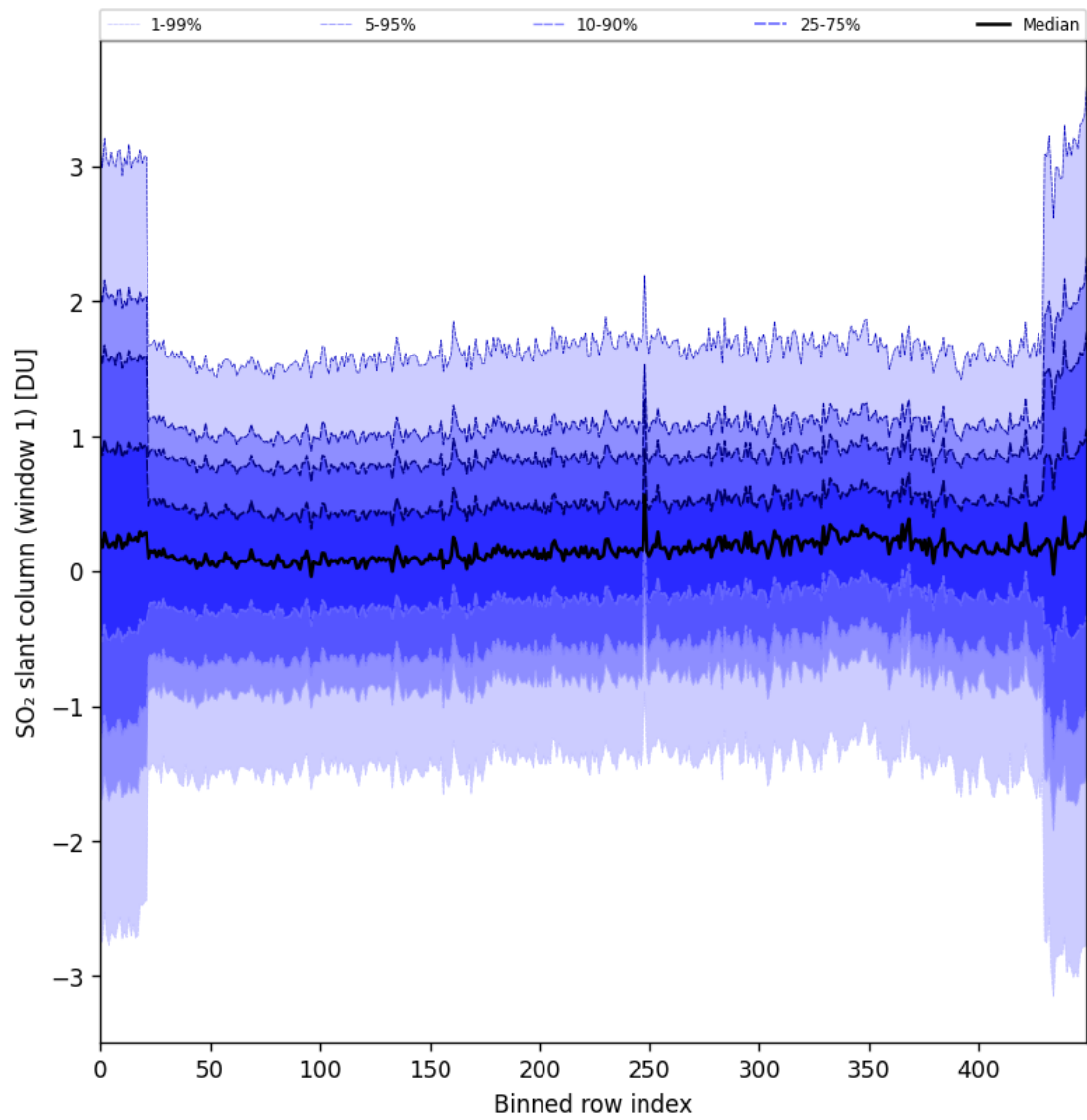
Figure 89: Along track statistics of “SO 2 slant column (window 1)” for 2025-10-17 to 2025-10-19
