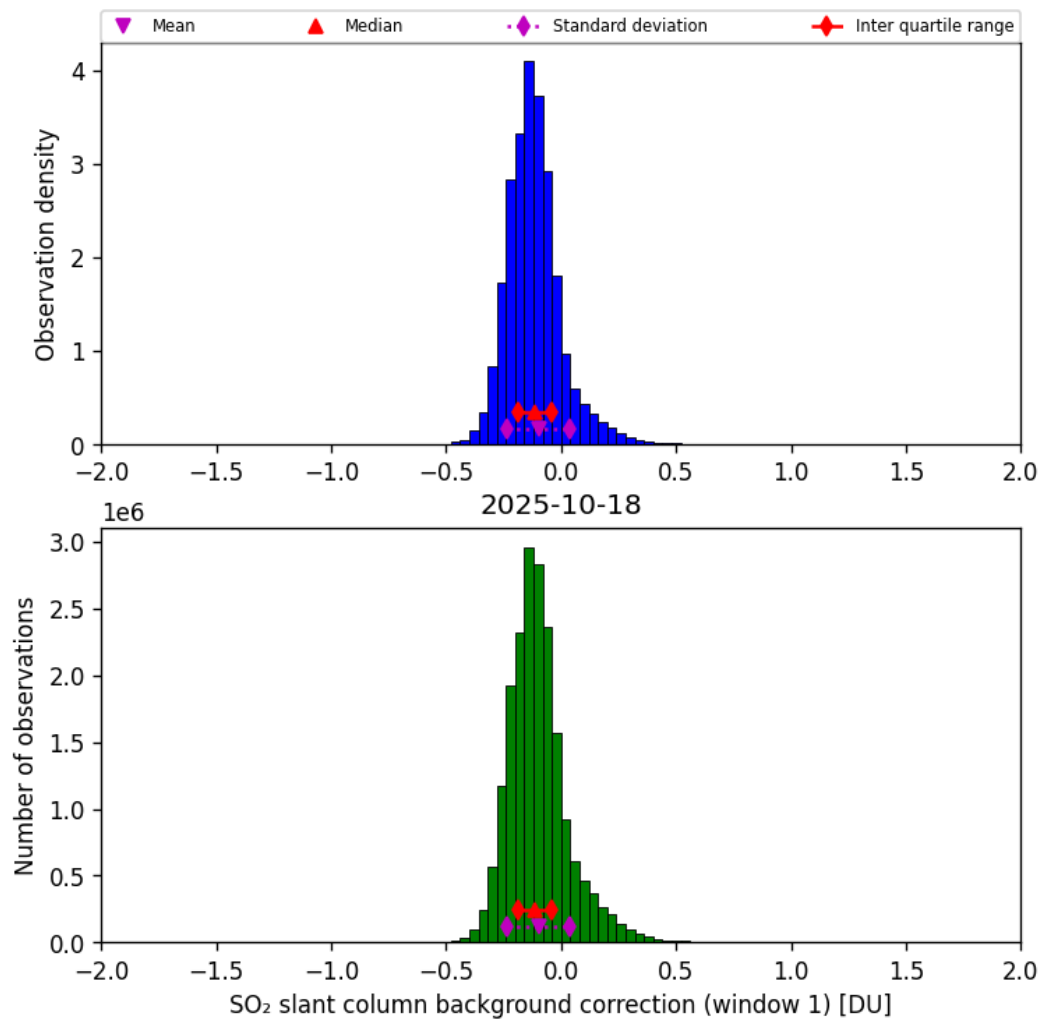
Figure 66: Histogram of “SO 2 slant column background correction (window 1)” for 2025-10-17 to 2025-10-19
