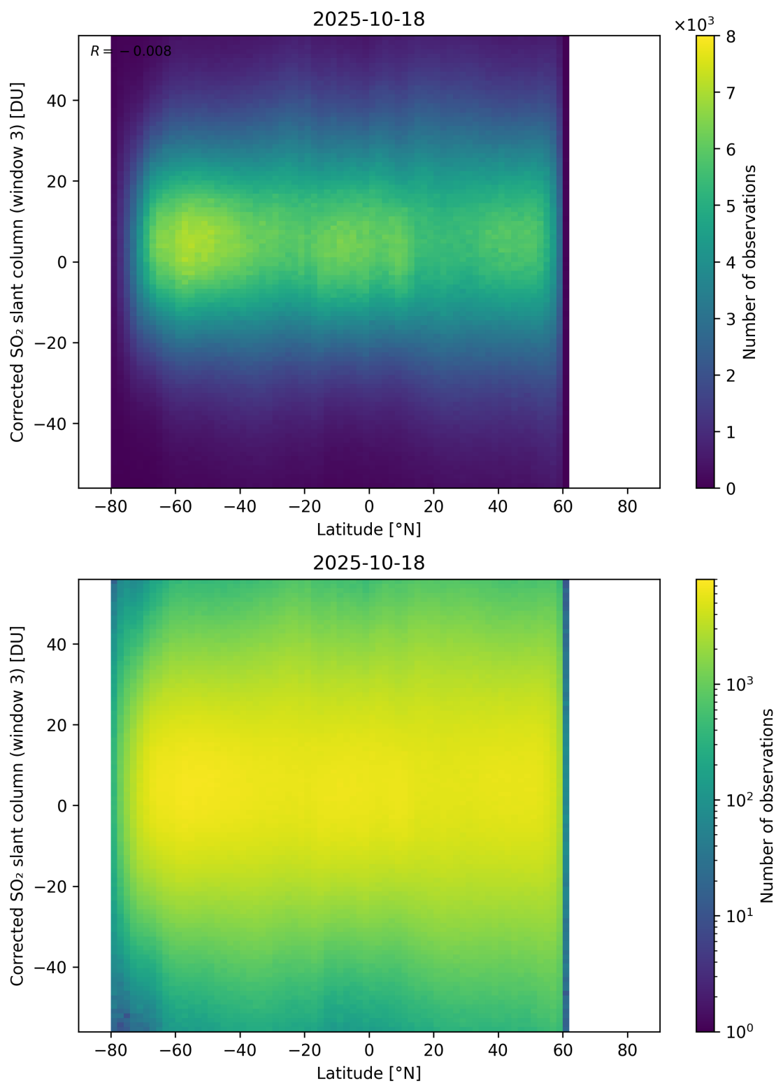
Figure 161: Scatter density plot of “Latitude” against “Corrected SO 2 slant column (window 3)” for 2025-10-17 to 2025-10-19.
