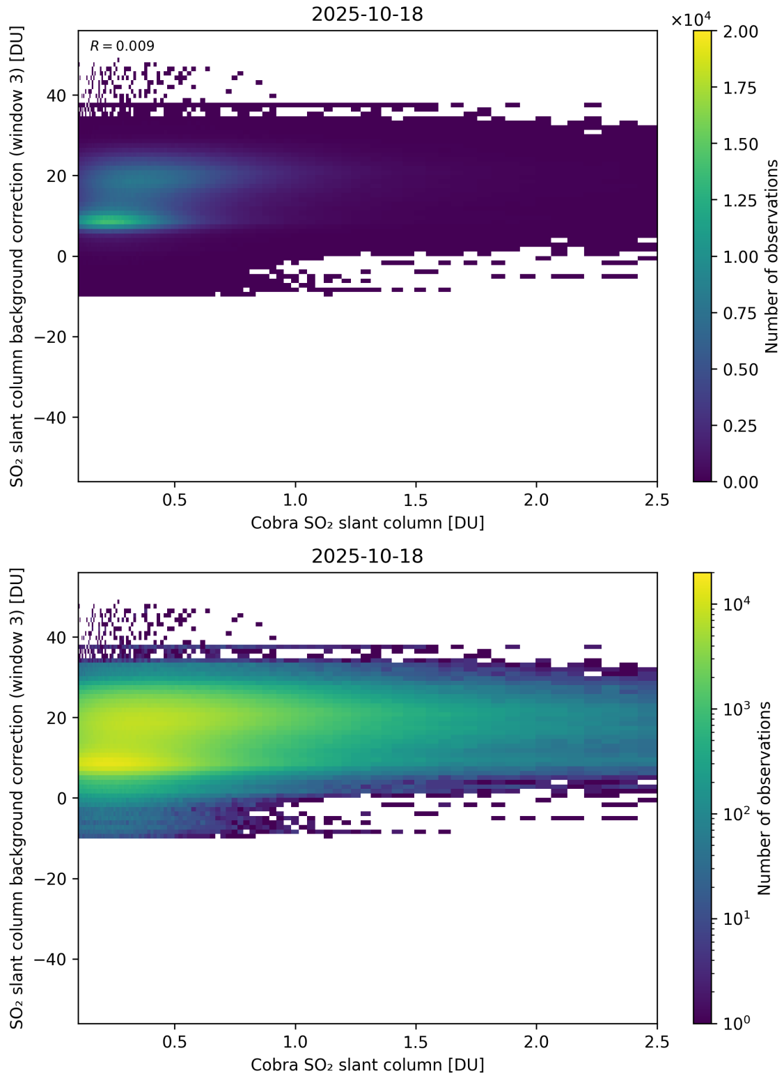
Figure 195: Scatter density plot of “Cobra SO 2 slant column” against “SO 2 slant column background correction (window 3)” for 2025-10-17 to 2025-10-19.
