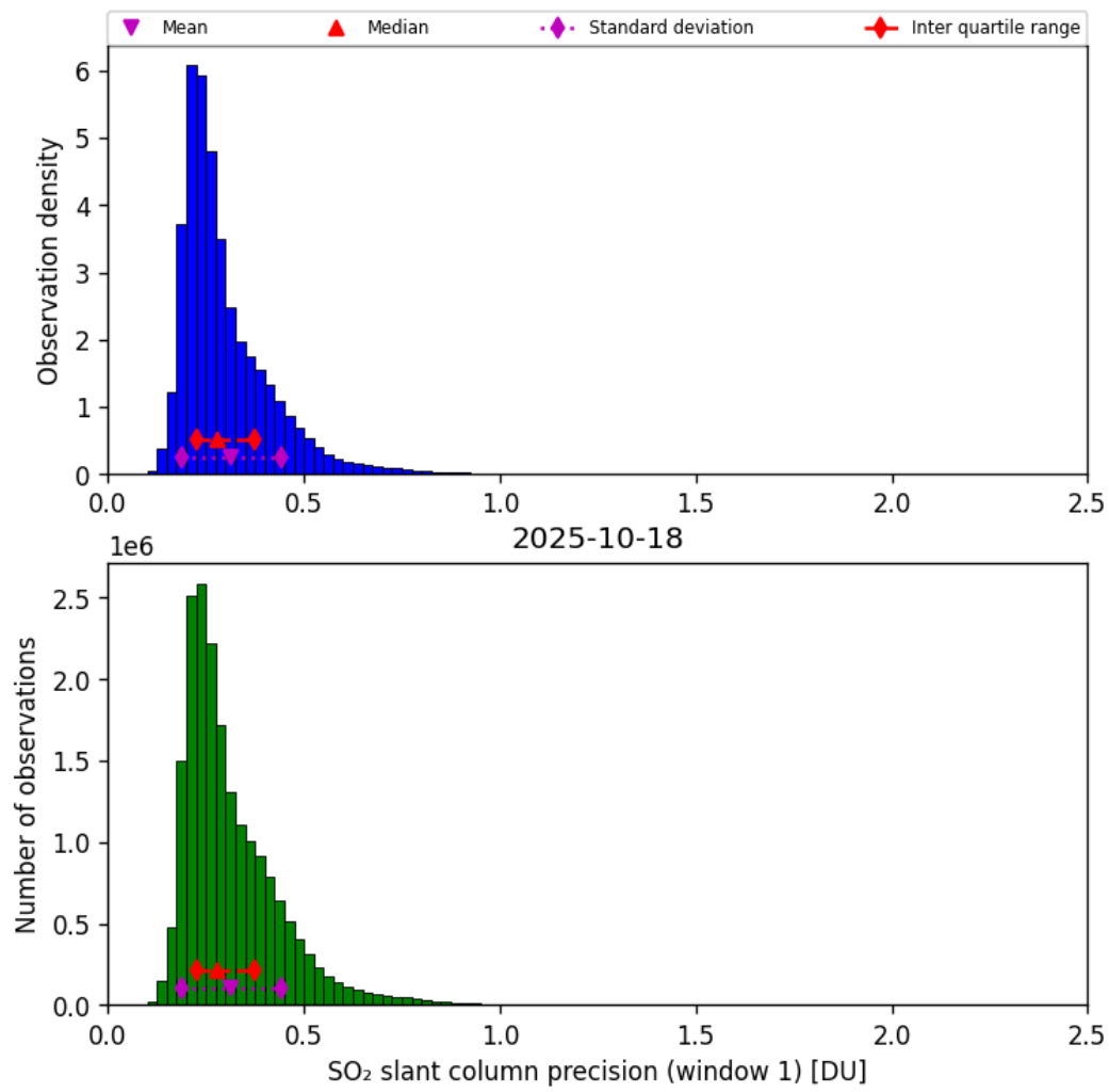
Figure 64: Histogram of “SO 2 slant column precision (window 1)” for 2025-10-17 to 2025-10-19
