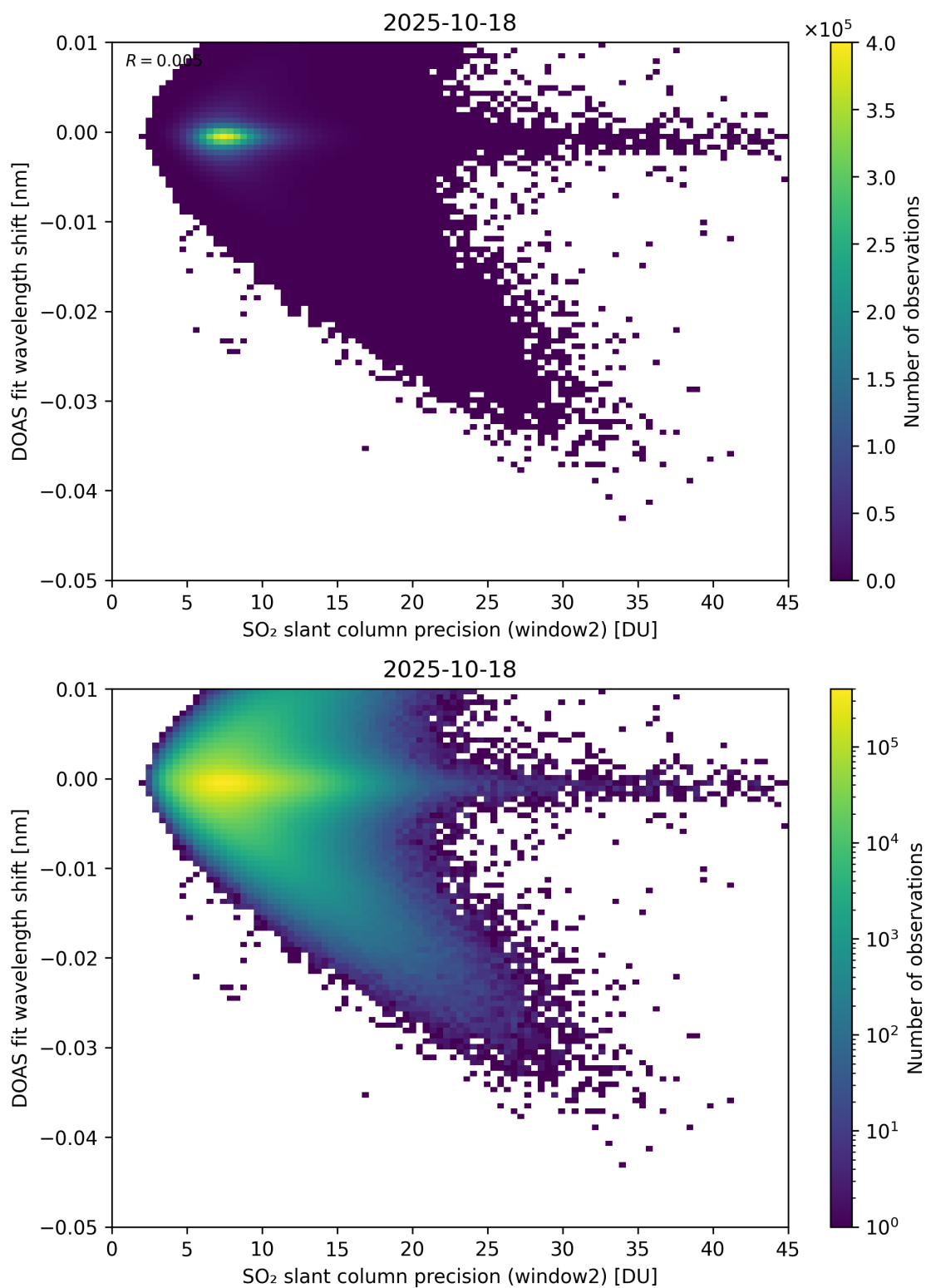
Figure 293: Scatter density plot of “SO 2 slant column precision (window2)” against “DOAS fit wavelength shift” for 2025-10-17 to 2025-10-19.
