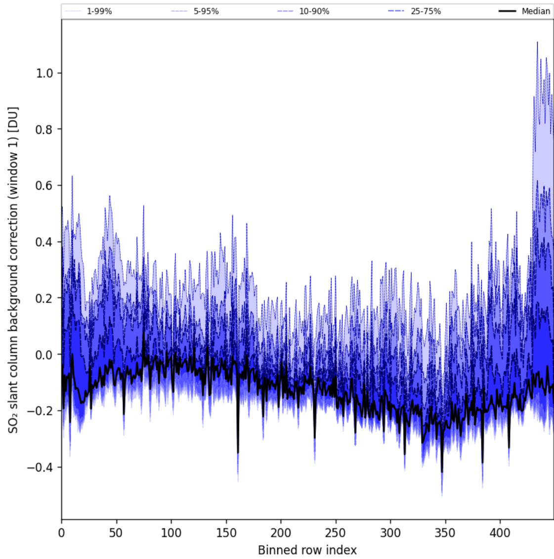
Figure 92: Along track statistics of “SO 2 slant column background correction (window 1)” for 2025-10-17 to 2025-10-19
