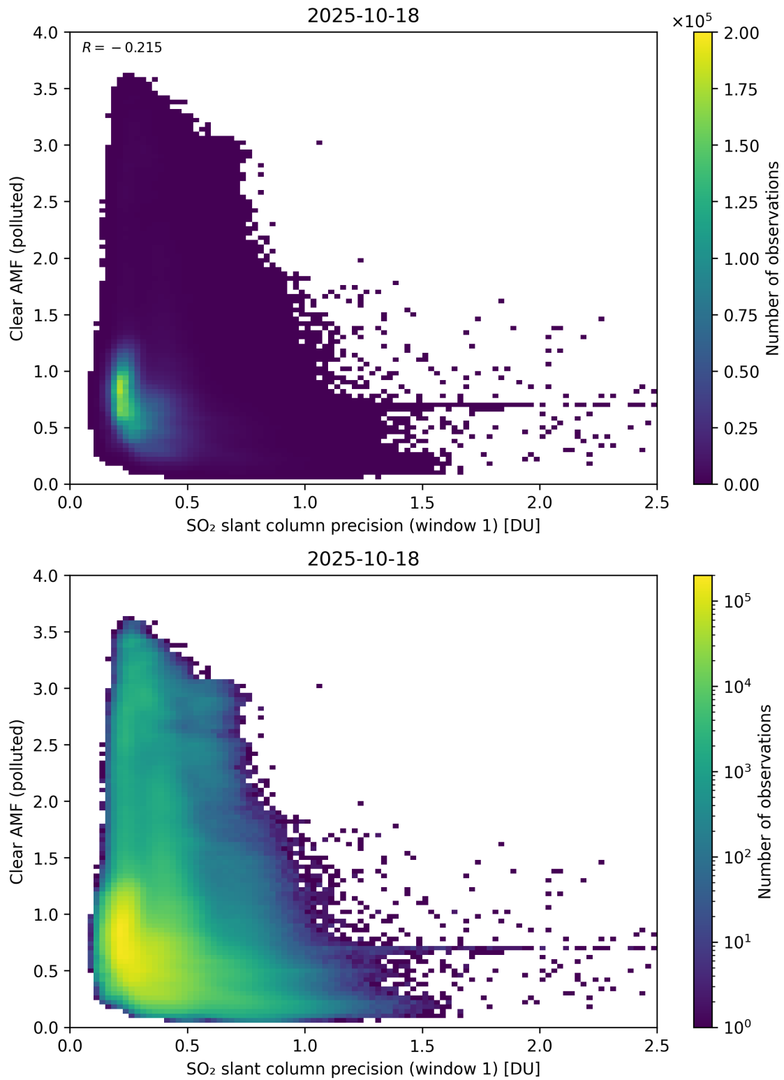
Figure 274: Scatter density plot of “SO 2 slant column precision (window 1)” against “Clear AMF (polluted)” for 2025-10-17 to 2025-10-19.
