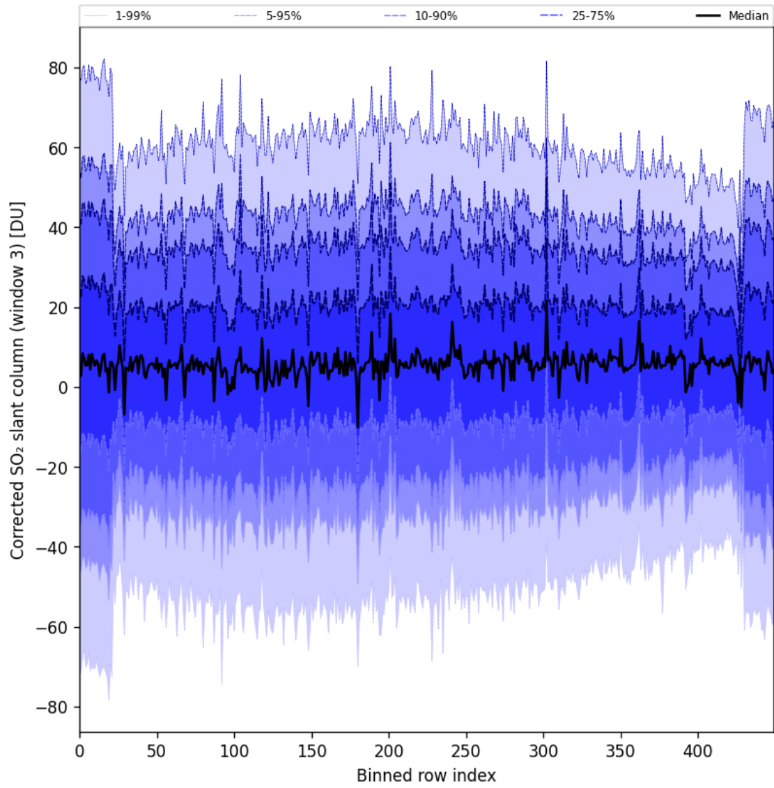
Figure 99: Along track statistics of “Corrected SO 2 slant column (window 3)” for 2025-10-17 to 2025-10-19
