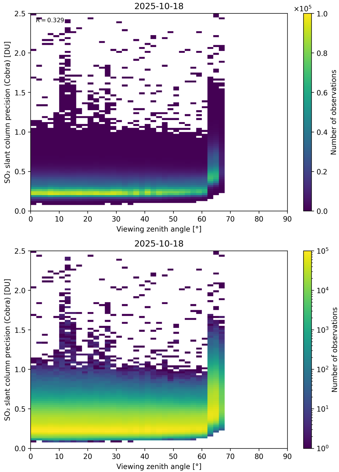
Figure 372: Scatter density plot of “Viewing zenith angle” against “SO 2 slant column precision (Cobra)” for 2025-10-17 to 2025-10-19.
