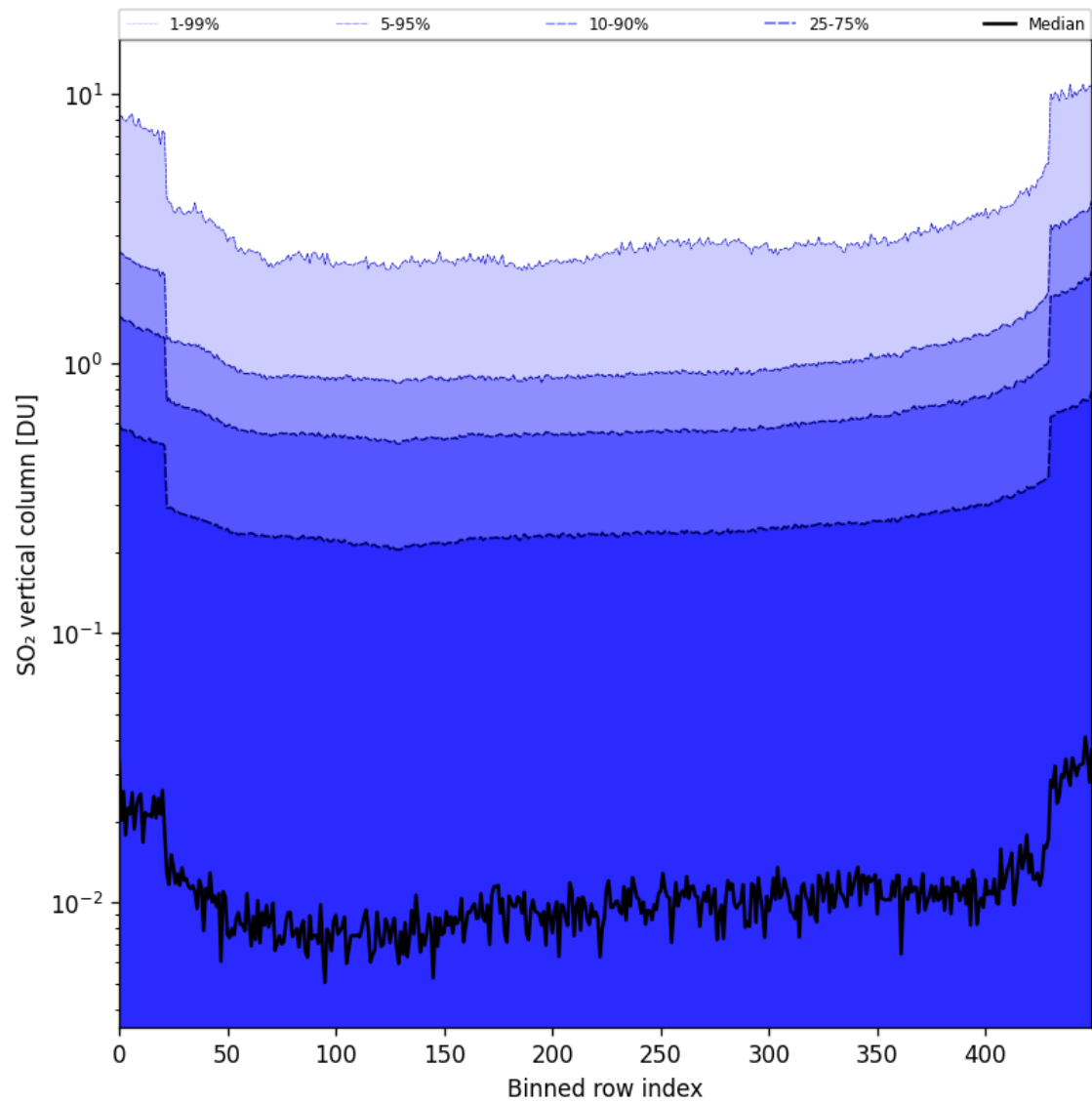
Figure 84: Along track statistics of “SO 2 vertical column” for 2025-10-17 to 2025-10-19
