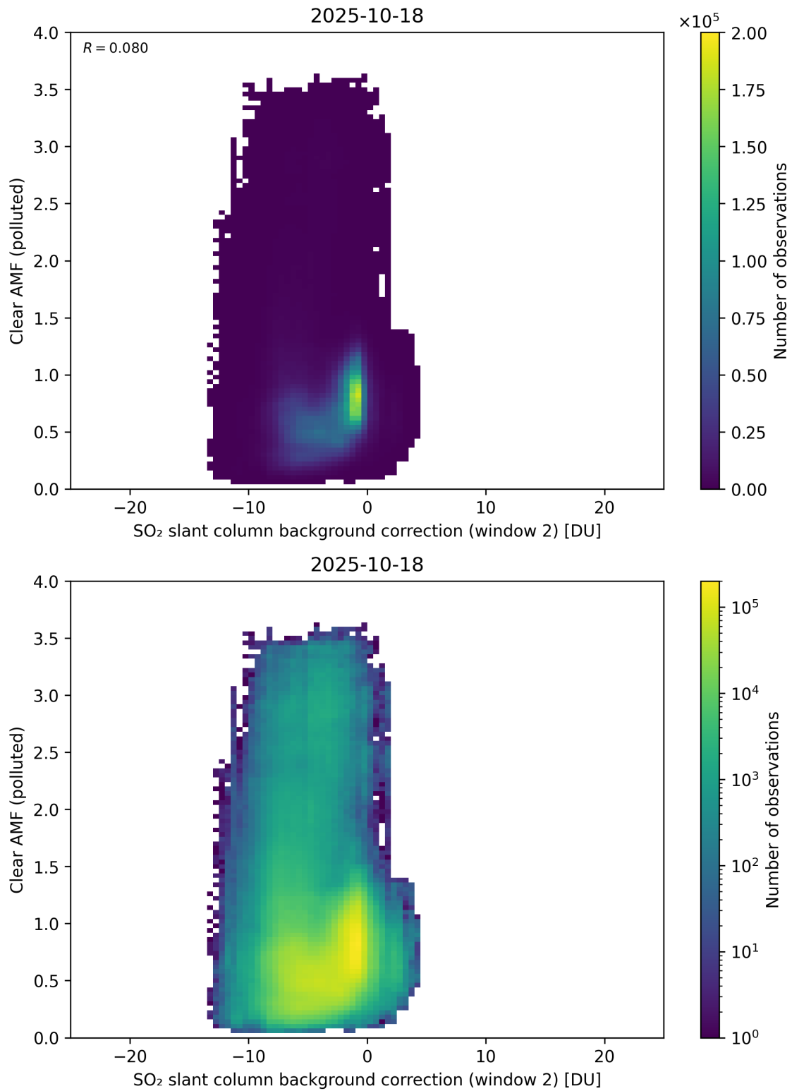
Figure 126: Scatter density plot of “SO 2 slant column background correction (window 2)” against “Clear AMF (polluted)” for 2025-10-17 to 2025-10-19.
