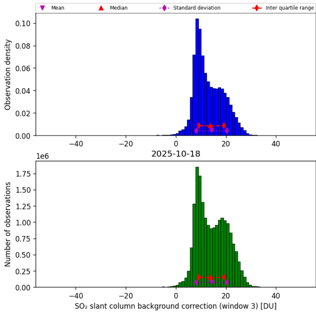
Figure 74: Histogram of “SO 2 slant column background correction (window 3)” for 2025-10-17 to 2025-10-19
