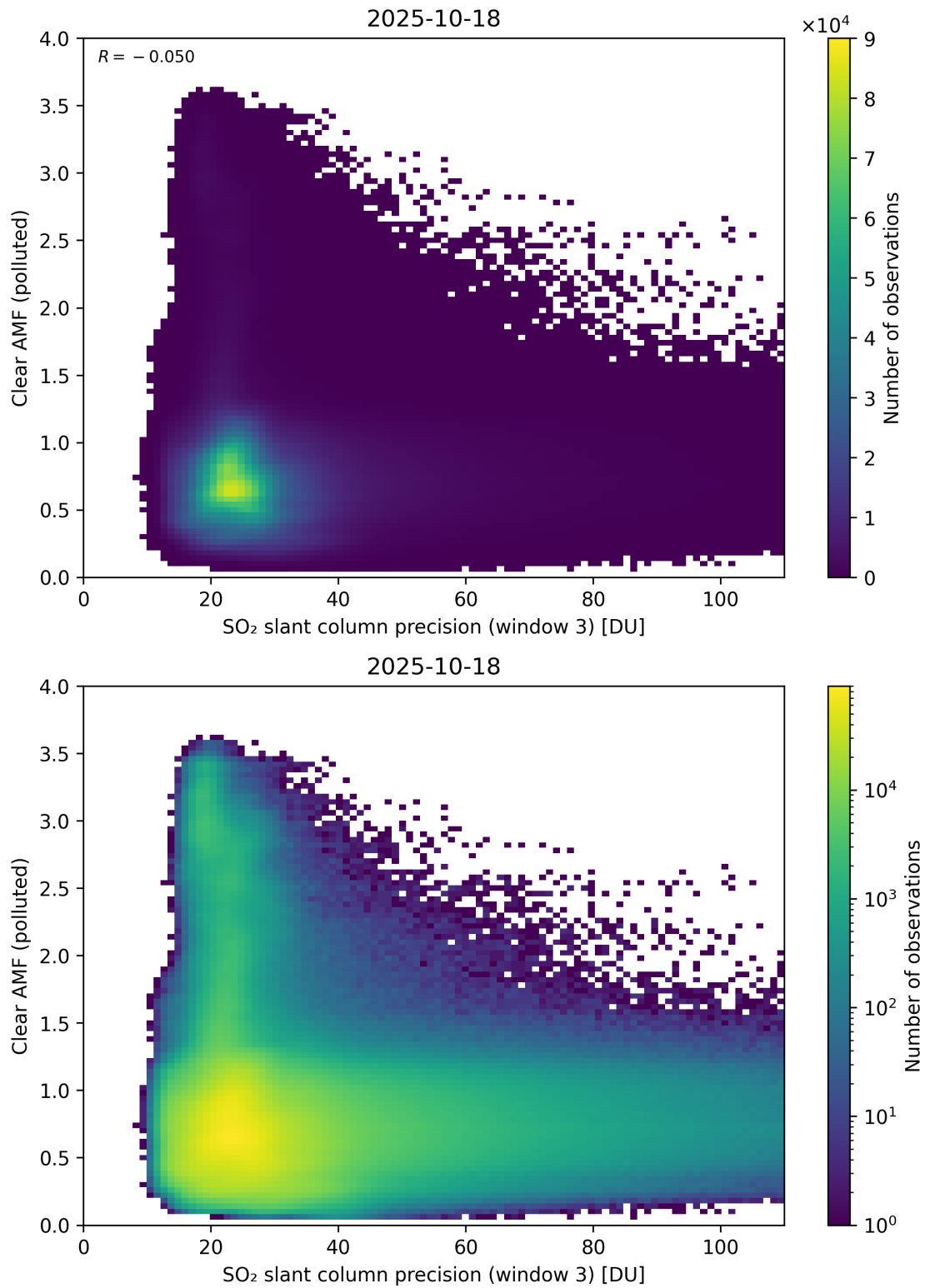
Figure 311: Scatter density plot of “SO 2 slant column precision (window 3)” against “Clear AMF (polluted)” for 2025-10-17 to 2025-10-19.
