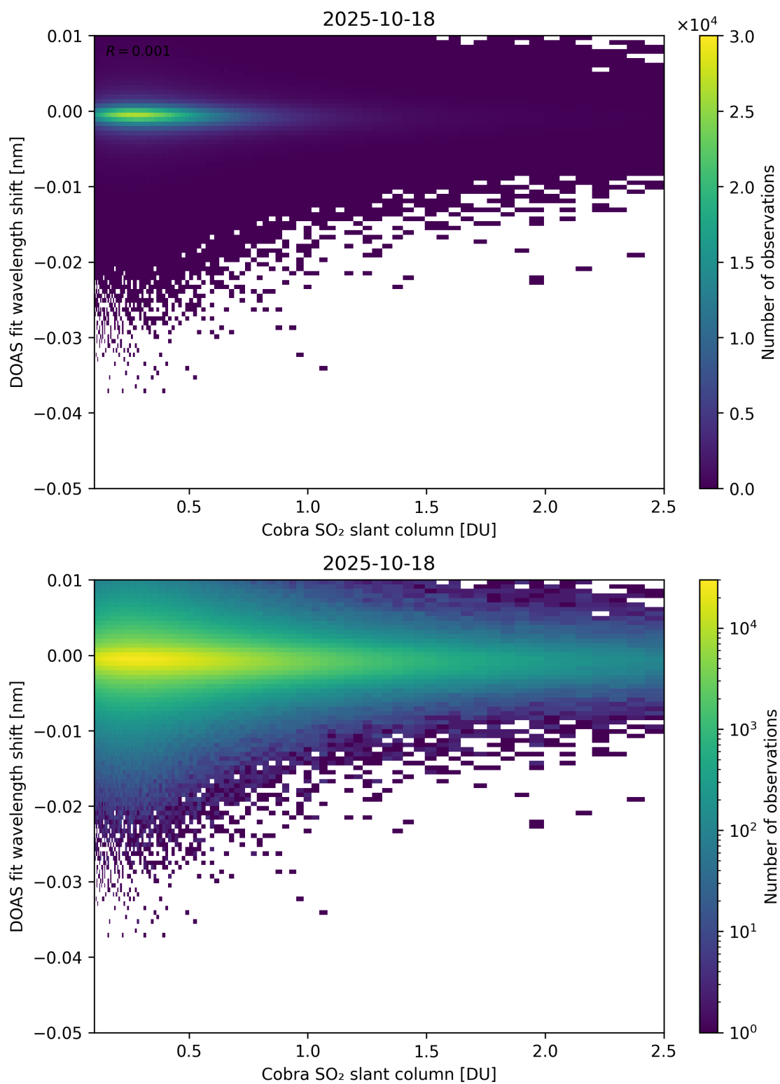
Figure 196: Scatter density plot of “Cobra SO 2 slant column” against “DOAS fit wavelength shift” for 2025-10-17 to 2025-10-19.
