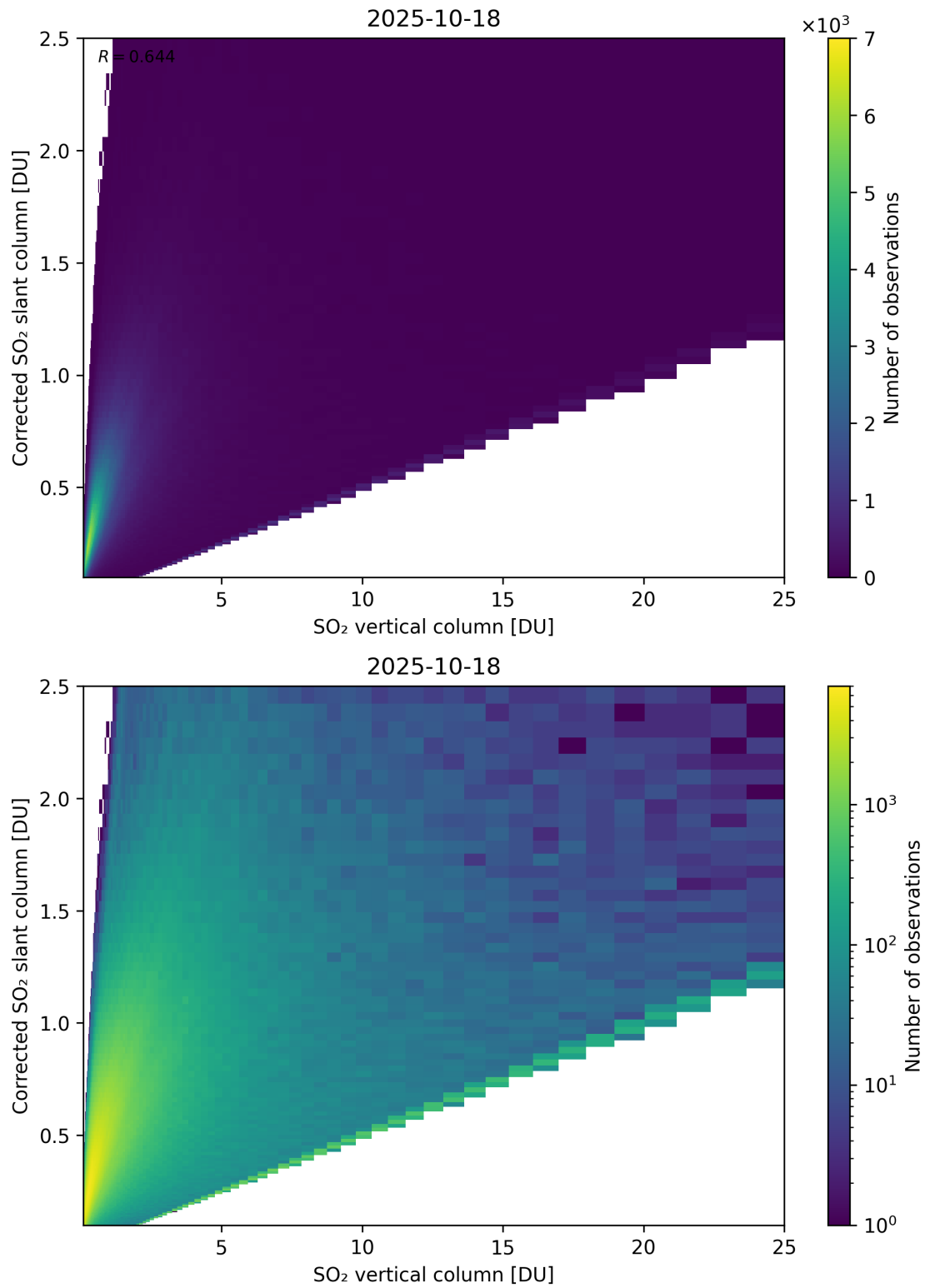
Figure 351: Scatter density plot of “SO 2 vertical column” against “Corrected SO 2 slant column” for 2025-10-17 to 2025-10-19.
