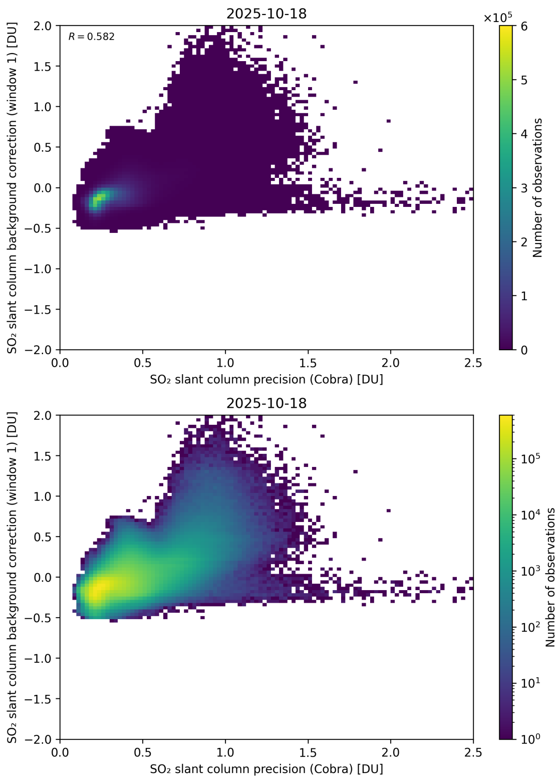
Figure 199: Scatter density plot of “SO 2 slant column precision (Cobra)” against “SO 2 slant column background correction (window 1)” for 2025-10-17 to 2025-10-19.
