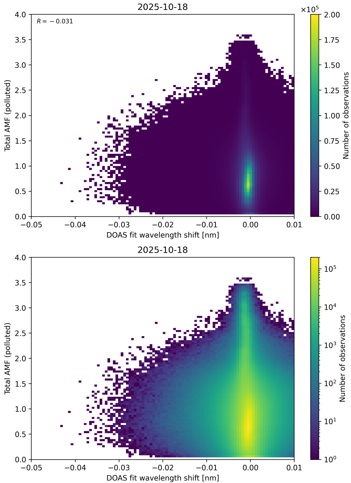
Figure 141: Scatter density plot of “DOAS fit wavelength shift” against “Total AMF (polluted)” for 2025-10-17 to 2025-10-19.
