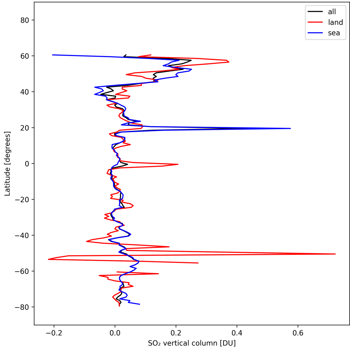
Figure 32: Zonal average of “SO 2 vertical column” for 2025-10-17 to 2025-10-19.
