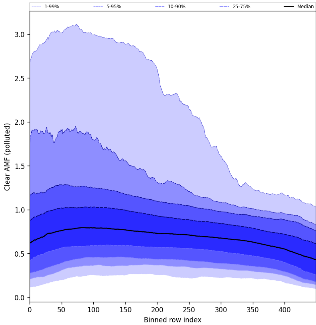
Figure 107: Along track statistics of “Clear AMF (polluted)” for 2025-10-17 to 2025-10-19
