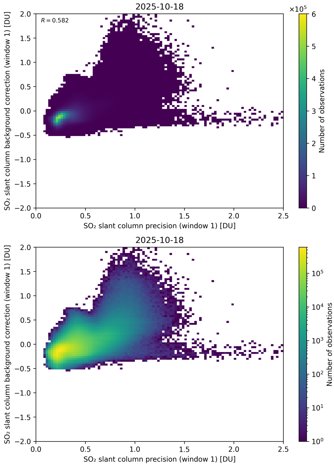
Figure 268: Scatter density plot of “SO 2 slant column precision (window 1)” against “SO 2 slant column background correction (window 1)” for 2025-10-17 to 2025-10-19.
