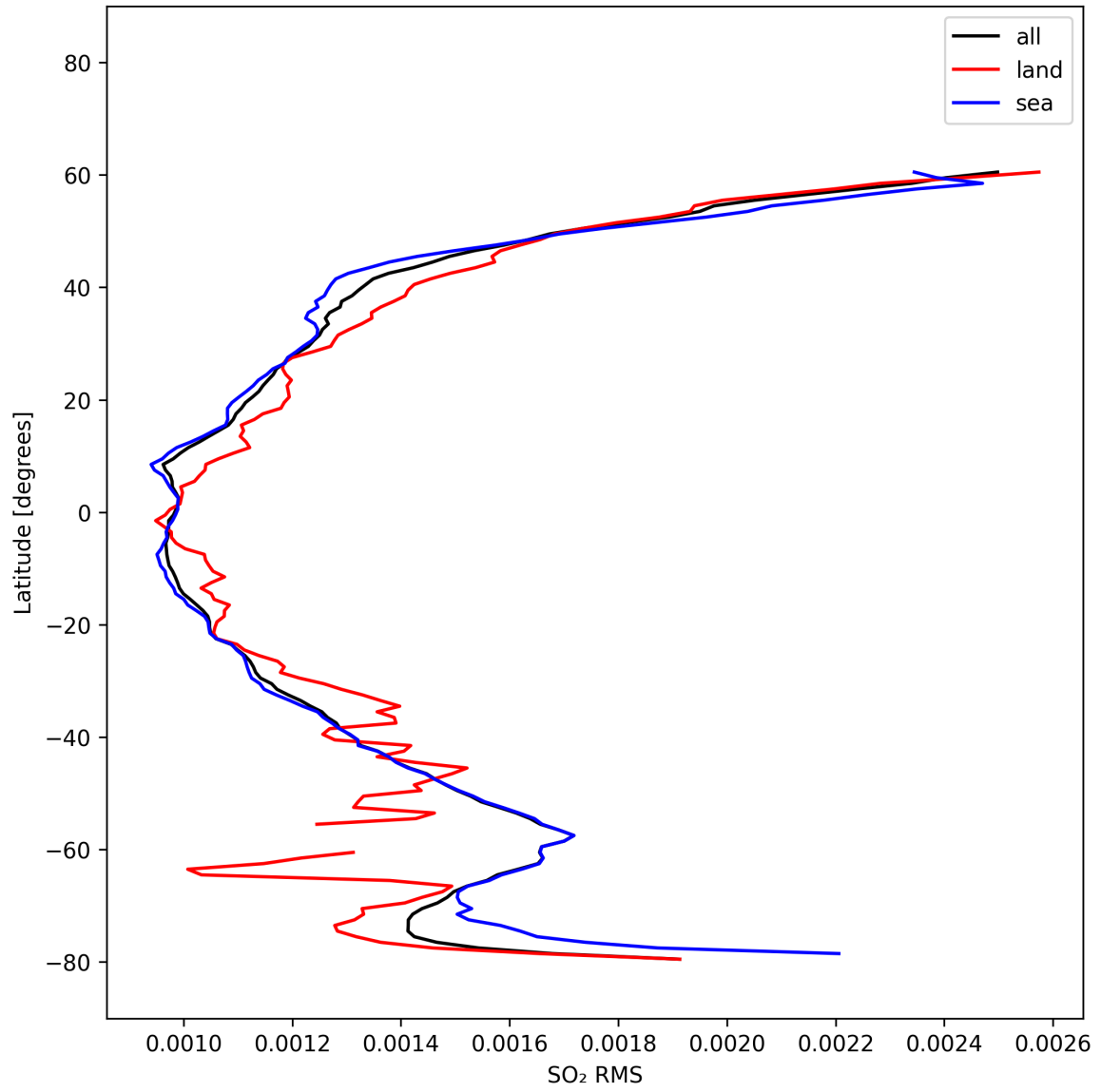
Figure 52: Zonal average of “SO 2 RMS” for 2025-10-17 to 2025-10-19.
