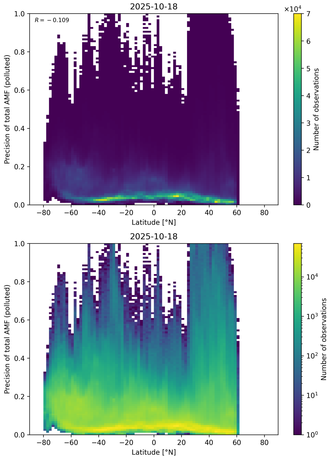
Figure 168: Scatter density plot of “Latitude” against “Precision of total AMF (polluted)” for 2025-10-17 to 2025-10-19.
