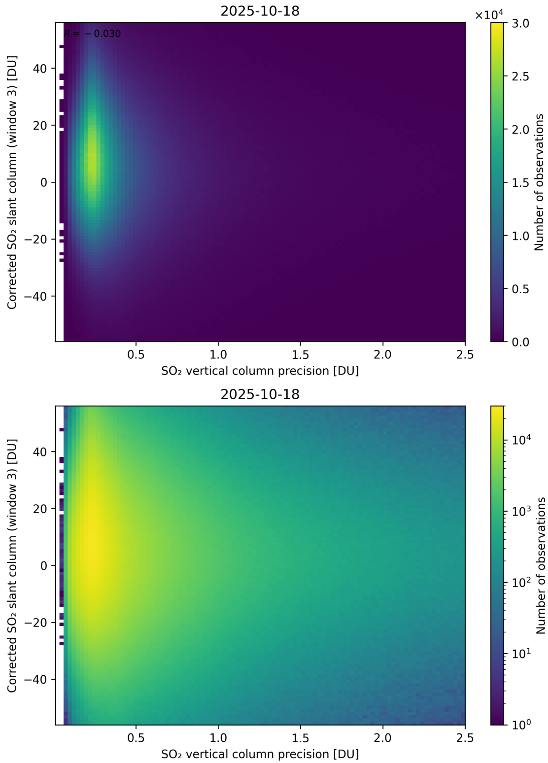
Figure 340: Scatter density plot of “SO 2 vertical column precision” against “Corrected SO 2 slant column (window 3)” for 2025-10-17 to 2025-10-19.
