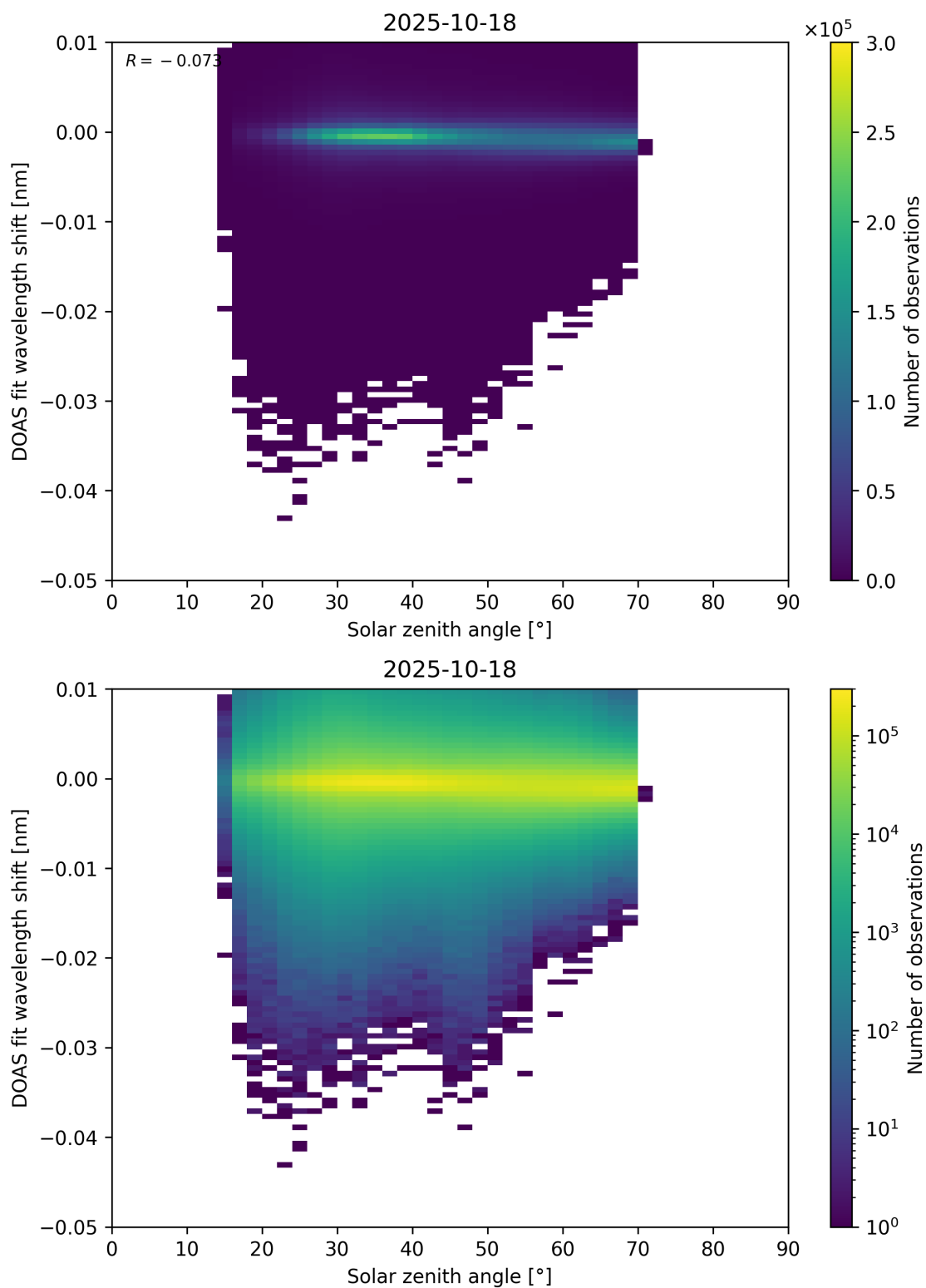
Figure 174: Scatter density plot of “Solar zenith angle” against “DOAS fit wavelength shift” for 2025-10-17 to 2025-10-19.
