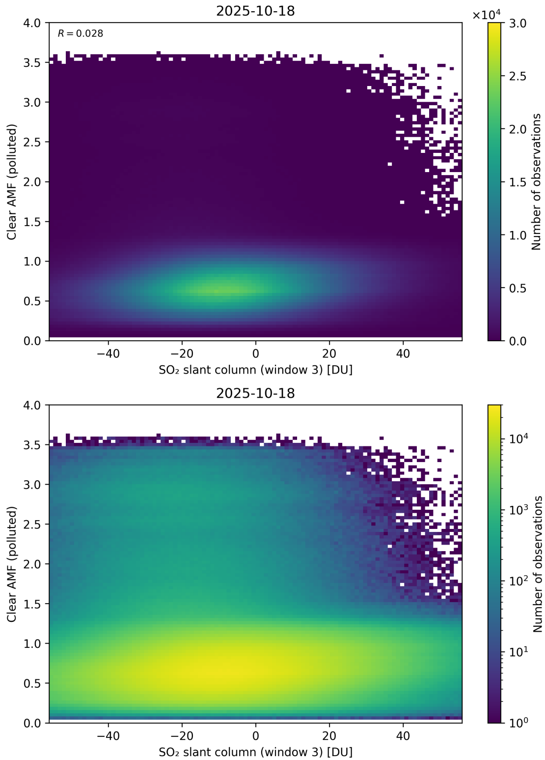
Figure 315: Scatter density plot of “SO 2 slant column (window 3)” against “Clear AMF (polluted)” for 2025-10-17 to 2025-10-19.
