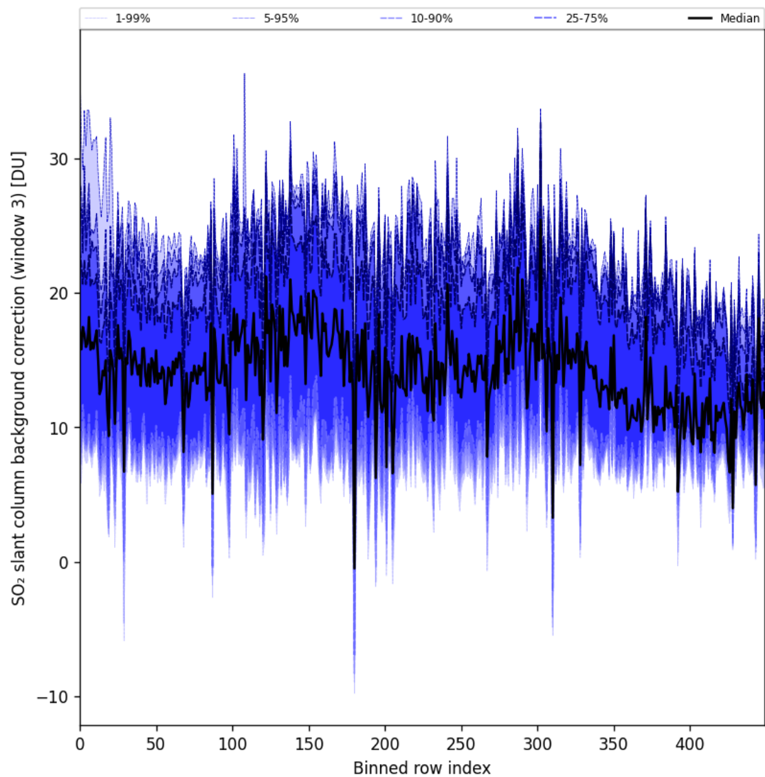
Figure 100: Along track statistics of “SO 2 slant column background correction (window 3)” for 2025-10-17 to 2025-10-19
