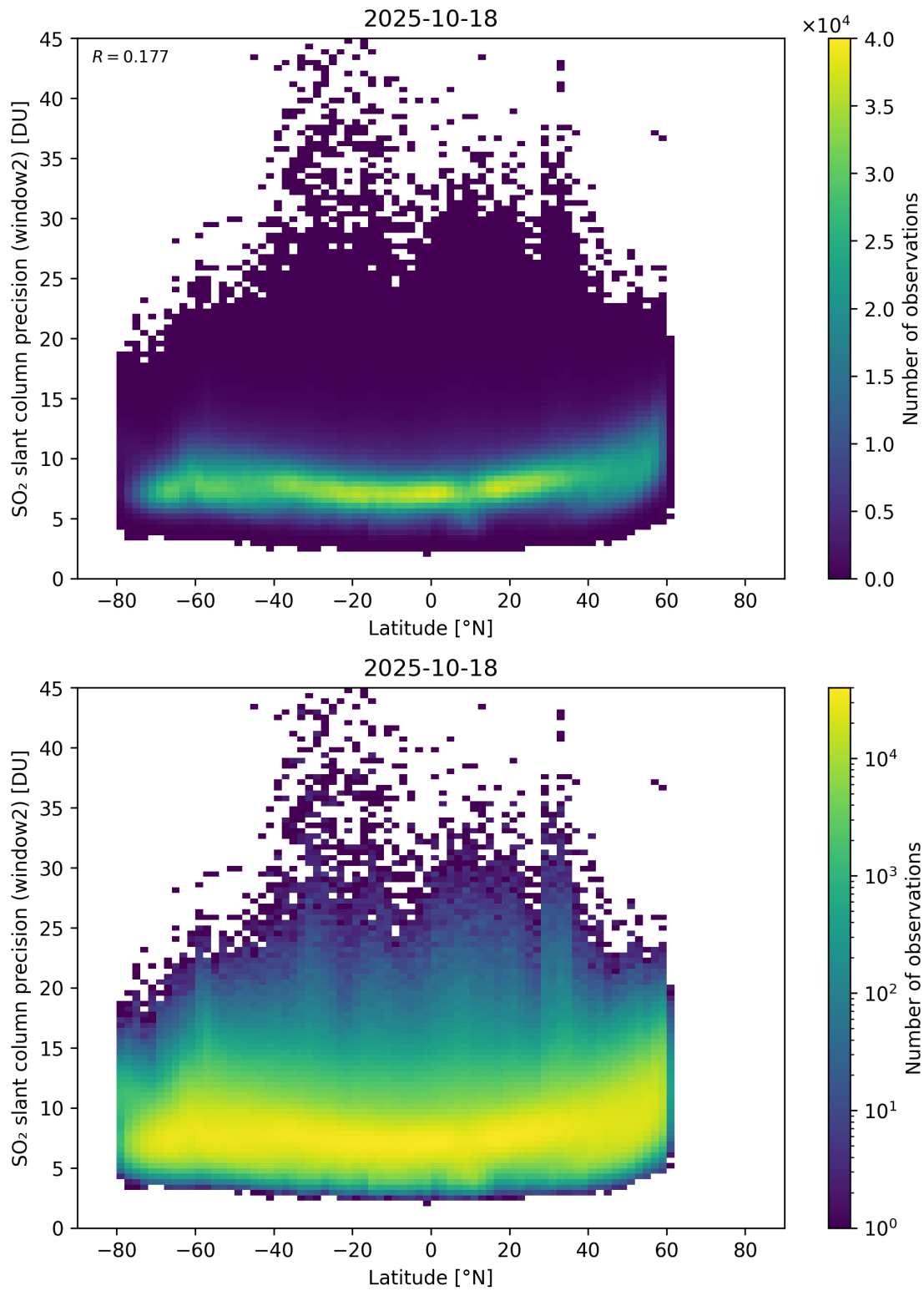
Figure 164: Scatter density plot of “Latitude” against “SO 2 slant column precision (window2)” for 2025-10-17 to 2025-10-19.
