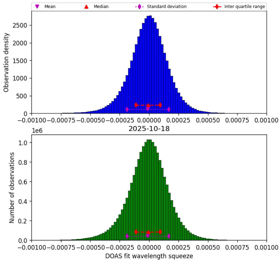
Figure 77: Histogram of “DOAS fit wavelength squeeze” for 2025-10-17 to 2025-10-19
