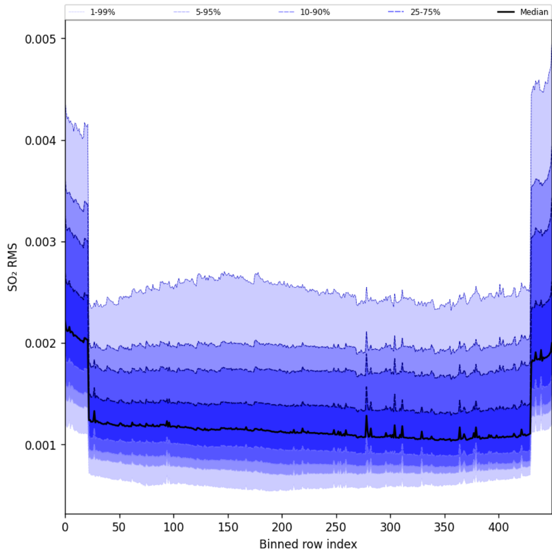
Figure 104: Along track statistics of “SO 2 RMS” for 2025-10-17 to 2025-10-19
