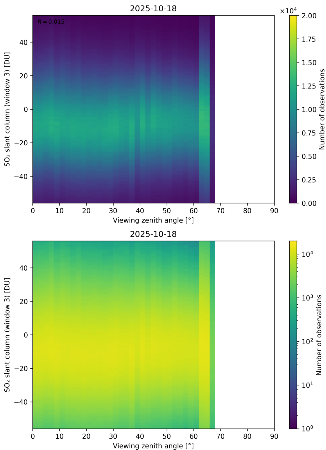
Figure 379: Scatter density plot of “Viewing zenith angle” against “SO 2 slant column (window 3)” for 2025-10-17 to 2025-10-19.
