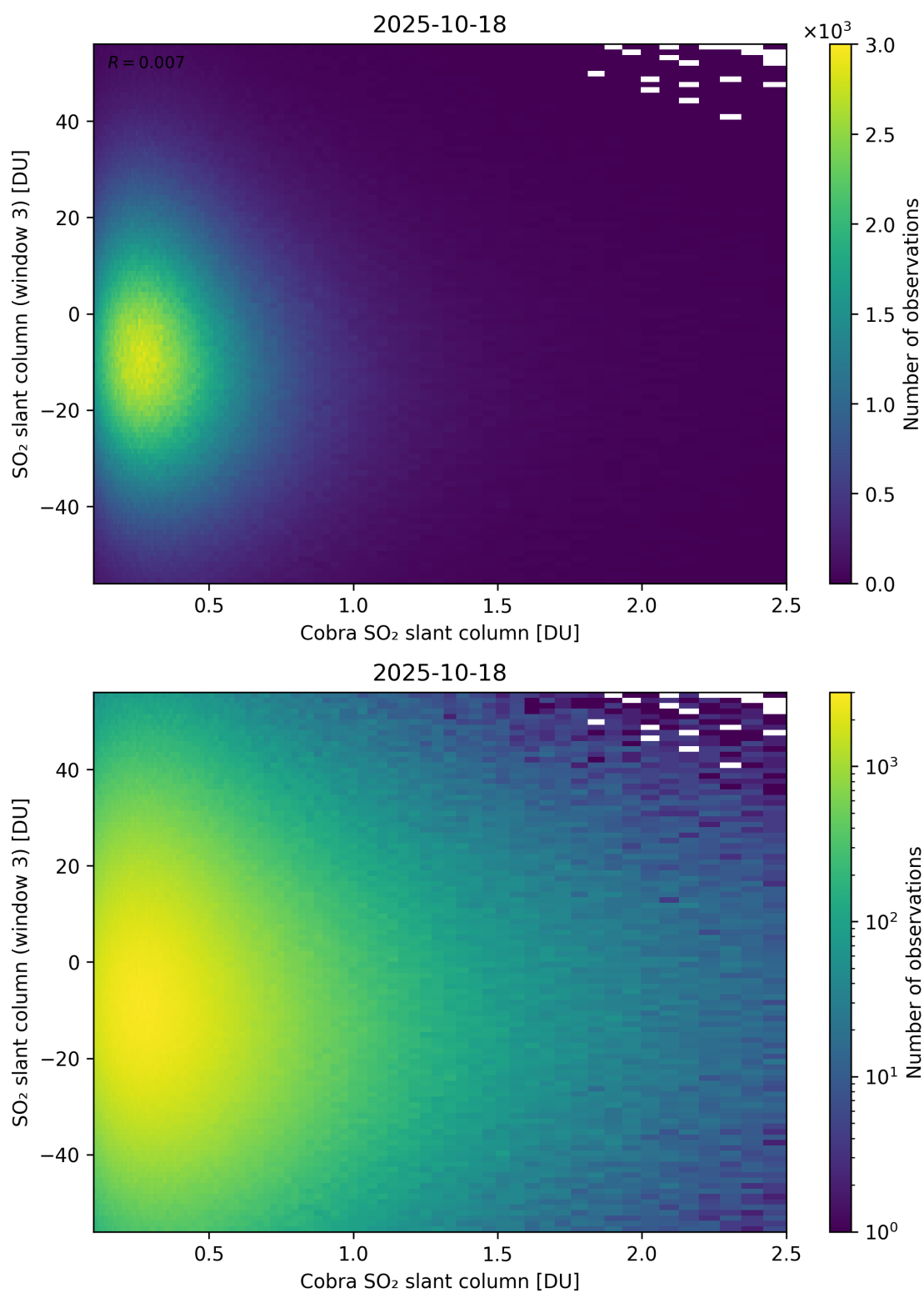
Figure 222: Scatter density plot of “Cobra SO 2 slant column” against “SO 2 slant column (window 3)” for 2025-10-17 to 2025-10-19.
