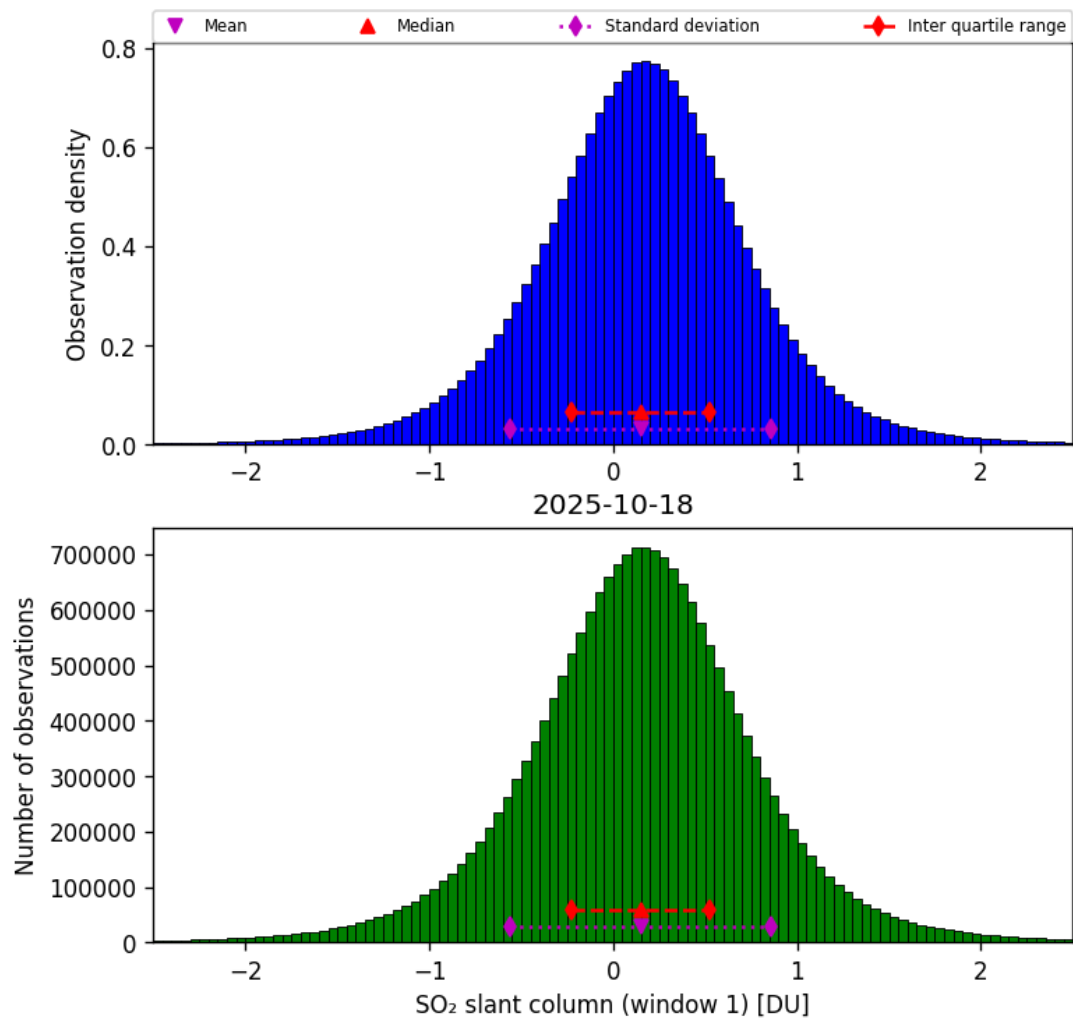
Figure 63: Histogram of “SO 2 slant column (window 1)” for 2025-10-17 to 2025-10-19
