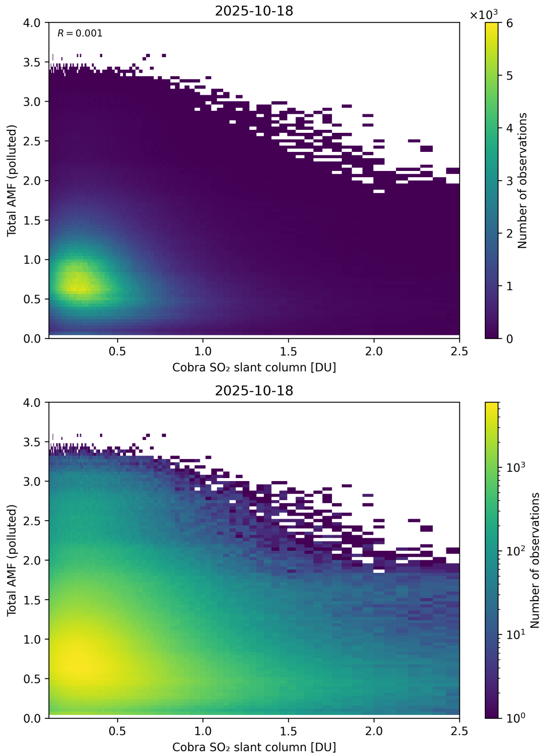
Figure 224: Scatter density plot of “Cobra SO 2 slant column” against “Total AMF (polluted)” for 2025-10-17 to 2025-10-19.
