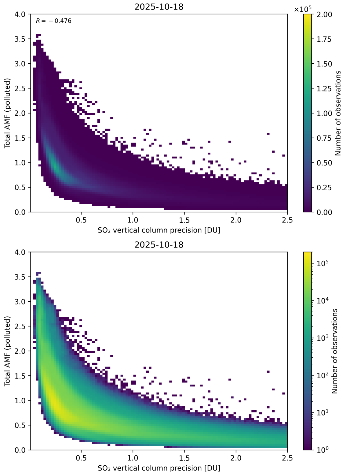
Figure 346: Scatter density plot of “SO 2 vertical column precision” against “Total AMF (polluted)” for 2025-10-17 to 2025-10-19.
