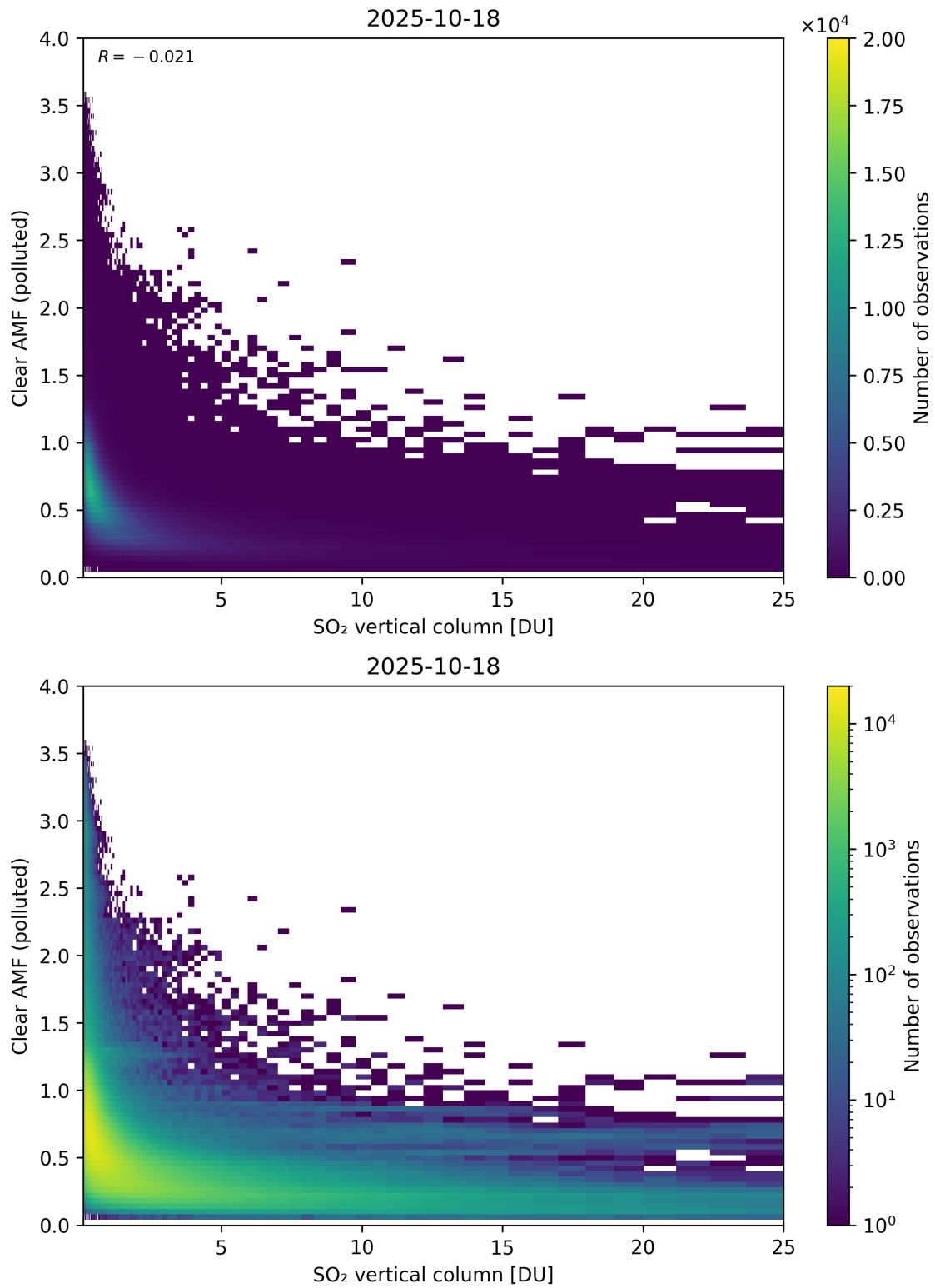
Figure 348: Scatter density plot of “SO 2 vertical column” against “Clear AMF (polluted)” for 2025-10-17 to 2025-10-19.
