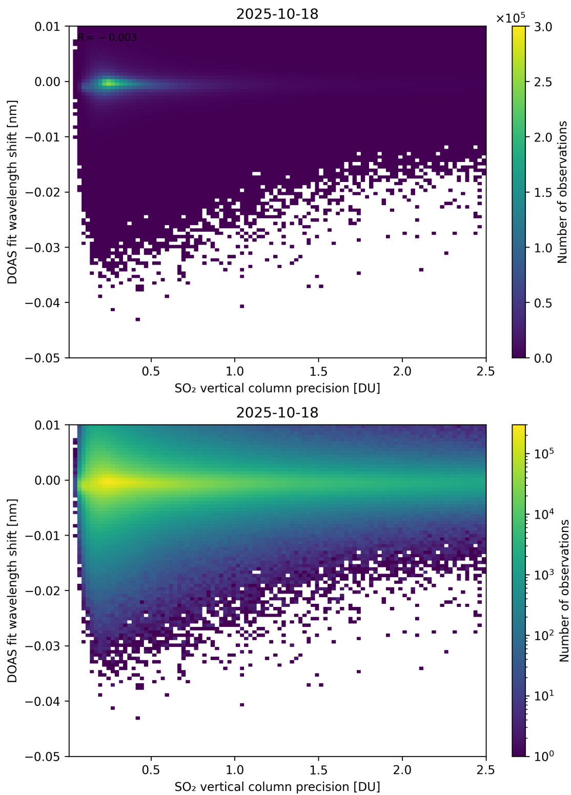
Figure 332: Scatter density plot of “SO 2 vertical column precision” against “DOAS fit wavelength shift” for 2025-10-17 to 2025-10-19.
