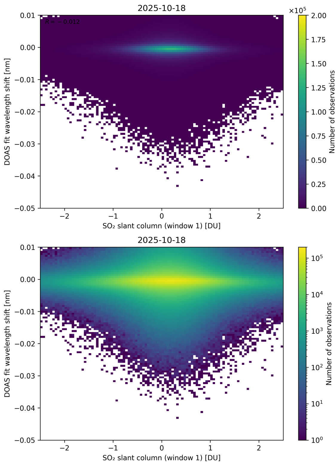
Figure 265: Scatter density plot of “SO 2 slant column (window 1)” against “DOAS fit wavelength shift” for 2025-10-17 to 2025-10-19.
