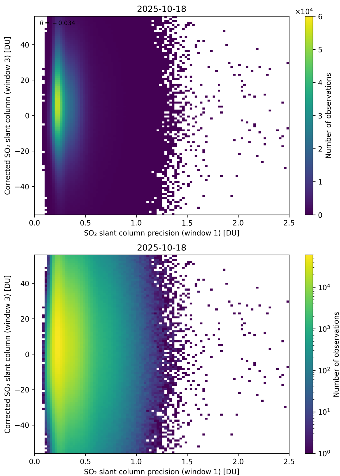
Figure 276: Scatter density plot of “SO 2 slant column precision (window 1)” against “Corrected SO 2 slant column (window 3)” for 2025-10-17 to 2025-10-19.
