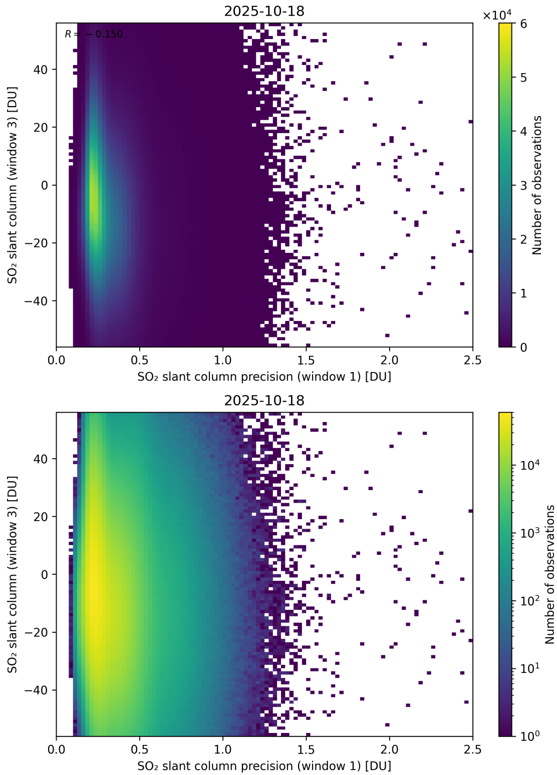
Figure 278: Scatter density plot of “SO 2 slant column precision (window 1)” against “SO 2 slant column (window 3)” for 2025-10-17 to 2025-10-19.
