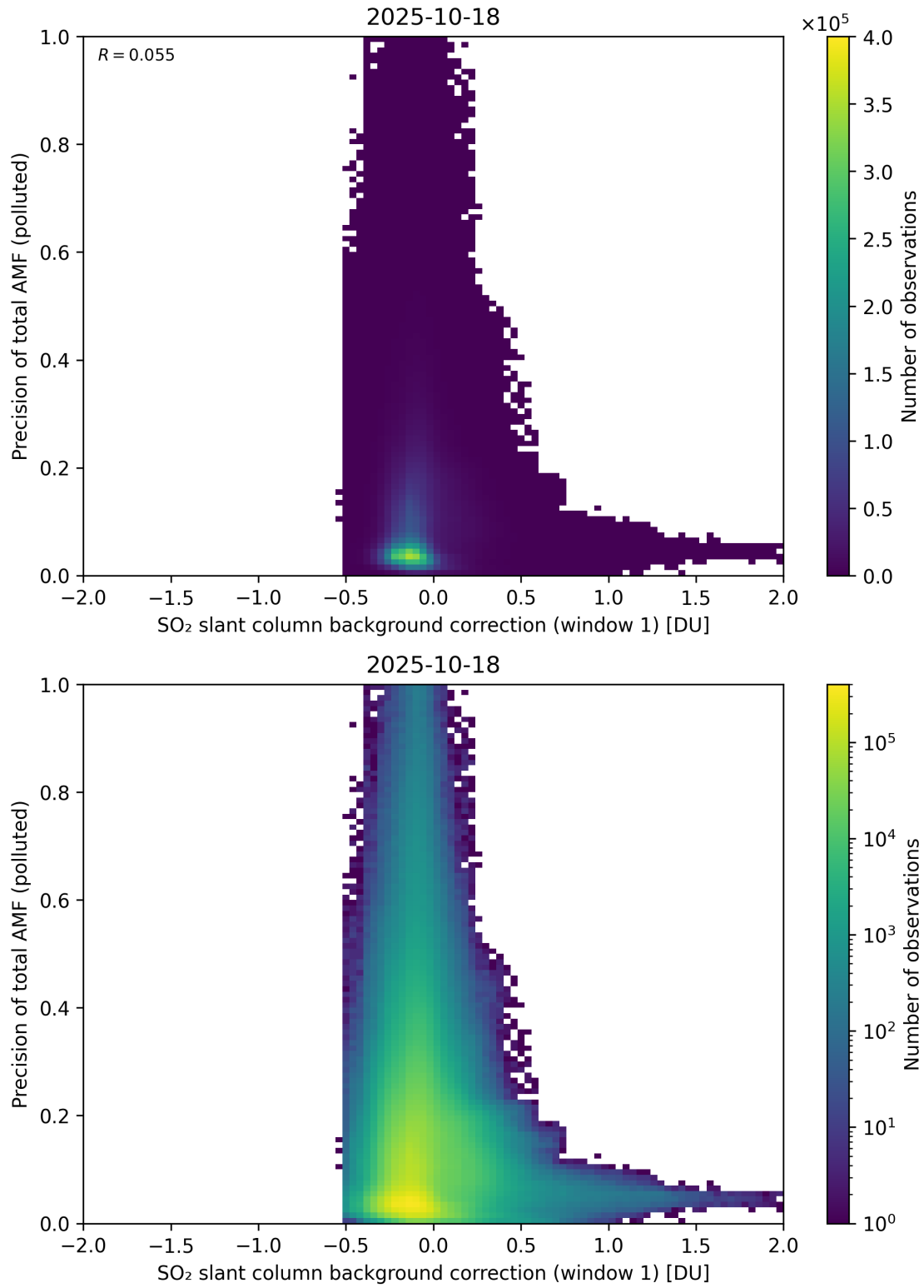
Figure 121: Scatter density plot of “SO 2 slant column background correction (window 1)” against “Precision of total AMF (polluted)” for 2025-10-17 to 2025-10-19.
