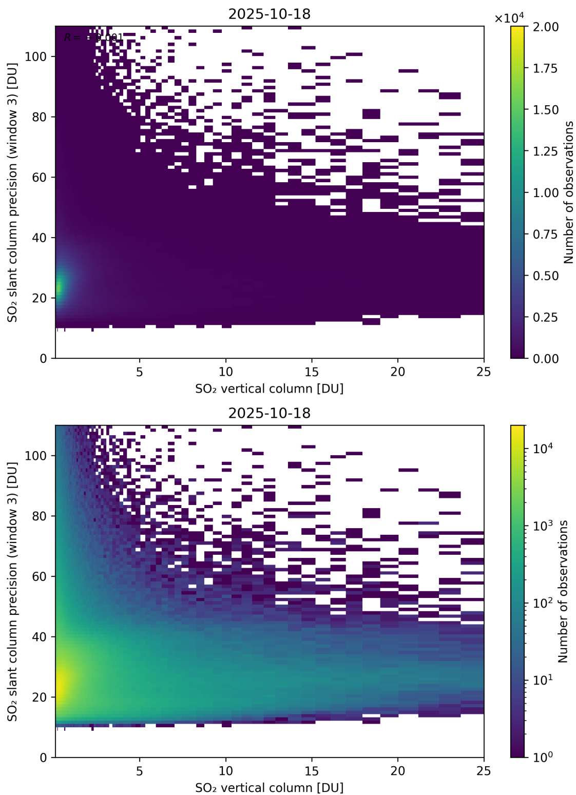
Figure 358: Scatter density plot of “SO 2 vertical column” against “SO 2 slant column precision (window 3)” for 2025-10-17 to 2025-10-19.
