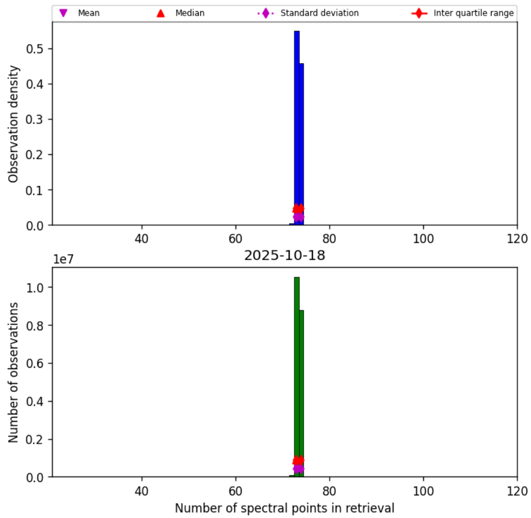
Figure 82: Histogram of “Number of spectral points in retrieval” for 2025-10-17 to 2025-10-19
