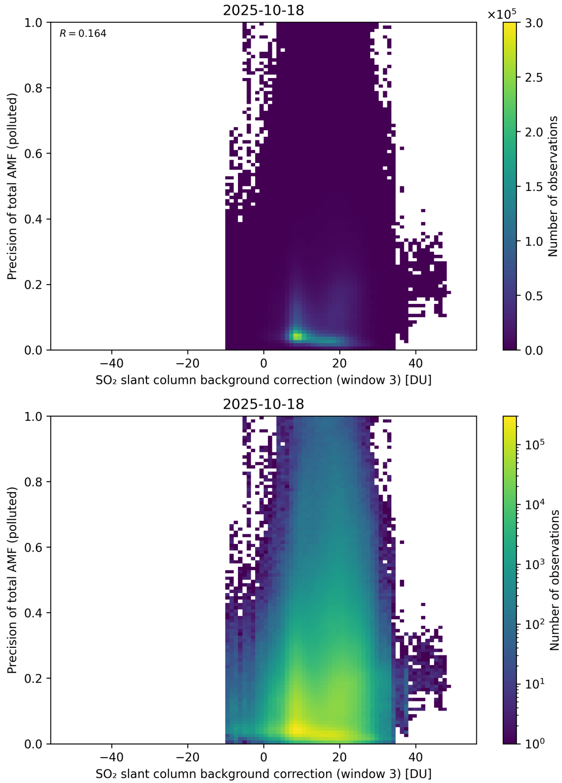
Figure 137: Scatter density plot of “SO 2 slant column background correction (window 3)” against “Precision of total AMF (polluted)” for 2025-10-17 to 2025-10-19.
