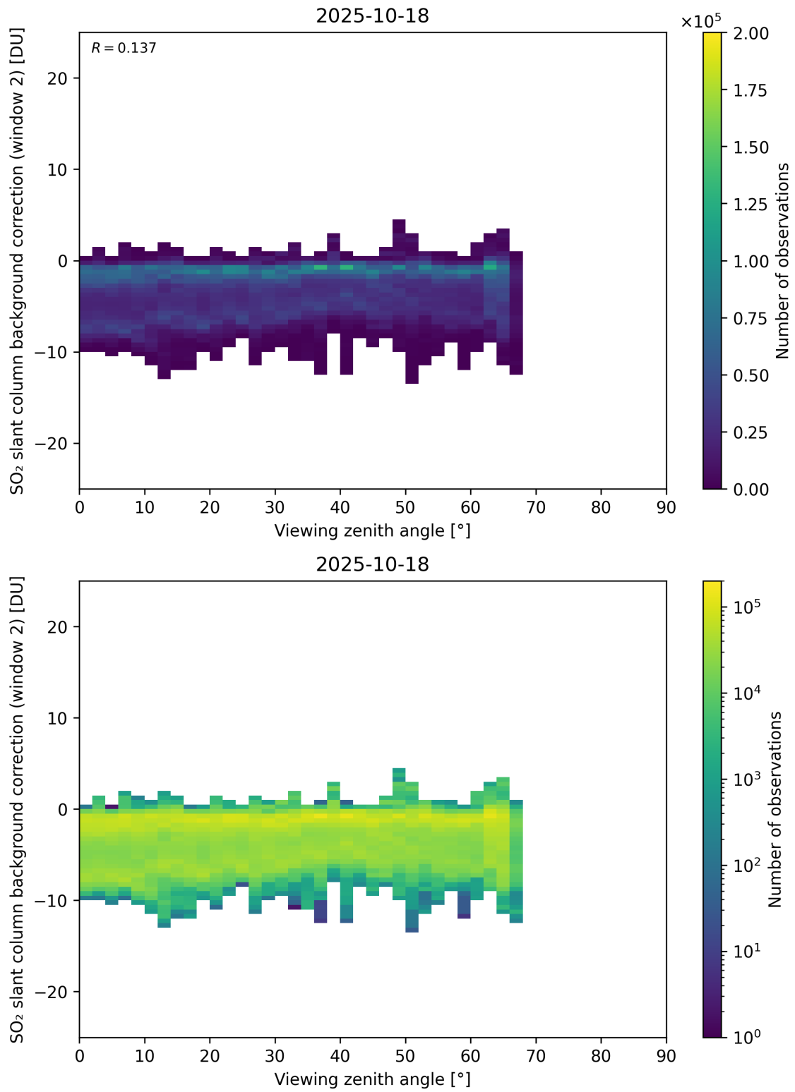
Figure 363: Scatter density plot of “Viewing zenith angle” against “SO 2 slant column background correction (window 2)” for 2025-10-17 to 2025-10-19.
