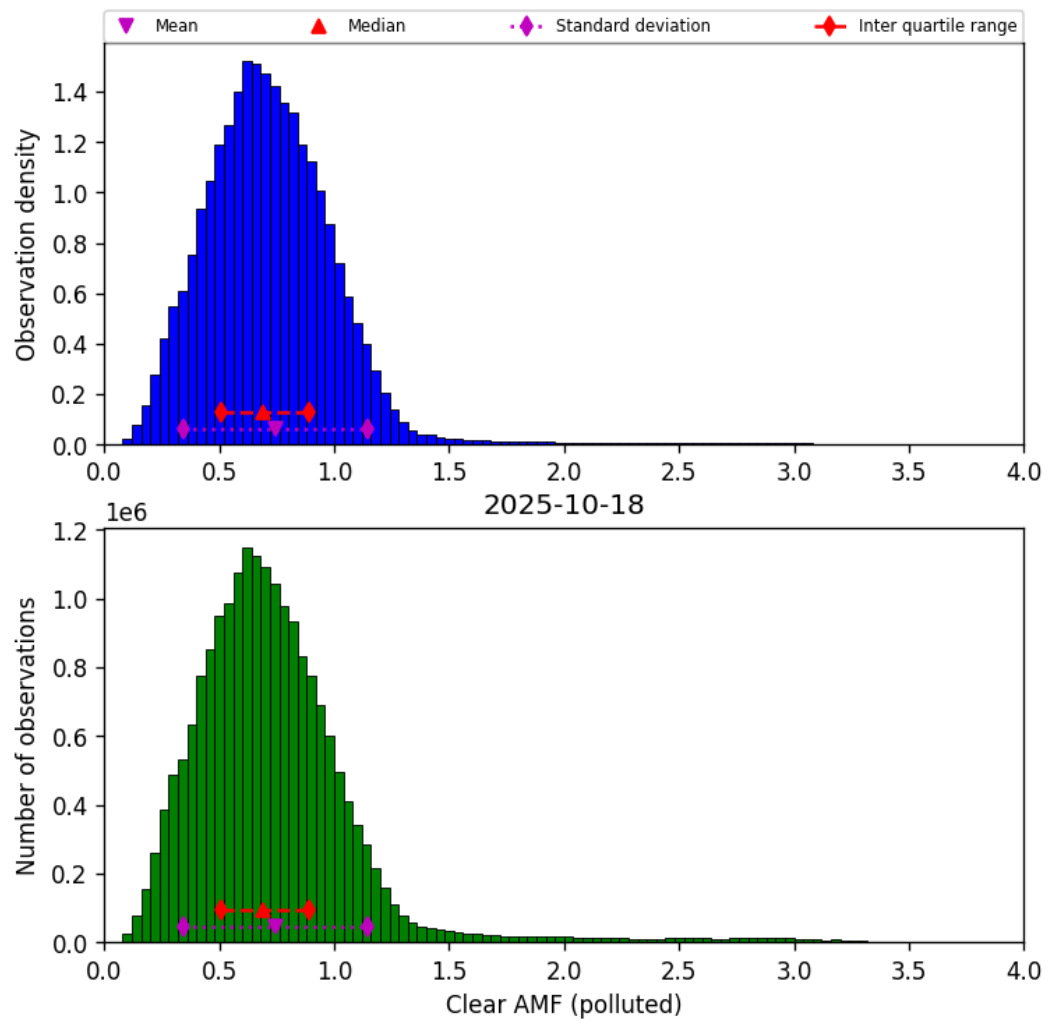
Figure 81: Histogram of “Clear AMF (polluted)” for 2025-10-17 to 2025-10-19
