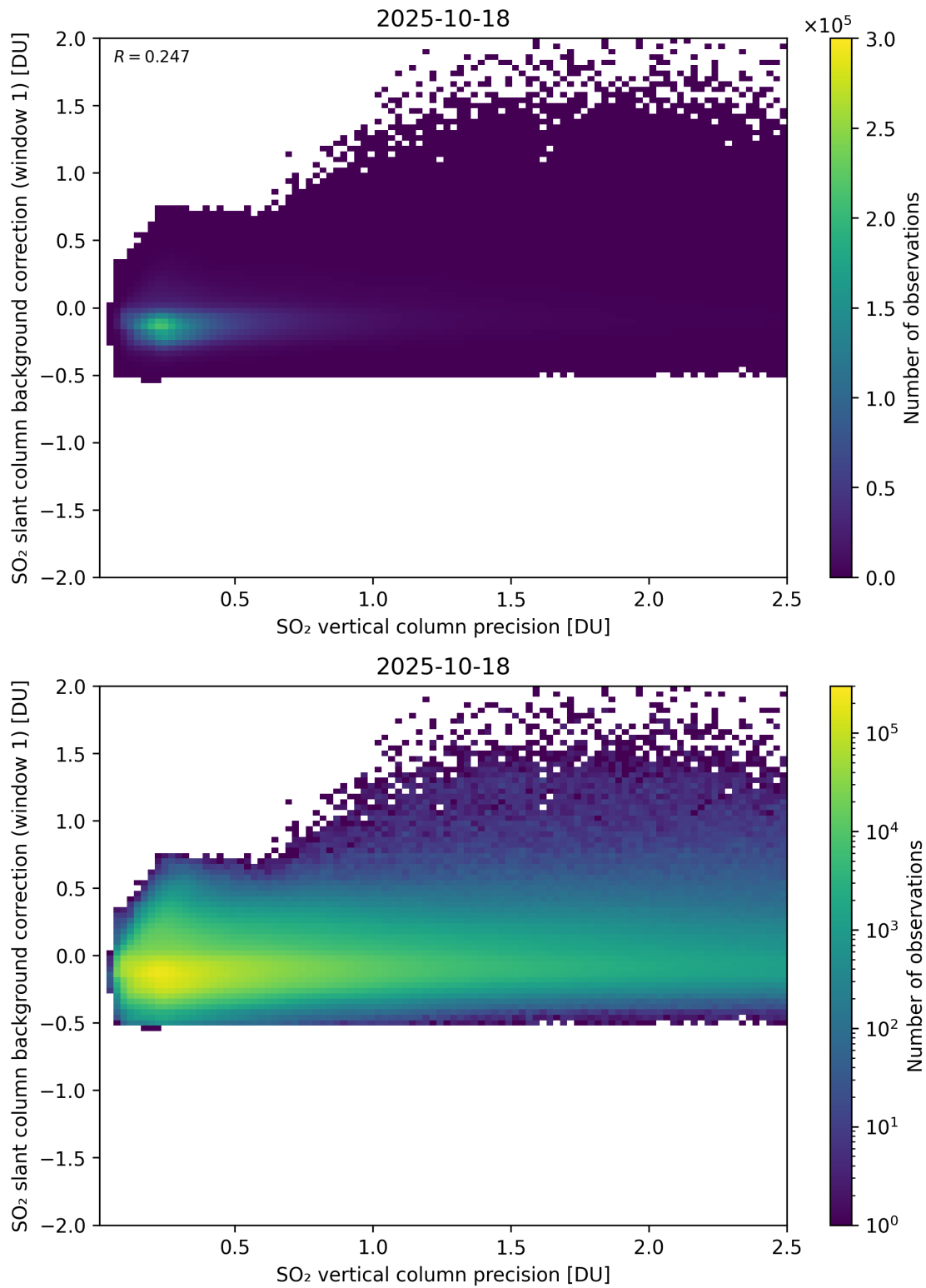
Figure 329: Scatter density plot of “SO 2 vertical column precision” against “SO 2 slant column background correction (window 1)” for 2025-10-17 to 2025-10-19.
