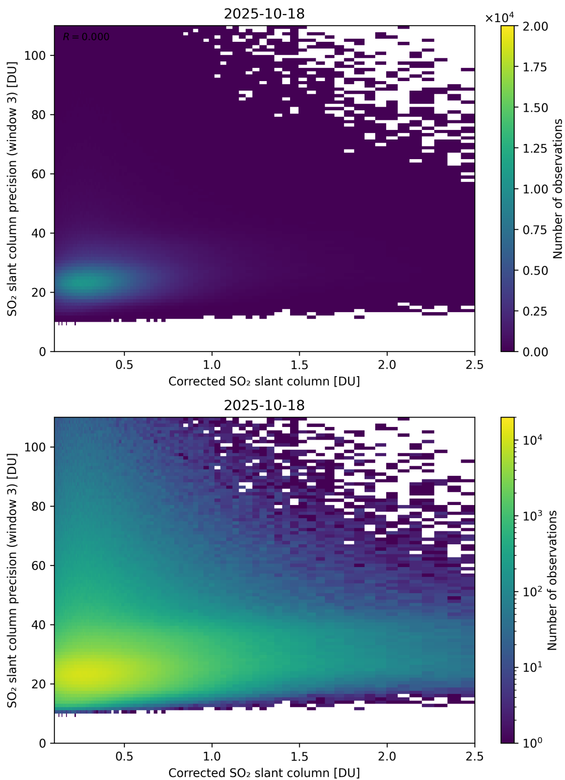
Figure 241: Scatter density plot of “Corrected SO 2 slant column” against “SO 2 slant column precision (window 3)” for 2025-10-17 to 2025-10-19.
