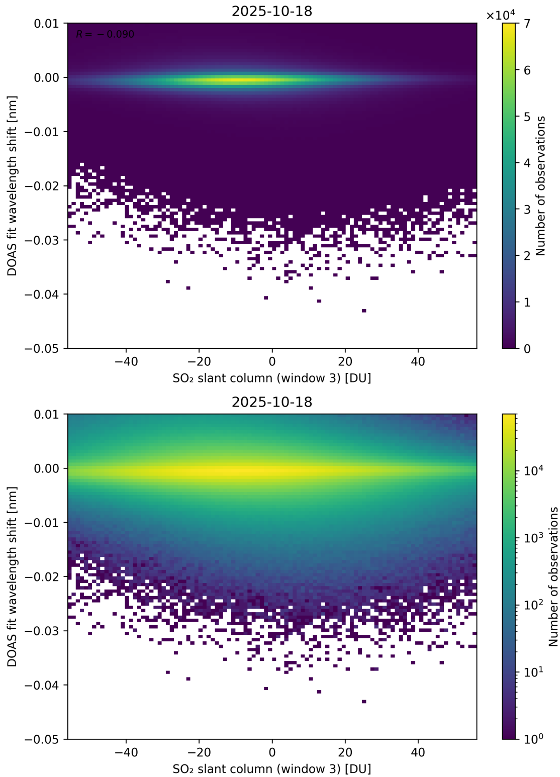
Figure 304: Scatter density plot of “SO 2 slant column (window 3)” against “DOAS fit wavelength shift” for 2025-10-17 to 2025-10-19.
