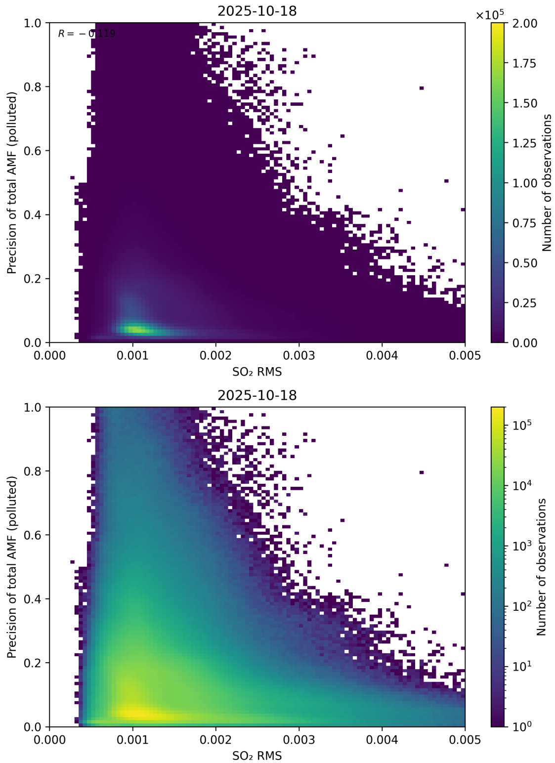
Figure 149: Scatter density plot of “SO 2 RMS” against “Precision of total AMF (polluted)” for 2025-10-17 to 2025-10-19.
