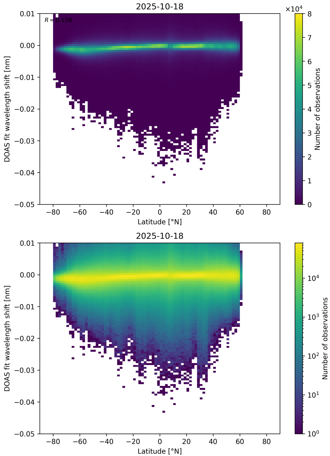
Figure 153: Scatter density plot of “Latitude” against “DOAS fit wavelength shift” for 2025-10-17 to 2025-10-19.
