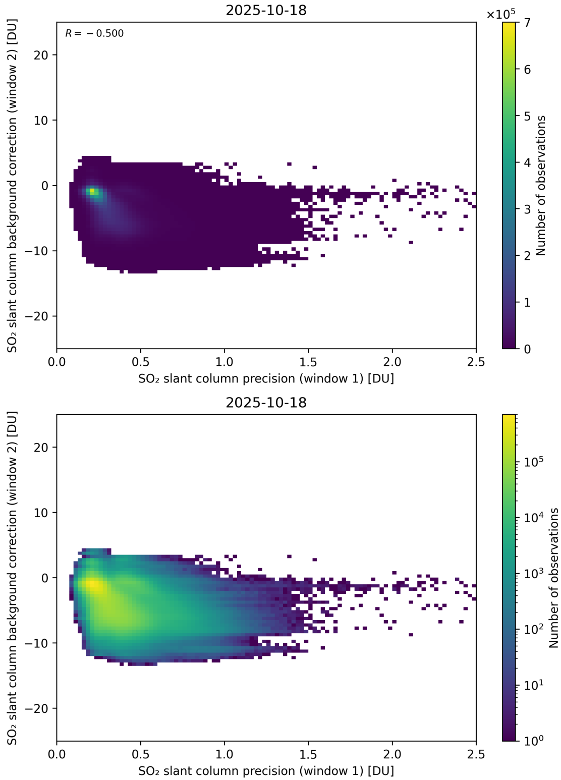
Figure 269: Scatter density plot of “SO 2 slant column precision (window 1)” against “SO 2 slant column background correction (window 2)” for 2025-10-17 to 2025-10-19.
