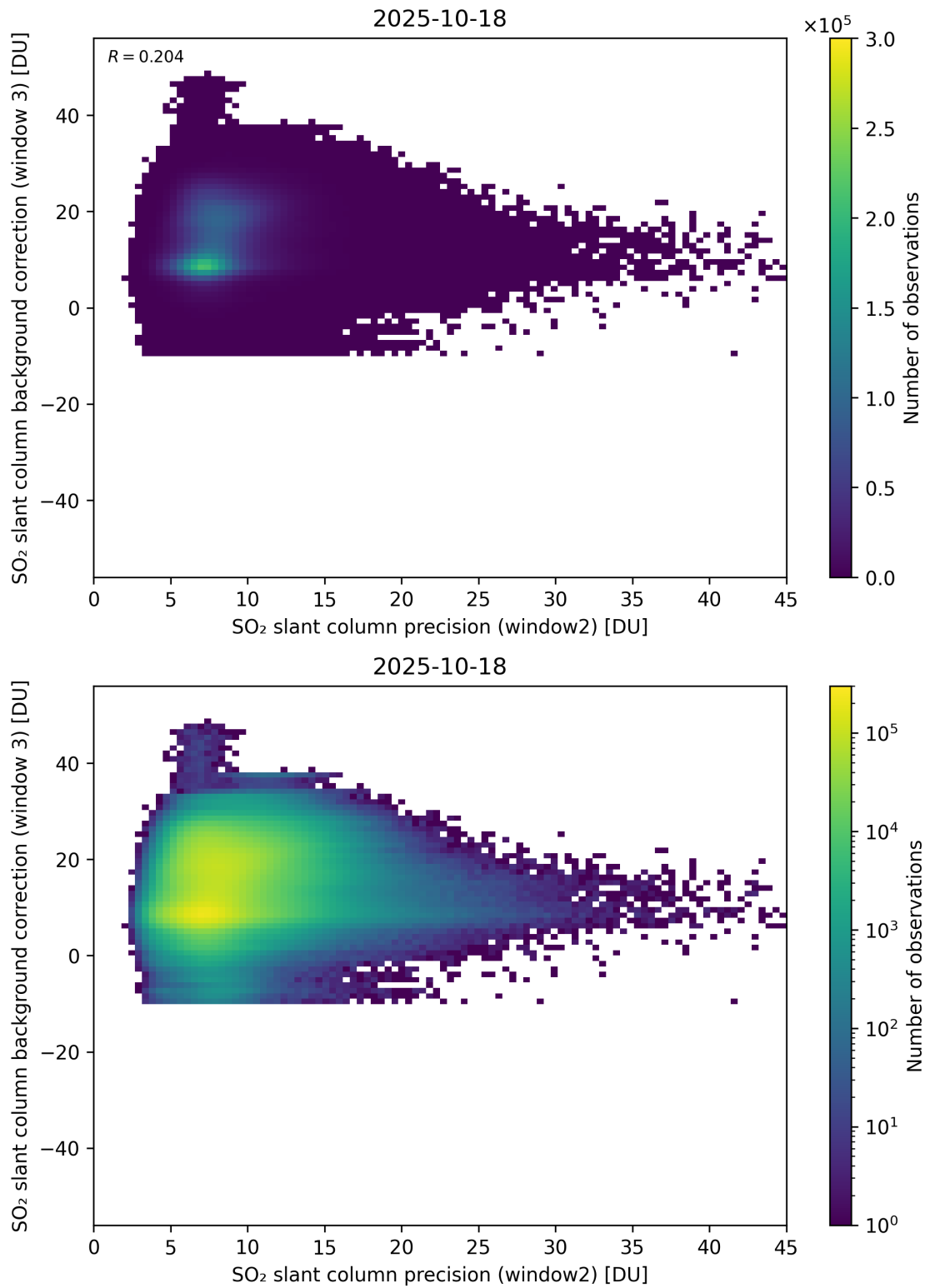
Figure 292: Scatter density plot of “SO 2 slant column precision (window2)” against “SO 2 slant column background correction (window 3)” for 2025-10-17 to 2025-10-19.
