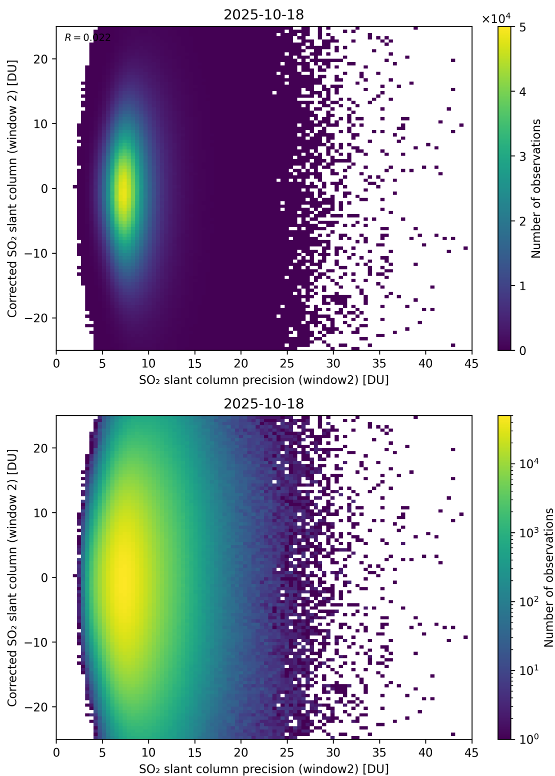
Figure 297: Scatter density plot of “SO 2 slant column precision (window2)” against “Corrected SO 2 slant column (window 2)” for 2025-10-17 to 2025-10-19.
