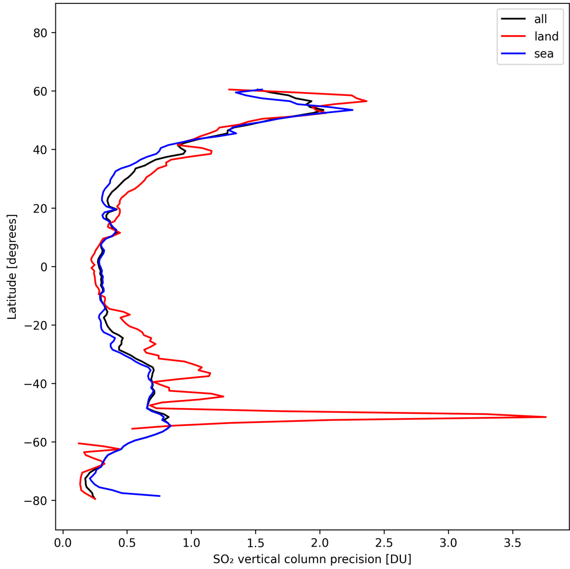
Figure 33: Zonal average of “SO 2 vertical column precision” for 2025-10-17 to 2025-10-19.
