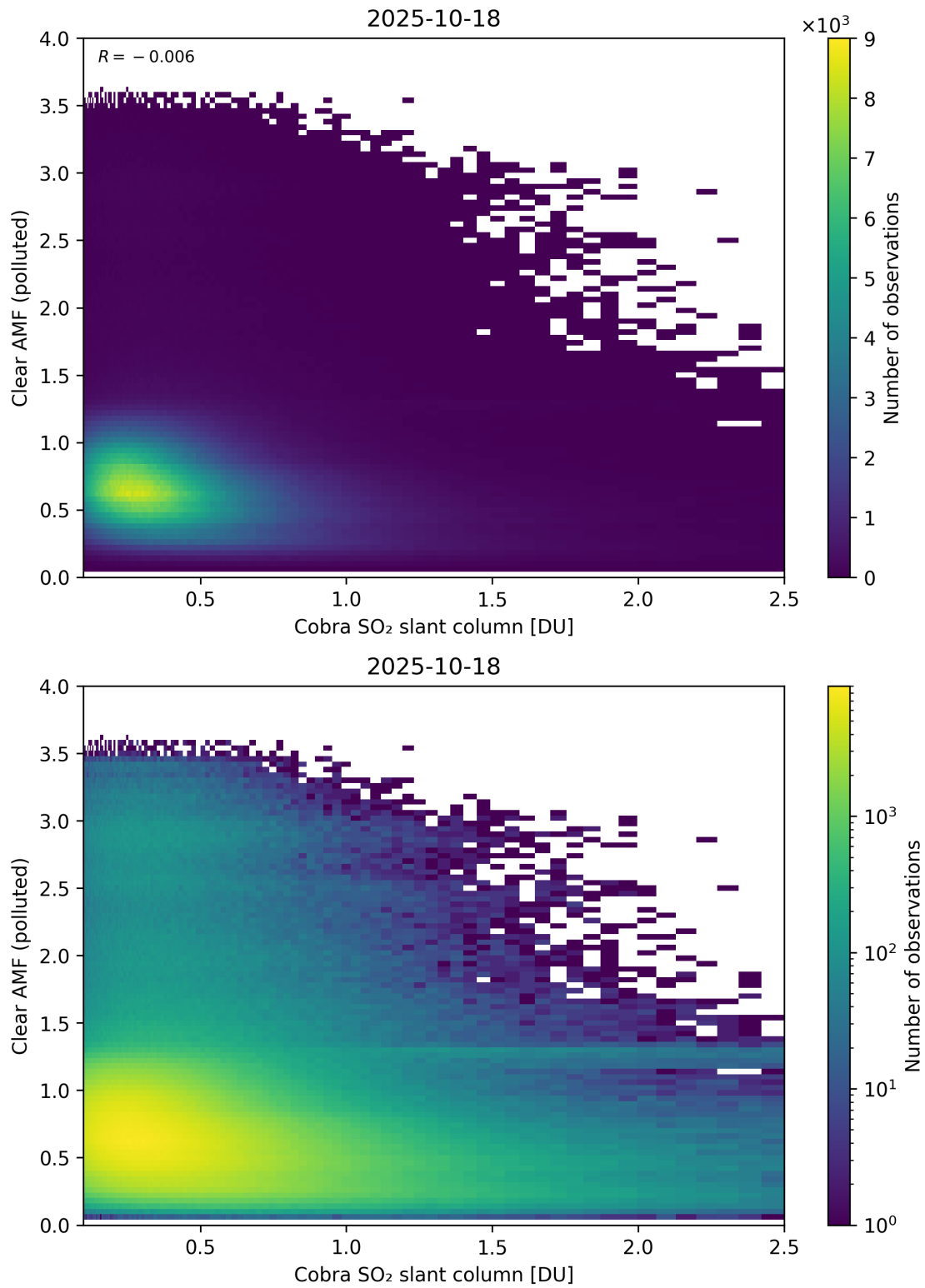
Figure 215: Scatter density plot of “Cobra SO 2 slant column” against “Clear AMF (polluted)” for 2025-10-17 to 2025-10-19.
