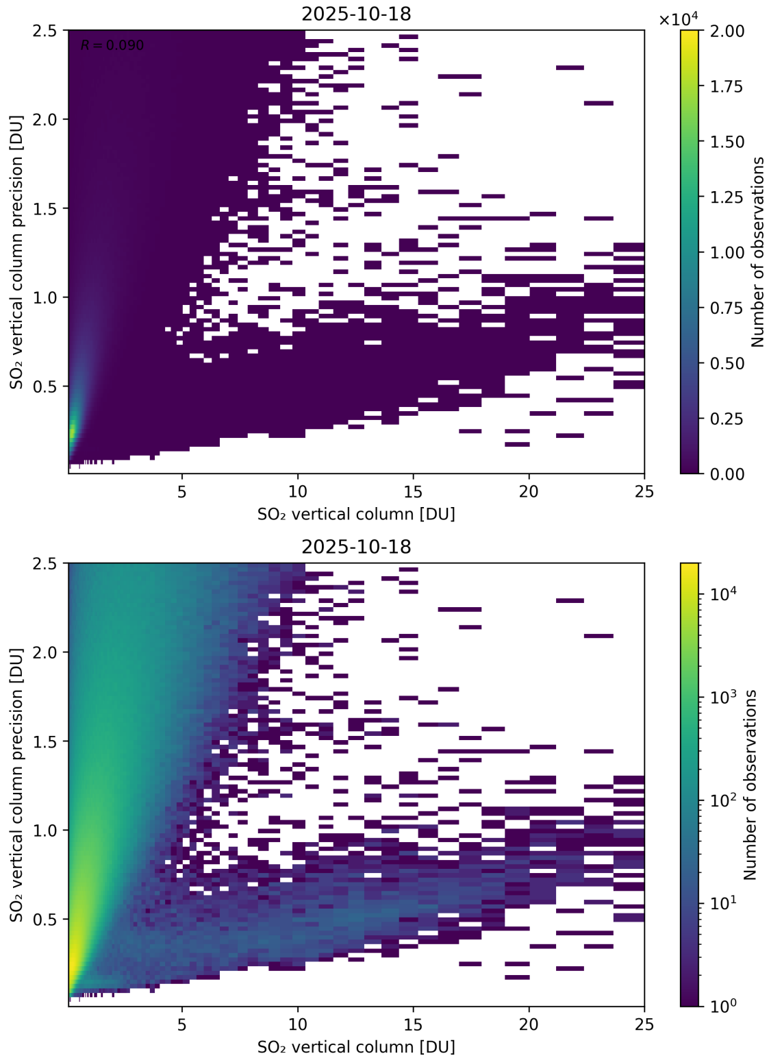
Figure 361: Scatter density plot of “SO 2 vertical column” against “SO 2 vertical column precision” for 2025-10-17 to 2025-10-19.
