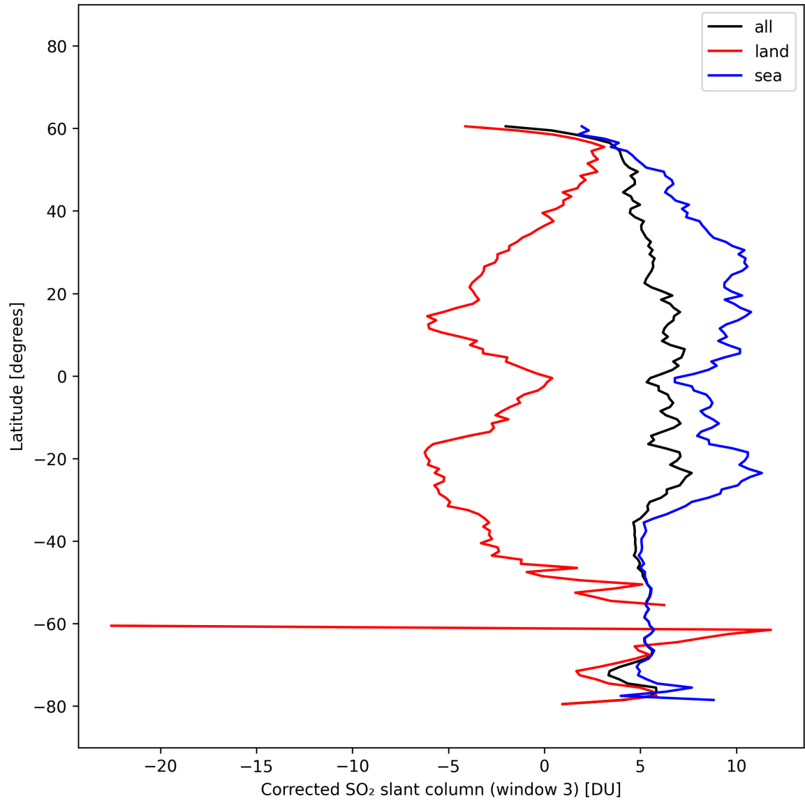
Figure 47: Zonal average of “Corrected SO 2 slant column (window 3)” for 2025-10-17 to 2025-10-19.
