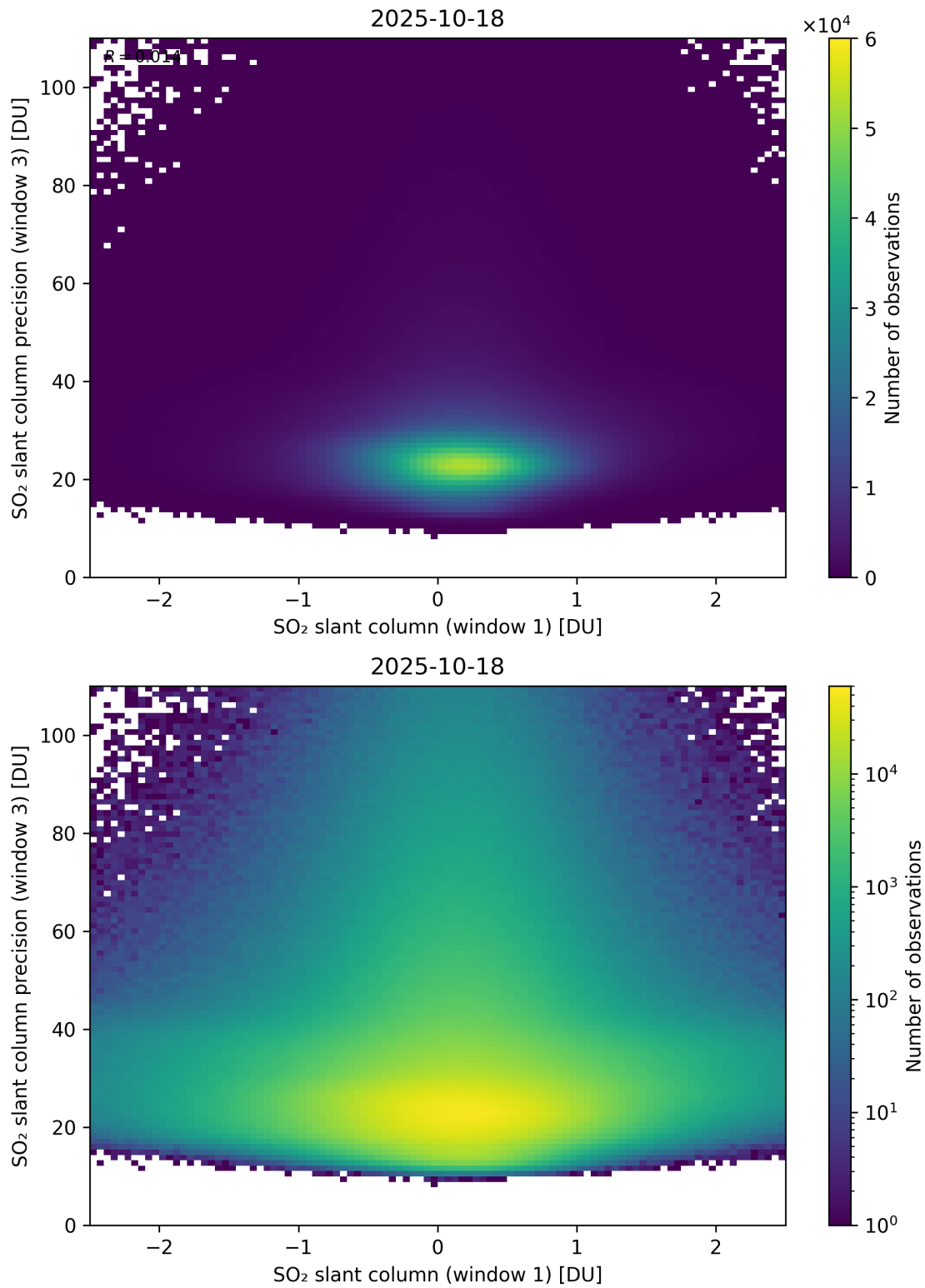
Figure 288: Scatter density plot of “SO 2 slant column (window 1)” against “SO 2 slant column precision (window 3)” for 2025-10-17 to 2025-10-19.
