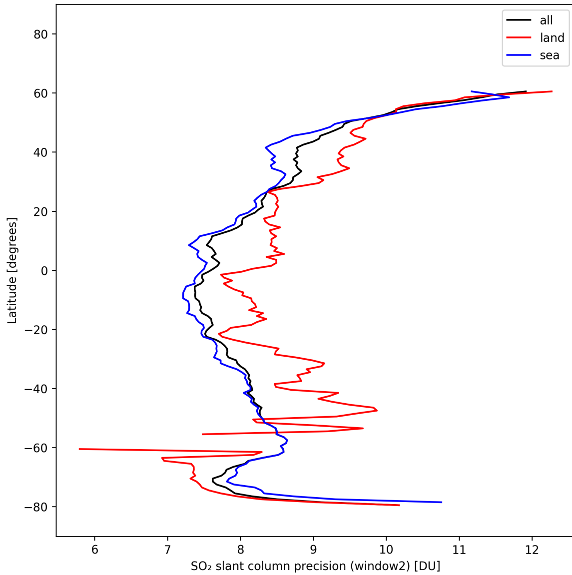
Figure 42: Zonal average of "SO 2 slant column precision (window2)" for 2025-10-17 to 2025-10-19.
