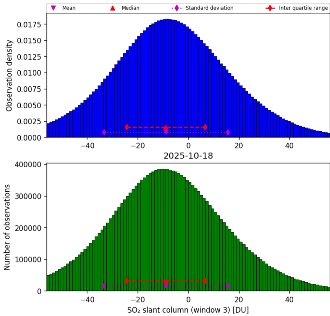
Figure 71: Histogram of “SO 2 slant column (window 3)” for 2025-10-17 to 2025-10-19
