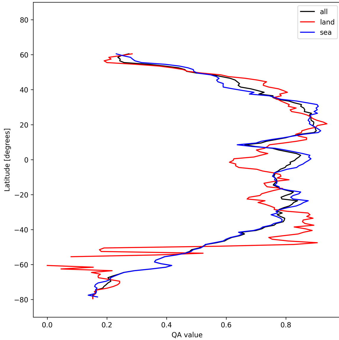
Figure 31: Zonal average of “QA value” for 2025-10-17 to 2025-10-19.
