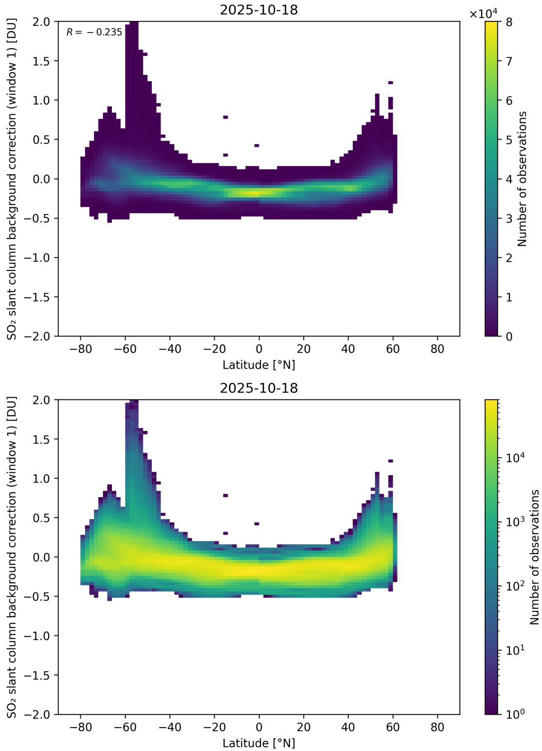
Figure 150: Scatter density plot of “Latitude” against “SO 2 slant column background correction (window 1)” for 2025-10-17 to 2025-10-19.
