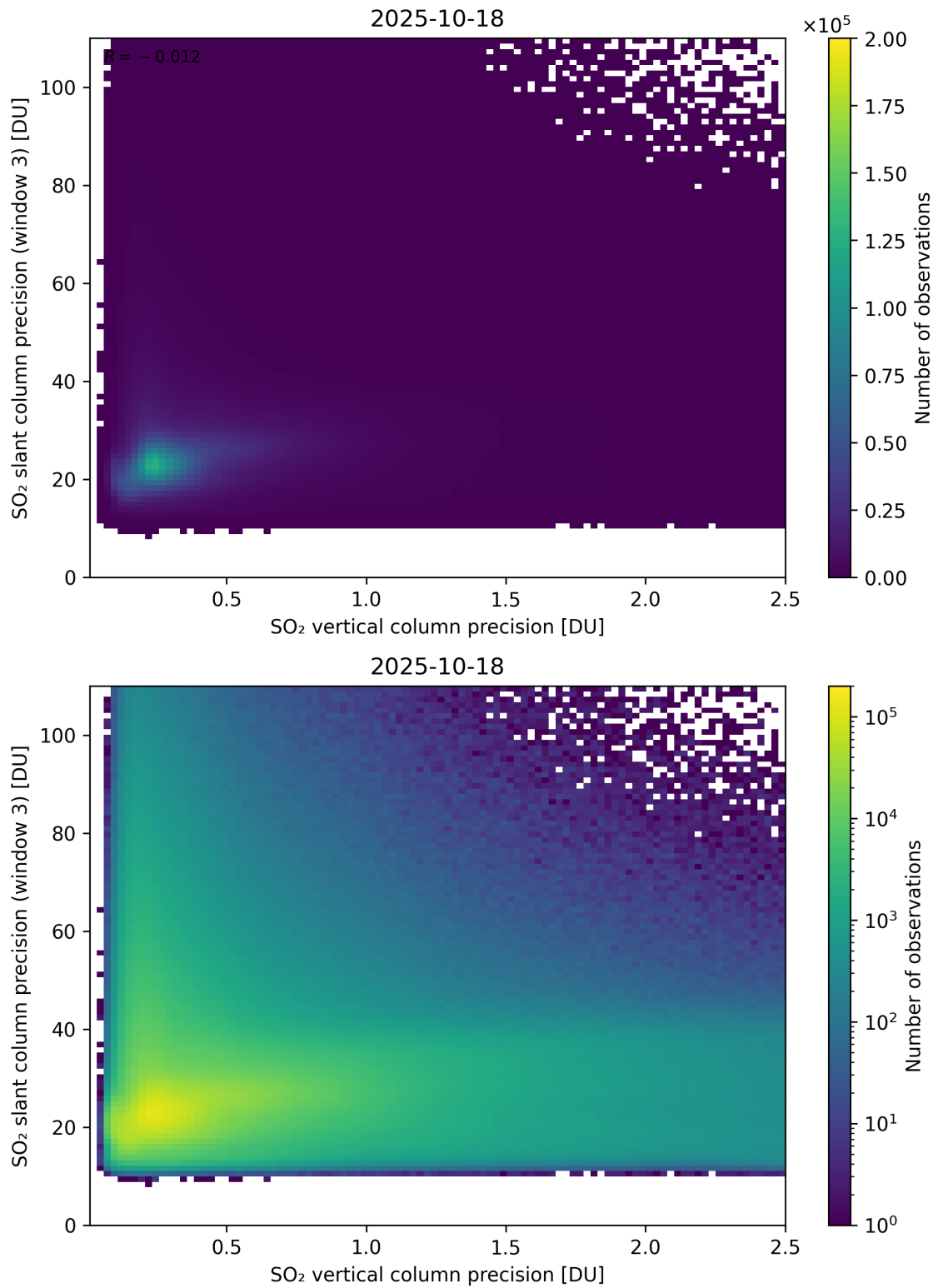
Figure 345: Scatter density plot of “SO 2 vertical column precision” against “SO 2 slant column precision (window 3)” for 2025-10-17 to 2025-10-19.
