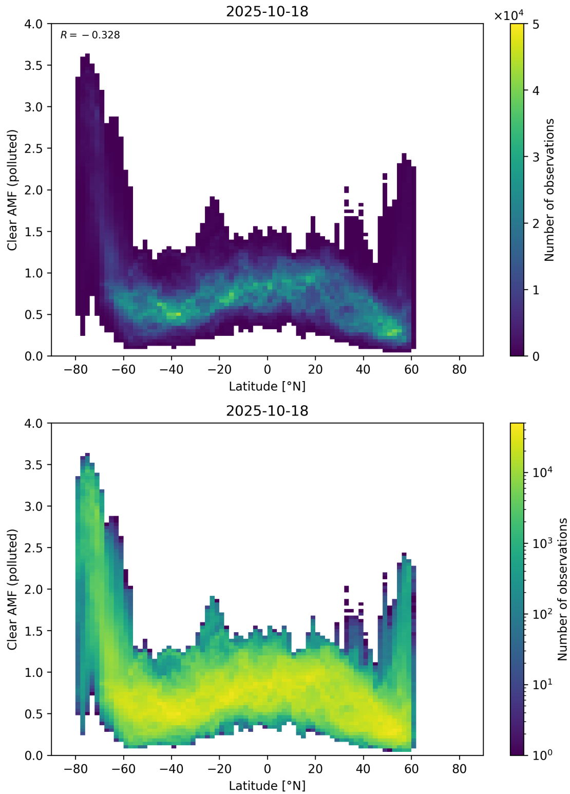
Figure 156: Scatter density plot of “Latitude” against “Clear AMF (polluted)” for 2025-10-17 to 2025-10-19.
