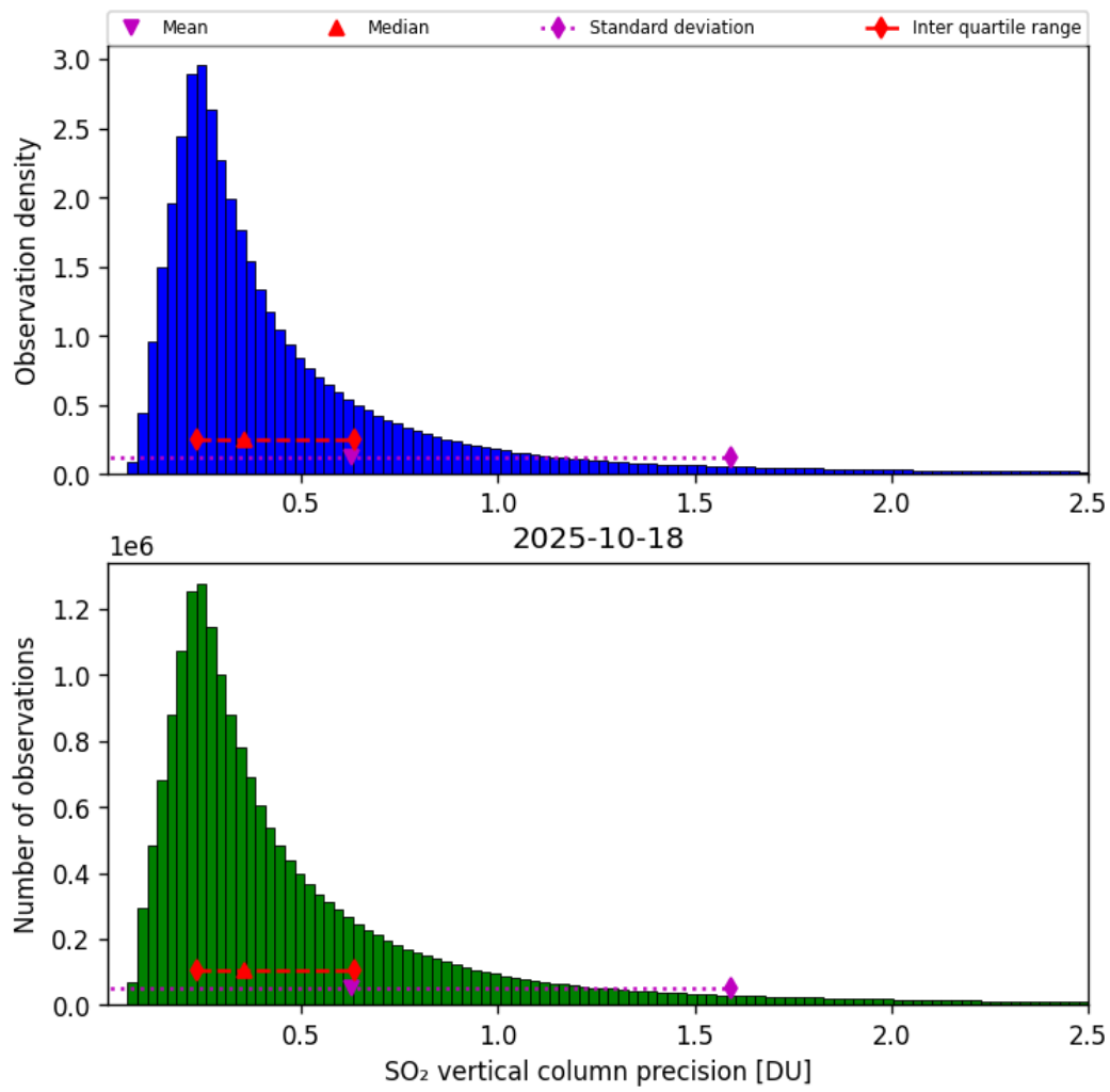
Figure 59: Histogram of “SO 2 vertical column precision” for 2025-10-17 to 2025-10-19
