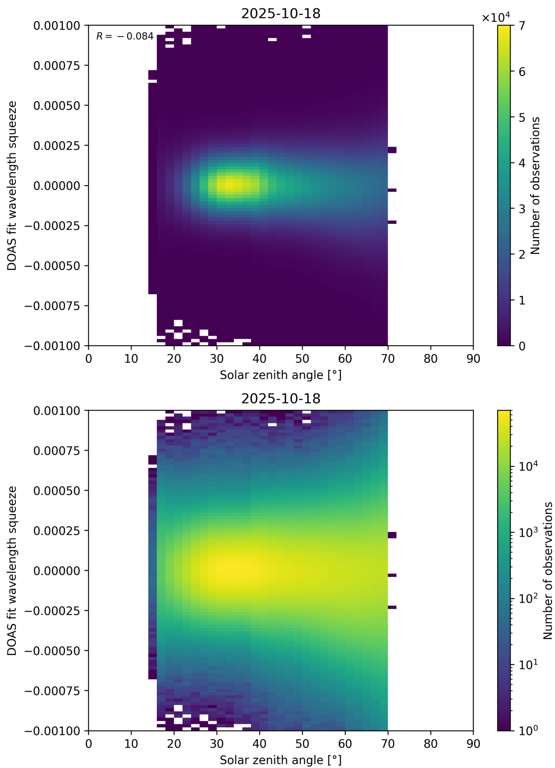
Figure 175: Scatter density plot of “Solar zenith angle” against “DOAS fit wavelength squeeze” for 2025-10-17 to 2025-10-19.
