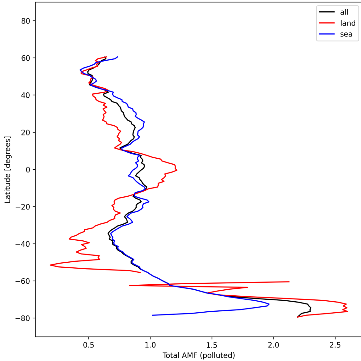
Figure 53: Zonal average of “Total AMF (polluted)” for 2025-10-17 to 2025-10-19.
