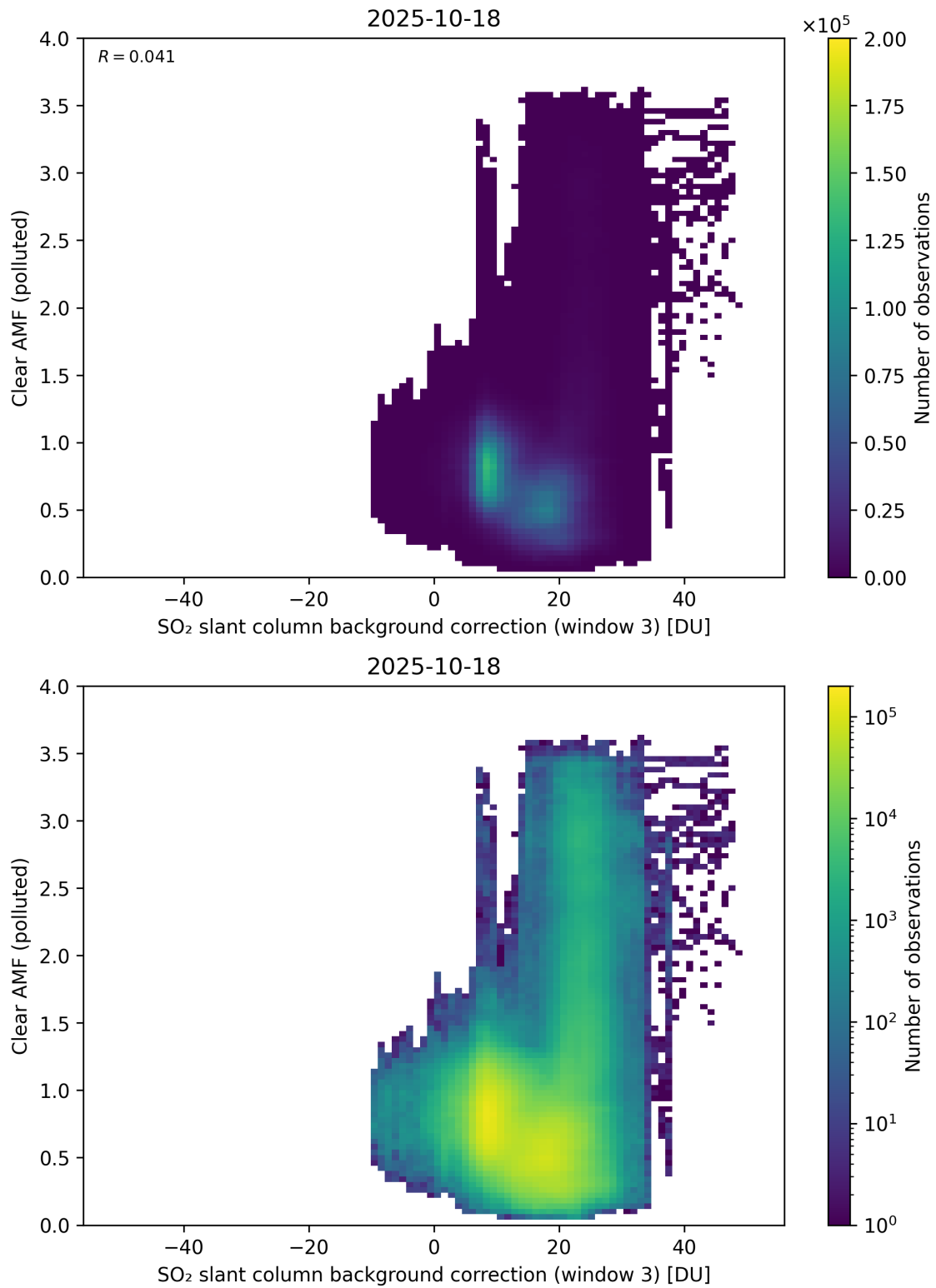
Figure 135: Scatter density plot of “SO 2 slant column background correction (window 3)” against “Clear AMF (polluted)” for 2025-10-17 to 2025-10-19.
