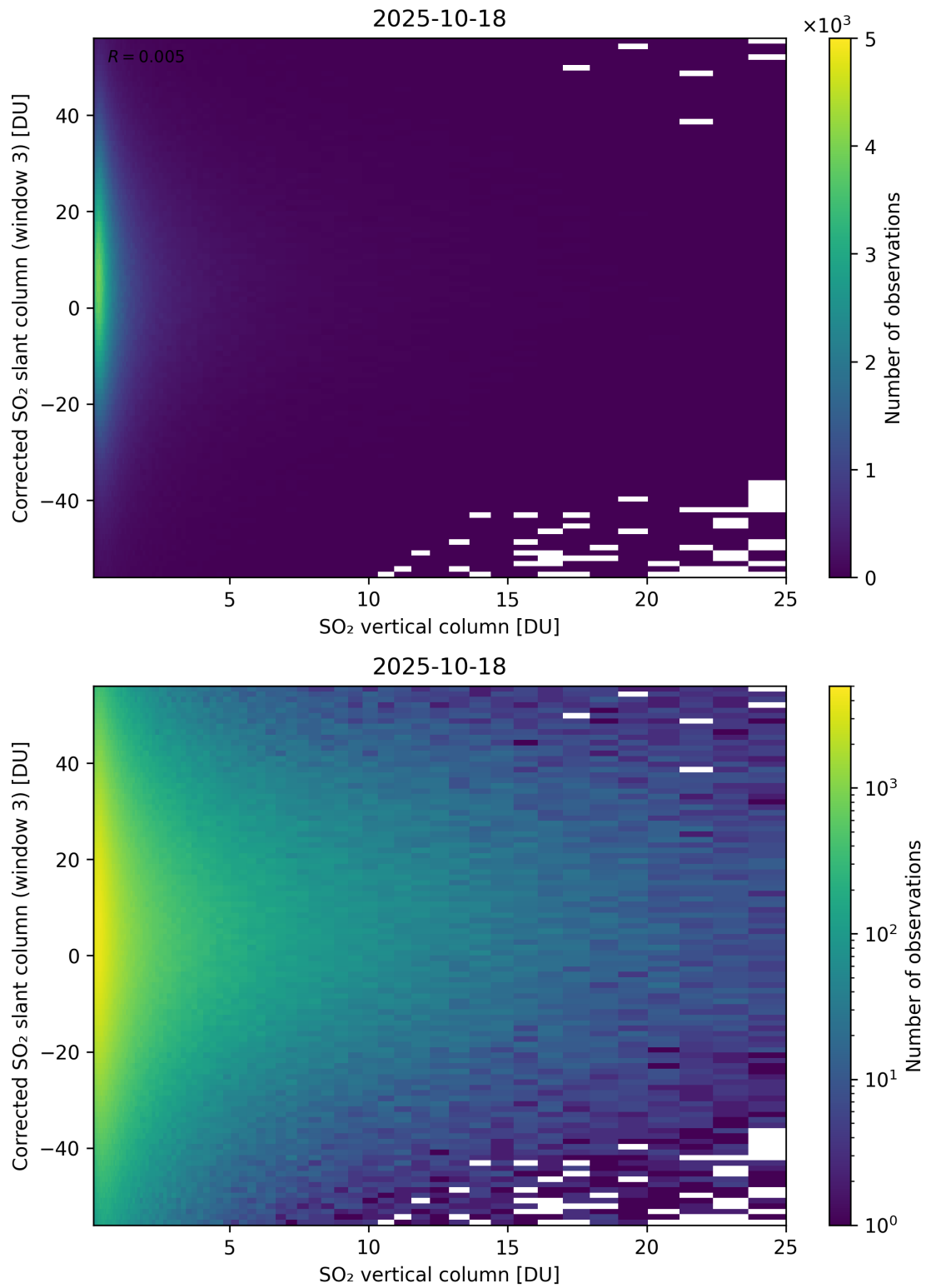
Figure 353: Scatter density plot of “SO 2 vertical column” against “Corrected SO 2 slant column (window 3)” for 2025-10-17 to 2025-10-19.
