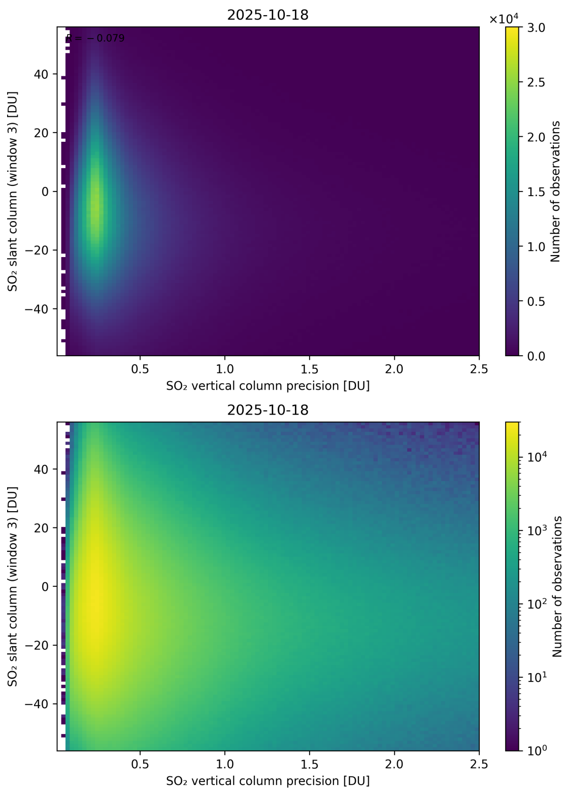
Figure 344: Scatter density plot of “SO 2 vertical column precision” against “SO 2 slant column (window 3)” for 2025-10-17 to 2025-10-19.
