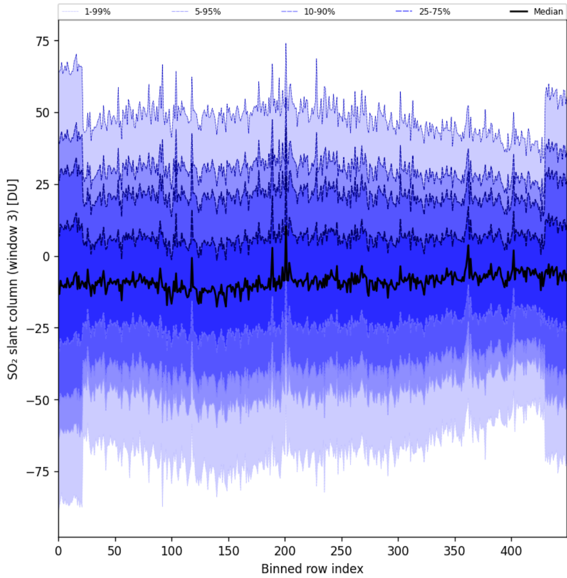
Figure 97: Along track statistics of “SO 2 slant column (window 3)” for 2025-10-17 to 2025-10-19
