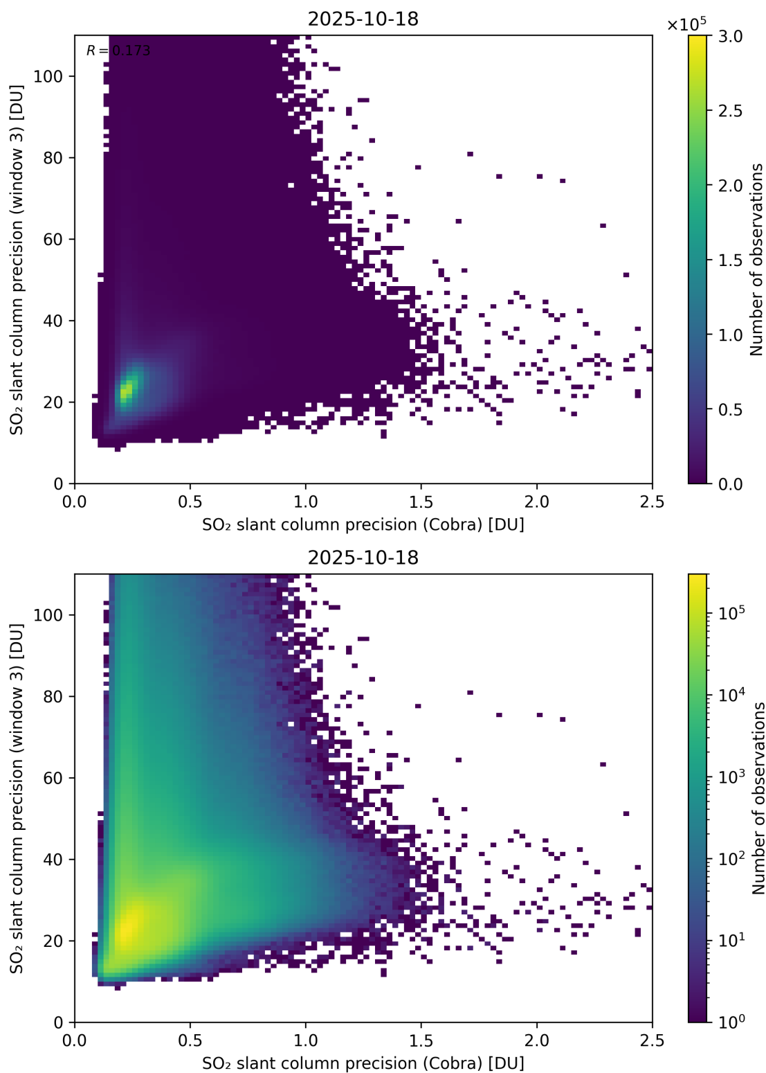
Figure 212: Scatter density plot of “SO 2 slant column precision (Cobra)” against “SO 2 slant column precision (window 3)” for 2025-10-17 to 2025-10-19.
