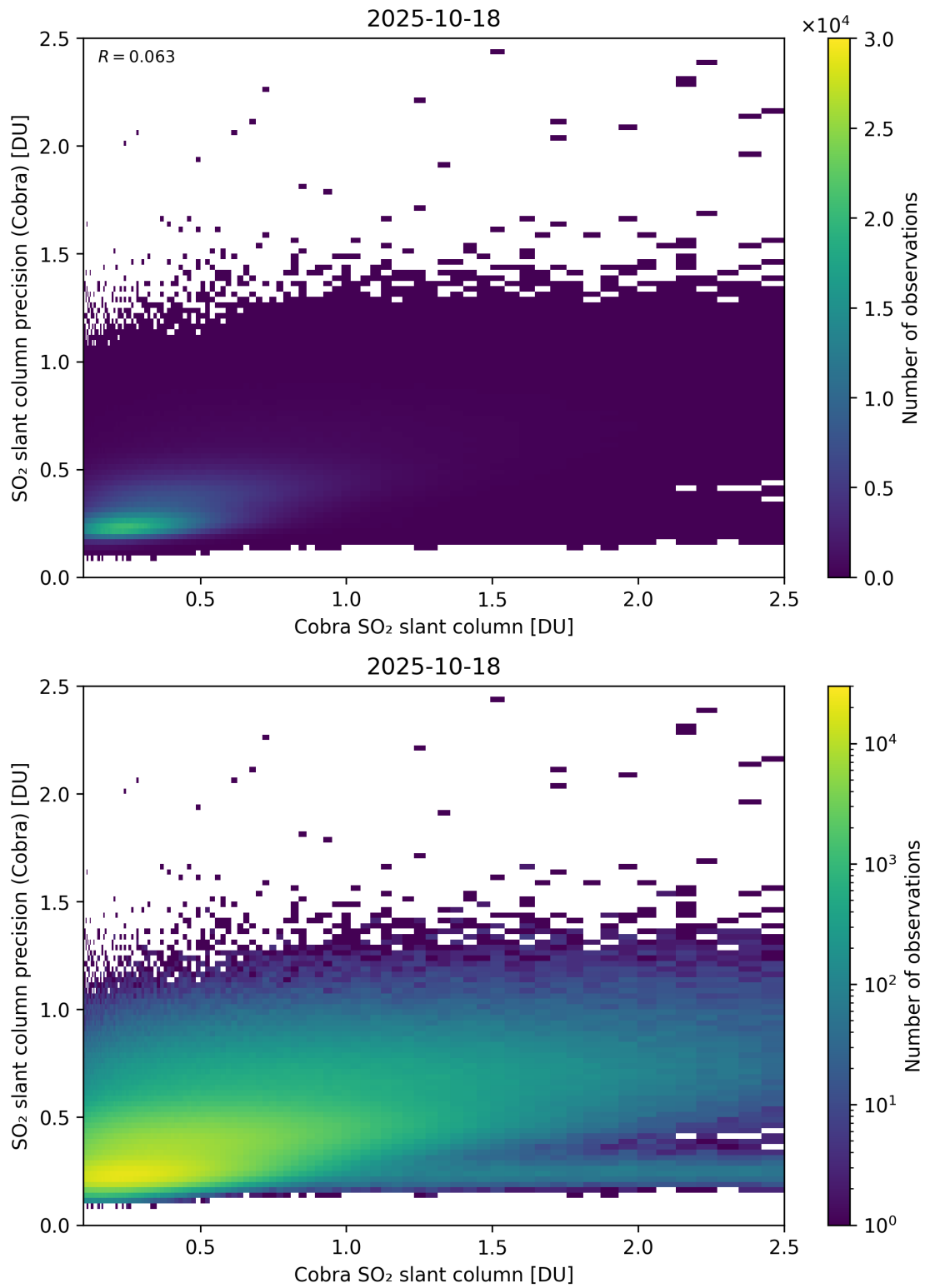
Figure 216: Scatter density plot of “Cobra SO 2 slant column” against “SO 2 slant column precision (Cobra)” for 2025-10-17 to 2025-10-19.
