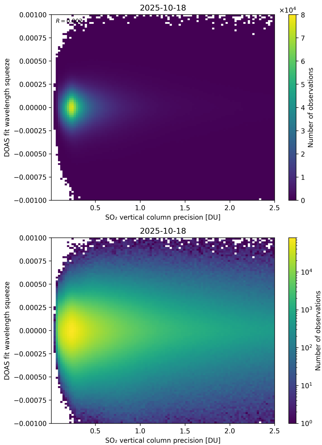
Figure 333: Scatter density plot of “SO 2 vertical column precision” against “DOAS fit wavelength squeeze” for 2025-10-17 to 2025-10-19.
