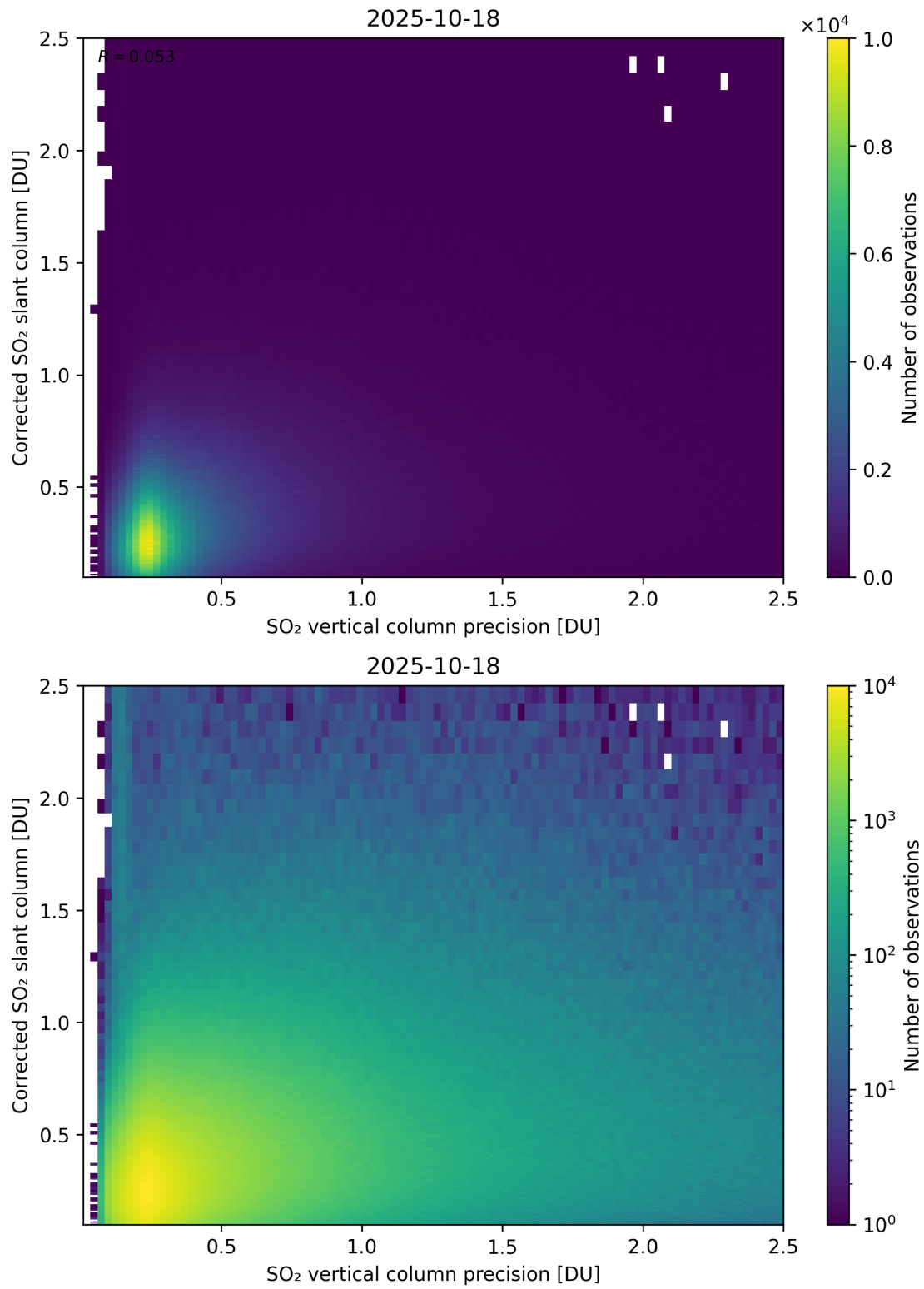
Figure 338: Scatter density plot of “SO 2 vertical column precision” against “Corrected SO 2 slant column” for 2025-10-17 to 2025-10-19.
