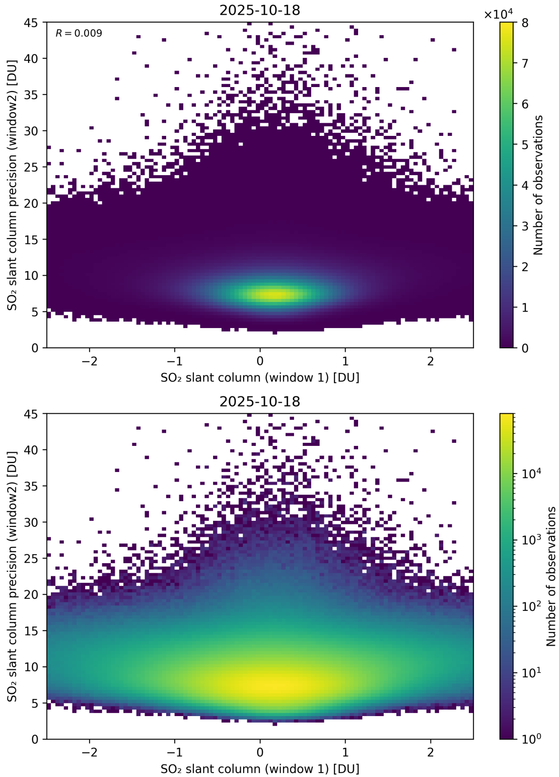
Figure 286: Scatter density plot of “SO 2 slant column (window 1)” against “SO 2 slant column precision (window2)” for 2025-10-17 to 2025-10-19.
