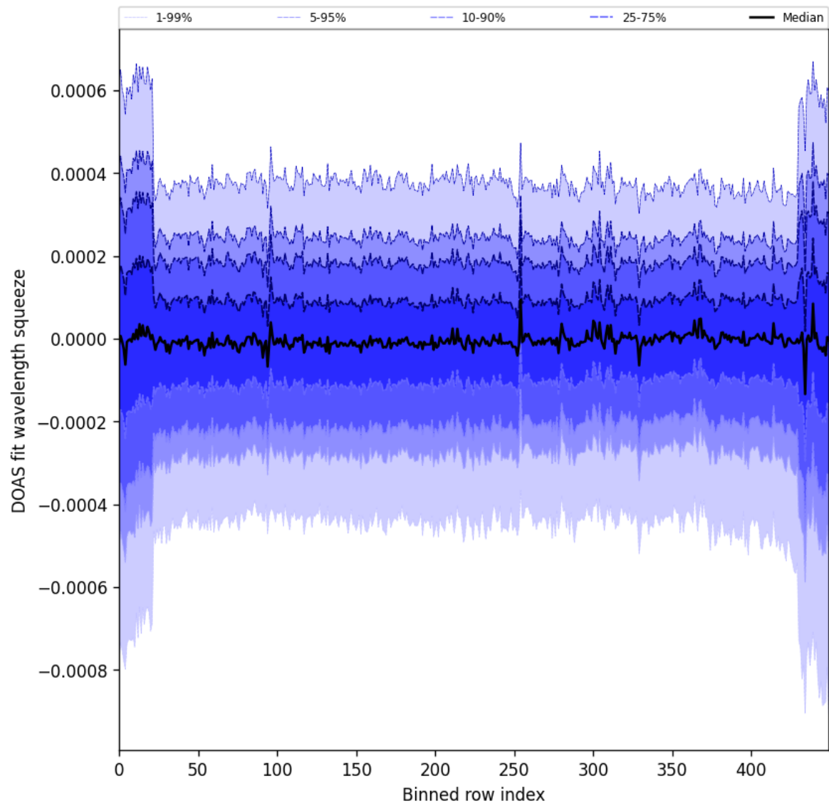
Figure 103: Along track statistics of “DOAS fit wavelength squeeze” for 2025-10-17 to 2025-10-19
