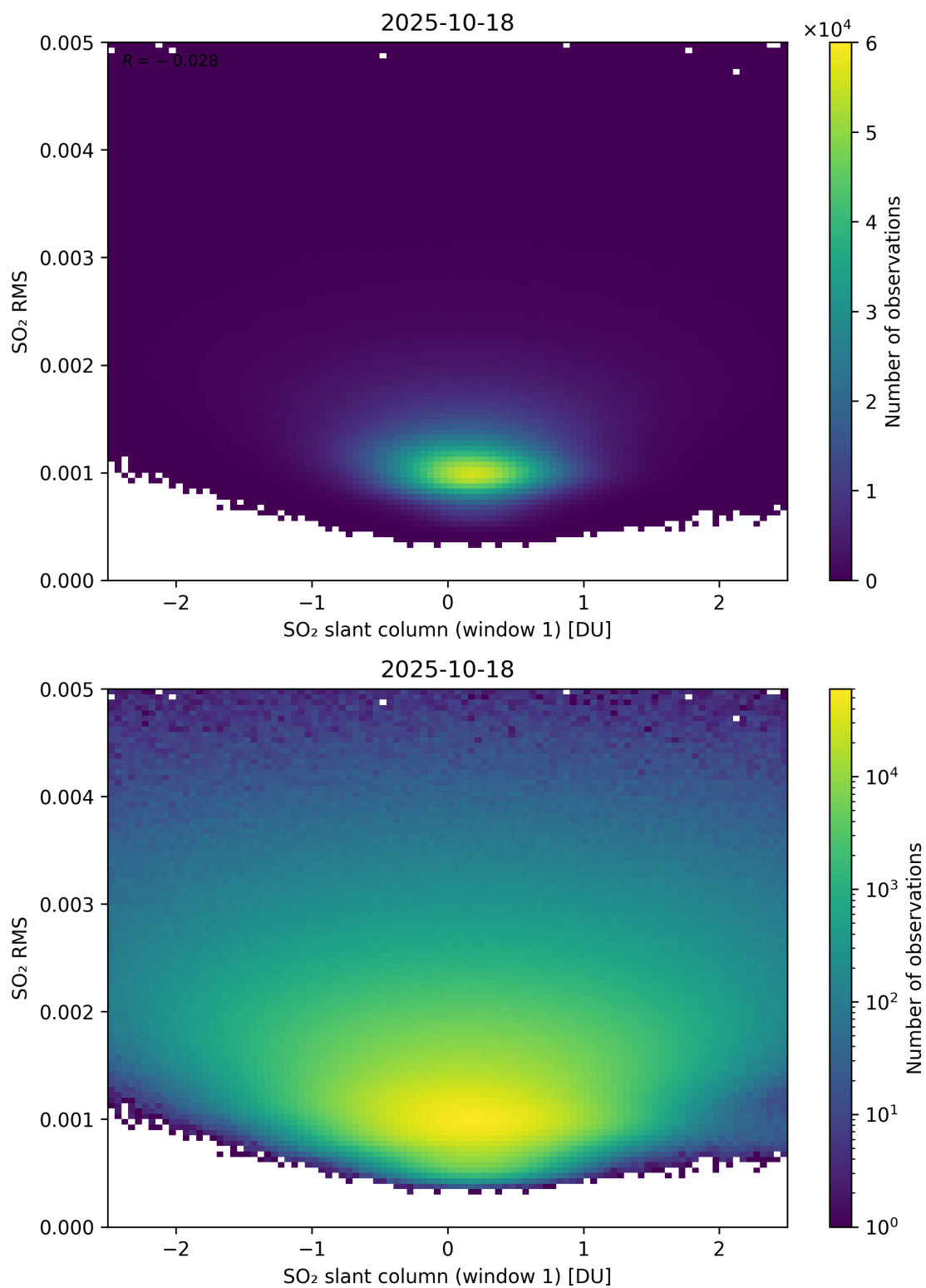
Figure 267: Scatter density plot of “SO 2 slant column (window 1)” against “SO 2 RMS” for 2025-10-17 to 2025-10-19.
