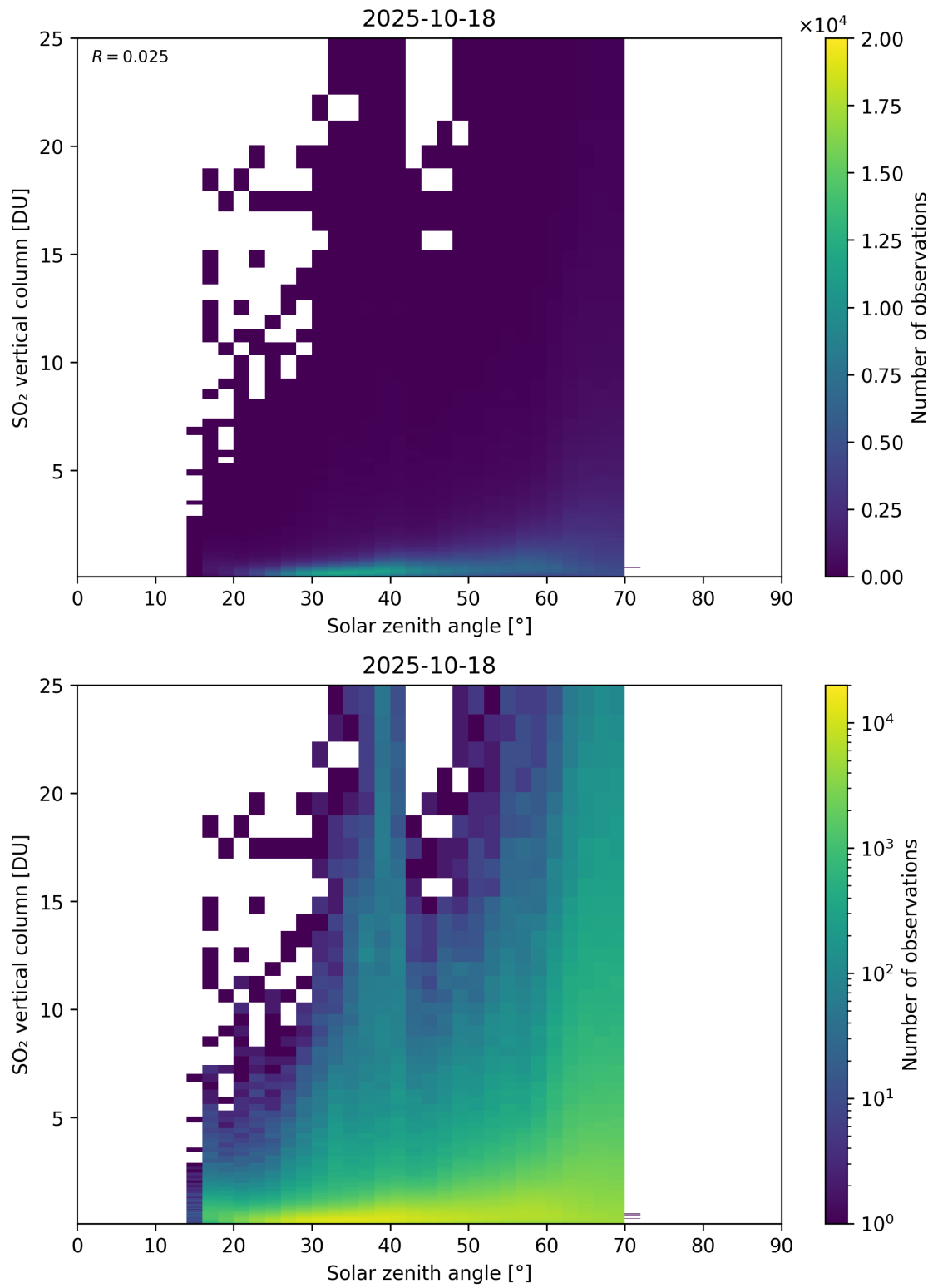
Figure 191: Scatter density plot of “Solar zenith angle” against “SO 2 vertical column” for 2025-10-17 to 2025-10-19.
