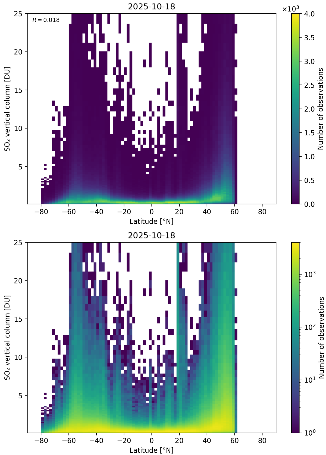
Figure 169: Scatter density plot of “Latitude” against “SO 2 vertical column” for 2025-10-17 to 2025-10-19.
