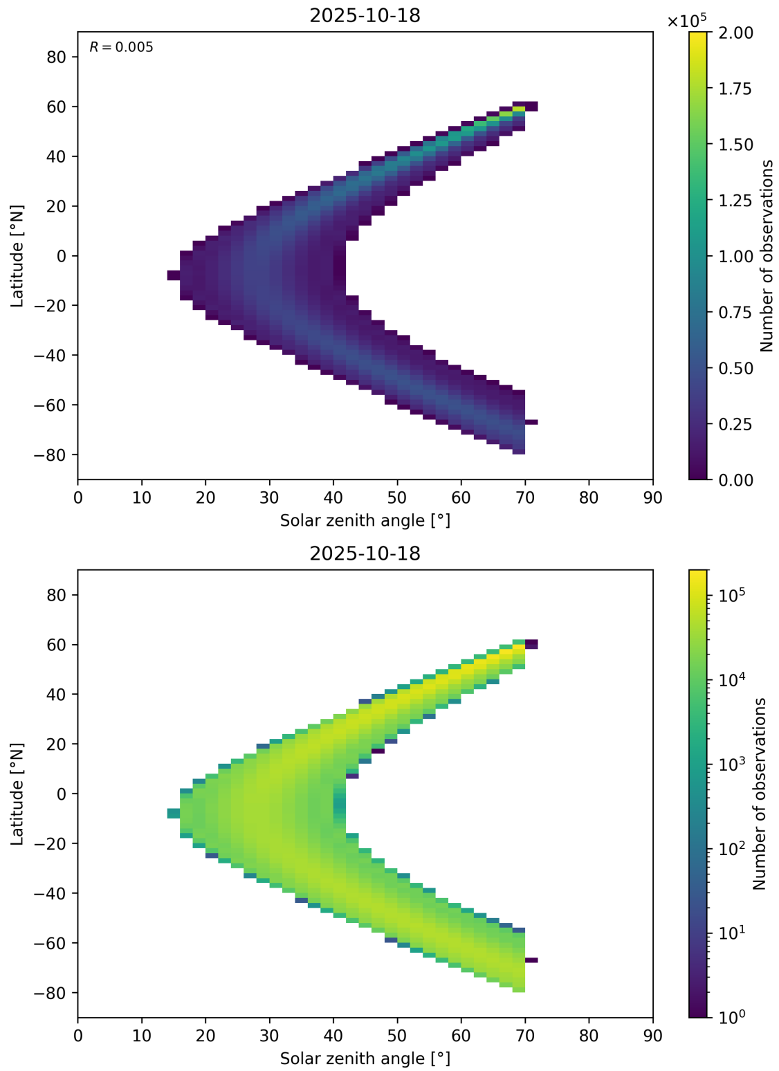
Figure 177: Scatter density plot of “Solar zenith angle” against “Latitude” for 2025-10-17 to 2025-10-19.
