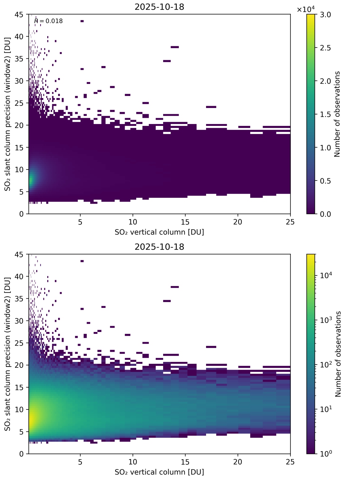
Figure 356: Scatter density plot of “SO 2 vertical column” against “SO 2 slant column precision (window2)” for 2025-10-17 to 2025-10-19.
