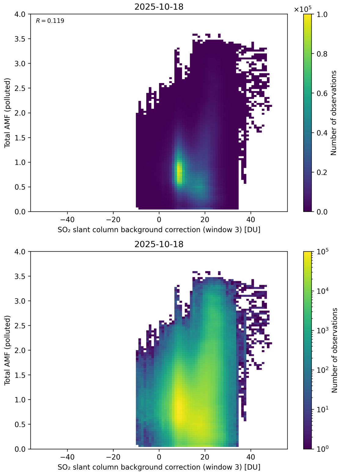
Figure 136: Scatter density plot of “SO 2 slant column background correction (window 3)” against “Total AMF (polluted)” for 2025-10-17 to 2025-10-19.
