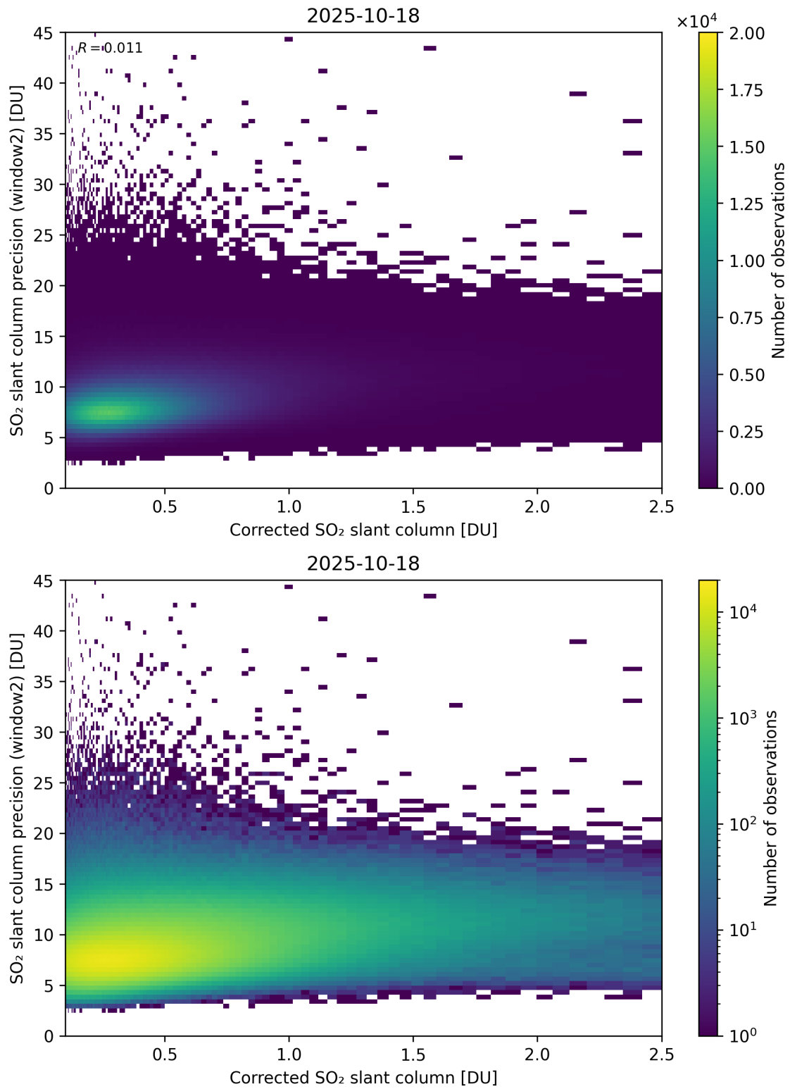
Figure 239: Scatter density plot of “Corrected SO 2 slant column” against “SO 2 slant column precision (window2)” for 2025-10-17 to 2025-10-19.
