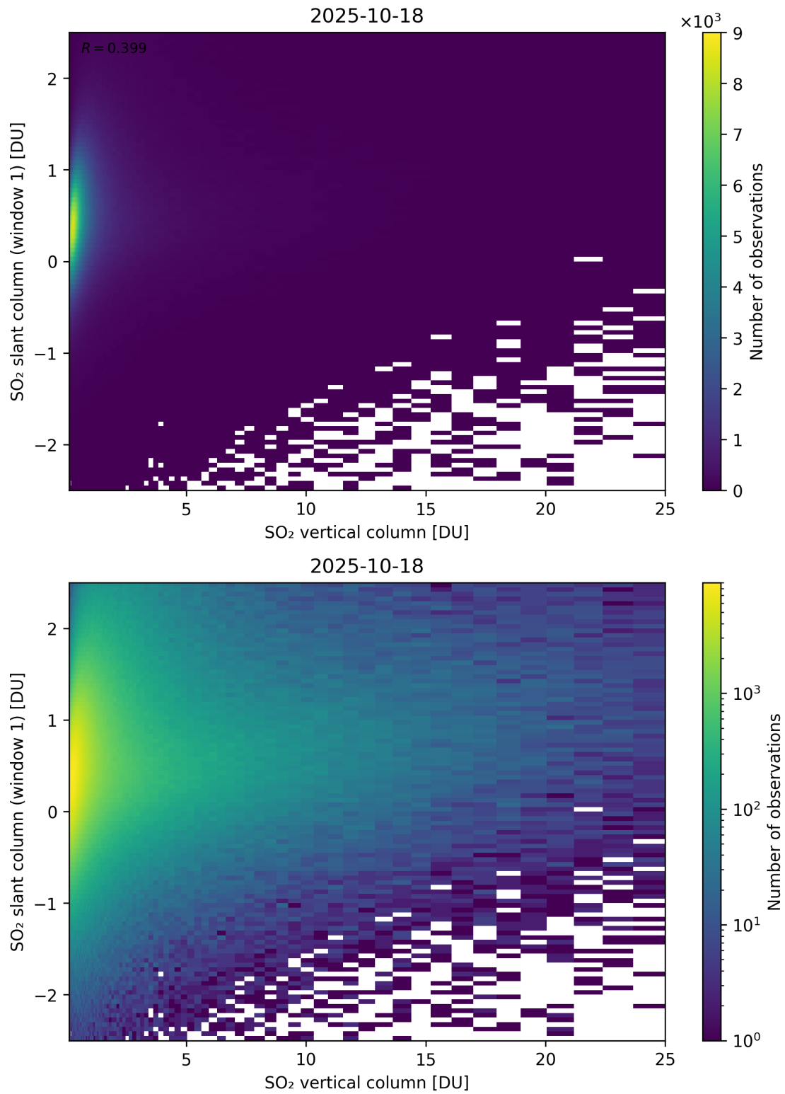
Figure 354: Scatter density plot of “SO 2 vertical column” against “SO 2 slant column (window 1)” for 2025-10-17 to 2025-10-19.
