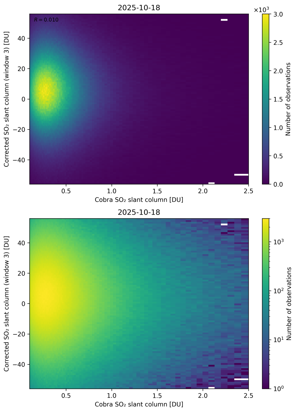
Figure 218: Scatter density plot of “Cobra SO 2 slant column” against “Corrected SO 2 slant column (window 3)” for 2025-10-17 to 2025-10-19.
