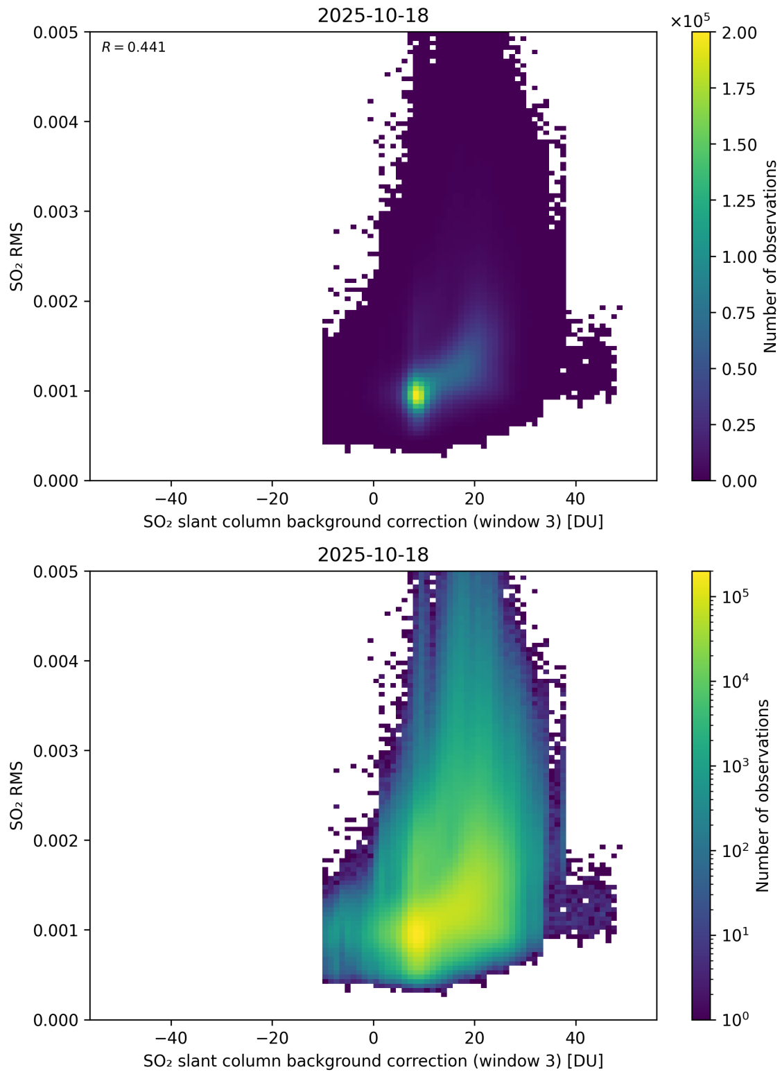
Figure 134: Scatter density plot of “SO 2 slant column background correction (window 3)” against “SO 2 RMS” for 2025-10-17 to 2025-10-19.
