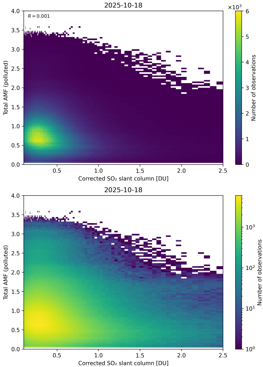
Figure 242: Scatter density plot of “Corrected SO 2 slant column” against “Total AMF (polluted)” for 2025-10-17 to 2025-10-19.
