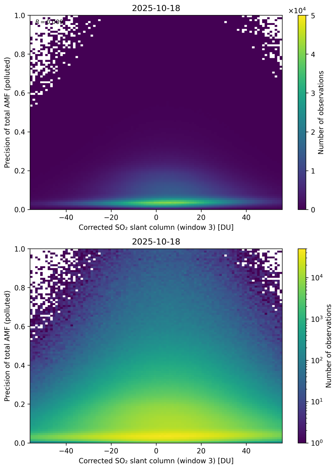
Figure 261: Scatter density plot of “Corrected SO 2 slant column (window 3)” against “Precision of total AMF (polluted)” for 2025-10-17 to 2025-10-19.
