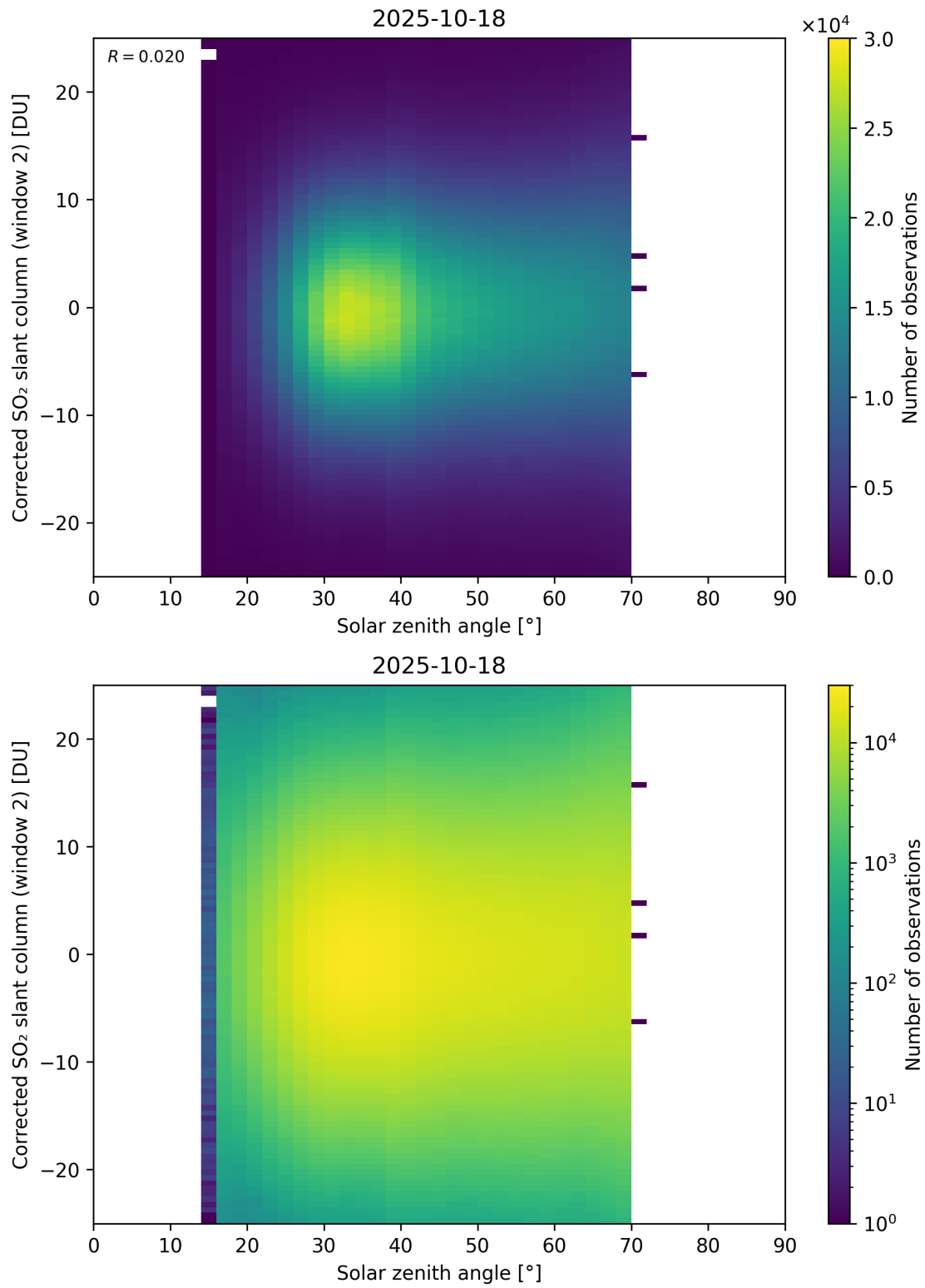
Figure 182: Scatter density plot of “Solar zenith angle” against “Corrected SO 2 slant column (window 2)” for 2025-10-17 to 2025-10-19.
