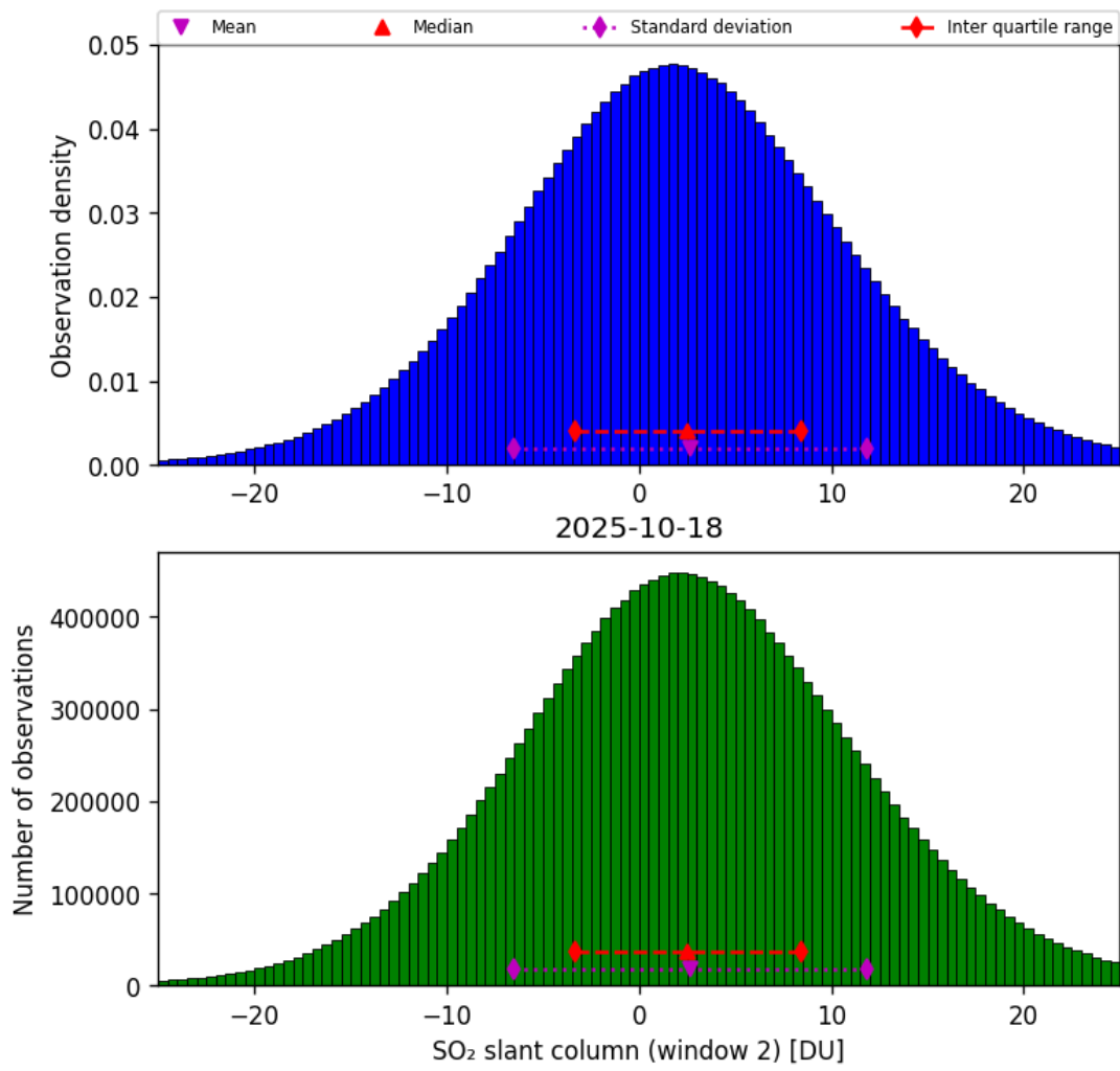
Figure 67: Histogram of “SO 2 slant column (window 2)” for 2025-10-17 to 2025-10-19
