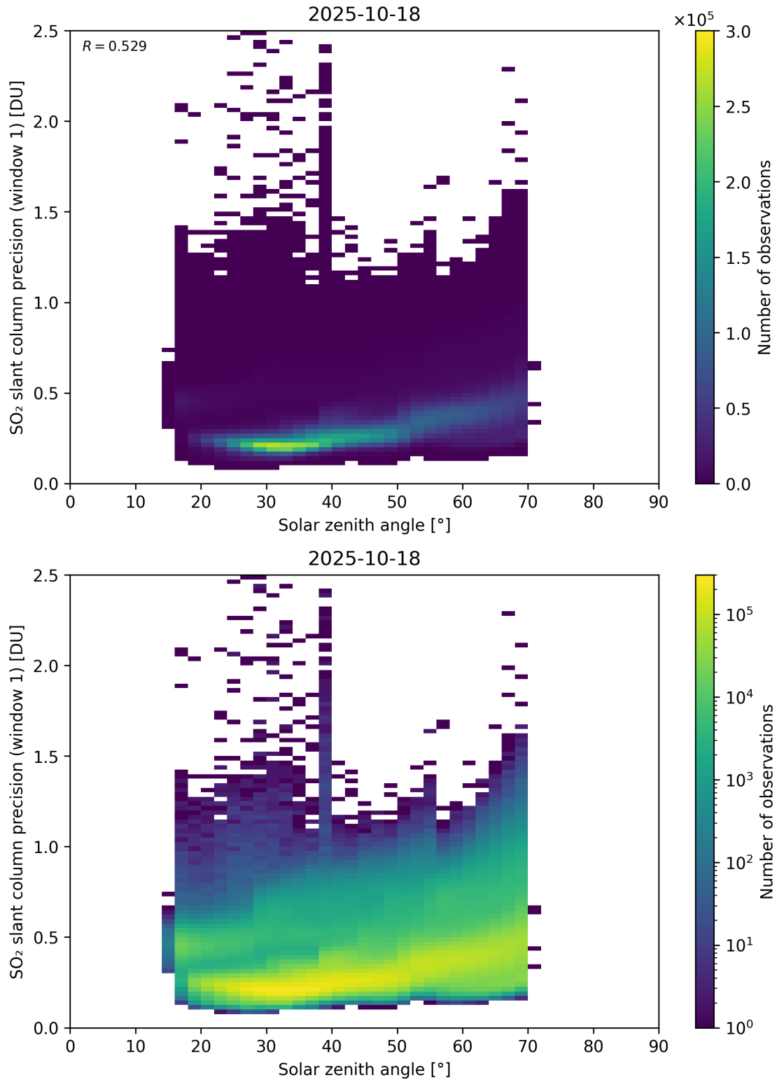
Figure 185: Scatter density plot of “Solar zenith angle” against “SO 2 slant column precision (window 1)” for 2025-10-17 to 2025-10-19.
