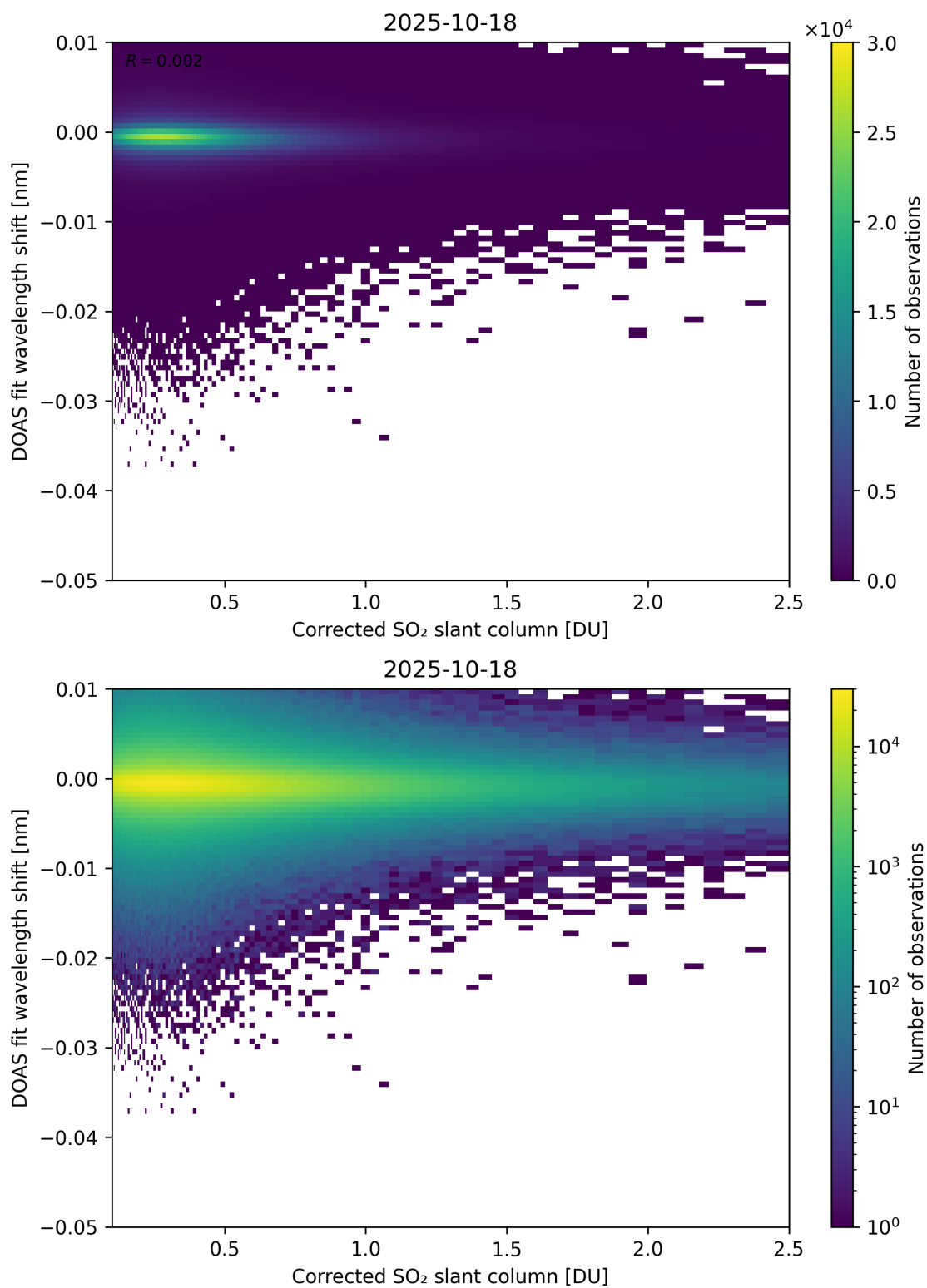
Figure 229: Scatter density plot of “Corrected SO 2 slant column” against “DOAS fit wavelength shift” for 2025-10-17 to 2025-10-19.
