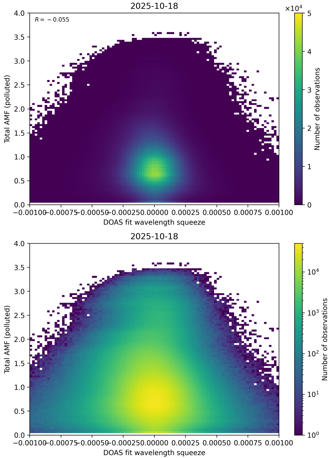
Figure 145: Scatter density plot of “DOAS fit wavelength squeeze” against “Total AMF (polluted)” for 2025-10-17 to 2025-10-19.
