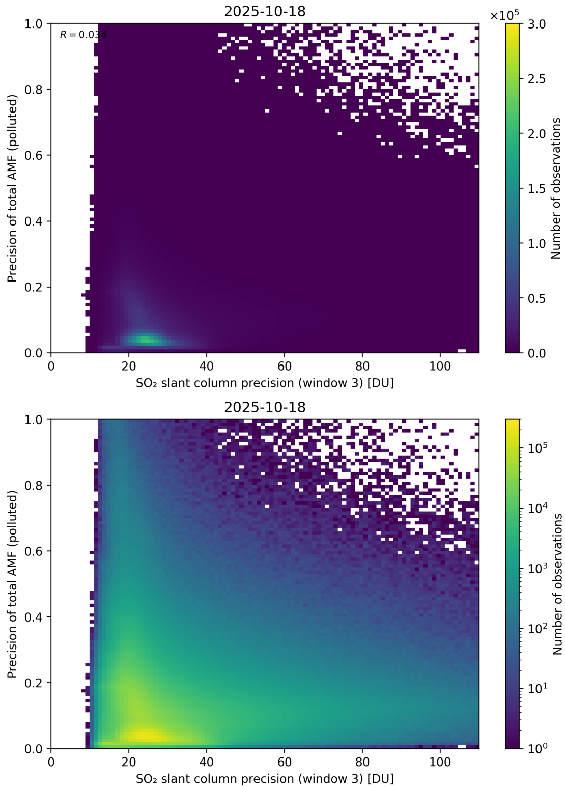
Figure 314: Scatter density plot of “SO 2 slant column precision (window 3)” against “Precision of total AMF (polluted)” for 2025-10-17 to 2025-10-19.
