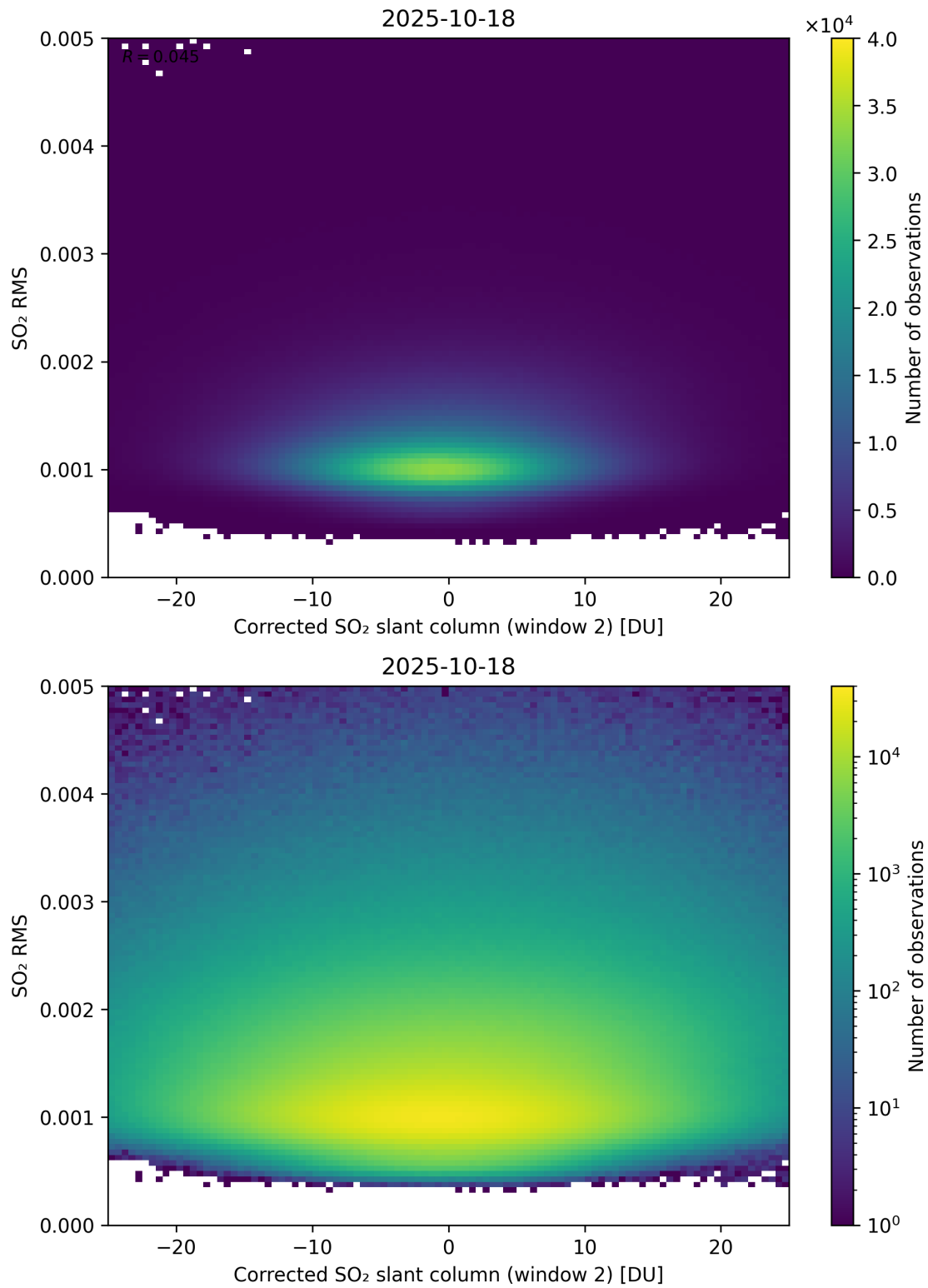
Figure 248: Scatter density plot of “Corrected SO 2 slant column (window 2)” against “SO 2 RMS” for 2025-10-17 to 2025-10-19.
