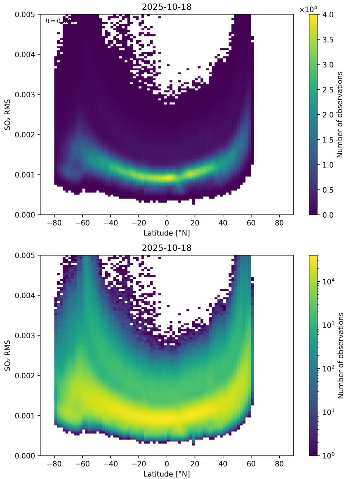
Figure 155: Scatter density plot of “Latitude” against “SO 2 RMS” for 2025-10-17 to 2025-10-19.
