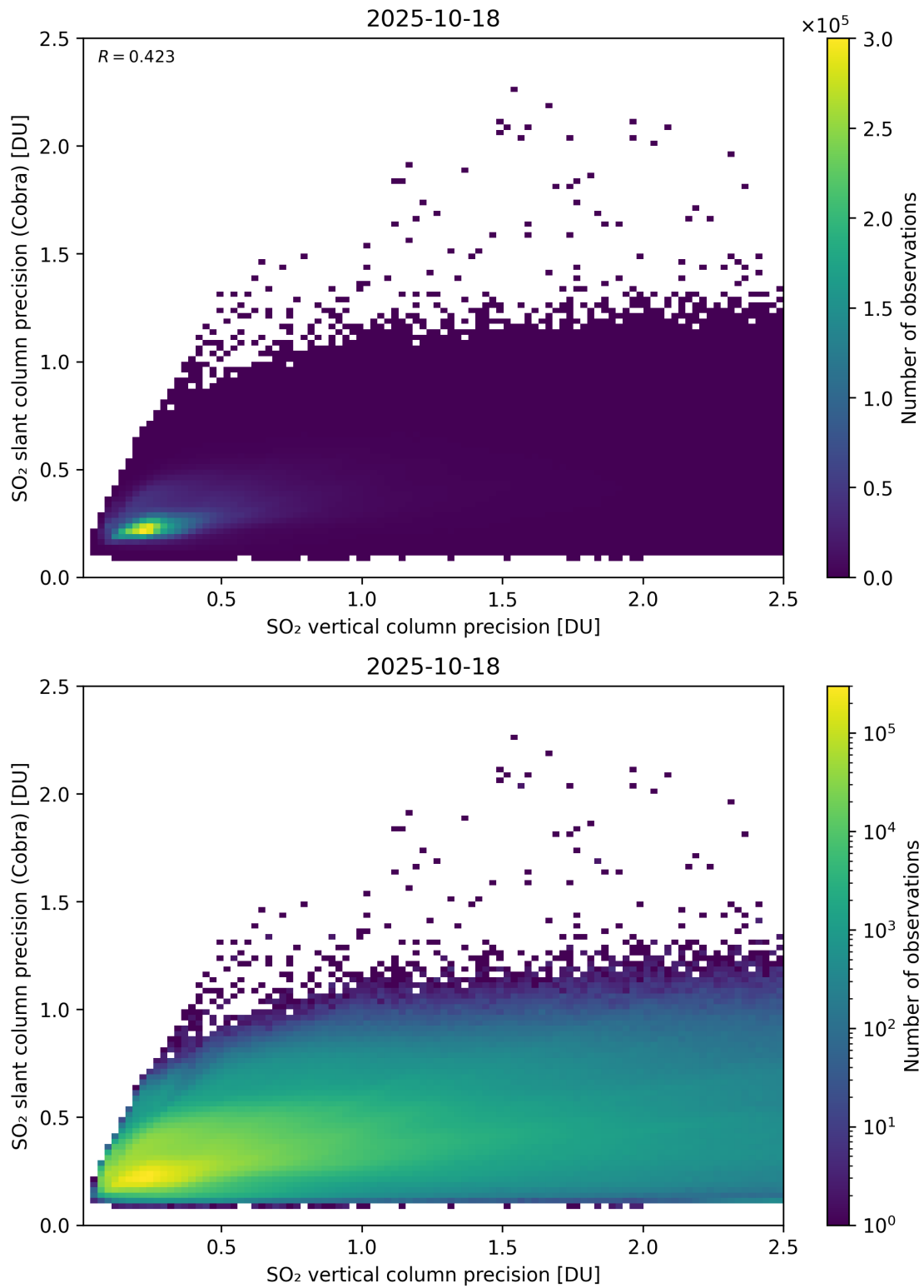
Figure 337: Scatter density plot of “SO 2 vertical column precision” against “SO 2 slant column precision (Cobra)” for 2025-10-17 to 2025-10-19.
