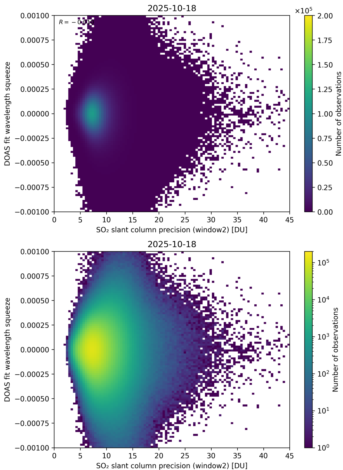
Figure 294: Scatter density plot of “SO 2 slant column precision (window2)” against “DOAS fit wavelength squeeze” for 2025-10-17 to 2025-10-19.
