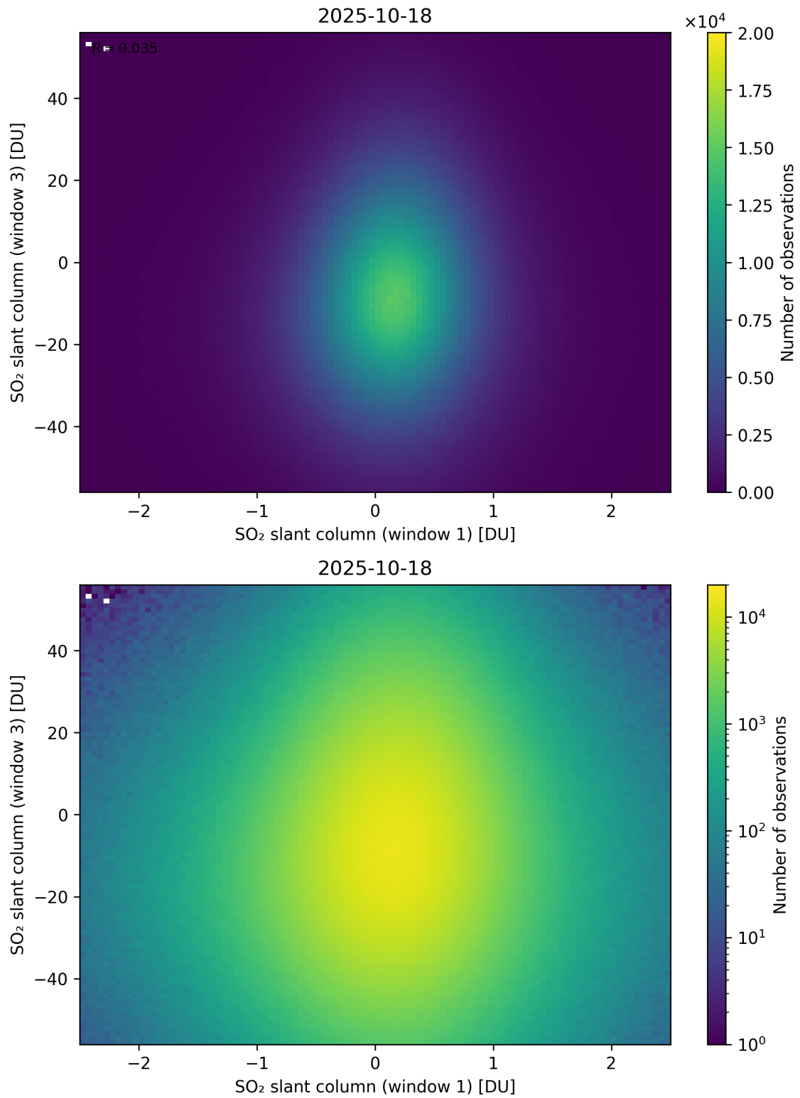
Figure 287: Scatter density plot of “SO 2 slant column (window 1)” against “SO 2 slant column (window 3)” for 2025-10-17 to 2025-10-19.
