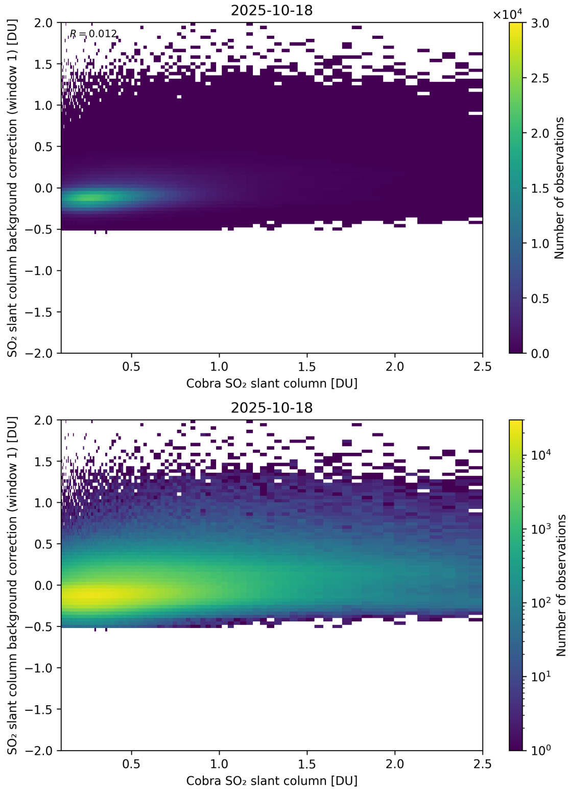
Figure 193: Scatter density plot of “Cobra SO 2 slant column” against “SO 2 slant column background correction (window 1)” for 2025-10-17 to 2025-10-19.
