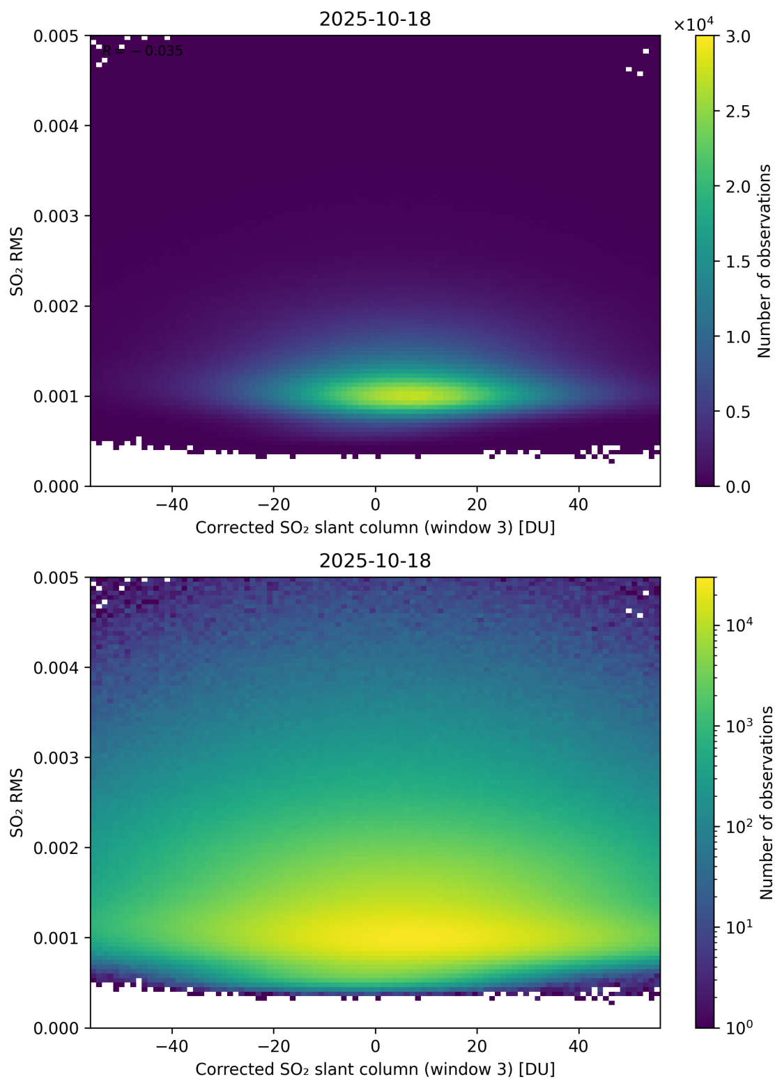
Figure 258: Scatter density plot of “Corrected SO 2 slant column (window 3)” against “SO 2 RMS” for 2025-10-17 to 2025-10-19.
