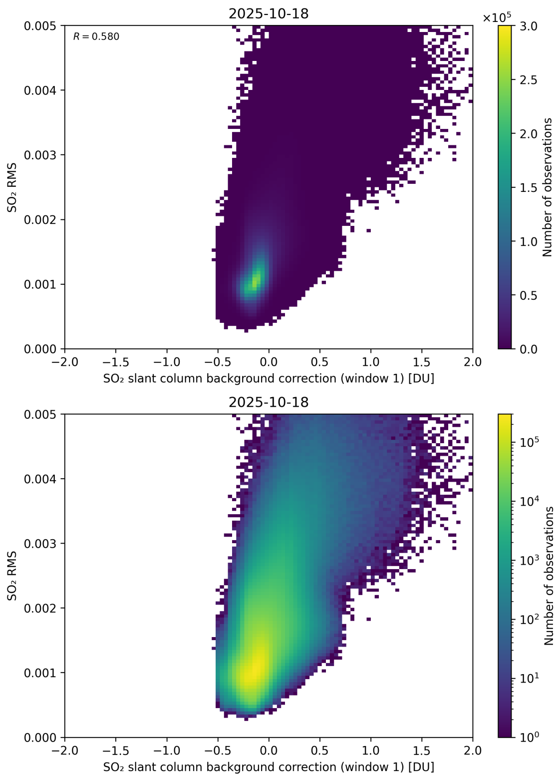
Figure 113: Scatter density plot of “SO 2 slant column background correction (window 1)” against “SO 2 RMS” for 2025-10-17 to 2025-10-19.
