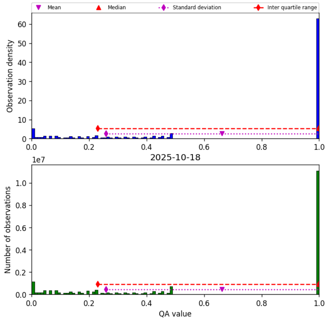
Figure 57: Histogram of “QA value” for 2025-10-17 to 2025-10-19
