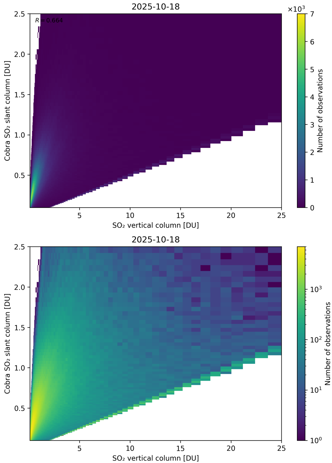
Figure 349: Scatter density plot of “SO 2 vertical column” against “Cobra SO 2 slant column” for 2025-10-17 to 2025-10-19.
