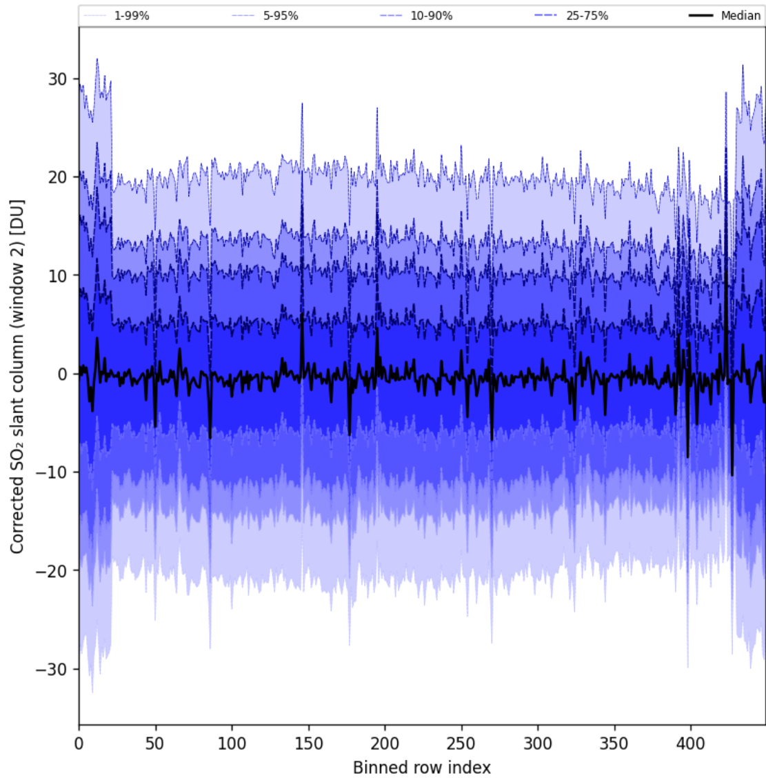
Figure 95: Along track statistics of “Corrected SO 2 slant column (window 2)” for 2025-10-17 to 2025-10-19
