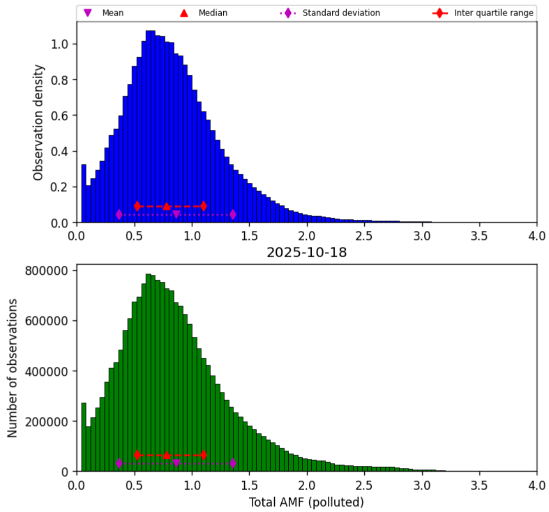
Figure 79: Histogram of “Total AMF (polluted)” for 2025-10-17 to 2025-10-19
