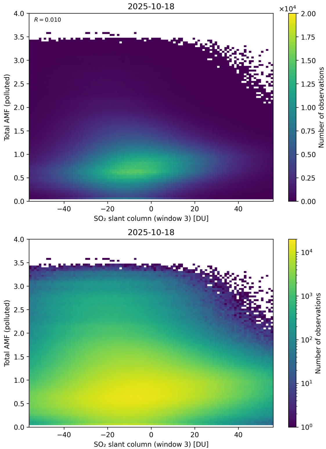
Figure 318: Scatter density plot of “SO 2 slant column (window 3)” against “Total AMF (polluted)” for 2025-10-17 to 2025-10-19.
