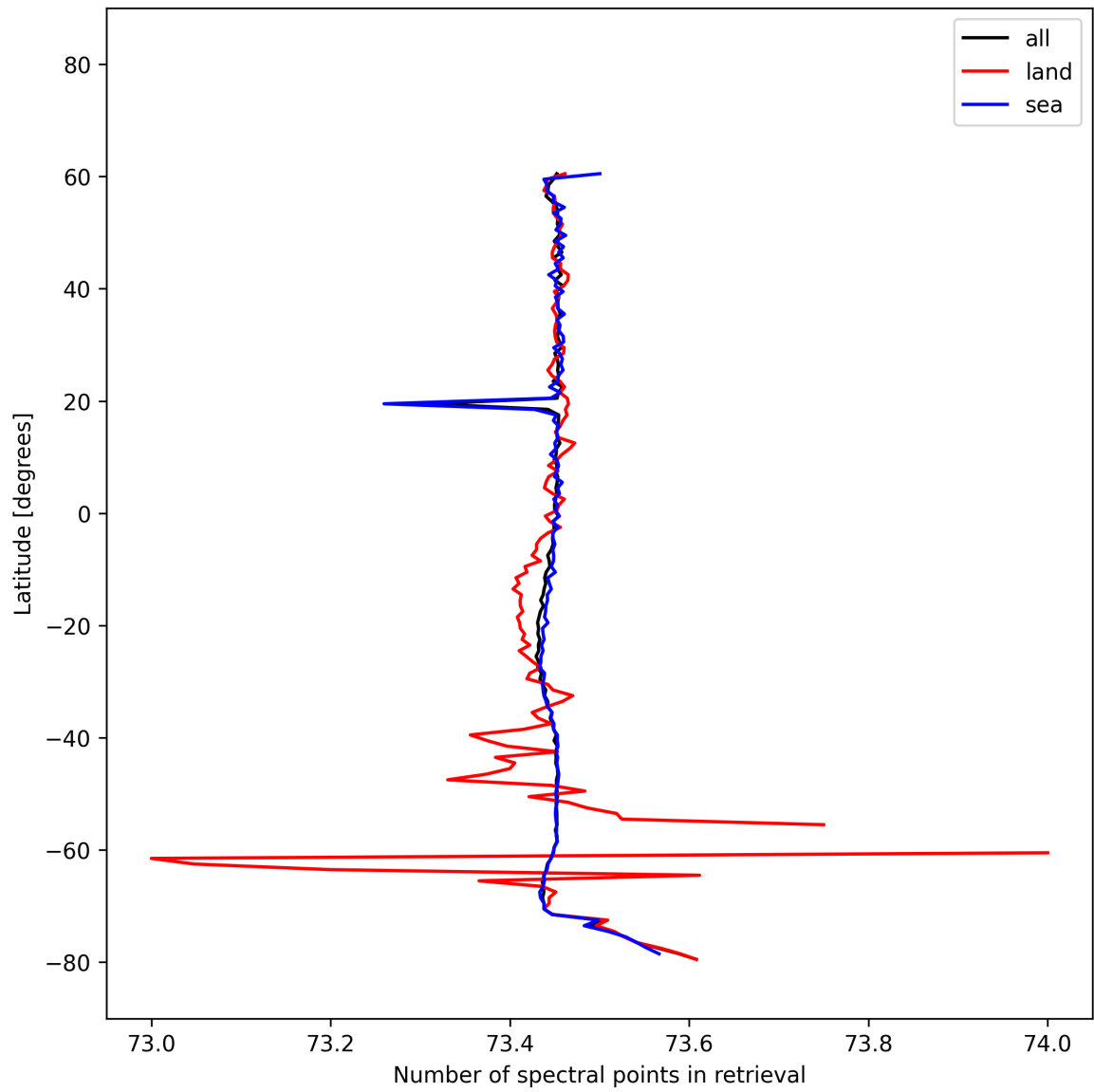
Figure 56: Zonal average of “Number of spectral points in retrieval” for 2025-10-17 to 2025-10-19.
