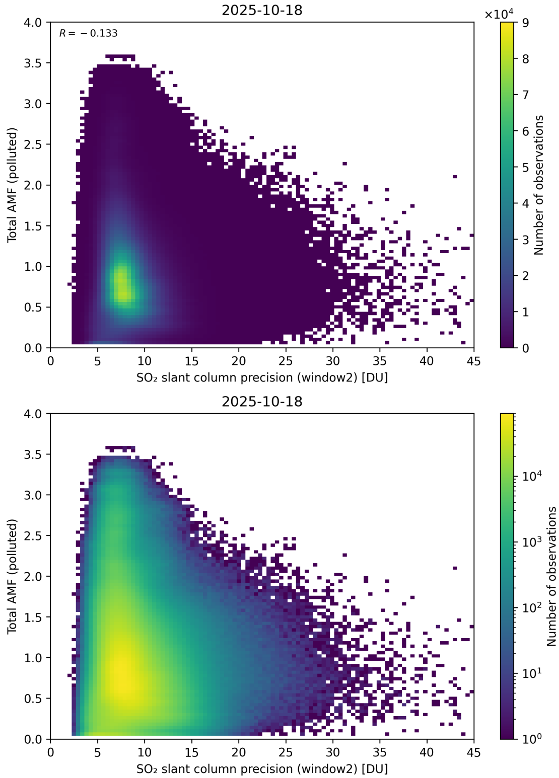
Figure 301: Scatter density plot of “SO 2 slant column precision (window2)” against “Total AMF (polluted)” for 2025-10-17 to 2025-10-19.
