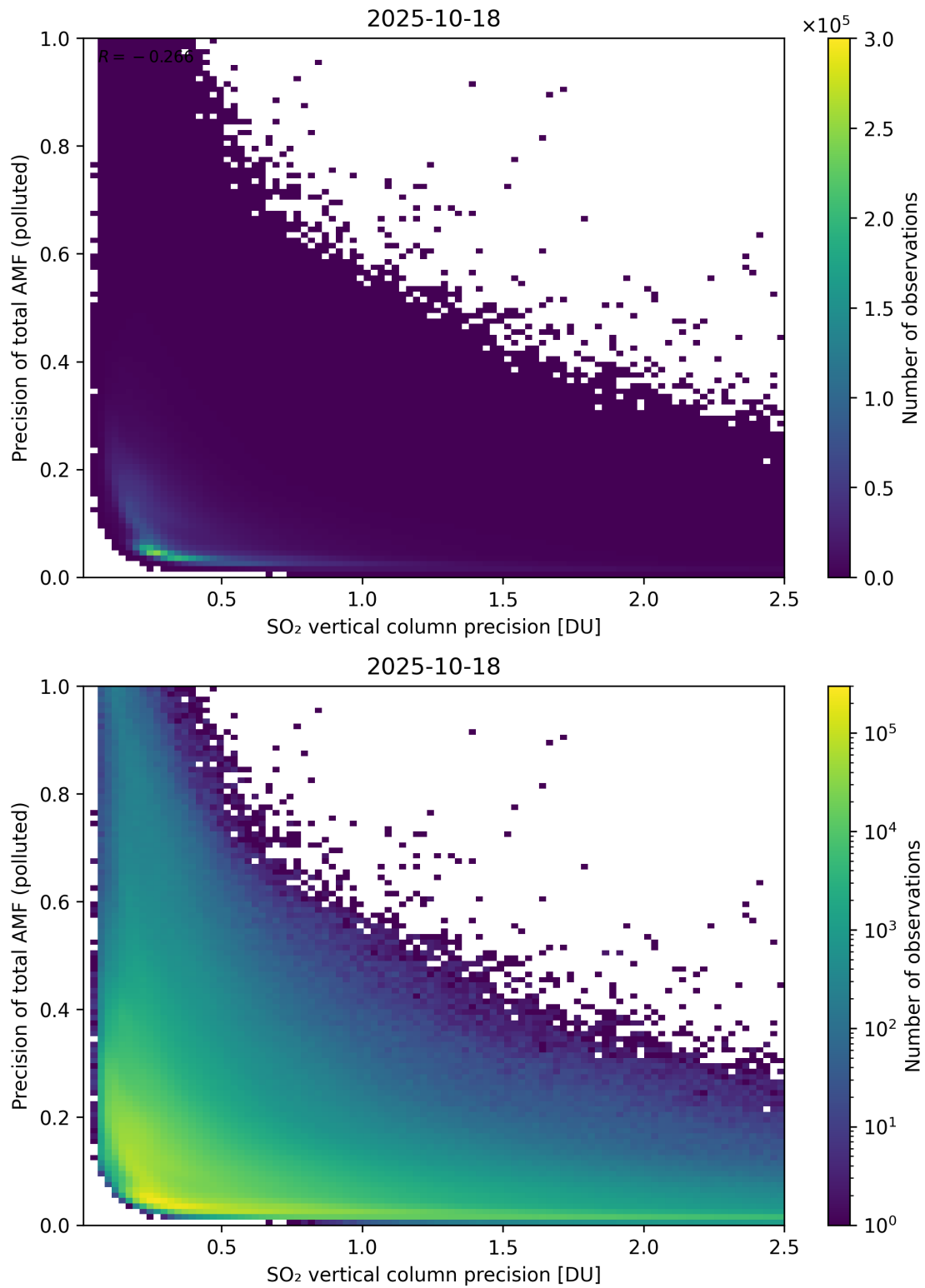
Figure 347: Scatter density plot of “SO 2 vertical column precision” against “Precision of total AMF (polluted)” for 2025-10-17 to 2025-10-19.
