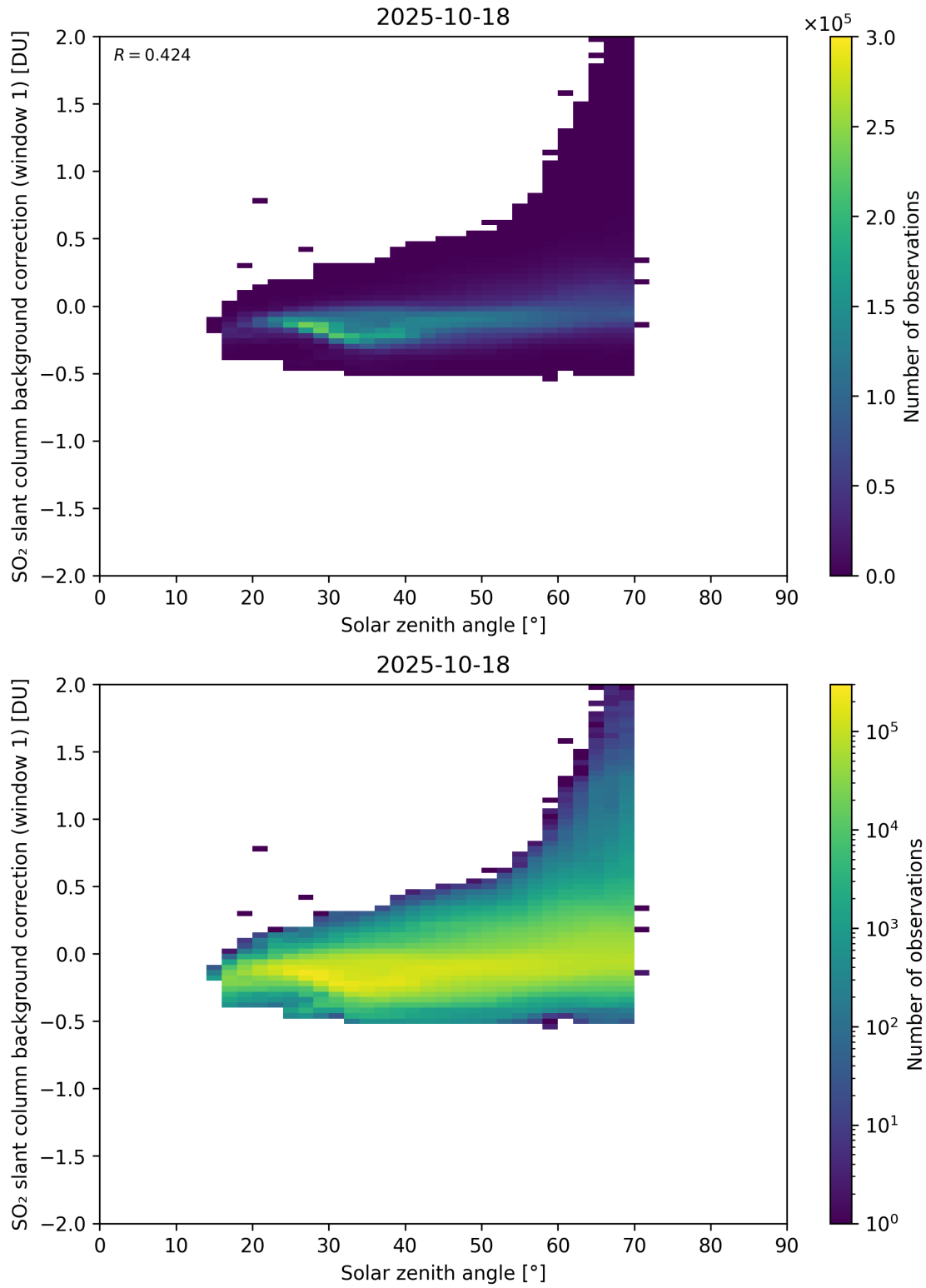
Figure 171: Scatter density plot of “Solar zenith angle” against “SO 2 slant column background correction (window 1)” for 2025-10-17 to 2025-10-19.
