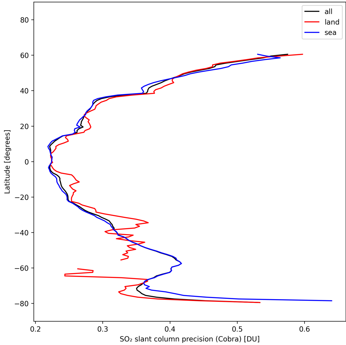
Figure 36: Zonal average of “SO 2 slant column precision (Cobra)” for 2025-10-17 to 2025-10-19.
