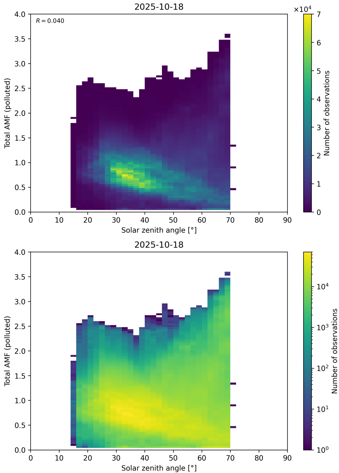
Figure 189: Scatter density plot of “Solar zenith angle” against “Total AMF (polluted)” for 2025-10-17 to 2025-10-19.
