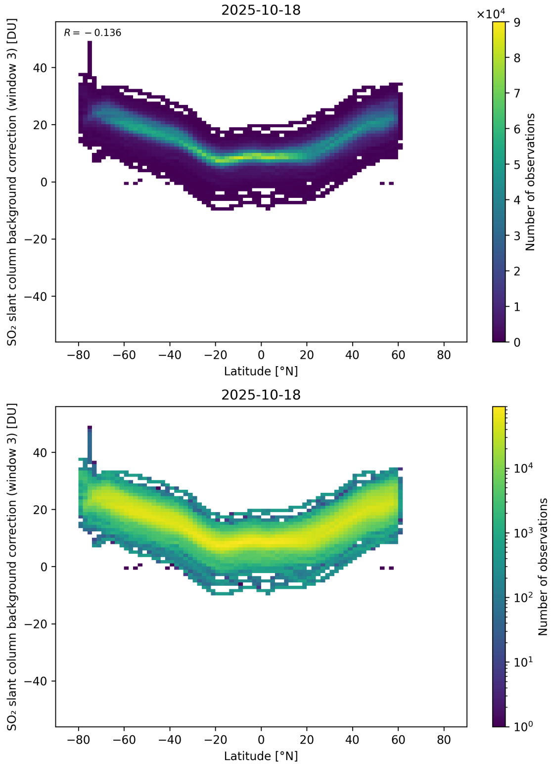
Figure 152: Scatter density plot of “Latitude” against “SO 2 slant column background correction (window 3)” for 2025-10-17 to 2025-10-19.
