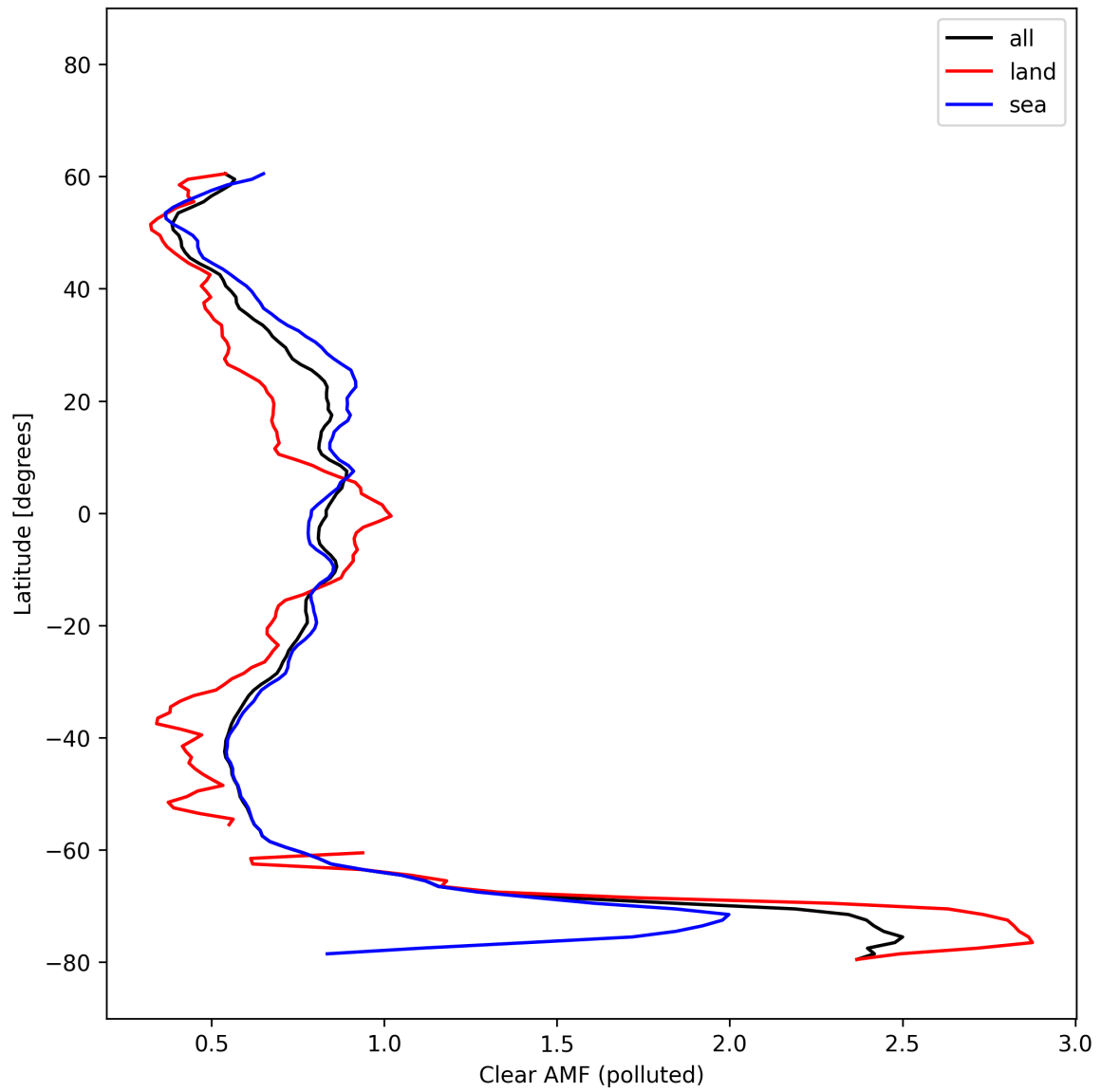
Figure 55: Zonal average of “Clear AMF (polluted)” for 2025-10-17 to 2025-10-19.
