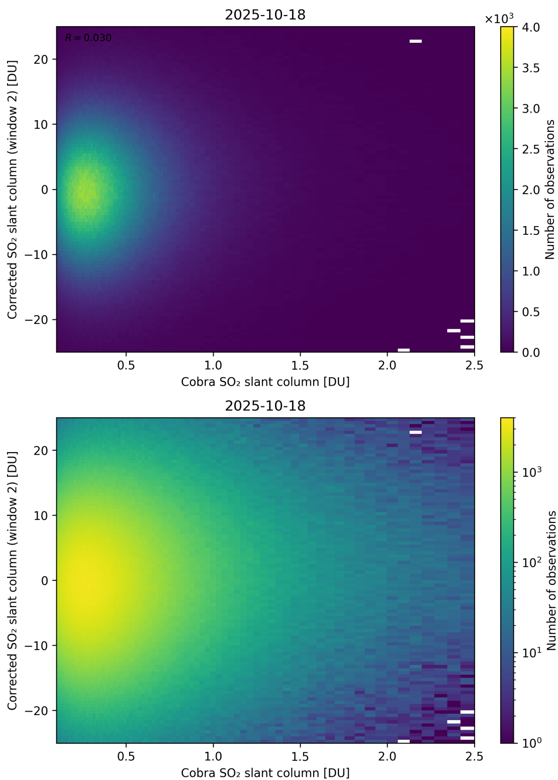
Figure 217: Scatter density plot of “Cobra SO 2 slant column” against “Corrected SO 2 slant column (window 2)” for 2025-10-17 to 2025-10-19.
