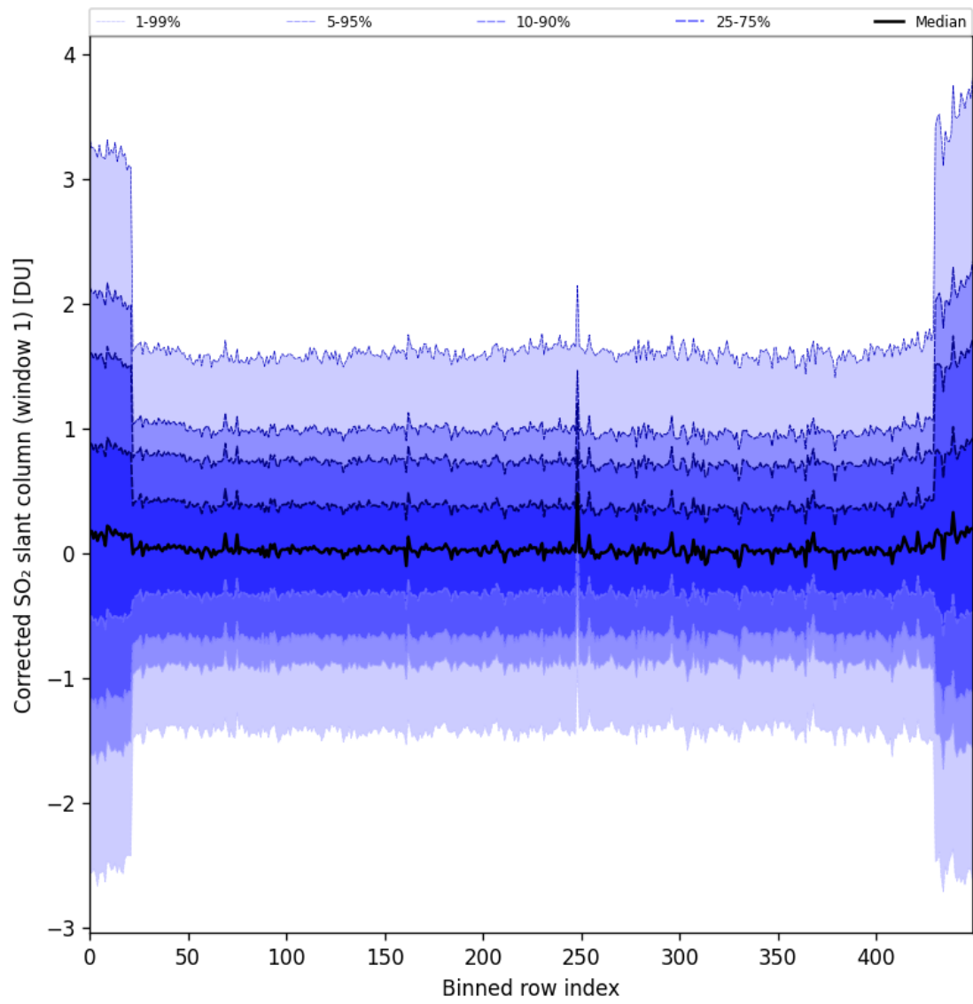
Figure 91: Along track statistics of “Corrected SO 2 slant column (window 1)” for 2025-10-17 to 2025-10-19
