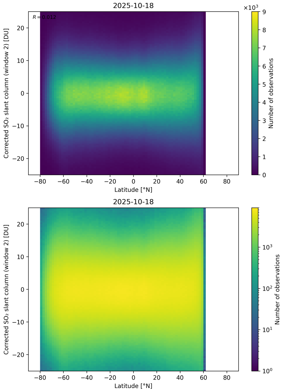
Figure 160: Scatter density plot of “Latitude” against “Corrected SO 2 slant column (window 2)” for 2025-10-17 to 2025-10-19.
