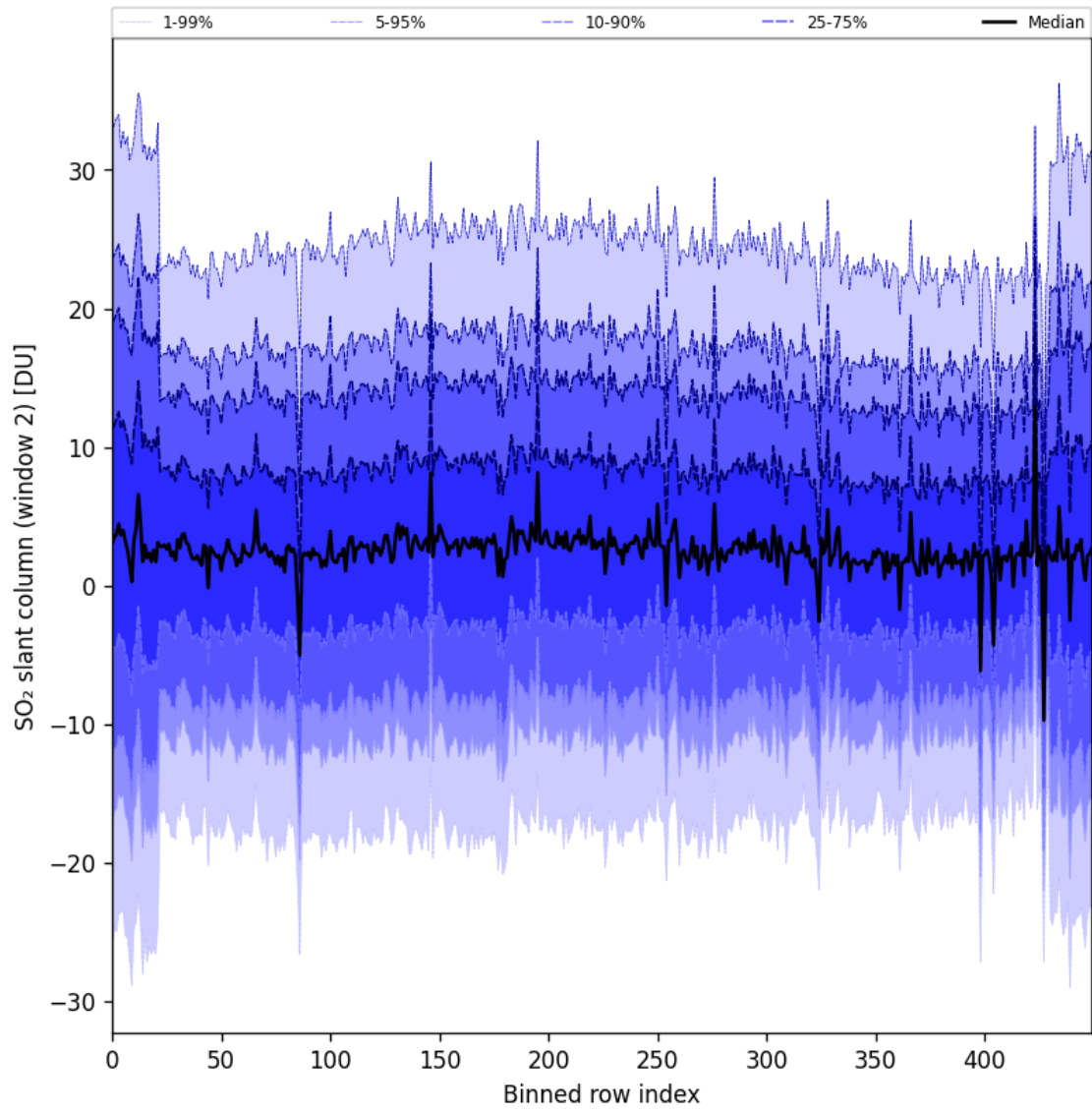
Figure 93: Along track statistics of “SO 2 slant column (window 2)” for 2025-10-17 to 2025-10-19
