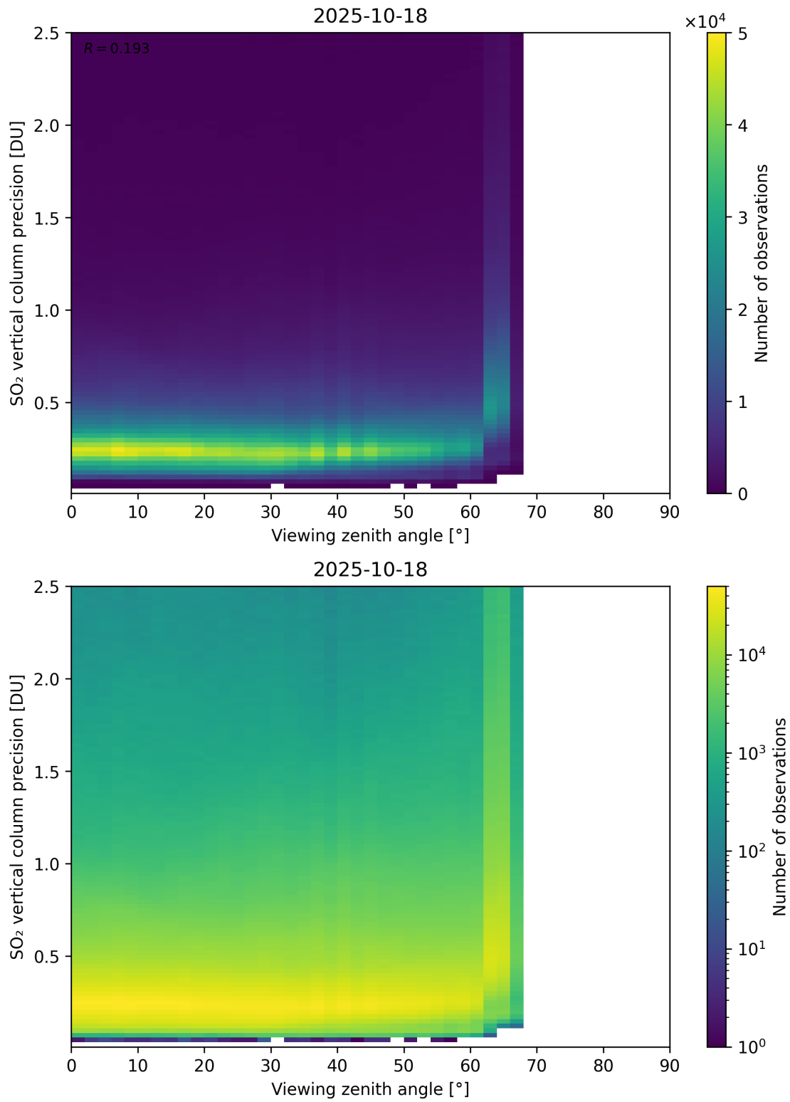
Figure 384: Scatter density plot of “Viewing zenith angle” against “SO 2 vertical column precision” for 2025-10-17 to 2025-10-19.
