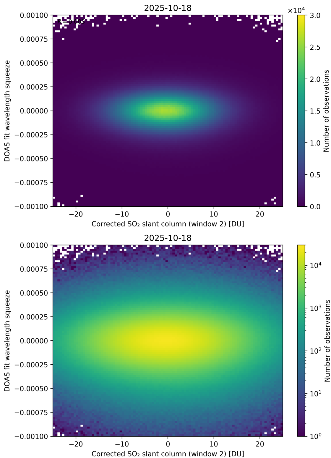
Figure 247: Scatter density plot of “Corrected SO 2 slant column (window 2)” against “DOAS fit wavelength squeeze” for 2025-10-17 to 2025-10-19.
