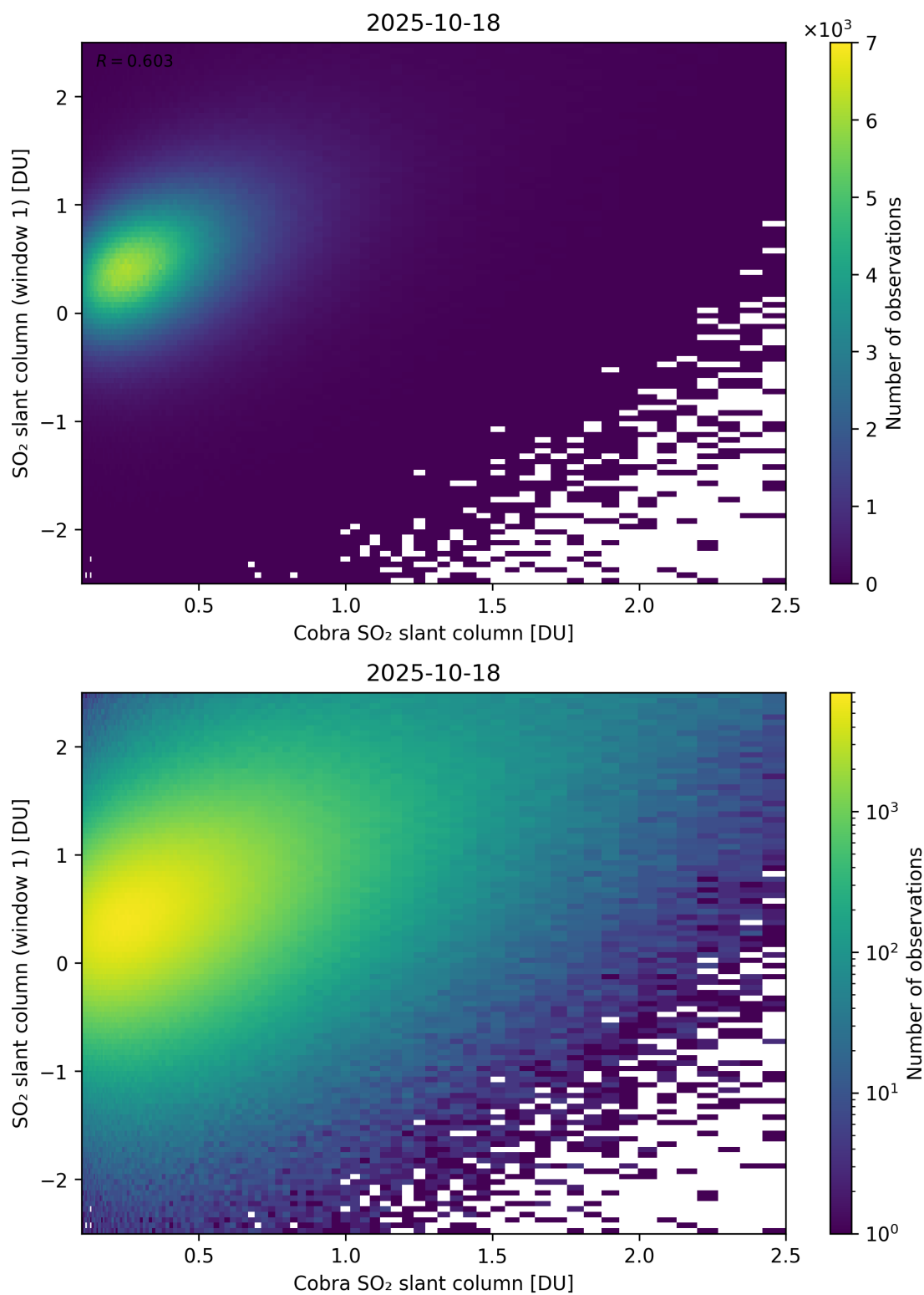
Figure 219: Scatter density plot of “Cobra SO 2 slant column” against “SO 2 slant column (window 1)” for 2025-10-17 to 2025-10-19.
