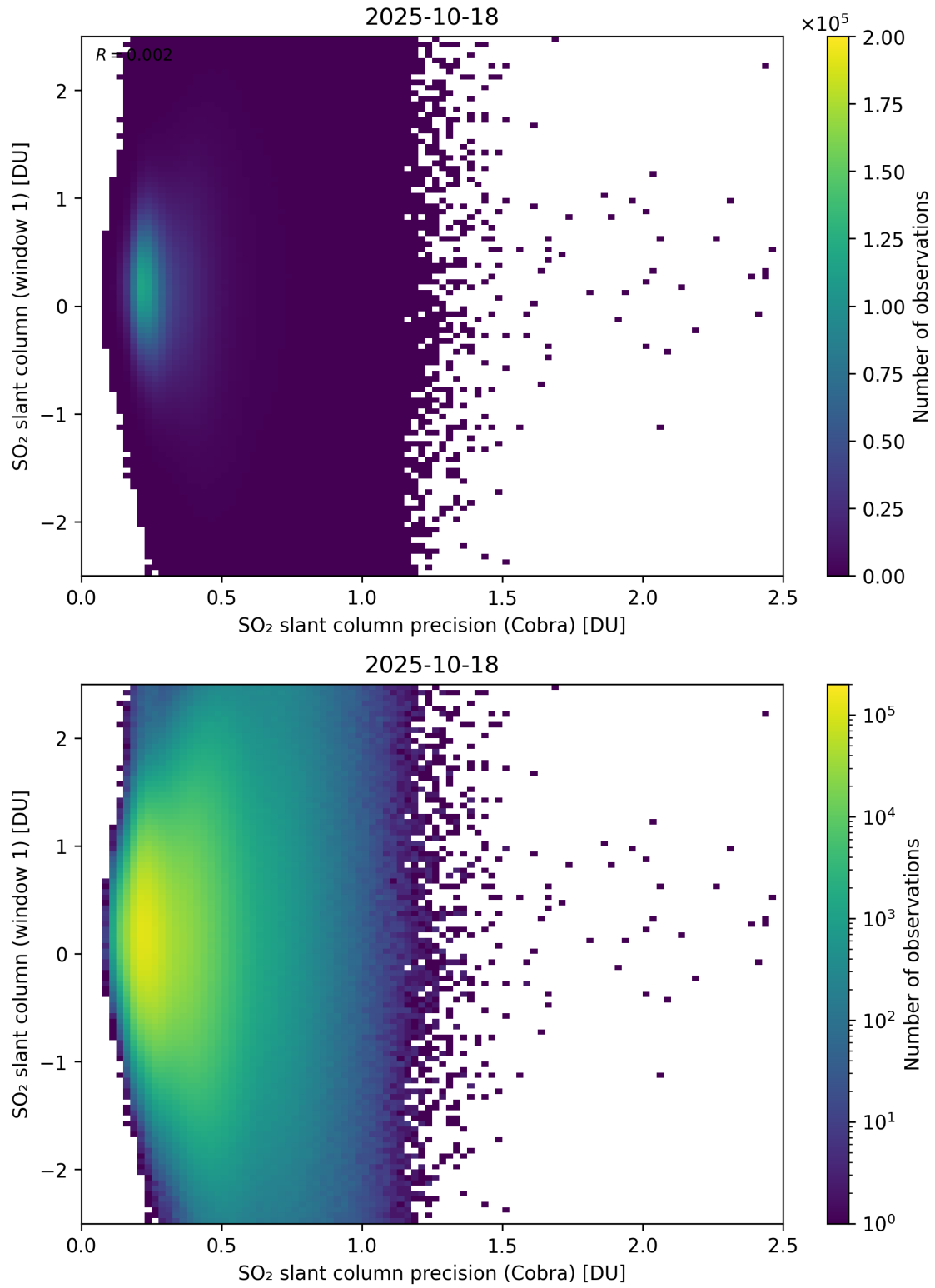
Figure 208: Scatter density plot of “SO 2 slant column precision (Cobra)” against “SO 2 slant column (window 1)” for 2025-10-17 to 2025-10-19.
