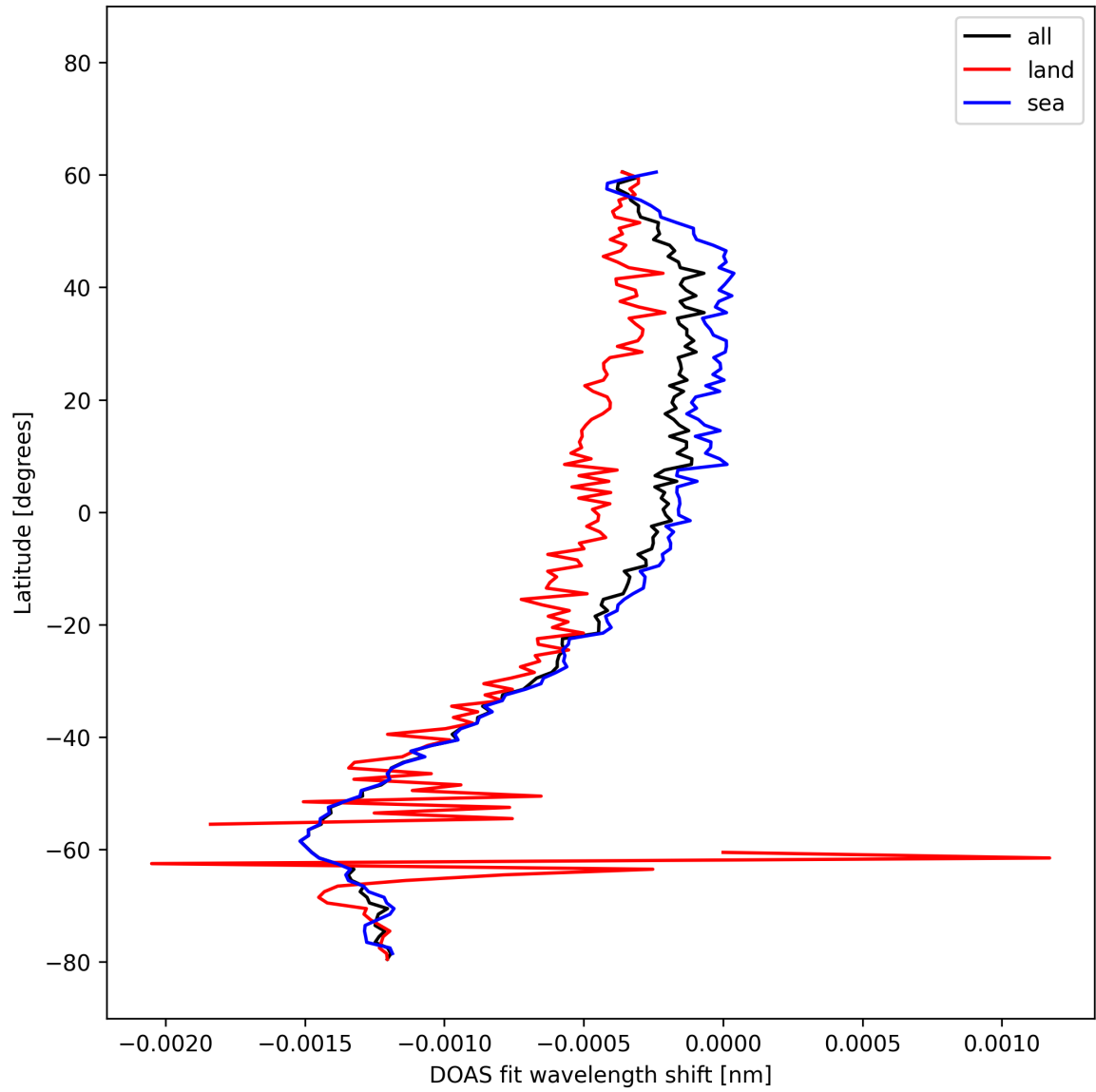
Figure 50: Zonal average of "DOAS fit wavelength shift" for 2025-10-17 to 2025-10-19.
