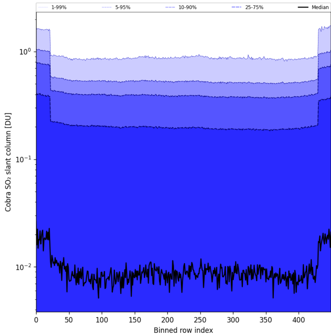
Figure 87: Along track statistics of "Cobra SO 2 slant column" for 2025-10-17 to 2025-10-19
