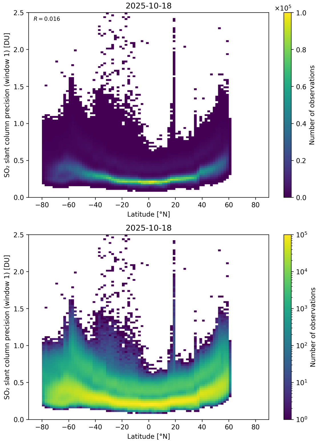
Figure 163: Scatter density plot of “Latitude” against “SO 2 slant column precision (window 1)” for 2025-10-17 to 2025-10-19.
