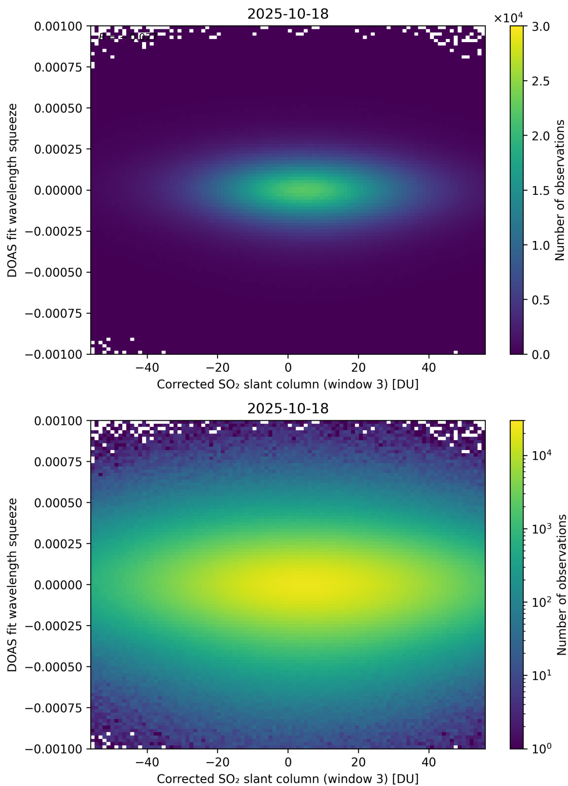
Figure 257: Scatter density plot of “Corrected SO 2 slant column (window 3)” against “DOAS fit wavelength squeeze” for 2025-10-17 to 2025-10-19.
