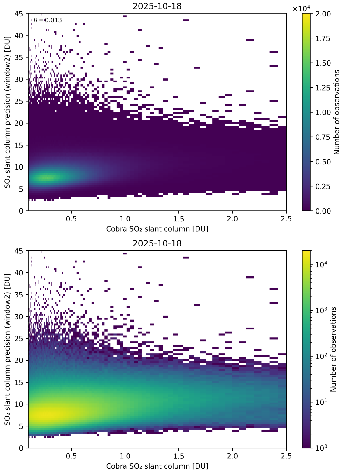
Figure 221: Scatter density plot of “Cobra SO 2 slant column” against “SO 2 slant column precision (window2)” for 2025-10-17 to 2025-10-19.
