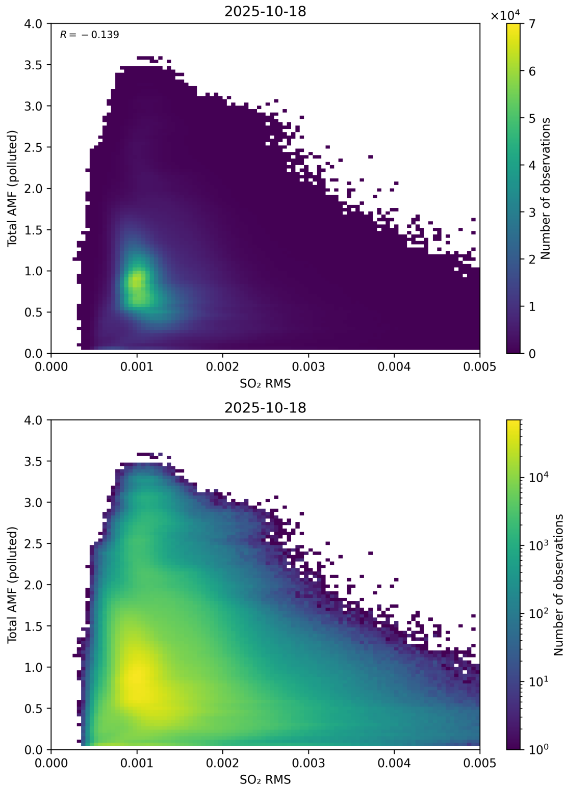
Figure 148: Scatter density plot of “SO 2 RMS” against “Total AMF (polluted)” for 2025-10-17 to 2025-10-19.
