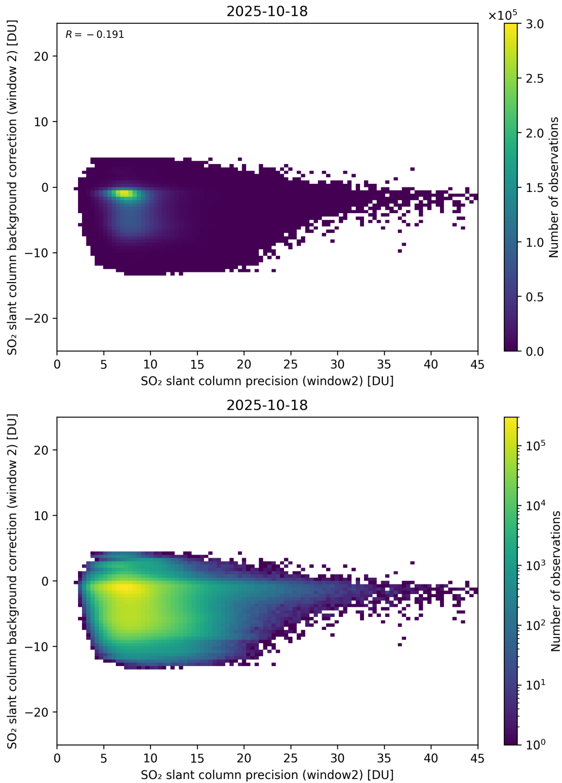
Figure 291: Scatter density plot of “SO 2 slant column precision (window2)” against “SO 2 slant column background correction (window 2)” for 2025-10-17 to 2025-10-19.
