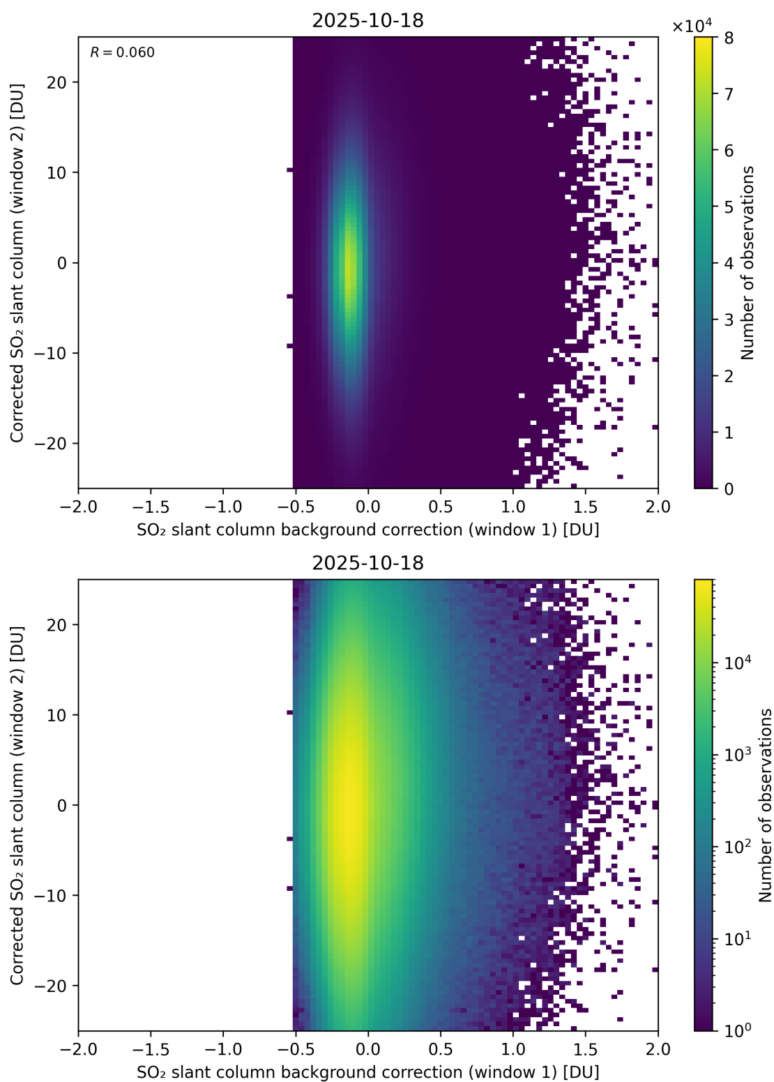
Figure 115: Scatter density plot of “SO 2 slant column background correction (window 1)” against “Corrected SO 2 slant column (window 2)” for 2025-10-17 to 2025-10-19.
