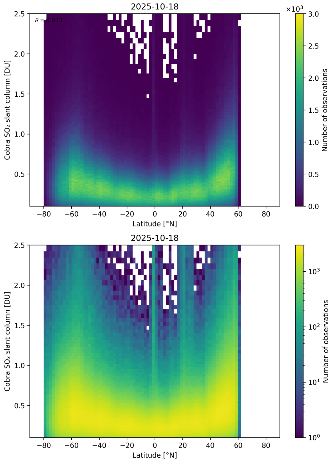
Figure 157: Scatter density plot of “Latitude” against “Cobra SO 2 slant column” for 2025-10-17 to 2025-10-19.
