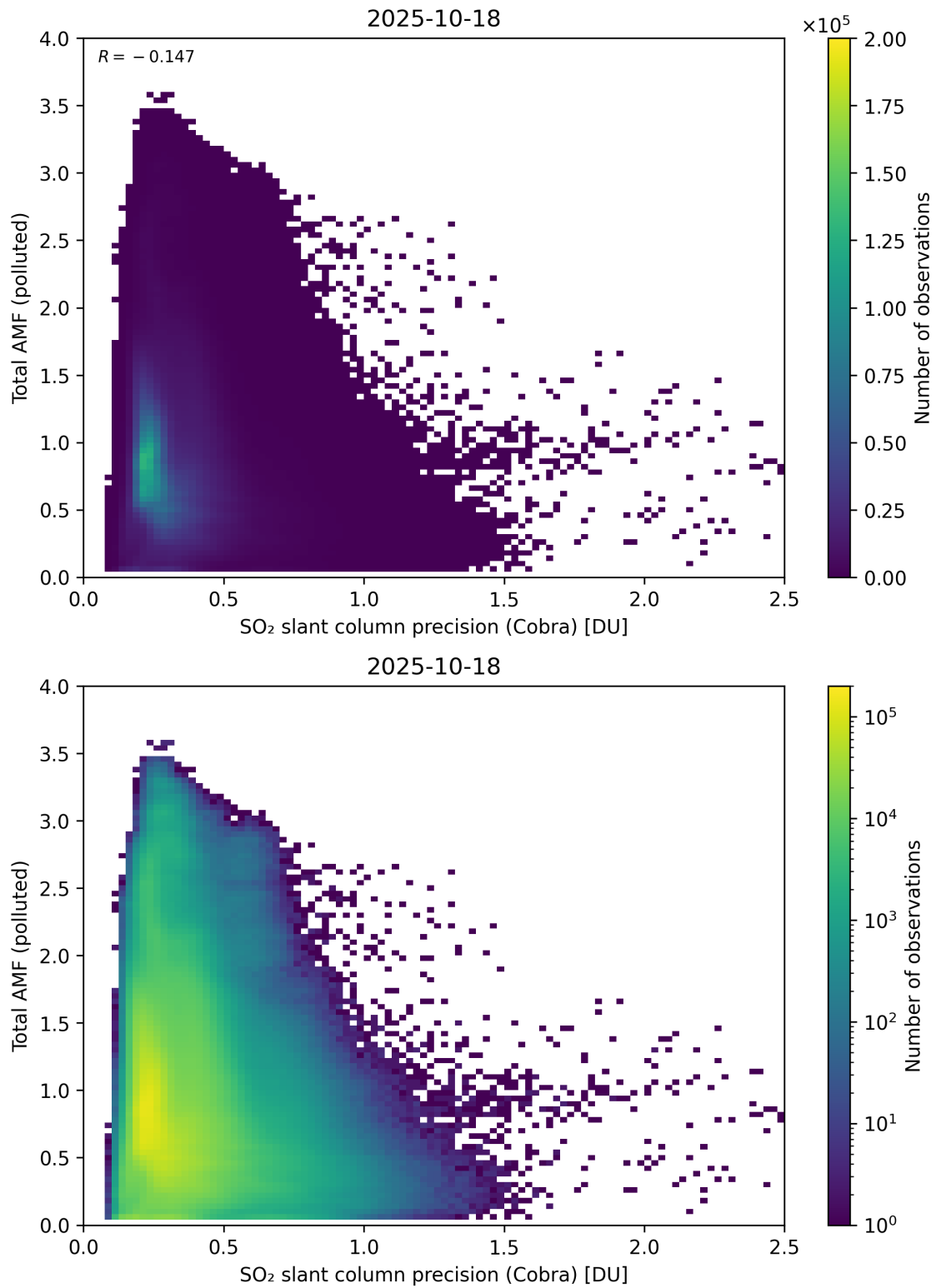
Figure 213: Scatter density plot of “SO 2 slant column precision (Cobra)” against “Total AMF (polluted)” for 2025-10-17 to 2025-10-19.
