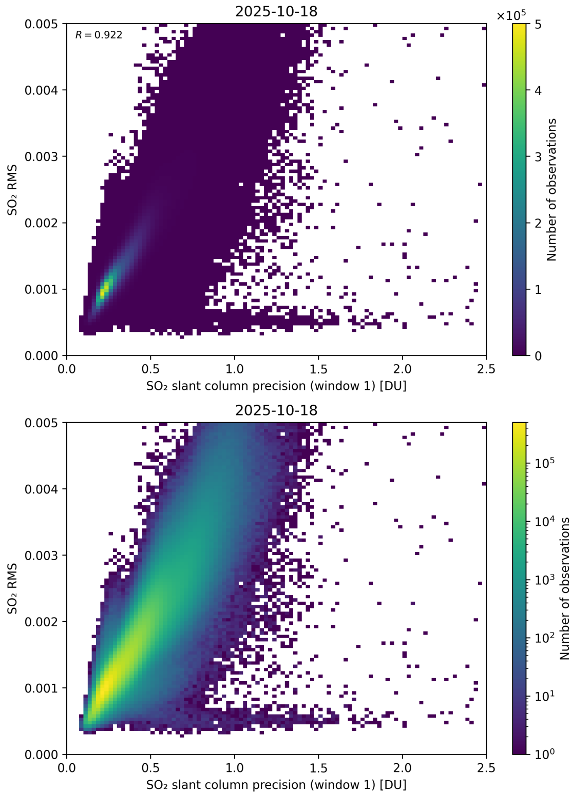
Figure 273: Scatter density plot of “SO 2 slant column precision (window 1)” against “SO 2 RMS” for 2025-10-17 to 2025-10-19.
