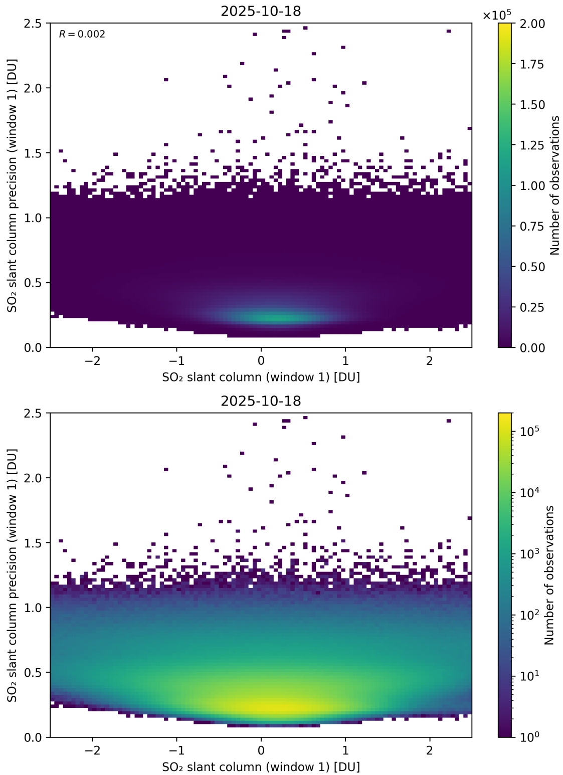
Figure 285: Scatter density plot of “SO 2 slant column (window 1)” against “SO 2 slant column precision (window 1)” for 2025-10-17 to 2025-10-19.
