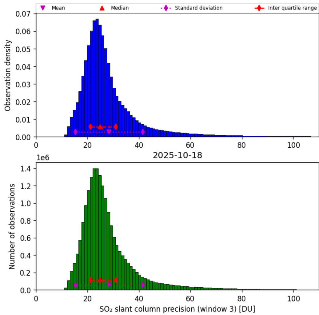
Figure 72: Histogram of “SO 2 slant column precision (window 3)” for 2025-10-17 to 2025-10-19
