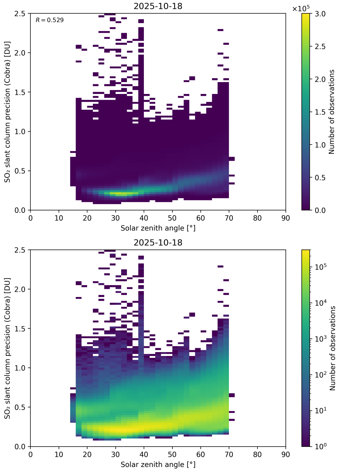
Figure 180: Scatter density plot of “Solar zenith angle” against “SO 2 slant column precision (Cobra)” for 2025-10-17 to 2025-10-19.
