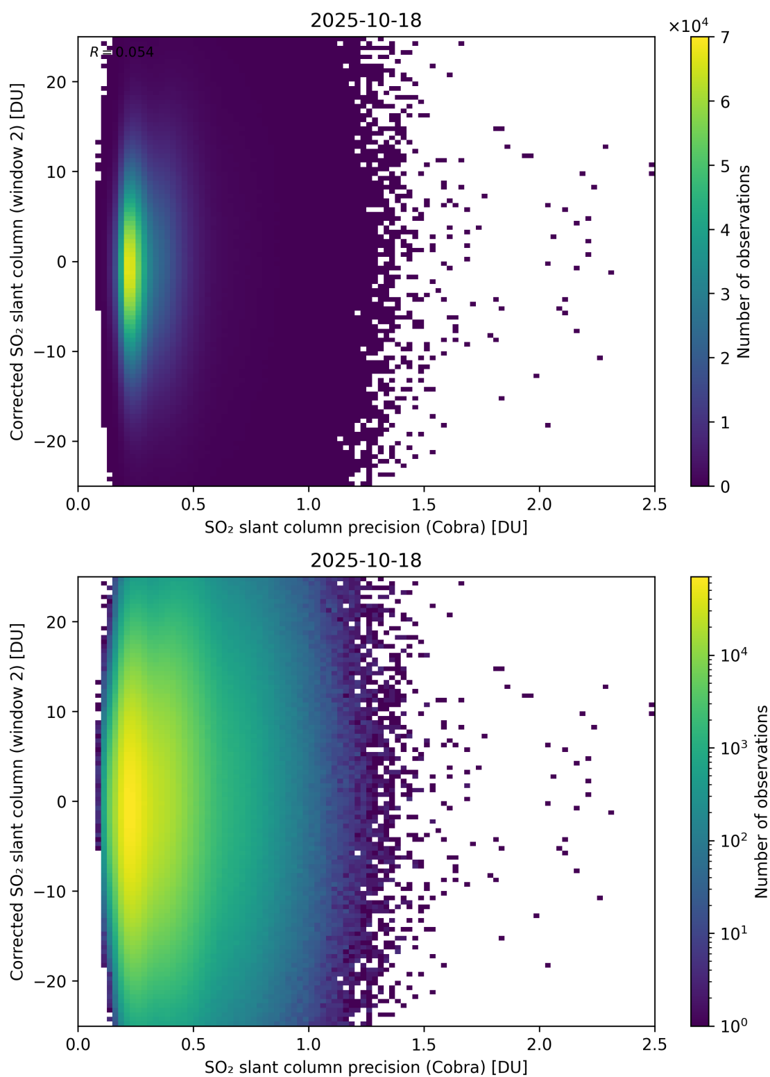
Figure 206: Scatter density plot of “SO 2 slant column precision (Cobra)” against “Corrected SO 2 slant column (window 2)” for 2025-10-17 to 2025-10-19.
