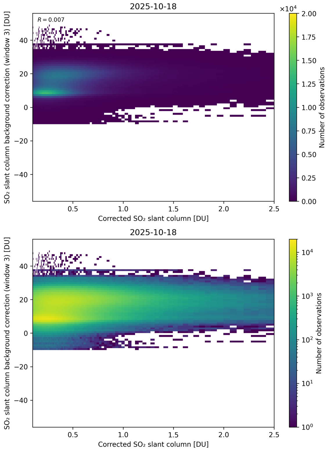
Figure 228: Scatter density plot of “Corrected SO 2 slant column” against “SO 2 slant column background correction (window 3)” for 2025-10-17 to 2025-10-19.
