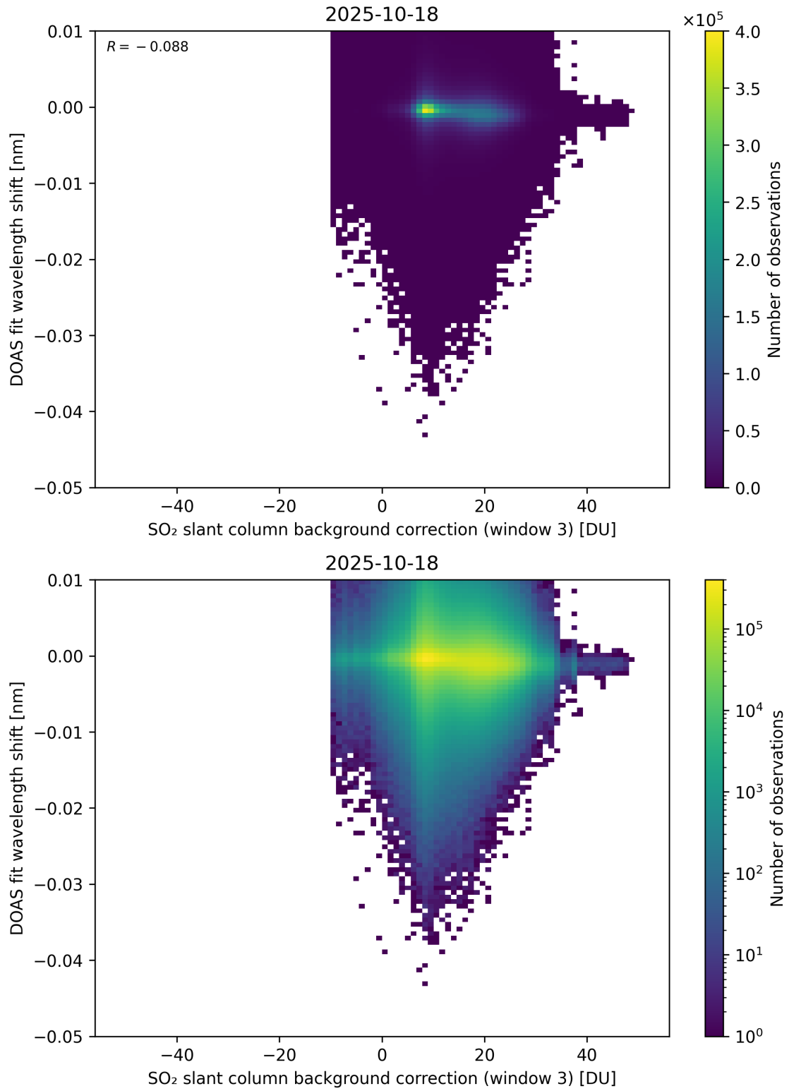
Figure 132: Scatter density plot of “SO 2 slant column background correction (window 3)” against “DOAS fit wavelength shift” for 2025-10-17 to 2025-10-19.
