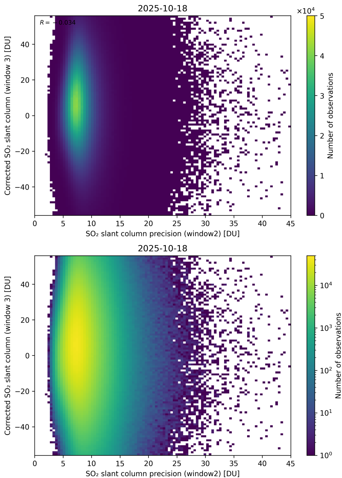
Figure 298: Scatter density plot of “SO 2 slant column precision (window2)” against “Corrected SO 2 slant column (window 3)” for 2025-10-17 to 2025-10-19.
