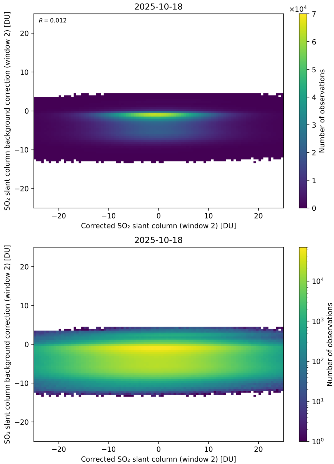
Figure 244: Scatter density plot of “Corrected SO 2 slant column (window 2)” against “SO 2 slant column background correction (window 2)” for 2025-10-17 to 2025-10-19.
