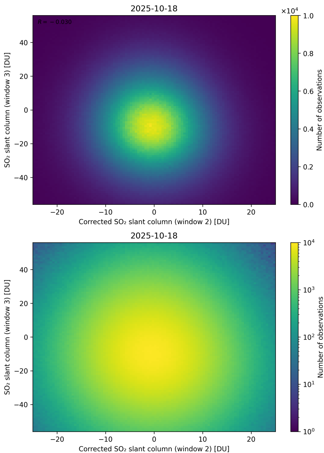
Figure 251: Scatter density plot of “Corrected SO 2 slant column (window 2)” against “SO 2 slant column (window 3)” for 2025-10-17 to 2025-10-19.
