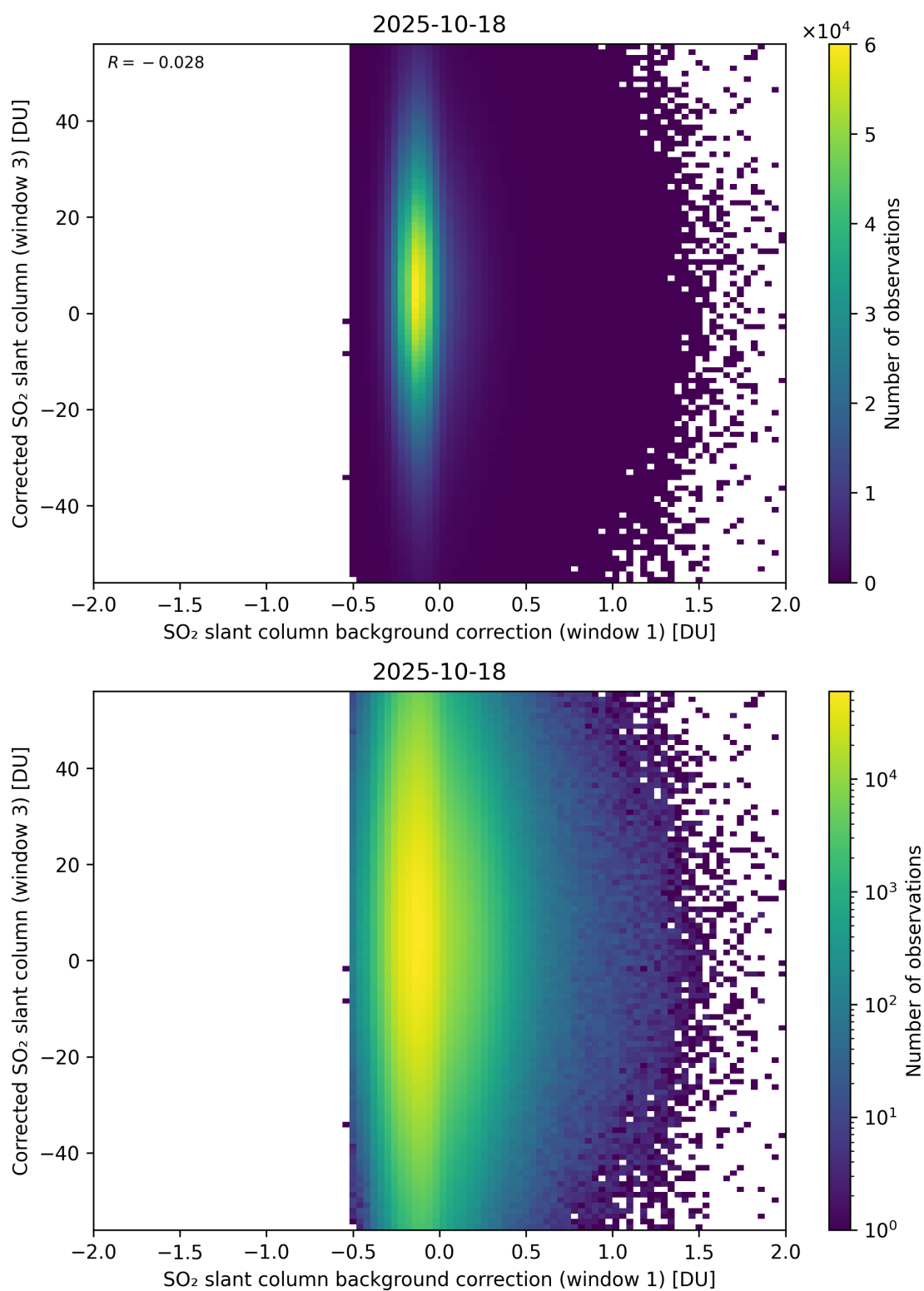
Figure 116: Scatter density plot of “SO 2 slant column background correction (window 1)” against “Corrected SO 2 slant column (window 3)” for 2025-10-17 to 2025-10-19.
