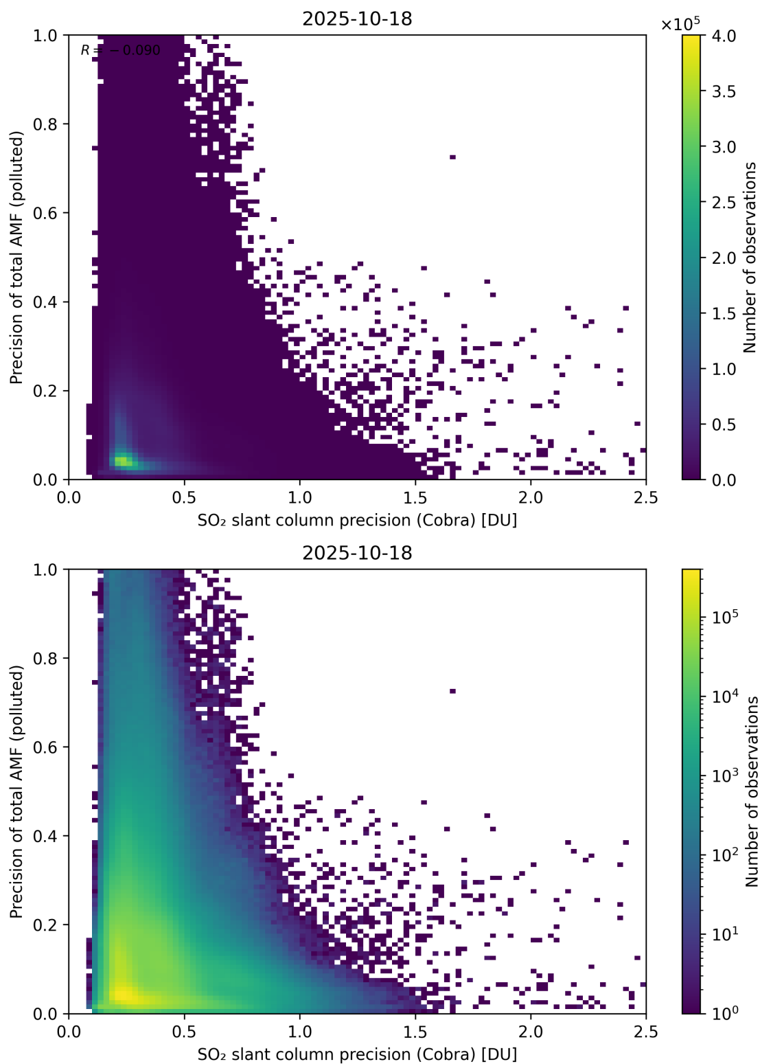
Figure 214: Scatter density plot of “SO 2 slant column precision (Cobra)” against “Precision of total AMF (polluted)” for 2025-10-17 to 2025-10-19.
