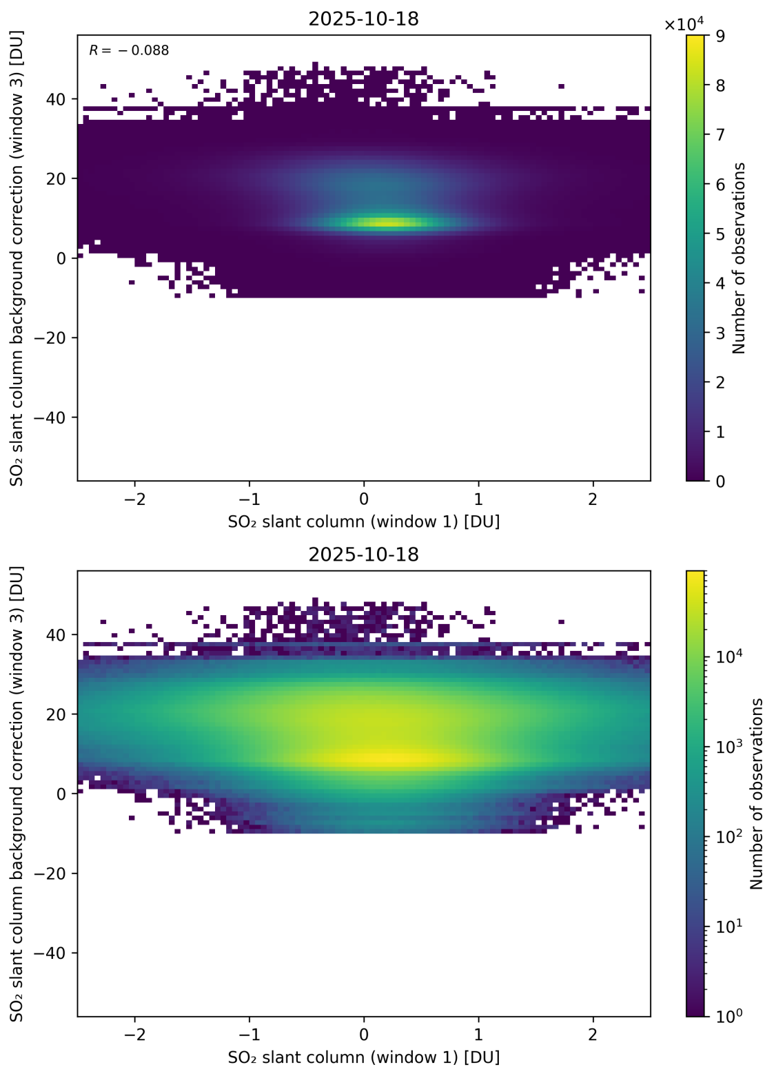
Figure 264: Scatter density plot of “SO 2 slant column (window 1)” against “SO 2 slant column background correction (window 3)” for 2025-10-17 to 2025-10-19.
