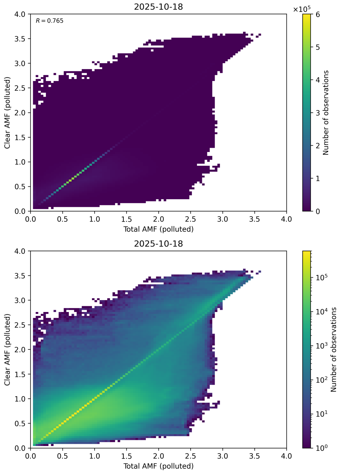
Figure 321: Scatter density plot of “Total AMF (polluted)” against “Clear AMF (polluted)” for 2025-10-17 to 2025-10-19.
