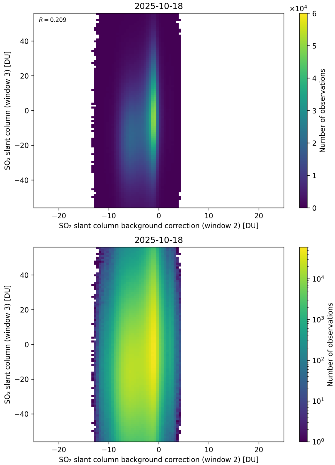
Figure 128: Scatter density plot of “SO 2 slant column background correction (window 2)” against “SO 2 slant column (window 3)” for 2025-10-17 to 2025-10-19.
