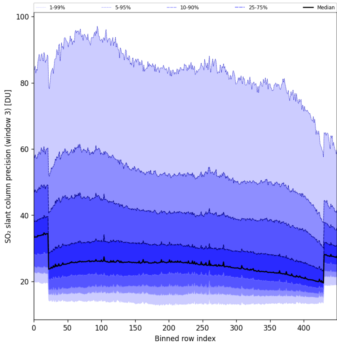
Figure 98: Along track statistics of “SO 2 slant column precision (window 3)” for 2025-10-17 to 2025-10-19
