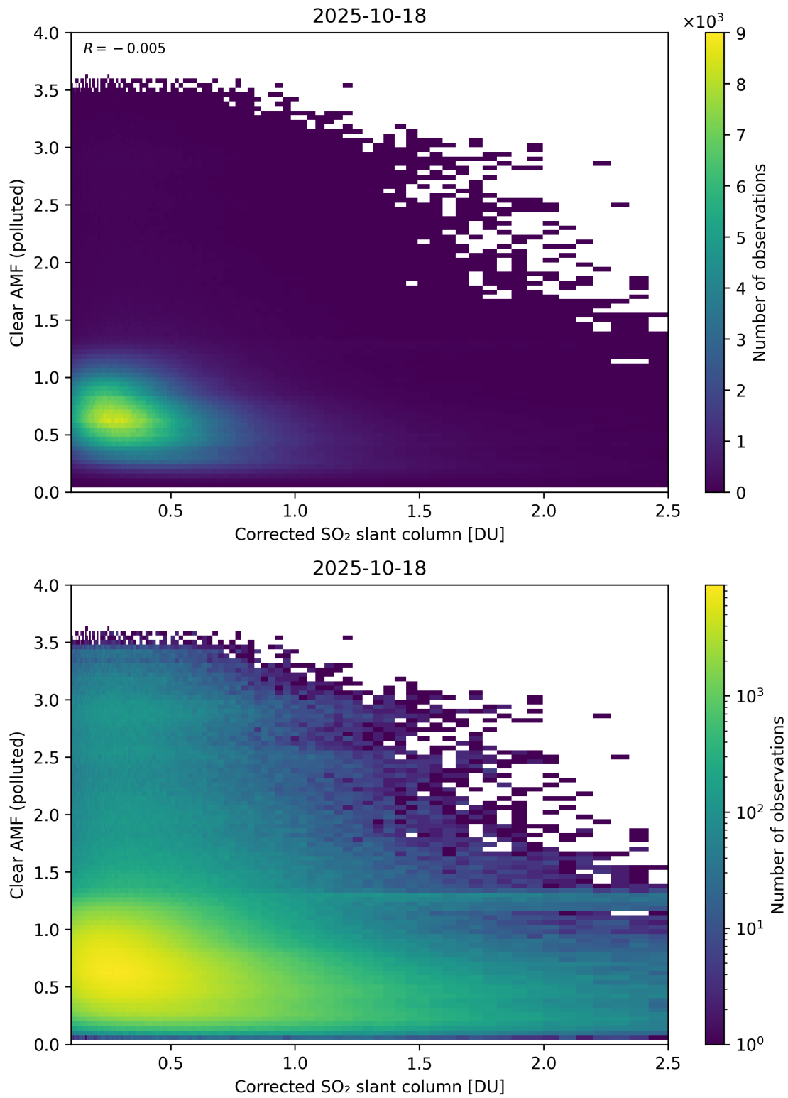
Figure 232: Scatter density plot of “Corrected SO 2 slant column” against “Clear AMF (polluted)” for 2025-10-17 to 2025-10-19.
