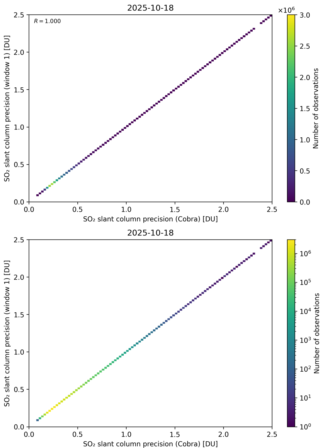
Figure 209: Scatter density plot of “SO 2 slant column precision (Cobra)” against “SO 2 slant column precision (window 1)” for 2025-10-17 to 2025-10-19.
