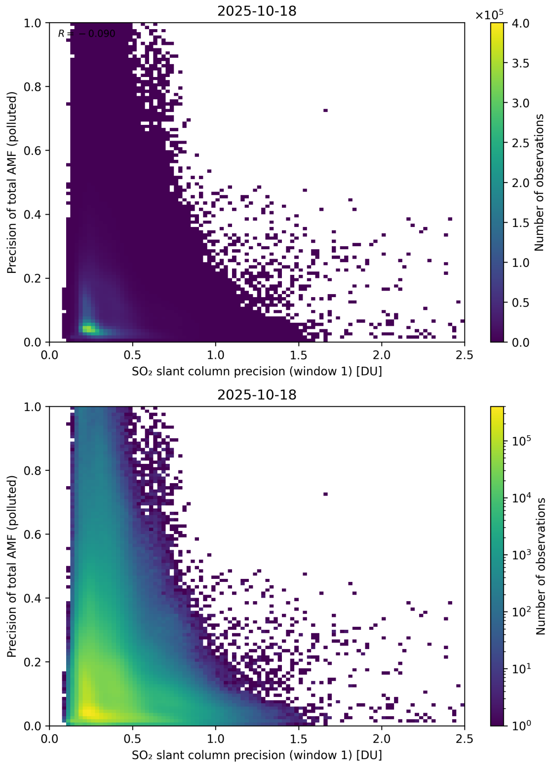
Figure 281: Scatter density plot of “SO 2 slant column precision (window 1)” against “Precision of total AMF (polluted)” for 2025-10-17 to 2025-10-19.
