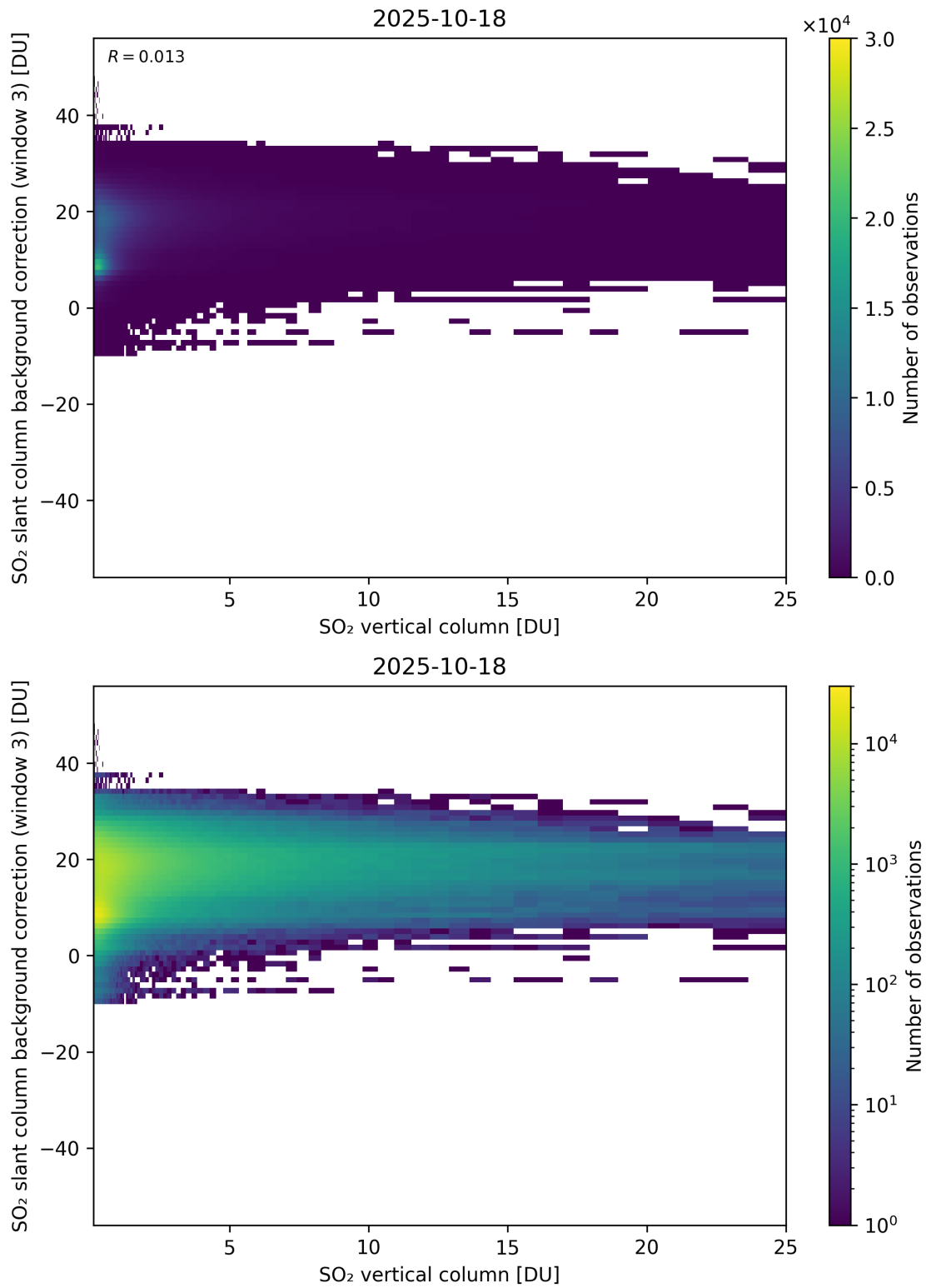
Figure 325: Scatter density plot of “SO 2 vertical column” against “SO 2 slant column background correction (window 3)” for 2025-10-17 to 2025-10-19.
