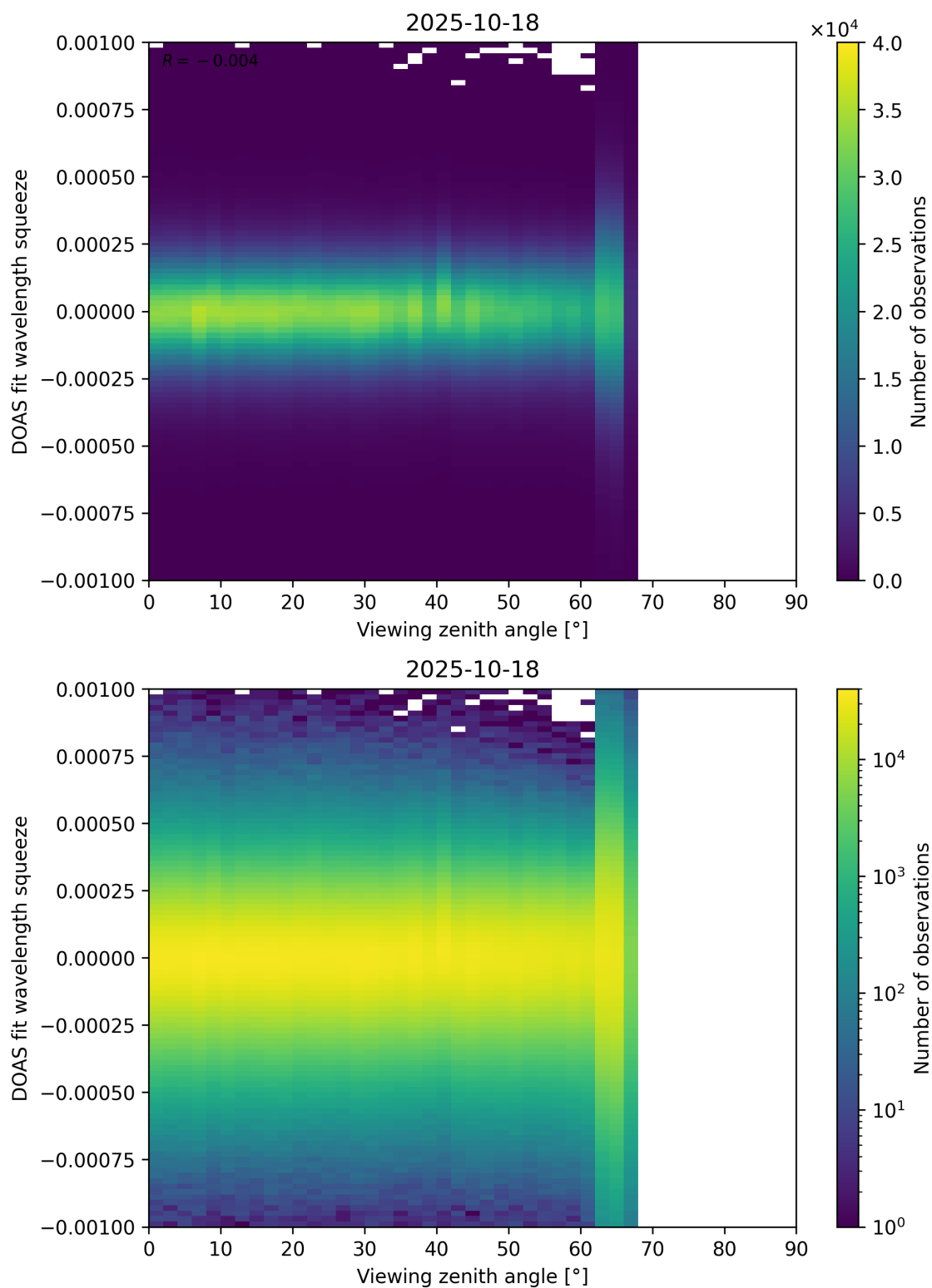
Figure 366: Scatter density plot of “Viewing zenith angle” against “DOAS fit wavelength squeeze” for 2025-10-17 to 2025-10-19.
