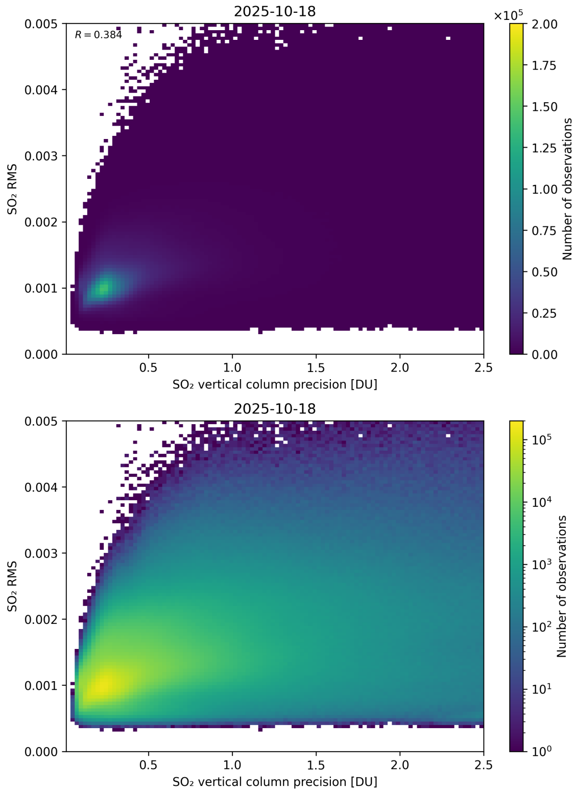
Figure 334: Scatter density plot of “SO 2 vertical column precision” against “SO 2 RMS” for 2025-10-17 to 2025-10-19.
