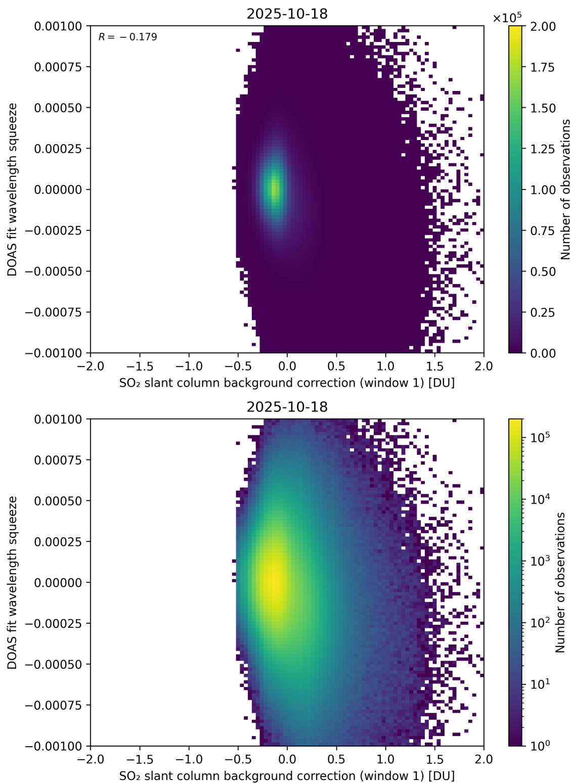
Figure 112: Scatter density plot of “SO 2 slant column background correction (window 1)” against “DOAS fit wavelength squeeze” for 2025-10-17 to 2025-10-19.
