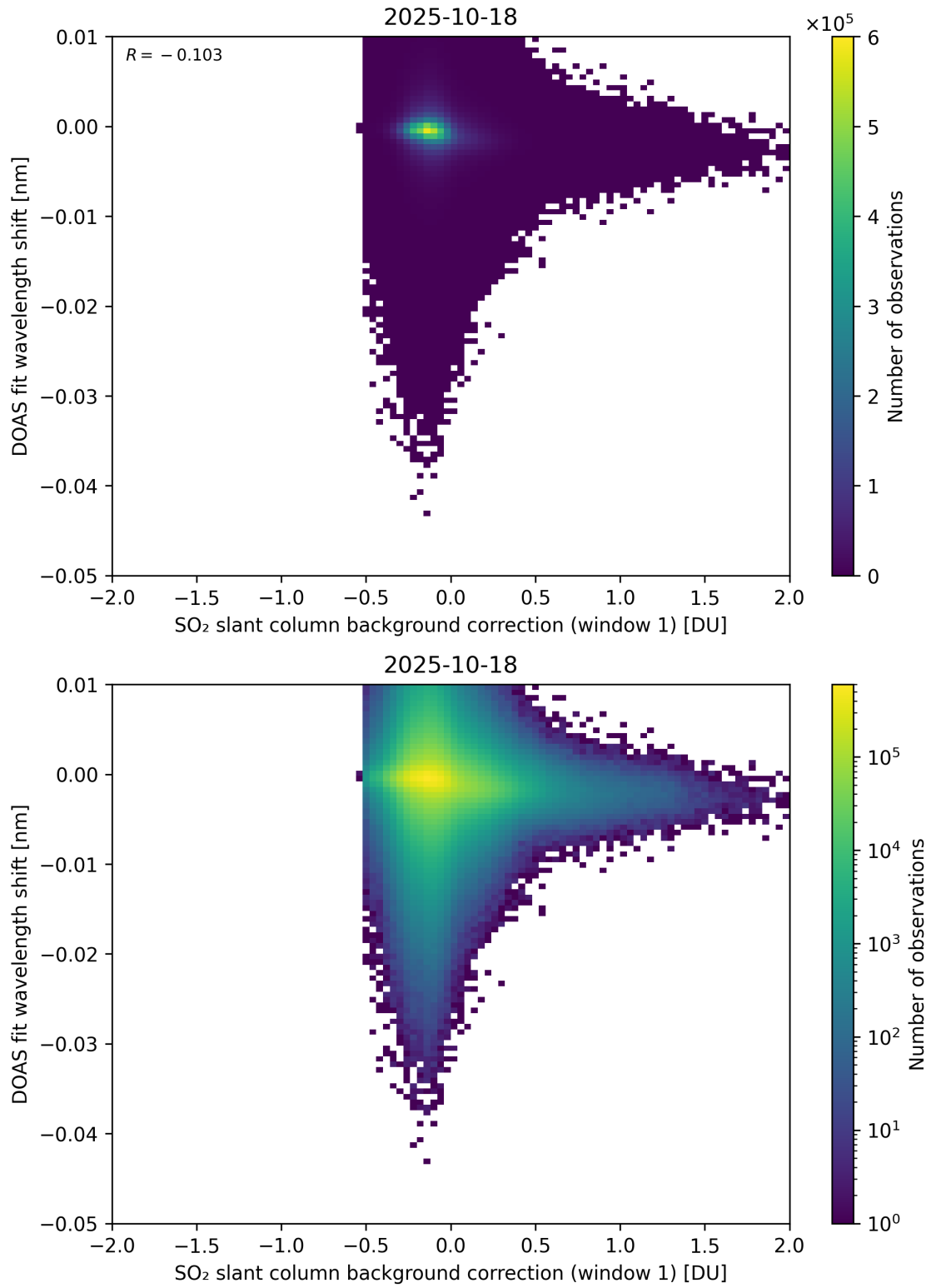
Figure 111: Scatter density plot of “SO 2 slant column background correction (window 1)” against “DOAS fit wavelength shift” for 2025-10-17 to 2025-10-19.
