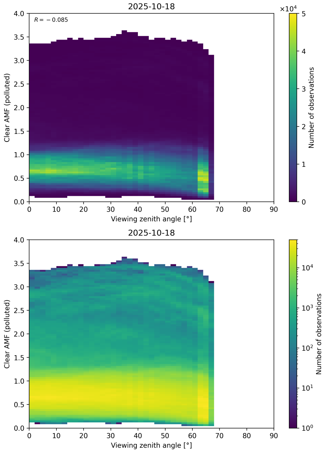
Figure 370: Scatter density plot of “Viewing zenith angle” against “Clear AMF (polluted)” for 2025-10-17 to 2025-10-19.
