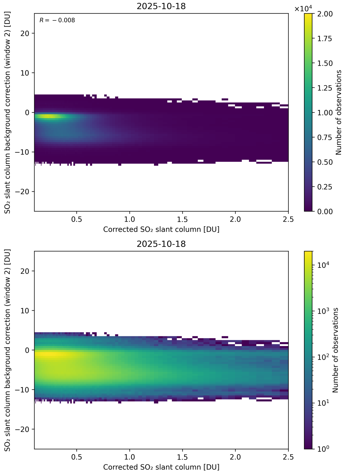
Figure 227: Scatter density plot of “Corrected SO 2 slant column” against “SO 2 slant column background correction (window 2)” for 2025-10-17 to 2025-10-19.
