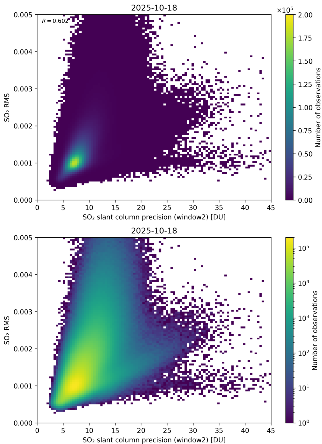
Figure 295: Scatter density plot of “SO 2 slant column precision (window2)” against “SO 2 RMS” for 2025-10-17 to 2025-10-19.
