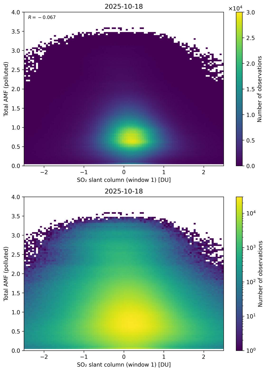
Figure 289: Scatter density plot of “SO 2 slant column (window 1)” against “Total AMF (polluted)” for 2025-10-17 to 2025-10-19.
