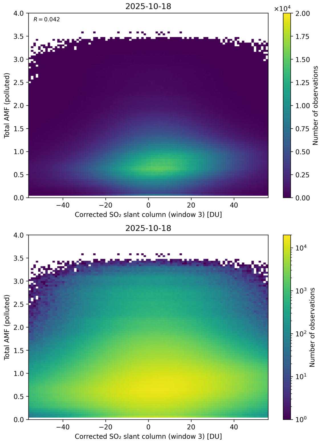
Figure 260: Scatter density plot of “Corrected SO 2 slant column (window 3)” against “Total AMF (polluted)” for 2025-10-17 to 2025-10-19.
