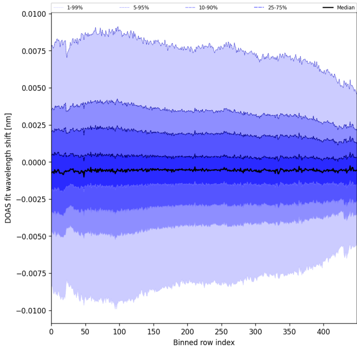
Figure 102: Along track statistics of “DOAS fit wavelength shift” for 2025-10-17 to 2025-10-19
