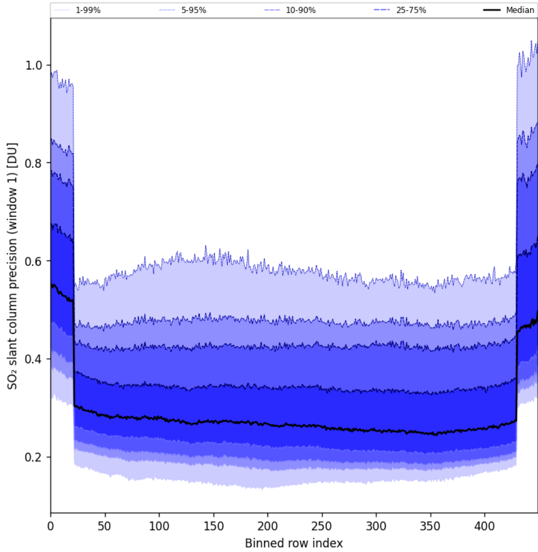
Figure 90: Along track statistics of “SO 2 slant column precision (window 1)” for 2025-10-17 to 2025-10-19
