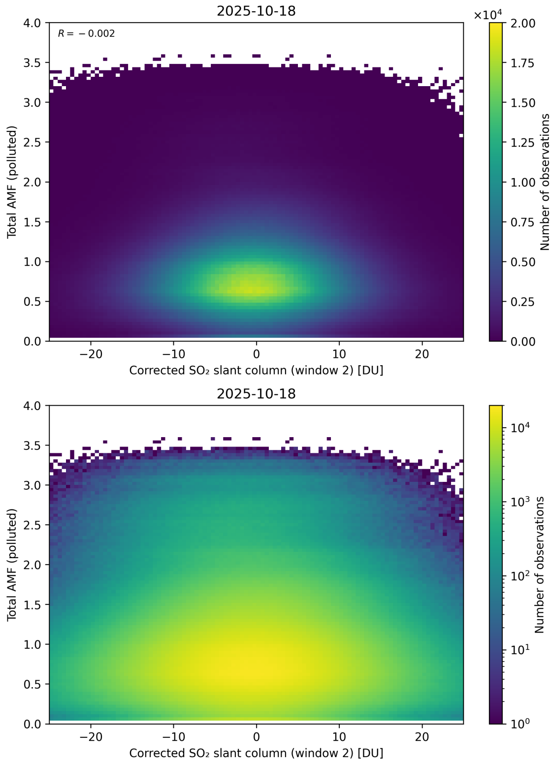
Figure 253: Scatter density plot of “Corrected SO 2 slant column (window 2)” against “Total AMF (polluted)” for 2025-10-17 to 2025-10-19.
