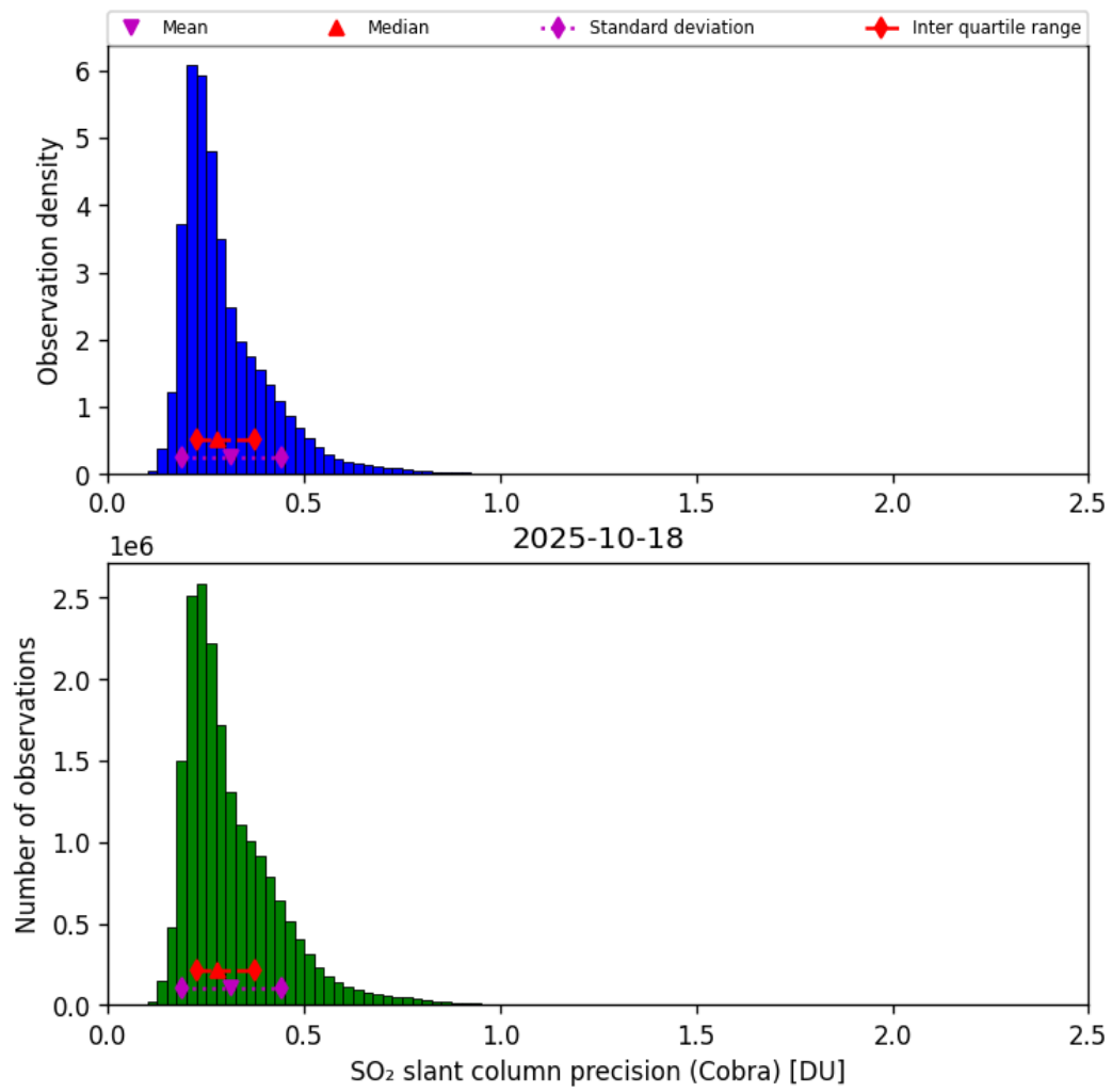
Figure 62: Histogram of “SO 2 slant column precision (Cobra)” for 2025-10-17 to 2025-10-19
