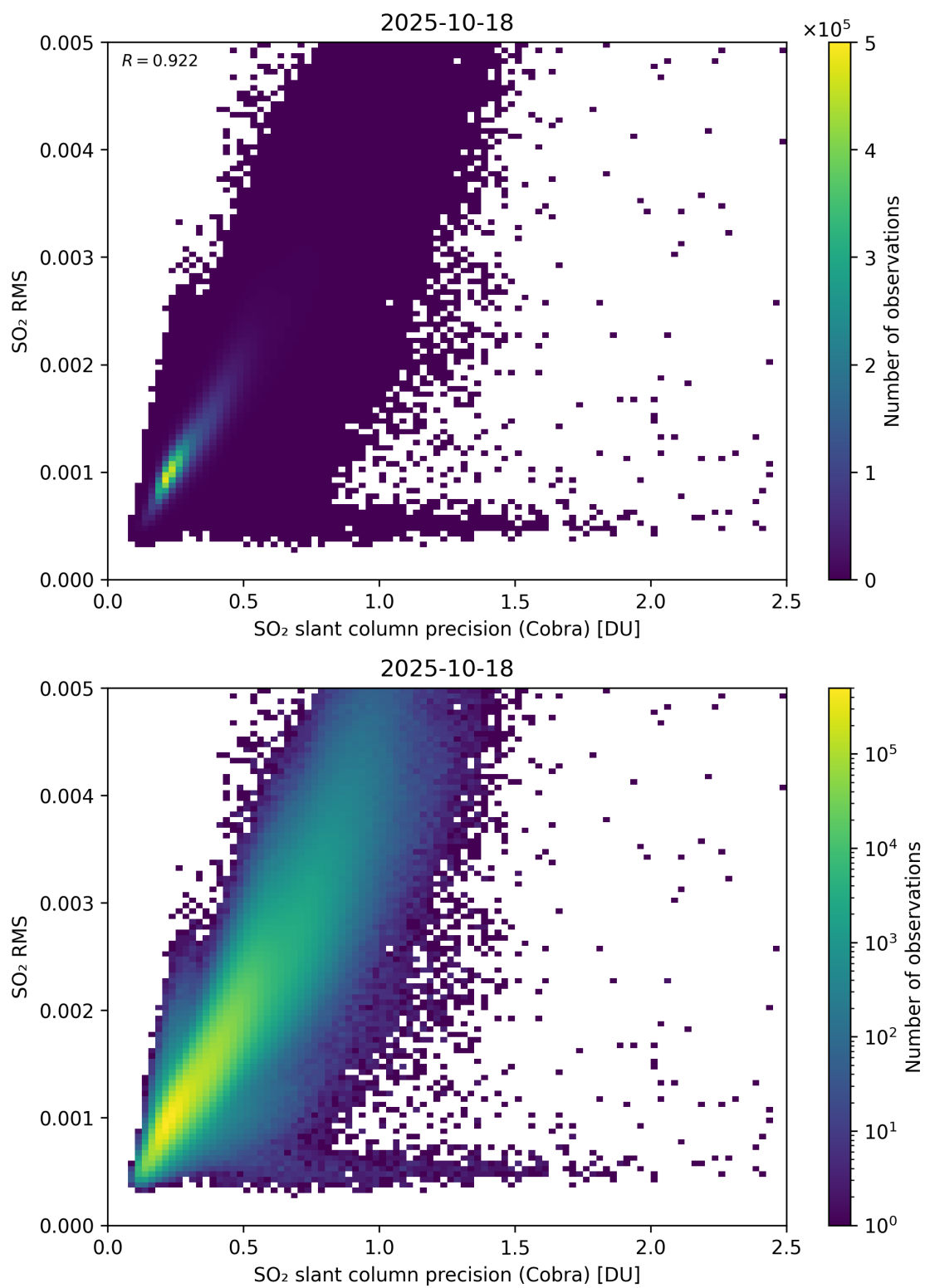
Figure 204: Scatter density plot of “SO 2 slant column precision (Cobra)” against “SO 2 RMS” for 2025-10-17 to 2025-10-19.
