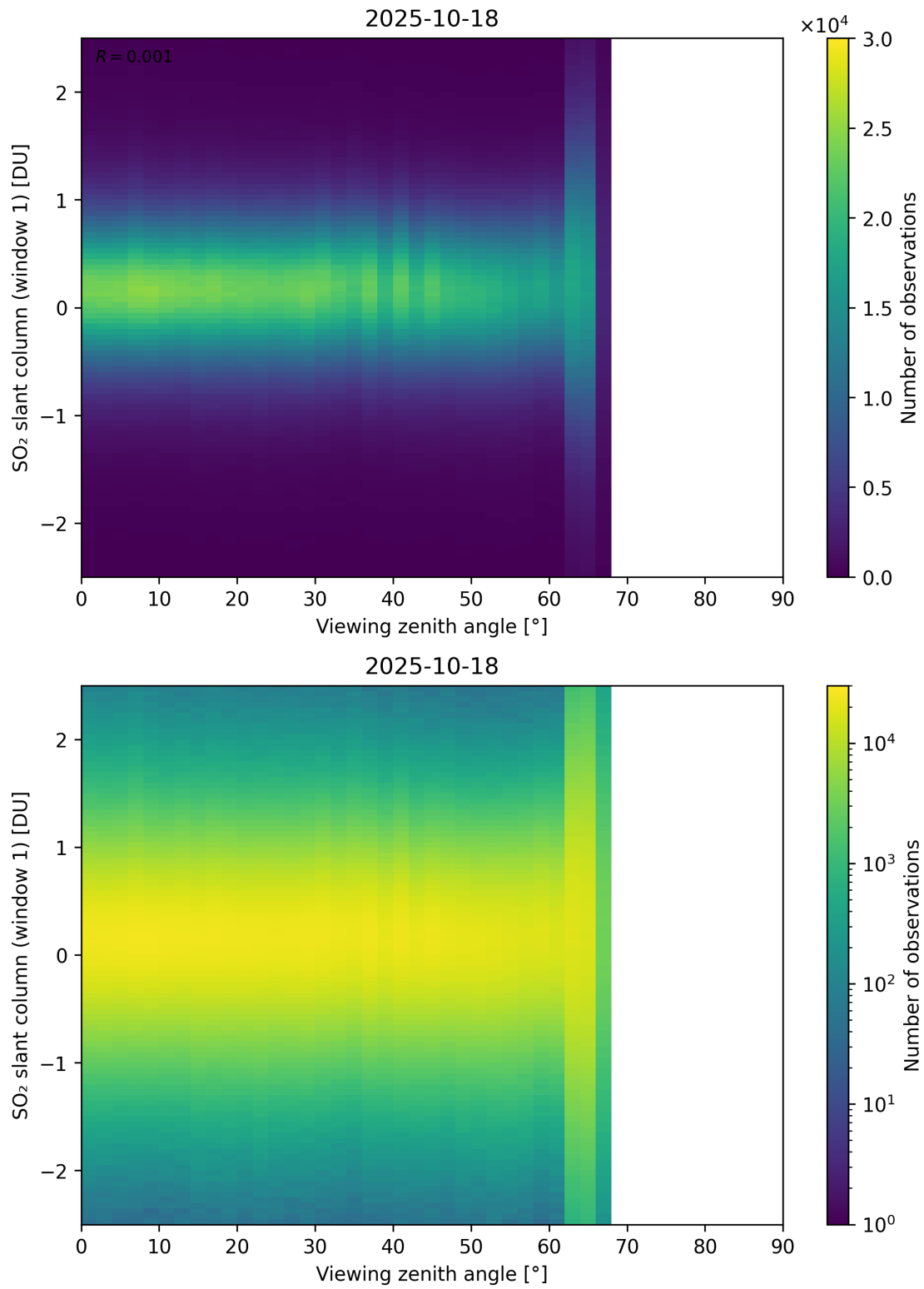
Figure 376: Scatter density plot of “Viewing zenith angle” against “SO 2 slant column (window 1)” for 2025-10-17 to 2025-10-19.
