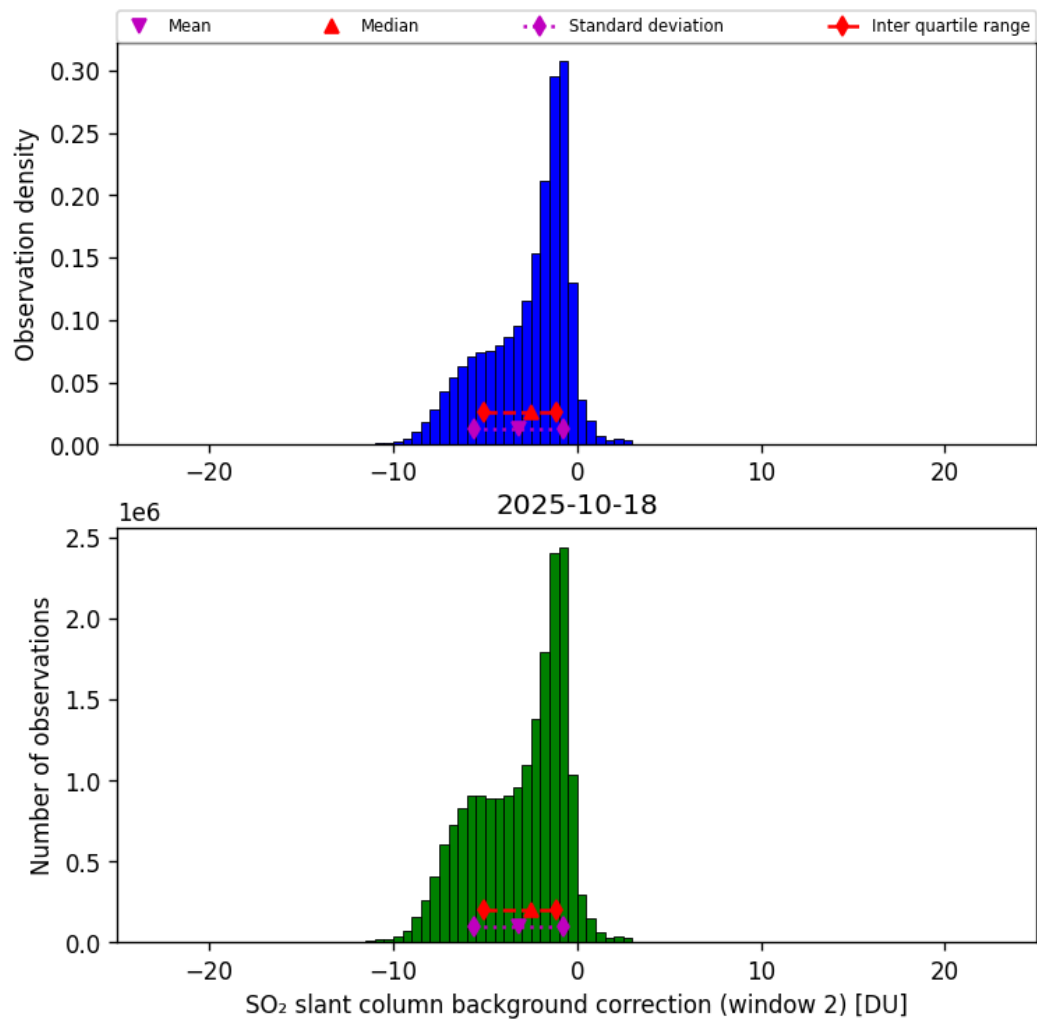
Figure 70: Histogram of “SO 2 slant column background correction (window 2)” for 2025-10-17 to 2025-10-19
