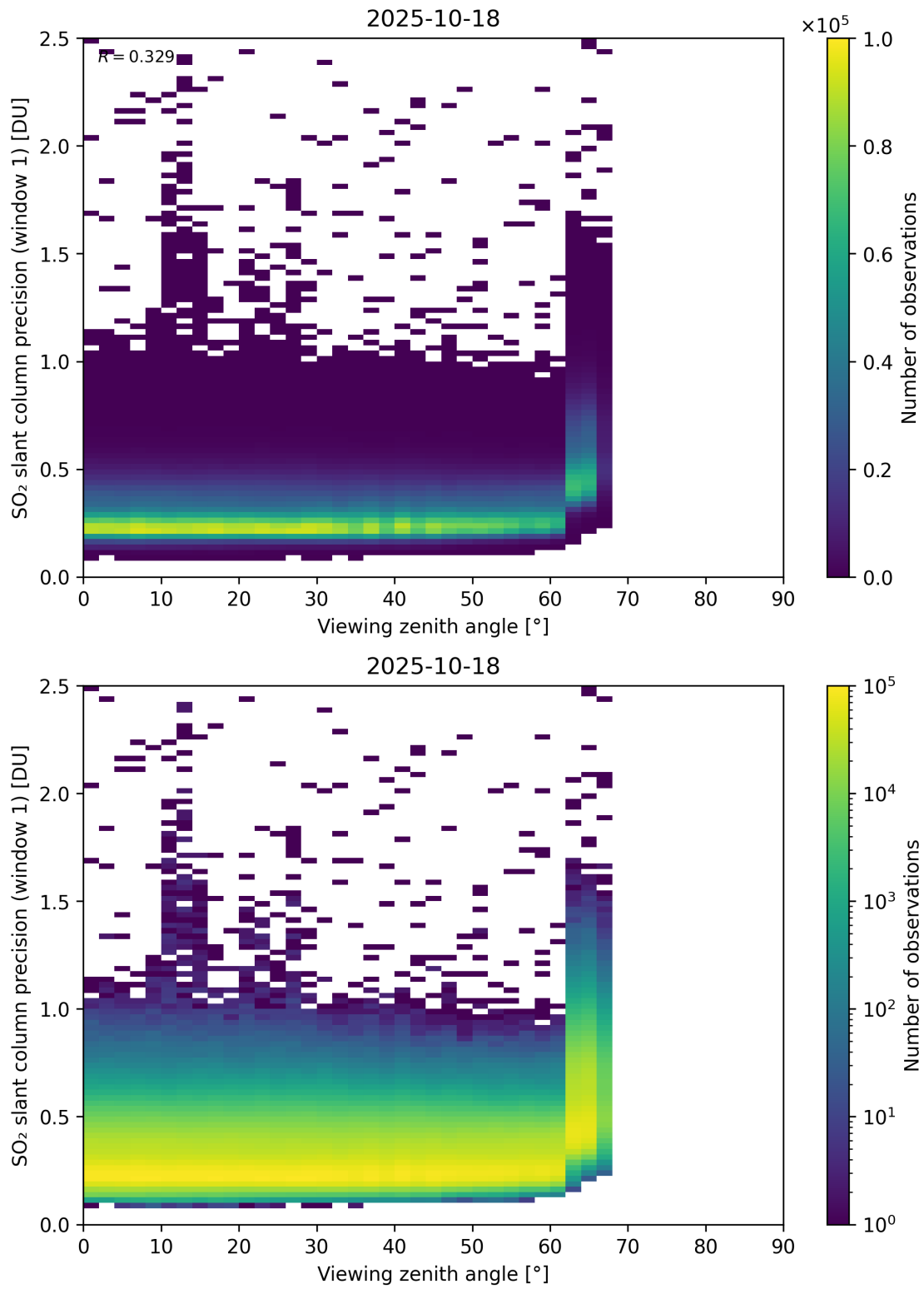
Figure 377: Scatter density plot of “Viewing zenith angle” against “SO 2 slant column precision (window 1)” for 2025-10-17 to 2025-10-19.
