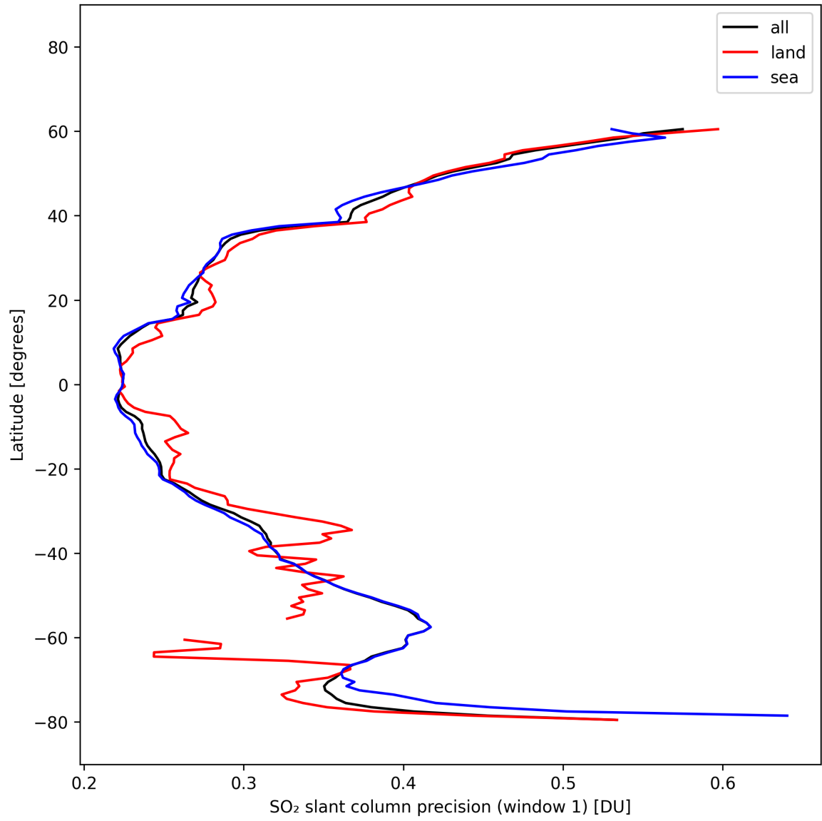
Figure 38: Zonal average of “SO 2 slant column precision (window 1)” for 2025-10-17 to 2025-10-19.
