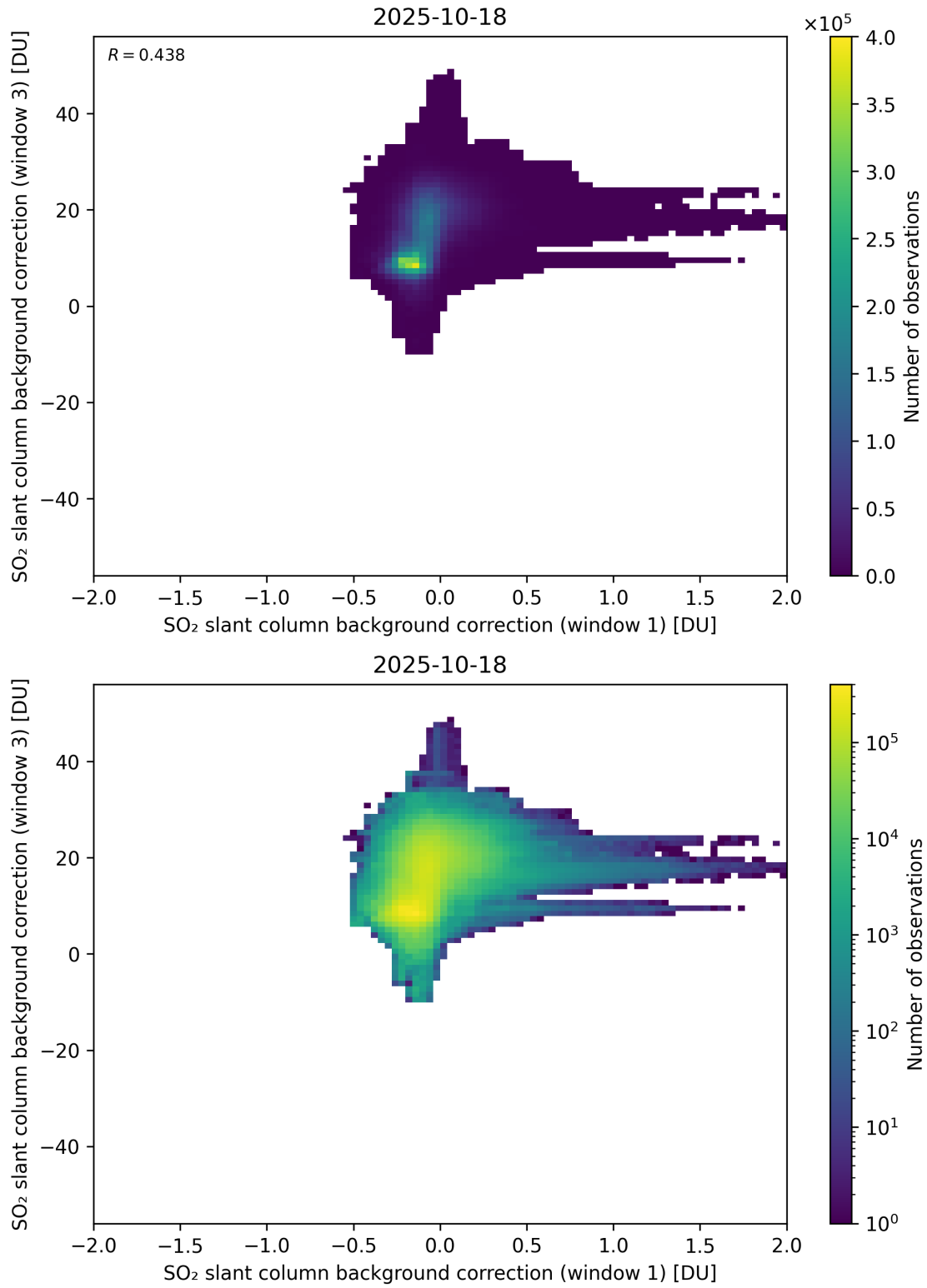
Figure 110: Scatter density plot of “SO 2 slant column background correction (window 1)” against “SO 2 slant column background correction (window 3)” for 2025-10-17 to 2025-10-19.
