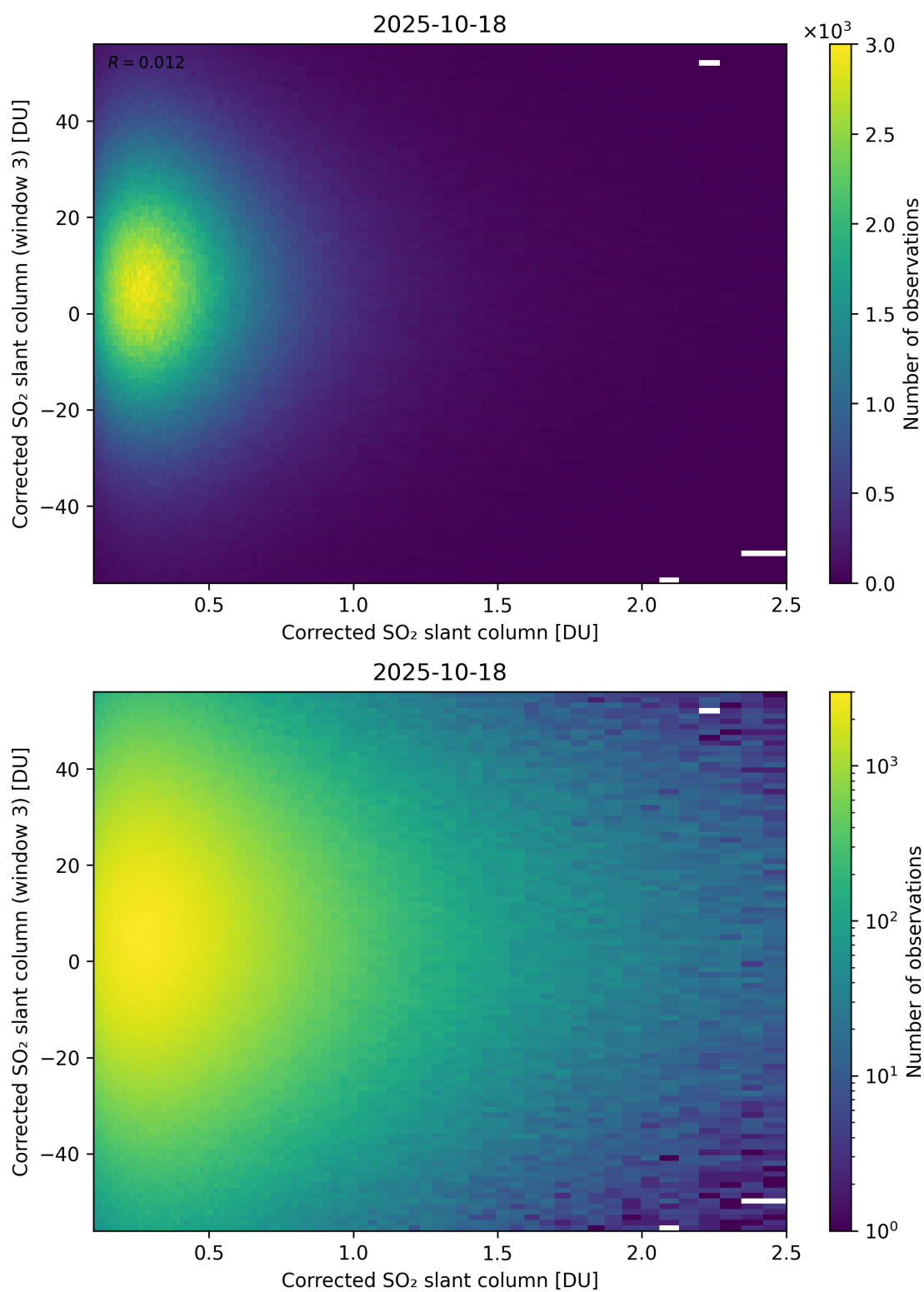
Figure 236: Scatter density plot of “Corrected SO 2 slant column” against “Corrected SO 2 slant column (window 3)” for 2025-10-17 to 2025-10-19.
