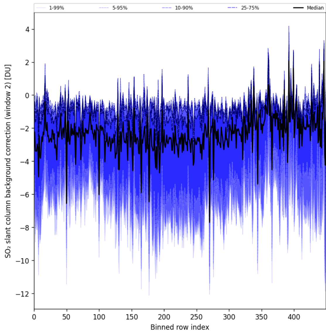
Figure 96: Along track statistics of “SO 2 slant column background correction (window 2)” for 2025-10-17 to 2025-10-19
