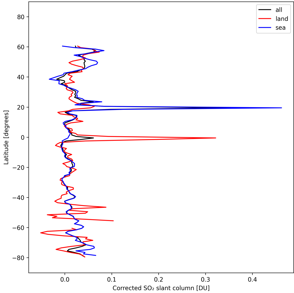
Figure 34: Zonal average of “Corrected SO 2 slant column” for 2025-10-17 to 2025-10-19.
