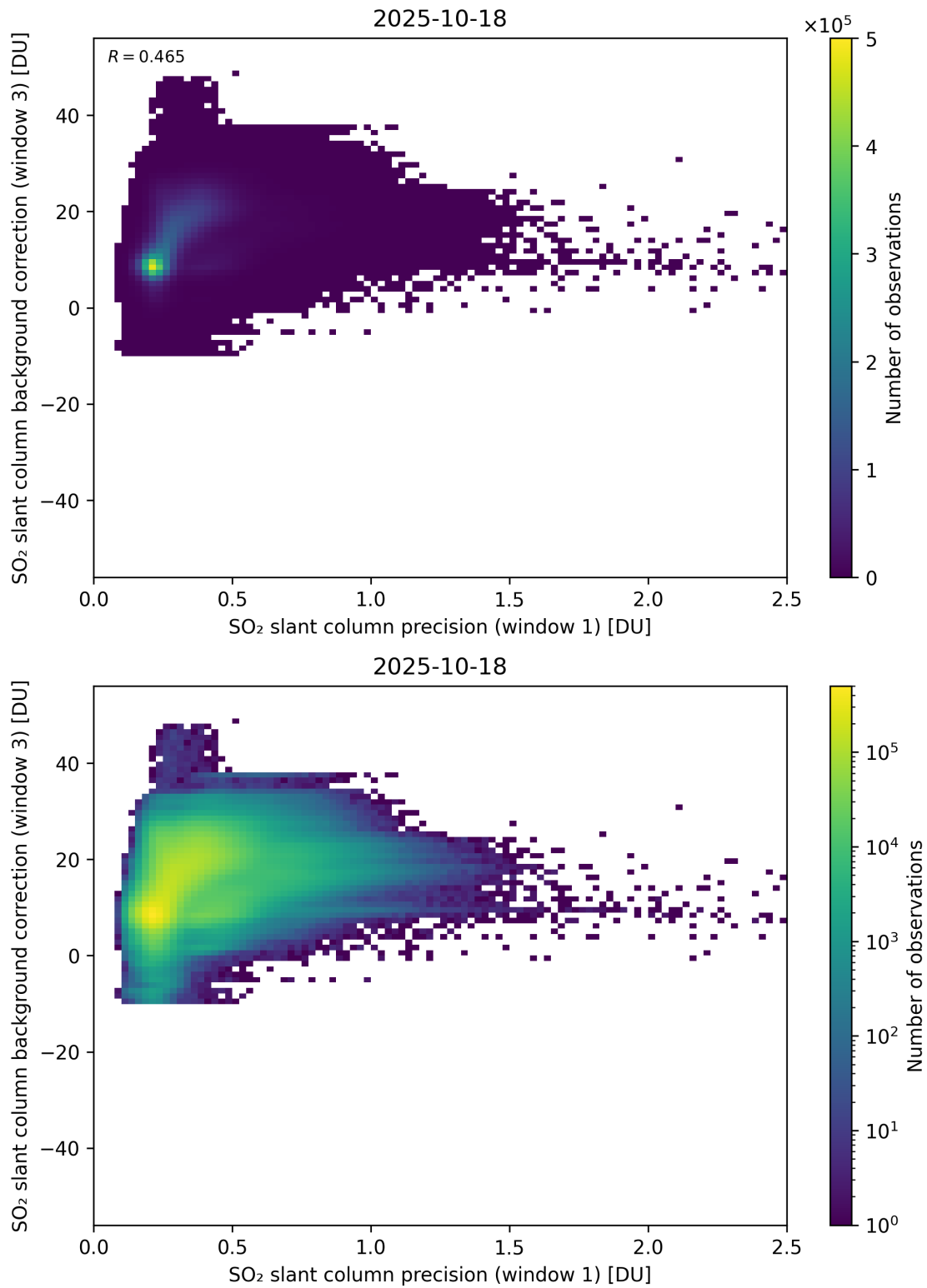
Figure 270: Scatter density plot of “SO 2 slant column precision (window 1)” against “SO 2 slant column background correction (window 3)” for 2025-10-17 to 2025-10-19.
