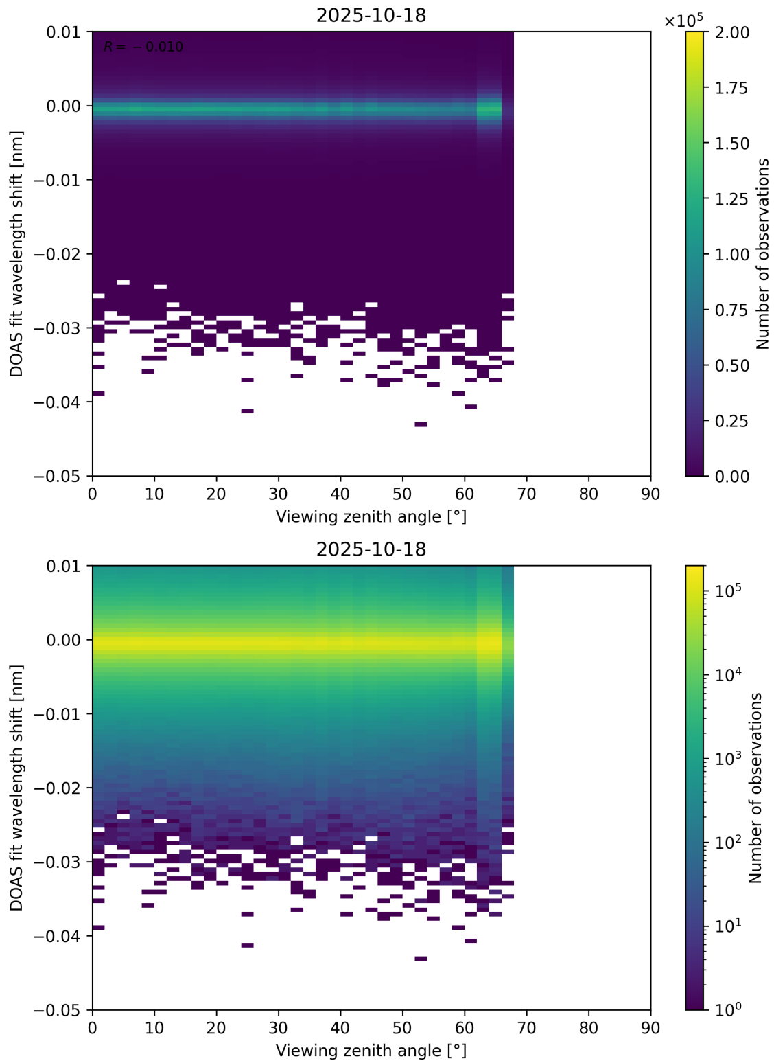
Figure 365: Scatter density plot of “Viewing zenith angle” against “DOAS fit wavelength shift” for 2025-10-17 to 2025-10-19.
