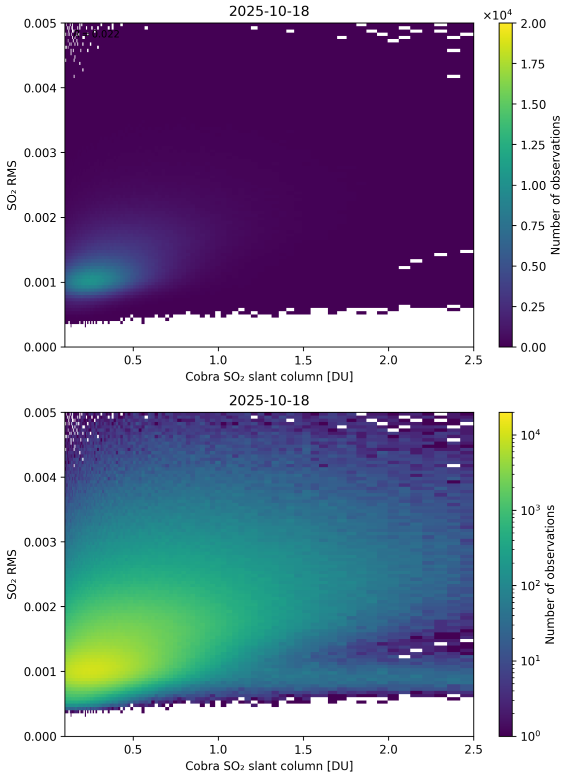
Figure 198: Scatter density plot of “Cobra SO 2 slant column” against “SO 2 RMS” for 2025-10-17 to 2025-10-19.
