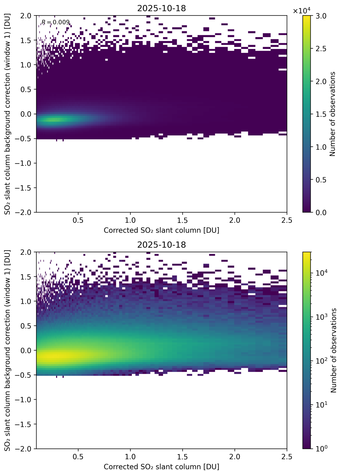
Figure 226: Scatter density plot of “Corrected SO 2 slant column” against “SO 2 slant column background correction (window 1)” for 2025-10-17 to 2025-10-19.
