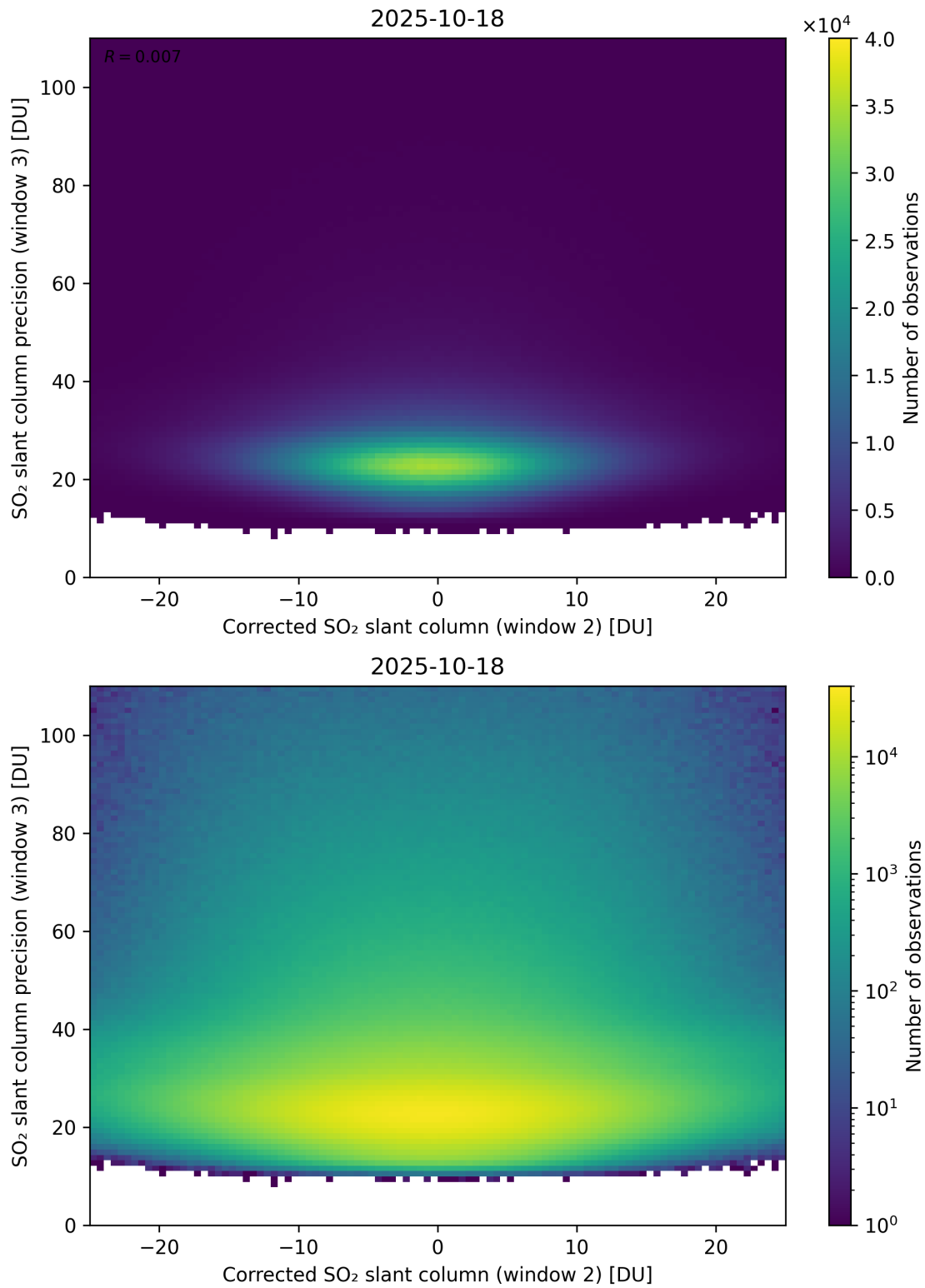
Figure 252: Scatter density plot of “Corrected SO 2 slant column (window 2)” against “SO 2 slant column precision (window 3)” for 2025-10-17 to 2025-10-19.
