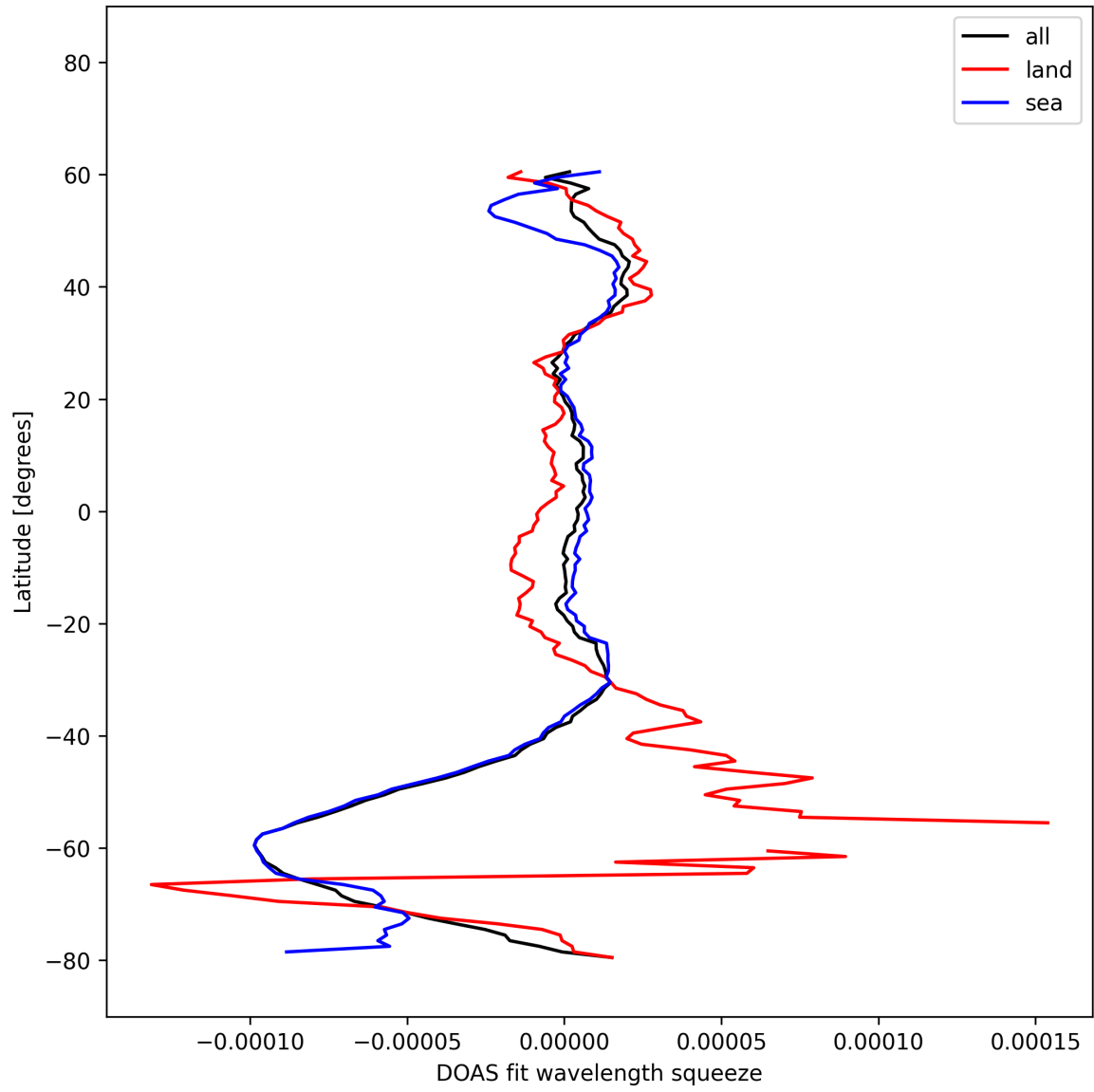
Figure 51: Zonal average of “DOAS fit wavelength squeeze” for 2025-10-17 to 2025-10-19.
