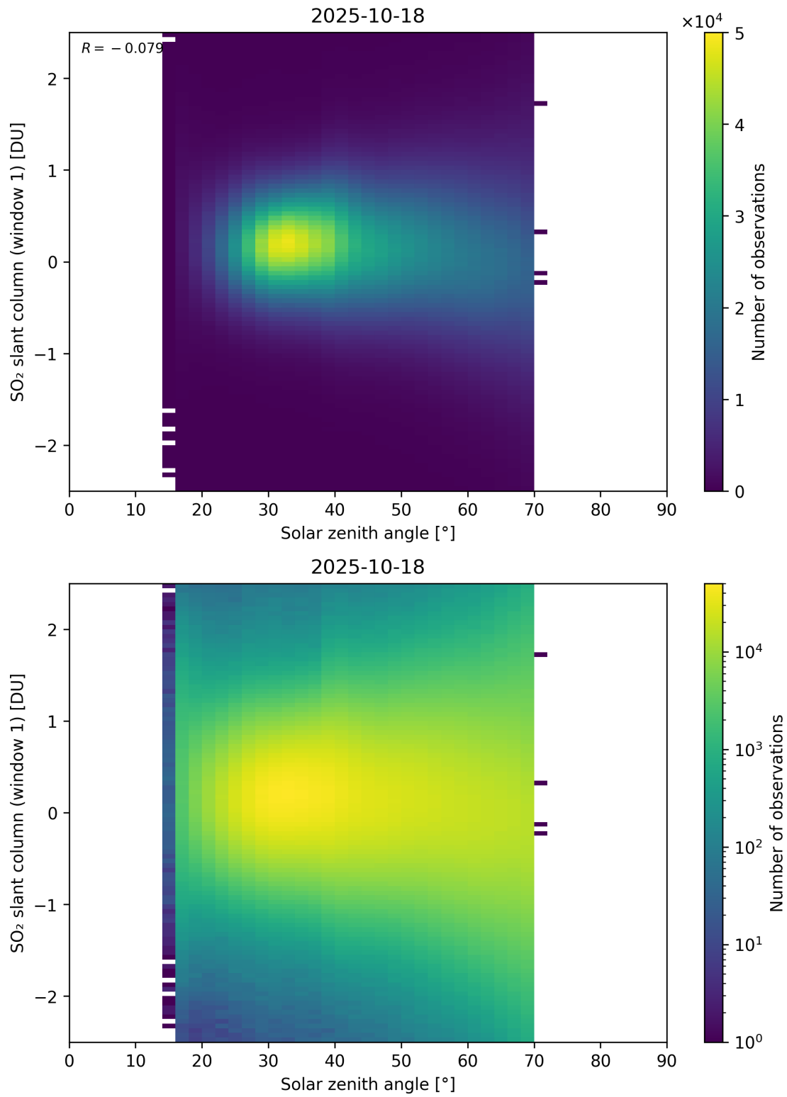
Figure 184: Scatter density plot of “Solar zenith angle” against “SO 2 slant column (window 1)” for 2025-10-17 to 2025-10-19.
