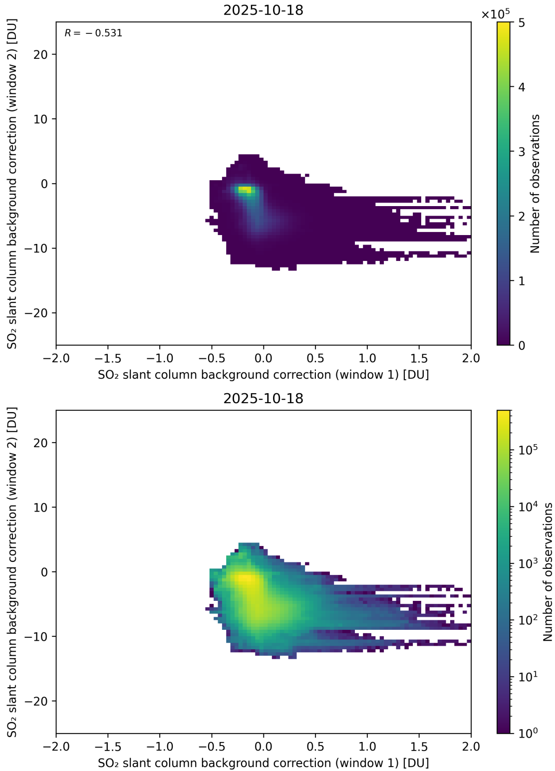
Figure 109: Scatter density plot of “SO 2 slant column background correction (window 1)” against “SO 2 slant column background correction (window 2)” for 2025-10-17 to 2025-10-19.
