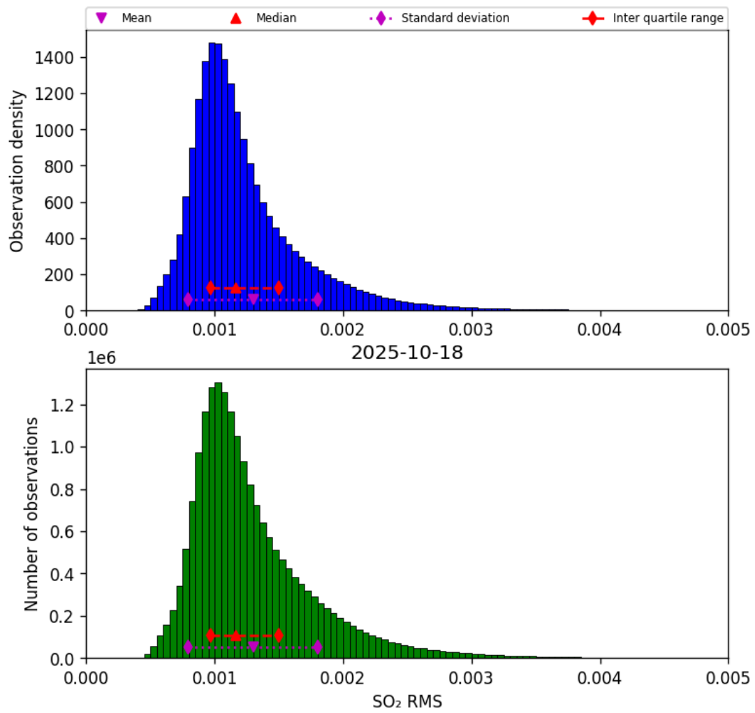
Figure 78: Histogram of “SO 2 RMS” for 2025-10-17 to 2025-10-19
