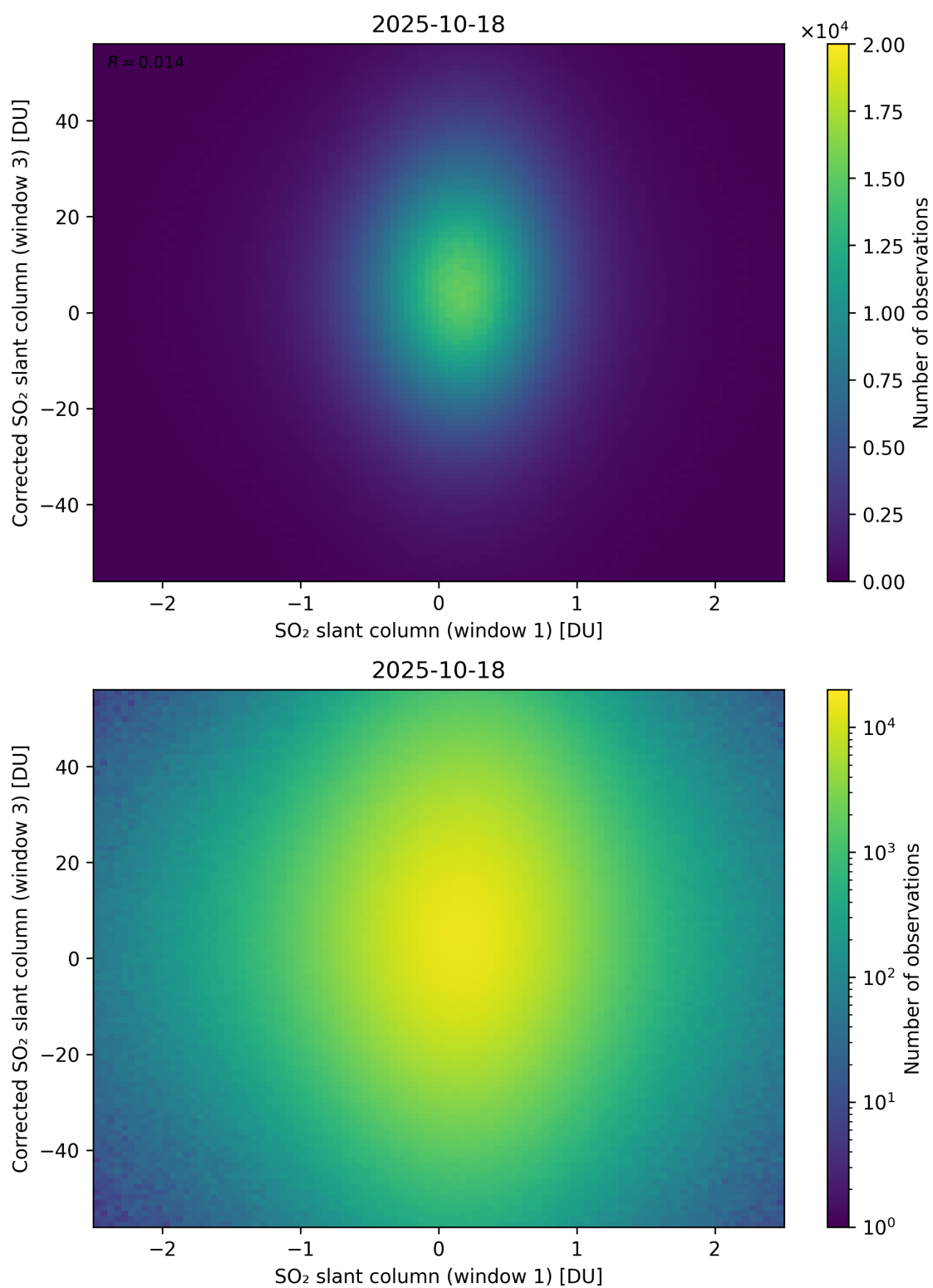
Figure 284: Scatter density plot of “SO 2 slant column (window 1)” against “Corrected SO 2 slant column (window 3)” for 2025-10-17 to 2025-10-19.
