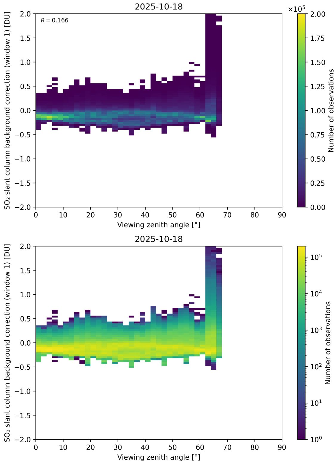
Figure 362: Scatter density plot of “Viewing zenith angle” against “SO 2 slant column background correction (window 1)” for 2025-10-17 to 2025-10-19.
