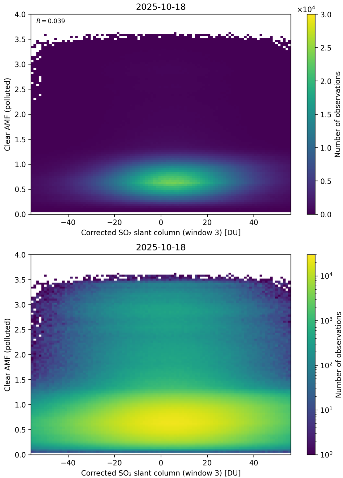
Figure 259: Scatter density plot of “Corrected SO 2 slant column (window 3)” against “Clear AMF (polluted)” for 2025-10-17 to 2025-10-19.
