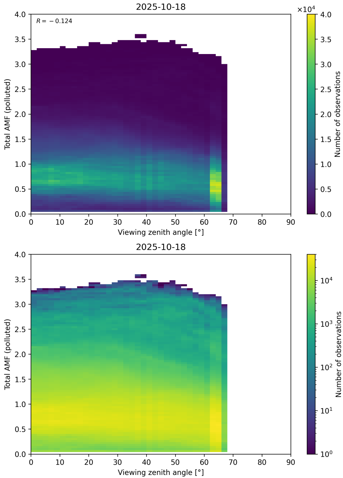
Figure 381: Scatter density plot of “Viewing zenith angle” against “Total AMF (polluted)” for 2025-10-17 to 2025-10-19.
