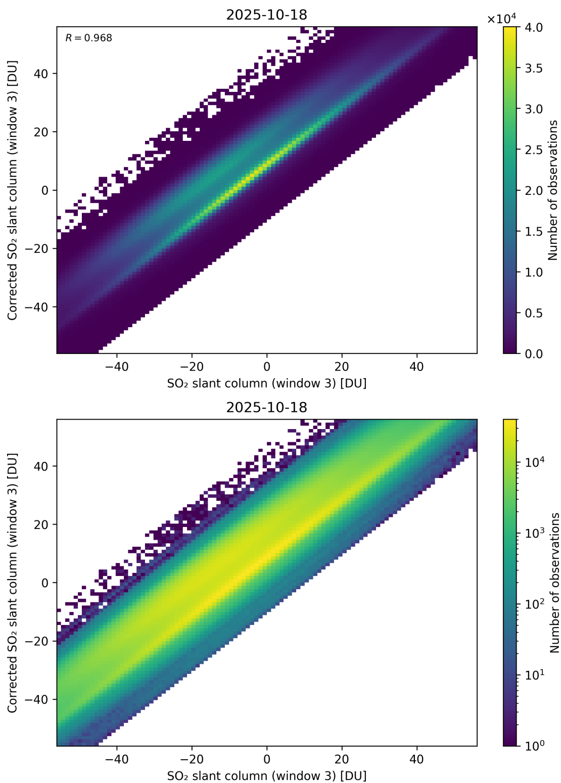
Figure 316: Scatter density plot of “SO 2 slant column (window 3)” against “Corrected SO 2 slant column (window 3)” for 2025-10-17 to 2025-10-19.
