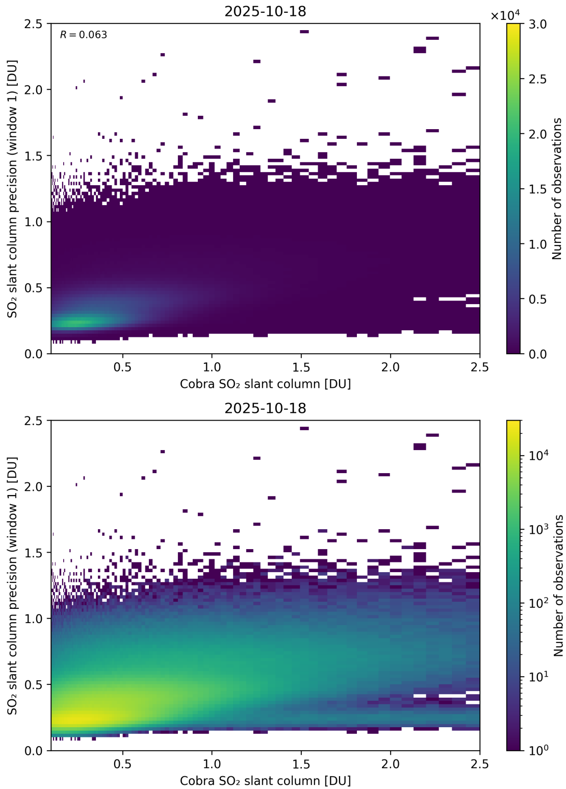
Figure 220: Scatter density plot of “Cobra SO 2 slant column” against “SO 2 slant column precision (window 1)” for 2025-10-17 to 2025-10-19.
