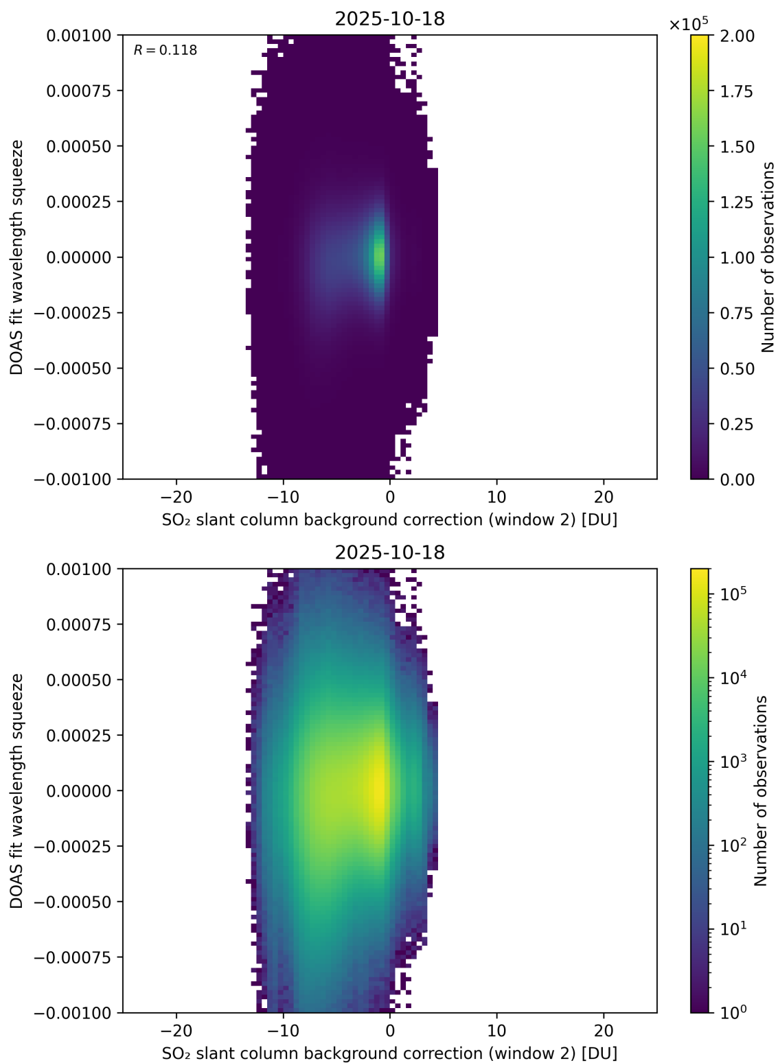
Figure 124: Scatter density plot of “SO 2 slant column background correction (window 2)” against “DOAS fit wavelength squeeze” for 2025-10-17 to 2025-10-19.
