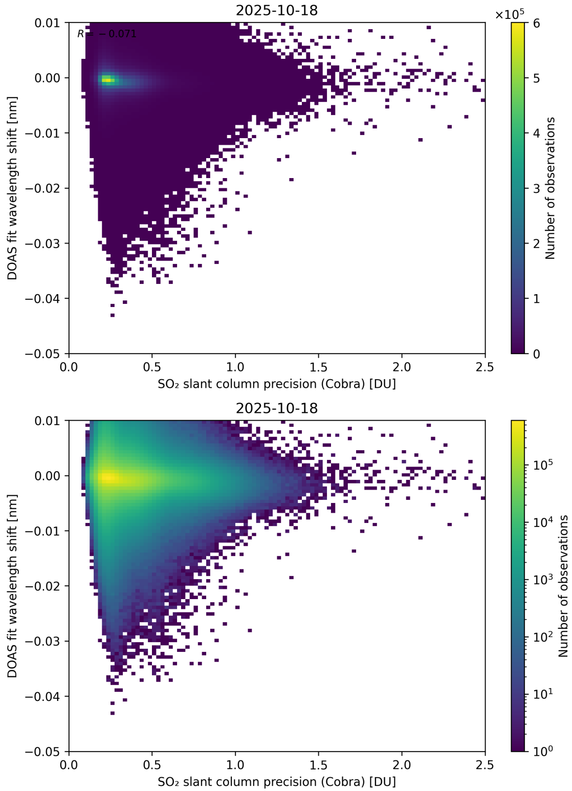
Figure 202: Scatter density plot of “SO 2 slant column precision (Cobra)” against “DOAS fit wavelength shift” for 2025-10-17 to 2025-10-19.
