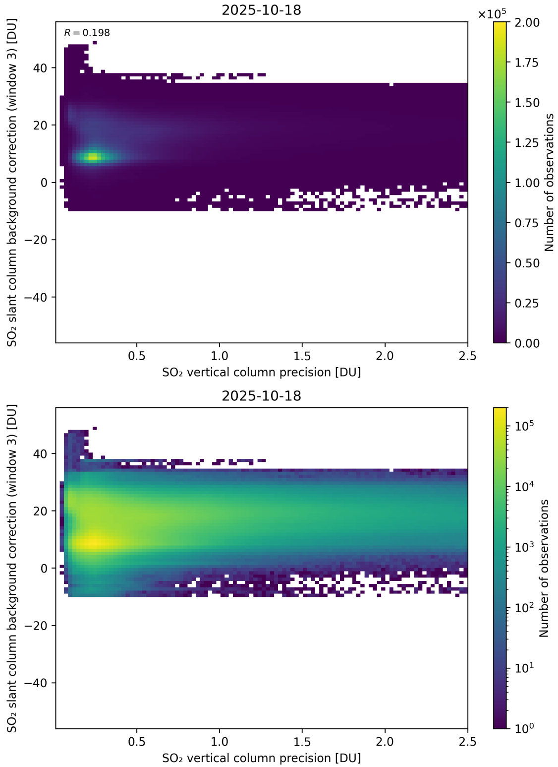
Figure 331: Scatter density plot of “SO 2 vertical column precision” against “SO 2 slant column background correction (window 3)” for 2025-10-17 to 2025-10-19.
