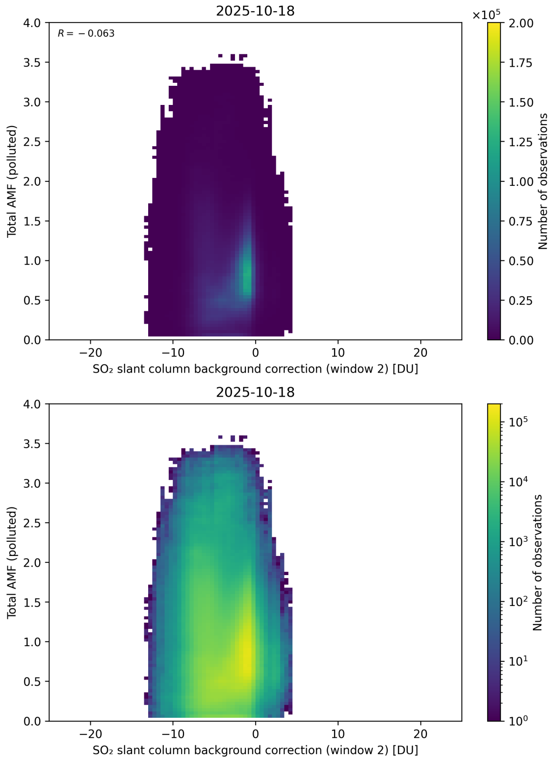
Figure 130: Scatter density plot of “SO 2 slant column background correction (window 2)” against “Total AMF (polluted)” for 2025-10-17 to 2025-10-19.
