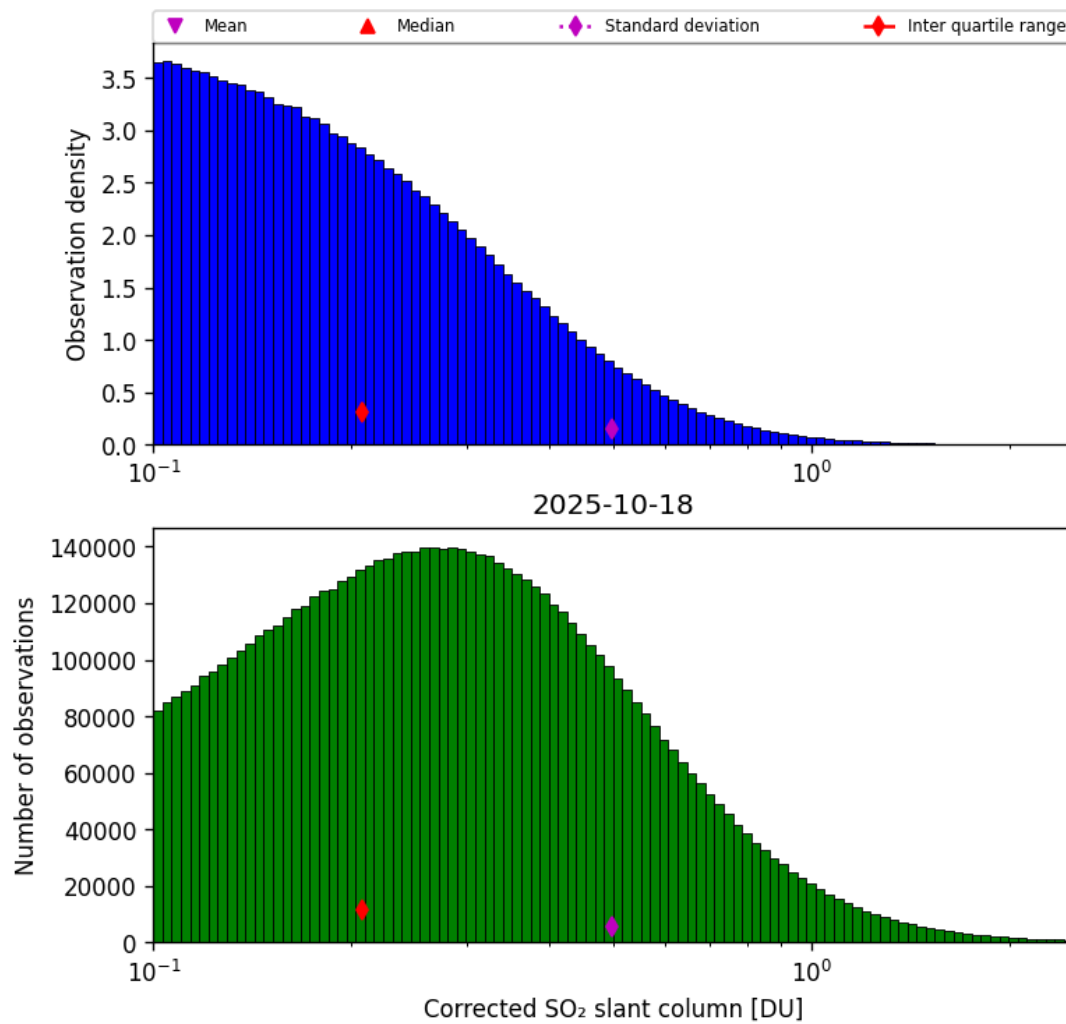
Figure 60: Histogram of “Corrected SO 2 slant column” for 2025-10-17 to 2025-10-19
