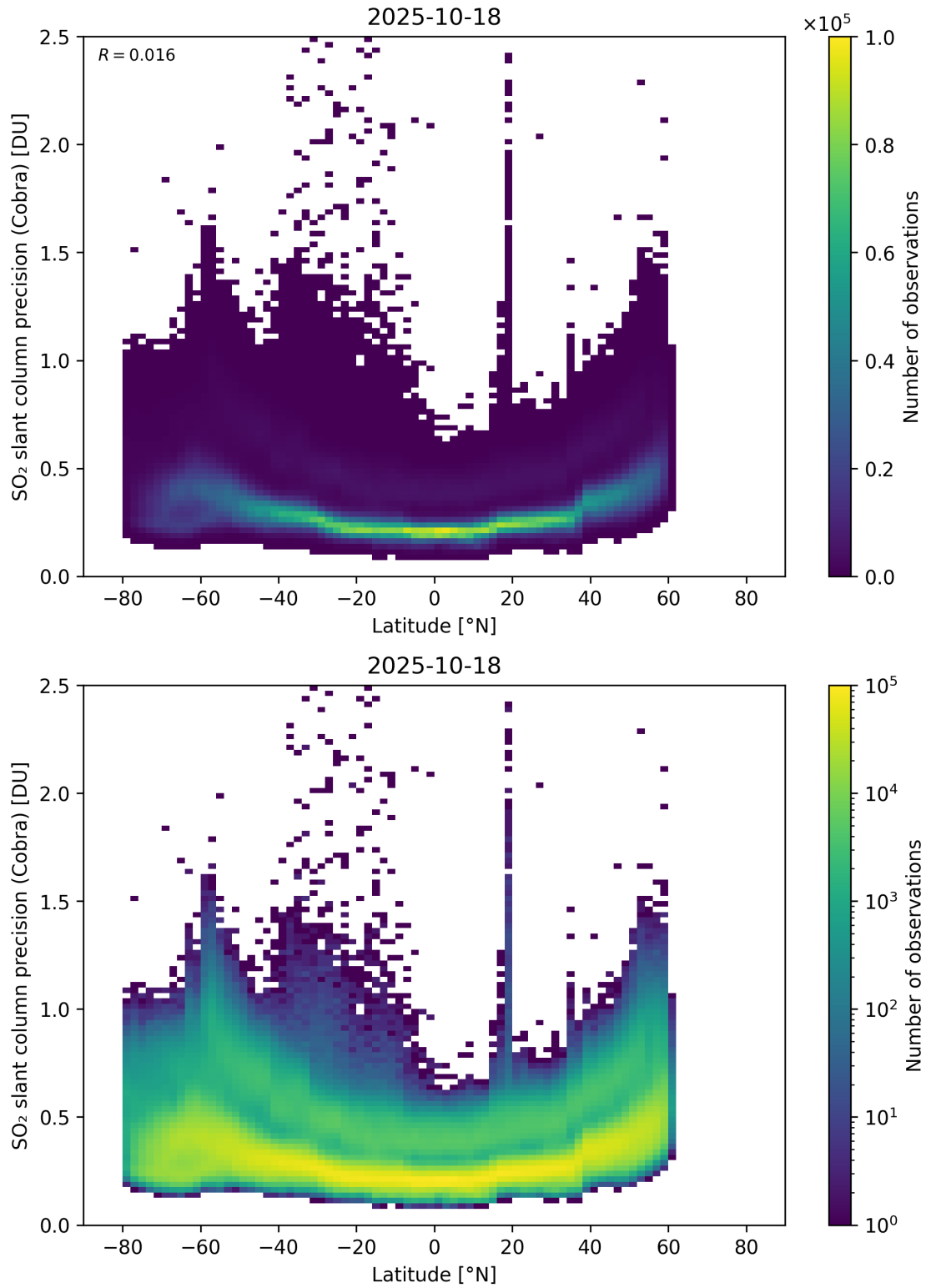
Figure 158: Scatter density plot of “Latitude” against “SO 2 slant column precision (Cobra)” for 2025-10-17 to 2025-10-19.
