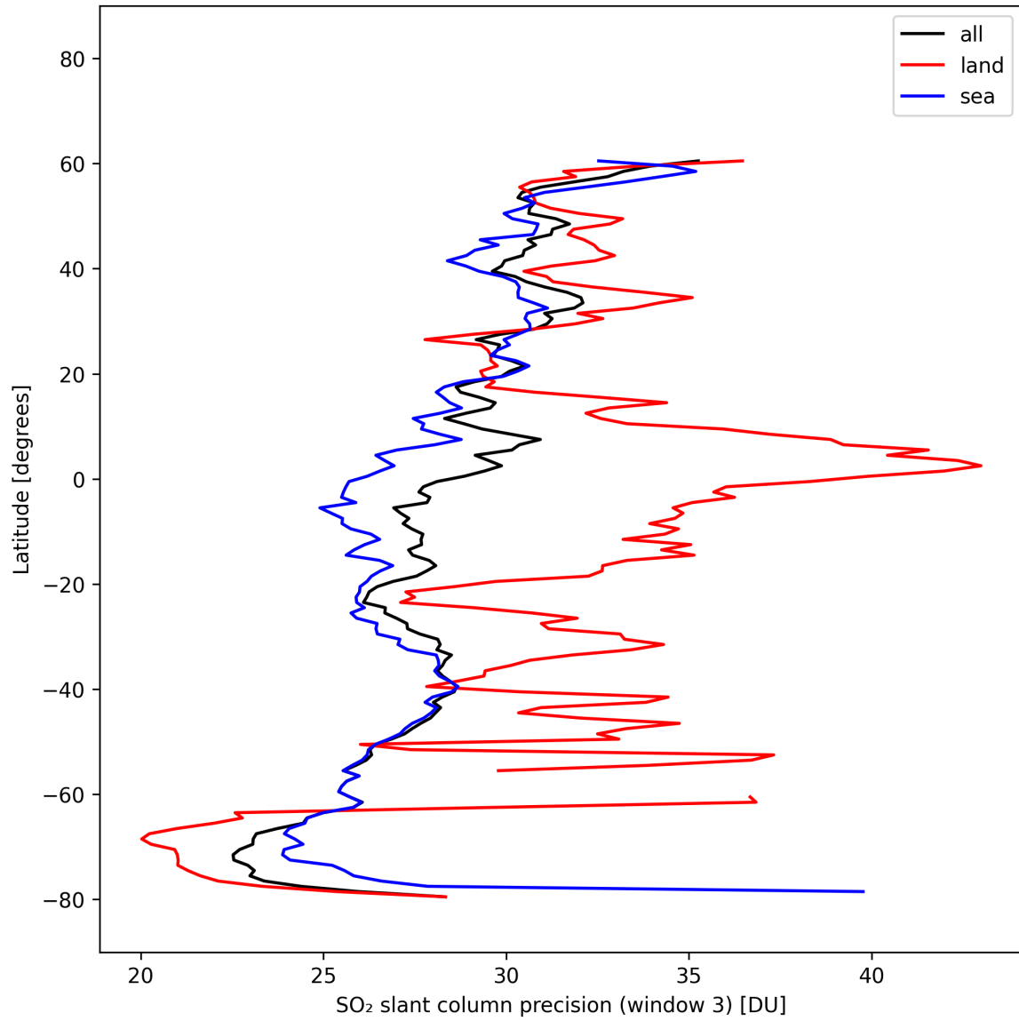
Figure 46: Zonal average of “SO 2 slant column precision (window 3)” for 2025-10-17 to 2025-10-19.
