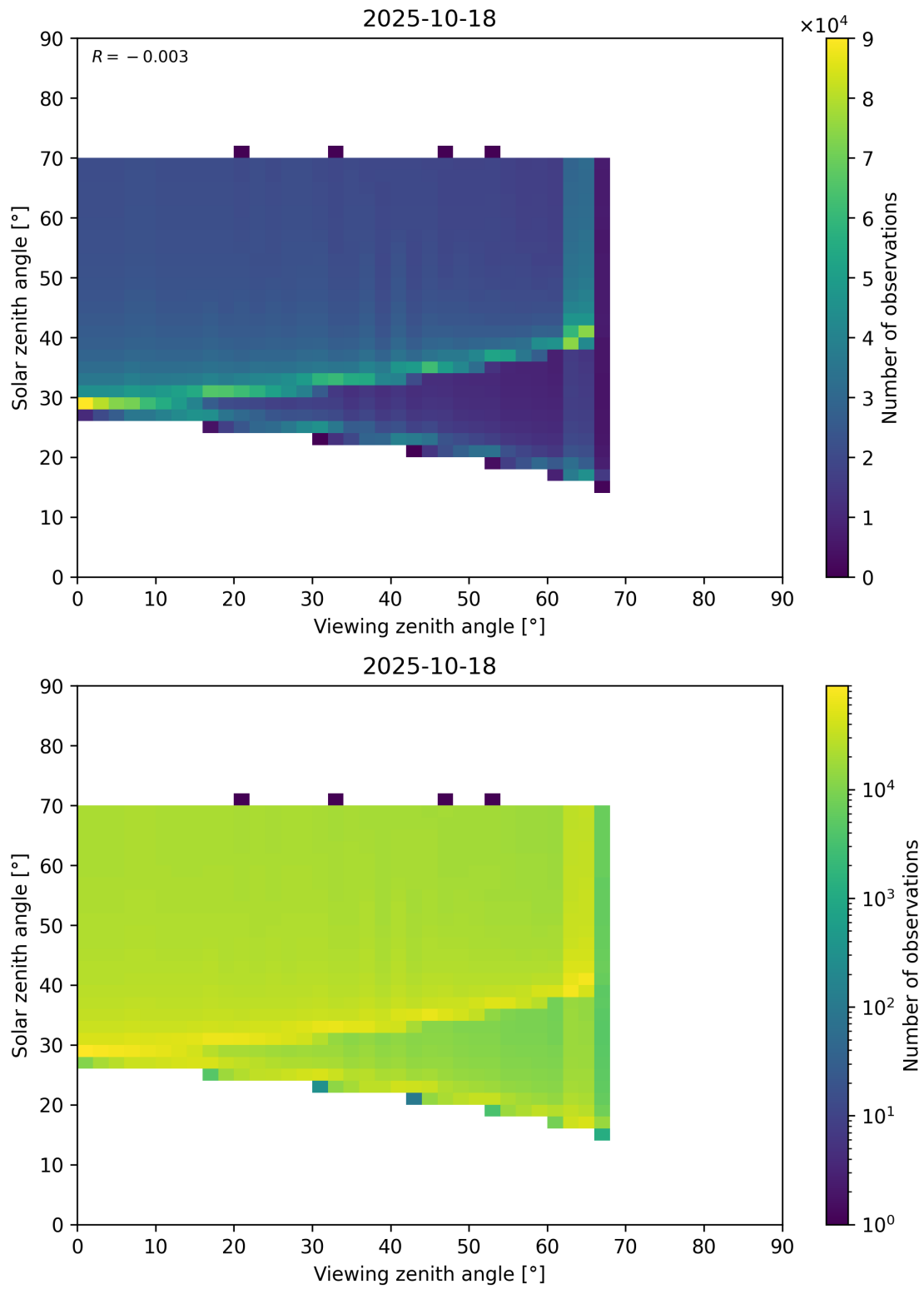
Figure 369: Scatter density plot of “Viewing zenith angle” against “Solar zenith angle” for 2025-10-17 to 2025-10-19.
