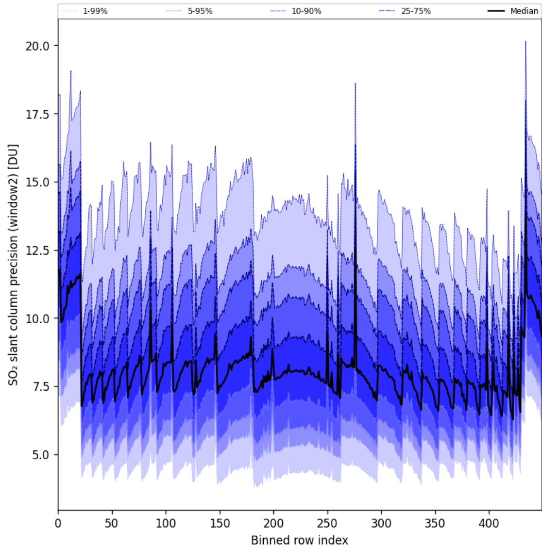
Figure 94: Along track statistics of “SO 2 slant column precision (window2)” for 2025-10-17 to 2025-10-19
