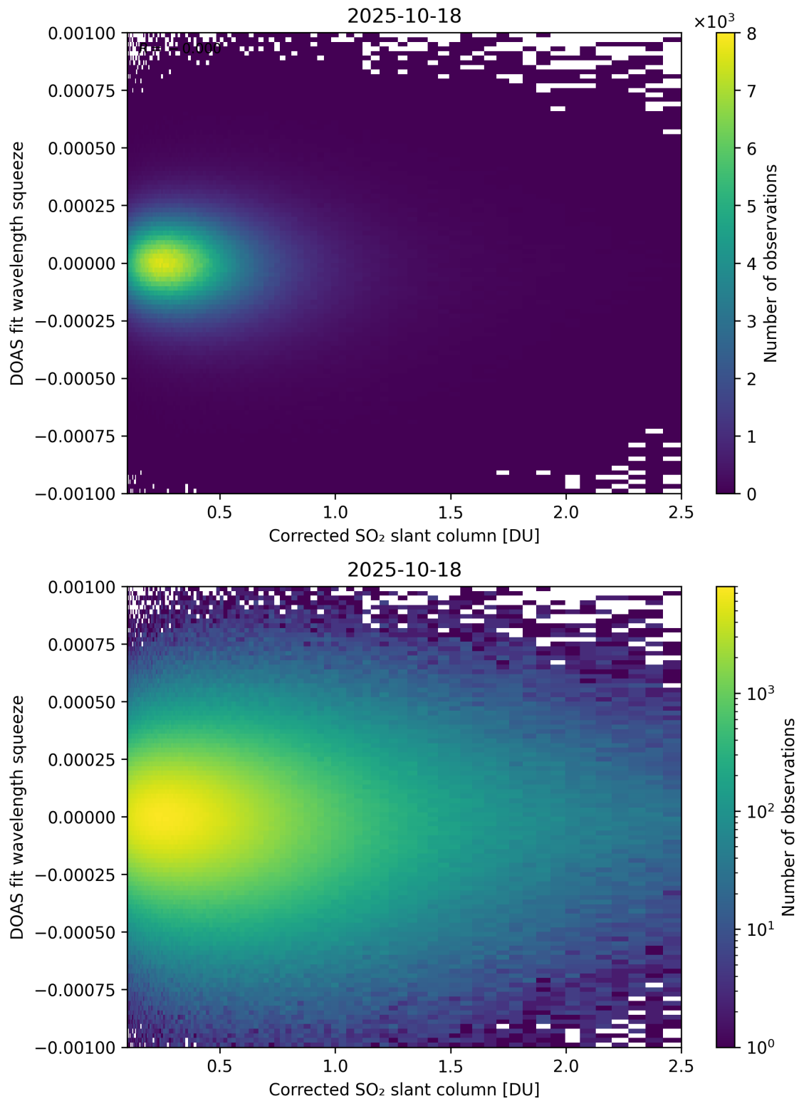
Figure 230: Scatter density plot of "Corrected SO 2 slant column" against "DOAS fit wavelength squeeze" for 2025-10-17 to 2025-10-19.
