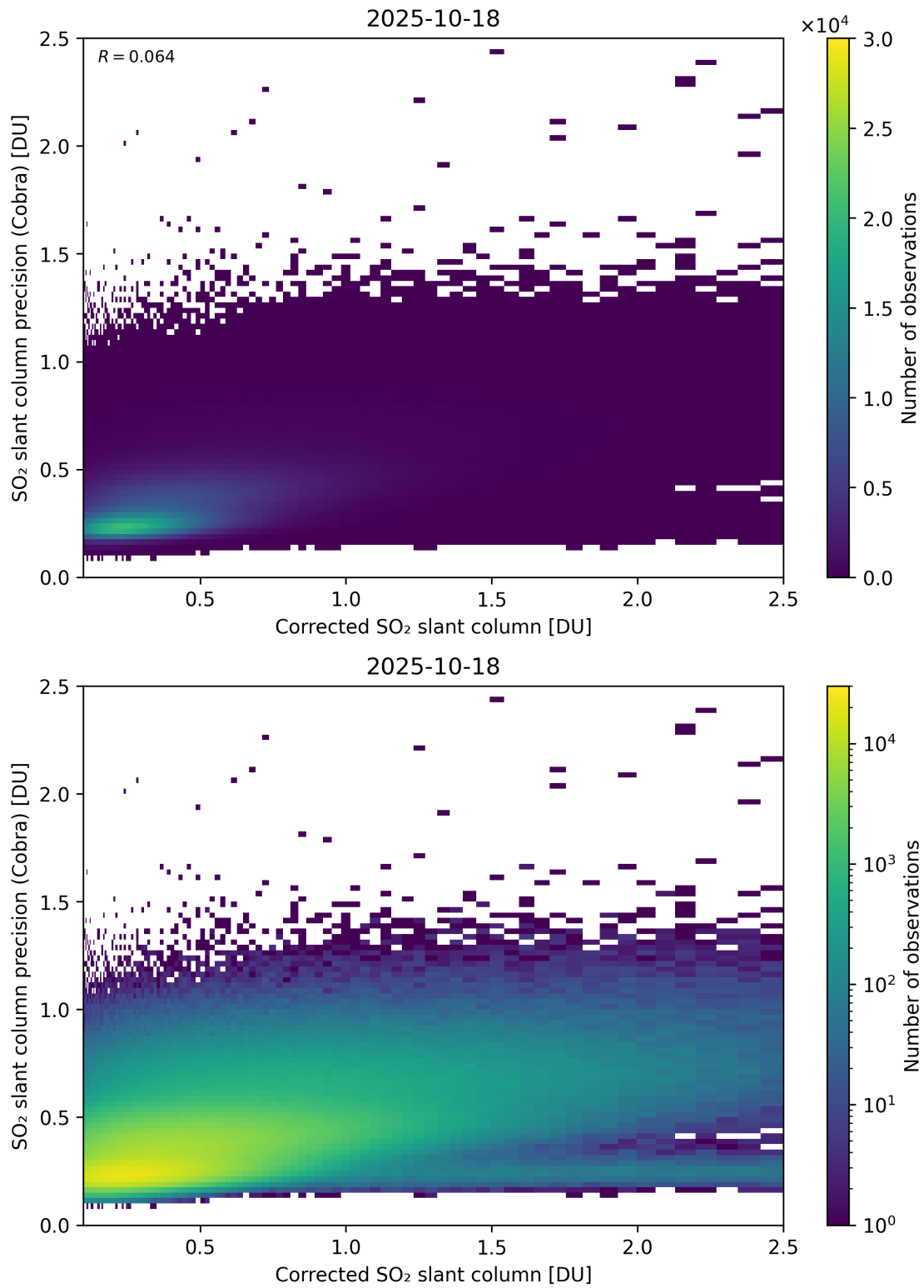
Figure 234: Scatter density plot of “Corrected SO 2 slant column” against “SO 2 slant column precision (Cobra)” for 2025-10-17 to 2025-10-19.
