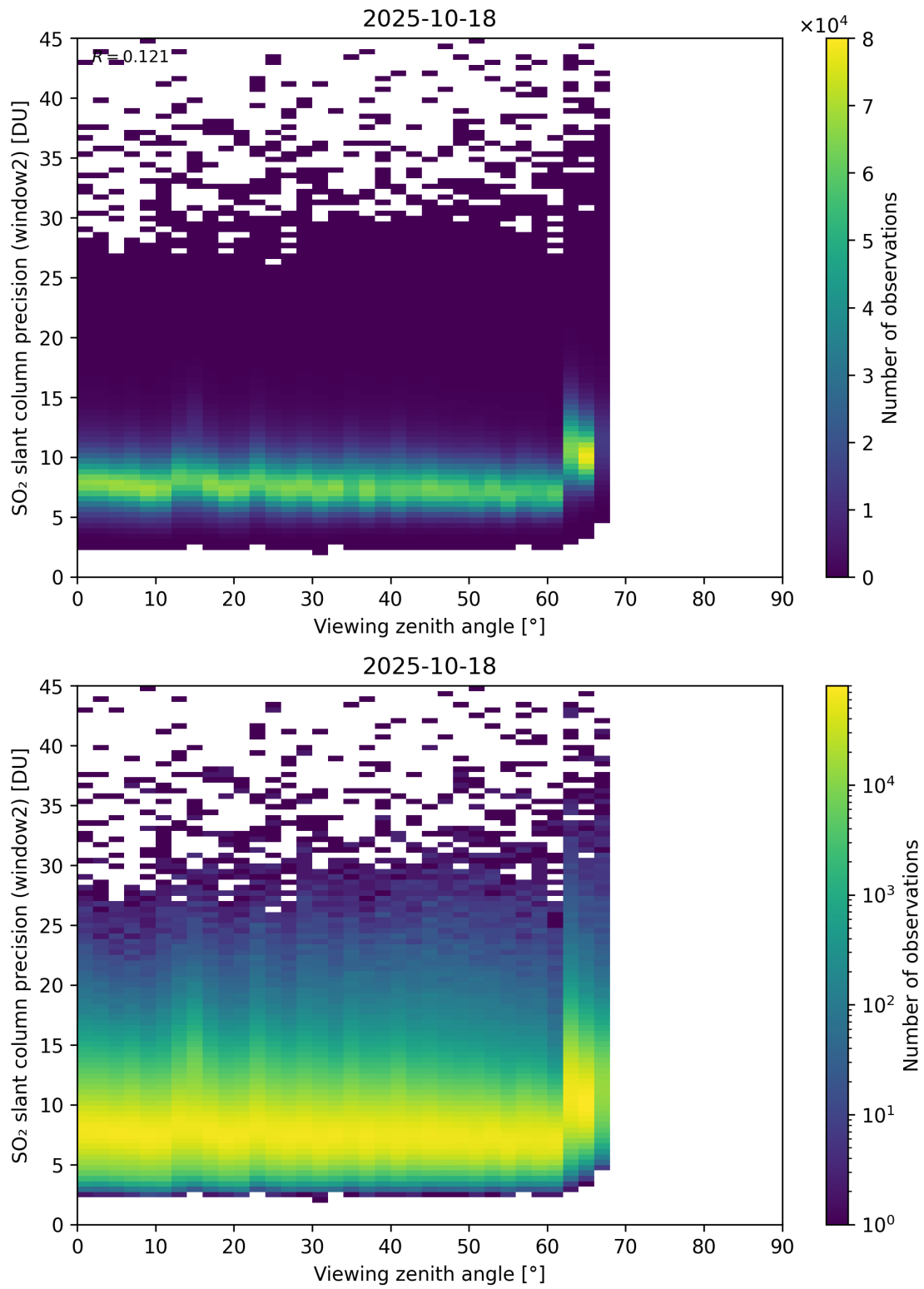
Figure 378: Scatter density plot of “Viewing zenith angle” against “SO 2 slant column precision (window2)” for 2025-10-17 to 2025-10-19.
