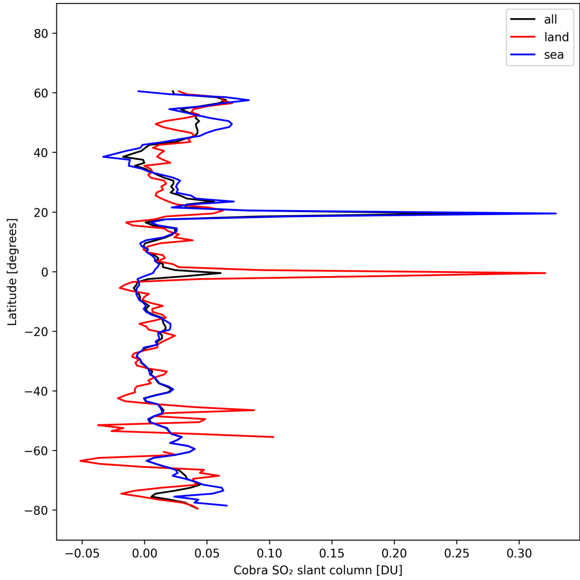
Figure 35: Zonal average of “Cobra SO 2 slant column” for 2025-10-17 to 2025-10-19.
