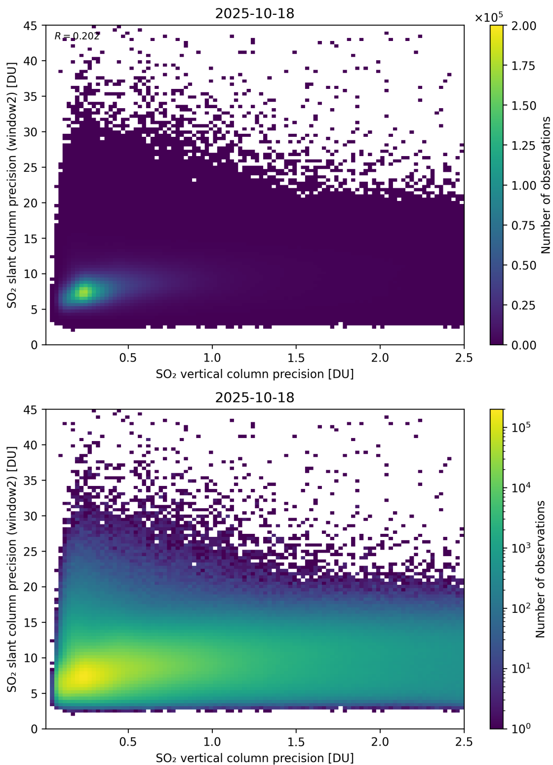
Figure 343: Scatter density plot of “SO 2 vertical column precision” against “SO 2 slant column precision (window2)” for 2025-10-17 to 2025-10-19.
