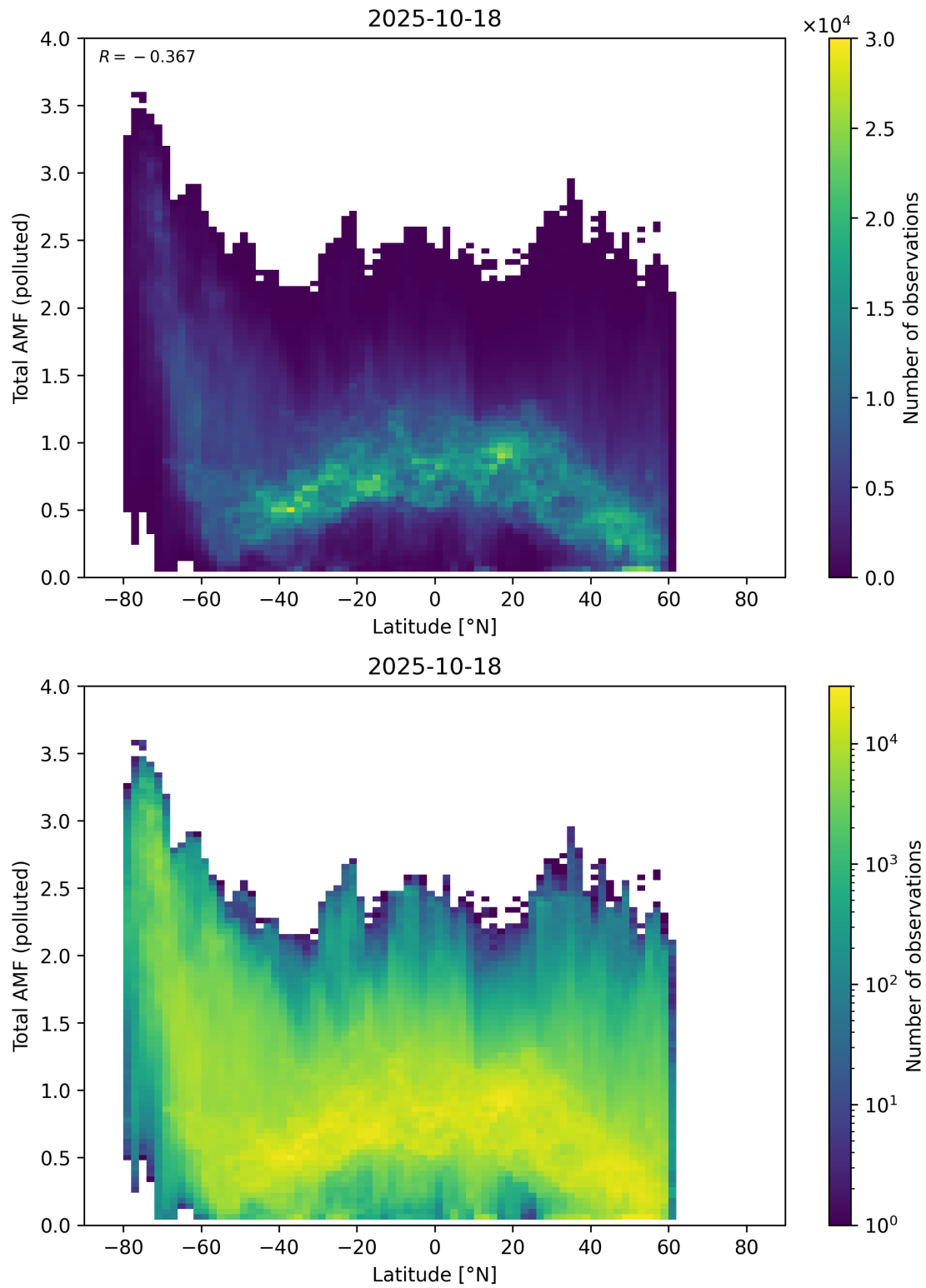
Figure 167: Scatter density plot of “Latitude” against “Total AMF (polluted)” for 2025-10-17 to 2025-10-19.
