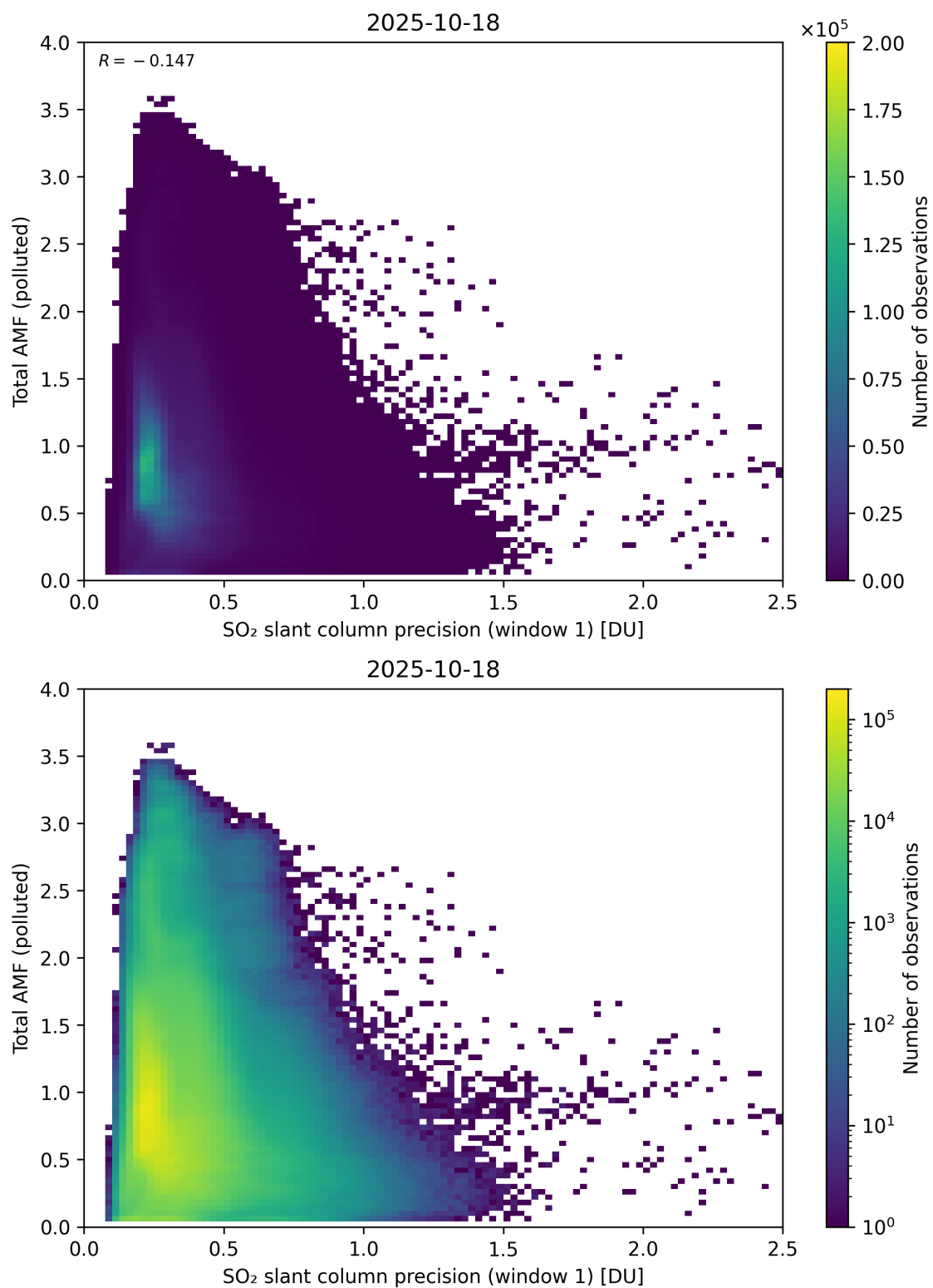
Figure 280: Scatter density plot of “SO 2 slant column precision (window 1)” against “Total AMF (polluted)” for 2025-10-17 to 2025-10-19.
