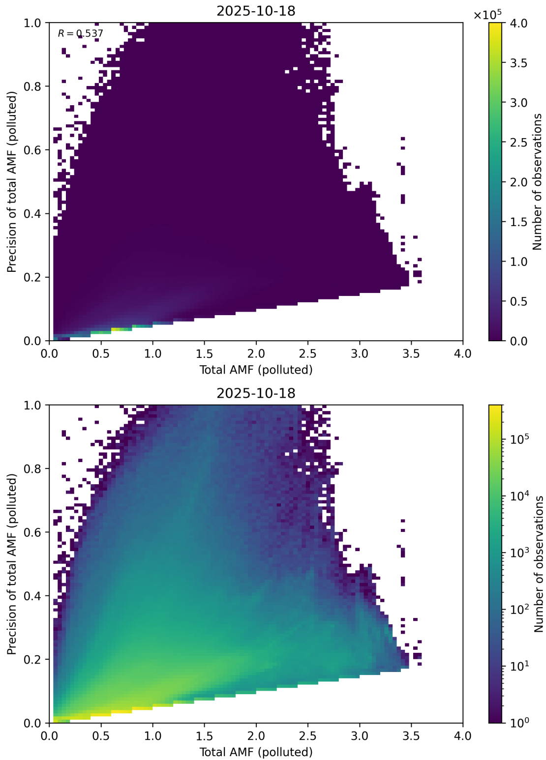
Figure 322: Scatter density plot of “Total AMF (polluted)” against “Precision of total AMF (polluted)” for 2025-10-17 to 2025-10-19.
