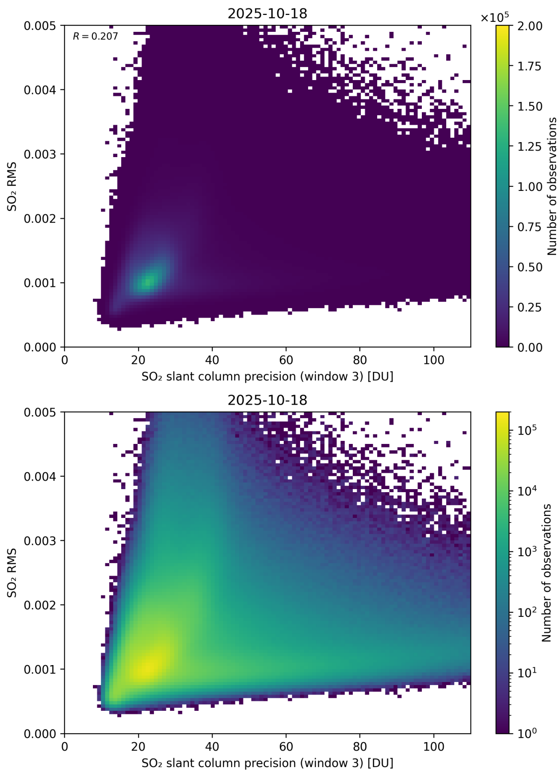
Figure 310: Scatter density plot of “SO 2 slant column precision (window 3)” against “SO 2 RMS” for 2025-10-17 to 2025-10-19.
