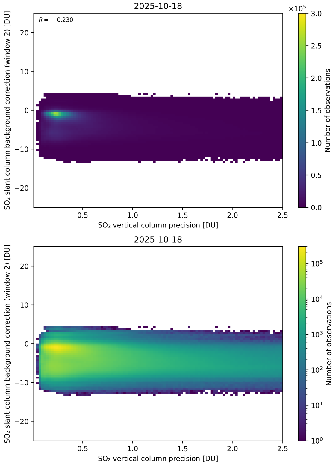
Figure 330: Scatter density plot of “SO 2 vertical column precision” against “SO 2 slant column background correction (window 2)” for 2025-10-17 to 2025-10-19.
