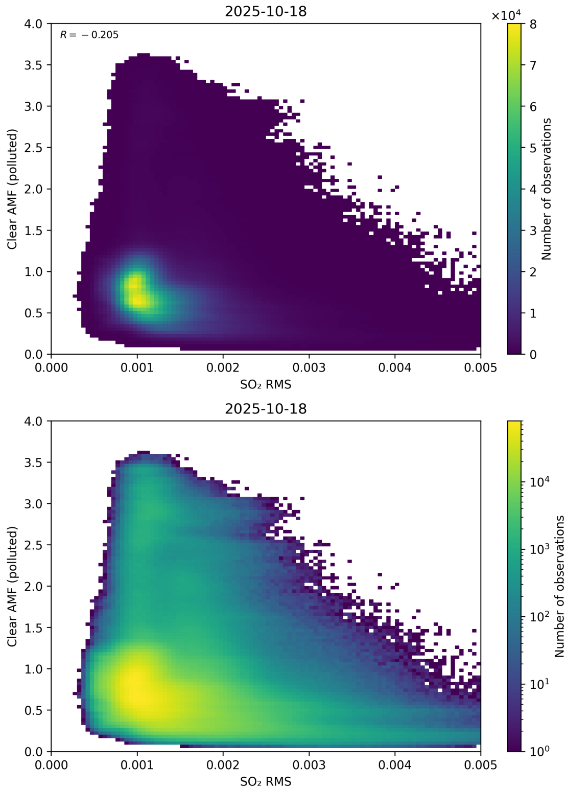
Figure 147: Scatter density plot of “SO 2 RMS” against “Clear AMF (polluted)” for 2025-10-17 to 2025-10-19.
