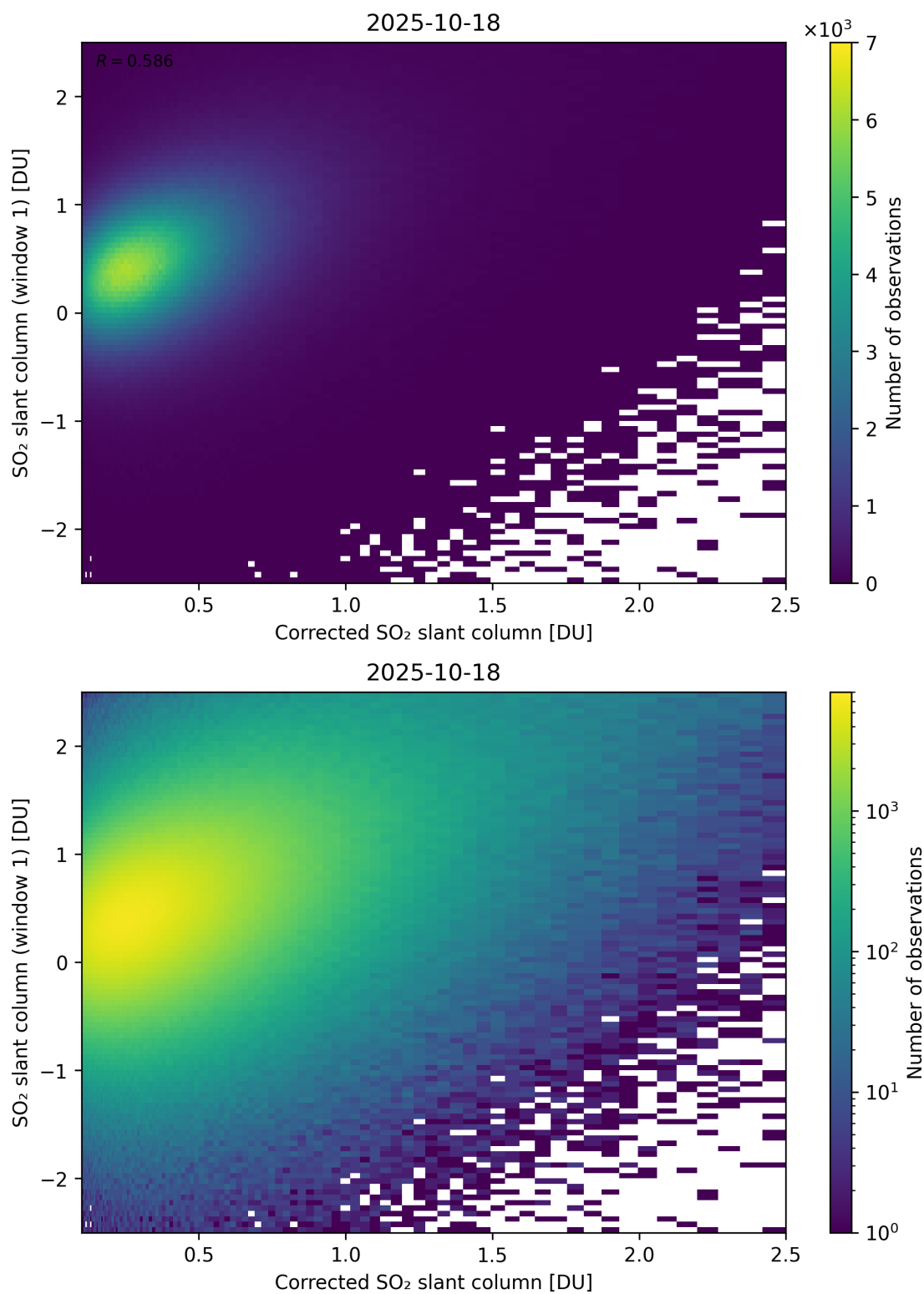
Figure 237: Scatter density plot of “Corrected SO 2 slant column” against “SO 2 slant column (window 1)” for 2025-10-17 to 2025-10-19.
