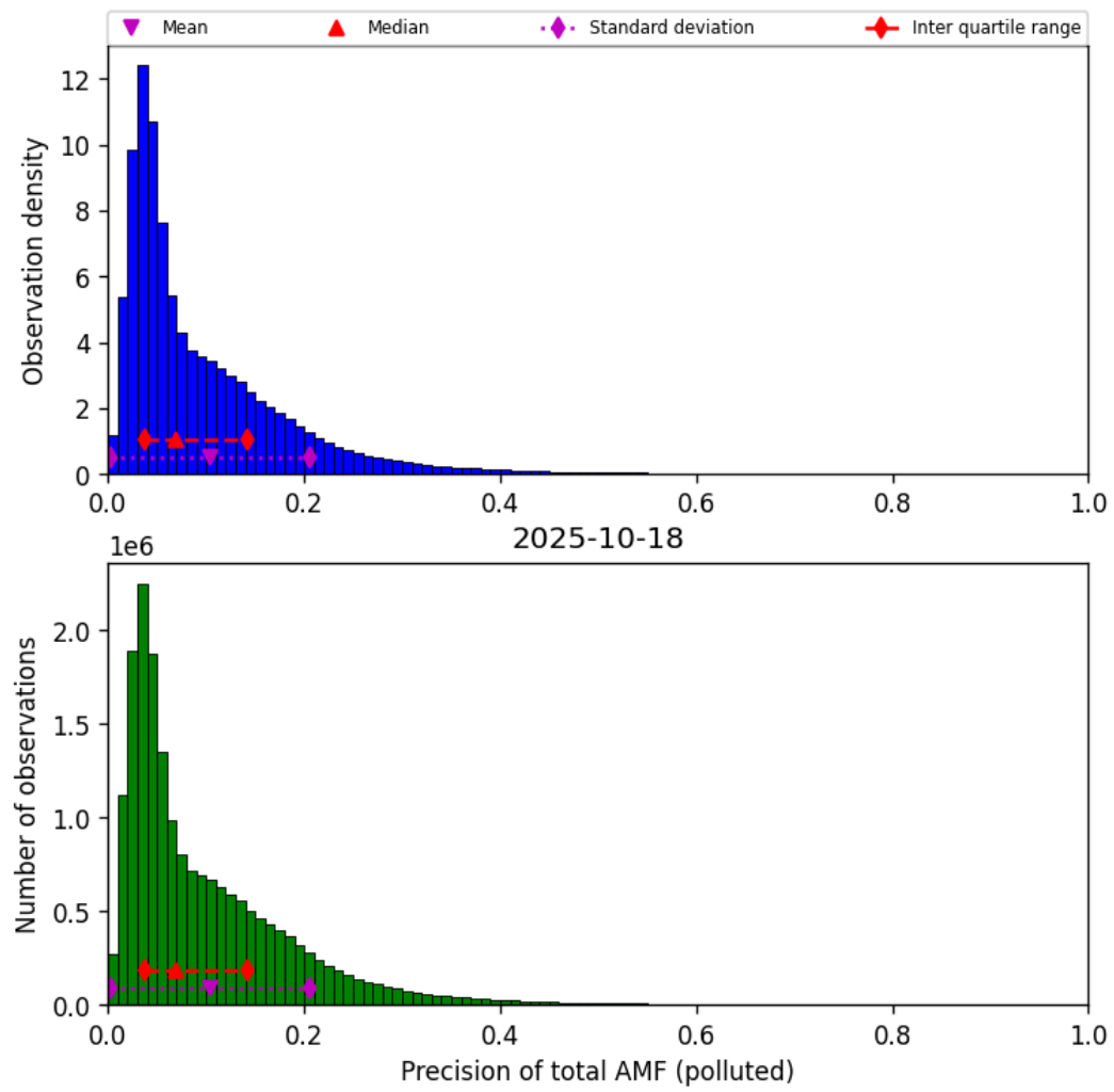
Figure 80: Histogram of “Precision of total AMF (polluted)” for 2025-10-17 to 2025-10-19
