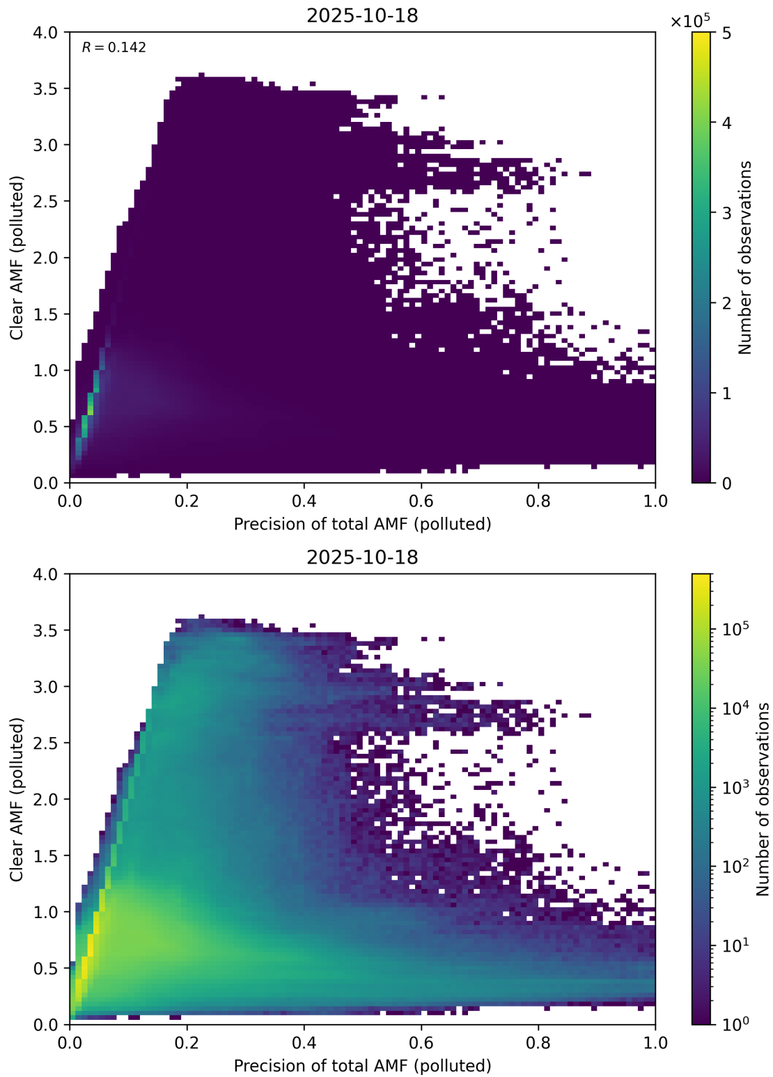
Figure 320: Scatter density plot of “Precision of total AMF (polluted)” against “Clear AMF (polluted)” for 2025-10-17 to 2025-10-19.
