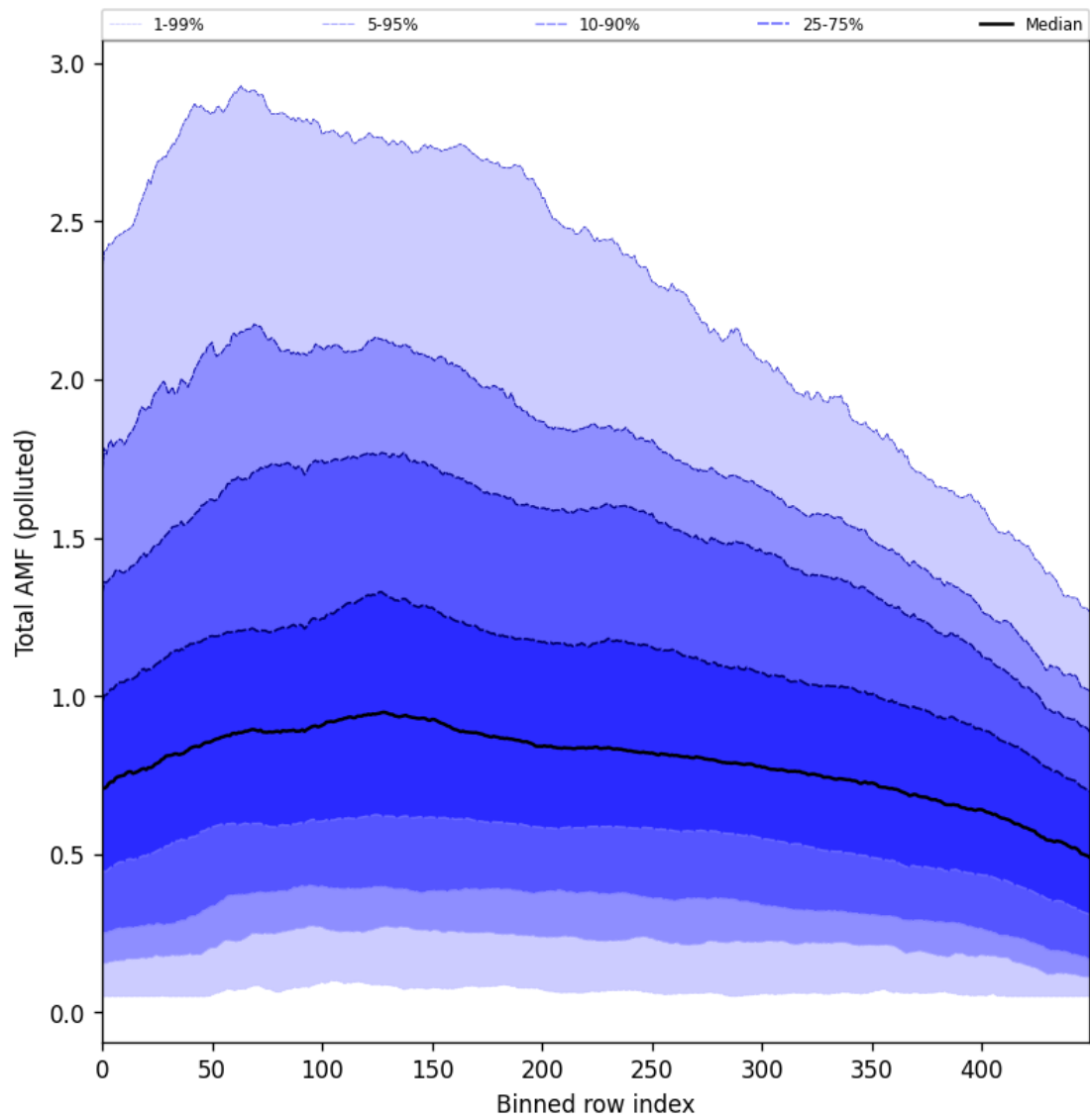
Figure 105: Along track statistics of “Total AMF (polluted)” for 2025-10-17 to 2025-10-19
