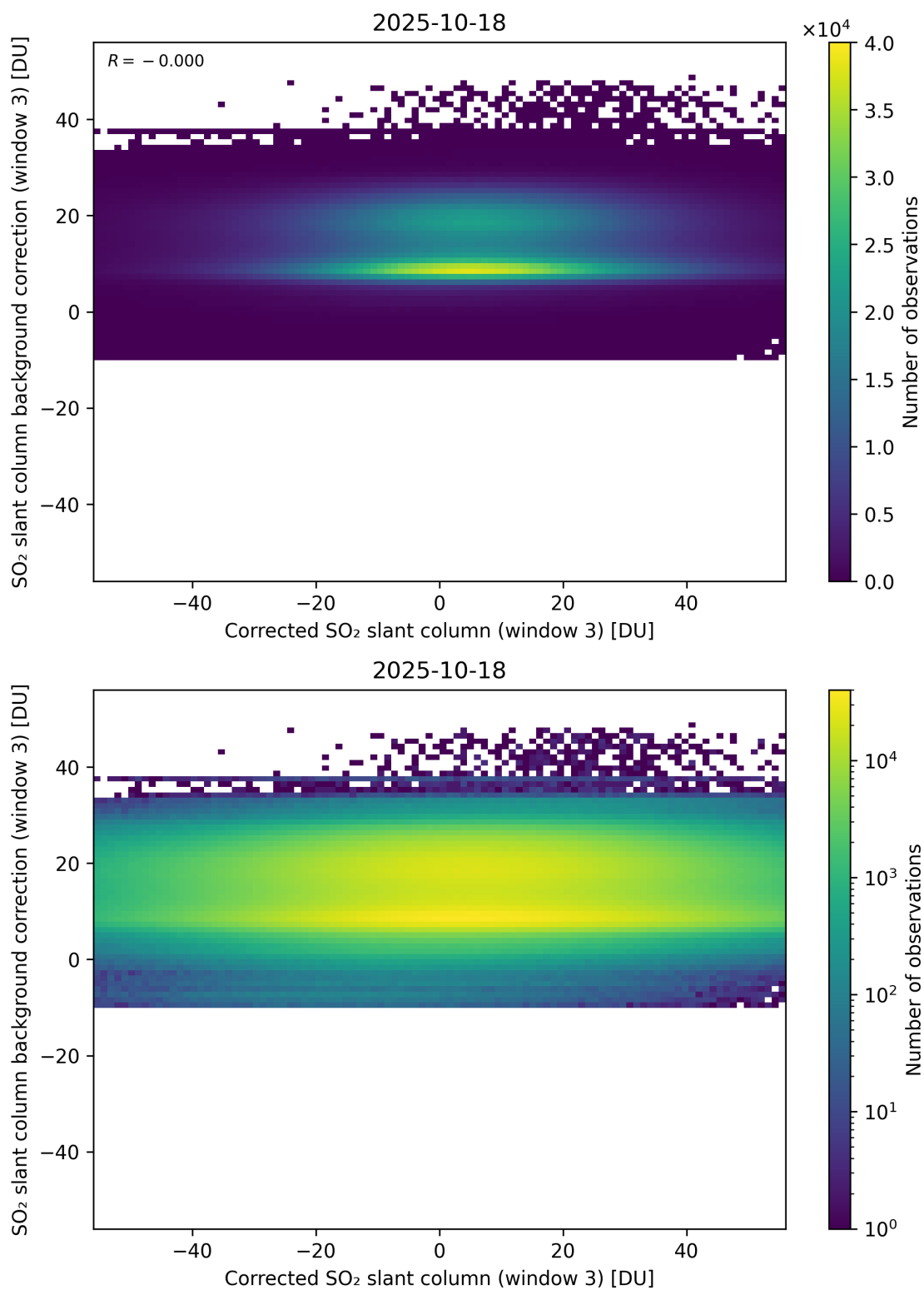
Figure 255: Scatter density plot of “Corrected SO 2 slant column (window 3)” against “SO 2 slant column background correction (window 3)” for 2025-10-17 to 2025-10-19.
