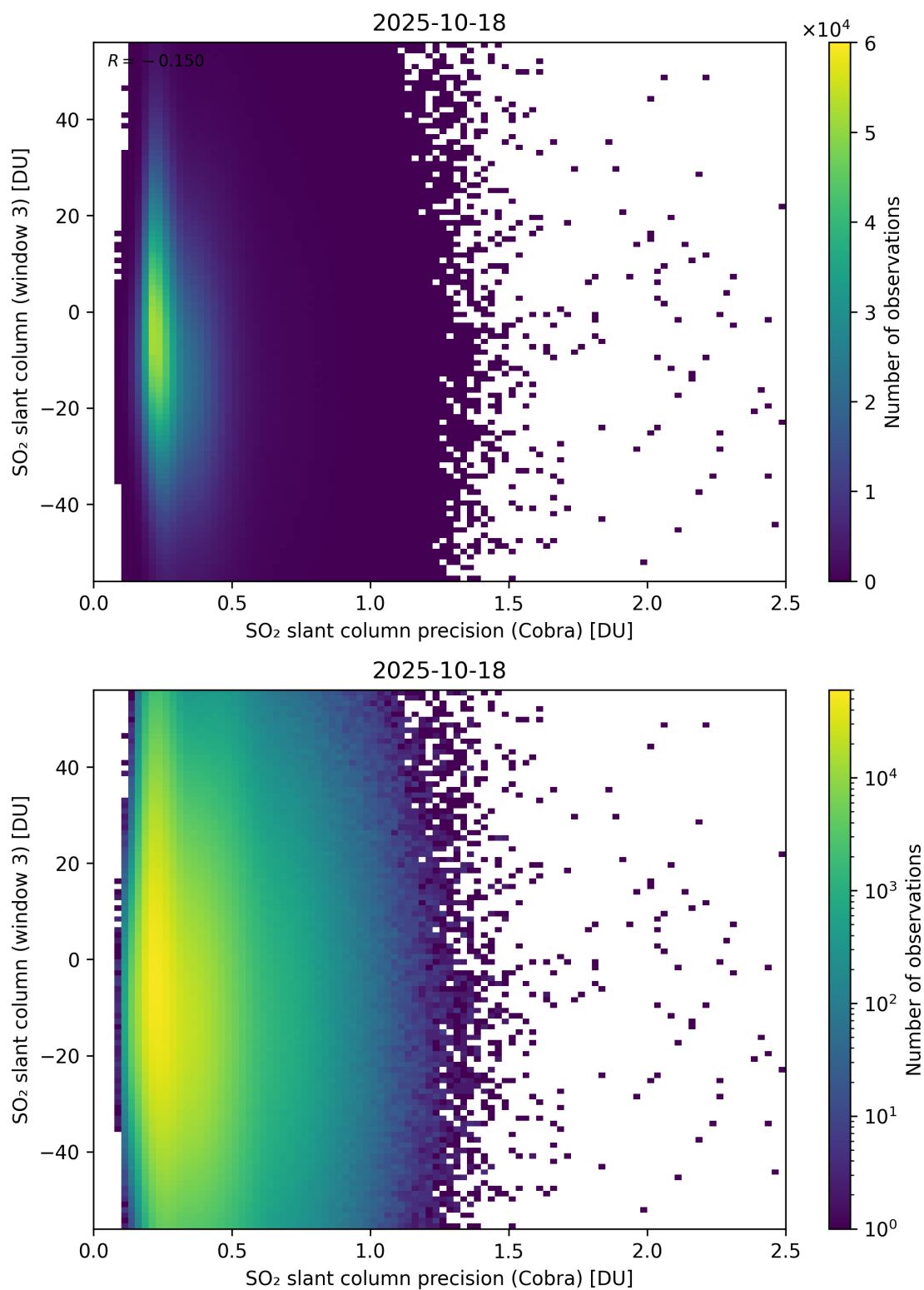
Figure 211: Scatter density plot of “SO 2 slant column precision (Cobra)” against “SO 2 slant column (window 3)” for 2025-10-17 to 2025-10-19.
