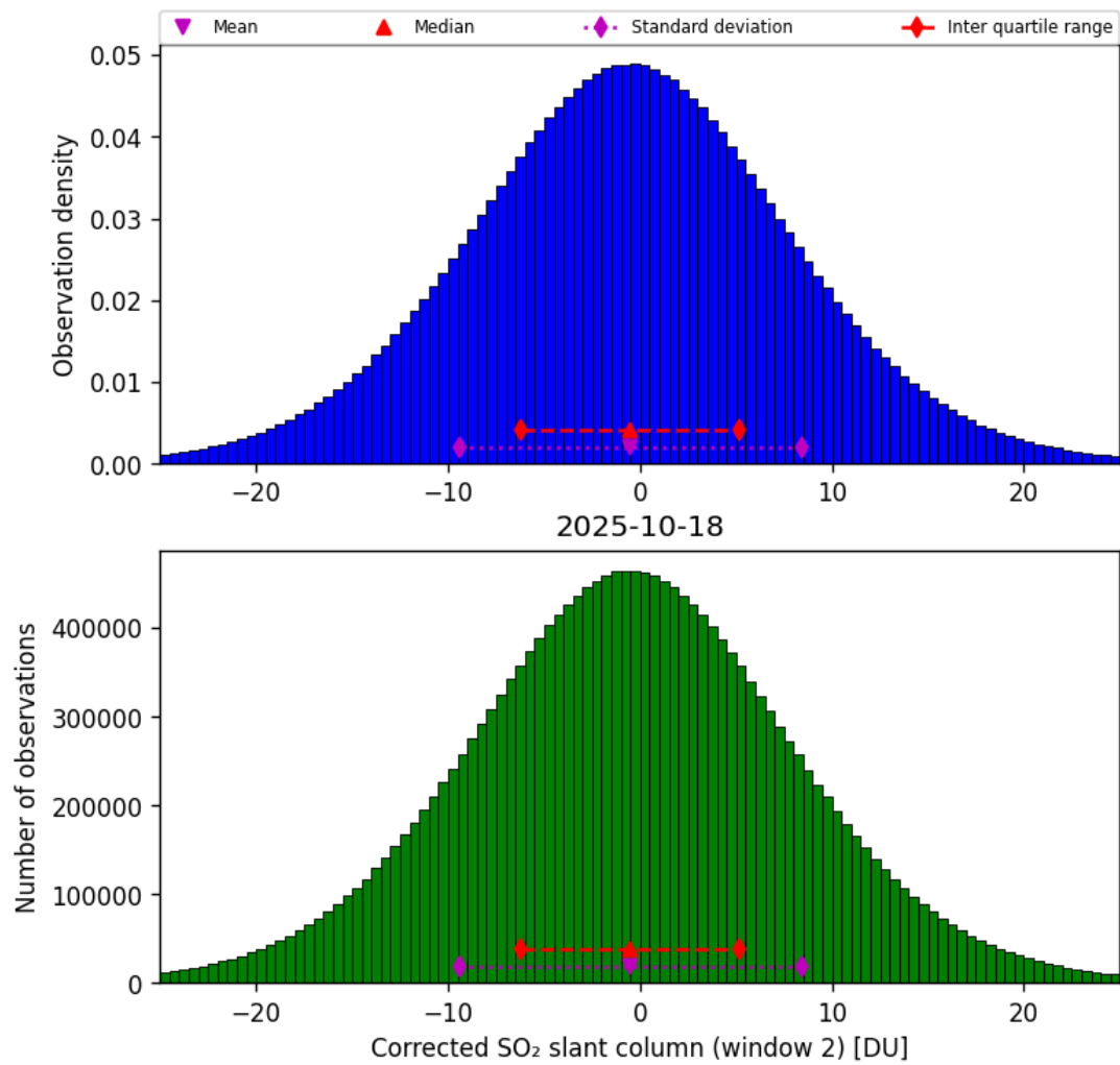
Figure 69: Histogram of “Corrected SO 2 slant column (window 2)” for 2025-10-17 to 2025-10-19
