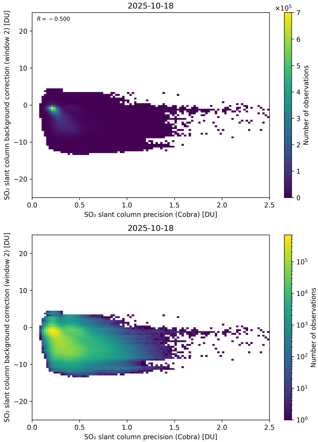
Figure 200: Scatter density plot of “SO 2 slant column precision (Cobra)” against “SO 2 slant column background correction (window 2)” for 2025-10-17 to 2025-10-19.
