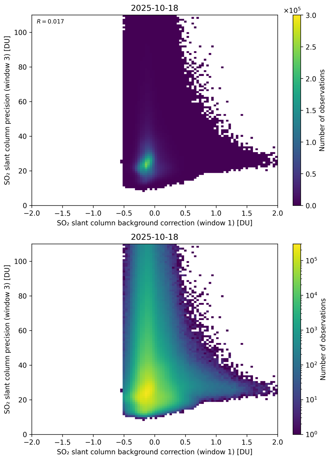
Figure 119: Scatter density plot of “SO 2 slant column background correction (window 1)” against “SO 2 slant column precision (window 3)” for 2025-10-17 to 2025-10-19.
