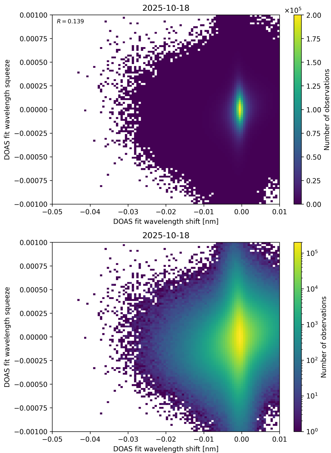
Figure 138: Scatter density plot of “DOAS fit wavelength shift” against “DOAS fit wavelength squeeze” for 2025-10-17 to 2025-10-19.
