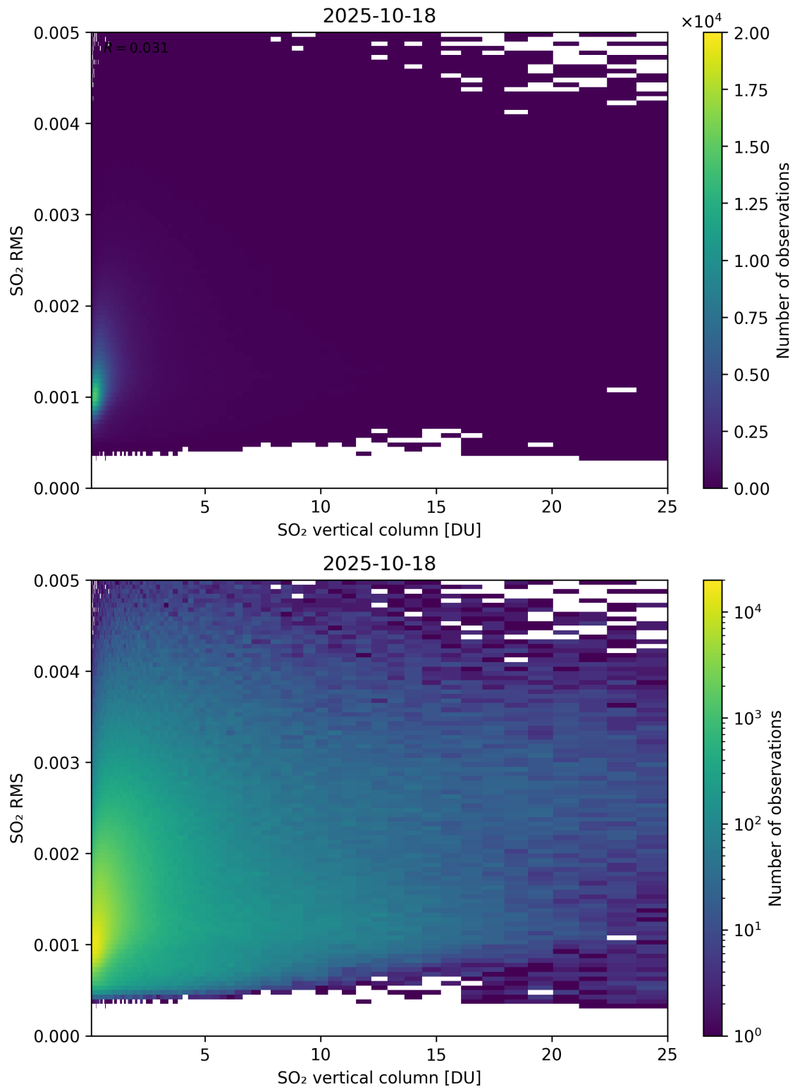
Figure 328: Scatter density plot of “SO 2 vertical column” against “SO 2 RMS” for 2025-10-17 to 2025-10-19.
