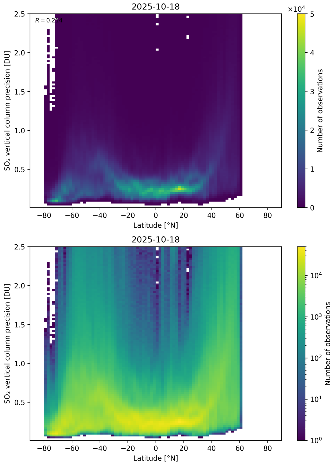
Figure 170: Scatter density plot of “Latitude” against “SO 2 vertical column precision” for 2025-10-17 to 2025-10-19.
