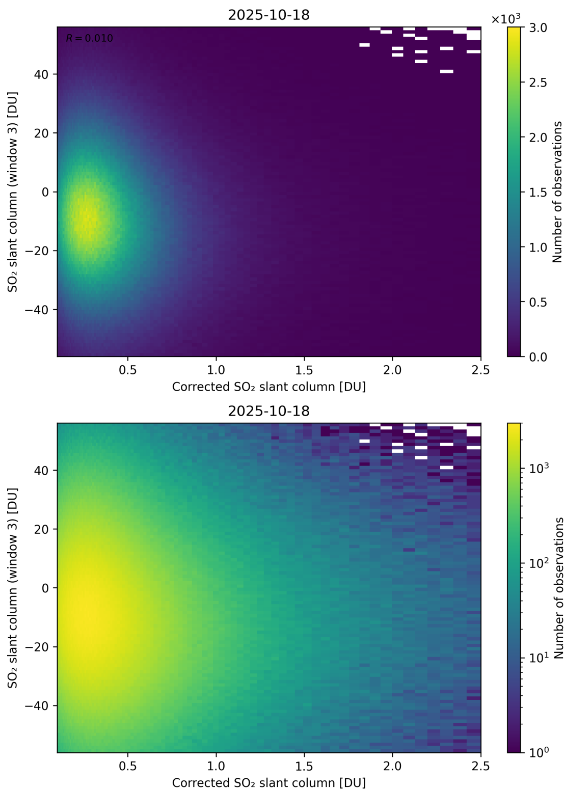
Figure 240: Scatter density plot of “Corrected SO 2 slant column” against “SO 2 slant column (window 3)” for 2025-10-17 to 2025-10-19.
