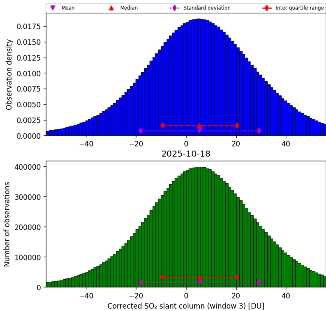
Figure 73: Histogram of “Corrected SO 2 slant column (window 3)” for 2025-10-17 to 2025-10-19
