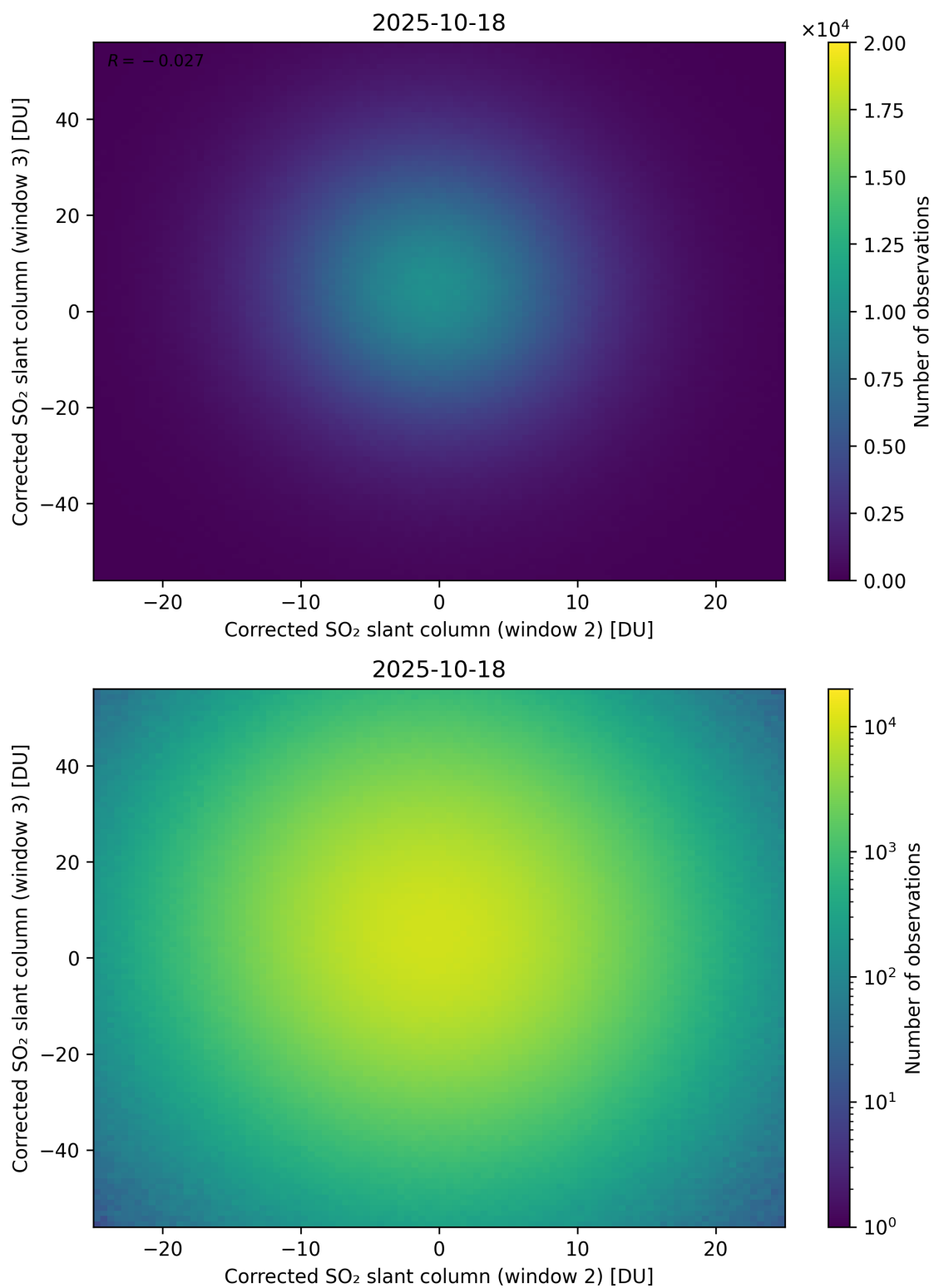
Figure 250: Scatter density plot of “Corrected SO 2 slant column (window 2)” against “Corrected SO 2 slant column (window 3)” for 2025-10-17 to 2025-10-19.
