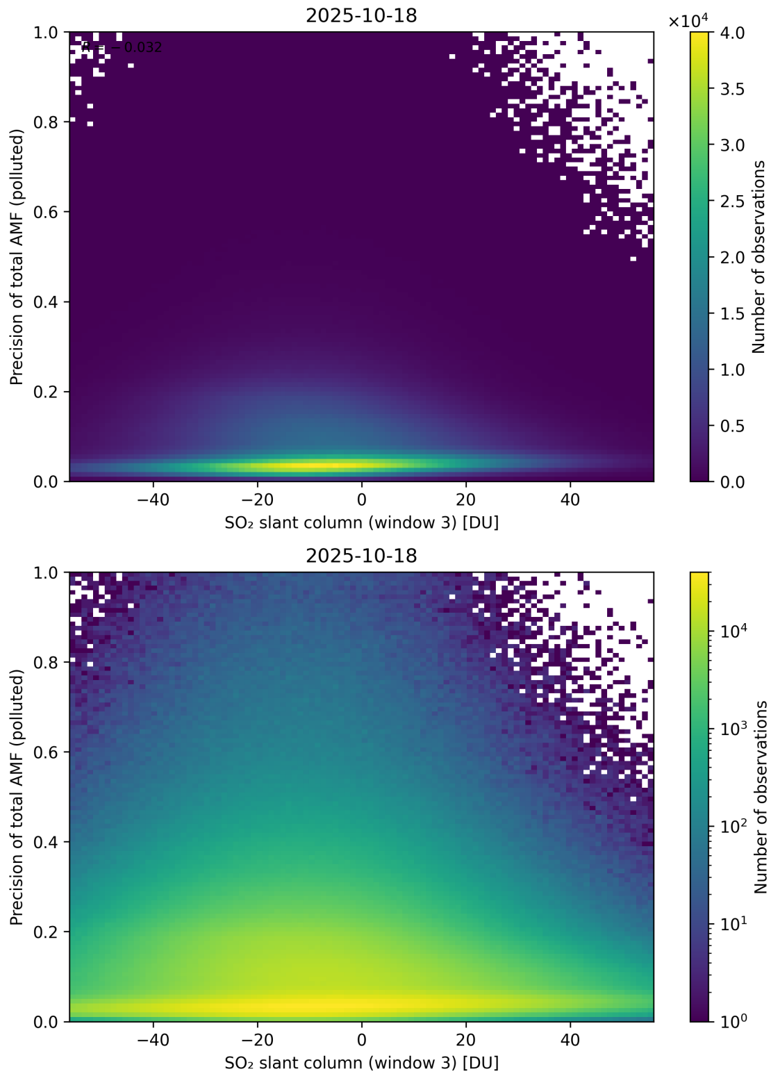
Figure 319: Scatter density plot of “SO 2 slant column (window 3)” against “Precision of total AMF (polluted)” for 2025-10-17 to 2025-10-19.
