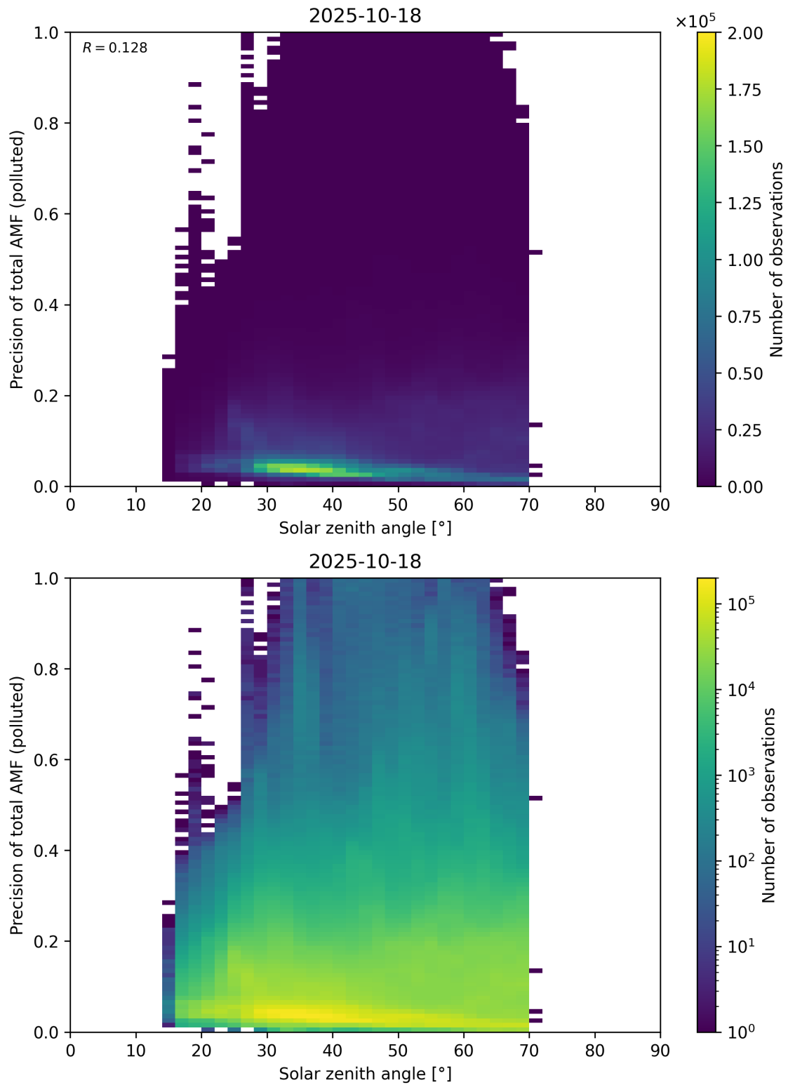
Figure 190: Scatter density plot of “Solar zenith angle” against “Precision of total AMF (polluted)” for 2025-10-17 to 2025-10-19.
