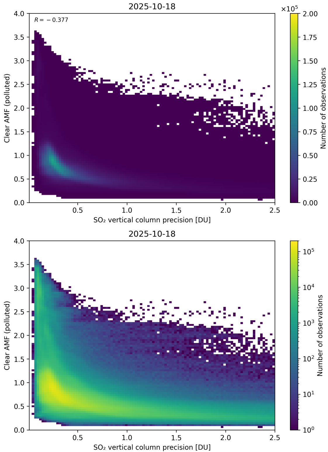
Figure 335: Scatter density plot of “SO 2 vertical column precision” against “Clear AMF (polluted)” for 2025-10-17 to 2025-10-19.
