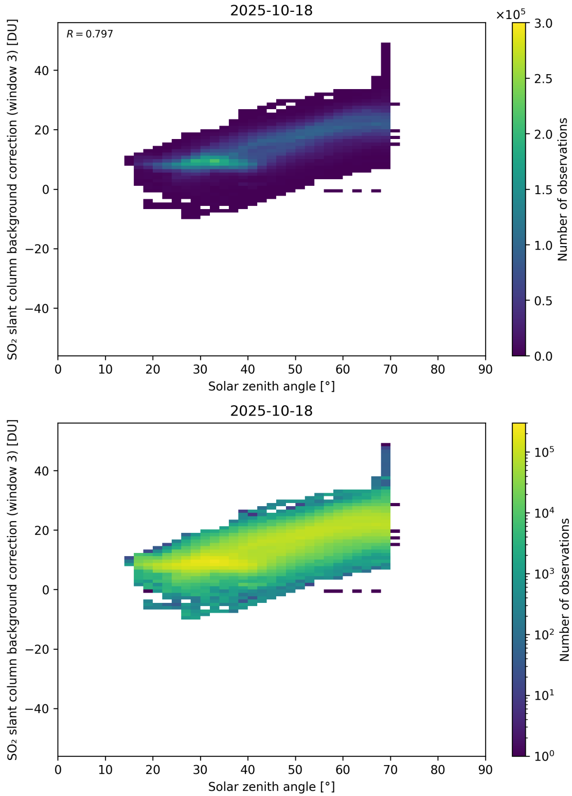
Figure 173: Scatter density plot of “Solar zenith angle” against “SO 2 slant column background correction (window 3)” for 2025-10-17 to 2025-10-19.
