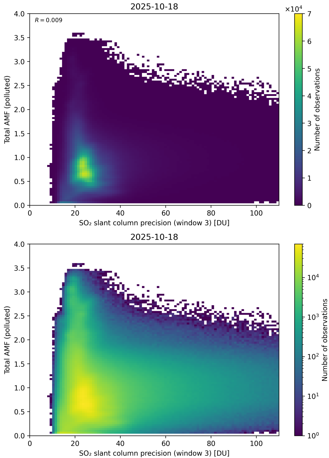
Figure 313: Scatter density plot of “SO 2 slant column precision (window 3)” against “Total AMF (polluted)” for 2025-10-17 to 2025-10-19.
