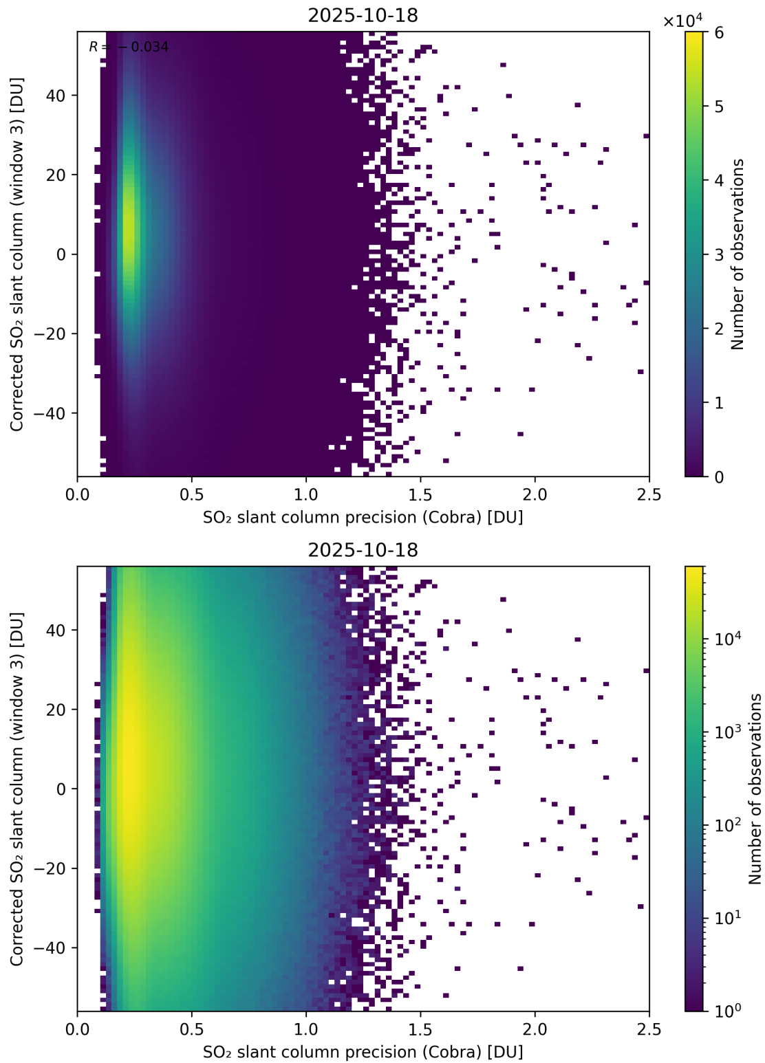
Figure 207: Scatter density plot of “SO 2 slant column precision (Cobra)” against “Corrected SO 2 slant column (window 3)” for 2025-10-17 to 2025-10-19.
