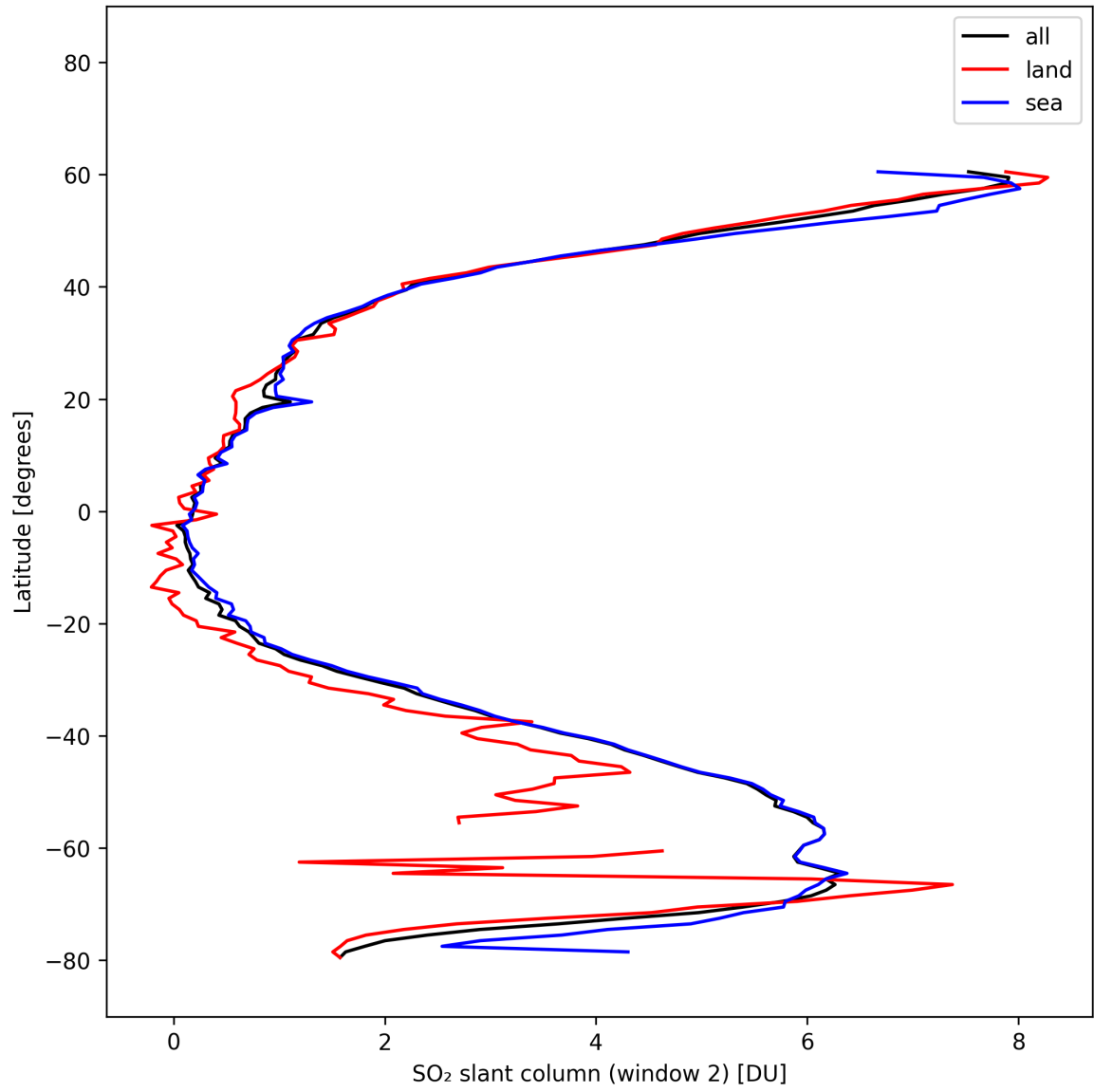
Figure 41: Zonal average of “SO 2 slant column (window 2)” for 2025-10-17 to 2025-10-19.
