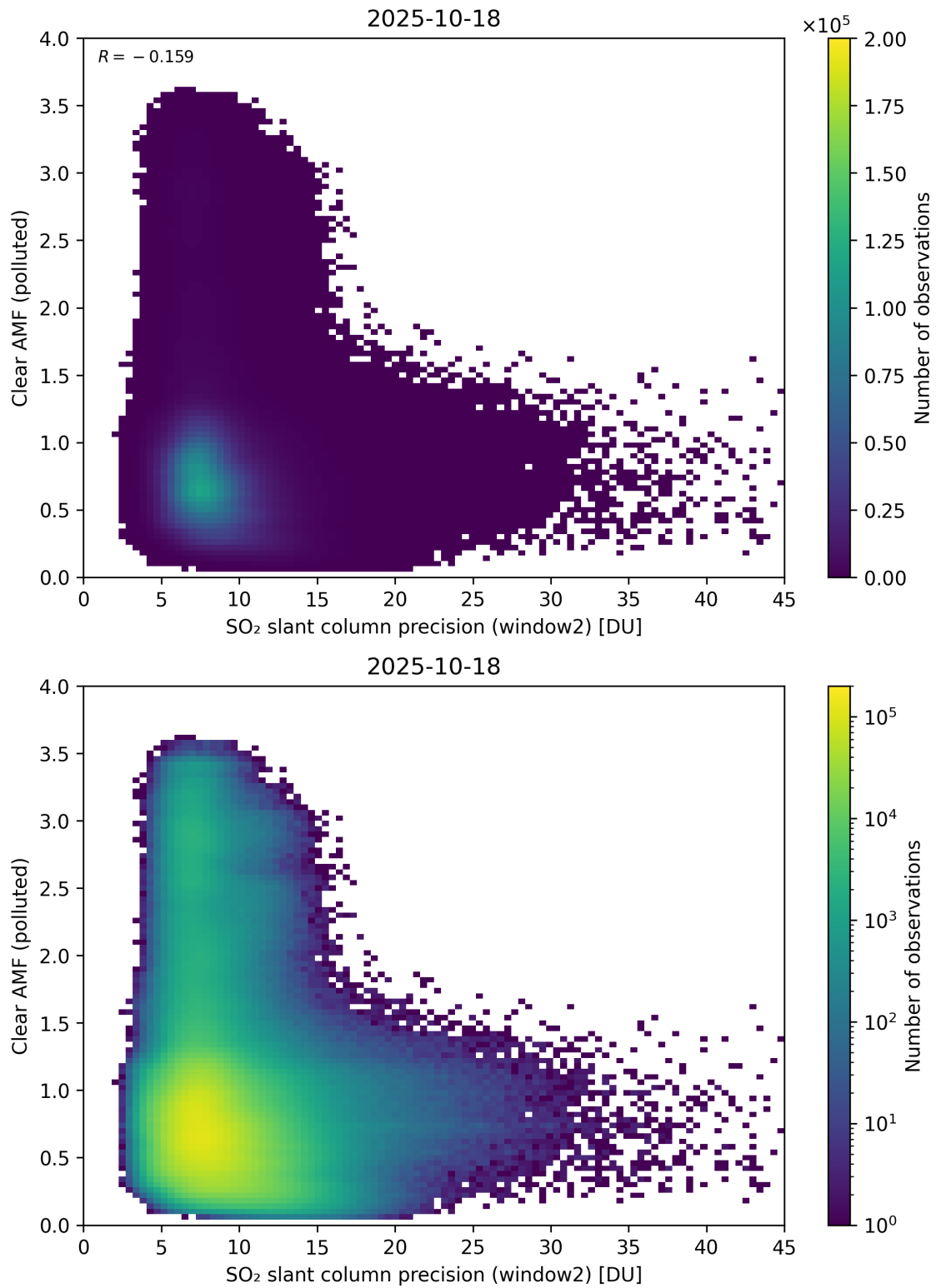
Figure 296: Scatter density plot of “SO 2 slant column precision (window2)” against “Clear AMF (polluted)” for 2025-10-17 to 2025-10-19.
