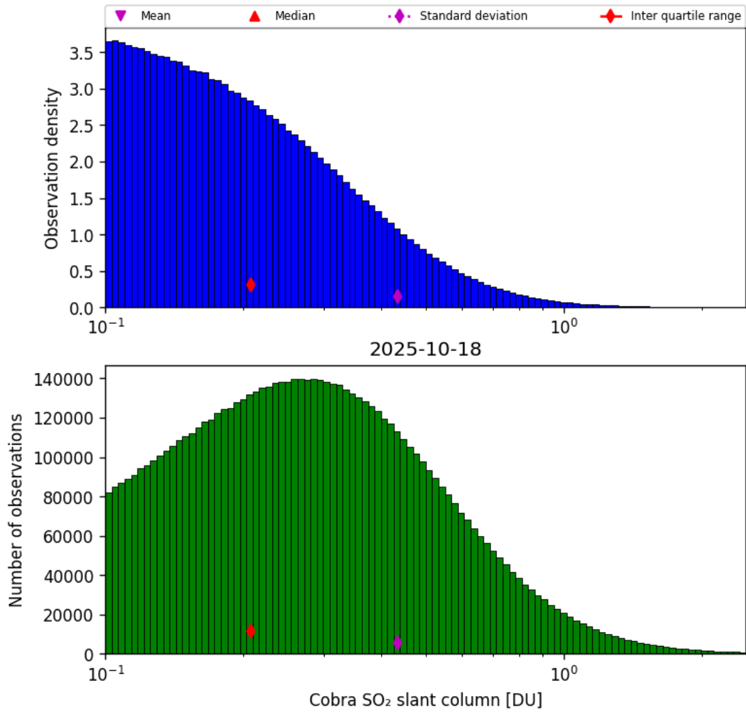
Figure 61: Histogram of “Cobra SO 2 slant column” for 2025-10-17 to 2025-10-19
