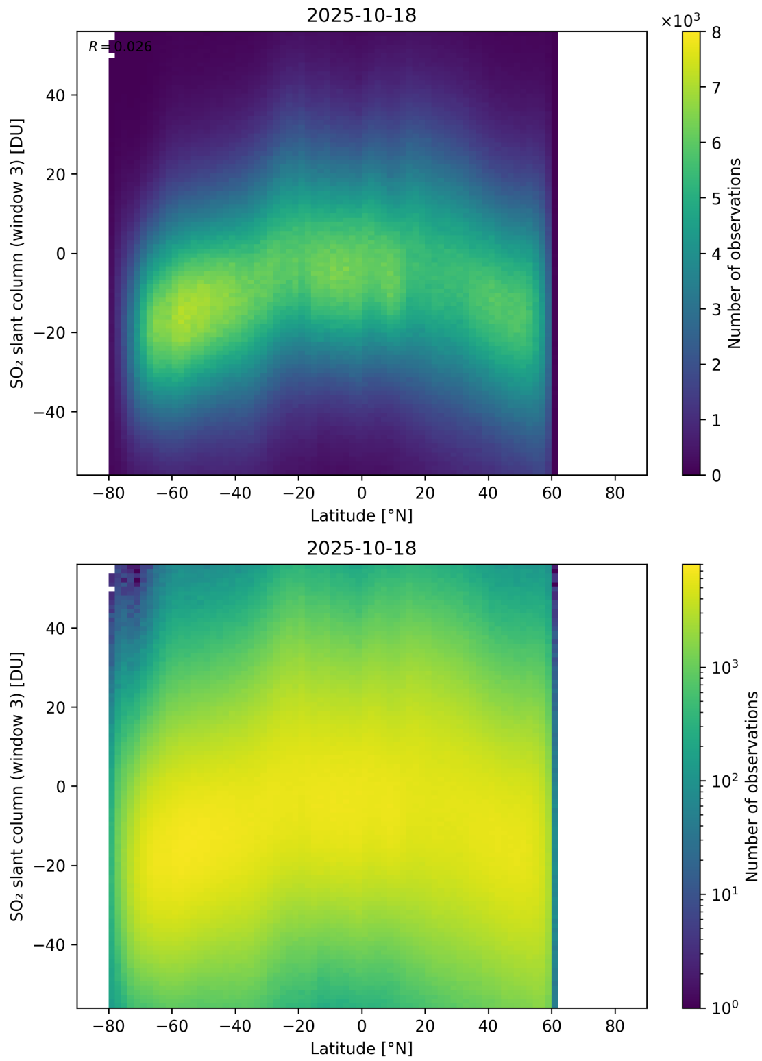
Figure 165: Scatter density plot of “Latitude” against “SO 2 slant column (window 3)” for 2025-10-17 to 2025-10-19.
