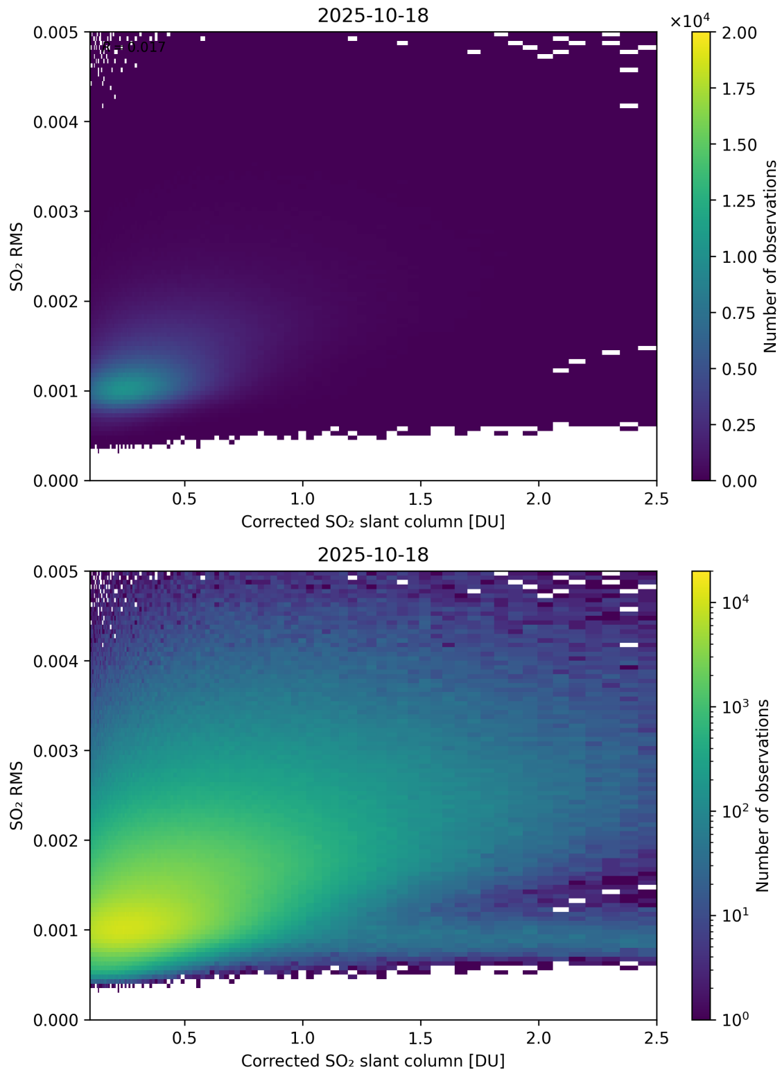
Figure 231: Scatter density plot of “Corrected SO 2 slant column” against “SO 2 RMS” for 2025-10-17 to 2025-10-19.
