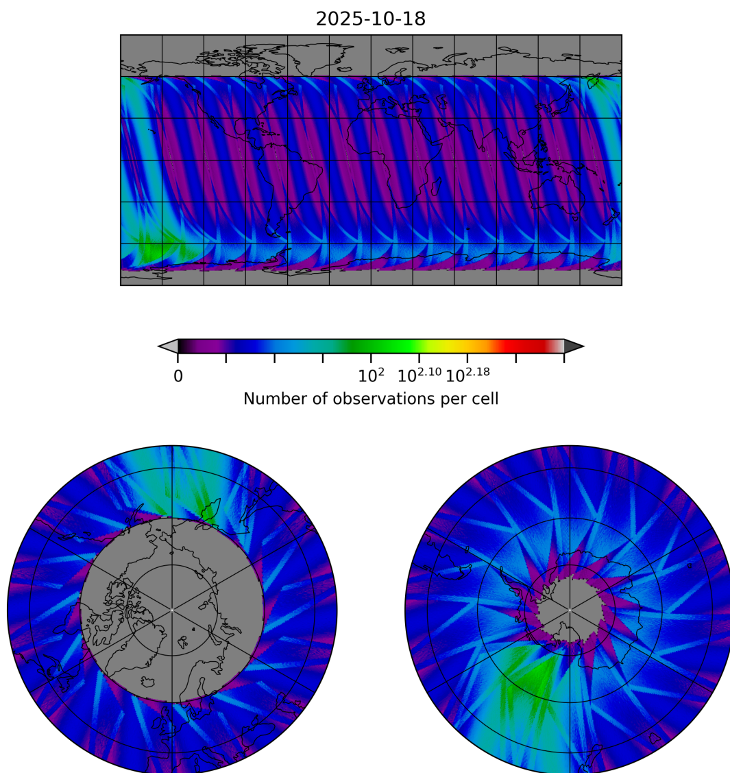
Figure 30: Map of the number of observations for 2025-10-17 to 2025-10-19
