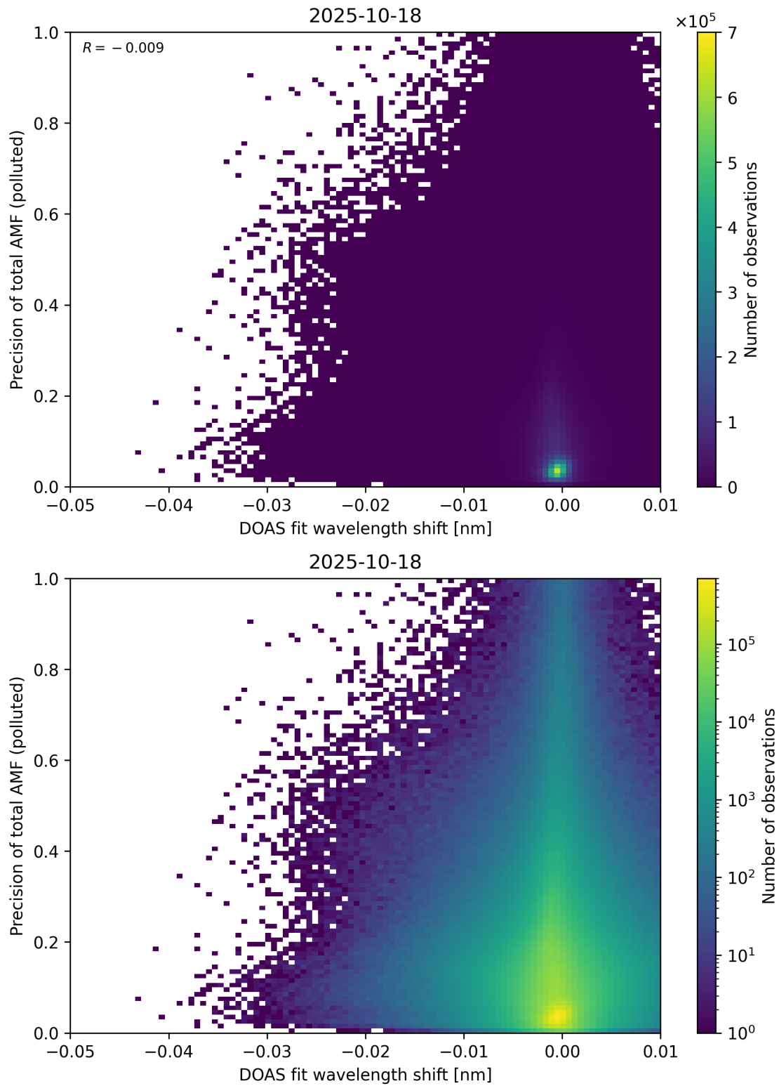
Figure 142: Scatter density plot of “DOAS fit wavelength shift” against “Precision of total AMF (polluted)” for 2025-10-17 to 2025-10-19.
