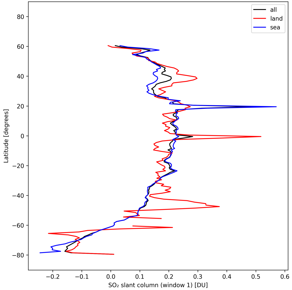
Figure 37: Zonal average of “SO 2 slant column (window 1)” for 2025-10-17 to 2025-10-19.
