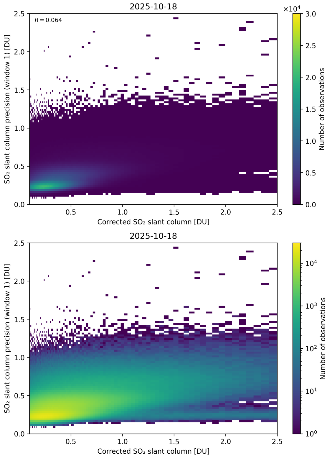
Figure 238: Scatter density plot of “Corrected SO 2 slant column” against “SO 2 slant column precision (window 1)” for 2025-10-17 to 2025-10-19.
