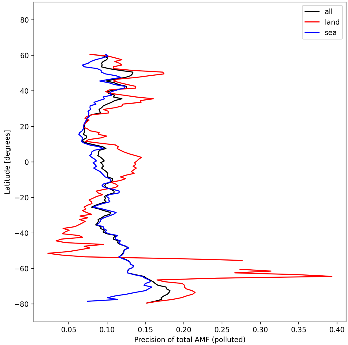
Figure 54: Zonal average of “Precision of total AMF (polluted)” for 2025-10-17 to 2025-10-19.
