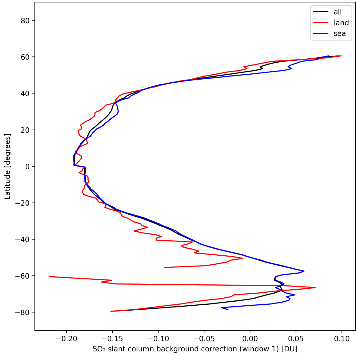
Figure 40: Zonal average of “SO 2 slant column background correction (window 1)” for 2025-10-17 to 2025-10-19.
