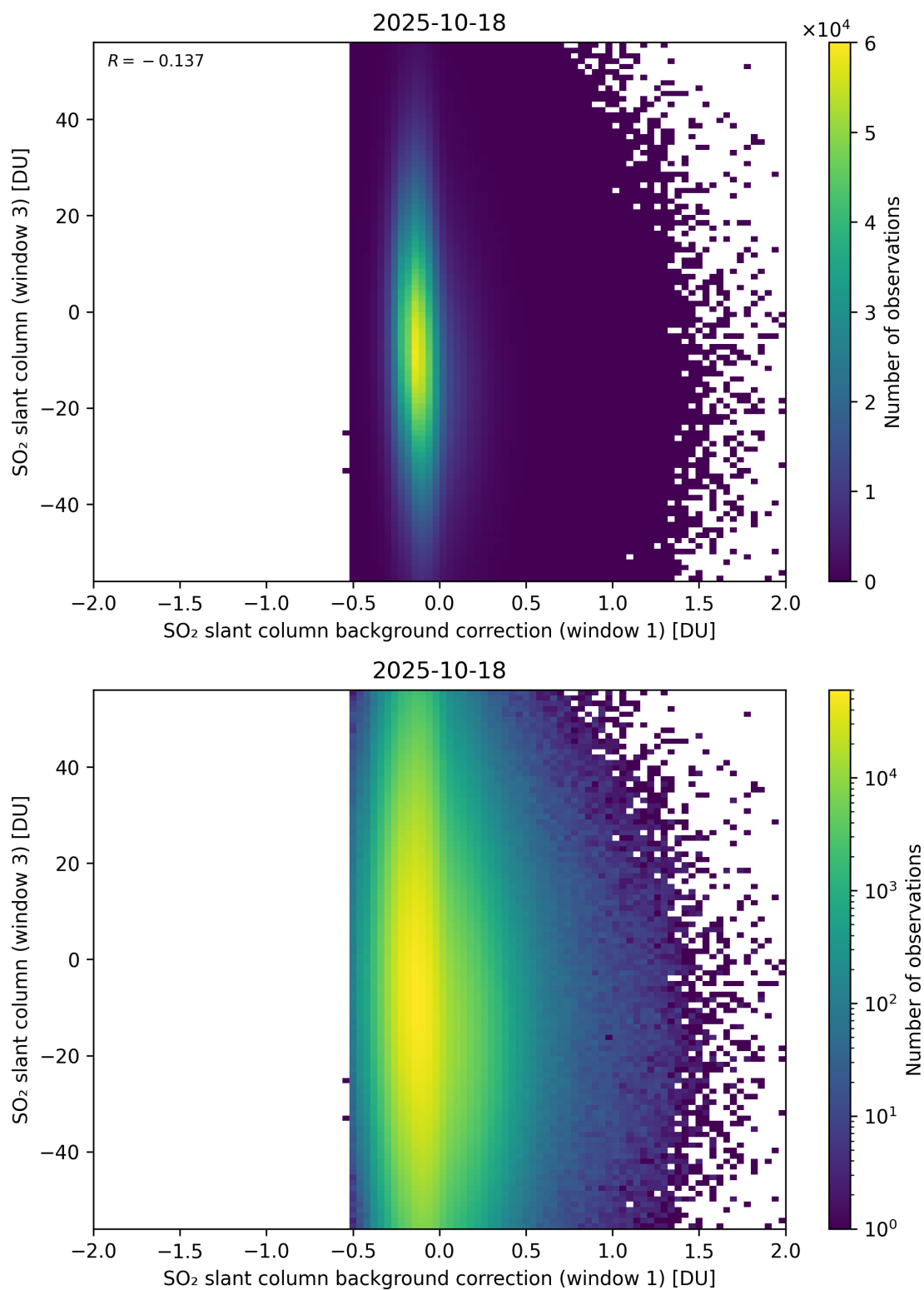
Figure 118: Scatter density plot of “SO 2 slant column background correction (window 1)” against “SO 2 slant column (window 3)” for 2025-10-17 to 2025-10-19.
