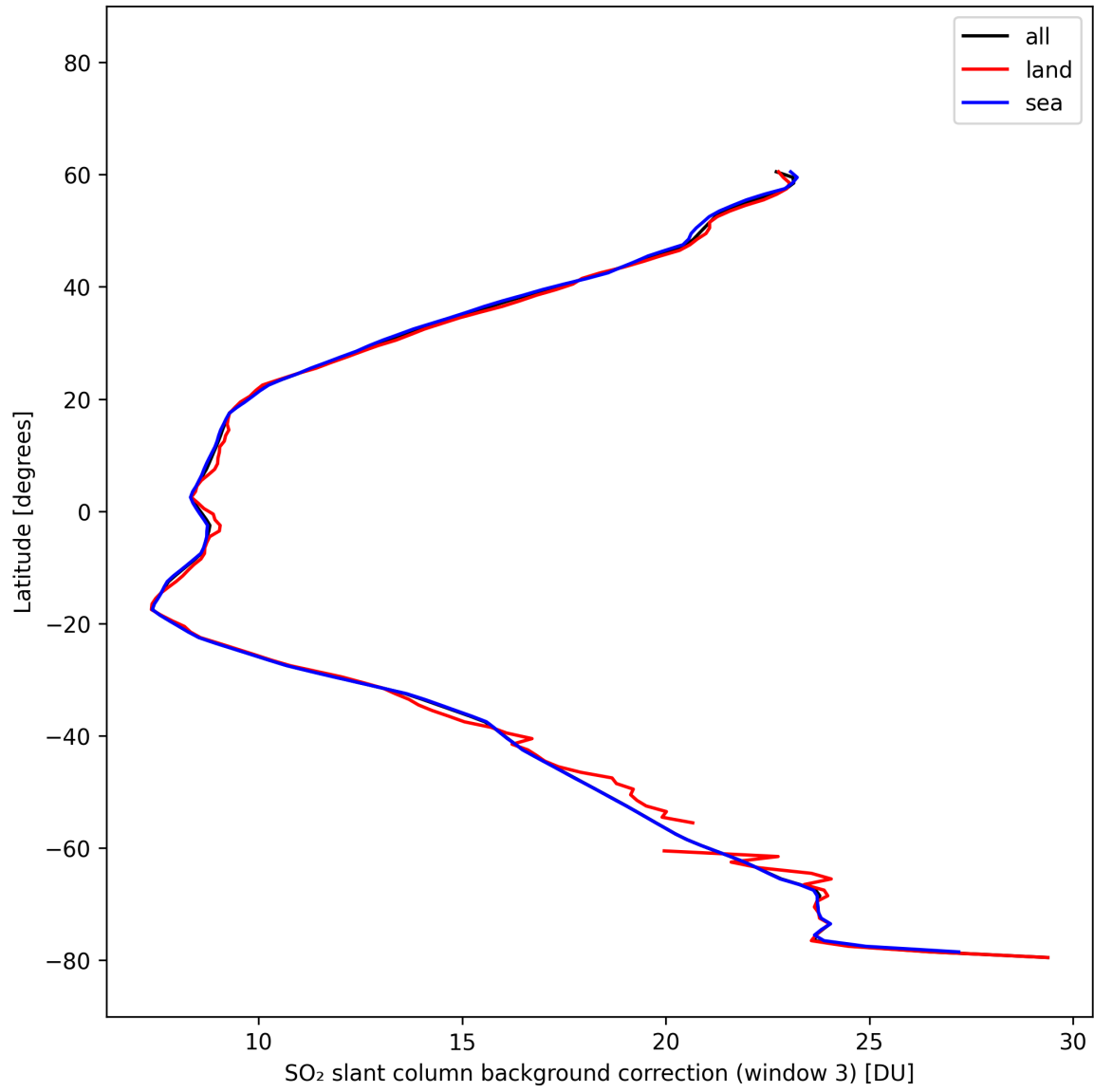
Figure 48: Zonal average of “SO 2 slant column background correction (window 3)” for 2025-10-17 to 2025-10-19.
