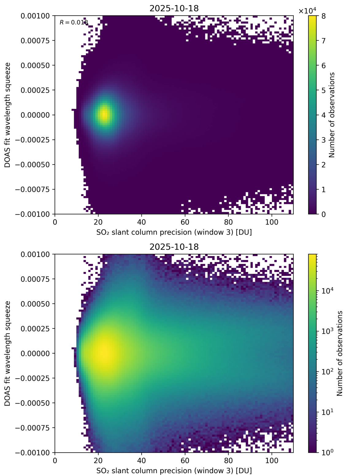
Figure 309: Scatter density plot of “SO 2 slant column precision (window 3)” against “DOAS fit wavelength squeeze” for 2025-10-17 to 2025-10-19.
