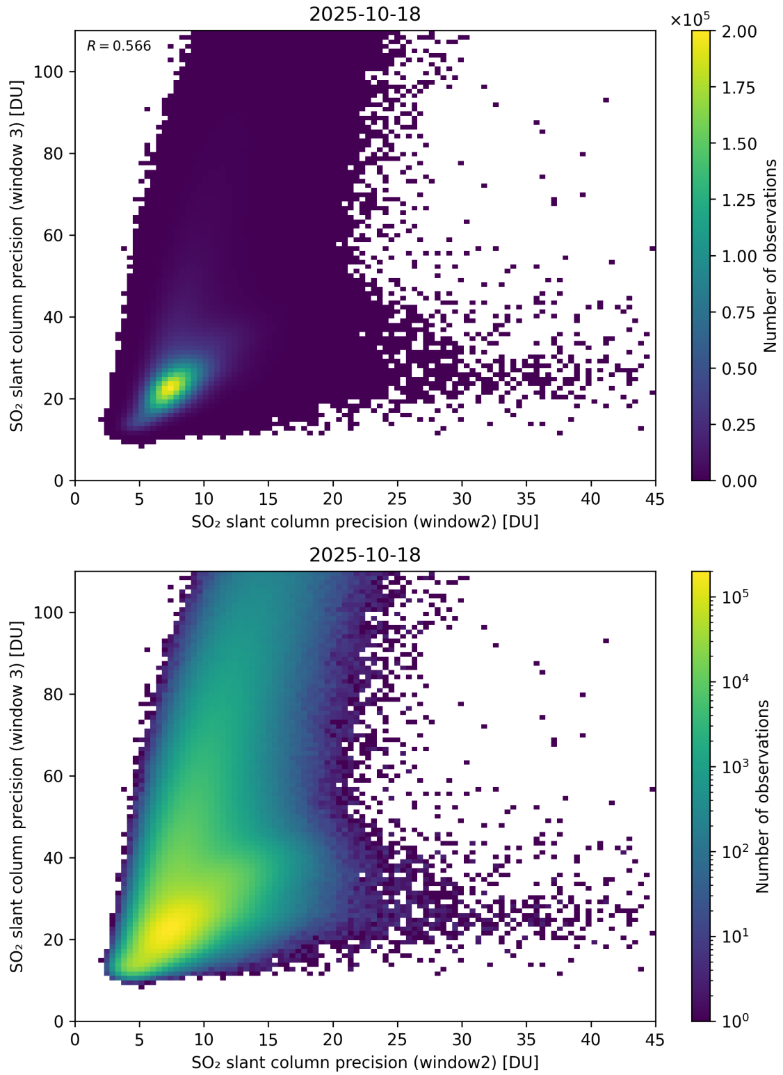
Figure 300: Scatter density plot of “SO 2 slant column precision (window2)” against “SO 2 slant column precision (window 3)” for 2025-10-17 to 2025-10-19.
