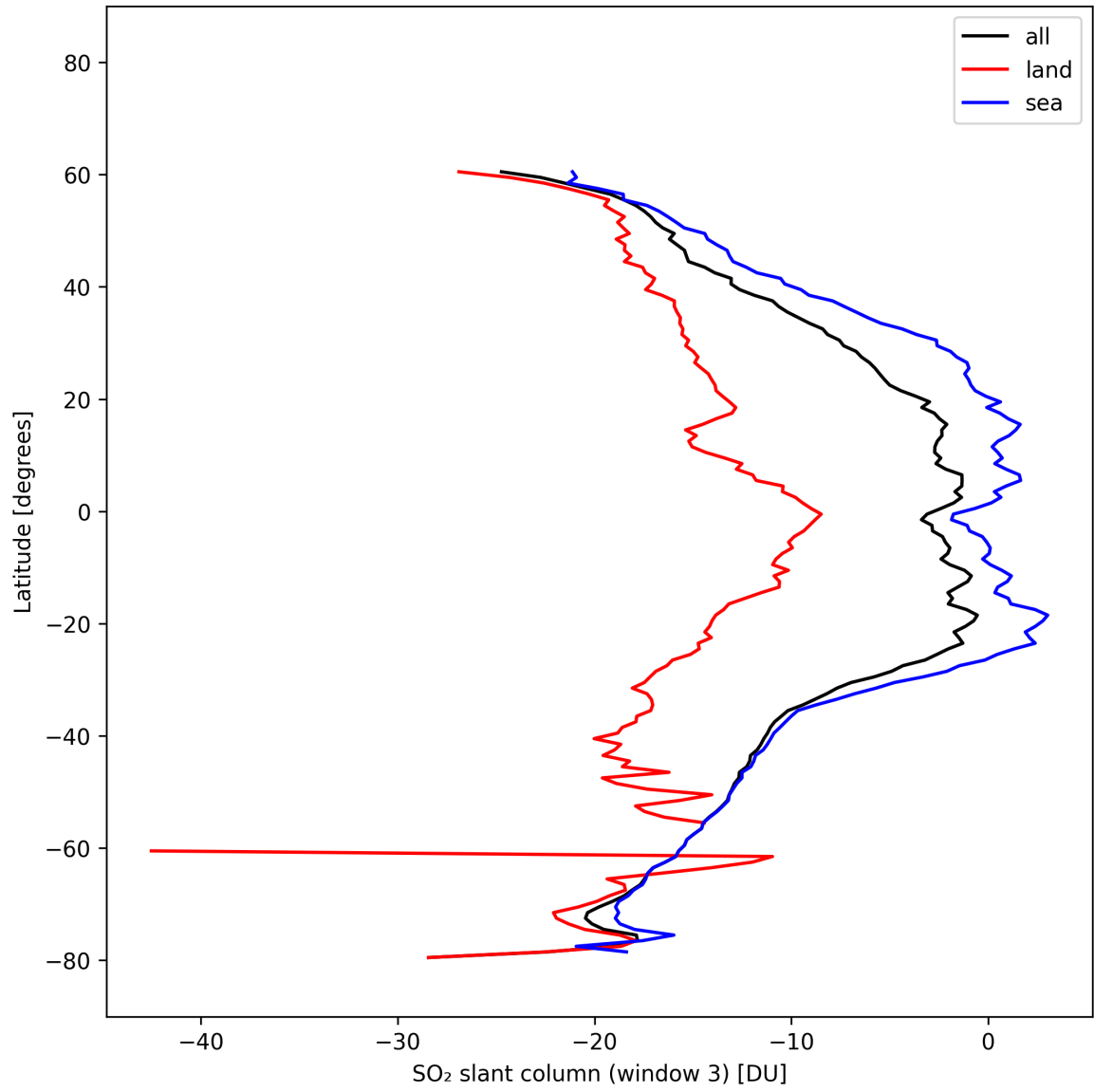
Figure 45: Zonal average of “SO 2 slant column (window 3)” for 2025-10-17 to 2025-10-19.
