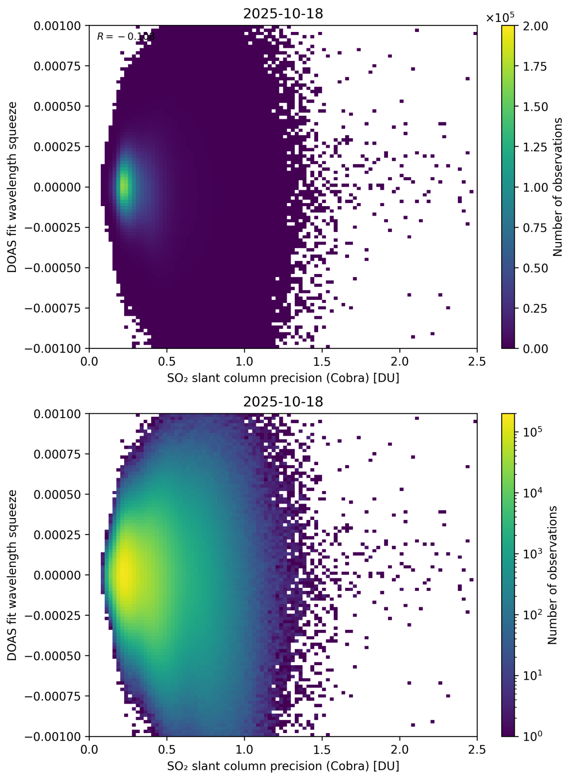
Figure 203: Scatter density plot of “SO 2 slant column precision (Cobra)” against “DOAS fit wavelength squeeze” for 2025-10-17 to 2025-10-19.
