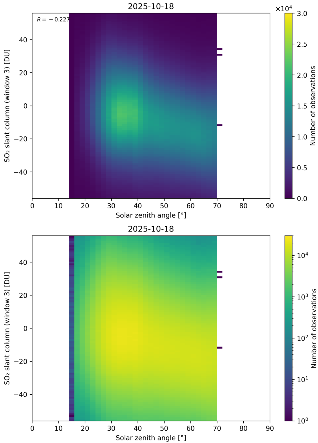
Figure 187: Scatter density plot of “Solar zenith angle” against “SO 2 slant column (window 3)” for 2025-10-17 to 2025-10-19.
