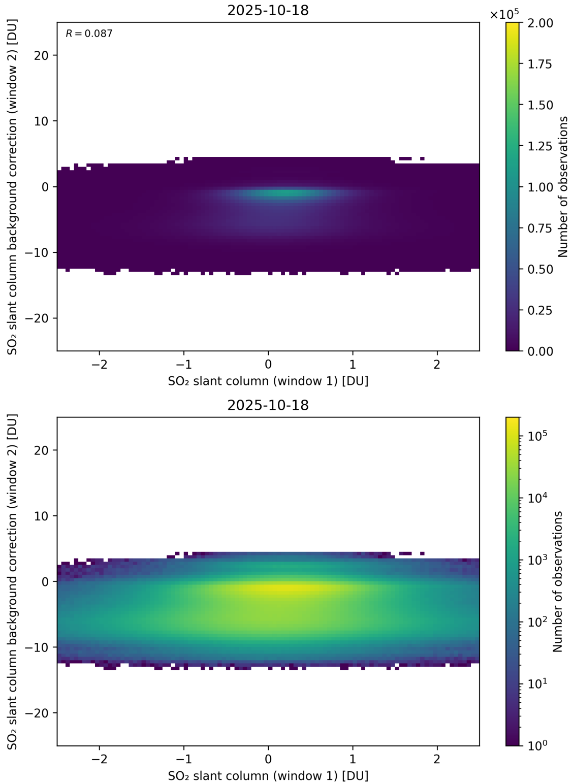
Figure 263: Scatter density plot of “SO 2 slant column (window 1)” against “SO 2 slant column background correction (window 2)” for 2025-10-17 to 2025-10-19.
