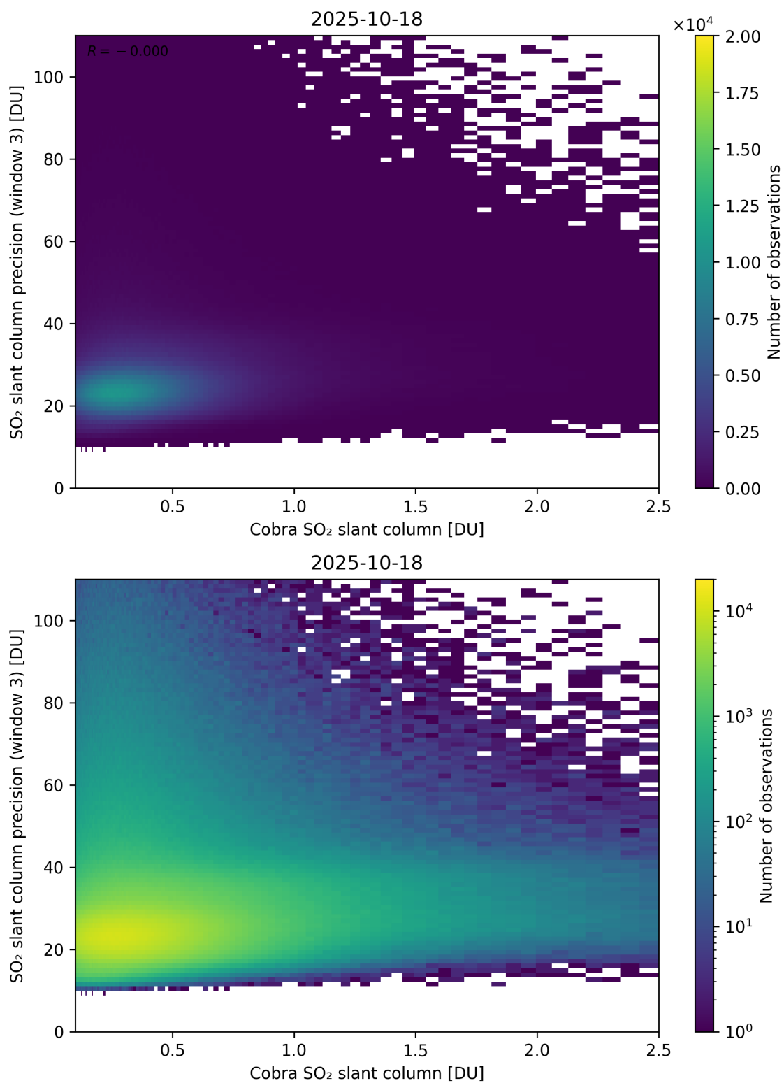
Figure 223: Scatter density plot of “Cobra SO 2 slant column” against “SO 2 slant column precision (window 3)” for 2025-10-17 to 2025-10-19.
