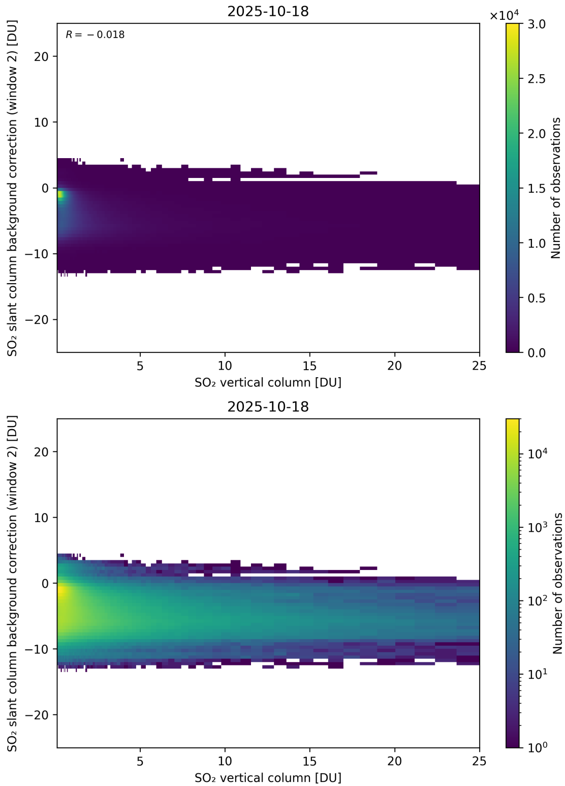
Figure 324: Scatter density plot of “SO 2 vertical column” against “SO 2 slant column background correction (window 2)” for 2025-10-17 to 2025-10-19.
