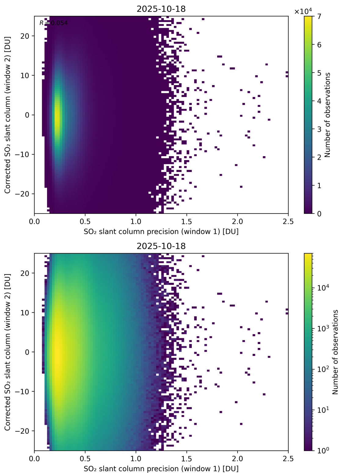
Figure 275: Scatter density plot of “SO 2 slant column precision (window 1)” against “Corrected SO 2 slant column (window 2)” for 2025-10-17 to 2025-10-19.
