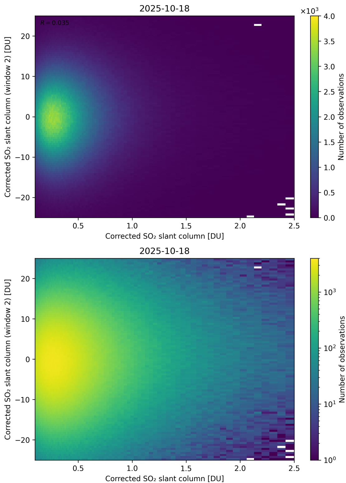
Figure 235: Scatter density plot of “Corrected SO 2 slant column” against “Corrected SO 2 slant column (window 2)” for 2025-10-17 to 2025-10-19.
