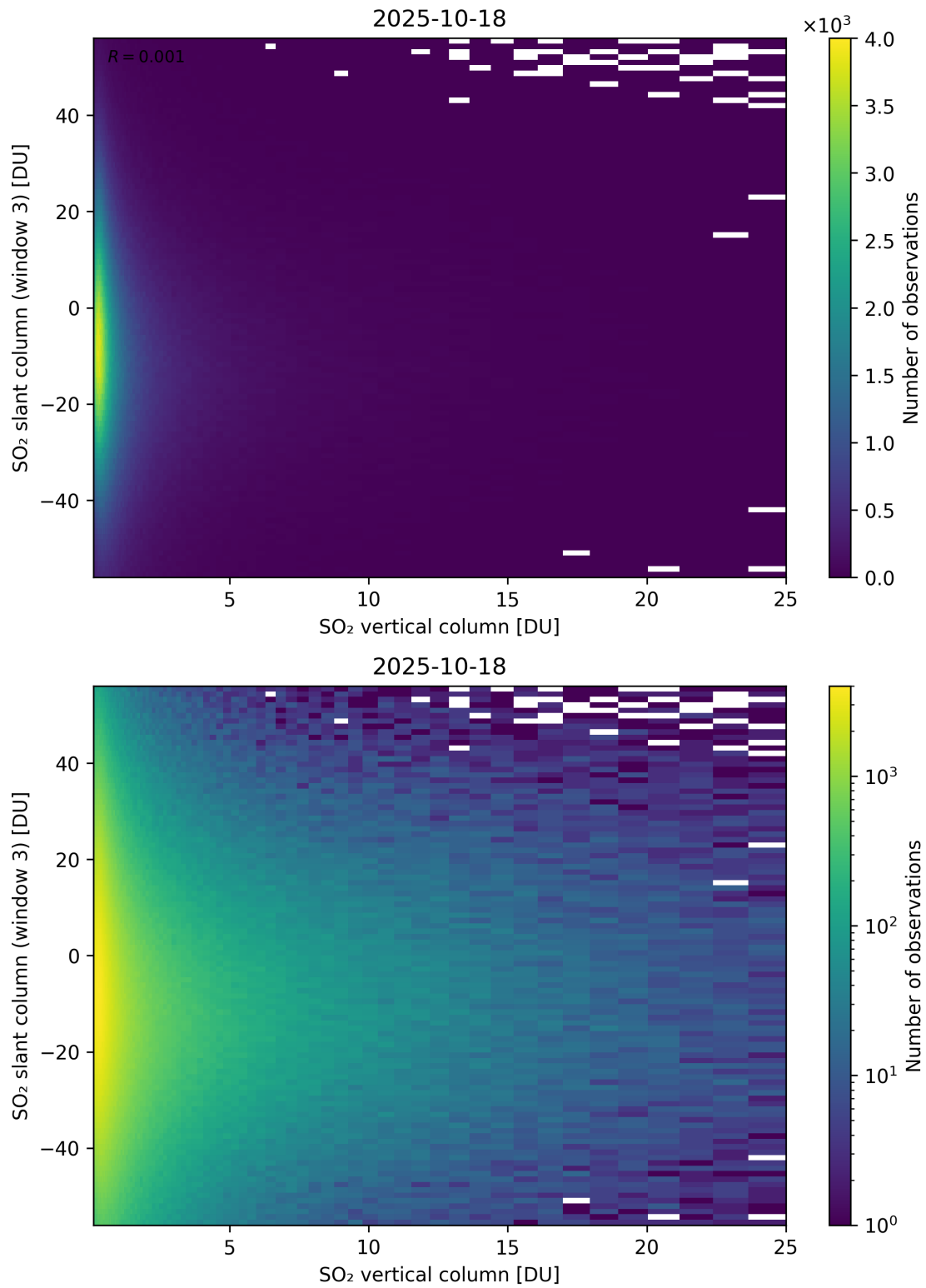
Figure 357: Scatter density plot of “SO 2 vertical column” against “SO 2 slant column (window 3)” for 2025-10-17 to 2025-10-19.
