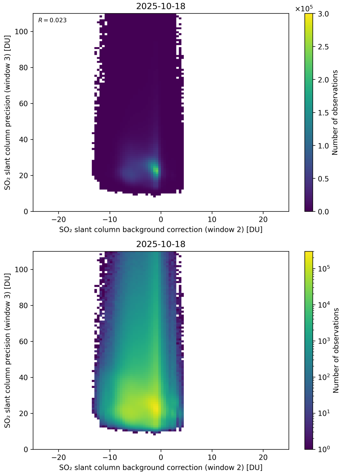
Figure 129: Scatter density plot of “SO 2 slant column background correction (window 2)” against “SO 2 slant column precision (window 3)” for 2025-10-17 to 2025-10-19.
