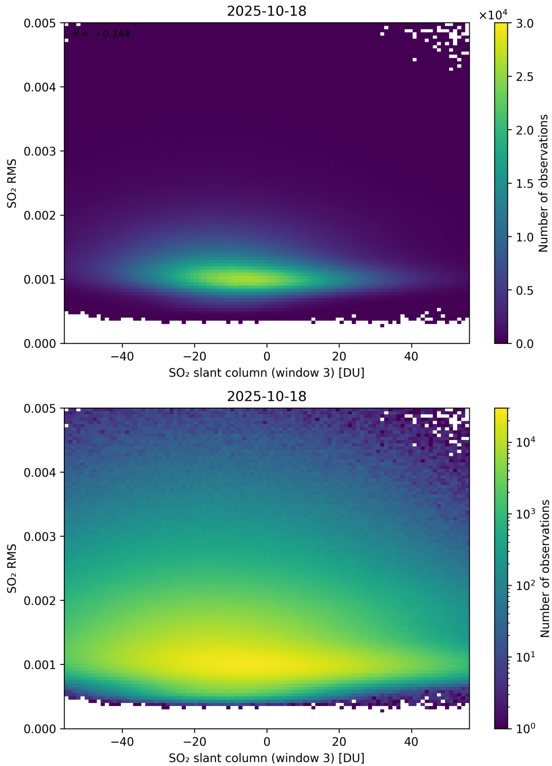
Figure 306: Scatter density plot of “SO 2 slant column (window 3)” against “SO 2 RMS” for 2025-10-17 to 2025-10-19.
