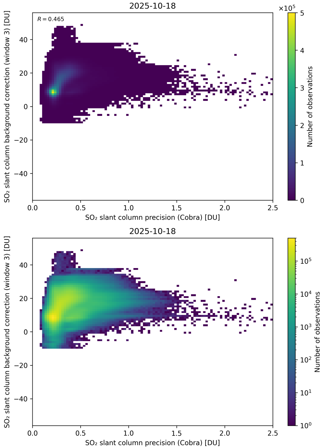
Figure 201: Scatter density plot of “SO 2 slant column precision (Cobra)” against “SO 2 slant column background correction (window 3)” for 2025-10-17 to 2025-10-19.
