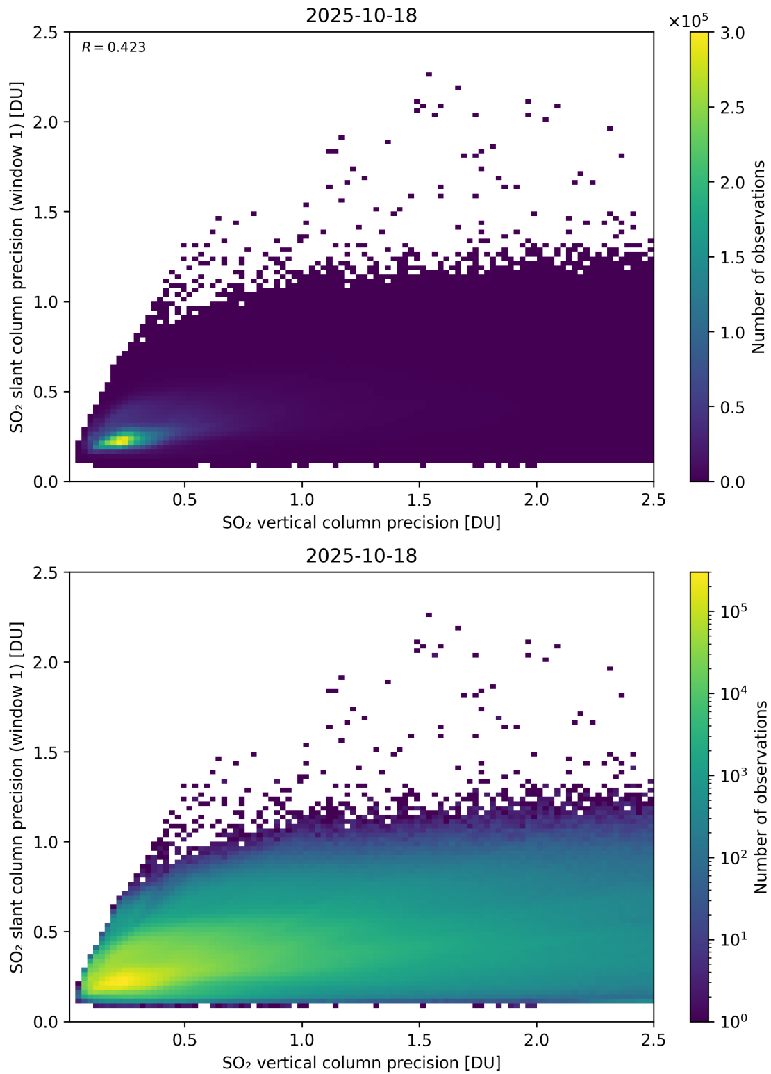
Figure 342: Scatter density plot of “SO 2 vertical column precision” against “SO 2 slant column precision (window 1)” for 2025-10-17 to 2025-10-19.
