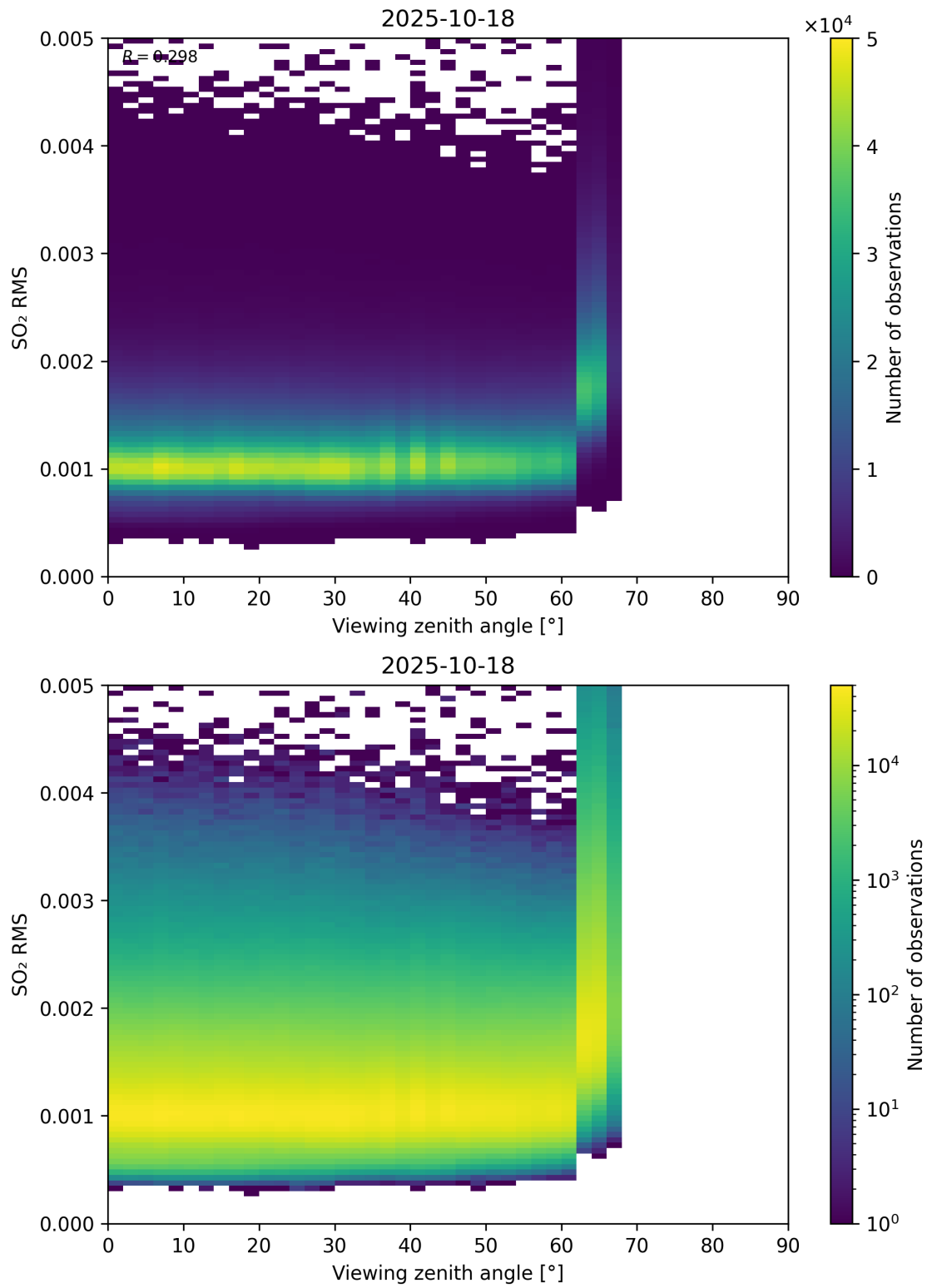
Figure 367: Scatter density plot of “Viewing zenith angle” against “SO 2 RMS” for 2025-10-17 to 2025-10-19.
