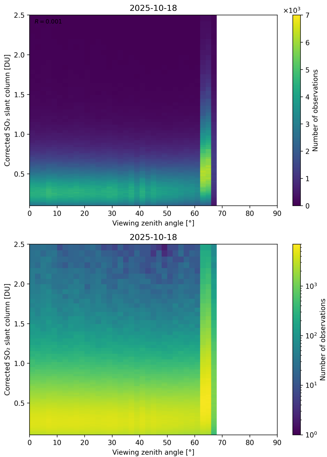
Figure 373: Scatter density plot of “Viewing zenith angle” against “Corrected SO 2 slant column” for 2025-10-17 to 2025-10-19.
