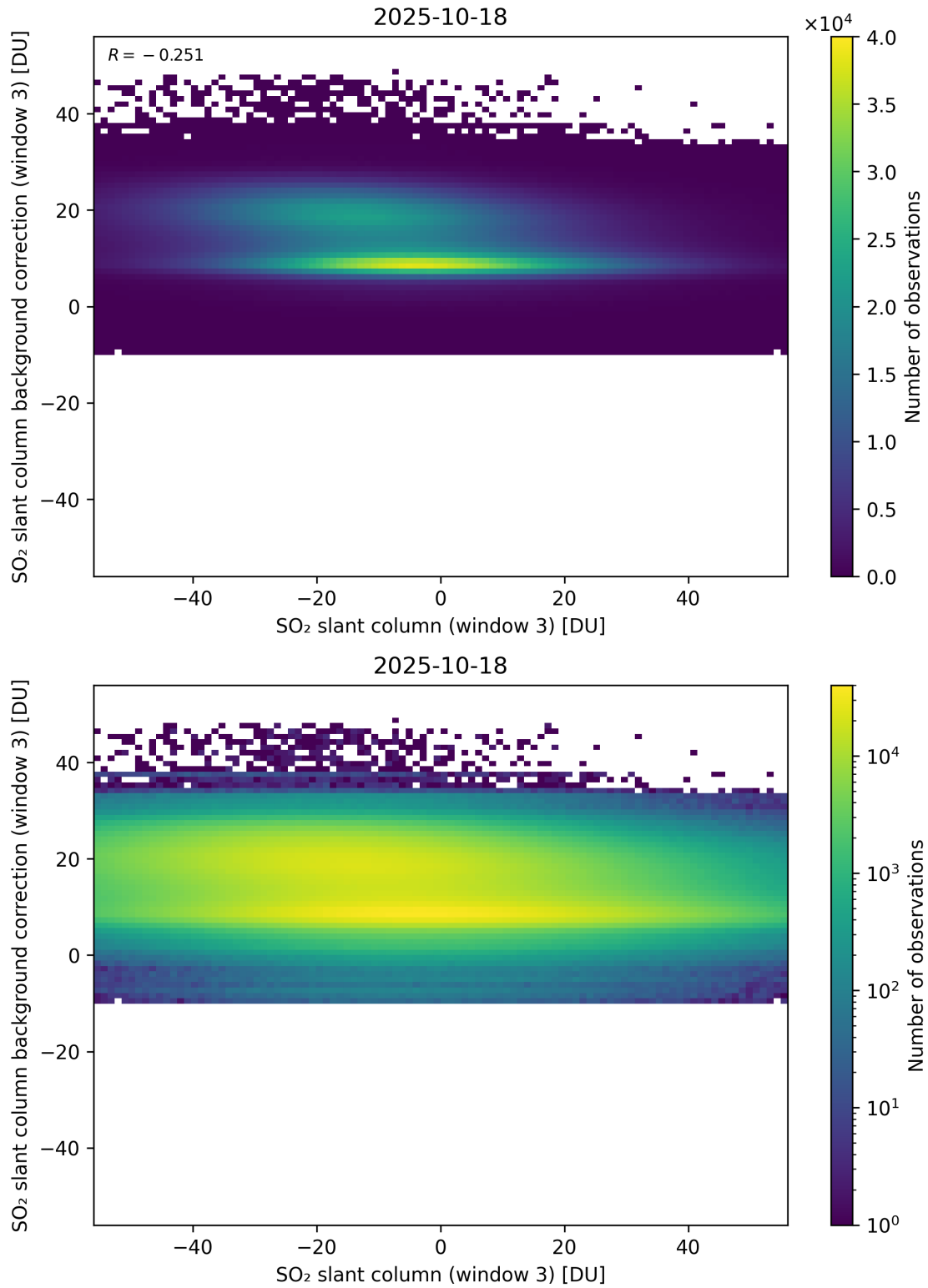
Figure 303: Scatter density plot of “SO 2 slant column (window 3)” against “SO 2 slant column background correction (window 3)” for 2025-10-17 to 2025-10-19.
