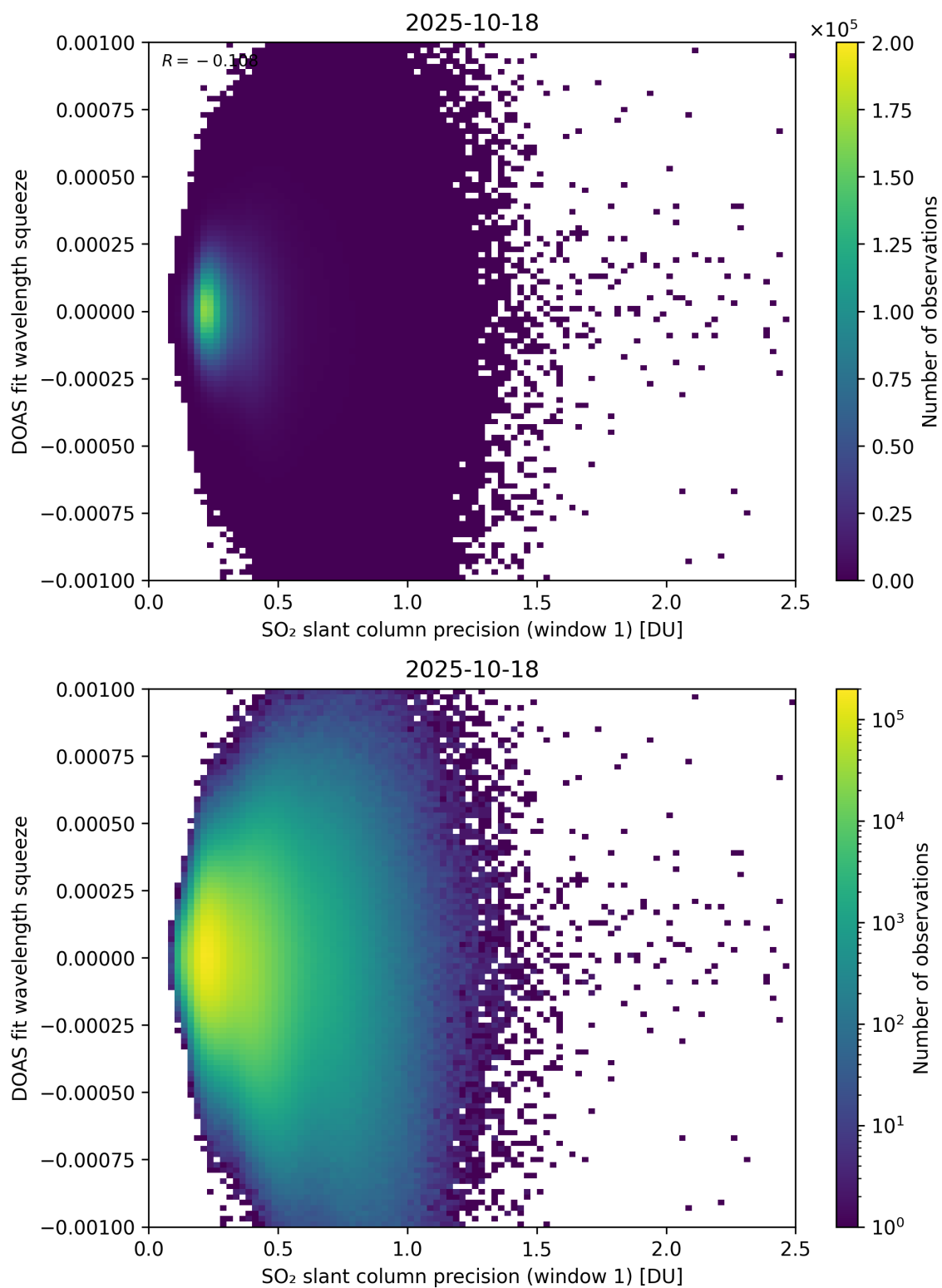
Figure 272: Scatter density plot of “SO 2 slant column precision (window 1)” against “DOAS fit wavelength squeeze” for 2025-10-17 to 2025-10-19.
