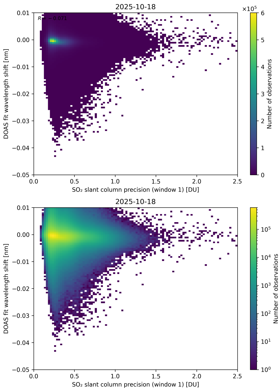
Figure 271: Scatter density plot of “SO 2 slant column precision (window 1)” against “DOAS fit wavelength shift” for 2025-10-17 to 2025-10-19.
