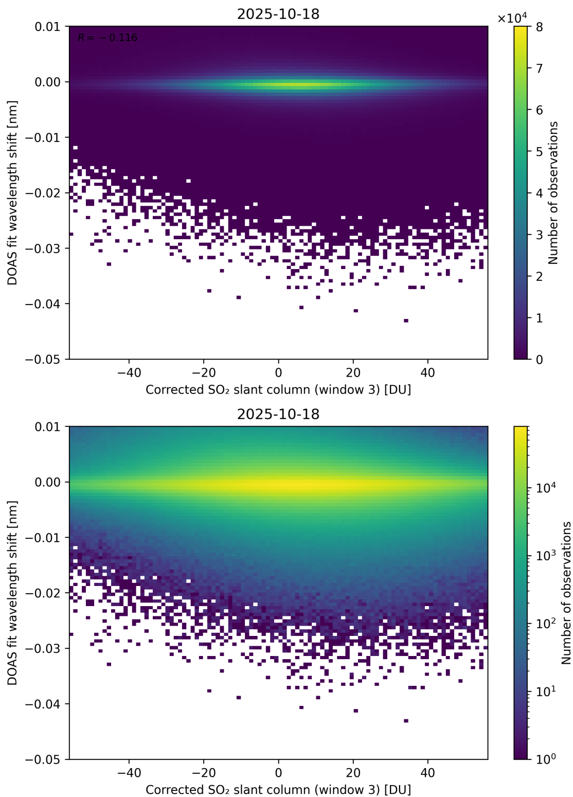
Figure 256: Scatter density plot of “Corrected SO 2 slant column (window 3)” against “DOAS fit wavelength shift” for 2025-10-17 to 2025-10-19.
