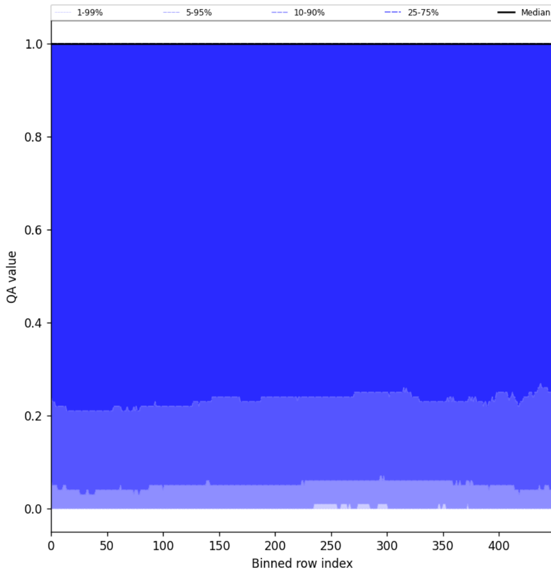
Figure 83: Along track statistics of “QA value” for 2025-10-17 to 2025-10-19
