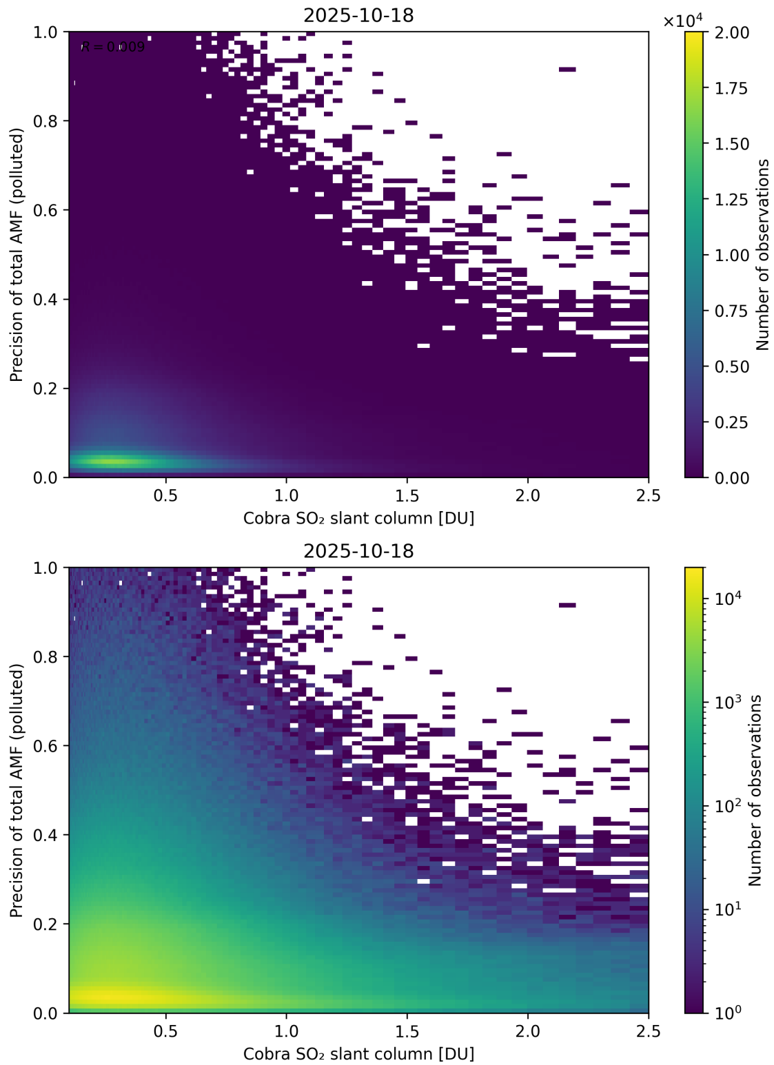
Figure 225: Scatter density plot of “Cobra SO 2 slant column” against “Precision of total AMF (polluted)” for 2025-10-17 to 2025-10-19.
