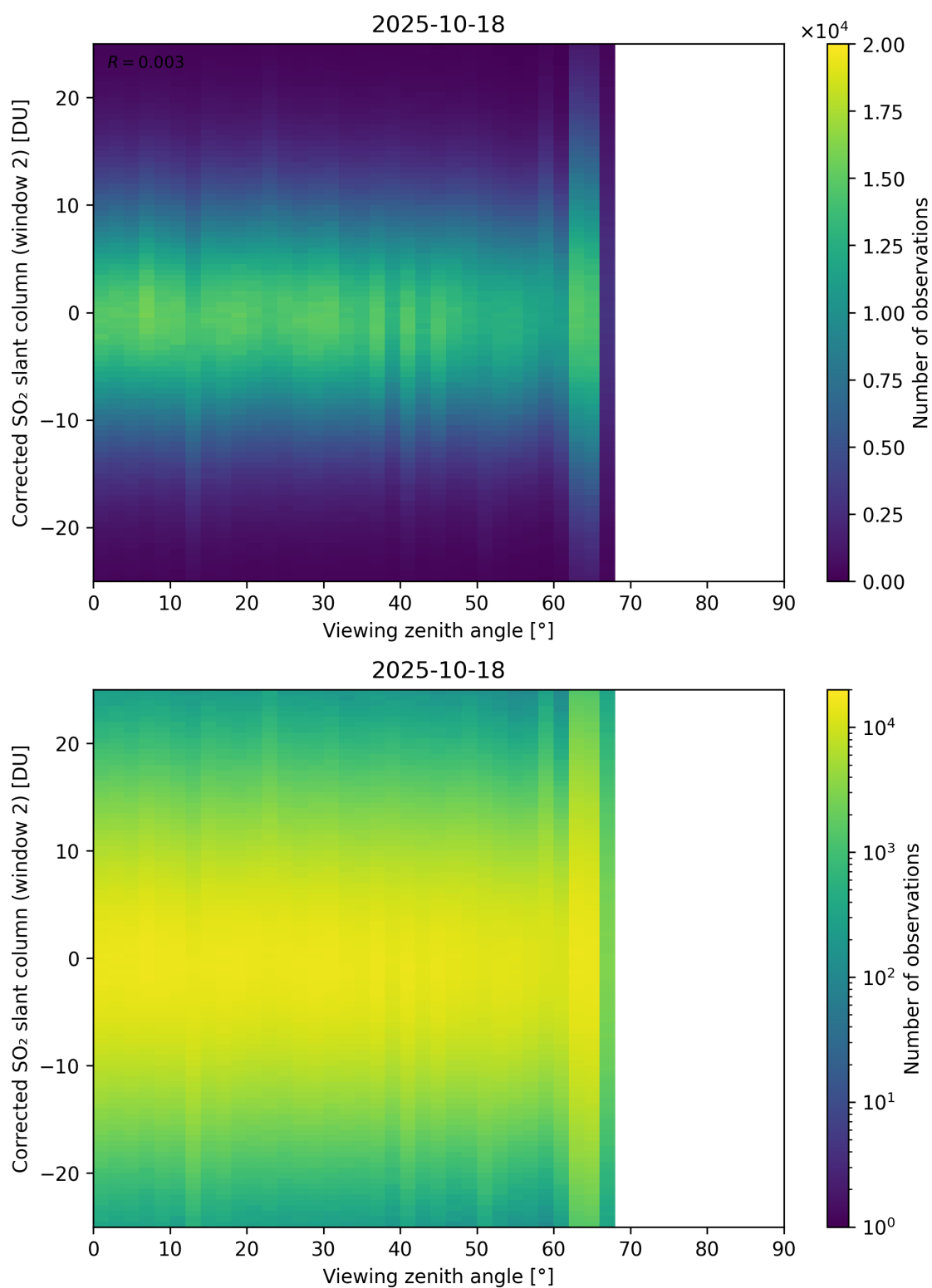
Figure 374: Scatter density plot of “Viewing zenith angle” against “Corrected SO 2 slant column (window 2)” for 2025-10-17 to 2025-10-19.
