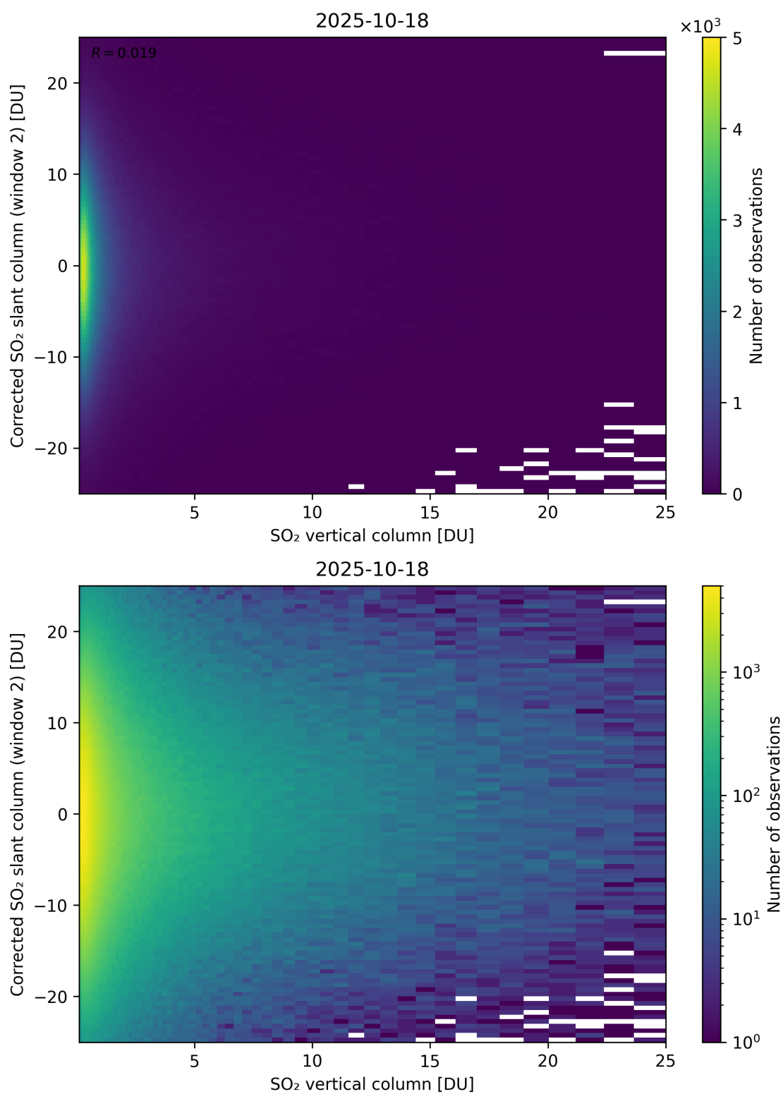
Figure 352: Scatter density plot of “SO 2 vertical column” against “Corrected SO 2 slant column (window 2)” for 2025-10-17 to 2025-10-19.
