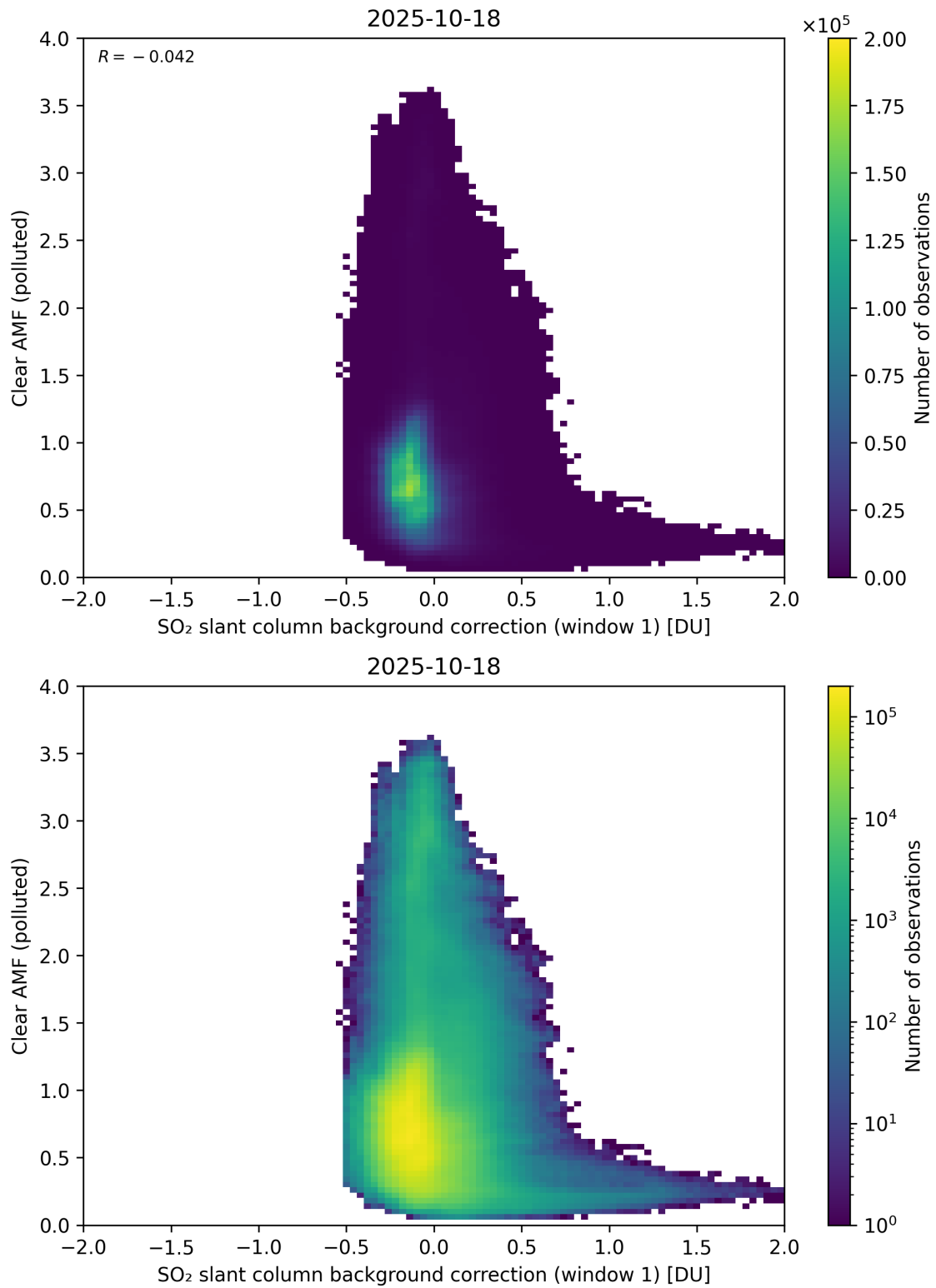
Figure 114: Scatter density plot of “SO 2 slant column background correction (window 1)” against “Clear AMF (polluted)” for 2025-10-17 to 2025-10-19.
