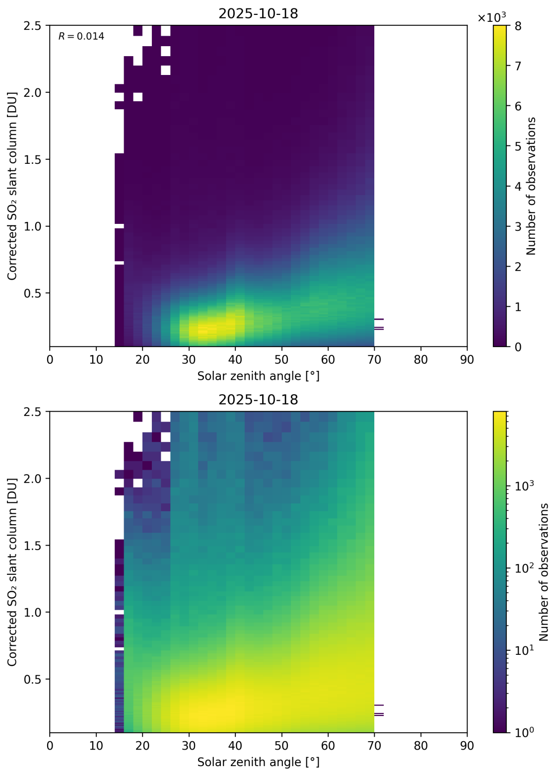
Figure 181: Scatter density plot of “Solar zenith angle” against “Corrected SO 2 slant column” for 2025-10-17 to 2025-10-19.
