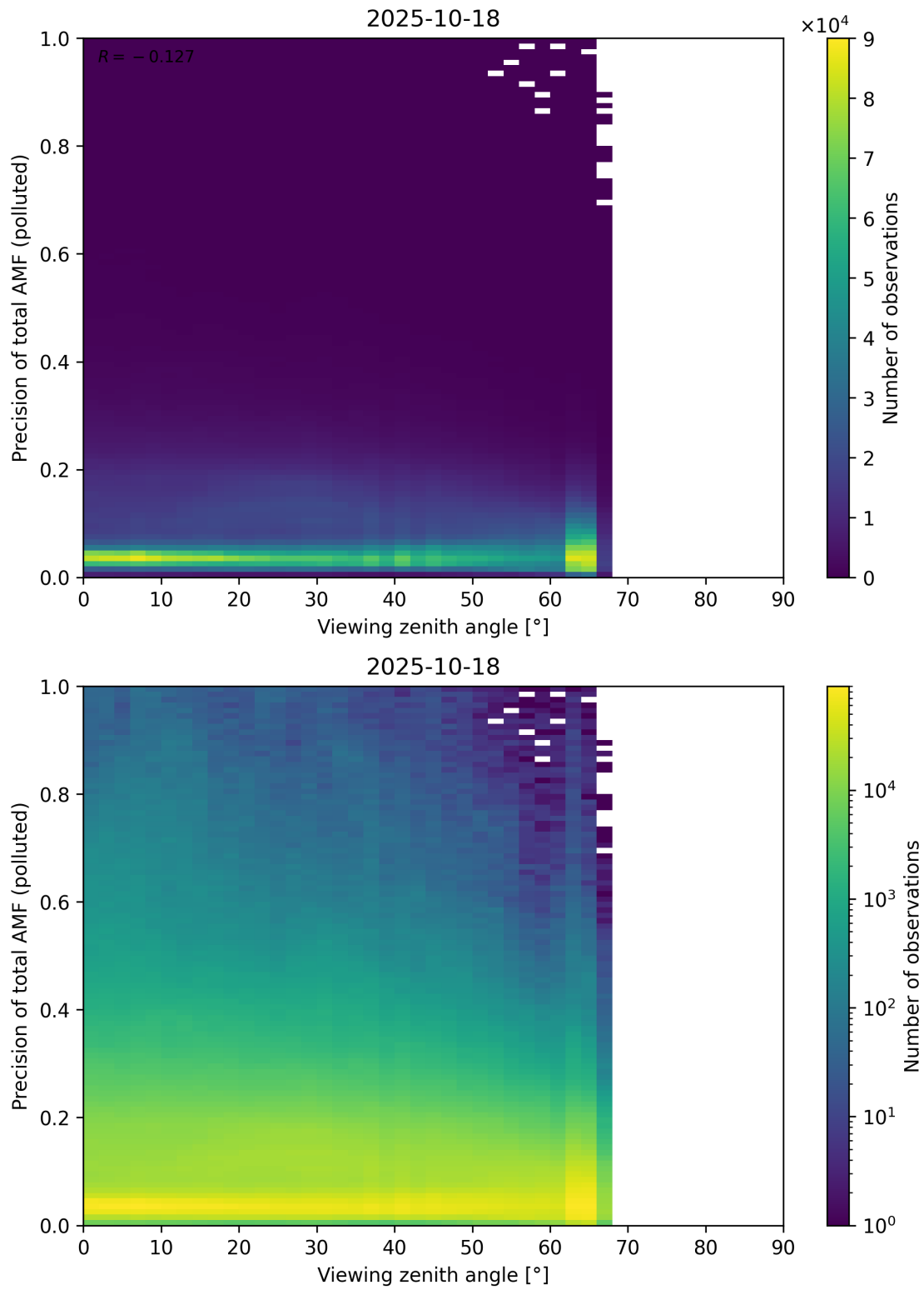
Figure 382: Scatter density plot of “Viewing zenith angle” against “Precision of total AMF (polluted)” for 2025-10-17 to 2025-10-19.
