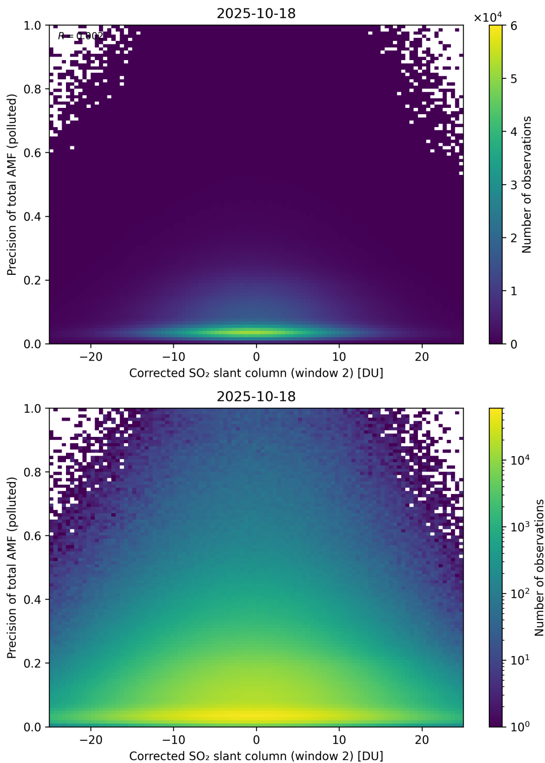
Figure 254: Scatter density plot of “Corrected SO 2 slant column (window 2)” against “Precision of total AMF (polluted)” for 2025-10-17 to 2025-10-19.
