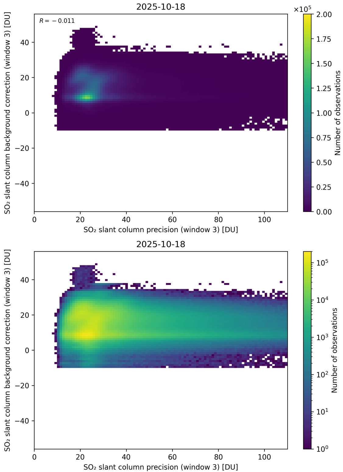
Figure 307: Scatter density plot of “SO 2 slant column precision (window 3)” against “SO 2 slant column background correction (window 3)” for 2025-10-17 to 2025-10-19.
