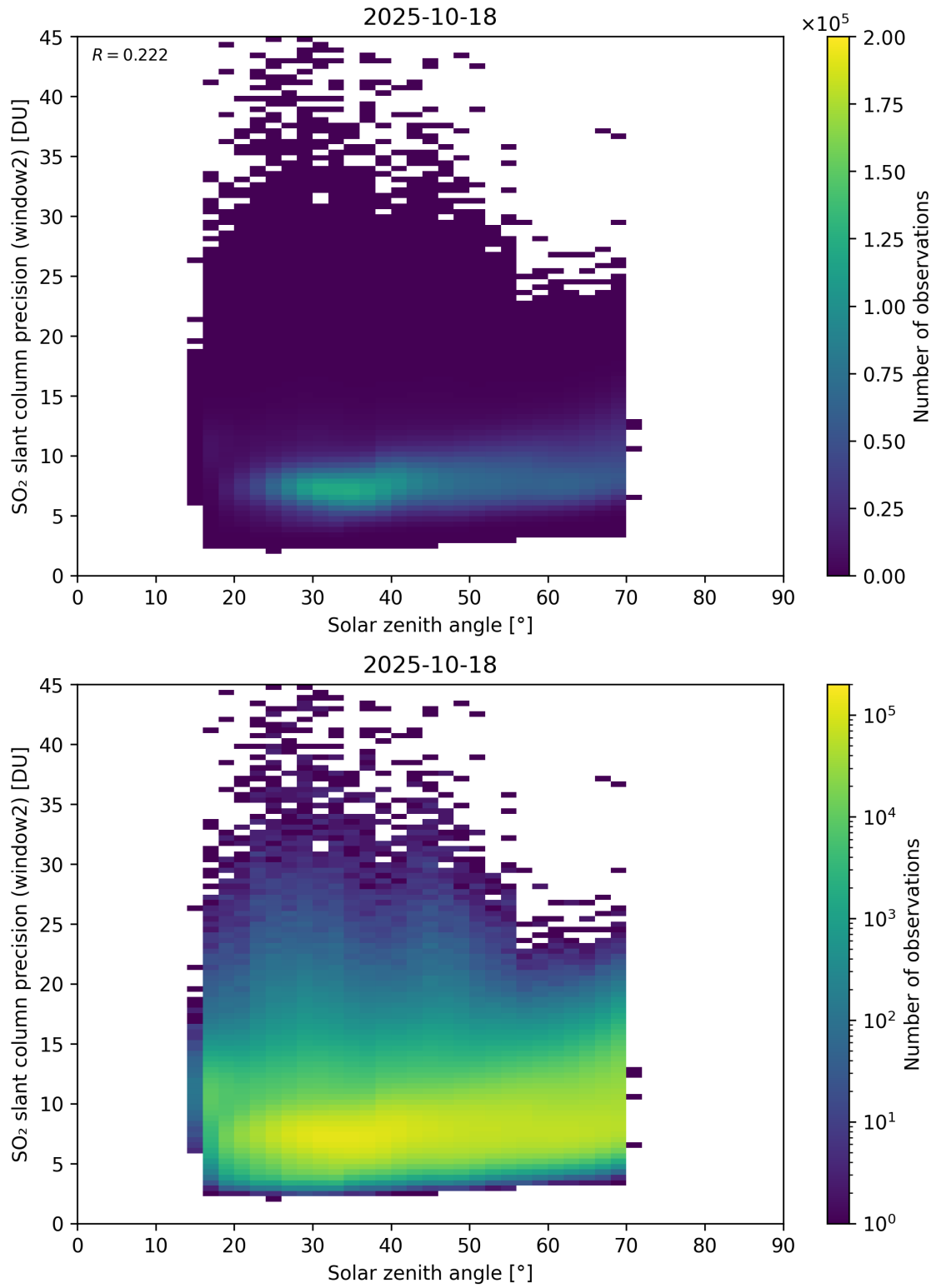
Figure 186: Scatter density plot of “Solar zenith angle” against “SO 2 slant column precision (window2)” for 2025-10-17 to 2025-10-19.
