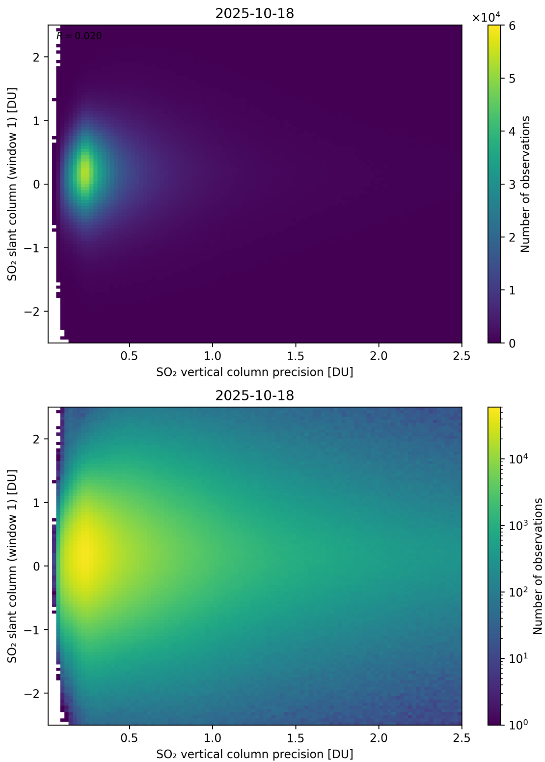
Figure 341: Scatter density plot of “SO 2 vertical column precision” against “SO 2 slant column (window 1)” for 2025-10-17 to 2025-10-19.
