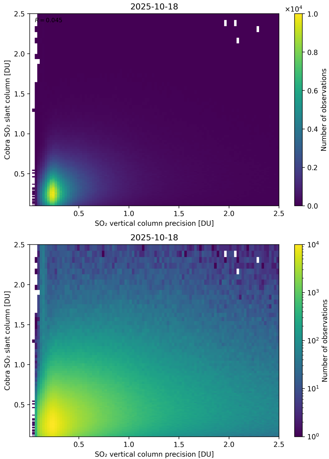
Figure 336: Scatter density plot of “SO 2 vertical column precision” against “Cobra SO 2 slant column” for 2025-10-17 to 2025-10-19.
