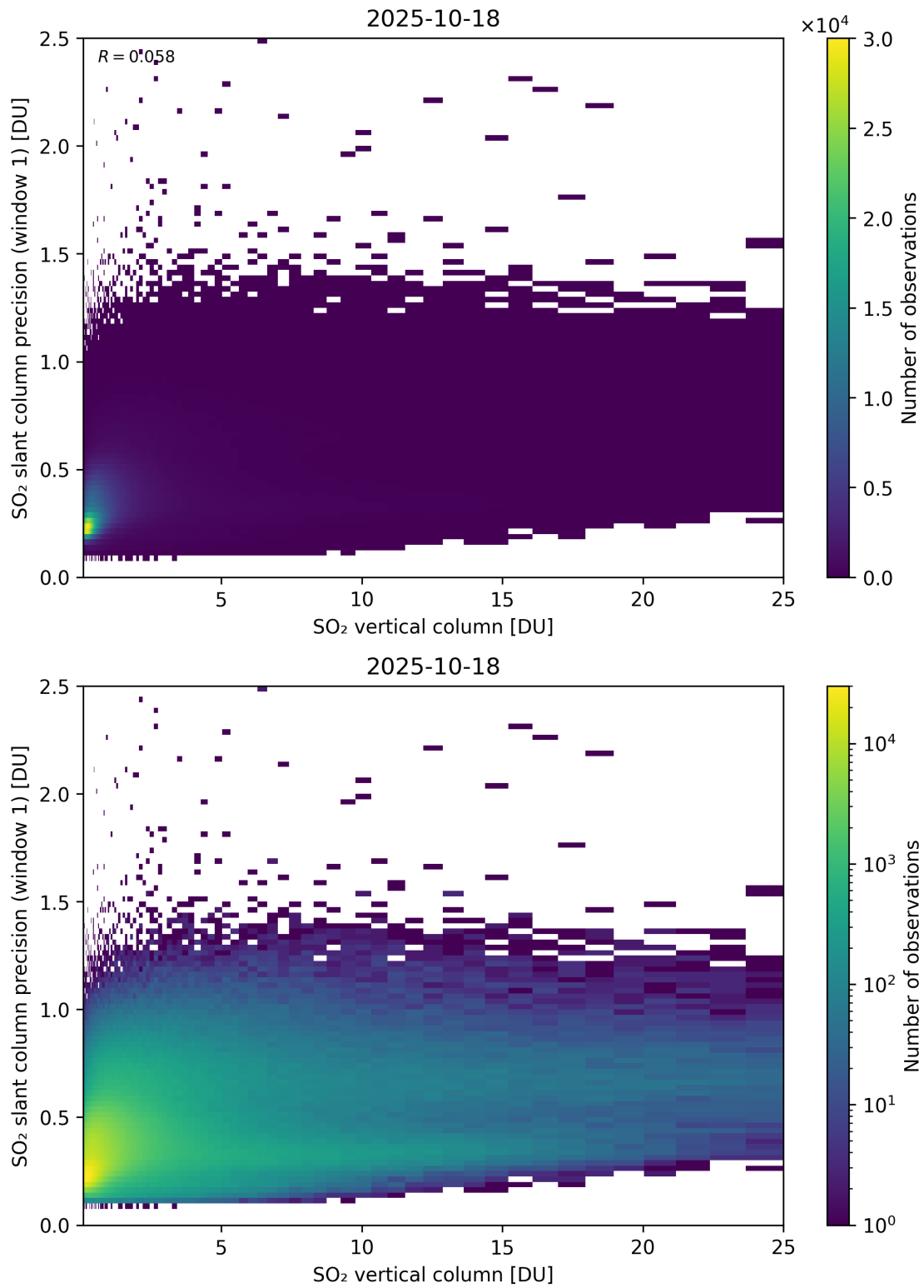
Figure 355: Scatter density plot of “SO 2 vertical column” against “SO 2 slant column precision (window 1)” for 2025-10-17 to 2025-10-19.
