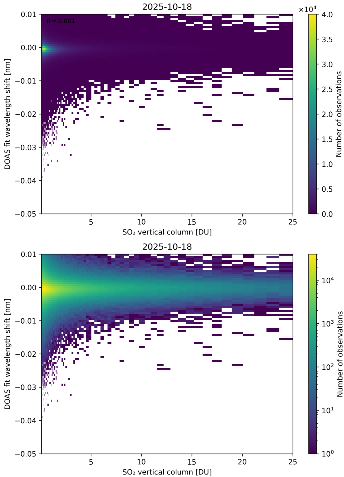
Figure 326: Scatter density plot of “SO 2 vertical column” against “DOAS fit wavelength shift” for 2025-10-17 to 2025-10-19.
