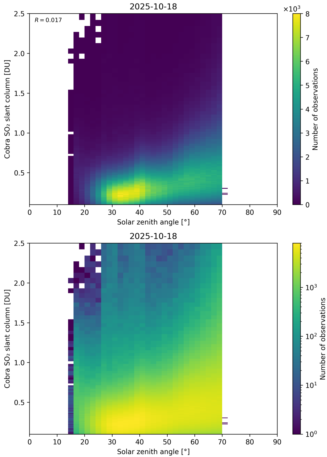
Figure 179: Scatter density plot of “Solar zenith angle” against “Cobra SO 2 slant column” for 2025-10-17 to 2025-10-19.
