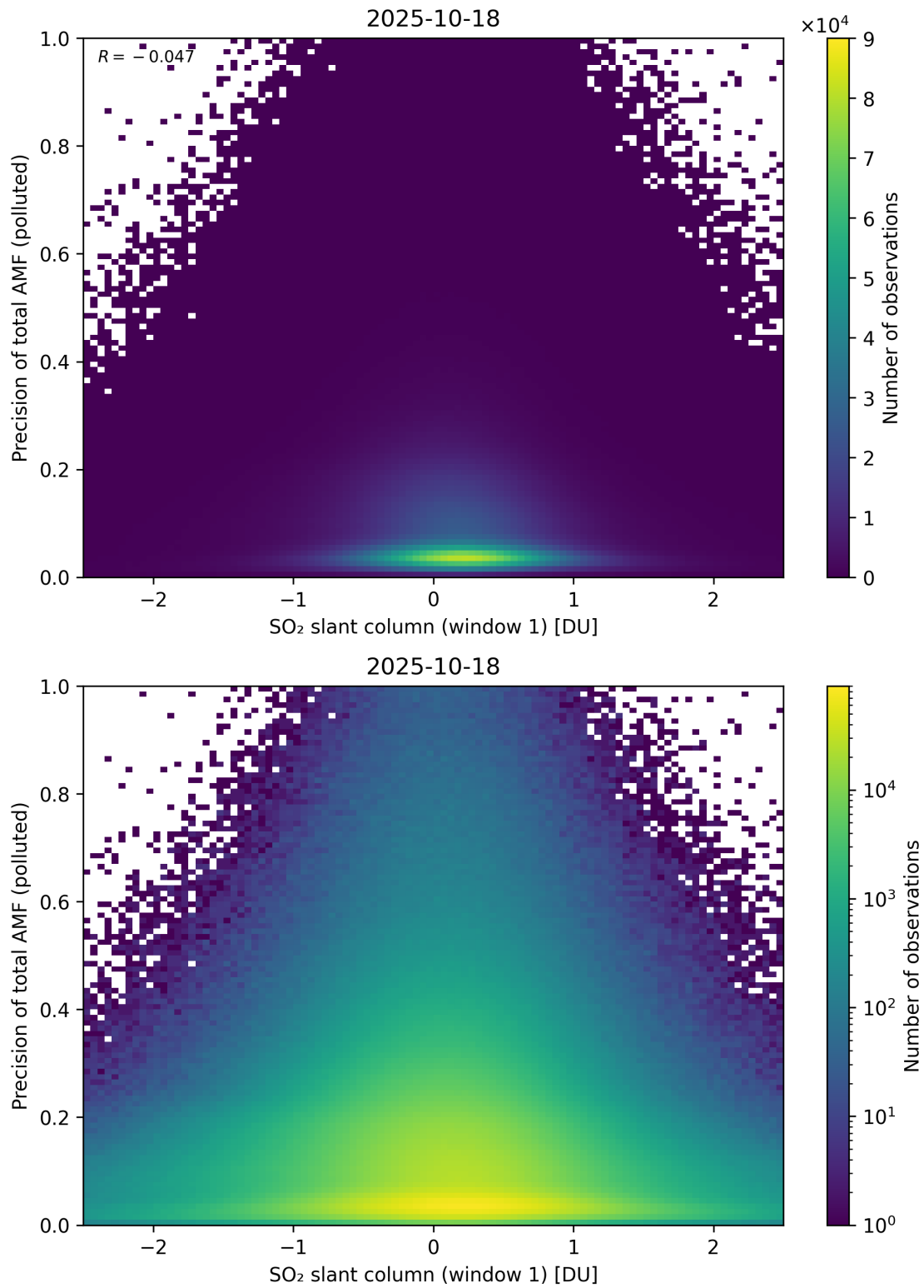
Figure 290: Scatter density plot of “SO 2 slant column (window 1)” against “Precision of total AMF (polluted)” for 2025-10-17 to 2025-10-19.
