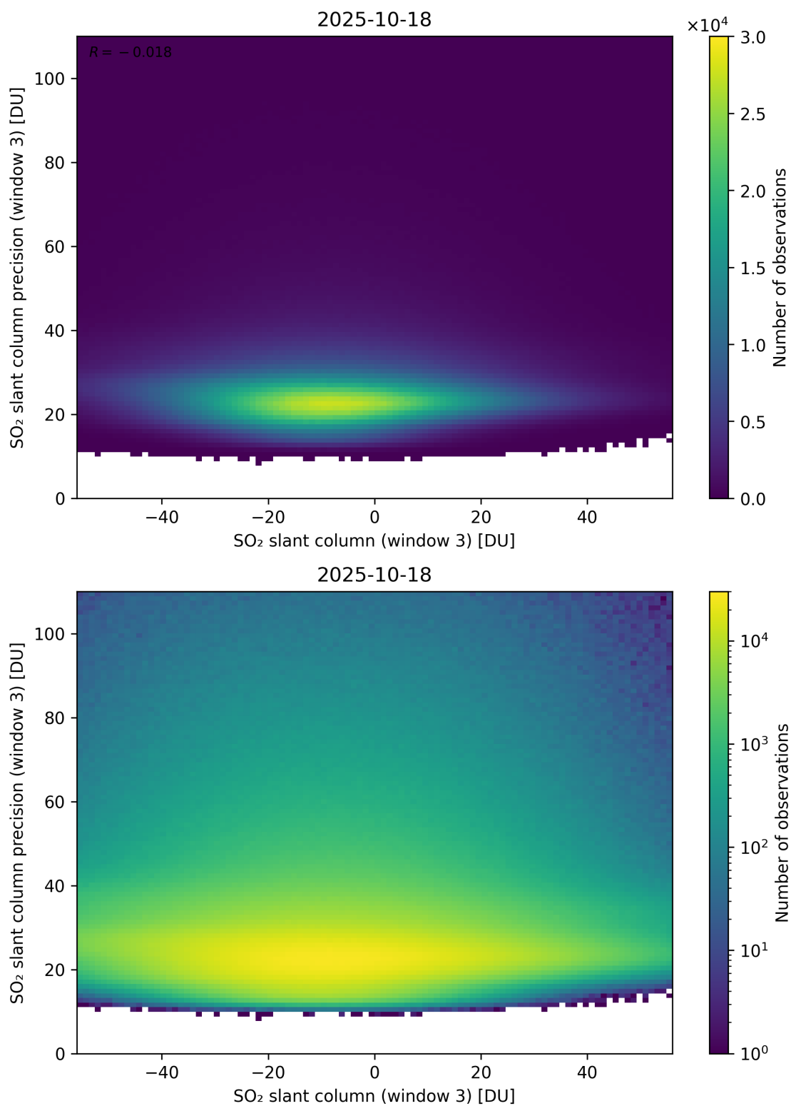
Figure 317: Scatter density plot of “SO 2 slant column (window 3)” against “SO 2 slant column precision (window 3)” for 2025-10-17 to 2025-10-19.
