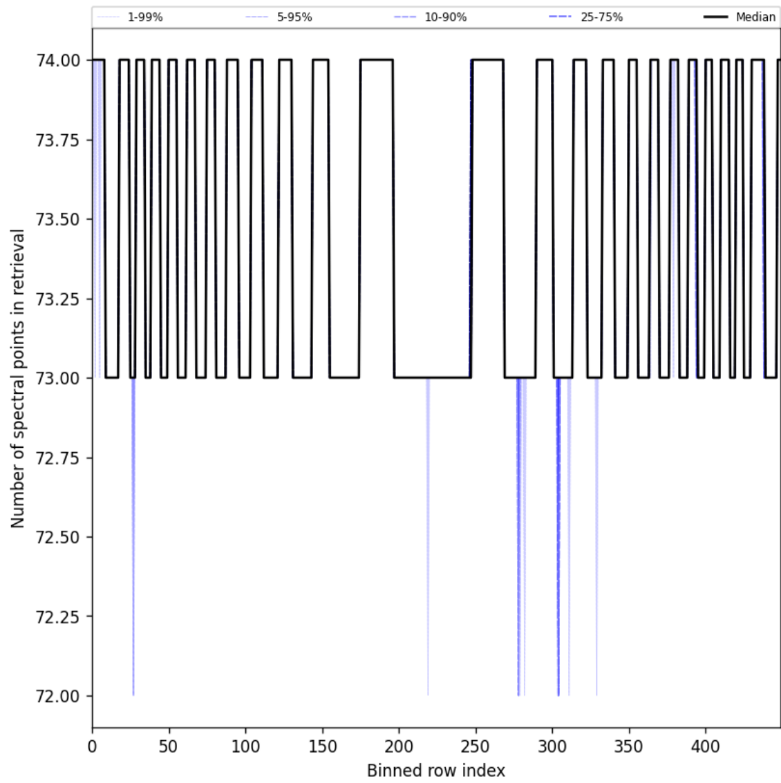
Figure 108: Along track statistics of “Number of spectral points in retrieval” for 2025-10-17 to 2025-10-19
