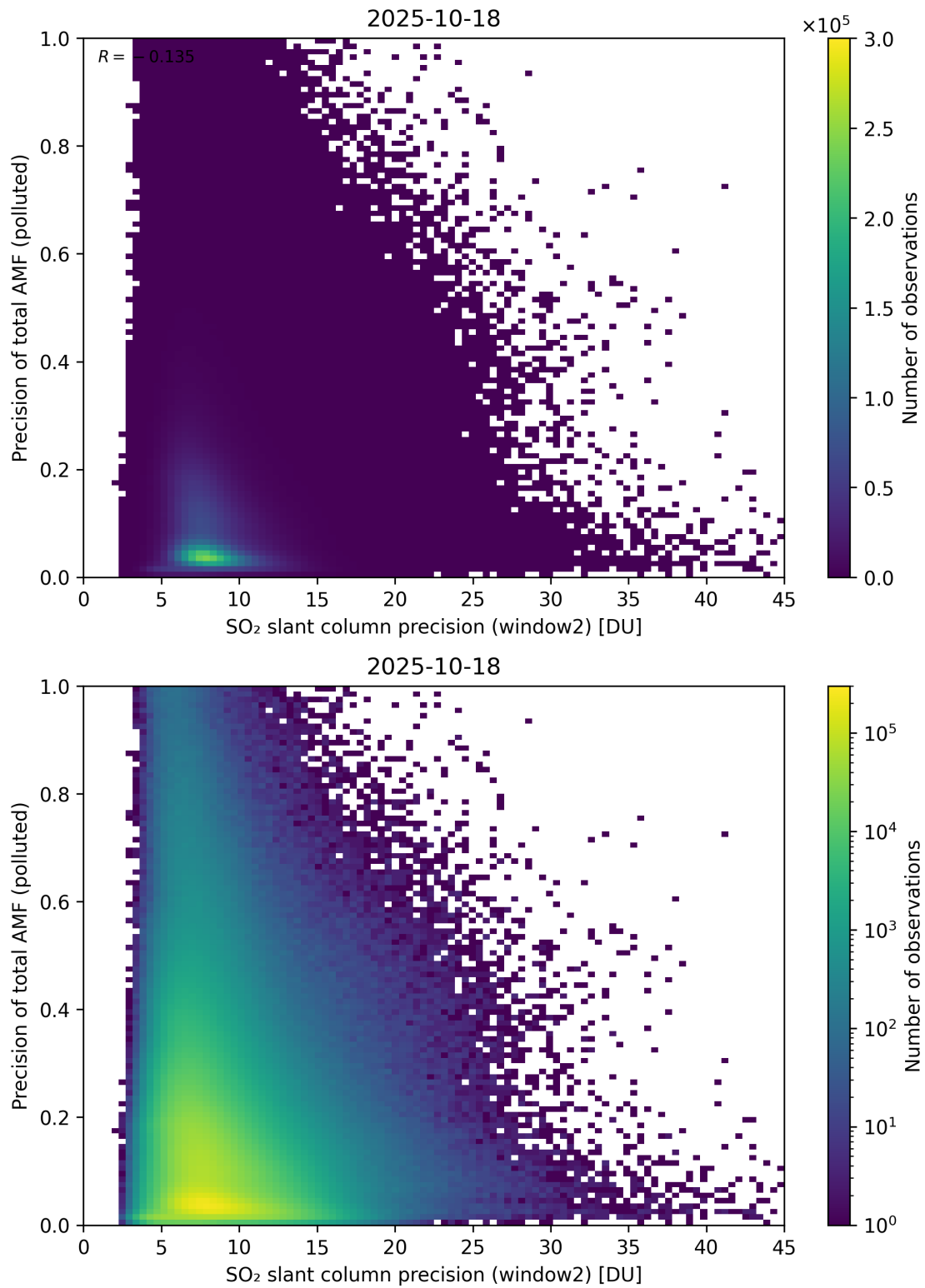
Figure 302: Scatter density plot of “SO 2 slant column precision (window2)” against “Precision of total AMF (polluted)” for 2025-10-17 to 2025-10-19.
