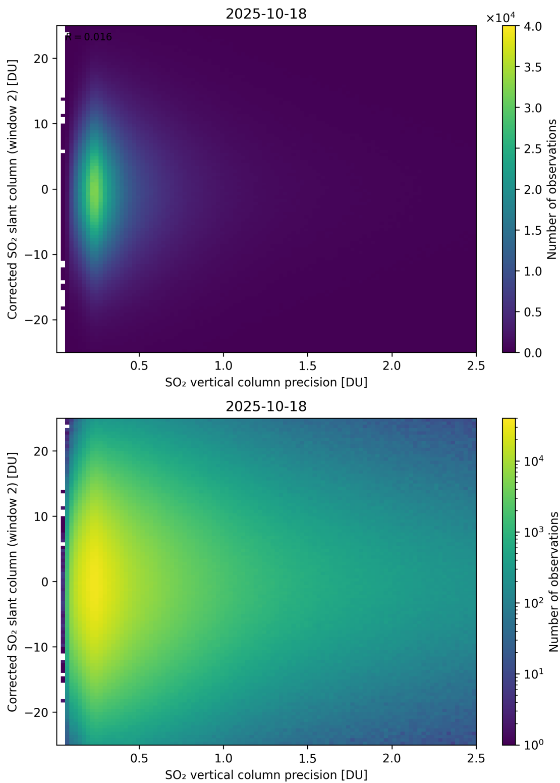
Figure 339: Scatter density plot of “SO 2 vertical column precision” against “Corrected SO 2 slant column (window 2)” for 2025-10-17 to 2025-10-19.
