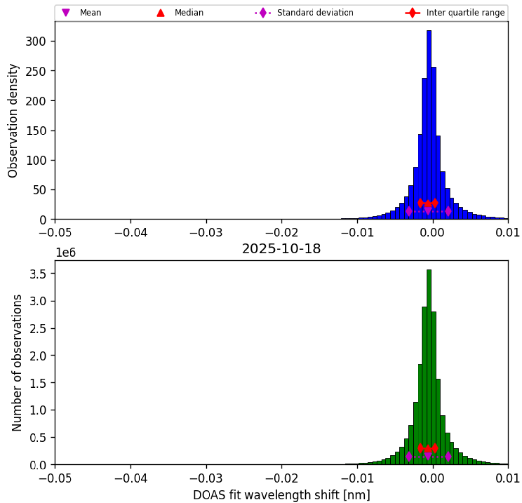
Figure 76: Histogram of “DOAS fit wavelength shift” for 2025-10-17 to 2025-10-19
