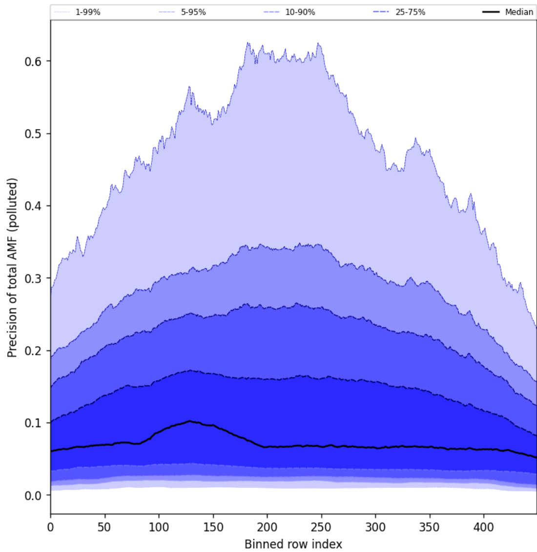
Figure 106: Along track statistics of “Precision of total AMF (polluted)” for 2025-10-17 to 2025-10-19
