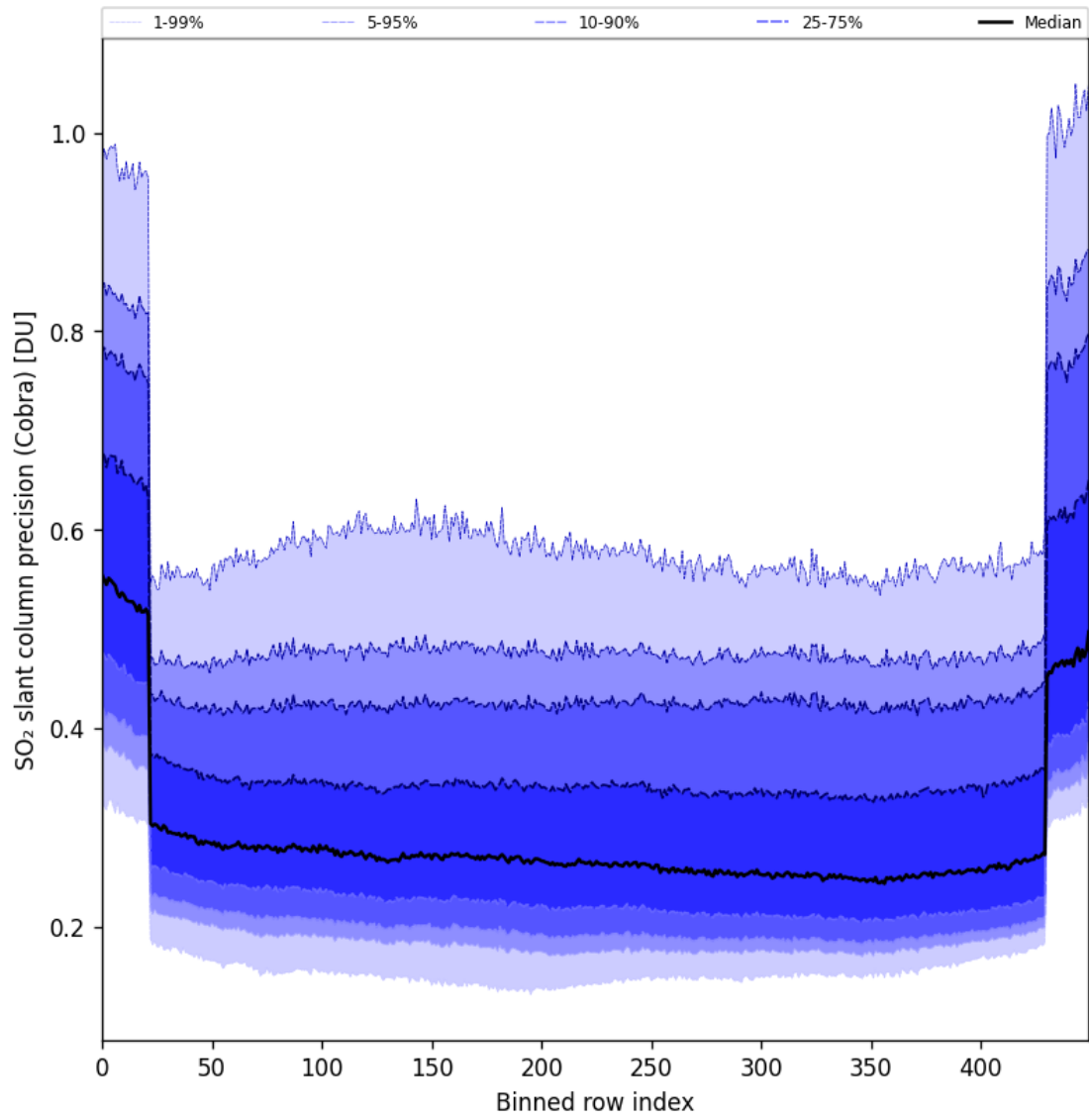
Figure 88: Along track statistics of “SO 2 slant column precision (Cobra)” for 2025-10-17 to 2025-10-19
