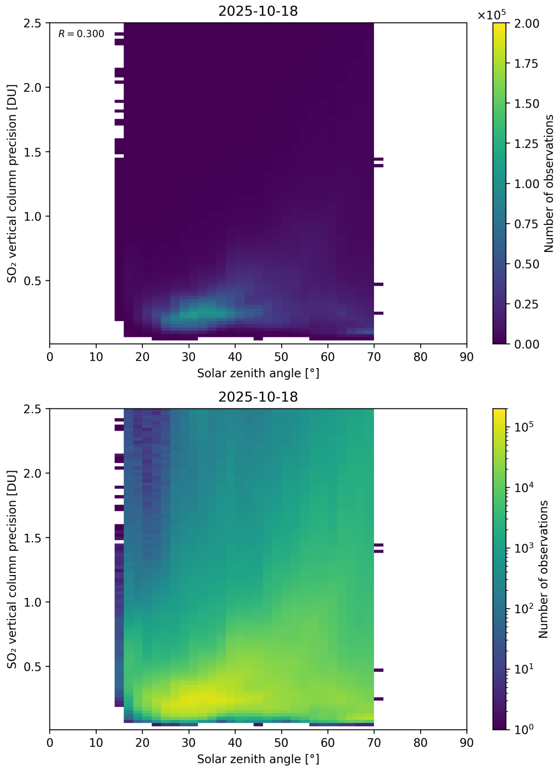
Figure 192: Scatter density plot of “Solar zenith angle” against “SO 2 vertical column precision” for 2025-10-17 to 2025-10-19.
