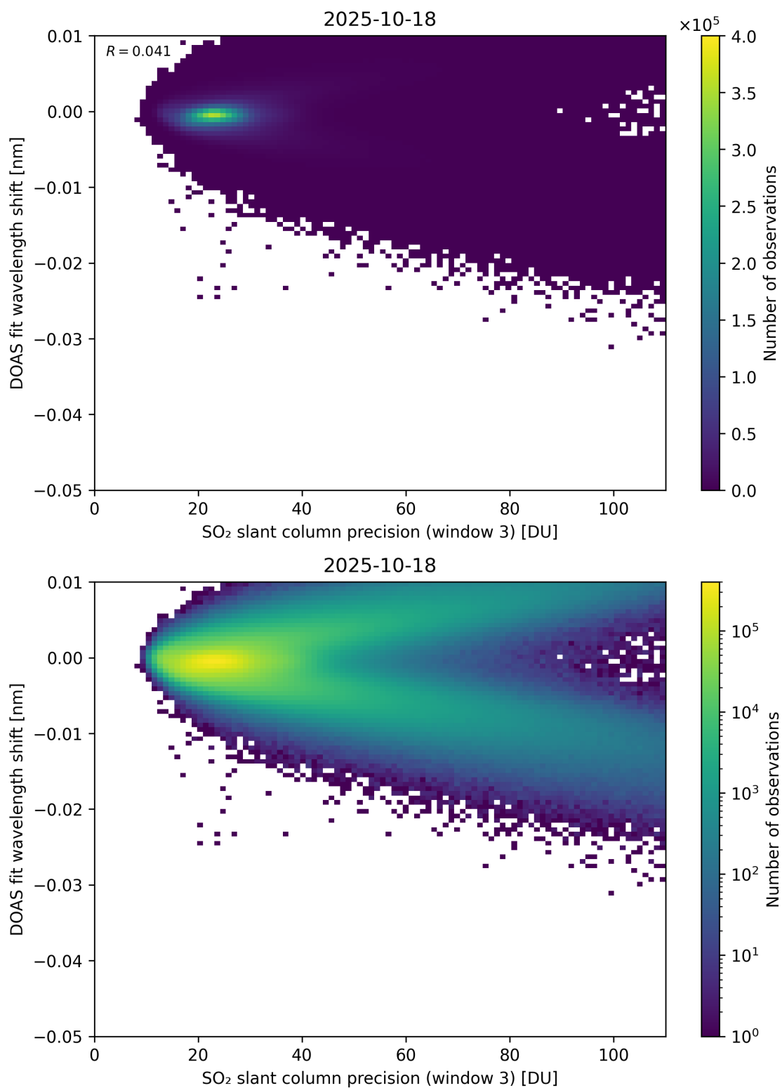
Figure 308: Scatter density plot of “SO 2 slant column precision (window 3)” against “DOAS fit wavelength shift” for 2025-10-17 to 2025-10-19.
