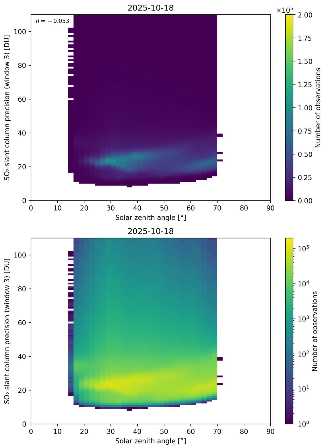
Figure 188: Scatter density plot of “Solar zenith angle” against “SO 2 slant column precision (window 3)” for 2025-10-17 to 2025-10-19.
