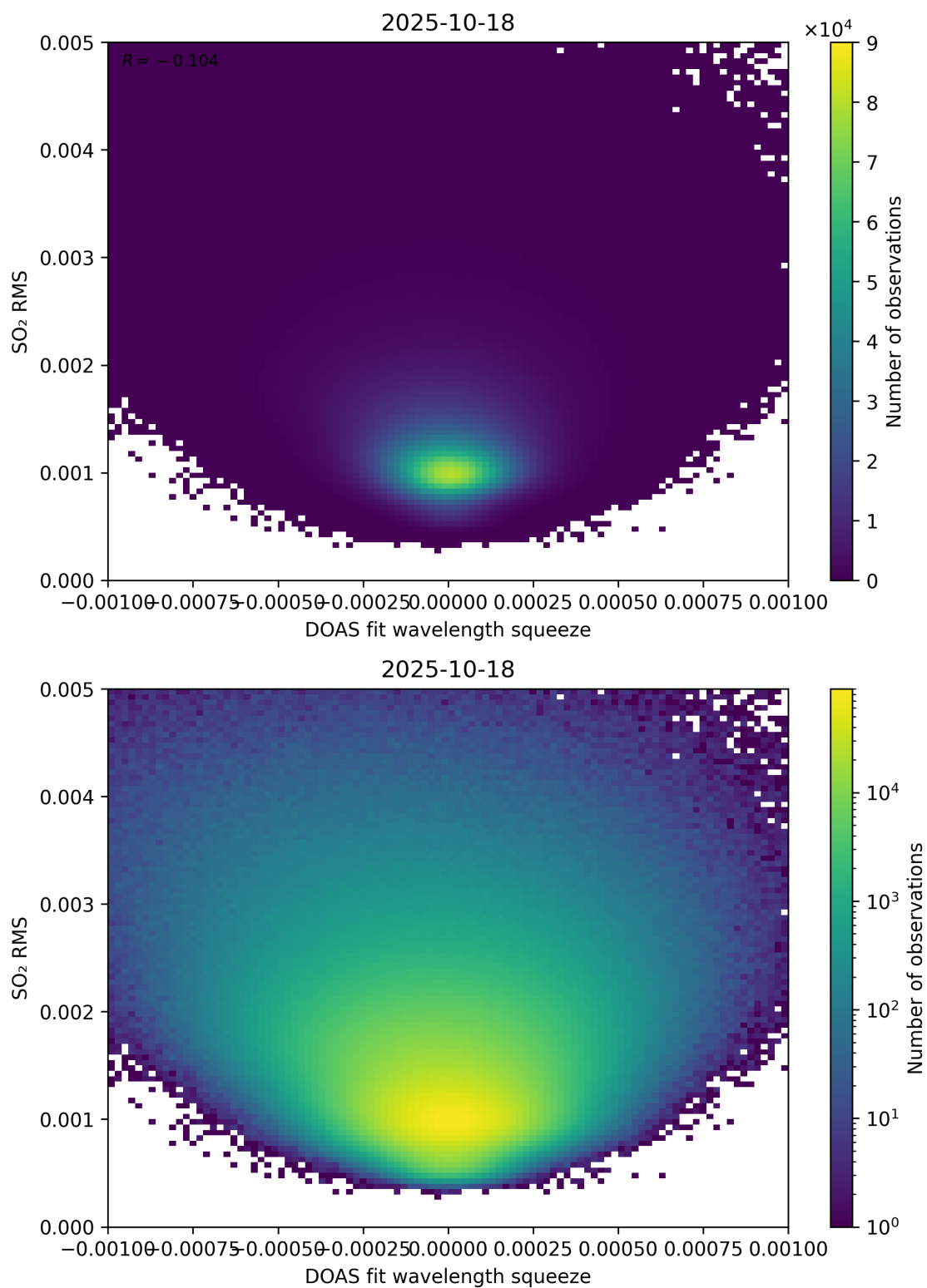
Figure 143: Scatter density plot of “DOAS fit wavelength squeeze” against “SO 2 RMS” for 2025-10-17 to 2025-10-19.
