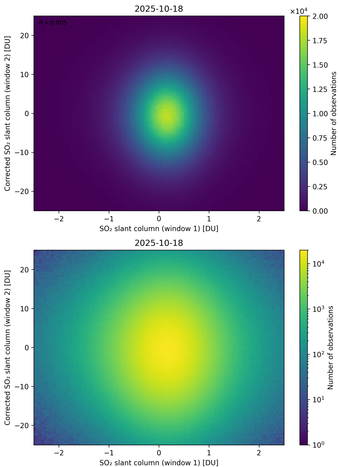
Figure 283: Scatter density plot of “SO 2 slant column (window 1)” against “Corrected SO 2 slant column (window 2)” for 2025-10-17 to 2025-10-19.
