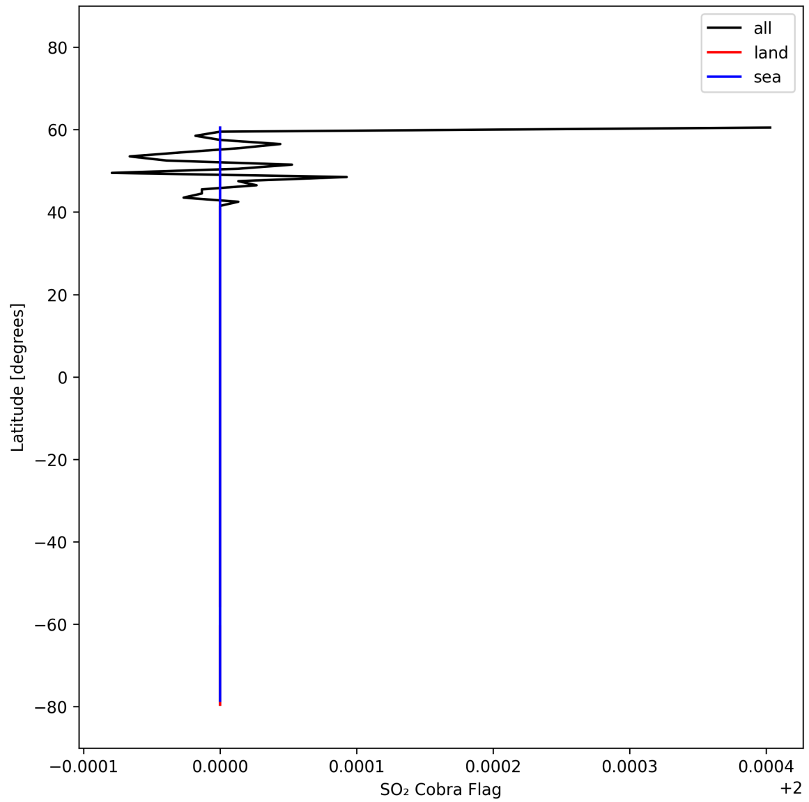
Figure 49: Zonal average of “SO 2 Cobra Flag” for 2025-10-17 to 2025-10-19.
