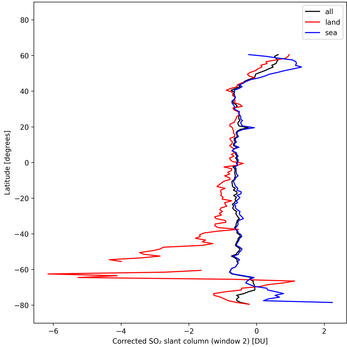
Figure 43: Zonal average of “Corrected SO 2 slant column (window 2)” for 2025-10-17 to 2025-10-19.
