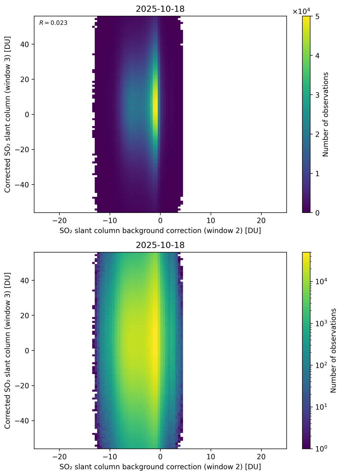
Figure 127: Scatter density plot of “SO 2 slant column background correction (window 2)” against “Corrected SO 2 slant column (window 3)” for 2025-10-17 to 2025-10-19.
