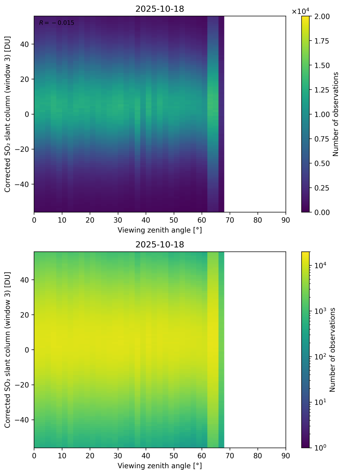
Figure 375: Scatter density plot of “Viewing zenith angle” against “Corrected SO 2 slant column (window 3)” for 2025-10-17 to 2025-10-19.
